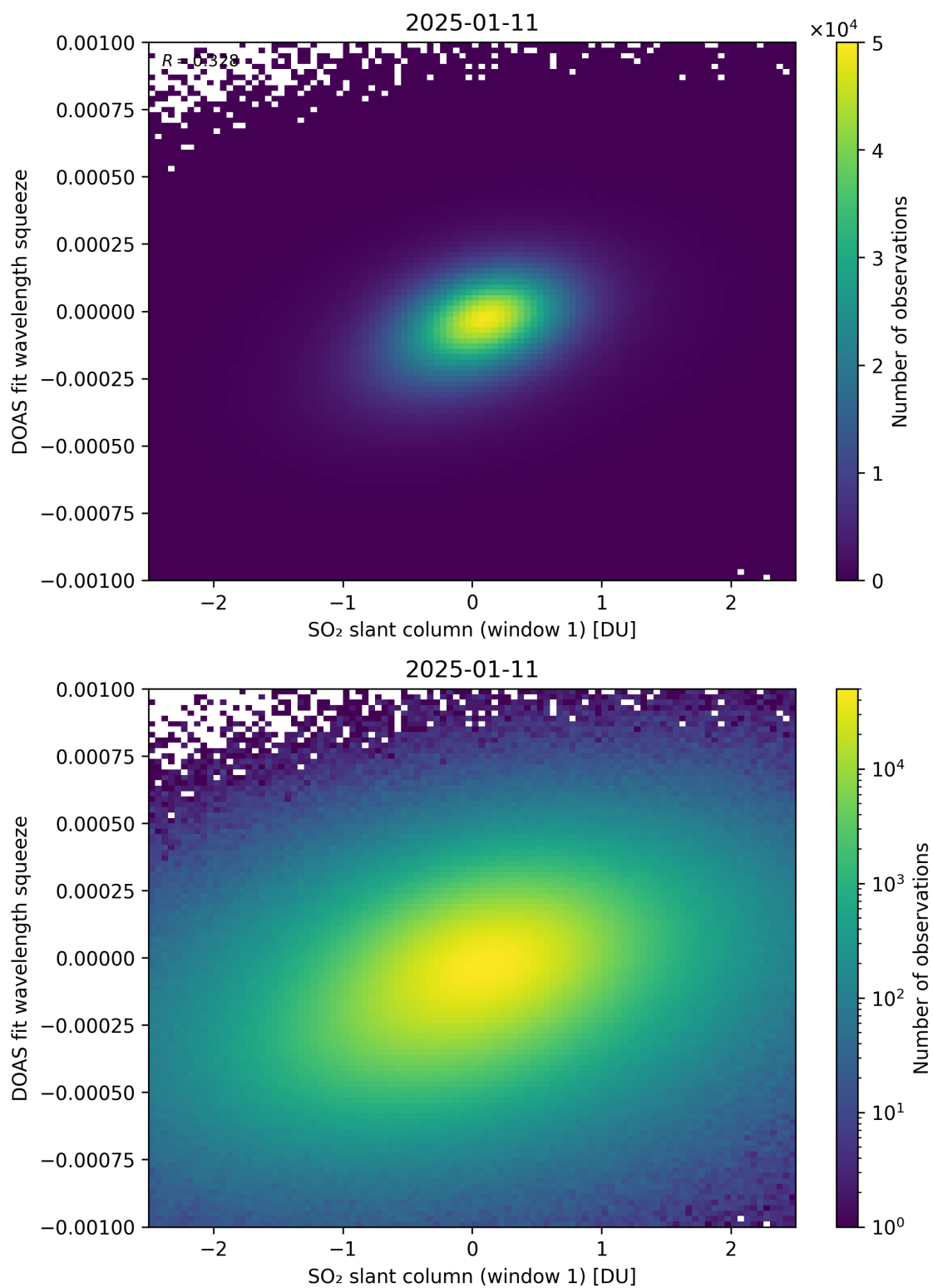
Figure 266: Scatter density plot of “SO 2 slant column (window 1)” against “DOAS fit wavelength squeeze” for 2025-01-10 to 2025-01-12.
