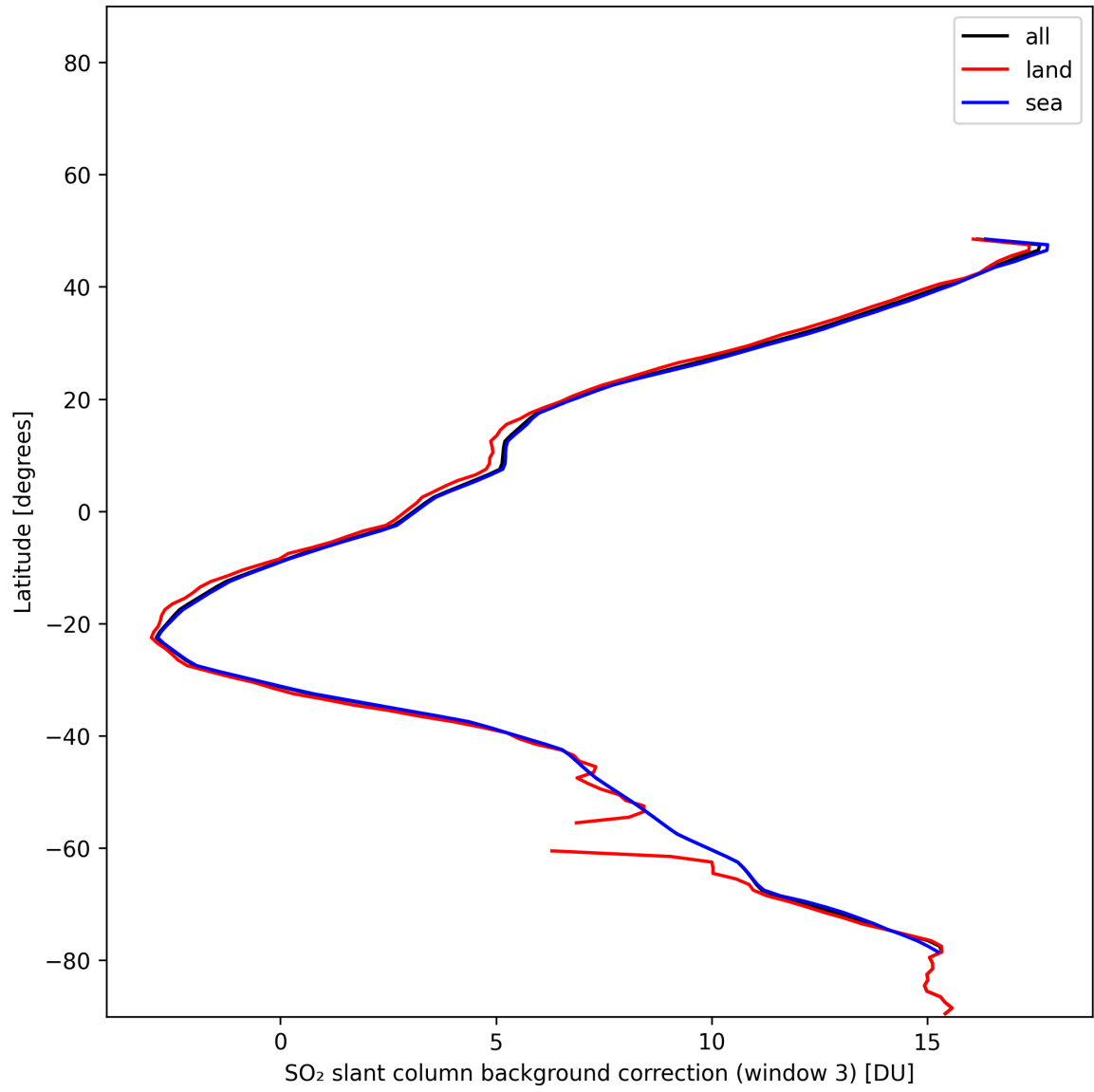
Figure 48: Zonal average of “SO 2 slant column background correction (window 3)” for 2025-01-10 to 2025-01-12.
