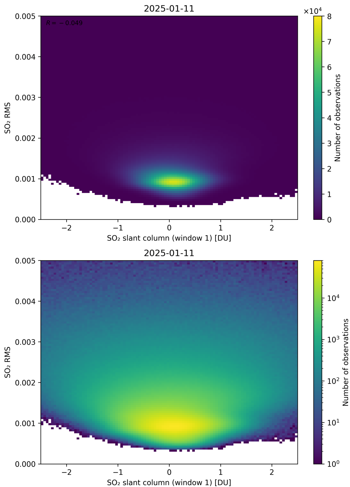
Figure 267: Scatter density plot of “SO 2 slant column (window 1)” against “SO 2 RMS” for 2025-01-10 to 2025-01-12.
