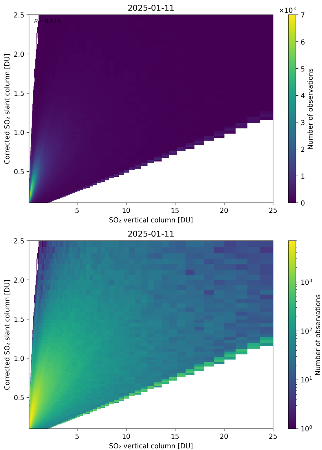
Figure 351: Scatter density plot of “SO 2 vertical column” against “Corrected SO 2 slant column” for 2025-01-10 to 2025-01-12.
