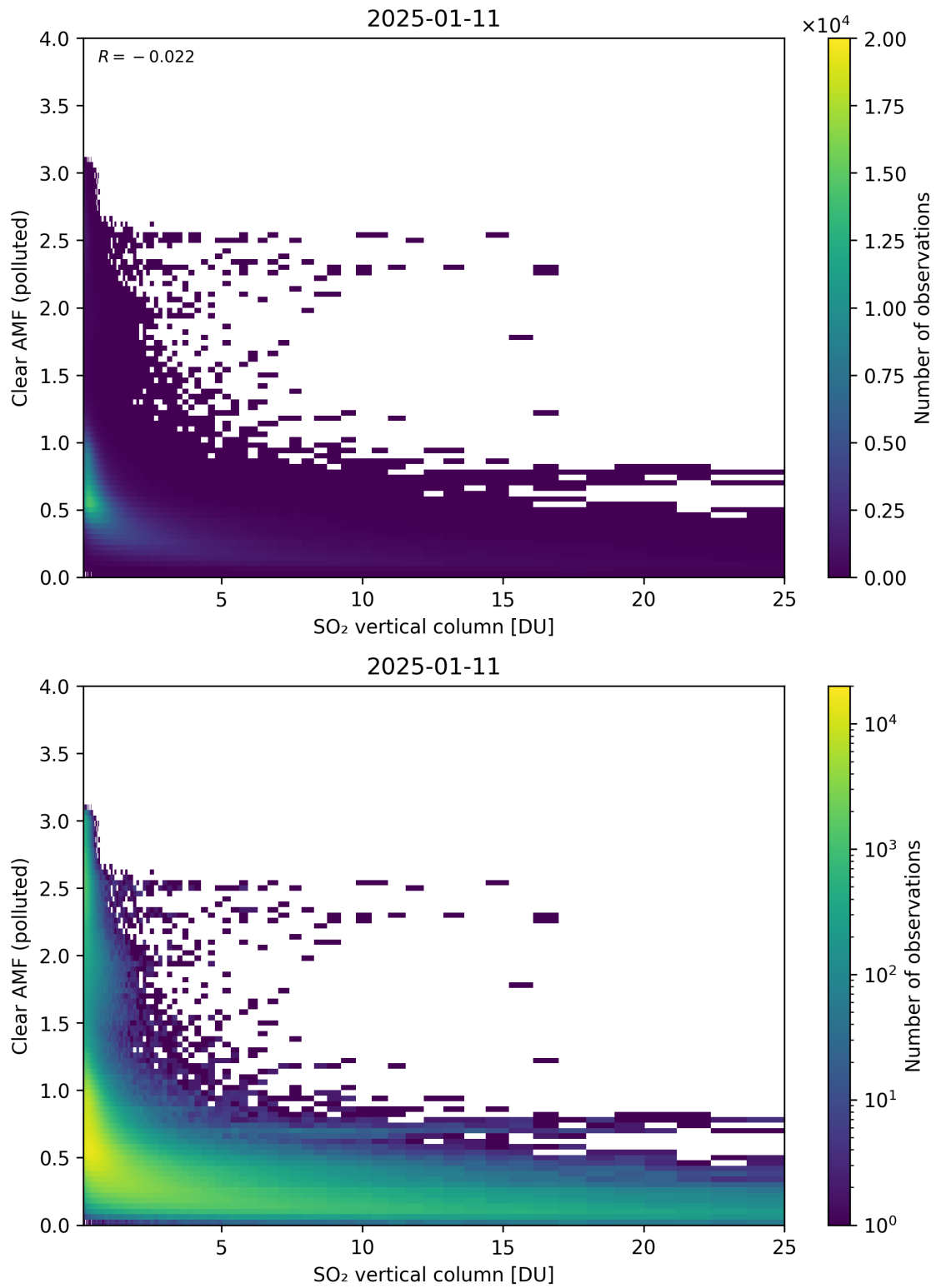
Figure 348: Scatter density plot of “SO 2 vertical column” against “Clear AMF (polluted)” for 2025-01-10 to 2025-01-12.
