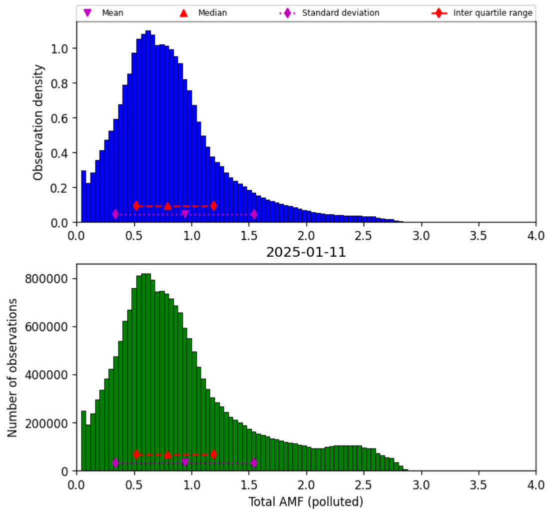
Figure 79: Histogram of “Total AMF (polluted)” for 2025-01-10 to 2025-01-12
