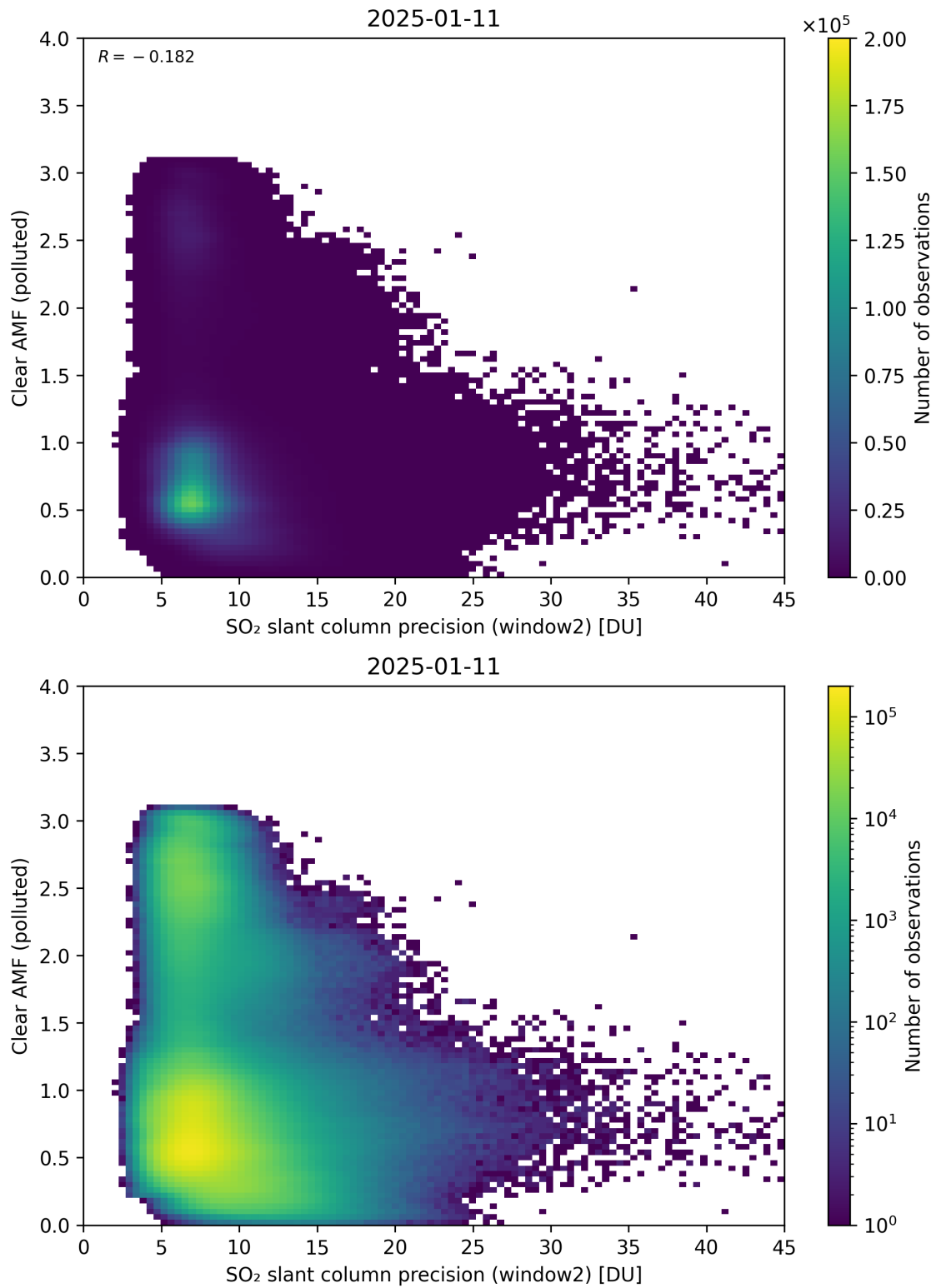
Figure 296: Scatter density plot of “SO 2 slant column precision (window2)” against “Clear AMF (polluted)” for 2025-01-10 to 2025-01-12.
