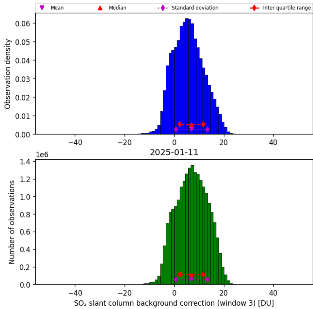
Figure 74: Histogram of “SO 2 slant column background correction (window 3)” for 2025-01-10 to 2025-01-12
