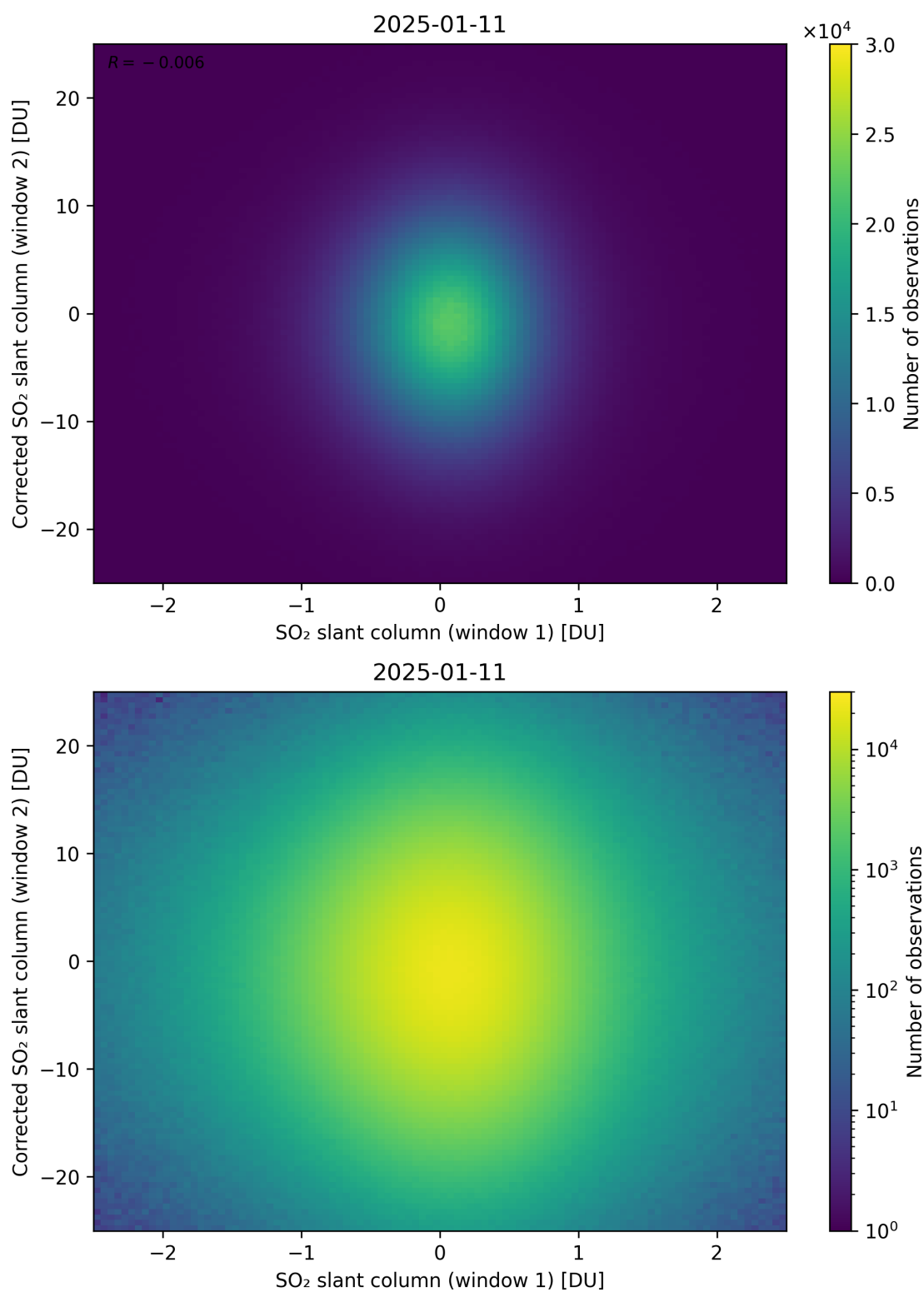
Figure 283: Scatter density plot of “SO 2 slant column (window 1)” against “Corrected SO 2 slant column (window 2)” for 2025-01-10 to 2025-01-12.
