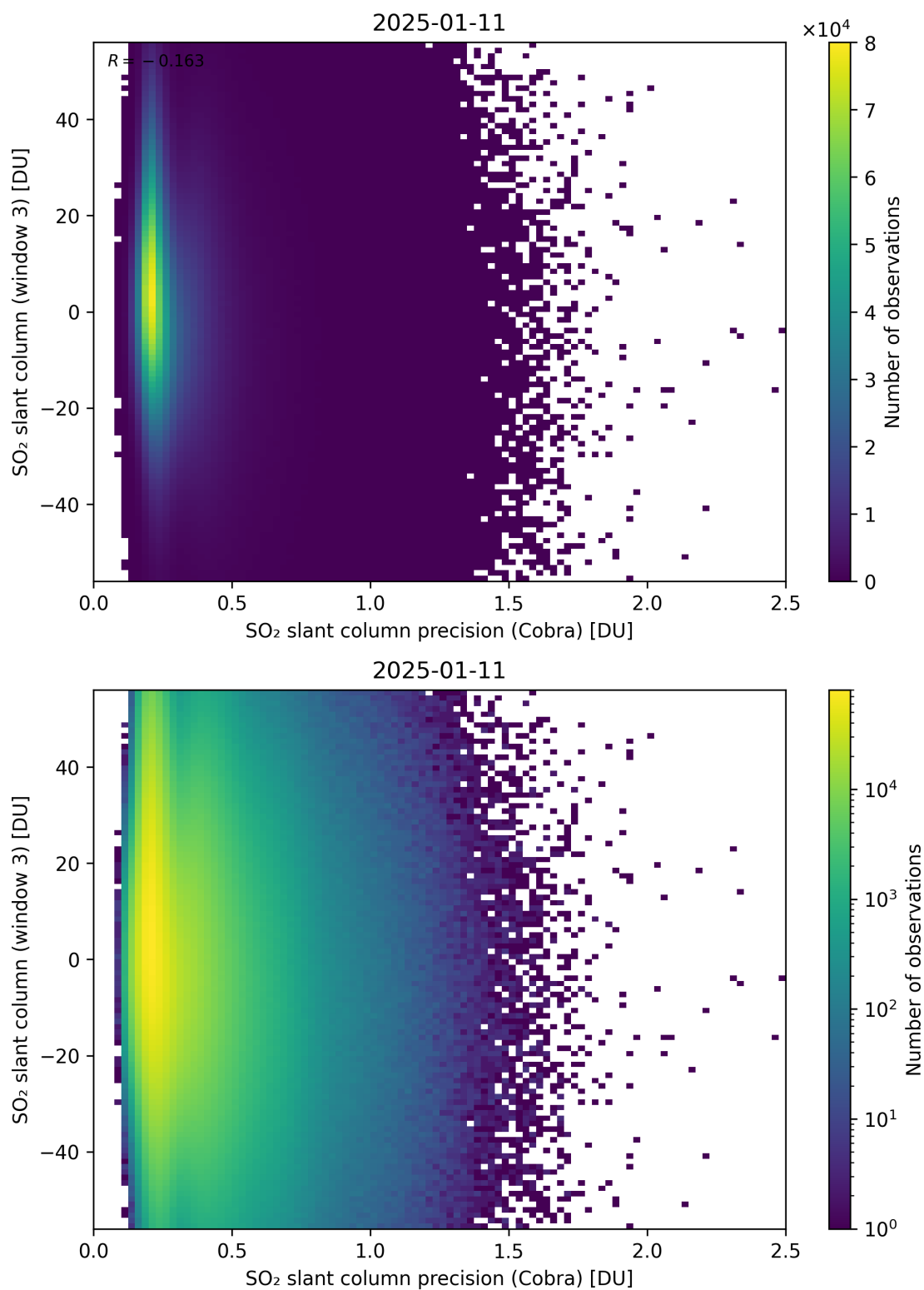
Figure 211: Scatter density plot of “SO 2 slant column precision (Cobra)” against “SO 2 slant column (window 3)” for 2025-01-10 to 2025-01-12.
