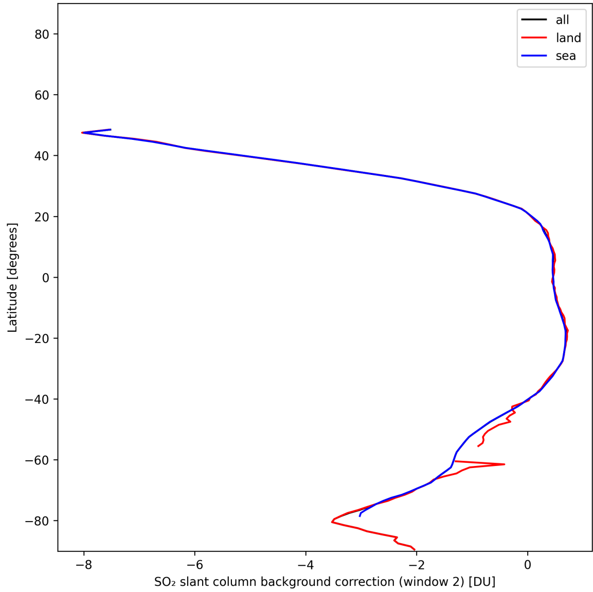
Figure 44: Zonal average of “SO 2 slant column background correction (window 2)” for 2025-01-10 to 2025-01-12.
