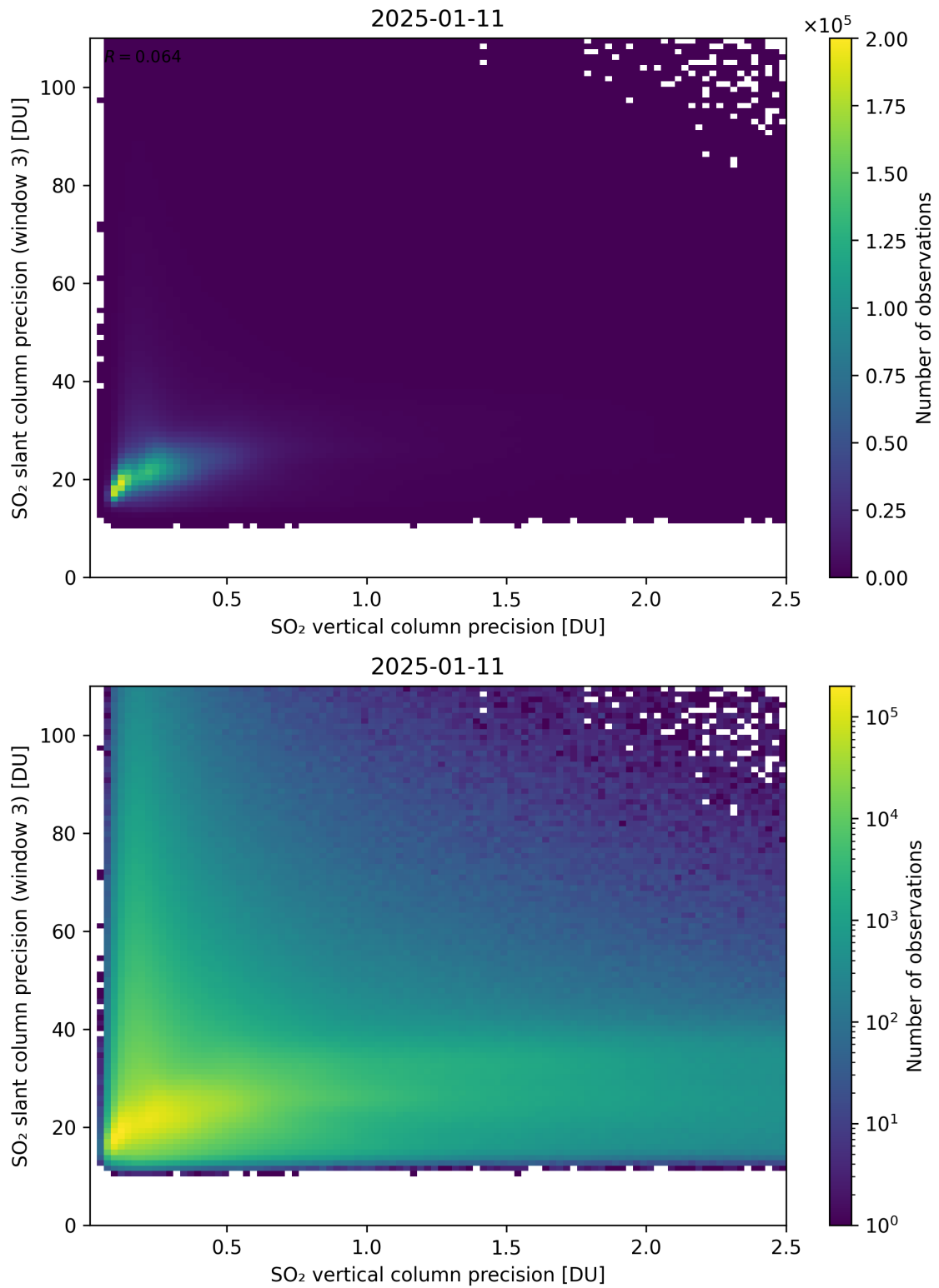
Figure 345: Scatter density plot of “SO 2 vertical column precision” against “SO 2 slant column precision (window 3)” for 2025-01-10 to 2025-01-12.
