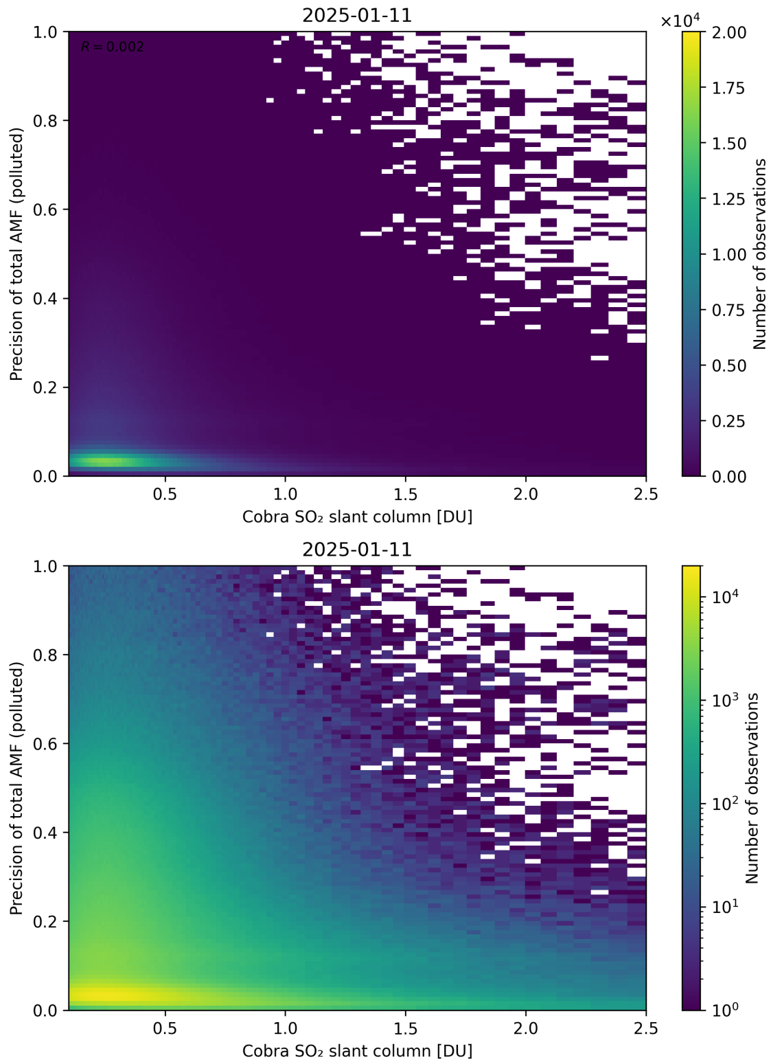
Figure 225: Scatter density plot of “Cobra SO 2 slant column” against “Precision of total AMF (polluted)” for 2025-01-10 to 2025-01-12.
