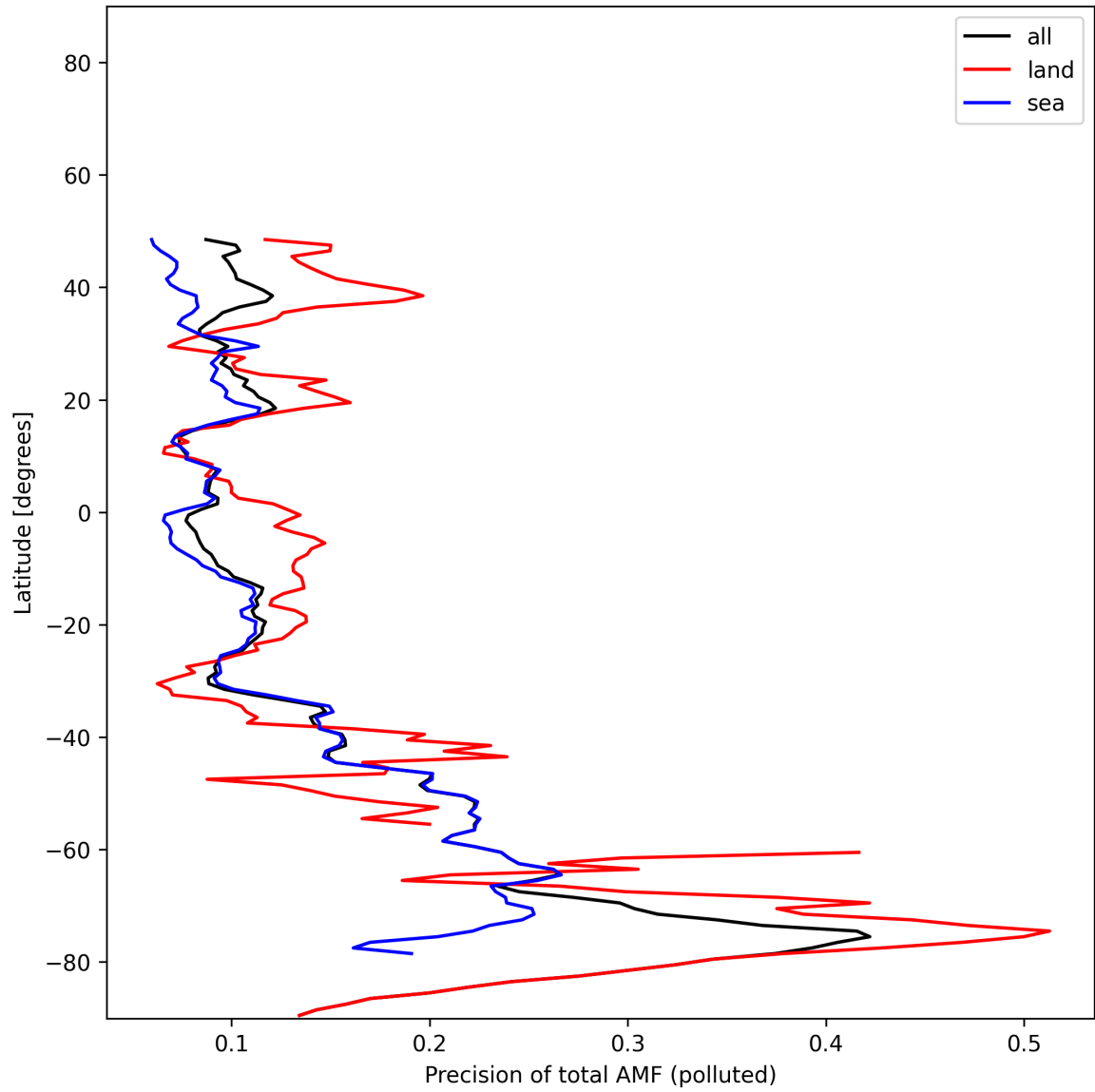
Figure 54: Zonal average of “Precision of total AMF (polluted)” for 2025-01-10 to 2025-01-12.
