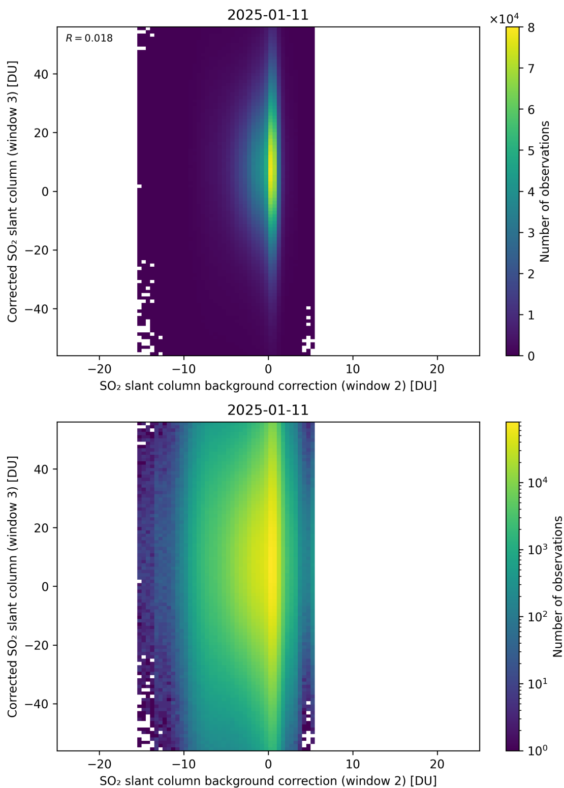
Figure 127: Scatter density plot of “SO 2 slant column background correction (window 2)” against “Corrected SO 2 slant column (window 3)” for 2025-01-10 to 2025-01-12.
