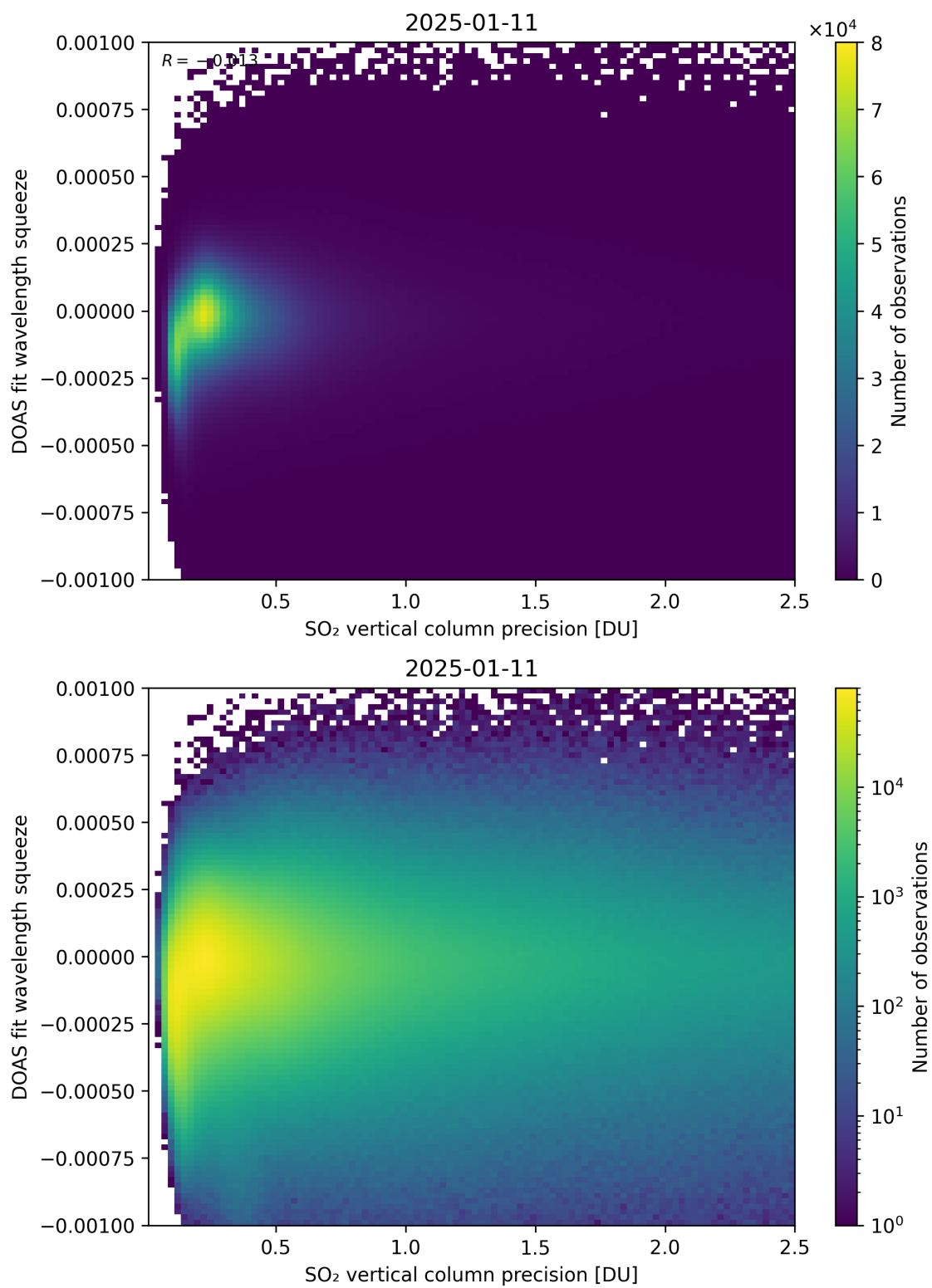
Figure 333: Scatter density plot of “SO 2 vertical column precision” against “DOAS fit wavelength squeeze” for 2025-01-10 to 2025-01-12.
