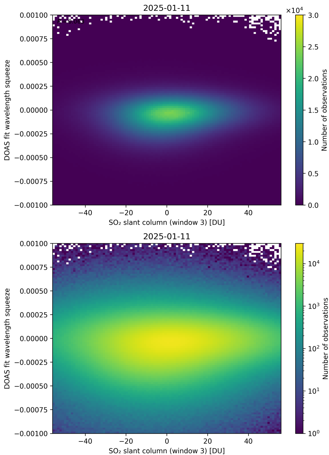
Figure 305: Scatter density plot of “SO 2 slant column (window 3)” against “DOAS fit wavelength squeeze” for 2025-01-10 to 2025-01-12.
