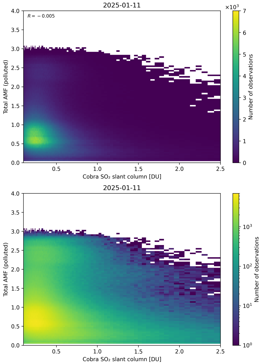
Figure 224: Scatter density plot of “Cobra SO 2 slant column” against “Total AMF (polluted)” for 2025-01-10 to 2025-01-12.
