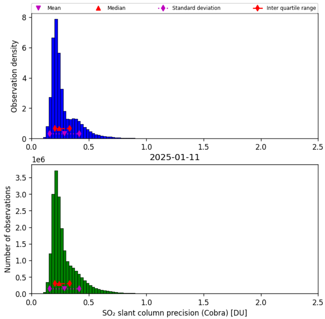
Figure 62: Histogram of “SO 2 slant column precision (Cobra)” for 2025-01-10 to 2025-01-12
