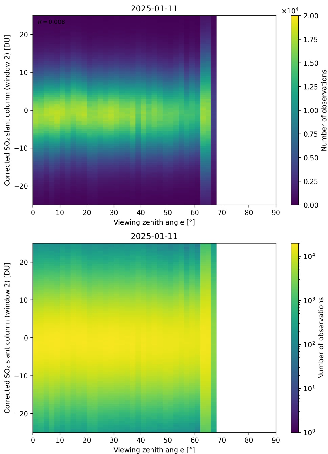
Figure 374: Scatter density plot of “Viewing zenith angle” against “Corrected SO 2 slant column (window 2)” for 2025-01-10 to 2025-01-12.
