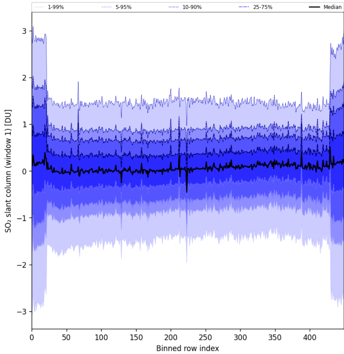
Figure 89: Along track statistics of “SO 2 slant column (window 1)” for 2025-01-10 to 2025-01-12
