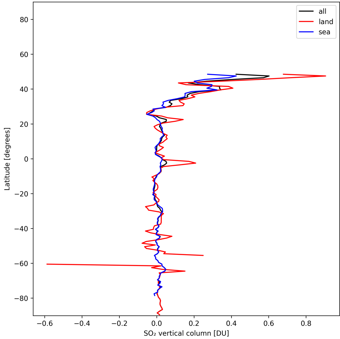
Figure 32: Zonal average of “SO 2 vertical column” for 2025-01-10 to 2025-01-12.
