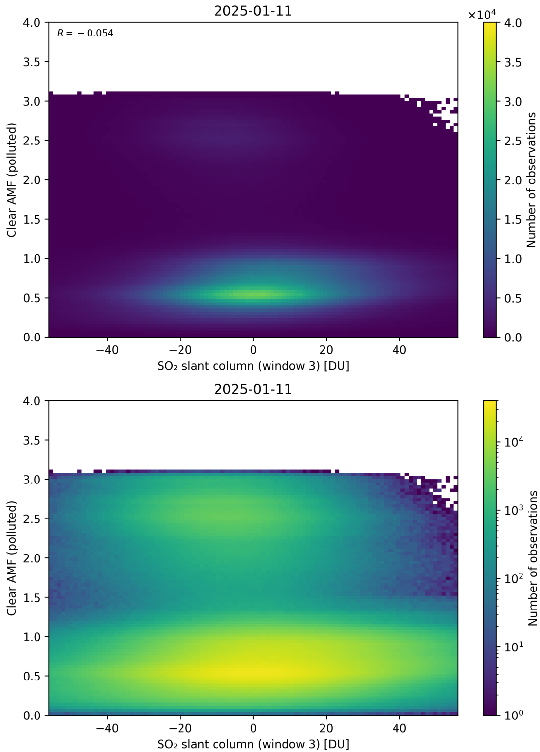
Figure 315: Scatter density plot of “SO 2 slant column (window 3)” against “Clear AMF (polluted)” for 2025-01-10 to 2025-01-12.
