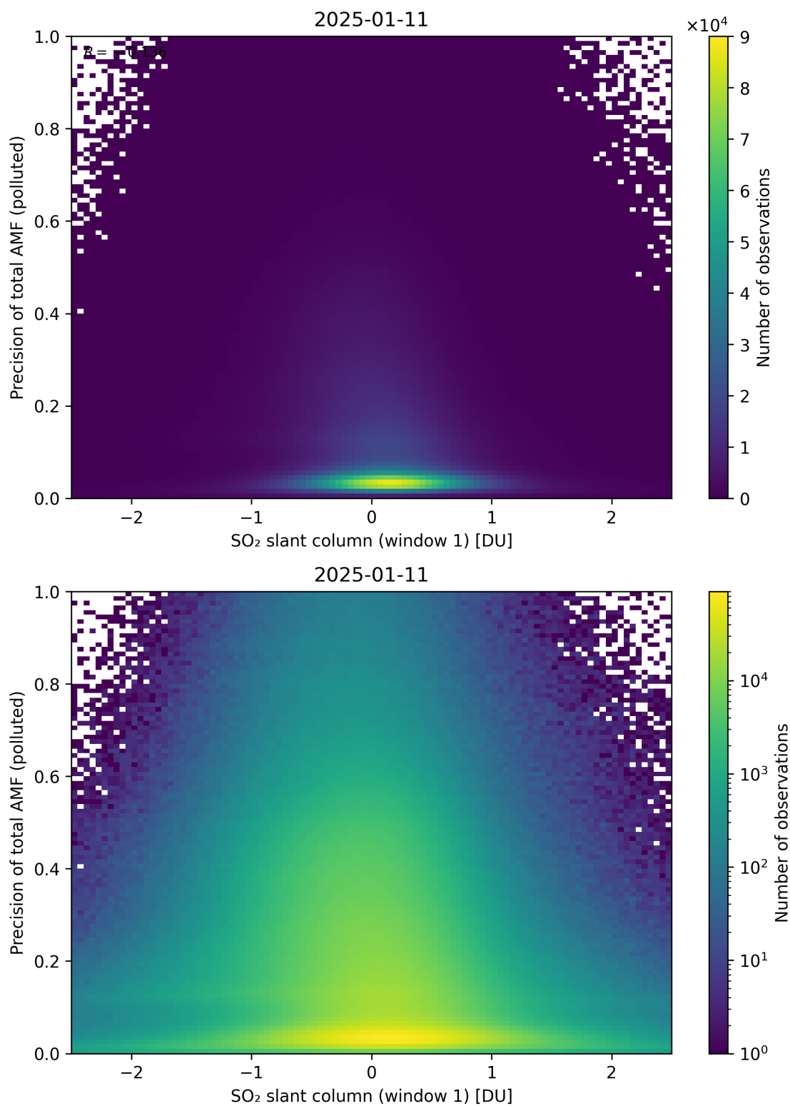
Figure 290: Scatter density plot of “SO 2 slant column (window 1)” against “Precision of total AMF (polluted)” for 2025-01-10 to 2025-01-12.
