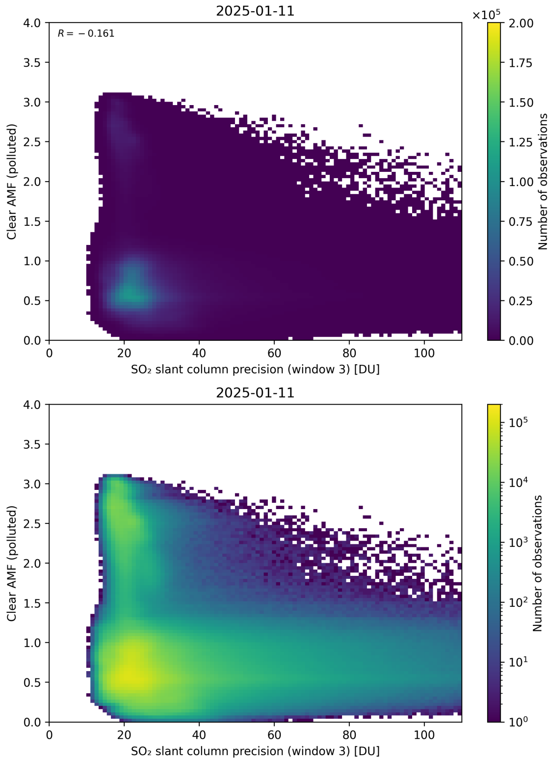
Figure 311: Scatter density plot of “SO 2 slant column precision (window 3)” against “Clear AMF (polluted)” for 2025-01-10 to 2025-01-12.
