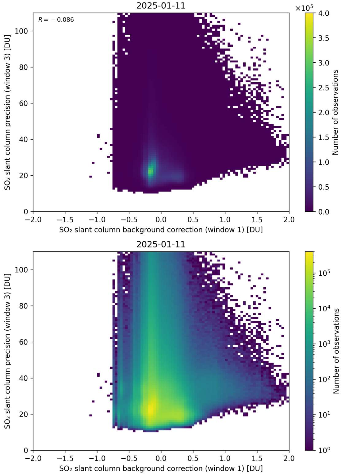
Figure 119: Scatter density plot of “SO 2 slant column background correction (window 1)” against “SO 2 slant column precision (window 3)” for 2025-01-10 to 2025-01-12.
