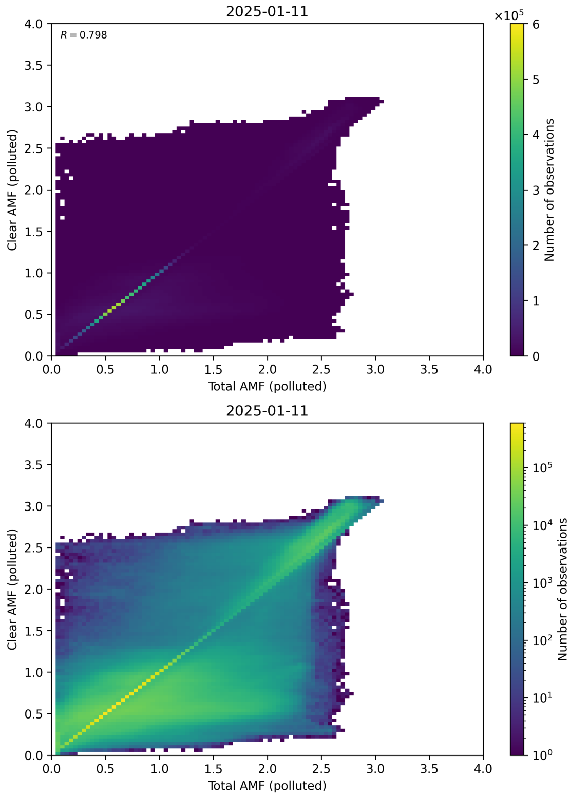
Figure 321: Scatter density plot of “Total AMF (polluted)” against “Clear AMF (polluted)” for 2025-01-10 to 2025-01-12.
