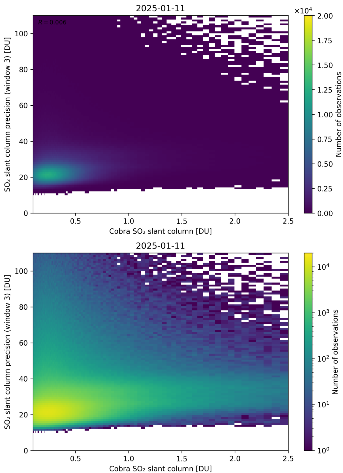
Figure 223: Scatter density plot of “Cobra SO 2 slant column” against “SO 2 slant column precision (window 3)” for 2025-01-10 to 2025-01-12.
