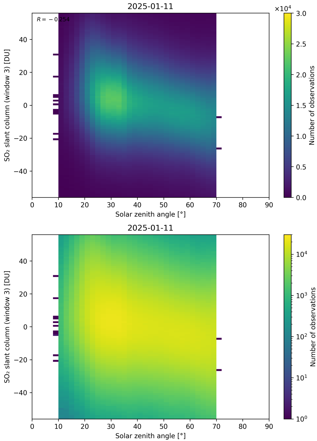
Figure 187: Scatter density plot of “Solar zenith angle” against “SO 2 slant column (window 3)” for 2025-01-10 to 2025-01-12.
