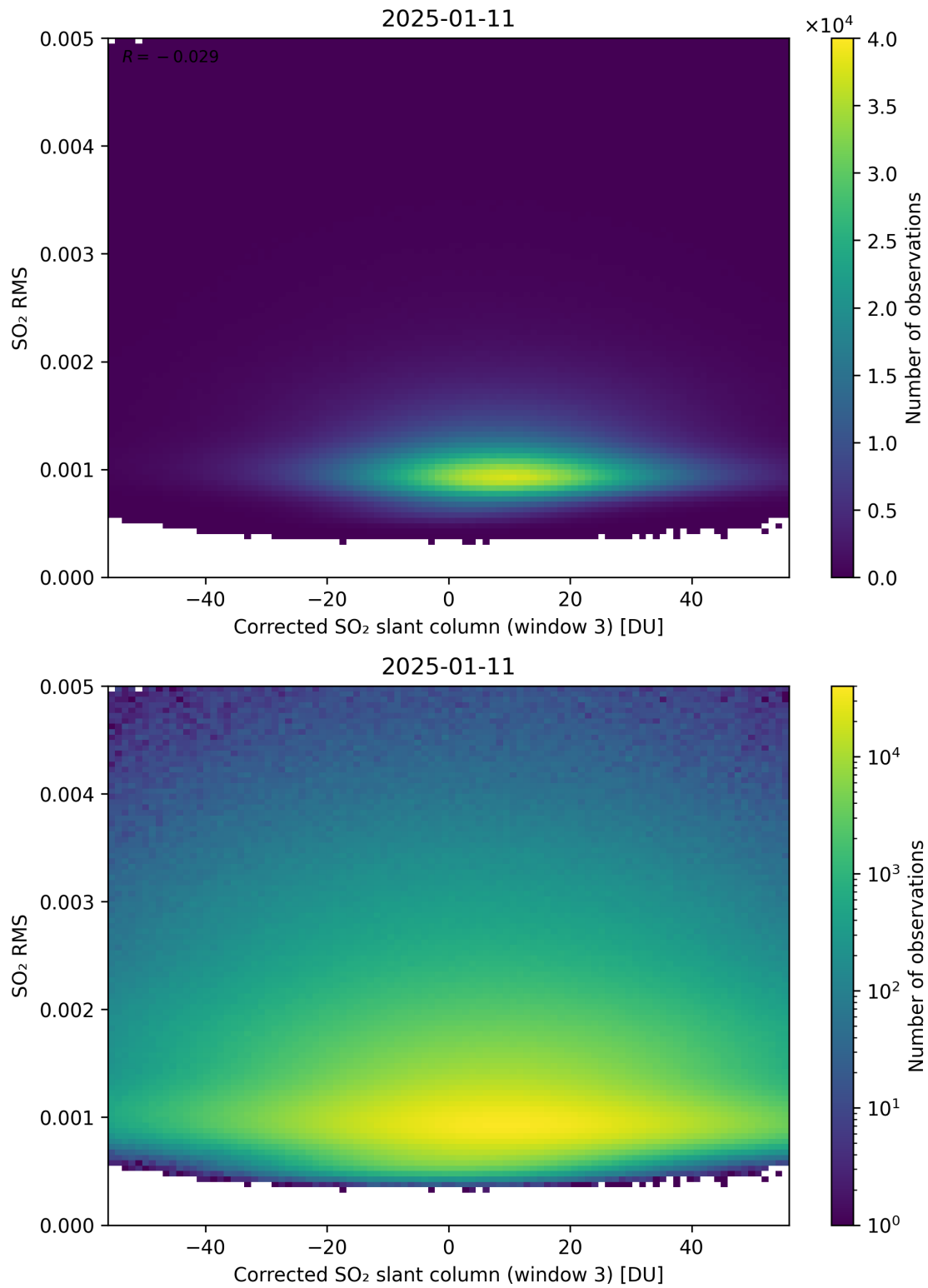
Figure 258: Scatter density plot of “Corrected SO 2 slant column (window 3)” against “SO 2 RMS” for 2025-01-10 to 2025-01-12.
