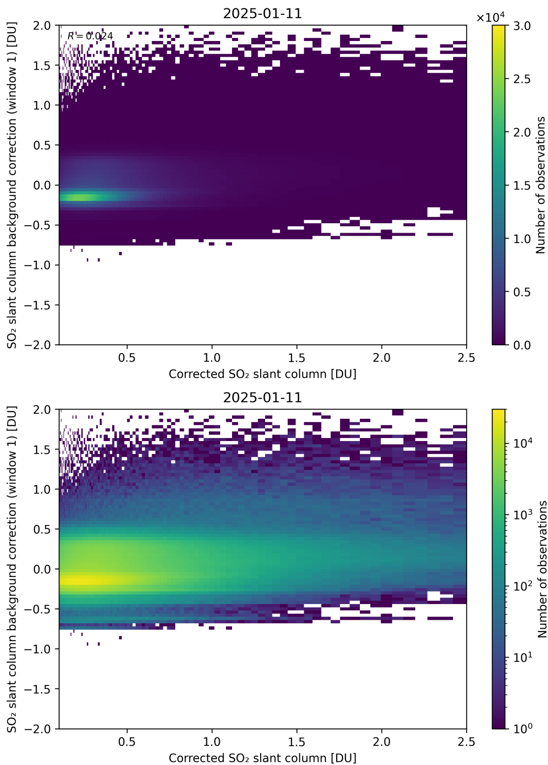
Figure 226: Scatter density plot of “Corrected SO 2 slant column” against “SO 2 slant column background correction (window 1)” for 2025-01-10 to 2025-01-12.
