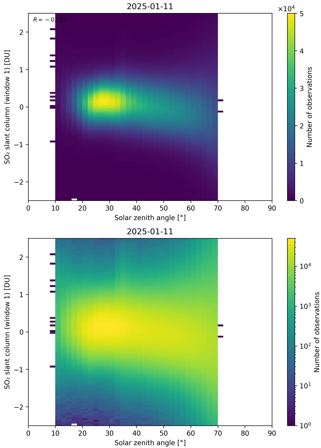
Figure 184: Scatter density plot of “Solar zenith angle” against “SO 2 slant column (window 1)” for 2025-01-10 to 2025-01-12.
