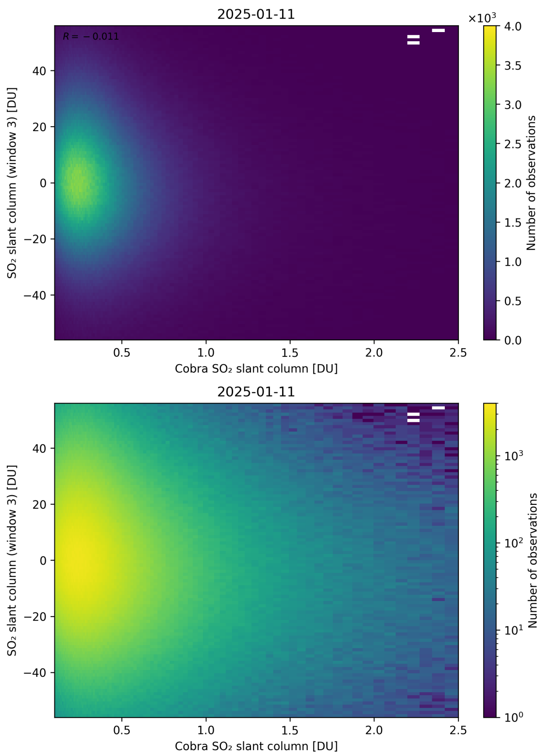
Figure 222: Scatter density plot of “Cobra SO 2 slant column” against “SO 2 slant column (window 3)” for 2025-01-10 to 2025-01-12.
