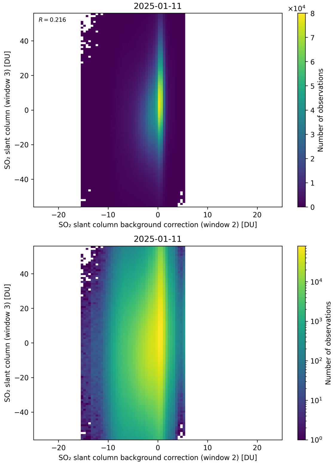
Figure 128: Scatter density plot of “SO 2 slant column background correction (window 2)” against “SO 2 slant column (window 3)” for 2025-01-10 to 2025-01-12.
