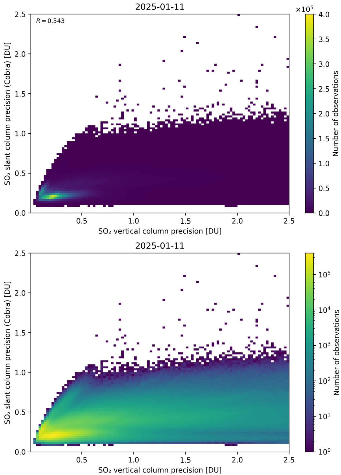
Figure 337: Scatter density plot of “SO 2 vertical column precision” against “SO 2 slant column precision (Cobra)” for 2025-01-10 to 2025-01-12.
