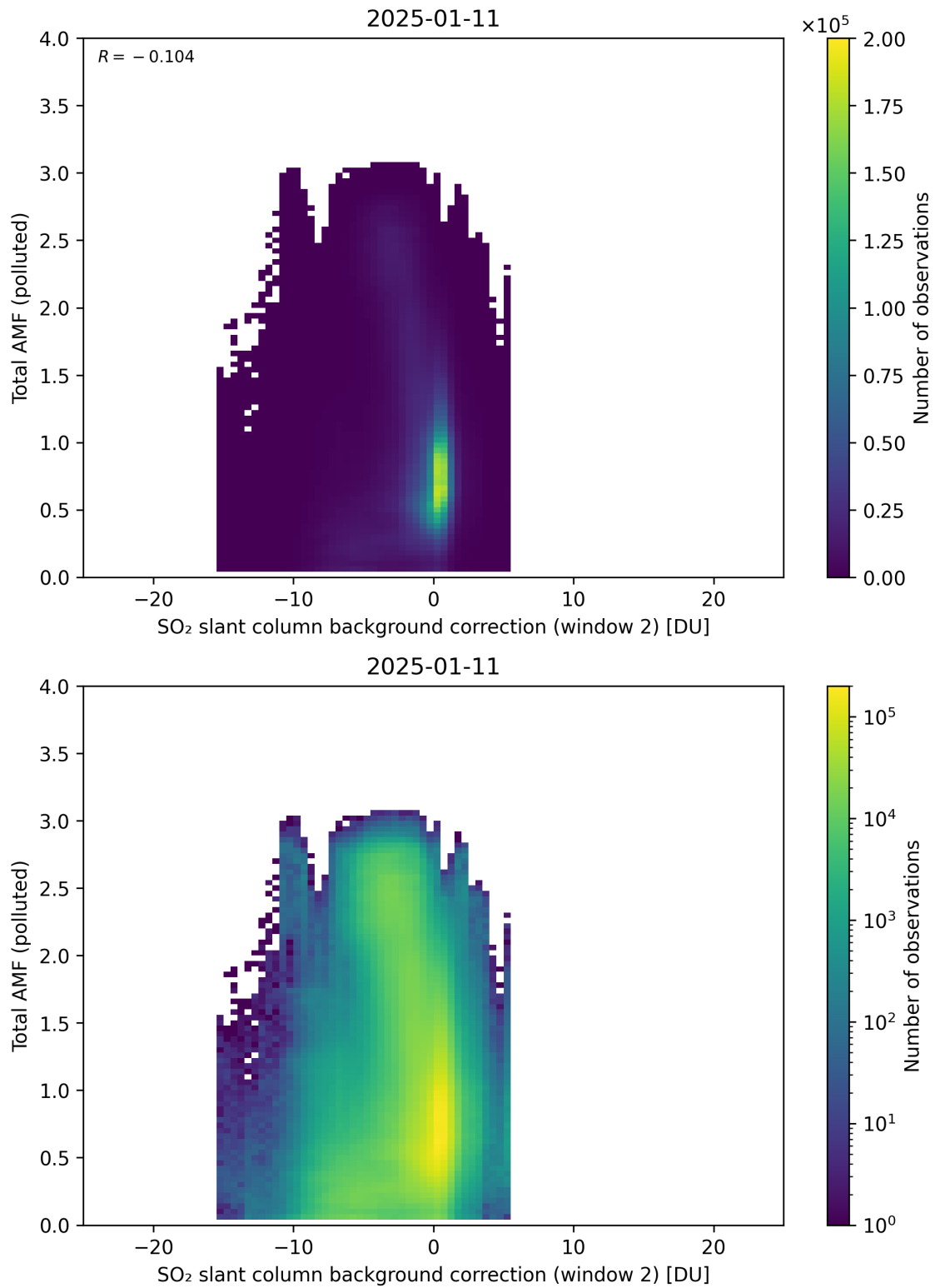
Figure 130: Scatter density plot of “SO 2 slant column background correction (window 2)” against “Total AMF (polluted)” for 2025-01-10 to 2025-01-12.
