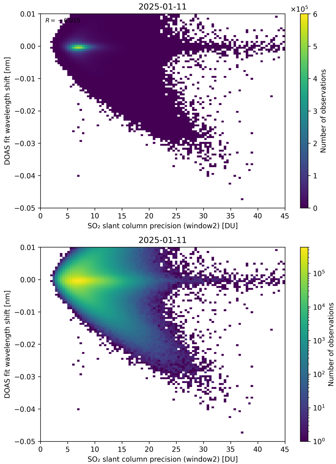
Figure 293: Scatter density plot of “SO 2 slant column precision (window2)” against “DOAS fit wavelength shift” for 2025-01-10 to 2025-01-12.
