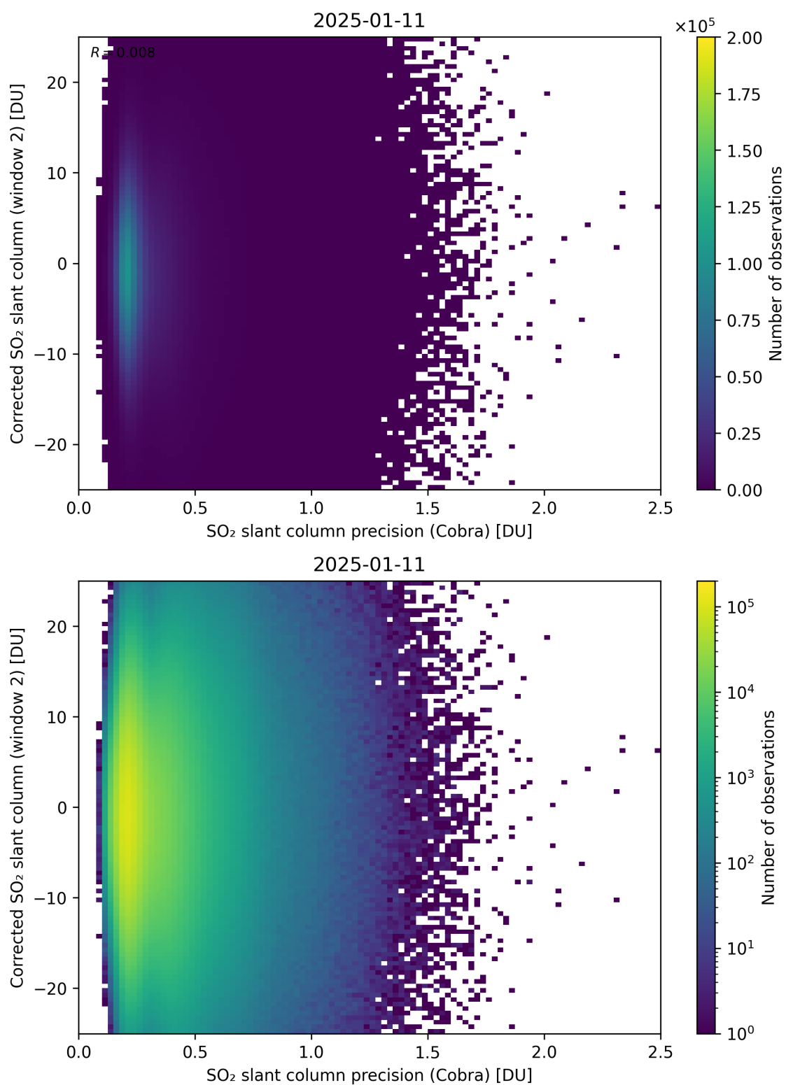
Figure 206: Scatter density plot of “SO 2 slant column precision (Cobra)” against “Corrected SO 2 slant column (window 2)” for 2025-01-10 to 2025-01-12.
