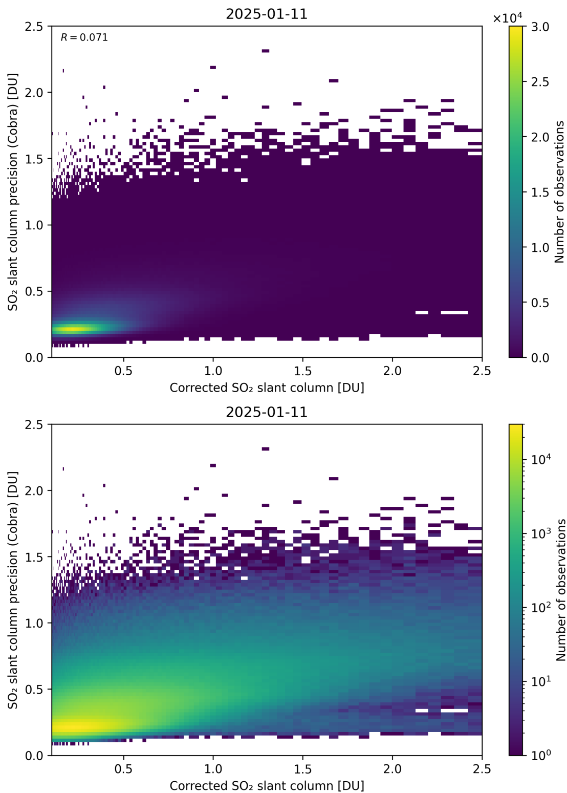
Figure 234: Scatter density plot of “Corrected SO 2 slant column” against “SO 2 slant column precision (Cobra)” for 2025-01-10 to 2025-01-12.
