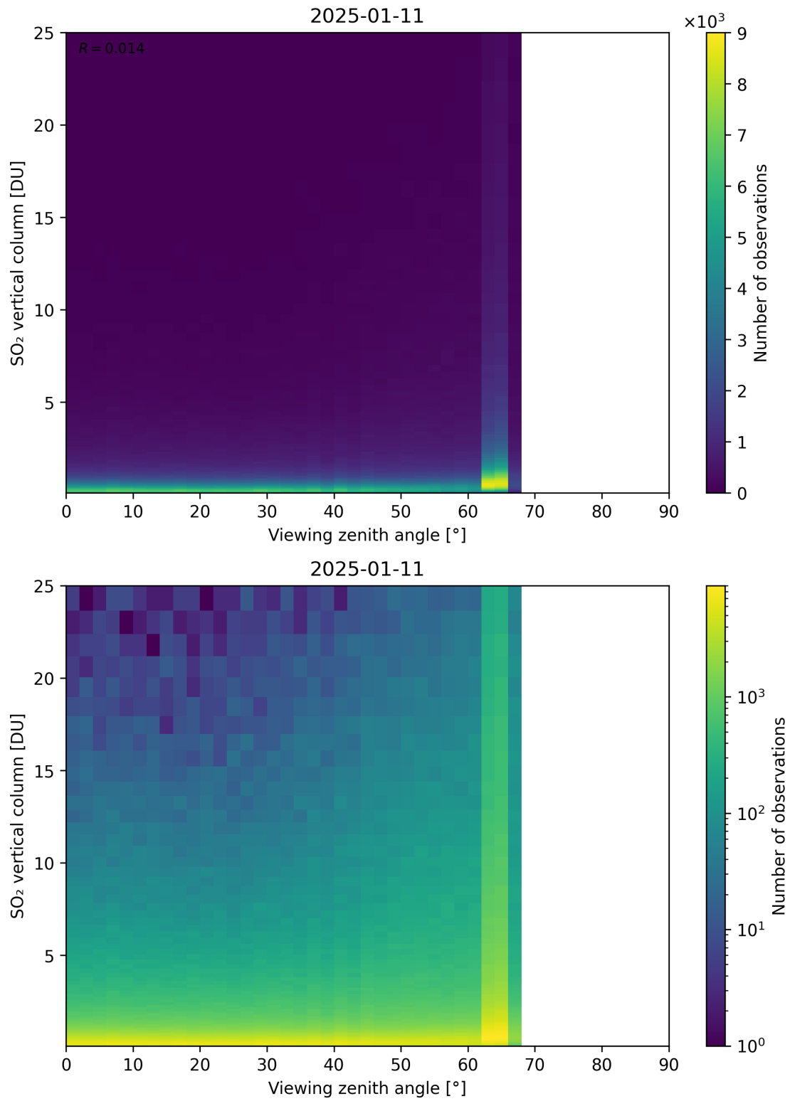
Figure 383: Scatter density plot of “Viewing zenith angle” against “SO 2 vertical column” for 2025-01-10 to 2025-01-12.
