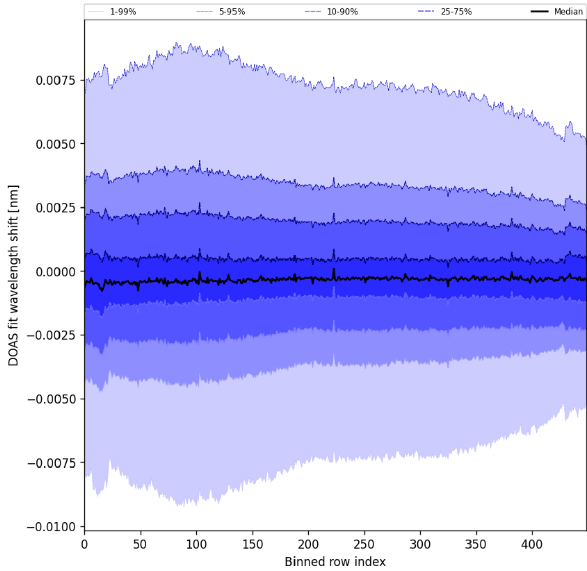
Figure 102: Along track statistics of “DOAS fit wavelength shift” for 2025-01-10 to 2025-01-12
