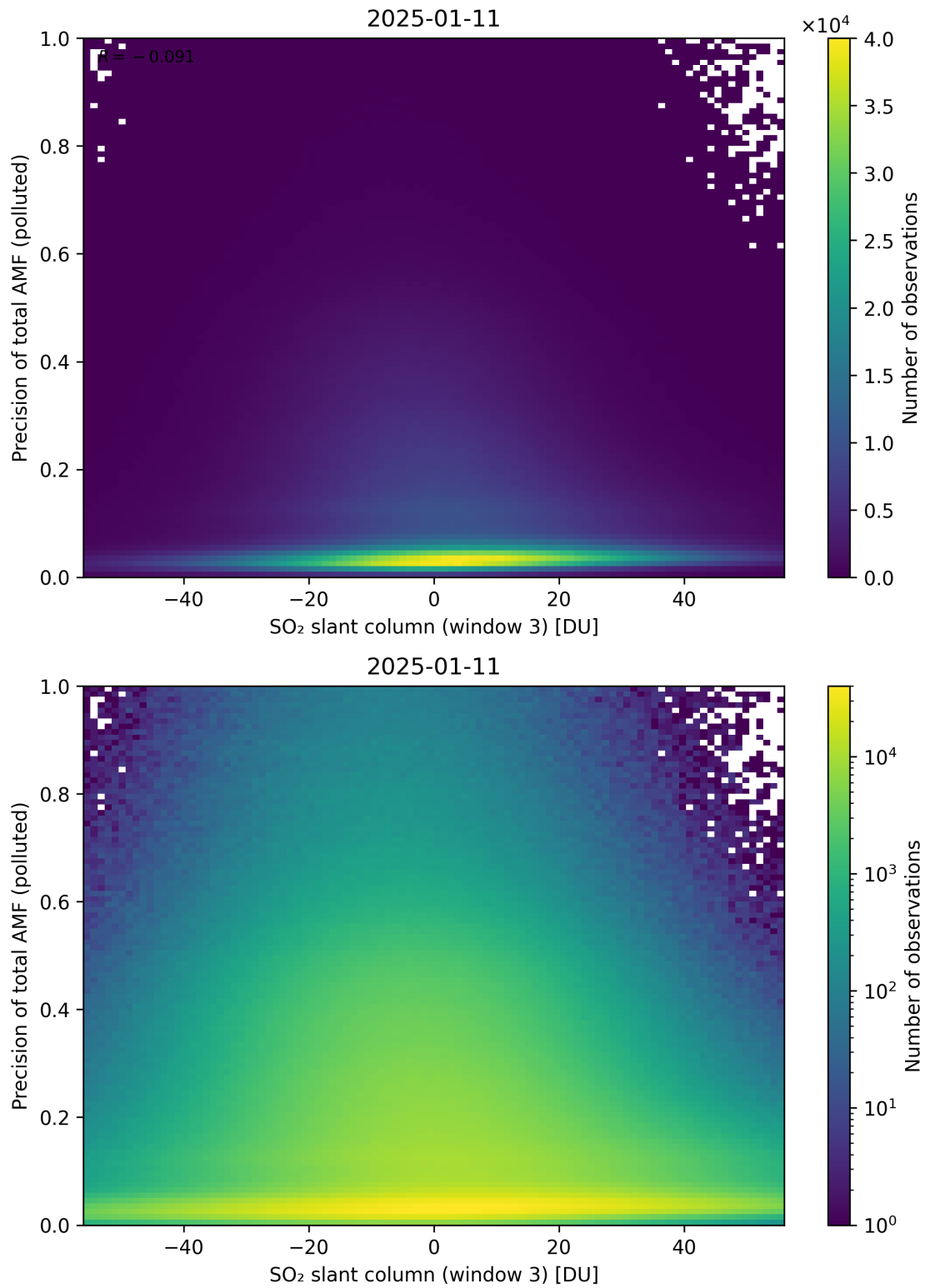
Figure 319: Scatter density plot of “SO 2 slant column (window 3)” against “Precision of total AMF (polluted)” for 2025-01-10 to 2025-01-12.
