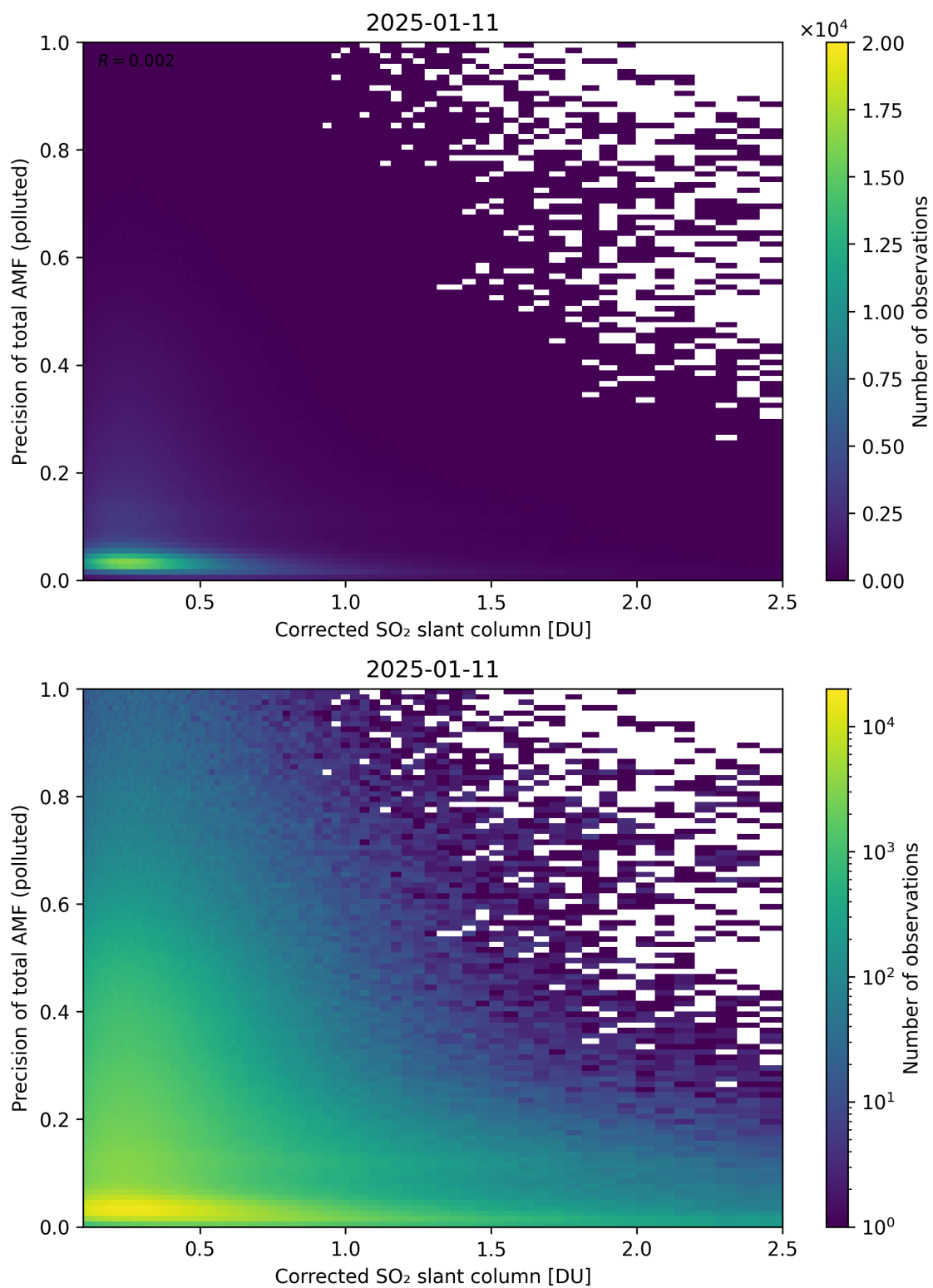
Figure 243: Scatter density plot of “Corrected SO 2 slant column” against “Precision of total AMF (polluted)” for 2025-01-10 to 2025-01-12.
