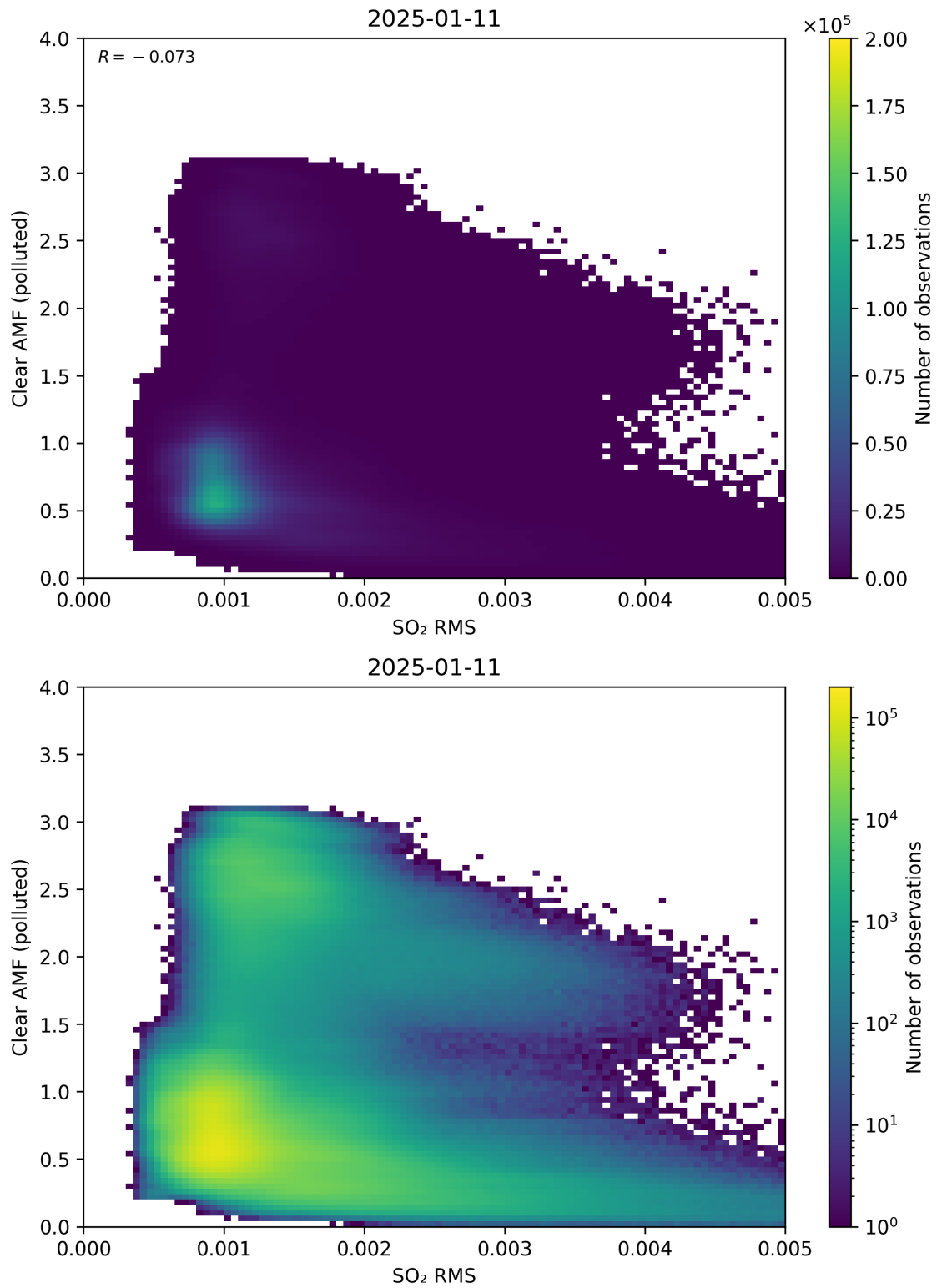
Figure 147: Scatter density plot of “SO 2 RMS” against “Clear AMF (polluted)” for 2025-01-10 to 2025-01-12.
