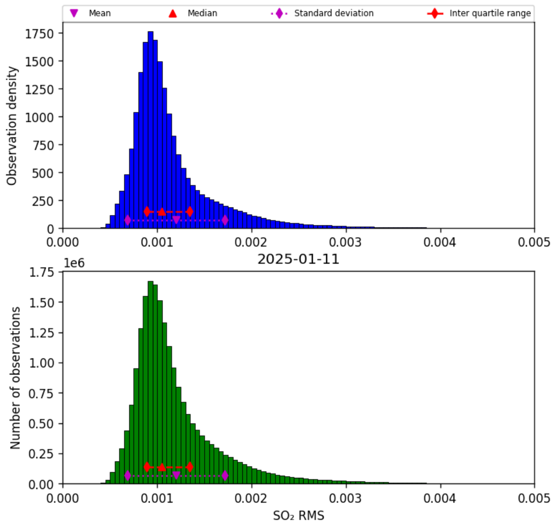
Figure 78: Histogram of “SO 2 RMS” for 2025-01-10 to 2025-01-12
