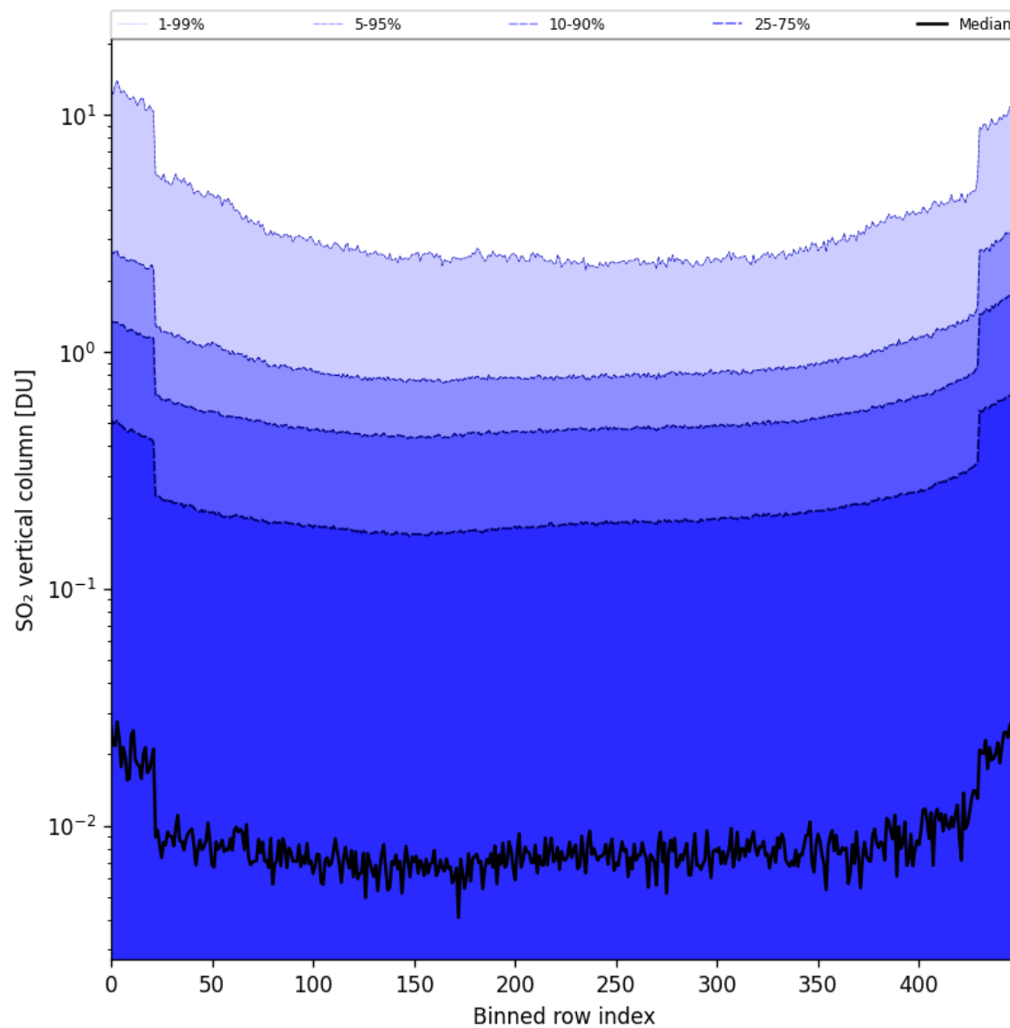
Figure 84: Along track statistics of “SO 2 vertical column” for 2025-01-10 to 2025-01-12
