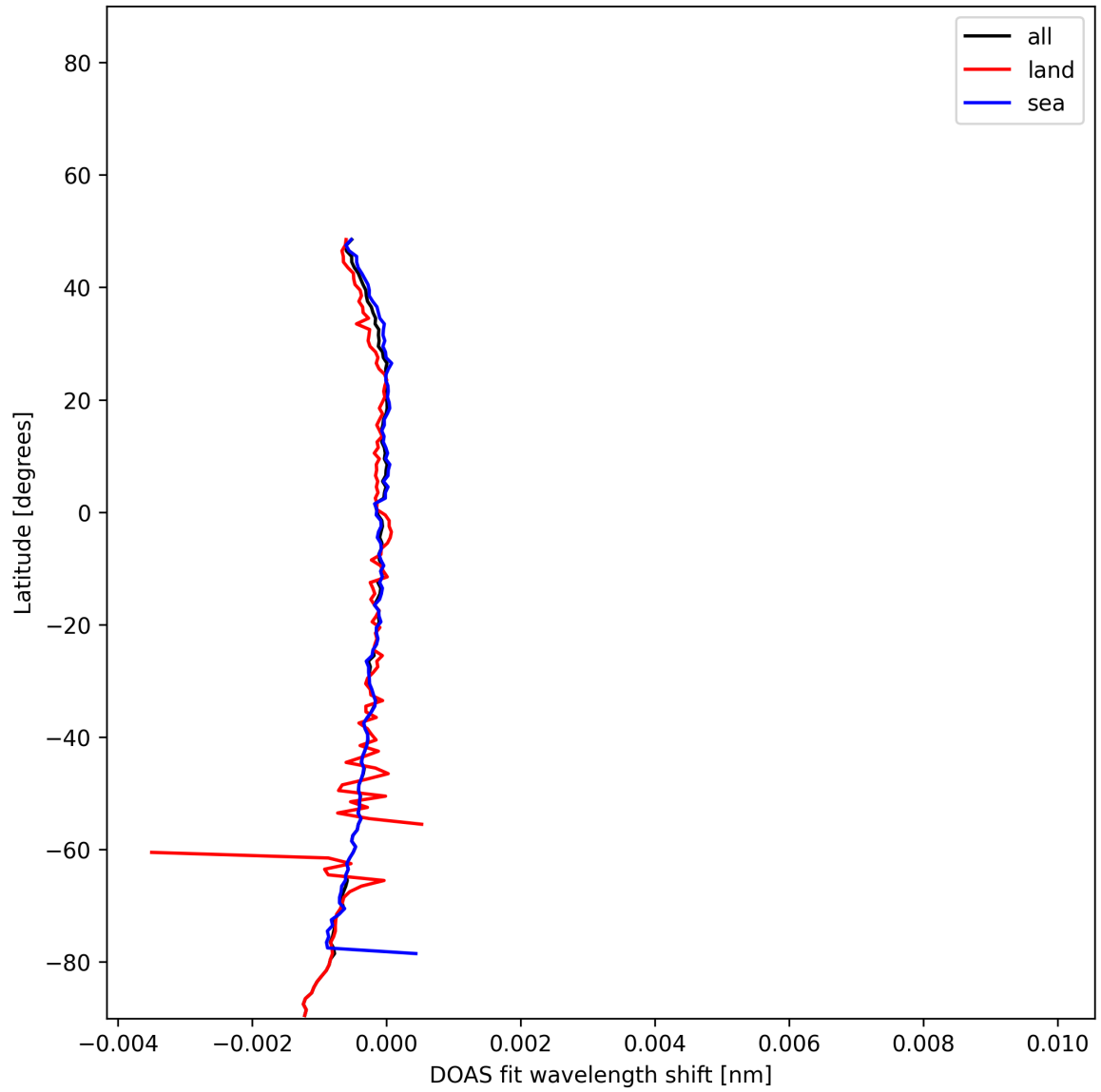
Figure 50: Zonal average of “DOAS fit wavelength shift” for 2025-01-10 to 2025-01-12.
