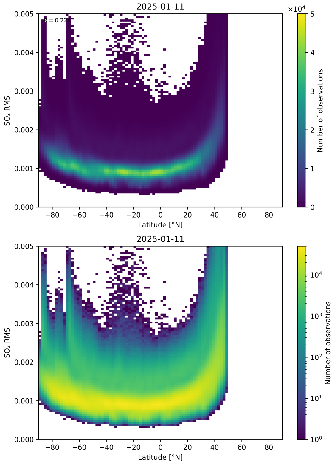
Figure 155: Scatter density plot of “Latitude” against “SO 2 RMS” for 2025-01-10 to 2025-01-12.
