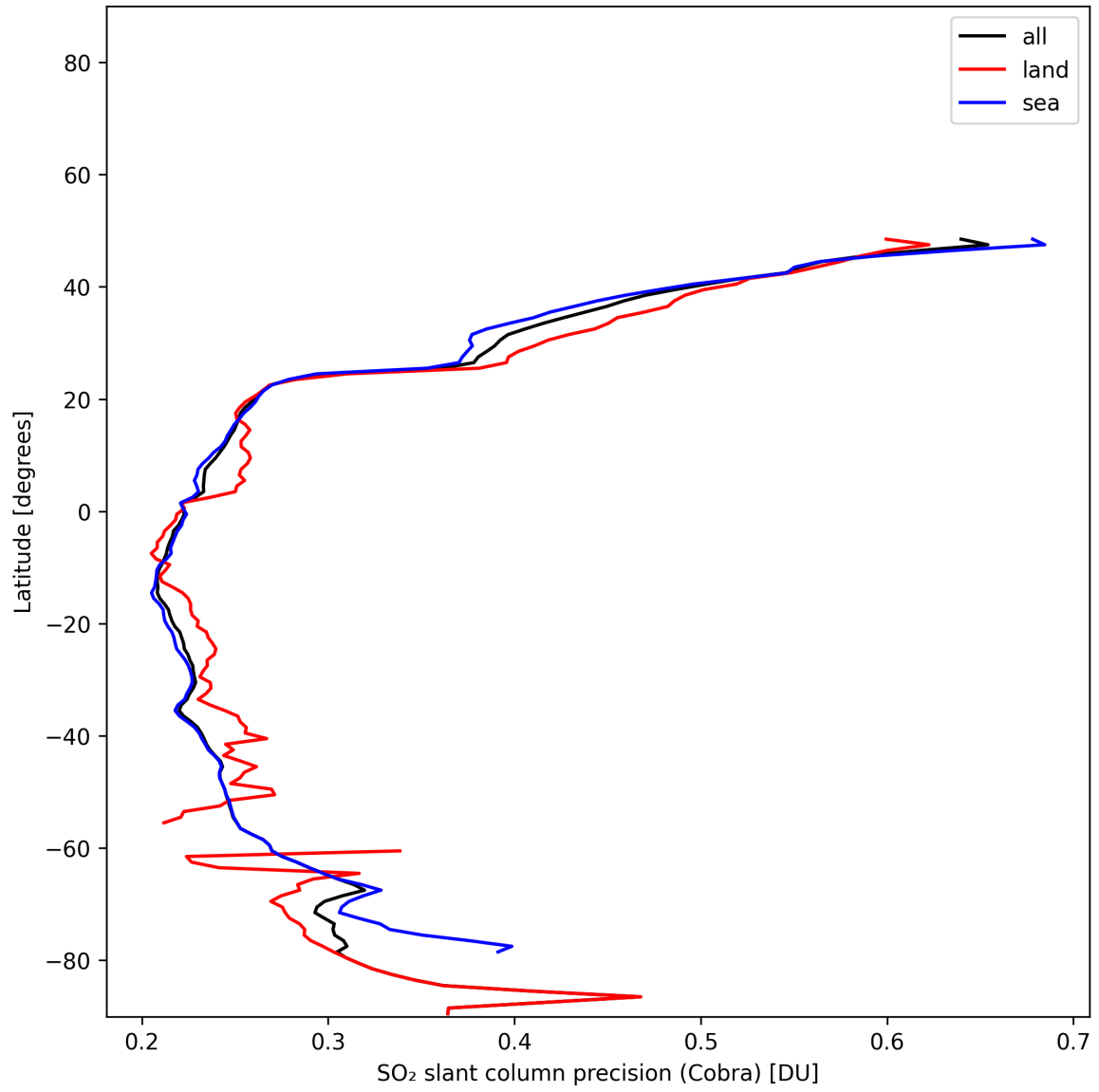
Figure 36: Zonal average of “SO 2 slant column precision (Cobra)” for 2025-01-10 to 2025-01-12.
