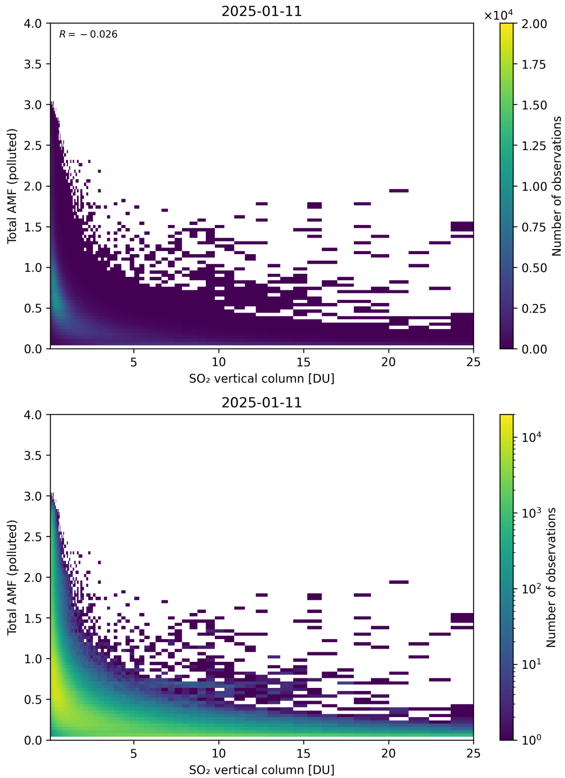
Figure 359: Scatter density plot of “SO 2 vertical column” against “Total AMF (polluted)” for 2025-01-10 to 2025-01-12.
