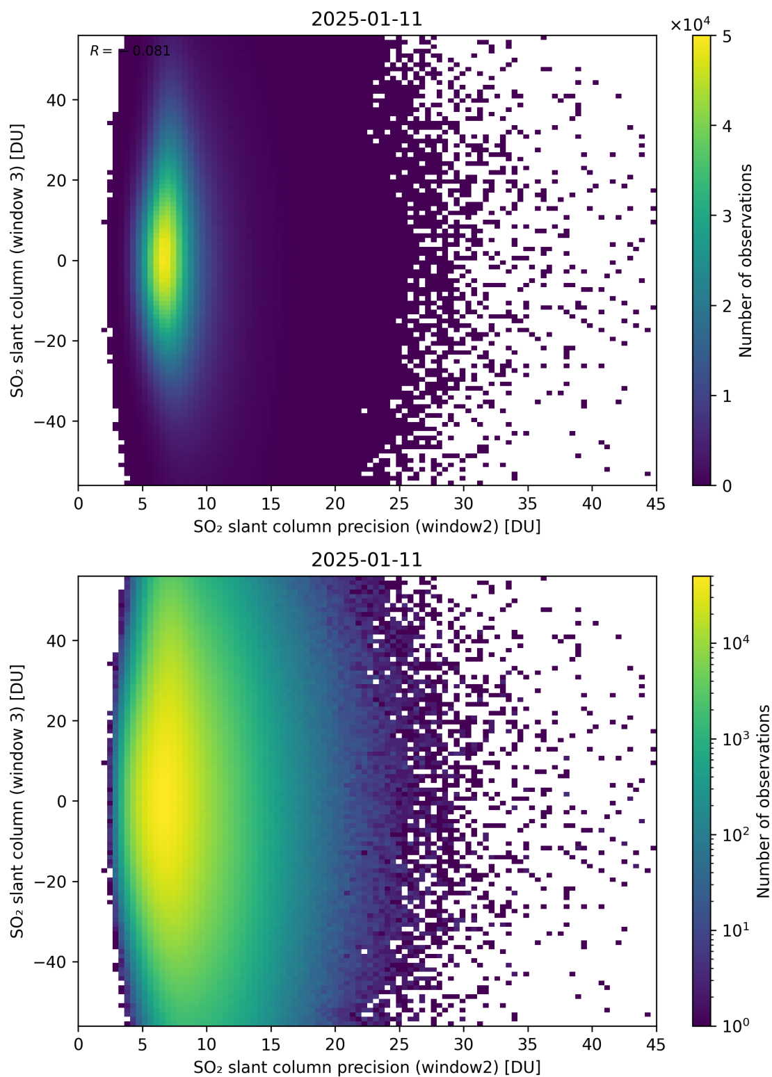
Figure 299: Scatter density plot of “SO 2 slant column precision (window2)” against “SO 2 slant column (window 3)” for 2025-01-10 to 2025-01-12.
