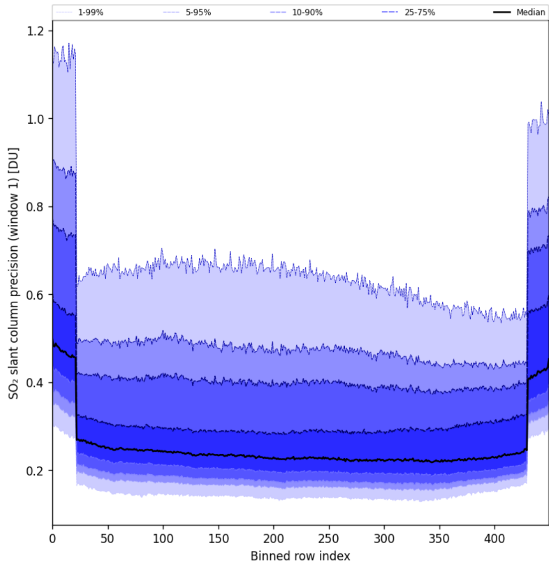
Figure 90: Along track statistics of “SO 2 slant column precision (window 1)” for 2025-01-10 to 2025-01-12
