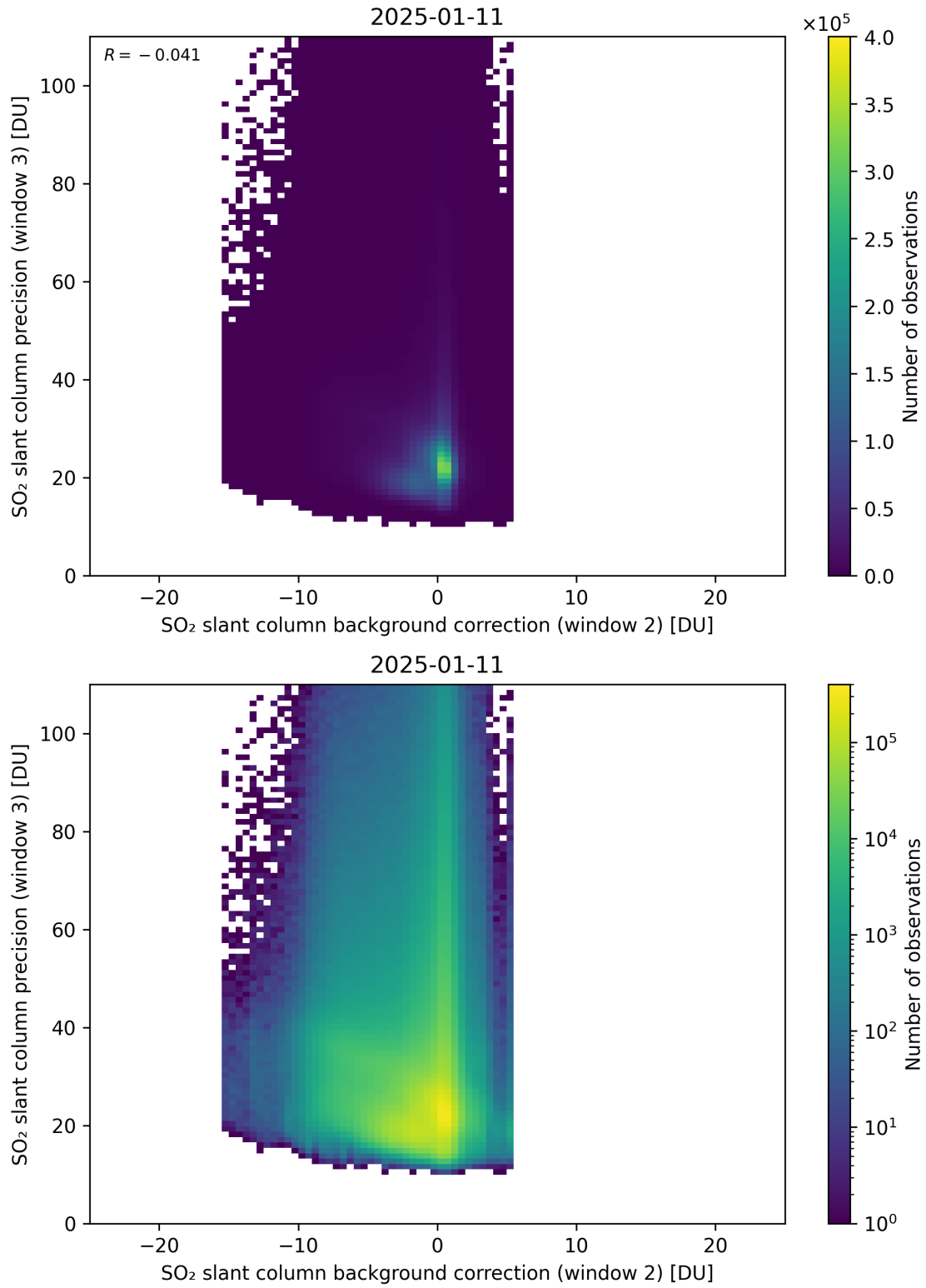
Figure 129: Scatter density plot of “SO 2 slant column background correction (window 2)” against “SO 2 slant column precision (window 3)” for 2025-01-10 to 2025-01-12.
