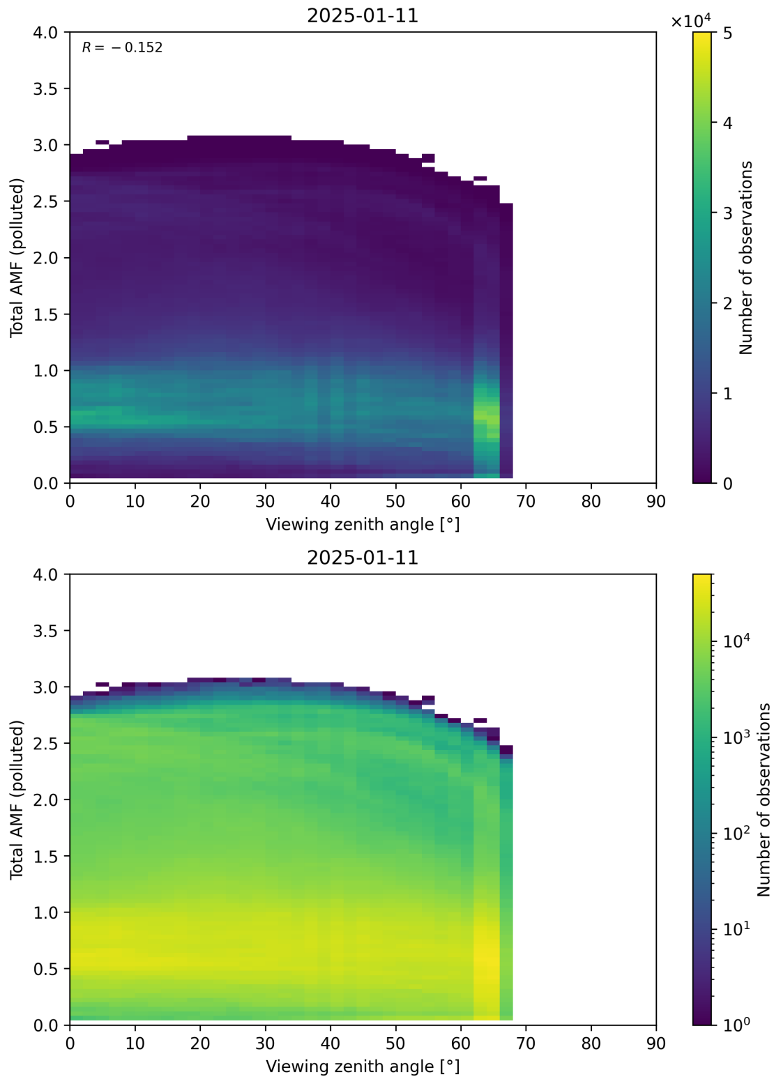
Figure 381: Scatter density plot of “Viewing zenith angle” against “Total AMF (polluted)” for 2025-01-10 to 2025-01-12.
