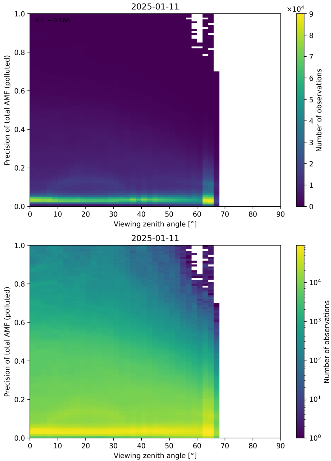
Figure 382: Scatter density plot of “Viewing zenith angle” against “Precision of total AMF (polluted)” for 2025-01-10 to 2025-01-12.
