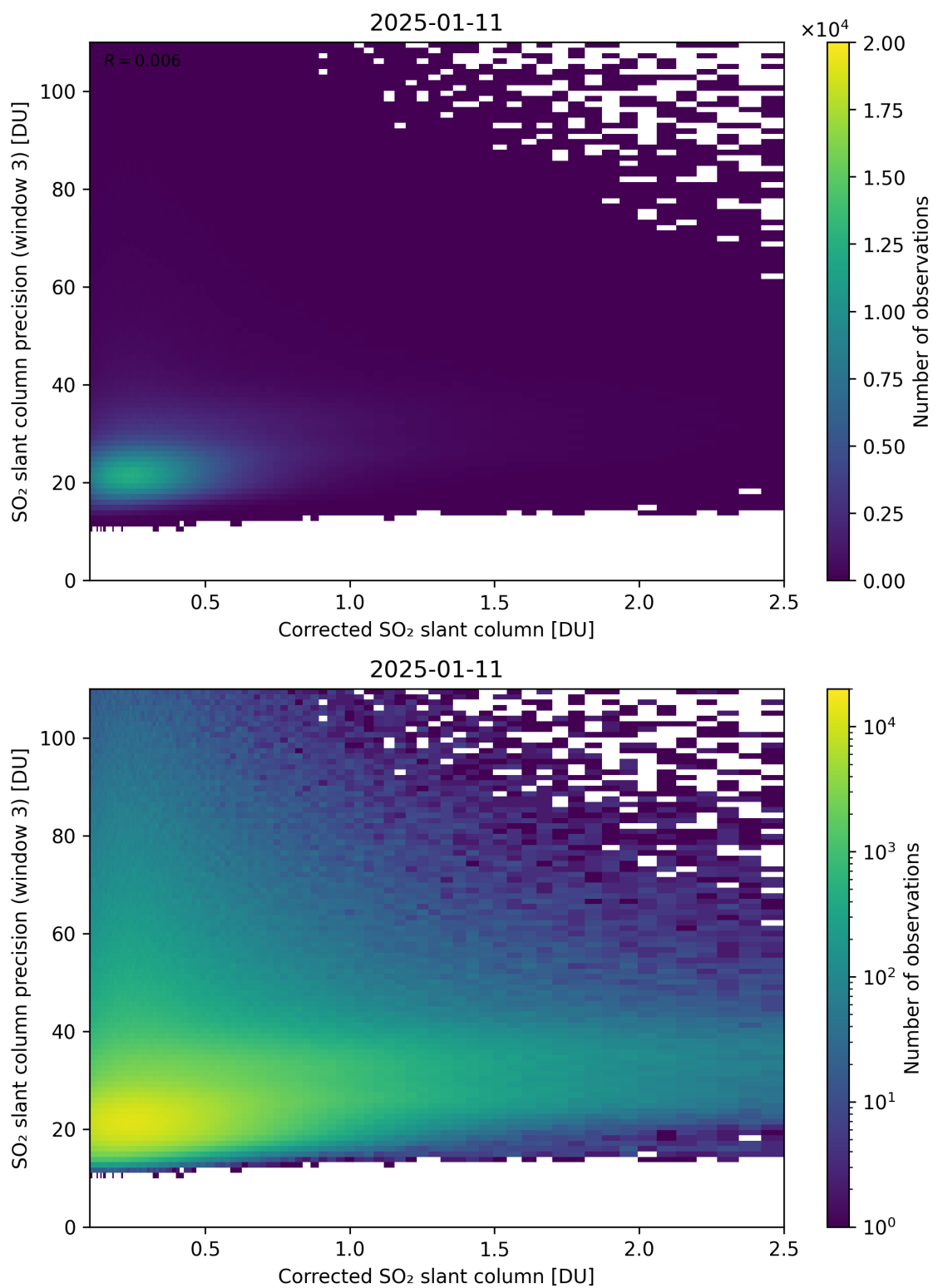
Figure 241: Scatter density plot of “Corrected SO 2 slant column” against “SO 2 slant column precision (window 3)” for 2025-01-10 to 2025-01-12.
