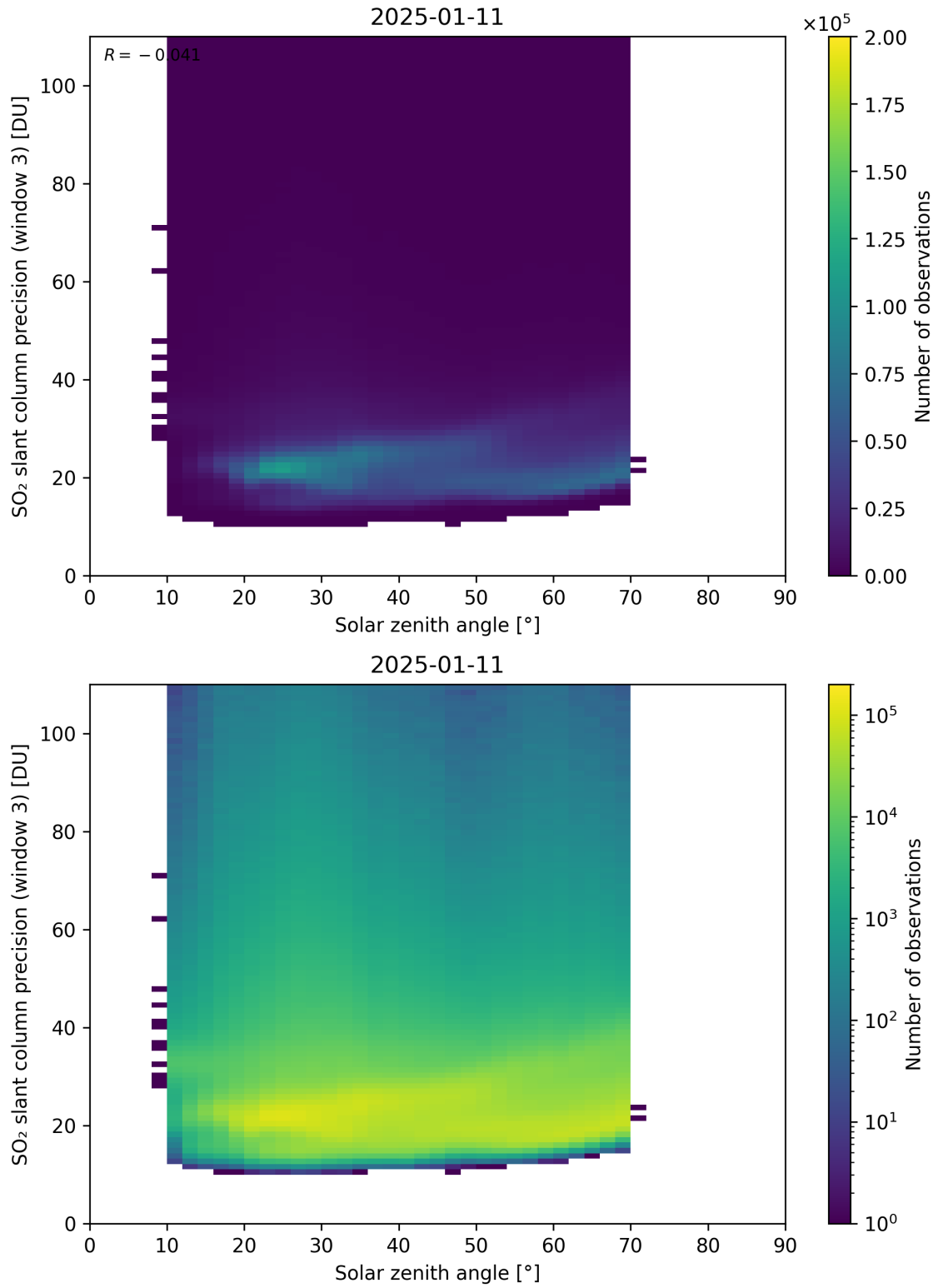
Figure 188: Scatter density plot of “Solar zenith angle” against “SO 2 slant column precision (window 3)” for 2025-01-10 to 2025-01-12.
