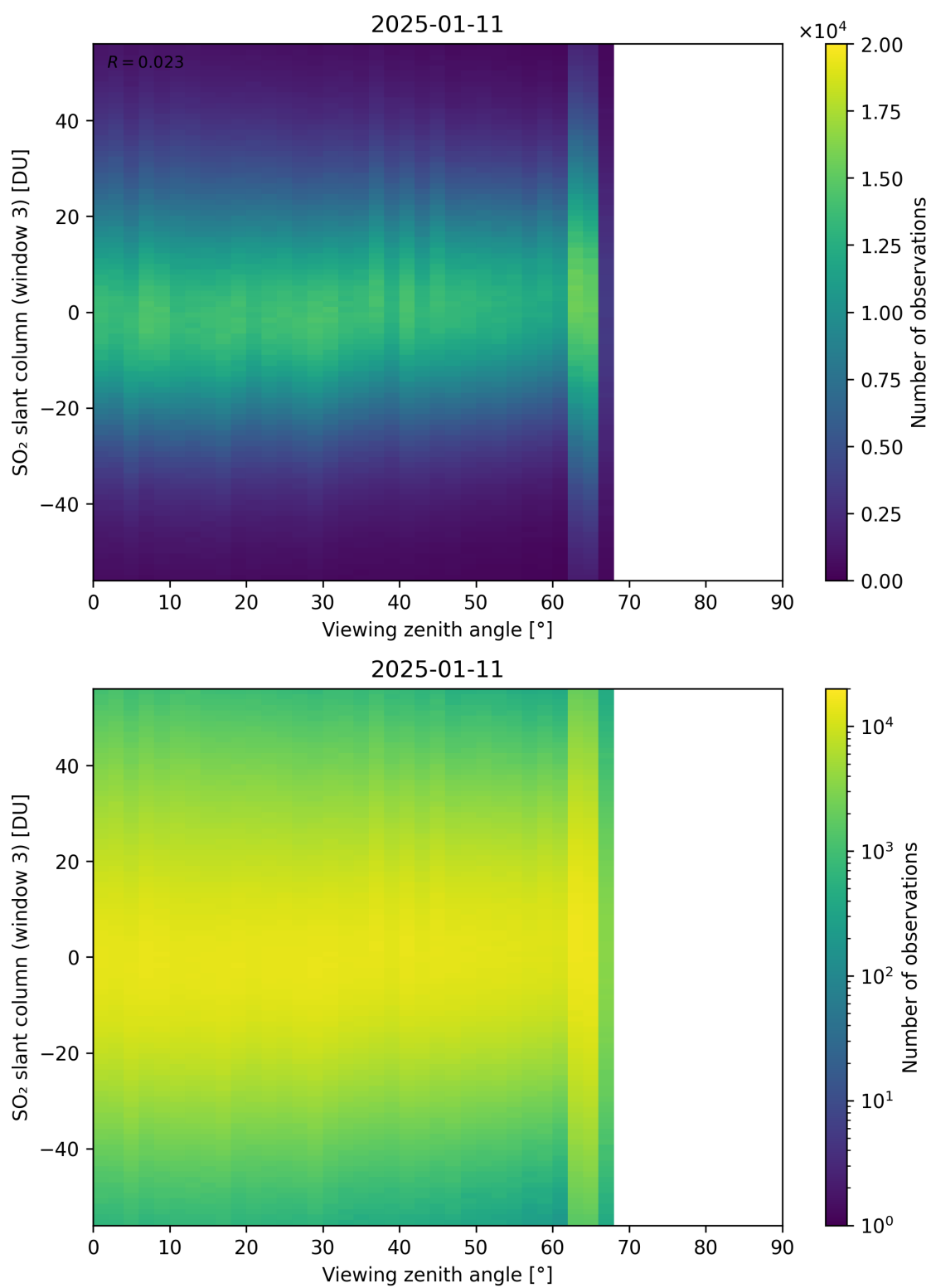
Figure 379: Scatter density plot of “Viewing zenith angle” against “SO 2 slant column (window 3)” for 2025-01-10 to 2025-01-12.
