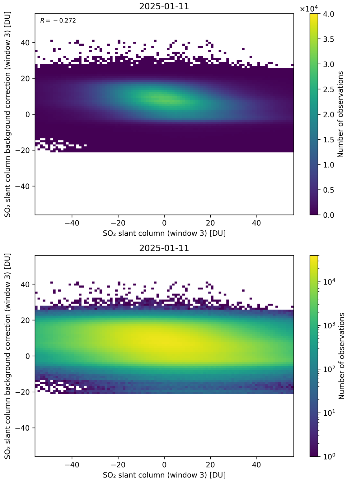
Figure 303: Scatter density plot of “SO 2 slant column (window 3)” against “SO 2 slant column background correction (window 3)” for 2025-01-10 to 2025-01-12.
