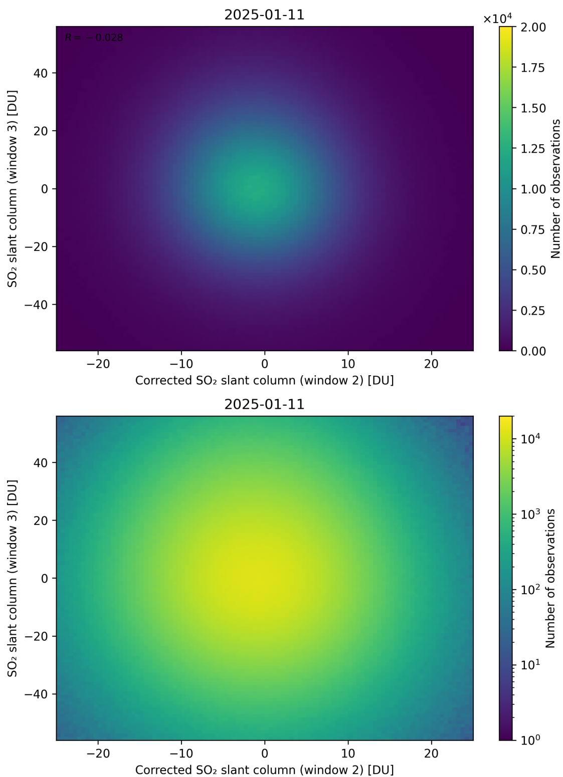
Figure 251: Scatter density plot of “Corrected SO 2 slant column (window 2)” against “SO 2 slant column (window 3)” for 2025-01-10 to 2025-01-12.
