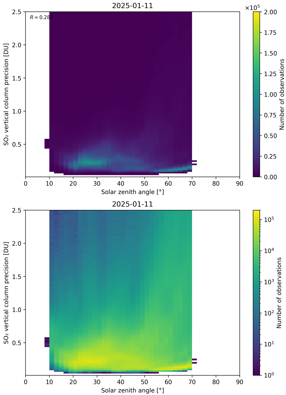
Figure 192: Scatter density plot of “Solar zenith angle” against “SO 2 vertical column precision” for 2025-01-10 to 2025-01-12.
