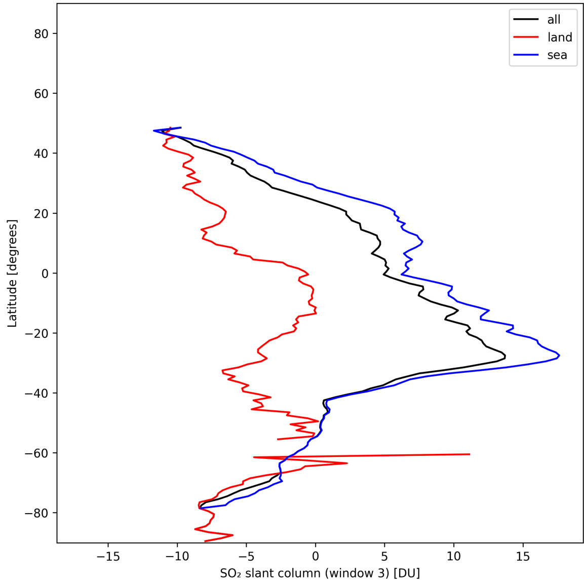
Figure 45: Zonal average of “SO 2 slant column (window 3)” for 2025-01-10 to 2025-01-12.
