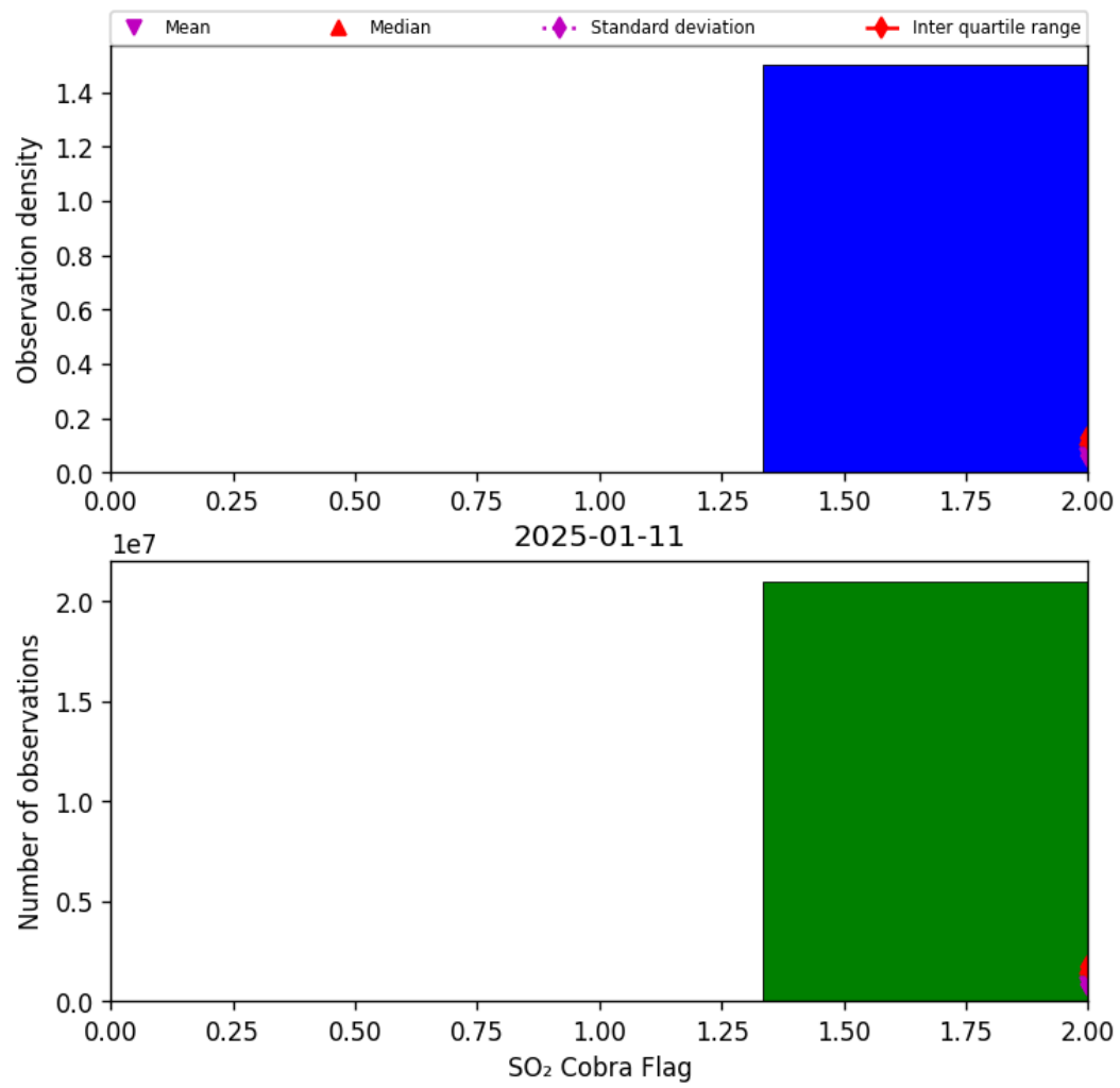
Figure 75: Histogram of “SO 2 Cobra Flag” for 2025-01-10 to 2025-01-12
