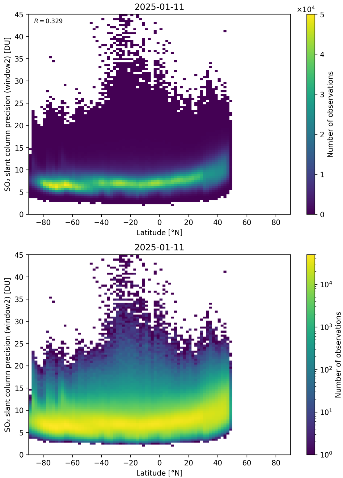
Figure 164: Scatter density plot of “Latitude” against “SO 2 slant column precision (window2)” for 2025-01-10 to 2025-01-12.
