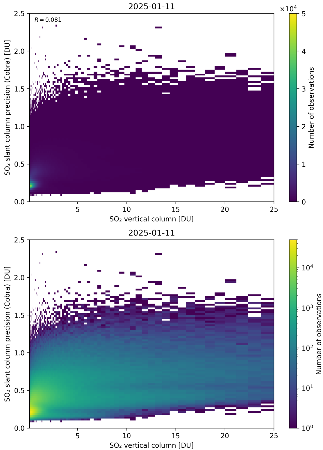
Figure 350: Scatter density plot of “SO 2 vertical column” against “SO 2 slant column precision (Cobra)” for 2025-01-10 to 2025-01-12.
