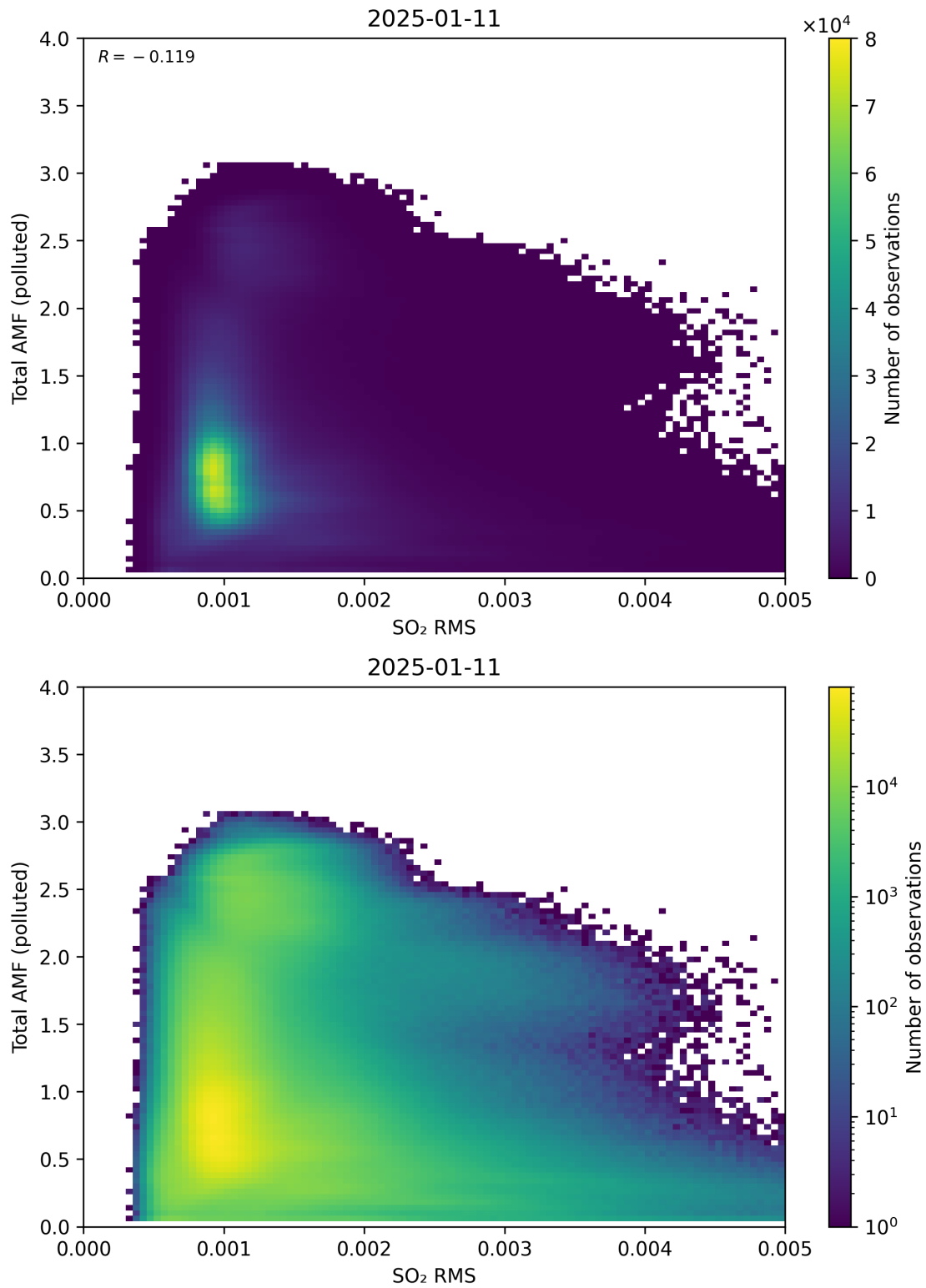
Figure 148: Scatter density plot of “SO 2 RMS” against “Total AMF (polluted)” for 2025-01-10 to 2025-01-12.
