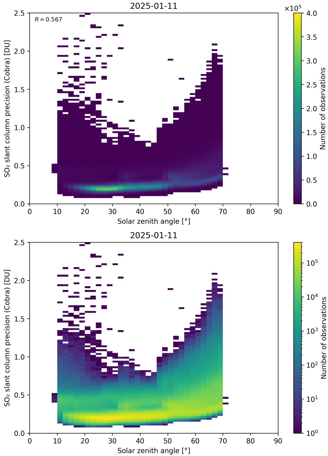
Figure 180: Scatter density plot of “Solar zenith angle” against “SO 2 slant column precision (Cobra)” for 2025-01-10 to 2025-01-12.
