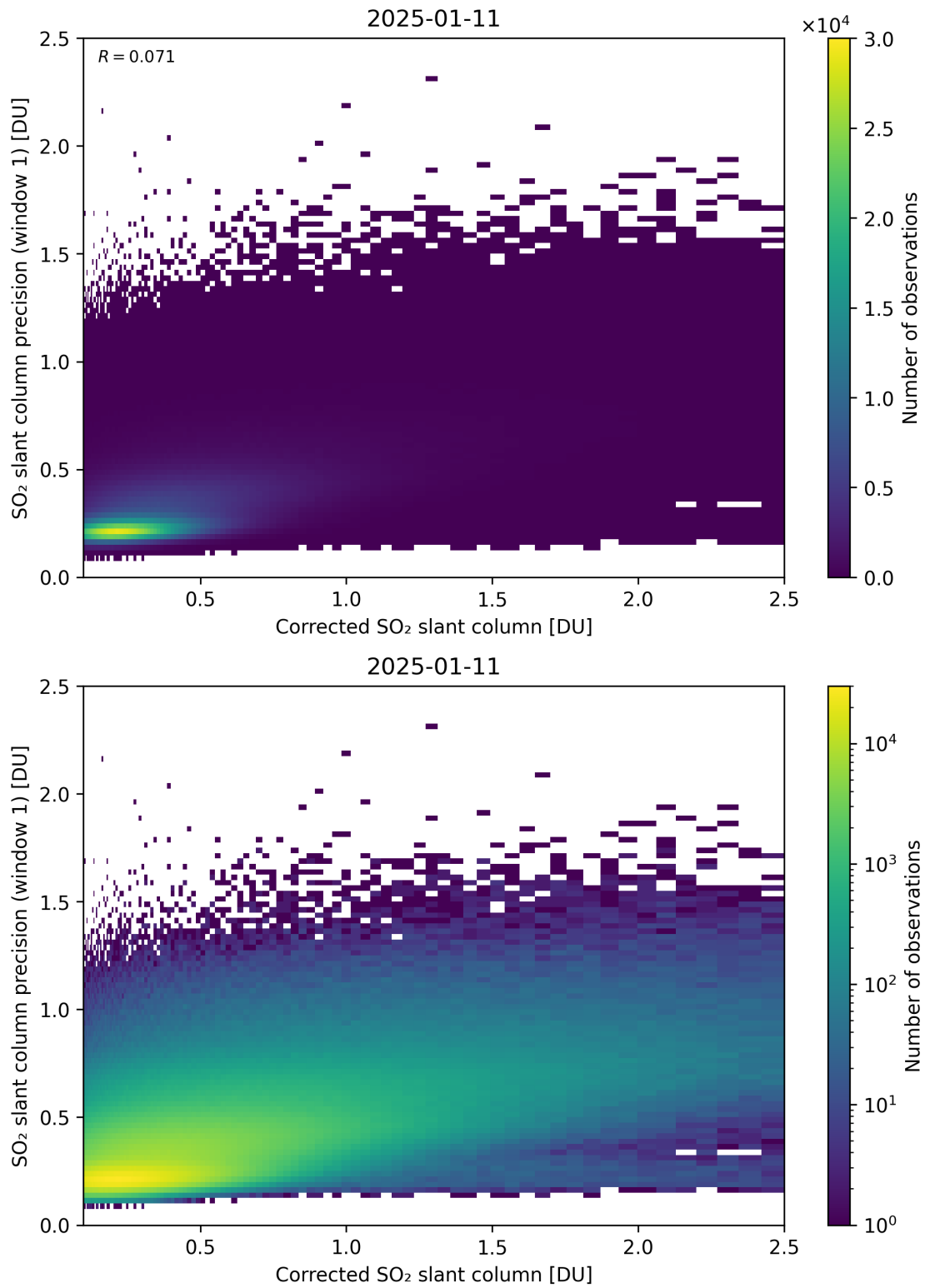
Figure 238: Scatter density plot of “Corrected SO 2 slant column” against “SO 2 slant column precision (window 1)” for 2025-01-10 to 2025-01-12.
