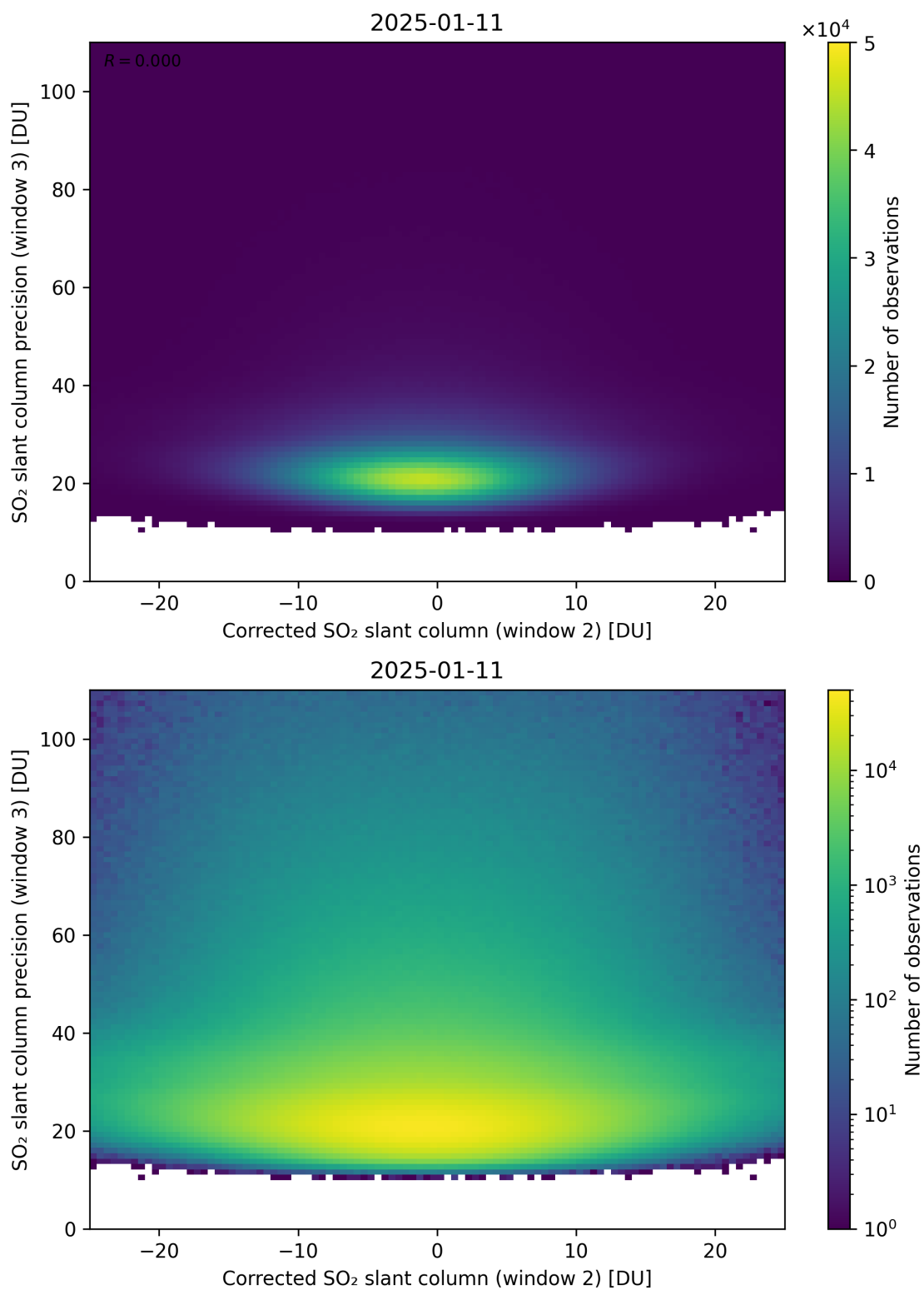
Figure 252: Scatter density plot of “Corrected SO 2 slant column (window 2)” against “SO 2 slant column precision (window 3)” for 2025-01-10 to 2025-01-12.
