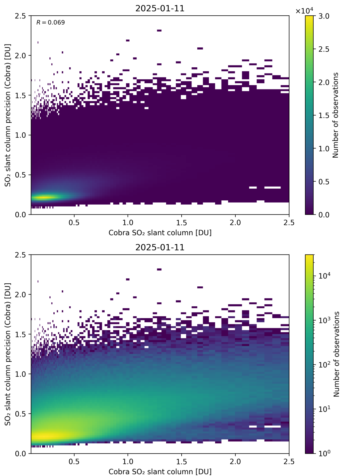
Figure 216: Scatter density plot of “Cobra SO 2 slant column” against “SO 2 slant column precision (Cobra)” for 2025-01-10 to 2025-01-12.
