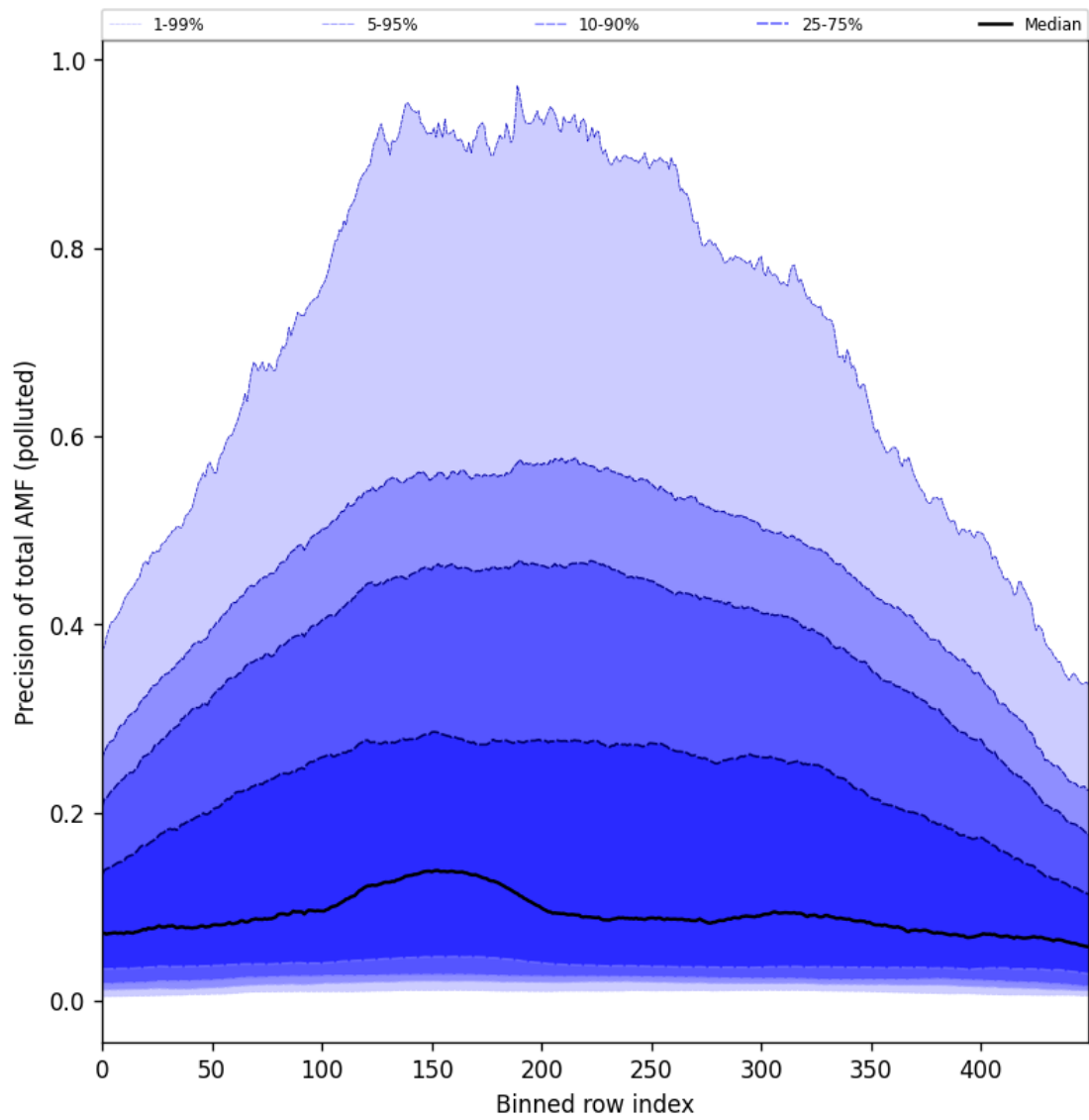
Figure 106: Along track statistics of “Precision of total AMF (polluted)” for 2025-01-10 to 2025-01-12
