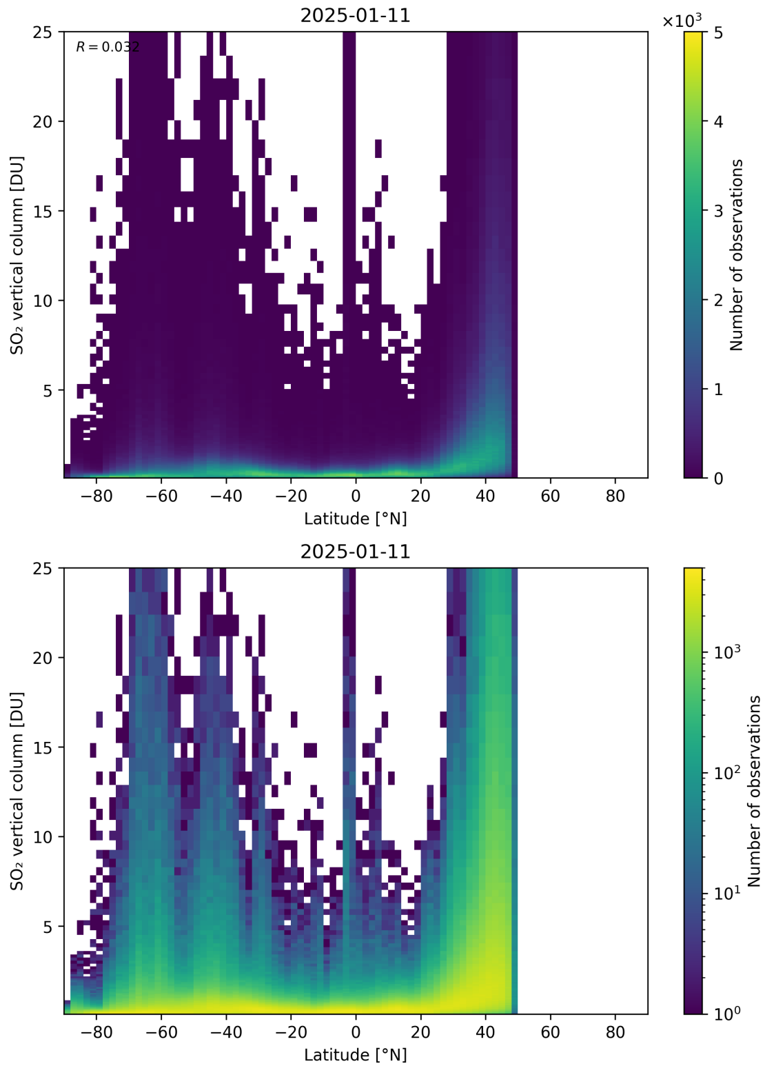
Figure 169: Scatter density plot of “Latitude” against “SO 2 vertical column” for 2025-01-10 to 2025-01-12.
