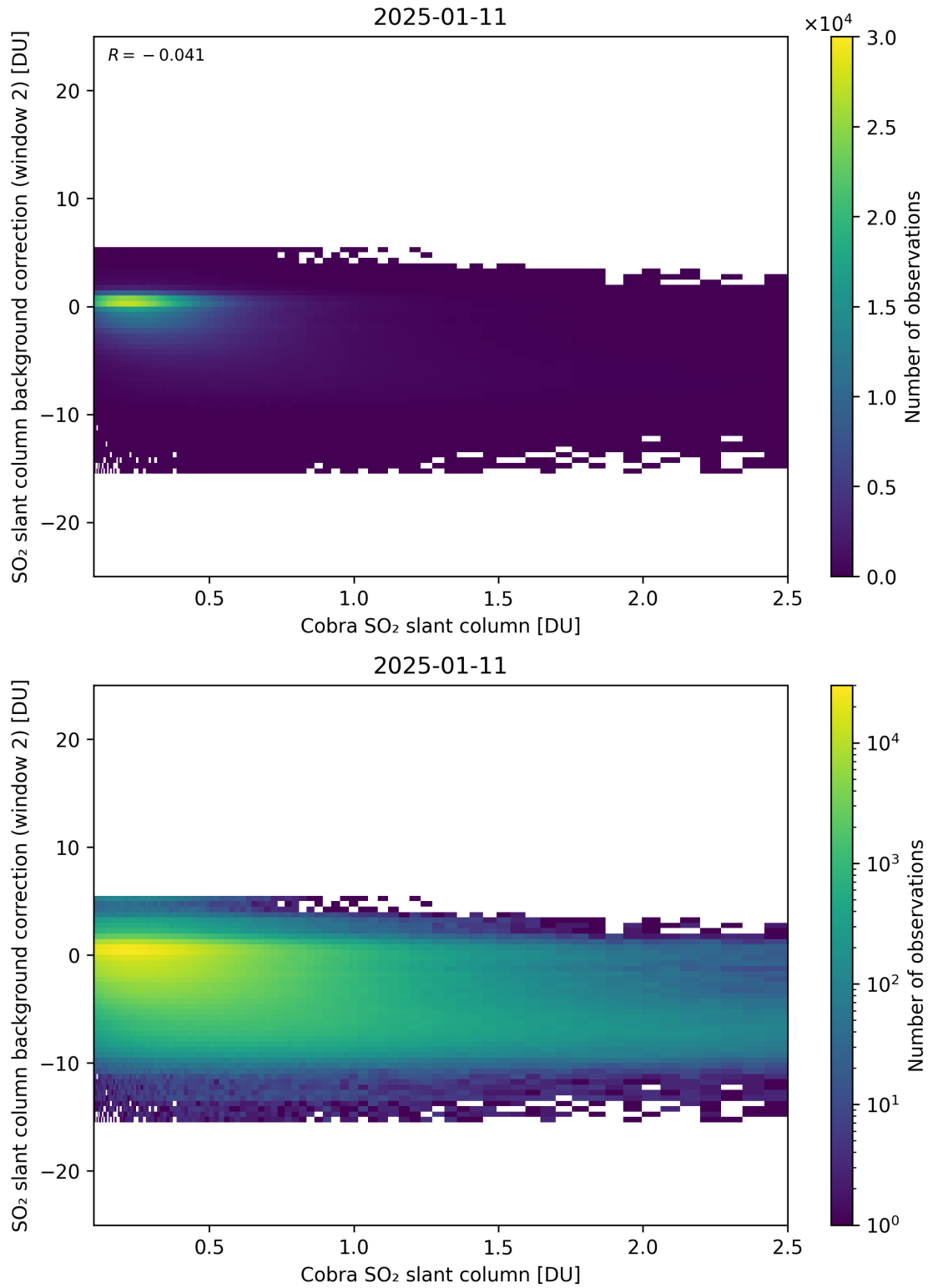
Figure 194: Scatter density plot of “Cobra SO 2 slant column” against “SO 2 slant column background correction (window 2)” for 2025-01-10 to 2025-01-12.
