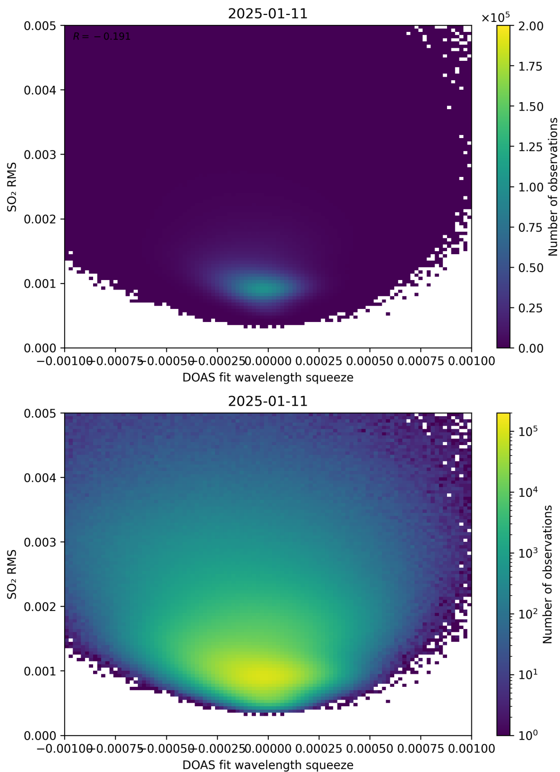
Figure 143: Scatter density plot of “DOAS fit wavelength squeeze” against “SO 2 RMS” for 2025-01-10 to 2025-01-12.
