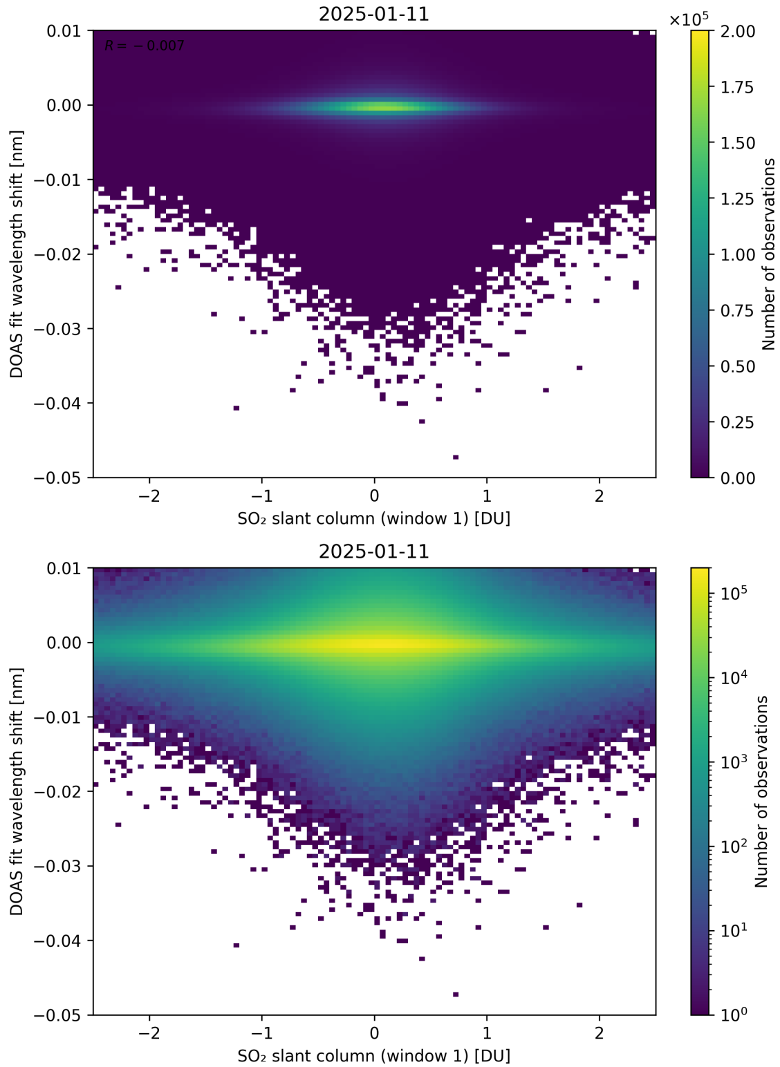
Figure 265: Scatter density plot of “SO 2 slant column (window 1)” against “DOAS fit wavelength shift” for 2025-01-10 to 2025-01-12.
