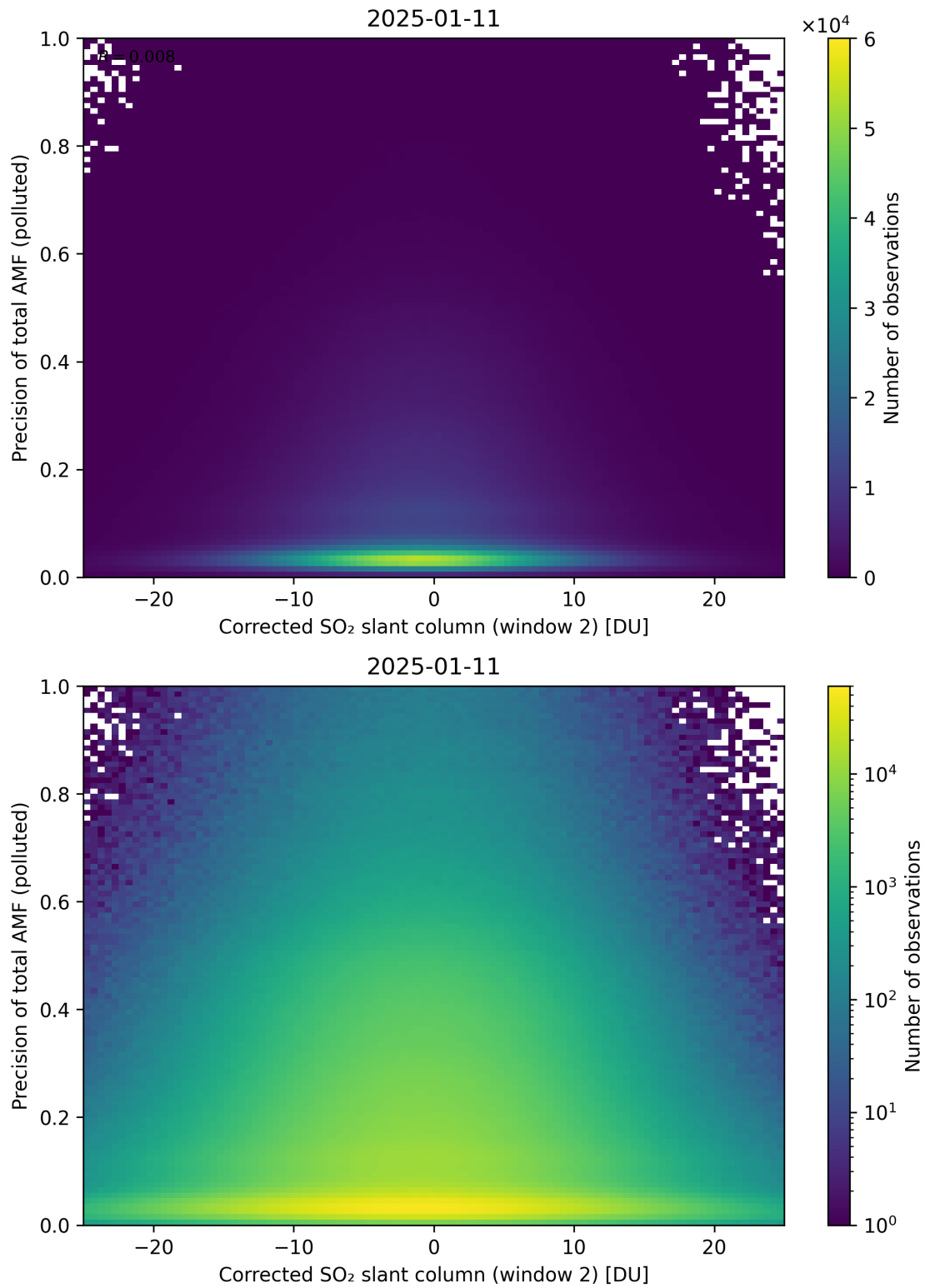
Figure 254: Scatter density plot of “Corrected SO 2 slant column (window 2)” against “Precision of total AMF (polluted)” for 2025-01-10 to 2025-01-12.
