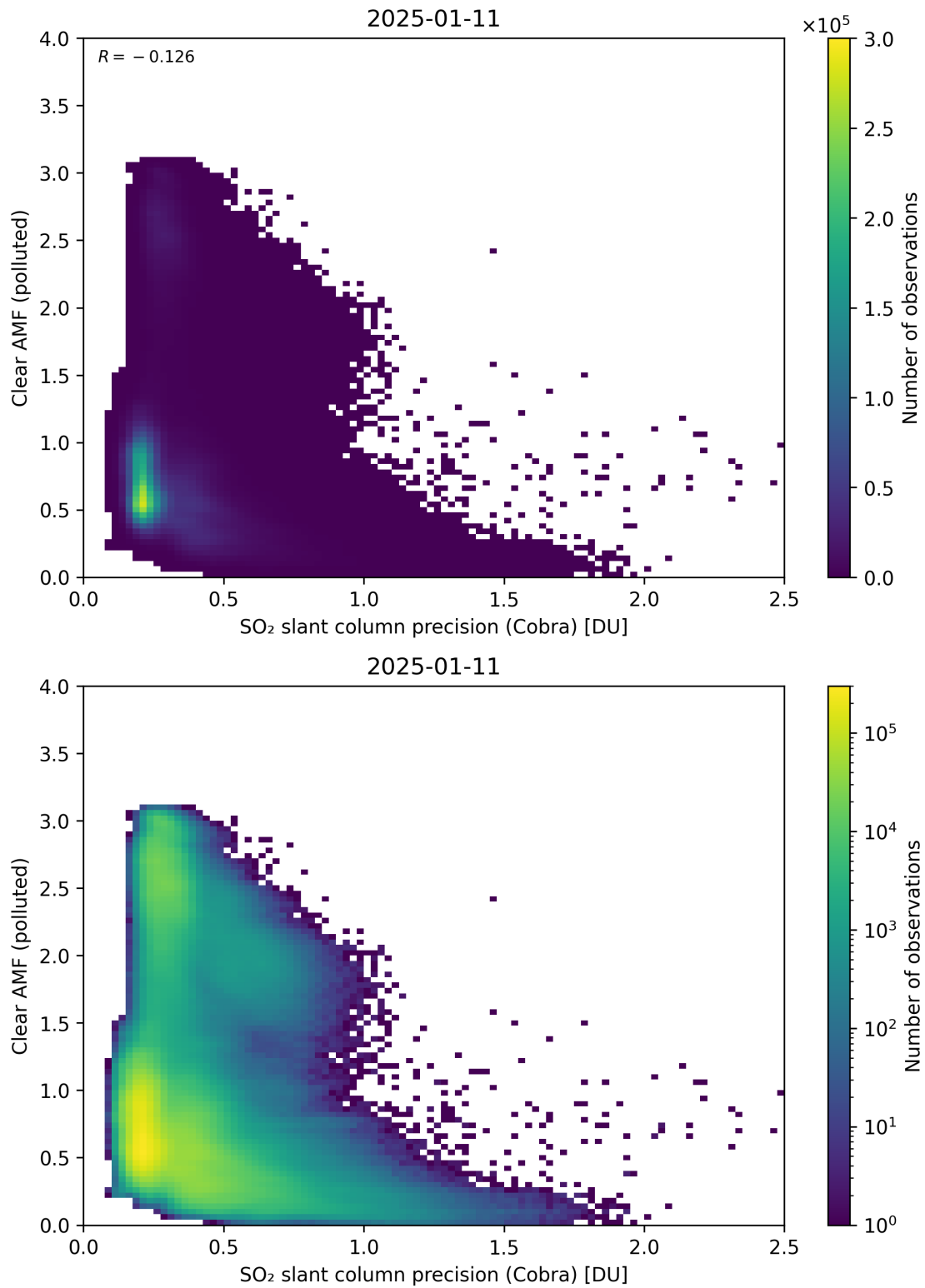
Figure 205: Scatter density plot of “SO 2 slant column precision (Cobra)” against “Clear AMF (polluted)” for 2025-01-10 to 2025-01-12.
