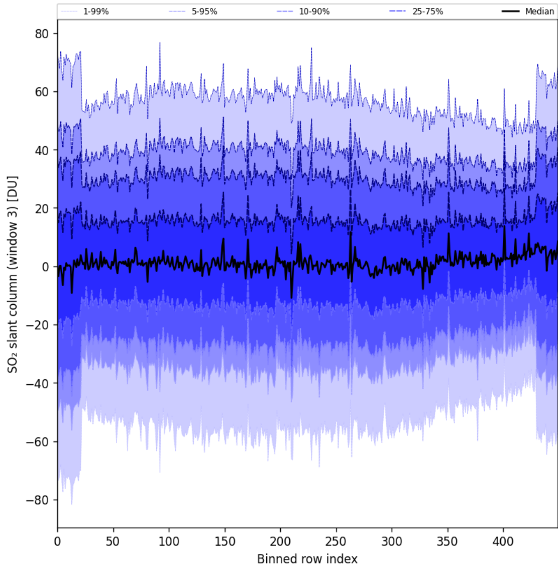
Figure 97: Along track statistics of “SO 2 slant column (window 3)” for 2025-01-10 to 2025-01-12
