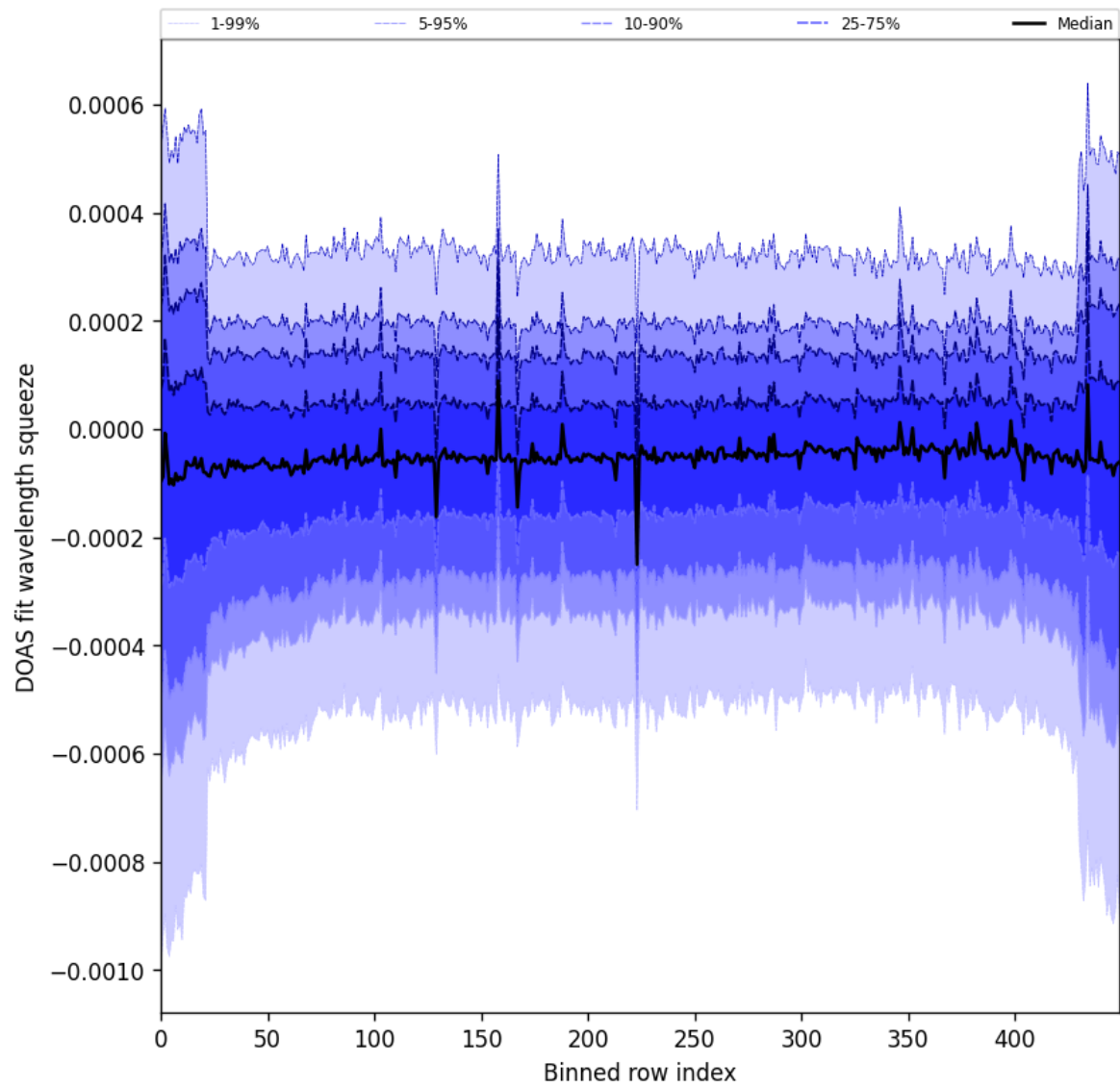
Figure 103: Along track statistics of “DOAS fit wavelength squeeze” for 2025-01-10 to 2025-01-12
