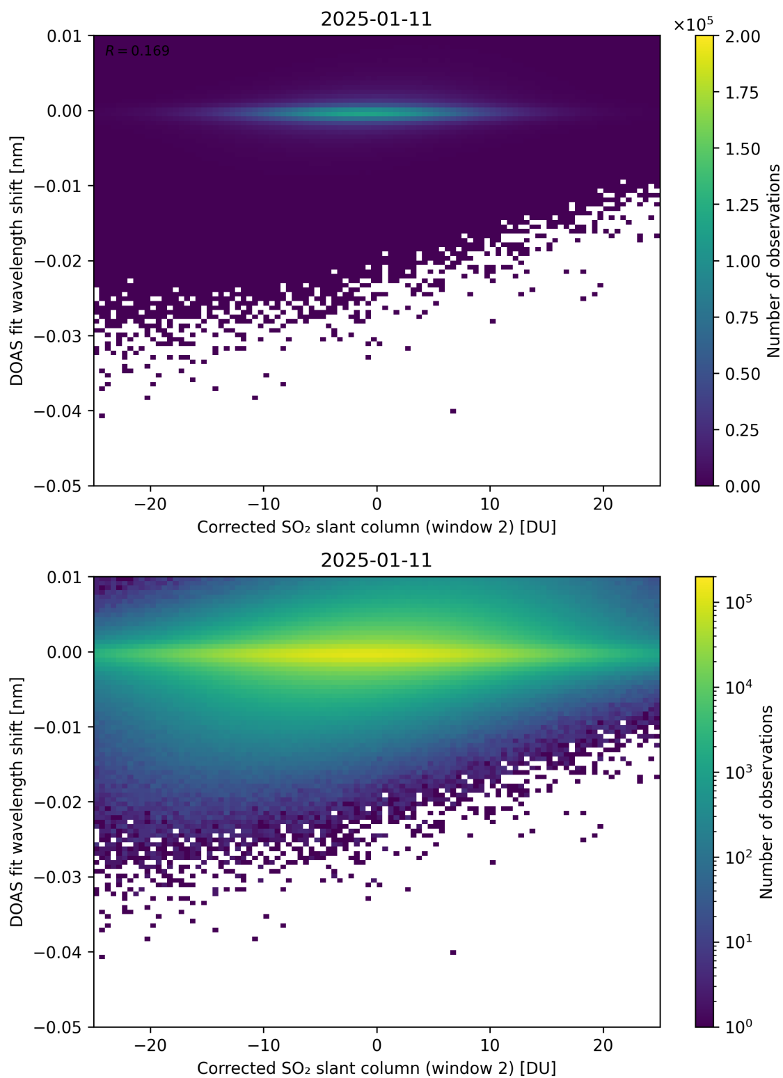
Figure 246: Scatter density plot of “Corrected SO 2 slant column (window 2)” against “DOAS fit wavelength shift” for 2025-01-10 to 2025-01-12.
