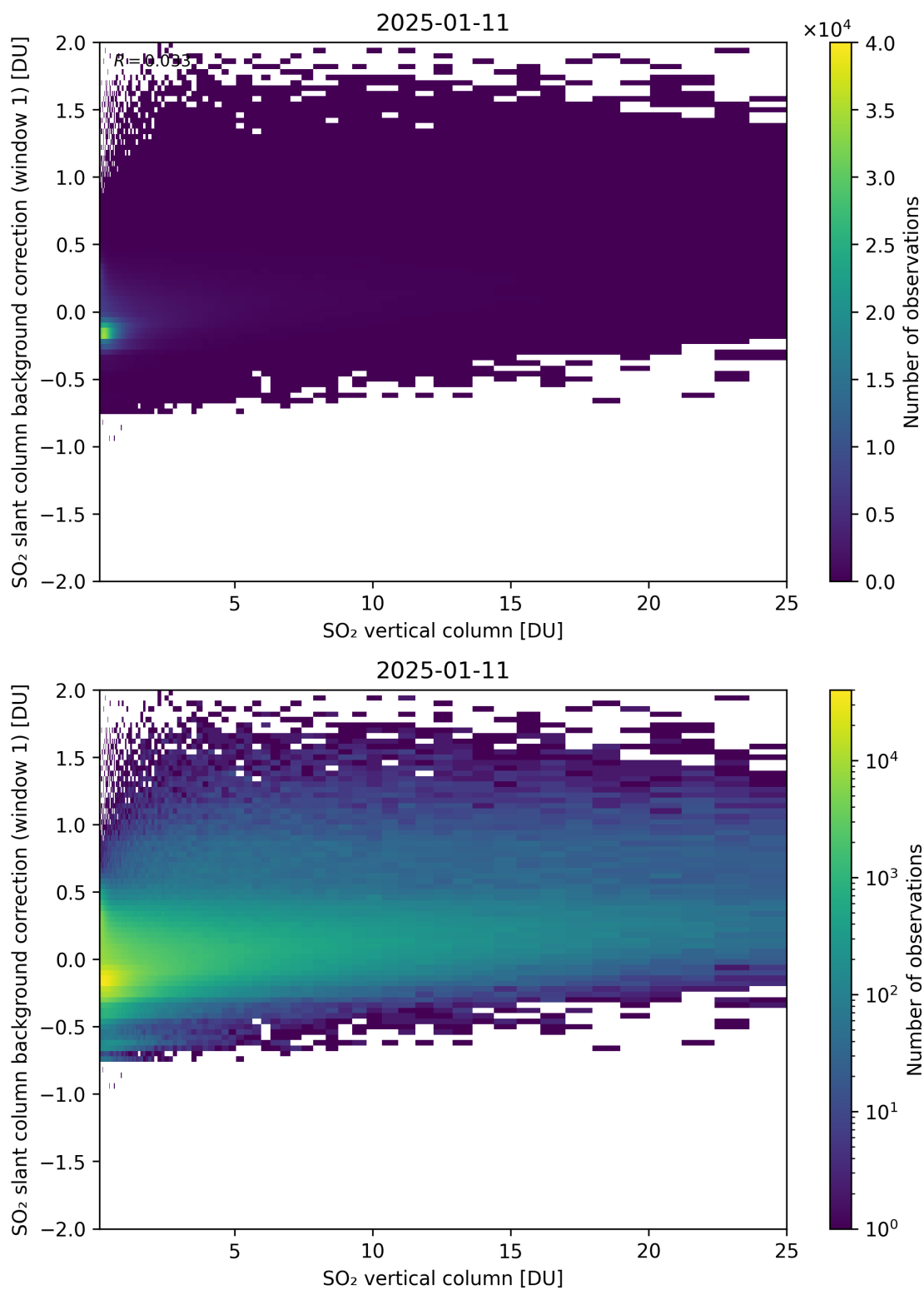
Figure 323: Scatter density plot of “SO 2 vertical column” against “SO 2 slant column background correction (window 1)” for 2025-01-10 to 2025-01-12.
