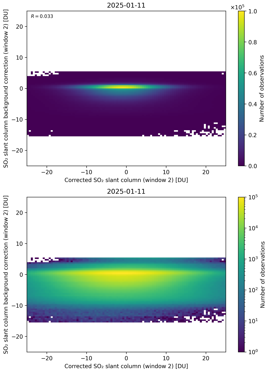
Figure 244: Scatter density plot of “Corrected SO 2 slant column (window 2)” against “SO 2 slant column background correction (window 2)” for 2025-01-10 to 2025-01-12.
