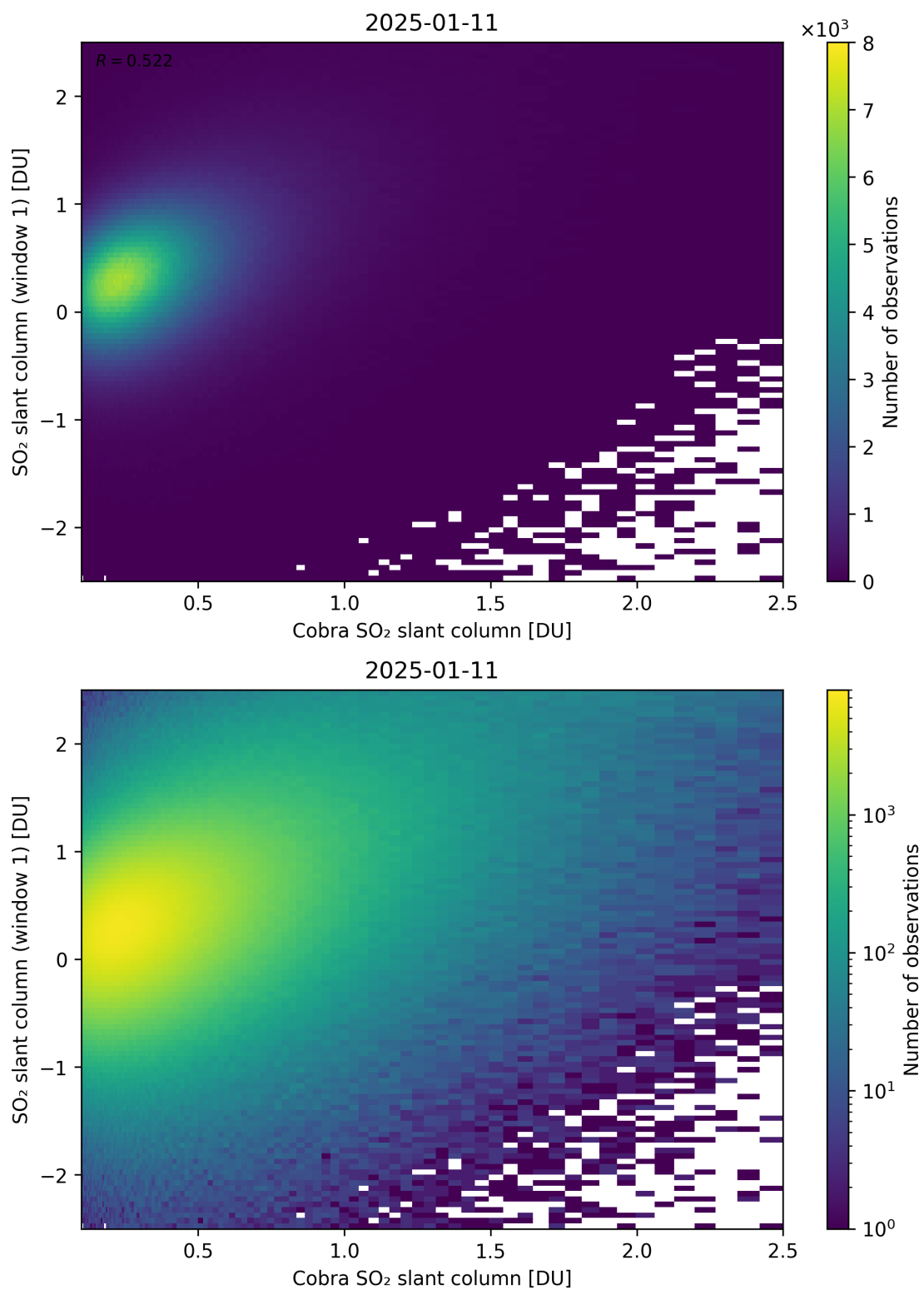
Figure 219: Scatter density plot of “Cobra SO 2 slant column” against “SO 2 slant column (window 1)” for 2025-01-10 to 2025-01-12.
