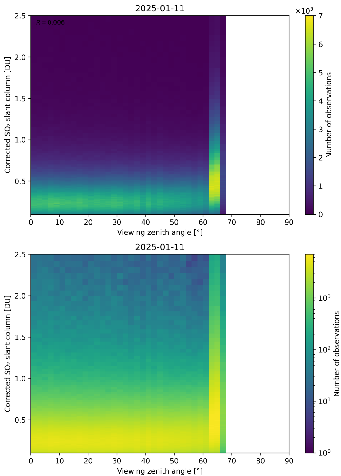
Figure 373: Scatter density plot of “Viewing zenith angle” against “Corrected SO 2 slant column” for 2025-01-10 to 2025-01-12.
