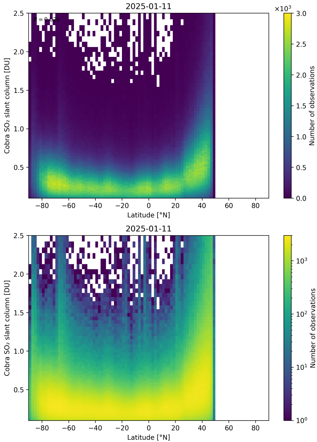
Figure 157: Scatter density plot of “Latitude” against “Cobra SO 2 slant column” for 2025-01-10 to 2025-01-12.
