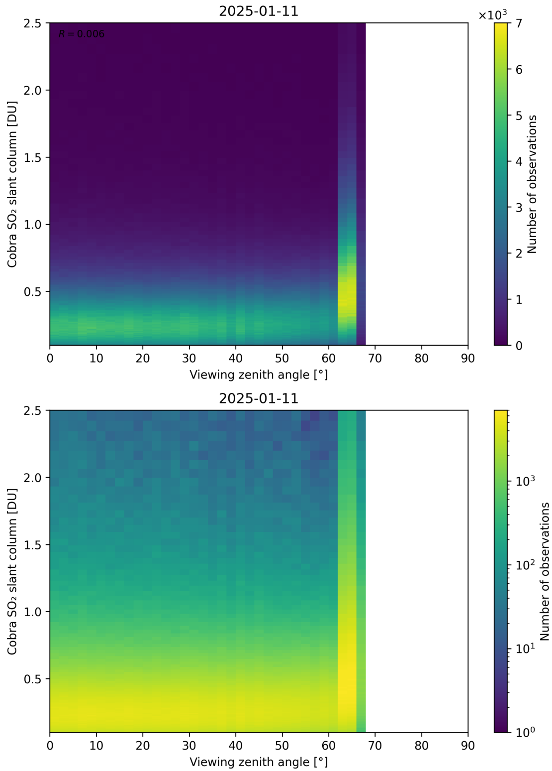
Figure 371: Scatter density plot of “Viewing zenith angle” against “Cobra SO 2 slant column” for 2025-01-10 to 2025-01-12.
