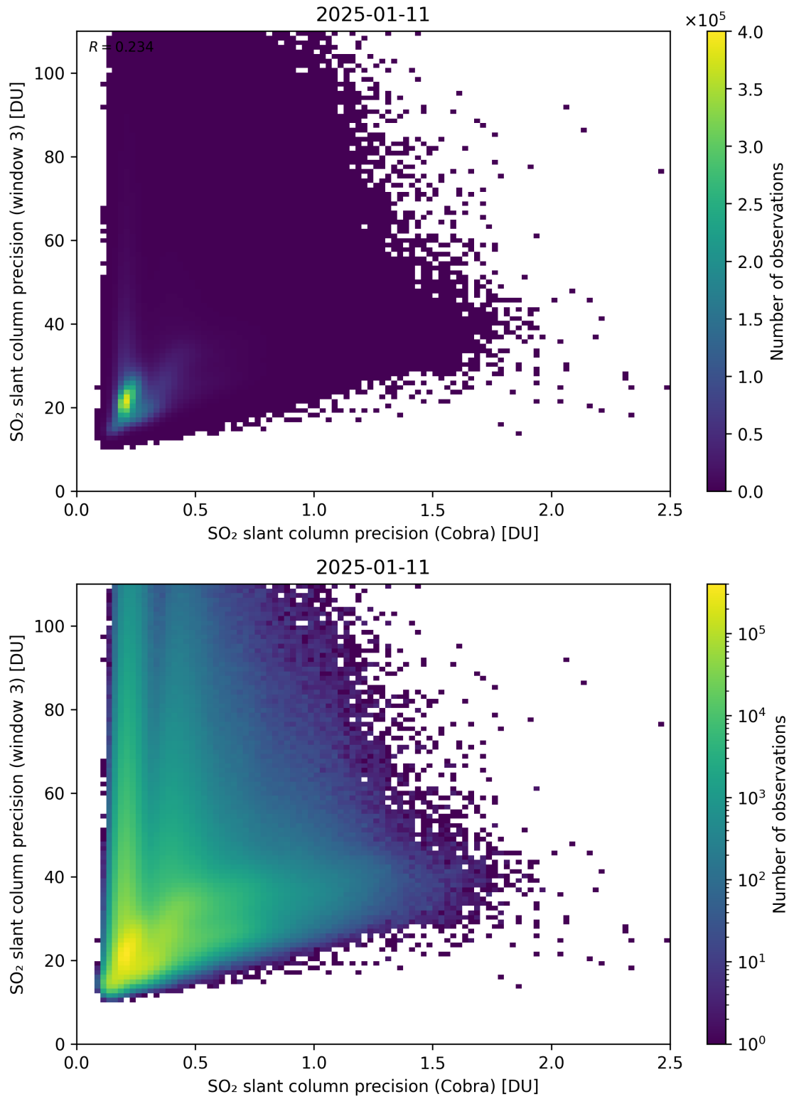
Figure 212: Scatter density plot of “SO 2 slant column precision (Cobra)” against “SO 2 slant column precision (window 3)” for 2025-01-10 to 2025-01-12.
