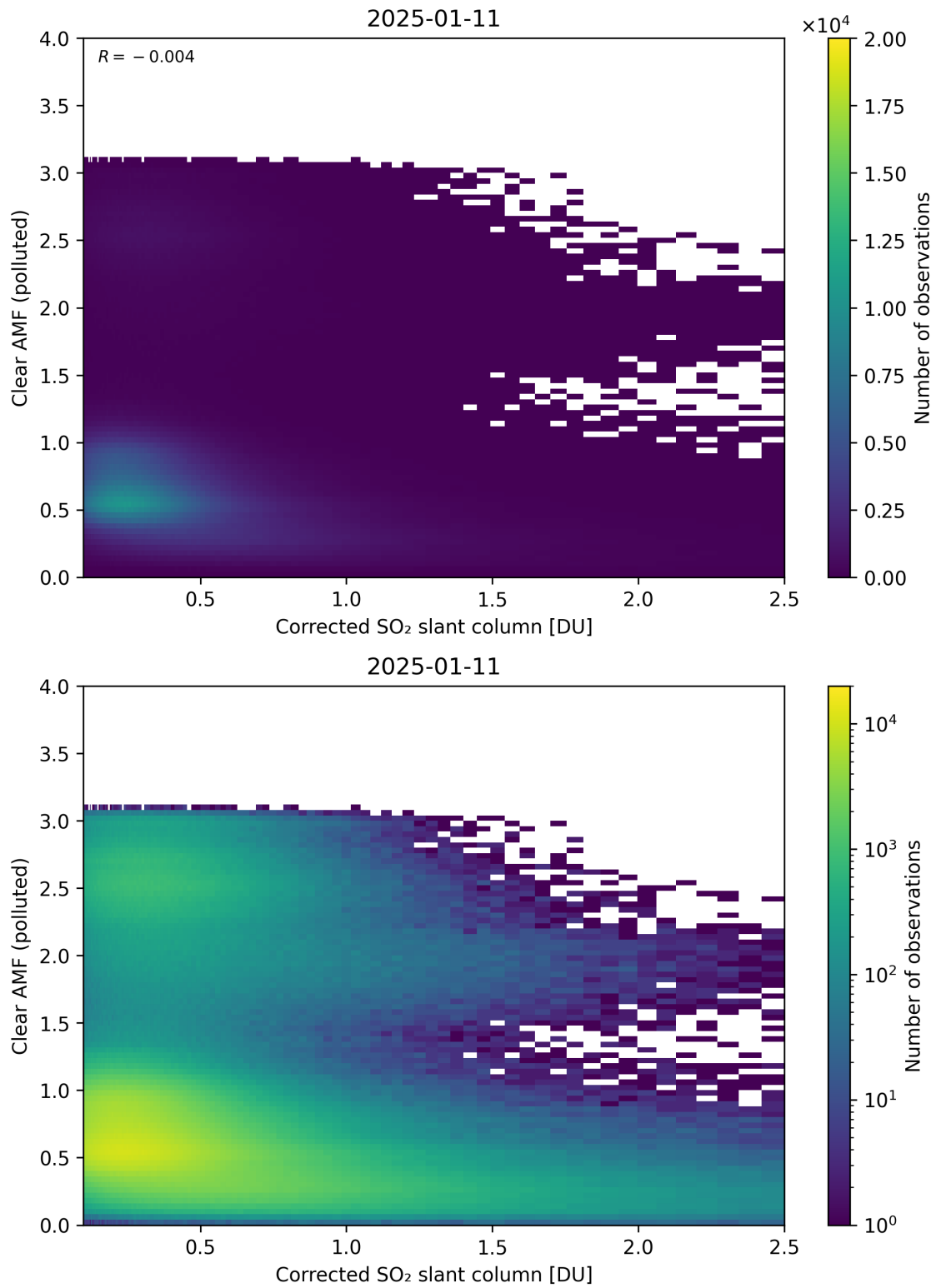
Figure 232: Scatter density plot of “Corrected SO 2 slant column” against “Clear AMF (polluted)” for 2025-01-10 to 2025-01-12.
