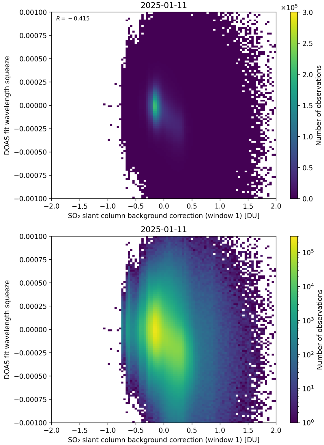
Figure 112: Scatter density plot of “SO 2 slant column background correction (window 1)” against “DOAS fit wavelength squeeze” for 2025-01-10 to 2025-01-12.
