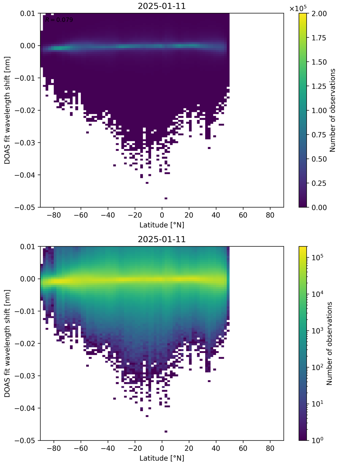
Figure 153: Scatter density plot of “Latitude” against “DOAS fit wavelength shift” for 2025-01-10 to 2025-01-12.
