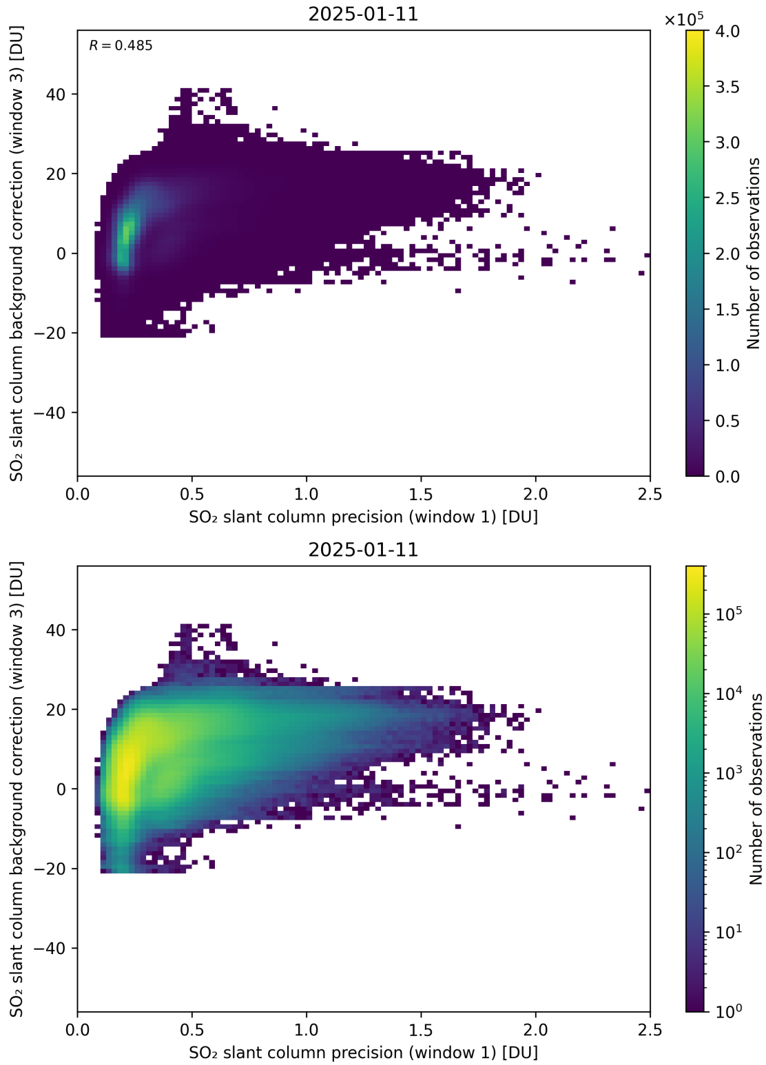
Figure 270: Scatter density plot of “SO 2 slant column precision (window 1)” against “SO 2 slant column background correction (window 3)” for 2025-01-10 to 2025-01-12.
