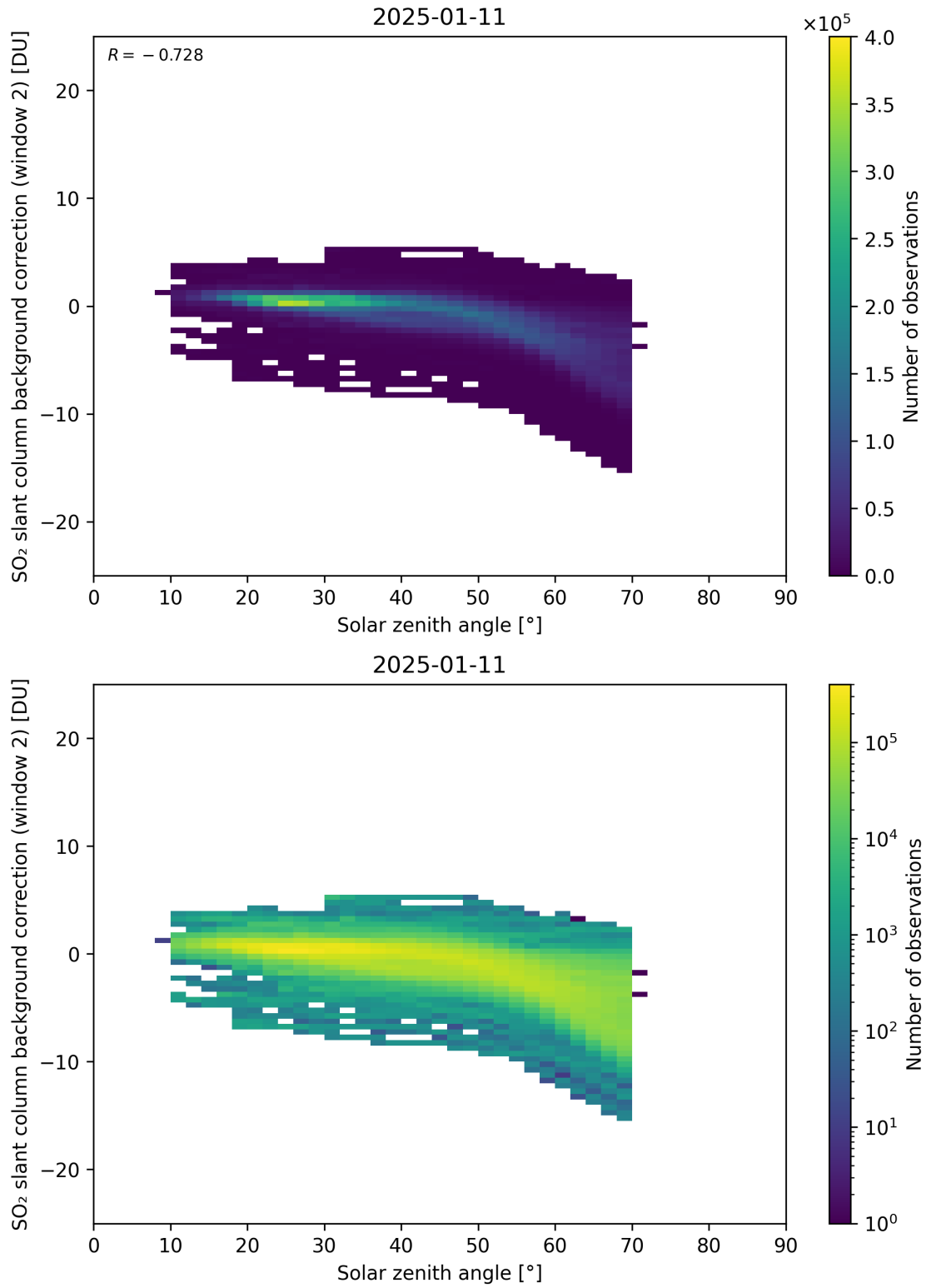
Figure 172: Scatter density plot of “Solar zenith angle” against “SO 2 slant column background correction (window 2)” for 2025-01-10 to 2025-01-12.
