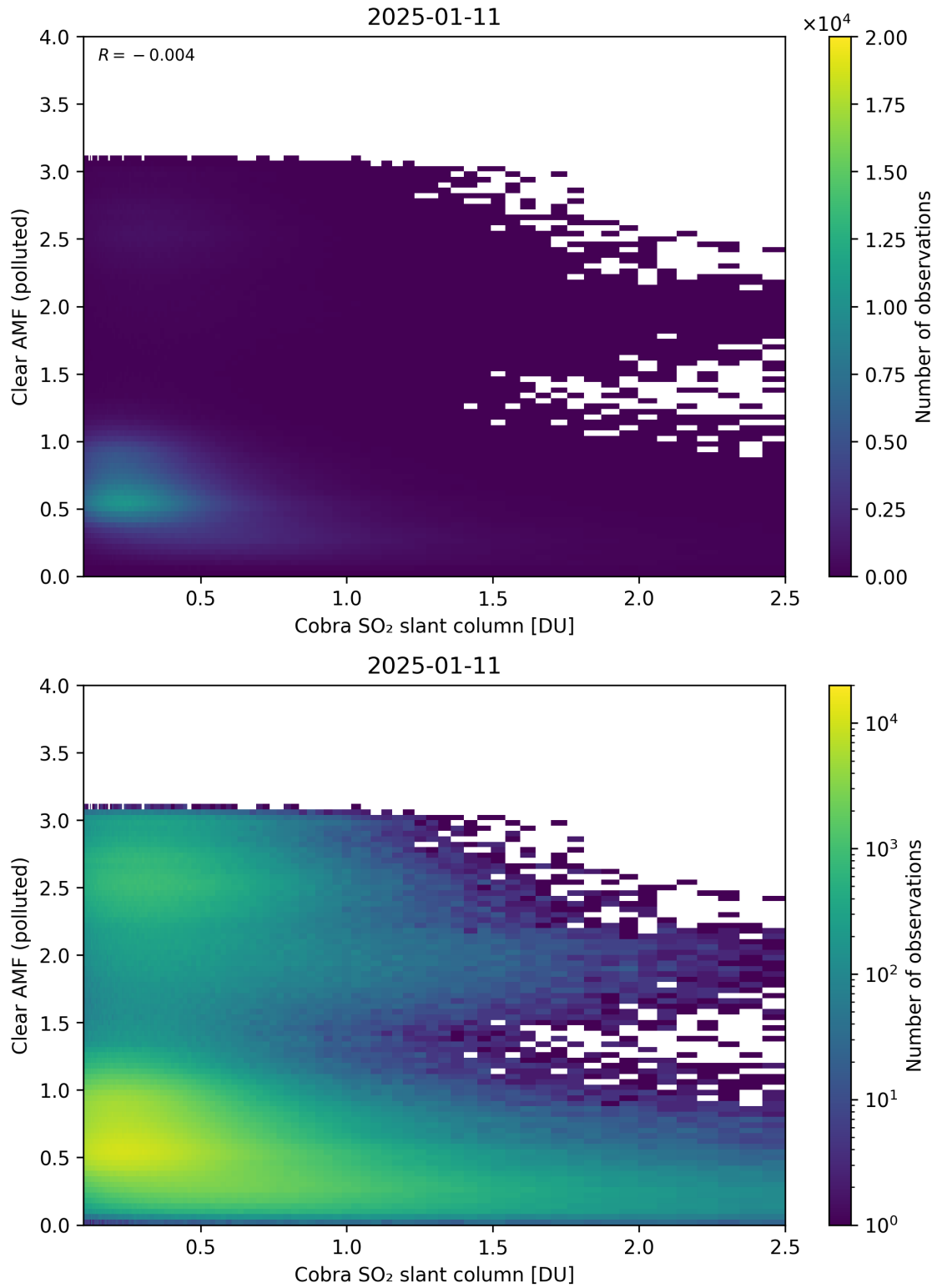
Figure 215: Scatter density plot of “Cobra SO 2 slant column” against “Clear AMF (polluted)” for 2025-01-10 to 2025-01-12.
