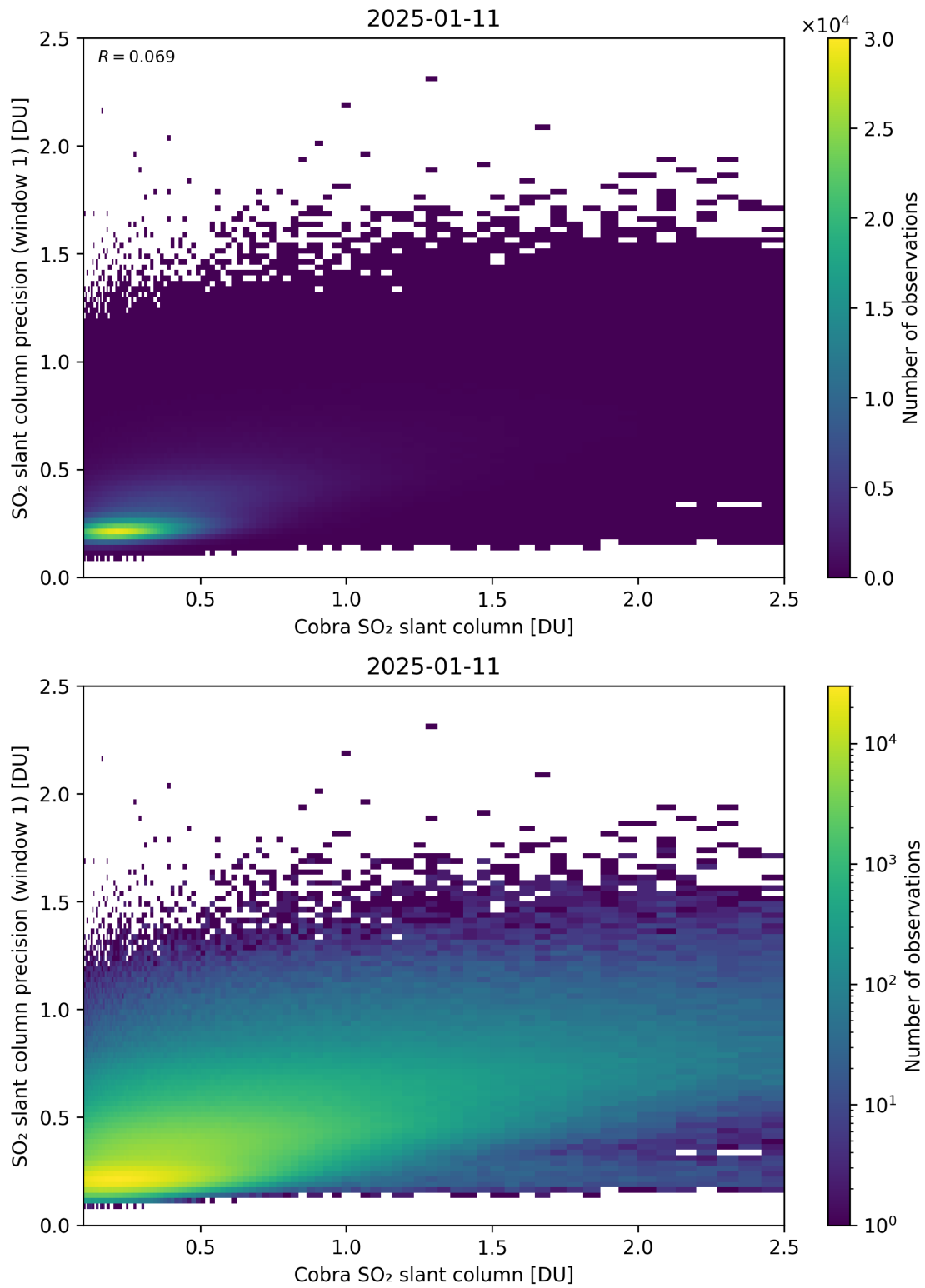
Figure 220: Scatter density plot of “Cobra SO 2 slant column” against “SO 2 slant column precision (window 1)” for 2025-01-10 to 2025-01-12.
