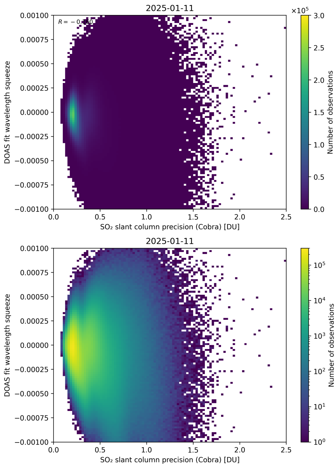
Figure 203: Scatter density plot of “SO 2 slant column precision (Cobra)” against “DOAS fit wavelength squeeze” for 2025-01-10 to 2025-01-12.
