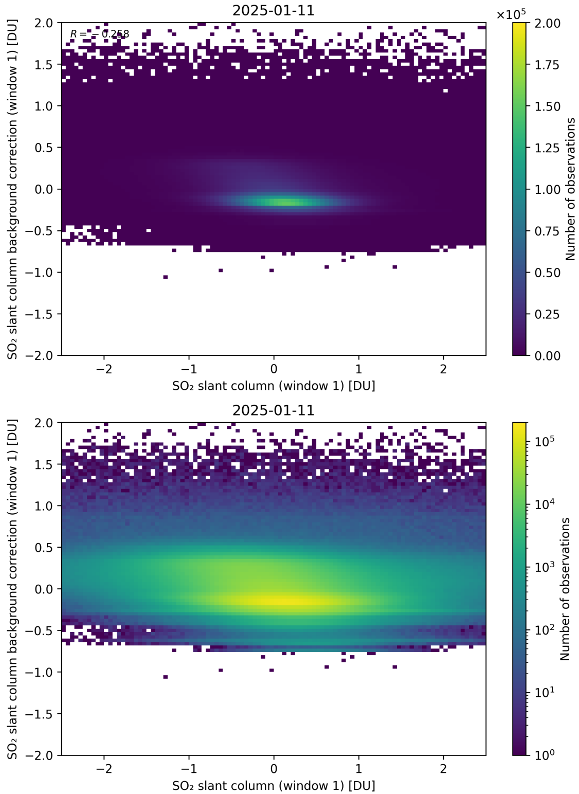
Figure 262: Scatter density plot of “SO 2 slant column (window 1)” against “SO 2 slant column background correction (window 1)” for 2025-01-10 to 2025-01-12.
