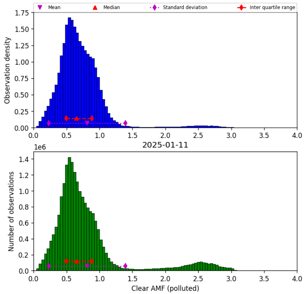
Figure 81: Histogram of “Clear AMF (polluted)” for 2025-01-10 to 2025-01-12
