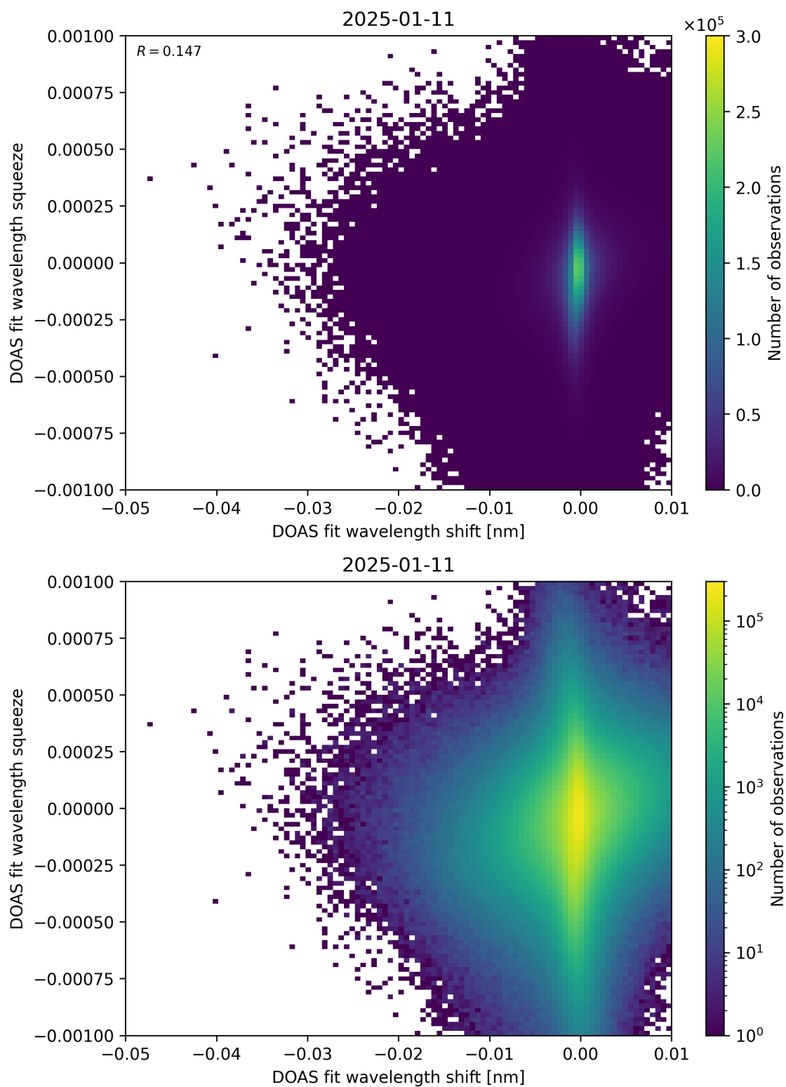
Figure 138: Scatter density plot of “DOAS fit wavelength shift” against “DOAS fit wavelength squeeze” for 2025-01-10 to 2025-01-12.
