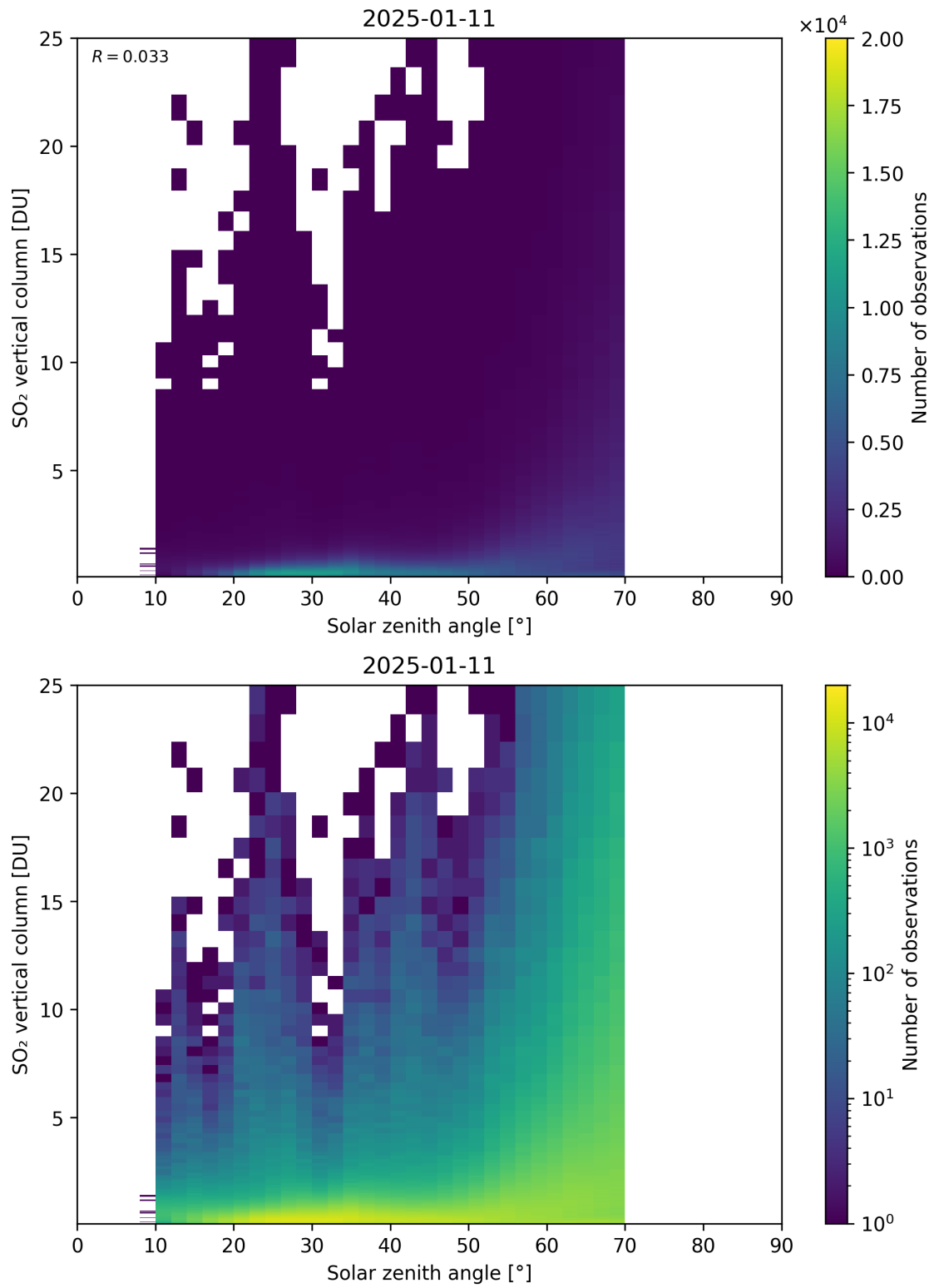
Figure 191: Scatter density plot of “Solar zenith angle” against “SO 2 vertical column” for 2025-01-10 to 2025-01-12.
