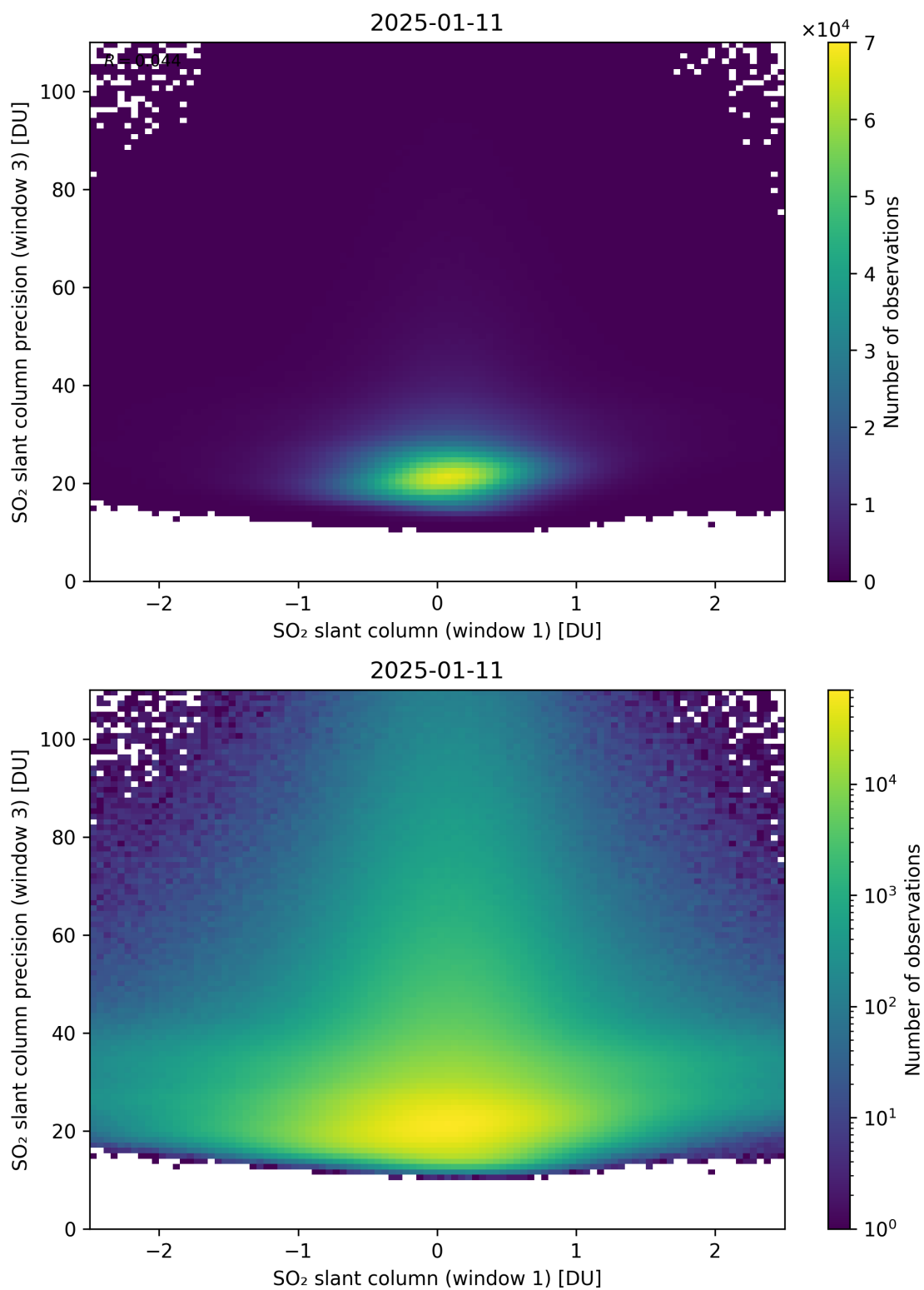
Figure 288: Scatter density plot of “SO 2 slant column (window 1)” against “SO 2 slant column precision (window 3)” for 2025-01-10 to 2025-01-12.
