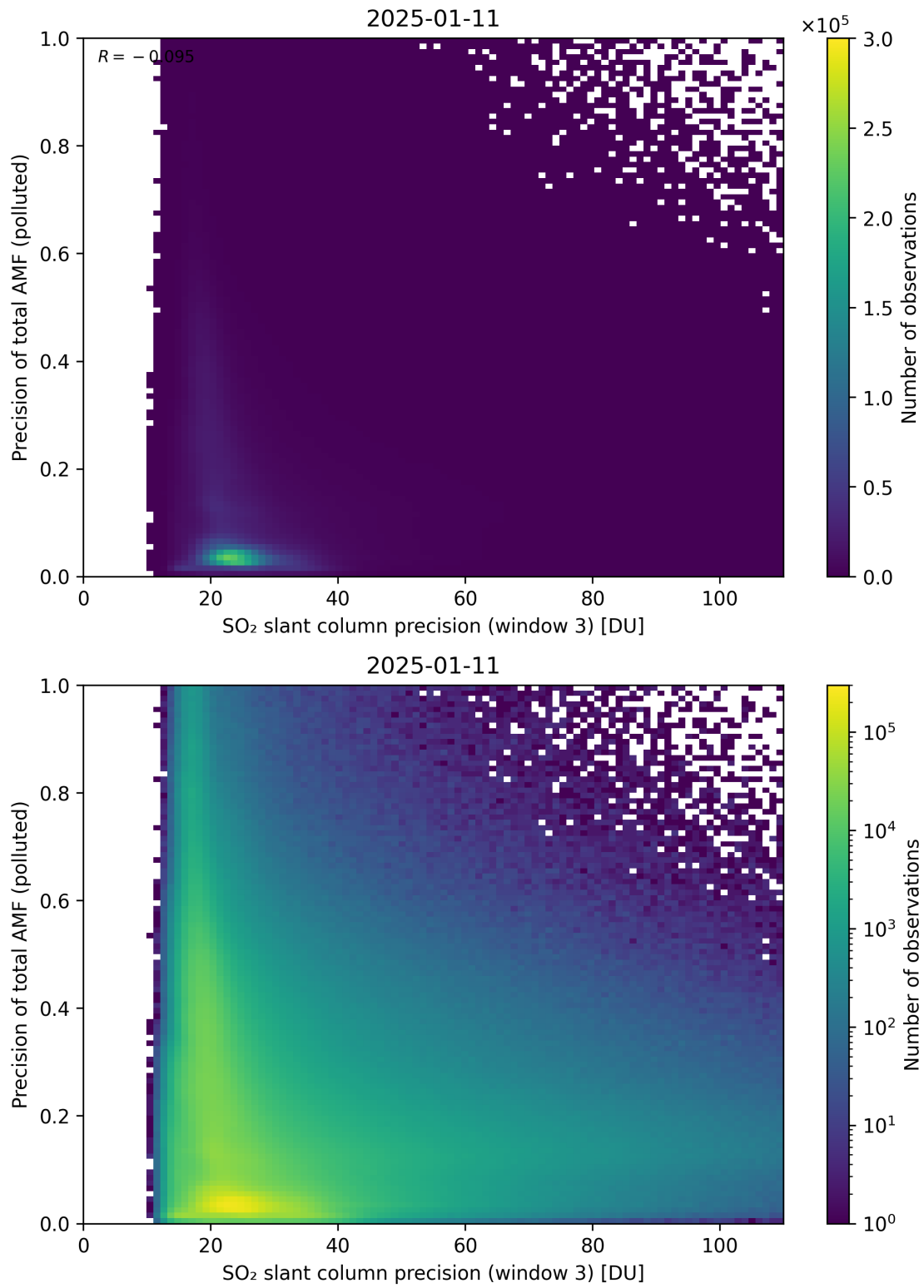
Figure 314: Scatter density plot of “SO 2 slant column precision (window 3)” against “Precision of total AMF (polluted)” for 2025-01-10 to 2025-01-12.
