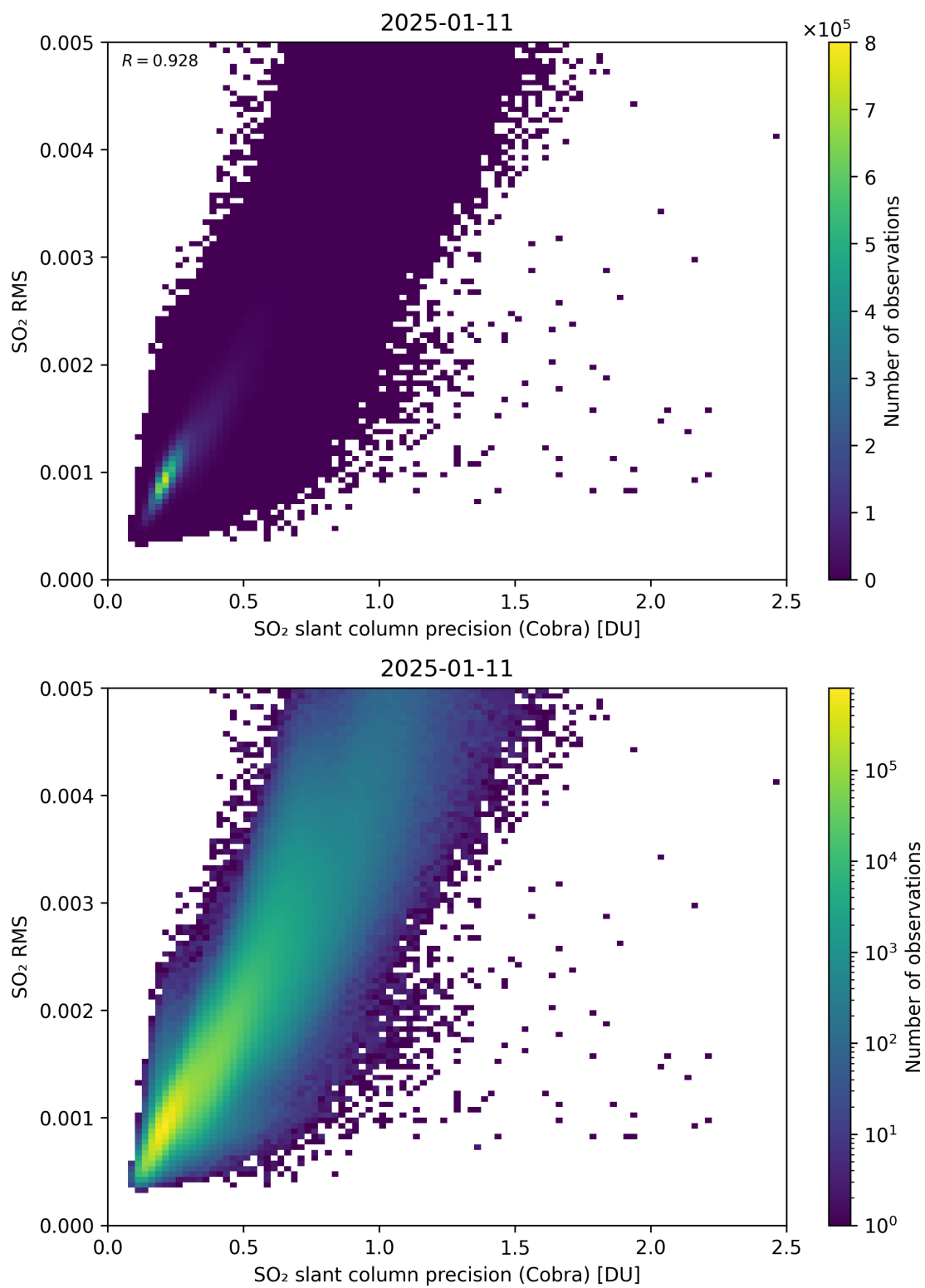
Figure 204: Scatter density plot of “SO 2 slant column precision (Cobra)” against “SO 2 RMS” for 2025-01-10 to 2025-01-12.
