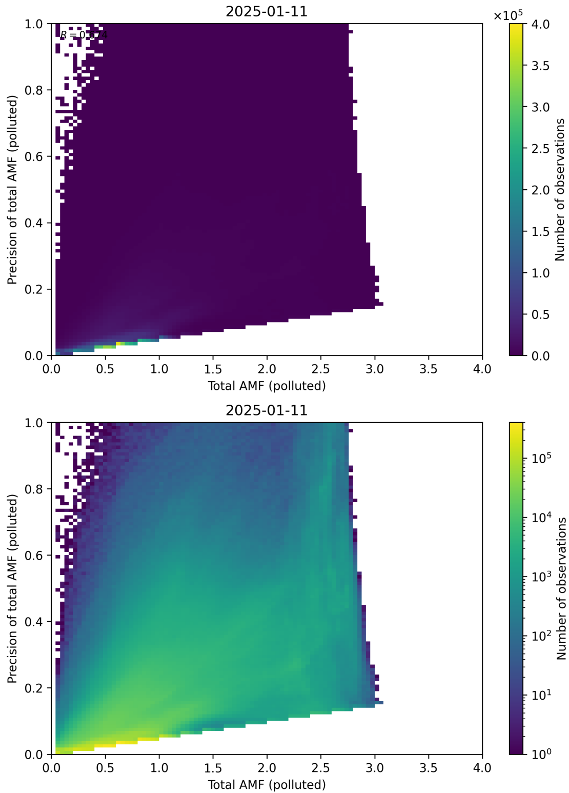
Figure 322: Scatter density plot of “Total AMF (polluted)” against “Precision of total AMF (polluted)” for 2025-01-10 to 2025-01-12.
