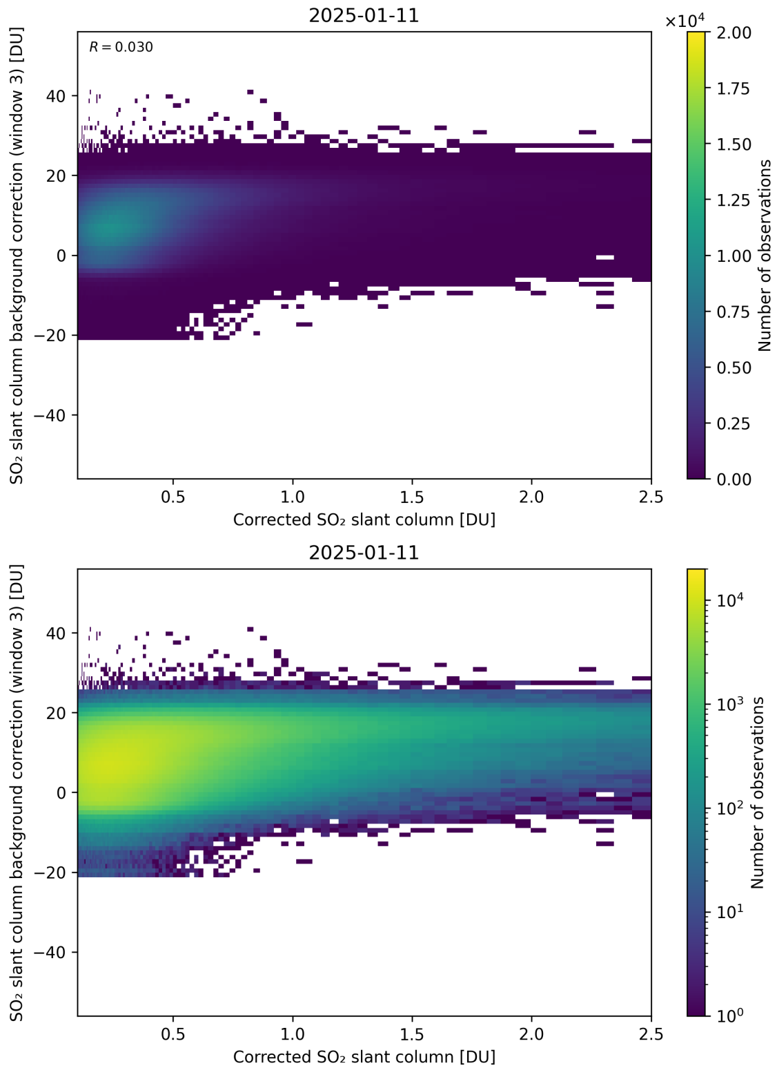
Figure 228: Scatter density plot of “Corrected SO 2 slant column” against “SO 2 slant column background correction (window 3)” for 2025-01-10 to 2025-01-12.
