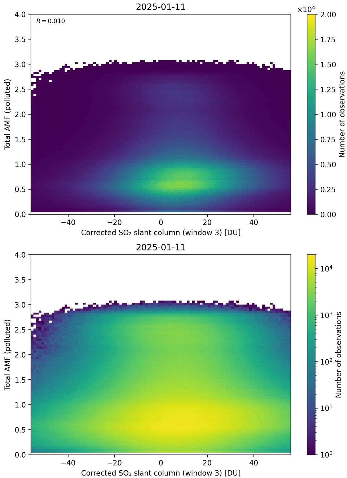
Figure 260: Scatter density plot of “Corrected SO 2 slant column (window 3)” against “Total AMF (polluted)” for 2025-01-10 to 2025-01-12.
