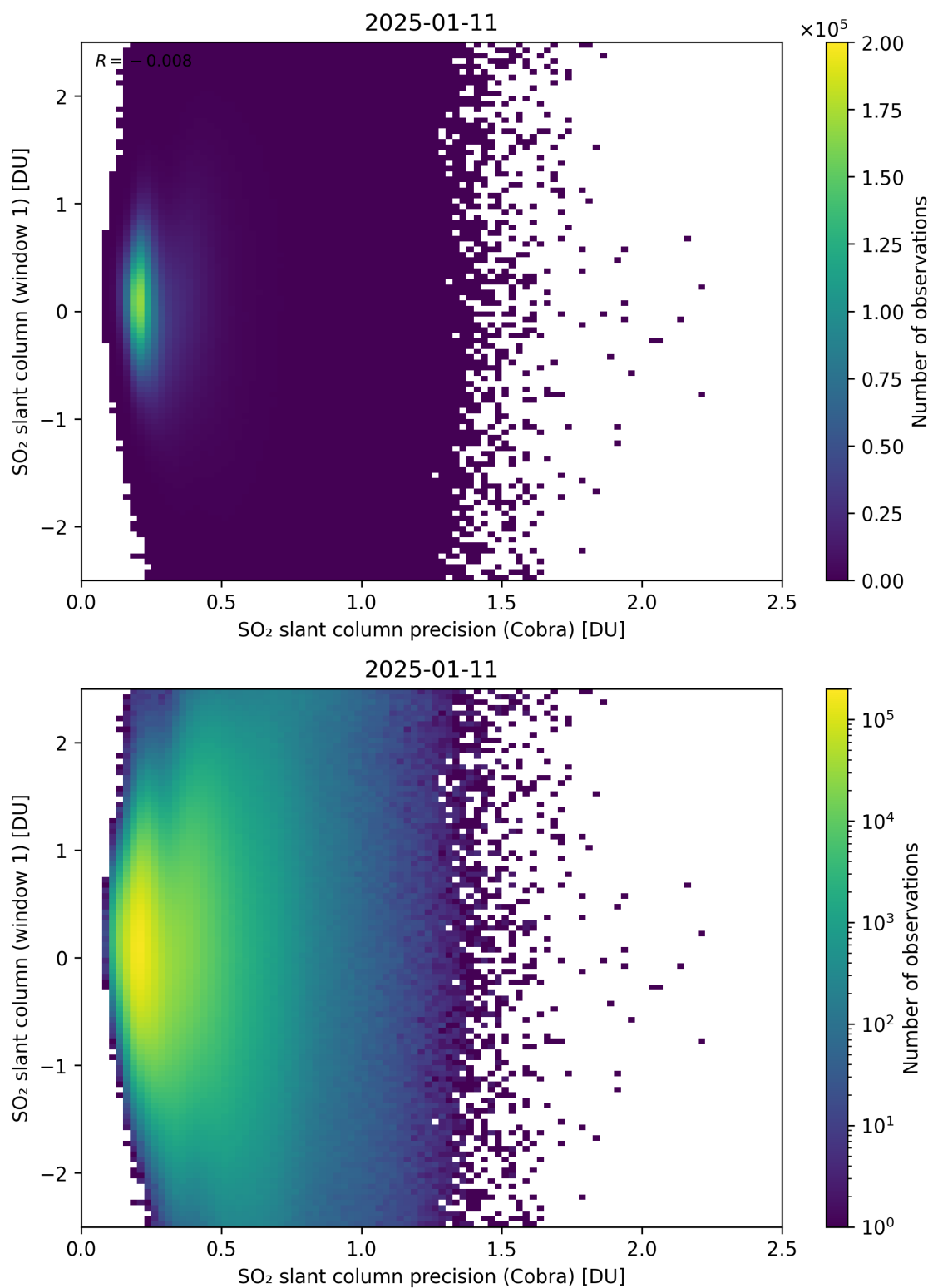
Figure 208: Scatter density plot of “SO 2 slant column precision (Cobra)” against “SO 2 slant column (window 1)” for 2025-01-10 to 2025-01-12.
