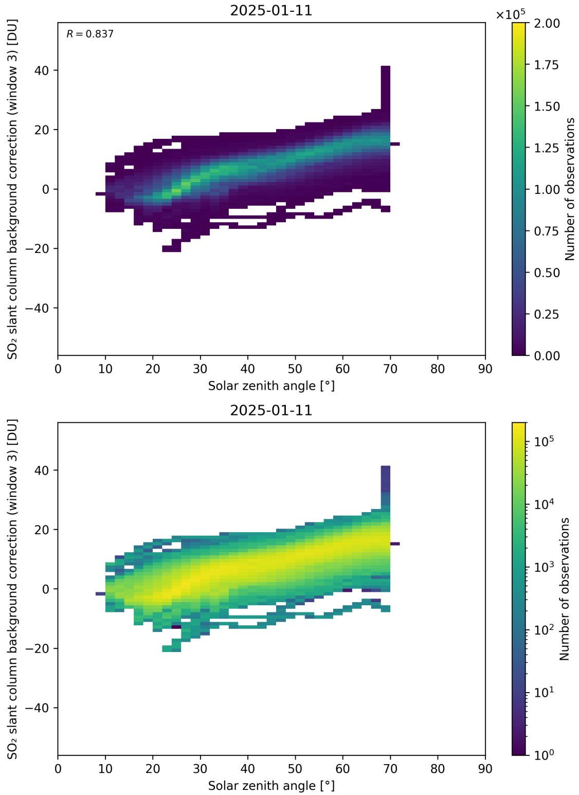
Figure 173: Scatter density plot of “Solar zenith angle” against “SO 2 slant column background correction (window 3)” for 2025-01-10 to 2025-01-12.
