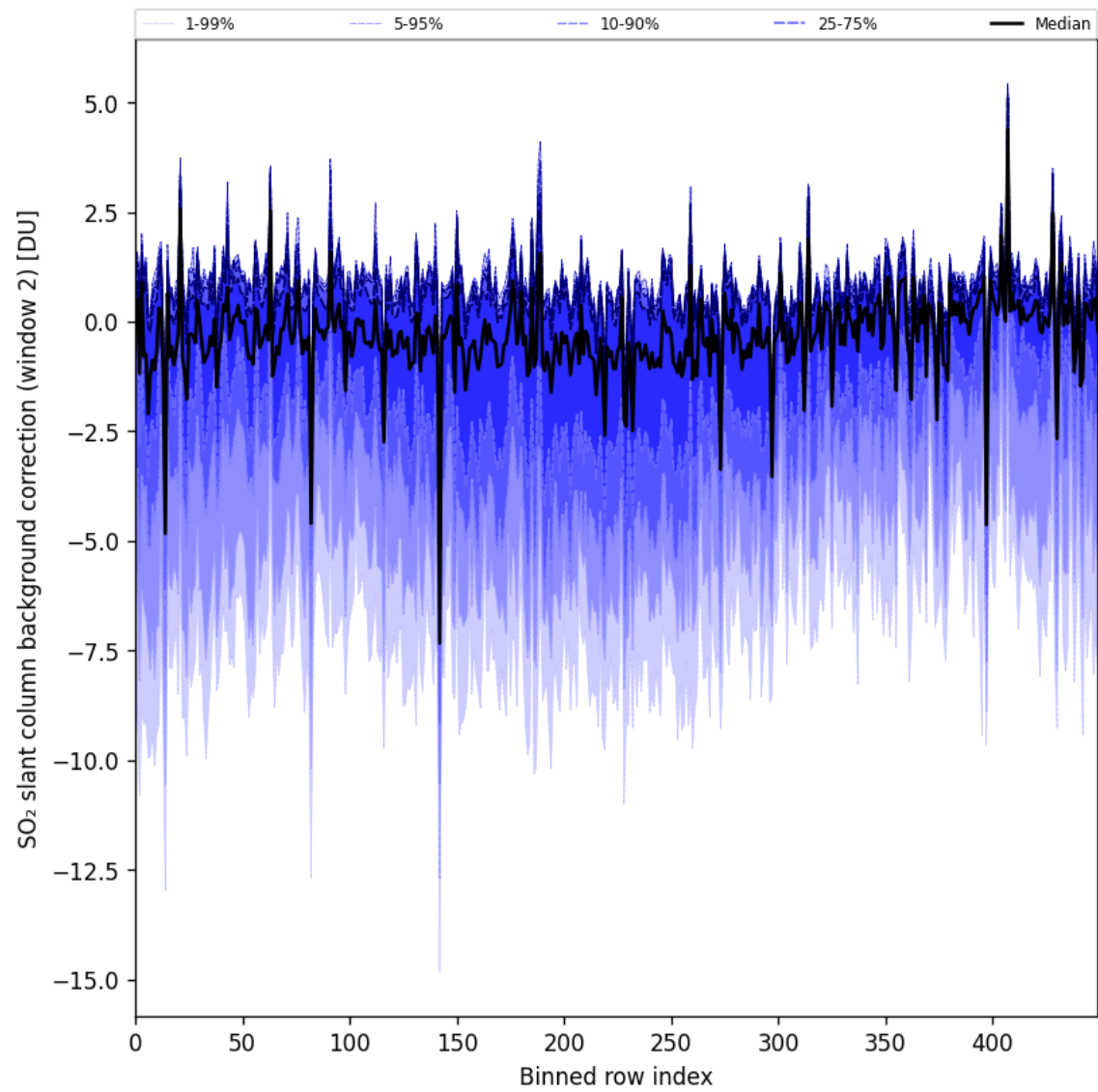
Figure 96: Along track statistics of “SO 2 slant column background correction (window 2)” for 2025-01-10 to 2025-01-12
