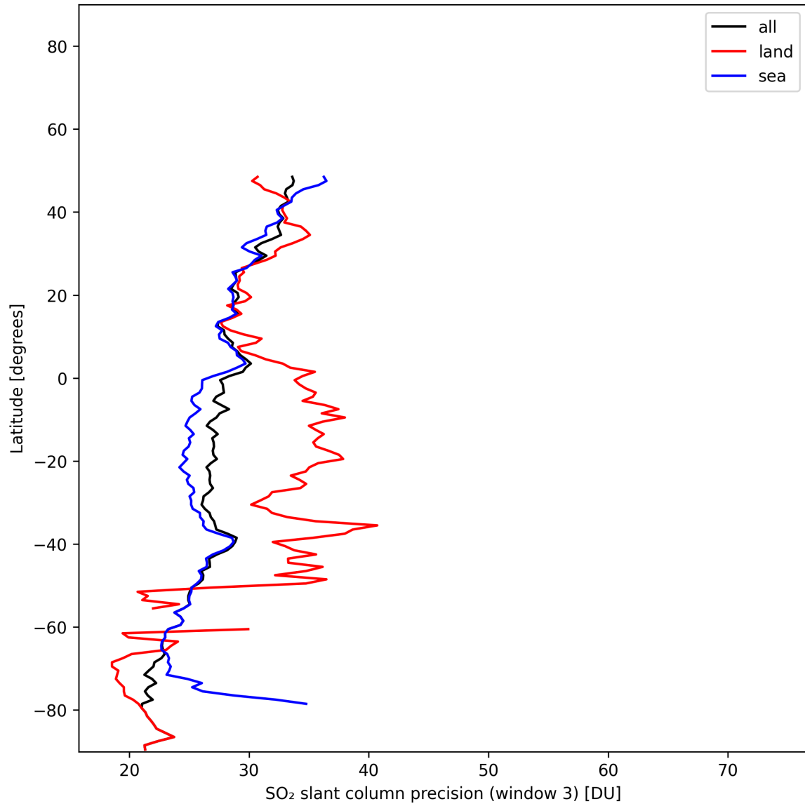
Figure 46: Zonal average of “SO 2 slant column precision (window 3)” for 2025-01-10 to 2025-01-12.
