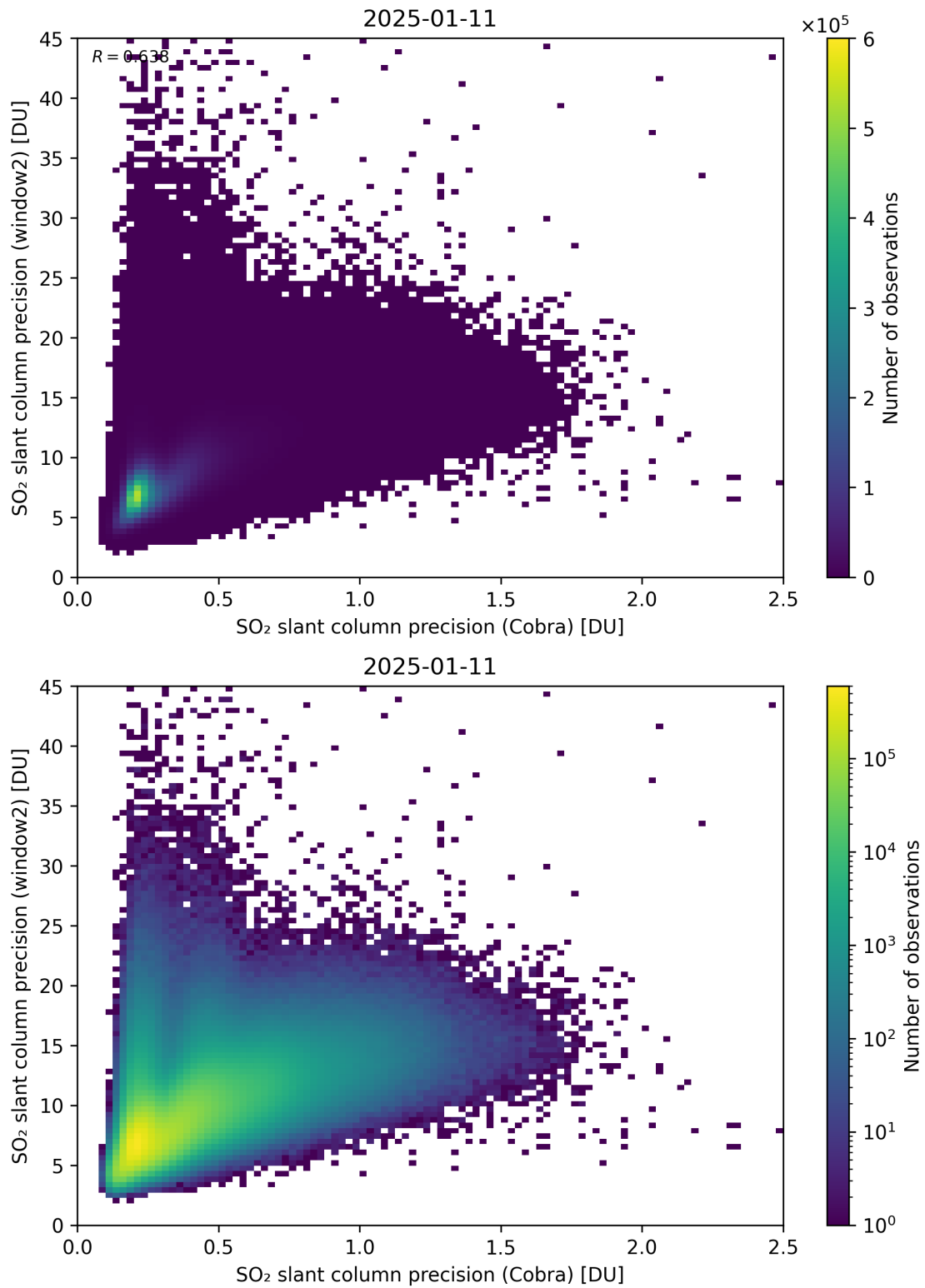
Figure 210: Scatter density plot of “SO 2 slant column precision (Cobra)” against “SO 2 slant column precision (window2)” for 2025-01-10 to 2025-01-12.
