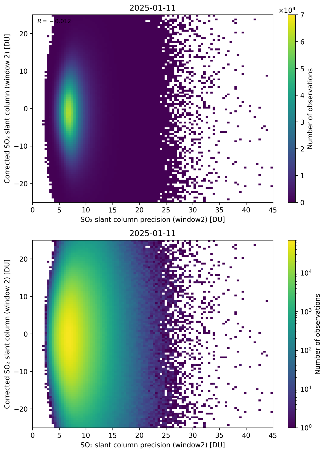
Figure 297: Scatter density plot of “SO 2 slant column precision (window2)” against “Corrected SO 2 slant column (window 2)” for 2025-01-10 to 2025-01-12.
