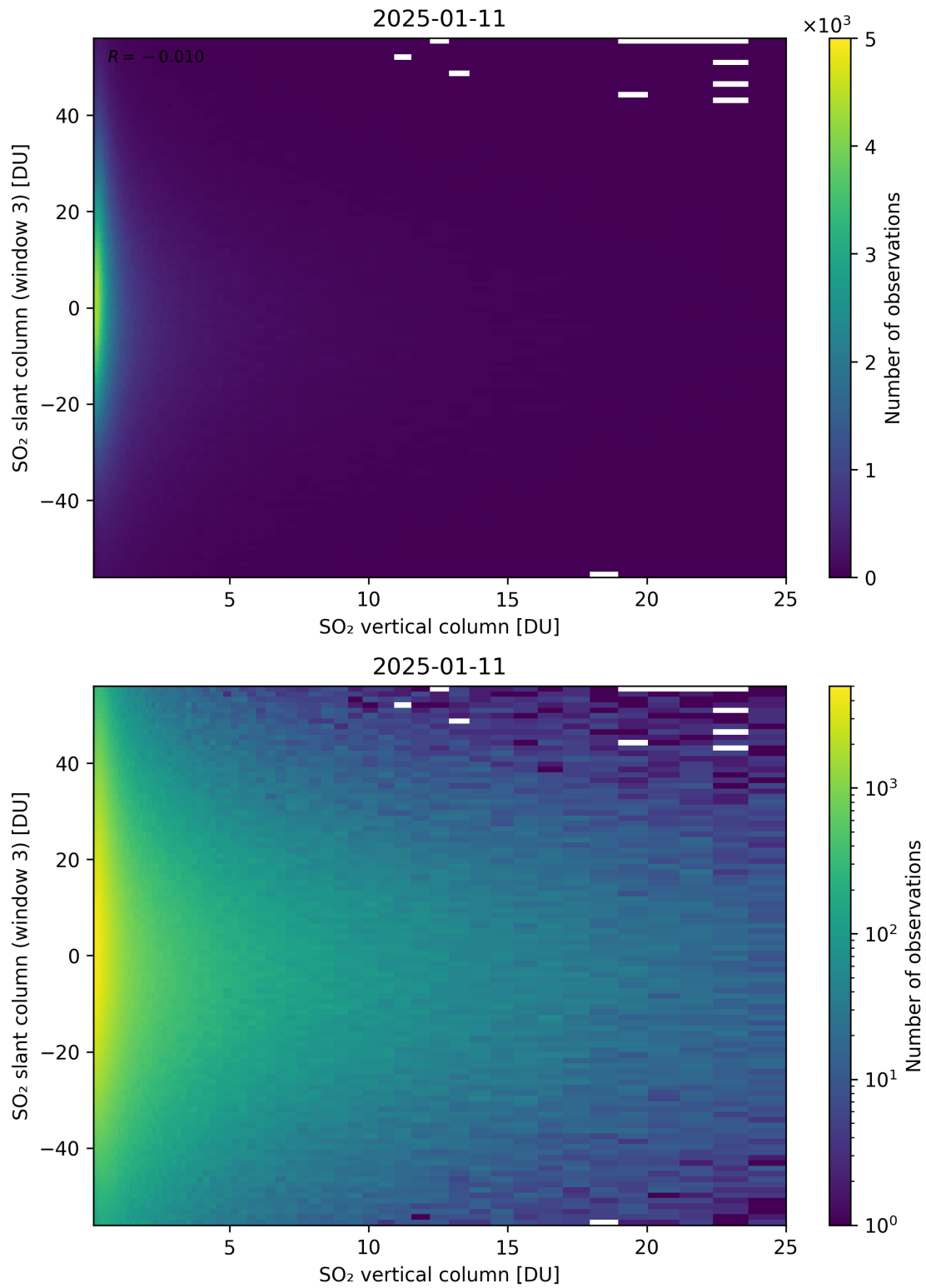
Figure 357: Scatter density plot of “SO 2 vertical column” against “SO 2 slant column (window 3)” for 2025-01-10 to 2025-01-12.
