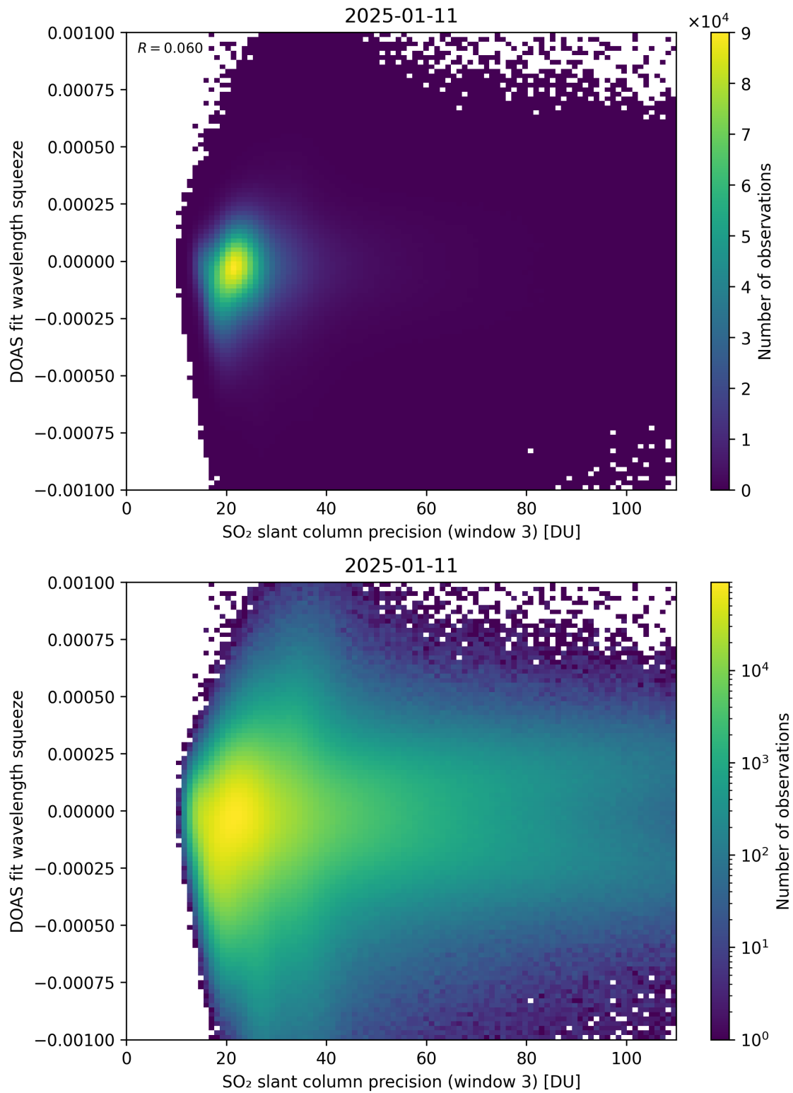
Figure 309: Scatter density plot of “SO 2 slant column precision (window 3)” against “DOAS fit wavelength squeeze” for 2025-01-10 to 2025-01-12.
