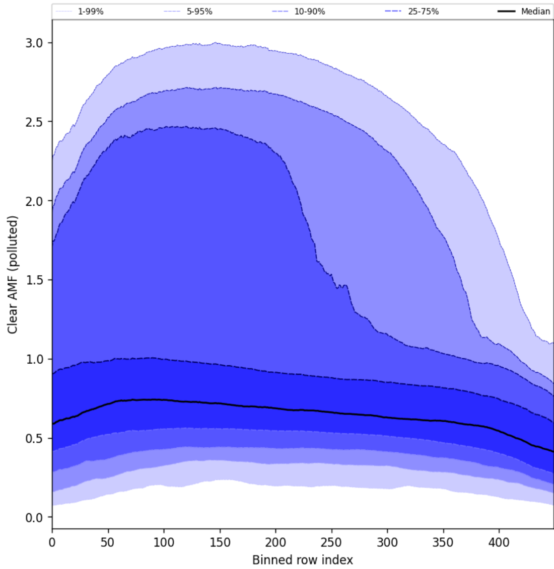
Figure 107: Along track statistics of “Clear AMF (polluted)” for 2025-01-10 to 2025-01-12
