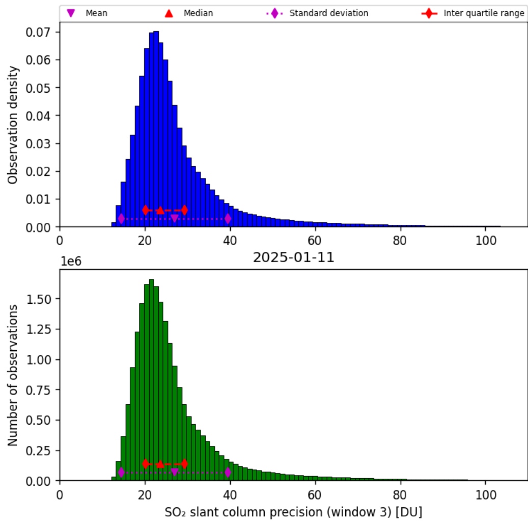
Figure 72: Histogram of “SO 2 slant column precision (window 3)” for 2025-01-10 to 2025-01-12
