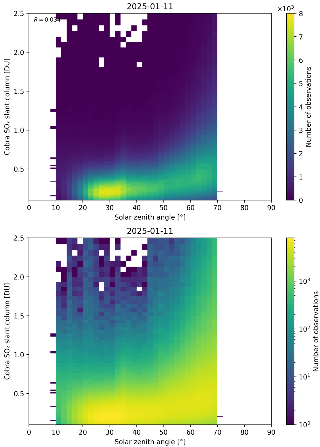
Figure 179: Scatter density plot of “Solar zenith angle” against “Cobra SO 2 slant column” for 2025-01-10 to 2025-01-12.
