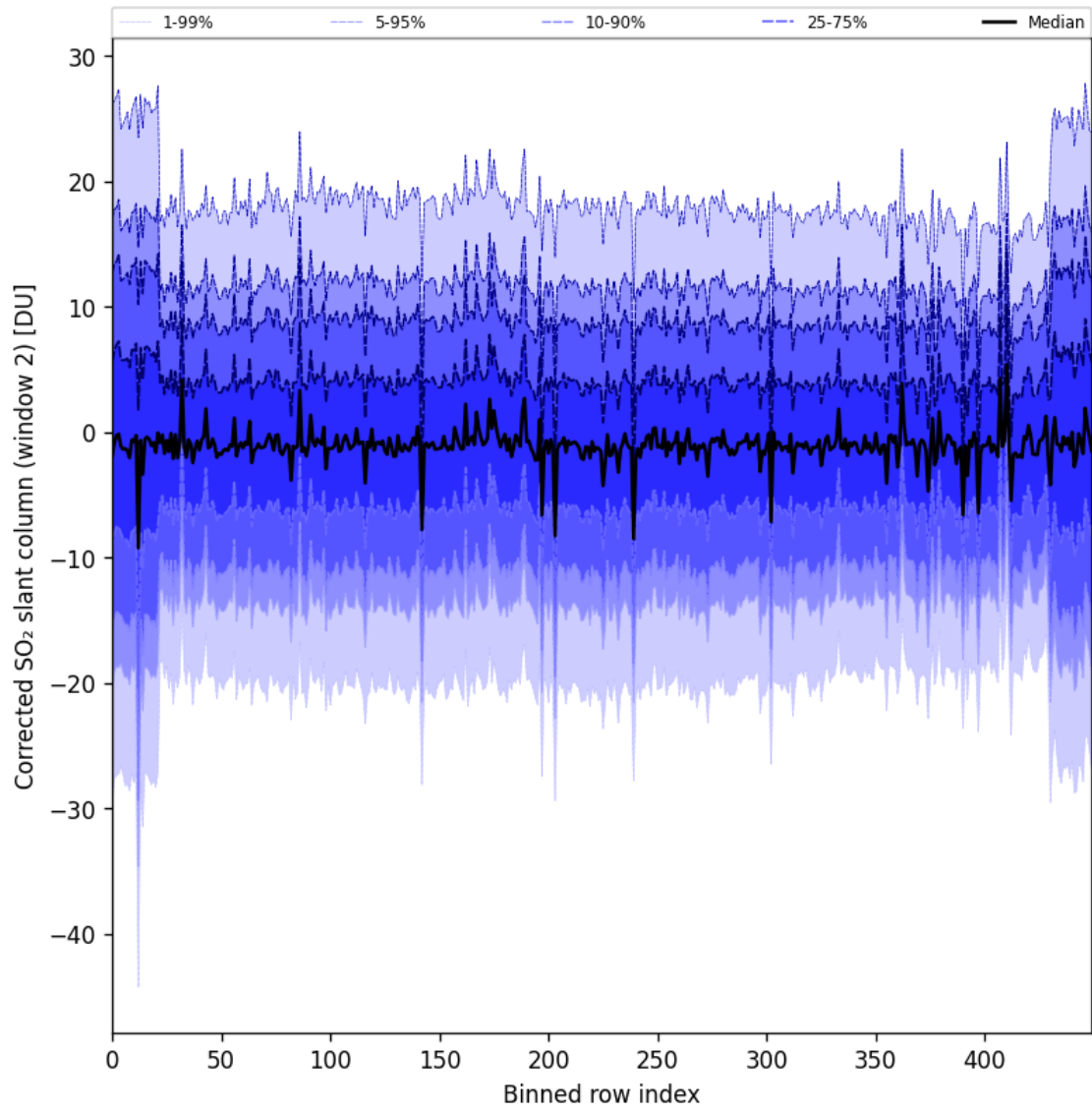
Figure 95: Along track statistics of “Corrected SO 2 slant column (window 2)” for 2025-01-10 to 2025-01-12
