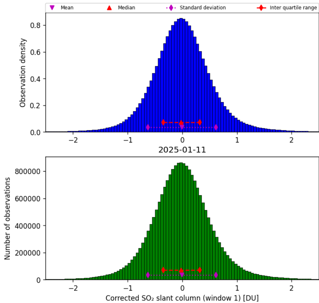
Figure 65: Histogram of “Corrected SO 2 slant column (window 1)” for 2025-01-10 to 2025-01-12
