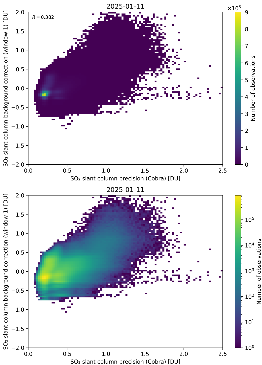
Figure 199: Scatter density plot of “SO 2 slant column precision (Cobra)” against “SO 2 slant column background correction (window 1)” for 2025-01-10 to 2025-01-12.
