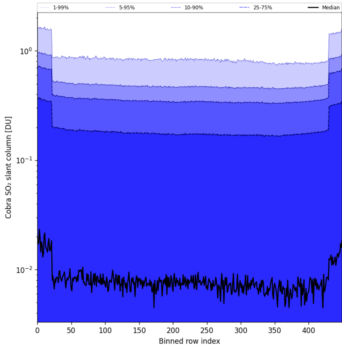
Figure 87: Along track statistics of “Cobra SO 2 slant column” for 2025-01-10 to 2025-01-12
