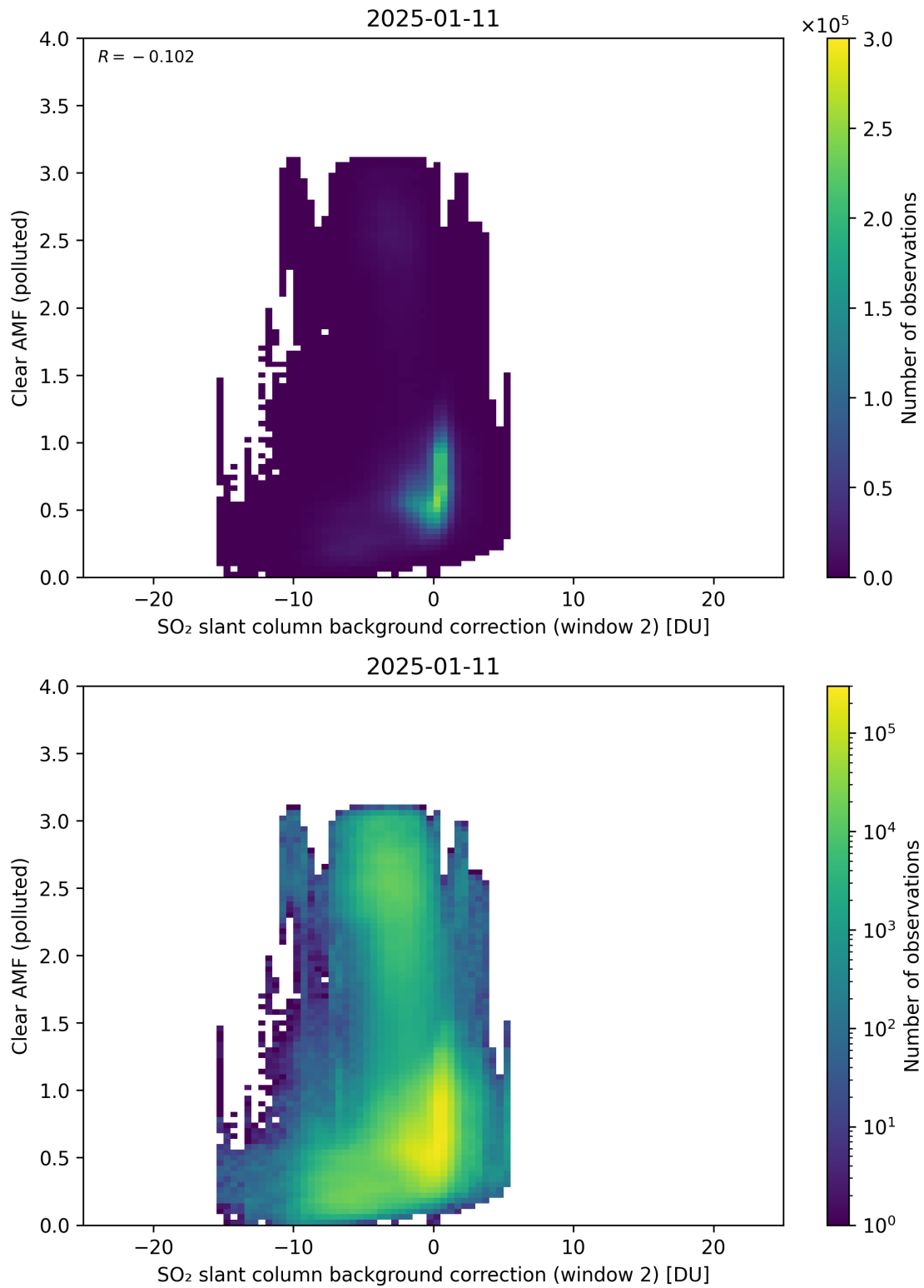
Figure 126: Scatter density plot of “SO 2 slant column background correction (window 2)” against “Clear AMF (polluted)” for 2025-01-10 to 2025-01-12.
