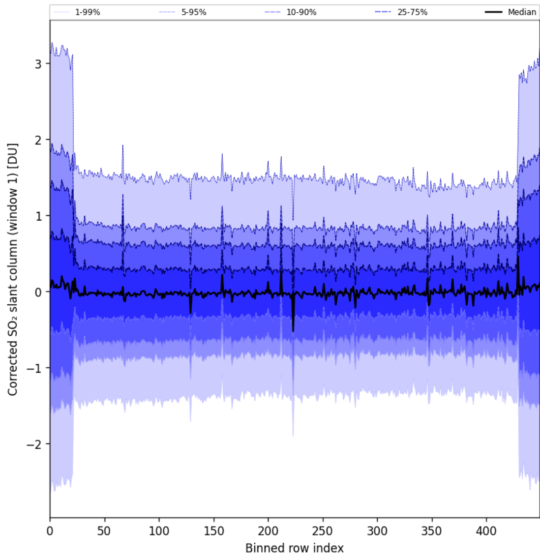
Figure 91: Along track statistics of “Corrected SO 2 slant column (window 1)” for 2025-01-10 to 2025-01-12
