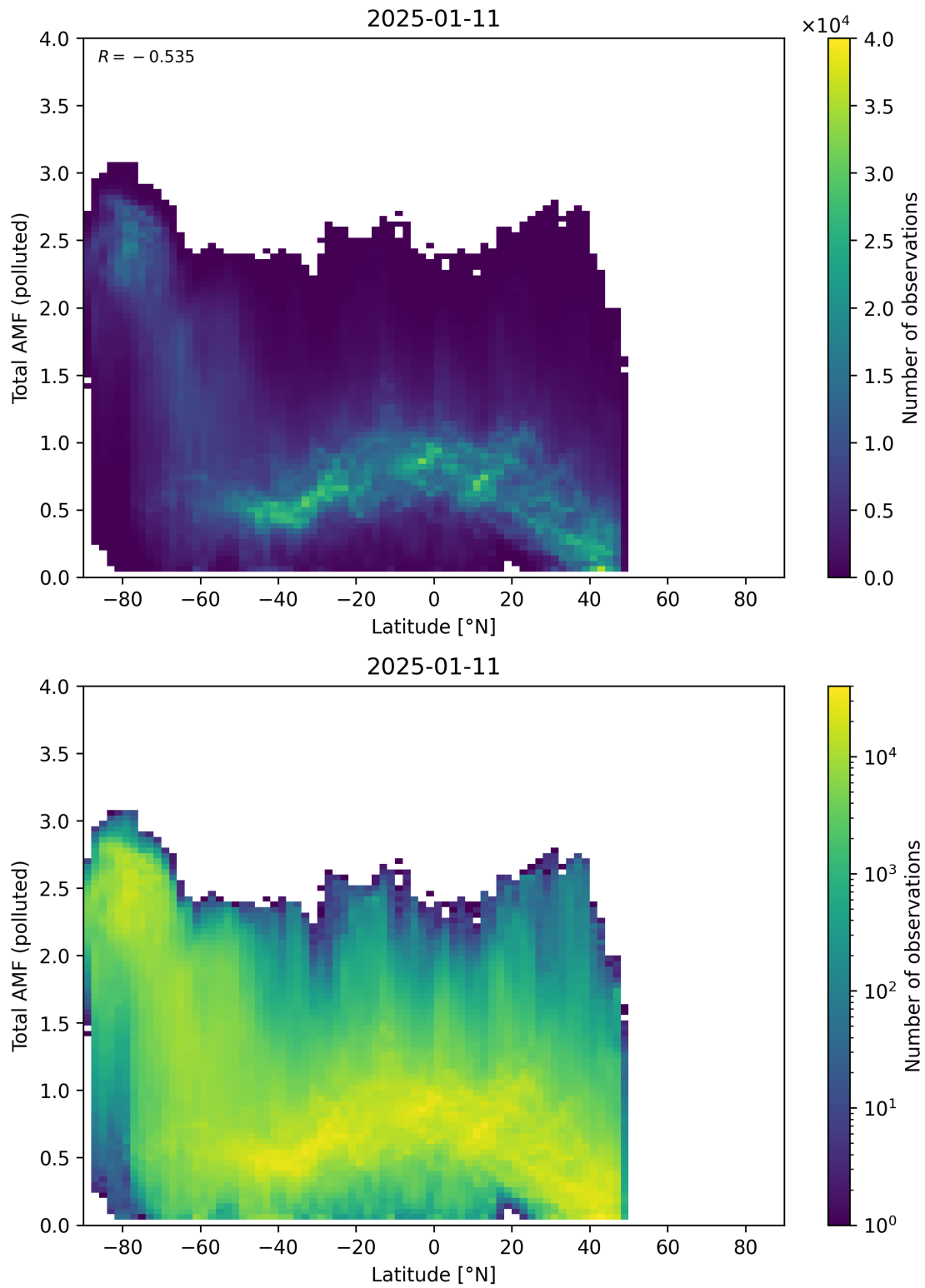
Figure 167: Scatter density plot of “Latitude” against “Total AMF (polluted)” for 2025-01-10 to 2025-01-12.
