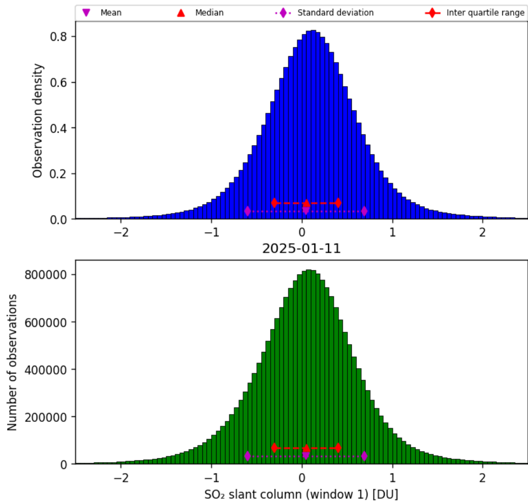
Figure 63: Histogram of “SO 2 slant column (window 1)” for 2025-01-10 to 2025-01-12
