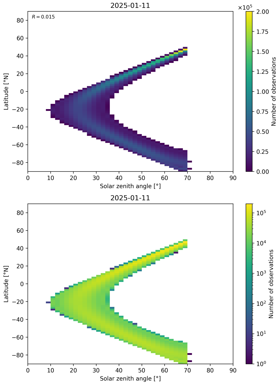
Figure 177: Scatter density plot of “Solar zenith angle” against “Latitude” for 2025-01-10 to 2025-01-12.
