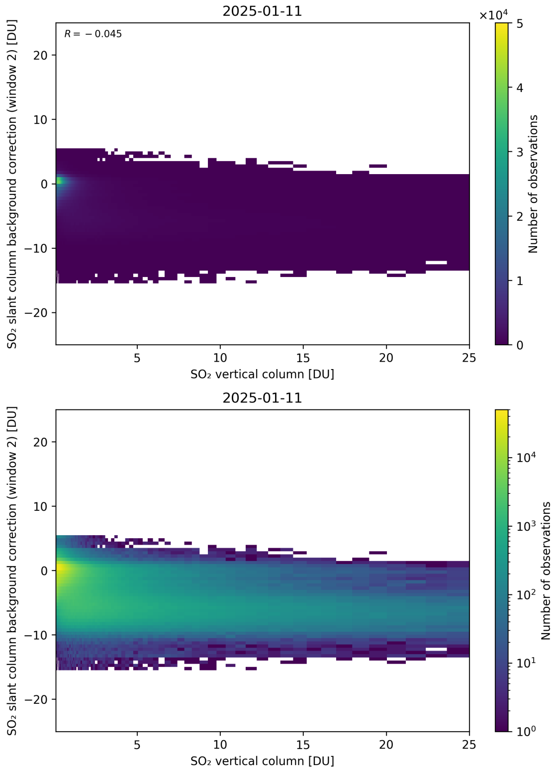
Figure 324: Scatter density plot of “SO 2 vertical column” against “SO 2 slant column background correction (window 2)” for 2025-01-10 to 2025-01-12.
