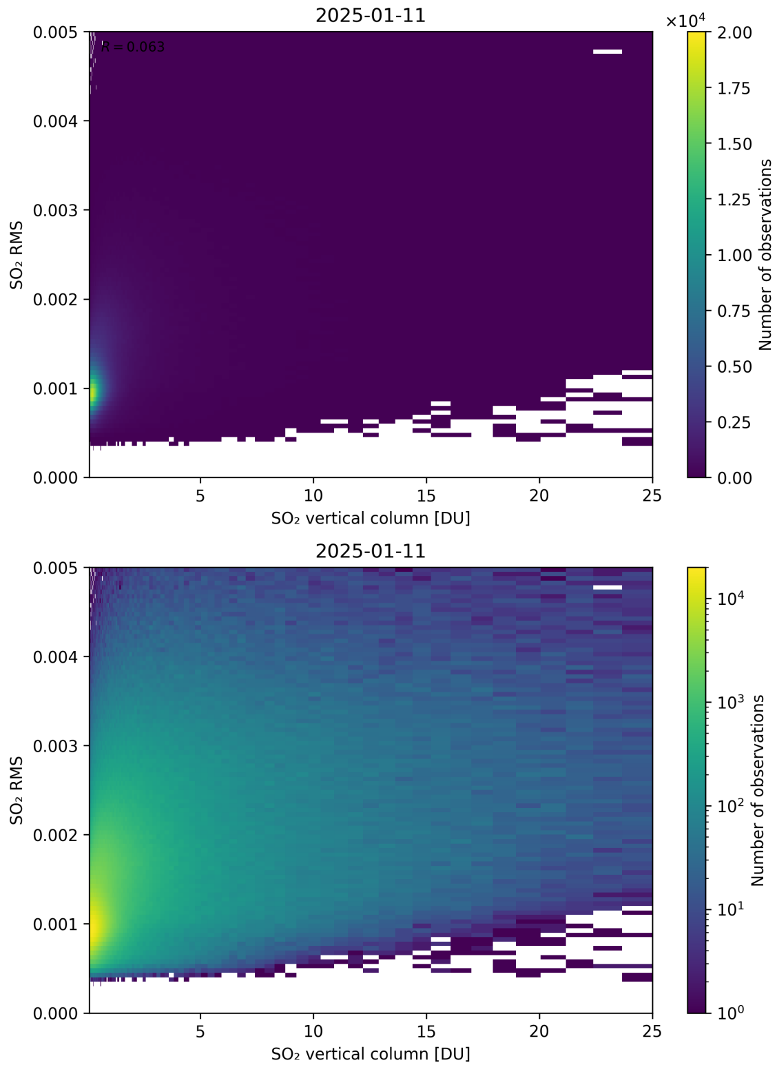
Figure 328: Scatter density plot of “SO 2 vertical column” against “SO 2 RMS” for 2025-01-10 to 2025-01-12.
