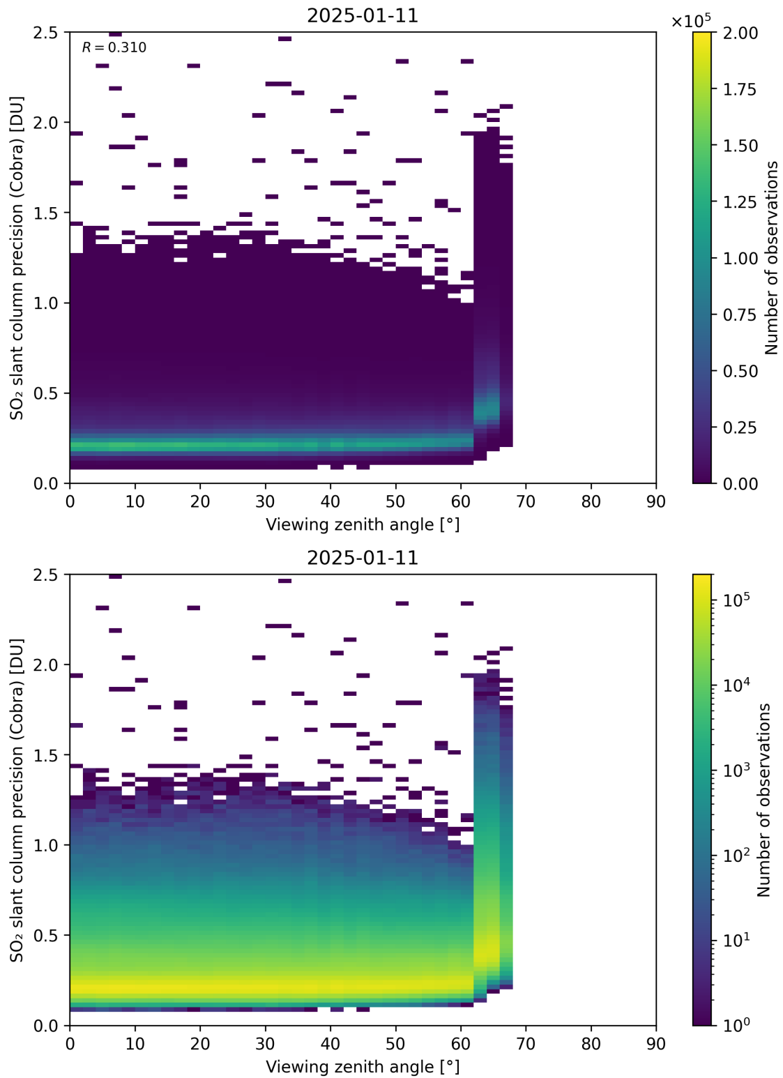
Figure 372: Scatter density plot of “Viewing zenith angle” against “SO 2 slant column precision (Cobra)” for 2025-01-10 to 2025-01-12.
