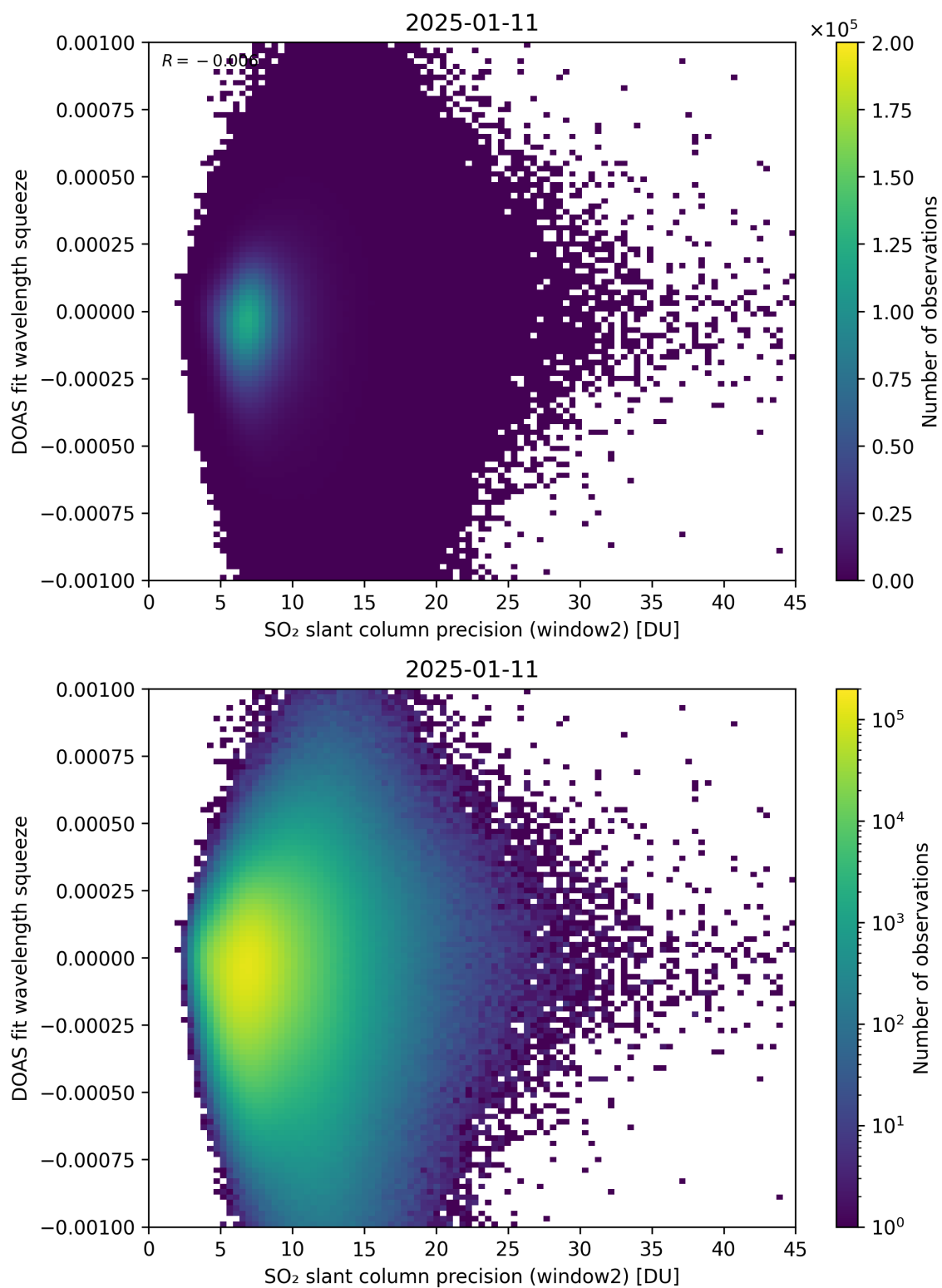
Figure 294: Scatter density plot of “SO 2 slant column precision (window2)” against “DOAS fit wavelength squeeze” for 2025-01-10 to 2025-01-12.
