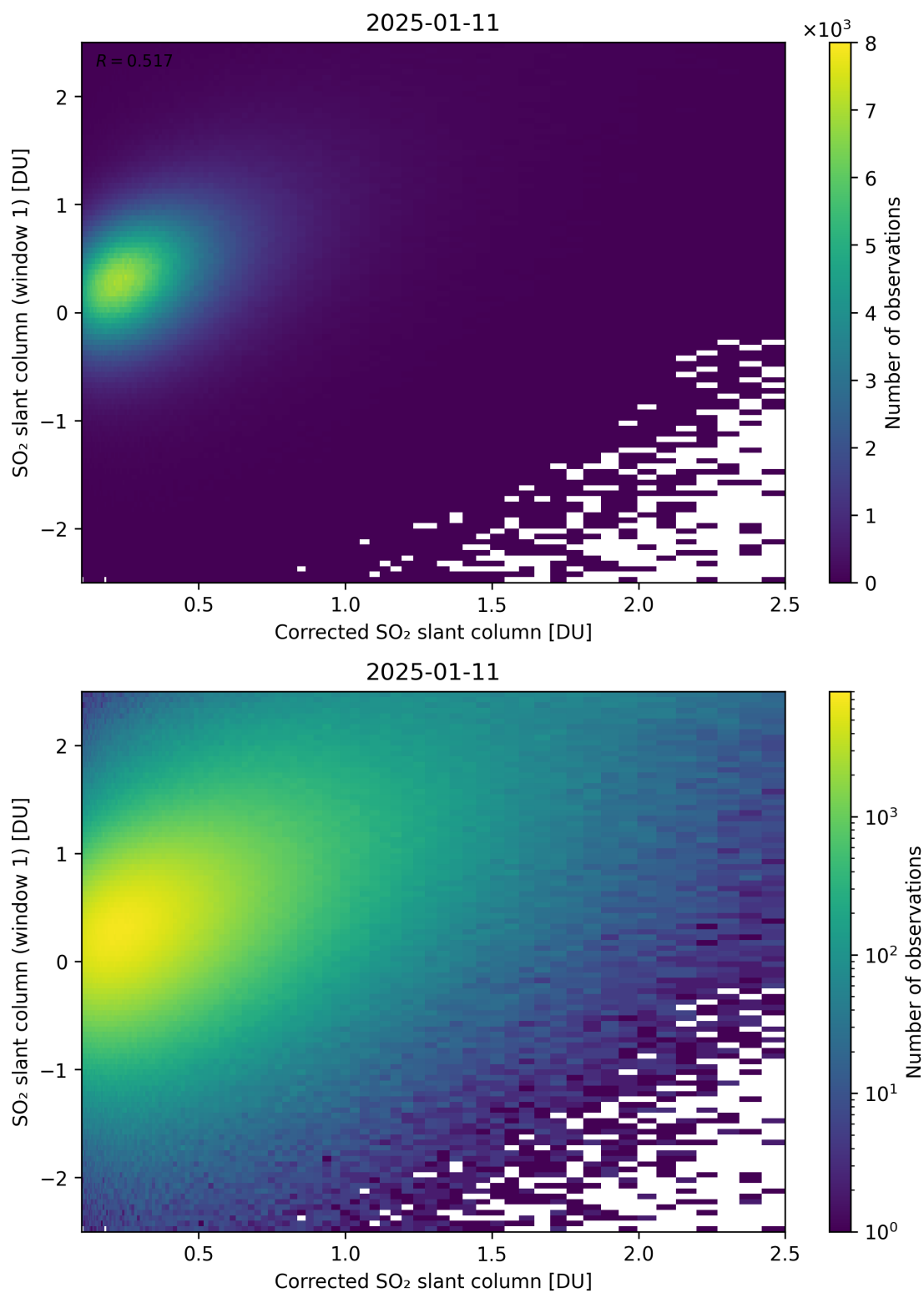
Figure 237: Scatter density plot of “Corrected SO 2 slant column” against “SO 2 slant column (window 1)” for 2025-01-10 to 2025-01-12.
