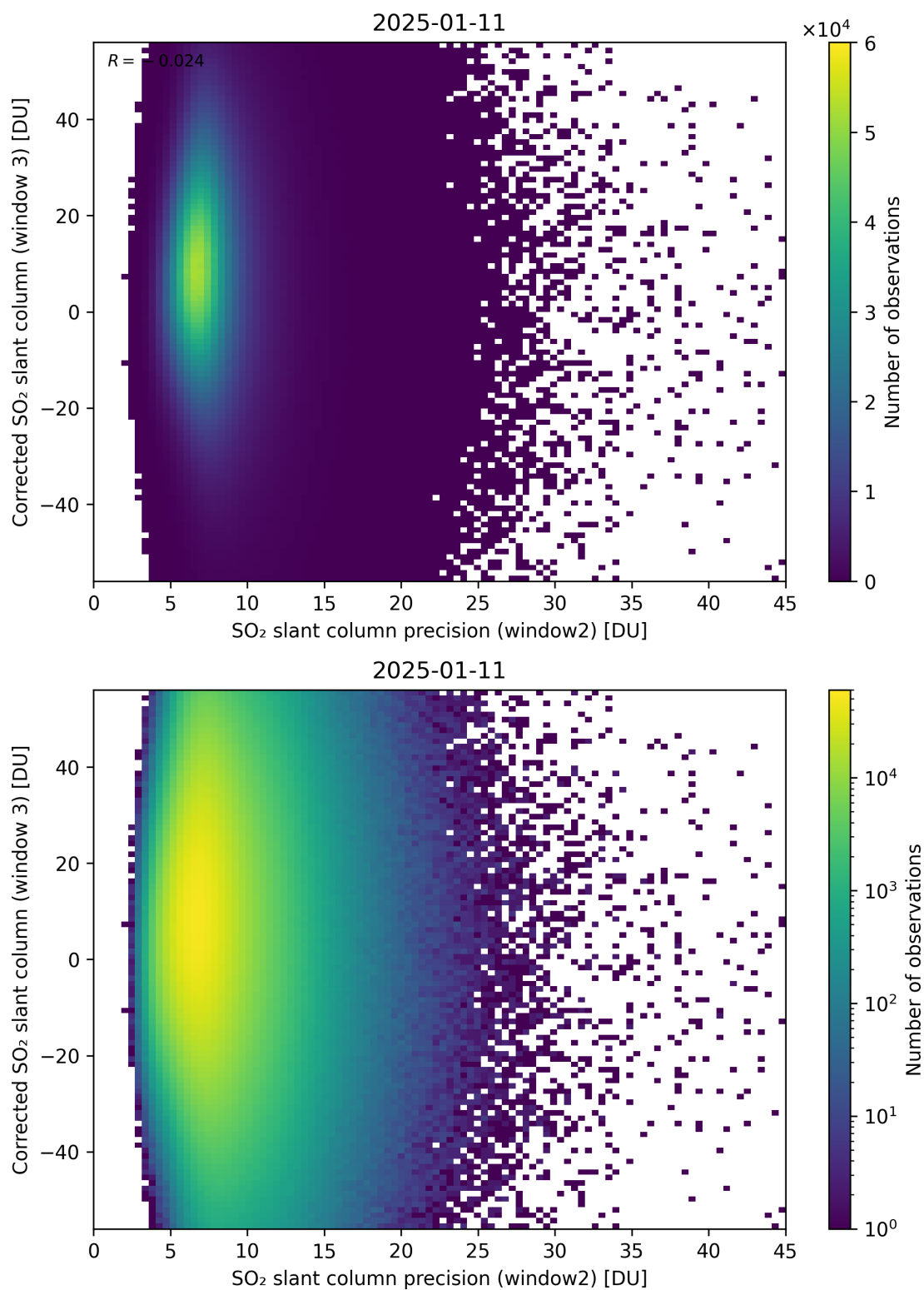
Figure 298: Scatter density plot of “SO 2 slant column precision (window2)” against “Corrected SO 2 slant column (window 3)” for 2025-01-10 to 2025-01-12.
