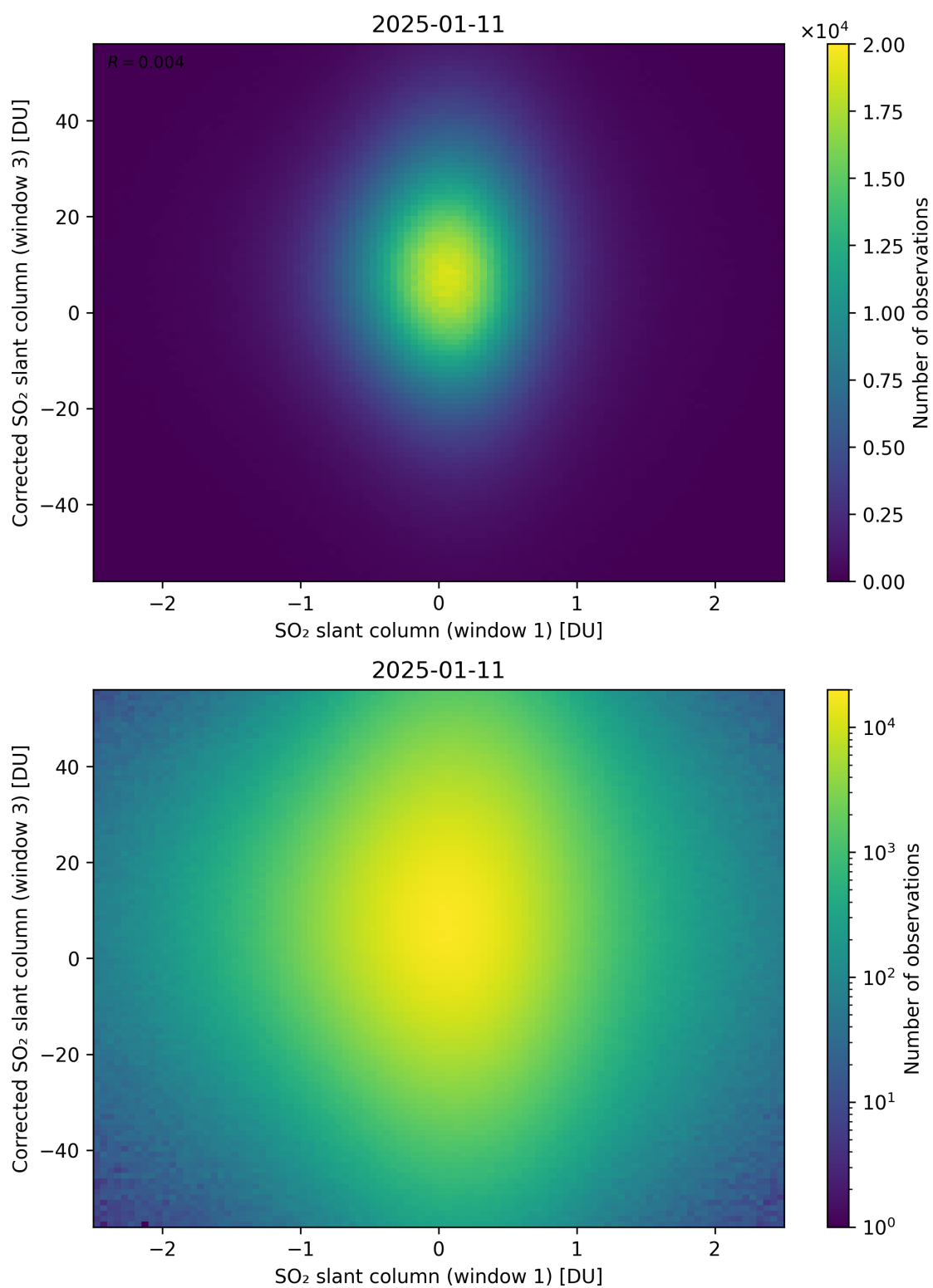
Figure 284: Scatter density plot of “SO 2 slant column (window 1)” against “Corrected SO 2 slant column (window 3)” for 2025-01-10 to 2025-01-12.
