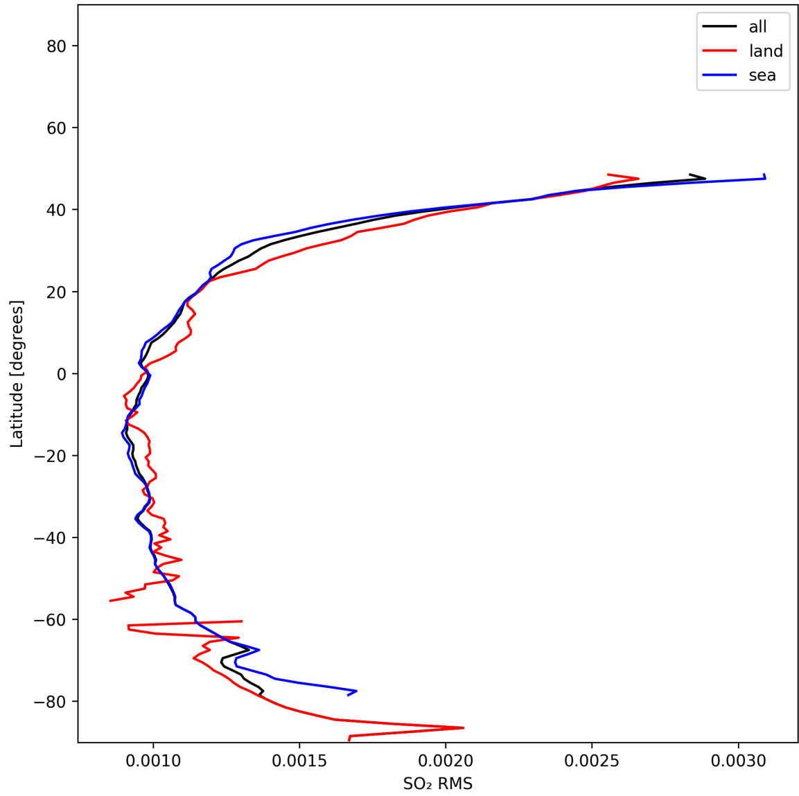
Figure 52: Zonal average of “SO 2 RMS” for 2025-01-10 to 2025-01-12.
