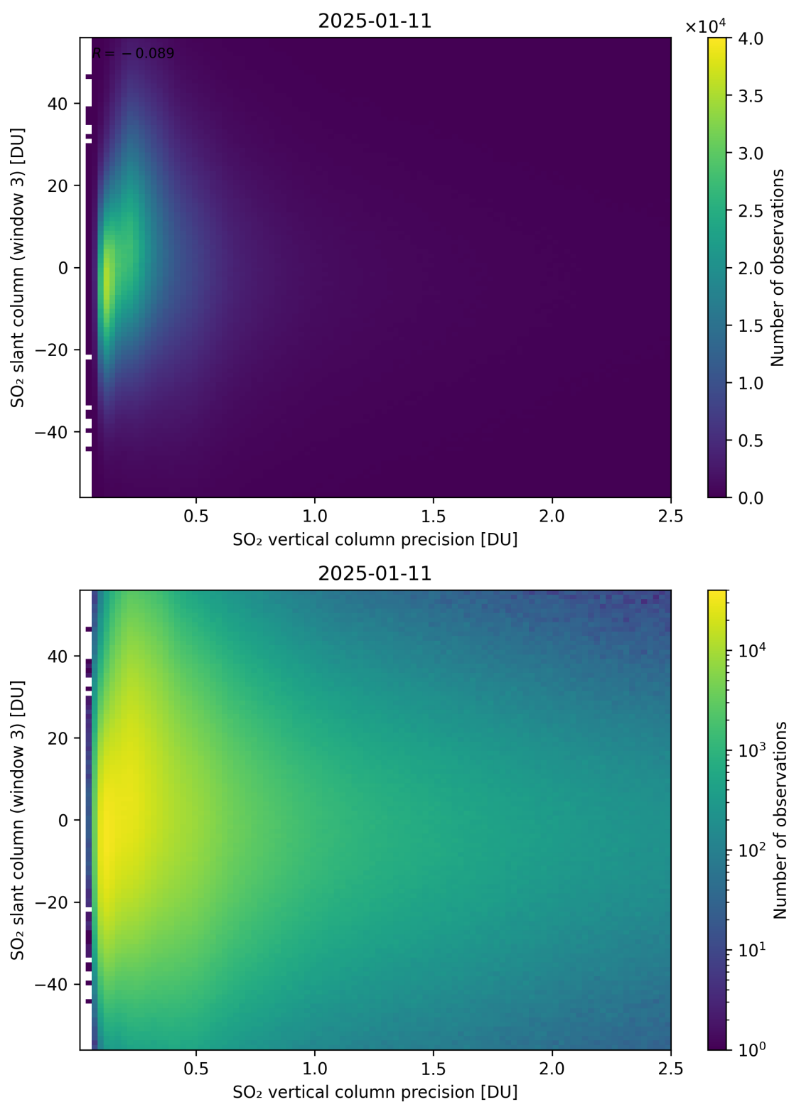
Figure 344: Scatter density plot of “SO 2 vertical column precision” against “SO 2 slant column (window 3)” for 2025-01-10 to 2025-01-12.
