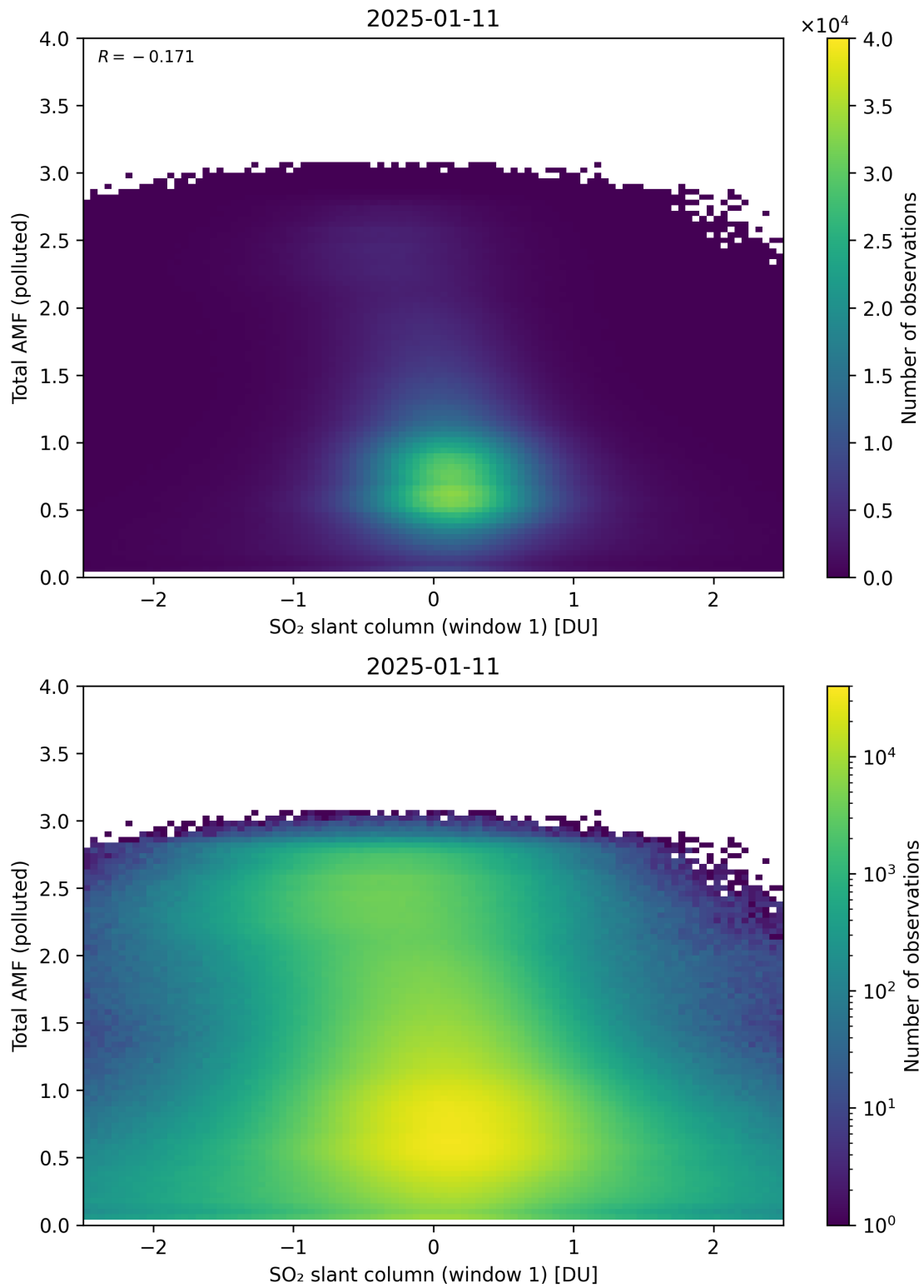
Figure 289: Scatter density plot of “SO 2 slant column (window 1)” against “Total AMF (polluted)” for 2025-01-10 to 2025-01-12.
