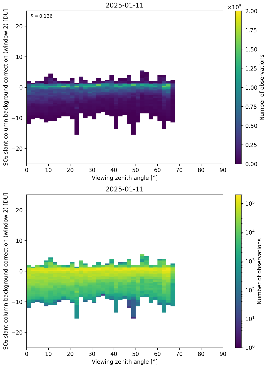
Figure 363: Scatter density plot of “Viewing zenith angle” against “SO 2 slant column background correction (window 2)” for 2025-01-10 to 2025-01-12.
