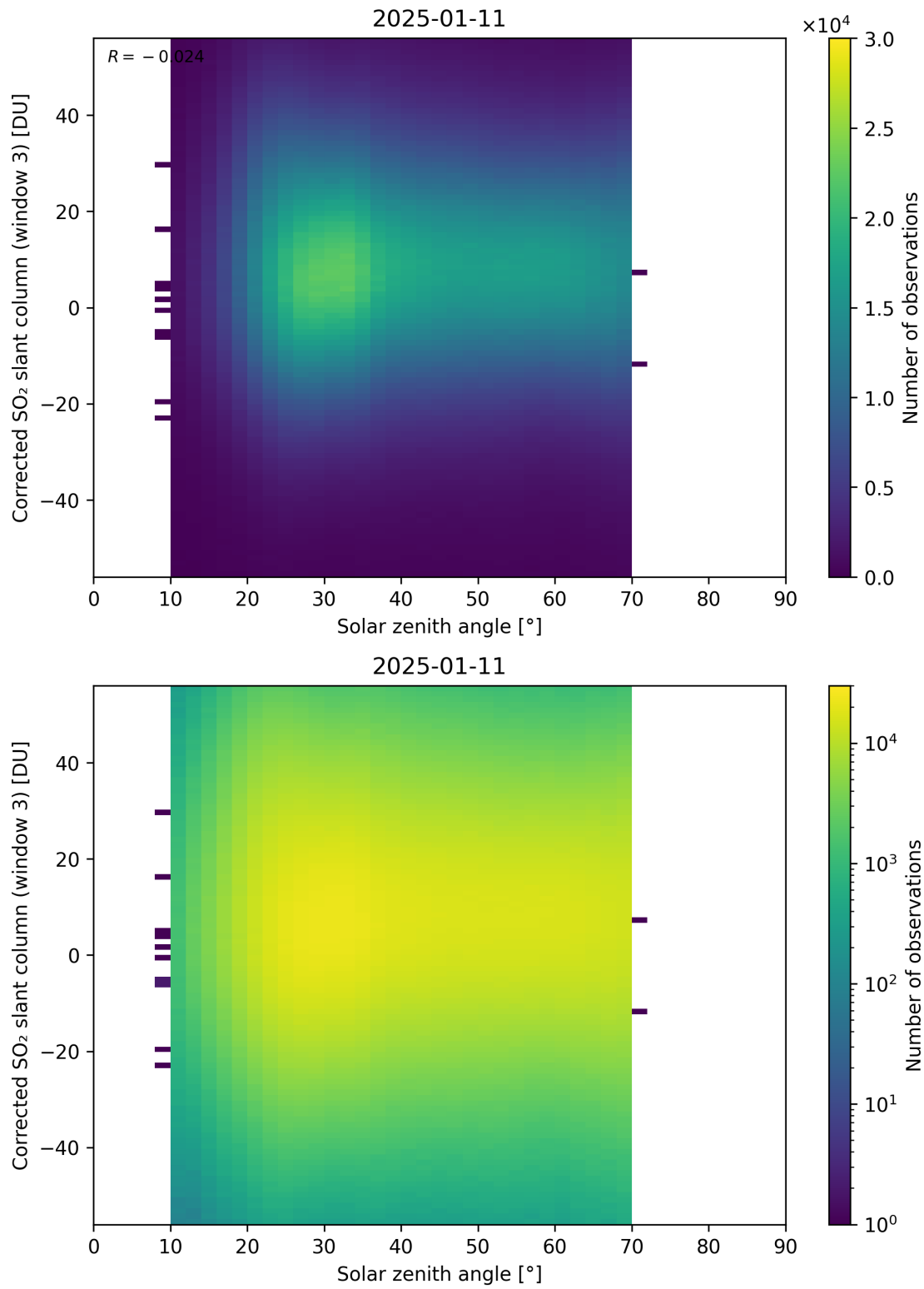
Figure 183: Scatter density plot of “Solar zenith angle” against “Corrected SO 2 slant column (window 3)” for 2025-01-10 to 2025-01-12.
