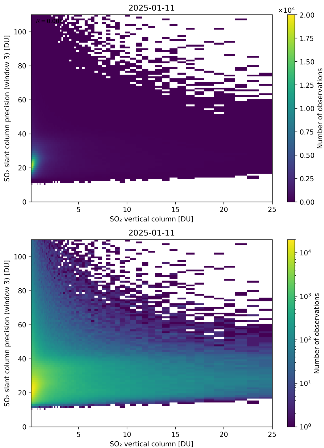
Figure 358: Scatter density plot of “SO 2 vertical column” against “SO 2 slant column precision (window 3)” for 2025-01-10 to 2025-01-12.
