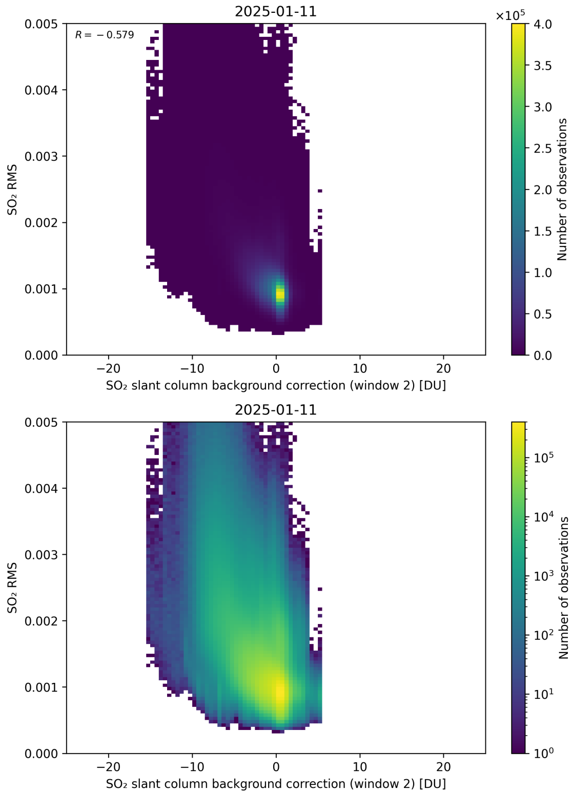
Figure 125: Scatter density plot of “SO 2 slant column background correction (window 2)” against “SO 2 RMS” for 2025-01-10 to 2025-01-12.
