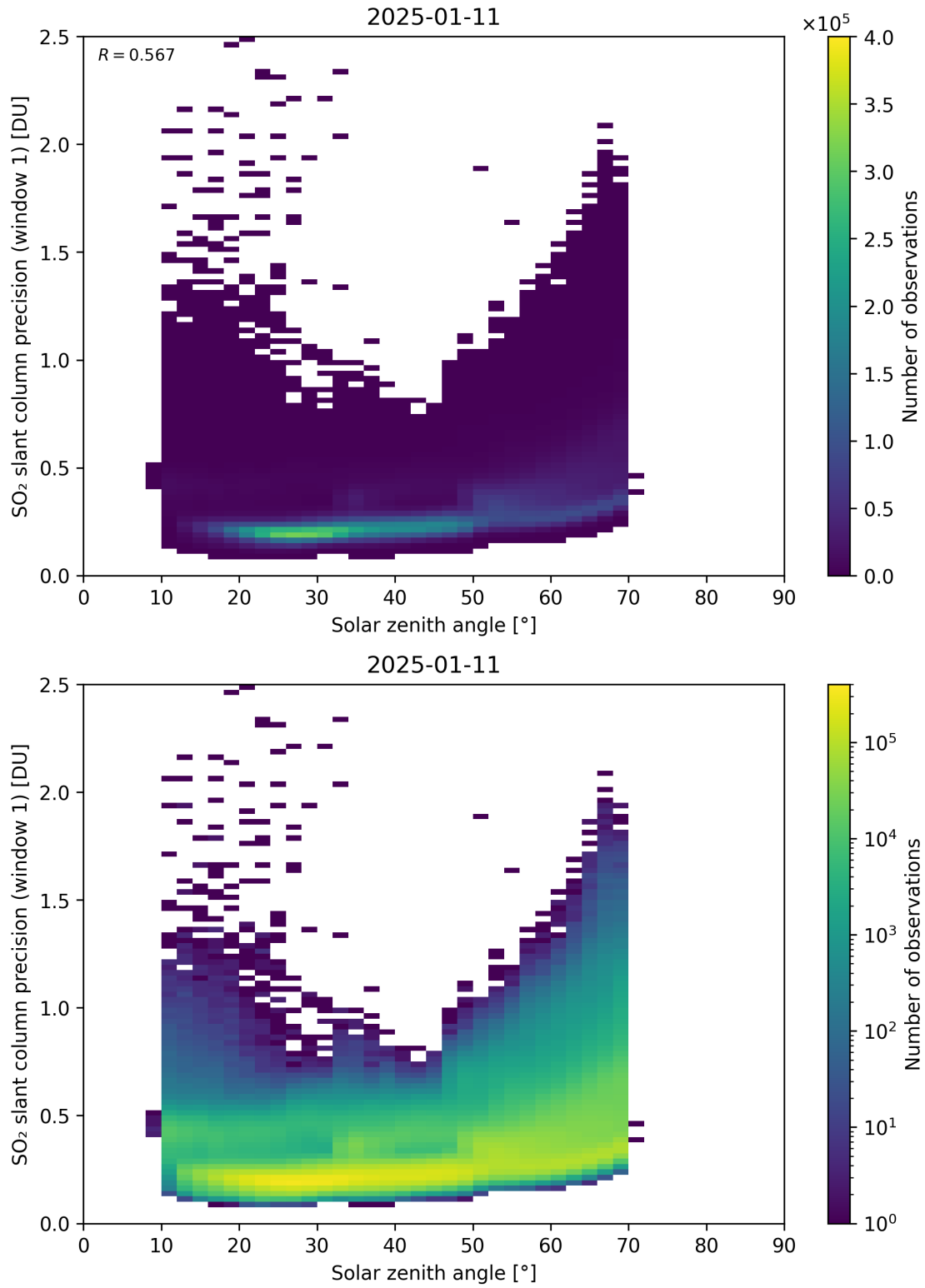
Figure 185: Scatter density plot of “Solar zenith angle” against “SO 2 slant column precision (window 1)” for 2025-01-10 to 2025-01-12.
