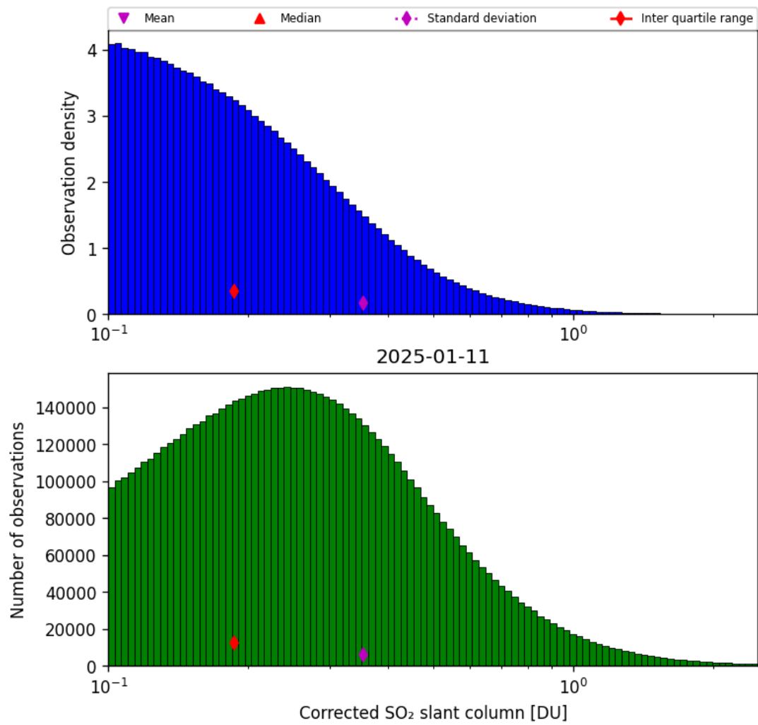
Figure 60: Histogram of "Corrected SO 2 slant column" for 2025-01-10 to 2025-01-12
