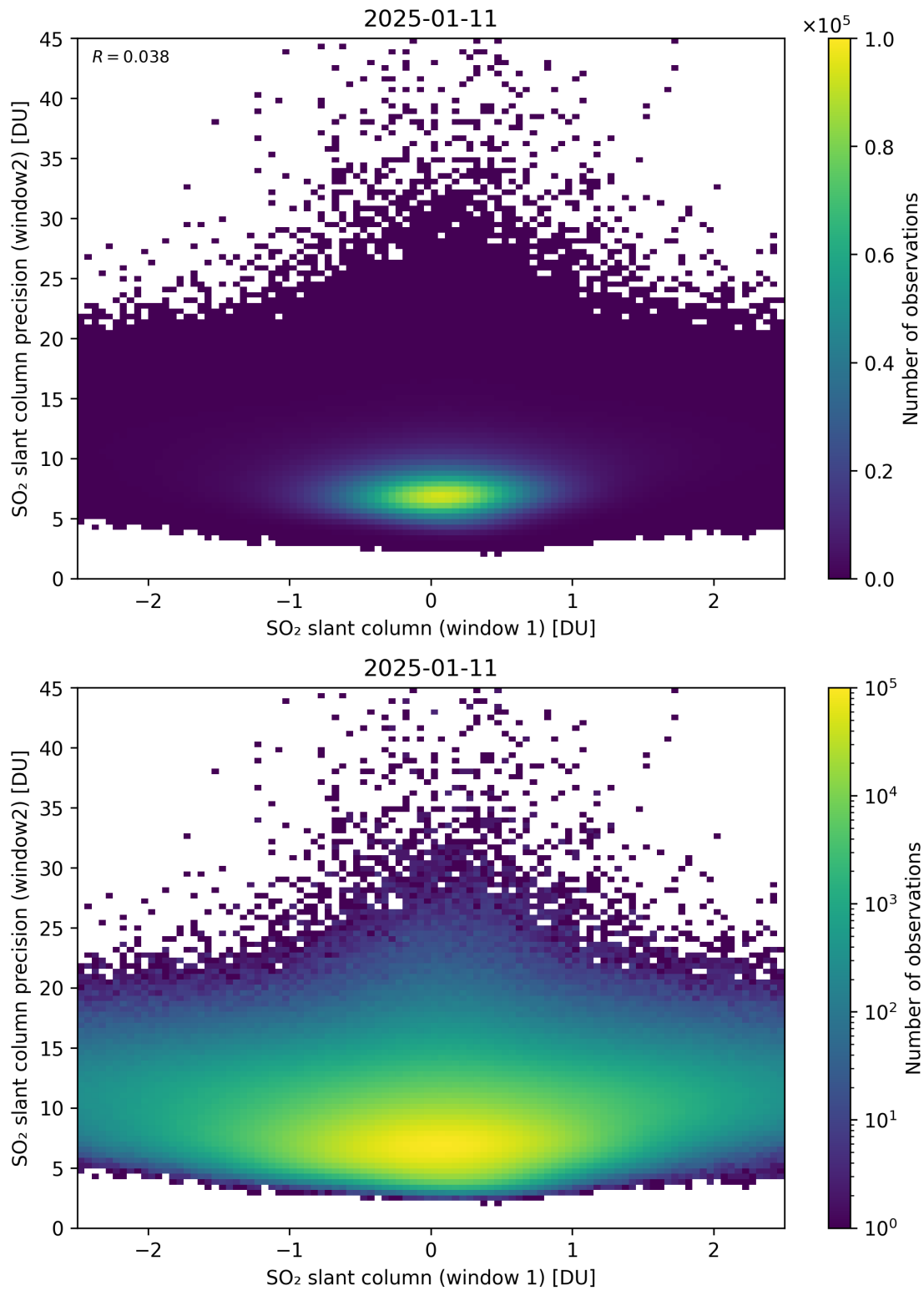
Figure 286: Scatter density plot of “SO 2 slant column (window 1)” against “SO 2 slant column precision (window2)” for 2025-01-10 to 2025-01-12.
