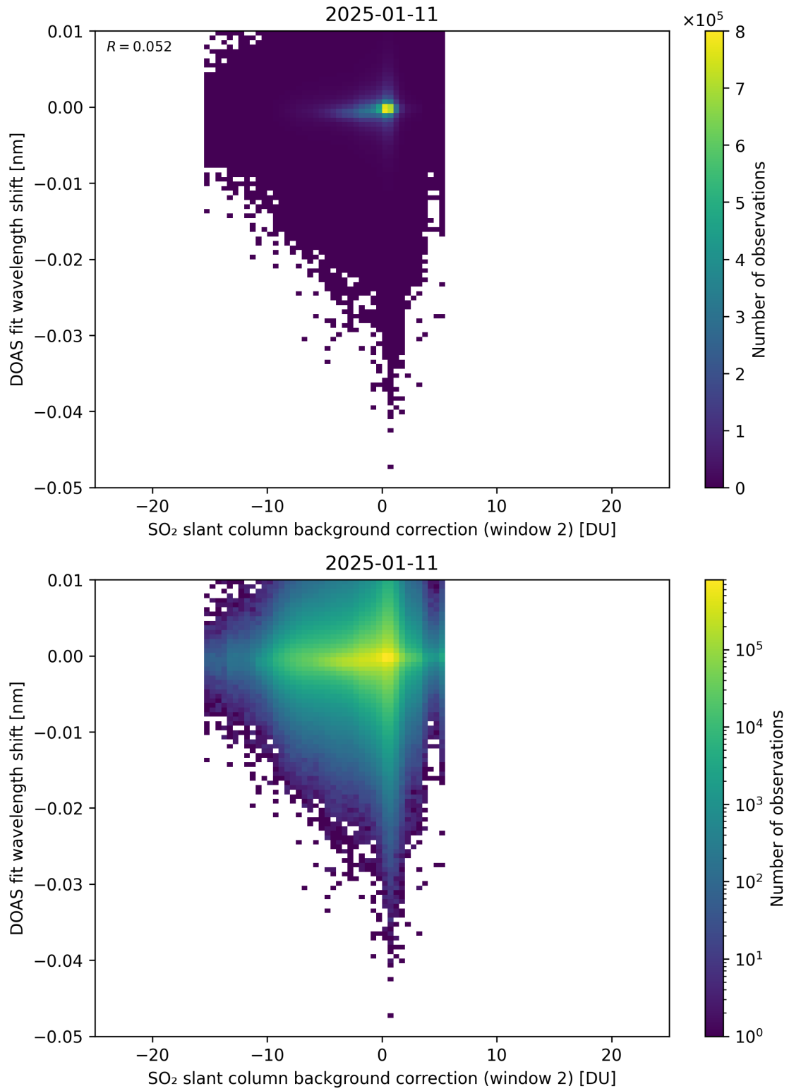
Figure 123: Scatter density plot of “SO 2 slant column background correction (window 2)” against “DOAS fit wavelength shift” for 2025-01-10 to 2025-01-12.
