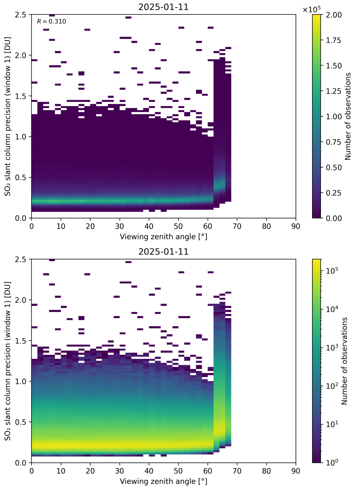
Figure 377: Scatter density plot of “Viewing zenith angle” against “SO 2 slant column precision (window 1)” for 2025-01-10 to 2025-01-12.
