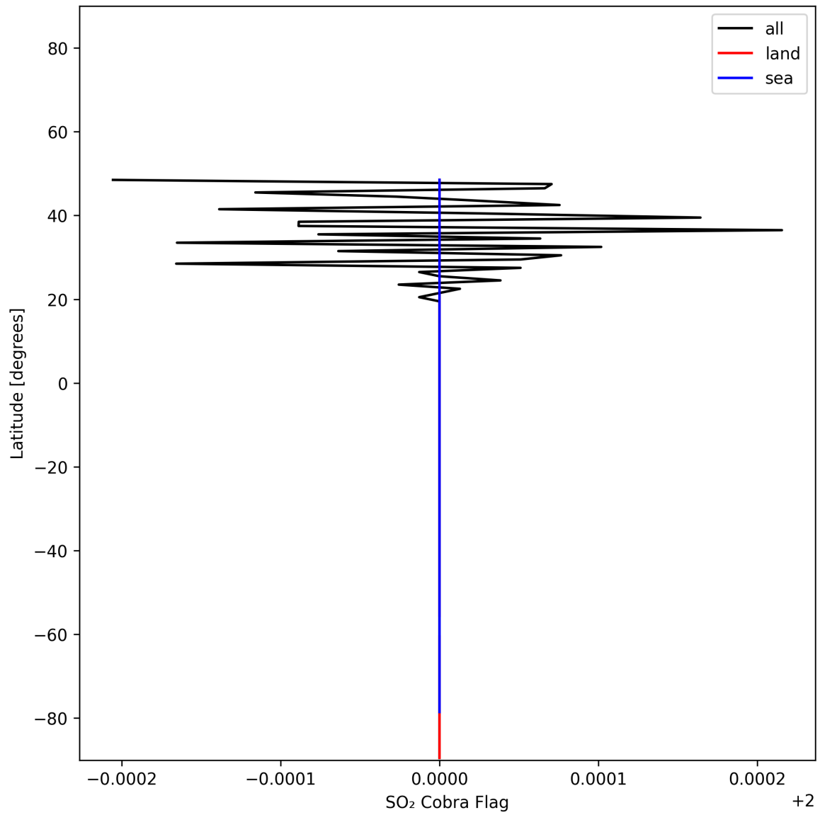
Figure 49: Zonal average of “SO 2 Cobra Flag” for 2025-01-10 to 2025-01-12.
