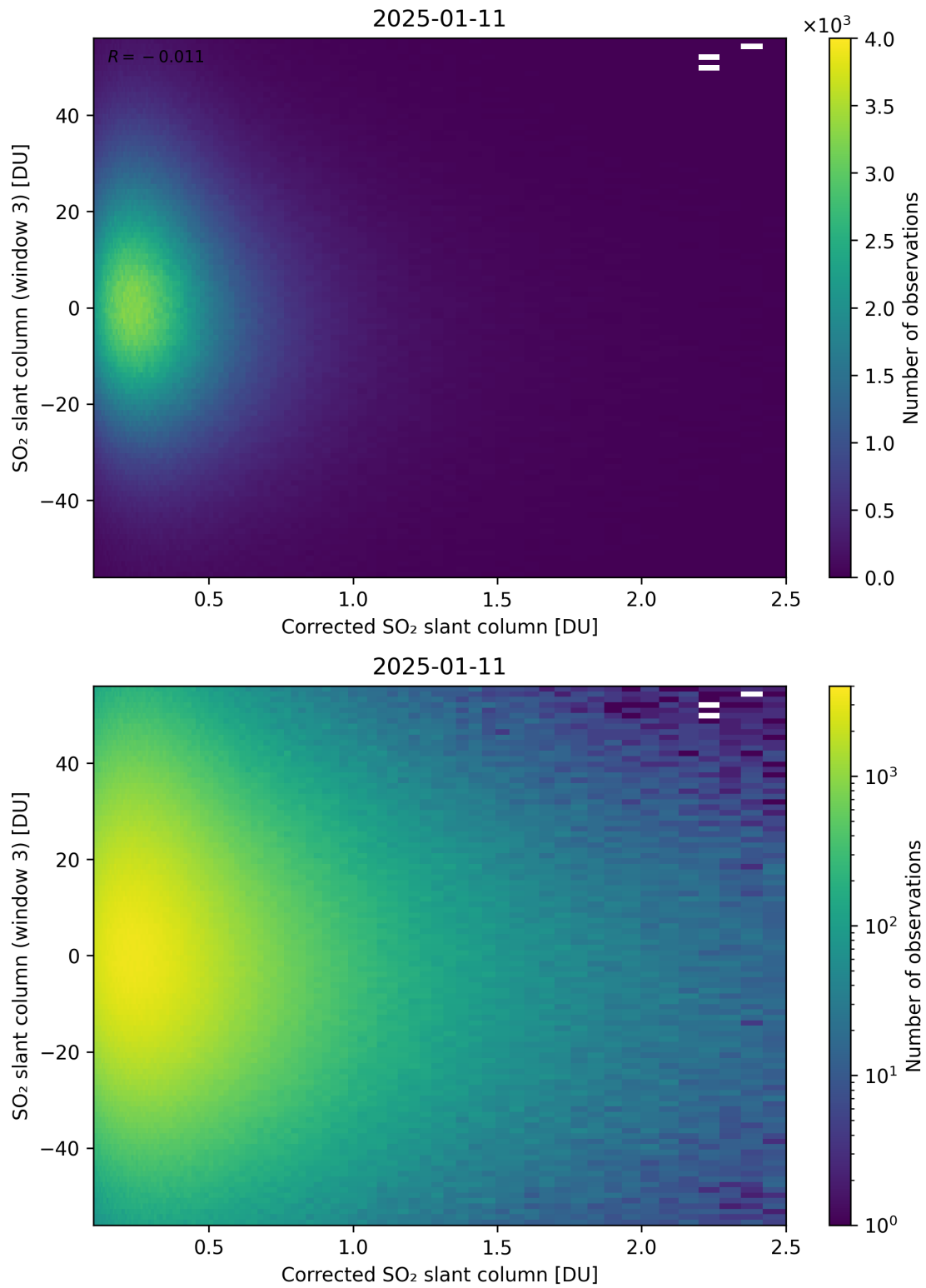
Figure 240: Scatter density plot of “Corrected SO 2 slant column” against “SO 2 slant column (window 3)” for 2025-01-10 to 2025-01-12.
