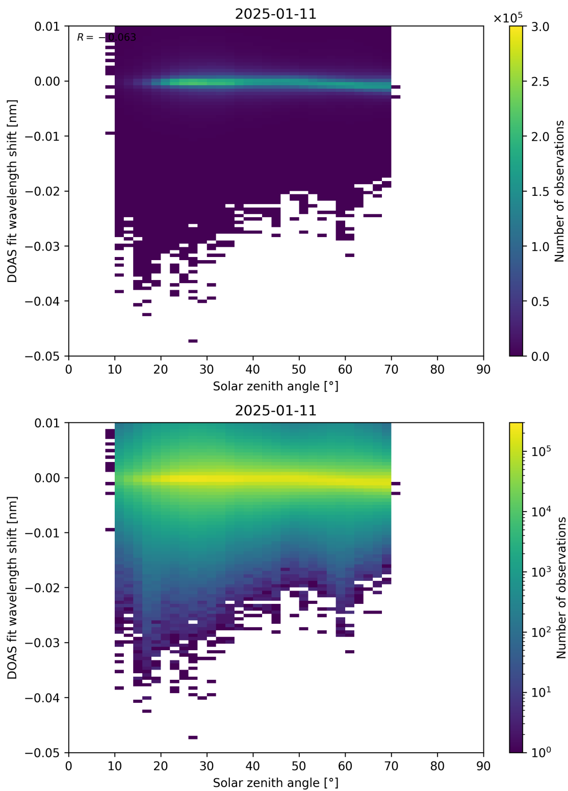
Figure 174: Scatter density plot of “Solar zenith angle” against “DOAS fit wavelength shift” for 2025-01-10 to 2025-01-12.
