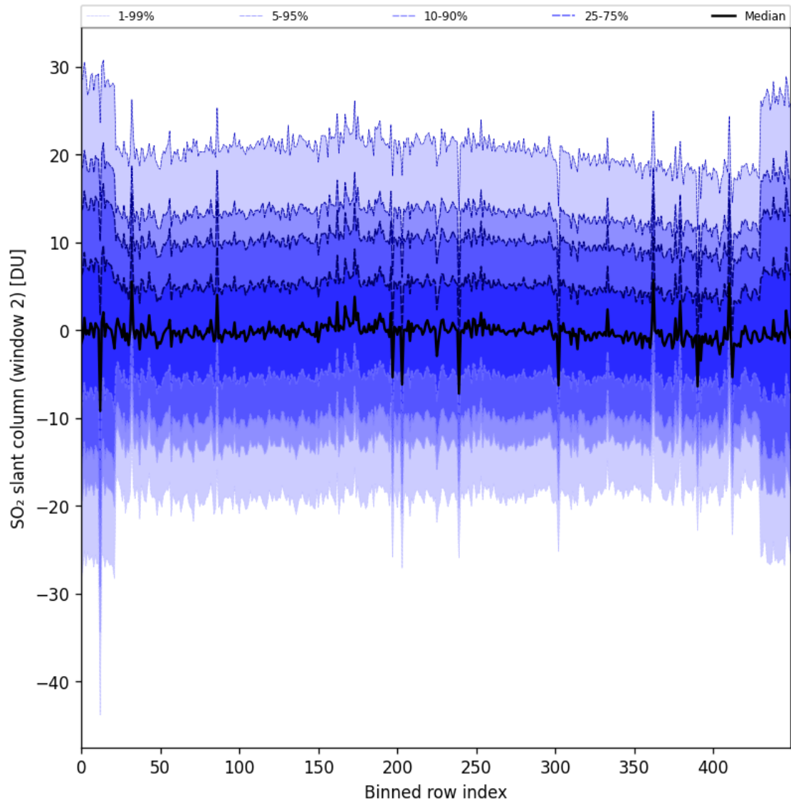
Figure 93: Along track statistics of “SO 2 slant column (window 2)” for 2025-01-10 to 2025-01-12
