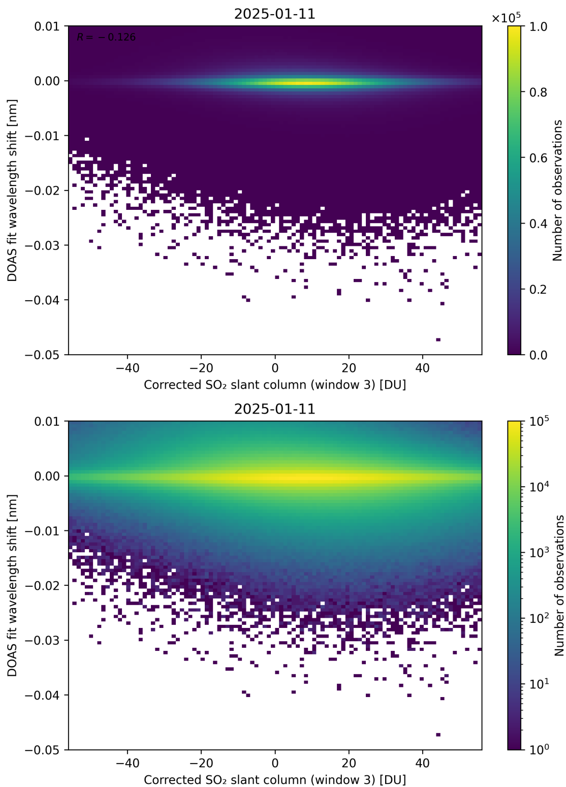
Figure 256: Scatter density plot of “Corrected SO 2 slant column (window 3)” against “DOAS fit wavelength shift” for 2025-01-10 to 2025-01-12.
