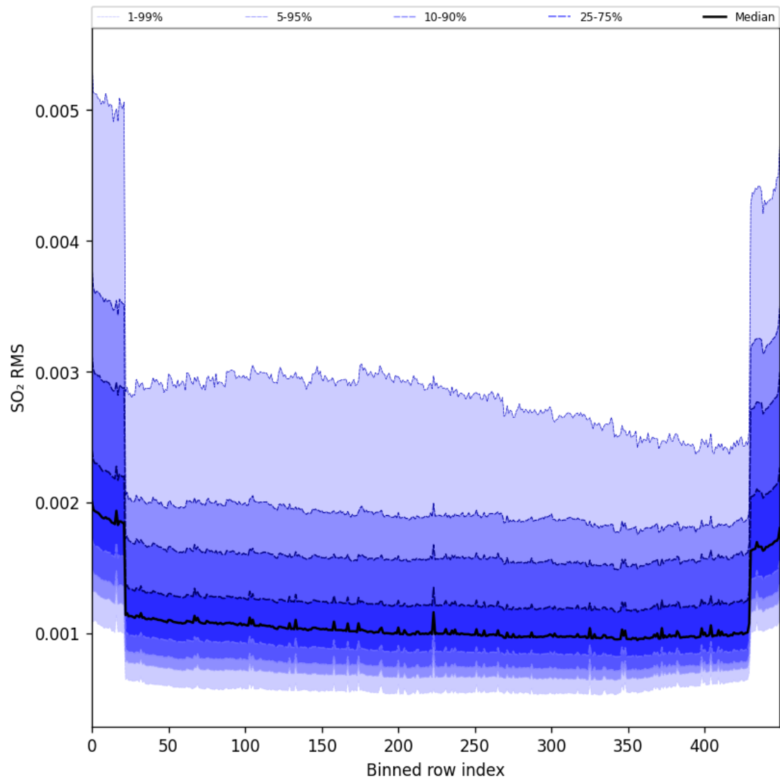
Figure 104: Along track statistics of “SO 2 RMS” for 2025-01-10 to 2025-01-12
