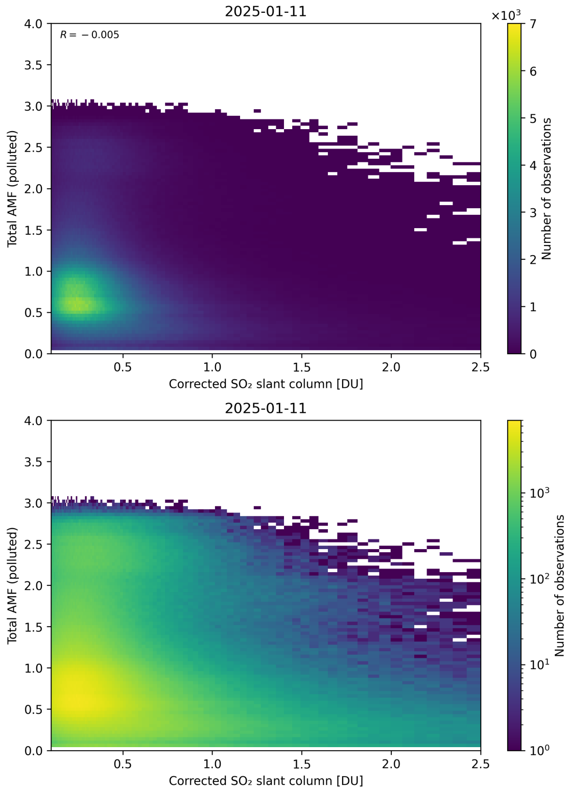
Figure 242: Scatter density plot of “Corrected SO 2 slant column” against “Total AMF (polluted)” for 2025-01-10 to 2025-01-12.
