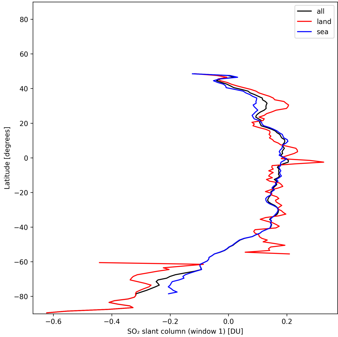
Figure 37: Zonal average of “SO 2 slant column (window 1)” for 2025-01-10 to 2025-01-12.
