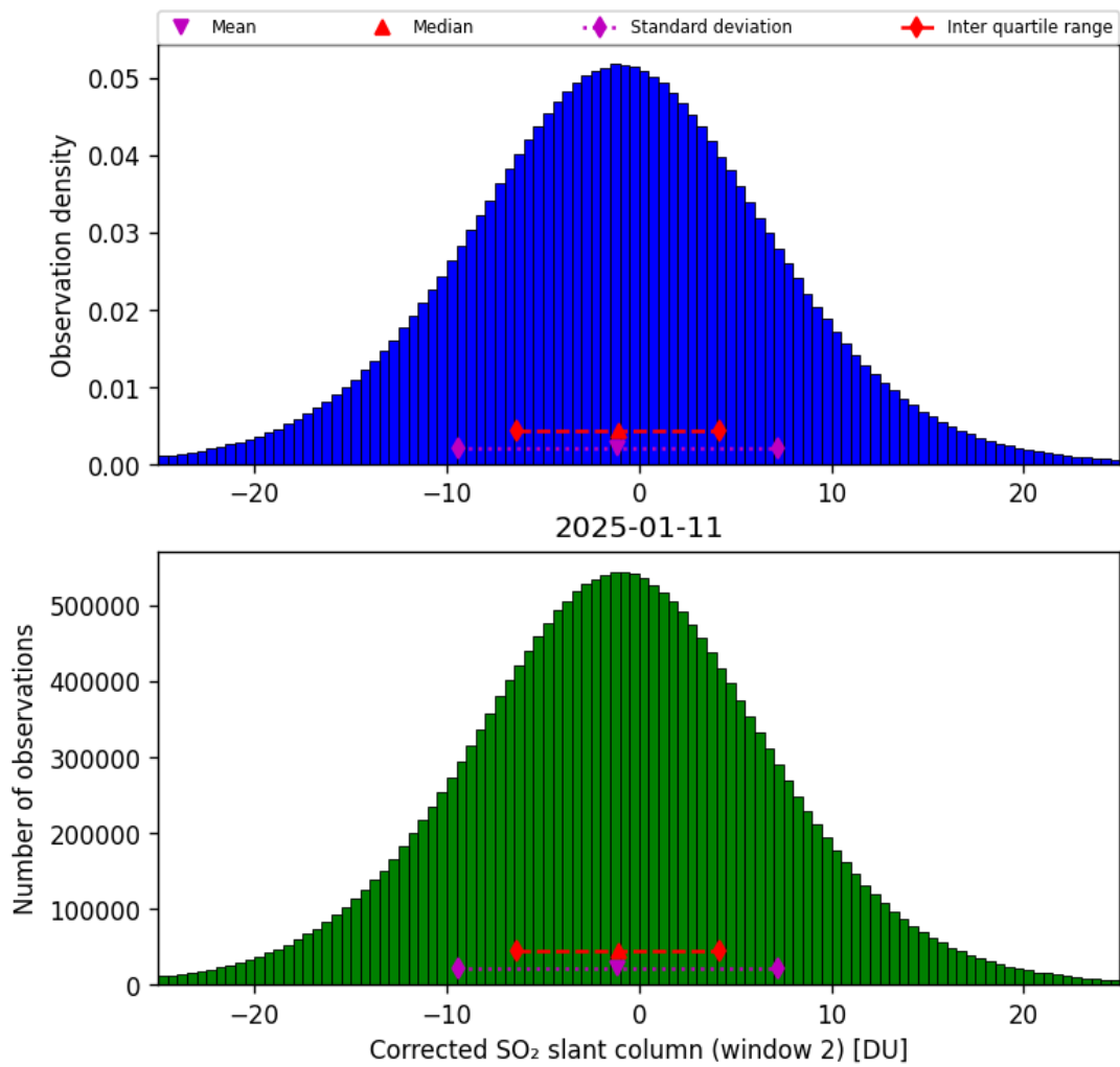
Figure 69: Histogram of “Corrected SO 2 slant column (window 2)” for 2025-01-10 to 2025-01-12
