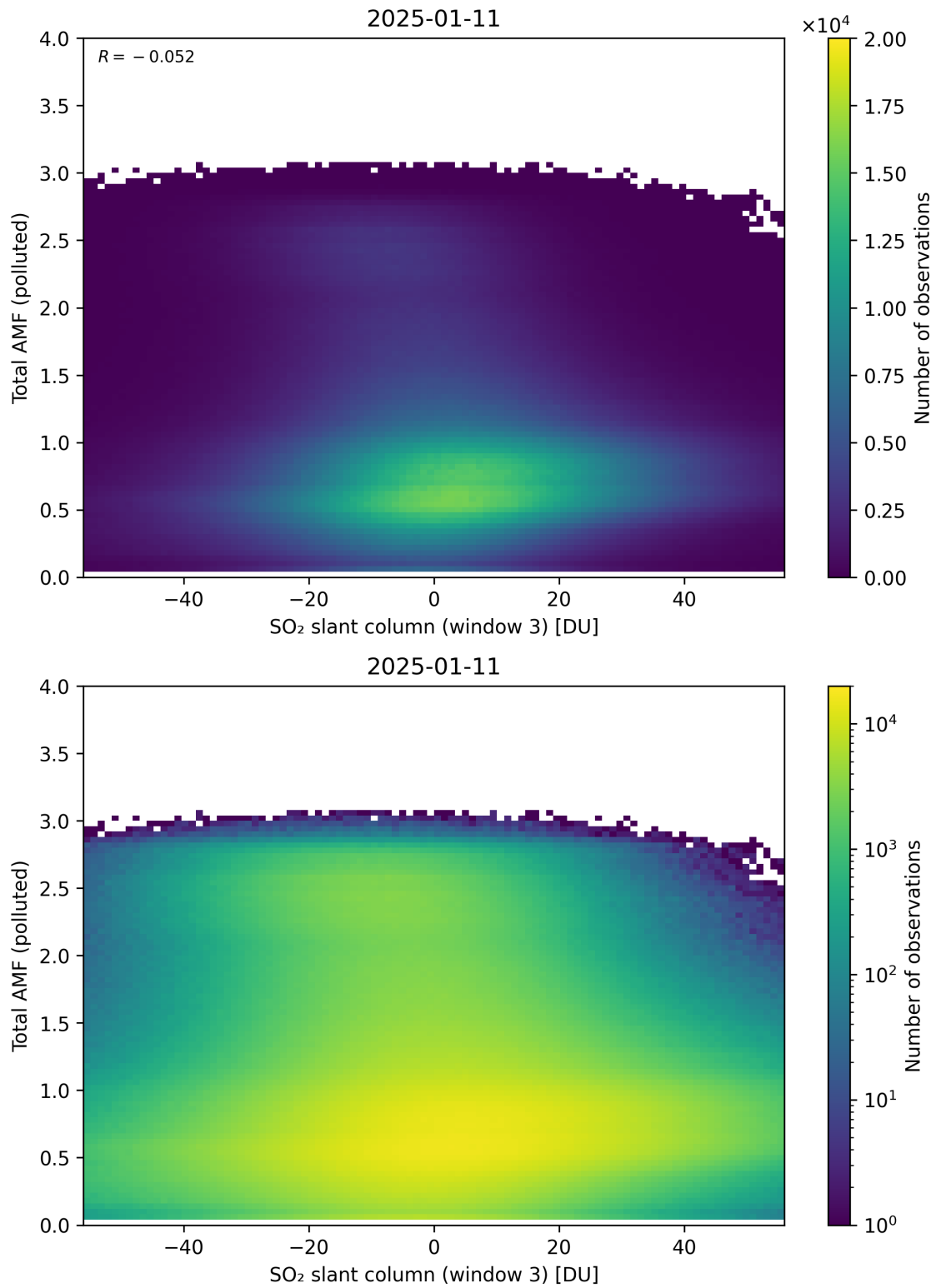
Figure 318: Scatter density plot of “SO 2 slant column (window 3)” against “Total AMF (polluted)” for 2025-01-10 to 2025-01-12.
