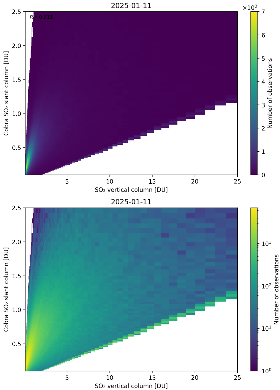
Figure 349: Scatter density plot of “SO 2 vertical column” against “Cobra SO 2 slant column” for 2025-01-10 to 2025-01-12.
