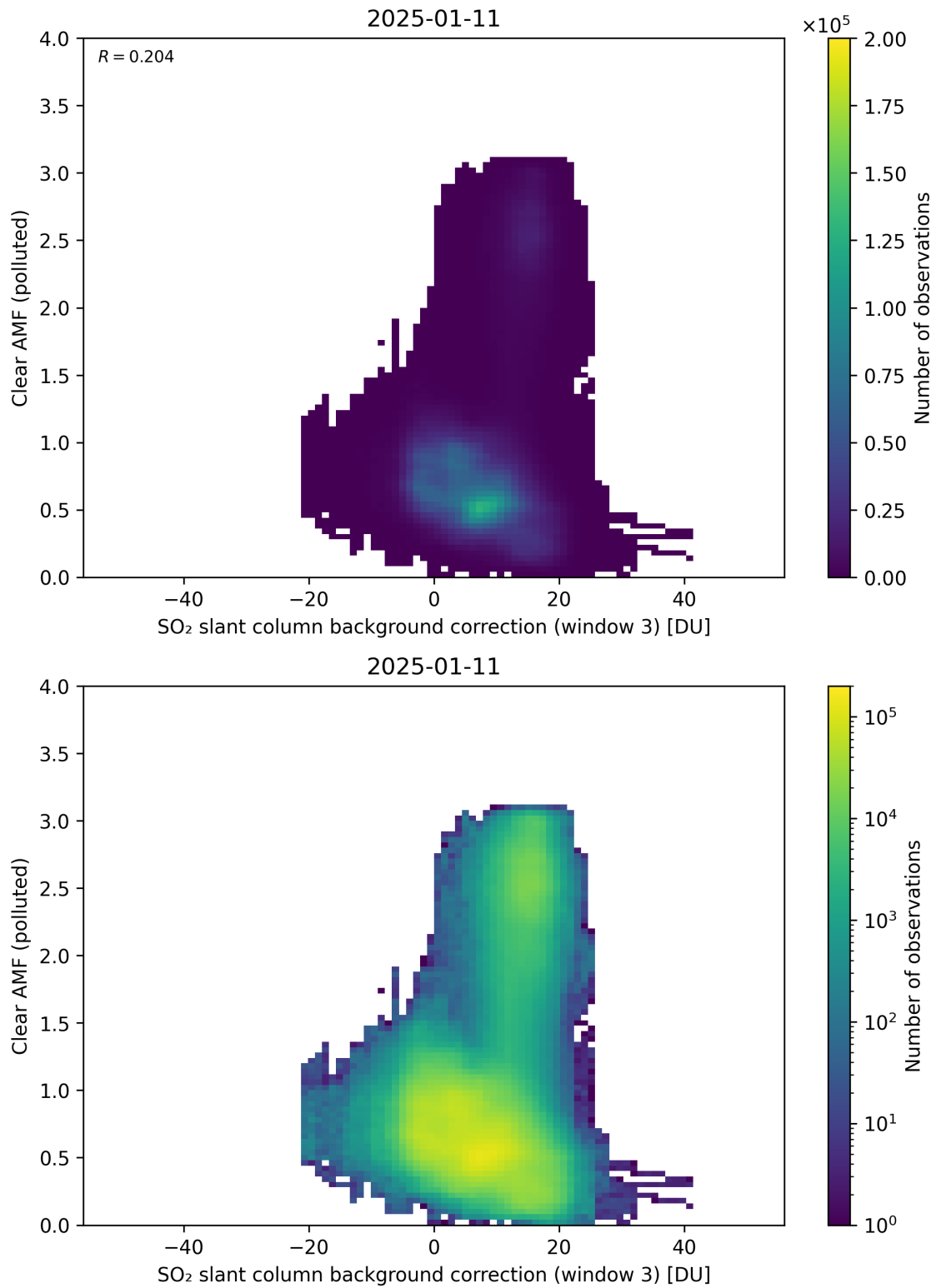
Figure 135: Scatter density plot of “SO 2 slant column background correction (window 3)” against “Clear AMF (polluted)” for 2025-01-10 to 2025-01-12.
