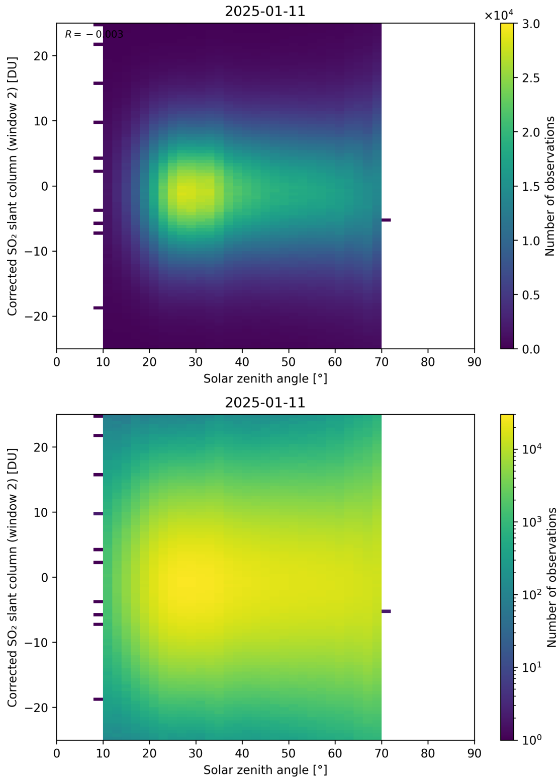
Figure 182: Scatter density plot of “Solar zenith angle” against “Corrected SO 2 slant column (window 2)” for 2025-01-10 to 2025-01-12.
