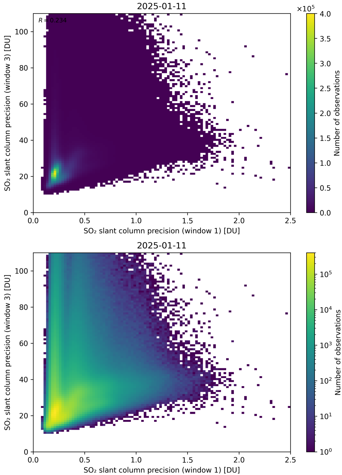
Figure 279: Scatter density plot of “SO 2 slant column precision (window 1)” against “SO 2 slant column precision (window 3)” for 2025-01-10 to 2025-01-12.
