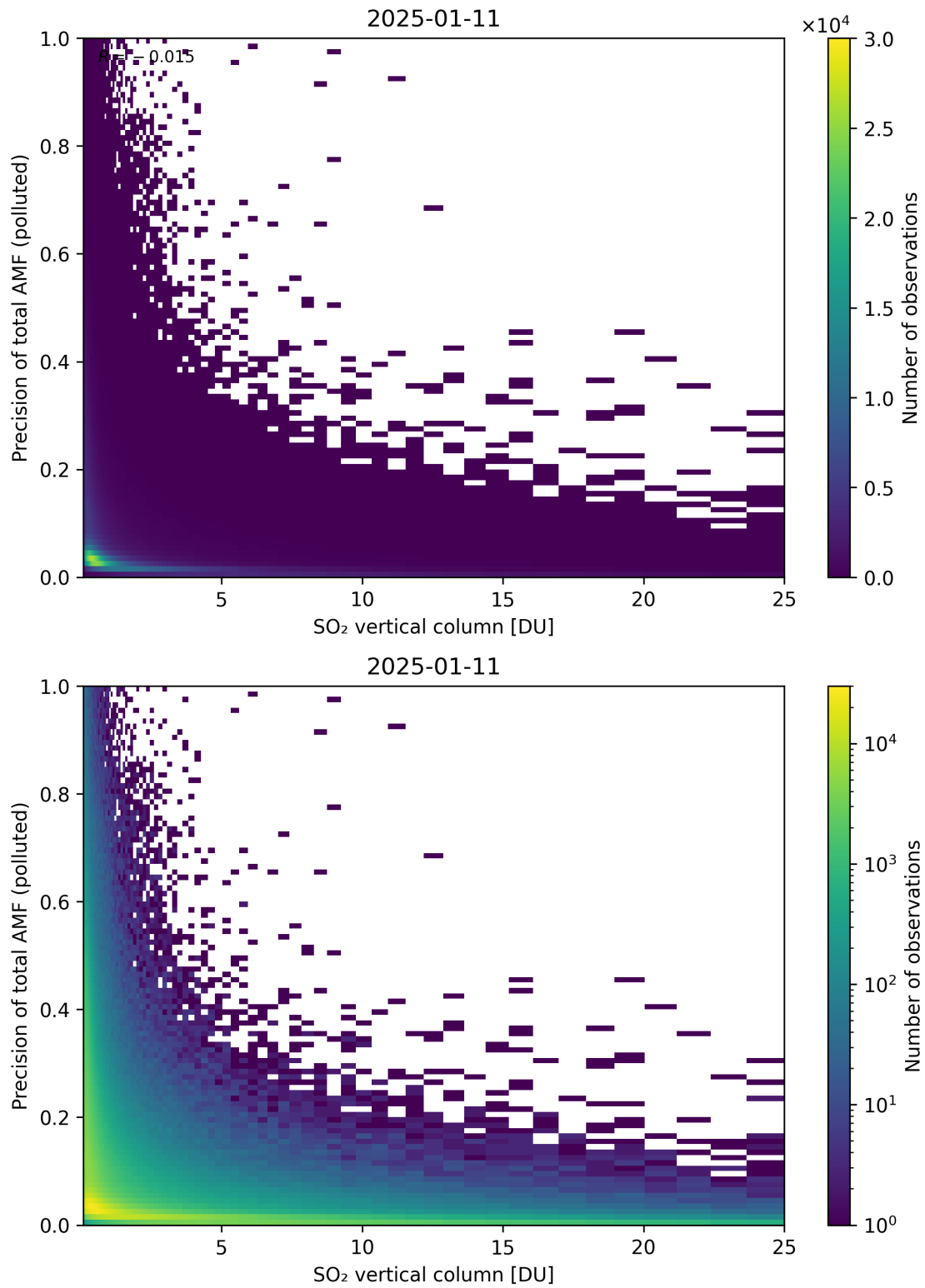
Figure 360: Scatter density plot of “SO 2 vertical column” against “Precision of total AMF (polluted)” for 2025-01-10 to 2025-01-12.
