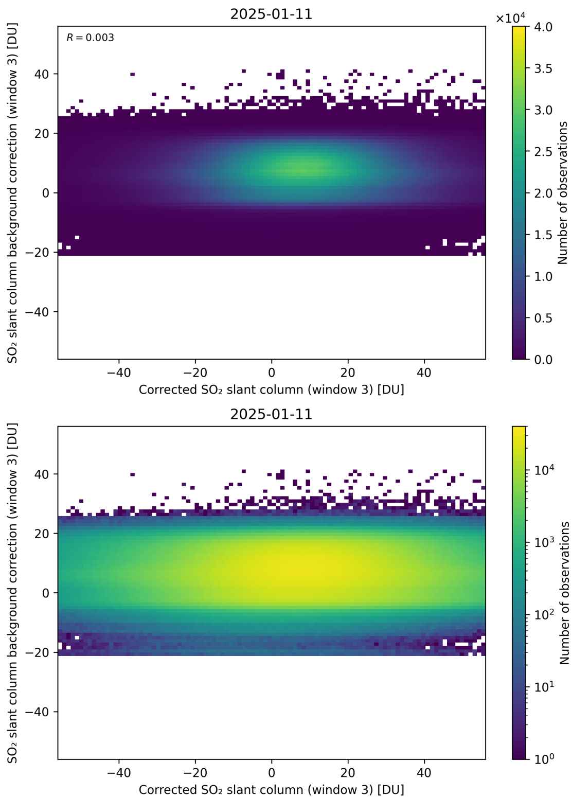
Figure 255: Scatter density plot of “Corrected SO 2 slant column (window 3)” against “SO 2 slant column background correction (window 3)” for 2025-01-10 to 2025-01-12.
