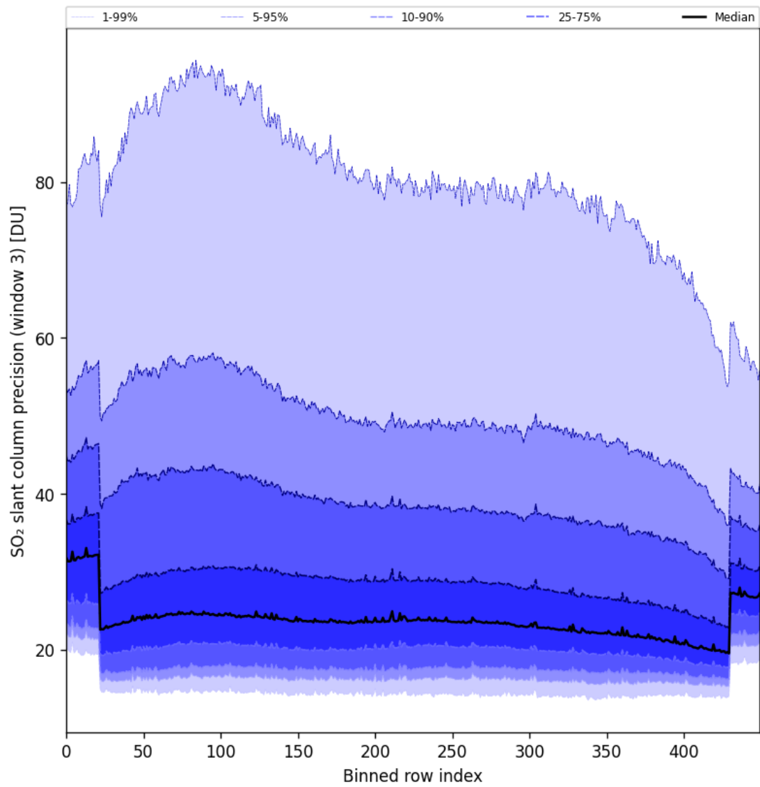
Figure 98: Along track statistics of “SO 2 slant column precision (window 3)” for 2025-01-10 to 2025-01-12
