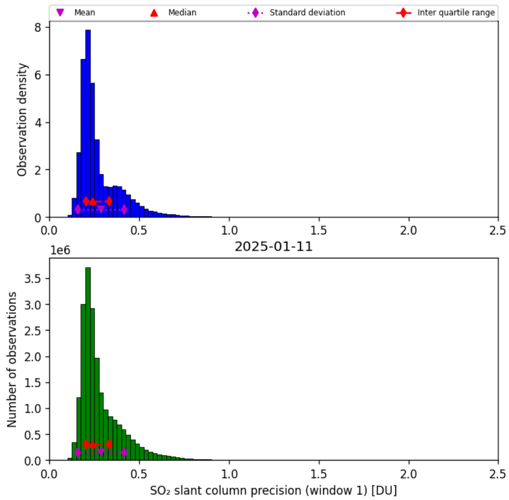
Figure 64: Histogram of “SO 2 slant column precision (window 1)” for 2025-01-10 to 2025-01-12
