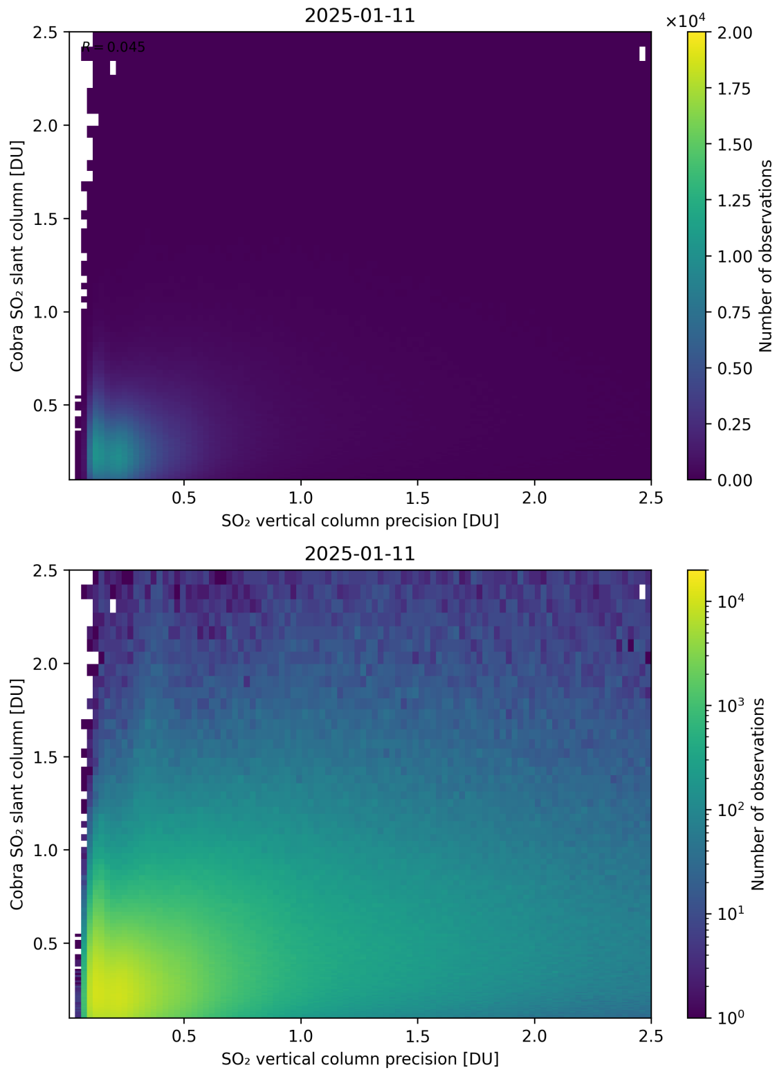
Figure 336: Scatter density plot of “SO 2 vertical column precision” against “Cobra SO 2 slant column” for 2025-01-10 to 2025-01-12.
