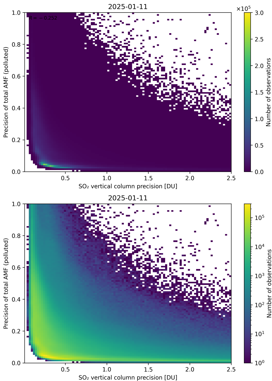
Figure 347: Scatter density plot of “SO 2 vertical column precision” against “Precision of total AMF (polluted)” for 2025-01-10 to 2025-01-12.
