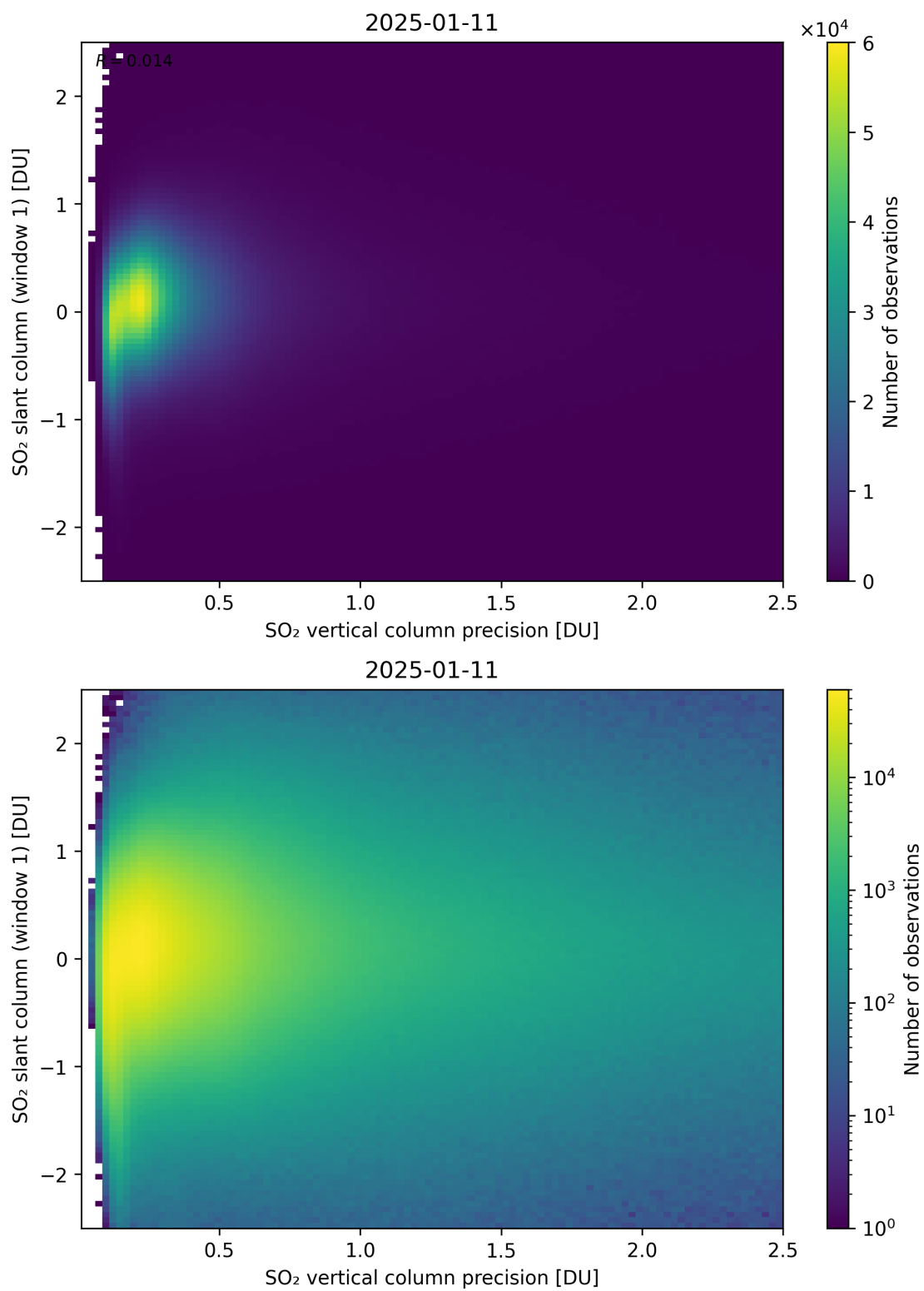
Figure 341: Scatter density plot of “SO 2 vertical column precision” against “SO 2 slant column (window 1)” for 2025-01-10 to 2025-01-12.
