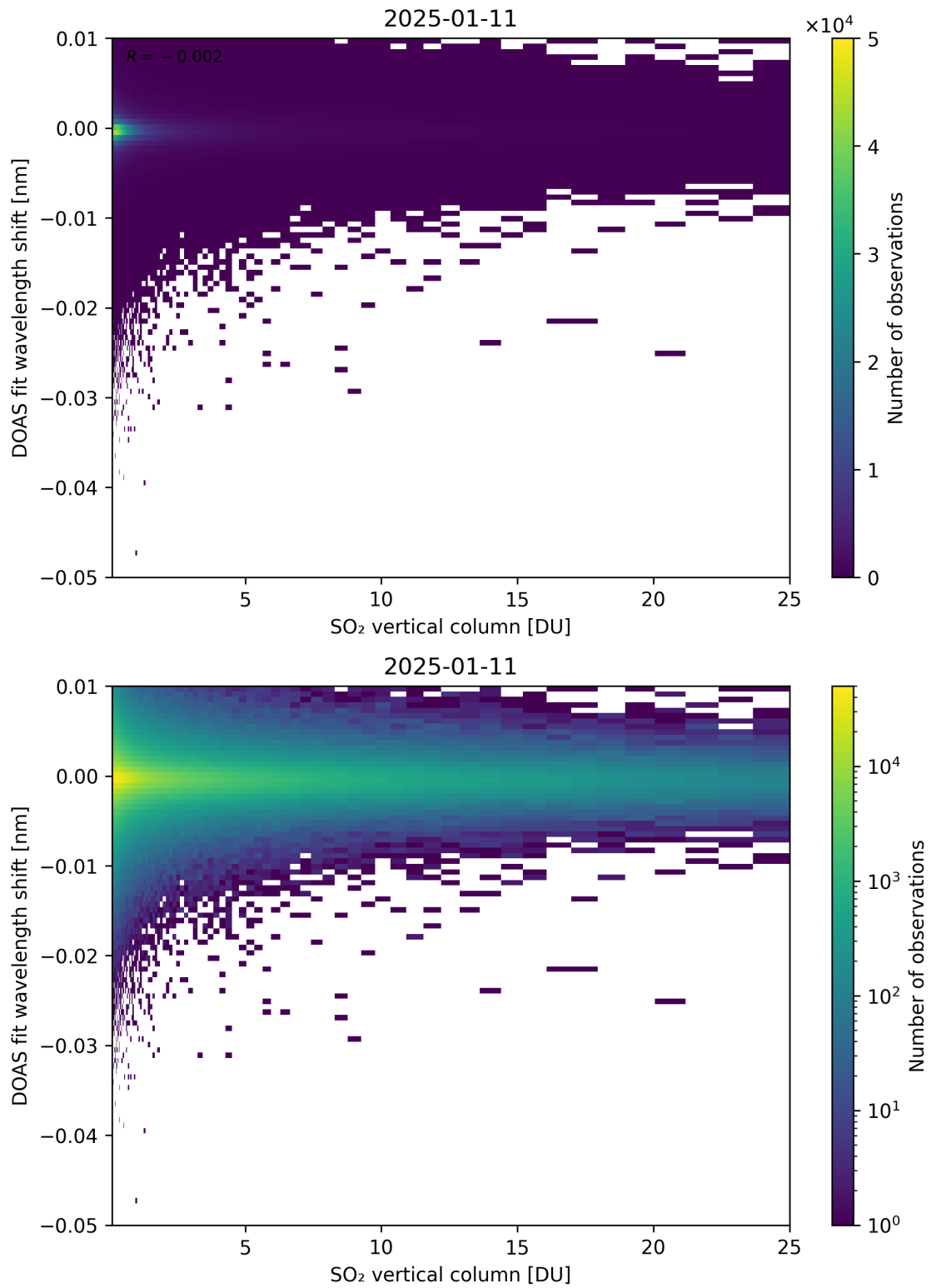
Figure 326: Scatter density plot of “SO 2 vertical column” against “DOAS fit wavelength shift” for 2025-01-10 to 2025-01-12.
