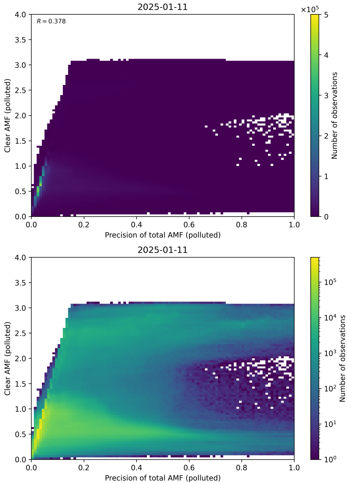
Figure 320: Scatter density plot of “Precision of total AMF (polluted)” against “Clear AMF (polluted)” for 2025-01-10 to 2025-01-12.
