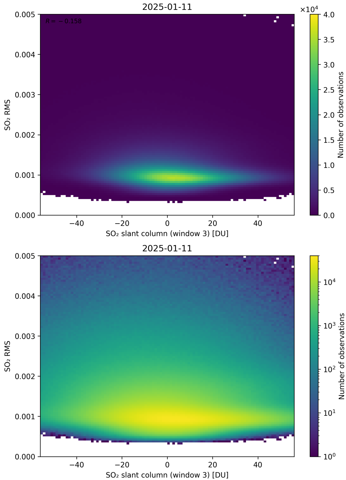
Figure 306: Scatter density plot of “SO 2 slant column (window 3)” against “SO 2 RMS” for 2025-01-10 to 2025-01-12.
