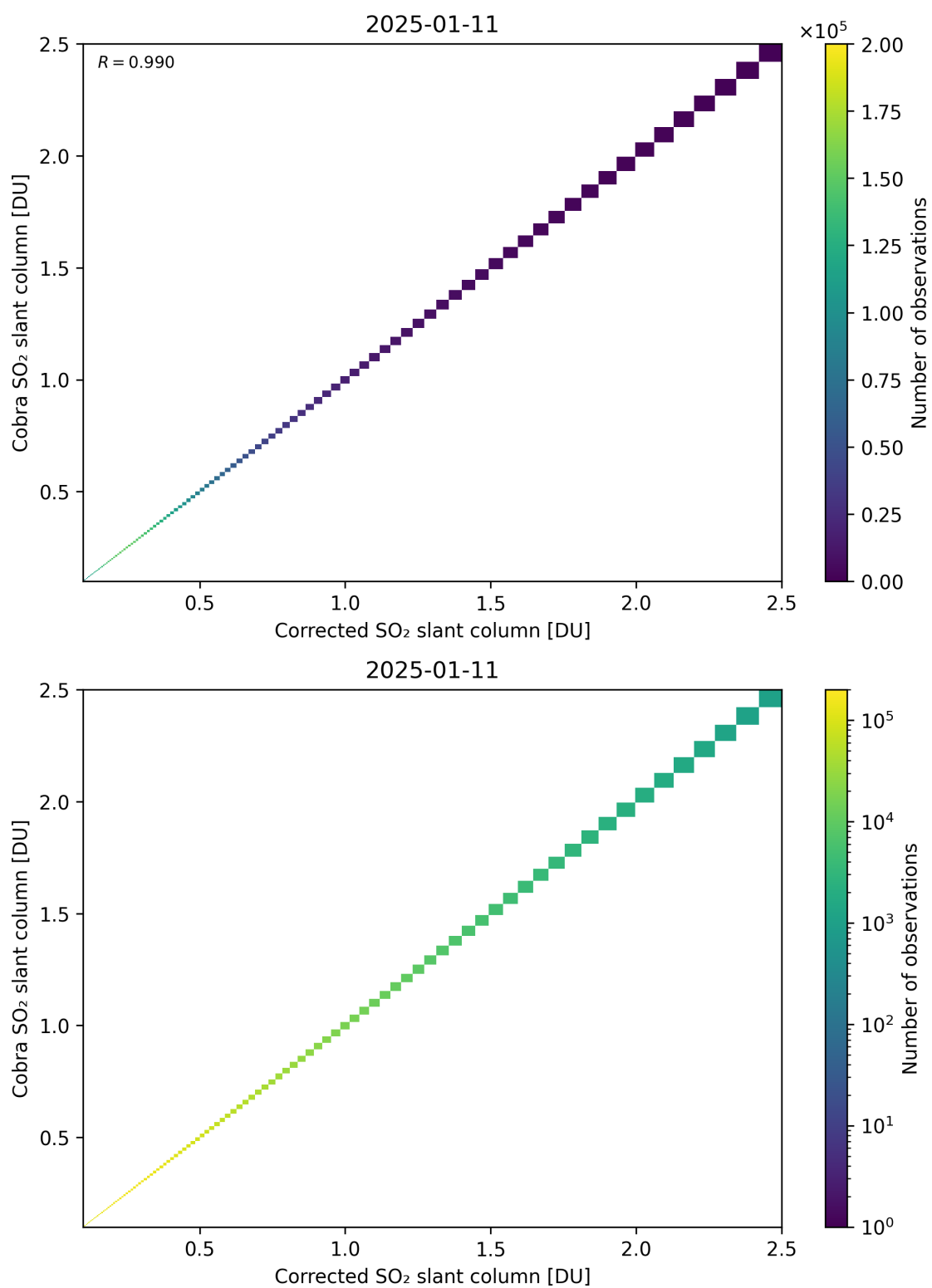
Figure 233: Scatter density plot of “Corrected SO 2 slant column” against “Cobra SO 2 slant column” for 2025-01-10 to 2025-01-12.
