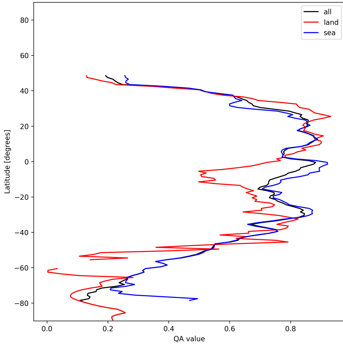
Figure 31: Zonal average of “QA value” for 2025-01-10 to 2025-01-12.
