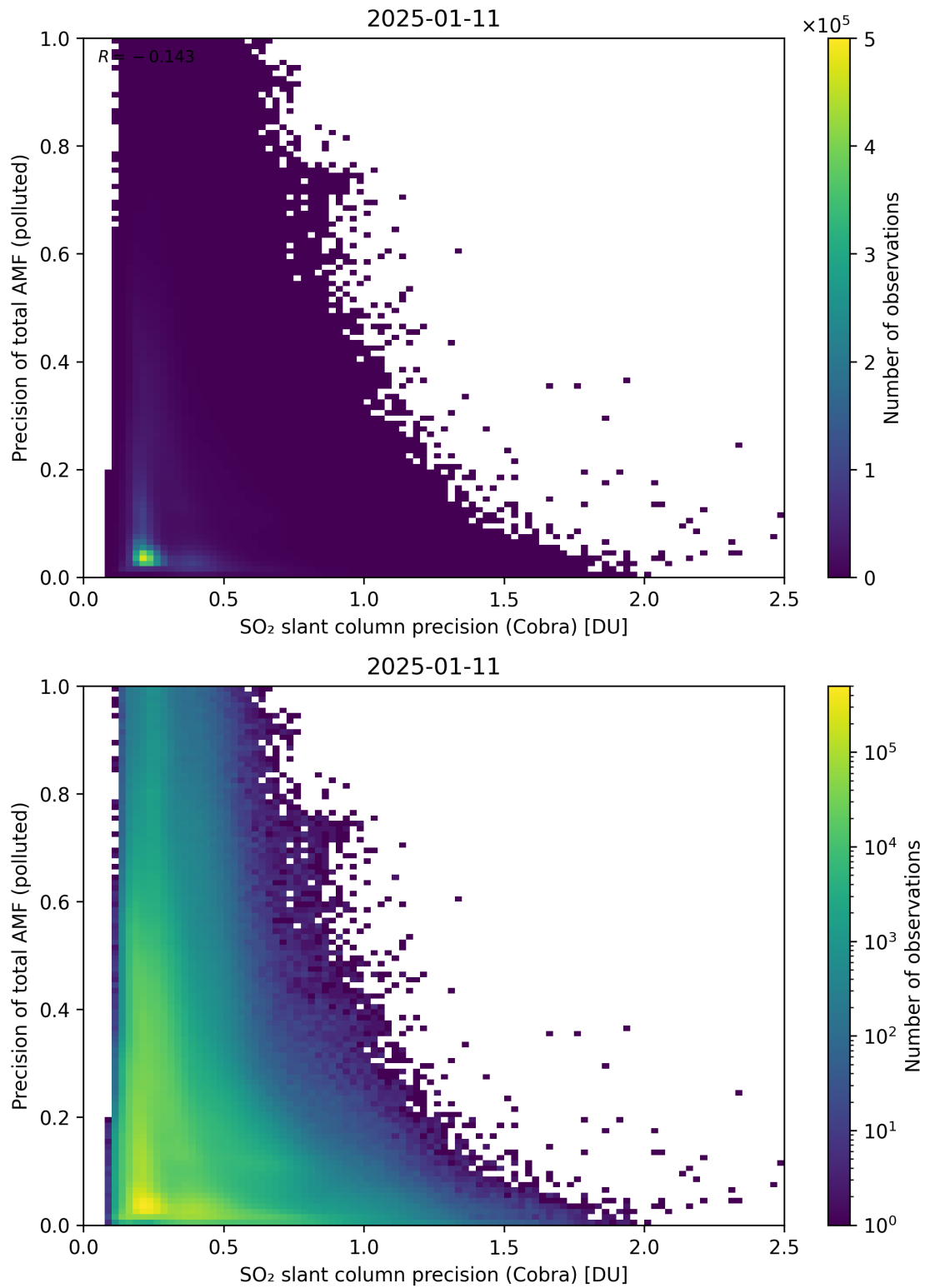
Figure 214: Scatter density plot of “SO 2 slant column precision (Cobra)” against “Precision of total AMF (polluted)” for 2025-01-10 to 2025-01-12.
