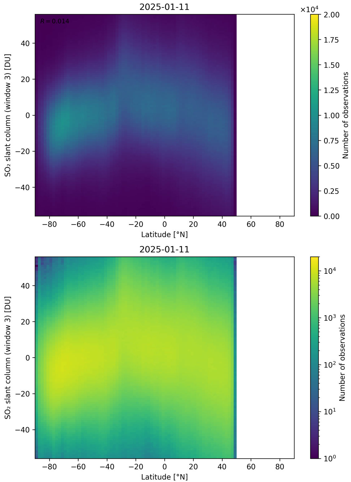
Figure 165: Scatter density plot of “Latitude” against “SO 2 slant column (window 3)” for 2025-01-10 to 2025-01-12.
