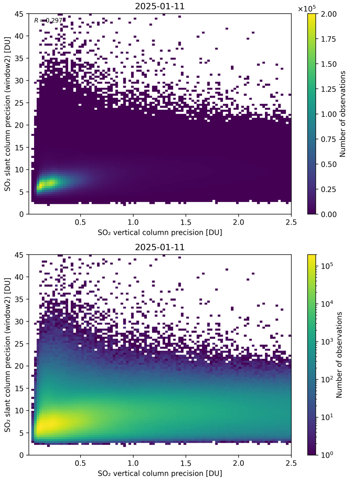
Figure 343: Scatter density plot of “SO 2 vertical column precision” against “SO 2 slant column precision (window2)” for 2025-01-10 to 2025-01-12.
