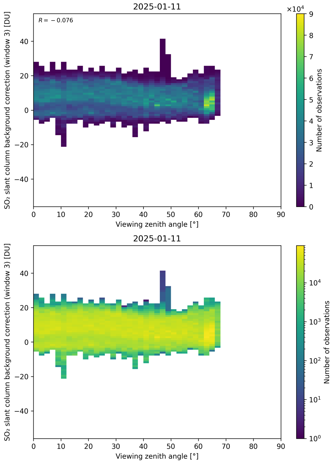
Figure 364: Scatter density plot of “Viewing zenith angle” against “SO 2 slant column background correction (window 3)” for 2025-01-10 to 2025-01-12.
