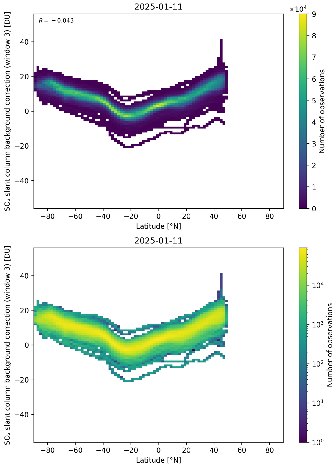
Figure 152: Scatter density plot of “Latitude” against “SO 2 slant column background correction (window 3)” for 2025-01-10 to 2025-01-12.
