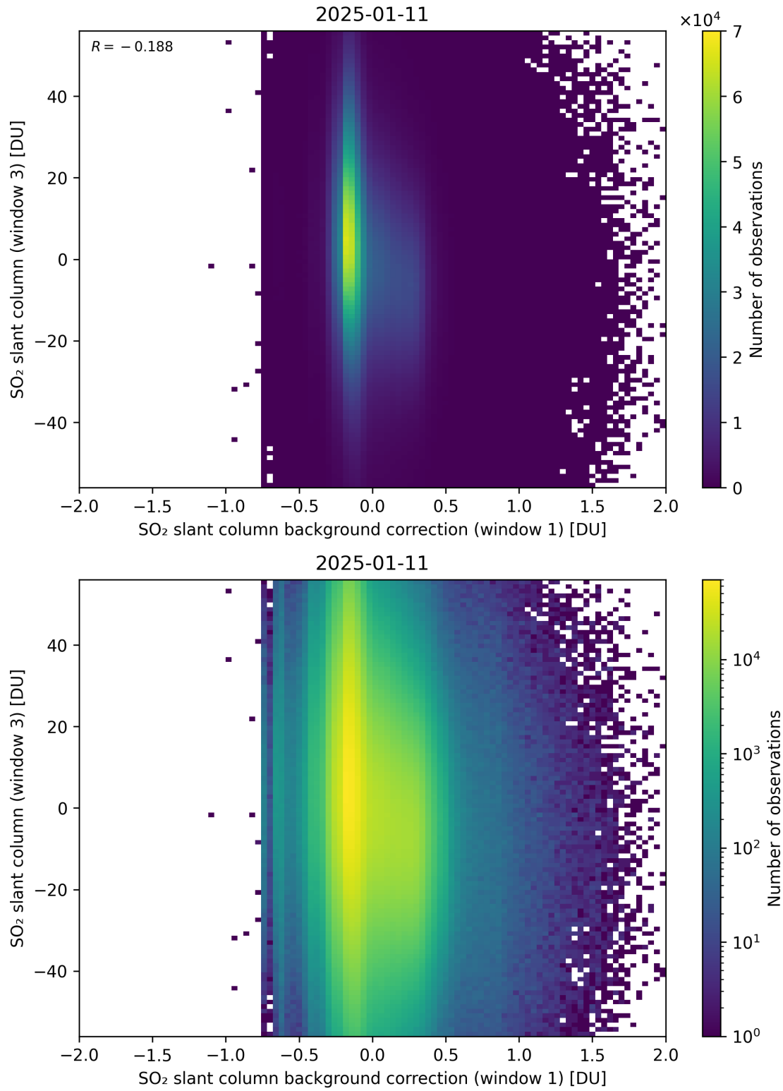
Figure 118: Scatter density plot of “SO 2 slant column background correction (window 1)” against “SO 2 slant column (window 3)” for 2025-01-10 to 2025-01-12.
