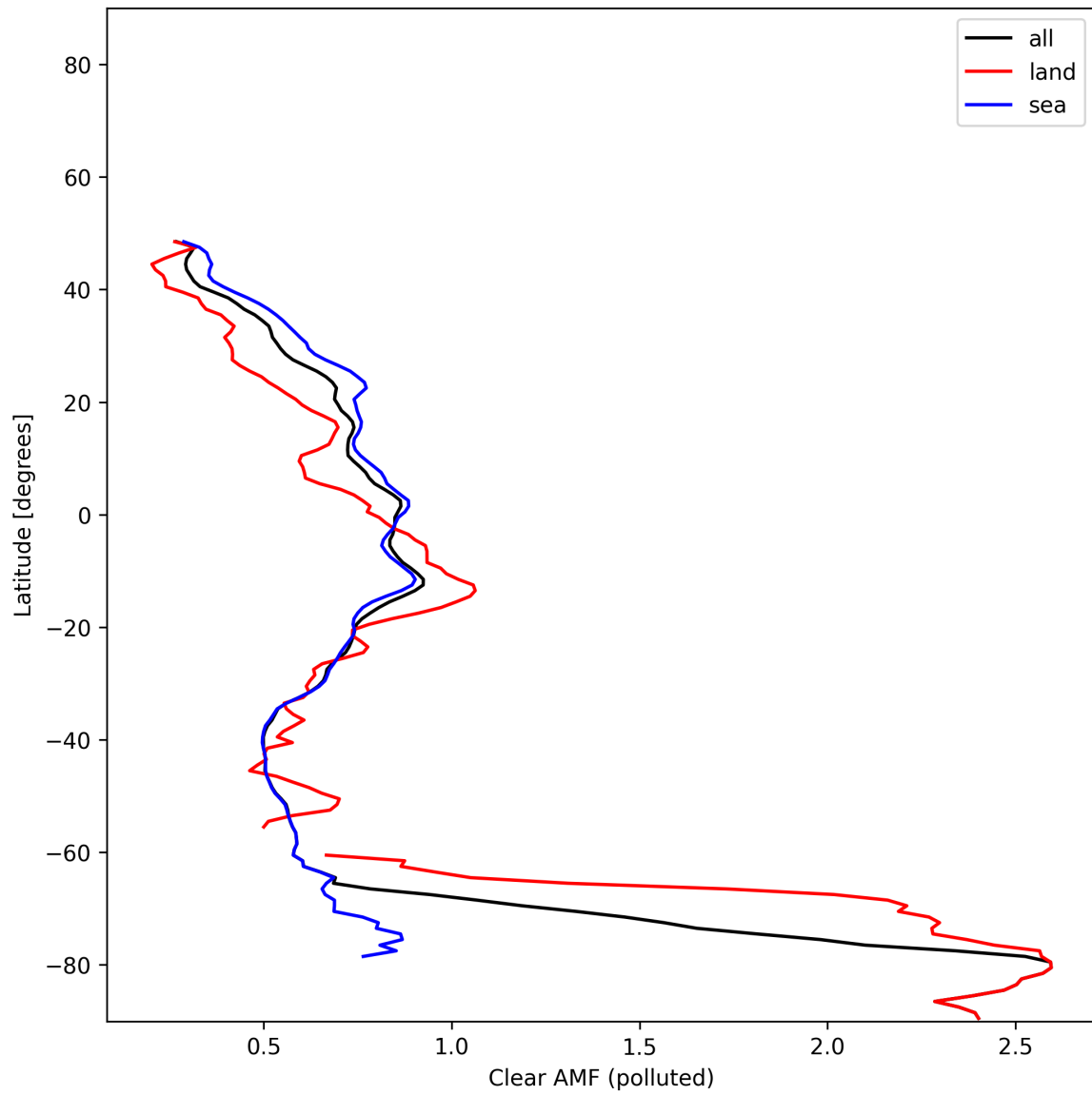
Figure 55: Zonal average of “Clear AMF (polluted)” for 2025-01-10 to 2025-01-12.
