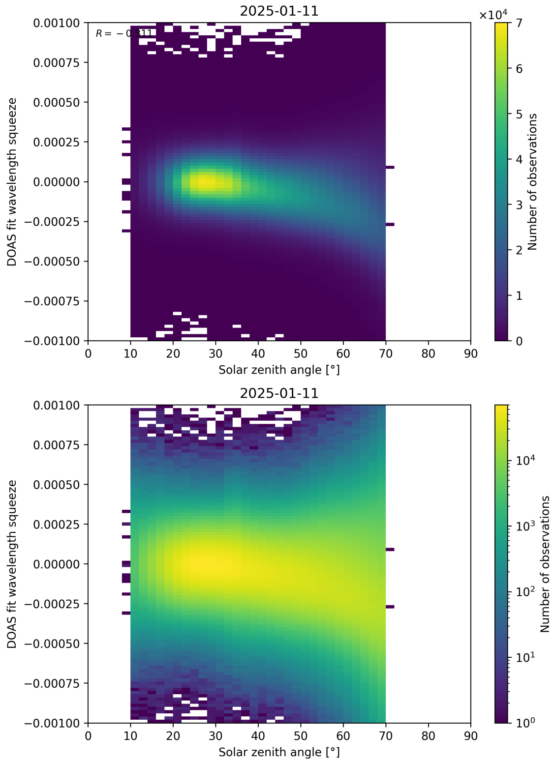
Figure 175: Scatter density plot of “Solar zenith angle” against “DOAS fit wavelength squeeze” for 2025-01-10 to 2025-01-12.
