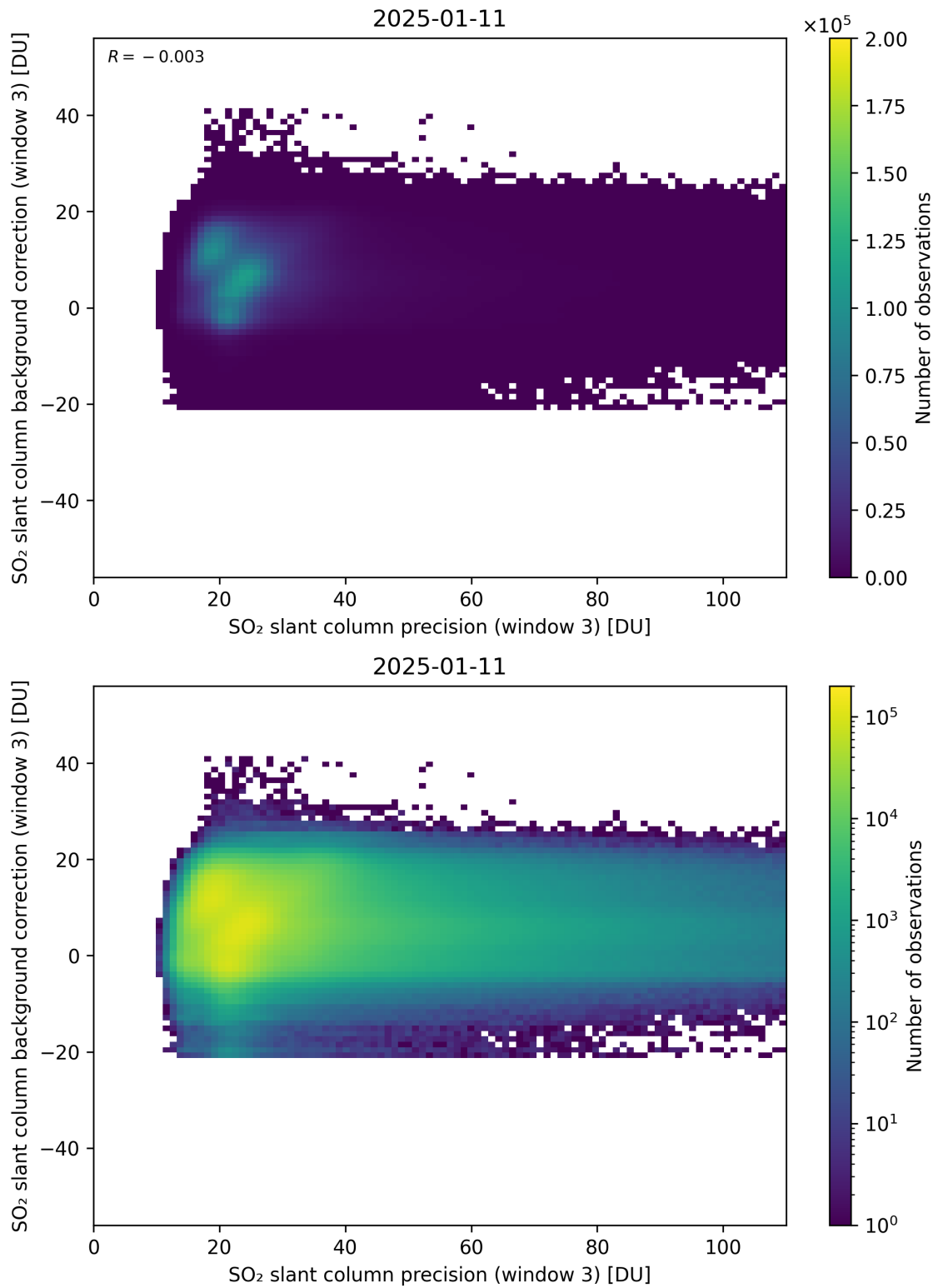
Figure 307: Scatter density plot of “SO 2 slant column precision (window 3)” against “SO 2 slant column background correction (window 3)” for 2025-01-10 to 2025-01-12.
