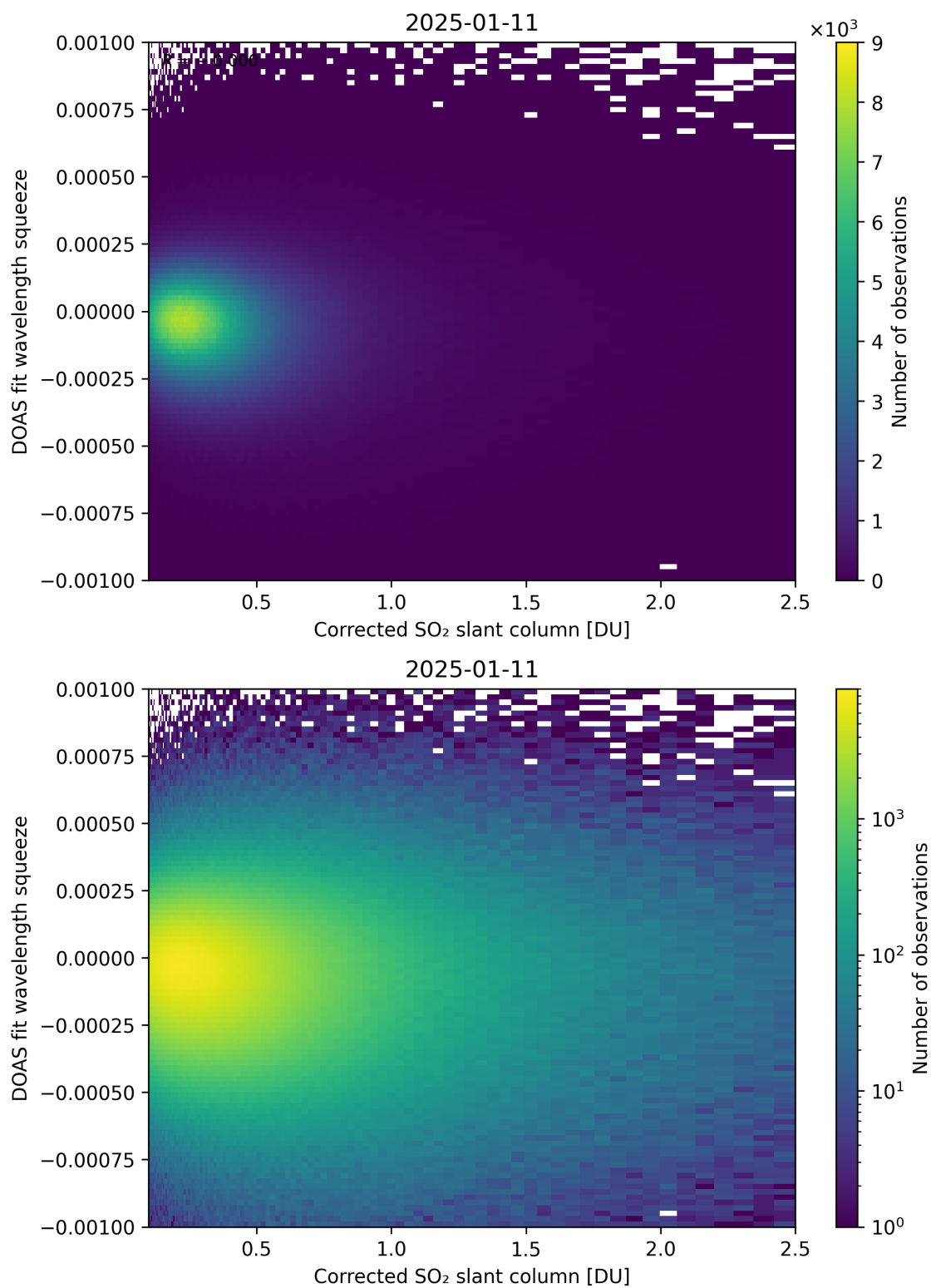
Figure 230: Scatter density plot of “Corrected SO 2 slant column” against “DOAS fit wavelength squeeze” for 2025-01-10 to 2025-01-12.
