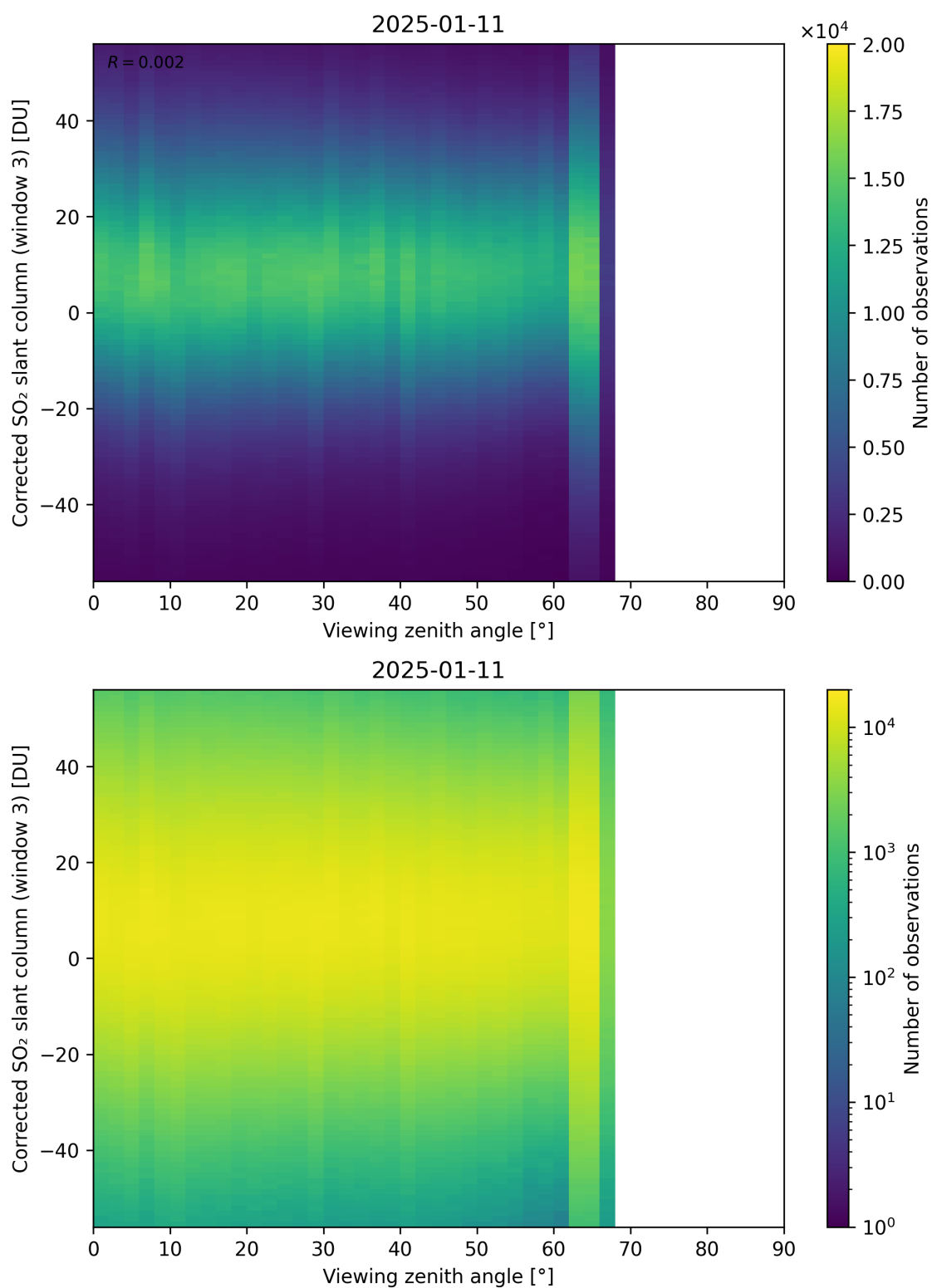
Figure 375: Scatter density plot of “Viewing zenith angle” against “Corrected SO 2 slant column (window 3)” for 2025-01-10 to 2025-01-12.
