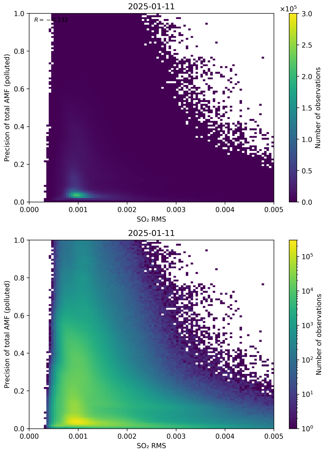
Figure 149: Scatter density plot of “SO 2 RMS” against “Precision of total AMF (polluted)” for 2025-01-10 to 2025-01-12.
