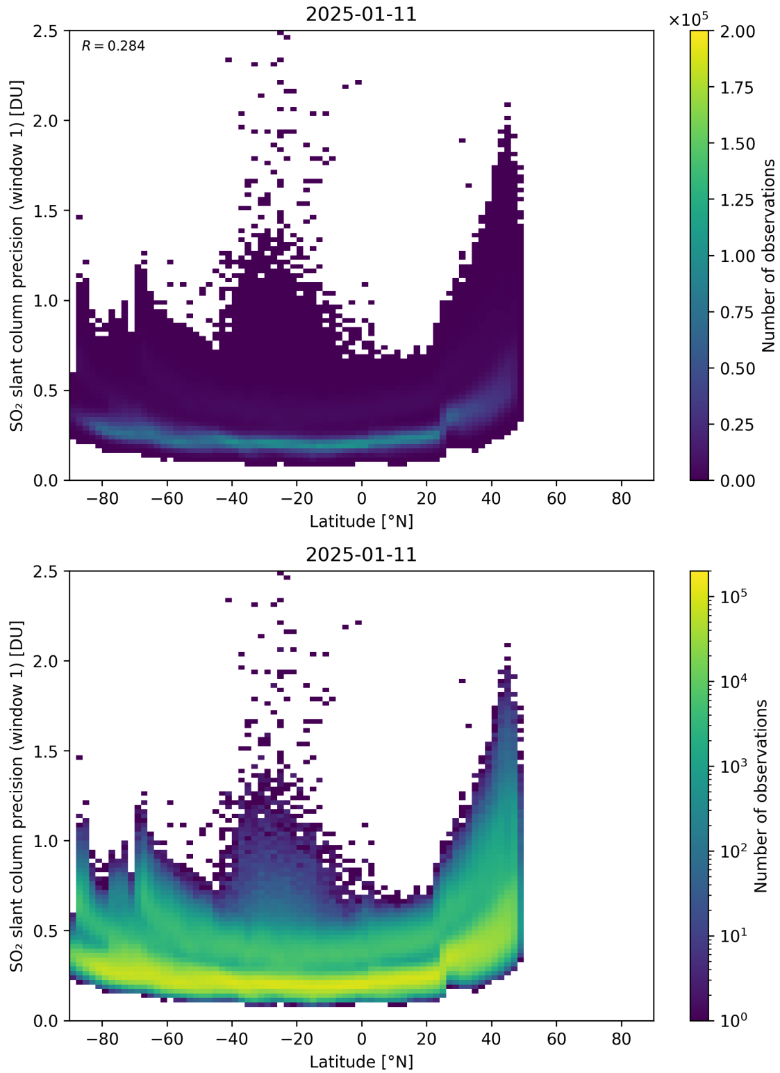
Figure 163: Scatter density plot of “Latitude” against “SO 2 slant column precision (window 1)” for 2025-01-10 to 2025-01-12.
