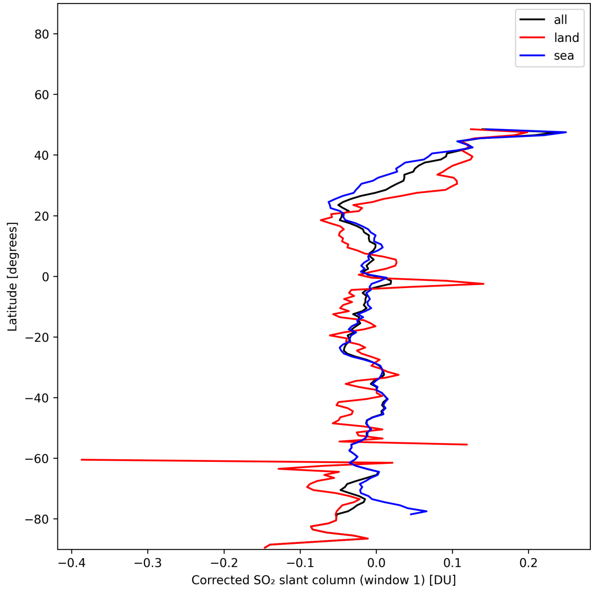
Figure 39: Zonal average of “Corrected SO 2 slant column (window 1)” for 2025-01-10 to 2025-01-12.
