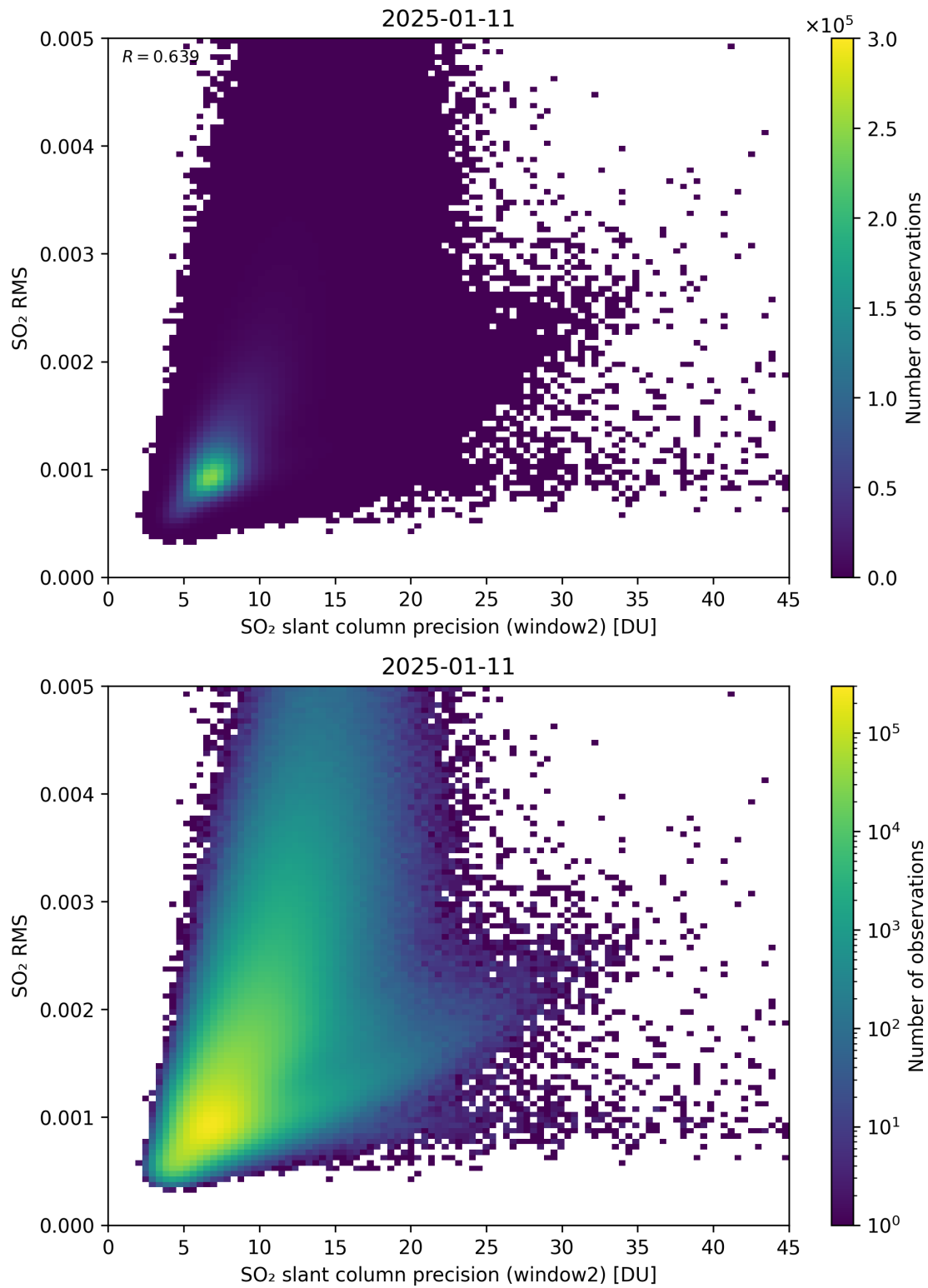
Figure 295: Scatter density plot of “SO 2 slant column precision (window2)” against “SO 2 RMS” for 2025-01-10 to 2025-01-12.
