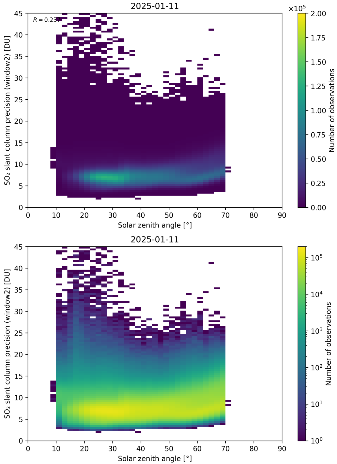
Figure 186: Scatter density plot of “Solar zenith angle” against “SO 2 slant column precision (window2)” for 2025-01-10 to 2025-01-12.
