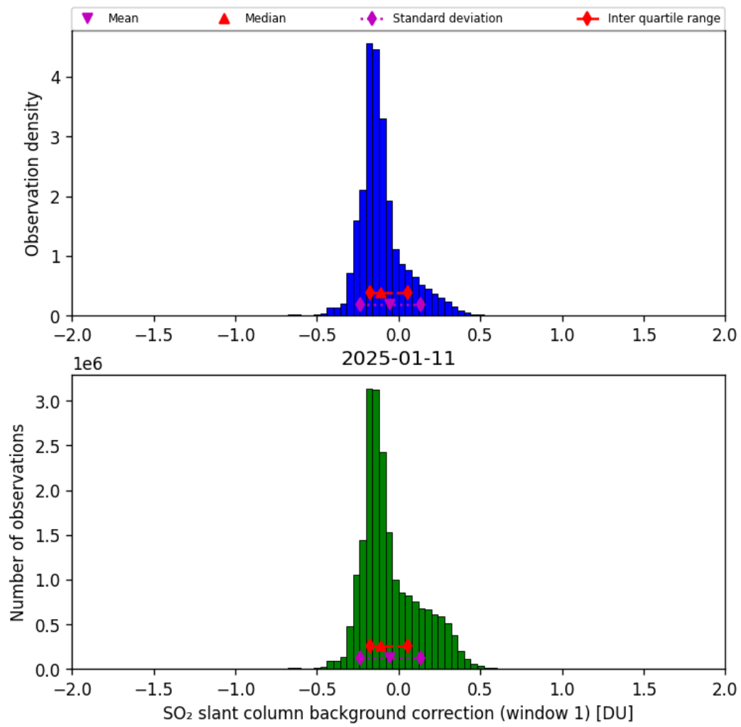
Figure 66: Histogram of “SO 2 slant column background correction (window 1)” for 2025-01-10 to 2025-01-12
