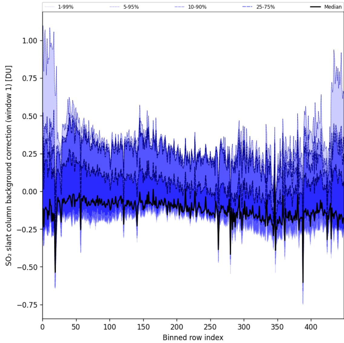
Figure 92: Along track statistics of “SO 2 slant column background correction (window 1)” for 2025-01-10 to 2025-01-12
