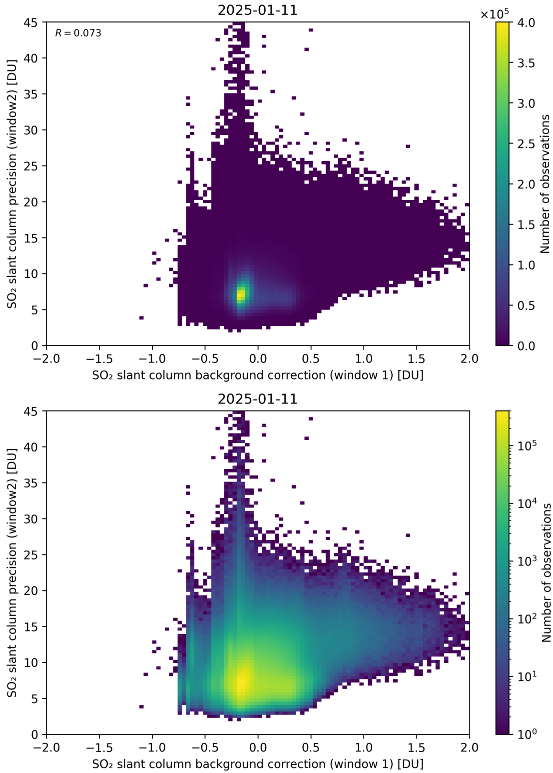
Figure 117: Scatter density plot of “SO 2 slant column background correction (window 1)” against “SO 2 slant column precision (window2)” for 2025-01-10 to 2025-01-12.
