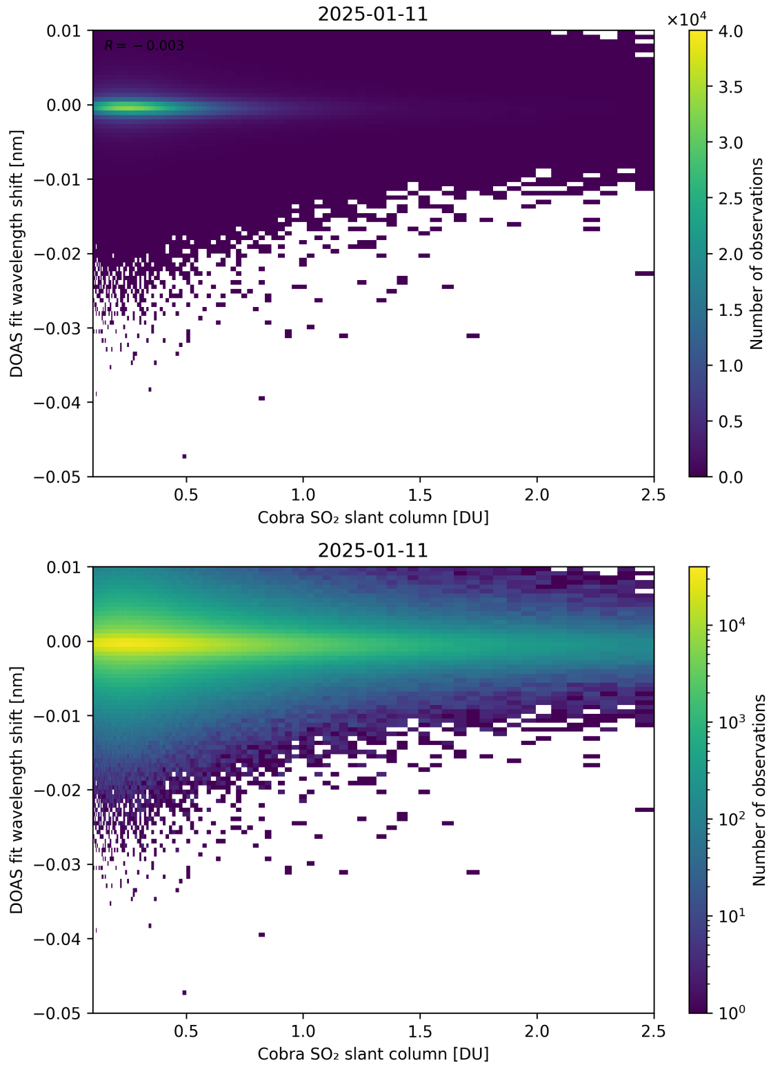
Figure 196: Scatter density plot of “Cobra SO 2 slant column” against “DOAS fit wavelength shift” for 2025-01-10 to 2025-01-12.
