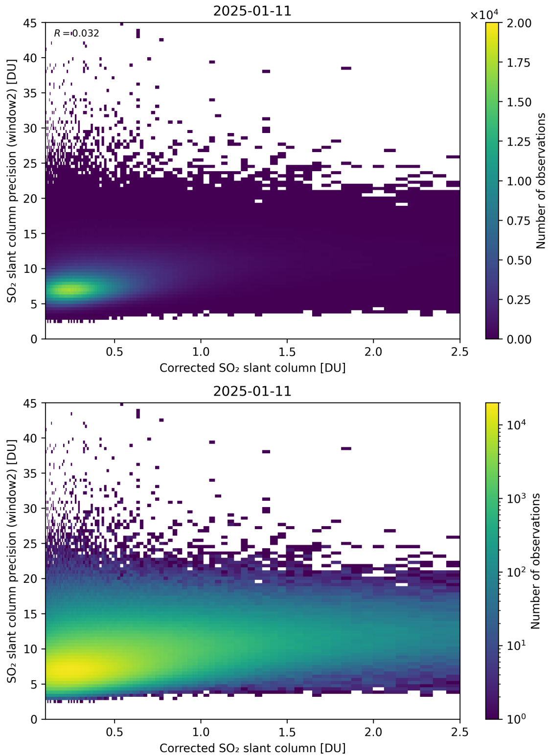
Figure 239: Scatter density plot of “Corrected SO 2 slant column” against “SO 2 slant column precision (window2)” for 2025-01-10 to 2025-01-12.
