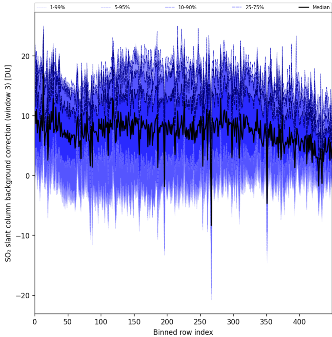
Figure 100: Along track statistics of “SO 2 slant column background correction (window 3)” for 2025-01-10 to 2025-01-12
