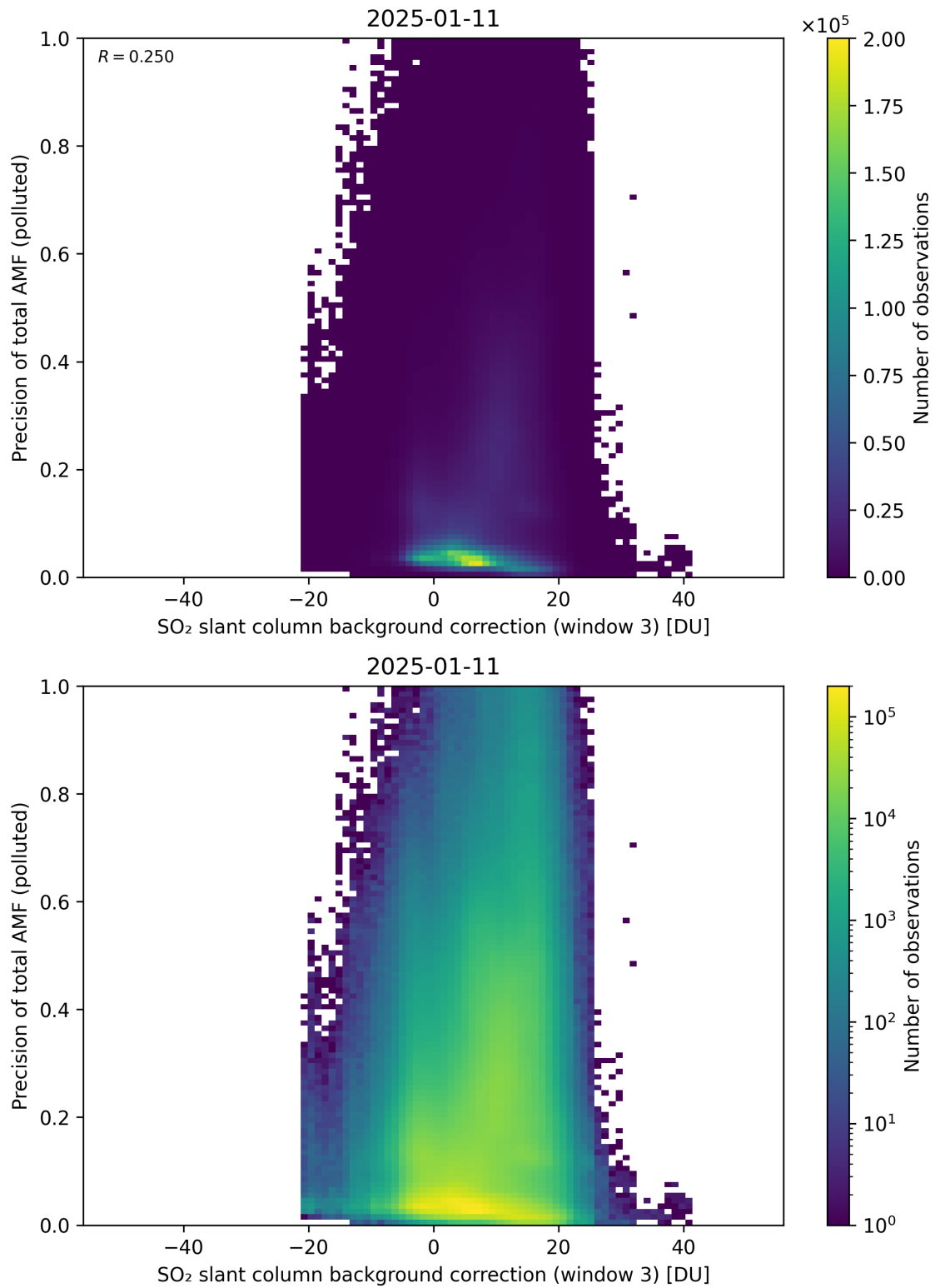
Figure 137: Scatter density plot of “SO 2 slant column background correction (window 3)” against “Precision of total AMF (polluted)” for 2025-01-10 to 2025-01-12.
