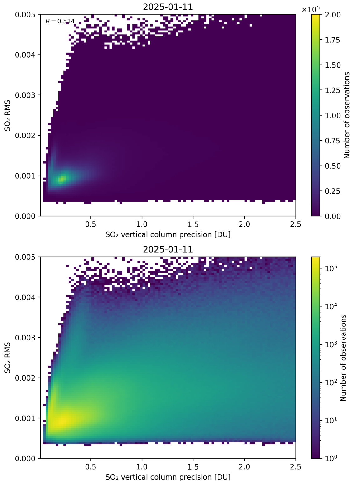
Figure 334: Scatter density plot of “SO 2 vertical column precision” against “SO 2 RMS” for 2025-01-10 to 2025-01-12.
