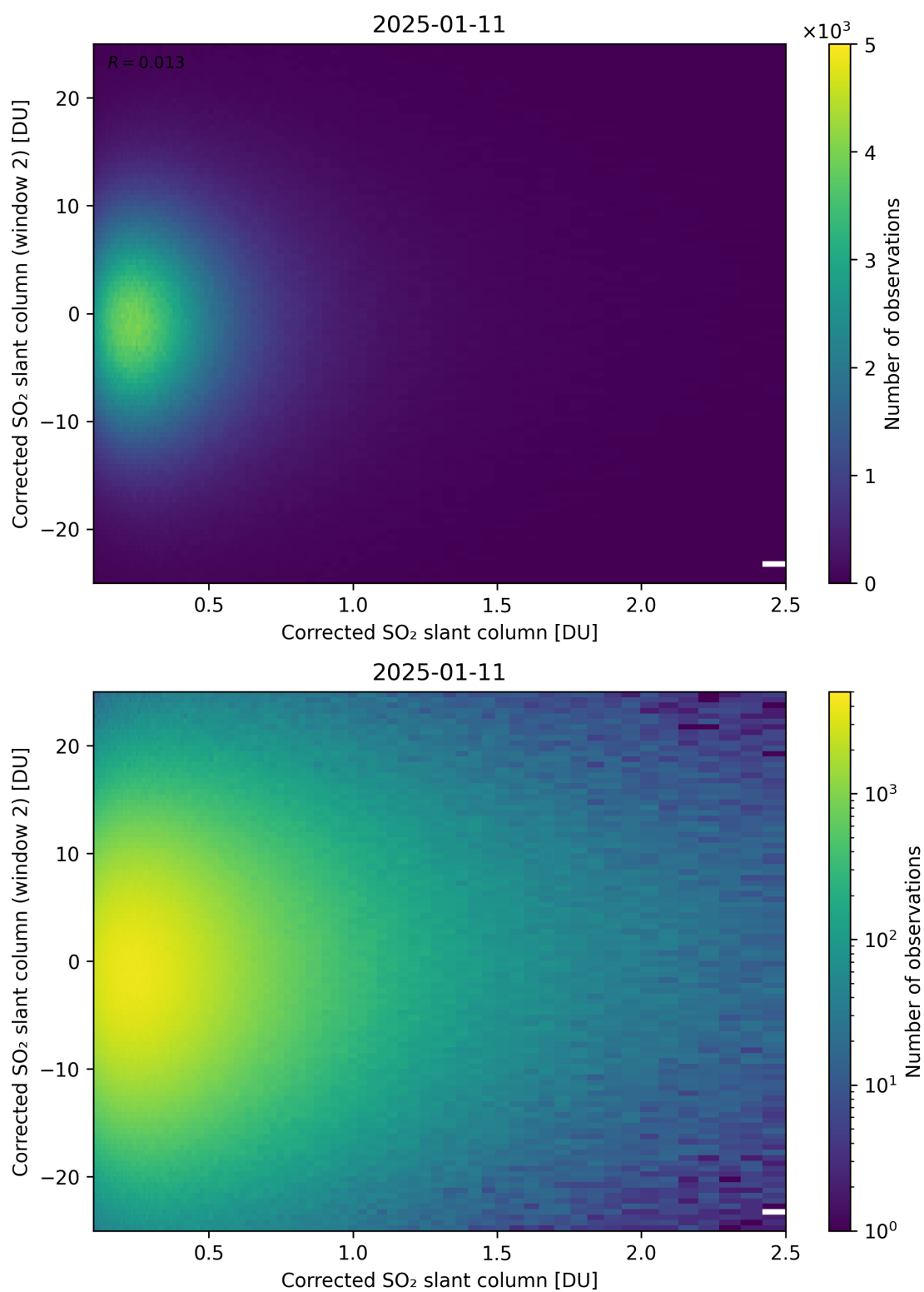
Figure 235: Scatter density plot of “Corrected SO 2 slant column” against “Corrected SO 2 slant column (window 2)” for 2025-01-10 to 2025-01-12.
