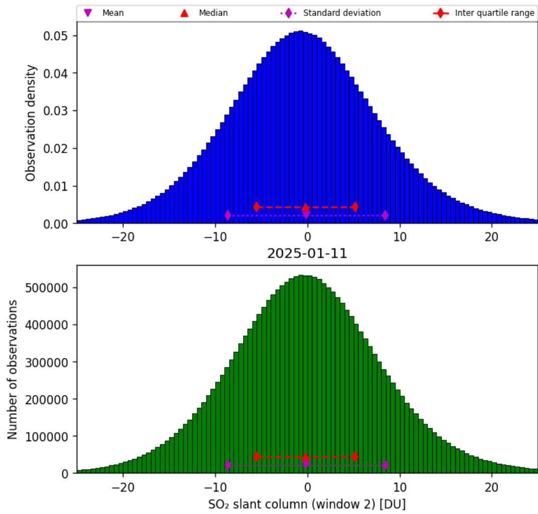
Figure 67: Histogram of “SO 2 slant column (window 2)” for 2025-01-10 to 2025-01-12
