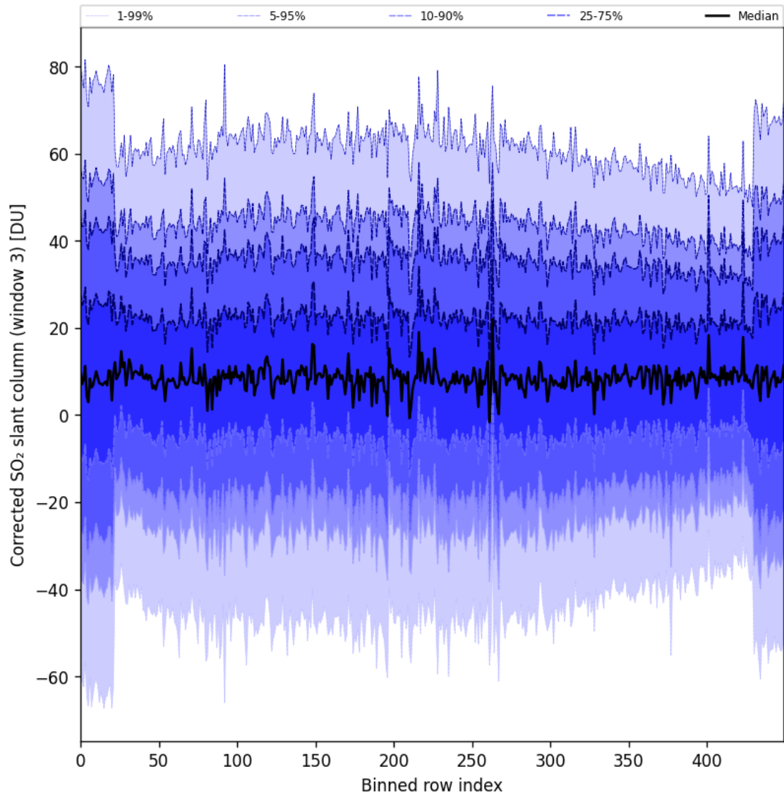
Figure 99: Along track statistics of “Corrected SO 2 slant column (window 3)” for 2025-01-10 to 2025-01-12
