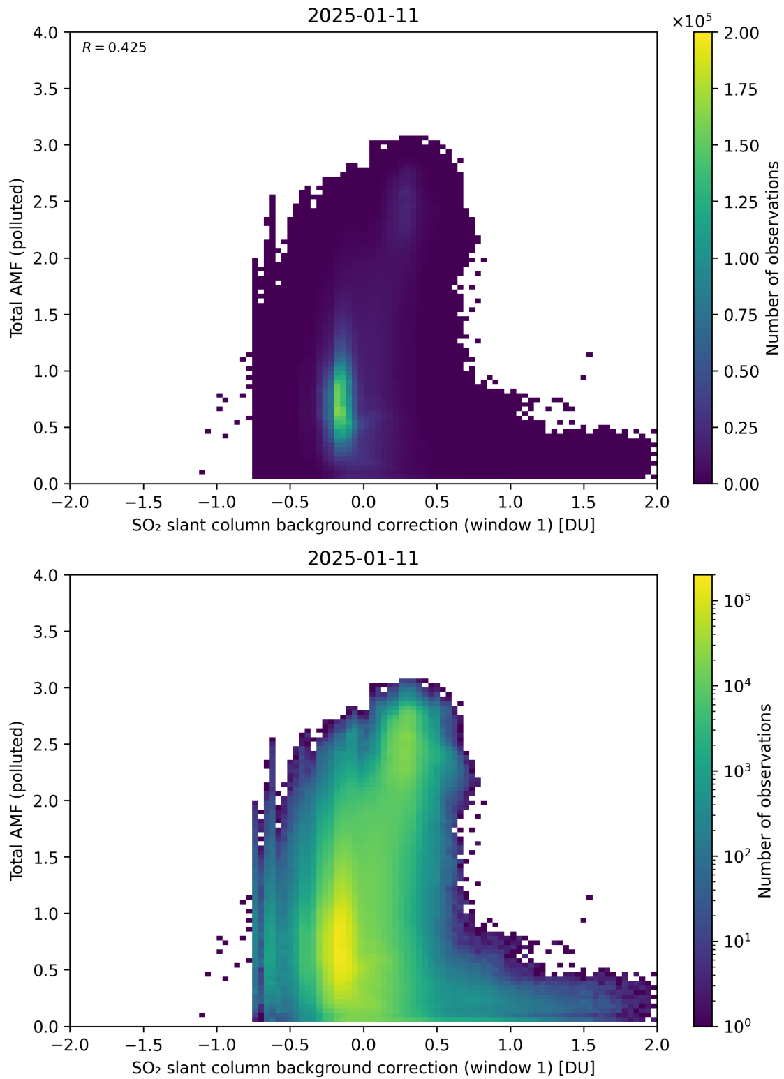
Figure 120: Scatter density plot of “SO 2 slant column background correction (window 1)” against “Total AMF (polluted)” for 2025-01-10 to 2025-01-12.
