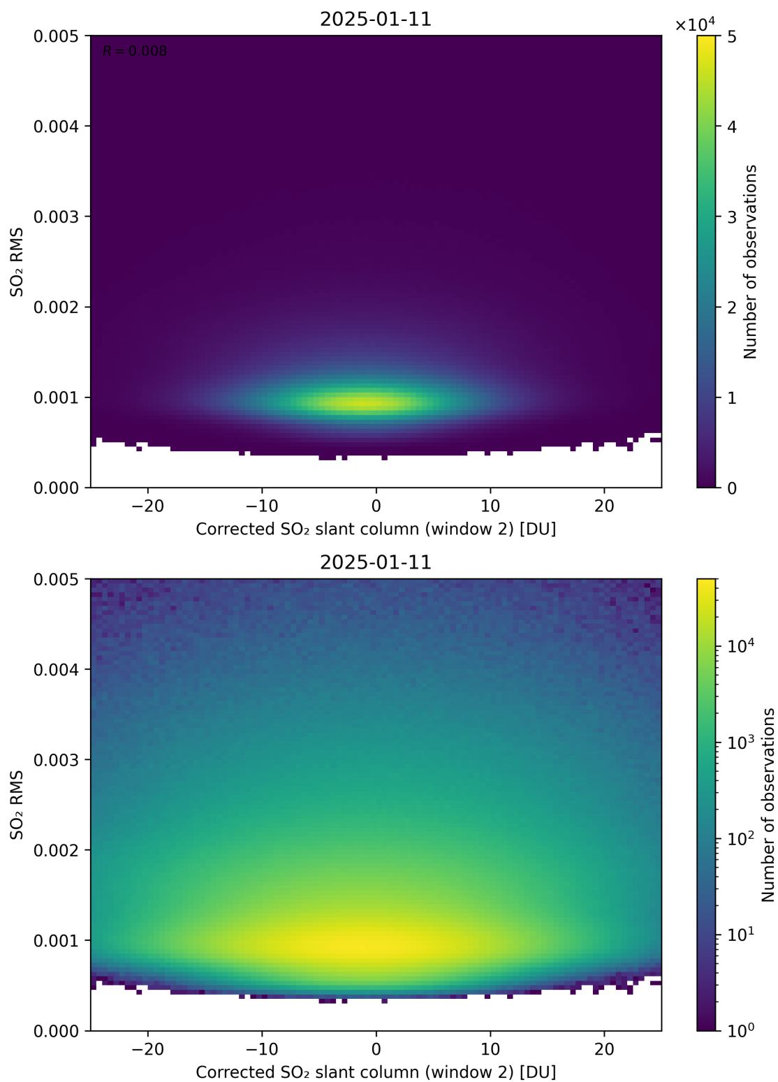
Figure 248: Scatter density plot of “Corrected SO 2 slant column (window 2)” against “SO 2 RMS” for 2025-01-10 to 2025-01-12.
