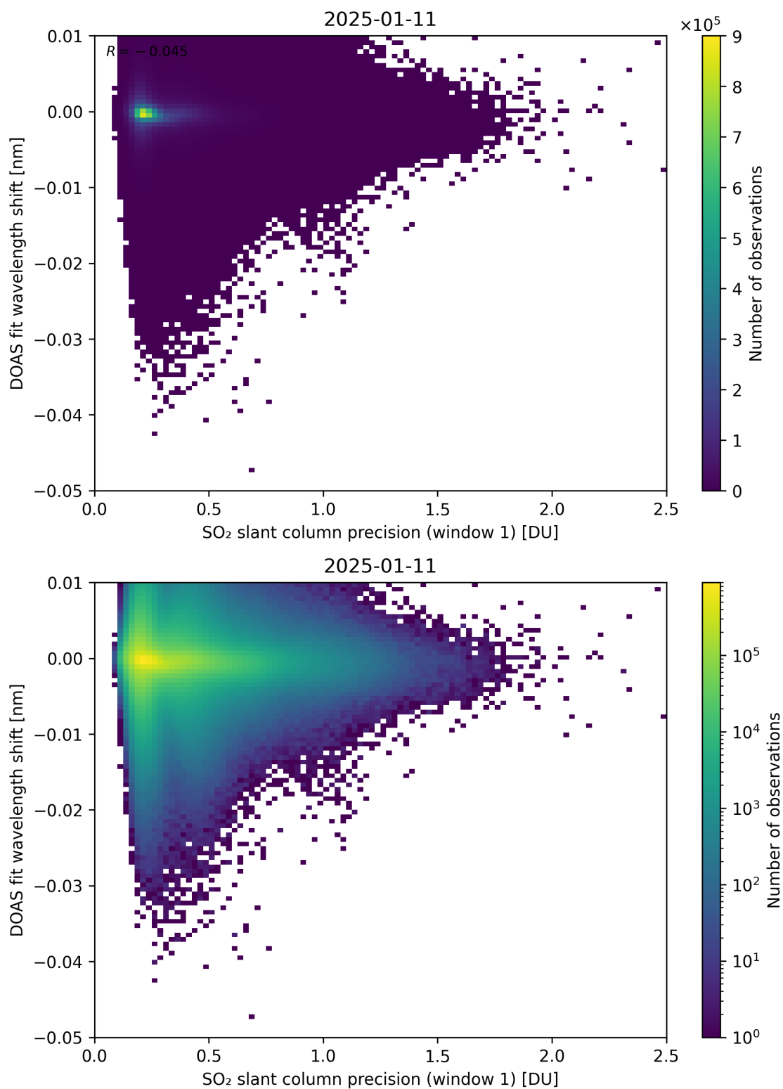
Figure 271: Scatter density plot of “SO 2 slant column precision (window 1)” against “DOAS fit wavelength shift” for 2025-01-10 to 2025-01-12.
