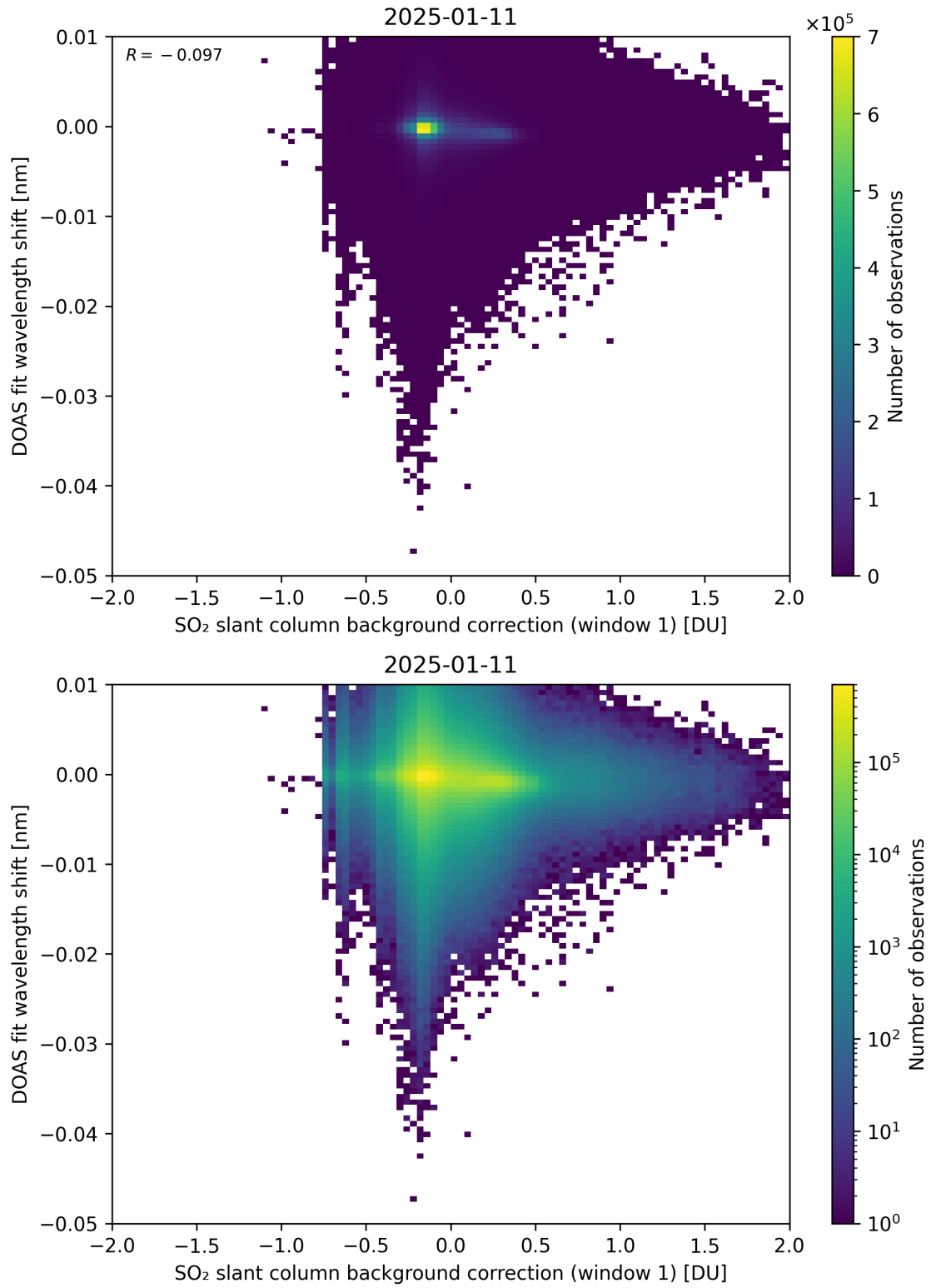
Figure 111: Scatter density plot of “SO 2 slant column background correction (window 1)” against “DOAS fit wavelength shift” for 2025-01-10 to 2025-01-12.
