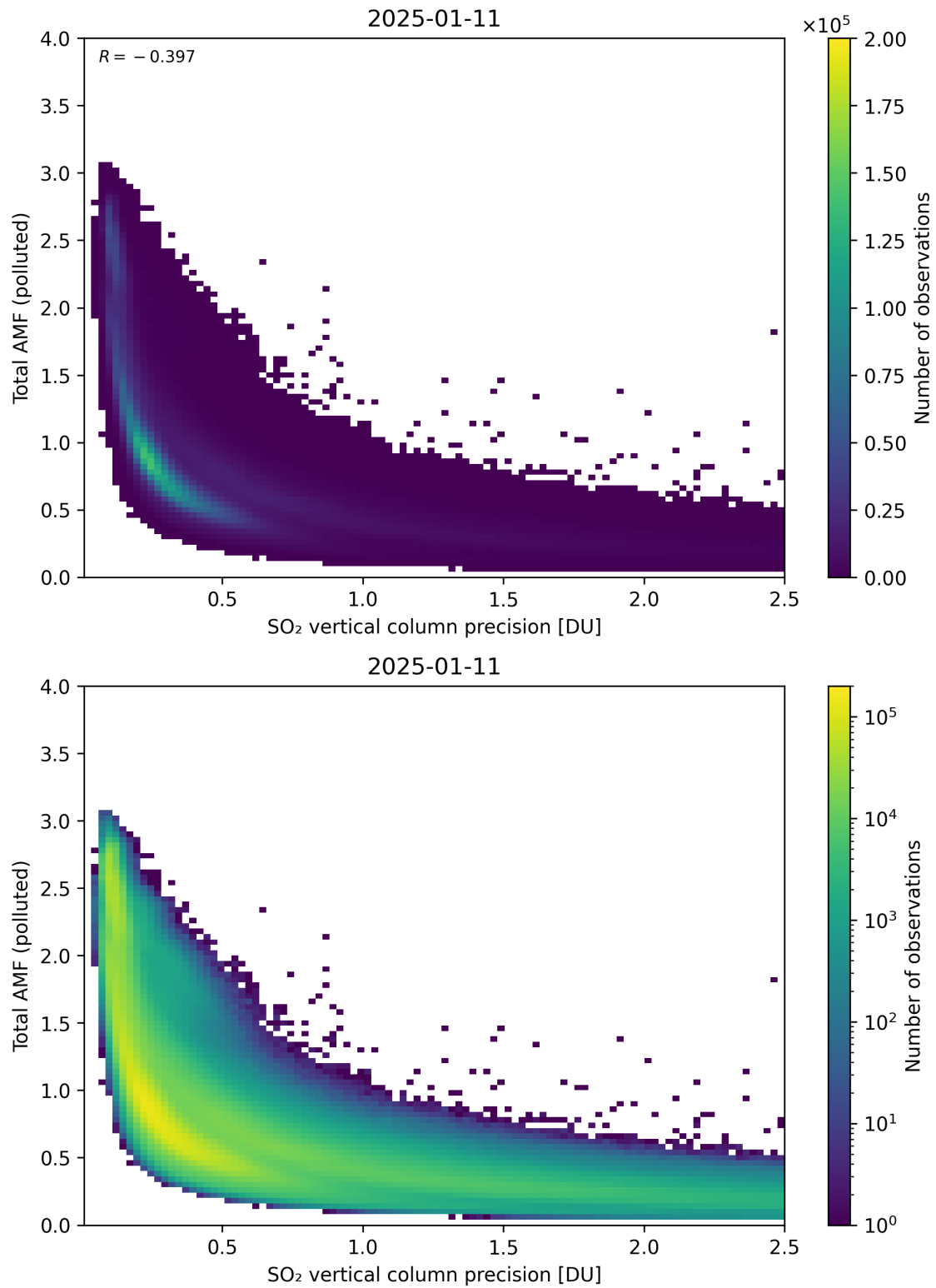
Figure 346: Scatter density plot of “SO 2 vertical column precision” against “Total AMF (polluted)” for 2025-01-10 to 2025-01-12.
