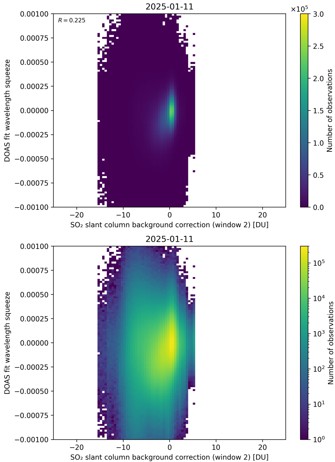
Figure 124: Scatter density plot of “SO 2 slant column background correction (window 2)” against “DOAS fit wavelength squeeze” for 2025-01-10 to 2025-01-12.
