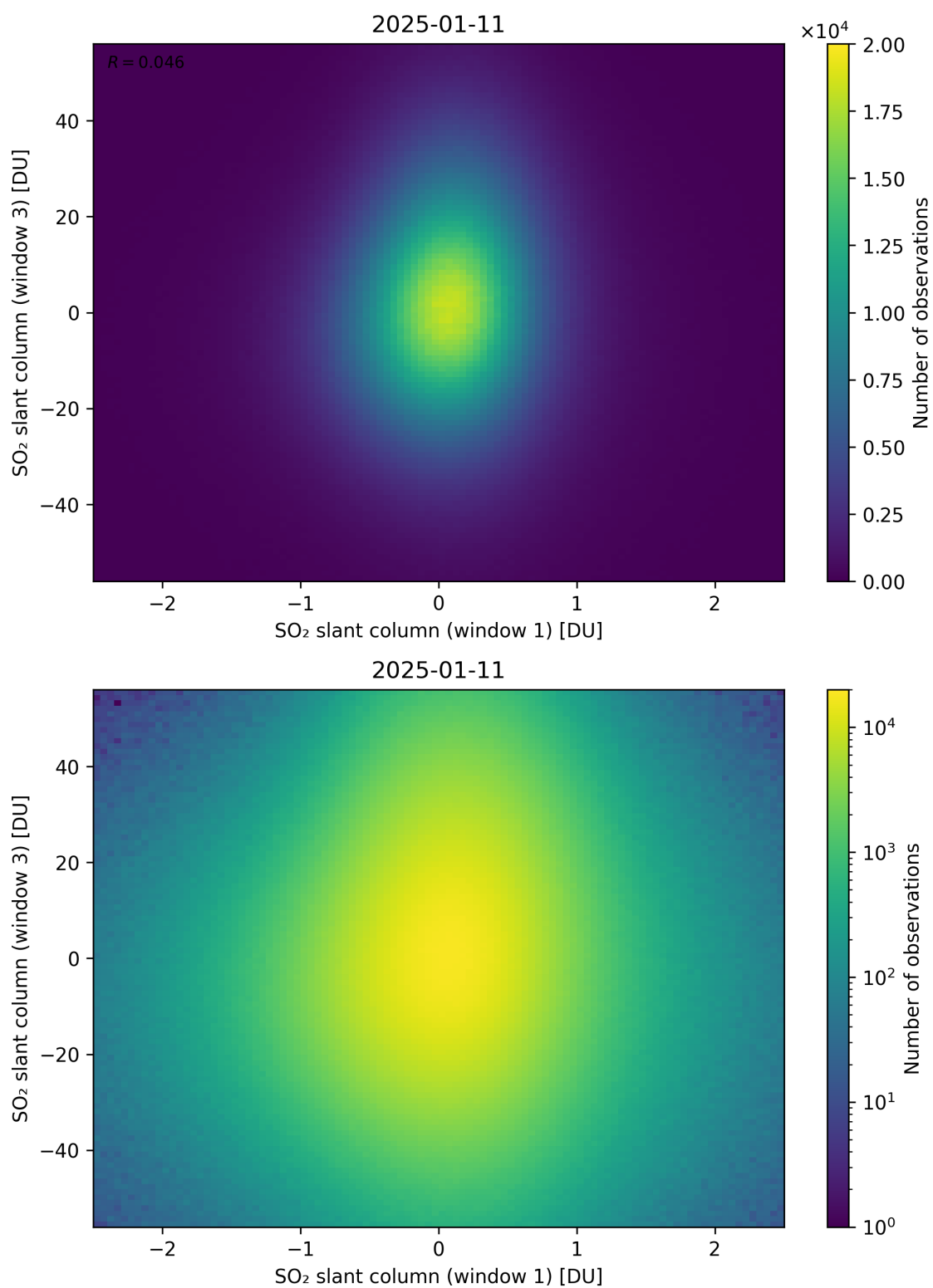
Figure 287: Scatter density plot of “SO 2 slant column (window 1)” against “SO 2 slant column (window 3)” for 2025-01-10 to 2025-01-12.
