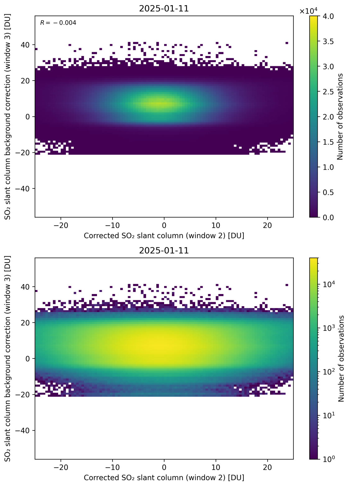
Figure 245: Scatter density plot of “Corrected SO 2 slant column (window 2)” against “SO 2 slant column background correction (window 3)” for 2025-01-10 to 2025-01-12.
