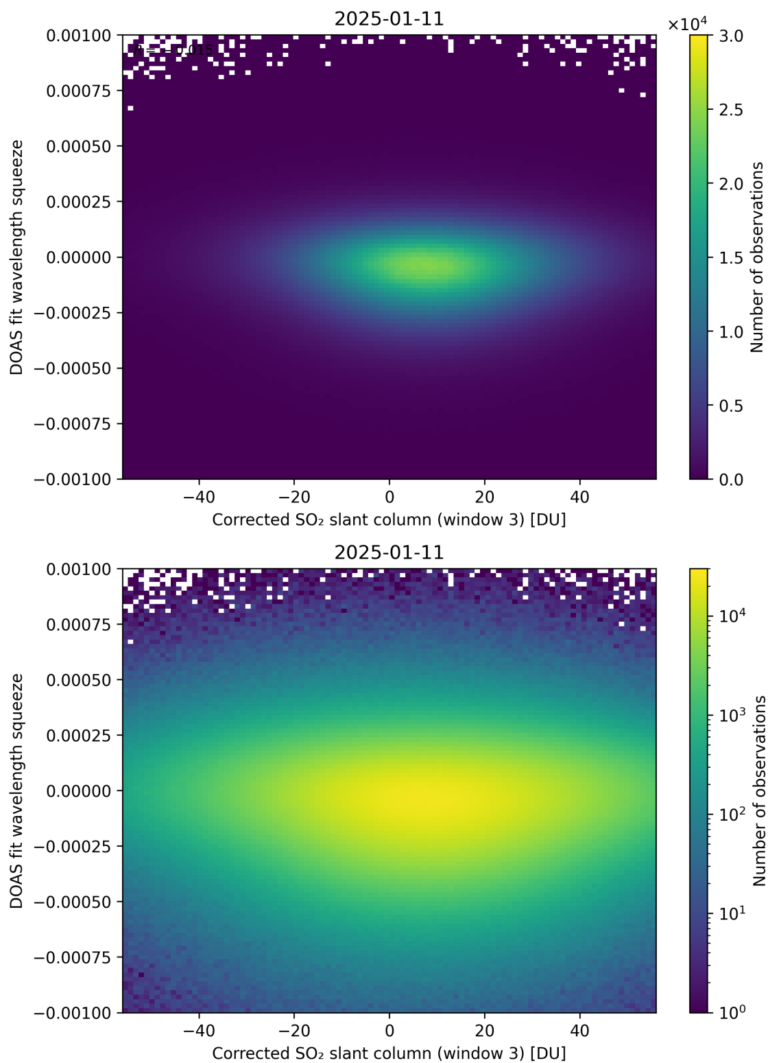
Figure 257: Scatter density plot of “Corrected SO 2 slant column (window 3)” against “DOAS fit wavelength squeeze” for 2025-01-10 to 2025-01-12.
