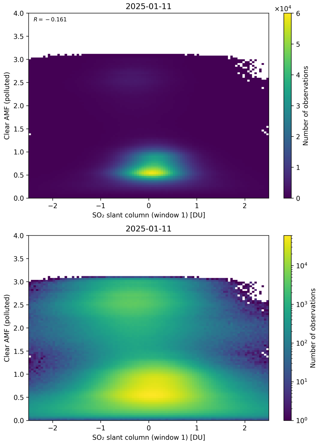
Figure 282: Scatter density plot of “SO 2 slant column (window 1)” against “Clear AMF (polluted)” for 2025-01-10 to 2025-01-12.
