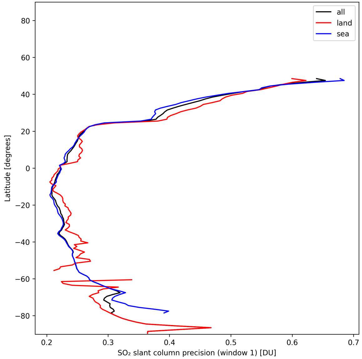
Figure 38: Zonal average of “SO 2 slant column precision (window 1)” for 2025-01-10 to 2025-01-12.
