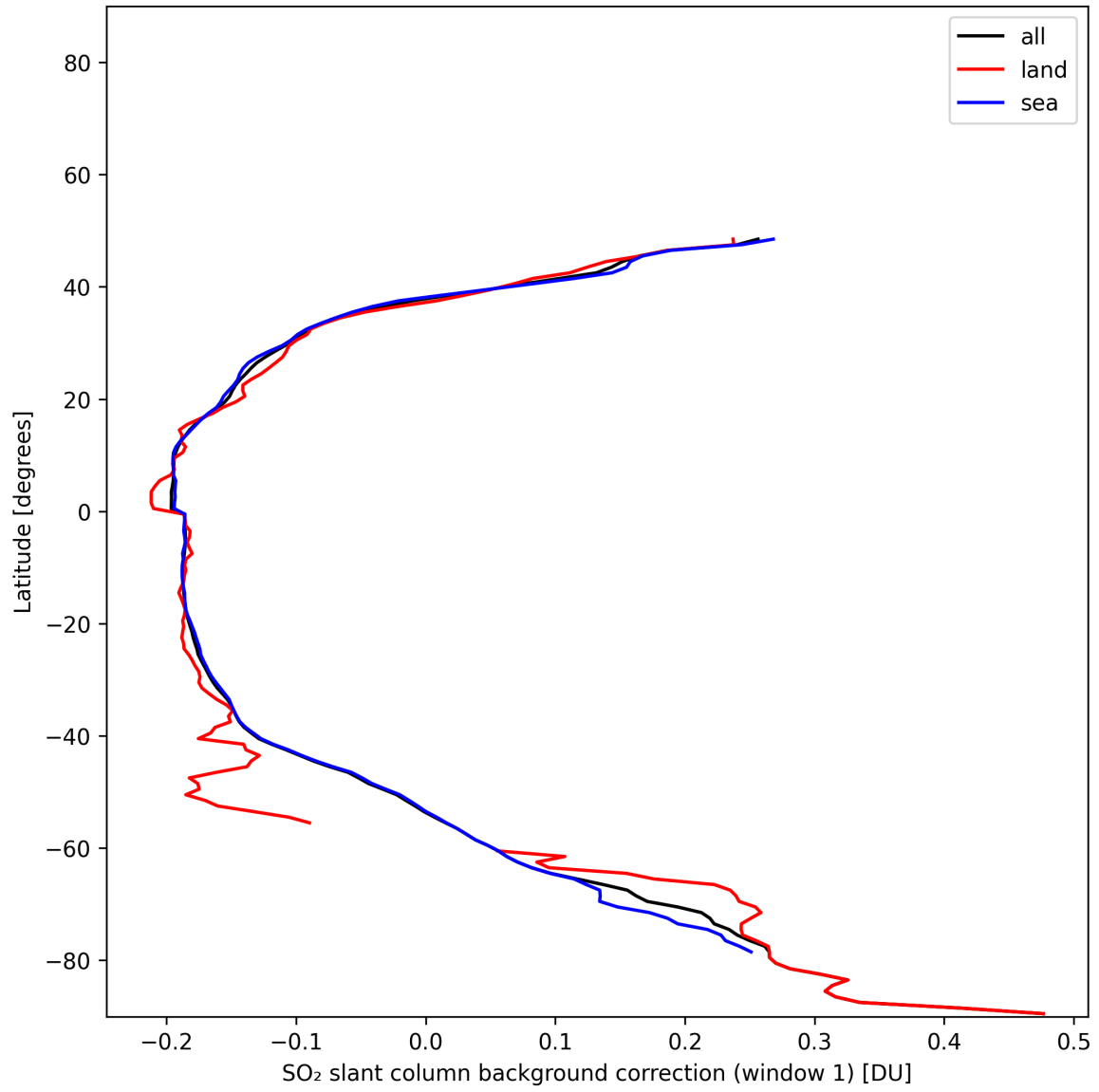
Figure 40: Zonal average of “SO 2 slant column background correction (window 1)” for 2025-01-10 to 2025-01-12.
