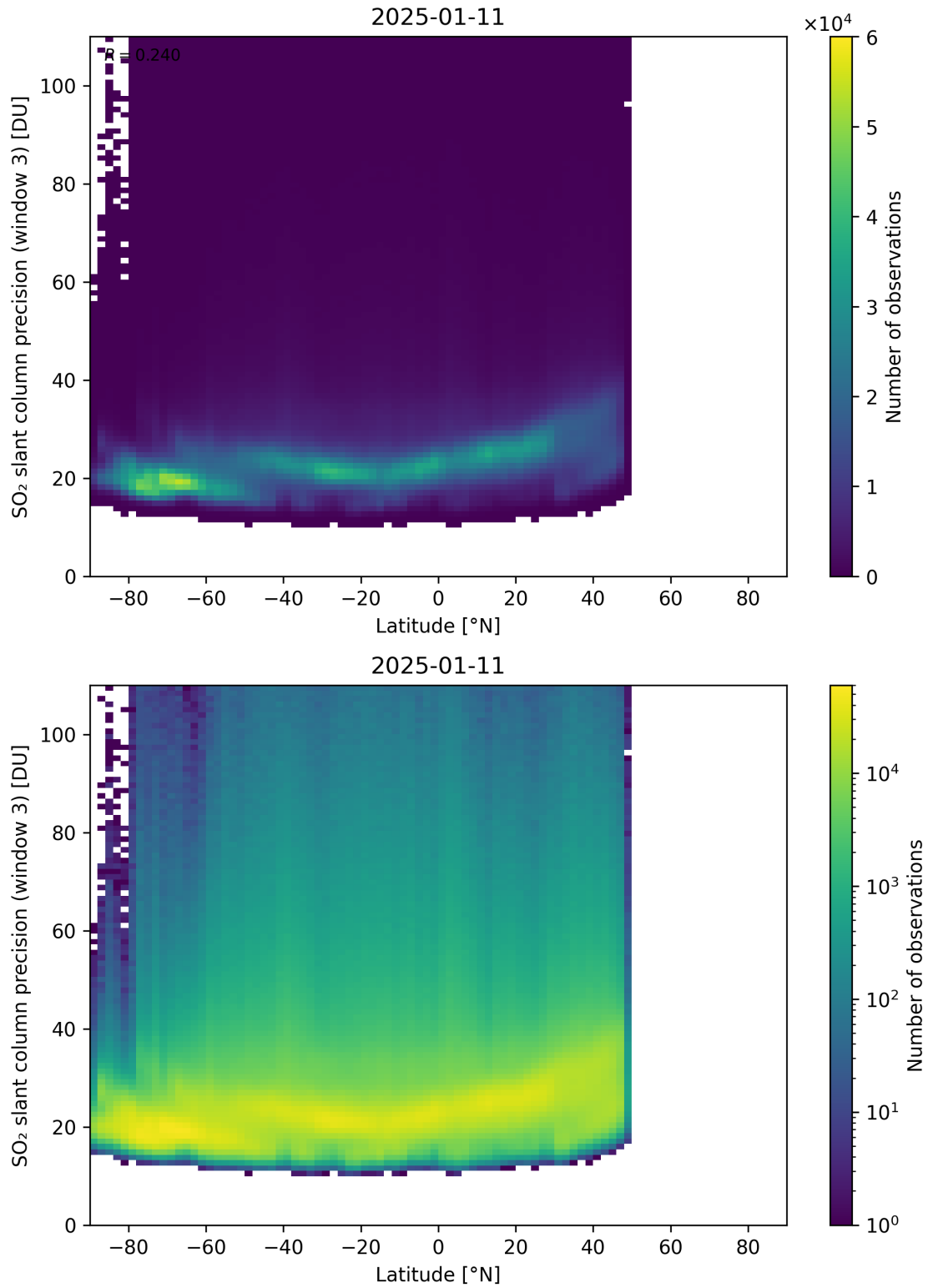
Figure 166: Scatter density plot of “Latitude” against “SO 2 slant column precision (window 3)” for 2025-01-10 to 2025-01-12.
