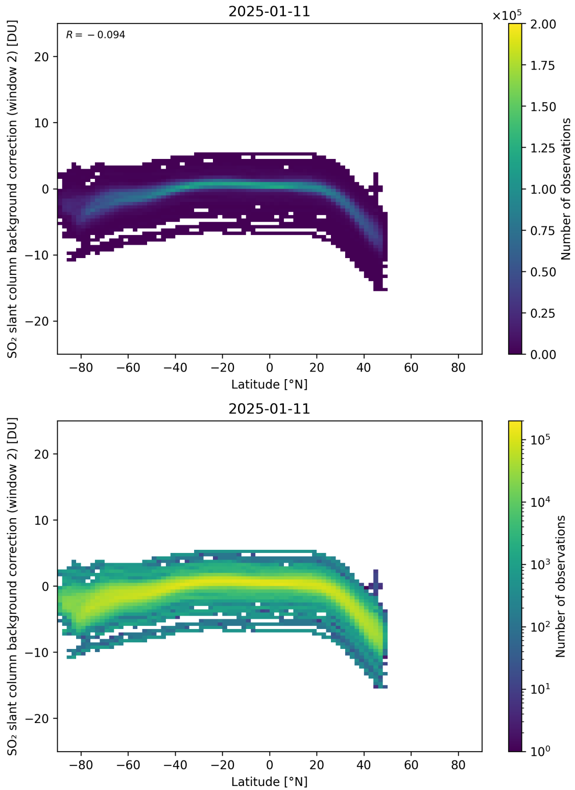
Figure 151: Scatter density plot of “Latitude” against “SO 2 slant column background correction (window 2)” for 2025-01-10 to 2025-01-12.
