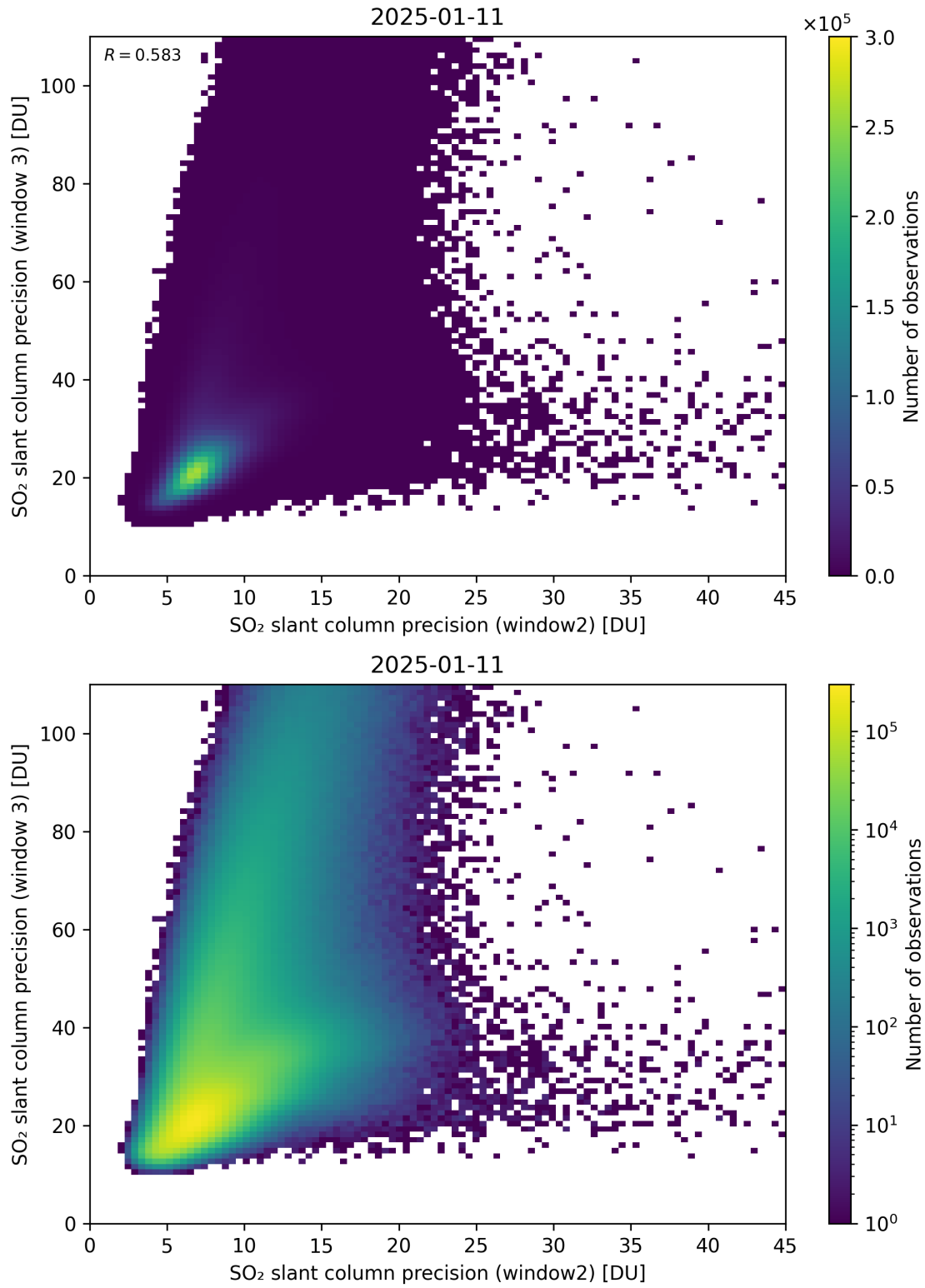
Figure 300: Scatter density plot of “SO 2 slant column precision (window2)” against “SO 2 slant column precision (window 3)” for 2025-01-10 to 2025-01-12.
