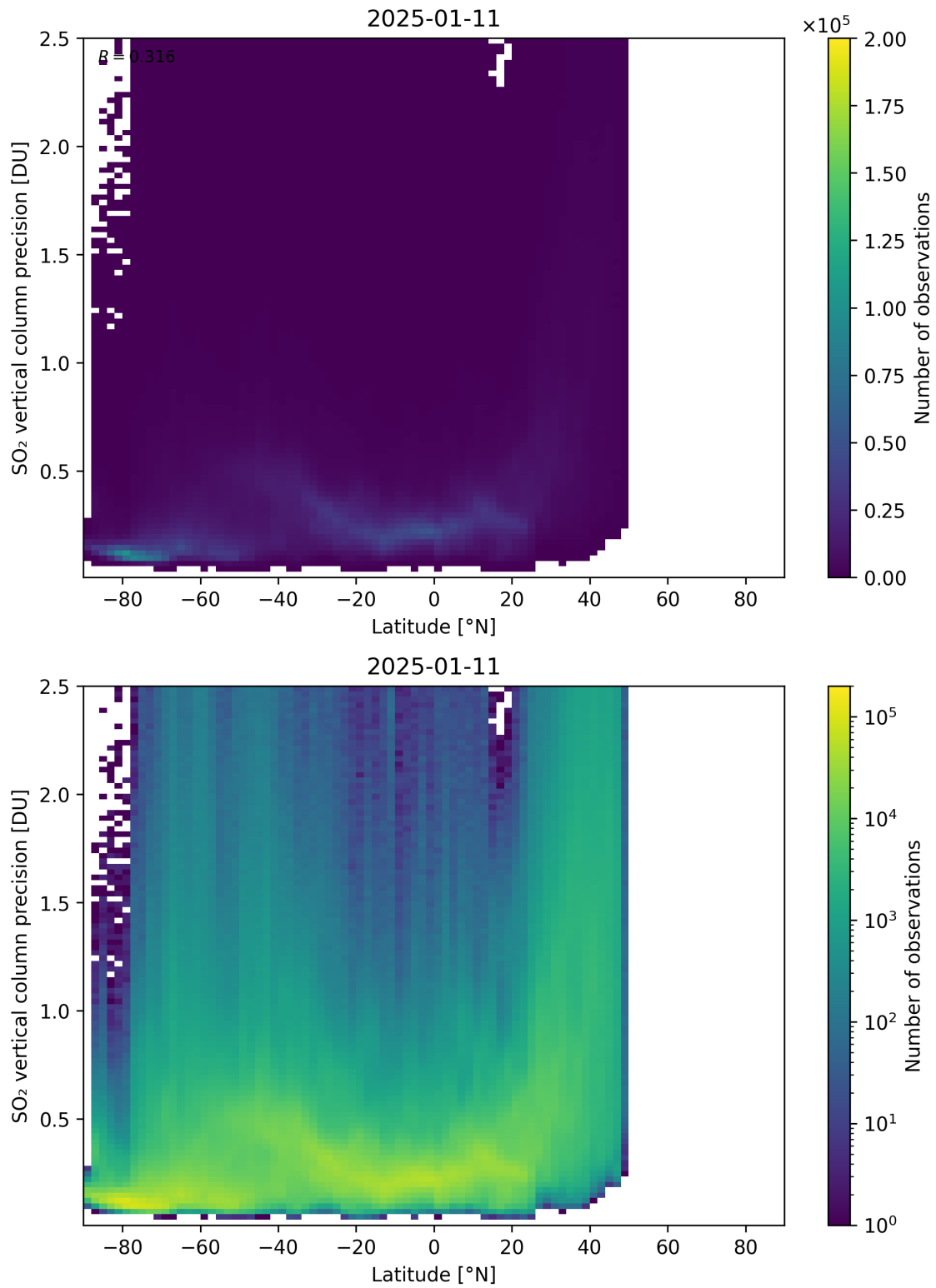
Figure 170: Scatter density plot of “Latitude” against “SO 2 vertical column precision” for 2025-01-10 to 2025-01-12.
