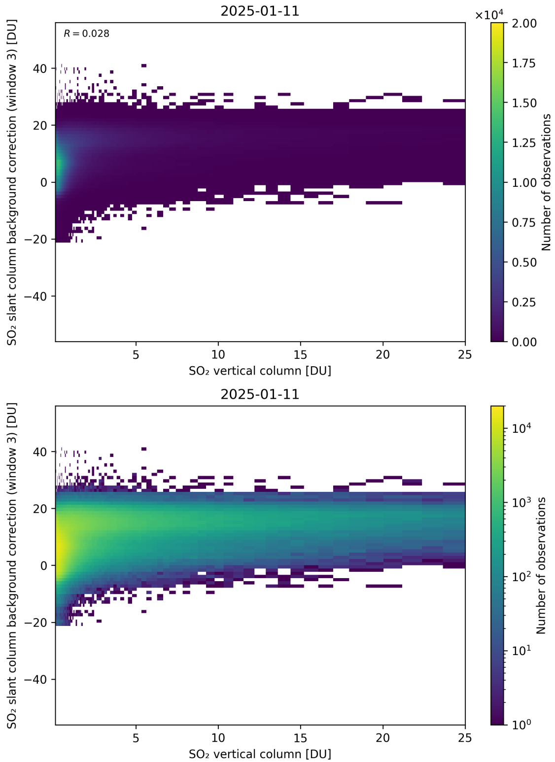
Figure 325: Scatter density plot of “SO 2 vertical column” against “SO 2 slant column background correction (window 3)” for 2025-01-10 to 2025-01-12.
