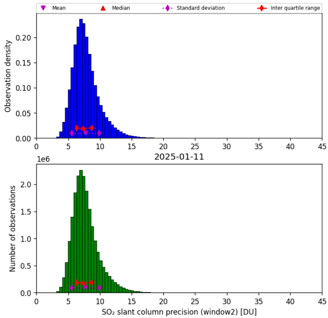
Figure 68: Histogram of “SO 2 slant column precision (window2)” for 2025-01-10 to 2025-01-12
