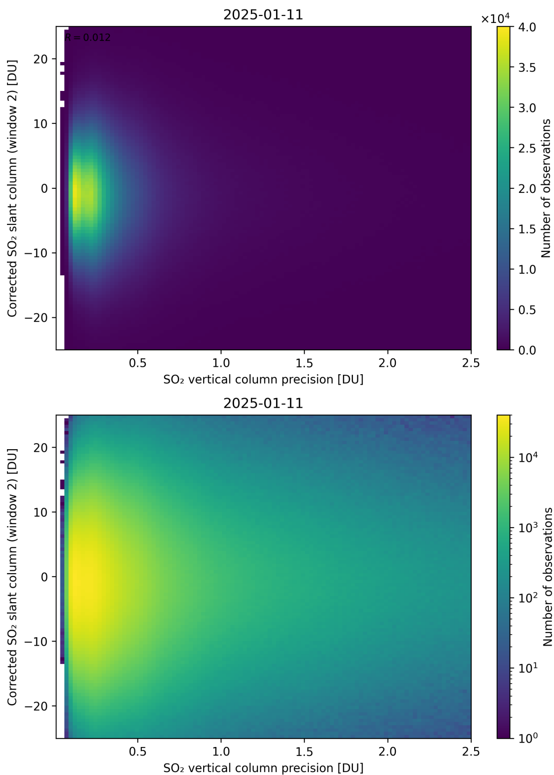
Figure 339: Scatter density plot of “SO 2 vertical column precision” against “Corrected SO 2 slant column (window 2)” for 2025-01-10 to 2025-01-12.
