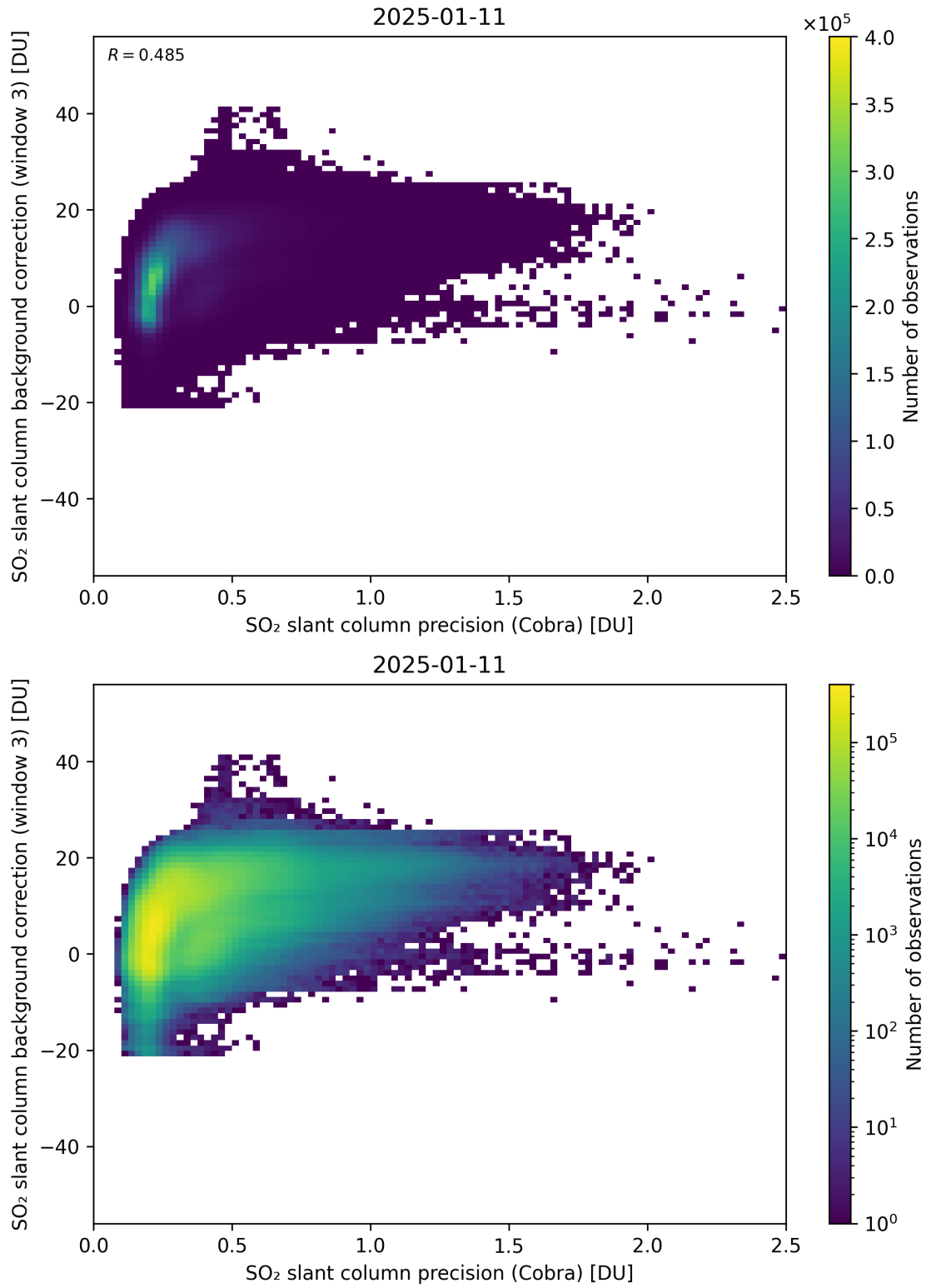
Figure 201: Scatter density plot of “SO 2 slant column precision (Cobra)” against “SO 2 slant column background correction (window 3)” for 2025-01-10 to 2025-01-12.
