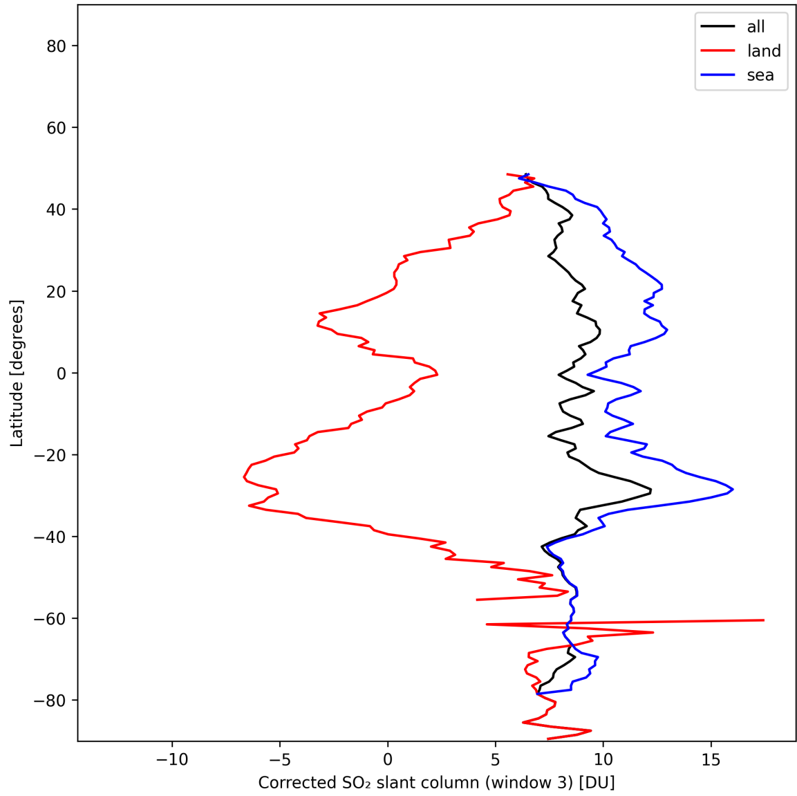
Figure 47: Zonal average of “Corrected SO 2 slant column (window 3)” for 2025-01-10 to 2025-01-12.
