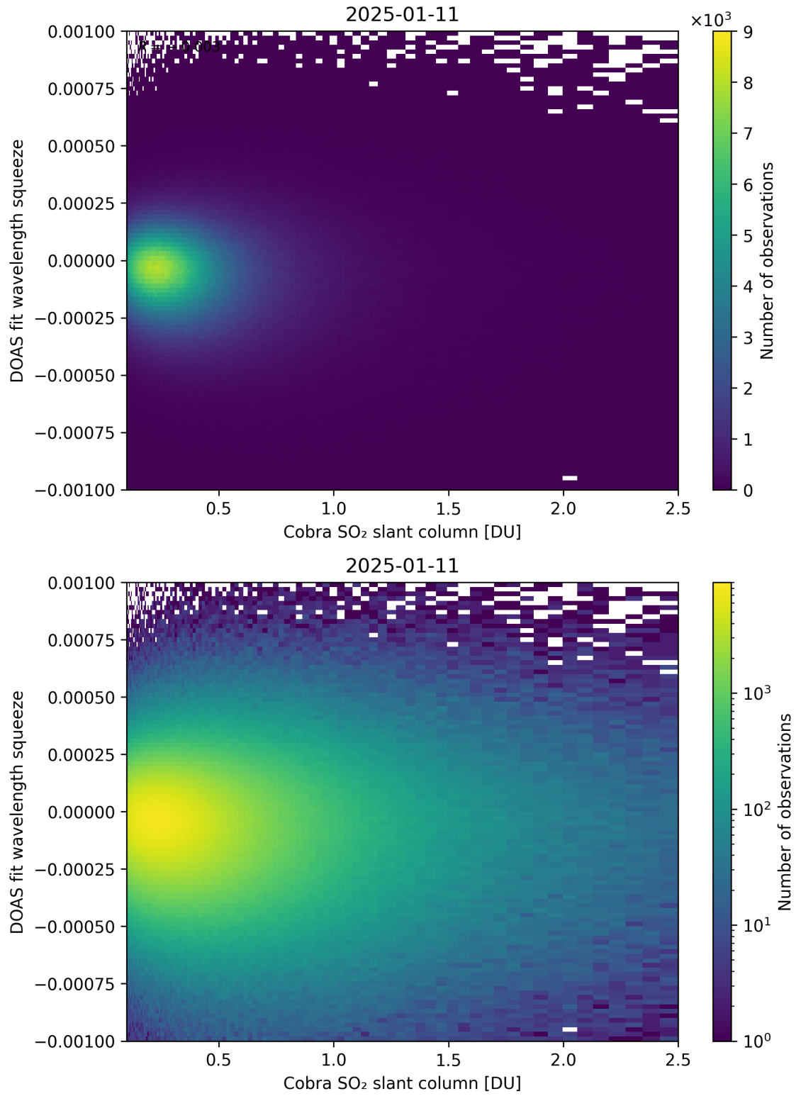
Figure 197: Scatter density plot of “Cobra SO 2 slant column” against “DOAS fit wavelength squeeze” for 2025-01-10 to 2025-01-12.
