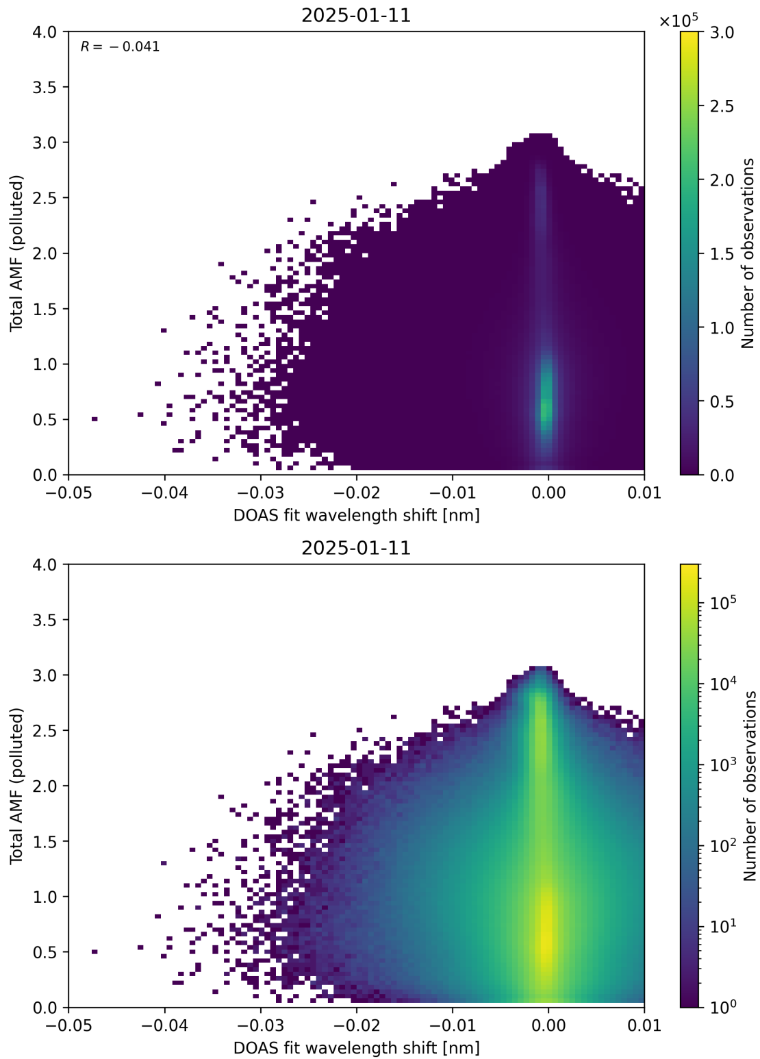
Figure 141: Scatter density plot of “DOAS fit wavelength shift” against “Total AMF (polluted)” for 2025-01-10 to 2025-01-12.
