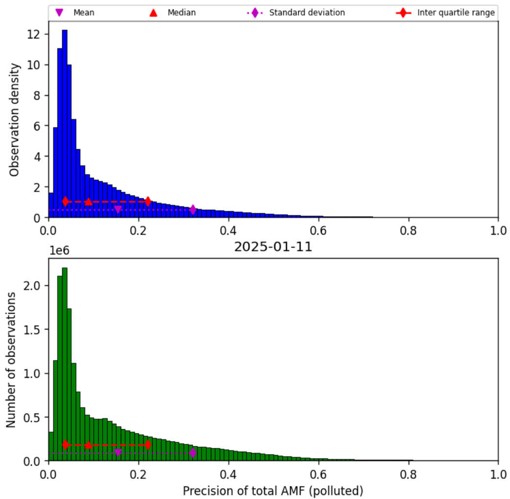
Figure 80: Histogram of “Precision of total AMF (polluted)” for 2025-01-10 to 2025-01-12
