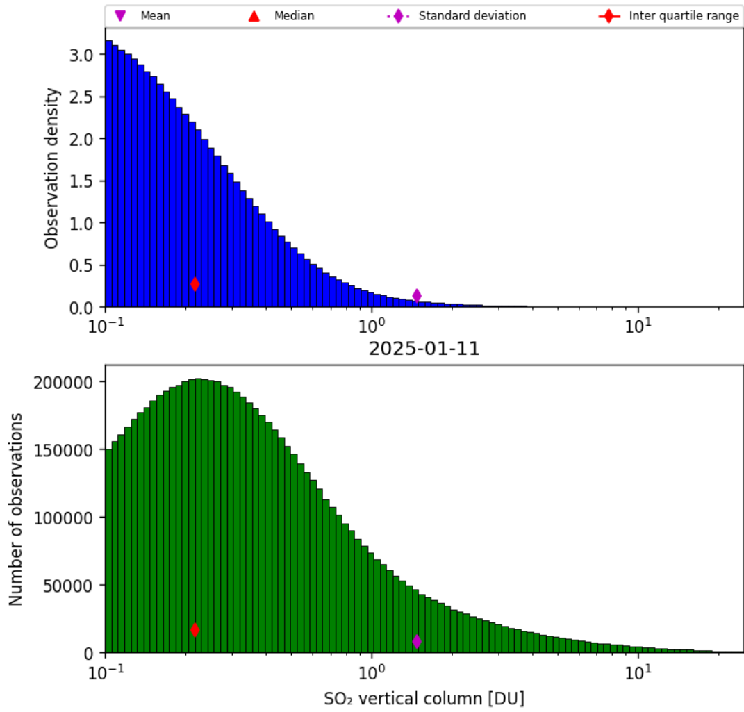
Figure 58: Histogram of “SO 2 vertical column” for 2025-01-10 to 2025-01-12
