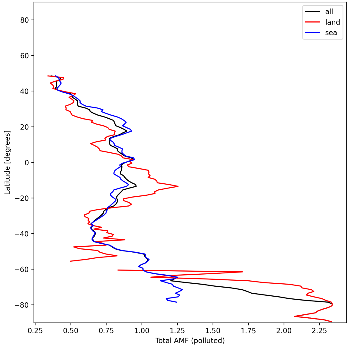
Figure 53: Zonal average of “Total AMF (polluted)” for 2025-01-10 to 2025-01-12.
