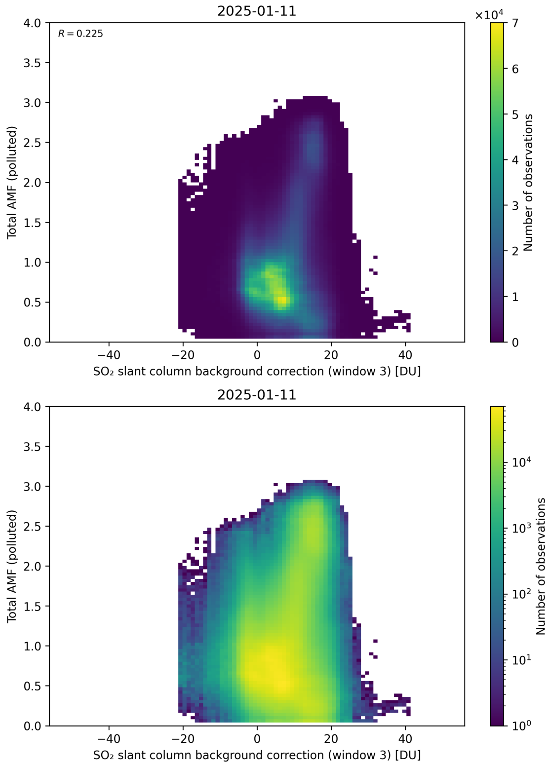
Figure 136: Scatter density plot of “SO 2 slant column background correction (window 3)” against “Total AMF (polluted)” for 2025-01-10 to 2025-01-12.
