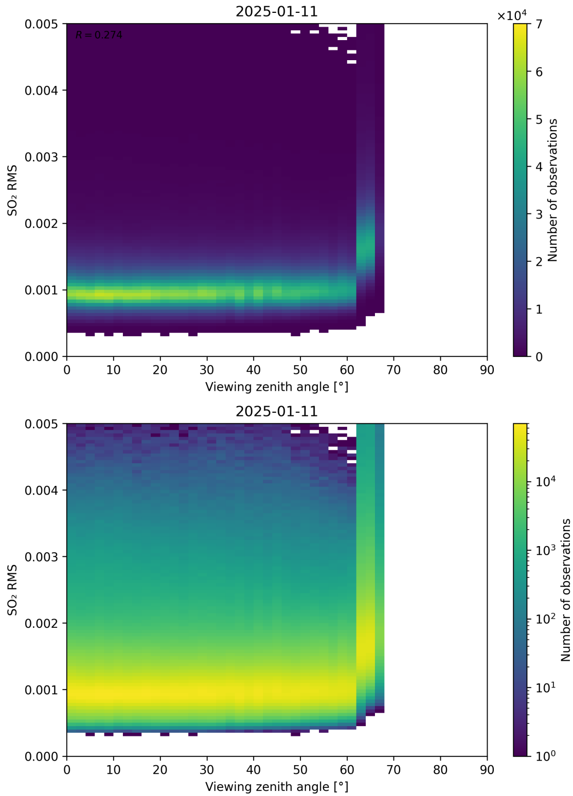
Figure 367: Scatter density plot of “Viewing zenith angle” against “SO 2 RMS” for 2025-01-10 to 2025-01-12.
