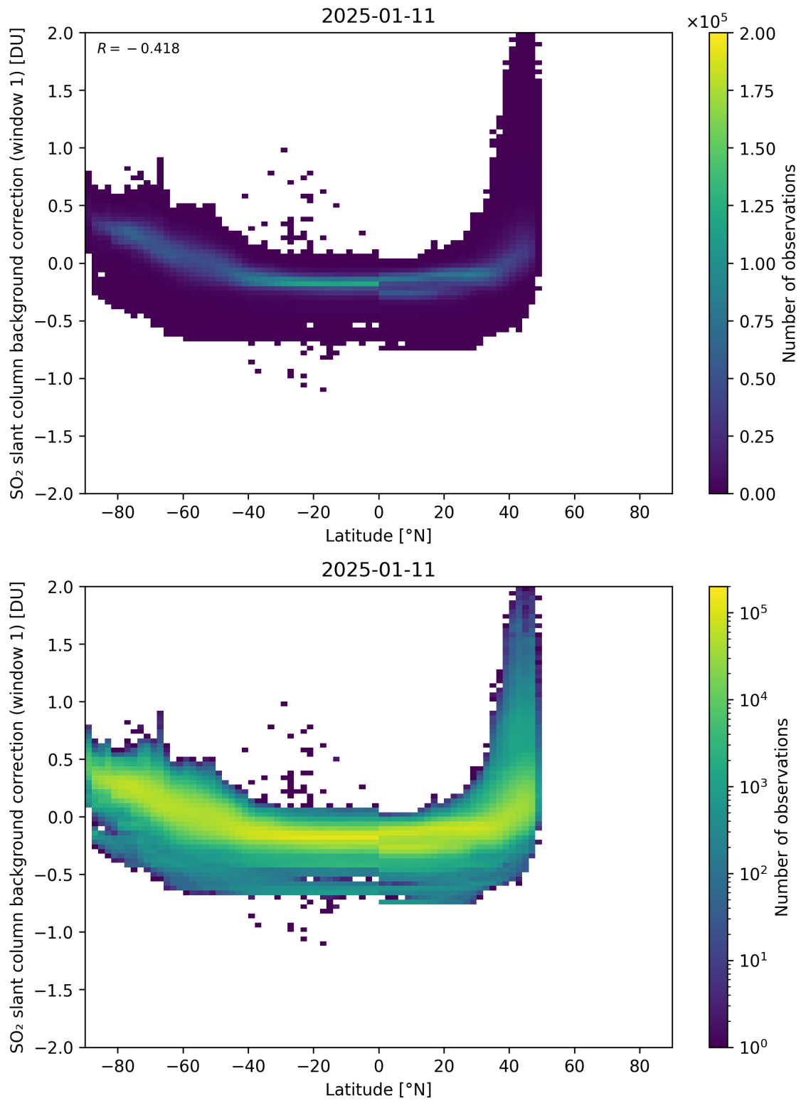
Figure 150: Scatter density plot of “Latitude” against “SO 2 slant column background correction (window 1)” for 2025-01-10 to 2025-01-12.
