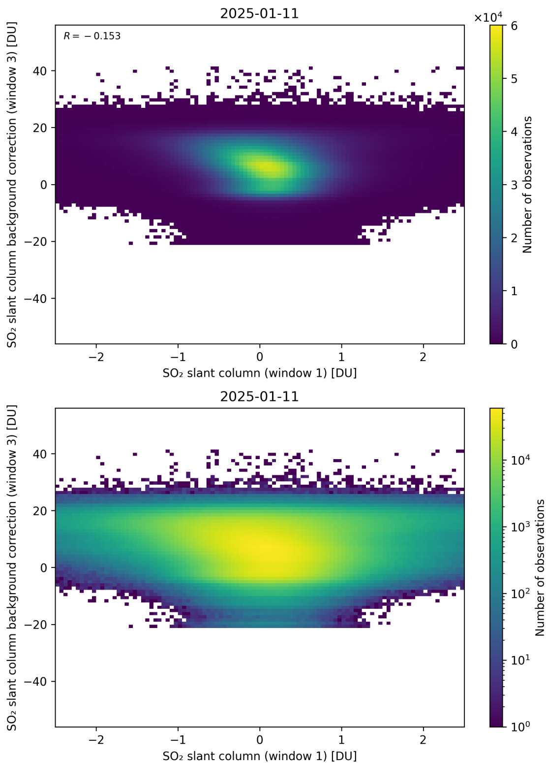
Figure 264: Scatter density plot of “SO 2 slant column (window 1)” against “SO 2 slant column background correction (window 3)” for 2025-01-10 to 2025-01-12.
