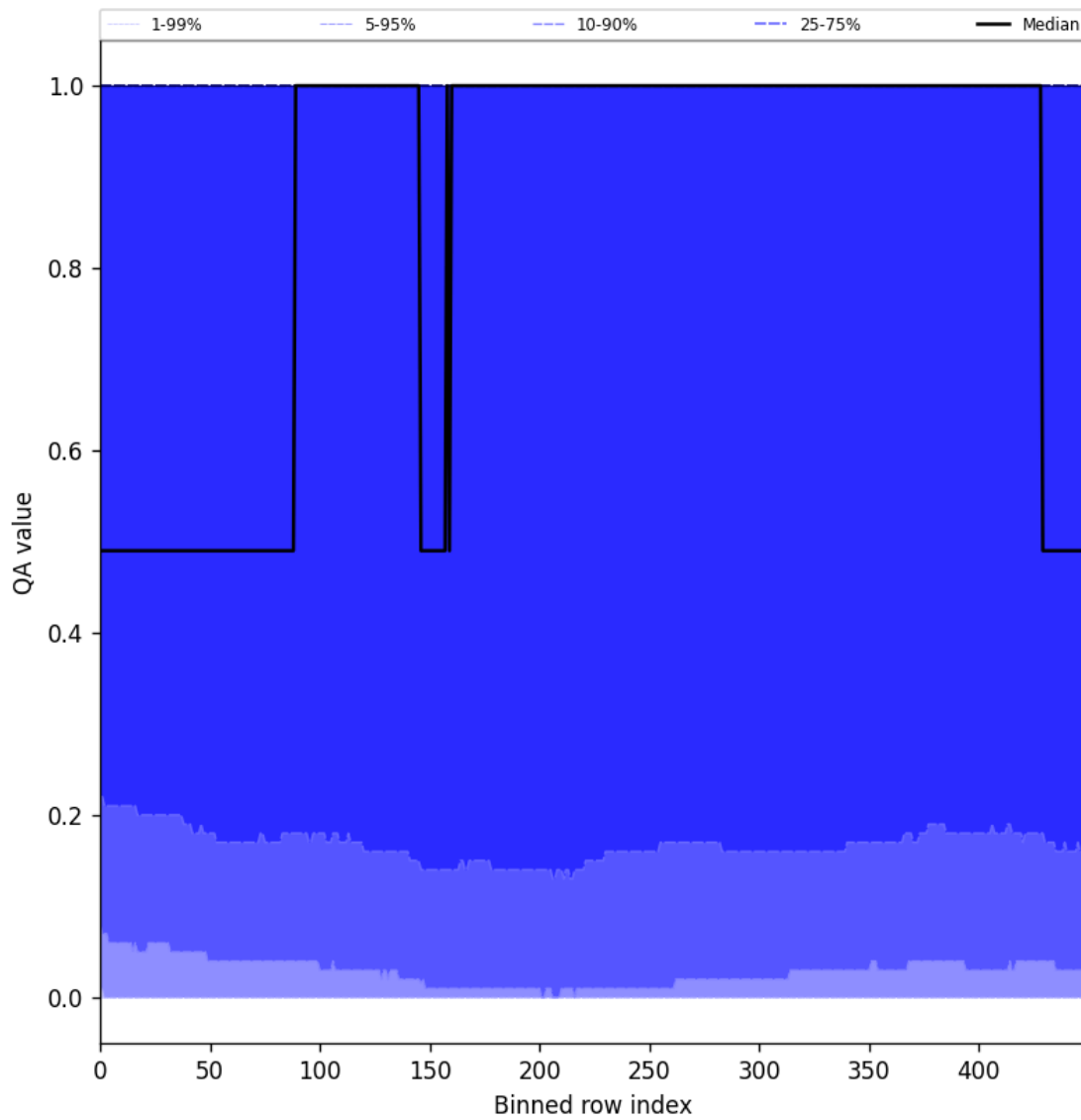
Figure 83: Along track statistics of “QA value” for 2025-01-10 to 2025-01-12
