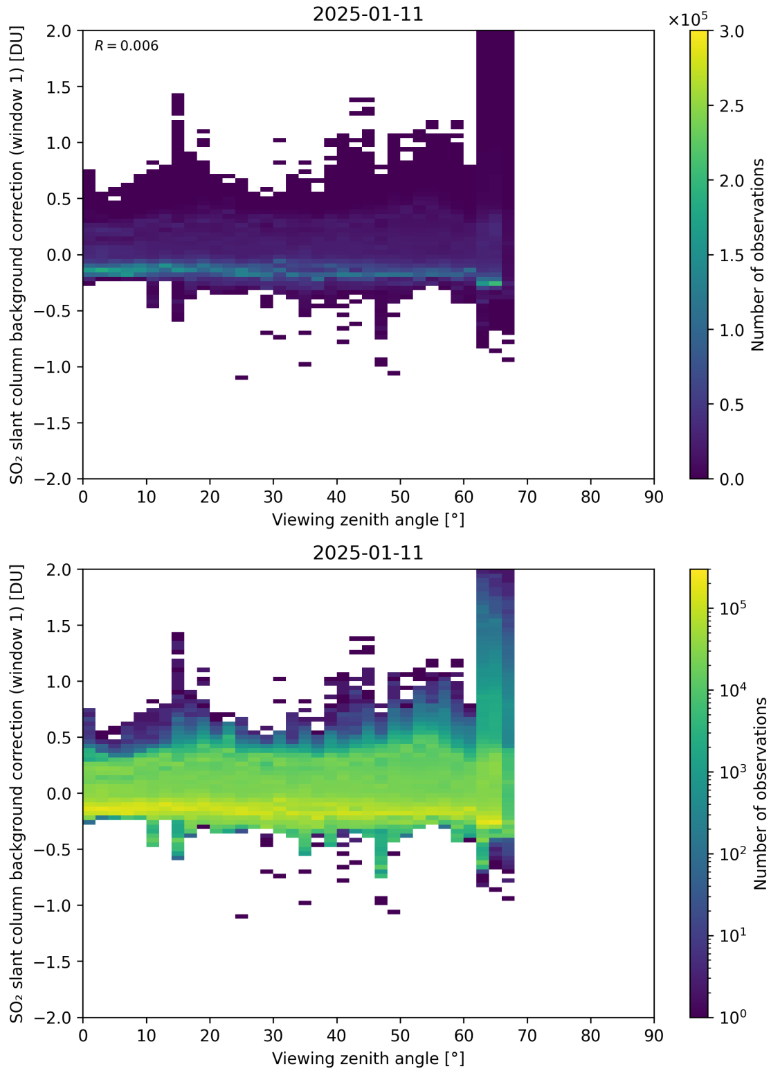
Figure 362: Scatter density plot of “Viewing zenith angle” against “SO 2 slant column background correction (window 1)” for 2025-01-10 to 2025-01-12.
