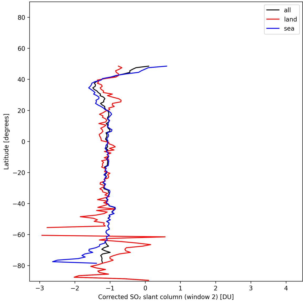
Figure 43: Zonal average of “Corrected SO 2 slant column (window 2)” for 2025-01-10 to 2025-01-12.
