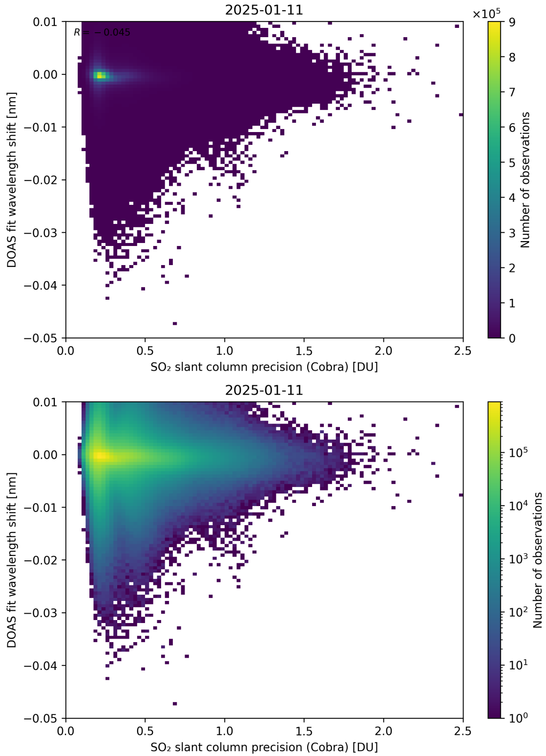
Figure 202: Scatter density plot of “SO 2 slant column precision (Cobra)” against “DOAS fit wavelength shift” for 2025-01-10 to 2025-01-12.
