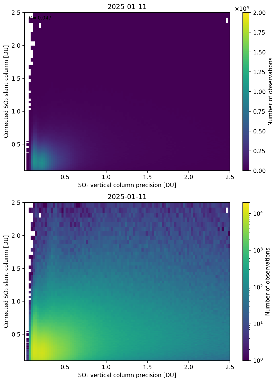
Figure 338: Scatter density plot of “SO 2 vertical column precision” against “Corrected SO 2 slant column” for 2025-01-10 to 2025-01-12.
