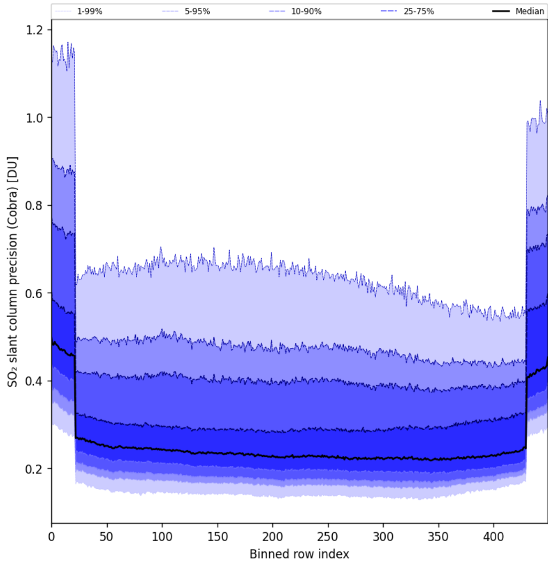
Figure 88: Along track statistics of “SO 2 slant column precision (Cobra)” for 2025-01-10 to 2025-01-12
