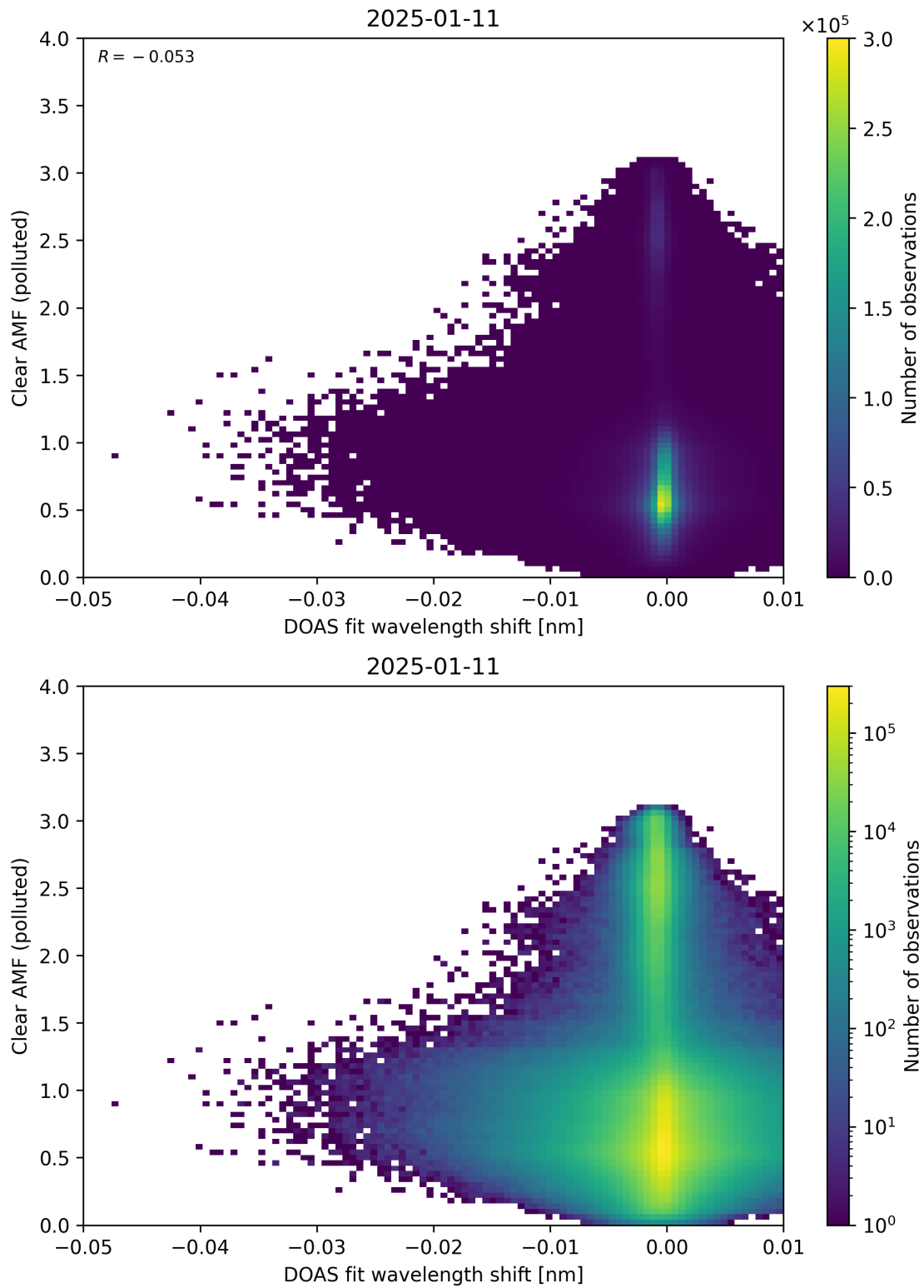
Figure 140: Scatter density plot of “DOAS fit wavelength shift” against “Clear AMF (polluted)” for 2025-01-10 to 2025-01-12.
