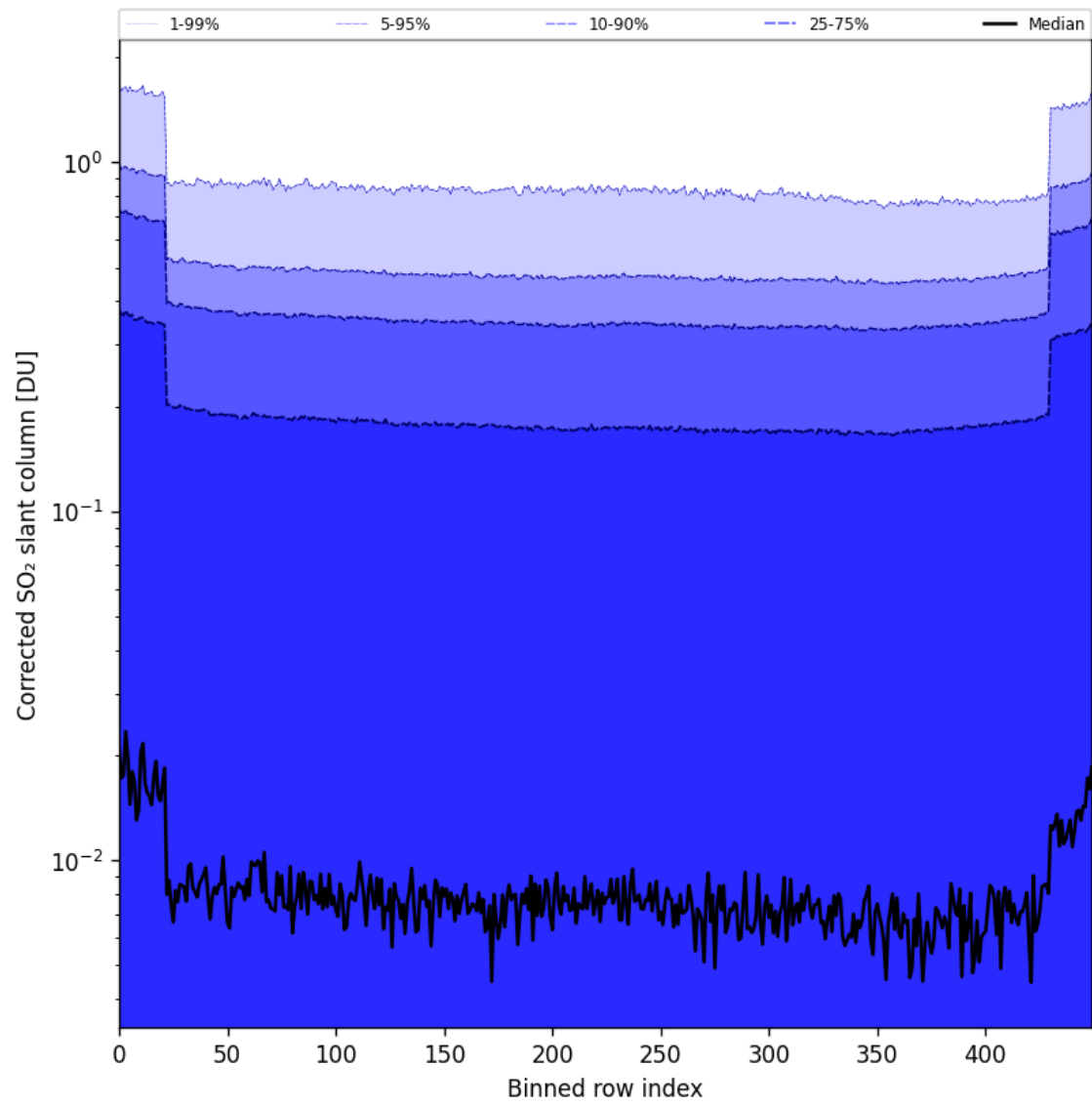
Figure 86: Along track statistics of "Corrected SO 2 slant column" for 2025-01-10 to 2025-01-12
