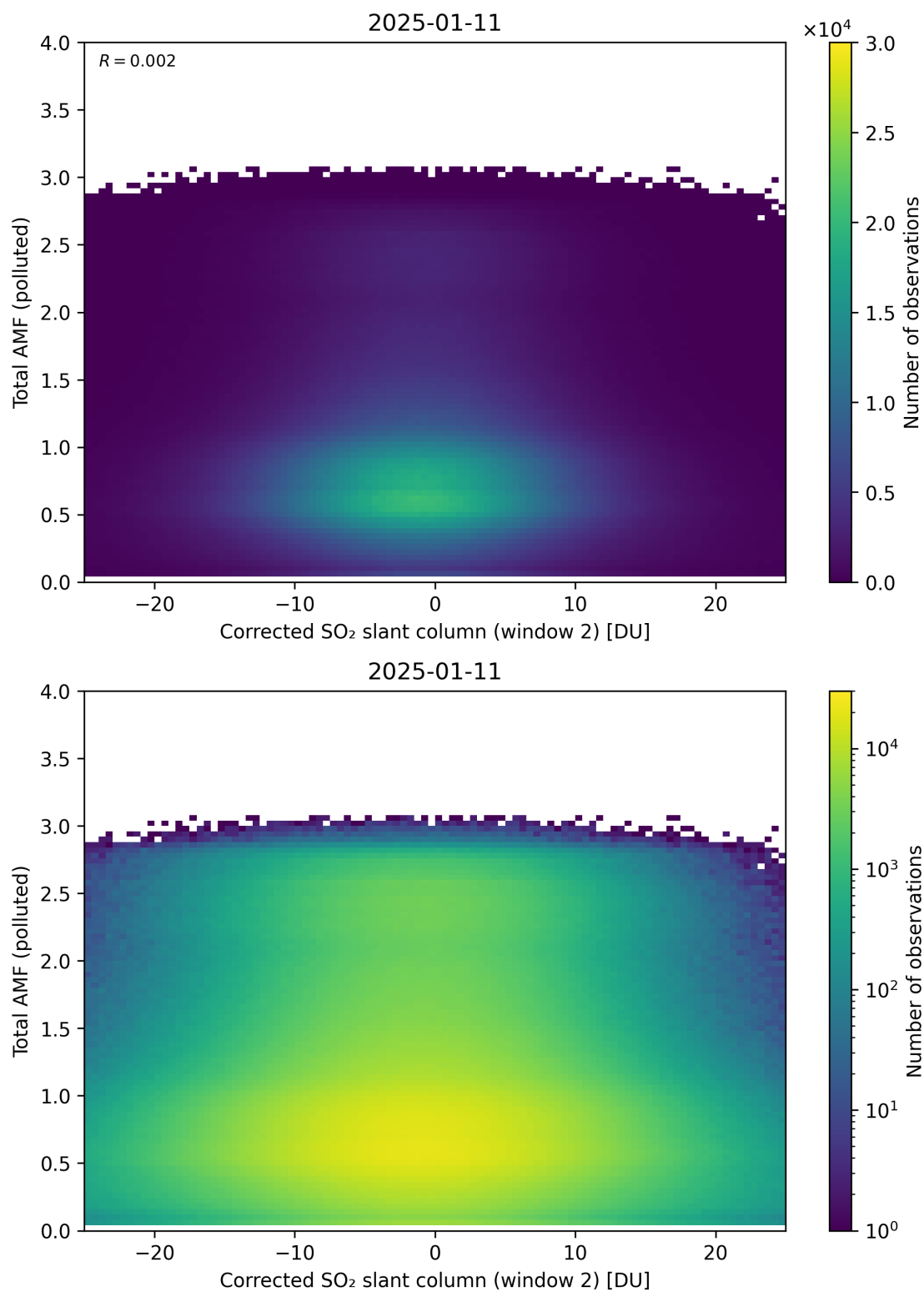
Figure 253: Scatter density plot of “Corrected SO 2 slant column (window 2)” against “Total AMF (polluted)” for 2025-01-10 to 2025-01-12.
