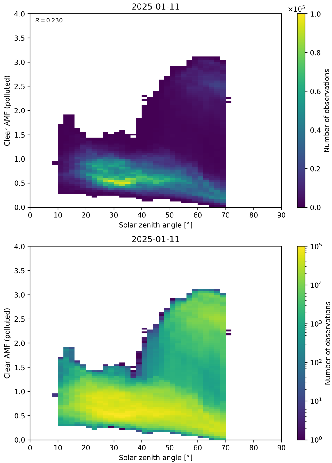
Figure 178: Scatter density plot of “Solar zenith angle” against “Clear AMF (polluted)” for 2025-01-10 to 2025-01-12.
