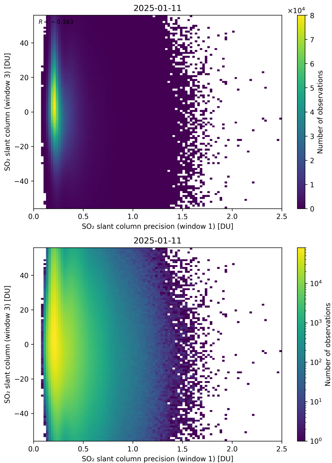
Figure 278: Scatter density plot of “SO 2 slant column precision (window 1)” against “SO 2 slant column (window 3)” for 2025-01-10 to 2025-01-12.
