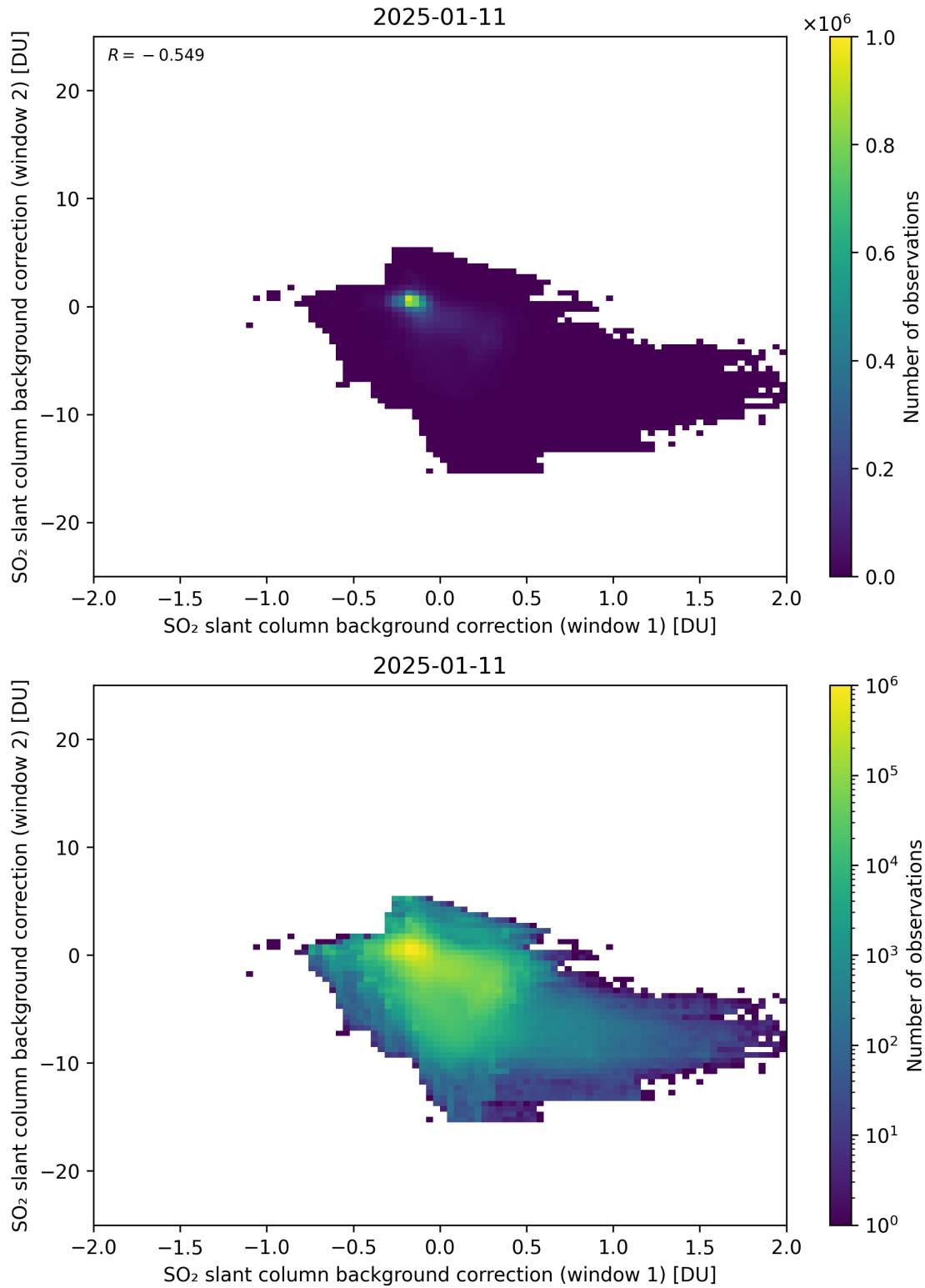
Figure 109: Scatter density plot of “SO 2 slant column background correction (window 1)” against “SO 2 slant column background correction (window 2)” for 2025-01-10 to 2025-01-12.
