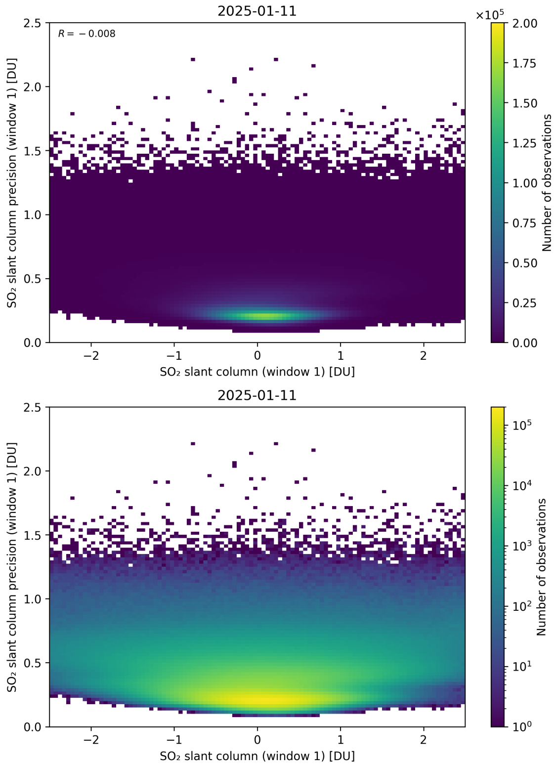
Figure 285: Scatter density plot of “SO 2 slant column (window 1)” against “SO 2 slant column precision (window 1)” for 2025-01-10 to 2025-01-12.
