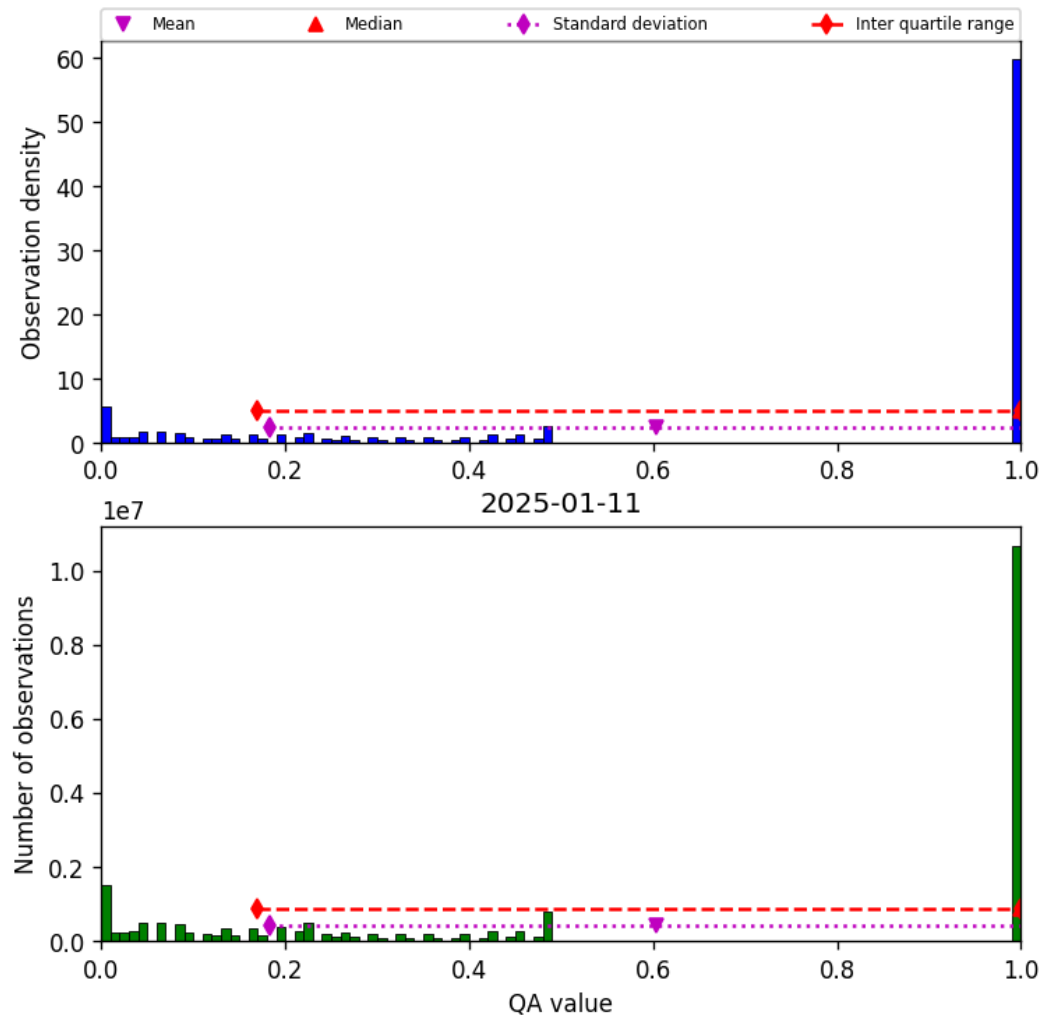
Figure 57: Histogram of “QA value” for 2025-01-10 to 2025-01-12
