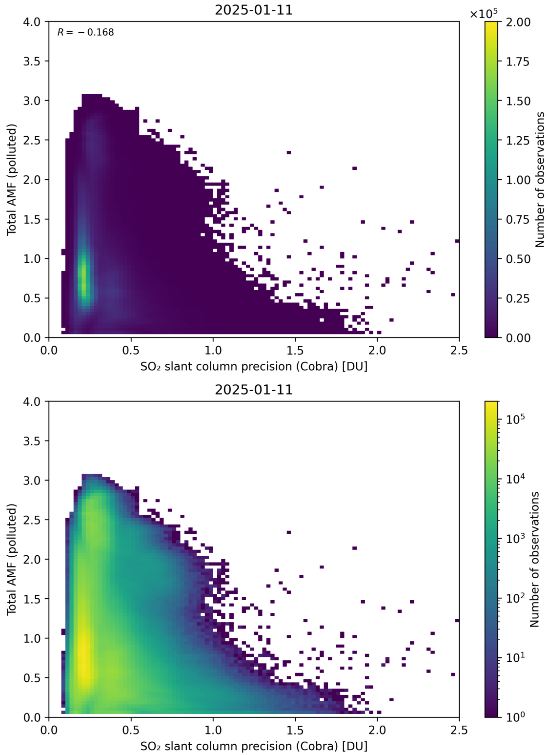
Figure 213: Scatter density plot of “SO 2 slant column precision (Cobra)” against “Total AMF (polluted)” for 2025-01-10 to 2025-01-12.
