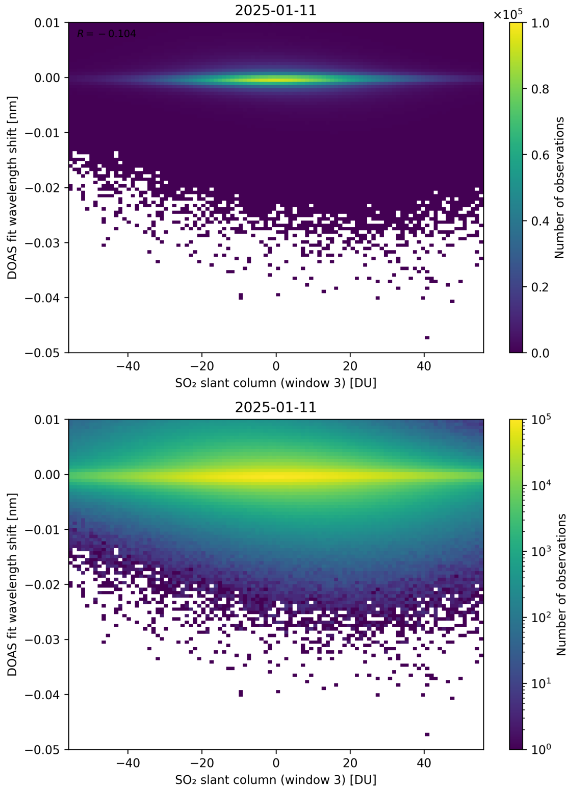
Figure 304: Scatter density plot of “SO 2 slant column (window 3)” against “DOAS fit wavelength shift” for 2025-01-10 to 2025-01-12.
