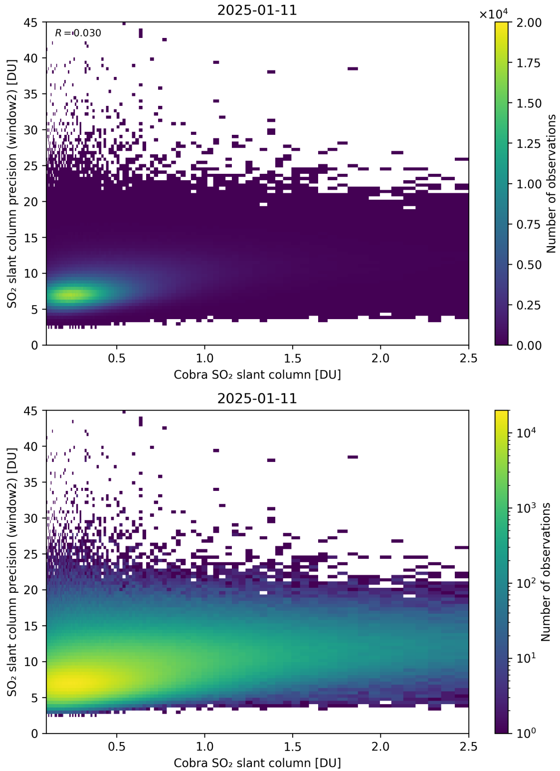
Figure 221: Scatter density plot of “Cobra SO 2 slant column” against “SO 2 slant column precision (window2)” for 2025-01-10 to 2025-01-12.
