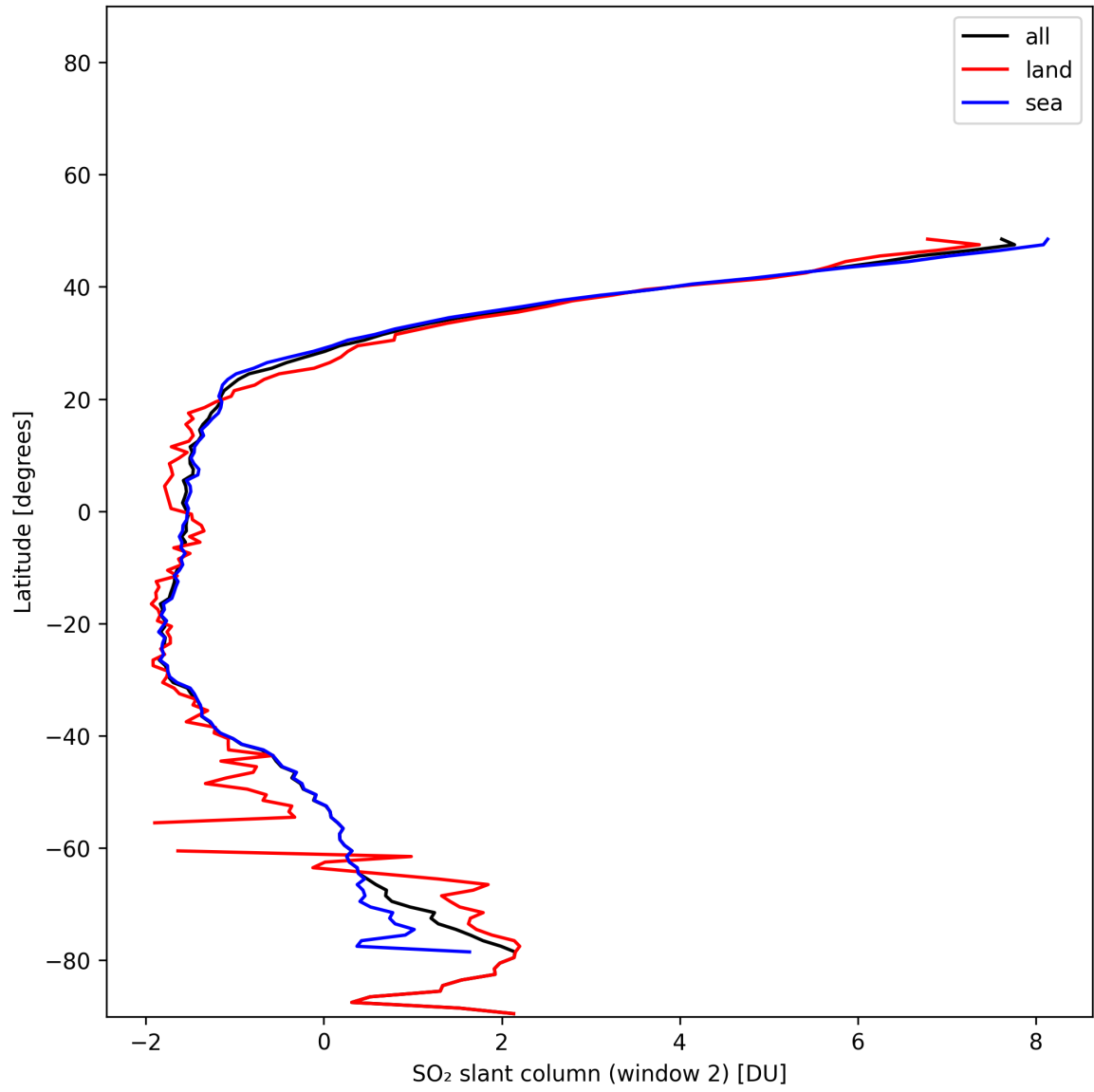
Figure 41: Zonal average of “SO 2 slant column (window 2)” for 2025-01-10 to 2025-01-12.
