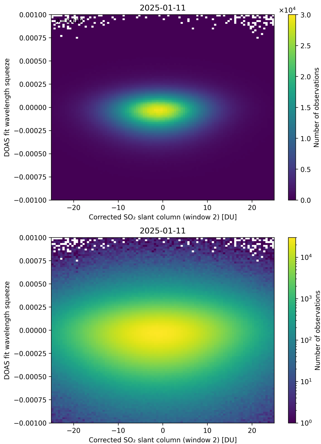
Figure 247: Scatter density plot of “Corrected SO 2 slant column (window 2)” against “DOAS fit wavelength squeeze” for 2025-01-10 to 2025-01-12.
