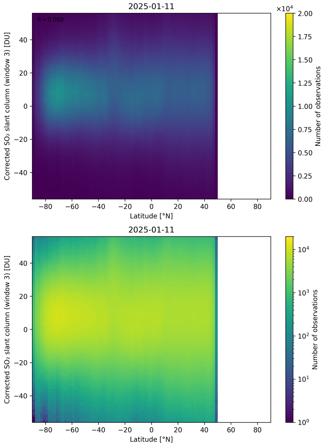
Figure 161: Scatter density plot of “Latitude” against “Corrected SO 2 slant column (window 3)” for 2025-01-10 to 2025-01-12.
