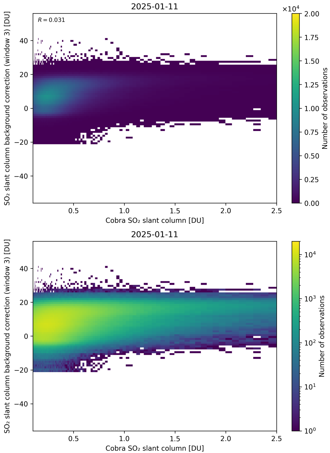
Figure 195: Scatter density plot of “Cobra SO 2 slant column” against “SO 2 slant column background correction (window 3)” for 2025-01-10 to 2025-01-12.
