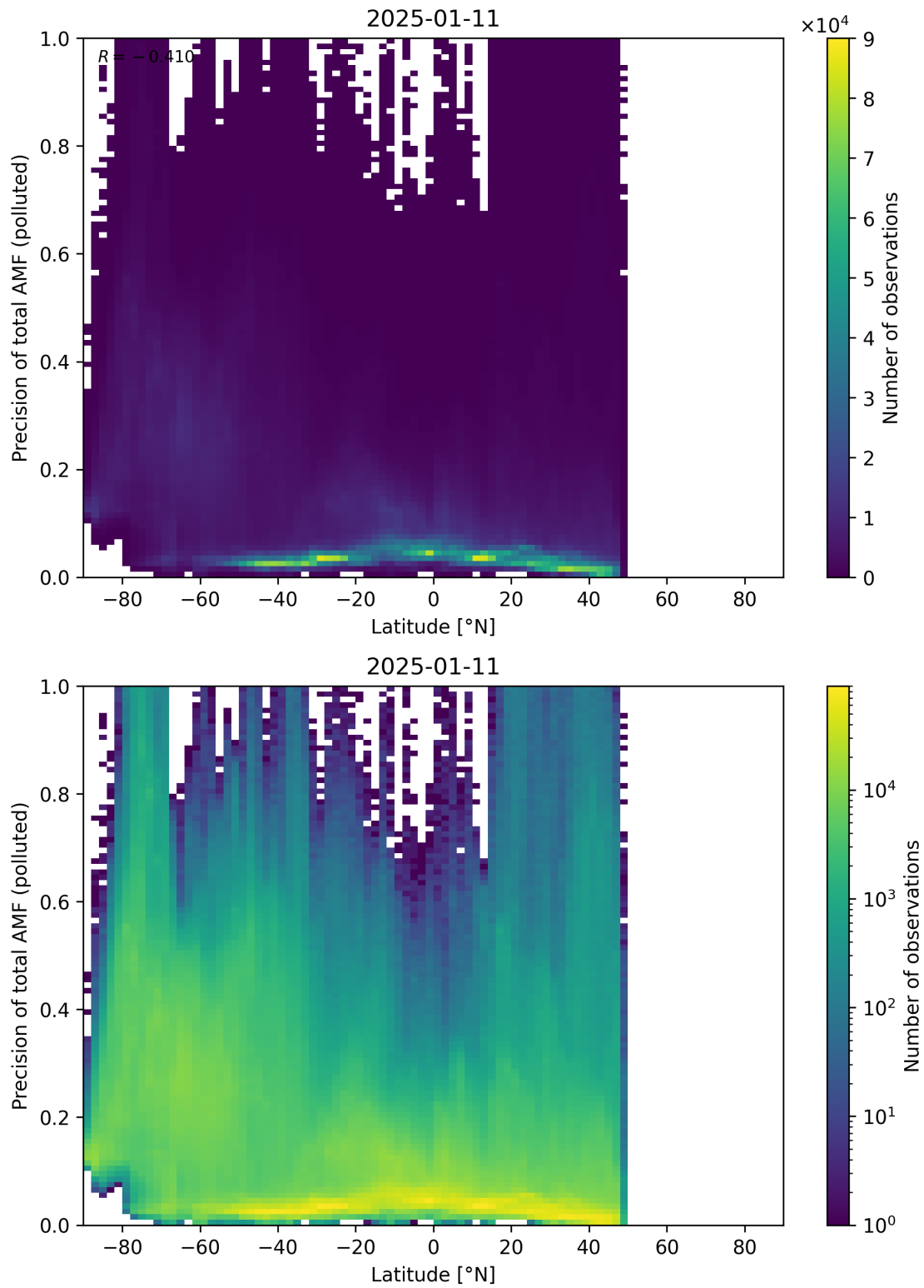
Figure 168: Scatter density plot of “Latitude” against “Precision of total AMF (polluted)” for 2025-01-10 to 2025-01-12.
