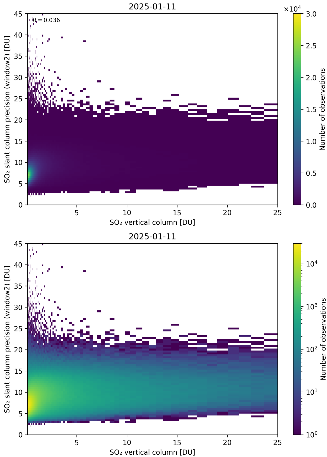
Figure 356: Scatter density plot of “SO 2 vertical column” against “SO 2 slant column precision (window2)” for 2025-01-10 to 2025-01-12.
