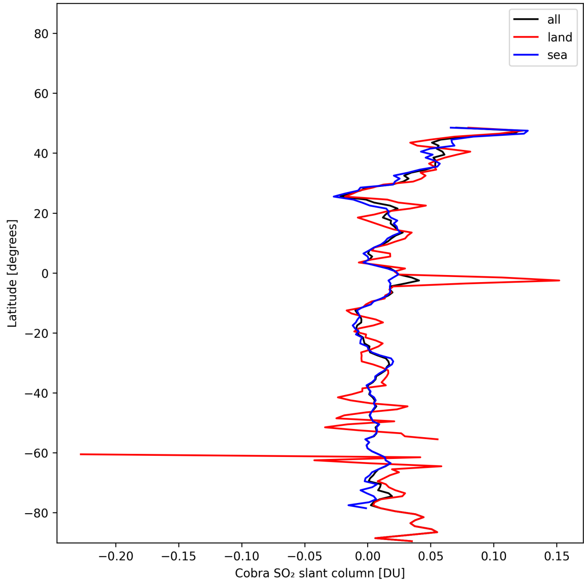
Figure 35: Zonal average of “Cobra SO 2 slant column” for 2025-01-10 to 2025-01-12.
