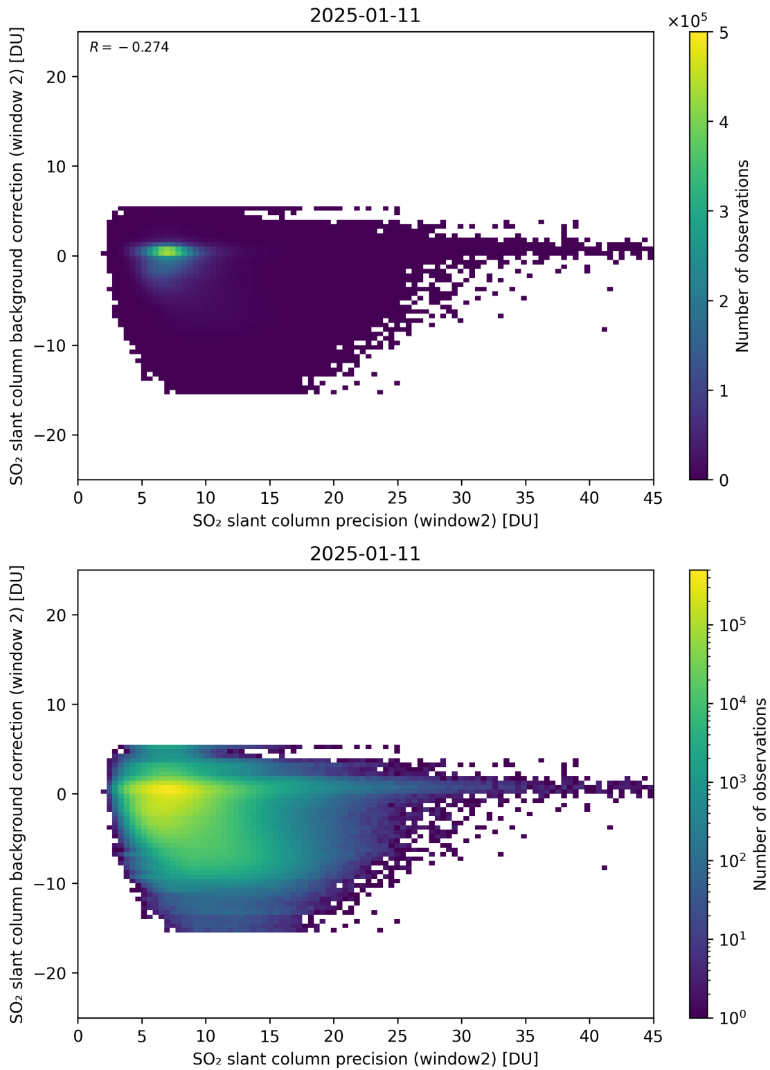
Figure 291: Scatter density plot of “SO 2 slant column precision (window2)” against “SO 2 slant column background correction (window 2)” for 2025-01-10 to 2025-01-12.
