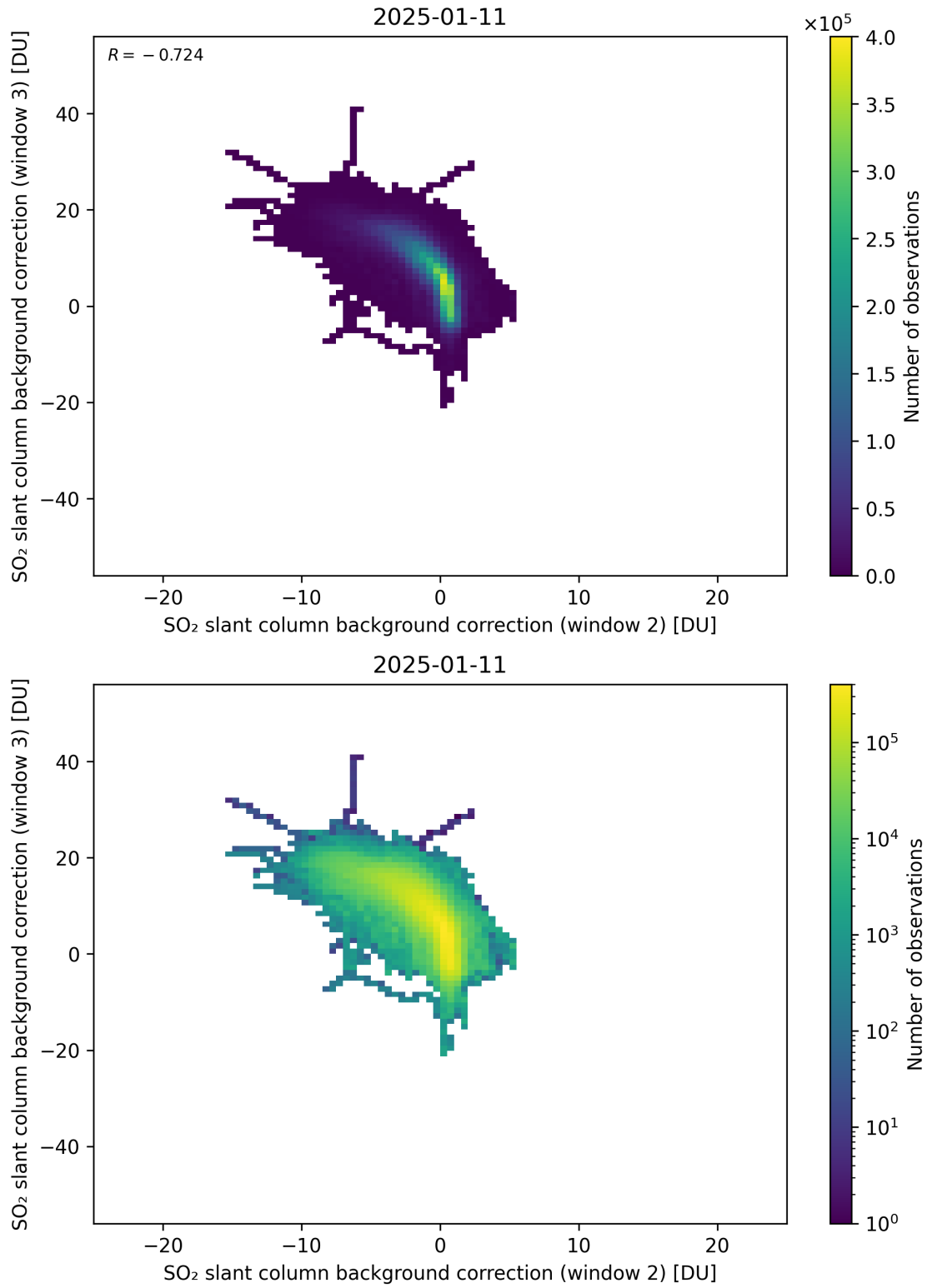
Figure 122: Scatter density plot of “SO 2 slant column background correction (window 2)” against “SO 2 slant column background correction (window 3)” for 2025-01-10 to 2025-01-12.
