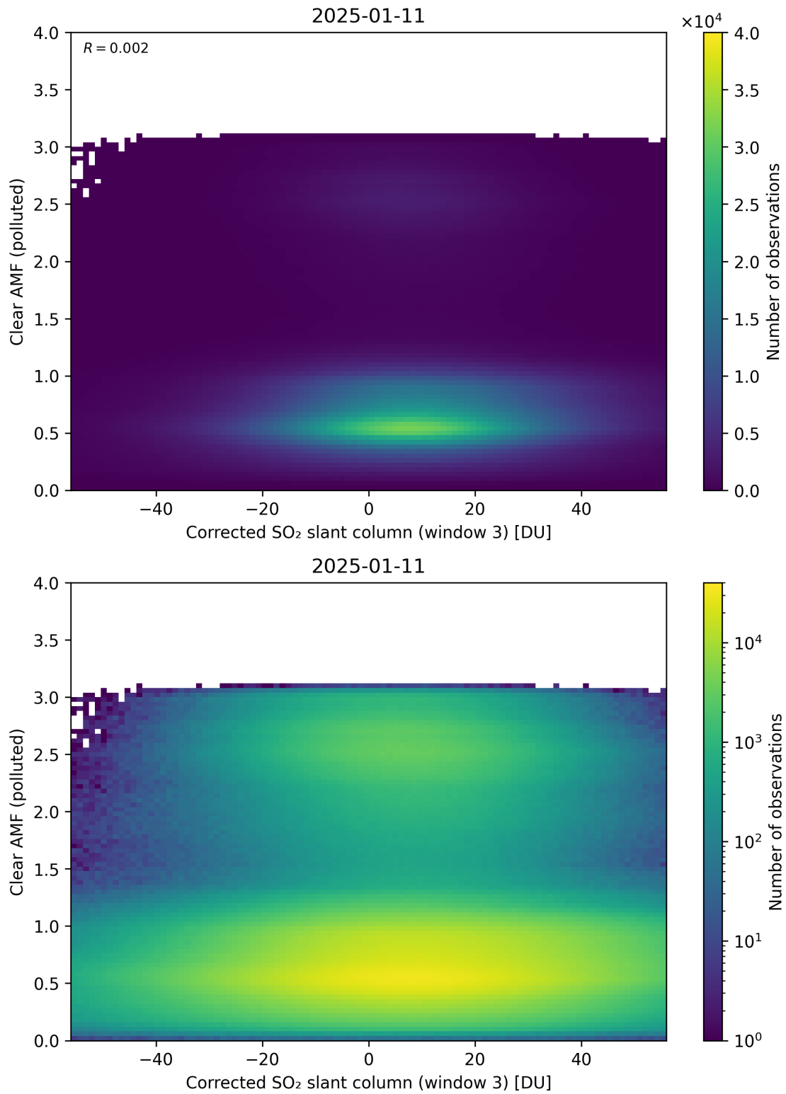
Figure 259: Scatter density plot of “Corrected SO 2 slant column (window 3)” against “Clear AMF (polluted)” for 2025-01-10 to 2025-01-12.
