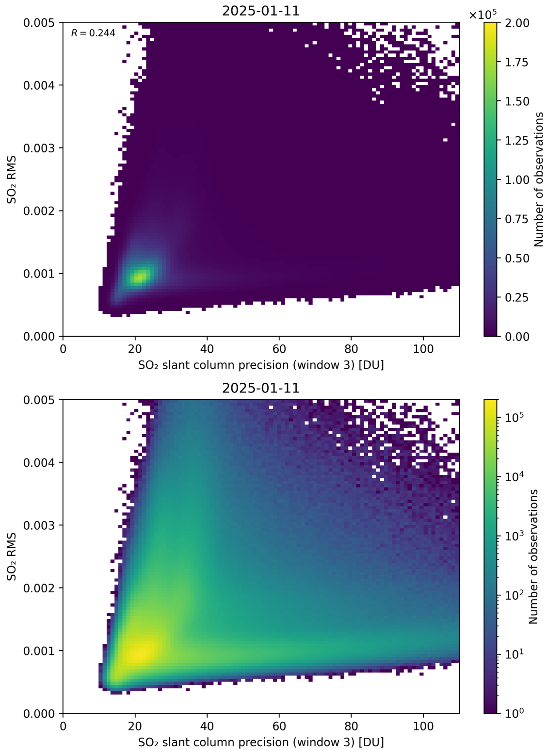
Figure 310: Scatter density plot of “SO 2 slant column precision (window 3)” against “SO 2 RMS” for 2025-01-10 to 2025-01-12.
