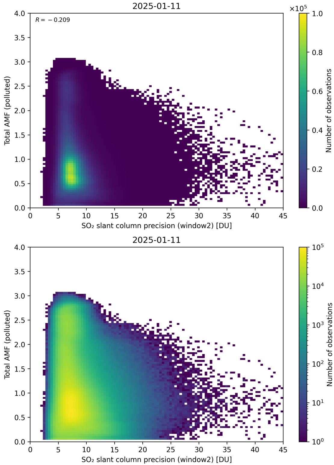
Figure 301: Scatter density plot of “SO 2 slant column precision (window2)” against “Total AMF (polluted)” for 2025-01-10 to 2025-01-12.
