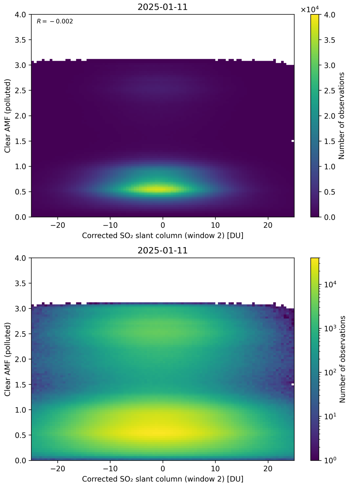
Figure 249: Scatter density plot of “Corrected SO 2 slant column (window 2)” against “Clear AMF (polluted)” for 2025-01-10 to 2025-01-12.
