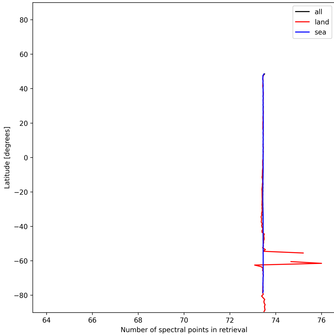
Figure 56: Zonal average of “Number of spectral points in retrieval” for 2025-01-10 to 2025-01-12.
