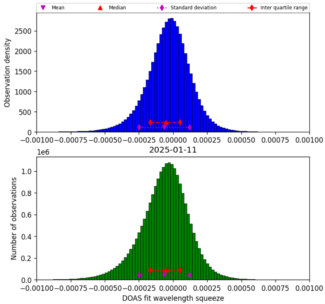
Figure 77: Histogram of “DOAS fit wavelength squeeze” for 2025-01-10 to 2025-01-12
