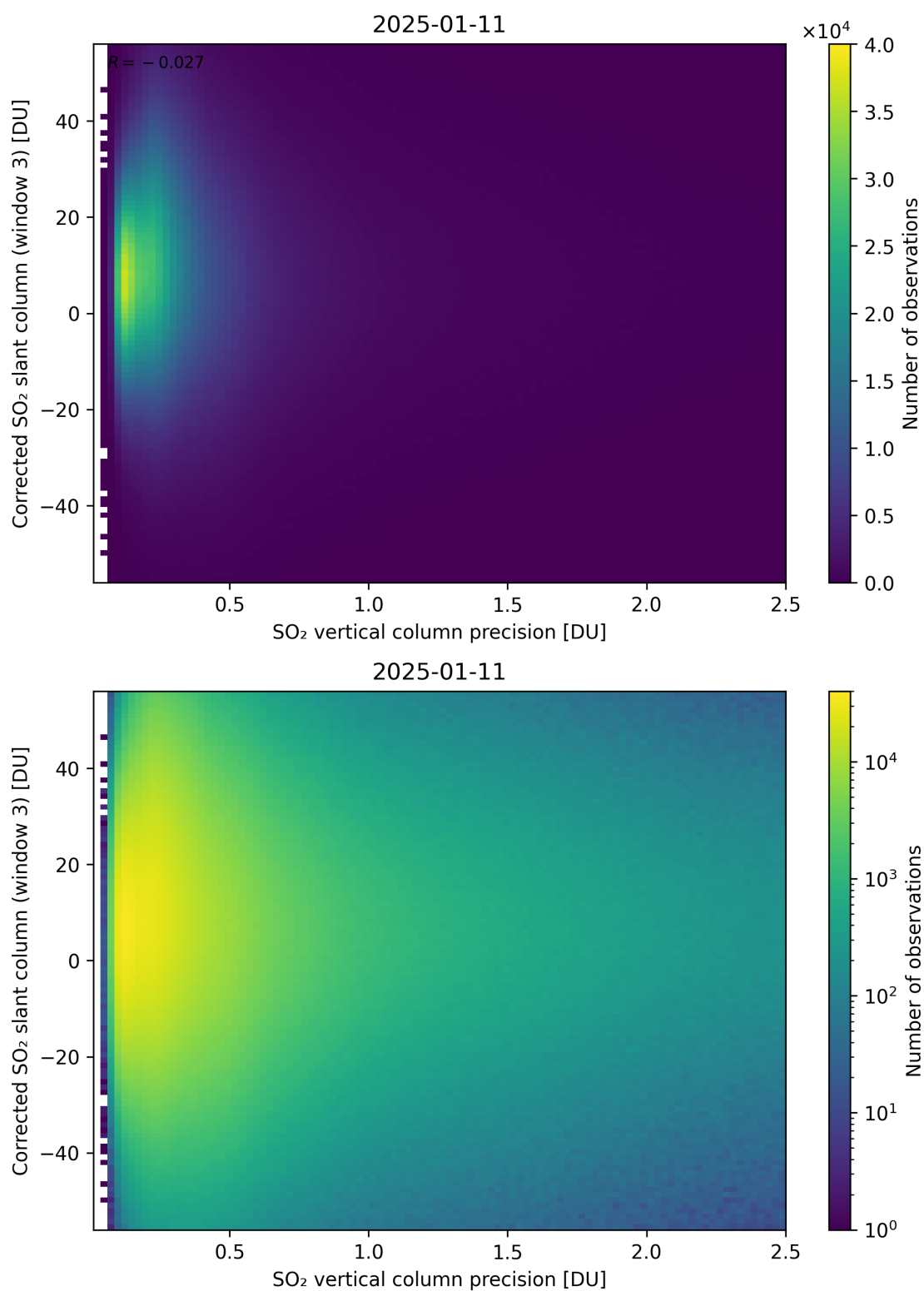
Figure 340: Scatter density plot of “SO 2 vertical column precision” against “Corrected SO 2 slant column (window 3)” for 2025-01-10 to 2025-01-12.
