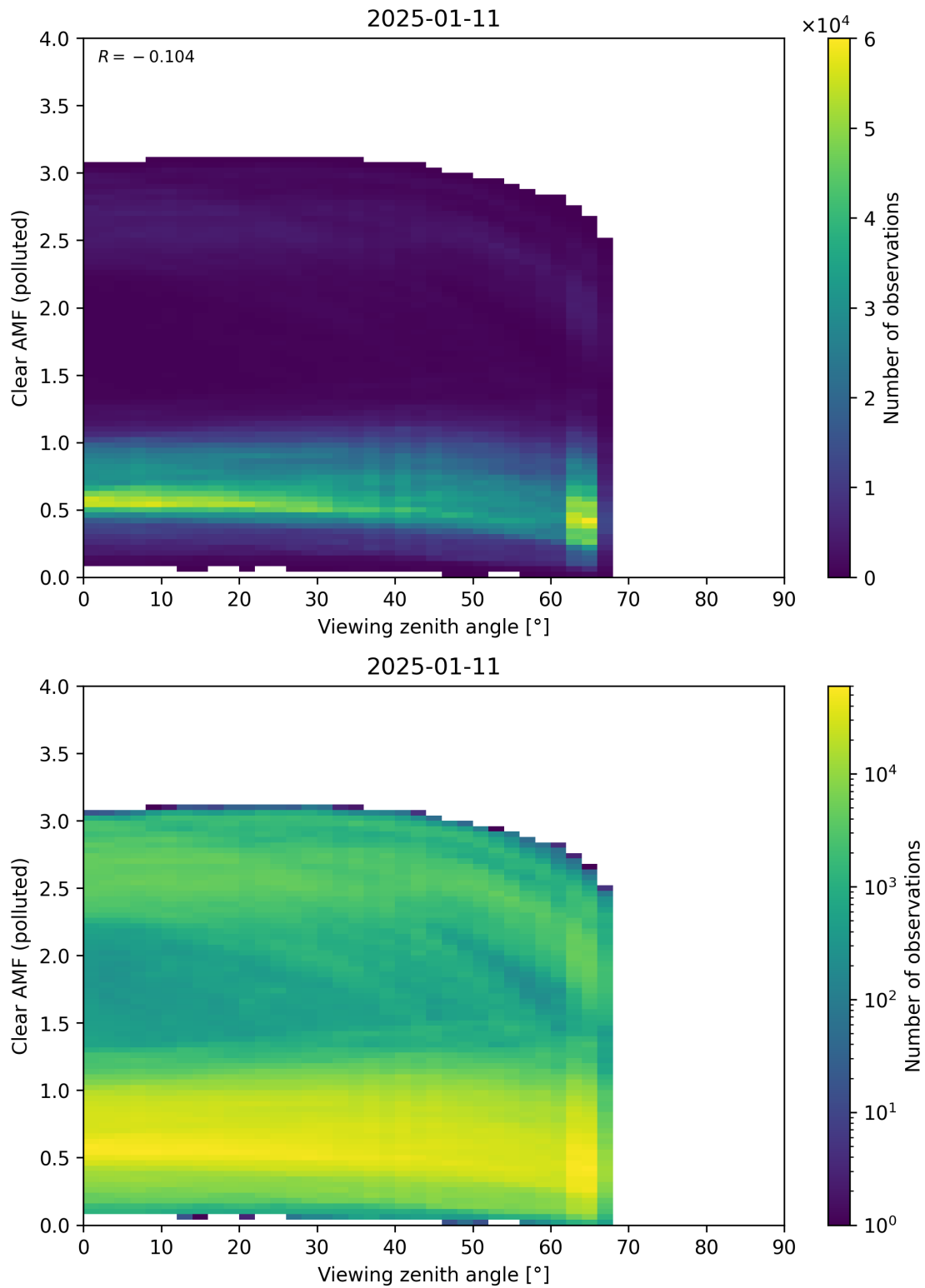
Figure 370: Scatter density plot of “Viewing zenith angle” against “Clear AMF (polluted)” for 2025-01-10 to 2025-01-12.
