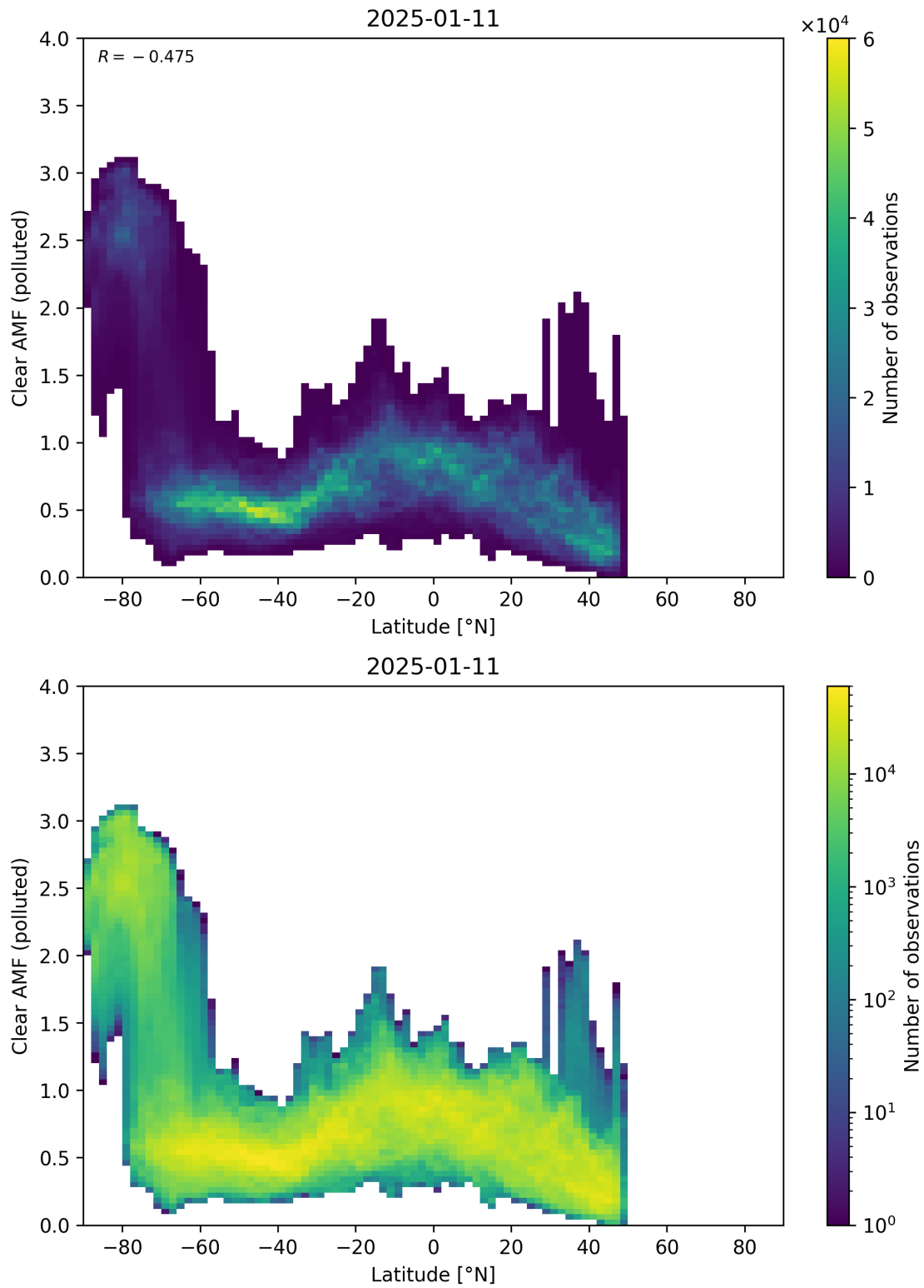
Figure 156: Scatter density plot of “Latitude” against “Clear AMF (polluted)” for 2025-01-10 to 2025-01-12.
