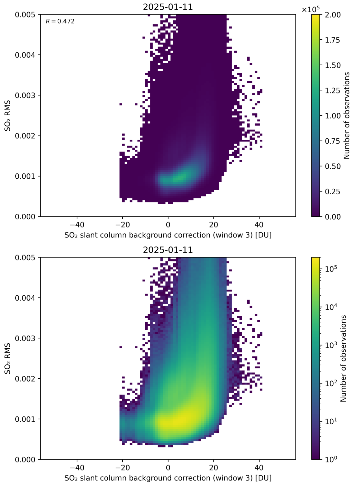
Figure 134: Scatter density plot of “SO 2 slant column background correction (window 3)” against “SO 2 RMS” for 2025-01-10 to 2025-01-12.
