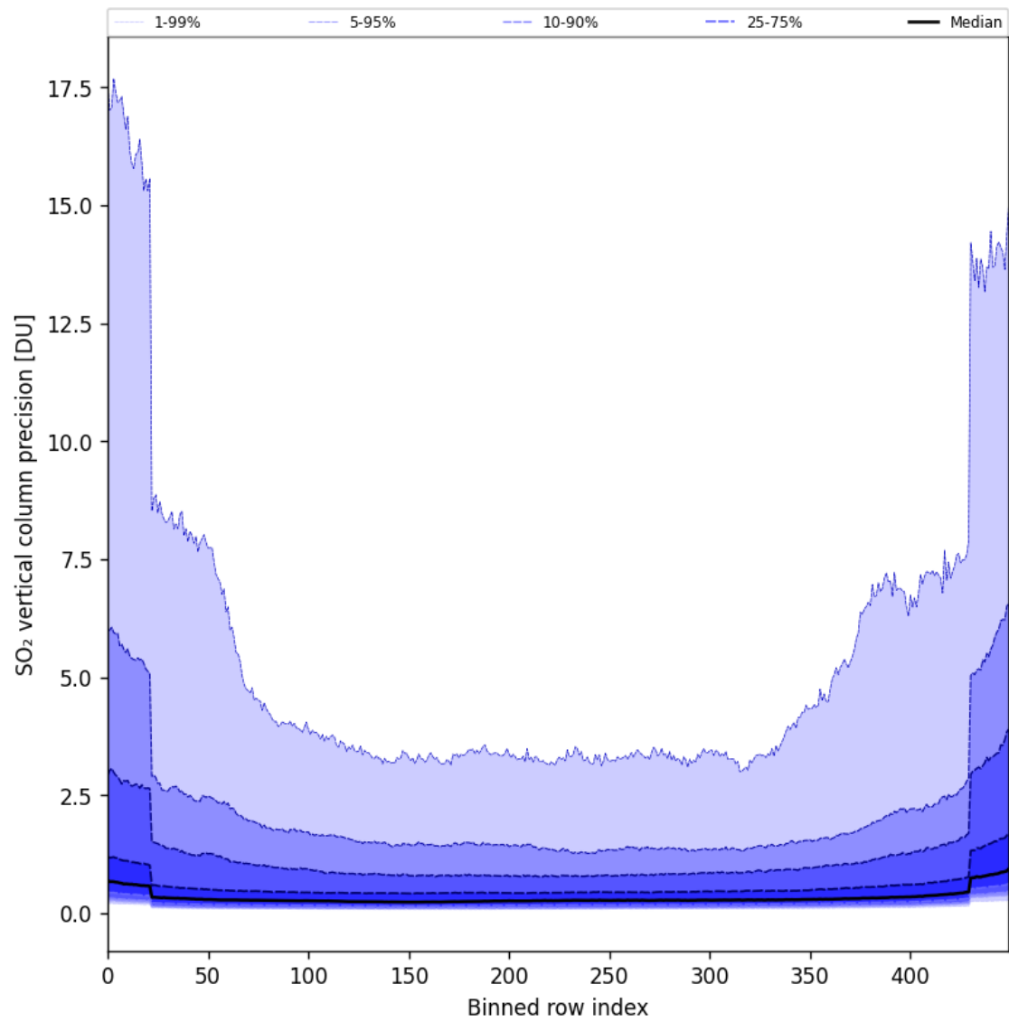
Figure 85: Along track statistics of “SO 2 vertical column precision” for 2025-01-10 to 2025-01-12
