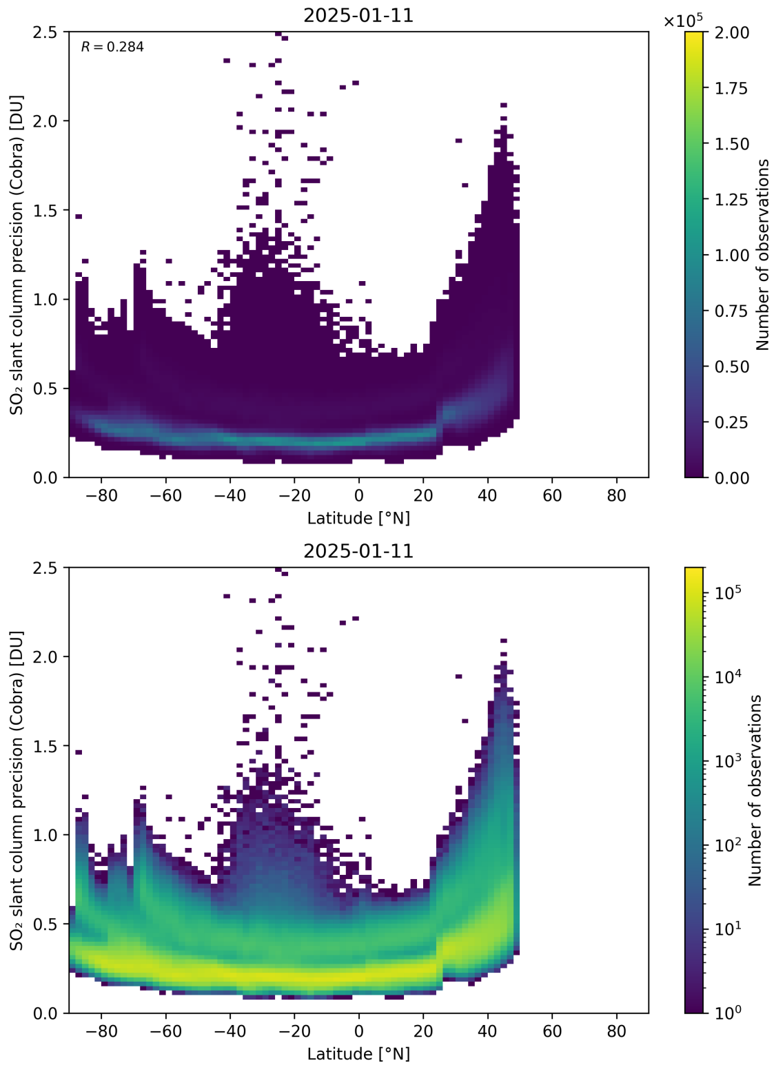
Figure 158: Scatter density plot of “Latitude” against “SO 2 slant column precision (Cobra)” for 2025-01-10 to 2025-01-12.
