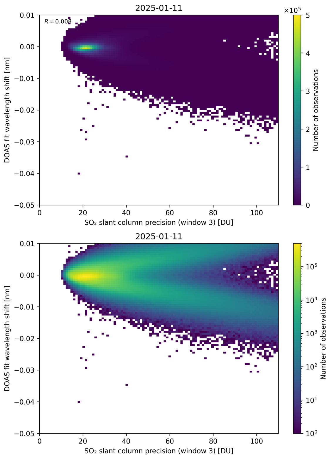
Figure 308: Scatter density plot of “SO 2 slant column precision (window 3)” against “DOAS fit wavelength shift” for 2025-01-10 to 2025-01-12.
