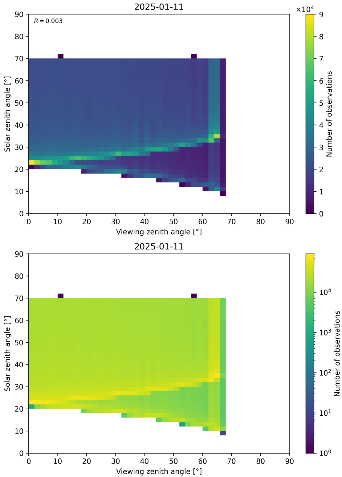
Figure 369: Scatter density plot of “Viewing zenith angle” against “Solar zenith angle” for 2025-01-10 to 2025-01-12.
