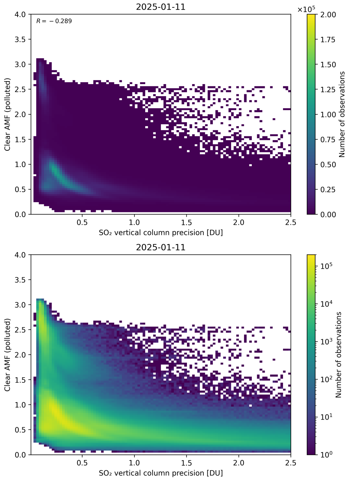
Figure 335: Scatter density plot of “SO 2 vertical column precision” against “Clear AMF (polluted)” for 2025-01-10 to 2025-01-12.
