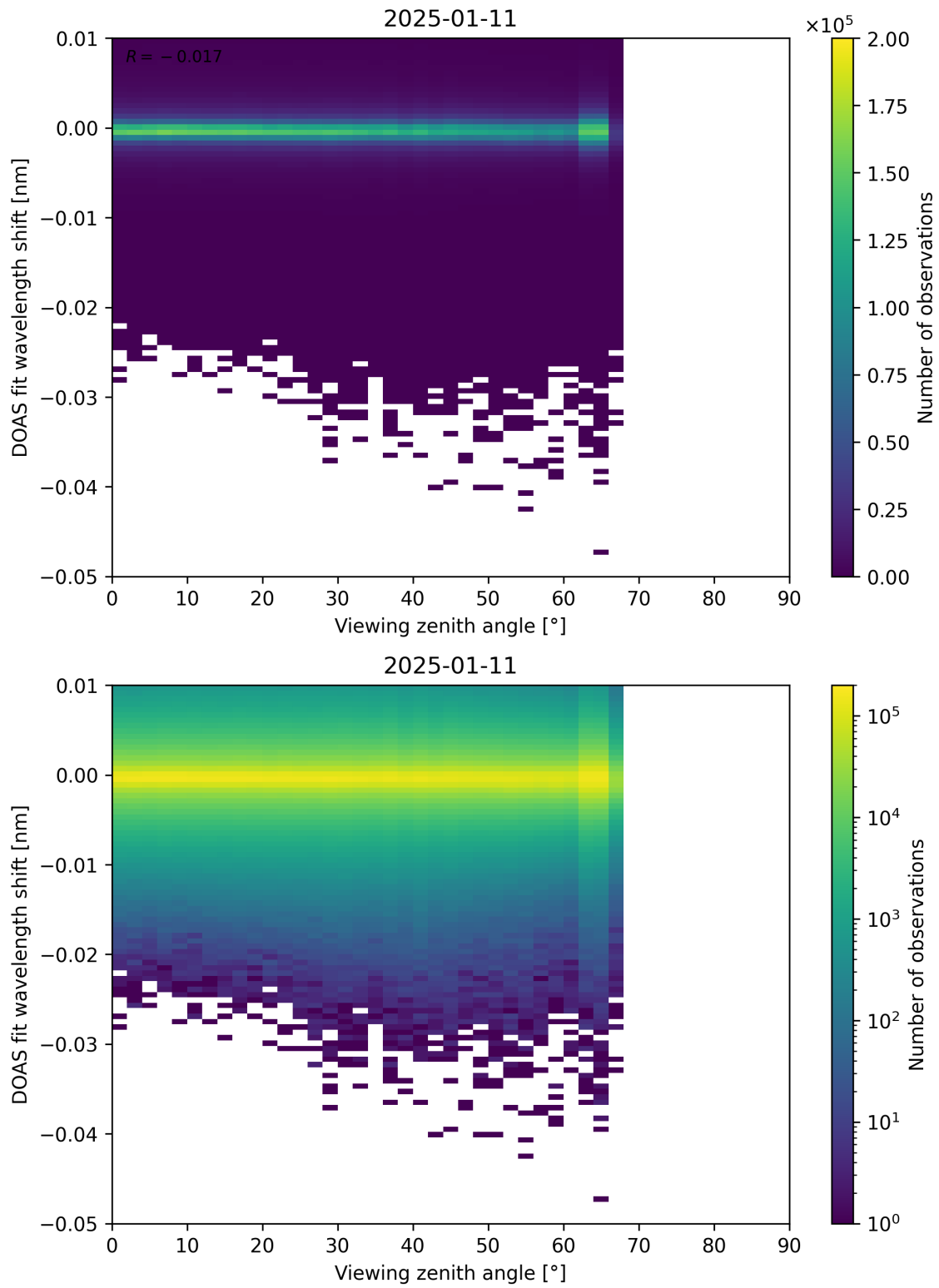
Figure 365: Scatter density plot of “Viewing zenith angle” against “DOAS fit wavelength shift” for 2025-01-10 to 2025-01-12.
