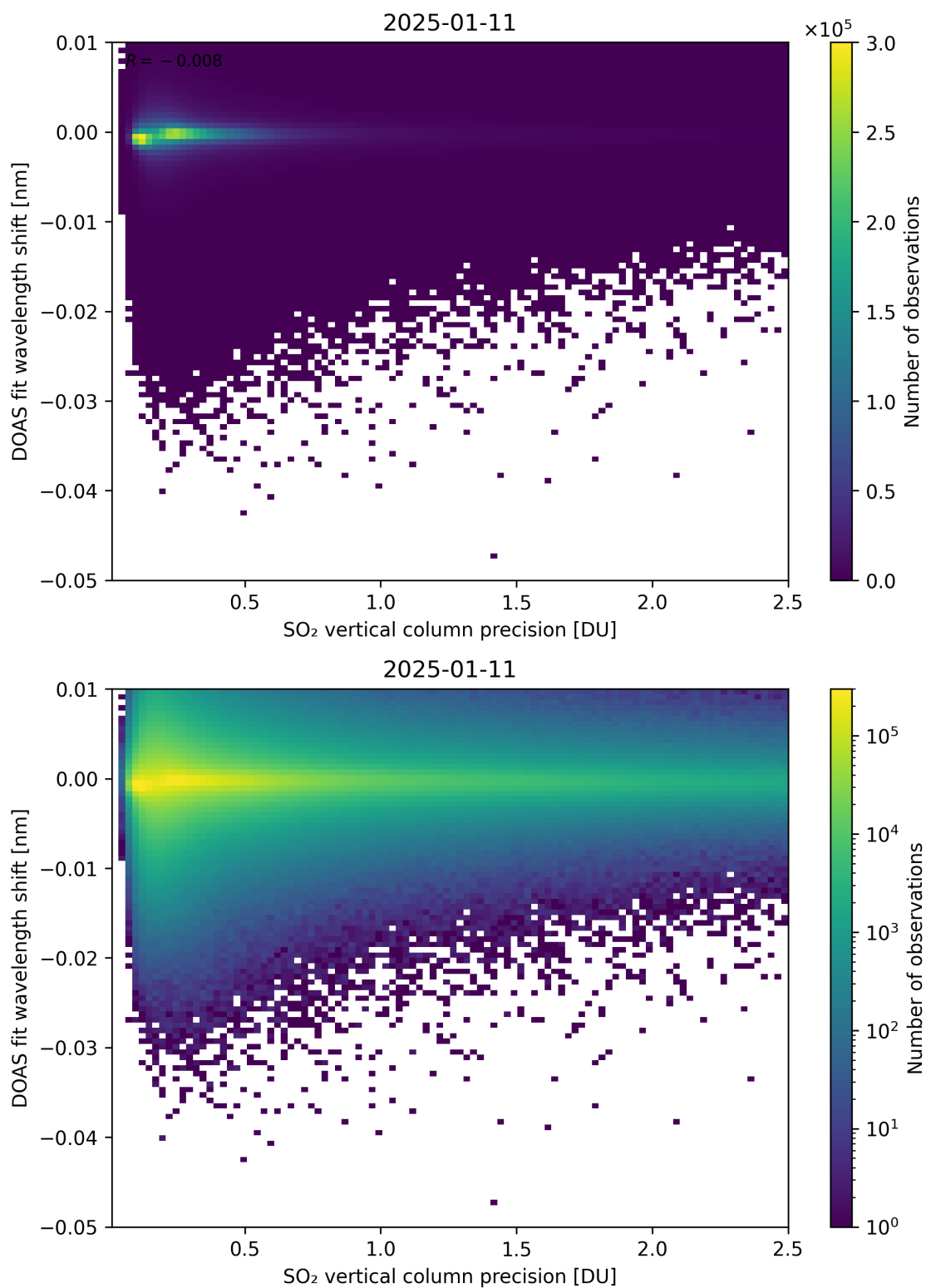
Figure 332: Scatter density plot of “SO 2 vertical column precision” against “DOAS fit wavelength shift” for 2025-01-10 to 2025-01-12.
