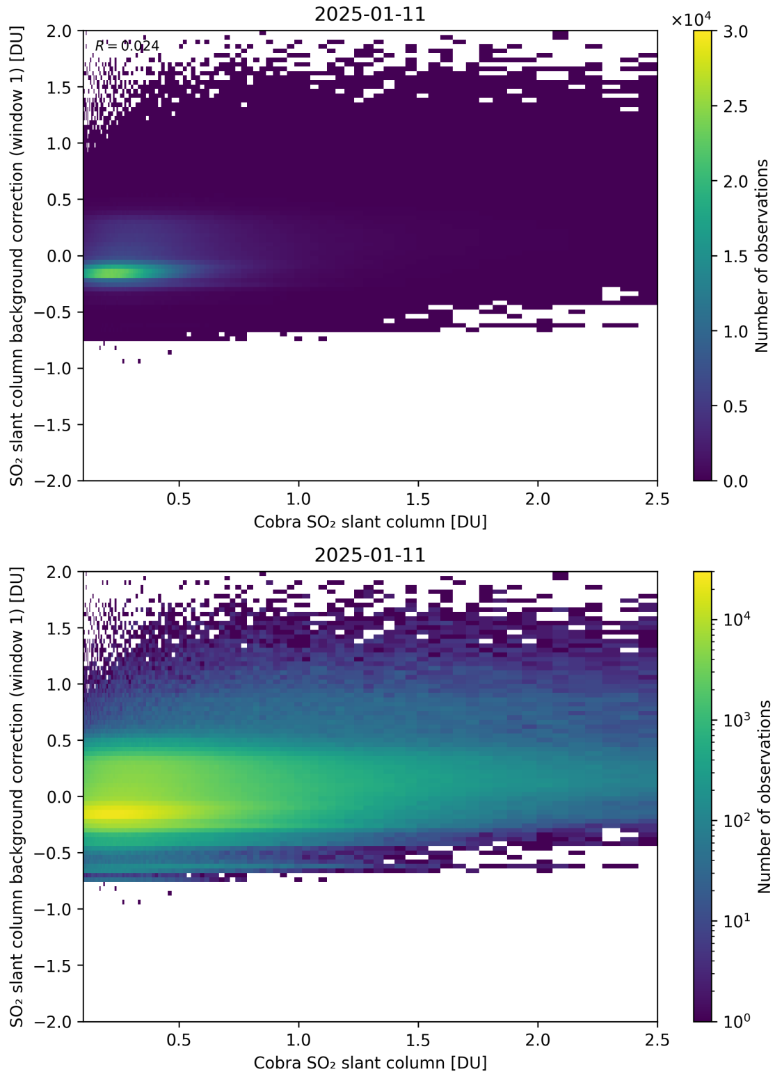
Figure 193: Scatter density plot of “Cobra SO 2 slant column” against “SO 2 slant column background correction (window 1)” for 2025-01-10 to 2025-01-12.
