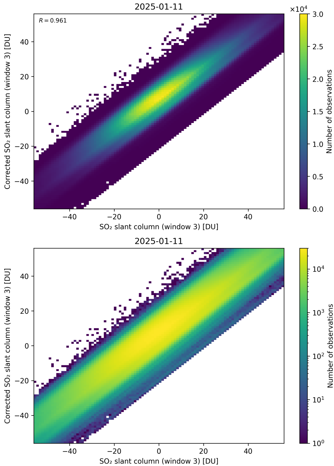
Figure 316: Scatter density plot of “SO 2 slant column (window 3)” against “Corrected SO 2 slant column (window 3)” for 2025-01-10 to 2025-01-12.
