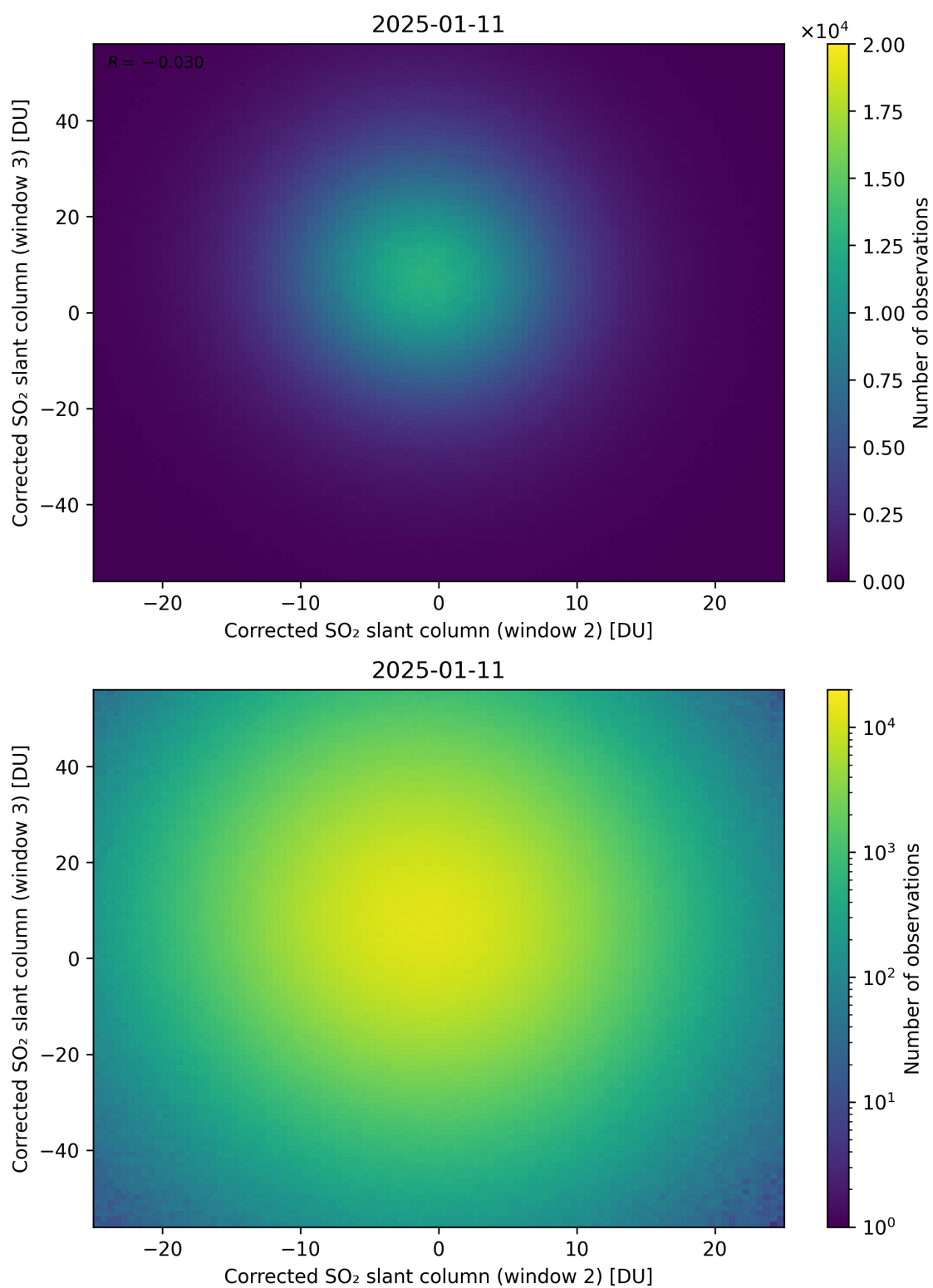
Figure 250: Scatter density plot of “Corrected SO 2 slant column (window 2)” against “Corrected SO 2 slant column (window 3)” for 2025-01-10 to 2025-01-12.
