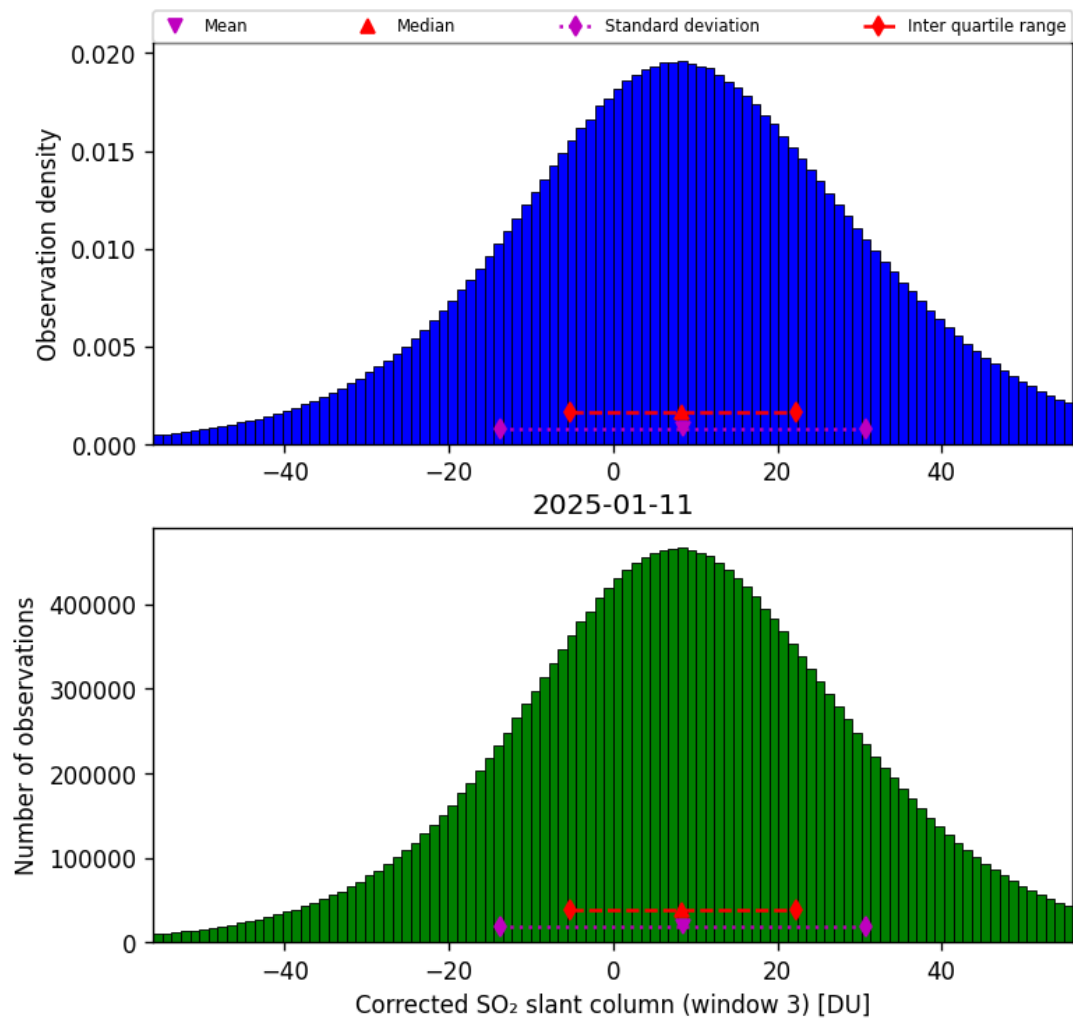
Figure 73: Histogram of “Corrected SO 2 slant column (window 3)” for 2025-01-10 to 2025-01-12
