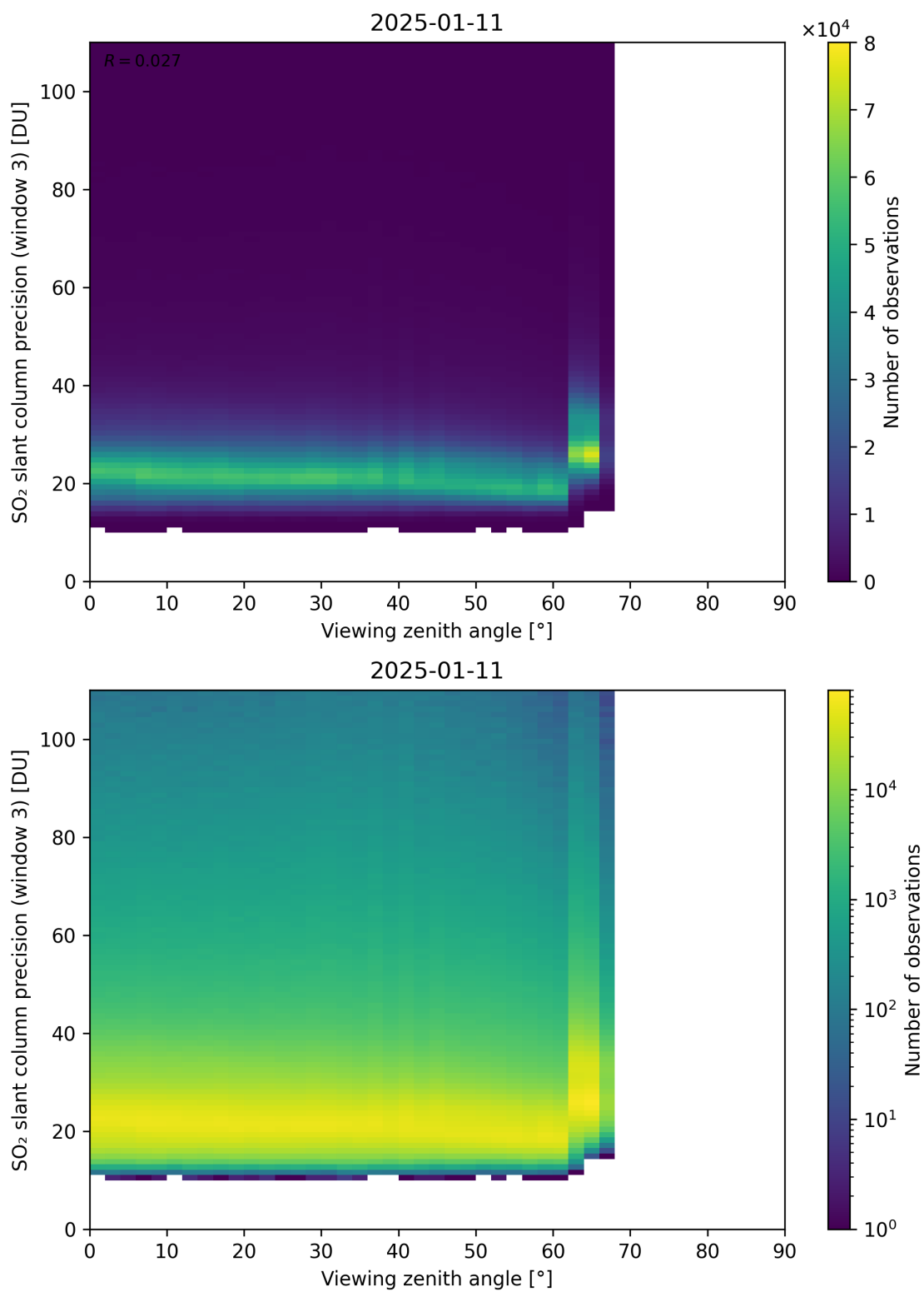
Figure 380: Scatter density plot of “Viewing zenith angle” against “SO 2 slant column precision (window 3)” for 2025-01-10 to 2025-01-12.
