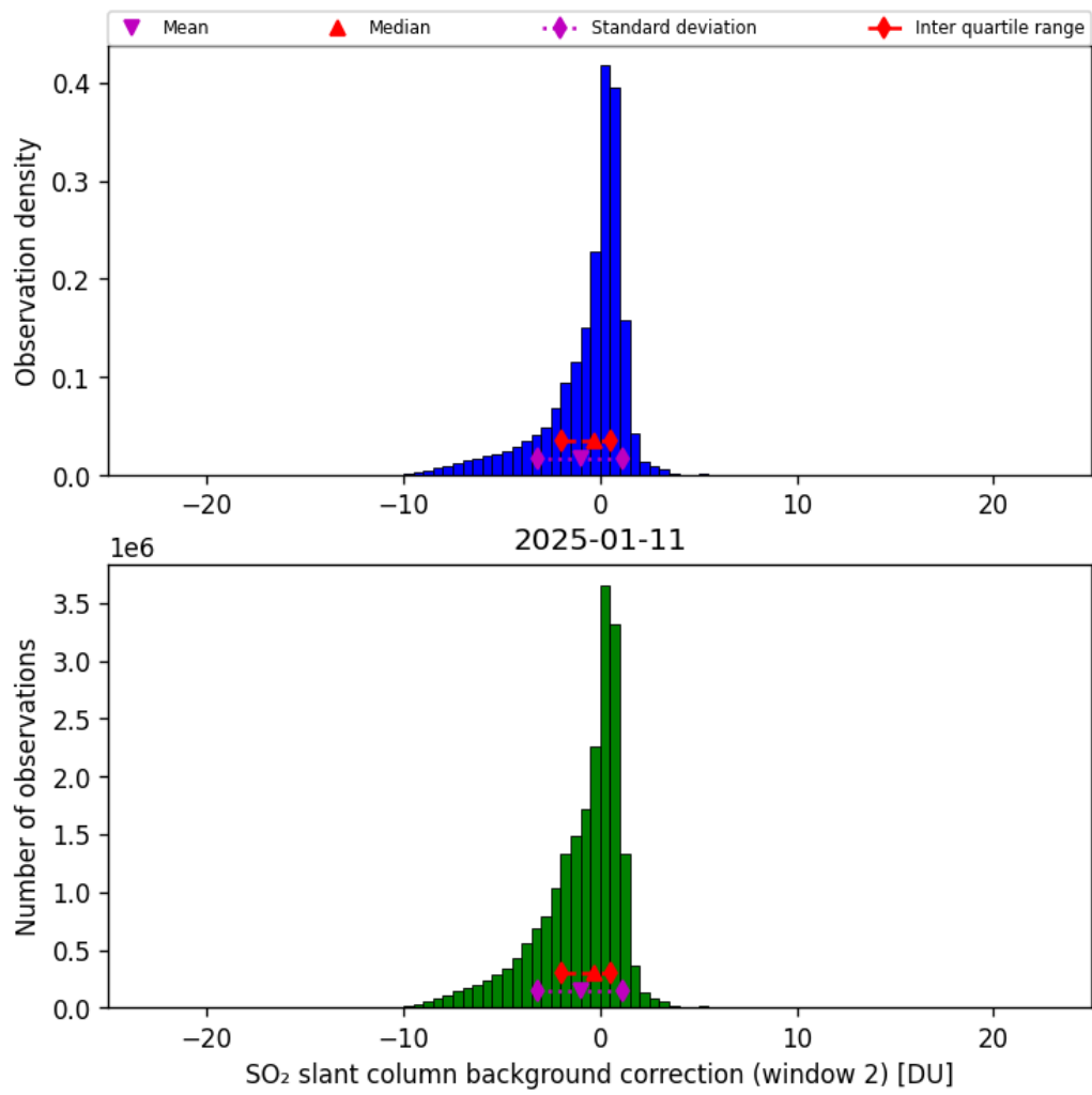
Figure 70: Histogram of “SO 2 slant column background correction (window 2)” for 2025-01-10 to 2025-01-12
