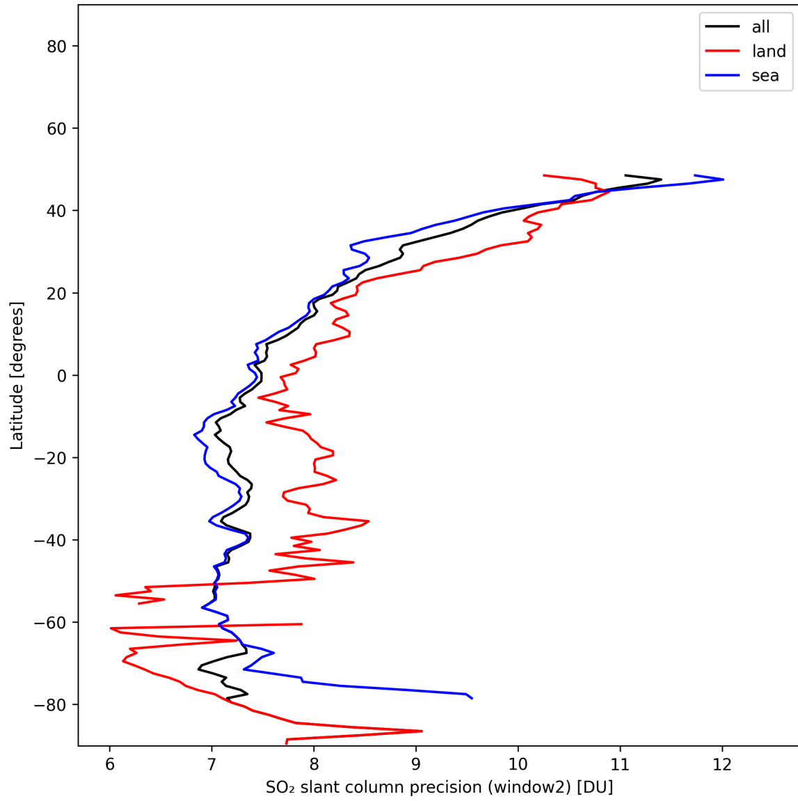
Figure 42: Zonal average of “SO 2 slant column precision (window2)” for 2025-01-10 to 2025-01-12.
