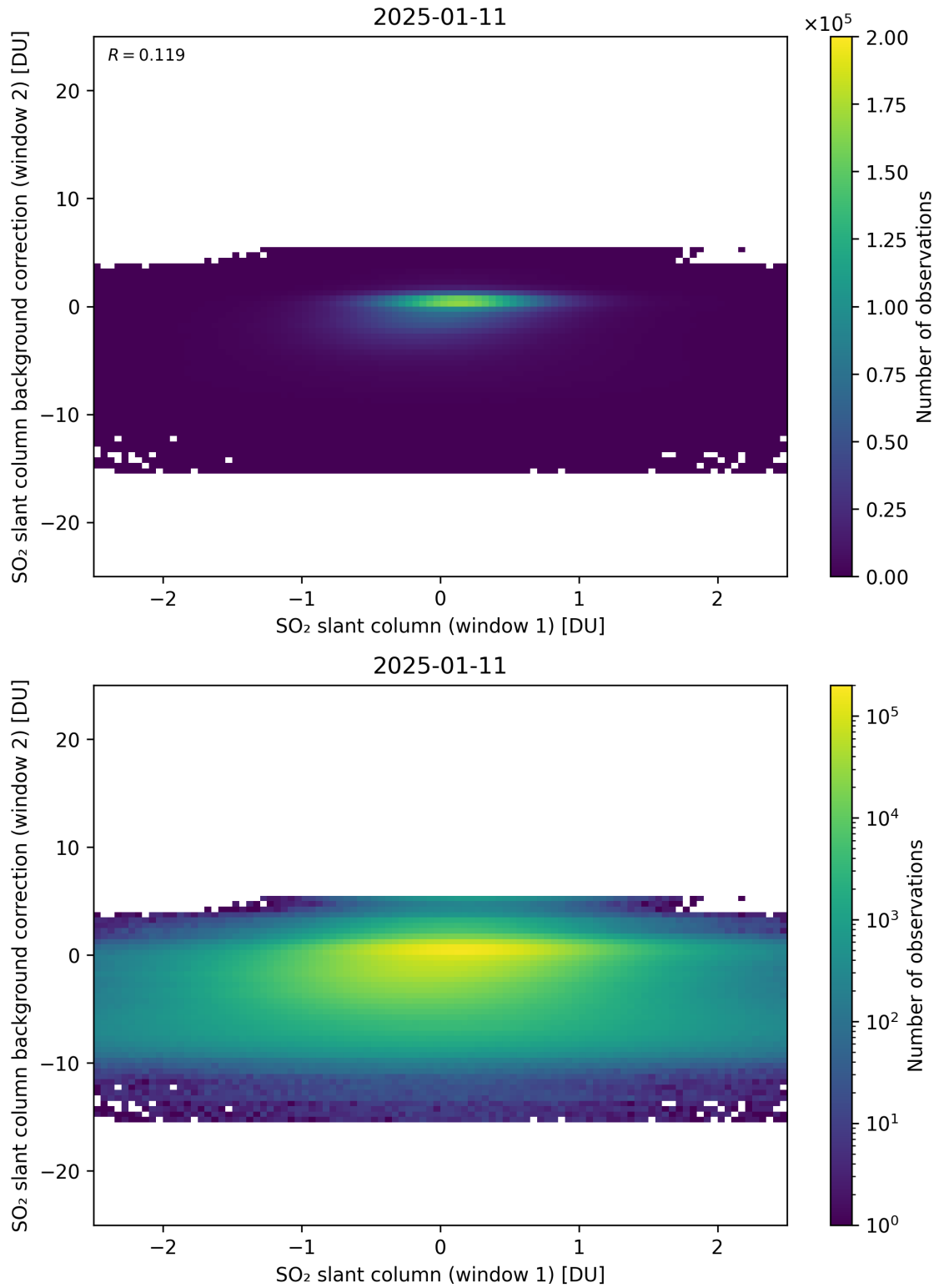
Figure 263: Scatter density plot of “SO 2 slant column (window 1)” against “SO 2 slant column background correction (window 2)” for 2025-01-10 to 2025-01-12.
