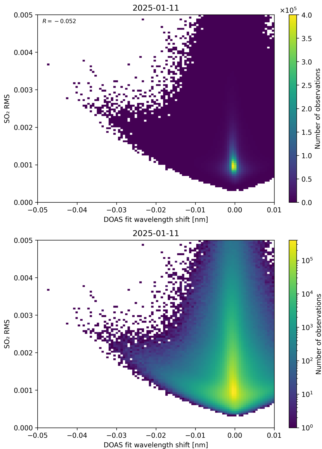
Figure 139: Scatter density plot of “DOAS fit wavelength shift” against “SO 2 RMS” for 2025-01-10 to 2025-01-12.
