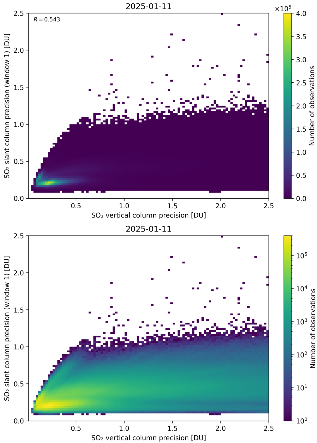
Figure 342: Scatter density plot of “SO 2 vertical column precision” against “SO 2 slant column precision (window 1)” for 2025-01-10 to 2025-01-12.
