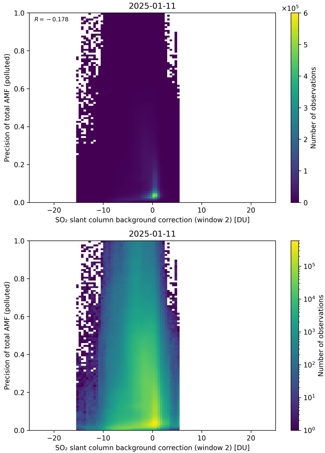
Figure 131: Scatter density plot of “SO 2 slant column background correction (window 2)” against “Precision of total AMF (polluted)” for 2025-01-10 to 2025-01-12.
