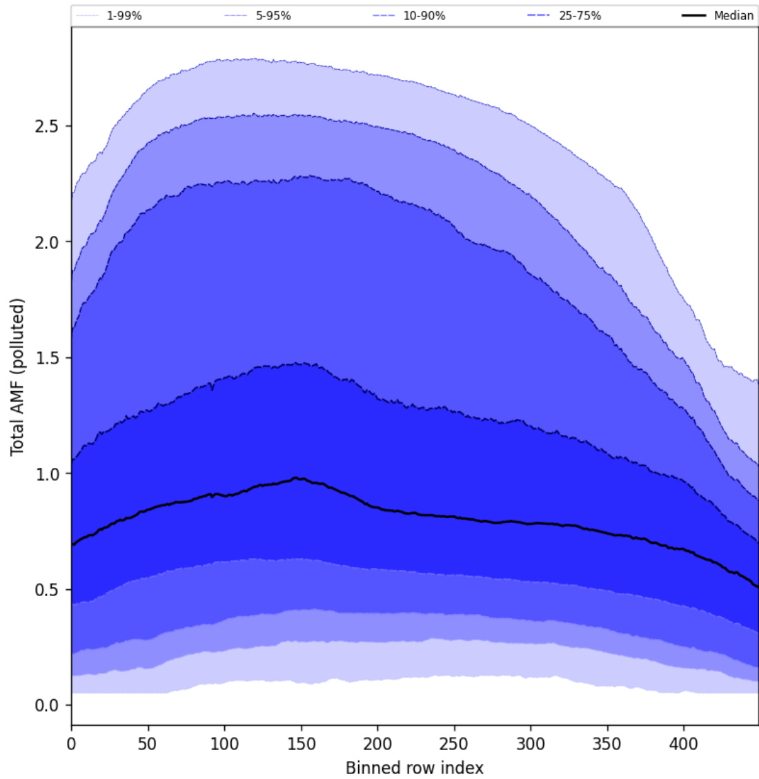
Figure 105: Along track statistics of “Total AMF (polluted)” for 2025-01-10 to 2025-01-12
