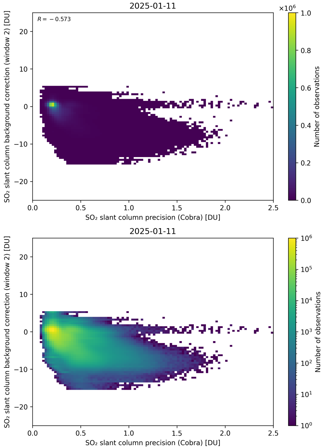
Figure 200: Scatter density plot of “SO 2 slant column precision (Cobra)” against “SO 2 slant column background correction (window 2)” for 2025-01-10 to 2025-01-12.
