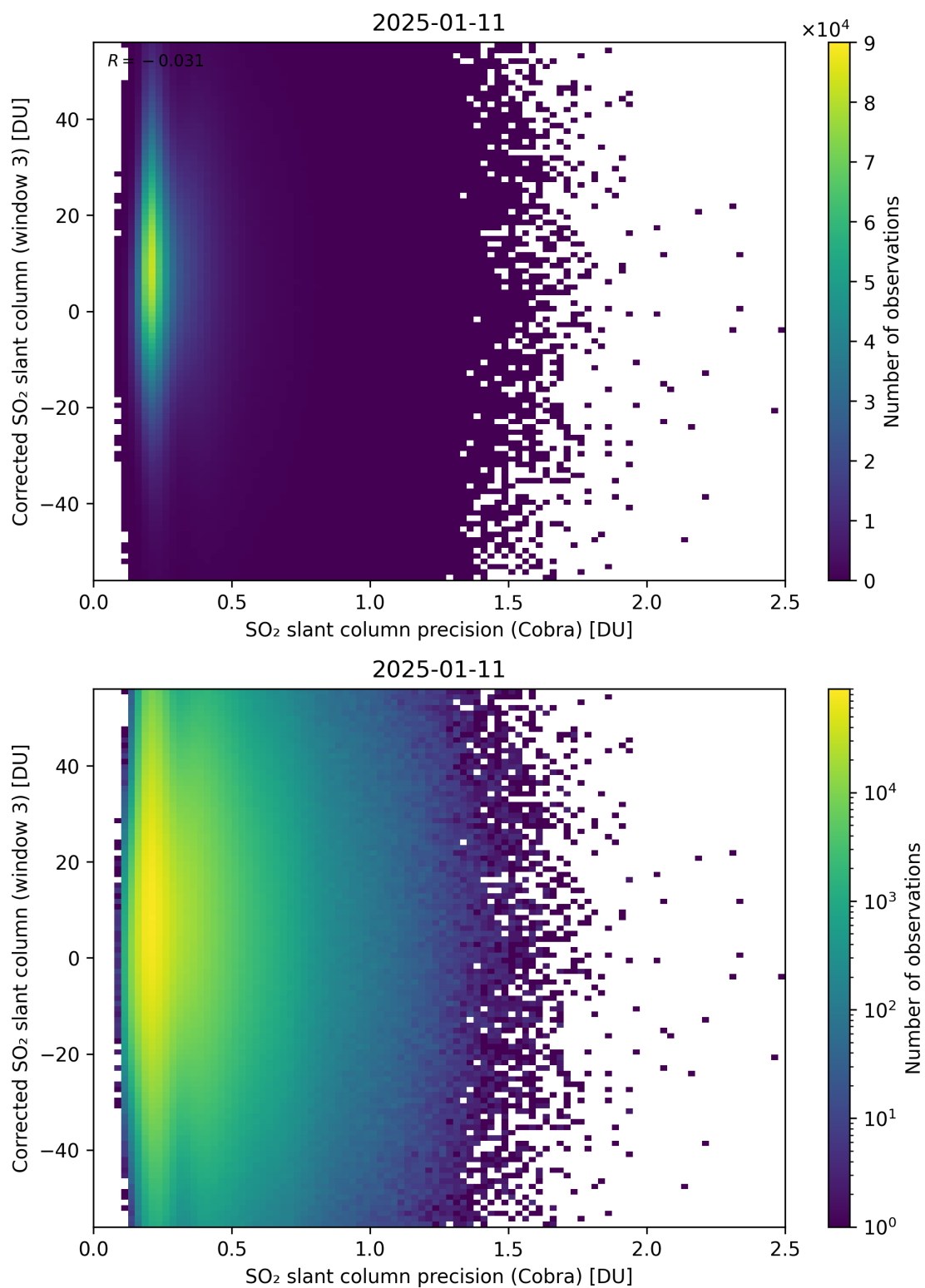
Figure 207: Scatter density plot of “SO 2 slant column precision (Cobra)” against “Corrected SO 2 slant column (window 3)” for 2025-01-10 to 2025-01-12.
