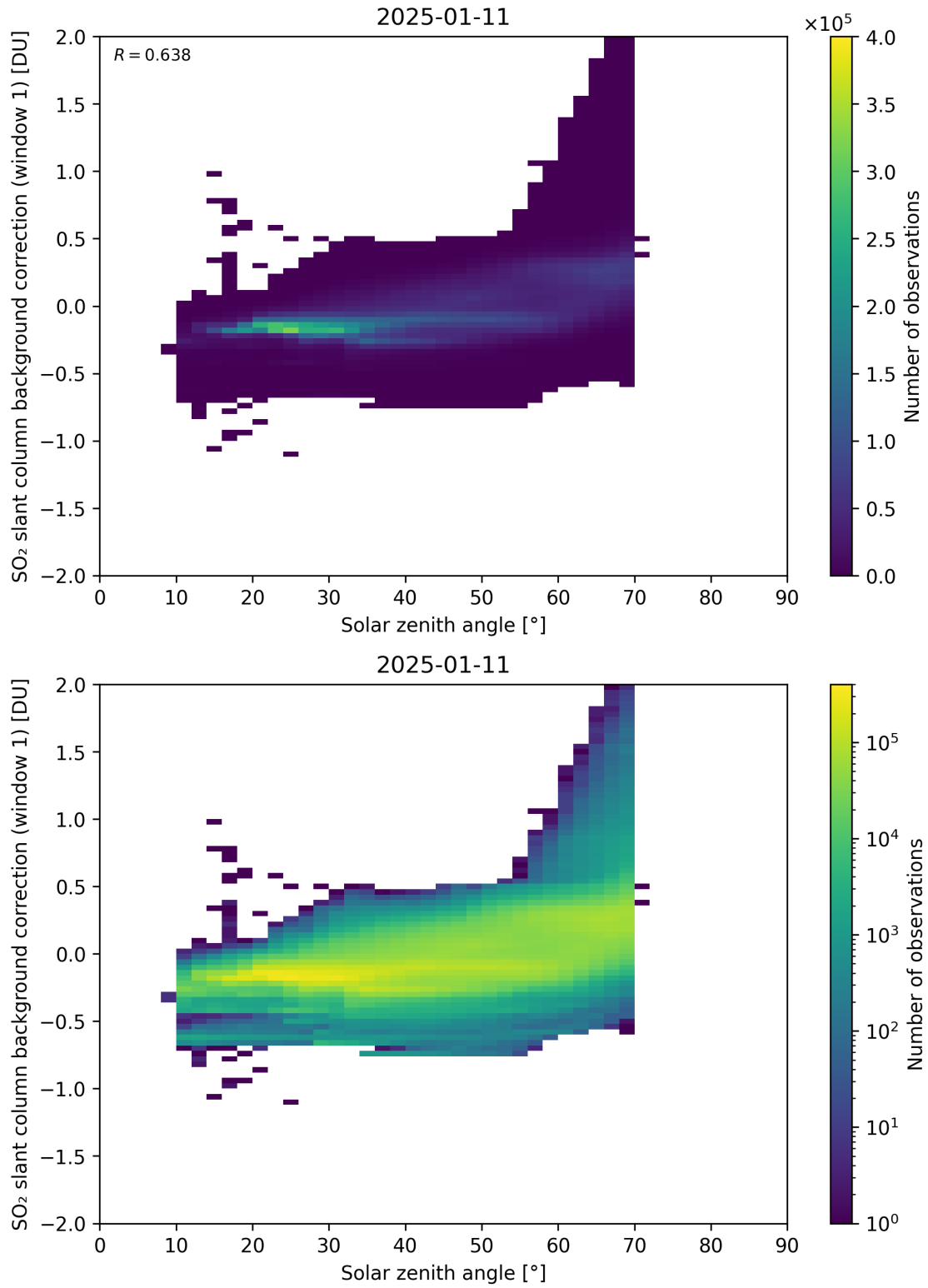
Figure 171: Scatter density plot of “Solar zenith angle” against “SO 2 slant column background correction (window 1)” for 2025-01-10 to 2025-01-12.
