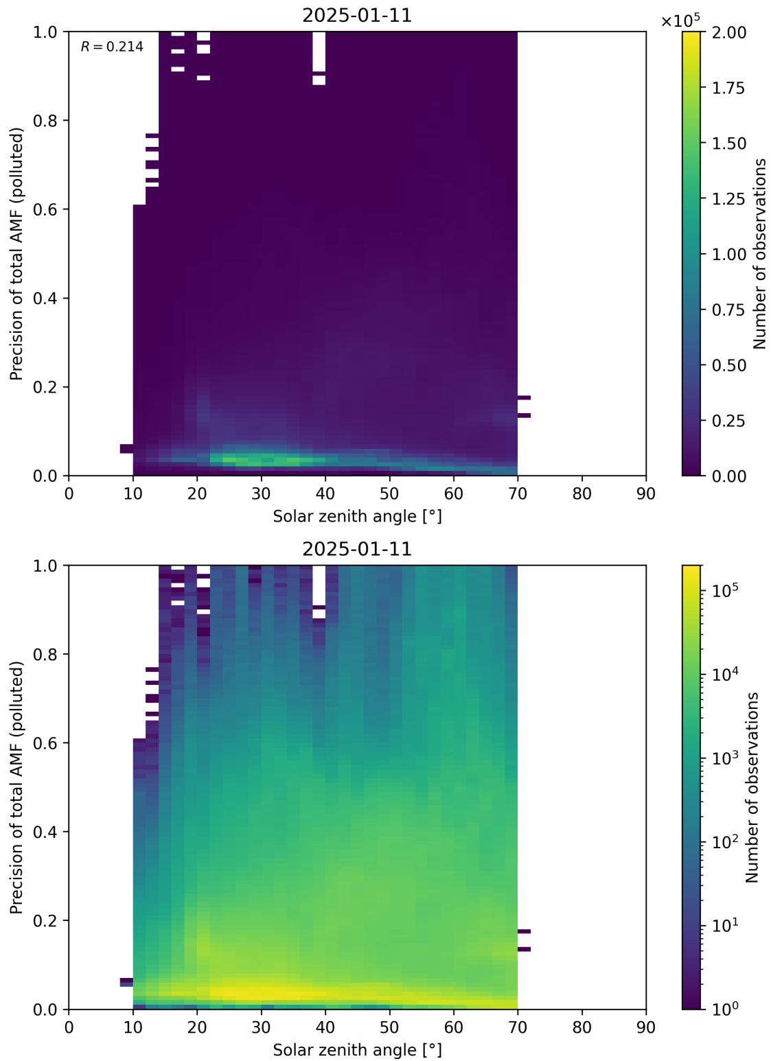
Figure 190: Scatter density plot of “Solar zenith angle” against “Precision of total AMF (polluted)” for 2025-01-10 to 2025-01-12.
