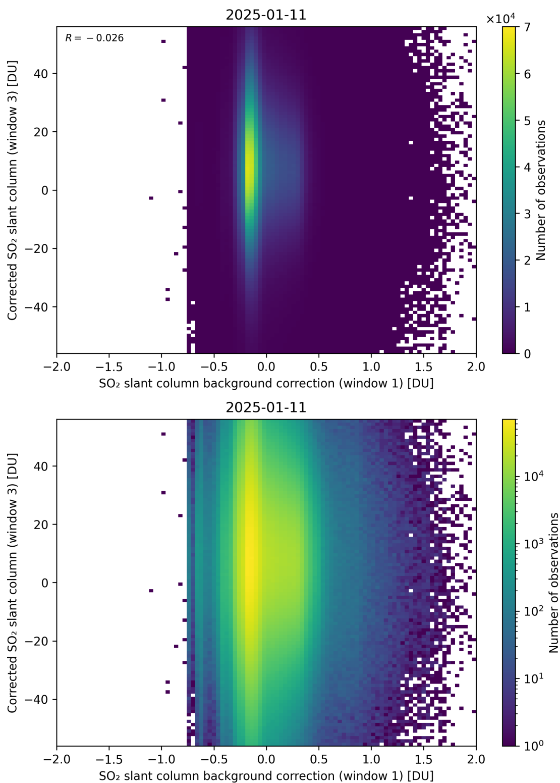
Figure 116: Scatter density plot of “SO 2 slant column background correction (window 1)” against “Corrected SO 2 slant column (window 3)” for 2025-01-10 to 2025-01-12.
