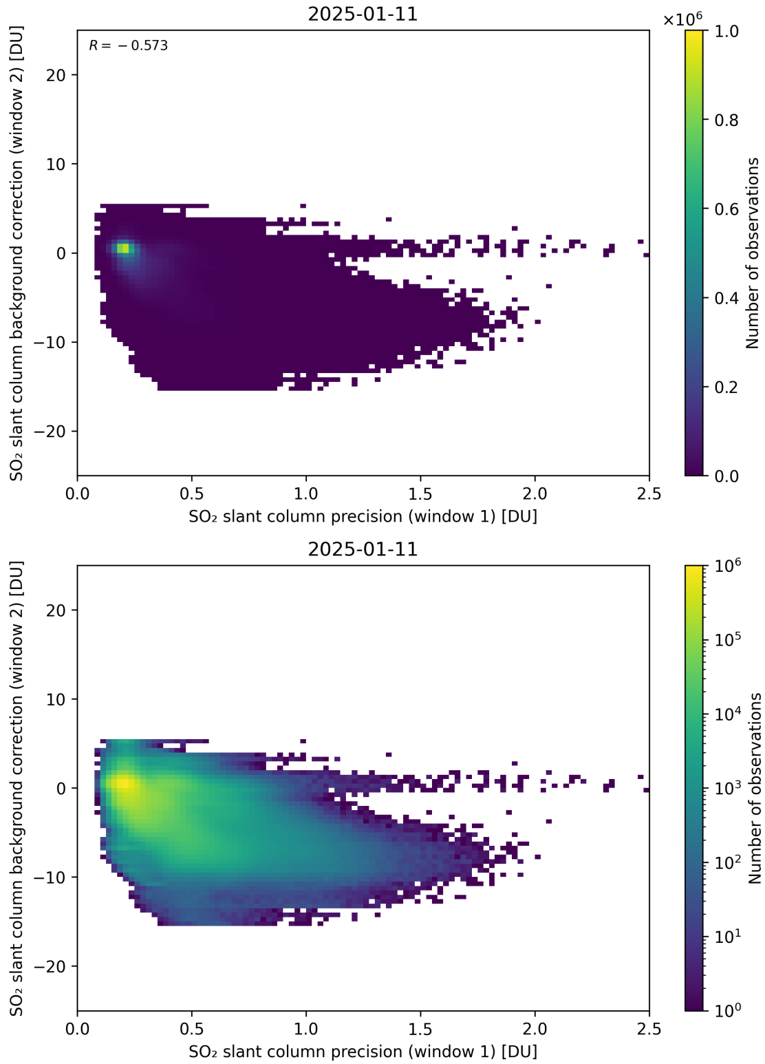
Figure 269: Scatter density plot of “SO 2 slant column precision (window 1)” against “SO 2 slant column background correction (window 2)” for 2025-01-10 to 2025-01-12.
