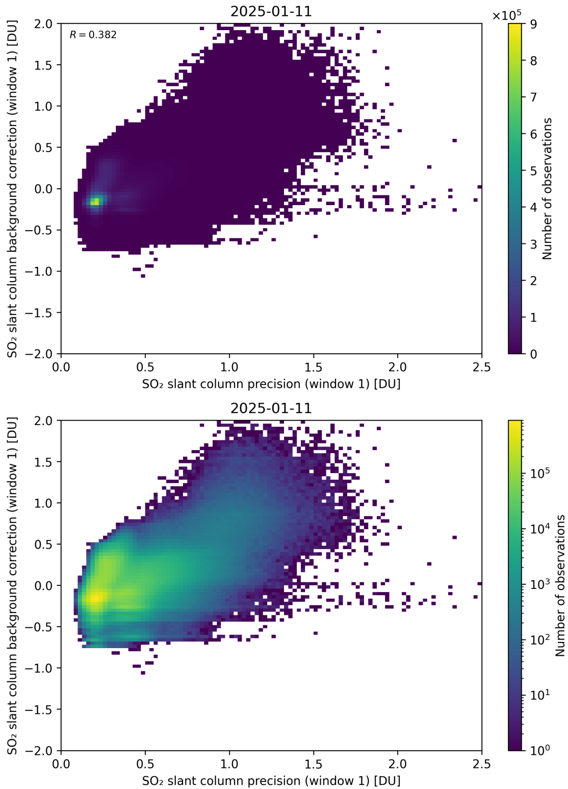
Figure 268: Scatter density plot of “SO 2 slant column precision (window 1)” against “SO 2 slant column background correction (window 1)” for 2025-01-10 to 2025-01-12.
