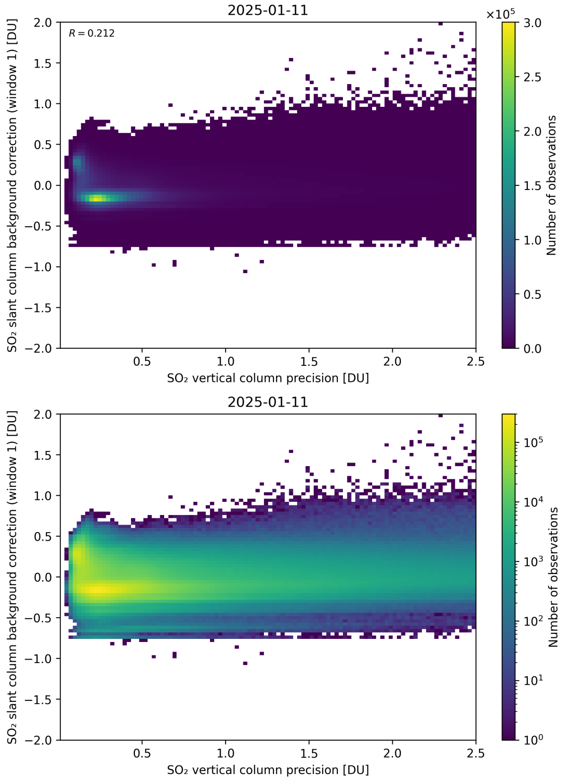
Figure 329: Scatter density plot of “SO 2 vertical column precision” against “SO 2 slant column background correction (window 1)” for 2025-01-10 to 2025-01-12.
