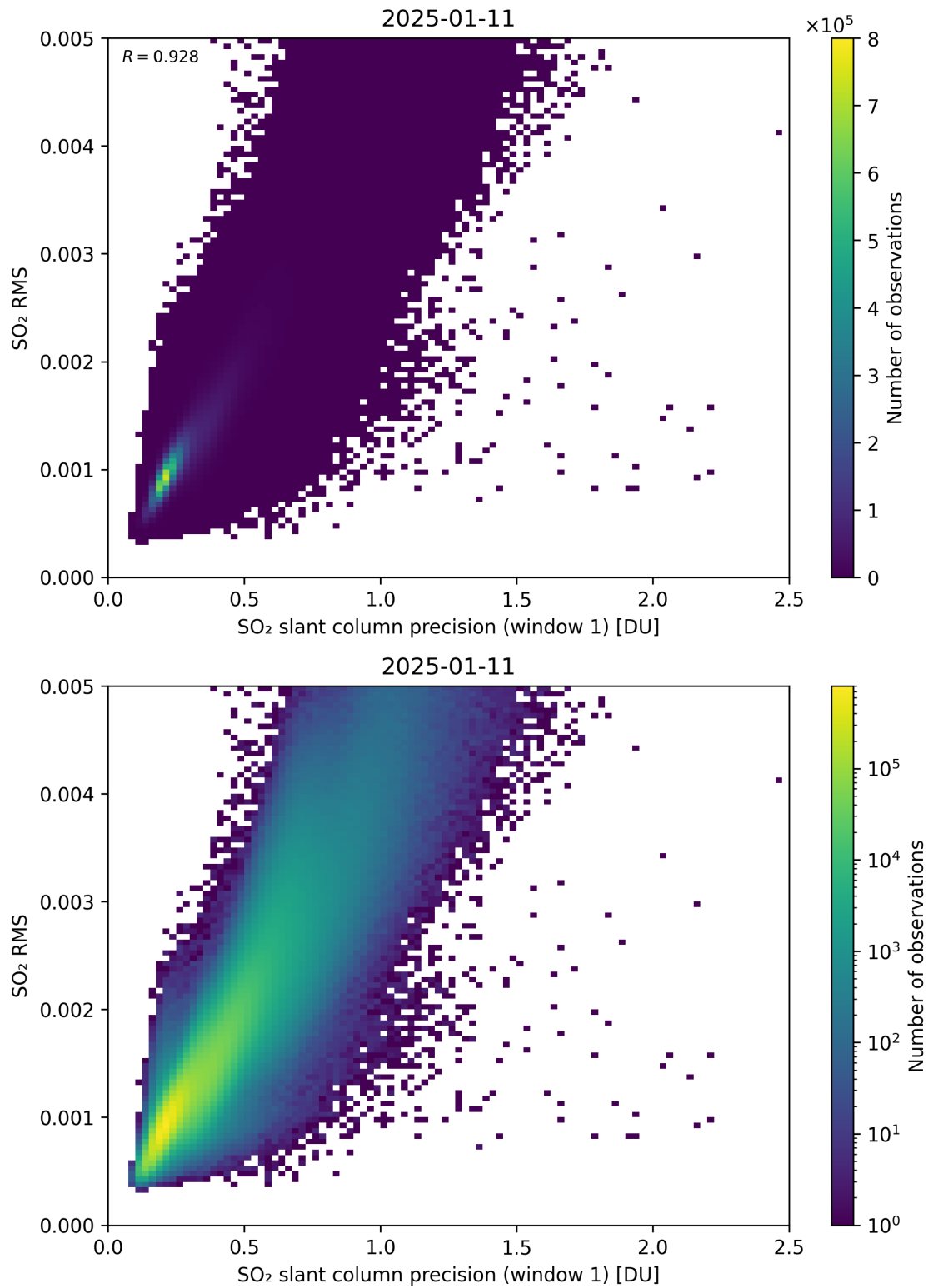
Figure 273: Scatter density plot of “SO 2 slant column precision (window 1)” against “SO 2 RMS” for 2025-01-10 to 2025-01-12.
