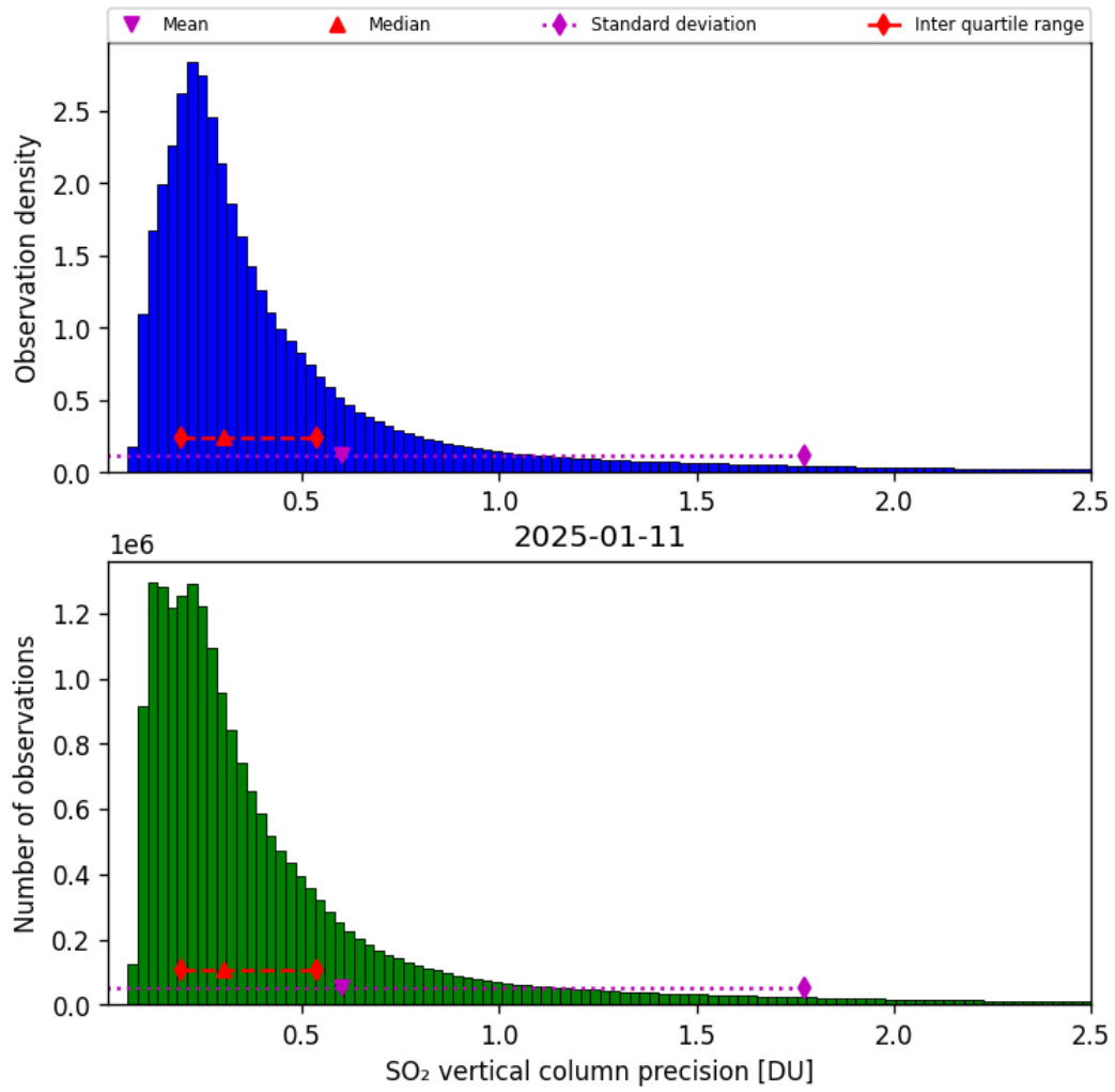
Figure 59: Histogram of “SO 2 vertical column precision” for 2025-01-10 to 2025-01-12
