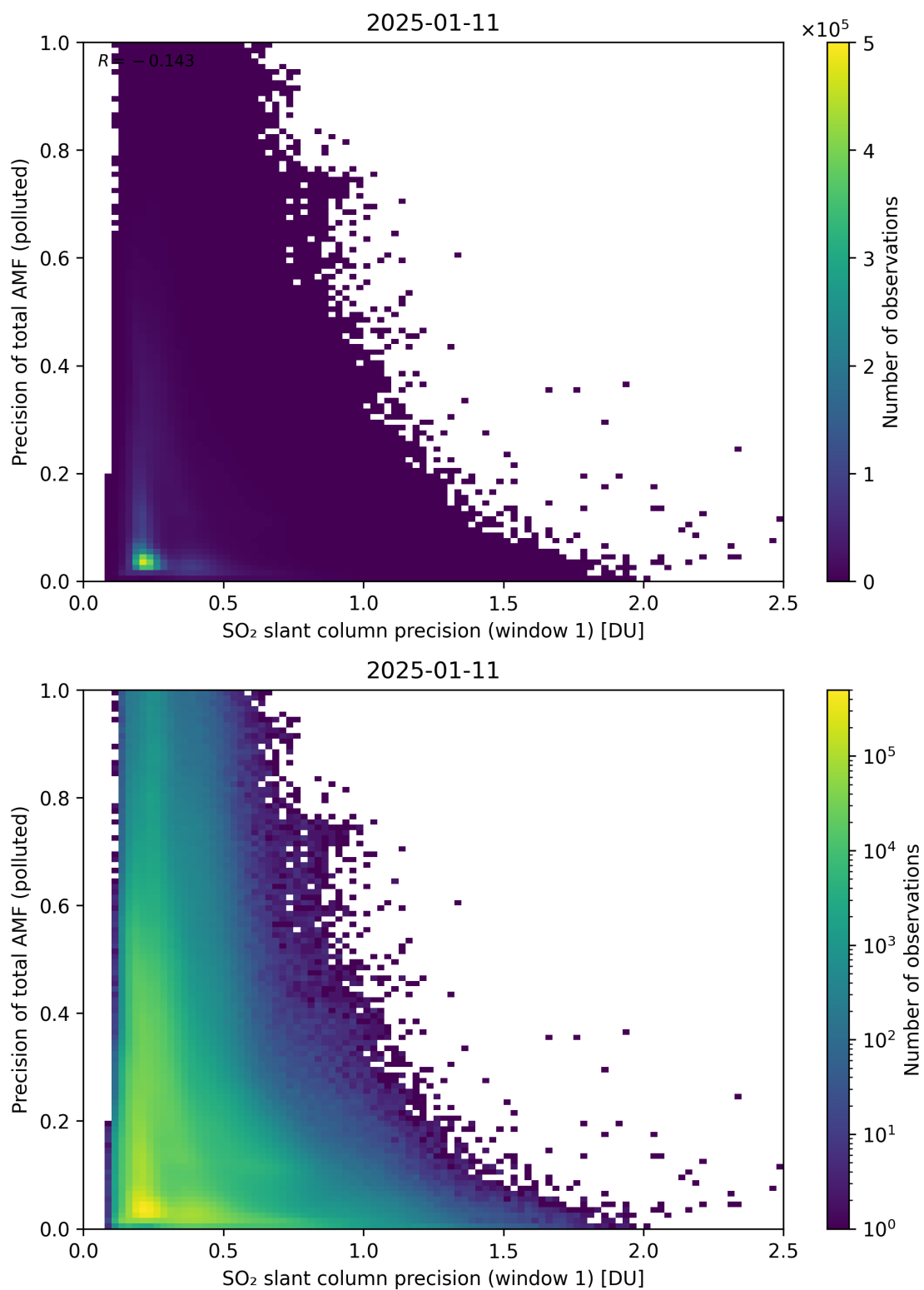
Figure 281: Scatter density plot of “SO 2 slant column precision (window 1)” against “Precision of total AMF (polluted)” for 2025-01-10 to 2025-01-12.
