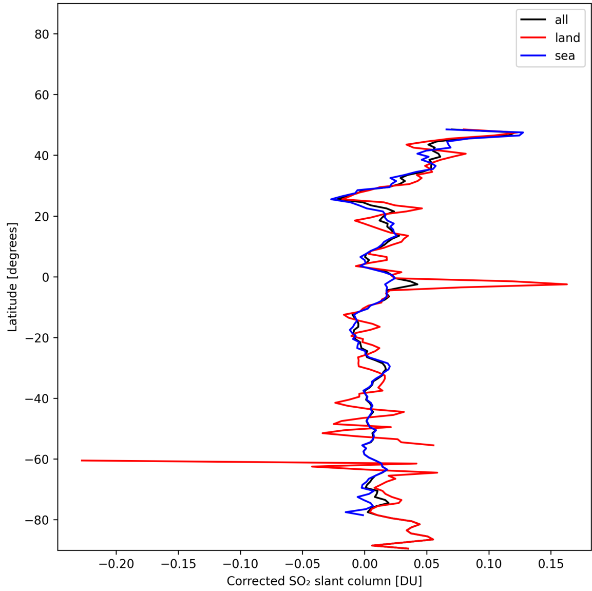
Figure 34: Zonal average of “Corrected SO 2 slant column” for 2025-01-10 to 2025-01-12.
