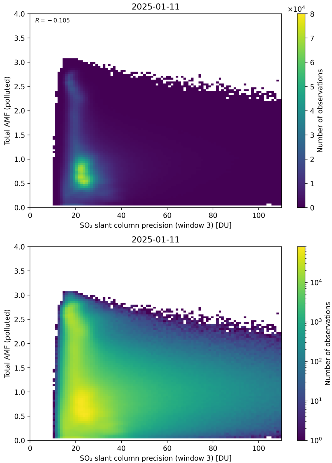
Figure 313: Scatter density plot of “SO 2 slant column precision (window 3)” against “Total AMF (polluted)” for 2025-01-10 to 2025-01-12.
