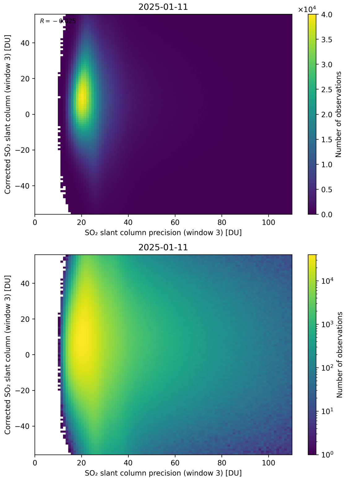
Figure 312: Scatter density plot of “SO 2 slant column precision (window 3)” against “Corrected SO 2 slant column (window 3)” for 2025-01-10 to 2025-01-12.
