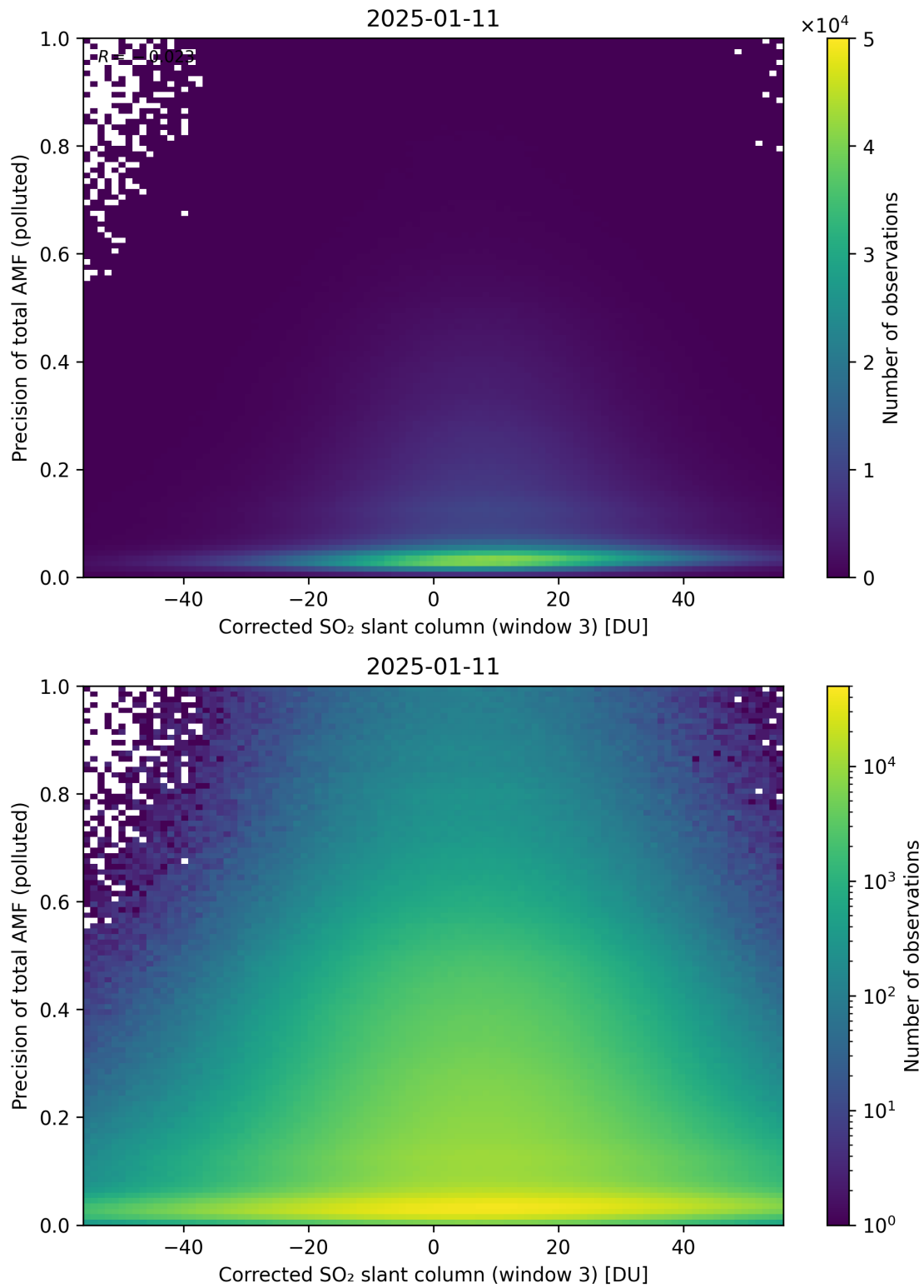
Figure 261: Scatter density plot of “Corrected SO 2 slant column (window 3)” against “Precision of total AMF (polluted)” for 2025-01-10 to 2025-01-12.
