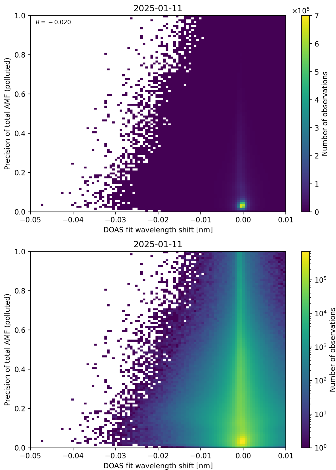
Figure 142: Scatter density plot of “DOAS fit wavelength shift” against “Precision of total AMF (polluted)” for 2025-01-10 to 2025-01-12.
