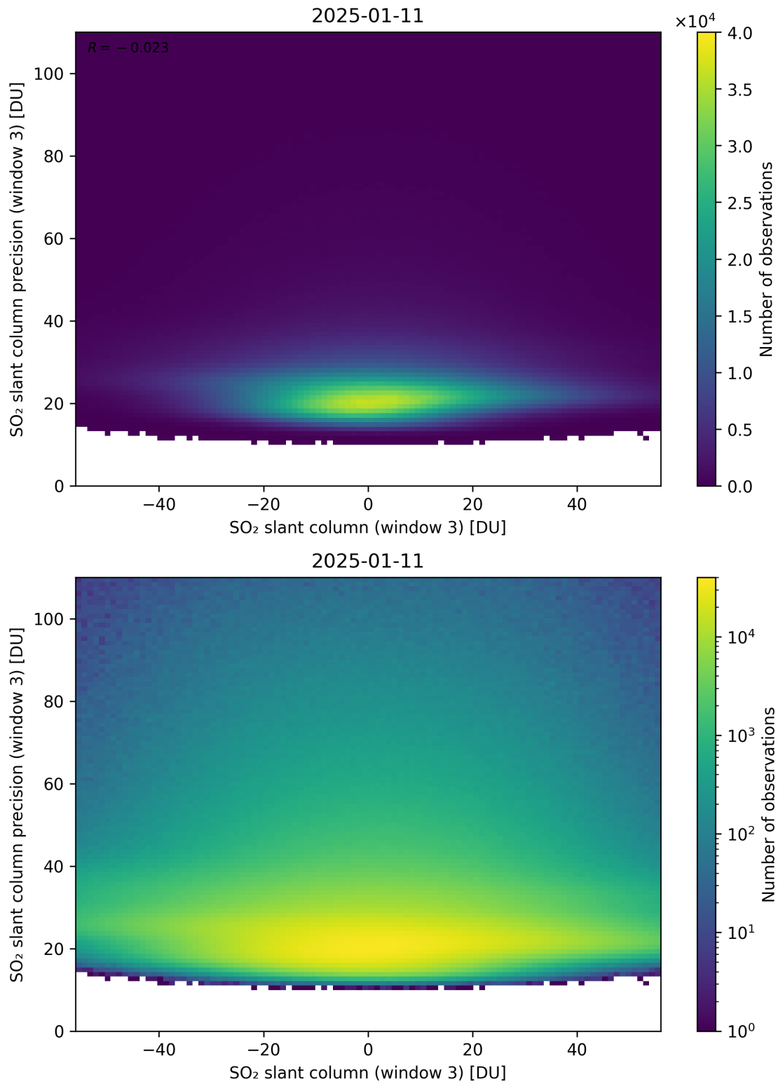
Figure 317: Scatter density plot of “SO 2 slant column (window 3)” against “SO 2 slant column precision (window 3)” for 2025-01-10 to 2025-01-12.
