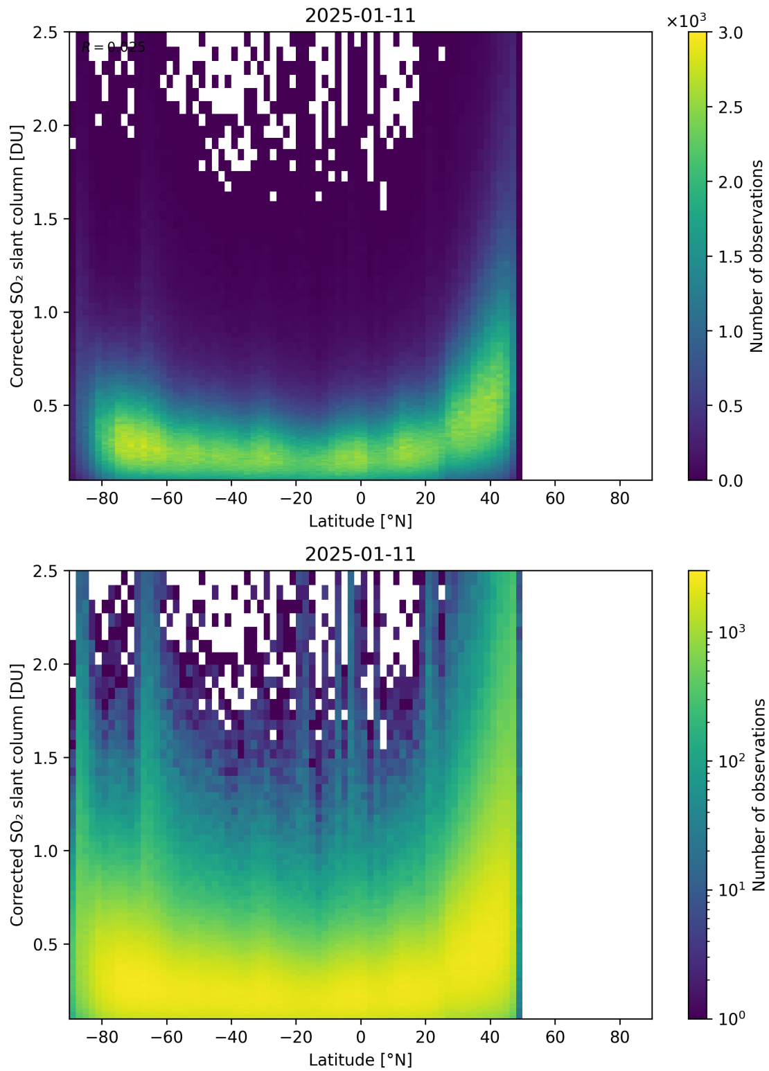
Figure 159: Scatter density plot of “Latitude” against “Corrected SO 2 slant column” for 2025-01-10 to 2025-01-12.
