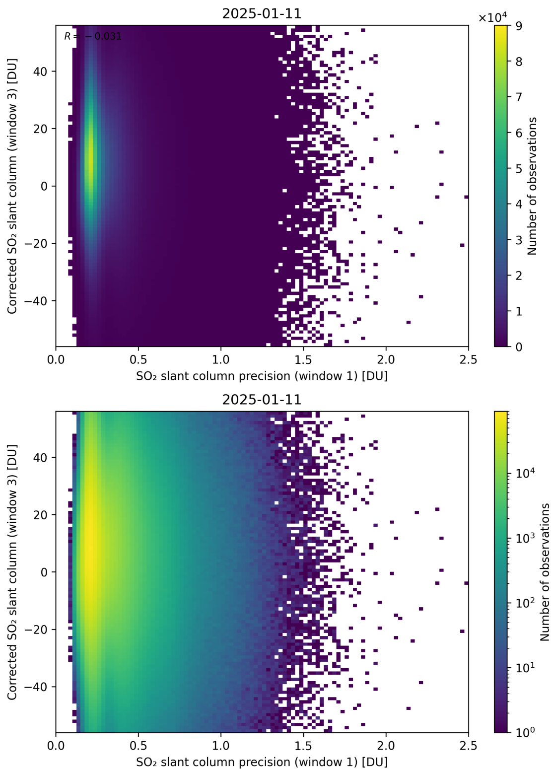
Figure 276: Scatter density plot of “SO 2 slant column precision (window 1)” against “Corrected SO 2 slant column (window 3)” for 2025-01-10 to 2025-01-12.
