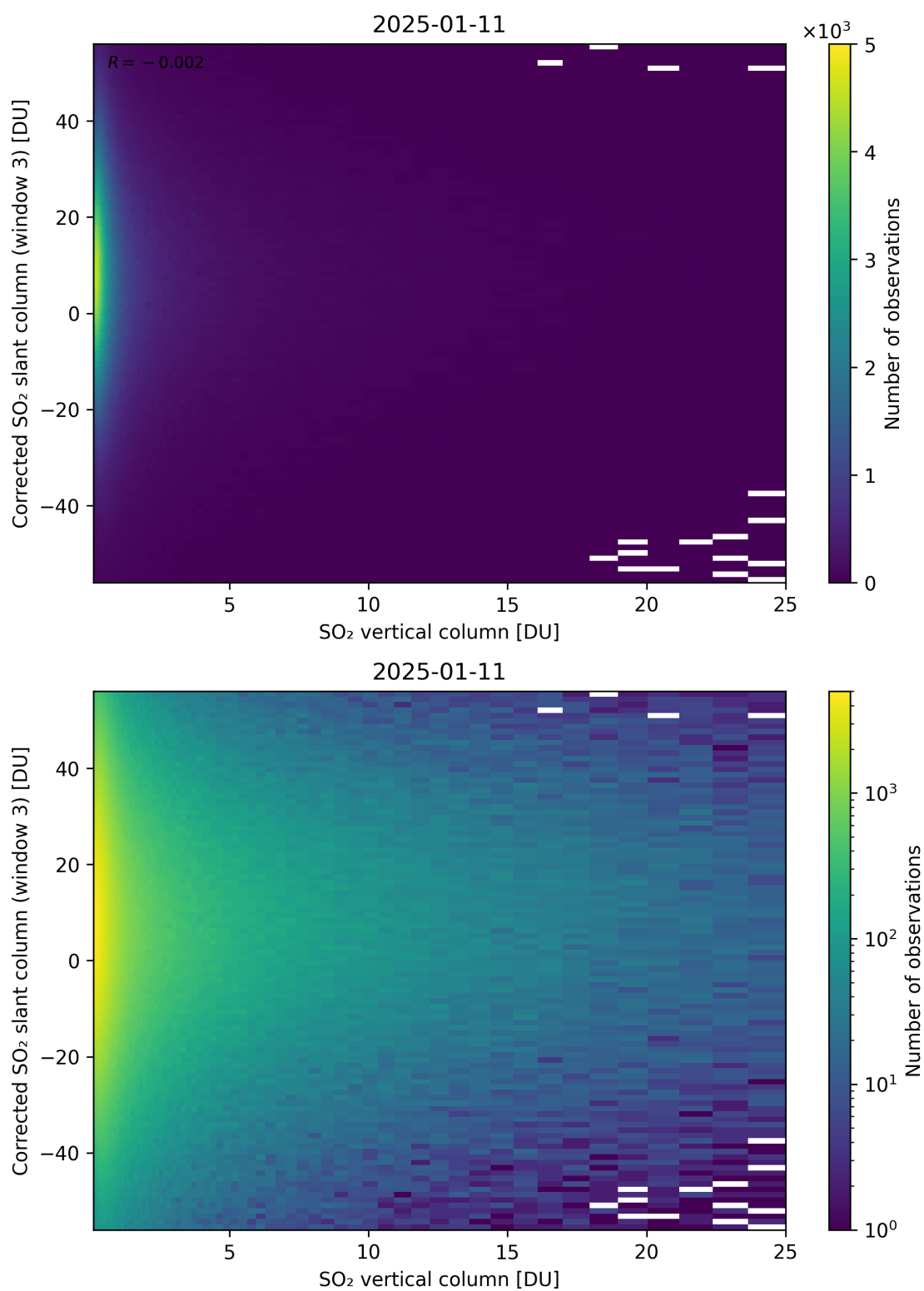
Figure 353: Scatter density plot of “SO 2 vertical column” against “Corrected SO 2 slant column (window 3)” for 2025-01-10 to 2025-01-12.
