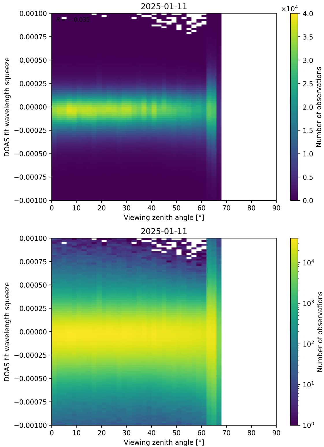
Figure 366: Scatter density plot of “Viewing zenith angle” against “DOAS fit wavelength squeeze” for 2025-01-10 to 2025-01-12.
