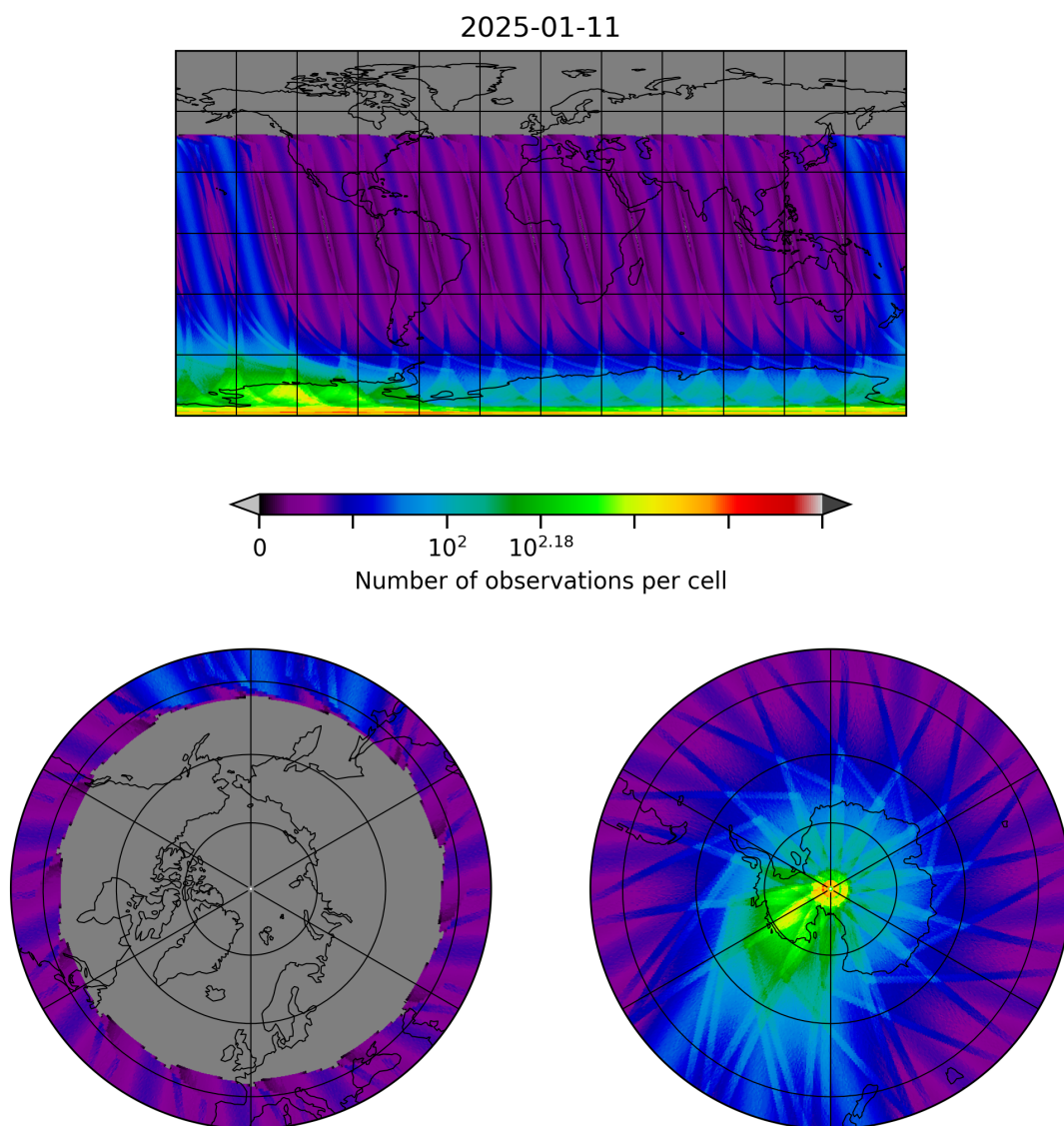
Figure 30: Map of the number of observations for 2025-01-10 to 2025-01-12
