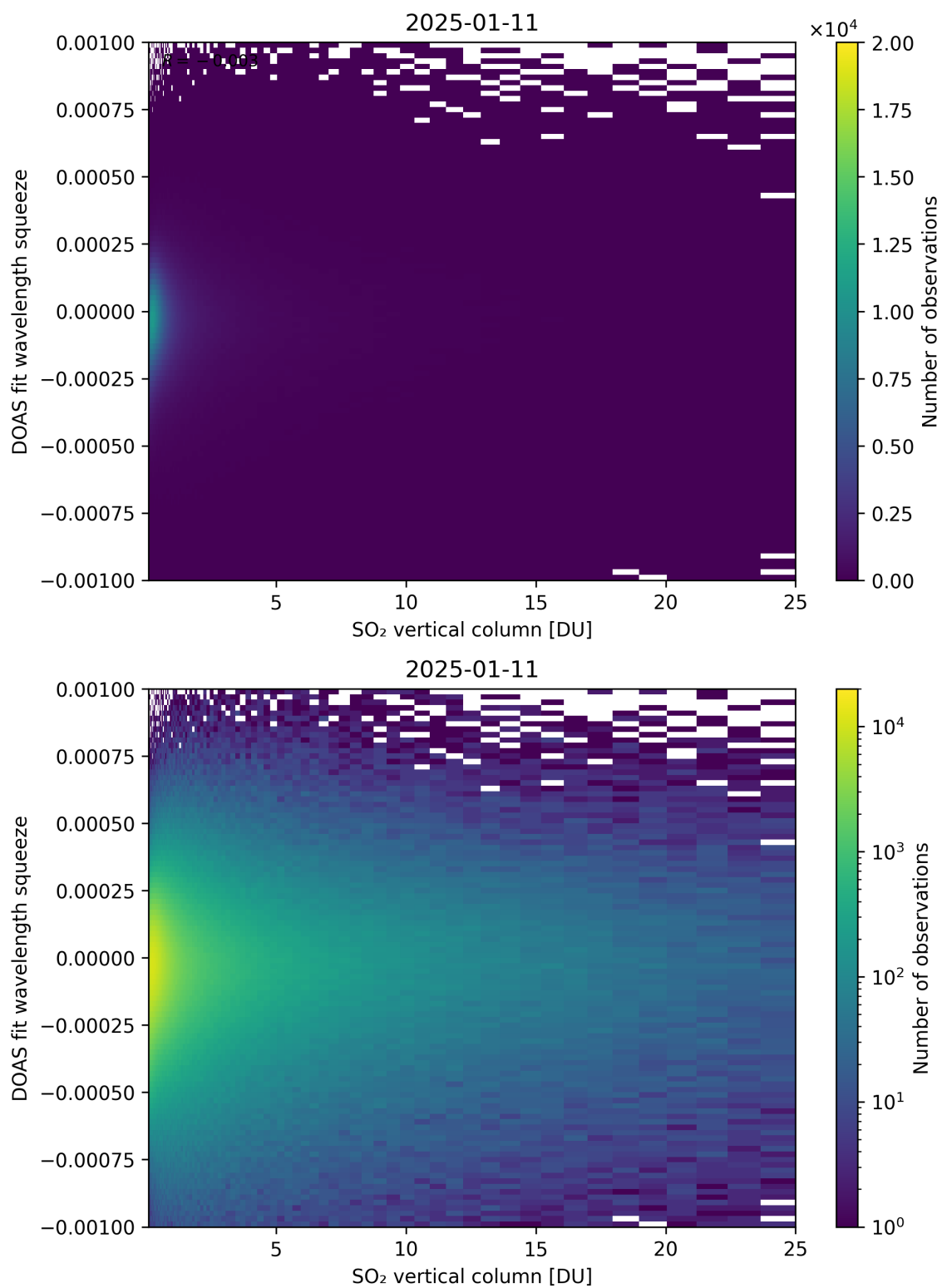
Figure 327: Scatter density plot of “SO 2 vertical column” against “DOAS fit wavelength squeeze” for 2025-01-10 to 2025-01-12.
