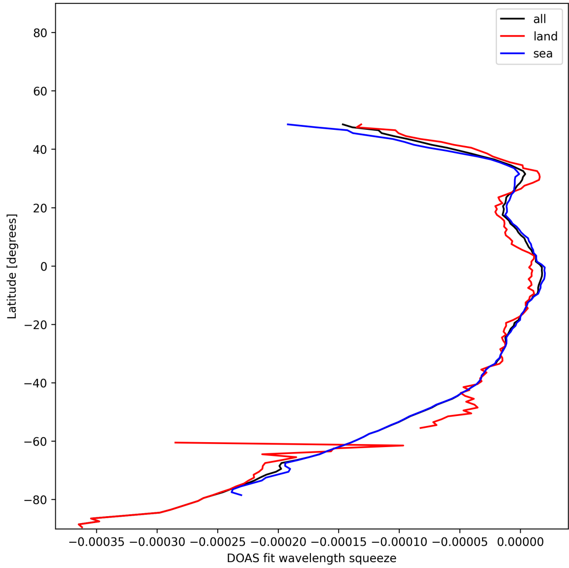
Figure 51: Zonal average of “DOAS fit wavelength squeeze” for 2025-01-10 to 2025-01-12.
