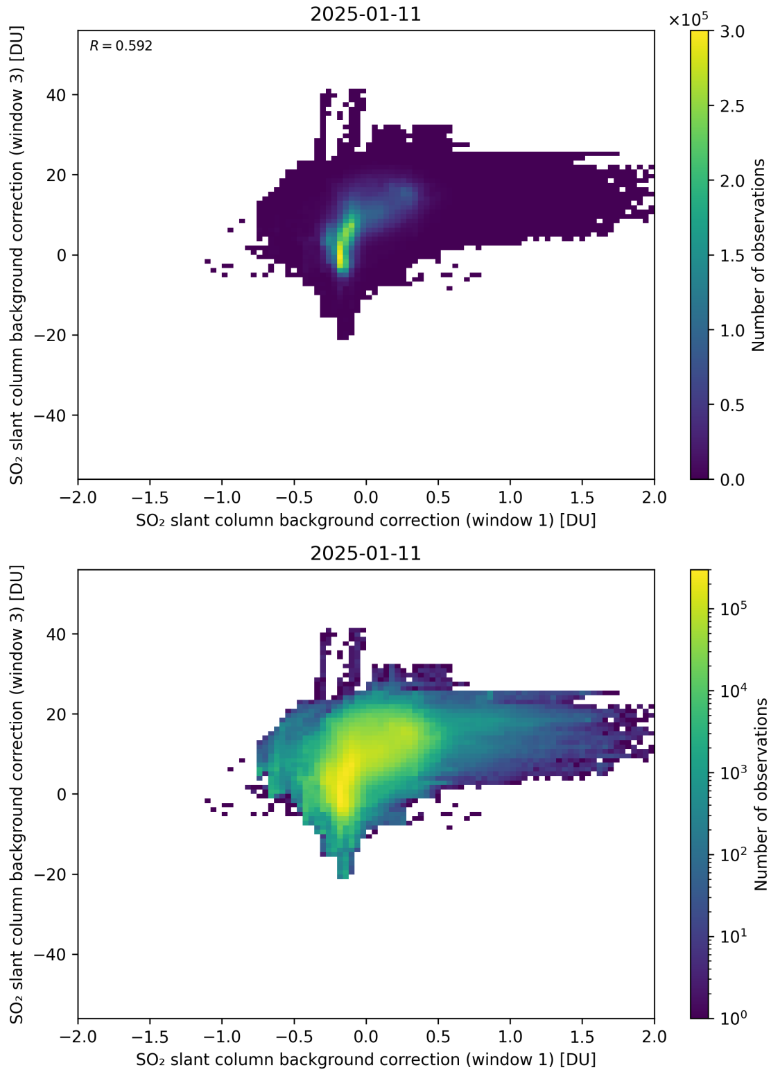
Figure 110: Scatter density plot of “SO 2 slant column background correction (window 1)” against “SO 2 slant column background correction (window 3)” for 2025-01-10 to 2025-01-12.
