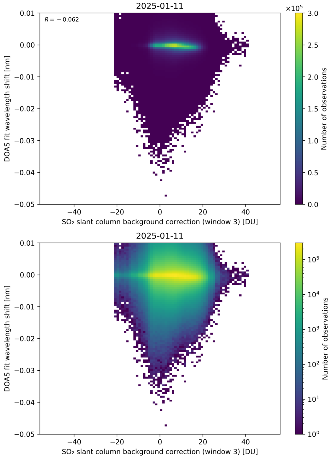
Figure 132: Scatter density plot of “SO 2 slant column background correction (window 3)” against “DOAS fit wavelength shift” for 2025-01-10 to 2025-01-12.
