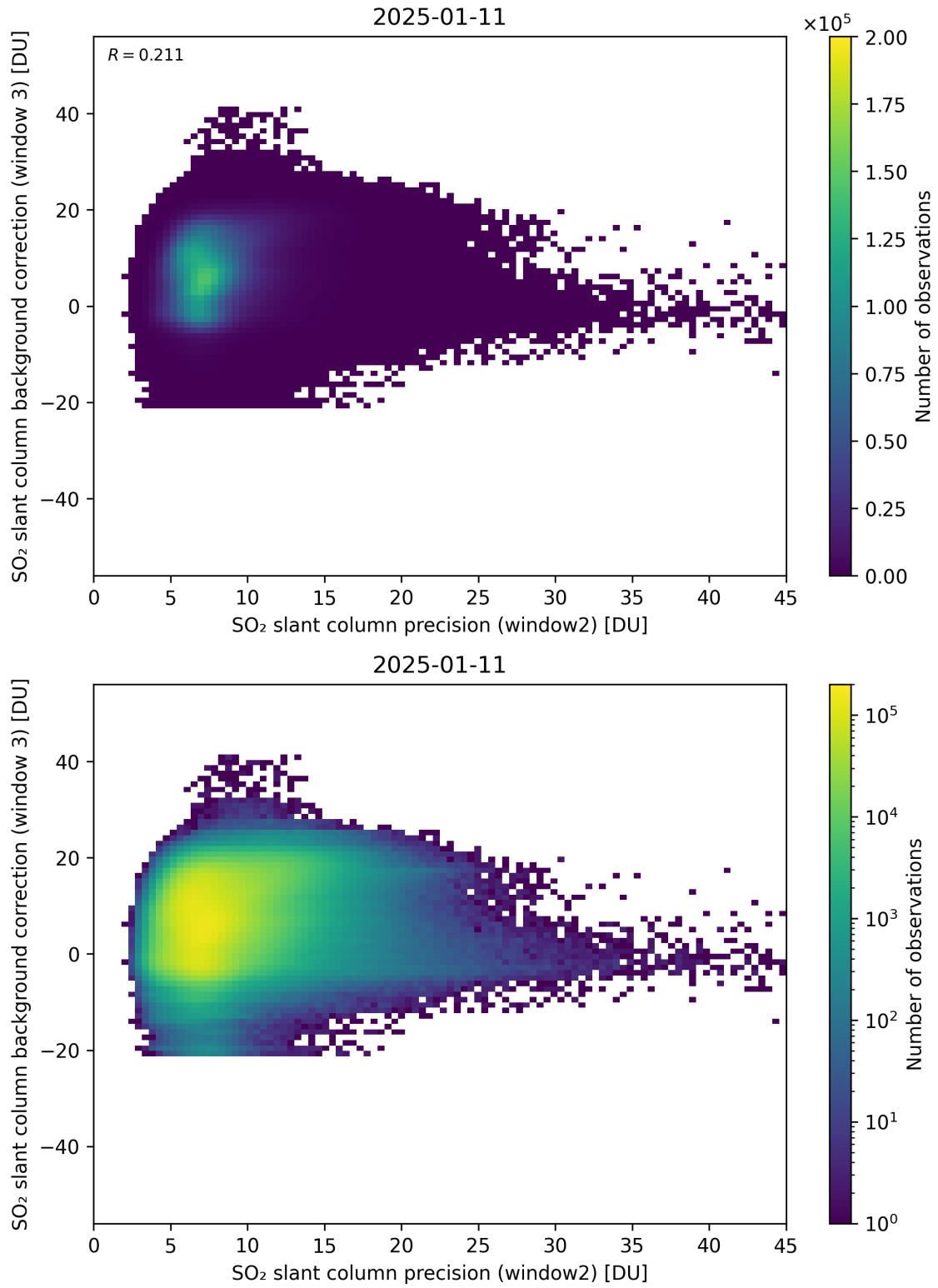
Figure 292: Scatter density plot of “SO 2 slant column precision (window2)” against “SO 2 slant column background correction (window 3)” for 2025-01-10 to 2025-01-12.
