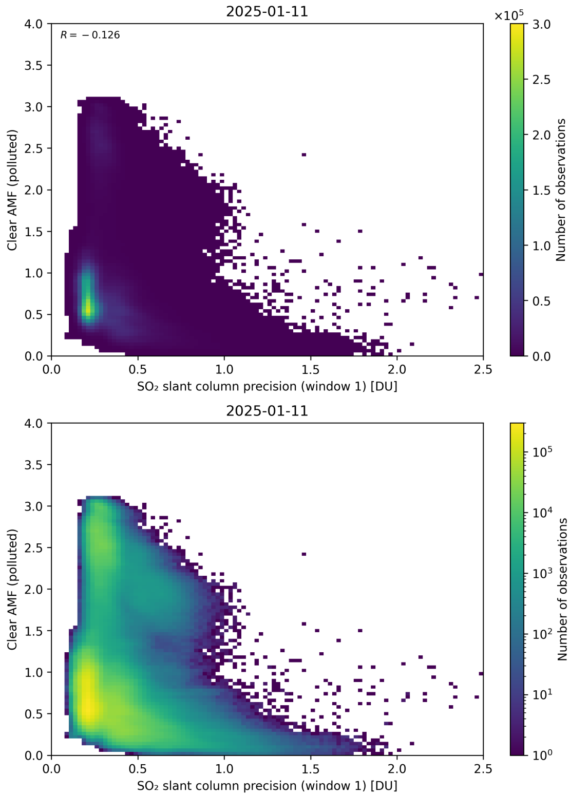
Figure 274: Scatter density plot of “SO 2 slant column precision (window 1)” against “Clear AMF (polluted)” for 2025-01-10 to 2025-01-12.
