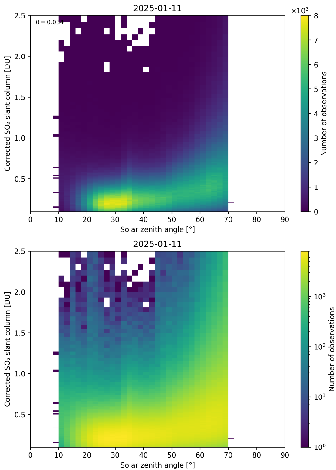
Figure 181: Scatter density plot of “Solar zenith angle” against “Corrected SO 2 slant column” for 2025-01-10 to 2025-01-12.
