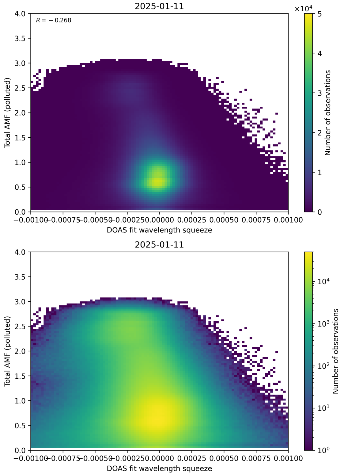
Figure 145: Scatter density plot of “DOAS fit wavelength squeeze” against “Total AMF (polluted)” for 2025-01-10 to 2025-01-12.
