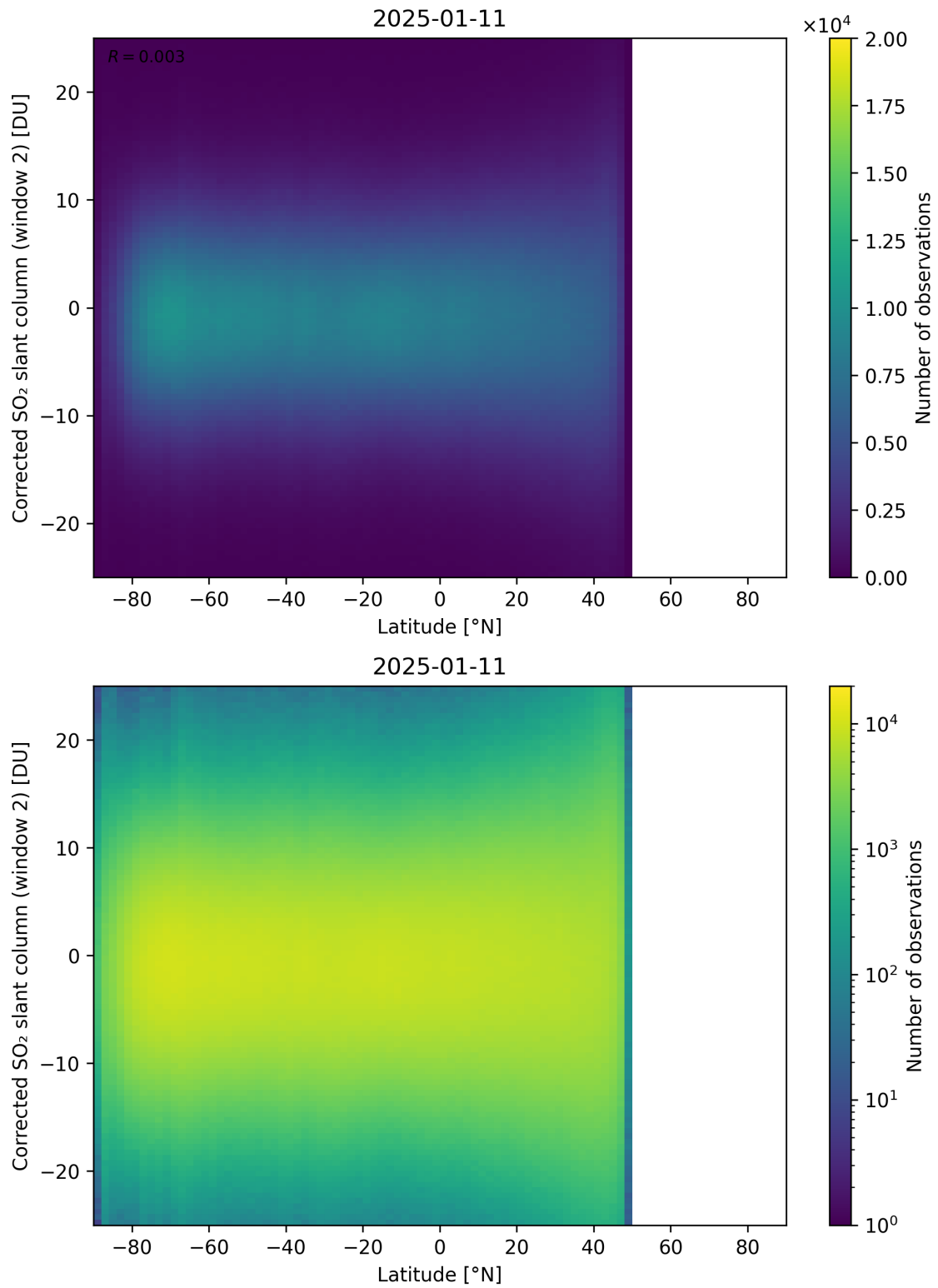
Figure 160: Scatter density plot of “Latitude” against “Corrected SO 2 slant column (window 2)” for 2025-01-10 to 2025-01-12.
