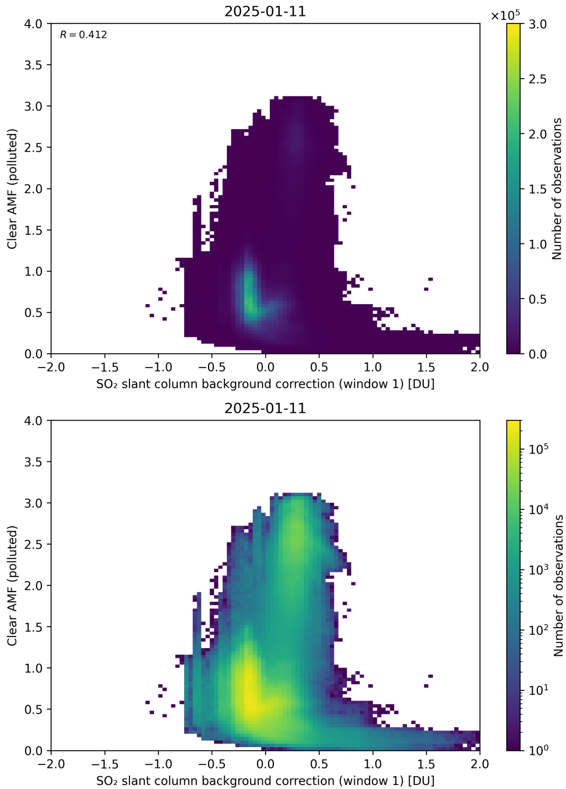
Figure 114: Scatter density plot of “SO 2 slant column background correction (window 1)” against “Clear AMF (polluted)” for 2025-01-10 to 2025-01-12.
