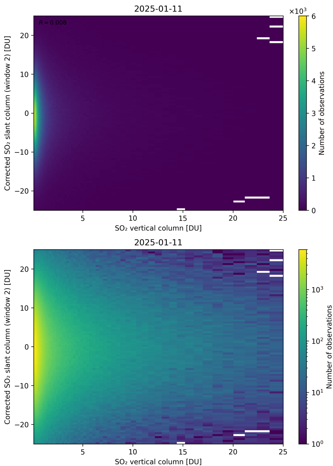
Figure 352: Scatter density plot of “SO 2 vertical column” against “Corrected SO 2 slant column (window 2)” for 2025-01-10 to 2025-01-12.
