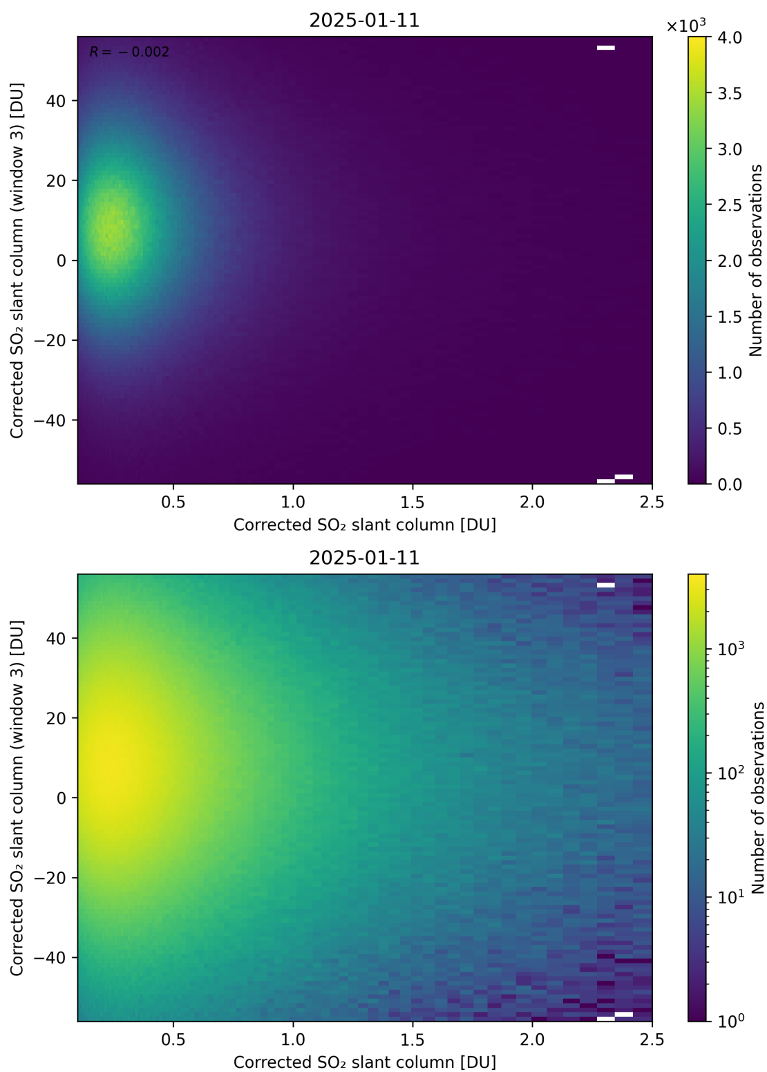
Figure 236: Scatter density plot of “Corrected SO 2 slant column” against “Corrected SO 2 slant column (window 3)” for 2025-01-10 to 2025-01-12.
