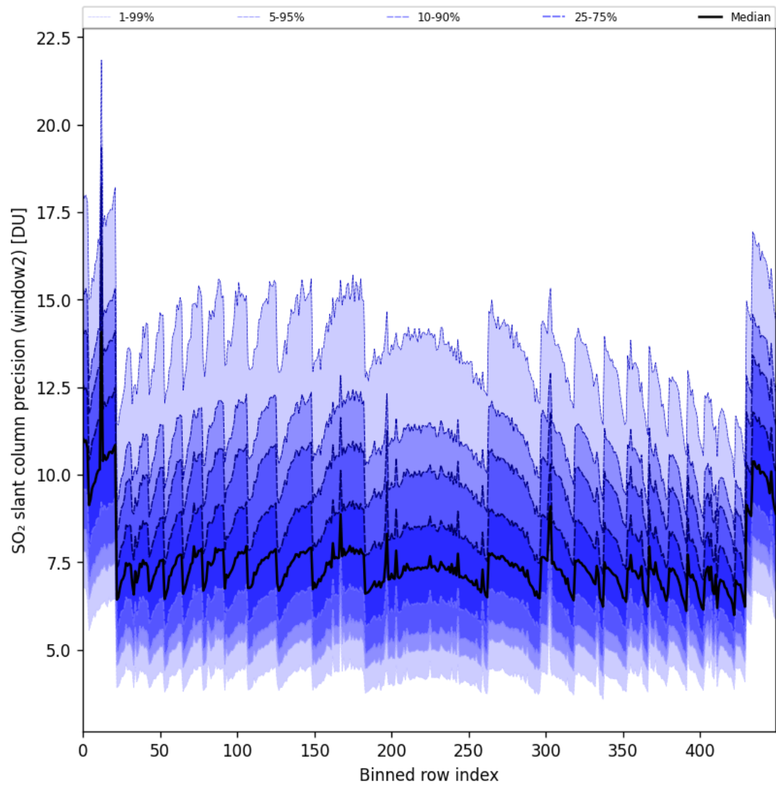
Figure 94: Along track statistics of “SO 2 slant column precision (window2)” for 2025-01-10 to 2025-01-12
