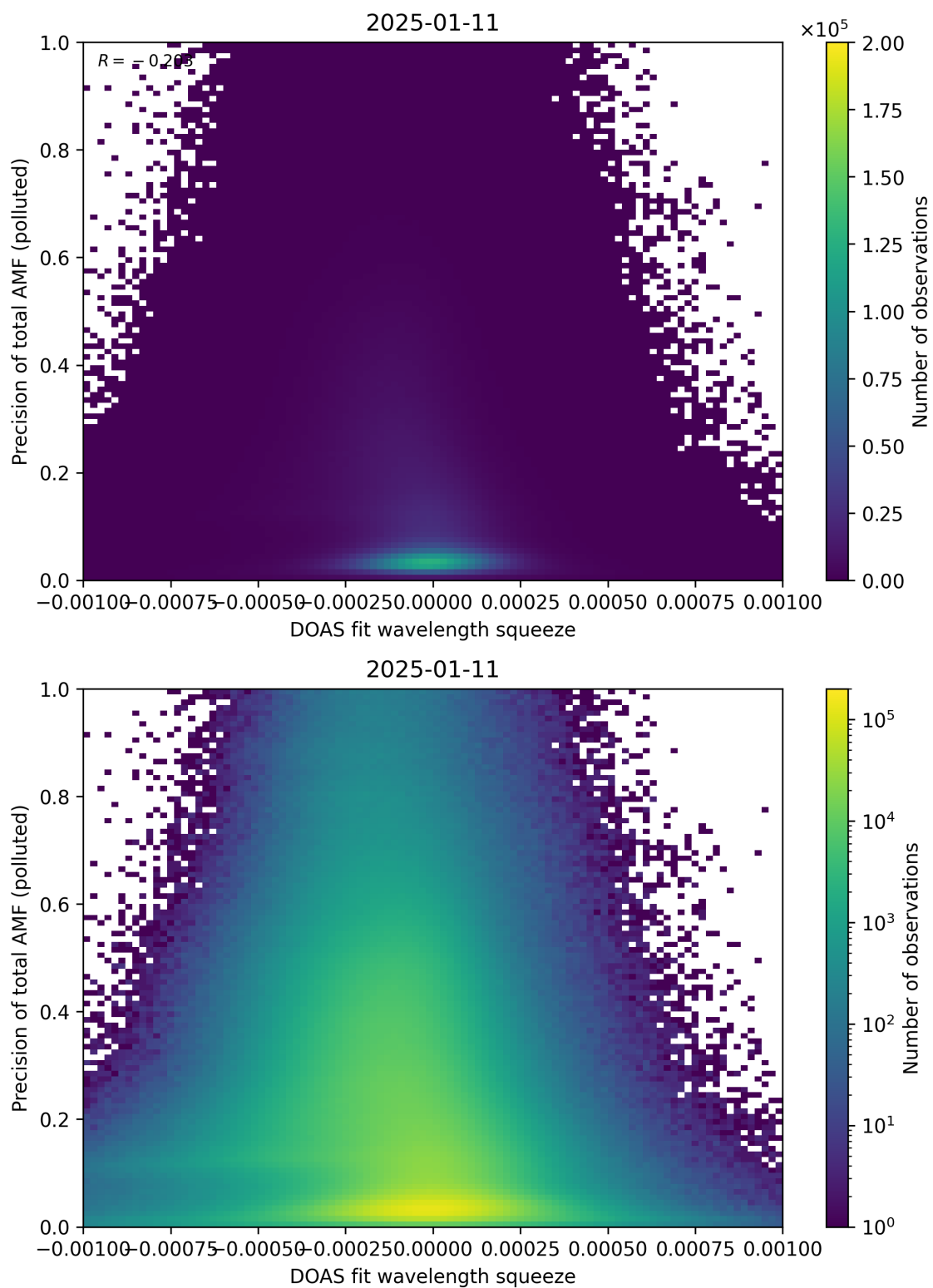
Figure 146: Scatter density plot of “DOAS fit wavelength squeeze” against “Precision of total AMF (polluted)” for 2025-01-10 to 2025-01-12.
