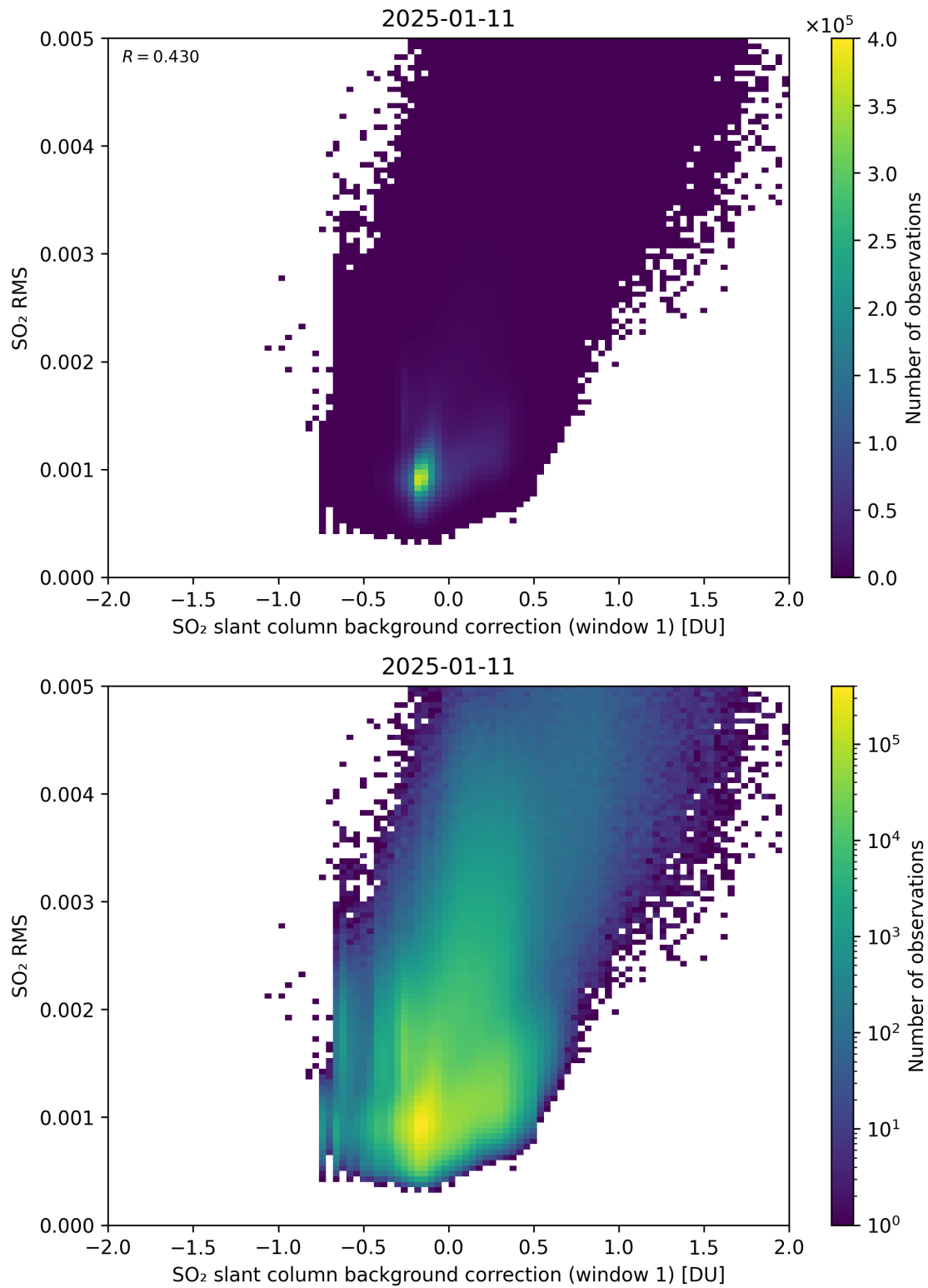
Figure 113: Scatter density plot of “SO 2 slant column background correction (window 1)” against “SO 2 RMS” for 2025-01-10 to 2025-01-12.
