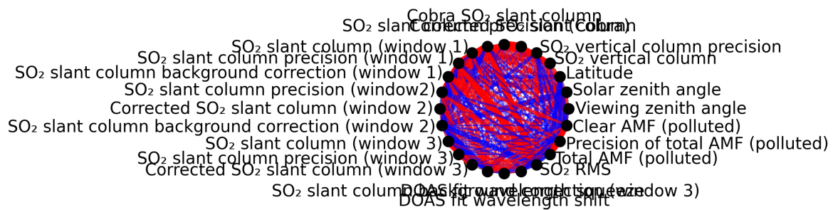
Figure 1: Map of correlation graph for 2025-01-10 to 2025-01-12.
