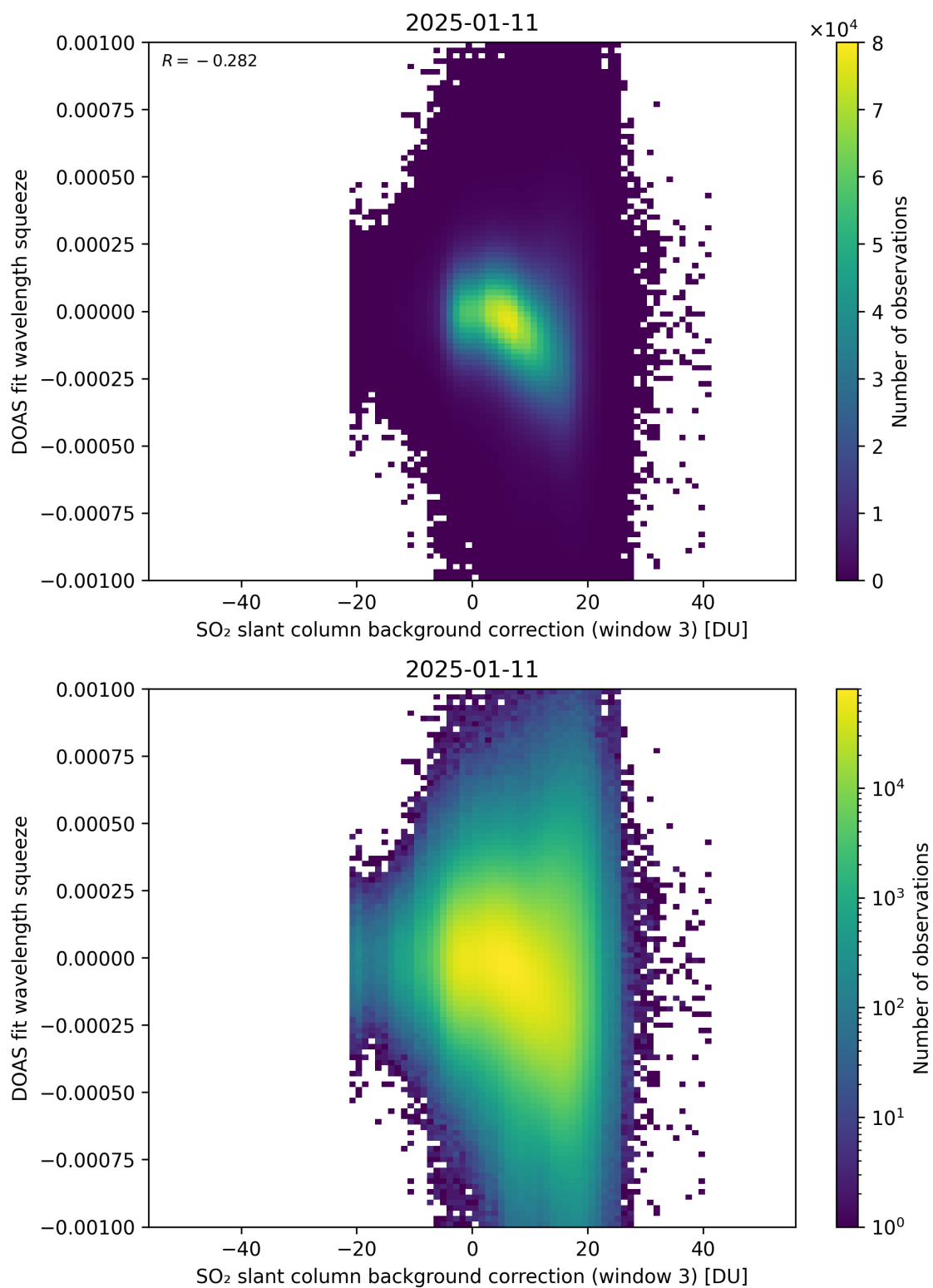
Figure 133: Scatter density plot of “SO 2 slant column background correction (window 3)” against “DOAS fit wavelength squeeze” for 2025-01-10 to 2025-01-12.
