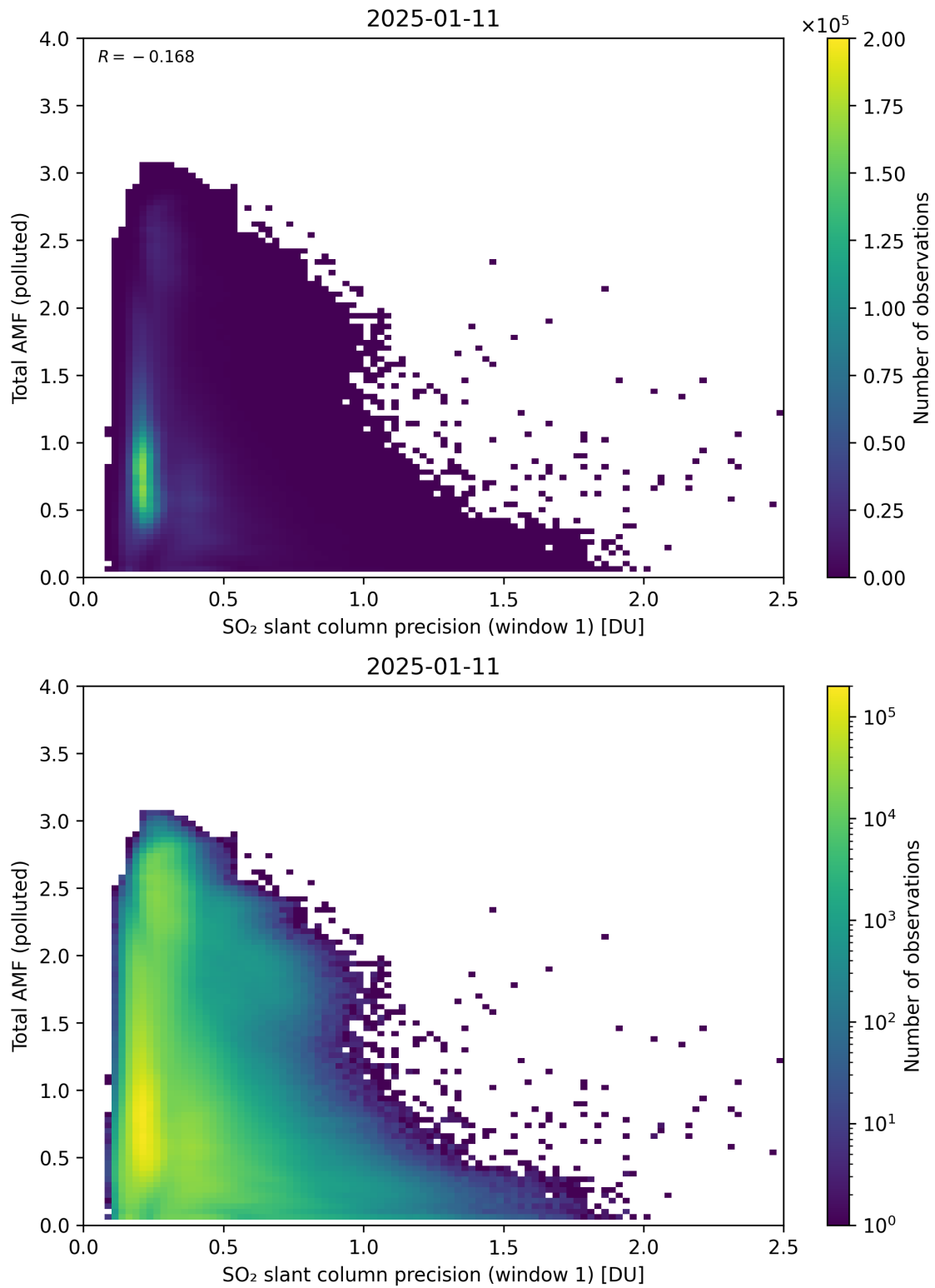
Figure 280: Scatter density plot of “SO 2 slant column precision (window 1)” against “Total AMF (polluted)” for 2025-01-10 to 2025-01-12.
