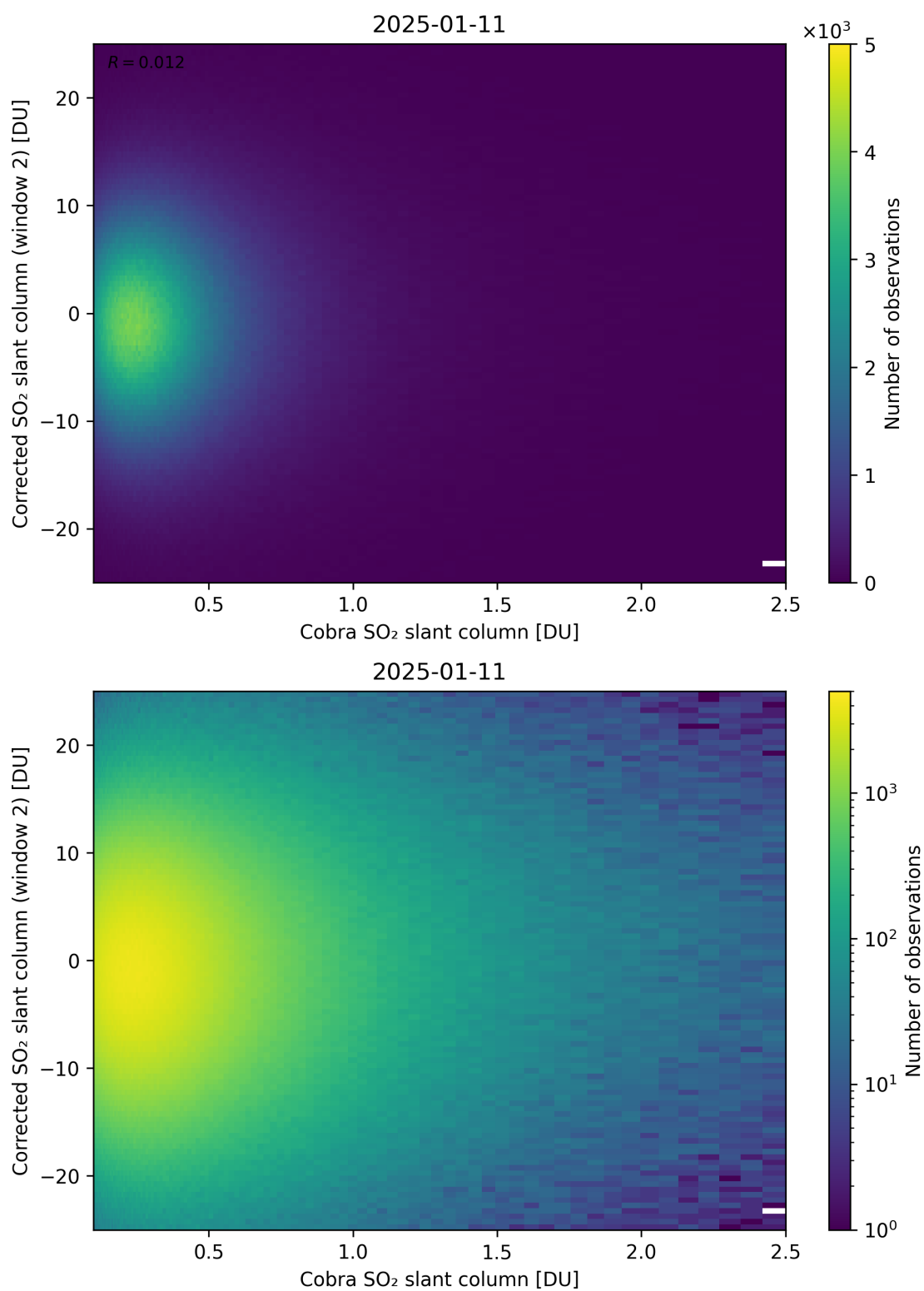
Figure 217: Scatter density plot of “Cobra SO 2 slant column” against “Corrected SO 2 slant column (window 2)” for 2025-01-10 to 2025-01-12.
