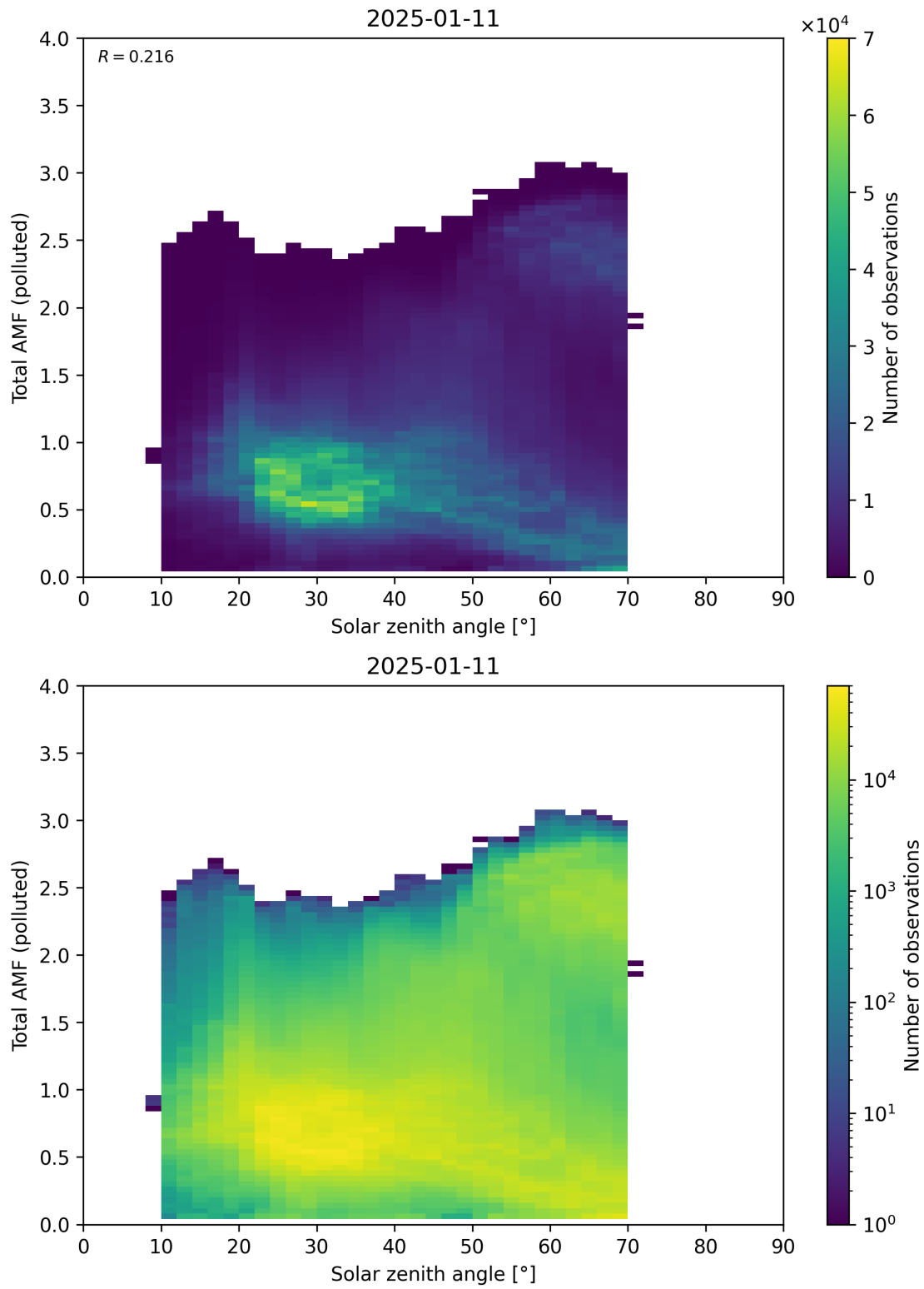
Figure 189: Scatter density plot of “Solar zenith angle” against “Total AMF (polluted)” for 2025-01-10 to 2025-01-12.
