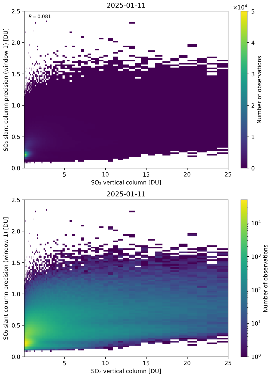
Figure 355: Scatter density plot of “SO 2 vertical column” against “SO 2 slant column precision (window 1)” for 2025-01-10 to 2025-01-12.
