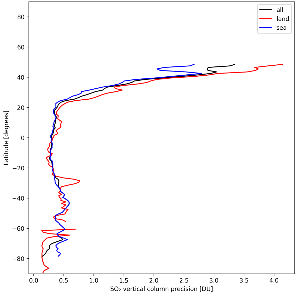
Figure 33: Zonal average of “SO 2 vertical column precision” for 2025-01-10 to 2025-01-12.
