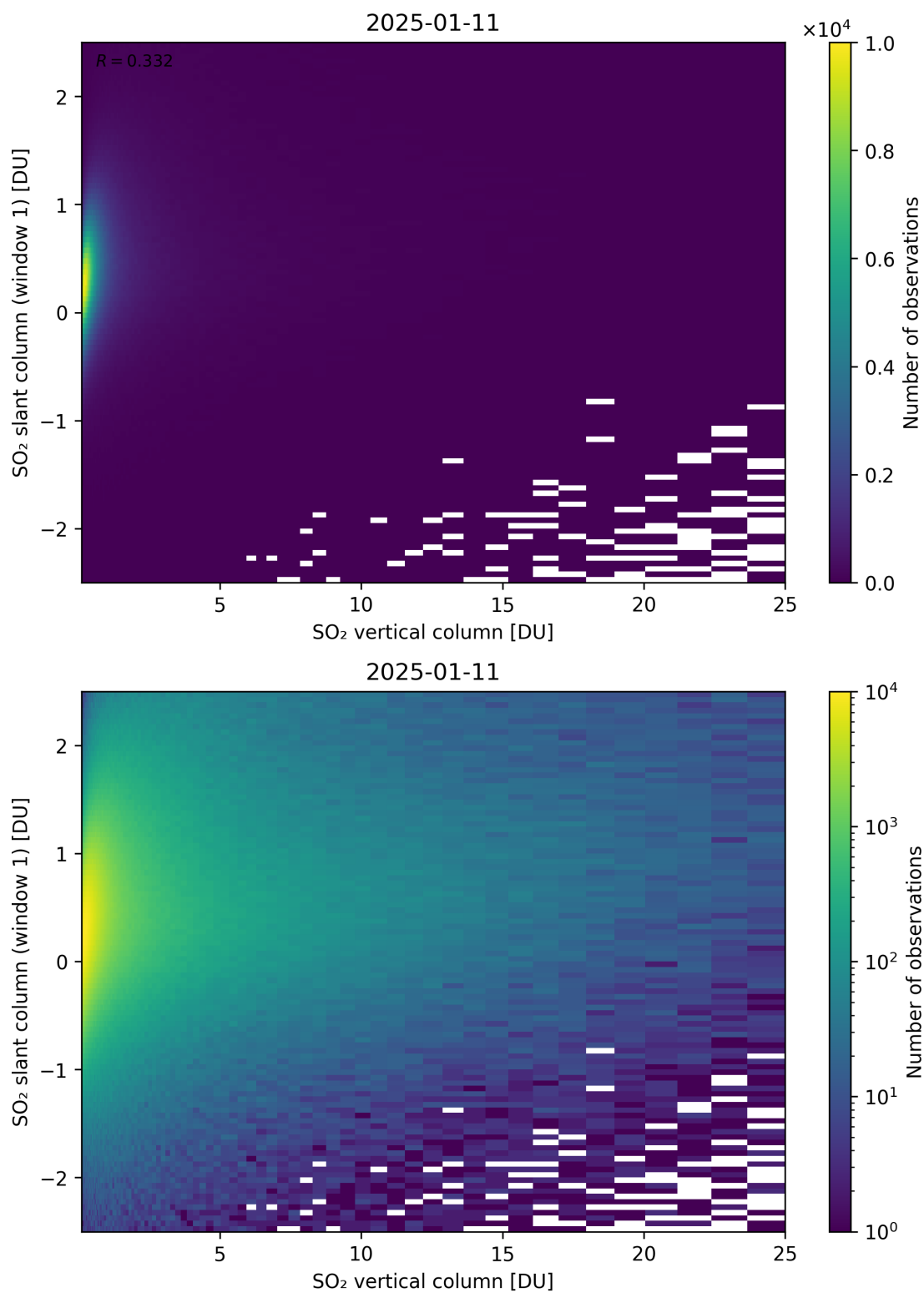
Figure 354: Scatter density plot of “SO 2 vertical column” against “SO 2 slant column (window 1)” for 2025-01-10 to 2025-01-12.
