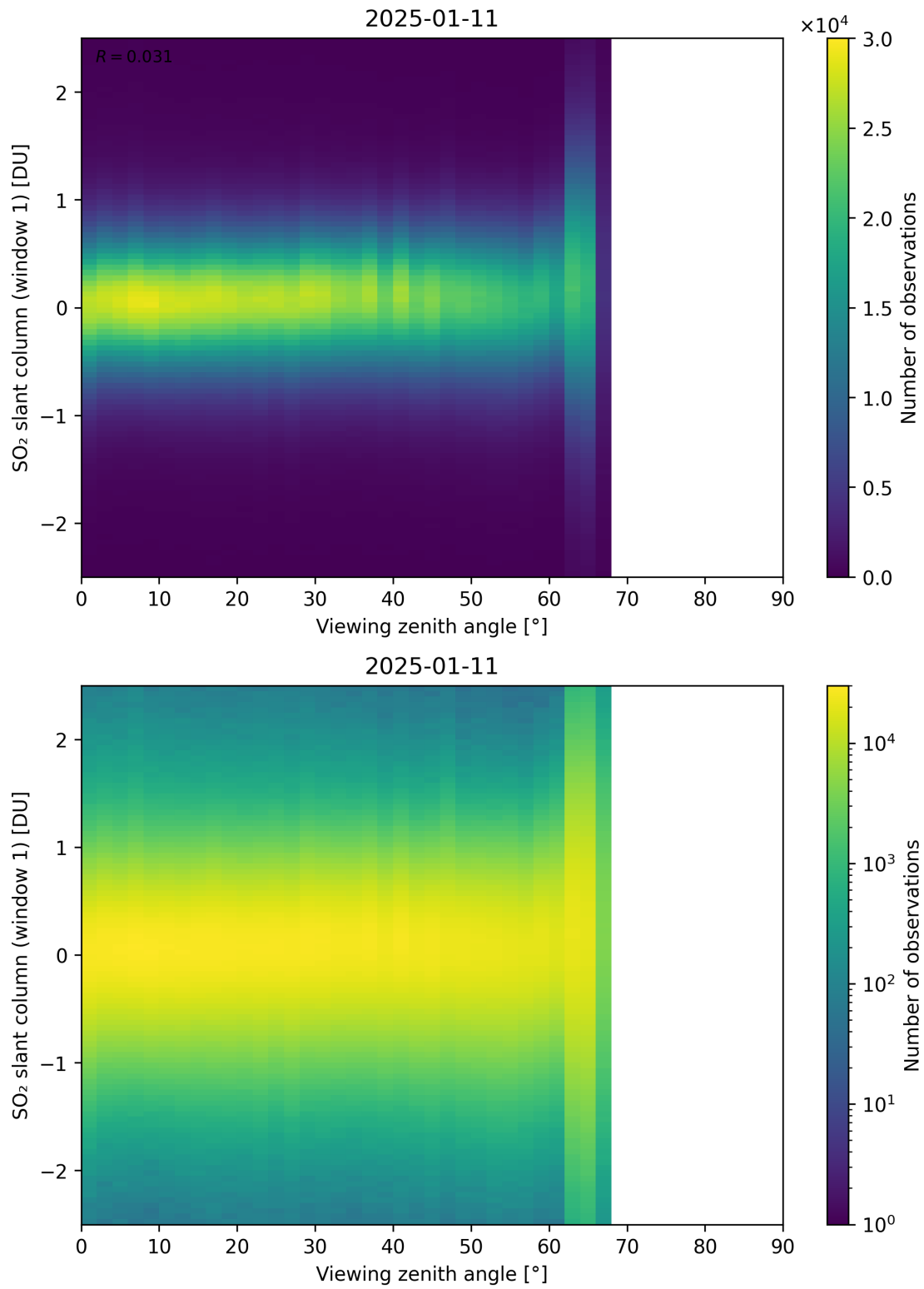
Figure 376: Scatter density plot of “Viewing zenith angle” against “SO 2 slant column (window 1)” for 2025-01-10 to 2025-01-12.
