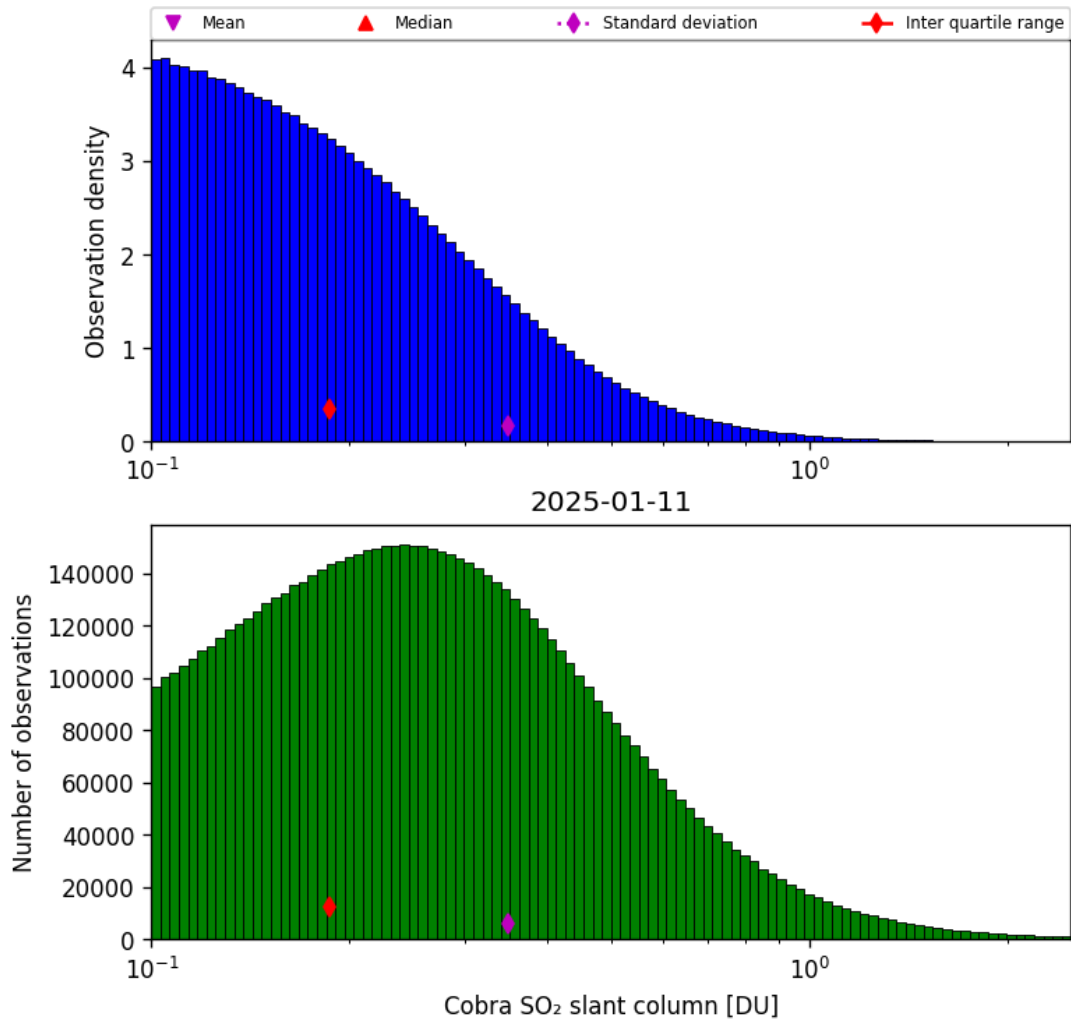
Figure 61: Histogram of “Cobra SO 2 slant column” for 2025-01-10 to 2025-01-12
