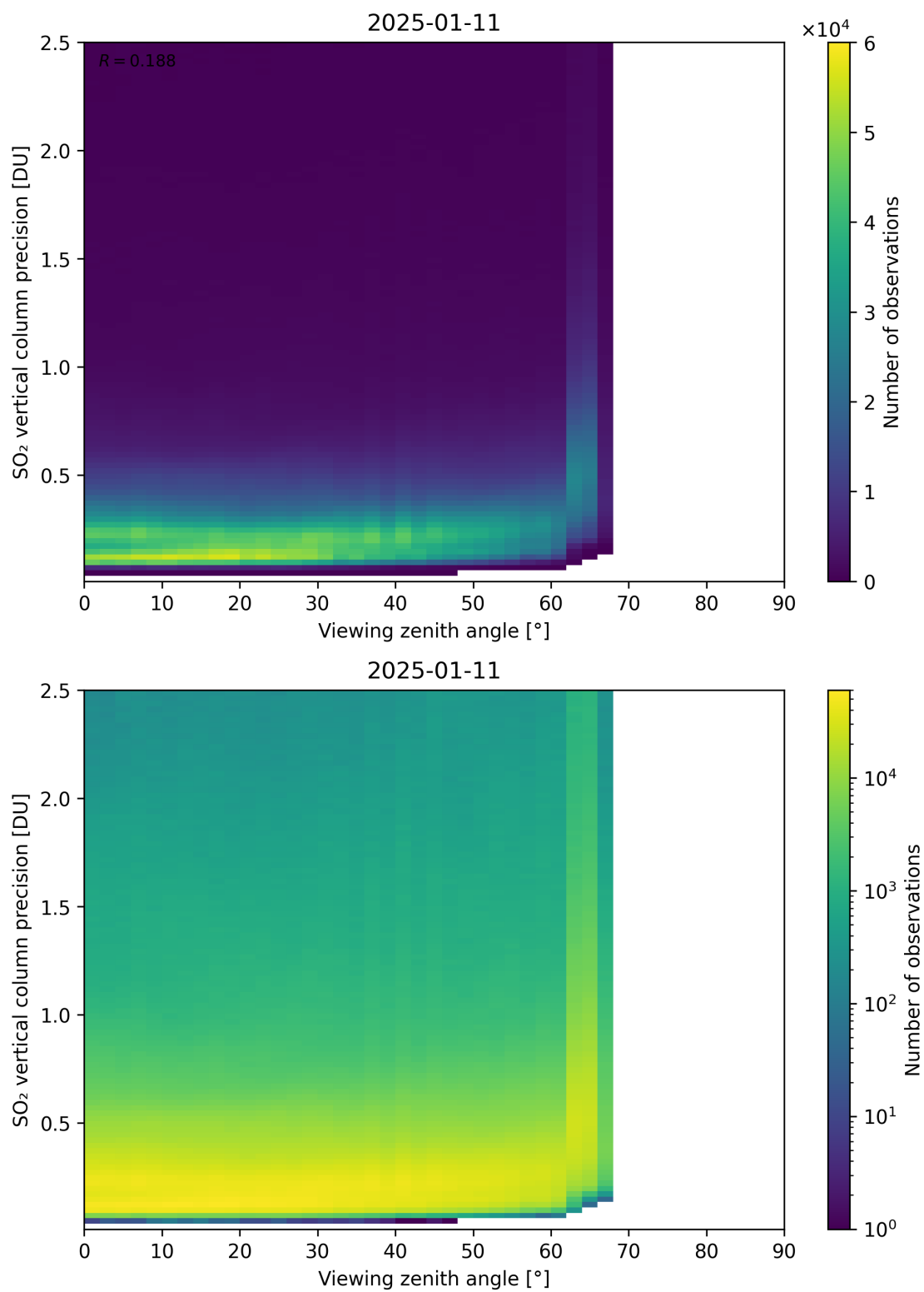
Figure 384: Scatter density plot of “Viewing zenith angle” against “SO 2 vertical column precision” for 2025-01-10 to 2025-01-12.
