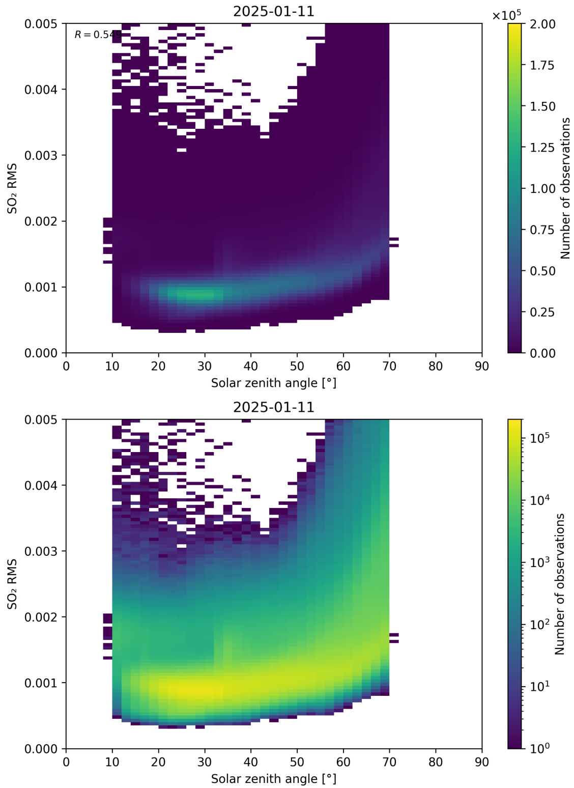
Figure 176: Scatter density plot of “Solar zenith angle” against “SO 2 RMS” for 2025-01-10 to 2025-01-12.
