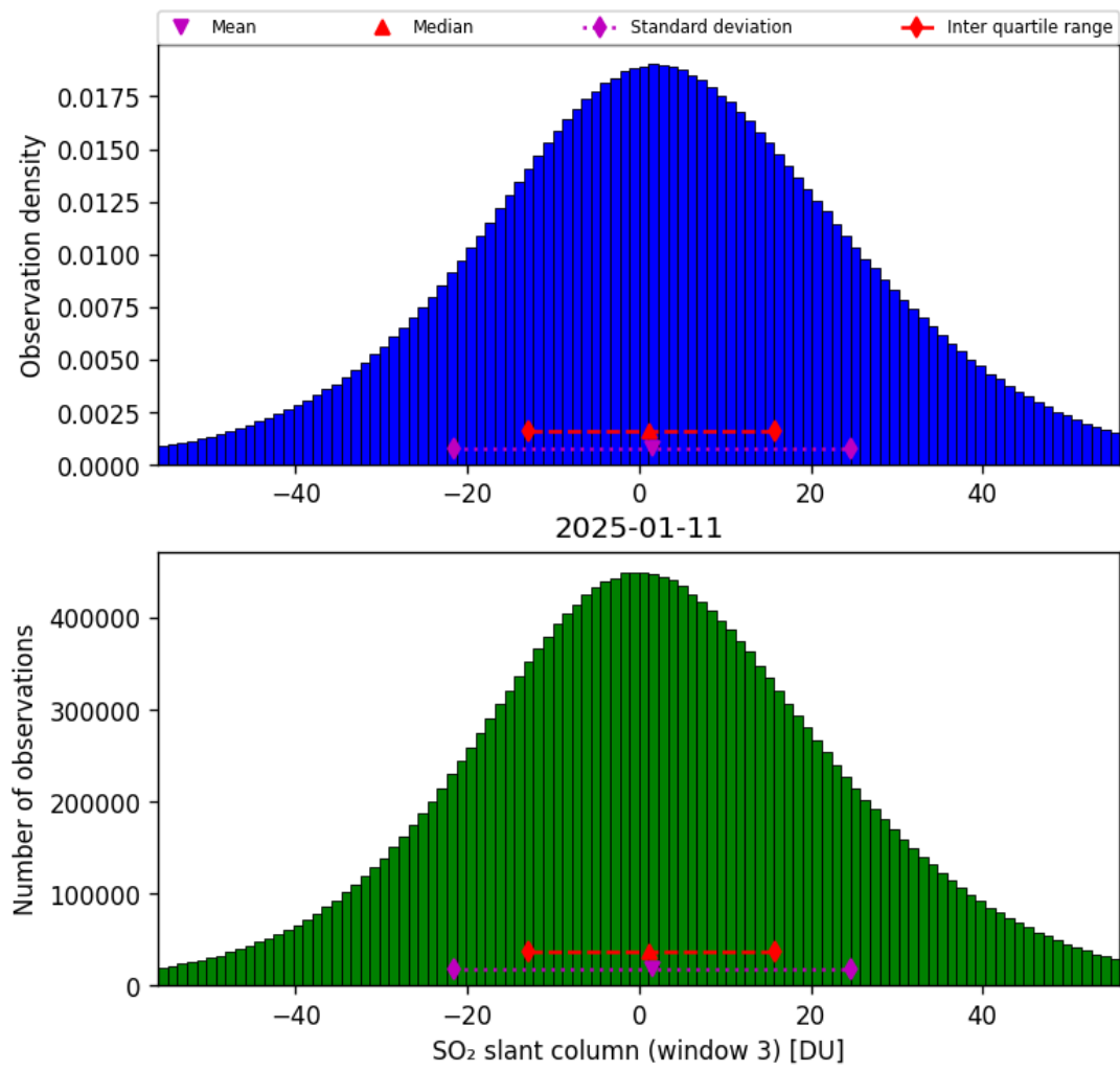
Figure 71: Histogram of “SO 2 slant column (window 3)” for 2025-01-10 to 2025-01-12
