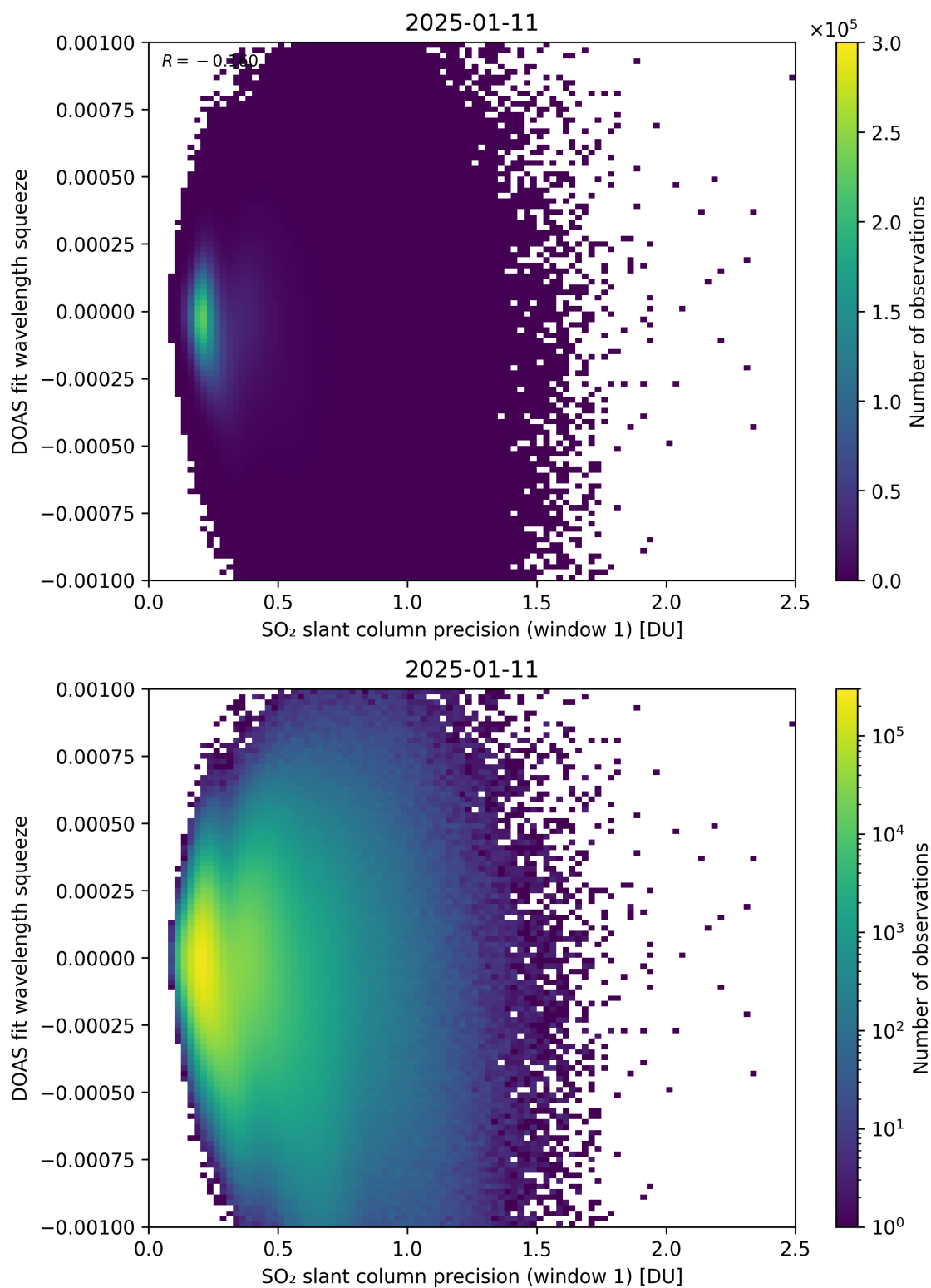
Figure 272: Scatter density plot of “SO 2 slant column precision (window 1)” against “DOAS fit wavelength squeeze” for 2025-01-10 to 2025-01-12.
