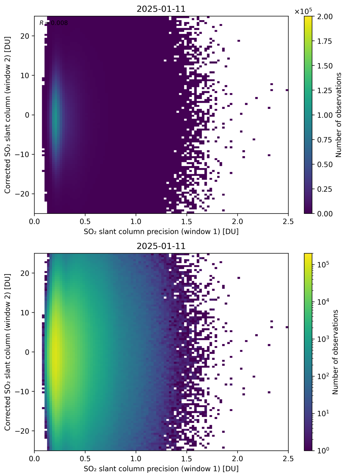
Figure 275: Scatter density plot of “SO 2 slant column precision (window 1)” against “Corrected SO 2 slant column (window 2)” for 2025-01-10 to 2025-01-12.
