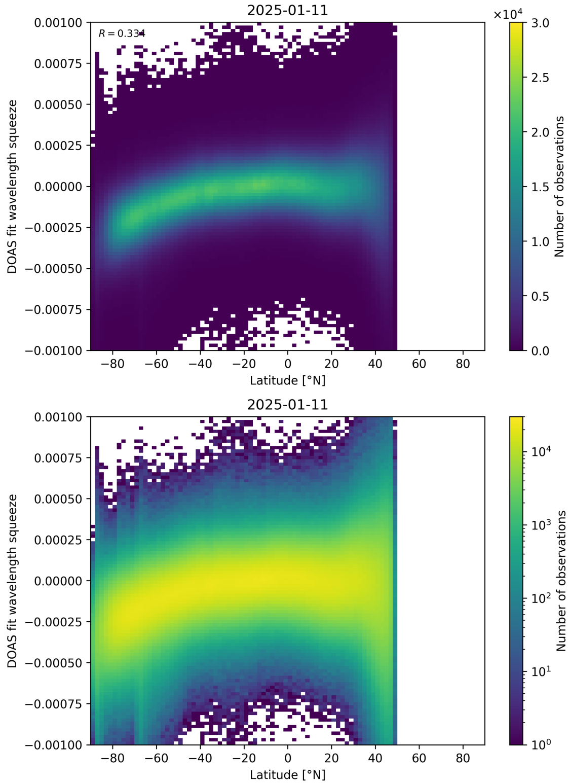
Figure 154: Scatter density plot of “Latitude” against “DOAS fit wavelength squeeze” for 2025-01-10 to 2025-01-12.
