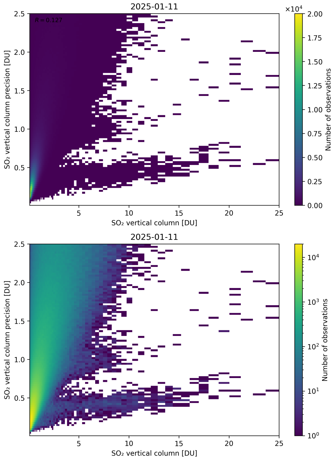
Figure 361: Scatter density plot of “SO 2 vertical column” against “SO 2 vertical column precision” for 2025-01-10 to 2025-01-12.
