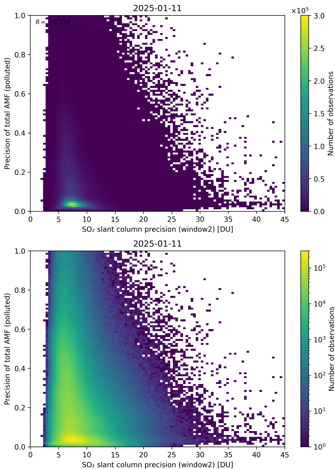
Figure 302: Scatter density plot of “SO 2 slant column precision (window2)” against “Precision of total AMF (polluted)” for 2025-01-10 to 2025-01-12.
