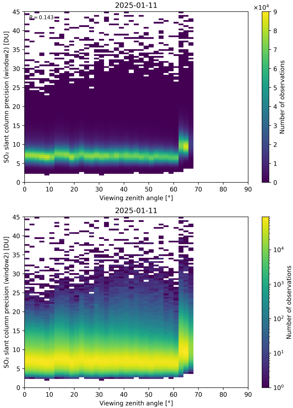
Figure 378: Scatter density plot of “Viewing zenith angle” against “SO 2 slant column precision (window2)” for 2025-01-10 to 2025-01-12.
