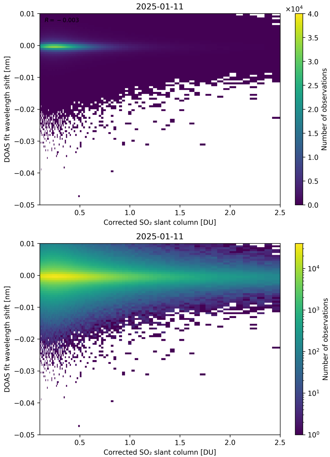
Figure 229: Scatter density plot of “Corrected SO 2 slant column” against “DOAS fit wavelength shift” for 2025-01-10 to 2025-01-12.
