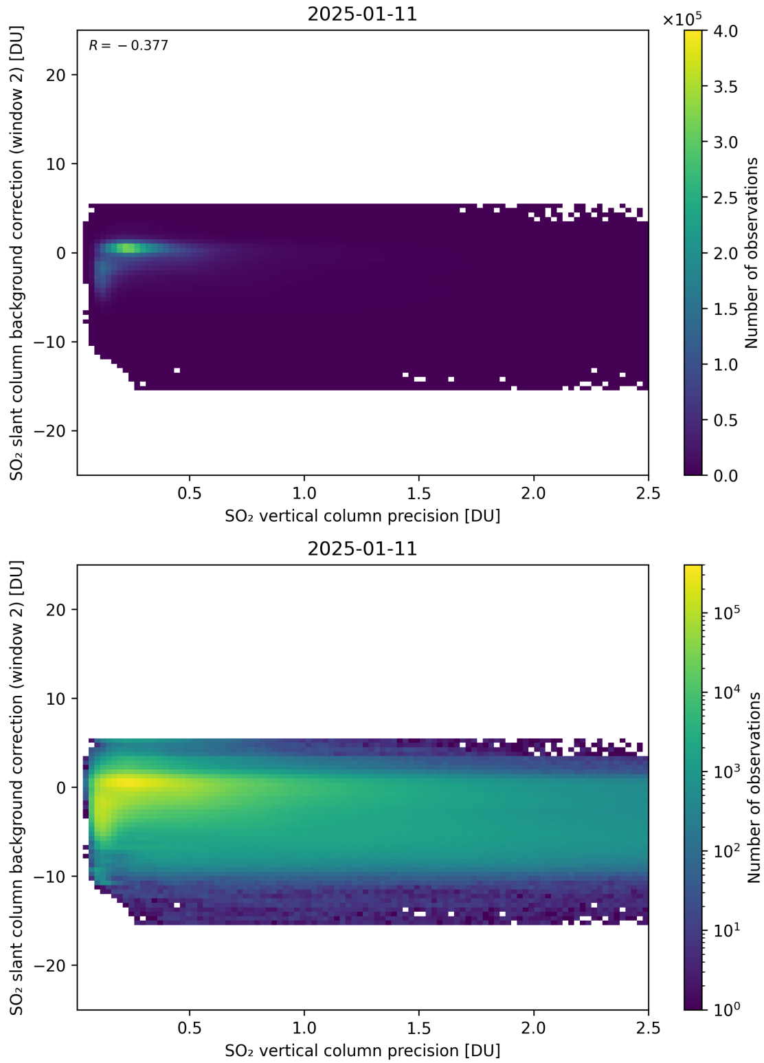
Figure 330: Scatter density plot of “SO 2 vertical column precision” against “SO 2 slant column background correction (window 2)” for 2025-01-10 to 2025-01-12.
