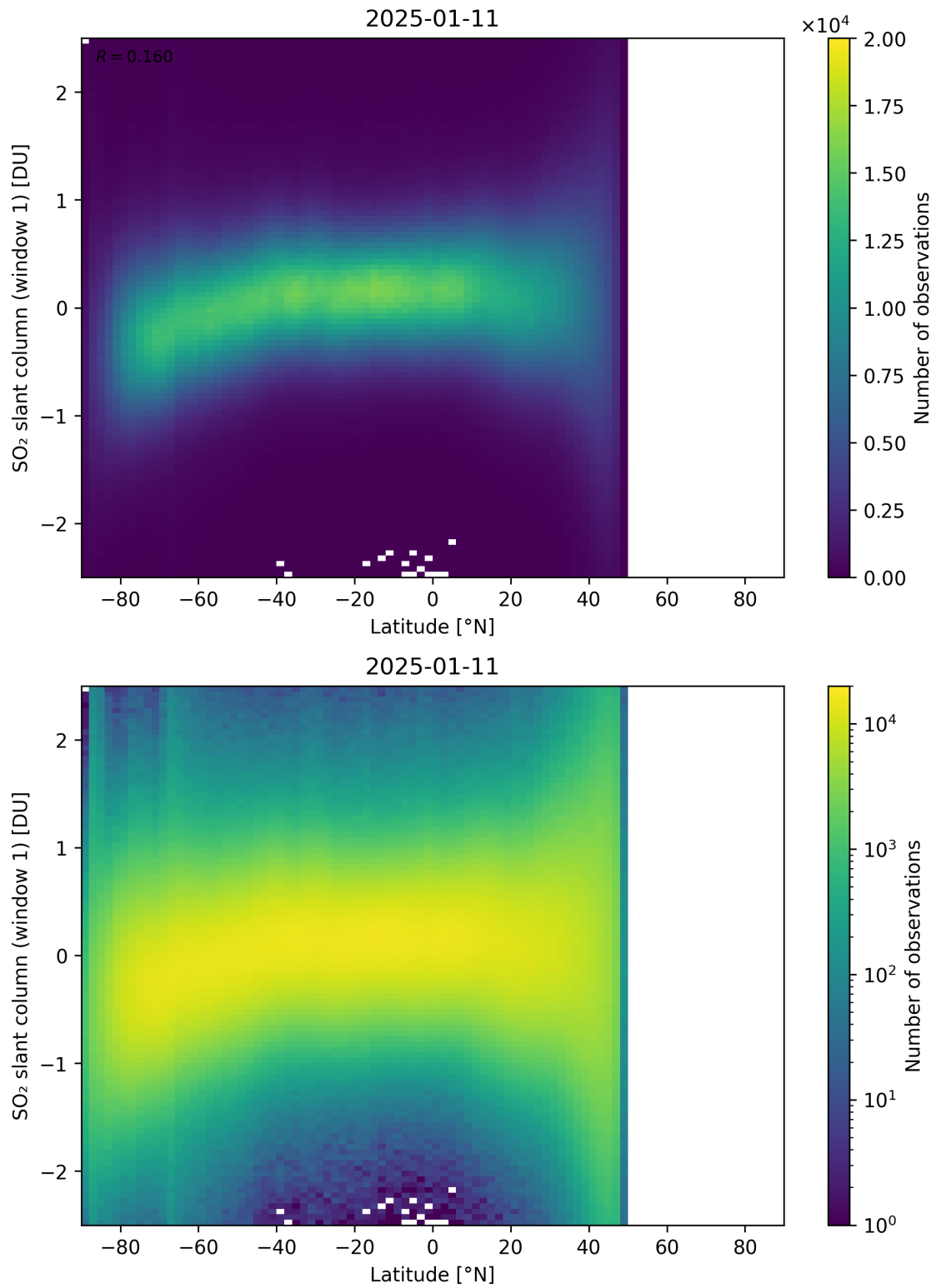
Figure 162: Scatter density plot of “Latitude” against “SO 2 slant column (window 1)” for 2025-01-10 to 2025-01-12.
