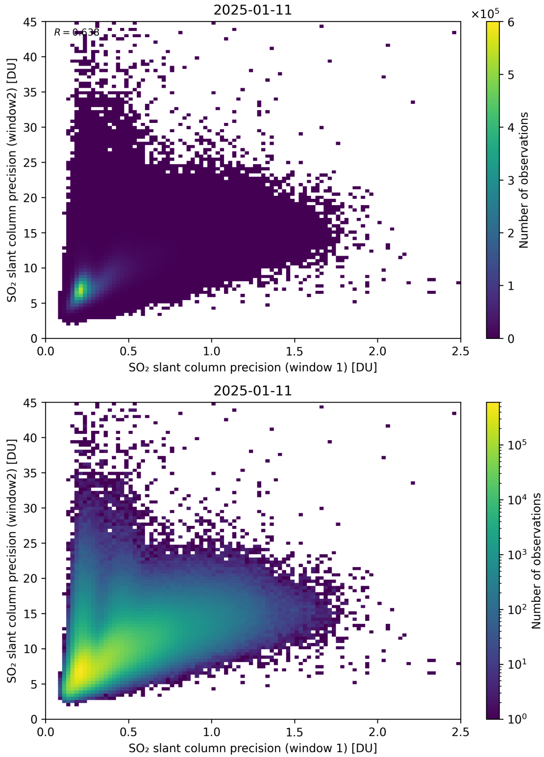
Figure 277: Scatter density plot of “SO 2 slant column precision (window 1)” against “SO 2 slant column precision (window 2)” for 2025-01-10 to 2025-01-12.
