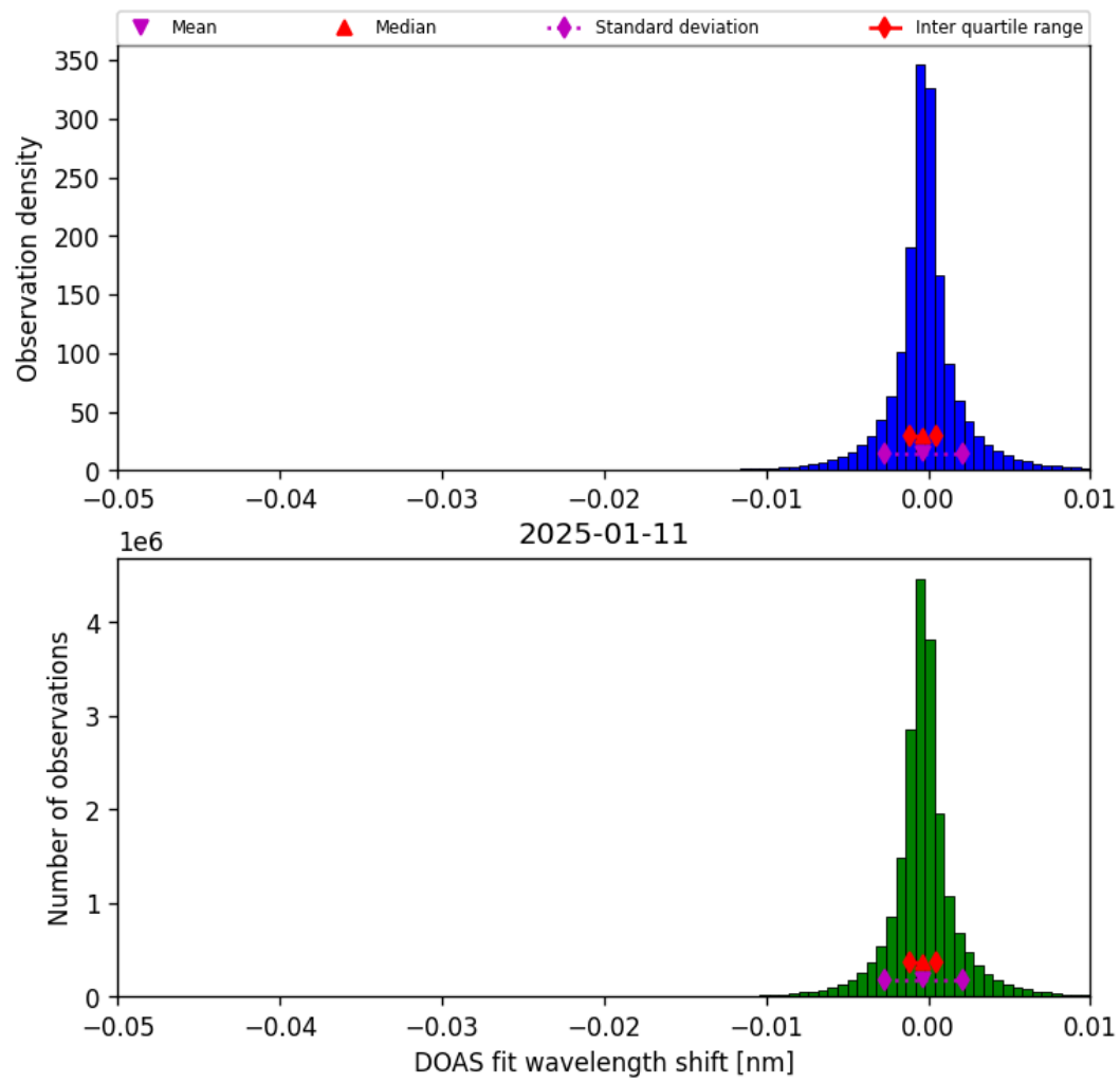
Figure 76: Histogram of “DOAS fit wavelength shift” for 2025-01-10 to 2025-01-12
