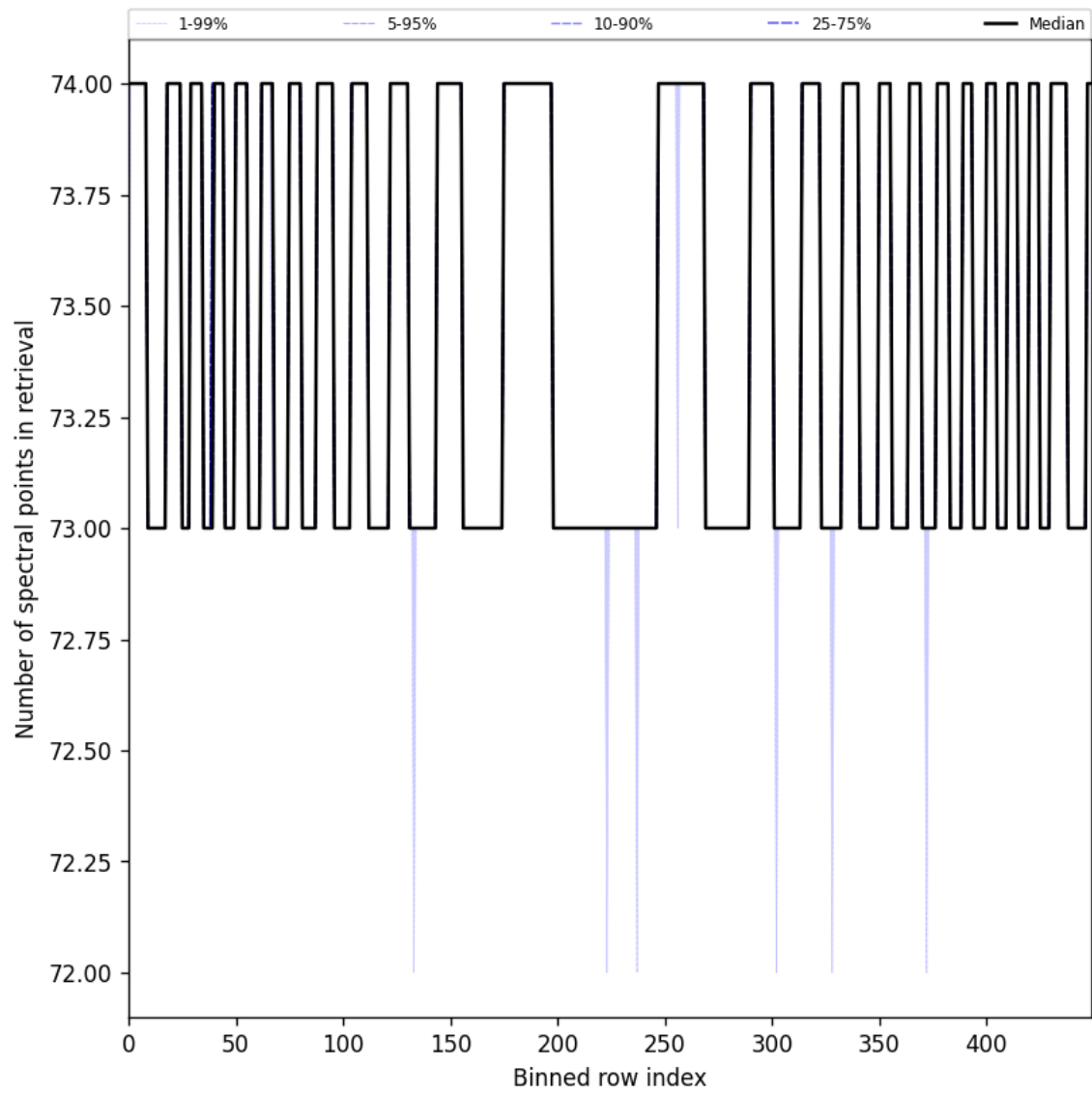
Figure 108: Along track statistics of “Number of spectral points in retrieval” for 2025-01-10 to 2025-01-12
