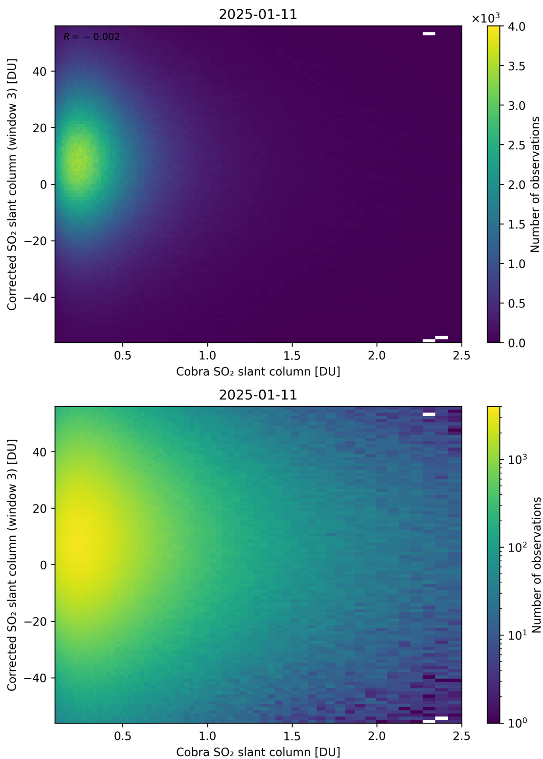
Figure 218: Scatter density plot of “Cobra SO 2 slant column” against “Corrected SO 2 slant column (window 3)” for 2025-01-10 to 2025-01-12.
