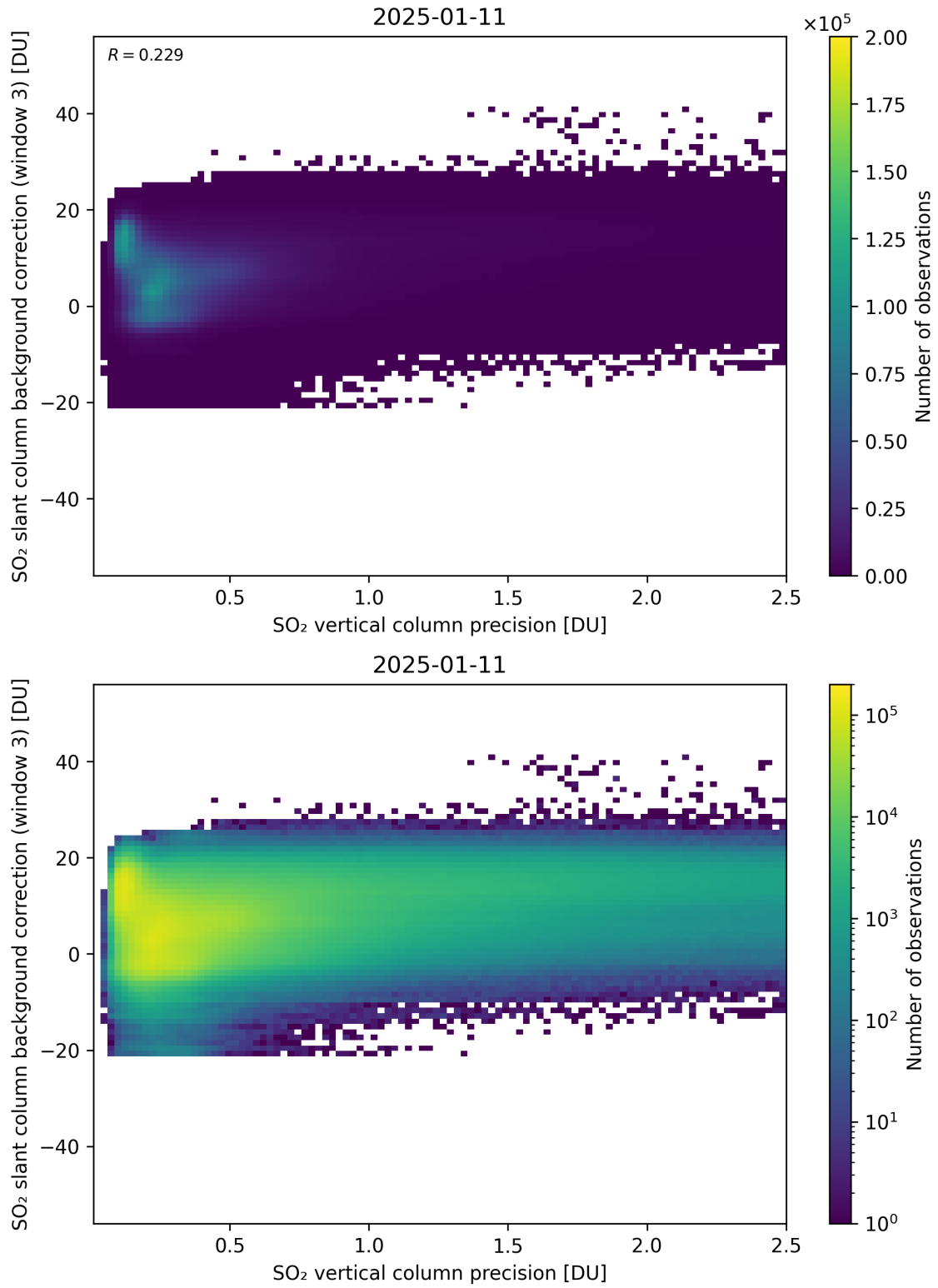
Figure 331: Scatter density plot of “SO 2 vertical column precision” against “SO 2 slant column background correction (window 3)” for 2025-01-10 to 2025-01-12.
