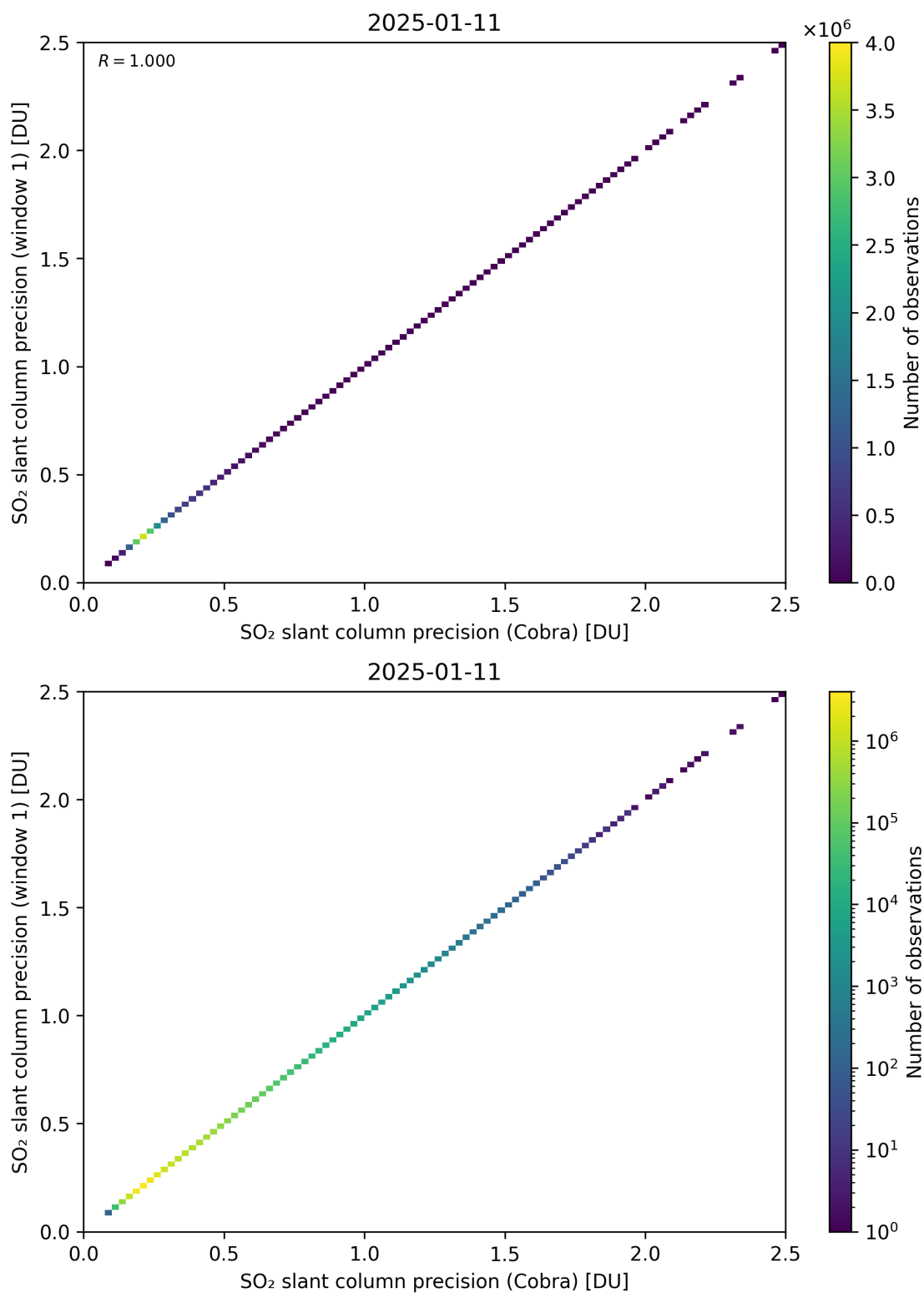
Figure 209: Scatter density plot of “SO 2 slant column precision (Cobra)” against “SO 2 slant column precision (window 1)” for 2025-01-10 to 2025-01-12.
