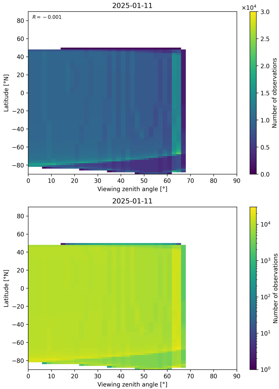
Figure 368: Scatter density plot of “Viewing zenith angle” against “Latitude” for 2025-01-10 to 2025-01-12.
