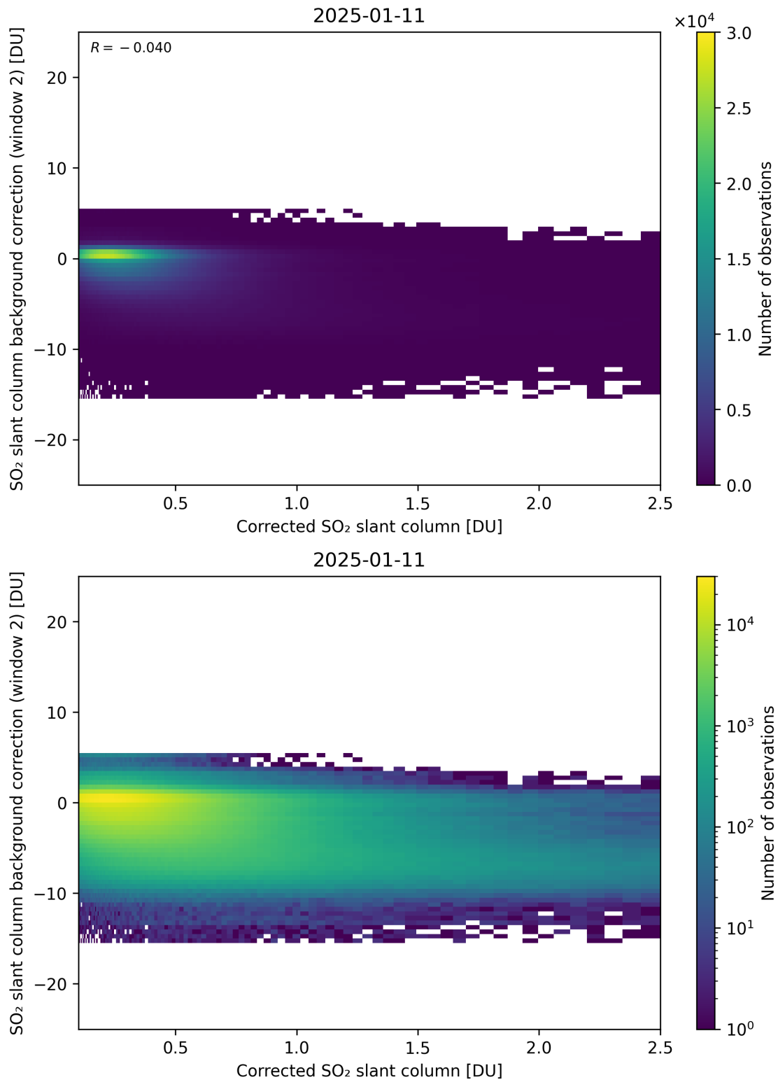
Figure 227: Scatter density plot of “Corrected SO 2 slant column” against “SO 2 slant column background correction (window 2)” for 2025-01-10 to 2025-01-12.
