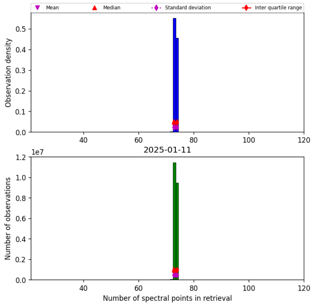
Figure 82: Histogram of “Number of spectral points in retrieval” for 2025-01-10 to 2025-01-12
