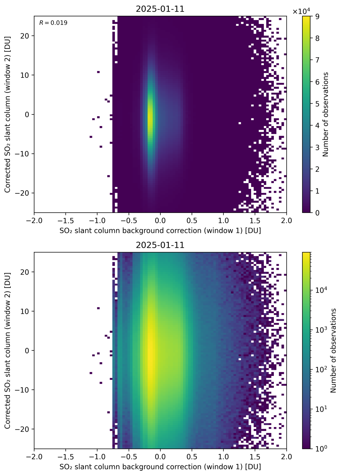
Figure 115: Scatter density plot of “SO 2 slant column background correction (window 1)” against “Corrected SO 2 slant column (window 2)” for 2025-01-10 to 2025-01-12.
