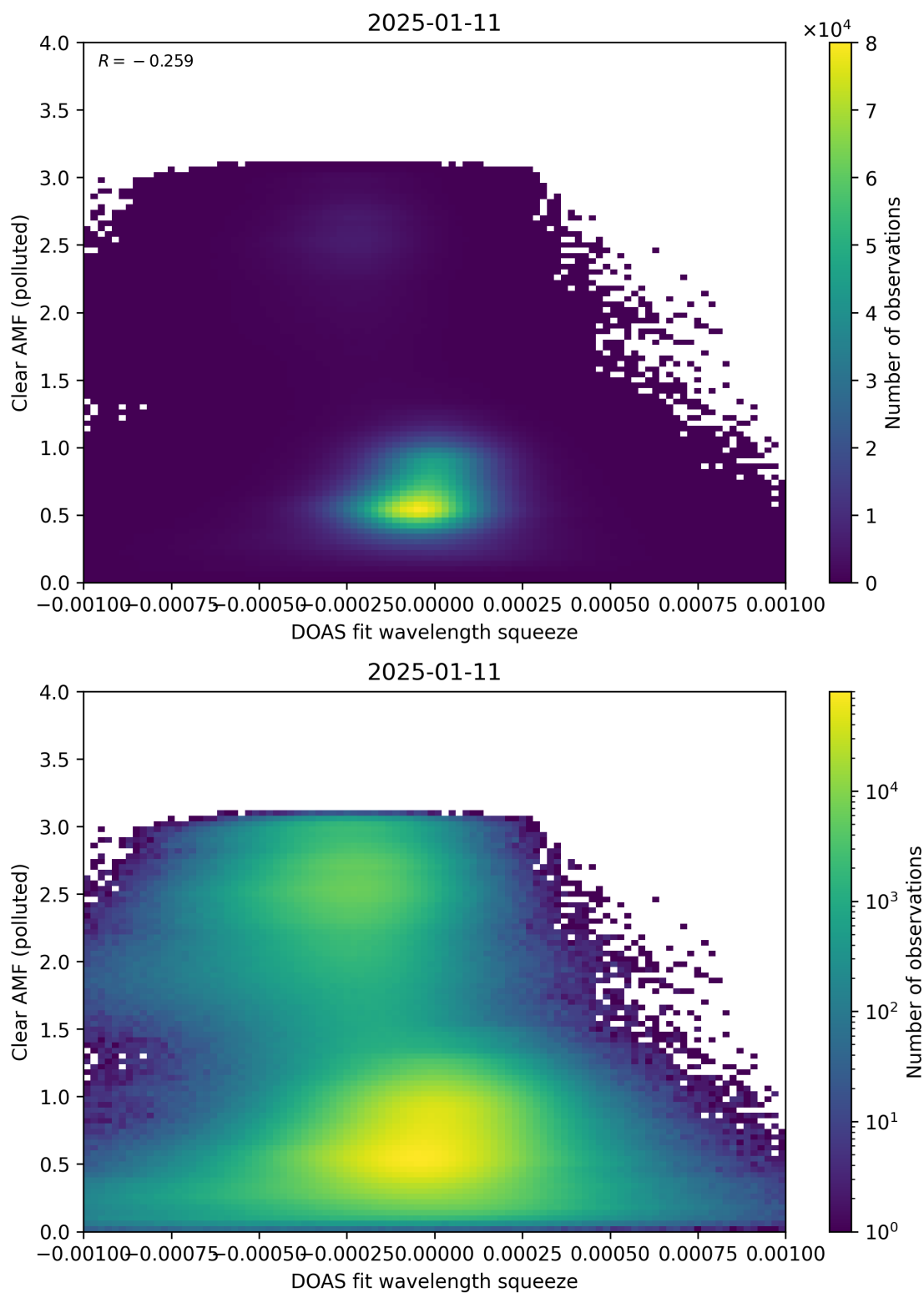
Figure 144: Scatter density plot of “DOAS fit wavelength squeeze” against “Clear AMF (polluted)” for 2025-01-10 to 2025-01-12.
