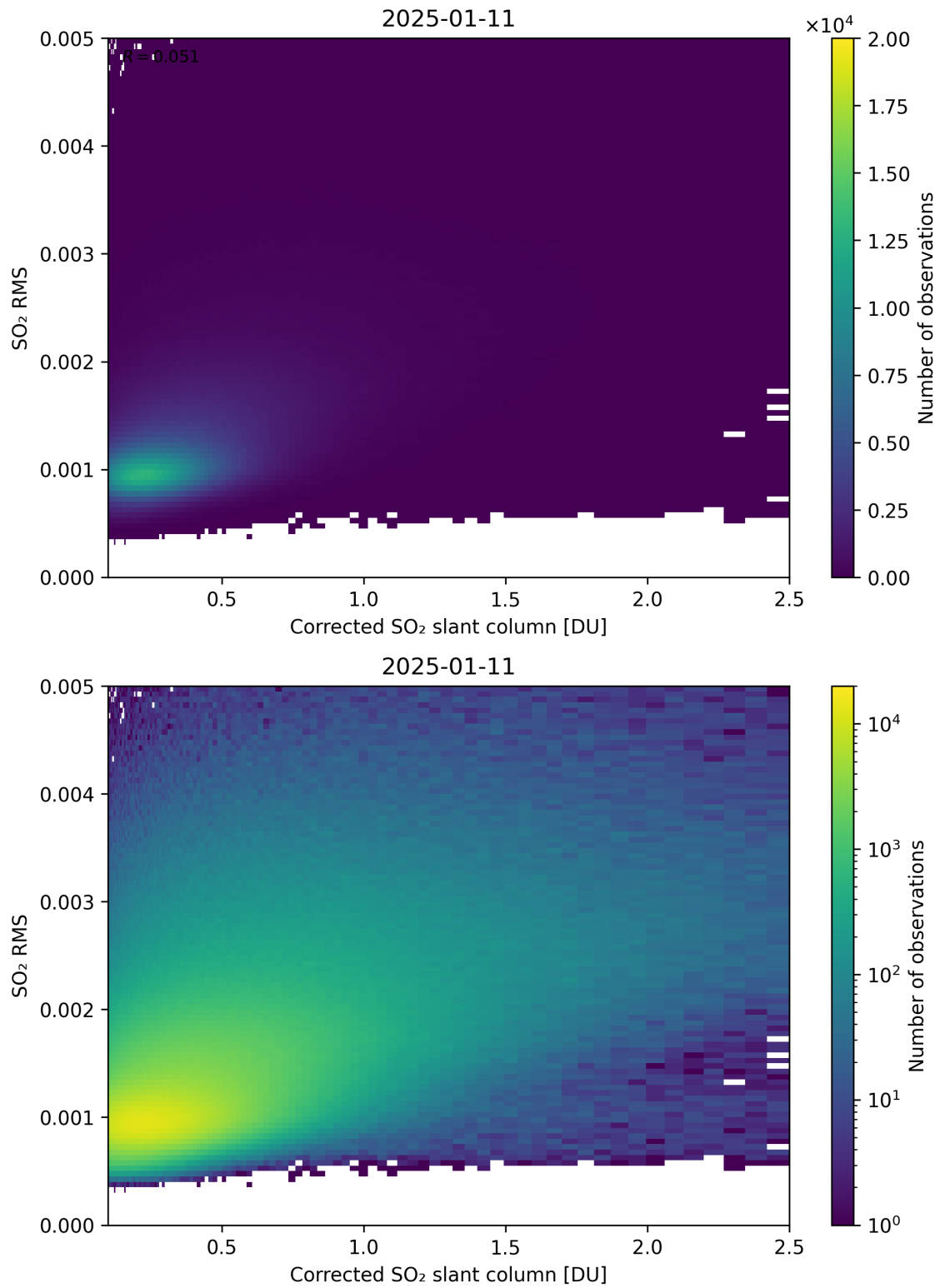
Figure 231: Scatter density plot of “Corrected SO 2 slant column” against “SO 2 RMS” for 2025-01-10 to 2025-01-12.
