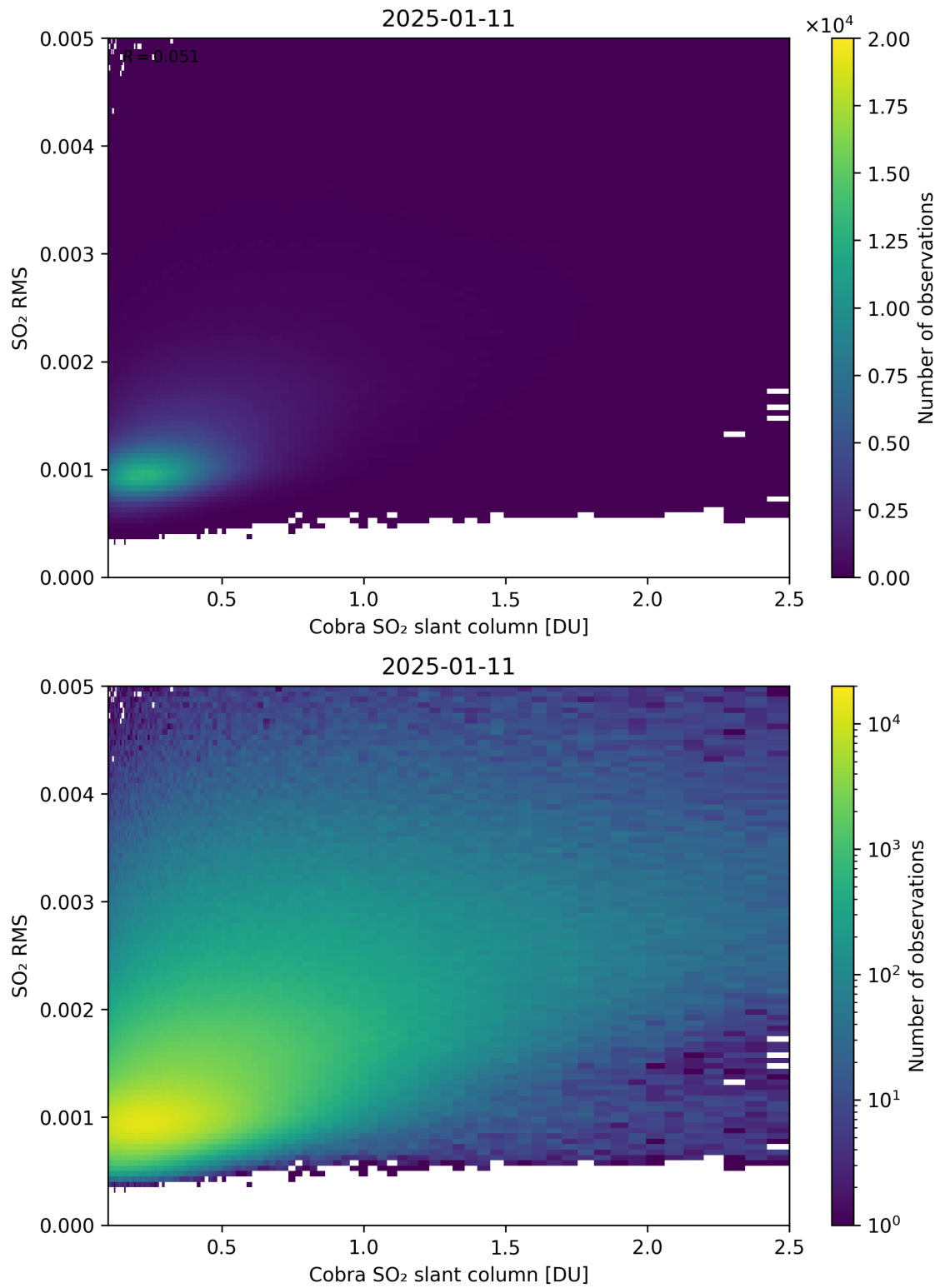
Figure 198: Scatter density plot of “Cobra SO 2 slant column” against “SO 2 RMS” for 2025-01-10 to 2025-01-12.
