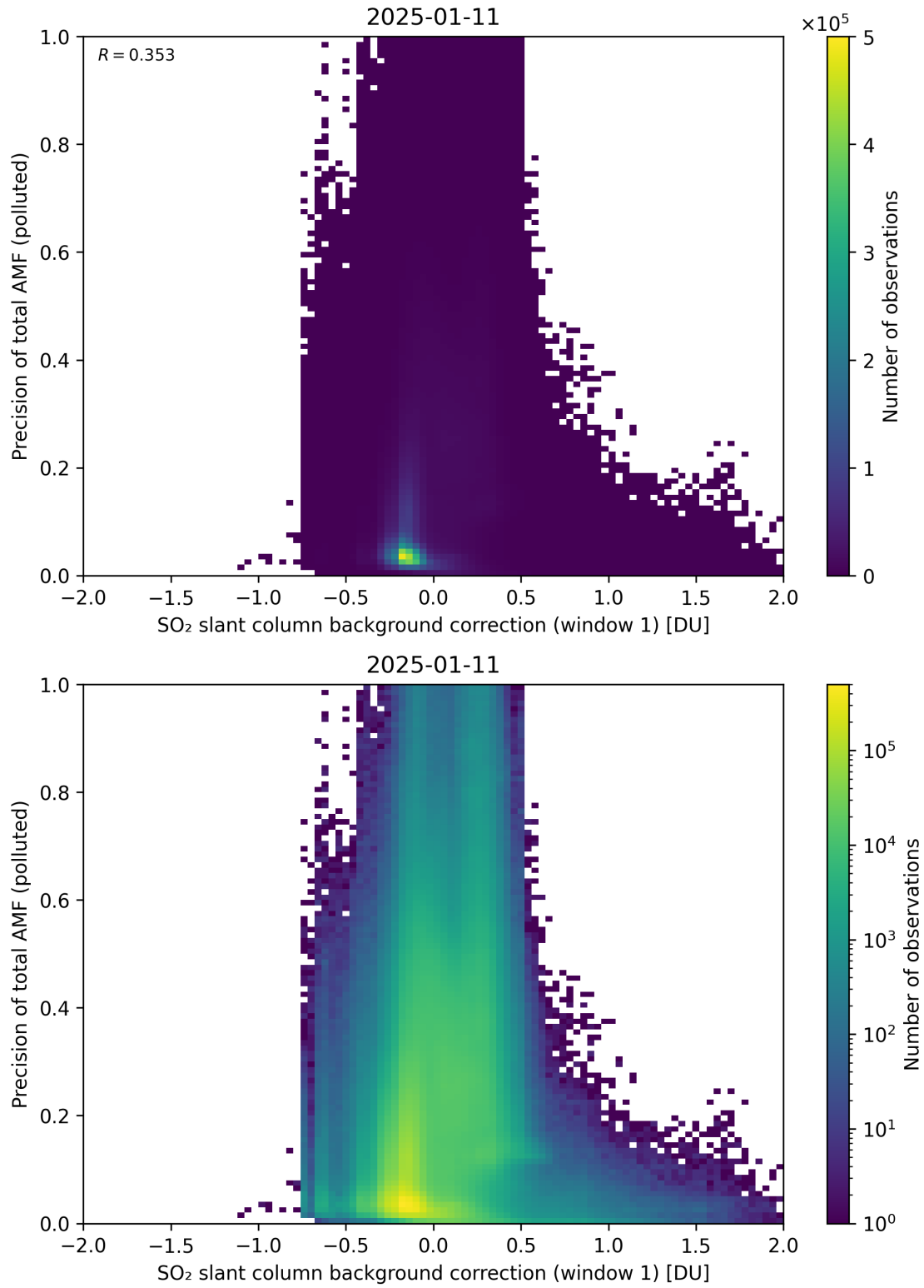
Figure 121: Scatter density plot of “SO 2 slant column background correction (window 1)” against “Precision of total AMF (polluted)” for 2025-01-10 to 2025-01-12.
