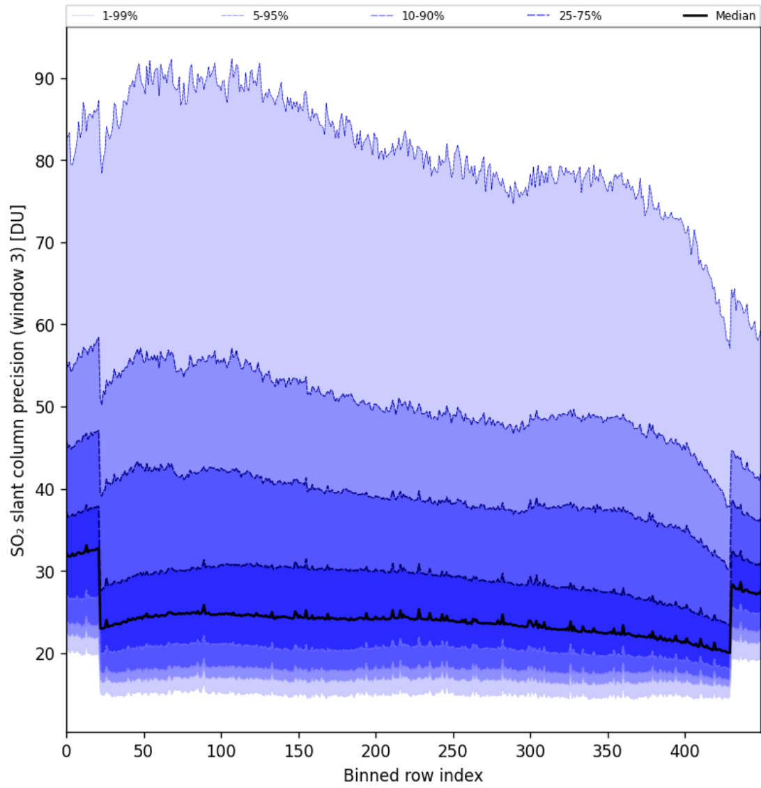
Figure 98: Along track statistics of “SO 2 slant column precision (window 3)” for 2025-01-12 to 2025-01-13
