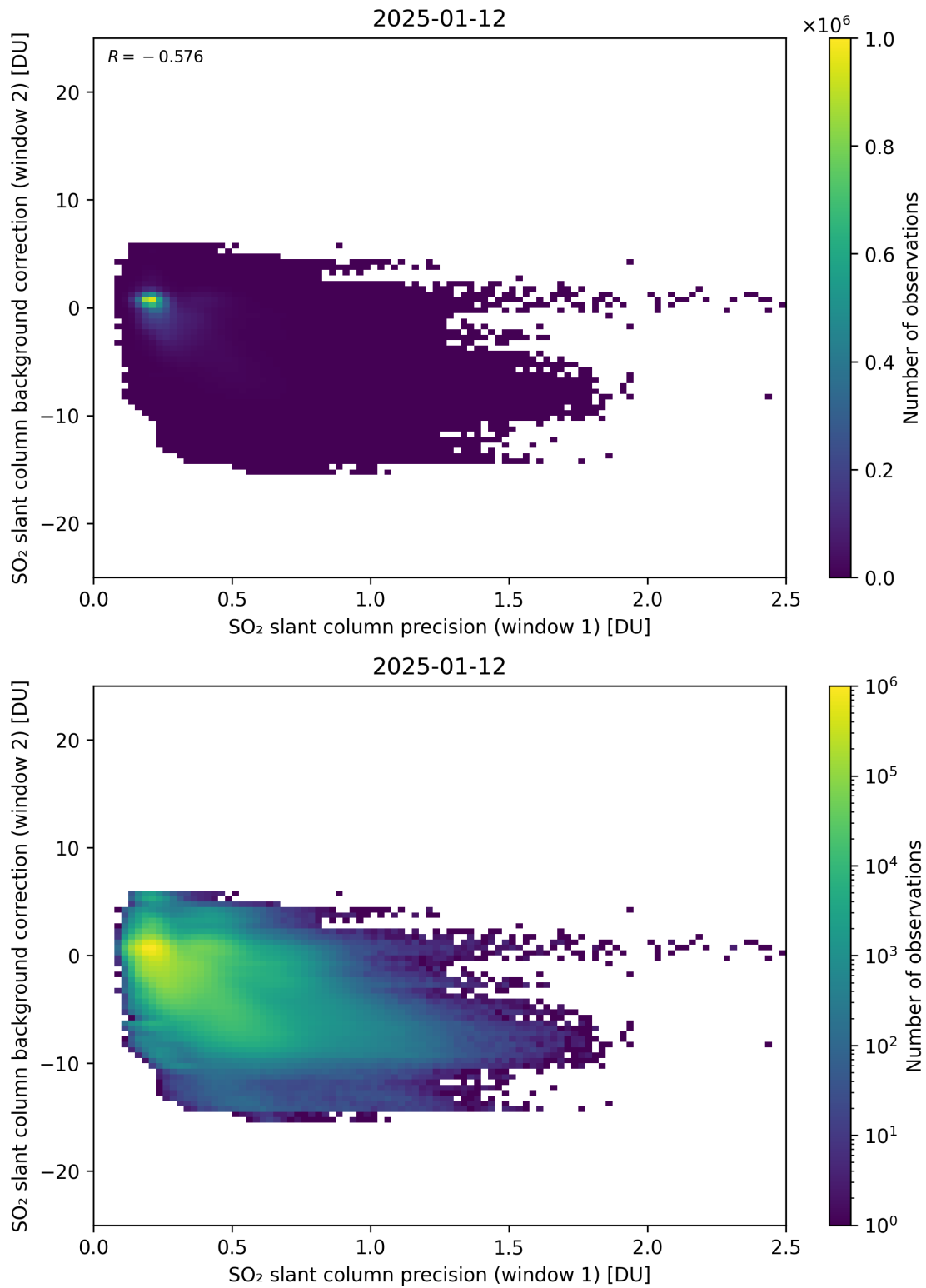
Figure 269: Scatter density plot of “SO 2 slant column precision (window 1)” against “SO 2 slant column background correction (window 2)” for 2025-01-12 to 2025-01-13.
