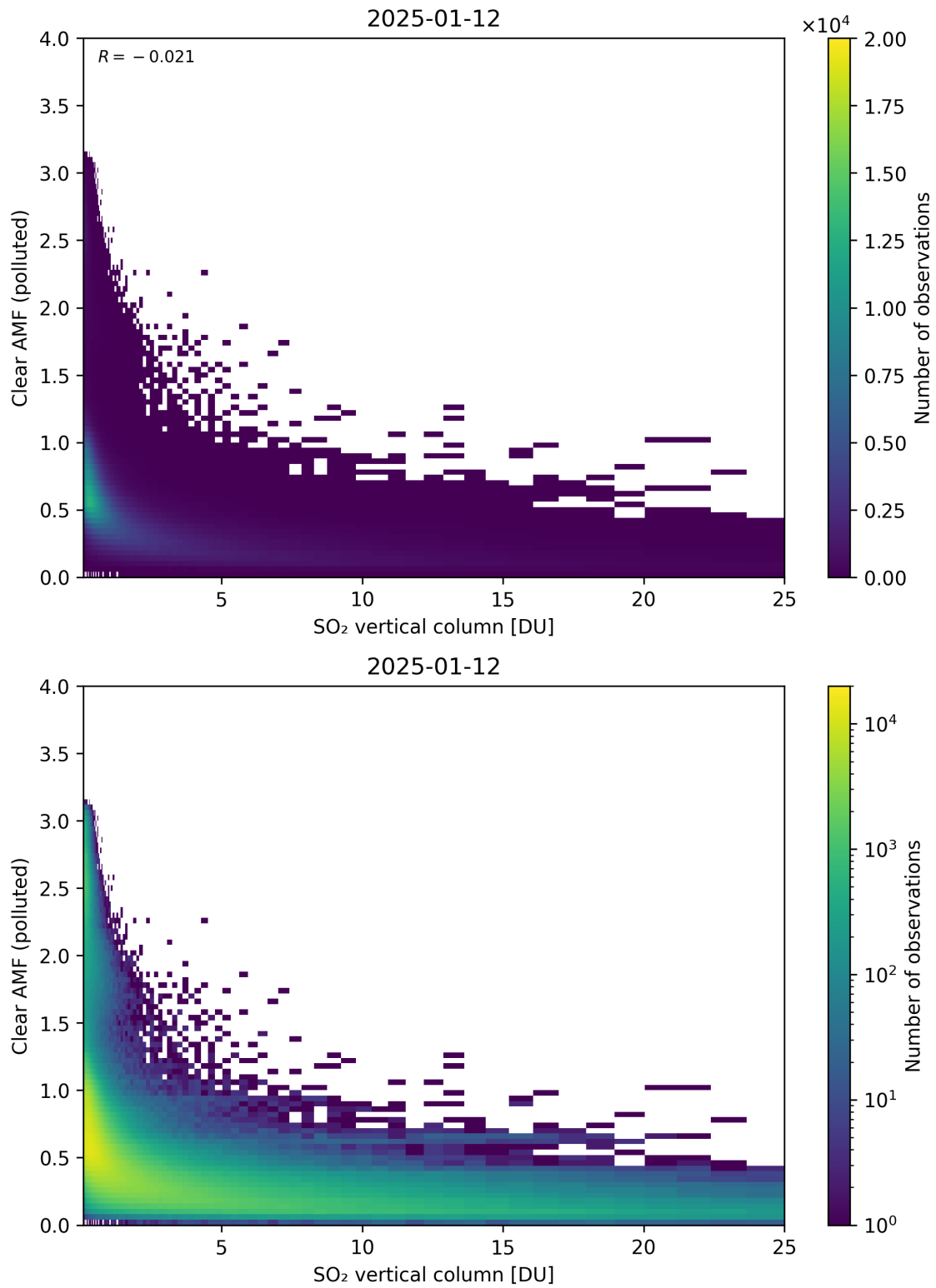
Figure 348: Scatter density plot of “SO 2 vertical column” against “Clear AMF (polluted)” for 2025-01-12 to 2025-01-13.
