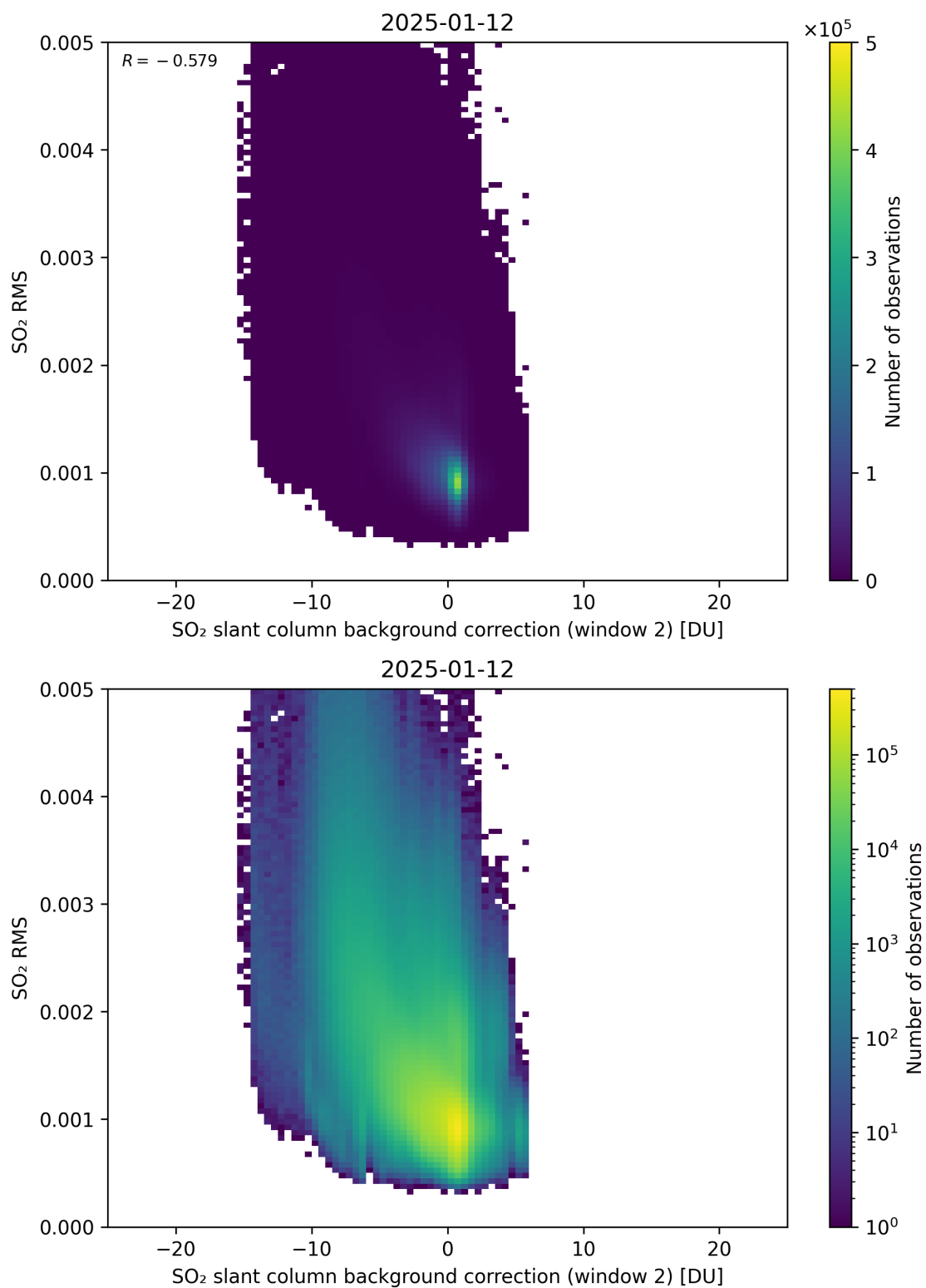
Figure 125: Scatter density plot of “SO 2 slant column background correction (window 2)” against “SO 2 RMS” for 2025-01-12 to 2025-01-13.
