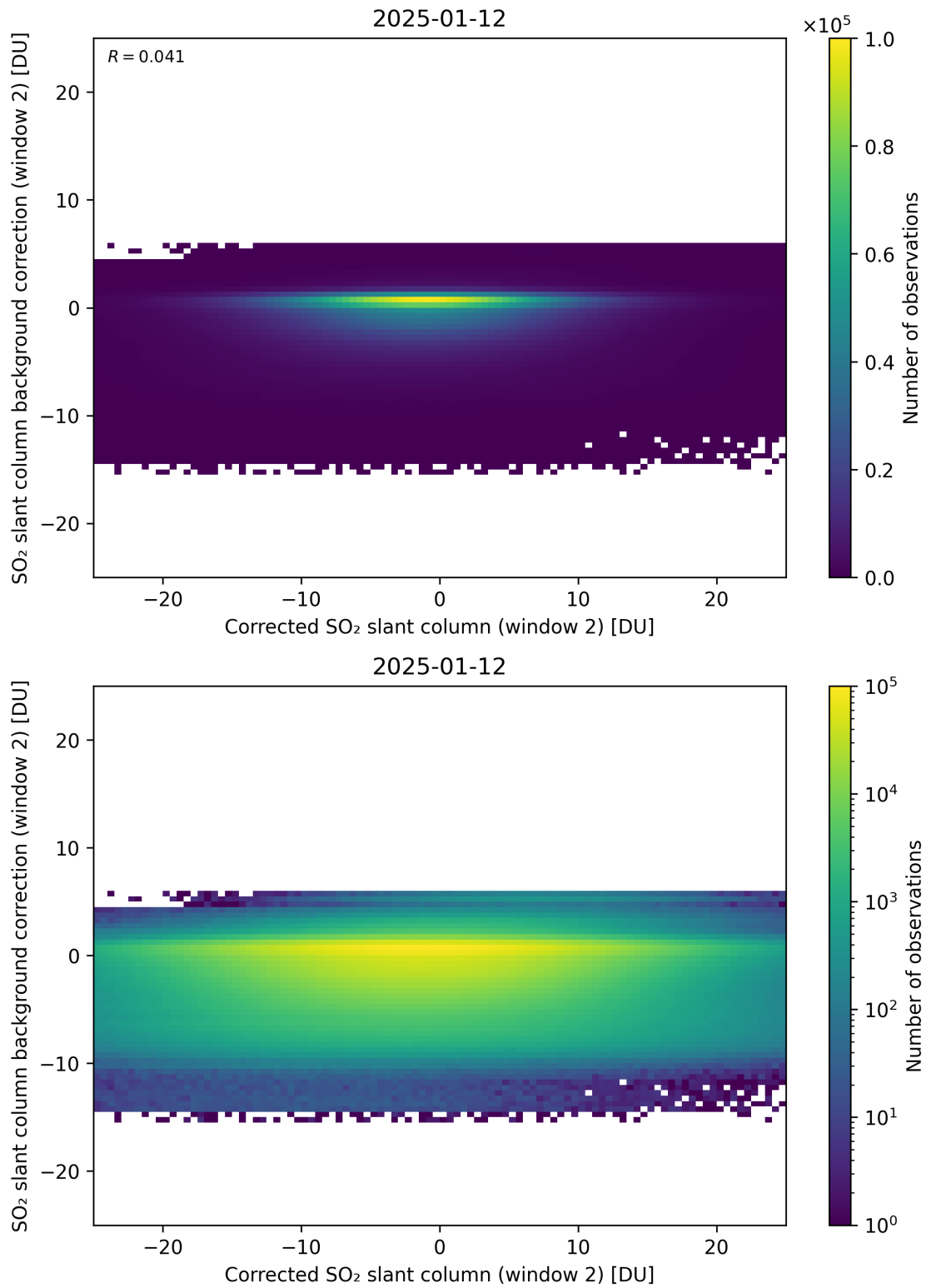
Figure 244: Scatter density plot of “Corrected SO 2 slant column (window 2)” against “SO 2 slant column background correction (window 2)” for 2025-01-12 to 2025-01-13.
