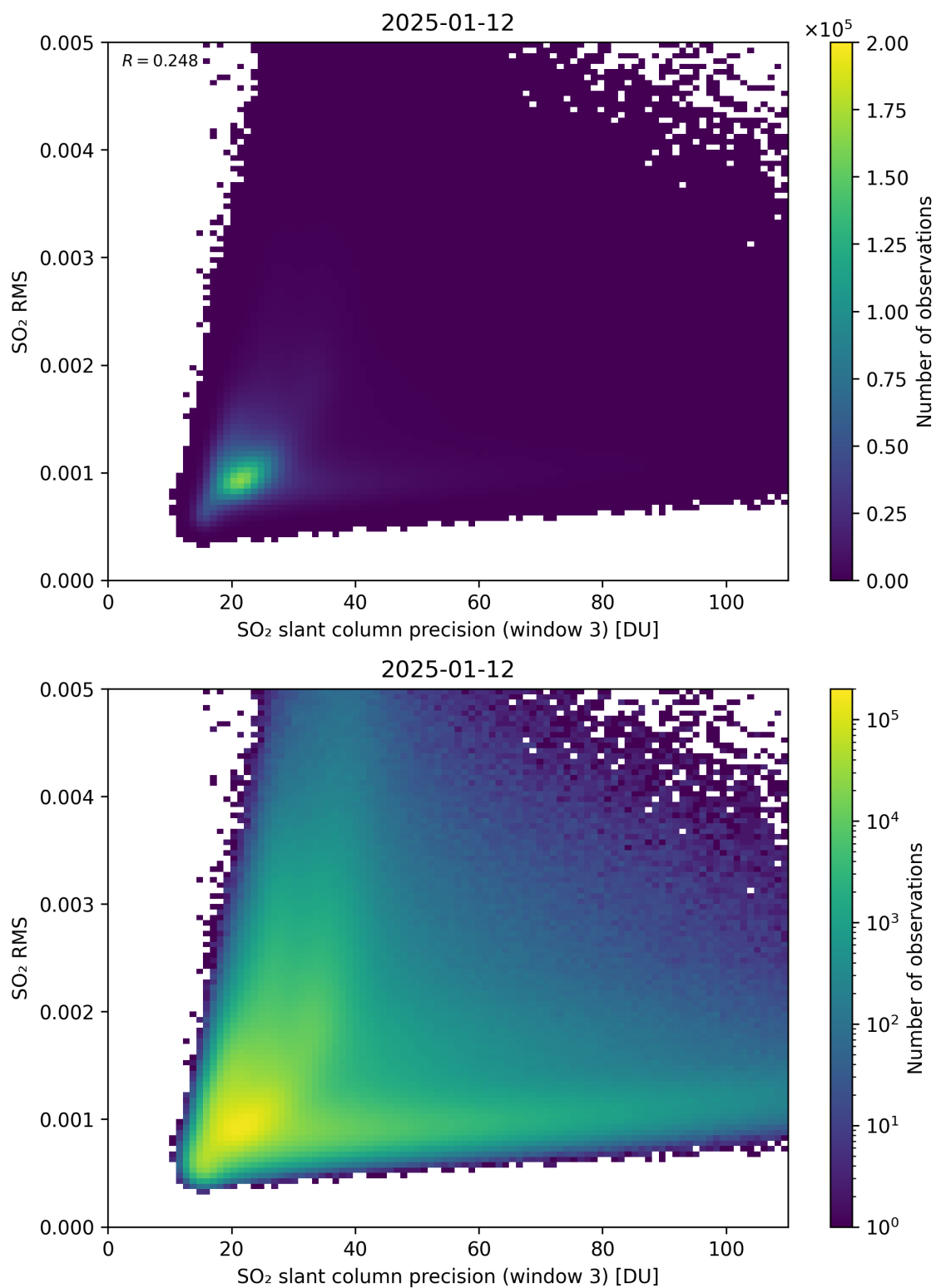
Figure 310: Scatter density plot of “SO 2 slant column precision (window 3)” against “SO 2 RMS” for 2025-01-12 to 2025-01-13.
