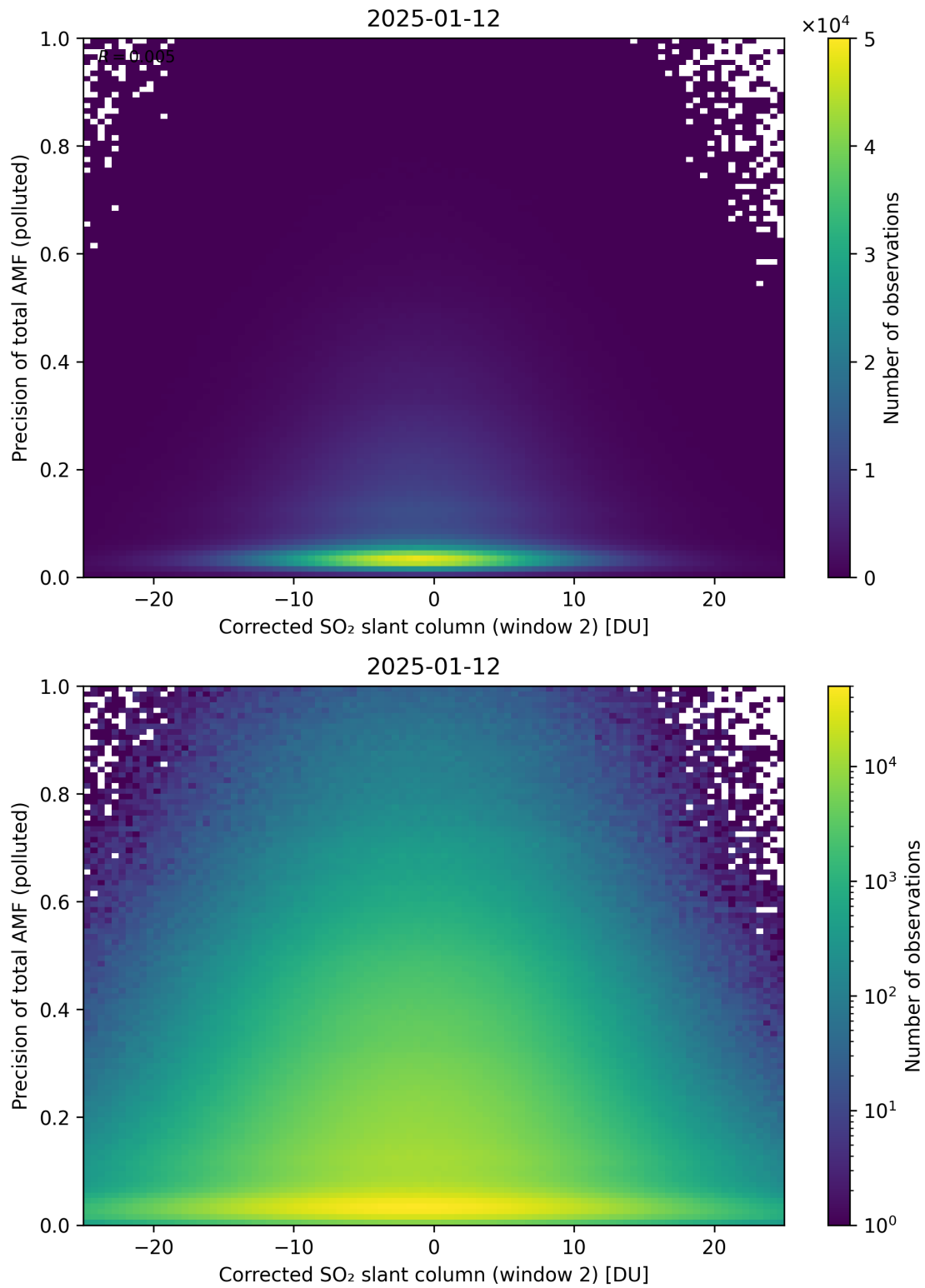
Figure 254: Scatter density plot of “Corrected SO 2 slant column (window 2)” against “Precision of total AMF (polluted)” for 2025-01-12 to 2025-01-13.
