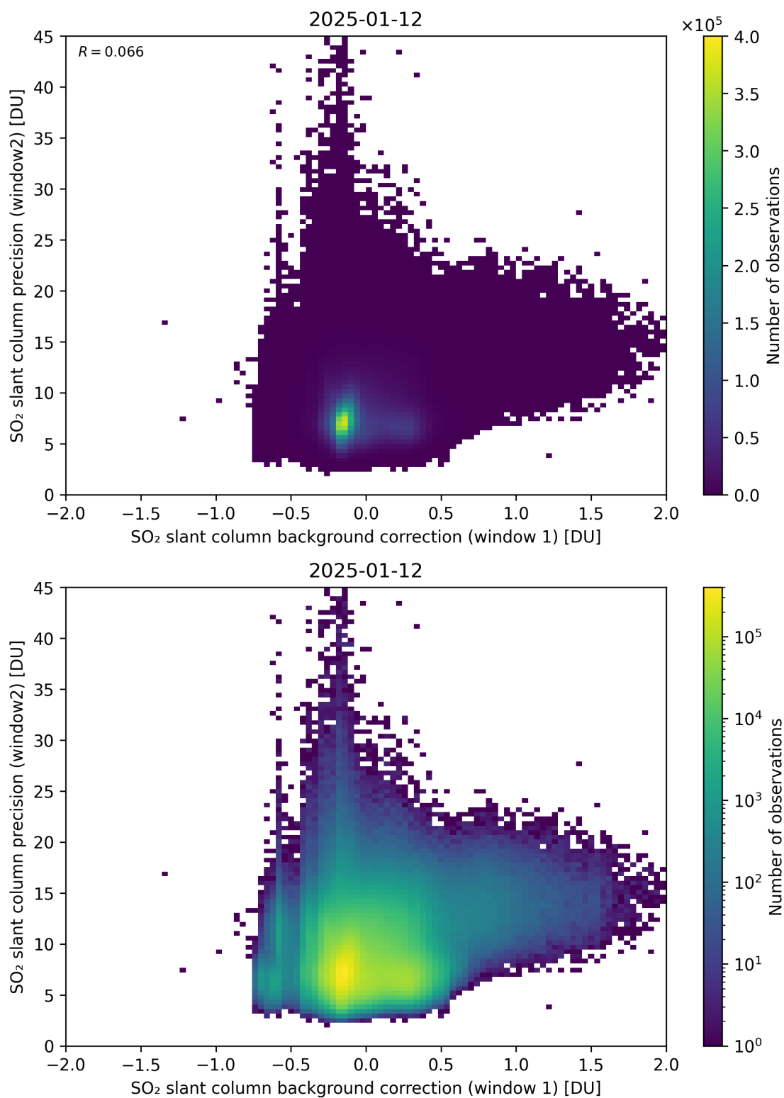
Figure 117: Scatter density plot of “SO 2 slant column background correction (window 1)” against “SO 2 slant column precision (window2)” for 2025-01-12 to 2025-01-13.
