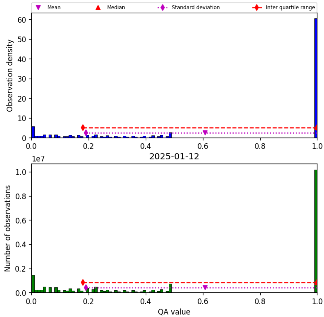
Figure 57: Histogram of “QA value” for 2025-01-12 to 2025-01-13
