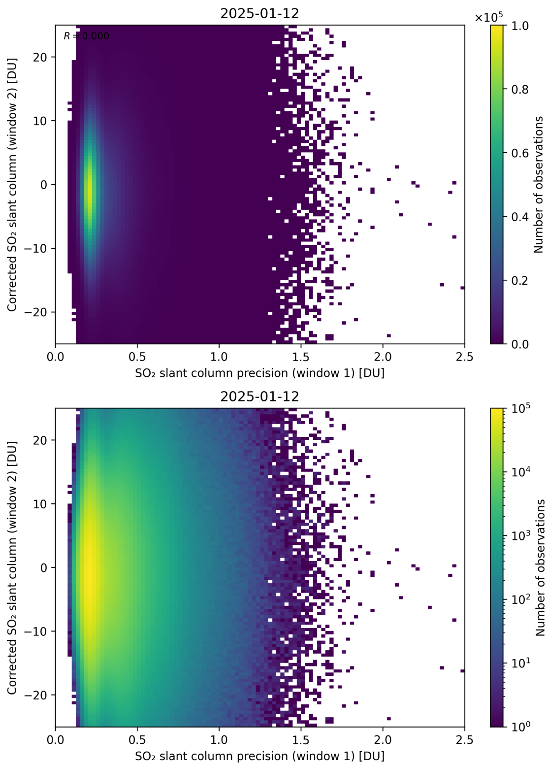
Figure 275: Scatter density plot of “SO 2 slant column precision (window 1)” against “Corrected SO 2 slant column (window 2)” for 2025-01-12 to 2025-01-13.
