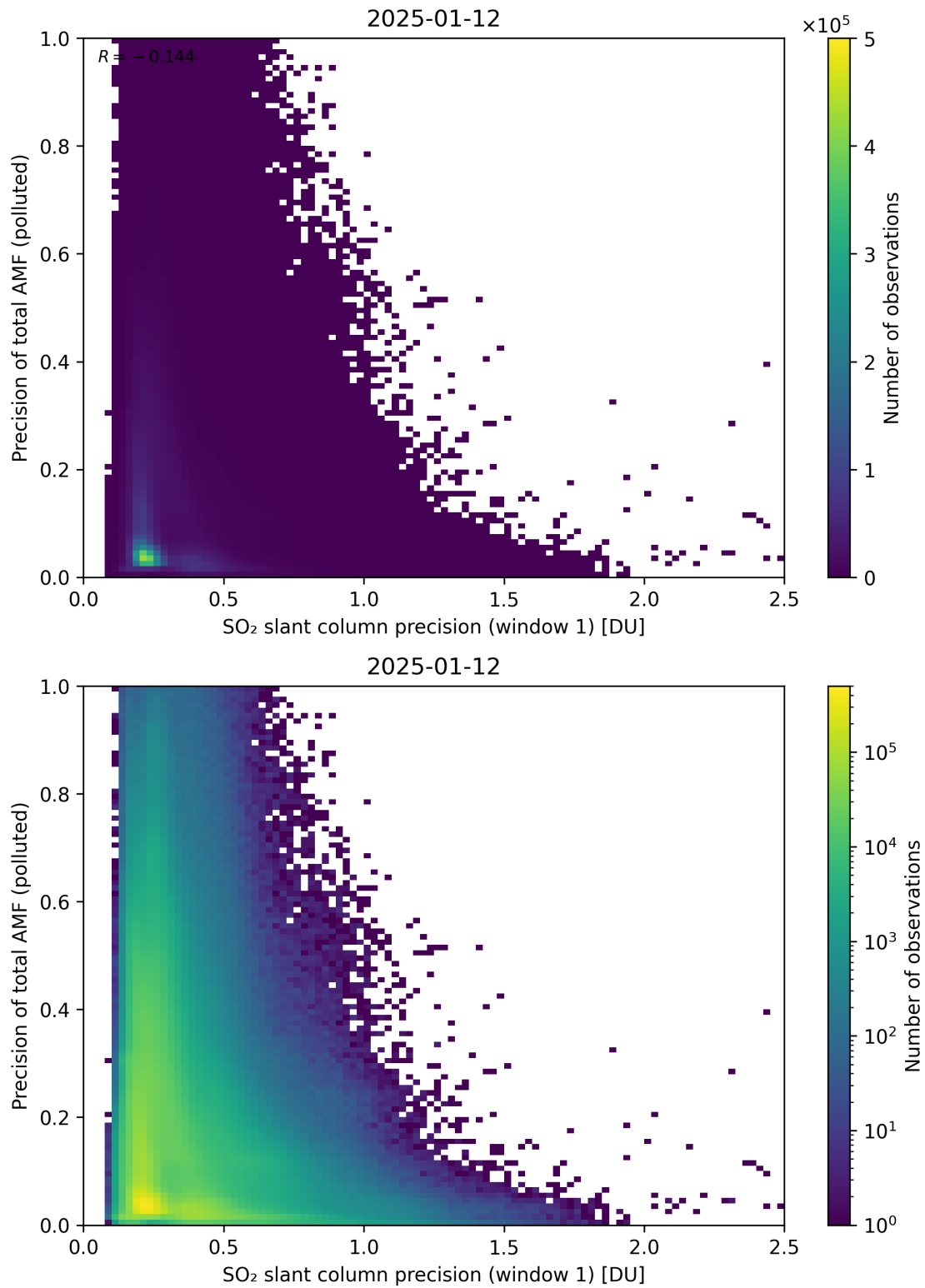
Figure 281: Scatter density plot of “SO 2 slant column precision (window 1)” against “Precision of total AMF (polluted)” for 2025-01-12 to 2025-01-13.
