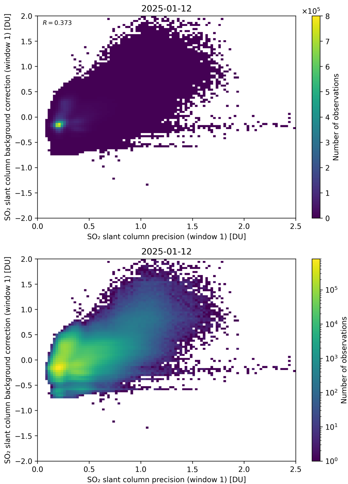
Figure 268: Scatter density plot of “SO 2 slant column precision (window 1)” against “SO 2 slant column background correction (window 1)” for 2025-01-12 to 2025-01-13.
