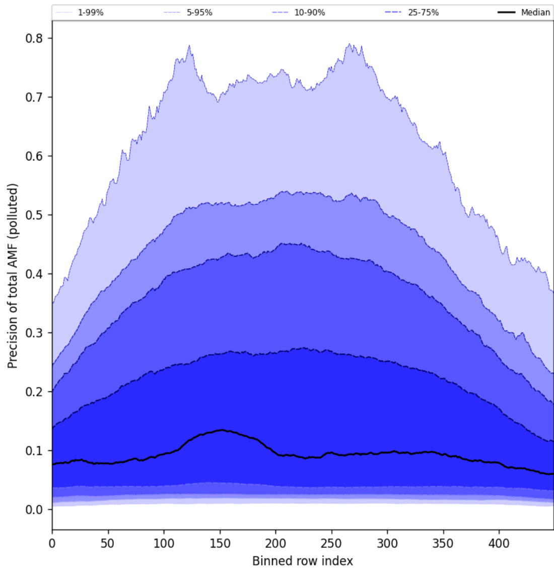
Figure 106: Along track statistics of “Precision of total AMF (polluted)” for 2025-01-12 to 2025-01-13
