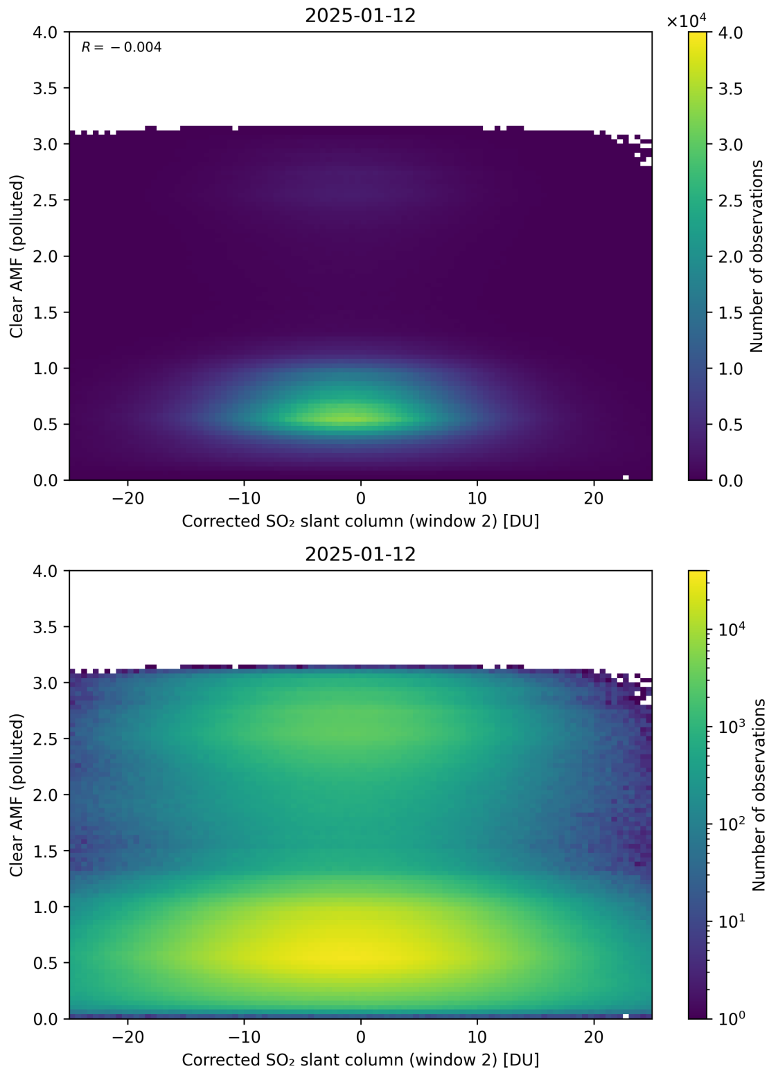
Figure 249: Scatter density plot of “Corrected SO 2 slant column (window 2)” against “Clear AMF (polluted)” for 2025-01-12 to 2025-01-13.
