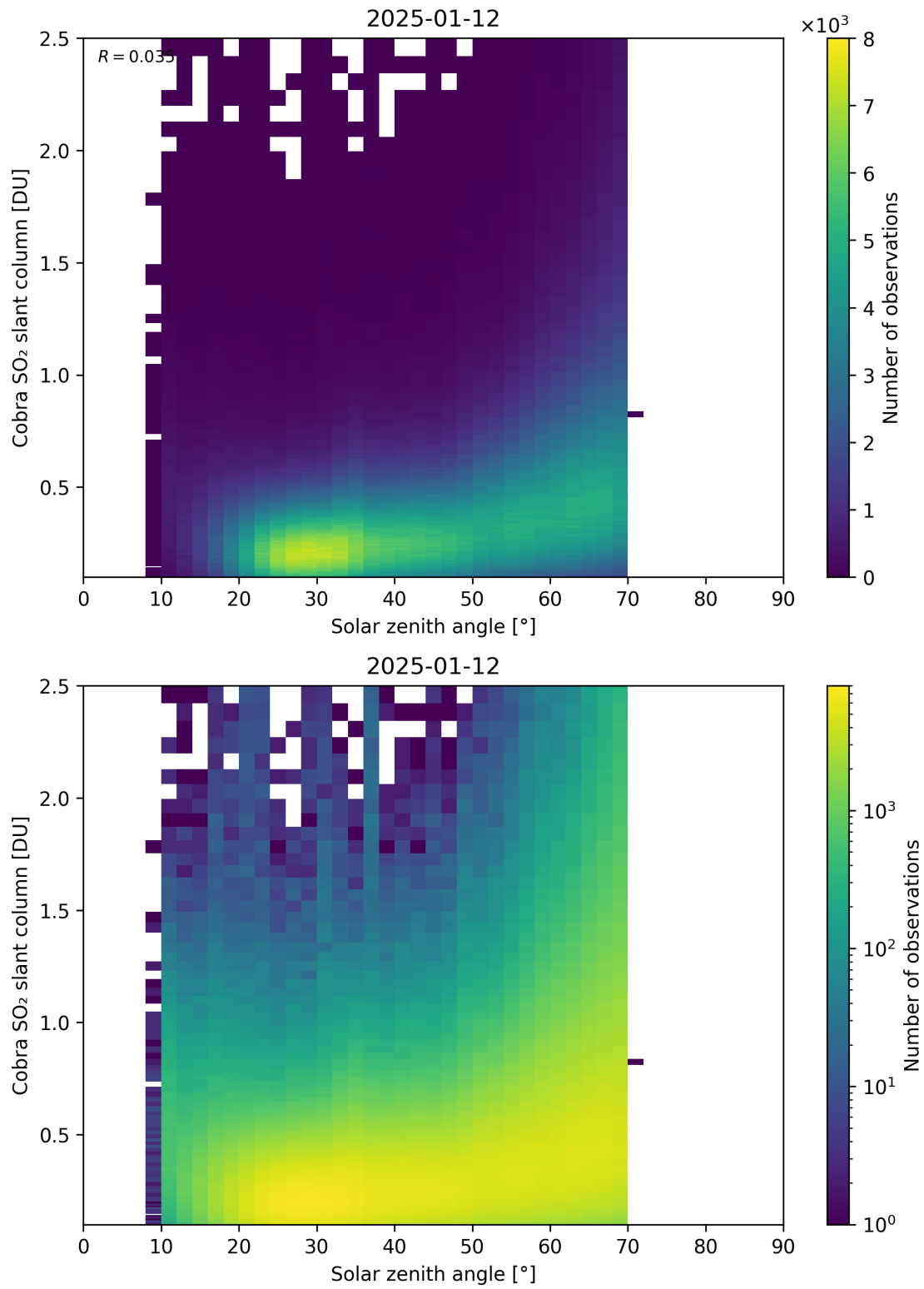
Figure 179: Scatter density plot of “Solar zenith angle” against “Cobra SO 2 slant column” for 2025-01-12 to 2025-01-13.
