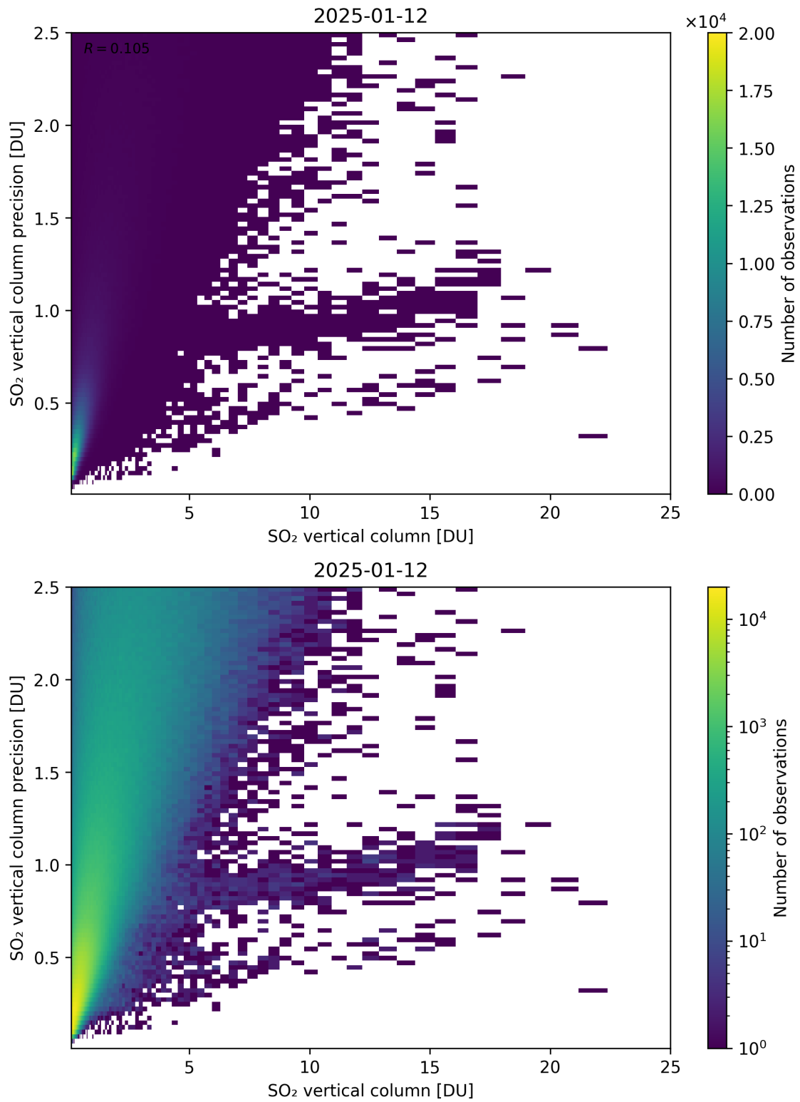
Figure 361: Scatter density plot of “SO 2 vertical column” against “SO 2 vertical column precision” for 2025-01-12 to 2025-01-13.
