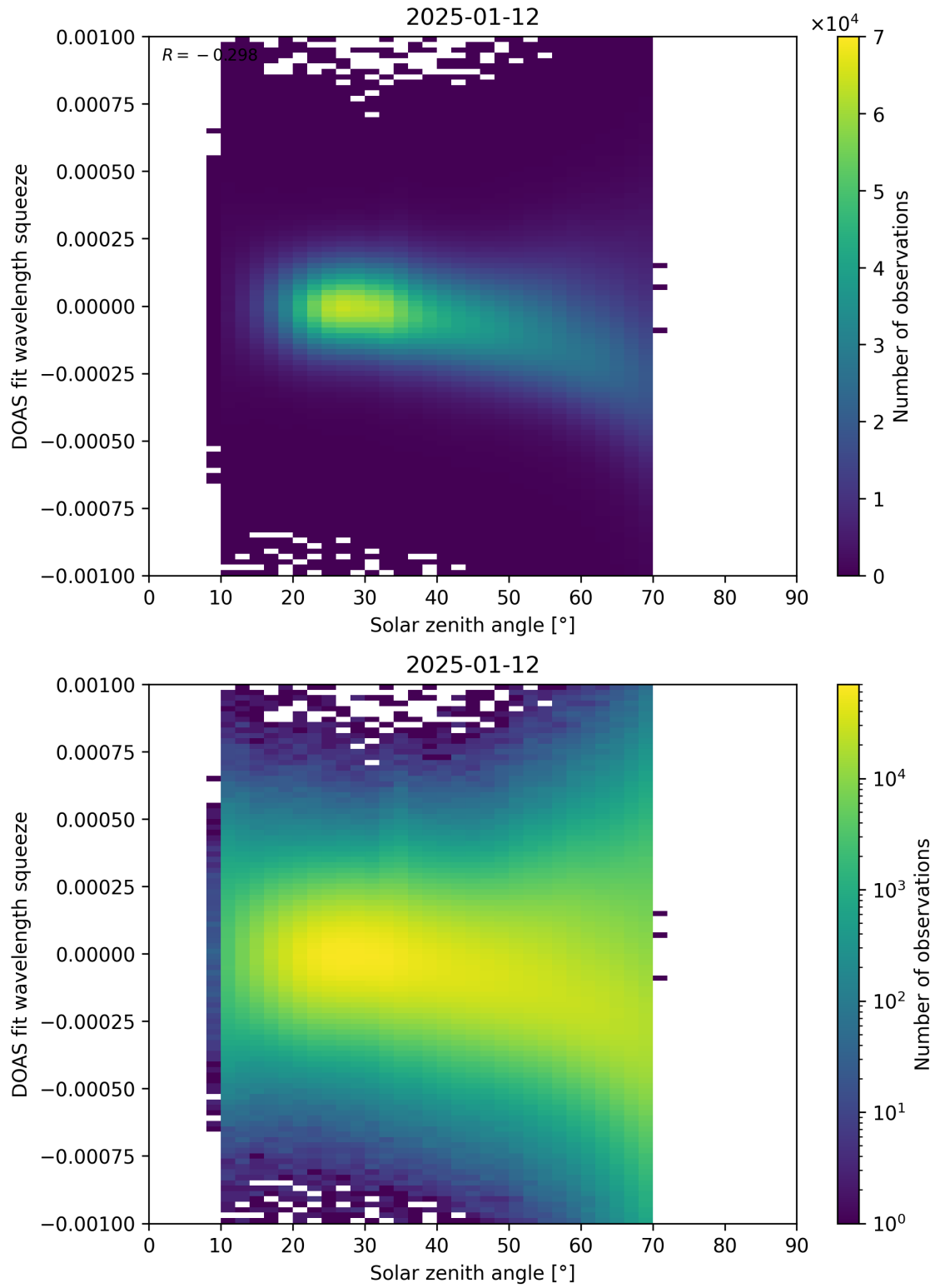
Figure 175: Scatter density plot of “Solar zenith angle” against “DOAS fit wavelength squeeze” for 2025-01-12 to 2025-01-13.
