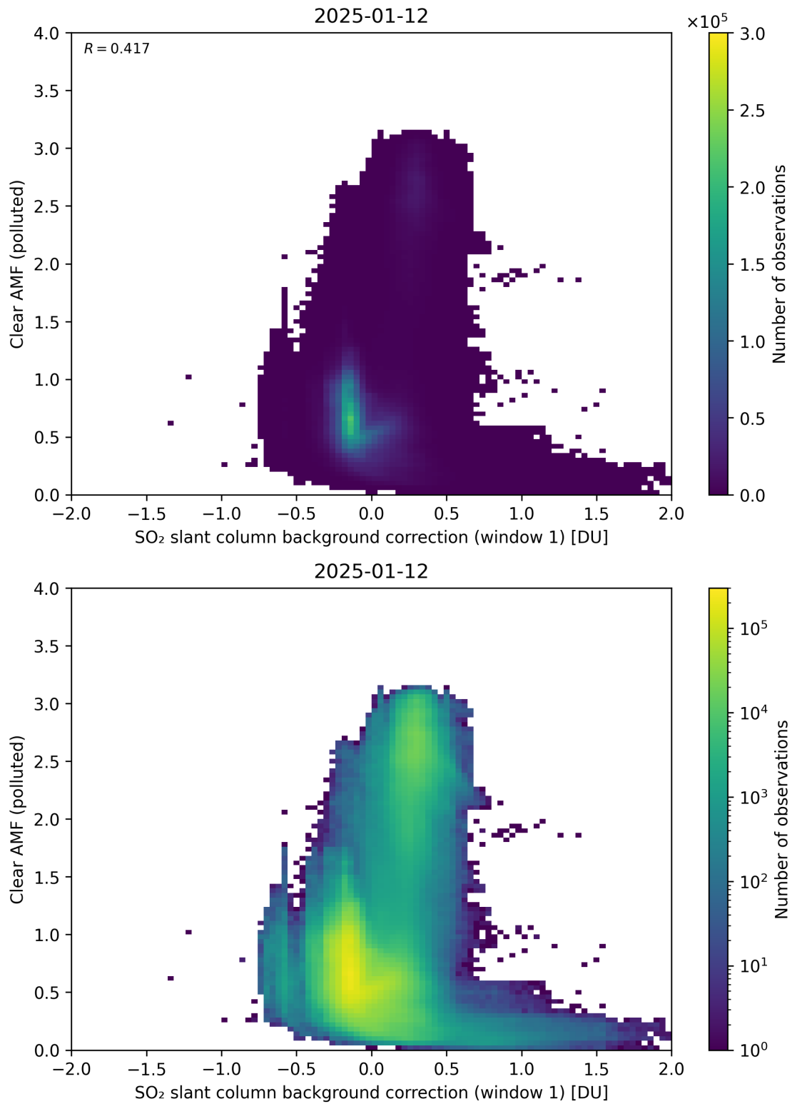
Figure 114: Scatter density plot of “SO 2 slant column background correction (window 1)” against “Clear AMF (polluted)” for 2025-01-12 to 2025-01-13.
