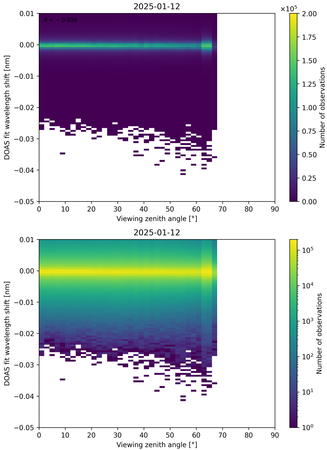
Figure 365: Scatter density plot of “Viewing zenith angle” against “DOAS fit wavelength shift” for 2025-01-12 to 2025-01-13.
