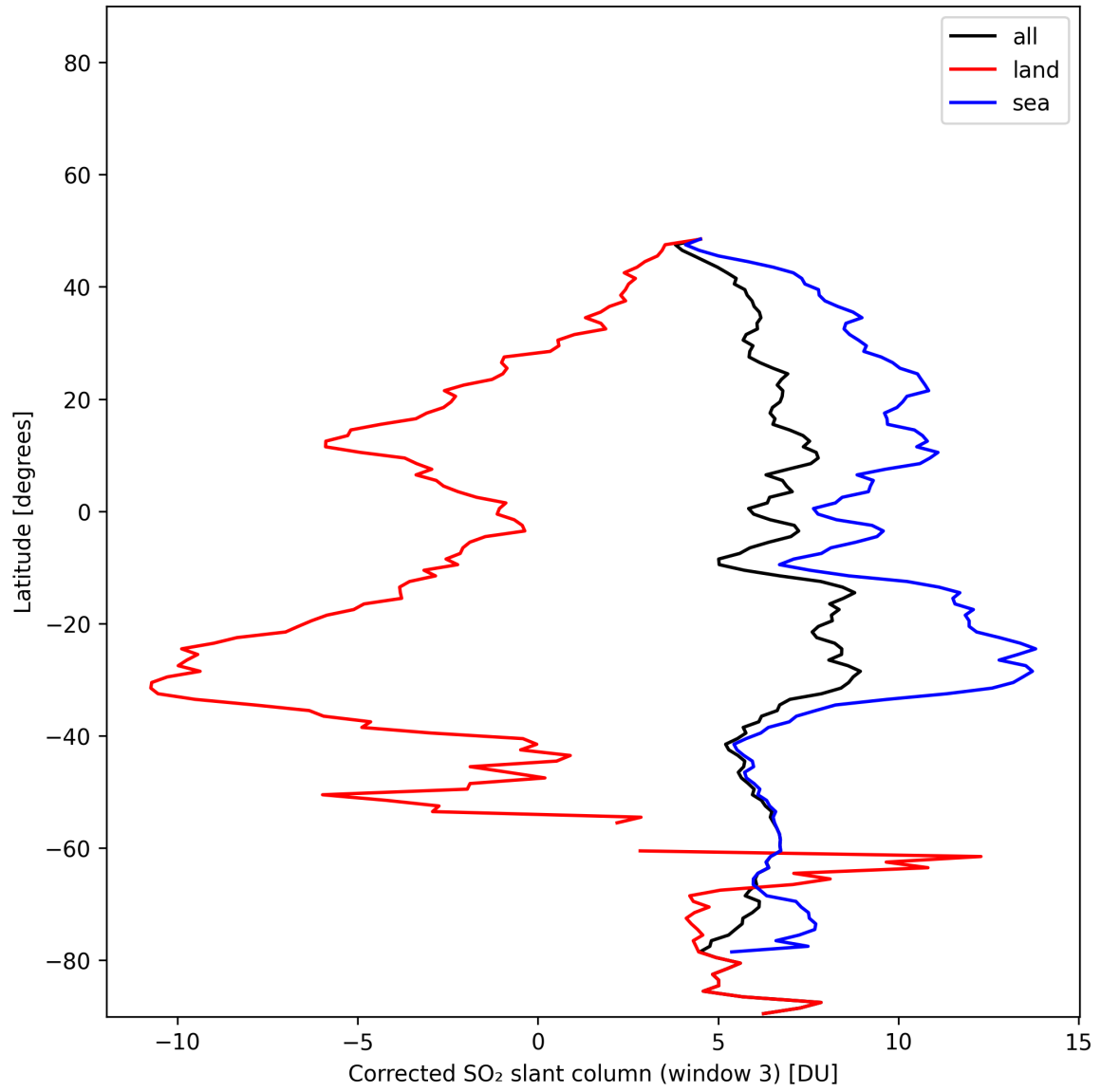
Figure 47: Zonal average of “Corrected SO 2 slant column (window 3)” for 2025-01-12 to 2025-01-13.
