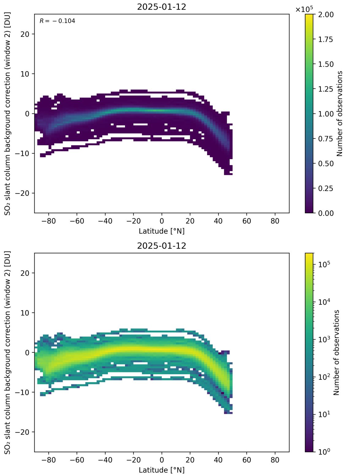
Figure 151: Scatter density plot of “Latitude” against “SO 2 slant column background correction (window 2)” for 2025-01-12 to 2025-01-13.
