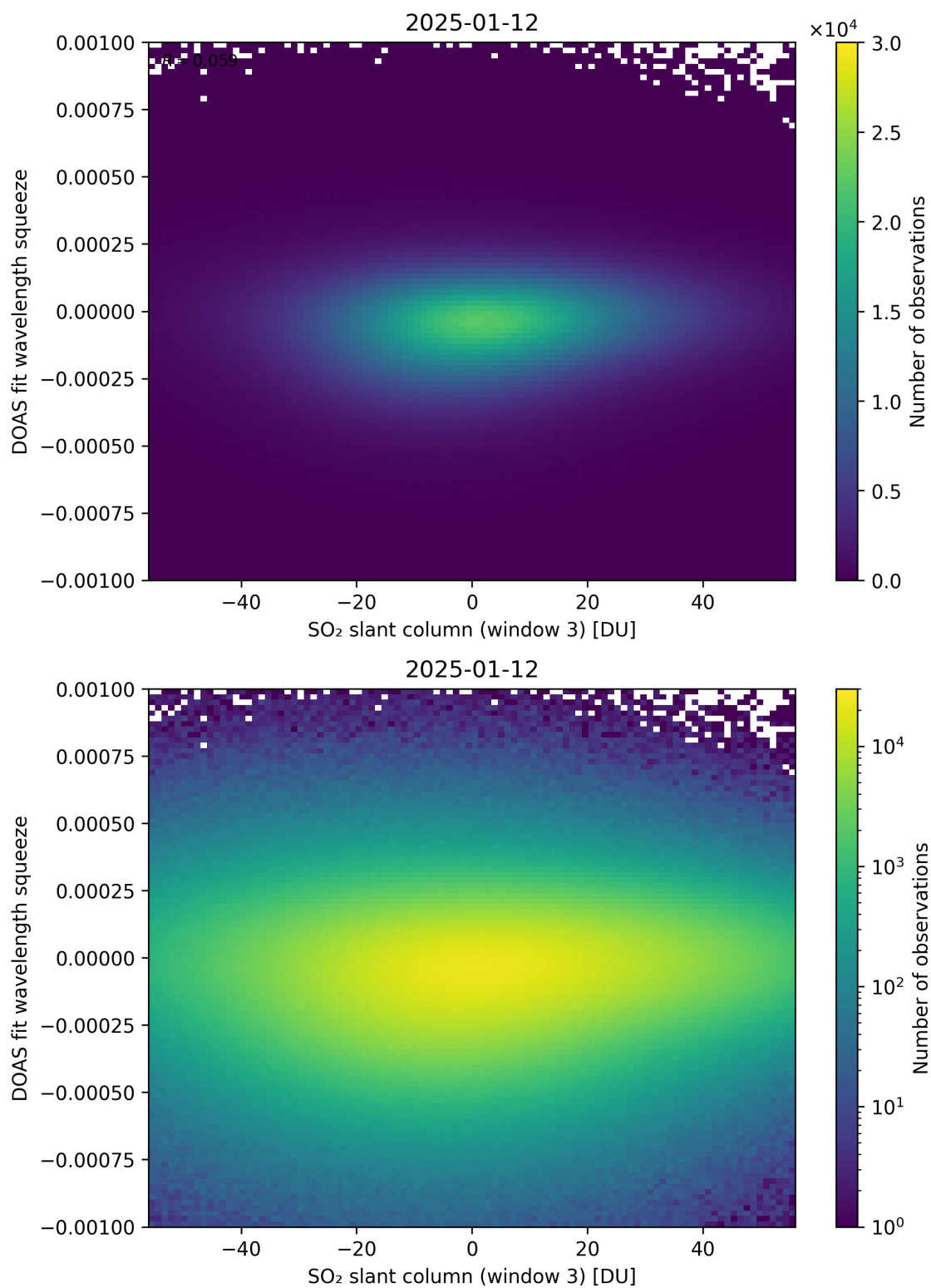
Figure 305: Scatter density plot of “SO 2 slant column (window 3)” against “DOAS fit wavelength squeeze” for 2025-01-12 to 2025-01-13.
