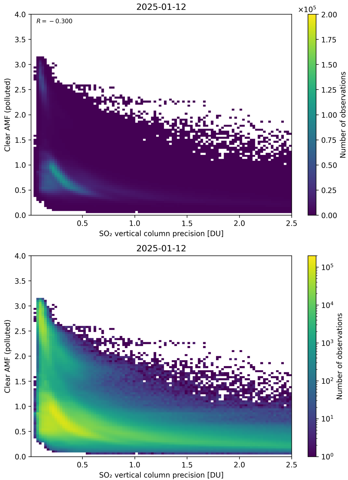
Figure 335: Scatter density plot of “SO 2 vertical column precision” against “Clear AMF (polluted)” for 2025-01-12 to 2025-01-13.
