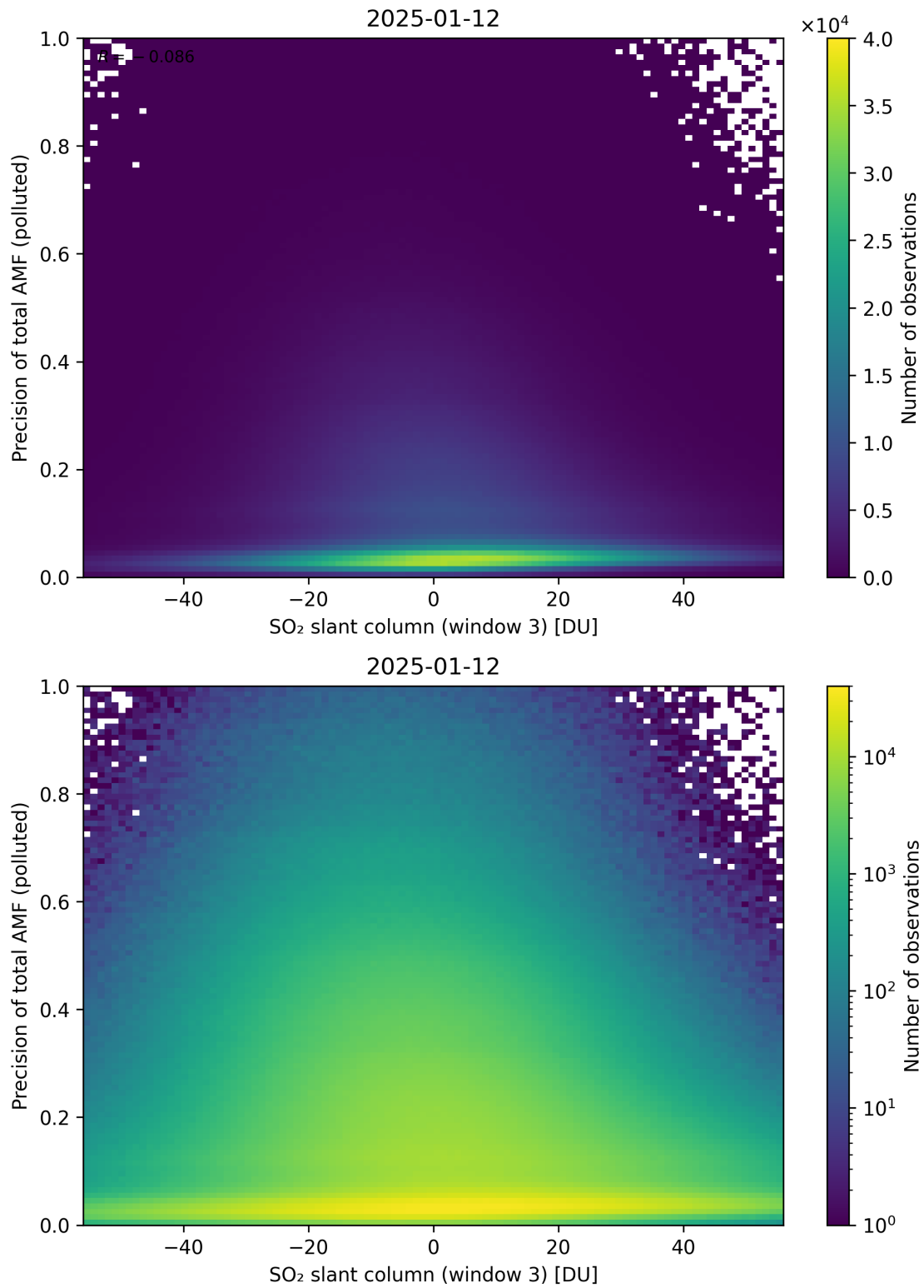
Figure 319: Scatter density plot of “SO 2 slant column (window 3)” against “Precision of total AMF (polluted)” for 2025-01-12 to 2025-01-13.
