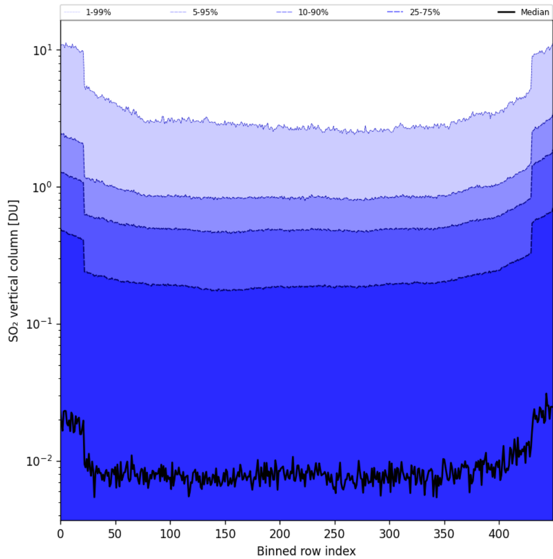
Figure 84: Along track statistics of “SO 2 vertical column” for 2025-01-12 to 2025-01-13
