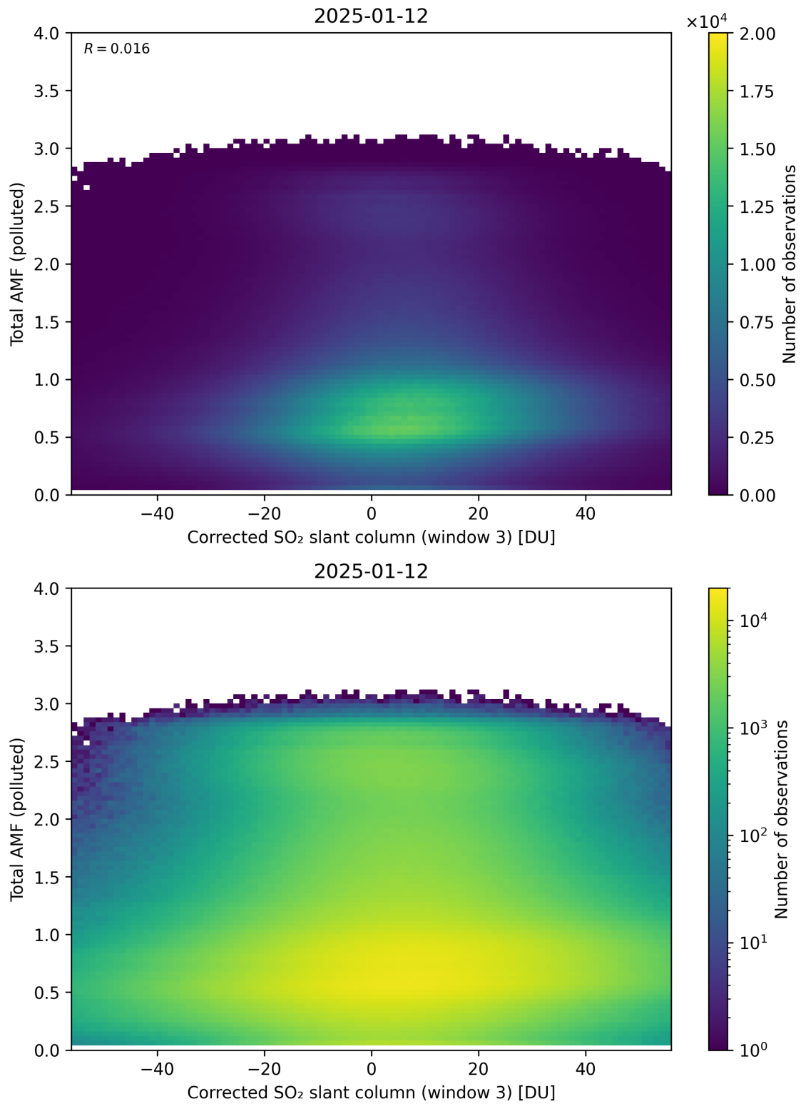
Figure 260: Scatter density plot of “Corrected SO 2 slant column (window 3)” against “Total AMF (polluted)” for 2025-01-12 to 2025-01-13.
