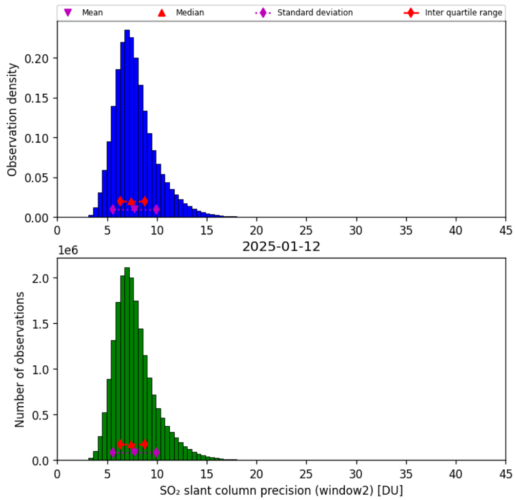
Figure 68: Histogram of “SO 2 slant column precision (window2)” for 2025-01-12 to 2025-01-13
