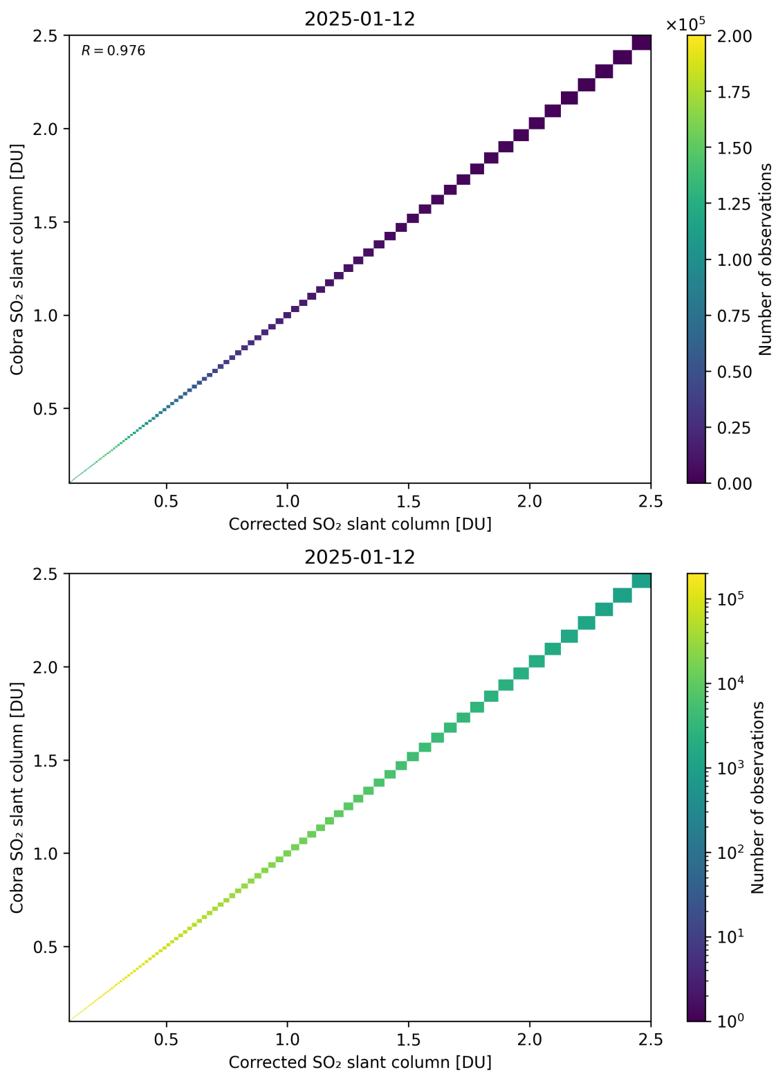
Figure 233: Scatter density plot of “Corrected SO 2 slant column” against “Cobra SO 2 slant column” for 2025-01-12 to 2025-01-13.
