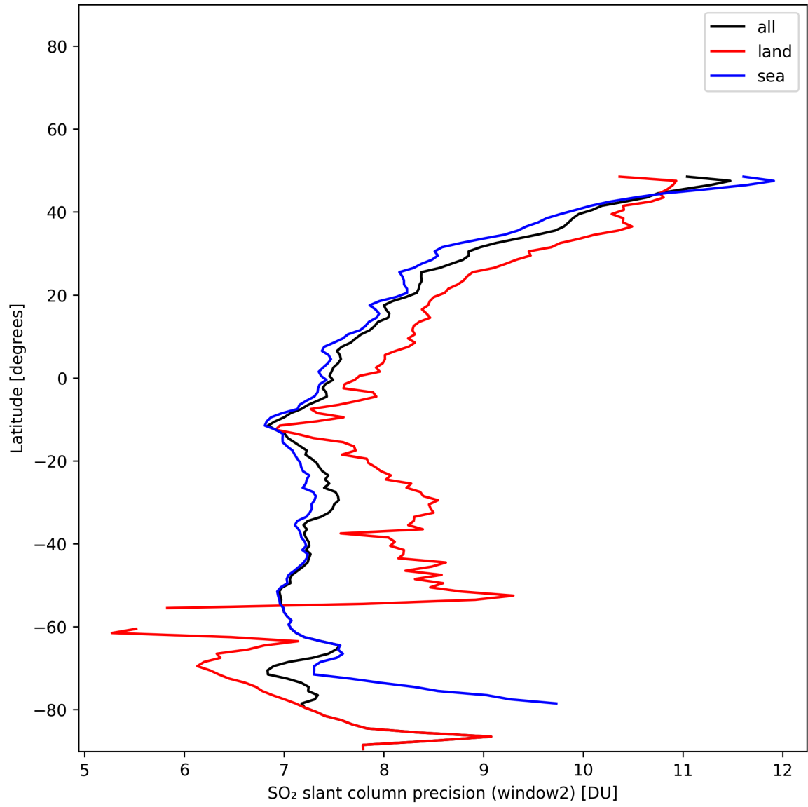
Figure 42: Zonal average of “SO 2 slant column precision (window2)” for 2025-01-12 to 2025-01-13.
