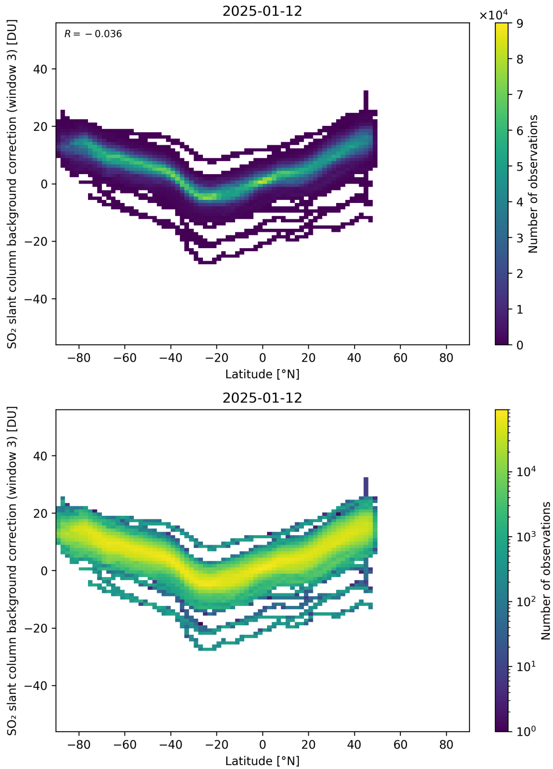
Figure 152: Scatter density plot of “Latitude” against “SO 2 slant column background correction (window 3)” for 2025-01-12 to 2025-01-13.
