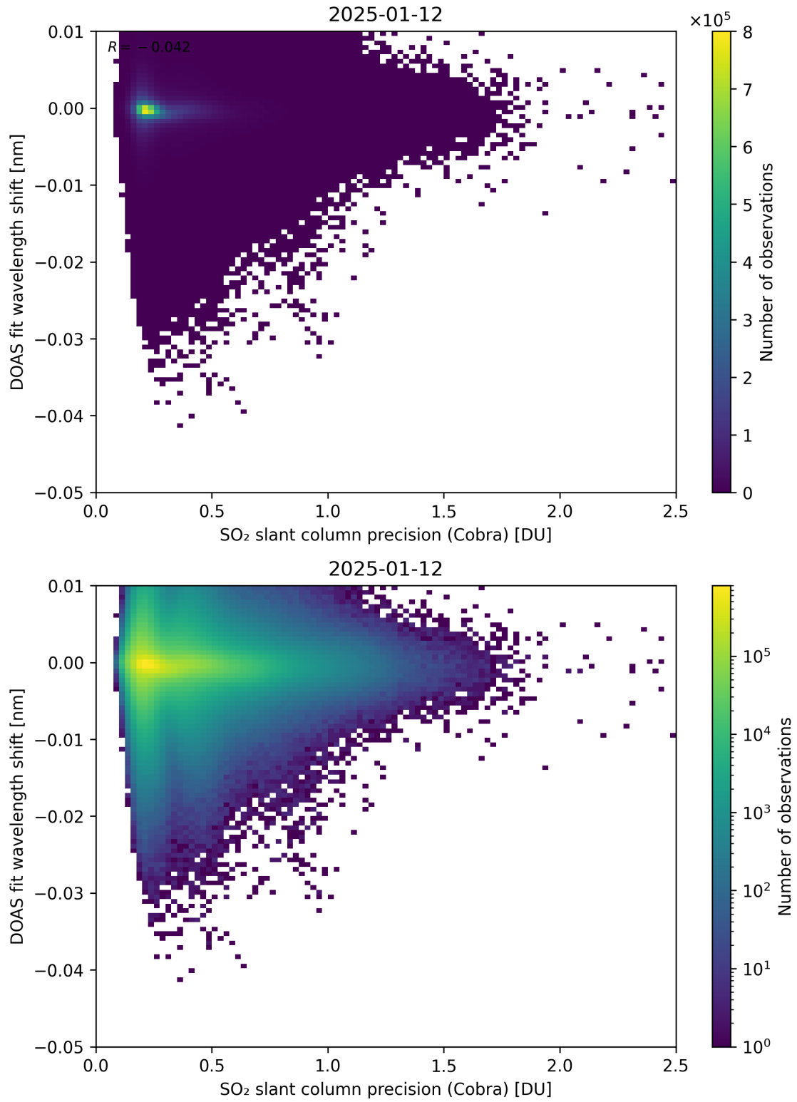
Figure 202: Scatter density plot of “SO 2 slant column precision (Cobra)” against “DOAS fit wavelength shift” for 2025-01-12 to 2025-01-13.
