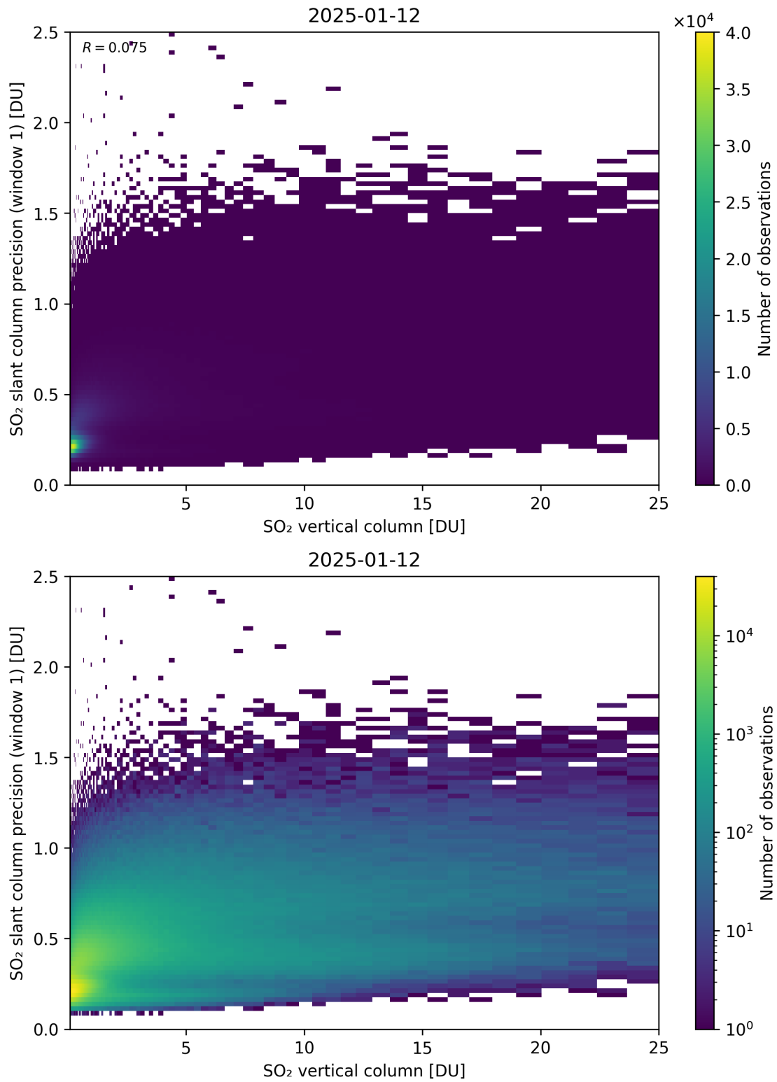
Figure 355: Scatter density plot of “SO 2 vertical column” against “SO 2 slant column precision (window 1)” for 2025-01-12 to 2025-01-13.
