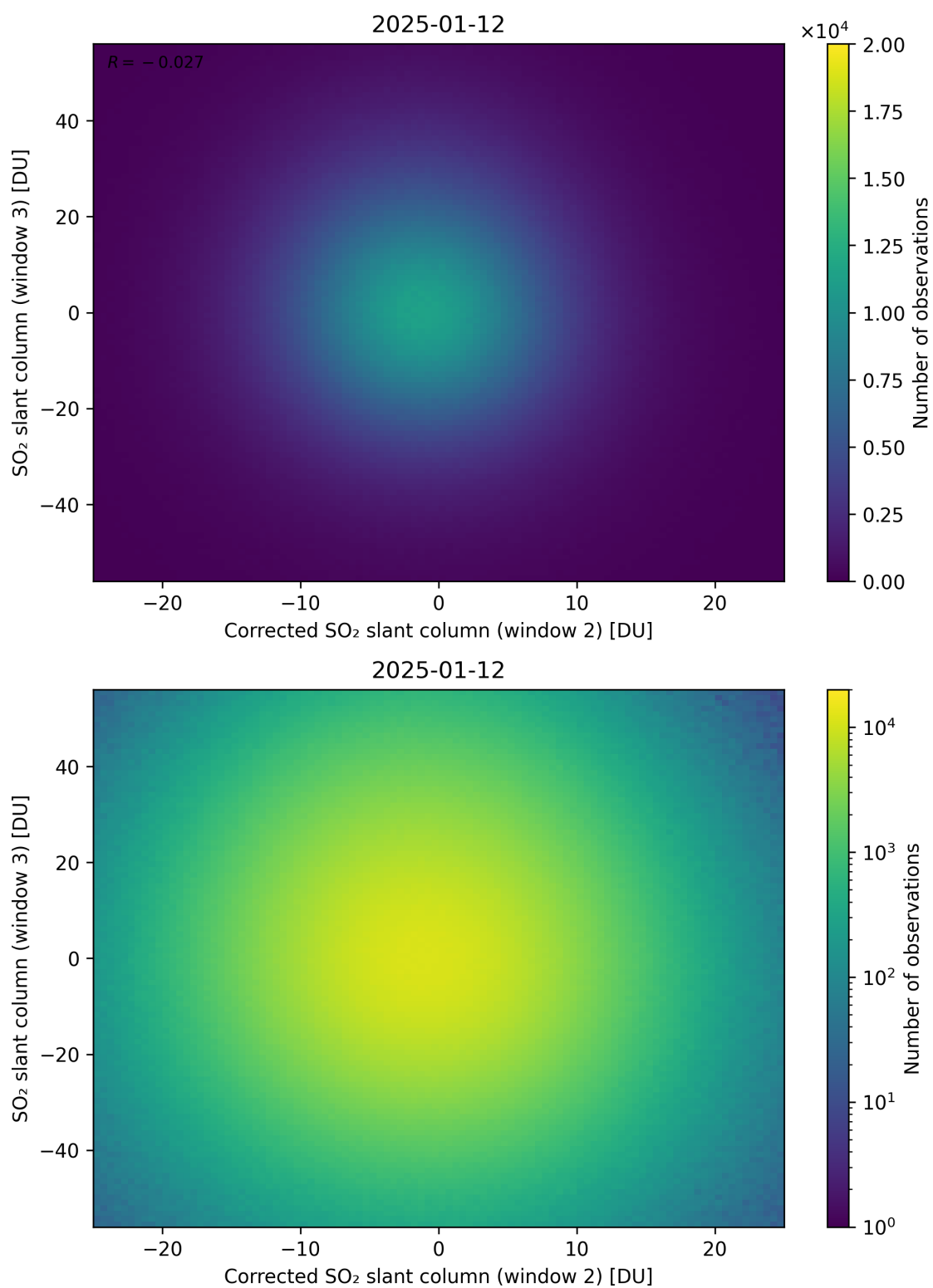
Figure 251: Scatter density plot of “Corrected SO 2 slant column (window 2)” against “SO 2 slant column (window 3)” for 2025-01-12 to 2025-01-13.
