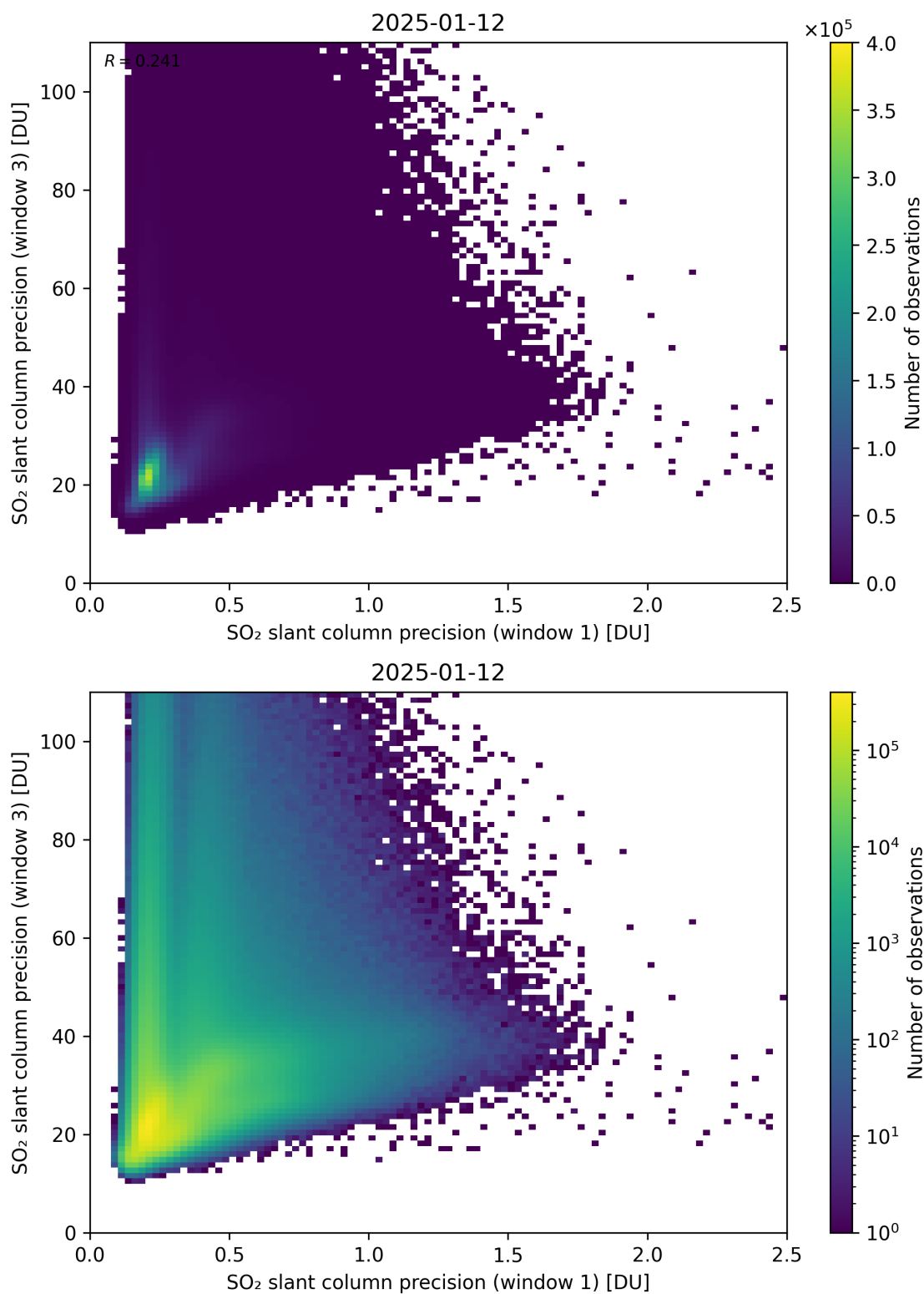
Figure 279: Scatter density plot of “SO 2 slant column precision (window 1)” against “SO 2 slant column precision (window 3)” for 2025-01-12 to 2025-01-13.
