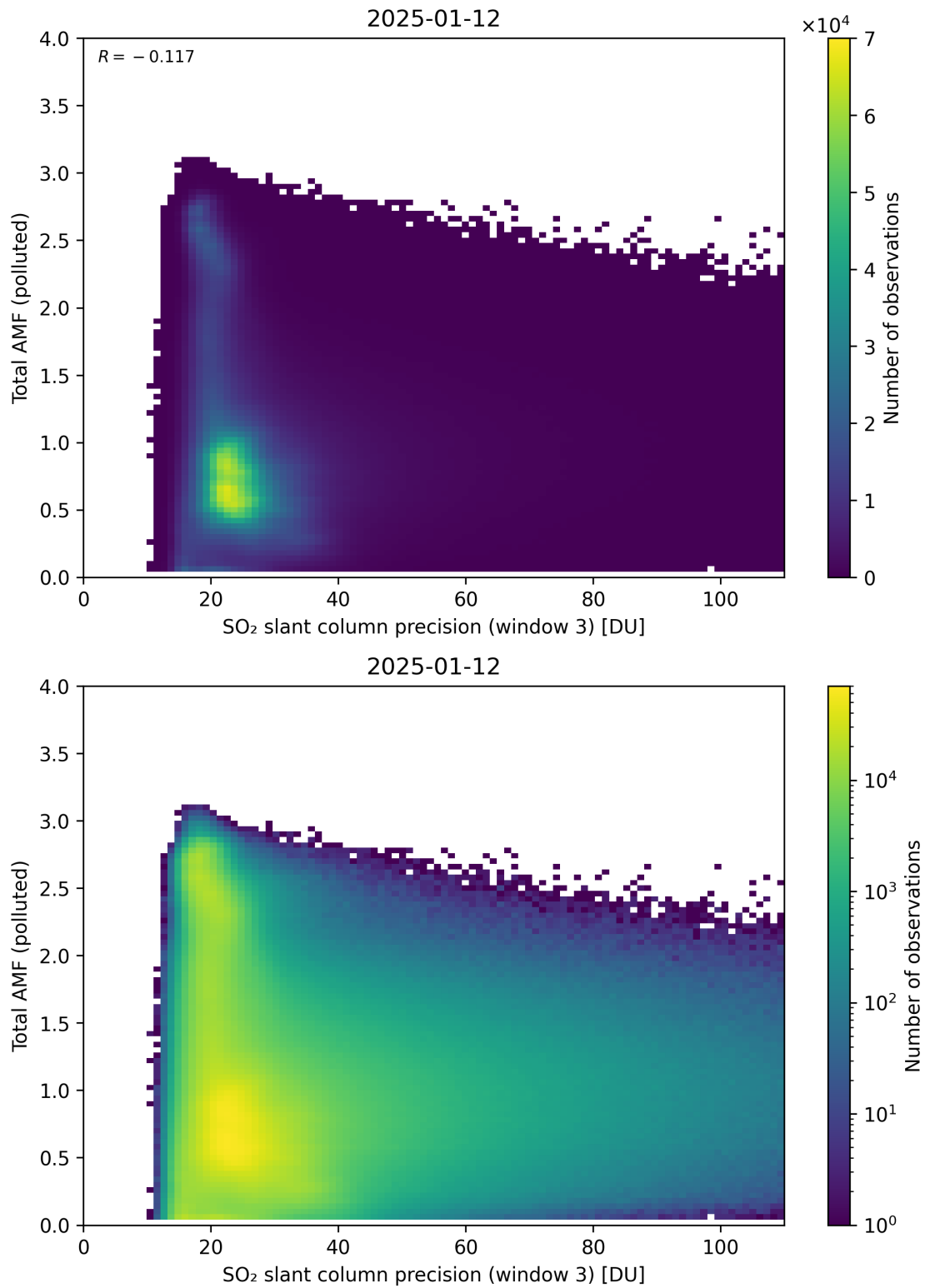
Figure 313: Scatter density plot of “SO 2 slant column precision (window 3)” against “Total AMF (polluted)” for 2025-01-12 to 2025-01-13.
