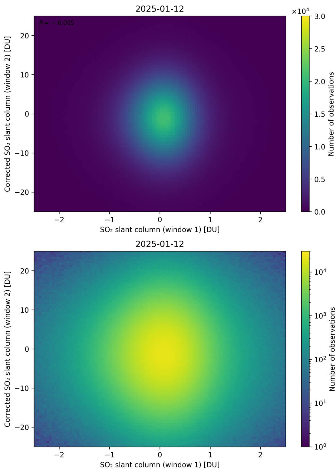
Figure 283: Scatter density plot of “SO 2 slant column (window 1)” against “Corrected SO 2 slant column (window 2)” for 2025-01-12 to 2025-01-13.
