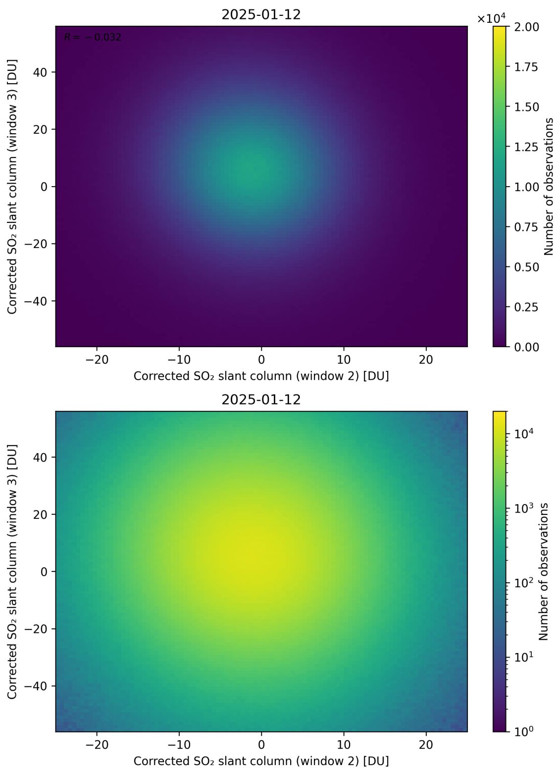
Figure 250: Scatter density plot of “Corrected SO 2 slant column (window 2)” against “Corrected SO 2 slant column (window 3)” for 2025-01-12 to 2025-01-13.
