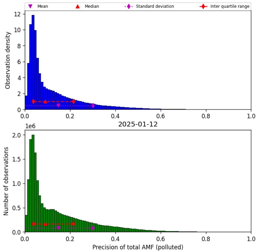
Figure 80: Histogram of “Precision of total AMF (polluted)” for 2025-01-12 to 2025-01-13
