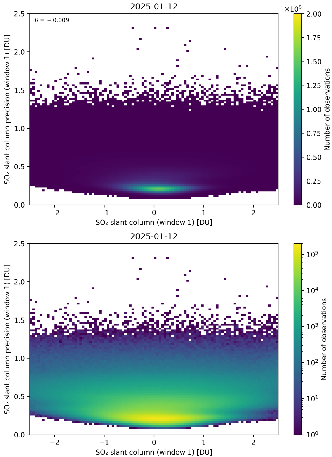
Figure 285: Scatter density plot of “SO 2 slant column (window 1)” against “SO 2 slant column precision (window 1)” for 2025-01-12 to 2025-01-13.
