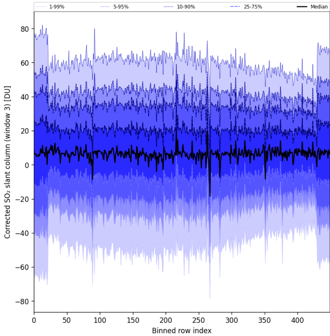
Figure 99: Along track statistics of “Corrected SO 2 slant column (window 3)” for 2025-01-12 to 2025-01-13
