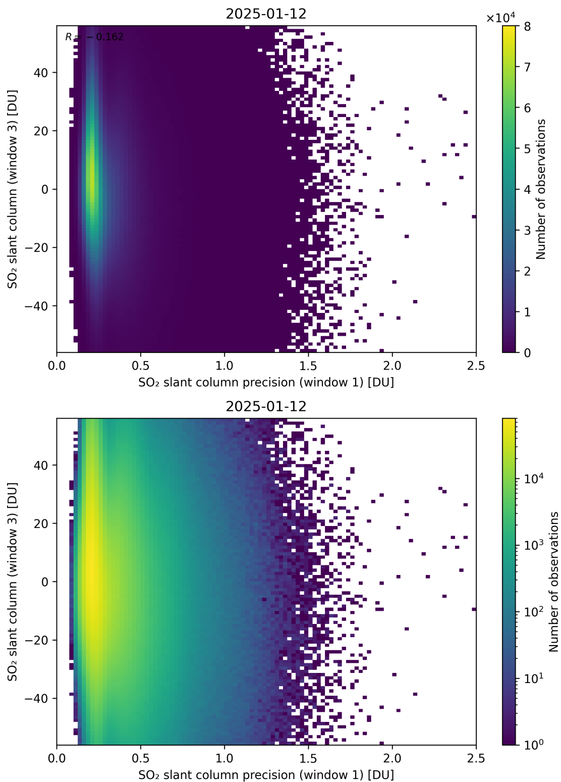
Figure 278: Scatter density plot of “SO 2 slant column precision (window 1)” against “SO 2 slant column (window 3)” for 2025-01-12 to 2025-01-13.
