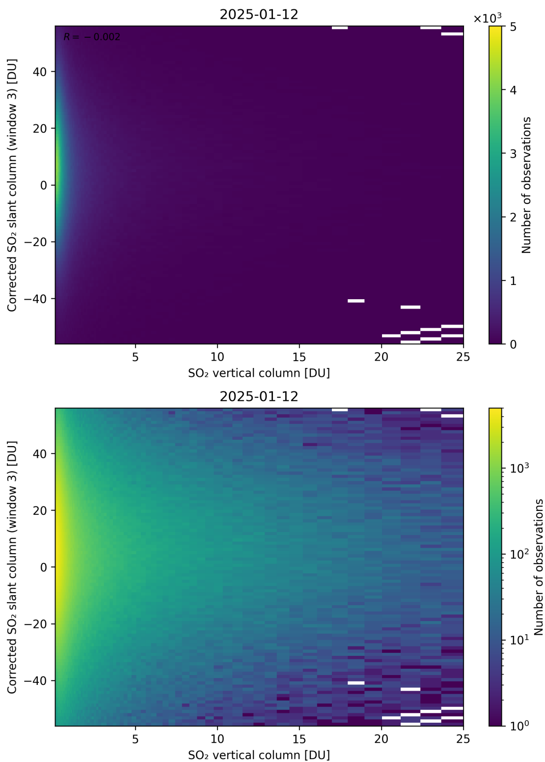
Figure 353: Scatter density plot of “SO 2 vertical column” against “Corrected SO 2 slant column (window 3)” for 2025-01-12 to 2025-01-13.
