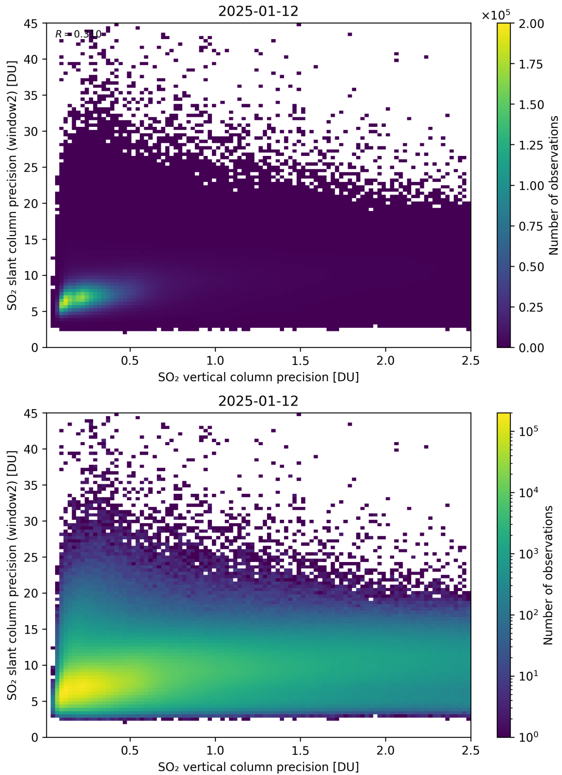
Figure 343: Scatter density plot of “SO 2 vertical column precision” against “SO 2 slant column precision (window2)” for 2025-01-12 to 2025-01-13.
