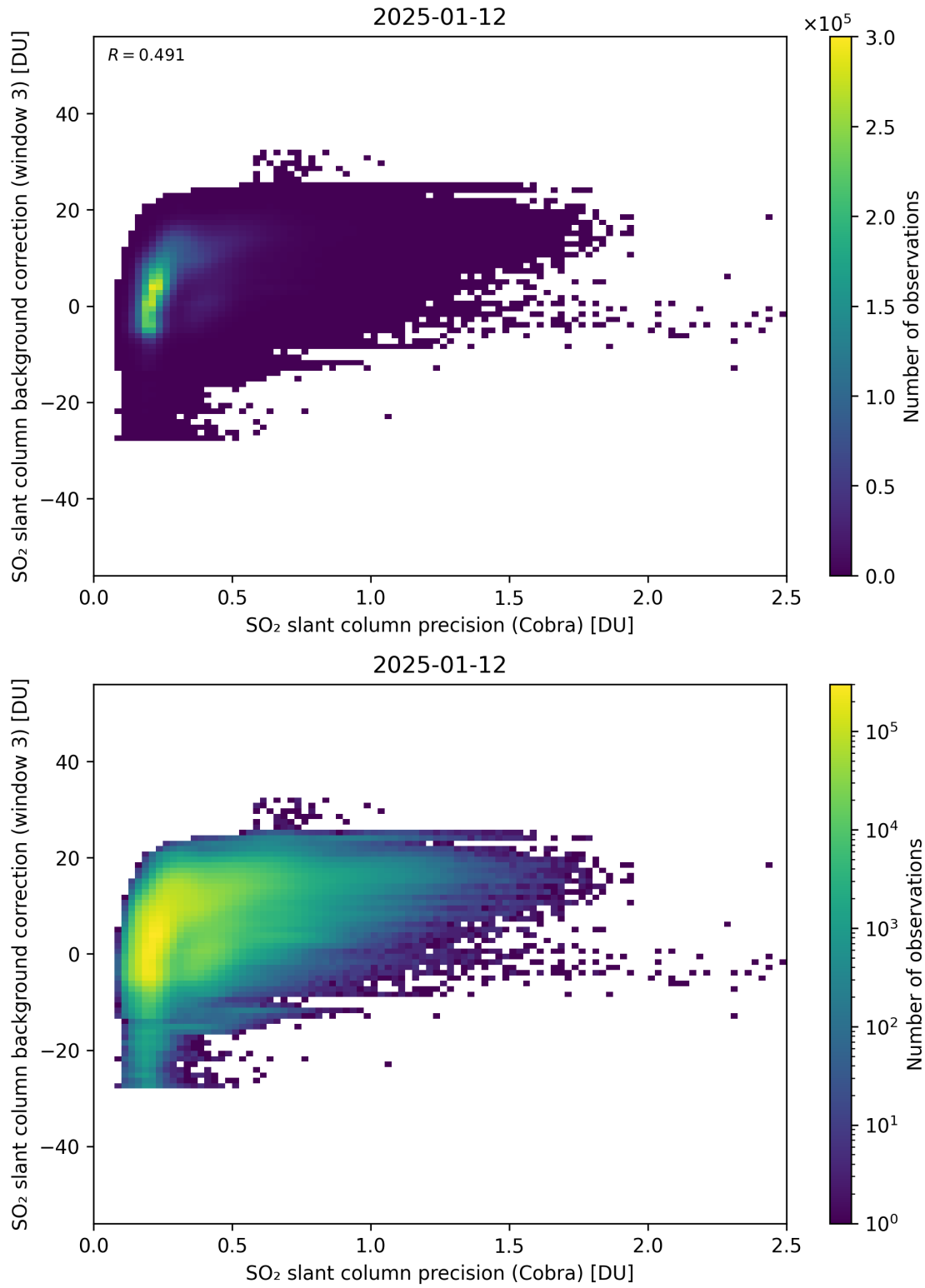
Figure 201: Scatter density plot of “SO 2 slant column precision (Cobra)” against “SO 2 slant column background correction (window 3)” for 2025-01-12 to 2025-01-13.
