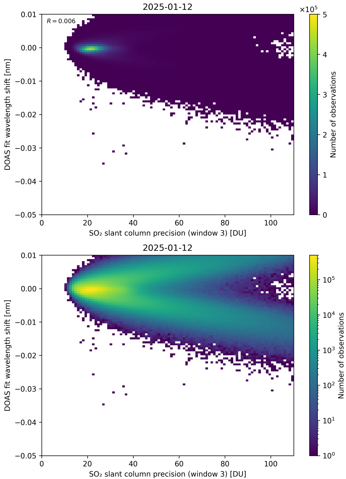
Figure 308: Scatter density plot of “SO 2 slant column precision (window 3)” against “DOAS fit wavelength shift” for 2025-01-12 to 2025-01-13.
