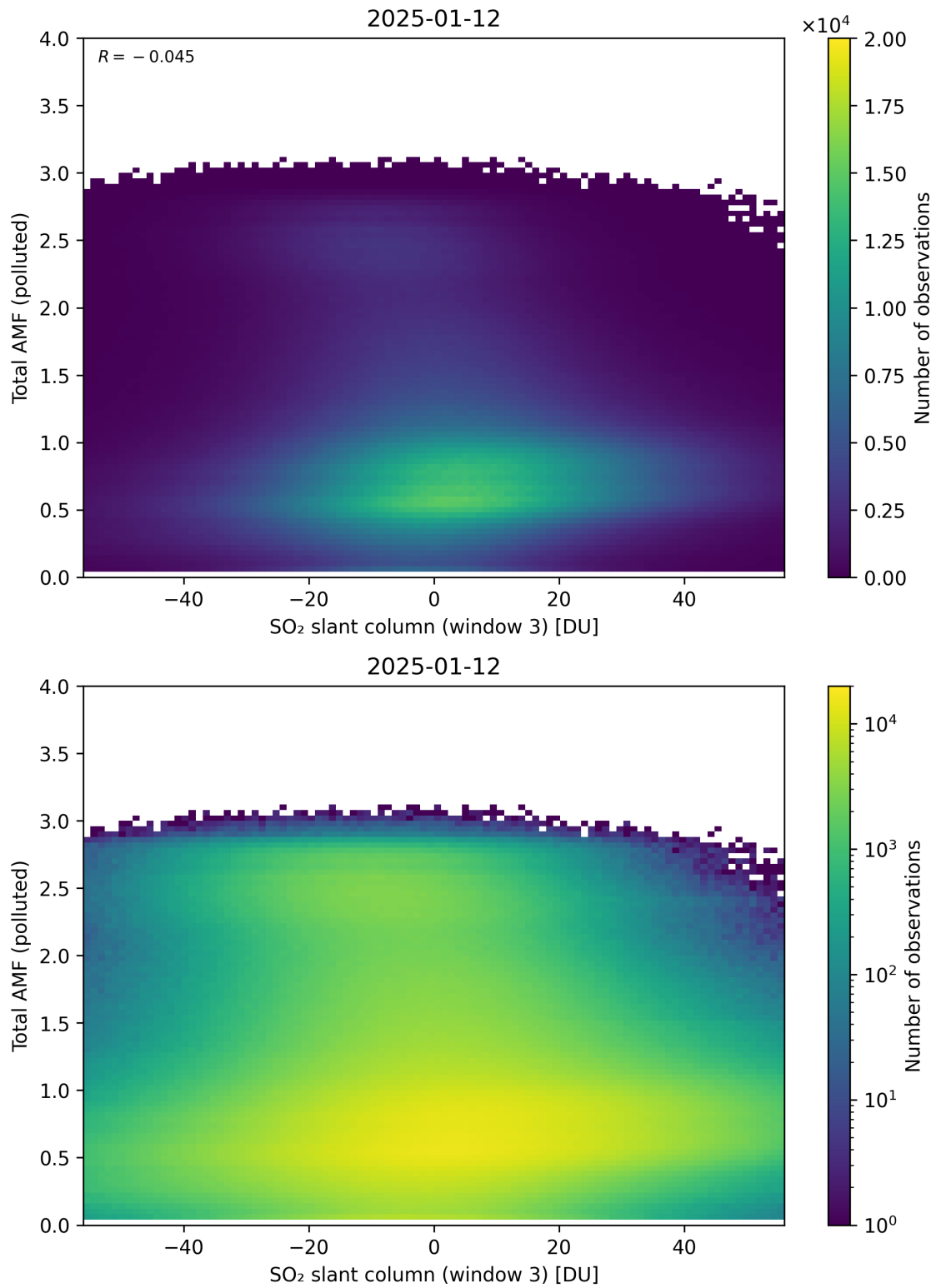
Figure 318: Scatter density plot of “SO 2 slant column (window 3)” against “Total AMF (polluted)” for 2025-01-12 to 2025-01-13.
