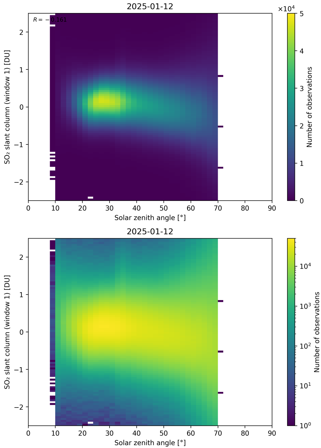
Figure 184: Scatter density plot of “Solar zenith angle” against “SO 2 slant column (window 1)” for 2025-01-12 to 2025-01-13.
