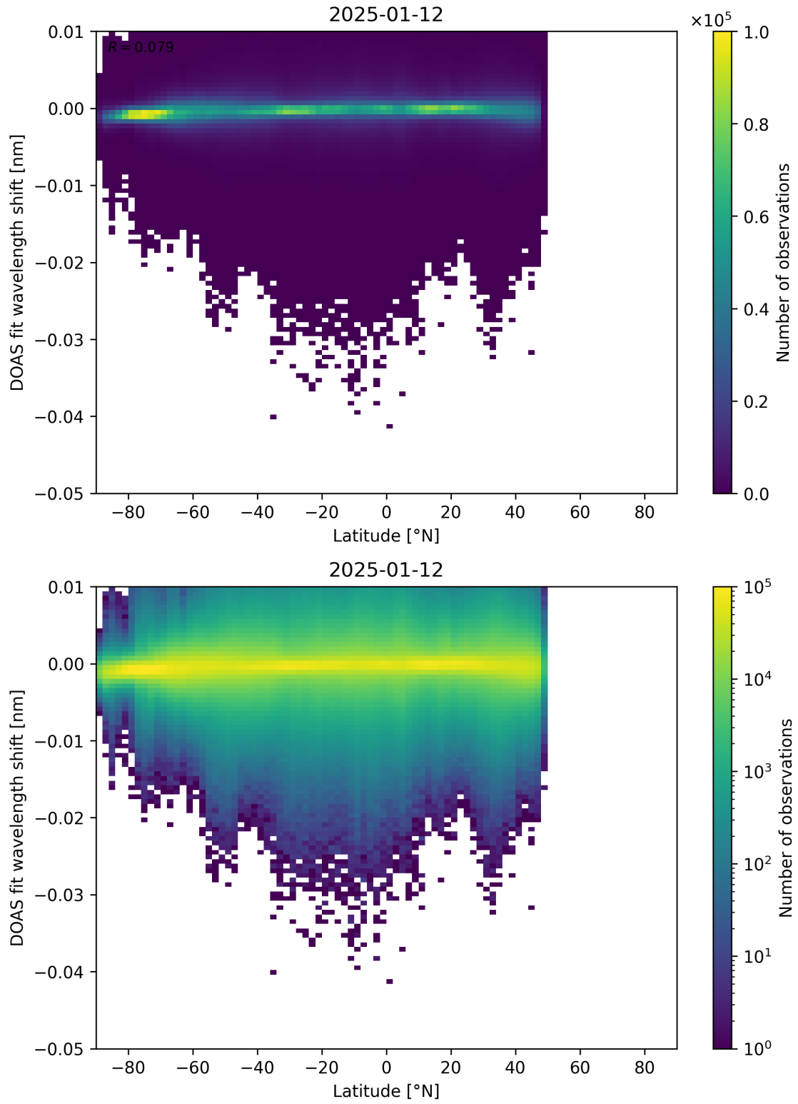
Figure 153: Scatter density plot of “Latitude” against “DOAS fit wavelength shift” for 2025-01-12 to 2025-01-13.
