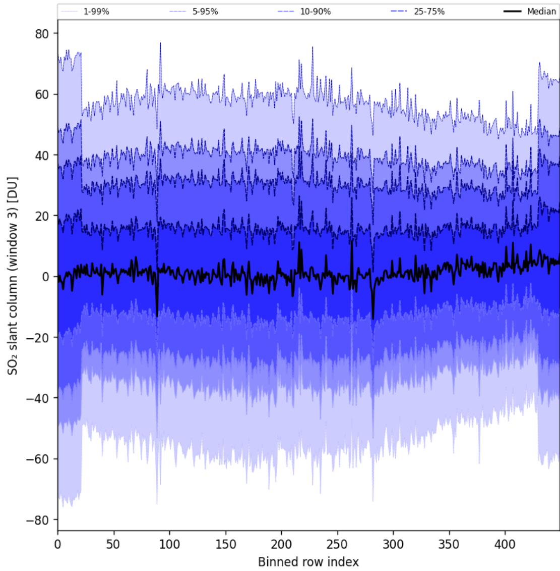
Figure 97: Along track statistics of “SO 2 slant column (window 3)” for 2025-01-12 to 2025-01-13
