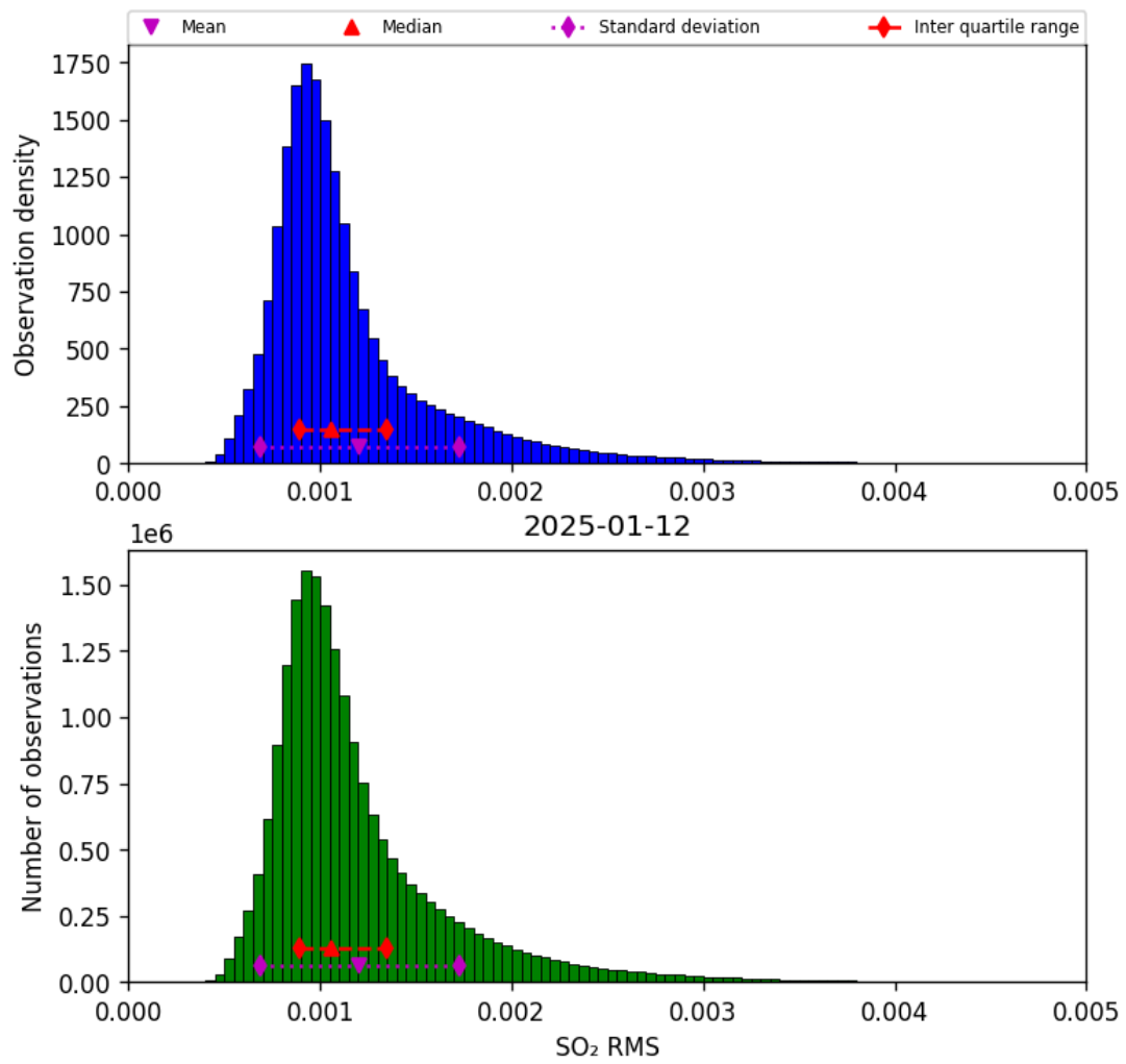
Figure 78: Histogram of “SO 2 RMS” for 2025-01-12 to 2025-01-13
