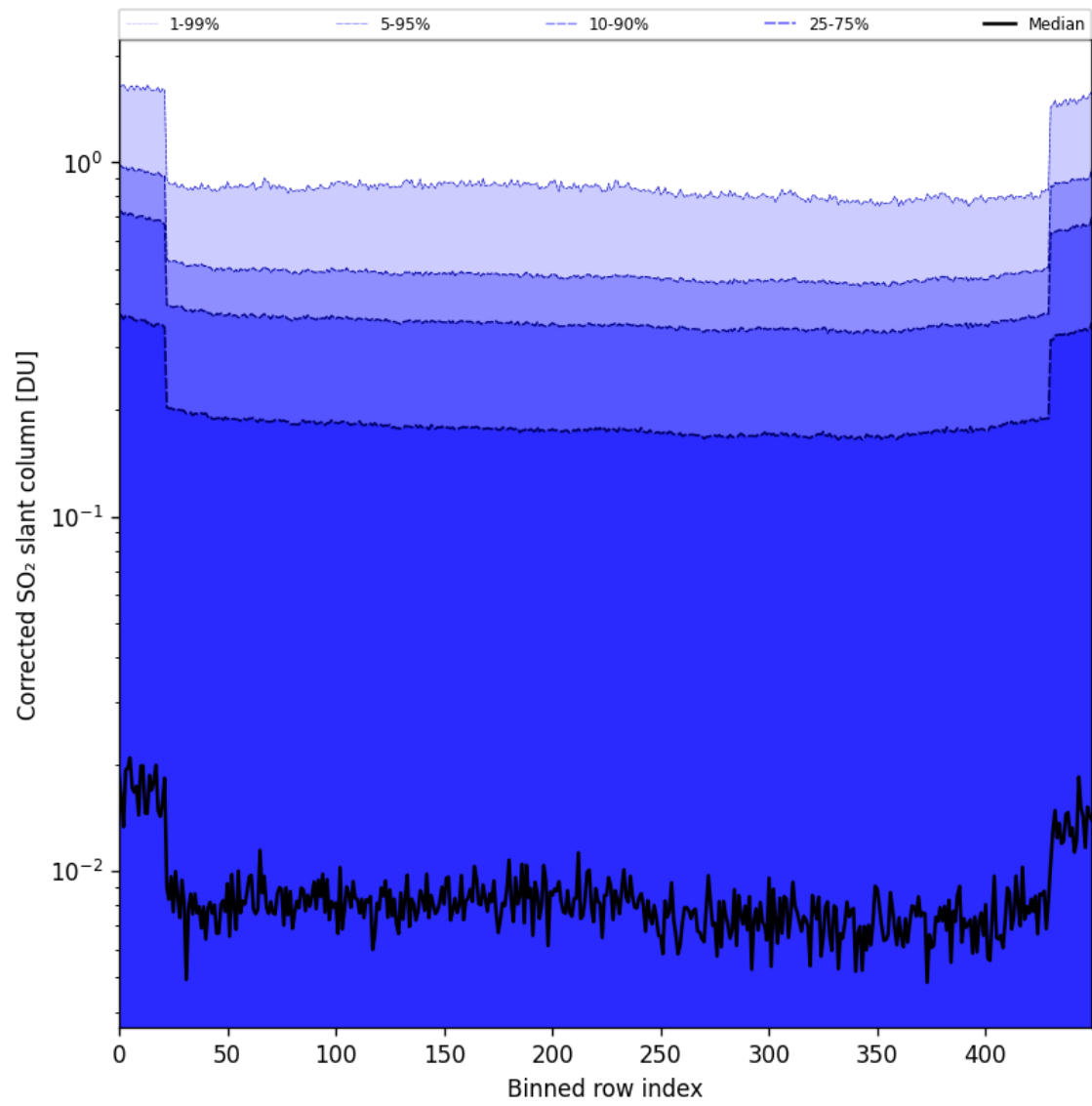
Figure 86: Along track statistics of “Corrected SO 2 slant column” for 2025-01-12 to 2025-01-13
