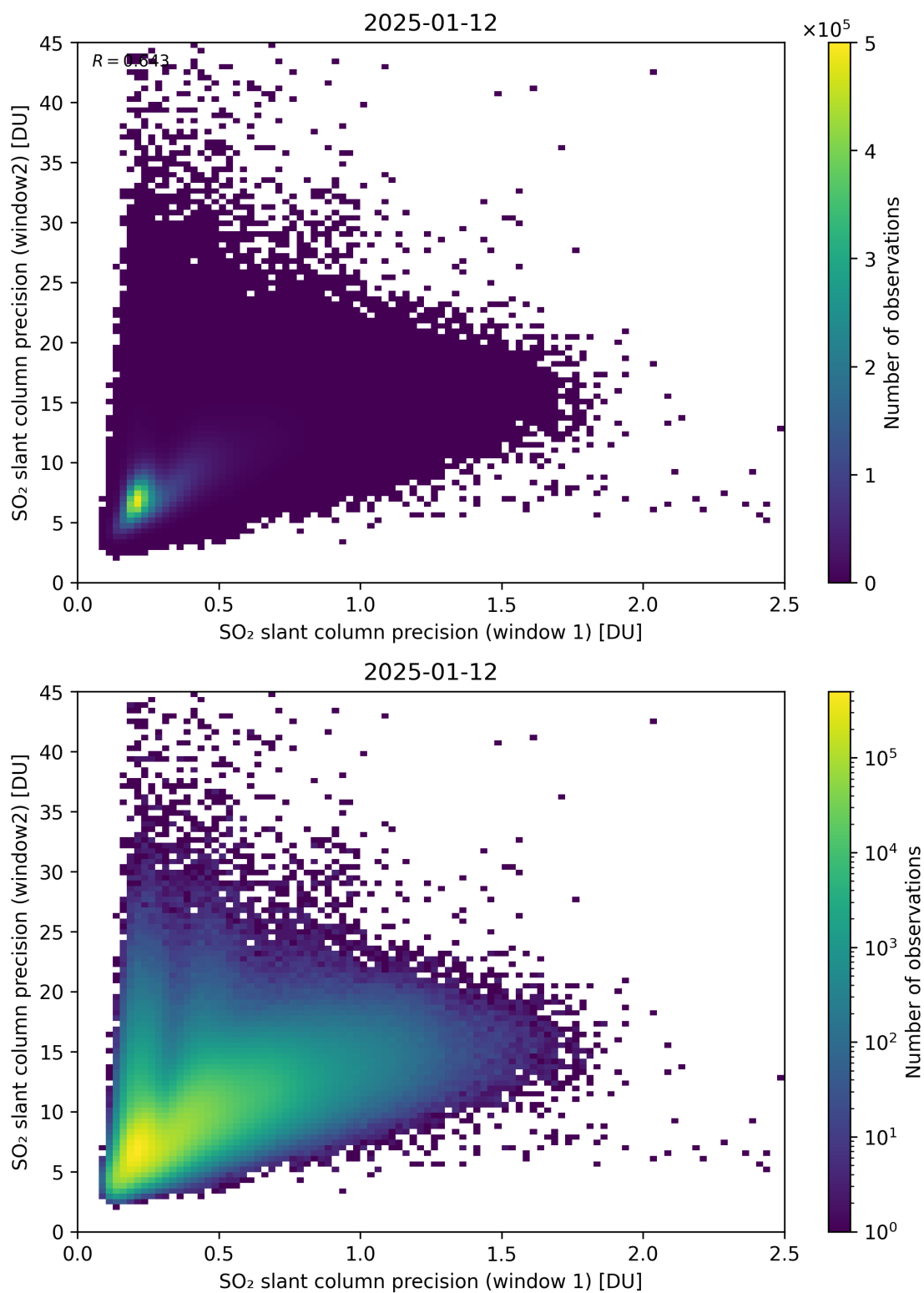
Figure 277: Scatter density plot of “SO 2 slant column precision (window 1)” against “SO 2 slant column precision (window2)” for 2025-01-12 to 2025-01-13.
