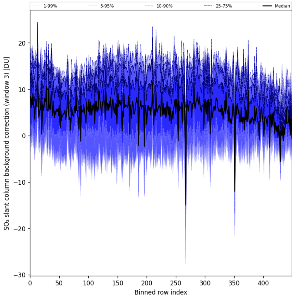
Figure 100: Along track statistics of “SO 2 slant column background correction (window 3)” for 2025-01-12 to 2025-01-13
