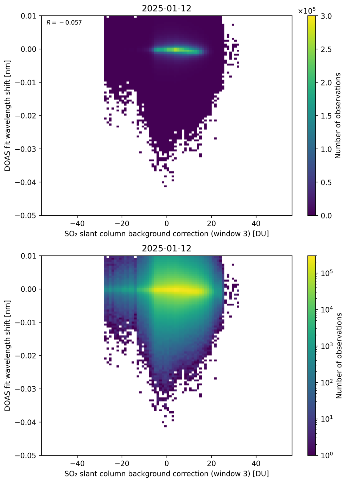
Figure 132: Scatter density plot of “SO 2 slant column background correction (window 3)” against “DOAS fit wavelength shift” for 2025-01-12 to 2025-01-13.
