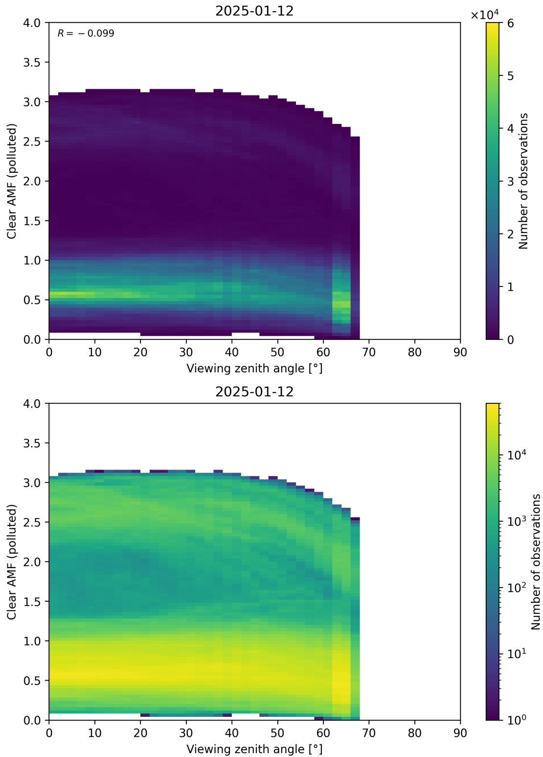
Figure 370: Scatter density plot of “Viewing zenith angle” against “Clear AMF (polluted)” for 2025-01-12 to 2025-01-13.
