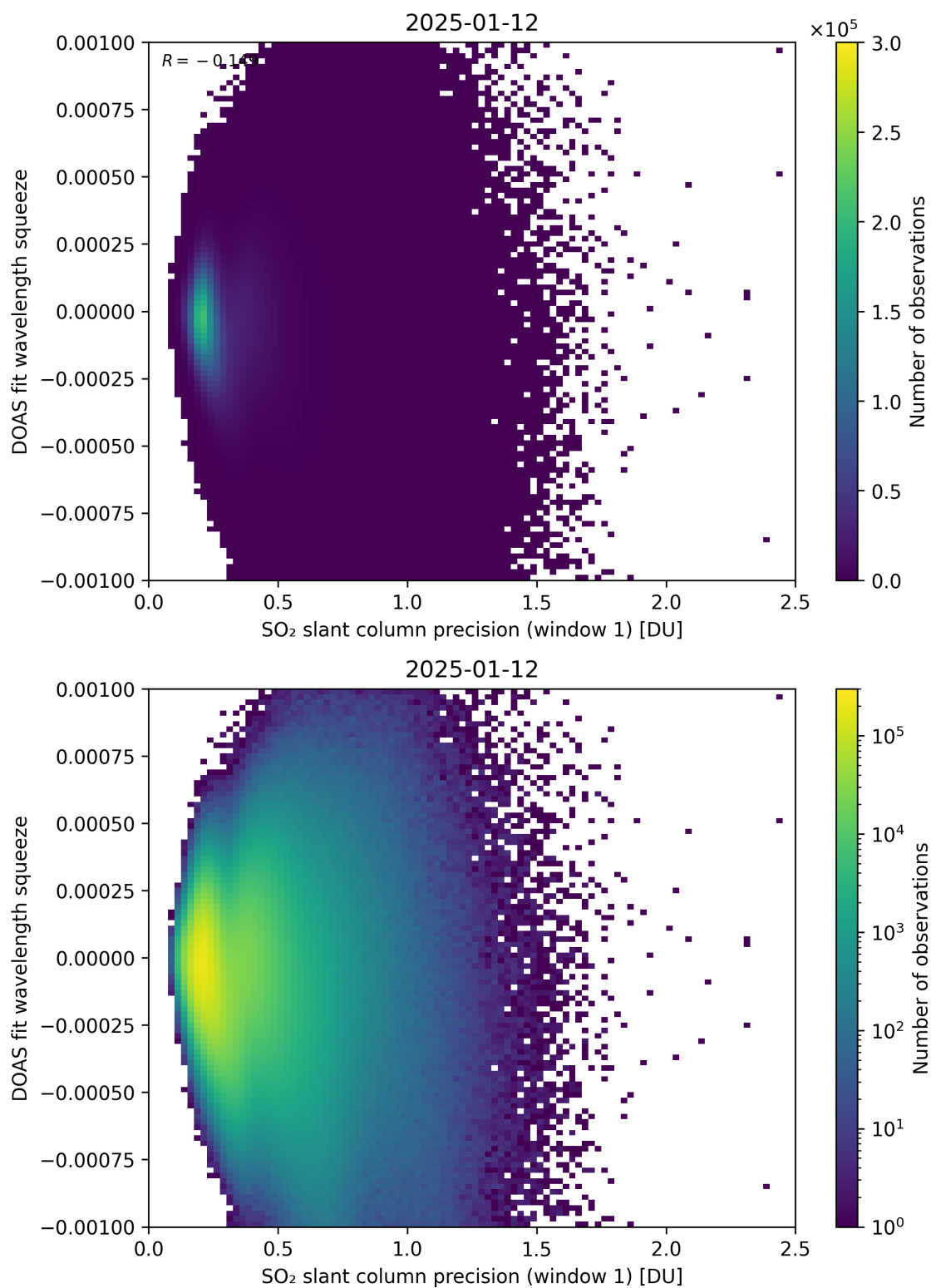
Figure 272: Scatter density plot of “SO 2 slant column precision (window 1)” against “DOAS fit wavelength squeeze” for 2025-01-12 to 2025-01-13.
