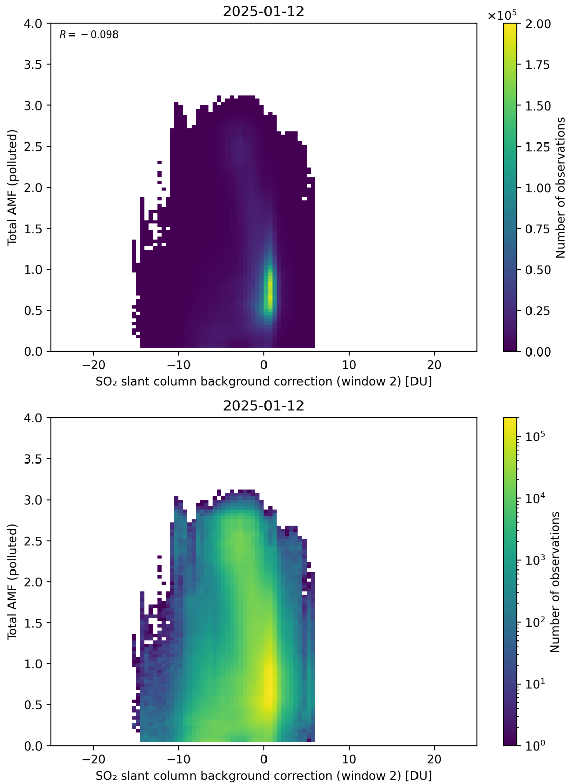
Figure 130: Scatter density plot of “SO 2 slant column background correction (window 2)” against “Total AMF (polluted)” for 2025-01-12 to 2025-01-13.
