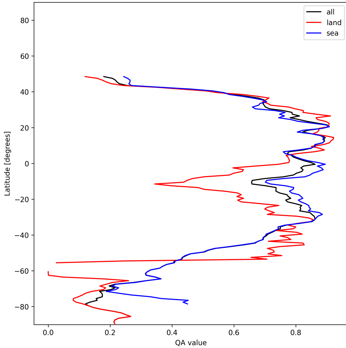
Figure 31: Zonal average of “QA value” for 2025-01-12 to 2025-01-13.
