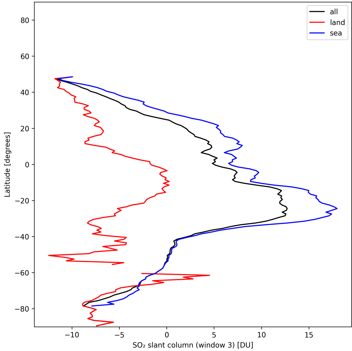
Figure 45: Zonal average of “SO 2 slant column (window 3)” for 2025-01-12 to 2025-01-13.
