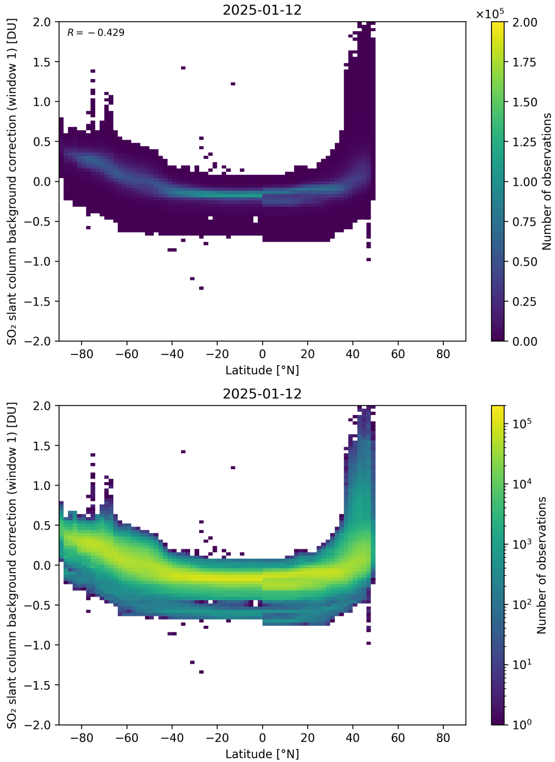
Figure 150: Scatter density plot of “Latitude” against “SO 2 slant column background correction (window 1)” for 2025-01-12 to 2025-01-13.
