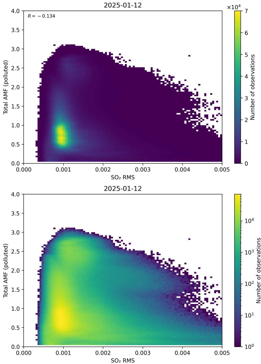
Figure 148: Scatter density plot of “SO 2 RMS” against “Total AMF (polluted)” for 2025-01-12 to 2025-01-13.
