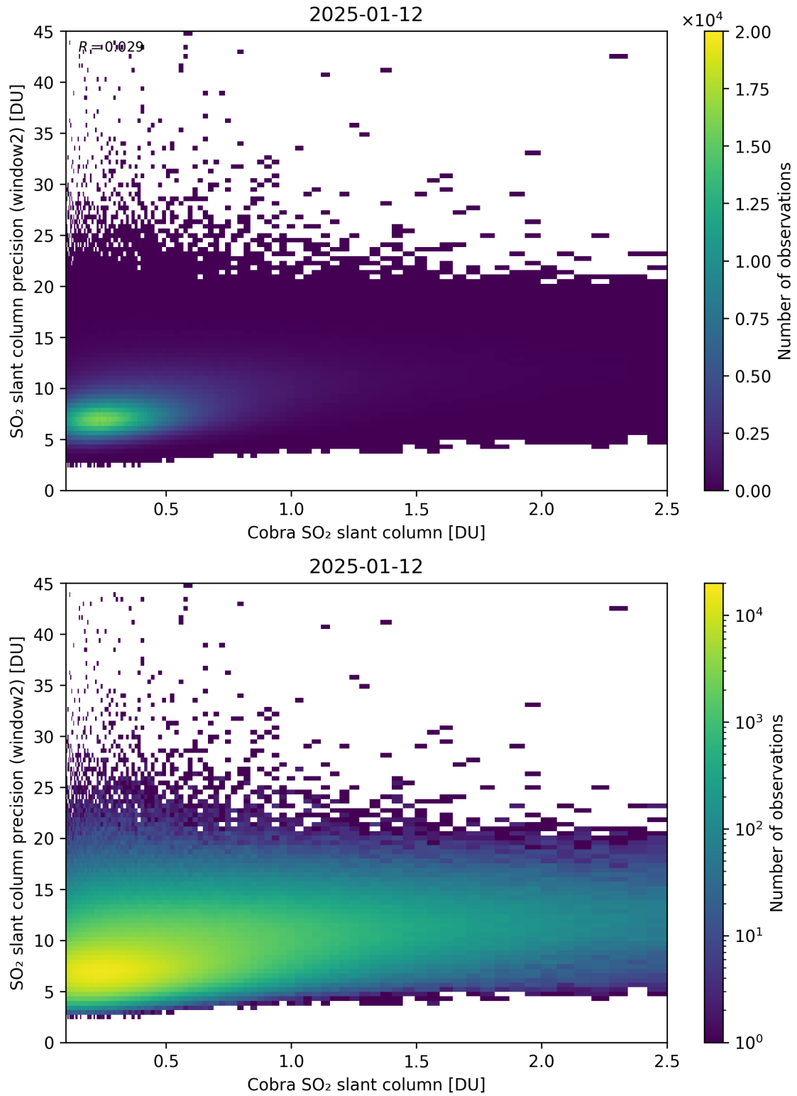
Figure 221: Scatter density plot of “Cobra SO 2 slant column” against “SO 2 slant column precision (window2)” for 2025-01-12 to 2025-01-13.
