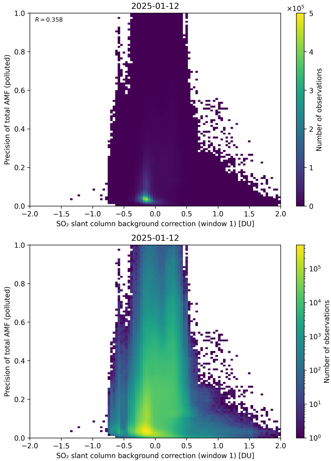
Figure 121: Scatter density plot of “SO 2 slant column background correction (window 1)” against “Precision of total AMF (polluted)” for 2025-01-12 to 2025-01-13.
