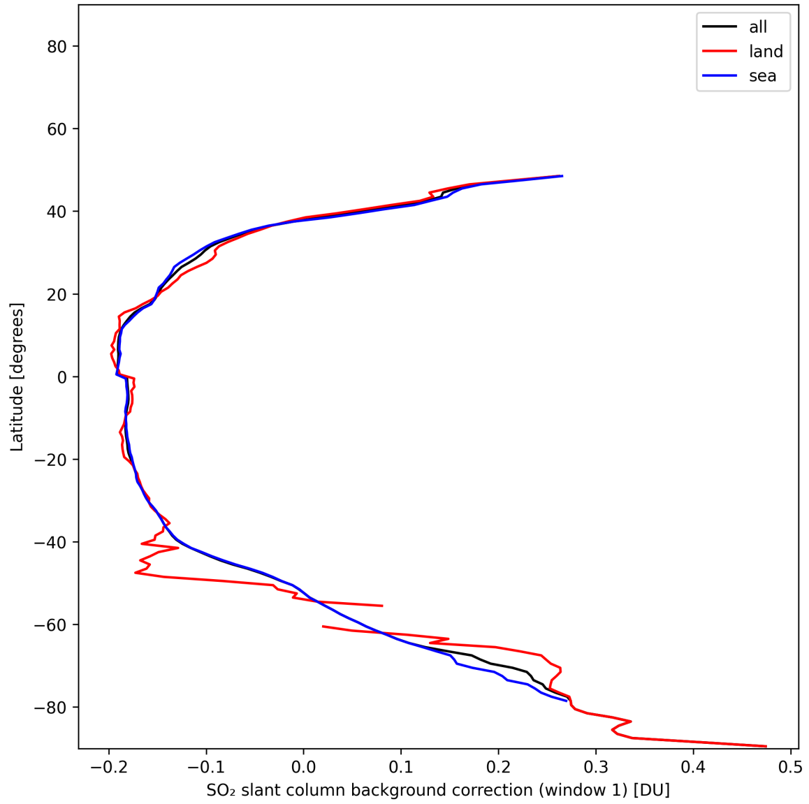
Figure 40: Zonal average of “SO 2 slant column background correction (window 1)” for 2025-01-12 to 2025-01-13.
