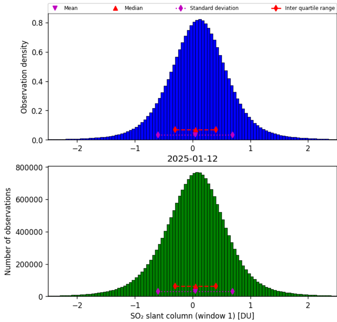
Figure 63: Histogram of “SO 2 slant column (window 1)” for 2025-01-12 to 2025-01-13
