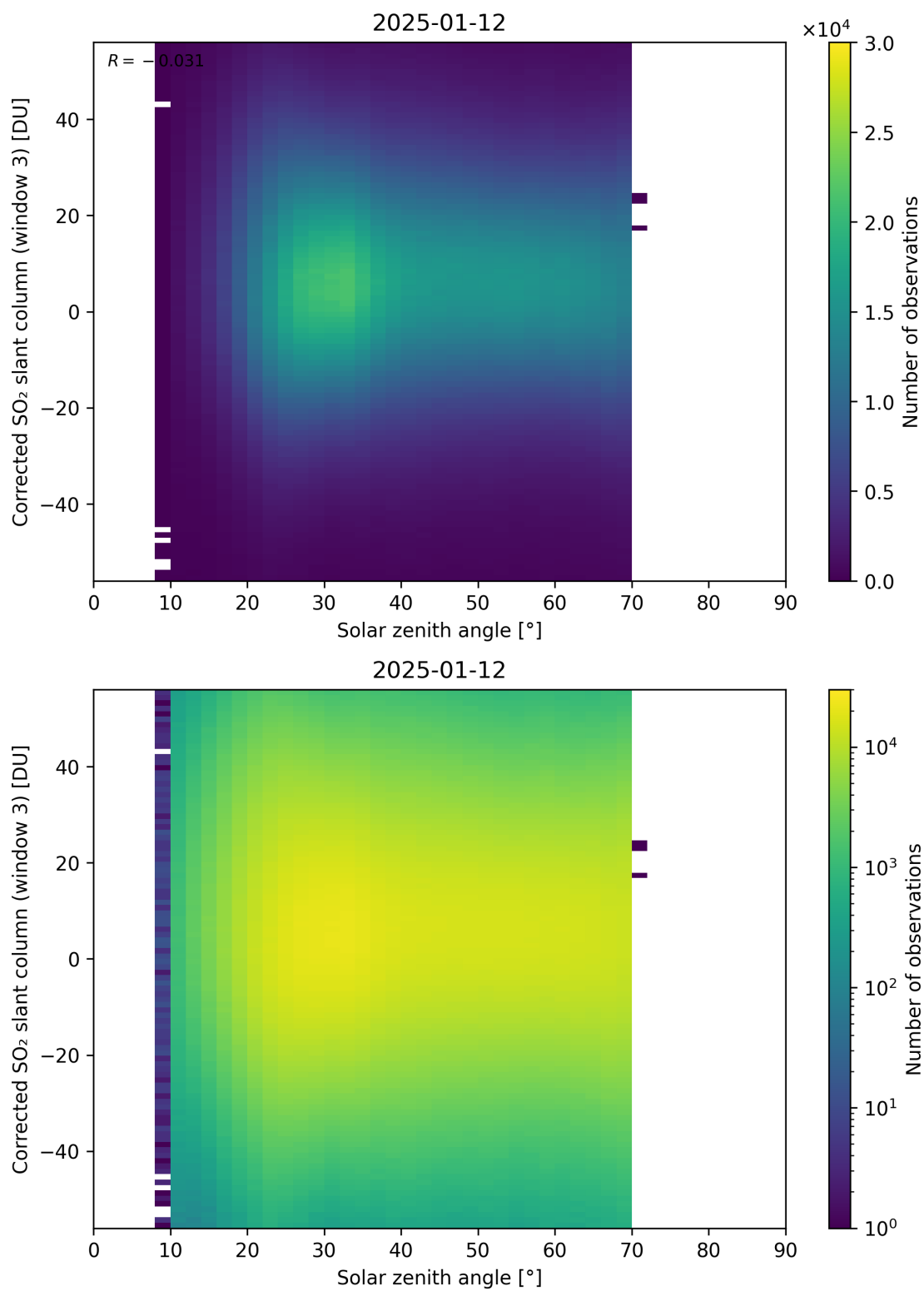
Figure 183: Scatter density plot of “Solar zenith angle” against “Corrected SO 2 slant column (window 3)” for 2025-01-12 to 2025-01-13.
