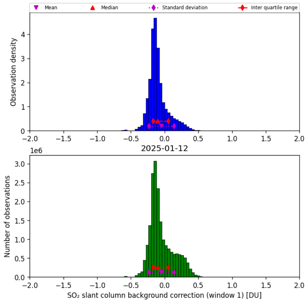
Figure 66: Histogram of “SO 2 slant column background correction (window 1)” for 2025-01-12 to 2025-01-13
