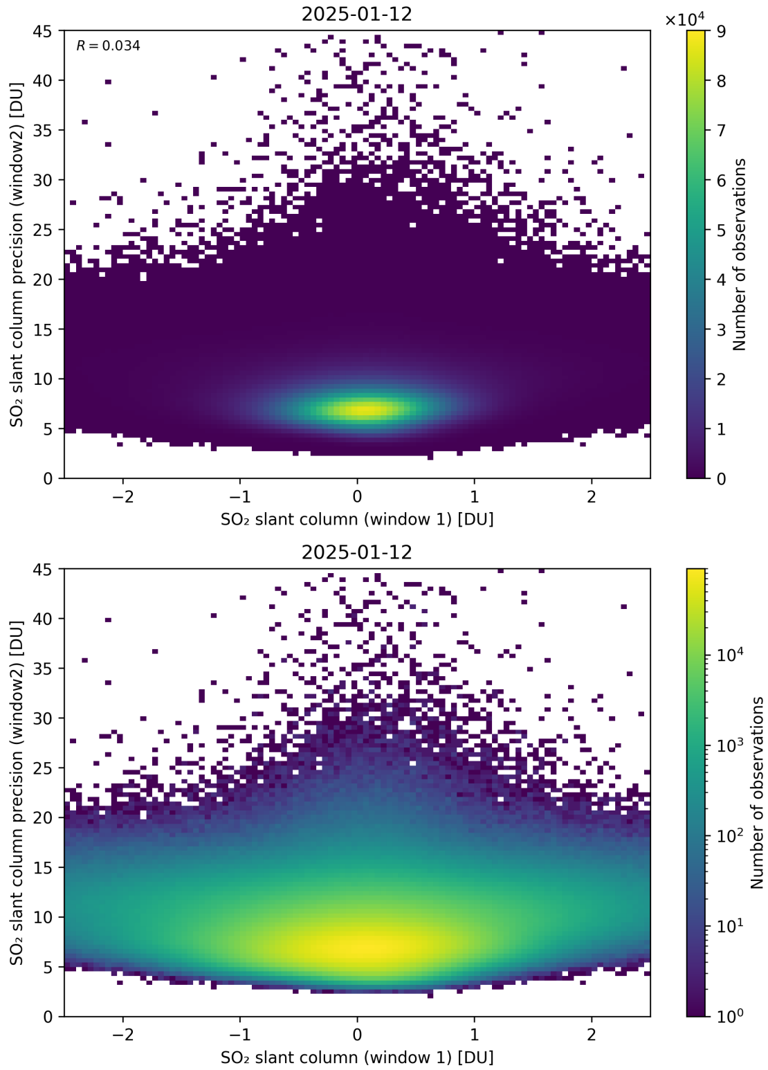
Figure 286: Scatter density plot of “SO 2 slant column (window 1)” against “SO 2 slant column precision (window2)” for 2025-01-12 to 2025-01-13.
