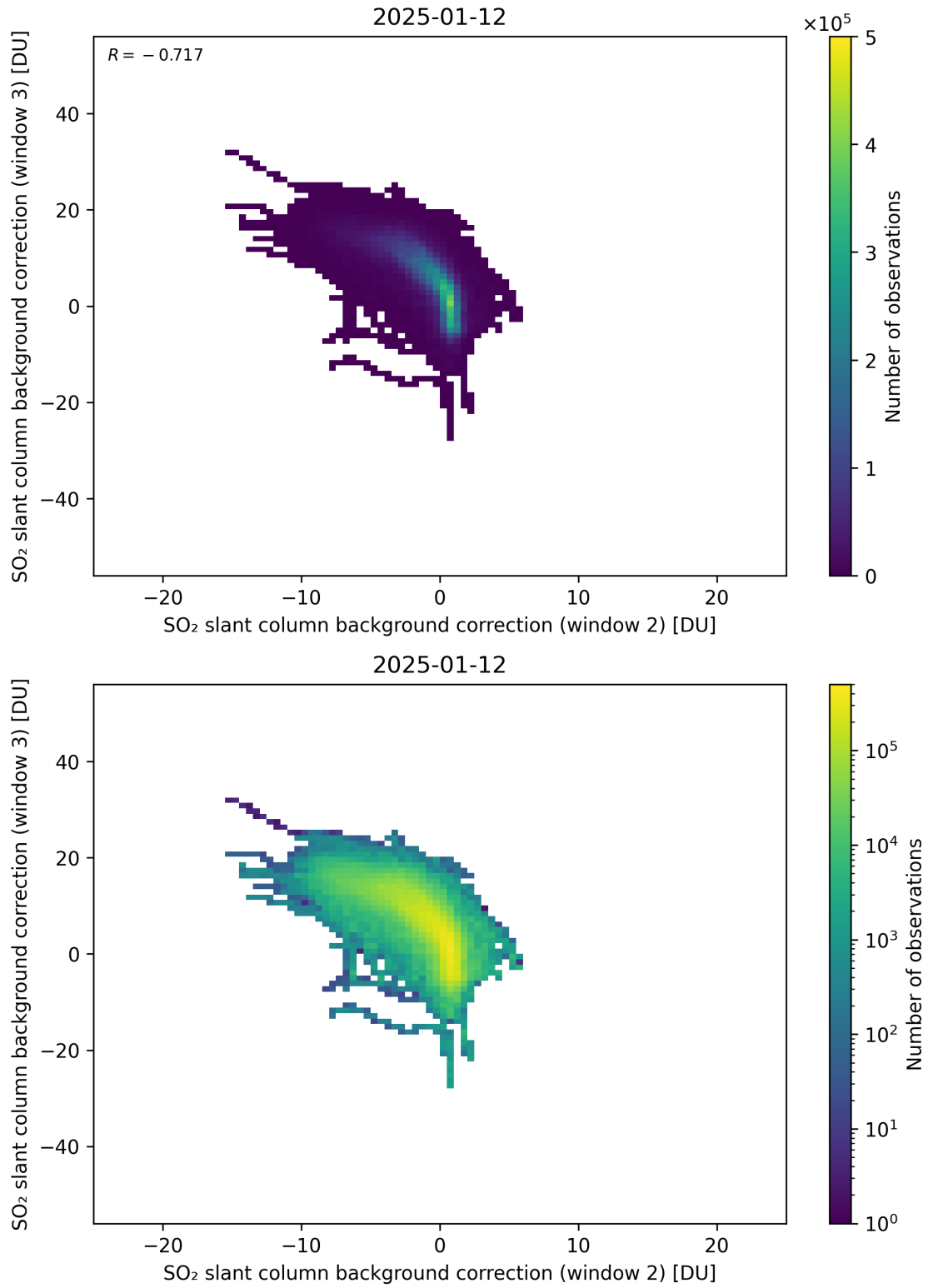
Figure 122: Scatter density plot of “SO 2 slant column background correction (window 2)” against “SO 2 slant column background correction (window 3)” for 2025-01-12 to 2025-01-13.
