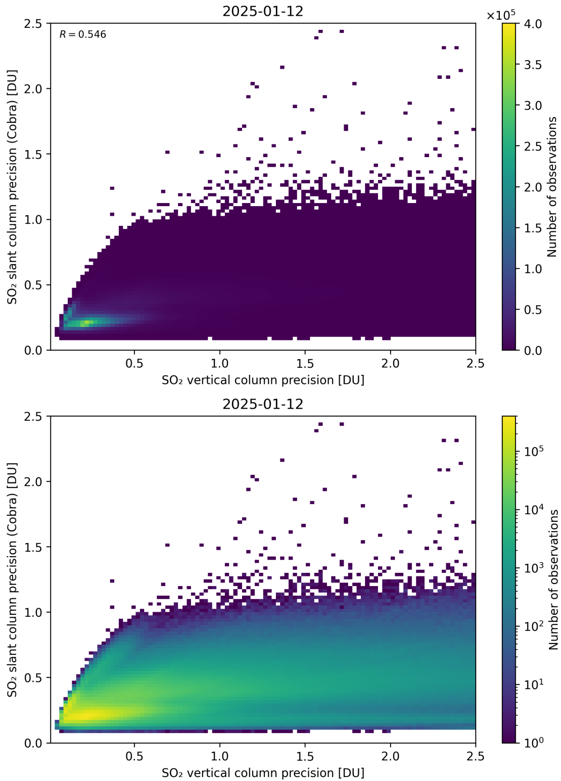
Figure 337: Scatter density plot of “SO 2 vertical column precision” against “SO 2 slant column precision (Cobra)” for 2025-01-12 to 2025-01-13.
