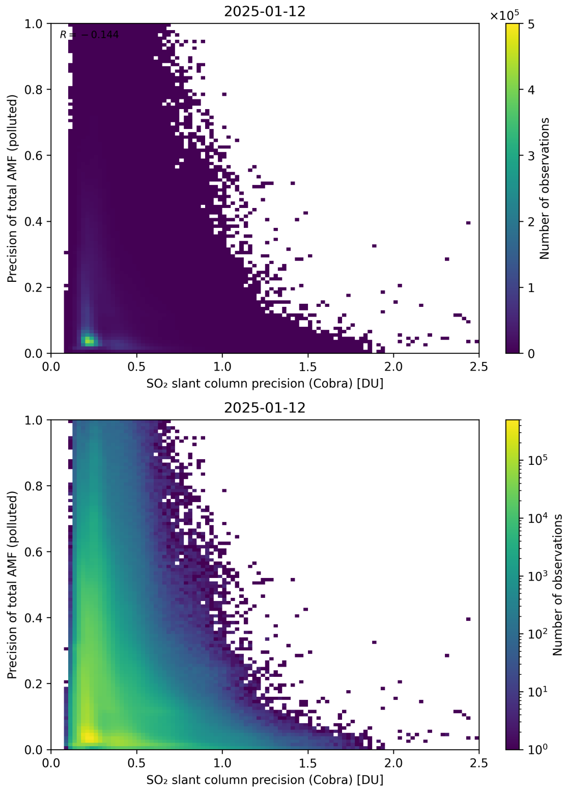
Figure 214: Scatter density plot of “SO 2 slant column precision (Cobra)” against “Precision of total AMF (polluted)” for 2025-01-12 to 2025-01-13.
