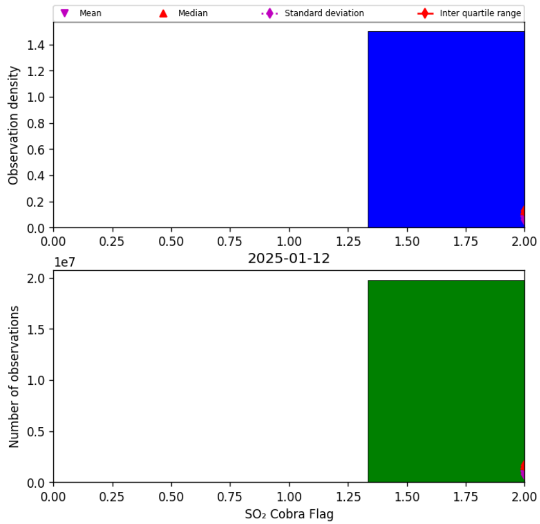
Figure 75: Histogram of “SO 2 Cobra Flag” for 2025-01-12 to 2025-01-13
