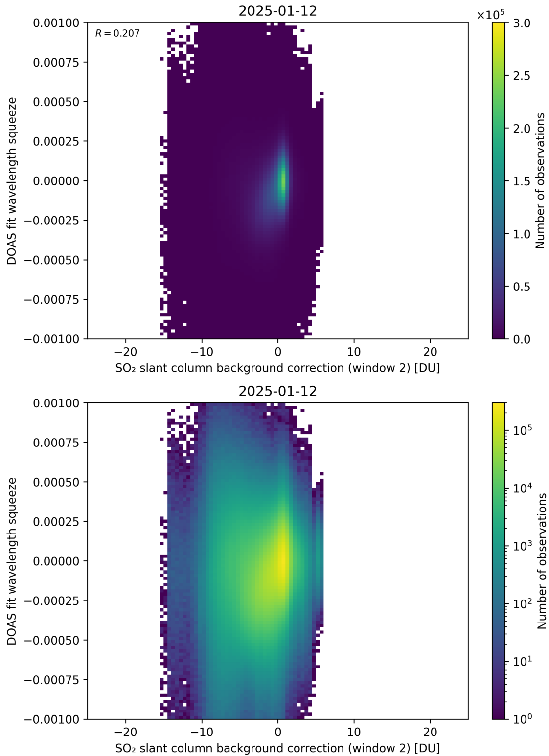
Figure 124: Scatter density plot of “SO 2 slant column background correction (window 2)” against “DOAS fit wavelength squeeze” for 2025-01-12 to 2025-01-13.
