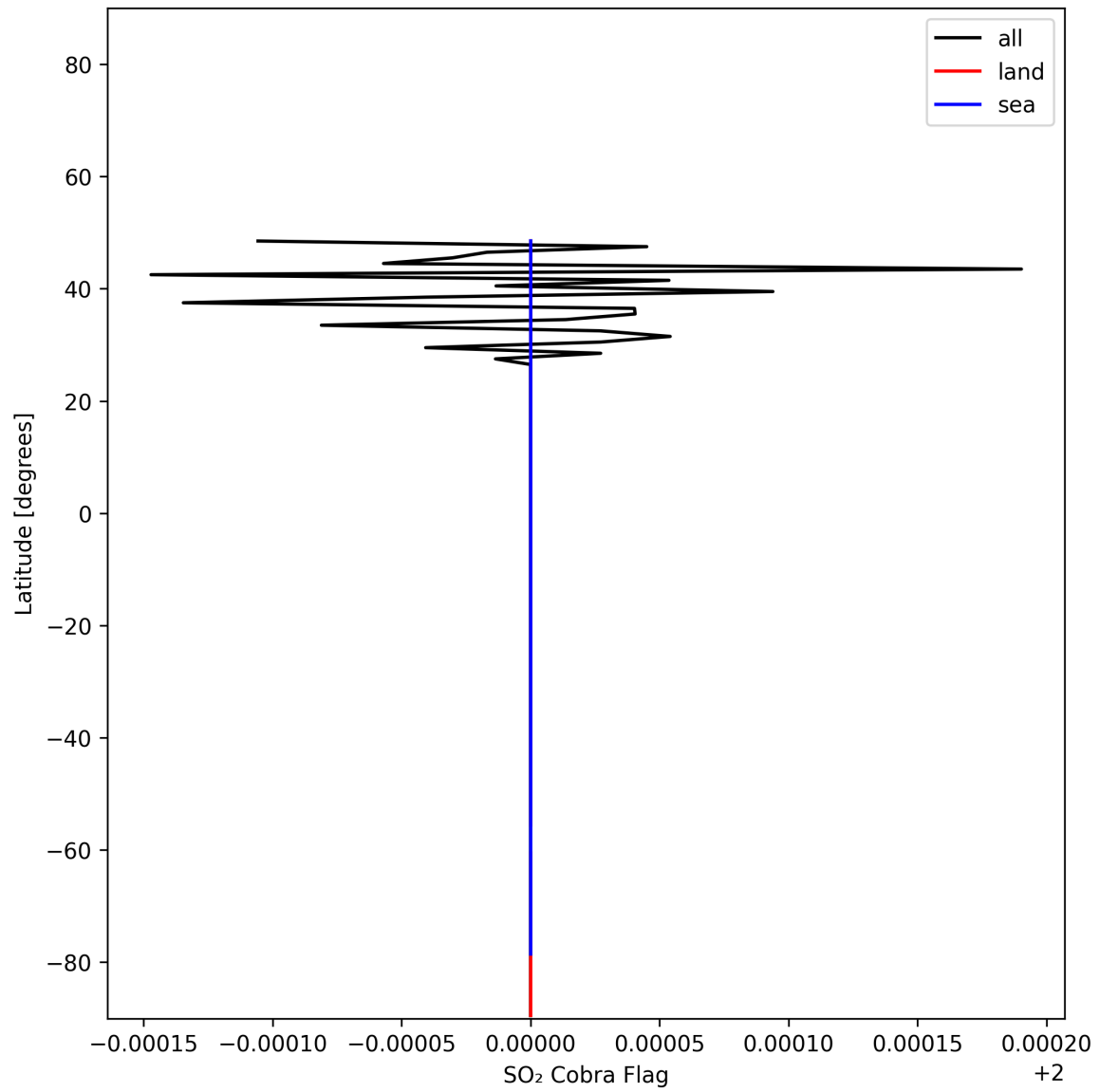
Figure 49: Zonal average of “SO 2 Cobra Flag” for 2025-01-12 to 2025-01-13.
