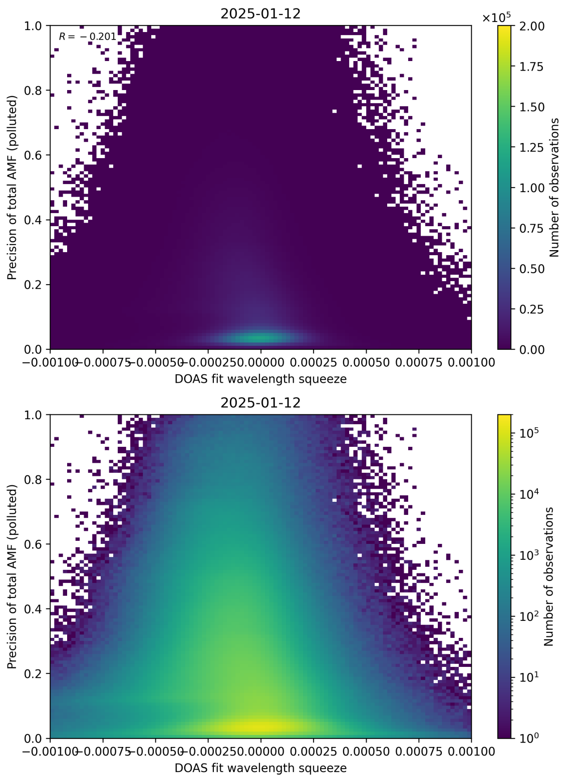
Figure 146: Scatter density plot of “DOAS fit wavelength squeeze” against “Precision of total AMF (polluted)” for 2025-01-12 to 2025-01-13.
