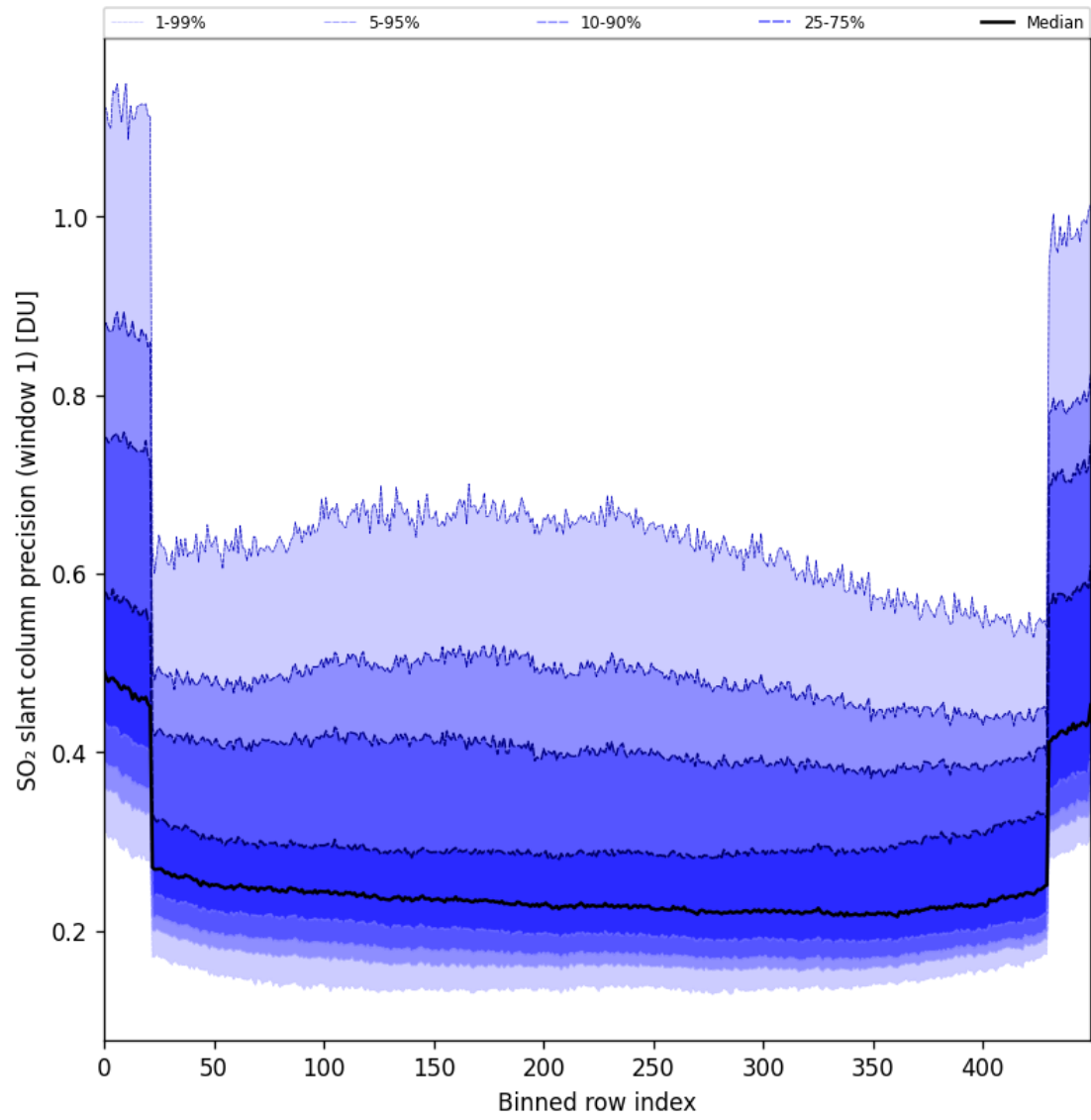
Figure 90: Along track statistics of “SO 2 slant column precision (window 1)” for 2025-01-12 to 2025-01-13
