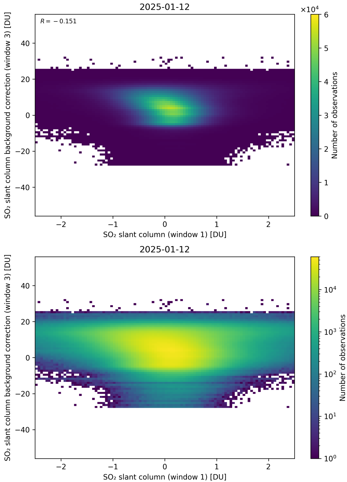
Figure 264: Scatter density plot of “SO 2 slant column (window 1)” against “SO 2 slant column background correction (window 3)” for 2025-01-12 to 2025-01-13.
