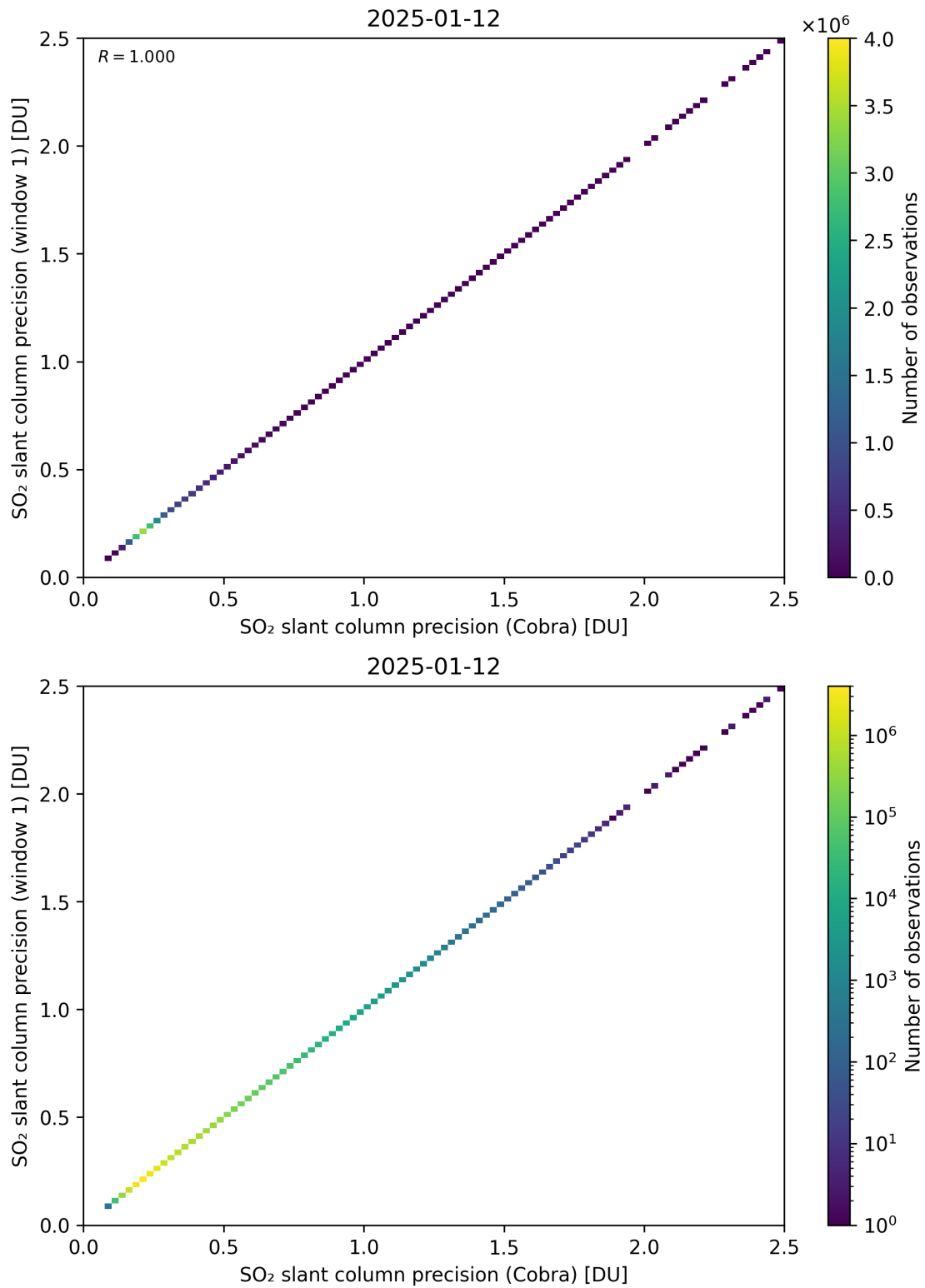
Figure 209: Scatter density plot of “SO 2 slant column precision (Cobra)” against “SO 2 slant column precision (window 1)” for 2025-01-12 to 2025-01-13.
