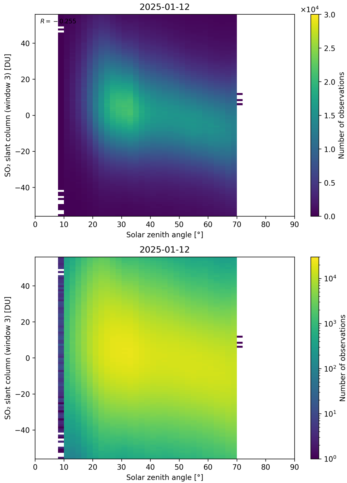
Figure 187: Scatter density plot of “Solar zenith angle” against “SO 2 slant column (window 3)” for 2025-01-12 to 2025-01-13.
