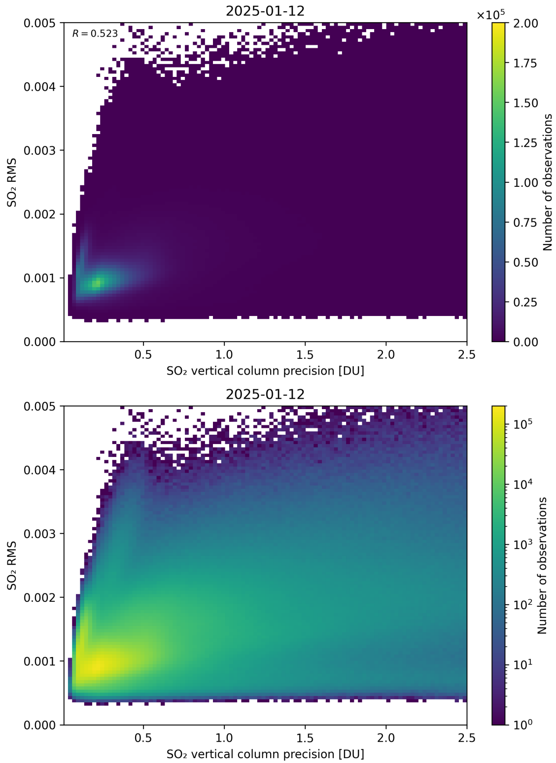
Figure 334: Scatter density plot of “SO 2 vertical column precision” against “SO 2 RMS” for 2025-01-12 to 2025-01-13.
