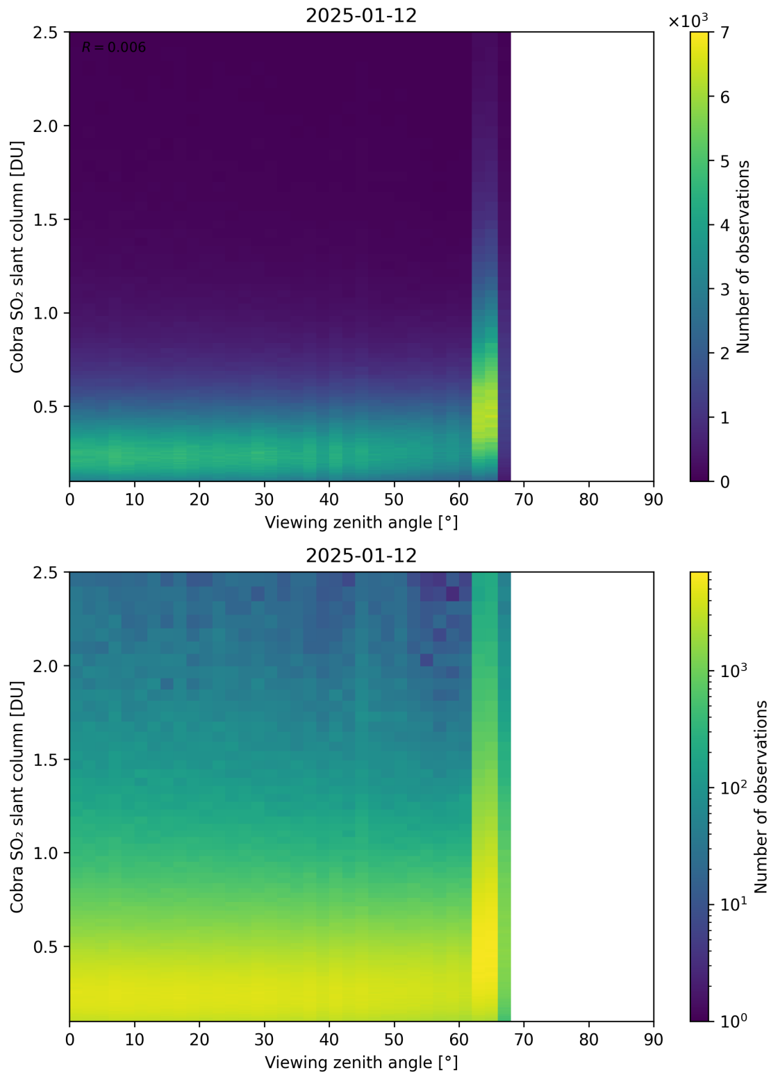
Figure 371: Scatter density plot of “Viewing zenith angle” against “Cobra SO 2 slant column” for 2025-01-12 to 2025-01-13.
