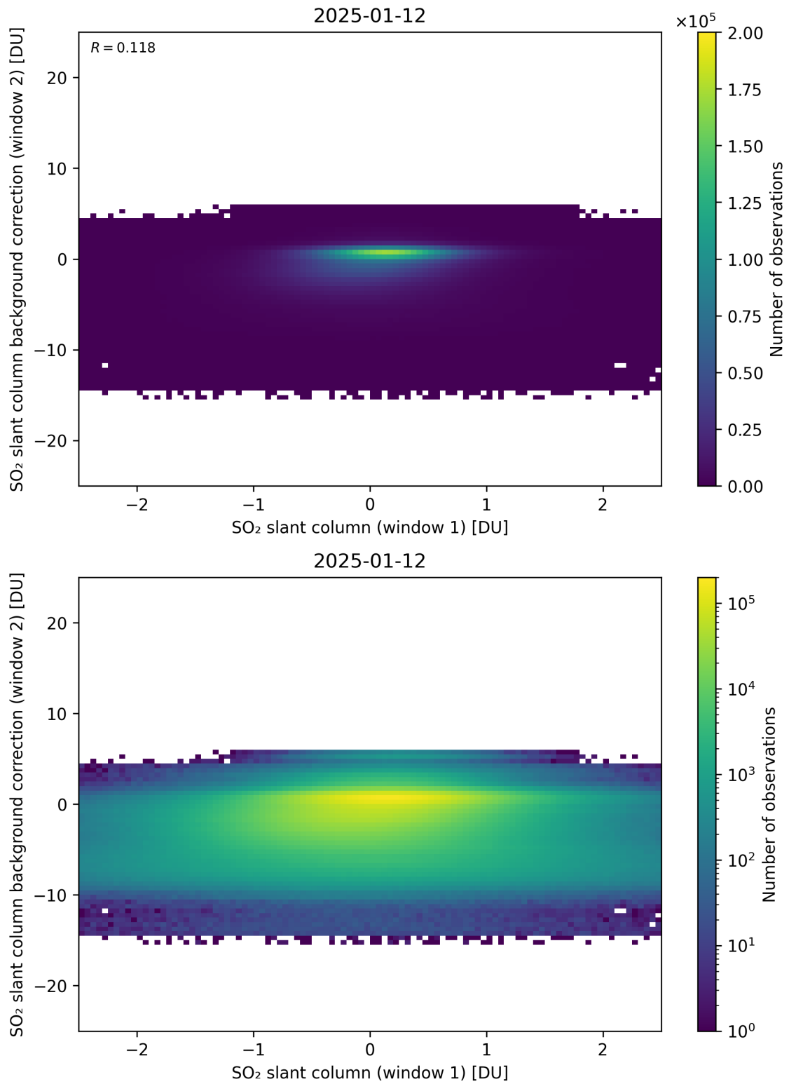
Figure 263: Scatter density plot of “SO 2 slant column (window 1)” against “SO 2 slant column background correction (window 2)” for 2025-01-12 to 2025-01-13.
