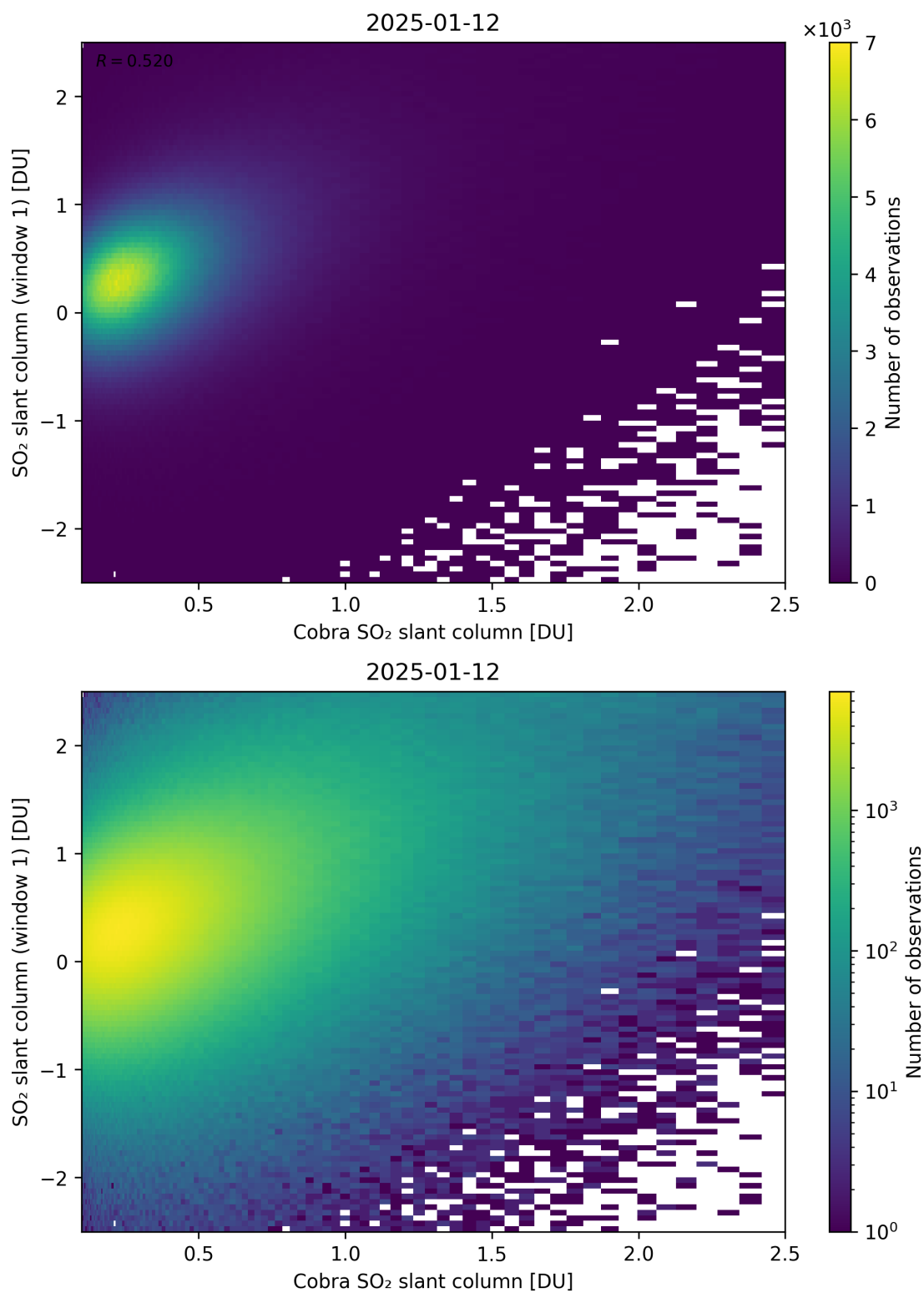
Figure 219: Scatter density plot of “Cobra SO 2 slant column” against “SO 2 slant column (window 1)” for 2025-01-12 to 2025-01-13.
