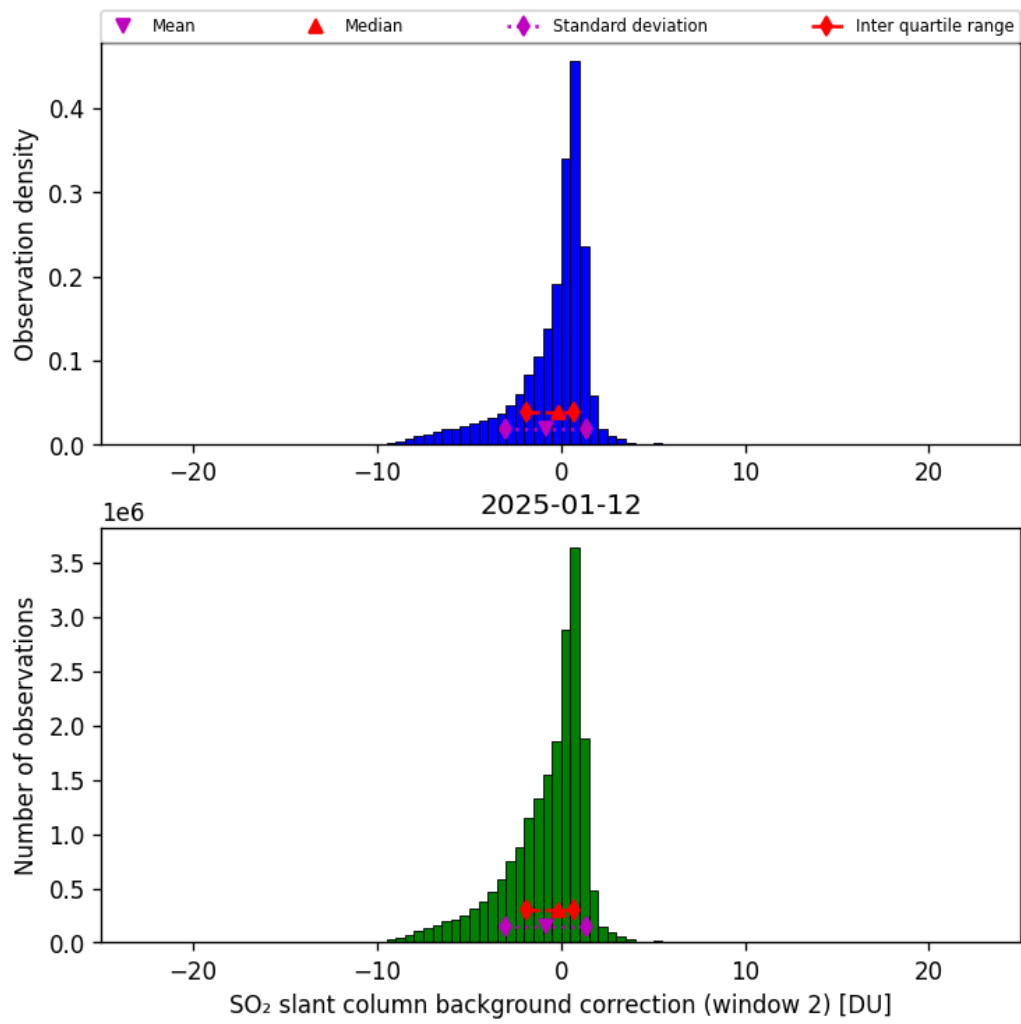
Figure 70: Histogram of “SO 2 slant column background correction (window 2)” for 2025-01-12 to 2025-01-13
