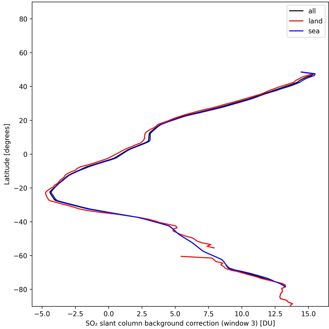
Figure 48: Zonal average of "SO 2 slant column background correction (window 3)" for 2025-01-12 to 2025-01-13.
