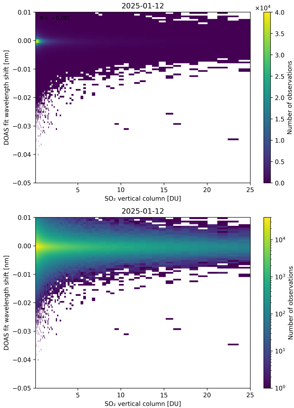
Figure 326: Scatter density plot of “SO 2 vertical column” against “DOAS fit wavelength shift” for 2025-01-12 to 2025-01-13.
