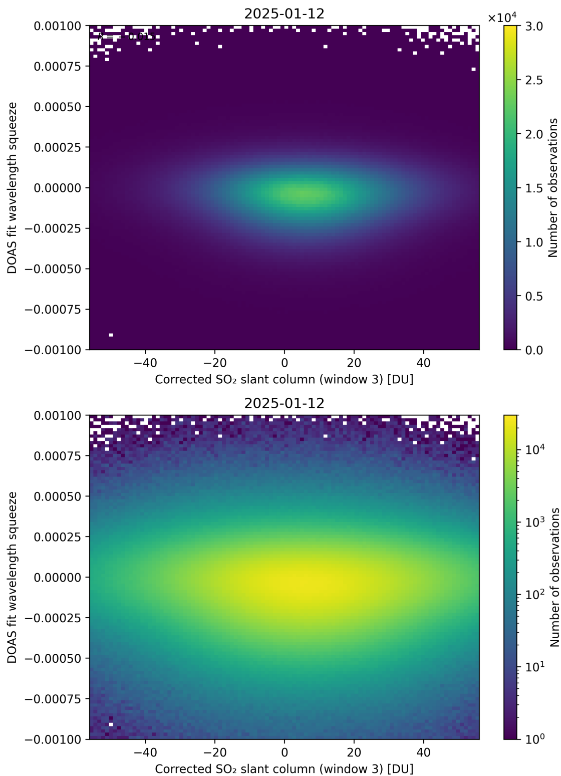
Figure 257: Scatter density plot of “Corrected SO 2 slant column (window 3)” against “DOAS fit wavelength squeeze” for 2025-01-12 to 2025-01-13.
