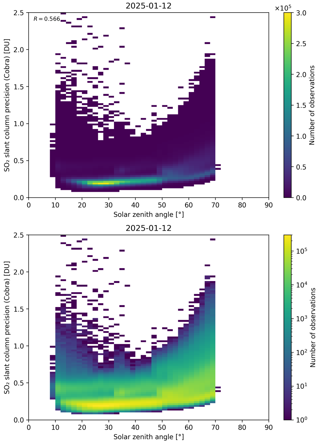
Figure 180: Scatter density plot of “Solar zenith angle” against “SO 2 slant column precision (Cobra)” for 2025-01-12 to 2025-01-13.
