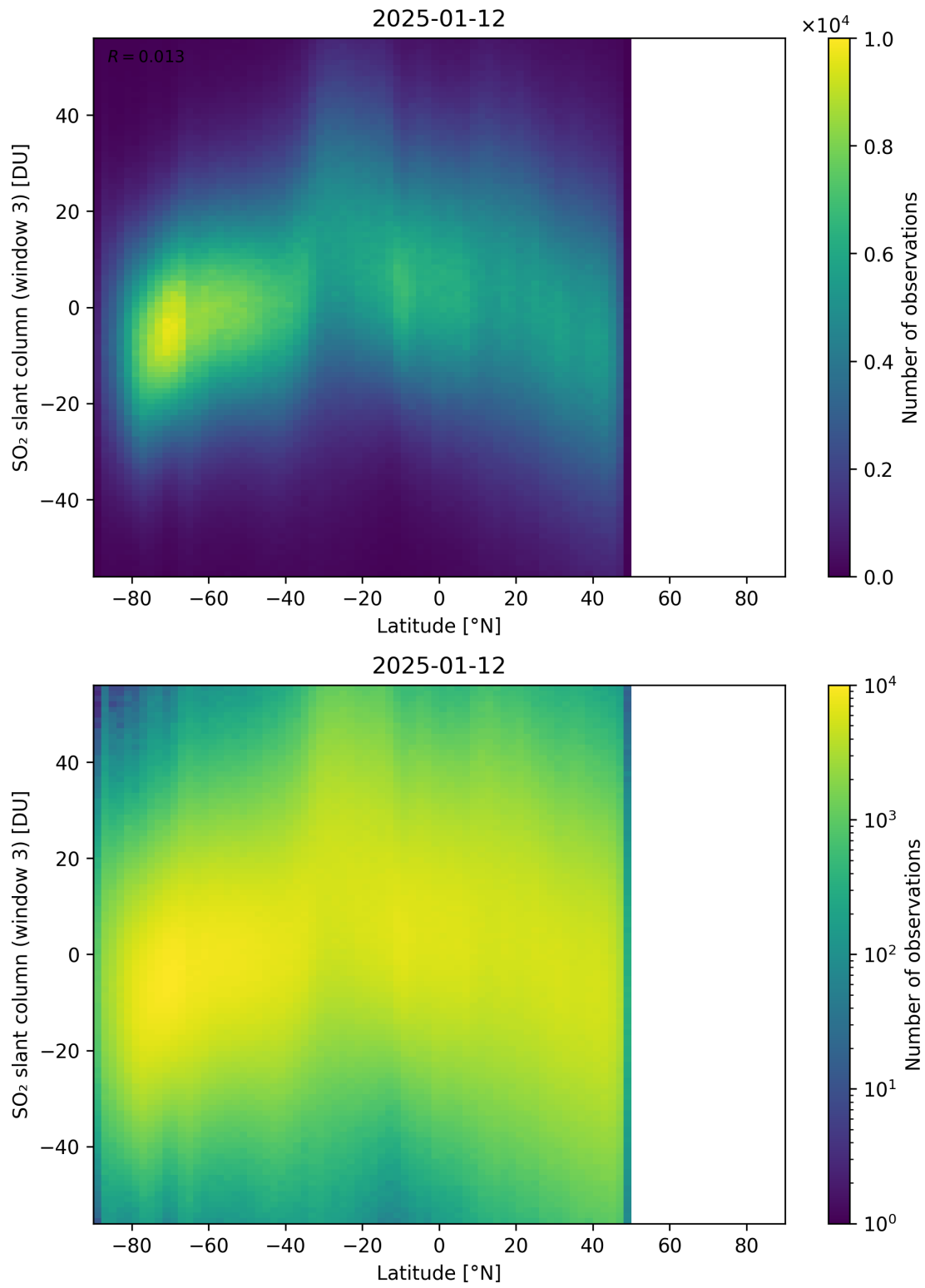
Figure 165: Scatter density plot of “Latitude” against “SO 2 slant column (window 3)” for 2025-01-12 to 2025-01-13.
