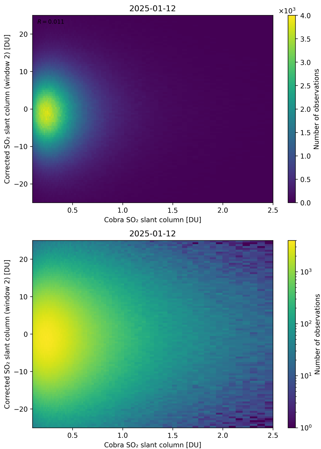
Figure 217: Scatter density plot of “Cobra SO 2 slant column” against “Corrected SO 2 slant column (window 2)” for 2025-01-12 to 2025-01-13.
