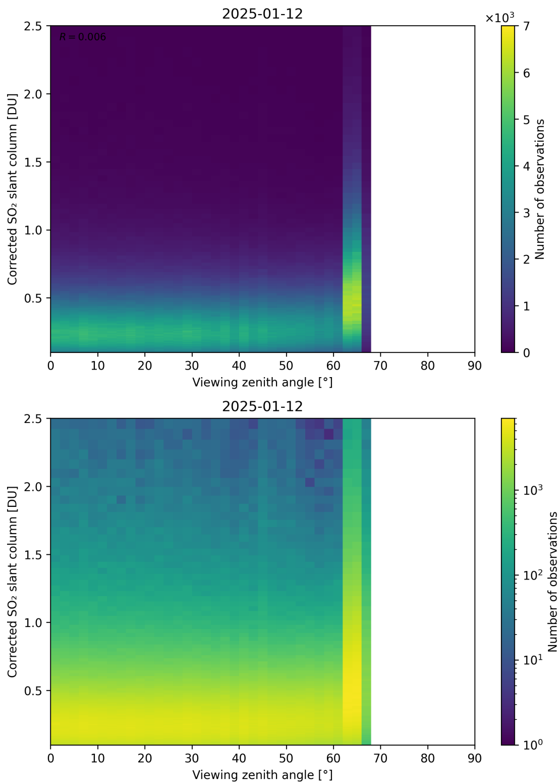
Figure 373: Scatter density plot of “Viewing zenith angle” against “Corrected SO 2 slant column” for 2025-01-12 to 2025-01-13.
