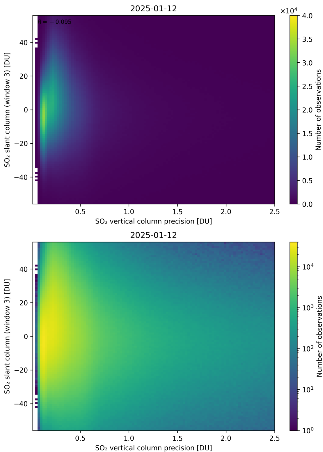
Figure 344: Scatter density plot of “SO 2 vertical column precision” against “SO 2 slant column (window 3)” for 2025-01-12 to 2025-01-13.
