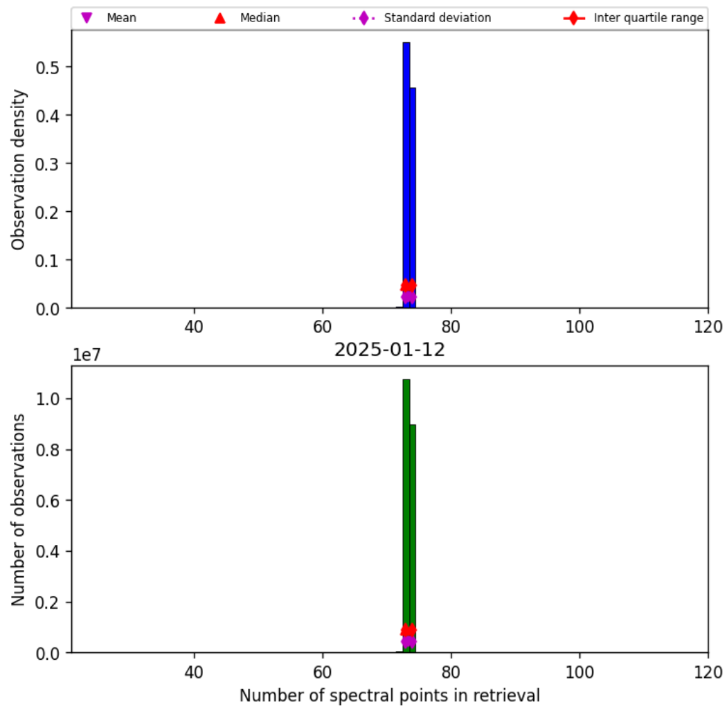
Figure 82: Histogram of “Number of spectral points in retrieval” for 2025-01-12 to 2025-01-13
