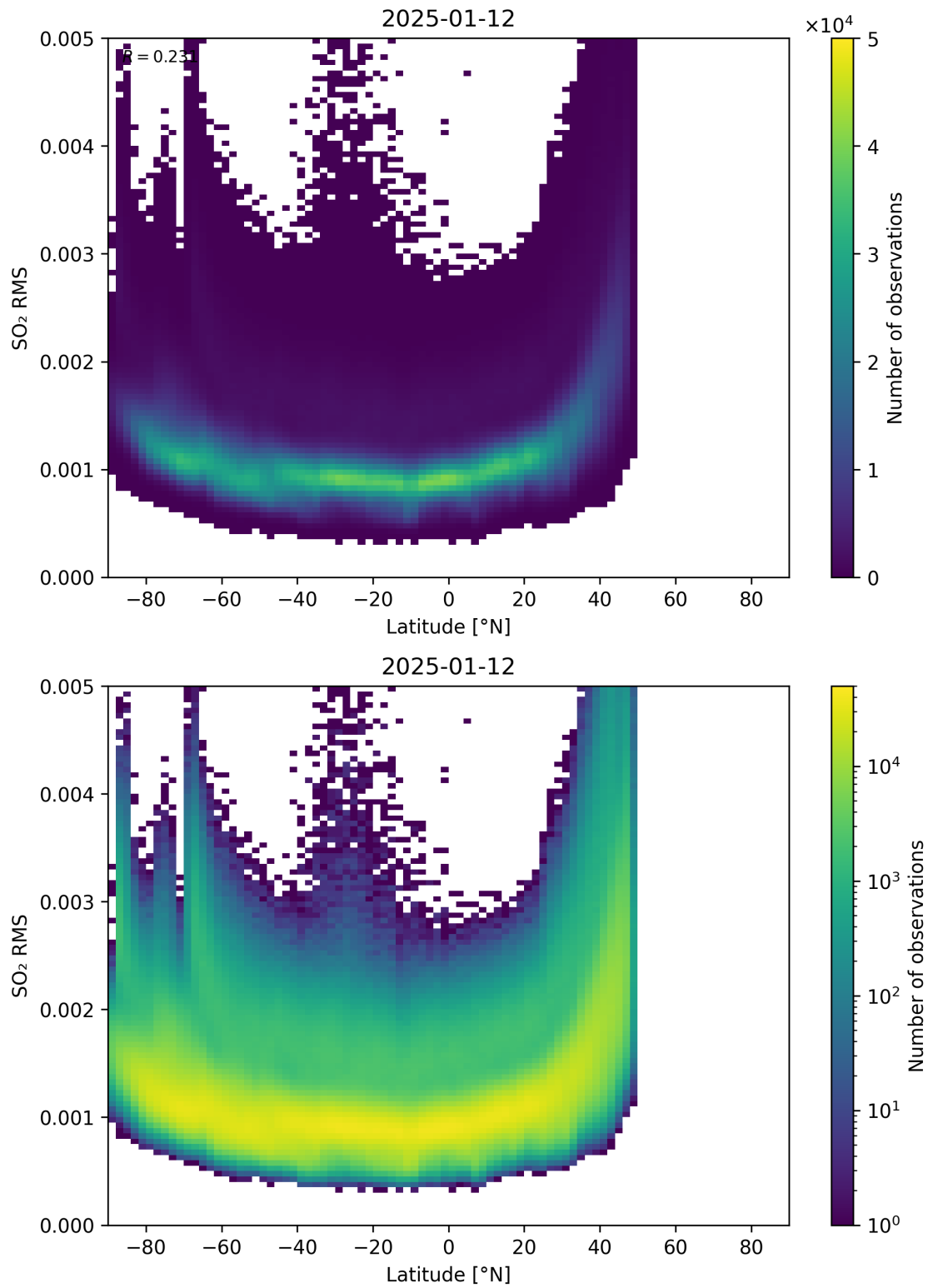
Figure 155: Scatter density plot of “Latitude” against “SO 2 RMS” for 2025-01-12 to 2025-01-13.
