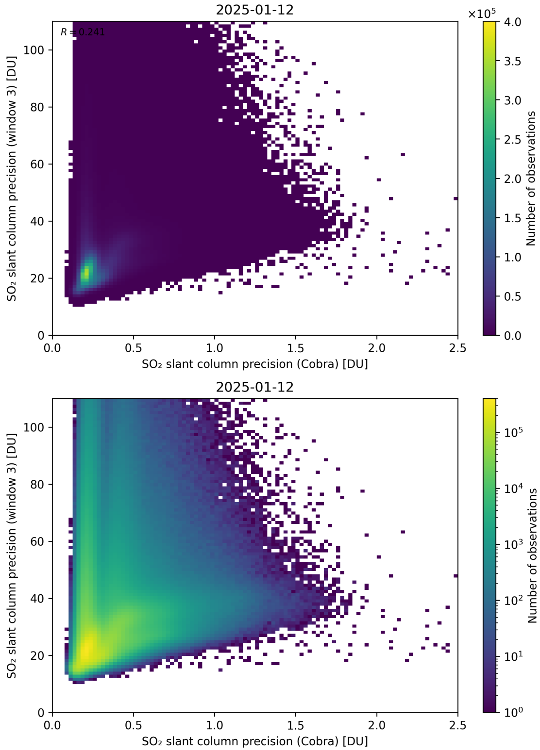
Figure 212: Scatter density plot of “SO 2 slant column precision (Cobra)” against “SO 2 slant column precision (window 3)” for 2025-01-12 to 2025-01-13.
