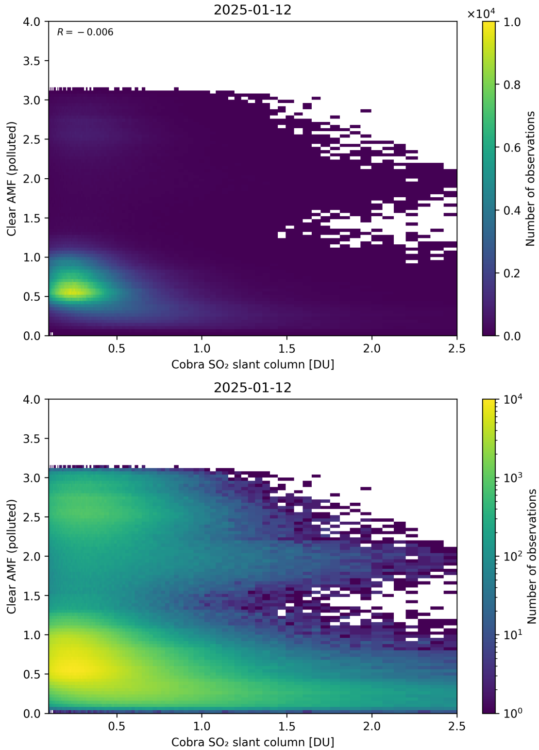
Figure 215: Scatter density plot of “Cobra SO 2 slant column” against “Clear AMF (polluted)” for 2025-01-12 to 2025-01-13.
