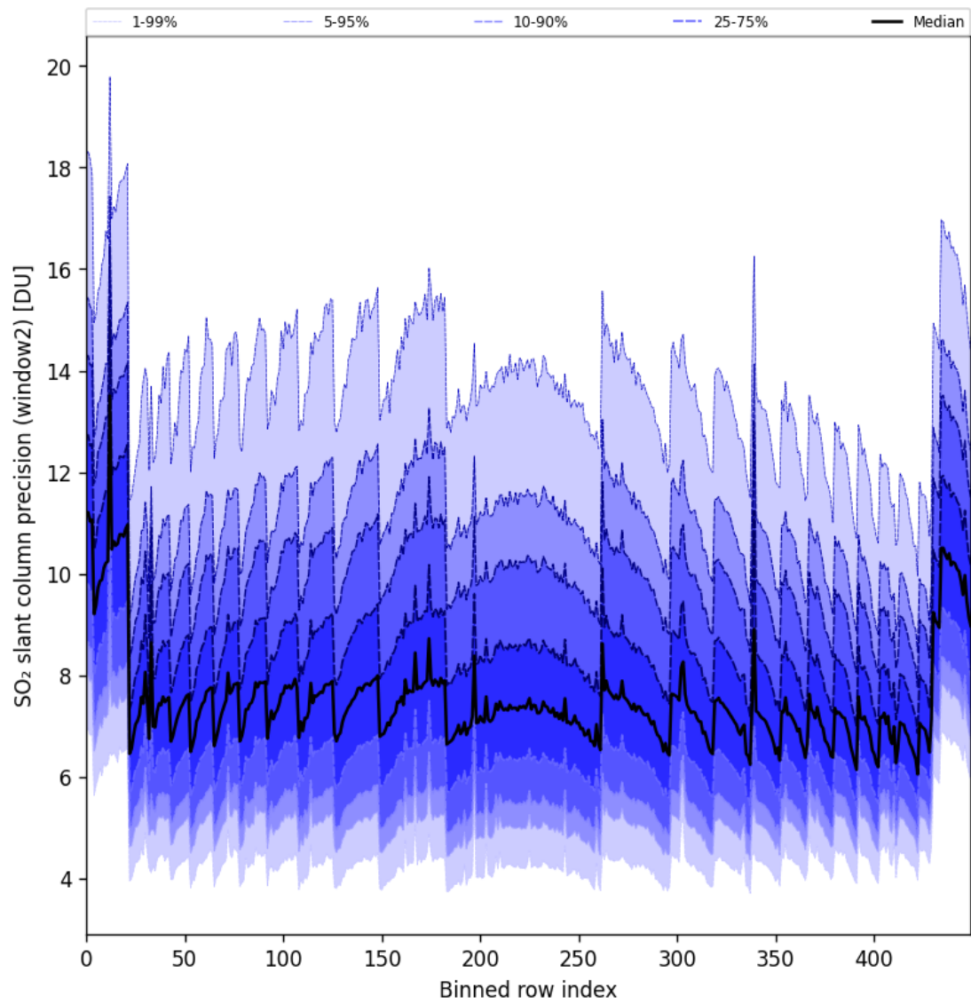
Figure 94: Along track statistics of “SO 2 slant column precision (window2)” for 2025-01-12 to 2025-01-13
