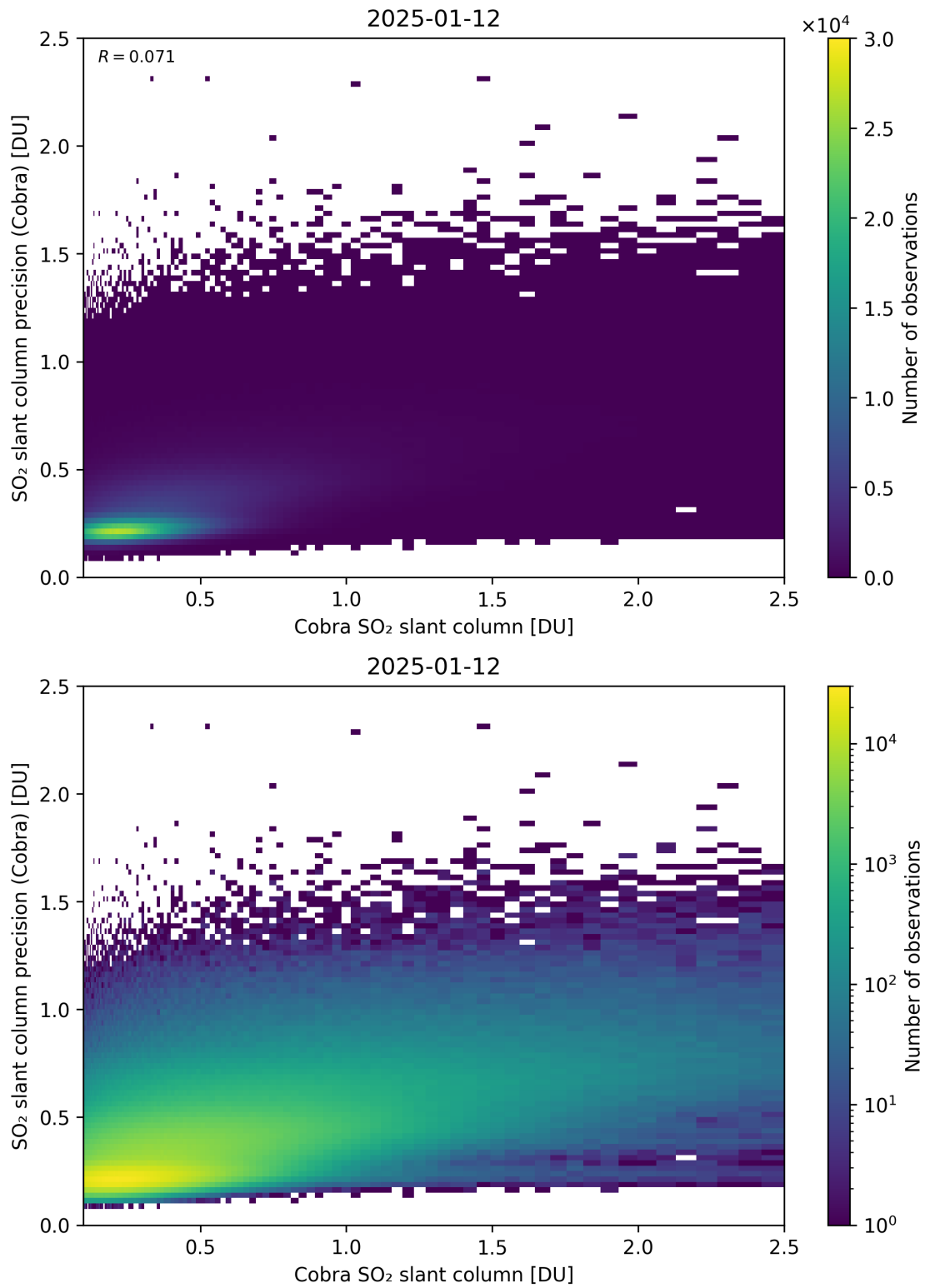
Figure 216: Scatter density plot of “Cobra SO 2 slant column” against “SO 2 slant column precision (Cobra)” for 2025-01-12 to 2025-01-13.
