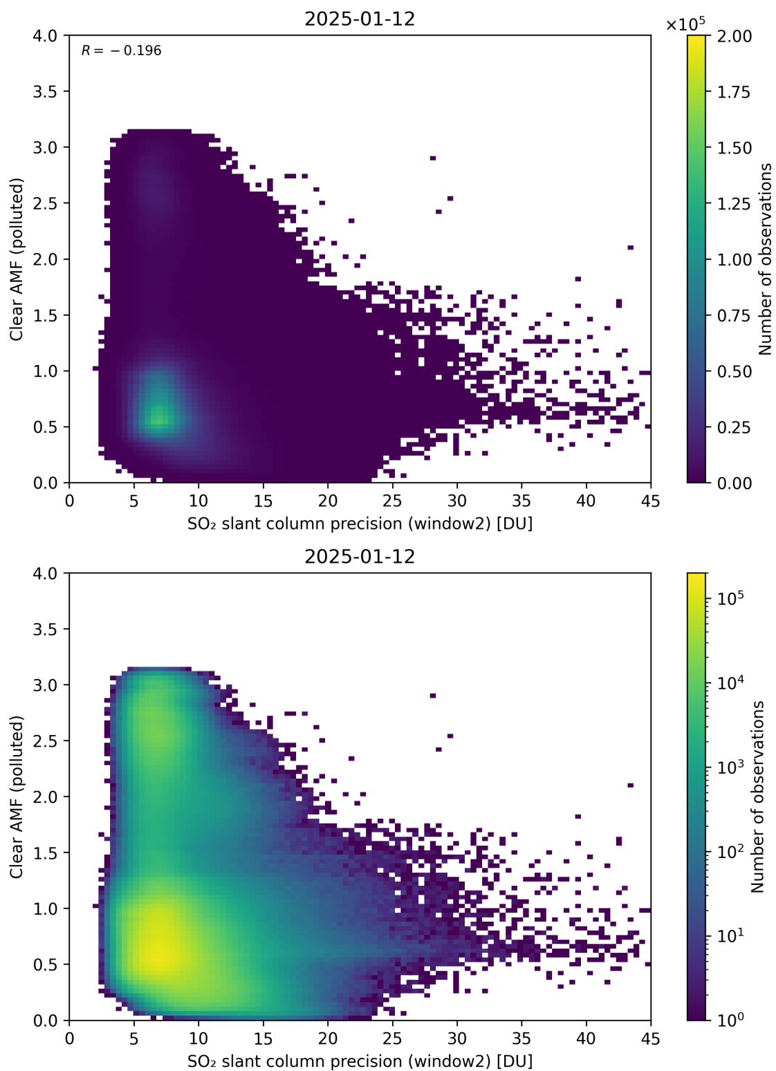
Figure 296: Scatter density plot of “SO 2 slant column precision (window2)” against “Clear AMF (polluted)” for 2025-01-12 to 2025-01-13.
