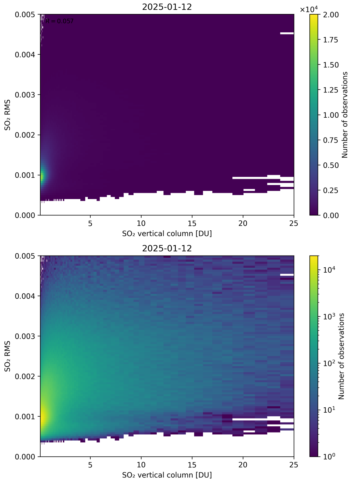
Figure 328: Scatter density plot of “SO 2 vertical column” against “SO 2 RMS” for 2025-01-12 to 2025-01-13.
