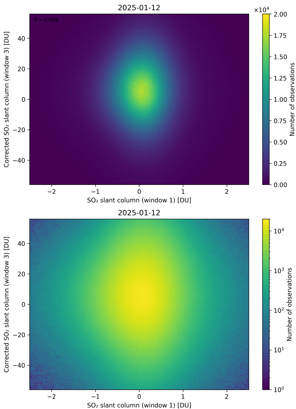
Figure 284: Scatter density plot of “SO 2 slant column (window 1)” against “Corrected SO 2 slant column (window 3)” for 2025-01-12 to 2025-01-13.
