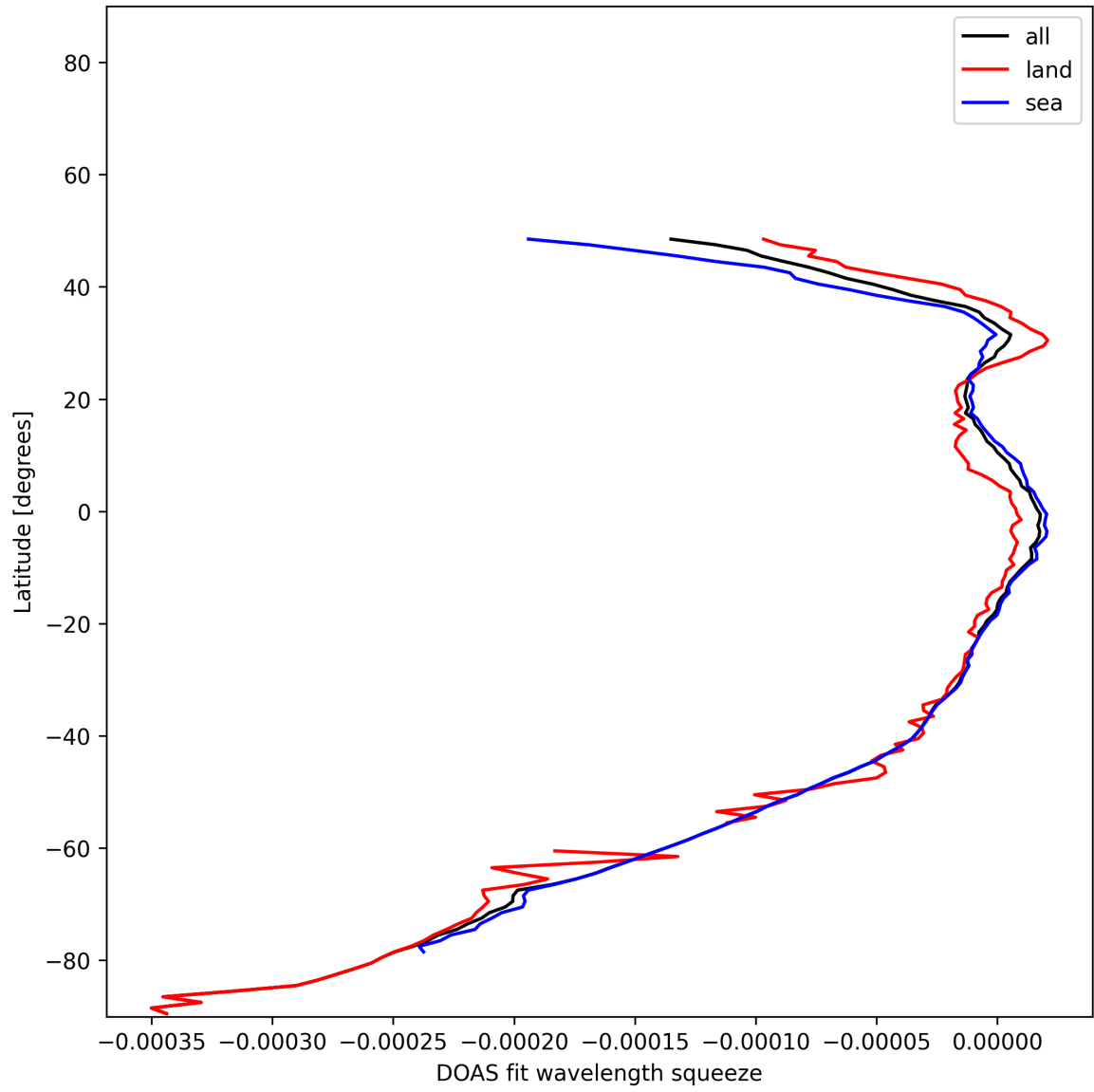
Figure 51: Zonal average of “DOAS fit wavelength squeeze” for 2025-01-12 to 2025-01-13.
