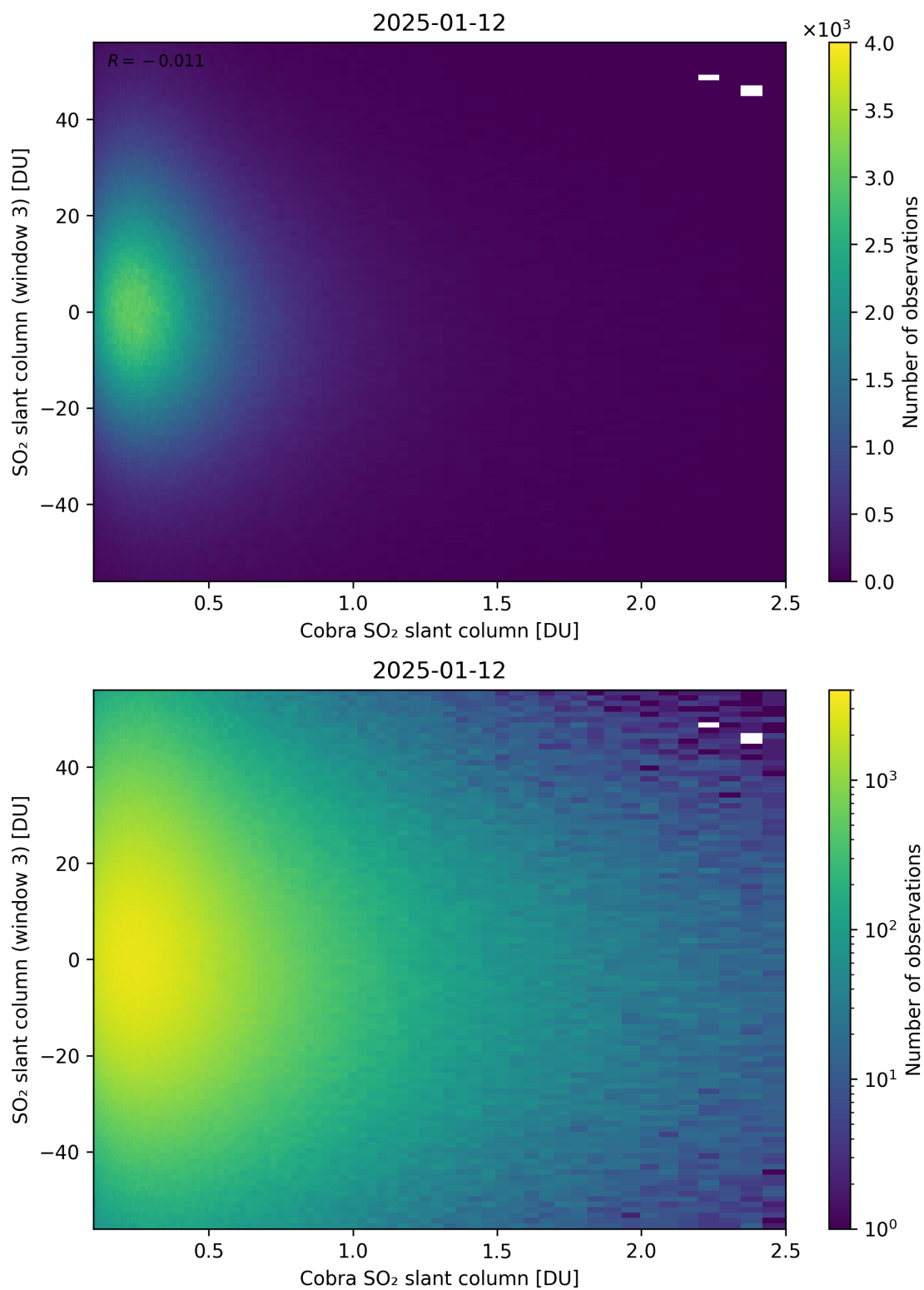
Figure 222: Scatter density plot of “Cobra SO 2 slant column” against “SO 2 slant column (window 3)” for 2025-01-12 to 2025-01-13.
