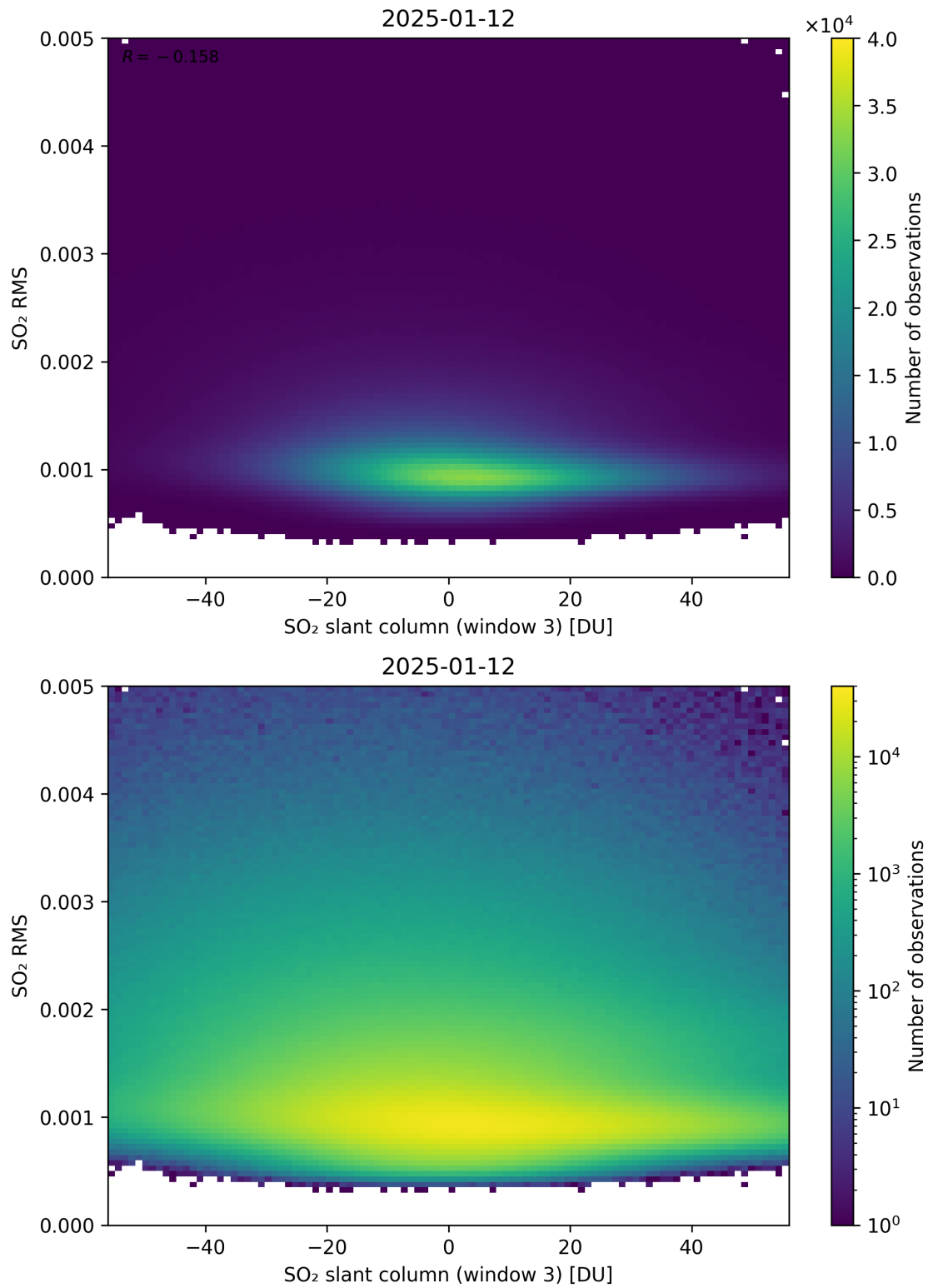
Figure 306: Scatter density plot of “SO 2 slant column (window 3)” against “SO 2 RMS” for 2025-01-12 to 2025-01-13.
