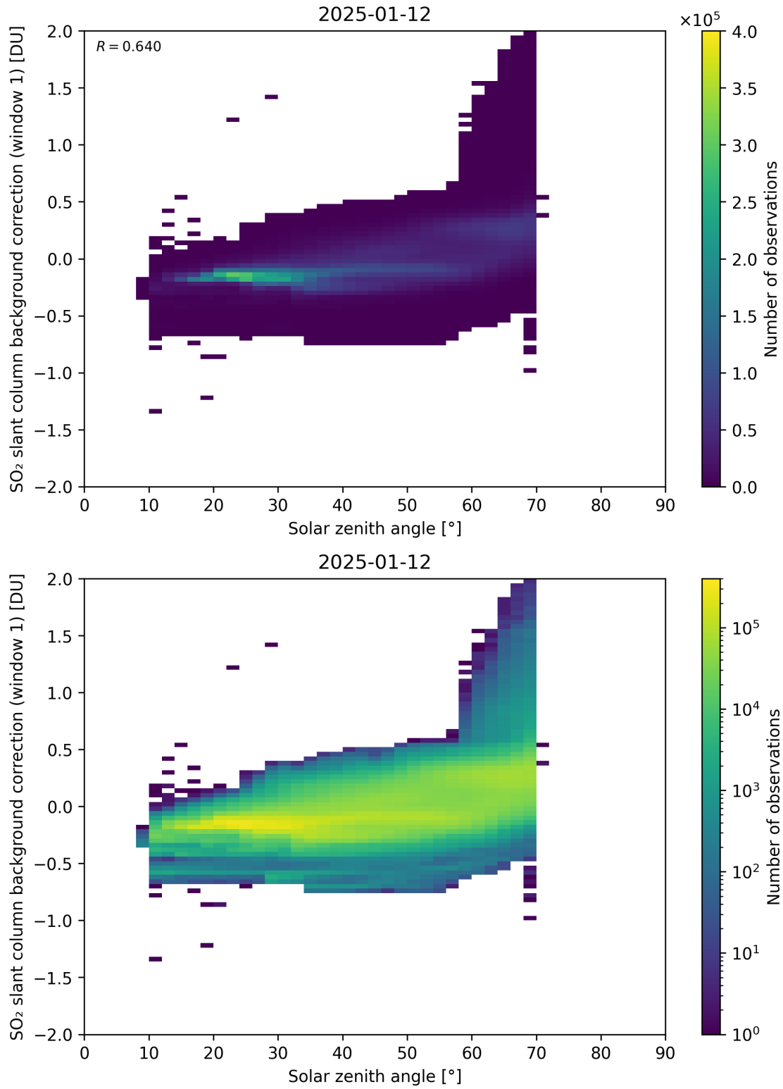
Figure 171: Scatter density plot of “Solar zenith angle” against “SO 2 slant column background correction (window 1)” for 2025-01-12 to 2025-01-13.
