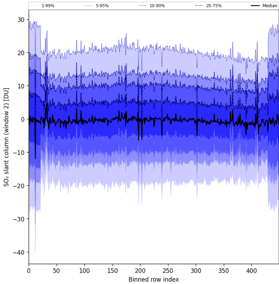
Figure 93: Along track statistics of “SO 2 slant column (window 2)” for 2025-01-12 to 2025-01-13
