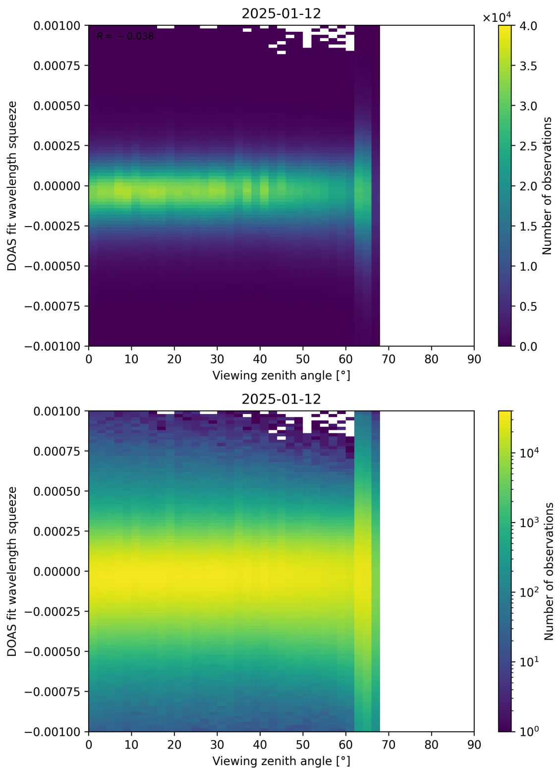
Figure 366: Scatter density plot of “Viewing zenith angle” against “DOAS fit wavelength squeeze” for 2025-01-12 to 2025-01-13.
