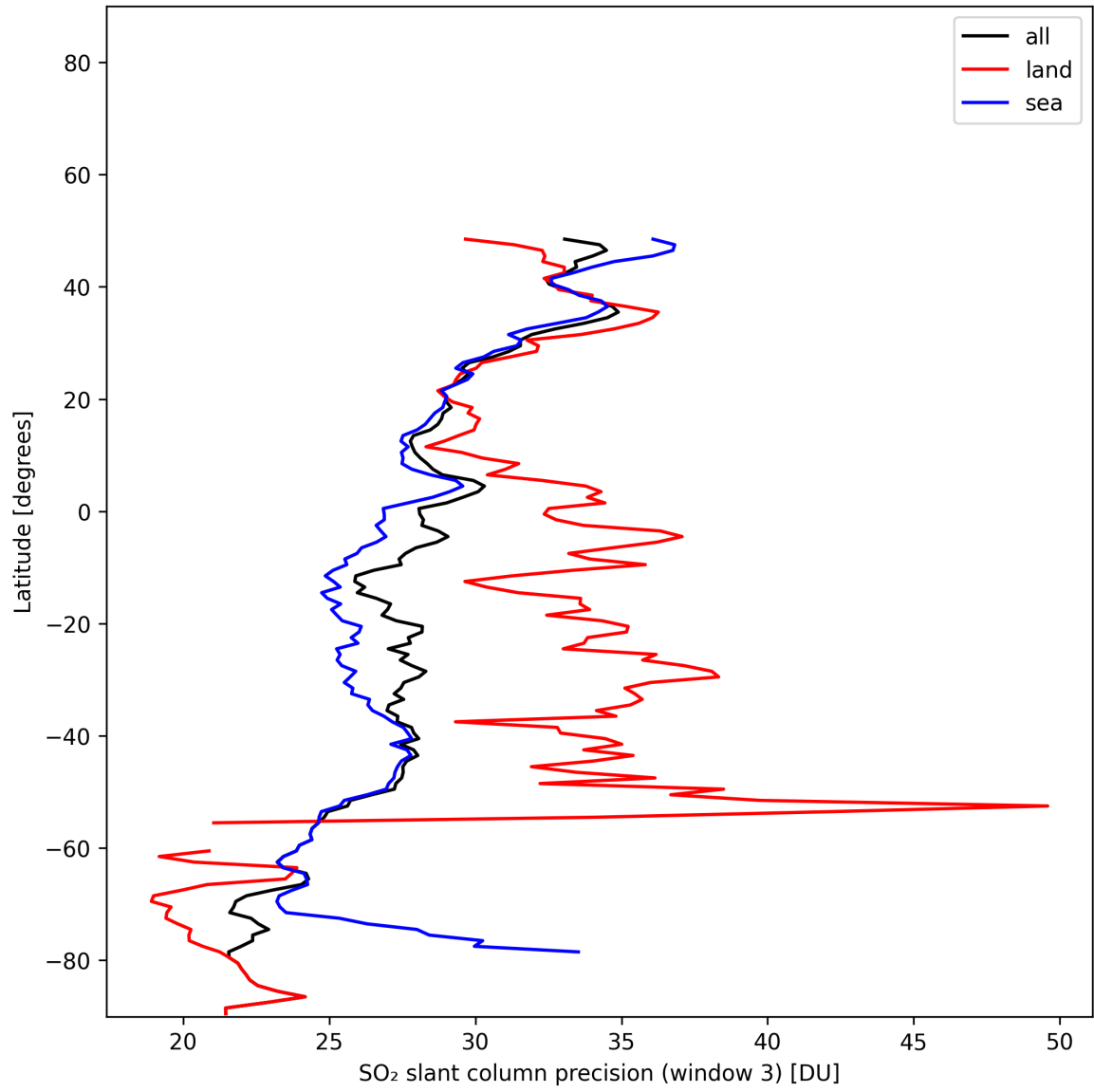
Figure 46: Zonal average of “SO 2 slant column precision (window 3)” for 2025-01-12 to 2025-01-13.
