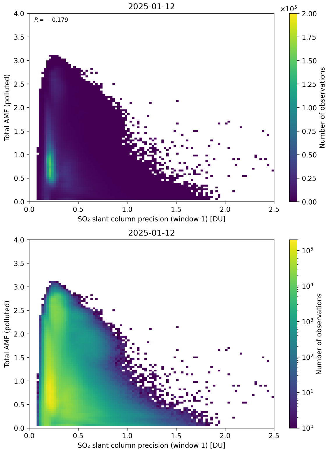
Figure 280: Scatter density plot of “SO 2 slant column precision (window 1)” against “Total AMF (polluted)” for 2025-01-12 to 2025-01-13.
