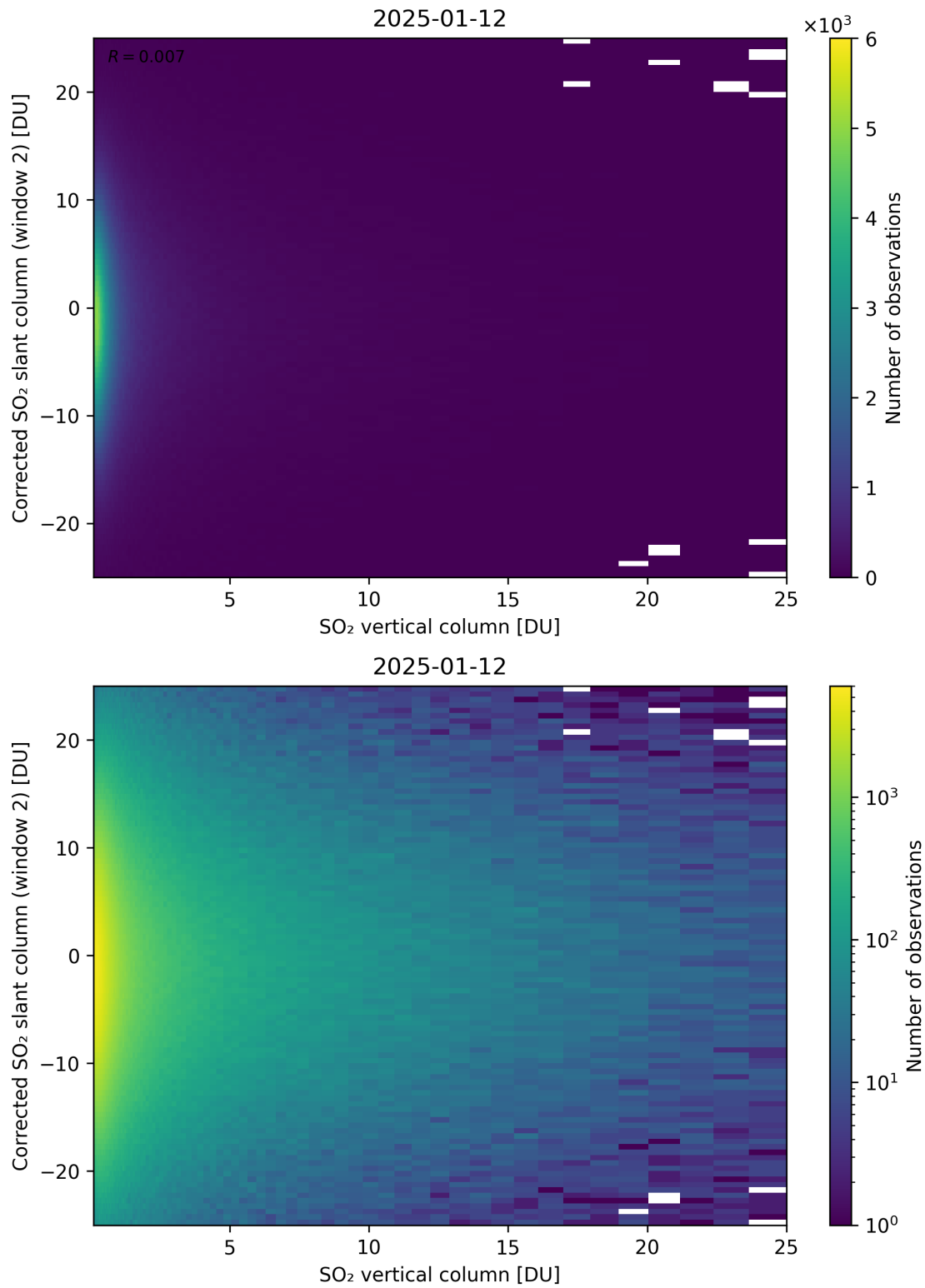
Figure 352: Scatter density plot of “SO 2 vertical column” against “Corrected SO 2 slant column (window 2)” for 2025-01-12 to 2025-01-13.
