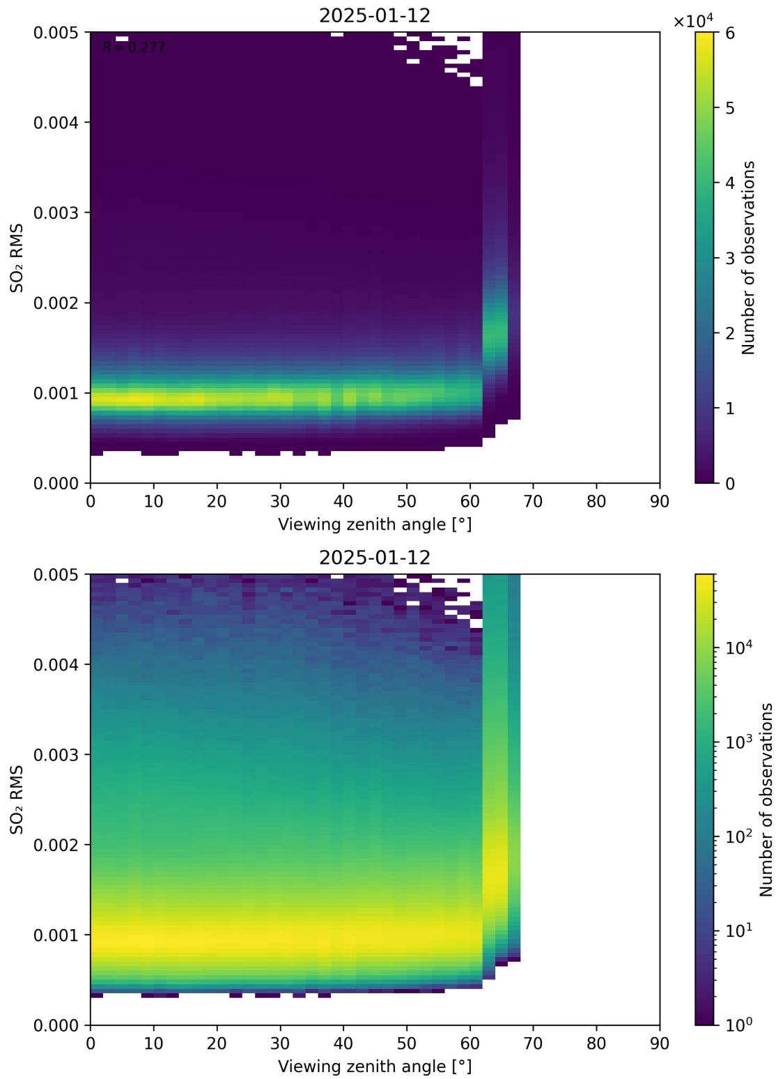
Figure 367: Scatter density plot of “Viewing zenith angle” against “SO 2 RMS” for 2025-01-12 to 2025-01-13.
