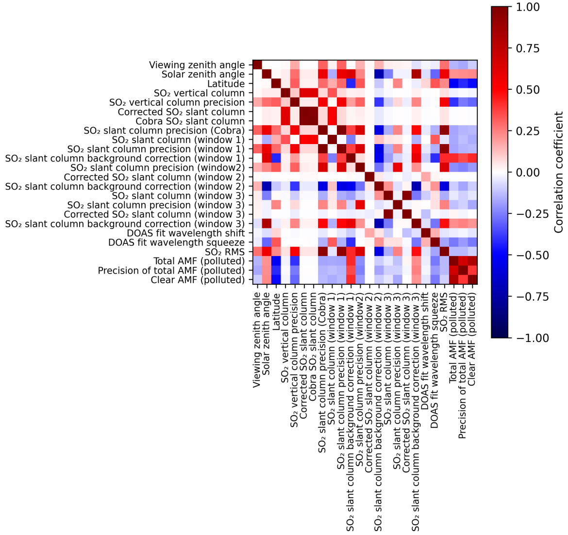
Figure 2: Map of correlation matrix for 2025-01-12 to 2025-01-13.
