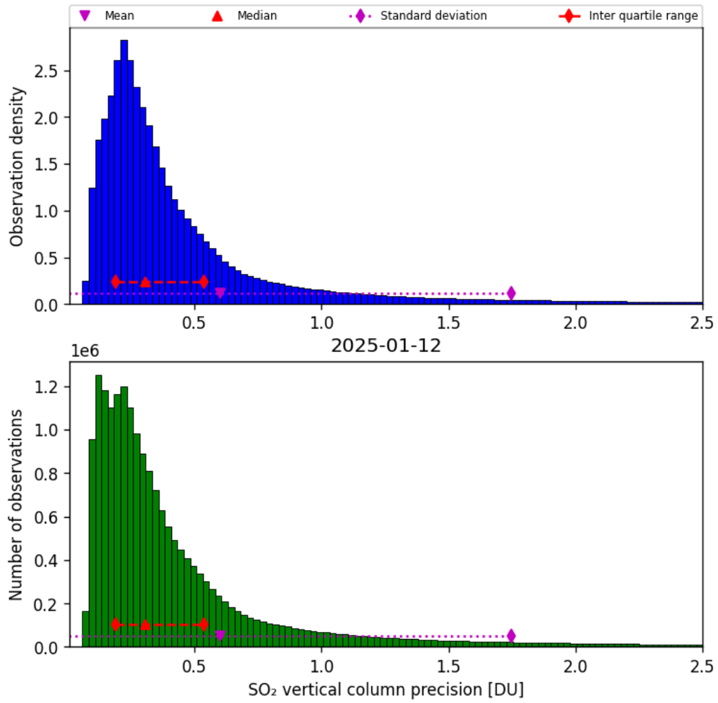
Figure 59: Histogram of “SO 2 vertical column precision” for 2025-01-12 to 2025-01-13
