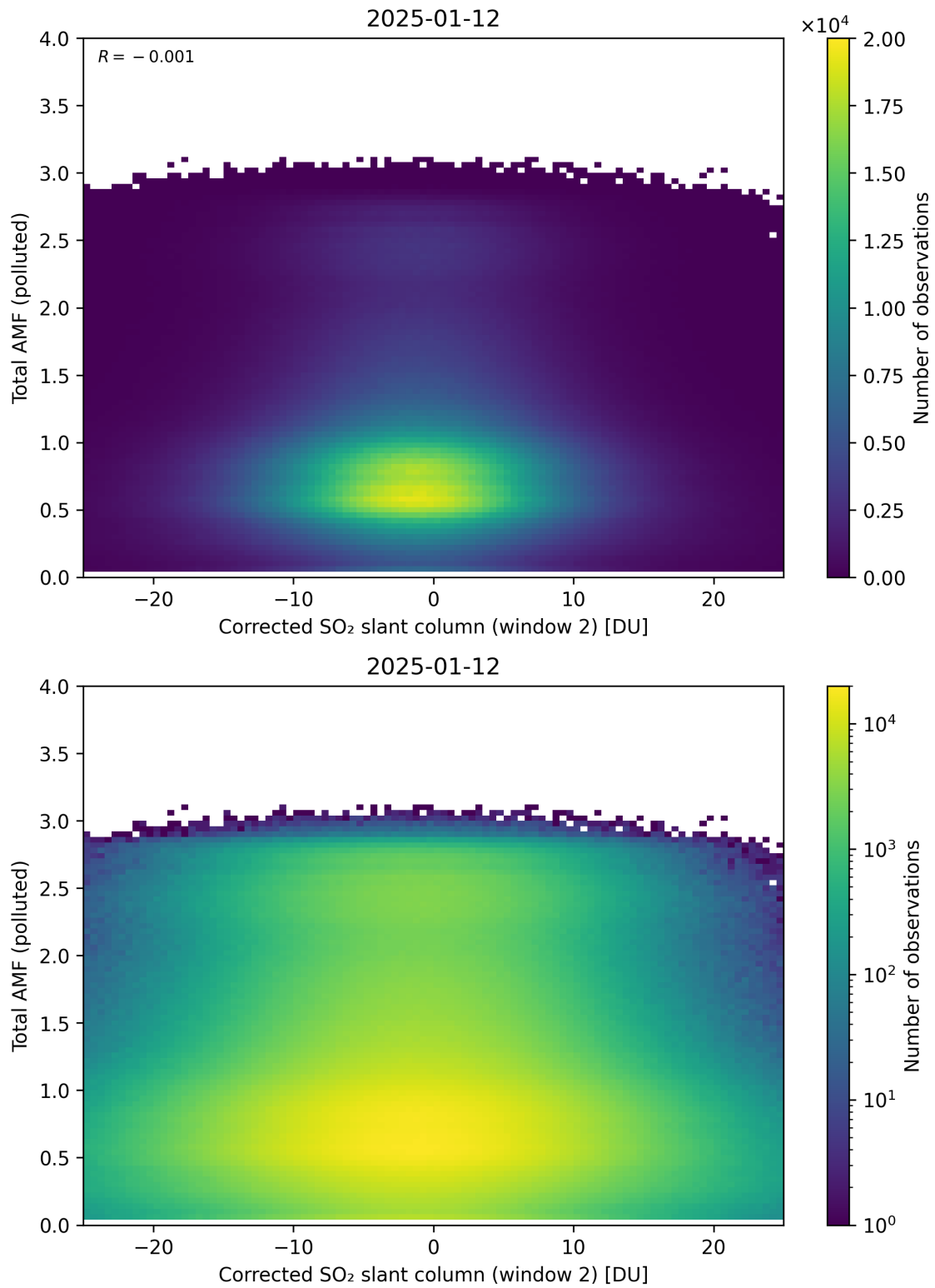
Figure 253: Scatter density plot of “Corrected SO 2 slant column (window 2)” against “Total AMF (polluted)” for 2025-01-12 to 2025-01-13.
