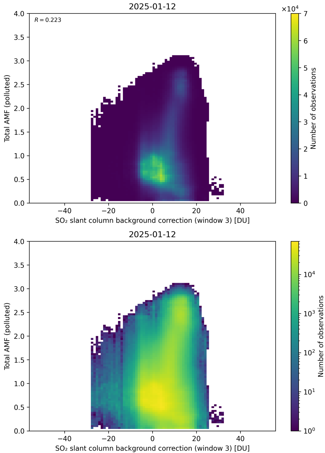
Figure 136: Scatter density plot of “SO 2 slant column background correction (window 3)” against “Total AMF (polluted)” for 2025-01-12 to 2025-01-13.
