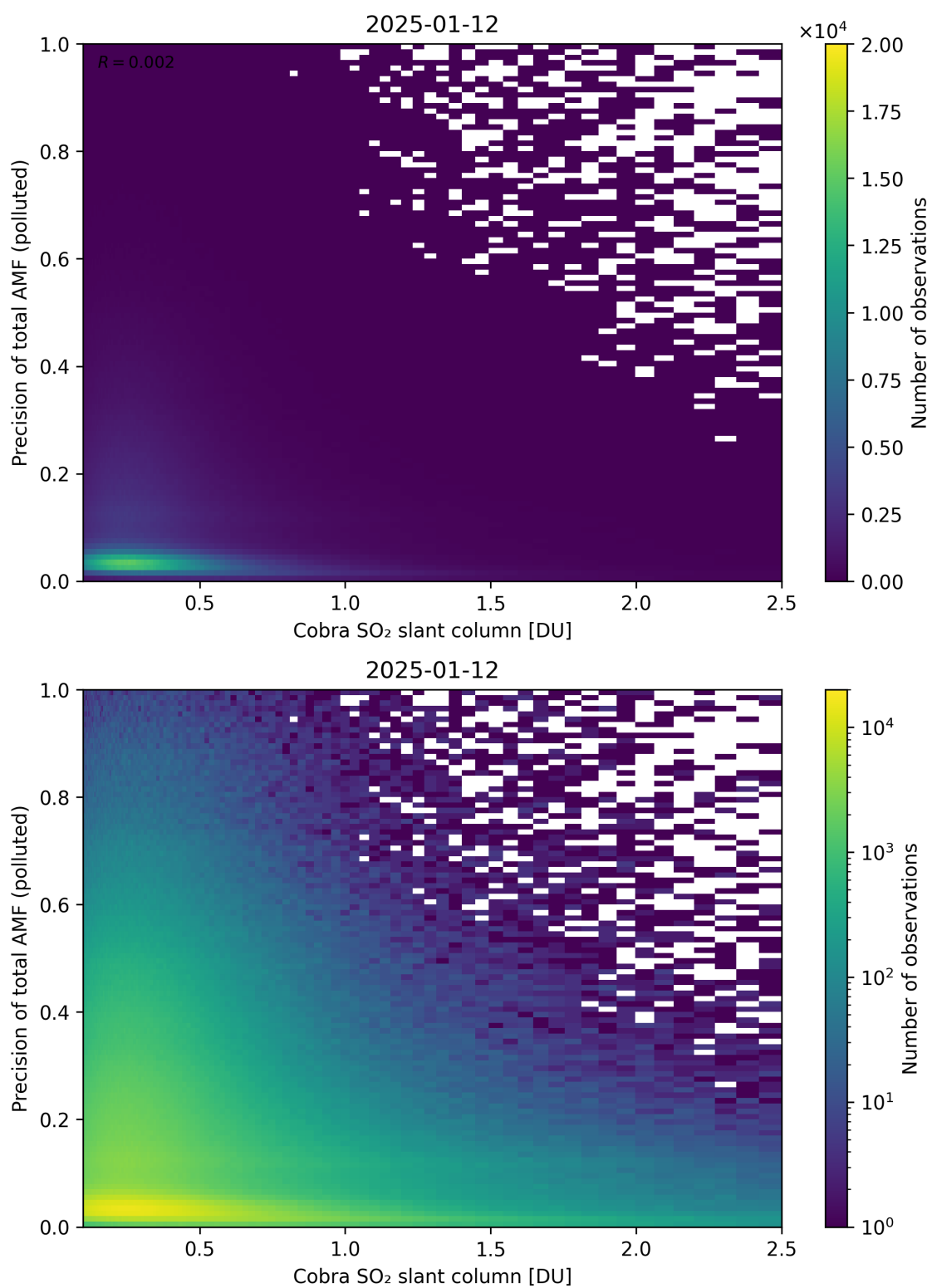
Figure 225: Scatter density plot of “Cobra SO 2 slant column” against “Precision of total AMF (polluted)” for 2025-01-12 to 2025-01-13.
