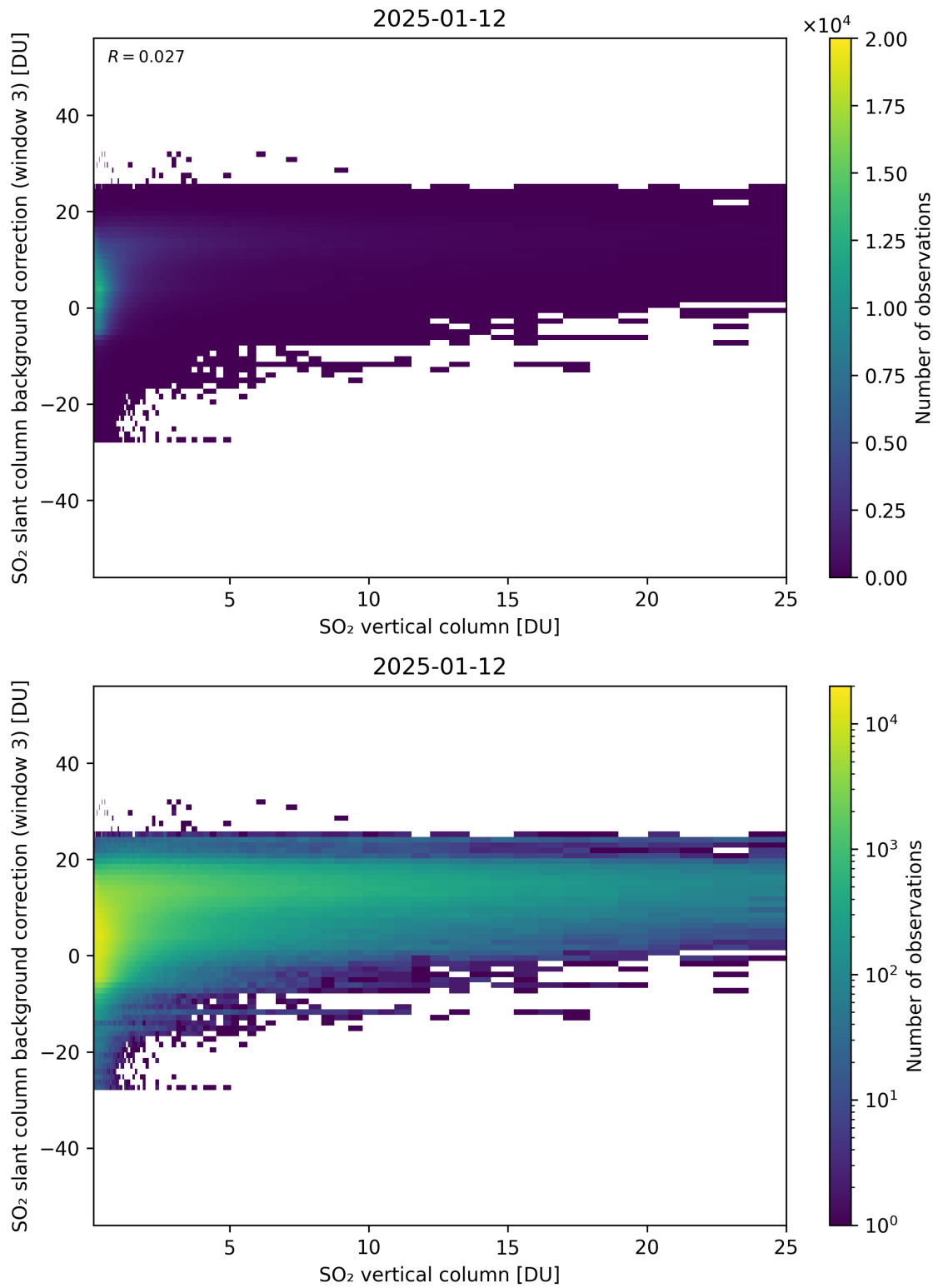
Figure 325: Scatter density plot of “SO 2 vertical column” against “SO 2 slant column background correction (window 3)” for 2025-01-12 to 2025-01-13.
