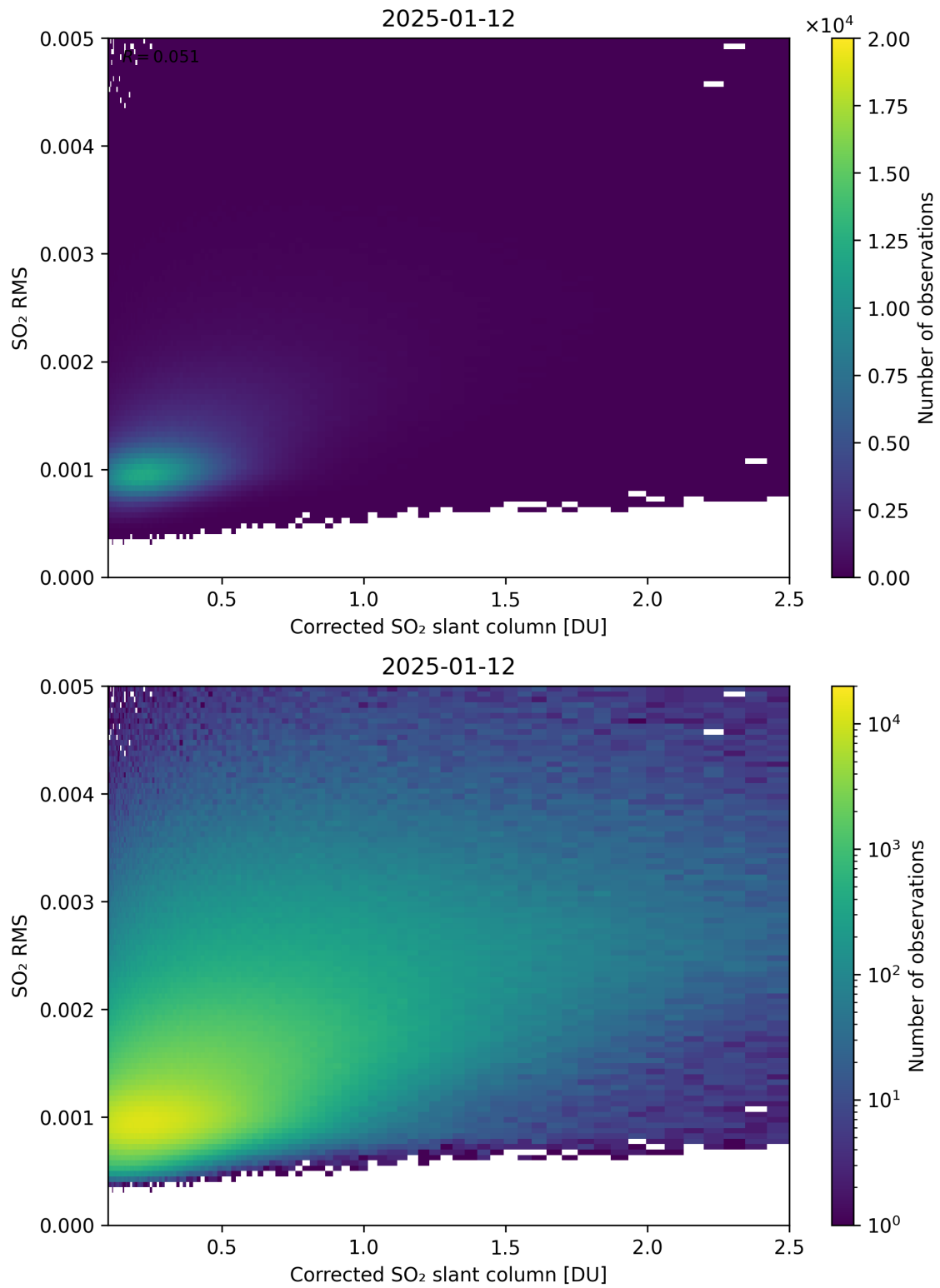
Figure 231: Scatter density plot of “Corrected SO 2 slant column” against “SO 2 RMS” for 2025-01-12 to 2025-01-13.
