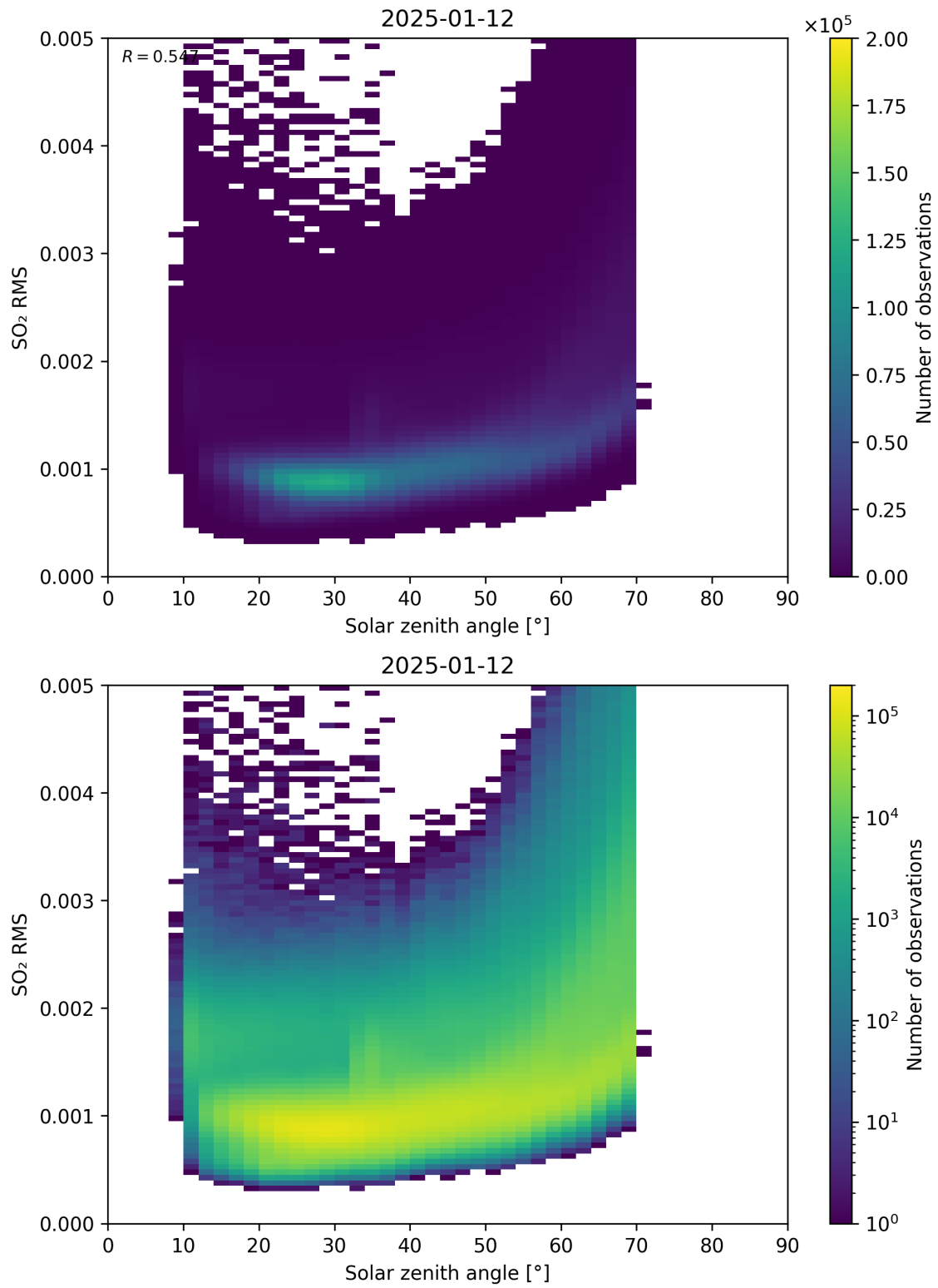
Figure 176: Scatter density plot of “Solar zenith angle” against “SO 2 RMS” for 2025-01-12 to 2025-01-13.
