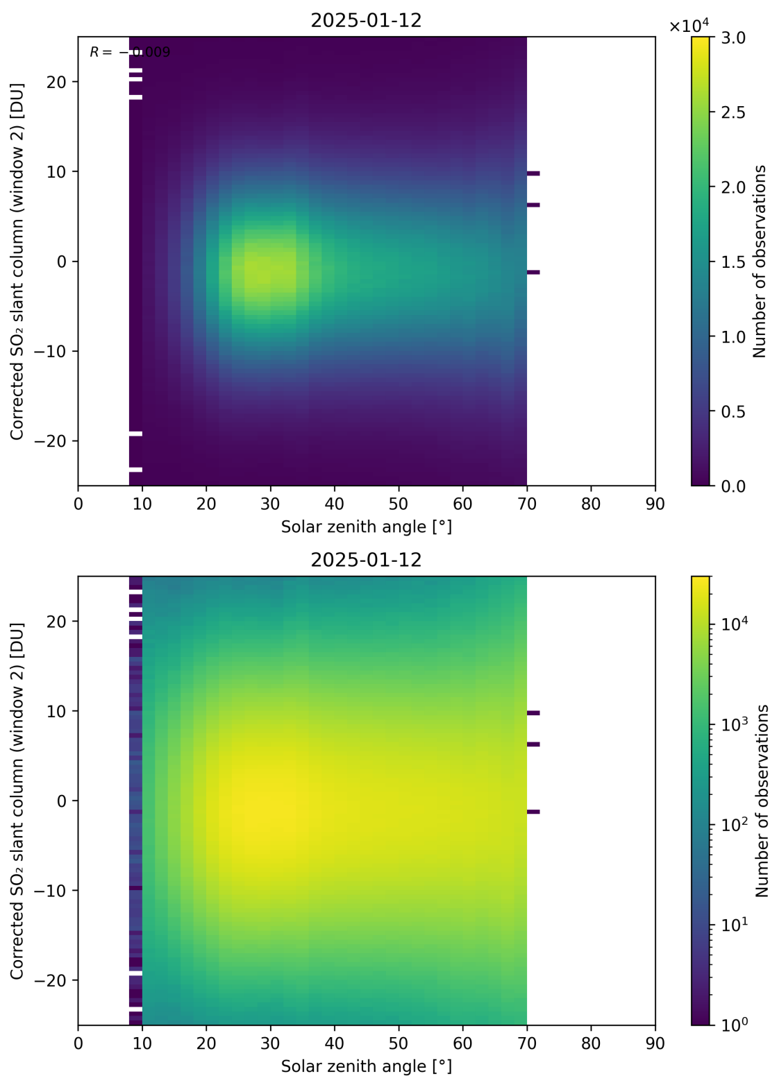
Figure 182: Scatter density plot of “Solar zenith angle” against “Corrected SO 2 slant column (window 2)” for 2025-01-12 to 2025-01-13.
