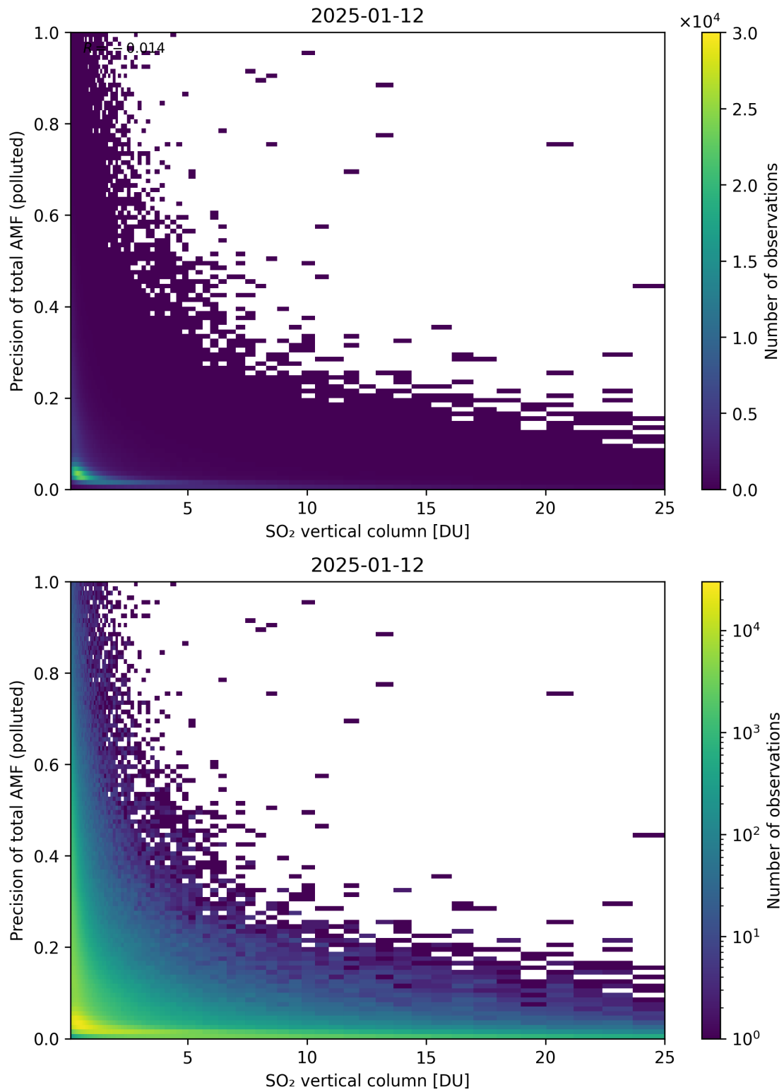
Figure 360: Scatter density plot of “SO 2 vertical column” against “Precision of total AMF (polluted)” for 2025-01-12 to 2025-01-13.
