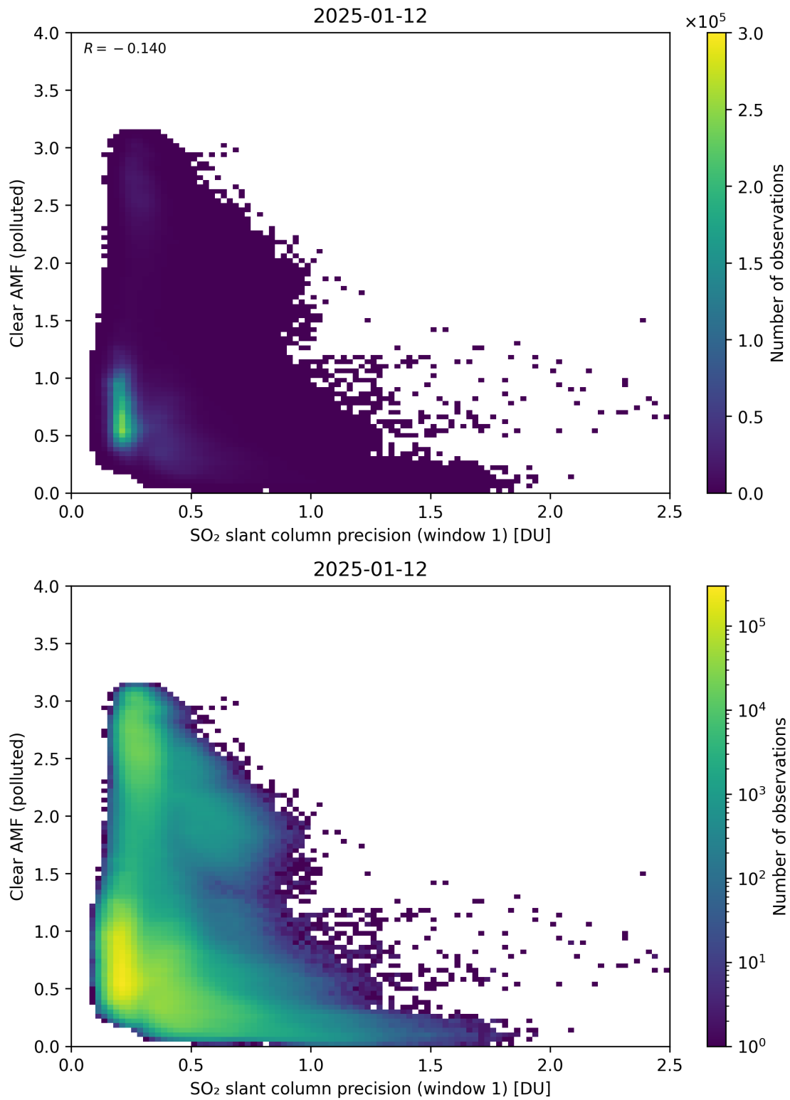
Figure 274: Scatter density plot of “SO 2 slant column precision (window 1)” against “Clear AMF (polluted)” for 2025-01-12 to 2025-01-13.
