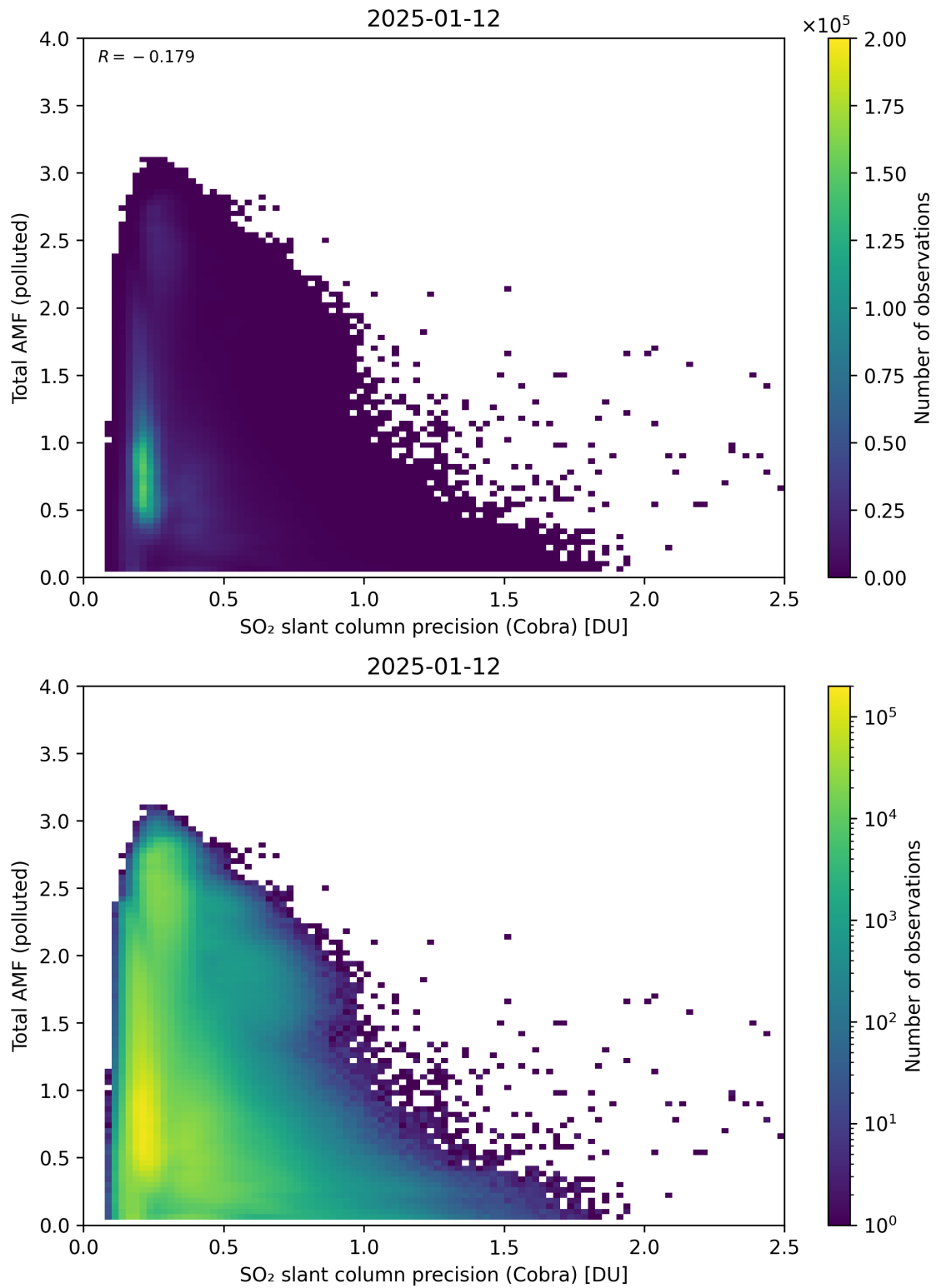
Figure 213: Scatter density plot of “SO 2 slant column precision (Cobra)” against “Total AMF (polluted)” for 2025-01-12 to 2025-01-13.
