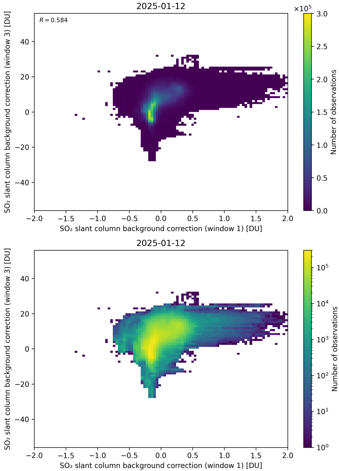
Figure 110: Scatter density plot of “SO 2 slant column background correction (window 1)” against “SO 2 slant column background correction (window 3)” for 2025-01-12 to 2025-01-13.
