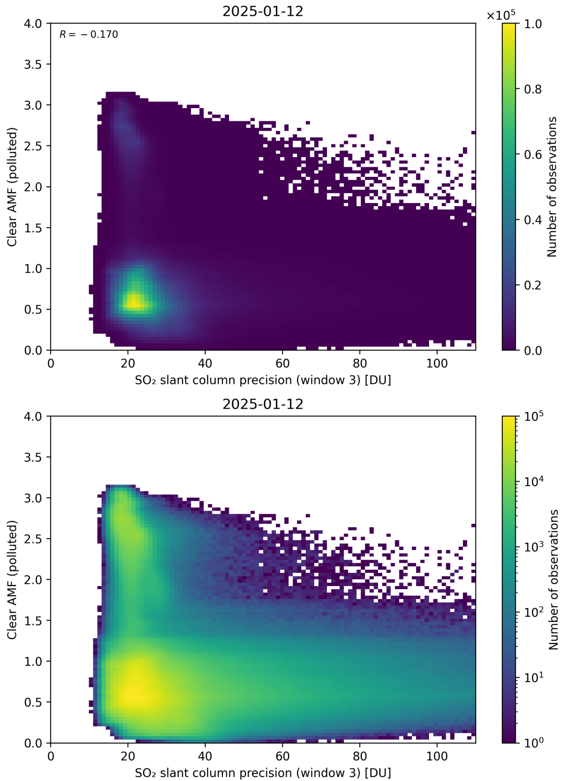
Figure 311: Scatter density plot of “SO 2 slant column precision (window 3)” against “Clear AMF (polluted)” for 2025-01-12 to 2025-01-13.
