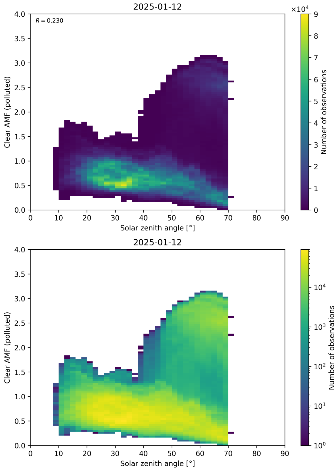
Figure 178: Scatter density plot of “Solar zenith angle” against “Clear AMF (polluted)” for 2025-01-12 to 2025-01-13.
