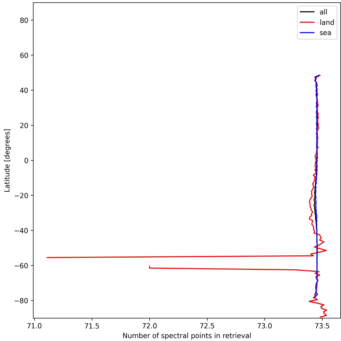
Figure 56: Zonal average of “Number of spectral points in retrieval” for 2025-01-12 to 2025-01-13.
