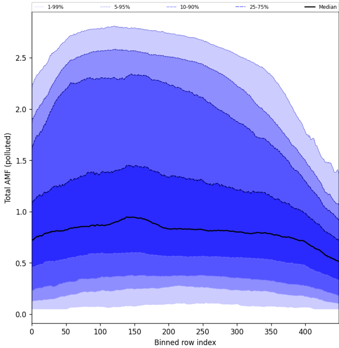
Figure 105: Along track statistics of “Total AMF (polluted)” for 2025-01-12 to 2025-01-13
