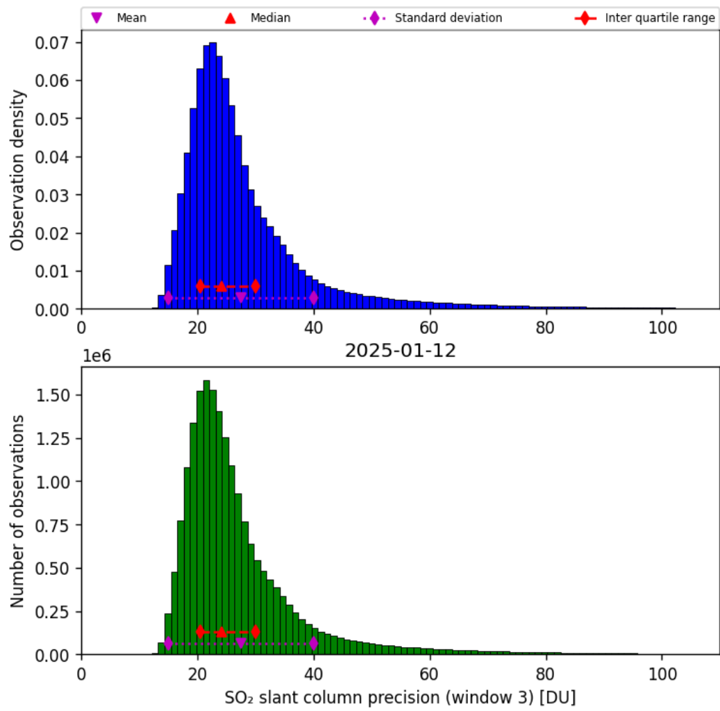
Figure 72: Histogram of “SO 2 slant column precision (window 3)” for 2025-01-12 to 2025-01-13
