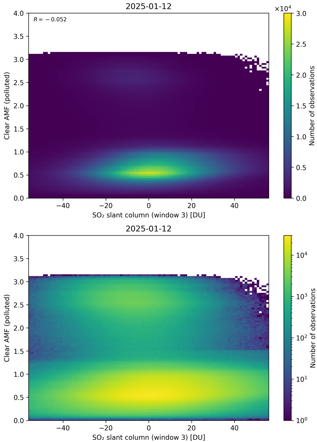
Figure 315: Scatter density plot of “SO 2 slant column (window 3)” against “Clear AMF (polluted)” for 2025-01-12 to 2025-01-13.
