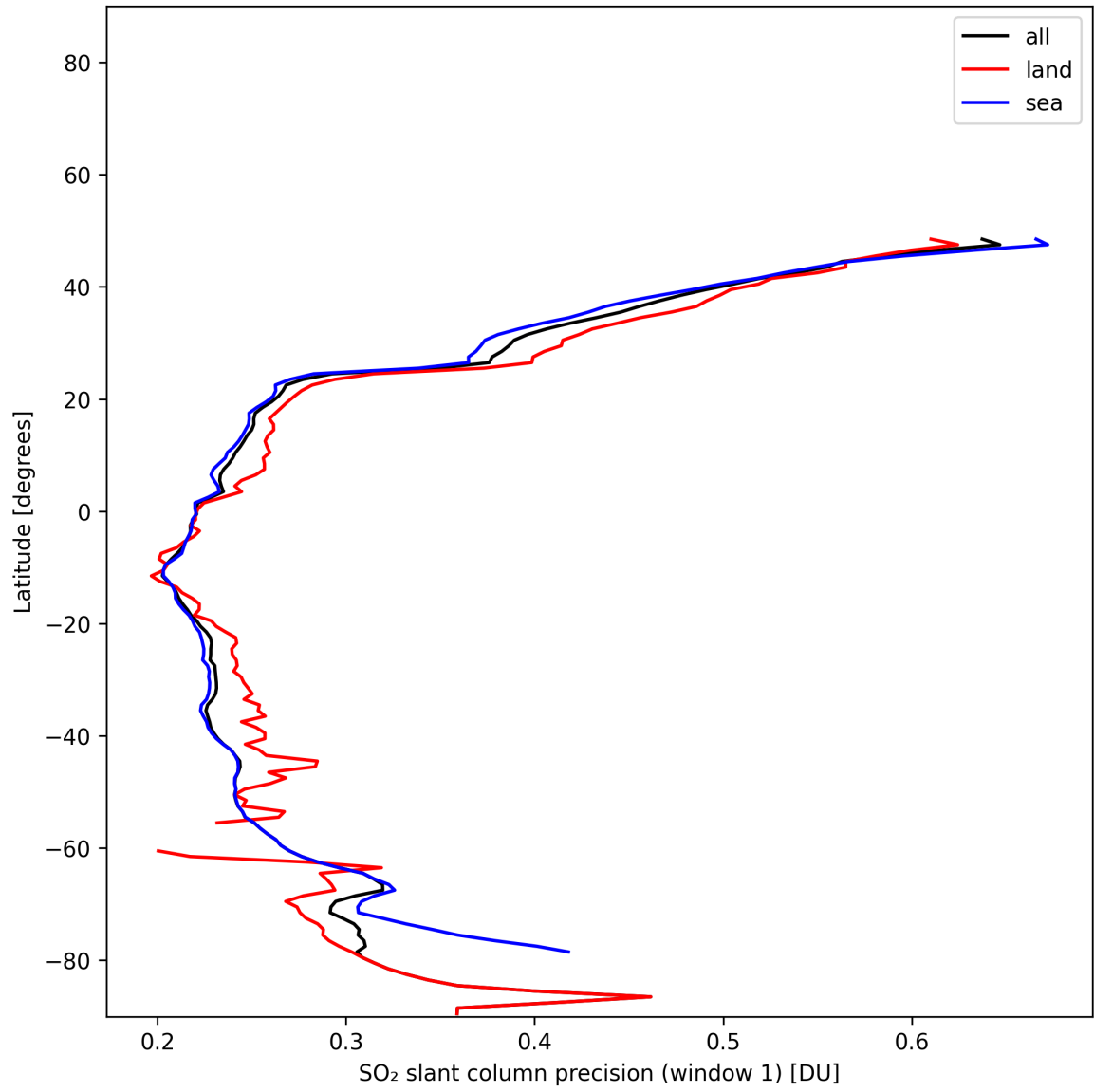
Figure 38: Zonal average of “SO 2 slant column precision (window 1)” for 2025-01-12 to 2025-01-13.
