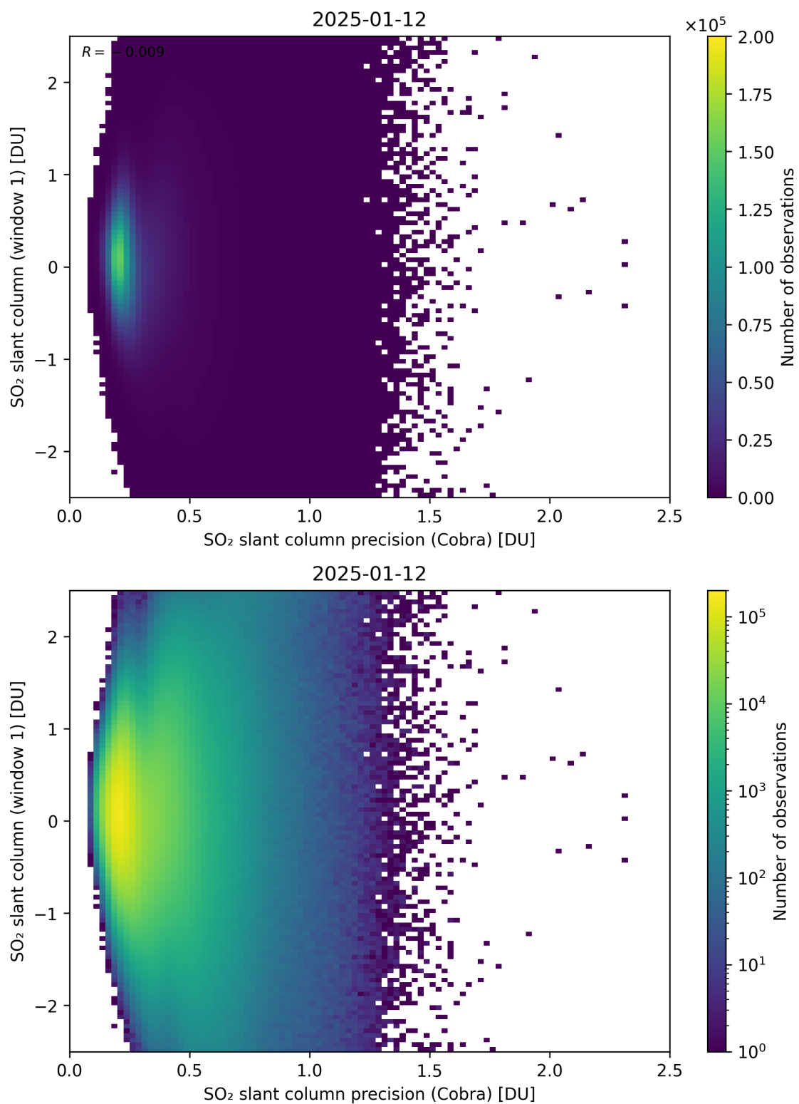
Figure 208: Scatter density plot of “SO 2 slant column precision (Cobra)” against “SO 2 slant column (window 1)” for 2025-01-12 to 2025-01-13.
