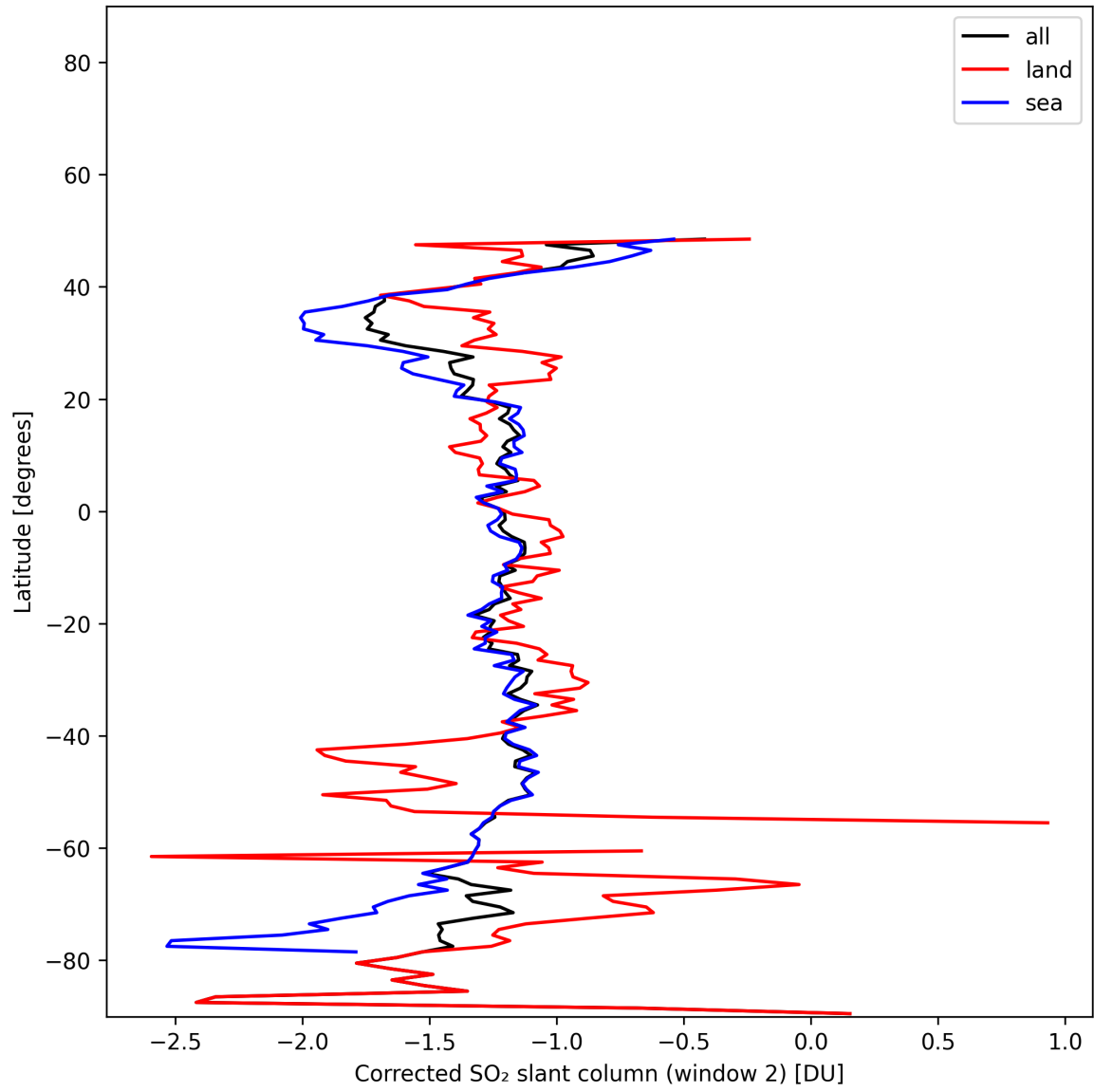
Figure 43: Zonal average of “Corrected SO 2 slant column (window 2)” for 2025-01-12 to 2025-01-13.
