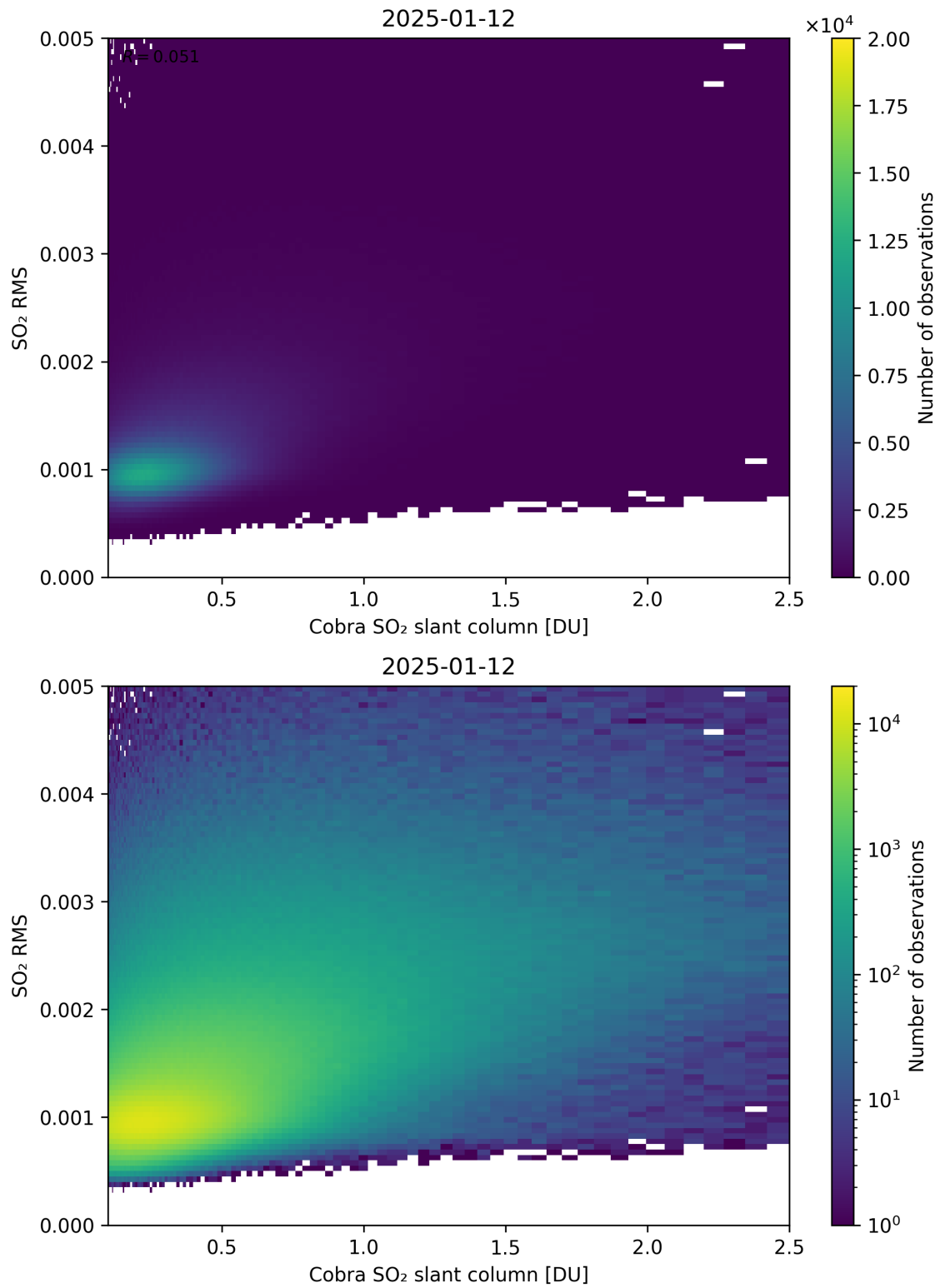
Figure 198: Scatter density plot of “Cobra SO 2 slant column” against “SO 2 RMS” for 2025-01-12 to 2025-01-13.
