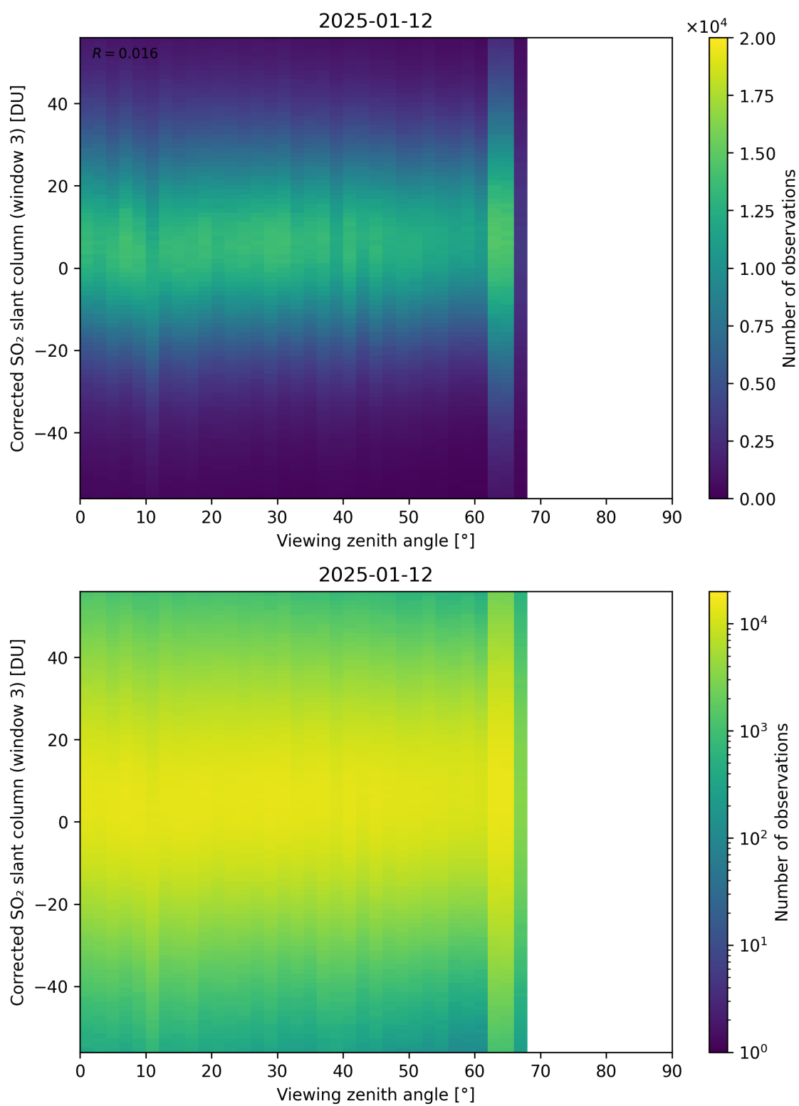
Figure 375: Scatter density plot of “Viewing zenith angle” against “Corrected SO 2 slant column (window 3)” for 2025-01-12 to 2025-01-13.
