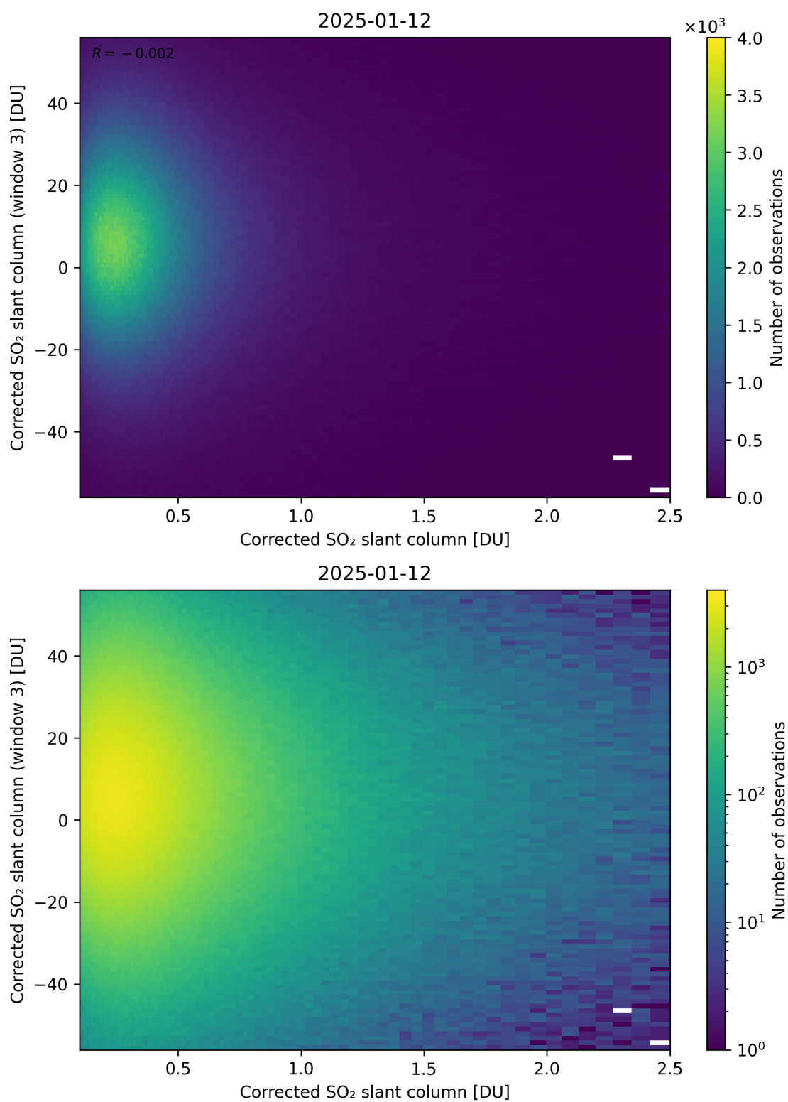
Figure 236: Scatter density plot of “Corrected SO 2 slant column” against “Corrected SO 2 slant column (window 3)” for 2025-01-12 to 2025-01-13.
