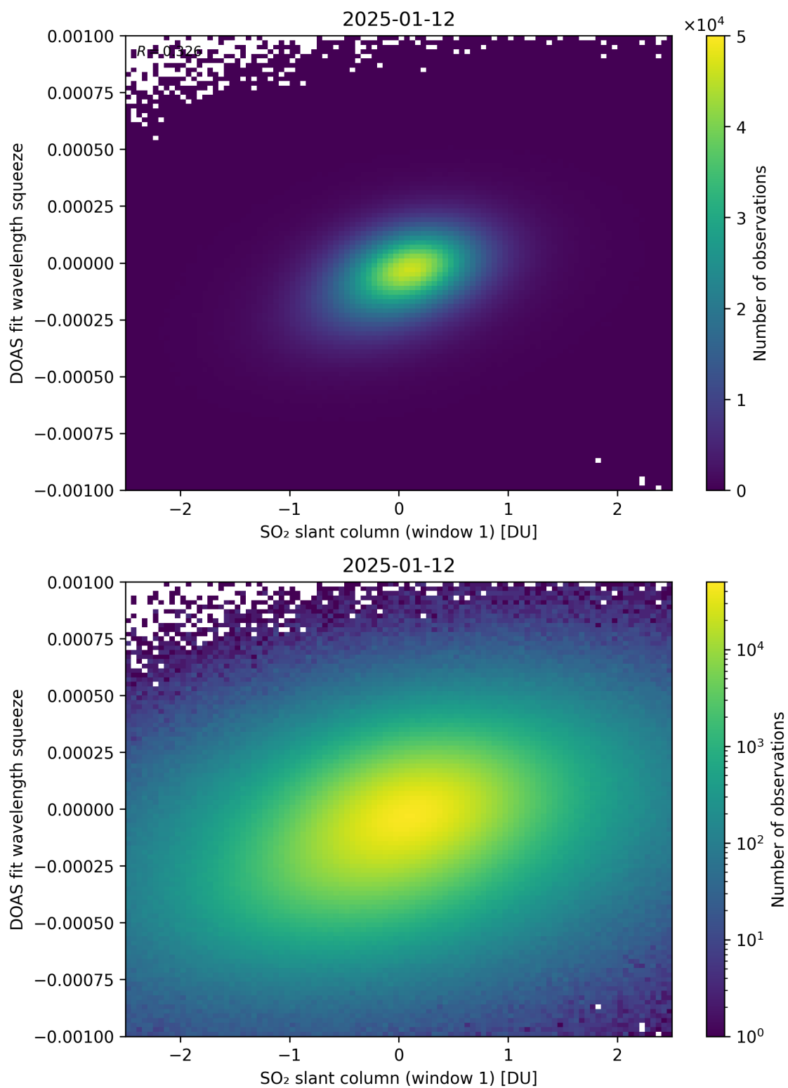
Figure 266: Scatter density plot of “SO 2 slant column (window 1)” against “DOAS fit wavelength squeeze” for 2025-01-12 to 2025-01-13.
