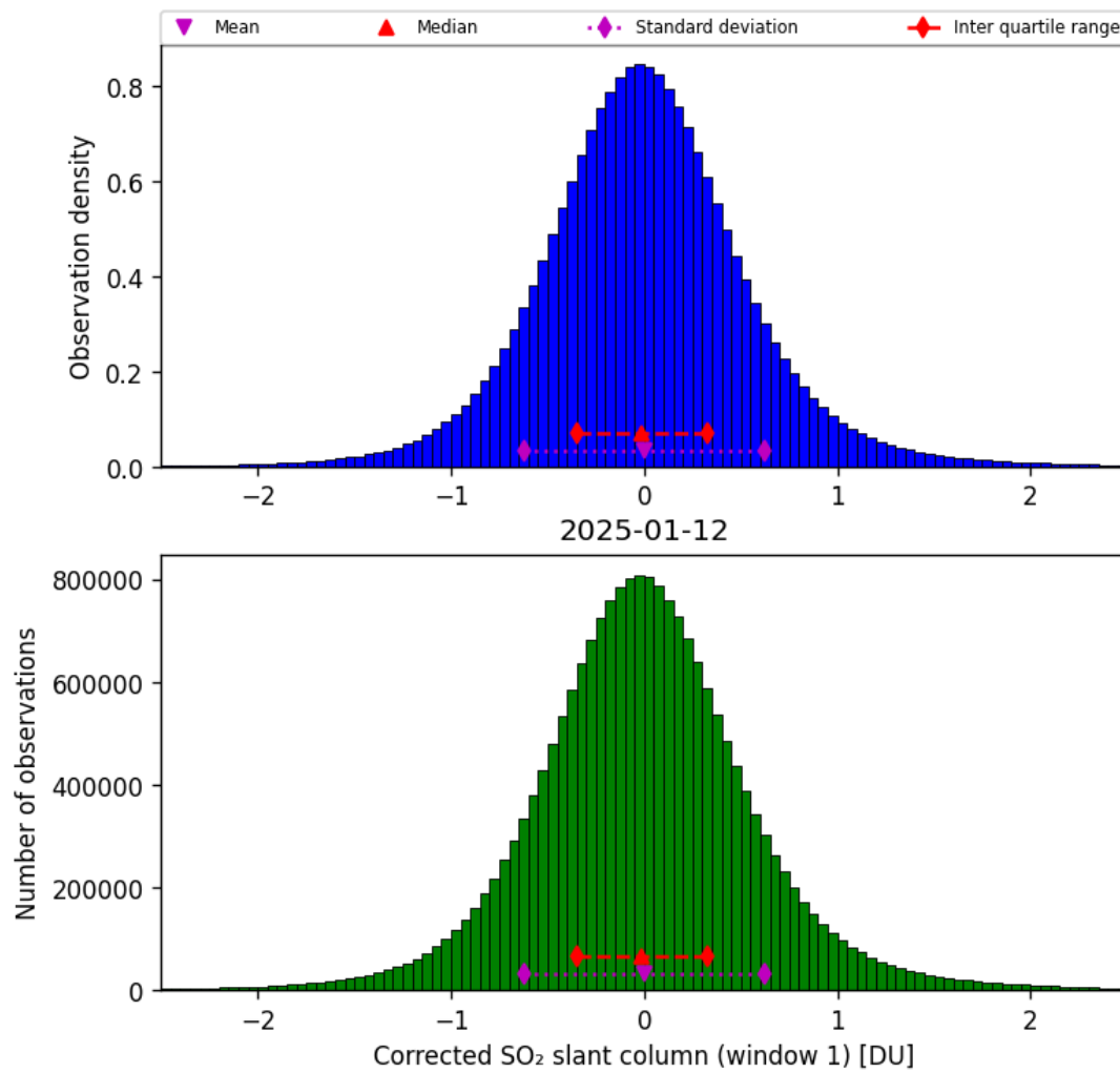
Figure 65: Histogram of “Corrected SO 2 slant column (window 1)” for 2025-01-12 to 2025-01-13
