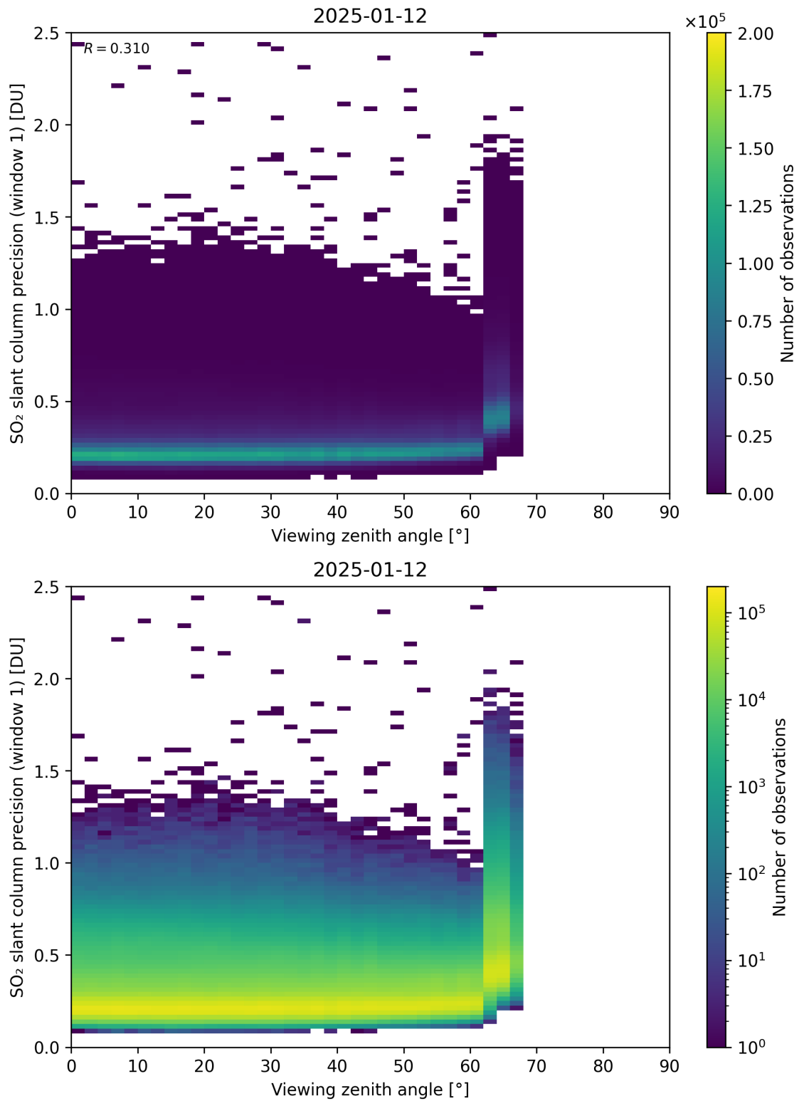
Figure 377: Scatter density plot of “Viewing zenith angle” against “SO 2 slant column precision (window 1)” for 2025-01-12 to 2025-01-13.
