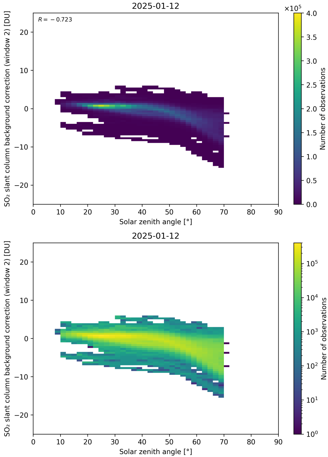
Figure 172: Scatter density plot of “Solar zenith angle” against “SO 2 slant column background correction (window 2)” for 2025-01-12 to 2025-01-13.
