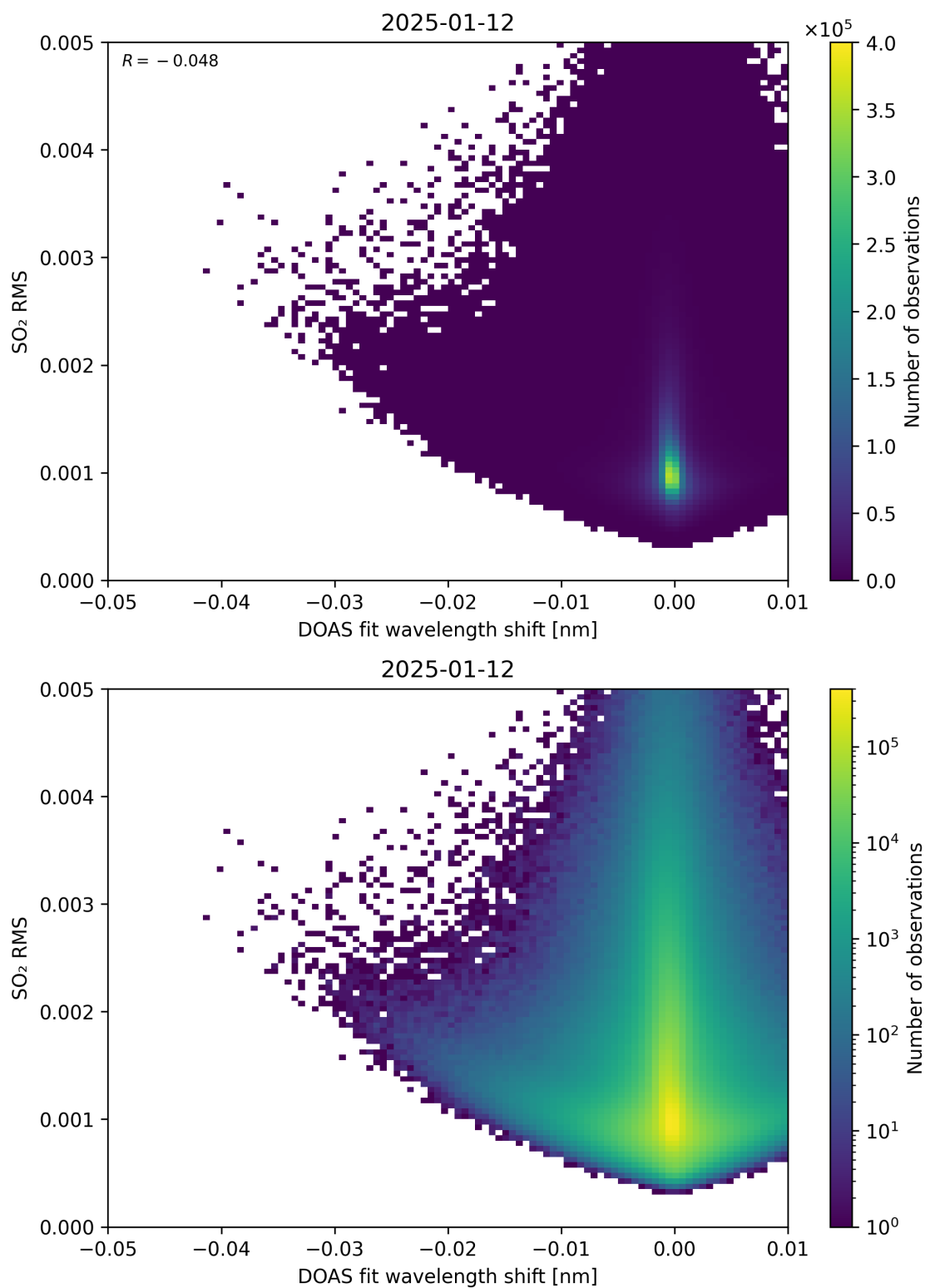
Figure 139: Scatter density plot of “DOAS fit wavelength shift” against “SO 2 RMS” for 2025-01-12 to 2025-01-13.
