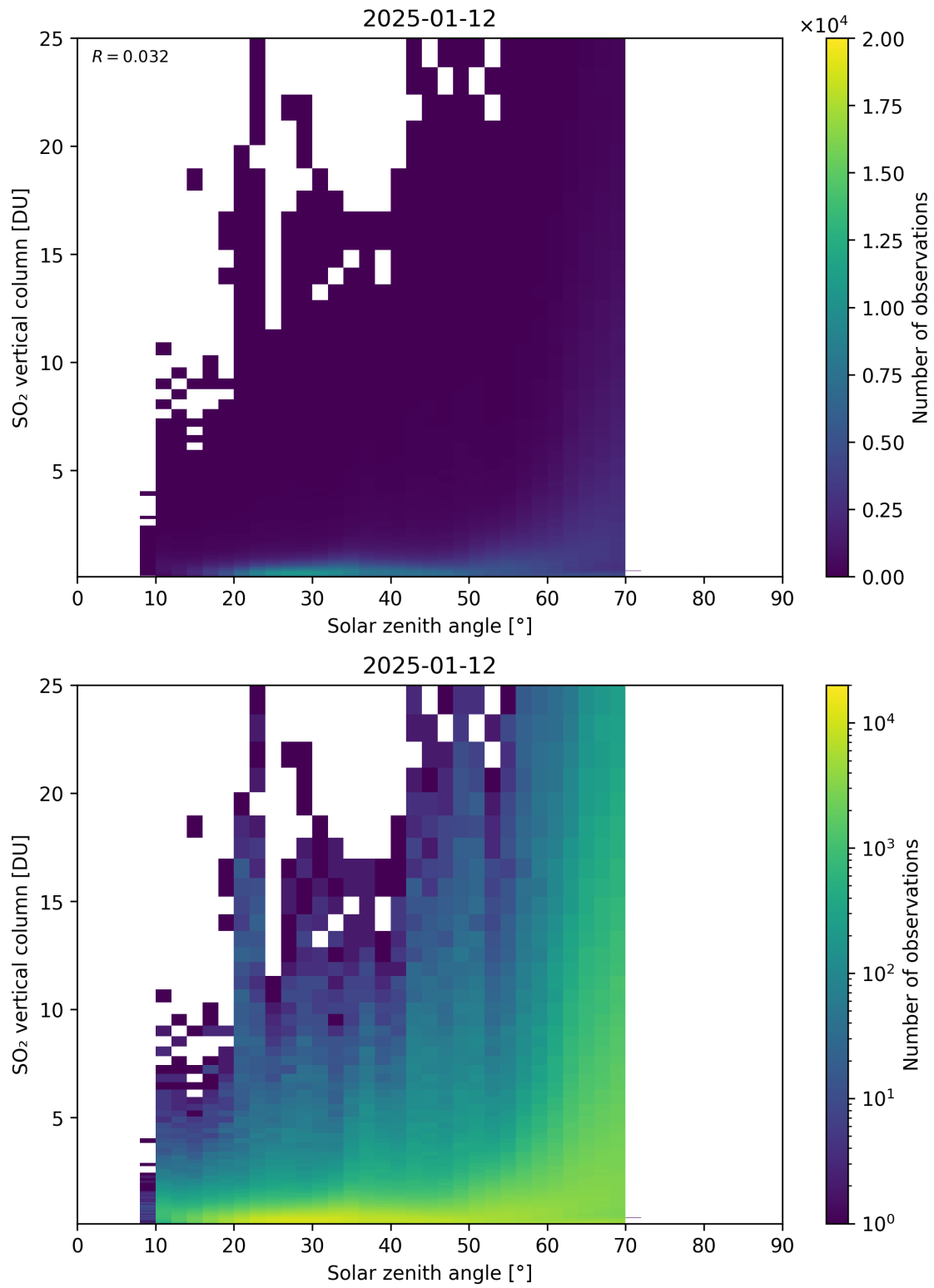
Figure 191: Scatter density plot of “Solar zenith angle” against “SO 2 vertical column” for 2025-01-12 to 2025-01-13.
