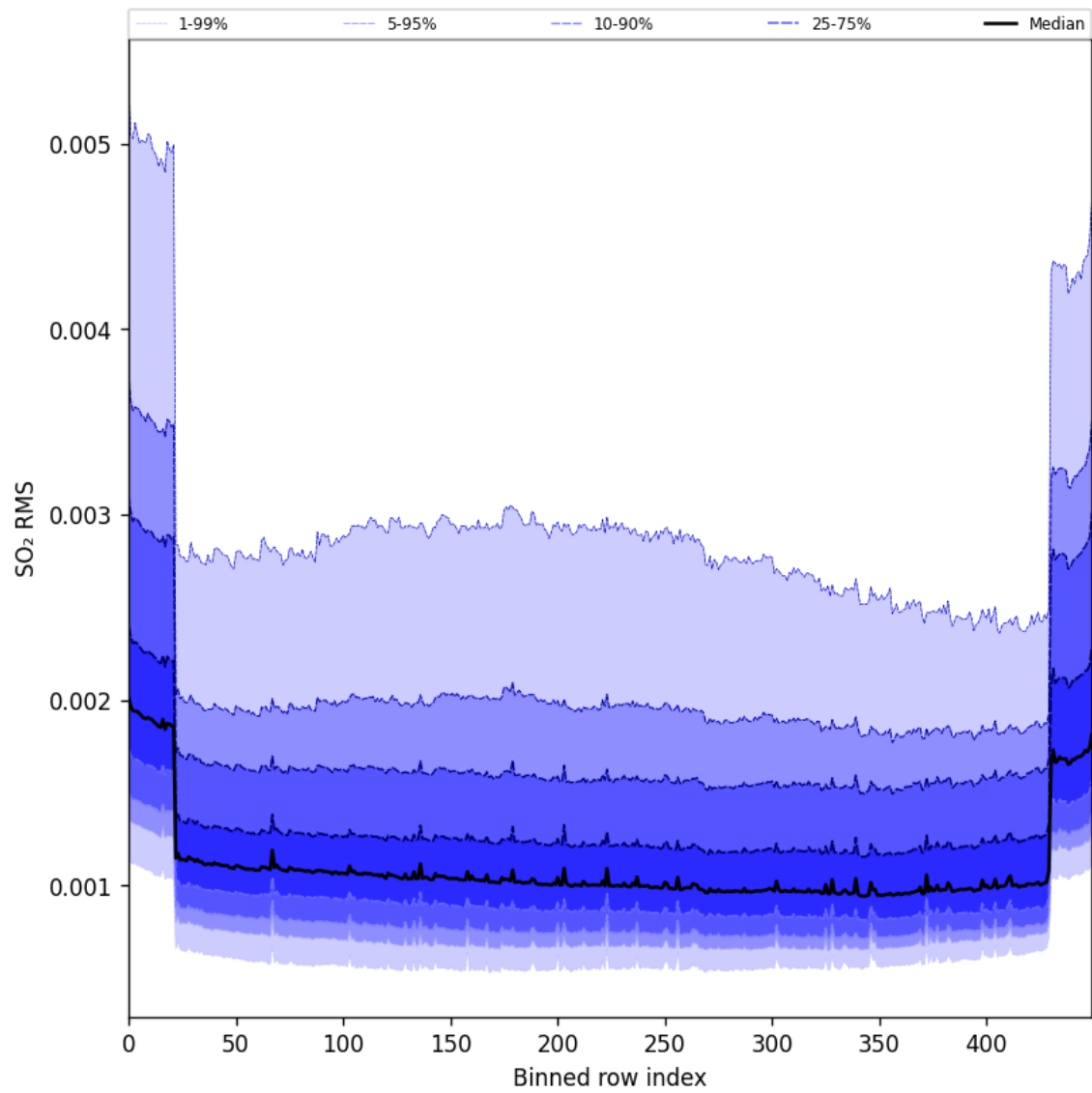
Figure 104: Along track statistics of “SO 2 RMS” for 2025-01-12 to 2025-01-13
