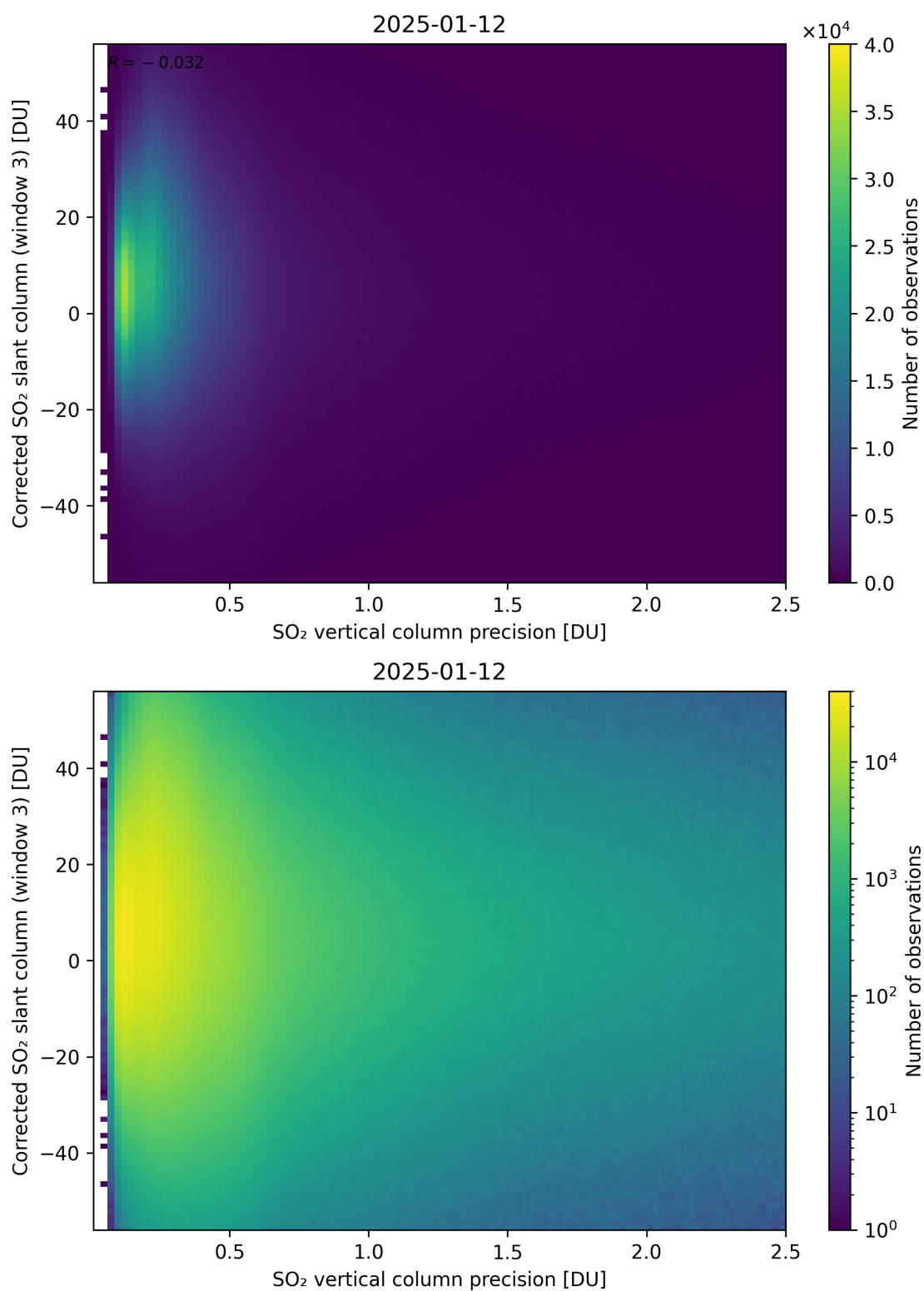
Figure 340: Scatter density plot of “SO 2 vertical column precision” against “Corrected SO 2 slant column (window 3)” for 2025-01-12 to 2025-01-13.
