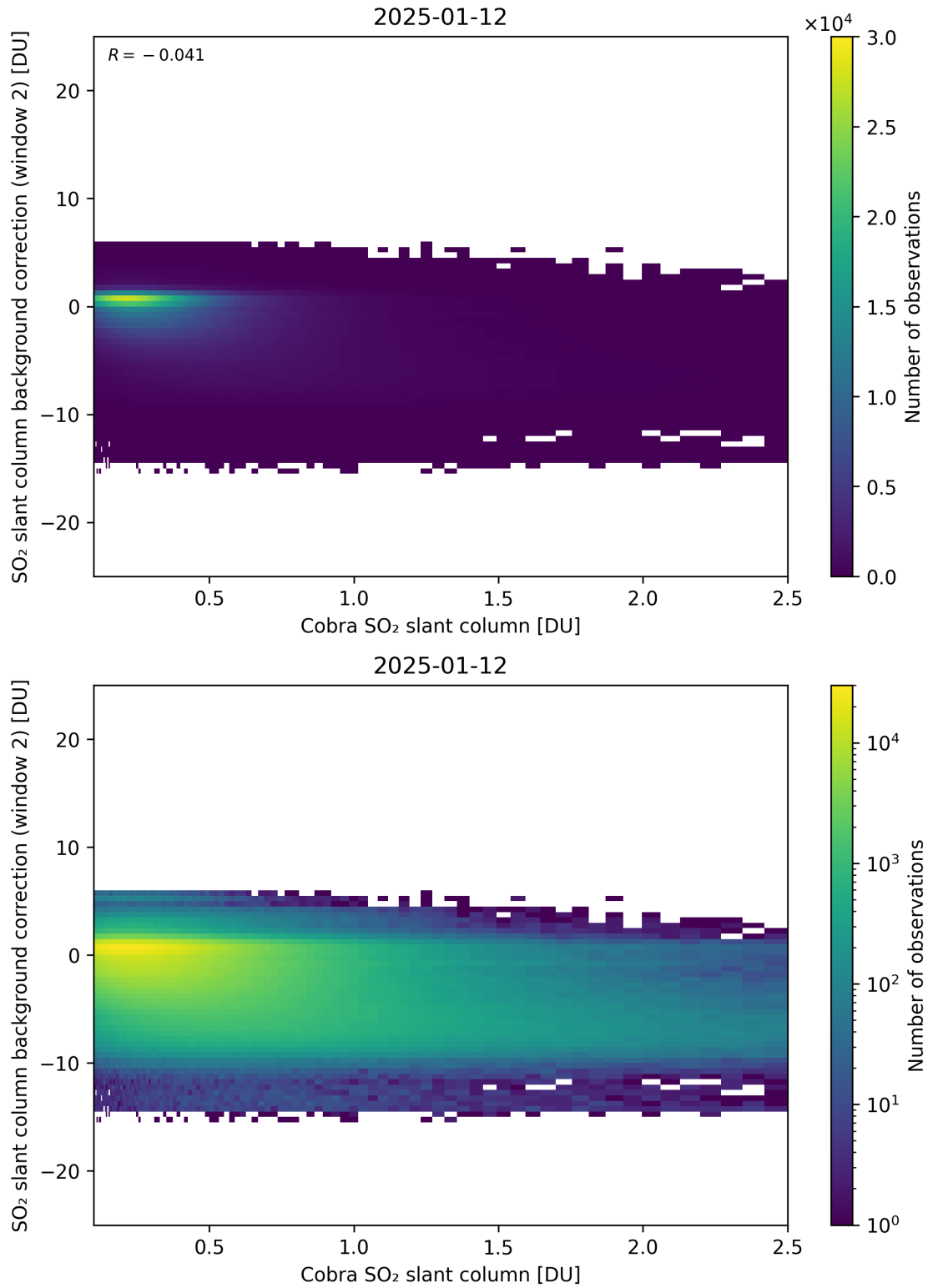
Figure 194: Scatter density plot of “Cobra SO 2 slant column” against “SO 2 slant column background correction (window 2)” for 2025-01-12 to 2025-01-13.
