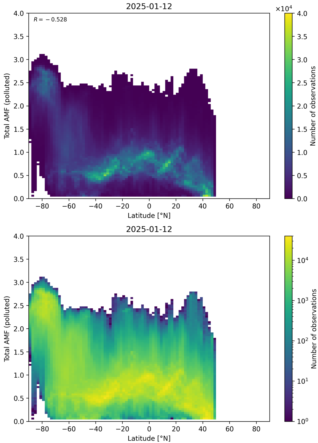
Figure 167: Scatter density plot of “Latitude” against “Total AMF (polluted)” for 2025-01-12 to 2025-01-13.
