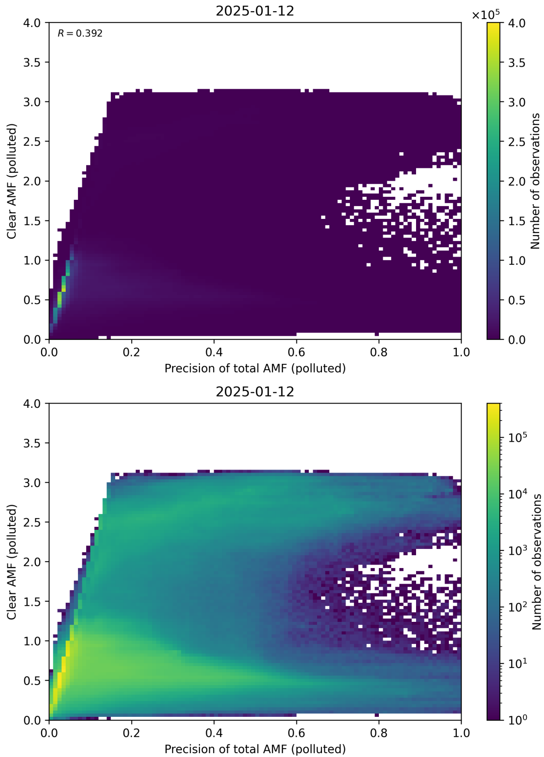
Figure 320: Scatter density plot of “Precision of total AMF (polluted)” against “Clear AMF (polluted)” for 2025-01-12 to 2025-01-13.
