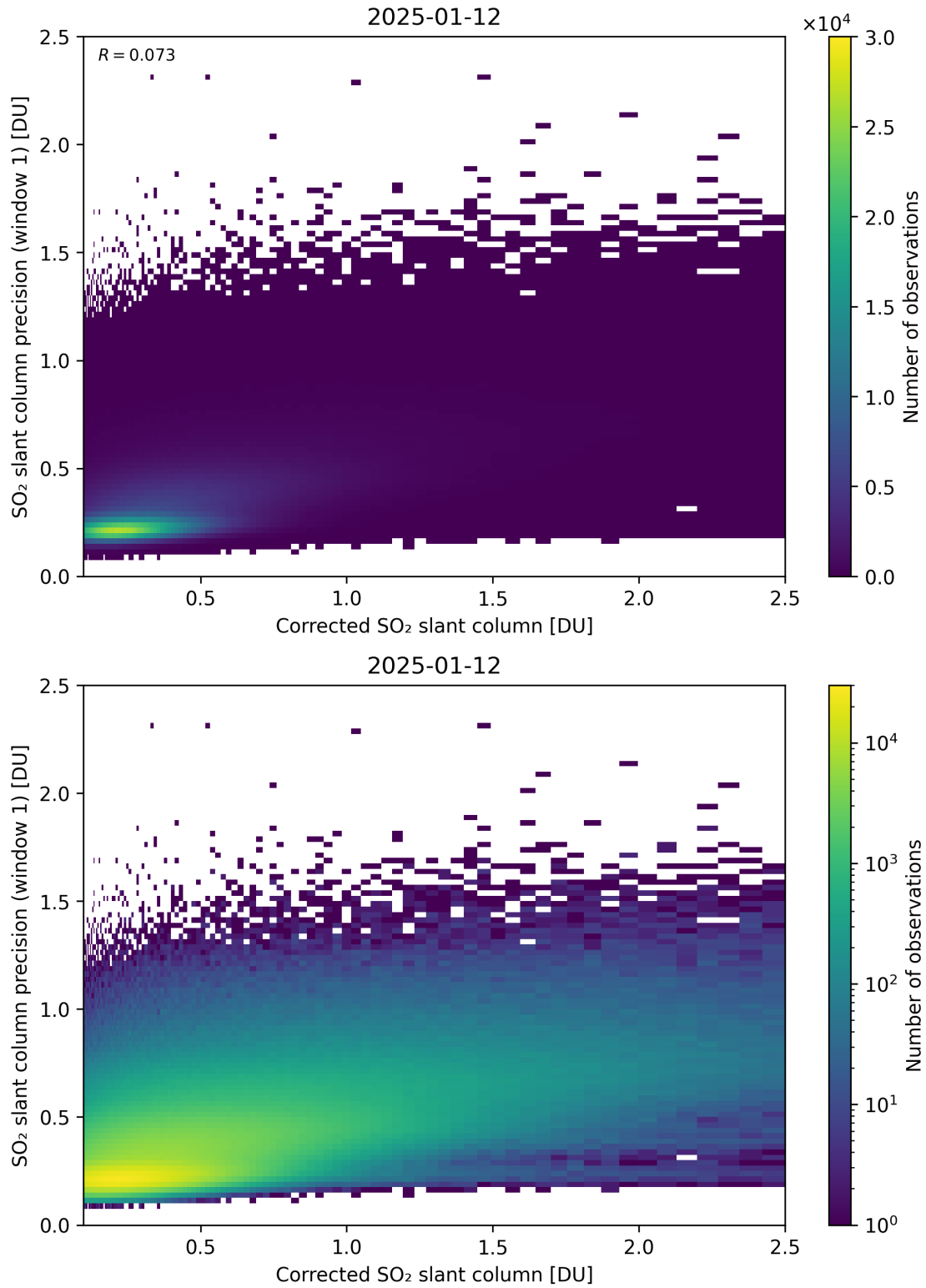
Figure 238: Scatter density plot of “Corrected SO 2 slant column” against “SO 2 slant column precision (window 1)” for 2025-01-12 to 2025-01-13.
