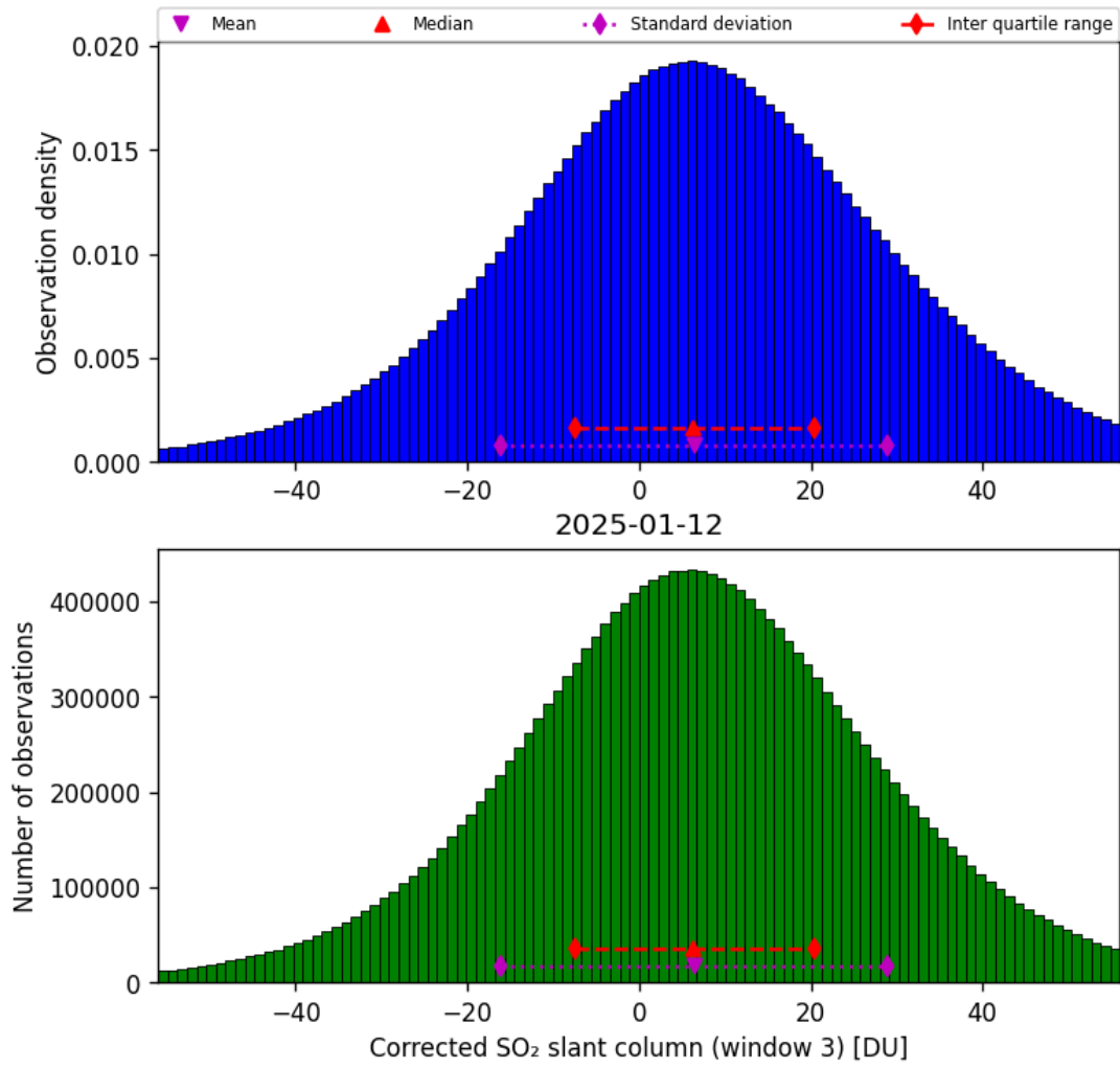
Figure 73: Histogram of “Corrected SO 2 slant column (window 3)” for 2025-01-12 to 2025-01-13
