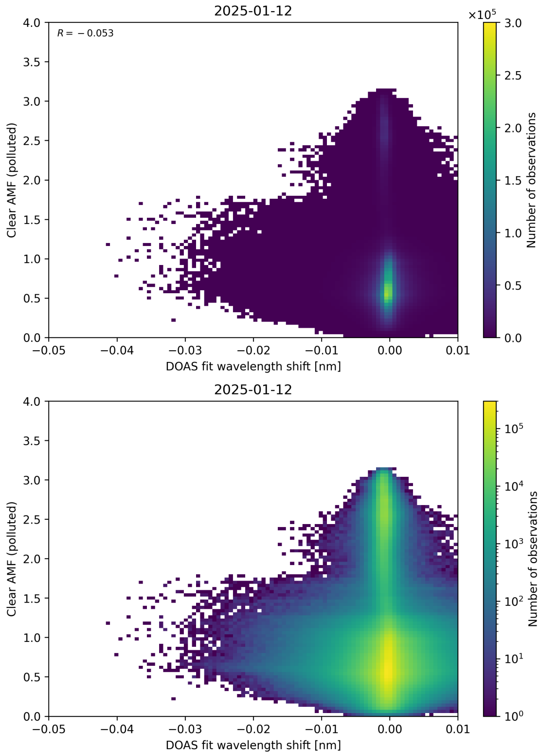
Figure 140: Scatter density plot of “DOAS fit wavelength shift” against “Clear AMF (polluted)” for 2025-01-12 to 2025-01-13.
