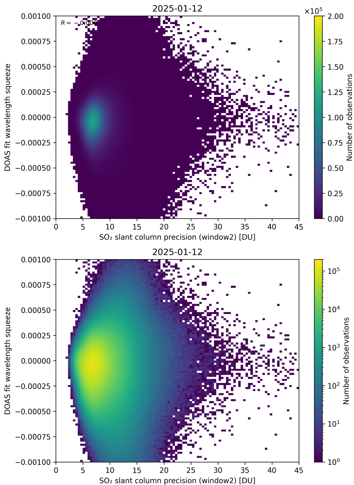
Figure 294: Scatter density plot of “SO 2 slant column precision (window2)” against “DOAS fit wavelength squeeze” for 2025-01-12 to 2025-01-13.
