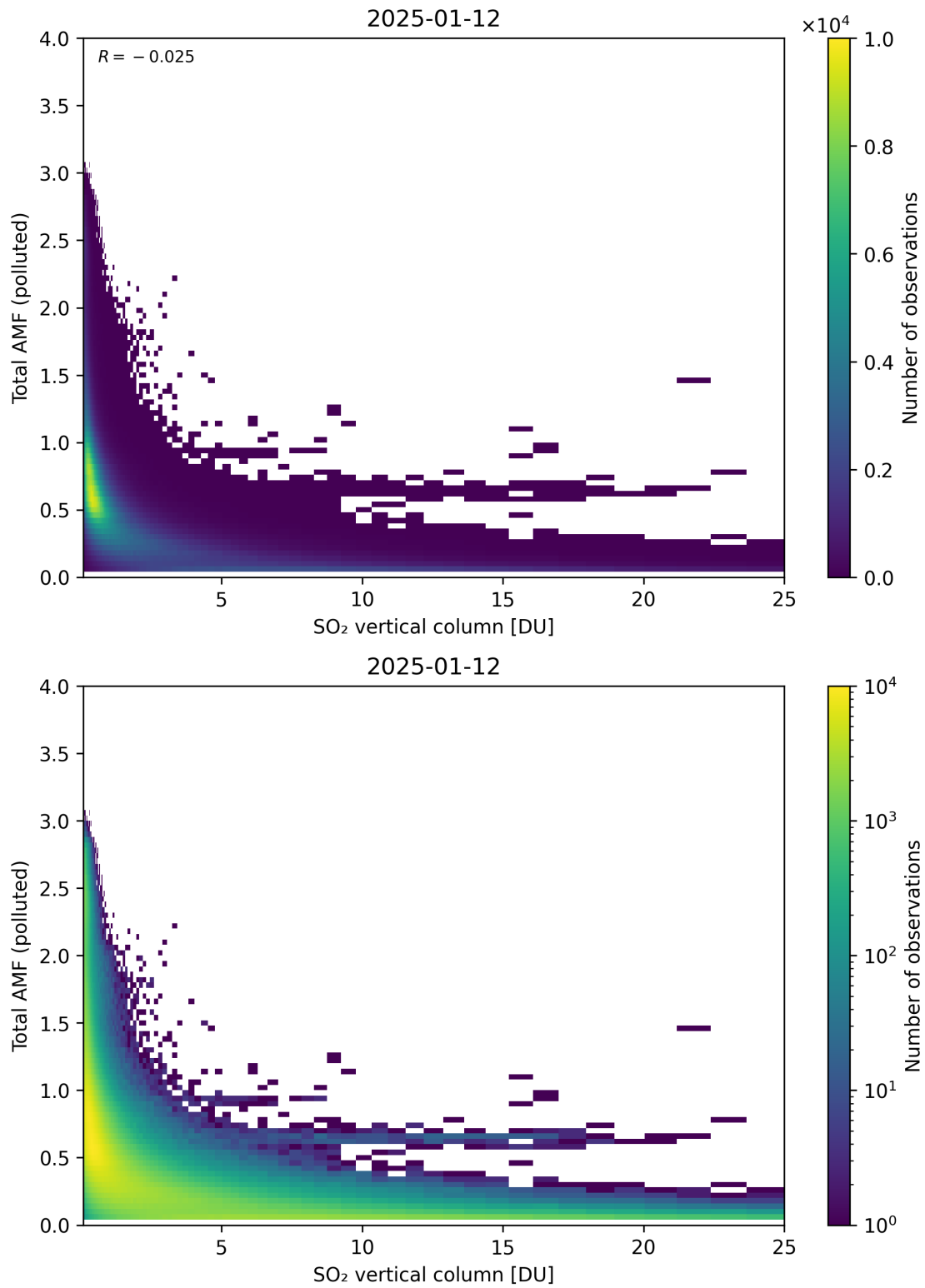
Figure 359: Scatter density plot of “SO 2 vertical column” against “Total AMF (polluted)” for 2025-01-12 to 2025-01-13.
