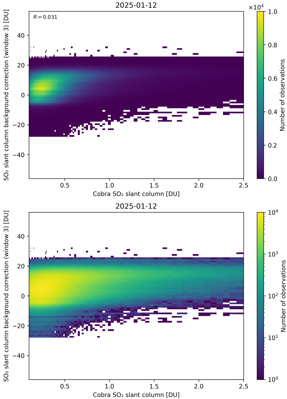
Figure 195: Scatter density plot of “Cobra SO 2 slant column” against “SO 2 slant column background correction (window 3)” for 2025-01-12 to 2025-01-13.
