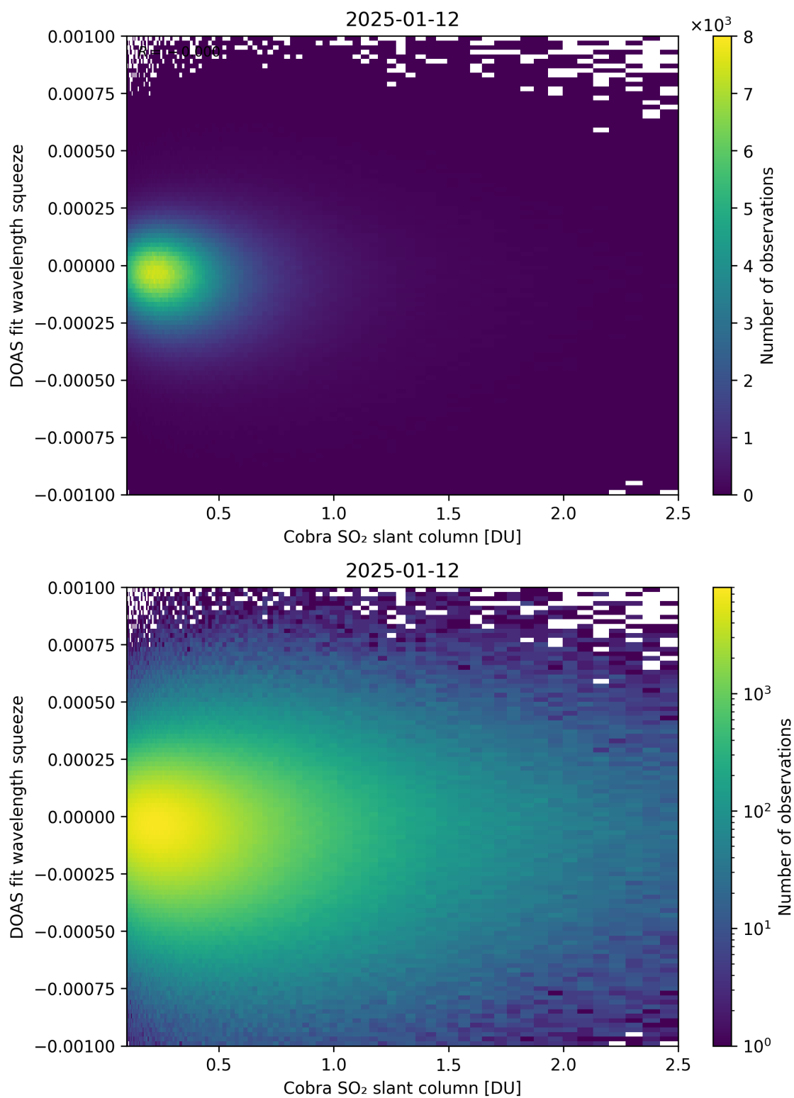
Figure 197: Scatter density plot of “Cobra SO 2 slant column” against “DOAS fit wavelength squeeze” for 2025-01-12 to 2025-01-13.
