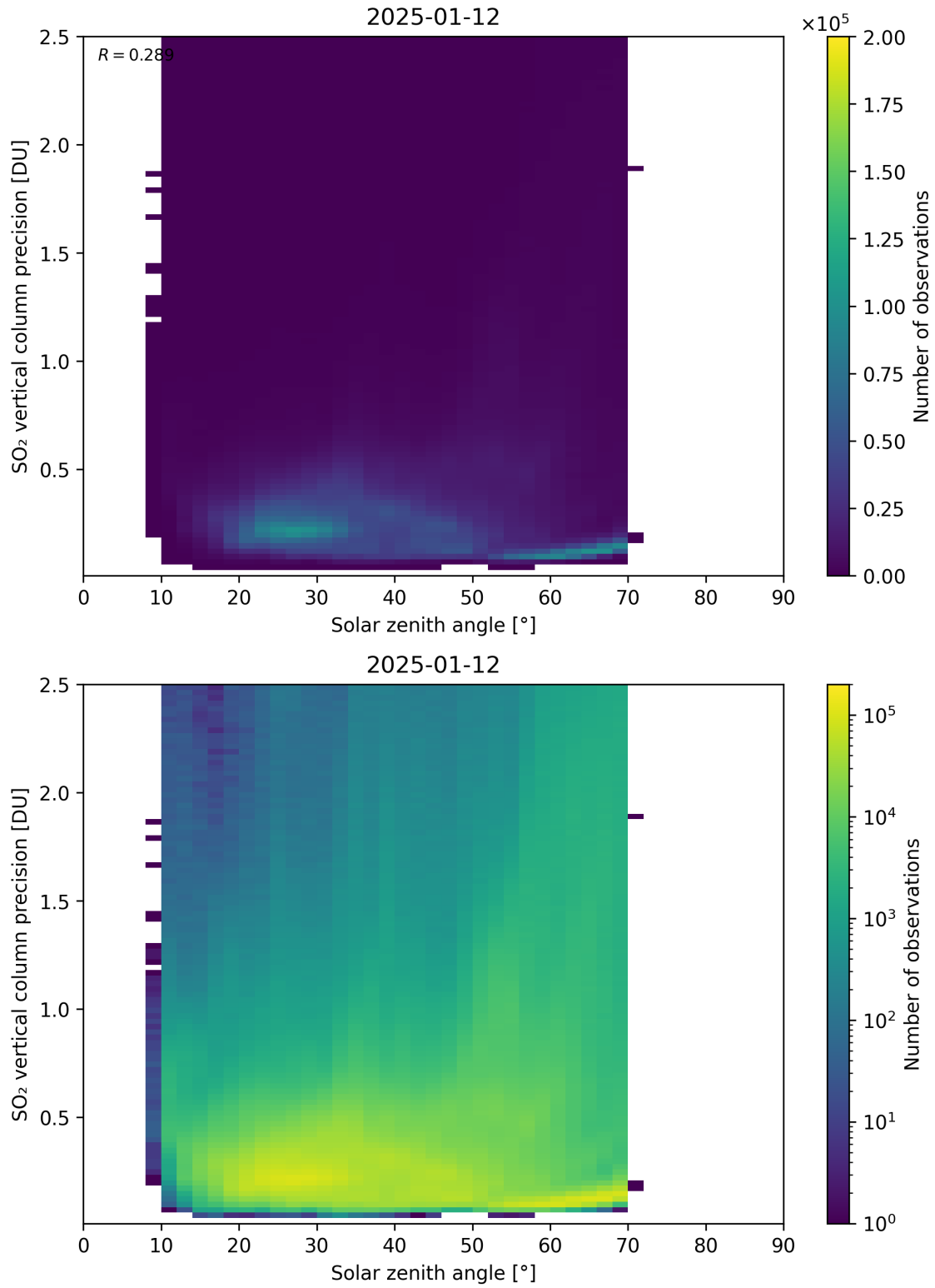
Figure 192: Scatter density plot of “Solar zenith angle” against “SO 2 vertical column precision” for 2025-01-12 to 2025-01-13.
