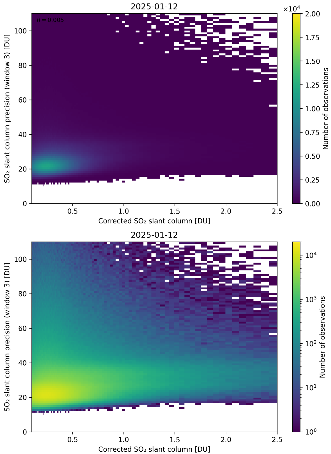
Figure 241: Scatter density plot of “Corrected SO 2 slant column” against “SO 2 slant column precision (window 3)” for 2025-01-12 to 2025-01-13.
