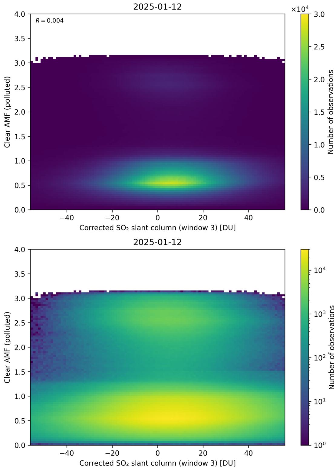
Figure 259: Scatter density plot of “Corrected SO 2 slant column (window 3)” against “Clear AMF (polluted)” for 2025-01-12 to 2025-01-13.
