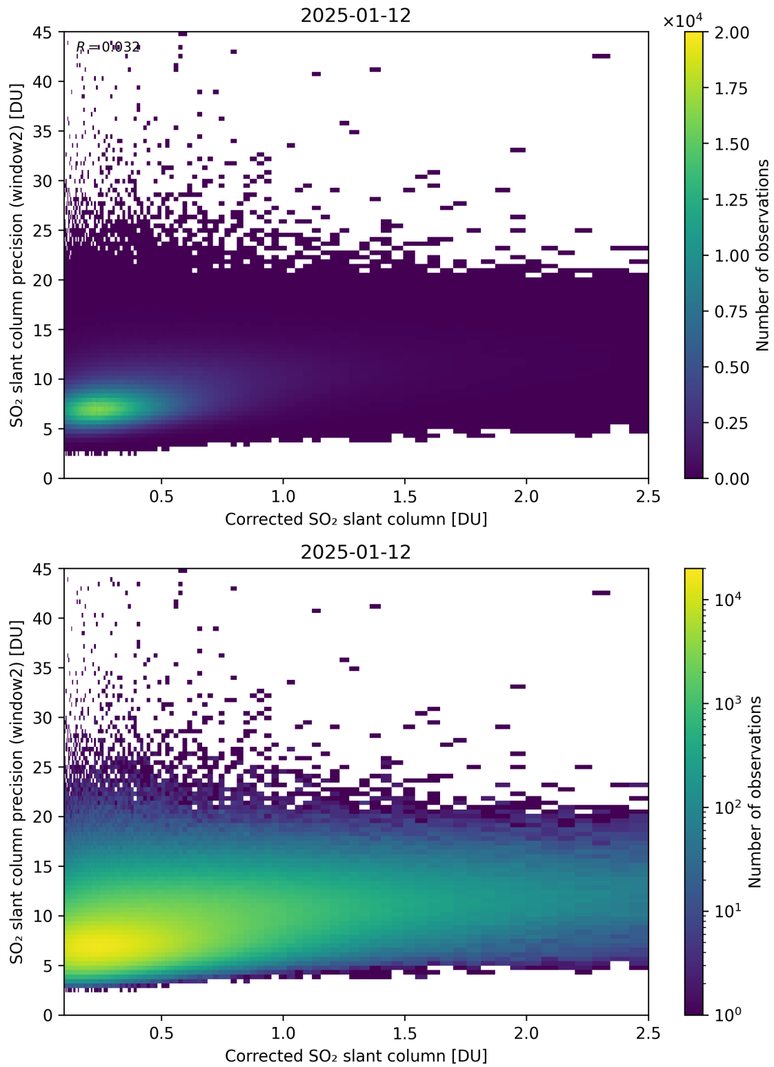
Figure 239: Scatter density plot of “Corrected SO 2 slant column” against “SO 2 slant column precision (window2)” for 2025-01-12 to 2025-01-13.
