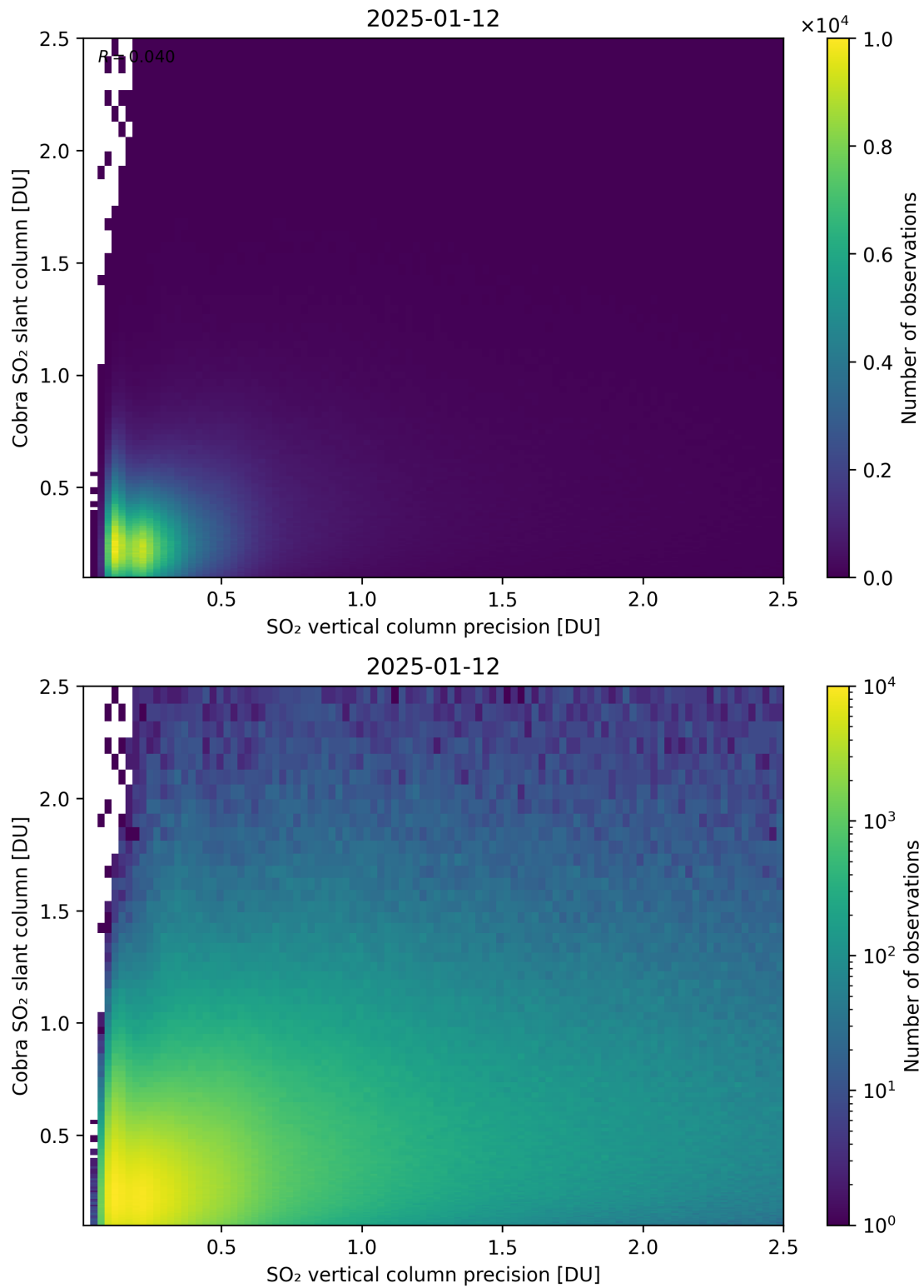
Figure 336: Scatter density plot of “SO 2 vertical column precision” against “Cobra SO 2 slant column” for 2025-01-12 to 2025-01-13.
