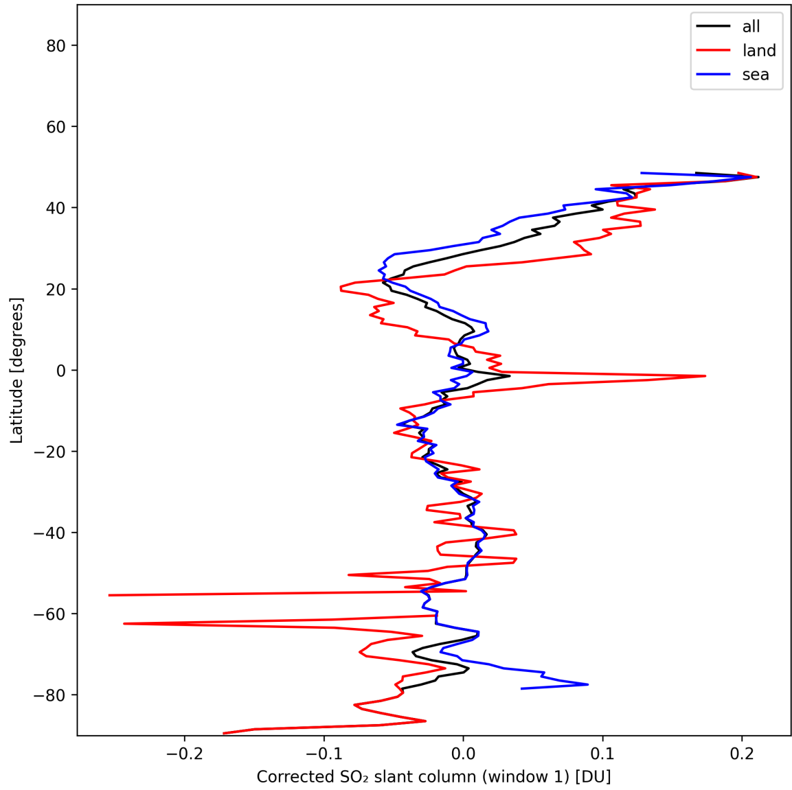
Figure 39: Zonal average of “Corrected SO 2 slant column (window 1)” for 2025-01-12 to 2025-01-13.
