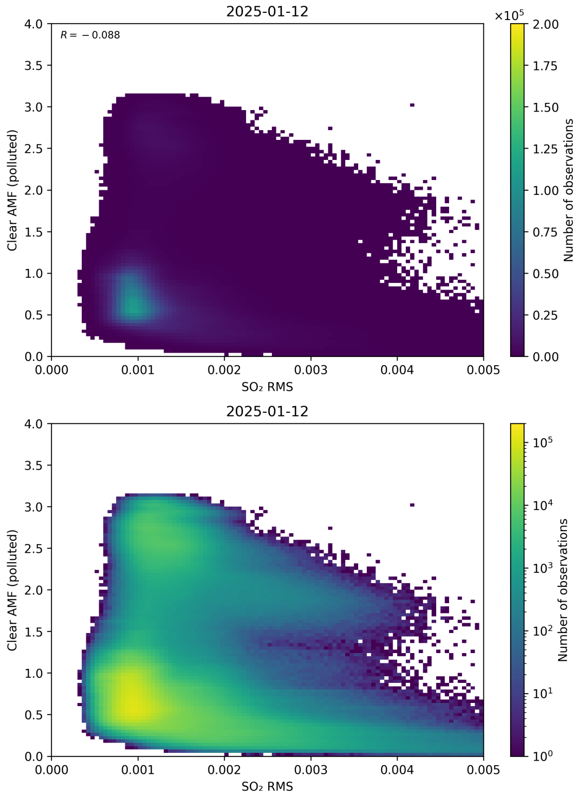
Figure 147: Scatter density plot of “SO 2 RMS” against “Clear AMF (polluted)” for 2025-01-12 to 2025-01-13.
