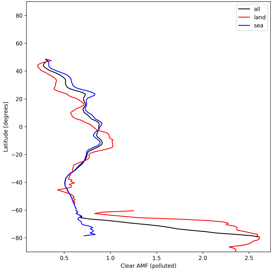
Figure 55: Zonal average of “Clear AMF (polluted)” for 2025-01-12 to 2025-01-13.
