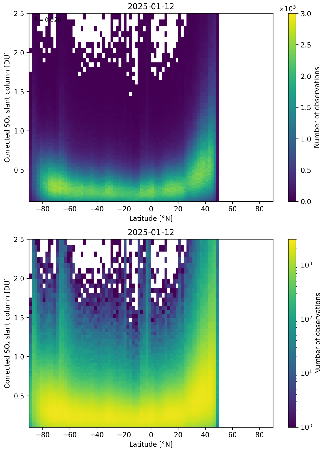
Figure 159: Scatter density plot of “Latitude” against “Corrected SO 2 slant column” for 2025-01-12 to 2025-01-13.
