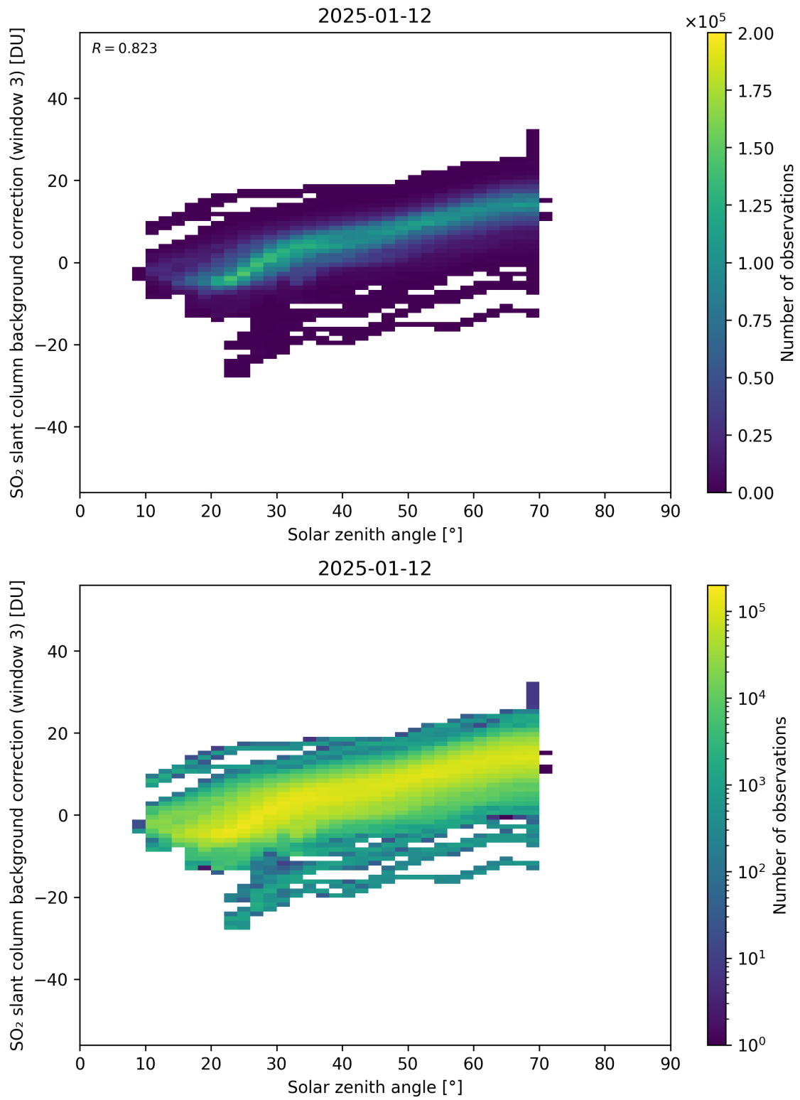
Figure 173: Scatter density plot of “Solar zenith angle” against “SO 2 slant column background correction (window 3)” for 2025-01-12 to 2025-01-13.
