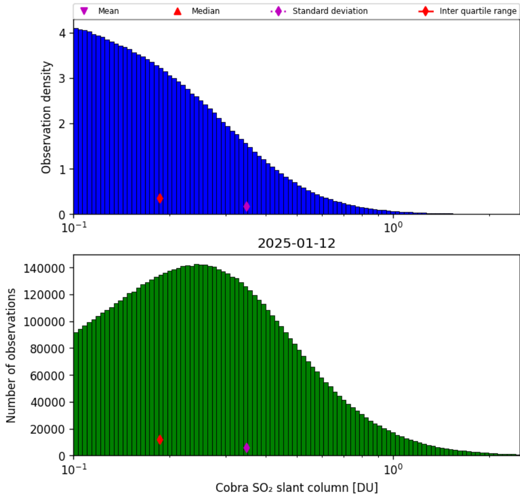
Figure 61: Histogram of “Cobra SO 2 slant column” for 2025-01-12 to 2025-01-13
