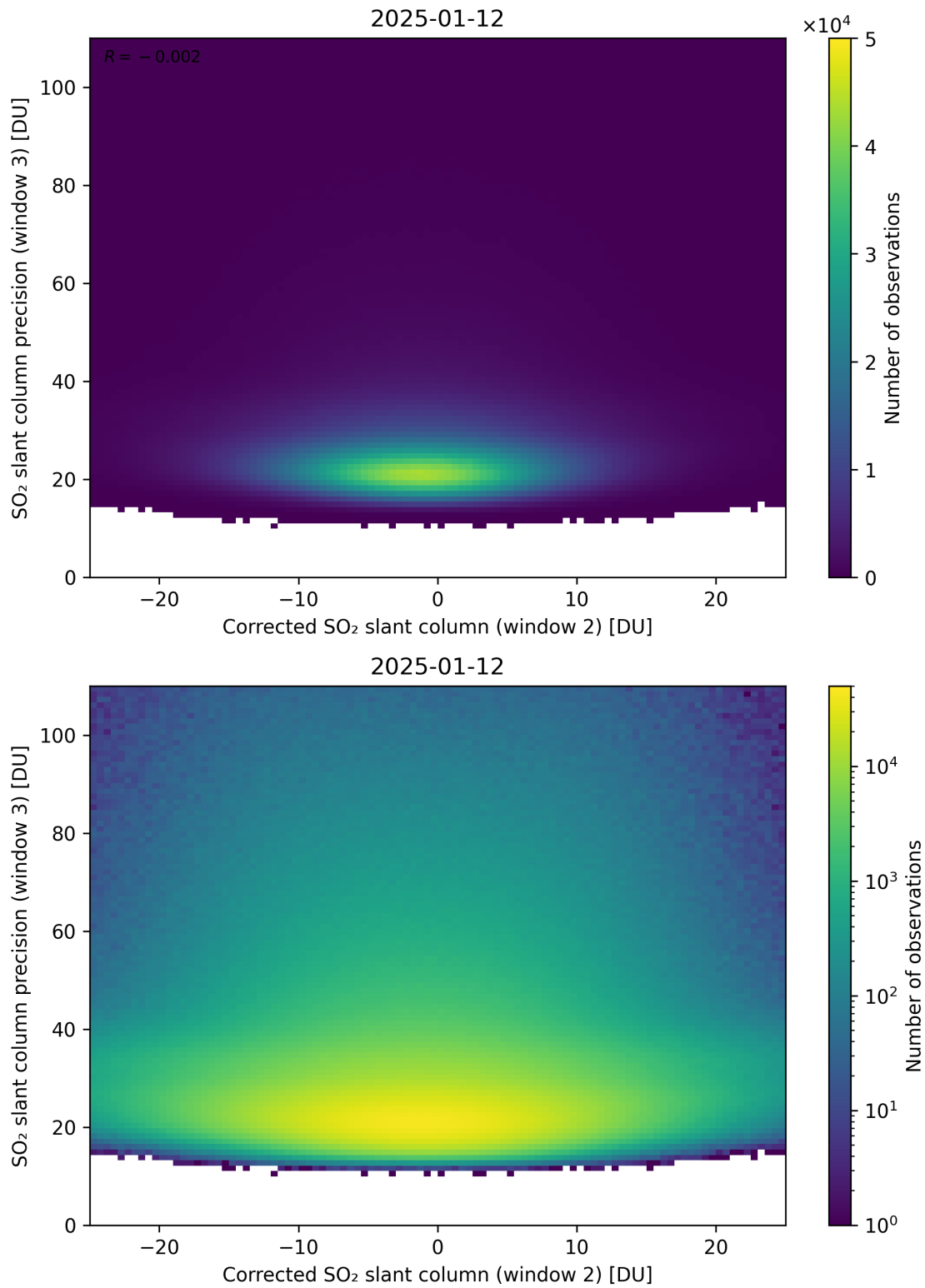
Figure 252: Scatter density plot of “Corrected SO 2 slant column (window 2)” against “SO 2 slant column precision (window 3)” for 2025-01-12 to 2025-01-13.
