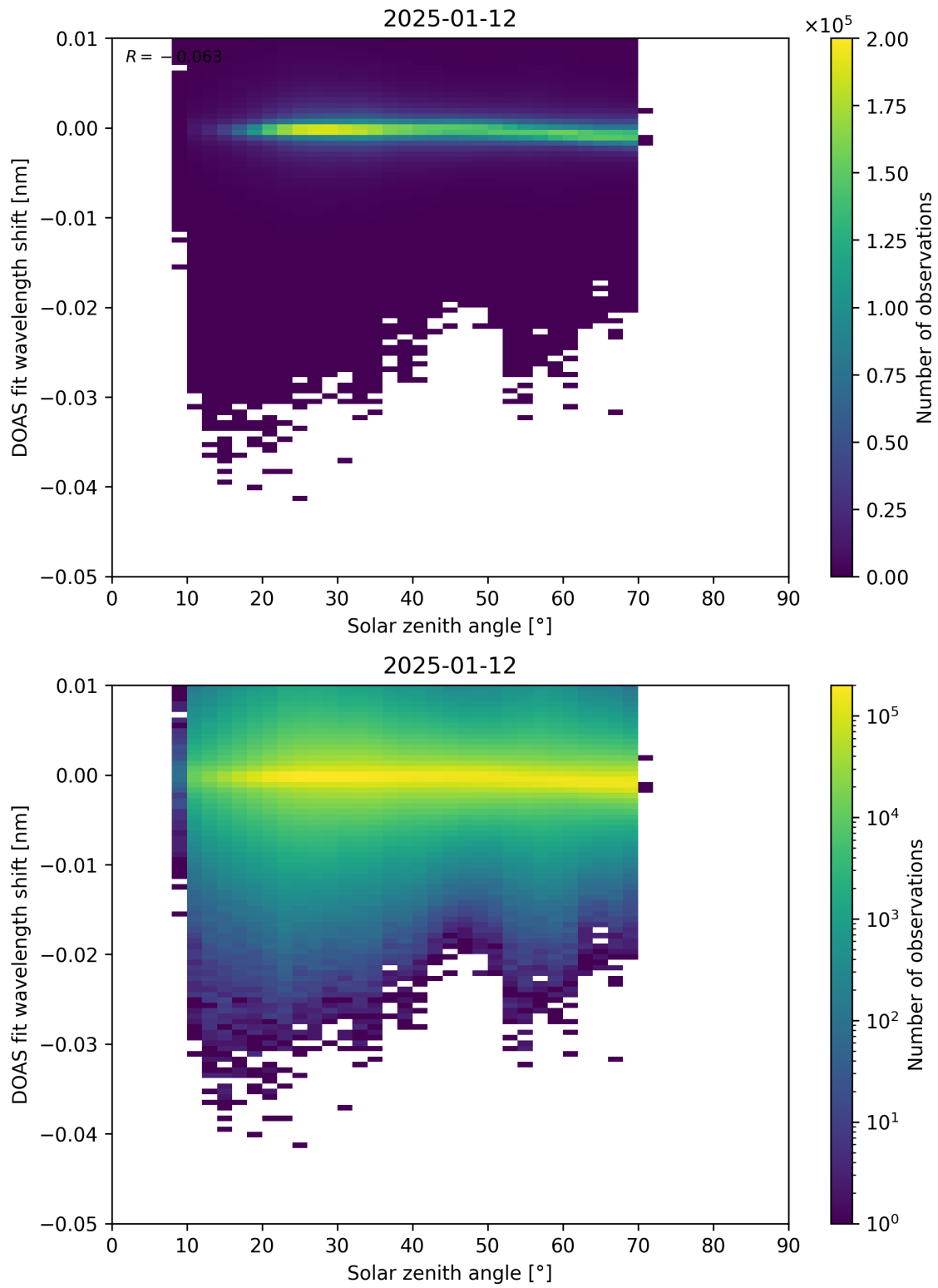
Figure 174: Scatter density plot of “Solar zenith angle” against “DOAS fit wavelength shift” for 2025-01-12 to 2025-01-13.
