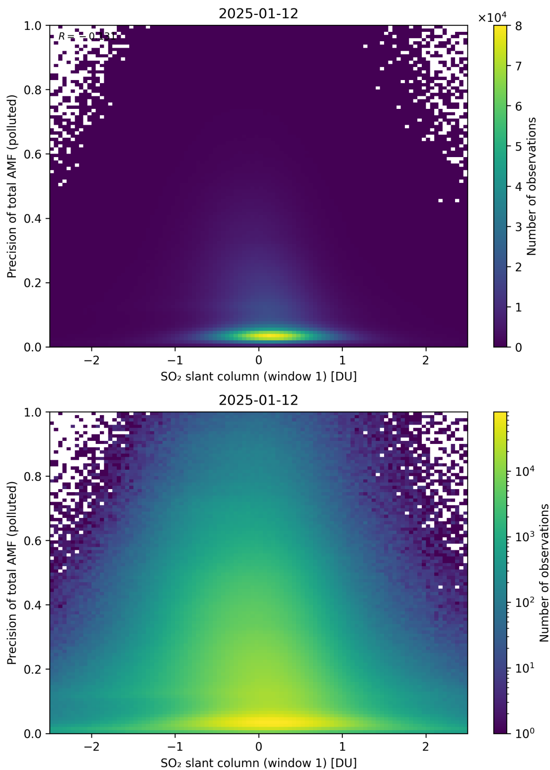
Figure 290: Scatter density plot of “SO 2 slant column (window 1)” against “Precision of total AMF (polluted)” for 2025-01-12 to 2025-01-13.
