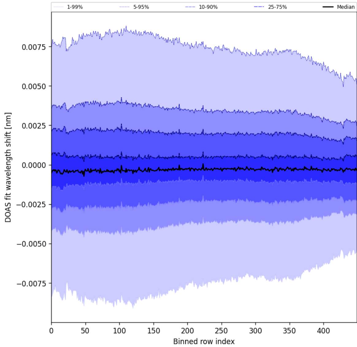
Figure 102: Along track statistics of “DOAS fit wavelength shift” for 2025-01-12 to 2025-01-13
