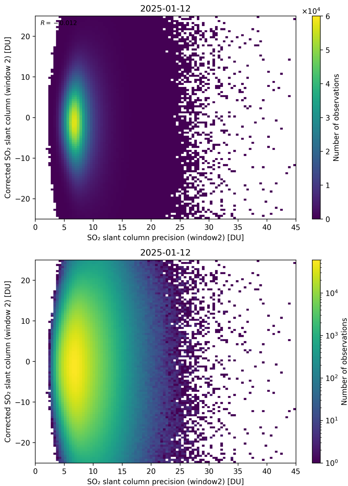
Figure 297: Scatter density plot of “SO 2 slant column precision (window2)” against “Corrected SO 2 slant column (window 2)” for 2025-01-12 to 2025-01-13.
