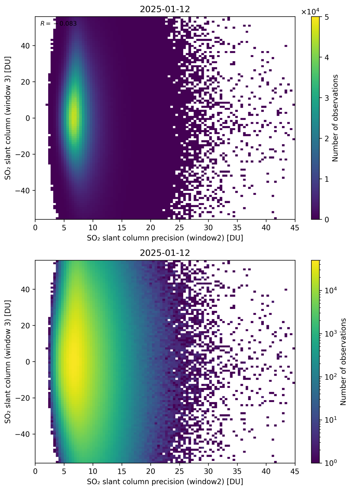
Figure 299: Scatter density plot of “SO 2 slant column precision (window2)” against “SO 2 slant column (window 3)” for 2025-01-12 to 2025-01-13.
