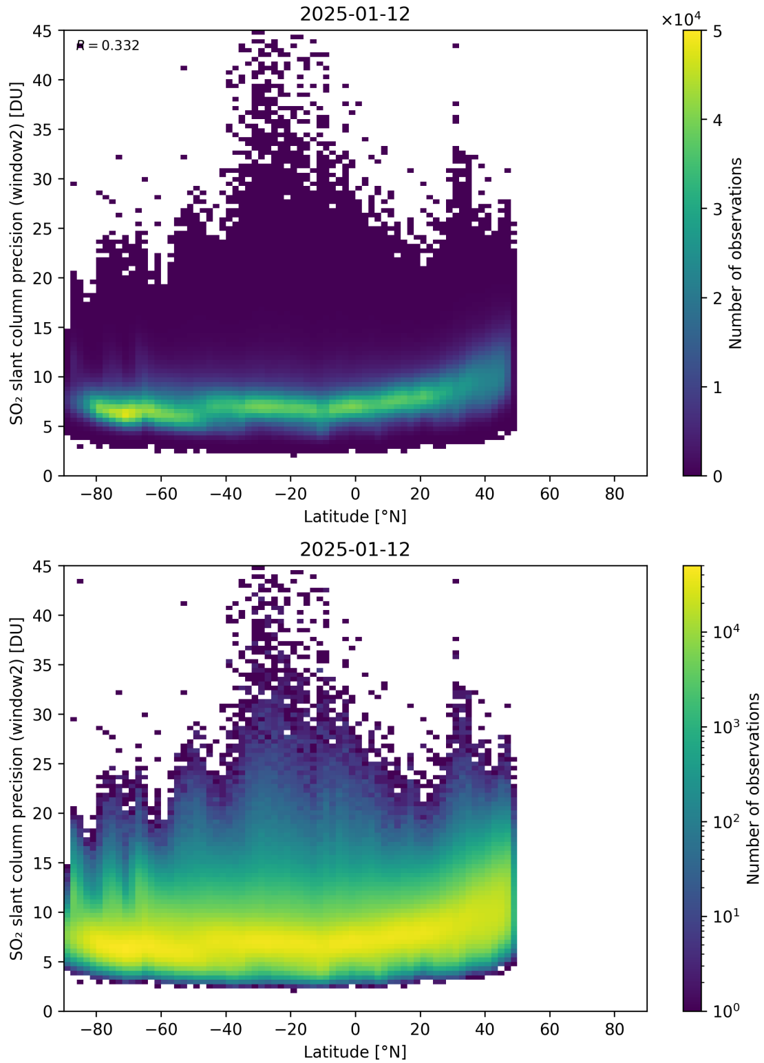
Figure 164: Scatter density plot of “Latitude” against “SO 2 slant column precision (window2)” for 2025-01-12 to 2025-01-13.
