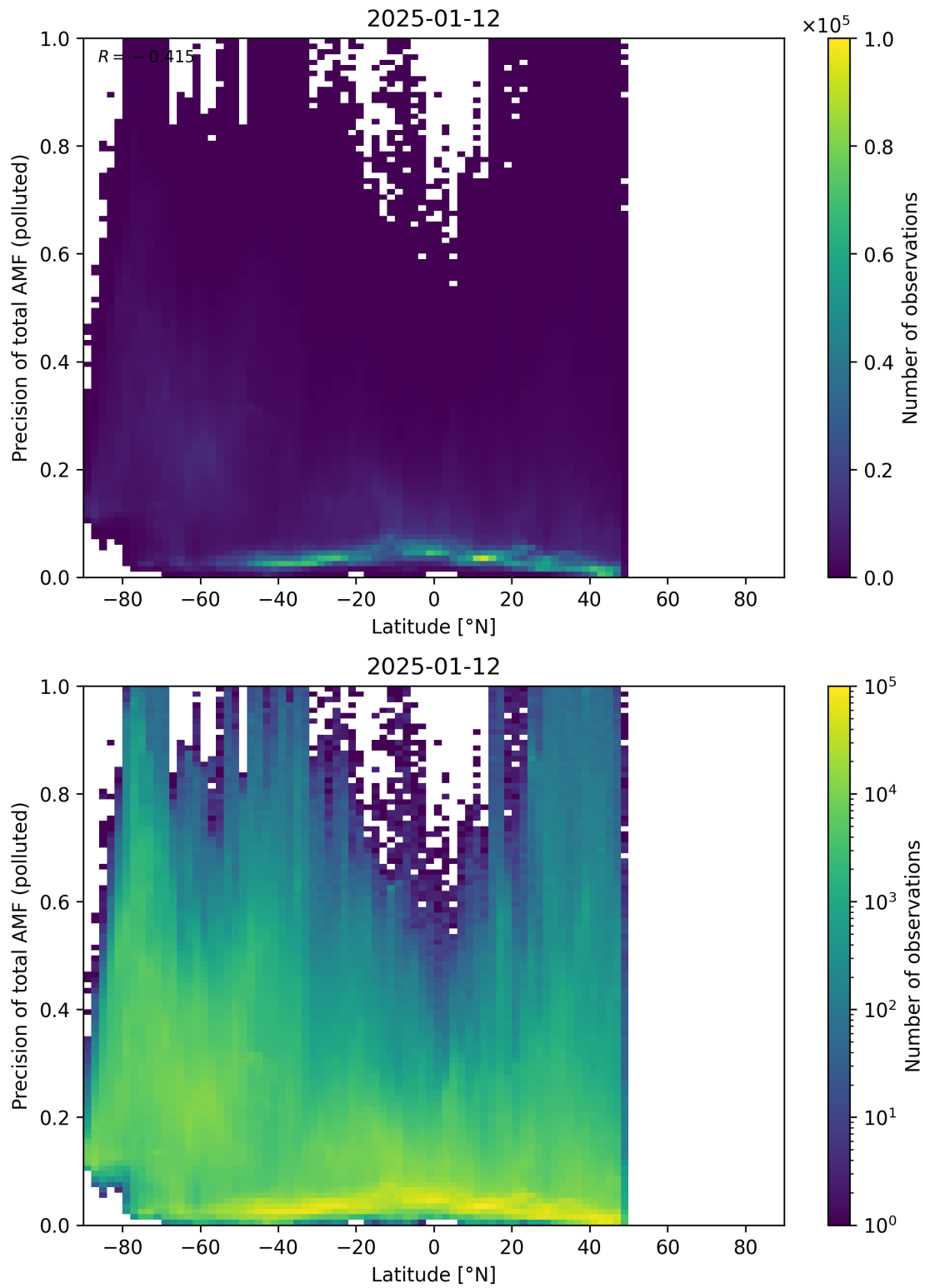
Figure 168: Scatter density plot of “Latitude” against “Precision of total AMF (polluted)” for 2025-01-12 to 2025-01-13.
