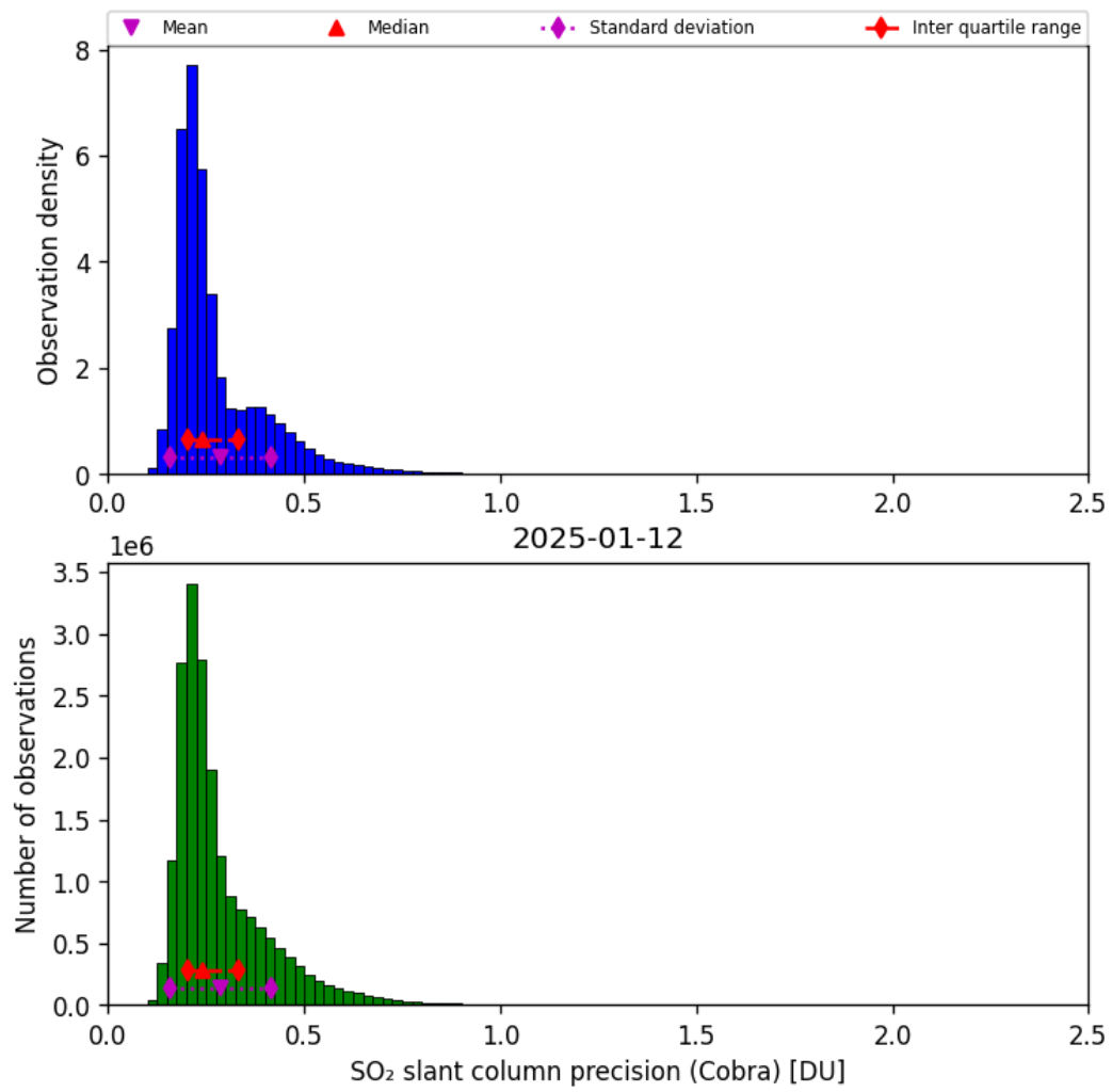
Figure 62: Histogram of “SO 2 slant column precision (Cobra)” for 2025-01-12 to 2025-01-13
