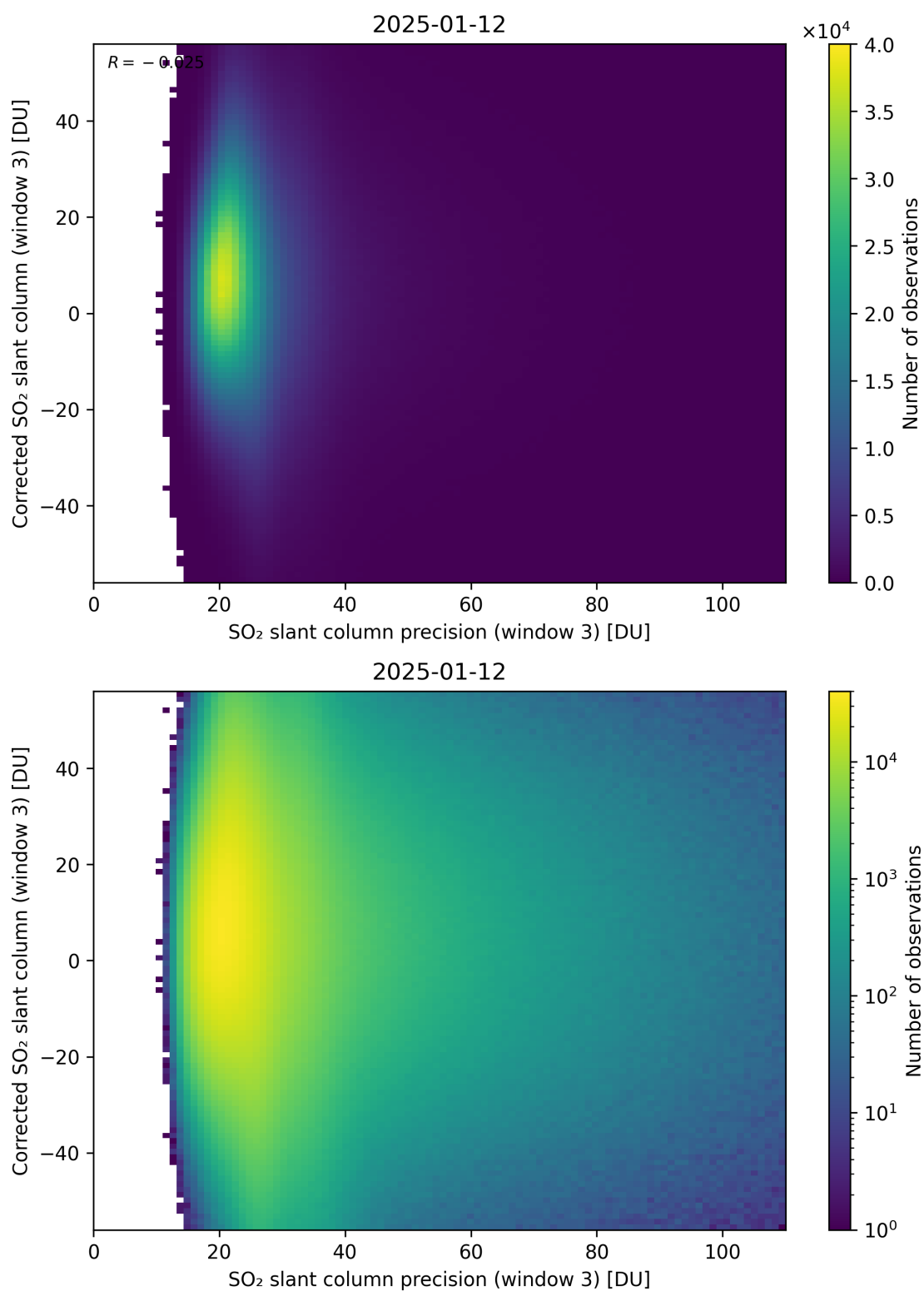
Figure 312: Scatter density plot of “SO 2 slant column precision (window 3)” against “Corrected SO 2 slant column (window 3)” for 2025-01-12 to 2025-01-13.
