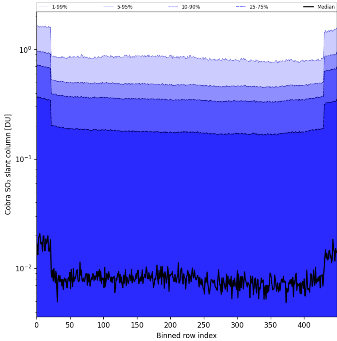
Figure 87: Along track statistics of "Cobra SO 2 slant column" for 2025-01-12 to 2025-01-13
