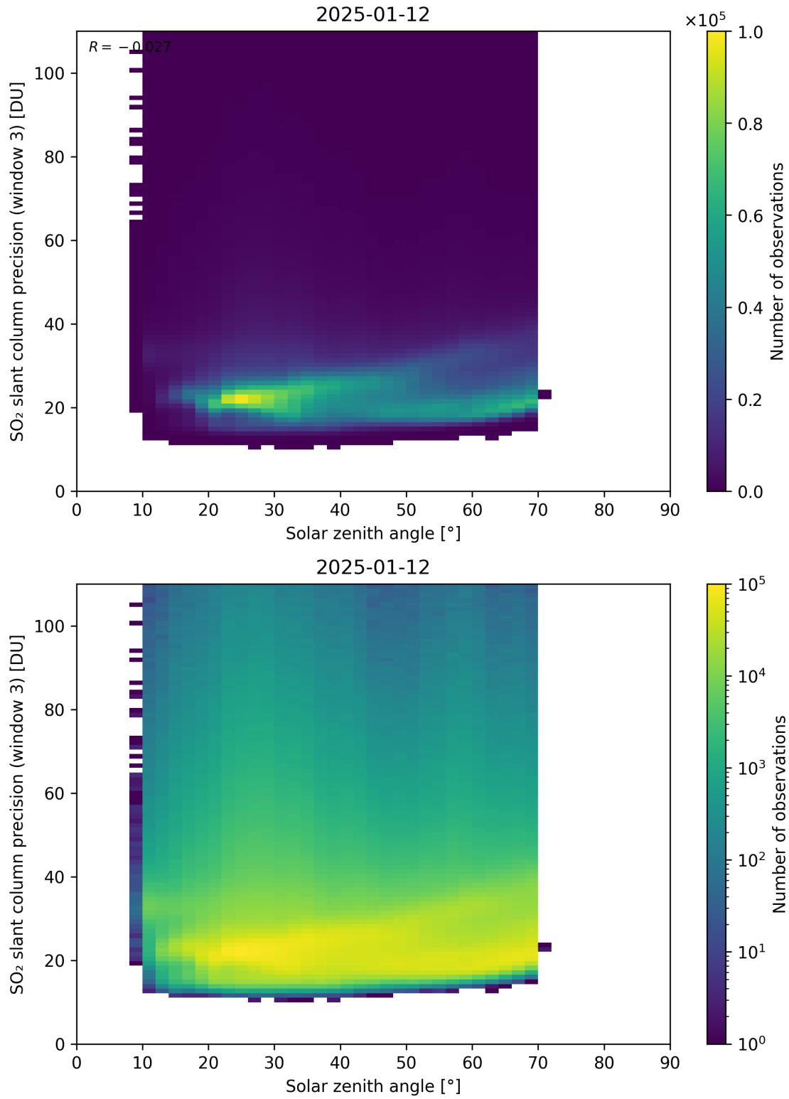
Figure 188: Scatter density plot of “Solar zenith angle” against “SO 2 slant column precision (window 3)” for 2025-01-12 to 2025-01-13.
