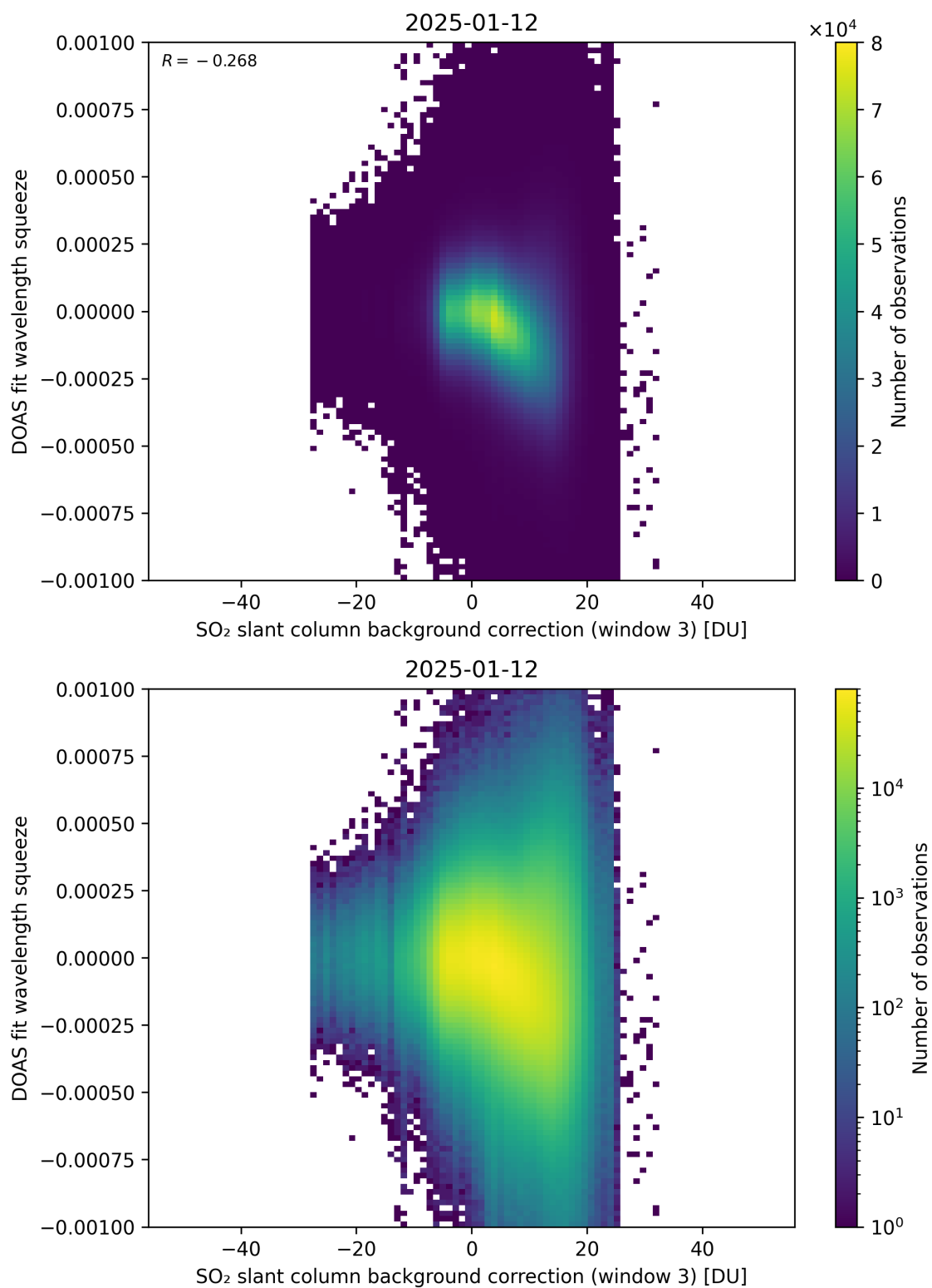
Figure 133: Scatter density plot of “SO 2 slant column background correction (window 3)” against “DOAS fit wavelength squeeze” for 2025-01-12 to 2025-01-13.
