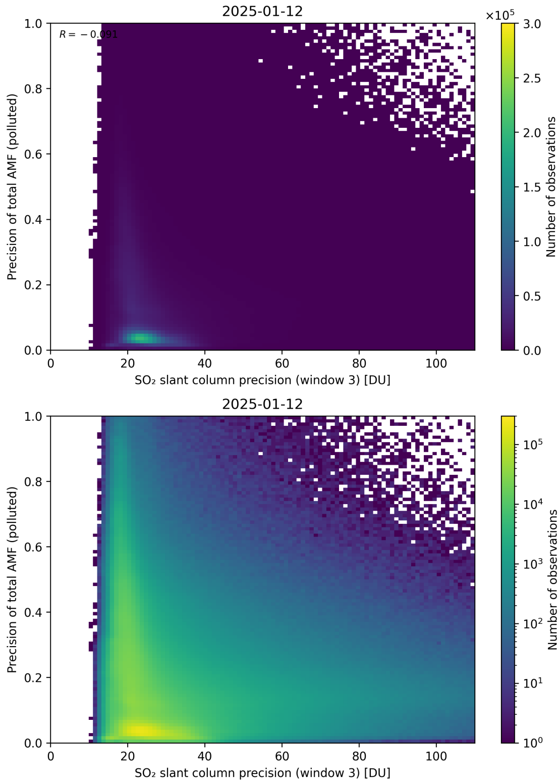
Figure 314: Scatter density plot of “SO 2 slant column precision (window 3)” against “Precision of total AMF (polluted)” for 2025-01-12 to 2025-01-13.
