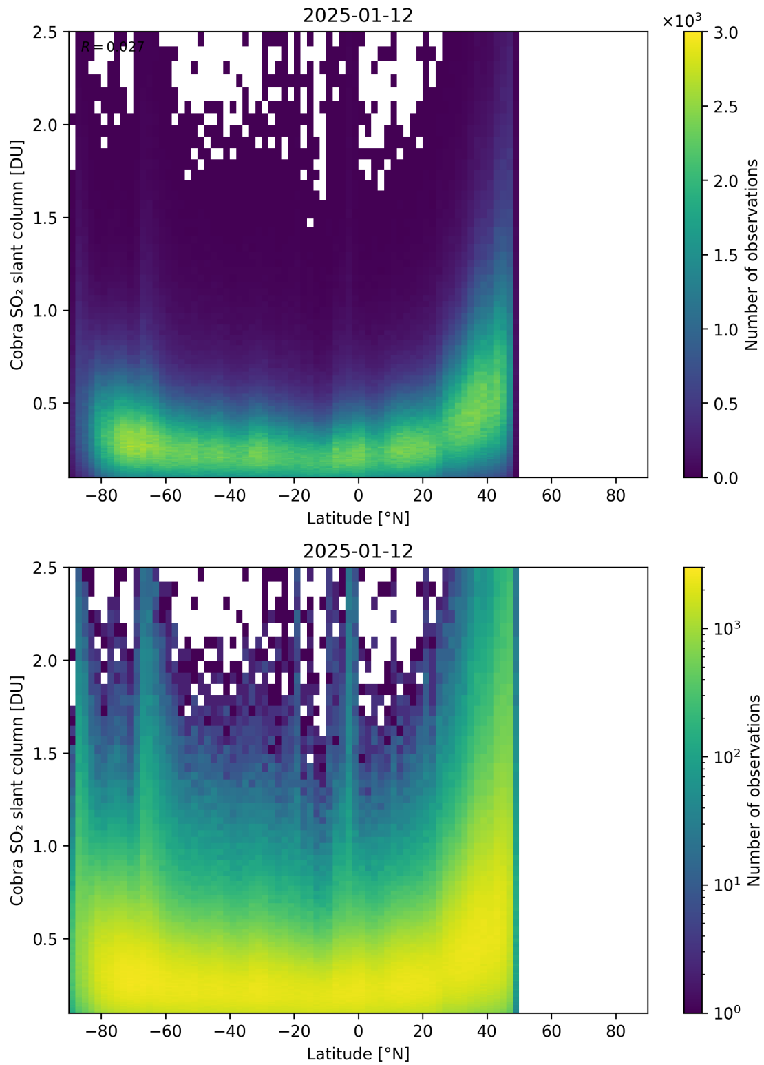
Figure 157: Scatter density plot of “Latitude” against “Cobra SO 2 slant column” for 2025-01-12 to 2025-01-13.
