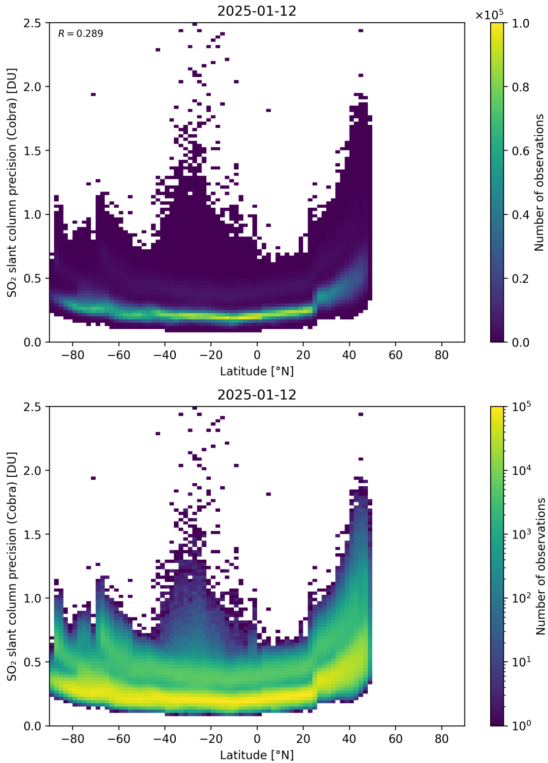
Figure 158: Scatter density plot of “Latitude” against “SO 2 slant column precision (Cobra)” for 2025-01-12 to 2025-01-13.
