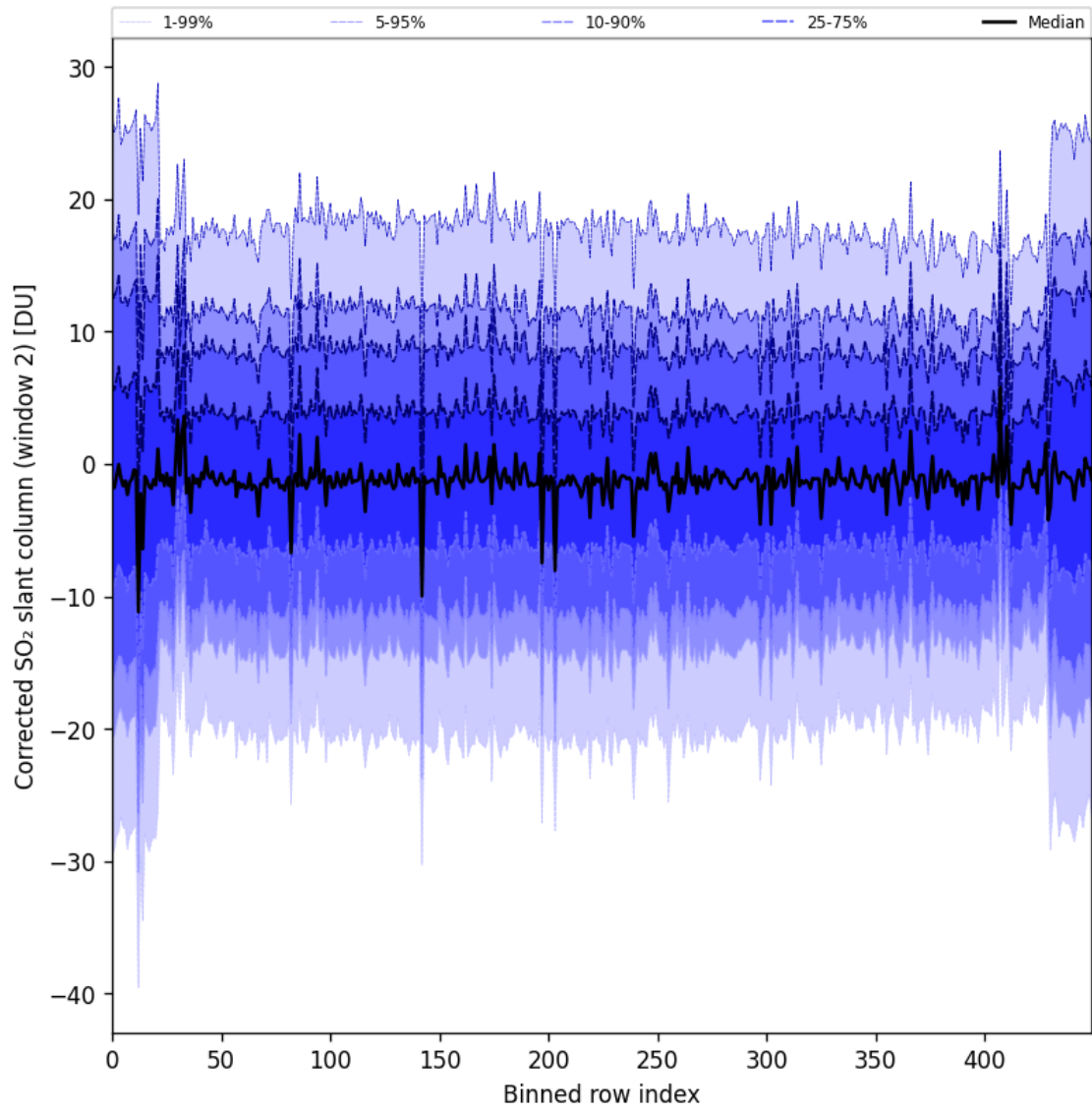
Figure 95: Along track statistics of “Corrected SO 2 slant column (window 2)” for 2025-01-12 to 2025-01-13
