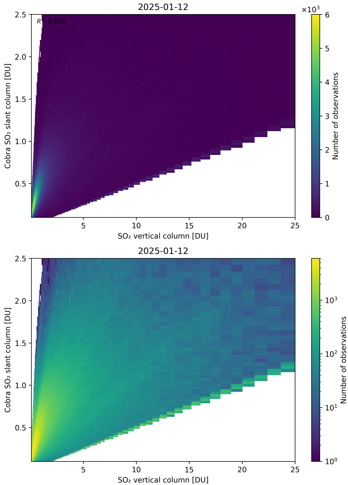
Figure 349: Scatter density plot of “SO 2 vertical column” against “Cobra SO 2 slant column” for 2025-01-12 to 2025-01-13.
