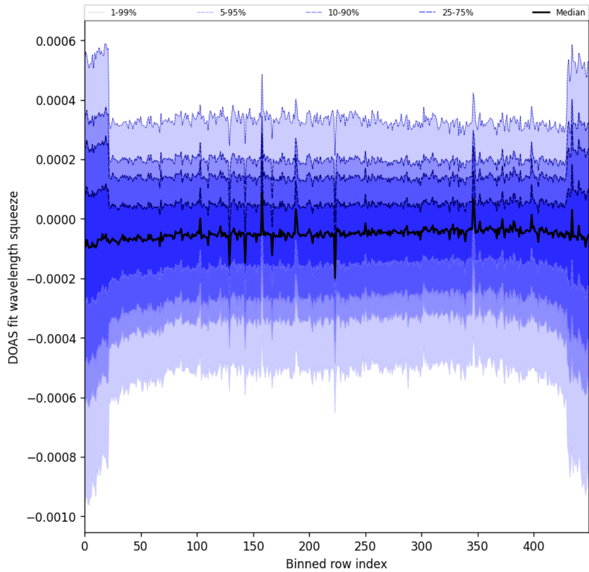
Figure 103: Along track statistics of “DOAS fit wavelength squeeze” for 2025-01-12 to 2025-01-13
