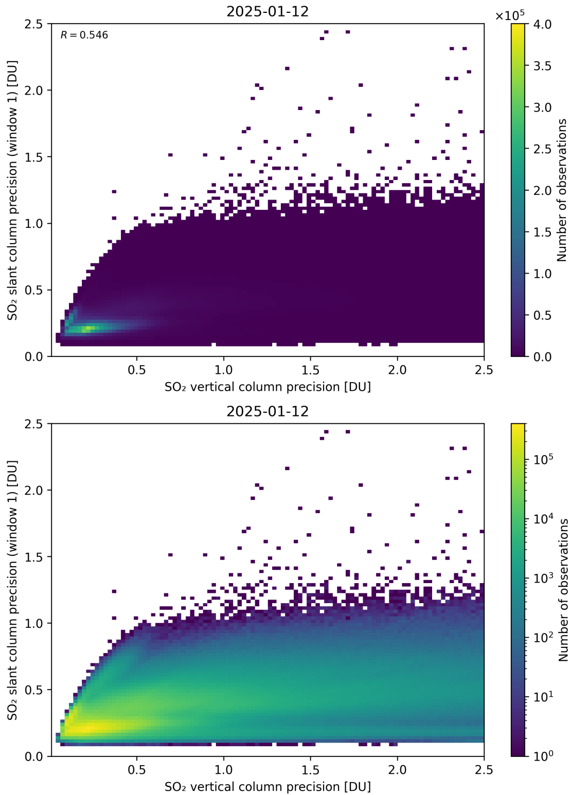
Figure 342: Scatter density plot of “SO 2 vertical column precision” against “SO 2 slant column precision (window 1)” for 2025-01-12 to 2025-01-13.
