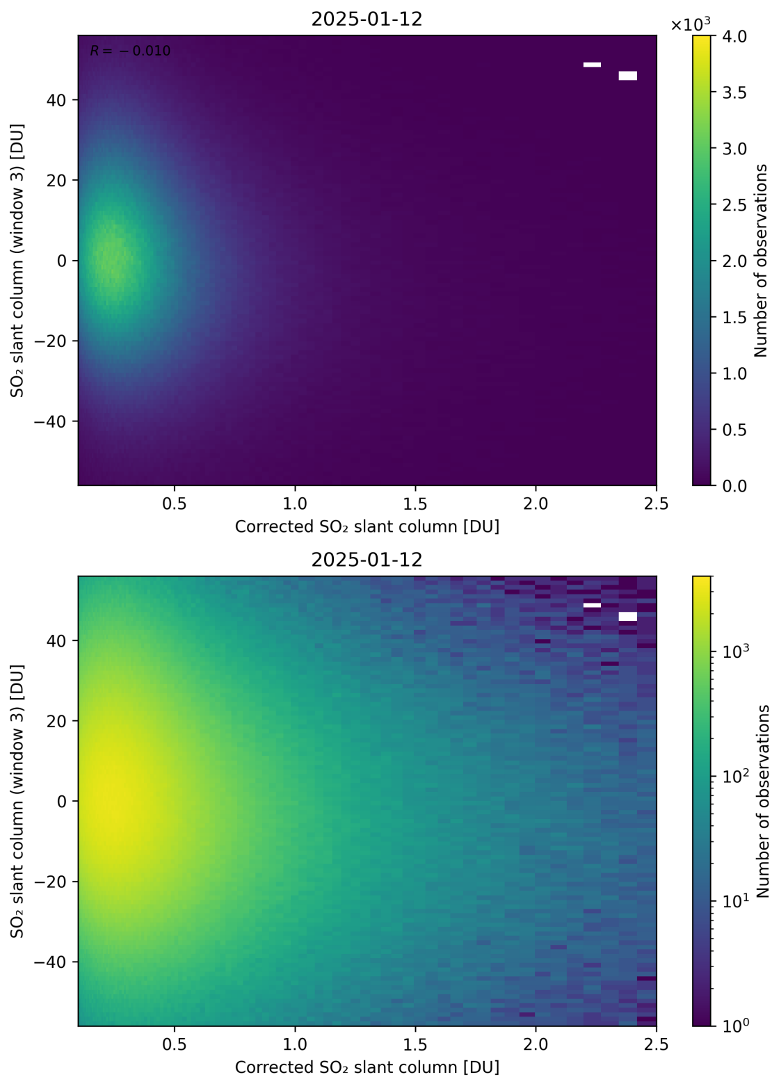
Figure 240: Scatter density plot of “Corrected SO 2 slant column” against “SO 2 slant column (window 3)” for 2025-01-12 to 2025-01-13.
