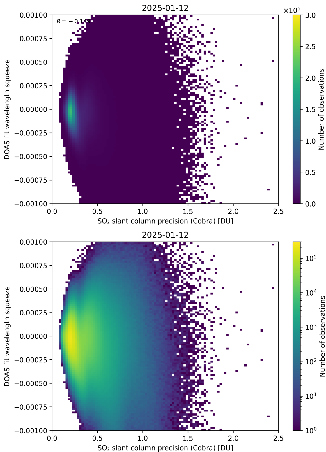
Figure 203: Scatter density plot of “SO 2 slant column precision (Cobra)” against “DOAS fit wavelength squeeze” for 2025-01-12 to 2025-01-13.
