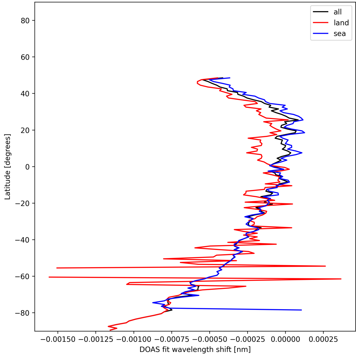
Figure 50: Zonal average of “DOAS fit wavelength shift” for 2025-01-12 to 2025-01-13.
