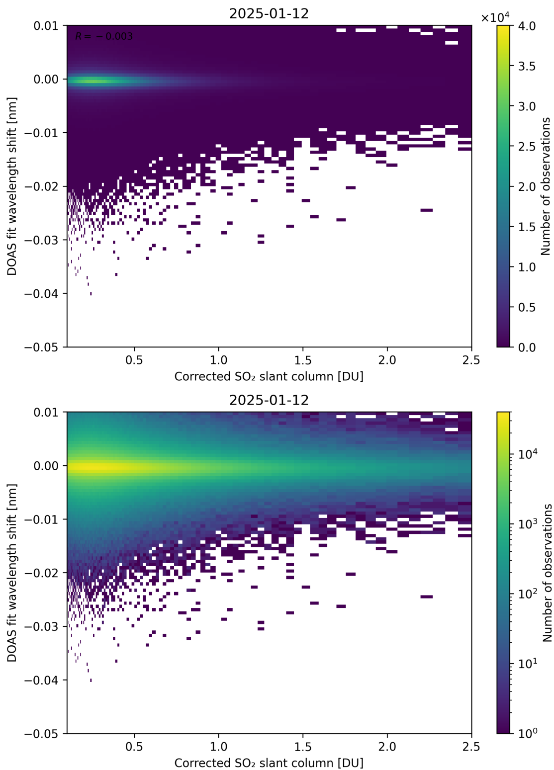
Figure 229: Scatter density plot of “Corrected SO 2 slant column” against “DOAS fit wavelength shift” for 2025-01-12 to 2025-01-13.
