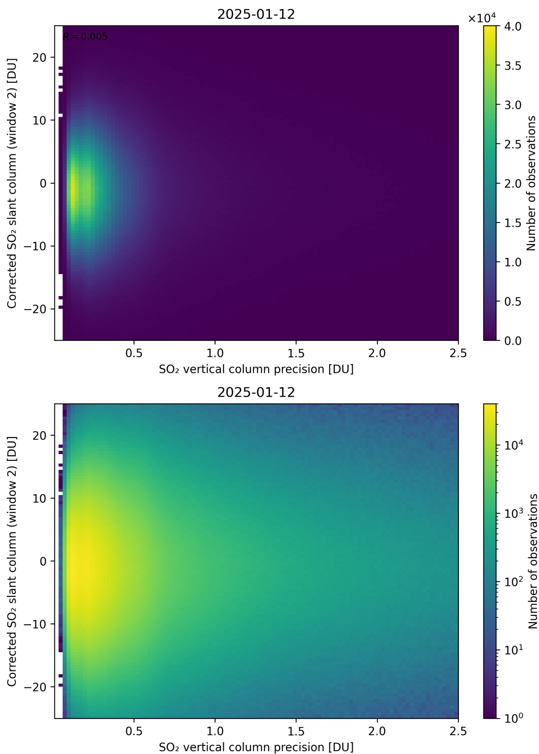
Figure 339: Scatter density plot of “SO 2 vertical column precision” against “Corrected SO 2 slant column (window 2)” for 2025-01-12 to 2025-01-13.
