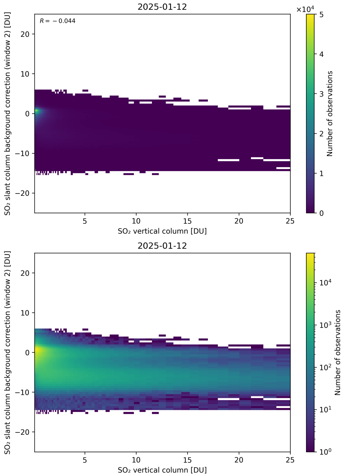
Figure 324: Scatter density plot of “SO 2 vertical column” against “SO 2 slant column background correction (window 2)” for 2025-01-12 to 2025-01-13.
