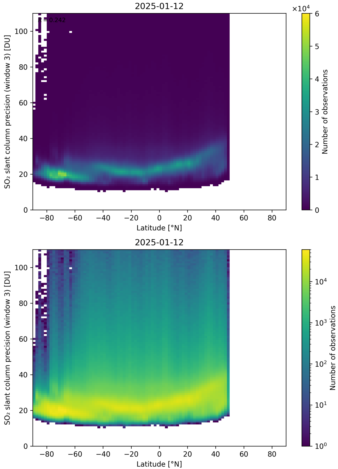
Figure 166: Scatter density plot of “Latitude” against “SO 2 slant column precision (window 3)” for 2025-01-12 to 2025-01-13.
