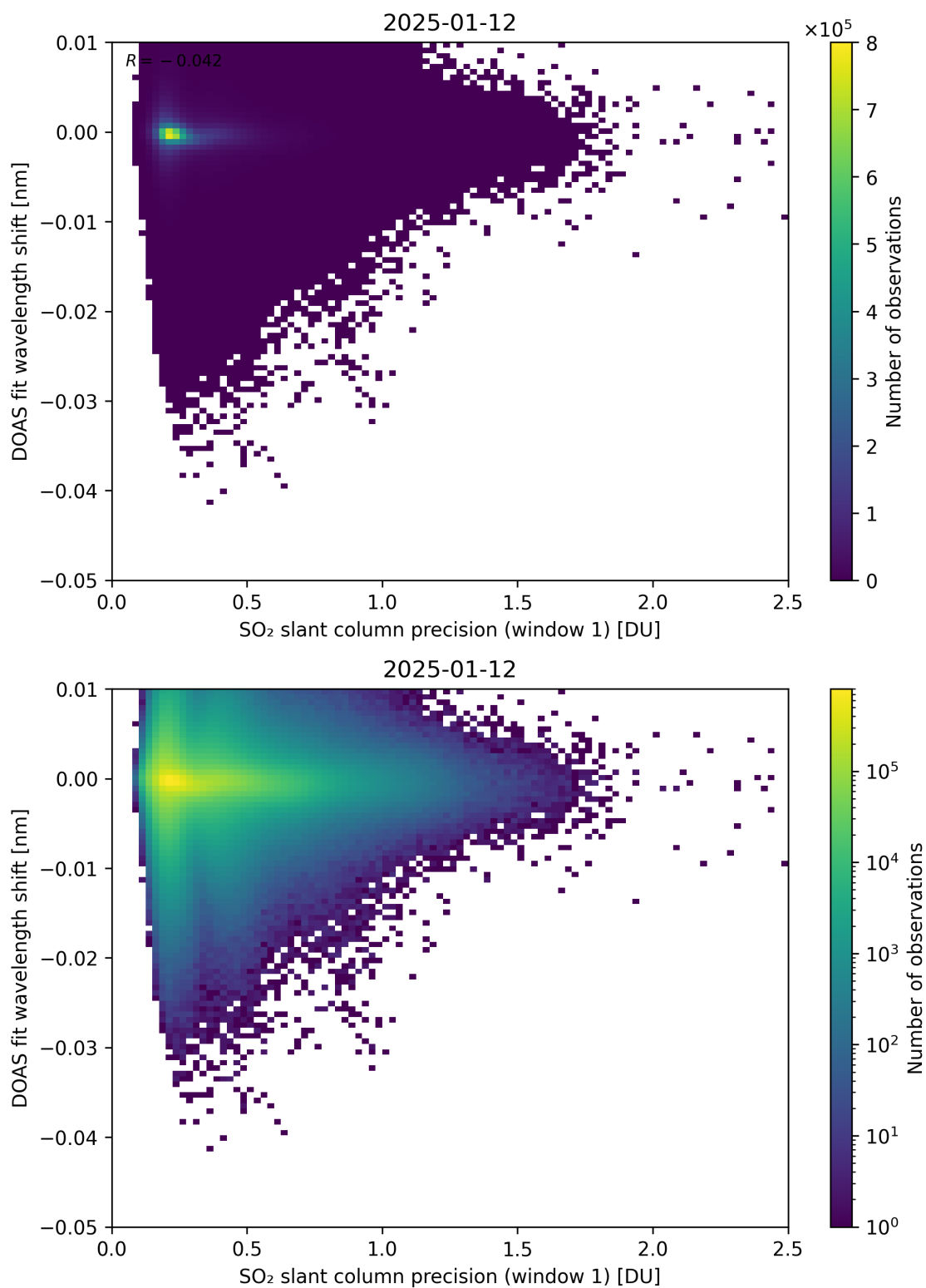
Figure 271: Scatter density plot of “SO 2 slant column precision (window 1)” against “DOAS fit wavelength shift” for 2025-01-12 to 2025-01-13.
