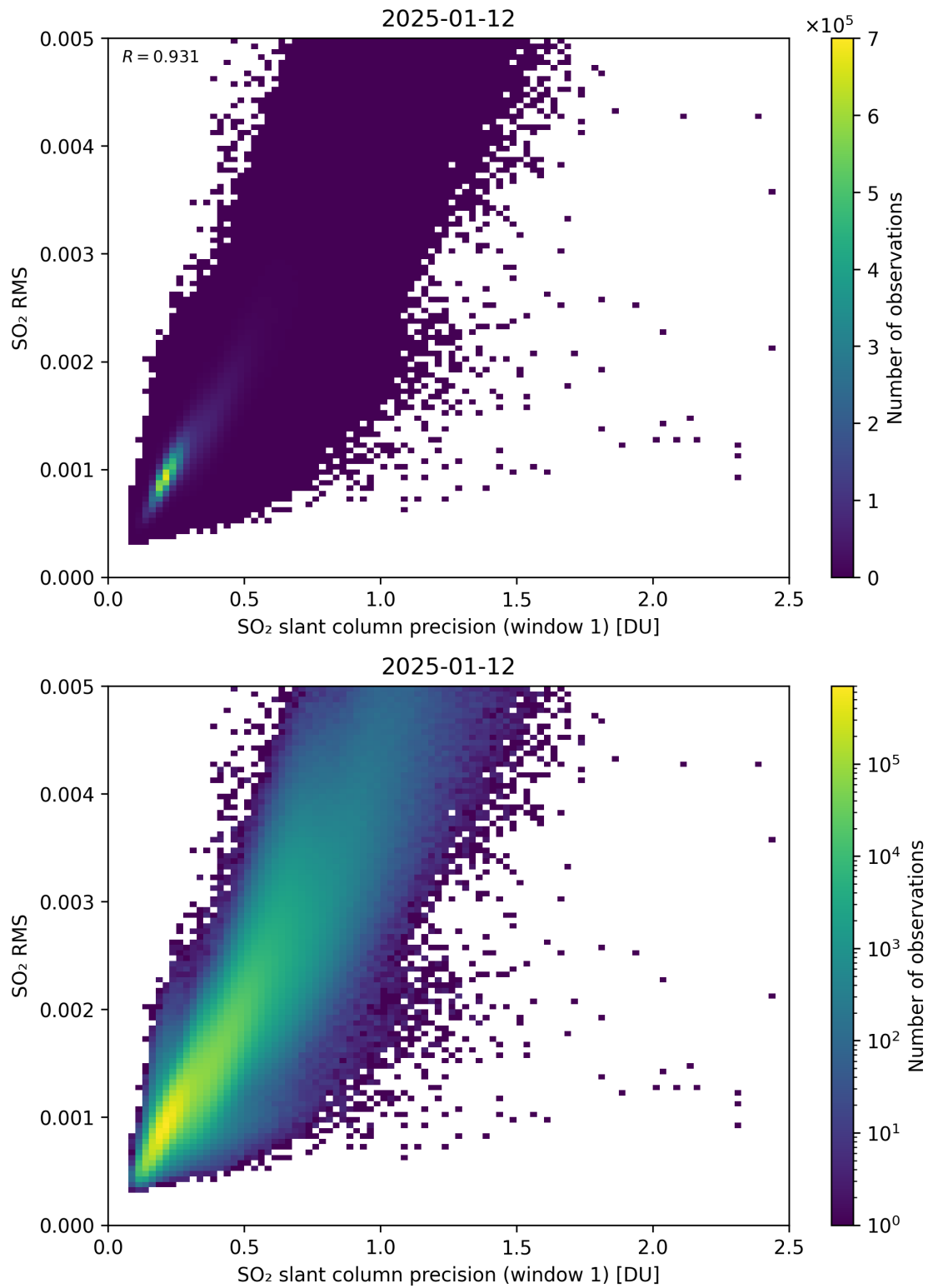
Figure 273: Scatter density plot of “SO 2 slant column precision (window 1)” against “SO 2 RMS” for 2025-01-12 to 2025-01-13.
