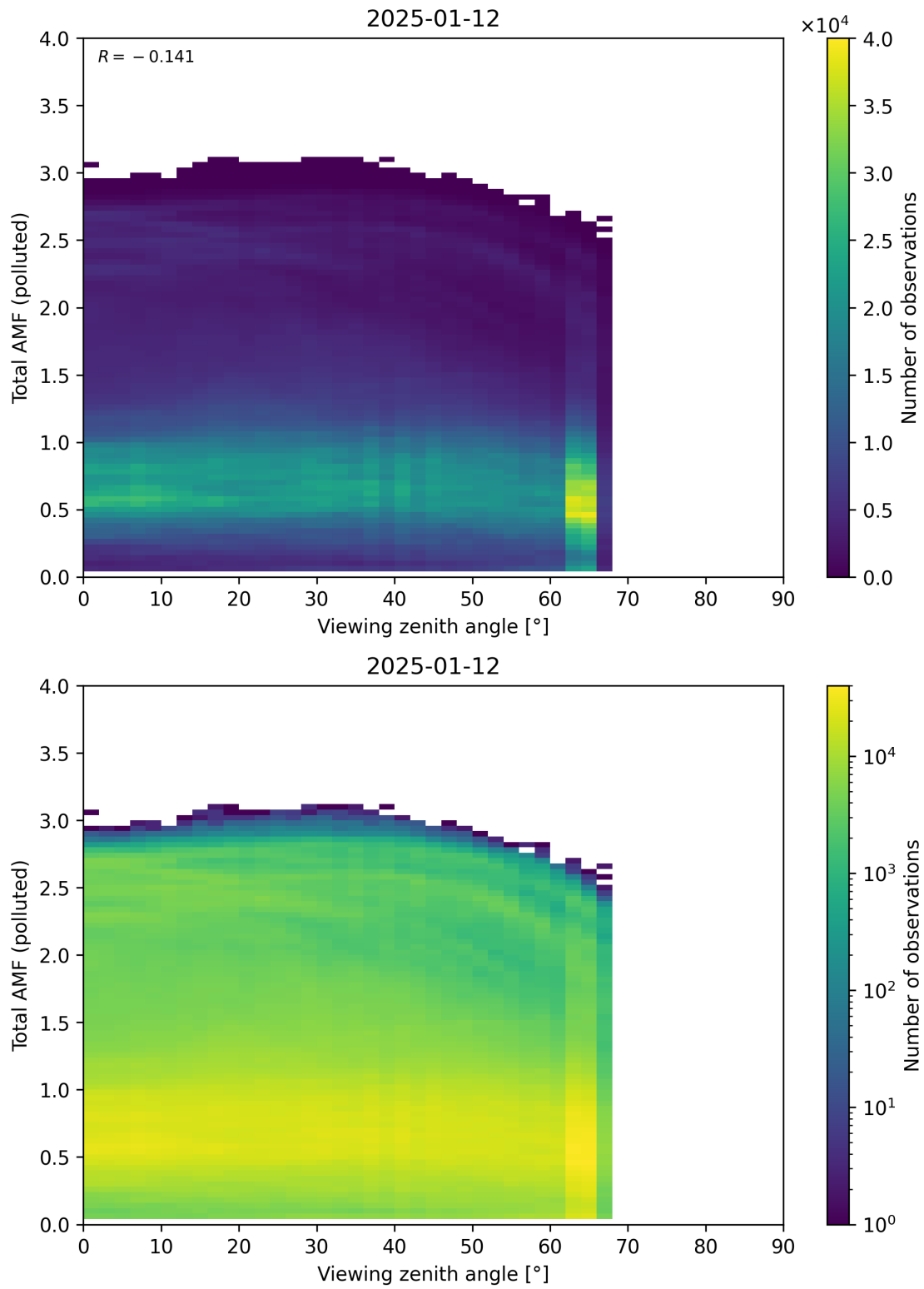
Figure 381: Scatter density plot of “Viewing zenith angle” against “Total AMF (polluted)” for 2025-01-12 to 2025-01-13.
