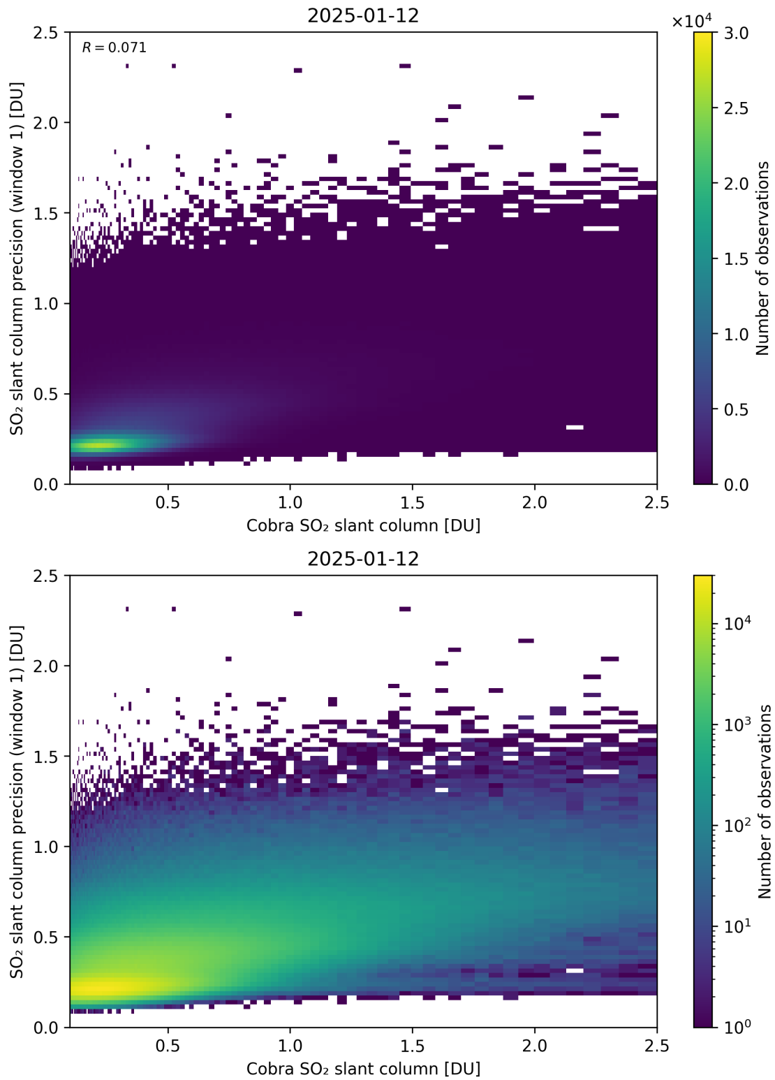
Figure 220: Scatter density plot of “Cobra SO 2 slant column” against “SO 2 slant column precision (window 1)” for 2025-01-12 to 2025-01-13.
