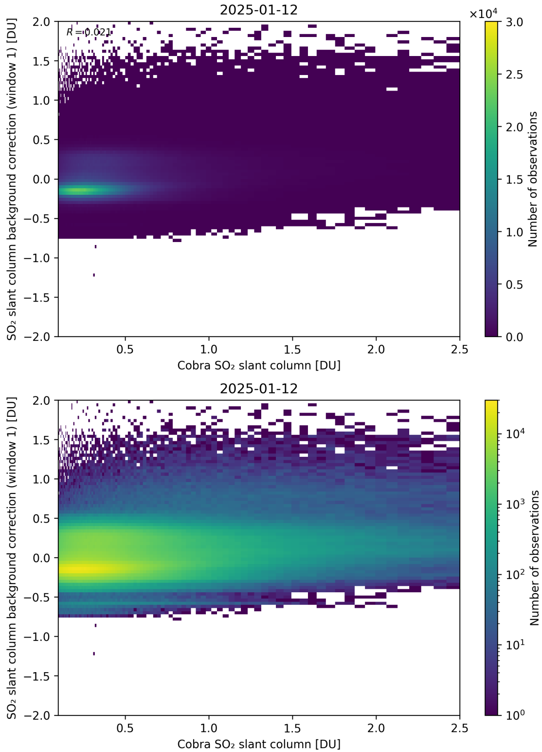
Figure 193: Scatter density plot of “Cobra SO 2 slant column” against “SO 2 slant column background correction (window 1)” for 2025-01-12 to 2025-01-13.
