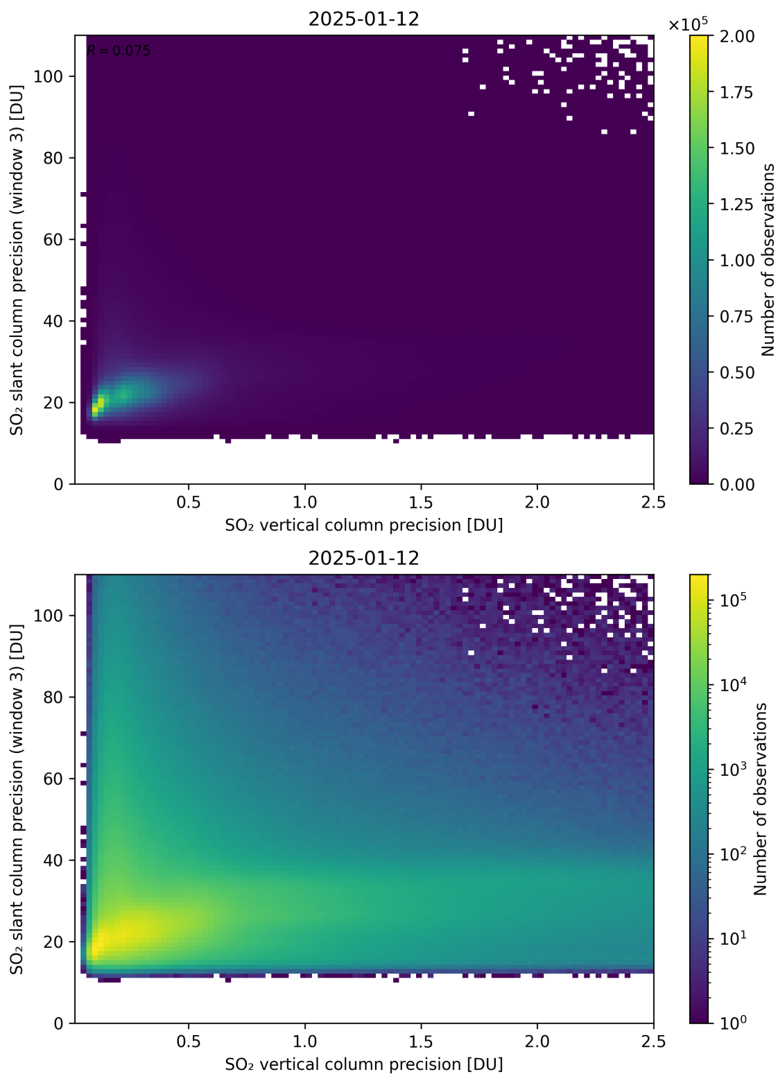
Figure 345: Scatter density plot of “SO 2 vertical column precision” against “SO 2 slant column precision (window 3)” for 2025-01-12 to 2025-01-13.
