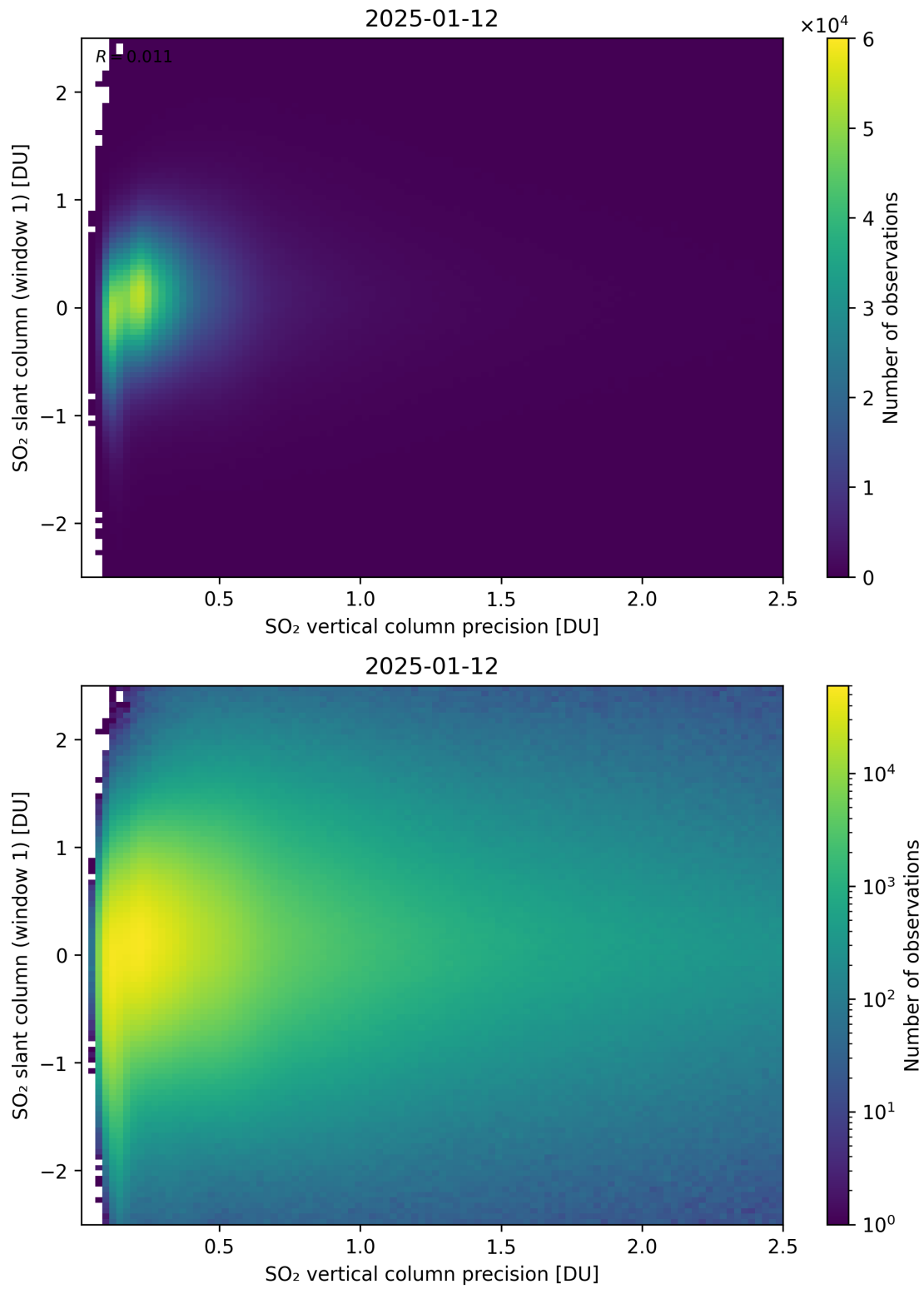
Figure 341: Scatter density plot of “SO 2 vertical column precision” against “SO 2 slant column (window 1)” for 2025-01-12 to 2025-01-13.
