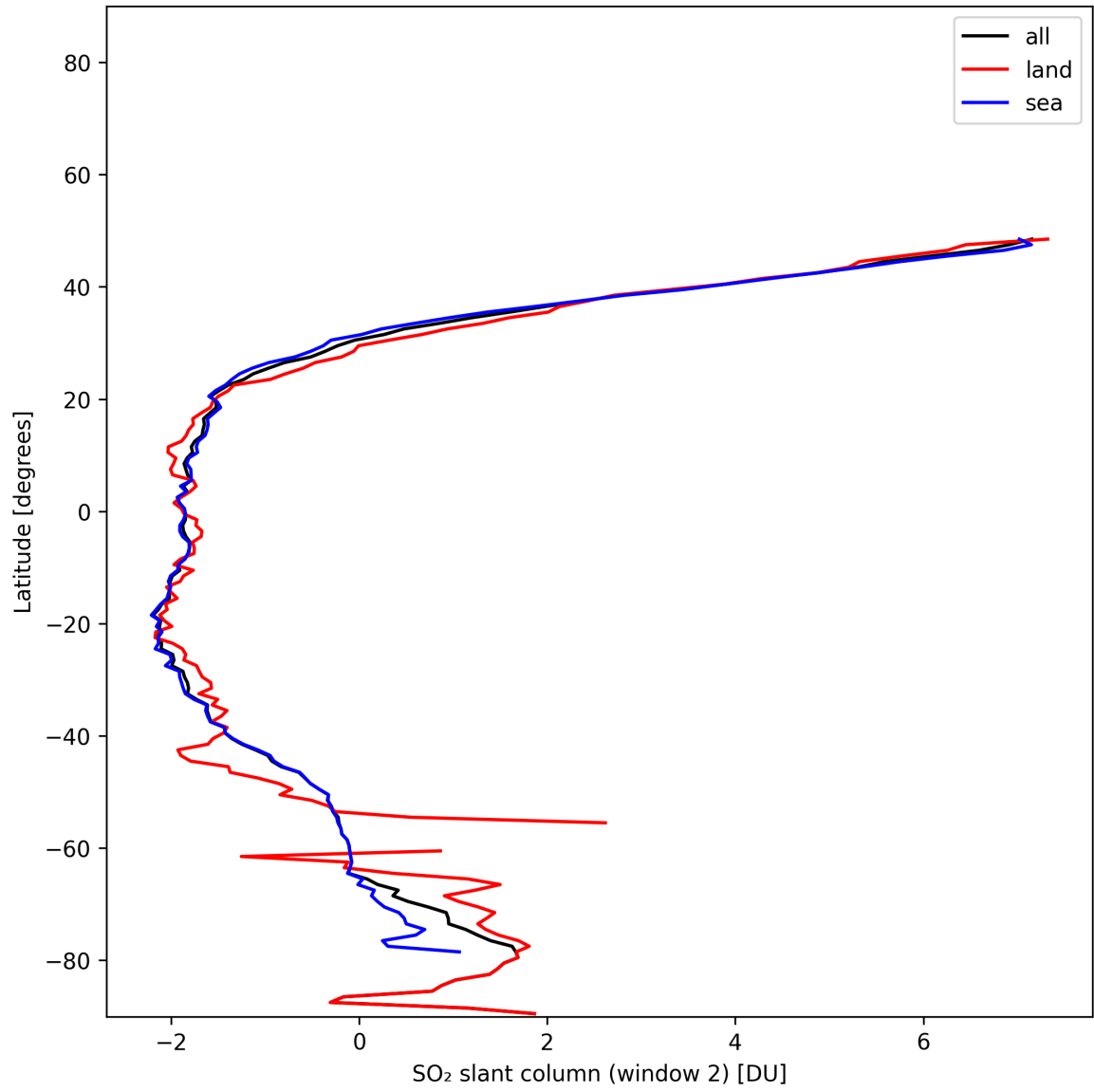
Figure 41: Zonal average of “SO 2 slant column (window 2)” for 2025-01-12 to 2025-01-13.
