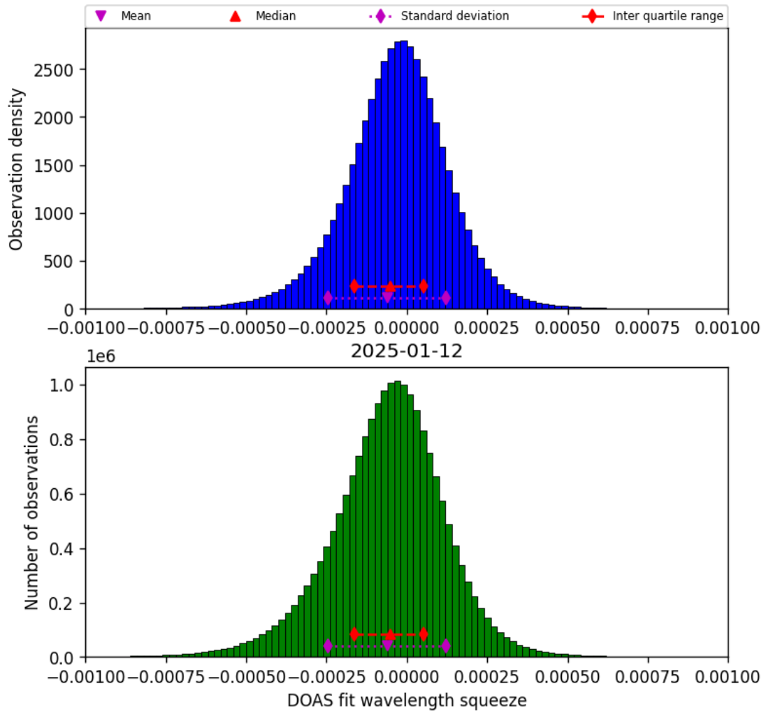
Figure 77: Histogram of “DOAS fit wavelength squeeze” for 2025-01-12 to 2025-01-13
