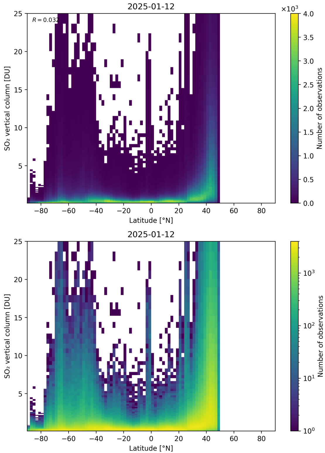
Figure 169: Scatter density plot of “Latitude” against “SO 2 vertical column” for 2025-01-12 to 2025-01-13.
