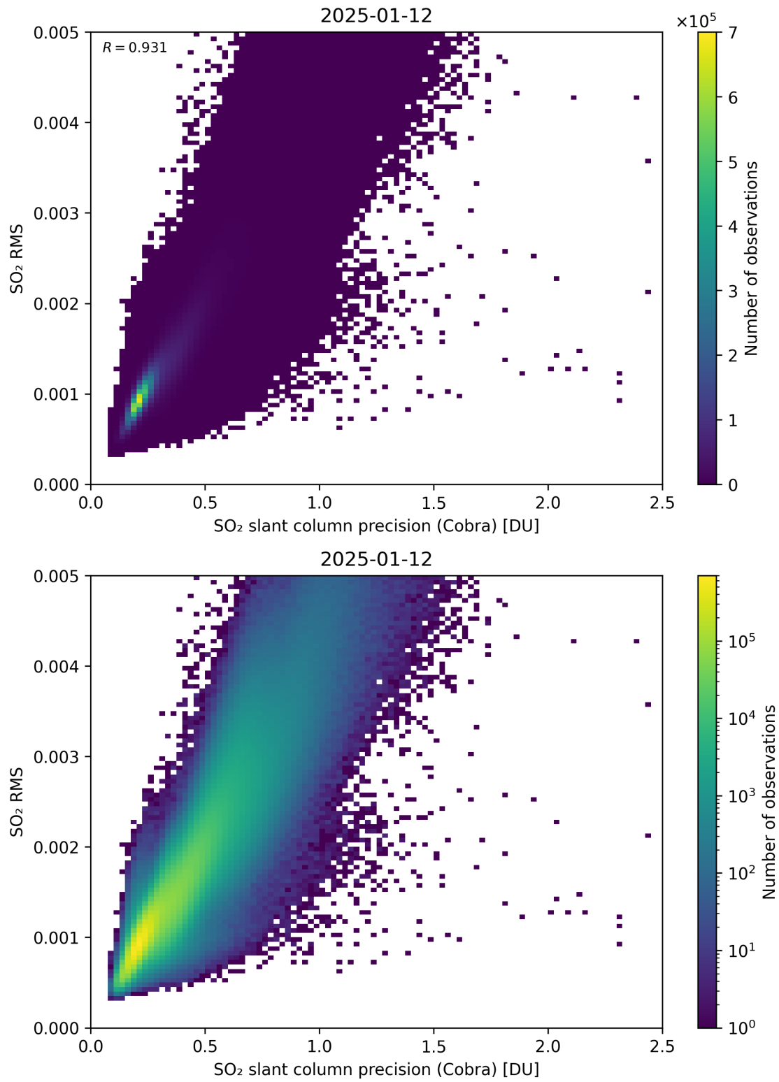
Figure 204: Scatter density plot of “SO 2 slant column precision (Cobra)” against “SO 2 RMS” for 2025-01-12 to 2025-01-13.
