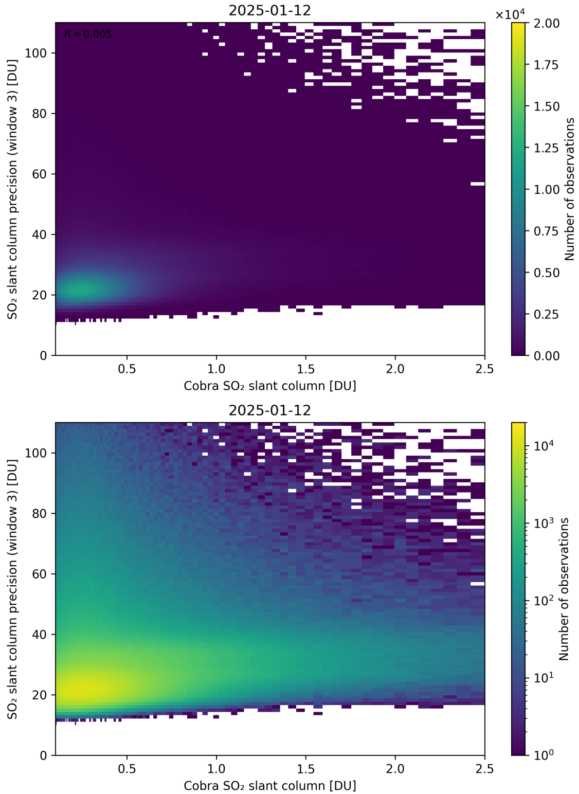
Figure 223: Scatter density plot of “Cobra SO 2 slant column” against “SO 2 slant column precision (window 3)” for 2025-01-12 to 2025-01-13.
