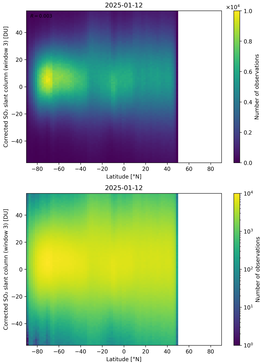
Figure 161: Scatter density plot of “Latitude” against “Corrected SO 2 slant column (window 3)” for 2025-01-12 to 2025-01-13.
