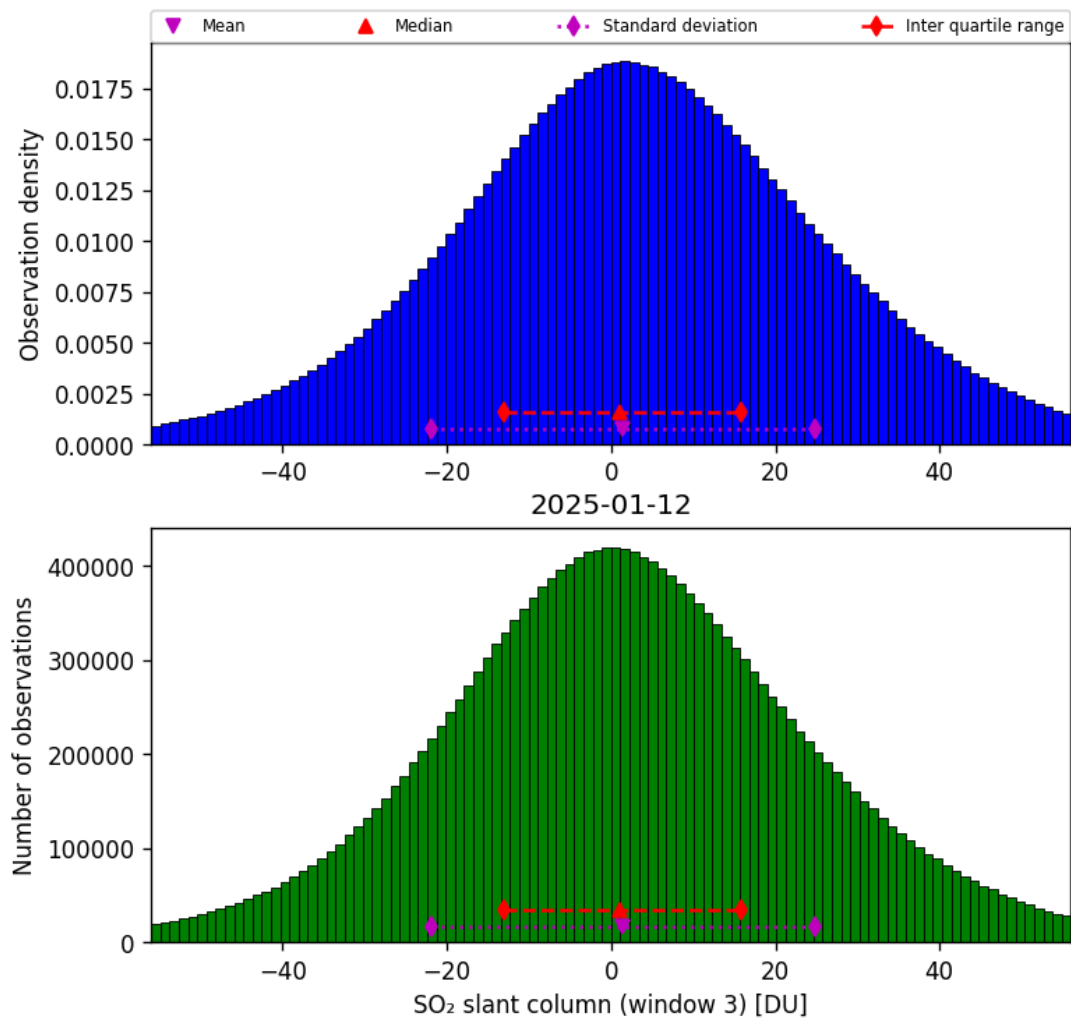
Figure 71: Histogram of “SO 2 slant column (window 3)” for 2025-01-12 to 2025-01-13
