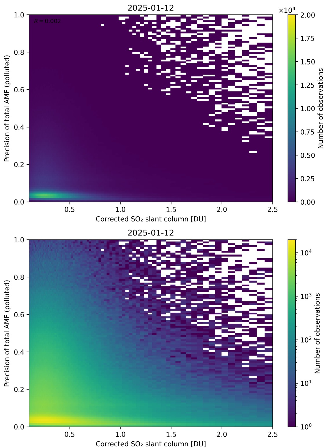
Figure 243: Scatter density plot of “Corrected SO 2 slant column” against “Precision of total AMF (polluted)” for 2025-01-12 to 2025-01-13.
