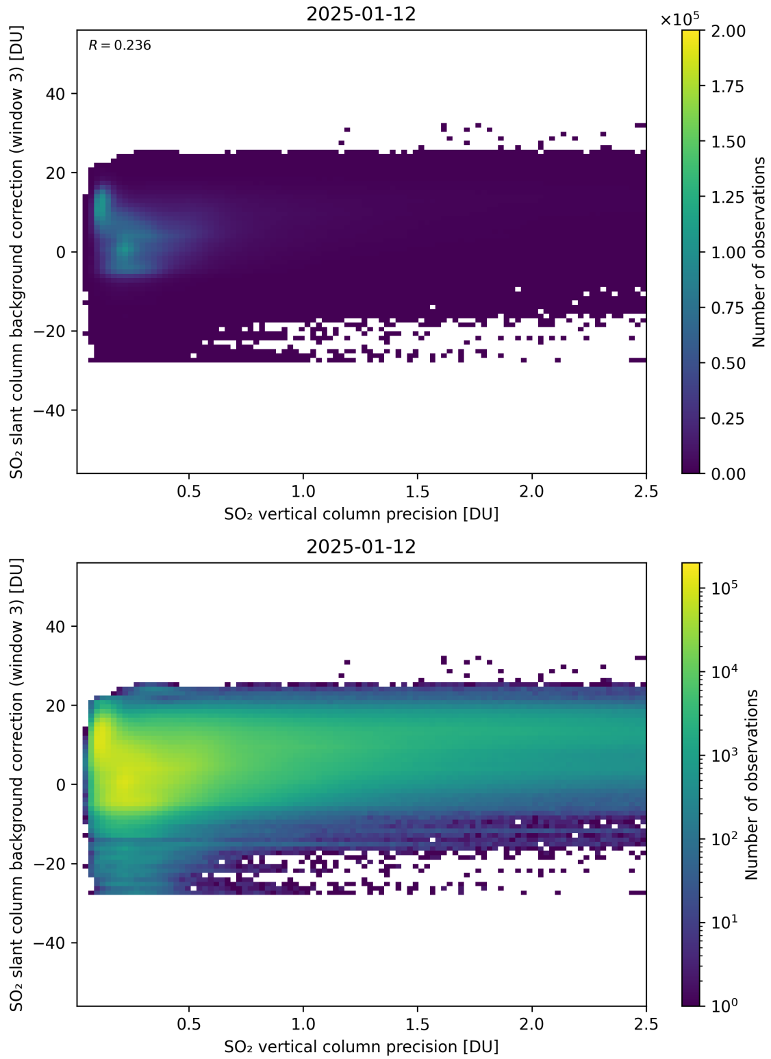
Figure 331: Scatter density plot of “SO 2 vertical column precision” against “SO 2 slant column background correction (window 3)” for 2025-01-12 to 2025-01-13.
