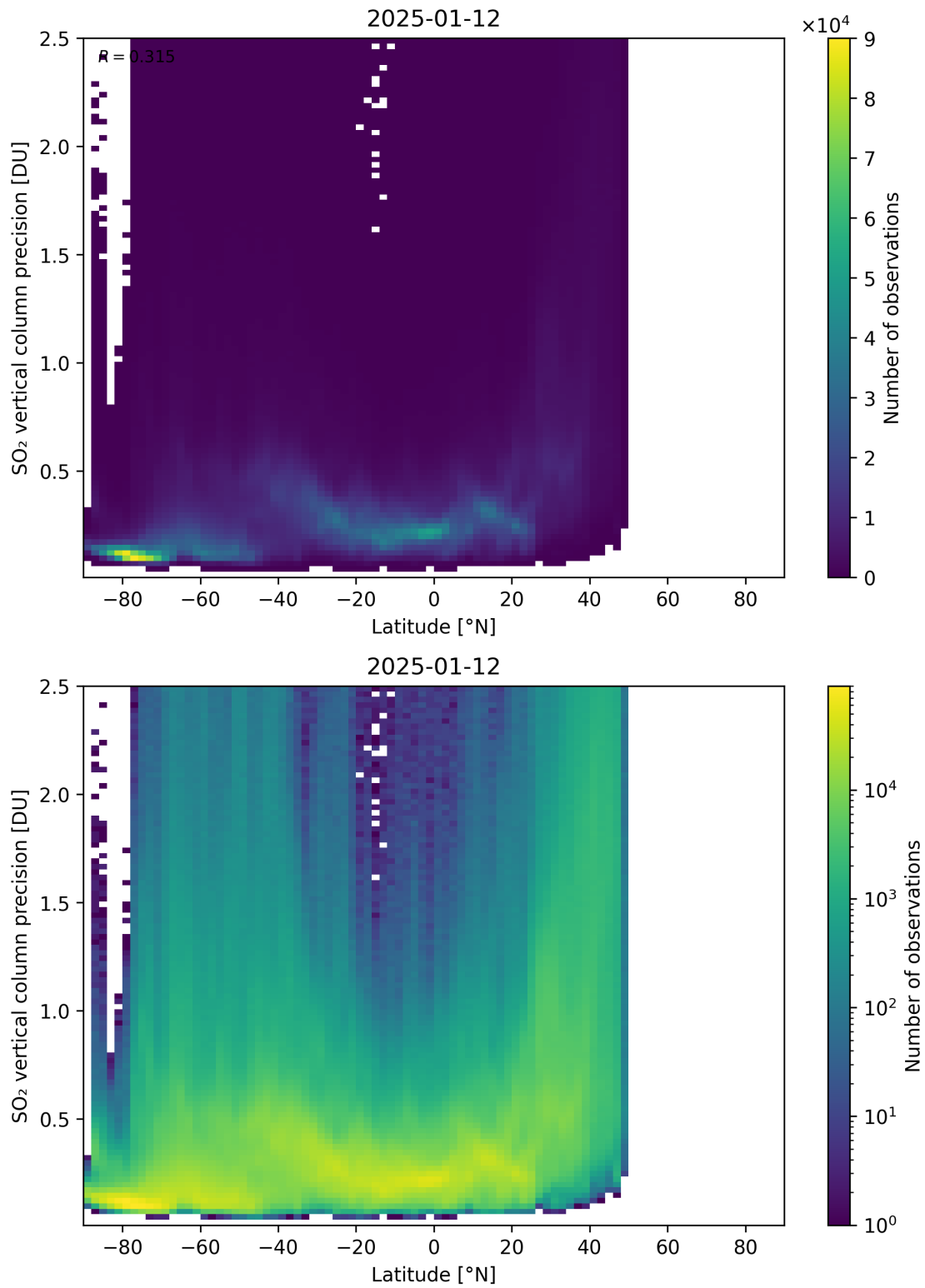
Figure 170: Scatter density plot of “Latitude” against “SO 2 vertical column precision” for 2025-01-12 to 2025-01-13.
