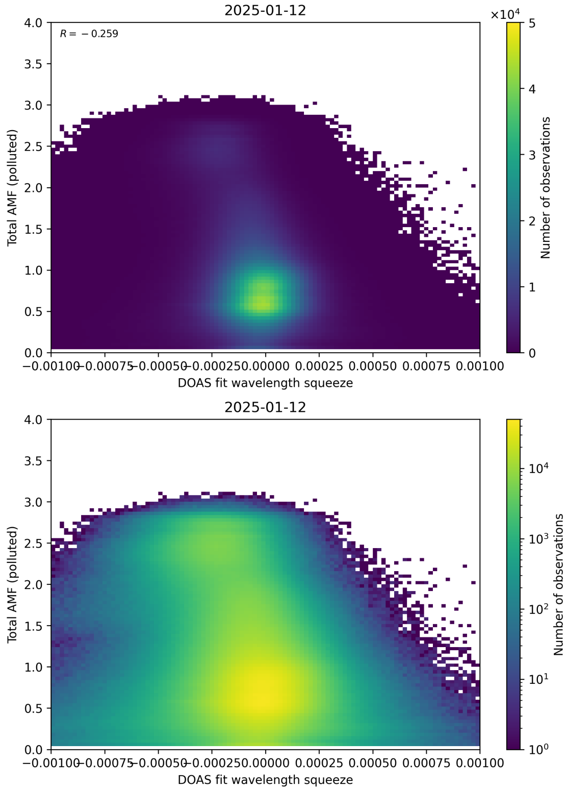
Figure 145: Scatter density plot of “DOAS fit wavelength squeeze” against “Total AMF (polluted)” for 2025-01-12 to 2025-01-13.
