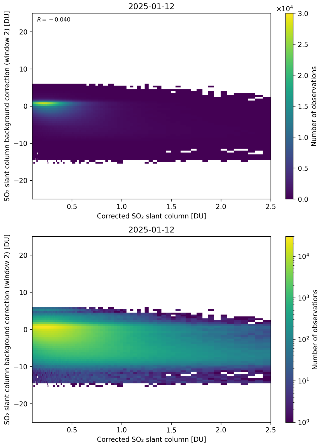
Figure 227: Scatter density plot of “Corrected SO 2 slant column” against “SO 2 slant column background correction (window 2)” for 2025-01-12 to 2025-01-13.
