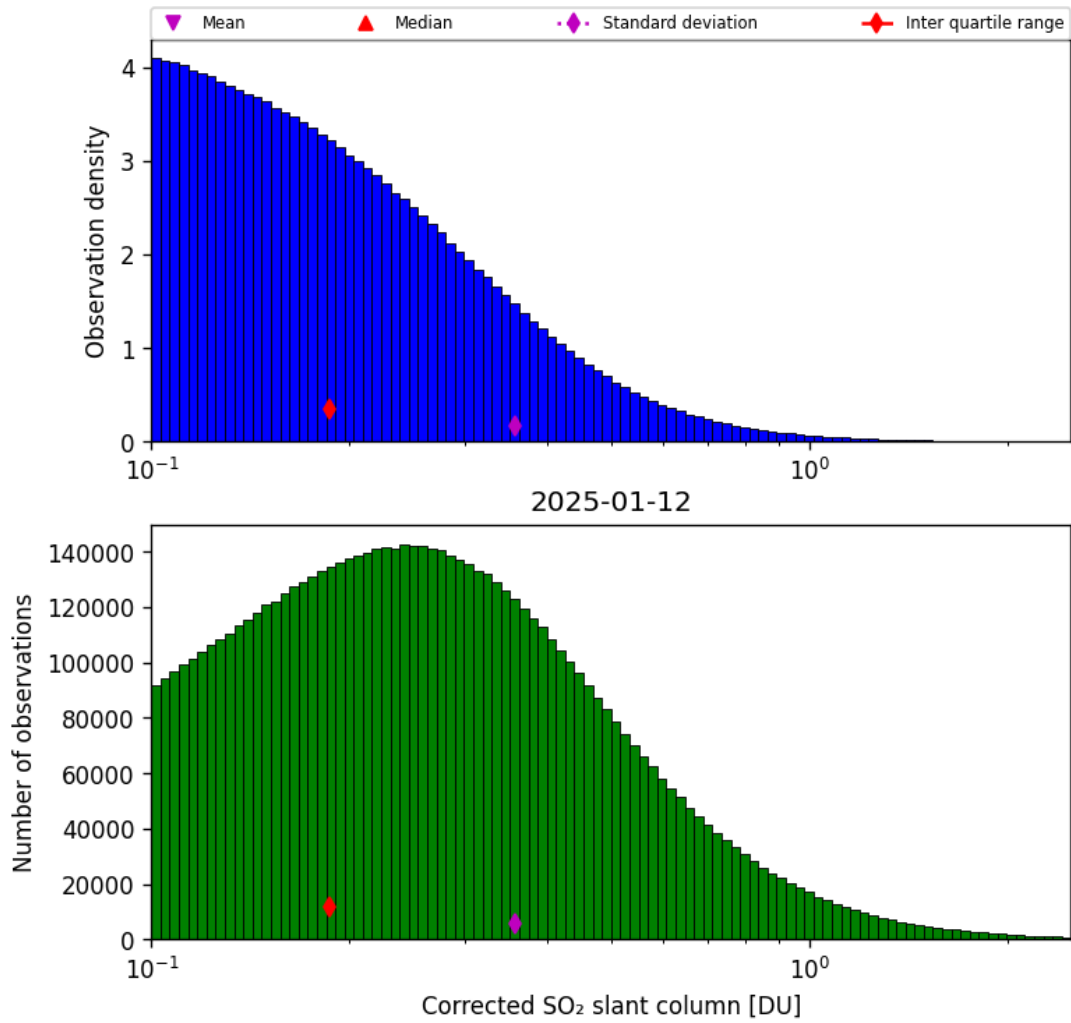
Figure 60: Histogram of “Corrected SO 2 slant column” for 2025-01-12 to 2025-01-13
