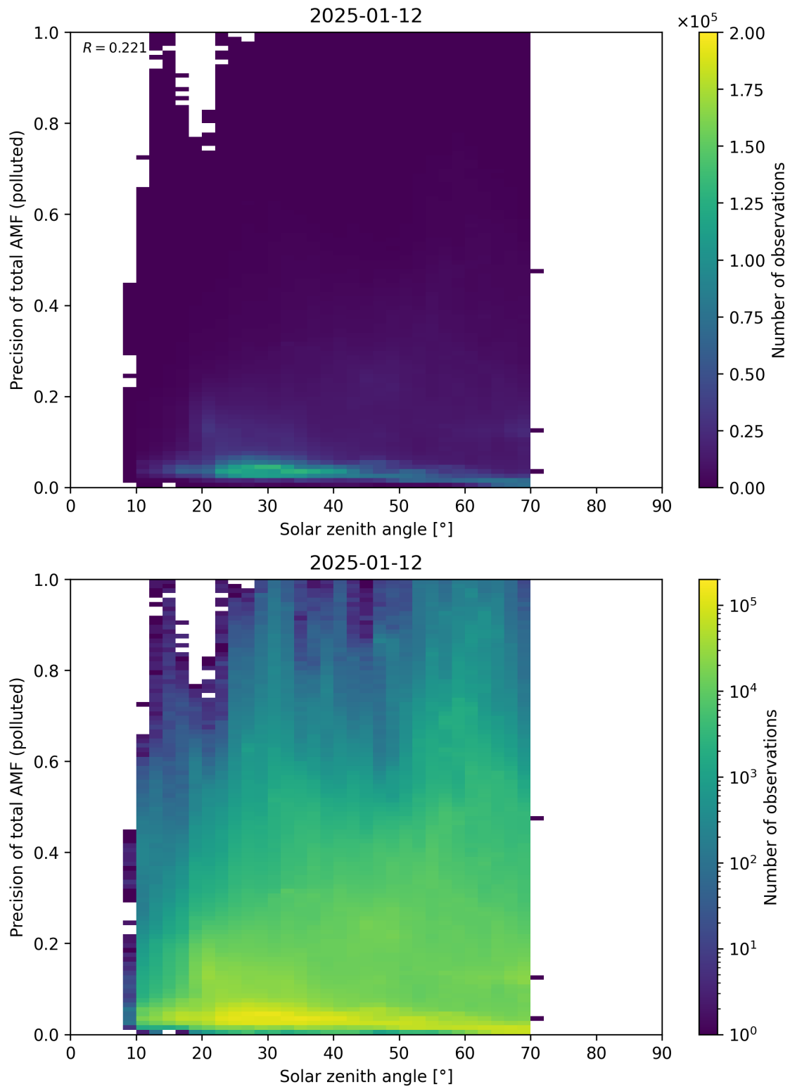
Figure 190: Scatter density plot of “Solar zenith angle” against “Precision of total AMF (polluted)” for 2025-01-12 to 2025-01-13.
