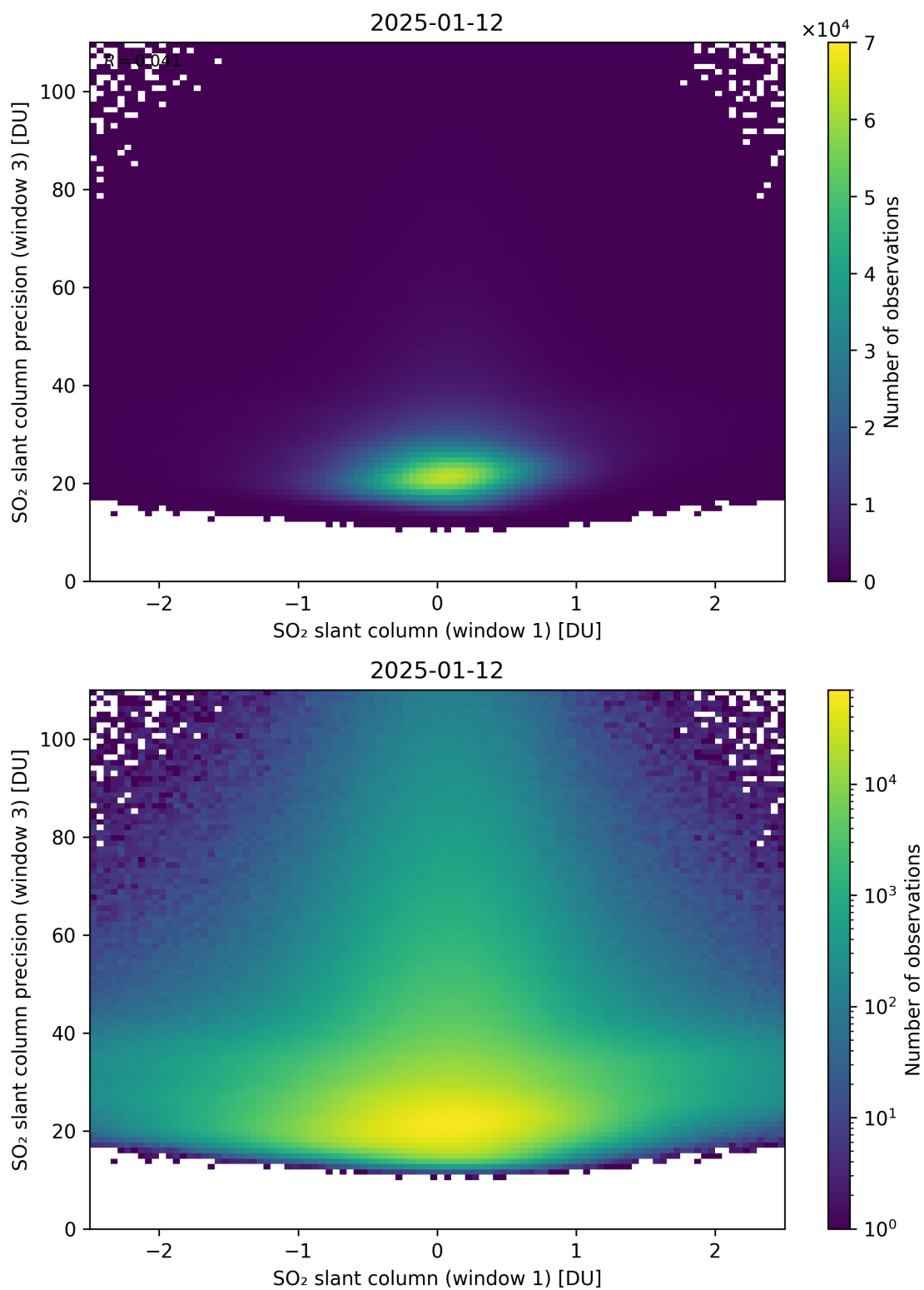
Figure 288: Scatter density plot of “SO 2 slant column (window 1)” against “SO 2 slant column precision (window 3)” for 2025-01-12 to 2025-01-13.
