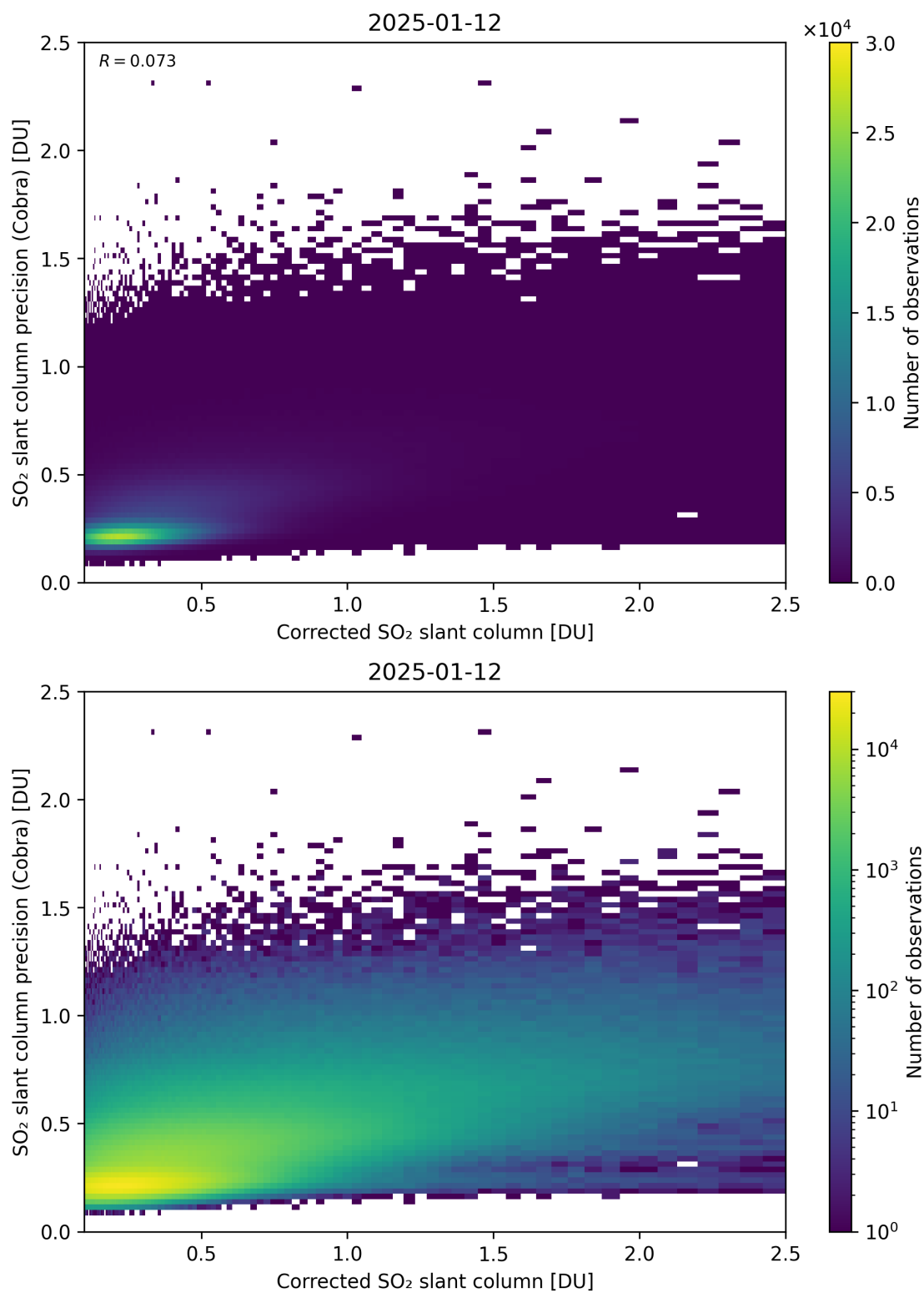
Figure 234: Scatter density plot of “Corrected SO 2 slant column” against “SO 2 slant column precision (Cobra)” for 2025-01-12 to 2025-01-13.
