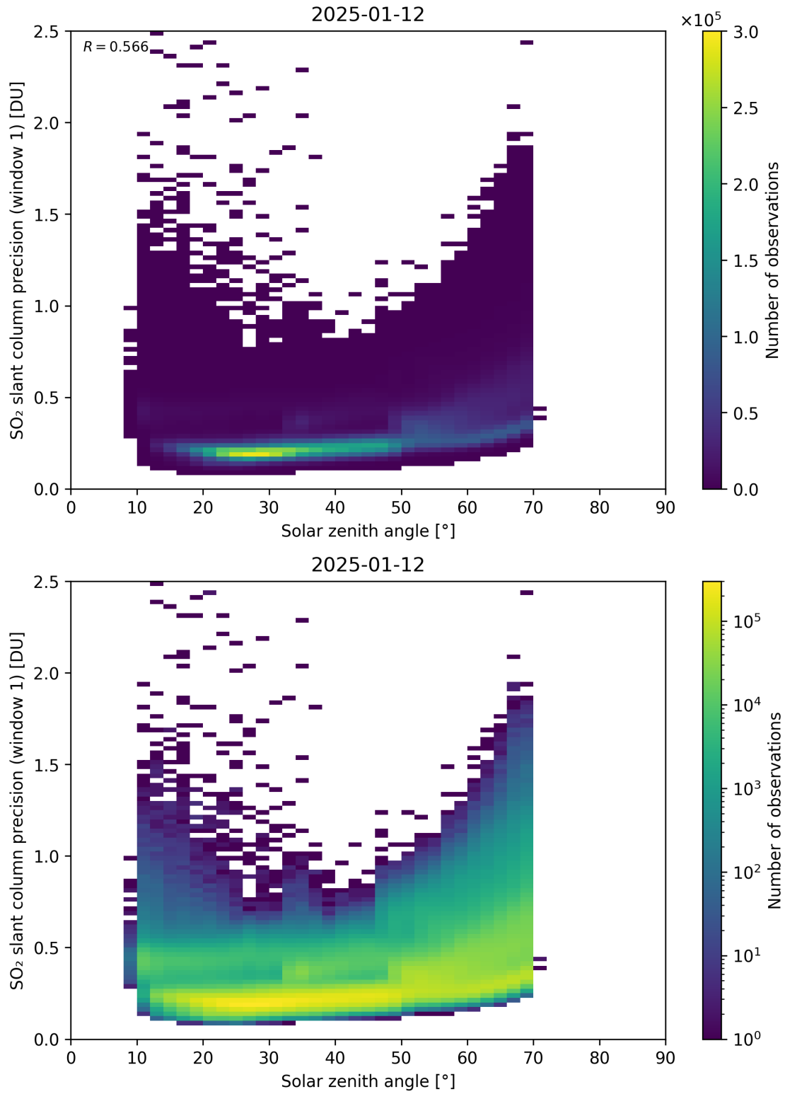
Figure 185: Scatter density plot of “Solar zenith angle” against “SO 2 slant column precision (window 1)” for 2025-01-12 to 2025-01-13.
