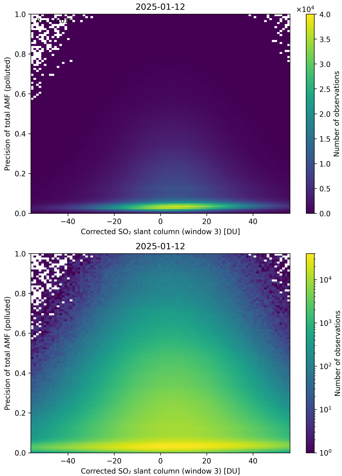
Figure 261: Scatter density plot of “Corrected SO 2 slant column (window 3)” against “Precision of total AMF (polluted)” for 2025-01-12 to 2025-01-13.
