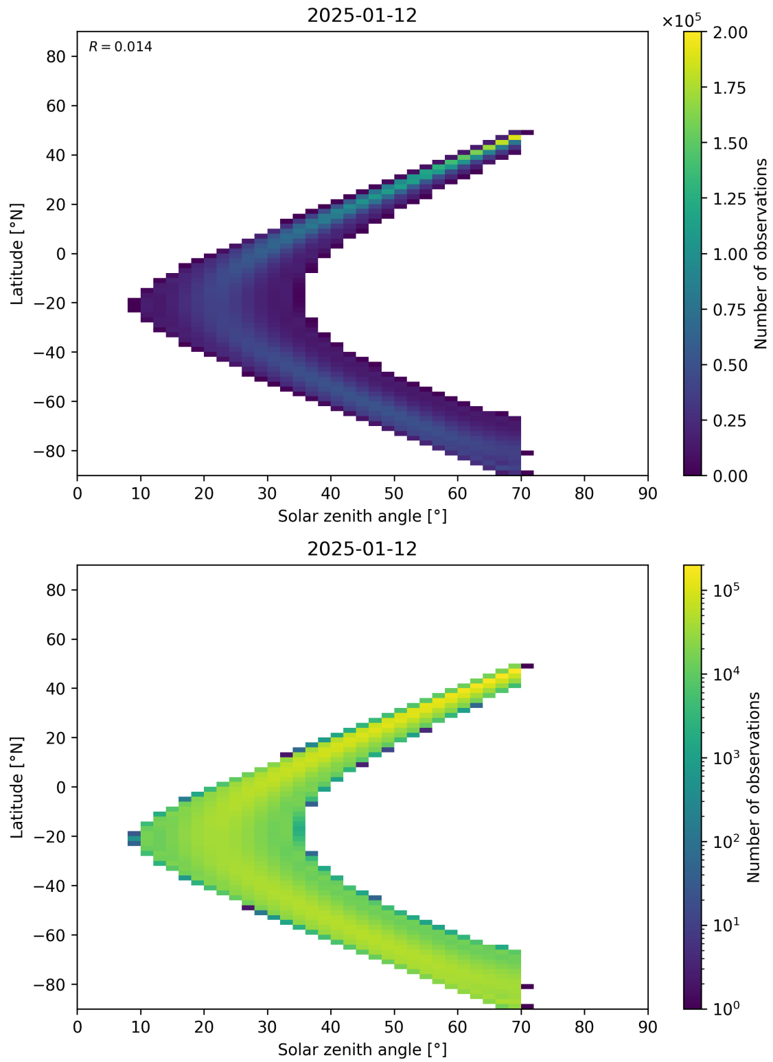
Figure 177: Scatter density plot of “Solar zenith angle” against “Latitude” for 2025-01-12 to 2025-01-13.
