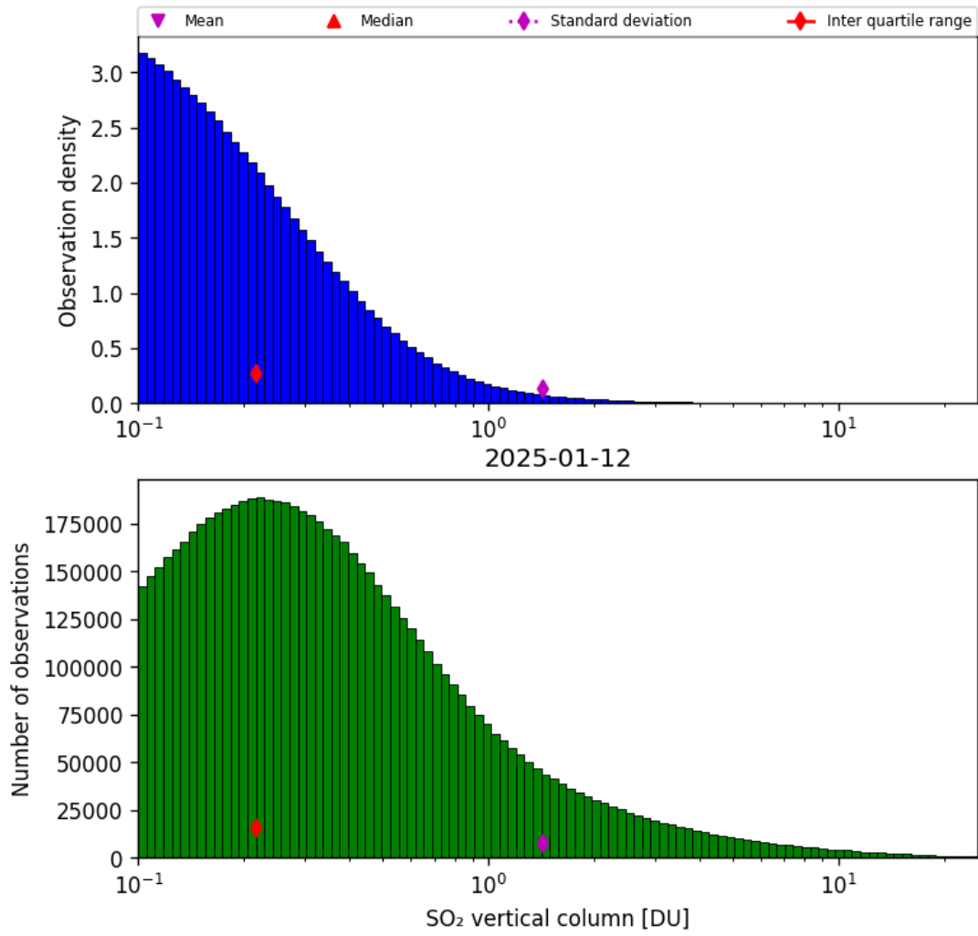
Figure 58: Histogram of “SO 2 vertical column” for 2025-01-12 to 2025-01-13
