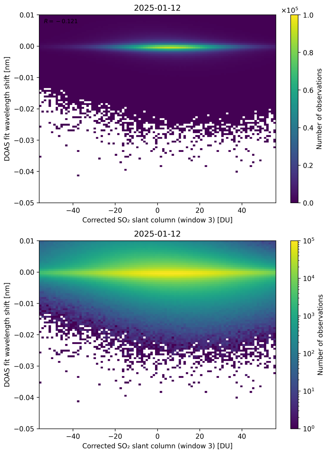
Figure 256: Scatter density plot of “Corrected SO 2 slant column (window 3)” against “DOAS fit wavelength shift” for 2025-01-12 to 2025-01-13.
