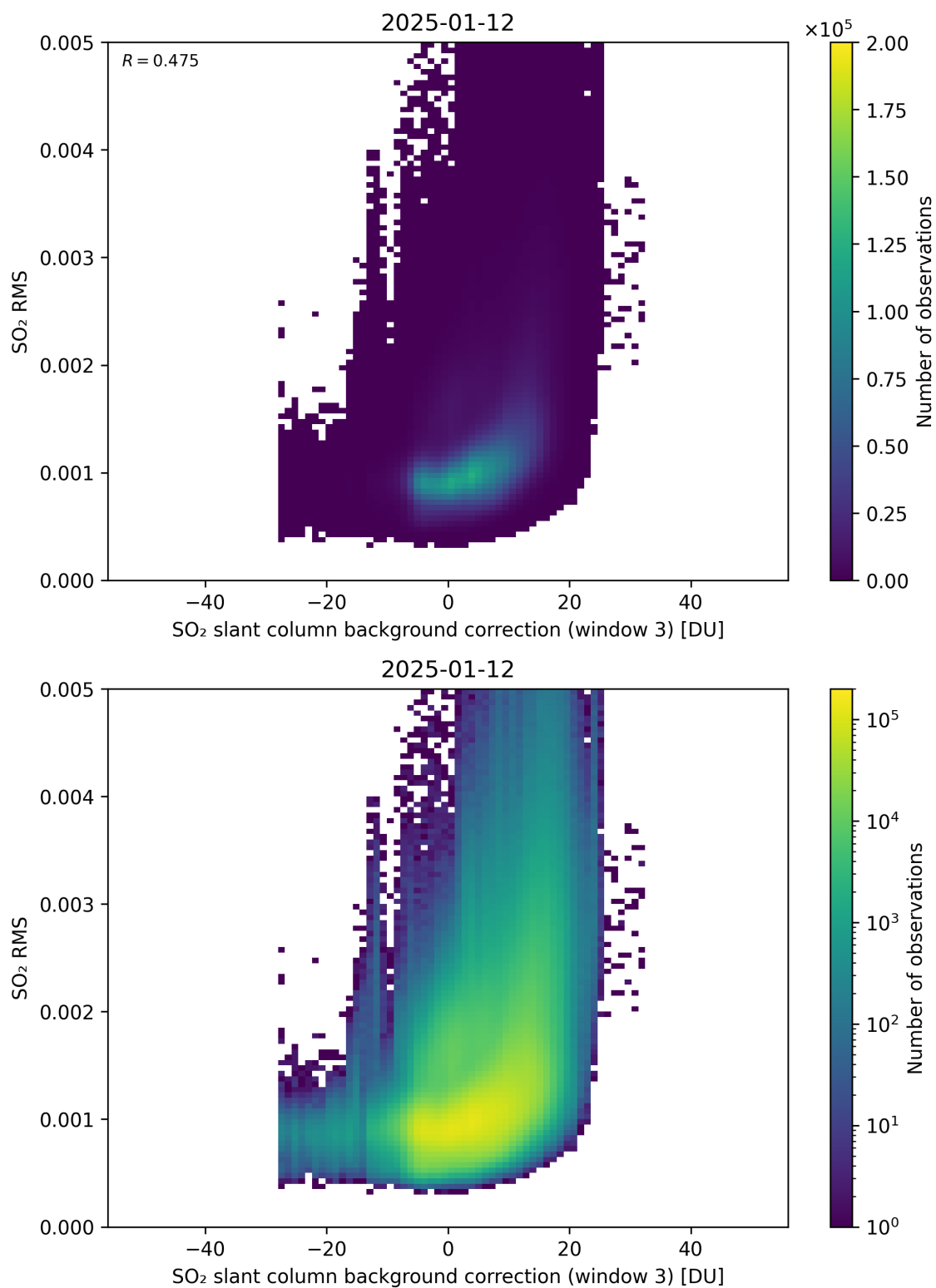
Figure 134: Scatter density plot of “SO 2 slant column background correction (window 3)” against “SO 2 RMS” for 2025-01-12 to 2025-01-13.
