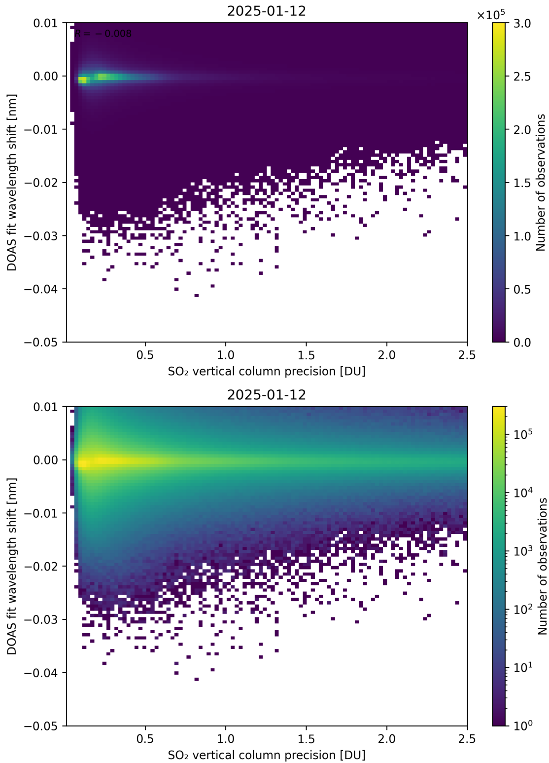
Figure 332: Scatter density plot of “SO 2 vertical column precision” against “DOAS fit wavelength shift” for 2025-01-12 to 2025-01-13.
