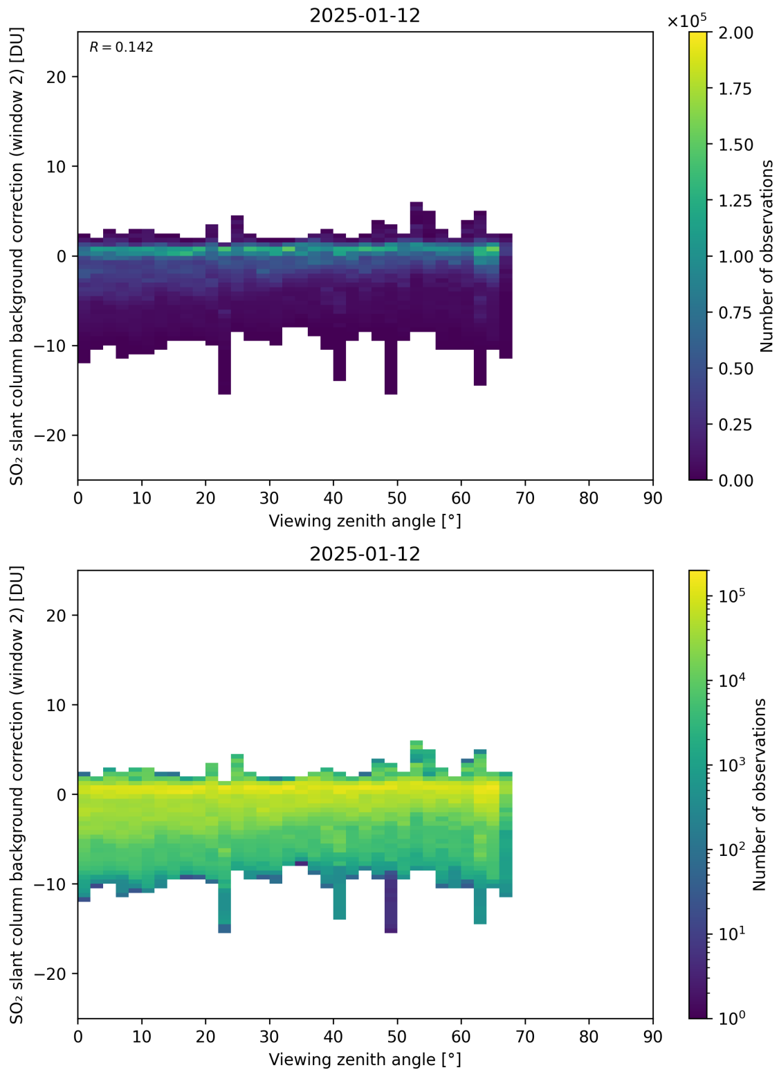
Figure 363: Scatter density plot of “Viewing zenith angle” against “SO 2 slant column background correction (window 2)” for 2025-01-12 to 2025-01-13.
