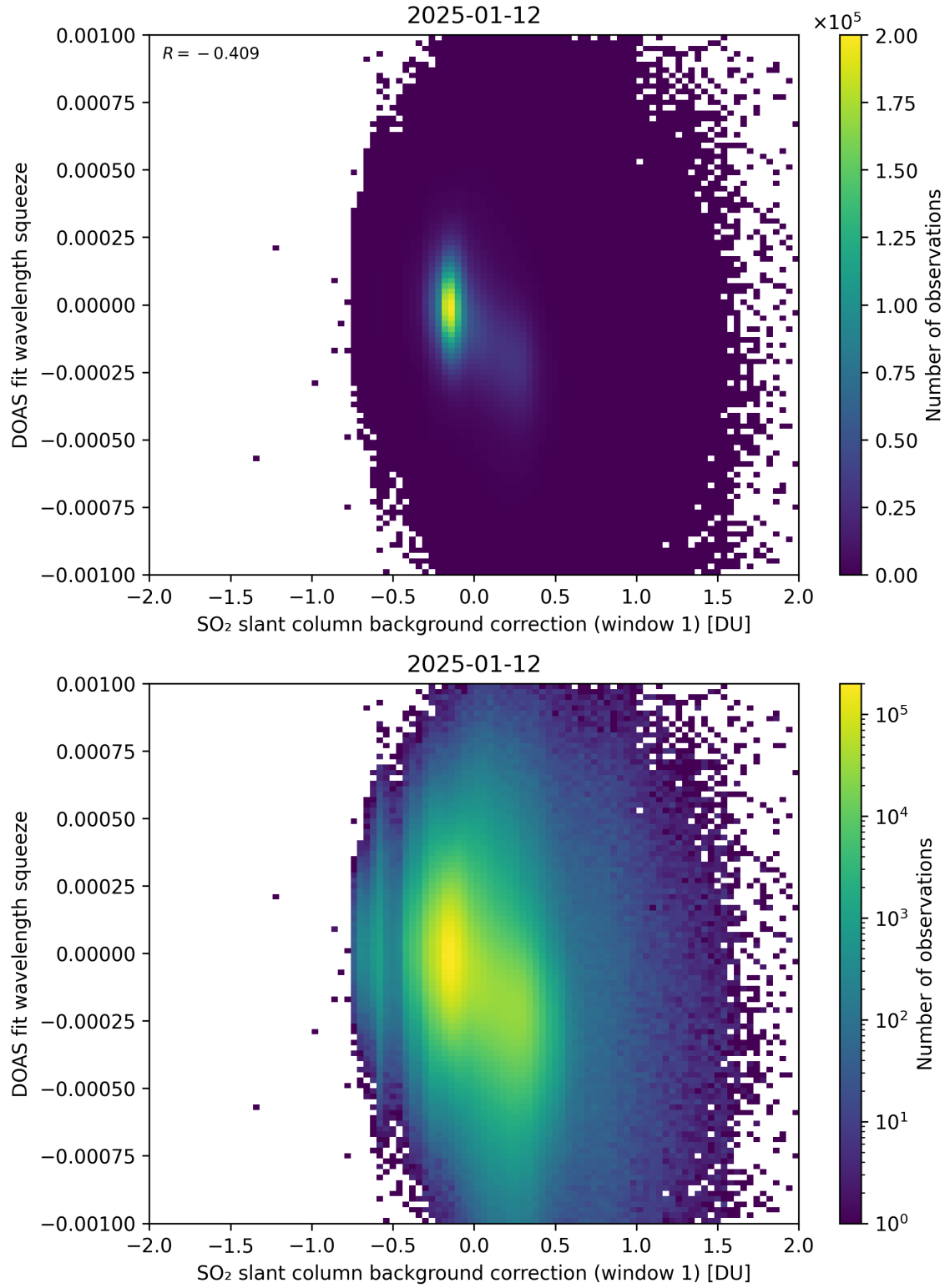
Figure 112: Scatter density plot of “SO 2 slant column background correction (window 1)” against “DOAS fit wavelength squeeze” for 2025-01-12 to 2025-01-13.
