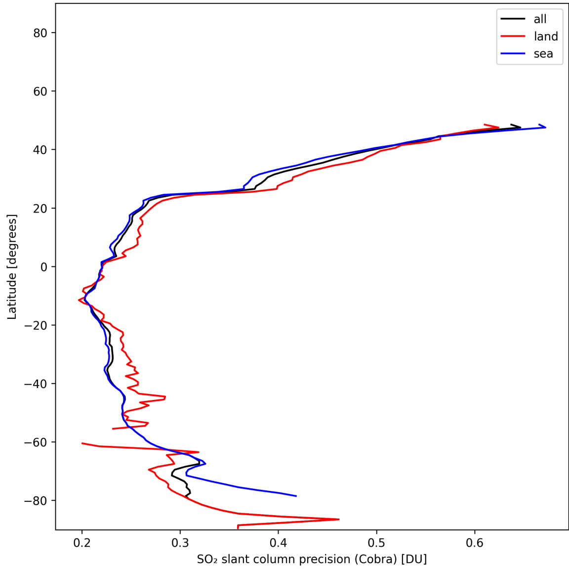
Figure 36: Zonal average of “SO 2 slant column precision (Cobra)” for 2025-01-12 to 2025-01-13.
