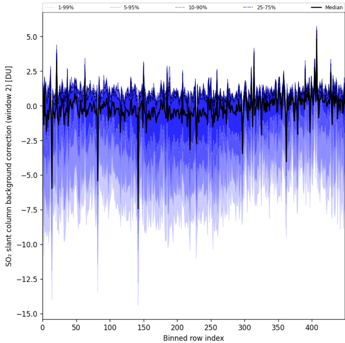
Figure 96: Along track statistics of “SO 2 slant column background correction (window 2)” for 2025-01-12 to 2025-01-13
