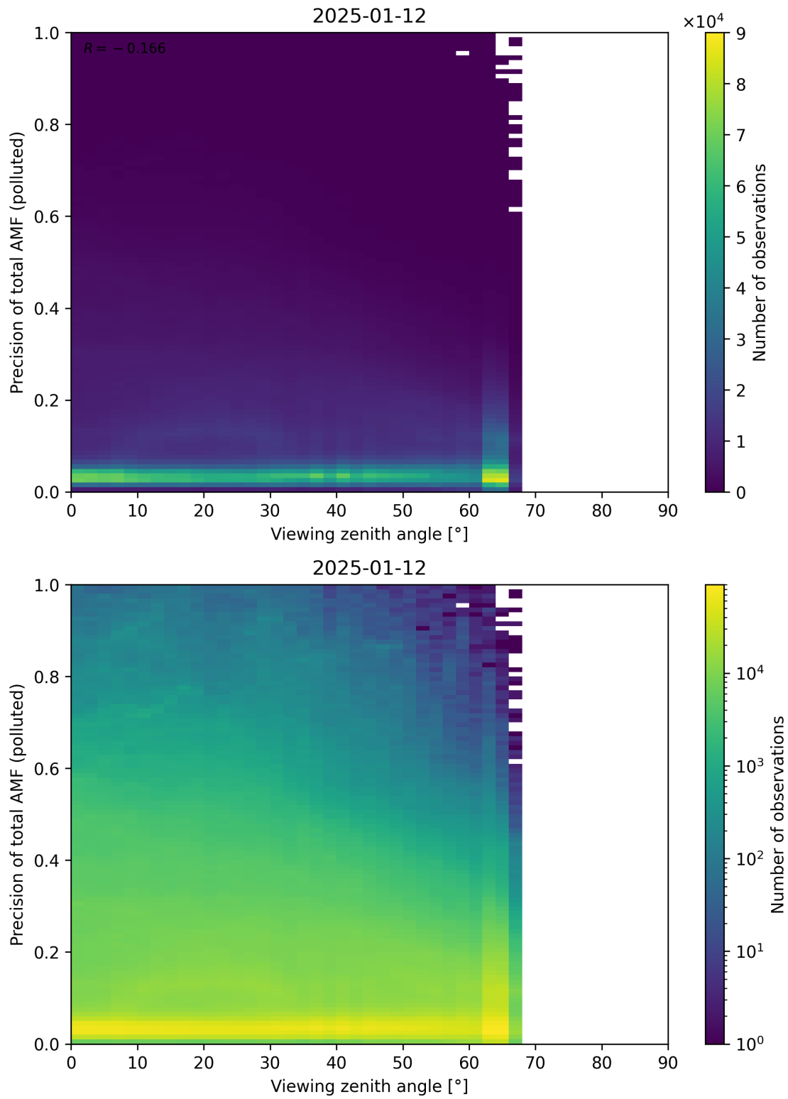
Figure 382: Scatter density plot of “Viewing zenith angle” against “Precision of total AMF (polluted)” for 2025-01-12 to 2025-01-13.
