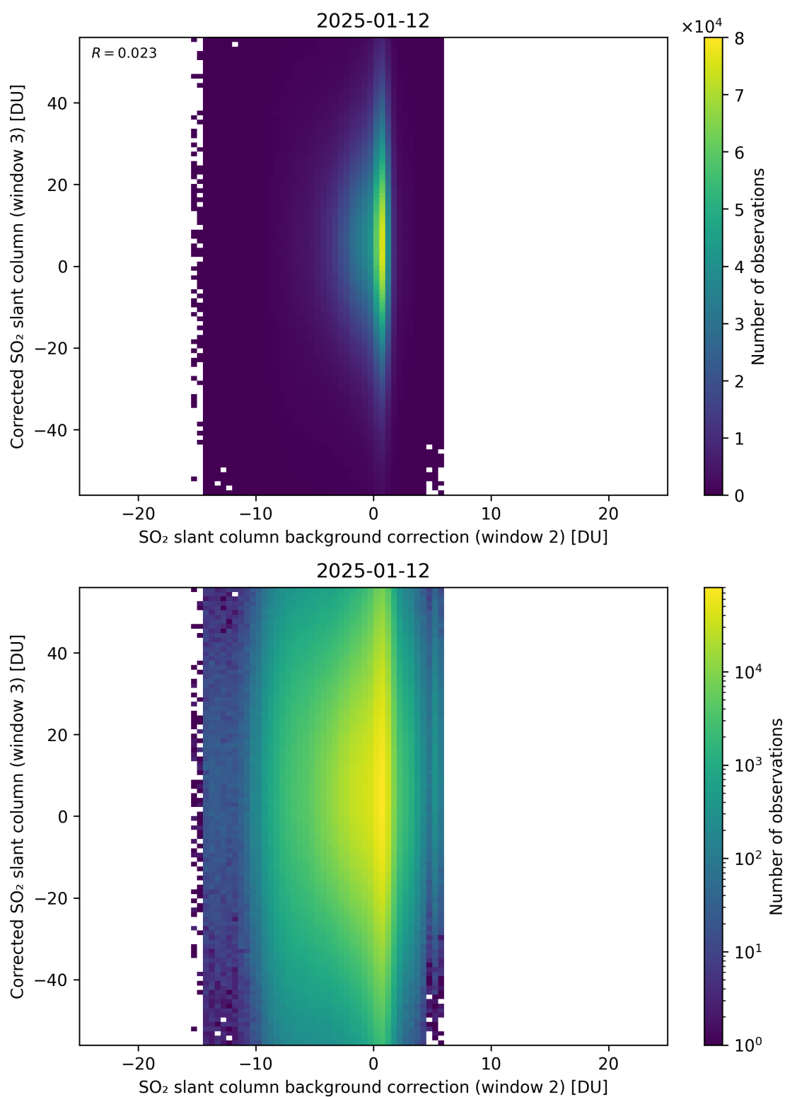
Figure 127: Scatter density plot of “SO 2 slant column background correction (window 2)” against “Corrected SO 2 slant column (window 3)” for 2025-01-12 to 2025-01-13.
