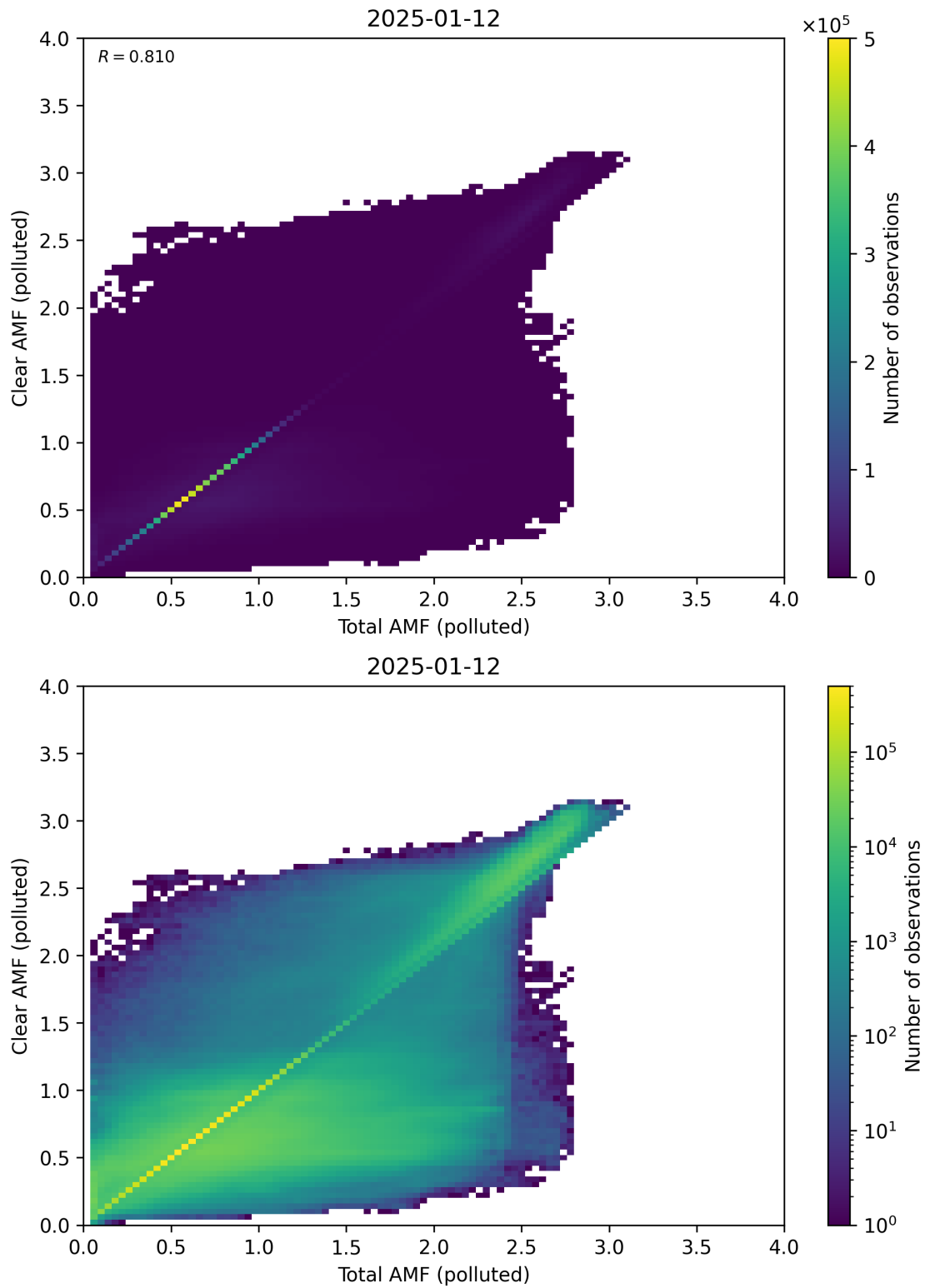
Figure 321: Scatter density plot of “Total AMF (polluted)” against “Clear AMF (polluted)” for 2025-01-12 to 2025-01-13.
