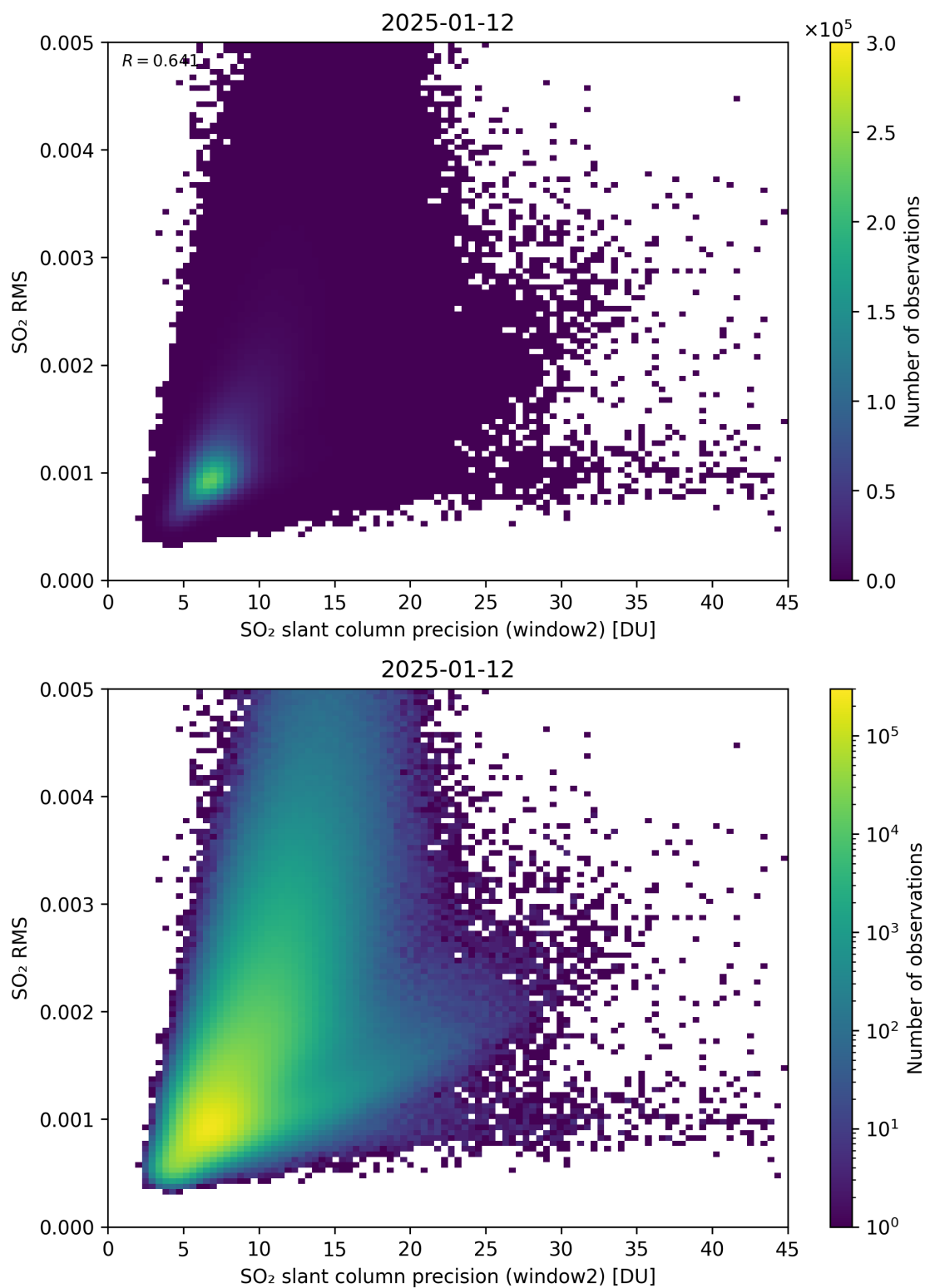
Figure 295: Scatter density plot of “SO 2 slant column precision (window2)” against “SO 2 RMS” for 2025-01-12 to 2025-01-13.
