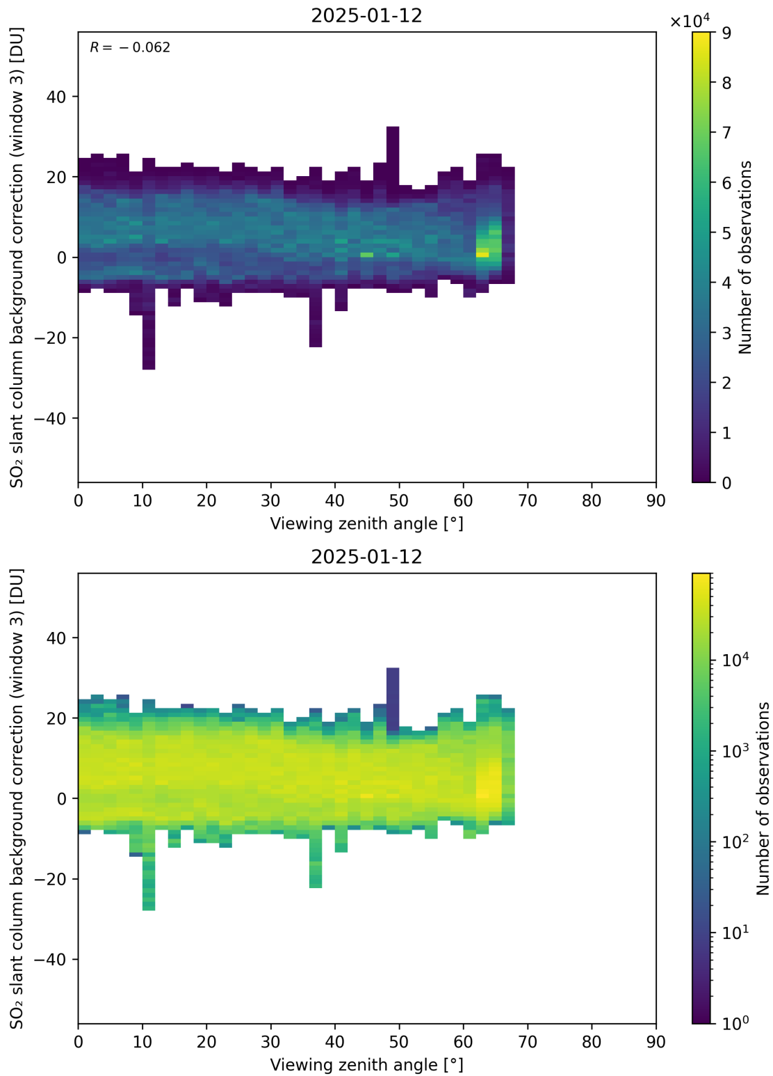
Figure 364: Scatter density plot of “Viewing zenith angle” against “SO 2 slant column background correction (window 3)” for 2025-01-12 to 2025-01-13.
