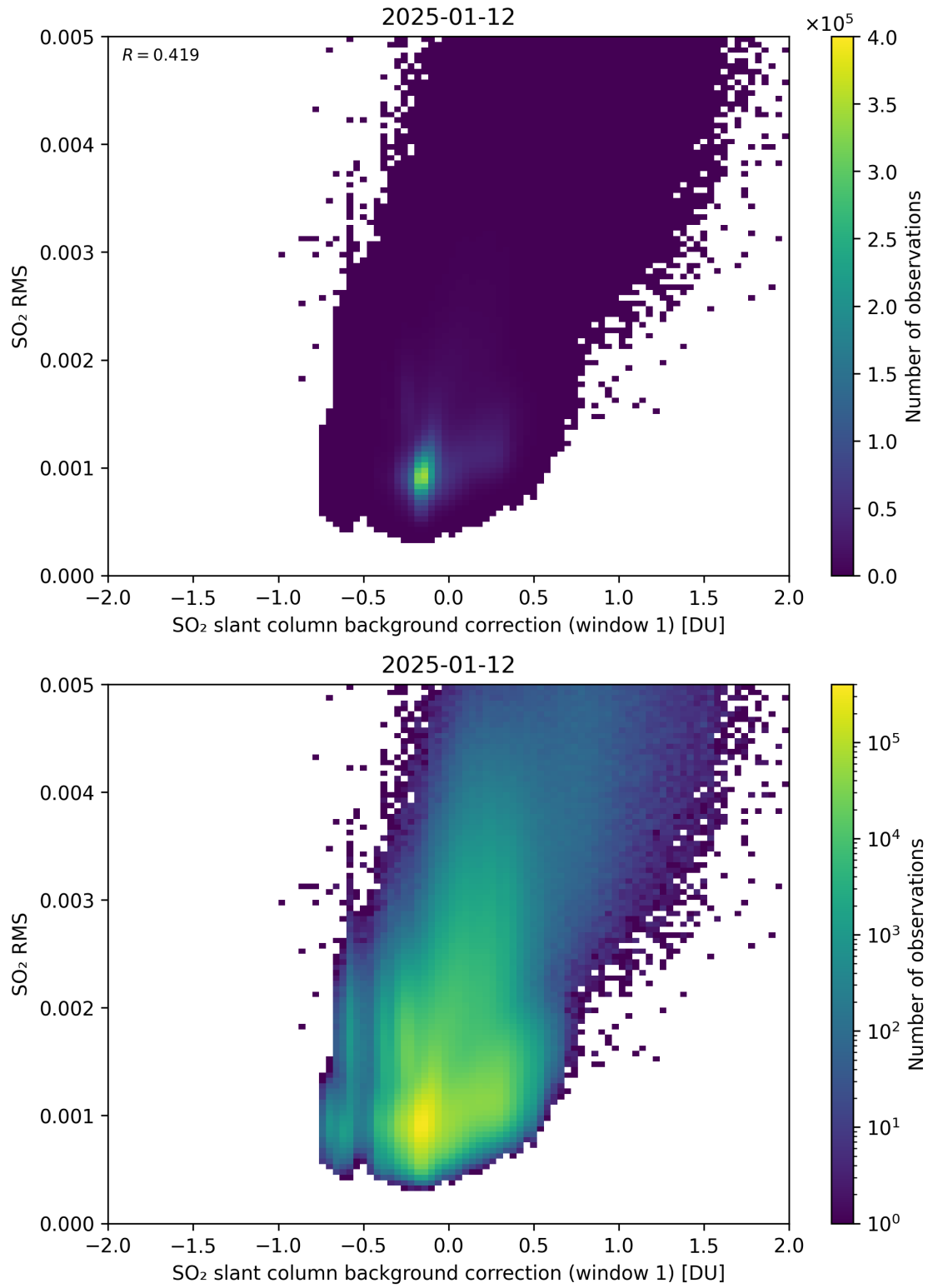
Figure 113: Scatter density plot of “SO 2 slant column background correction (window 1)” against “SO 2 RMS” for 2025-01-12 to 2025-01-13.
