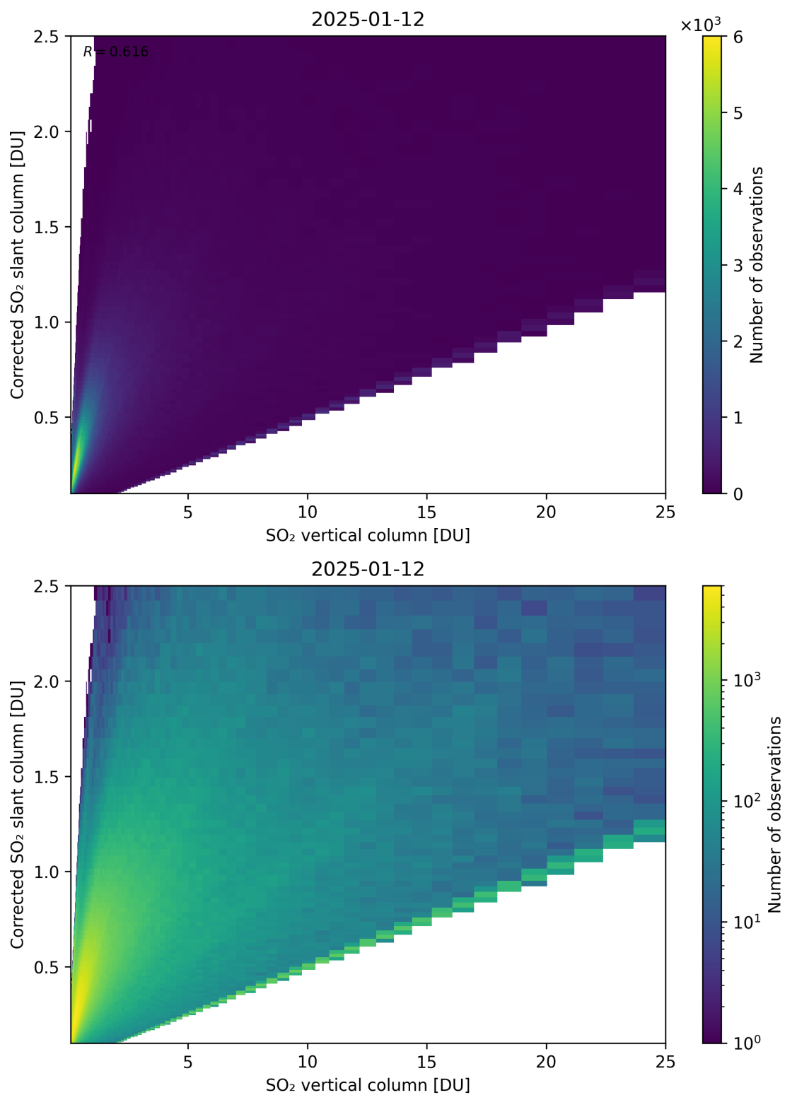
Figure 351: Scatter density plot of “SO 2 vertical column” against “Corrected SO 2 slant column” for 2025-01-12 to 2025-01-13.
