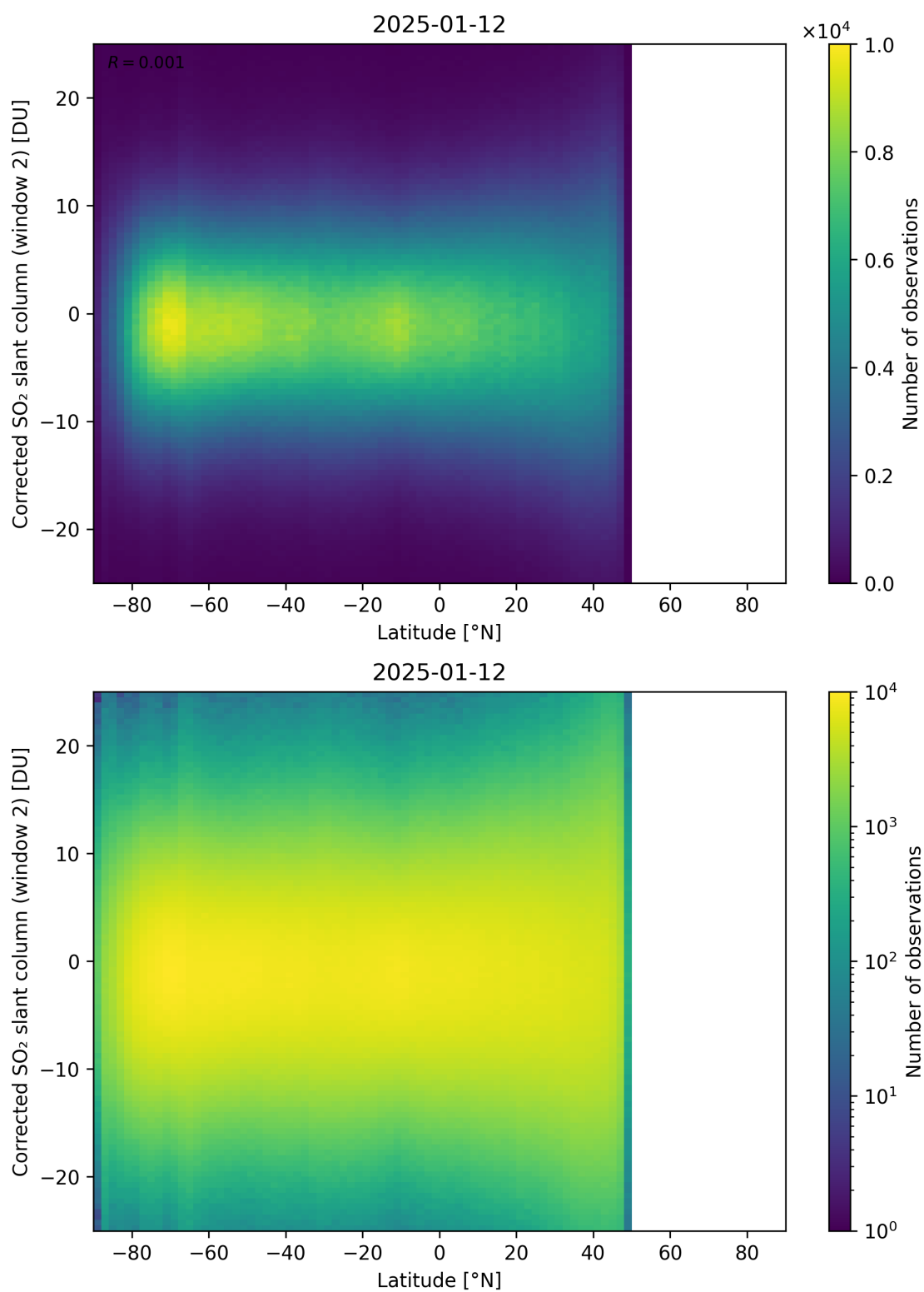
Figure 160: Scatter density plot of “Latitude” against “Corrected SO 2 slant column (window 2)” for 2025-01-12 to 2025-01-13.
