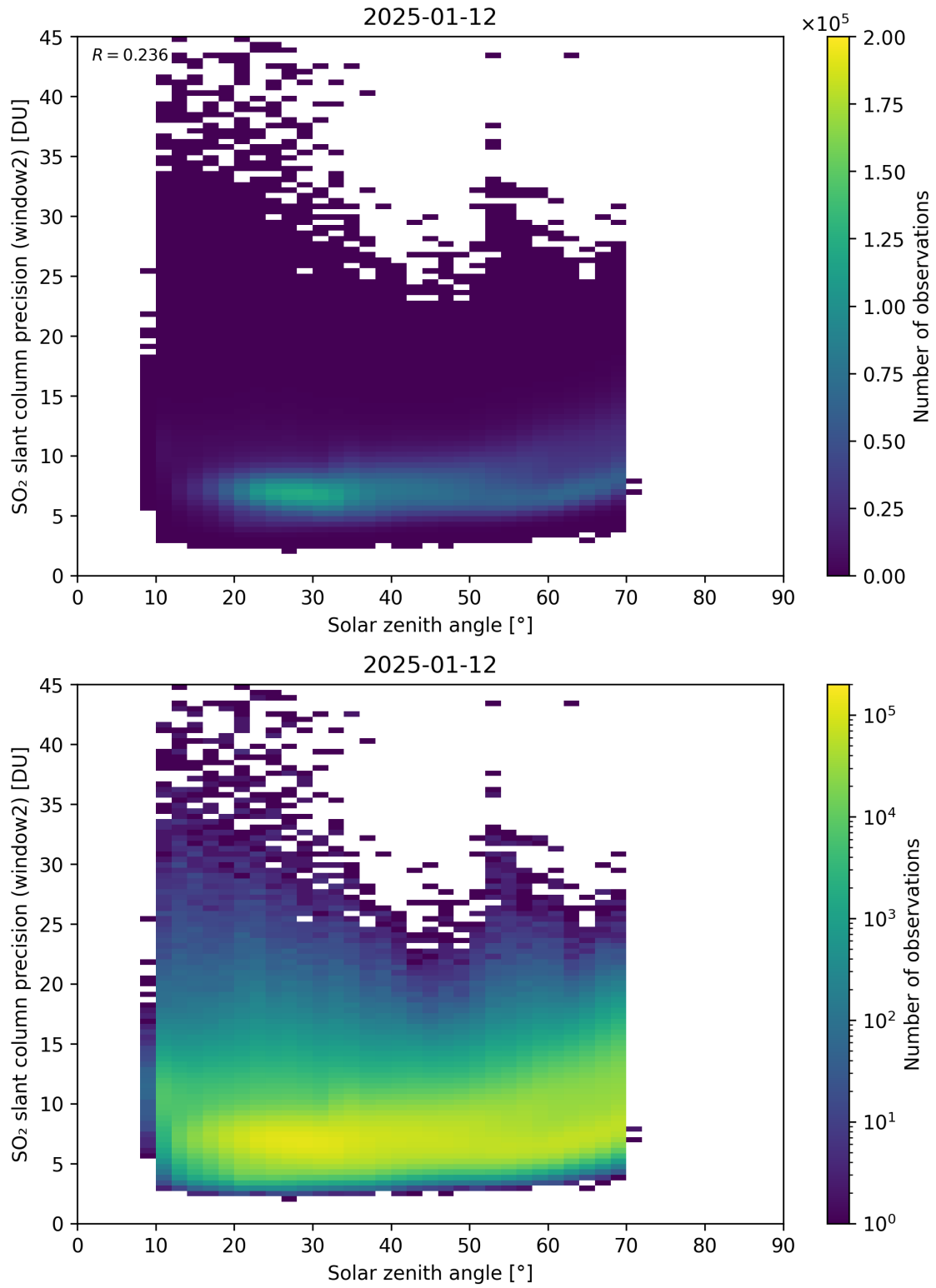
Figure 186: Scatter density plot of “Solar zenith angle” against “SO 2 slant column precision (window2)” for 2025-01-12 to 2025-01-13.
