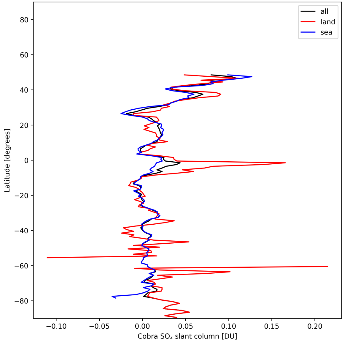
Figure 35: Zonal average of “Cobra SO 2 slant column” for 2025-01-12 to 2025-01-13.
