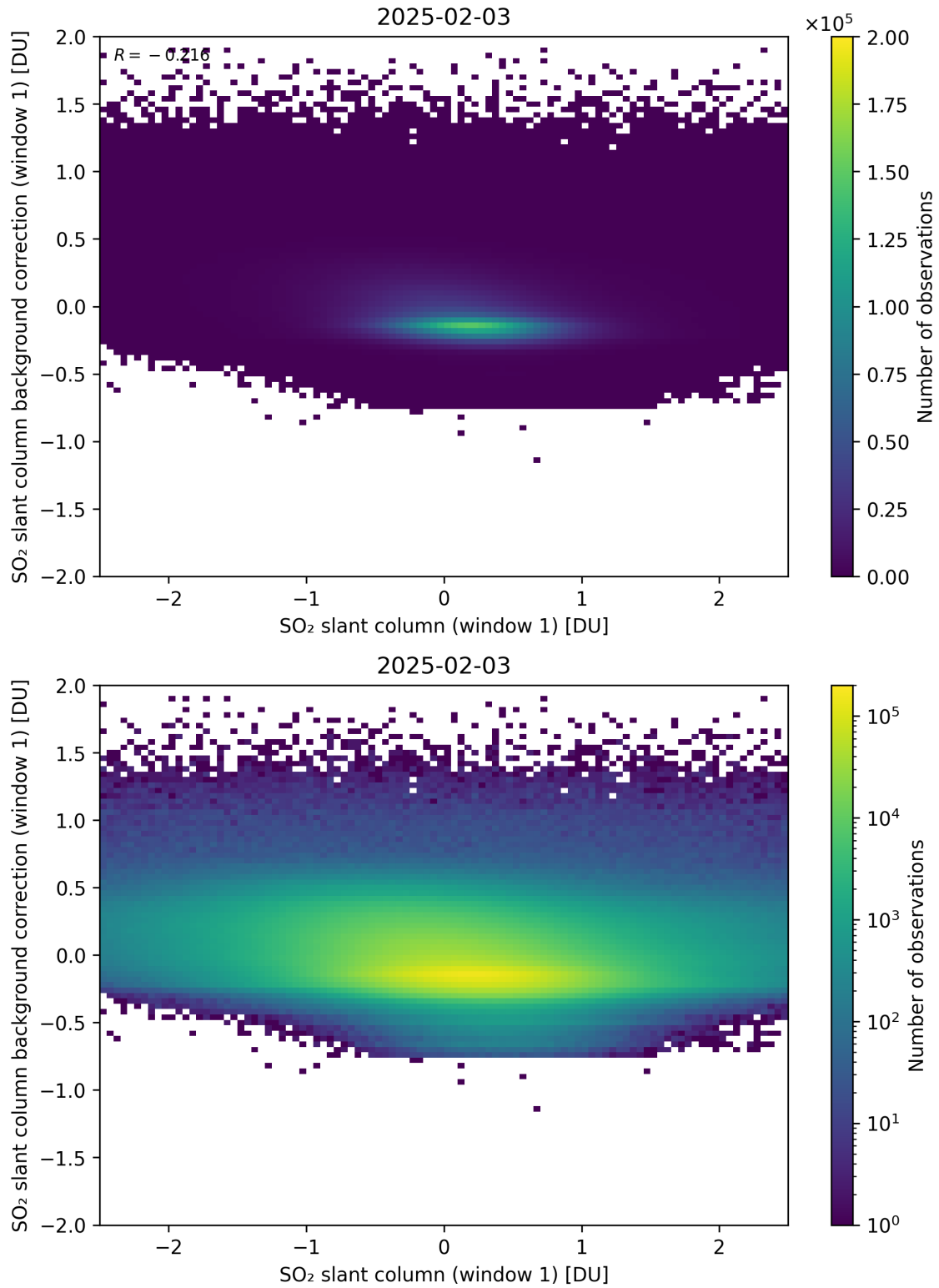
Figure 262: Scatter density plot of “SO 2 slant column (window 1)” against “SO 2 slant column background correction (window 1)” for 2025-02-03 to 2025-02-04.
