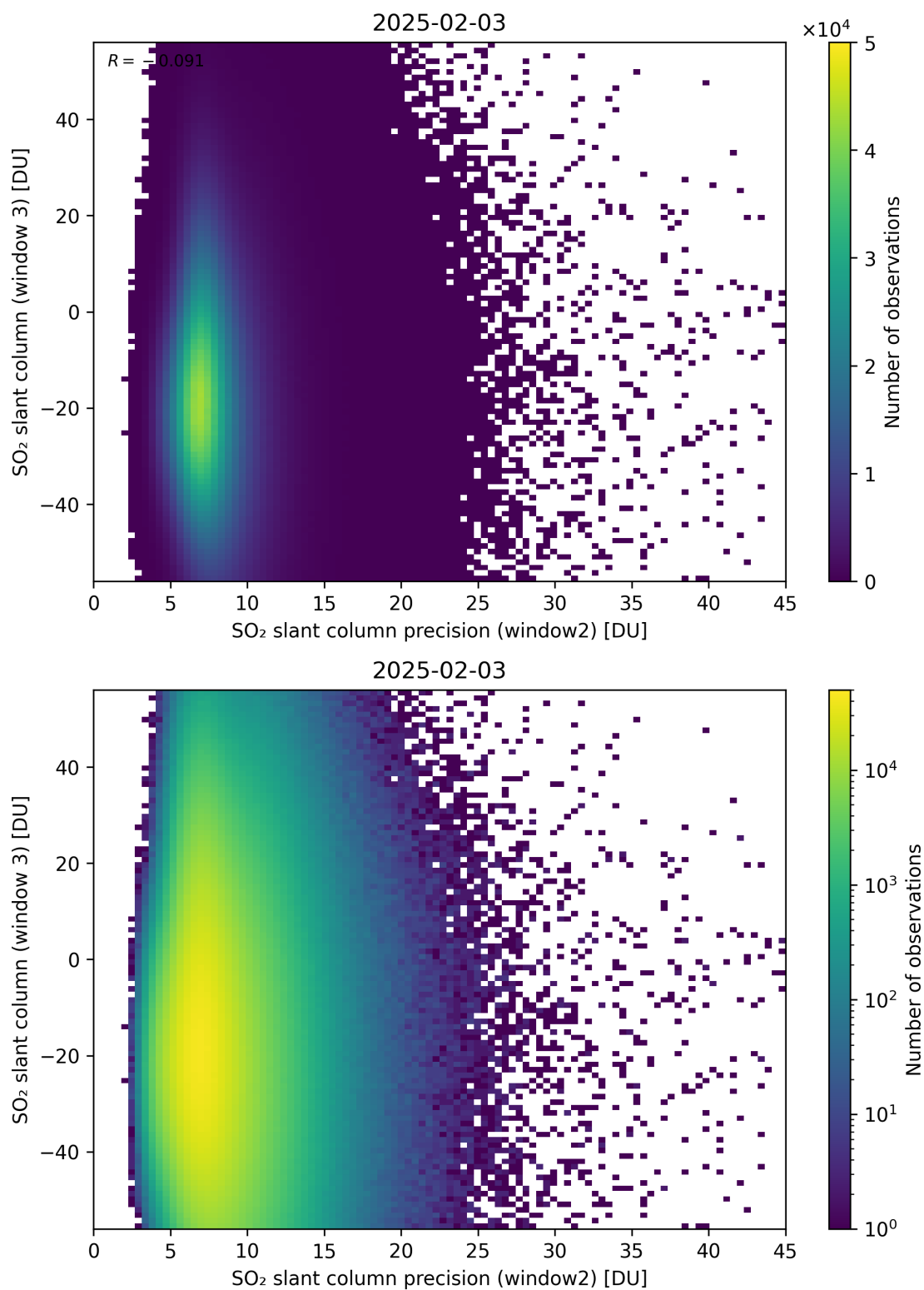
Figure 299: Scatter density plot of “SO 2 slant column precision (window2)” against “SO 2 slant column (window 3)” for 2025-02-03 to 2025-02-04.
