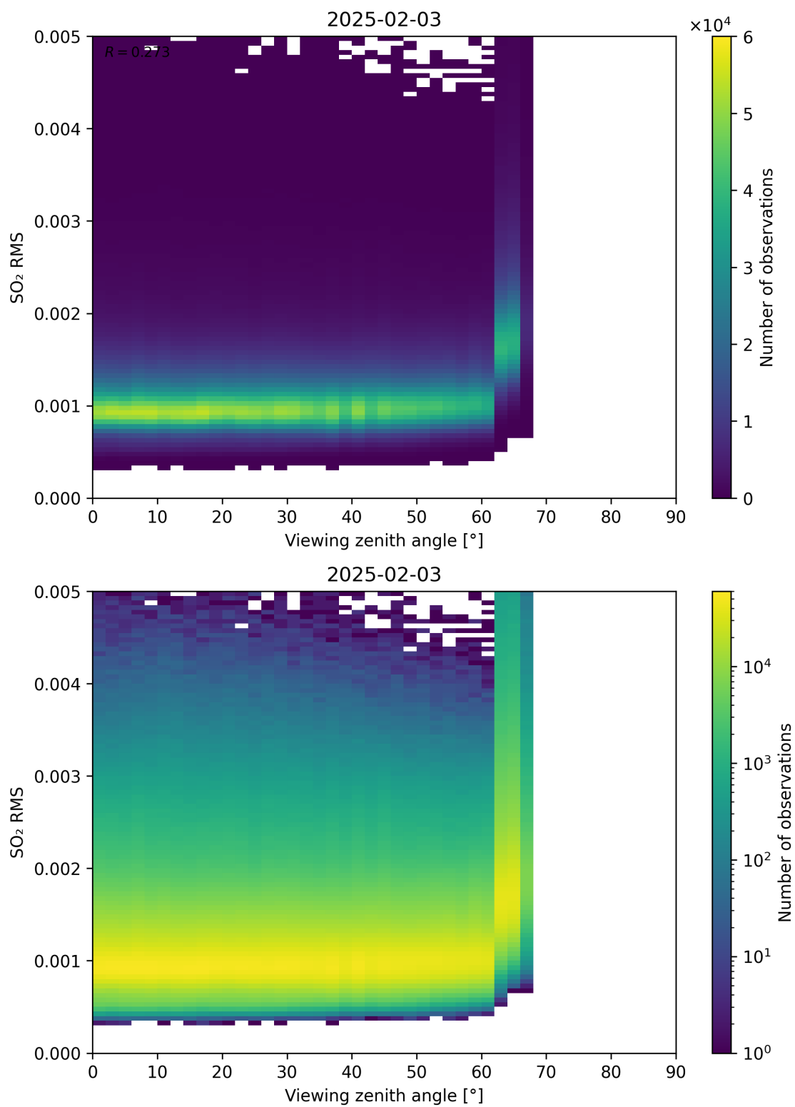
Figure 367: Scatter density plot of “Viewing zenith angle” against “SO 2 RMS” for 2025-02-03 to 2025-02-04.
