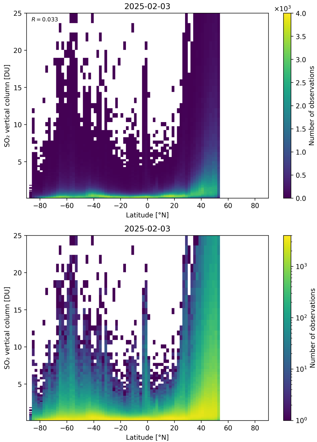
Figure 169: Scatter density plot of “Latitude” against “SO 2 vertical column” for 2025-02-03 to 2025-02-04.
