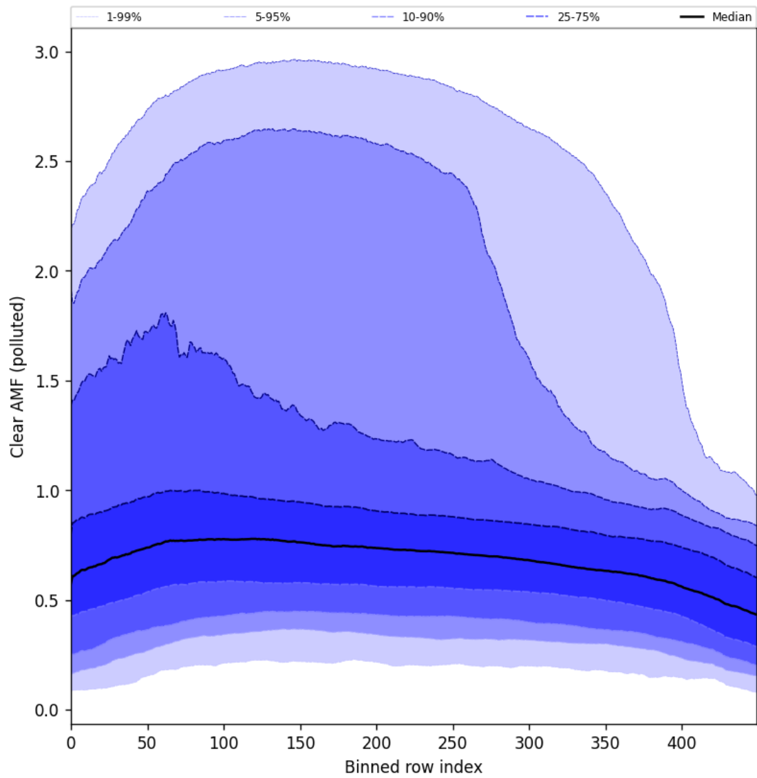
Figure 107: Along track statistics of “Clear AMF (polluted)” for 2025-02-03 to 2025-02-04
