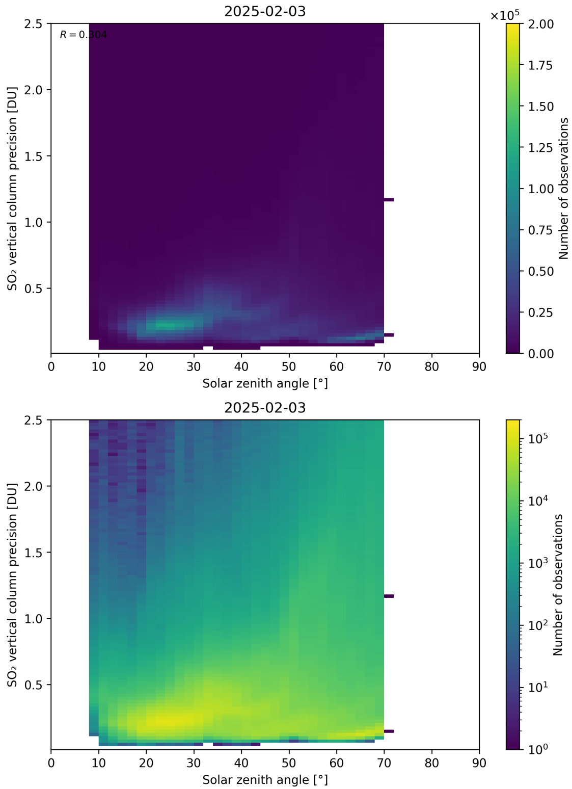
Figure 192: Scatter density plot of “Solar zenith angle” against “SO 2 vertical column precision” for 2025-02-03 to 2025-02-04.
