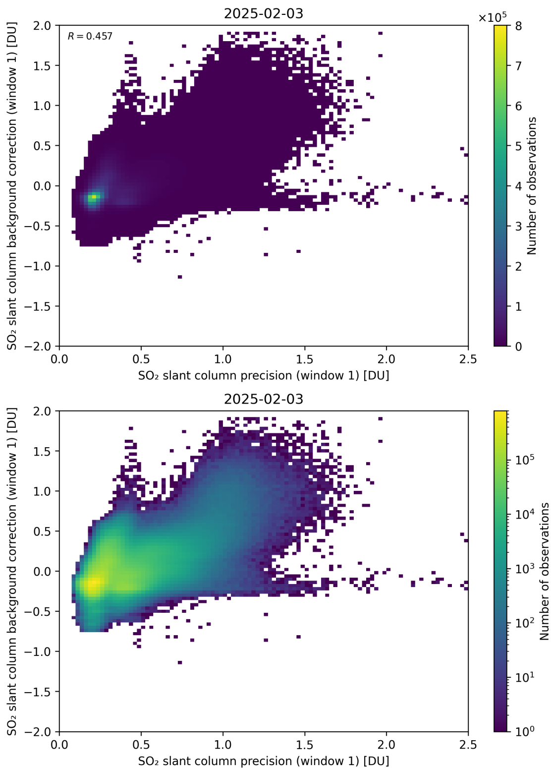
Figure 268: Scatter density plot of “SO 2 slant column precision (window 1)” against “SO 2 slant column background correction (window 1)” for 2025-02-03 to 2025-02-04.
