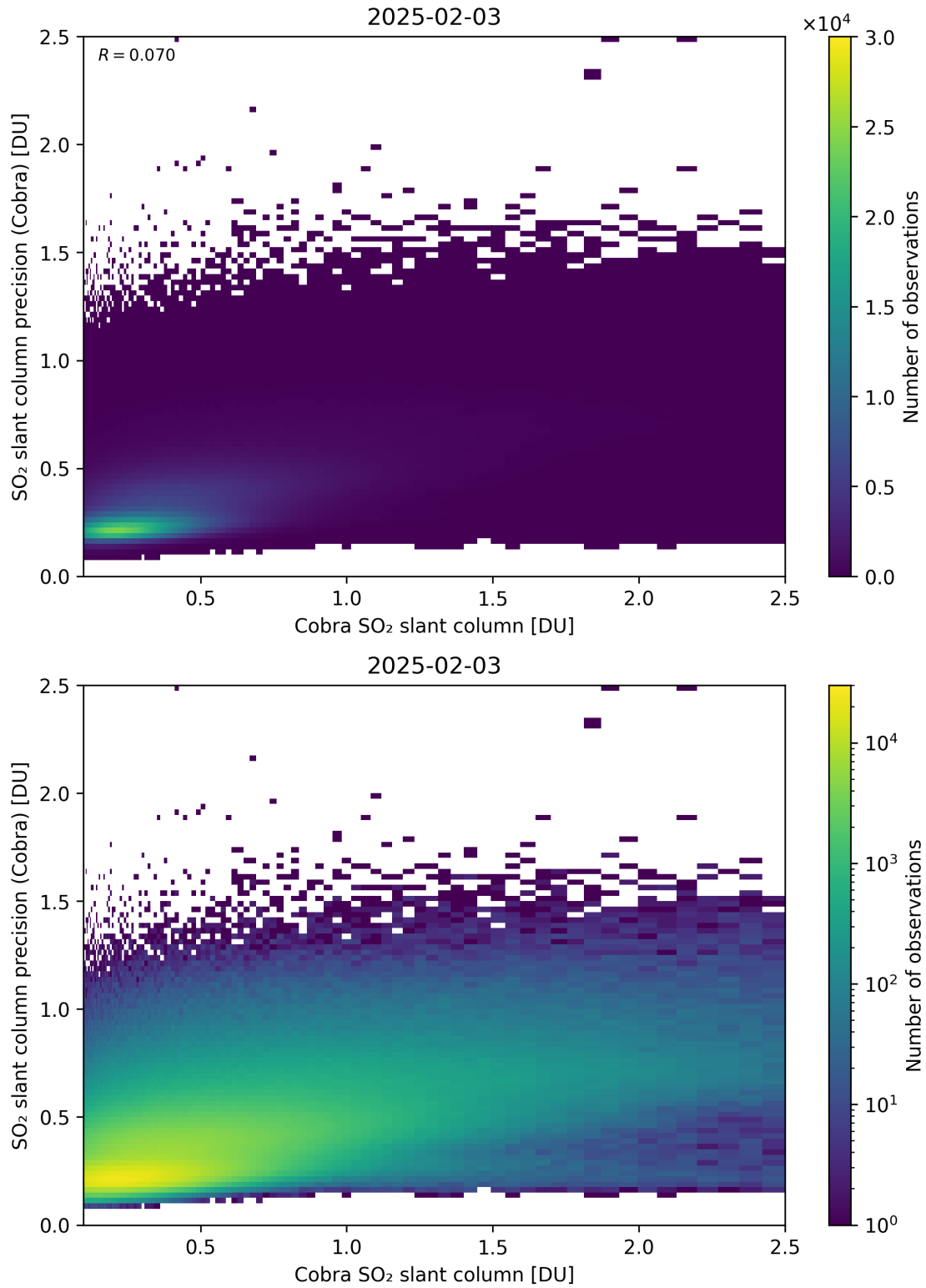
Figure 216: Scatter density plot of “Cobra SO 2 slant column” against “SO 2 slant column precision (Cobra)” for 2025-02-03 to 2025-02-04.
