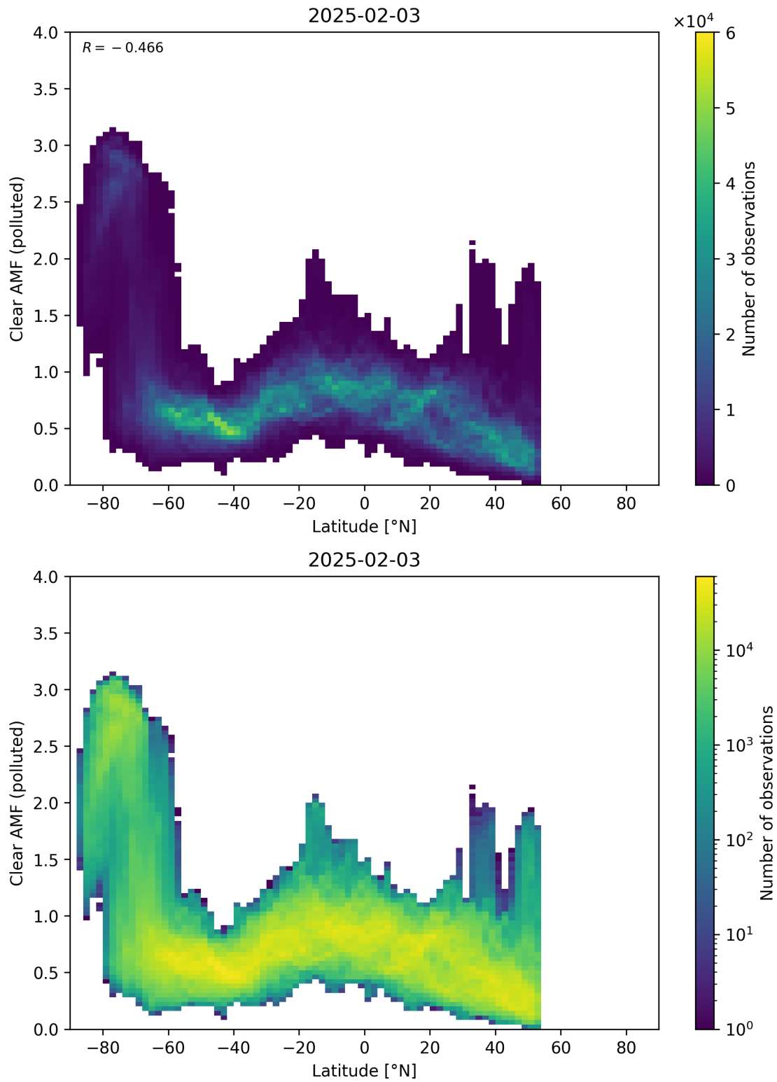
Figure 156: Scatter density plot of “Latitude” against “Clear AMF (polluted)” for 2025-02-03 to 2025-02-04.
