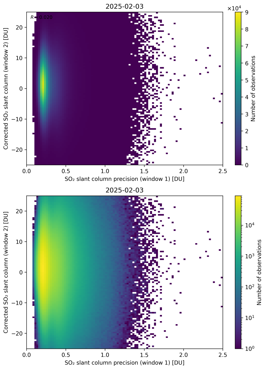
Figure 275: Scatter density plot of “SO 2 slant column precision (window 1)” against “Corrected SO 2 slant column (window 2)” for 2025-02-03 to 2025-02-04.
