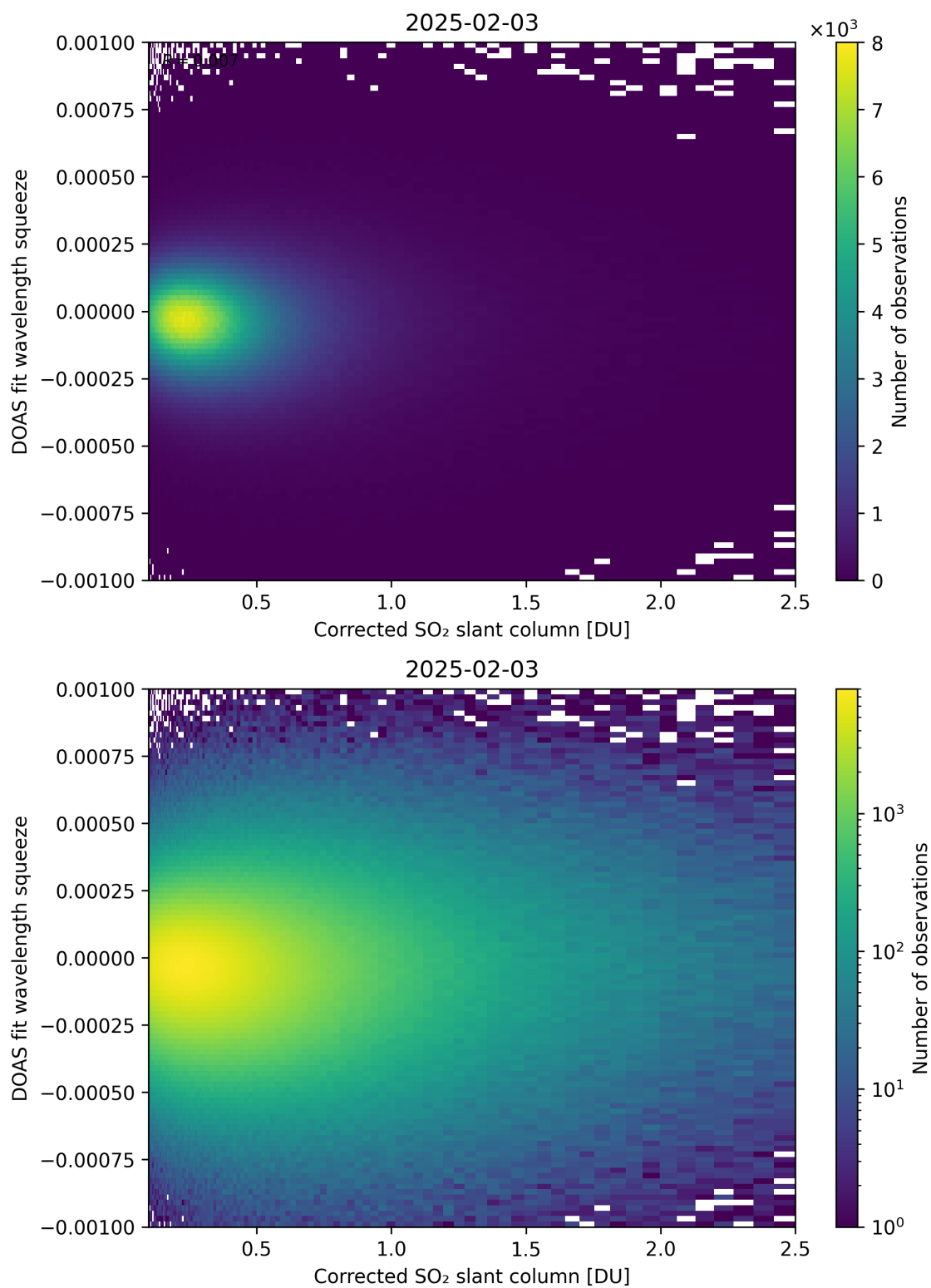
Figure 230: Scatter density plot of “Corrected SO 2 slant column” against “DOAS fit wavelength squeeze” for 2025-02-03 to 2025-02-04.
