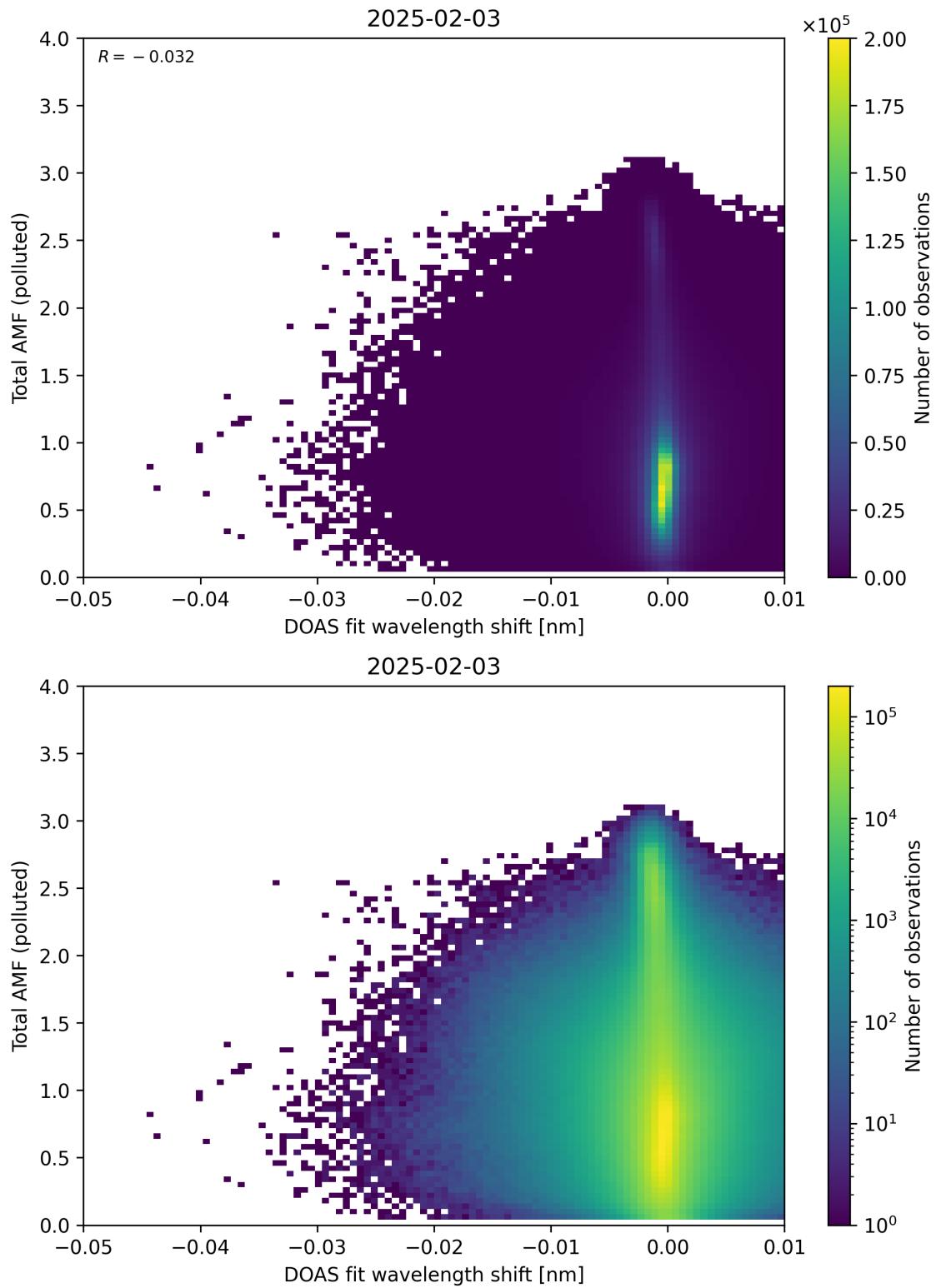
Figure 141: Scatter density plot of “DOAS fit wavelength shift” against “Total AMF (polluted)” for 2025-02-03 to 2025-02-04.
