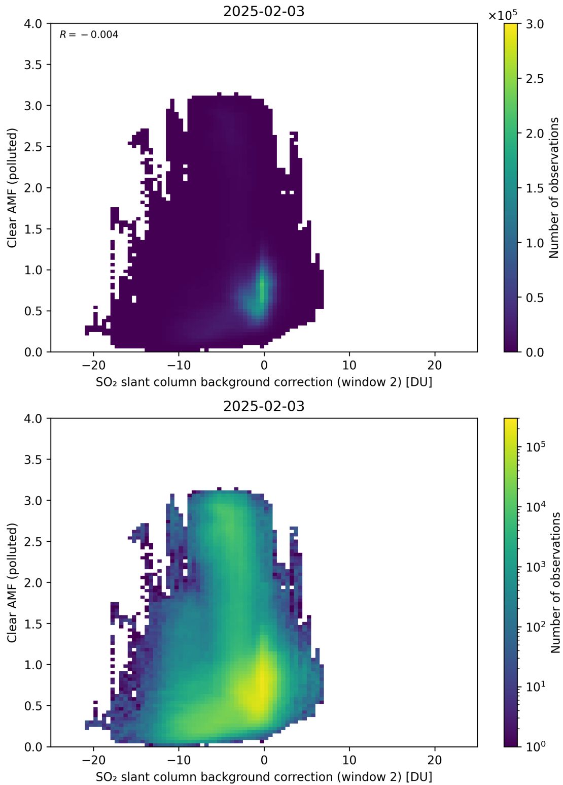
Figure 126: Scatter density plot of “SO 2 slant column background correction (window 2)” against “Clear AMF (polluted)” for 2025-02-03 to 2025-02-04.
