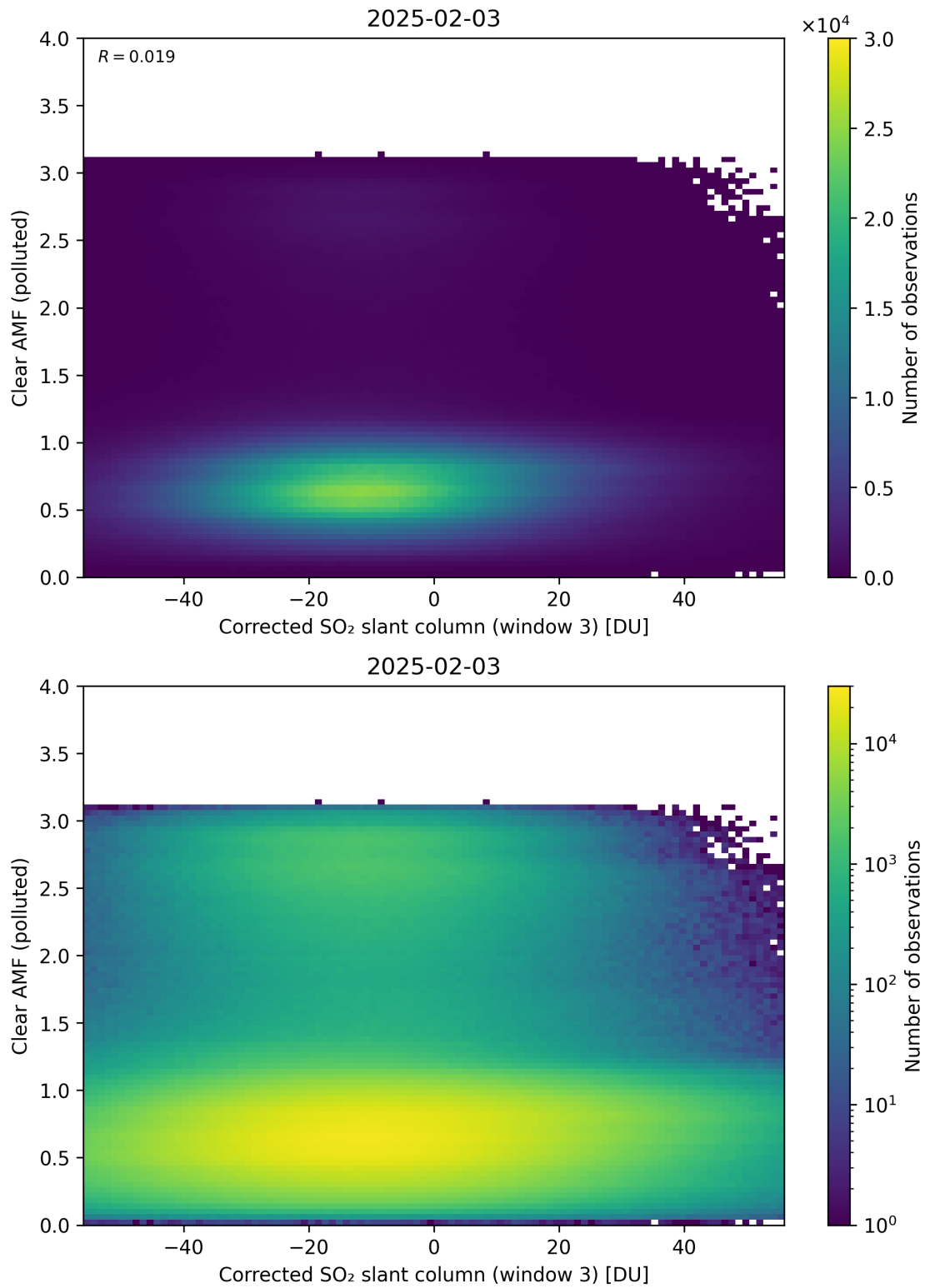
Figure 259: Scatter density plot of “Corrected SO 2 slant column (window 3)” against “Clear AMF (polluted)” for 2025-02-03 to 2025-02-04.
