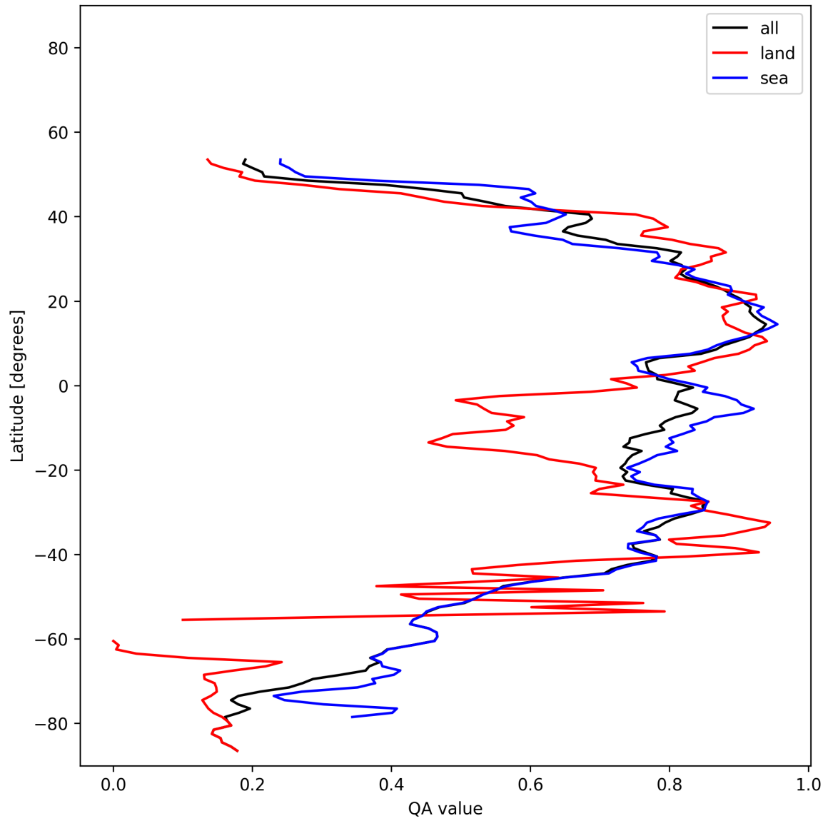
Figure 31: Zonal average of “QA value” for 2025-02-03 to 2025-02-04.
