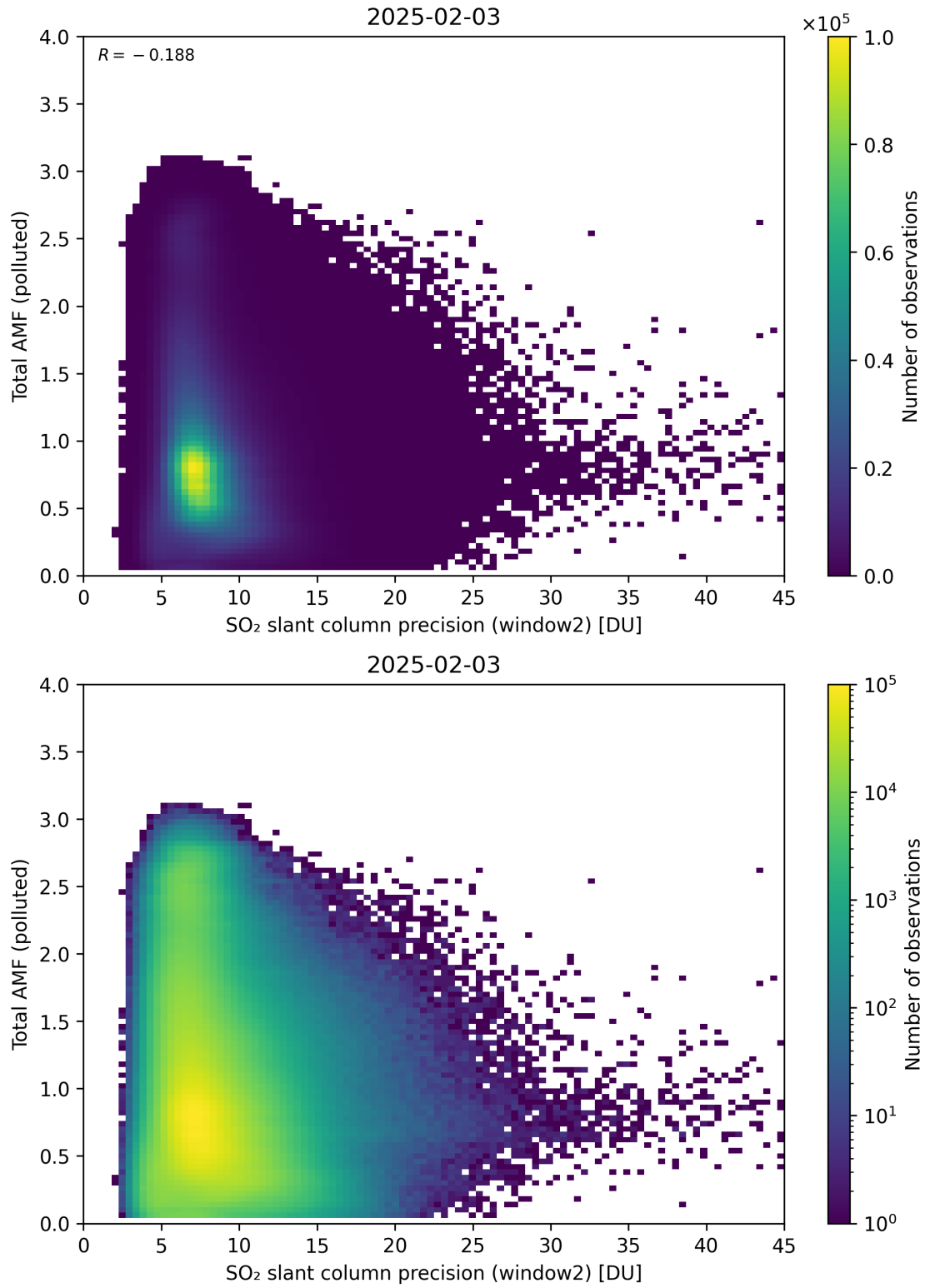
Figure 301: Scatter density plot of “SO 2 slant column precision (window2)” against “Total AMF (polluted)” for 2025-02-03 to 2025-02-04.
