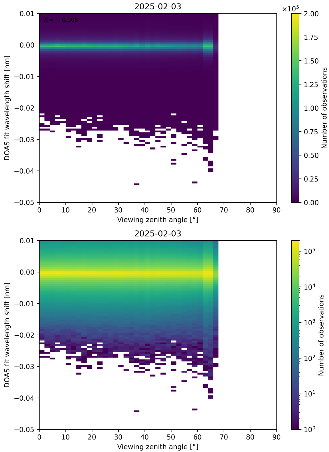
Figure 365: Scatter density plot of “Viewing zenith angle” against “DOAS fit wavelength shift” for 2025-02-03 to 2025-02-04.
