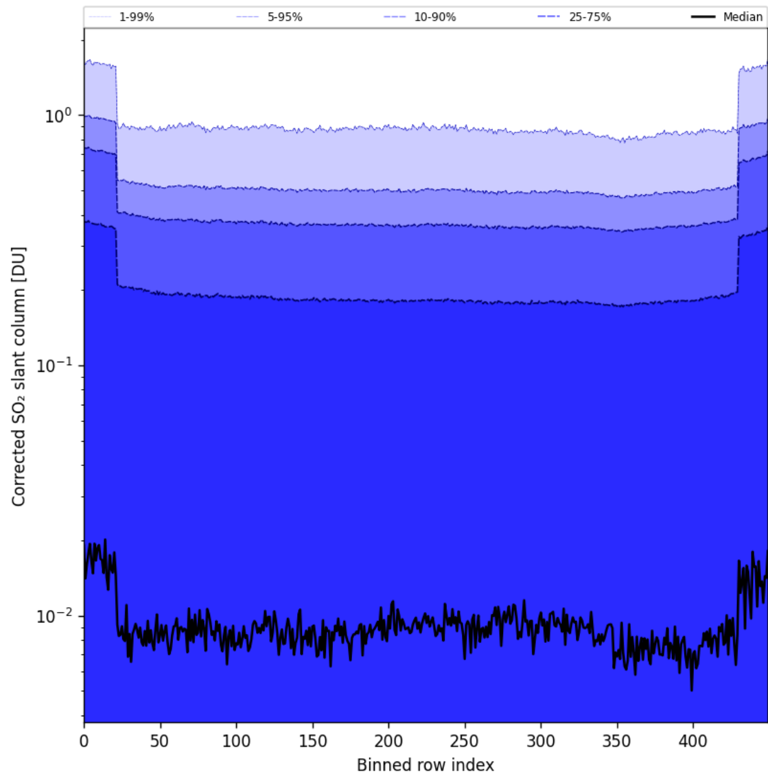
Figure 86: Along track statistics of “Corrected SO 2 slant column” for 2025-02-03 to 2025-02-04
