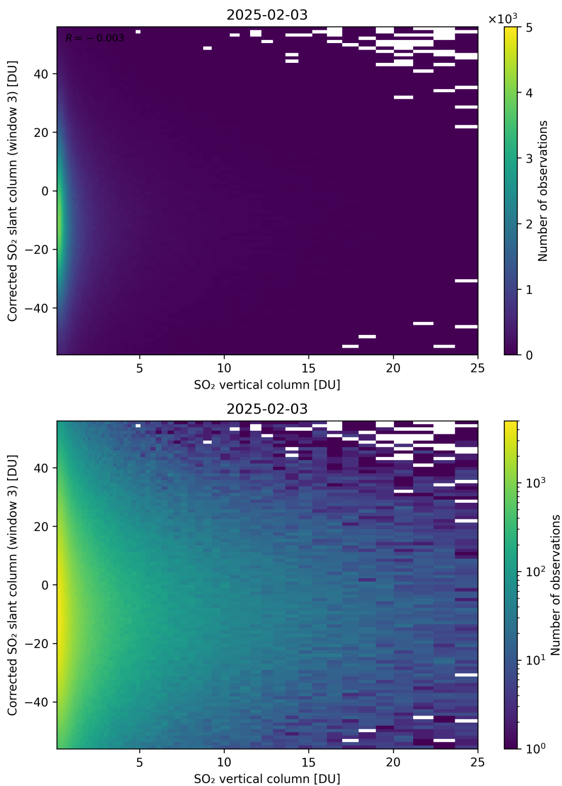
Figure 353: Scatter density plot of “SO 2 vertical column” against “Corrected SO 2 slant column (window 3)” for 2025-02-03 to 2025-02-04.
