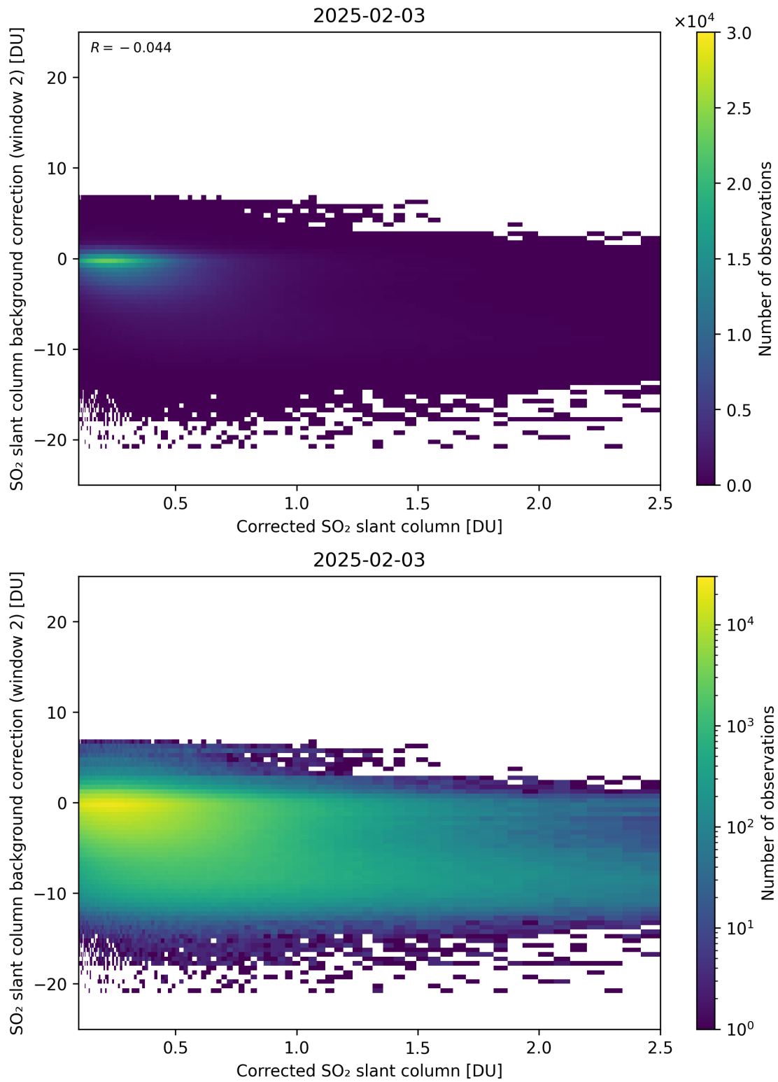
Figure 227: Scatter density plot of “Corrected SO 2 slant column” against “SO 2 slant column background correction (window 2)” for 2025-02-03 to 2025-02-04.
