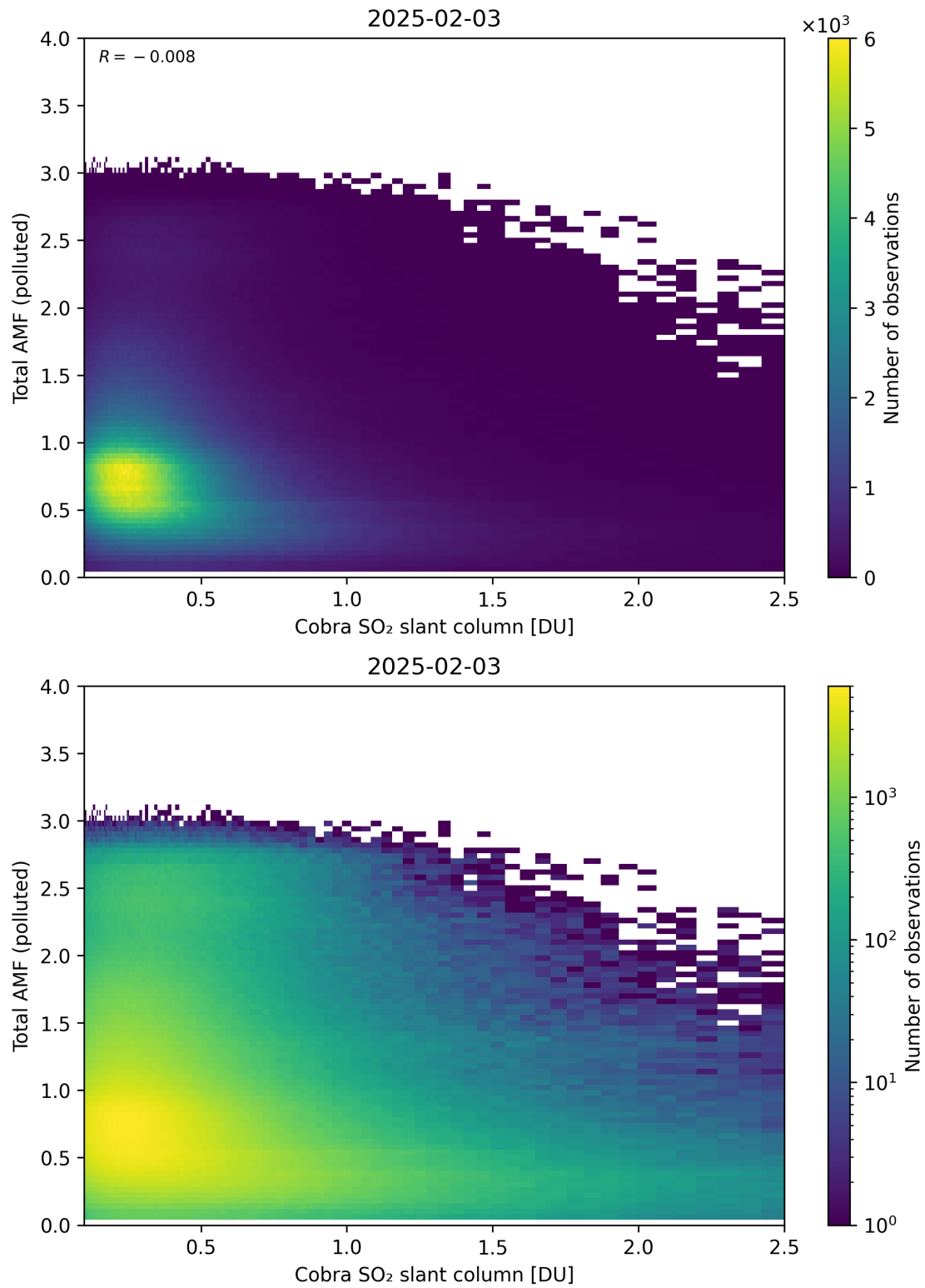
Figure 224: Scatter density plot of “Cobra SO 2 slant column” against “Total AMF (polluted)” for 2025-02-03 to 2025-02-04.
