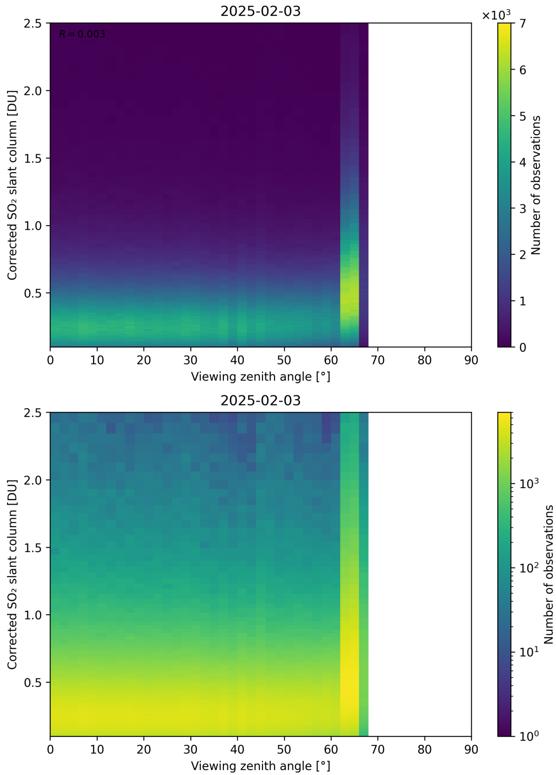
Figure 373: Scatter density plot of “Viewing zenith angle” against “Corrected SO 2 slant column” for 2025-02-03 to 2025-02-04.
