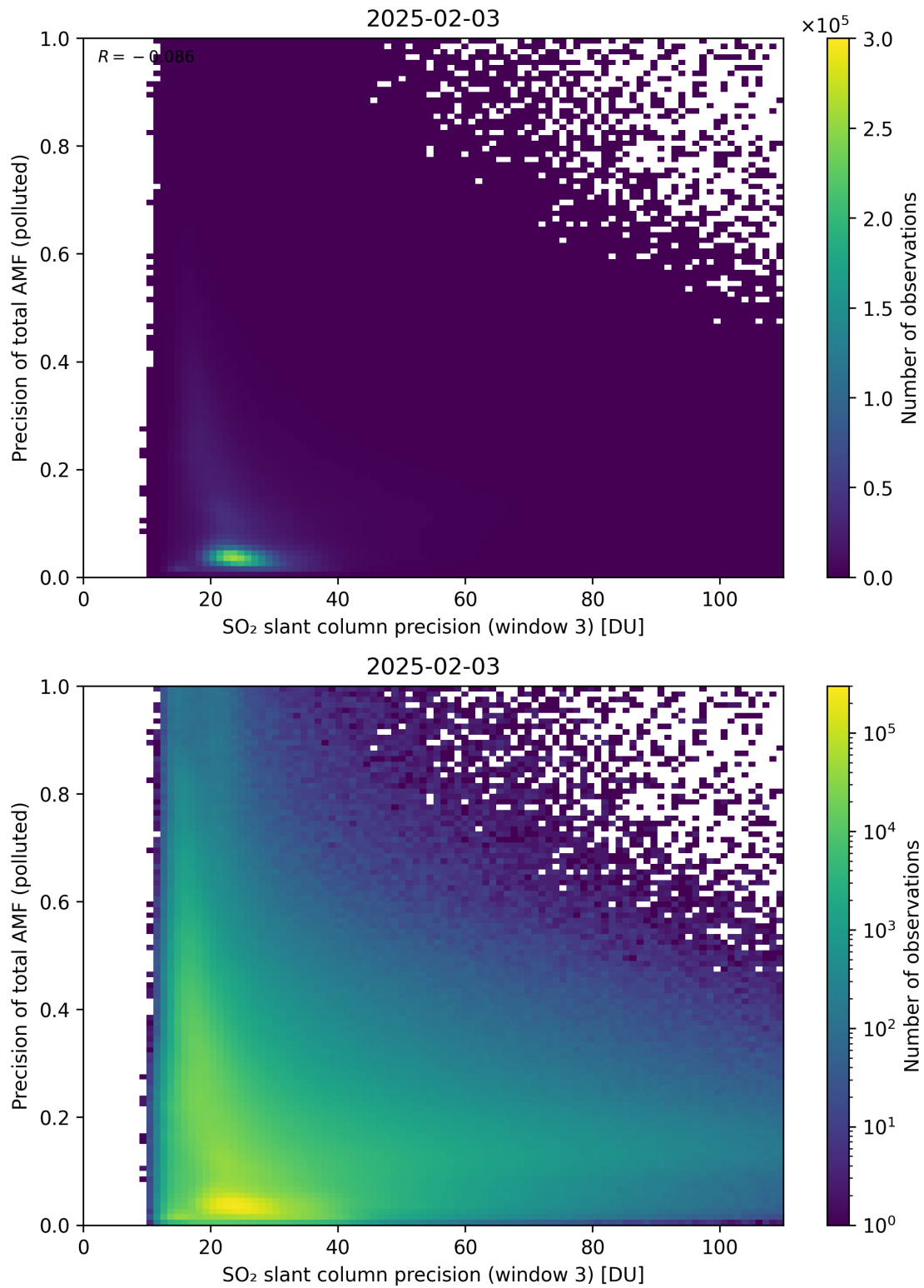
Figure 314: Scatter density plot of “SO 2 slant column precision (window 3)” against “Precision of total AMF (polluted)” for 2025-02-03 to 2025-02-04.
