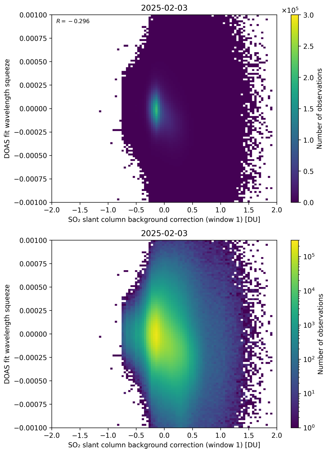
Figure 112: Scatter density plot of “SO 2 slant column background correction (window 1)” against “DOAS fit wavelength squeeze” for 2025-02-03 to 2025-02-04.
