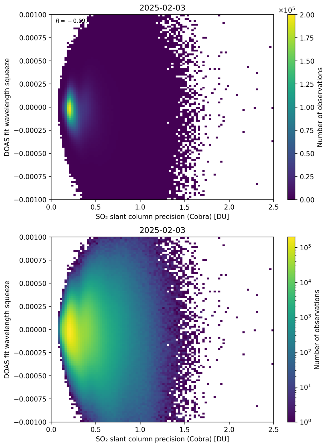
Figure 203: Scatter density plot of “SO 2 slant column precision (Cobra)” against “DOAS fit wavelength squeeze” for 2025-02-03 to 2025-02-04.
