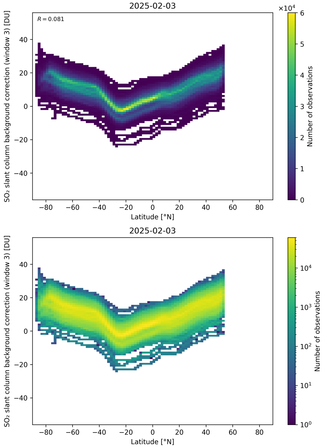
Figure 152: Scatter density plot of “Latitude” against “SO 2 slant column background correction (window 3)” for 2025-02-03 to 2025-02-04.
