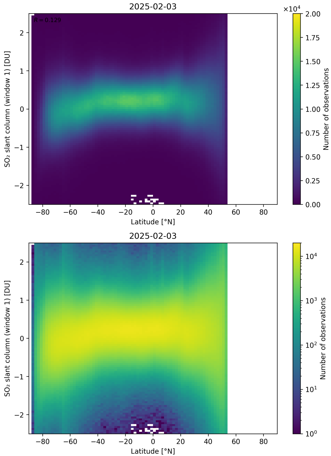
Figure 162: Scatter density plot of “Latitude” against “SO 2 slant column (window 1)” for 2025-02-03 to 2025-02-04.
