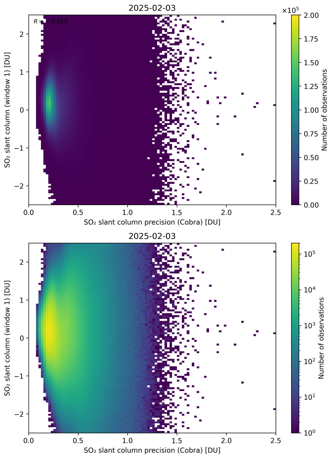
Figure 208: Scatter density plot of “SO 2 slant column precision (Cobra)” against “SO 2 slant column (window 1)” for 2025-02-03 to 2025-02-04.
