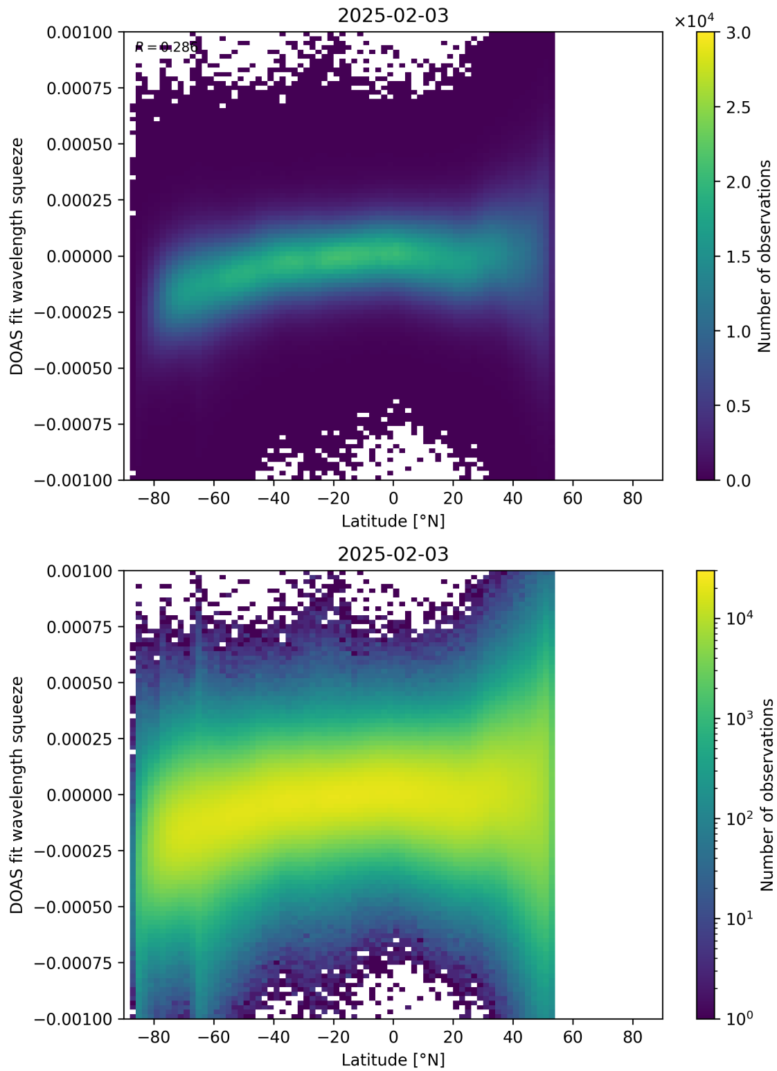
Figure 154: Scatter density plot of “Latitude” against “DOAS fit wavelength squeeze” for 2025-02-03 to 2025-02-04.
