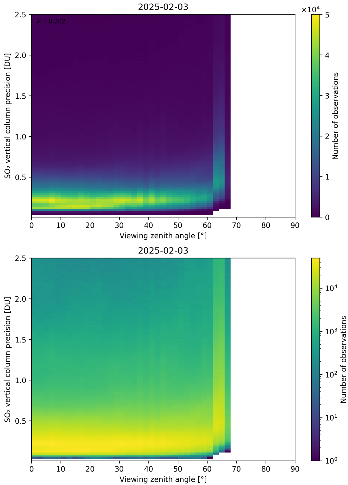
Figure 384: Scatter density plot of “Viewing zenith angle” against “SO 2 vertical column precision” for 2025-02-03 to 2025-02-04.
