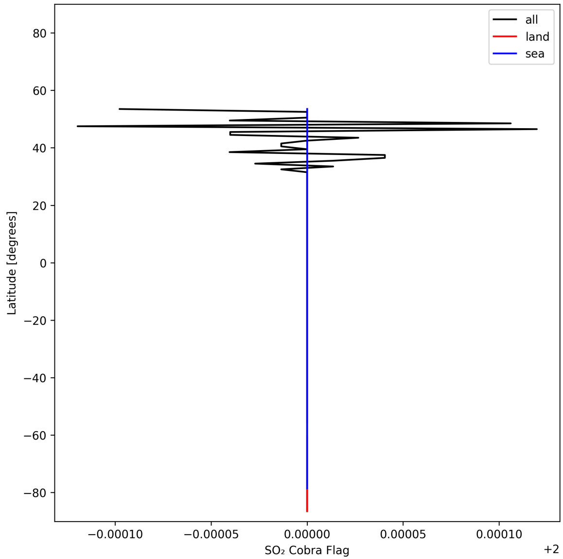
Figure 49: Zonal average of "SO 2 Cobra Flag" for 2025-02-03 to 2025-02-04.
