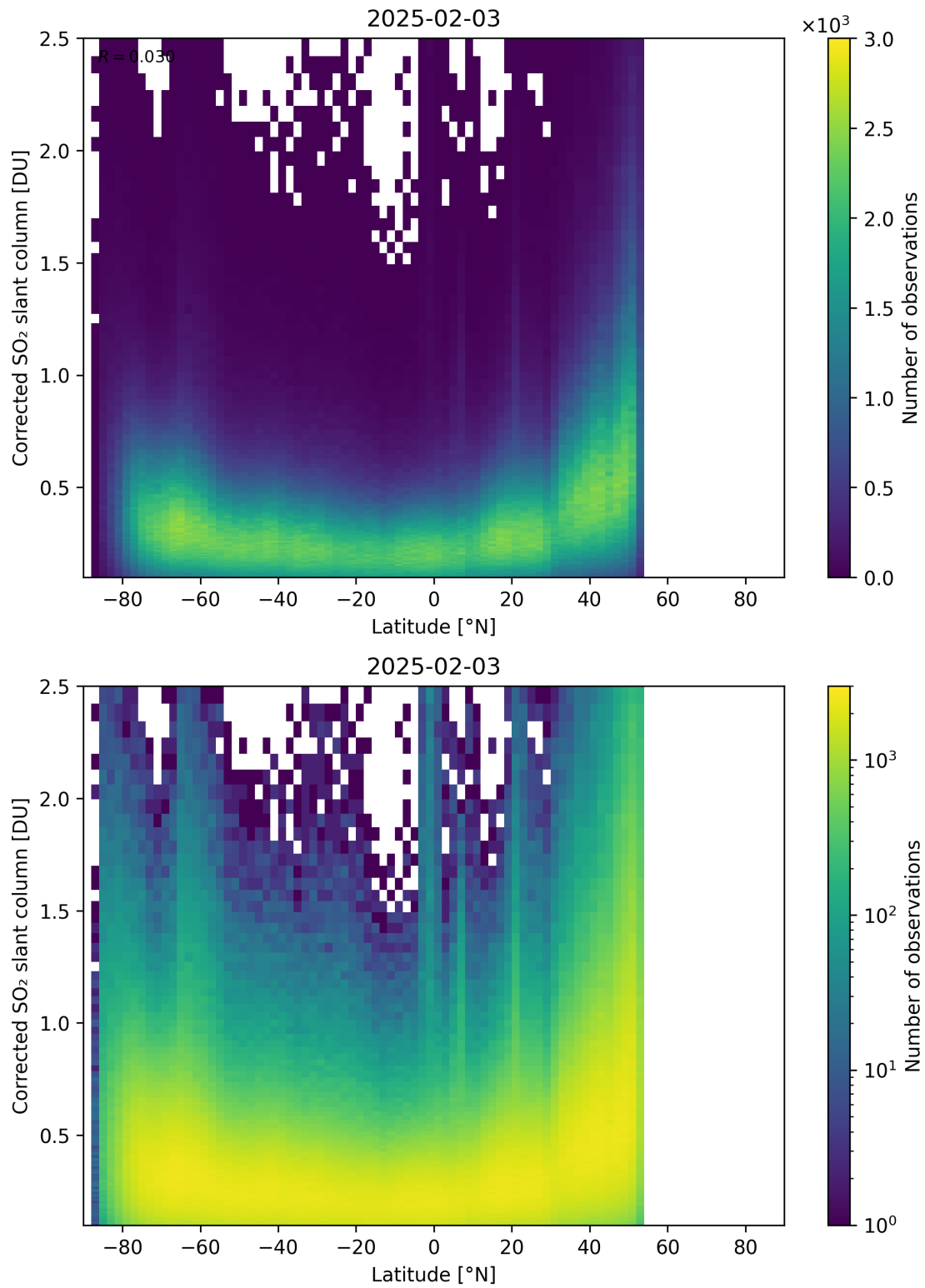
Figure 159: Scatter density plot of “Latitude” against “Corrected SO 2 slant column” for 2025-02-03 to 2025-02-04.
