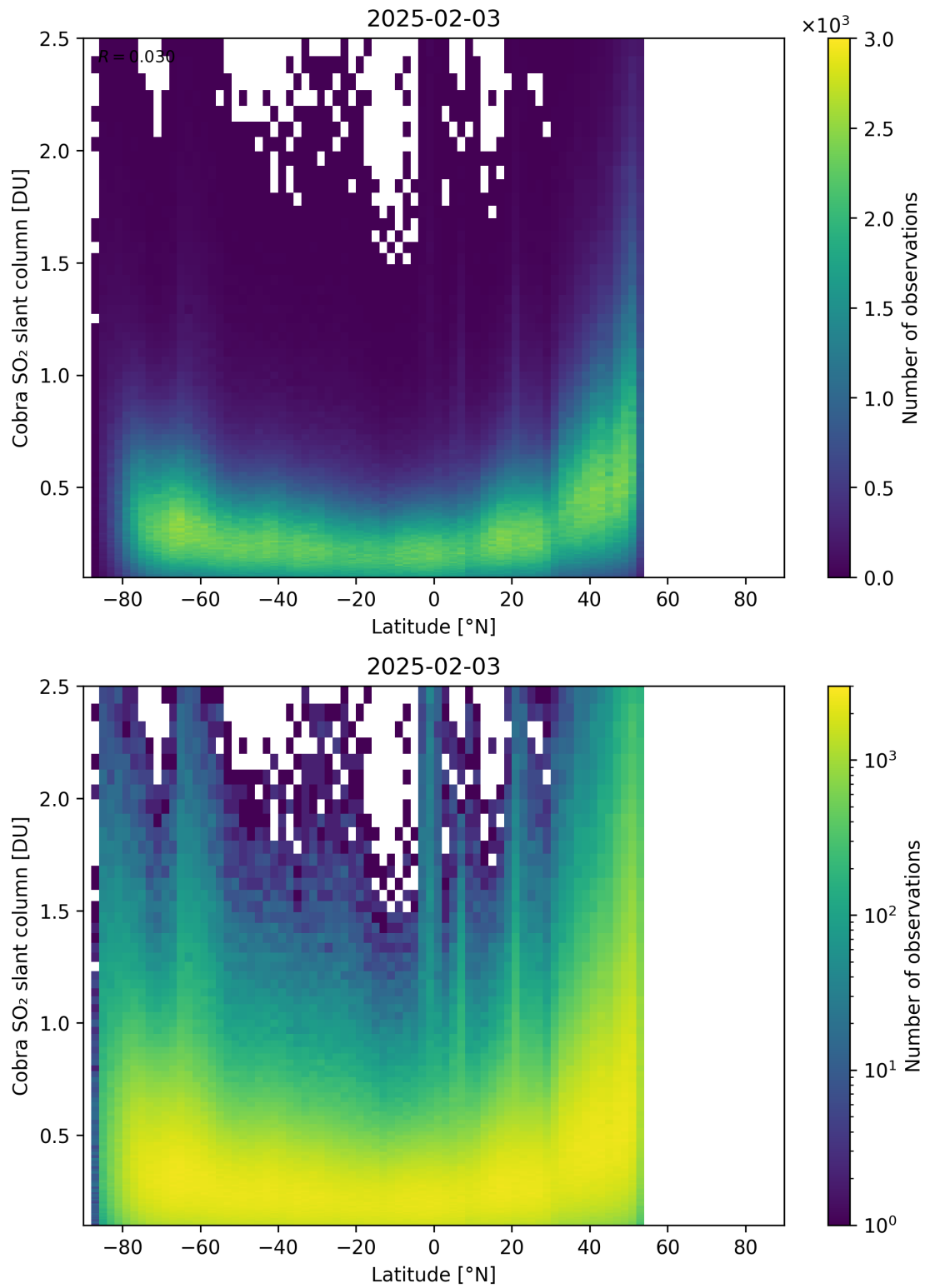
Figure 157: Scatter density plot of “Latitude” against “Cobra SO 2 slant column” for 2025-02-03 to 2025-02-04.
