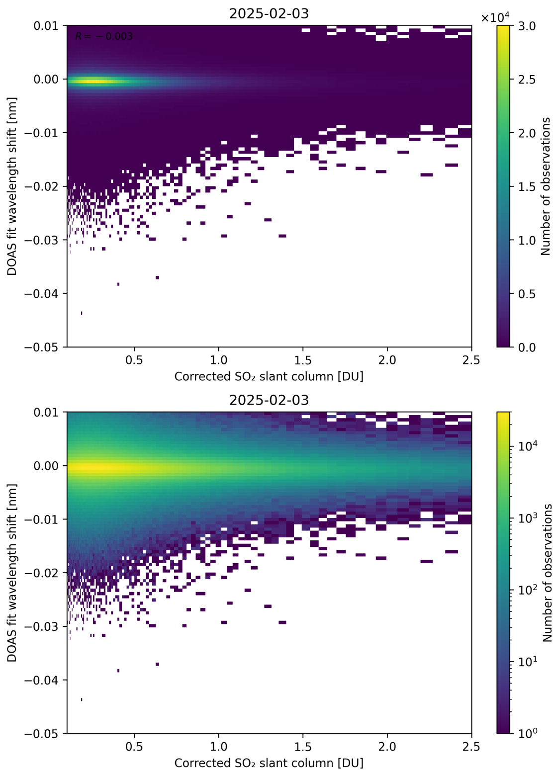
Figure 229: Scatter density plot of “Corrected SO 2 slant column” against “DOAS fit wavelength shift” for 2025-02-03 to 2025-02-04.
