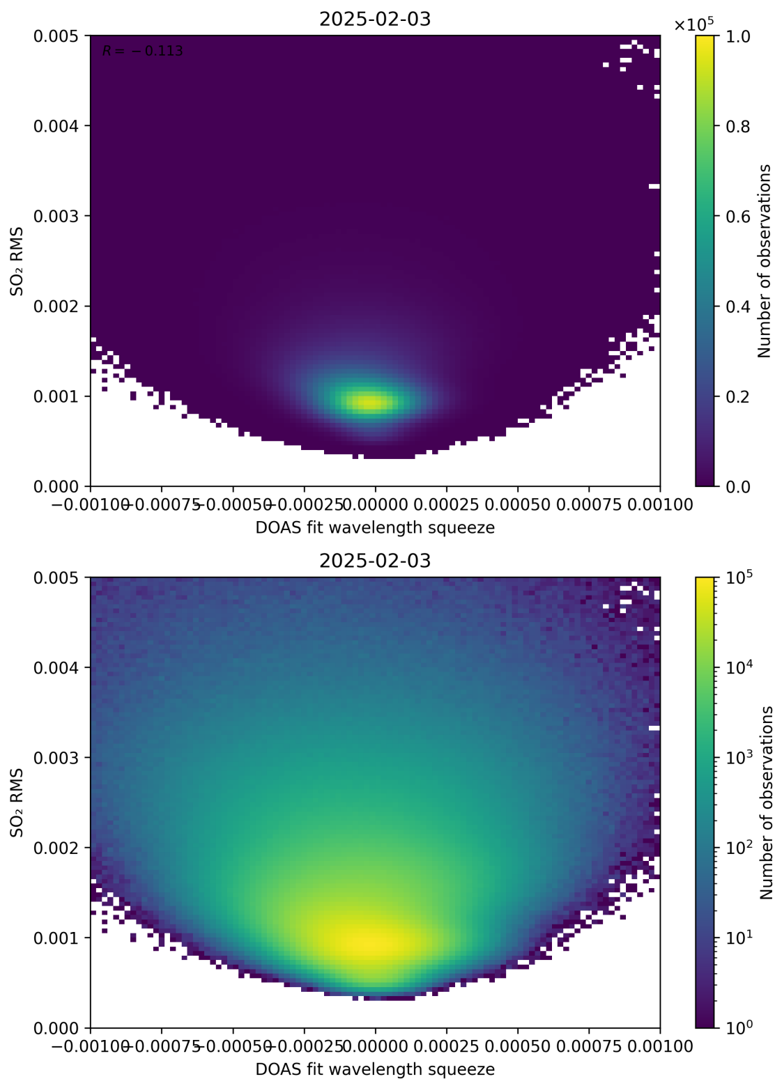
Figure 143: Scatter density plot of “DOAS fit wavelength squeeze” against “SO 2 RMS” for 2025-02-03 to 2025-02-04.
