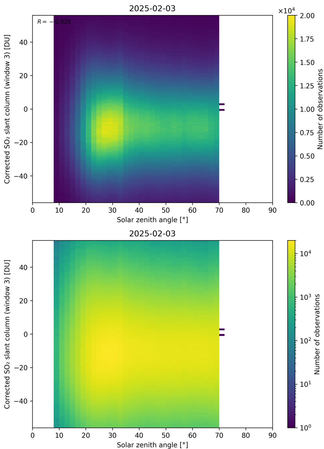
Figure 183: Scatter density plot of “Solar zenith angle” against “Corrected SO 2 slant column (window 3)” for 2025-02-03 to 2025-02-04.
