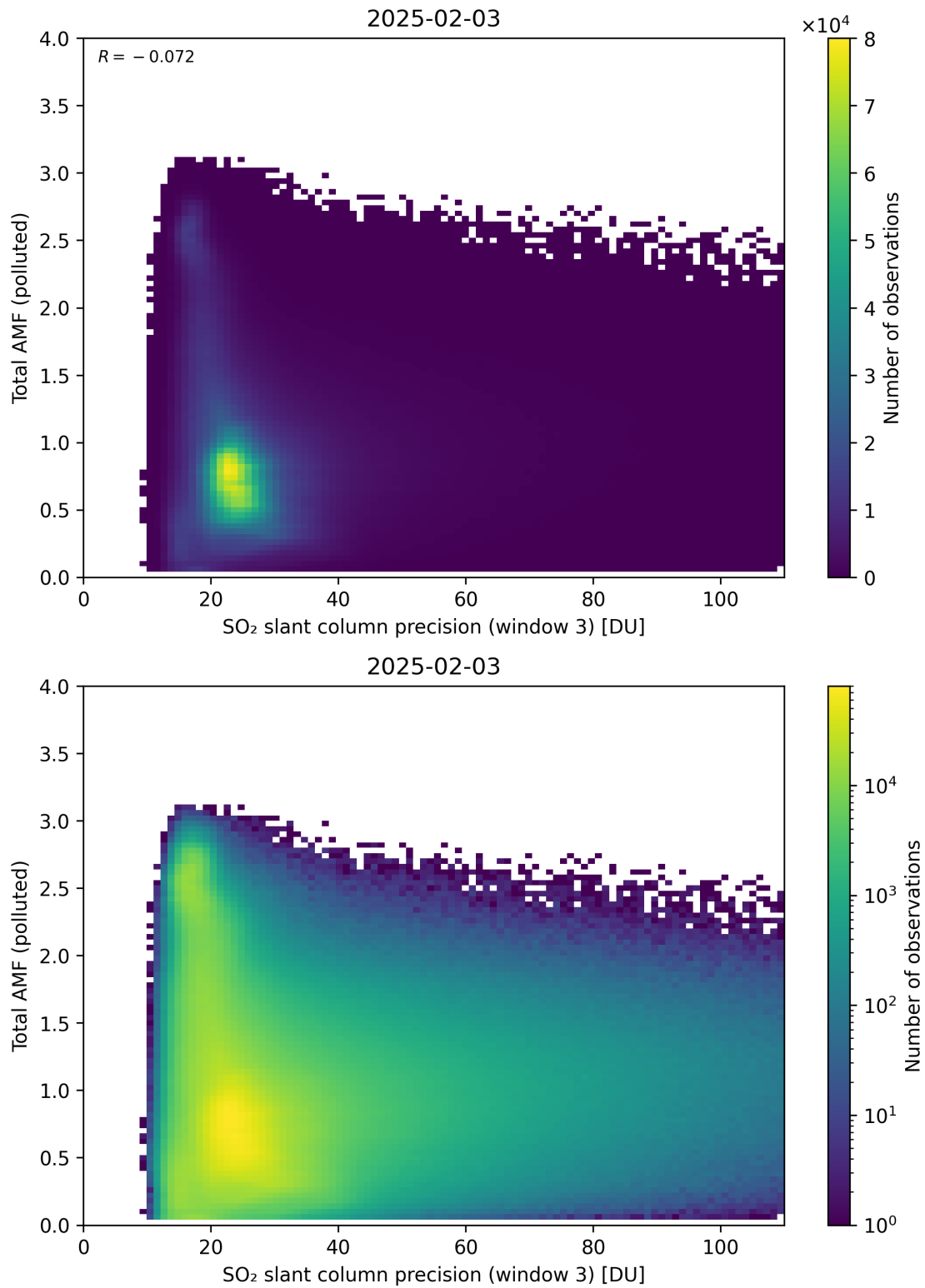
Figure 313: Scatter density plot of “SO 2 slant column precision (window 3)” against “Total AMF (polluted)” for 2025-02-03 to 2025-02-04.
