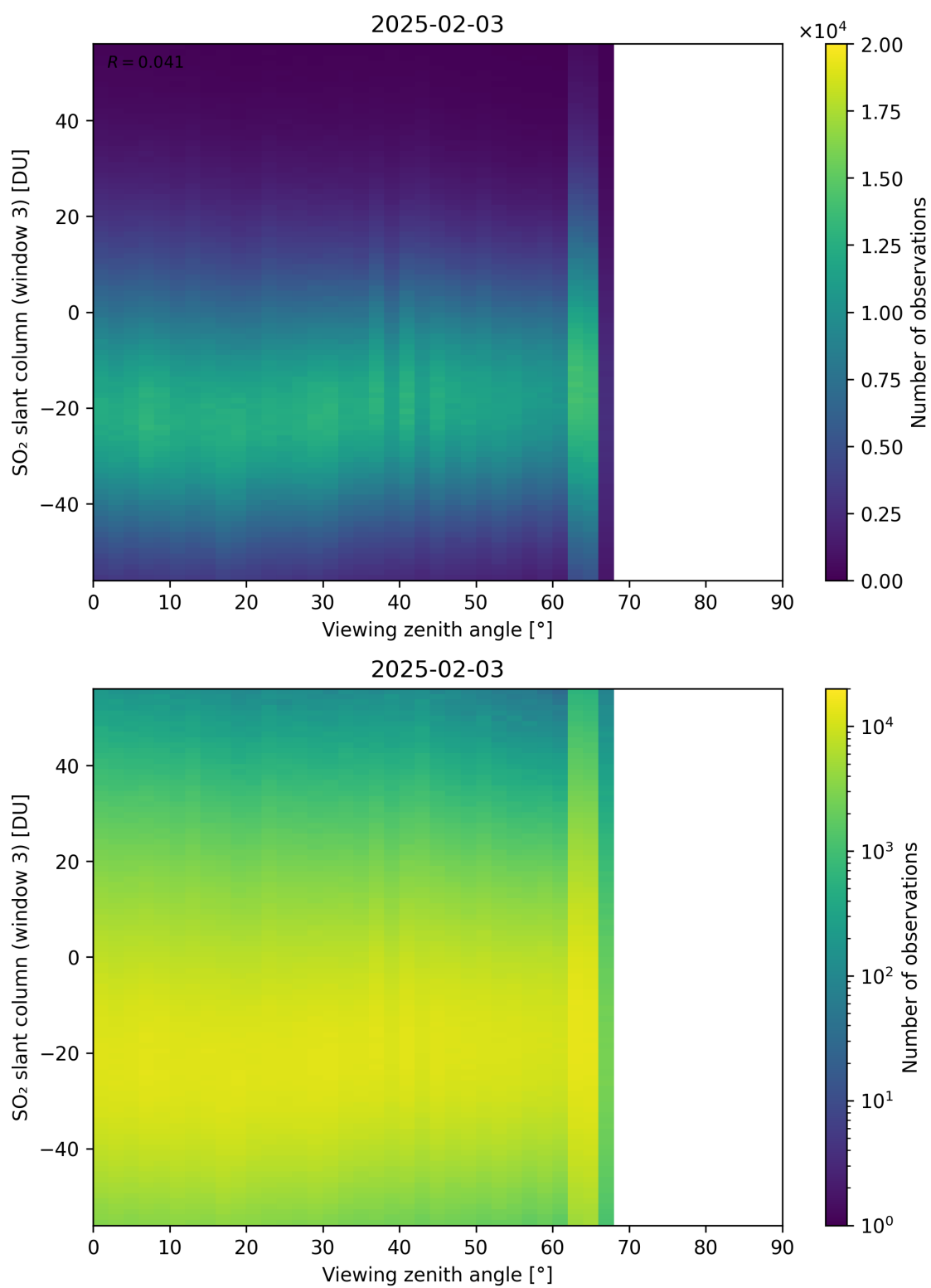
Figure 379: Scatter density plot of “Viewing zenith angle” against “SO 2 slant column (window 3)” for 2025-02-03 to 2025-02-04.
