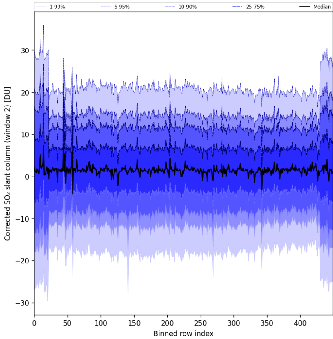
Figure 95: Along track statistics of “Corrected SO 2 slant column (window 2)” for 2025-02-03 to 2025-02-04
