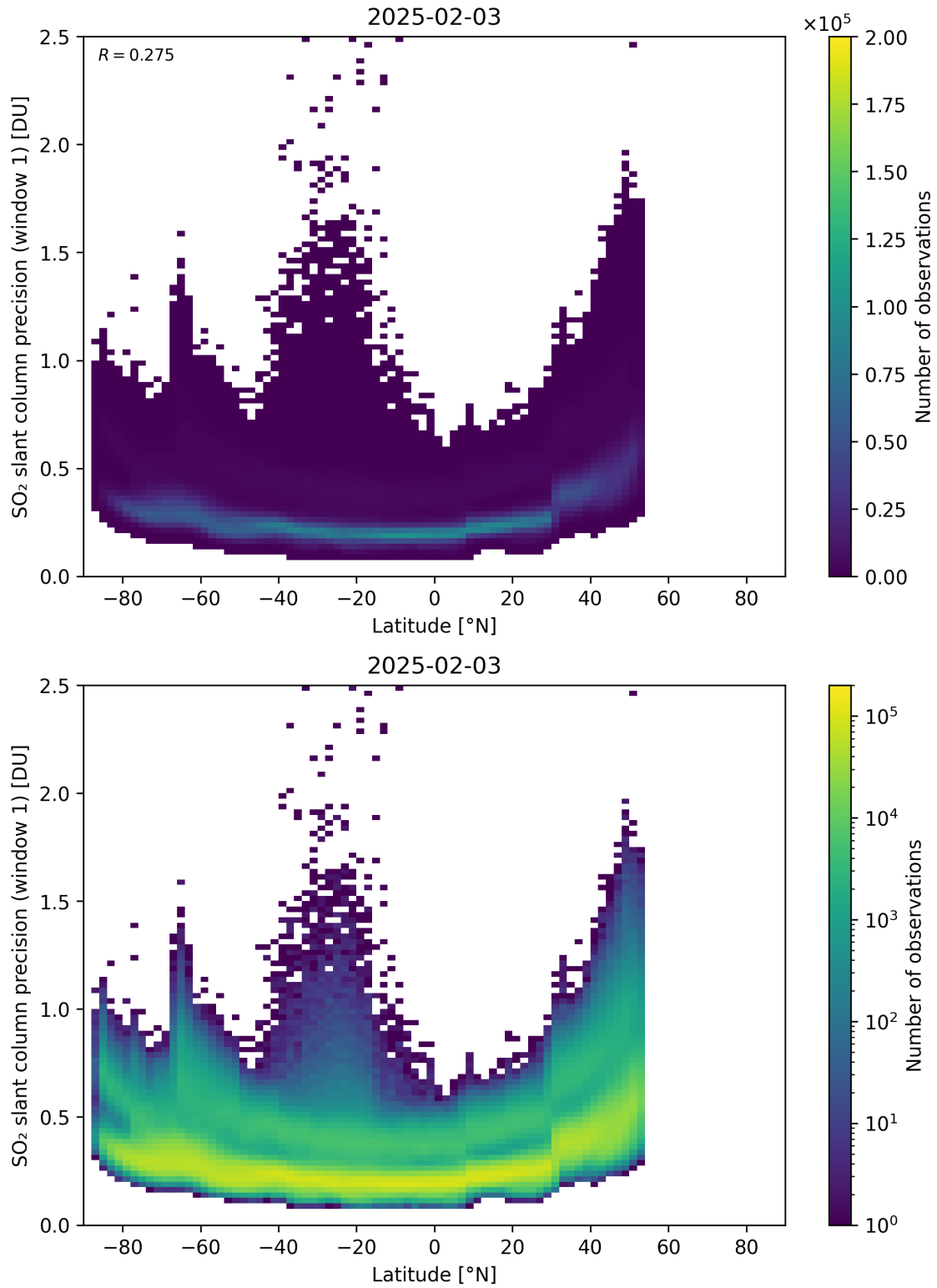
Figure 163: Scatter density plot of “Latitude” against “SO 2 slant column precision (window 1)” for 2025-02-03 to 2025-02-04.
