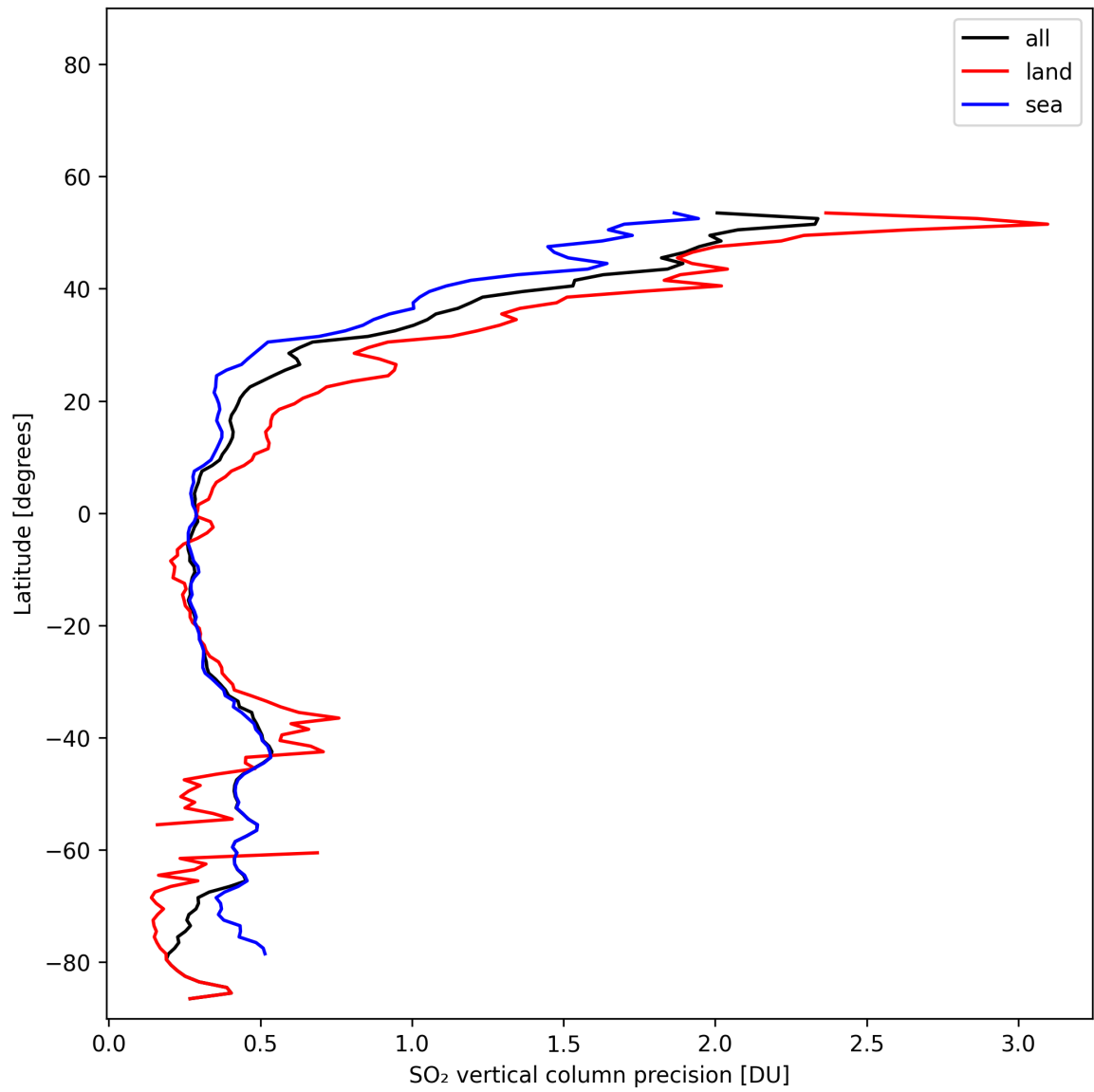
Figure 33: Zonal average of “SO 2 vertical column precision” for 2025-02-03 to 2025-02-04.
