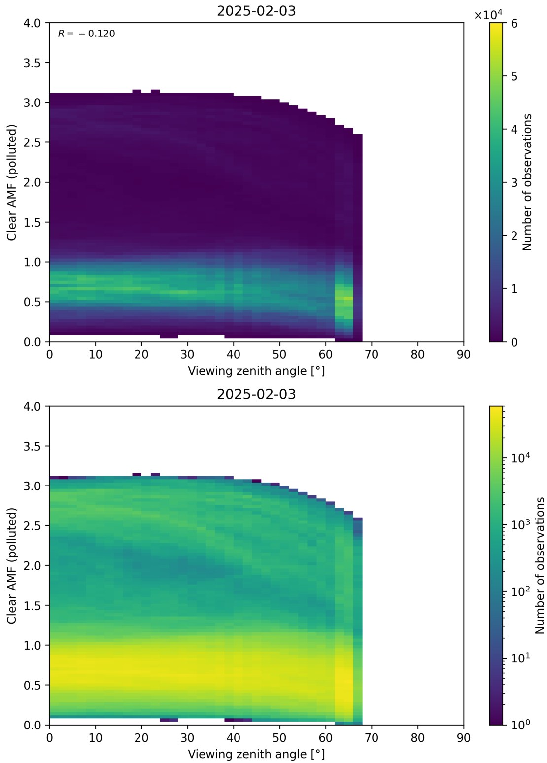
Figure 370: Scatter density plot of “Viewing zenith angle” against “Clear AMF (polluted)” for 2025-02-03 to 2025-02-04.
