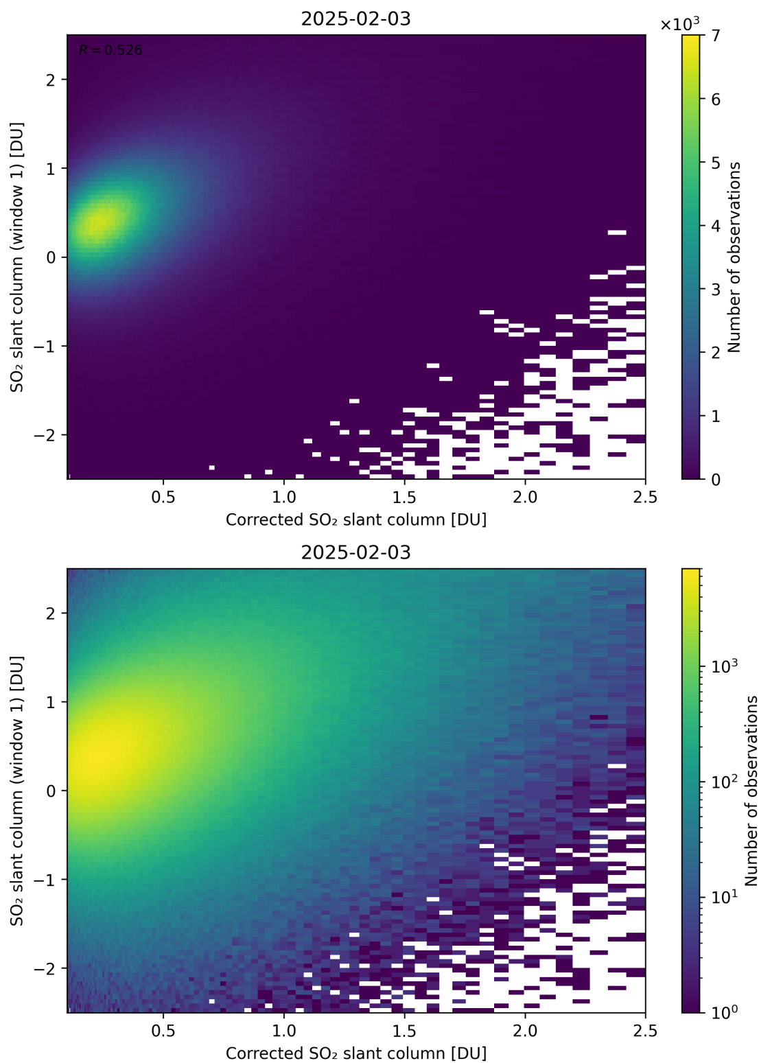
Figure 237: Scatter density plot of “Corrected SO 2 slant column” against “SO 2 slant column (window 1)” for 2025-02-03 to 2025-02-04.
