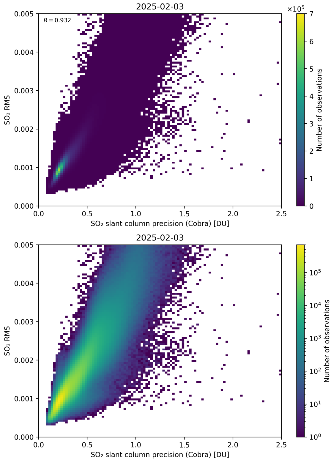
Figure 204: Scatter density plot of “SO 2 slant column precision (Cobra)” against “SO 2 RMS” for 2025-02-03 to 2025-02-04.
