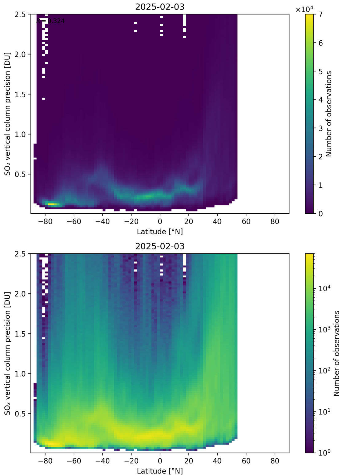
Figure 170: Scatter density plot of “Latitude” against “SO 2 vertical column precision” for 2025-02-03 to 2025-02-04.
