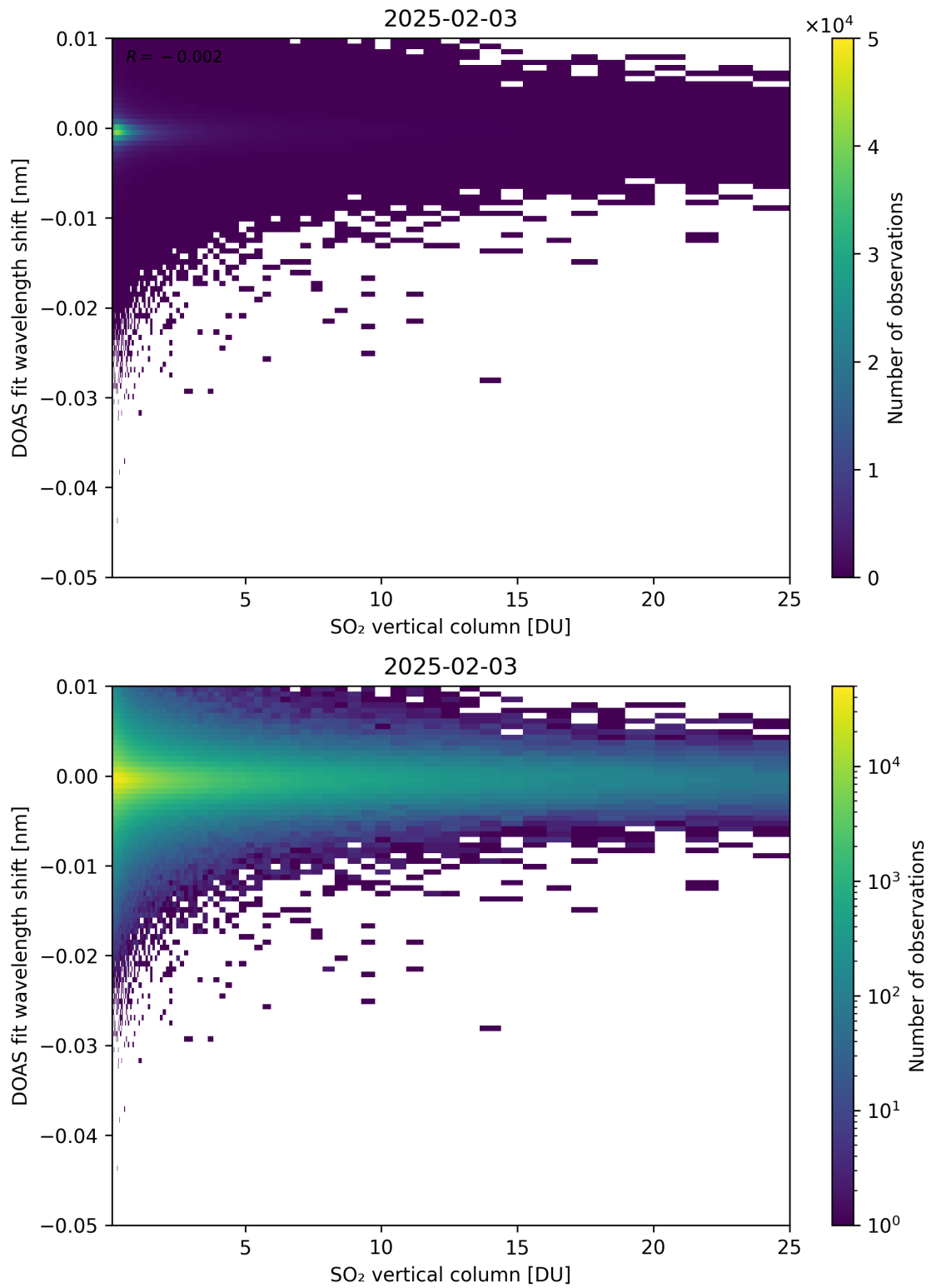
Figure 326: Scatter density plot of “SO 2 vertical column” against “DOAS fit wavelength shift” for 2025-02-03 to 2025-02-04.
