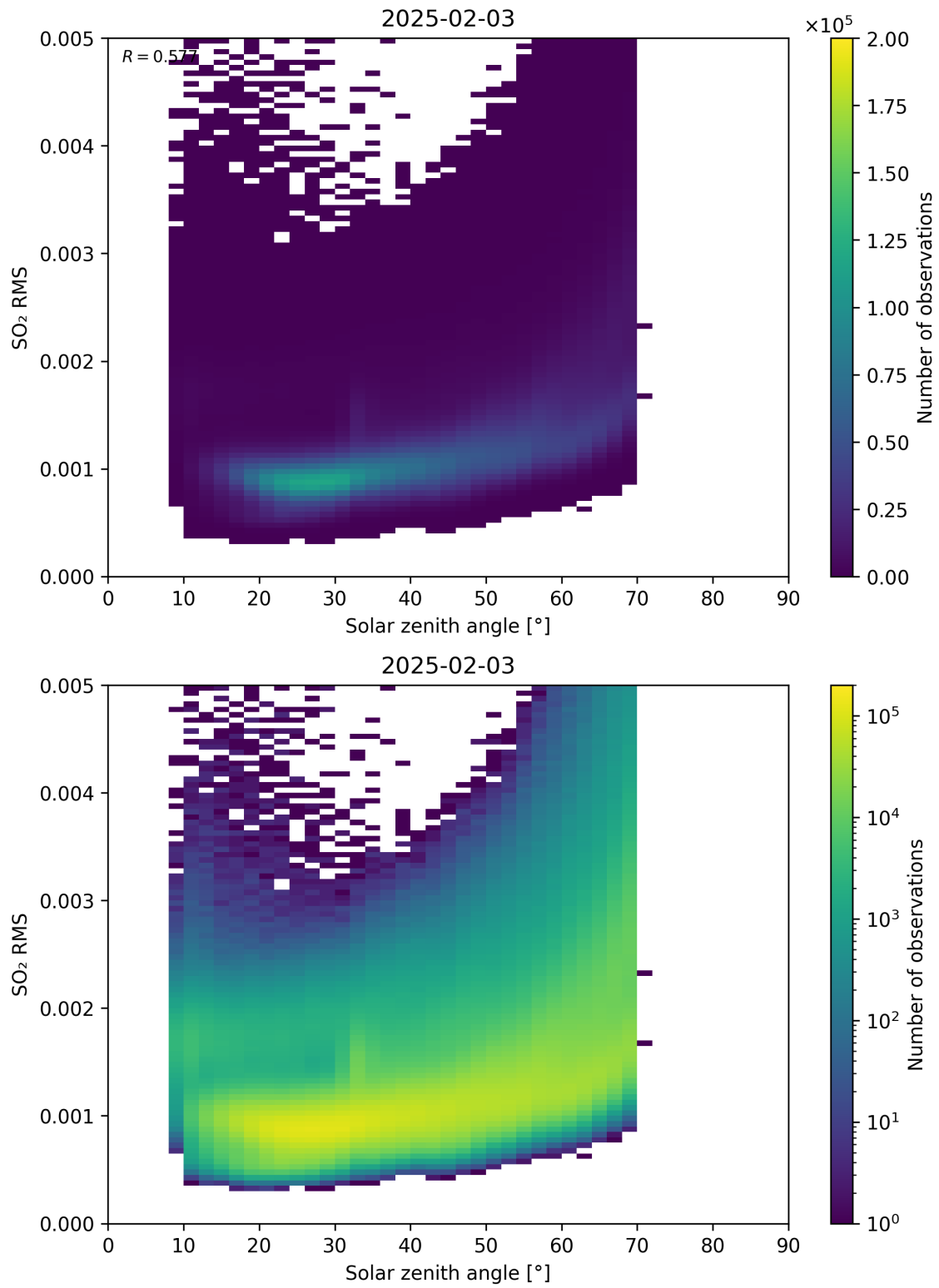
Figure 176: Scatter density plot of “Solar zenith angle” against “SO 2 RMS” for 2025-02-03 to 2025-02-04.
