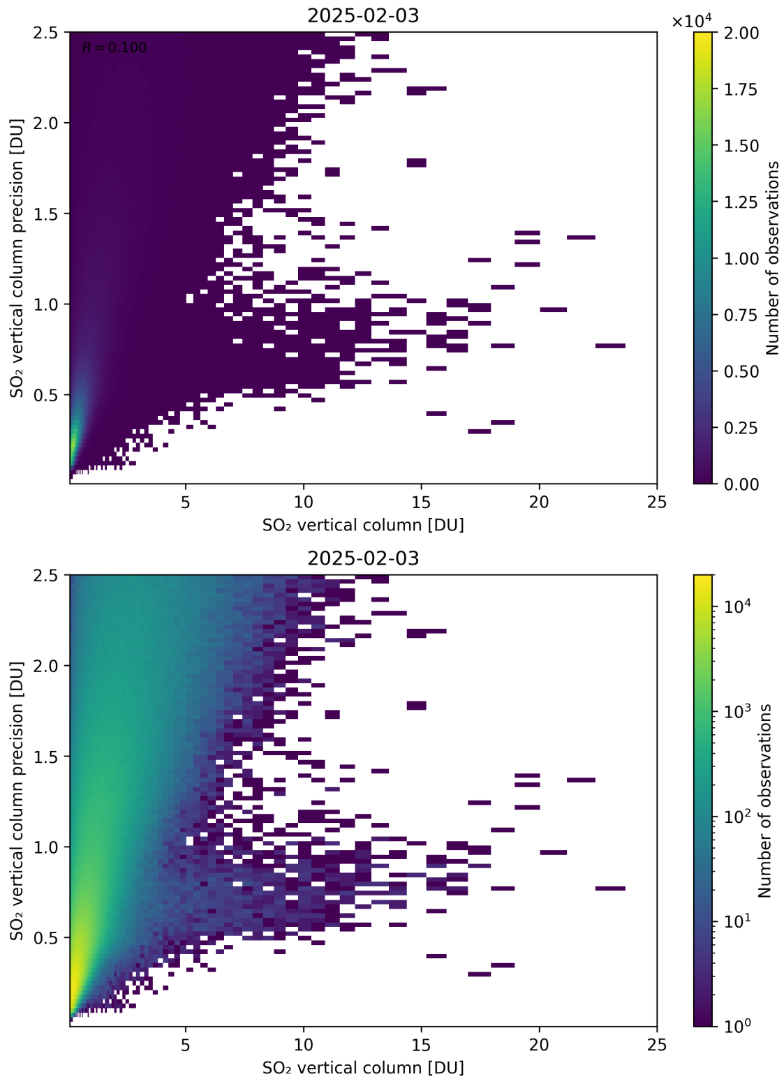
Figure 361: Scatter density plot of “SO 2 vertical column” against “SO 2 vertical column precision” for 2025-02-03 to 2025-02-04.
