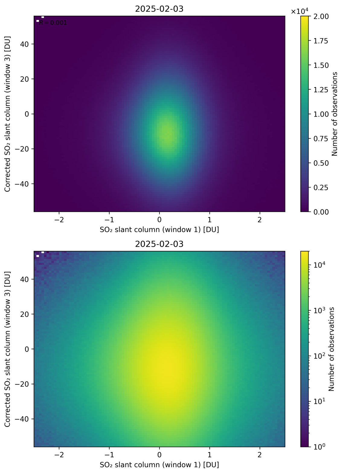
Figure 284: Scatter density plot of “SO 2 slant column (window 1)” against “Corrected SO 2 slant column (window 3)” for 2025-02-03 to 2025-02-04.
