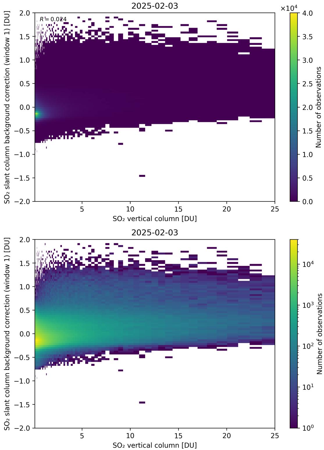
Figure 323: Scatter density plot of “SO 2 vertical column” against “SO 2 slant column background correction (window 1)” for 2025-02-03 to 2025-02-04.
