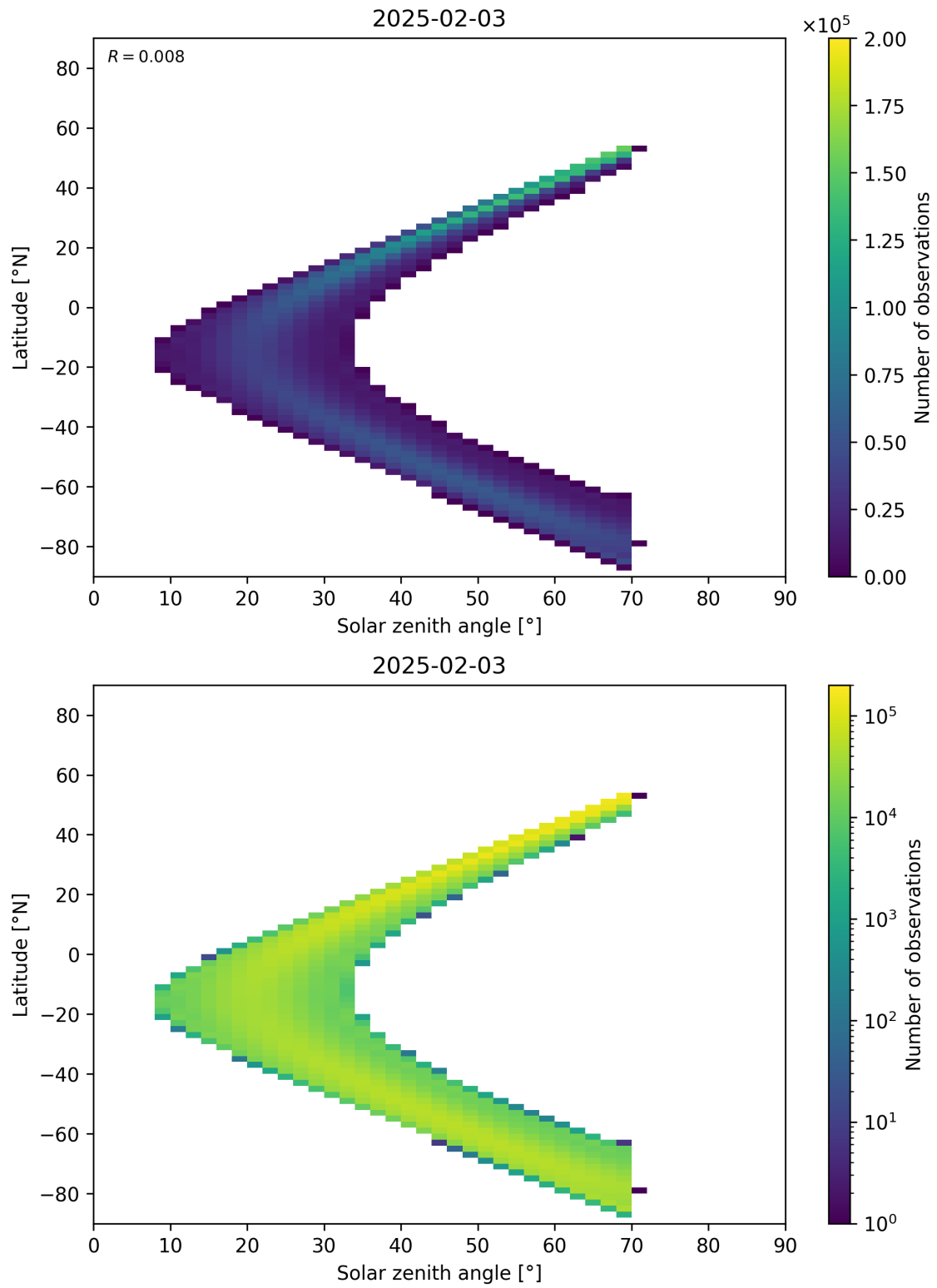
Figure 177: Scatter density plot of “Solar zenith angle” against “Latitude” for 2025-02-03 to 2025-02-04.
