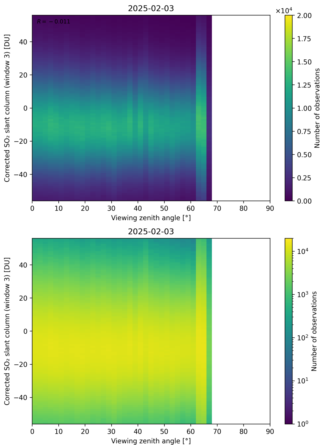
Figure 375: Scatter density plot of “Viewing zenith angle” against “Corrected SO 2 slant column (window 3)” for 2025-02-03 to 2025-02-04.
