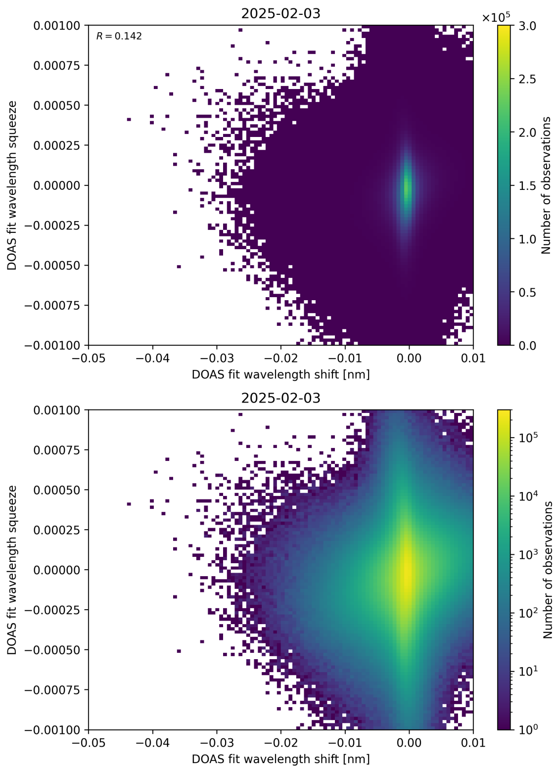
Figure 138: Scatter density plot of “DOAS fit wavelength shift” against “DOAS fit wavelength squeeze” for 2025-02-03 to 2025-02-04.
