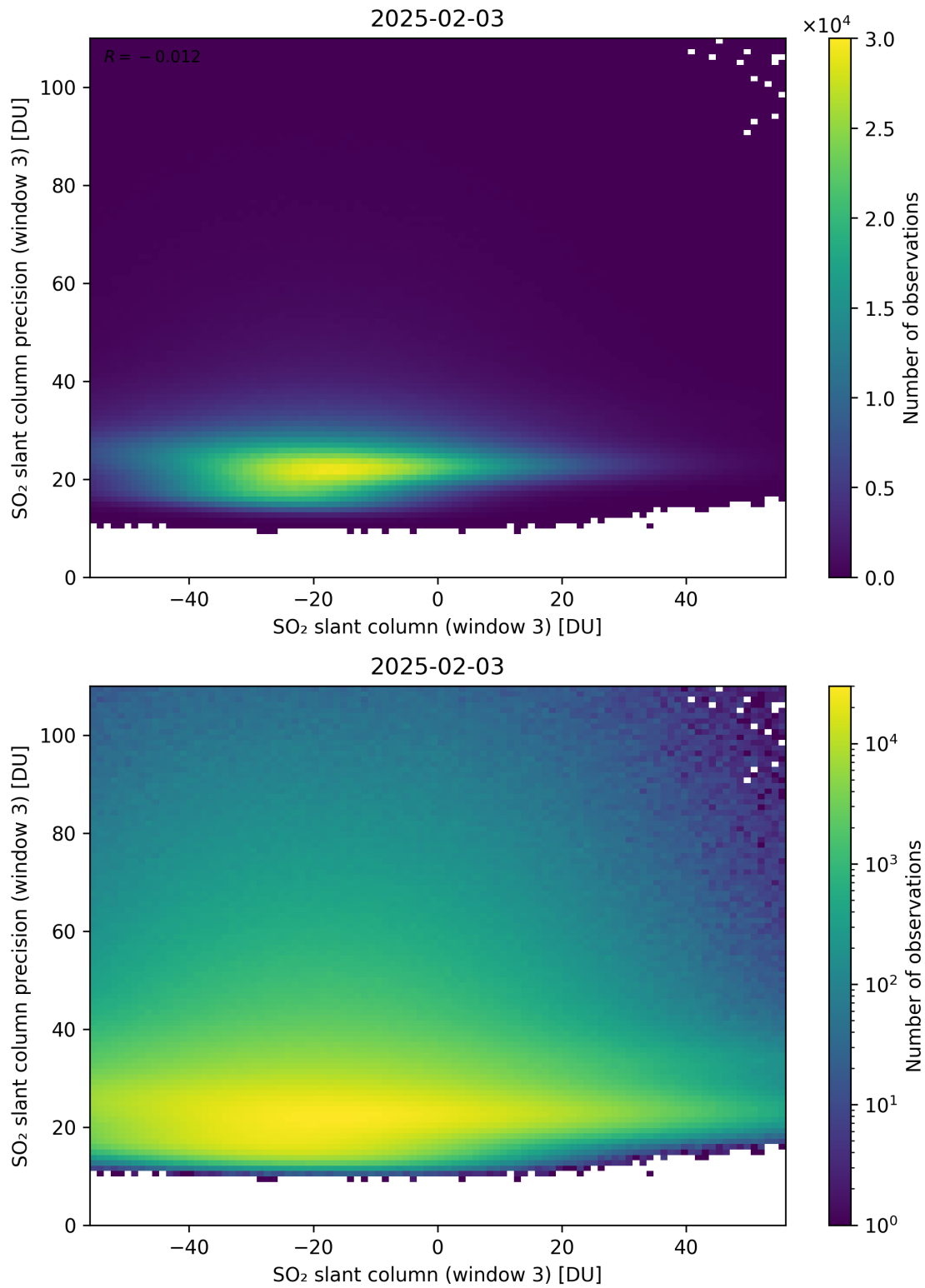
Figure 317: Scatter density plot of “SO 2 slant column (window 3)” against “SO 2 slant column precision (window 3)” for 2025-02-03 to 2025-02-04.
