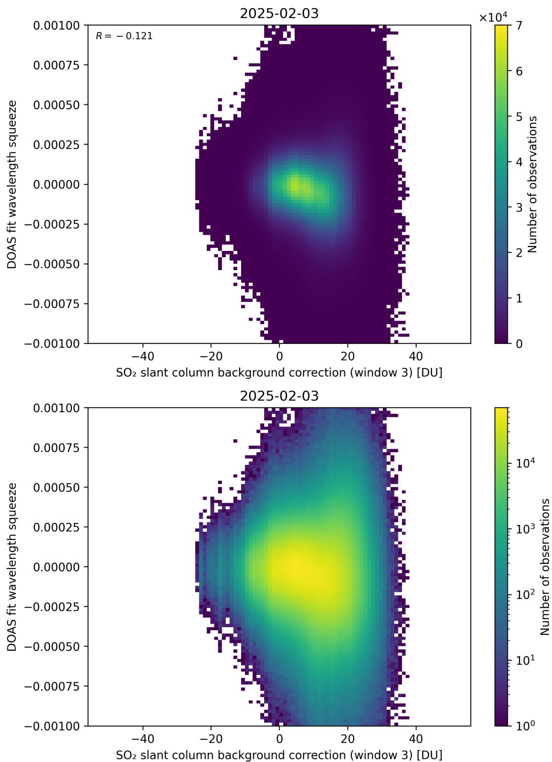
Figure 133: Scatter density plot of “SO 2 slant column background correction (window 3)” against “DOAS fit wavelength squeeze” for 2025-02-03 to 2025-02-04.
