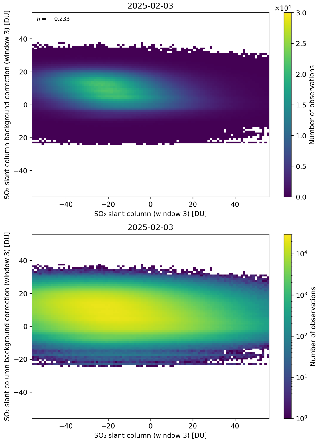
Figure 303: Scatter density plot of “SO 2 slant column (window 3)” against “SO 2 slant column background correction (window 3)” for 2025-02-03 to 2025-02-04.
