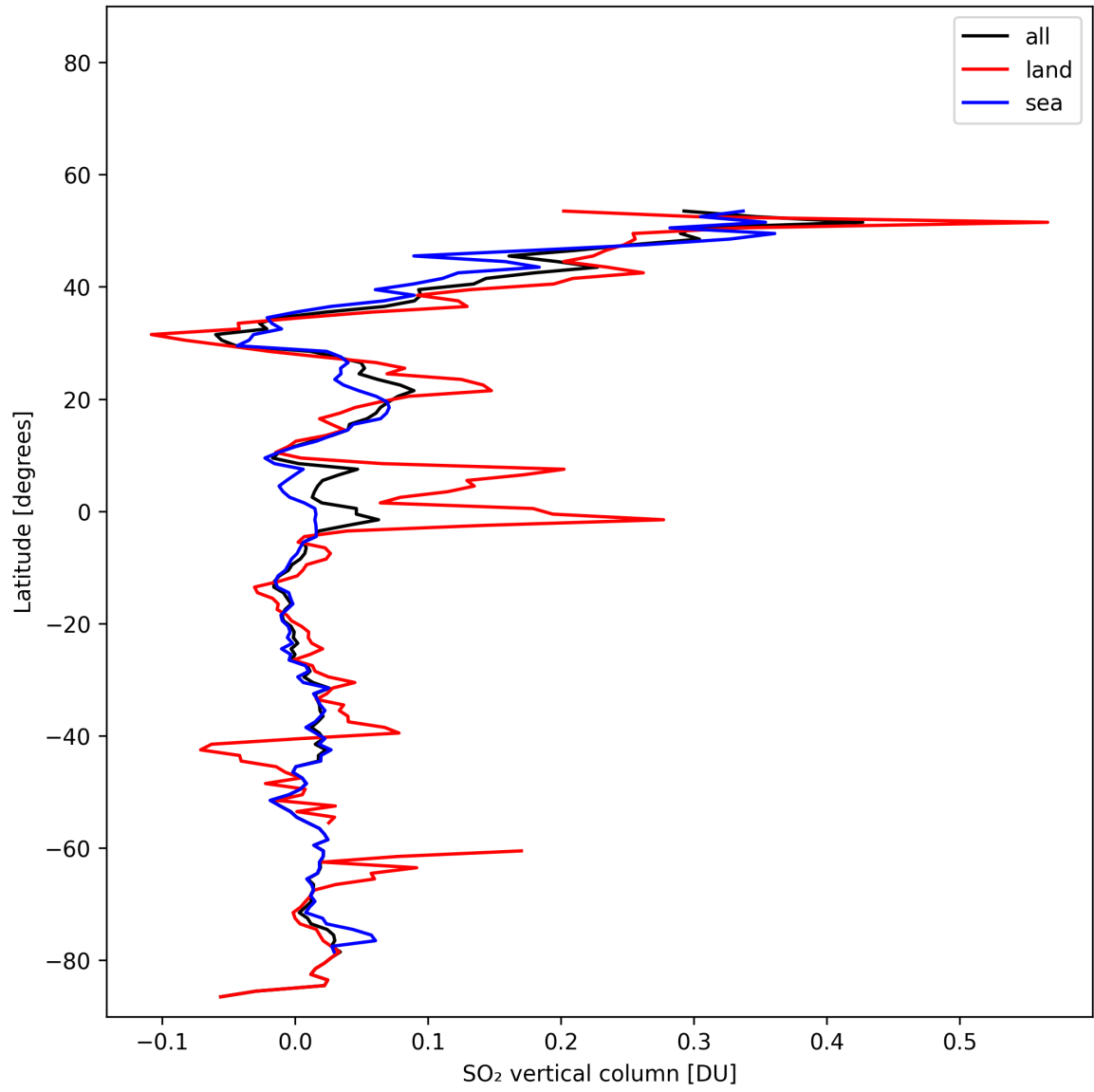
Figure 32: Zonal average of “SO 2 vertical column” for 2025-02-03 to 2025-02-04.
