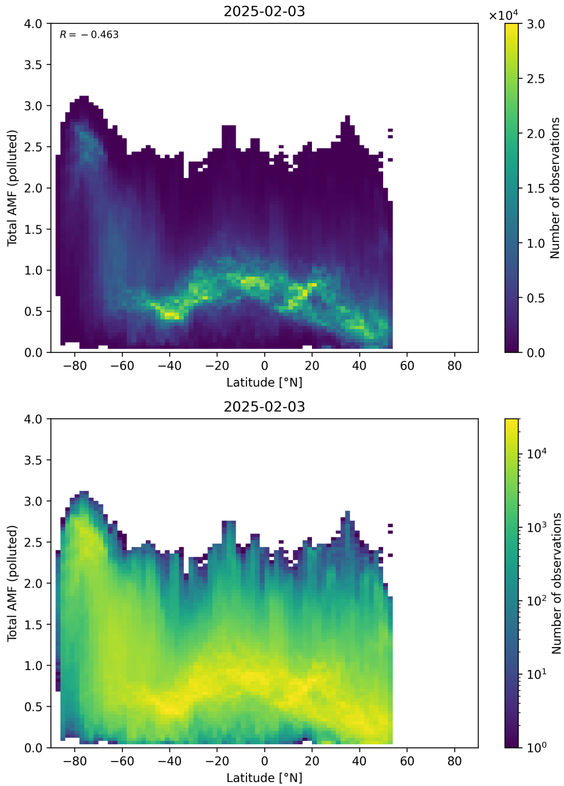
Figure 167: Scatter density plot of “Latitude” against “Total AMF (polluted)” for 2025-02-03 to 2025-02-04.
