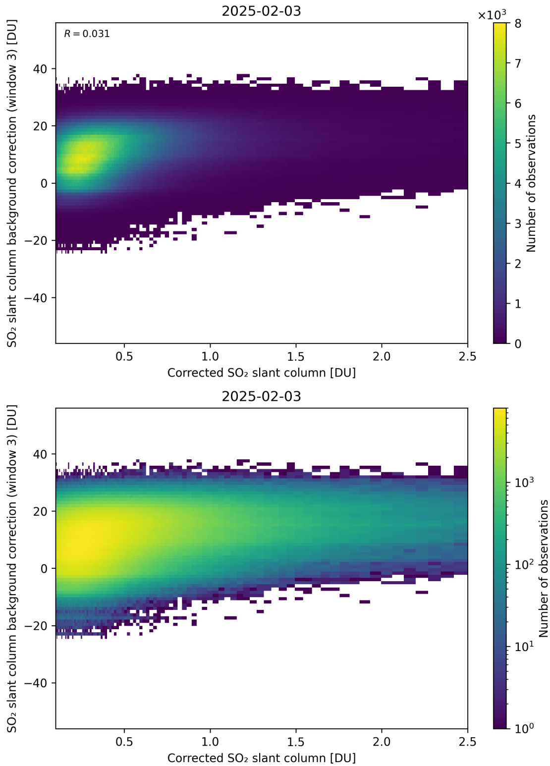
Figure 228: Scatter density plot of “Corrected SO 2 slant column” against “SO 2 slant column background correction (window 3)” for 2025-02-03 to 2025-02-04.
