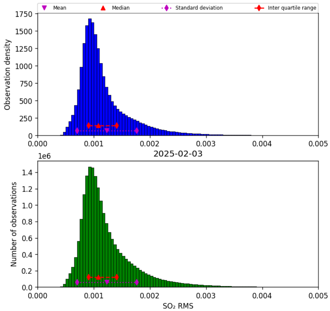
Figure 78: Histogram of “SO 2 RMS” for 2025-02-03 to 2025-02-04
