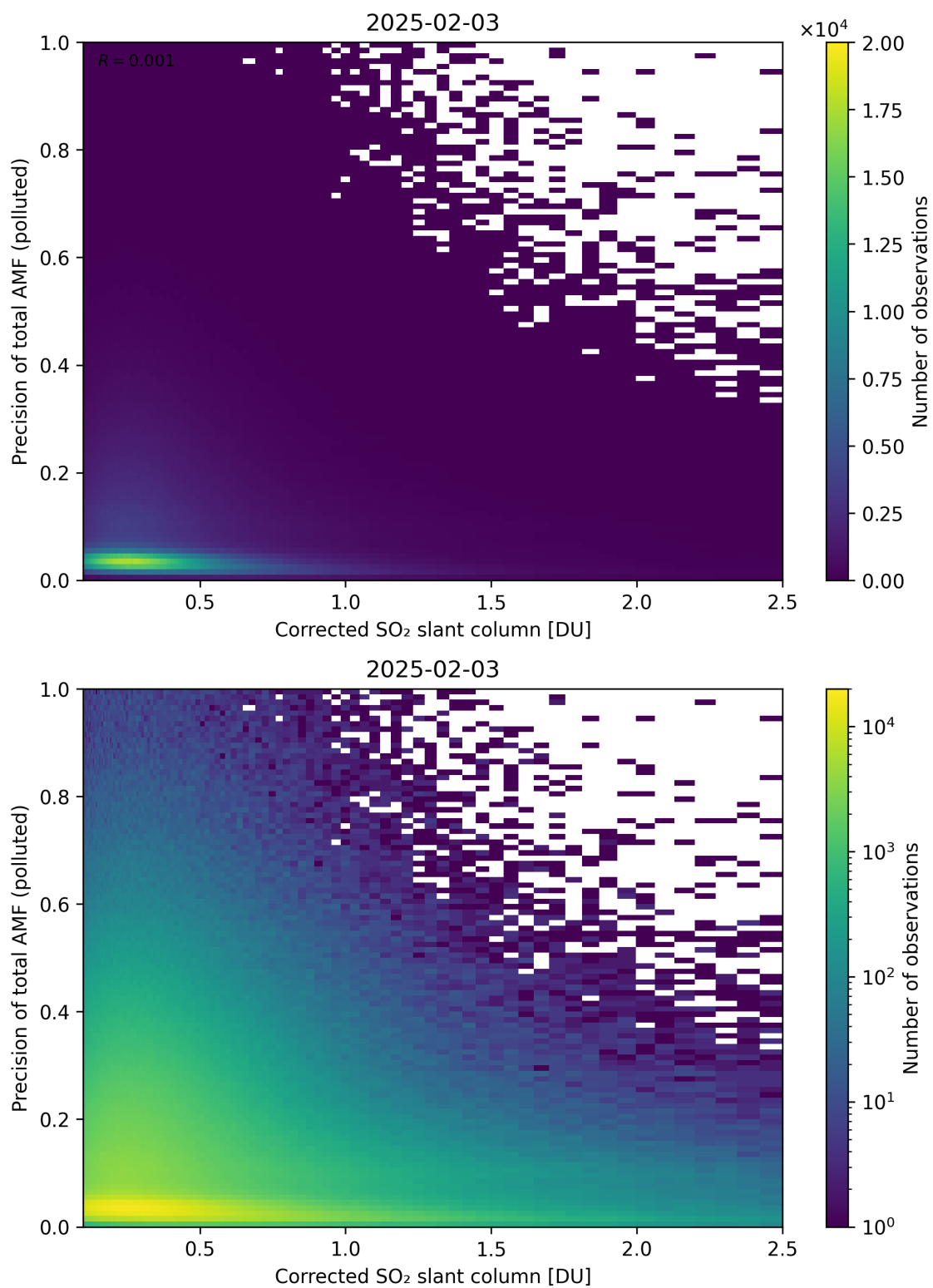
Figure 243: Scatter density plot of “Corrected SO 2 slant column” against “Precision of total AMF (polluted)” for 2025-02-03 to 2025-02-04.
