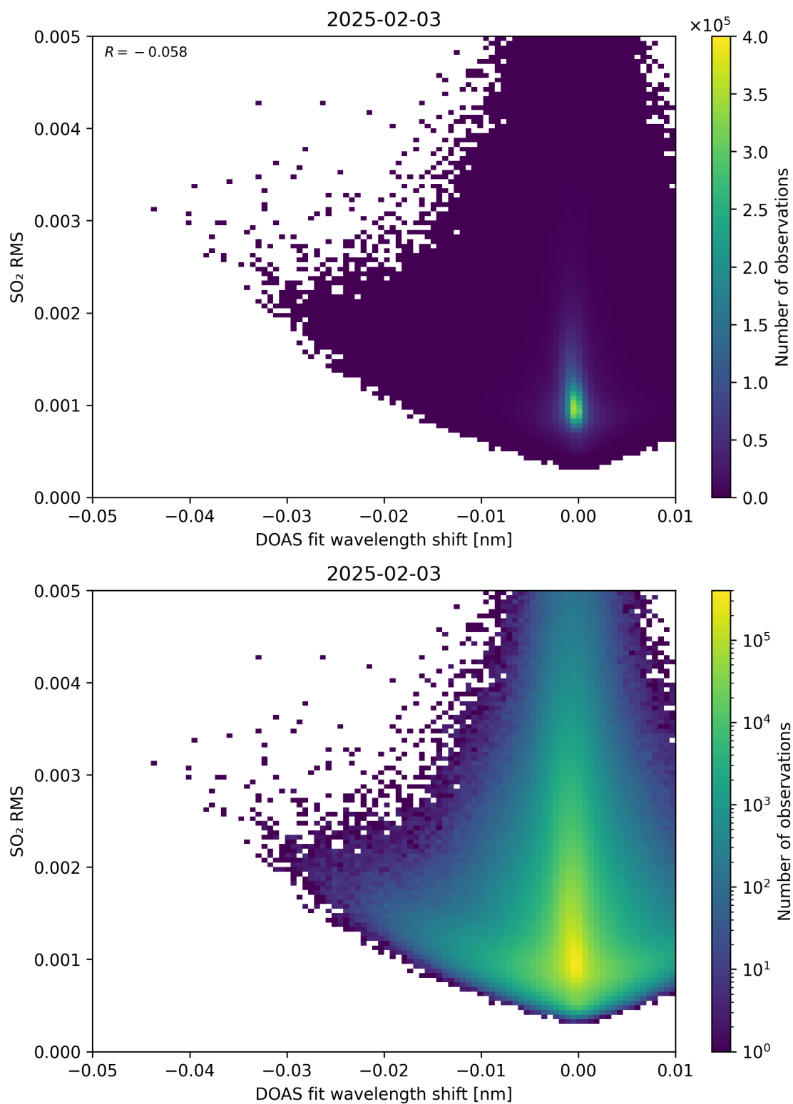
Figure 139: Scatter density plot of “DOAS fit wavelength shift” against “SO 2 RMS” for 2025-02-03 to 2025-02-04.
