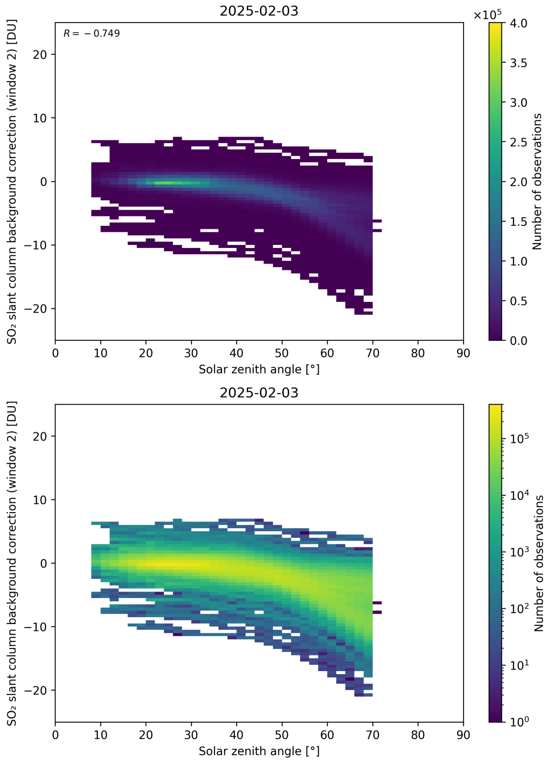
Figure 172: Scatter density plot of “Solar zenith angle” against “SO 2 slant column background correction (window 2)” for 2025-02-03 to 2025-02-04.
