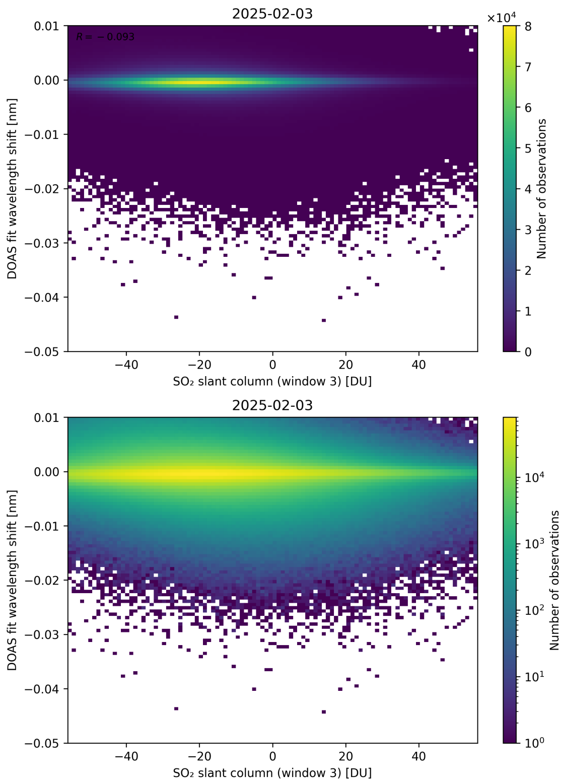
Figure 304: Scatter density plot of “SO 2 slant column (window 3)” against “DOAS fit wavelength shift” for 2025-02-03 to 2025-02-04.
