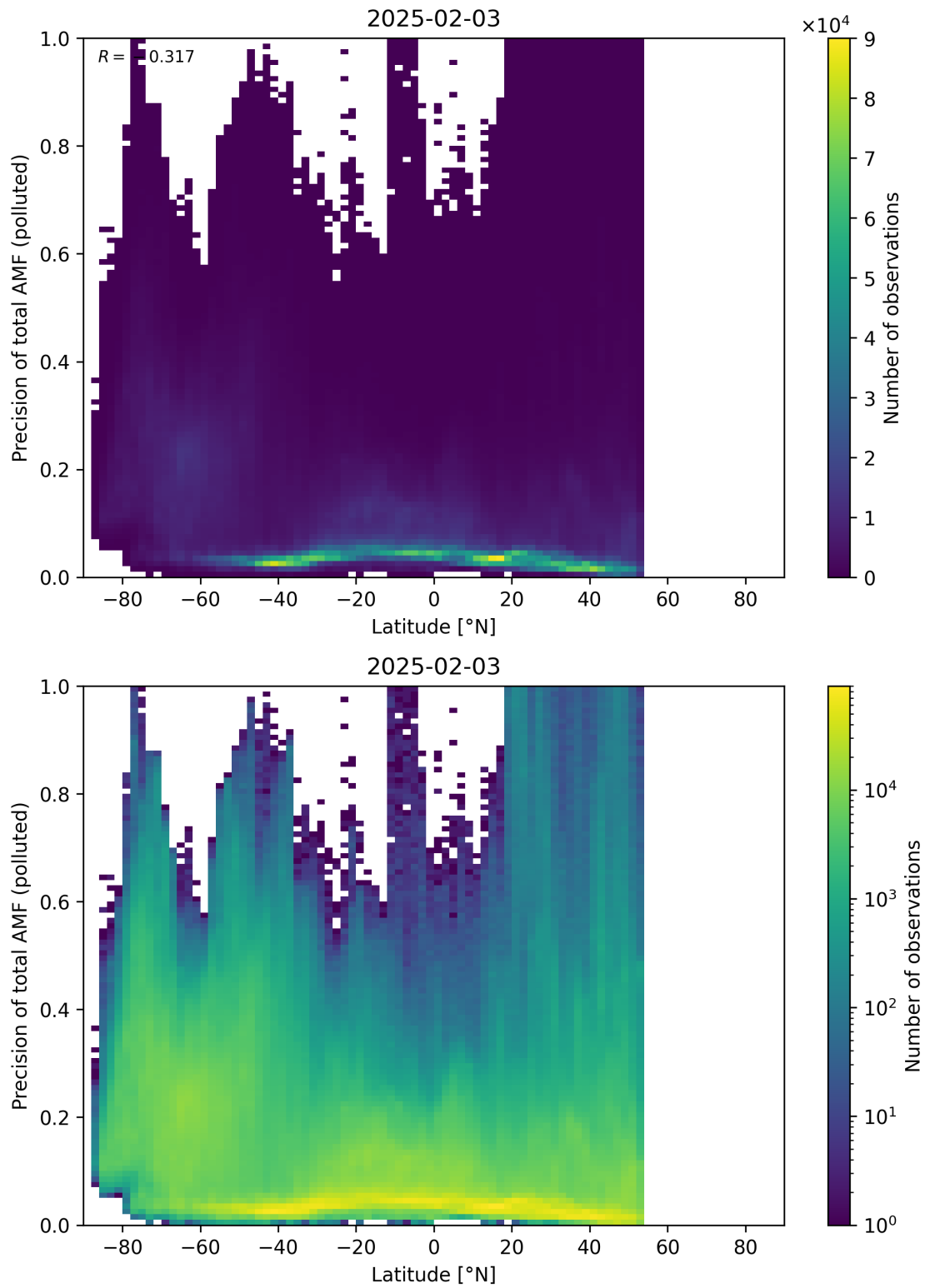
Figure 168: Scatter density plot of “Latitude” against “Precision of total AMF (polluted)” for 2025-02-03 to 2025-02-04.
