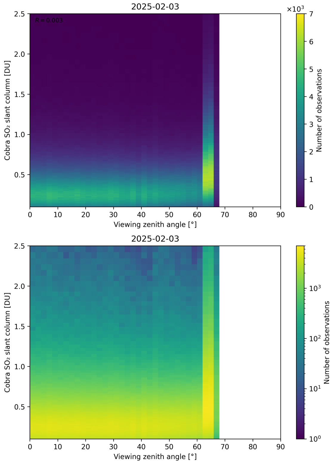
Figure 371: Scatter density plot of “Viewing zenith angle” against “Cobra SO 2 slant column” for 2025-02-03 to 2025-02-04.
