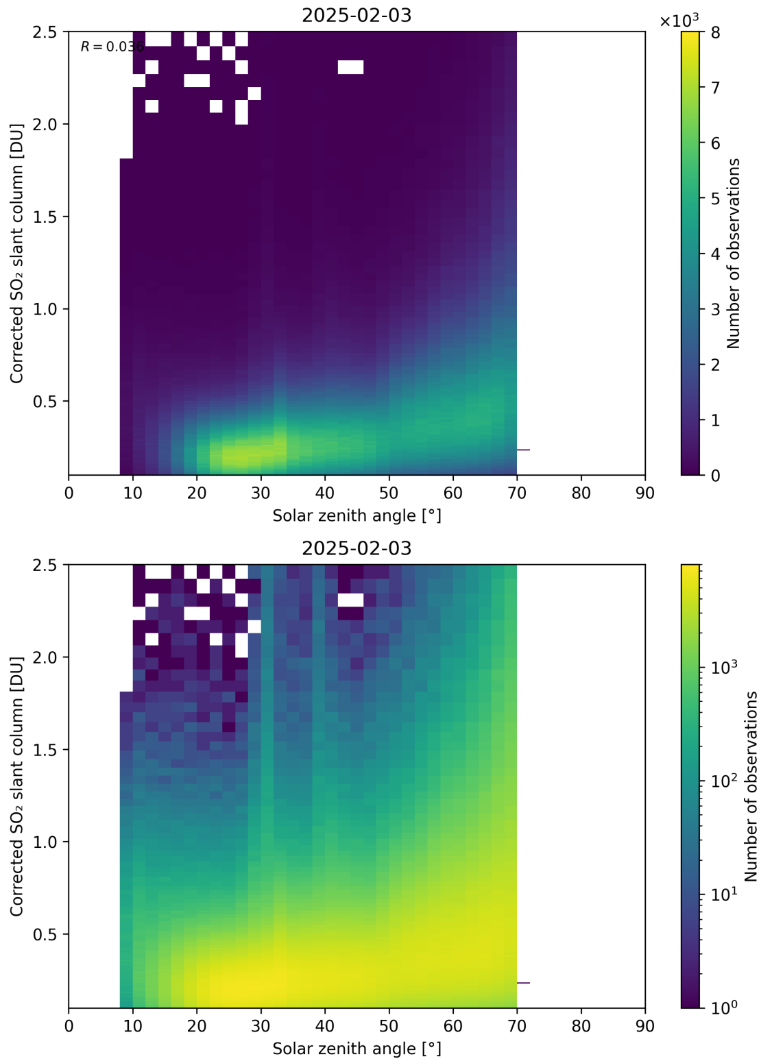
Figure 181: Scatter density plot of “Solar zenith angle” against “Corrected SO 2 slant column” for 2025-02-03 to 2025-02-04.
