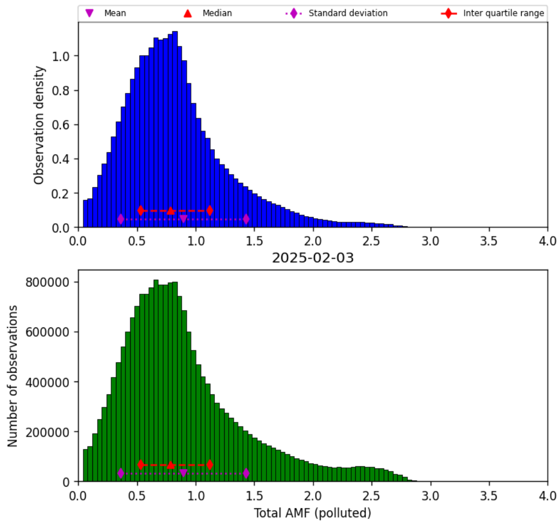
Figure 79: Histogram of “Total AMF (polluted)” for 2025-02-03 to 2025-02-04
