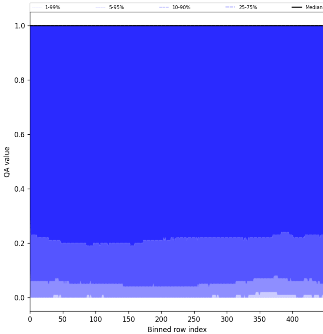
Figure 83: Along track statistics of “QA value” for 2025-02-03 to 2025-02-04
