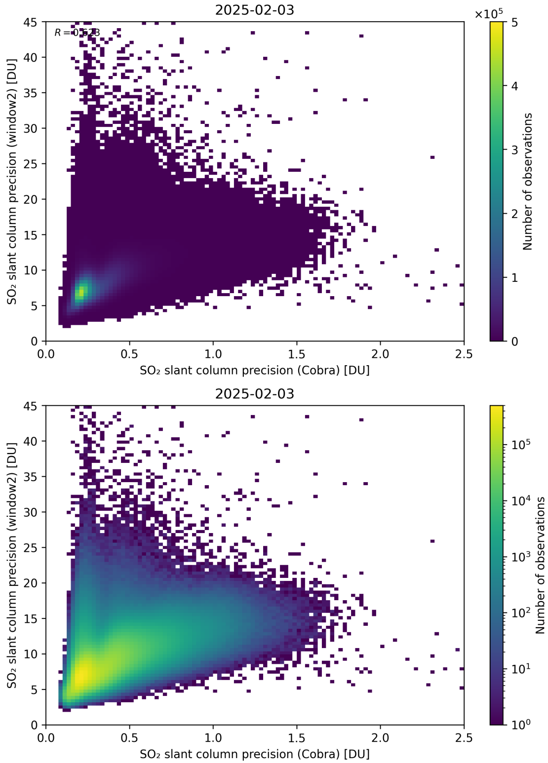
Figure 210: Scatter density plot of “SO 2 slant column precision (Cobra)” against “SO 2 slant column precision (window2)” for 2025-02-03 to 2025-02-04.
