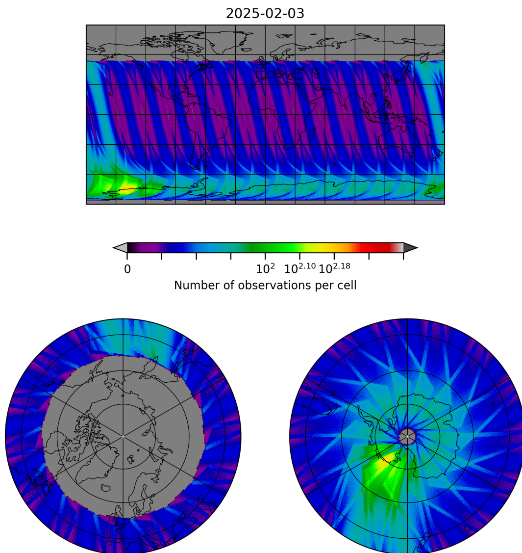
Figure 30: Map of the number of observations for 2025-02-03 to 2025-02-04
