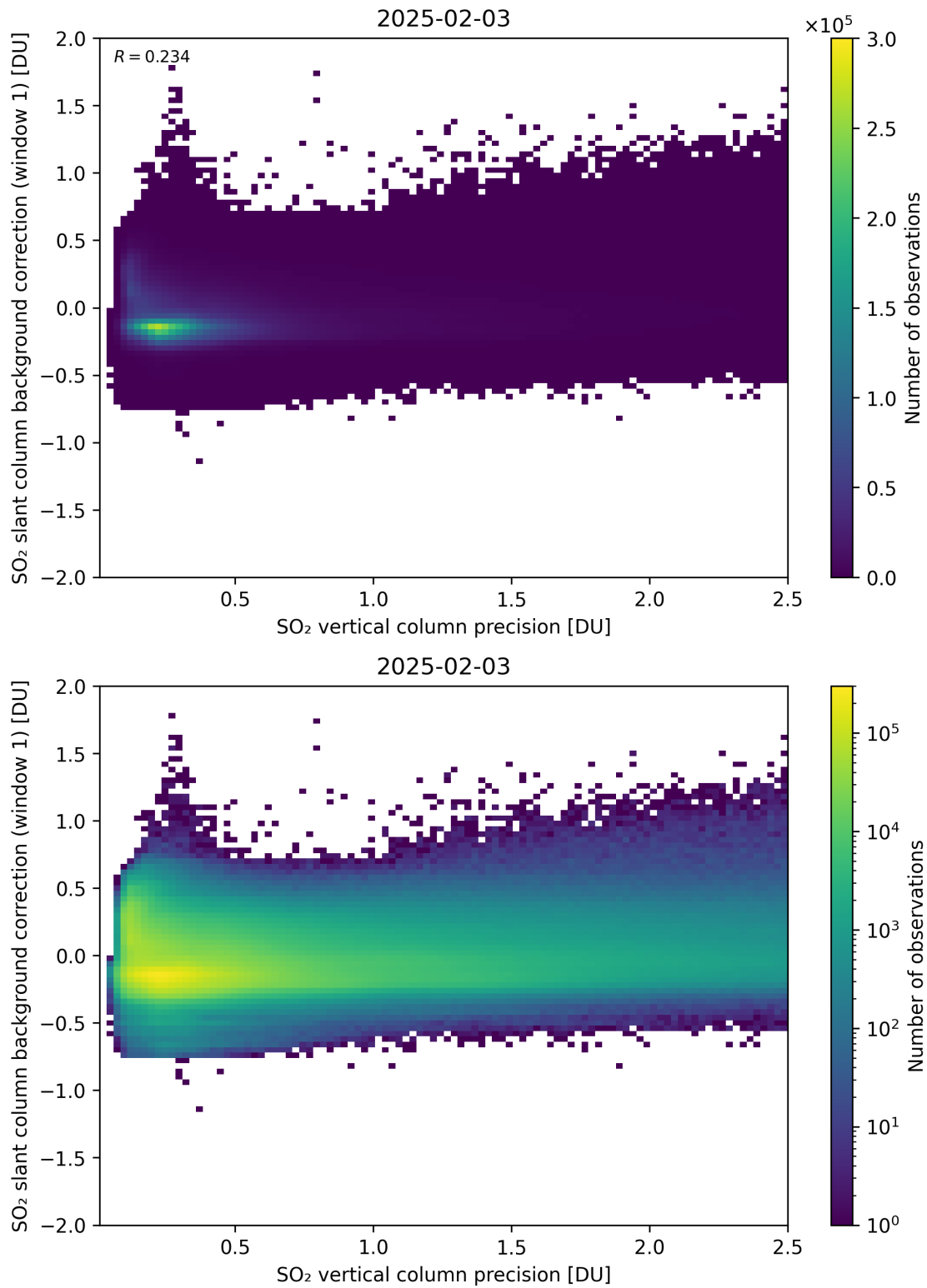
Figure 329: Scatter density plot of “SO 2 vertical column precision” against “SO 2 slant column background correction (window 1)” for 2025-02-03 to 2025-02-04.
