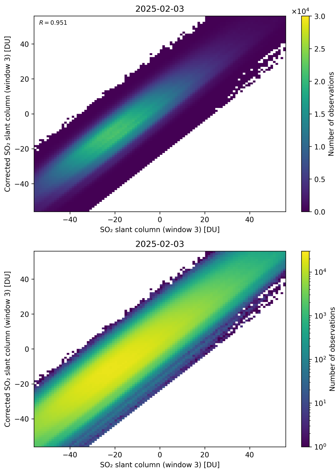
Figure 316: Scatter density plot of “SO 2 slant column (window 3)” against “Corrected SO 2 slant column (window 3)” for 2025-02-03 to 2025-02-04.
