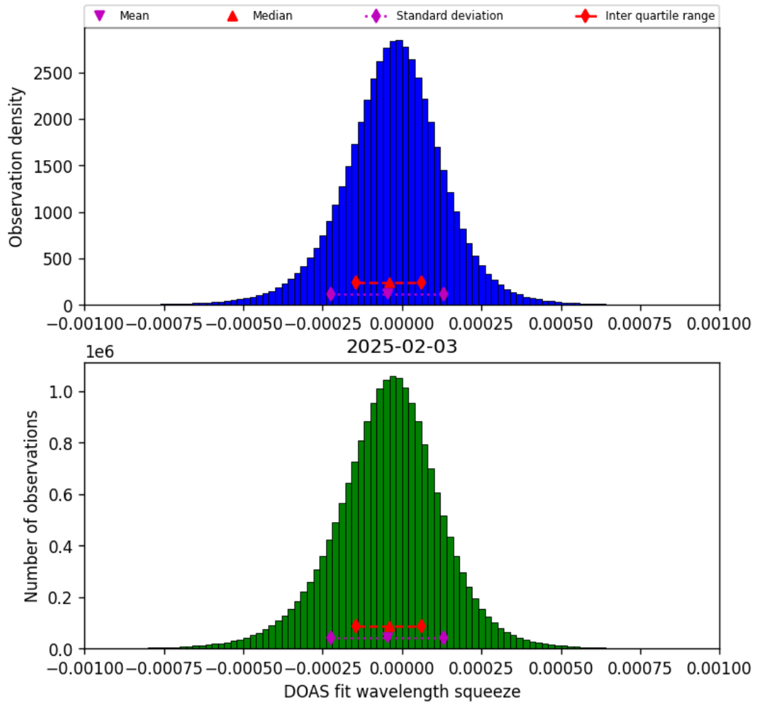
Figure 77: Histogram of “DOAS fit wavelength squeeze” for 2025-02-03 to 2025-02-04
