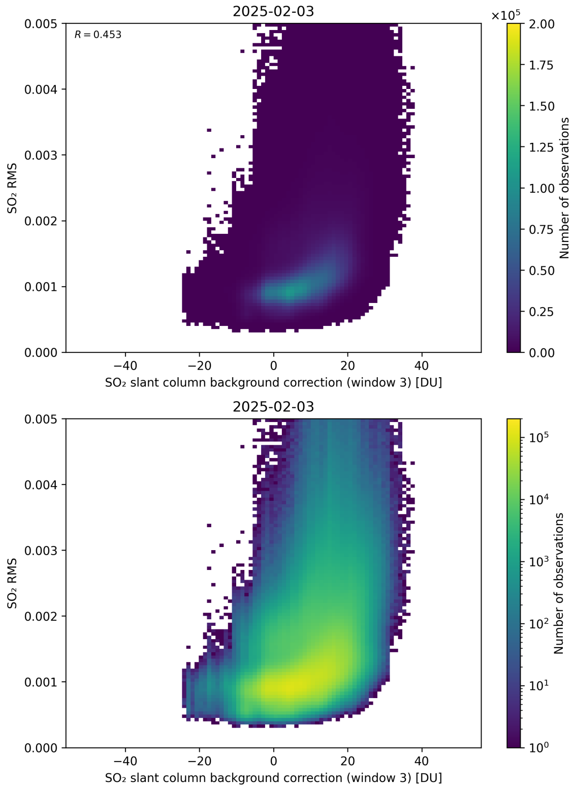
Figure 134: Scatter density plot of “SO 2 slant column background correction (window 3)” against “SO 2 RMS” for 2025-02-03 to 2025-02-04.
