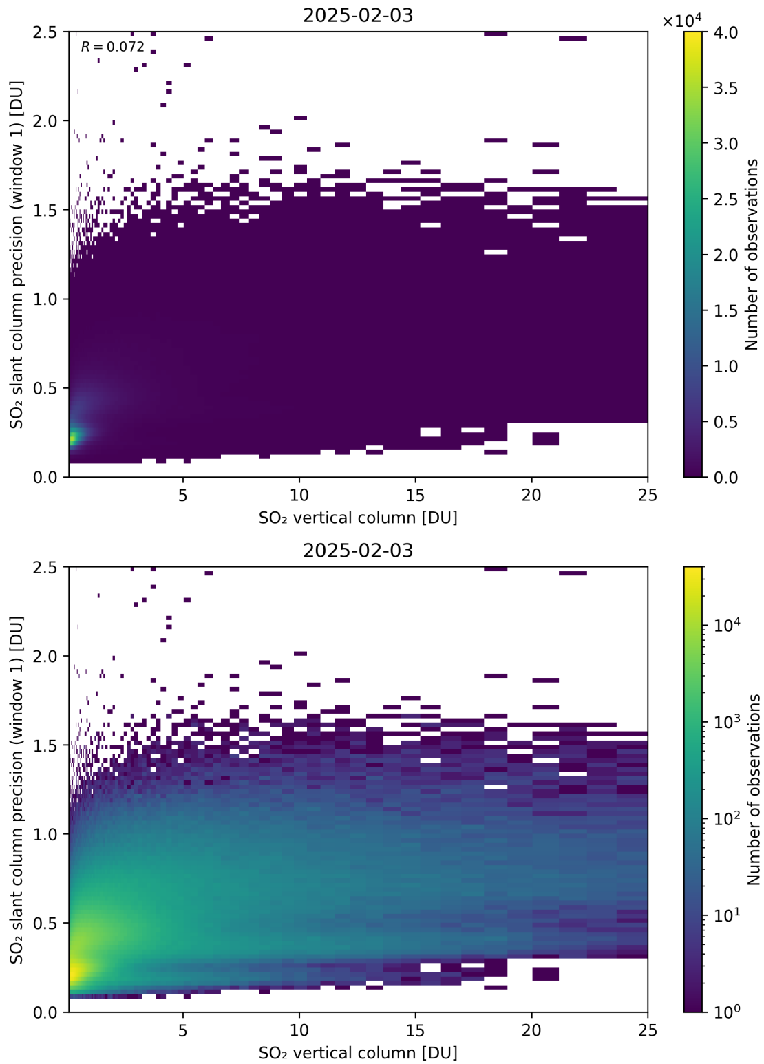
Figure 355: Scatter density plot of “SO 2 vertical column” against “SO 2 slant column precision (window 1)” for 2025-02-03 to 2025-02-04.
