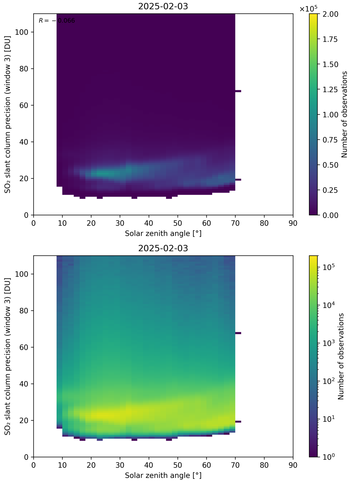
Figure 188: Scatter density plot of “Solar zenith angle” against “SO 2 slant column precision (window 3)” for 2025-02-03 to 2025-02-04.
