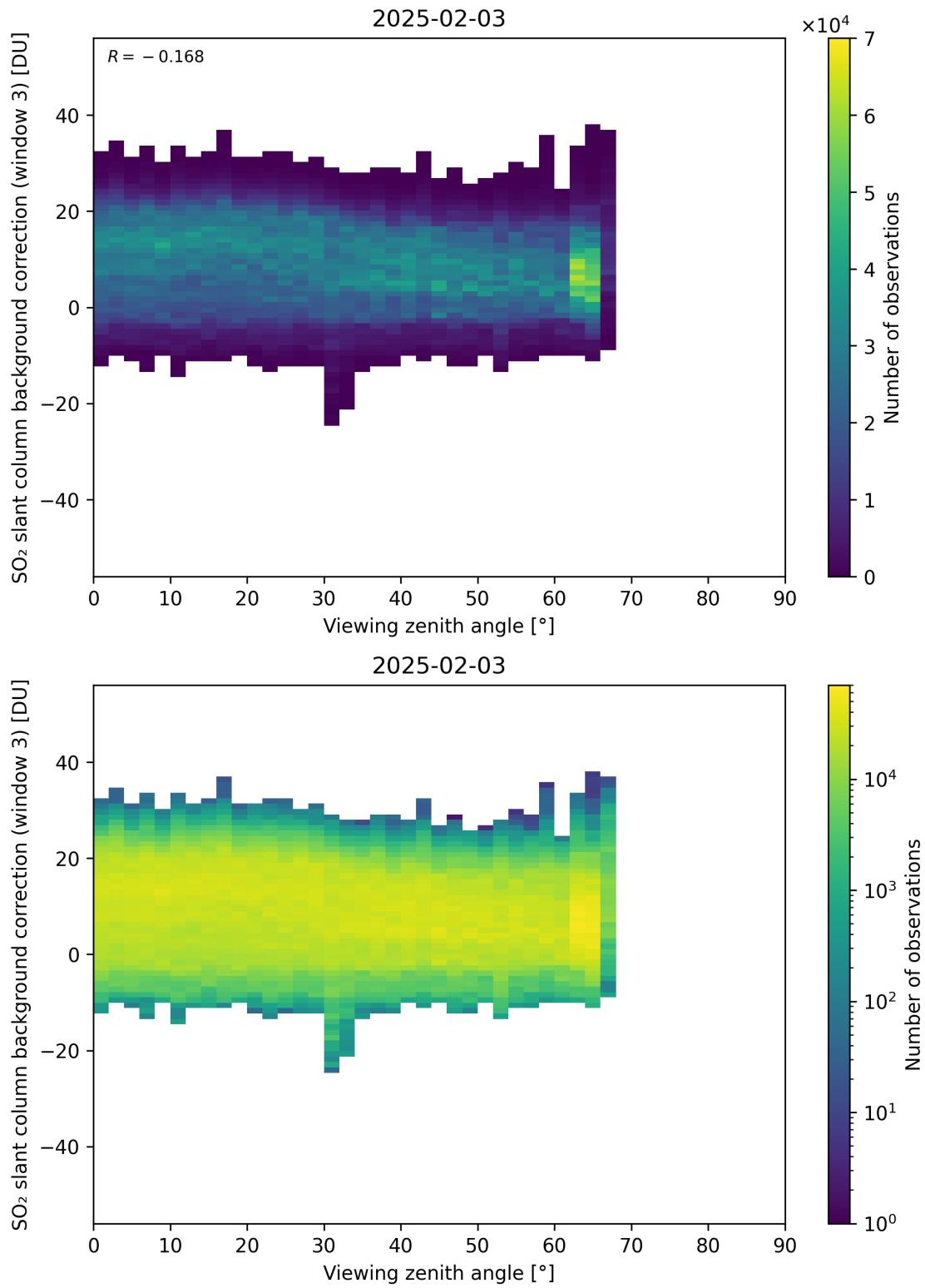
Figure 364: Scatter density plot of “Viewing zenith angle” against “SO 2 slant column background correction (window 3)” for 2025-02-03 to 2025-02-04.
