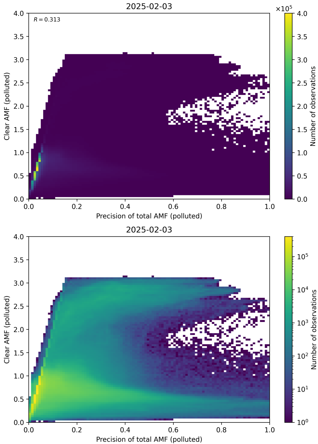
Figure 320: Scatter density plot of “Precision of total AMF (polluted)” against “Clear AMF (polluted)” for 2025-02-03 to 2025-02-04.
