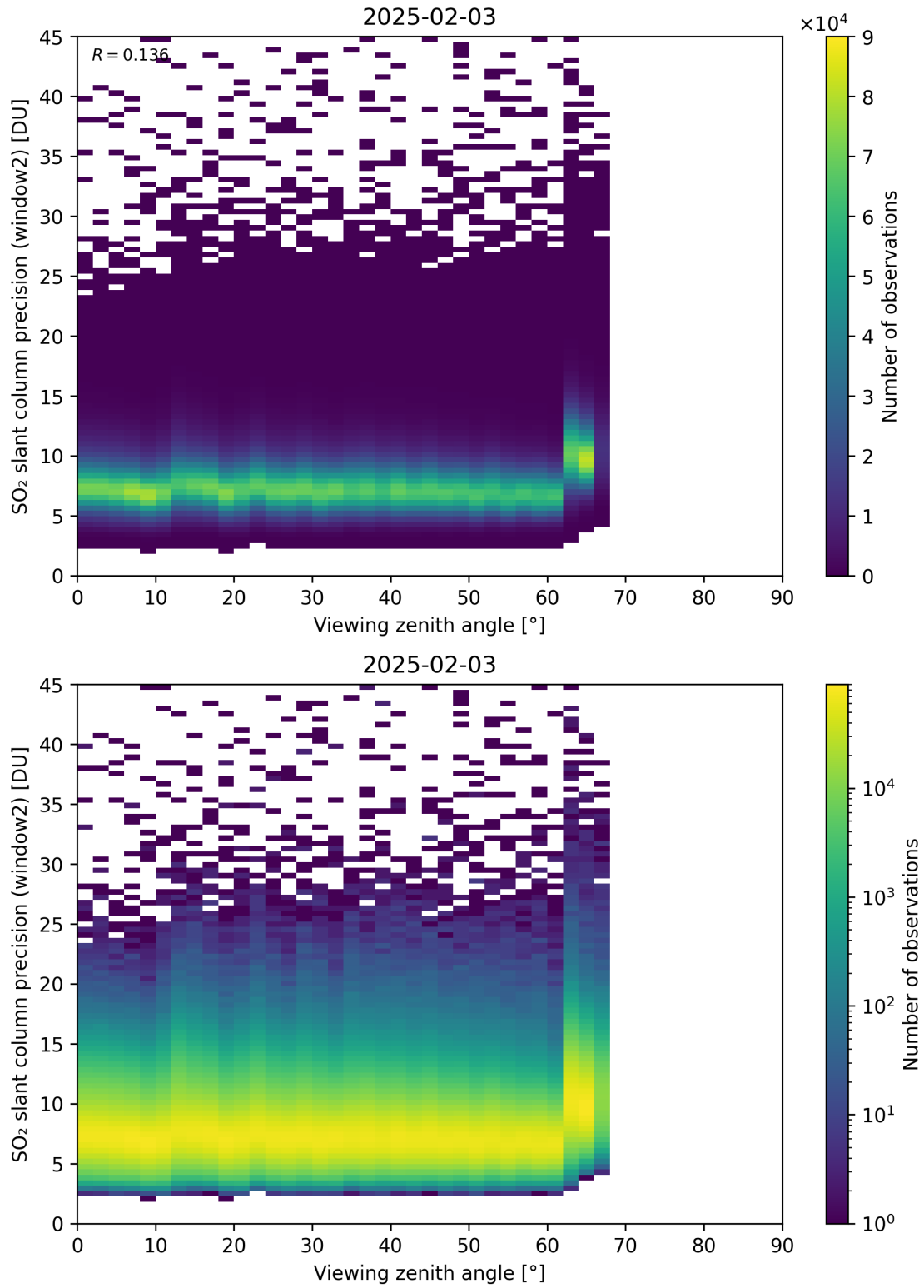
Figure 378: Scatter density plot of “Viewing zenith angle” against “SO 2 slant column precision (window2)” for 2025-02-03 to 2025-02-04.
