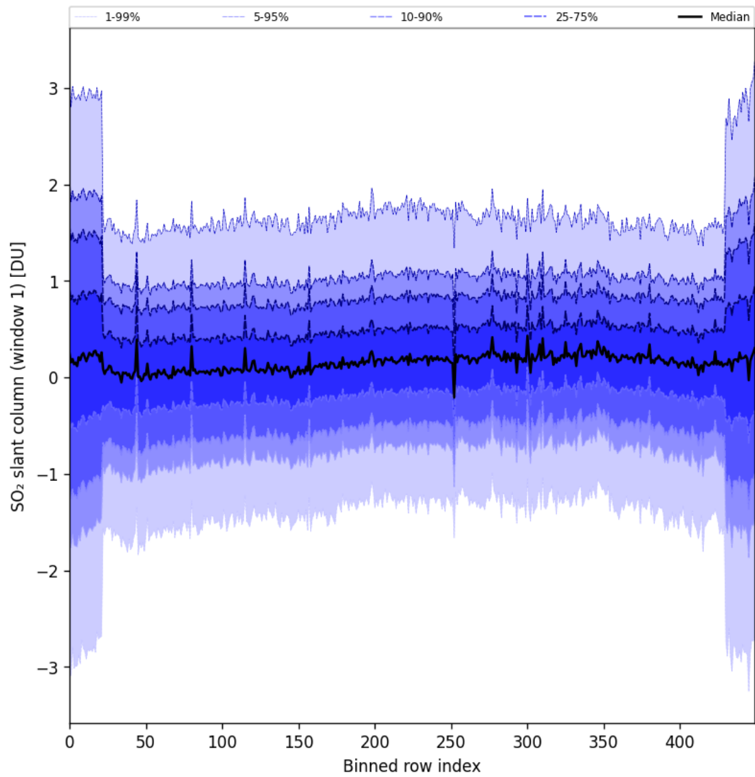
Figure 89: Along track statistics of "SO 2 slant column (window 1)" for 2025-02-03 to 2025-02-04
