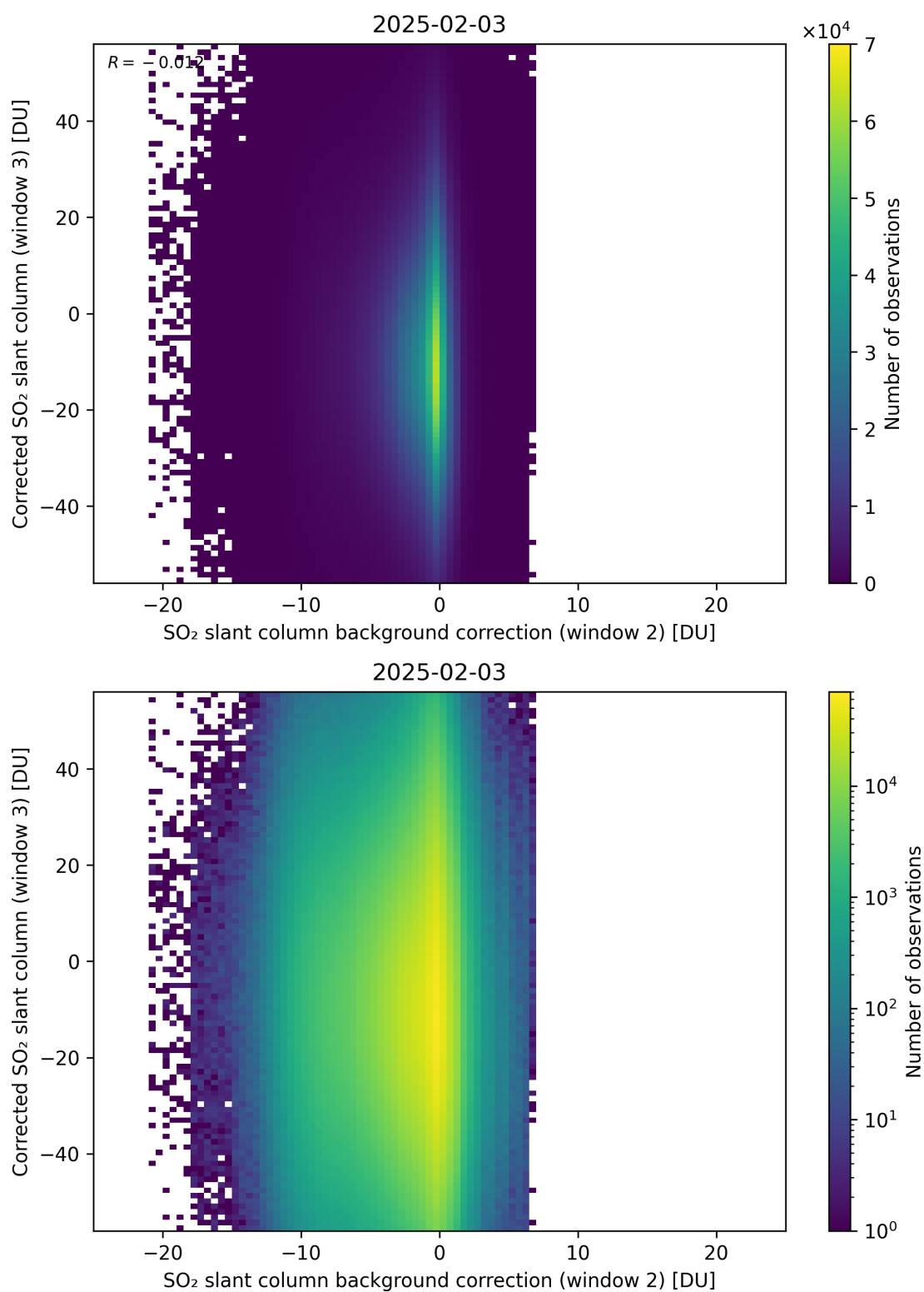
Figure 127: Scatter density plot of “SO 2 slant column background correction (window 2)” against “Corrected SO 2 slant column (window 3)” for 2025-02-03 to 2025-02-04.
