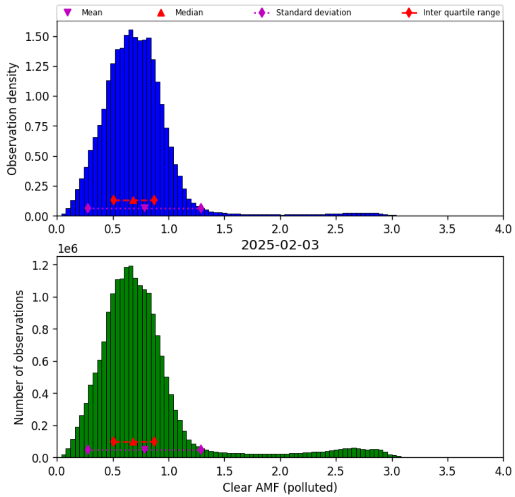
Figure 81: Histogram of “Clear AMF (polluted)” for 2025-02-03 to 2025-02-04
