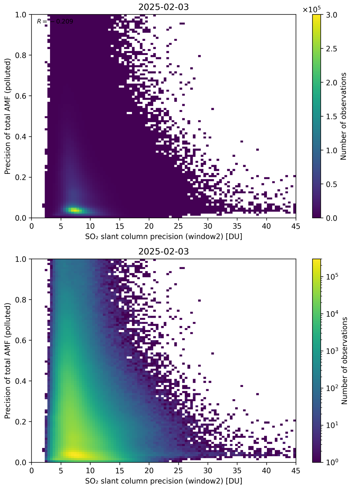
Figure 302: Scatter density plot of “SO 2 slant column precision (window2)” against “Precision of total AMF (polluted)” for 2025-02-03 to 2025-02-04.
