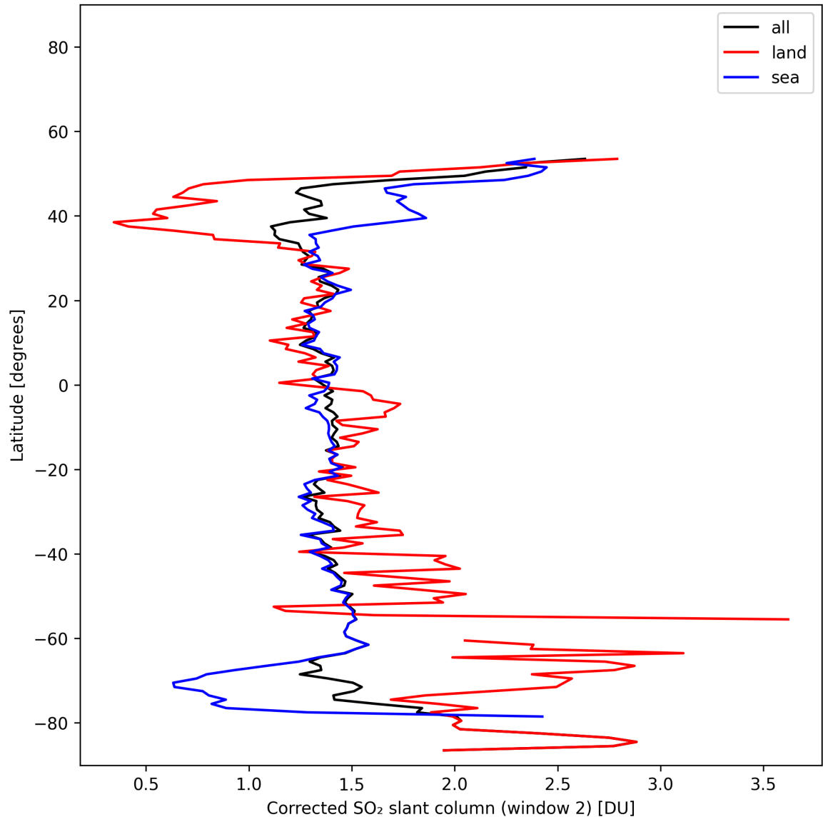
Figure 43: Zonal average of “Corrected SO 2 slant column (window 2)” for 2025-02-03 to 2025-02-04.
