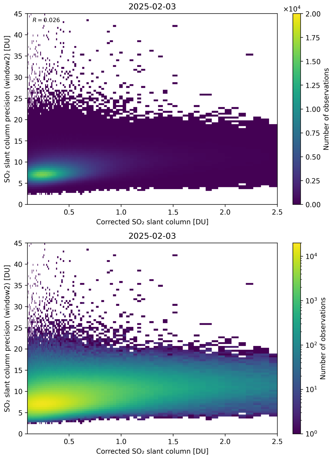
Figure 239: Scatter density plot of “Corrected SO 2 slant column” against “SO 2 slant column precision (window2)” for 2025-02-03 to 2025-02-04.
