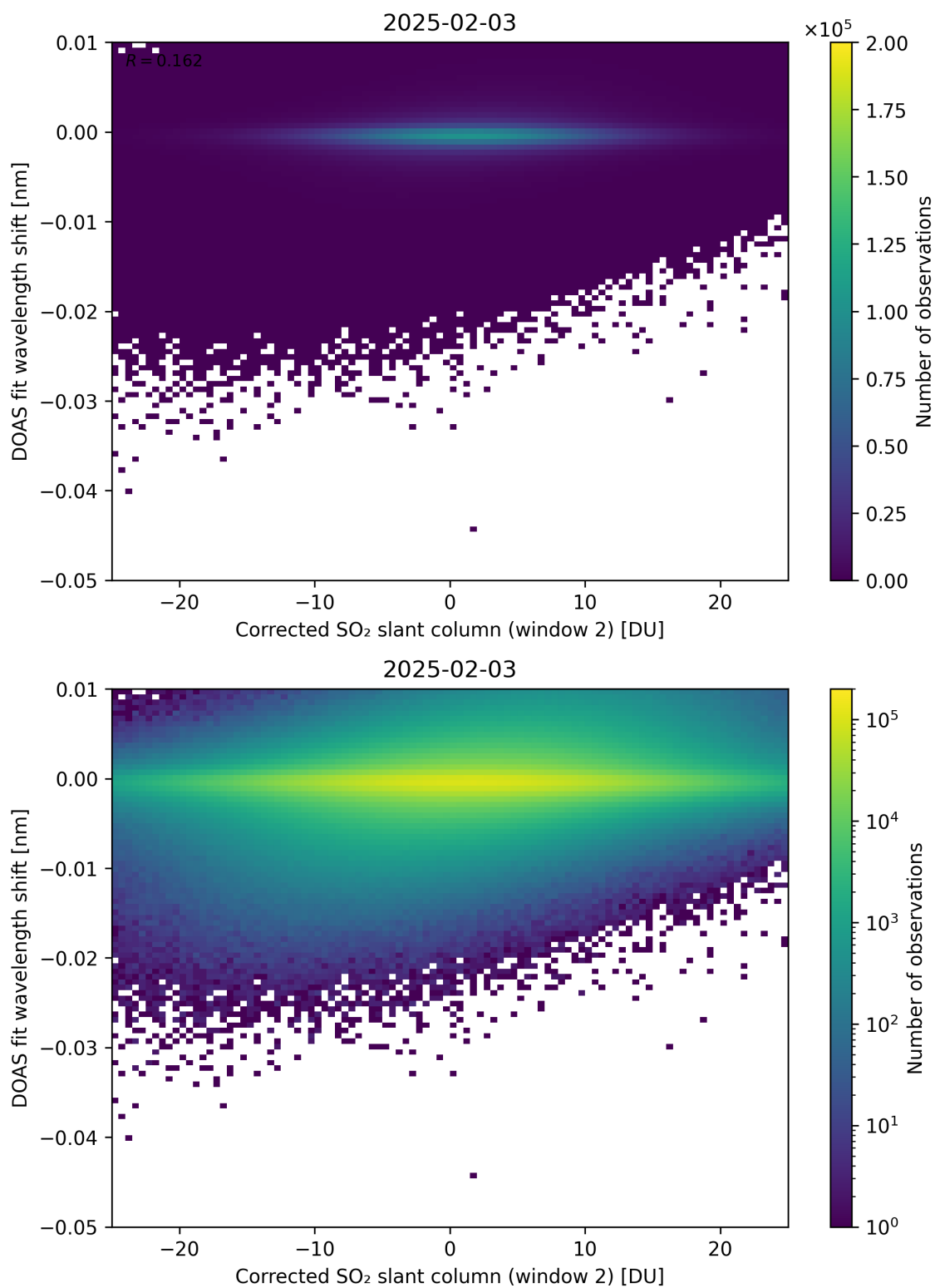
Figure 246: Scatter density plot of “Corrected SO 2 slant column (window 2)” against “DOAS fit wavelength shift” for 2025-02-03 to 2025-02-04.
