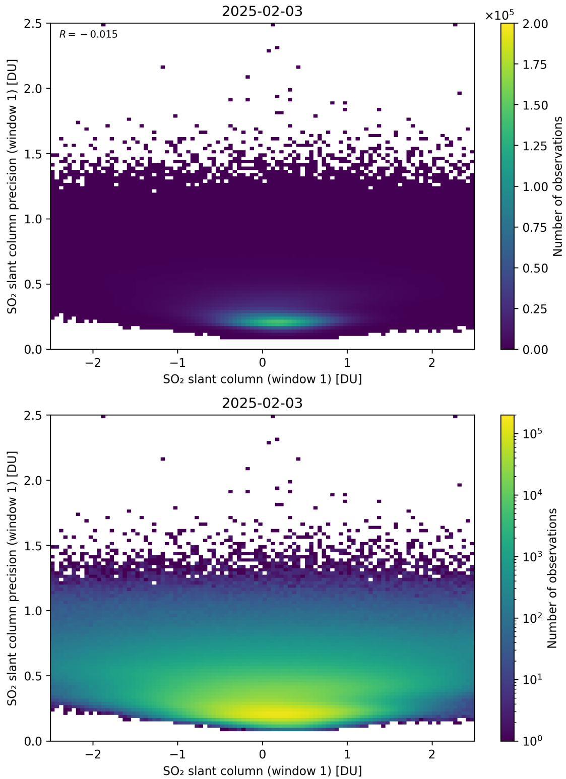
Figure 285: Scatter density plot of “SO 2 slant column (window 1)” against “SO 2 slant column precision (window 1)” for 2025-02-03 to 2025-02-04.
