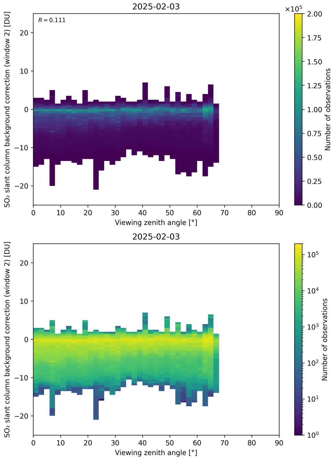
Figure 363: Scatter density plot of “Viewing zenith angle” against “SO 2 slant column background correction (window 2)” for 2025-02-03 to 2025-02-04.
