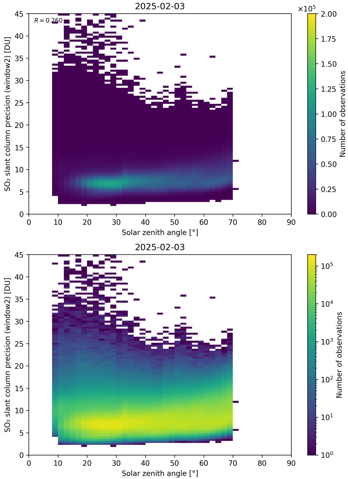
Figure 186: Scatter density plot of “Solar zenith angle” against “SO 2 slant column precision (window2)” for 2025-02-03 to 2025-02-04.
