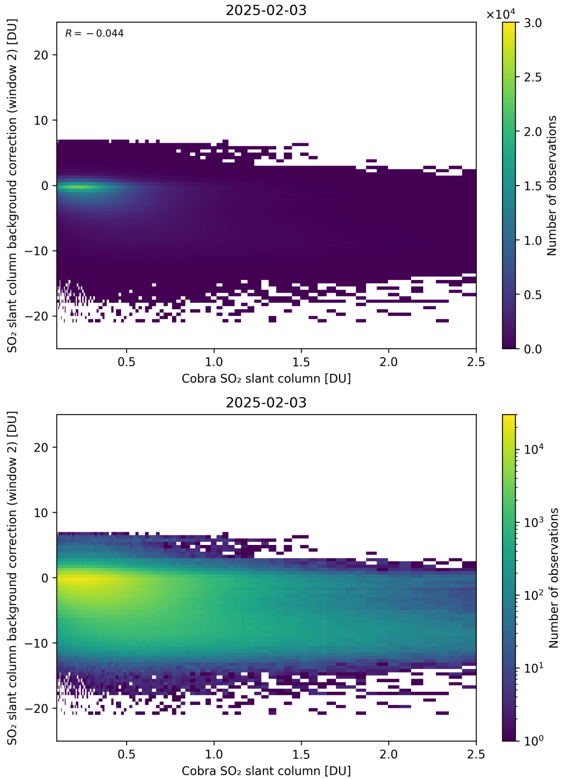
Figure 194: Scatter density plot of “Cobra SO 2 slant column” against “SO 2 slant column background correction (window 2)” for 2025-02-03 to 2025-02-04.
