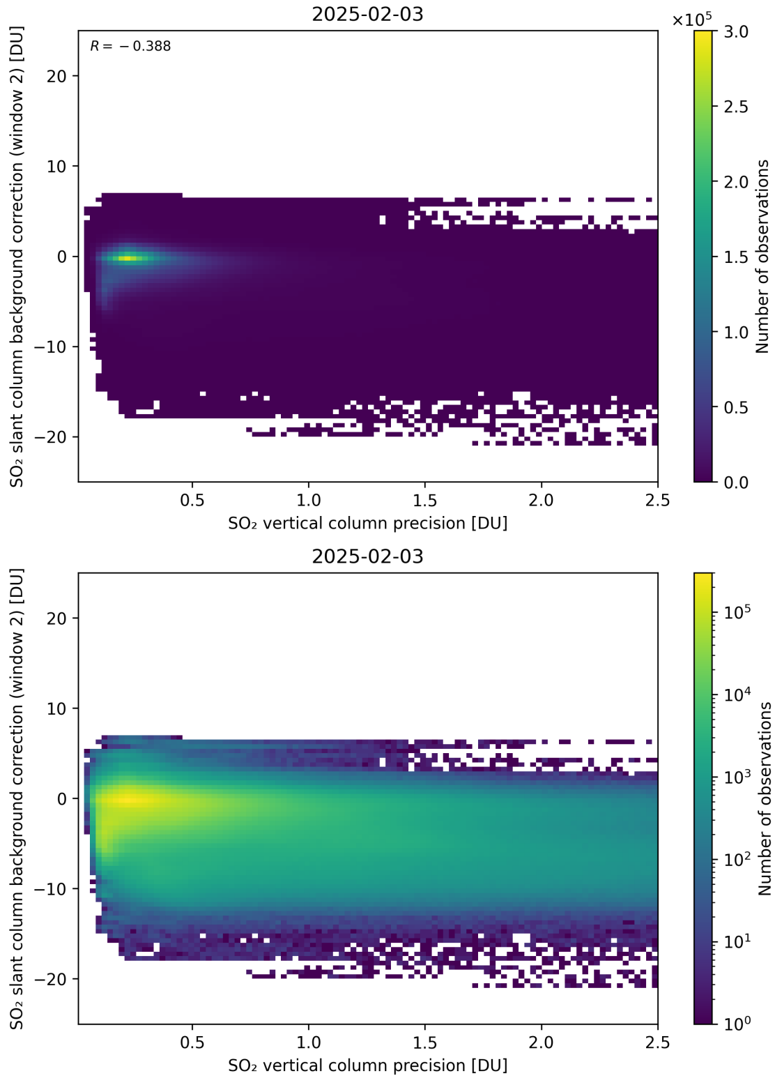
Figure 330: Scatter density plot of “SO 2 vertical column precision” against “SO 2 slant column background correction (window 2)” for 2025-02-03 to 2025-02-04.
