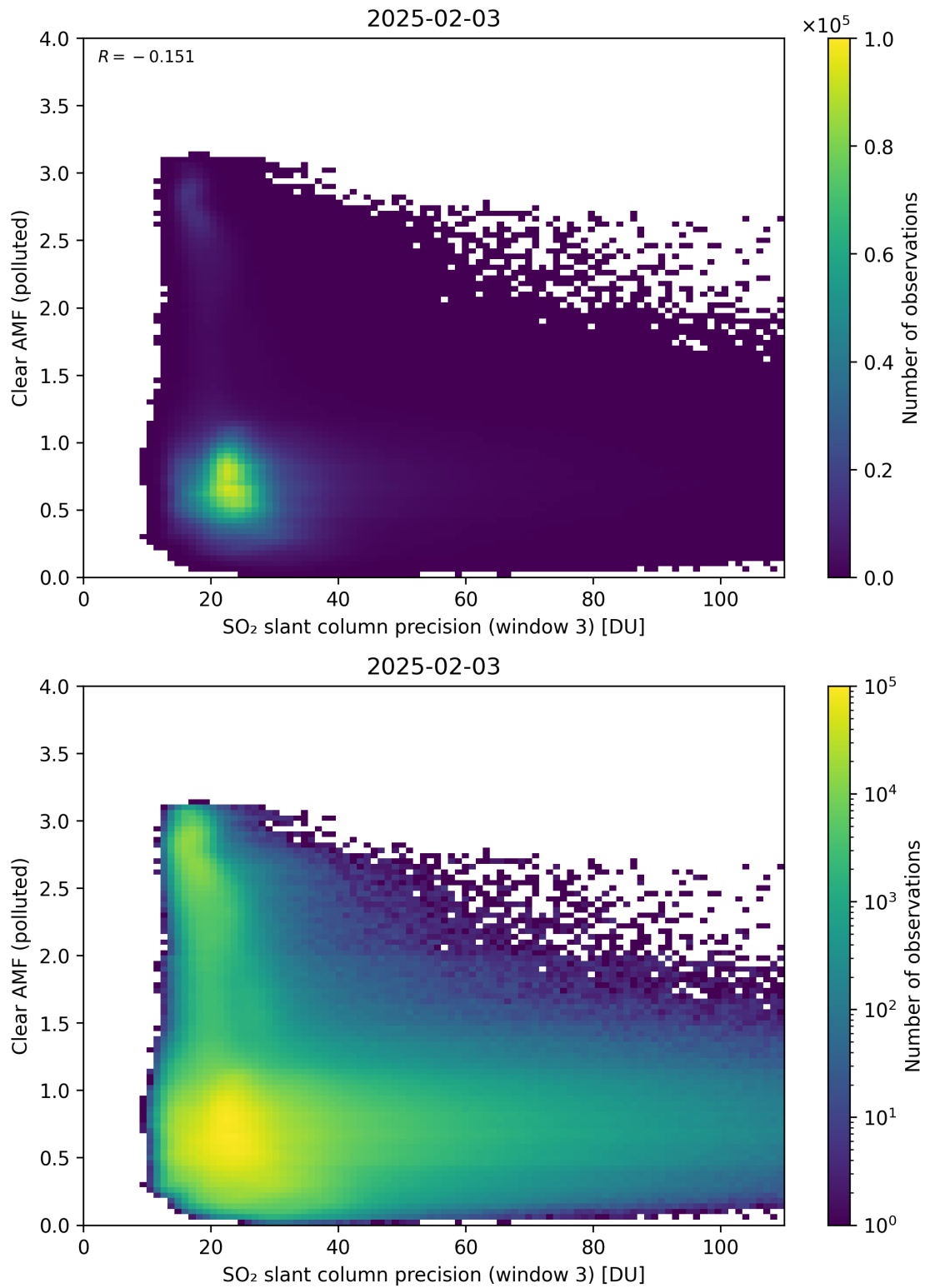
Figure 311: Scatter density plot of “SO 2 slant column precision (window 3)” against “Clear AMF (polluted)” for 2025-02-03 to 2025-02-04.
