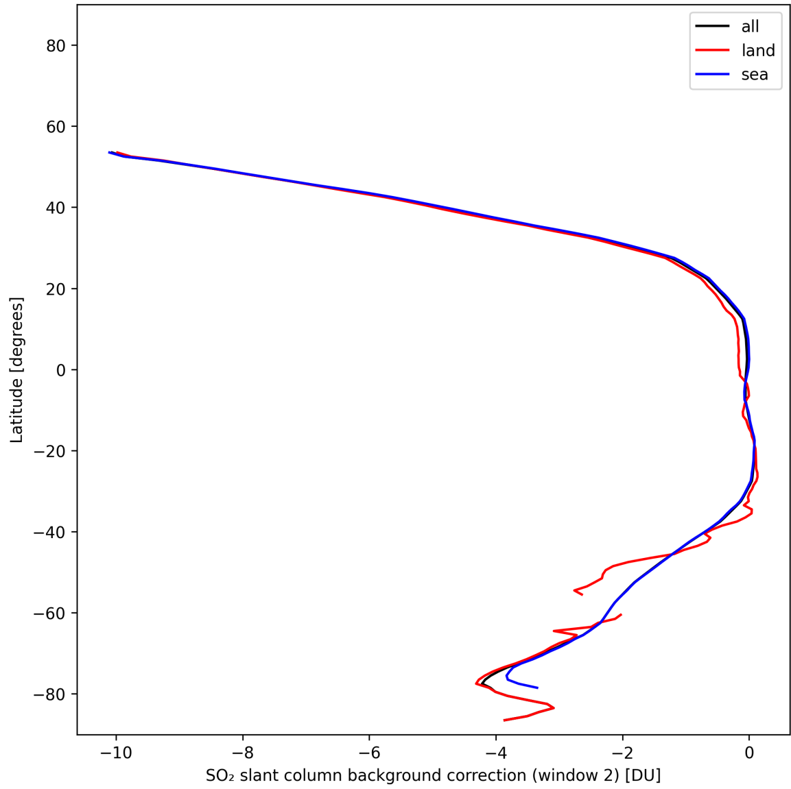
Figure 44: Zonal average of “SO 2 slant column background correction (window 2)” for 2025-02-03 to 2025-02-04.
