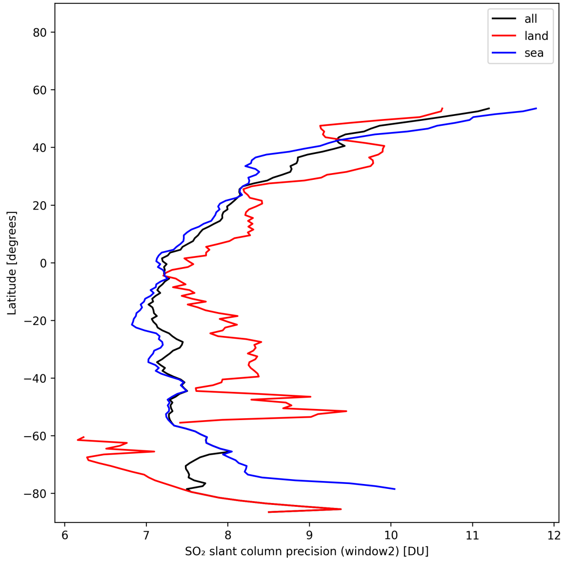
Figure 42: Zonal average of “SO 2 slant column precision (window2)” for 2025-02-03 to 2025-02-04.
