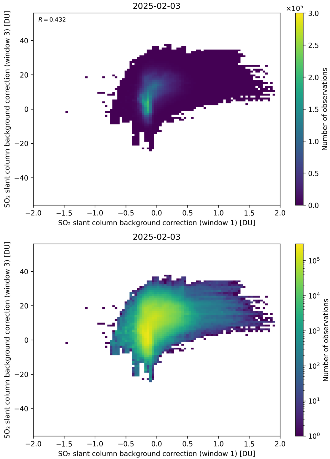
Figure 110: Scatter density plot of “SO 2 slant column background correction (window 1)” against “SO 2 slant column background correction (window 3)” for 2025-02-03 to 2025-02-04.
