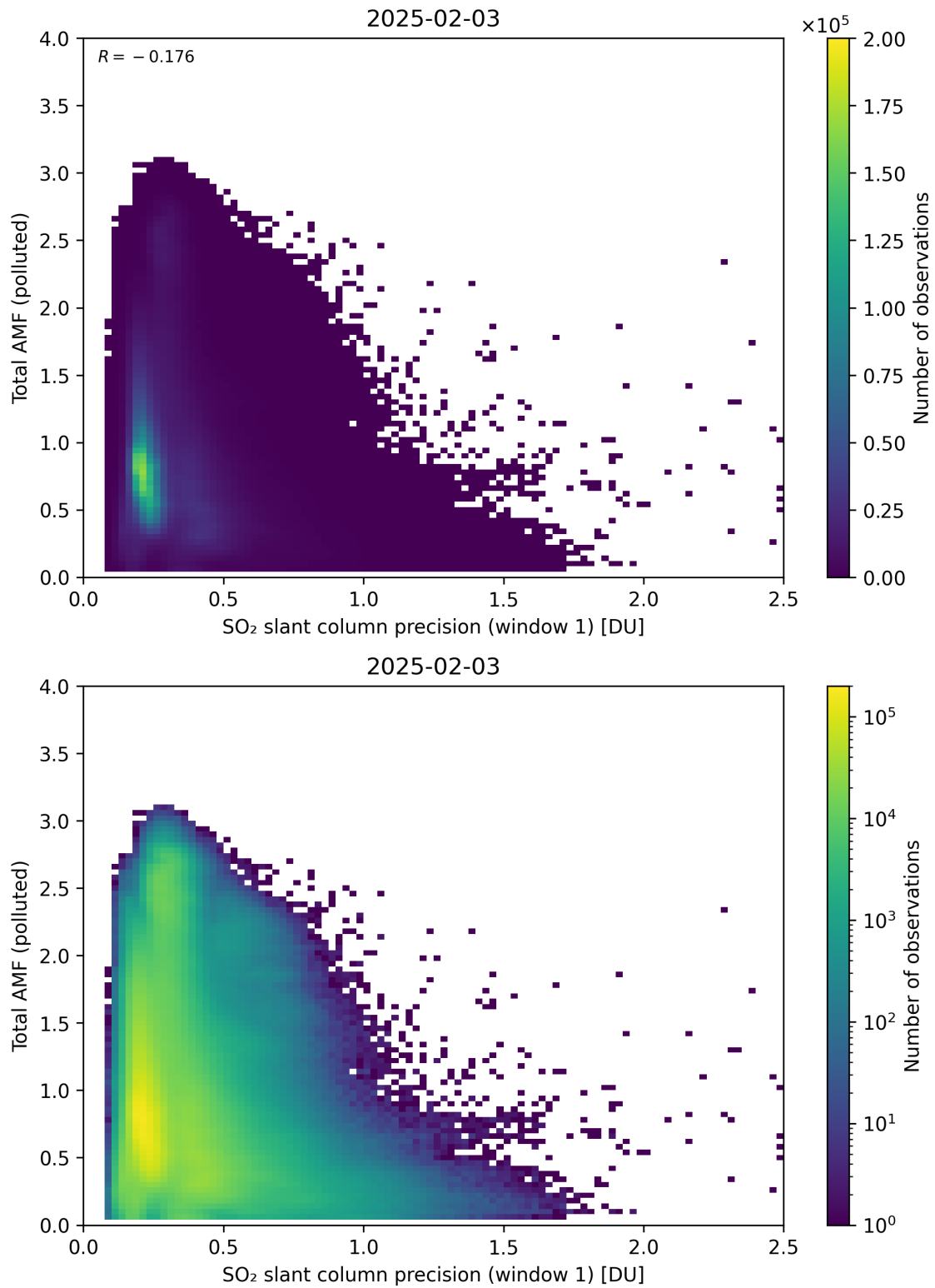
Figure 280: Scatter density plot of “SO 2 slant column precision (window 1)” against “Total AMF (polluted)” for 2025-02-03 to 2025-02-04.
