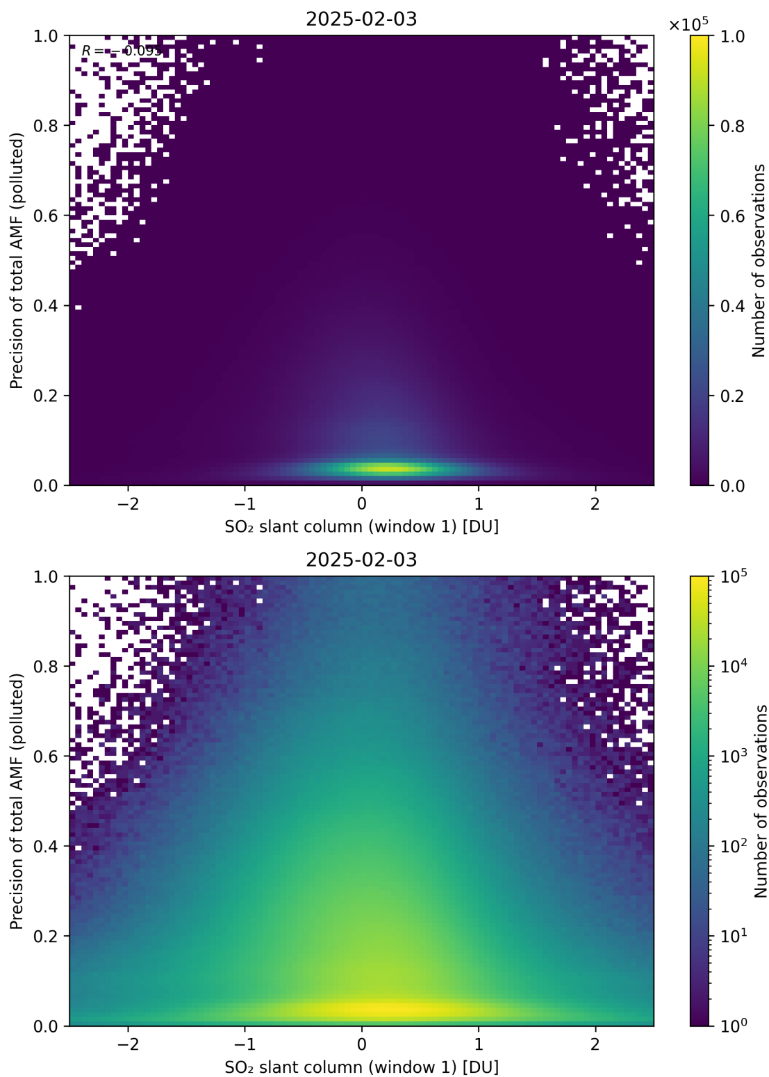
Figure 290: Scatter density plot of “SO 2 slant column (window 1)” against “Precision of total AMF (polluted)” for 2025-02-03 to 2025-02-04.
