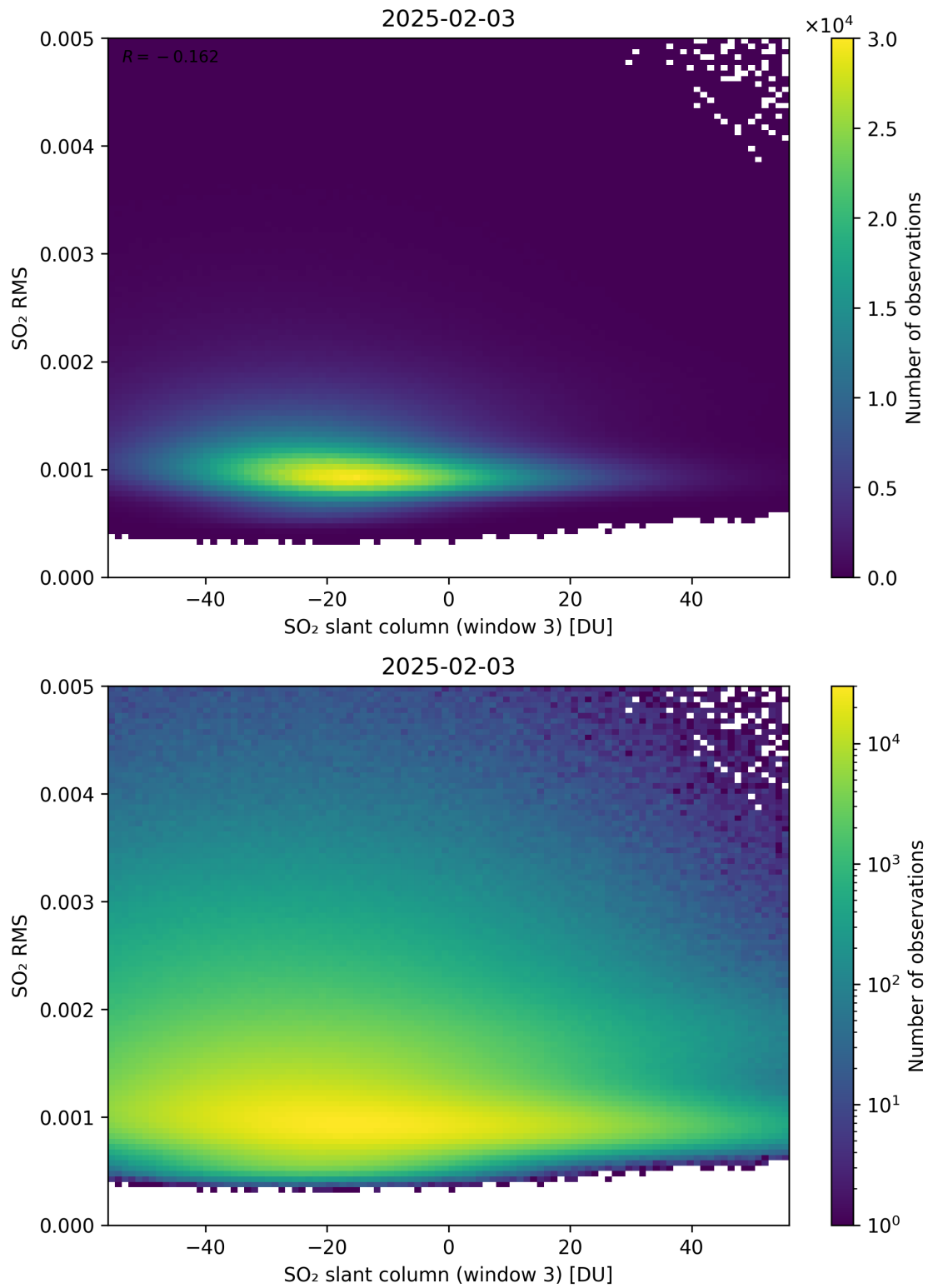
Figure 306: Scatter density plot of “SO 2 slant column (window 3)” against “SO 2 RMS” for 2025-02-03 to 2025-02-04.
