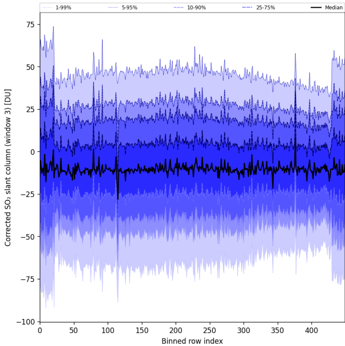
Figure 99: Along track statistics of “Corrected SO 2 slant column (window 3)” for 2025-02-03 to 2025-02-04
