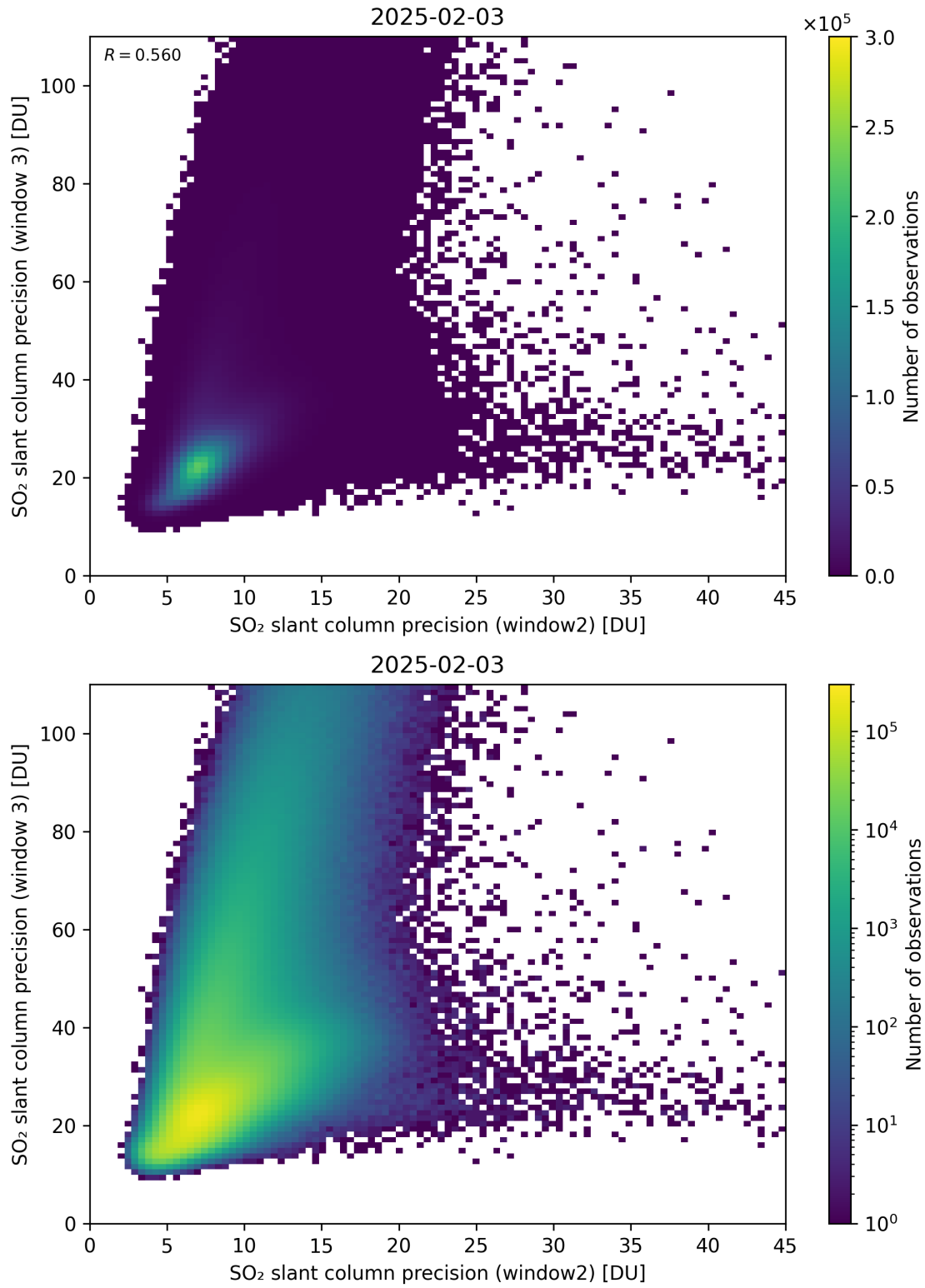
Figure 300: Scatter density plot of “SO 2 slant column precision (window2)” against “SO 2 slant column precision (window 3)” for 2025-02-03 to 2025-02-04.
