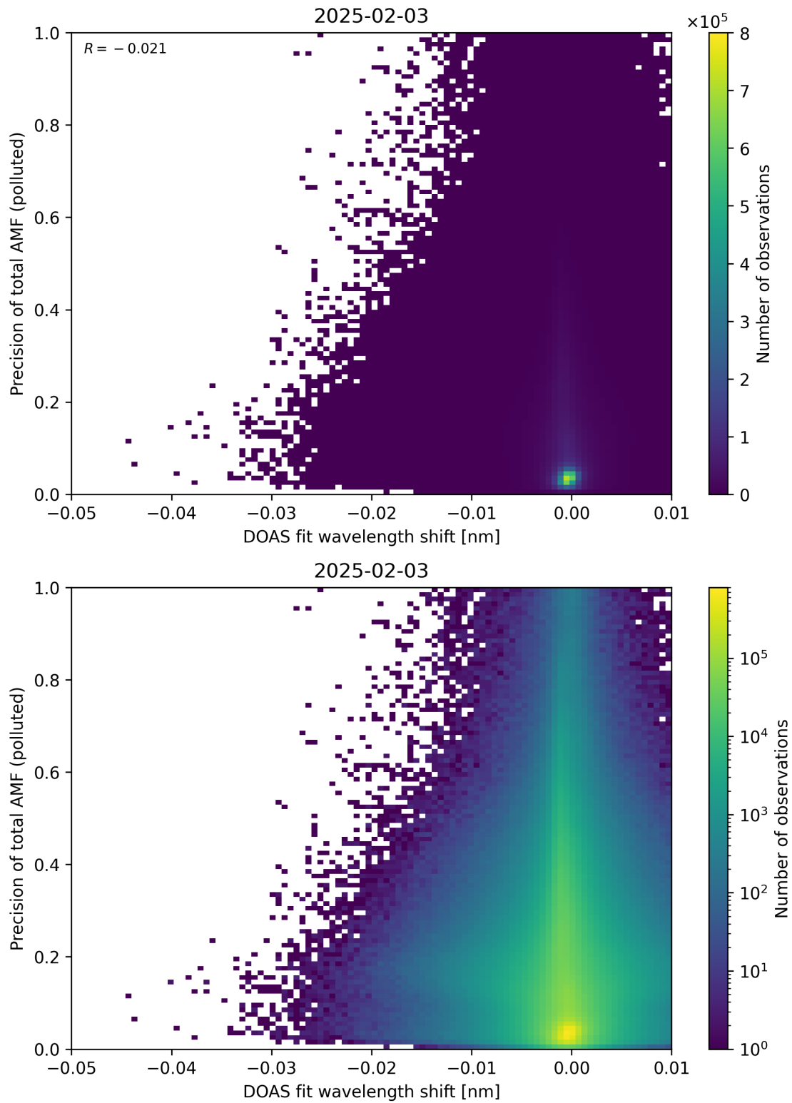
Figure 142: Scatter density plot of “DOAS fit wavelength shift” against “Precision of total AMF (polluted)” for 2025-02-03 to 2025-02-04.
