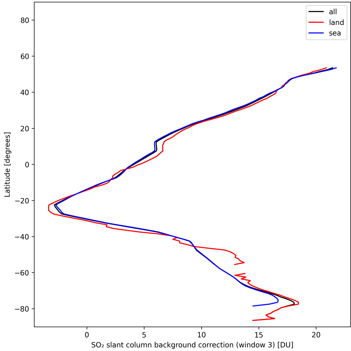
Figure 48: Zonal average of “SO 2 slant column background correction (window 3)” for 2025-02-03 to 2025-02-04.
