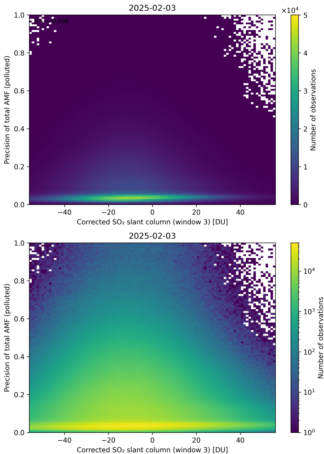
Figure 261: Scatter density plot of “Corrected SO 2 slant column (window 3)” against “Precision of total AMF (polluted)” for 2025-02-03 to 2025-02-04.
