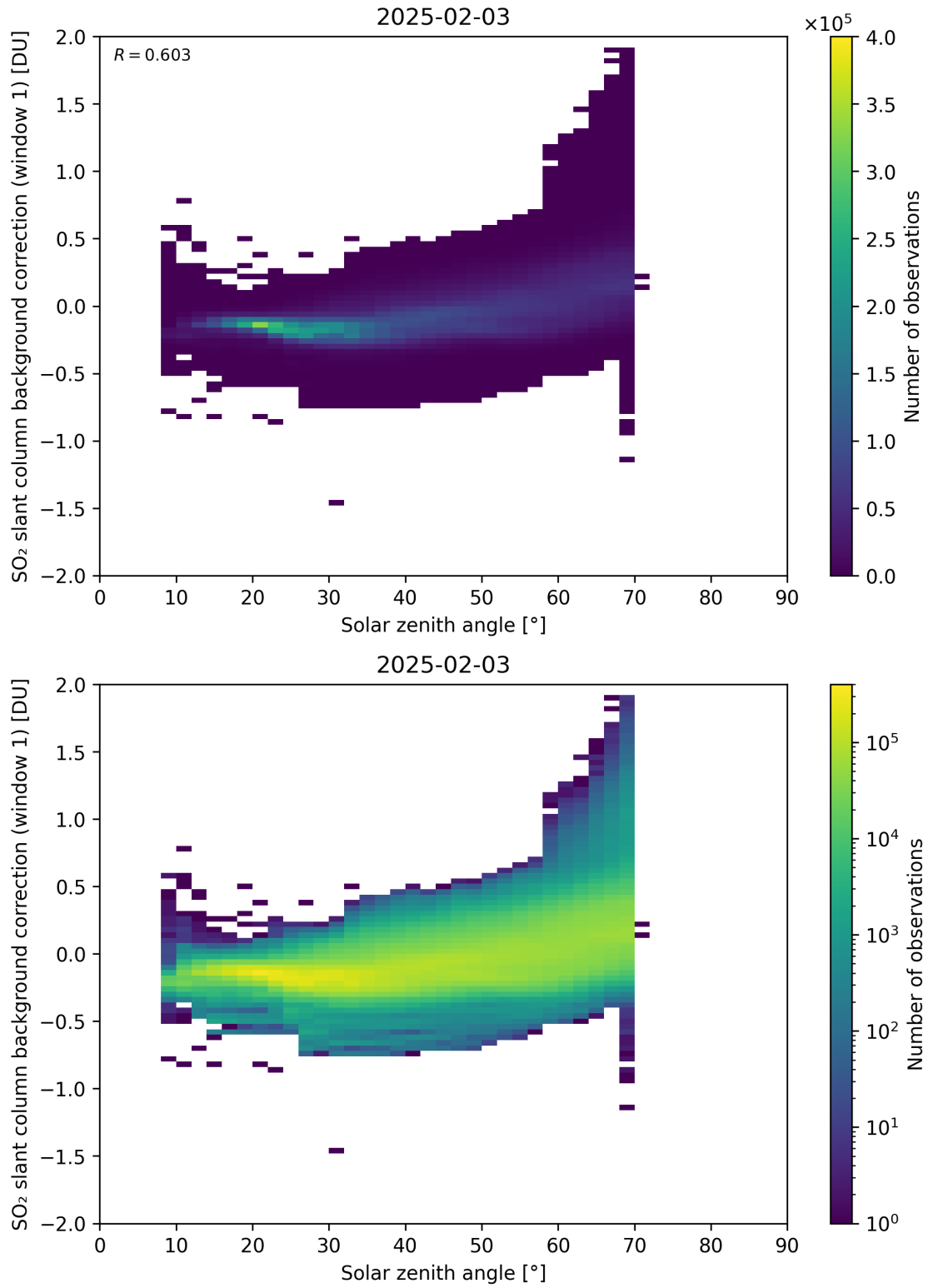
Figure 171: Scatter density plot of “Solar zenith angle” against “SO 2 slant column background correction (window 1)” for 2025-02-03 to 2025-02-04.
