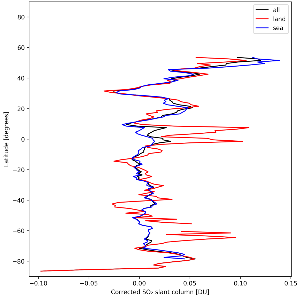
Figure 34: Zonal average of “Corrected SO 2 slant column” for 2025-02-03 to 2025-02-04.
