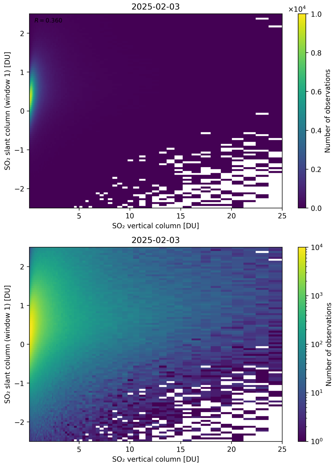
Figure 354: Scatter density plot of “SO 2 vertical column” against “SO 2 slant column (window 1)” for 2025-02-03 to 2025-02-04.
