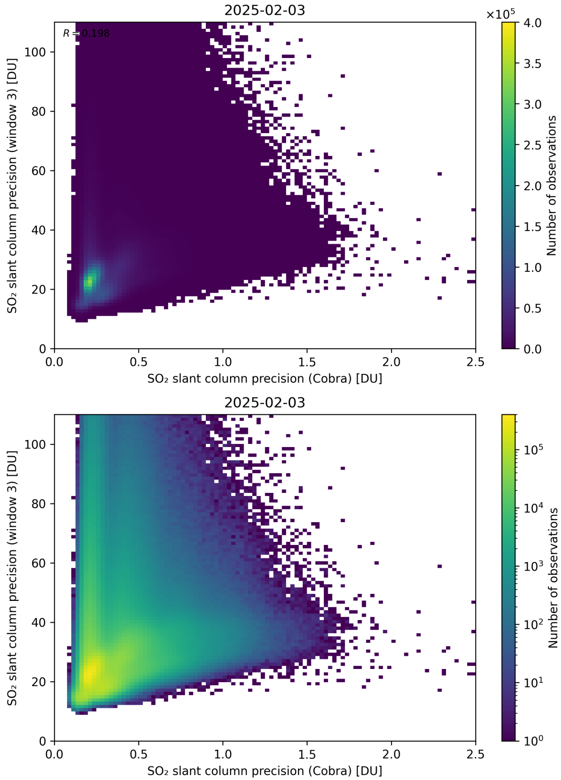
Figure 212: Scatter density plot of “SO 2 slant column precision (Cobra)” against “SO 2 slant column precision (window 3)” for 2025-02-03 to 2025-02-04.
