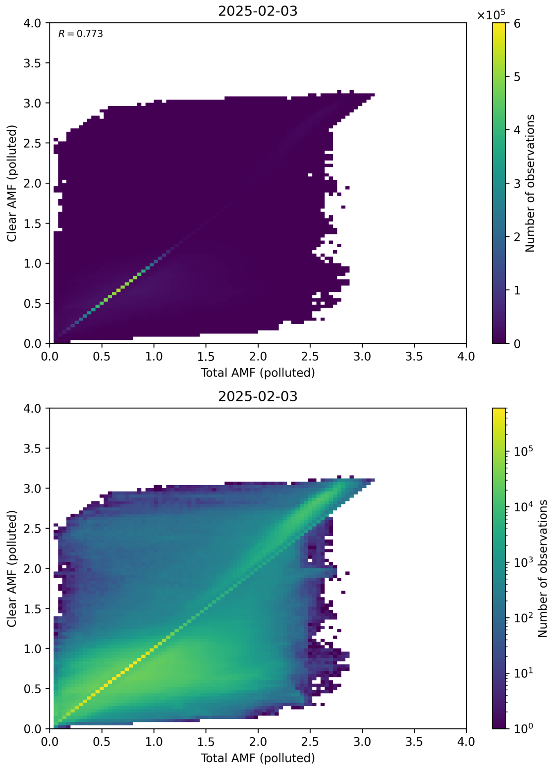
Figure 321: Scatter density plot of “Total AMF (polluted)” against “Clear AMF (polluted)” for 2025-02-03 to 2025-02-04.
