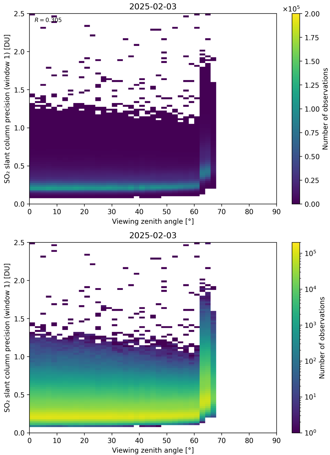
Figure 377: Scatter density plot of “Viewing zenith angle” against “SO 2 slant column precision (window 1)” for 2025-02-03 to 2025-02-04.
