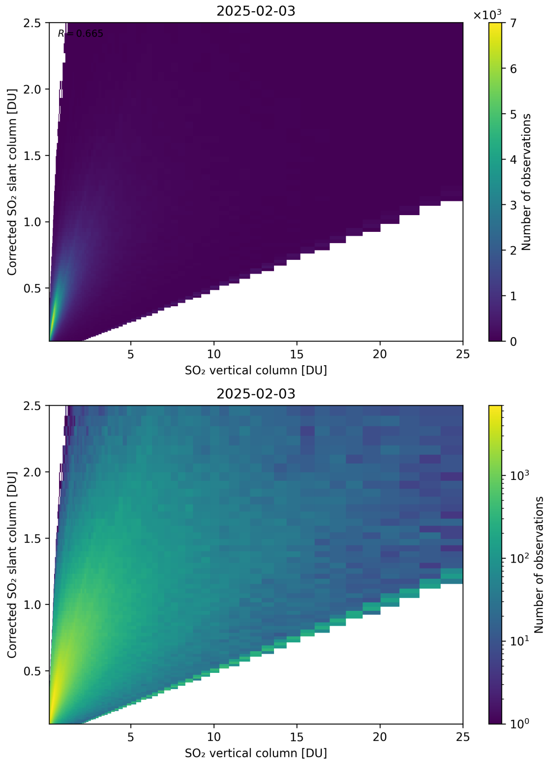
Figure 351: Scatter density plot of “SO 2 vertical column” against “Corrected SO 2 slant column” for 2025-02-03 to 2025-02-04.
