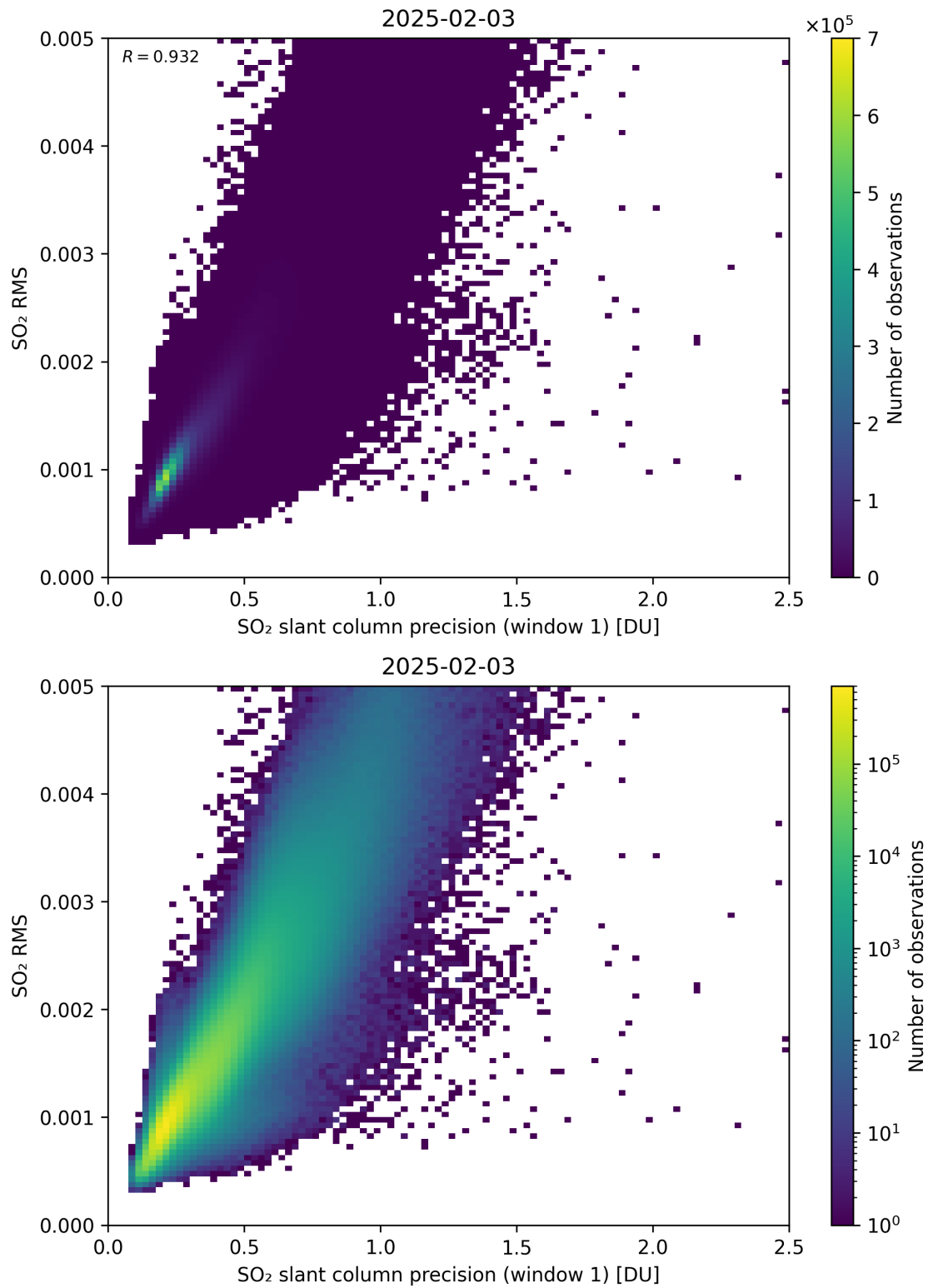
Figure 273: Scatter density plot of “SO 2 slant column precision (window 1)” against “SO 2 RMS” for 2025-02-03 to 2025-02-04.
