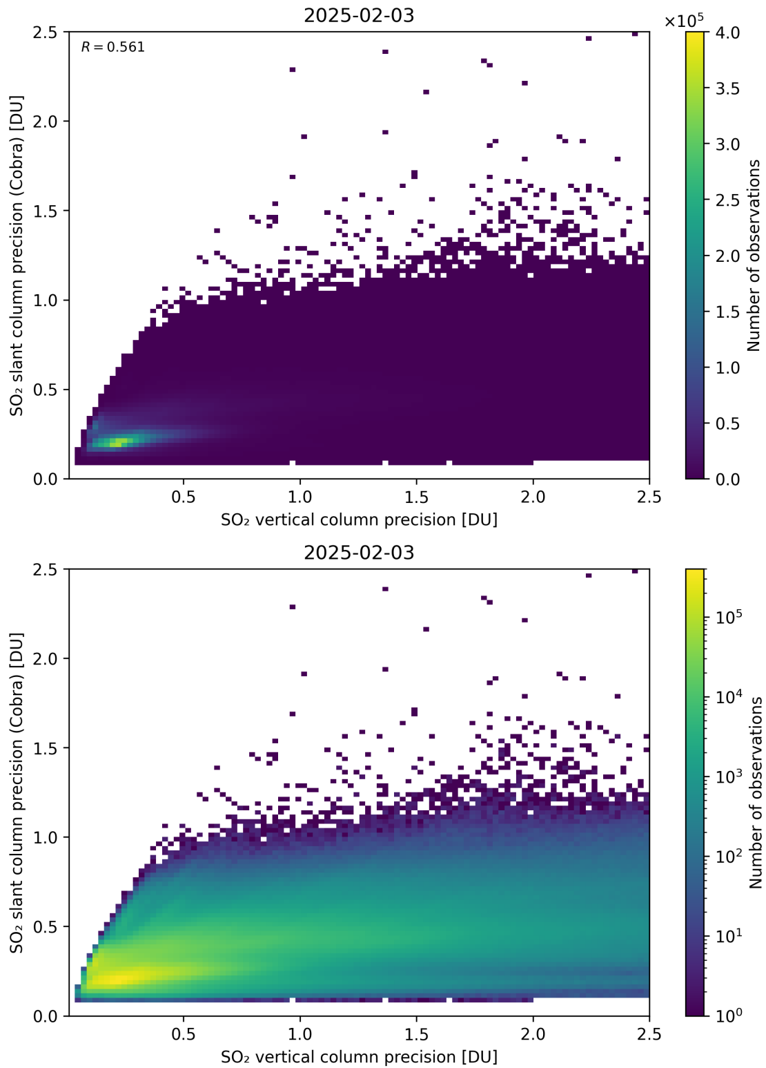
Figure 337: Scatter density plot of “SO 2 vertical column precision” against “SO 2 slant column precision (Cobra)” for 2025-02-03 to 2025-02-04.
