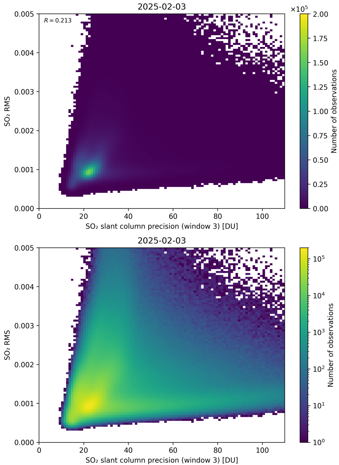
Figure 310: Scatter density plot of “SO 2 slant column precision (window 3)” against “SO 2 RMS” for 2025-02-03 to 2025-02-04.
