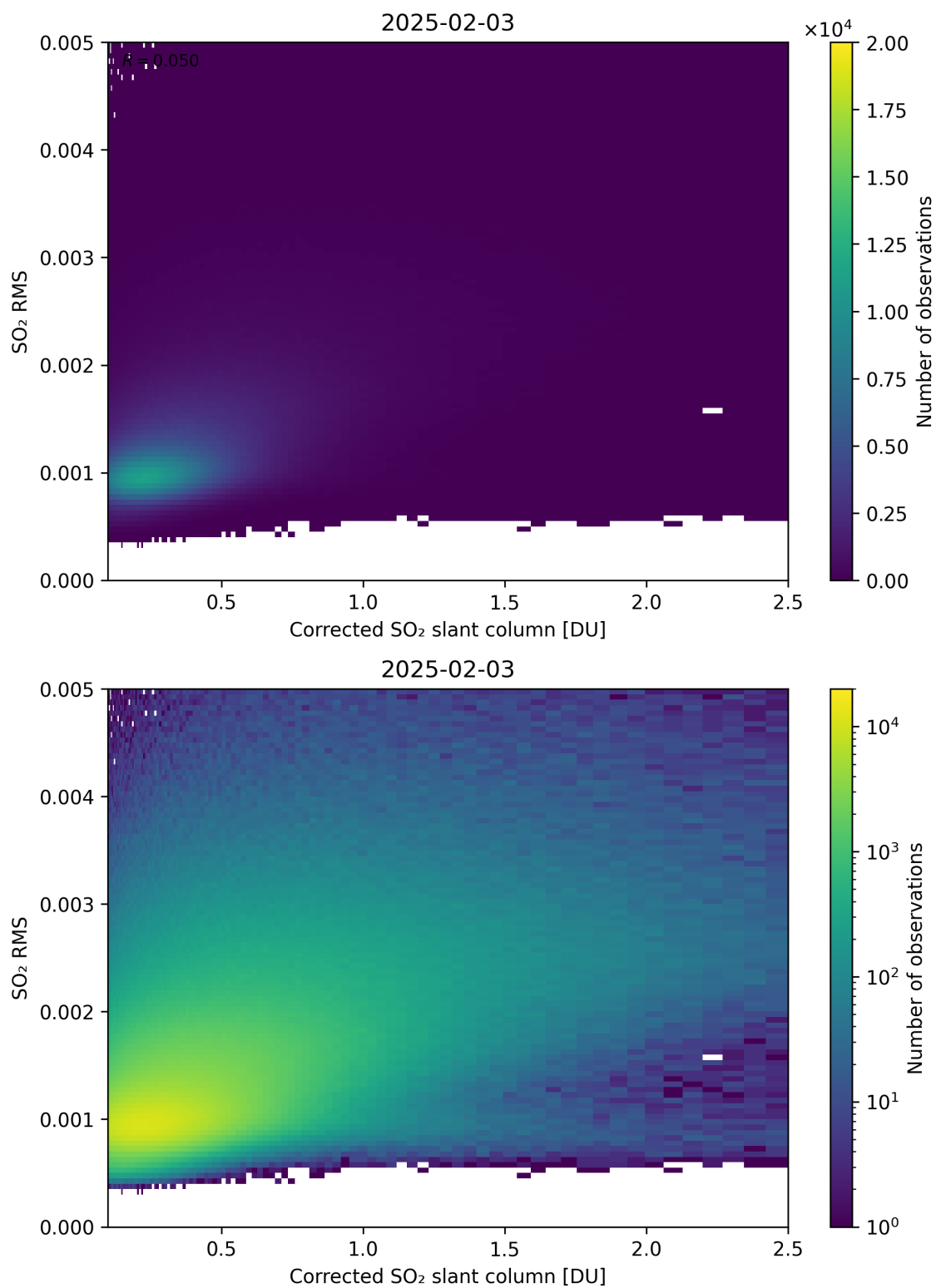
Figure 231: Scatter density plot of “Corrected SO 2 slant column” against “SO 2 RMS” for 2025-02-03 to 2025-02-04.
