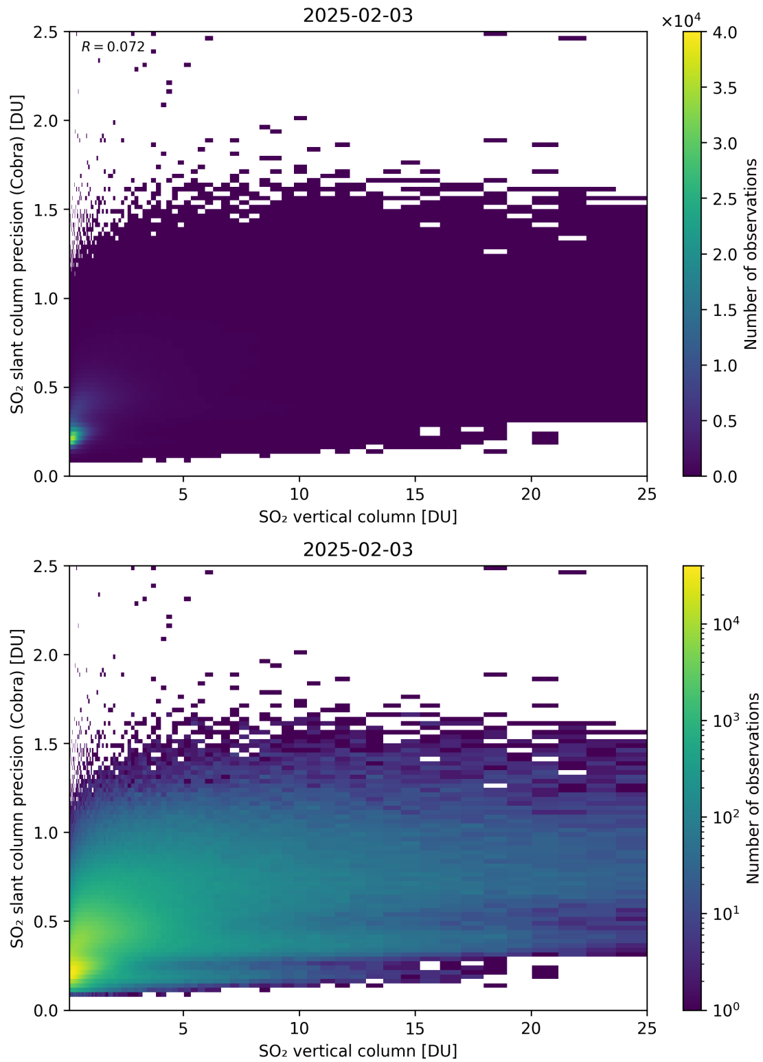
Figure 350: Scatter density plot of “SO 2 vertical column” against “SO 2 slant column precision (Cobra)” for 2025-02-03 to 2025-02-04.
