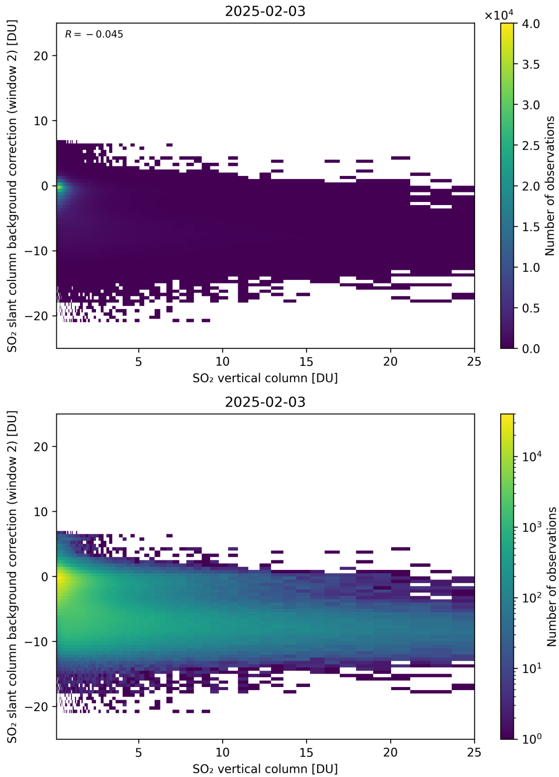
Figure 324: Scatter density plot of “SO 2 vertical column” against “SO 2 slant column background correction (window 2)” for 2025-02-03 to 2025-02-04.
