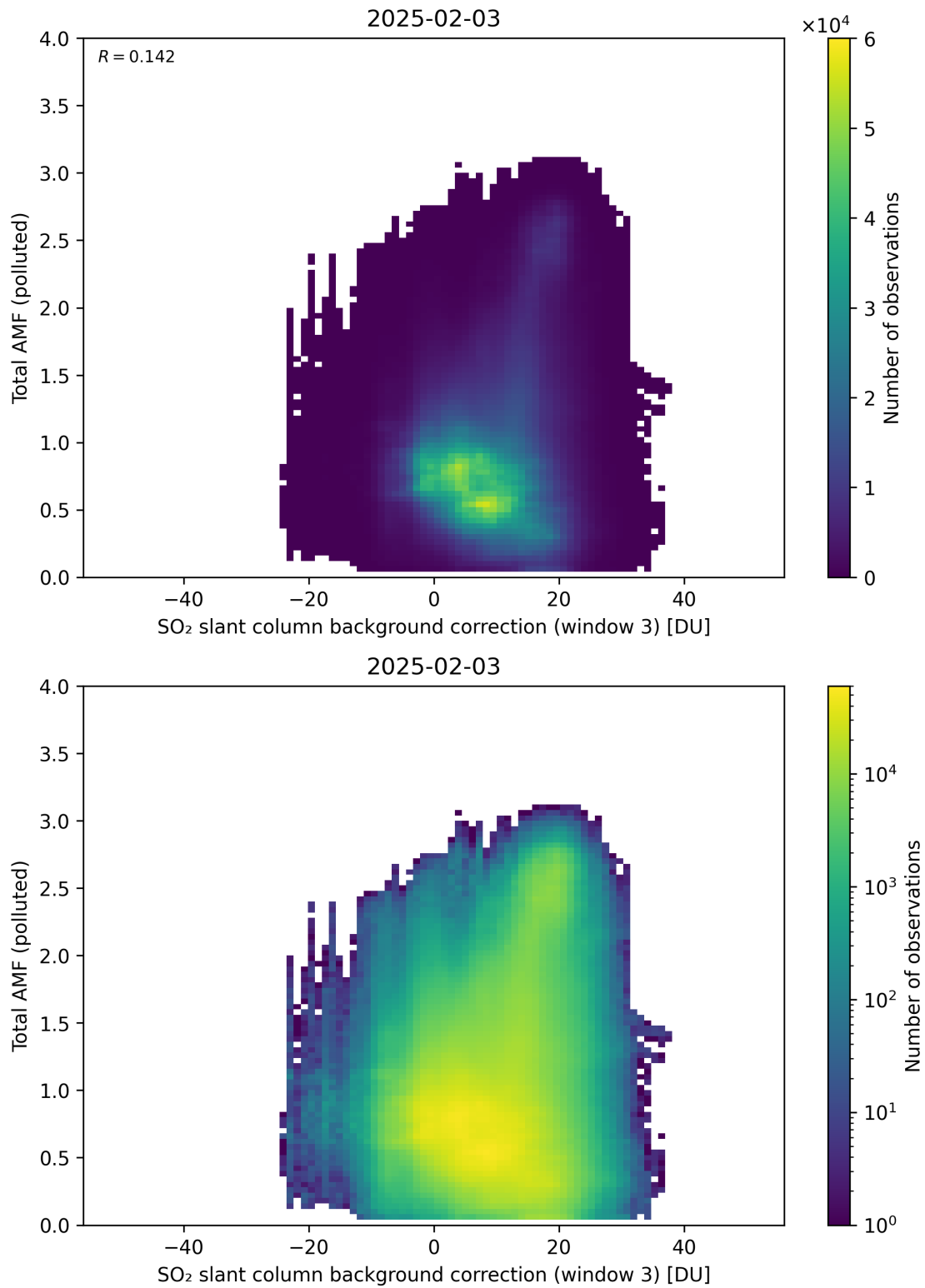
Figure 136: Scatter density plot of “SO 2 slant column background correction (window 3)” against “Total AMF (polluted)” for 2025-02-03 to 2025-02-04.
