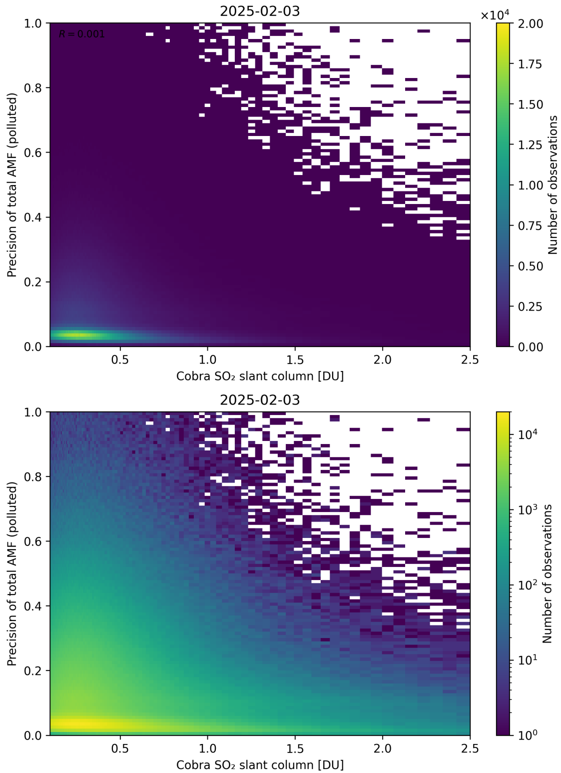
Figure 225: Scatter density plot of “Cobra SO 2 slant column” against “Precision of total AMF (polluted)” for 2025-02-03 to 2025-02-04.
