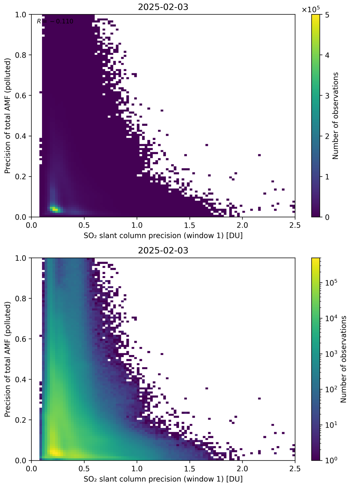
Figure 281: Scatter density plot of “SO 2 slant column precision (window 1)” against “Precision of total AMF (polluted)” for 2025-02-03 to 2025-02-04.
