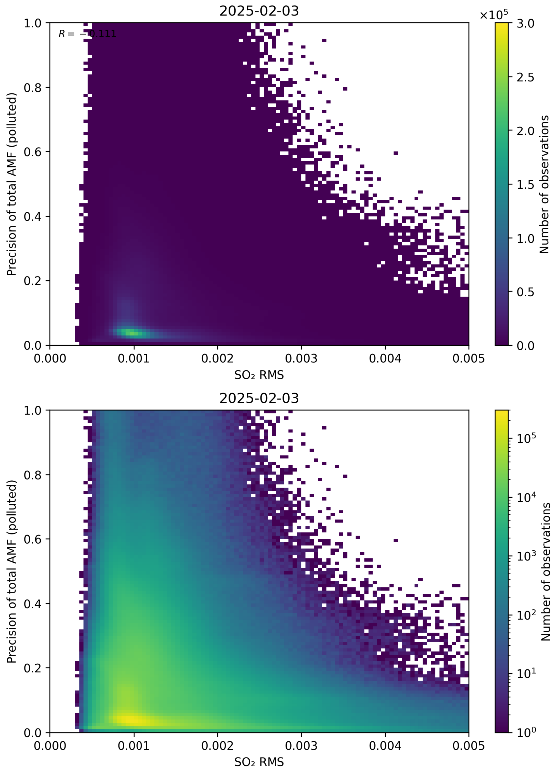
Figure 149: Scatter density plot of “SO 2 RMS” against “Precision of total AMF (polluted)” for 2025-02-03 to 2025-02-04.
