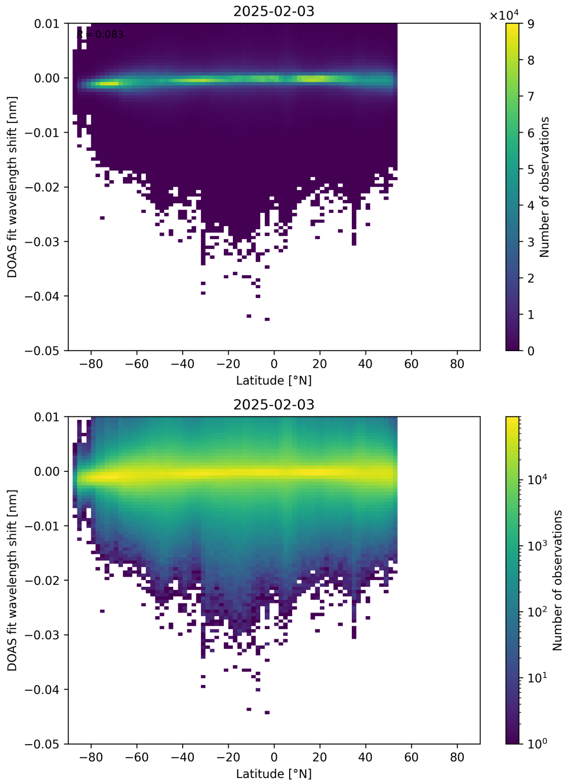
Figure 153: Scatter density plot of “Latitude” against “DOAS fit wavelength shift” for 2025-02-03 to 2025-02-04.
