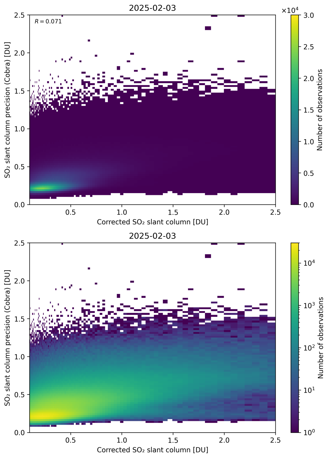
Figure 234: Scatter density plot of “Corrected SO 2 slant column” against “SO 2 slant column precision (Cobra)” for 2025-02-03 to 2025-02-04.
