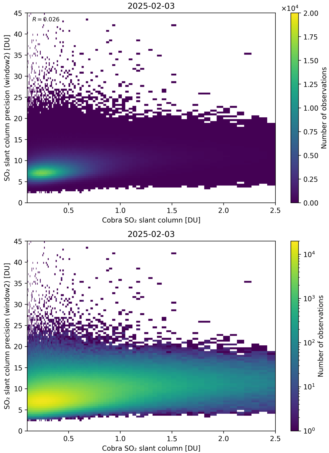
Figure 221: Scatter density plot of “Cobra SO 2 slant column” against “SO 2 slant column precision (window2)” for 2025-02-03 to 2025-02-04.
