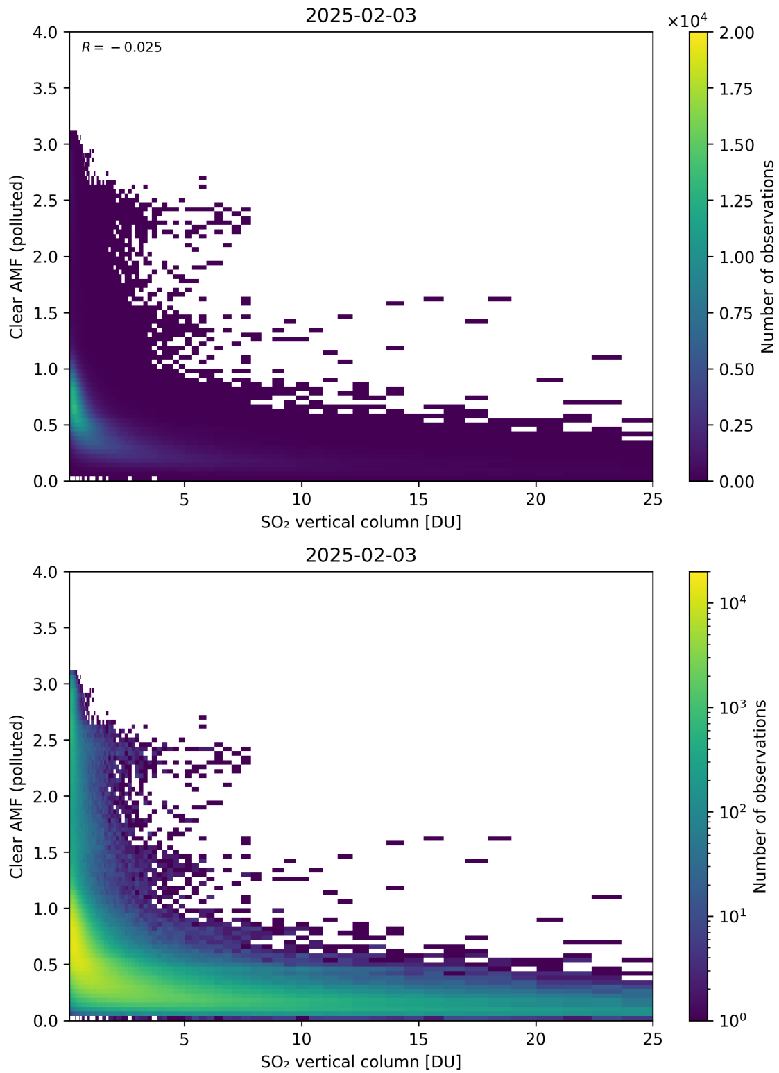
Figure 348: Scatter density plot of “SO 2 vertical column” against “Clear AMF (polluted)” for 2025-02-03 to 2025-02-04.
