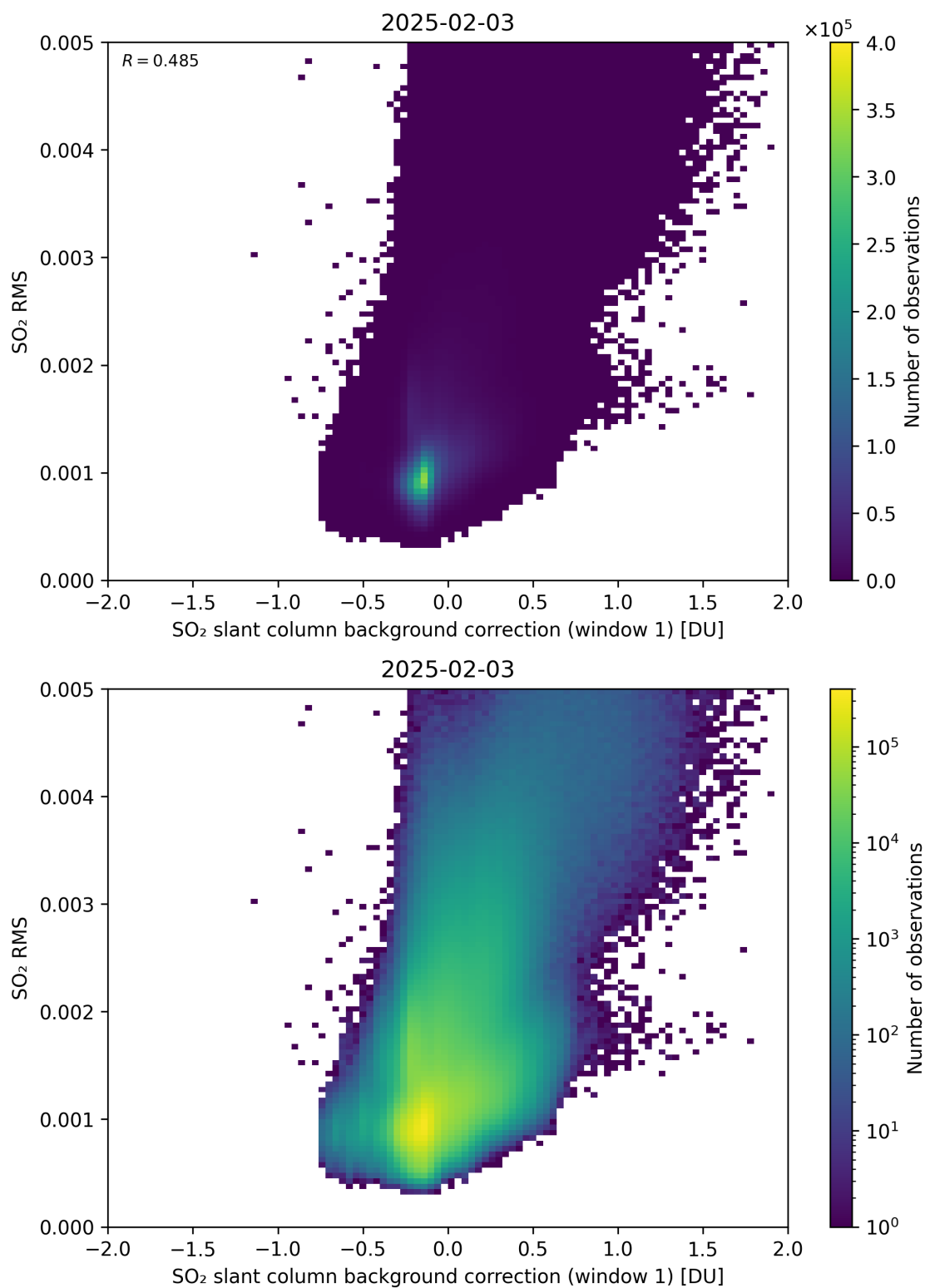
Figure 113: Scatter density plot of “SO 2 slant column background correction (window 1)” against “SO 2 RMS” for 2025-02-03 to 2025-02-04.
