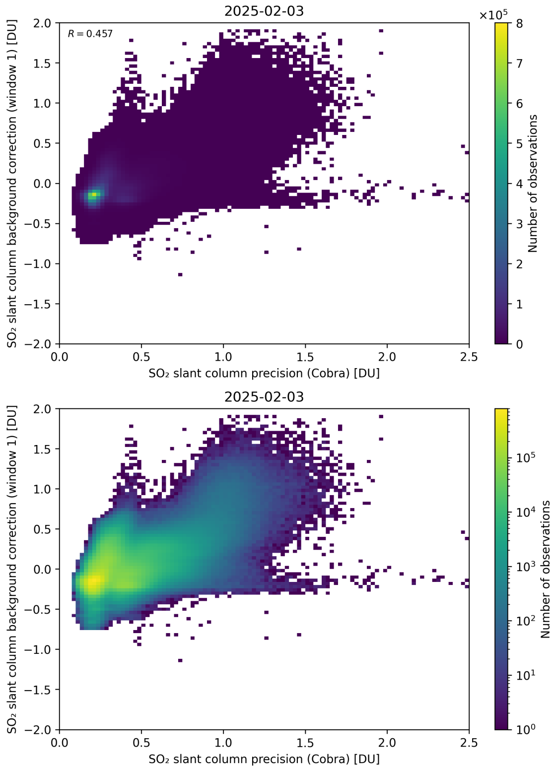
Figure 199: Scatter density plot of “SO 2 slant column precision (Cobra)” against “SO 2 slant column background correction (window 1)” for 2025-02-03 to 2025-02-04.
