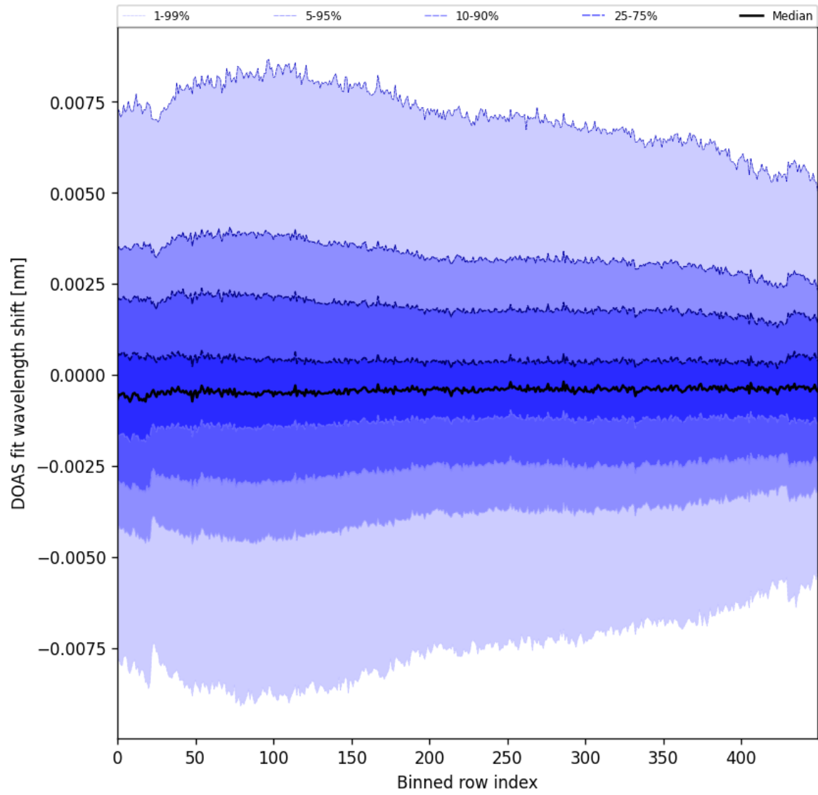
Figure 102: Along track statistics of “DOAS fit wavelength shift” for 2025-02-03 to 2025-02-04
