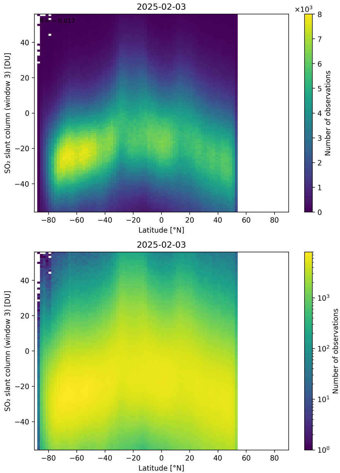
Figure 165: Scatter density plot of “Latitude” against “SO 2 slant column (window 3)” for 2025-02-03 to 2025-02-04.
