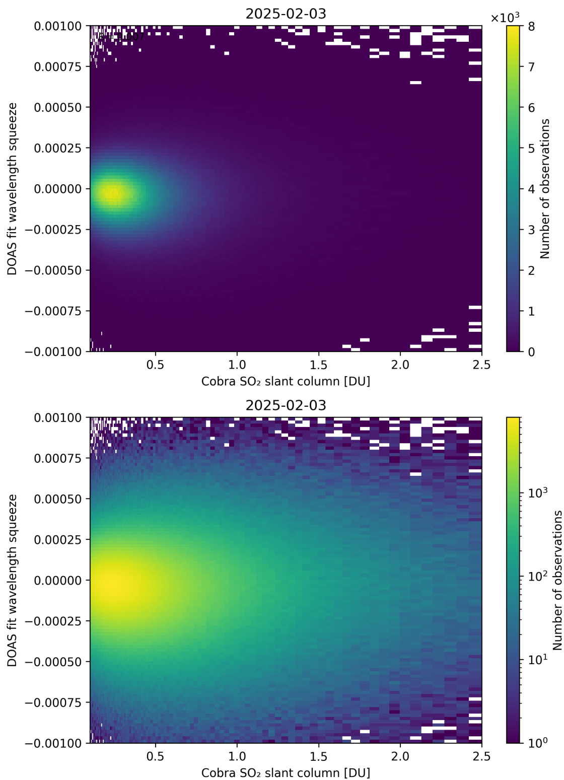
Figure 197: Scatter density plot of “Cobra SO 2 slant column” against “DOAS fit wavelength squeeze” for 2025-02-03 to 2025-02-04.
