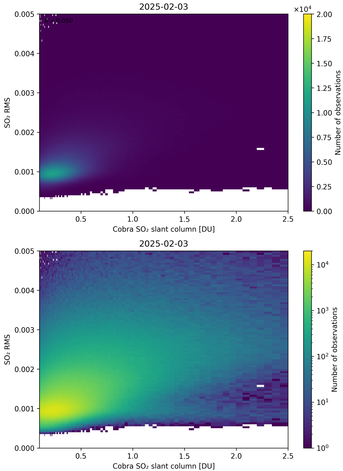
Figure 198: Scatter density plot of “Cobra SO 2 slant column” against “SO 2 RMS” for 2025-02-03 to 2025-02-04.
