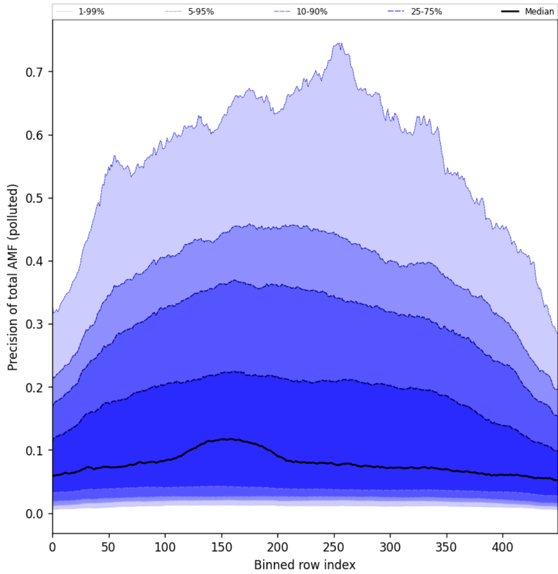
Figure 106: Along track statistics of “Precision of total AMF (polluted)” for 2025-02-03 to 2025-02-04
