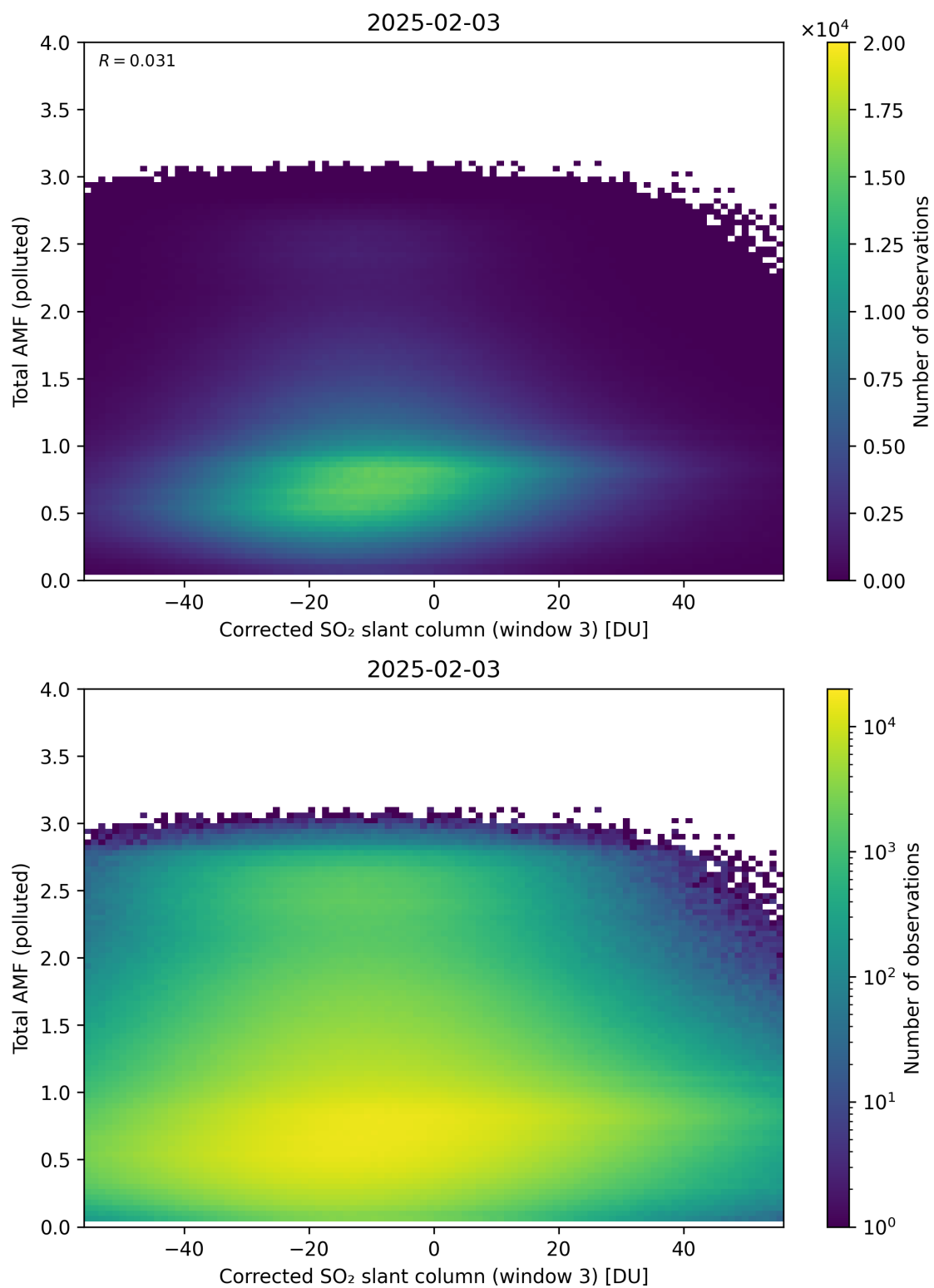
Figure 260: Scatter density plot of “Corrected SO 2 slant column (window 3)” against “Total AMF (polluted)” for 2025-02-03 to 2025-02-04.
