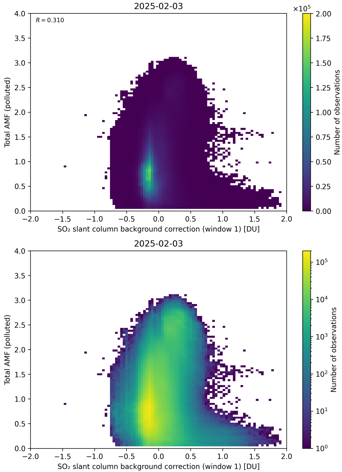
Figure 120: Scatter density plot of “SO 2 slant column background correction (window 1)” against “Total AMF (polluted)” for 2025-02-03 to 2025-02-04.
