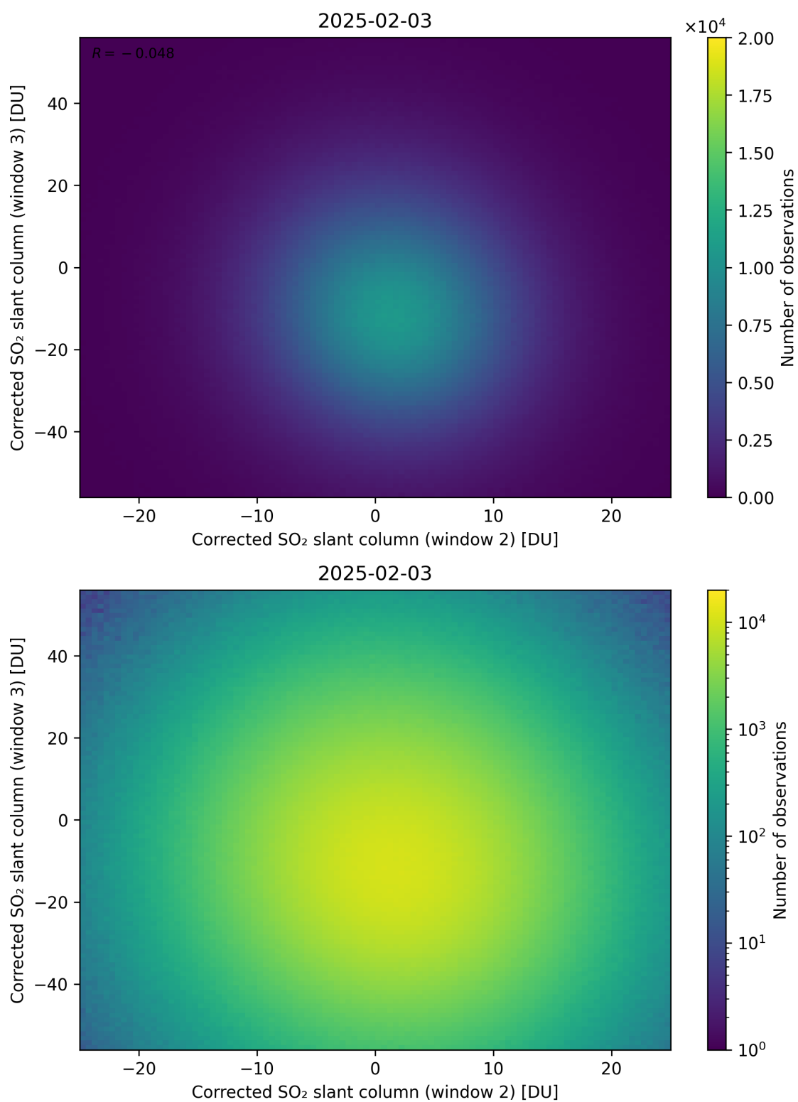
Figure 250: Scatter density plot of “Corrected SO 2 slant column (window 2)” against “Corrected SO 2 slant column (window 3)” for 2025-02-03 to 2025-02-04.
