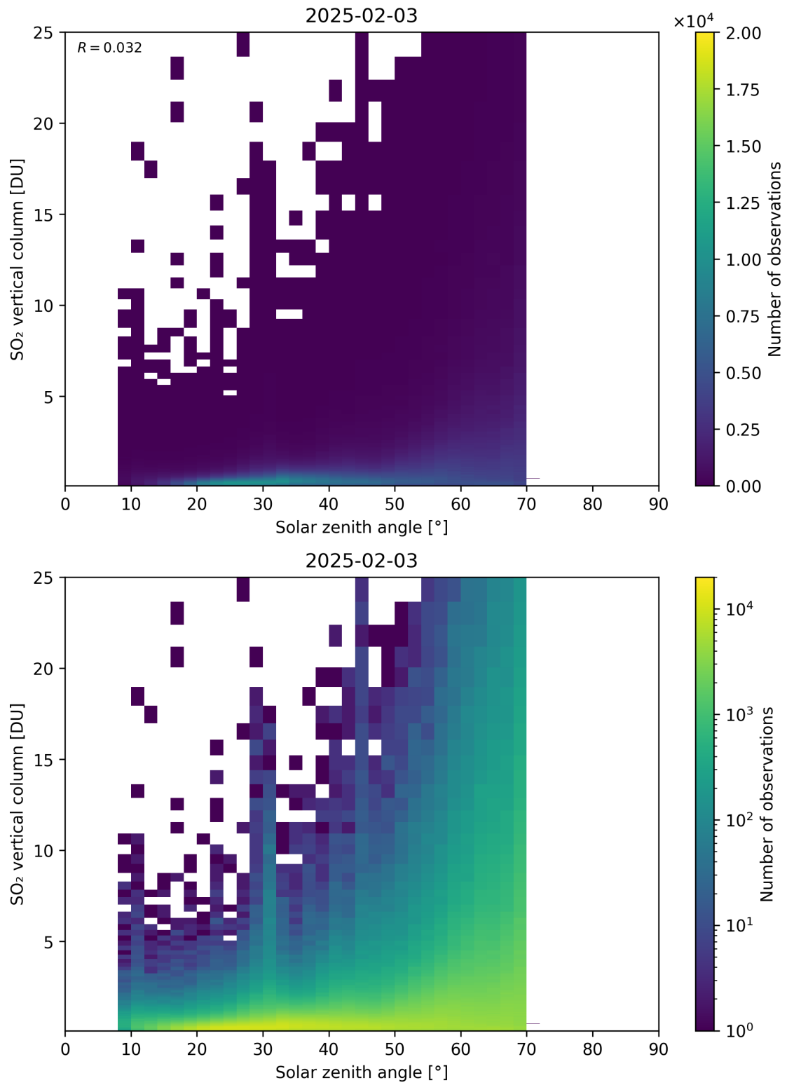
Figure 191: Scatter density plot of “Solar zenith angle” against “SO 2 vertical column” for 2025-02-03 to 2025-02-04.
