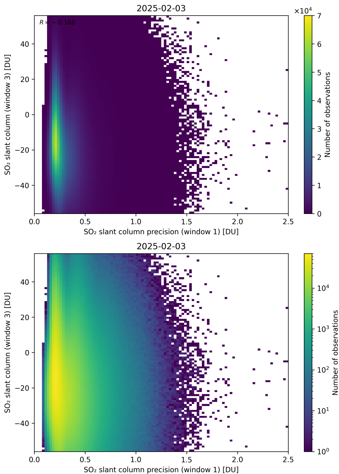
Figure 278: Scatter density plot of “SO 2 slant column precision (window 1)” against “SO 2 slant column (window 3)” for 2025-02-03 to 2025-02-04.
