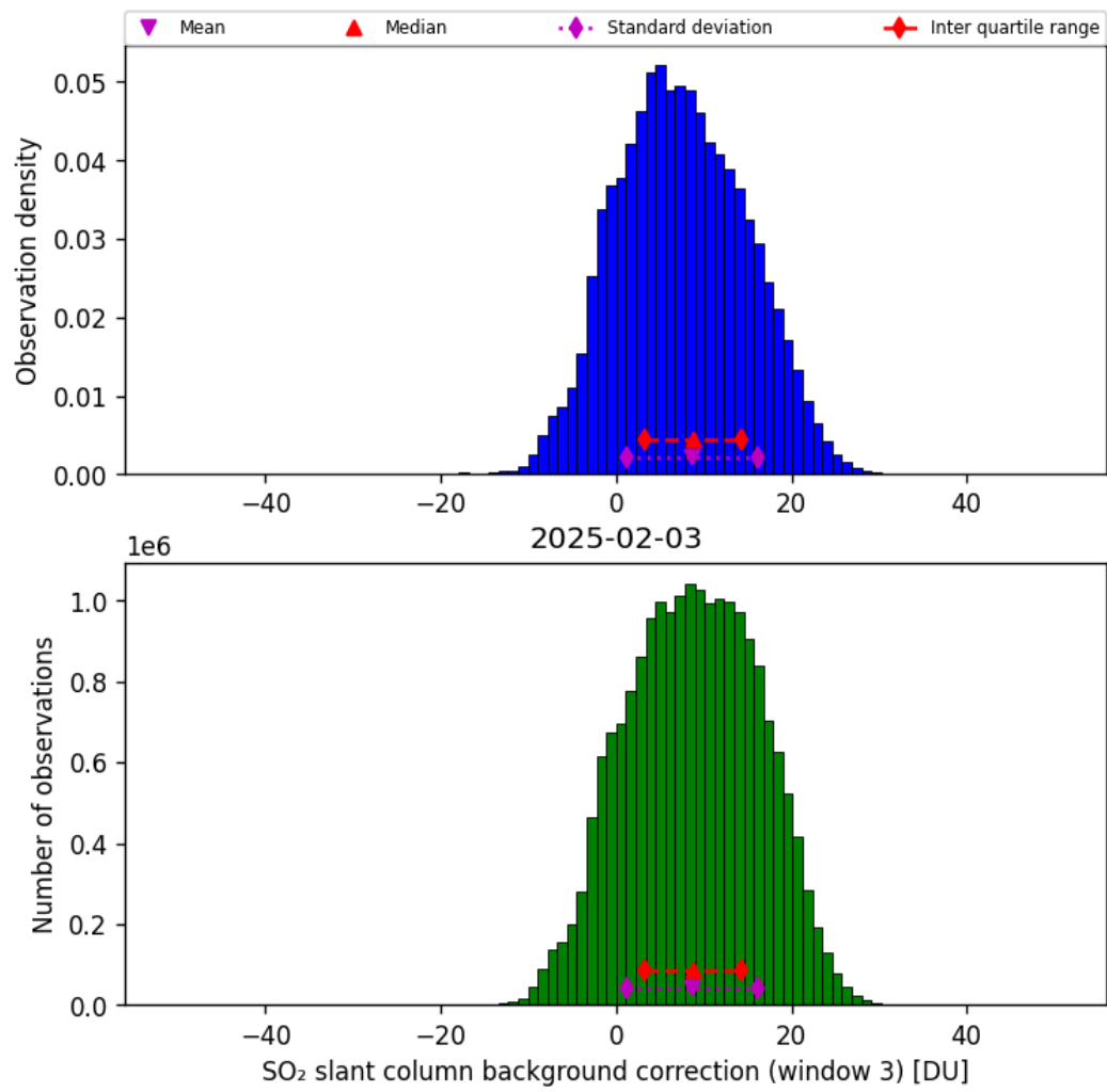
Figure 74: Histogram of “SO 2 slant column background correction (window 3)” for 2025-02-03 to 2025-02-04
