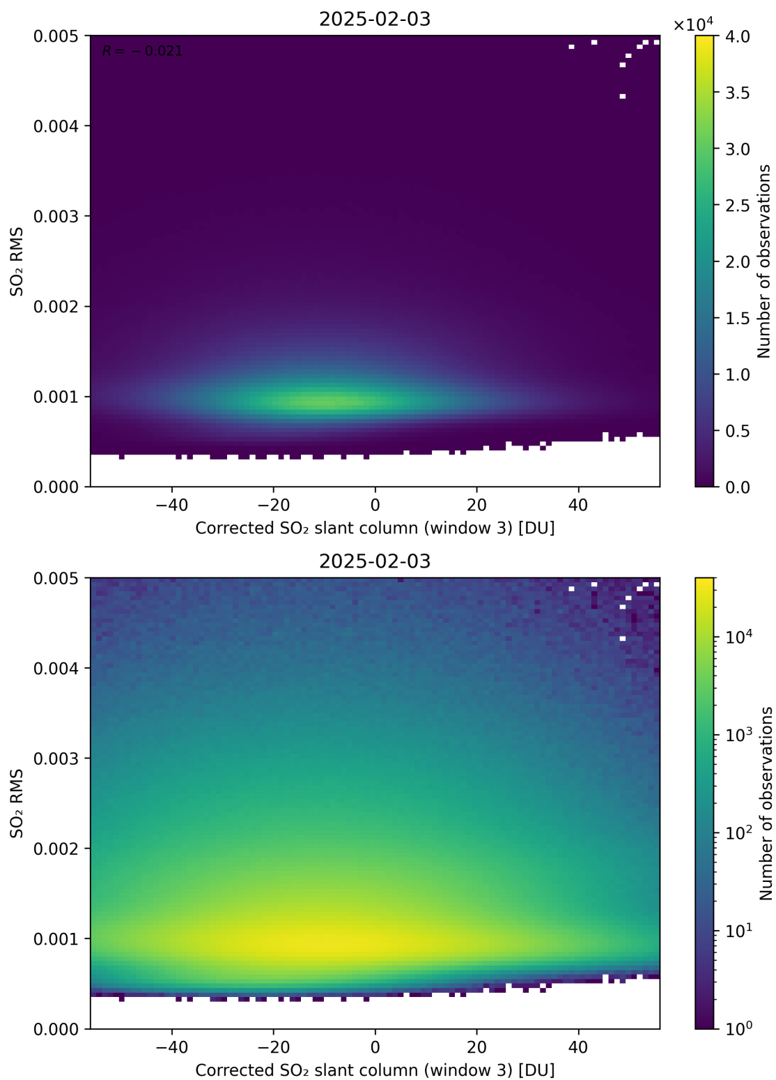
Figure 258: Scatter density plot of “Corrected SO 2 slant column (window 3)” against “SO 2 RMS” for 2025-02-03 to 2025-02-04.
