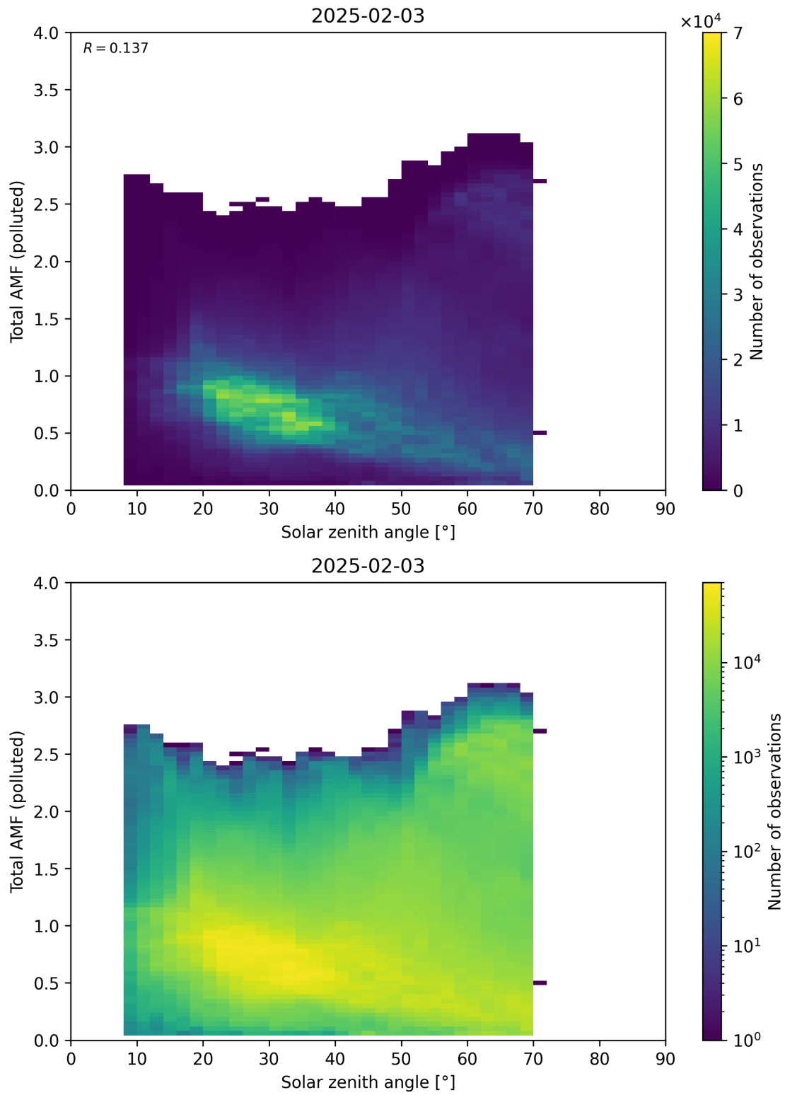
Figure 189: Scatter density plot of “Solar zenith angle” against “Total AMF (polluted)” for 2025-02-03 to 2025-02-04.
