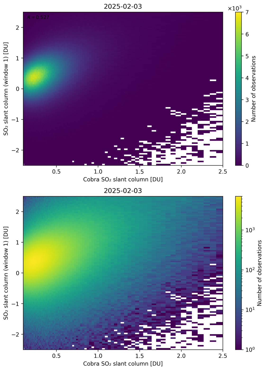
Figure 219: Scatter density plot of “Cobra SO 2 slant column” against “SO 2 slant column (window 1)” for 2025-02-03 to 2025-02-04.
