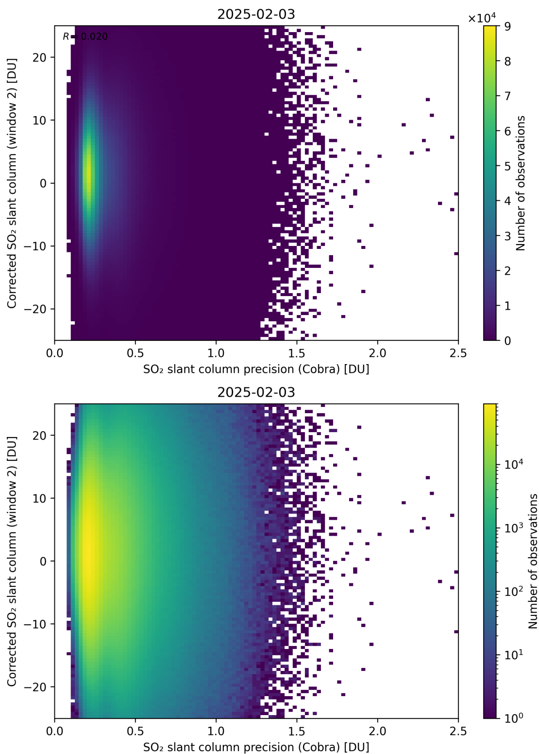
Figure 206: Scatter density plot of “SO 2 slant column precision (Cobra)” against “Corrected SO 2 slant column (window 2)” for 2025-02-03 to 2025-02-04.
