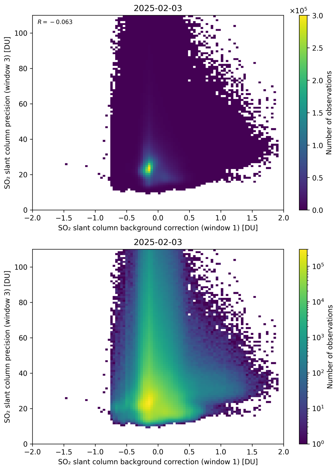
Figure 119: Scatter density plot of “SO 2 slant column background correction (window 1)” against “SO 2 slant column precision (window 3)” for 2025-02-03 to 2025-02-04.
