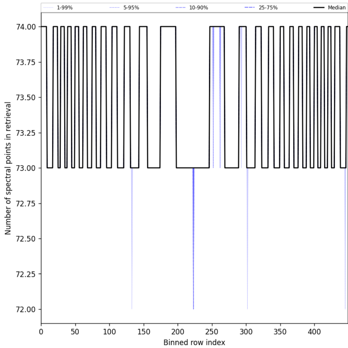
Figure 108: Along track statistics of “Number of spectral points in retrieval” for 2025-02-03 to 2025-02-04
