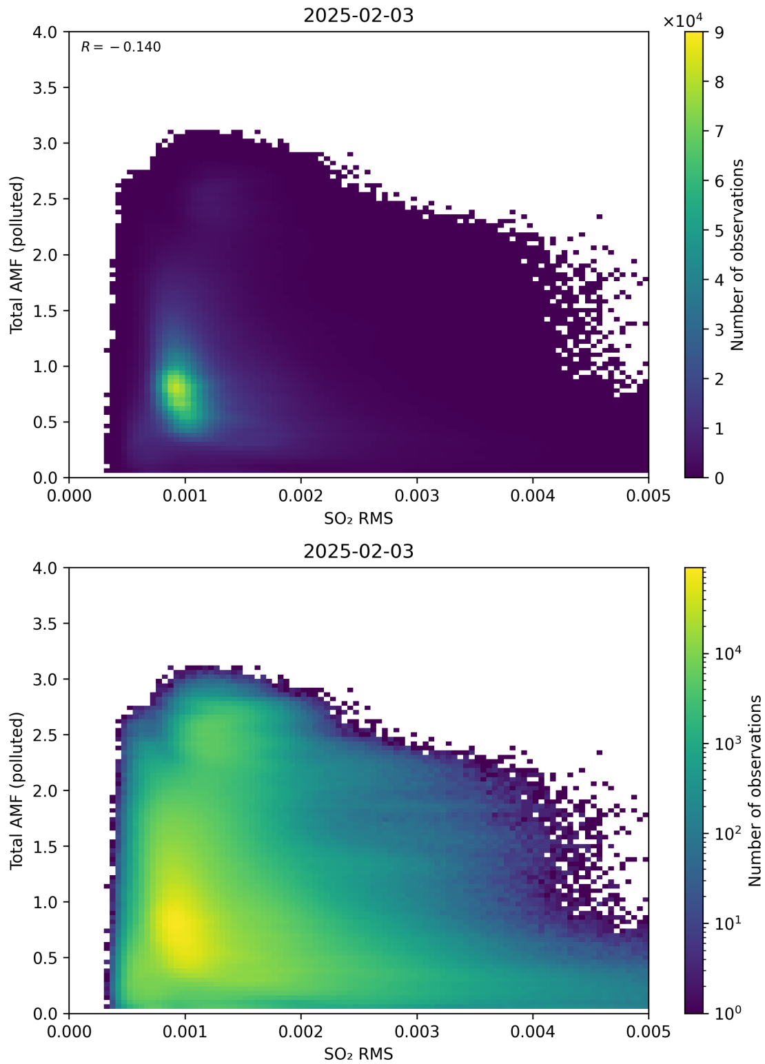
Figure 148: Scatter density plot of “SO 2 RMS” against “Total AMF (polluted)” for 2025-02-03 to 2025-02-04.
