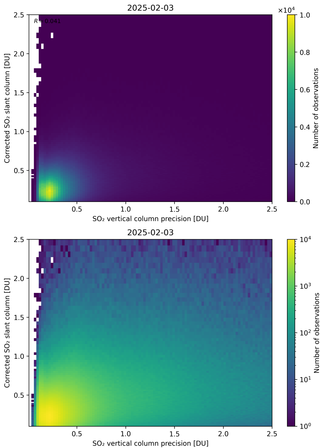
Figure 338: Scatter density plot of “SO 2 vertical column precision” against “Corrected SO 2 slant column” for 2025-02-03 to 2025-02-04.
