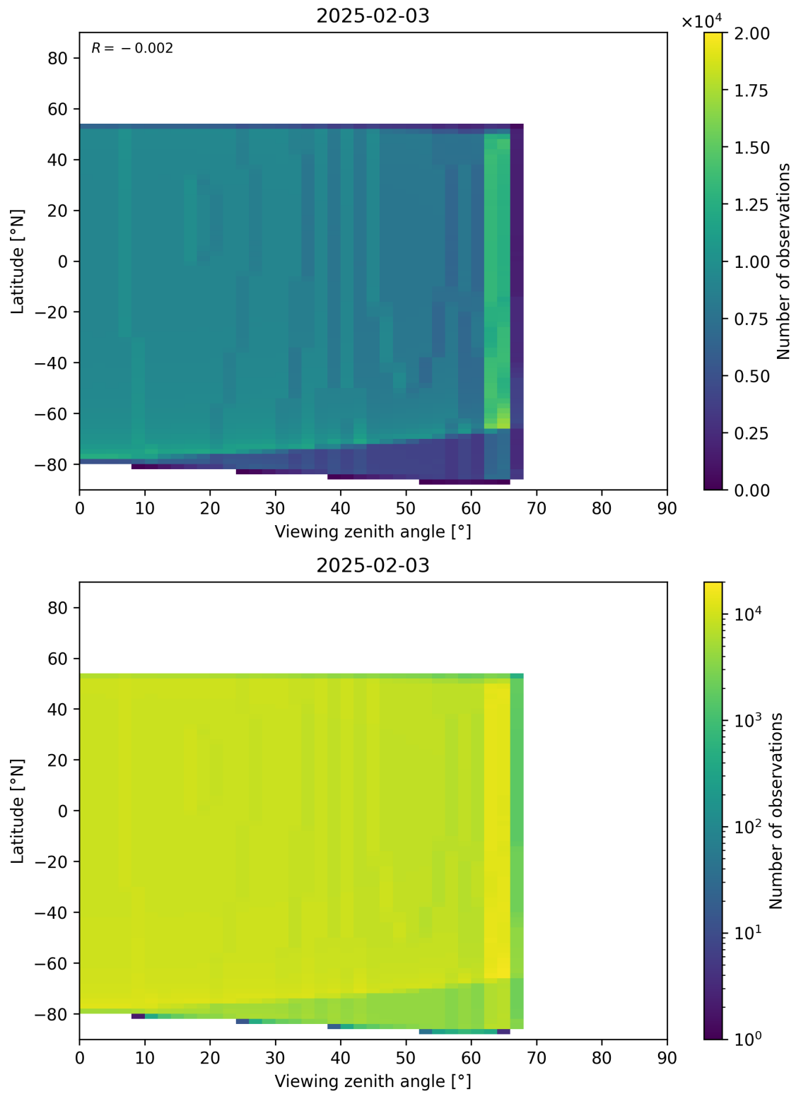
Figure 368: Scatter density plot of “Viewing zenith angle” against “Latitude” for 2025-02-03 to 2025-02-04.
