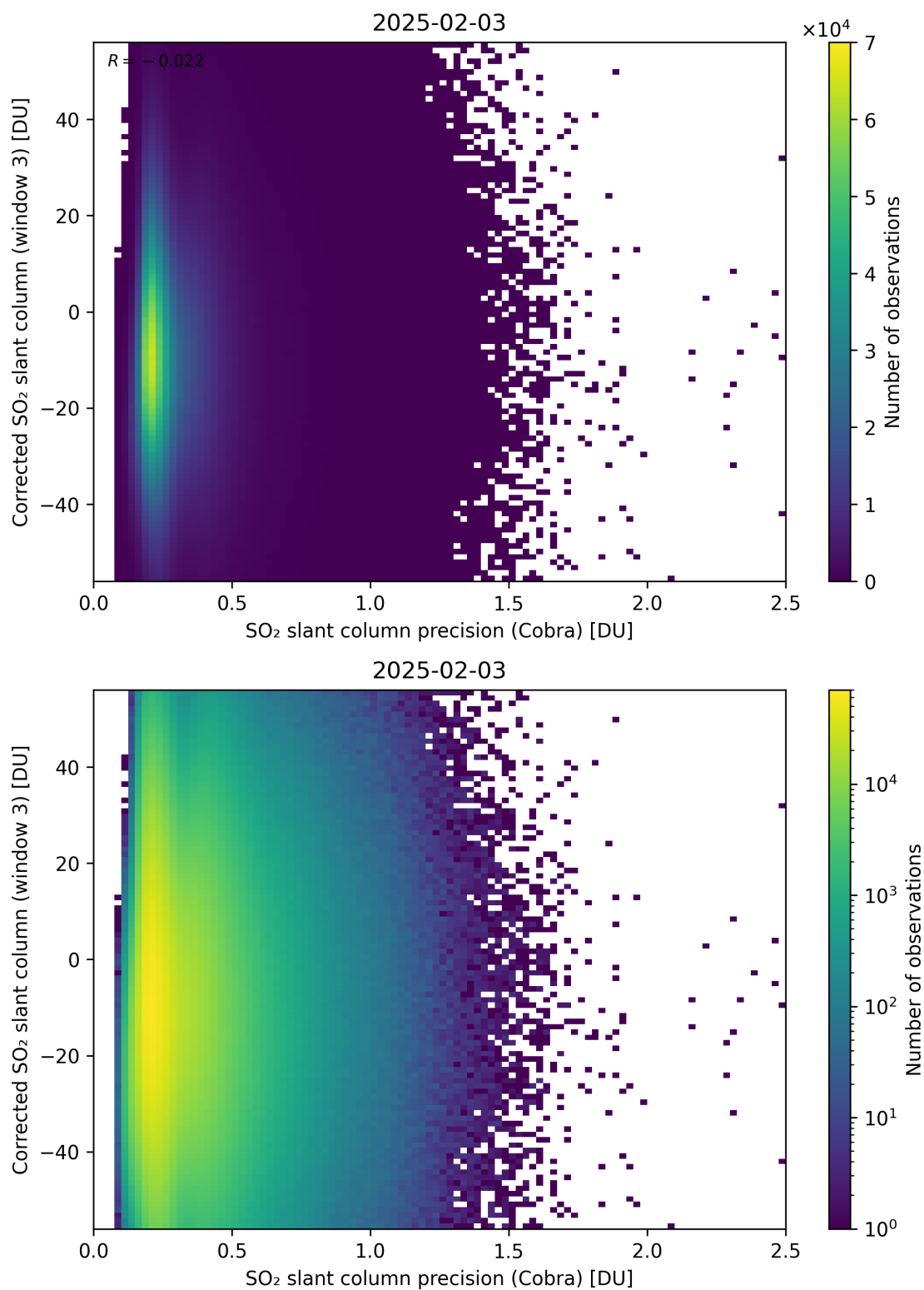
Figure 207: Scatter density plot of “SO 2 slant column precision (Cobra)” against “Corrected SO 2 slant column (window 3)” for 2025-02-03 to 2025-02-04.
