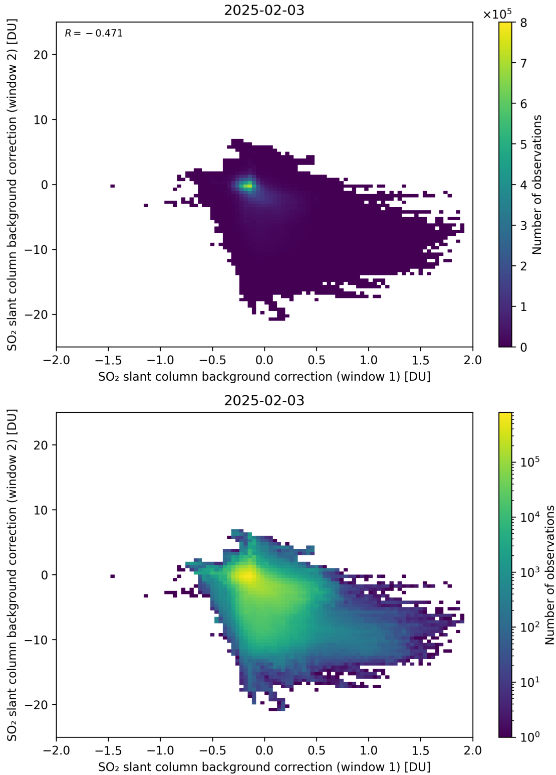
Figure 109: Scatter density plot of “SO 2 slant column background correction (window 1)” against “SO 2 slant column background correction (window 2)” for 2025-02-03 to 2025-02-04.
