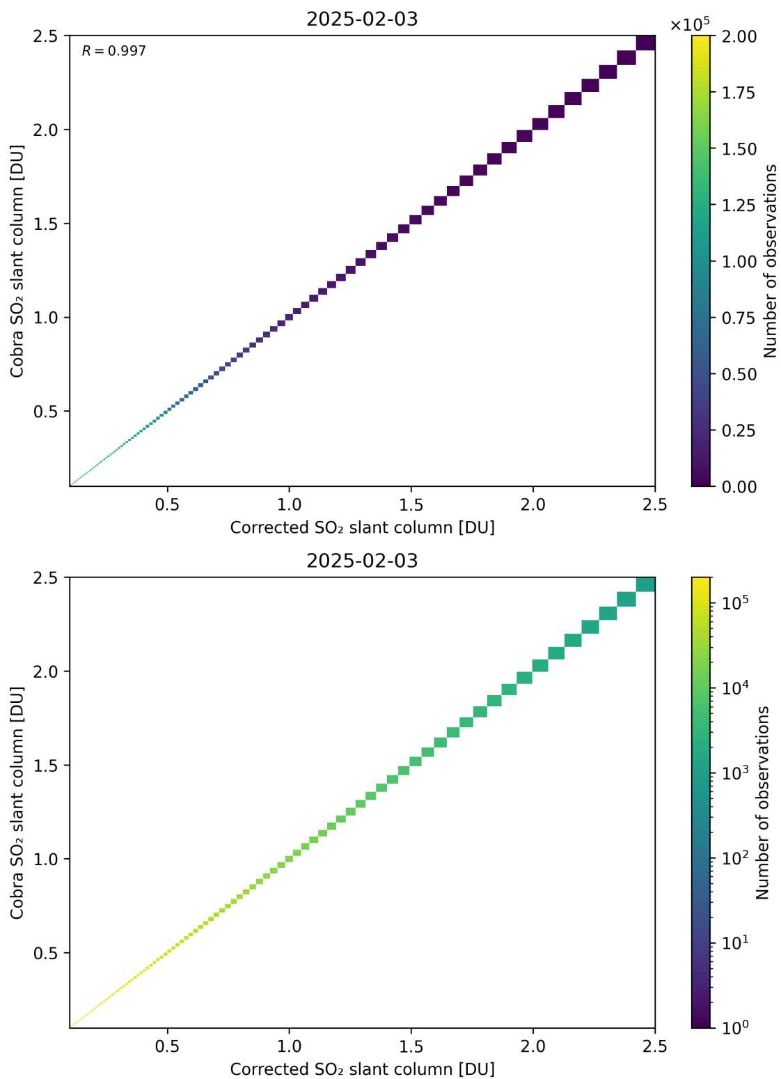
Figure 233: Scatter density plot of “Corrected SO 2 slant column” against “Cobra SO 2 slant column” for 2025-02-03 to 2025-02-04.
