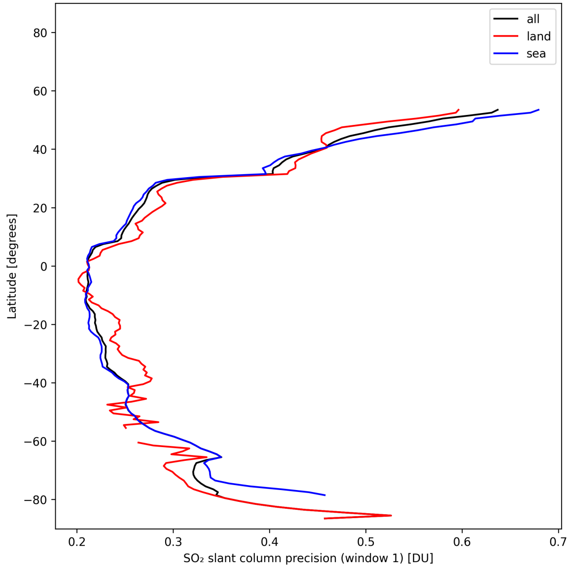
Figure 38: Zonal average of “SO 2 slant column precision (window 1)” for 2025-02-03 to 2025-02-04.
