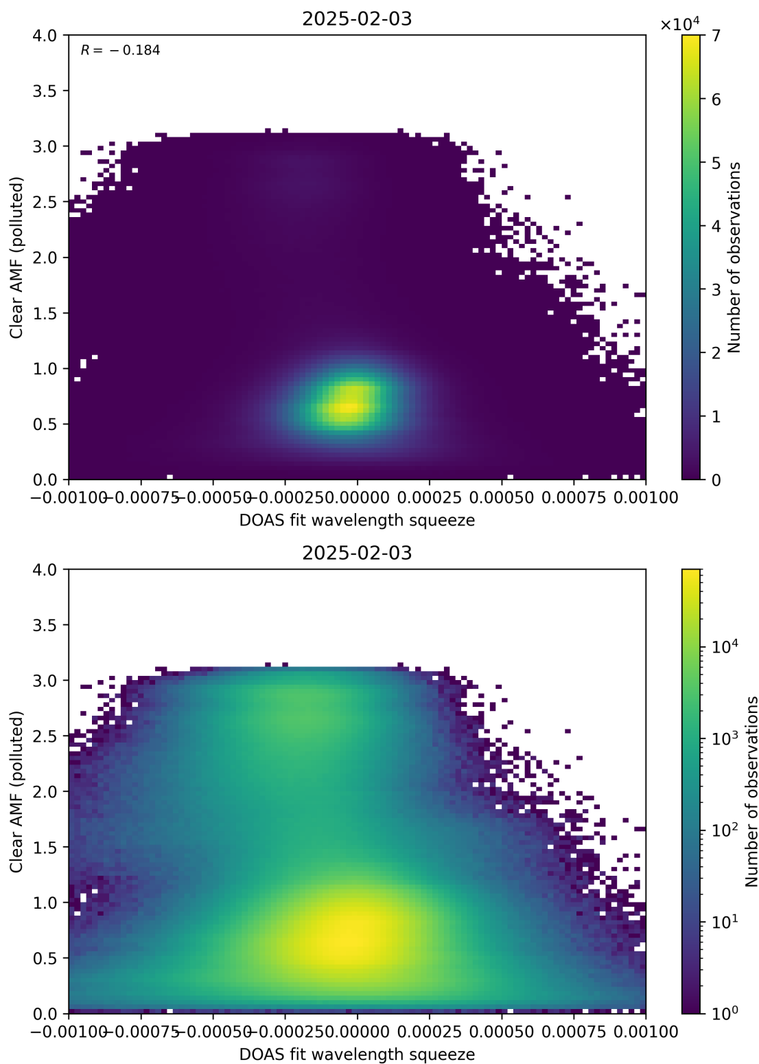
Figure 144: Scatter density plot of “DOAS fit wavelength squeeze” against “Clear AMF (polluted)” for 2025-02-03 to 2025-02-04.
