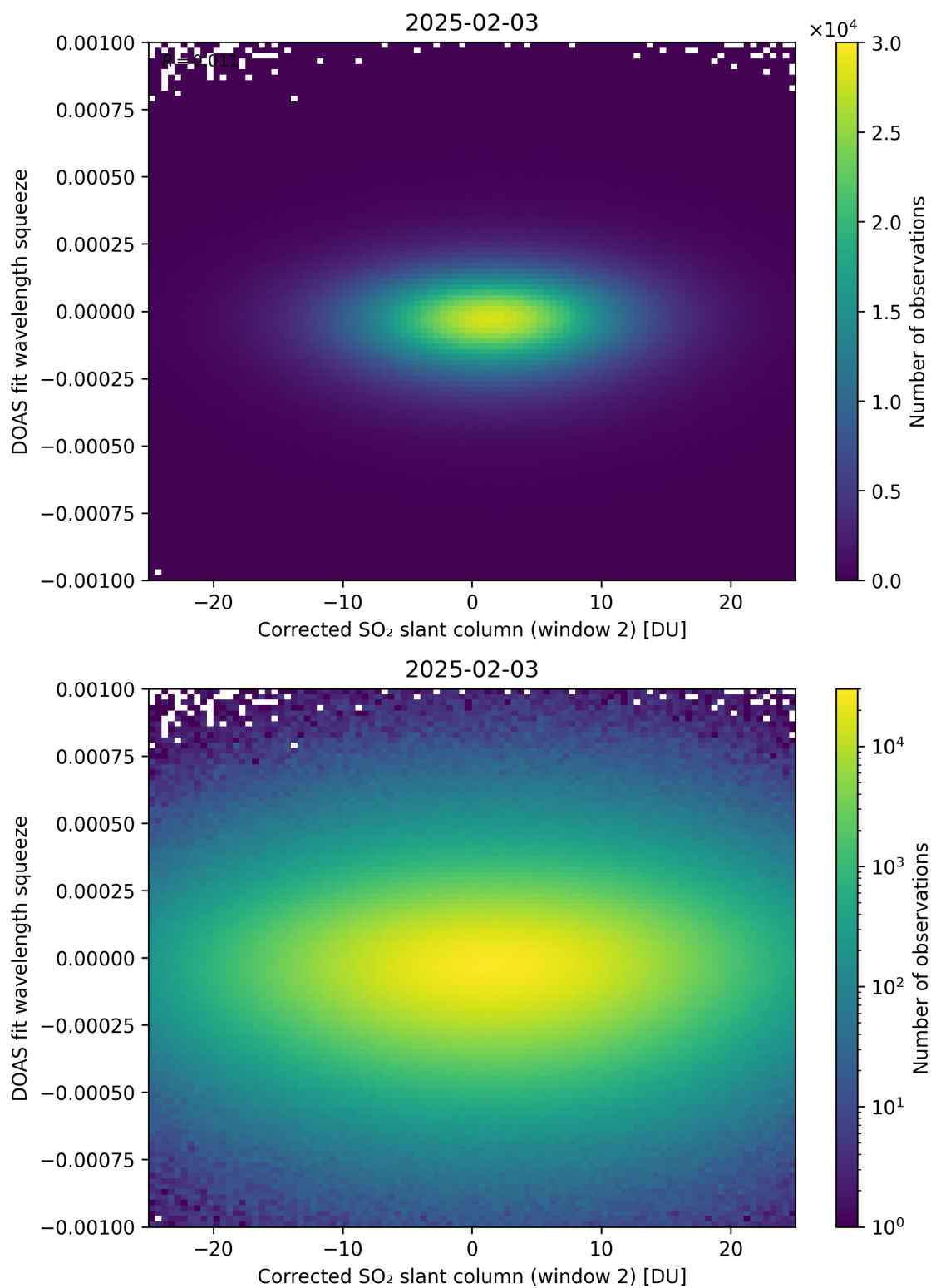
Figure 247: Scatter density plot of “Corrected SO 2 slant column (window 2)” against “DOAS fit wavelength squeeze” for 2025-02-03 to 2025-02-04.
