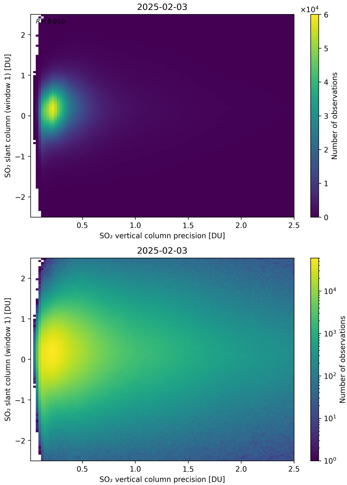
Figure 341: Scatter density plot of “SO 2 vertical column precision” against “SO 2 slant column (window 1)” for 2025-02-03 to 2025-02-04.
