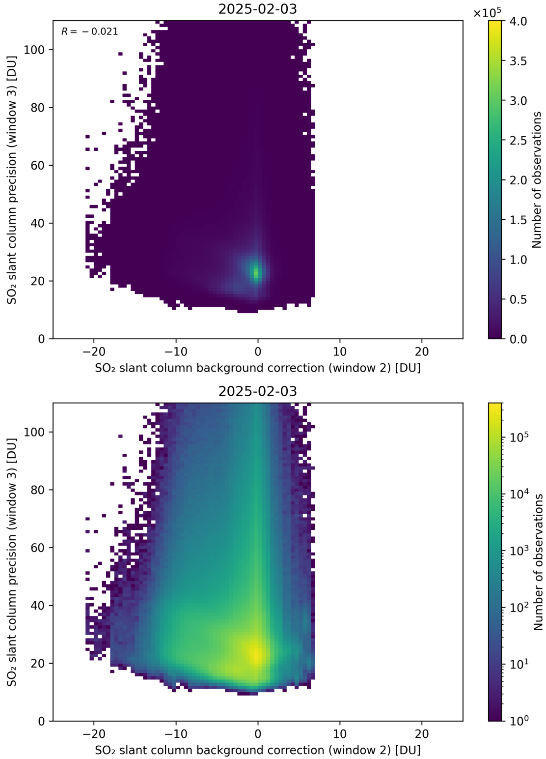
Figure 129: Scatter density plot of “SO 2 slant column background correction (window 2)” against “SO 2 slant column precision (window 3)” for 2025-02-03 to 2025-02-04.
