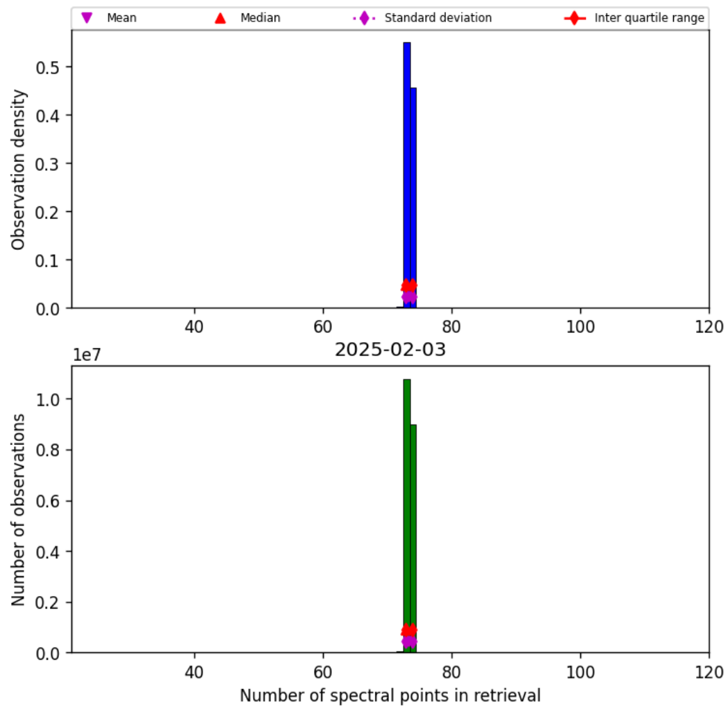
Figure 82: Histogram of “Number of spectral points in retrieval” for 2025-02-03 to 2025-02-04
