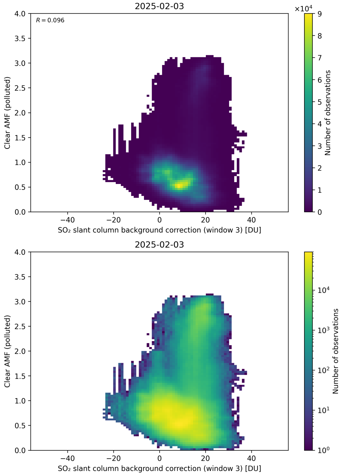
Figure 135: Scatter density plot of “SO 2 slant column background correction (window 3)” against “Clear AMF (polluted)” for 2025-02-03 to 2025-02-04.
