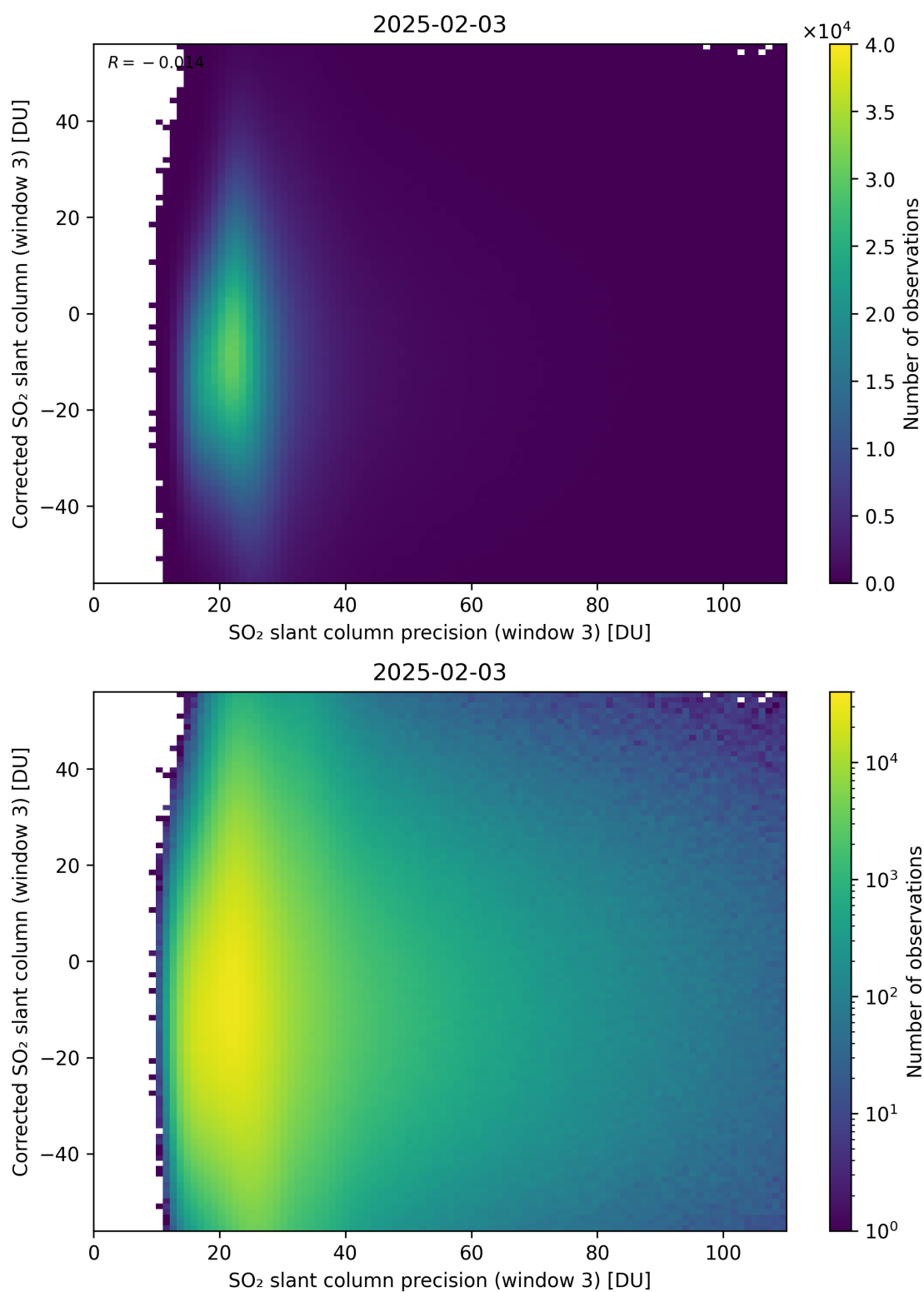
Figure 312: Scatter density plot of “SO 2 slant column precision (window 3)” against “Corrected SO 2 slant column (window 3)” for 2025-02-03 to 2025-02-04.
