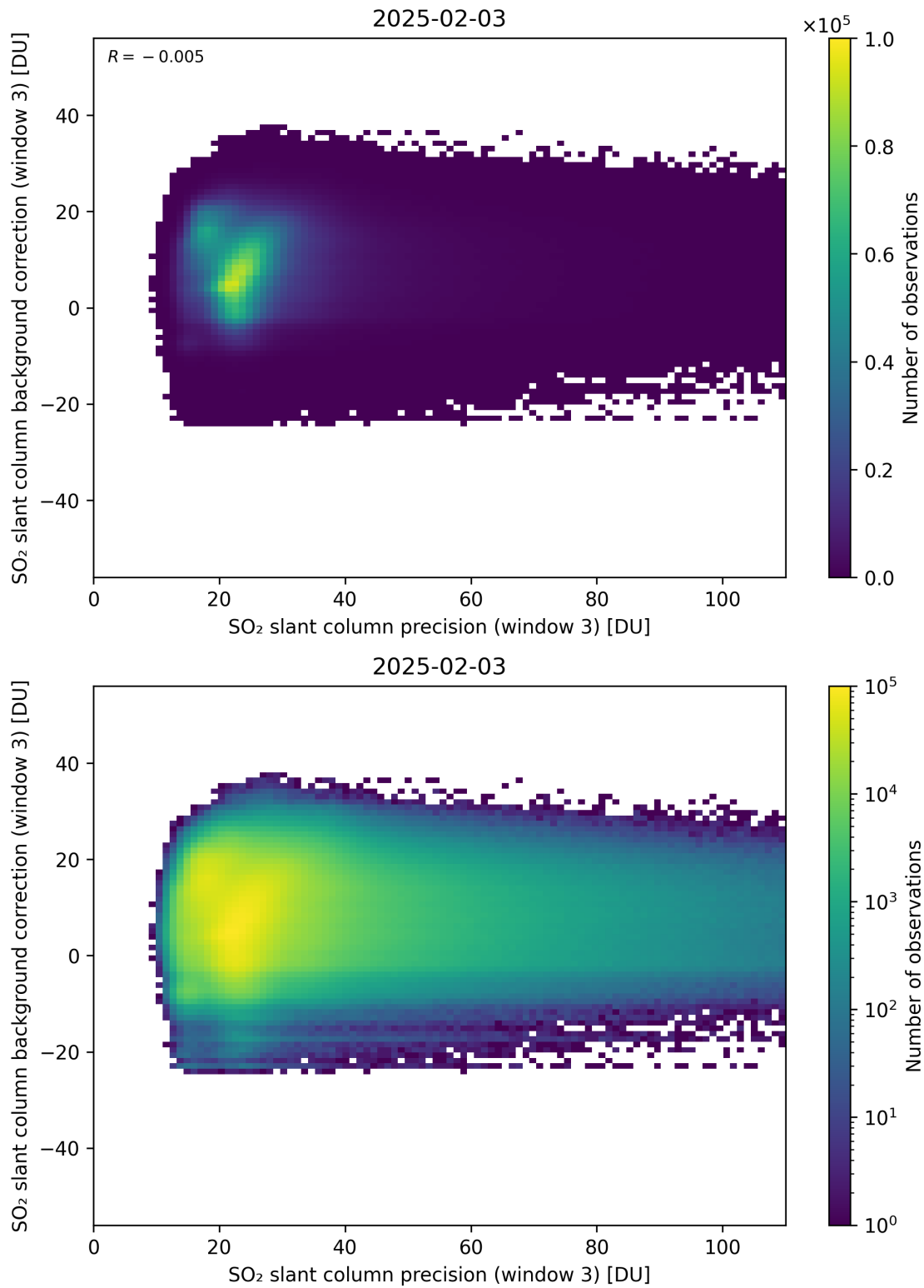
Figure 307: Scatter density plot of “SO 2 slant column precision (window 3)” against “SO 2 slant column background correction (window 3)” for 2025-02-03 to 2025-02-04.
