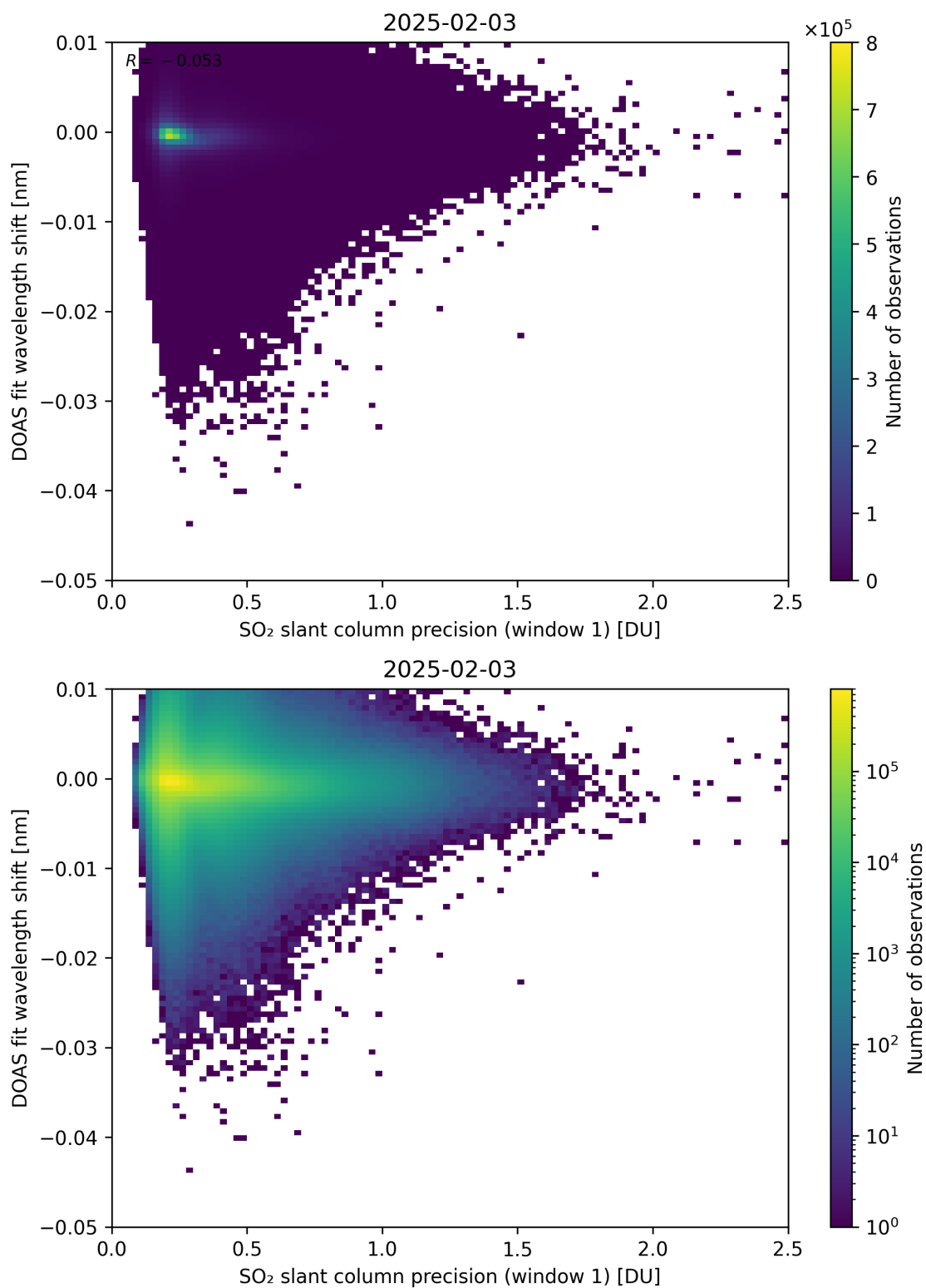
Figure 271: Scatter density plot of “SO 2 slant column precision (window 1)” against “DOAS fit wavelength shift” for 2025-02-03 to 2025-02-04.
