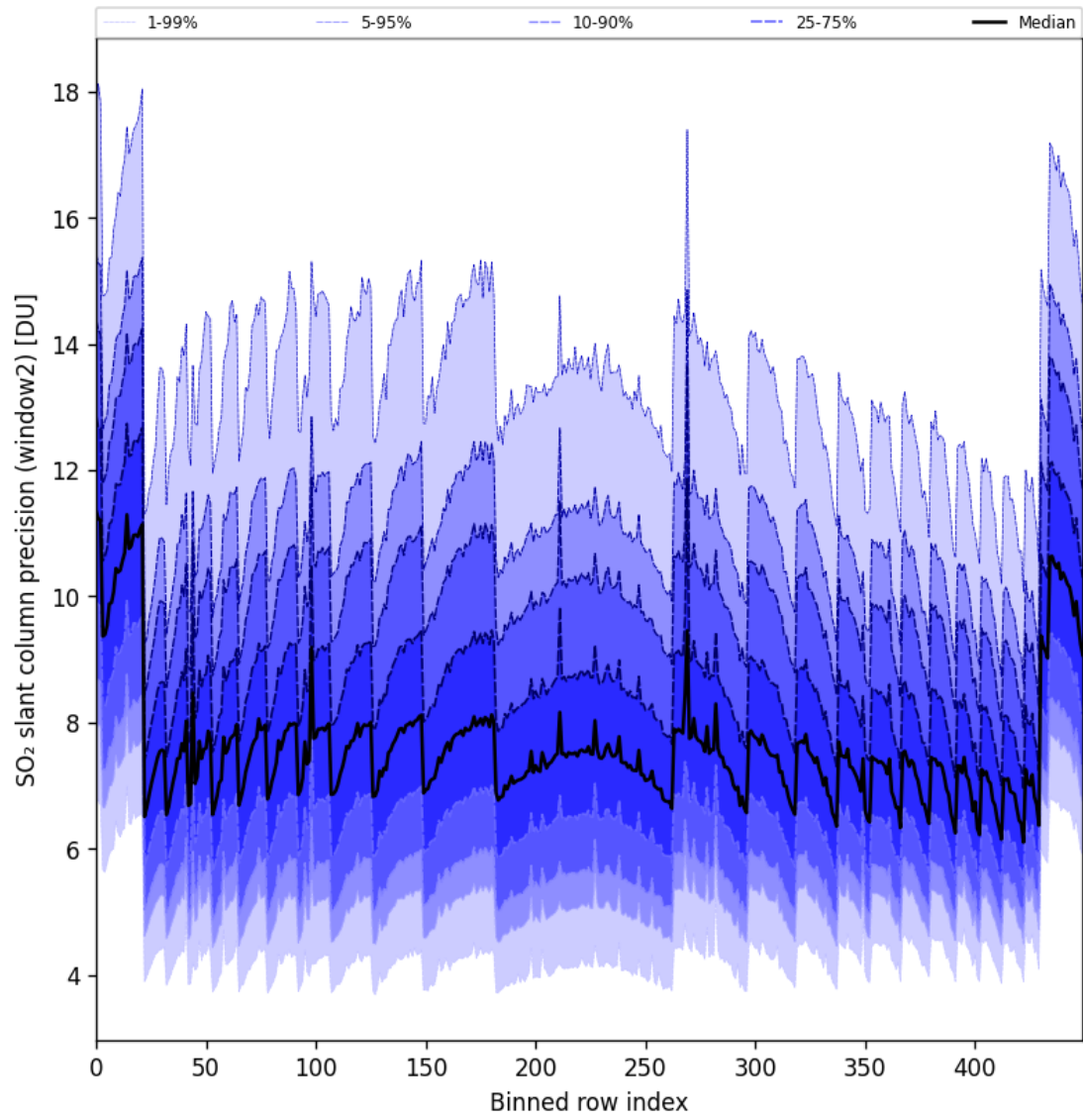
Figure 94: Along track statistics of “SO 2 slant column precision (window2)” for 2025-02-03 to 2025-02-04
