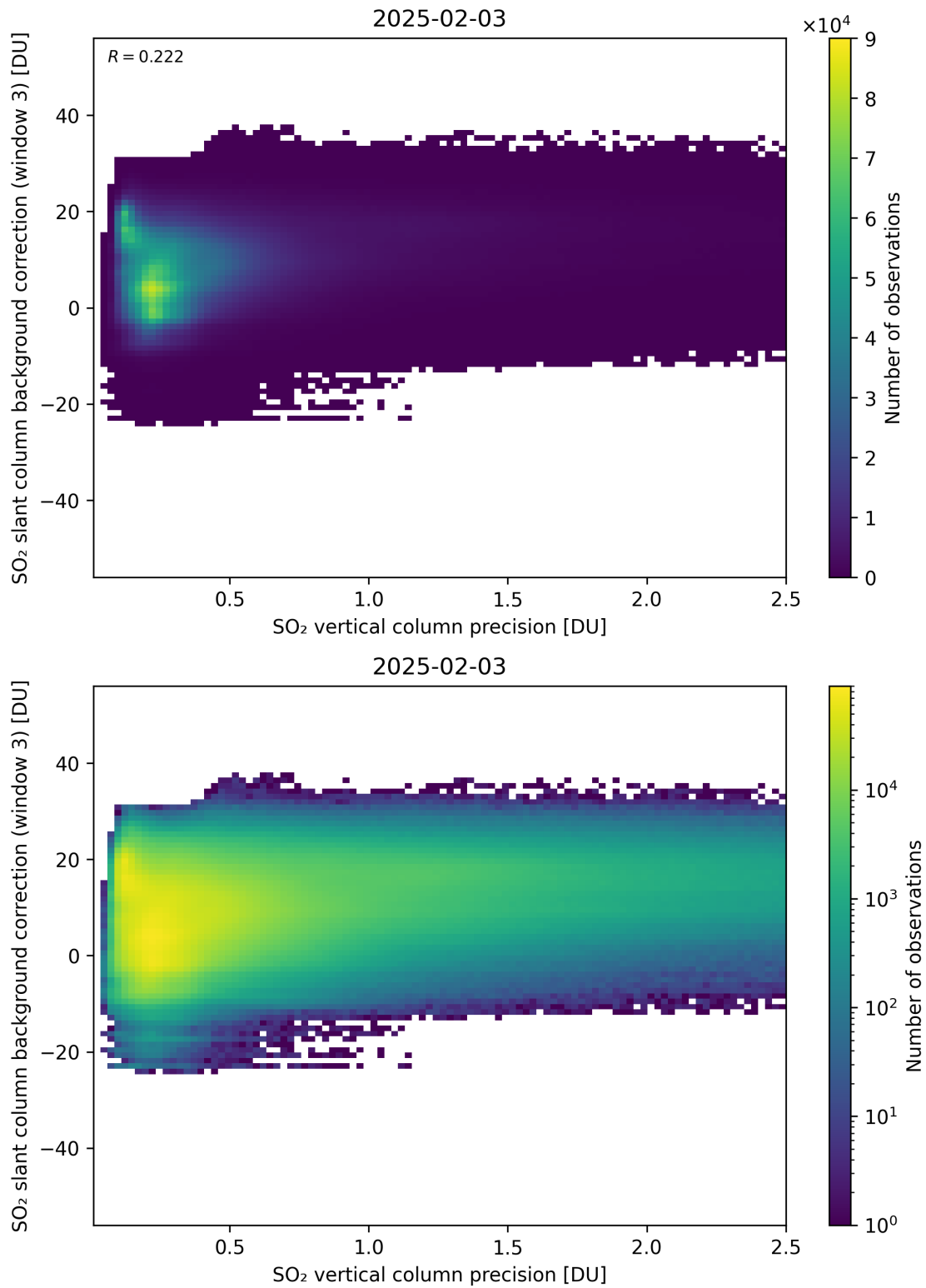
Figure 331: Scatter density plot of “SO 2 vertical column precision” against “SO 2 slant column background correction (window 3)” for 2025-02-03 to 2025-02-04.
