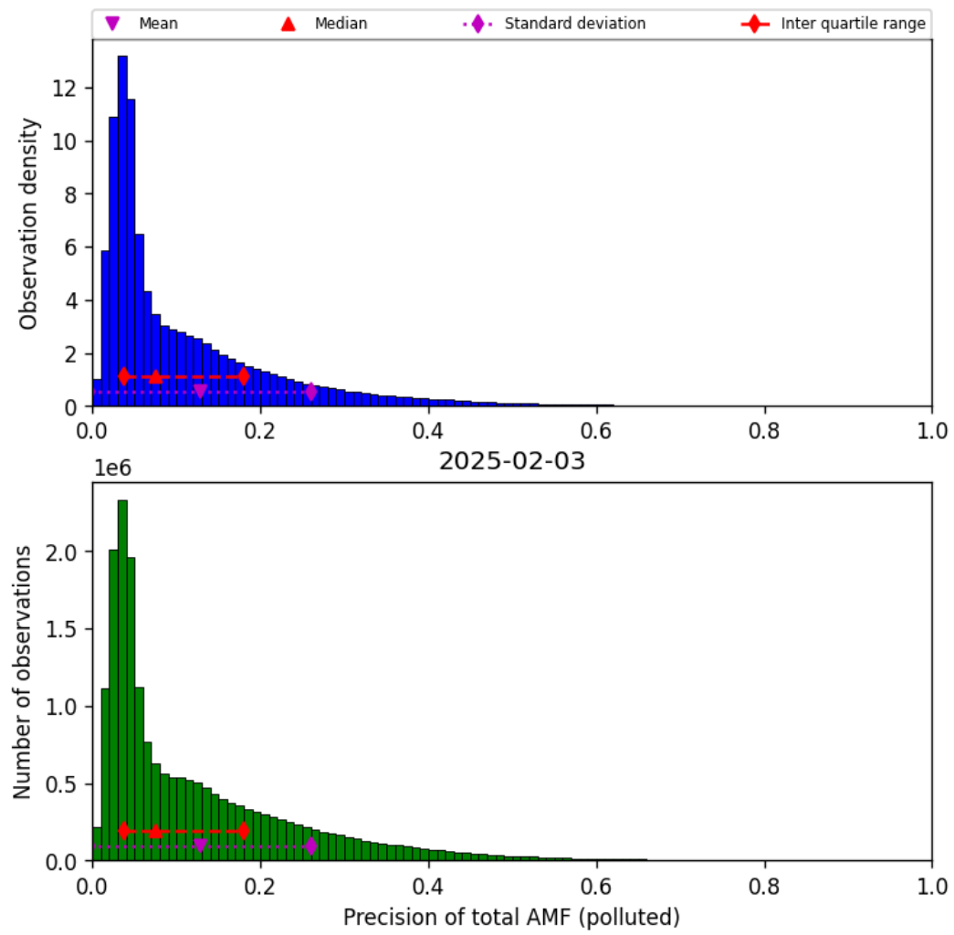
Figure 80: Histogram of “Precision of total AMF (polluted)” for 2025-02-03 to 2025-02-04
