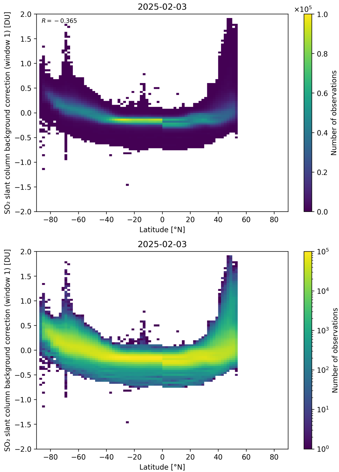
Figure 150: Scatter density plot of “Latitude” against “SO 2 slant column background correction (window 1)” for 2025-02-03 to 2025-02-04.
