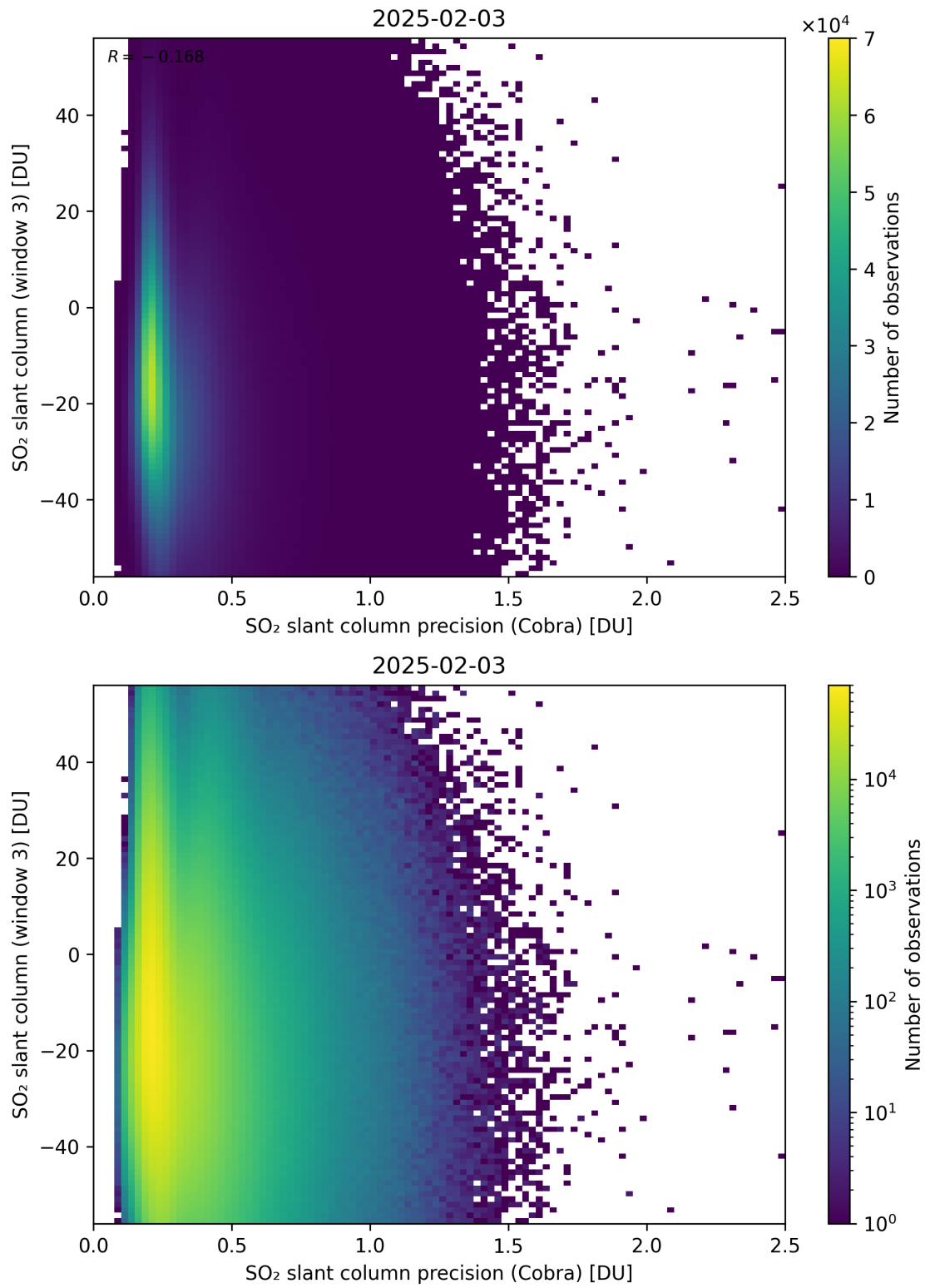
Figure 211: Scatter density plot of “SO 2 slant column precision (Cobra)” against “SO 2 slant column (window 3)” for 2025-02-03 to 2025-02-04.
