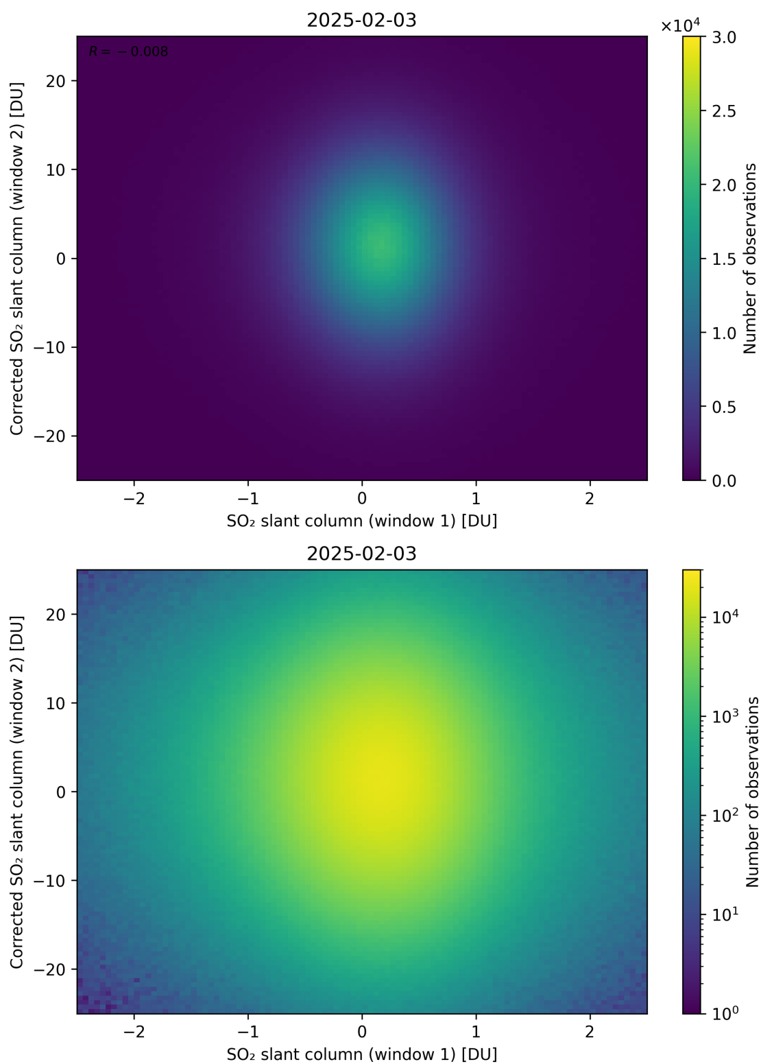
Figure 283: Scatter density plot of “SO 2 slant column (window 1)” against “Corrected SO 2 slant column (window 2)” for 2025-02-03 to 2025-02-04.
