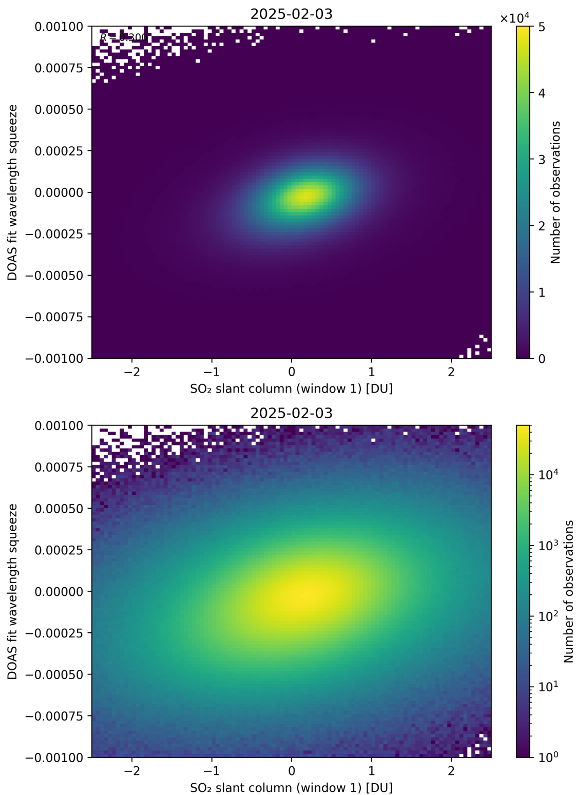
Figure 266: Scatter density plot of “SO 2 slant column (window 1)” against “DOAS fit wavelength squeeze” for 2025-02-03 to 2025-02-04.
