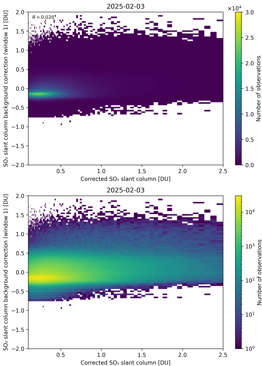
Figure 226: Scatter density plot of “Corrected SO 2 slant column” against “SO 2 slant column background correction (window 1)” for 2025-02-03 to 2025-02-04.
