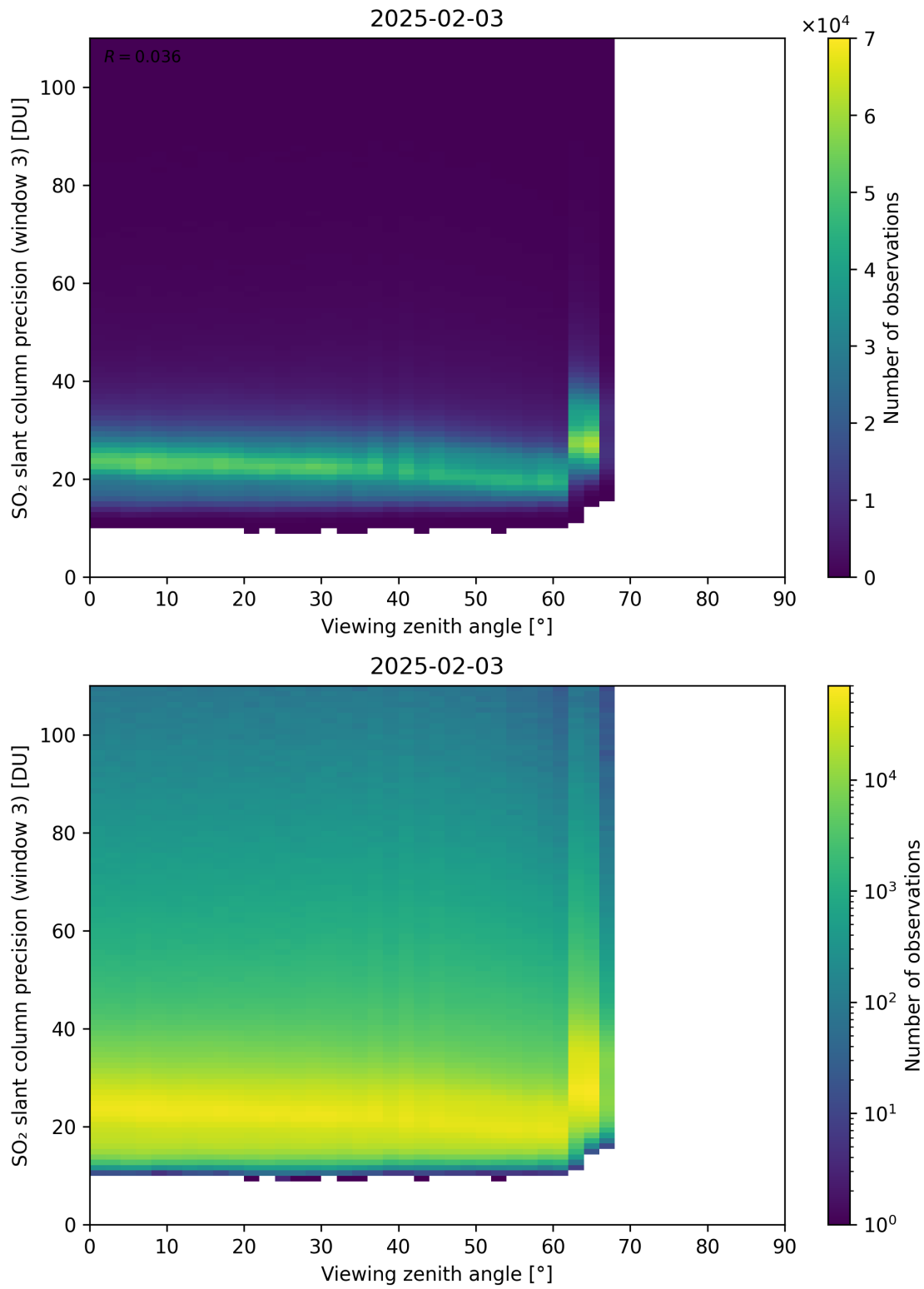
Figure 380: Scatter density plot of “Viewing zenith angle” against “SO 2 slant column precision (window 3)” for 2025-02-03 to 2025-02-04.
