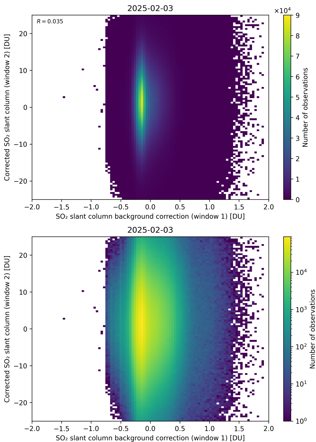
Figure 115: Scatter density plot of “SO 2 slant column background correction (window 1)” against “Corrected SO 2 slant column (window 2)” for 2025-02-03 to 2025-02-04.
