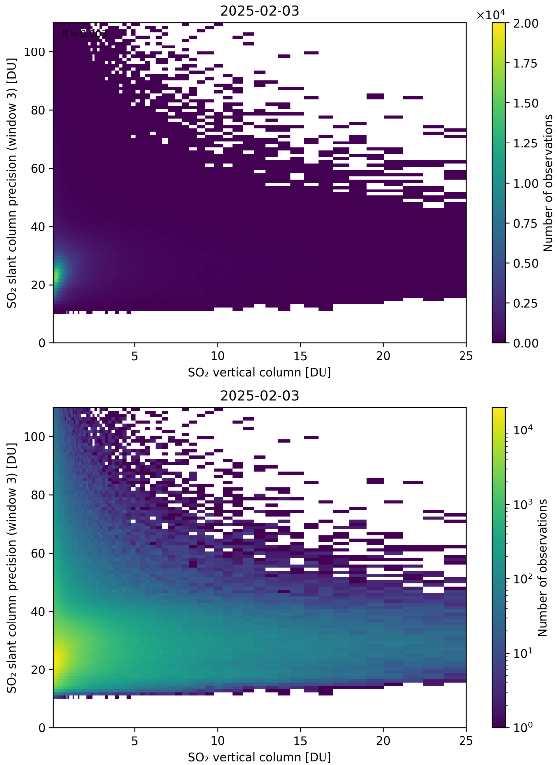
Figure 358: Scatter density plot of “SO 2 vertical column” against “SO 2 slant column precision (window 3)” for 2025-02-03 to 2025-02-04.
