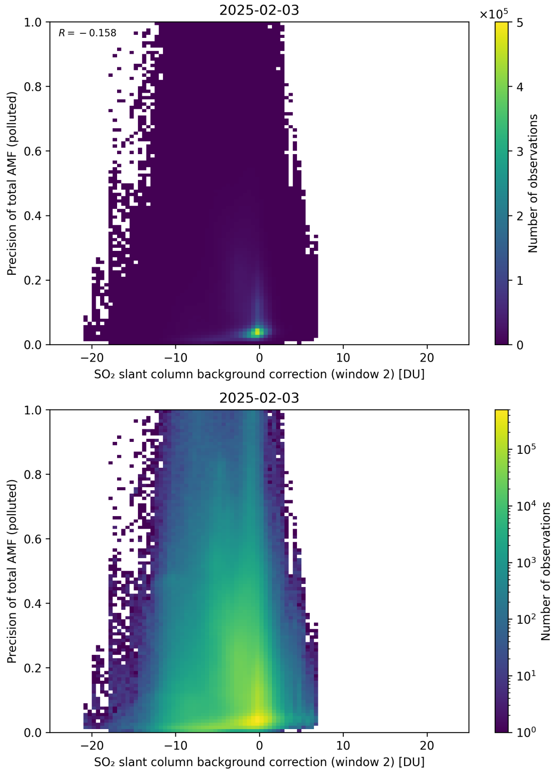
Figure 131: Scatter density plot of “SO 2 slant column background correction (window 2)” against “Precision of total AMF (polluted)” for 2025-02-03 to 2025-02-04.
