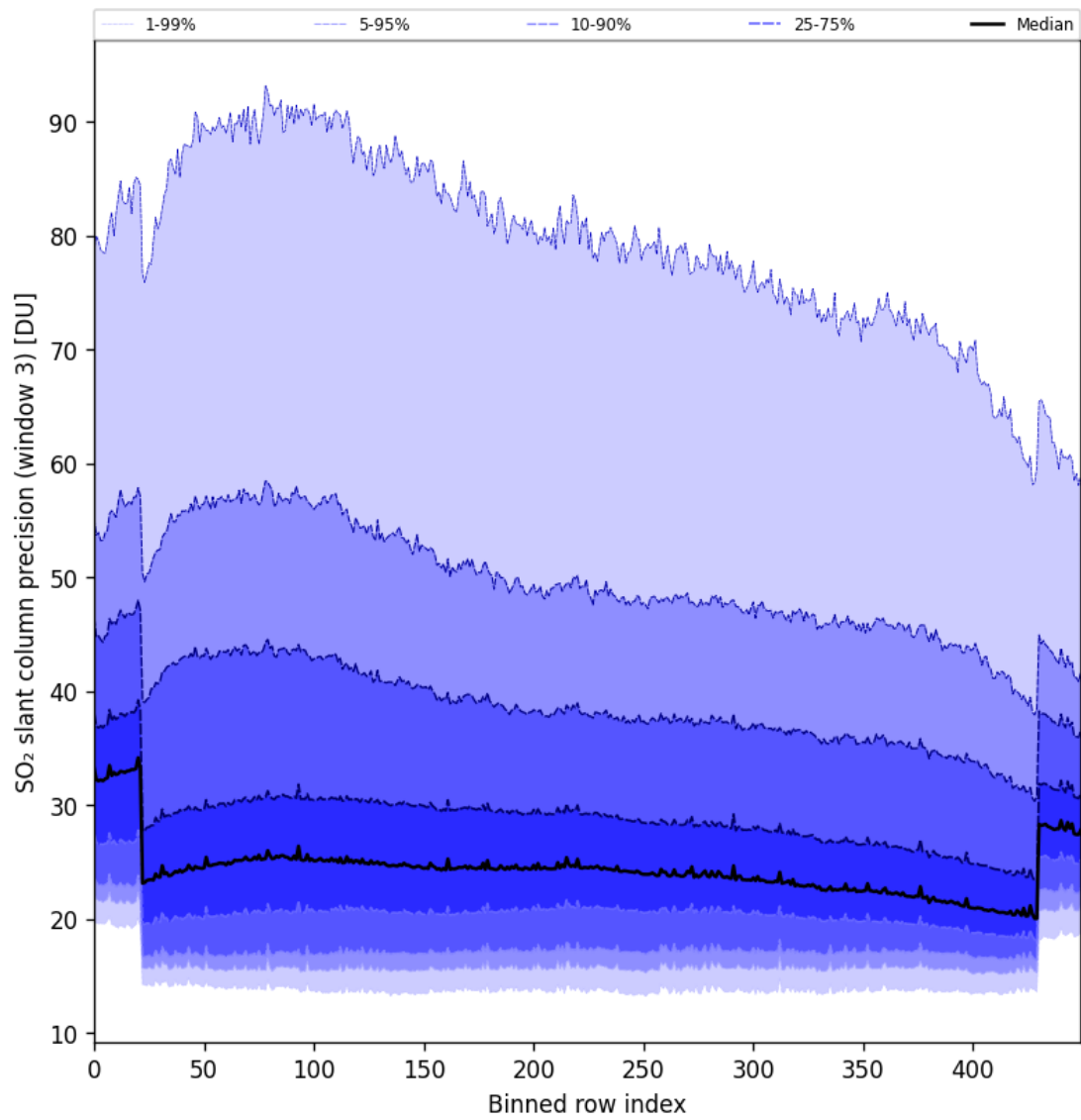
Figure 98: Along track statistics of “SO 2 slant column precision (window 3)” for 2025-02-03 to 2025-02-04
