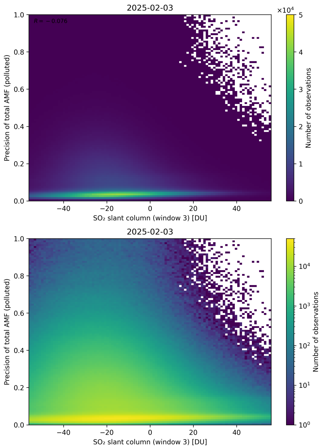
Figure 319: Scatter density plot of “SO 2 slant column (window 3)” against “Precision of total AMF (polluted)” for 2025-02-03 to 2025-02-04.
