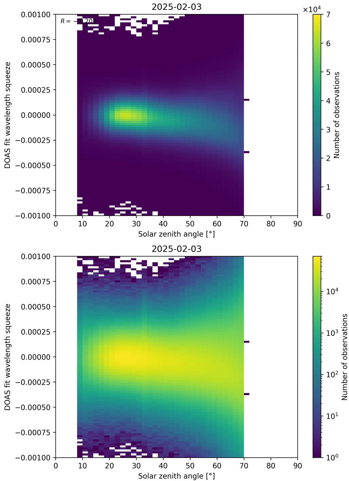
Figure 175: Scatter density plot of “Solar zenith angle” against “DOAS fit wavelength squeeze” for 2025-02-03 to 2025-02-04.
