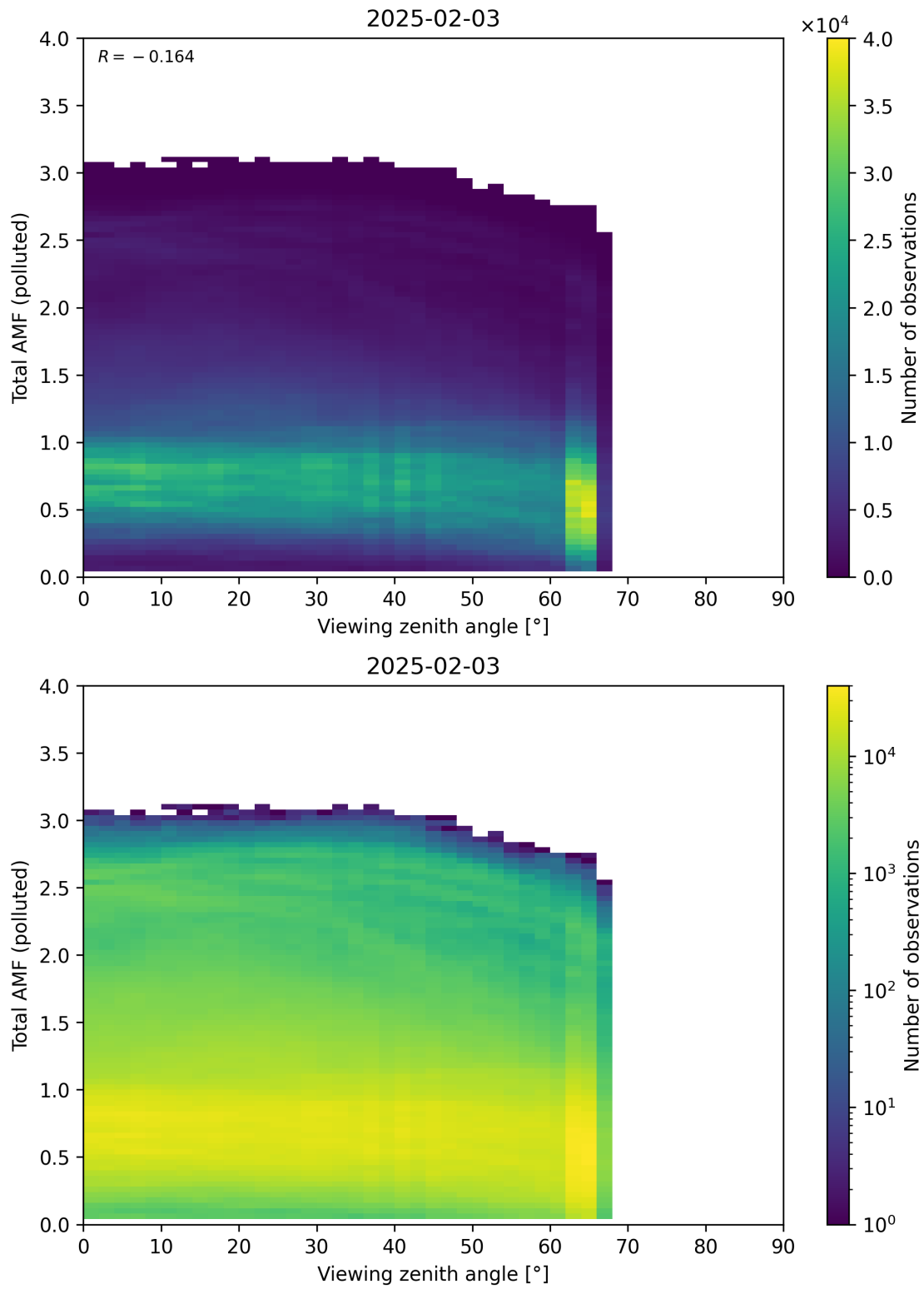
Figure 381: Scatter density plot of “Viewing zenith angle” against “Total AMF (polluted)” for 2025-02-03 to 2025-02-04.
