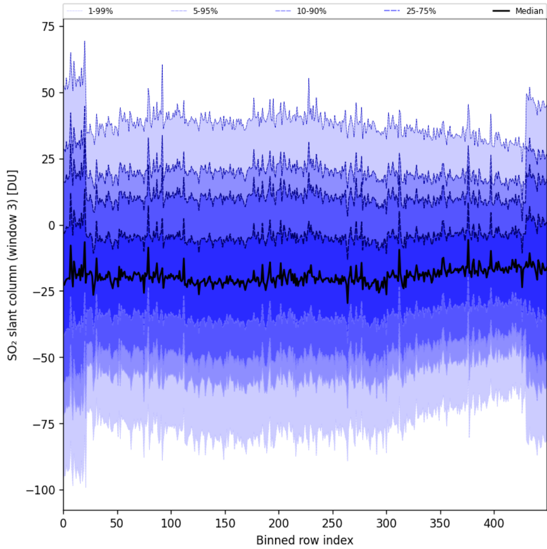
Figure 97: Along track statistics of “SO 2 slant column (window 3)” for 2025-02-03 to 2025-02-04
