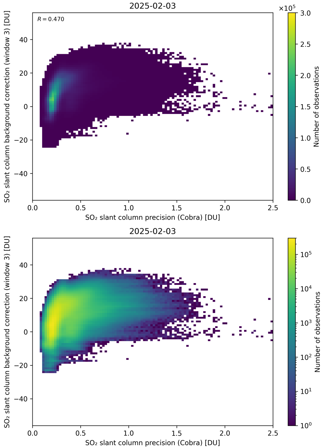
Figure 201: Scatter density plot of “SO 2 slant column precision (Cobra)” against “SO 2 slant column background correction (window 3)” for 2025-02-03 to 2025-02-04.
