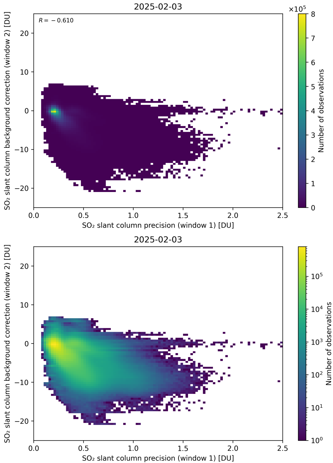
Figure 269: Scatter density plot of “SO 2 slant column precision (window 1)” against “SO 2 slant column background correction (window 2)” for 2025-02-03 to 2025-02-04.
