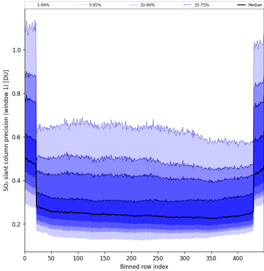
Figure 90: Along track statistics of “SO 2 slant column precision (window 1)” for 2025-02-03 to 2025-02-04
