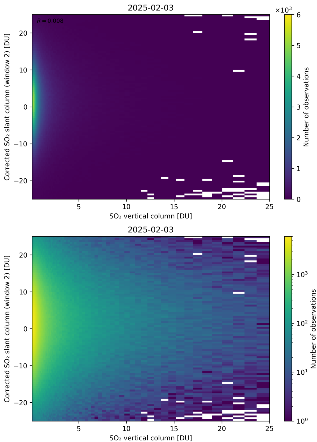
Figure 352: Scatter density plot of “SO 2 vertical column” against “Corrected SO 2 slant column (window 2)” for 2025-02-03 to 2025-02-04.
