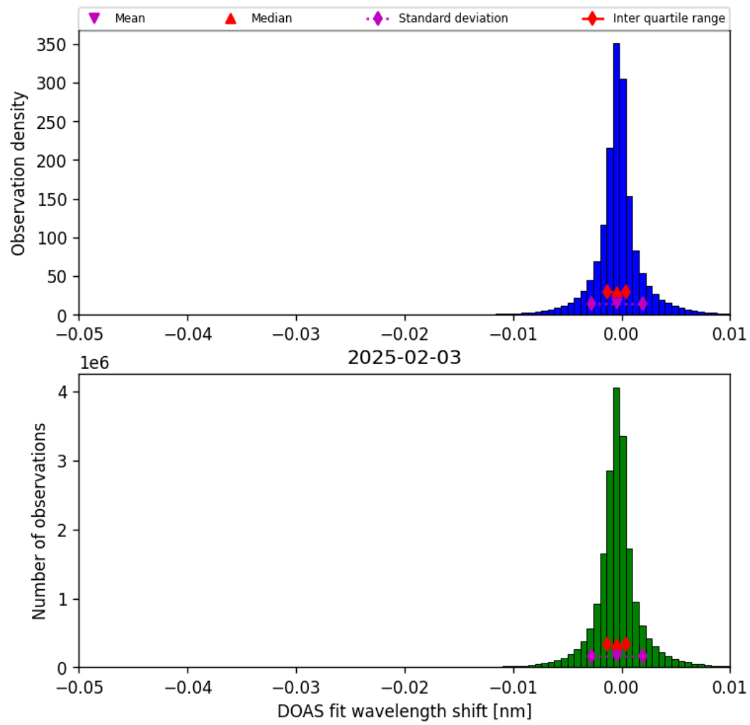
Figure 76: Histogram of “DOAS fit wavelength shift” for 2025-02-03 to 2025-02-04
