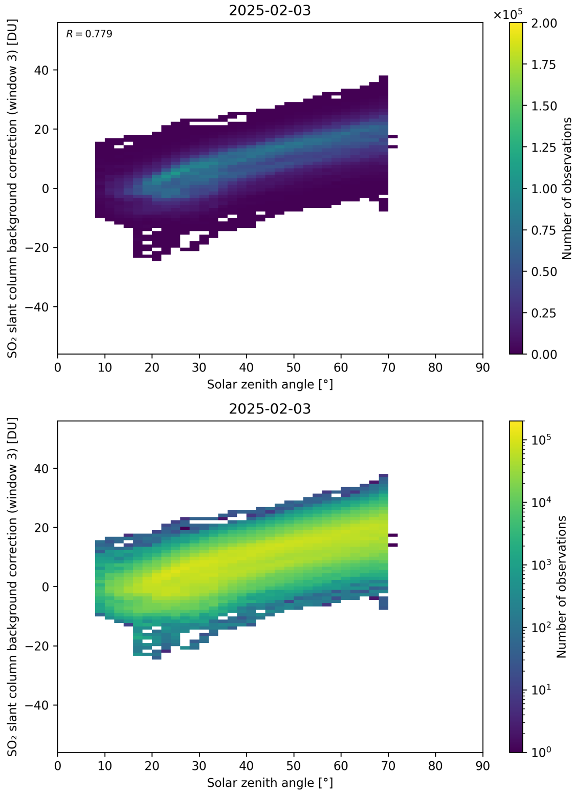
Figure 173: Scatter density plot of “Solar zenith angle” against “SO 2 slant column background correction (window 3)” for 2025-02-03 to 2025-02-04.
