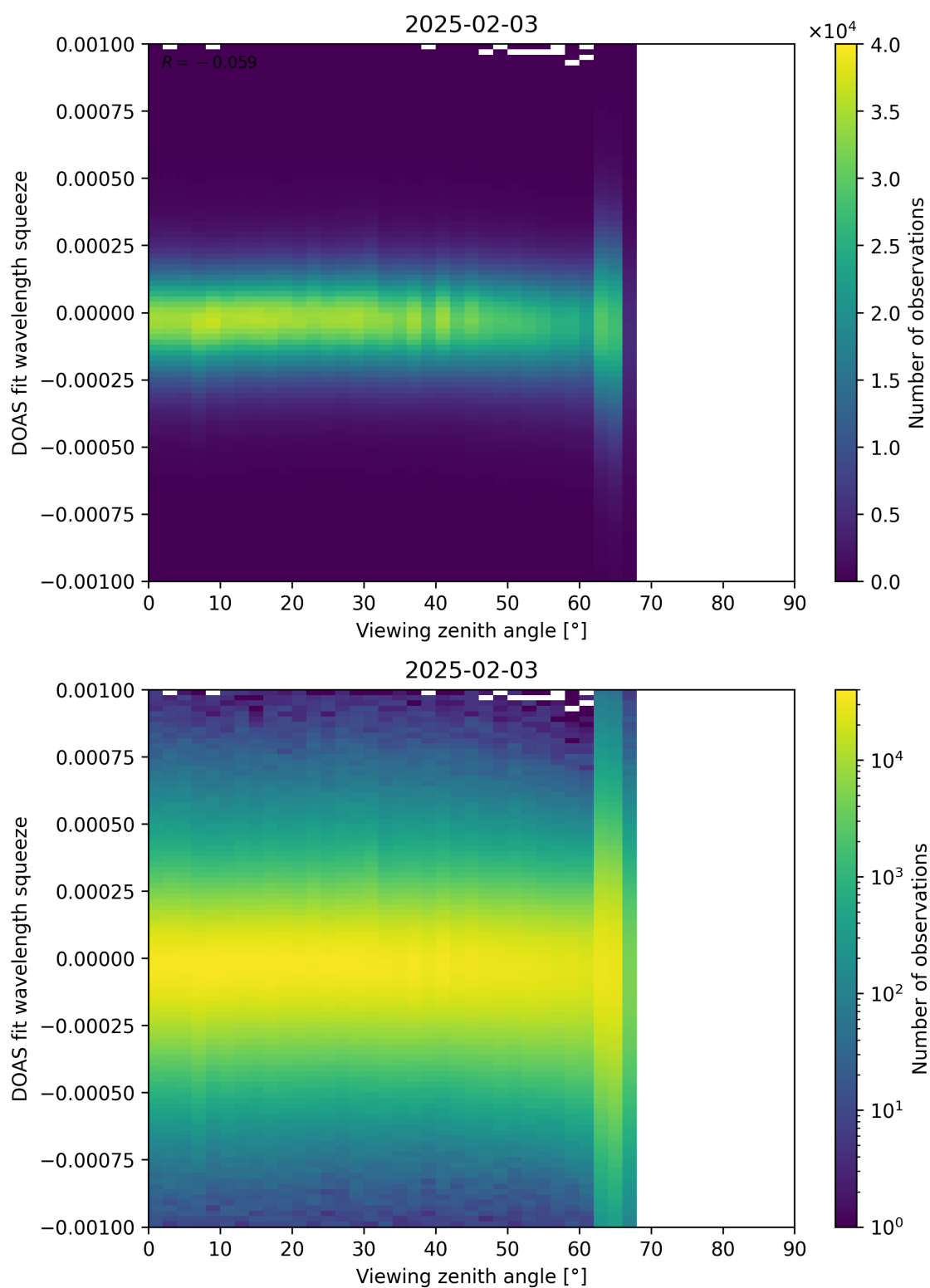
Figure 366: Scatter density plot of “Viewing zenith angle” against “DOAS fit wavelength squeeze” for 2025-02-03 to 2025-02-04.
