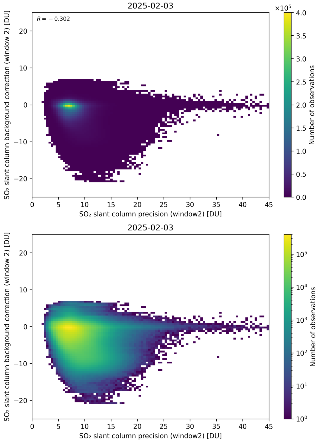
Figure 291: Scatter density plot of “SO 2 slant column precision (window2)” against “SO 2 slant column background correction (window 2)” for 2025-02-03 to 2025-02-04.
