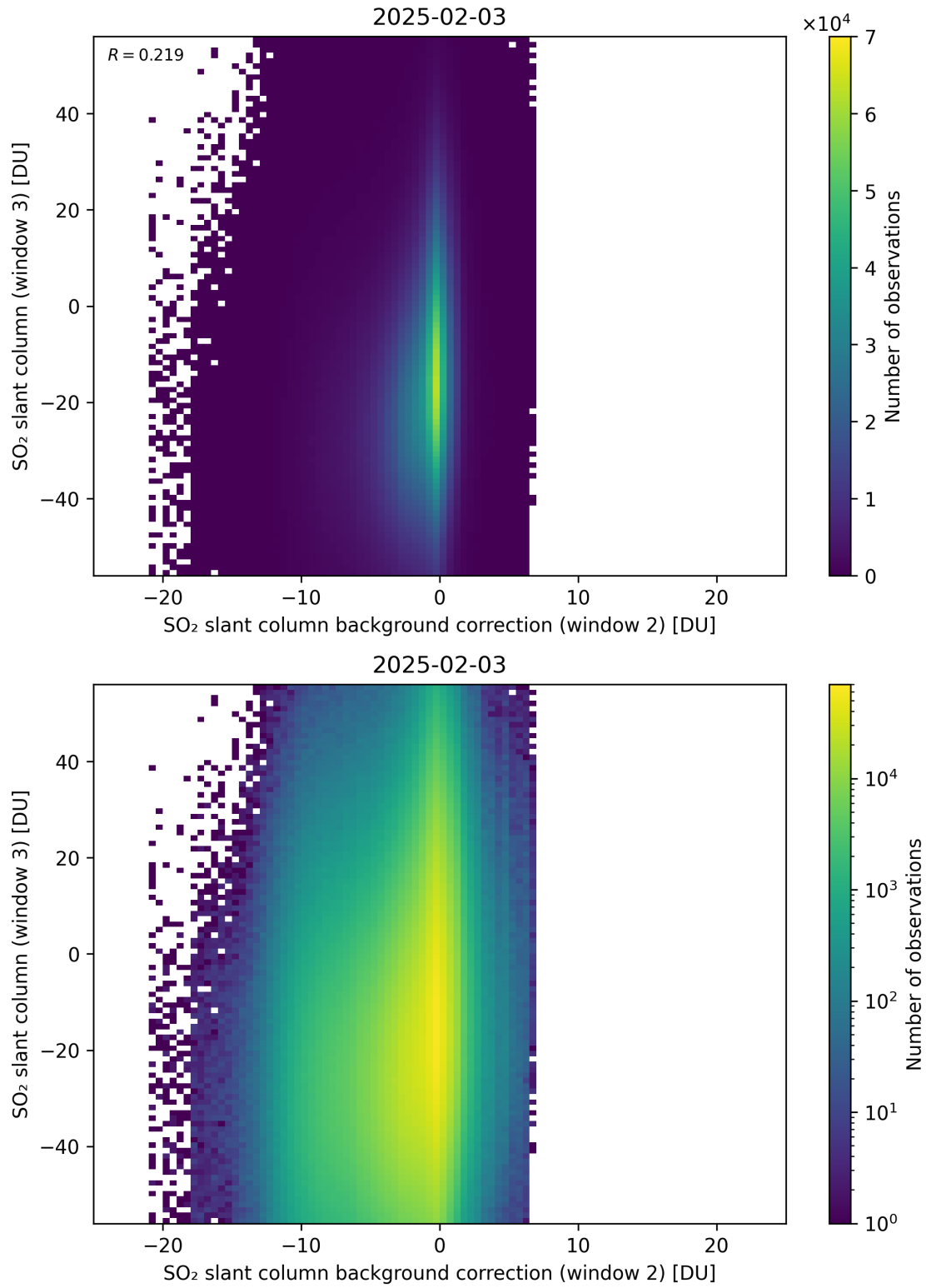
Figure 128: Scatter density plot of “SO 2 slant column background correction (window 2)” against “SO 2 slant column (window 3)” for 2025-02-03 to 2025-02-04.
