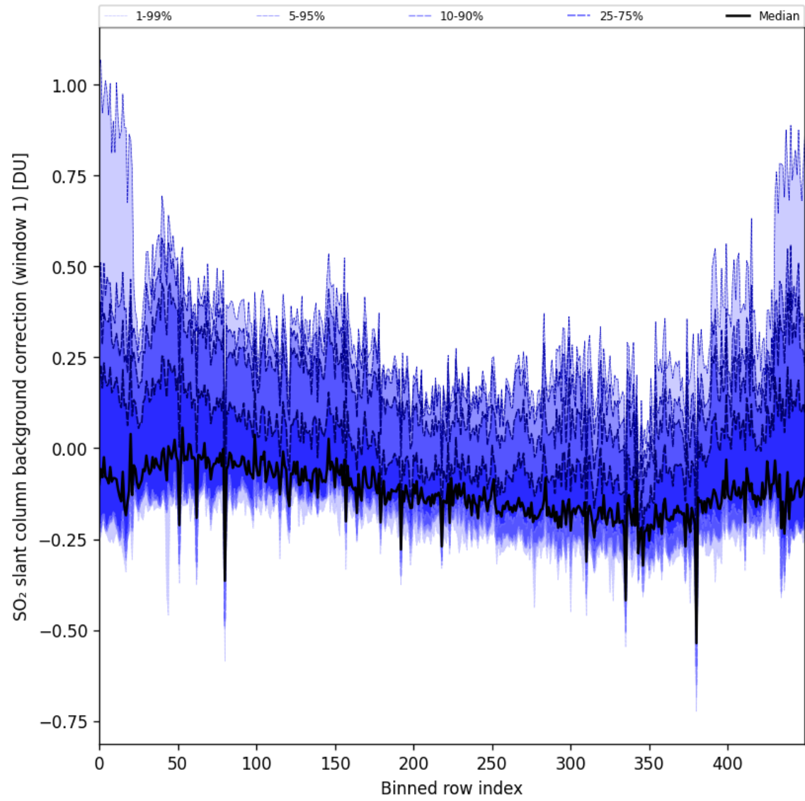
Figure 92: Along track statistics of “SO 2 slant column background correction (window 1)” for 2025-02-03 to 2025-02-04
