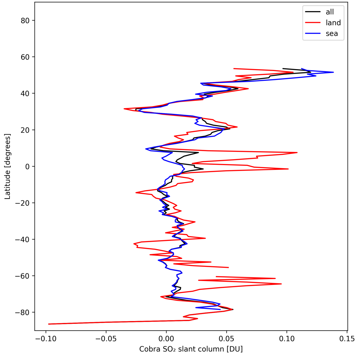
Figure 35: Zonal average of “Cobra SO 2 slant column” for 2025-02-03 to 2025-02-04.
