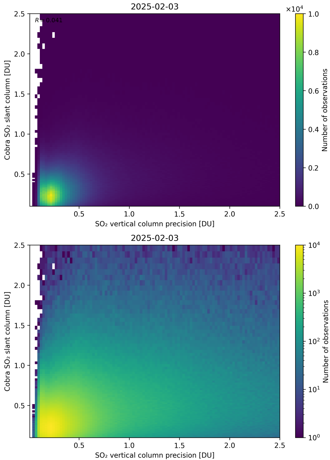
Figure 336: Scatter density plot of “SO 2 vertical column precision” against “Cobra SO 2 slant column” for 2025-02-03 to 2025-02-04.
