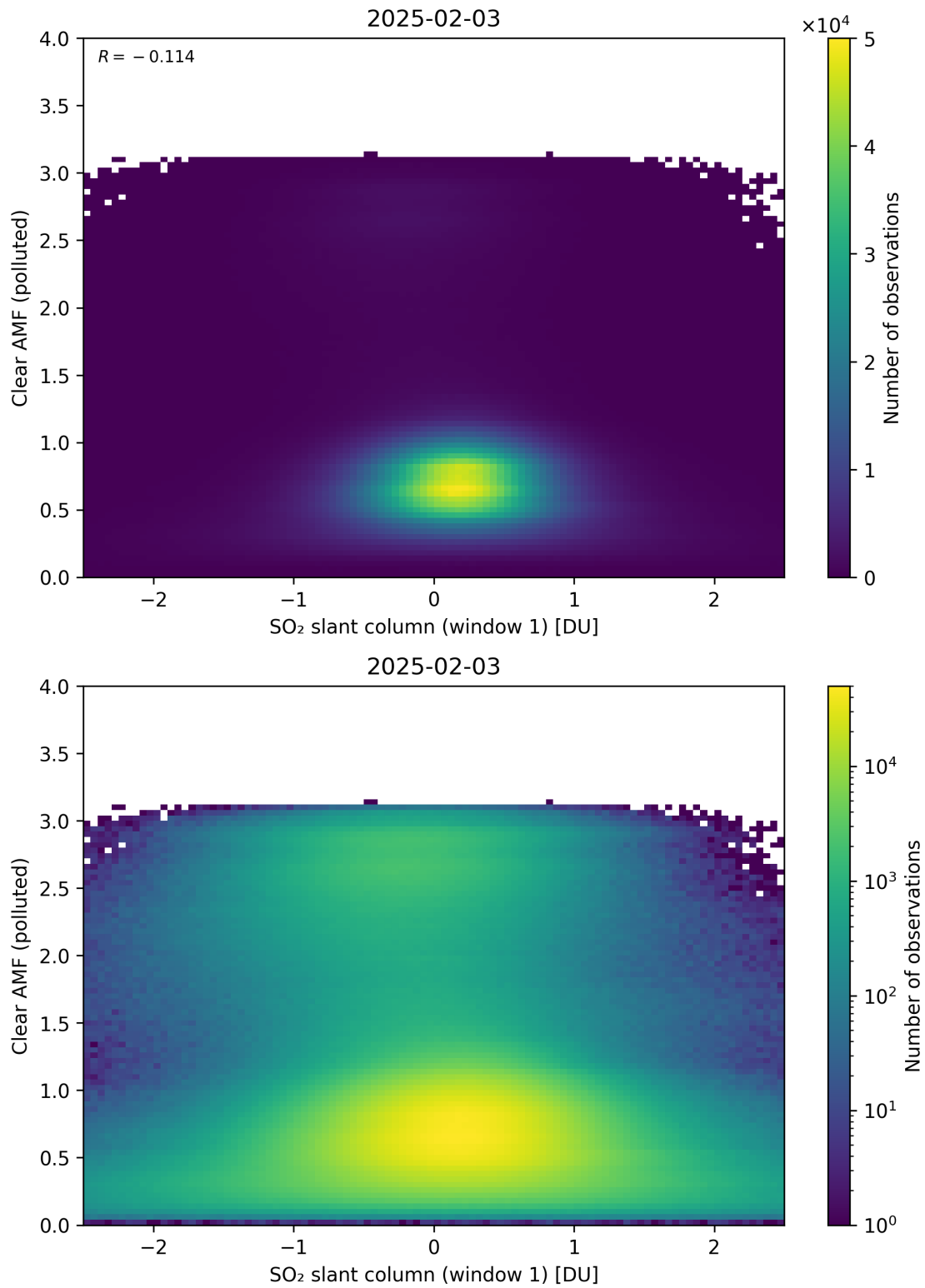
Figure 282: Scatter density plot of “SO 2 slant column (window 1)” against “Clear AMF (polluted)” for 2025-02-03 to 2025-02-04.
