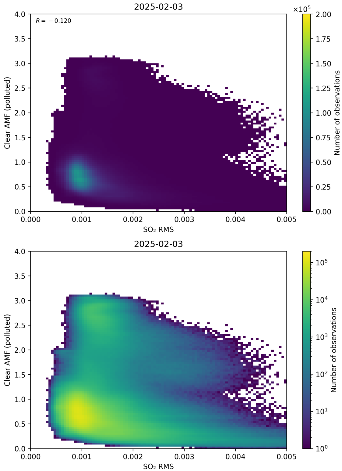
Figure 147: Scatter density plot of “SO 2 RMS” against “Clear AMF (polluted)” for 2025-02-03 to 2025-02-04.
