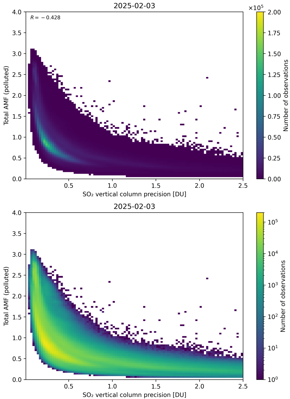
Figure 346: Scatter density plot of “SO 2 vertical column precision” against “Total AMF (polluted)” for 2025-02-03 to 2025-02-04.
