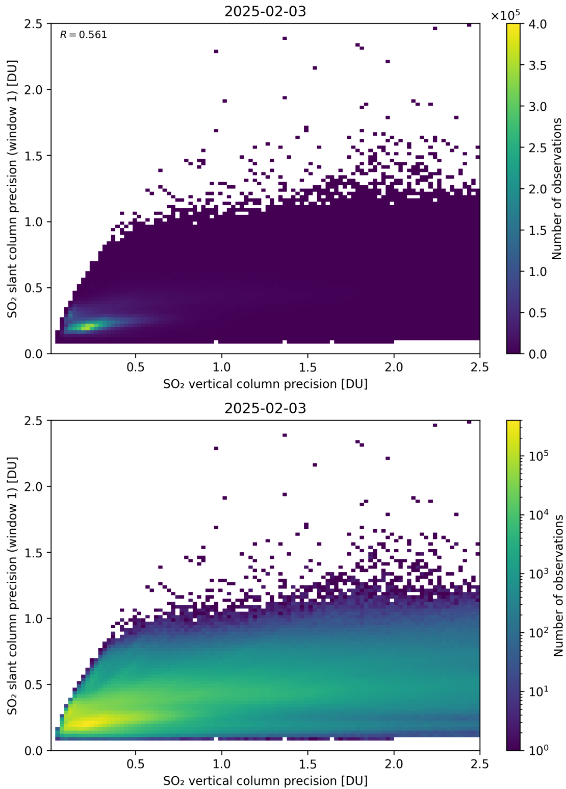
Figure 342: Scatter density plot of “SO 2 vertical column precision” against “SO 2 slant column precision (window 1)” for 2025-02-03 to 2025-02-04.
