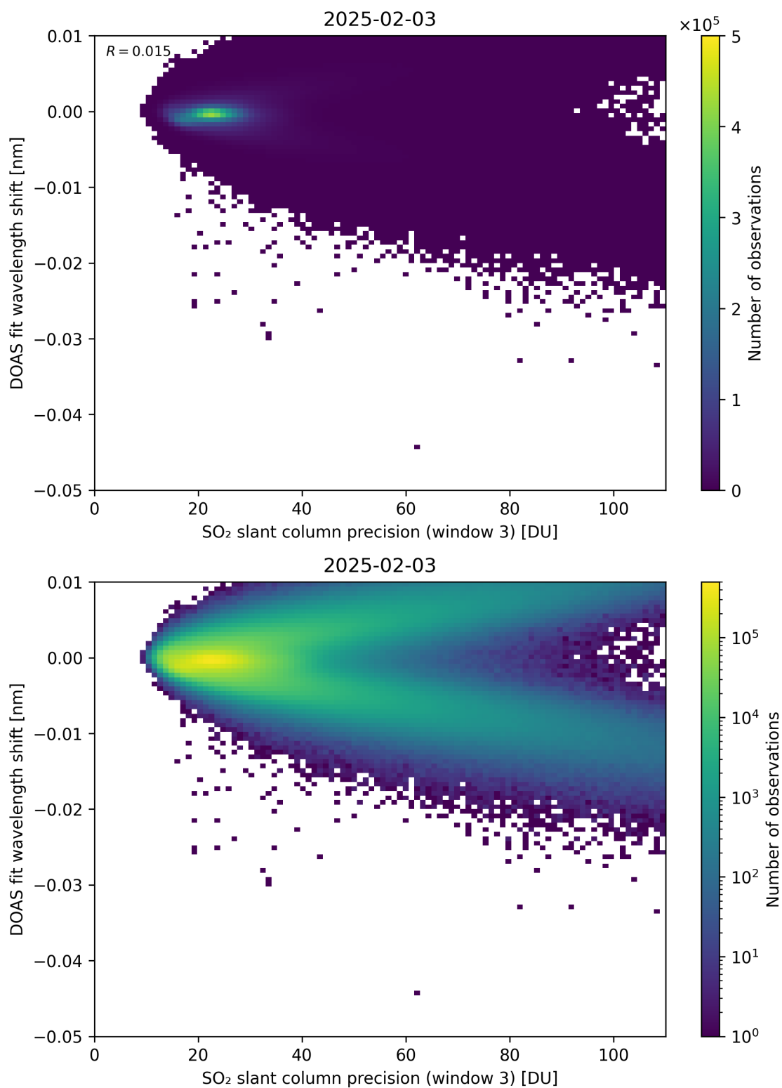
Figure 308: Scatter density plot of “SO 2 slant column precision (window 3)” against “DOAS fit wavelength shift” for 2025-02-03 to 2025-02-04.
