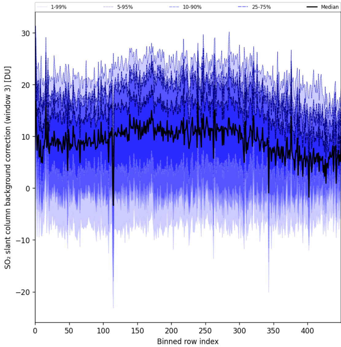
Figure 100: Along track statistics of “SO 2 slant column background correction (window 3)” for 2025-02-03 to 2025-02-04
