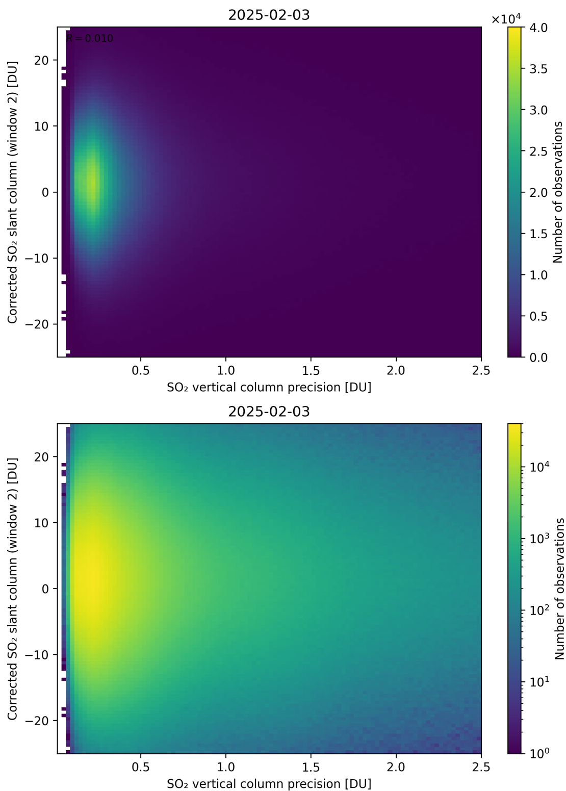
Figure 339: Scatter density plot of “SO 2 vertical column precision” against “Corrected SO 2 slant column (window 2)” for 2025-02-03 to 2025-02-04.
