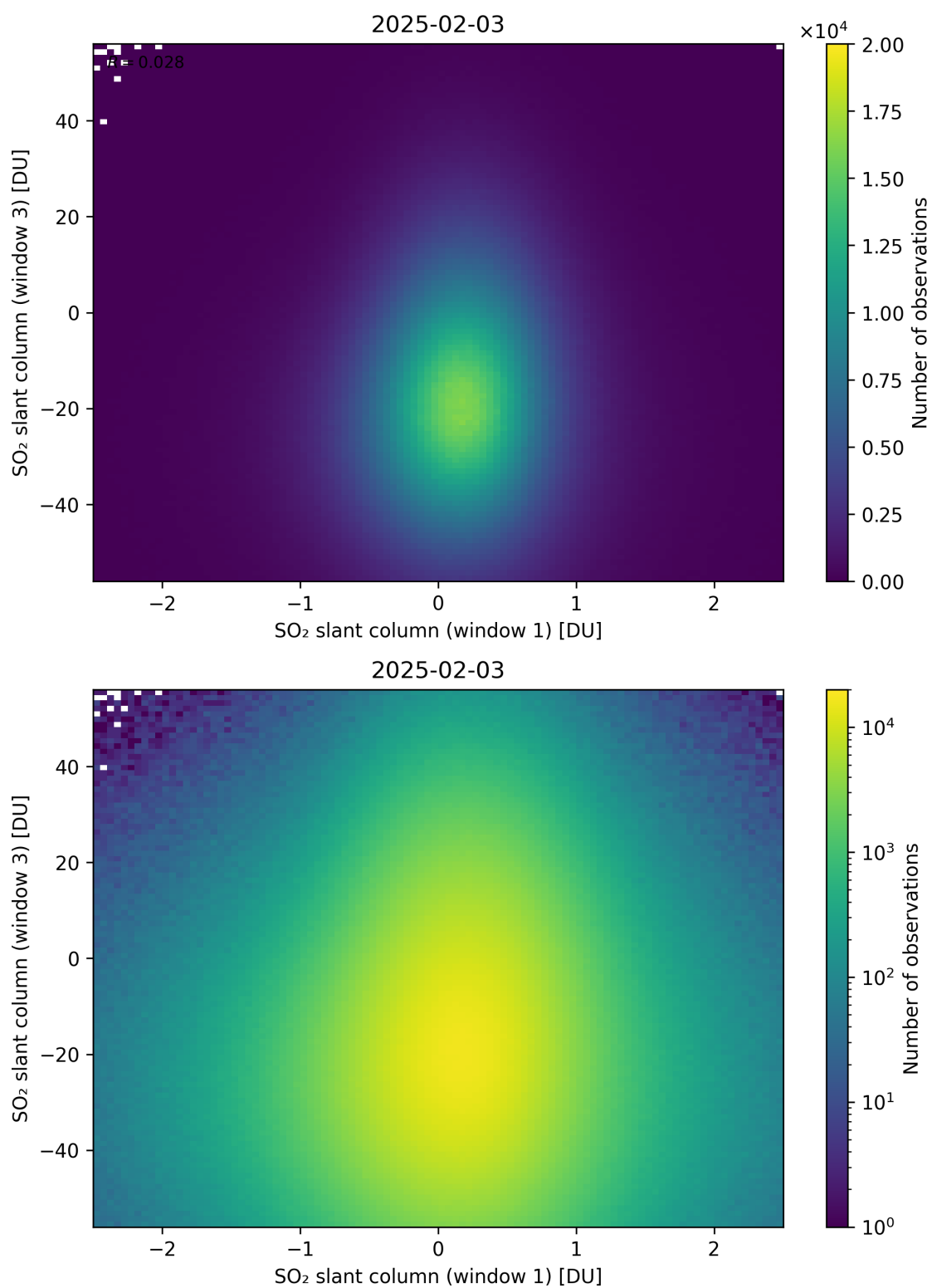
Figure 287: Scatter density plot of “SO 2 slant column (window 1)” against “SO 2 slant column (window 3)” for 2025-02-03 to 2025-02-04.
