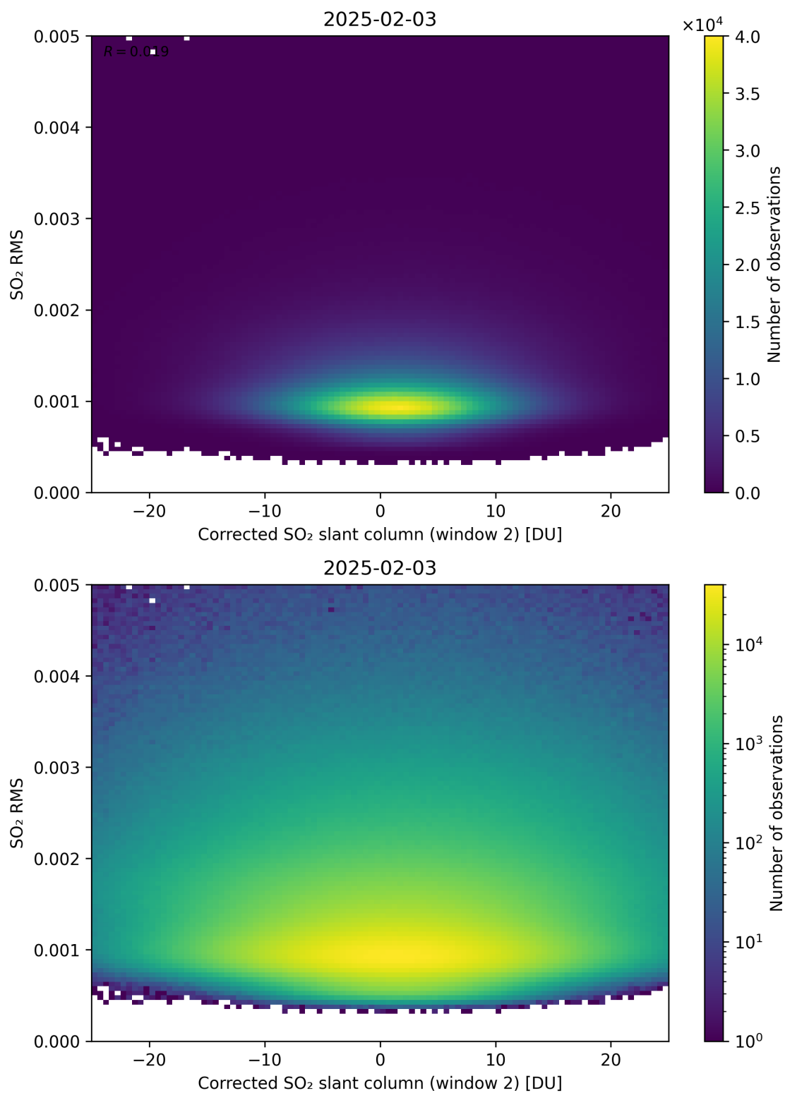
Figure 248: Scatter density plot of “Corrected SO 2 slant column (window 2)” against “SO 2 RMS” for 2025-02-03 to 2025-02-04.
