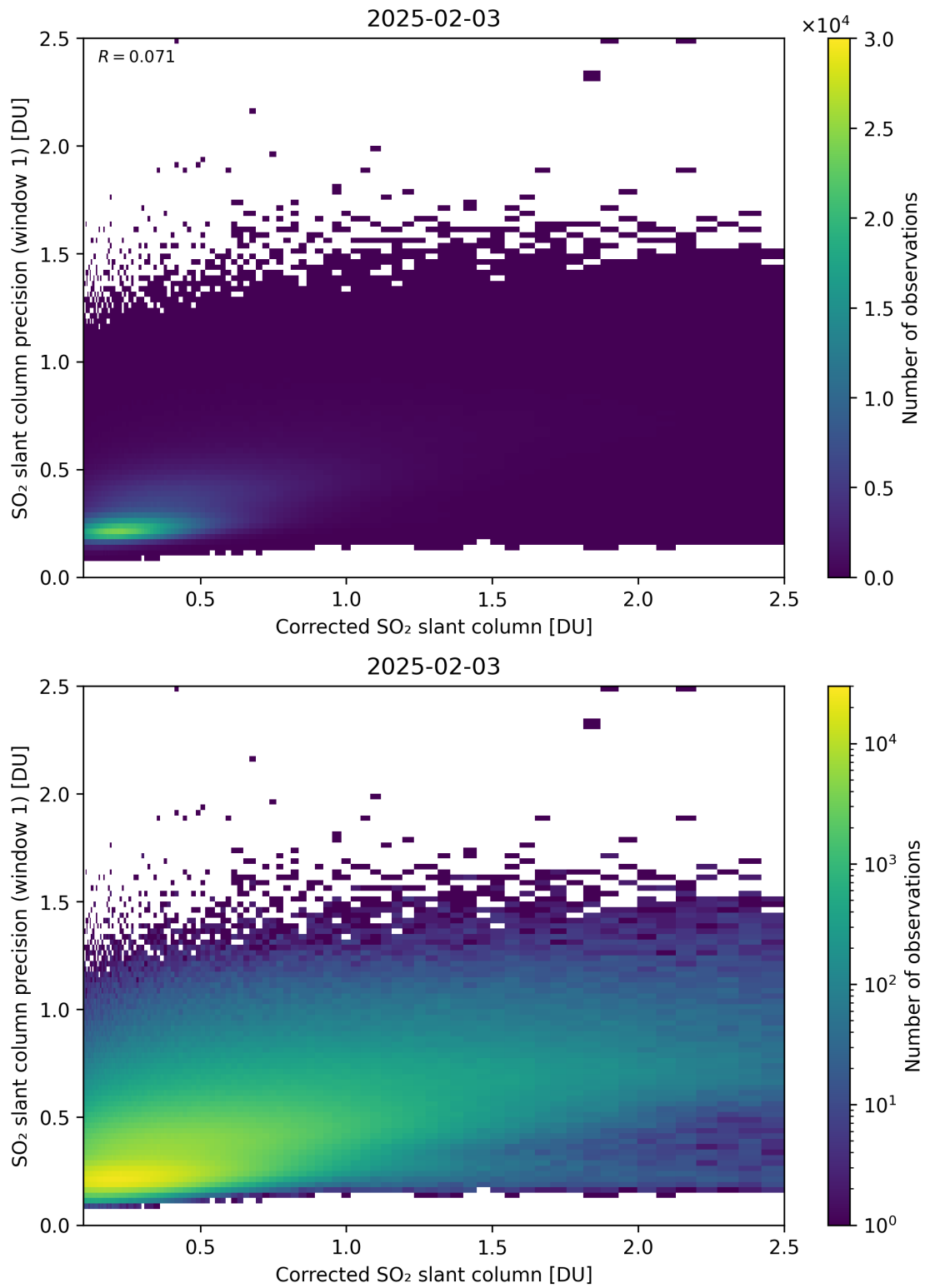
Figure 238: Scatter density plot of “Corrected SO 2 slant column” against “SO 2 slant column precision (window 1)” for 2025-02-03 to 2025-02-04.
