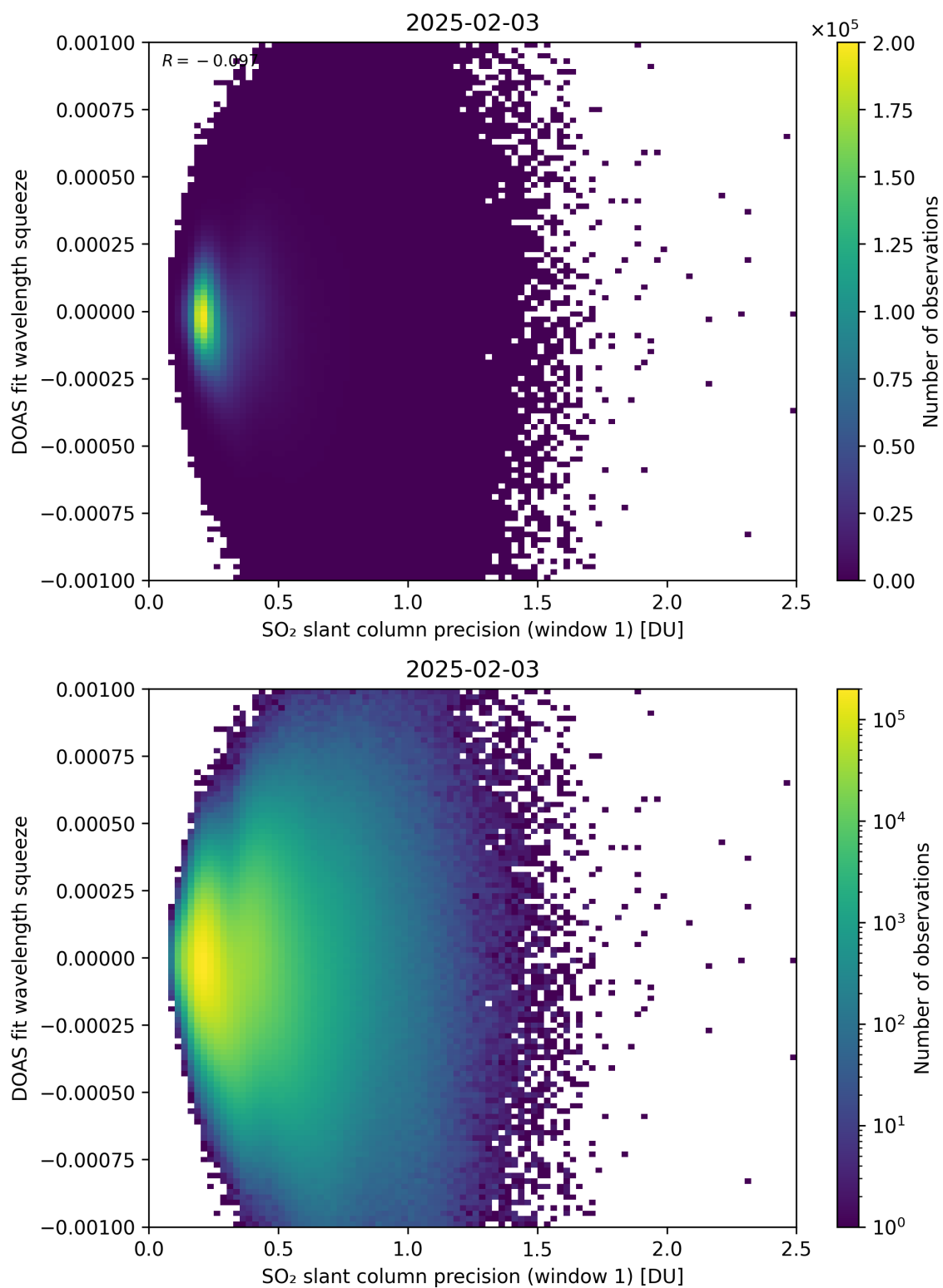
Figure 272: Scatter density plot of “SO 2 slant column precision (window 1)” against “DOAS fit wavelength squeeze” for 2025-02-03 to 2025-02-04.
