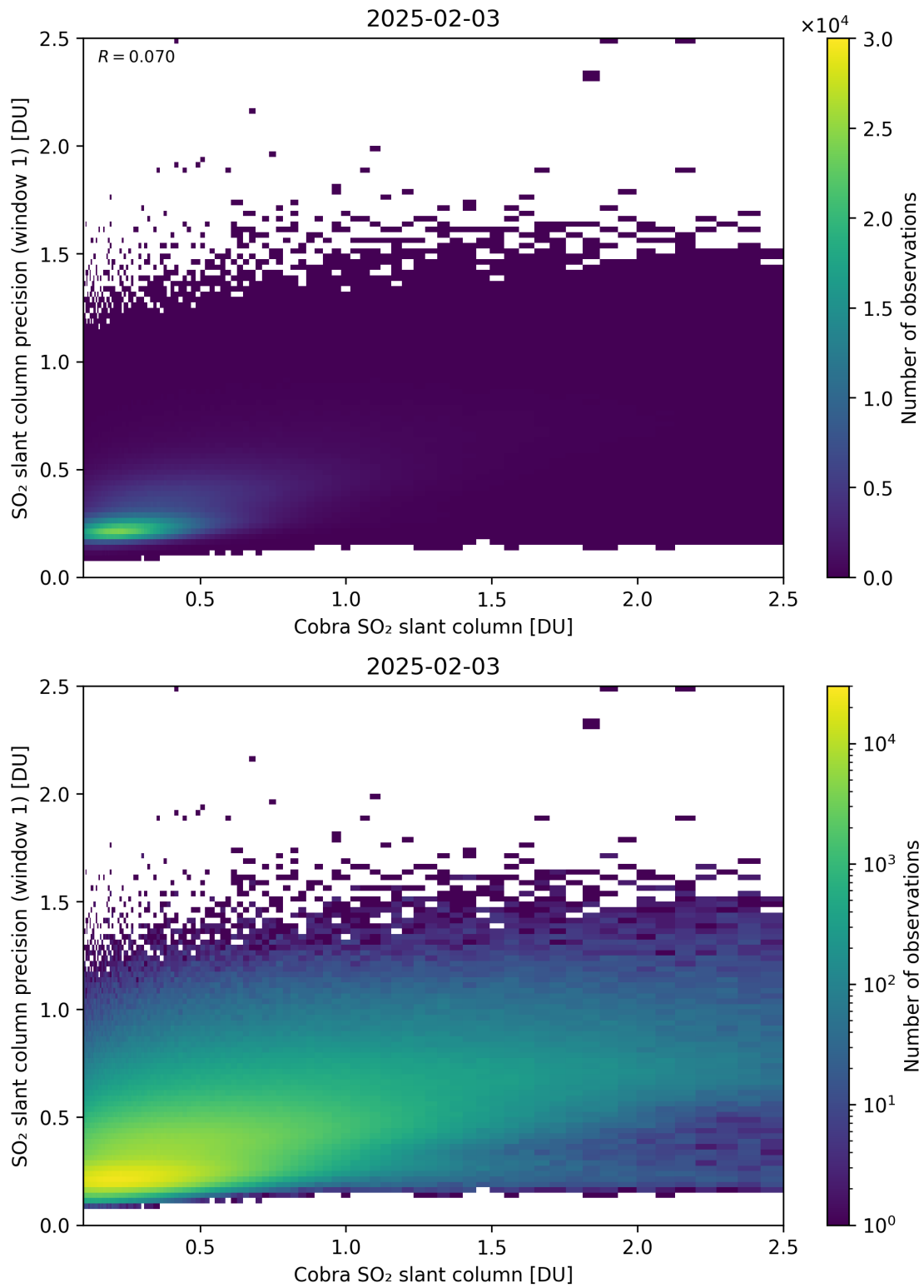
Figure 220: Scatter density plot of “Cobra SO 2 slant column” against “SO 2 slant column precision (window 1)” for 2025-02-03 to 2025-02-04.
