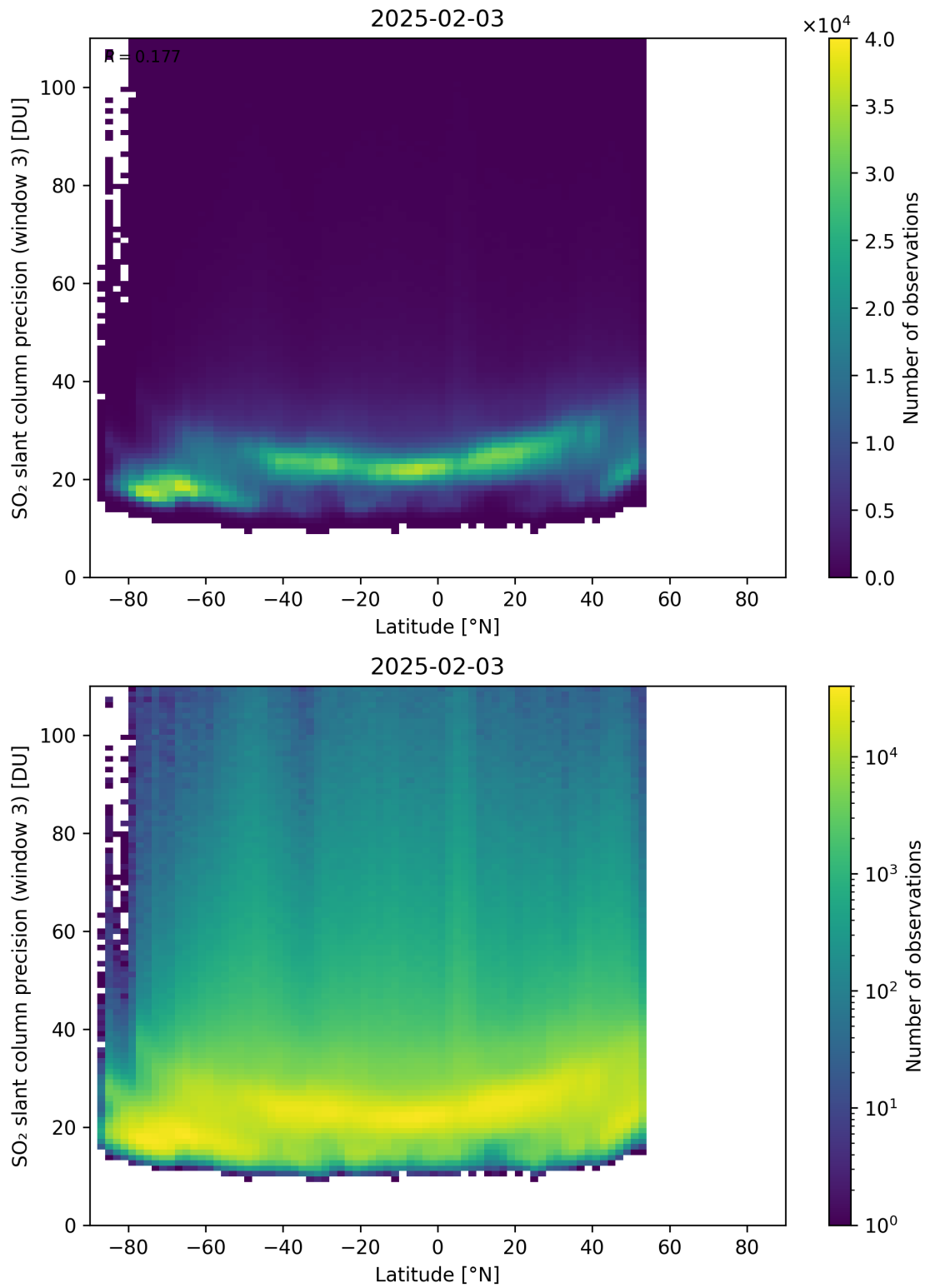
Figure 166: Scatter density plot of “Latitude” against “SO 2 slant column precision (window 3)” for 2025-02-03 to 2025-02-04.
