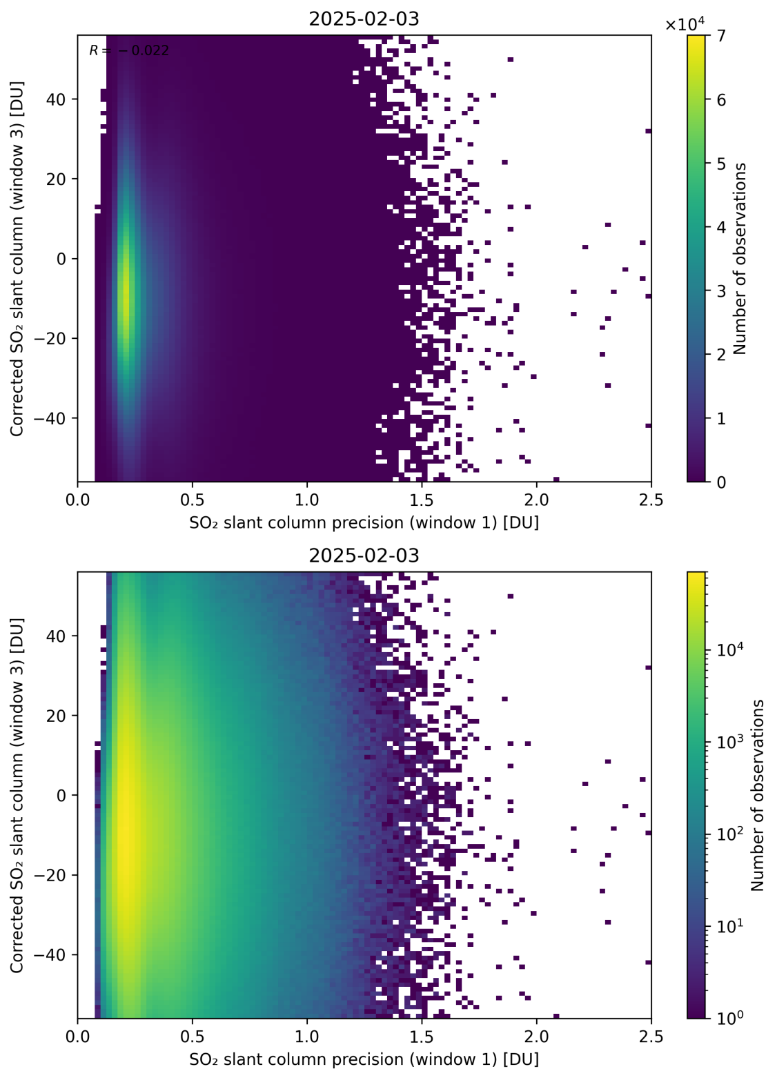
Figure 276: Scatter density plot of “SO 2 slant column precision (window 1)” against “Corrected SO 2 slant column (window 3)” for 2025-02-03 to 2025-02-04.
