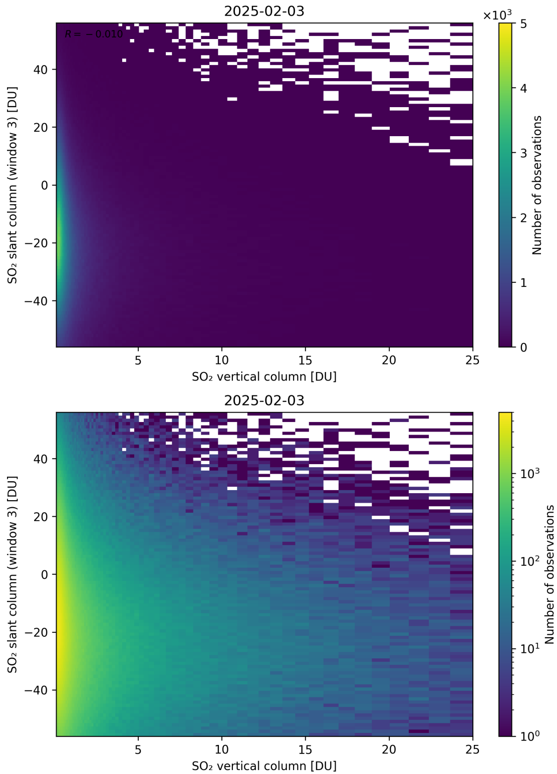
Figure 357: Scatter density plot of “SO 2 vertical column” against “SO 2 slant column (window 3)” for 2025-02-03 to 2025-02-04.
