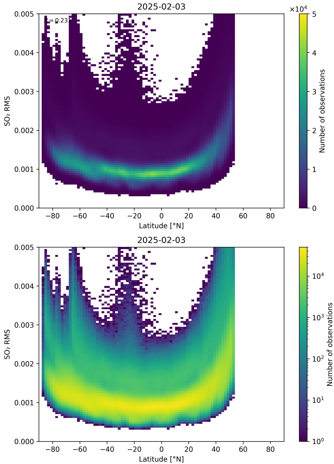
Figure 155: Scatter density plot of “Latitude” against “SO 2 RMS” for 2025-02-03 to 2025-02-04.
