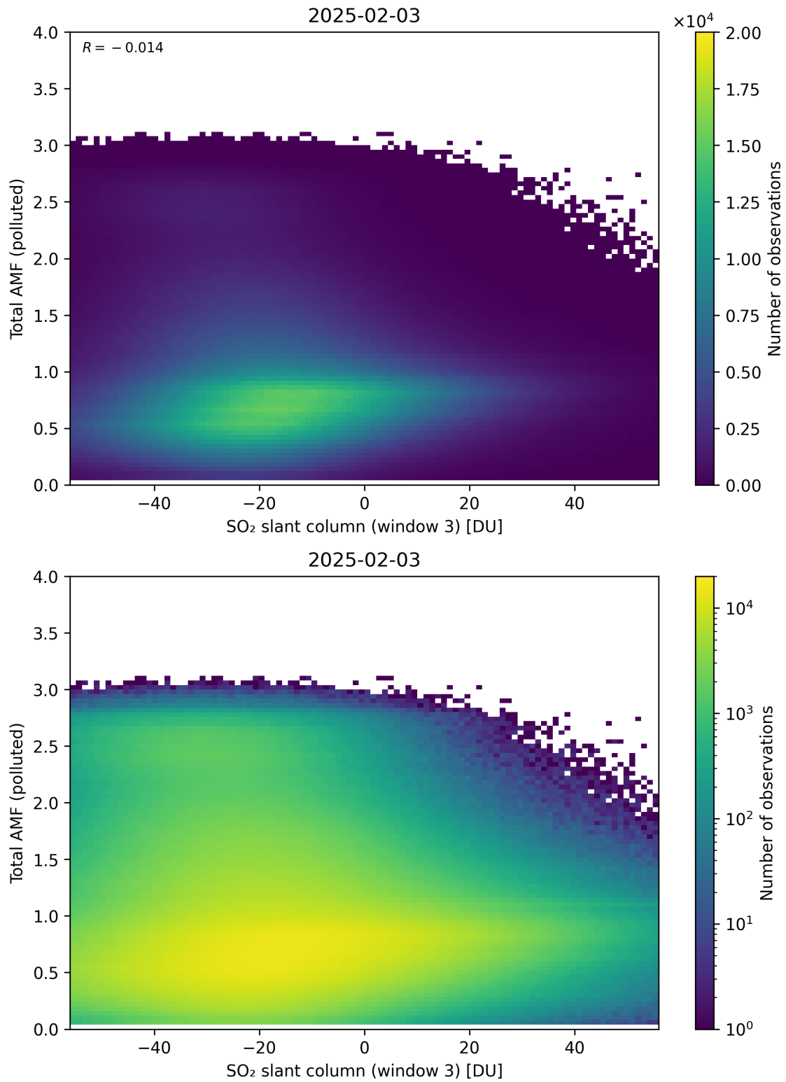
Figure 318: Scatter density plot of “SO 2 slant column (window 3)” against “Total AMF (polluted)” for 2025-02-03 to 2025-02-04.
