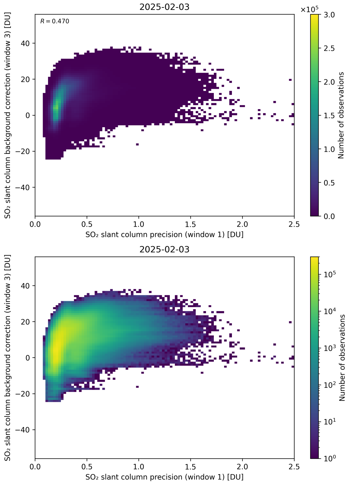
Figure 270: Scatter density plot of “SO 2 slant column precision (window 1)” against “SO 2 slant column background correction (window 3)” for 2025-02-03 to 2025-02-04.
