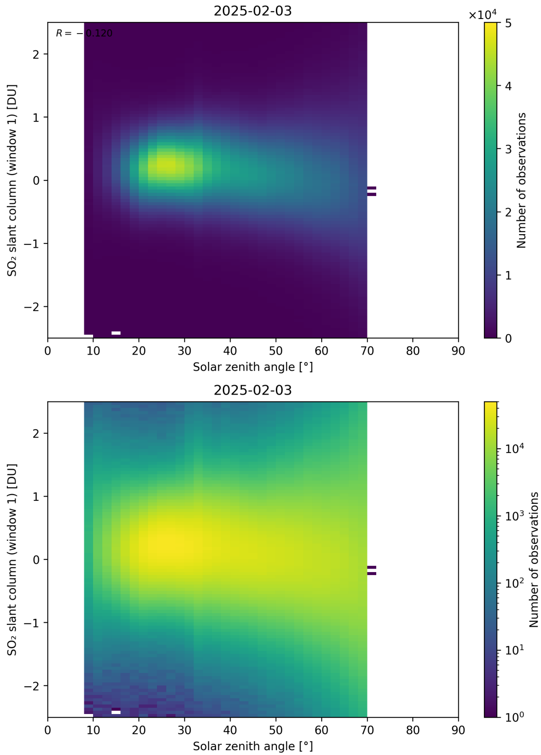
Figure 184: Scatter density plot of “Solar zenith angle” against “SO 2 slant column (window 1)” for 2025-02-03 to 2025-02-04.
