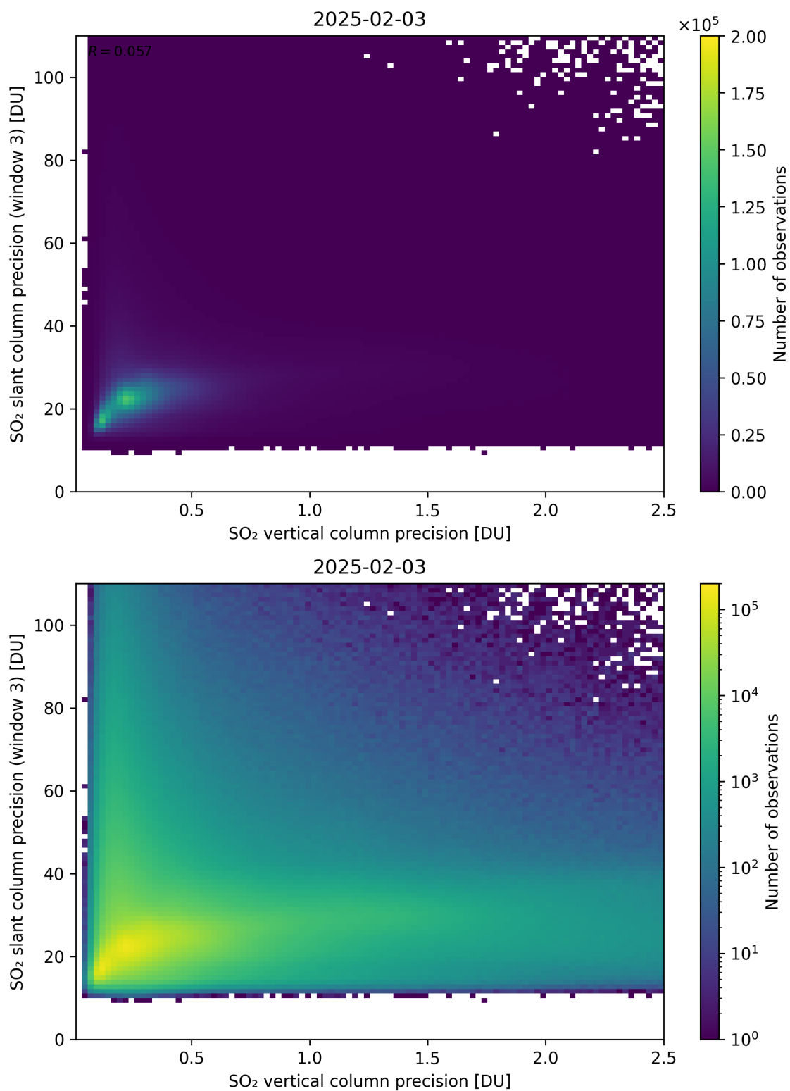
Figure 345: Scatter density plot of “SO 2 vertical column precision” against “SO 2 slant column precision (window 3)” for 2025-02-03 to 2025-02-04.
