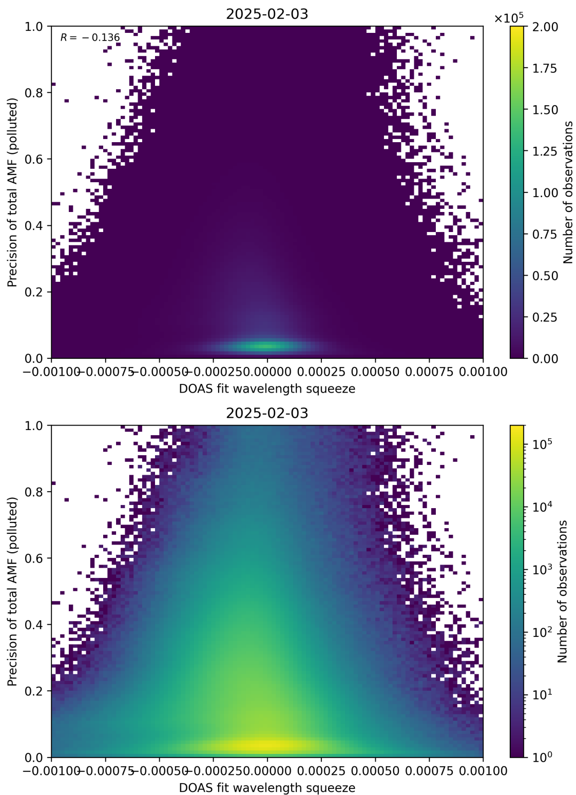
Figure 146: Scatter density plot of “DOAS fit wavelength squeeze” against “Precision of total AMF (polluted)” for 2025-02-03 to 2025-02-04.
