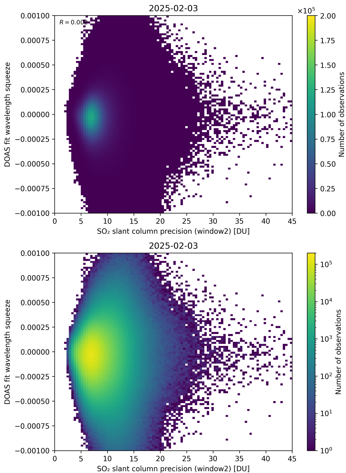
Figure 294: Scatter density plot of “SO 2 slant column precision (window2)” against “DOAS fit wavelength squeeze” for 2025-02-03 to 2025-02-04.
