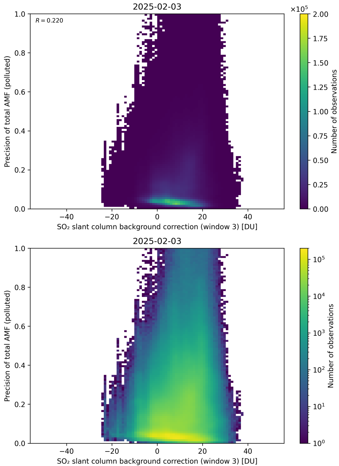
Figure 137: Scatter density plot of “SO 2 slant column background correction (window 3)” against “Precision of total AMF (polluted)” for 2025-02-03 to 2025-02-04.
