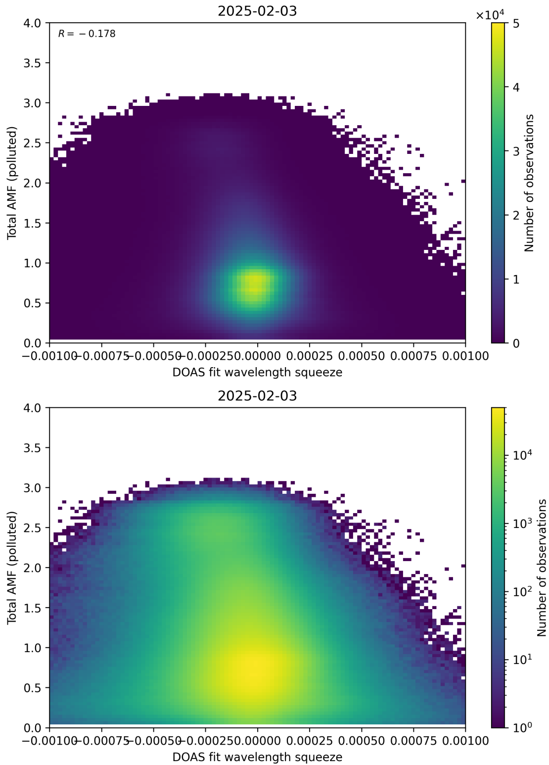
Figure 145: Scatter density plot of “DOAS fit wavelength squeeze” against “Total AMF (polluted)” for 2025-02-03 to 2025-02-04.
