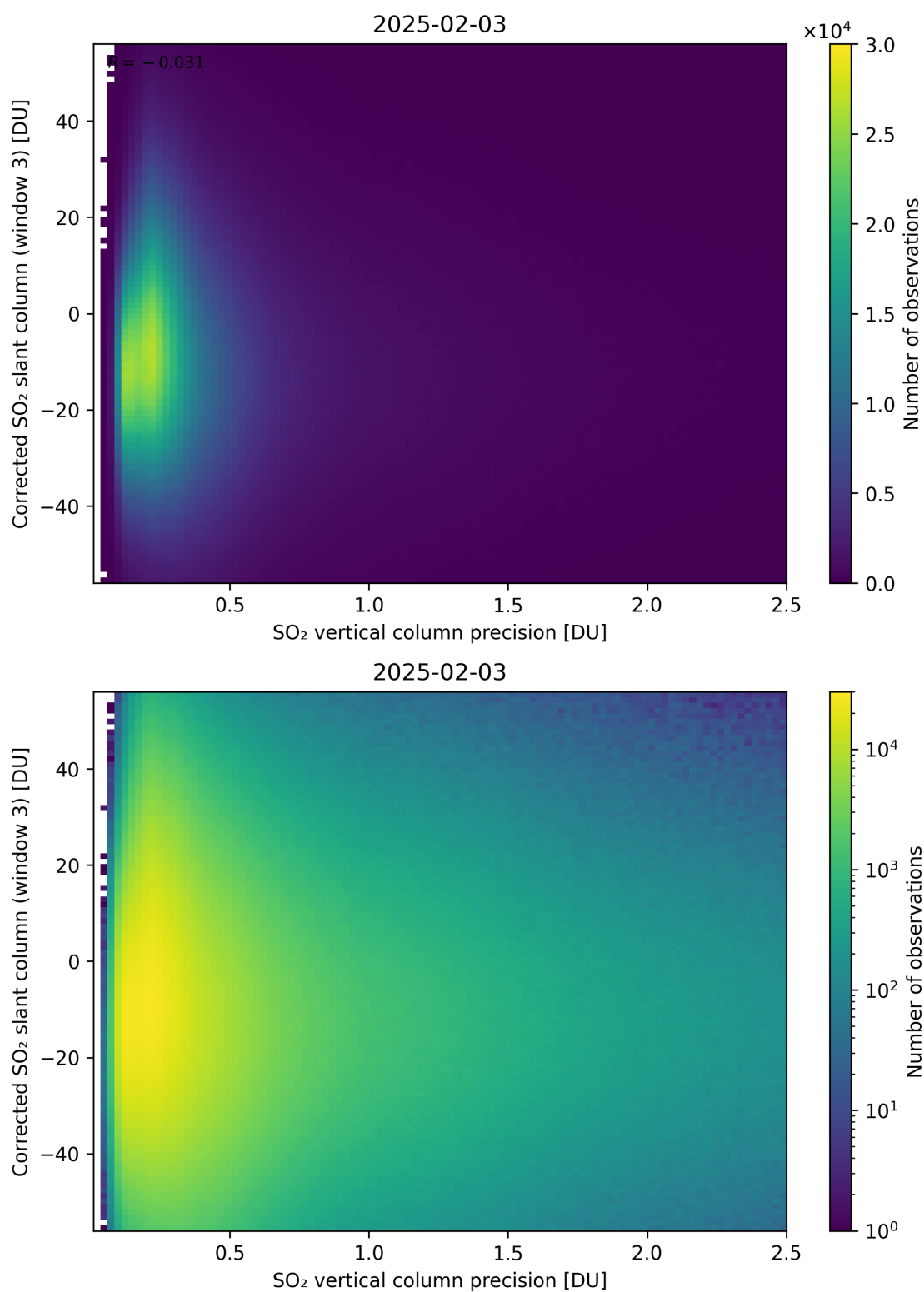
Figure 340: Scatter density plot of “SO 2 vertical column precision” against “Corrected SO 2 slant column (window 3)” for 2025-02-03 to 2025-02-04.
