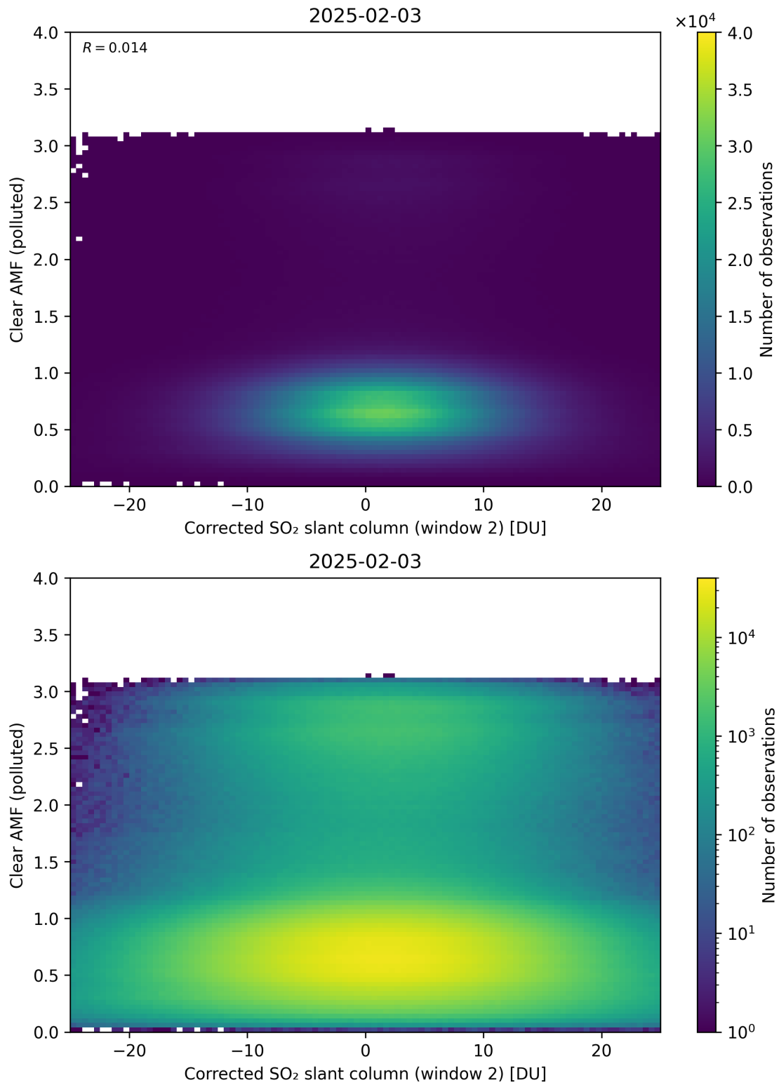
Figure 249: Scatter density plot of “Corrected SO 2 slant column (window 2)” against “Clear AMF (polluted)” for 2025-02-03 to 2025-02-04.
