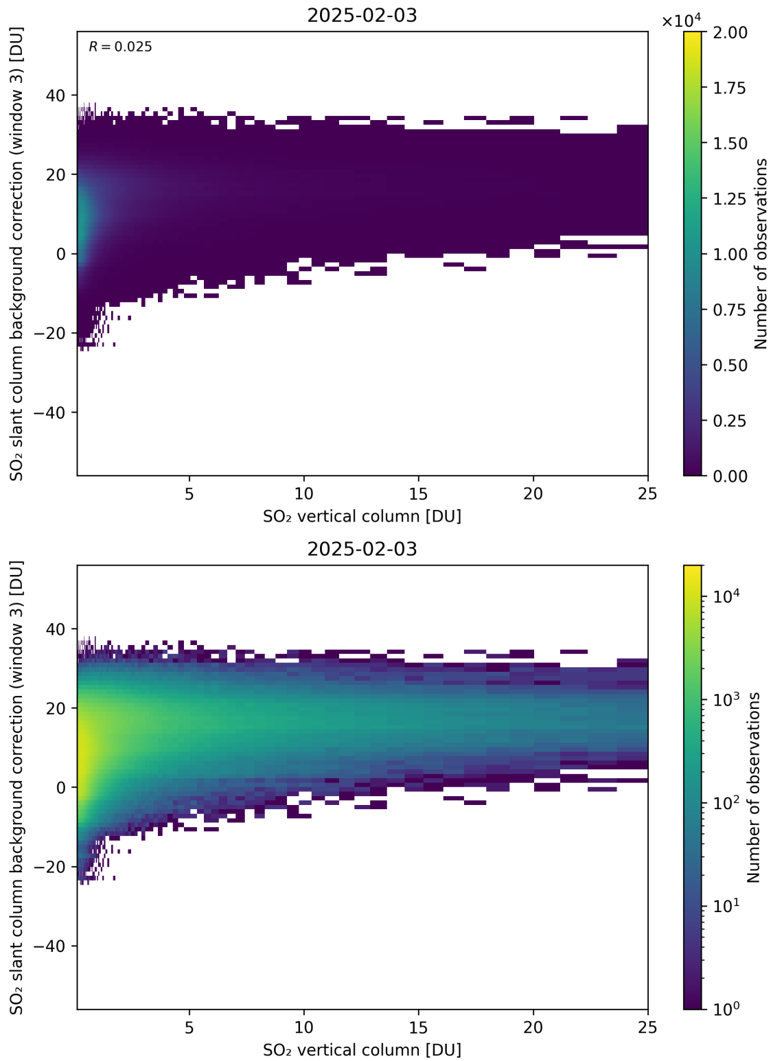
Figure 325: Scatter density plot of “SO 2 vertical column” against “SO 2 slant column background correction (window 3)” for 2025-02-03 to 2025-02-04.
