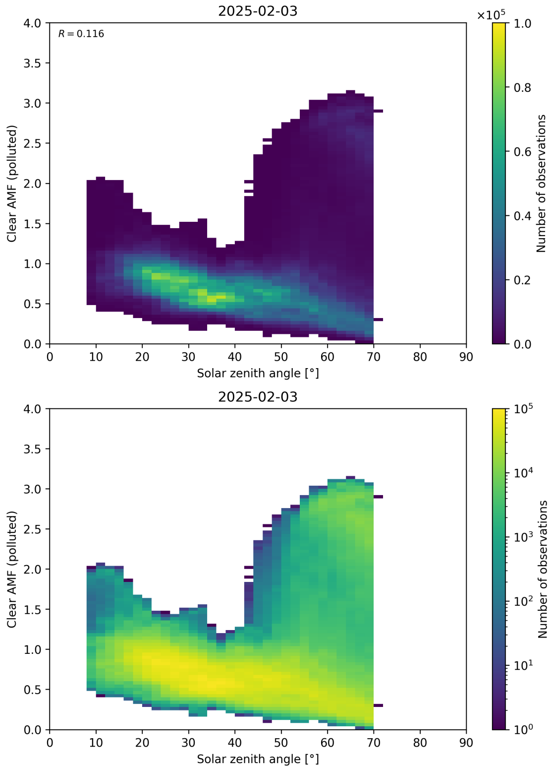
Figure 178: Scatter density plot of “Solar zenith angle” against “Clear AMF (polluted)” for 2025-02-03 to 2025-02-04.
