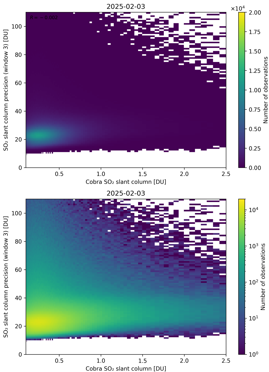
Figure 223: Scatter density plot of “Cobra SO 2 slant column” against “SO 2 slant column precision (window 3)” for 2025-02-03 to 2025-02-04.
