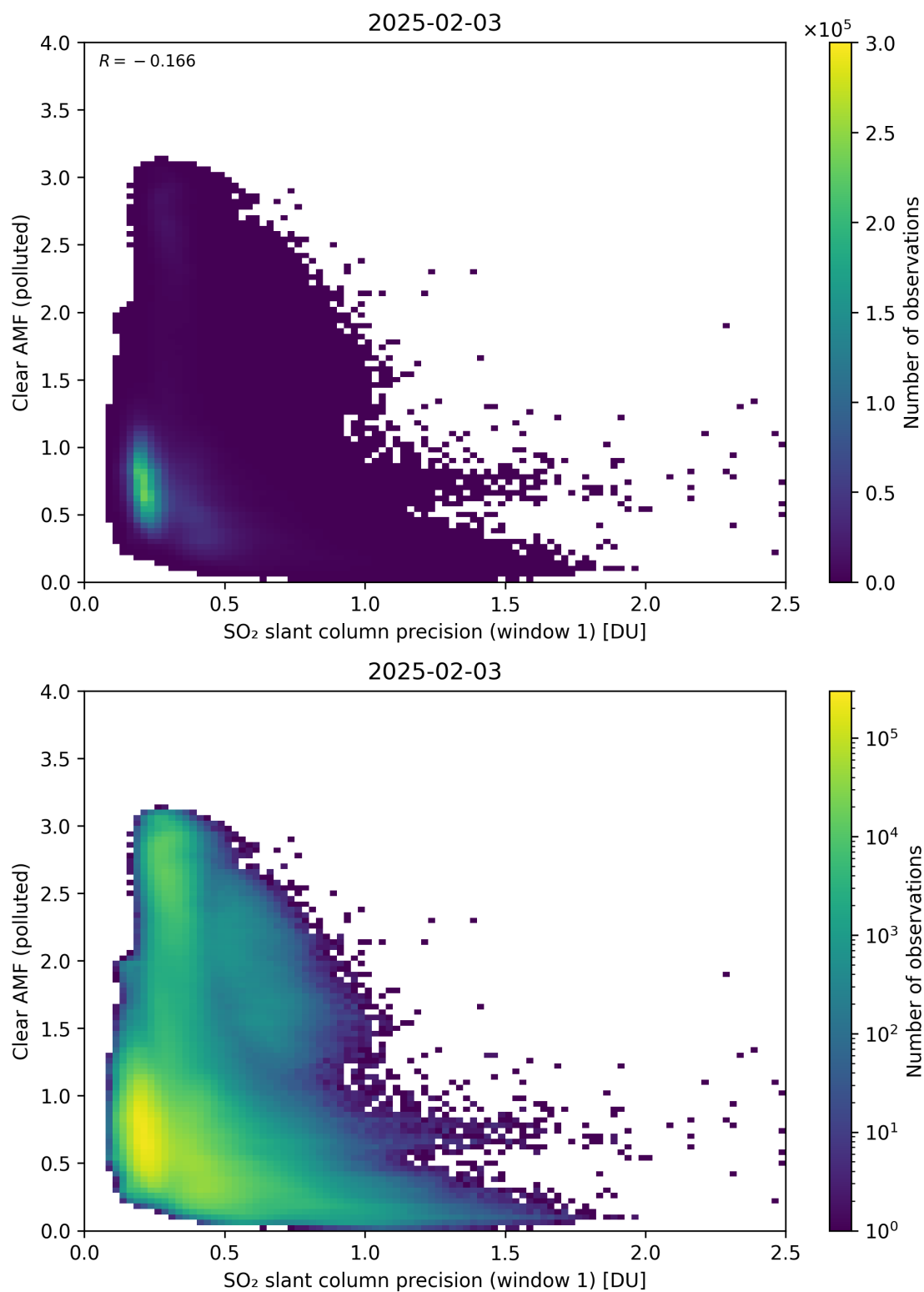
Figure 274: Scatter density plot of “SO 2 slant column precision (window 1)” against “Clear AMF (polluted)” for 2025-02-03 to 2025-02-04.
