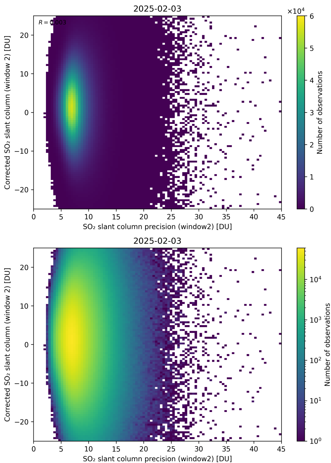
Figure 297: Scatter density plot of “SO 2 slant column precision (window2)” against “Corrected SO 2 slant column (window 2)” for 2025-02-03 to 2025-02-04.
