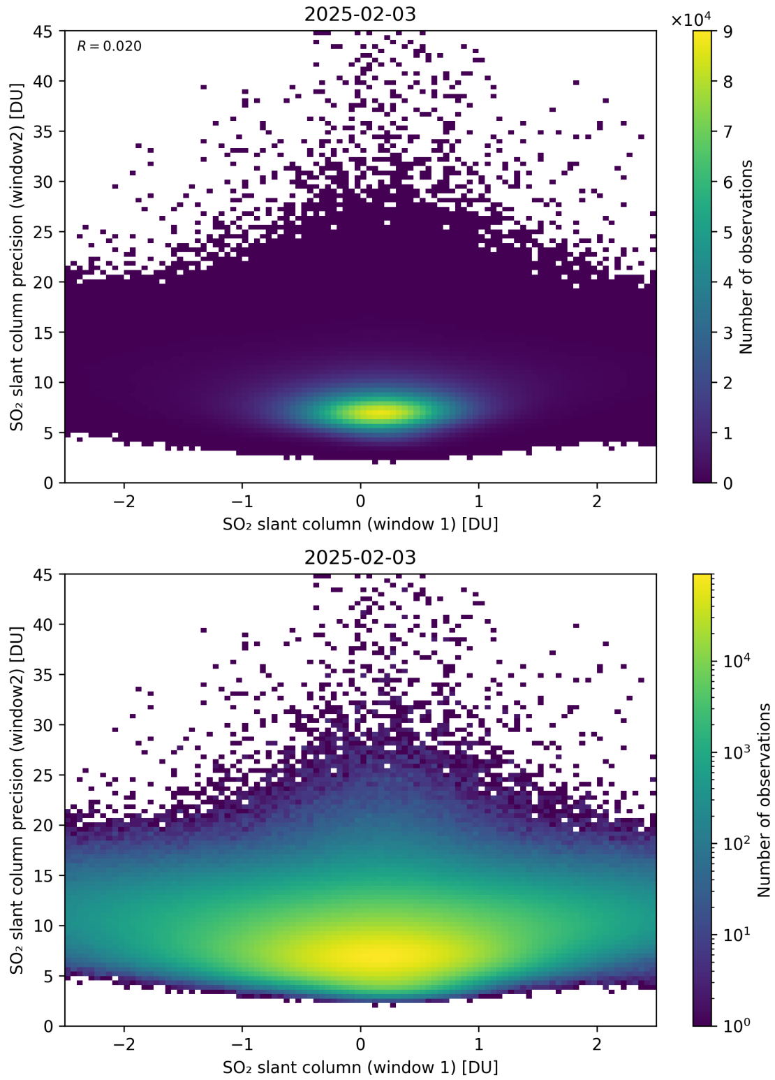
Figure 286: Scatter density plot of “SO 2 slant column (window 1)” against “SO 2 slant column precision (window2)” for 2025-02-03 to 2025-02-04.
