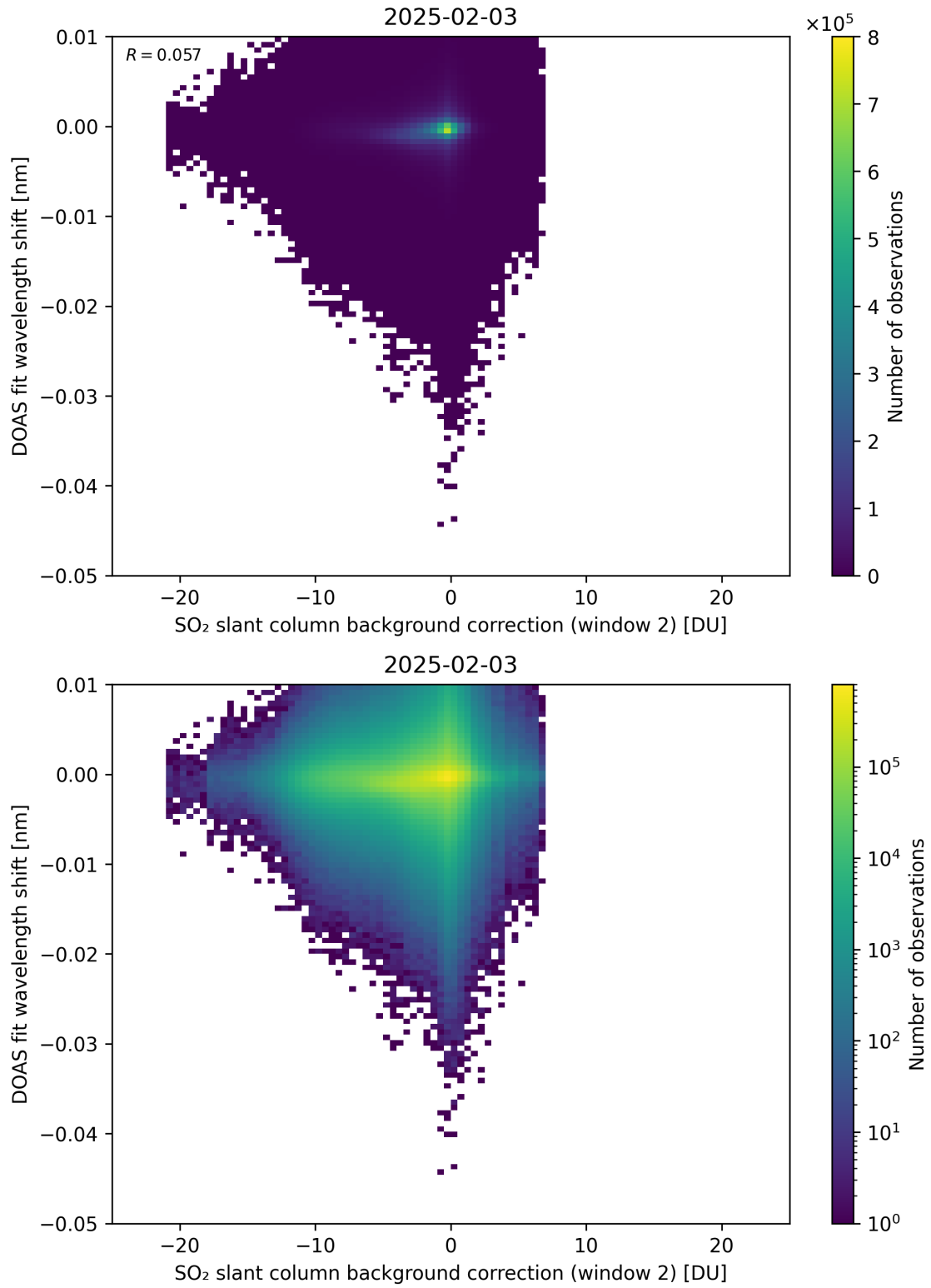
Figure 123: Scatter density plot of “SO 2 slant column background correction (window 2)” against “DOAS fit wavelength shift” for 2025-02-03 to 2025-02-04.
