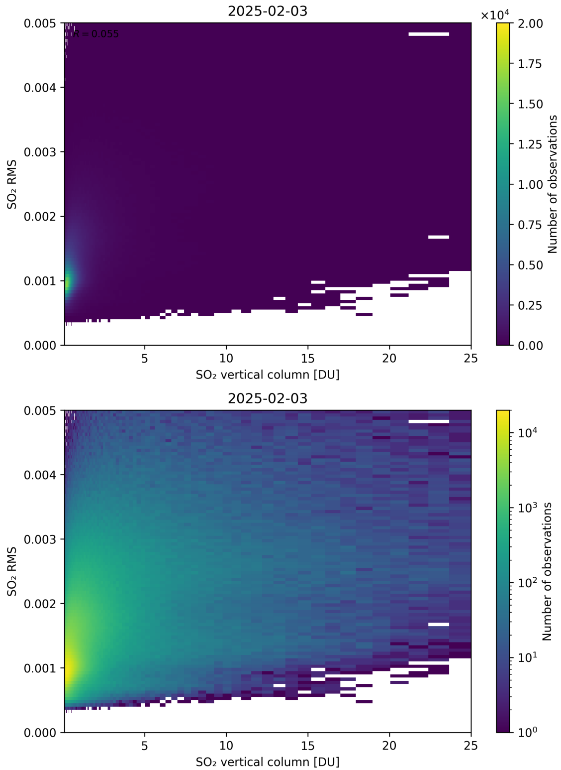
Figure 328: Scatter density plot of “SO 2 vertical column” against “SO 2 RMS” for 2025-02-03 to 2025-02-04.
