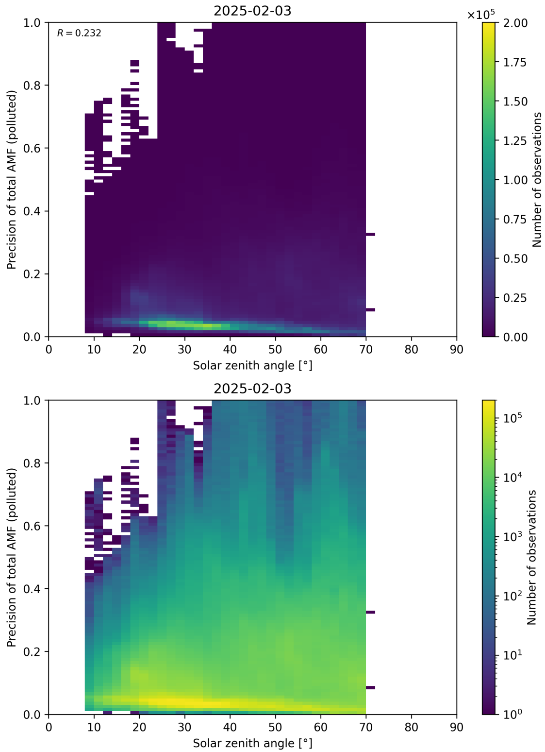
Figure 190: Scatter density plot of “Solar zenith angle” against “Precision of total AMF (polluted)” for 2025-02-03 to 2025-02-04.
