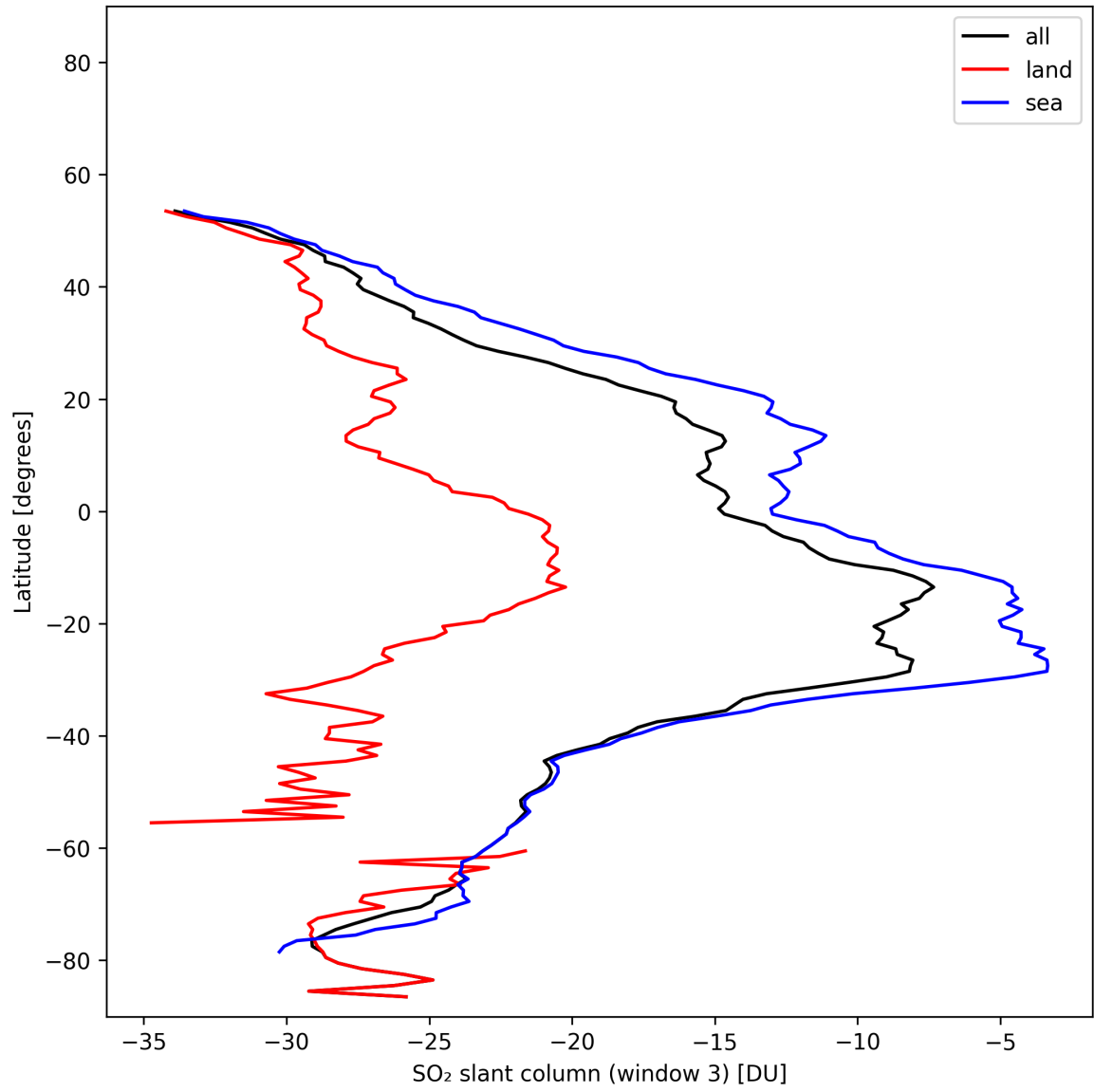
Figure 45: Zonal average of “SO 2 slant column (window 3)” for 2025-02-03 to 2025-02-04.
