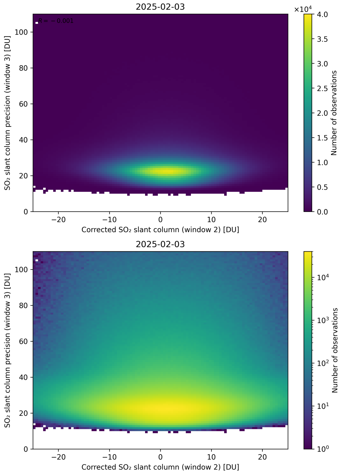
Figure 252: Scatter density plot of “Corrected SO 2 slant column (window 2)” against “SO 2 slant column precision (window 3)” for 2025-02-03 to 2025-02-04.
