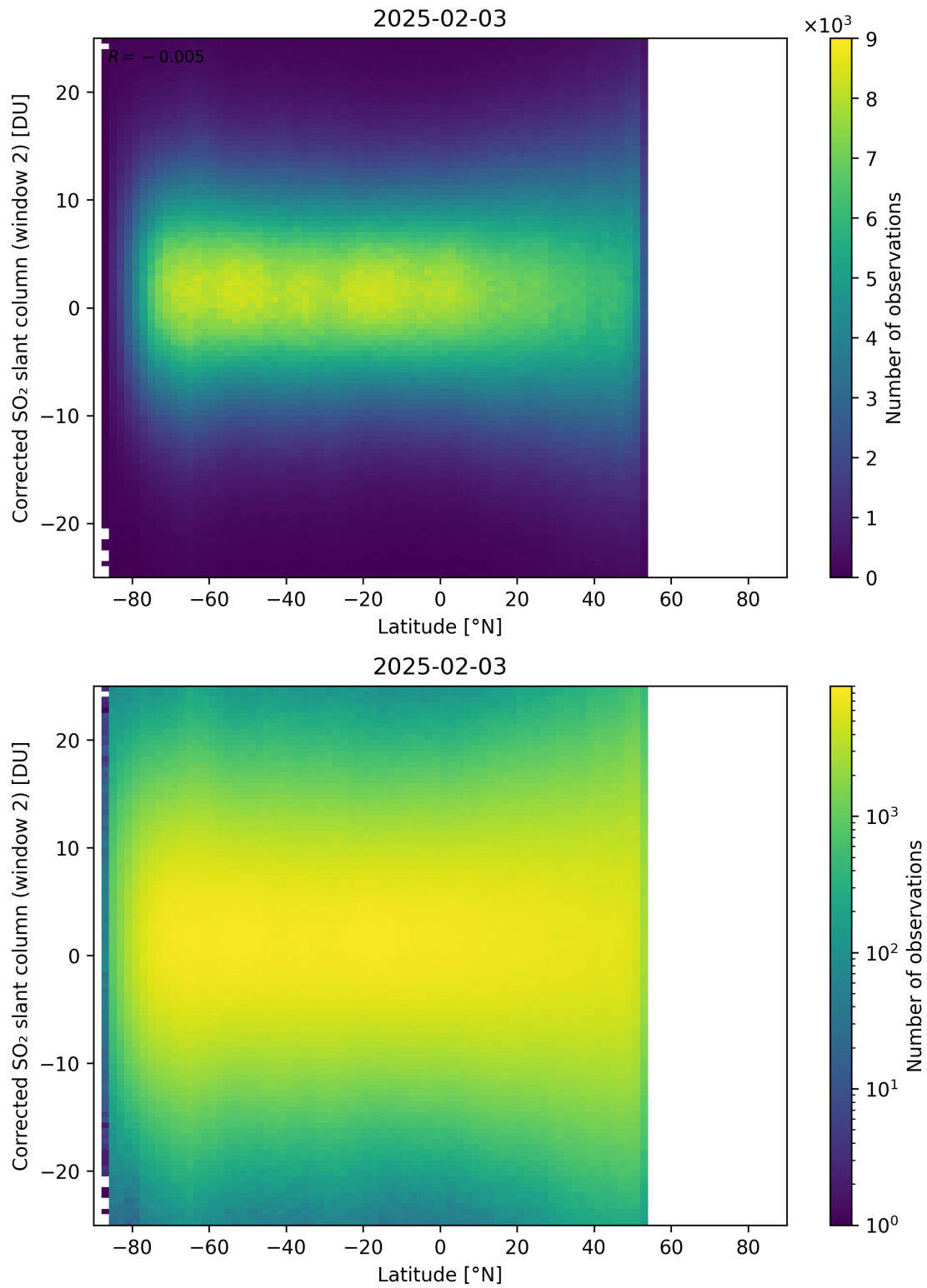
Figure 160: Scatter density plot of “Latitude” against “Corrected SO 2 slant column (window 2)” for 2025-02-03 to 2025-02-04.
