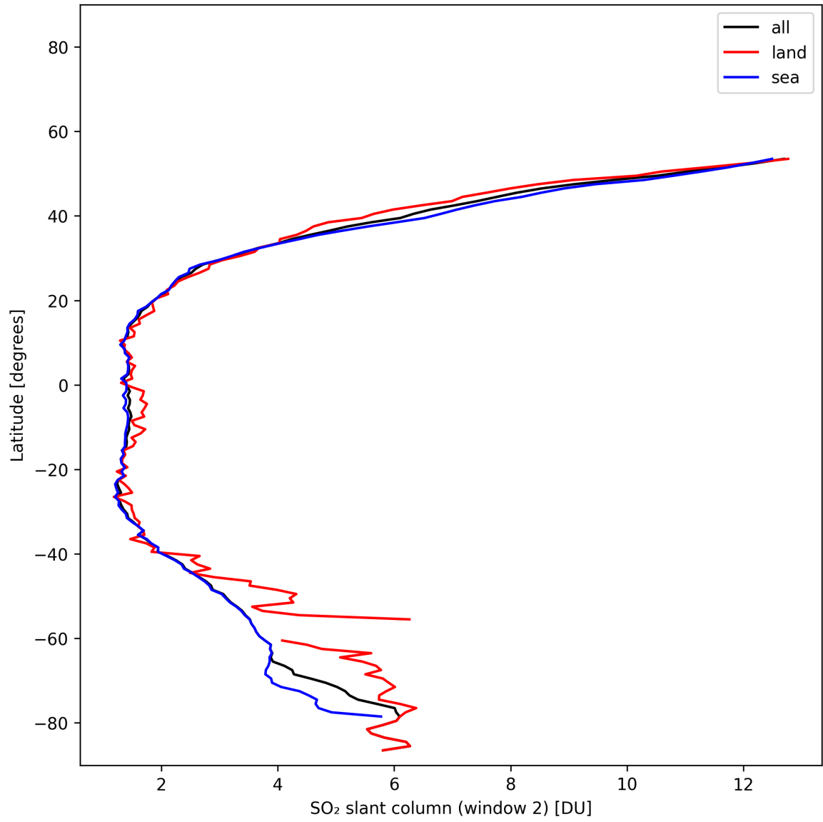
Figure 41: Zonal average of “SO 2 slant column (window 2)” for 2025-02-03 to 2025-02-04.
