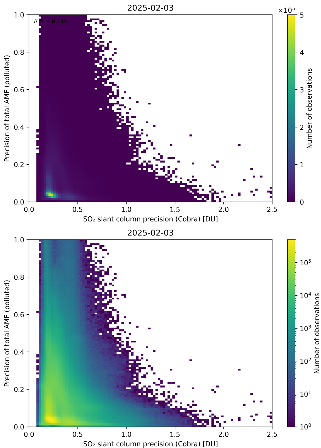
Figure 214: Scatter density plot of “SO 2 slant column precision (Cobra)” against “Precision of total AMF (polluted)” for 2025-02-03 to 2025-02-04.
