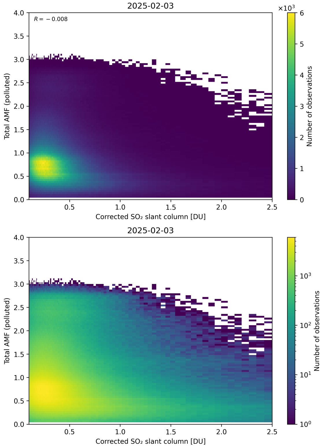
Figure 242: Scatter density plot of “Corrected SO 2 slant column” against “Total AMF (polluted)” for 2025-02-03 to 2025-02-04.
