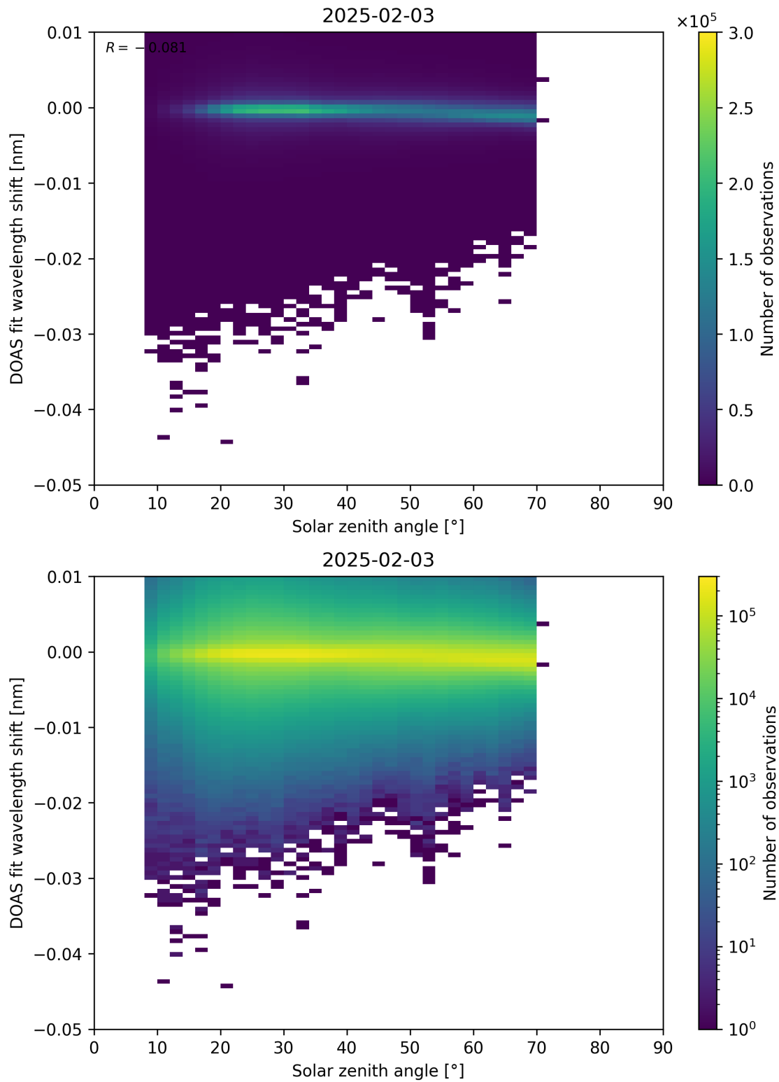
Figure 174: Scatter density plot of “Solar zenith angle” against “DOAS fit wavelength shift” for 2025-02-03 to 2025-02-04.
