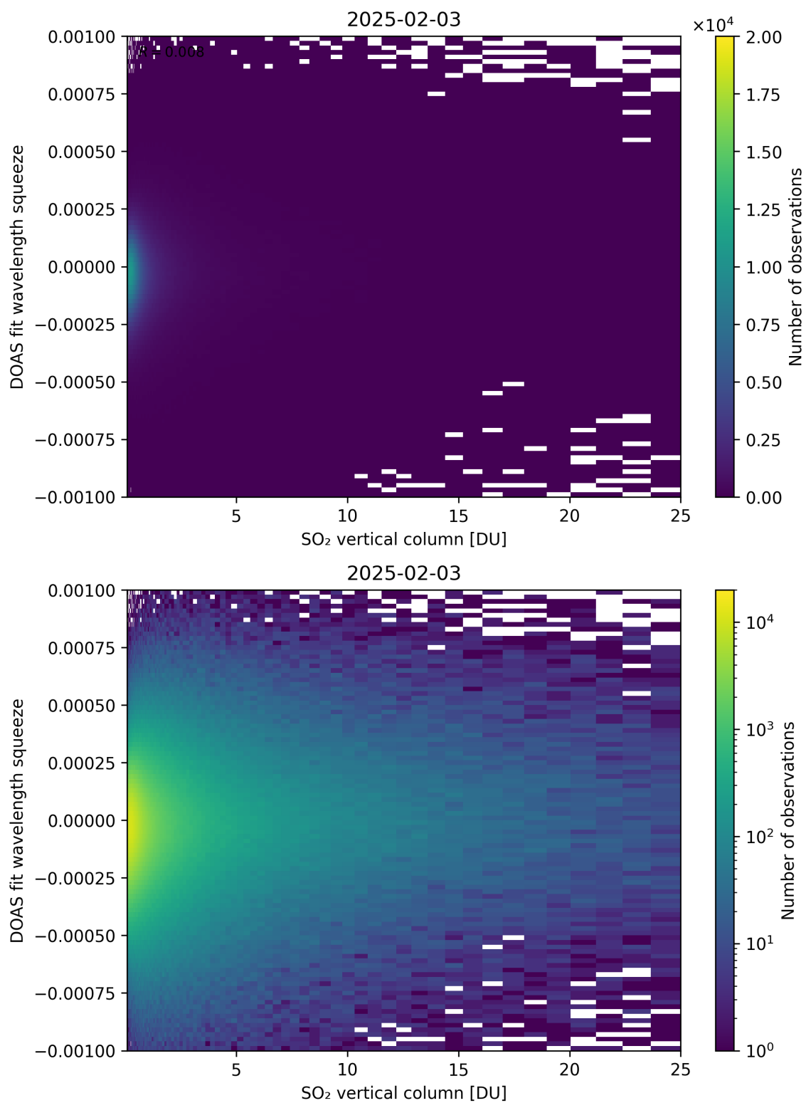
Figure 327: Scatter density plot of “SO 2 vertical column” against “DOAS fit wavelength squeeze” for 2025-02-03 to 2025-02-04.
