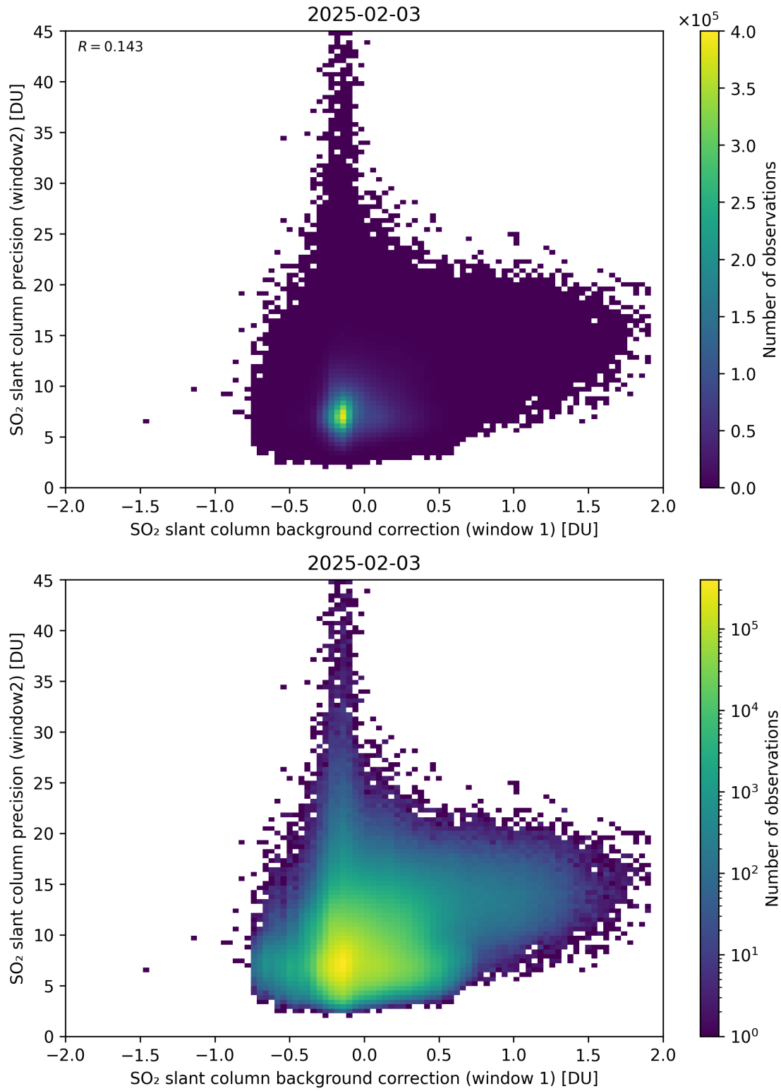
Figure 117: Scatter density plot of “SO 2 slant column background correction (window 1)” against “SO 2 slant column precision (window2)” for 2025-02-03 to 2025-02-04.
