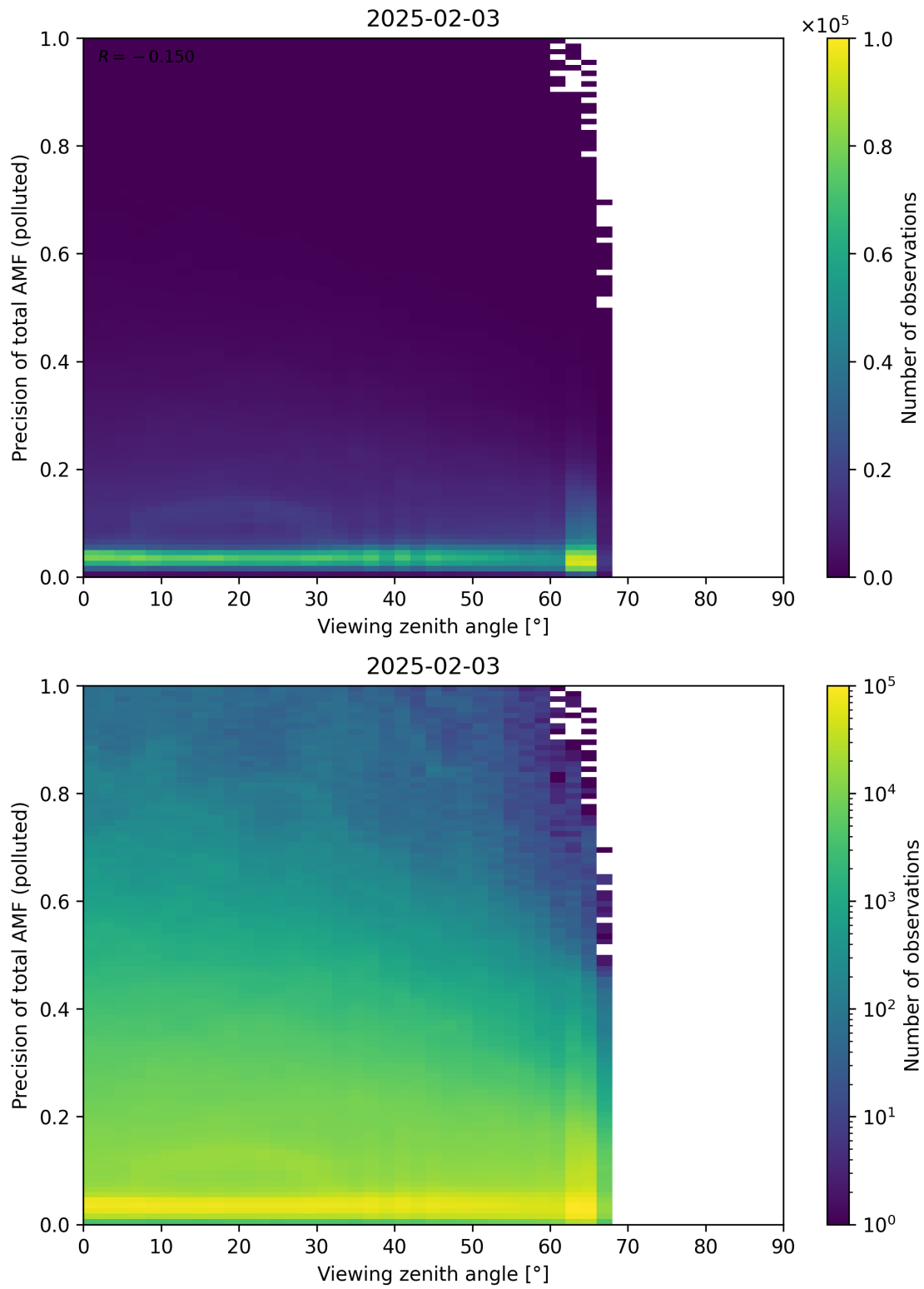
Figure 382: Scatter density plot of “Viewing zenith angle” against “Precision of total AMF (polluted)” for 2025-02-03 to 2025-02-04.
