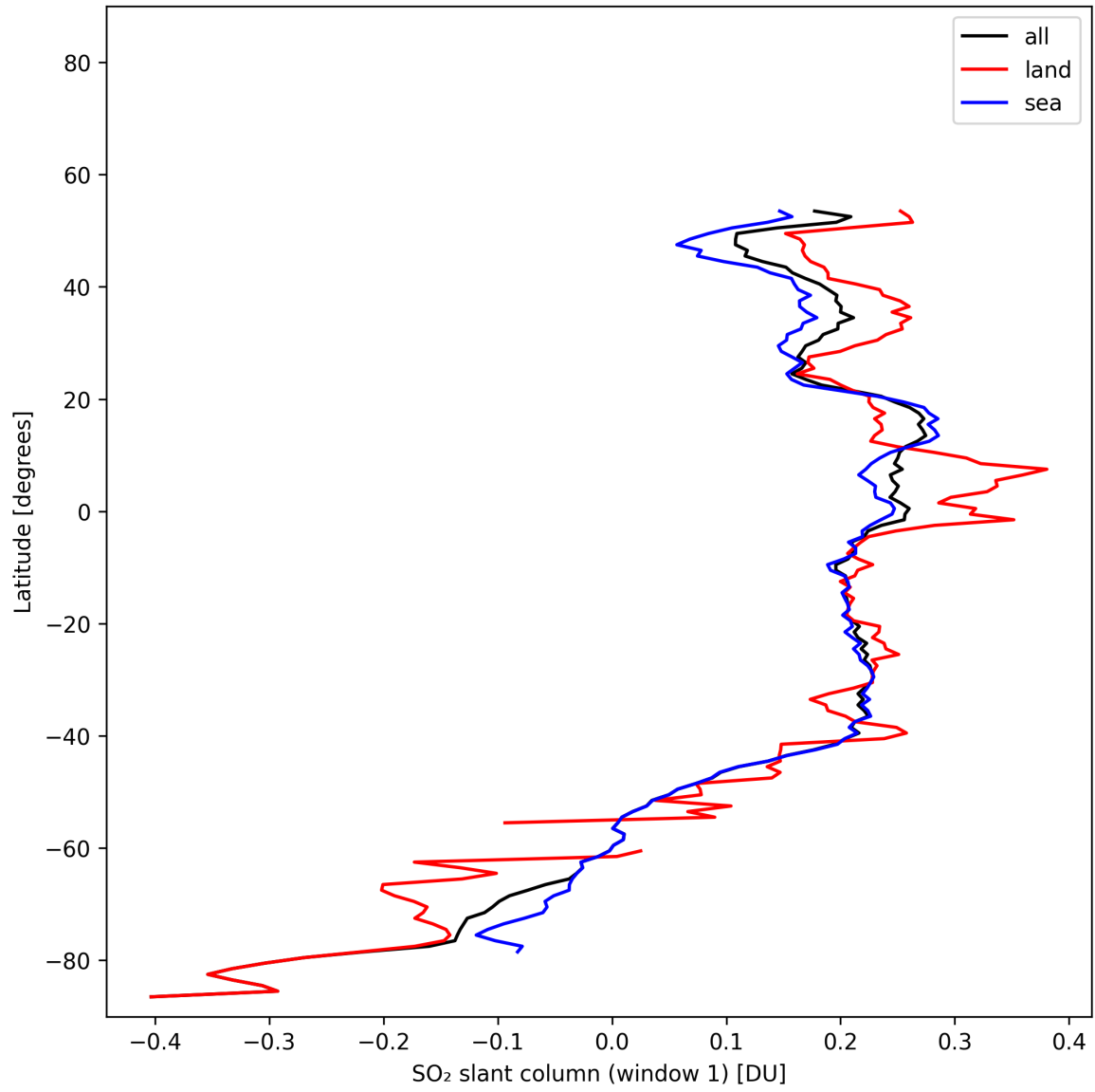
Figure 37: Zonal average of “SO 2 slant column (window 1)” for 2025-02-03 to 2025-02-04.
