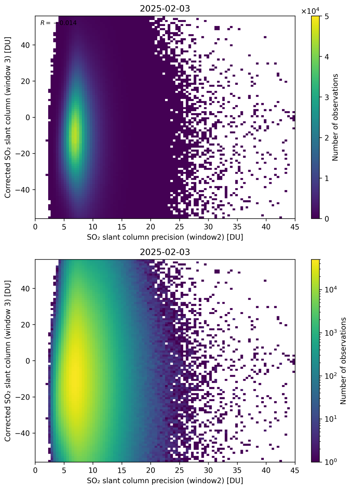
Figure 298: Scatter density plot of “SO 2 slant column precision (window2)” against “Corrected SO 2 slant column (window 3)” for 2025-02-03 to 2025-02-04.
