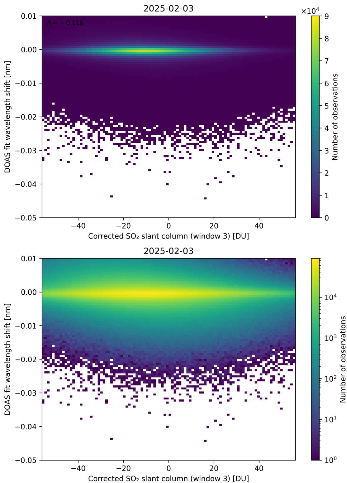
Figure 256: Scatter density plot of “Corrected SO 2 slant column (window 3)” against “DOAS fit wavelength shift” for 2025-02-03 to 2025-02-04.
