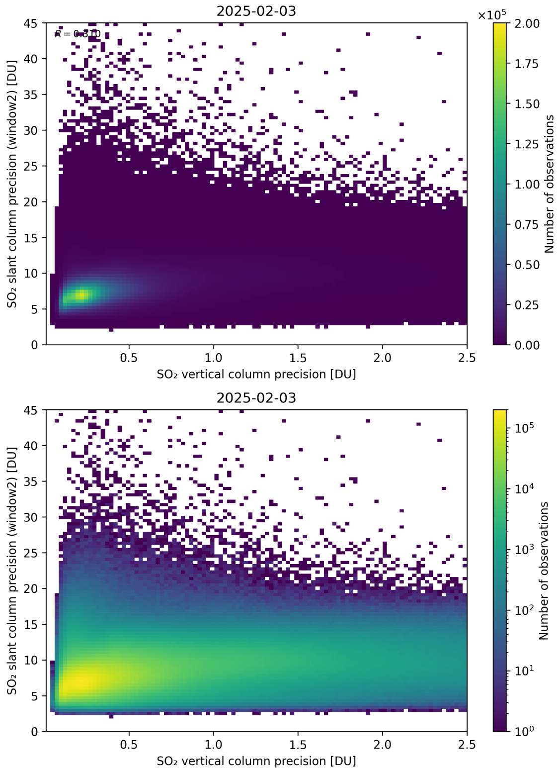
Figure 343: Scatter density plot of “SO 2 vertical column precision” against “SO 2 slant column precision (window2)” for 2025-02-03 to 2025-02-04.
