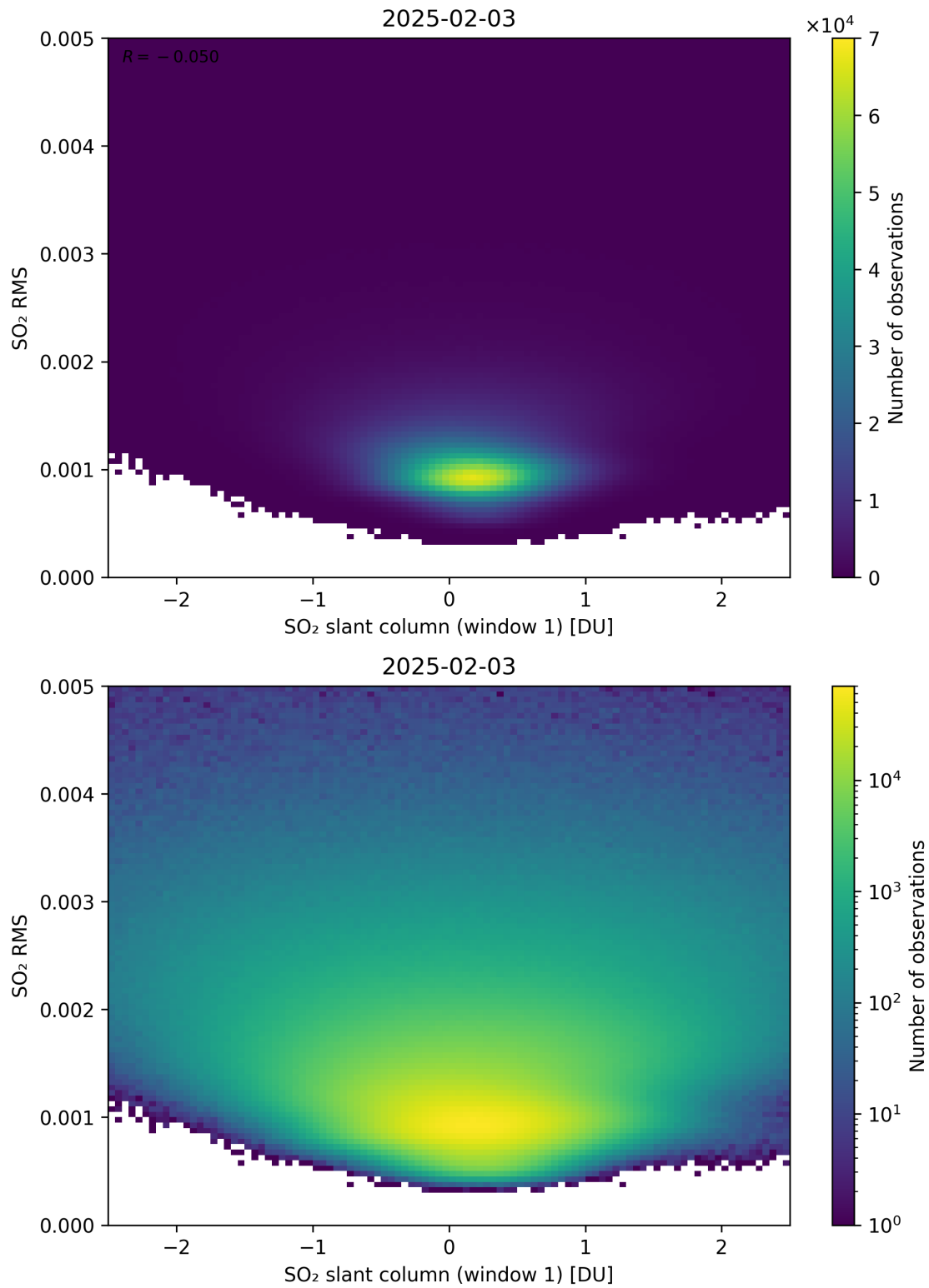
Figure 267: Scatter density plot of “SO 2 slant column (window 1)” against “SO 2 RMS” for 2025-02-03 to 2025-02-04.
