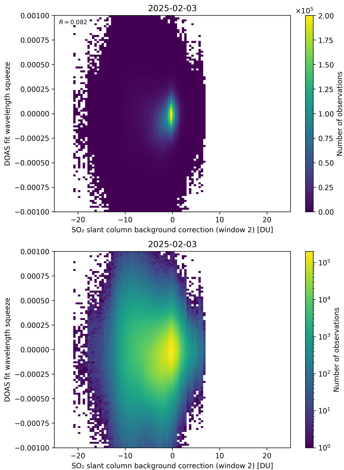
Figure 124: Scatter density plot of “SO 2 slant column background correction (window 2)” against “DOAS fit wavelength squeeze” for 2025-02-03 to 2025-02-04.
