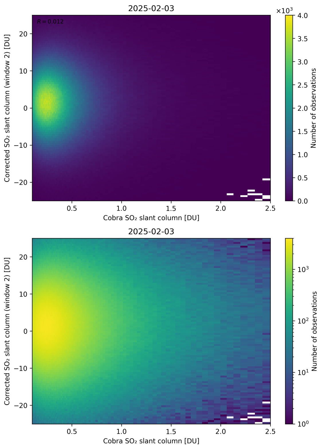
Figure 217: Scatter density plot of “Cobra SO 2 slant column” against “Corrected SO 2 slant column (window 2)” for 2025-02-03 to 2025-02-04.
