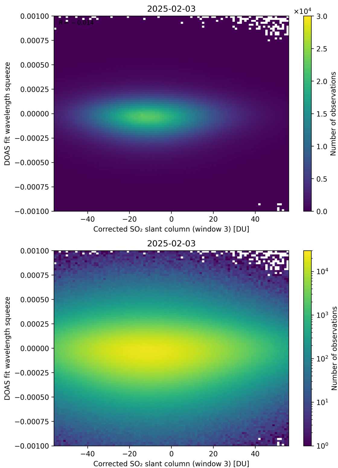
Figure 257: Scatter density plot of “Corrected SO 2 slant column (window 3)” against “DOAS fit wavelength squeeze” for 2025-02-03 to 2025-02-04.
