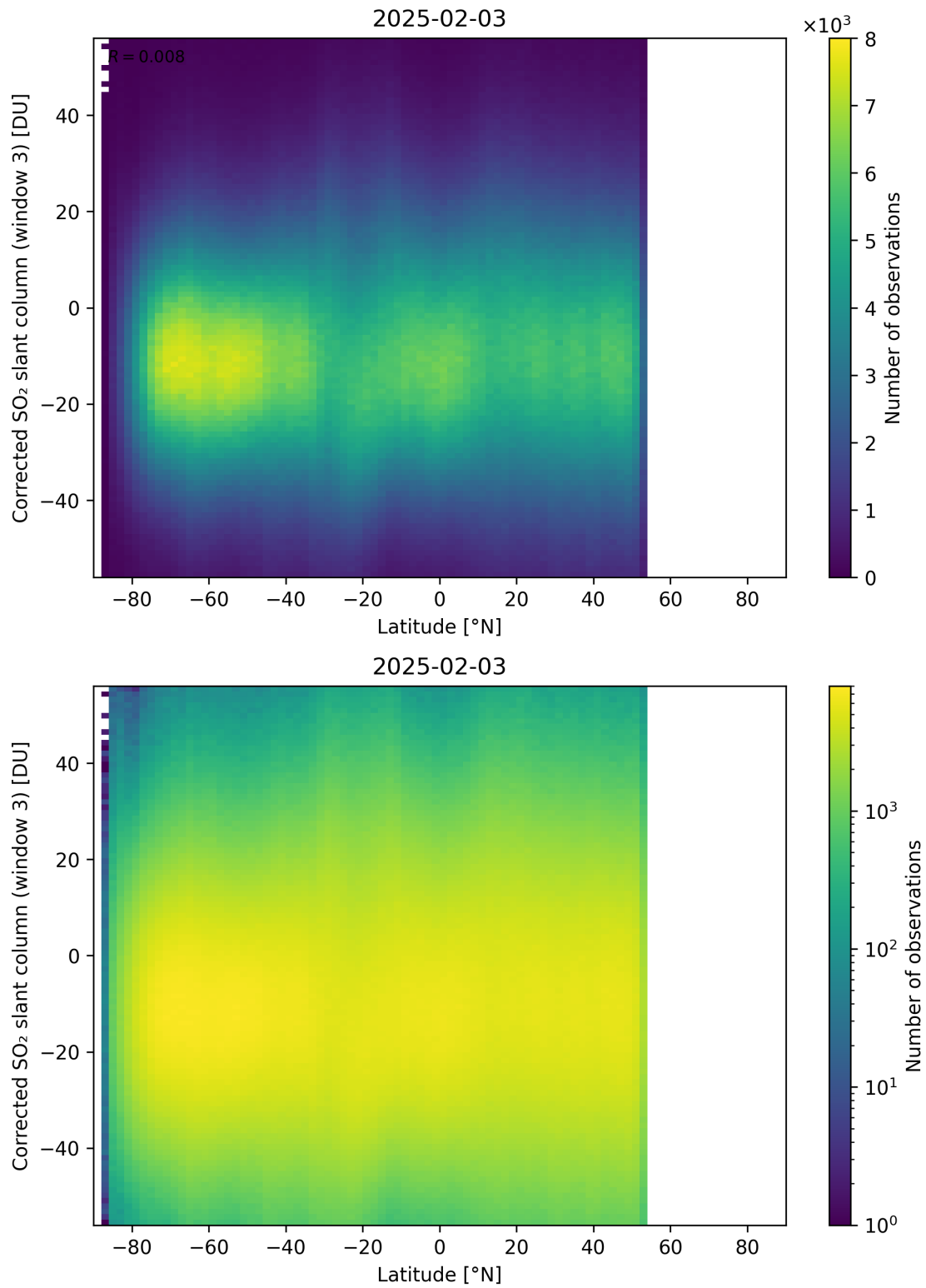
Figure 161: Scatter density plot of “Latitude” against “Corrected SO 2 slant column (window 3)” for 2025-02-03 to 2025-02-04.
