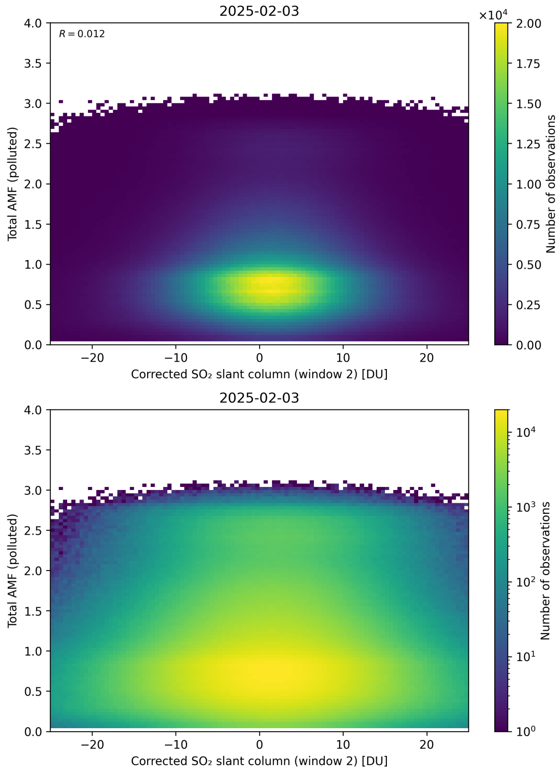
Figure 253: Scatter density plot of “Corrected SO 2 slant column (window 2)” against “Total AMF (polluted)” for 2025-02-03 to 2025-02-04.
