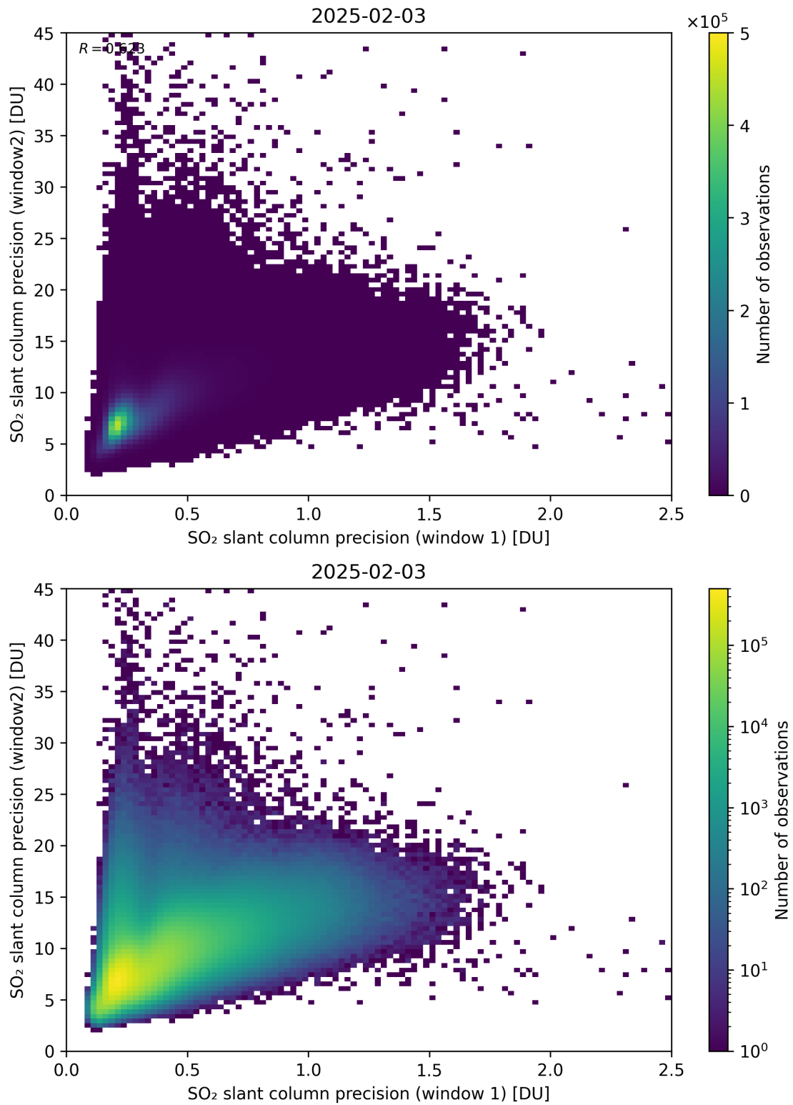
Figure 277: Scatter density plot of “SO 2 slant column precision (window 1)” against “SO 2 slant column precision (window2)” for 2025-02-03 to 2025-02-04.
