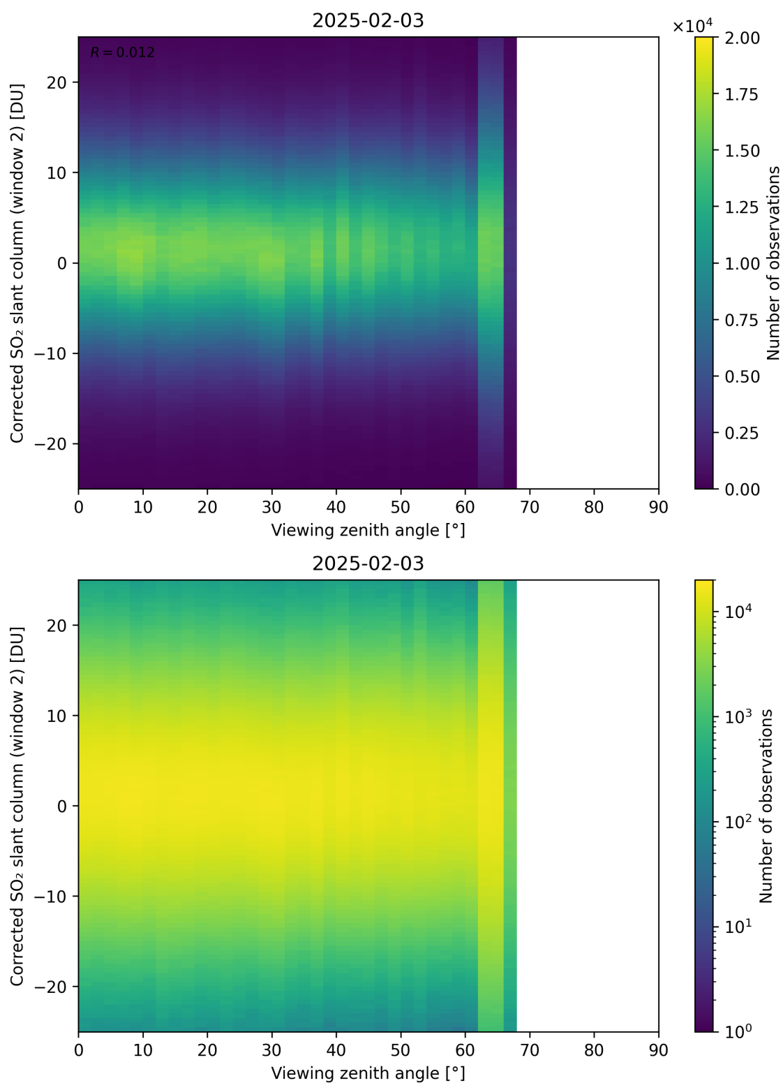
Figure 374: Scatter density plot of “Viewing zenith angle” against “Corrected SO 2 slant column (window 2)” for 2025-02-03 to 2025-02-04.
