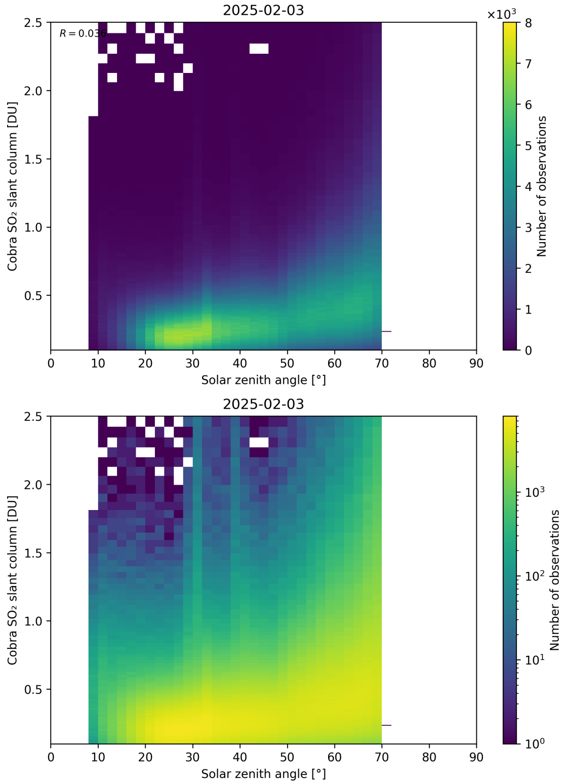
Figure 179: Scatter density plot of “Solar zenith angle” against “Cobra SO 2 slant column” for 2025-02-03 to 2025-02-04.
