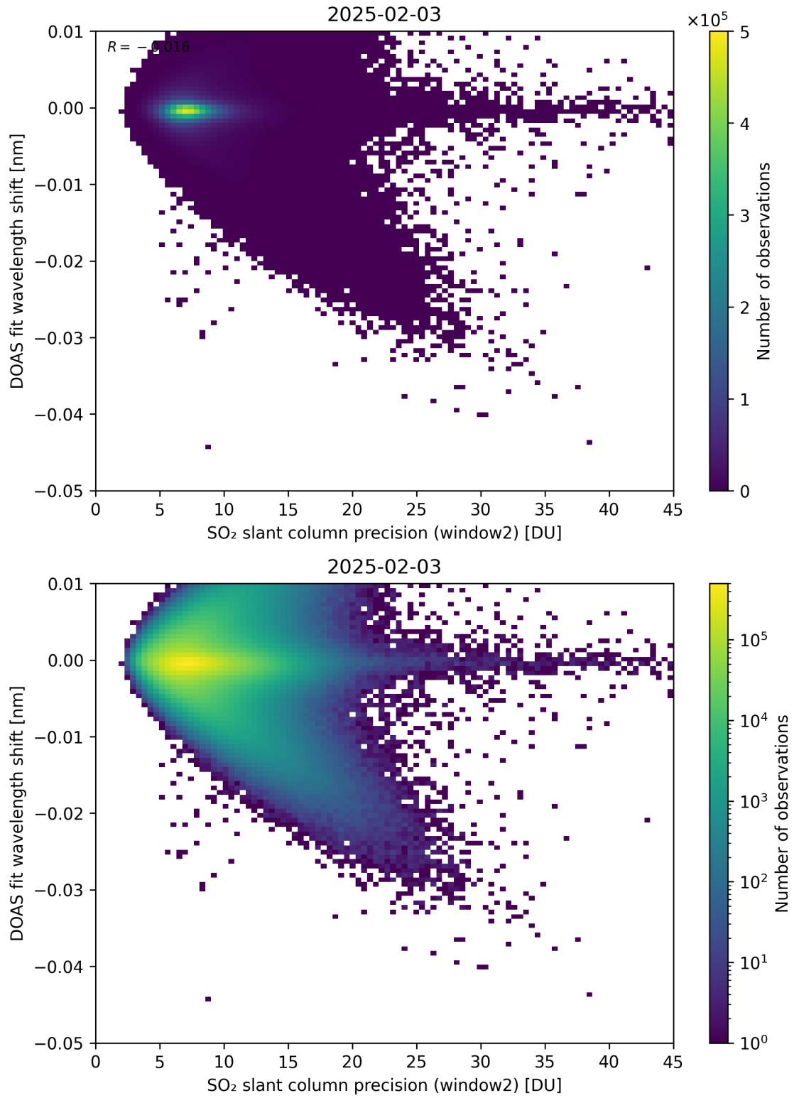
Figure 293: Scatter density plot of “SO 2 slant column precision (window2)” against “DOAS fit wavelength shift” for 2025-02-03 to 2025-02-04.
