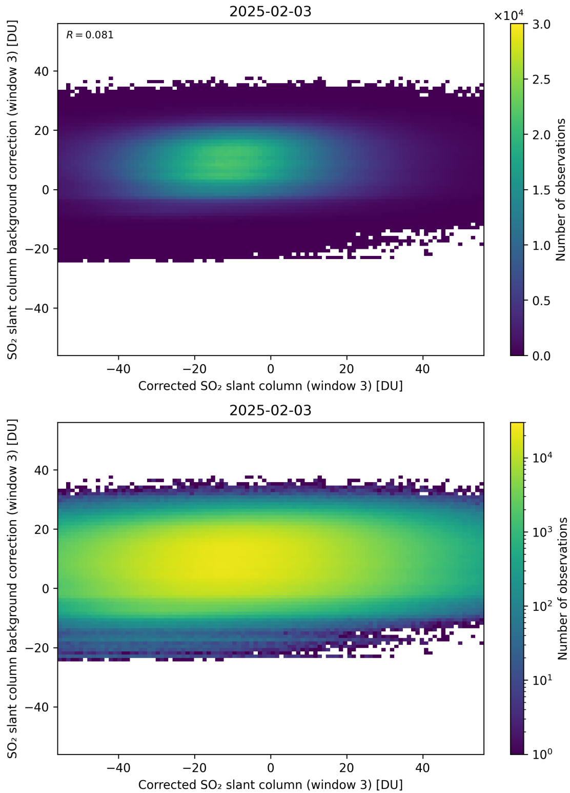
Figure 255: Scatter density plot of “Corrected SO 2 slant column (window 3)” against “SO 2 slant column background correction (window 3)” for 2025-02-03 to 2025-02-04.
