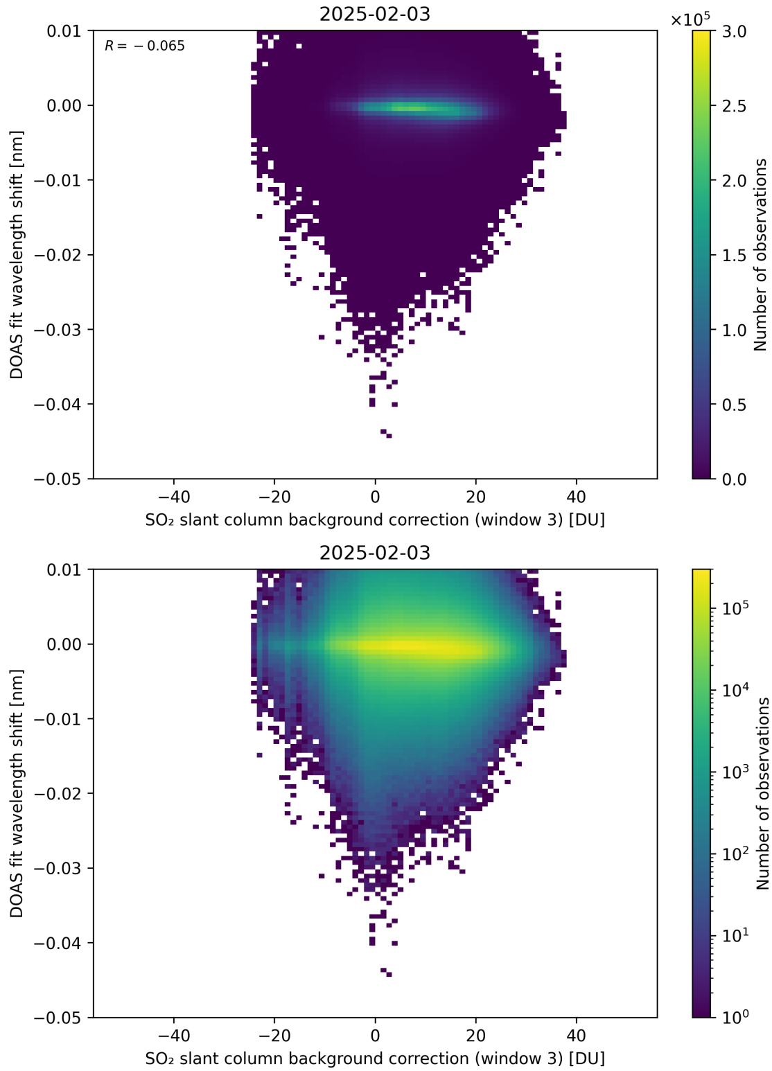
Figure 132: Scatter density plot of “SO 2 slant column background correction (window 3)” against “DOAS fit wavelength shift” for 2025-02-03 to 2025-02-04.
