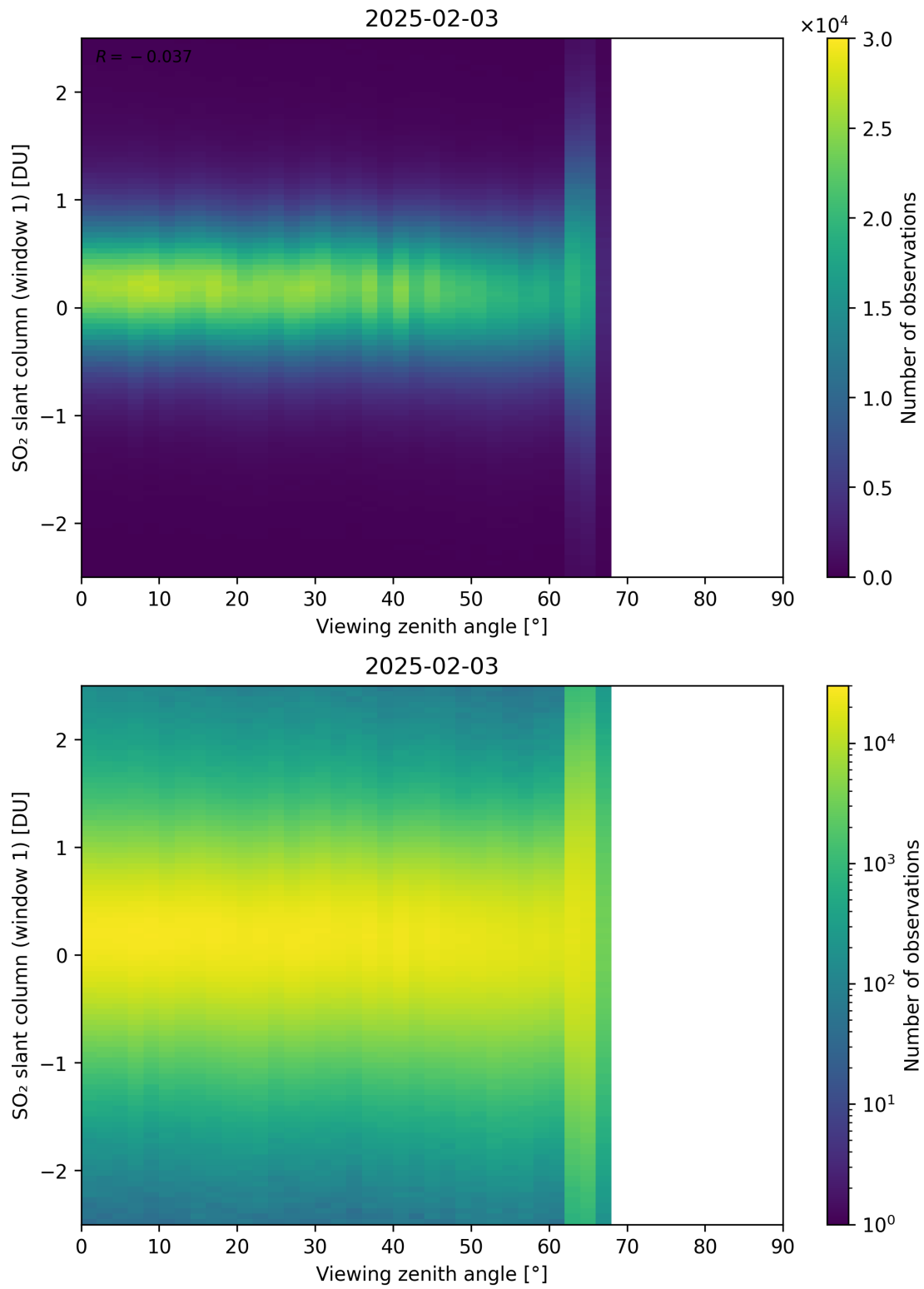
Figure 376: Scatter density plot of “Viewing zenith angle” against “SO 2 slant column (window 1)” for 2025-02-03 to 2025-02-04.
