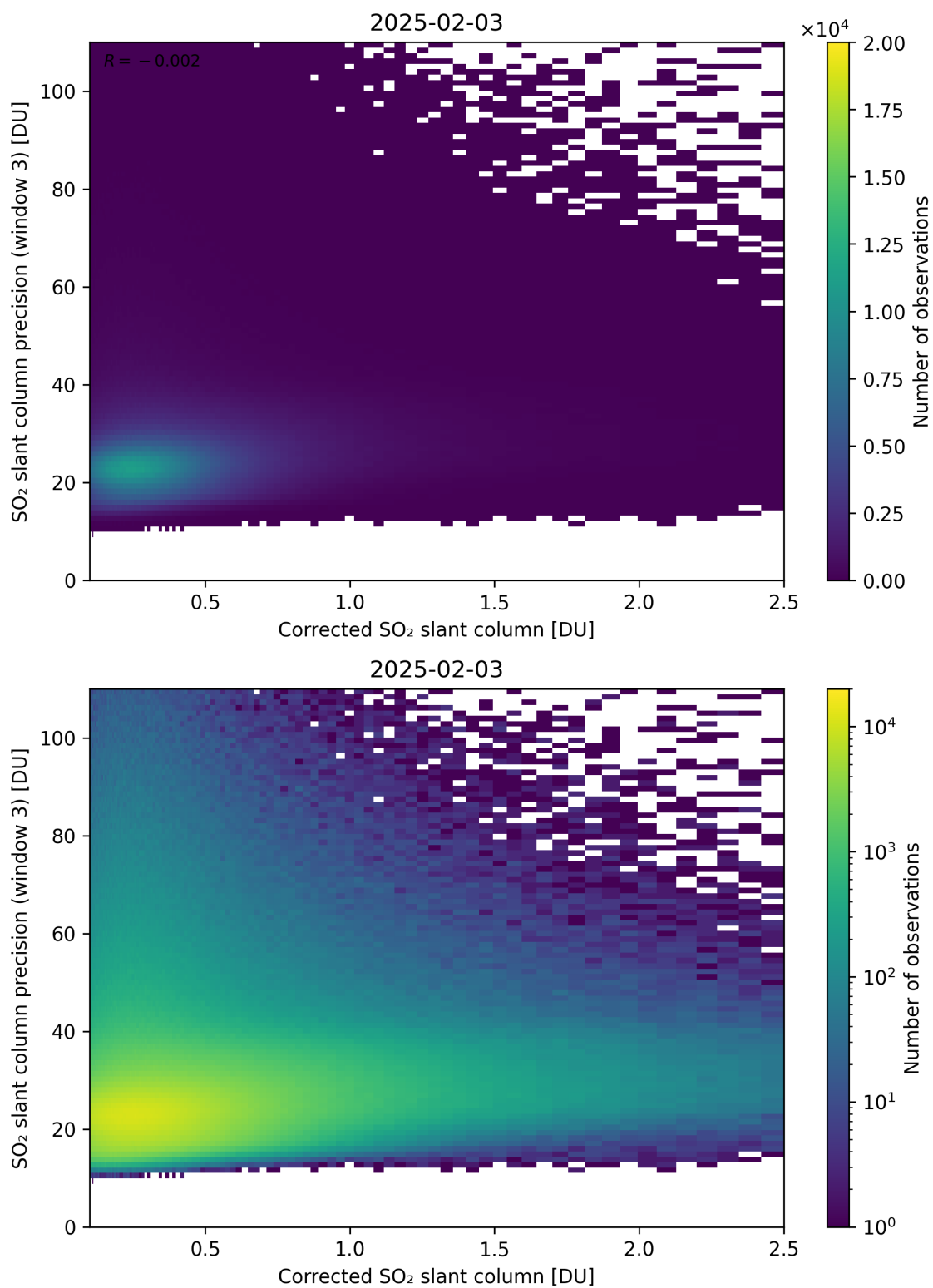
Figure 241: Scatter density plot of “Corrected SO 2 slant column” against “SO 2 slant column precision (window 3)” for 2025-02-03 to 2025-02-04.
