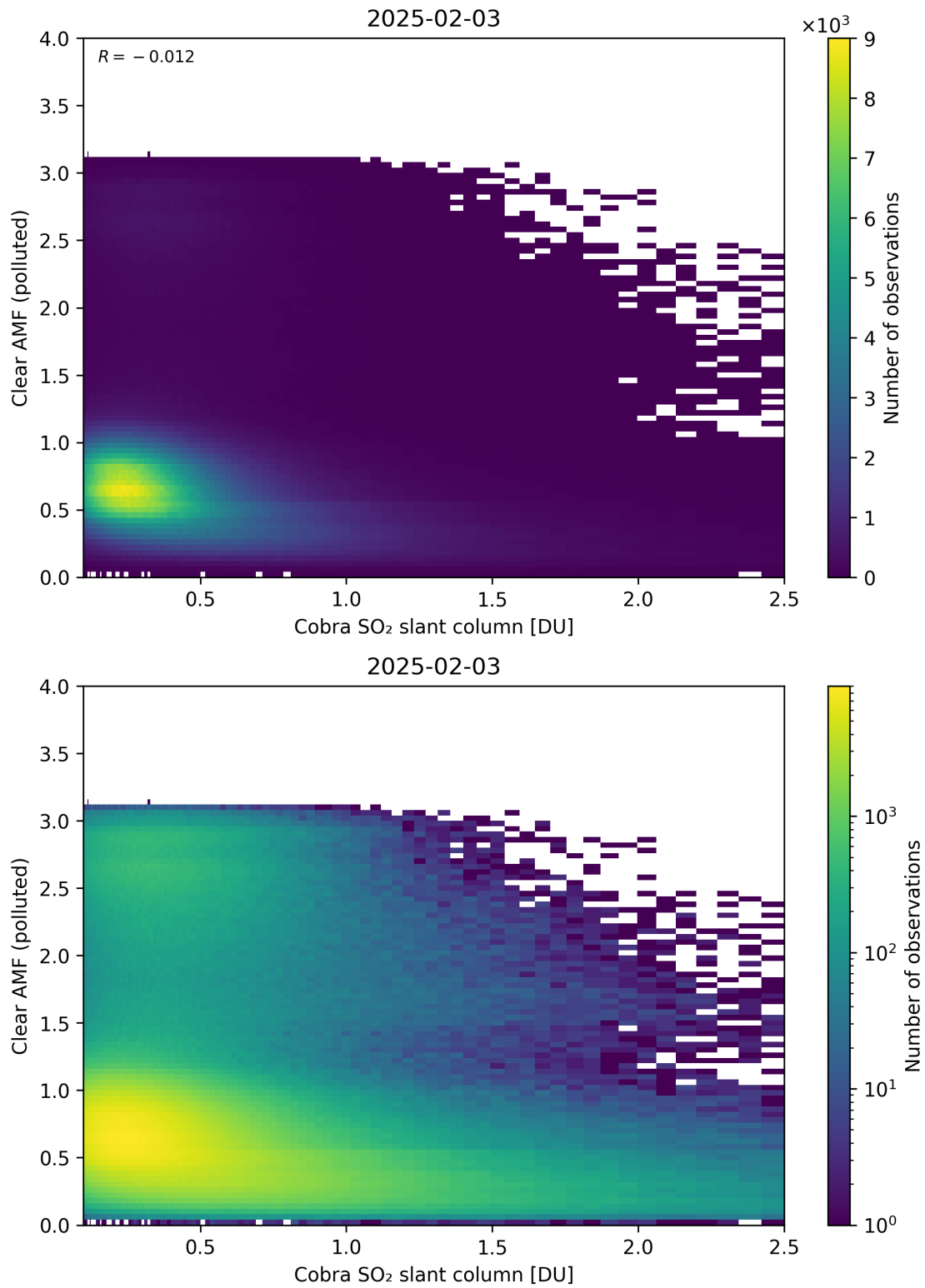
Figure 215: Scatter density plot of “Cobra SO 2 slant column” against “Clear AMF (polluted)” for 2025-02-03 to 2025-02-04.
