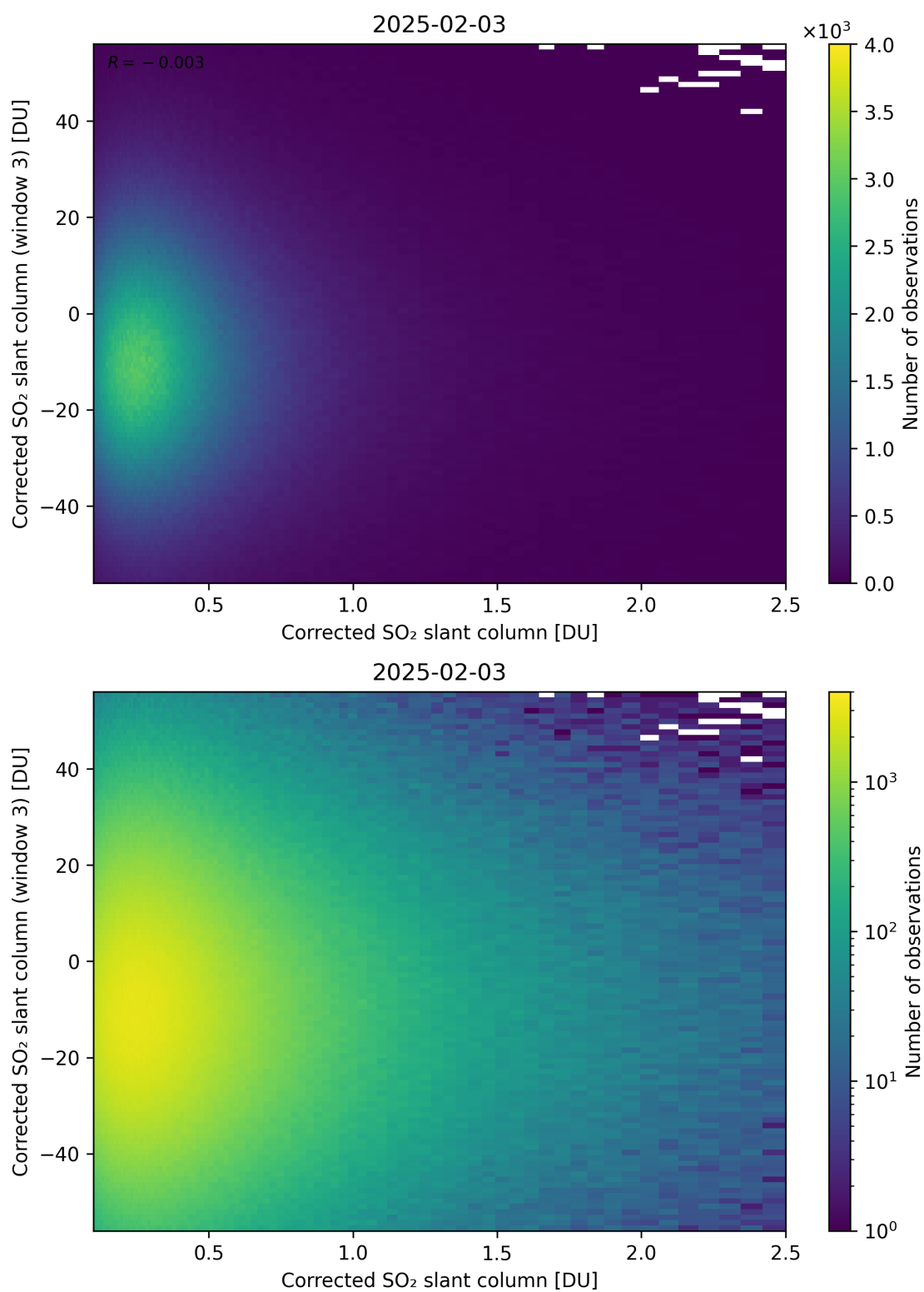
Figure 236: Scatter density plot of “Corrected SO 2 slant column” against “Corrected SO 2 slant column (window 3)” for 2025-02-03 to 2025-02-04.
