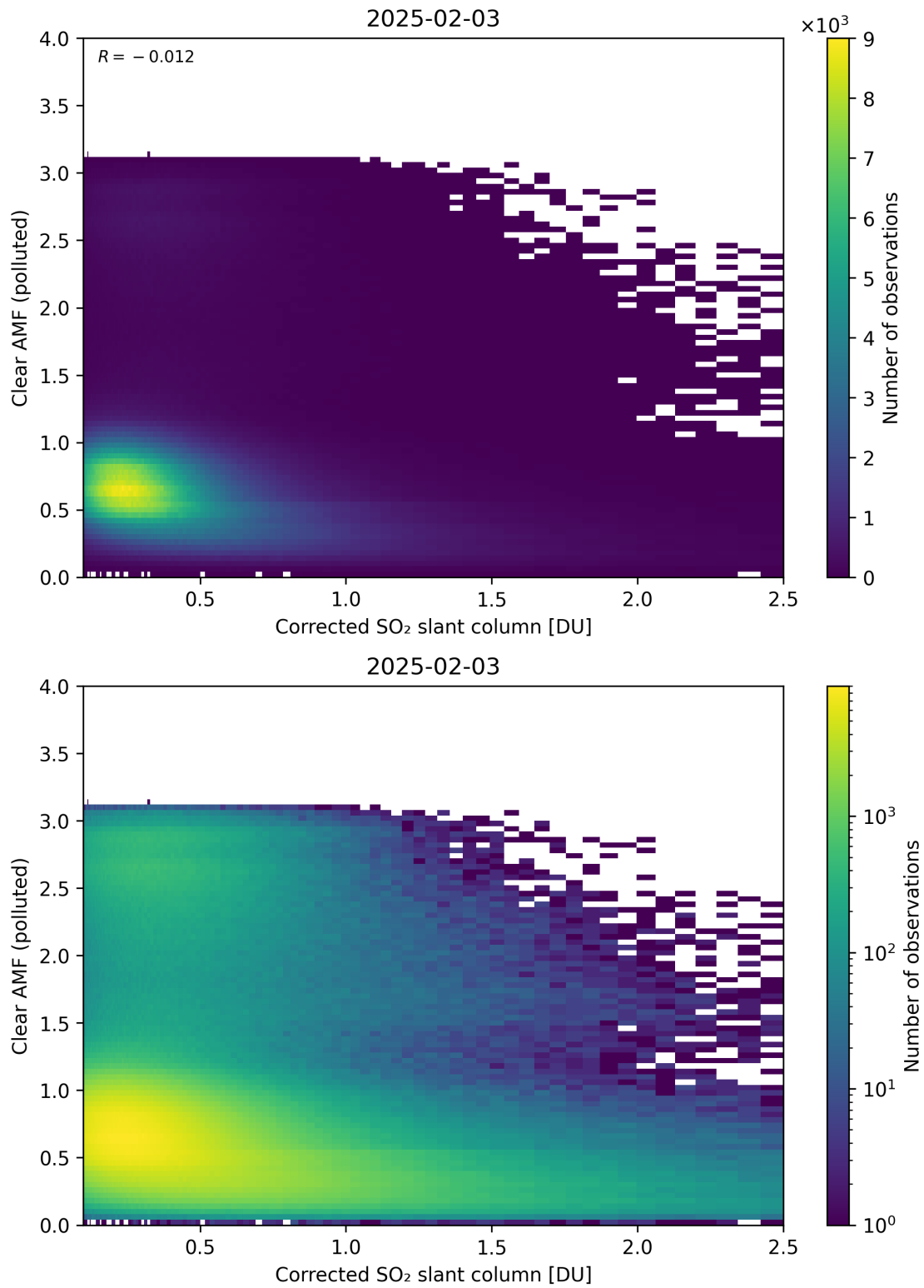
Figure 232: Scatter density plot of “Corrected SO 2 slant column” against “Clear AMF (polluted)” for 2025-02-03 to 2025-02-04.
