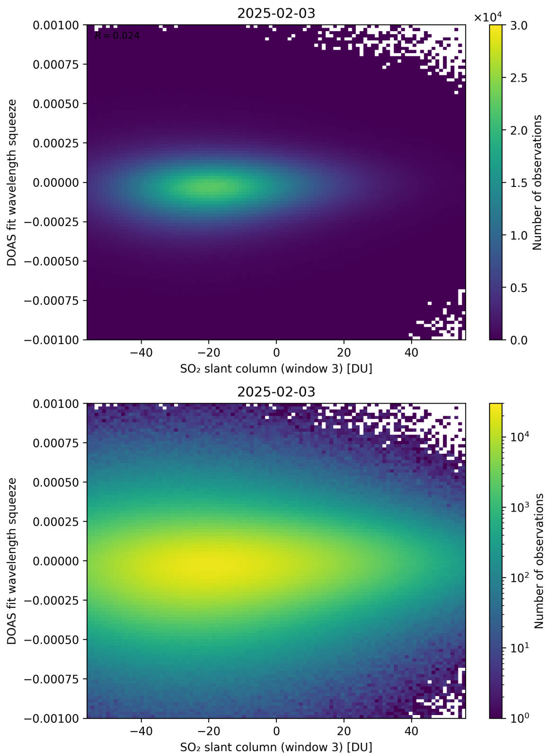
Figure 305: Scatter density plot of “SO 2 slant column (window 3)” against “DOAS fit wavelength squeeze” for 2025-02-03 to 2025-02-04.
