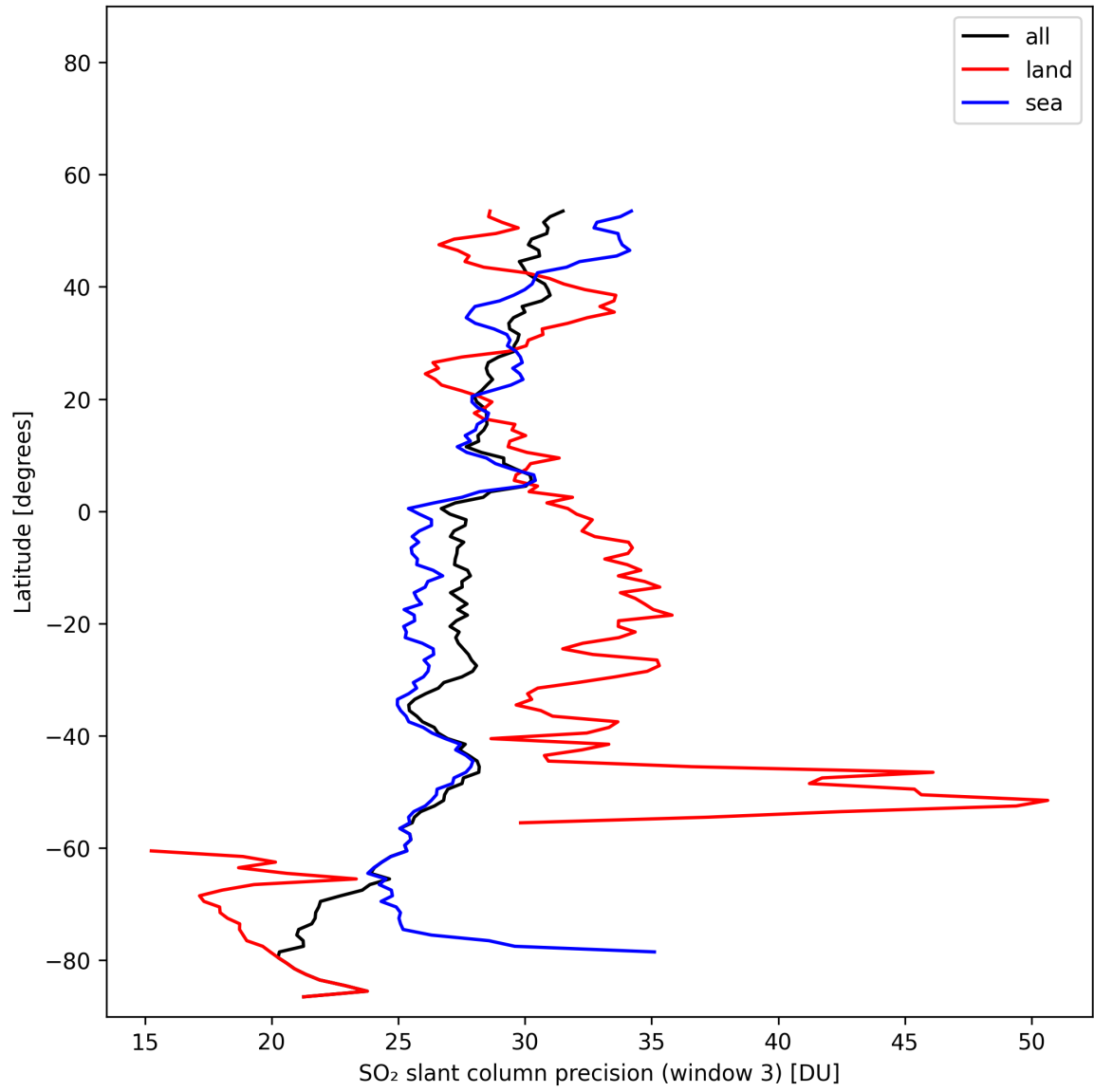
Figure 46: Zonal average of “SO 2 slant column precision (window 3)” for 2025-02-03 to 2025-02-04.
