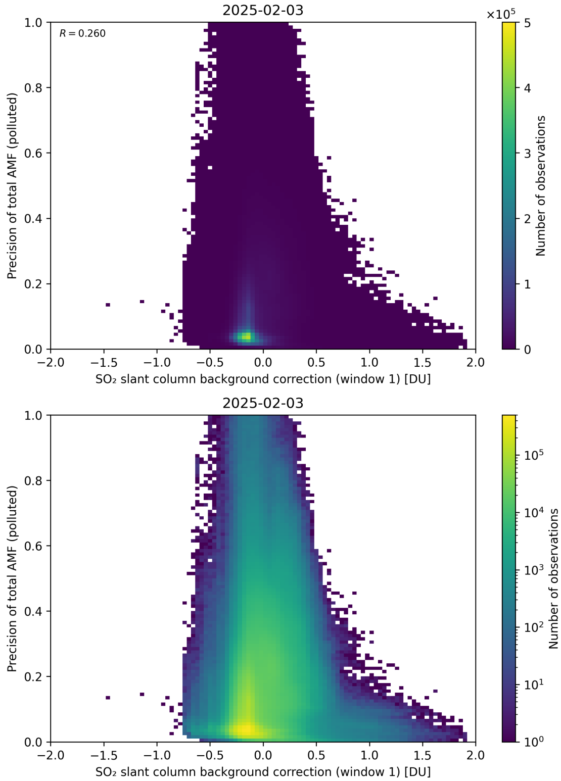
Figure 121: Scatter density plot of “SO 2 slant column background correction (window 1)” against “Precision of total AMF (polluted)” for 2025-02-03 to 2025-02-04.
