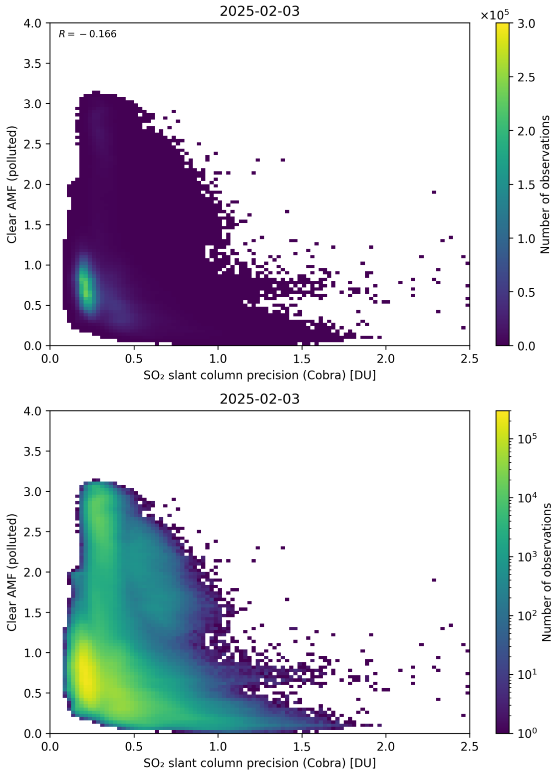
Figure 205: Scatter density plot of “SO 2 slant column precision (Cobra)” against “Clear AMF (polluted)” for 2025-02-03 to 2025-02-04.
