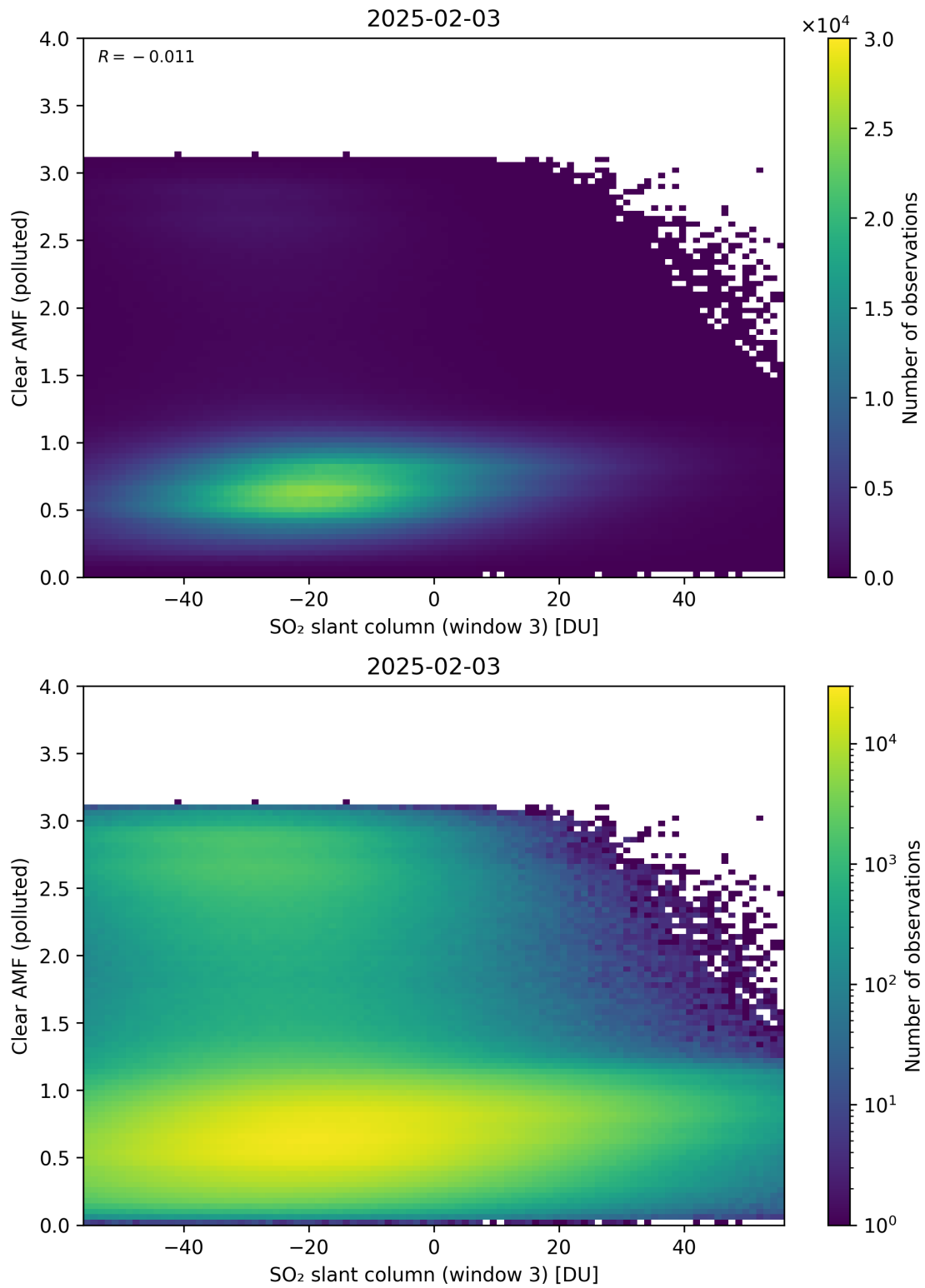
Figure 315: Scatter density plot of “SO 2 slant column (window 3)” against “Clear AMF (polluted)” for 2025-02-03 to 2025-02-04.
