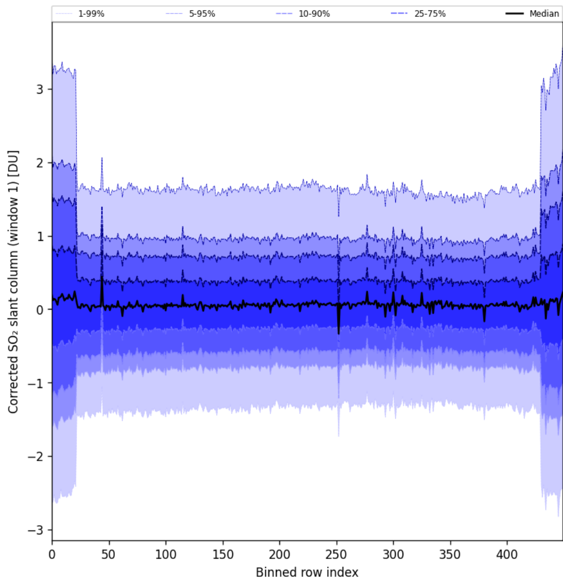
Figure 91: Along track statistics of “Corrected SO 2 slant column (window 1)” for 2025-02-03 to 2025-02-04
