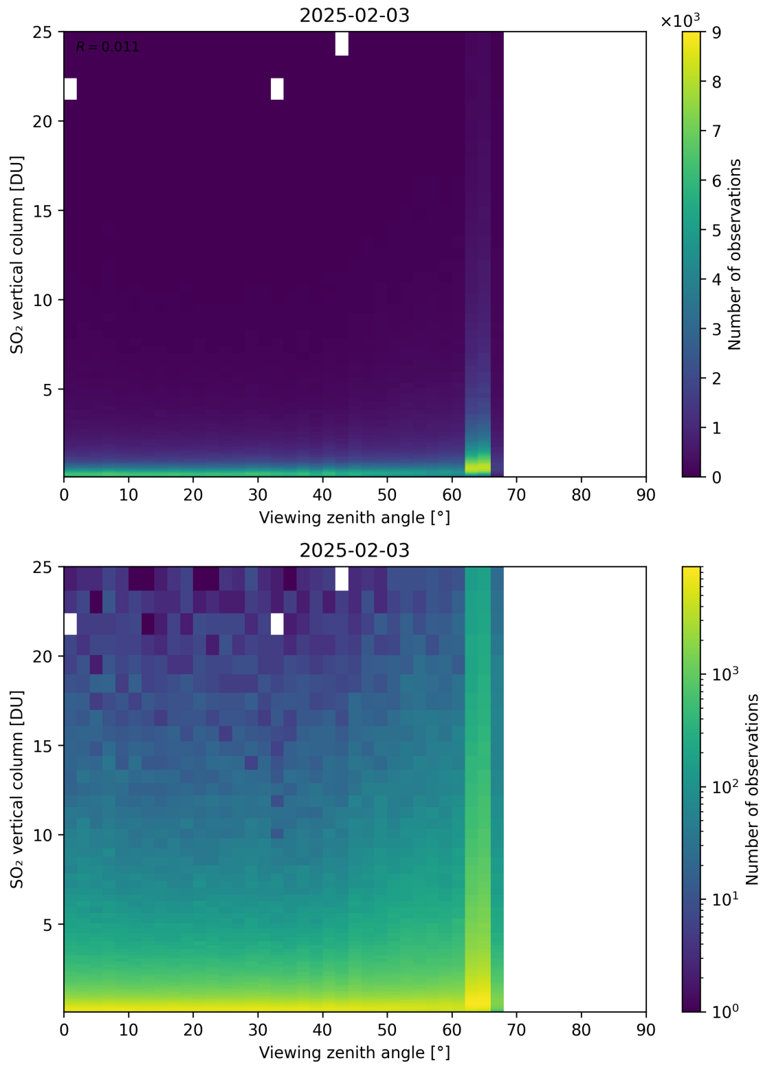
Figure 383: Scatter density plot of “Viewing zenith angle” against “SO 2 vertical column” for 2025-02-03 to 2025-02-04.
