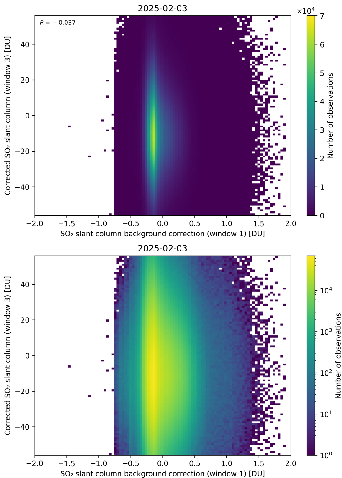
Figure 116: Scatter density plot of “SO 2 slant column background correction (window 1)” against “Corrected SO 2 slant column (window 3)” for 2025-02-03 to 2025-02-04.
