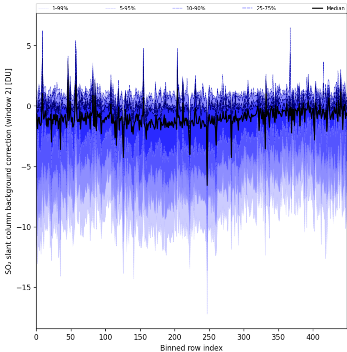
Figure 96: Along track statistics of “SO 2 slant column background correction (window 2)” for 2025-02-03 to 2025-02-04
