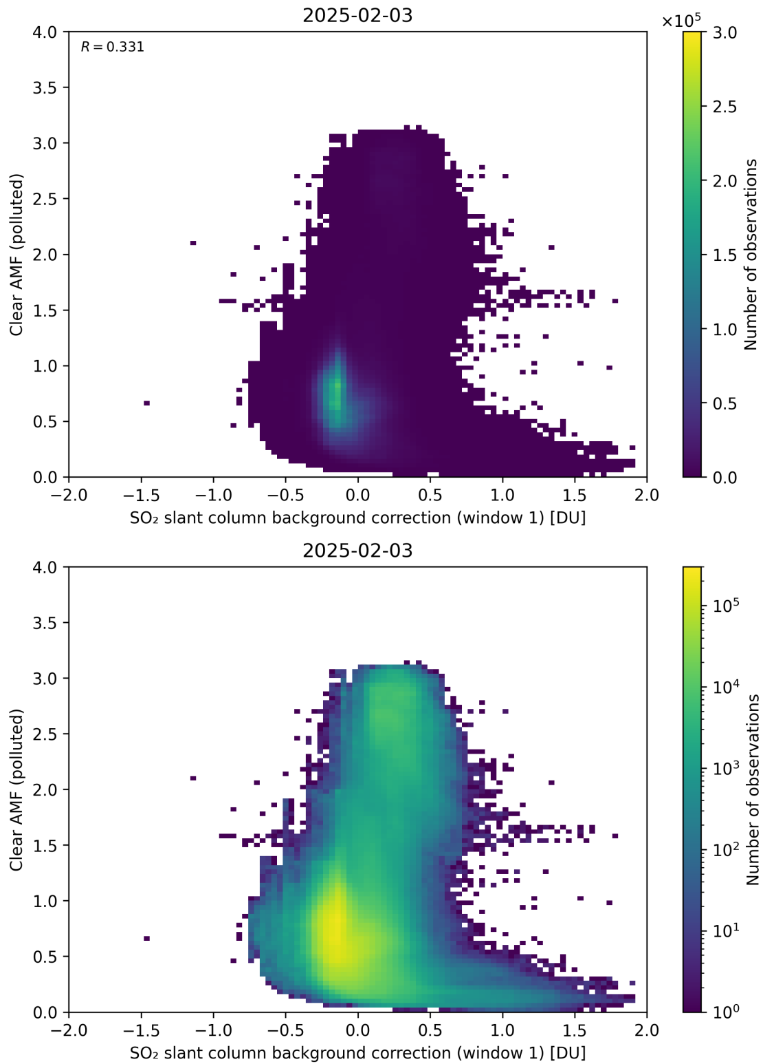
Figure 114: Scatter density plot of “SO 2 slant column background correction (window 1)” against “Clear AMF (polluted)” for 2025-02-03 to 2025-02-04.
