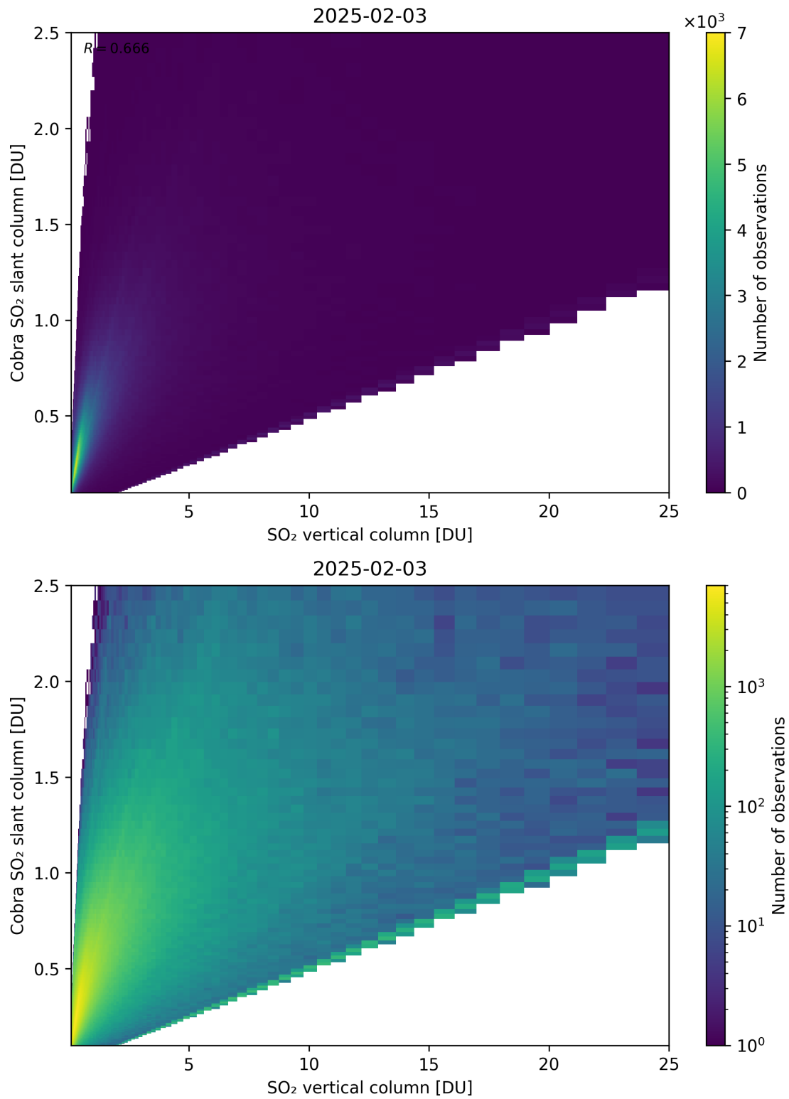
Figure 349: Scatter density plot of “SO 2 vertical column” against “Cobra SO 2 slant column” for 2025-02-03 to 2025-02-04.
