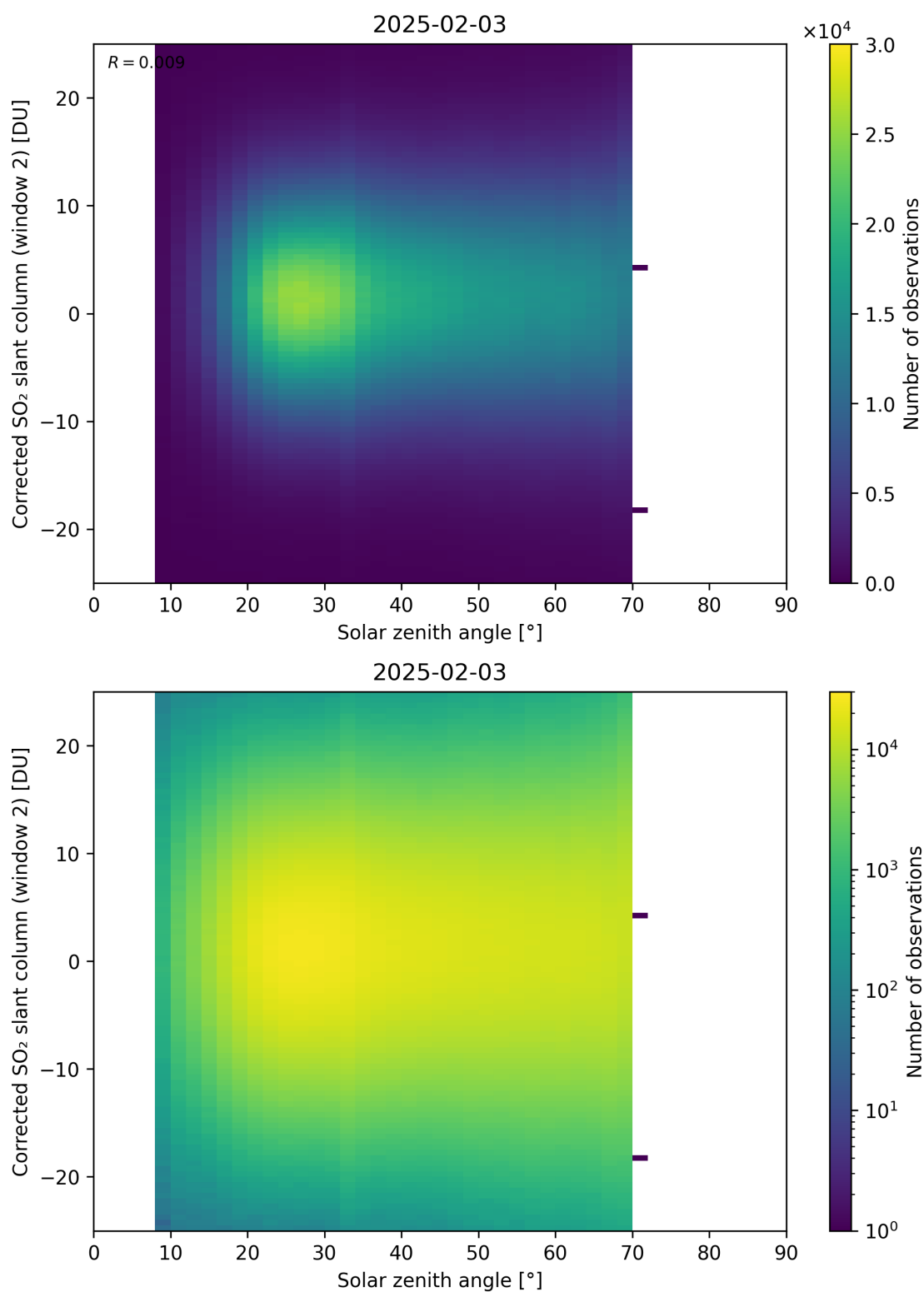
Figure 182: Scatter density plot of “Solar zenith angle” against “Corrected SO 2 slant column (window 2)” for 2025-02-03 to 2025-02-04.
