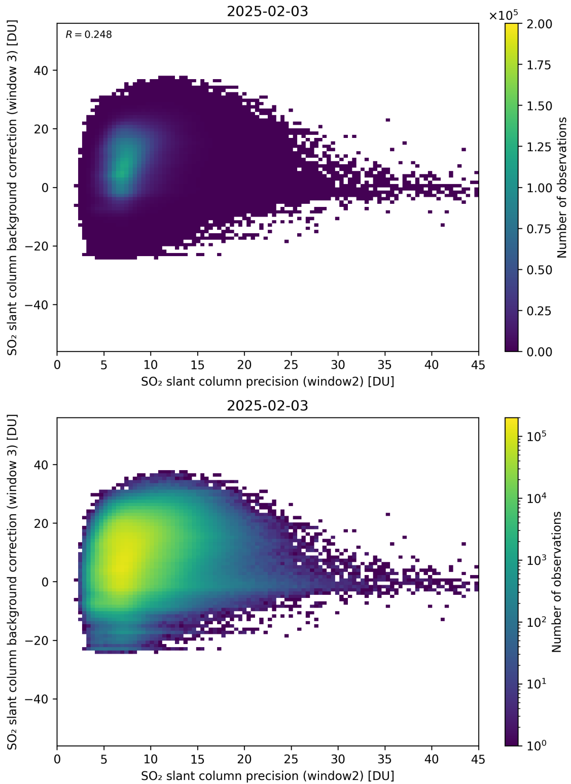
Figure 292: Scatter density plot of “SO 2 slant column precision (window2)” against “SO 2 slant column background correction (window 3)” for 2025-02-03 to 2025-02-04.
