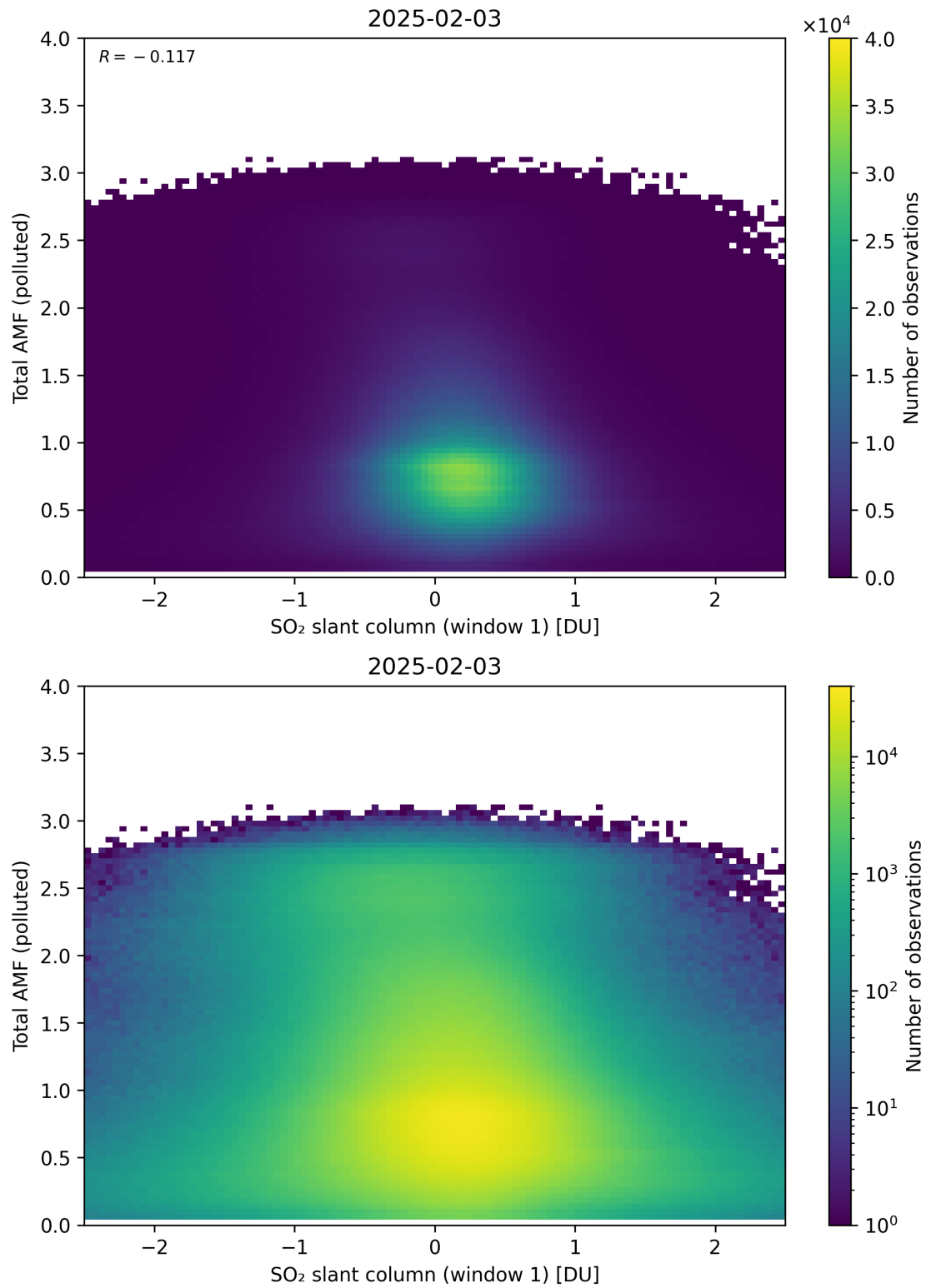
Figure 289: Scatter density plot of “SO 2 slant column (window 1)” against “Total AMF (polluted)” for 2025-02-03 to 2025-02-04.
