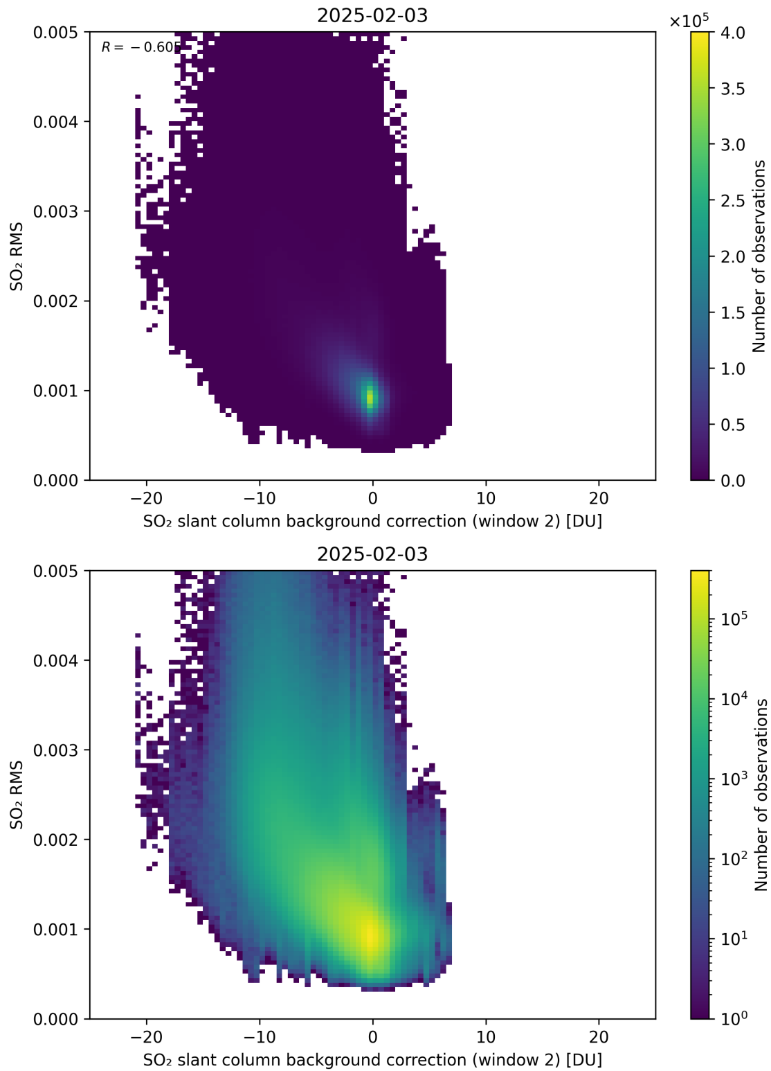
Figure 125: Scatter density plot of “SO 2 slant column background correction (window 2)” against “SO 2 RMS” for 2025-02-03 to 2025-02-04.
