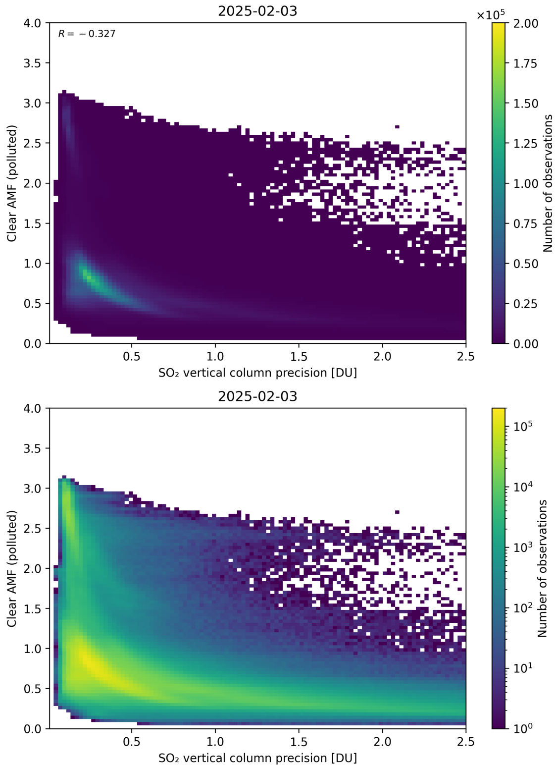
Figure 335: Scatter density plot of “SO 2 vertical column precision” against “Clear AMF (polluted)” for 2025-02-03 to 2025-02-04.
