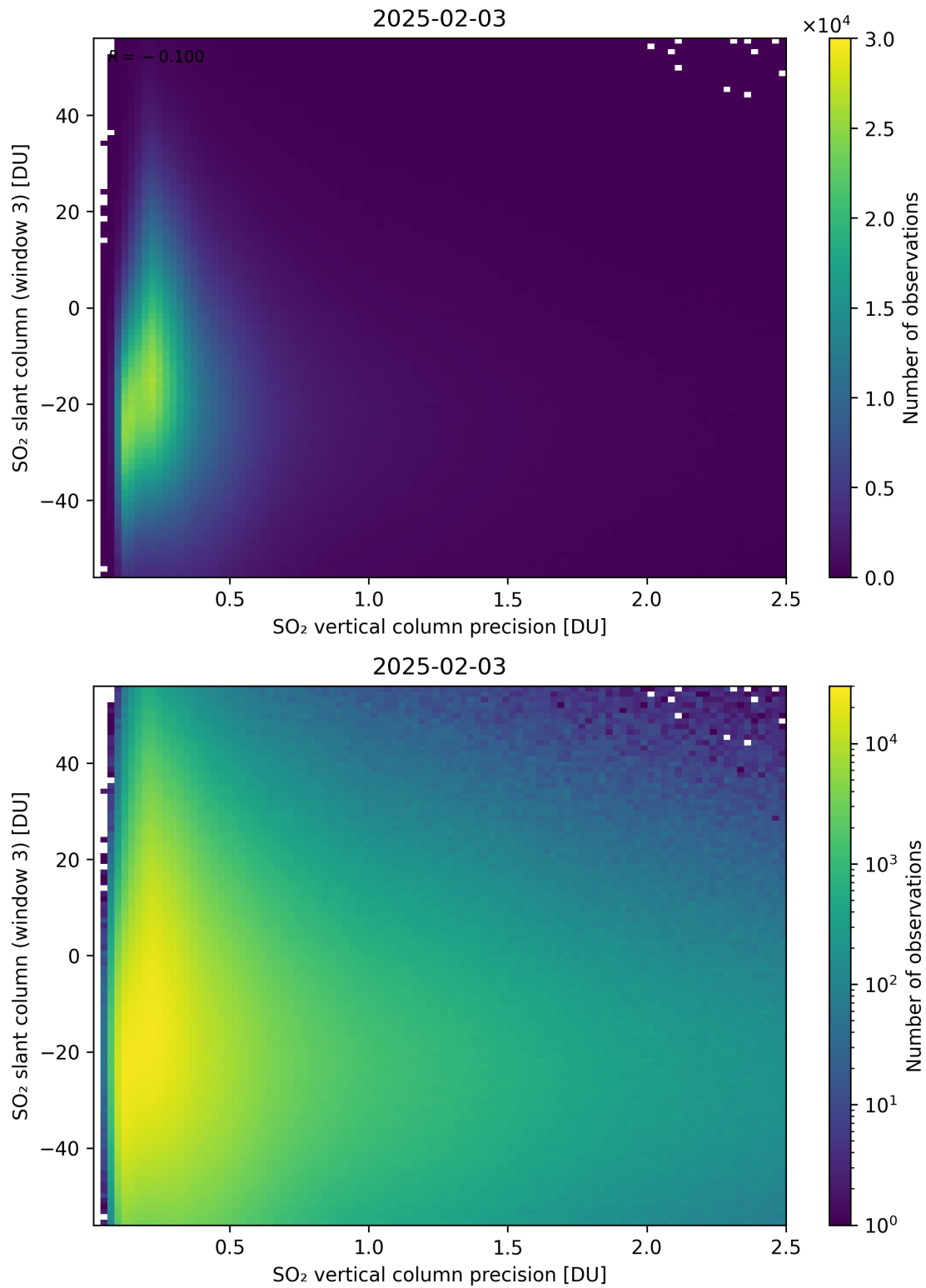
Figure 344: Scatter density plot of “SO 2 vertical column precision” against “SO 2 slant column (window 3)” for 2025-02-03 to 2025-02-04.
