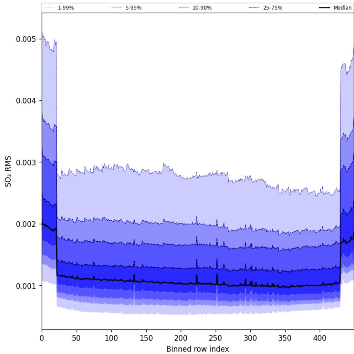
Figure 104: Along track statistics of “SO 2 RMS” for 2025-02-03 to 2025-02-04
