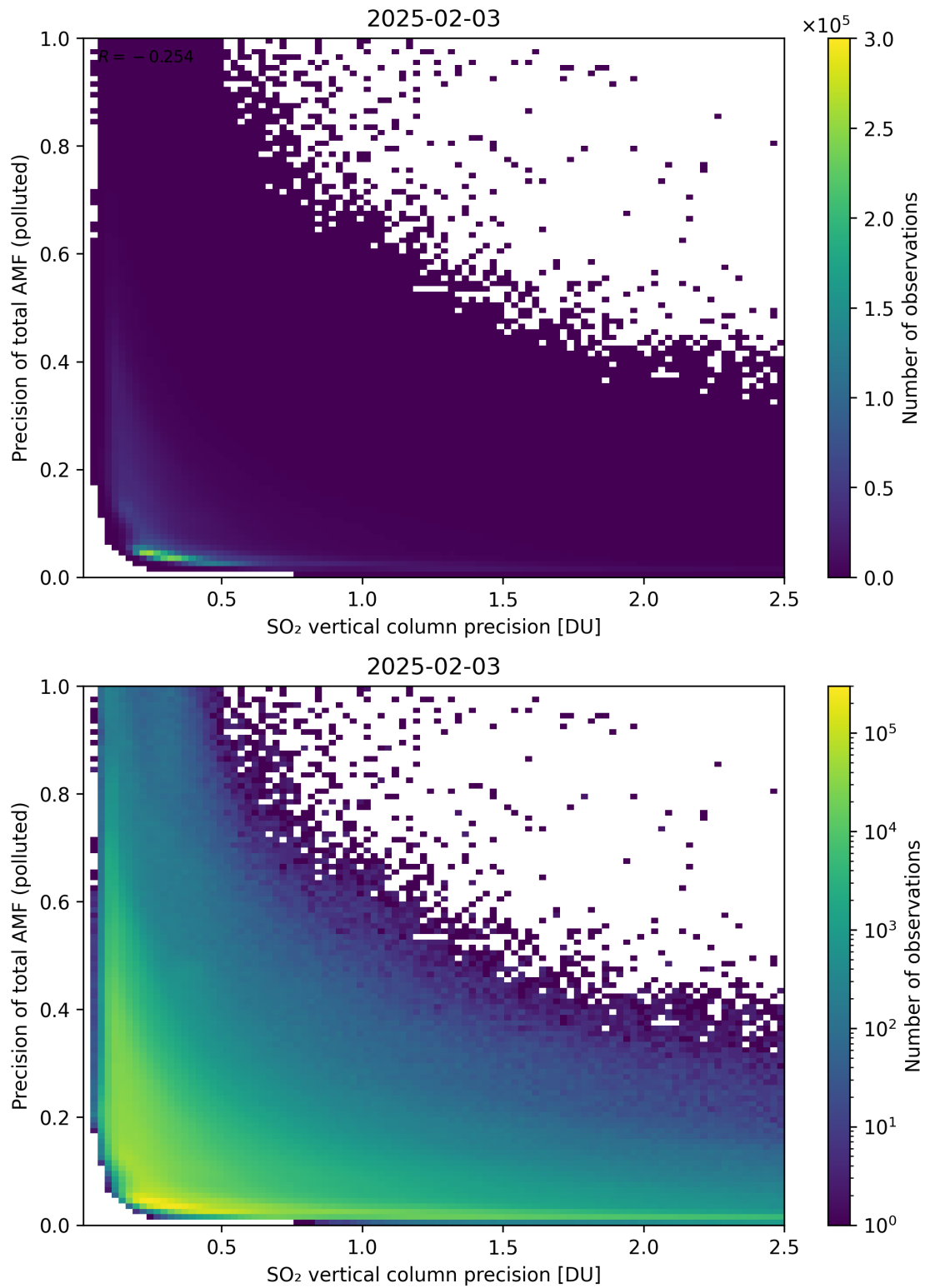
Figure 347: Scatter density plot of “SO 2 vertical column precision” against “Precision of total AMF (polluted)” for 2025-02-03 to 2025-02-04.
