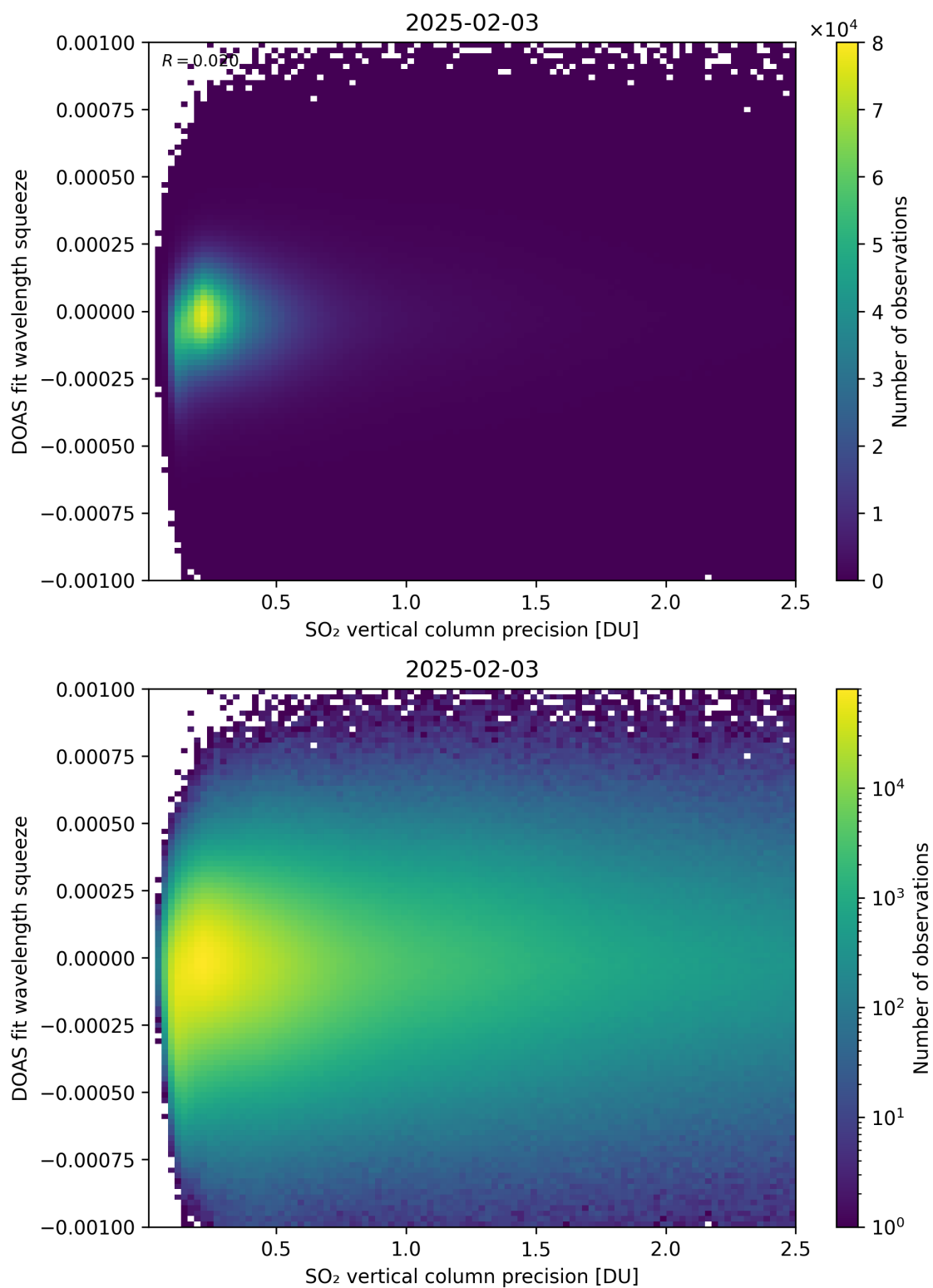
Figure 333: Scatter density plot of “SO 2 vertical column precision” against “DOAS fit wavelength squeeze” for 2025-02-03 to 2025-02-04.
