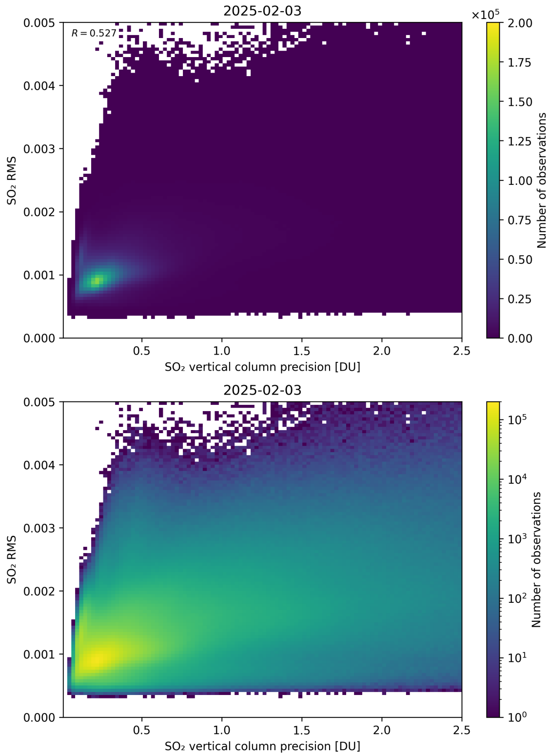
Figure 334: Scatter density plot of “SO 2 vertical column precision” against “SO 2 RMS” for 2025-02-03 to 2025-02-04.
