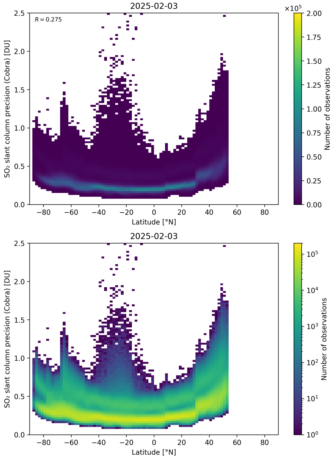
Figure 158: Scatter density plot of “Latitude” against “SO 2 slant column precision (Cobra)” for 2025-02-03 to 2025-02-04.
