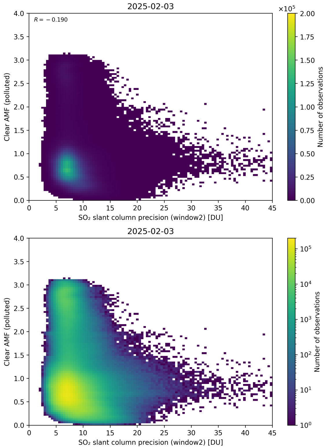
Figure 296: Scatter density plot of “SO 2 slant column precision (window2)” against “Clear AMF (polluted)” for 2025-02-03 to 2025-02-04.
