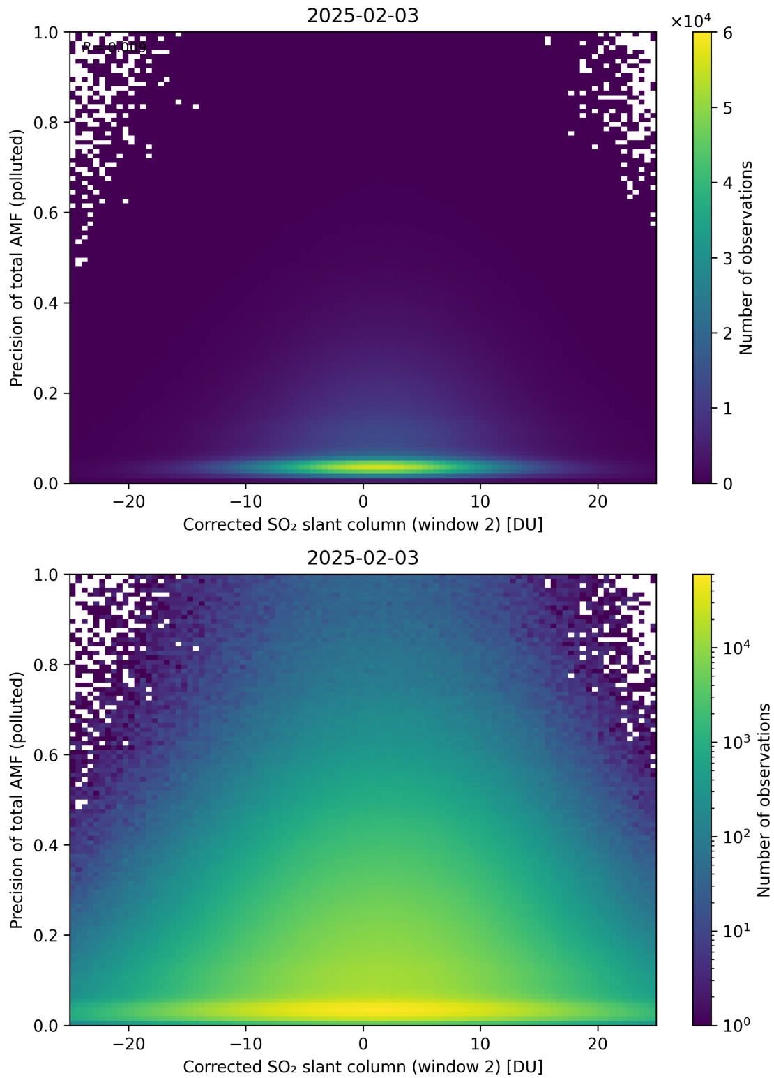
Figure 254: Scatter density plot of “Corrected SO 2 slant column (window 2)” against “Precision of total AMF (polluted)” for 2025-02-03 to 2025-02-04.
