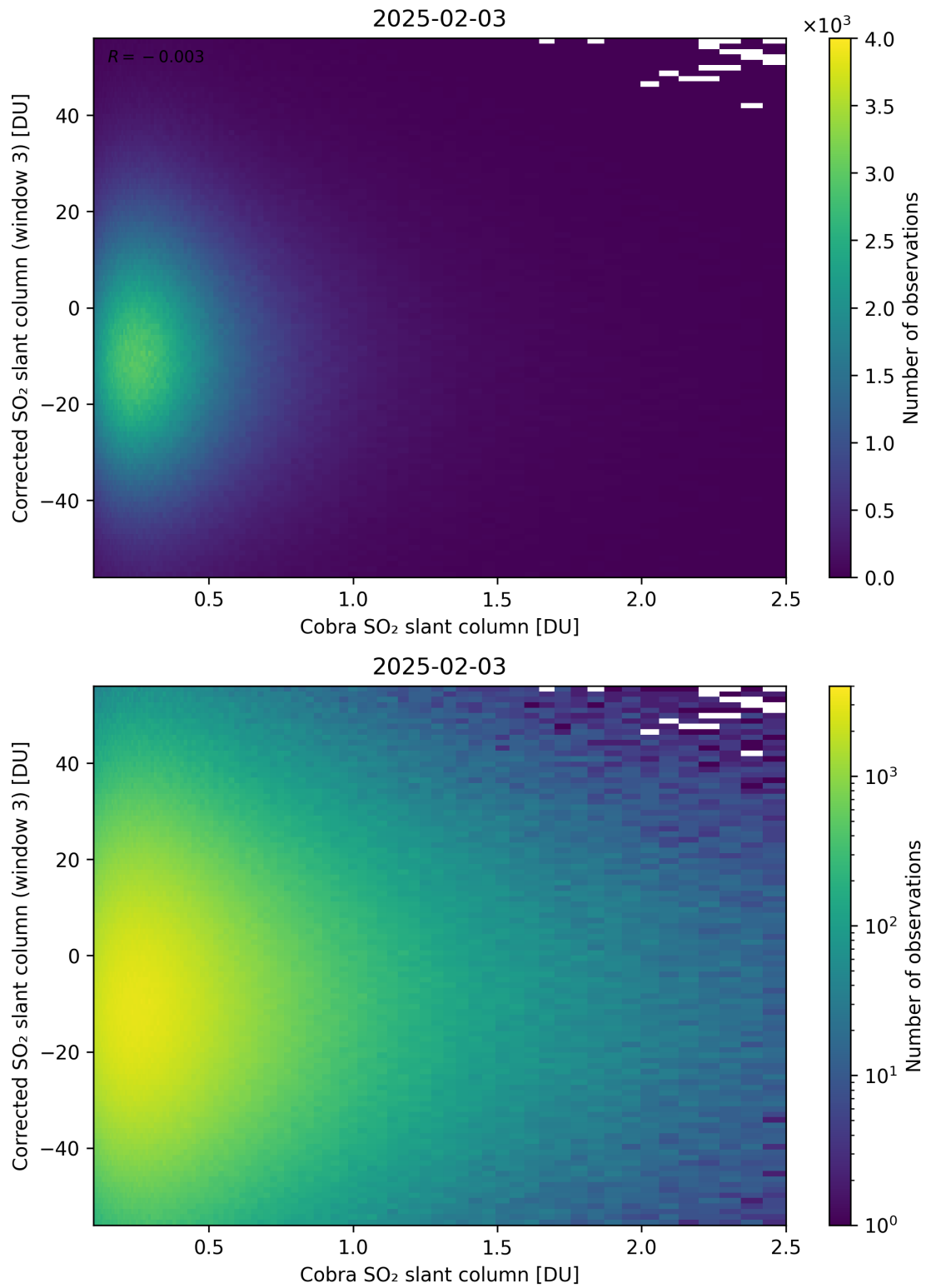
Figure 218: Scatter density plot of “Cobra SO 2 slant column” against “Corrected SO 2 slant column (window 3)” for 2025-02-03 to 2025-02-04.
