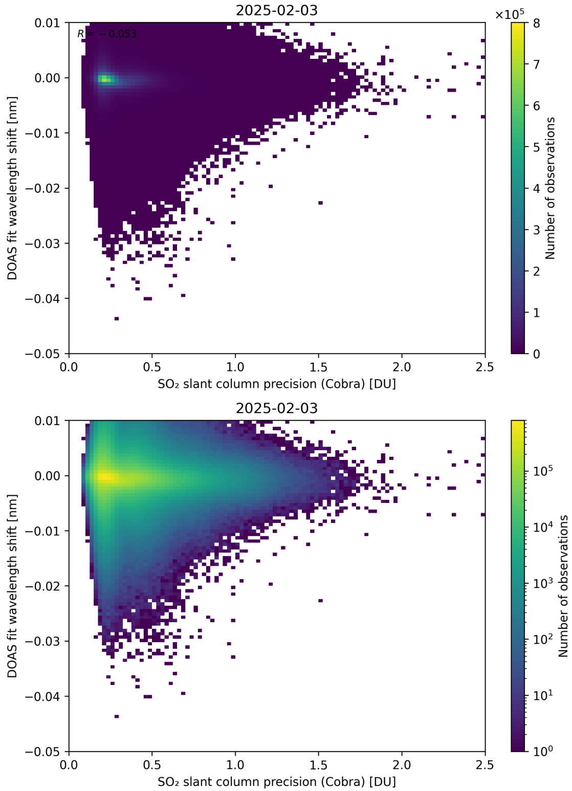
Figure 202: Scatter density plot of “SO 2 slant column precision (Cobra)” against “DOAS fit wavelength shift” for 2025-02-03 to 2025-02-04.
