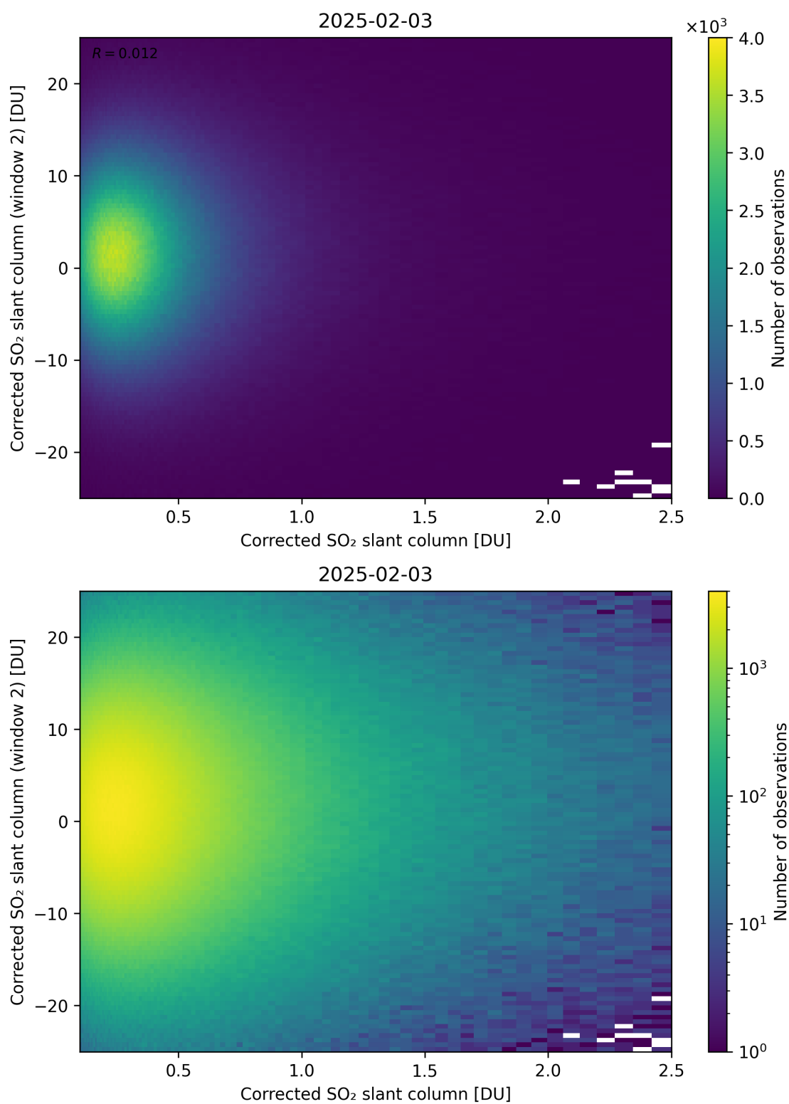
Figure 235: Scatter density plot of “Corrected SO 2 slant column” against “Corrected SO 2 slant column (window 2)” for 2025-02-03 to 2025-02-04.
