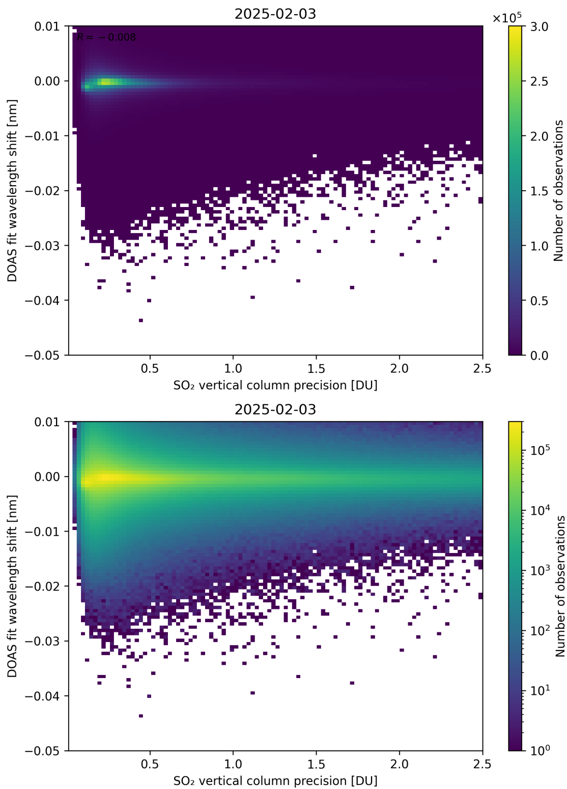
Figure 332: Scatter density plot of “SO 2 vertical column precision” against “DOAS fit wavelength shift” for 2025-02-03 to 2025-02-04.
