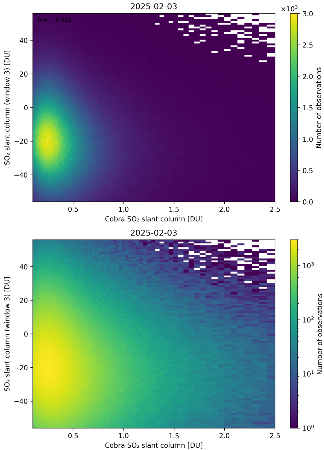
Figure 222: Scatter density plot of “Cobra SO 2 slant column” against “SO 2 slant column (window 3)” for 2025-02-03 to 2025-02-04.
