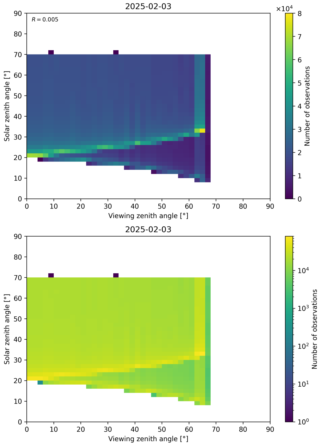
Figure 369: Scatter density plot of “Viewing zenith angle” against “Solar zenith angle” for 2025-02-03 to 2025-02-04.
