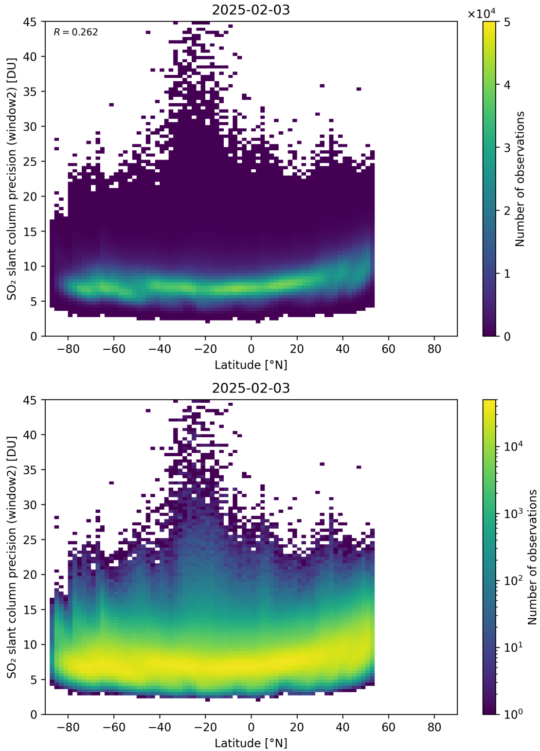
Figure 164: Scatter density plot of “Latitude” against “SO 2 slant column precision (window2)” for 2025-02-03 to 2025-02-04.
