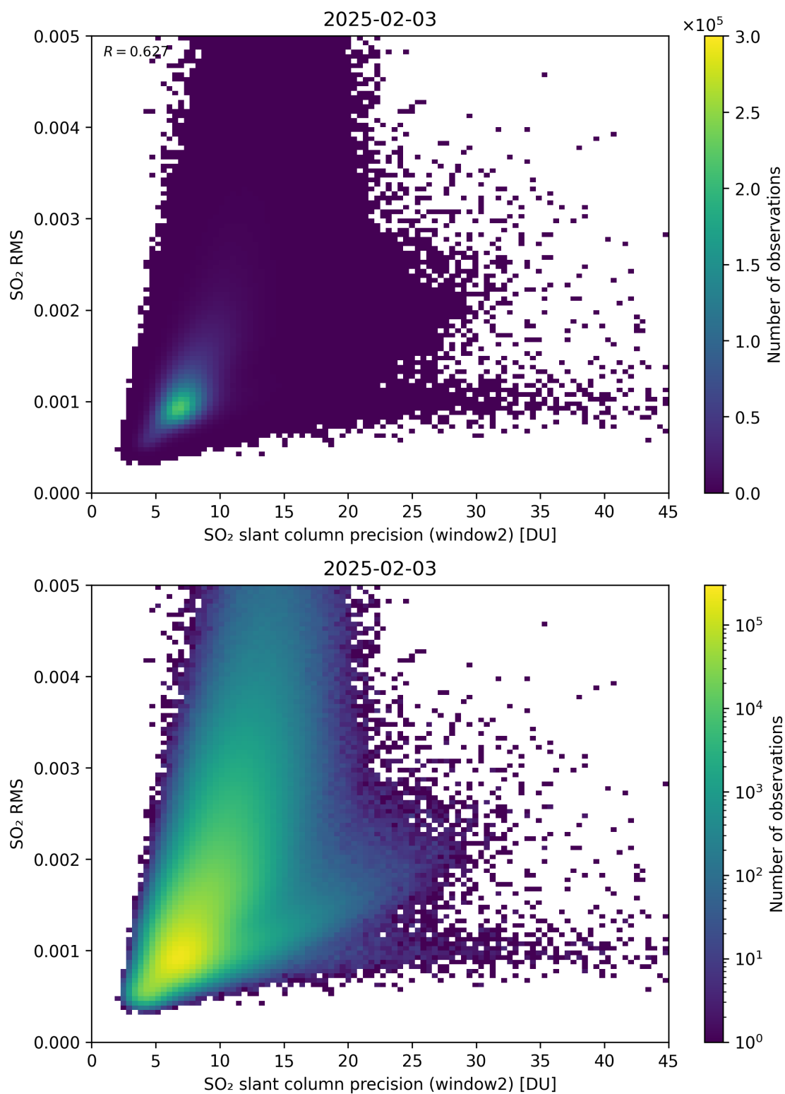
Figure 295: Scatter density plot of “SO 2 slant column precision (window2)” against “SO 2 RMS” for 2025-02-03 to 2025-02-04.
