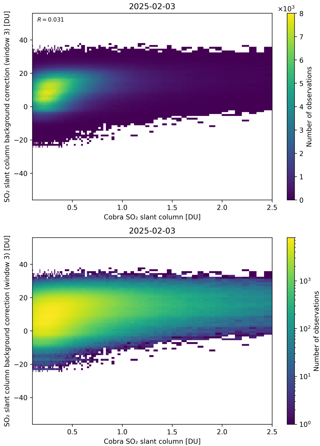
Figure 195: Scatter density plot of “Cobra SO 2 slant column” against “SO 2 slant column background correction (window 3)” for 2025-02-03 to 2025-02-04.
