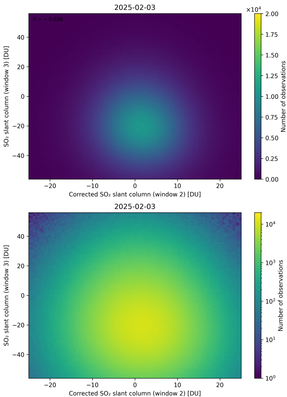
Figure 251: Scatter density plot of “Corrected SO 2 slant column (window 2)” against “SO 2 slant column (window 3)” for 2025-02-03 to 2025-02-04.
