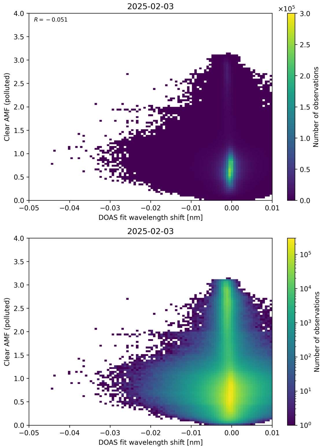
Figure 140: Scatter density plot of “DOAS fit wavelength shift” against “Clear AMF (polluted)” for 2025-02-03 to 2025-02-04.
