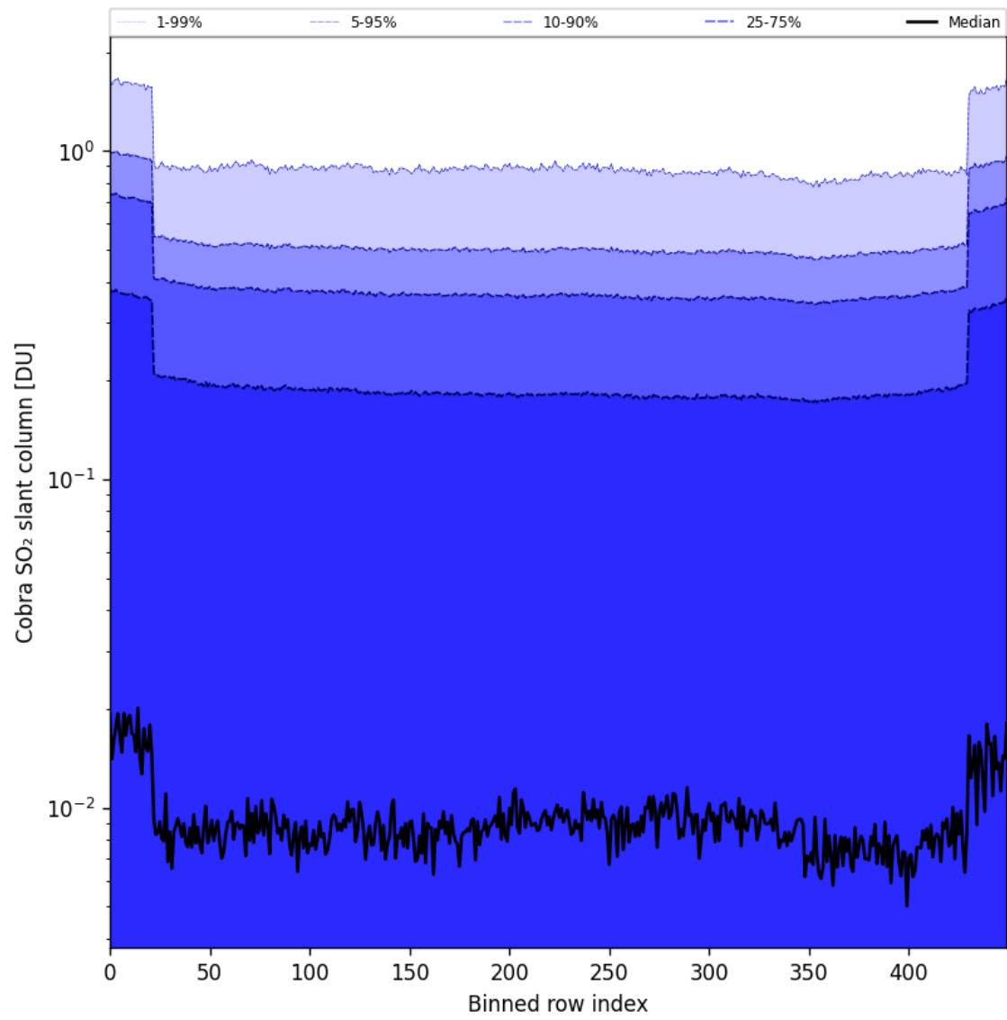
Figure 87: Along track statistics of "Cobra SO 2 slant column" for 2025-02-03 to 2025-02-04
