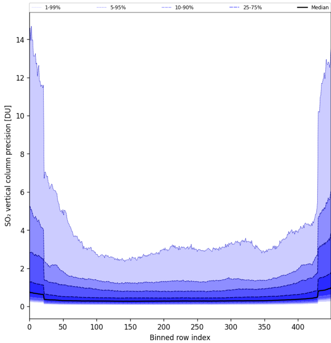
Figure 85: Along track statistics of “SO 2 vertical column precision” for 2025-02-03 to 2025-02-04
