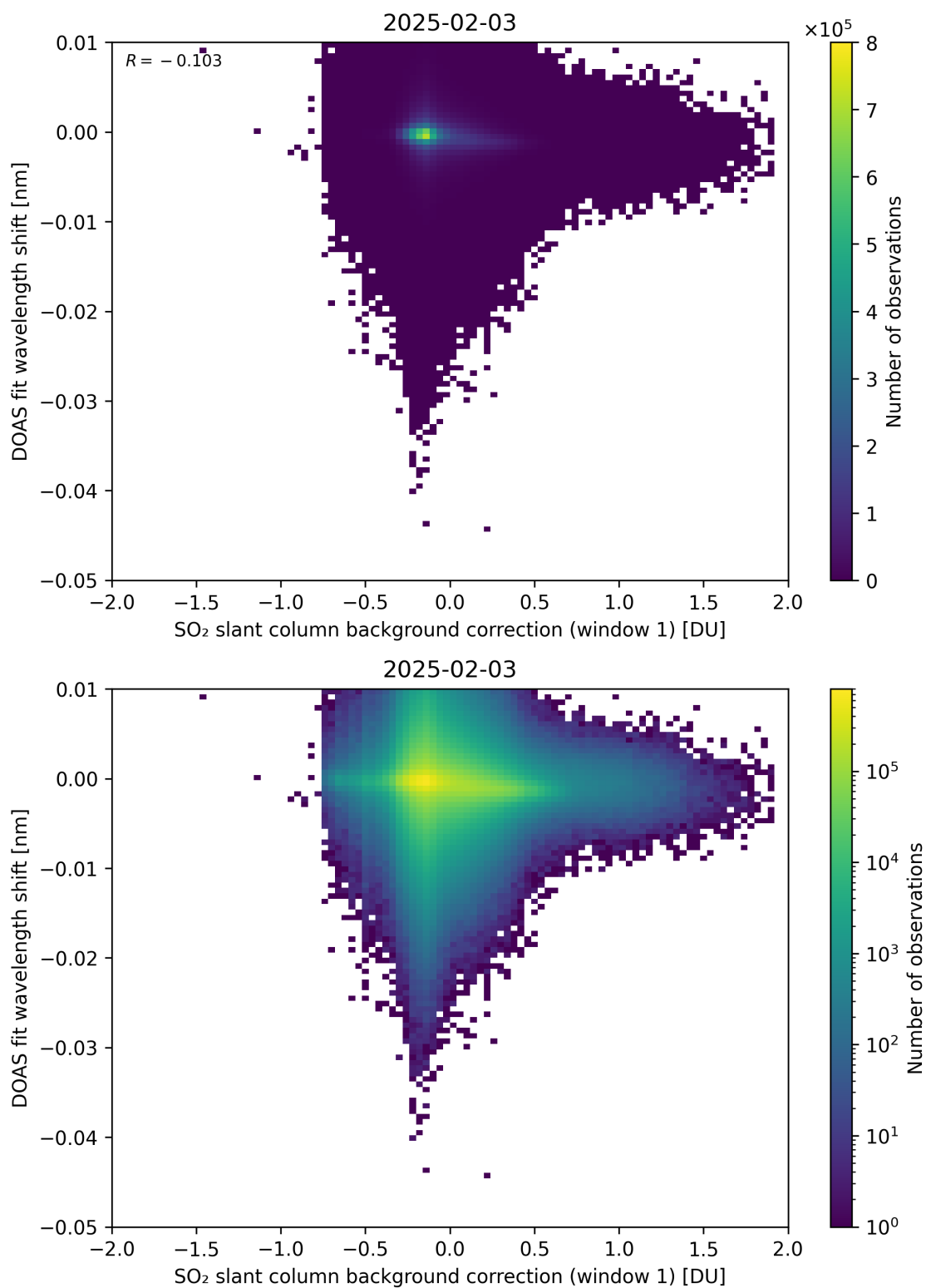
Figure 111: Scatter density plot of “SO 2 slant column background correction (window 1)” against “DOAS fit wavelength shift” for 2025-02-03 to 2025-02-04.
