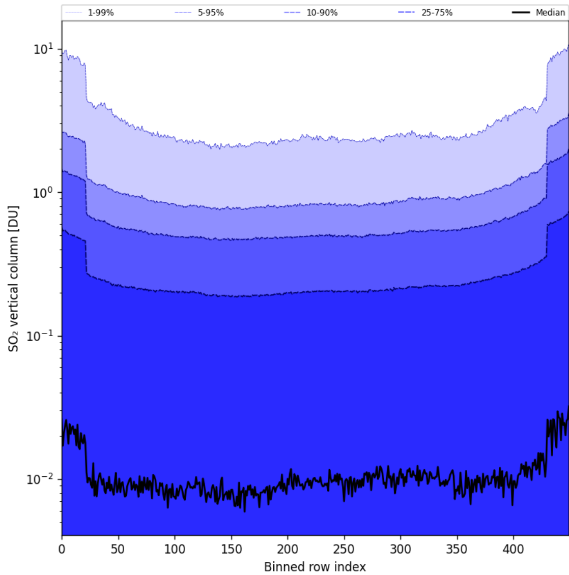
Figure 84: Along track statistics of “SO 2 vertical column” for 2025-02-03 to 2025-02-04
