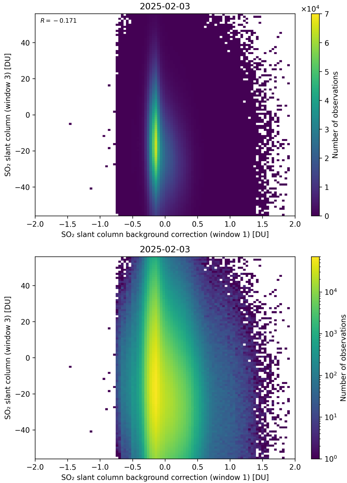
Figure 118: Scatter density plot of “SO 2 slant column background correction (window 1)” against “SO 2 slant column (window 3)” for 2025-02-03 to 2025-02-04.
