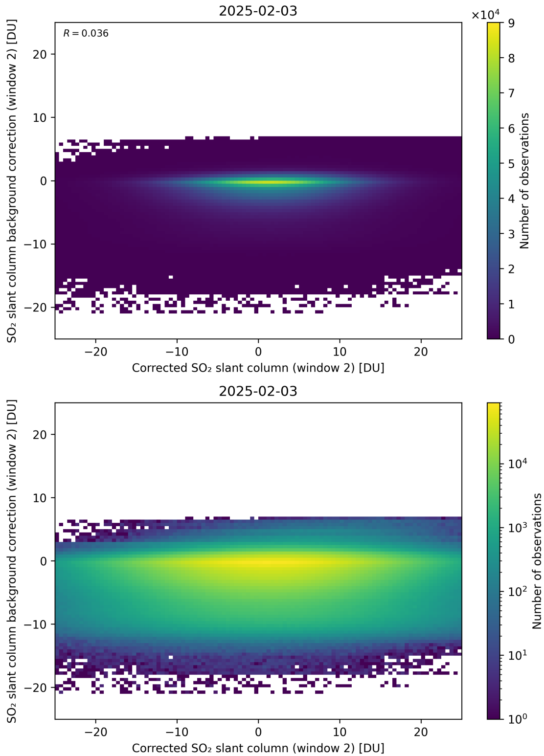
Figure 244: Scatter density plot of “Corrected SO 2 slant column (window 2)” against “SO 2 slant column background correction (window 2)” for 2025-02-03 to 2025-02-04.
