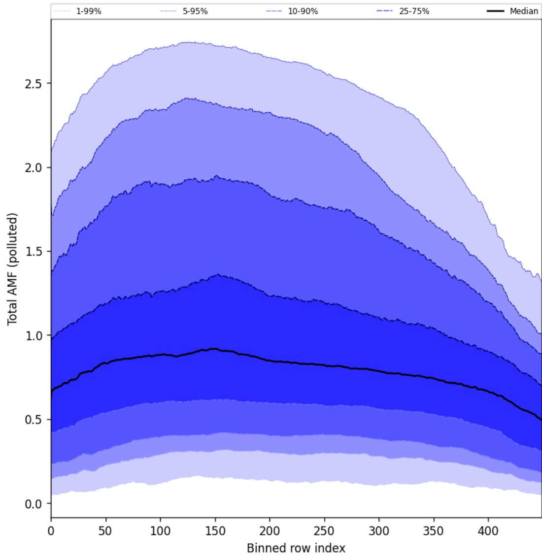
Figure 105: Along track statistics of “Total AMF (polluted)” for 2025-02-03 to 2025-02-04
