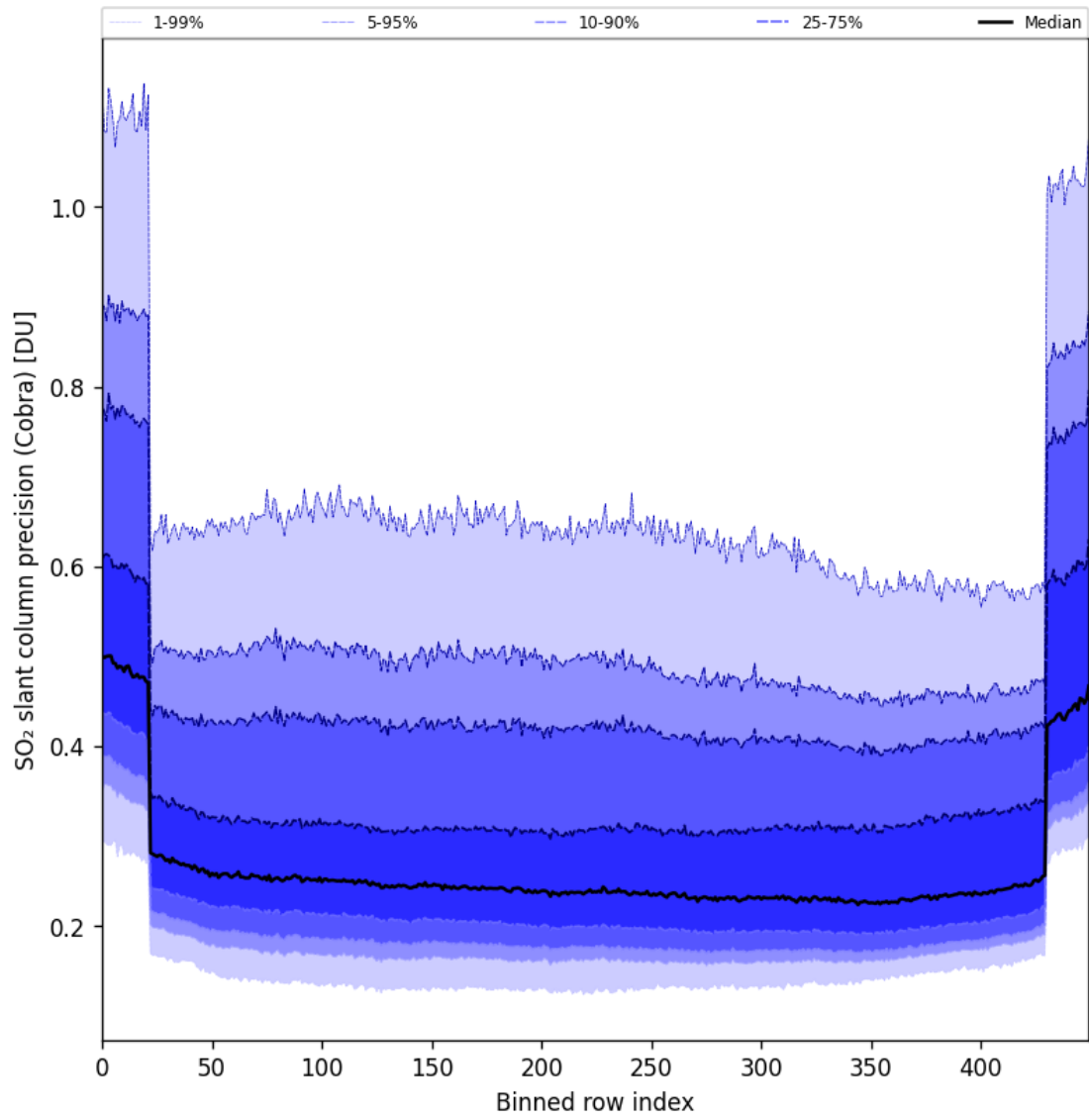
Figure 88: Along track statistics of “SO 2 slant column precision (Cobra)” for 2025-02-03 to 2025-02-04
