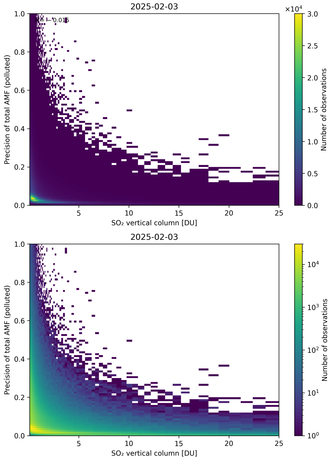
Figure 360: Scatter density plot of “SO 2 vertical column” against “Precision of total AMF (polluted)” for 2025-02-03 to 2025-02-04.
