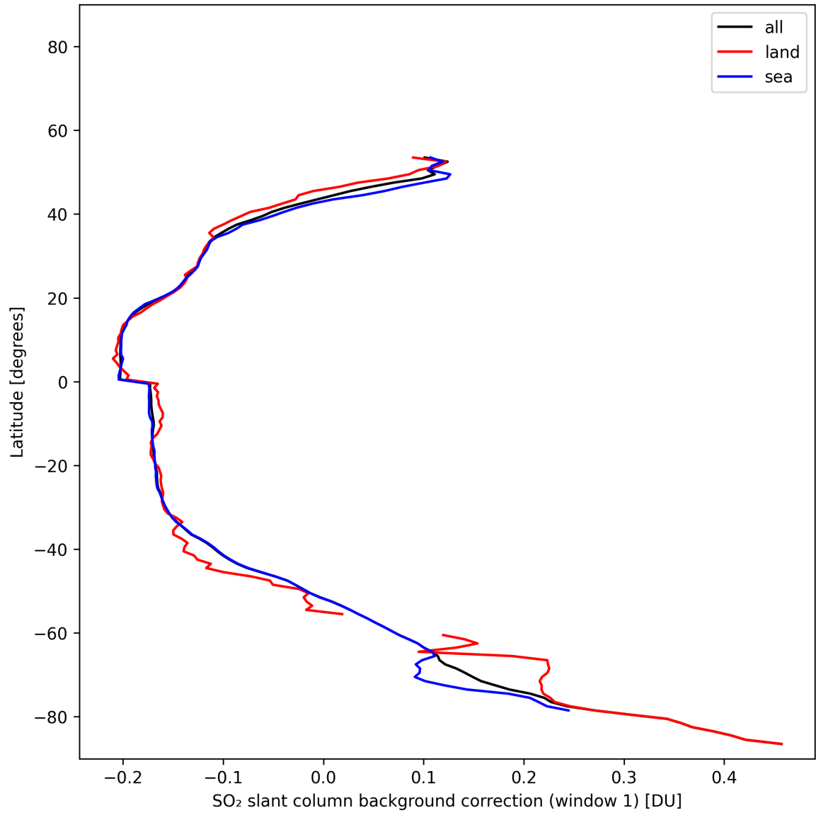
Figure 40: Zonal average of “SO 2 slant column background correction (window 1)” for 2025-02-03 to 2025-02-04.
