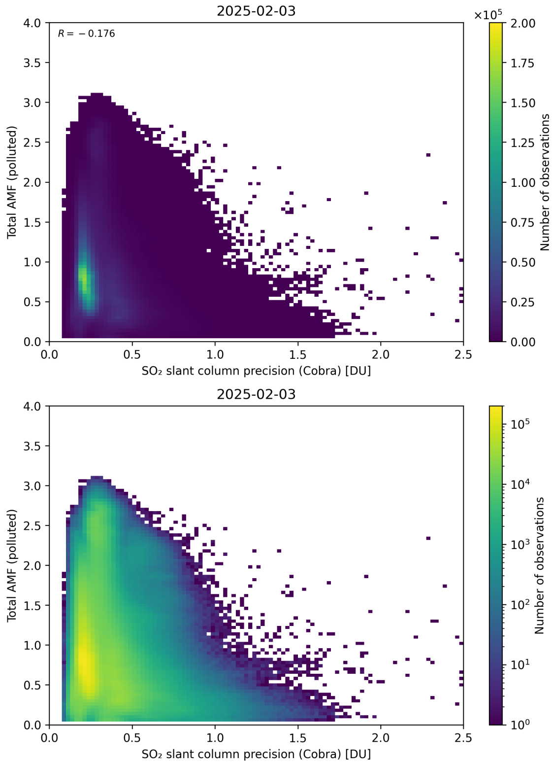
Figure 213: Scatter density plot of “SO 2 slant column precision (Cobra)” against “Total AMF (polluted)” for 2025-02-03 to 2025-02-04.
