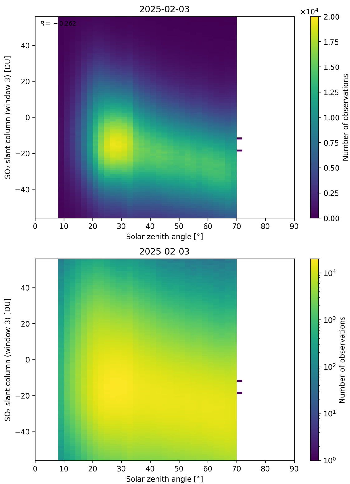
Figure 187: Scatter density plot of “Solar zenith angle” against “SO 2 slant column (window 3)” for 2025-02-03 to 2025-02-04.
