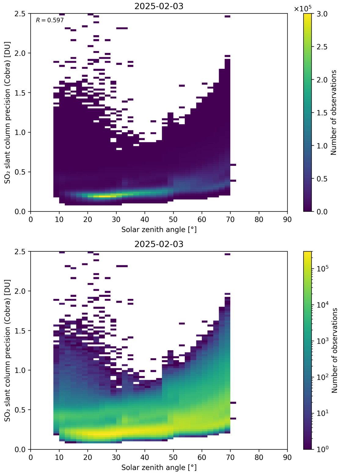
Figure 180: Scatter density plot of “Solar zenith angle” against “SO 2 slant column precision (Cobra)” for 2025-02-03 to 2025-02-04.
