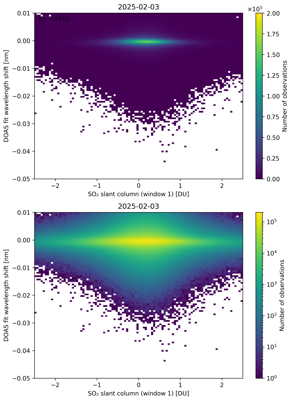
Figure 265: Scatter density plot of “SO 2 slant column (window 1)” against “DOAS fit wavelength shift” for 2025-02-03 to 2025-02-04.
