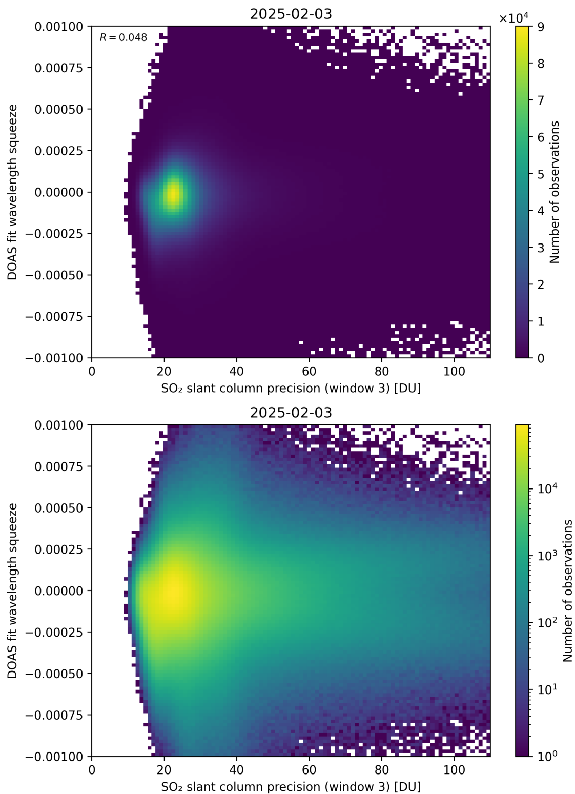
Figure 309: Scatter density plot of “SO 2 slant column precision (window 3)” against “DOAS fit wavelength squeeze” for 2025-02-03 to 2025-02-04.
