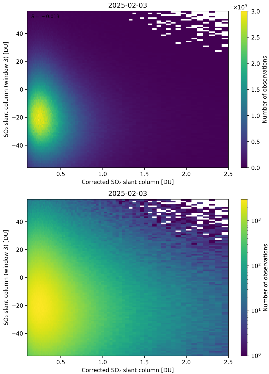
Figure 240: Scatter density plot of “Corrected SO 2 slant column” against “SO 2 slant column (window 3)” for 2025-02-03 to 2025-02-04.
