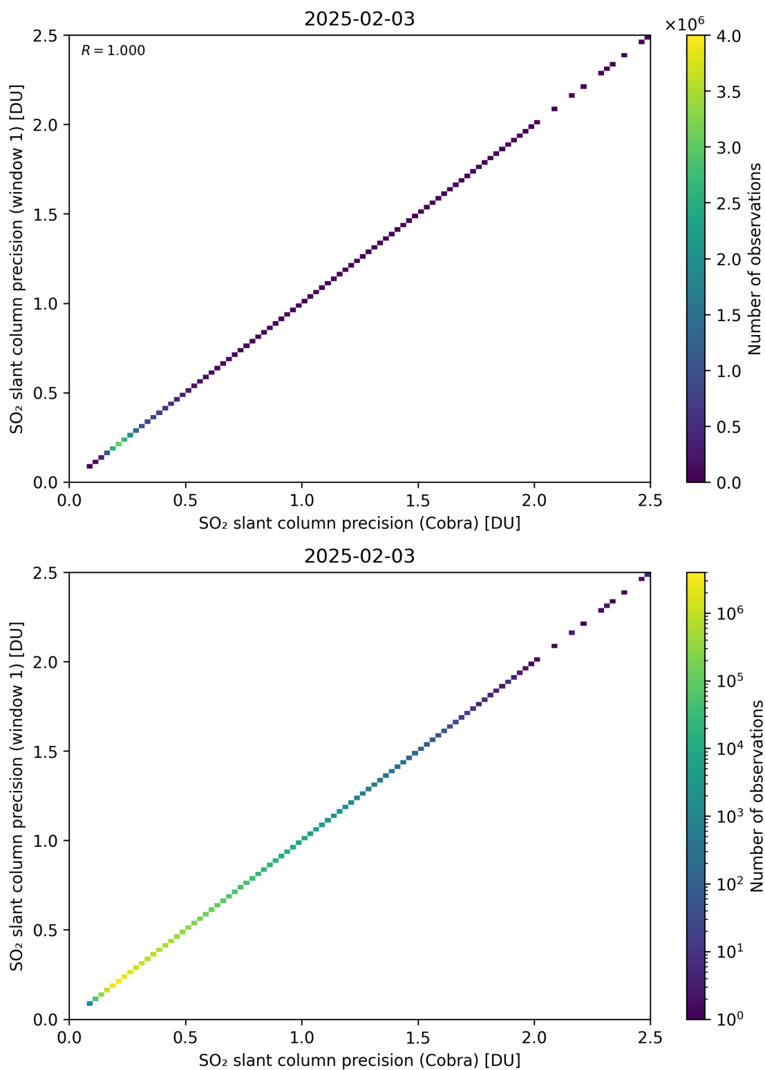
Figure 209: Scatter density plot of “SO 2 slant column precision (Cobra)” against “SO 2 slant column precision (window 1)” for 2025-02-03 to 2025-02-04.
