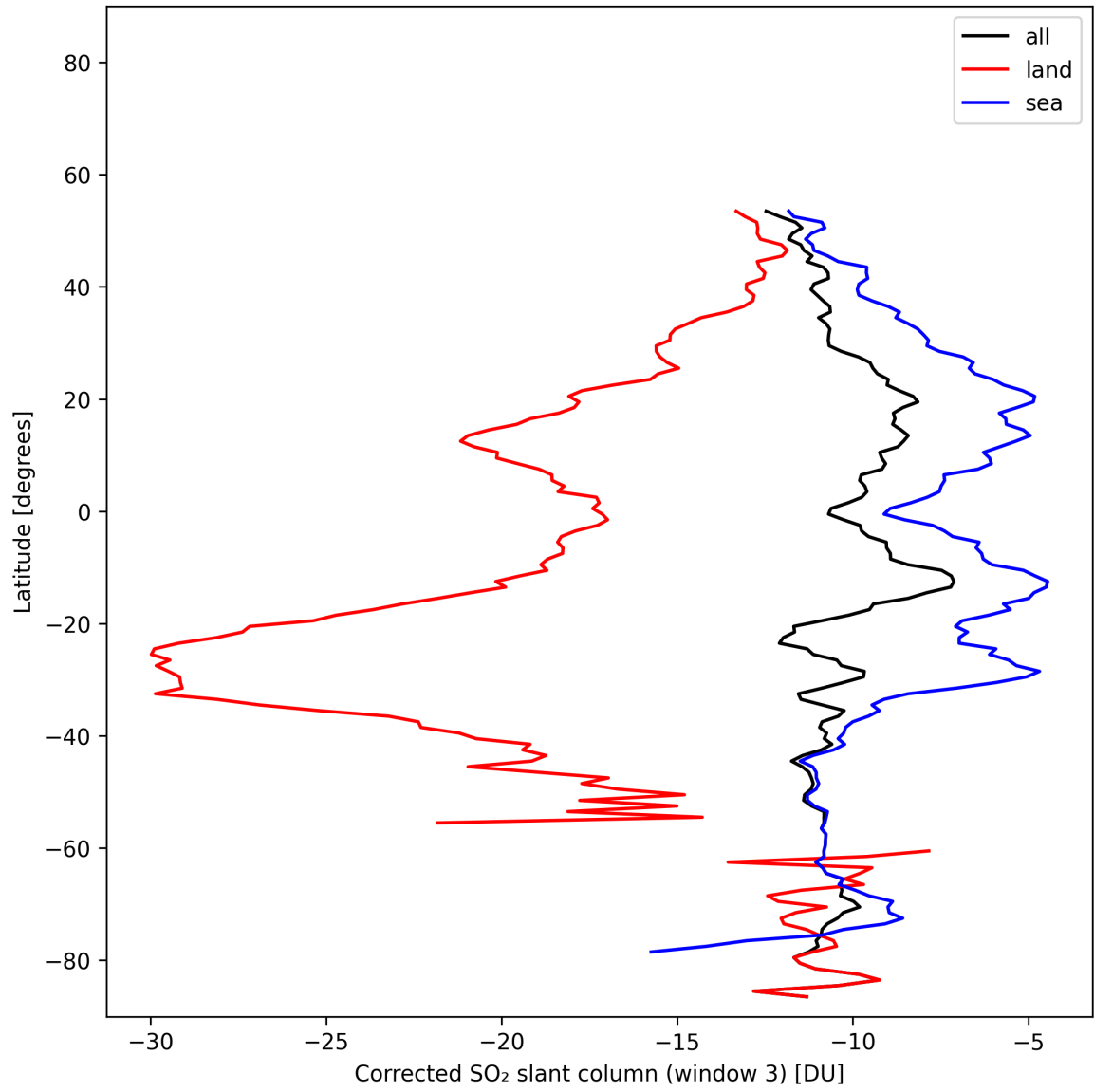
Figure 47: Zonal average of “Corrected SO 2 slant column (window 3)” for 2025-02-03 to 2025-02-04.
