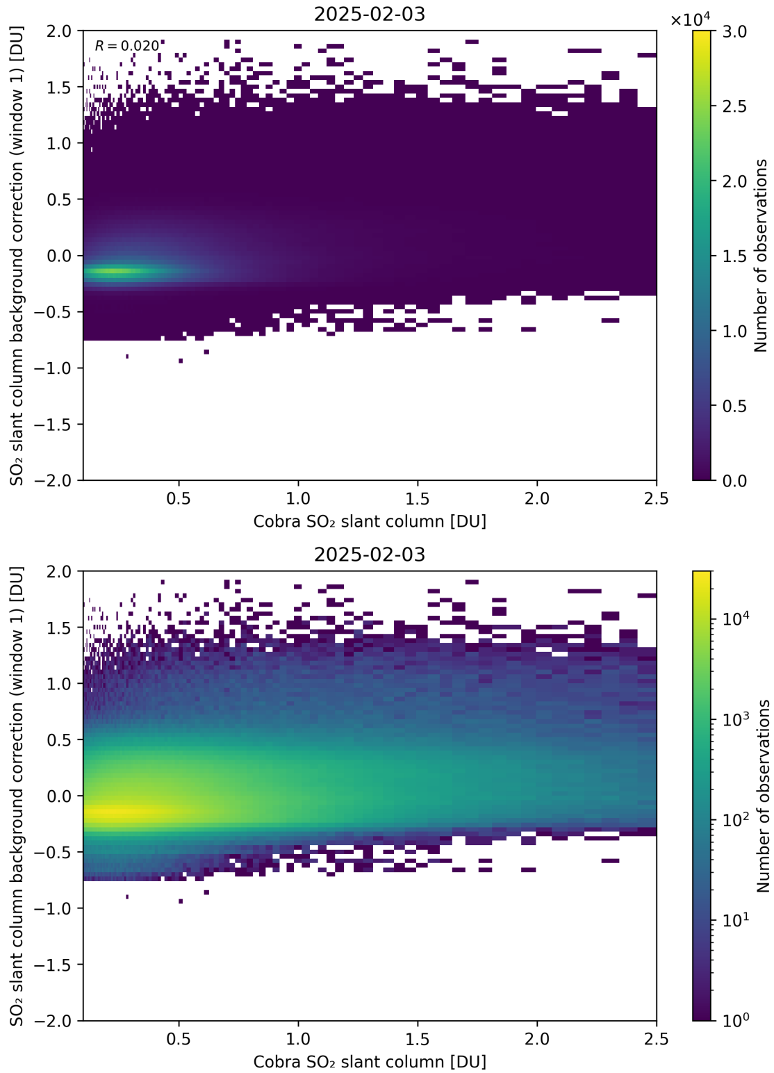
Figure 193: Scatter density plot of “Cobra SO 2 slant column” against “SO 2 slant column background correction (window 1)” for 2025-02-03 to 2025-02-04.
