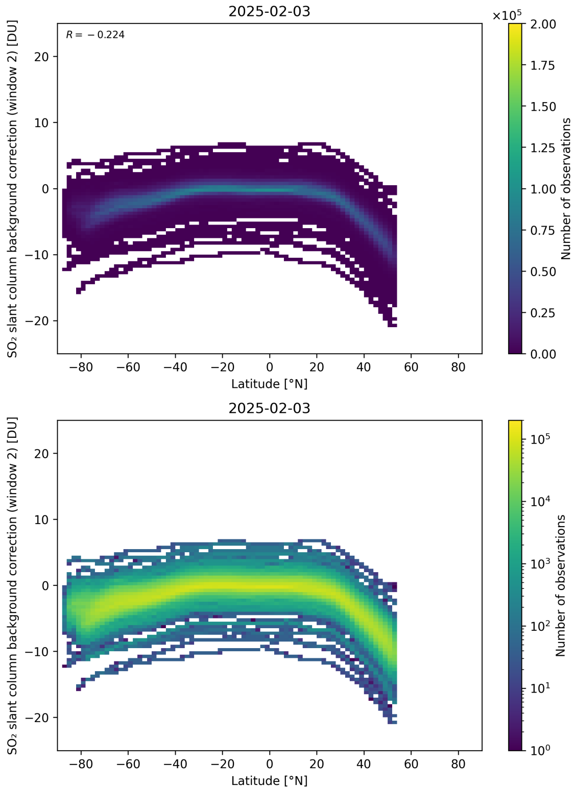
Figure 151: Scatter density plot of “Latitude” against “SO 2 slant column background correction (window 2)” for 2025-02-03 to 2025-02-04.
