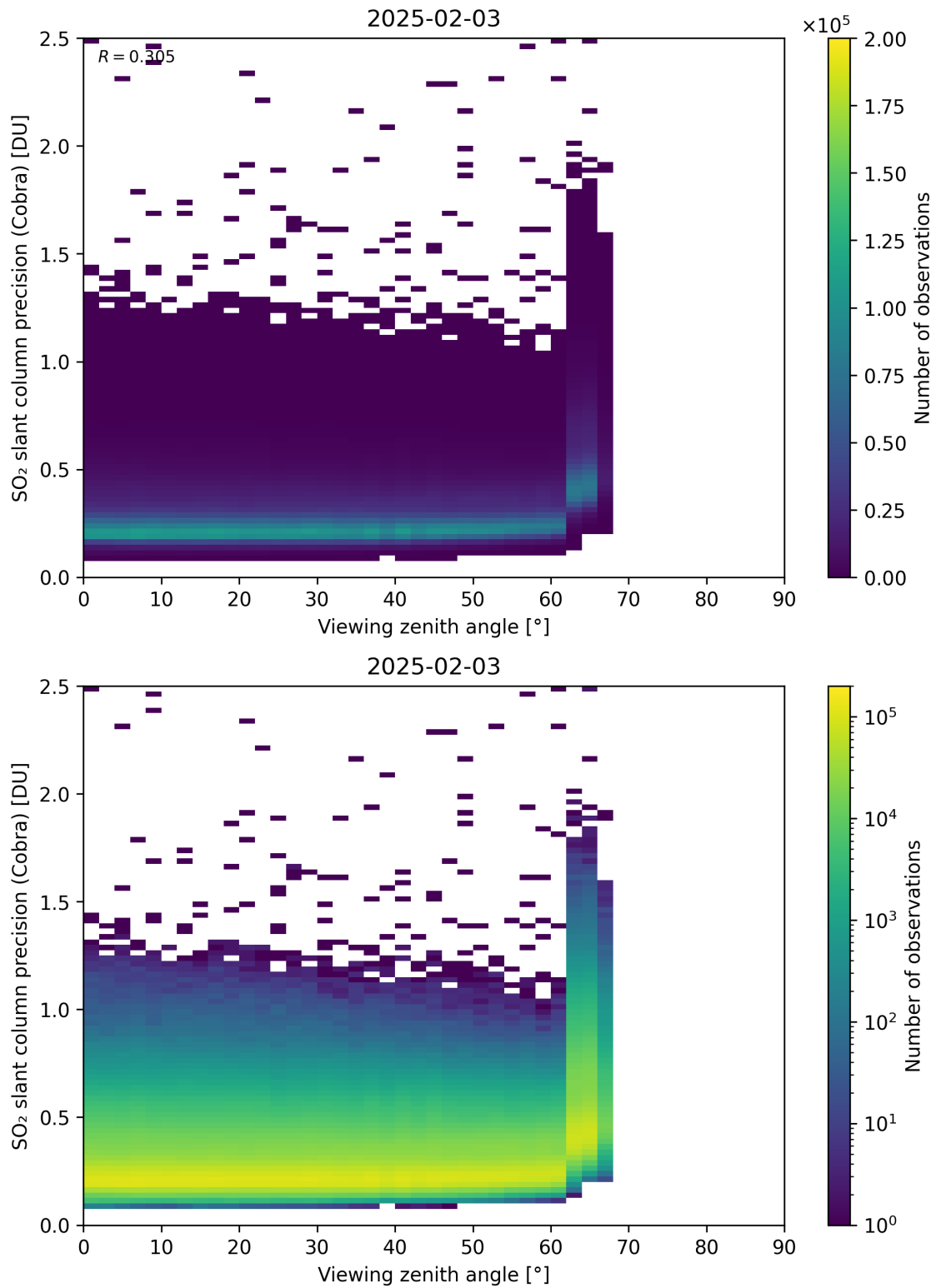
Figure 372: Scatter density plot of “Viewing zenith angle” against “SO 2 slant column precision (Cobra)” for 2025-02-03 to 2025-02-04.
