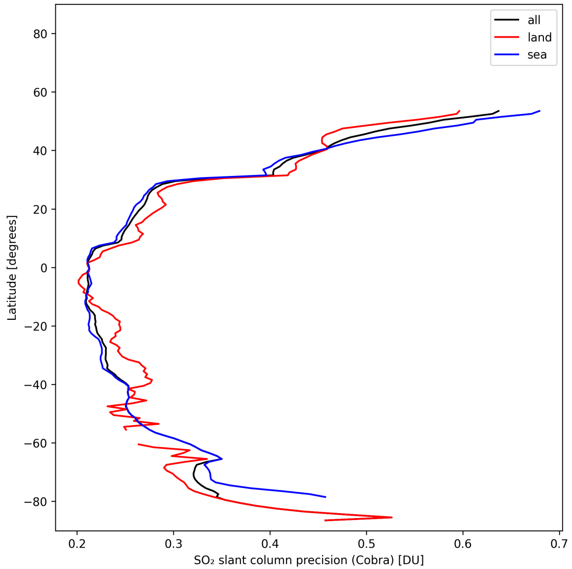
Figure 36: Zonal average of “SO 2 slant column precision (Cobra)” for 2025-02-03 to 2025-02-04.
