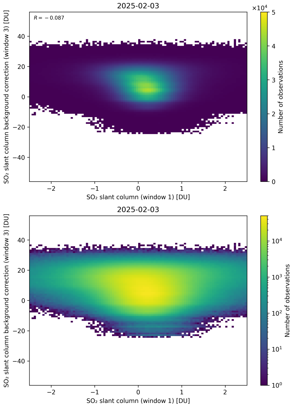
Figure 264: Scatter density plot of “SO 2 slant column (window 1)” against “SO 2 slant column background correction (window 3)” for 2025-02-03 to 2025-02-04.
