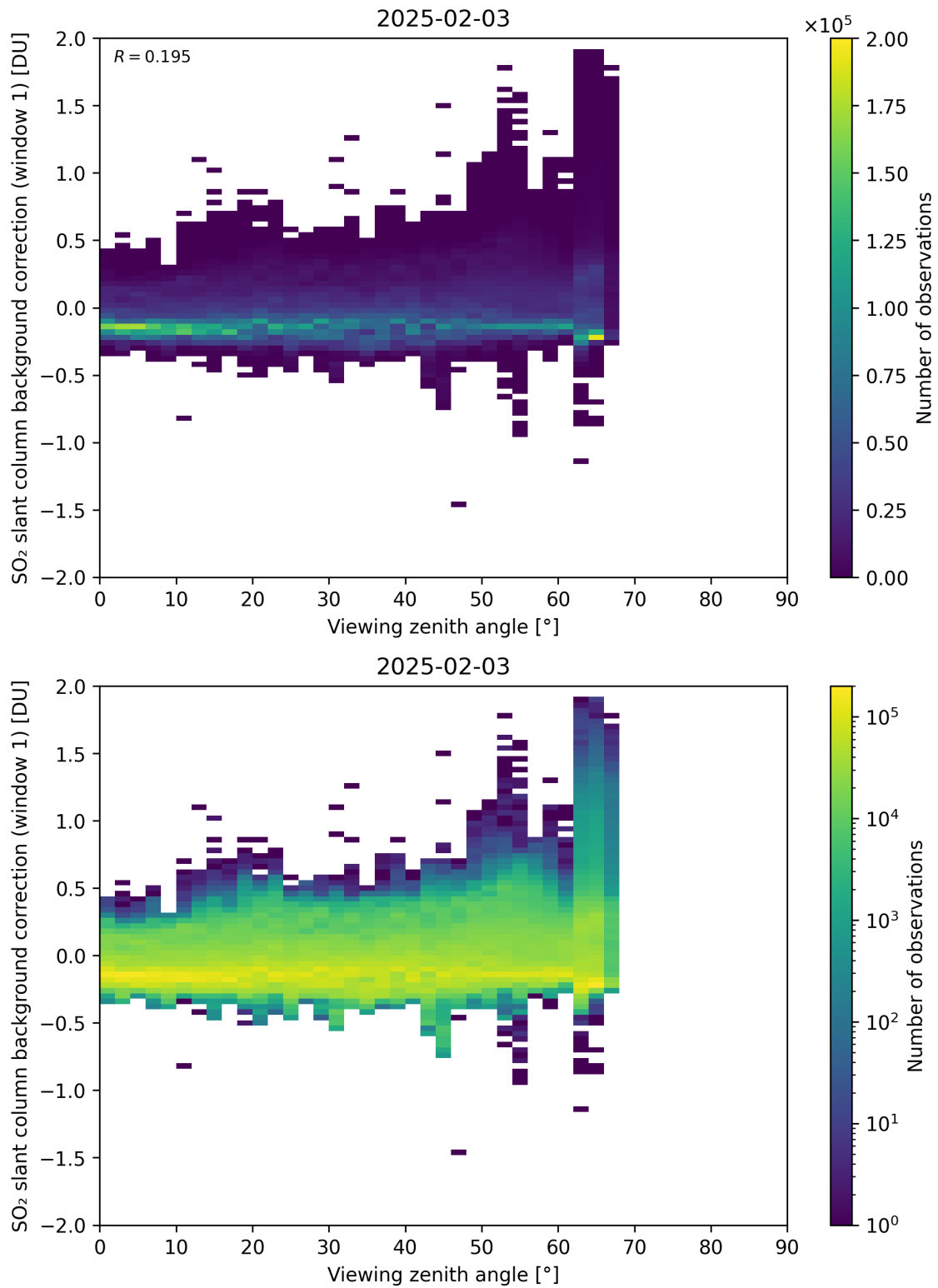
Figure 362: Scatter density plot of “Viewing zenith angle” against “SO 2 slant column background correction (window 1)” for 2025-02-03 to 2025-02-04.
