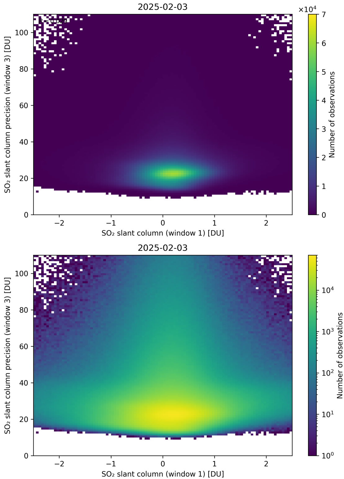
Figure 288: Scatter density plot of “SO 2 slant column (window 1)” against “SO 2 slant column precision (window 3)” for 2025-02-03 to 2025-02-04.
