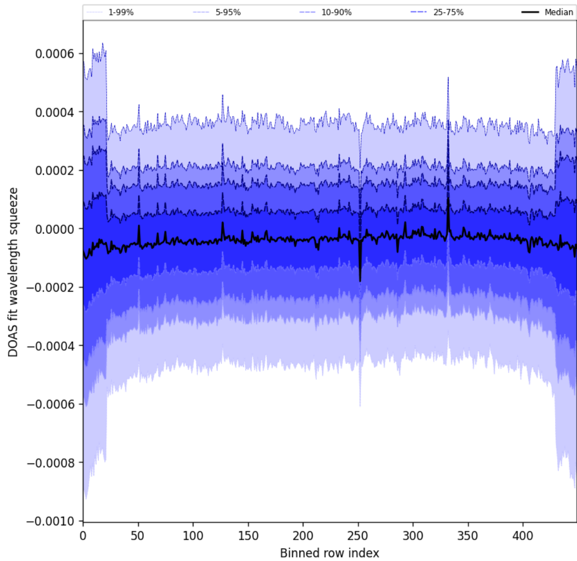
Figure 103: Along track statistics of “DOAS fit wavelength squeeze” for 2025-02-03 to 2025-02-04
