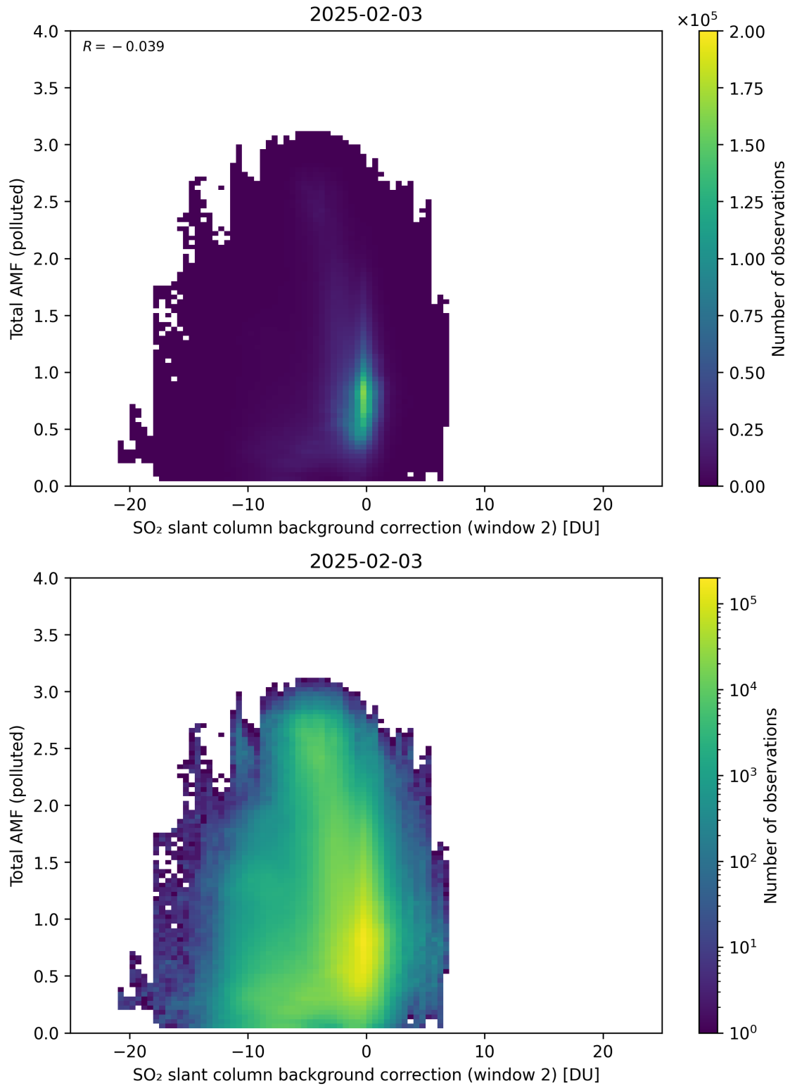
Figure 130: Scatter density plot of “SO 2 slant column background correction (window 2)” against “Total AMF (polluted)” for 2025-02-03 to 2025-02-04.
