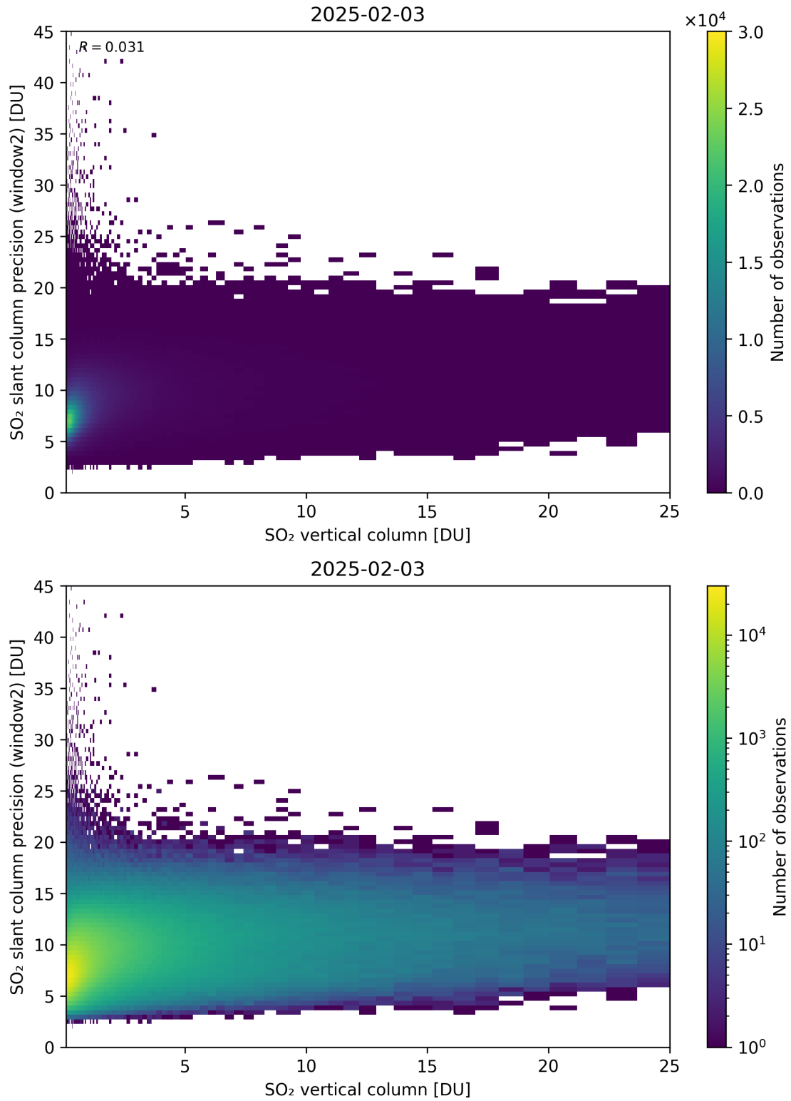
Figure 356: Scatter density plot of “SO 2 vertical column” against “SO 2 slant column precision (window2)” for 2025-02-03 to 2025-02-04.
