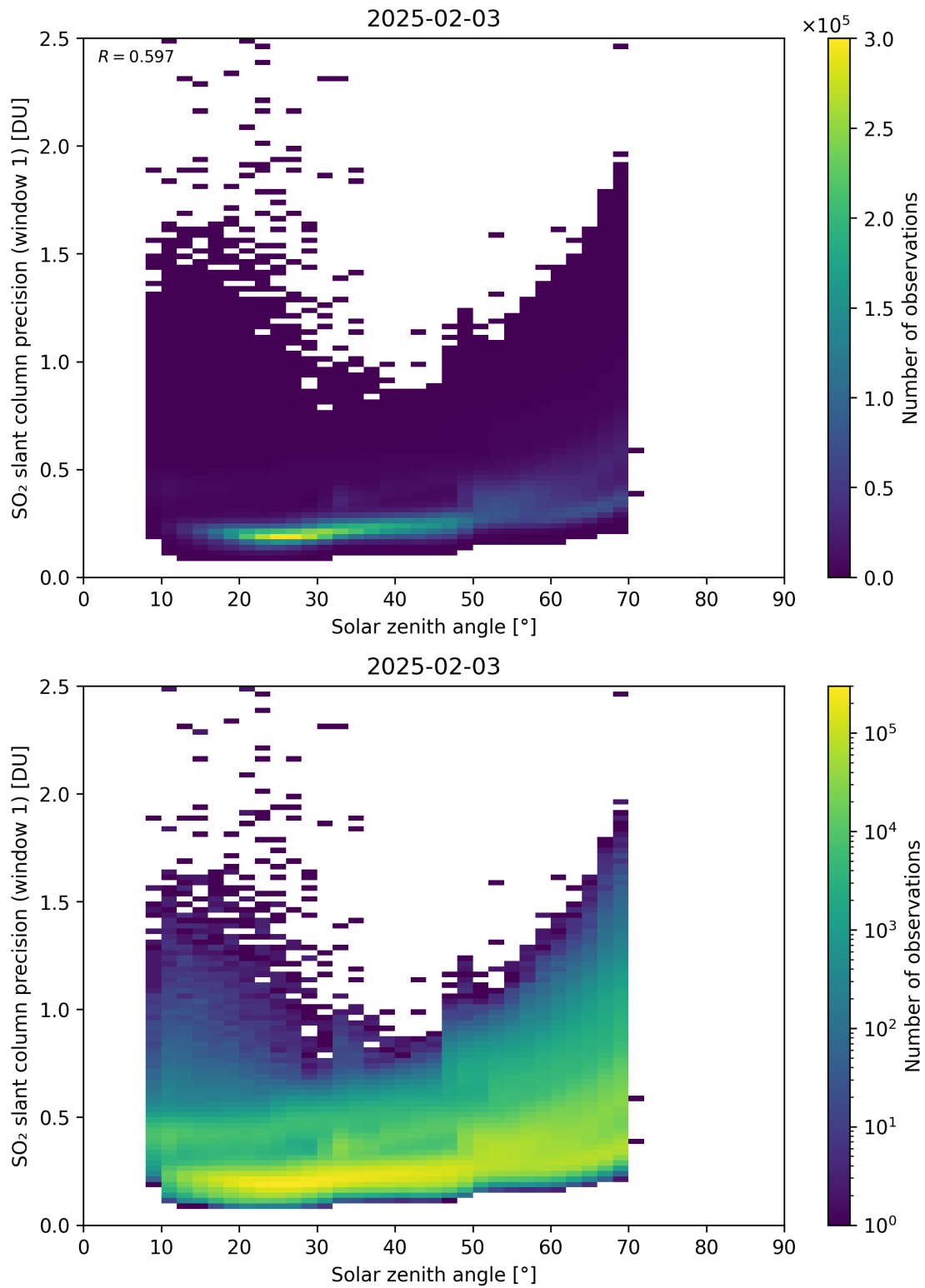
Figure 185: Scatter density plot of “Solar zenith angle” against “SO 2 slant column precision (window 1)” for 2025-02-03 to 2025-02-04.
