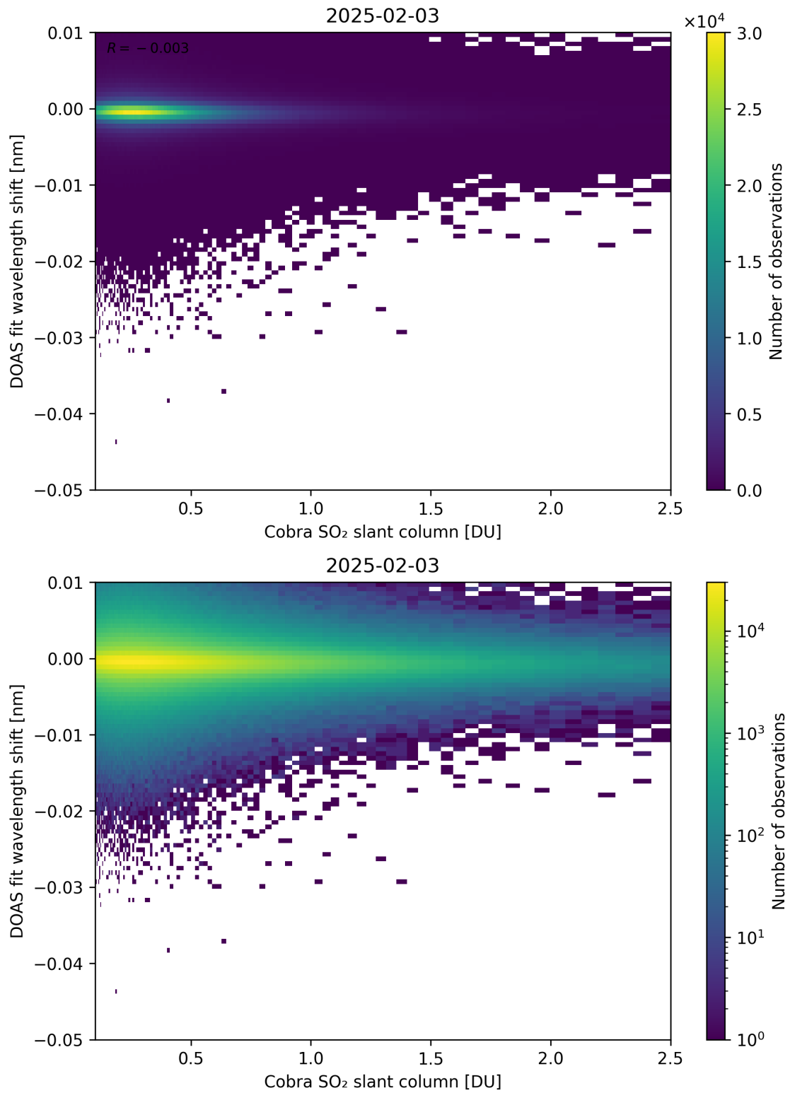
Figure 196: Scatter density plot of “Cobra SO 2 slant column” against “DOAS fit wavelength shift” for 2025-02-03 to 2025-02-04.
