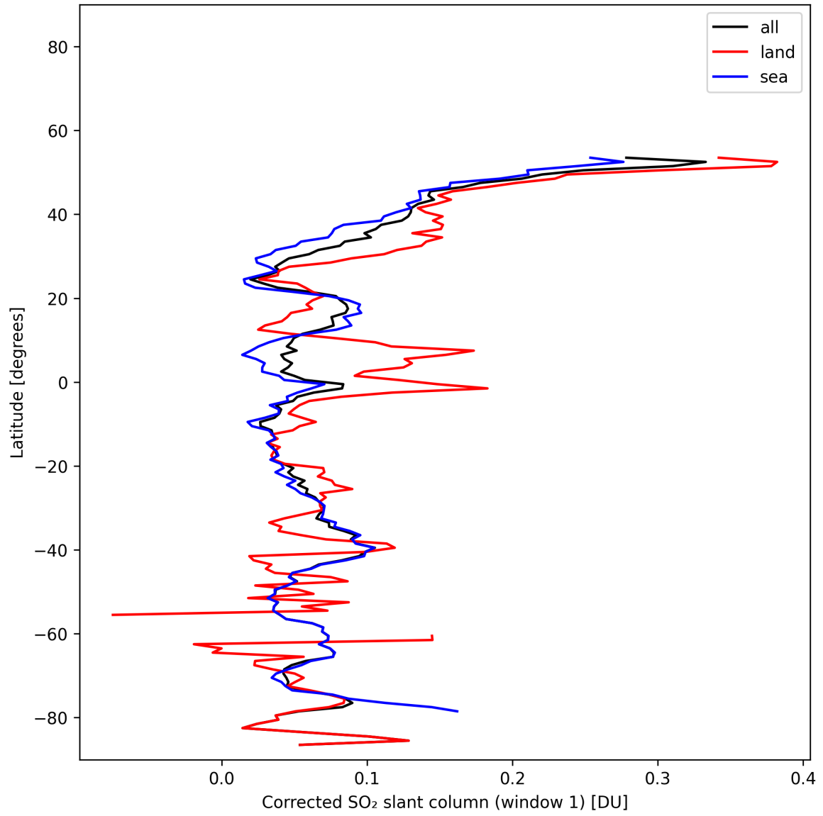
Figure 39: Zonal average of “Corrected SO 2 slant column (window 1)” for 2025-02-03 to 2025-02-04.
