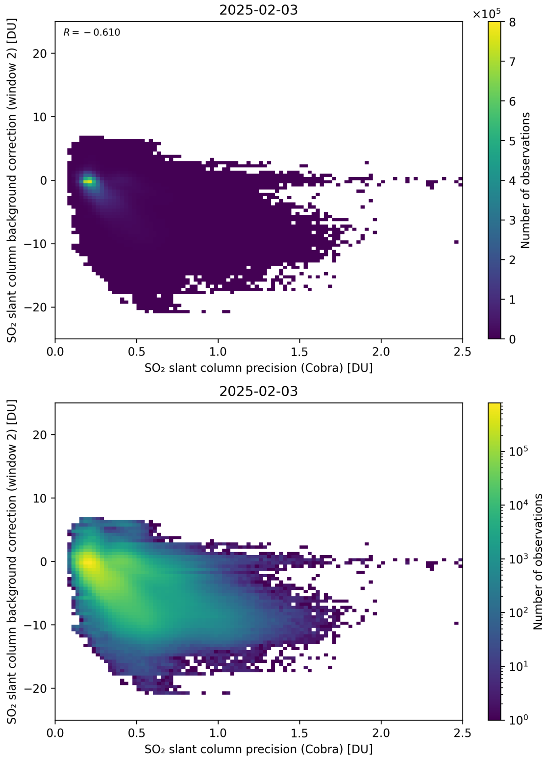
Figure 200: Scatter density plot of “SO 2 slant column precision (Cobra)” against “SO 2 slant column background correction (window 2)” for 2025-02-03 to 2025-02-04.
