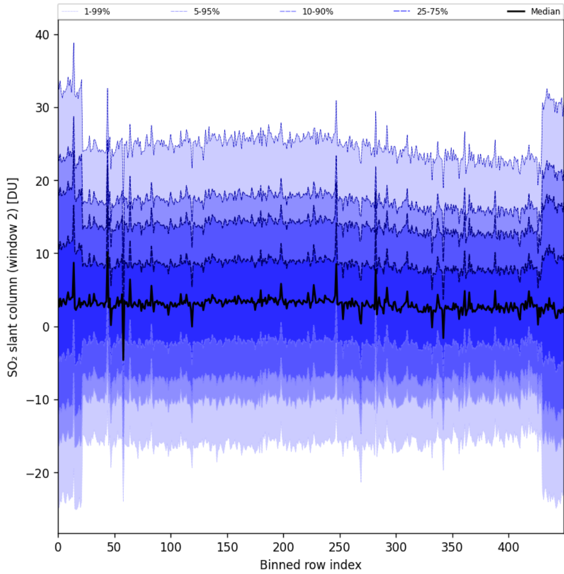
Figure 93: Along track statistics of “SO 2 slant column (window 2)” for 2025-02-03 to 2025-02-04
