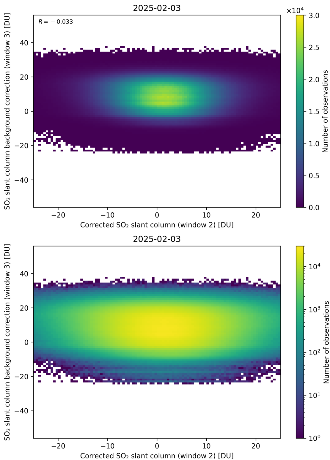
Figure 245: Scatter density plot of “Corrected SO 2 slant column (window 2)” against “SO 2 slant column background correction (window 3)” for 2025-02-03 to 2025-02-04.
