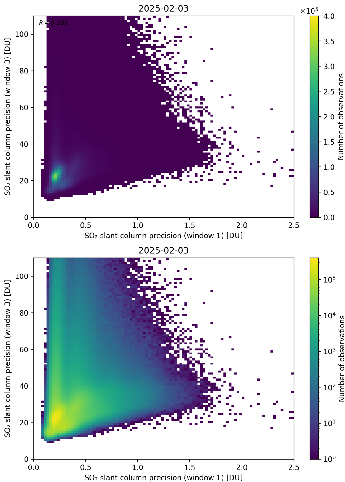
Figure 279: Scatter density plot of “SO 2 slant column precision (window 1)” against “SO 2 slant column precision (window 3)” for 2025-02-03 to 2025-02-04.
