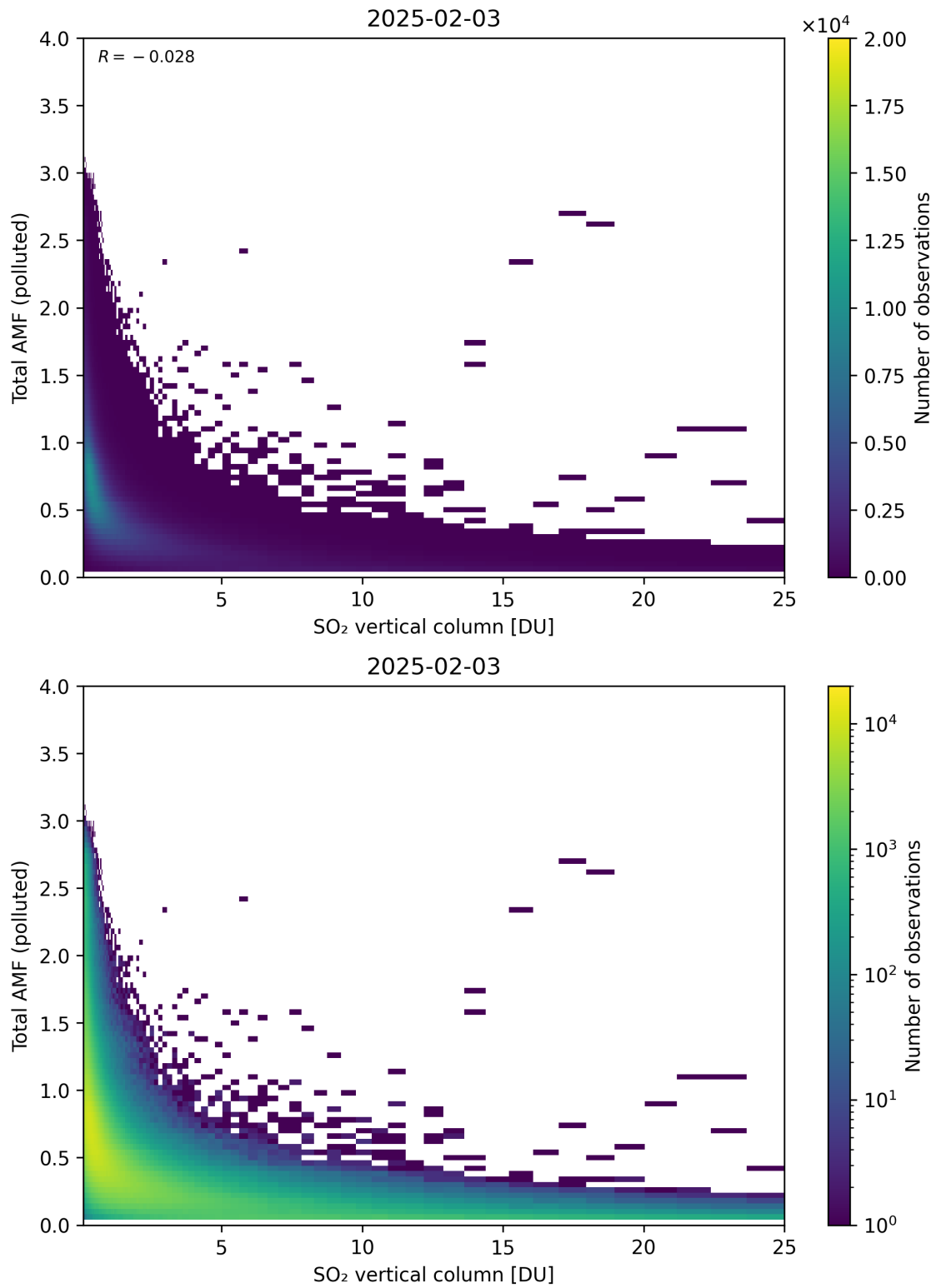
Figure 359: Scatter density plot of “SO 2 vertical column” against “Total AMF (polluted)” for 2025-02-03 to 2025-02-04.
