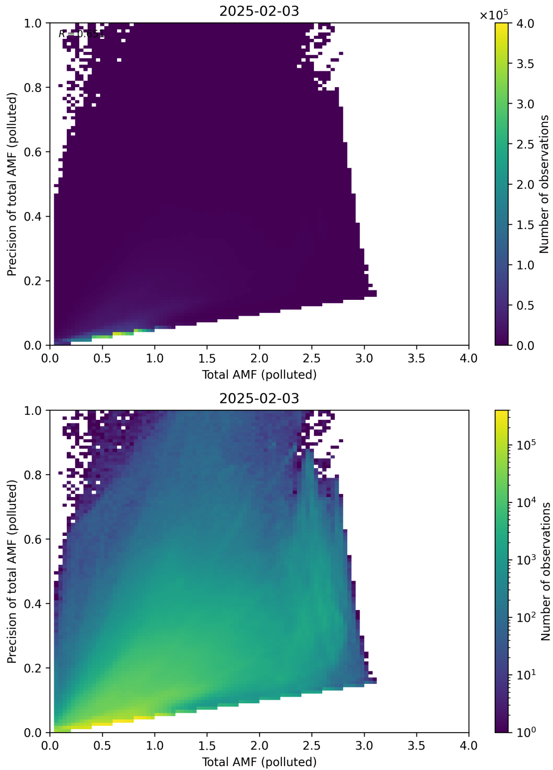
Figure 322: Scatter density plot of “Total AMF (polluted)” against “Precision of total AMF (polluted)” for 2025-02-03 to 2025-02-04.
