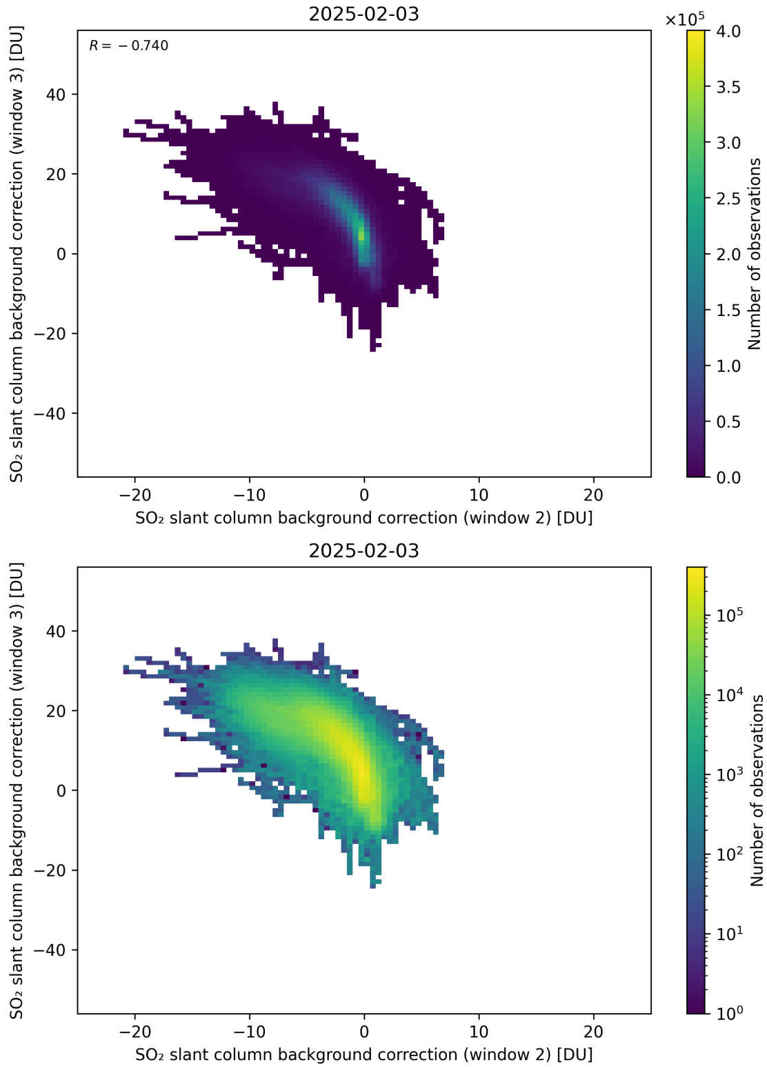
Figure 122: Scatter density plot of “SO 2 slant column background correction (window 2)” against “SO 2 slant column background correction (window 3)” for 2025-02-03 to 2025-02-04.
