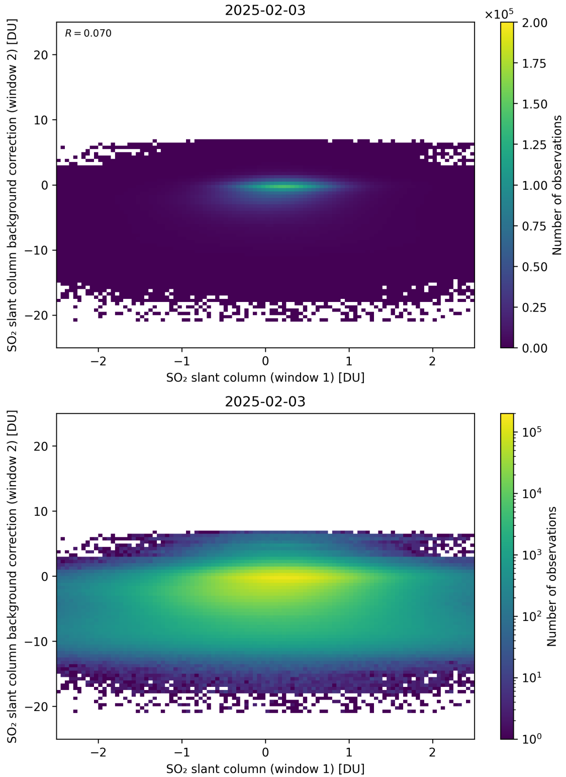
Figure 263: Scatter density plot of “SO 2 slant column (window 1)” against “SO 2 slant column background correction (window 2)” for 2025-02-03 to 2025-02-04.
