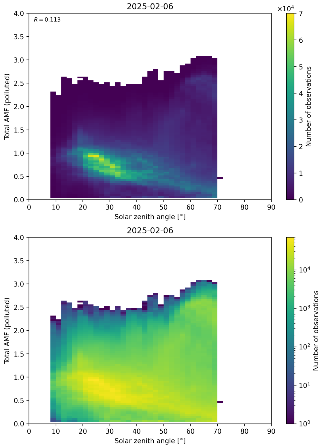
Figure 189: Scatter density plot of “Solar zenith angle” against “Total AMF (polluted)” for 2025-02-05 to 2025-02-07.
