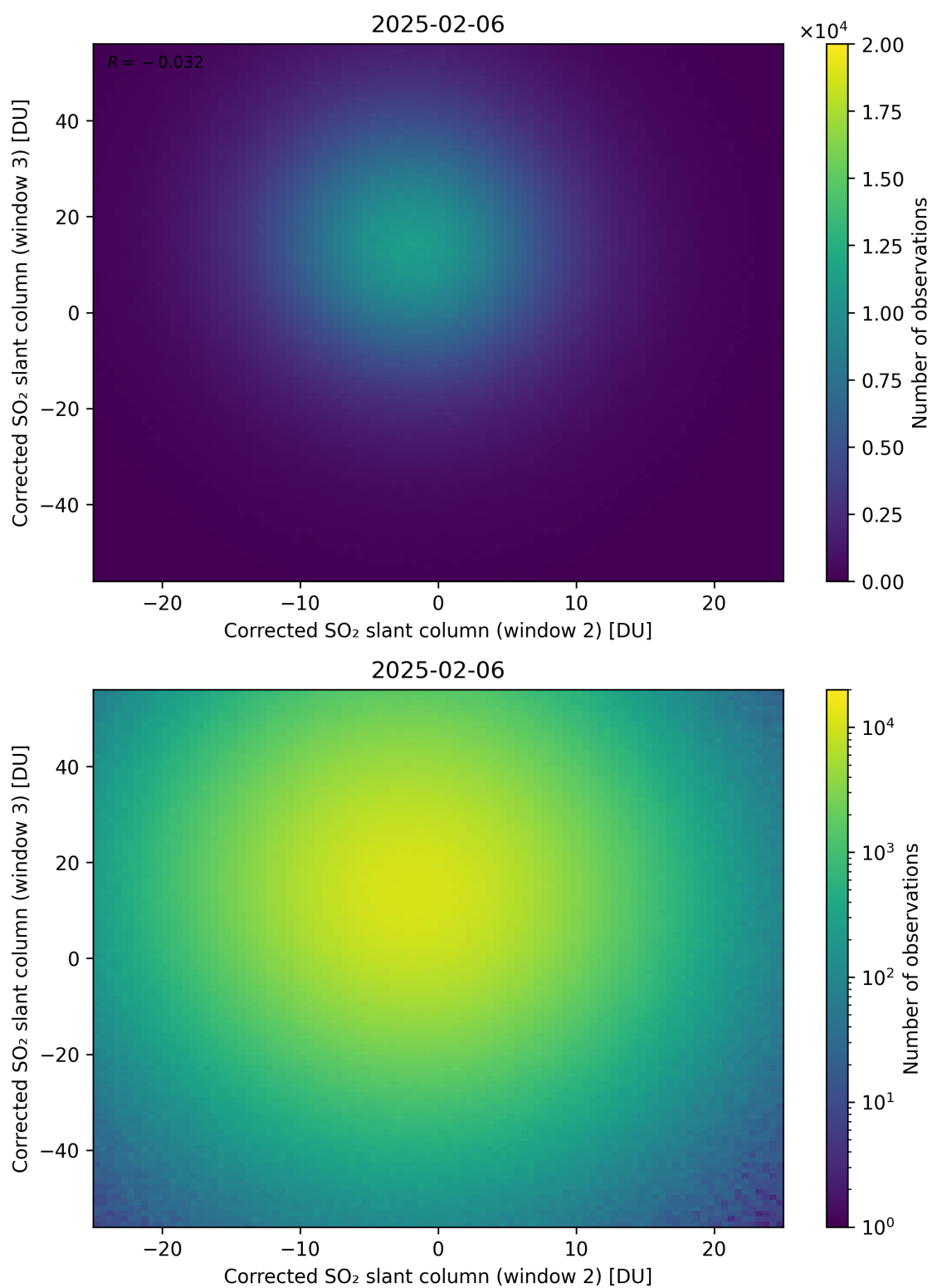
Figure 250: Scatter density plot of “Corrected SO 2 slant column (window 2)” against “Corrected SO 2 slant column (window 3)” for 2025-02-05 to 2025-02-07.
