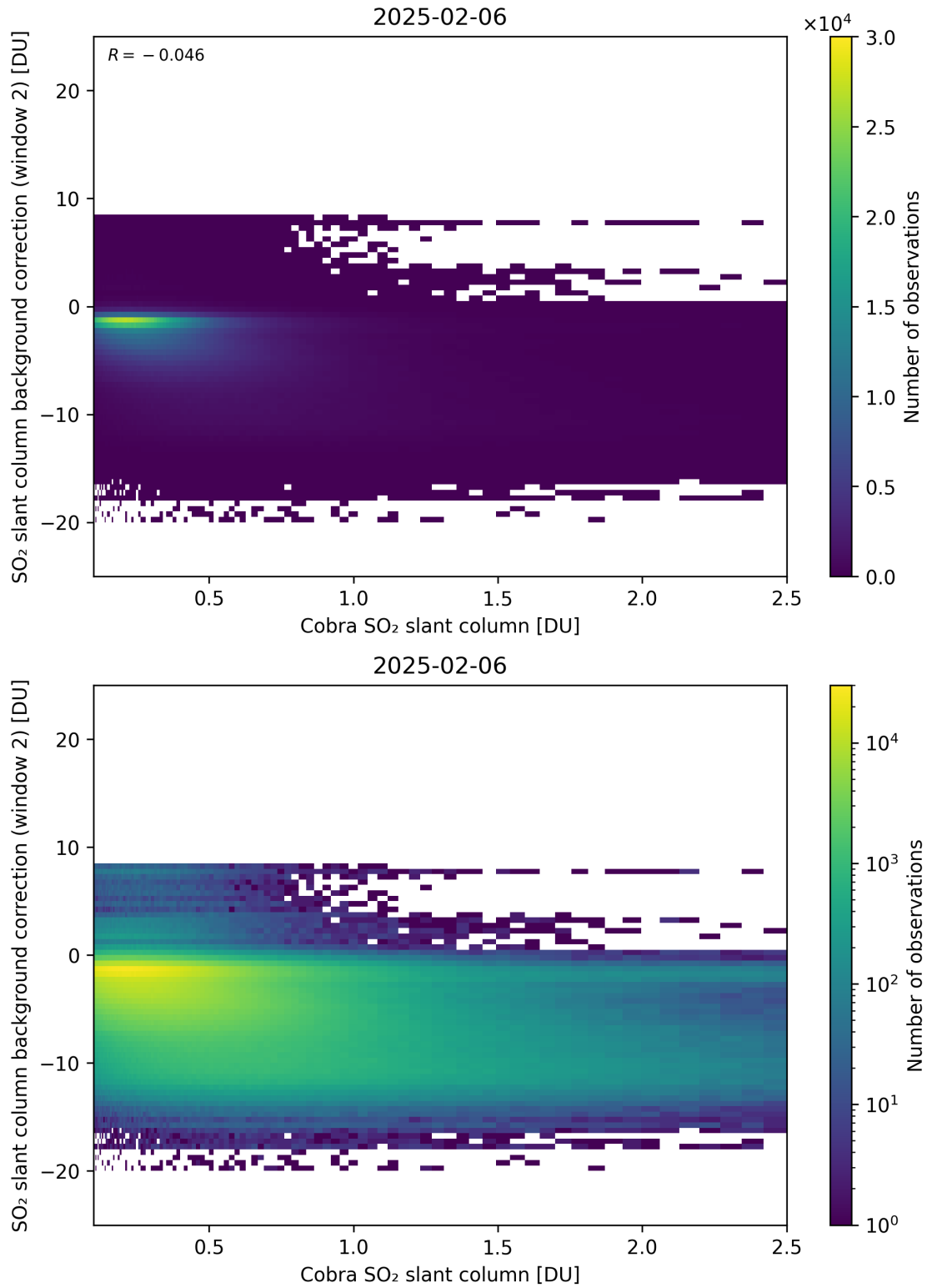
Figure 194: Scatter density plot of “Cobra SO 2 slant column” against “SO 2 slant column background correction (window 2)” for 2025-02-05 to 2025-02-07.
