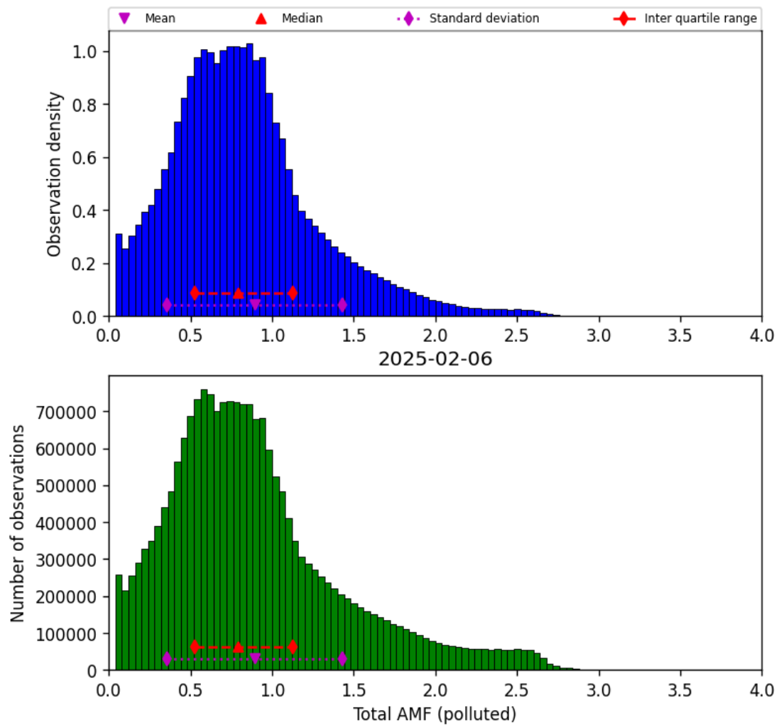
Figure 79: Histogram of “Total AMF (polluted)” for 2025-02-05 to 2025-02-07
