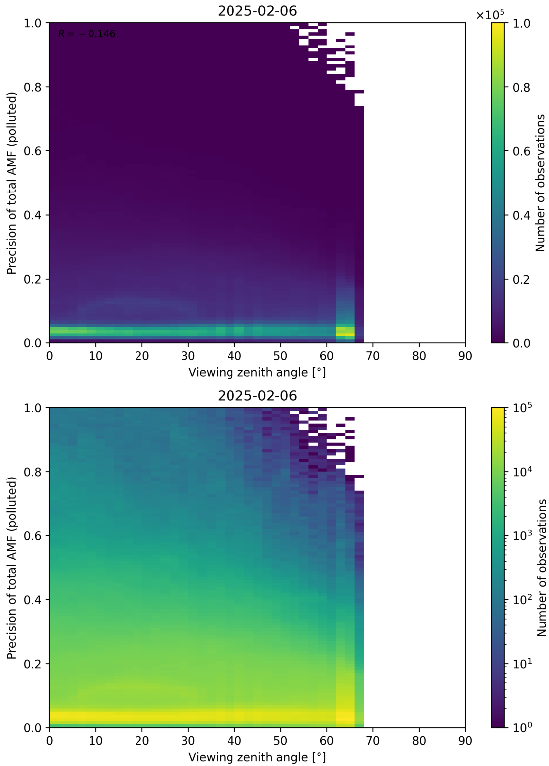
Figure 382: Scatter density plot of “Viewing zenith angle” against “Precision of total AMF (polluted)” for 2025-02-05 to 2025-02-07.
