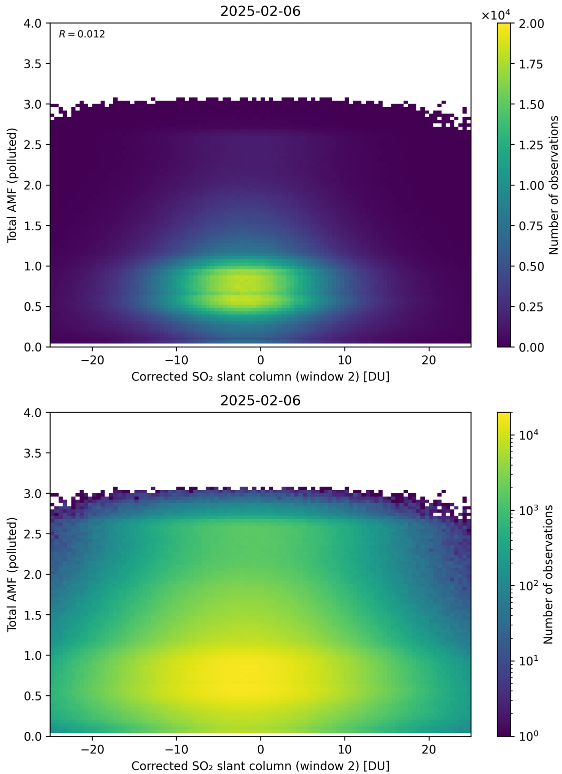
Figure 253: Scatter density plot of “Corrected SO 2 slant column (window 2)” against “Total AMF (polluted)” for 2025-02-05 to 2025-02-07.
