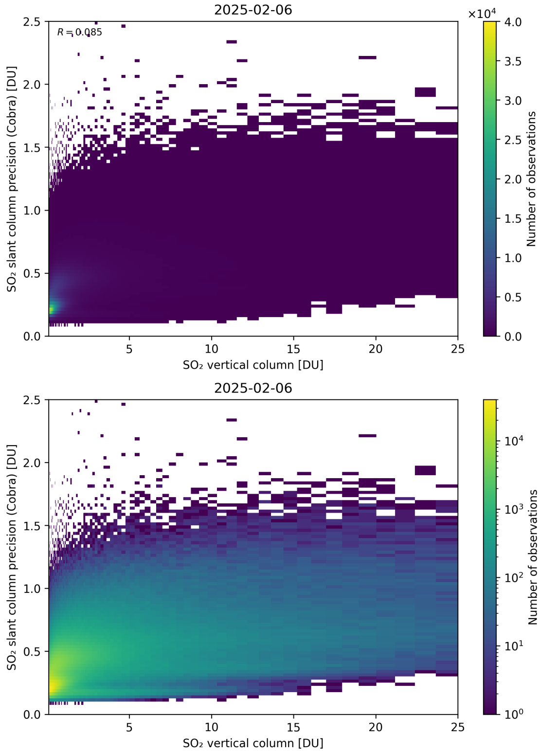
Figure 350: Scatter density plot of “SO 2 vertical column” against “SO 2 slant column precision (Cobra)” for 2025-02-05 to 2025-02-07.
