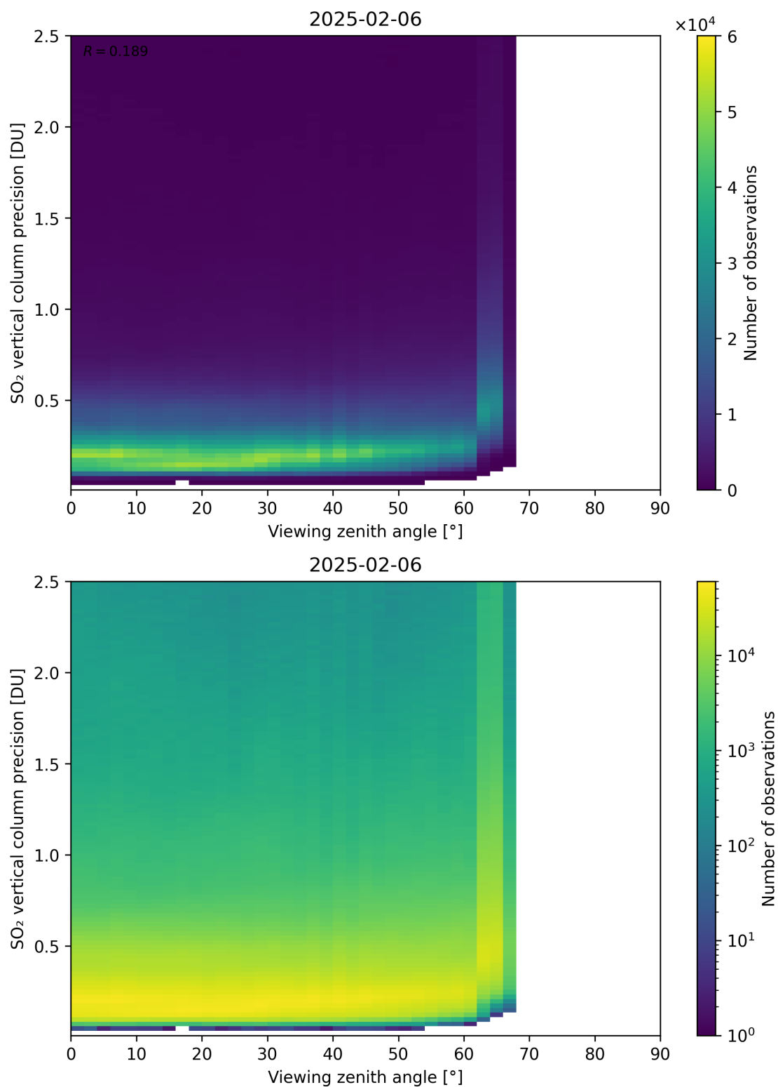
Figure 384: Scatter density plot of “Viewing zenith angle” against “SO 2 vertical column precision” for 2025-02-05 to 2025-02-07.
