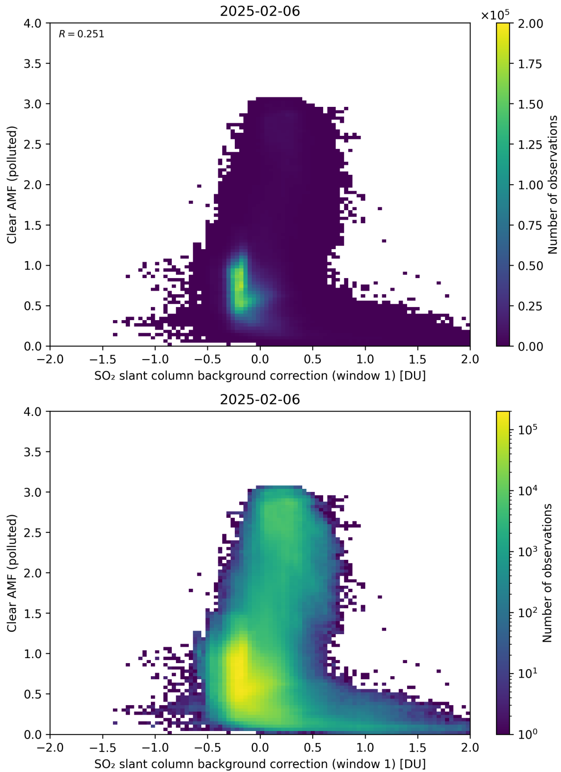
Figure 114: Scatter density plot of “SO 2 slant column background correction (window 1)” against “Clear AMF (polluted)” for 2025-02-05 to 2025-02-07.
