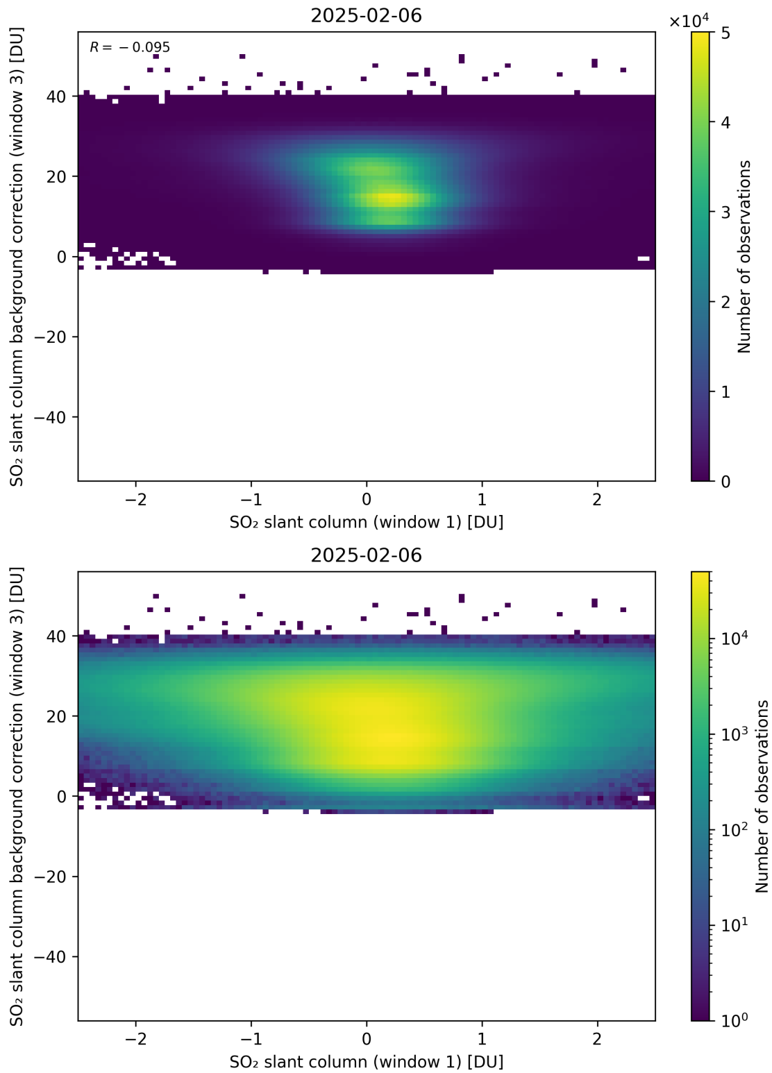
Figure 264: Scatter density plot of “SO 2 slant column (window 1)” against “SO 2 slant column background correction (window 3)” for 2025-02-05 to 2025-02-07.
