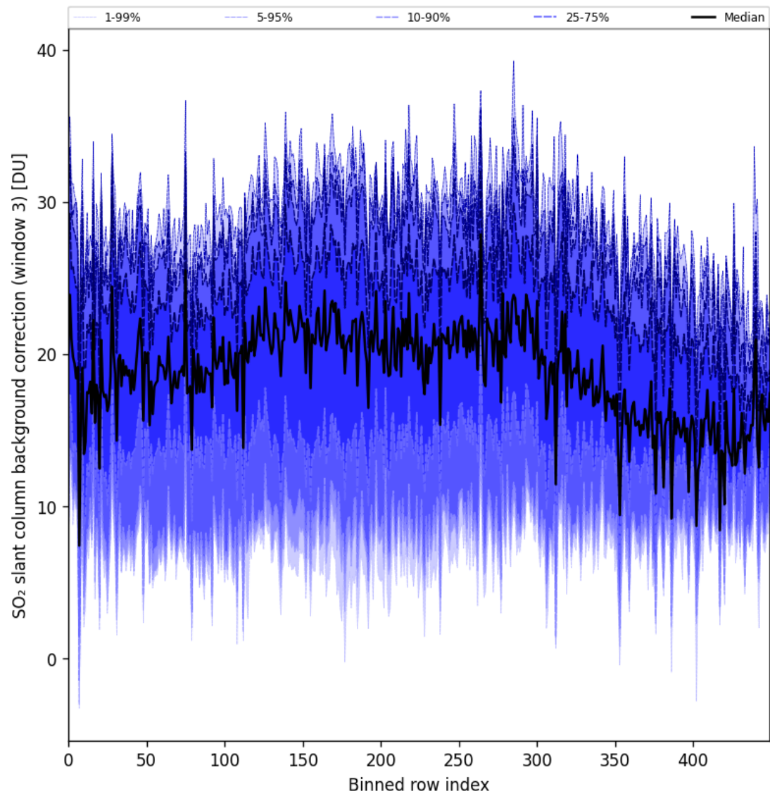
Figure 100: Along track statistics of “SO 2 slant column background correction (window 3)” for 2025-02-05 to 2025-02-07
