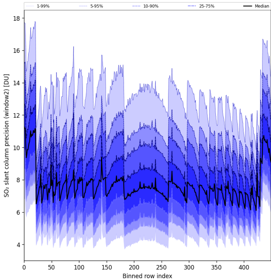
Figure 94: Along track statistics of “SO 2 slant column precision (window2)” for 2025-02-05 to 2025-02-07
