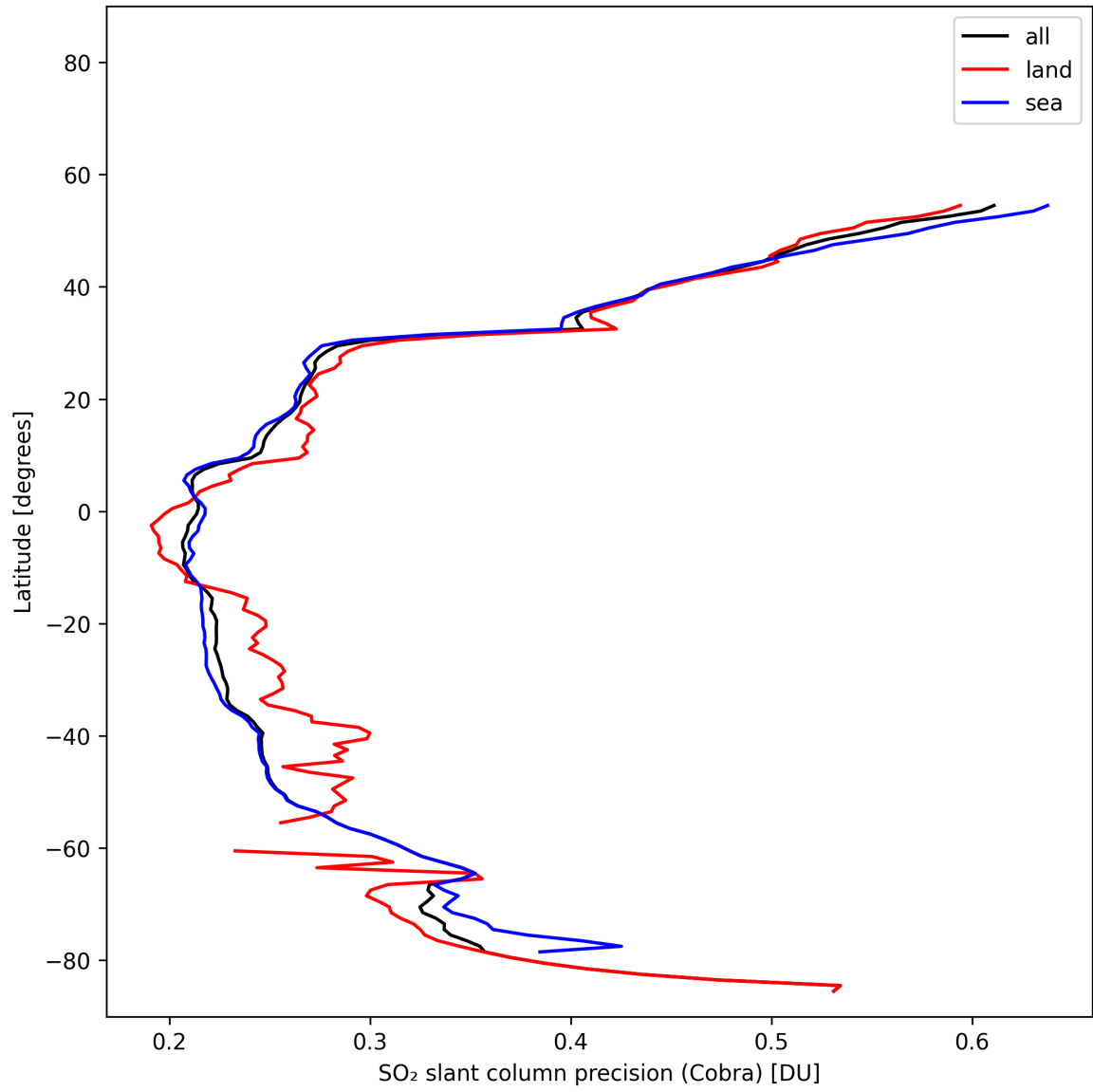
Figure 36: Zonal average of “SO 2 slant column precision (Cobra)” for 2025-02-05 to 2025-02-07.
