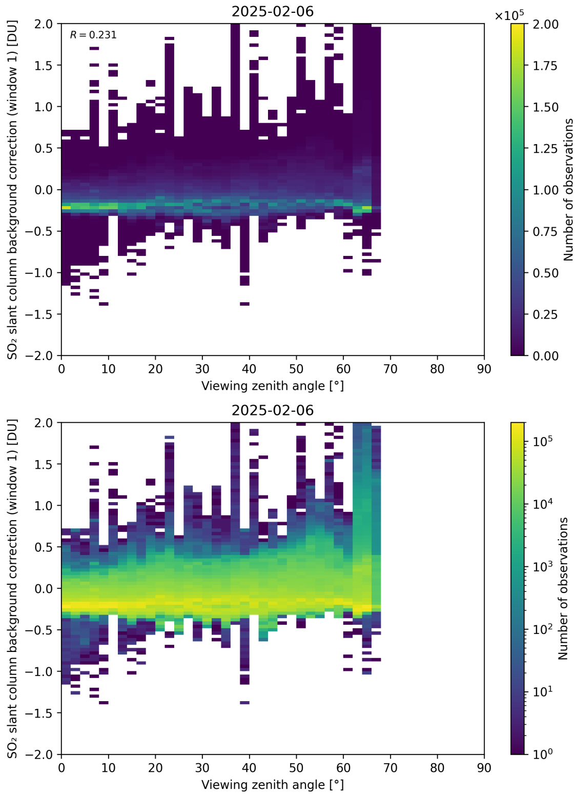
Figure 362: Scatter density plot of “Viewing zenith angle” against “SO 2 slant column background correction (window 1)” for 2025-02-05 to 2025-02-07.
