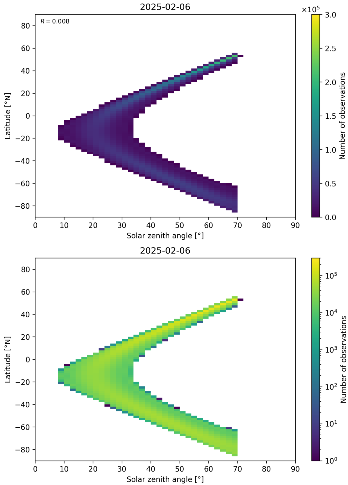
Figure 177: Scatter density plot of “Solar zenith angle” against “Latitude” for 2025-02-05 to 2025-02-07.
