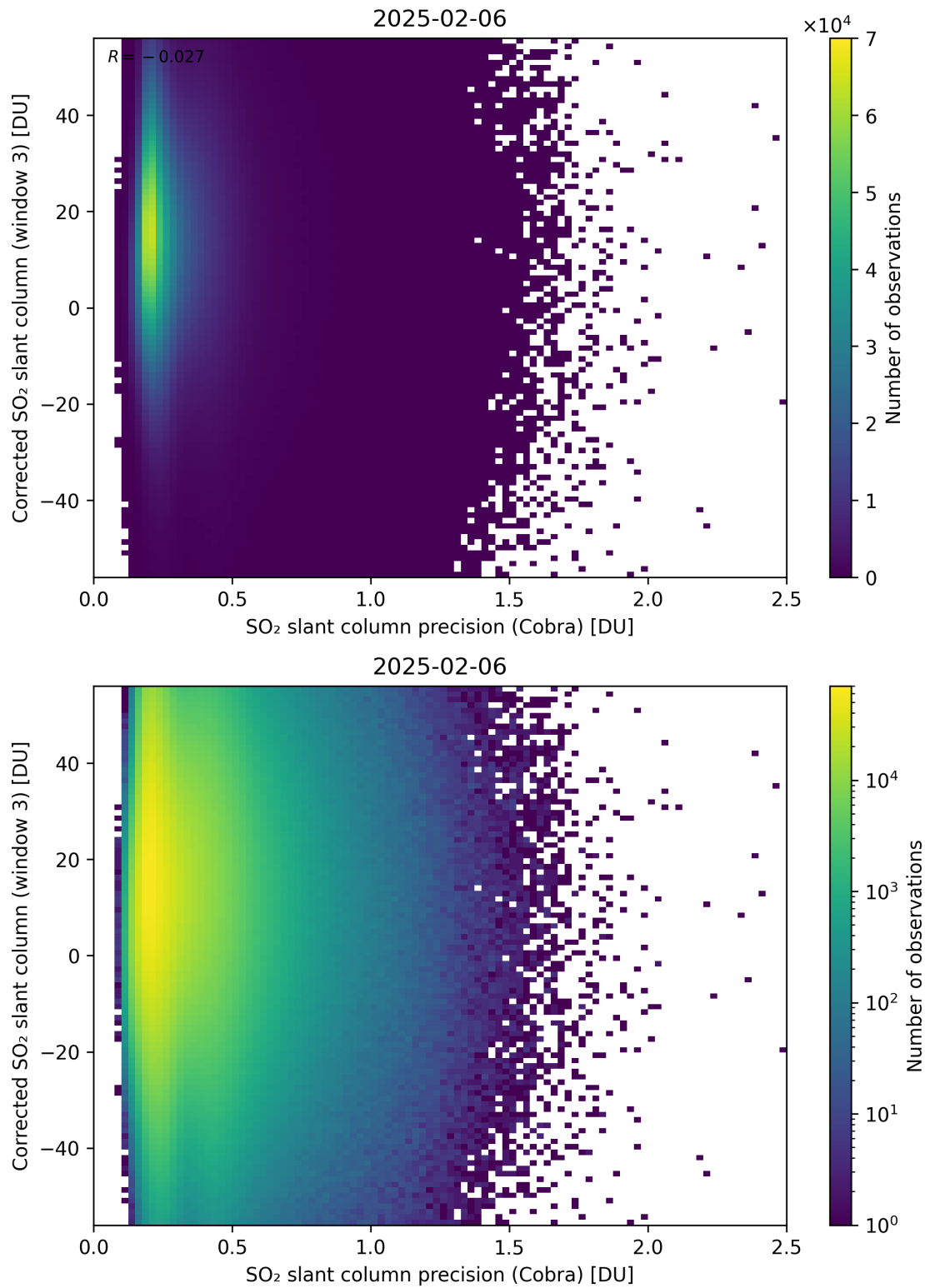
Figure 207: Scatter density plot of “SO 2 slant column precision (Cobra)” against “Corrected SO 2 slant column (window 3)” for 2025-02-05 to 2025-02-07.
