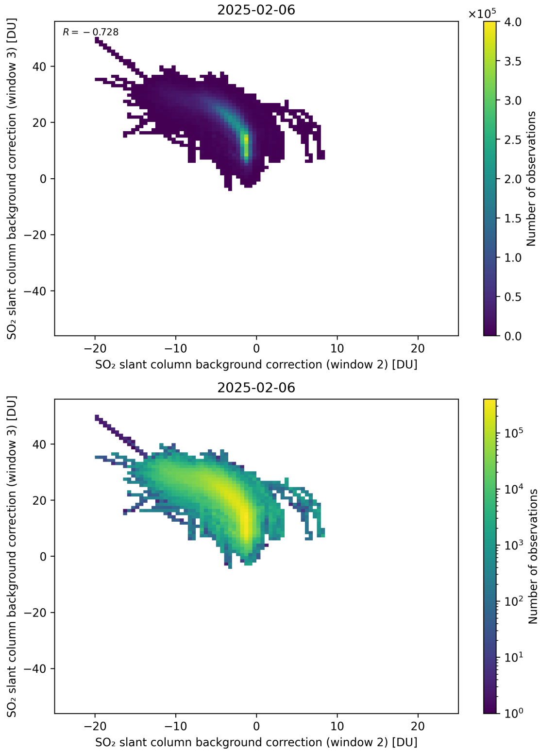
Figure 122: Scatter density plot of “SO 2 slant column background correction (window 2)” against “SO 2 slant column background correction (window 3)” for 2025-02-05 to 2025-02-07.
