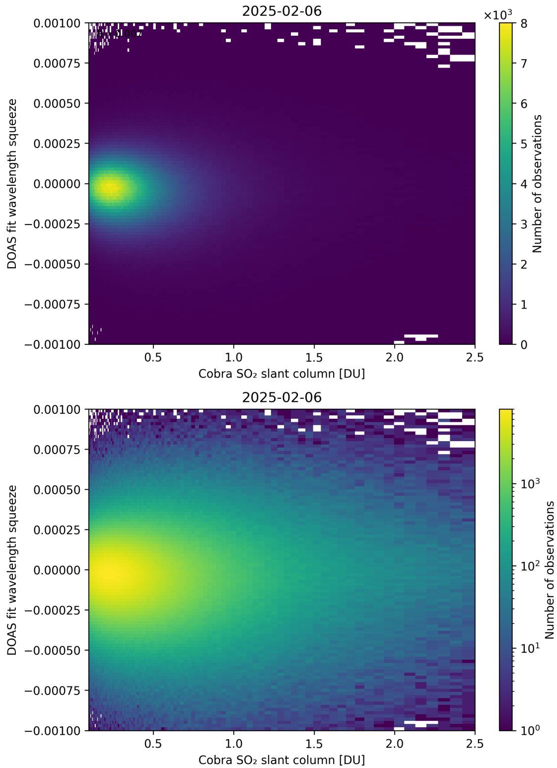
Figure 197: Scatter density plot of “Cobra SO 2 slant column” against “DOAS fit wavelength squeeze” for 2025-02-05 to 2025-02-07.
