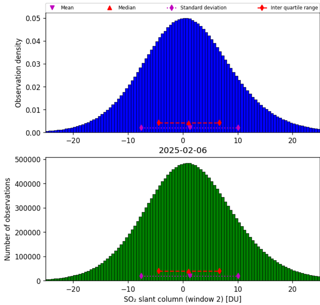
Figure 67: Histogram of “SO 2 slant column (window 2)” for 2025-02-05 to 2025-02-07
