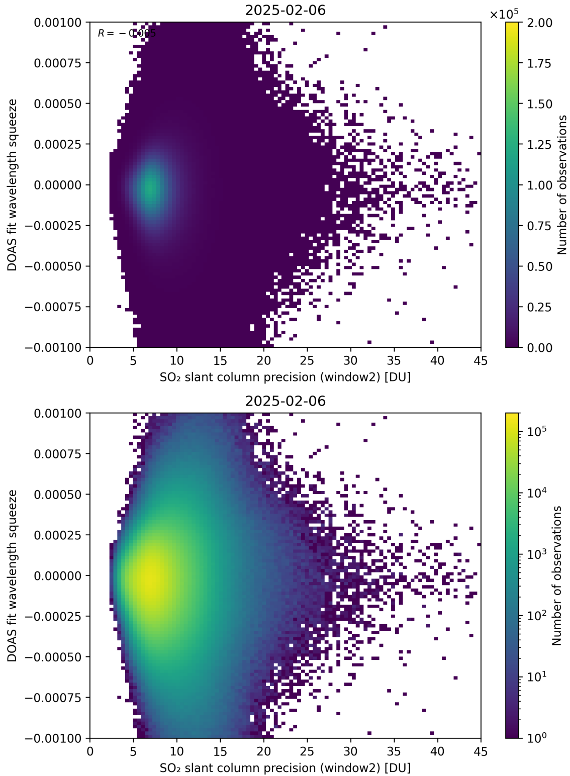
Figure 294: Scatter density plot of “SO 2 slant column precision (window2)” against “DOAS fit wavelength squeeze” for 2025-02-05 to 2025-02-07.
