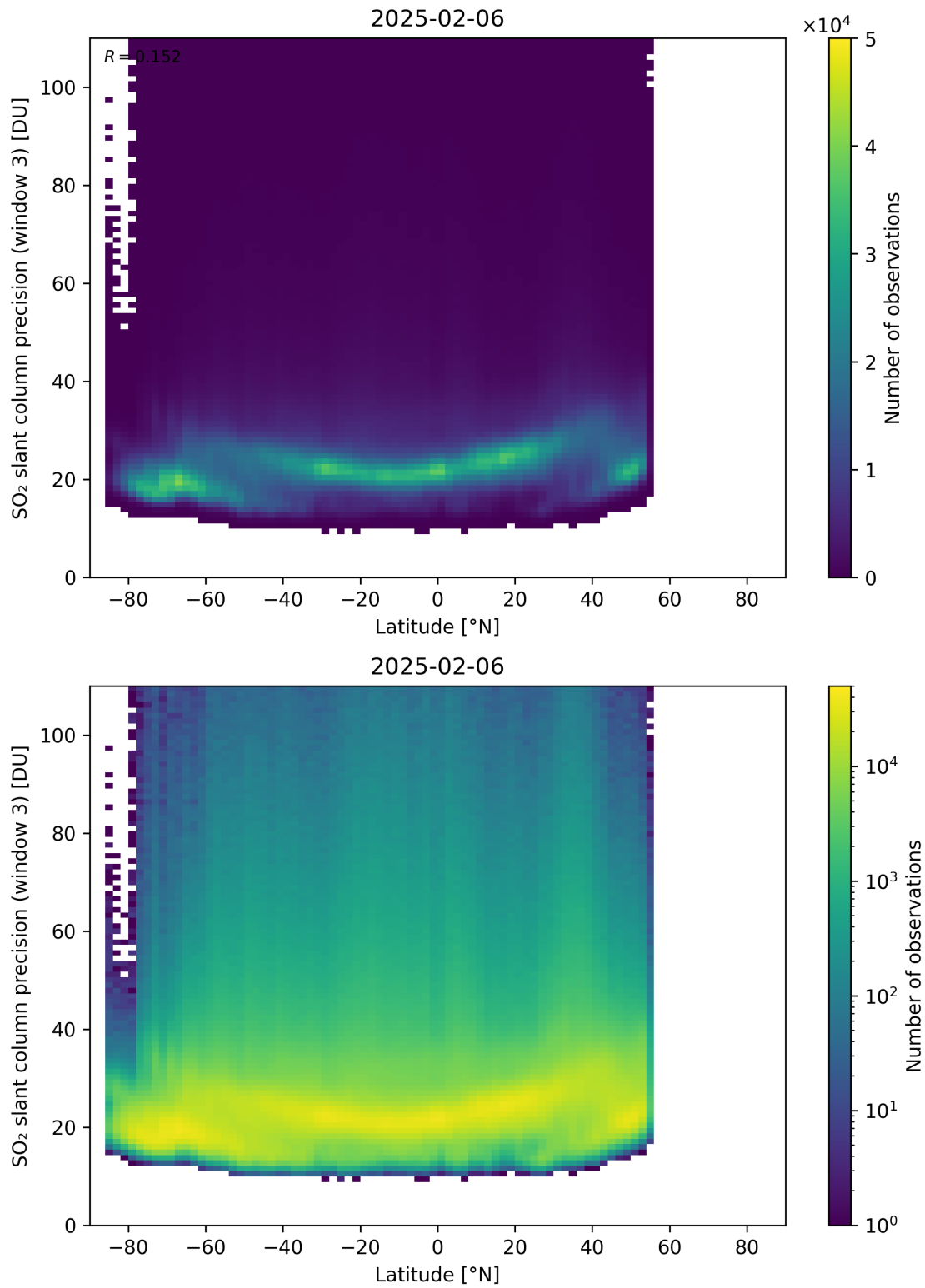
Figure 166: Scatter density plot of “Latitude” against “SO 2 slant column precision (window 3)” for 2025-02-05 to 2025-02-07.
