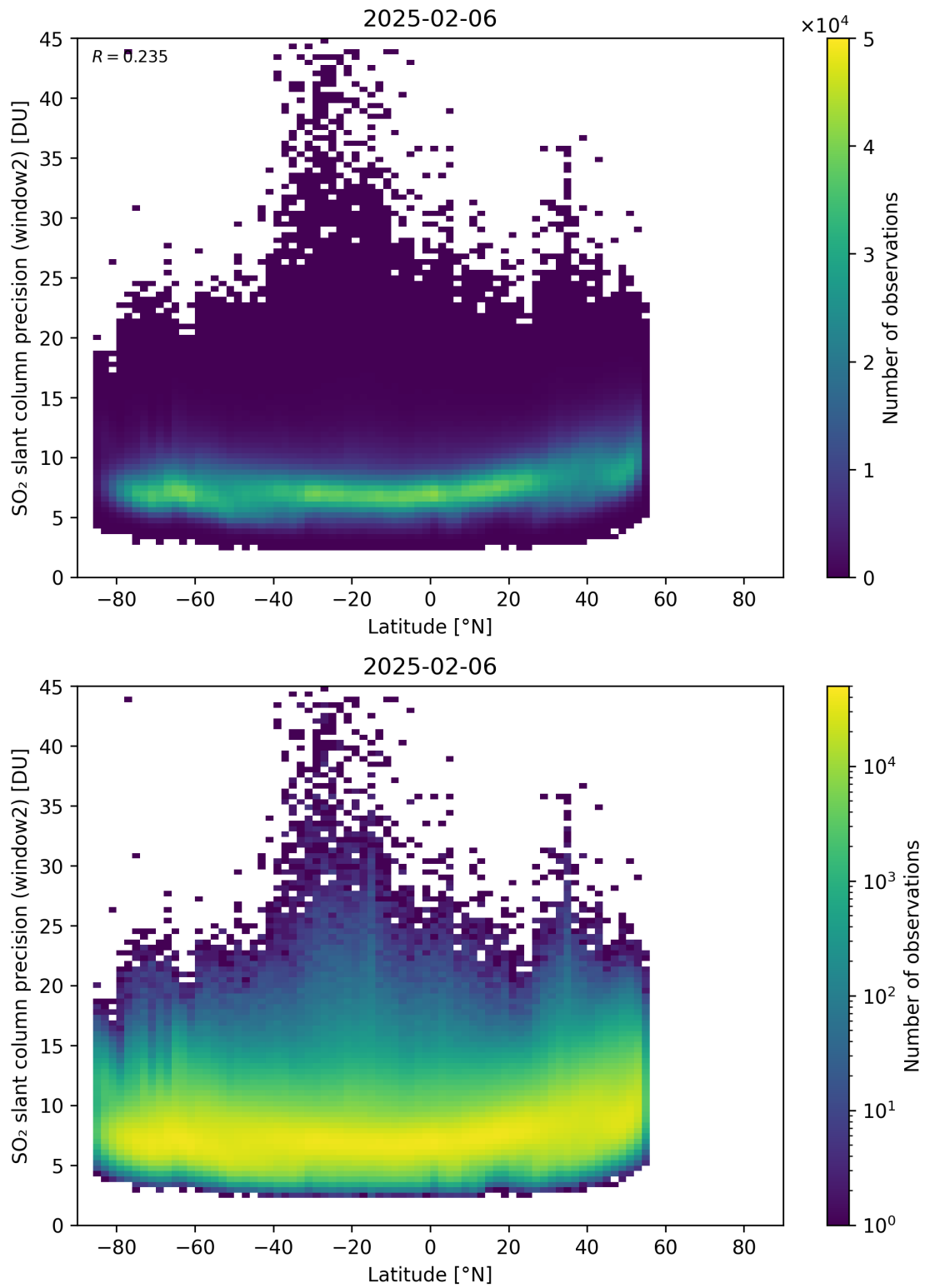
Figure 164: Scatter density plot of “Latitude” against “SO 2 slant column precision (window2)” for 2025-02-05 to 2025-02-07.
