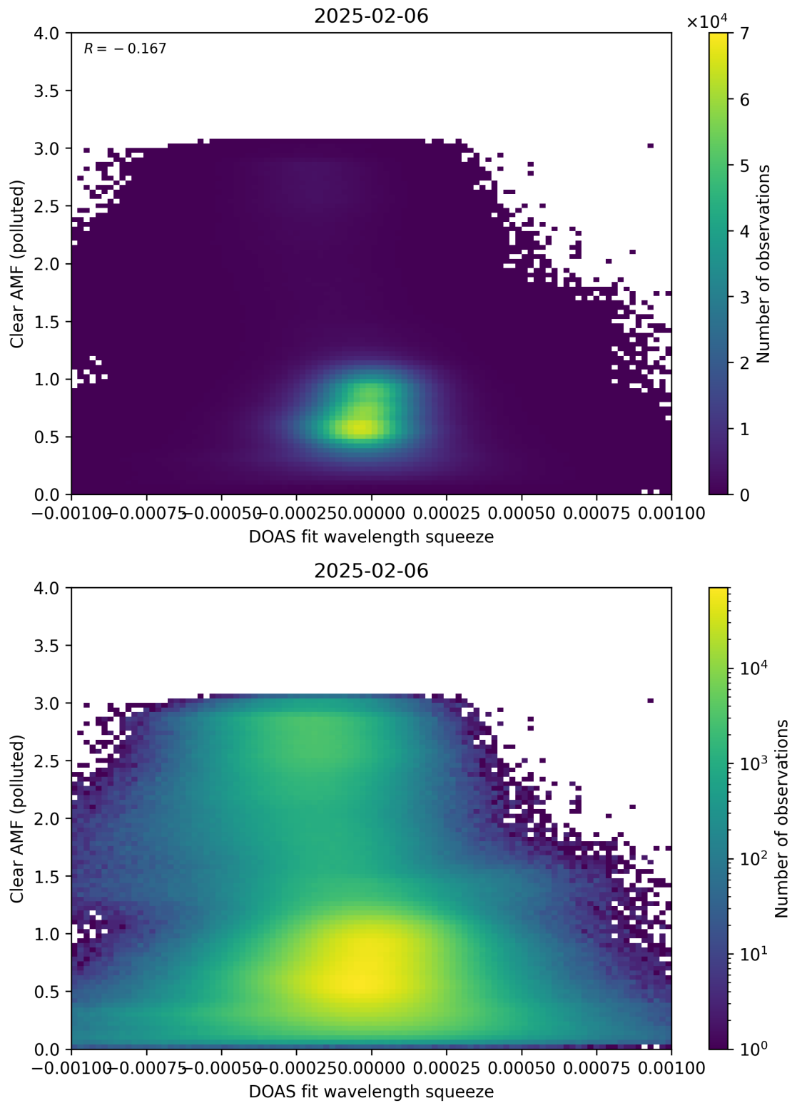
Figure 144: Scatter density plot of “DOAS fit wavelength squeeze” against “Clear AMF (polluted)” for 2025-02-05 to 2025-02-07.
