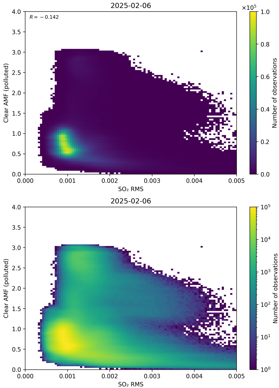
Figure 147: Scatter density plot of “SO 2 RMS” against “Clear AMF (polluted)” for 2025-02-05 to 2025-02-07.
