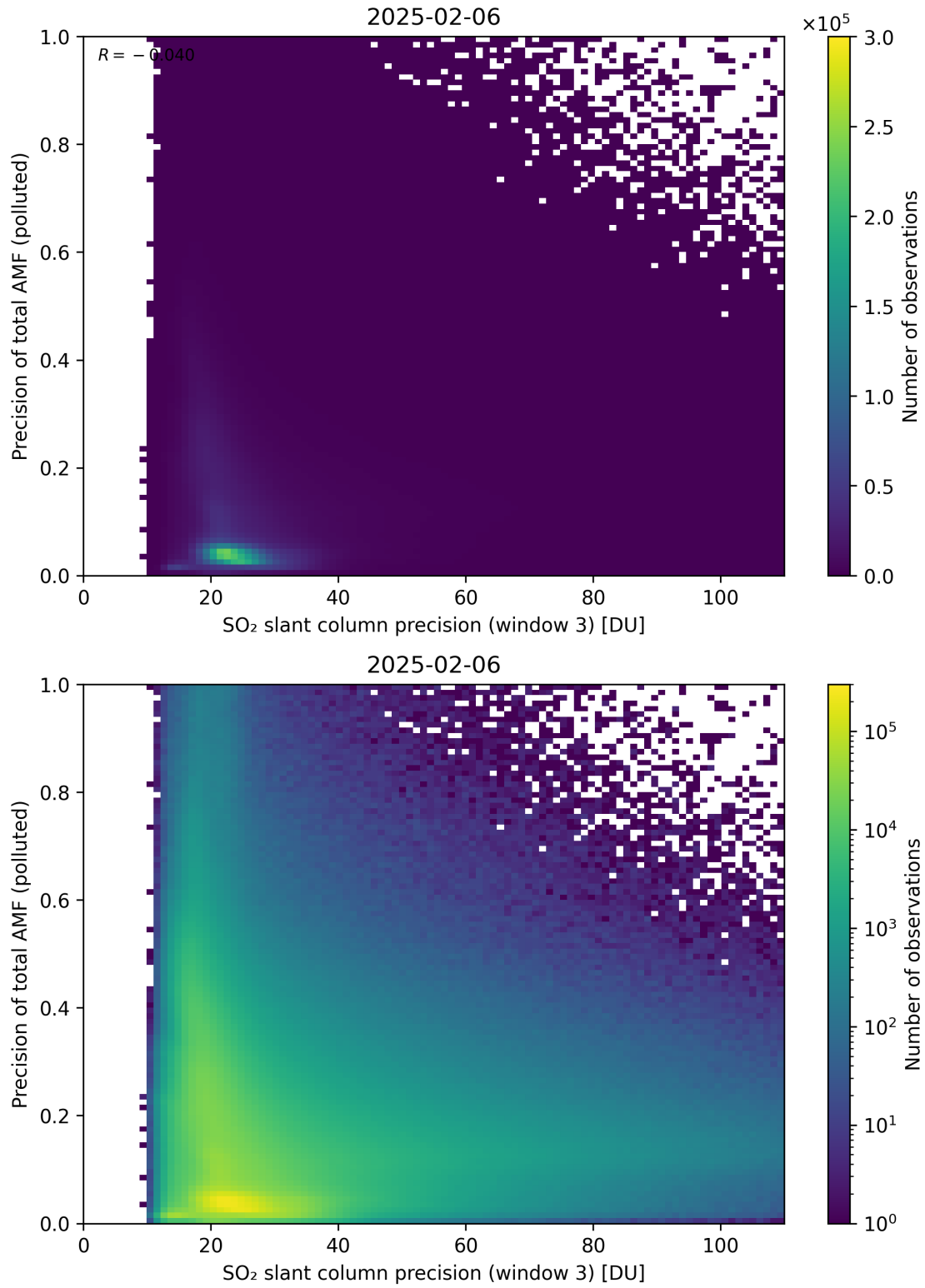
Figure 314: Scatter density plot of “SO 2 slant column precision (window 3)” against “Precision of total AMF (polluted)” for 2025-02-05 to 2025-02-07.
