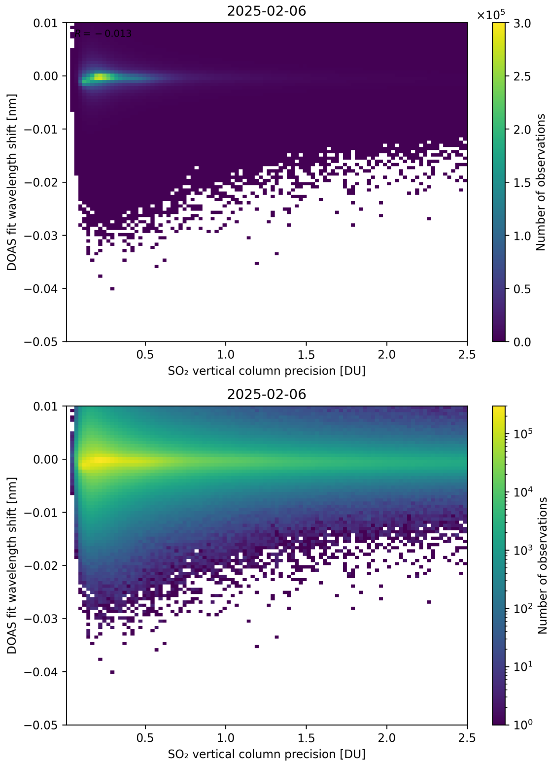
Figure 332: Scatter density plot of “SO 2 vertical column precision” against “DOAS fit wavelength shift” for 2025-02-05 to 2025-02-07.
