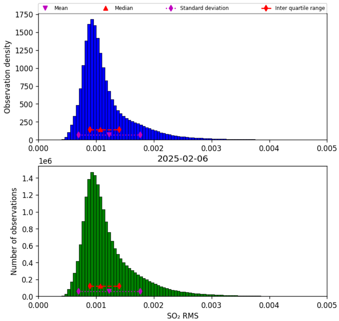
Figure 78: Histogram of “SO 2 RMS” for 2025-02-05 to 2025-02-07
