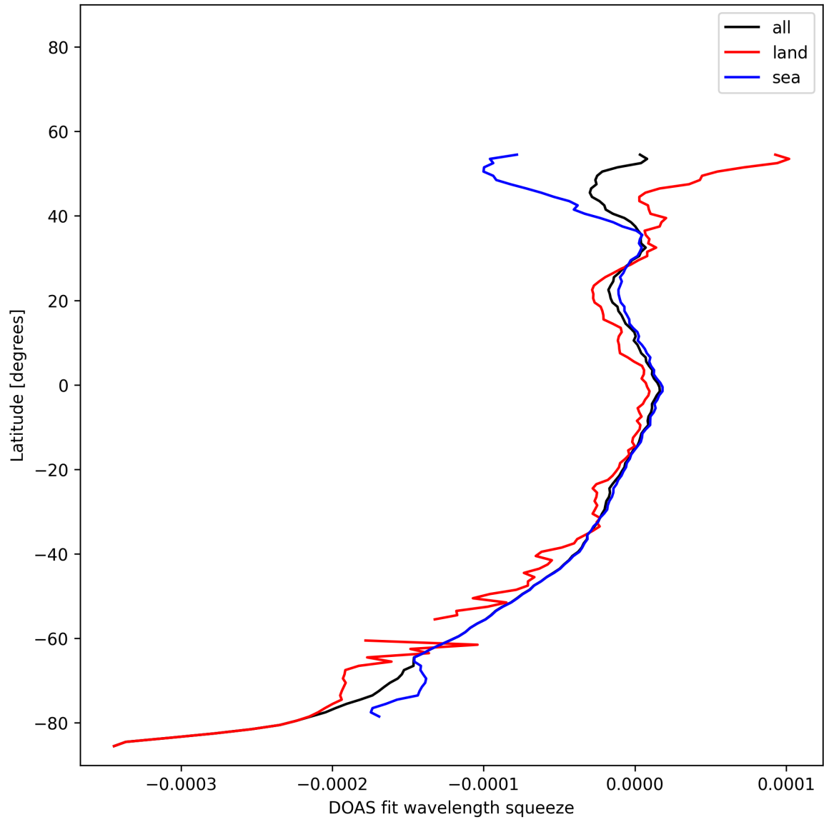
Figure 51: Zonal average of “DOAS fit wavelength squeeze” for 2025-02-05 to 2025-02-07.
