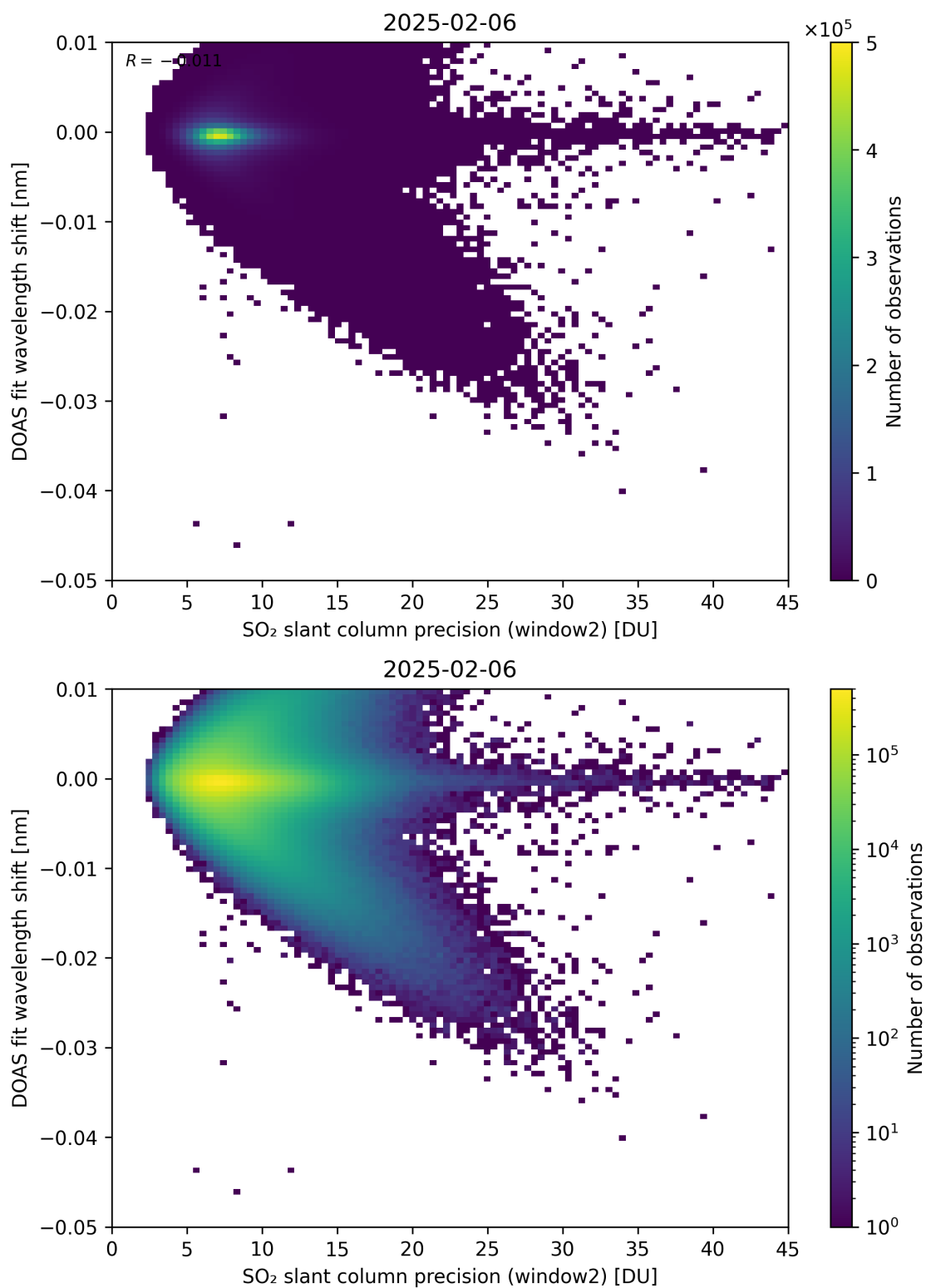
Figure 293: Scatter density plot of “SO 2 slant column precision (window2)” against “DOAS fit wavelength shift” for 2025-02-05 to 2025-02-07.
