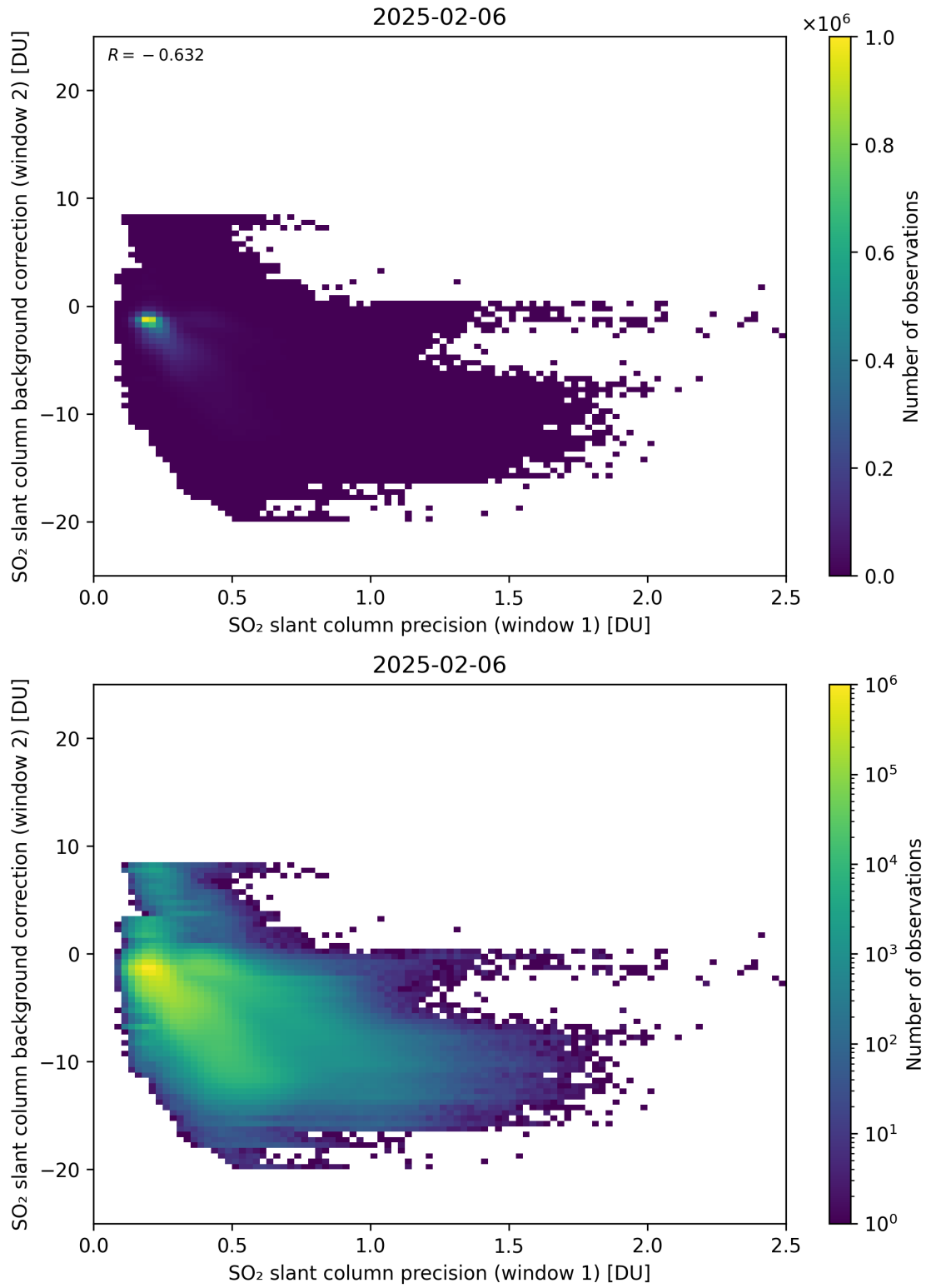
Figure 269: Scatter density plot of “SO 2 slant column precision (window 1)” against “SO 2 slant column background correction (window 2)” for 2025-02-05 to 2025-02-07.
