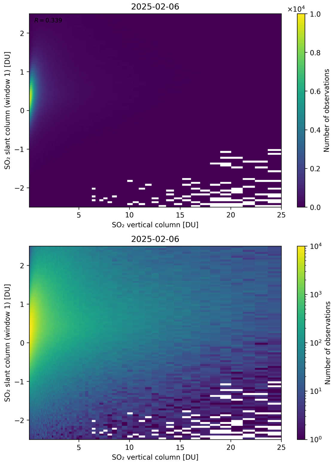
Figure 354: Scatter density plot of “SO 2 vertical column” against “SO 2 slant column (window 1)” for 2025-02-05 to 2025-02-07.
