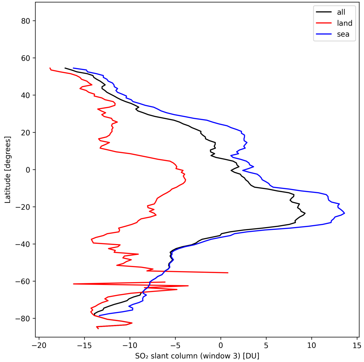
Figure 45: Zonal average of “SO 2 slant column (window 3)” for 2025-02-05 to 2025-02-07.
