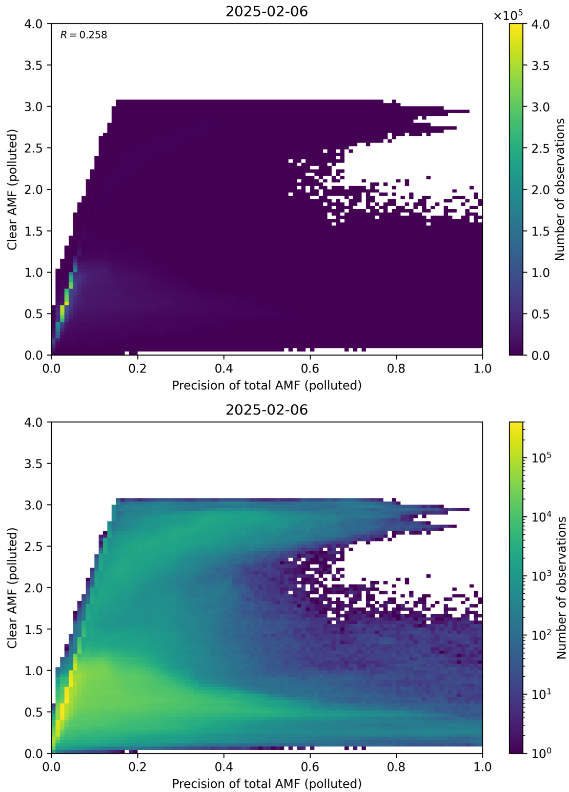
Figure 320: Scatter density plot of “Precision of total AMF (polluted)” against “Clear AMF (polluted)” for 2025-02-05 to 2025-02-07.
