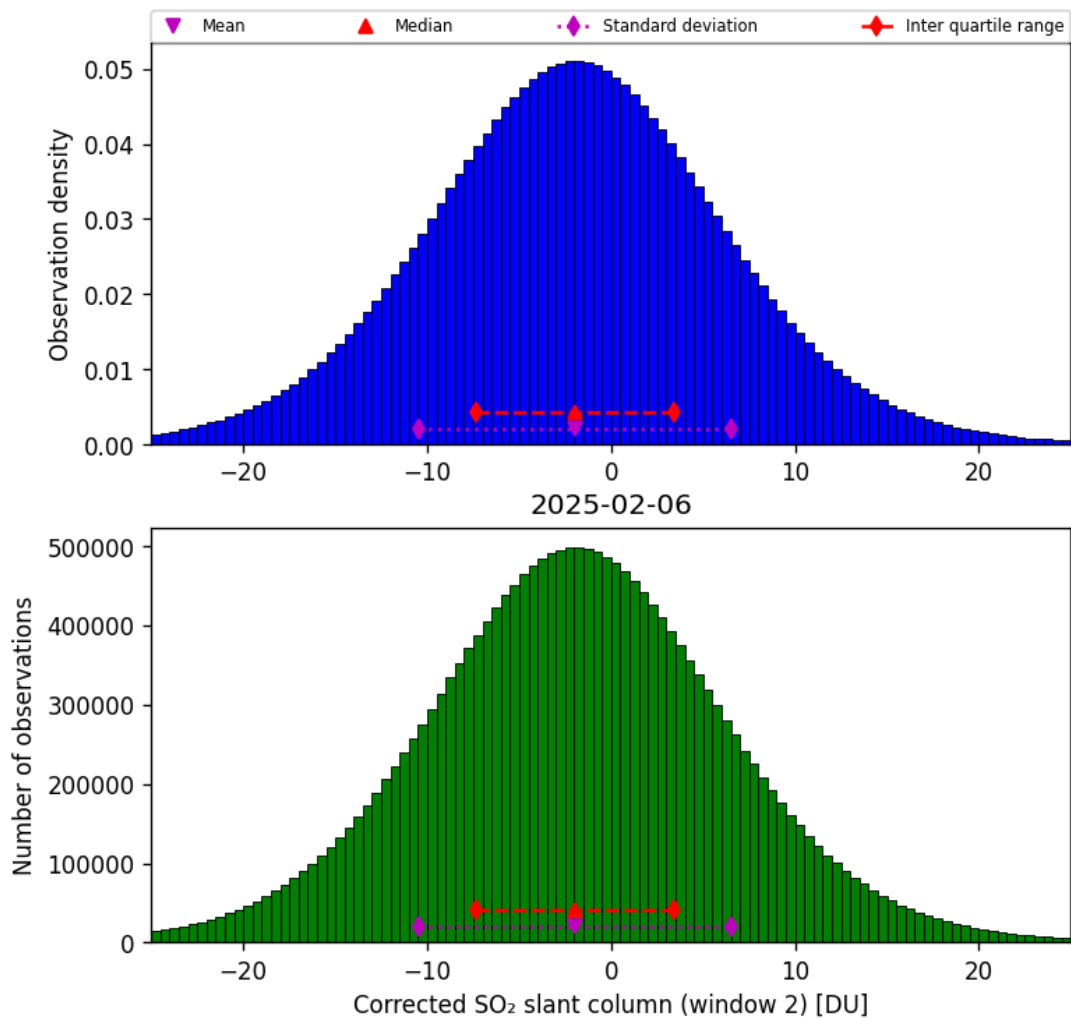
Figure 69: Histogram of “Corrected SO 2 slant column (window 2)” for 2025-02-05 to 2025-02-07
