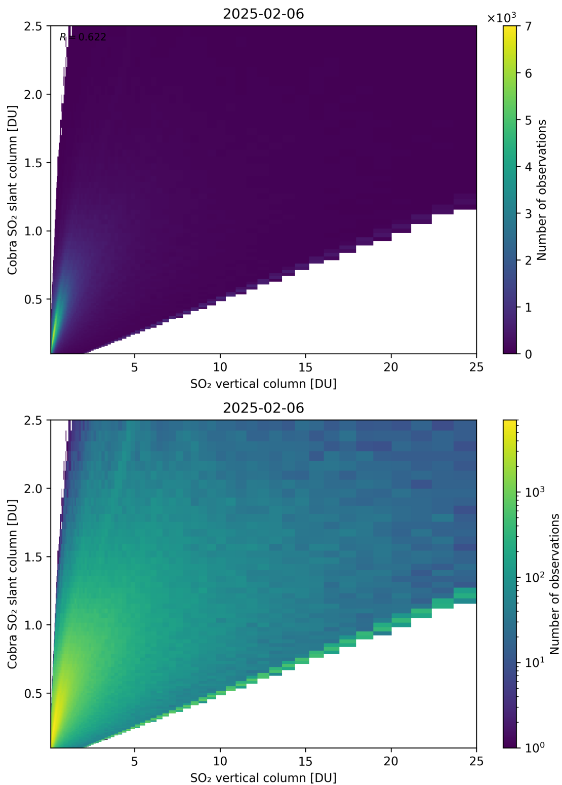
Figure 349: Scatter density plot of “SO 2 vertical column” against “Cobra SO 2 slant column” for 2025-02-05 to 2025-02-07.
