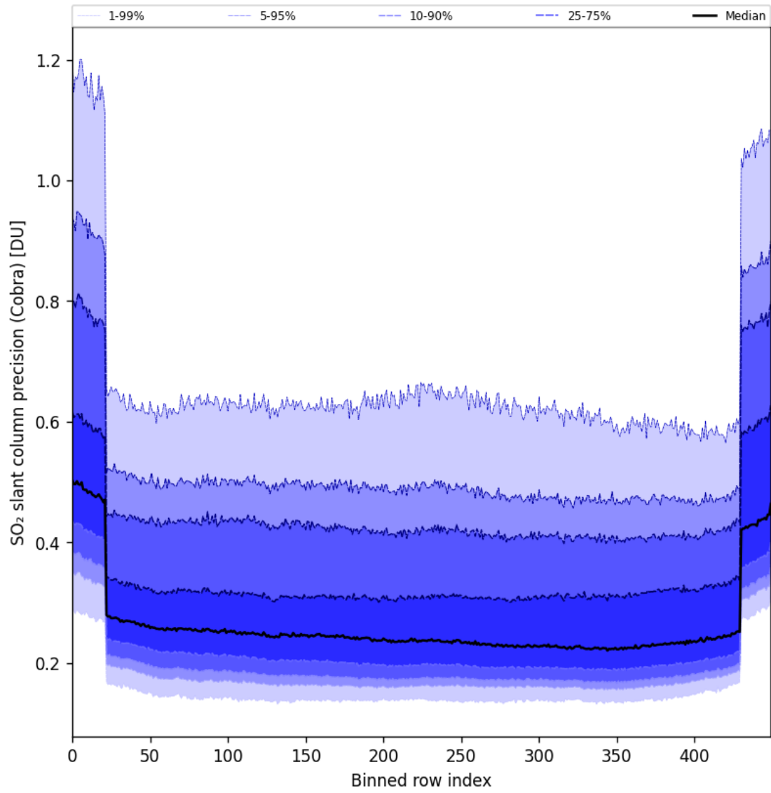
Figure 88: Along track statistics of “SO 2 slant column precision (Cobra)” for 2025-02-05 to 2025-02-07
