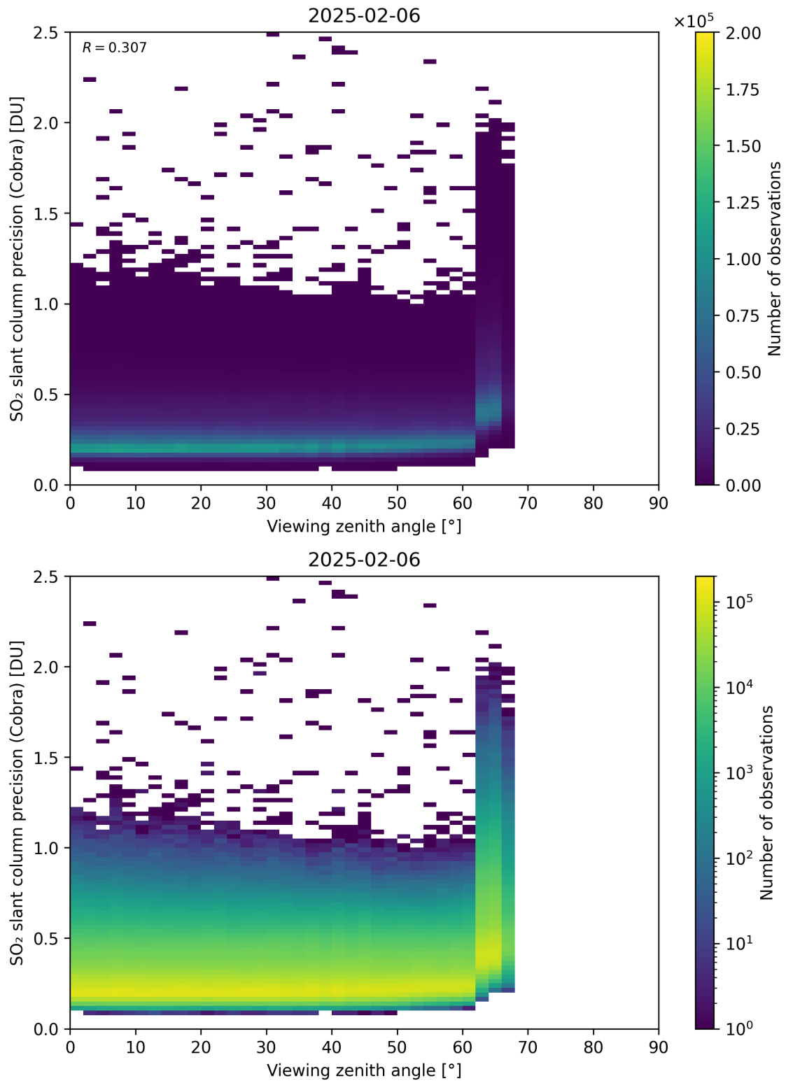
Figure 372: Scatter density plot of “Viewing zenith angle” against “SO 2 slant column precision (Cobra)” for 2025-02-05 to 2025-02-07.
