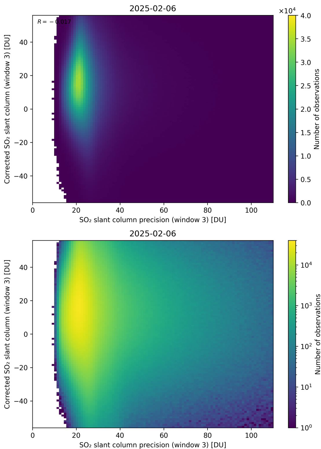
Figure 312: Scatter density plot of “SO 2 slant column precision (window 3)” against “Corrected SO 2 slant column (window 3)” for 2025-02-05 to 2025-02-07.
