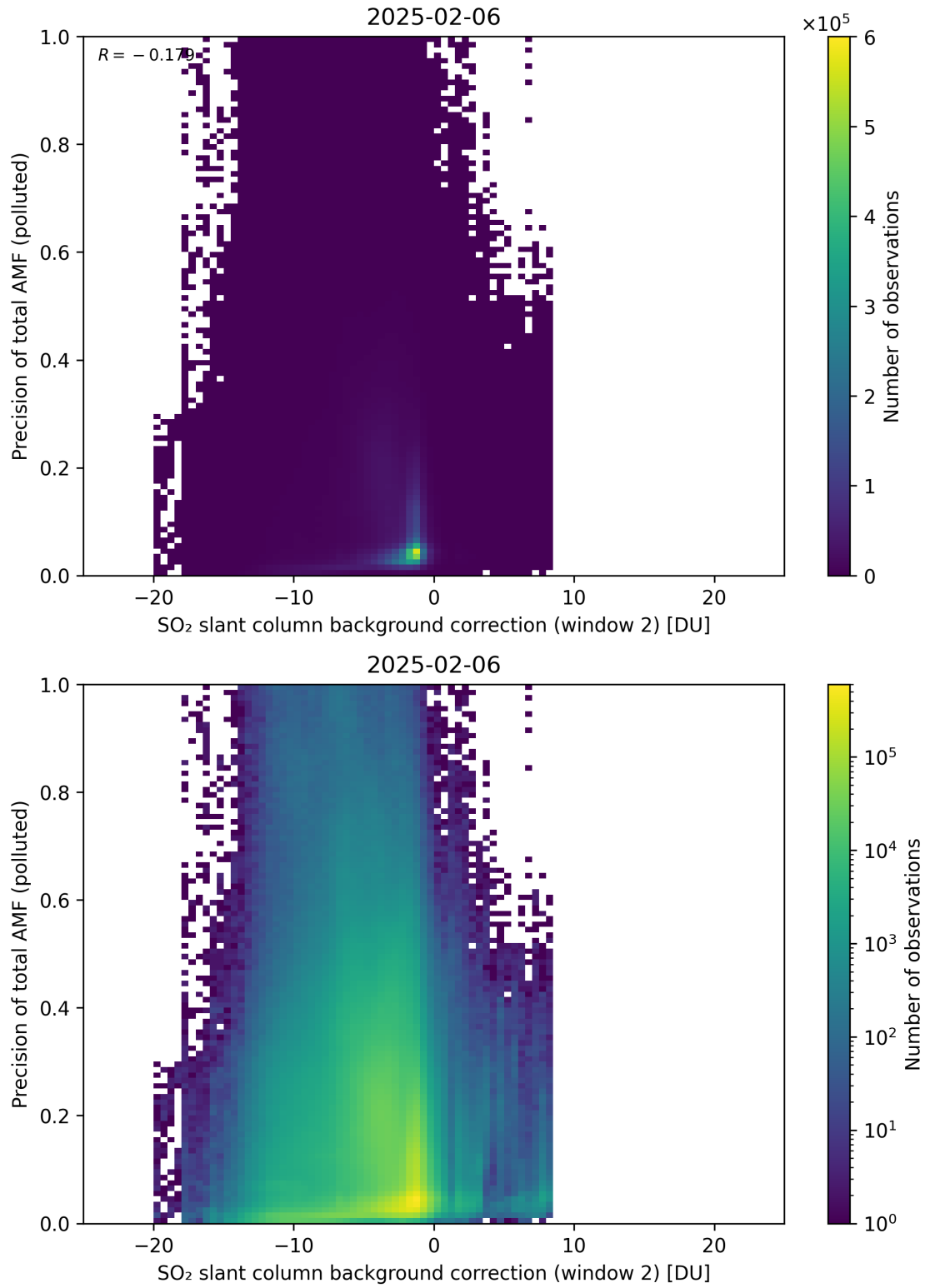
Figure 131: Scatter density plot of “SO 2 slant column background correction (window 2)” against “Precision of total AMF (polluted)” for 2025-02-05 to 2025-02-07.
