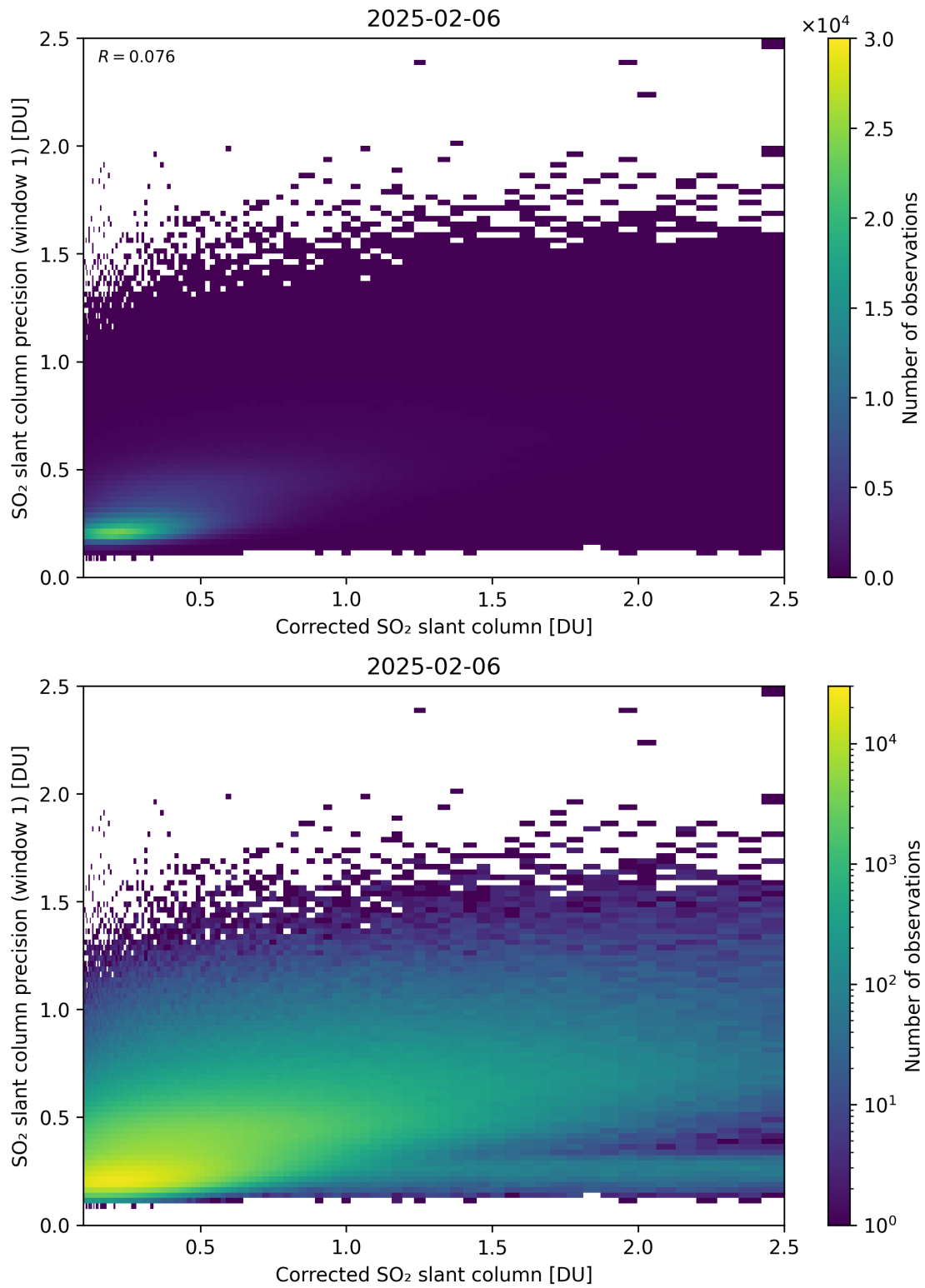
Figure 238: Scatter density plot of “Corrected SO 2 slant column” against “SO 2 slant column precision (window 1)” for 2025-02-05 to 2025-02-07.
