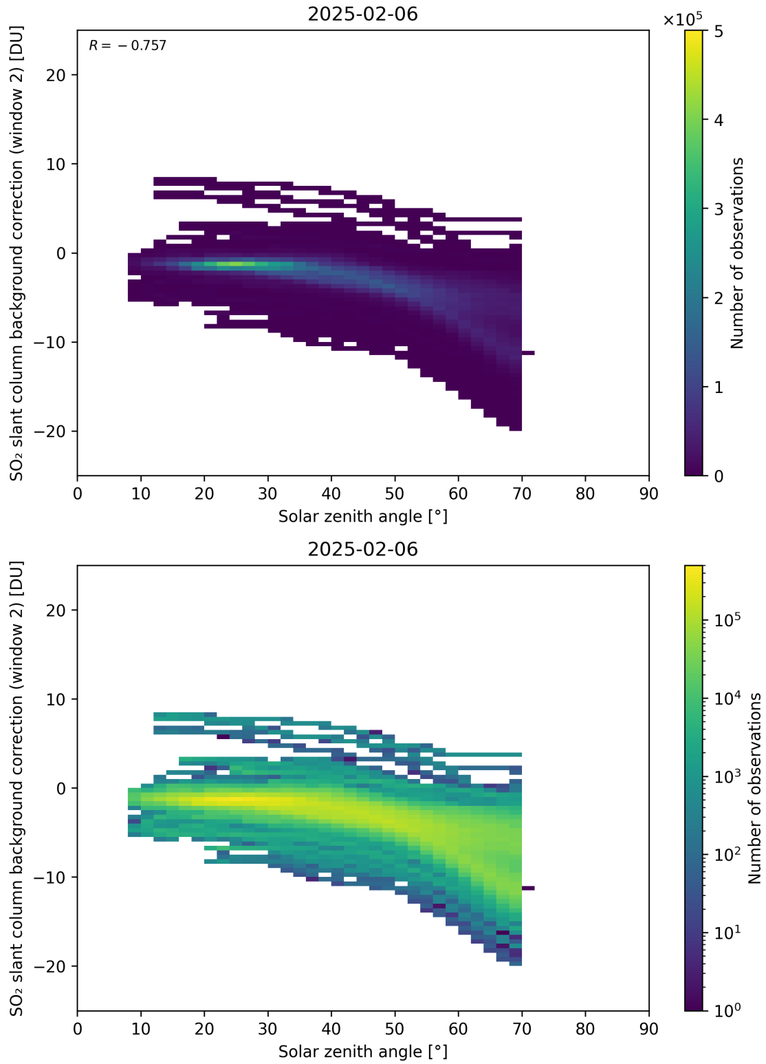
Figure 172: Scatter density plot of “Solar zenith angle” against “SO 2 slant column background correction (window 2)” for 2025-02-05 to 2025-02-07.
