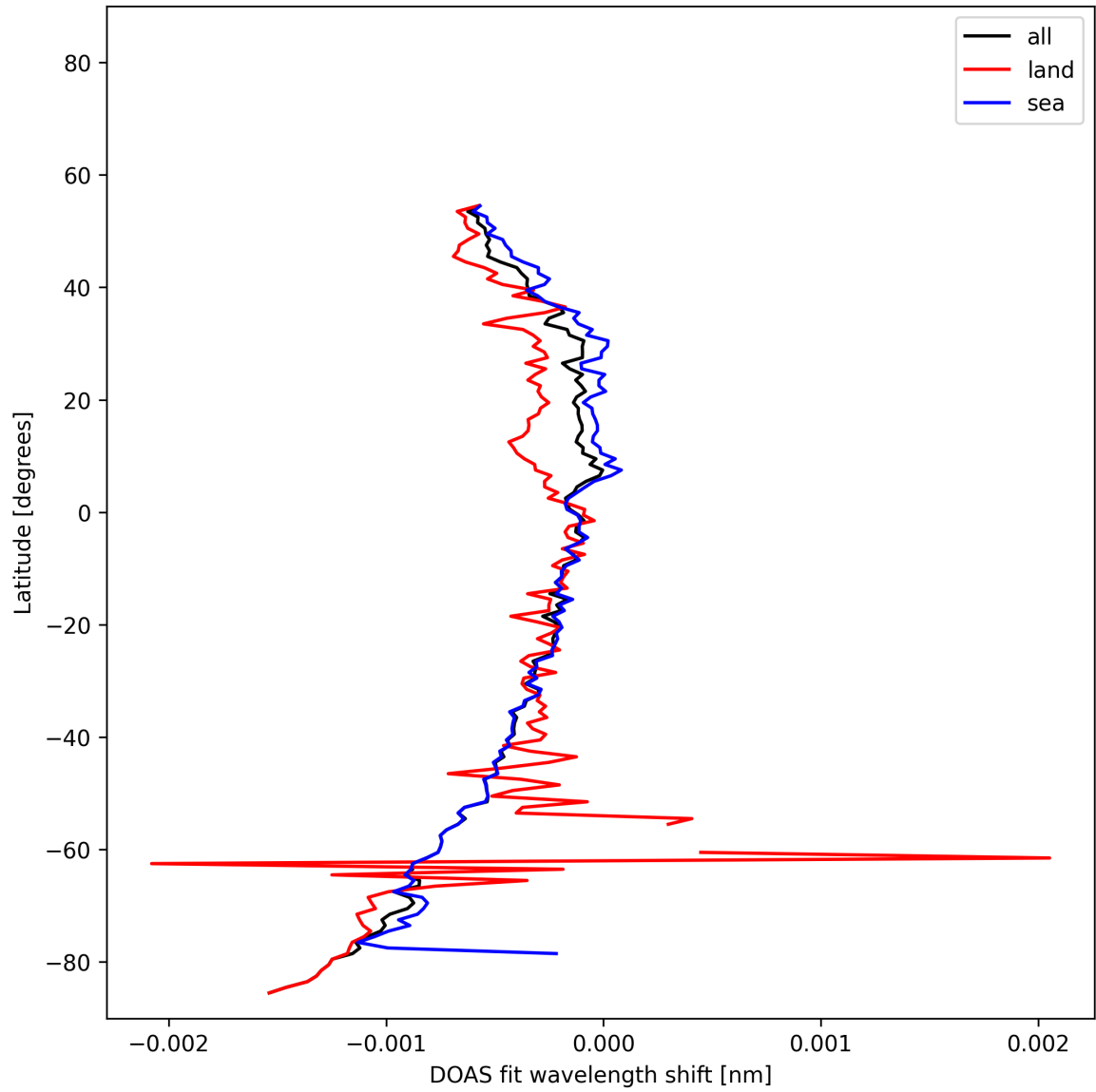
Figure 50: Zonal average of “DOAS fit wavelength shift” for 2025-02-05 to 2025-02-07.
