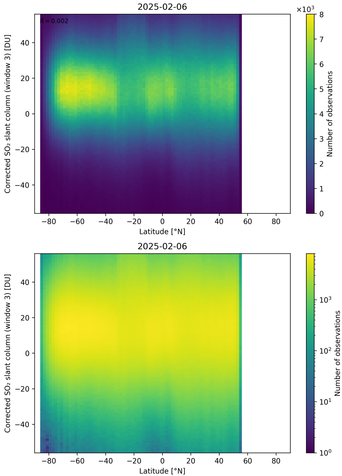
Figure 161: Scatter density plot of “Latitude” against “Corrected SO 2 slant column (window 3)” for 2025-02-05 to 2025-02-07.
