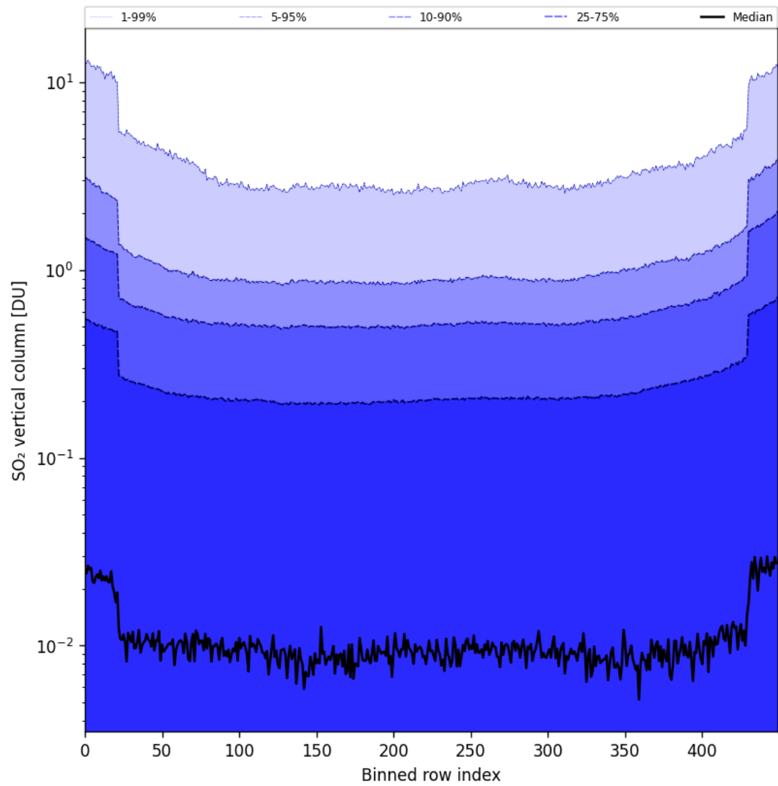
Figure 84: Along track statistics of “SO 2 vertical column” for 2025-02-05 to 2025-02-07
