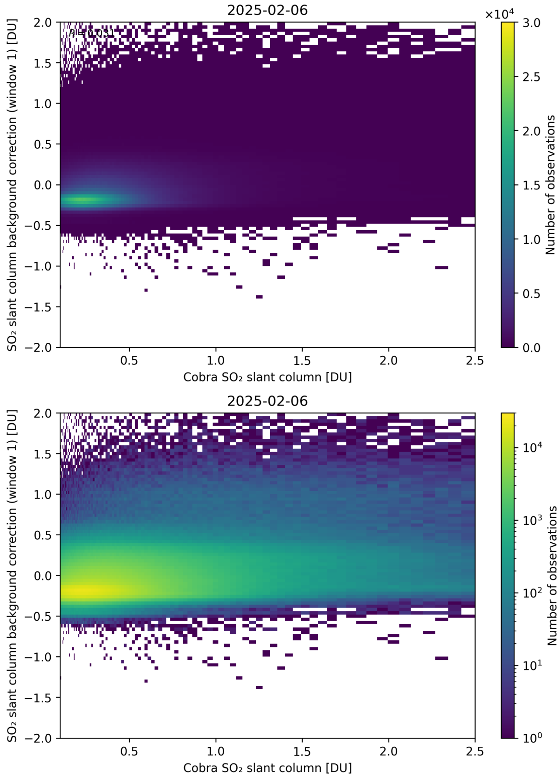
Figure 193: Scatter density plot of “Cobra SO 2 slant column” against “SO 2 slant column background correction (window 1)” for 2025-02-05 to 2025-02-07.
