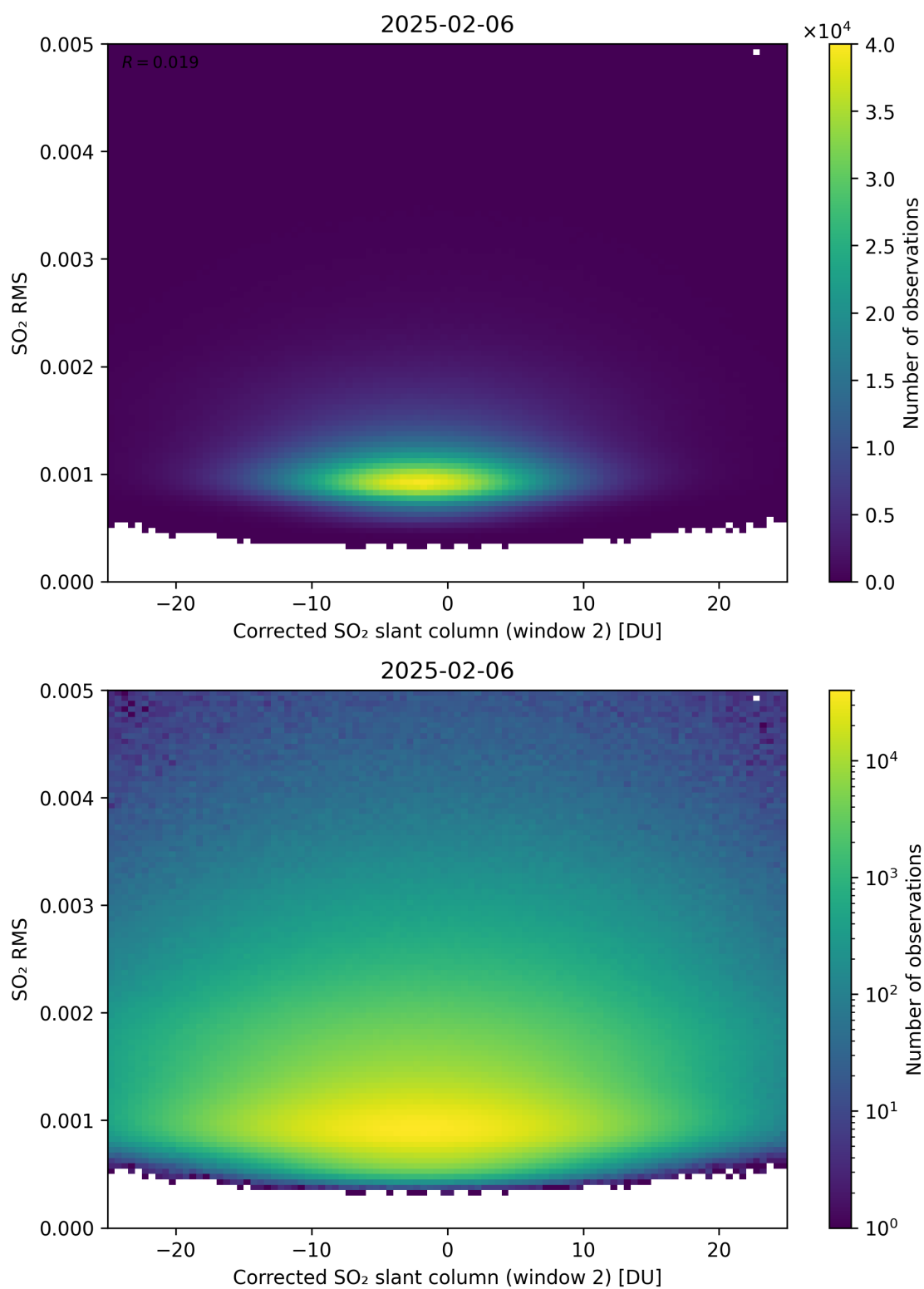
Figure 248: Scatter density plot of “Corrected SO 2 slant column (window 2)” against “SO 2 RMS” for 2025-02-05 to 2025-02-07.
