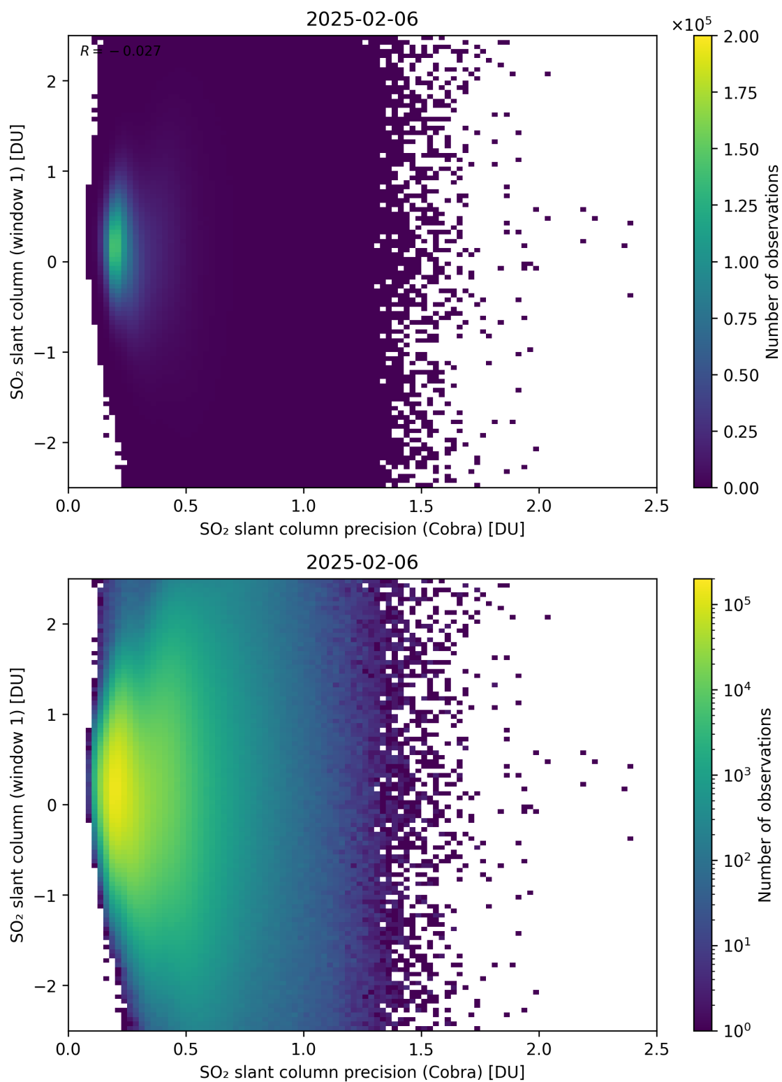
Figure 208: Scatter density plot of “SO 2 slant column precision (Cobra)” against “SO 2 slant column (window 1)” for 2025-02-05 to 2025-02-07.
