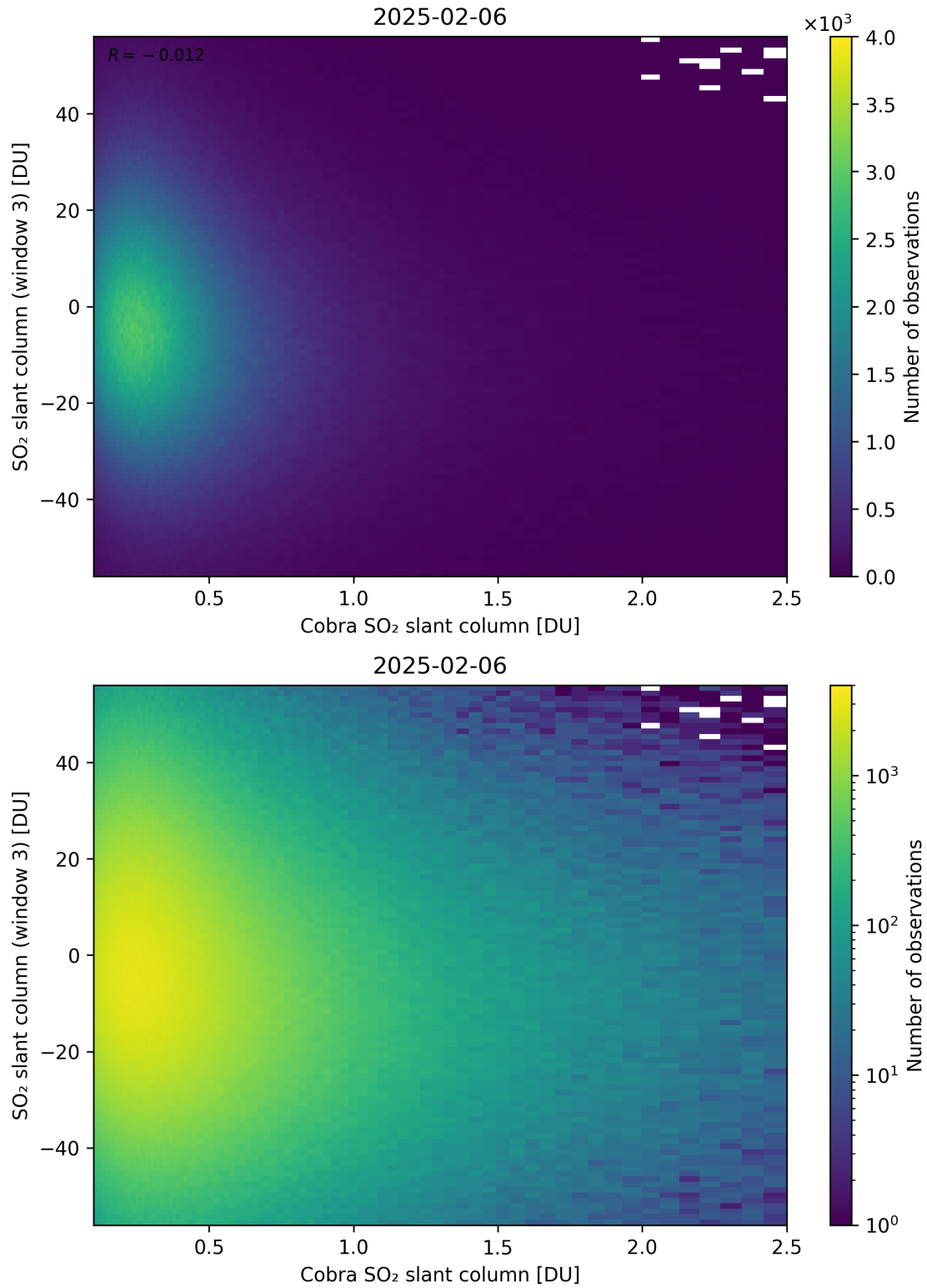
Figure 222: Scatter density plot of “Cobra SO 2 slant column” against “SO 2 slant column (window 3)” for 2025-02-05 to 2025-02-07.
