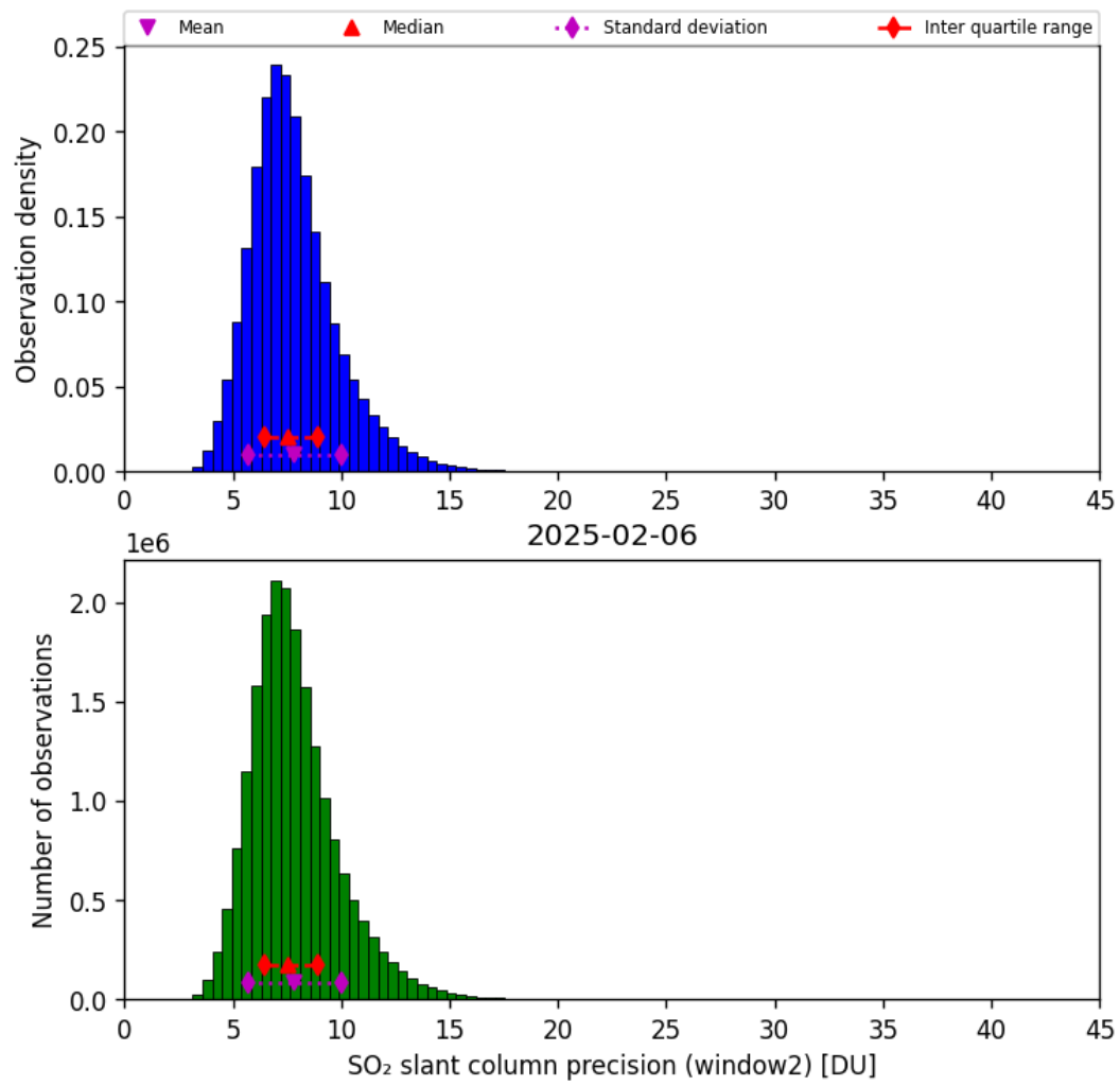
Figure 68: Histogram of “SO 2 slant column precision (window2)” for 2025-02-05 to 2025-02-07
