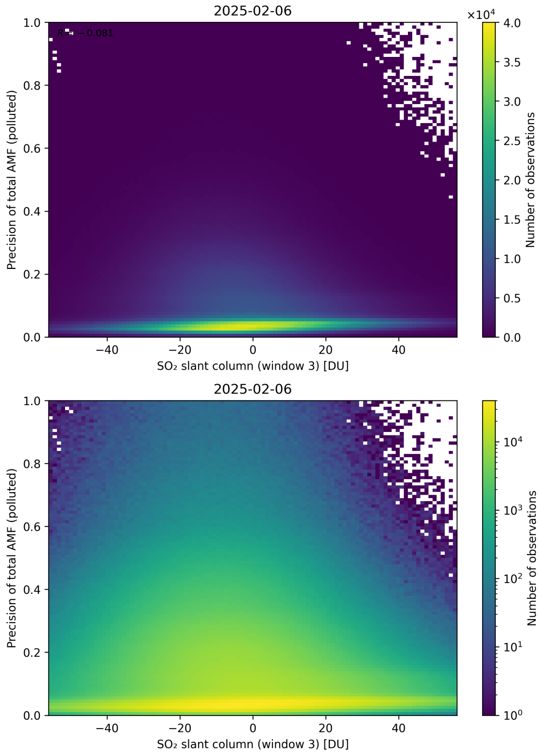
Figure 319: Scatter density plot of “SO 2 slant column (window 3)” against “Precision of total AMF (polluted)” for 2025-02-05 to 2025-02-07.
