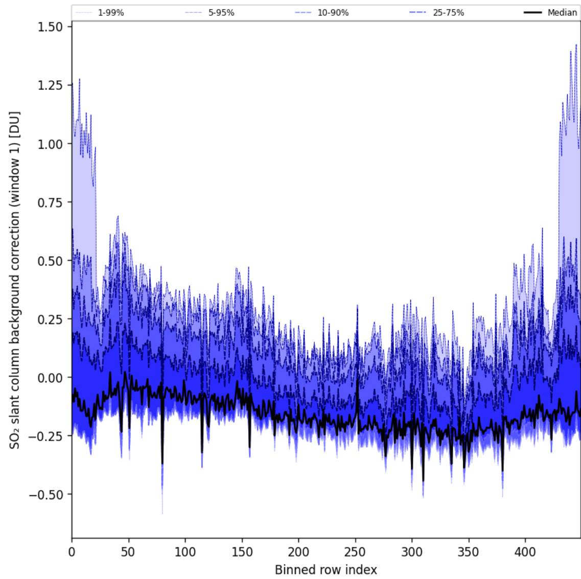
Figure 92: Along track statistics of “SO 2 slant column background correction (window 1)” for 2025-02-05 to 2025-02-07
