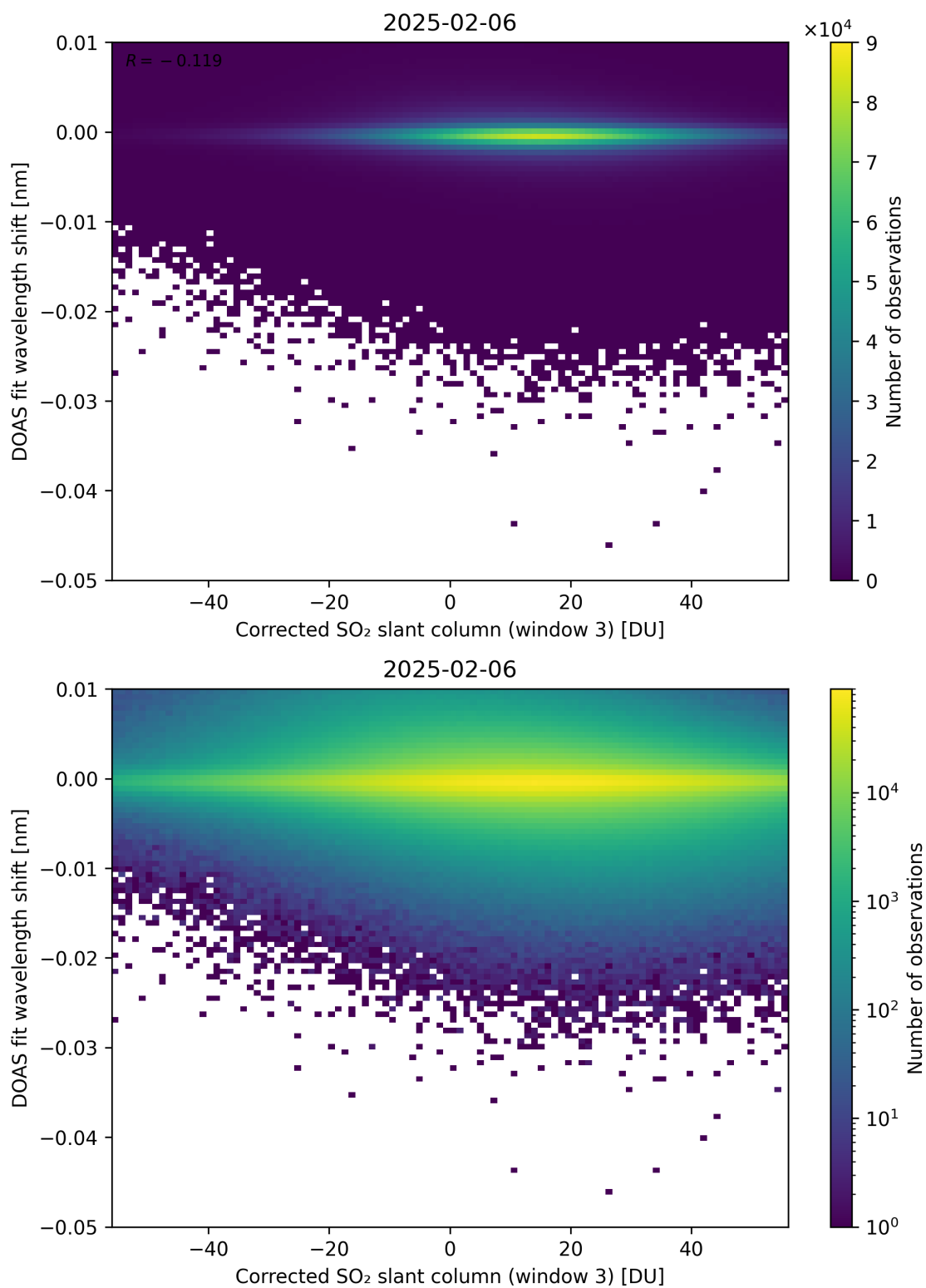
Figure 256: Scatter density plot of “Corrected SO 2 slant column (window 3)” against “DOAS fit wavelength shift” for 2025-02-05 to 2025-02-07.
