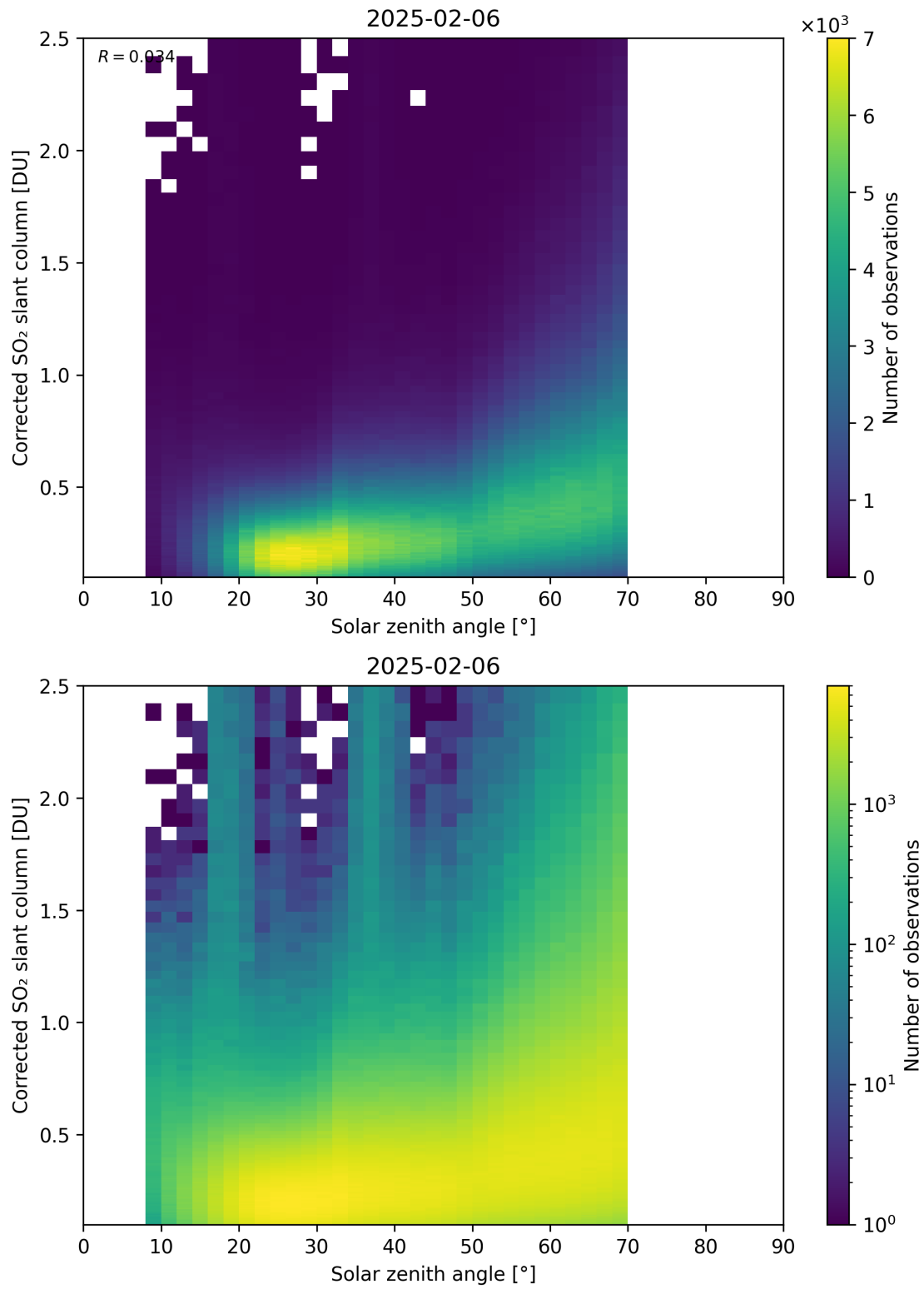
Figure 181: Scatter density plot of “Solar zenith angle” against “Corrected SO 2 slant column” for 2025-02-05 to 2025-02-07.
