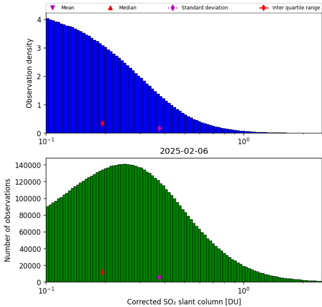
Figure 60: Histogram of "Corrected SO 2 slant column" for 2025-02-05 to 2025-02-07
