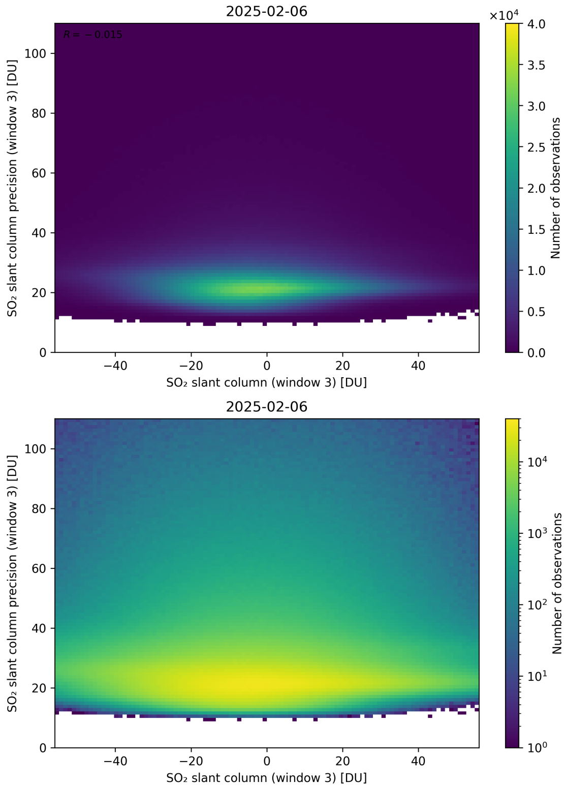
Figure 317: Scatter density plot of “SO 2 slant column (window 3)” against “SO 2 slant column precision (window 3)” for 2025-02-05 to 2025-02-07.
