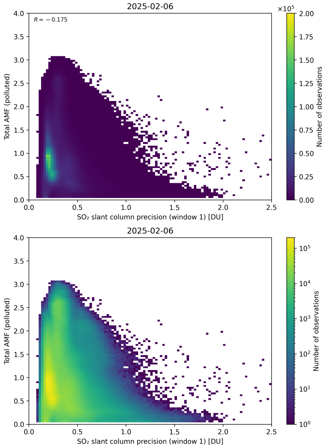
Figure 280: Scatter density plot of “SO 2 slant column precision (window 1)” against “Total AMF (polluted)” for 2025-02-05 to 2025-02-07.
