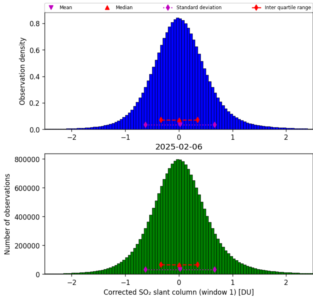
Figure 65: Histogram of “Corrected SO 2 slant column (window 1)” for 2025-02-05 to 2025-02-07
