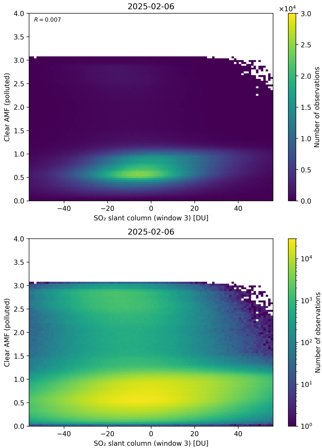
Figure 315: Scatter density plot of “SO 2 slant column (window 3)” against “Clear AMF (polluted)” for 2025-02-05 to 2025-02-07.
