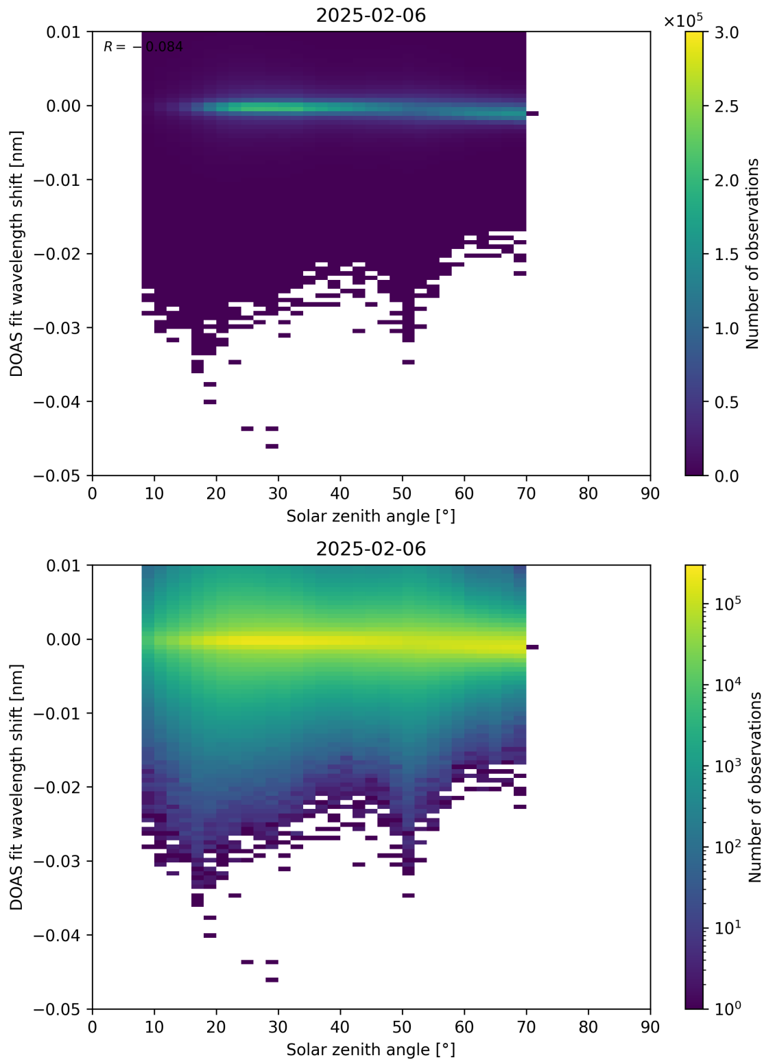
Figure 174: Scatter density plot of “Solar zenith angle” against “DOAS fit wavelength shift” for 2025-02-05 to 2025-02-07.
