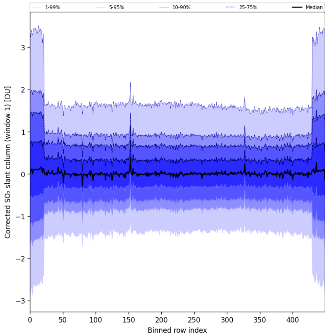
Figure 91: Along track statistics of “Corrected SO 2 slant column (window 1)” for 2025-02-05 to 2025-02-07
