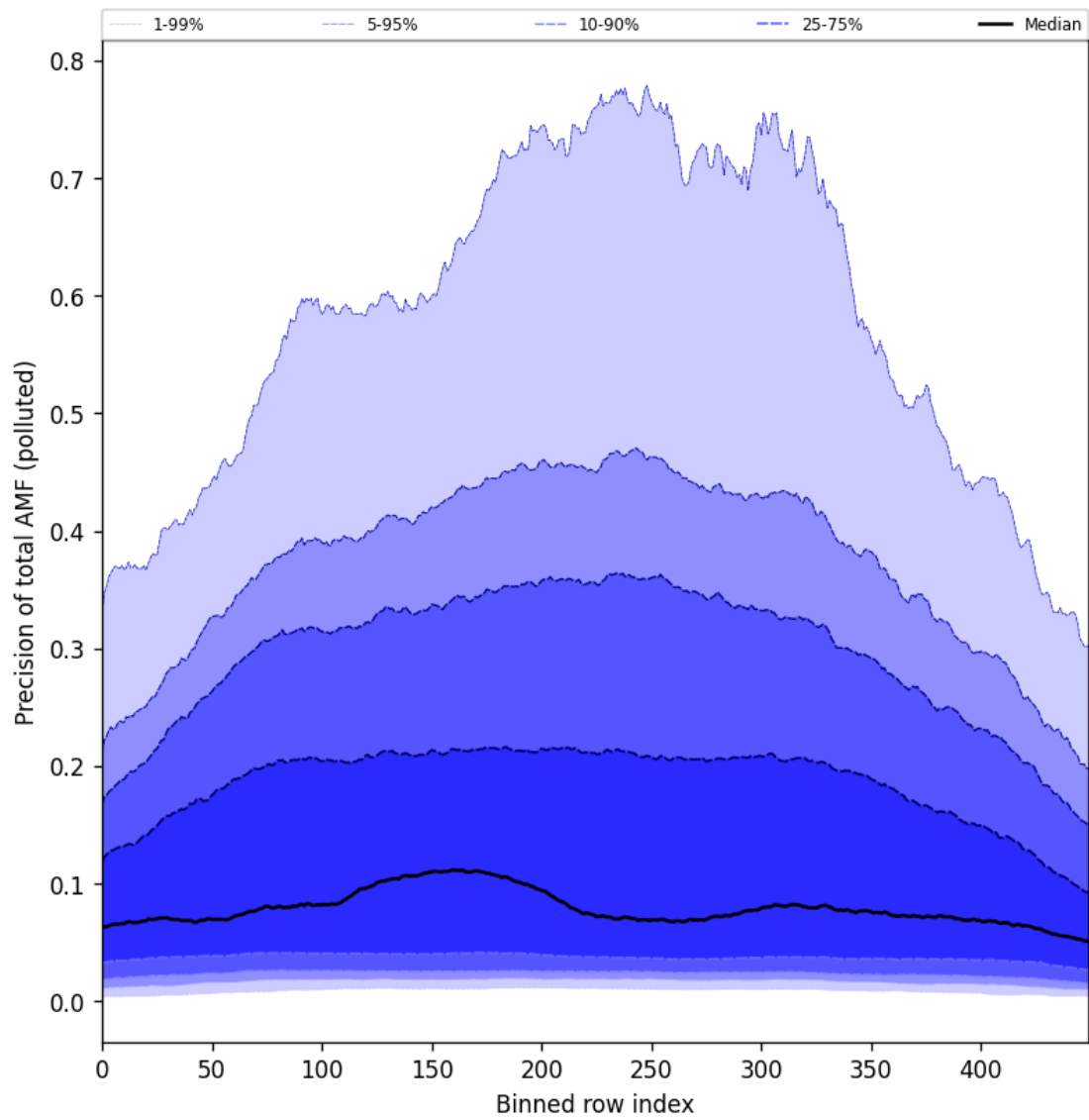
Figure 106: Along track statistics of “Precision of total AMF (polluted)” for 2025-02-05 to 2025-02-07
