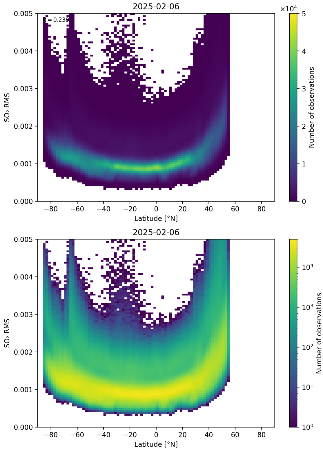
Figure 155: Scatter density plot of “Latitude” against “SO 2 RMS” for 2025-02-05 to 2025-02-07.
