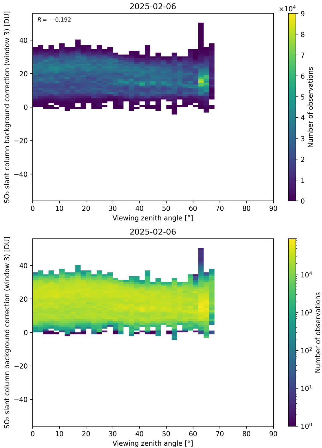
Figure 364: Scatter density plot of “Viewing zenith angle” against “SO 2 slant column background correction (window 3)” for 2025-02-05 to 2025-02-07.
