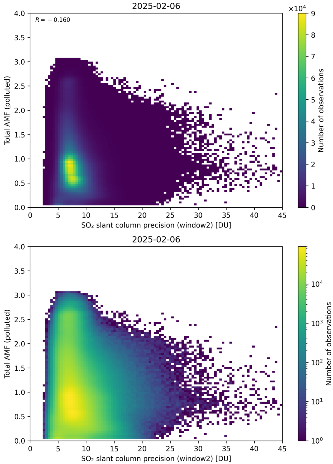
Figure 301: Scatter density plot of “SO 2 slant column precision (window2)” against “Total AMF (polluted)” for 2025-02-05 to 2025-02-07.
