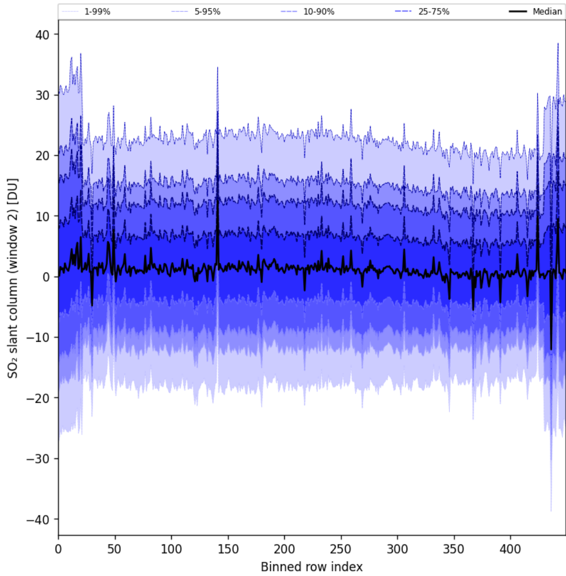
Figure 93: Along track statistics of "SO 2 slant column (window 2)" for 2025-02-05 to 2025-02-07
