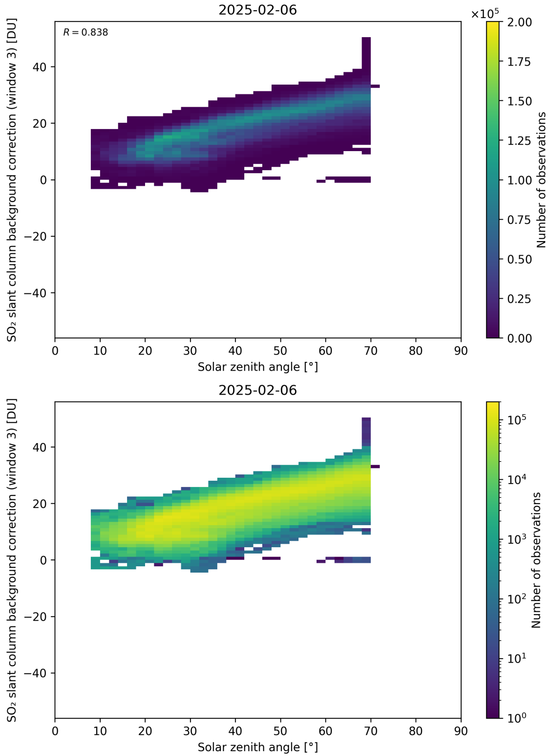
Figure 173: Scatter density plot of “Solar zenith angle” against “SO 2 slant column background correction (window 3)” for 2025-02-05 to 2025-02-07.
