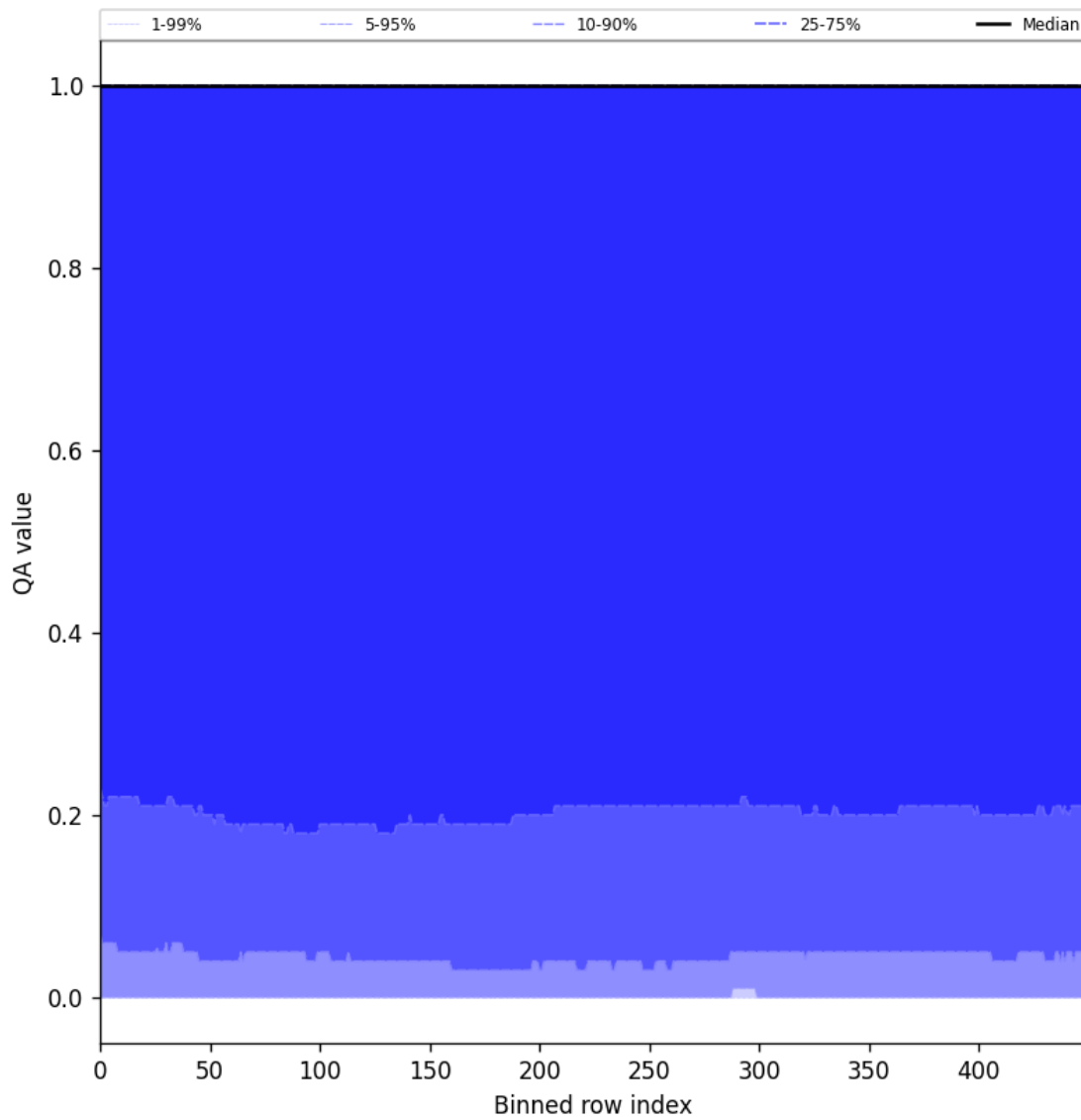
Figure 83: Along track statistics of “QA value” for 2025-02-05 to 2025-02-07
