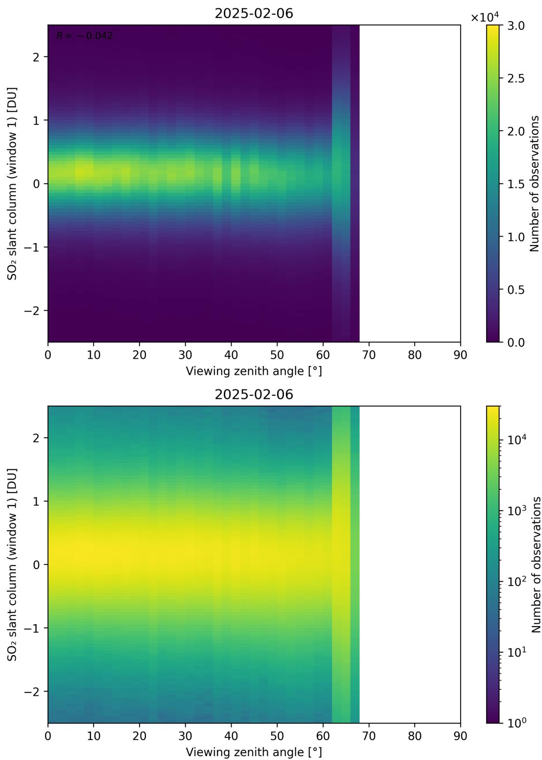
Figure 376: Scatter density plot of “Viewing zenith angle” against “SO 2 slant column (window 1)” for 2025-02-05 to 2025-02-07.
