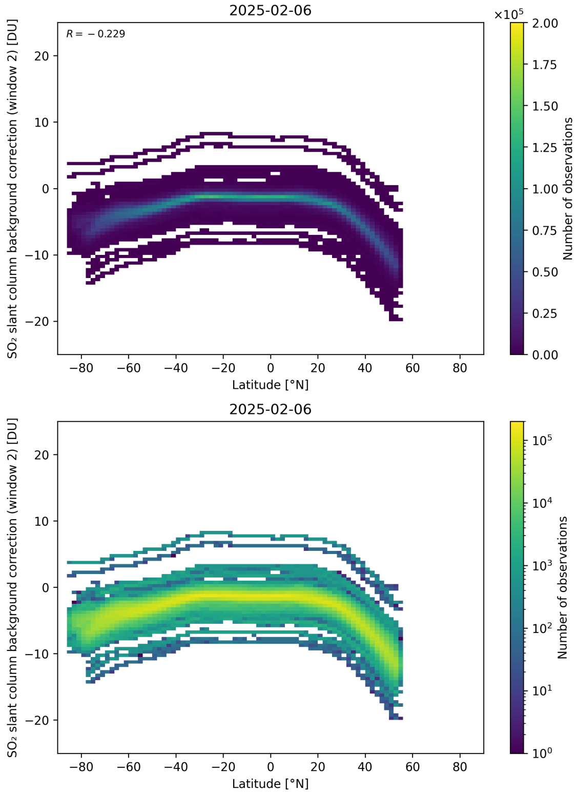
Figure 151: Scatter density plot of “Latitude” against “SO 2 slant column background correction (window 2)” for 2025-02-05 to 2025-02-07.
