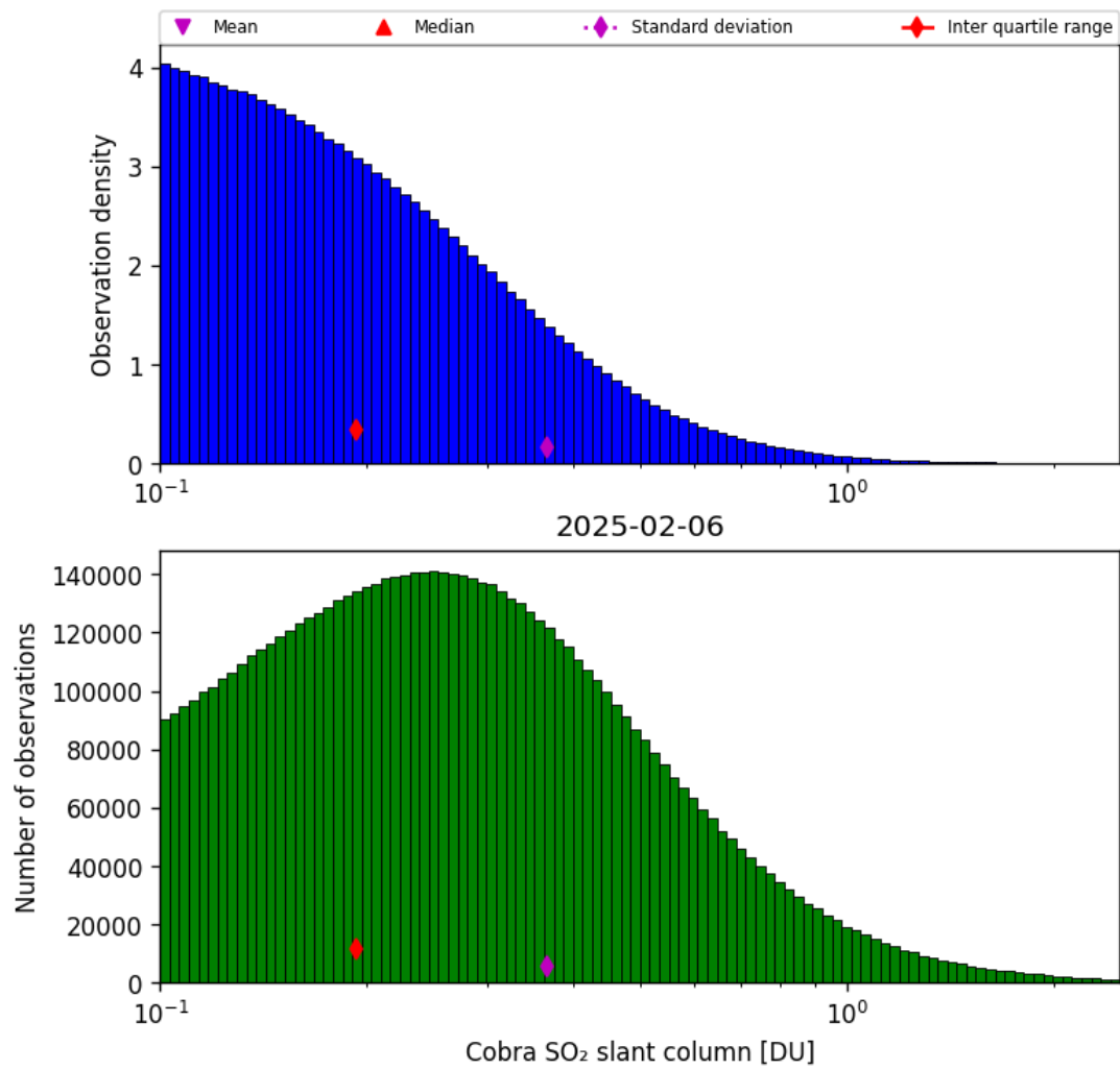
Figure 61: Histogram of “Cobra SO 2 slant column” for 2025-02-05 to 2025-02-07
