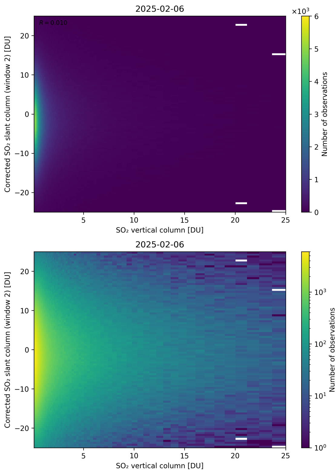
Figure 352: Scatter density plot of “SO 2 vertical column” against “Corrected SO 2 slant column (window 2)” for 2025-02-05 to 2025-02-07.
