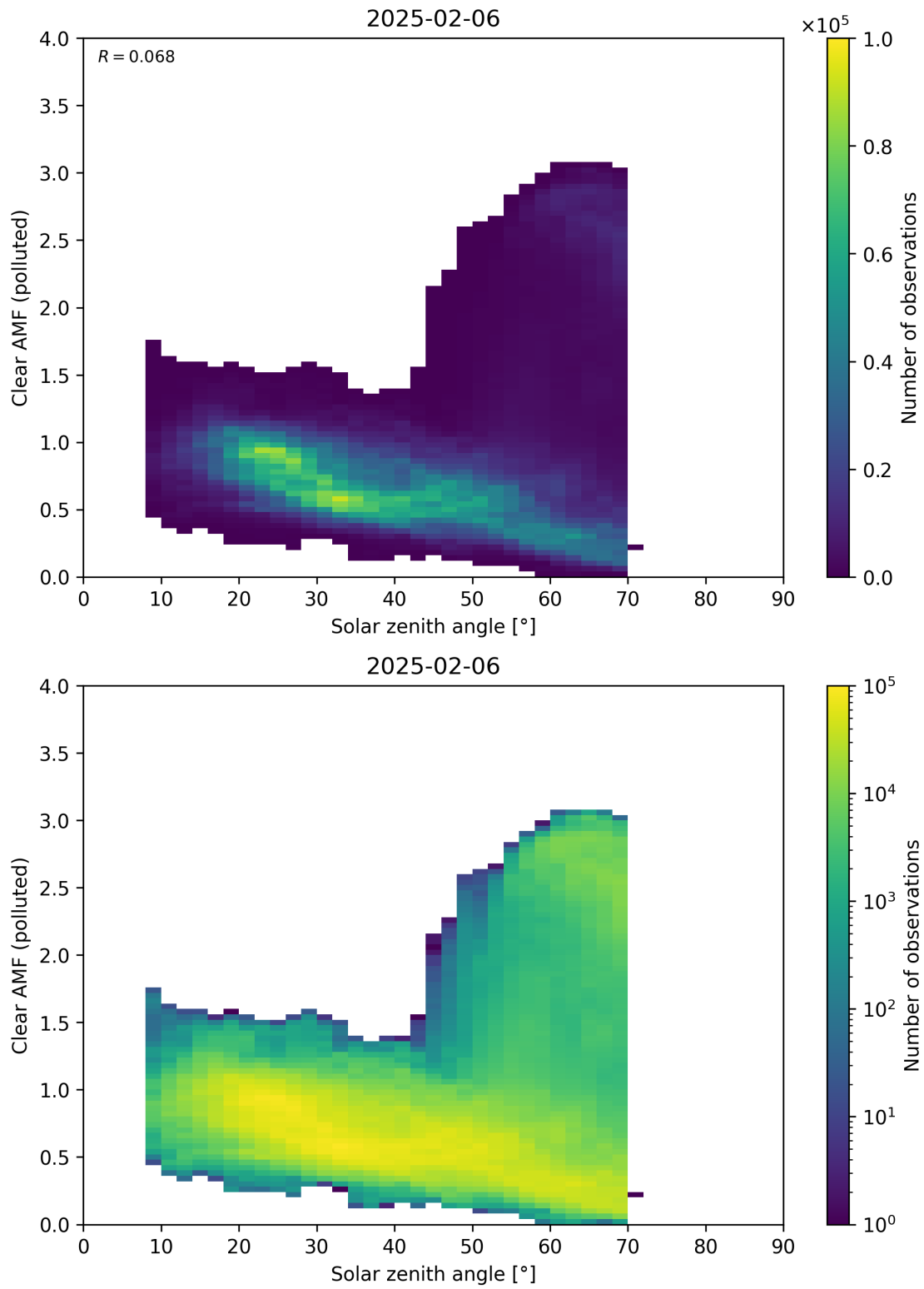
Figure 178: Scatter density plot of “Solar zenith angle” against “Clear AMF (polluted)” for 2025-02-05 to 2025-02-07.
