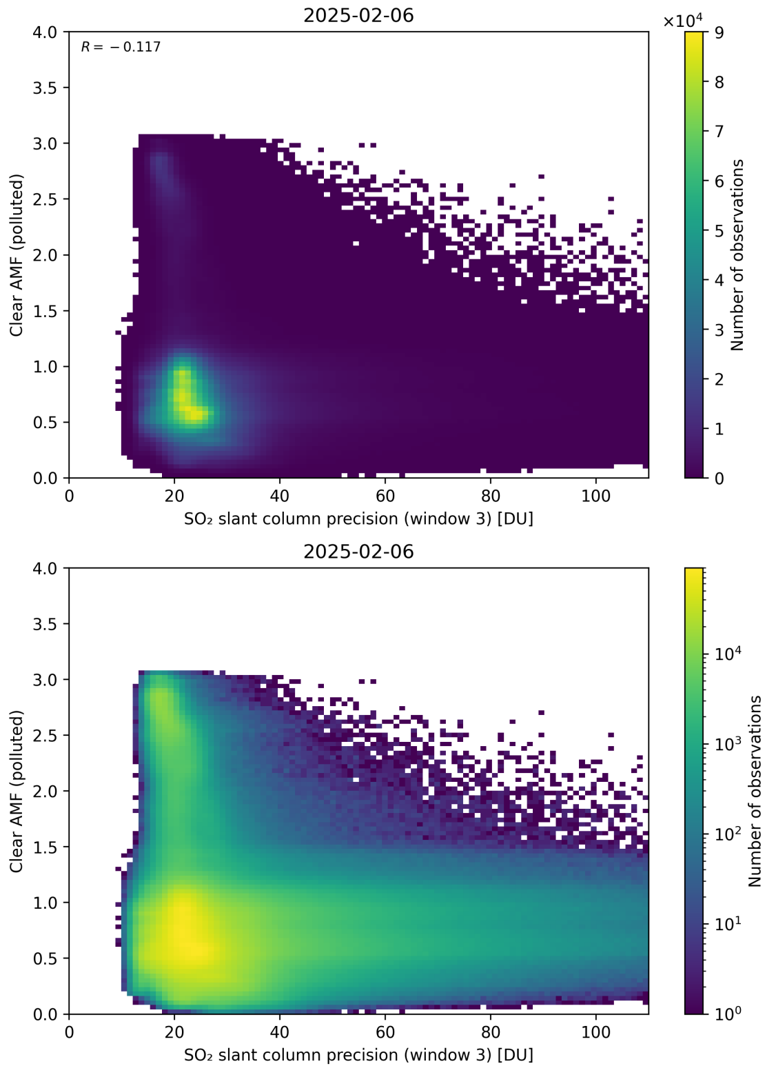
Figure 311: Scatter density plot of “SO 2 slant column precision (window 3)” against “Clear AMF (polluted)” for 2025-02-05 to 2025-02-07.
