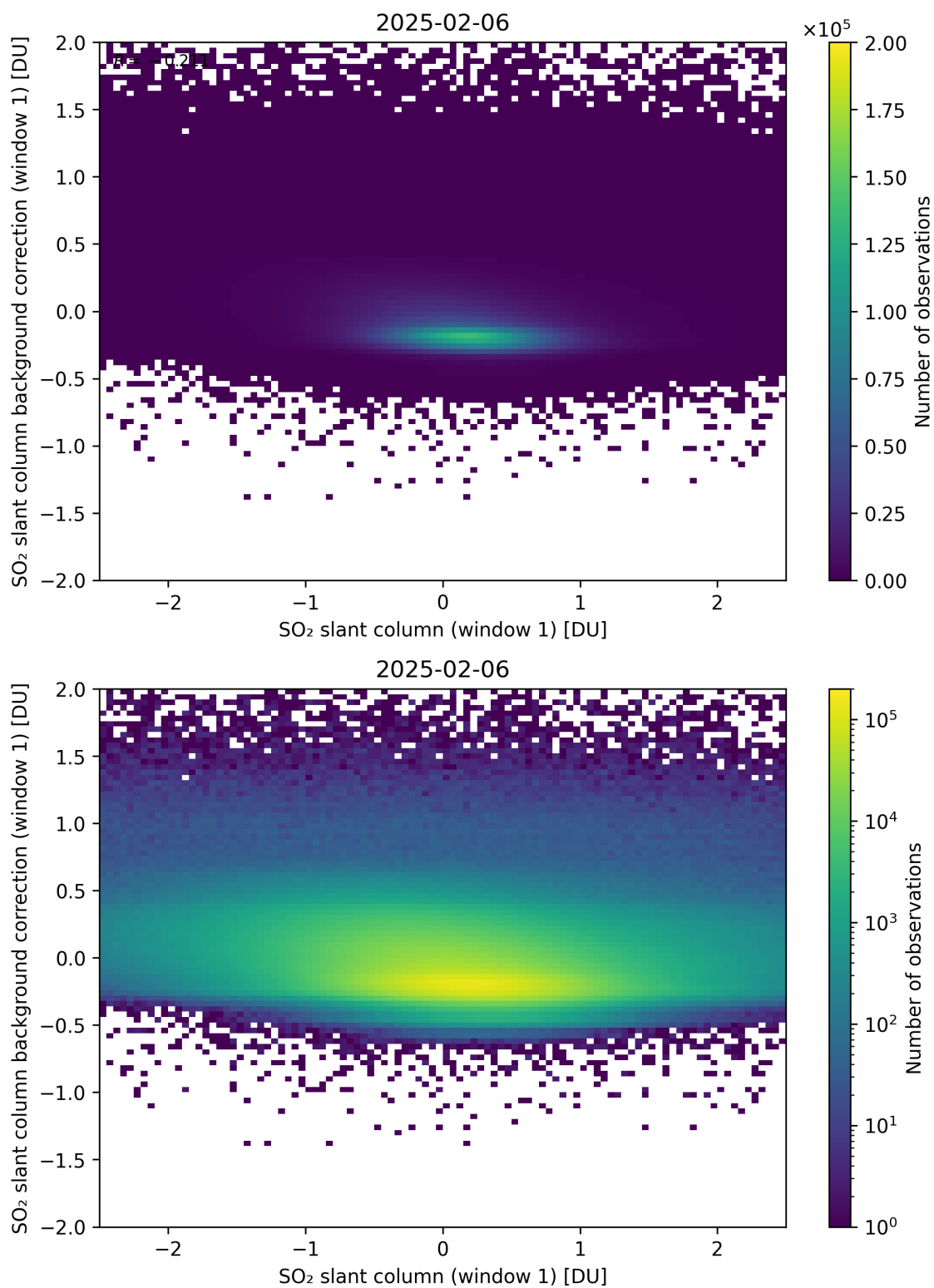
Figure 262: Scatter density plot of “SO 2 slant column (window 1)” against “SO 2 slant column background correction (window 1)” for 2025-02-05 to 2025-02-07.
