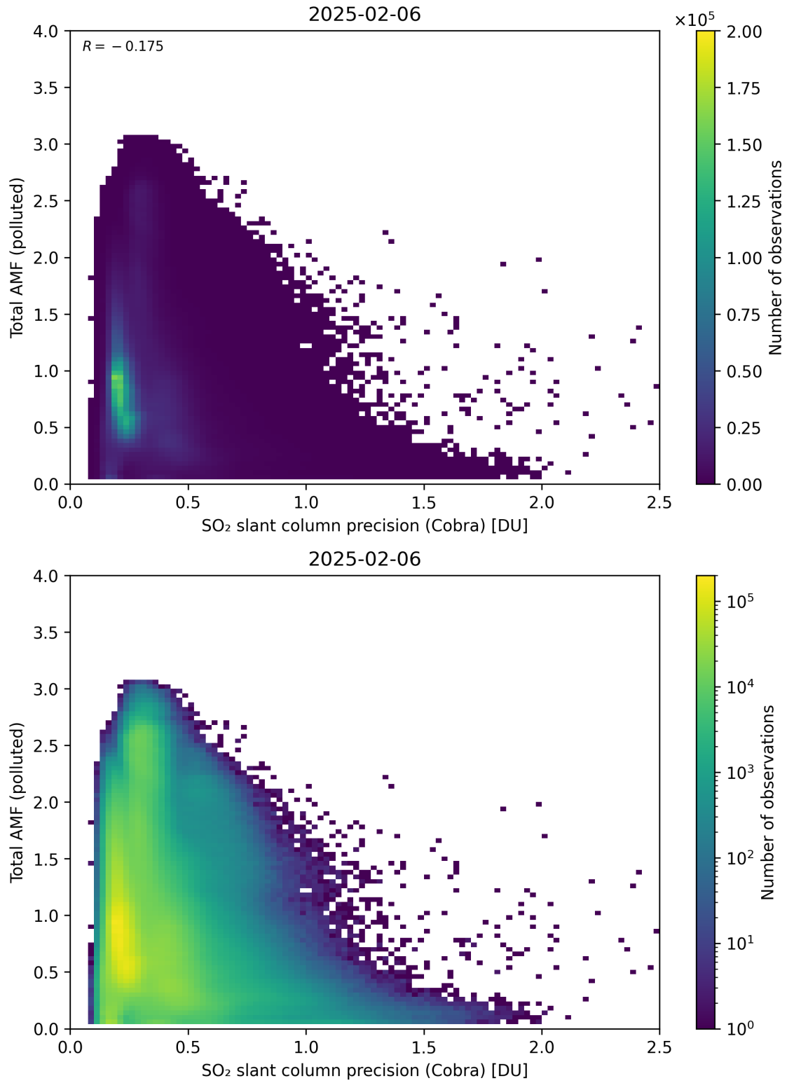
Figure 213: Scatter density plot of “SO 2 slant column precision (Cobra)” against “Total AMF (polluted)” for 2025-02-05 to 2025-02-07.
