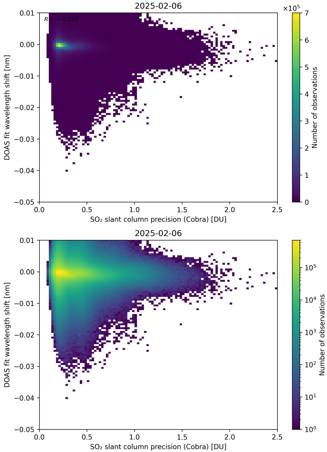
Figure 202: Scatter density plot of “SO 2 slant column precision (Cobra)” against “DOAS fit wavelength shift” for 2025-02-05 to 2025-02-07.
