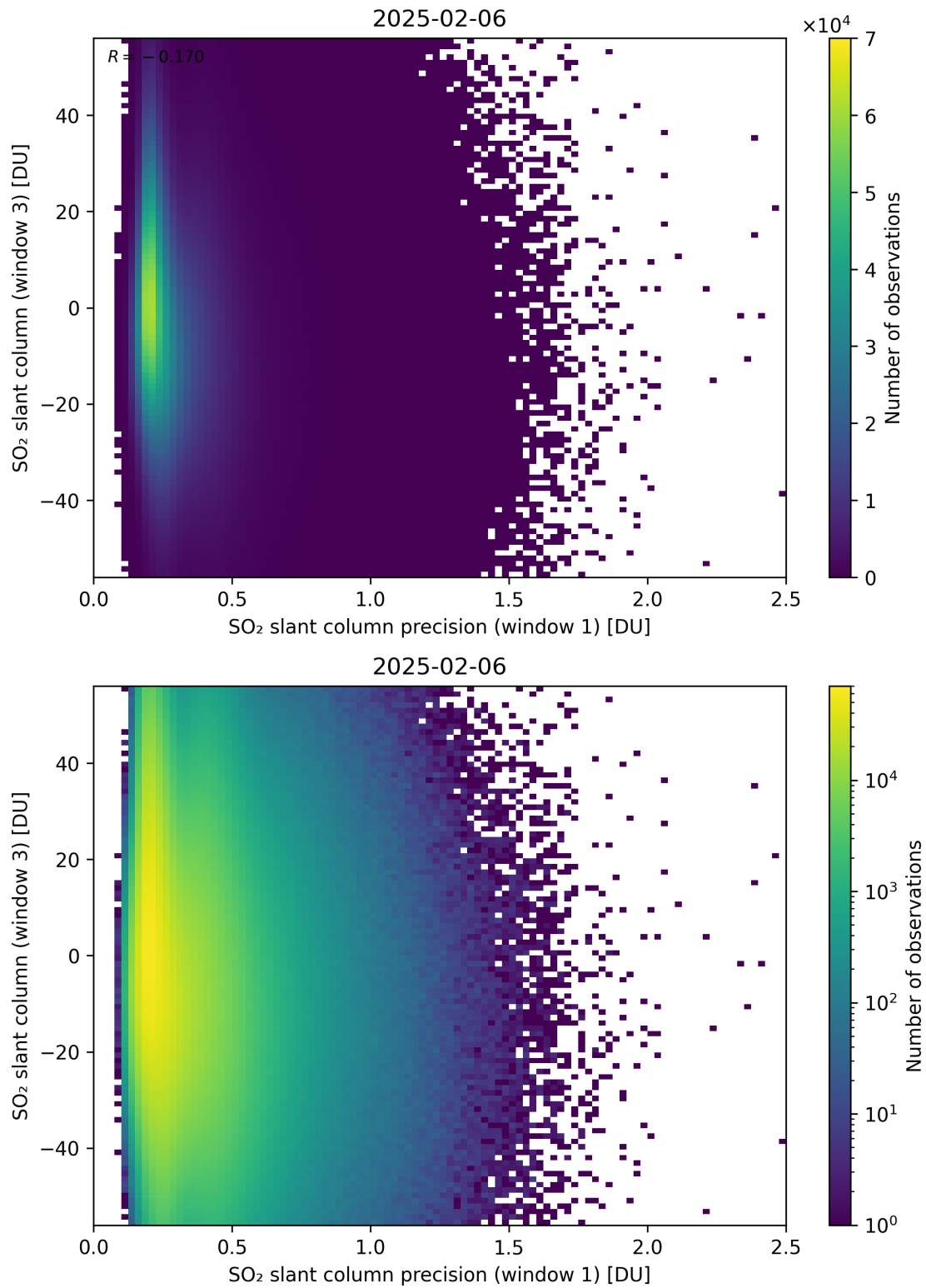
Figure 278: Scatter density plot of “SO 2 slant column precision (window 1)” against “SO 2 slant column (window 3)” for 2025-02-05 to 2025-02-07.
