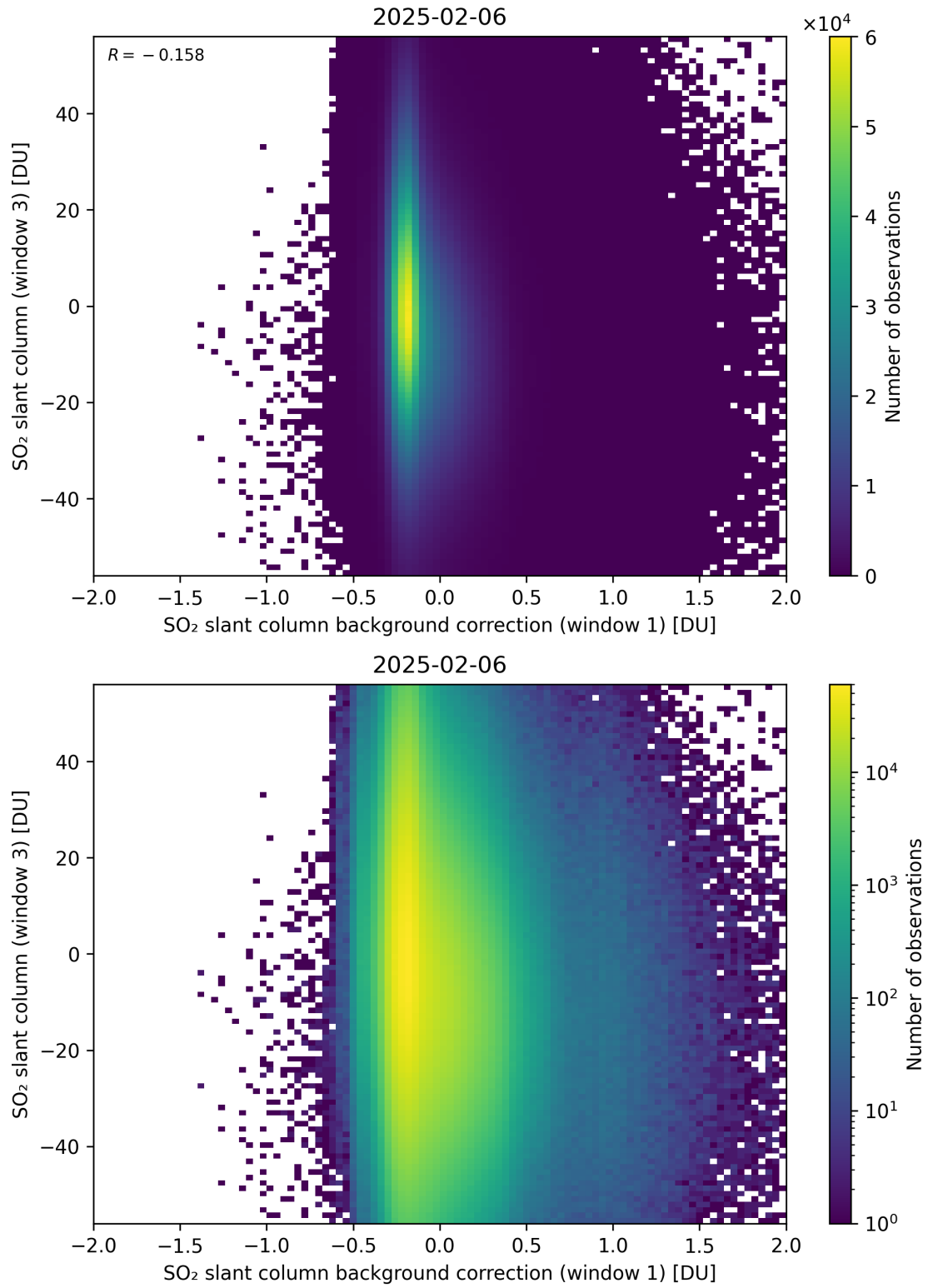
Figure 118: Scatter density plot of “SO 2 slant column background correction (window 1)” against “SO 2 slant column (window 3)” for 2025-02-05 to 2025-02-07.
