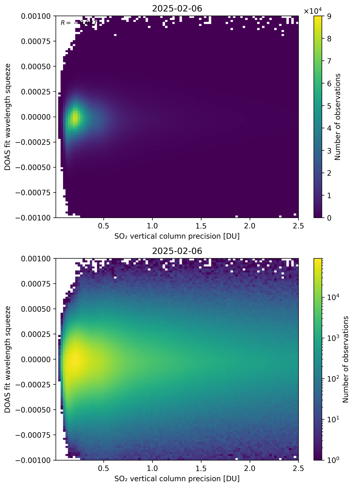
Figure 333: Scatter density plot of “SO 2 vertical column precision” against “DOAS fit wavelength squeeze” for 2025-02-05 to 2025-02-07.
