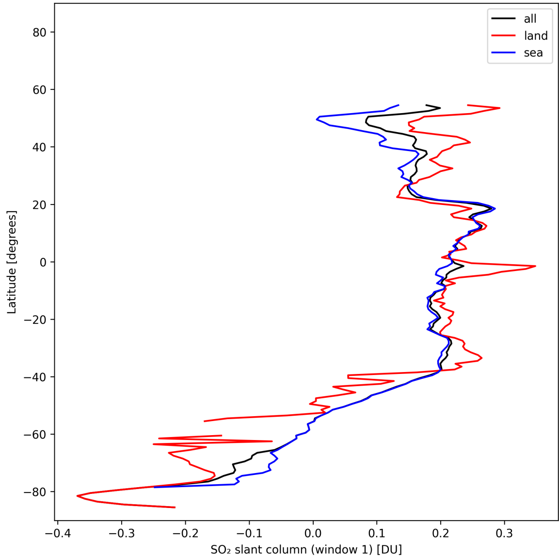
Figure 37: Zonal average of “SO 2 slant column (window 1)” for 2025-02-05 to 2025-02-07.
