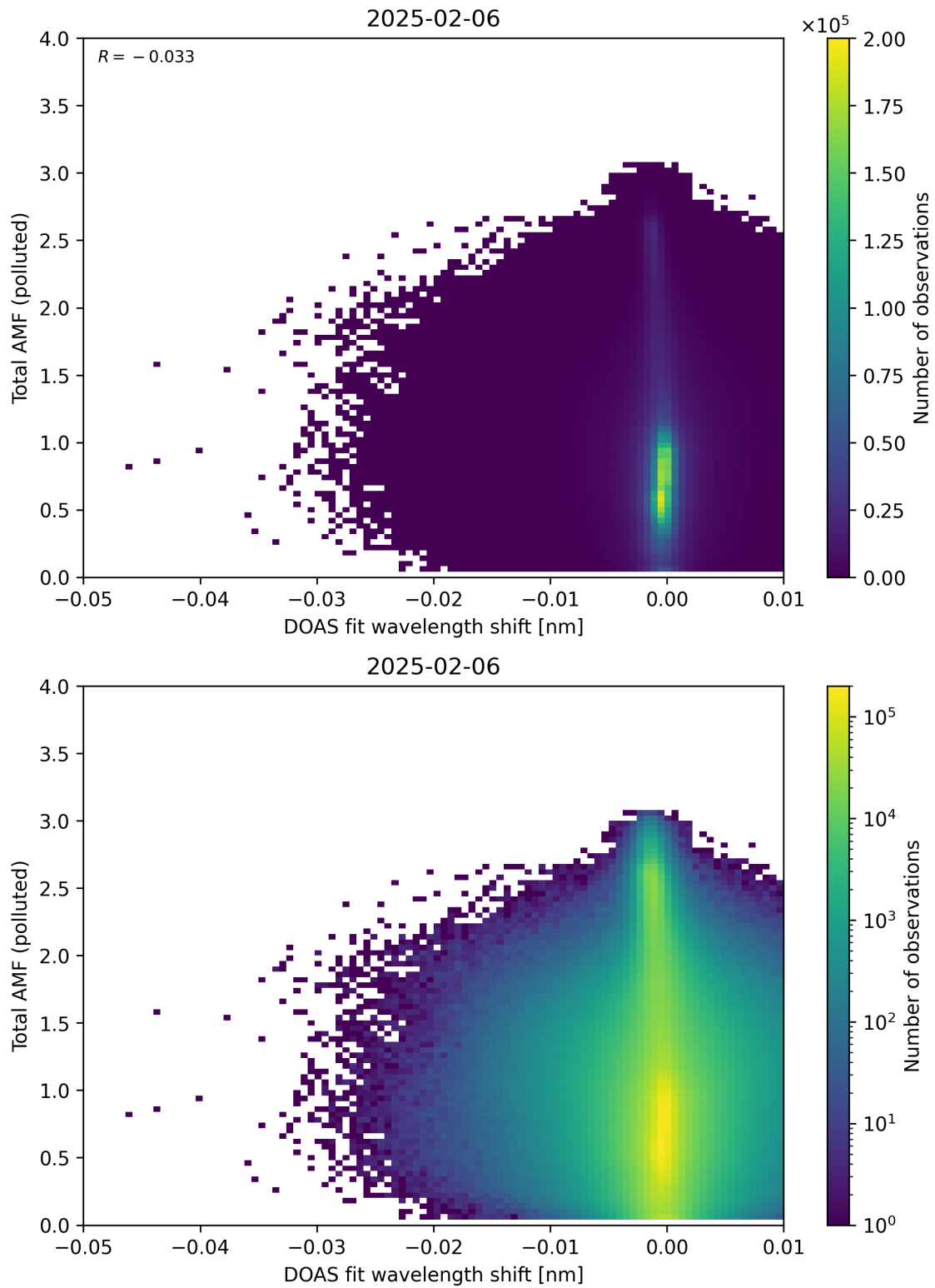
Figure 141: Scatter density plot of “DOAS fit wavelength shift” against “Total AMF (polluted)” for 2025-02-05 to 2025-02-07.
