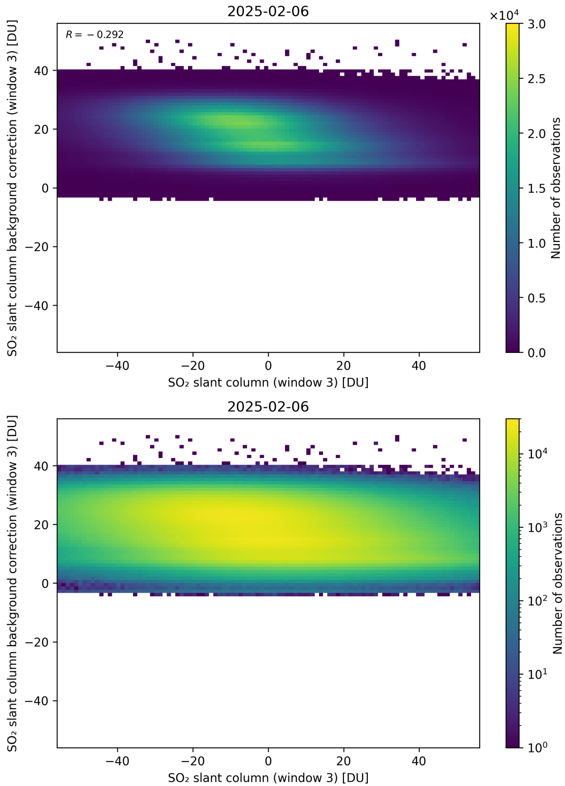
Figure 303: Scatter density plot of “SO 2 slant column (window 3)” against “SO 2 slant column background correction (window 3)” for 2025-02-05 to 2025-02-07.
