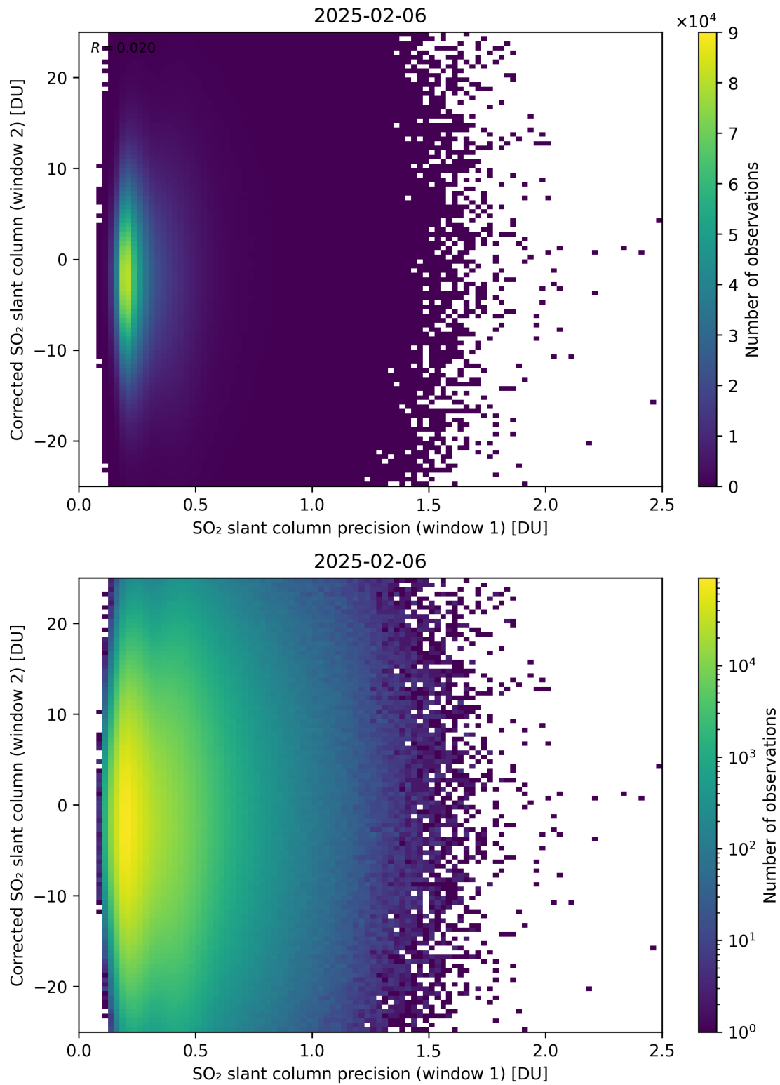
Figure 275: Scatter density plot of “SO 2 slant column precision (window 1)” against “Corrected SO 2 slant column (window 2)” for 2025-02-05 to 2025-02-07.
