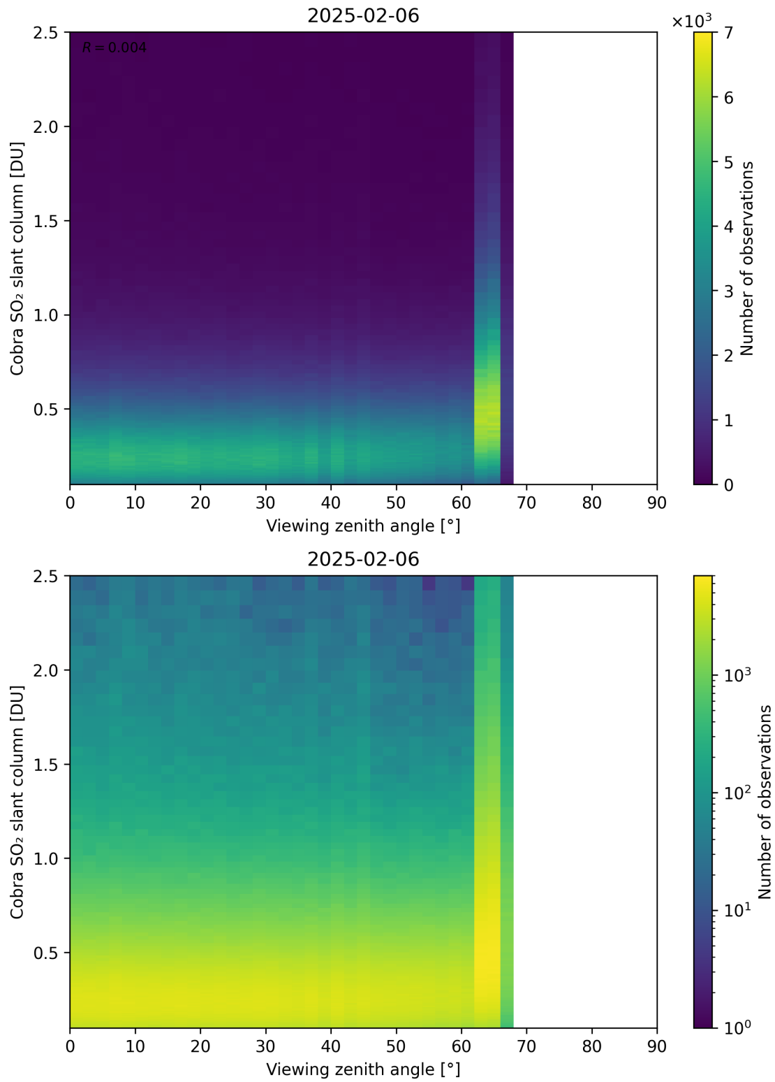
Figure 371: Scatter density plot of “Viewing zenith angle” against “Cobra SO 2 slant column” for 2025-02-05 to 2025-02-07.
