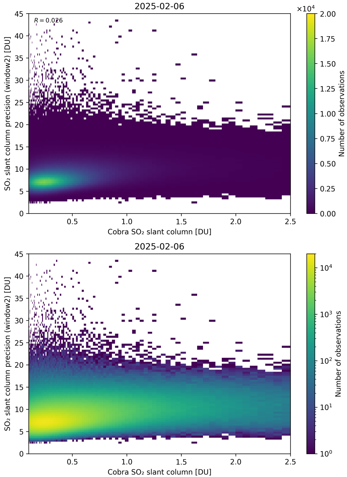
Figure 221: Scatter density plot of “Cobra SO 2 slant column” against “SO 2 slant column precision (window2)” for 2025-02-05 to 2025-02-07.
