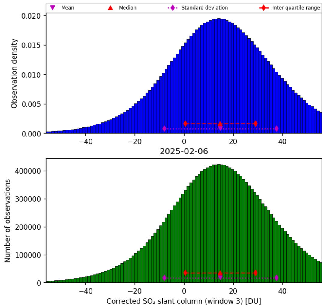
Figure 73: Histogram of “Corrected SO 2 slant column (window 3)” for 2025-02-05 to 2025-02-07
