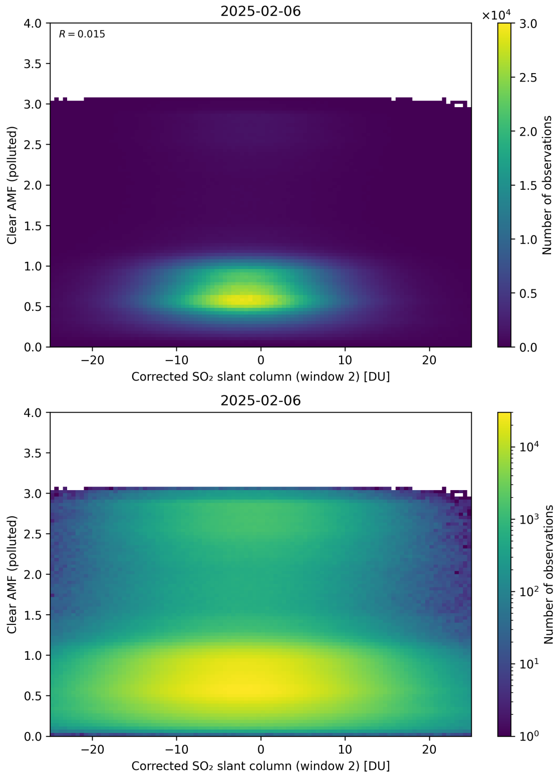
Figure 249: Scatter density plot of “Corrected SO 2 slant column (window 2)” against “Clear AMF (polluted)” for 2025-02-05 to 2025-02-07.
