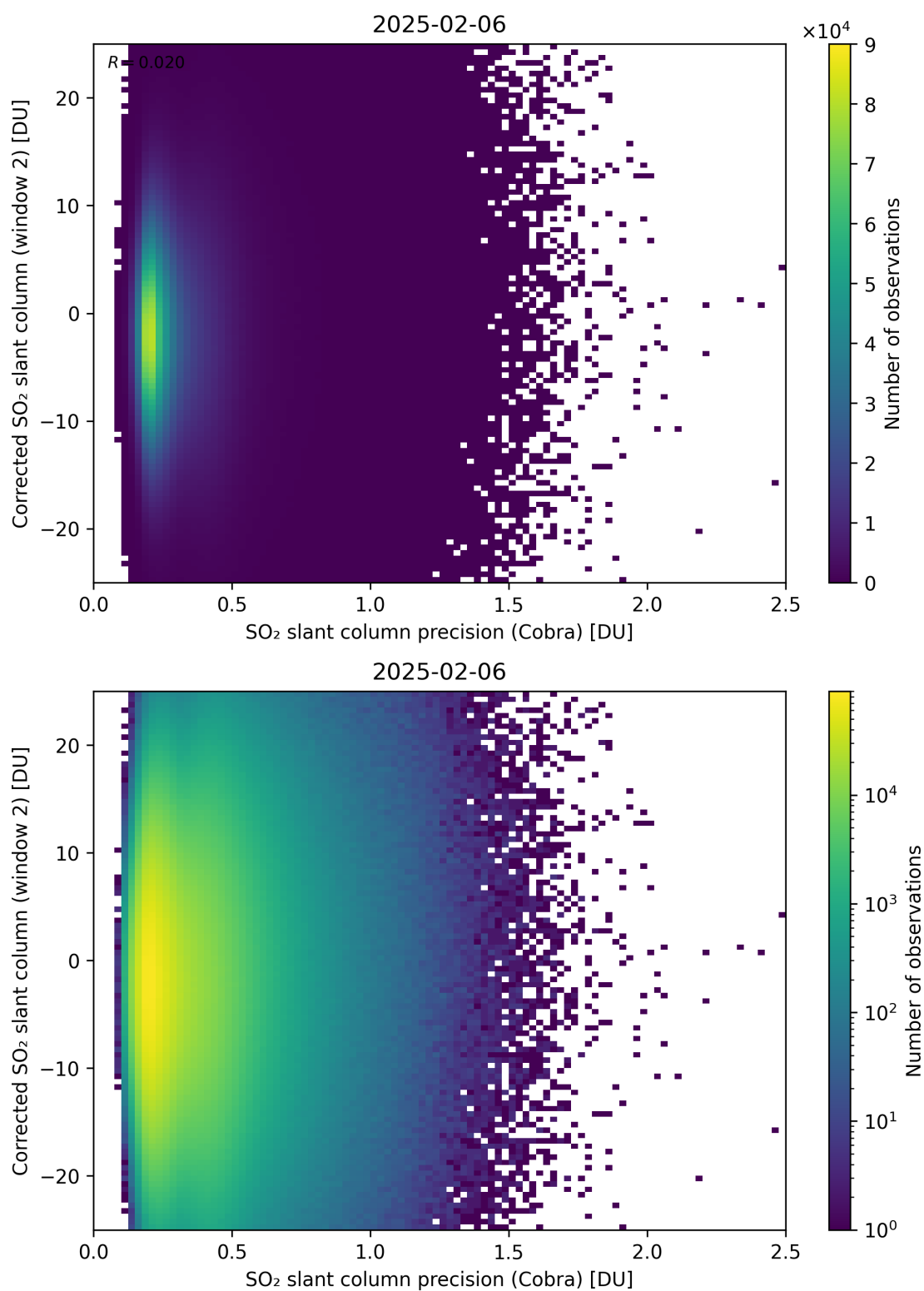
Figure 206: Scatter density plot of “SO 2 slant column precision (Cobra)” against “Corrected SO 2 slant column (window 2)” for 2025-02-05 to 2025-02-07.
