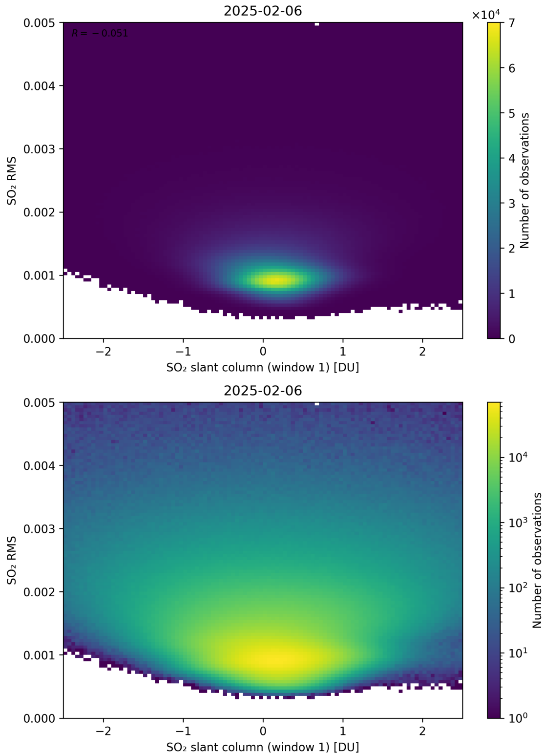
Figure 267: Scatter density plot of “SO 2 slant column (window 1)” against “SO 2 RMS” for 2025-02-05 to 2025-02-07.
