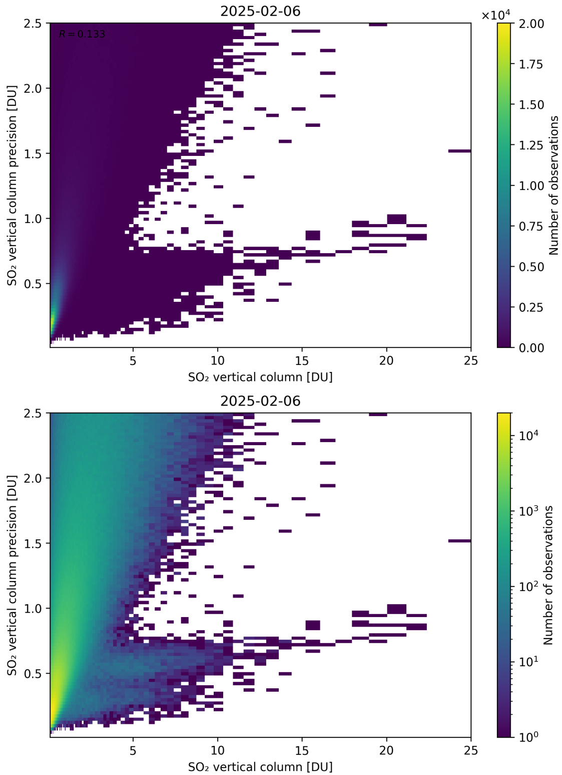
Figure 361: Scatter density plot of “SO 2 vertical column” against “SO 2 vertical column precision” for 2025-02-05 to 2025-02-07.
