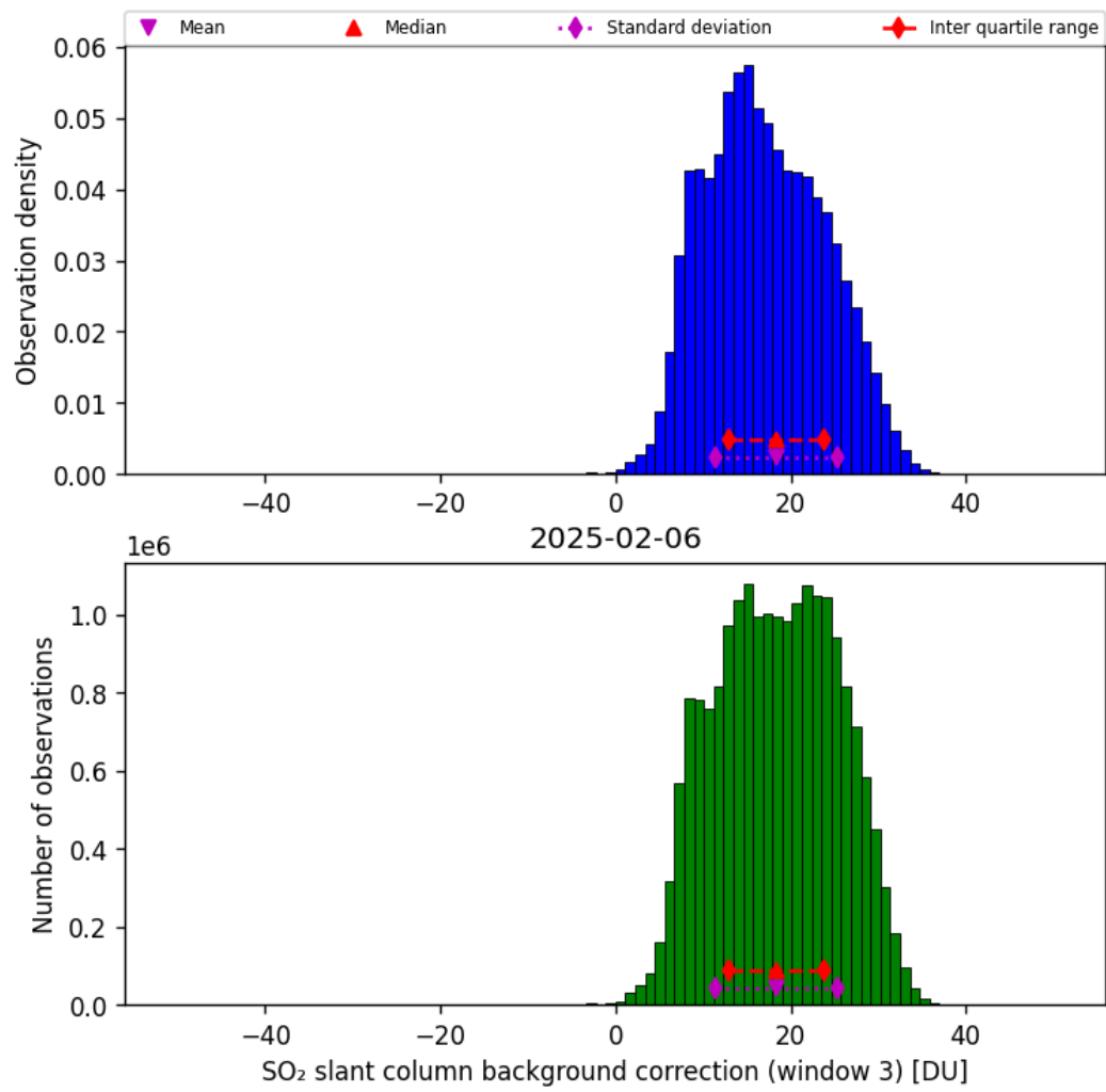
Figure 74: Histogram of “SO 2 slant column background correction (window 3)” for 2025-02-05 to 2025-02-07
