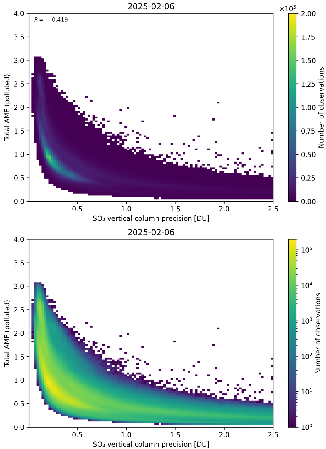
Figure 346: Scatter density plot of “SO 2 vertical column precision” against “Total AMF (polluted)” for 2025-02-05 to 2025-02-07.
