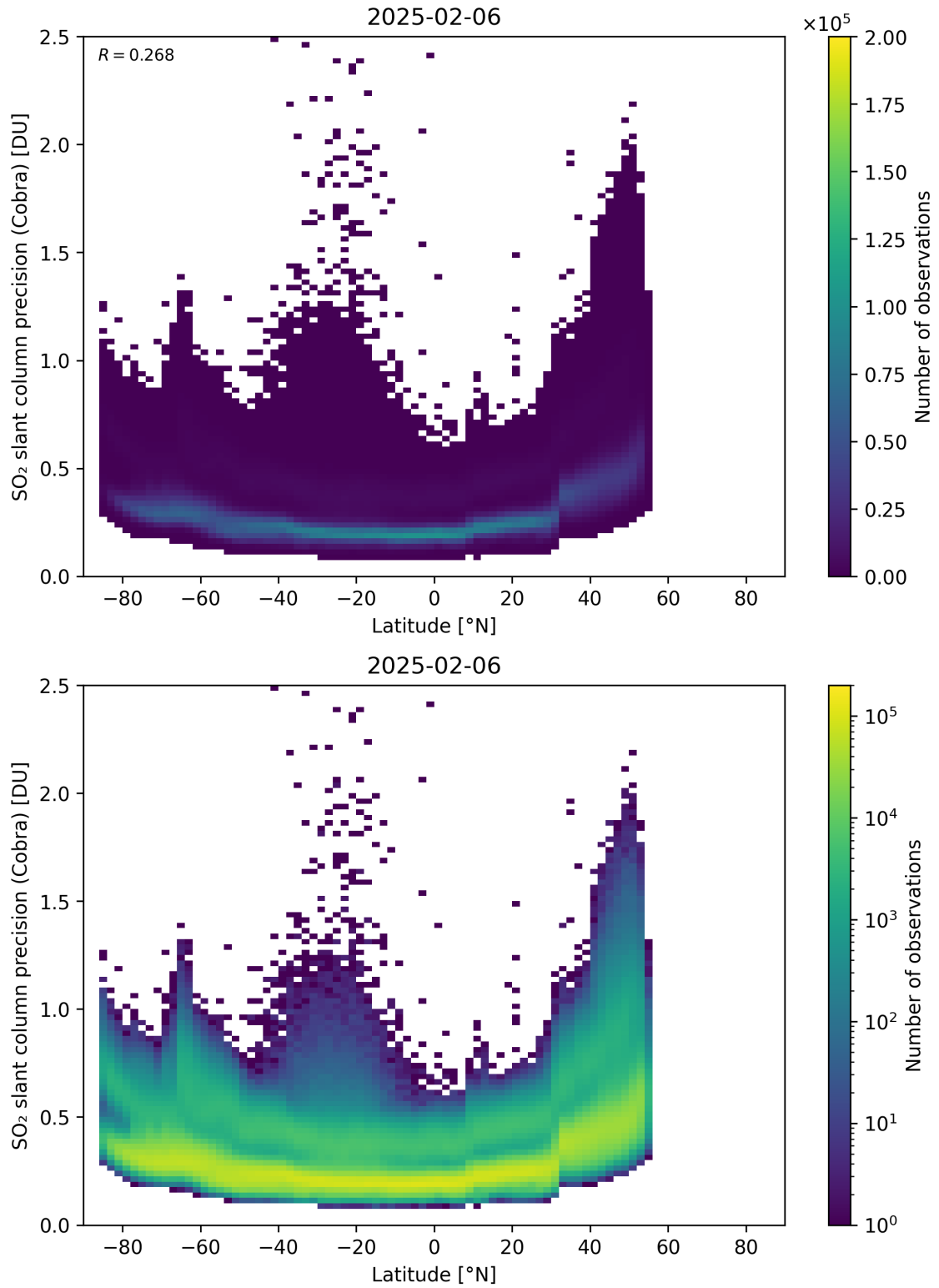
Figure 158: Scatter density plot of “Latitude” against “SO 2 slant column precision (Cobra)” for 2025-02-05 to 2025-02-07.
