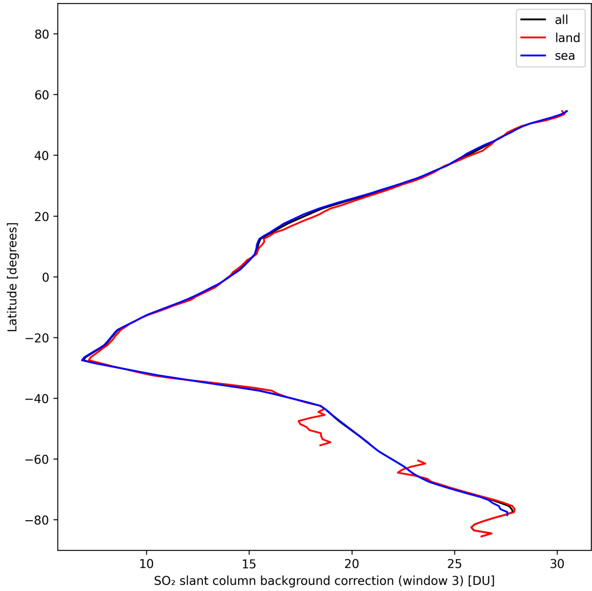
Figure 48: Zonal average of “SO 2 slant column background correction (window 3)” for 2025-02-05 to 2025-02-07.
