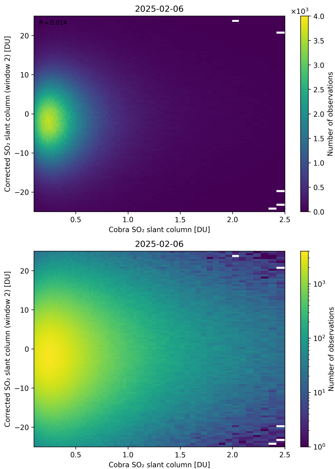
Figure 217: Scatter density plot of “Cobra SO 2 slant column” against “Corrected SO 2 slant column (window 2)” for 2025-02-05 to 2025-02-07.
