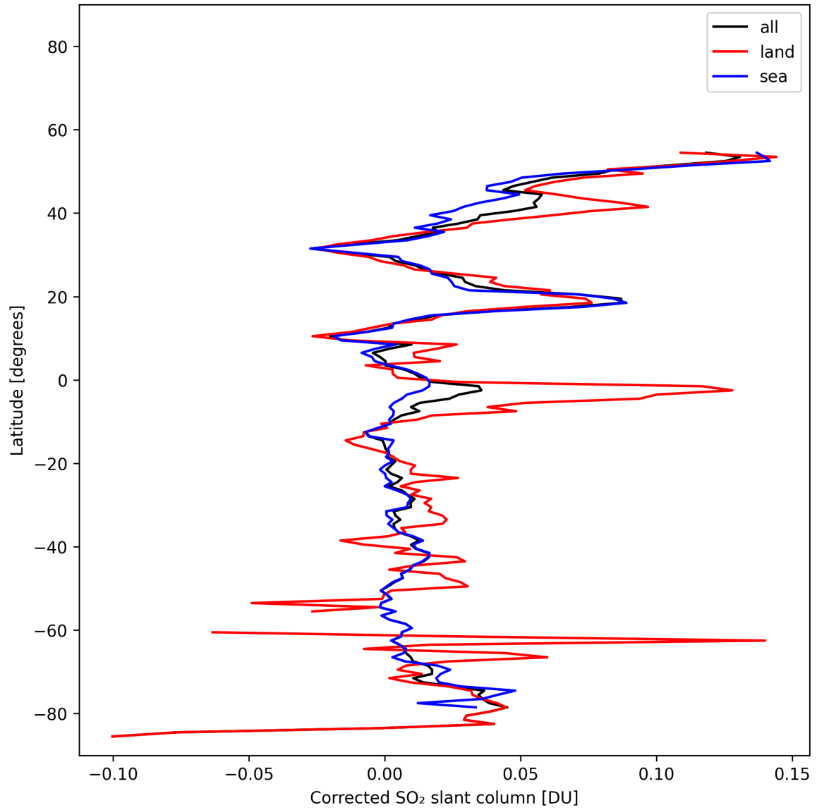
Figure 34: Zonal average of “Corrected SO 2 slant column” for 2025-02-05 to 2025-02-07.
