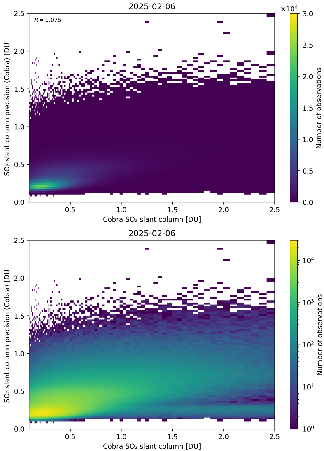
Figure 216: Scatter density plot of “Cobra SO 2 slant column” against “SO 2 slant column precision (Cobra)” for 2025-02-05 to 2025-02-07.
