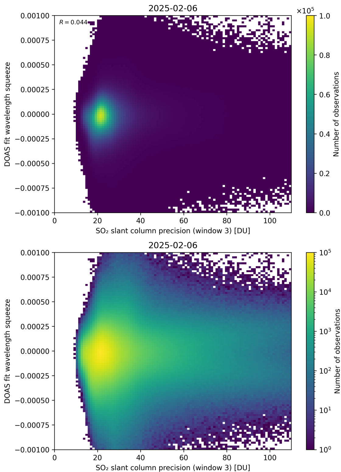
Figure 309: Scatter density plot of “SO 2 slant column precision (window 3)” against “DOAS fit wavelength squeeze” for 2025-02-05 to 2025-02-07.
