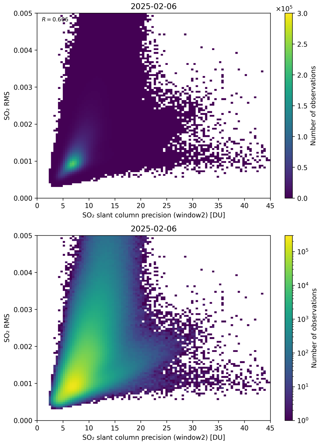
Figure 295: Scatter density plot of “SO 2 slant column precision (window2)” against “SO 2 RMS” for 2025-02-05 to 2025-02-07.
