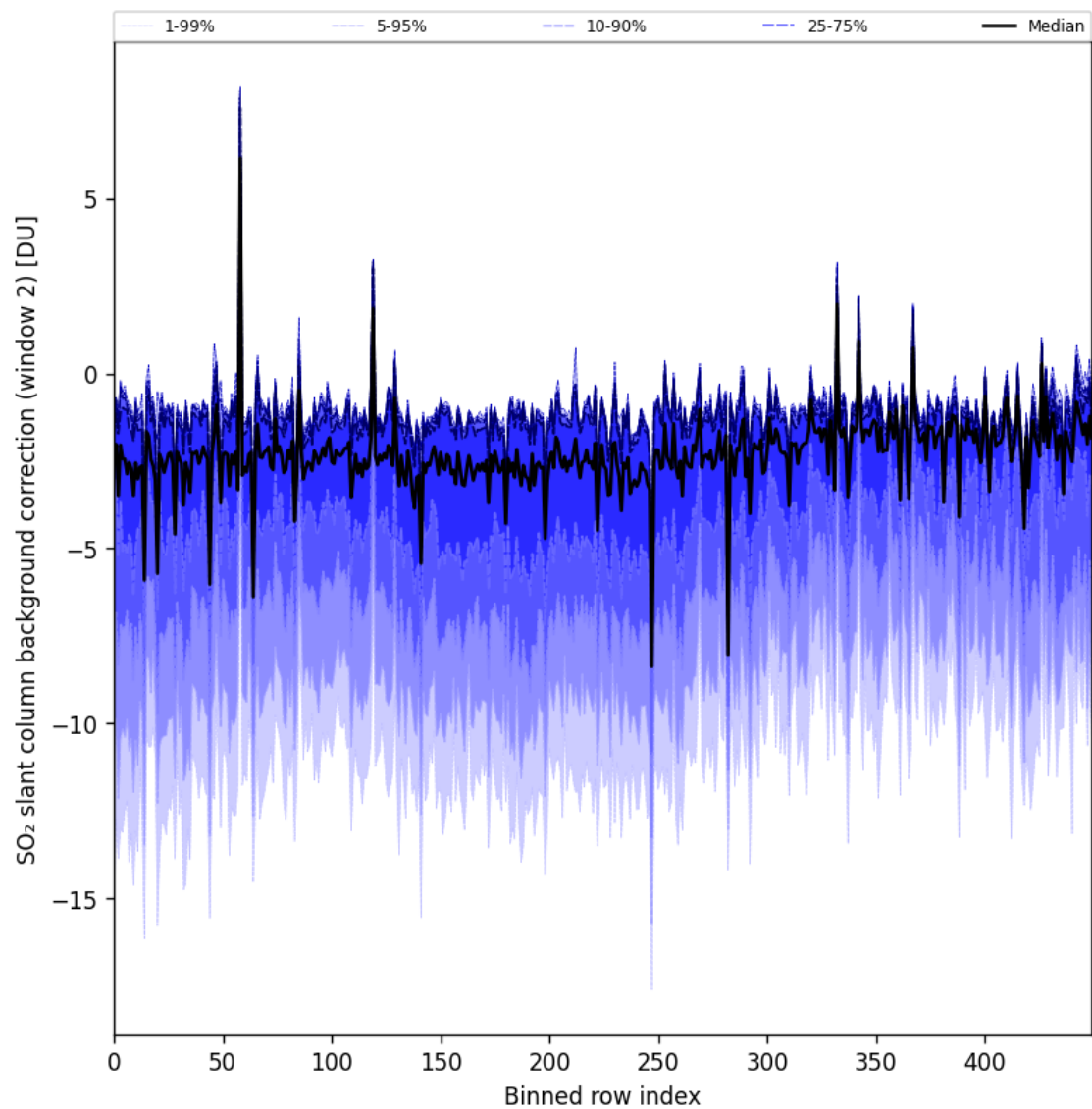
Figure 96: Along track statistics of “SO 2 slant column background correction (window 2)” for 2025-02-05 to 2025-02-07
