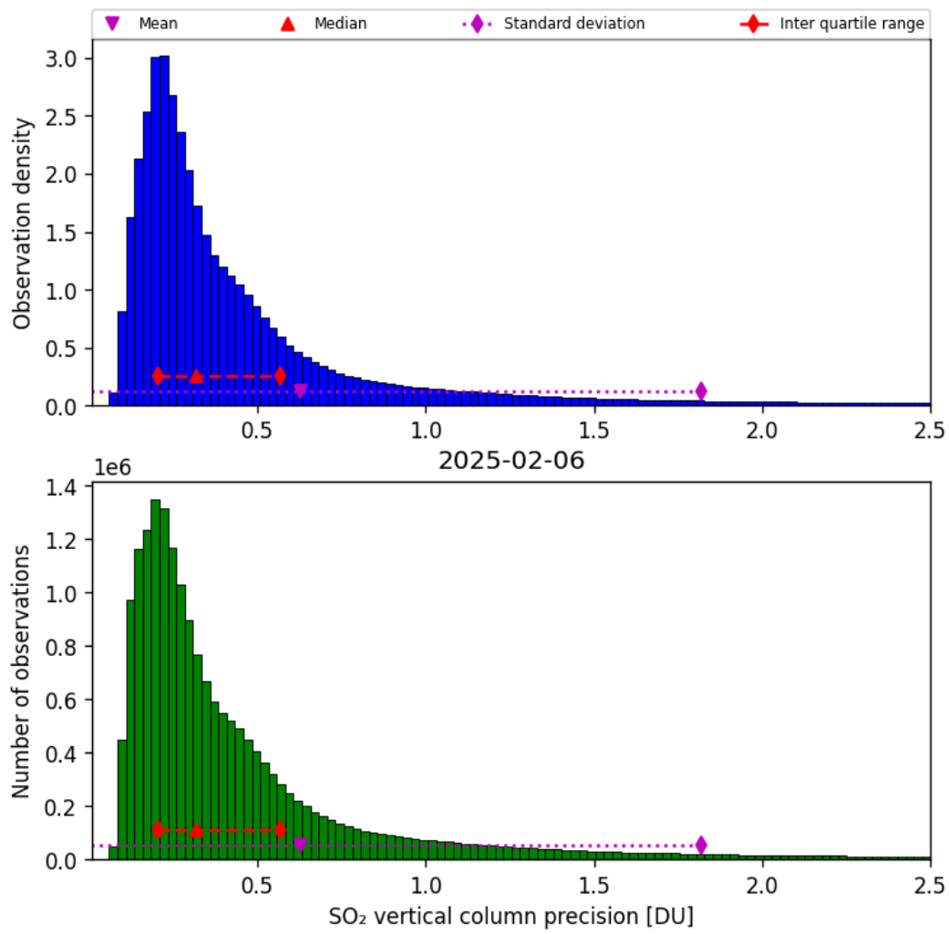
Figure 59: Histogram of “SO 2 vertical column precision” for 2025-02-05 to 2025-02-07
