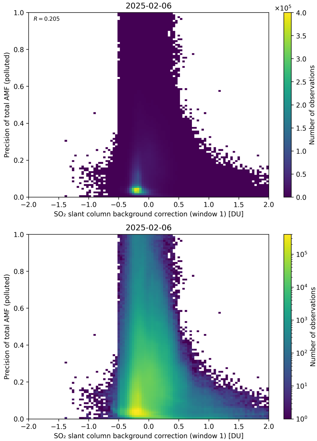
Figure 121: Scatter density plot of “SO 2 slant column background correction (window 1)” against “Precision of total AMF (polluted)” for 2025-02-05 to 2025-02-07.
