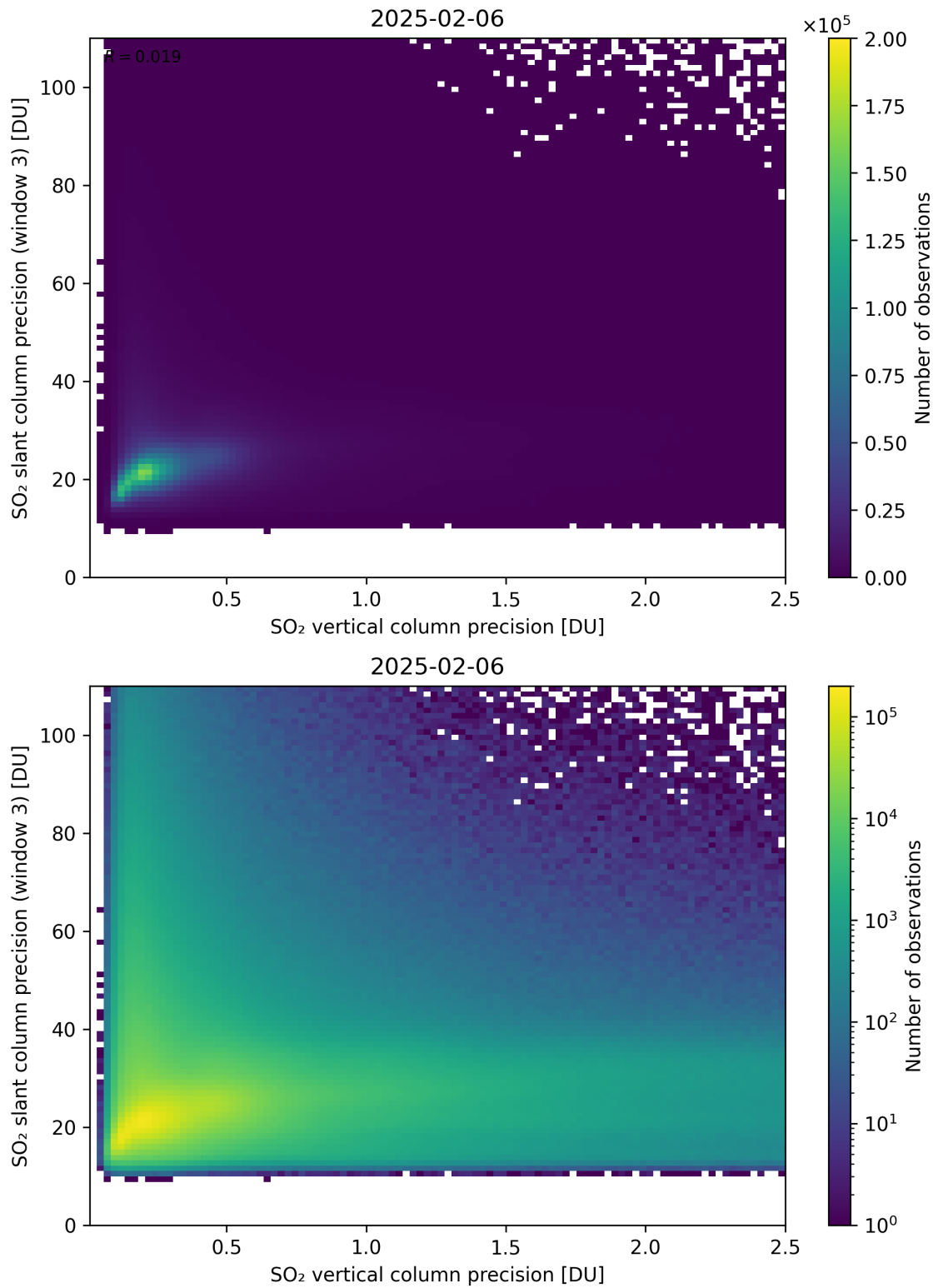
Figure 345: Scatter density plot of “SO 2 vertical column precision” against “SO 2 slant column precision (window 3)” for 2025-02-05 to 2025-02-07.
