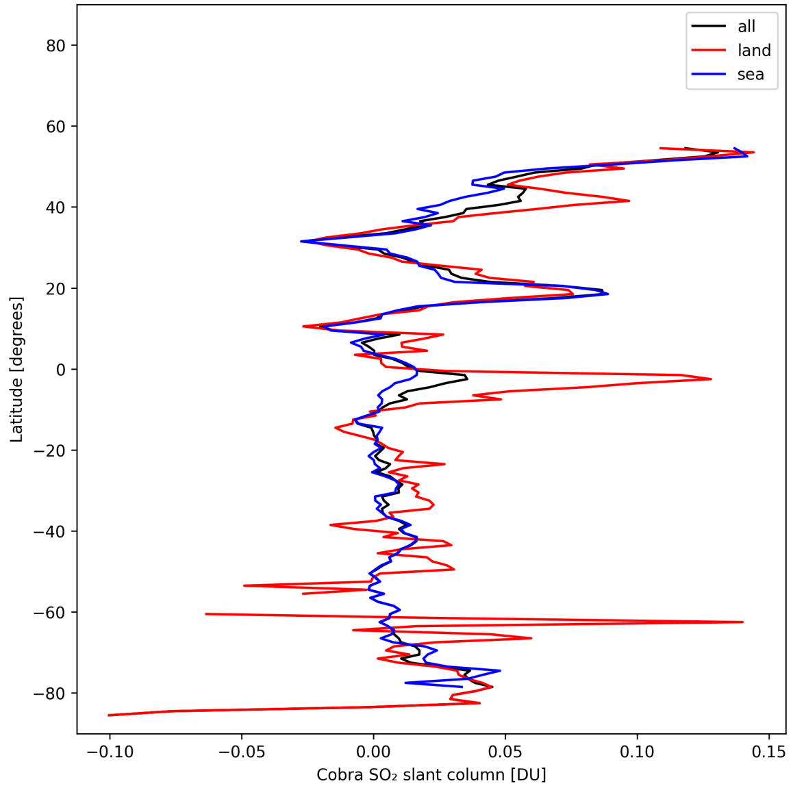
Figure 35: Zonal average of “Cobra SO 2 slant column” for 2025-02-05 to 2025-02-07.
