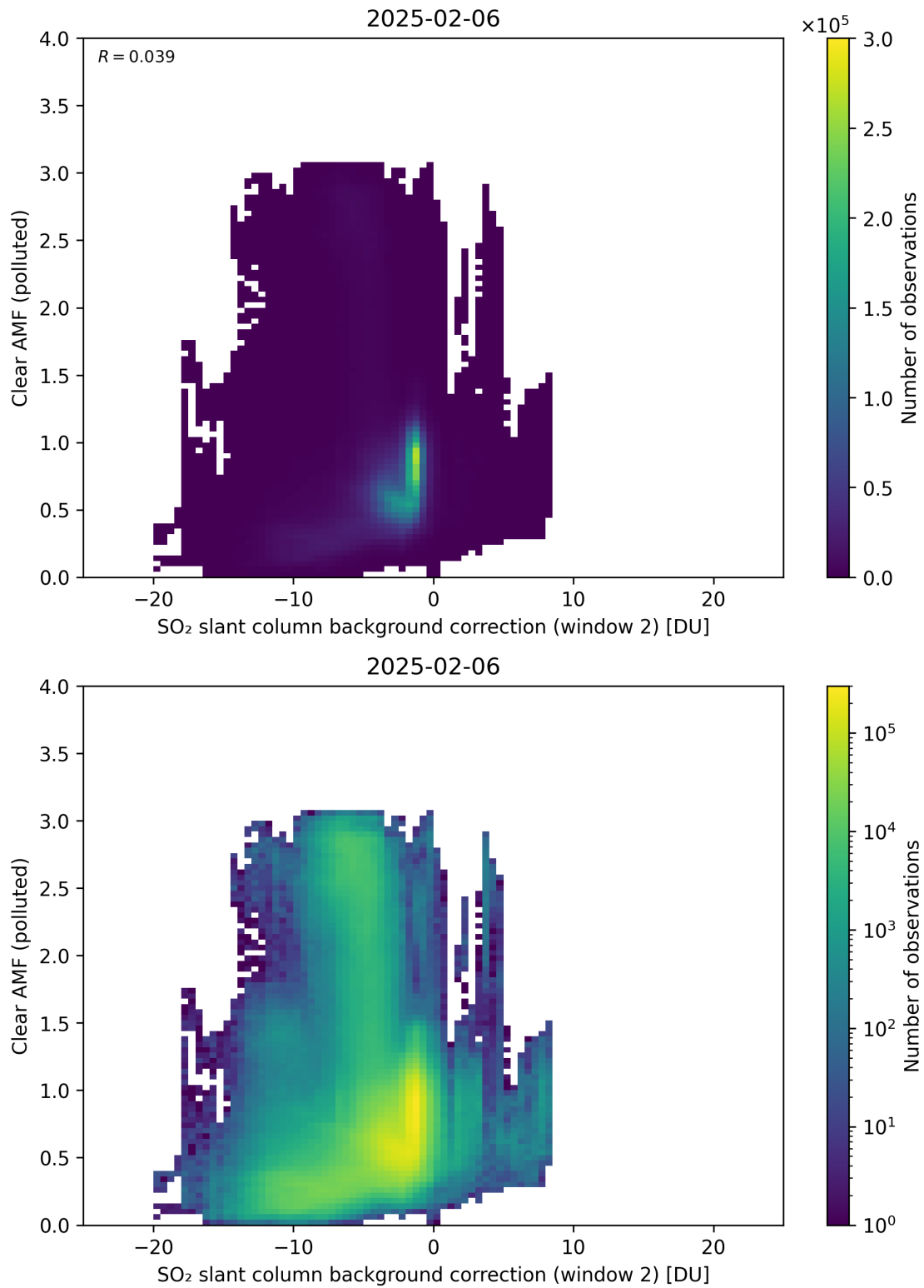
Figure 126: Scatter density plot of “SO 2 slant column background correction (window 2)” against “Clear AMF (polluted)” for 2025-02-05 to 2025-02-07.
