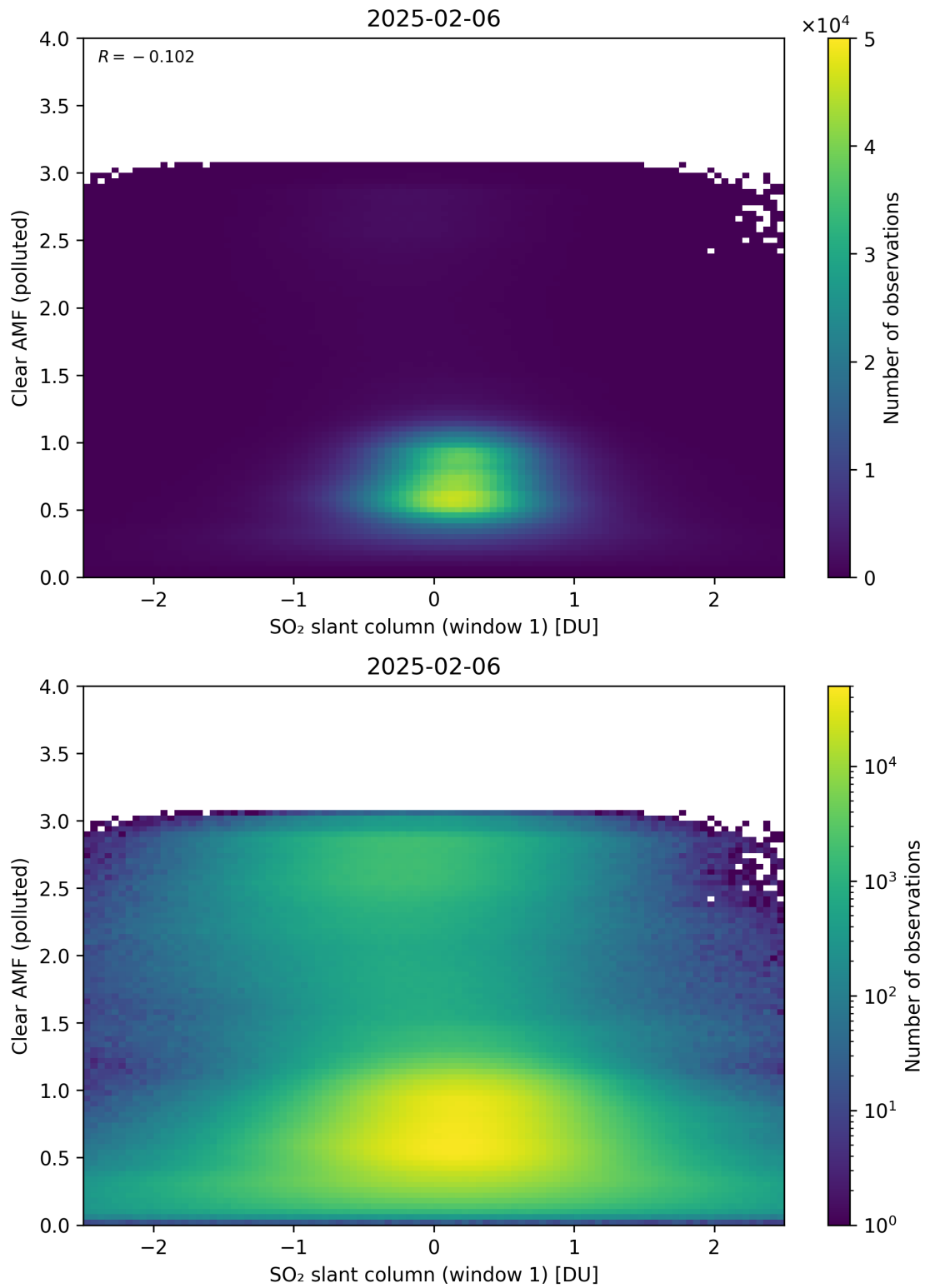
Figure 282: Scatter density plot of “SO 2 slant column (window 1)” against “Clear AMF (polluted)” for 2025-02-05 to 2025-02-07.
