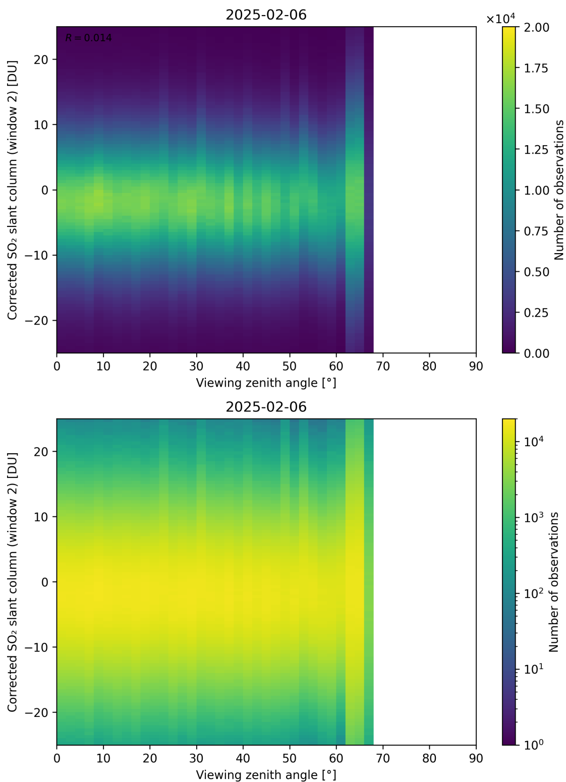
Figure 374: Scatter density plot of “Viewing zenith angle” against “Corrected SO 2 slant column (window 2)” for 2025-02-05 to 2025-02-07.
