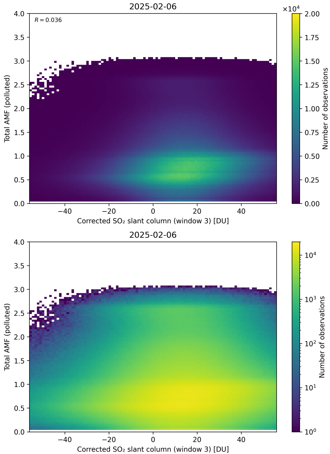
Figure 260: Scatter density plot of “Corrected SO 2 slant column (window 3)” against “Total AMF (polluted)” for 2025-02-05 to 2025-02-07.
