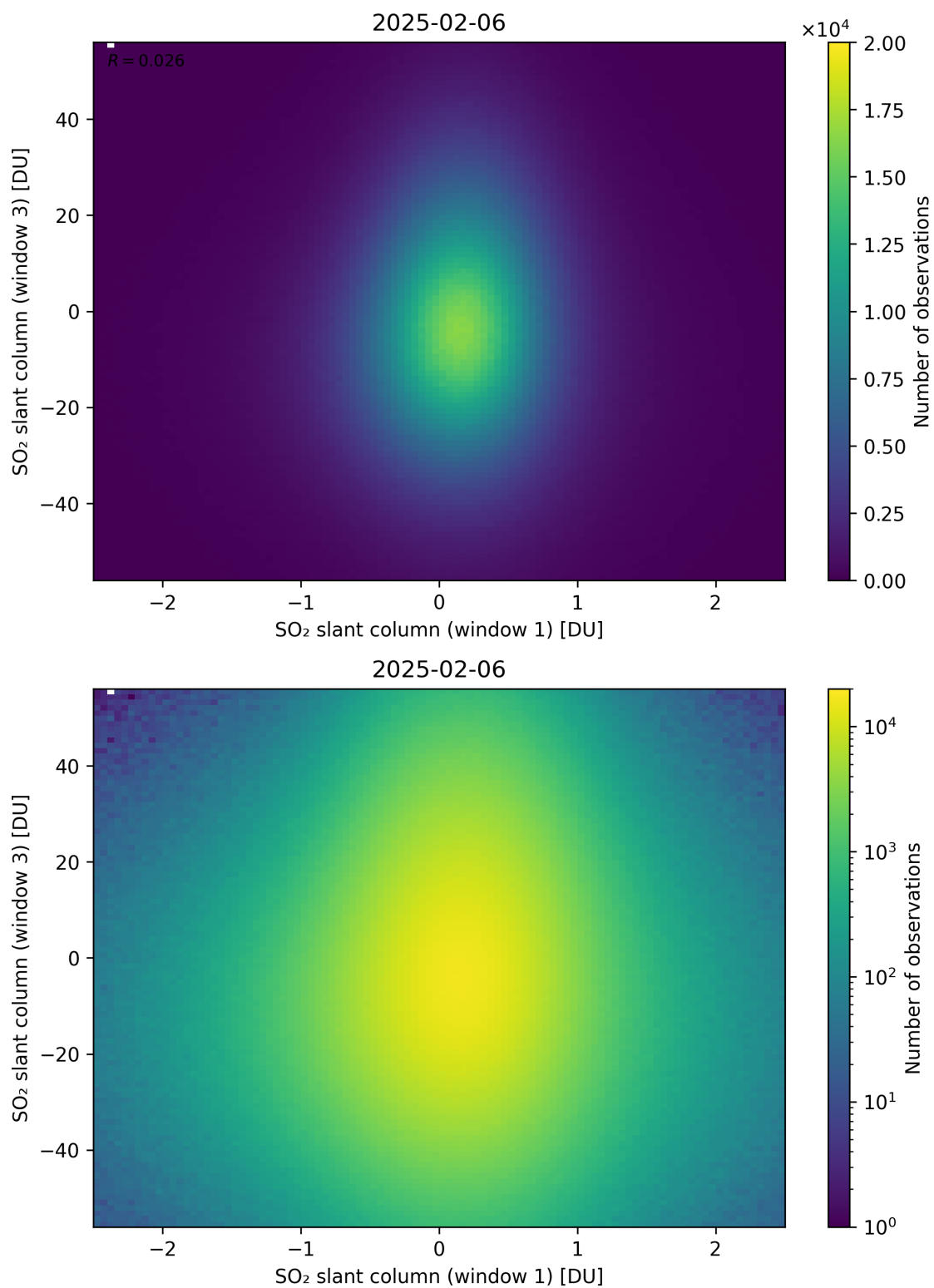
Figure 287: Scatter density plot of “SO 2 slant column (window 1)” against “SO 2 slant column (window 3)” for 2025-02-05 to 2025-02-07.
