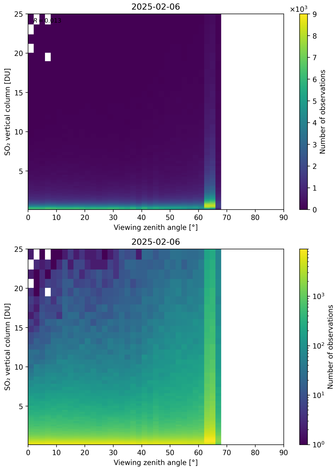
Figure 383: Scatter density plot of “Viewing zenith angle” against “SO 2 vertical column” for 2025-02-05 to 2025-02-07.
