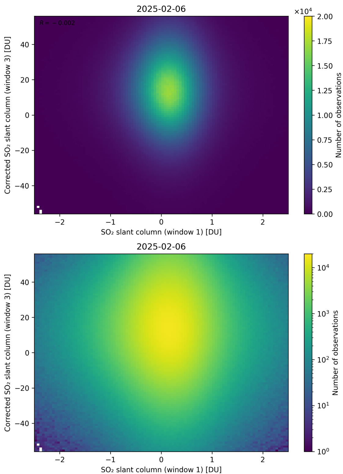
Figure 284: Scatter density plot of “SO 2 slant column (window 1)” against “Corrected SO 2 slant column (window 3)” for 2025-02-05 to 2025-02-07.
