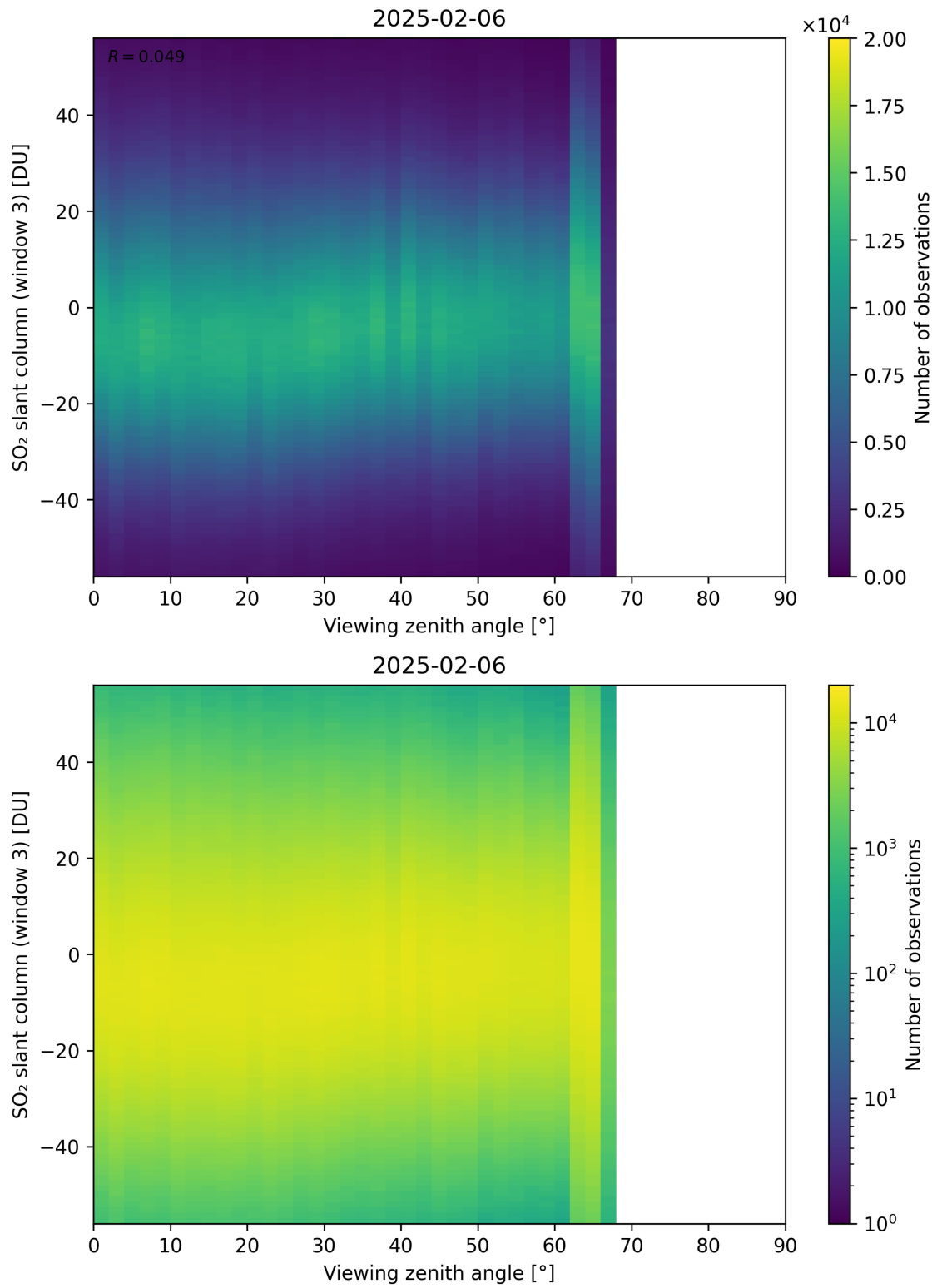
Figure 379: Scatter density plot of “Viewing zenith angle” against “SO 2 slant column (window 3)” for 2025-02-05 to 2025-02-07.
