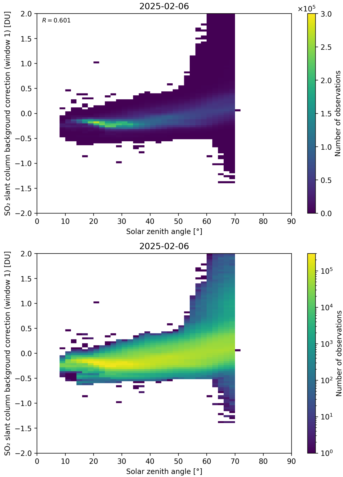
Figure 171: Scatter density plot of “Solar zenith angle” against “SO 2 slant column background correction (window 1)” for 2025-02-05 to 2025-02-07.
