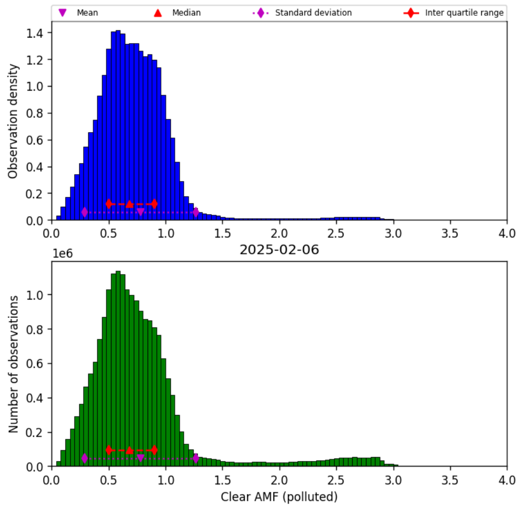
Figure 81: Histogram of “Clear AMF (polluted)” for 2025-02-05 to 2025-02-07
