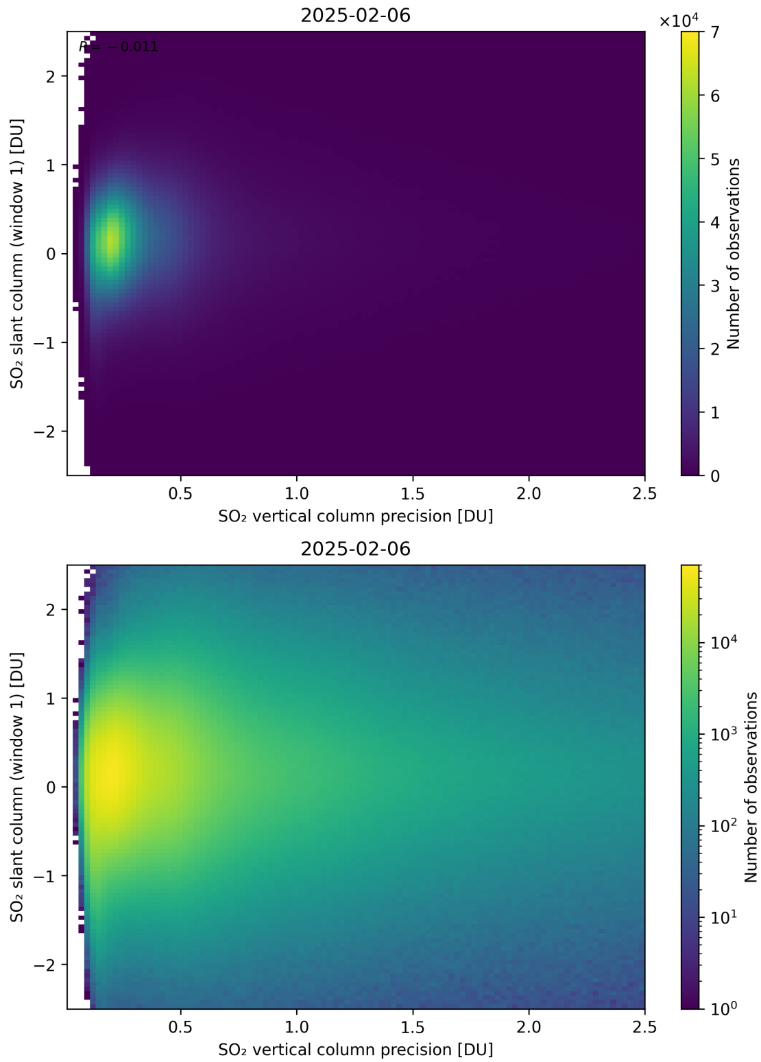
Figure 341: Scatter density plot of “SO 2 vertical column precision” against “SO 2 slant column (window 1)” for 2025-02-05 to 2025-02-07.
