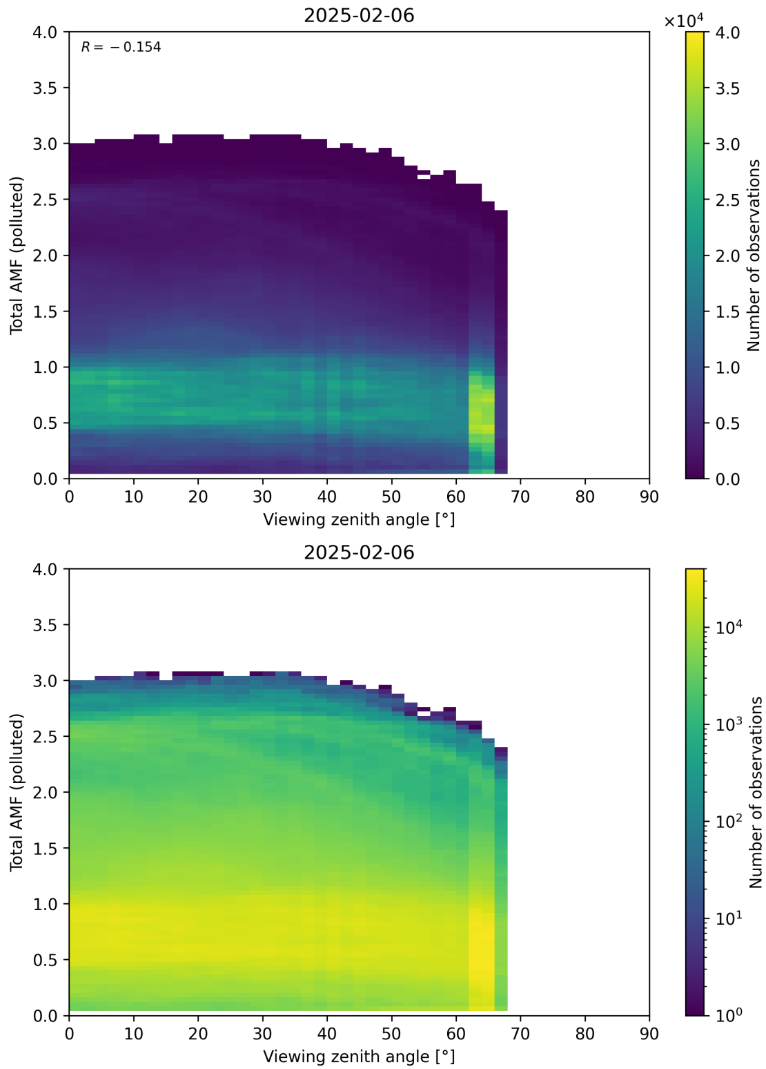
Figure 381: Scatter density plot of “Viewing zenith angle” against “Total AMF (polluted)” for 2025-02-05 to 2025-02-07.
