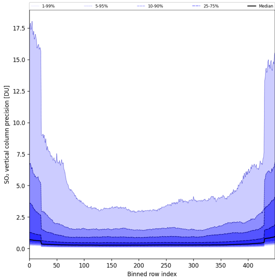
Figure 85: Along track statistics of “SO 2 vertical column precision” for 2025-02-05 to 2025-02-07
