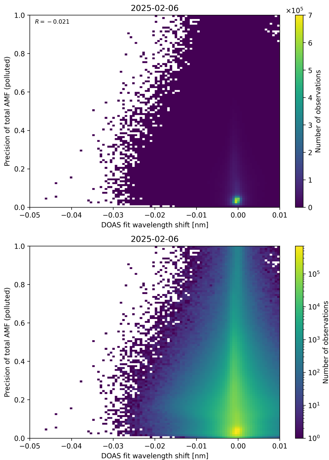
Figure 142: Scatter density plot of “DOAS fit wavelength shift” against “Precision of total AMF (polluted)” for 2025-02-05 to 2025-02-07.
