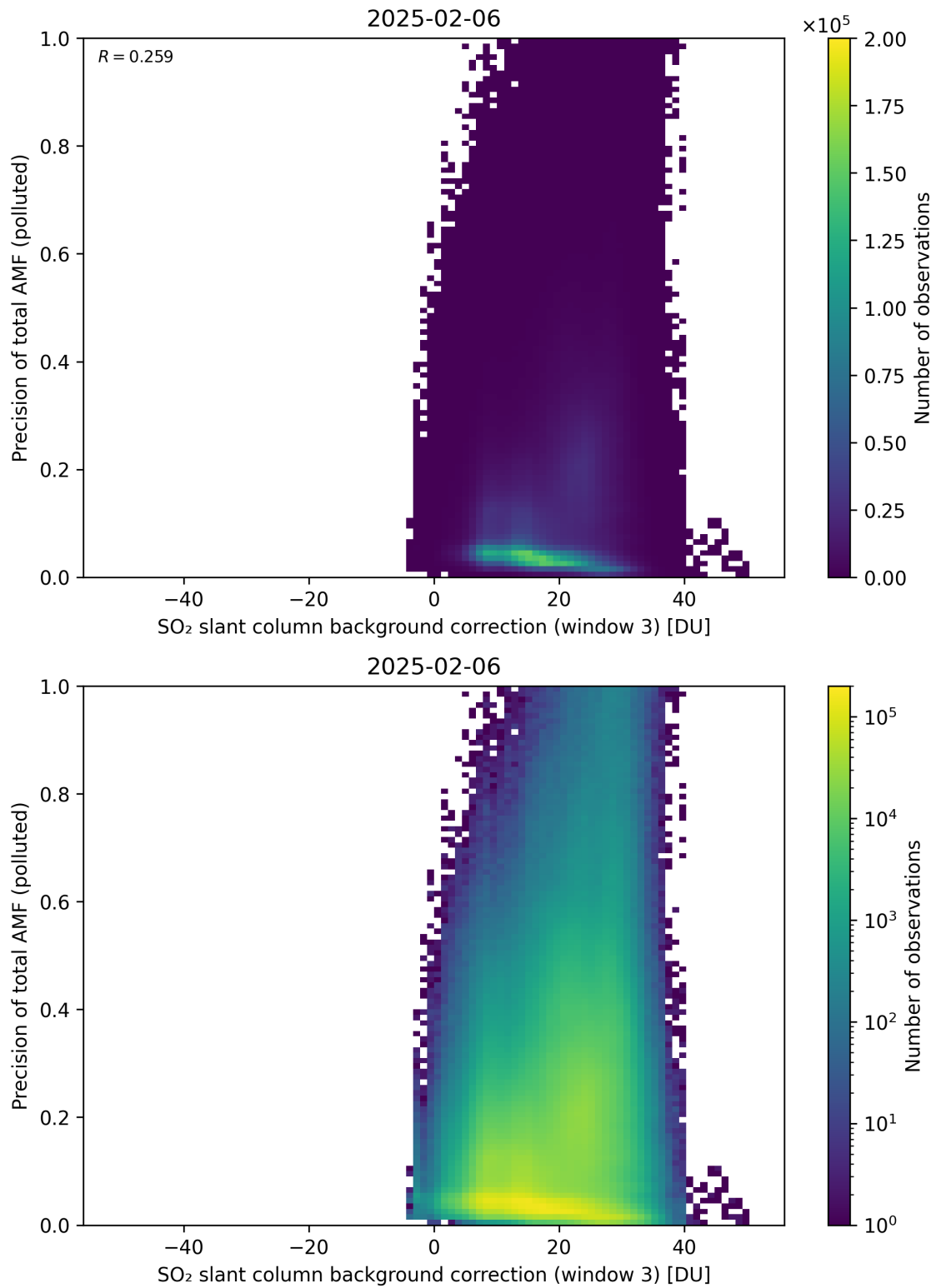
Figure 137: Scatter density plot of “SO 2 slant column background correction (window 3)” against “Precision of total AMF (polluted)” for 2025-02-05 to 2025-02-07.
