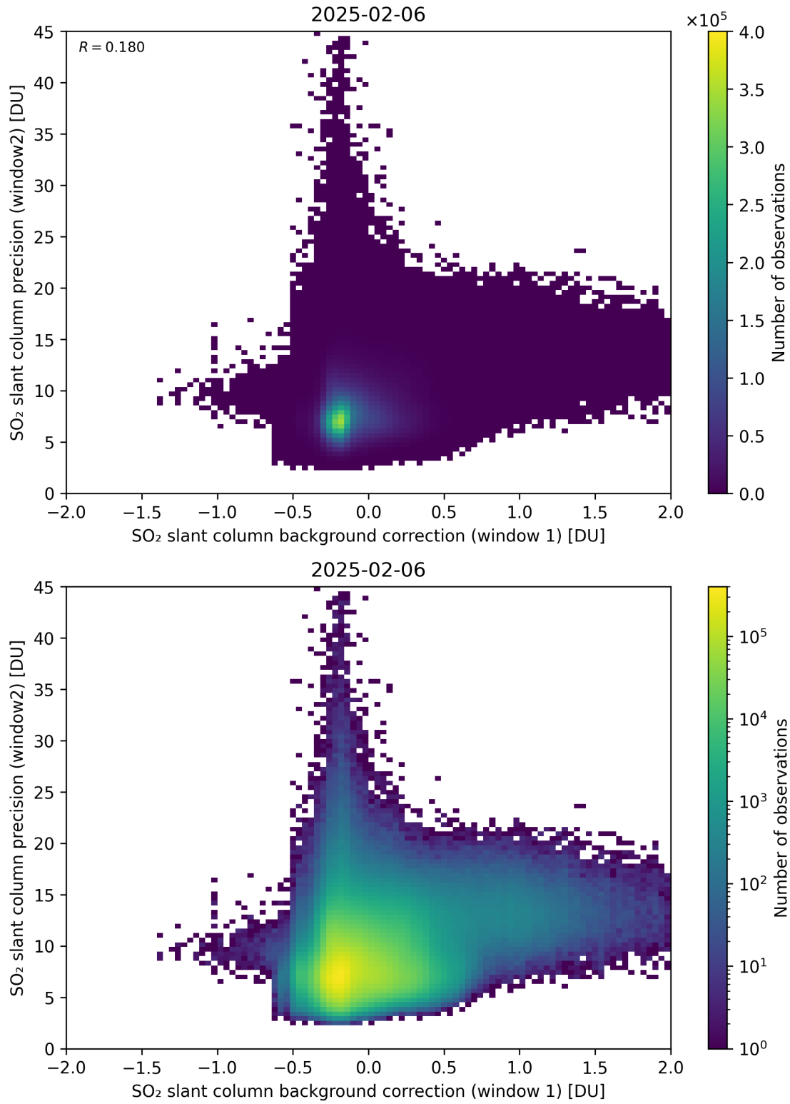
Figure 117: Scatter density plot of “SO 2 slant column background correction (window 1)” against “SO 2 slant column precision (window2)” for 2025-02-05 to 2025-02-07.
