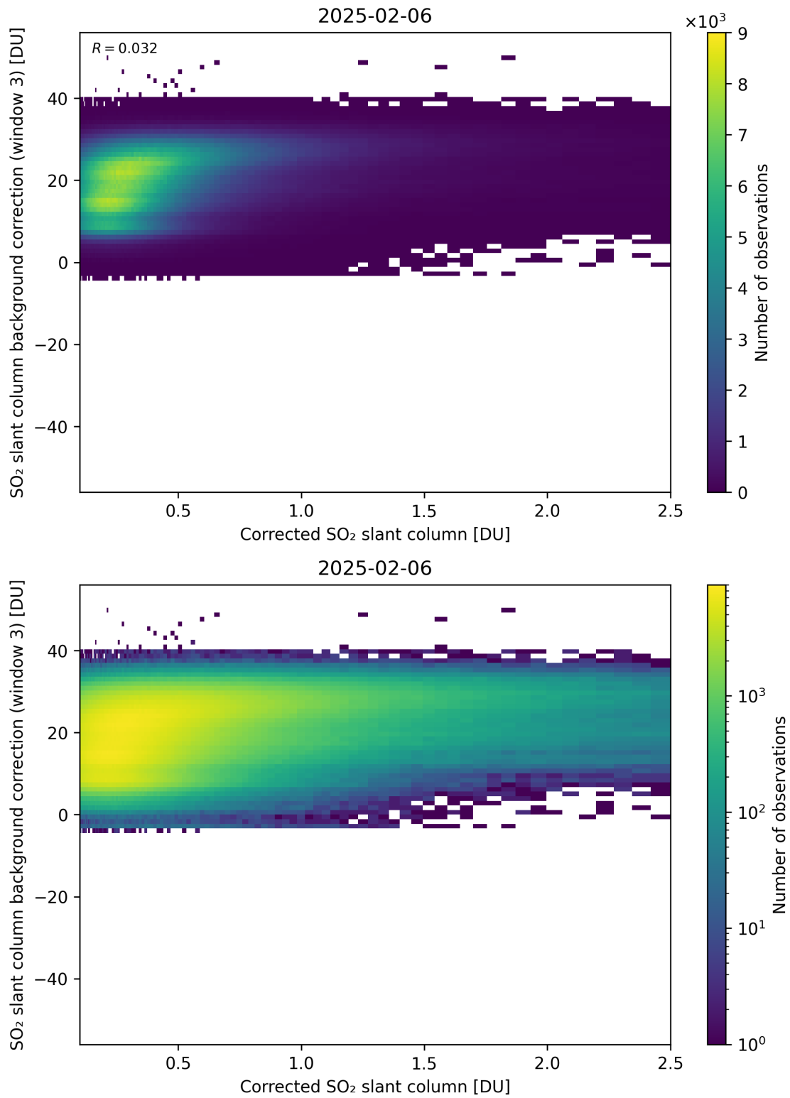
Figure 228: Scatter density plot of “Corrected SO 2 slant column” against “SO 2 slant column background correction (window 3)” for 2025-02-05 to 2025-02-07.
