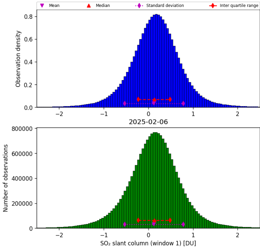
Figure 63: Histogram of “SO 2 slant column (window 1)” for 2025-02-05 to 2025-02-07
