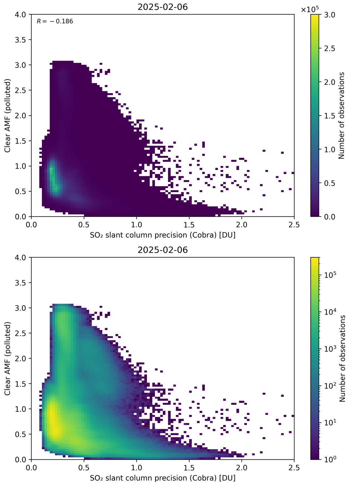
Figure 205: Scatter density plot of “SO 2 slant column precision (Cobra)” against “Clear AMF (polluted)” for 2025-02-05 to 2025-02-07.
