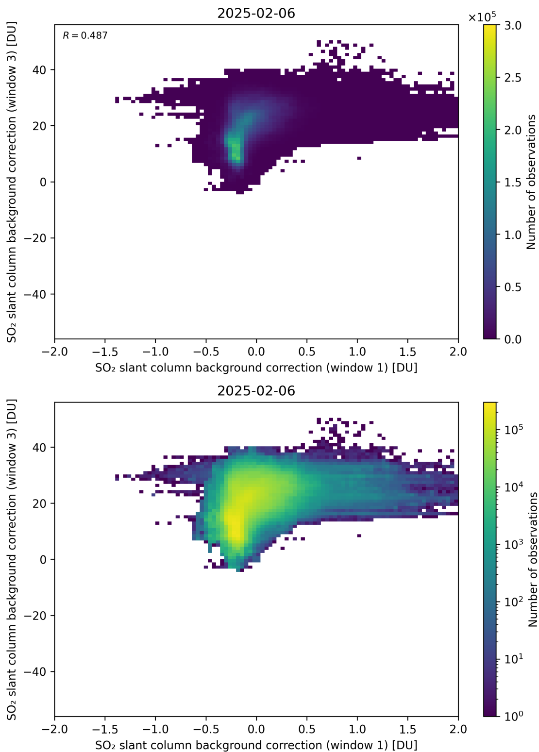
Figure 110: Scatter density plot of “SO 2 slant column background correction (window 1)” against “SO 2 slant column background correction (window 3)” for 2025-02-05 to 2025-02-07.
