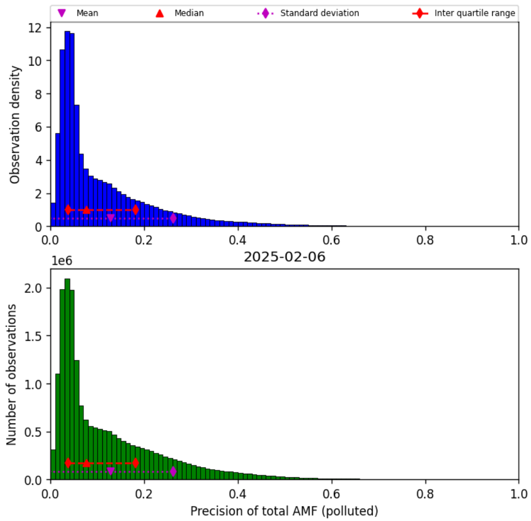
Figure 80: Histogram of “Precision of total AMF (polluted)” for 2025-02-05 to 2025-02-07
