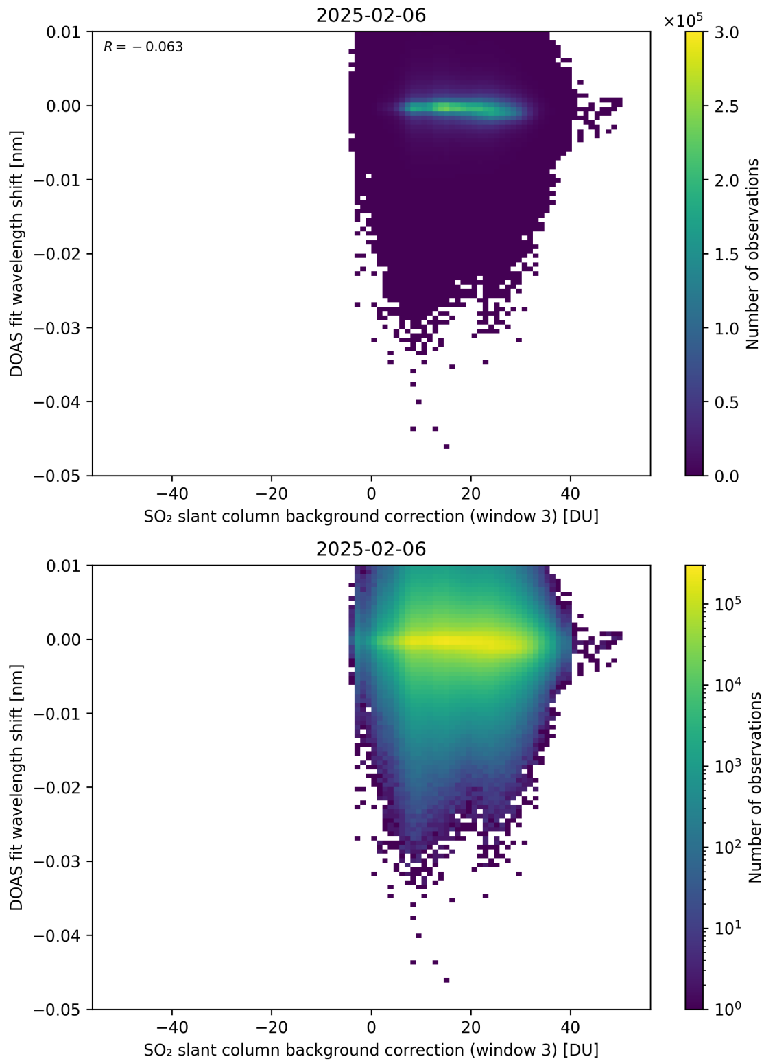
Figure 132: Scatter density plot of “SO 2 slant column background correction (window 3)” against “DOAS fit wavelength shift” for 2025-02-05 to 2025-02-07.
