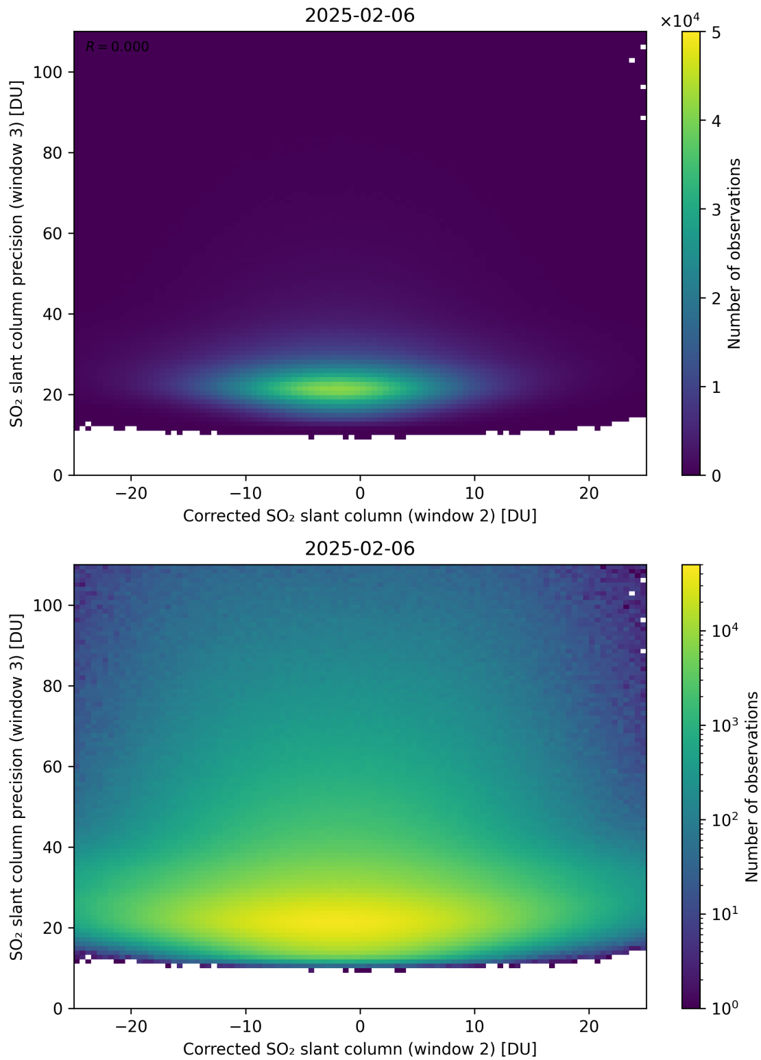
Figure 252: Scatter density plot of “Corrected SO 2 slant column (window 2)” against “SO 2 slant column precision (window 3)” for 2025-02-05 to 2025-02-07.
