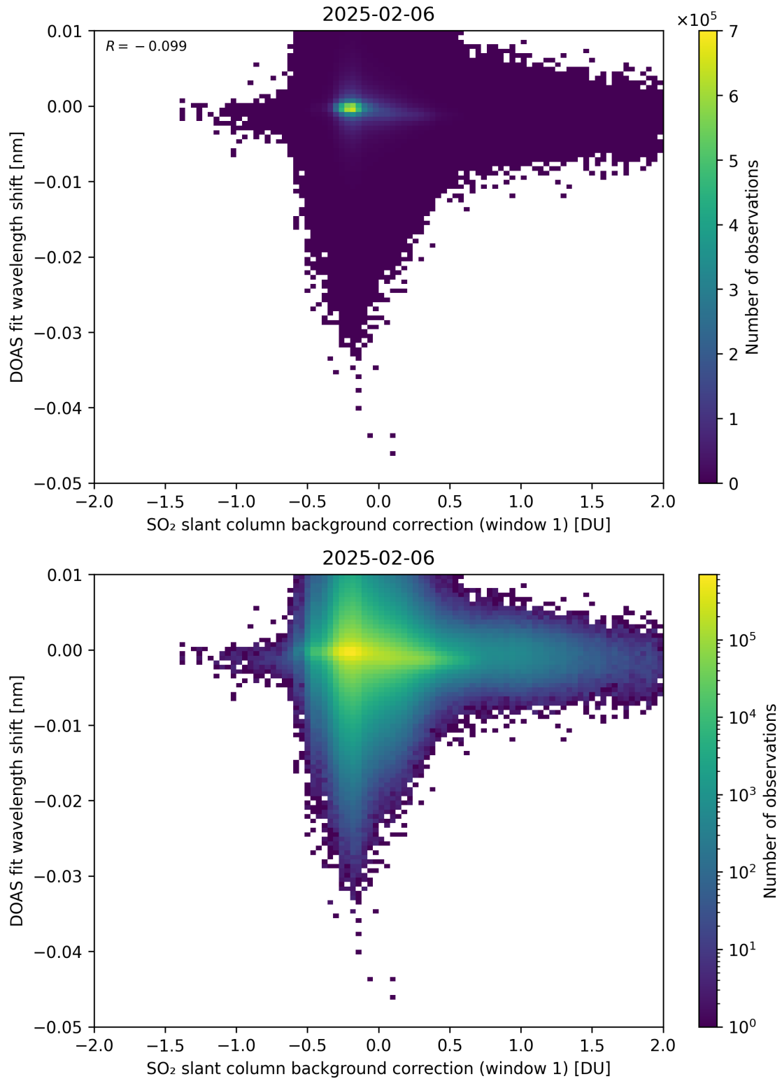
Figure 111: Scatter density plot of “SO 2 slant column background correction (window 1)” against “DOAS fit wavelength shift” for 2025-02-05 to 2025-02-07.
