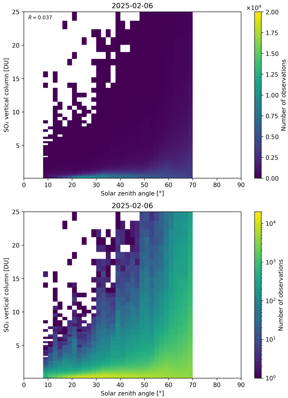
Figure 191: Scatter density plot of “Solar zenith angle” against “SO 2 vertical column” for 2025-02-05 to 2025-02-07.
