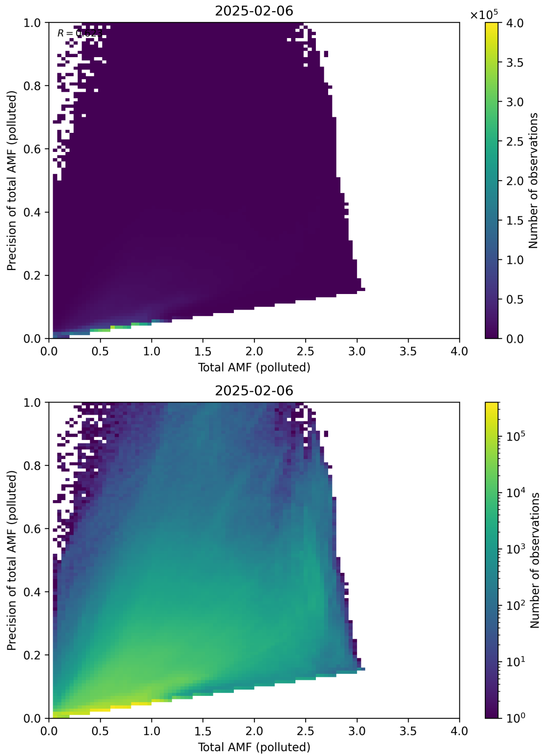
Figure 322: Scatter density plot of “Total AMF (polluted)” against “Precision of total AMF (polluted)” for 2025-02-05 to 2025-02-07.
