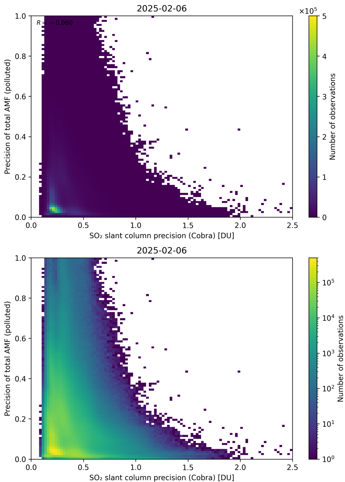
Figure 214: Scatter density plot of “SO 2 slant column precision (Cobra)” against “Precision of total AMF (polluted)” for 2025-02-05 to 2025-02-07.
