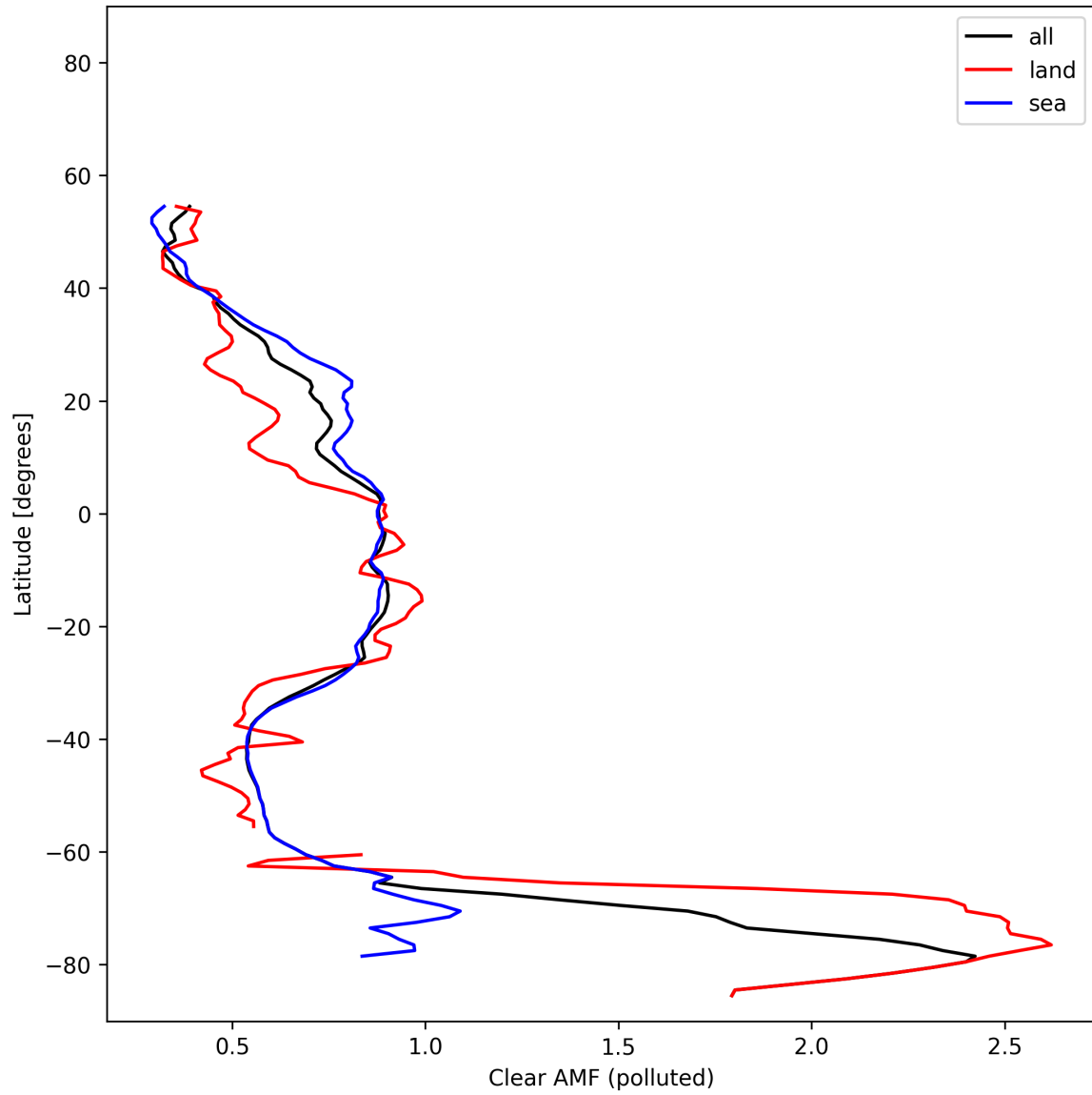
Figure 55: Zonal average of “Clear AMF (polluted)” for 2025-02-05 to 2025-02-07.
