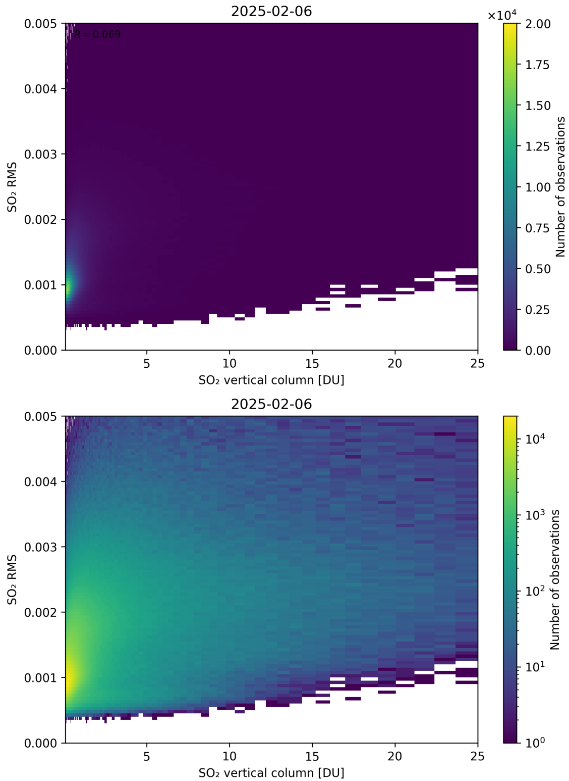
Figure 328: Scatter density plot of “SO 2 vertical column” against “SO 2 RMS” for 2025-02-05 to 2025-02-07.
