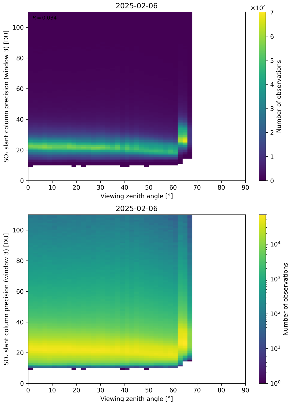
Figure 380: Scatter density plot of “Viewing zenith angle” against “SO 2 slant column precision (window 3)” for 2025-02-05 to 2025-02-07.
