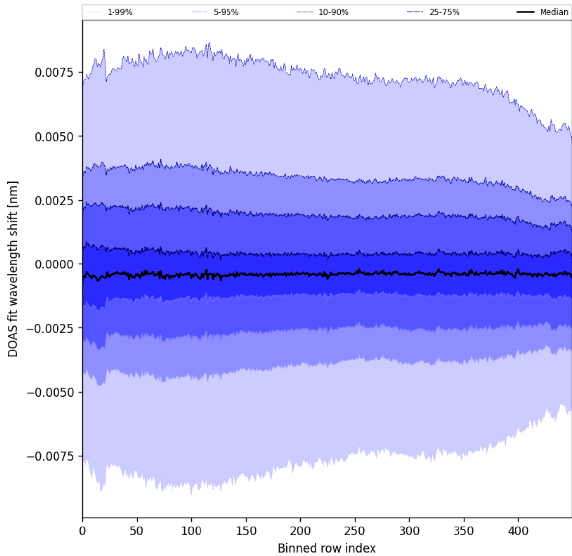
Figure 102: Along track statistics of “DOAS fit wavelength shift” for 2025-02-05 to 2025-02-07
