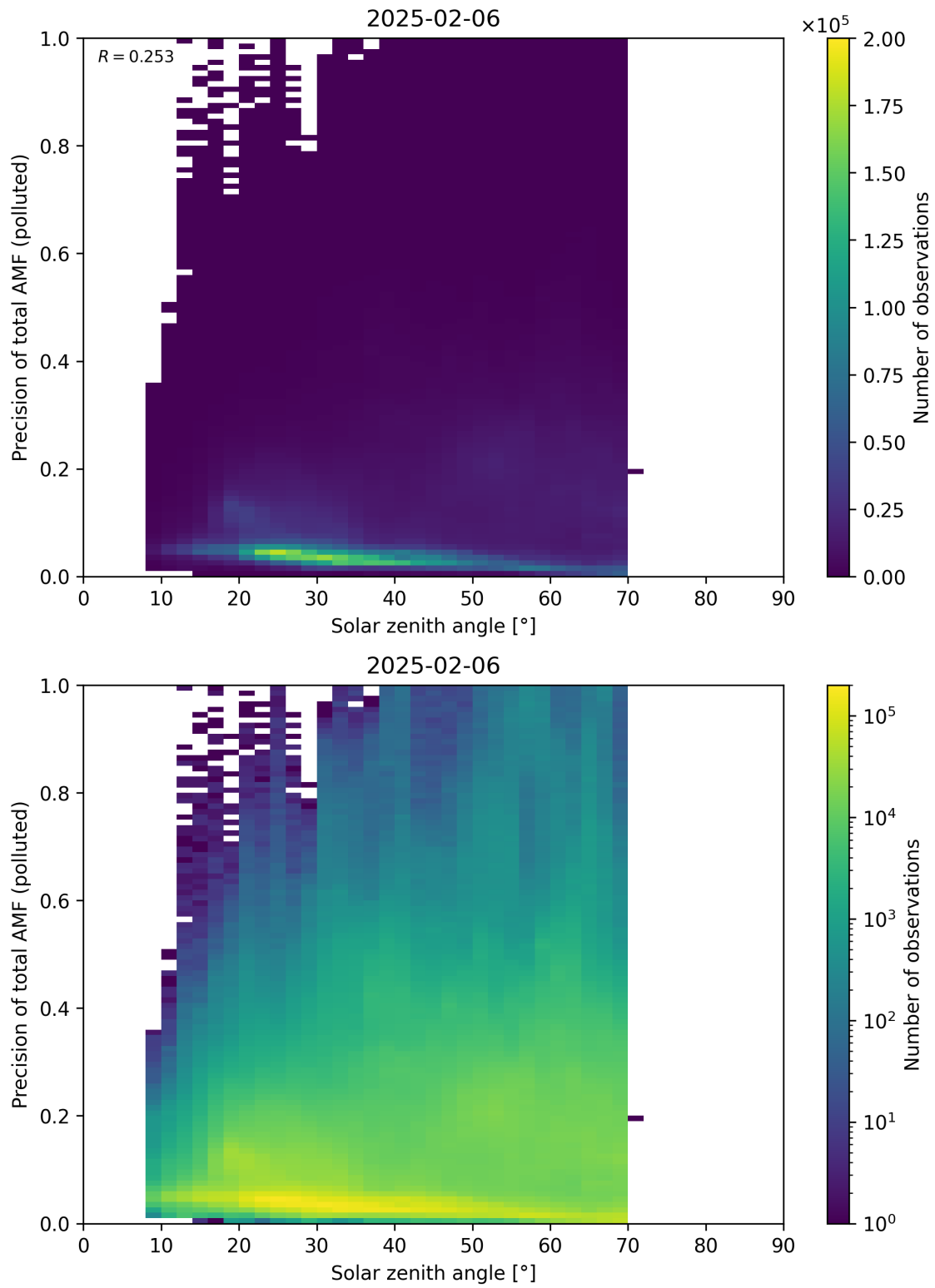
Figure 190: Scatter density plot of “Solar zenith angle” against “Precision of total AMF (polluted)” for 2025-02-05 to 2025-02-07.
