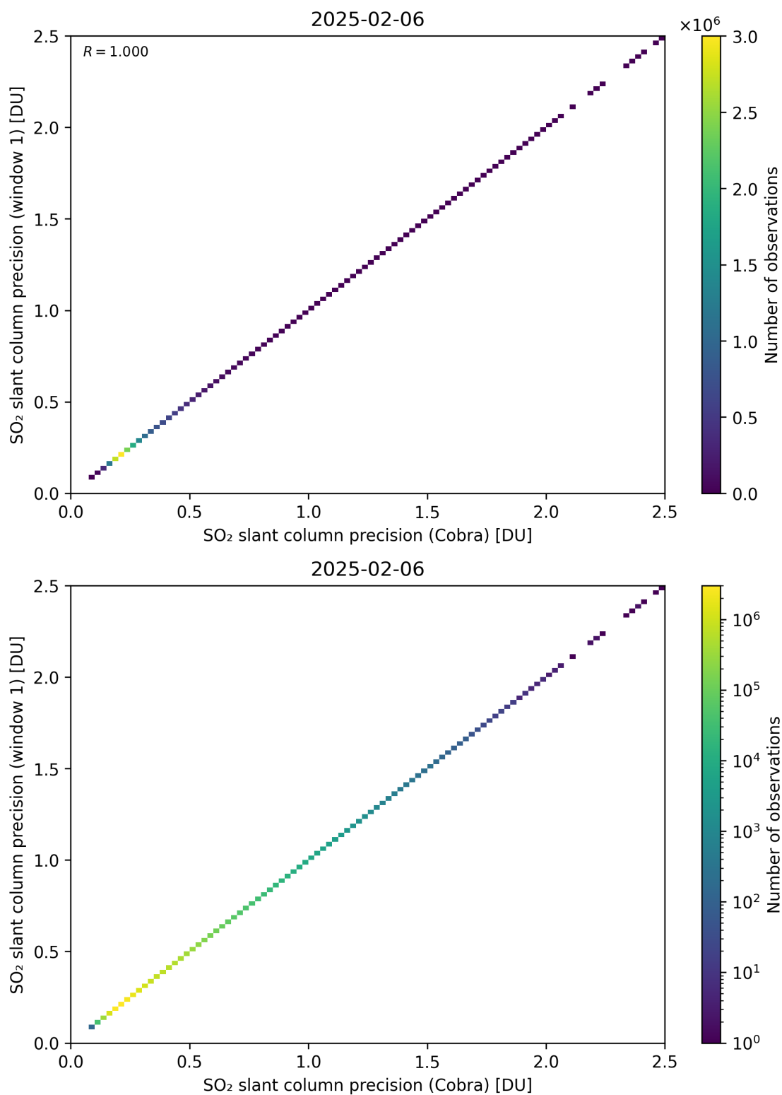
Figure 209: Scatter density plot of “SO 2 slant column precision (Cobra)” against “SO 2 slant column precision (window 1)” for 2025-02-05 to 2025-02-07.
