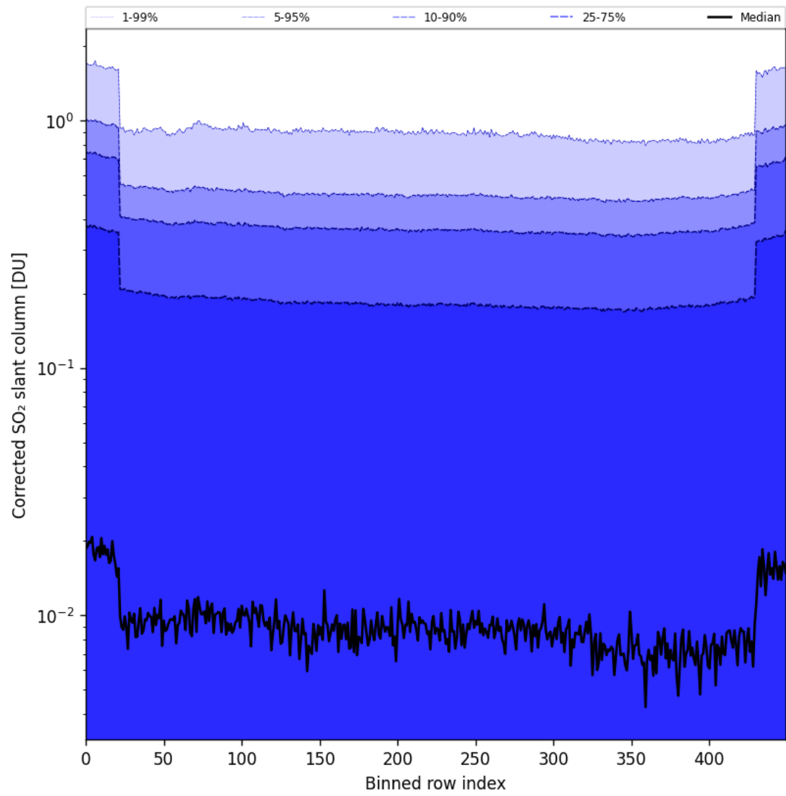
Figure 86: Along track statistics of “Corrected SO 2 slant column” for 2025-02-05 to 2025-02-07
