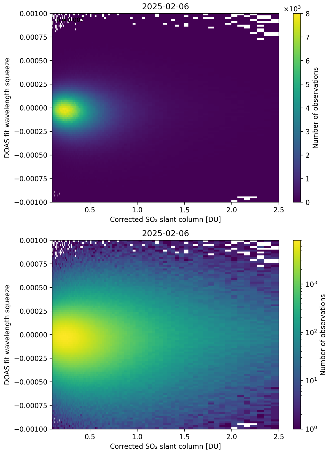
Figure 230: Scatter density plot of “Corrected SO 2 slant column” against “DOAS fit wavelength squeeze” for 2025-02-05 to 2025-02-07.
