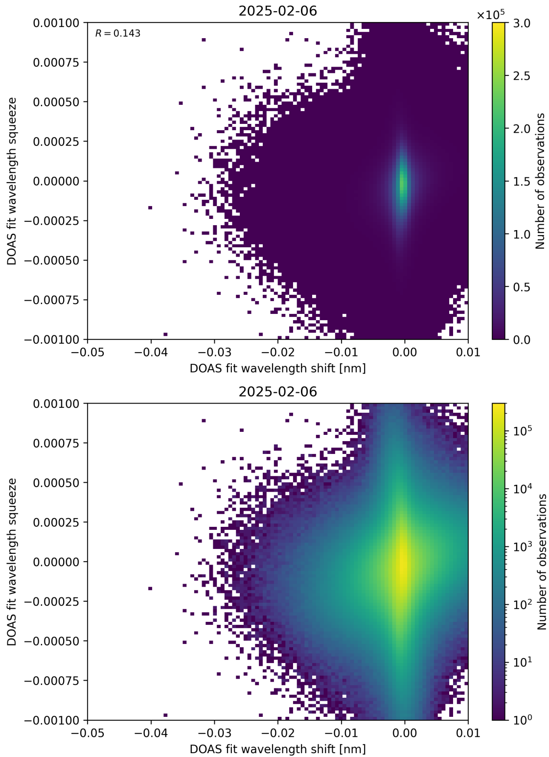
Figure 138: Scatter density plot of “DOAS fit wavelength shift” against “DOAS fit wavelength squeeze” for 2025-02-05 to 2025-02-07.
