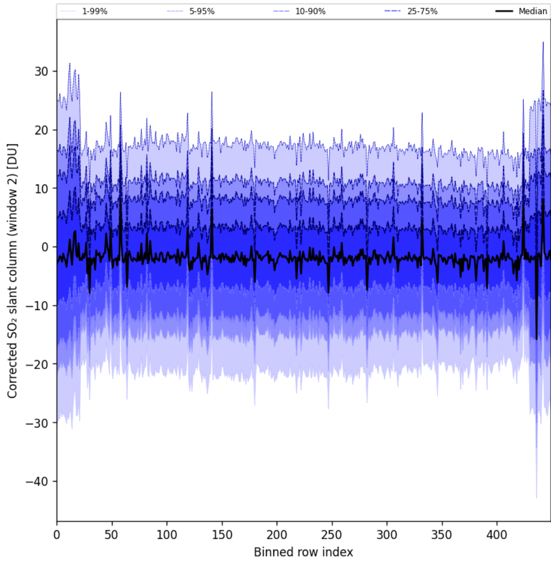
Figure 95: Along track statistics of “Corrected SO 2 slant column (window 2)” for 2025-02-05 to 2025-02-07
