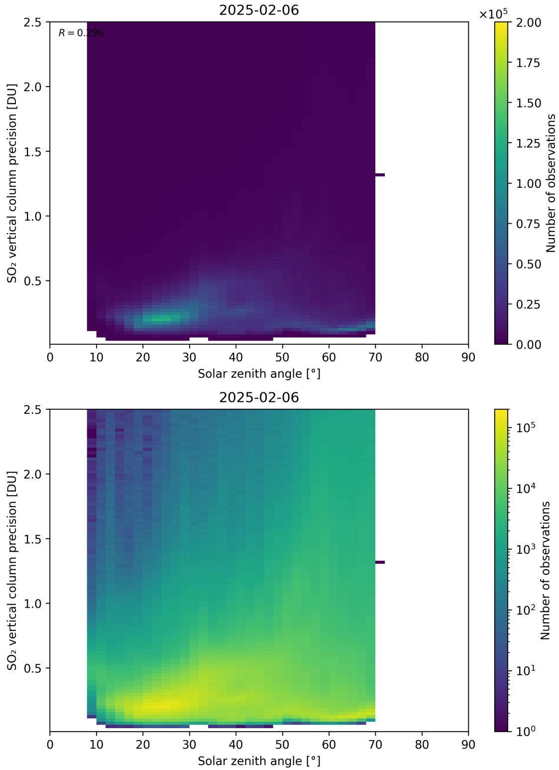
Figure 192: Scatter density plot of “Solar zenith angle” against “SO 2 vertical column precision” for 2025-02-05 to 2025-02-07.
