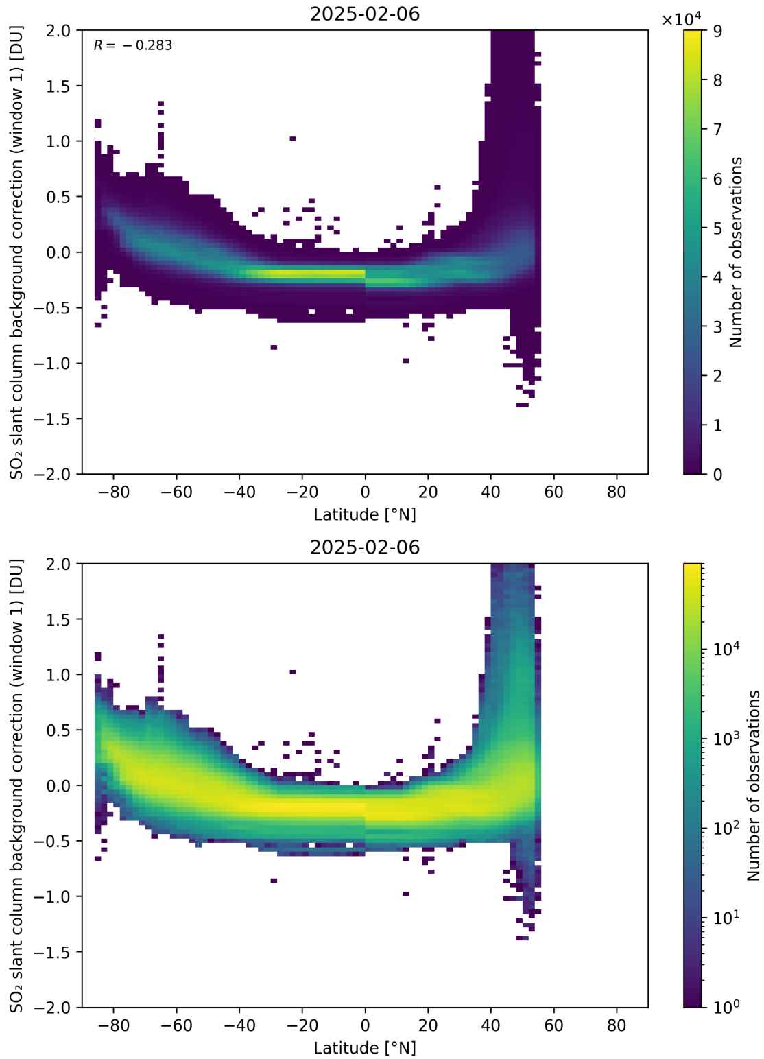
Figure 150: Scatter density plot of “Latitude” against “SO 2 slant column background correction (window 1)” for 2025-02-05 to 2025-02-07.
