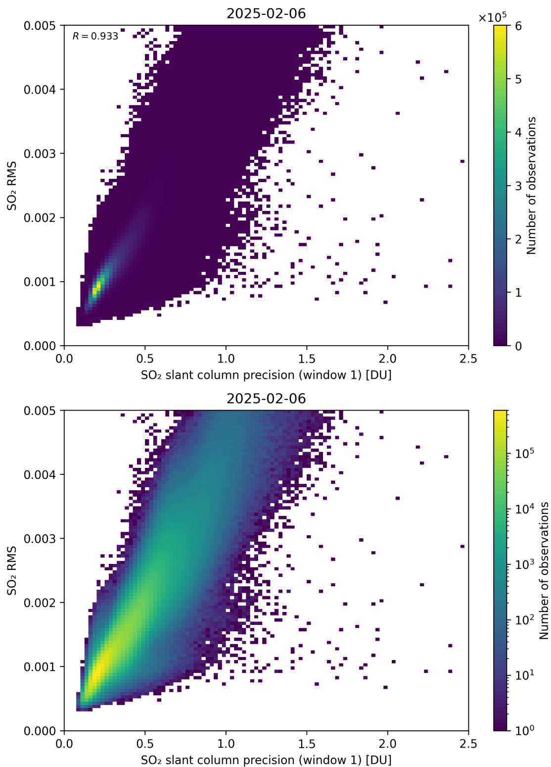
Figure 273: Scatter density plot of “SO 2 slant column precision (window 1)” against “SO 2 RMS” for 2025-02-05 to 2025-02-07.
