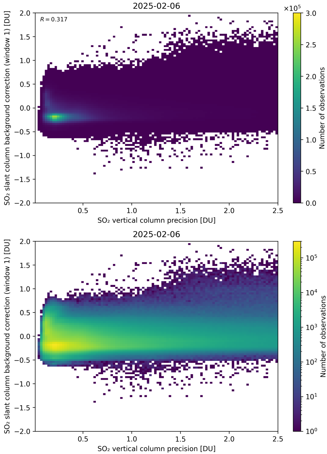
Figure 329: Scatter density plot of “SO 2 vertical column precision” against “SO 2 slant column background correction (window 1)” for 2025-02-05 to 2025-02-07.
