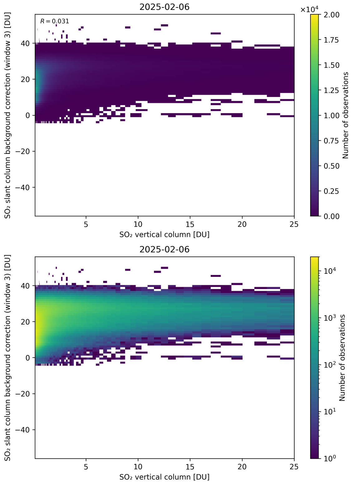
Figure 325: Scatter density plot of “SO 2 vertical column” against “SO 2 slant column background correction (window 3)” for 2025-02-05 to 2025-02-07.
