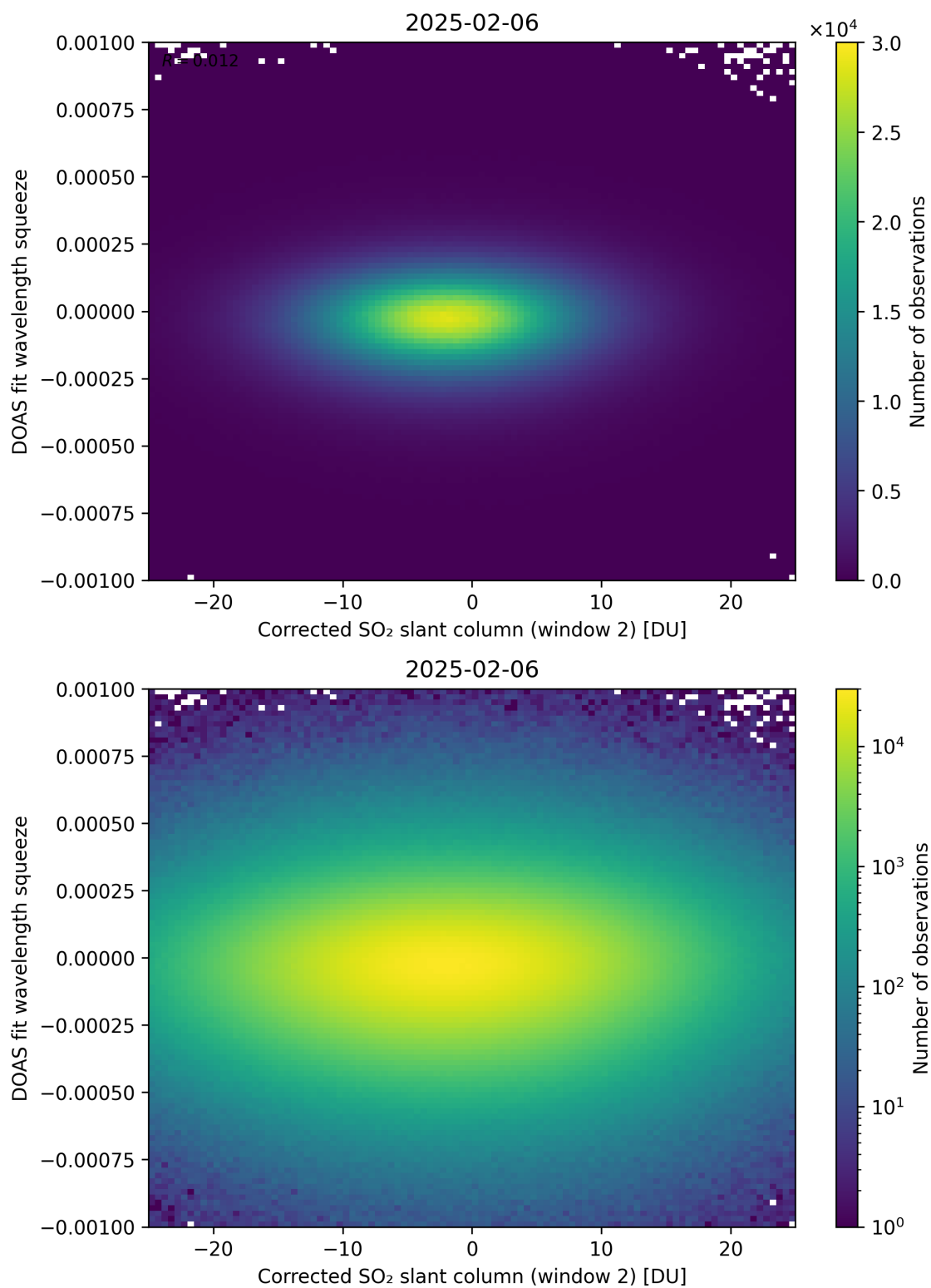
Figure 247: Scatter density plot of “Corrected SO 2 slant column (window 2)” against “DOAS fit wavelength squeeze” for 2025-02-05 to 2025-02-07.
