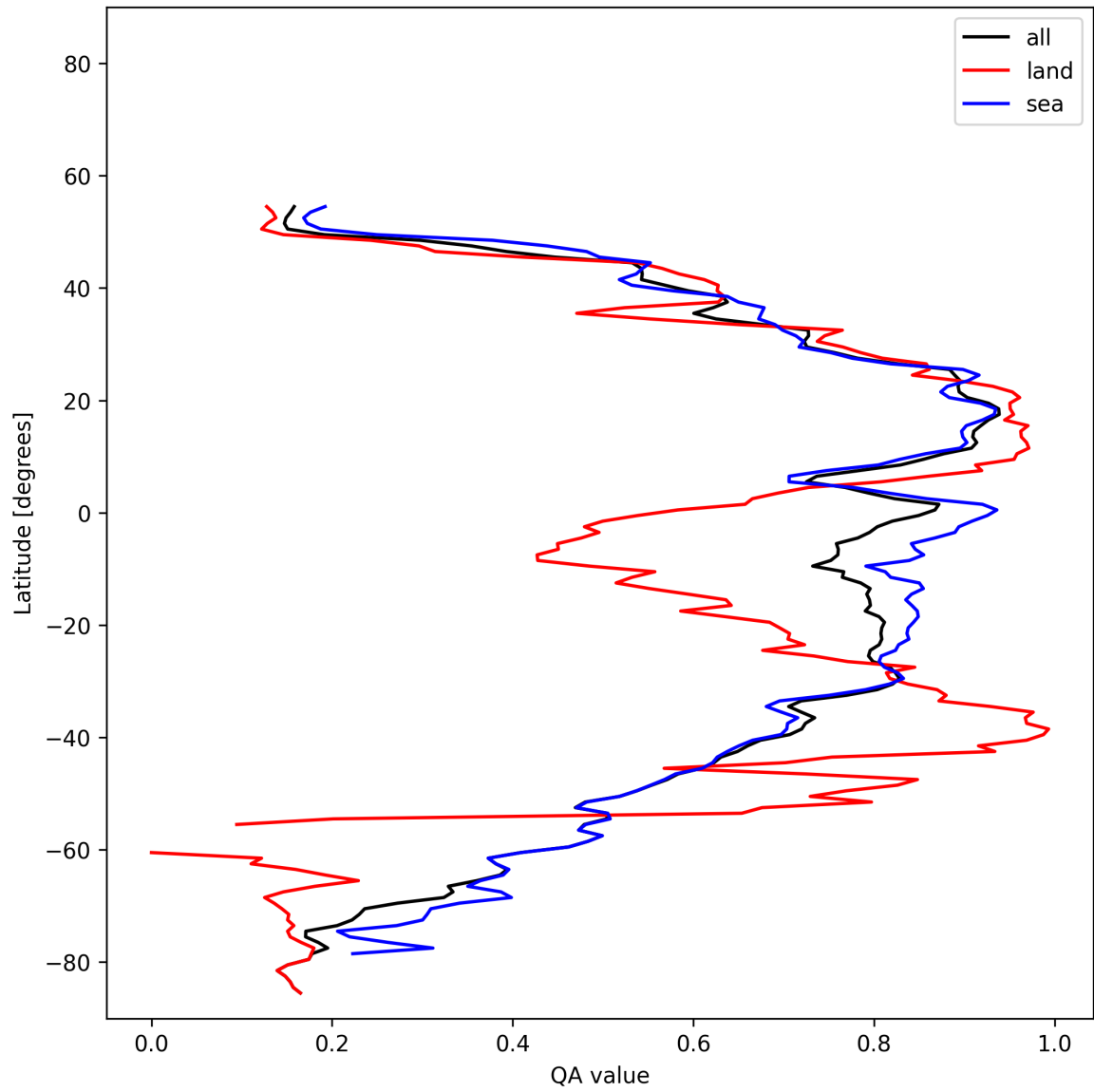
Figure 31: Zonal average of “QA value” for 2025-02-05 to 2025-02-07.
