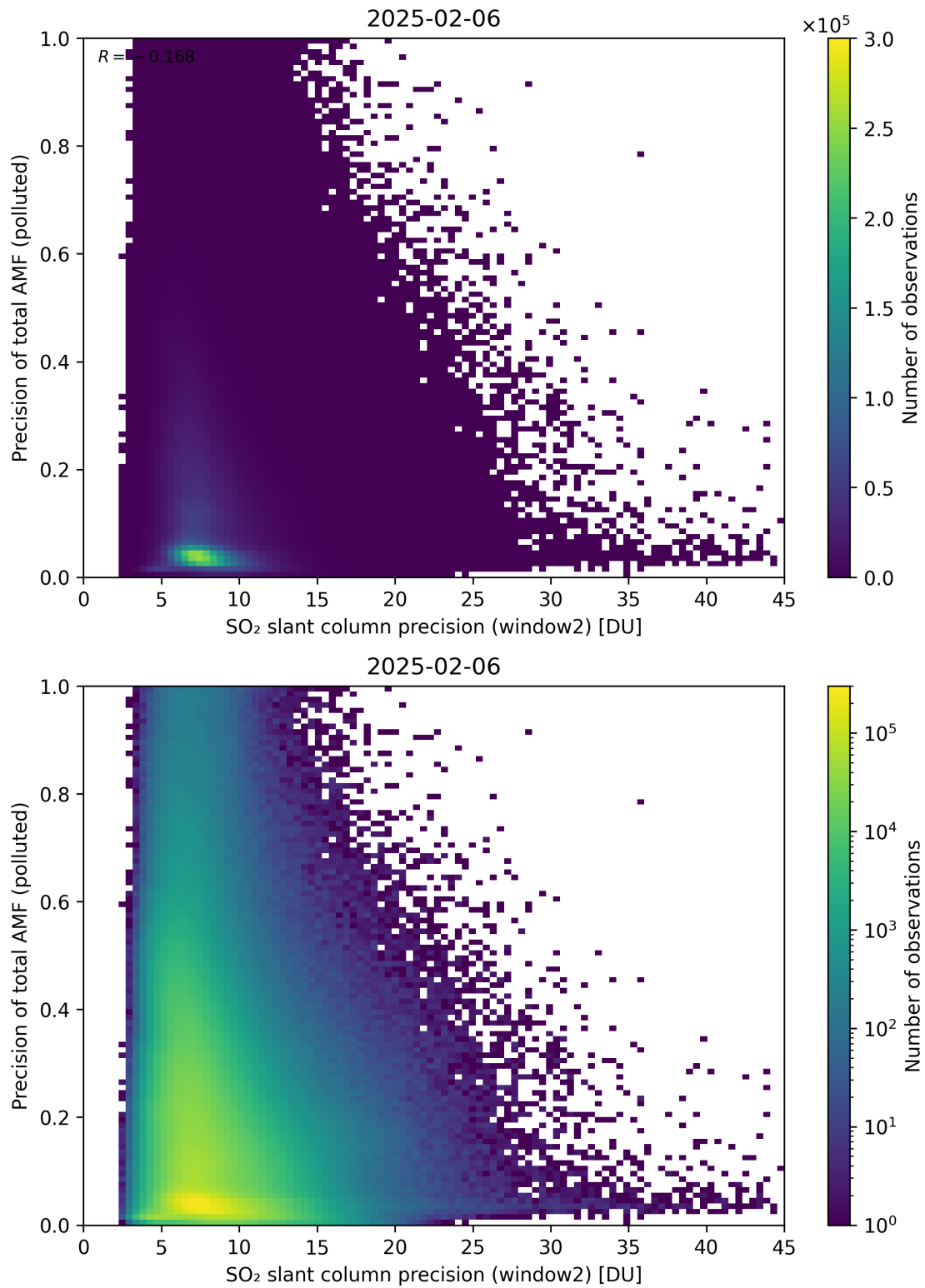
Figure 302: Scatter density plot of “SO 2 slant column precision (window2)” against “Precision of total AMF (polluted)” for 2025-02-05 to 2025-02-07.
