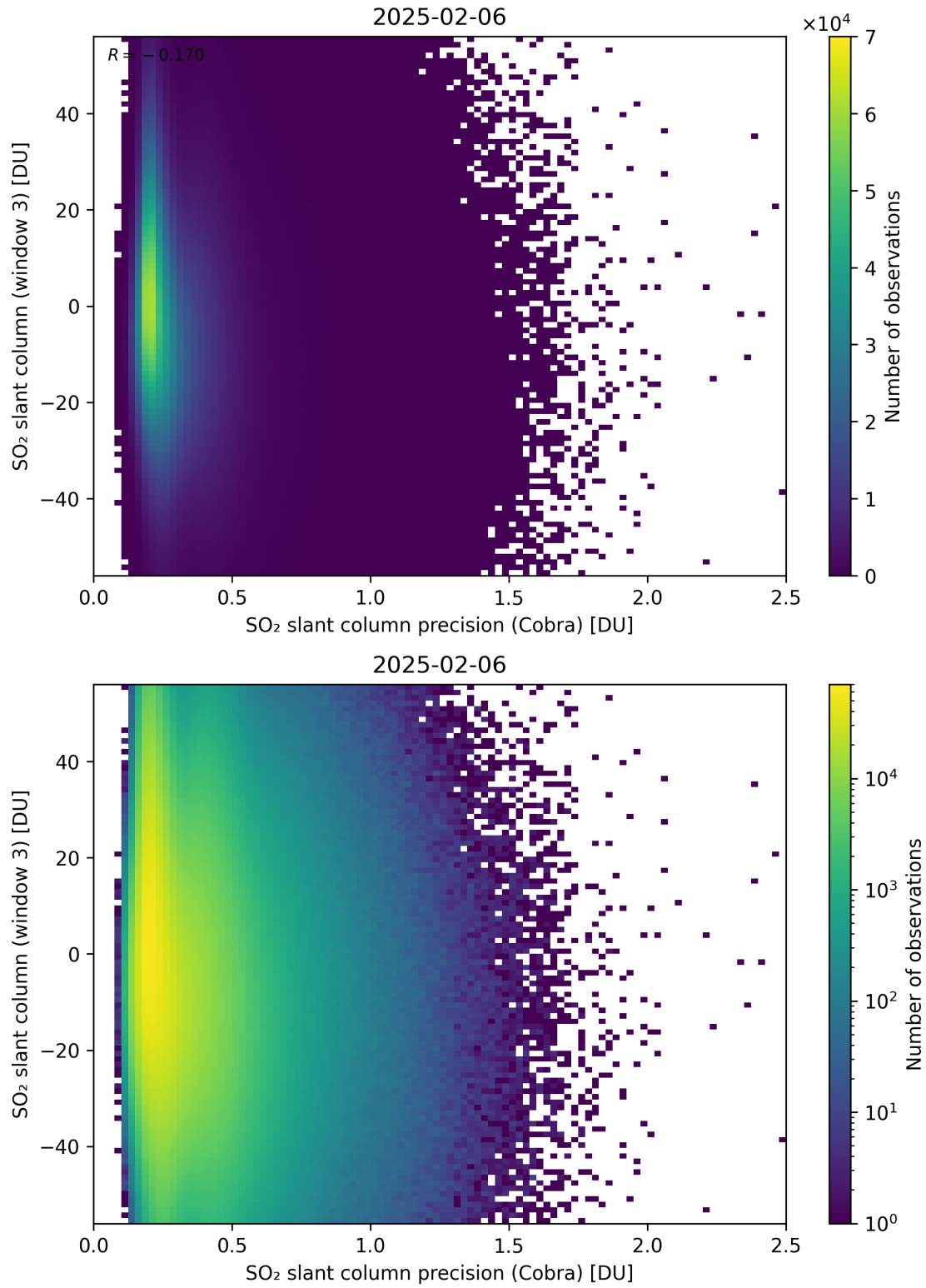
Figure 211: Scatter density plot of “SO 2 slant column precision (Cobra)” against “SO 2 slant column (window 3)” for 2025-02-05 to 2025-02-07.
