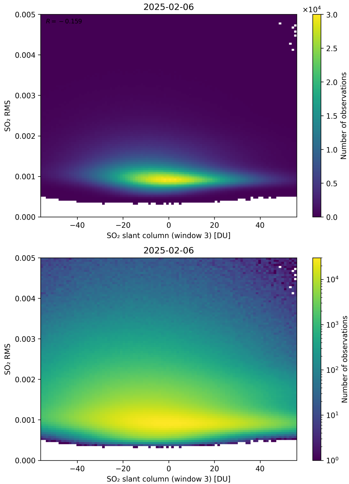
Figure 306: Scatter density plot of “SO 2 slant column (window 3)” against “SO 2 RMS” for 2025-02-05 to 2025-02-07.
