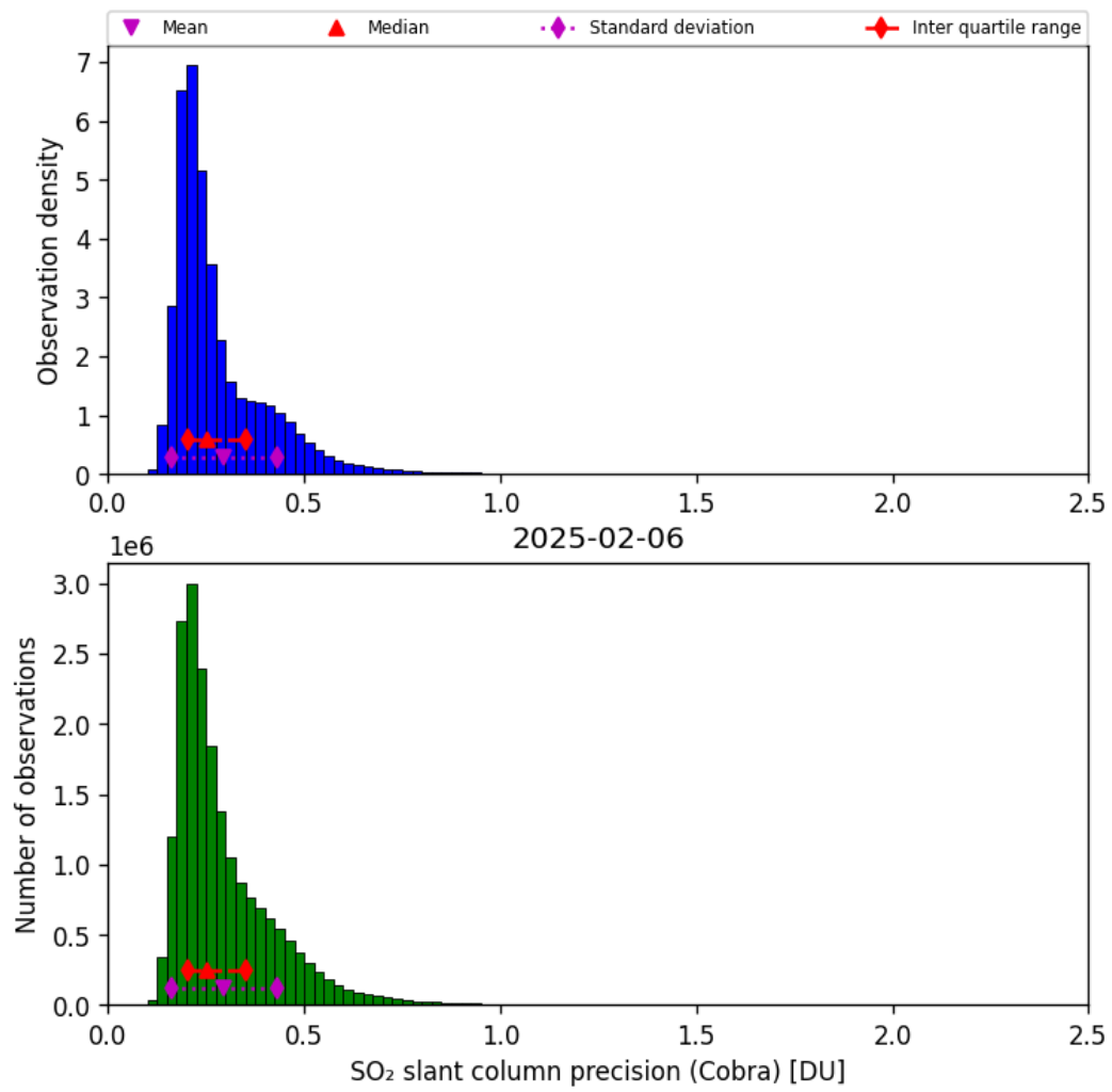
Figure 62: Histogram of “SO 2 slant column precision (Cobra)” for 2025-02-05 to 2025-02-07
