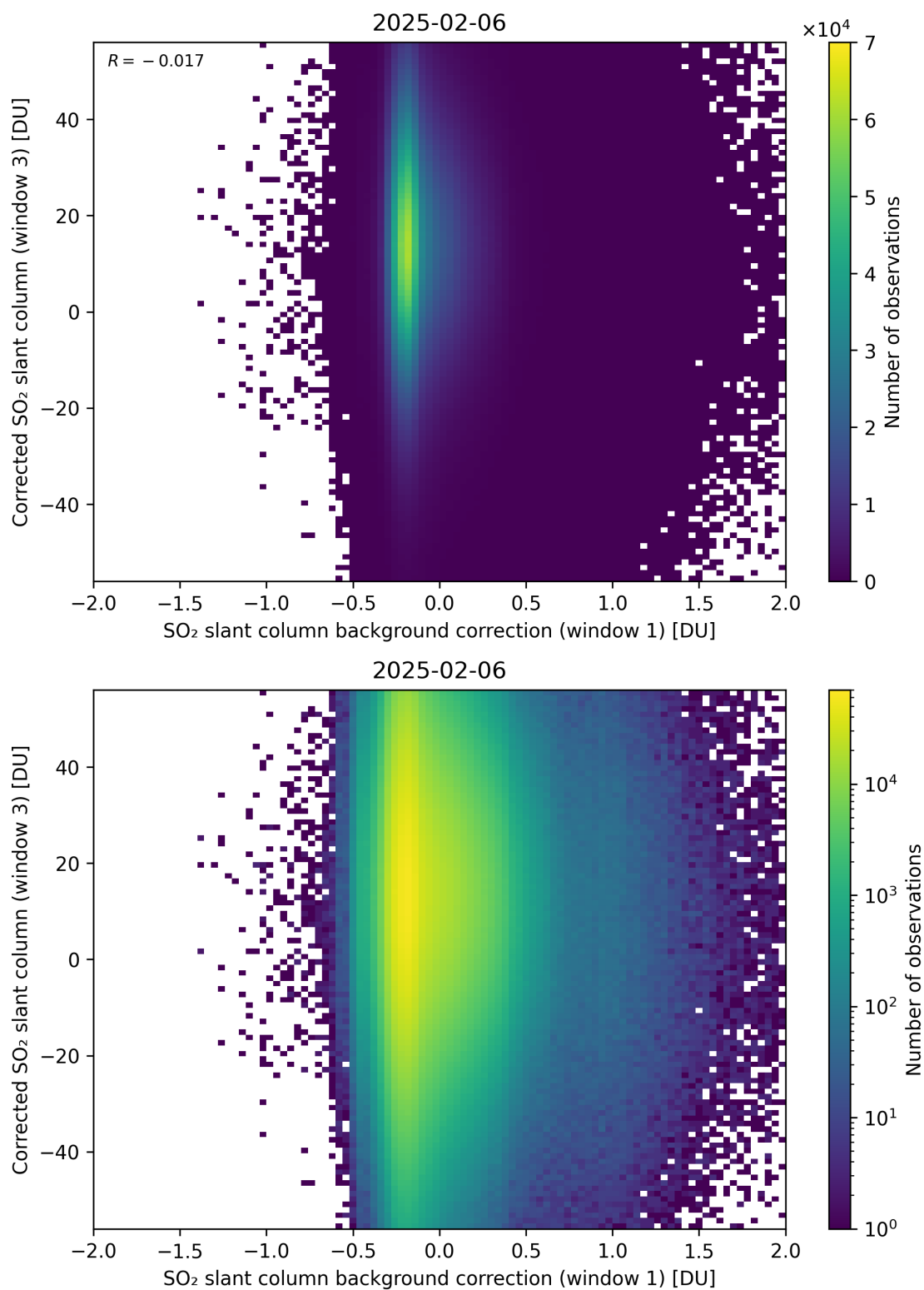
Figure 116: Scatter density plot of “SO 2 slant column background correction (window 1)” against “Corrected SO 2 slant column (window 3)” for 2025-02-05 to 2025-02-07.
