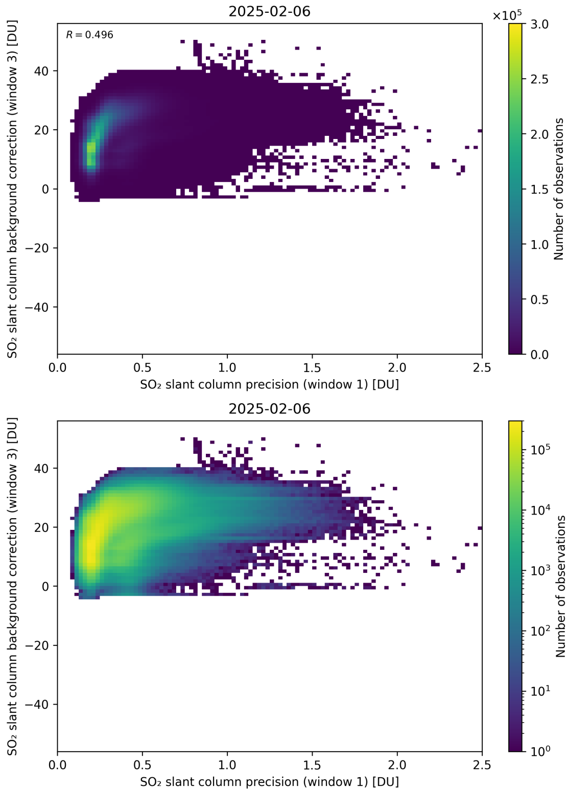
Figure 270: Scatter density plot of “SO 2 slant column precision (window 1)” against “SO 2 slant column background correction (window 3)” for 2025-02-05 to 2025-02-07.
