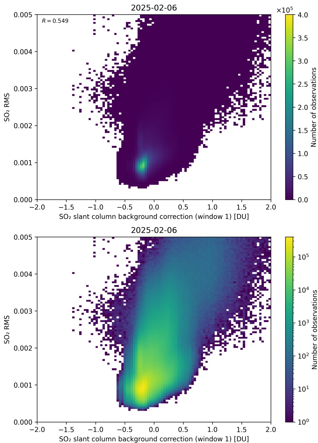
Figure 113: Scatter density plot of “SO 2 slant column background correction (window 1)” against “SO 2 RMS” for 2025-02-05 to 2025-02-07.
