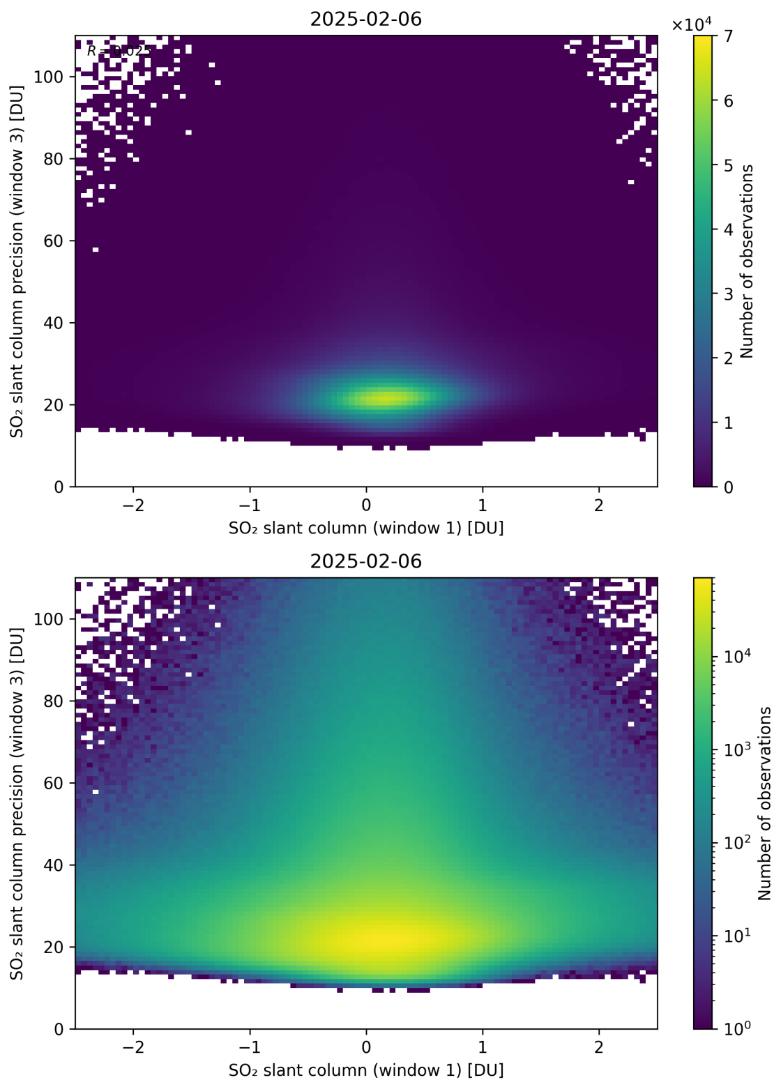
Figure 288: Scatter density plot of “SO 2 slant column (window 1)” against “SO 2 slant column precision (window 3)” for 2025-02-05 to 2025-02-07.
