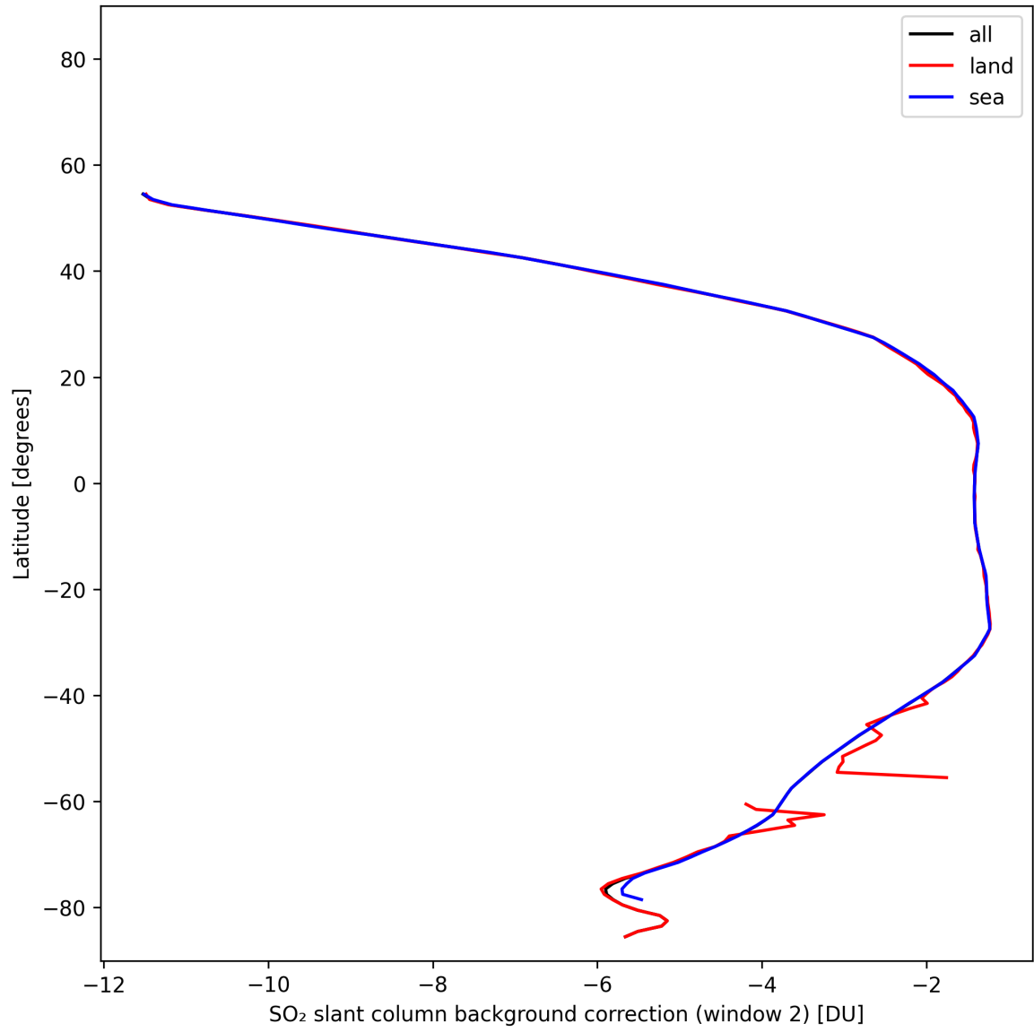
Figure 44: Zonal average of “SO 2 slant column background correction (window 2)” for 2025-02-05 to 2025-02-07.
