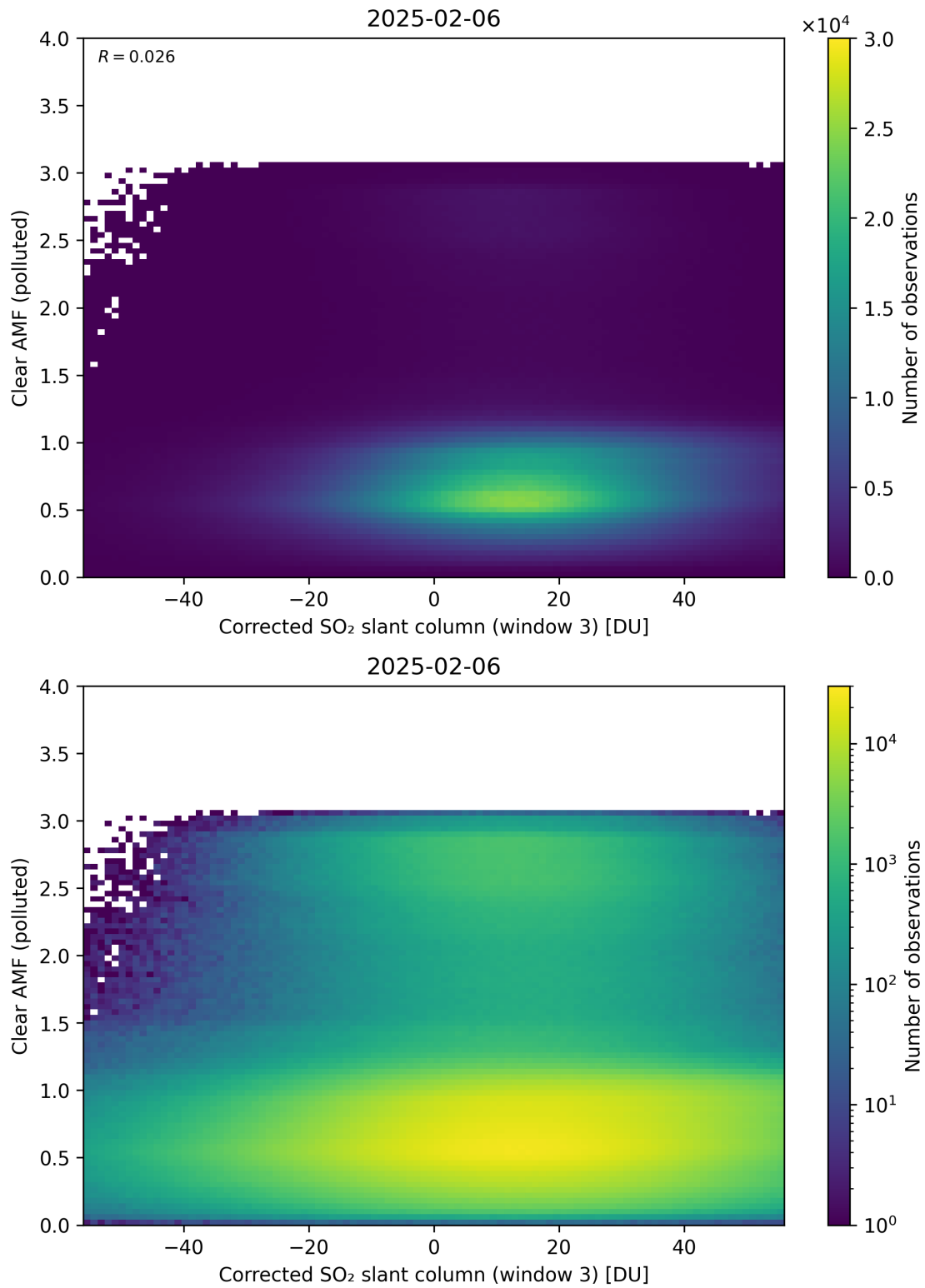
Figure 259: Scatter density plot of “Corrected SO 2 slant column (window 3)” against “Clear AMF (polluted)” for 2025-02-05 to 2025-02-07.
