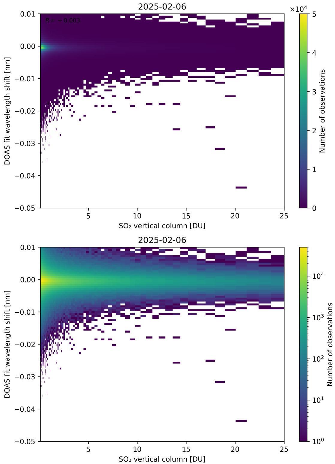
Figure 326: Scatter density plot of “SO 2 vertical column” against “DOAS fit wavelength shift” for 2025-02-05 to 2025-02-07.
