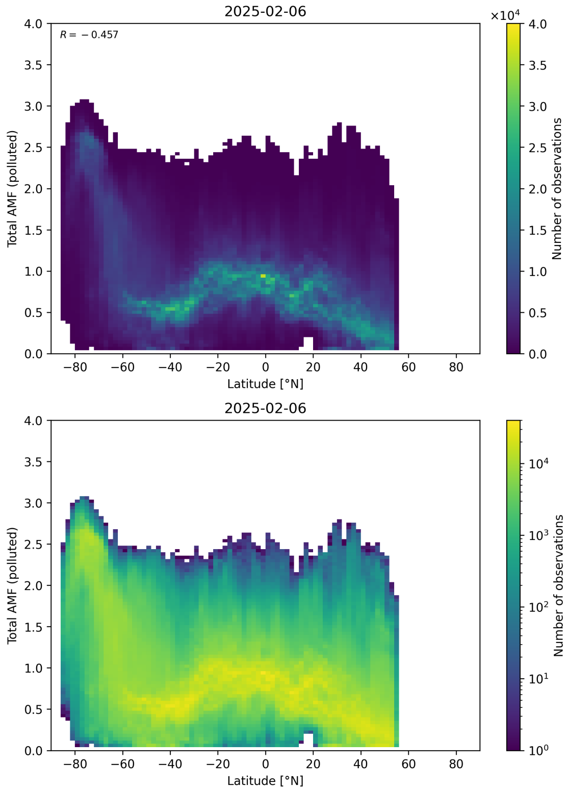
Figure 167: Scatter density plot of “Latitude” against “Total AMF (polluted)” for 2025-02-05 to 2025-02-07.
