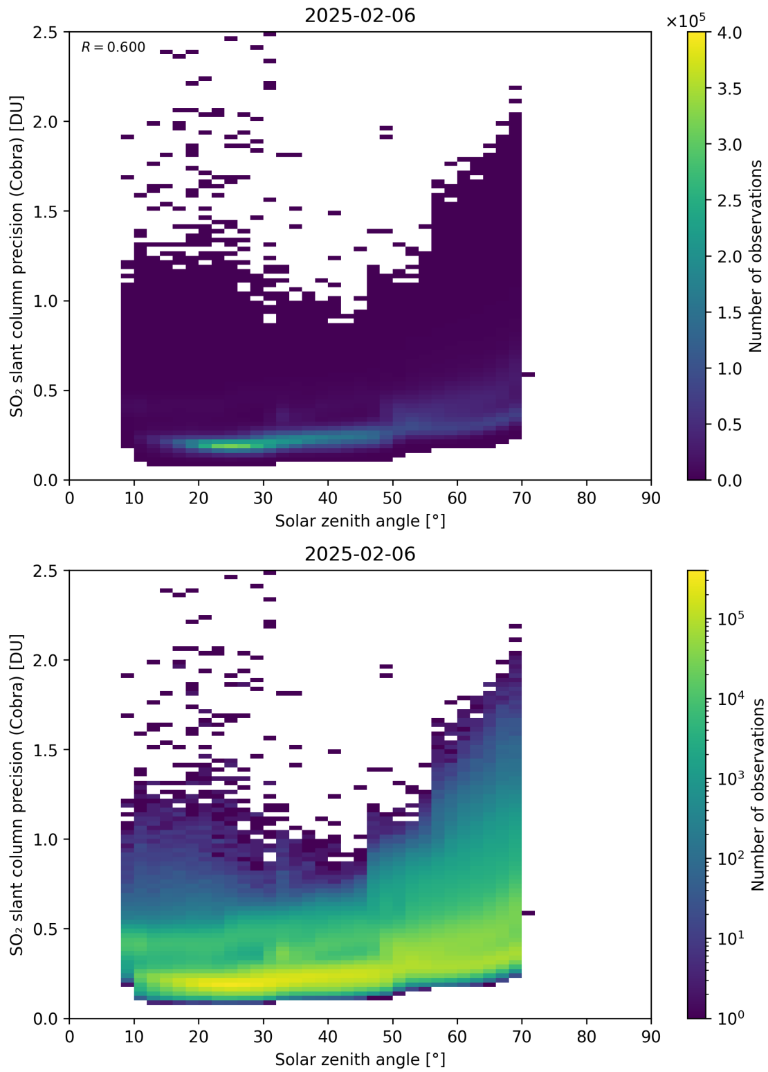
Figure 180: Scatter density plot of “Solar zenith angle” against “SO 2 slant column precision (Cobra)” for 2025-02-05 to 2025-02-07.
