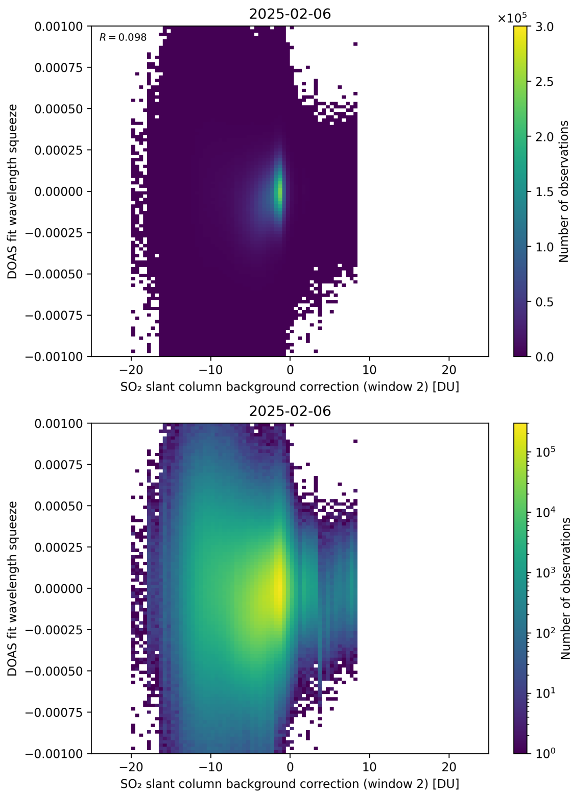
Figure 124: Scatter density plot of “SO 2 slant column background correction (window 2)” against “DOAS fit wavelength squeeze” for 2025-02-05 to 2025-02-07.
