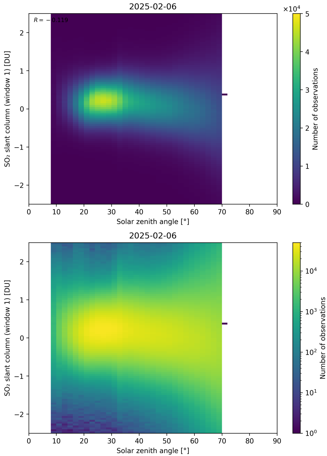
Figure 184: Scatter density plot of “Solar zenith angle” against “SO 2 slant column (window 1)” for 2025-02-05 to 2025-02-07.
