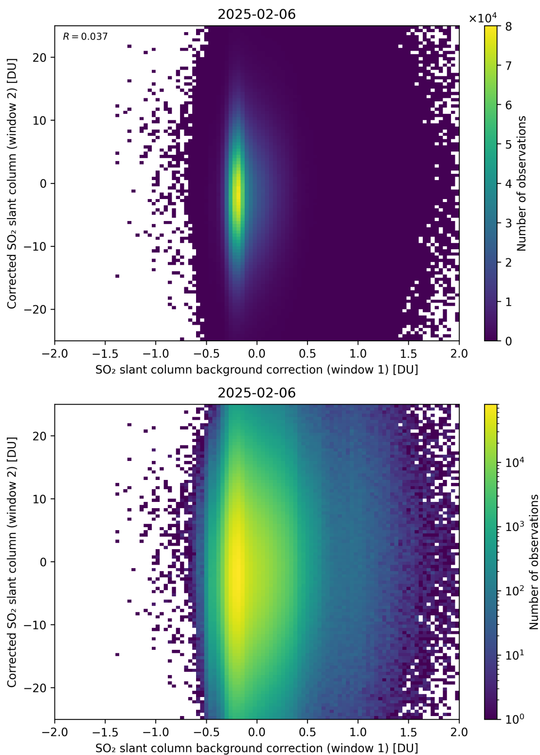
Figure 115: Scatter density plot of “SO 2 slant column background correction (window 1)” against “Corrected SO 2 slant column (window 2)” for 2025-02-05 to 2025-02-07.
