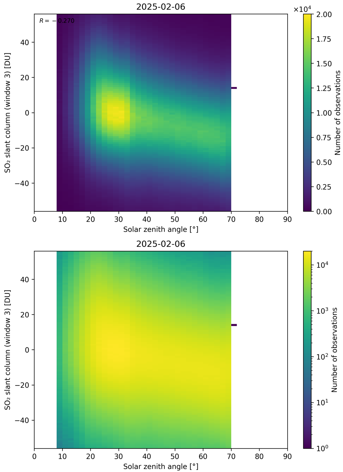
Figure 187: Scatter density plot of “Solar zenith angle” against “SO 2 slant column (window 3)” for 2025-02-05 to 2025-02-07.
