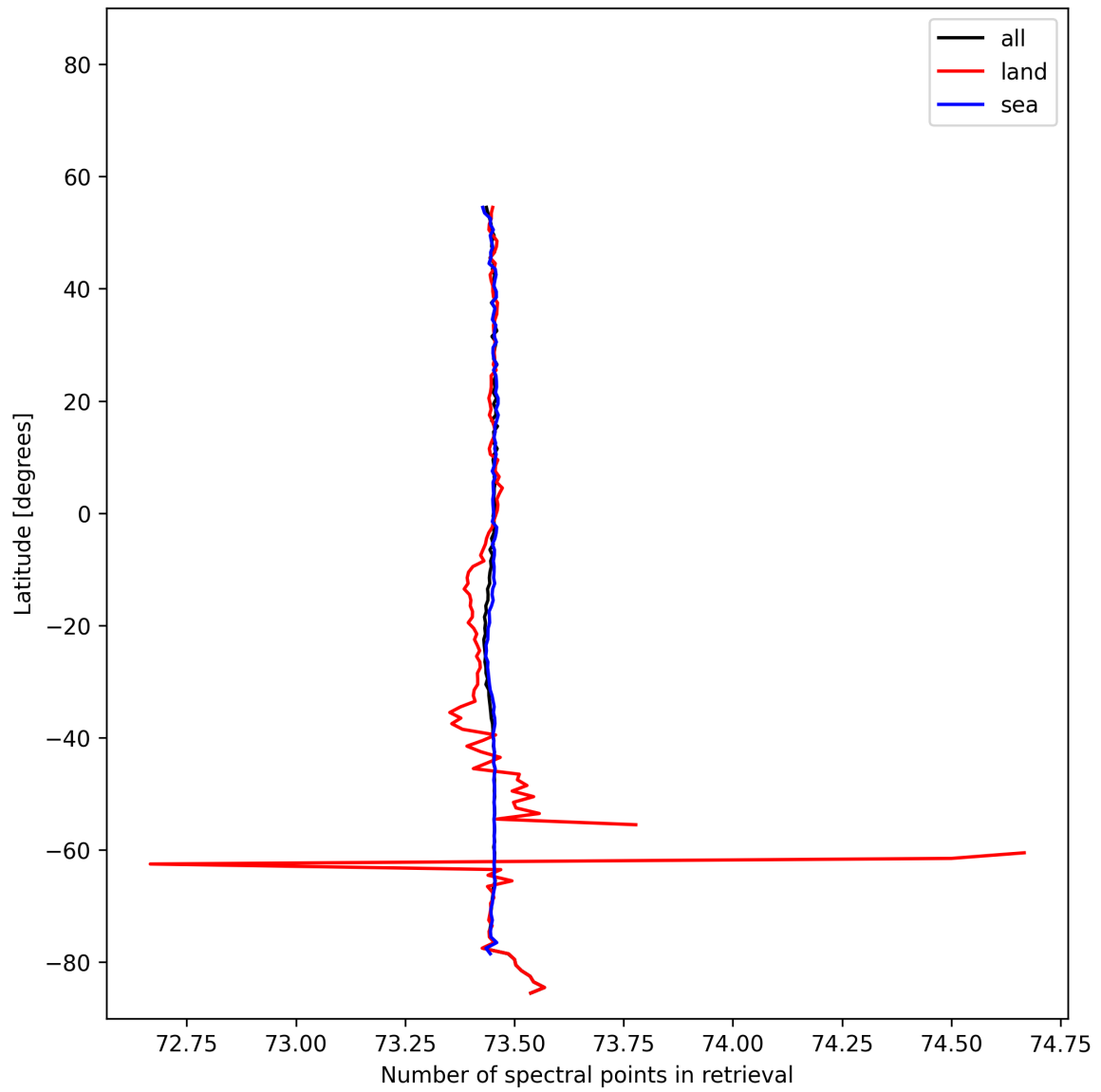
Figure 56: Zonal average of “Number of spectral points in retrieval” for 2025-02-05 to 2025-02-07.
