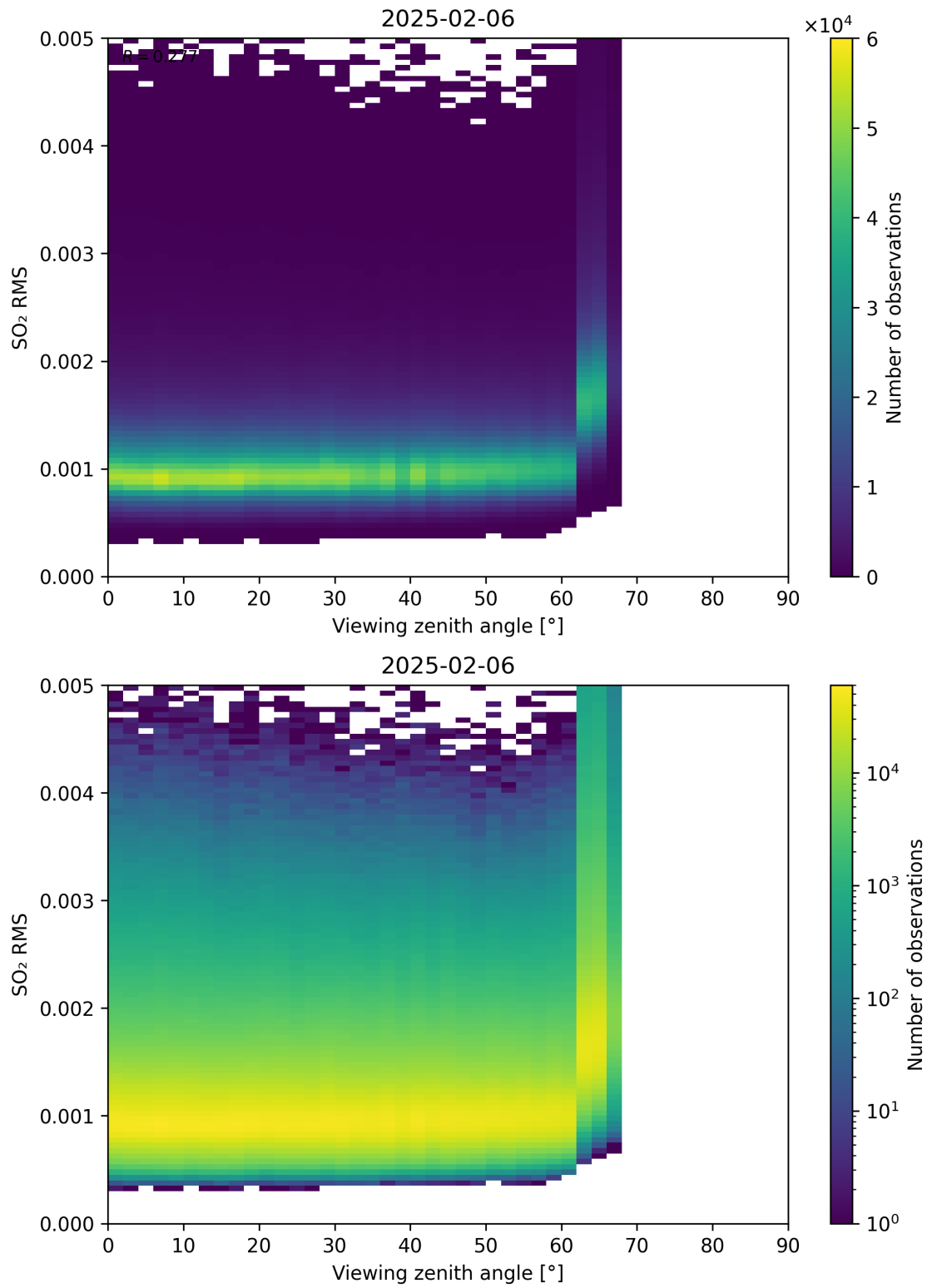
Figure 367: Scatter density plot of “Viewing zenith angle” against “SO 2 RMS” for 2025-02-05 to 2025-02-07.
