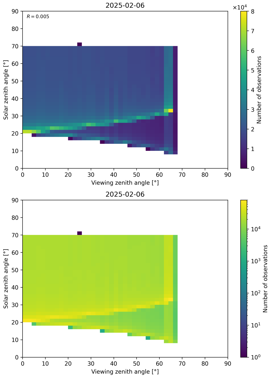
Figure 369: Scatter density plot of “Viewing zenith angle” against “Solar zenith angle” for 2025-02-05 to 2025-02-07.
