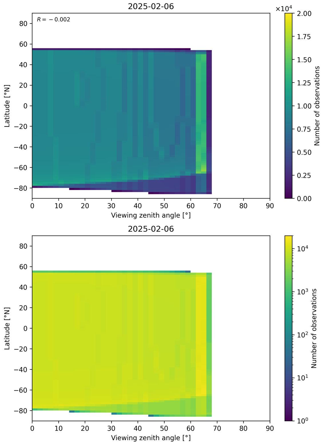
Figure 368: Scatter density plot of “Viewing zenith angle” against “Latitude” for 2025-02-05 to 2025-02-07.
