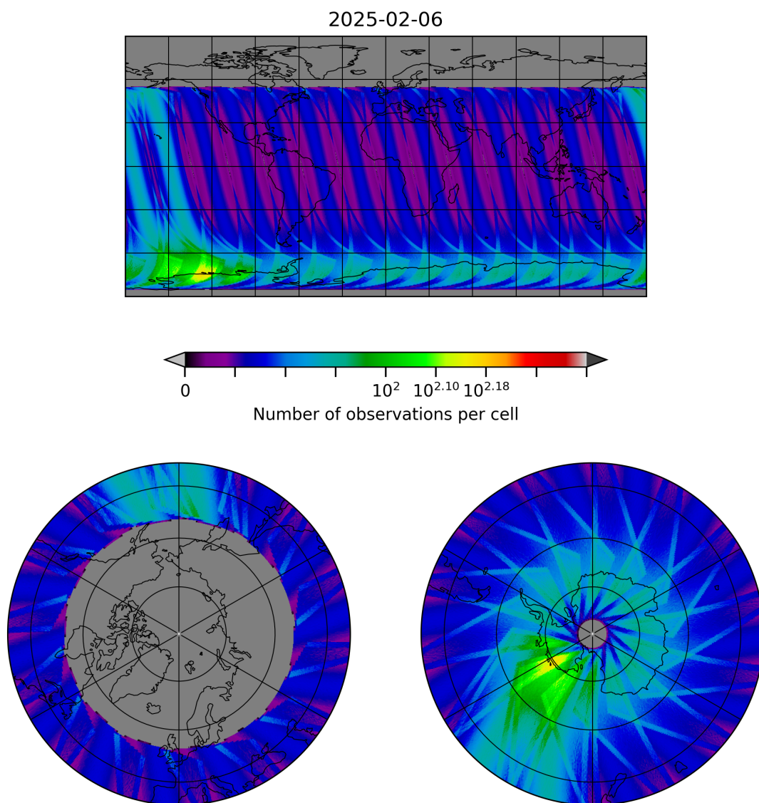
Figure 30: Map of the number of observations for 2025-02-05 to 2025-02-07
