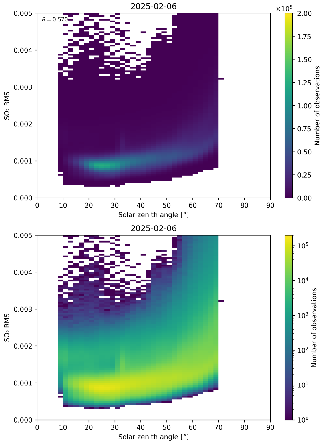
Figure 176: Scatter density plot of “Solar zenith angle” against “SO 2 RMS” for 2025-02-05 to 2025-02-07.
