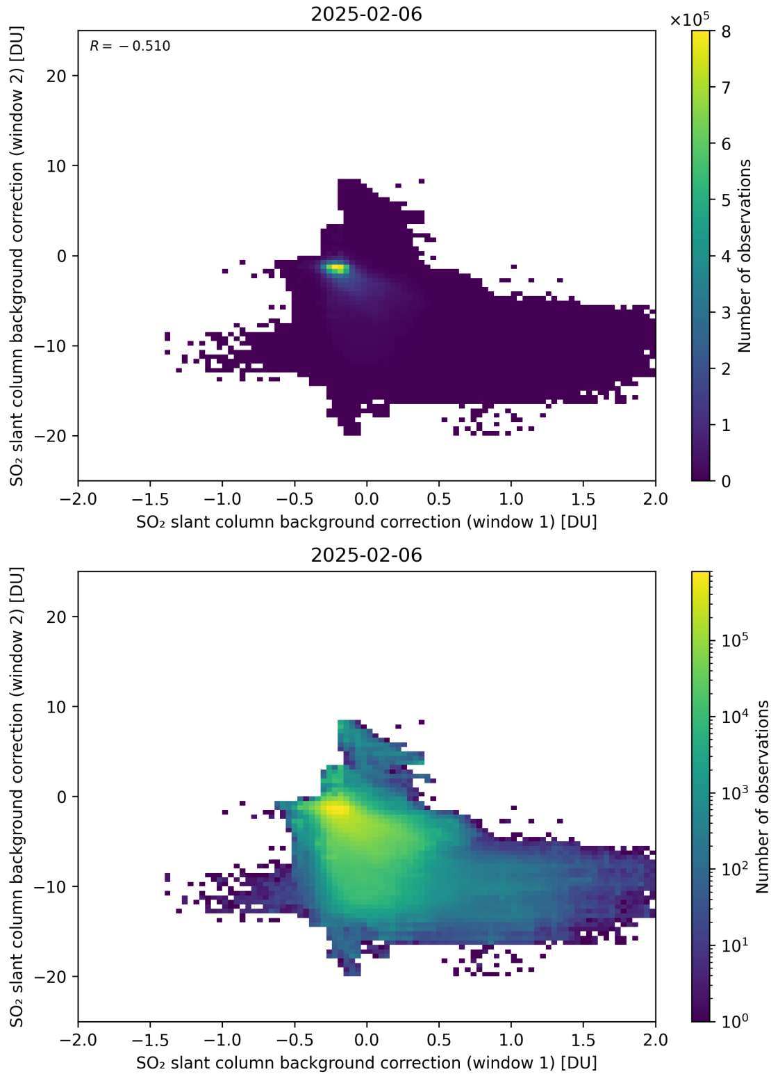
Figure 109: Scatter density plot of “SO 2 slant column background correction (window 1)” against “SO 2 slant column background correction (window 2)” for 2025-02-05 to 2025-02-07.
