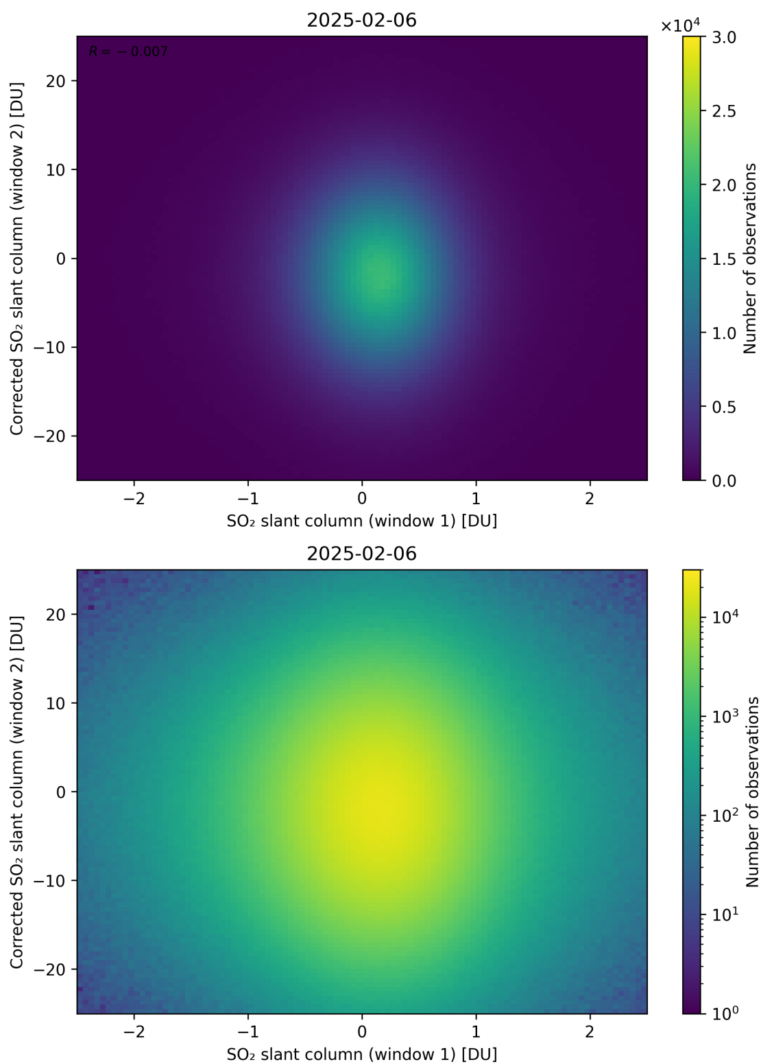
Figure 283: Scatter density plot of “SO 2 slant column (window 1)” against “Corrected SO 2 slant column (window 2)” for 2025-02-05 to 2025-02-07.
