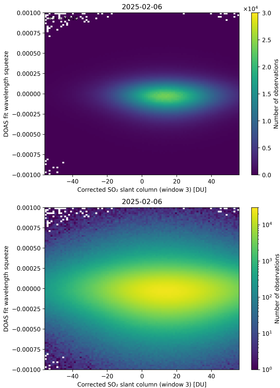
Figure 257: Scatter density plot of “Corrected SO 2 slant column (window 3)” against “DOAS fit wavelength squeeze” for 2025-02-05 to 2025-02-07.
