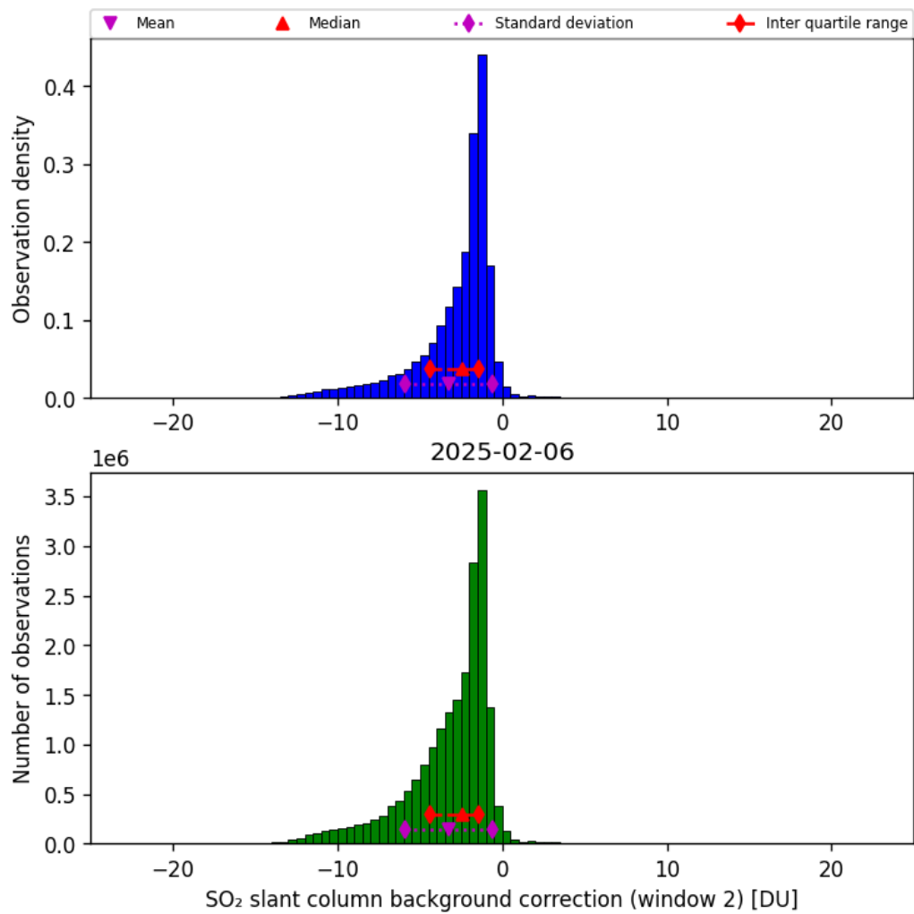
Figure 70: Histogram of “SO 2 slant column background correction (window 2)” for 2025-02-05 to 2025-02-07
