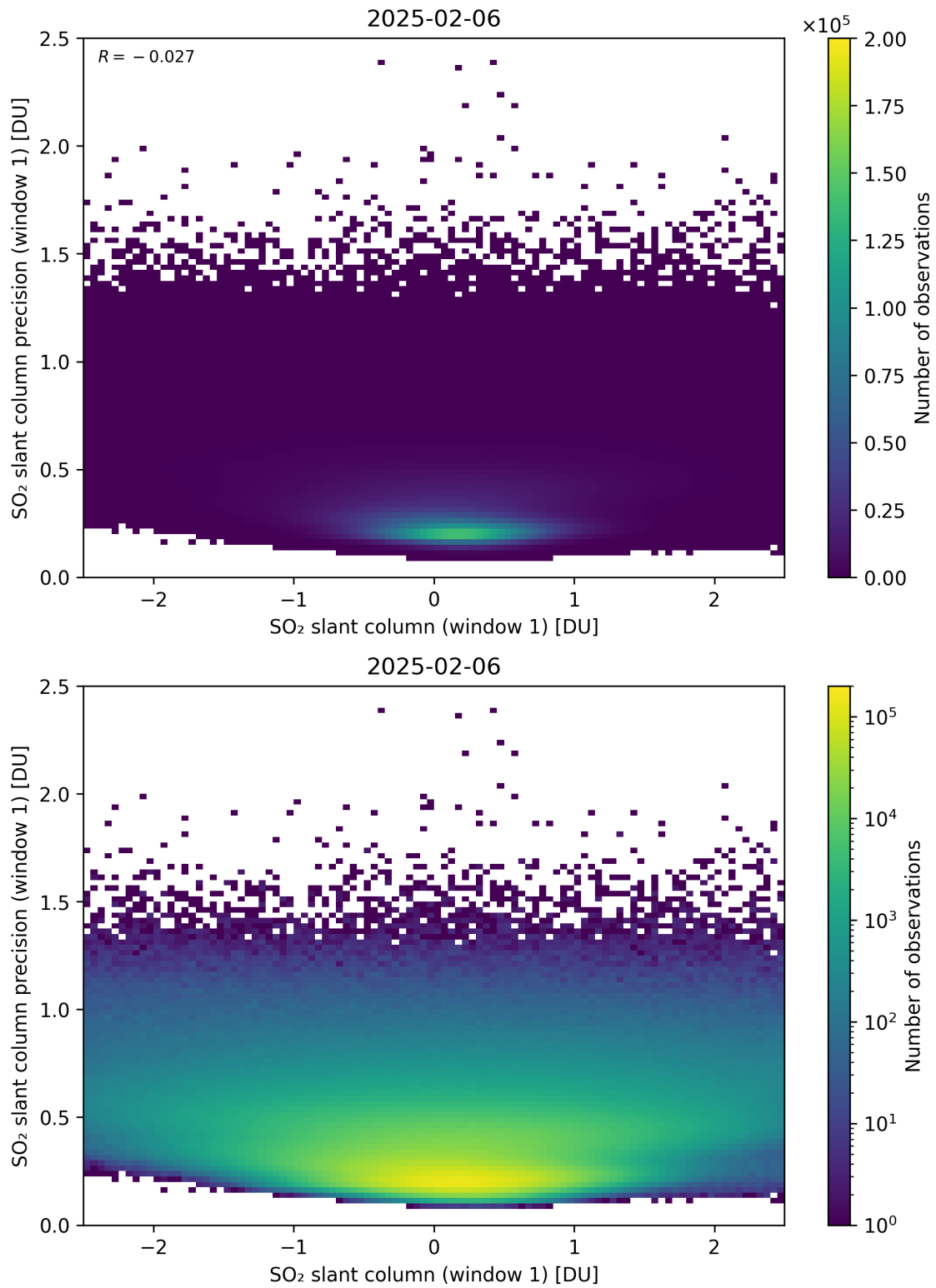
Figure 285: Scatter density plot of “SO 2 slant column (window 1)” against “SO 2 slant column precision (window 1)” for 2025-02-05 to 2025-02-07.
