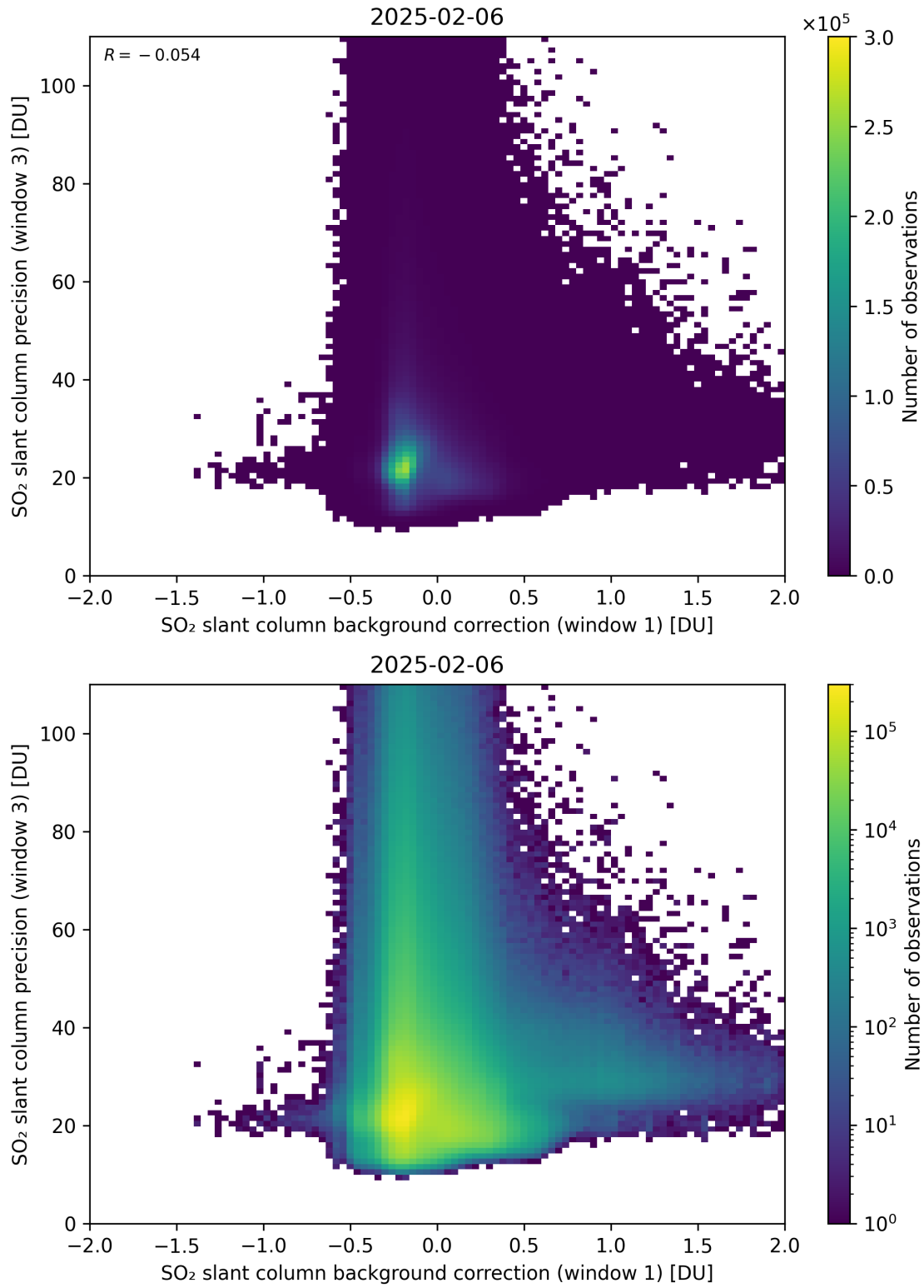
Figure 119: Scatter density plot of “SO 2 slant column background correction (window 1)” against “SO 2 slant column precision (window 3)” for 2025-02-05 to 2025-02-07.
