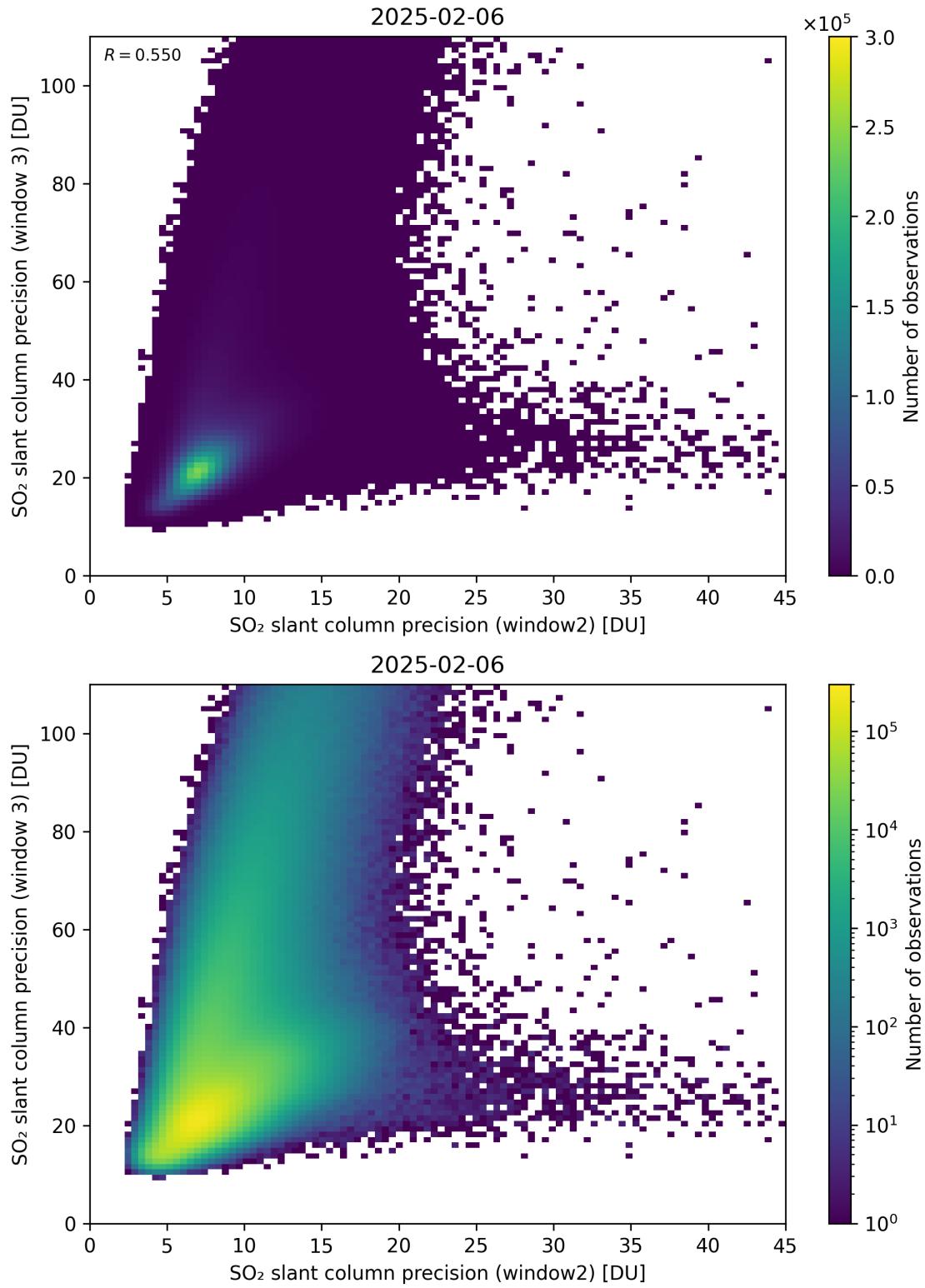
Figure 300: Scatter density plot of “SO 2 slant column precision (window2)” against “SO 2 slant column precision (window 3)” for 2025-02-05 to 2025-02-07.
