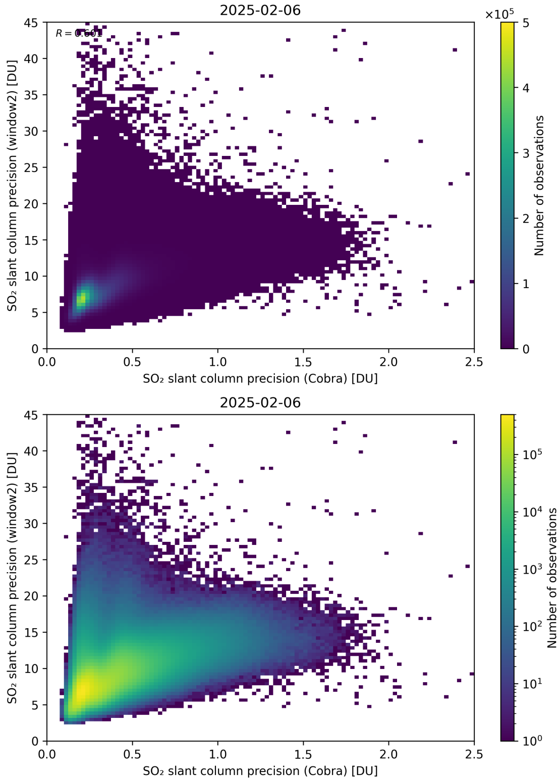
Figure 210: Scatter density plot of “SO 2 slant column precision (Cobra)” against “SO 2 slant column precision (window2)” for 2025-02-05 to 2025-02-07.
