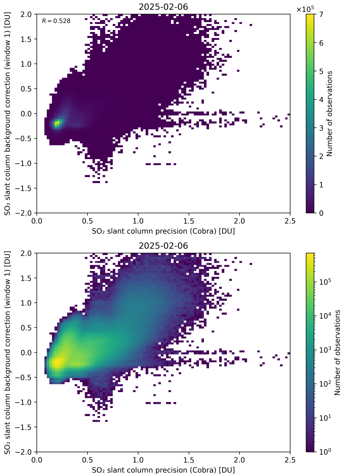
Figure 199: Scatter density plot of “SO 2 slant column precision (Cobra)” against “SO 2 slant column background correction (window 1)” for 2025-02-05 to 2025-02-07.
