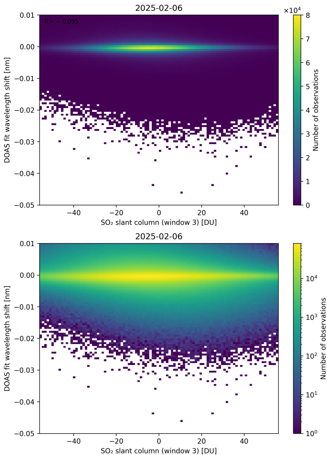
Figure 304: Scatter density plot of “SO 2 slant column (window 3)” against “DOAS fit wavelength shift” for 2025-02-05 to 2025-02-07.
