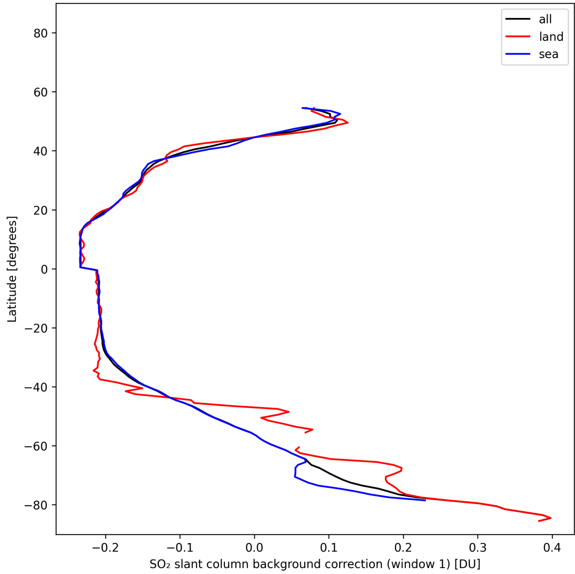
Figure 40: Zonal average of “SO 2 slant column background correction (window 1)” for 2025-02-05 to 2025-02-07.
