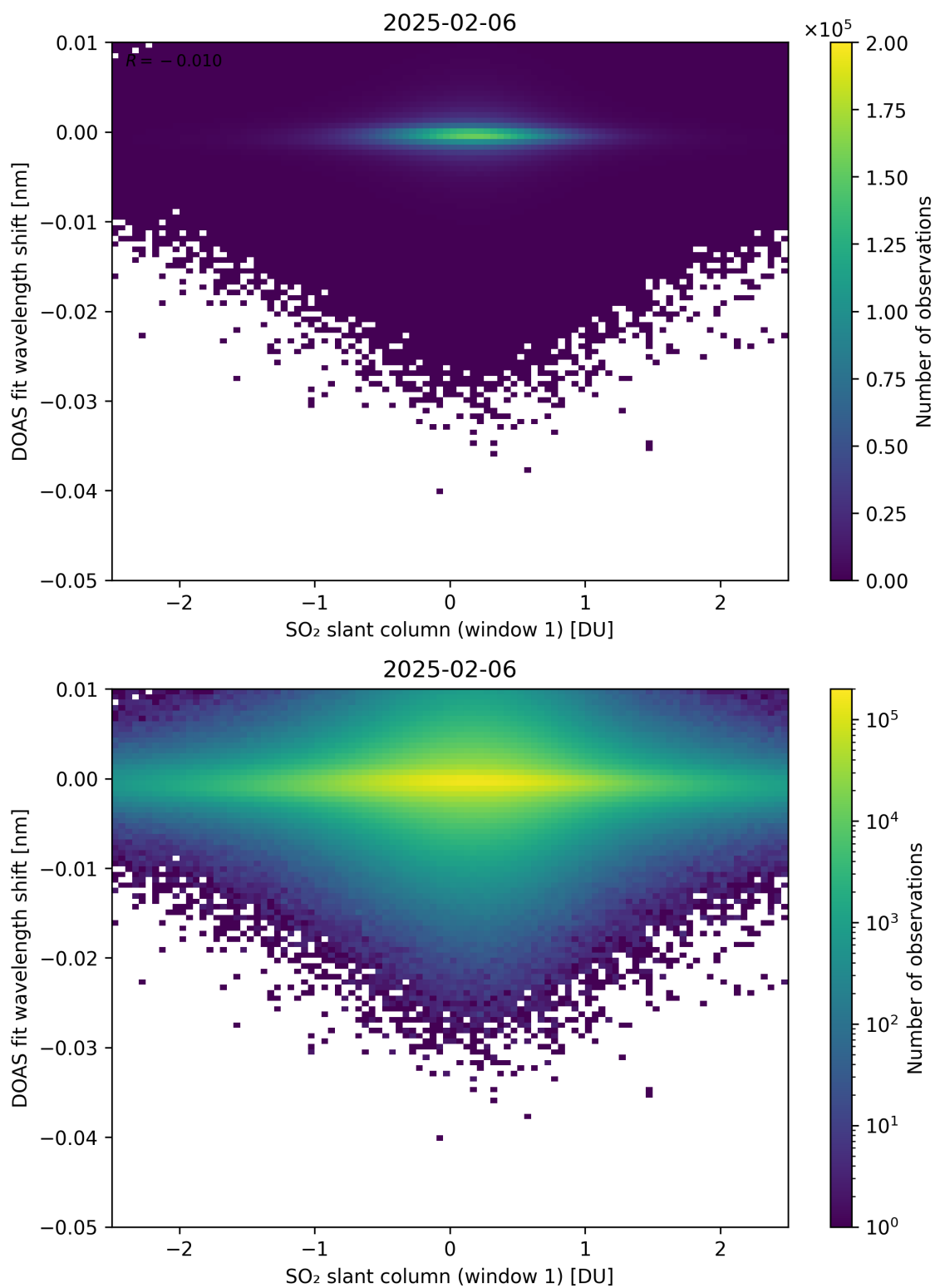
Figure 265: Scatter density plot of “SO 2 slant column (window 1)” against “DOAS fit wavelength shift” for 2025-02-05 to 2025-02-07.
