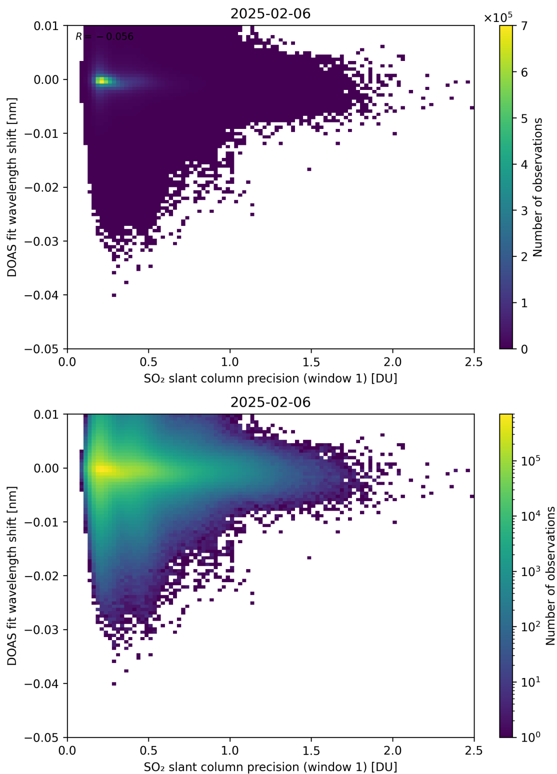
Figure 271: Scatter density plot of “SO 2 slant column precision (window 1)” against “DOAS fit wavelength shift” for 2025-02-05 to 2025-02-07.
