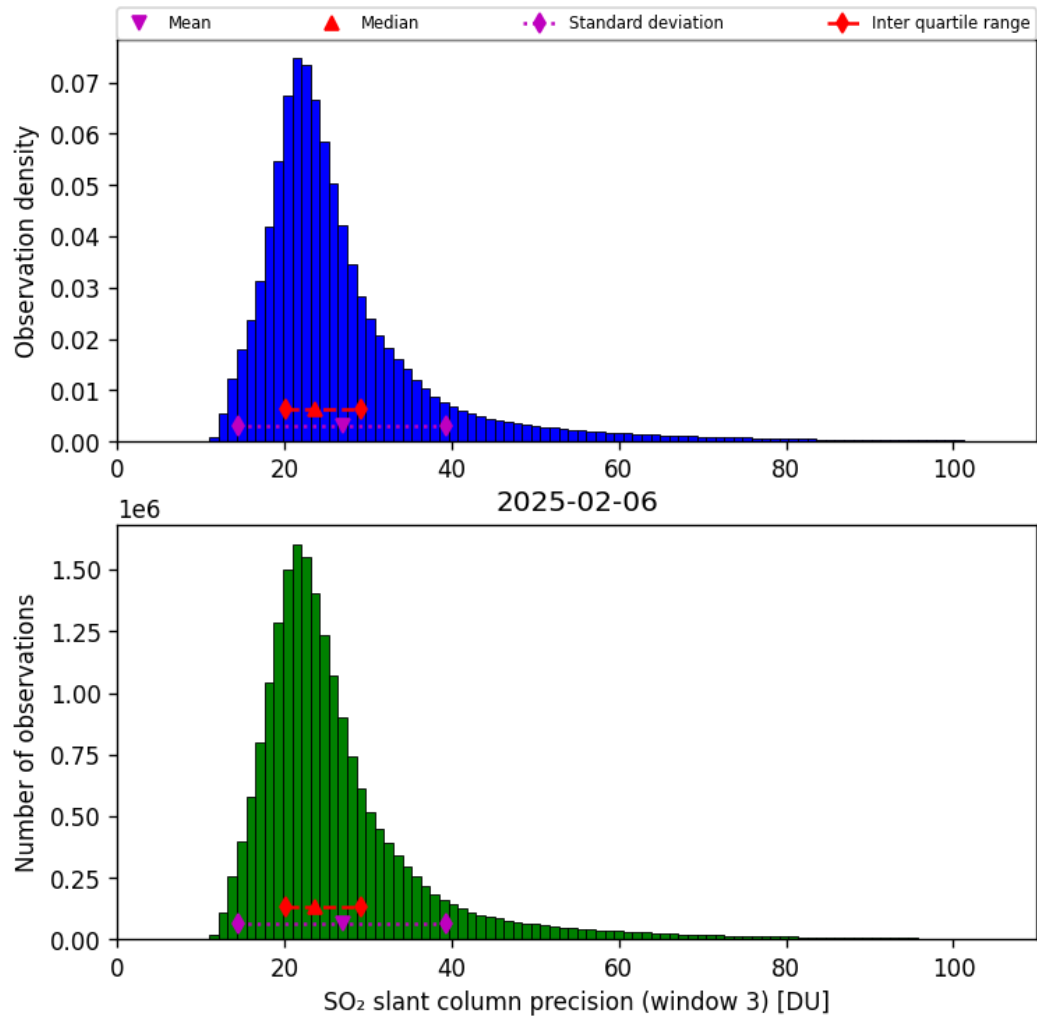
Figure 72: Histogram of “SO 2 slant column precision (window 3)” for 2025-02-05 to 2025-02-07
