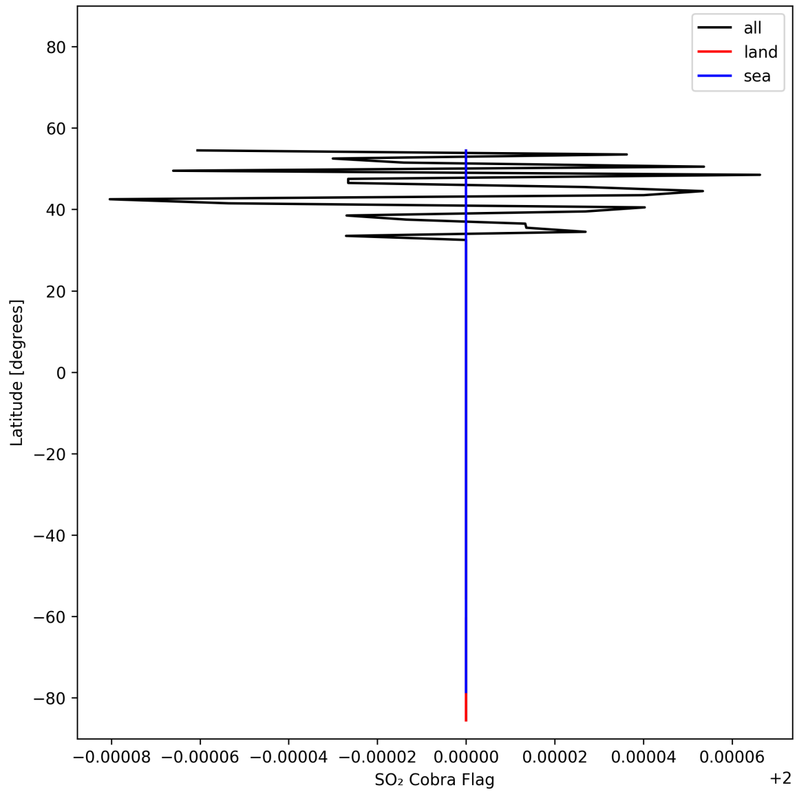
Figure 49: Zonal average of “SO 2 Cobra Flag” for 2025-02-05 to 2025-02-07.
