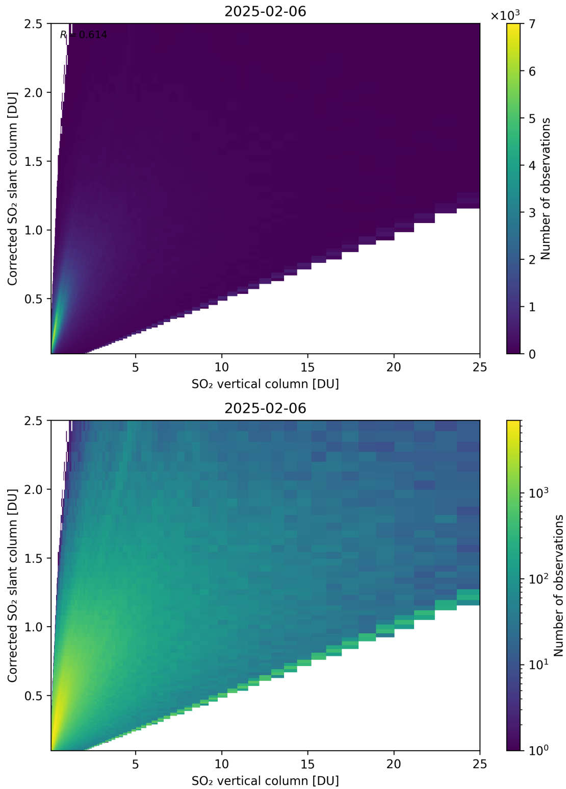
Figure 351: Scatter density plot of “SO 2 vertical column” against “Corrected SO 2 slant column” for 2025-02-05 to 2025-02-07.
