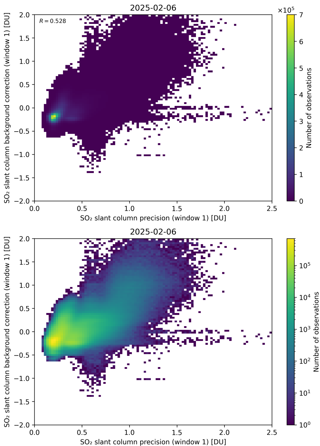
Figure 268: Scatter density plot of “SO 2 slant column precision (window 1)” against “SO 2 slant column background correction (window 1)” for 2025-02-05 to 2025-02-07.
