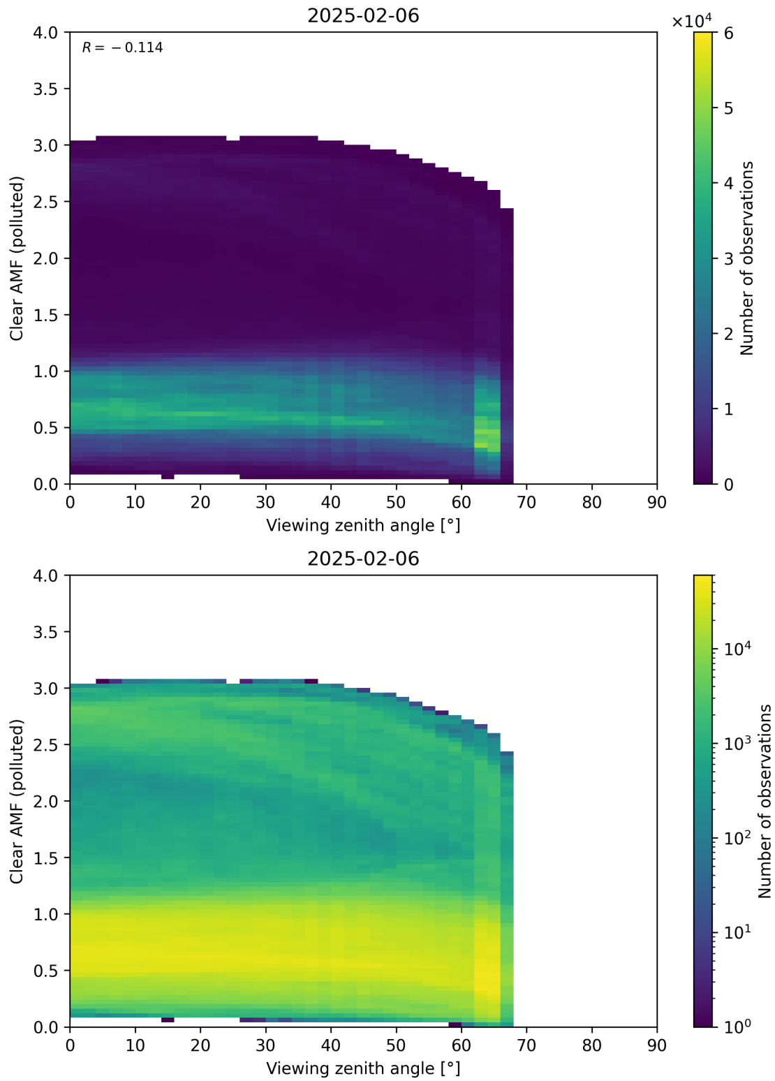
Figure 370: Scatter density plot of “Viewing zenith angle” against “Clear AMF (polluted)” for 2025-02-05 to 2025-02-07.
