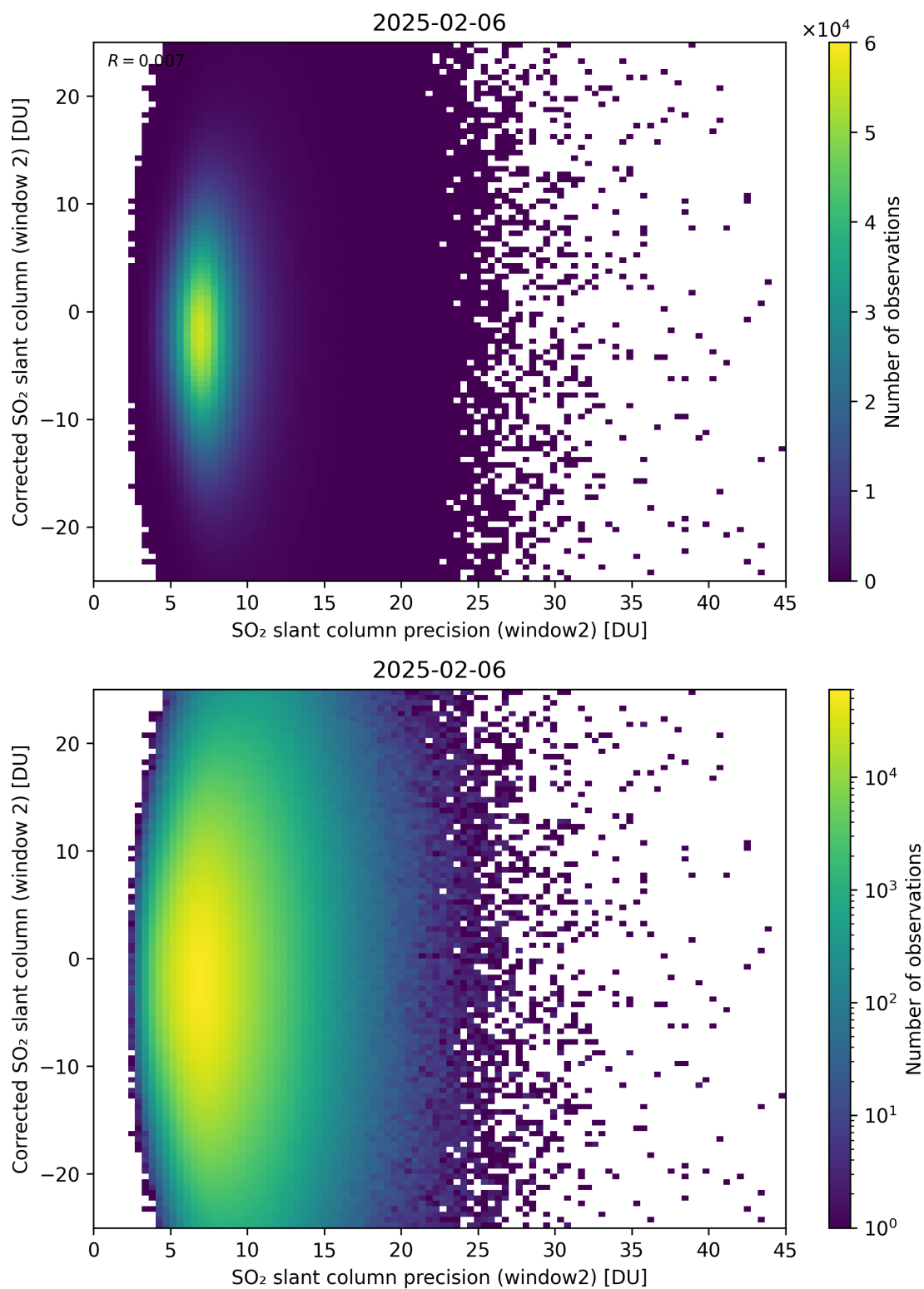
Figure 297: Scatter density plot of “SO 2 slant column precision (window2)” against “Corrected SO 2 slant column (window 2)” for 2025-02-05 to 2025-02-07.
