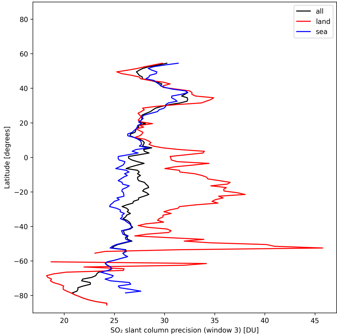
Figure 46: Zonal average of “SO 2 slant column precision (window 3)” for 2025-02-05 to 2025-02-07.
