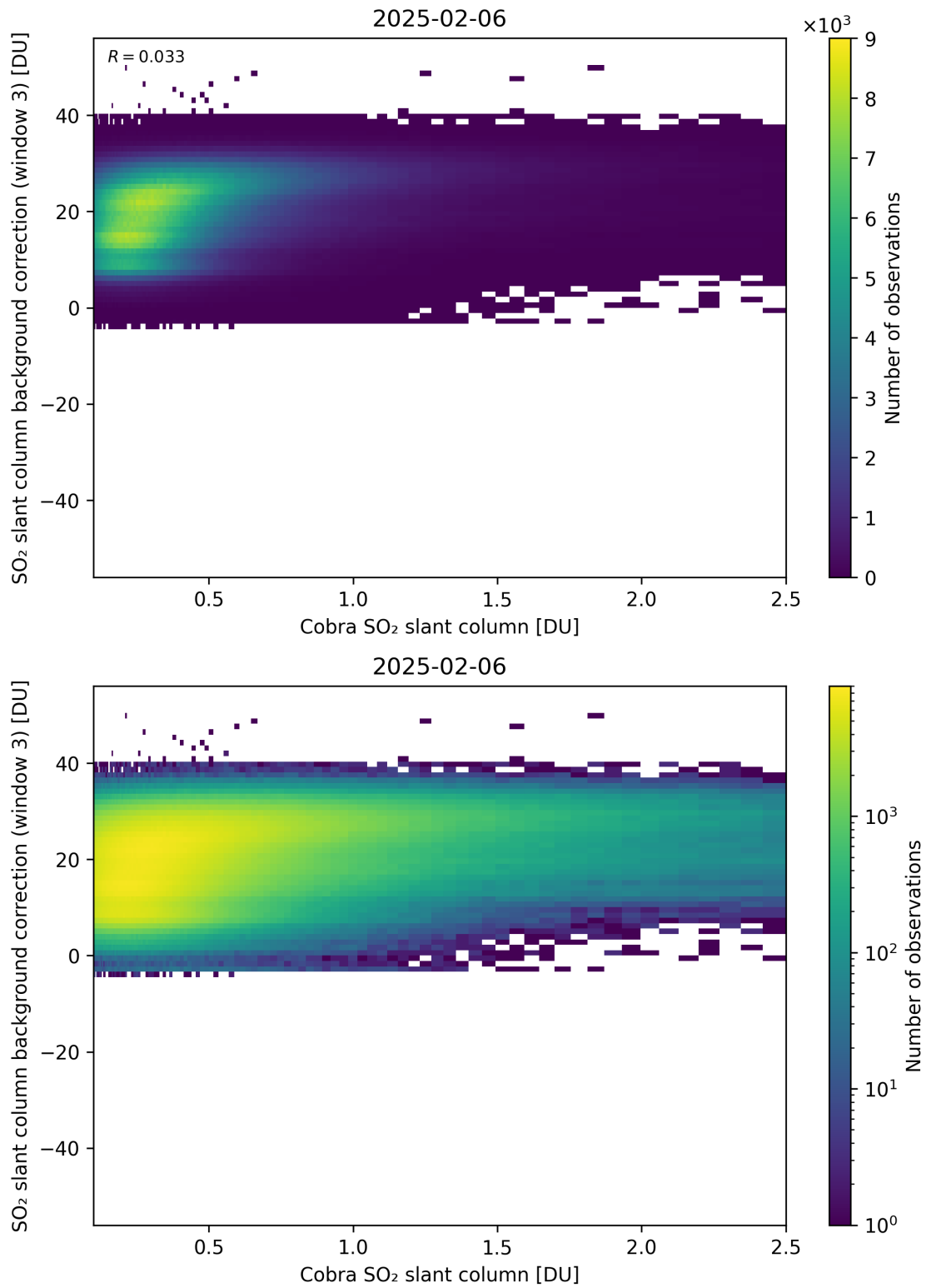
Figure 195: Scatter density plot of “Cobra SO 2 slant column” against “SO 2 slant column background correction (window 3)” for 2025-02-05 to 2025-02-07.
