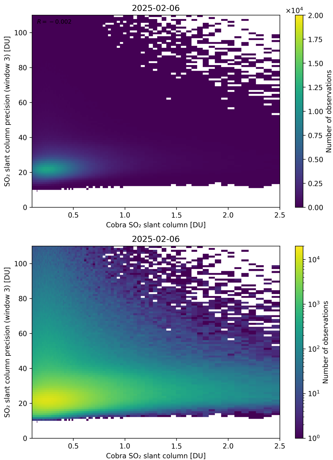
Figure 223: Scatter density plot of “Cobra SO 2 slant column” against “SO 2 slant column precision (window 3)” for 2025-02-05 to 2025-02-07.
