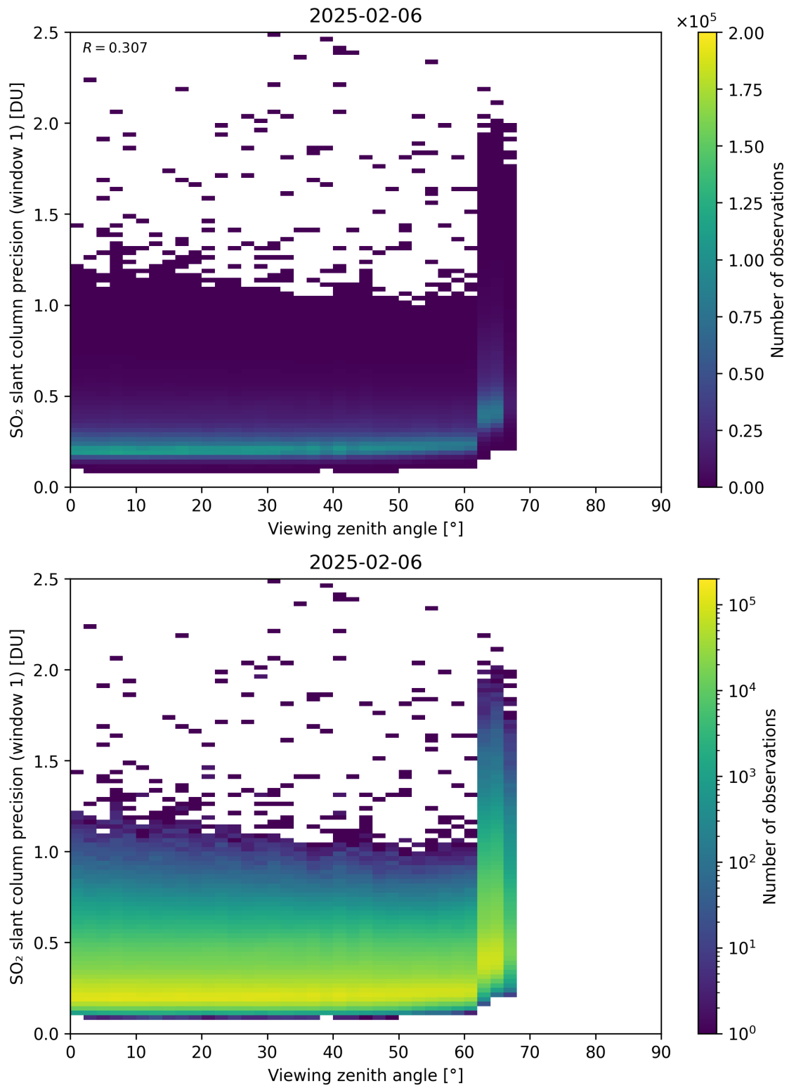
Figure 377: Scatter density plot of “Viewing zenith angle” against “SO 2 slant column precision (window 1)” for 2025-02-05 to 2025-02-07.
