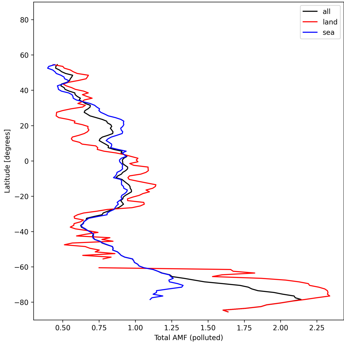
Figure 53: Zonal average of “Total AMF (polluted)” for 2025-02-05 to 2025-02-07.
