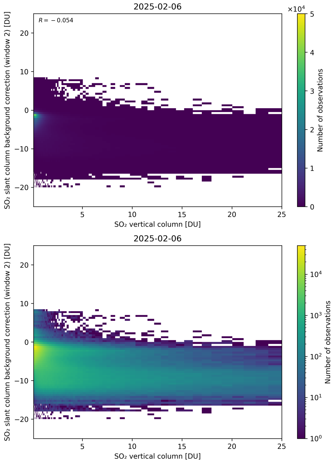
Figure 324: Scatter density plot of “SO 2 vertical column” against “SO 2 slant column background correction (window 2)” for 2025-02-05 to 2025-02-07.
