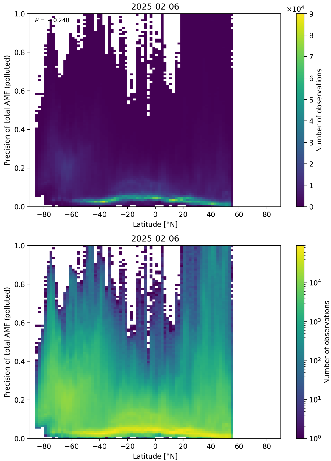
Figure 168: Scatter density plot of “Latitude” against “Precision of total AMF (polluted)” for 2025-02-05 to 2025-02-07.
