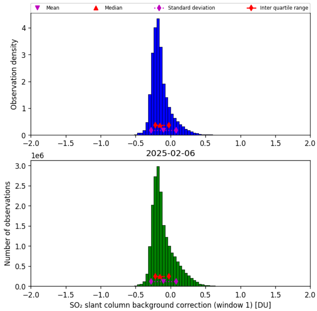
Figure 66: Histogram of “SO 2 slant column background correction (window 1)” for 2025-02-05 to 2025-02-07
