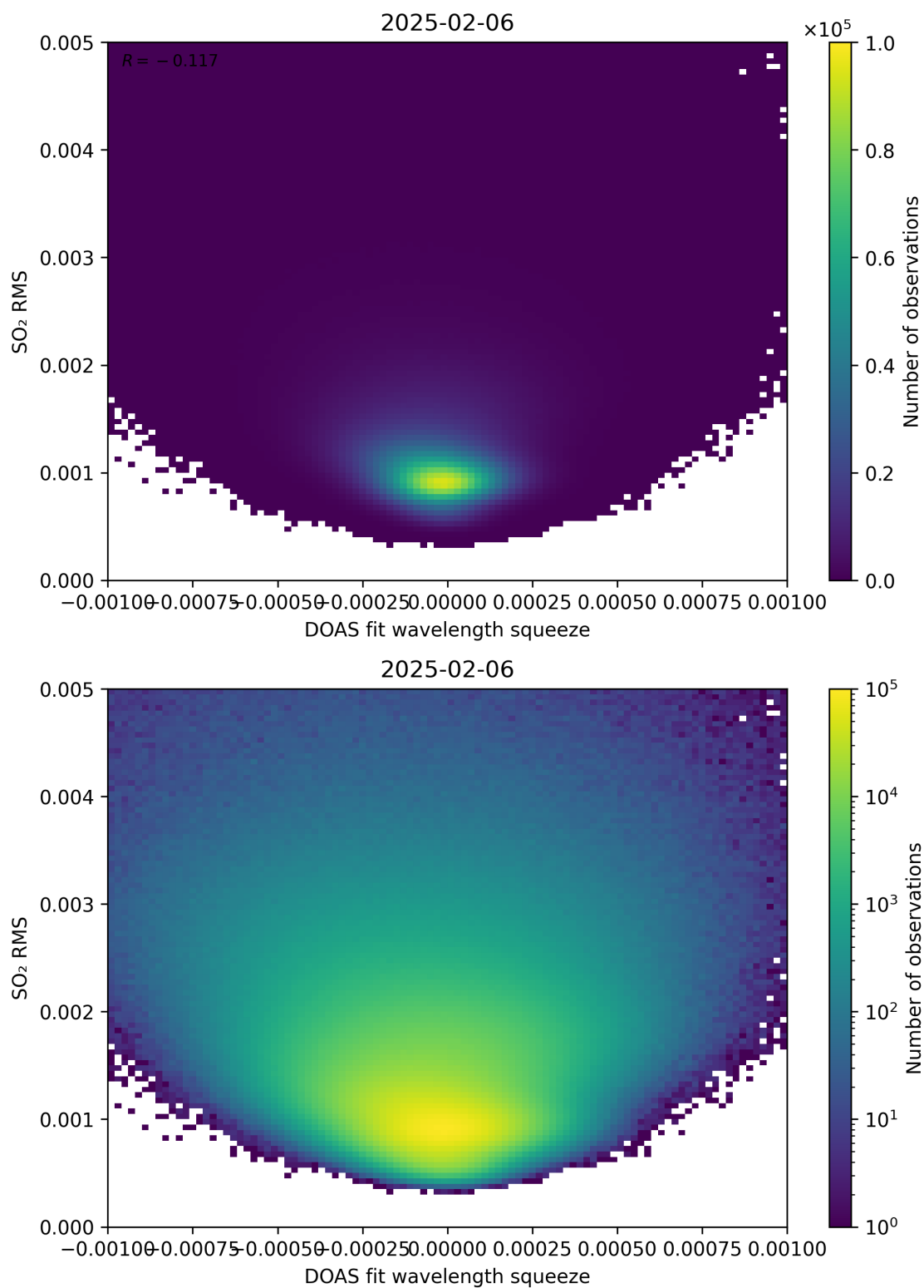
Figure 143: Scatter density plot of “DOAS fit wavelength squeeze” against “SO 2 RMS” for 2025-02-05 to 2025-02-07.
