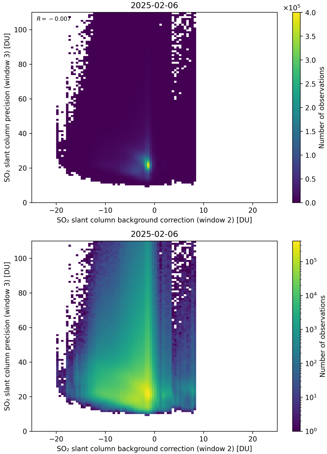
Figure 129: Scatter density plot of “SO 2 slant column background correction (window 2)” against “SO 2 slant column precision (window 3)” for 2025-02-05 to 2025-02-07.
