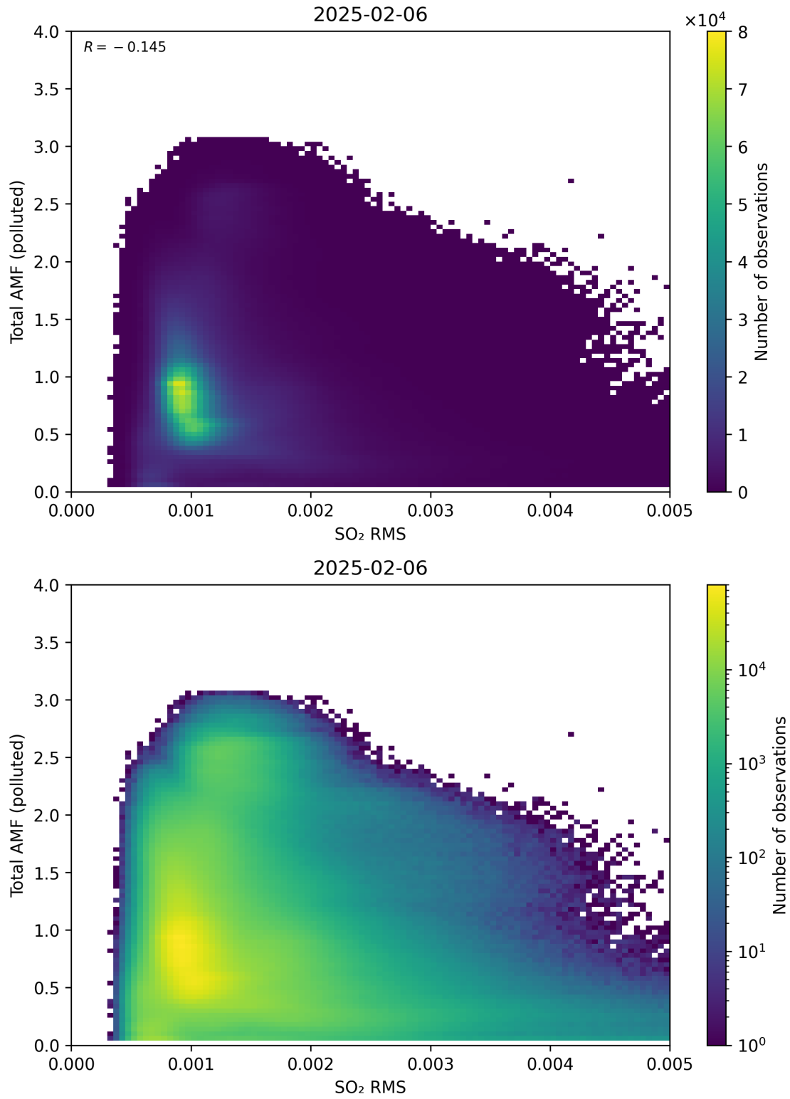
Figure 148: Scatter density plot of “SO 2 RMS” against “Total AMF (polluted)” for 2025-02-05 to 2025-02-07.
