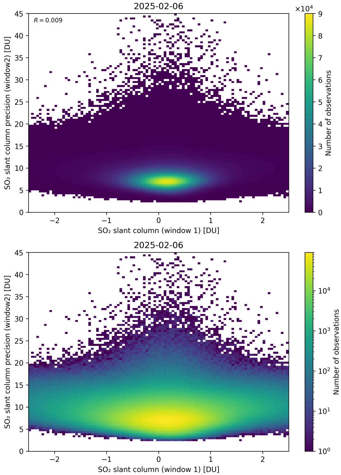
Figure 286: Scatter density plot of “SO 2 slant column (window 1)” against “SO 2 slant column precision (window2)” for 2025-02-05 to 2025-02-07.
