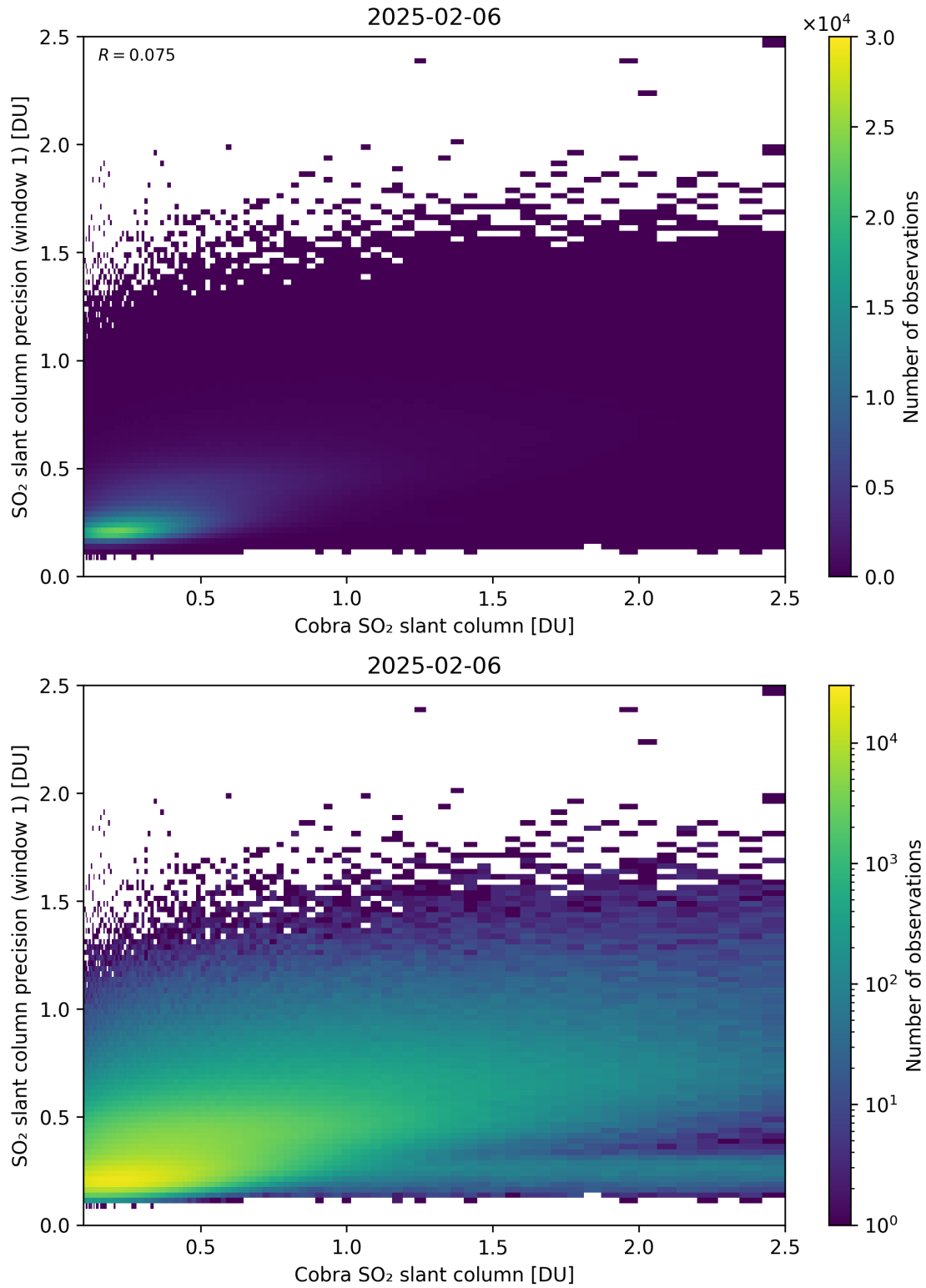
Figure 220: Scatter density plot of “Cobra SO 2 slant column” against “SO 2 slant column precision (window 1)” for 2025-02-05 to 2025-02-07.
