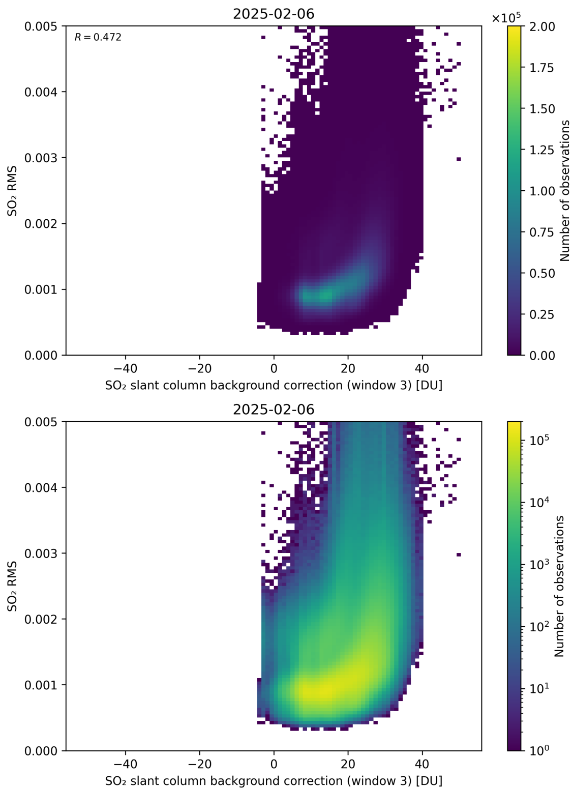
Figure 134: Scatter density plot of “SO 2 slant column background correction (window 3)” against “SO 2 RMS” for 2025-02-05 to 2025-02-07.
