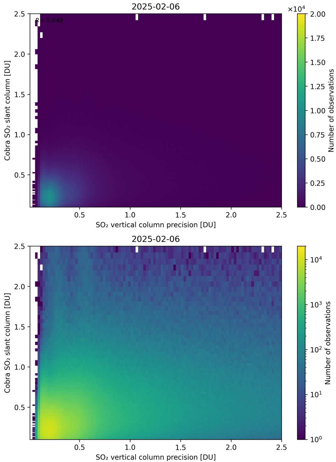
Figure 336: Scatter density plot of “SO 2 vertical column precision” against “Cobra SO 2 slant column” for 2025-02-05 to 2025-02-07.
