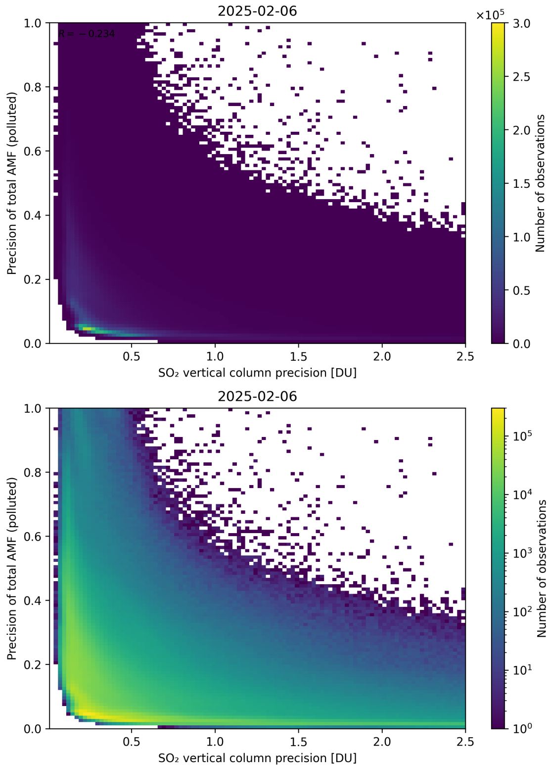
Figure 347: Scatter density plot of “SO 2 vertical column precision” against “Precision of total AMF (polluted)” for 2025-02-05 to 2025-02-07.
