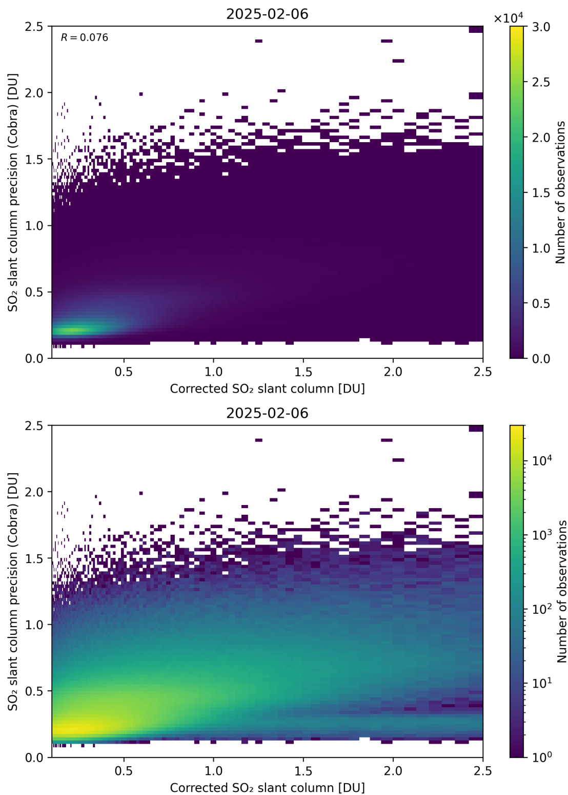
Figure 234: Scatter density plot of “Corrected SO 2 slant column” against “SO 2 slant column precision (Cobra)” for 2025-02-05 to 2025-02-07.
