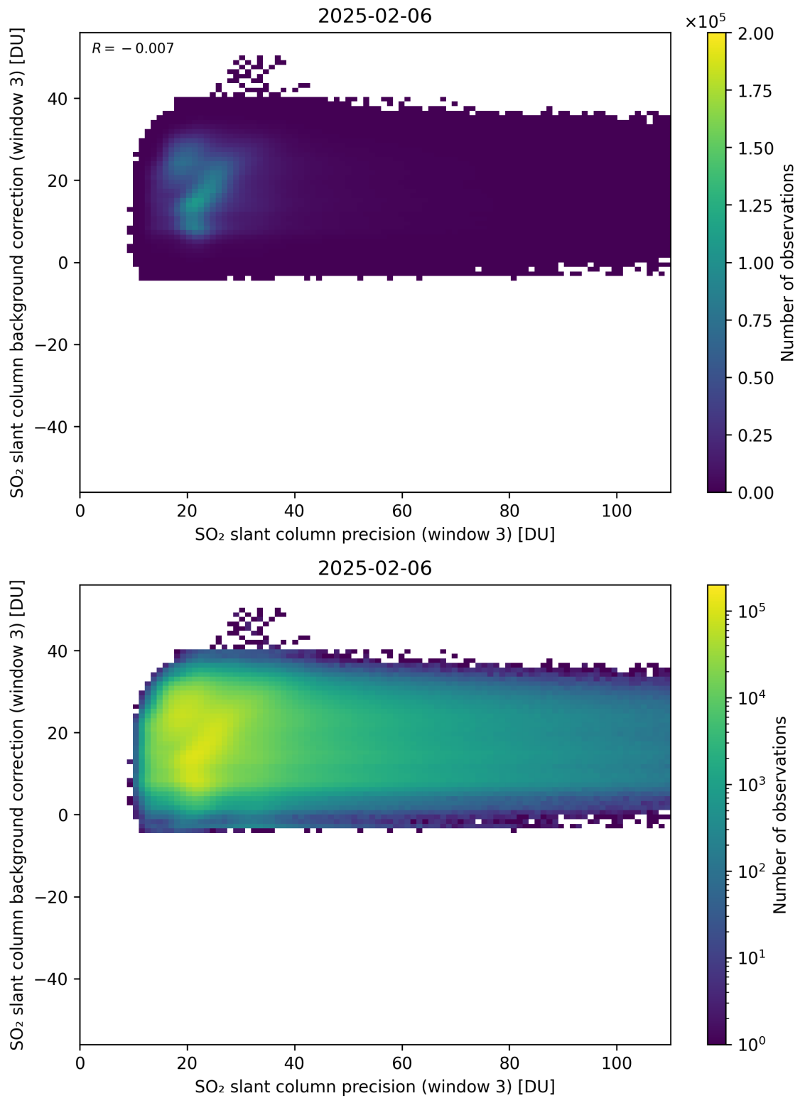
Figure 307: Scatter density plot of “SO 2 slant column precision (window 3)” against “SO 2 slant column background correction (window 3)” for 2025-02-05 to 2025-02-07.
