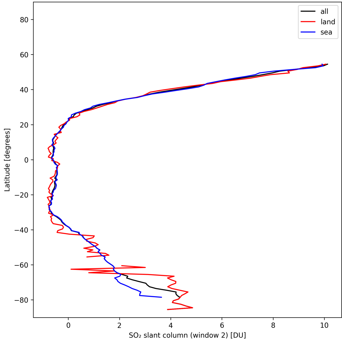
Figure 41: Zonal average of “SO 2 slant column (window 2)” for 2025-02-05 to 2025-02-07.
