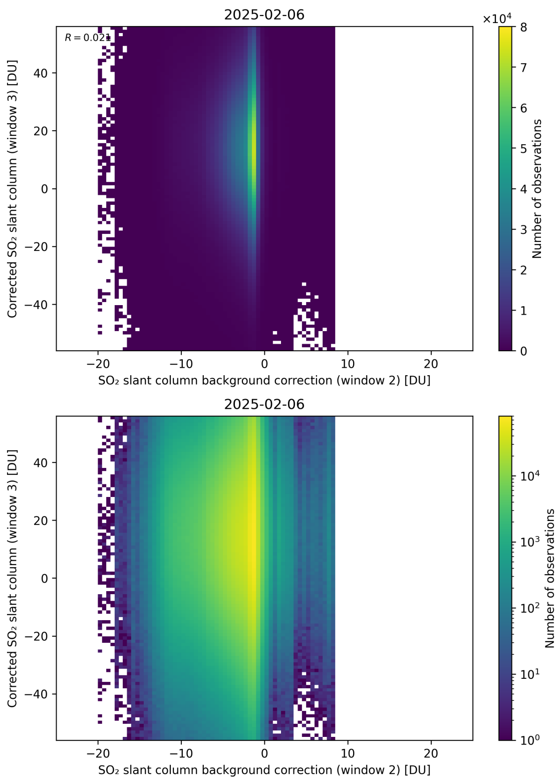
Figure 127: Scatter density plot of “SO 2 slant column background correction (window 2)” against “Corrected SO 2 slant column (window 3)” for 2025-02-05 to 2025-02-07.
