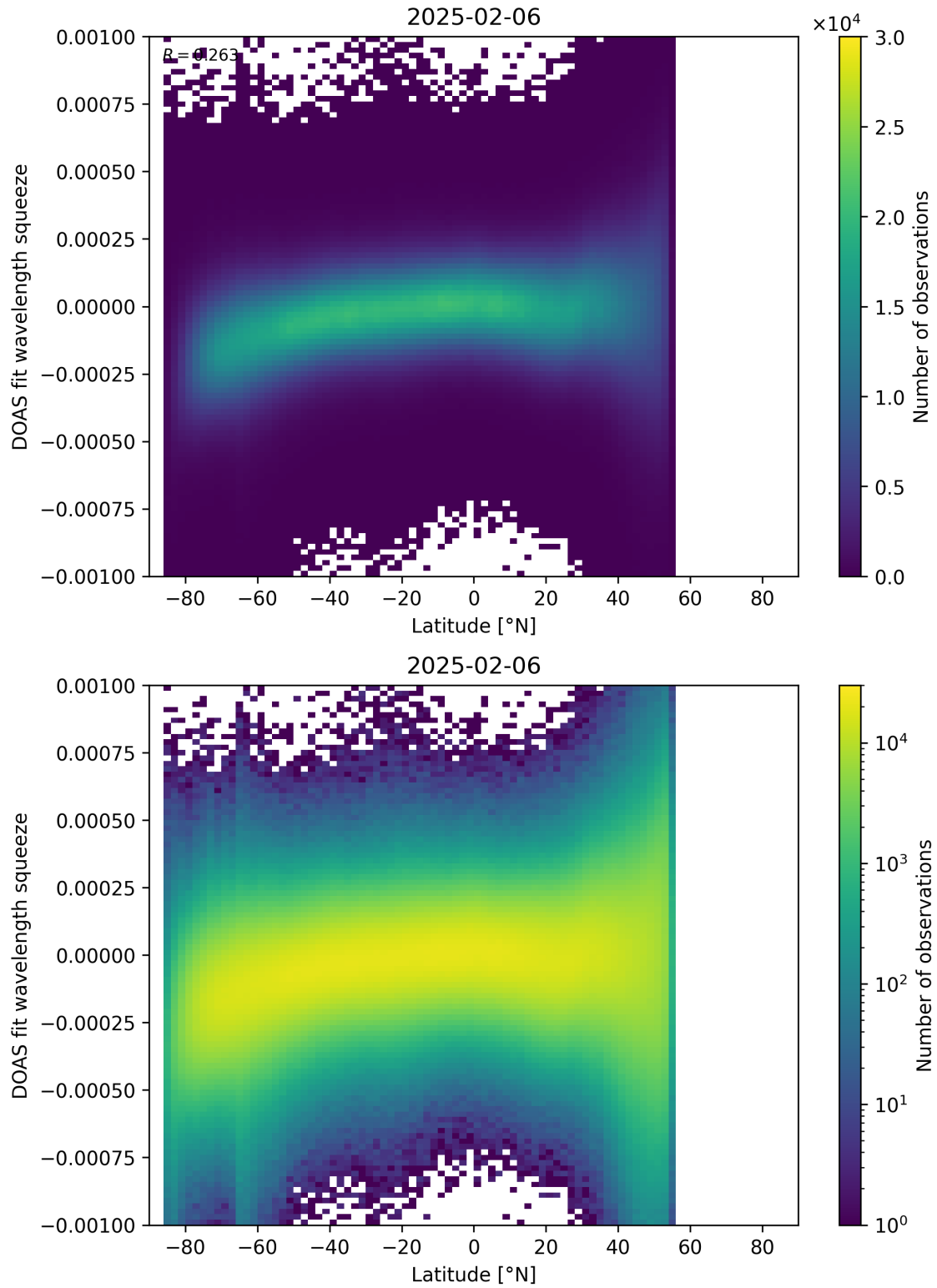
Figure 154: Scatter density plot of “Latitude” against “DOAS fit wavelength squeeze” for 2025-02-05 to 2025-02-07.
