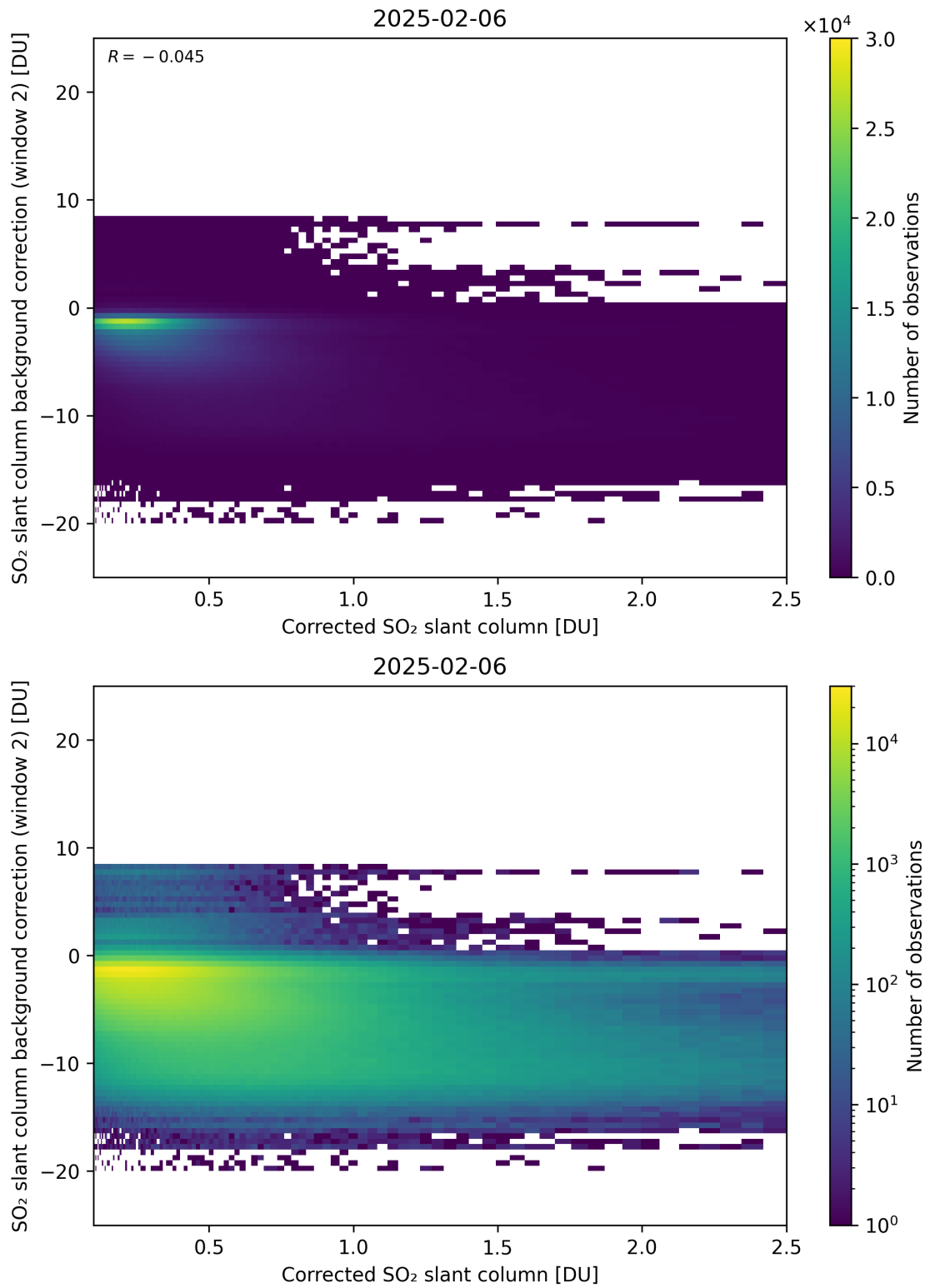
Figure 227: Scatter density plot of “Corrected SO 2 slant column” against “SO 2 slant column background correction (window 2)” for 2025-02-05 to 2025-02-07.
