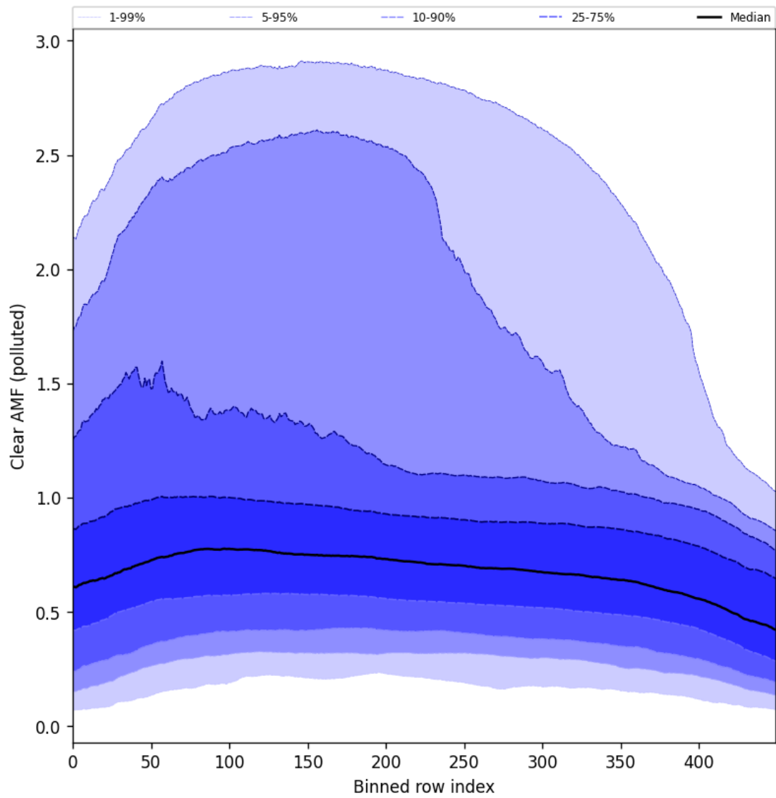
Figure 107: Along track statistics of “Clear AMF (polluted)” for 2025-02-05 to 2025-02-07
