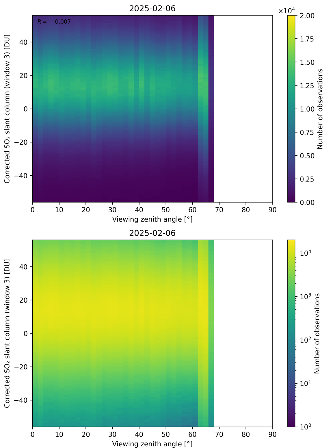
Figure 375: Scatter density plot of “Viewing zenith angle” against “Corrected SO 2 slant column (window 3)” for 2025-02-05 to 2025-02-07.
