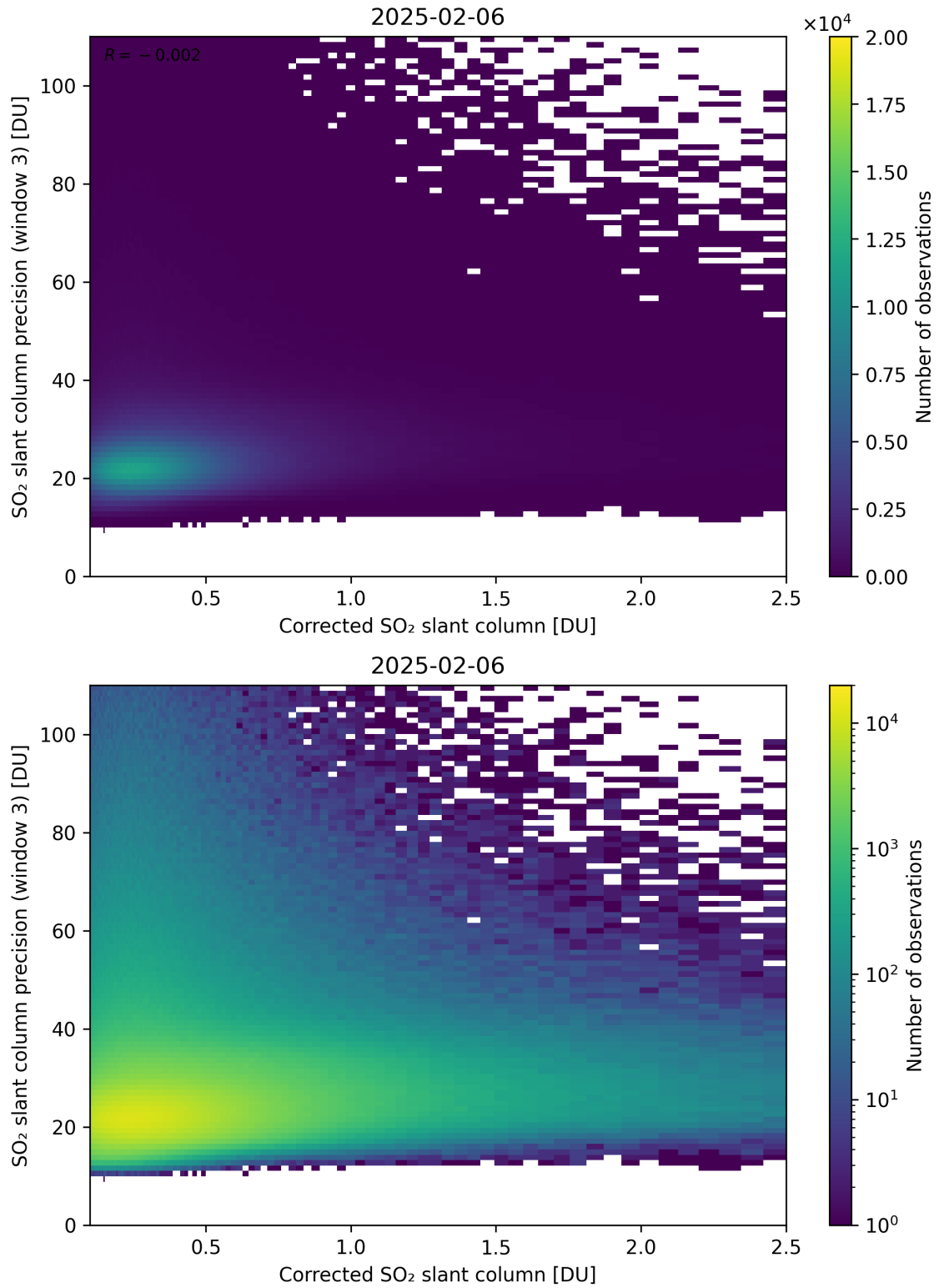
Figure 241: Scatter density plot of “Corrected SO 2 slant column” against “SO 2 slant column precision (window 3)” for 2025-02-05 to 2025-02-07.
