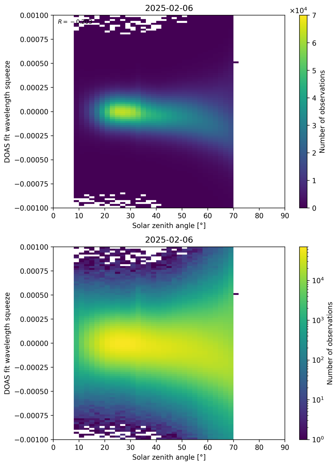
Figure 175: Scatter density plot of “Solar zenith angle” against “DOAS fit wavelength squeeze” for 2025-02-05 to 2025-02-07.
