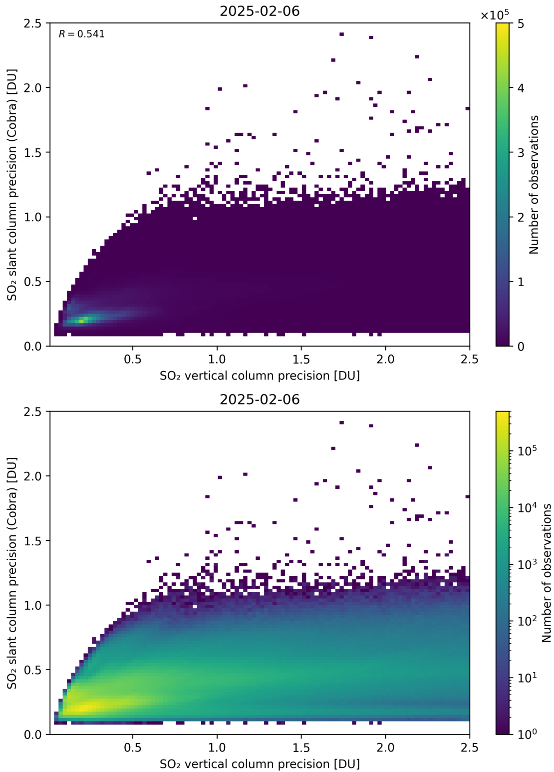
Figure 337: Scatter density plot of “SO 2 vertical column precision” against “SO 2 slant column precision (Cobra)” for 2025-02-05 to 2025-02-07.
