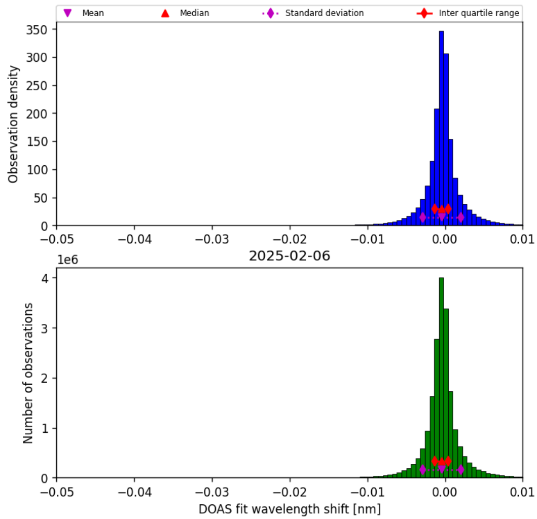
Figure 76: Histogram of “DOAS fit wavelength shift” for 2025-02-05 to 2025-02-07
