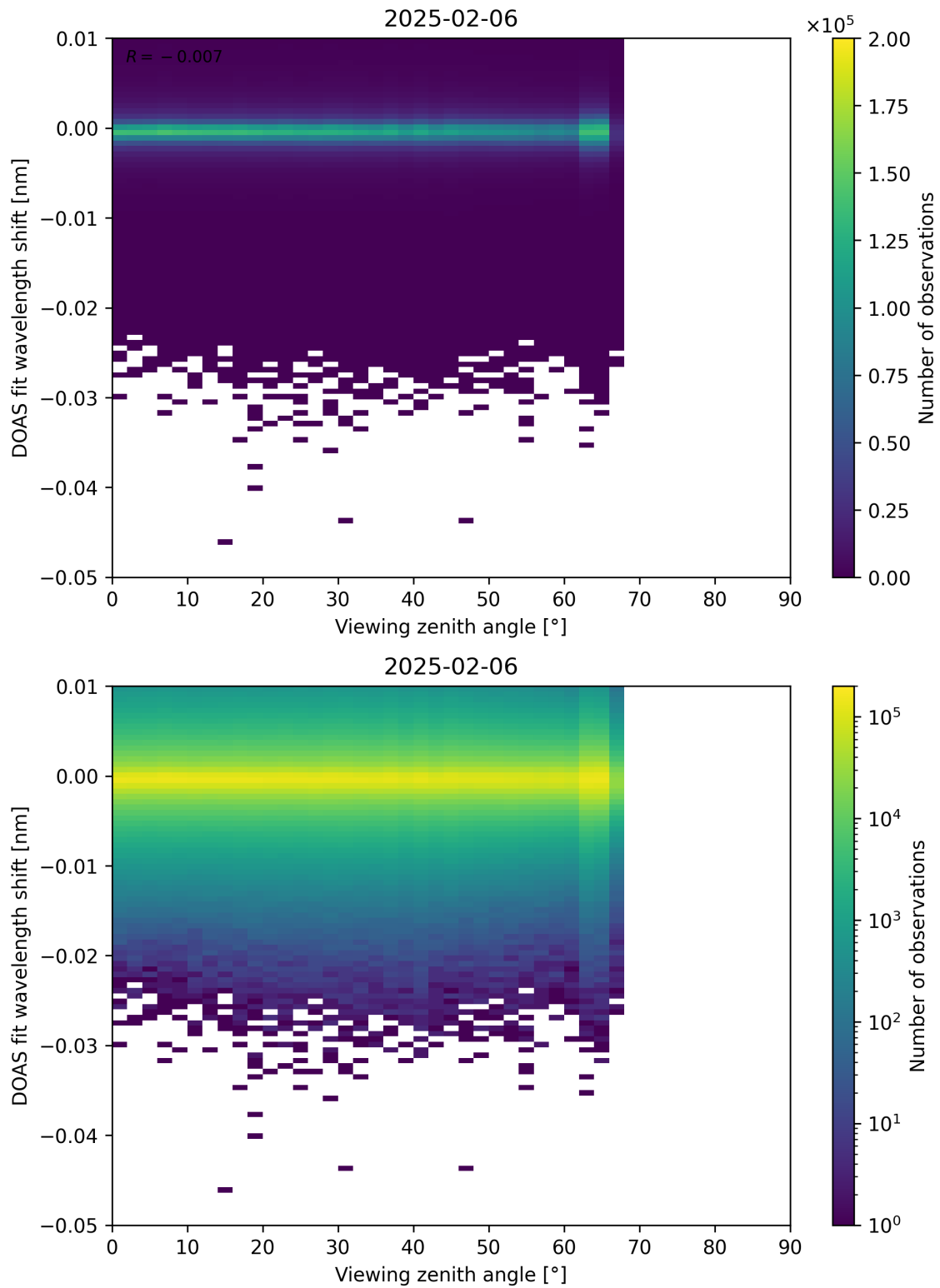
Figure 365: Scatter density plot of “Viewing zenith angle” against “DOAS fit wavelength shift” for 2025-02-05 to 2025-02-07.
