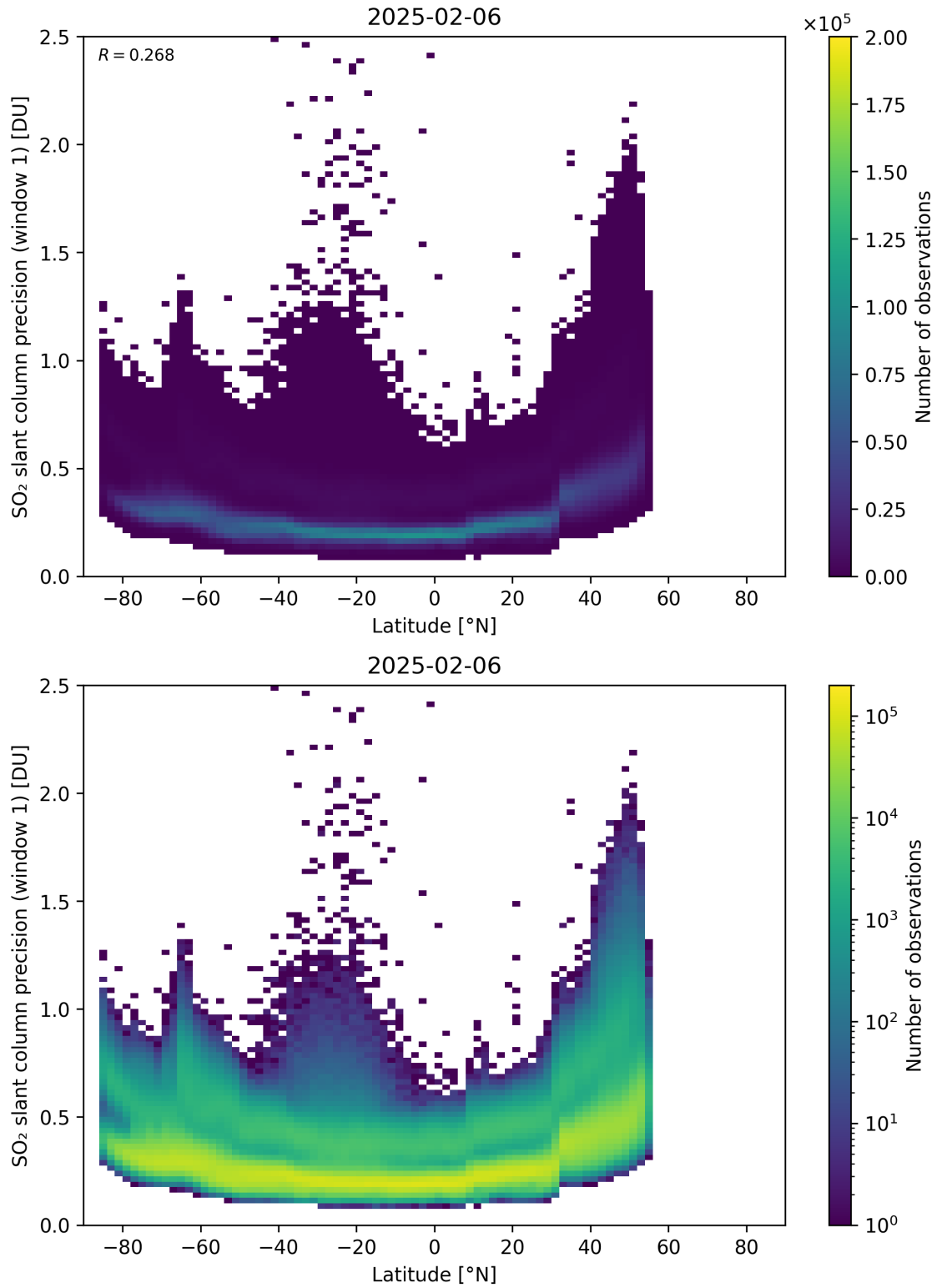
Figure 163: Scatter density plot of “Latitude” against “SO 2 slant column precision (window 1)” for 2025-02-05 to 2025-02-07.
