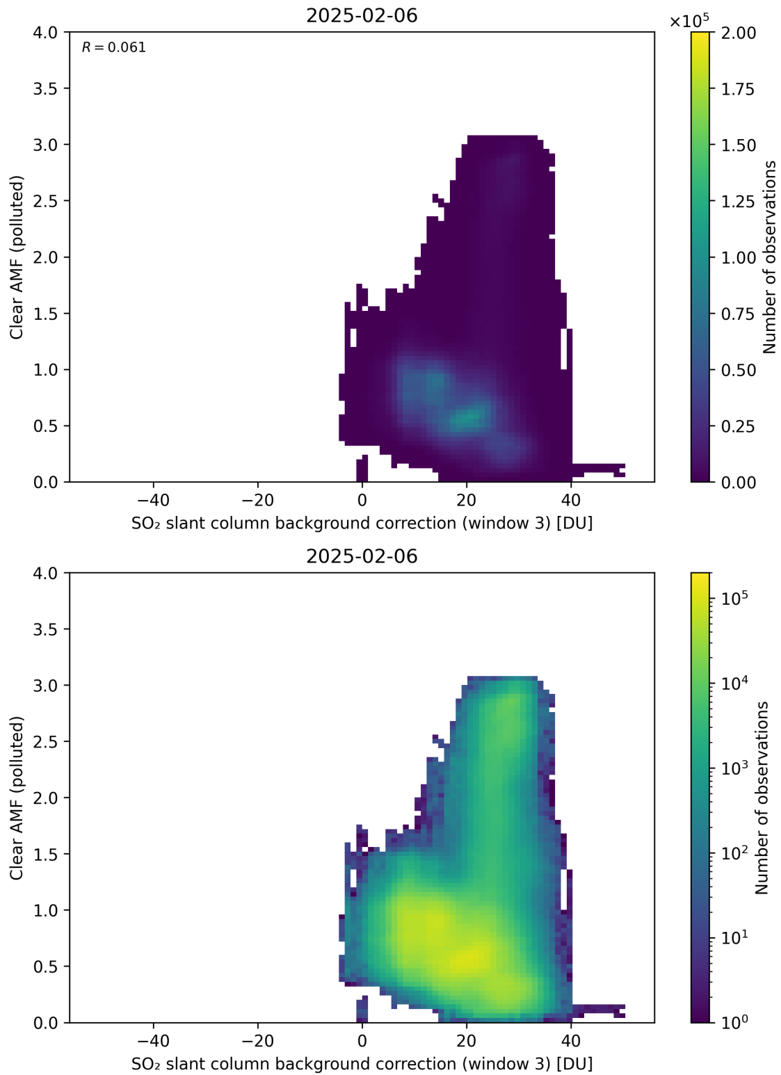
Figure 135: Scatter density plot of “SO 2 slant column background correction (window 3)” against “Clear AMF (polluted)” for 2025-02-05 to 2025-02-07.
