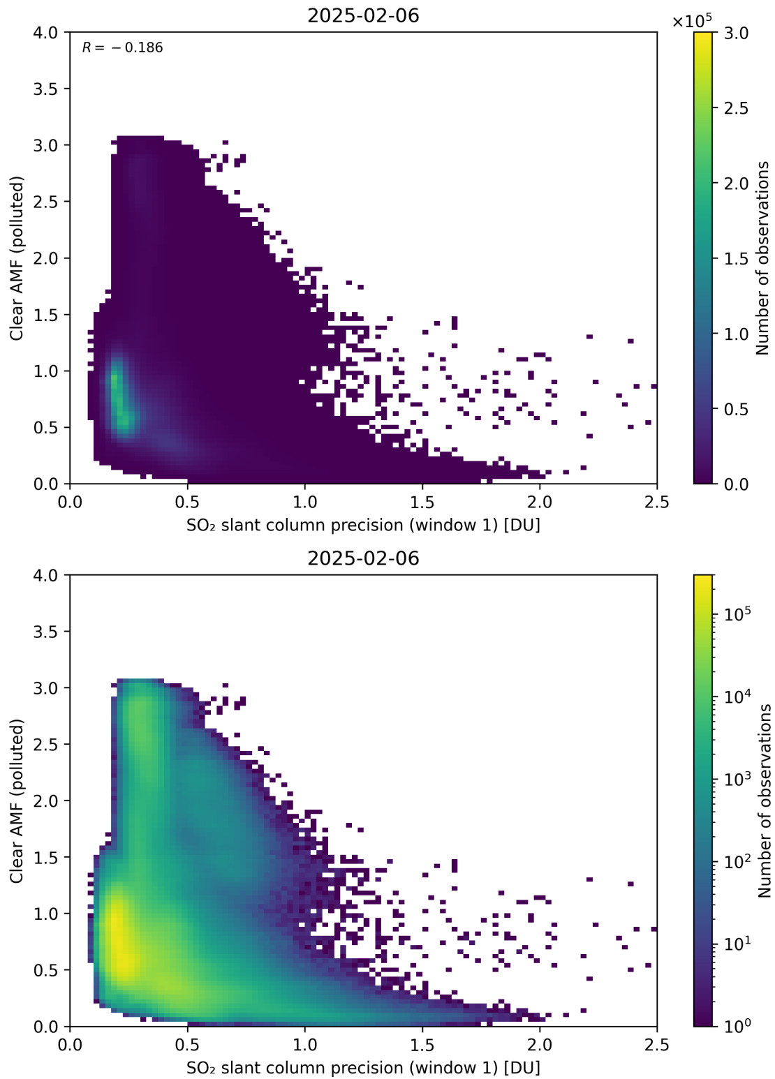
Figure 274: Scatter density plot of “SO 2 slant column precision (window 1)” against “Clear AMF (polluted)” for 2025-02-05 to 2025-02-07.
