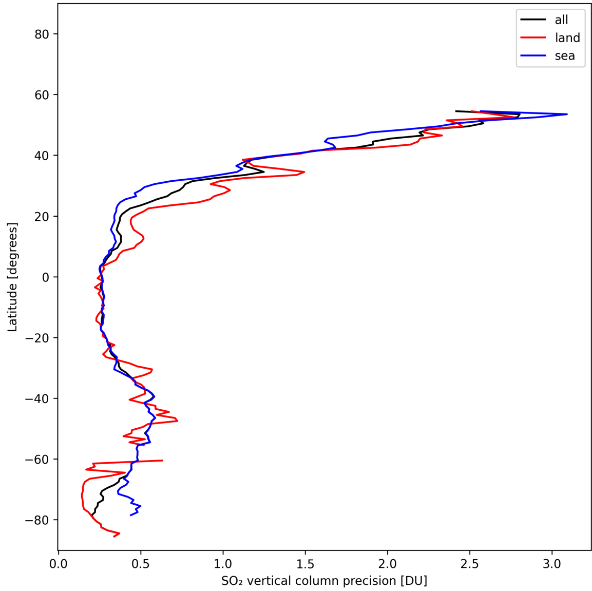
Figure 33: Zonal average of “SO 2 vertical column precision” for 2025-02-05 to 2025-02-07.
