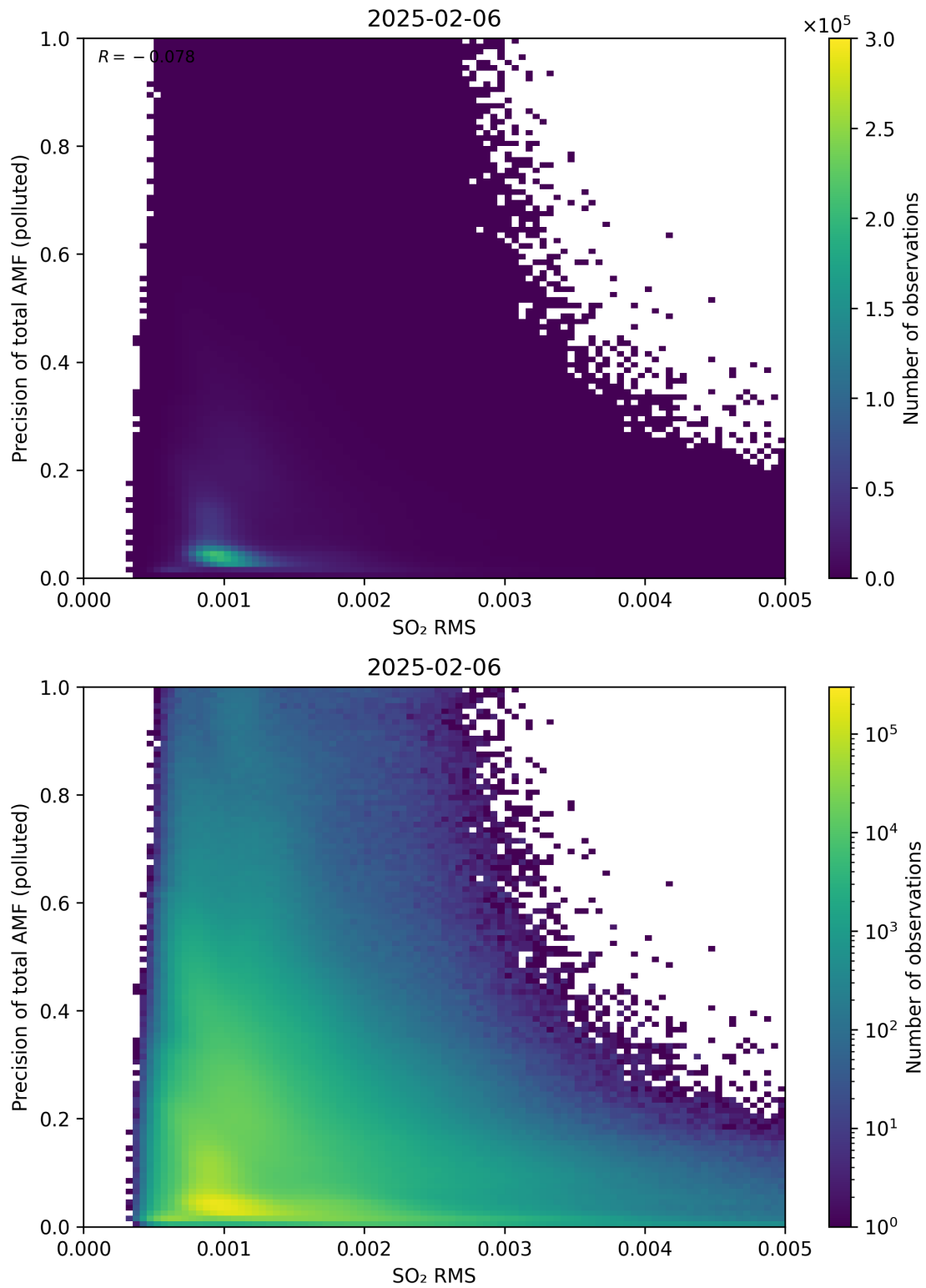
Figure 149: Scatter density plot of “SO 2 RMS” against “Precision of total AMF (polluted)” for 2025-02-05 to 2025-02-07.
