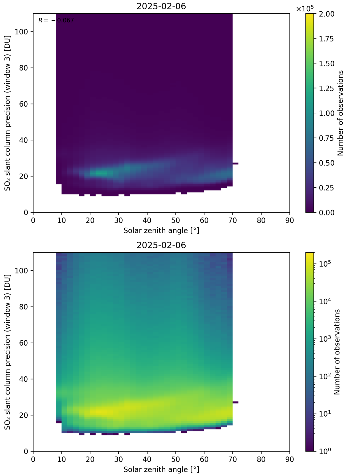
Figure 188: Scatter density plot of “Solar zenith angle” against “SO 2 slant column precision (window 3)” for 2025-02-05 to 2025-02-07.
