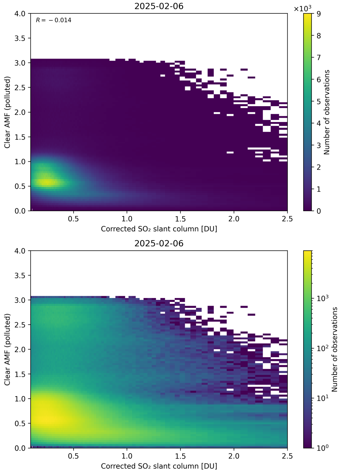
Figure 232: Scatter density plot of “Corrected SO 2 slant column” against “Clear AMF (polluted)” for 2025-02-05 to 2025-02-07.
