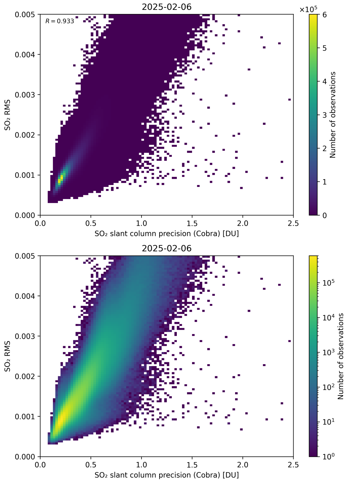
Figure 204: Scatter density plot of “SO 2 slant column precision (Cobra)” against “SO 2 RMS” for 2025-02-05 to 2025-02-07.
