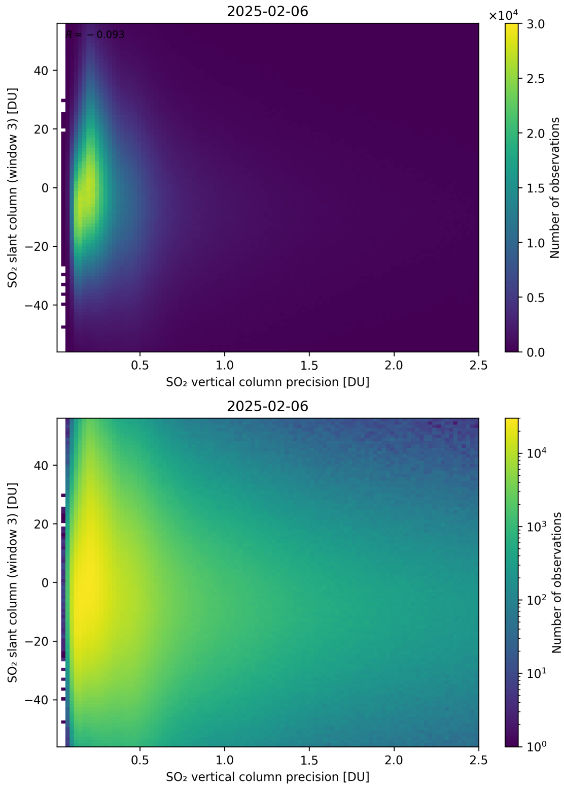
Figure 344: Scatter density plot of “SO 2 vertical column precision” against “SO 2 slant column (window 3)” for 2025-02-05 to 2025-02-07.
