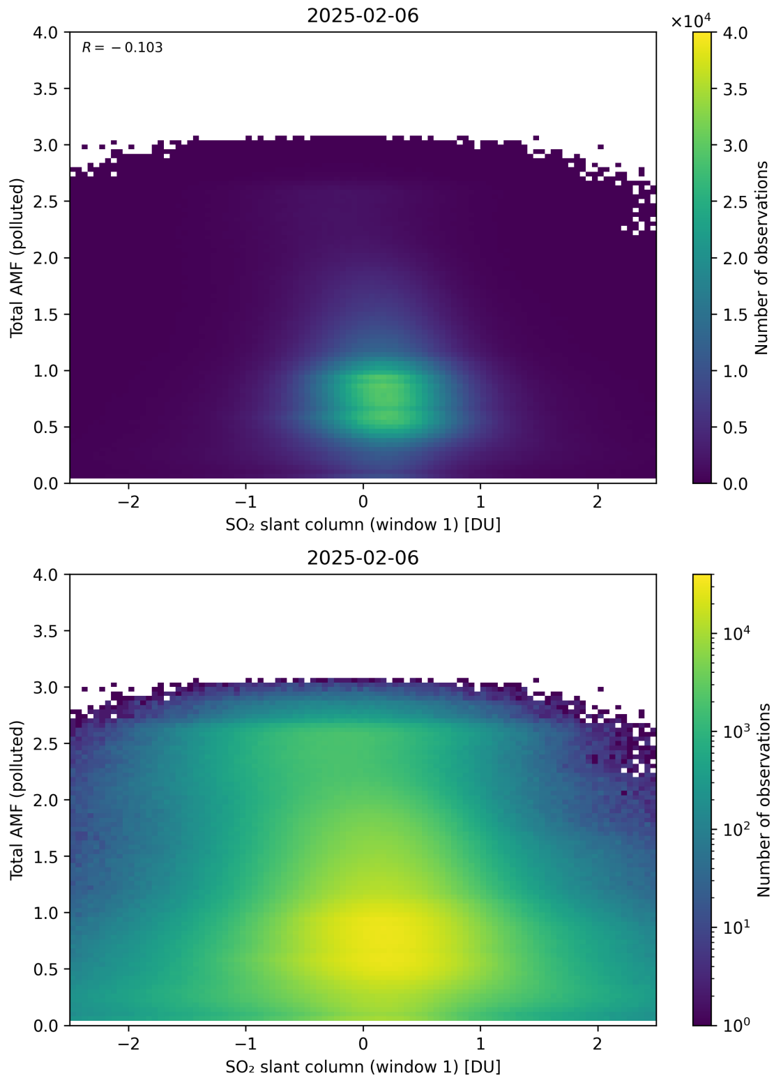
Figure 289: Scatter density plot of “SO 2 slant column (window 1)” against “Total AMF (polluted)” for 2025-02-05 to 2025-02-07.
