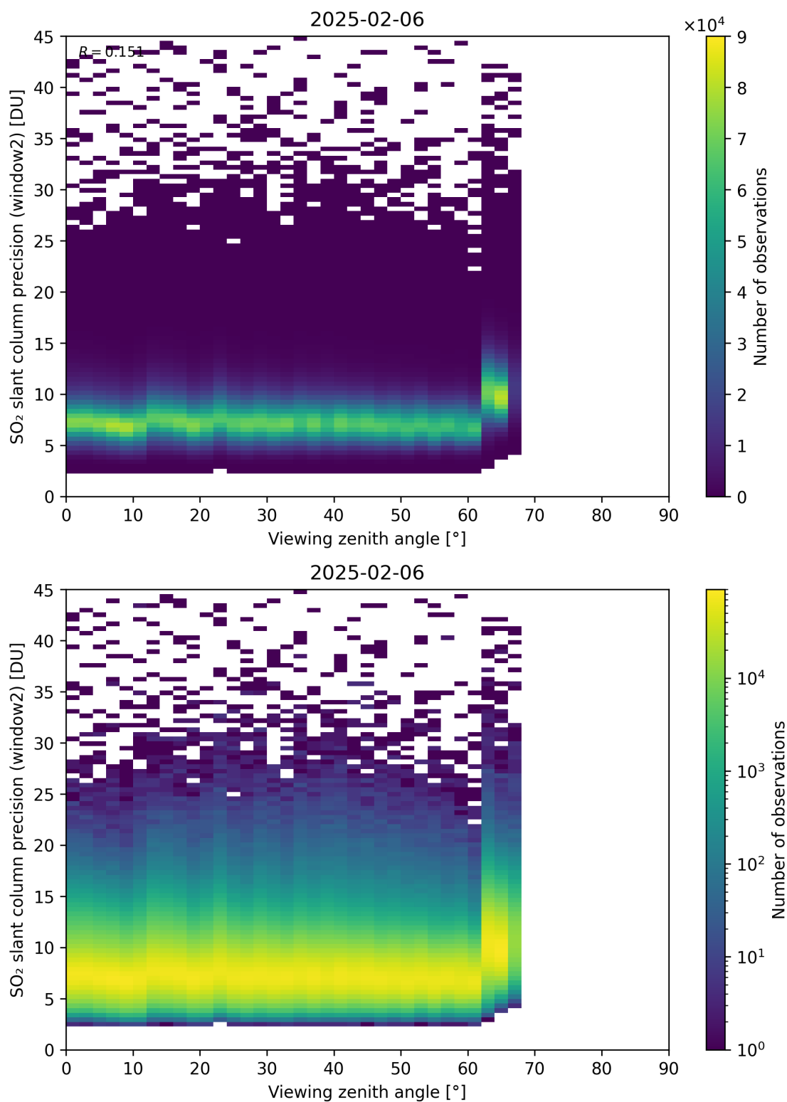
Figure 378: Scatter density plot of “Viewing zenith angle” against “SO 2 slant column precision (window2)” for 2025-02-05 to 2025-02-07.
