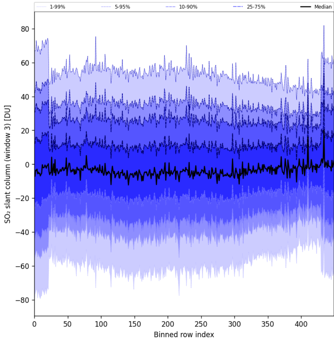
Figure 97: Along track statistics of “SO 2 slant column (window 3)” for 2025-02-05 to 2025-02-07
