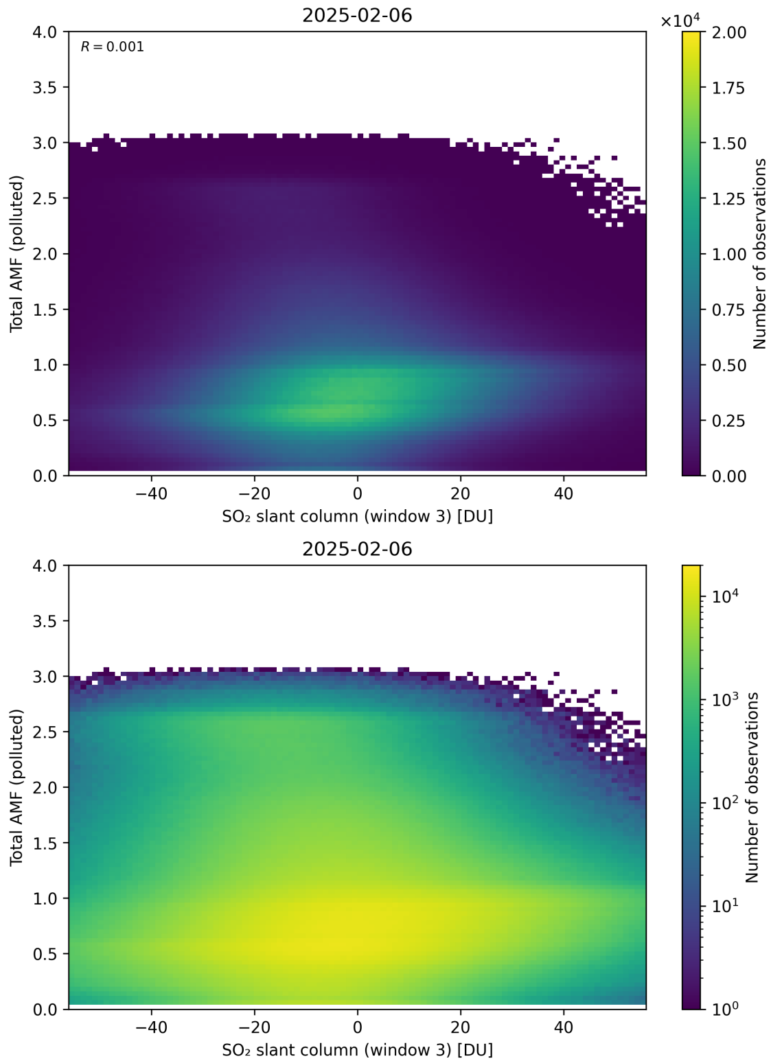
Figure 318: Scatter density plot of “SO 2 slant column (window 3)” against “Total AMF (polluted)” for 2025-02-05 to 2025-02-07.
