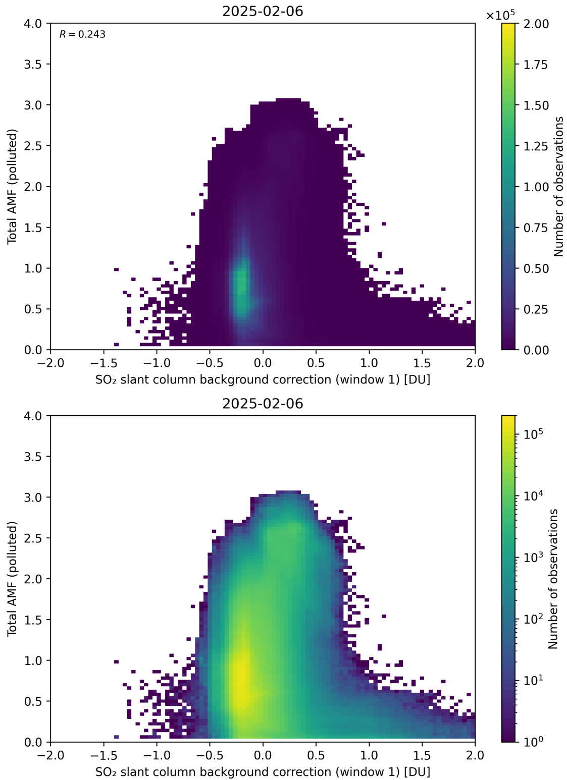
Figure 120: Scatter density plot of “SO 2 slant column background correction (window 1)” against “Total AMF (polluted)” for 2025-02-05 to 2025-02-07.
