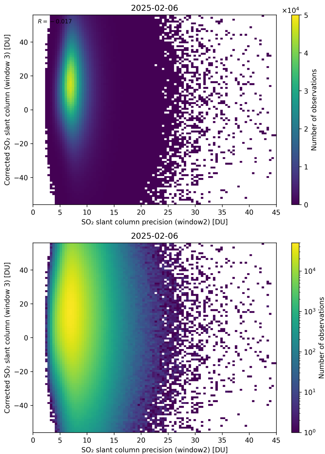
Figure 298: Scatter density plot of “SO 2 slant column precision (window2)” against “Corrected SO 2 slant column (window 3)” for 2025-02-05 to 2025-02-07.
