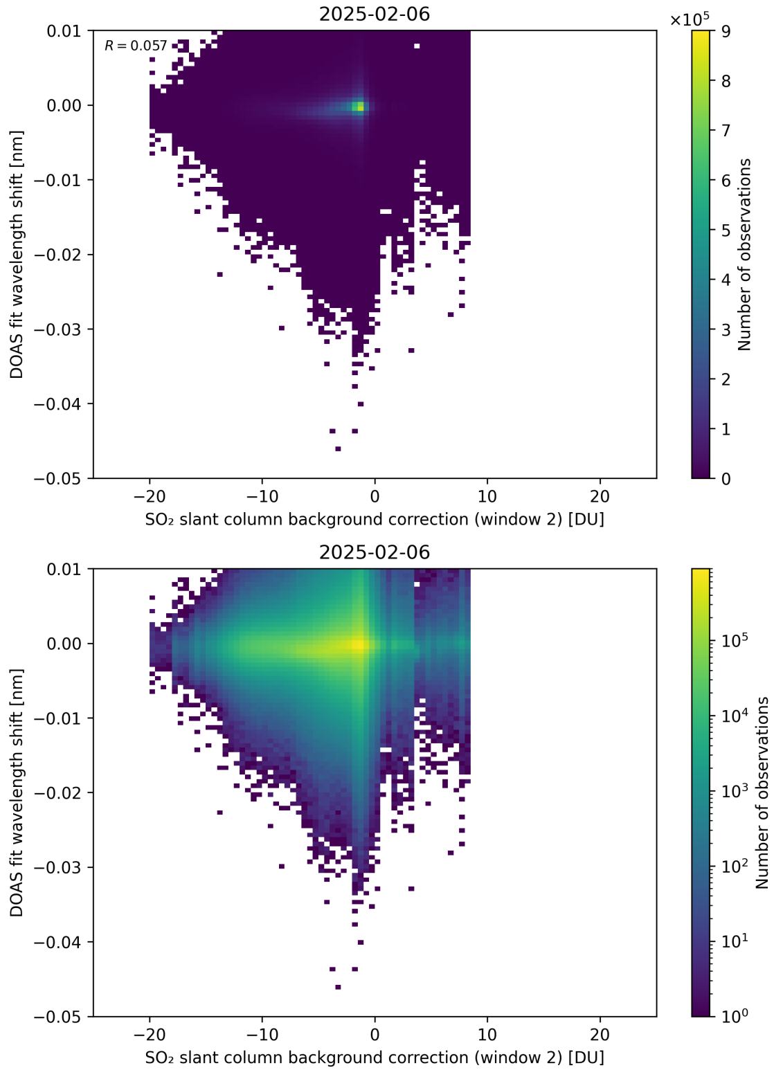
Figure 123: Scatter density plot of “SO 2 slant column background correction (window 2)” against “DOAS fit wavelength shift” for 2025-02-05 to 2025-02-07.
