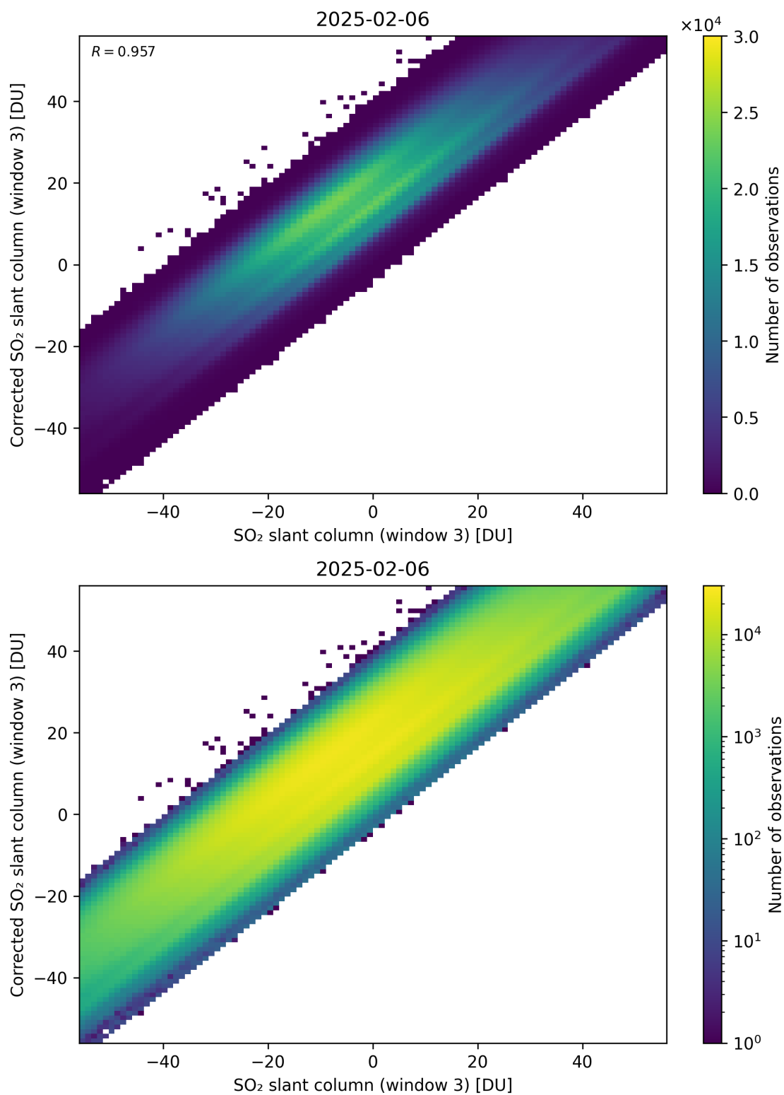
Figure 316: Scatter density plot of “SO 2 slant column (window 3)” against “Corrected SO 2 slant column (window 3)” for 2025-02-05 to 2025-02-07.
