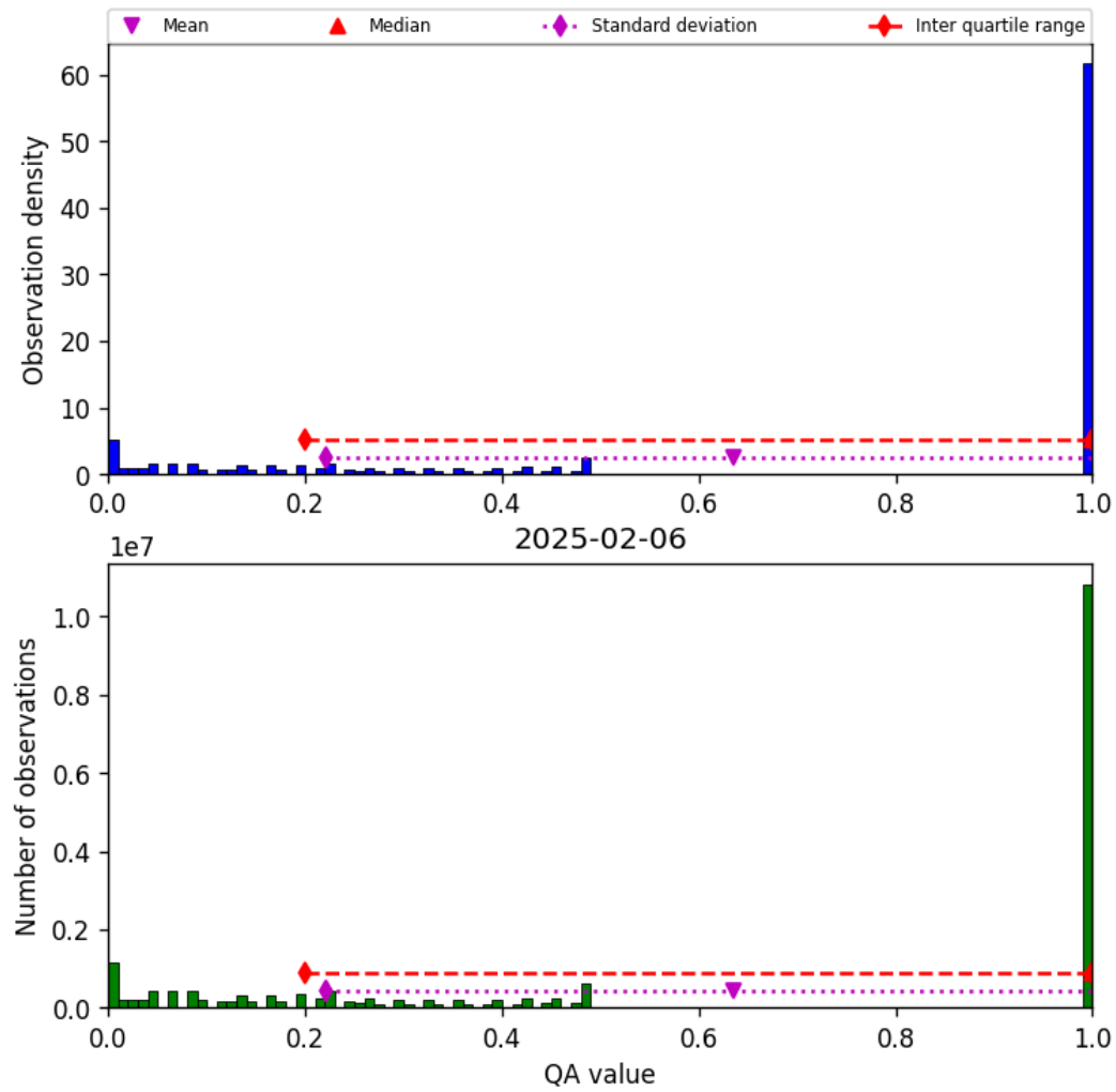
Figure 57: Histogram of “QA value” for 2025-02-05 to 2025-02-07
