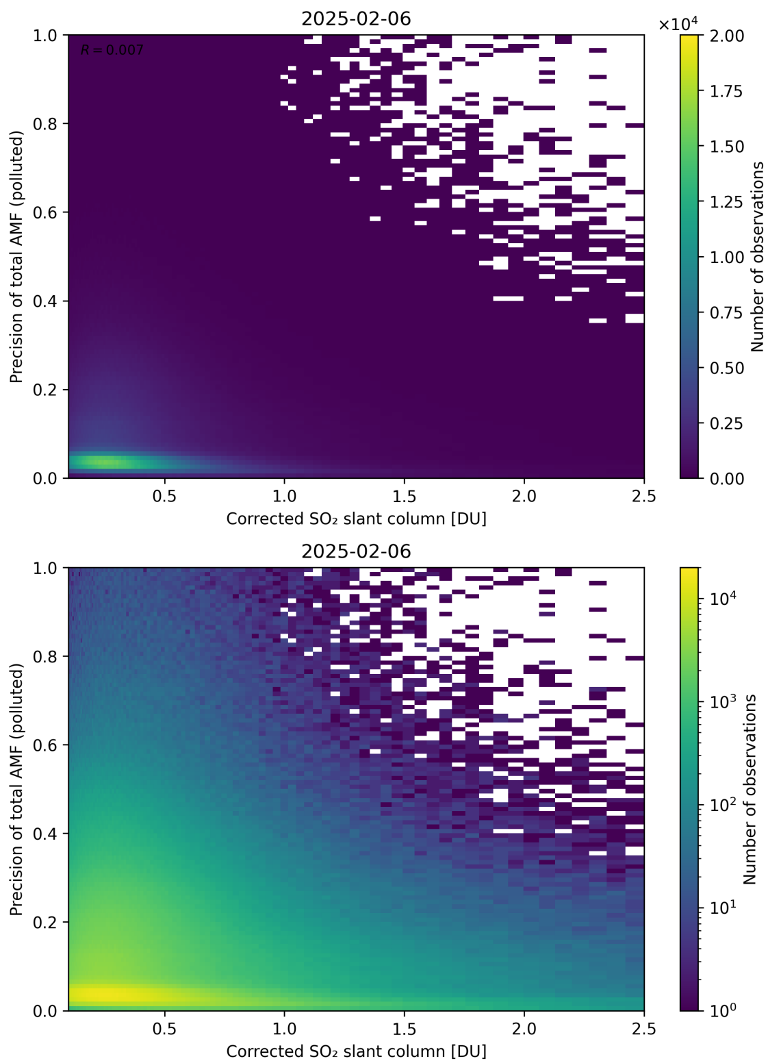
Figure 243: Scatter density plot of “Corrected SO 2 slant column” against “Precision of total AMF (polluted)” for 2025-02-05 to 2025-02-07.
