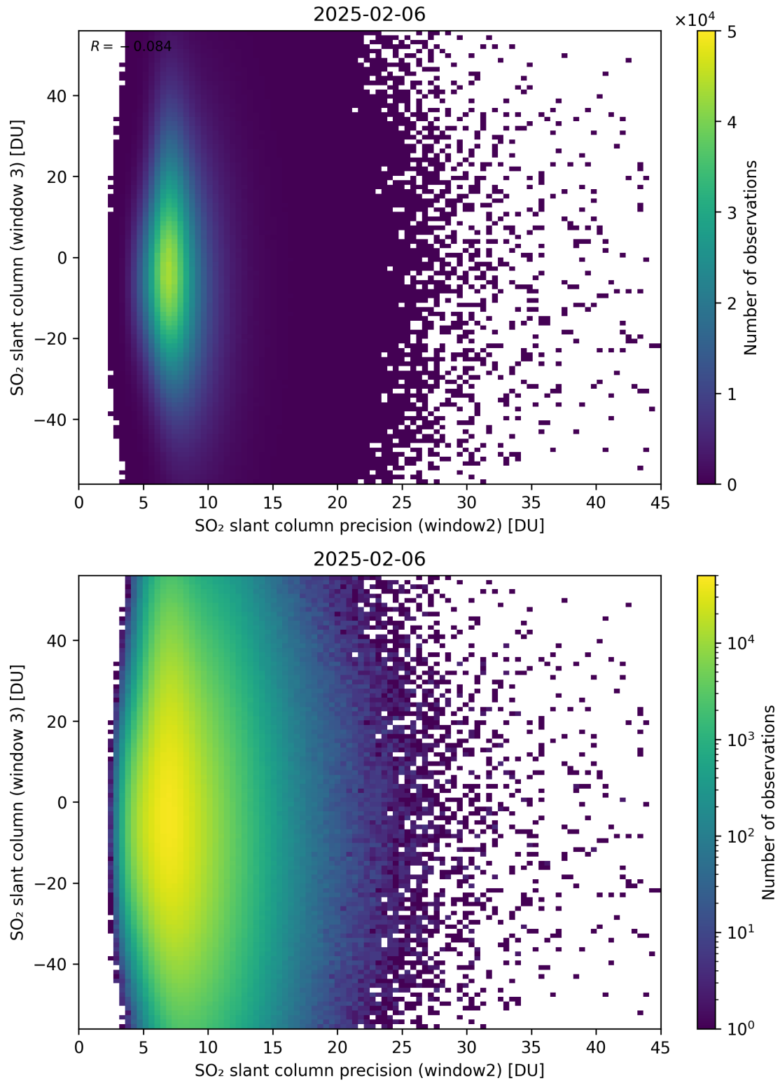
Figure 299: Scatter density plot of “SO 2 slant column precision (window2)” against “SO 2 slant column (window 3)” for 2025-02-05 to 2025-02-07.
