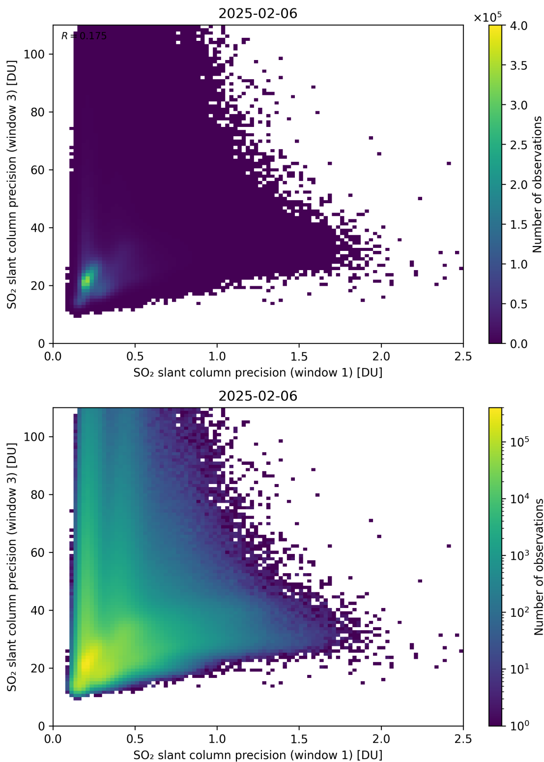
Figure 279: Scatter density plot of “SO 2 slant column precision (window 1)” against “SO 2 slant column precision (window 3)” for 2025-02-05 to 2025-02-07.
