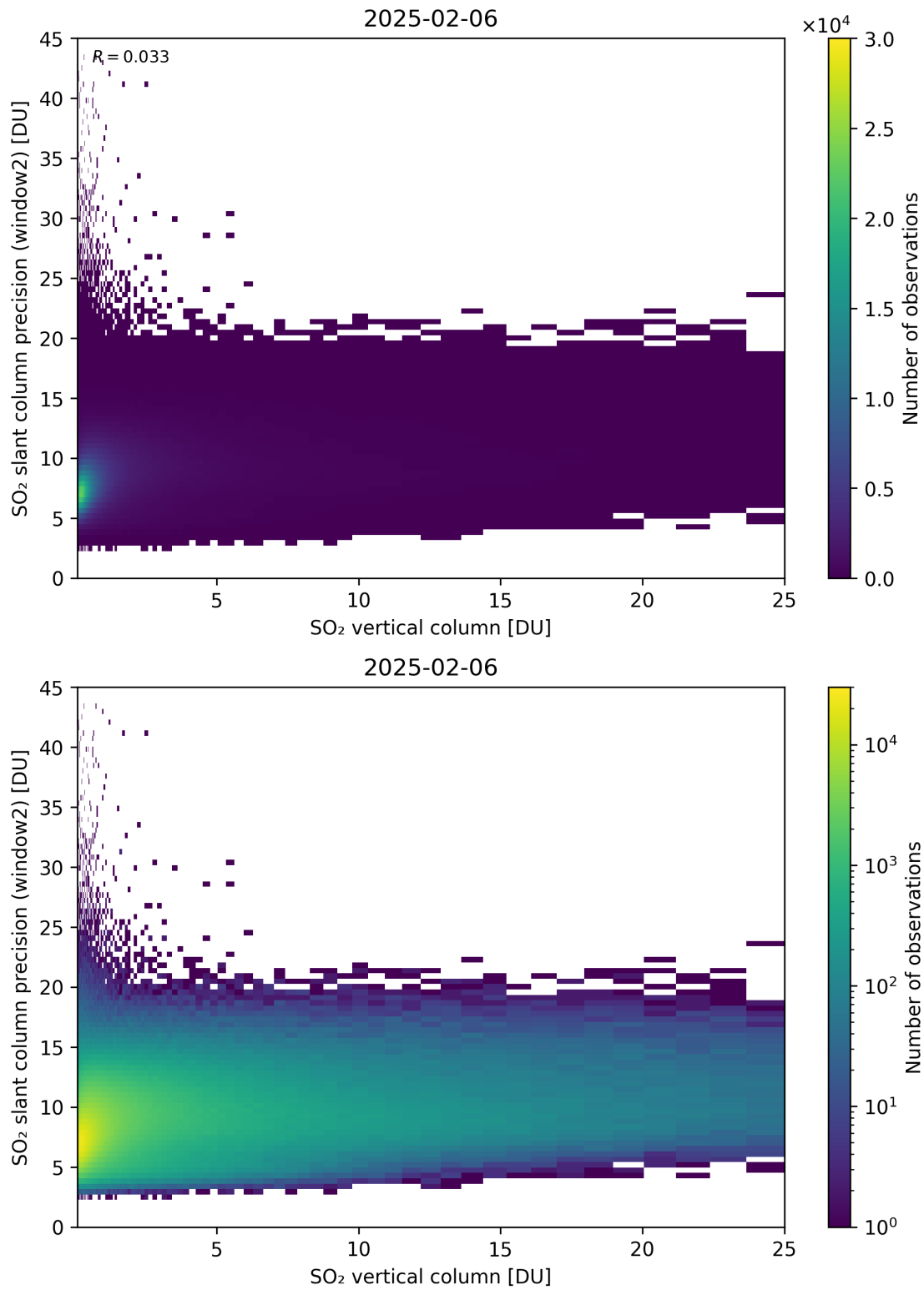
Figure 356: Scatter density plot of “SO 2 vertical column” against “SO 2 slant column precision (window2)” for 2025-02-05 to 2025-02-07.
