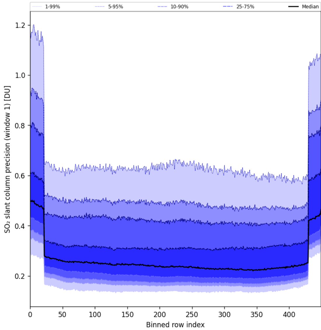
Figure 90: Along track statistics of “SO 2 slant column precision (window 1)” for 2025-02-05 to 2025-02-07
