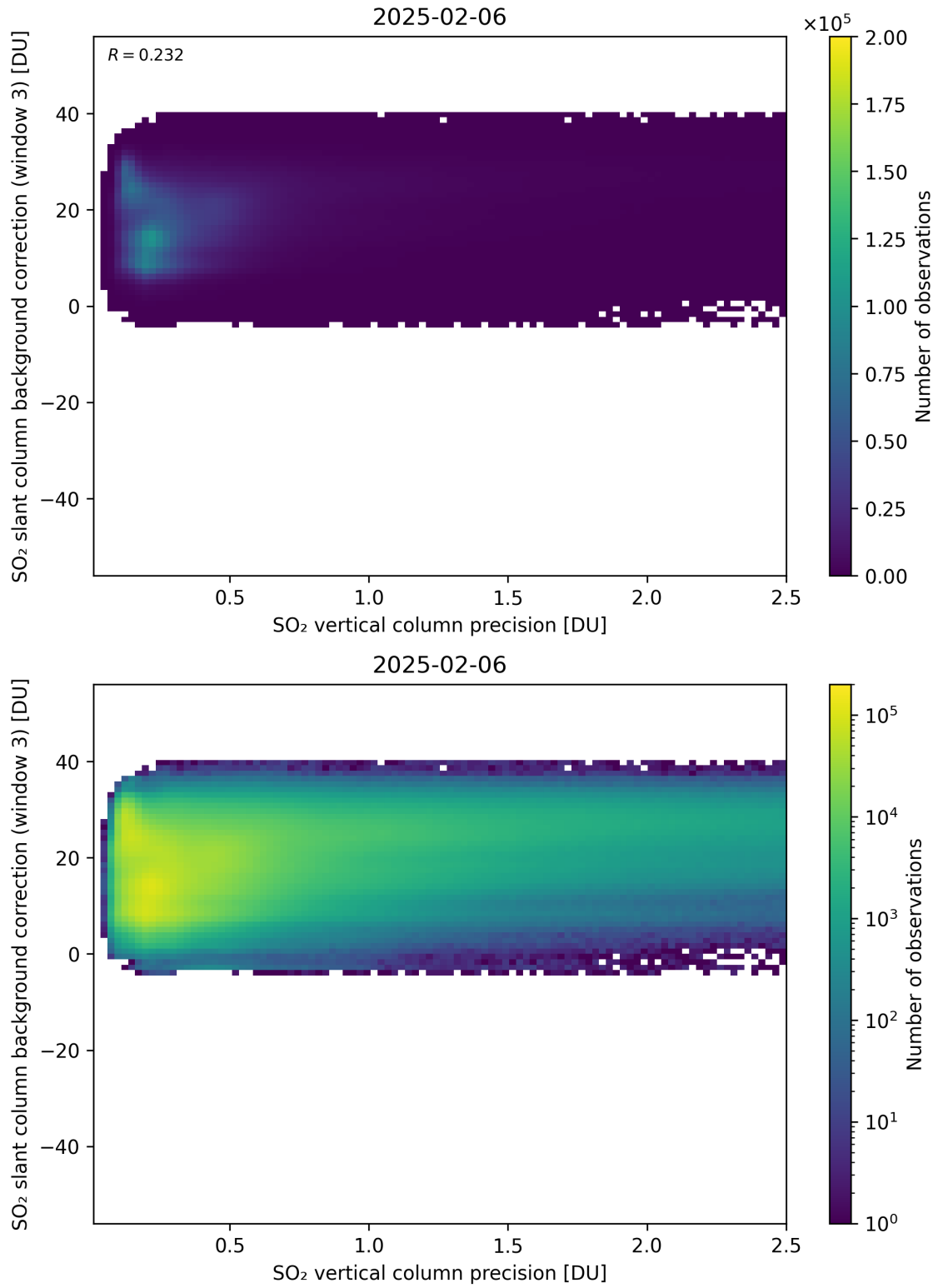
Figure 331: Scatter density plot of “SO 2 vertical column precision” against “SO 2 slant column background correction (window 3)” for 2025-02-05 to 2025-02-07.
