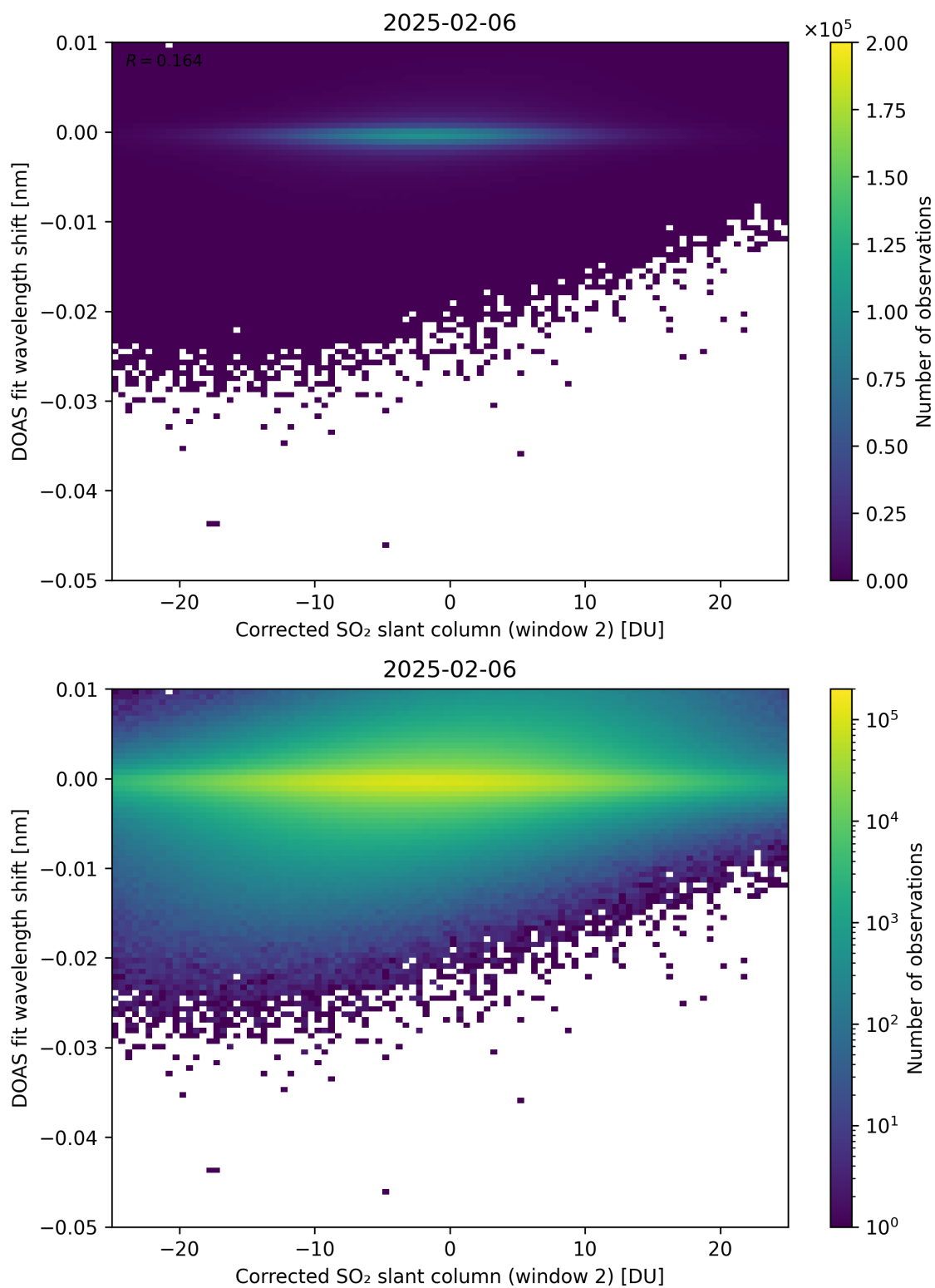
Figure 246: Scatter density plot of “Corrected SO 2 slant column (window 2)” against “DOAS fit wavelength shift” for 2025-02-05 to 2025-02-07.
