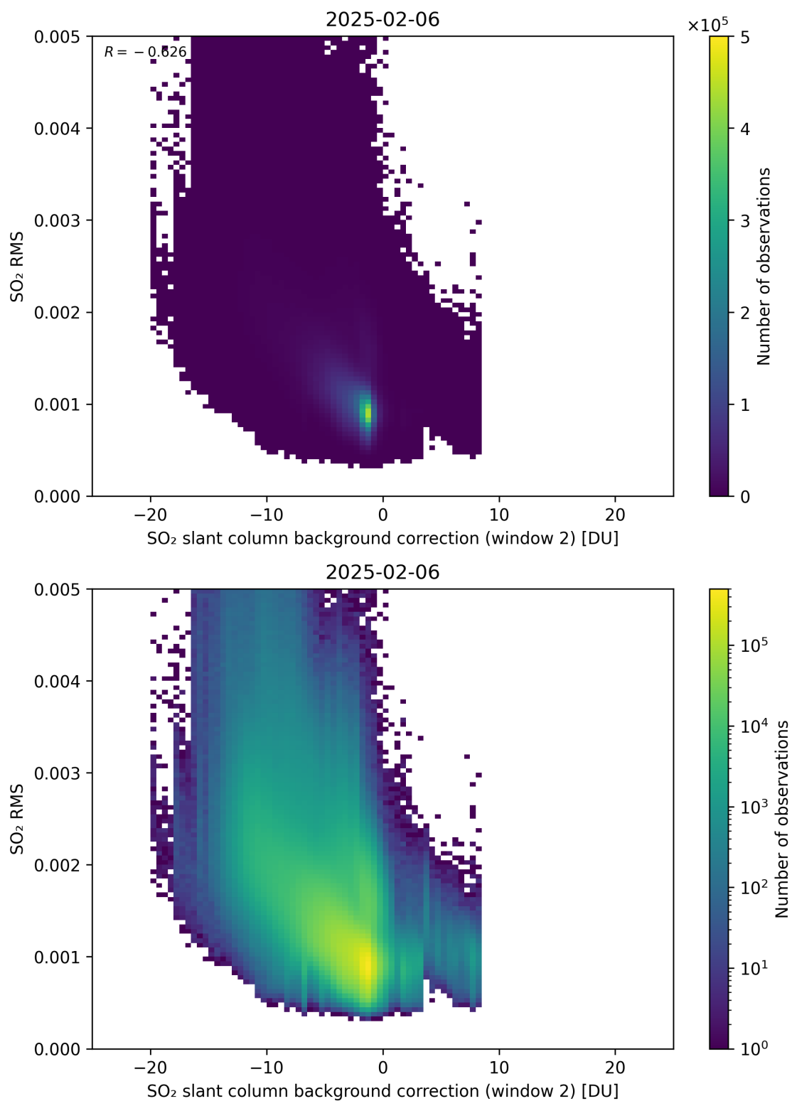
Figure 125: Scatter density plot of “SO 2 slant column background correction (window 2)” against “SO 2 RMS” for 2025-02-05 to 2025-02-07.
