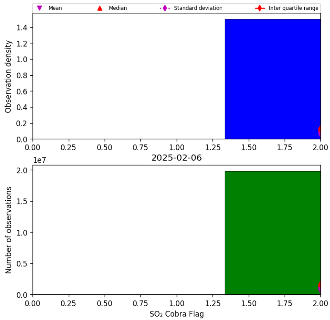
Figure 75: Histogram of “SO 2 Cobra Flag” for 2025-02-05 to 2025-02-07
