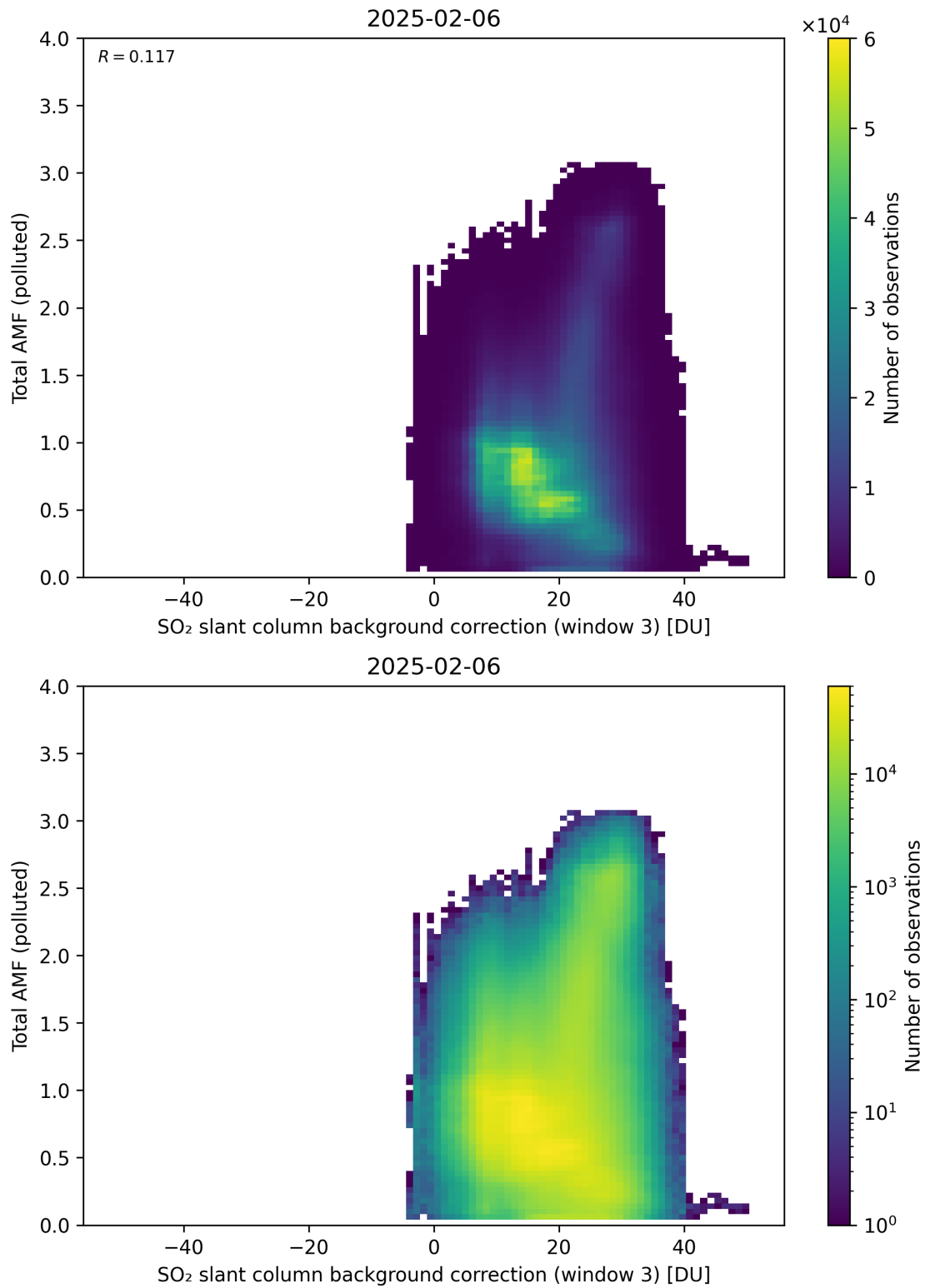
Figure 136: Scatter density plot of “SO 2 slant column background correction (window 3)” against “Total AMF (polluted)” for 2025-02-05 to 2025-02-07.
