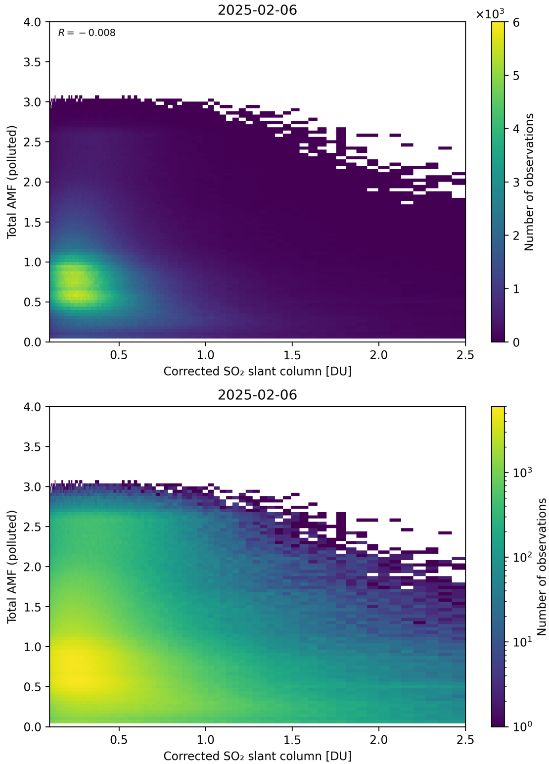
Figure 242: Scatter density plot of “Corrected SO 2 slant column” against “Total AMF (polluted)” for 2025-02-05 to 2025-02-07.
