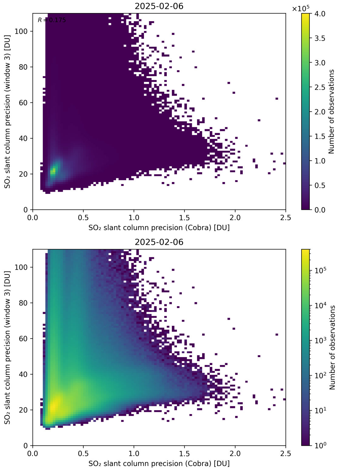
Figure 212: Scatter density plot of “SO 2 slant column precision (Cobra)” against “SO 2 slant column precision (window 3)” for 2025-02-05 to 2025-02-07.
