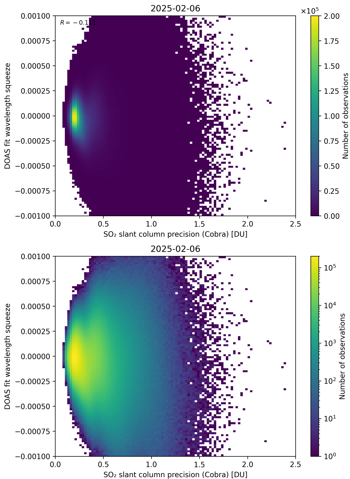
Figure 203: Scatter density plot of “SO 2 slant column precision (Cobra)” against “DOAS fit wavelength squeeze” for 2025-02-05 to 2025-02-07.
