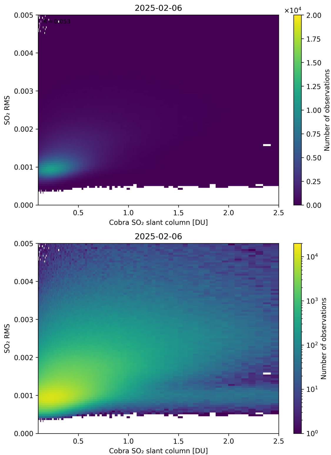
Figure 198: Scatter density plot of “Cobra SO 2 slant column” against “SO 2 RMS” for 2025-02-05 to 2025-02-07.
