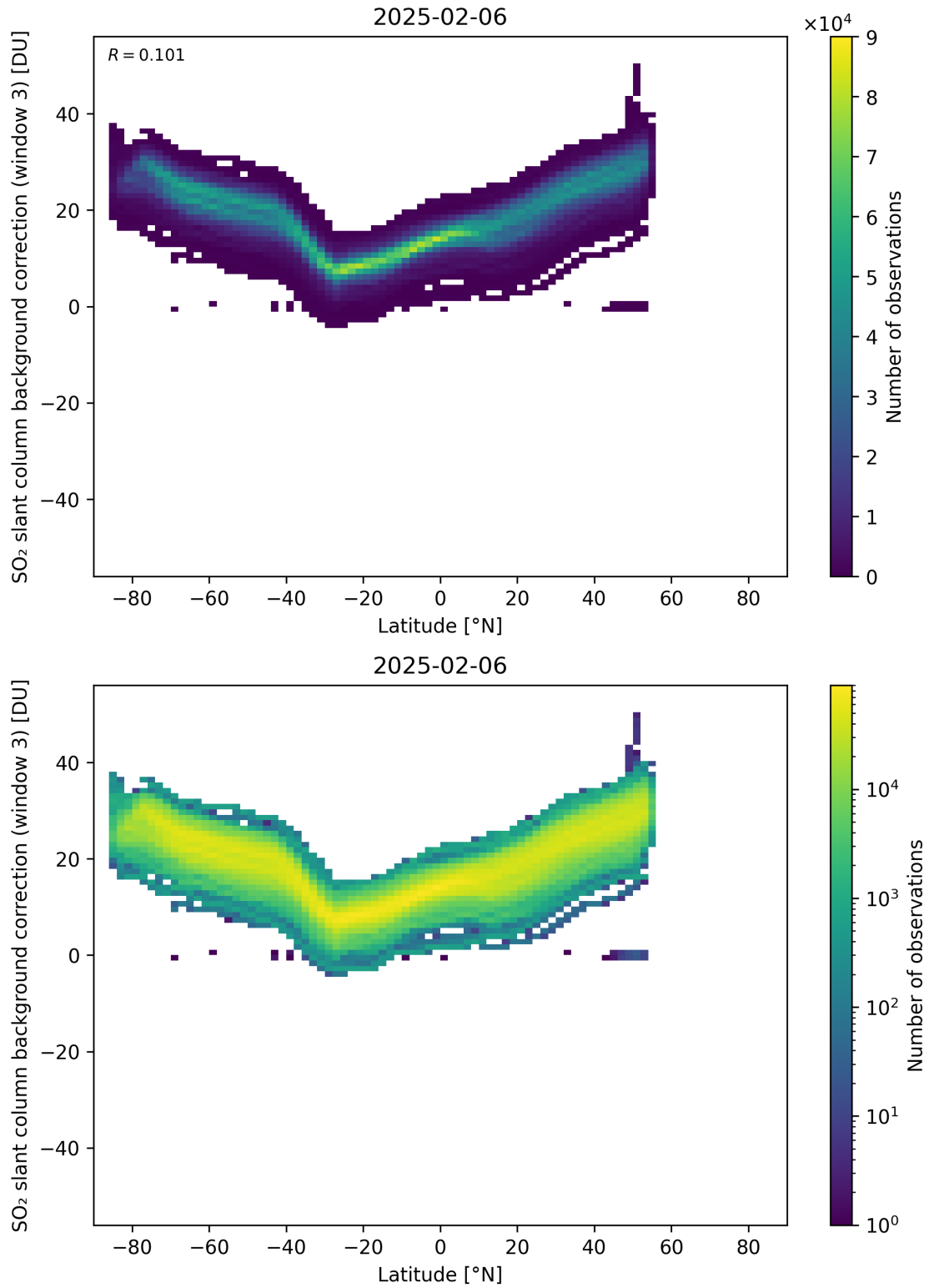
Figure 152: Scatter density plot of “Latitude” against “SO 2 slant column background correction (window 3)” for 2025-02-05 to 2025-02-07.
