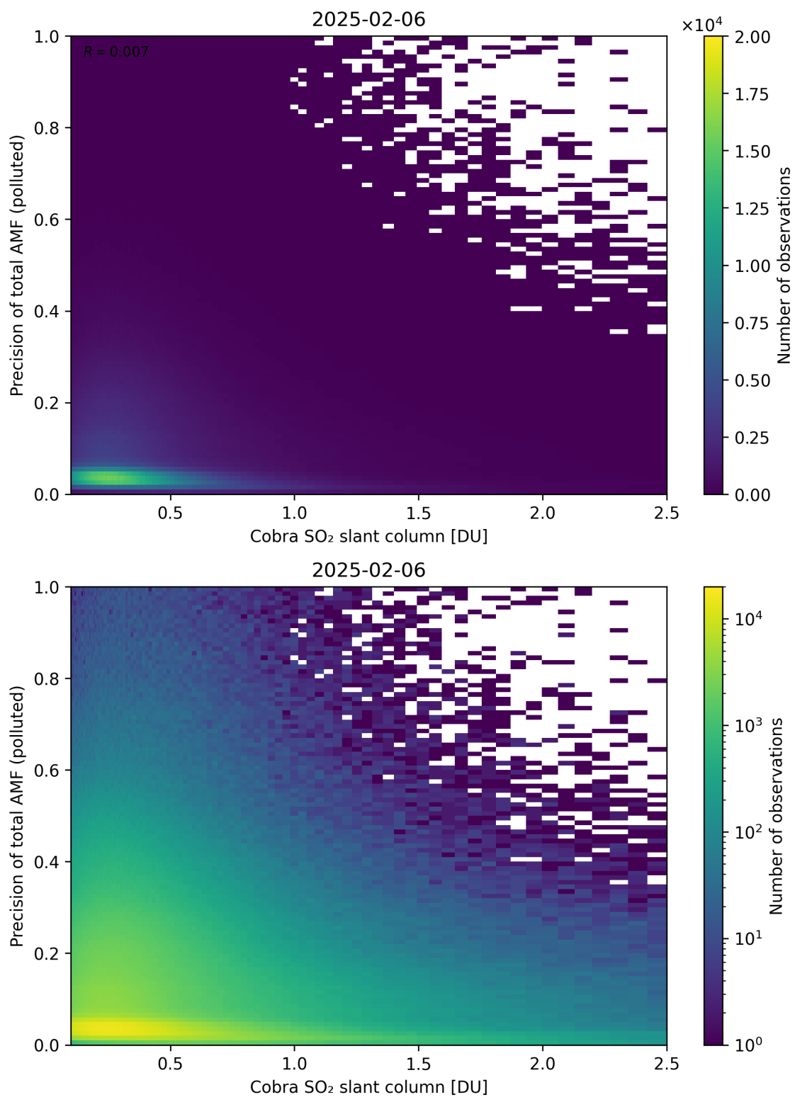
Figure 225: Scatter density plot of “Cobra SO 2 slant column” against “Precision of total AMF (polluted)” for 2025-02-05 to 2025-02-07.
