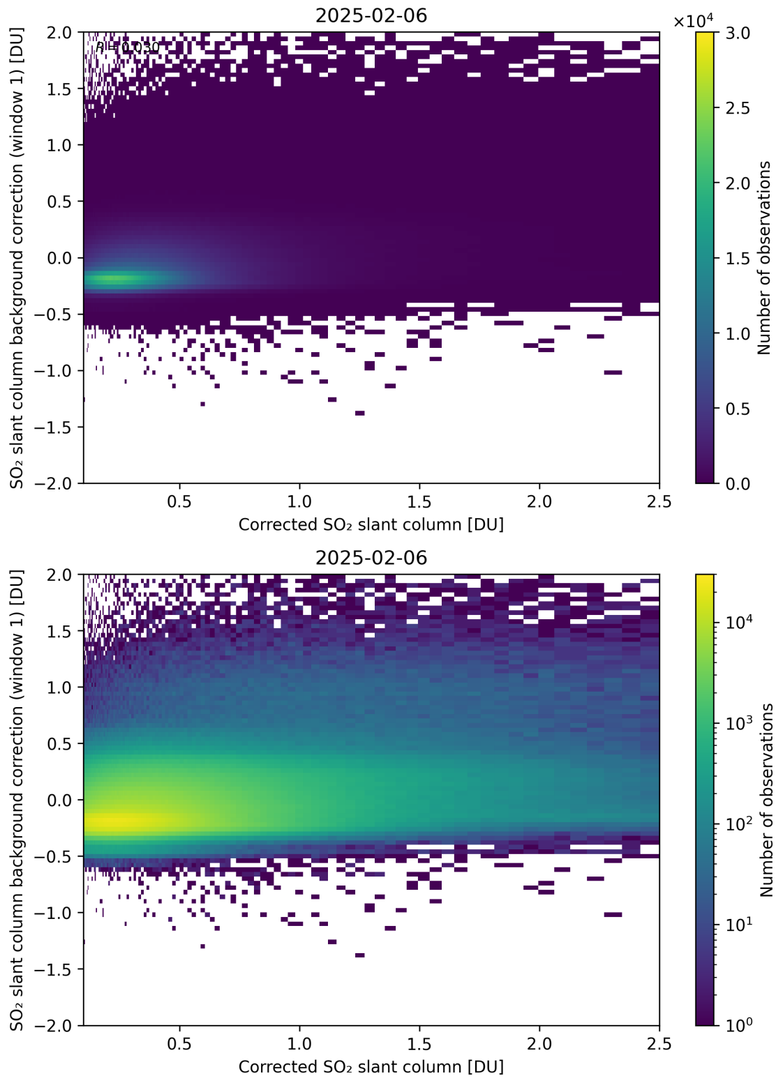
Figure 226: Scatter density plot of “Corrected SO 2 slant column” against “SO 2 slant column background correction (window 1)” for 2025-02-05 to 2025-02-07.
