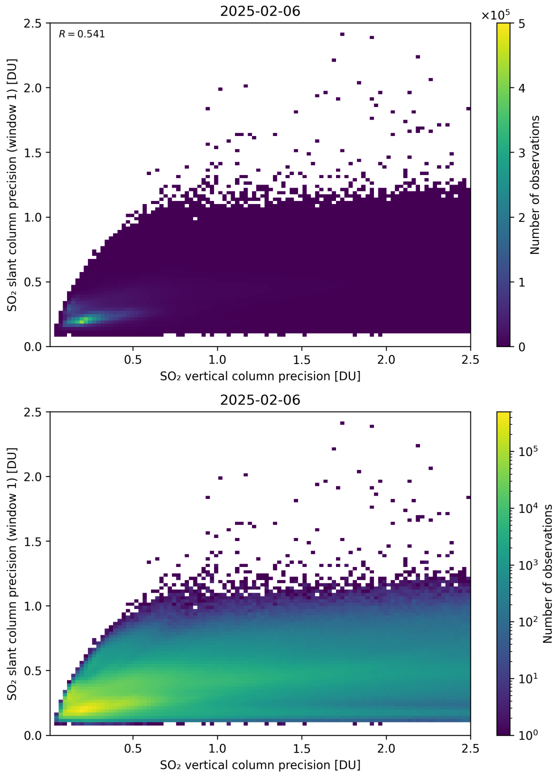
Figure 342: Scatter density plot of “SO 2 vertical column precision” against “SO 2 slant column precision (window 1)” for 2025-02-05 to 2025-02-07.
