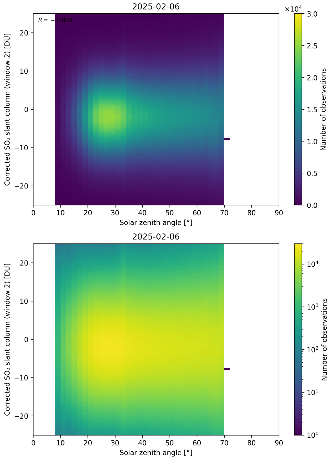
Figure 182: Scatter density plot of “Solar zenith angle” against “Corrected SO 2 slant column (window 2)” for 2025-02-05 to 2025-02-07.
