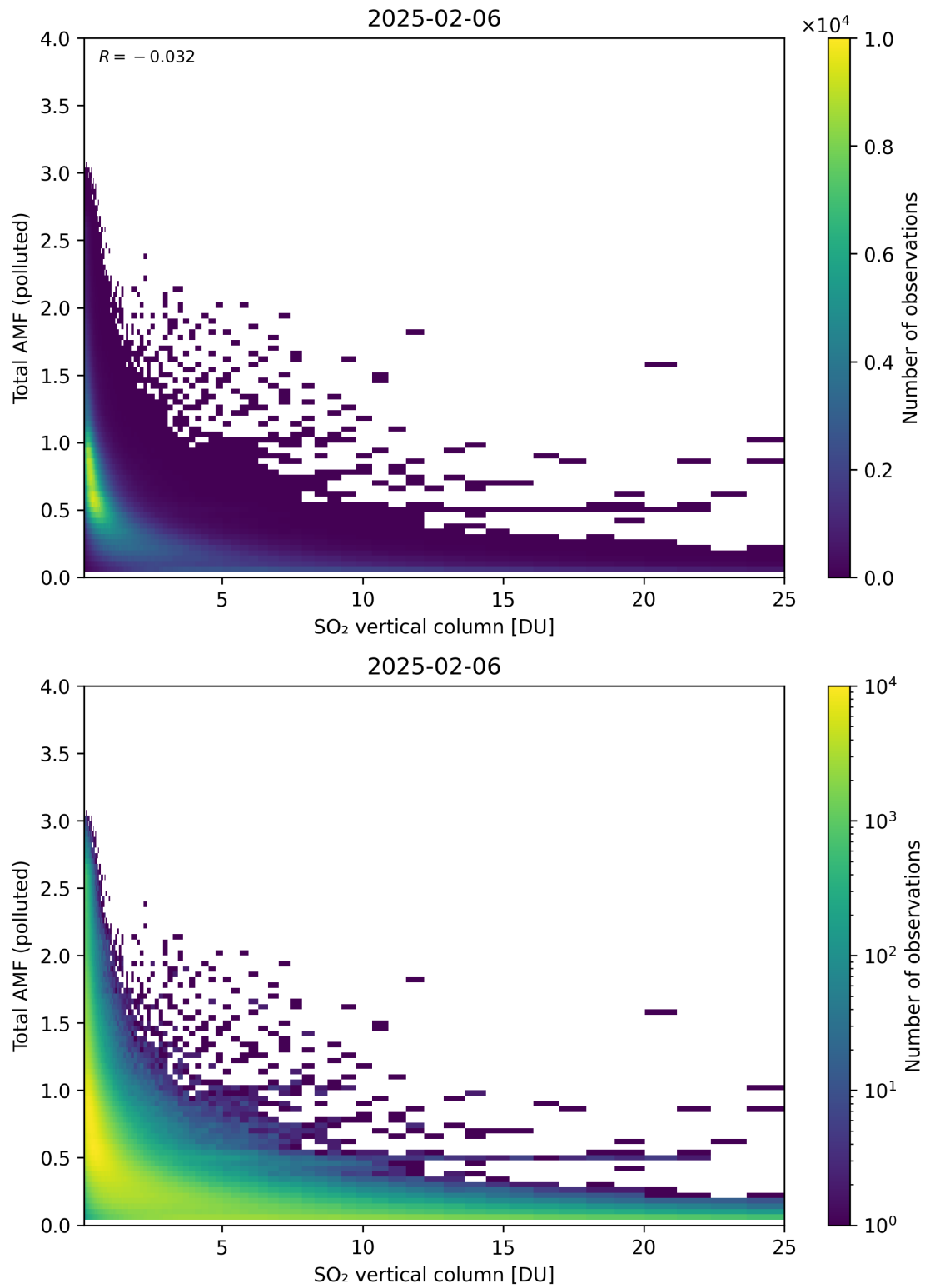
Figure 359: Scatter density plot of “SO 2 vertical column” against “Total AMF (polluted)” for 2025-02-05 to 2025-02-07.
