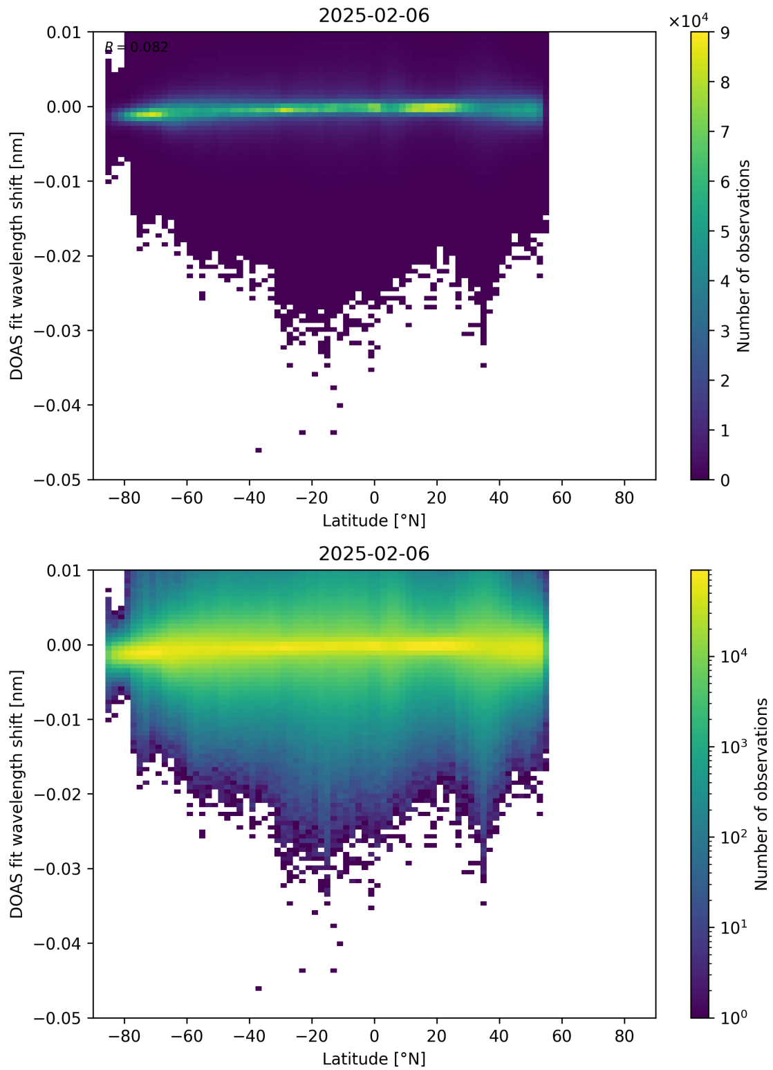
Figure 153: Scatter density plot of “Latitude” against “DOAS fit wavelength shift” for 2025-02-05 to 2025-02-07.
