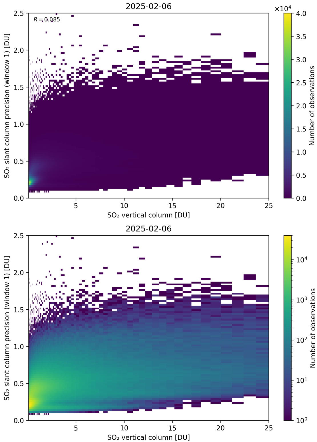
Figure 355: Scatter density plot of “SO 2 vertical column” against “SO 2 slant column precision (window 1)” for 2025-02-05 to 2025-02-07.
