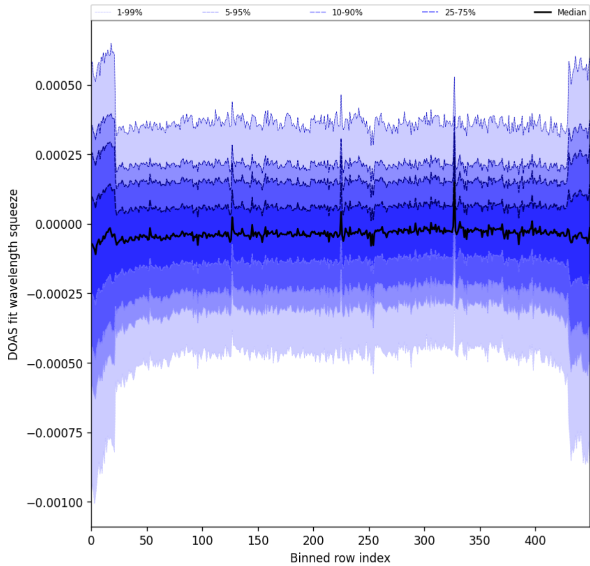
Figure 103: Along track statistics of “DOAS fit wavelength squeeze” for 2025-02-05 to 2025-02-07
