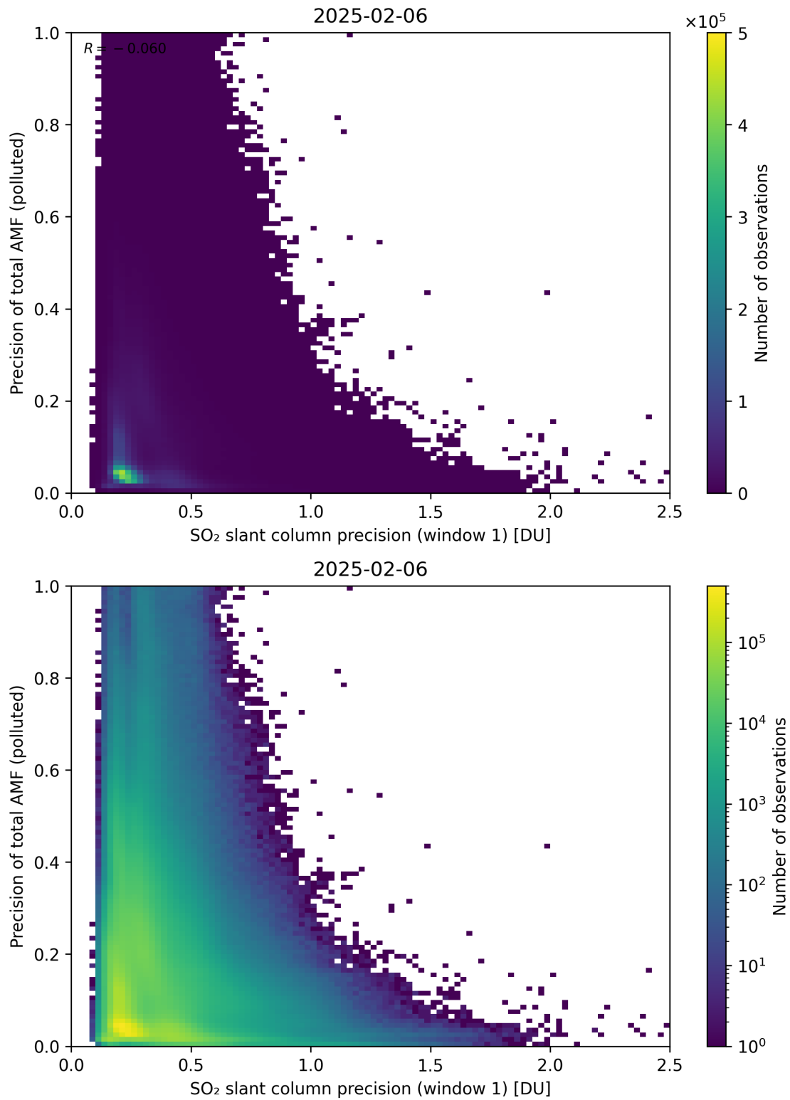
Figure 281: Scatter density plot of “SO 2 slant column precision (window 1)” against “Precision of total AMF (polluted)” for 2025-02-05 to 2025-02-07.
