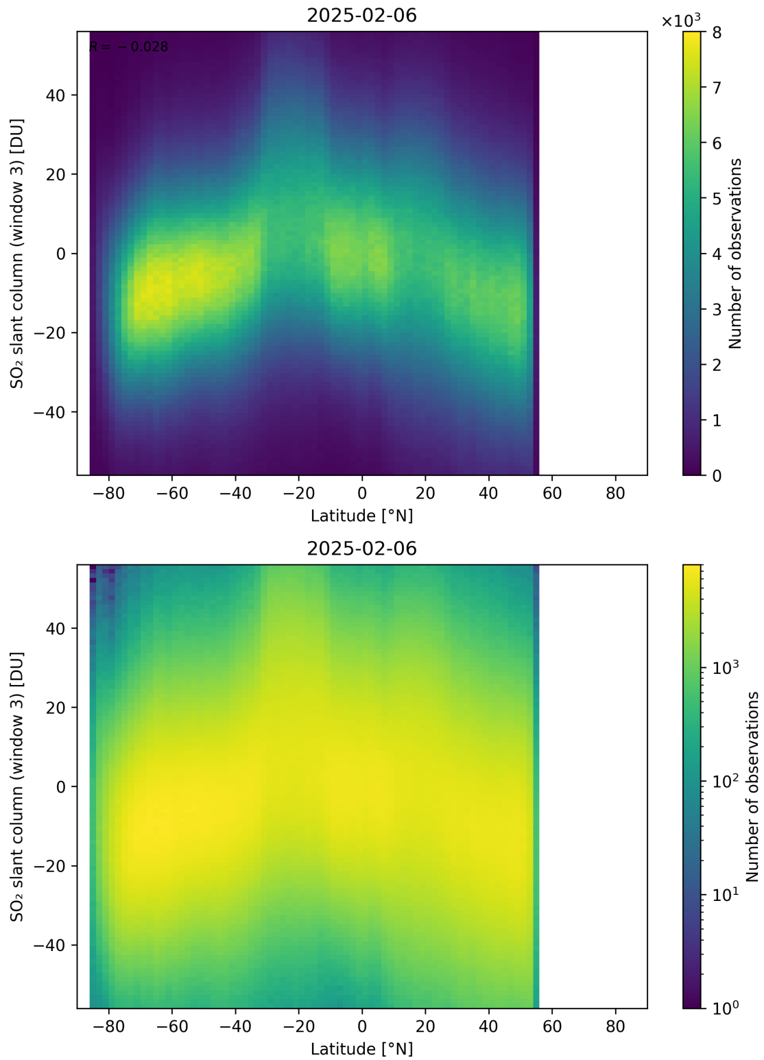
Figure 165: Scatter density plot of “Latitude” against “SO 2 slant column (window 3)” for 2025-02-05 to 2025-02-07.
