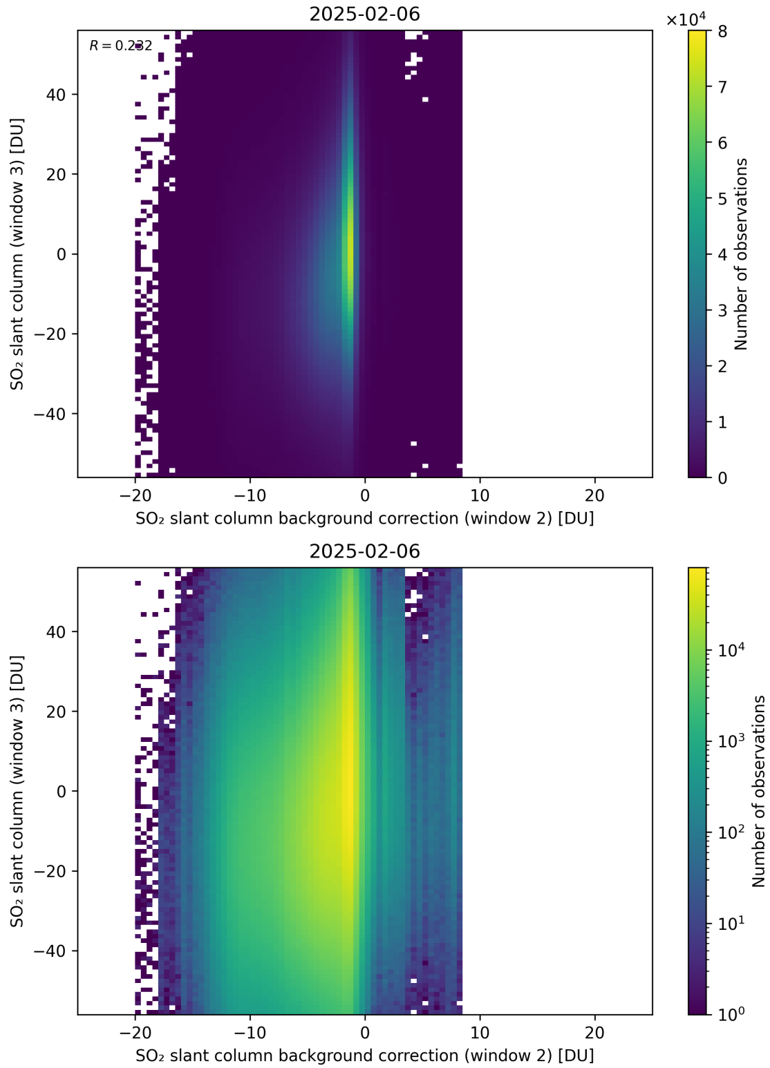
Figure 128: Scatter density plot of “SO 2 slant column background correction (window 2)” against “SO 2 slant column (window 3)” for 2025-02-05 to 2025-02-07.
