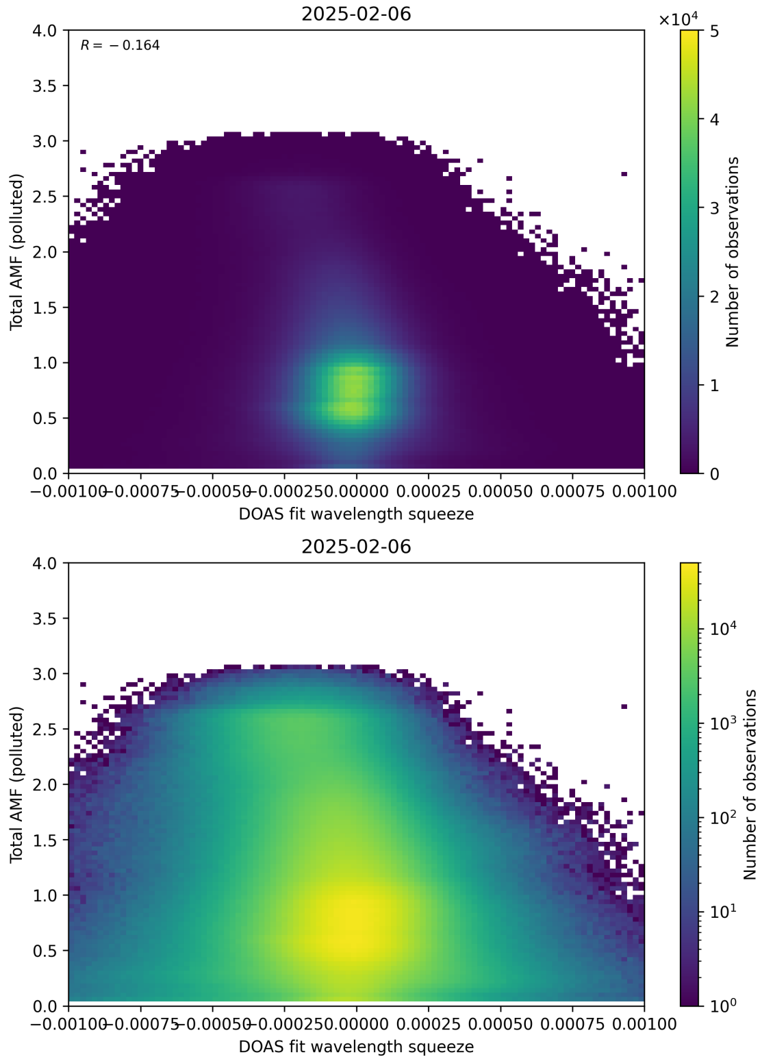
Figure 145: Scatter density plot of “DOAS fit wavelength squeeze” against “Total AMF (polluted)” for 2025-02-05 to 2025-02-07.
