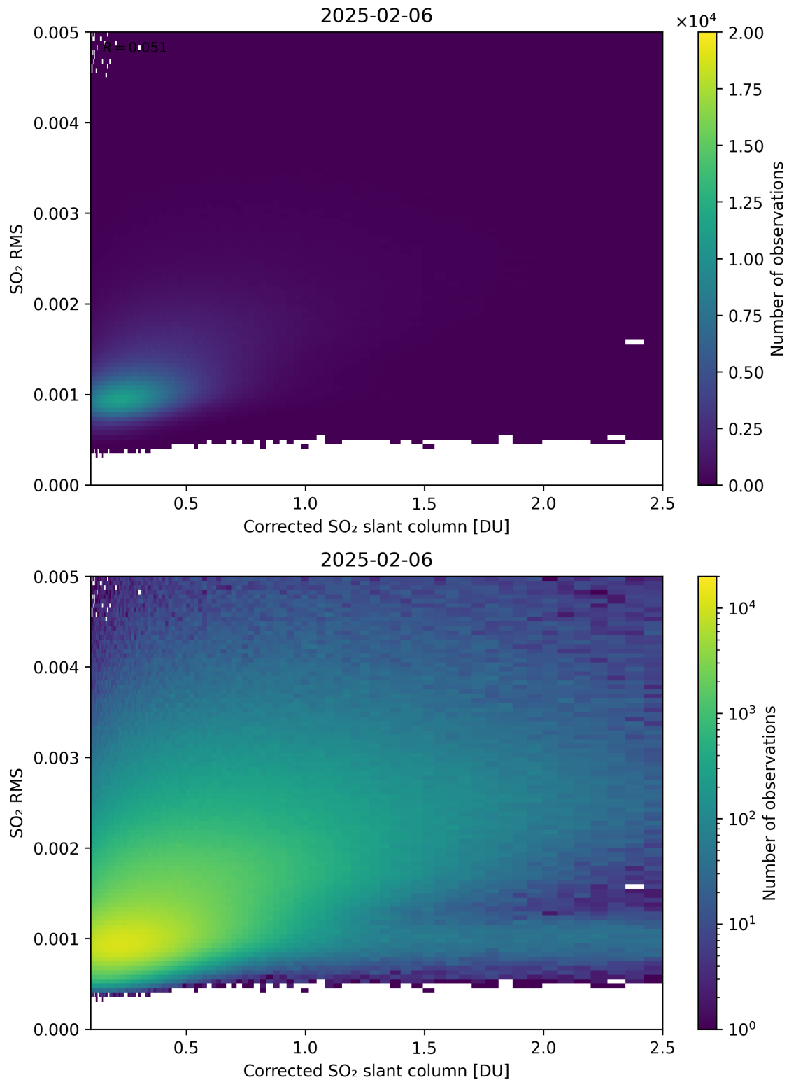
Figure 231: Scatter density plot of “Corrected SO 2 slant column” against “SO 2 RMS” for 2025-02-05 to 2025-02-07.
