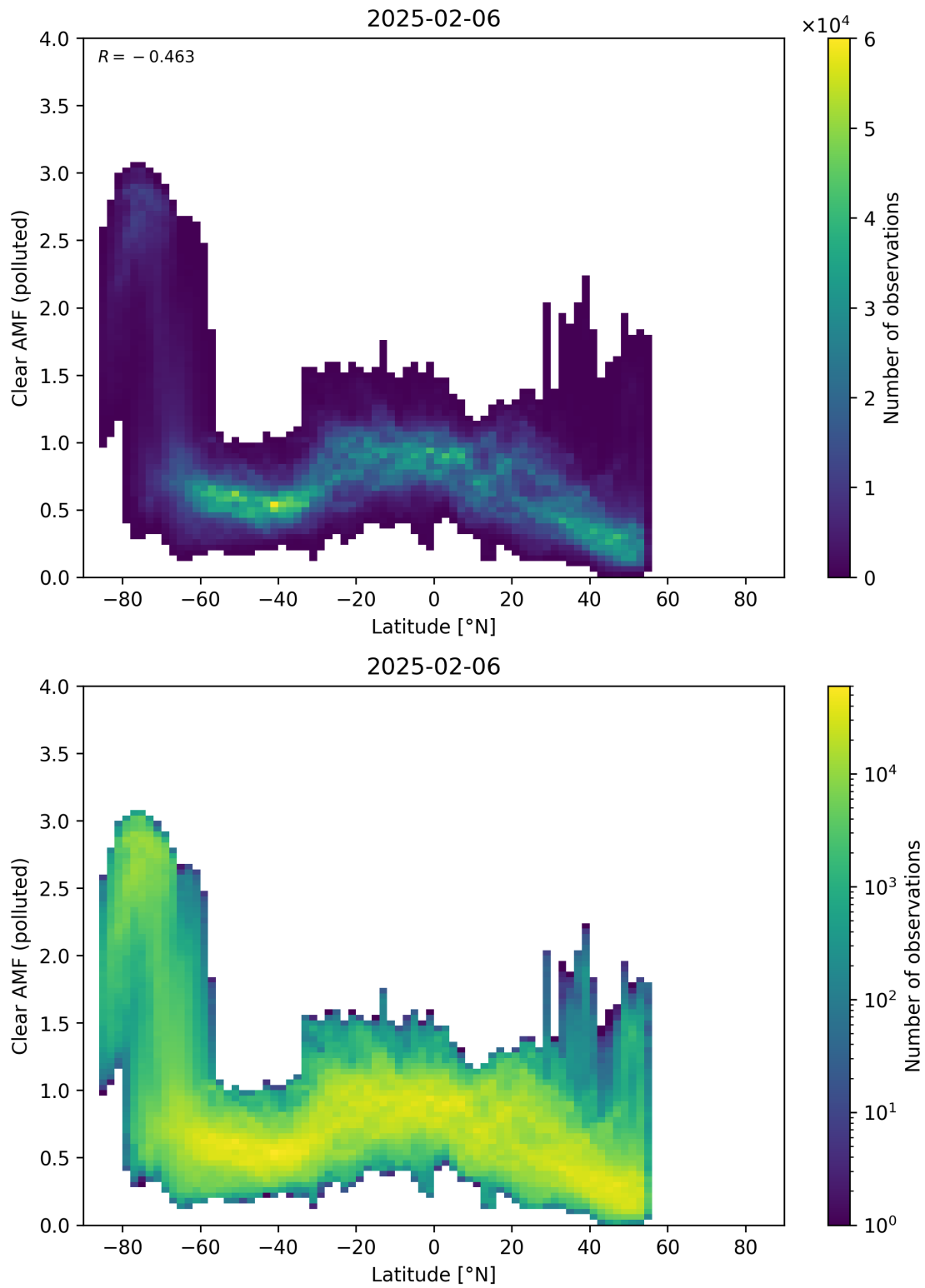
Figure 156: Scatter density plot of “Latitude” against “Clear AMF (polluted)” for 2025-02-05 to 2025-02-07.
