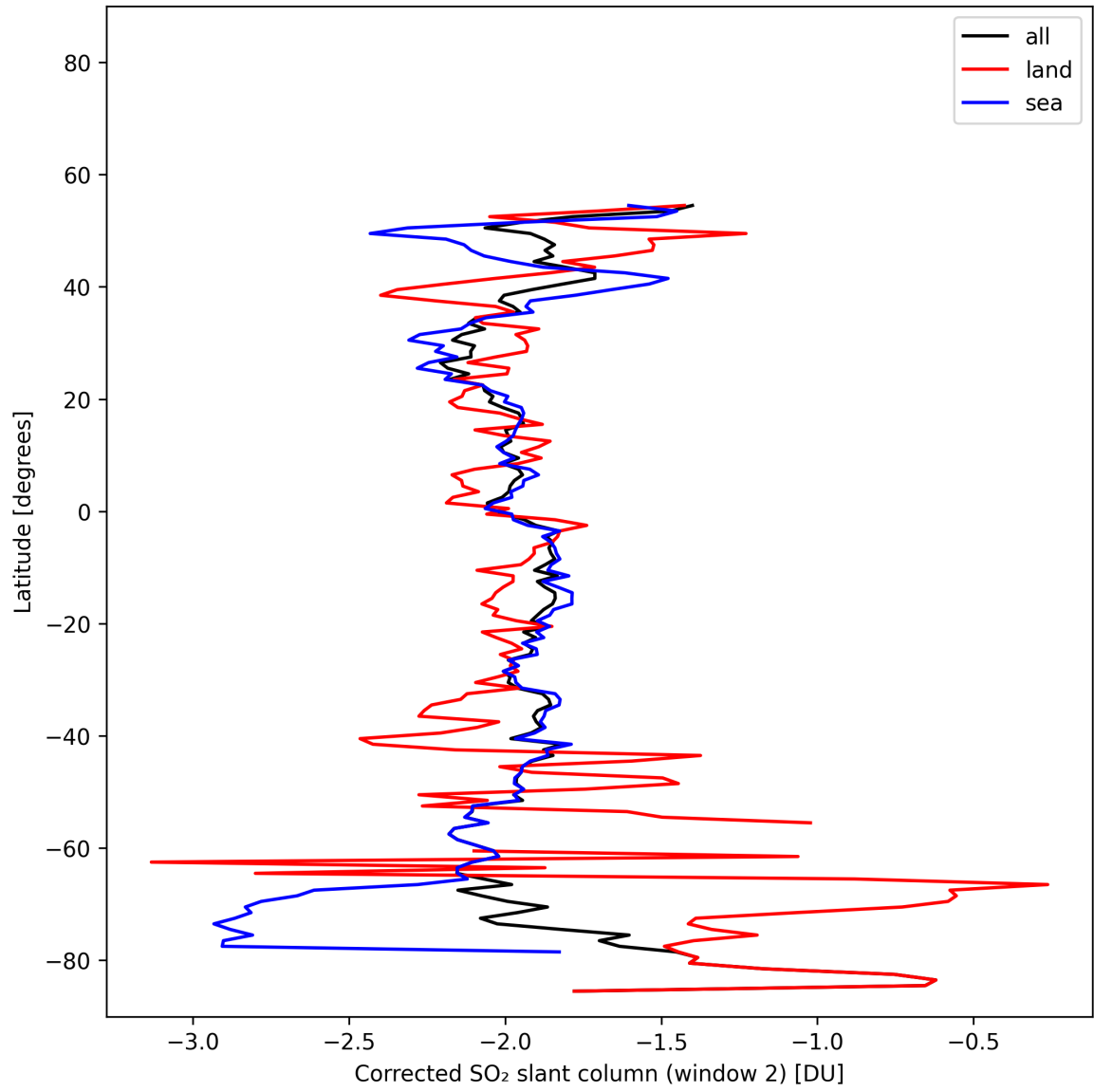
Figure 43: Zonal average of “Corrected SO 2 slant column (window 2)” for 2025-02-05 to 2025-02-07.
