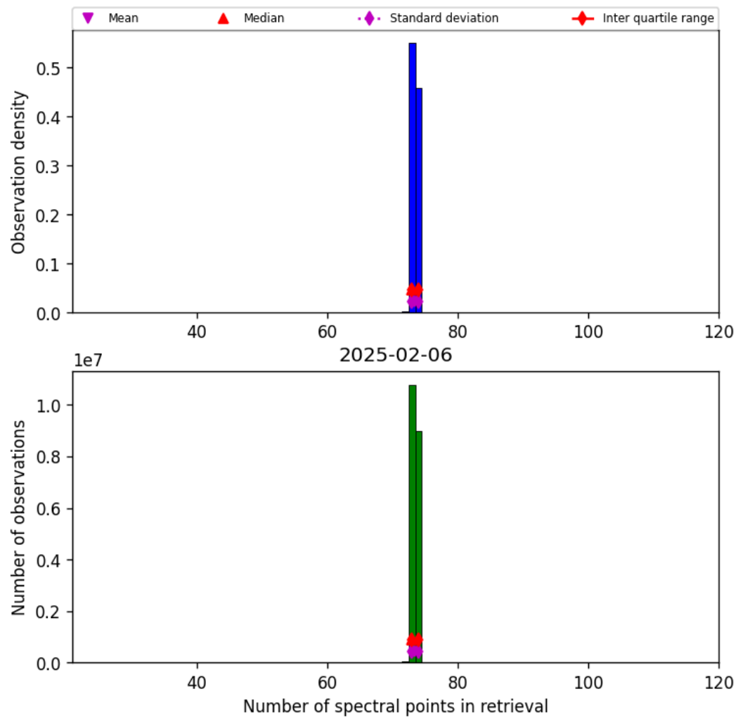
Figure 82: Histogram of “Number of spectral points in retrieval” for 2025-02-05 to 2025-02-07
