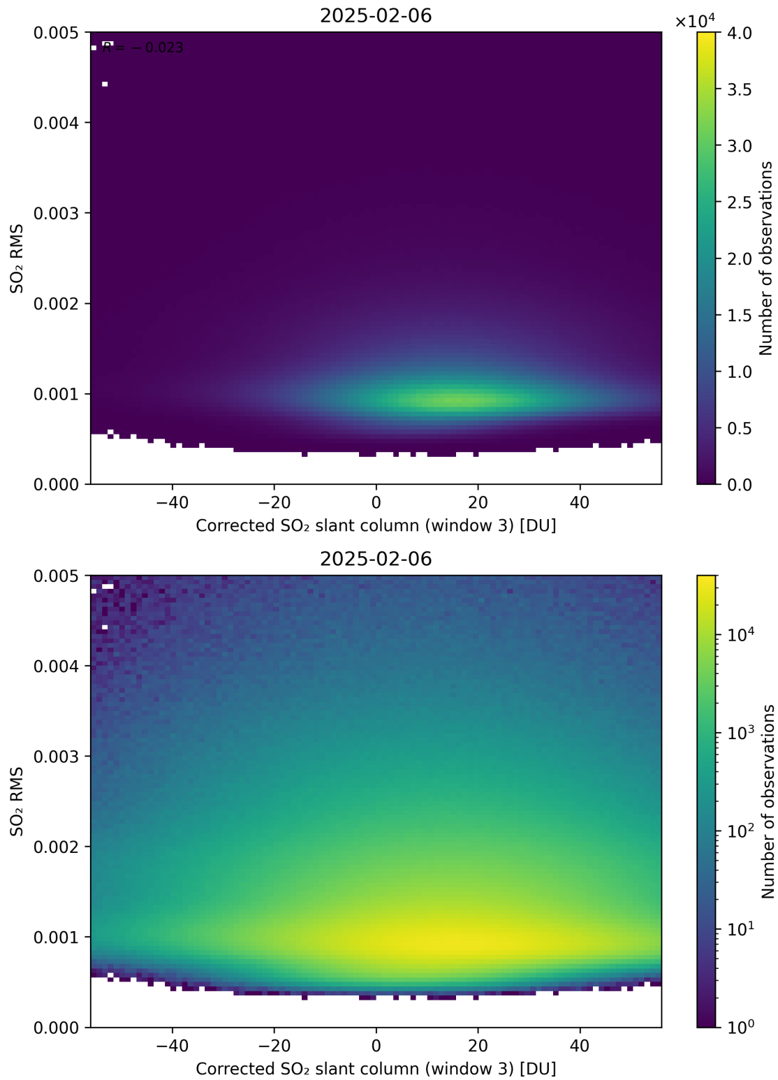
Figure 258: Scatter density plot of “Corrected SO 2 slant column (window 3)” against “SO 2 RMS” for 2025-02-05 to 2025-02-07.
