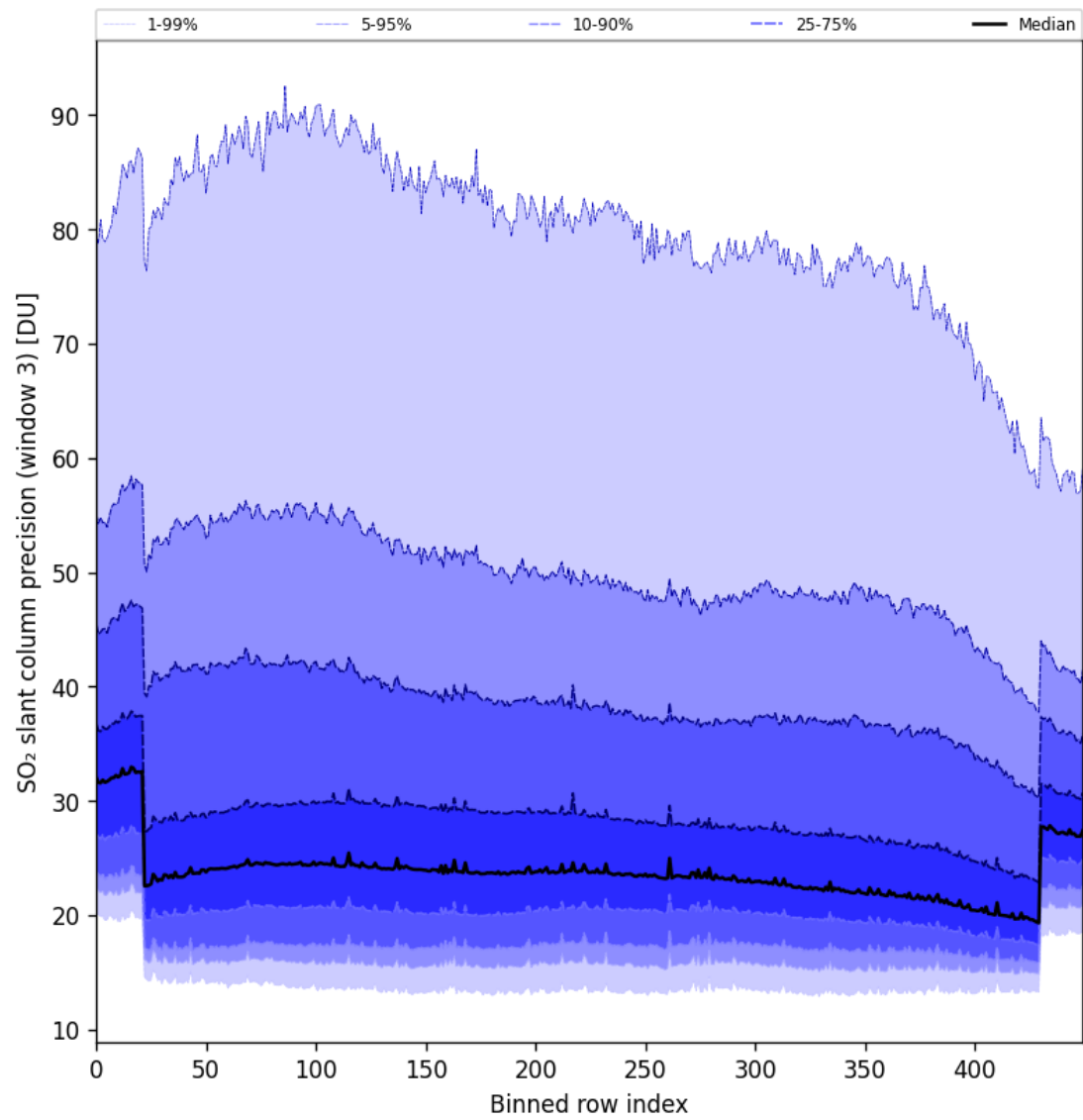
Figure 98: Along track statistics of “SO 2 slant column precision (window 3)” for 2025-02-05 to 2025-02-07
