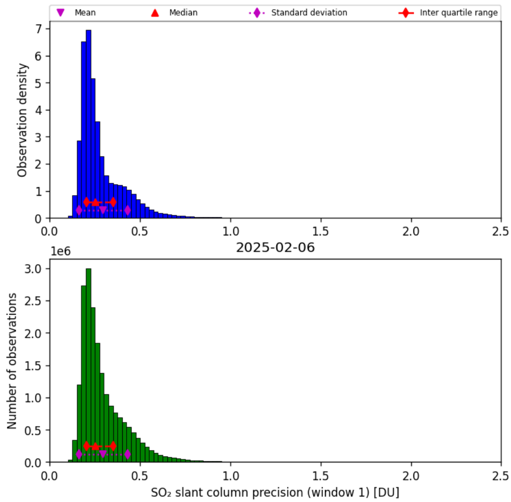
Figure 64: Histogram of “SO 2 slant column precision (window 1)” for 2025-02-05 to 2025-02-07
