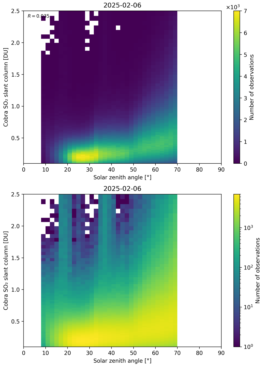
Figure 179: Scatter density plot of “Solar zenith angle” against “Cobra SO 2 slant column” for 2025-02-05 to 2025-02-07.
