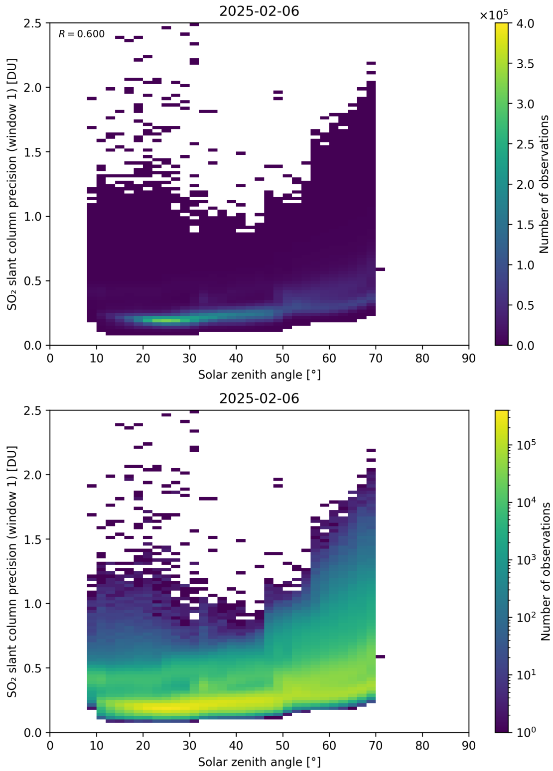
Figure 185: Scatter density plot of “Solar zenith angle” against “SO 2 slant column precision (window 1)” for 2025-02-05 to 2025-02-07.
