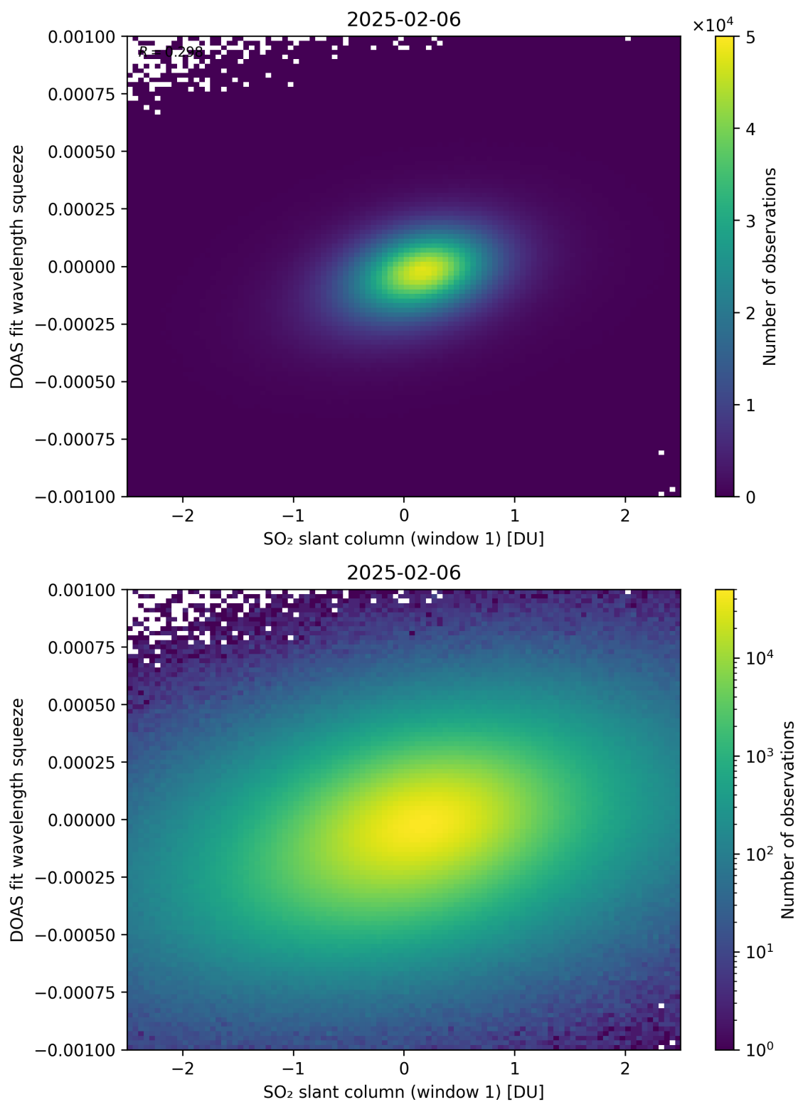
Figure 266: Scatter density plot of “SO 2 slant column (window 1)” against “DOAS fit wavelength squeeze” for 2025-02-05 to 2025-02-07.
