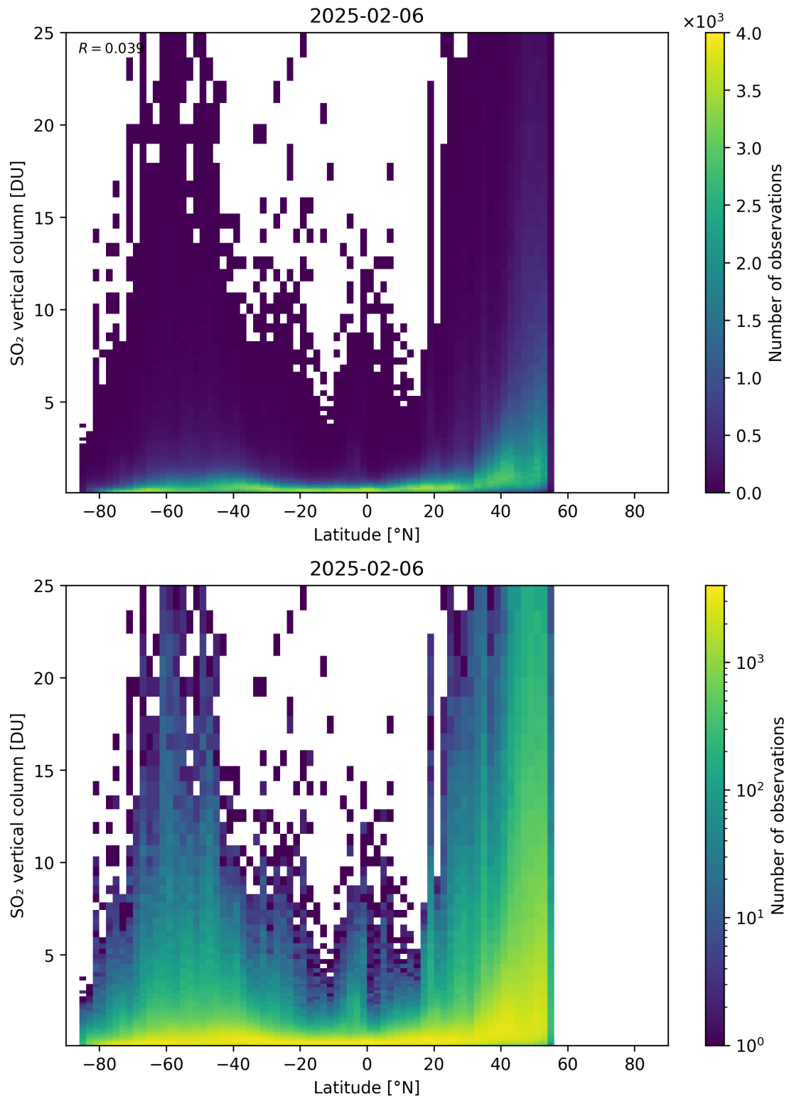
Figure 169: Scatter density plot of “Latitude” against “SO 2 vertical column” for 2025-02-05 to 2025-02-07.
