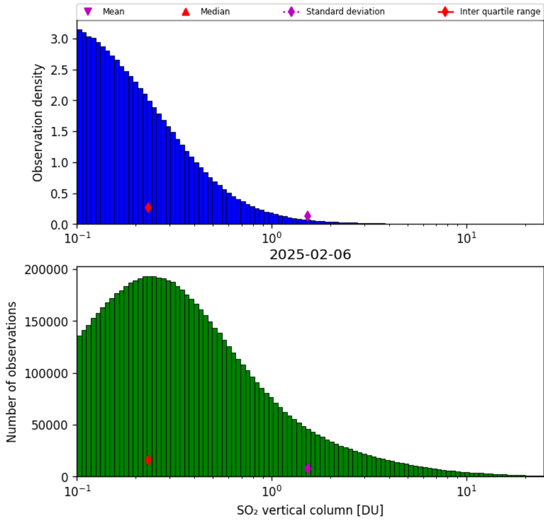
Figure 58: Histogram of “SO 2 vertical column” for 2025-02-05 to 2025-02-07
