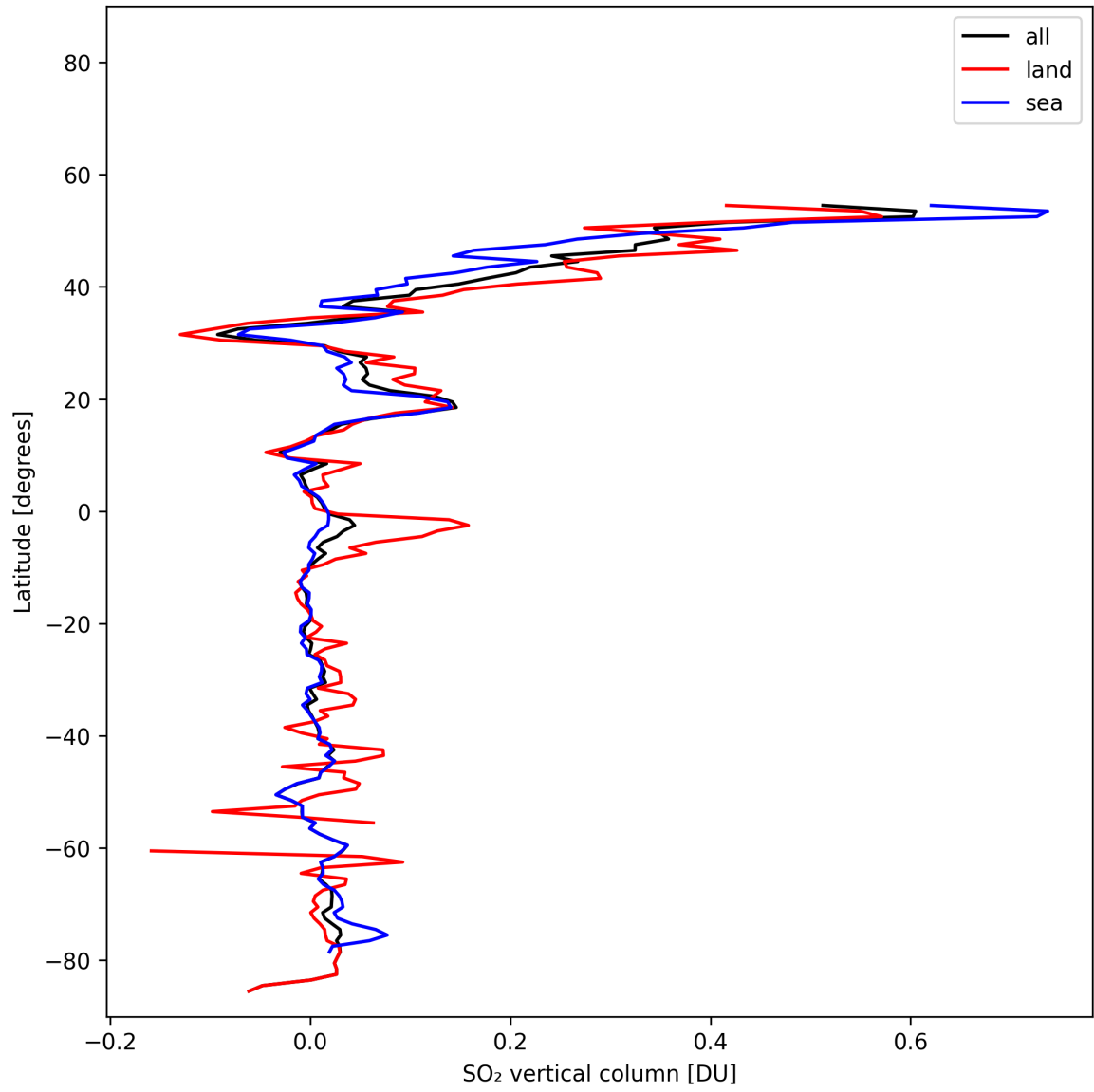
Figure 32: Zonal average of “SO 2 vertical column” for 2025-02-05 to 2025-02-07.
