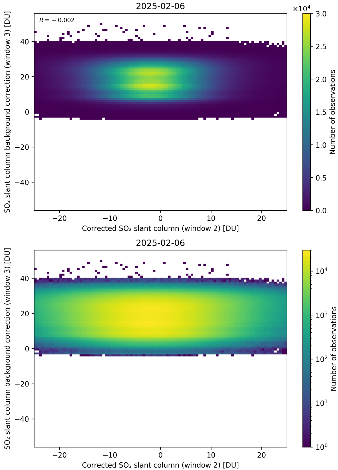
Figure 245: Scatter density plot of “Corrected SO 2 slant column (window 2)” against “SO 2 slant column background correction (window 3)” for 2025-02-05 to 2025-02-07.
