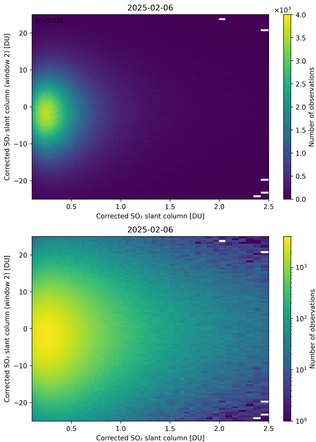
Figure 235: Scatter density plot of “Corrected SO 2 slant column” against “Corrected SO 2 slant column (window 2)” for 2025-02-05 to 2025-02-07.
