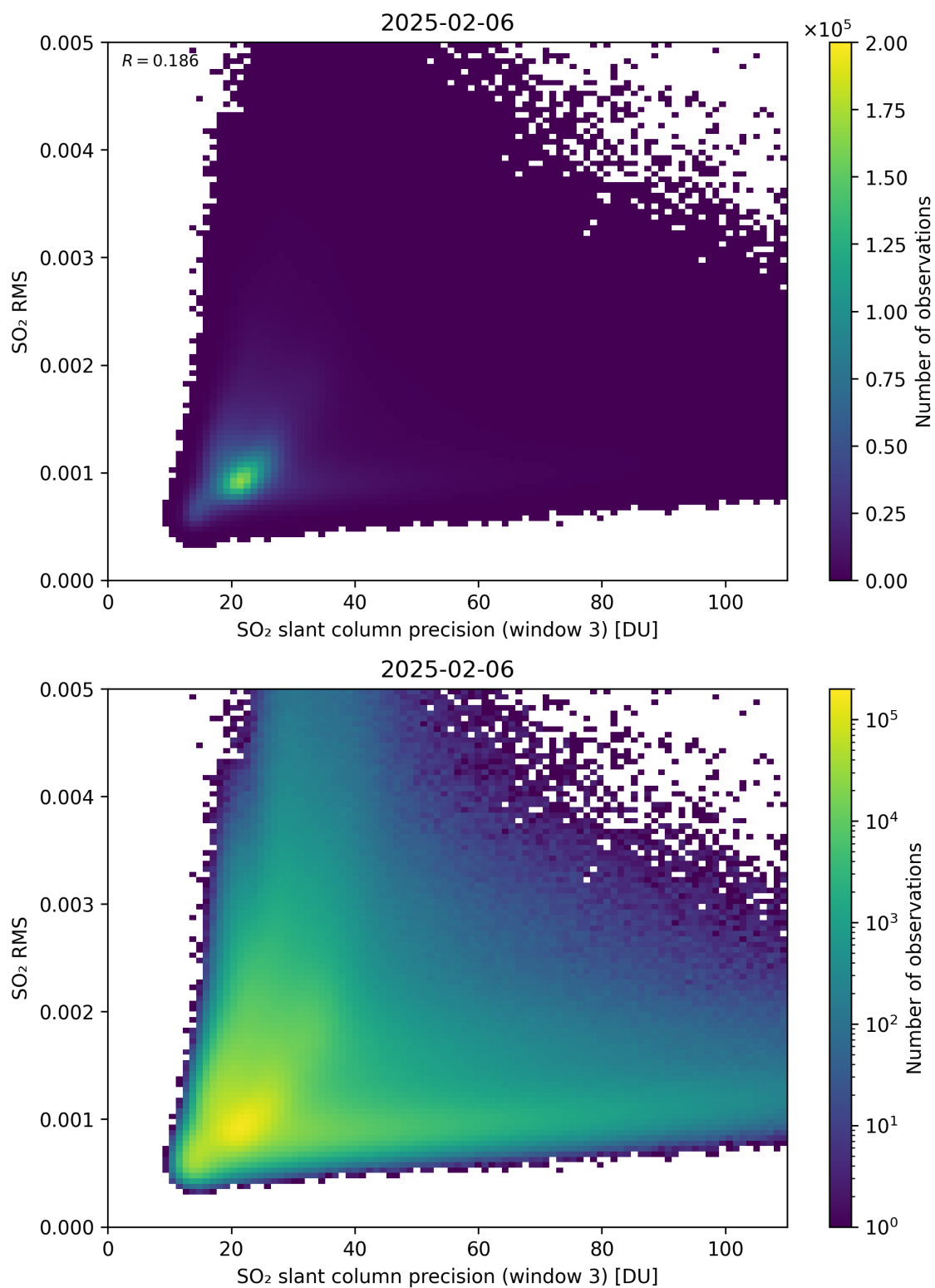
Figure 310: Scatter density plot of “SO 2 slant column precision (window 3)” against “SO 2 RMS” for 2025-02-05 to 2025-02-07.
