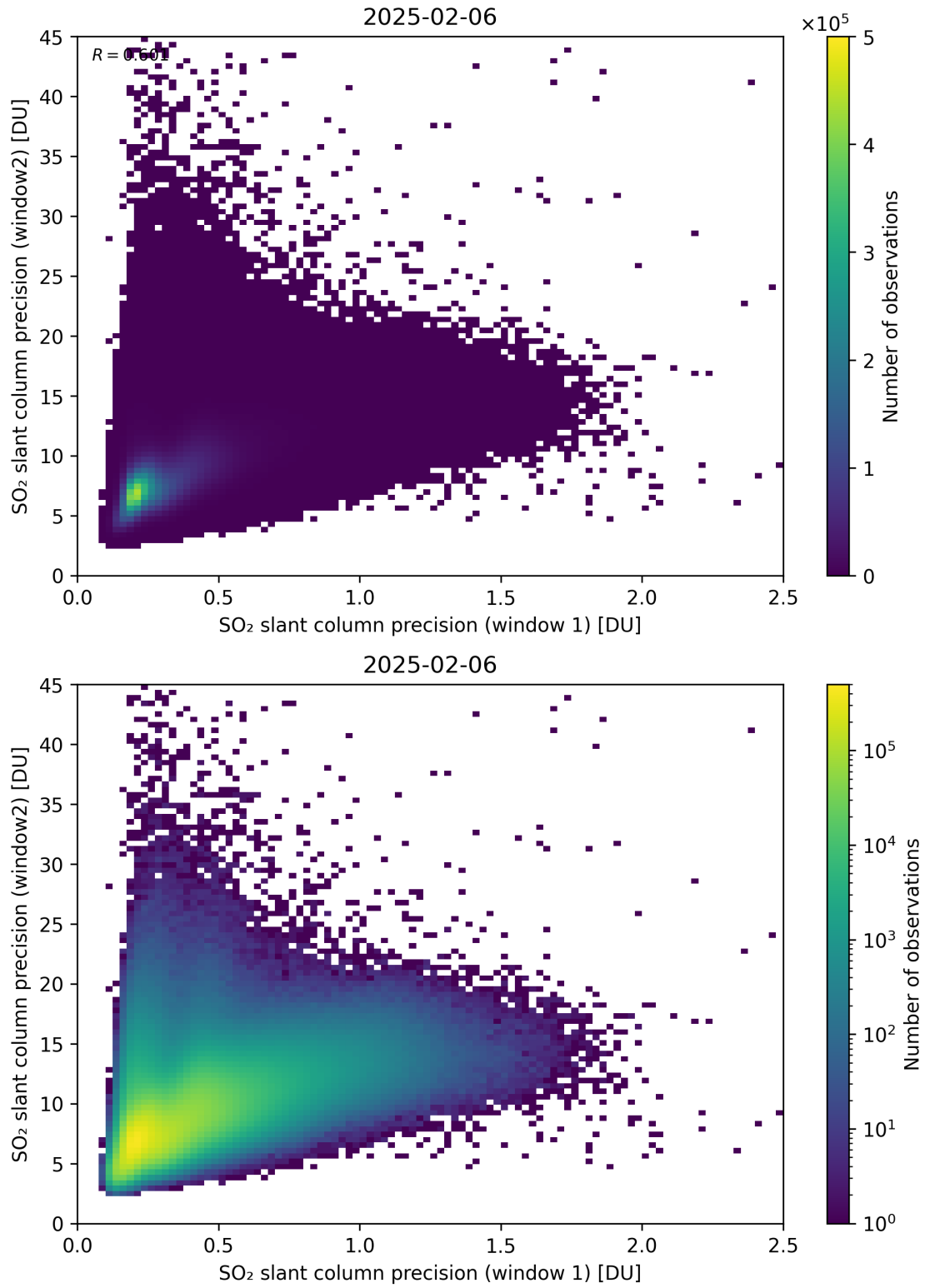
Figure 277: Scatter density plot of “SO 2 slant column precision (window 1)” against “SO 2 slant column precision (window2)” for 2025-02-05 to 2025-02-07.
