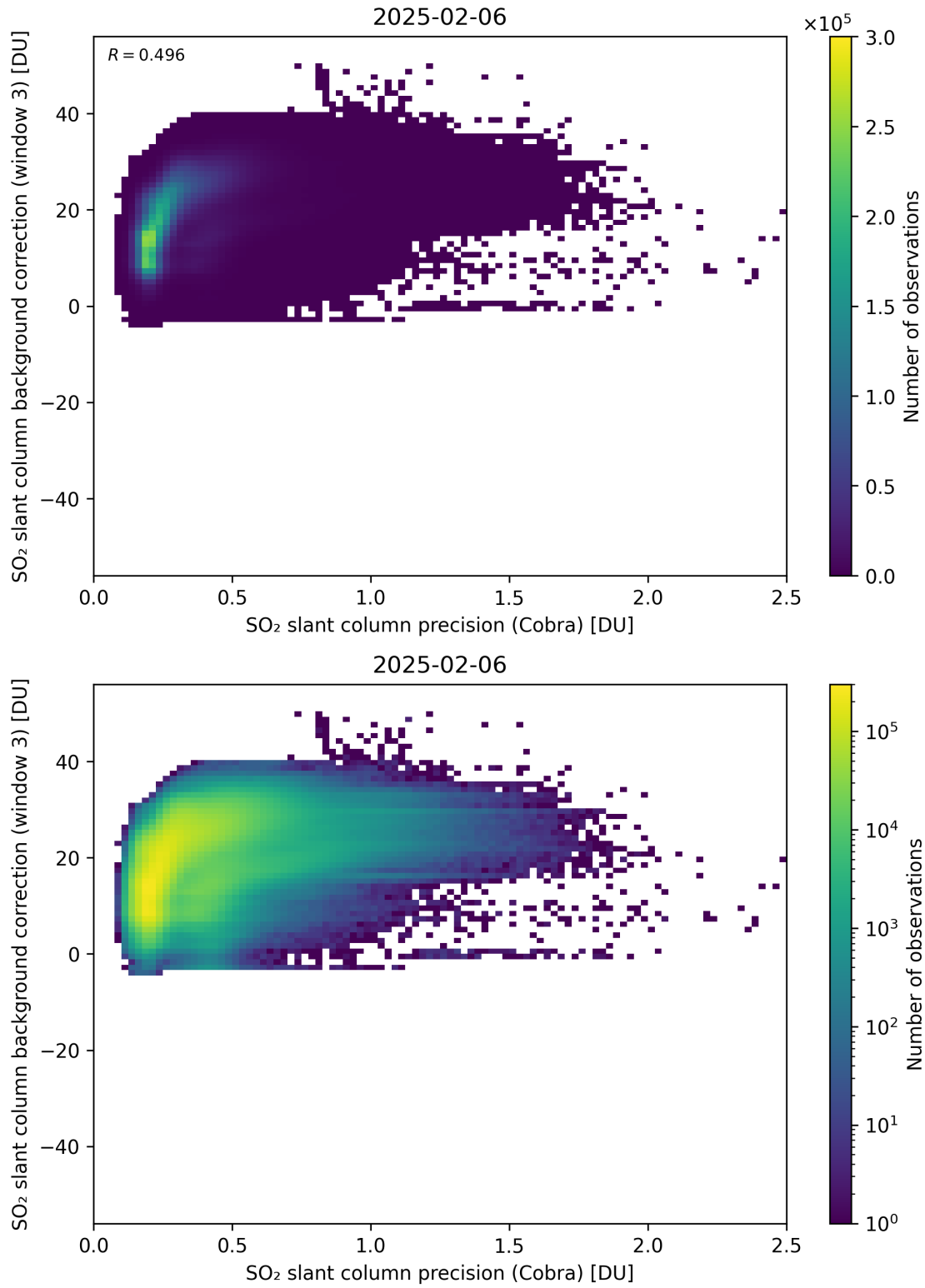
Figure 201: Scatter density plot of “SO 2 slant column precision (Cobra)” against “SO 2 slant column background correction (window 3)” for 2025-02-05 to 2025-02-07.
