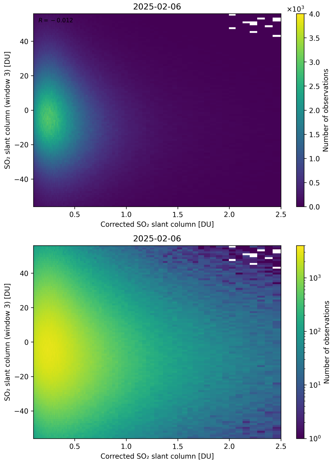
Figure 240: Scatter density plot of “Corrected SO 2 slant column” against “SO 2 slant column (window 3)” for 2025-02-05 to 2025-02-07.
