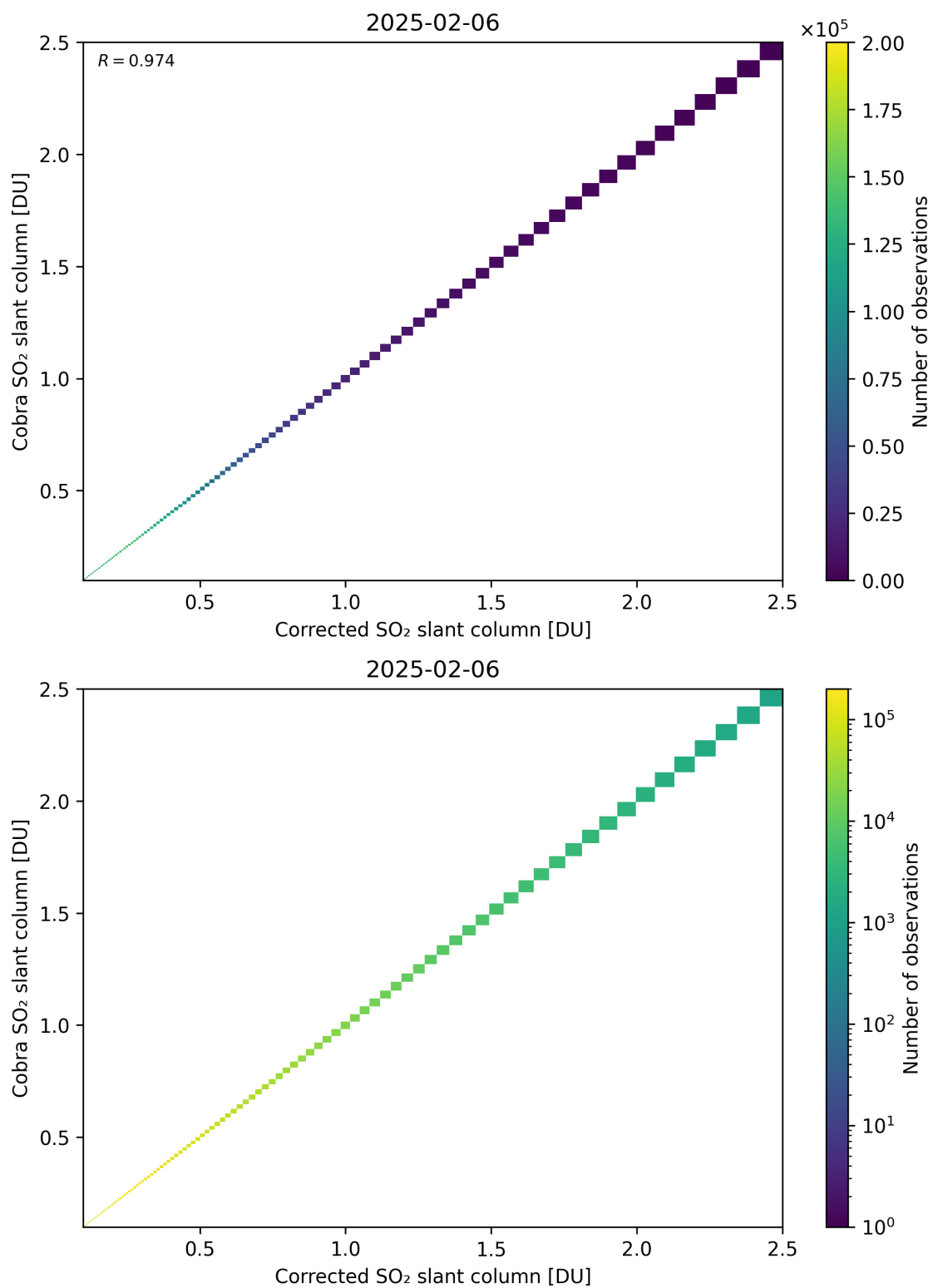
Figure 233: Scatter density plot of “Corrected SO 2 slant column” against “Cobra SO 2 slant column” for 2025-02-05 to 2025-02-07.
