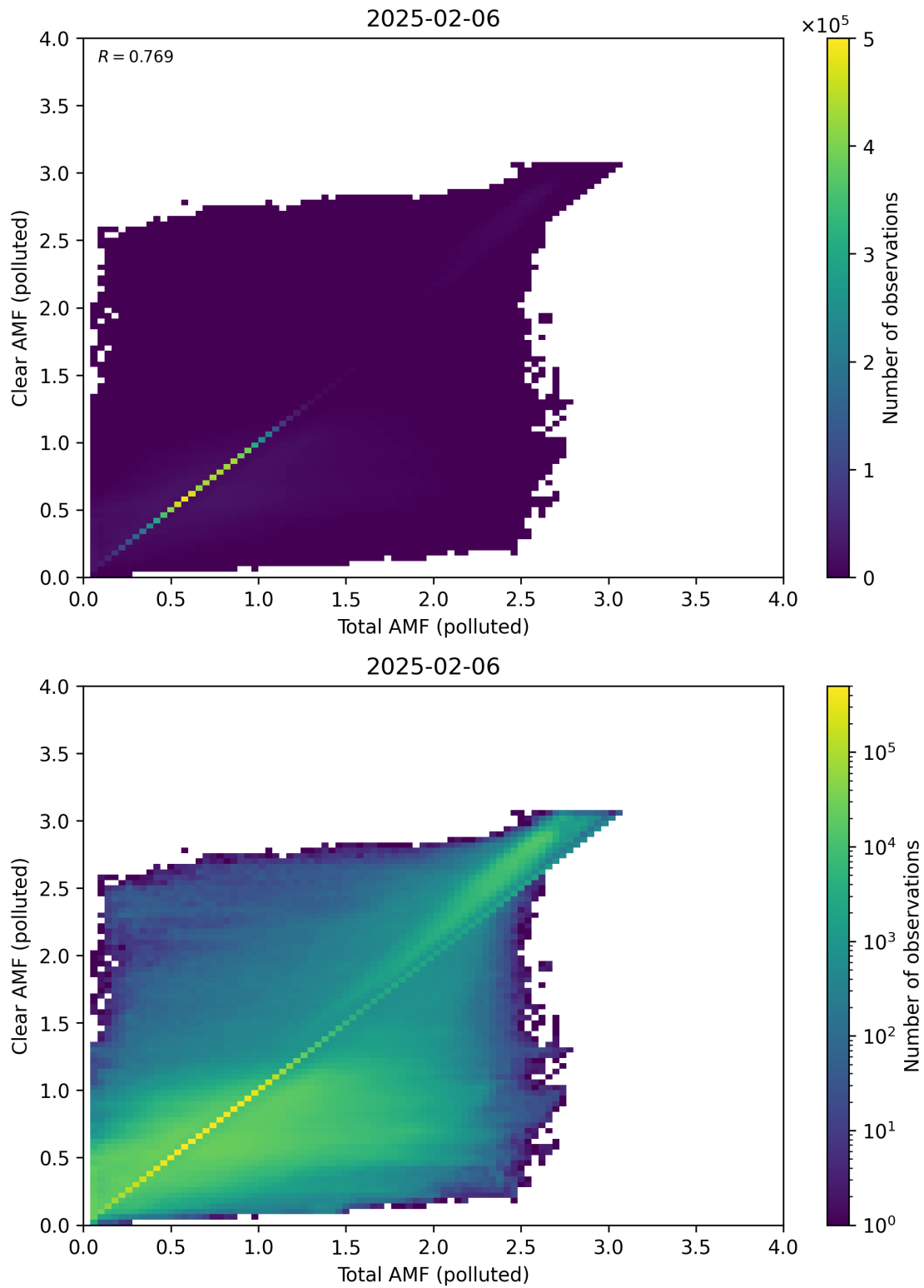
Figure 321: Scatter density plot of “Total AMF (polluted)” against “Clear AMF (polluted)” for 2025-02-05 to 2025-02-07.
