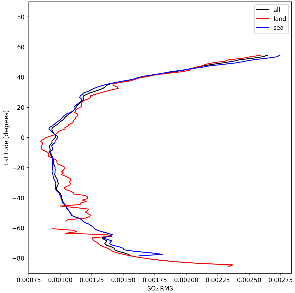
Figure 52: Zonal average of “SO 2 RMS” for 2025-02-05 to 2025-02-07.
