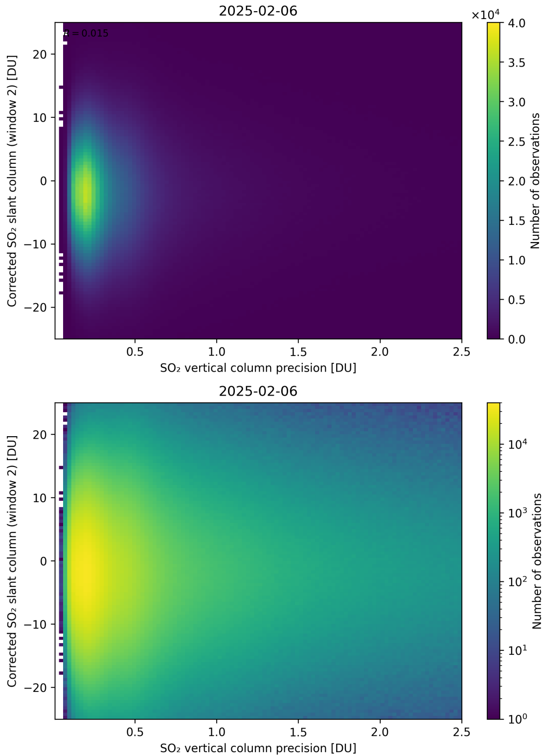
Figure 339: Scatter density plot of “SO 2 vertical column precision” against “Corrected SO 2 slant column (window 2)” for 2025-02-05 to 2025-02-07.
