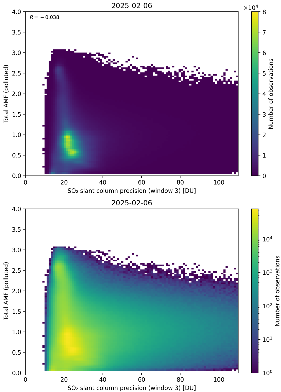
Figure 313: Scatter density plot of “SO 2 slant column precision (window 3)” against “Total AMF (polluted)” for 2025-02-05 to 2025-02-07.
