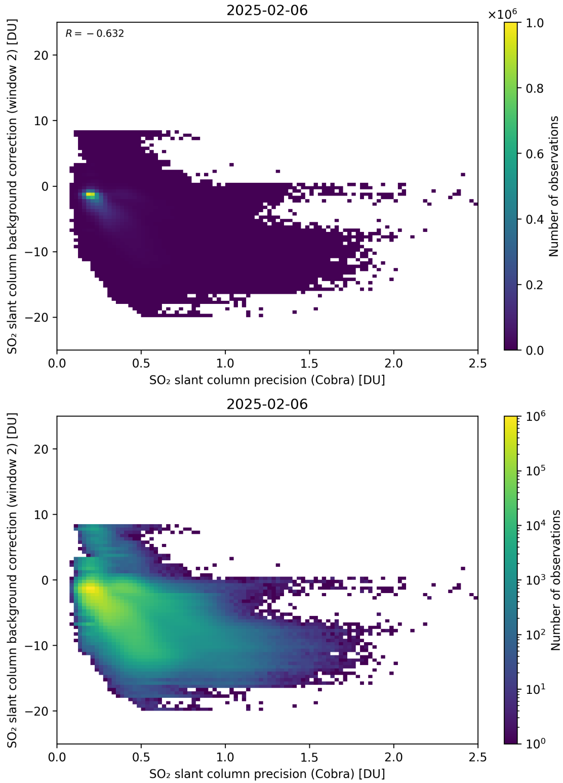
Figure 200: Scatter density plot of “SO 2 slant column precision (Cobra)” against “SO 2 slant column background correction (window 2)” for 2025-02-05 to 2025-02-07.
