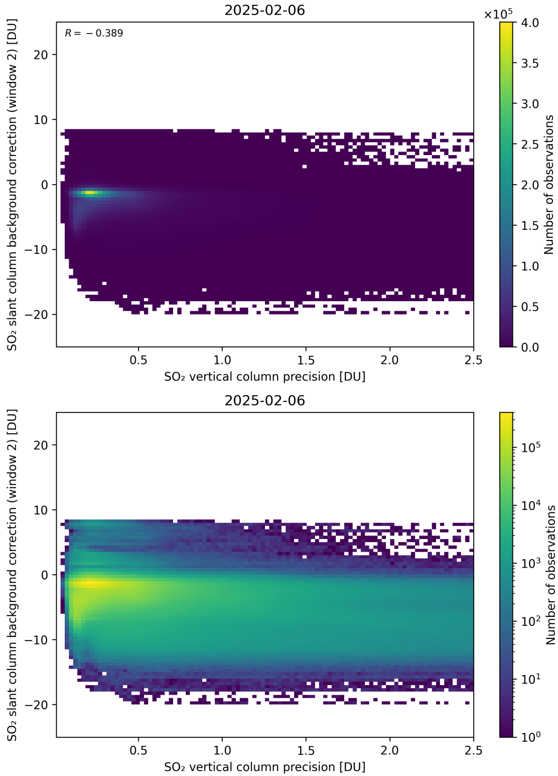
Figure 330: Scatter density plot of “SO 2 vertical column precision” against “SO 2 slant column background correction (window 2)” for 2025-02-05 to 2025-02-07.
