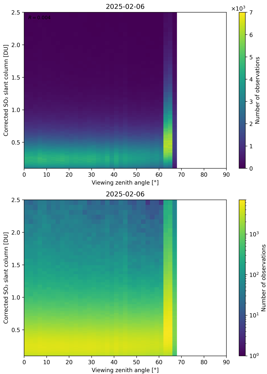
Figure 373: Scatter density plot of “Viewing zenith angle” against “Corrected SO 2 slant column” for 2025-02-05 to 2025-02-07.
