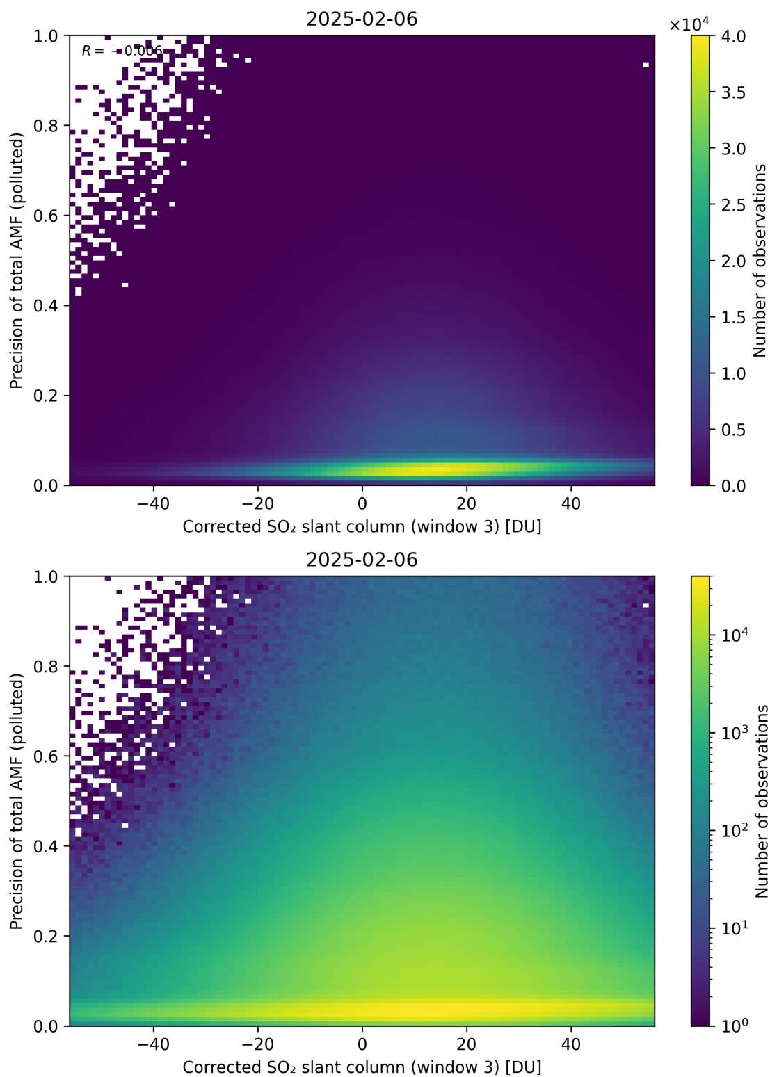
Figure 261: Scatter density plot of “Corrected SO 2 slant column (window 3)” against “Precision of total AMF (polluted)” for 2025-02-05 to 2025-02-07.
