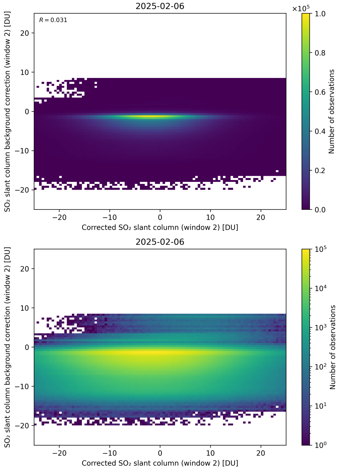
Figure 244: Scatter density plot of “Corrected SO 2 slant column (window 2)” against “SO 2 slant column background correction (window 2)” for 2025-02-05 to 2025-02-07.
