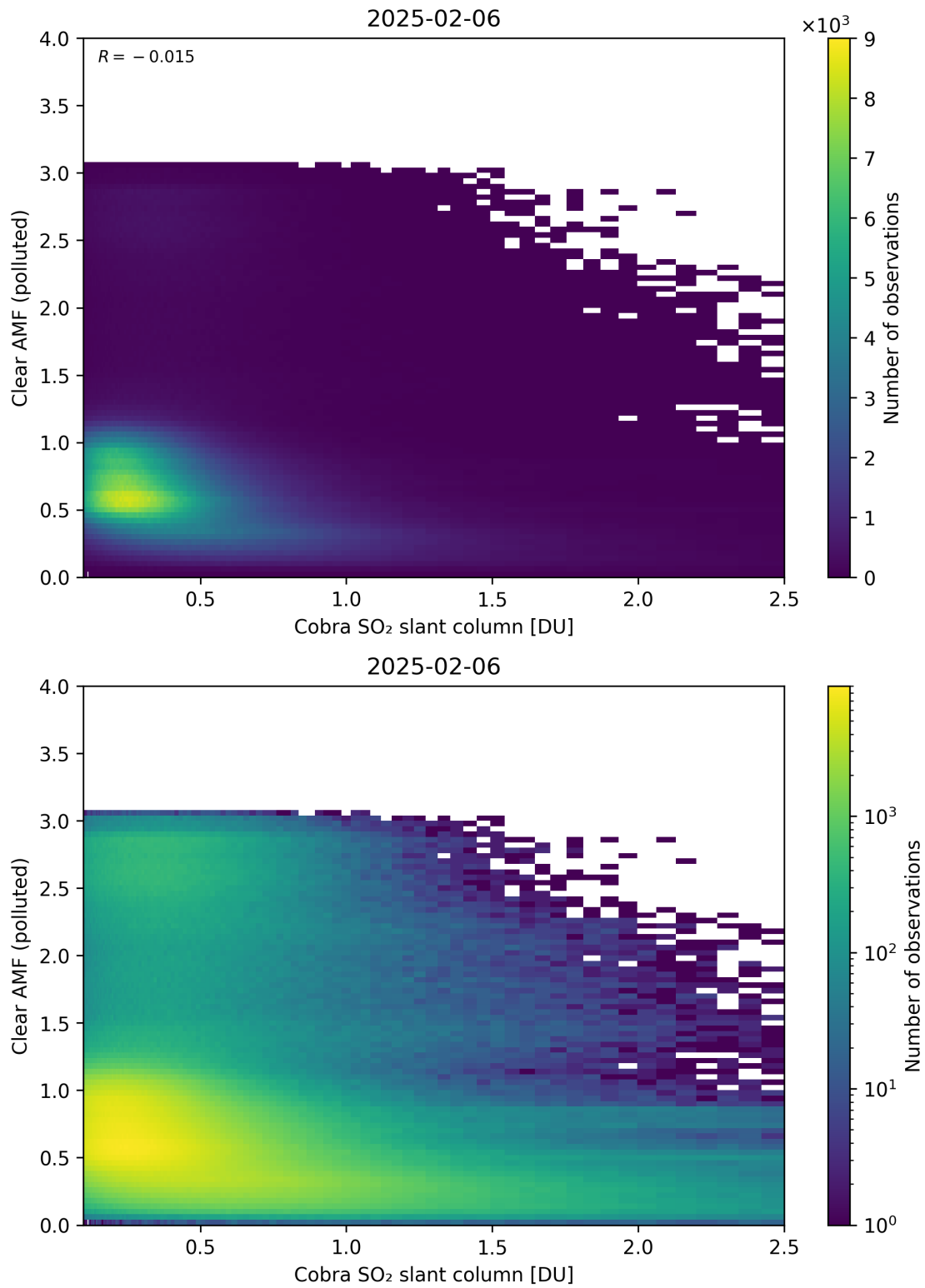
Figure 215: Scatter density plot of “Cobra SO 2 slant column” against “Clear AMF (polluted)” for 2025-02-05 to 2025-02-07.
