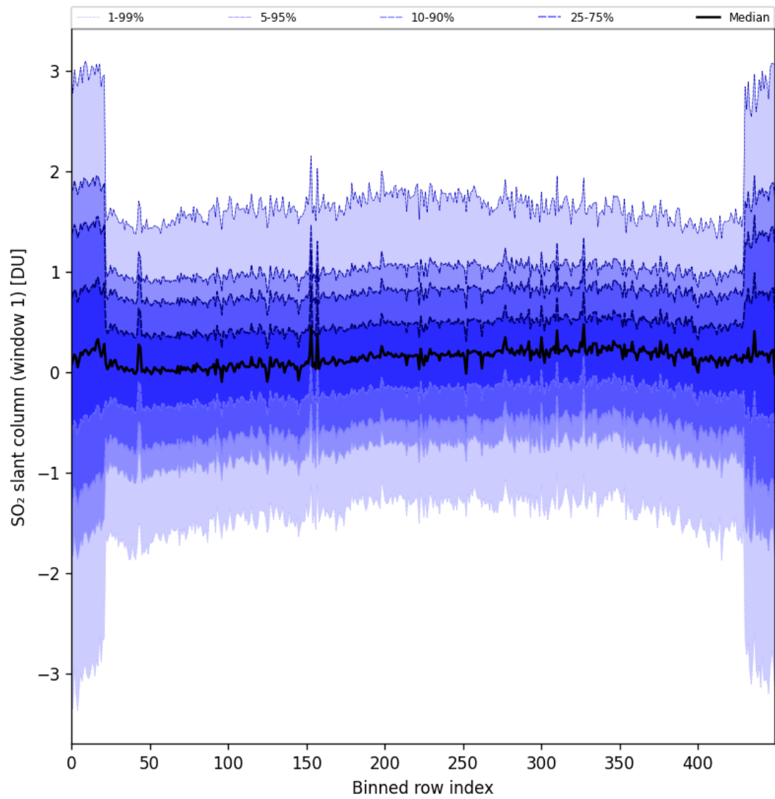
Figure 89: Along track statistics of “SO 2 slant column (window 1)” for 2025-02-05 to 2025-02-07
