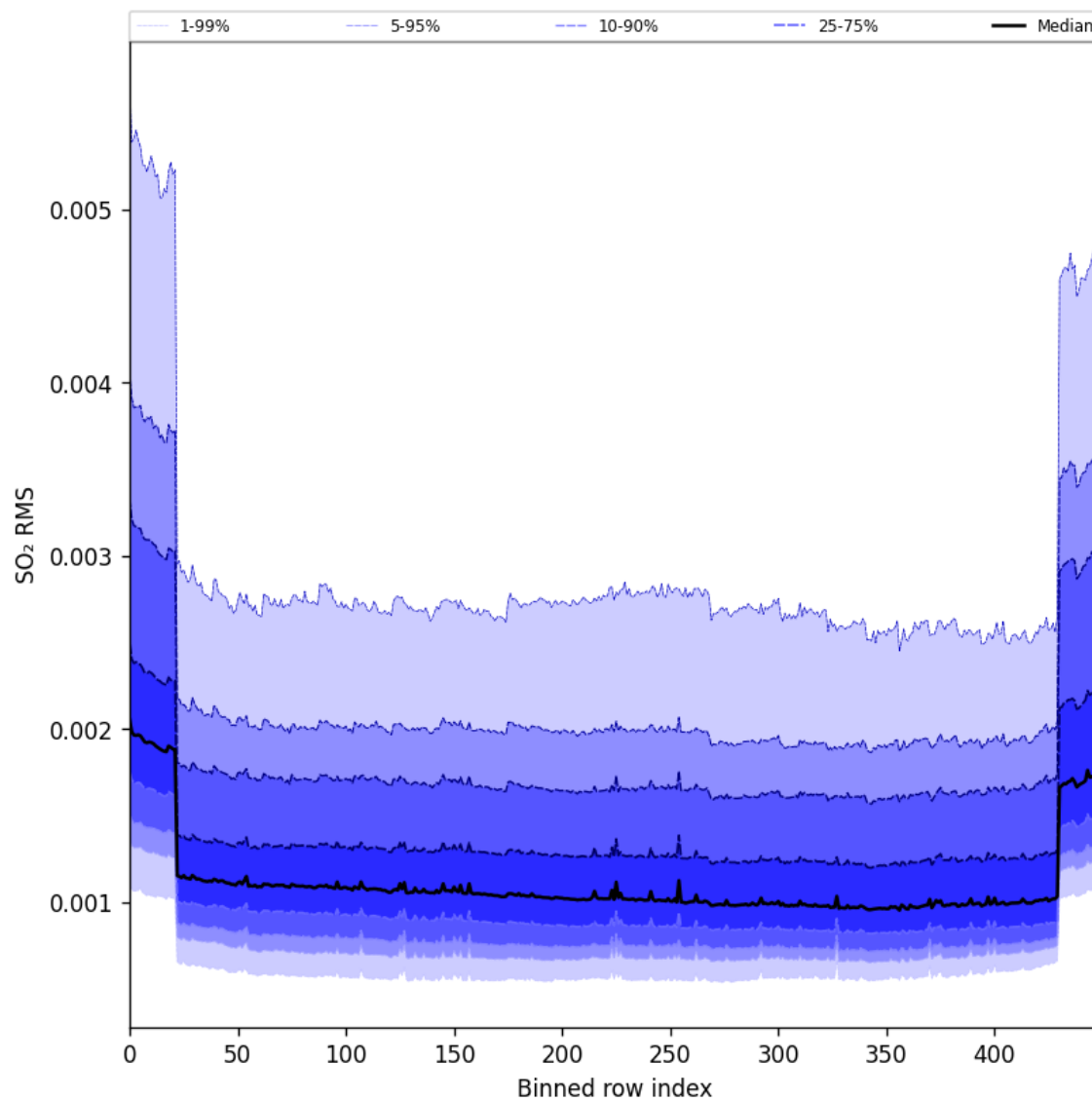
Figure 104: Along track statistics of “SO 2 RMS” for 2025-02-05 to 2025-02-07
