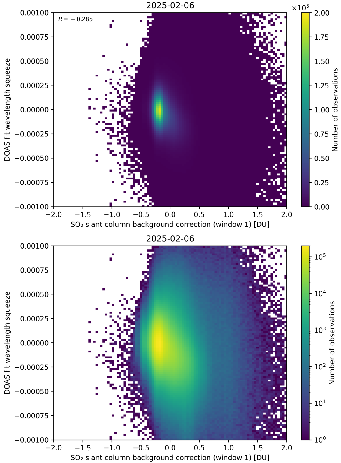
Figure 112: Scatter density plot of “SO 2 slant column background correction (window 1)” against “DOAS fit wavelength squeeze” for 2025-02-05 to 2025-02-07.
