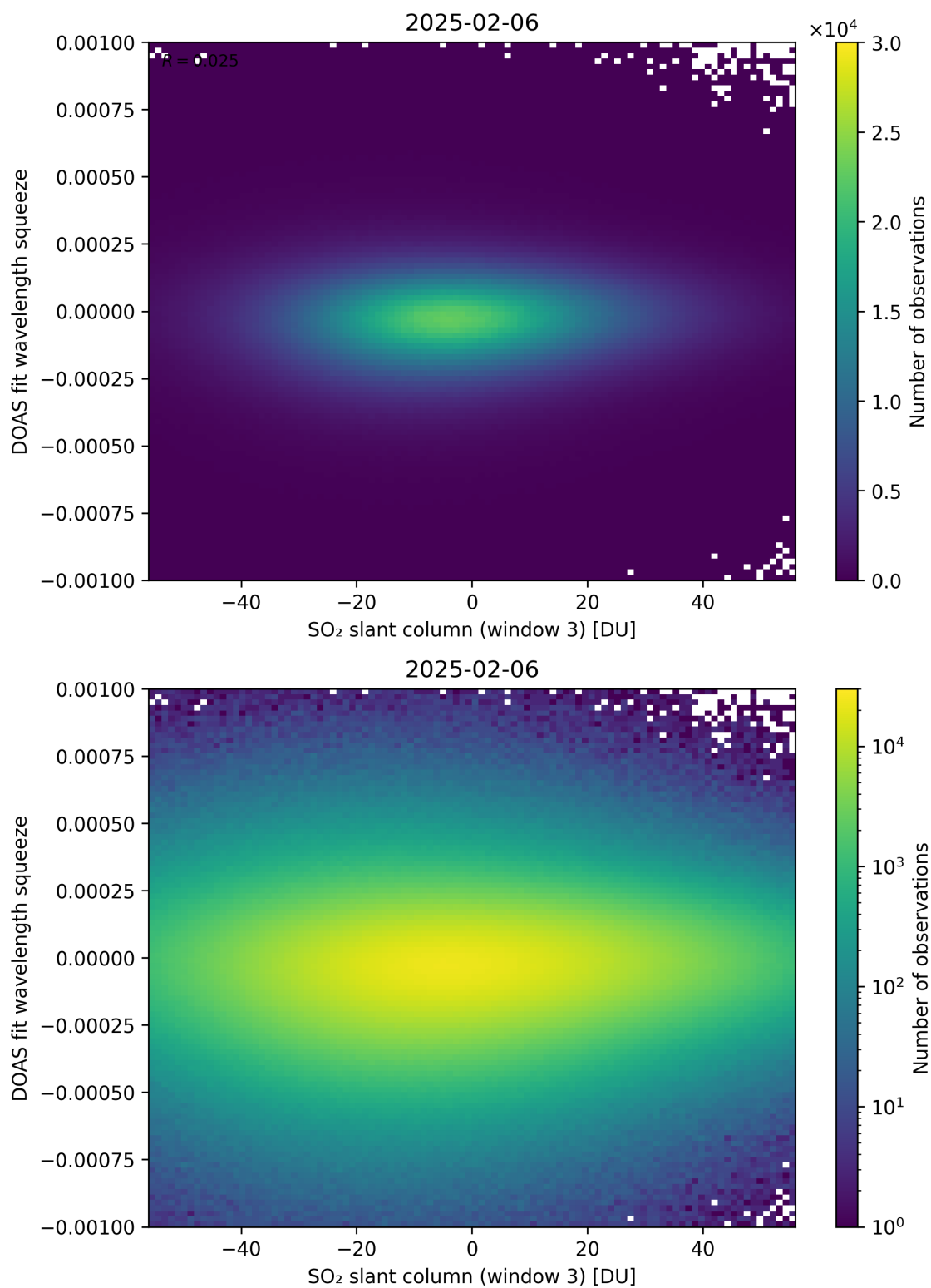
Figure 305: Scatter density plot of “SO 2 slant column (window 3)” against “DOAS fit wavelength squeeze” for 2025-02-05 to 2025-02-07.
