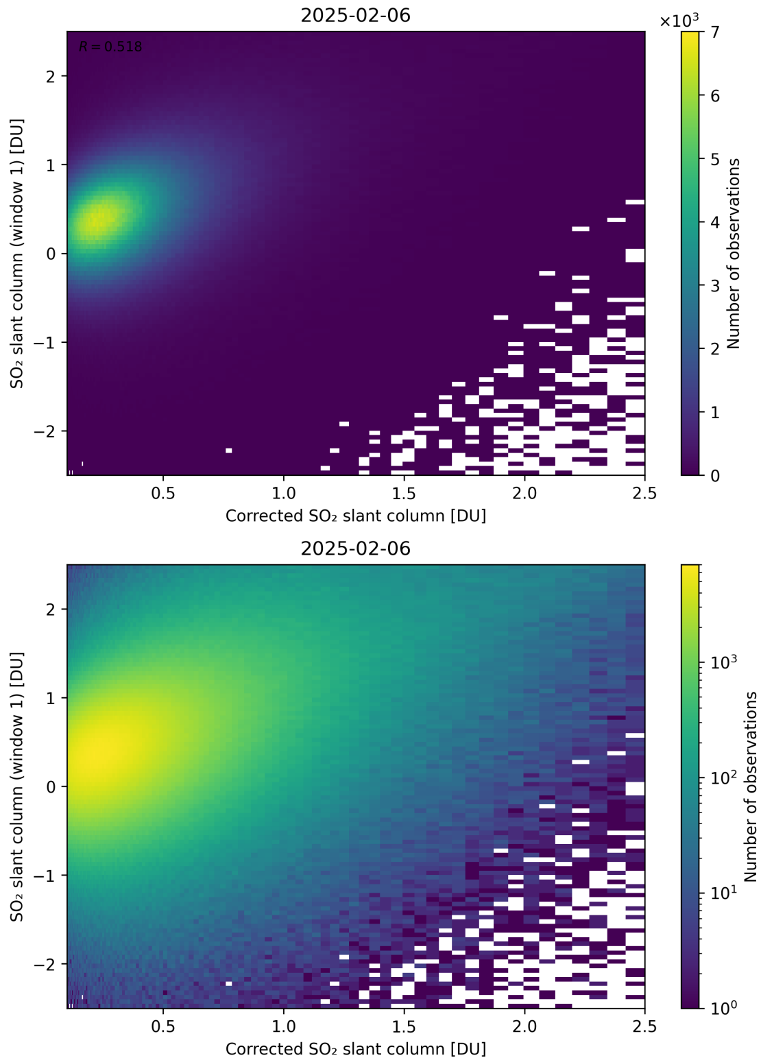
Figure 237: Scatter density plot of “Corrected SO 2 slant column” against “SO 2 slant column (window 1)” for 2025-02-05 to 2025-02-07.
