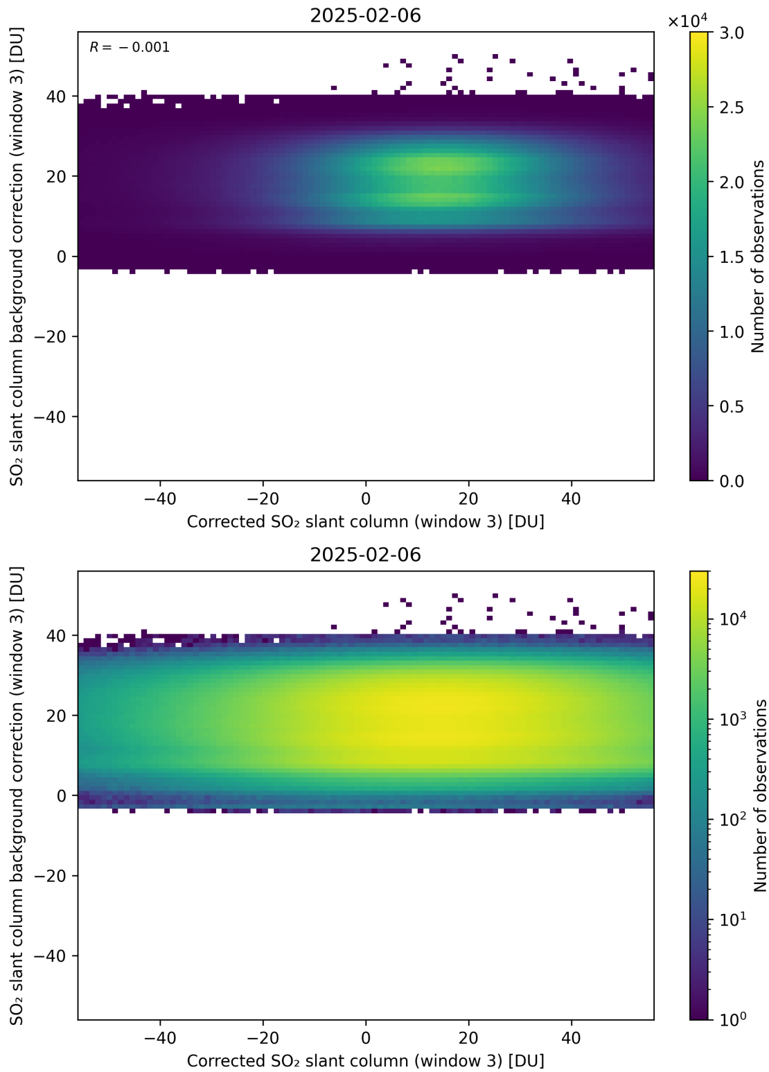
Figure 255: Scatter density plot of “Corrected SO 2 slant column (window 3)” against “SO 2 slant column background correction (window 3)” for 2025-02-05 to 2025-02-07.
