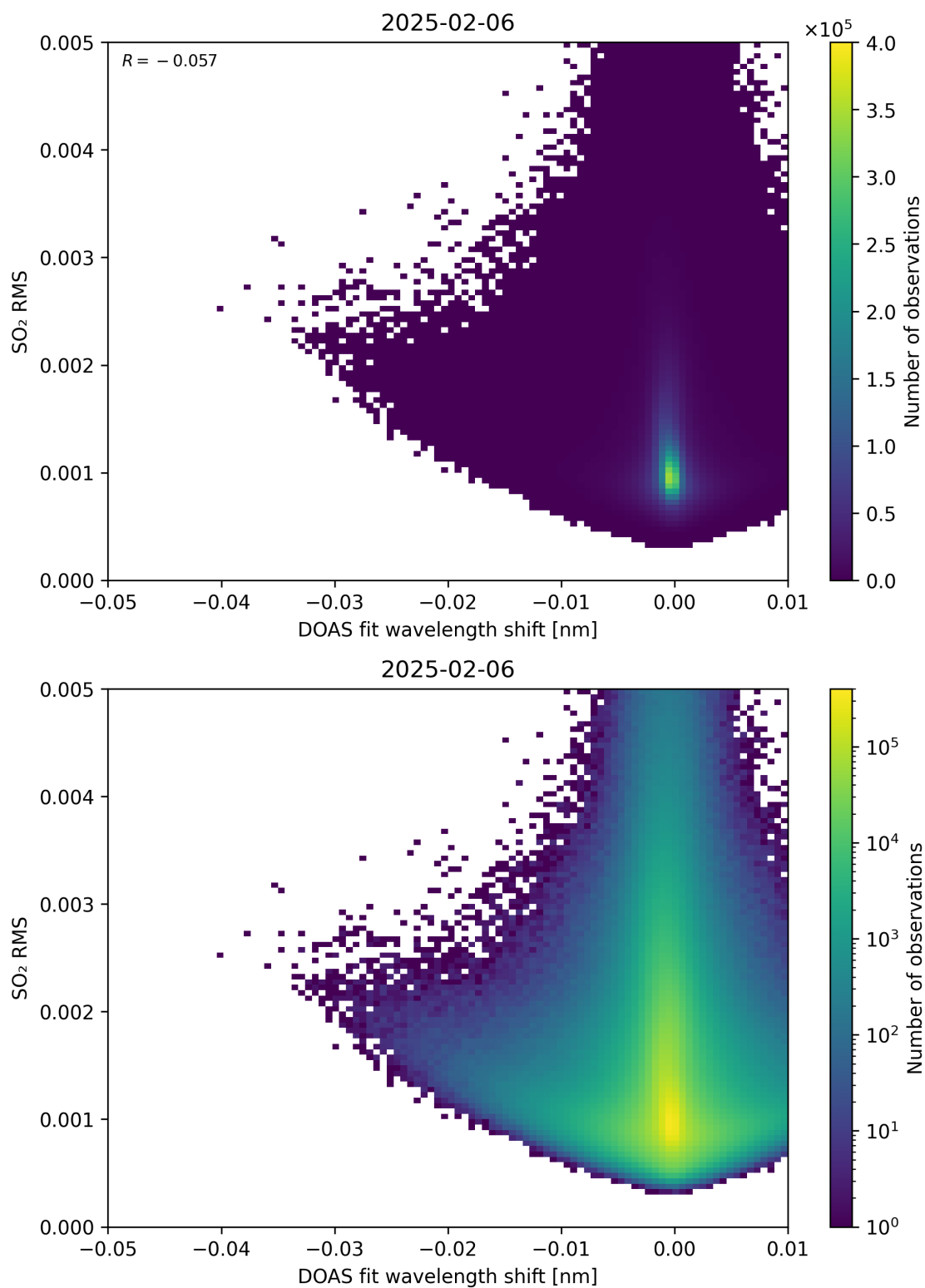
Figure 139: Scatter density plot of “DOAS fit wavelength shift” against “SO 2 RMS” for 2025-02-05 to 2025-02-07.
