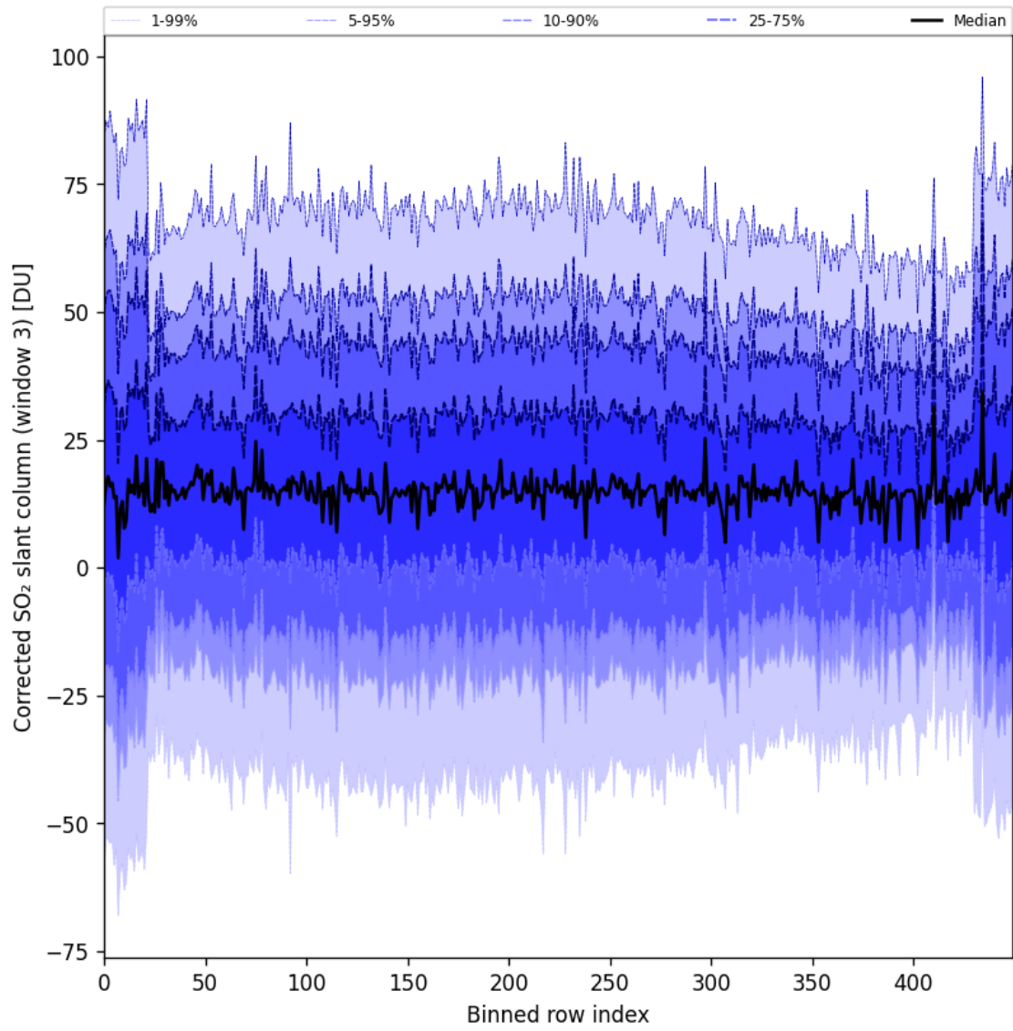
Figure 99: Along track statistics of “Corrected SO 2 slant column (window 3)” for 2025-02-05 to 2025-02-07
