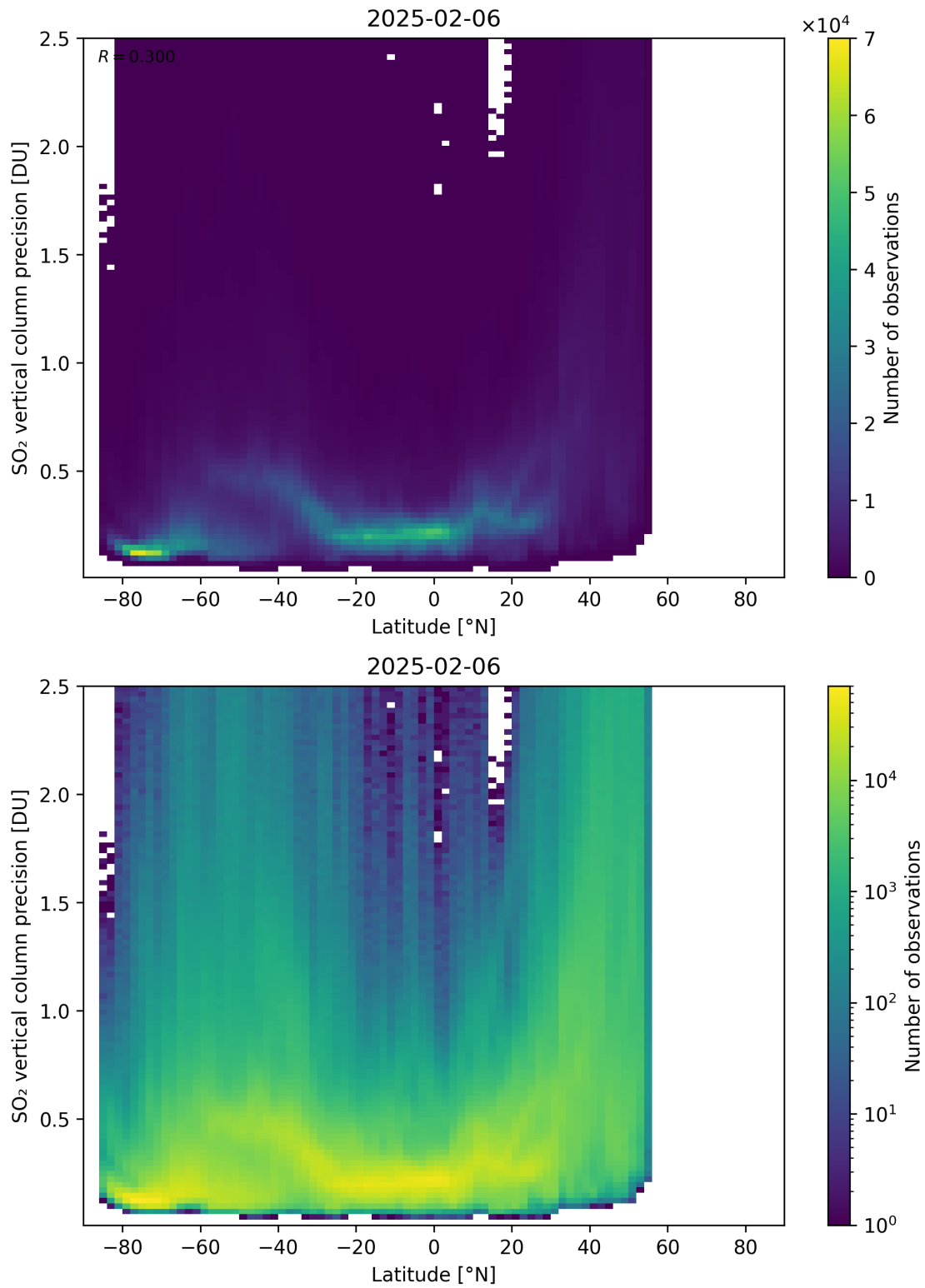
Figure 170: Scatter density plot of “Latitude” against “SO 2 vertical column precision” for 2025-02-05 to 2025-02-07.
