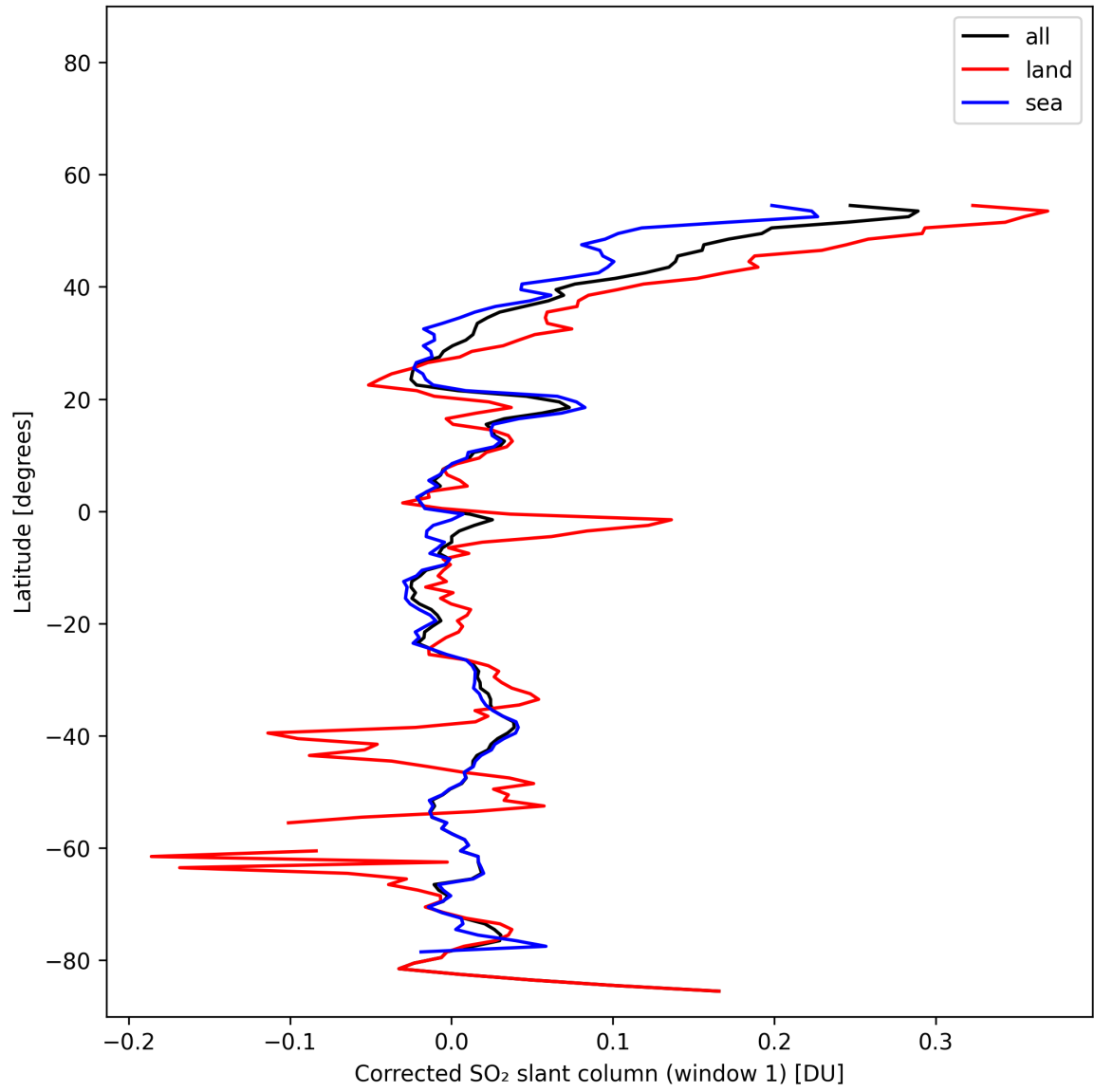
Figure 39: Zonal average of “Corrected SO 2 slant column (window 1)” for 2025-02-05 to 2025-02-07.
