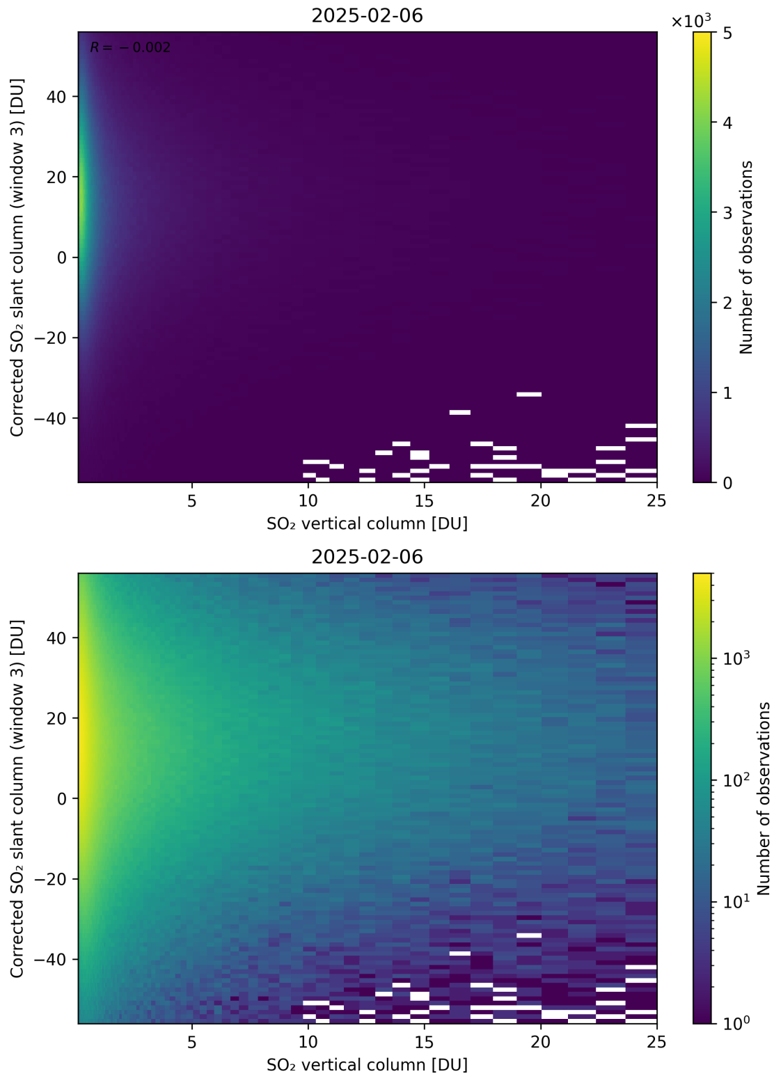
Figure 353: Scatter density plot of “SO 2 vertical column” against “Corrected SO 2 slant column (window 3)” for 2025-02-05 to 2025-02-07.
