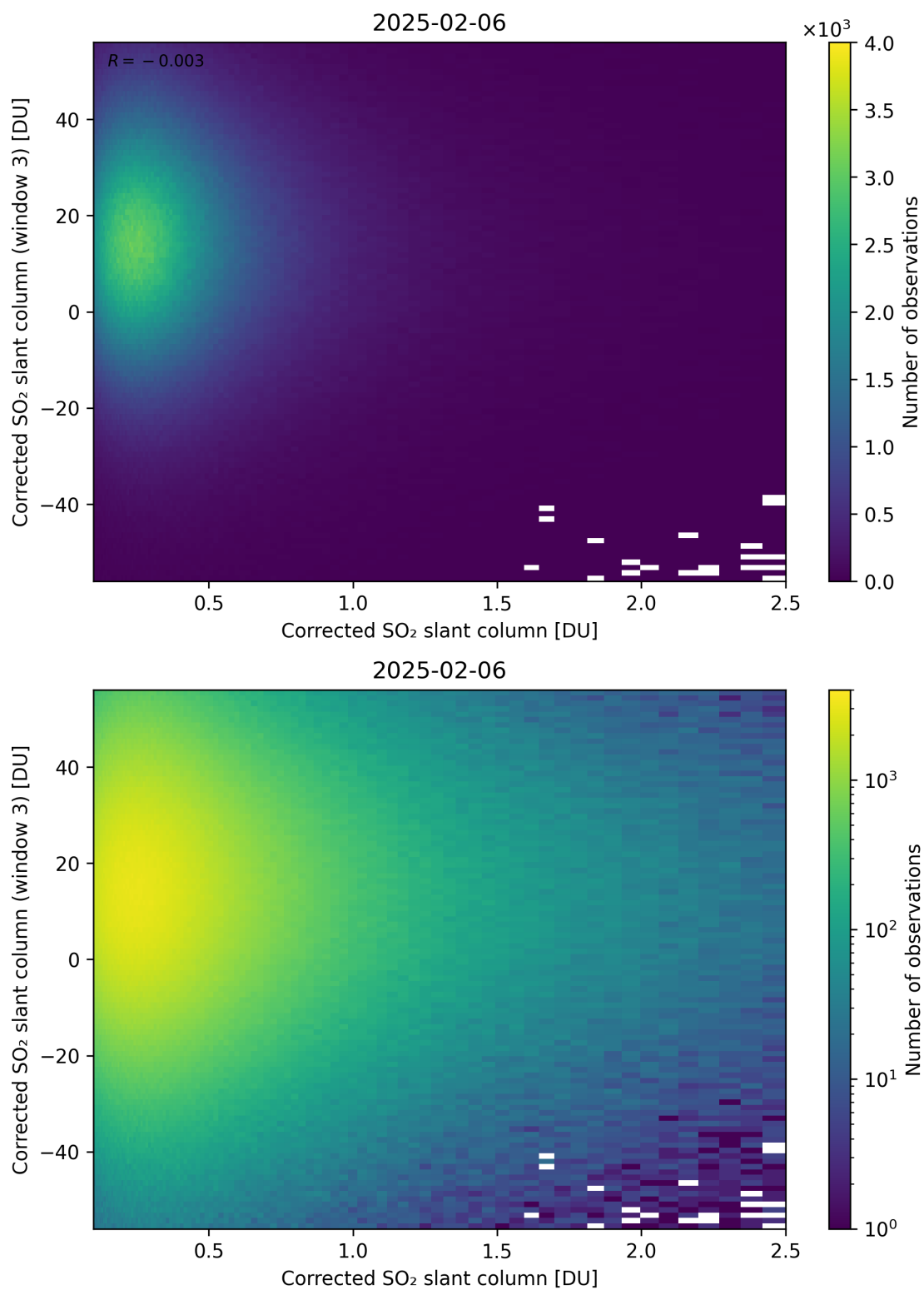
Figure 236: Scatter density plot of “Corrected SO 2 slant column” against “Corrected SO 2 slant column (window 3)” for 2025-02-05 to 2025-02-07.
