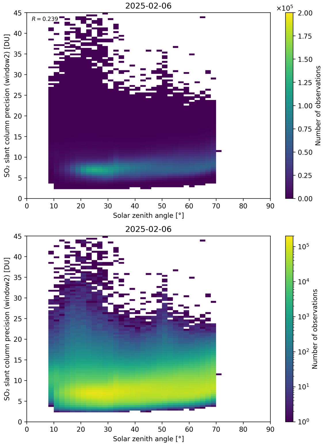
Figure 186: Scatter density plot of “Solar zenith angle” against “SO 2 slant column precision (window2)” for 2025-02-05 to 2025-02-07.
