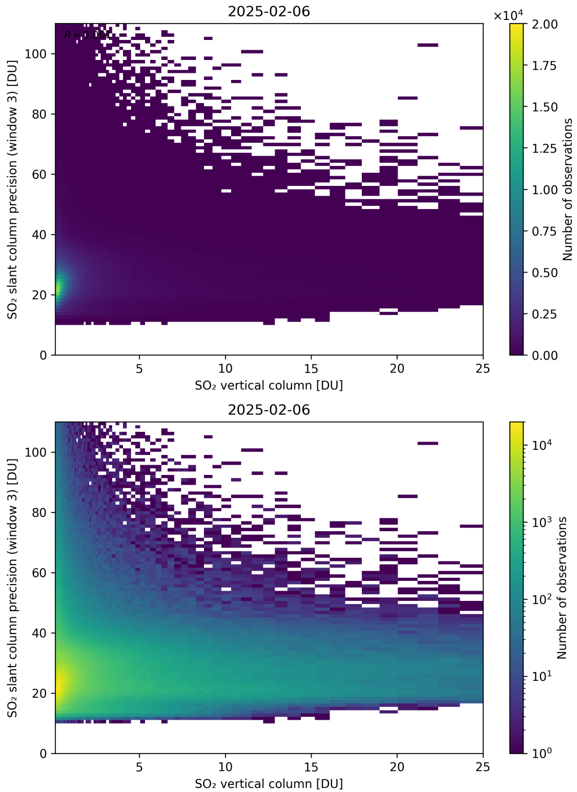
Figure 358: Scatter density plot of “SO 2 vertical column” against “SO 2 slant column precision (window 3)” for 2025-02-05 to 2025-02-07.
