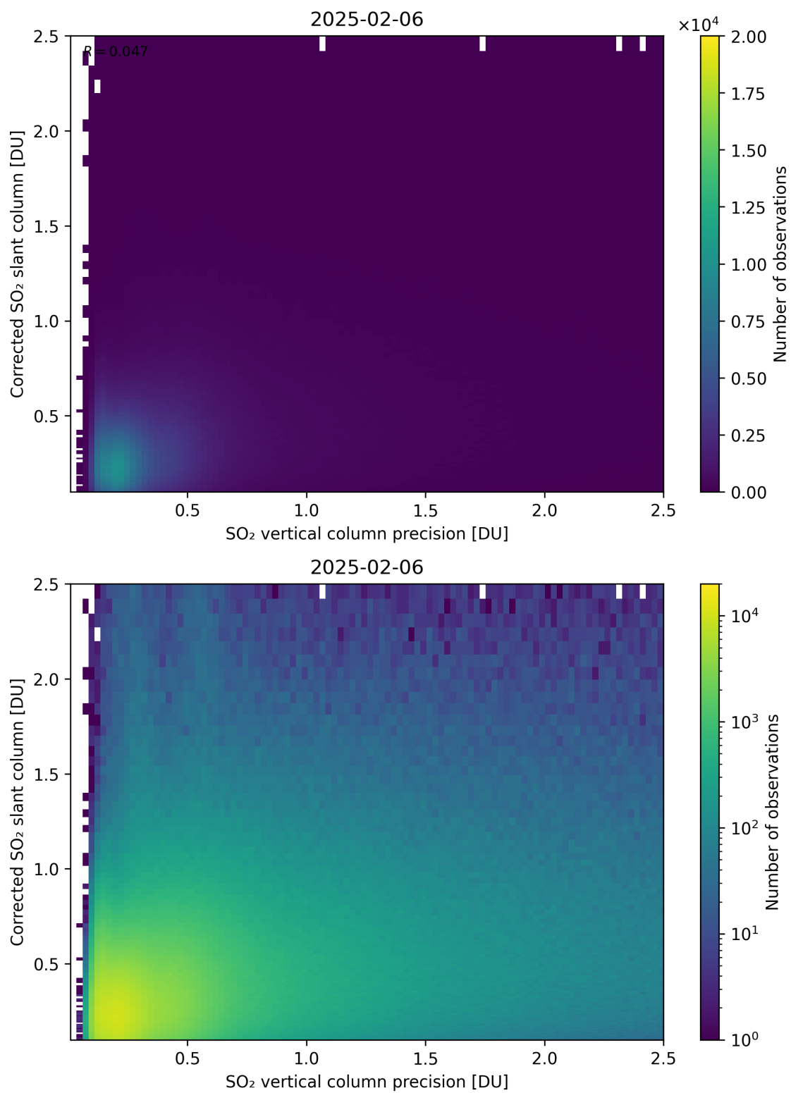
Figure 338: Scatter density plot of “SO 2 vertical column precision” against “Corrected SO 2 slant column” for 2025-02-05 to 2025-02-07.
