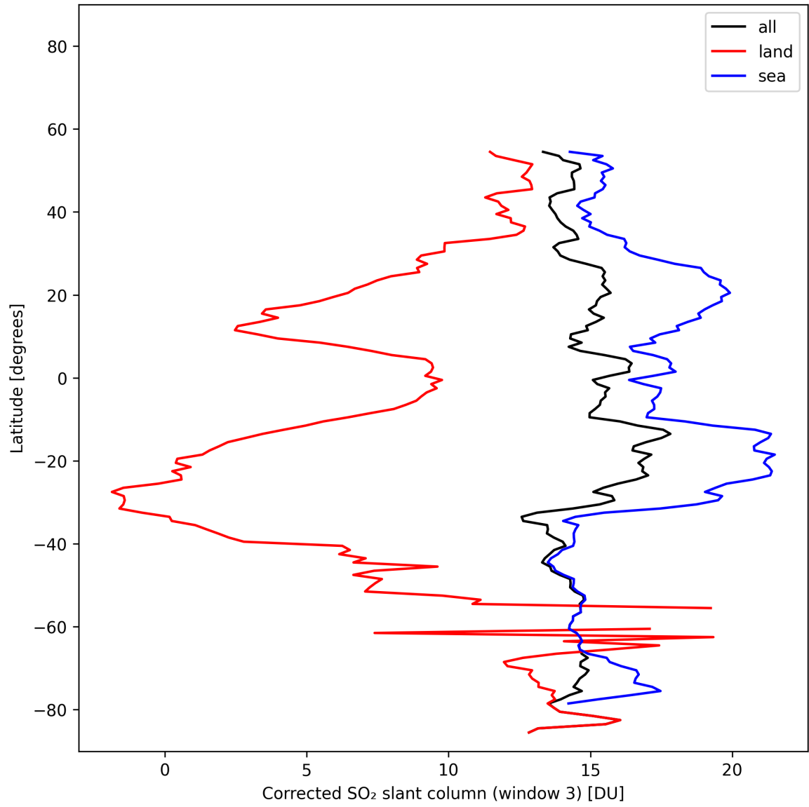
Figure 47: Zonal average of “Corrected SO 2 slant column (window 3)” for 2025-02-05 to 2025-02-07.
