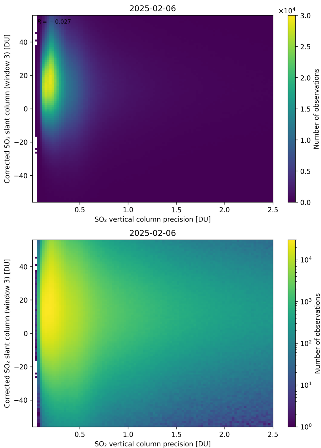
Figure 340: Scatter density plot of “SO 2 vertical column precision” against “Corrected SO 2 slant column (window 3)” for 2025-02-05 to 2025-02-07.
