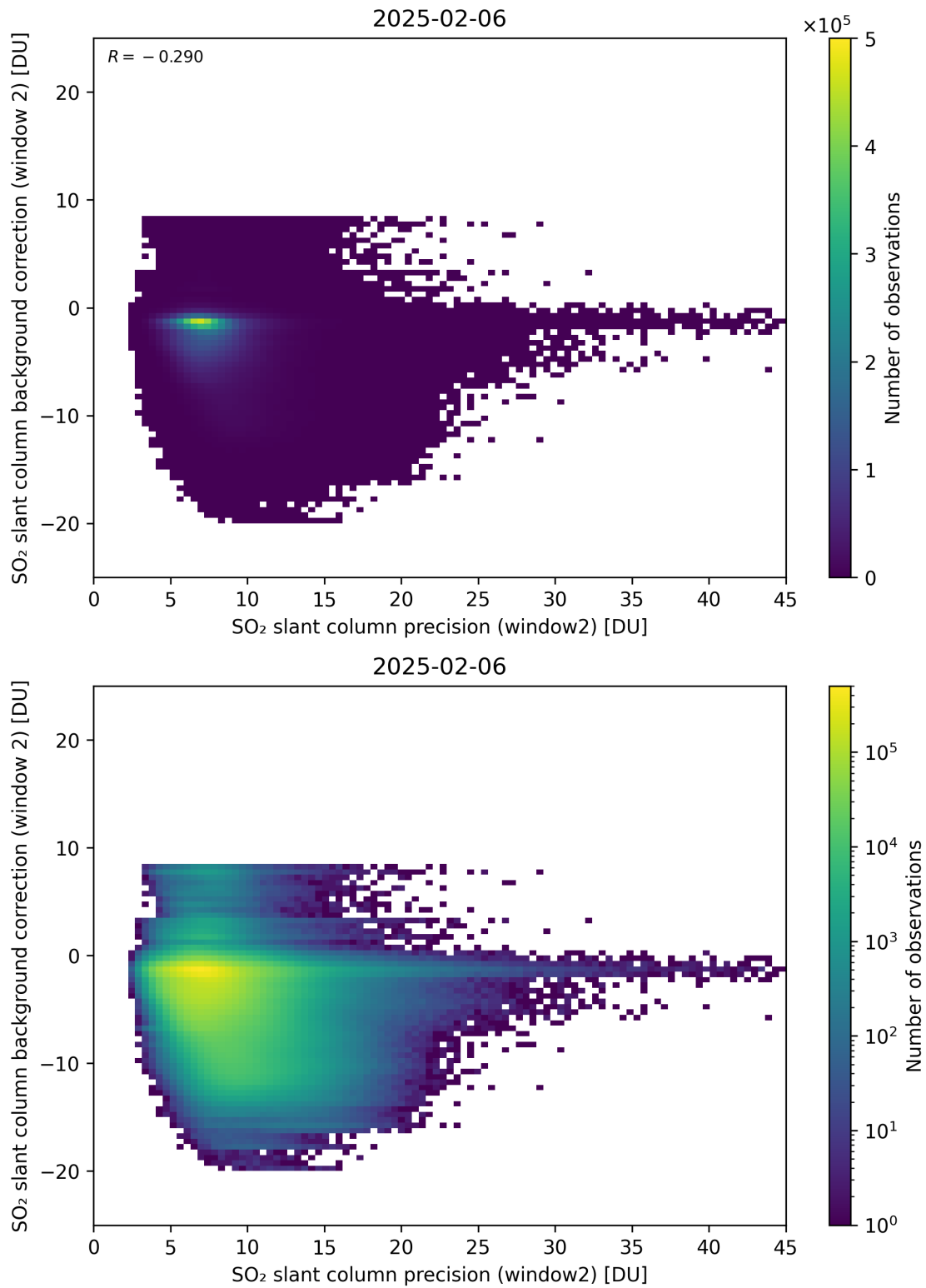
Figure 291: Scatter density plot of “SO 2 slant column precision (window2)” against “SO 2 slant column background correction (window 2)” for 2025-02-05 to 2025-02-07.
