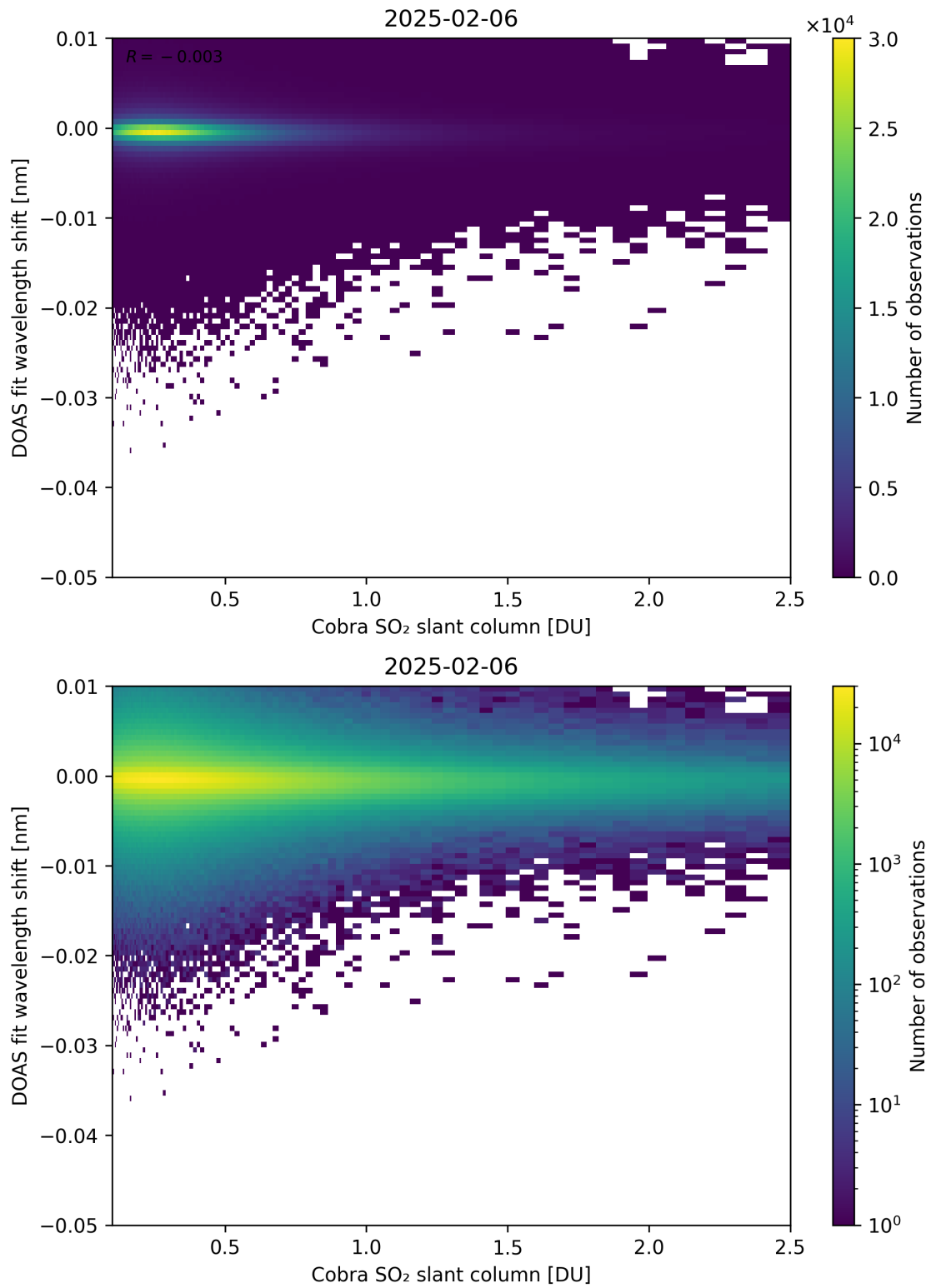
Figure 196: Scatter density plot of “Cobra SO 2 slant column” against “DOAS fit wavelength shift” for 2025-02-05 to 2025-02-07.
