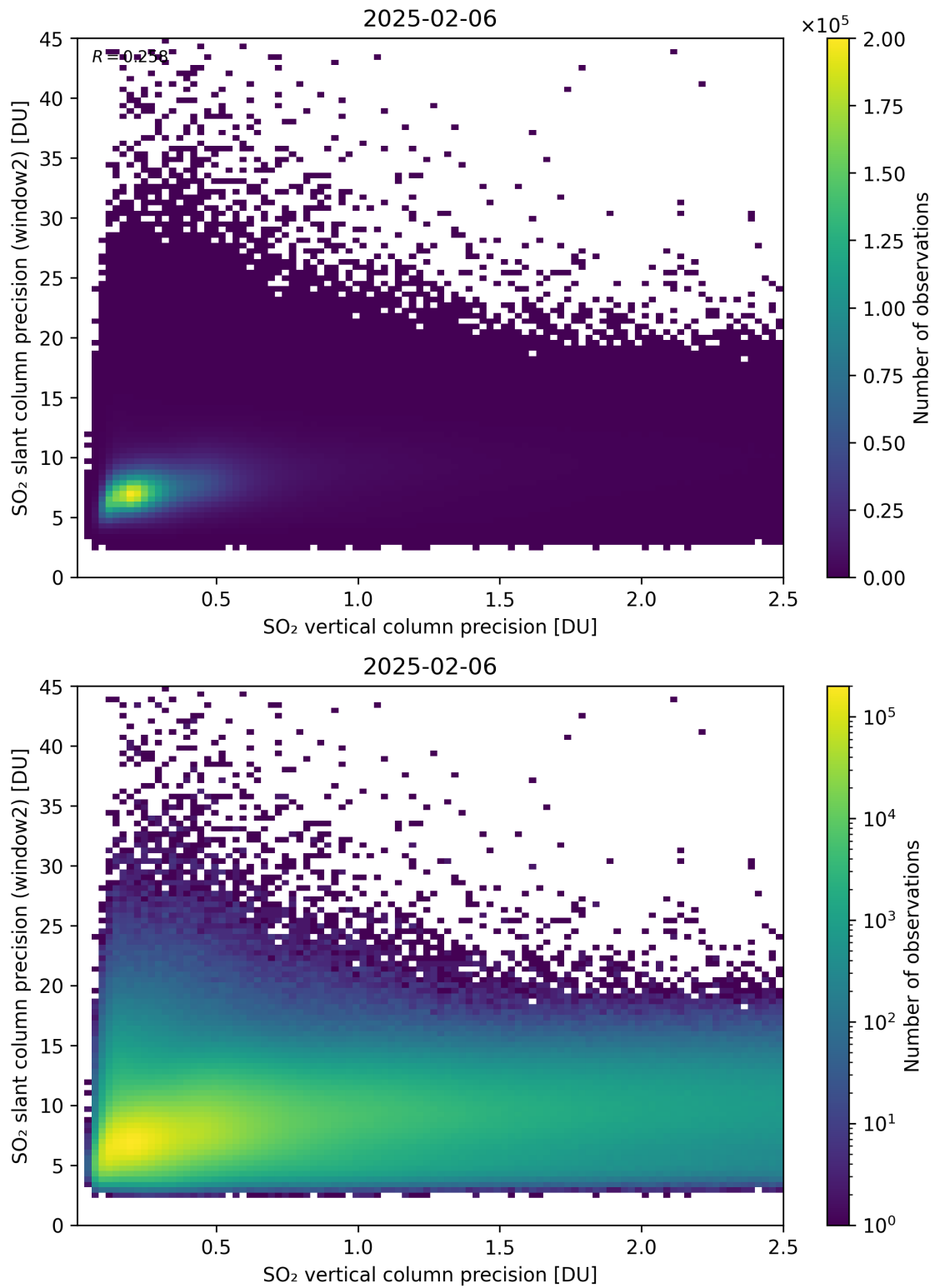
Figure 343: Scatter density plot of “SO 2 vertical column precision” against “SO 2 slant column precision (window2)” for 2025-02-05 to 2025-02-07.
