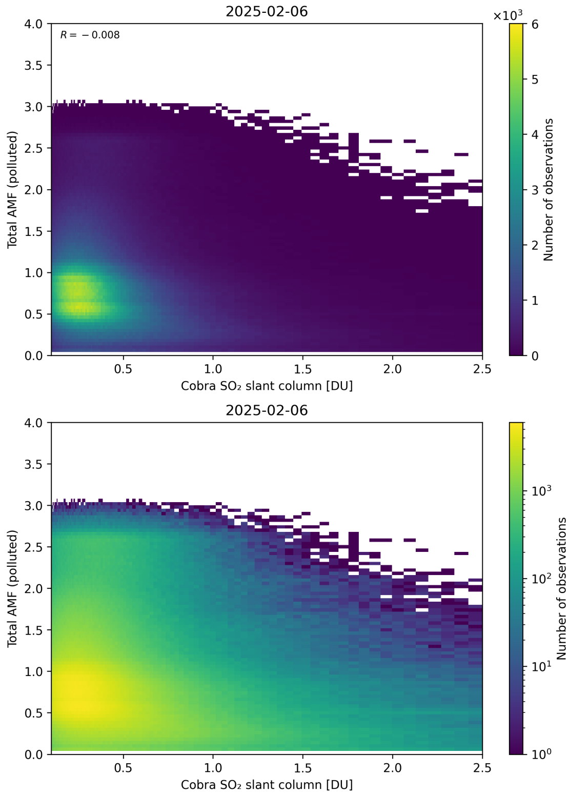
Figure 224: Scatter density plot of “Cobra SO 2 slant column” against “Total AMF (polluted)” for 2025-02-05 to 2025-02-07.
