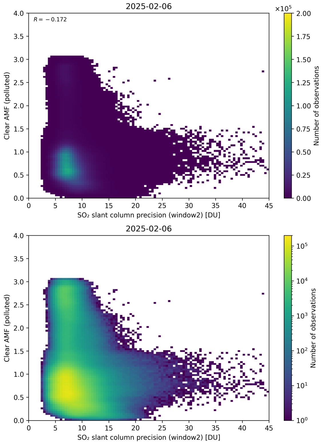
Figure 296: Scatter density plot of “SO 2 slant column precision (window2)” against “Clear AMF (polluted)” for 2025-02-05 to 2025-02-07.
