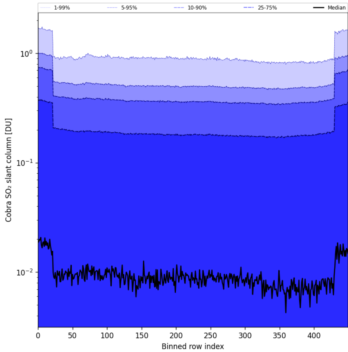
Figure 87: Along track statistics of “Cobra SO 2 slant column” for 2025-02-05 to 2025-02-07
