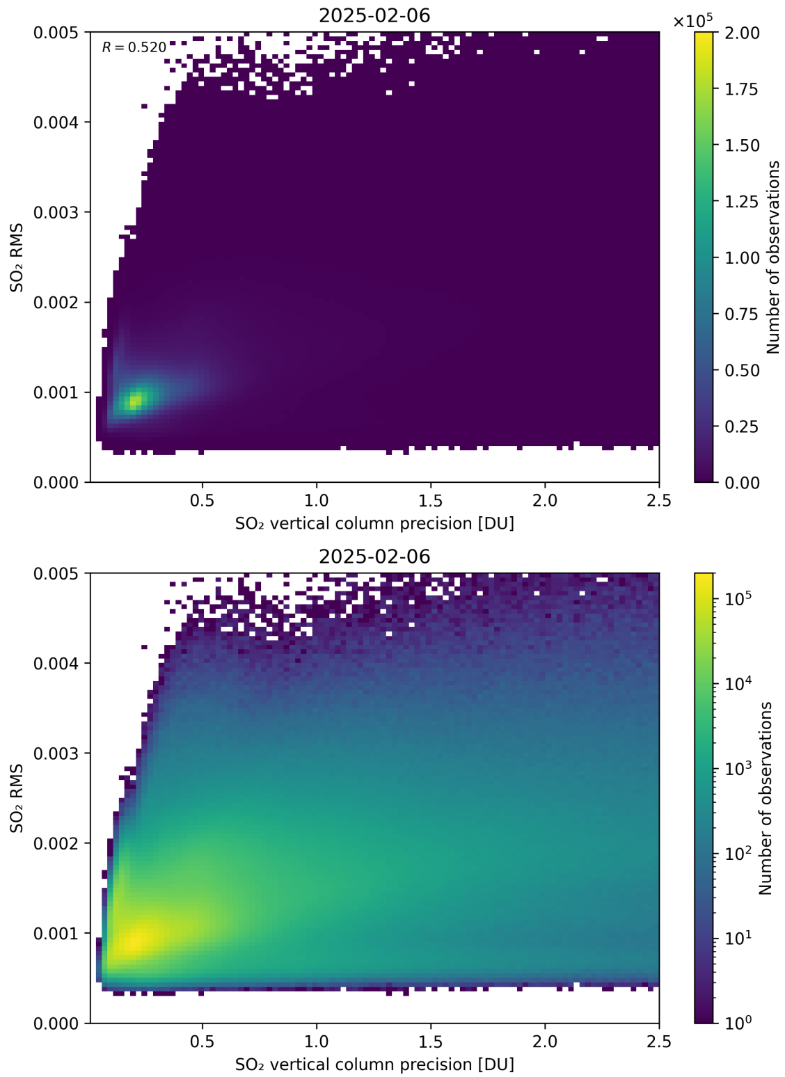
Figure 334: Scatter density plot of “SO 2 vertical column precision” against “SO 2 RMS” for 2025-02-05 to 2025-02-07.
