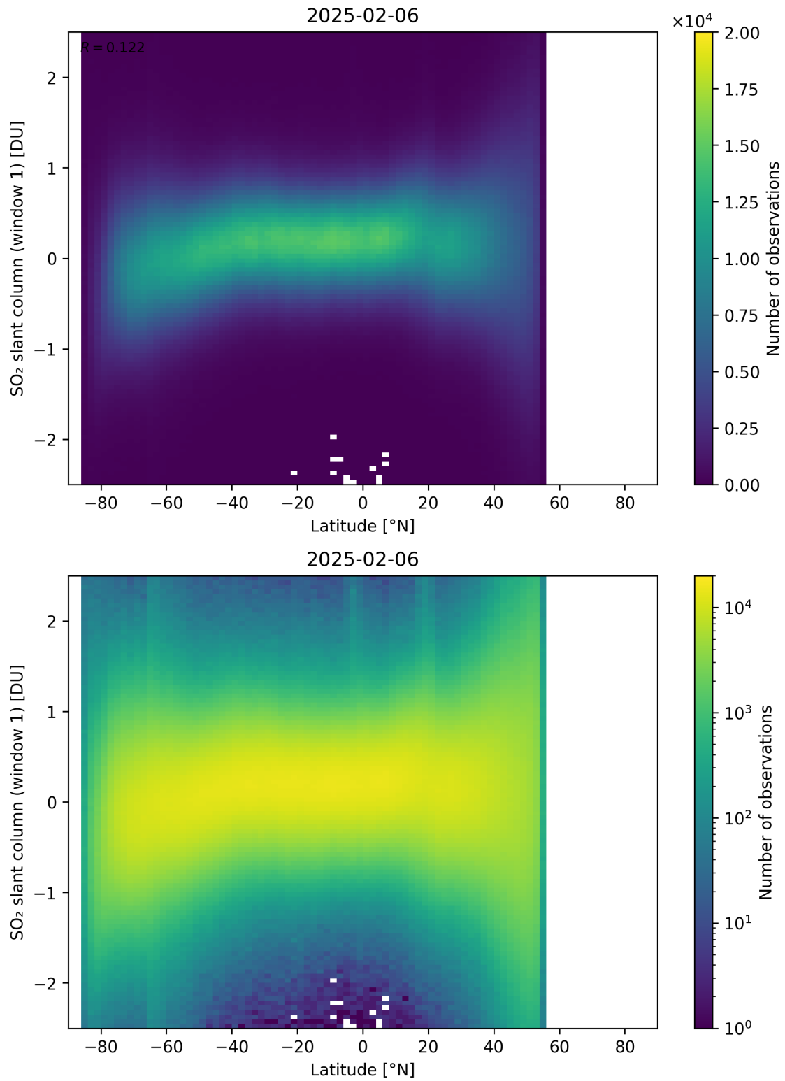
Figure 162: Scatter density plot of “Latitude” against “SO 2 slant column (window 1)” for 2025-02-05 to 2025-02-07.
