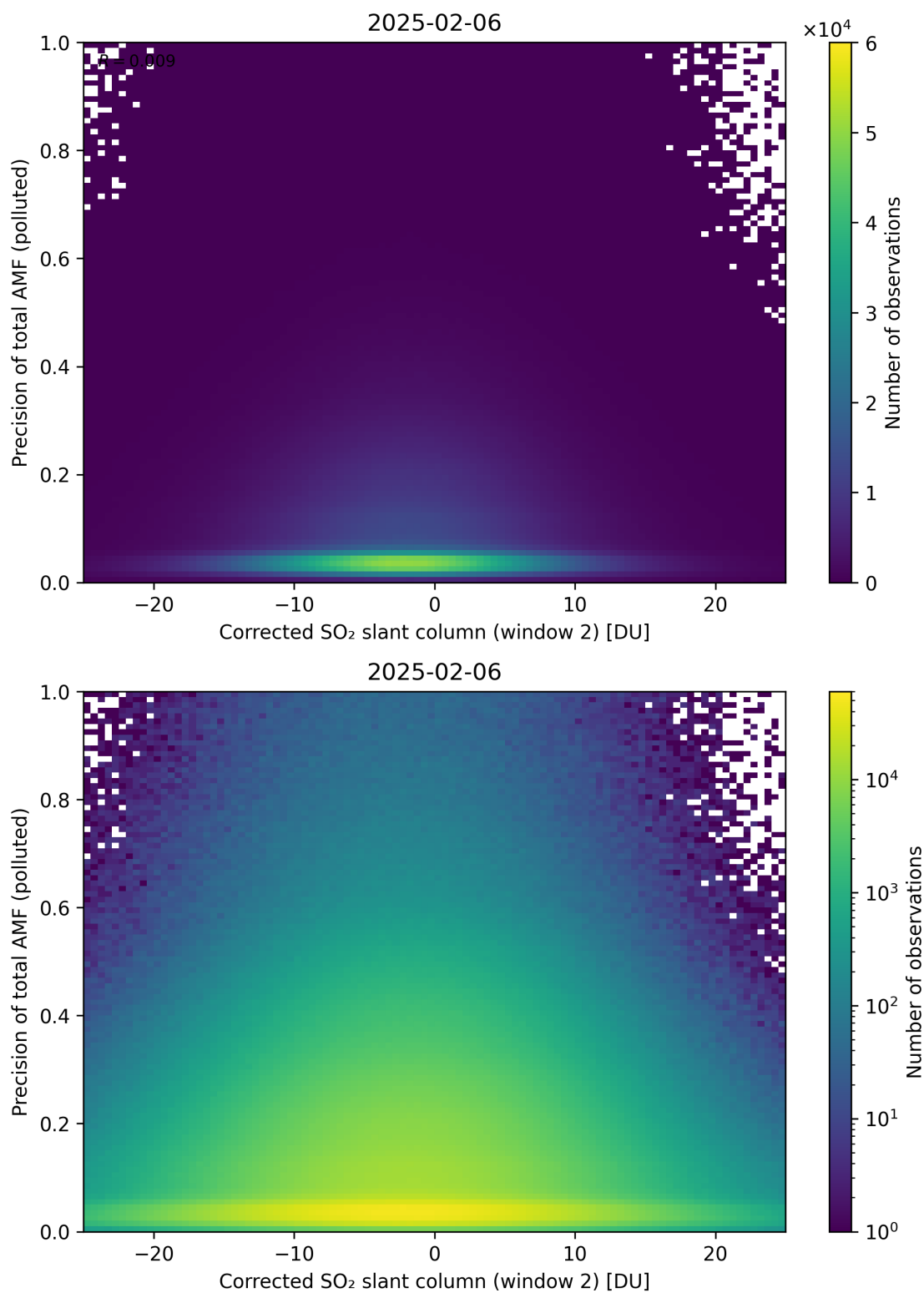
Figure 254: Scatter density plot of “Corrected SO 2 slant column (window 2)” against “Precision of total AMF (polluted)” for 2025-02-05 to 2025-02-07.
