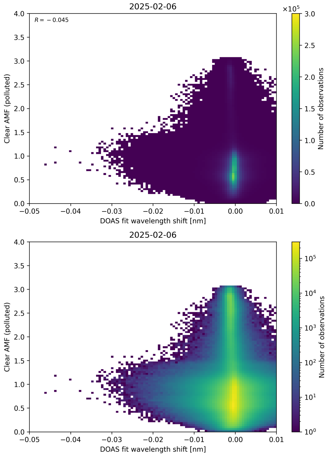
Figure 140: Scatter density plot of “DOAS fit wavelength shift” against “Clear AMF (polluted)” for 2025-02-05 to 2025-02-07.
