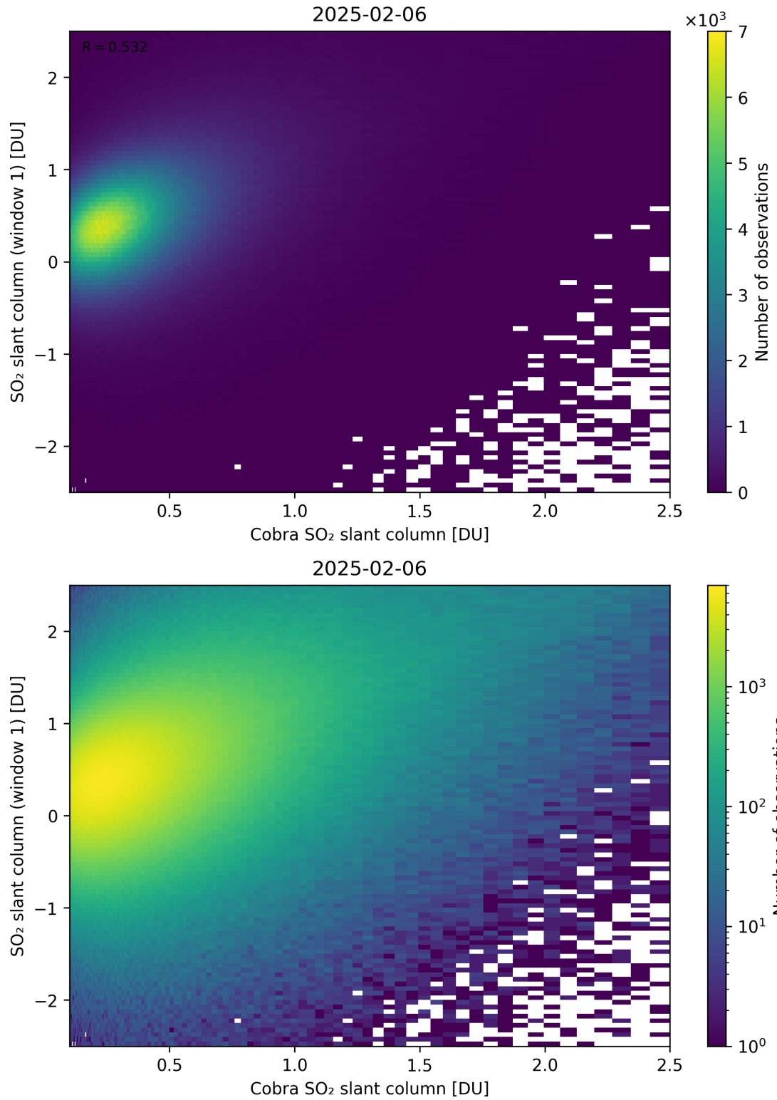
Figure 219: Scatter density plot of “Cobra SO 2 slant column” against “SO 2 slant column (window 1)” for 2025-02-05 to 2025-02-07.
