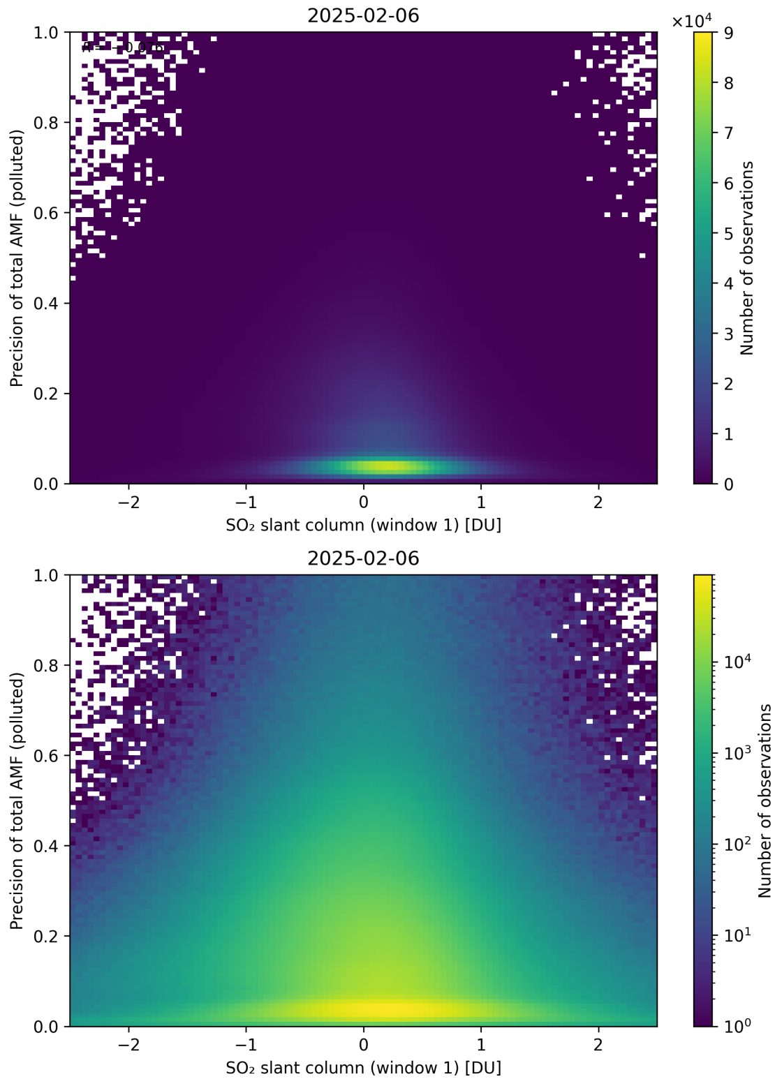
Figure 290: Scatter density plot of “SO 2 slant column (window 1)” against “Precision of total AMF (polluted)” for 2025-02-05 to 2025-02-07.
