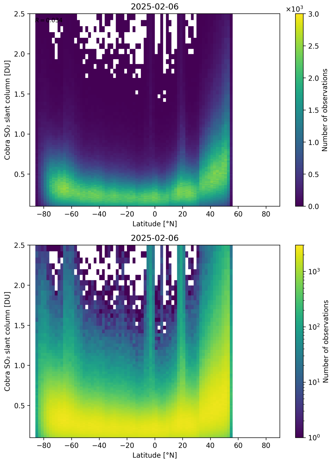
Figure 157: Scatter density plot of “Latitude” against “Cobra SO 2 slant column” for 2025-02-05 to 2025-02-07.
