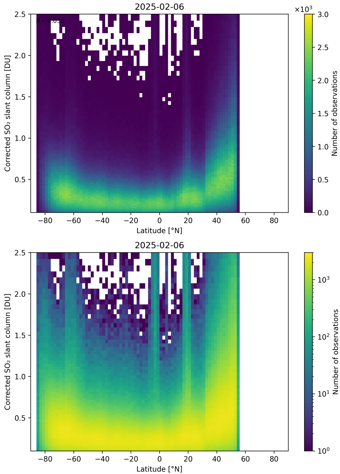
Figure 159: Scatter density plot of “Latitude” against “Corrected SO 2 slant column” for 2025-02-05 to 2025-02-07.
