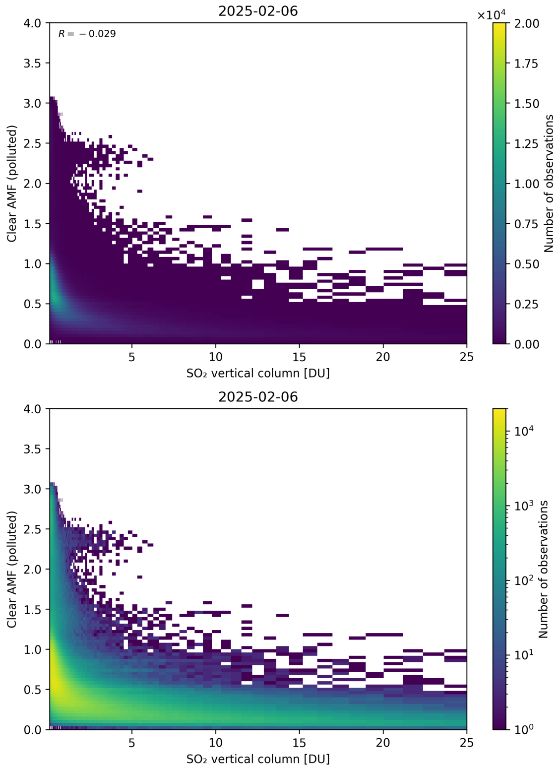
Figure 348: Scatter density plot of “SO 2 vertical column” against “Clear AMF (polluted)” for 2025-02-05 to 2025-02-07.
