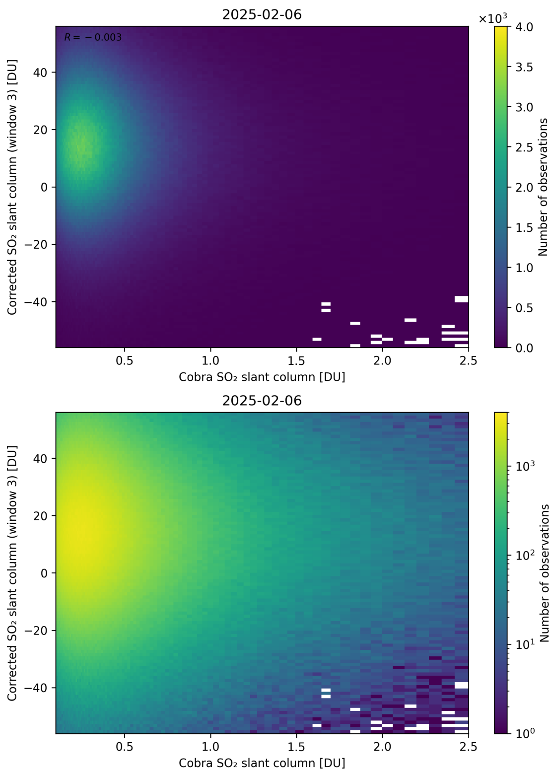
Figure 218: Scatter density plot of “Cobra SO 2 slant column” against “Corrected SO 2 slant column (window 3)” for 2025-02-05 to 2025-02-07.
