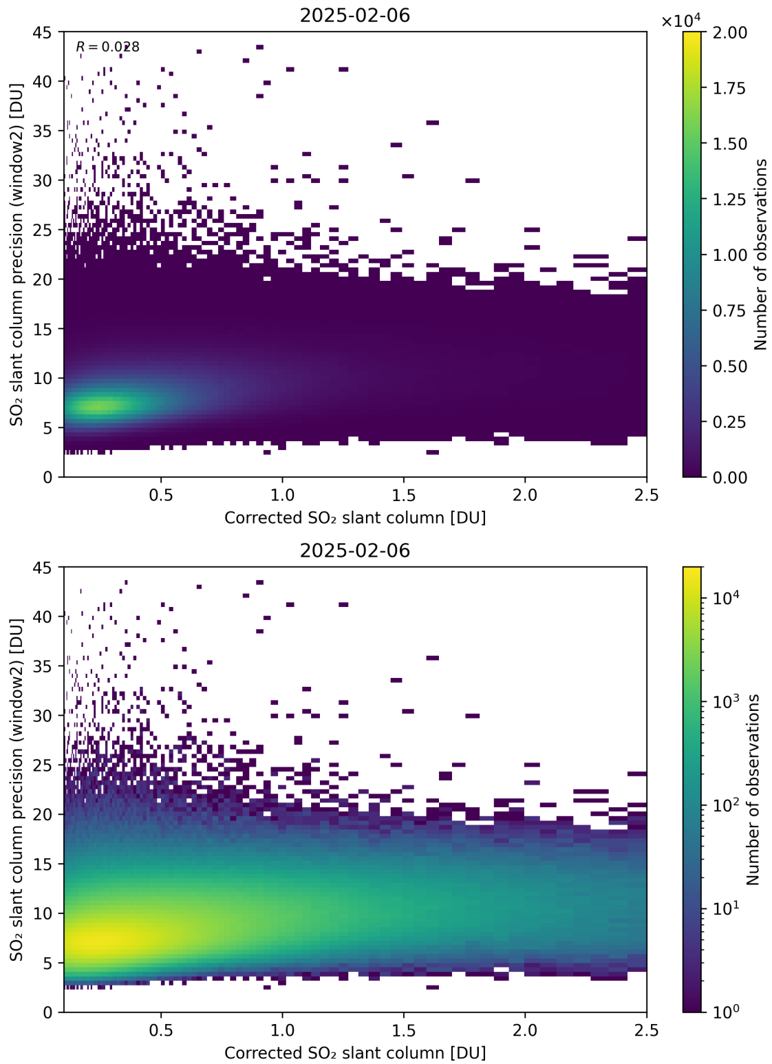
Figure 239: Scatter density plot of “Corrected SO 2 slant column” against “SO 2 slant column precision (window2)” for 2025-02-05 to 2025-02-07.
