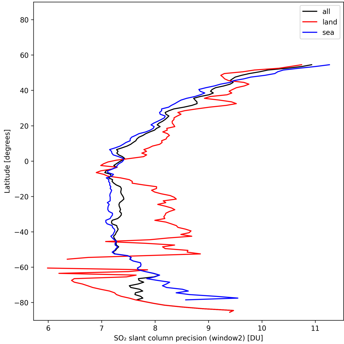
Figure 42: Zonal average of “SO 2 slant column precision (window2)” for 2025-02-05 to 2025-02-07.
