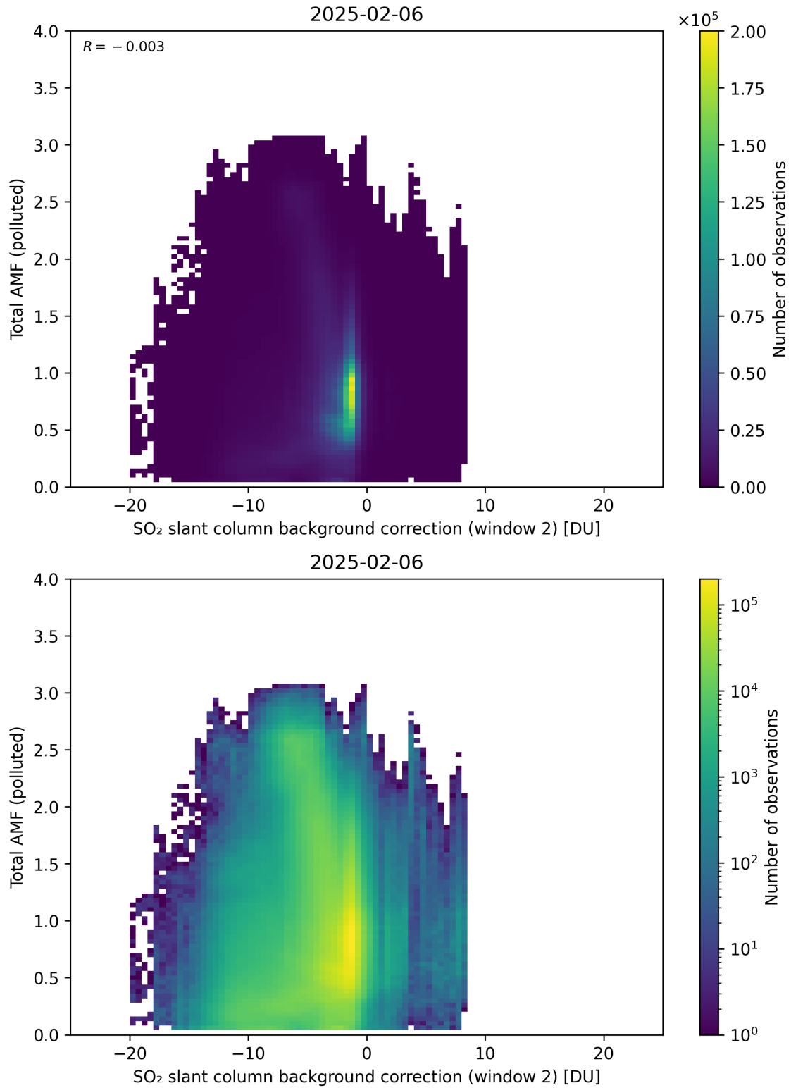
Figure 130: Scatter density plot of “SO 2 slant column background correction (window 2)” against “Total AMF (polluted)” for 2025-02-05 to 2025-02-07.
