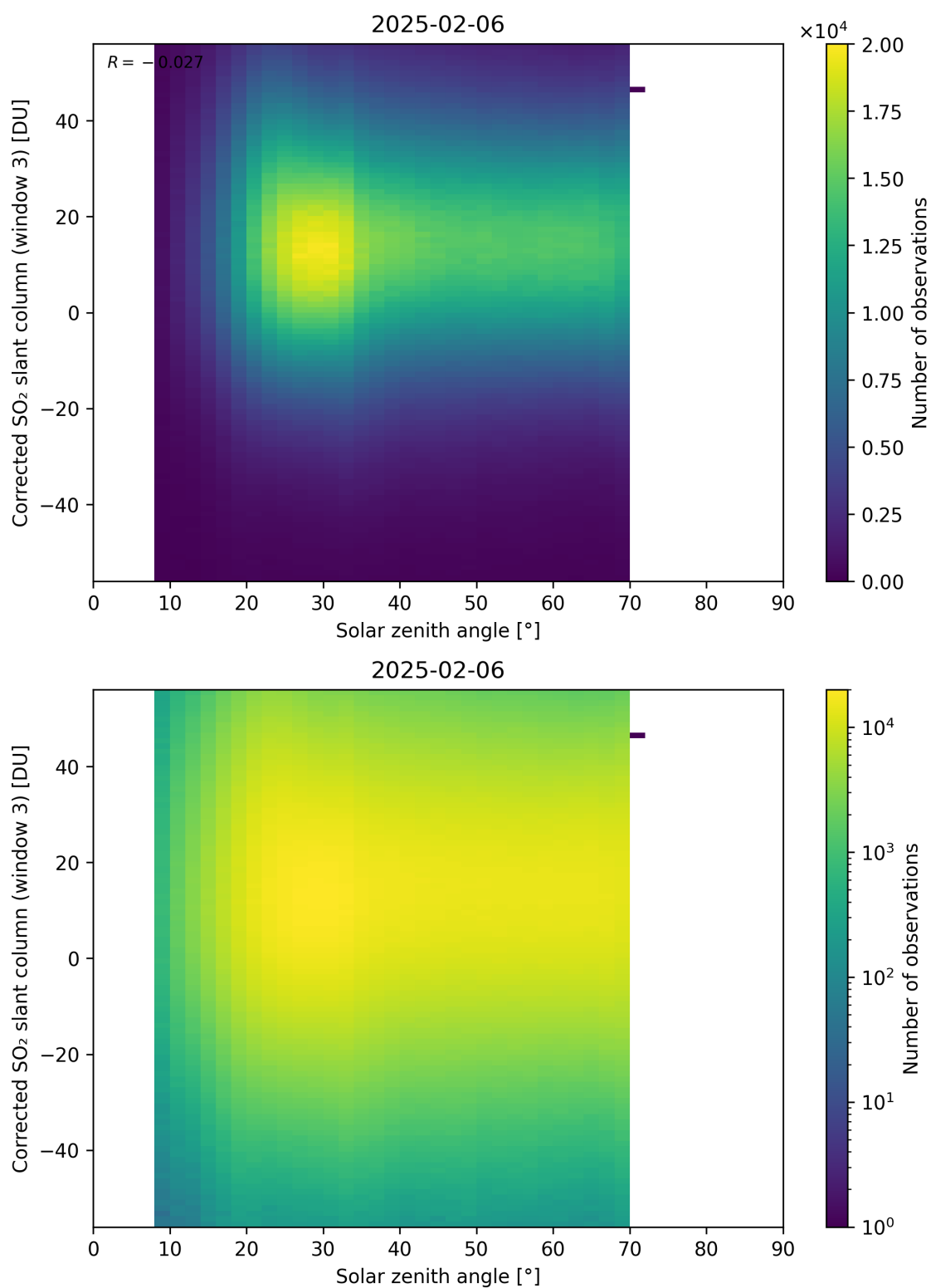
Figure 183: Scatter density plot of “Solar zenith angle” against “Corrected SO 2 slant column (window 3)” for 2025-02-05 to 2025-02-07.
