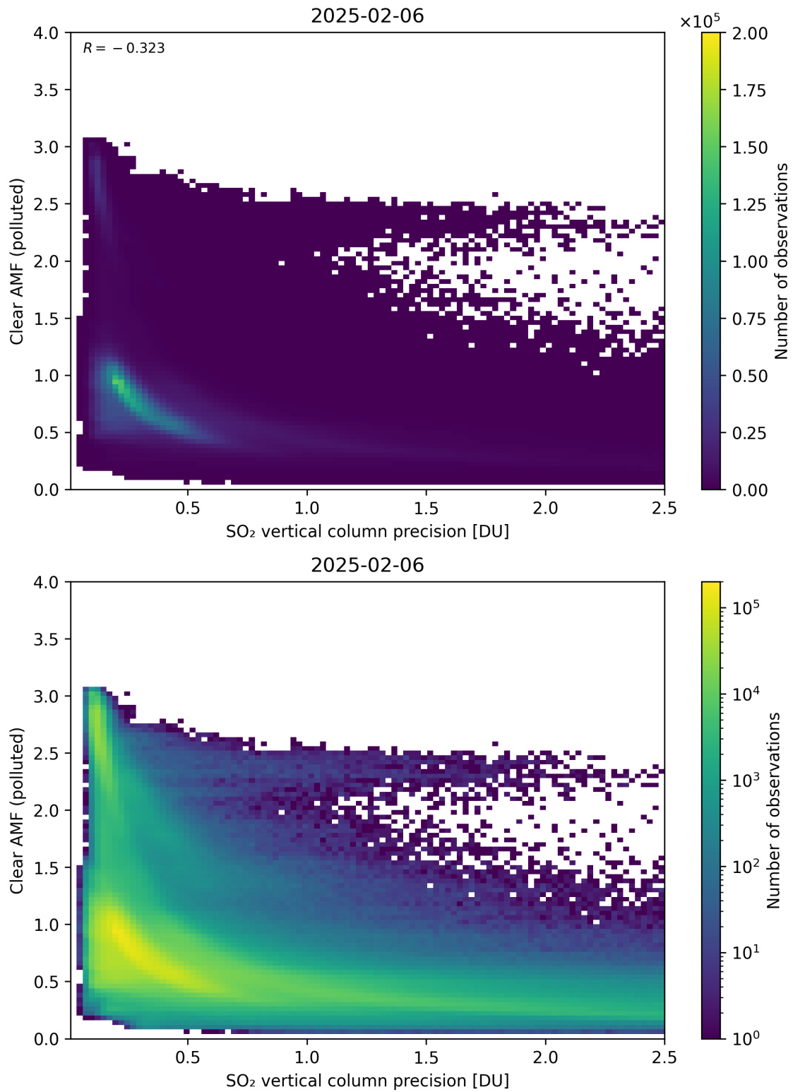
Figure 335: Scatter density plot of “SO 2 vertical column precision” against “Clear AMF (polluted)” for 2025-02-05 to 2025-02-07.
