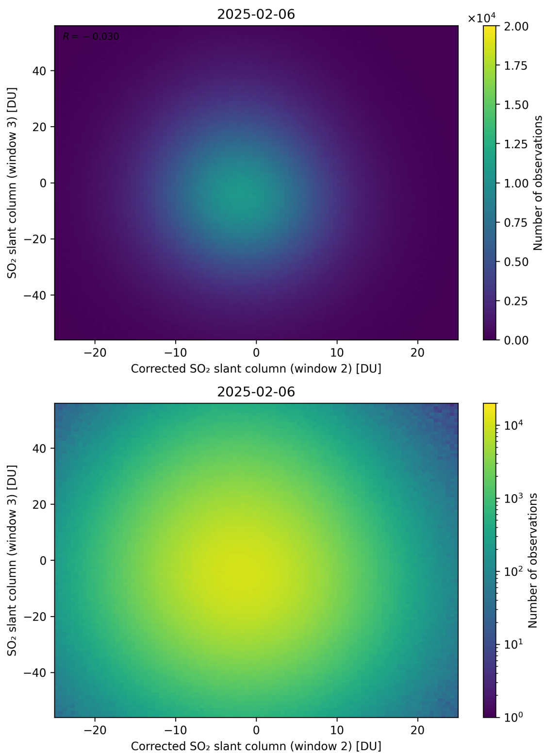
Figure 251: Scatter density plot of “Corrected SO 2 slant column (window 2)” against “SO 2 slant column (window 3)” for 2025-02-05 to 2025-02-07.
