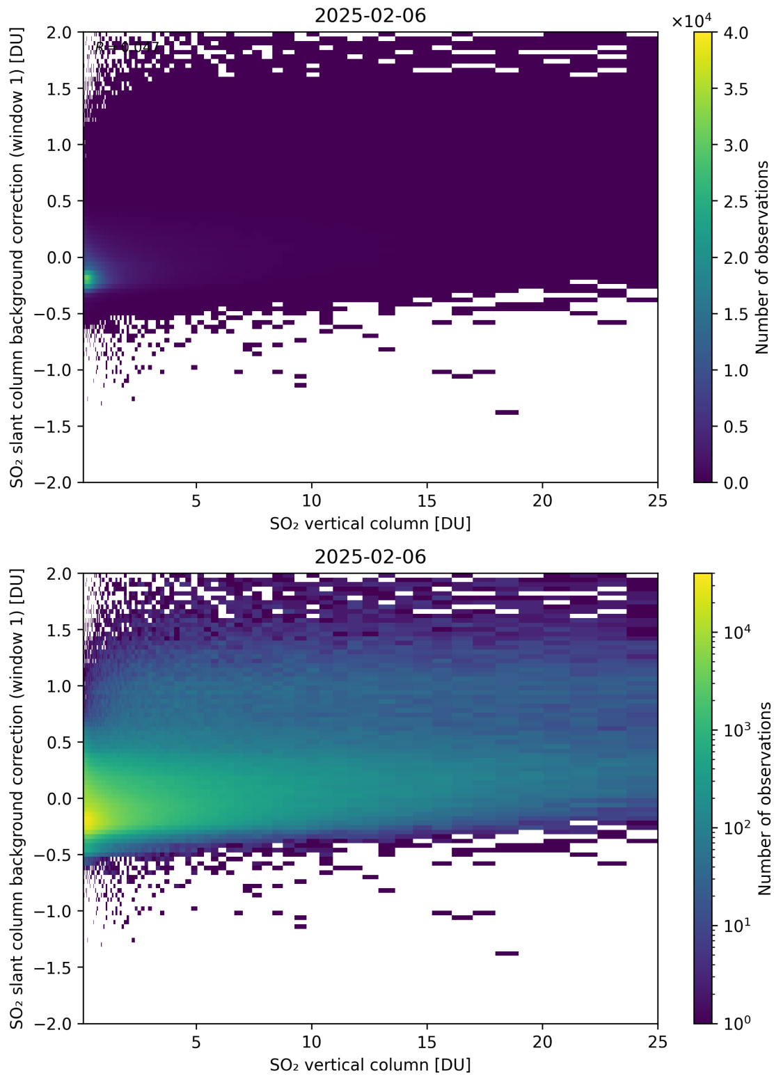
Figure 323: Scatter density plot of “SO 2 vertical column” against “SO 2 slant column background correction (window 1)” for 2025-02-05 to 2025-02-07.
