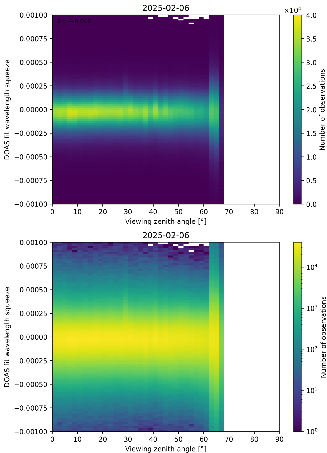
Figure 366: Scatter density plot of “Viewing zenith angle” against “DOAS fit wavelength squeeze” for 2025-02-05 to 2025-02-07.
