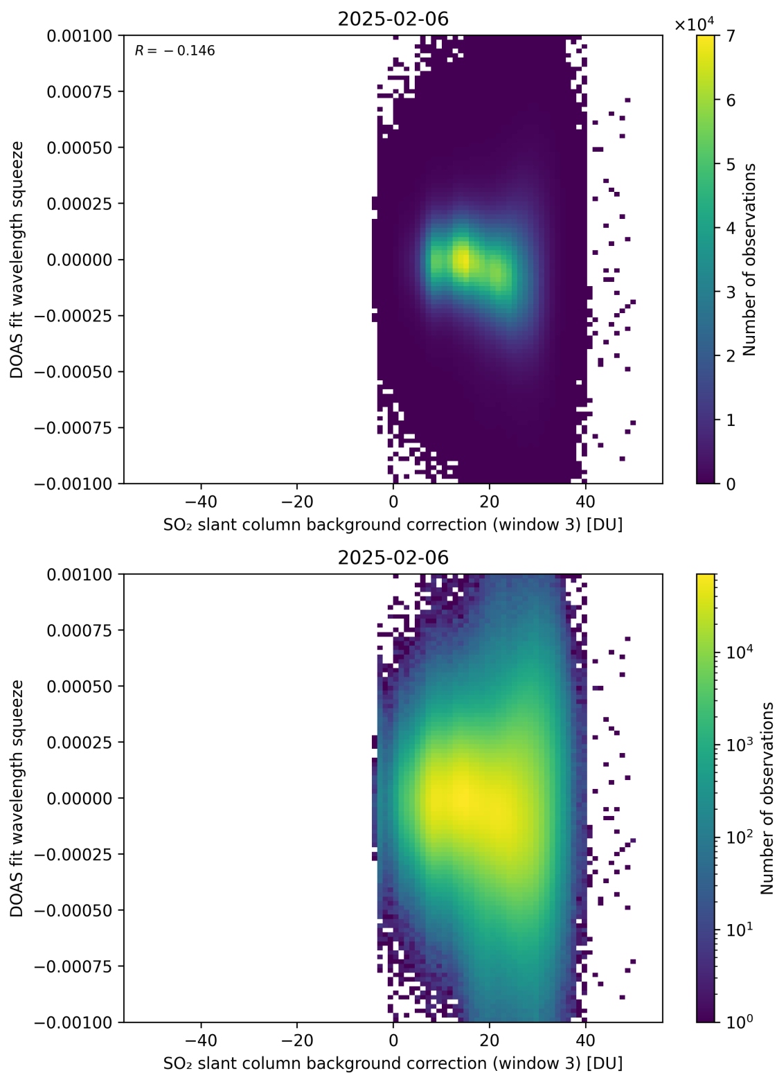
Figure 133: Scatter density plot of “SO 2 slant column background correction (window 3)” against “DOAS fit wavelength squeeze” for 2025-02-05 to 2025-02-07.
