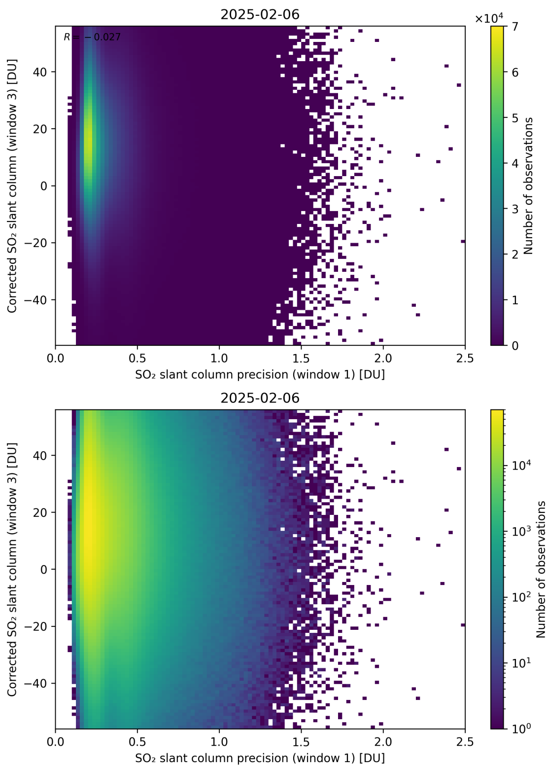
Figure 276: Scatter density plot of “SO 2 slant column precision (window 1)” against “Corrected SO 2 slant column (window 3)” for 2025-02-05 to 2025-02-07.
