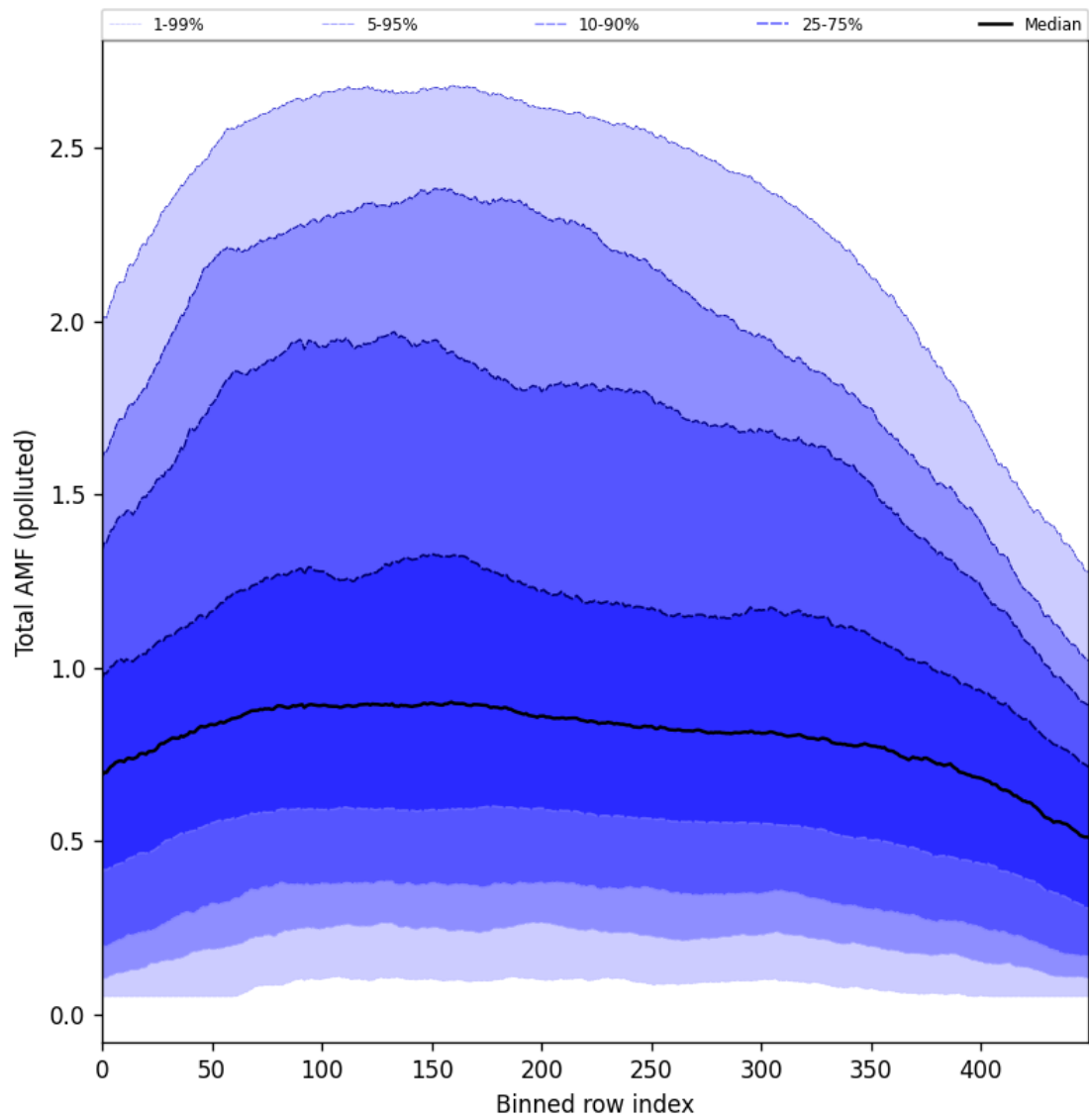
Figure 105: Along track statistics of “Total AMF (polluted)” for 2025-02-05 to 2025-02-07
