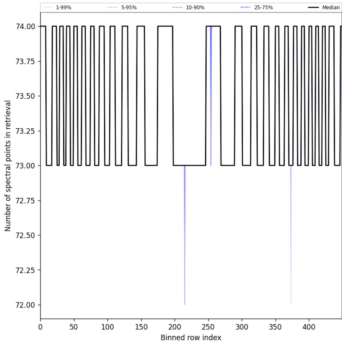
Figure 108: Along track statistics of “Number of spectral points in retrieval” for 2025-02-05 to 2025-02-07
