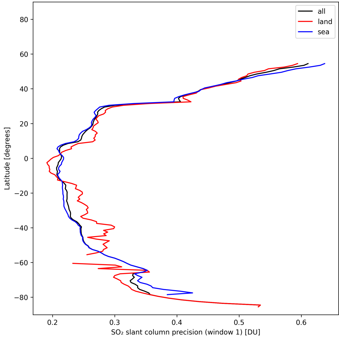
Figure 38: Zonal average of “SO 2 slant column precision (window 1)” for 2025-02-05 to 2025-02-07.
