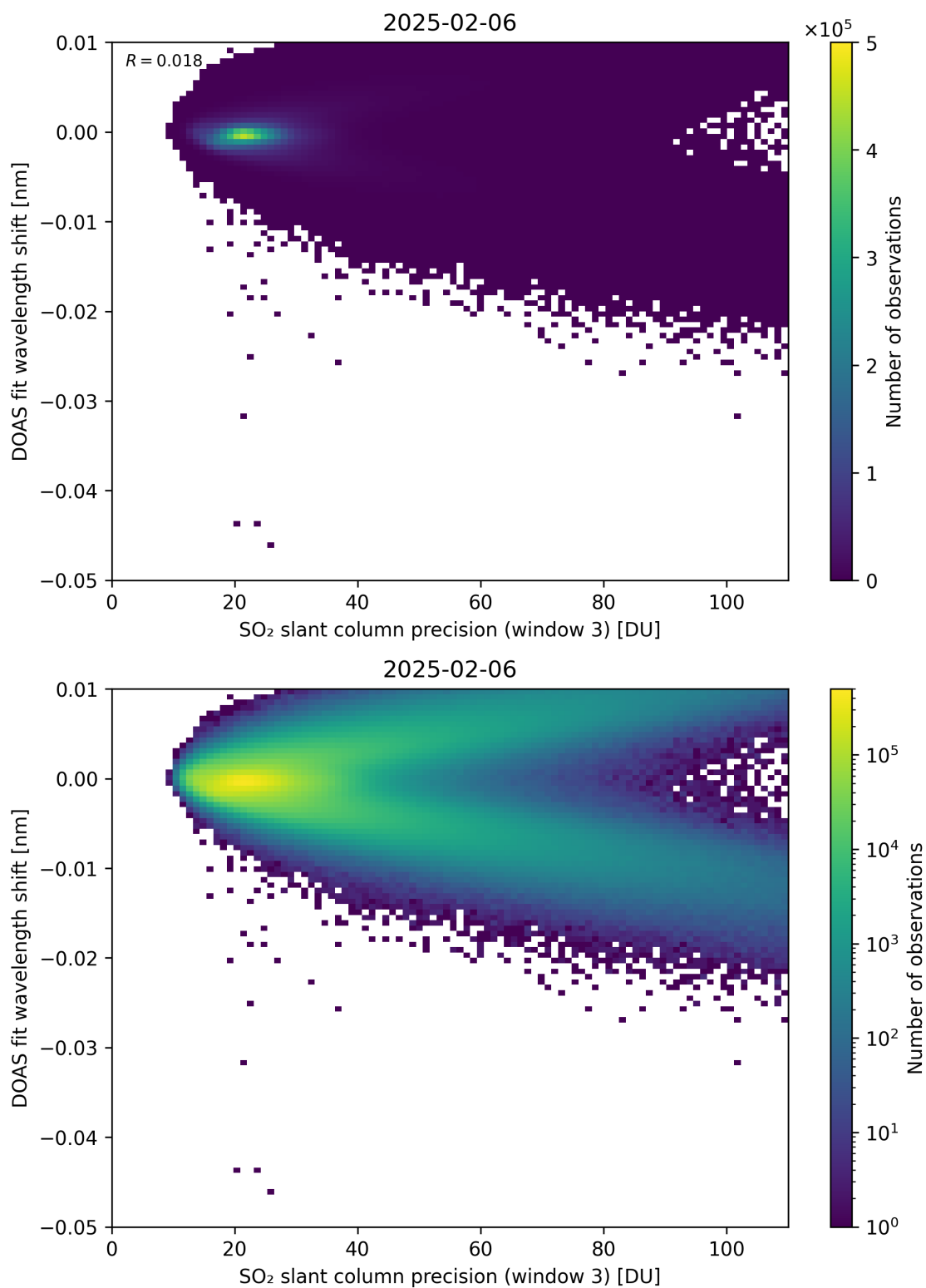
Figure 308: Scatter density plot of “SO 2 slant column precision (window 3)” against “DOAS fit wavelength shift” for 2025-02-05 to 2025-02-07.
