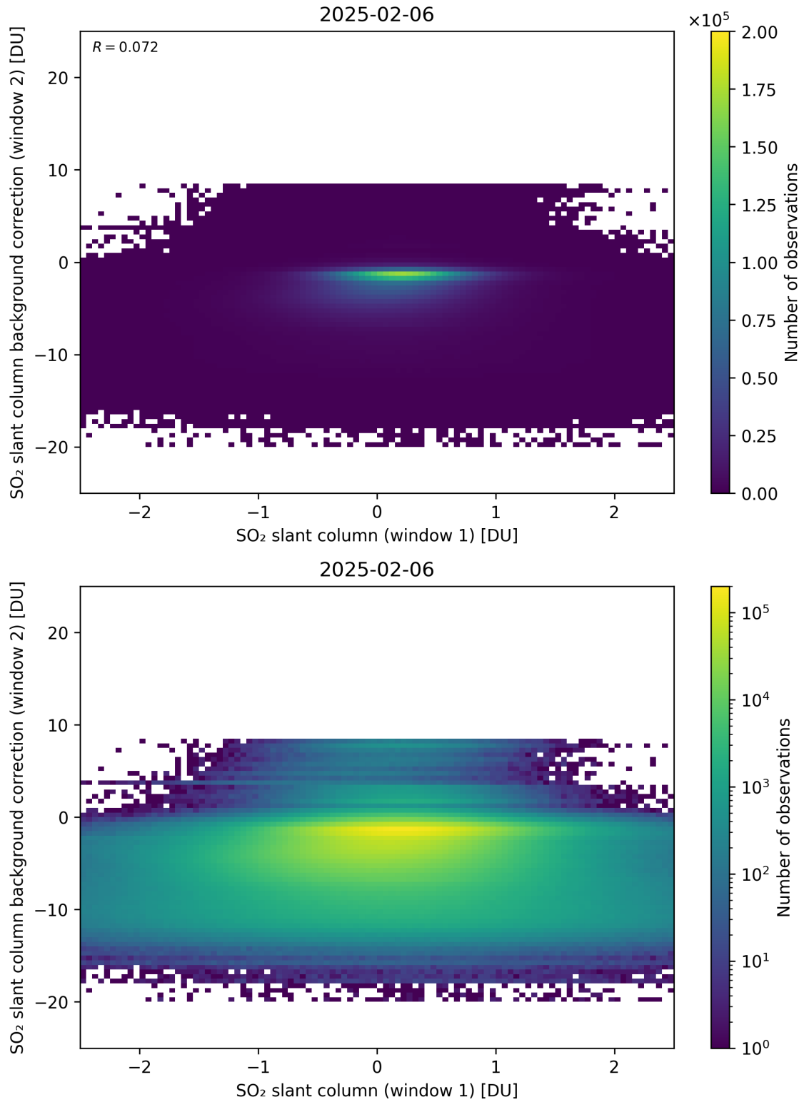
Figure 263: Scatter density plot of “SO 2 slant column (window 1)” against “SO 2 slant column background correction (window 2)” for 2025-02-05 to 2025-02-07.
