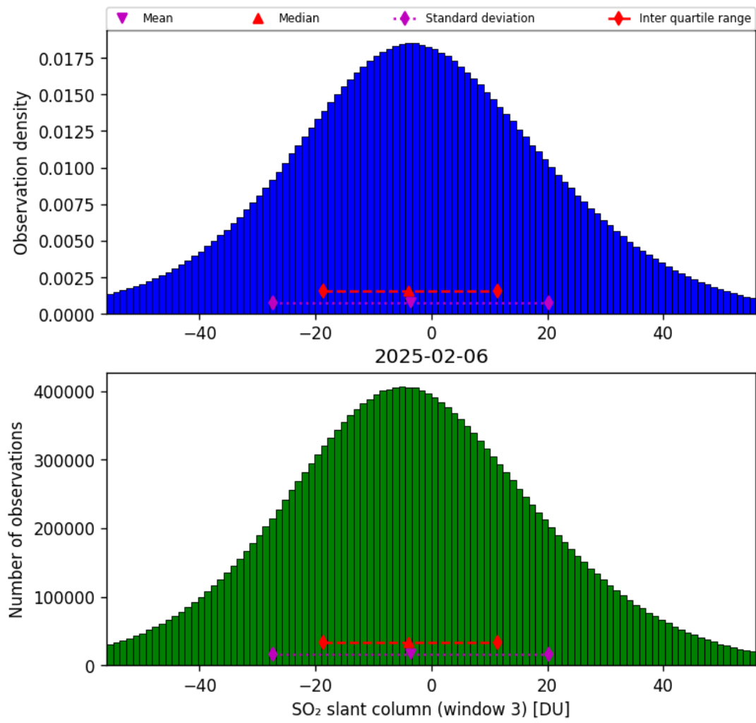
Figure 71: Histogram of “SO 2 slant column (window 3)” for 2025-02-05 to 2025-02-07
