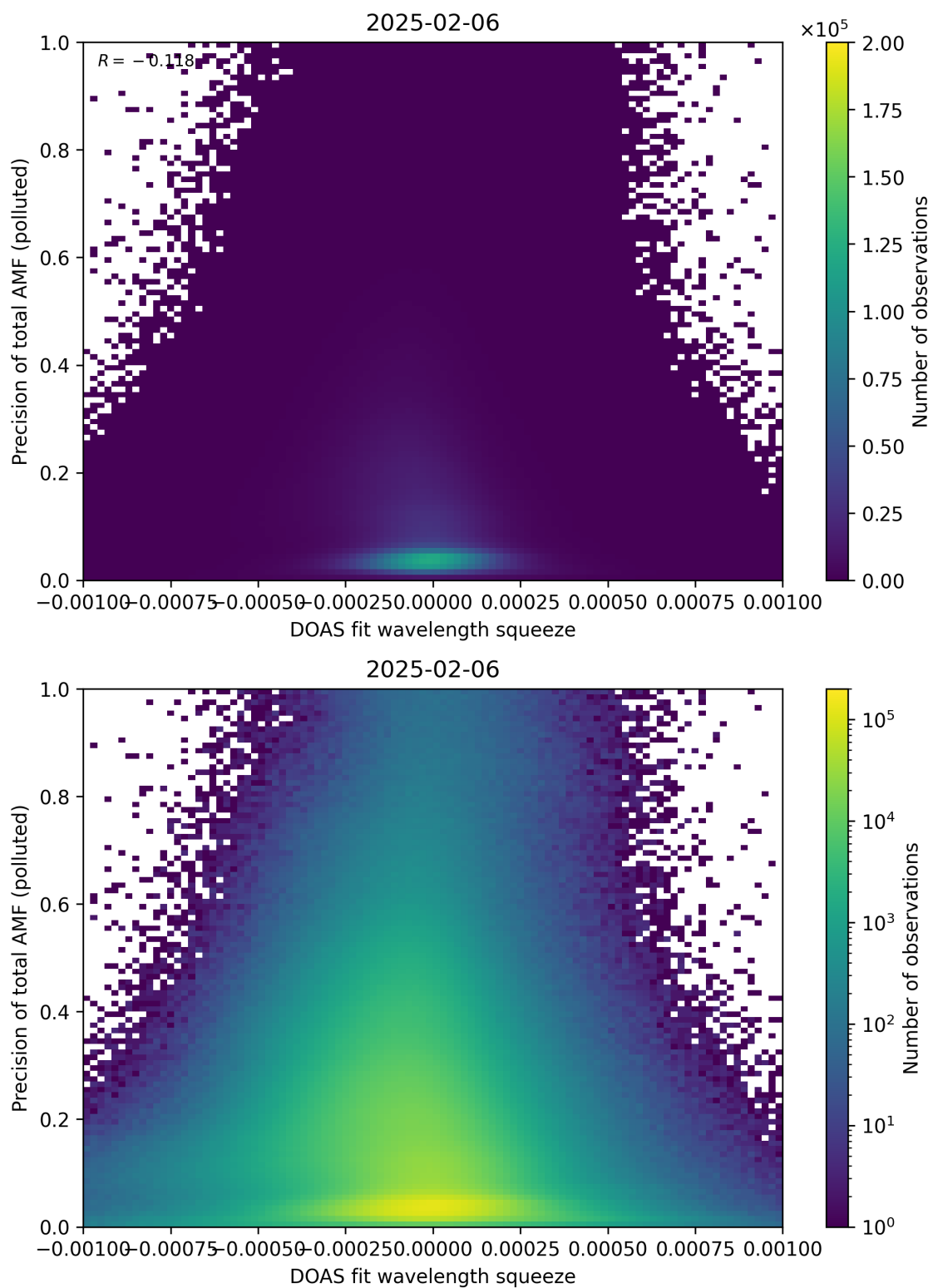
Figure 146: Scatter density plot of “DOAS fit wavelength squeeze” against “Precision of total AMF (polluted)” for 2025-02-05 to 2025-02-07.
