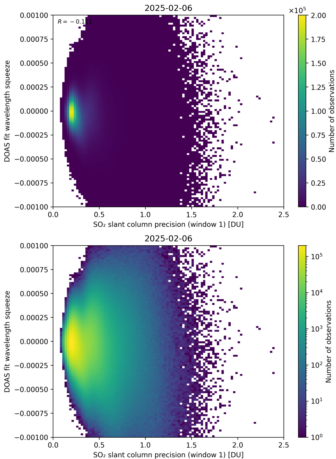
Figure 272: Scatter density plot of “SO 2 slant column precision (window 1)” against “DOAS fit wavelength squeeze” for 2025-02-05 to 2025-02-07.
