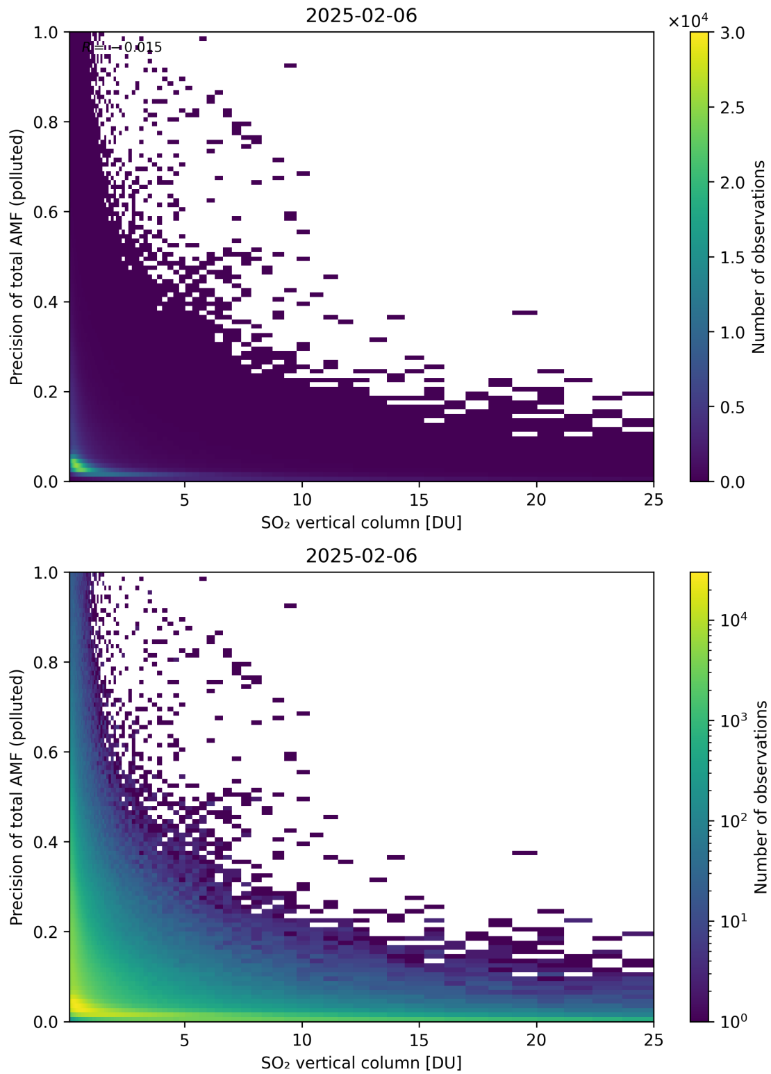
Figure 360: Scatter density plot of “SO 2 vertical column” against “Precision of total AMF (polluted)” for 2025-02-05 to 2025-02-07.
