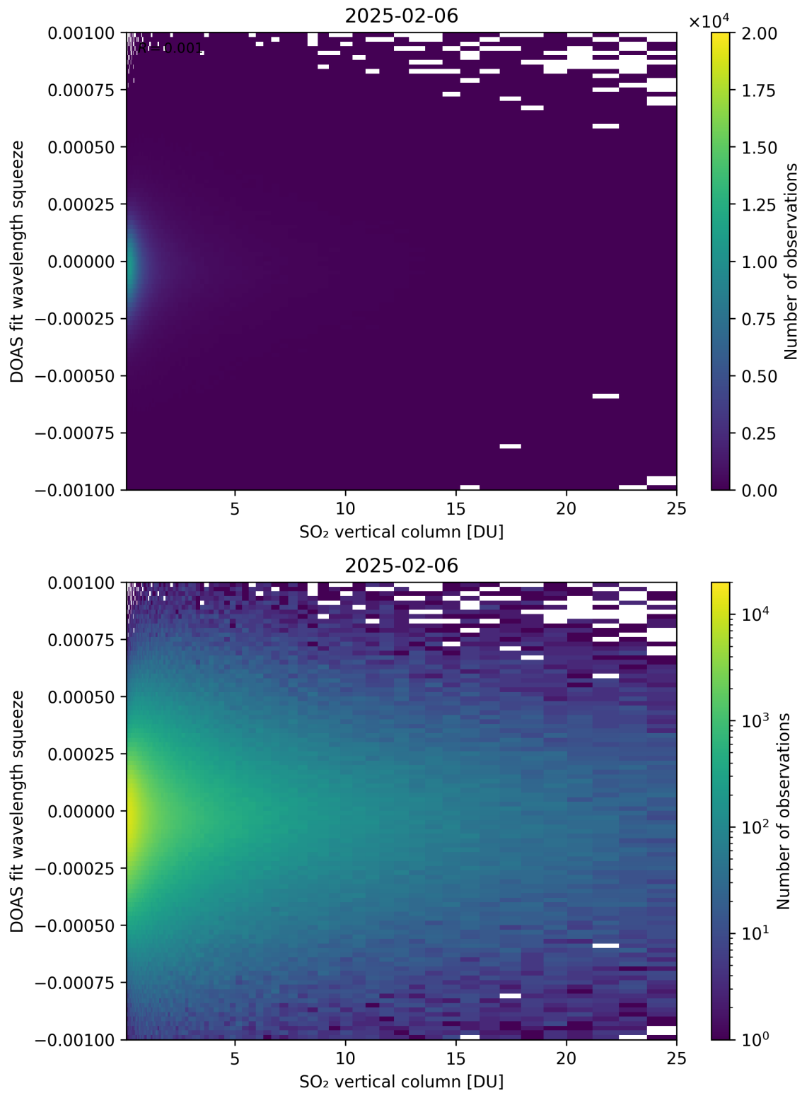
Figure 327: Scatter density plot of “SO 2 vertical column” against “DOAS fit wavelength squeeze” for 2025-02-05 to 2025-02-07.
