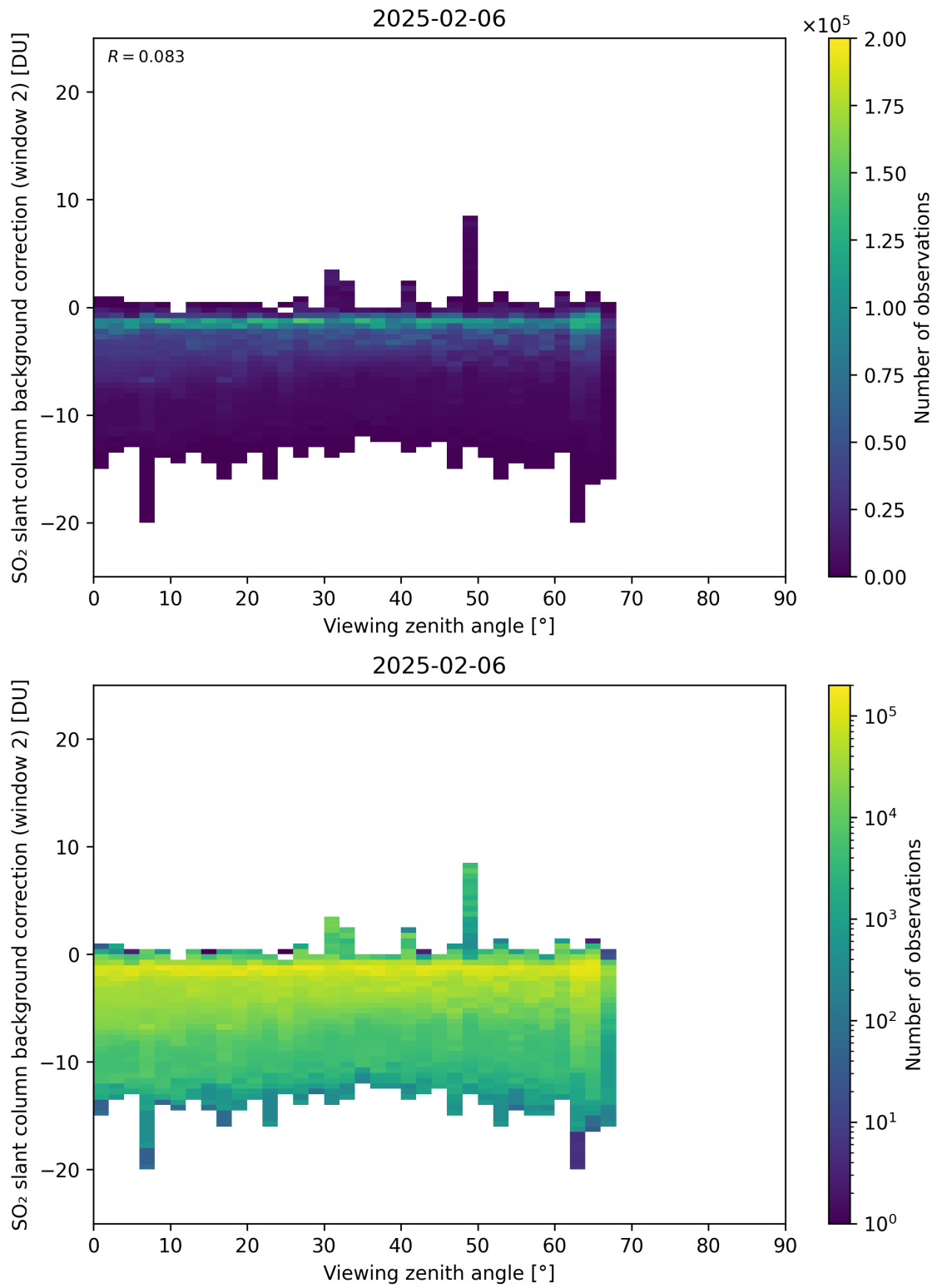
Figure 363: Scatter density plot of “Viewing zenith angle” against “SO 2 slant column background correction (window 2)” for 2025-02-05 to 2025-02-07.
