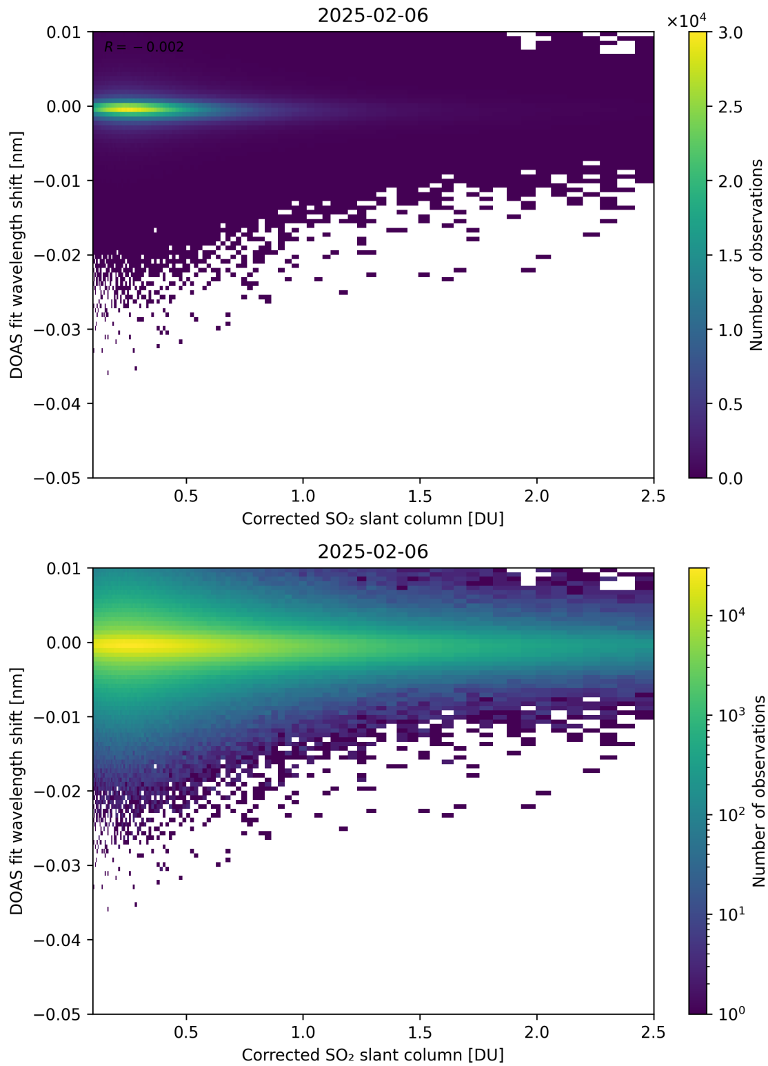
Figure 229: Scatter density plot of “Corrected SO 2 slant column” against “DOAS fit wavelength shift” for 2025-02-05 to 2025-02-07.
