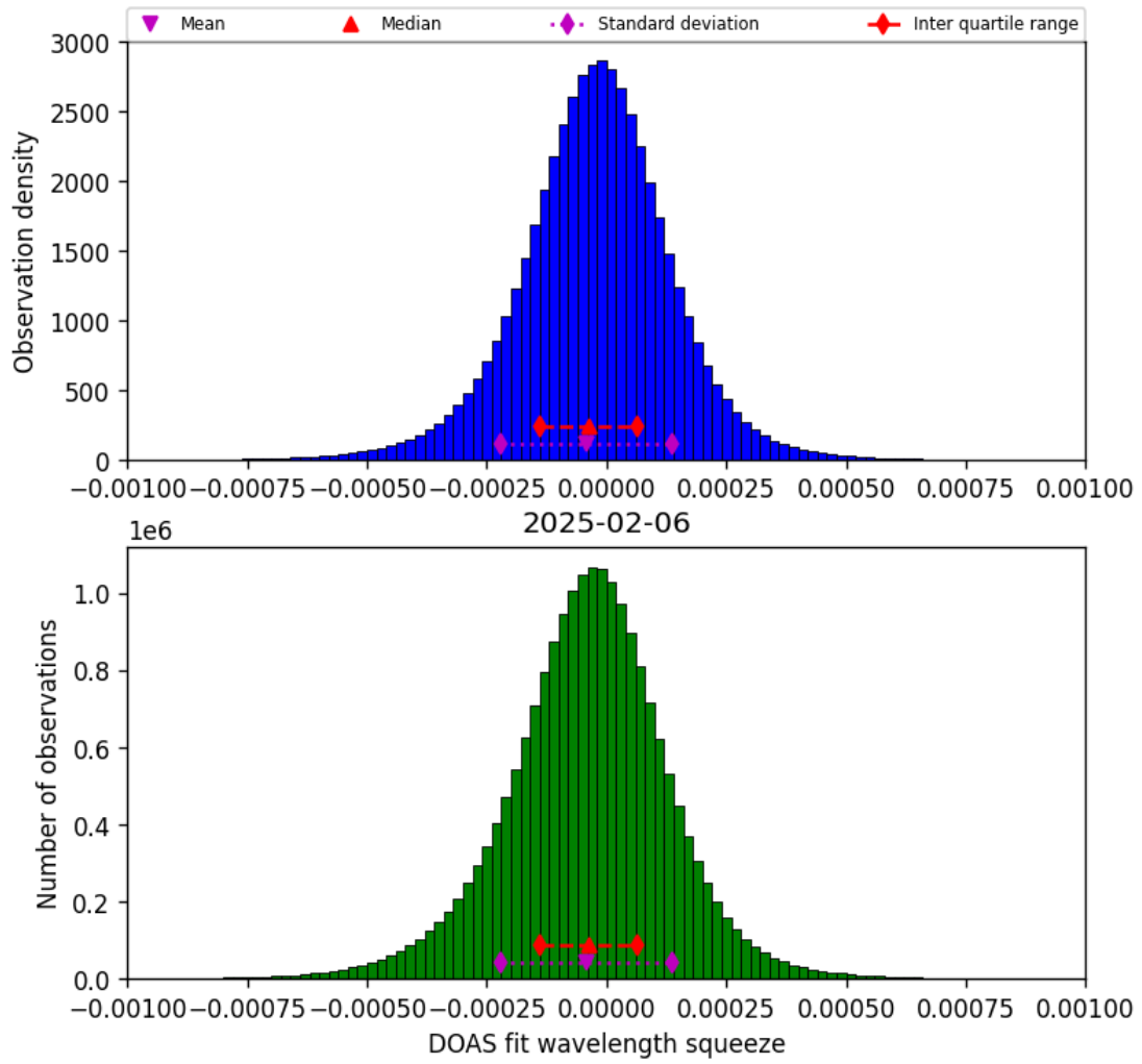
Figure 77: Histogram of “DOAS fit wavelength squeeze” for 2025-02-05 to 2025-02-07
