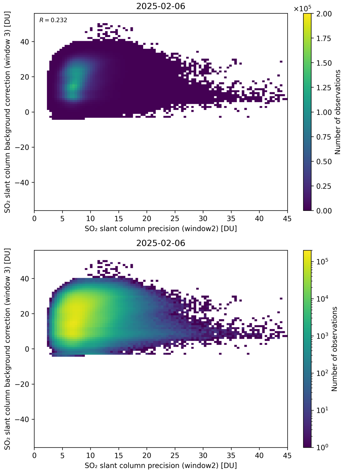
Figure 292: Scatter density plot of “SO 2 slant column precision (window2)” against “SO 2 slant column background correction (window 3)” for 2025-02-05 to 2025-02-07.
