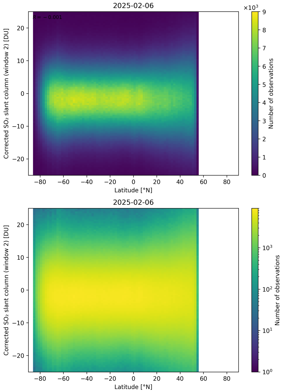
Figure 160: Scatter density plot of “Latitude” against “Corrected SO 2 slant column (window 2)” for 2025-02-05 to 2025-02-07.
