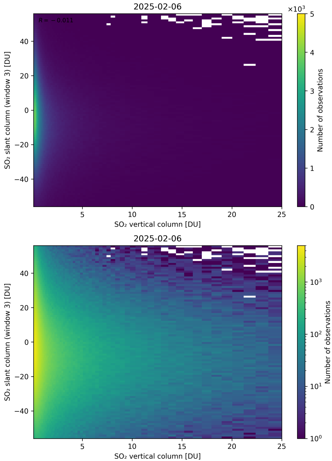
Figure 357: Scatter density plot of “SO 2 vertical column” against “SO 2 slant column (window 3)” for 2025-02-05 to 2025-02-07.
