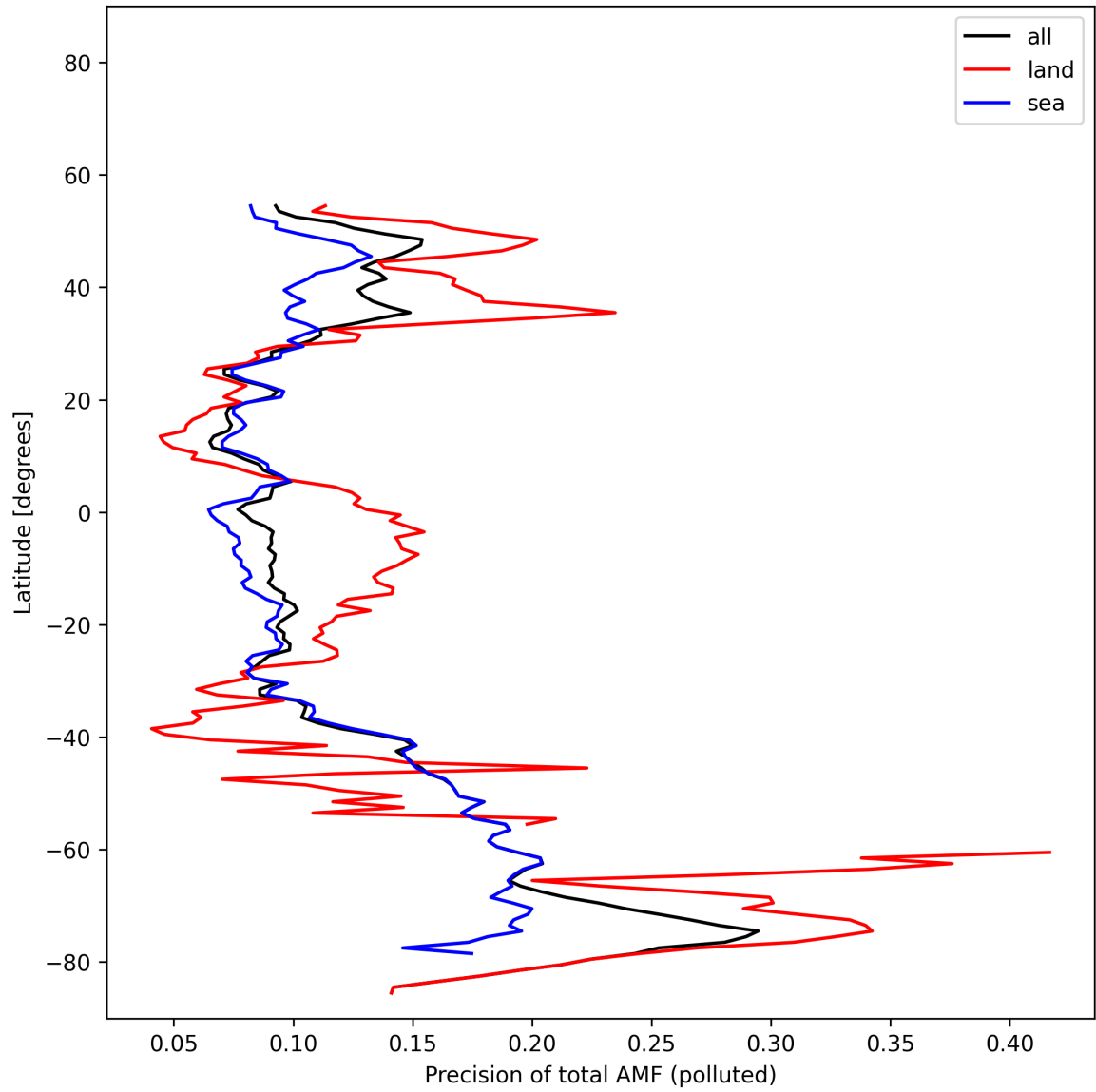
Figure 54: Zonal average of “Precision of total AMF (polluted)” for 2025-02-05 to 2025-02-07.
