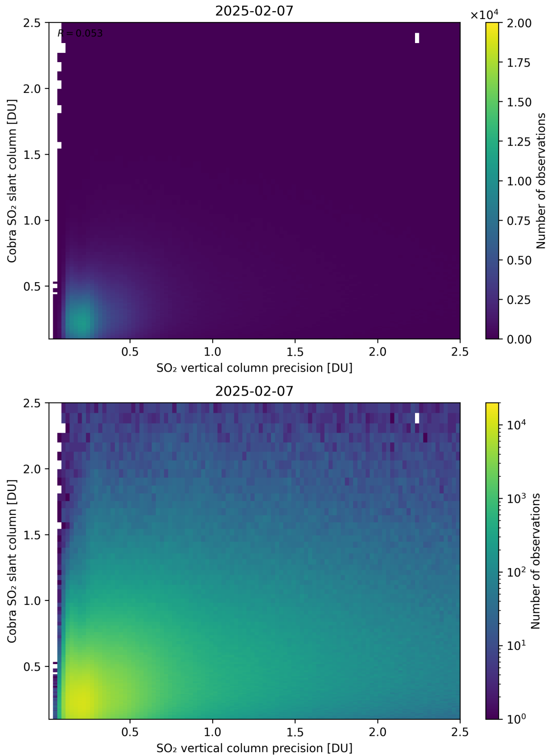
Figure 336: Scatter density plot of “SO 2 vertical column precision” against “Cobra SO 2 slant column” for 2025-02-06 to 2025-02-08.
