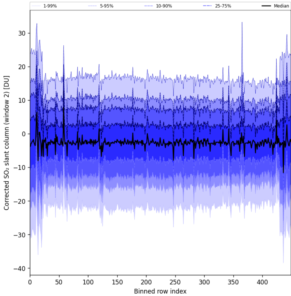
Figure 95: Along track statistics of “Corrected SO 2 slant column (window 2)” for 2025-02-06 to 2025-02-08
