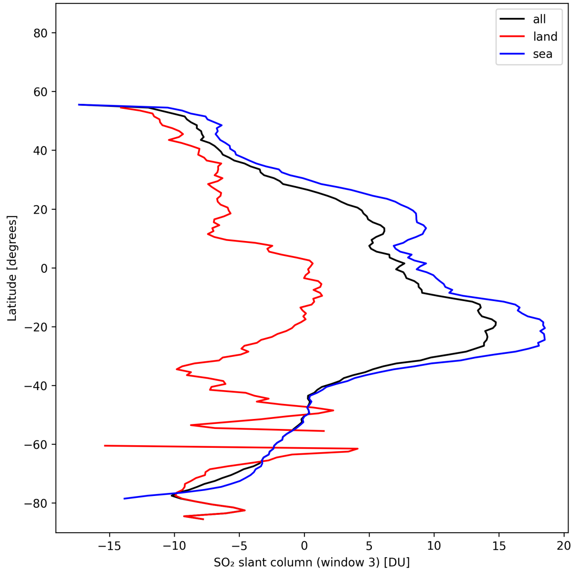
Figure 45: Zonal average of “SO 2 slant column (window 3)” for 2025-02-06 to 2025-02-08.
