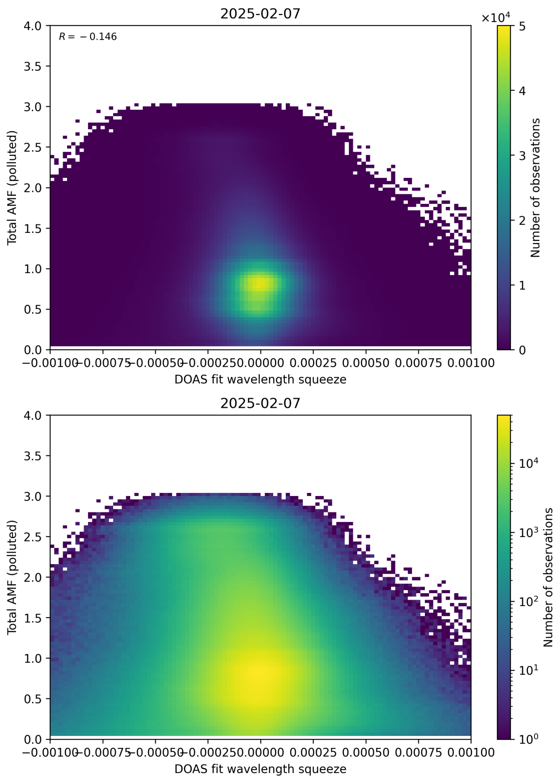
Figure 145: Scatter density plot of “DOAS fit wavelength squeeze” against “Total AMF (polluted)” for 2025-02-06 to 2025-02-08.
