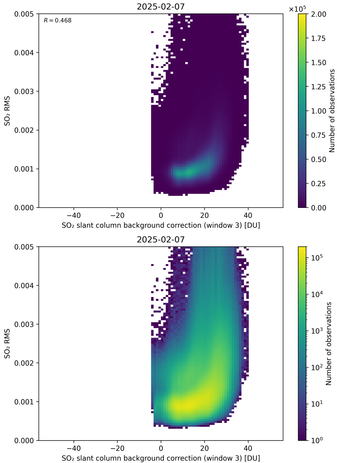
Figure 134: Scatter density plot of “SO 2 slant column background correction (window 3)” against “SO 2 RMS” for 2025-02-06 to 2025-02-08.
