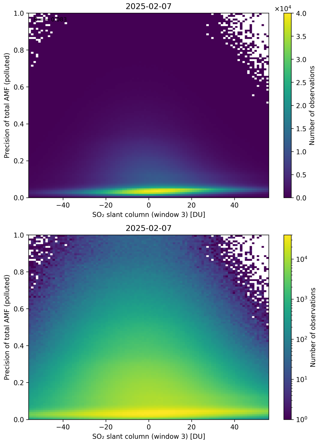
Figure 319: Scatter density plot of “SO 2 slant column (window 3)” against “Precision of total AMF (polluted)” for 2025-02-06 to 2025-02-08.
