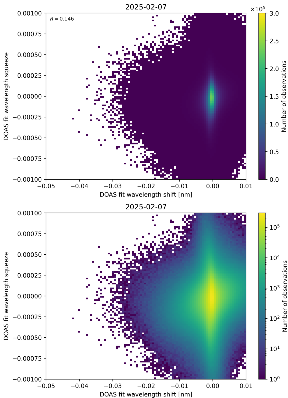
Figure 138: Scatter density plot of “DOAS fit wavelength shift” against “DOAS fit wavelength squeeze” for 2025-02-06 to 2025-02-08.
