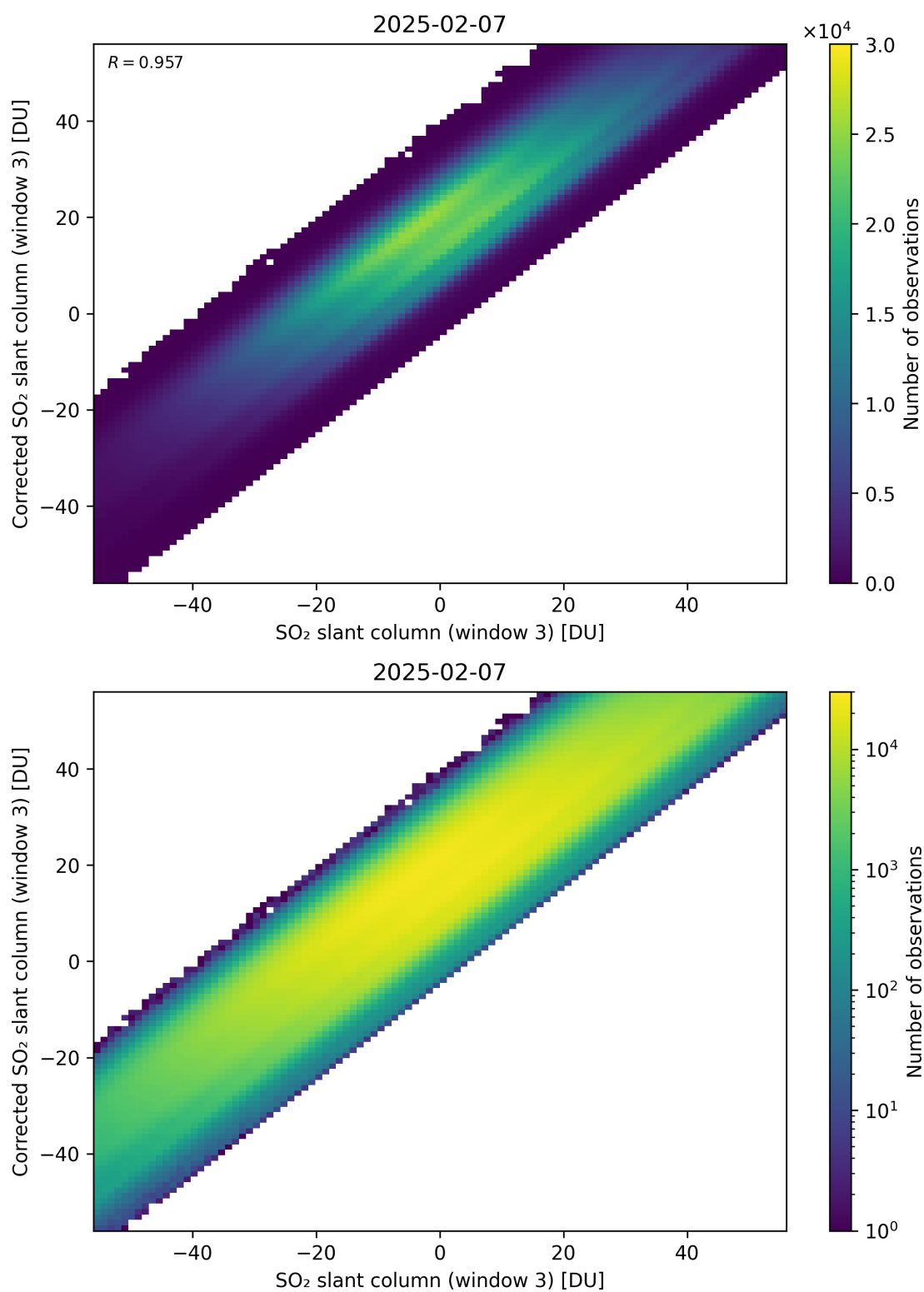
Figure 316: Scatter density plot of “SO 2 slant column (window 3)” against “Corrected SO 2 slant column (window 3)” for 2025-02-06 to 2025-02-08.
