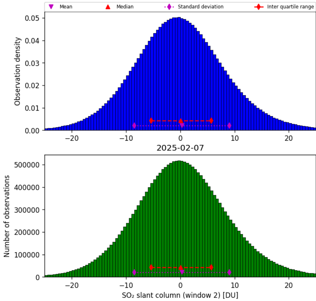
Figure 67: Histogram of “SO 2 slant column (window 2)” for 2025-02-06 to 2025-02-08
