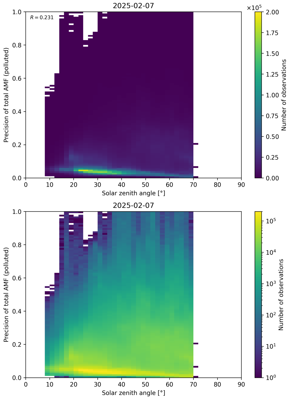
Figure 190: Scatter density plot of “Solar zenith angle” against “Precision of total AMF (polluted)” for 2025-02-06 to 2025-02-08.
