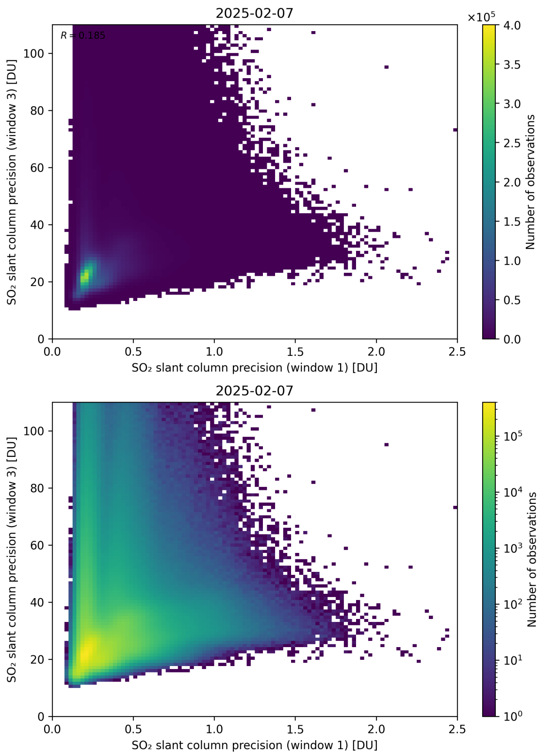
Figure 279: Scatter density plot of “SO 2 slant column precision (window 1)” against “SO 2 slant column precision (window 3)” for 2025-02-06 to 2025-02-08.
