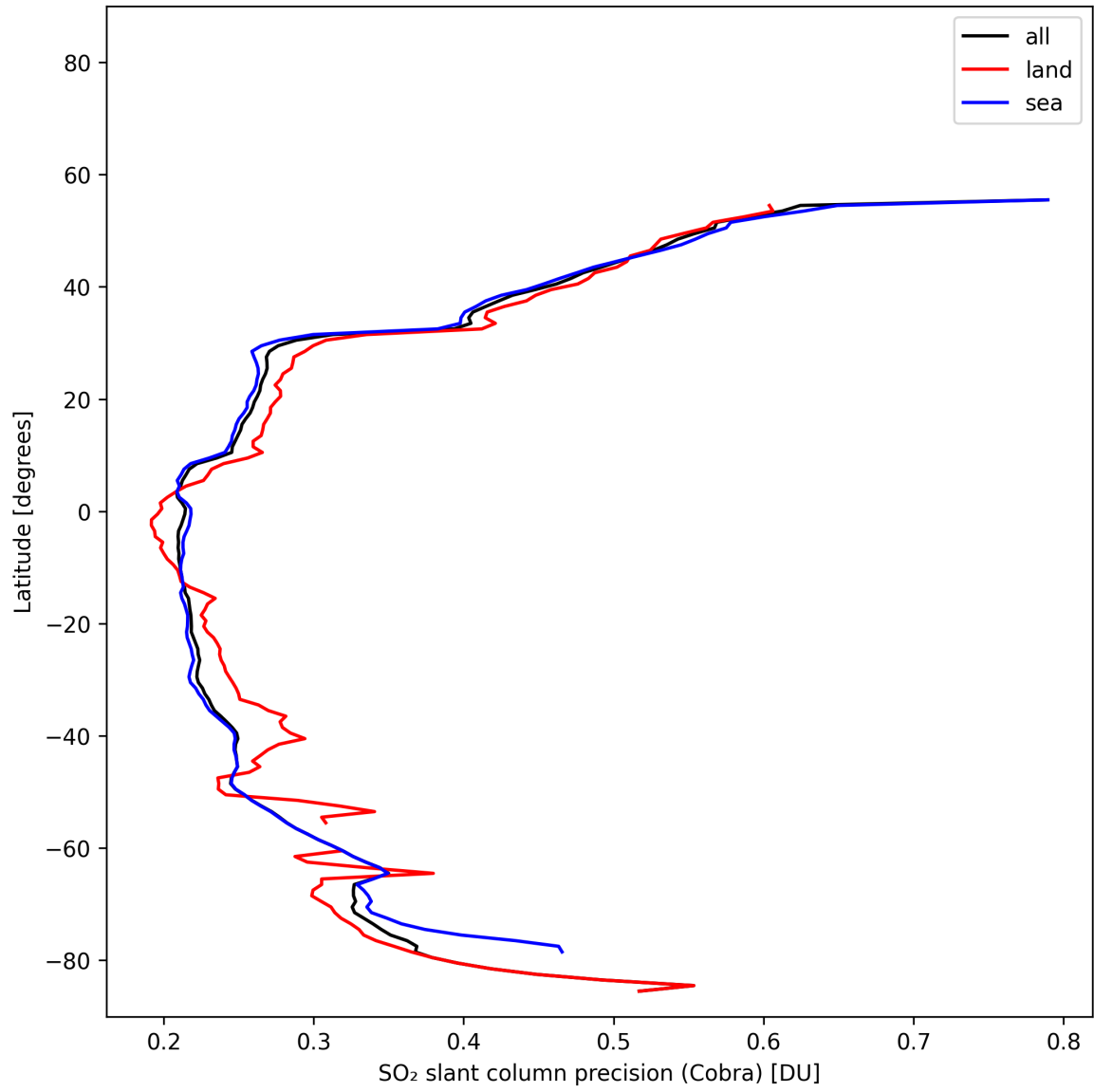
Figure 36: Zonal average of “SO 2 slant column precision (Cobra)” for 2025-02-06 to 2025-02-08.
