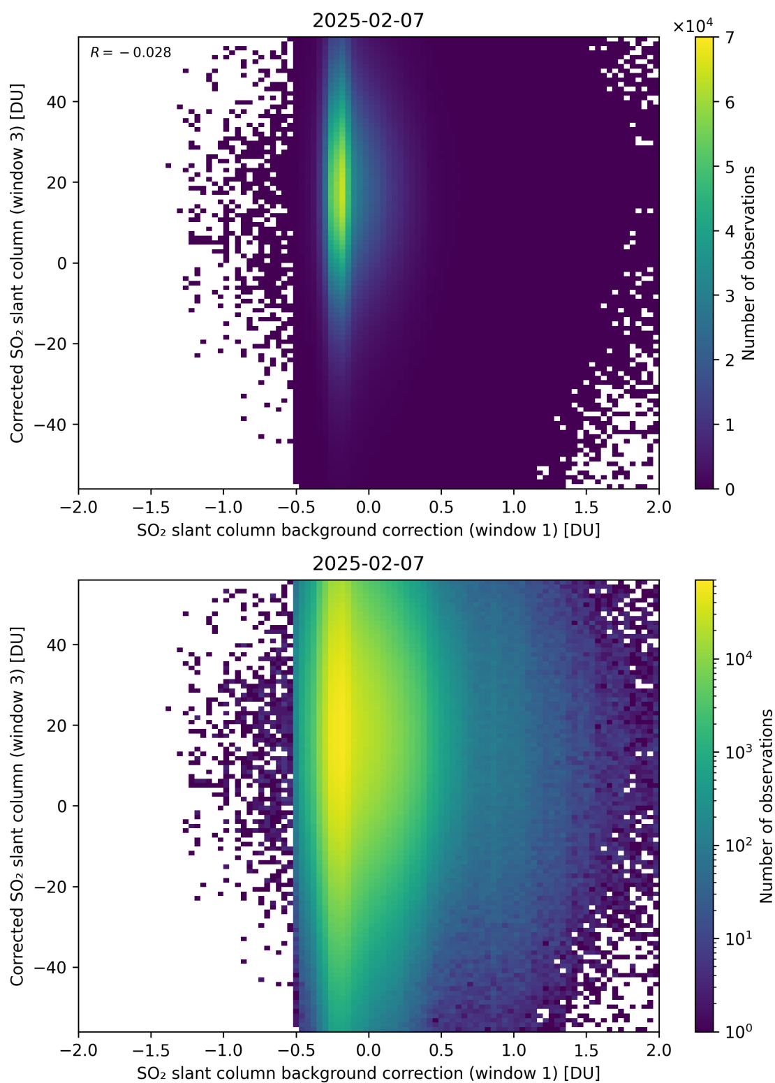
Figure 116: Scatter density plot of “SO 2 slant column background correction (window 1)” against “Corrected SO 2 slant column (window 3)” for 2025-02-06 to 2025-02-08.
