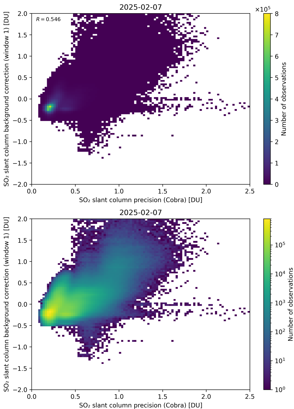
Figure 199: Scatter density plot of “SO 2 slant column precision (Cobra)” against “SO 2 slant column background correction (window 1)” for 2025-02-06 to 2025-02-08.
