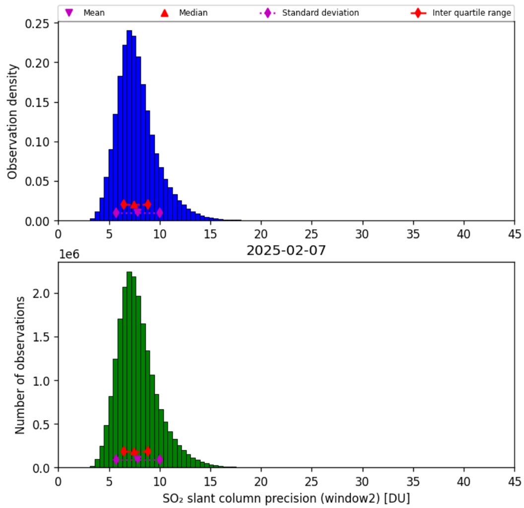
Figure 68: Histogram of “SO 2 slant column precision (window2)” for 2025-02-06 to 2025-02-08
