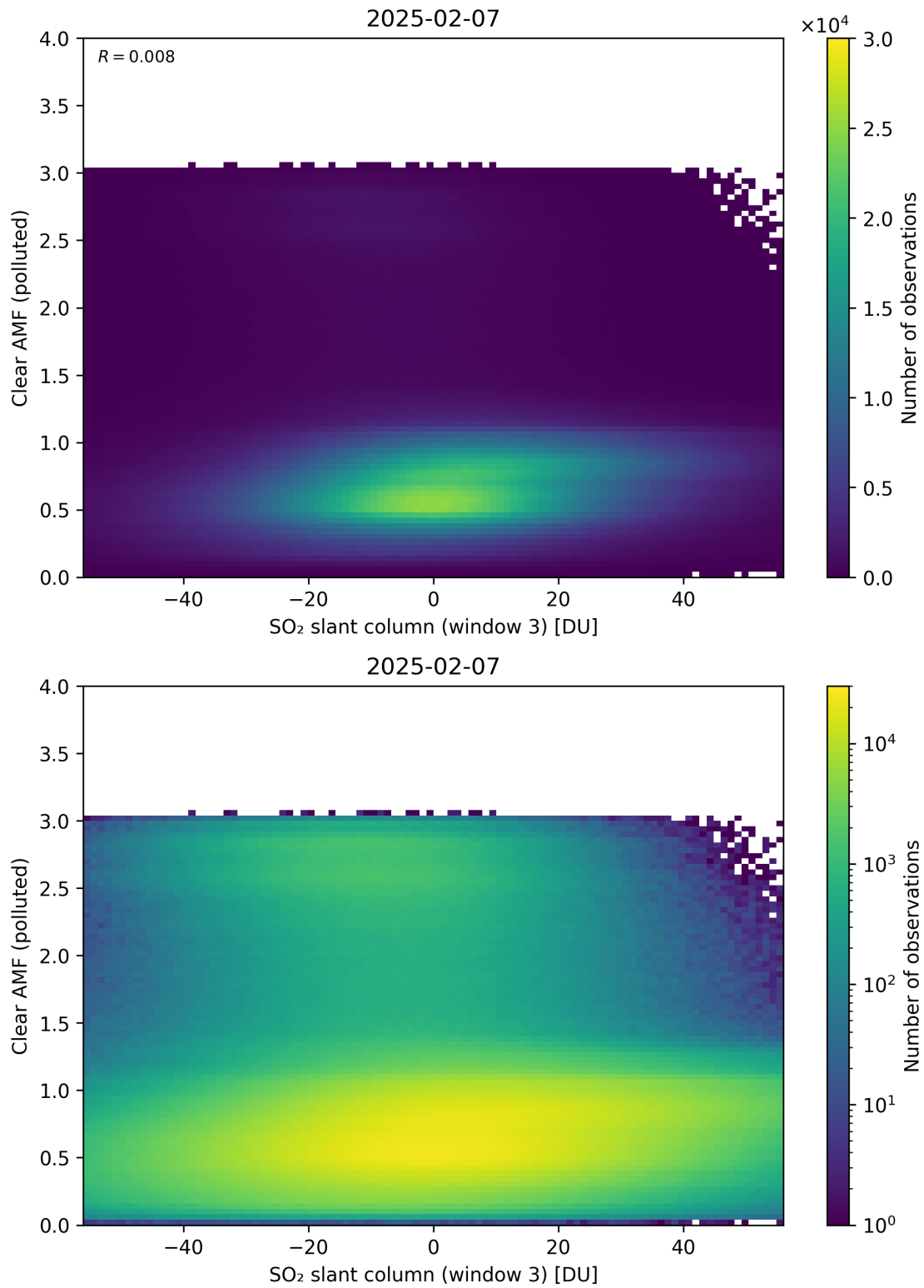
Figure 315: Scatter density plot of “SO 2 slant column (window 3)” against “Clear AMF (polluted)” for 2025-02-06 to 2025-02-08.
