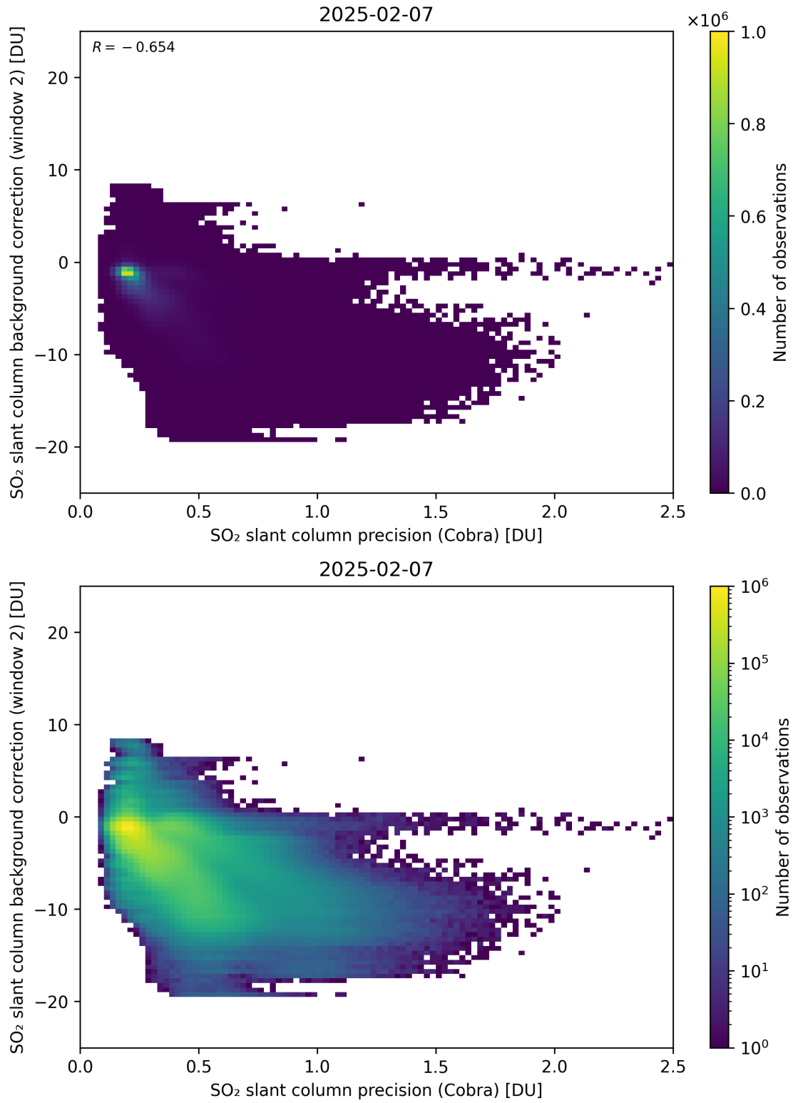
Figure 200: Scatter density plot of “SO 2 slant column precision (Cobra)” against “SO 2 slant column background correction (window 2)” for 2025-02-06 to 2025-02-08.
