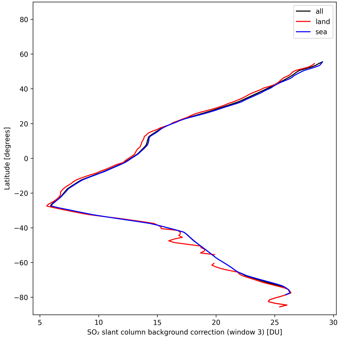
Figure 48: Zonal average of “SO 2 slant column background correction (window 3)” for 2025-02-06 to 2025-02-08.
