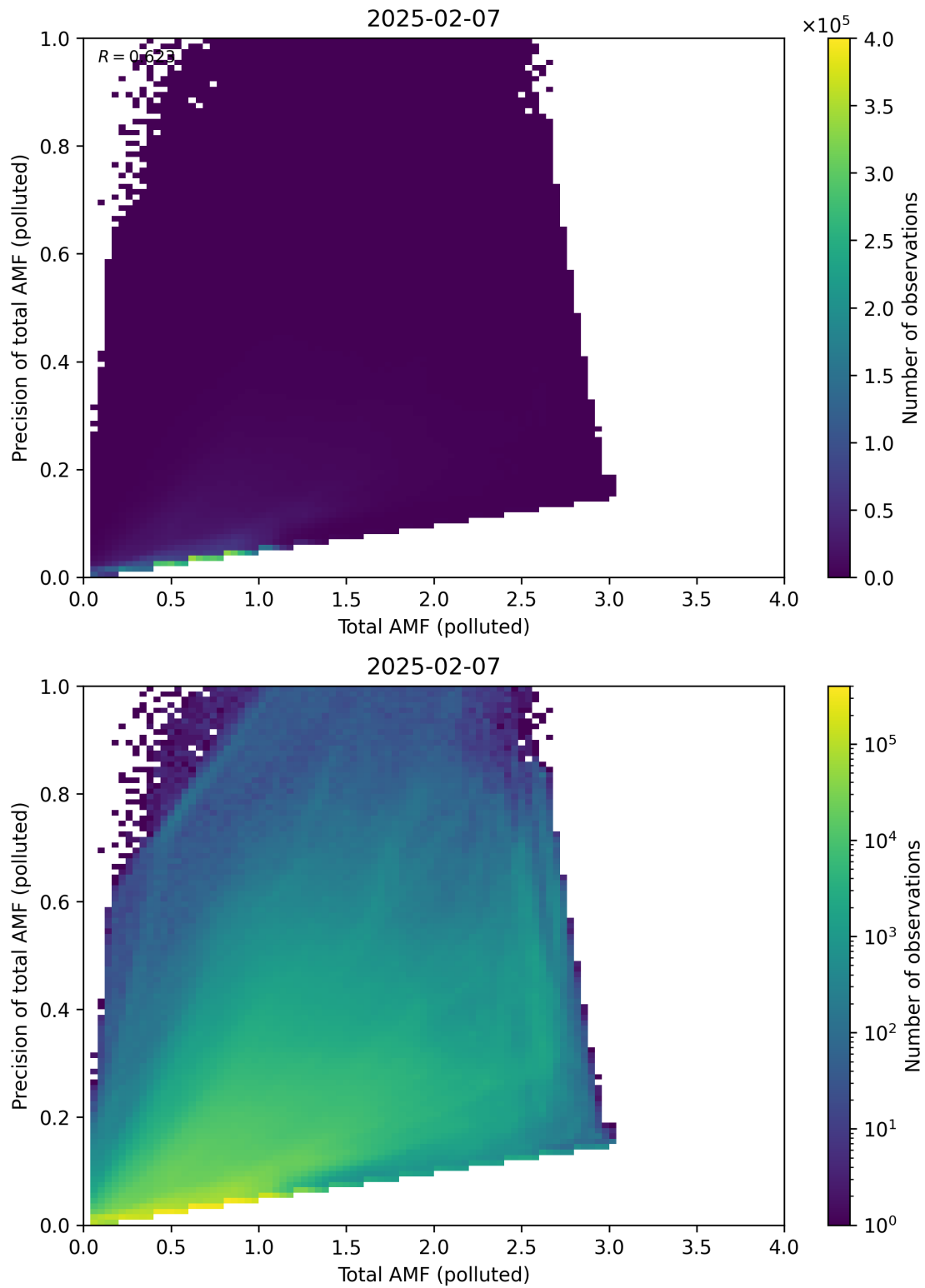
Figure 322: Scatter density plot of “Total AMF (polluted)” against “Precision of total AMF (polluted)” for 2025-02-06 to 2025-02-08.
