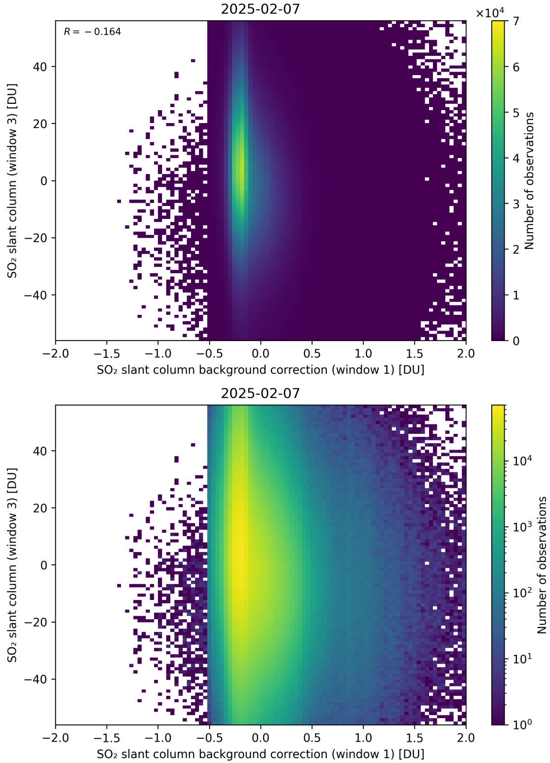
Figure 118: Scatter density plot of “SO 2 slant column background correction (window 1)” against “SO 2 slant column (window 3)” for 2025-02-06 to 2025-02-08.
