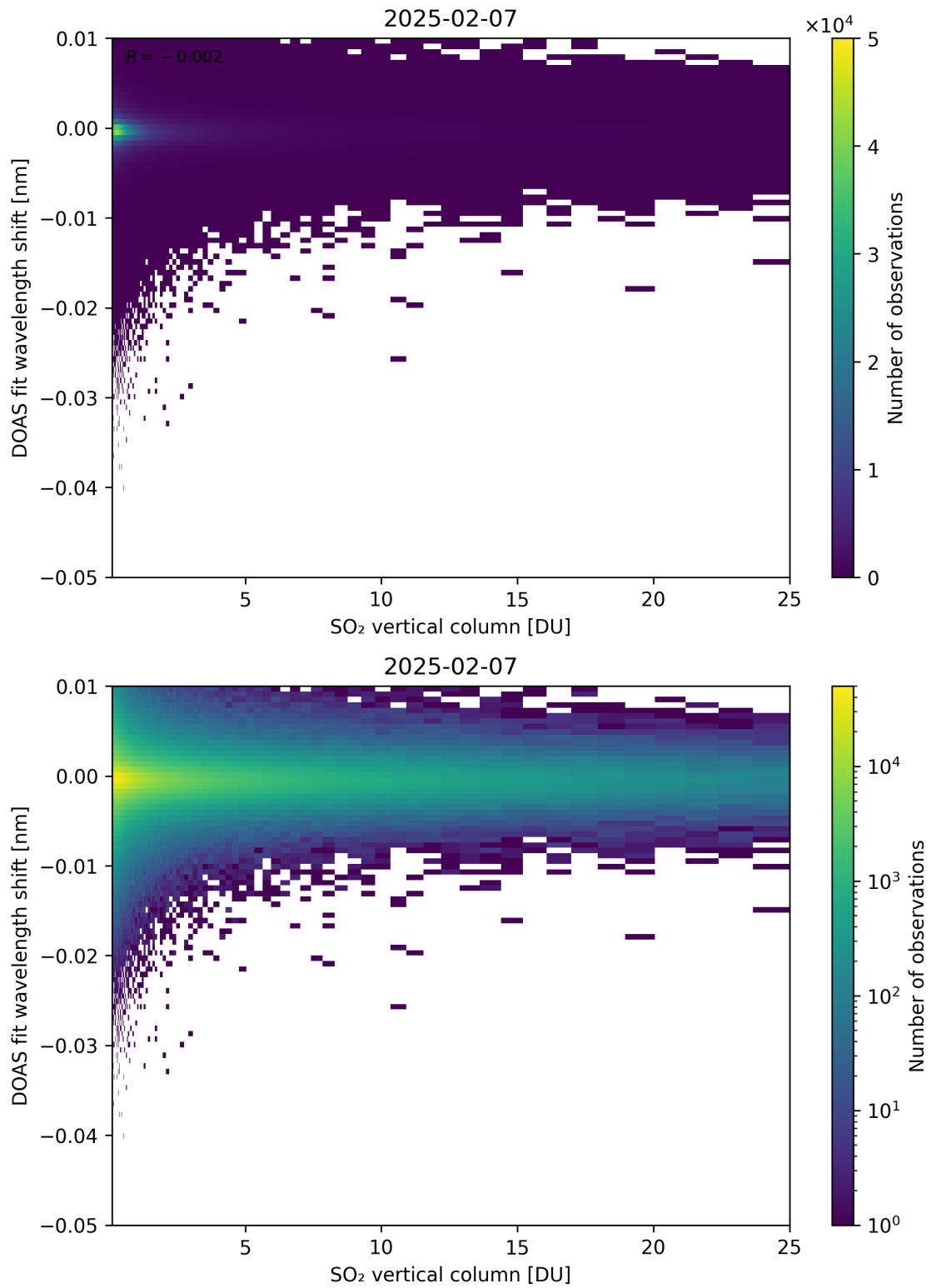
Figure 326: Scatter density plot of “SO 2 vertical column” against “DOAS fit wavelength shift” for 2025-02-06 to 2025-02-08.
