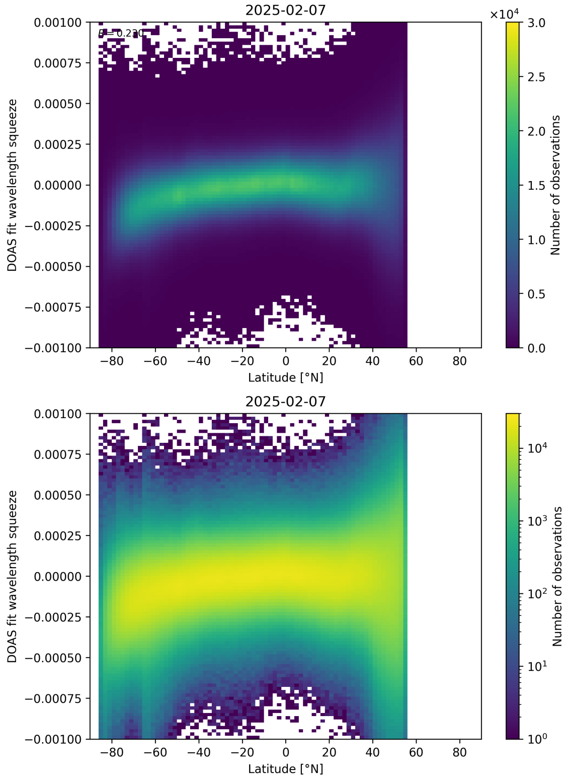
Figure 154: Scatter density plot of “Latitude” against “DOAS fit wavelength squeeze” for 2025-02-06 to 2025-02-08.
