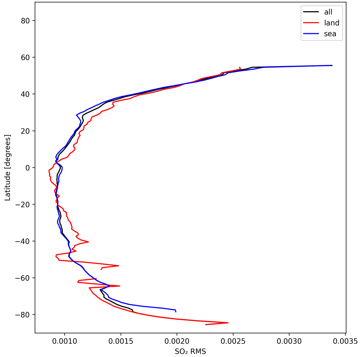
Figure 52: Zonal average of “SO 2 RMS” for 2025-02-06 to 2025-02-08.
