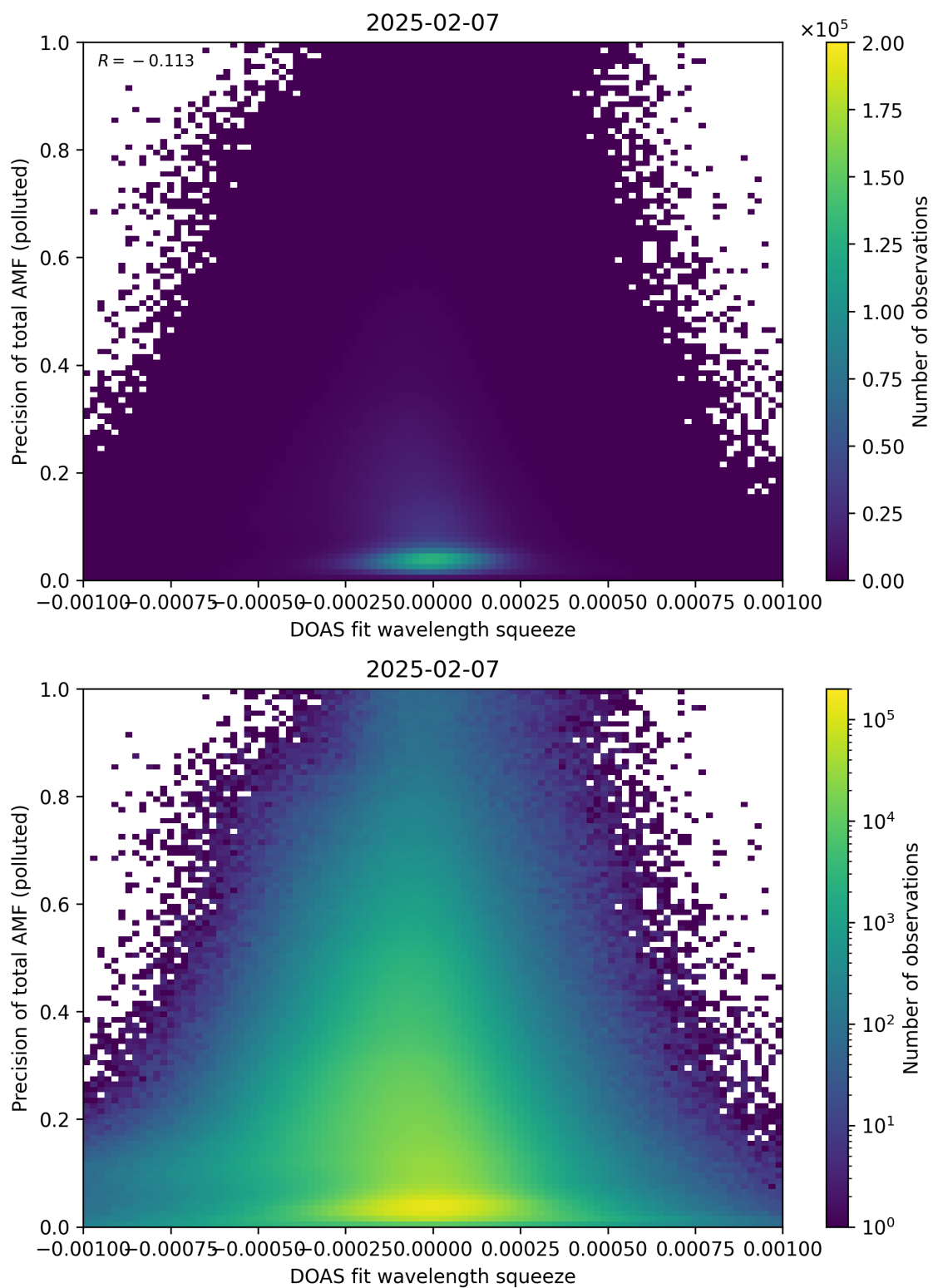
Figure 146: Scatter density plot of “DOAS fit wavelength squeeze” against “Precision of total AMF (polluted)” for 2025-02-06 to 2025-02-08.
