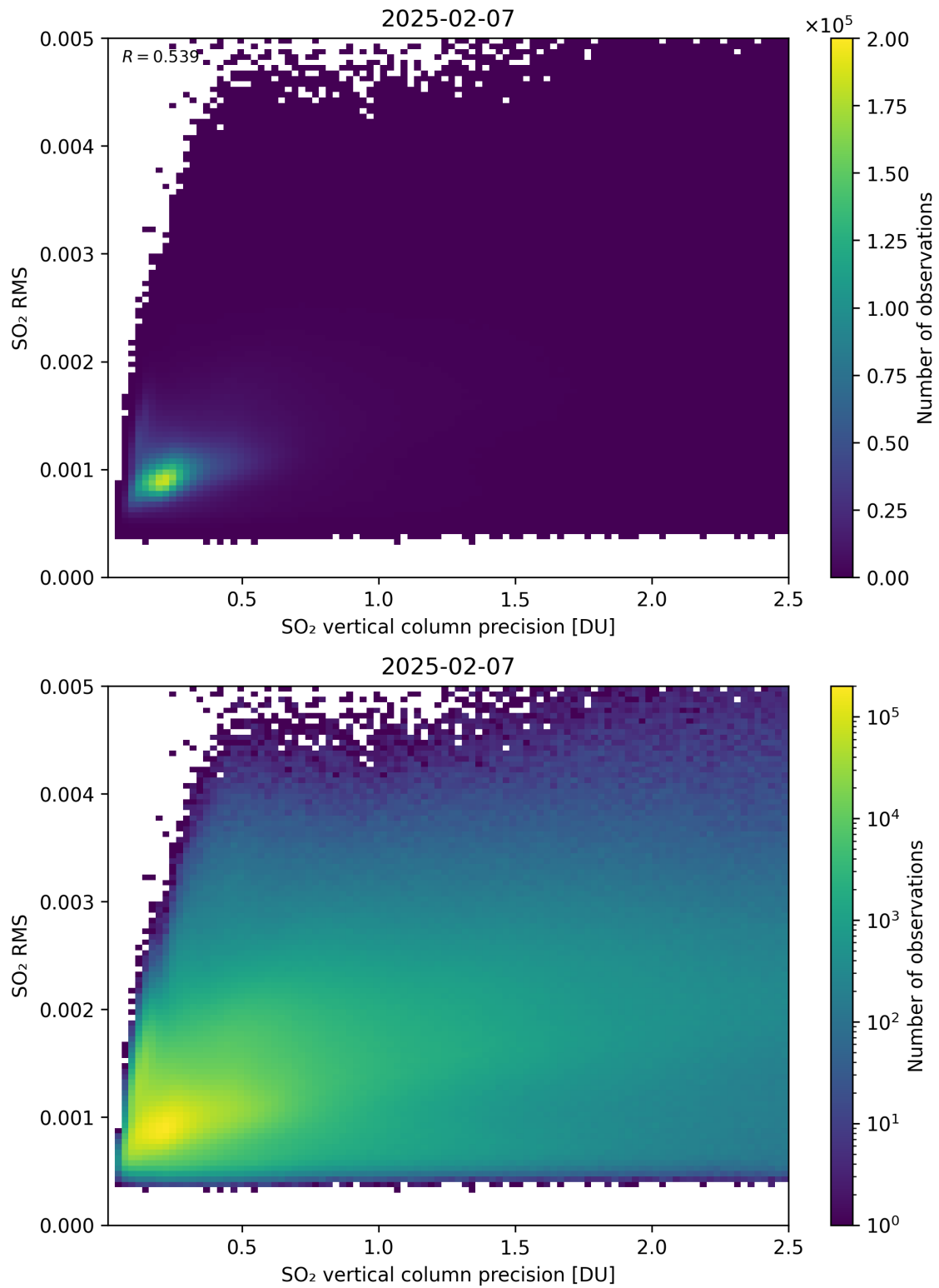
Figure 334: Scatter density plot of “SO 2 vertical column precision” against “SO 2 RMS” for 2025-02-06 to 2025-02-08.
