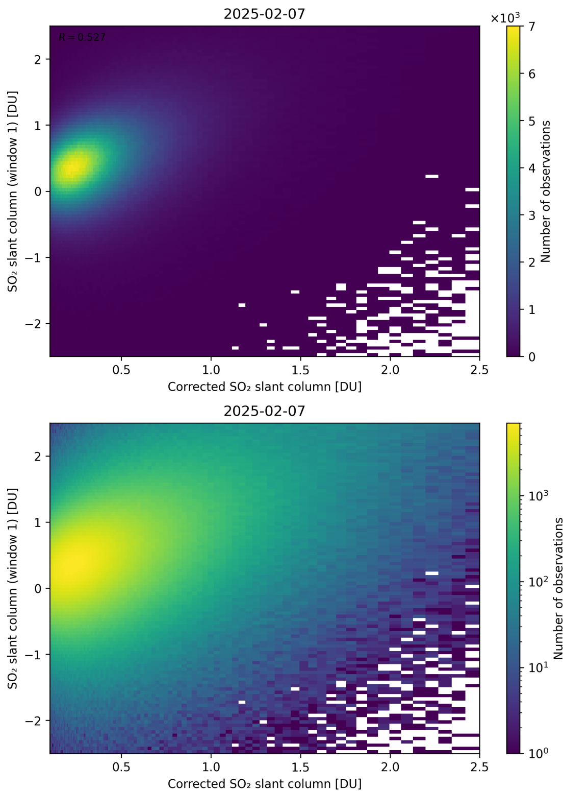
Figure 237: Scatter density plot of “Corrected SO 2 slant column” against “SO 2 slant column (window 1)” for 2025-02-06 to 2025-02-08.
