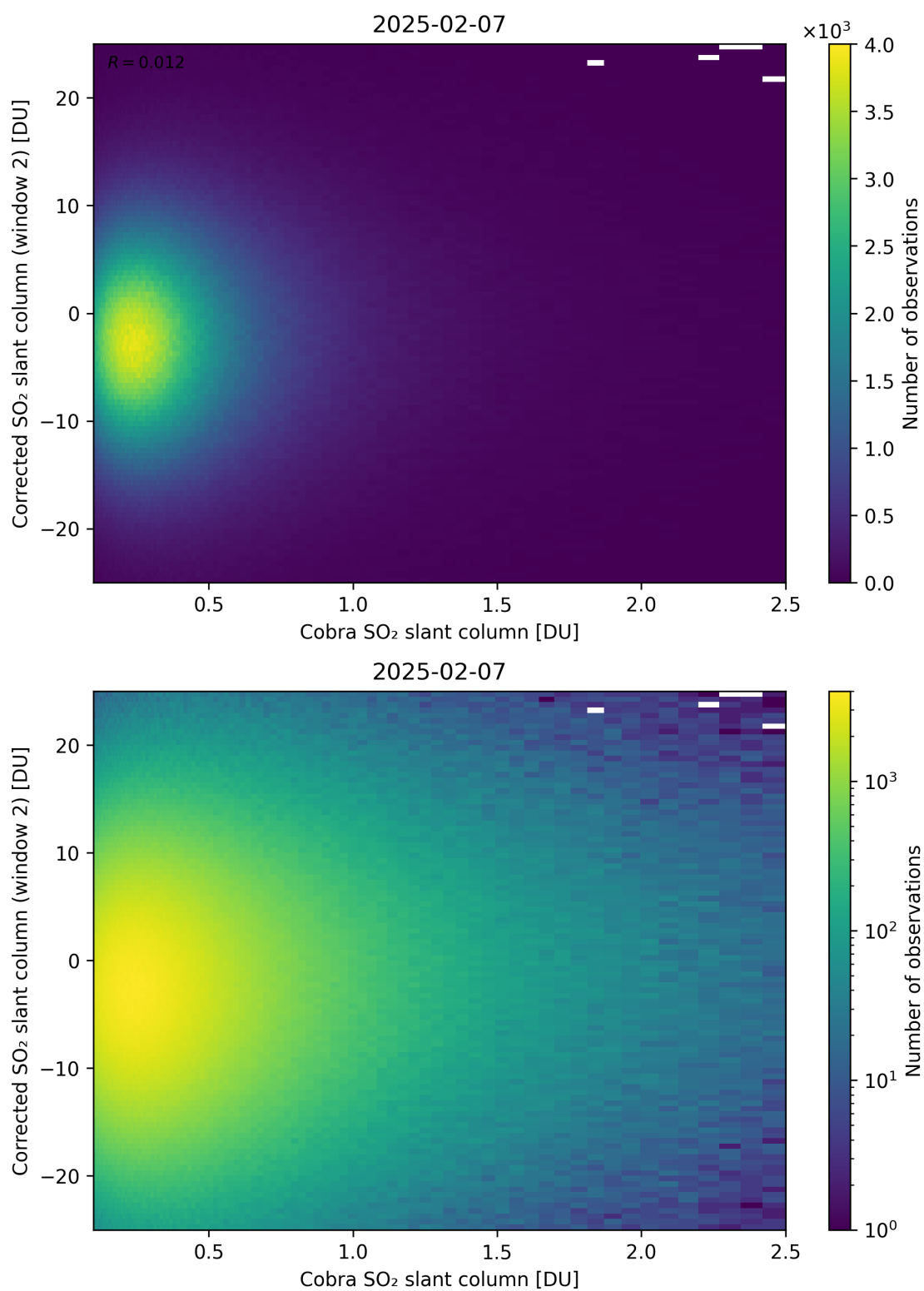
Figure 217: Scatter density plot of “Cobra SO 2 slant column” against “Corrected SO 2 slant column (window 2)” for 2025-02-06 to 2025-02-08.
