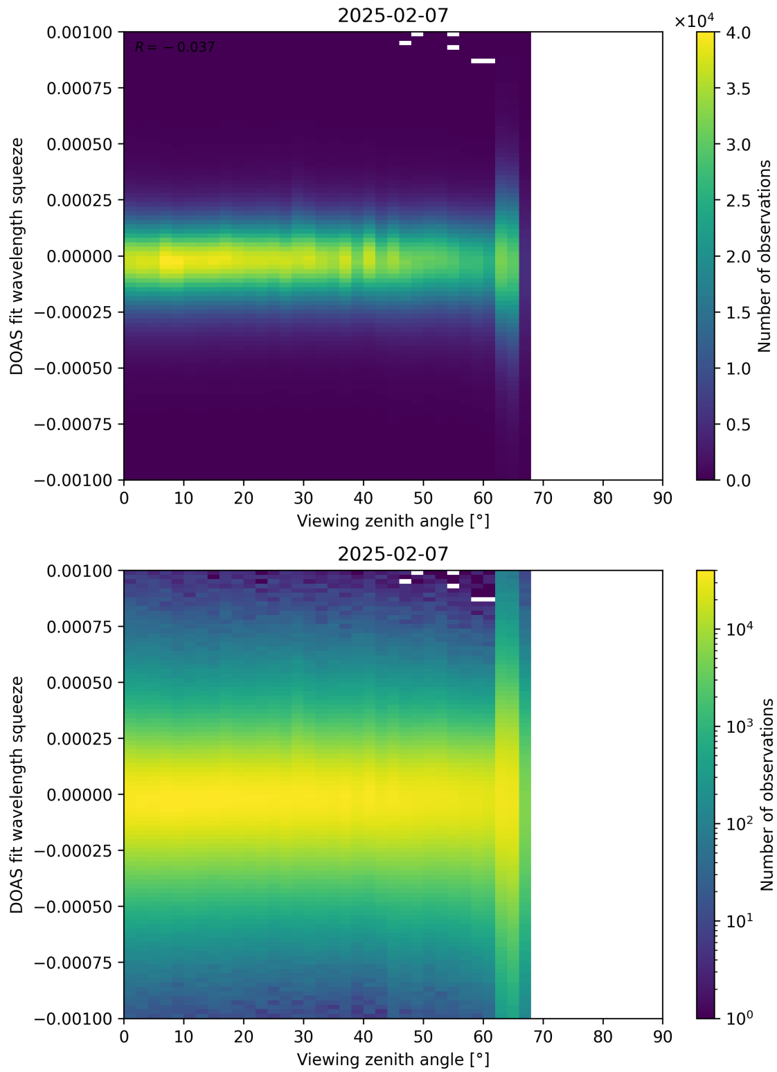
Figure 366: Scatter density plot of “Viewing zenith angle” against “DOAS fit wavelength squeeze” for 2025-02-06 to 2025-02-08.
