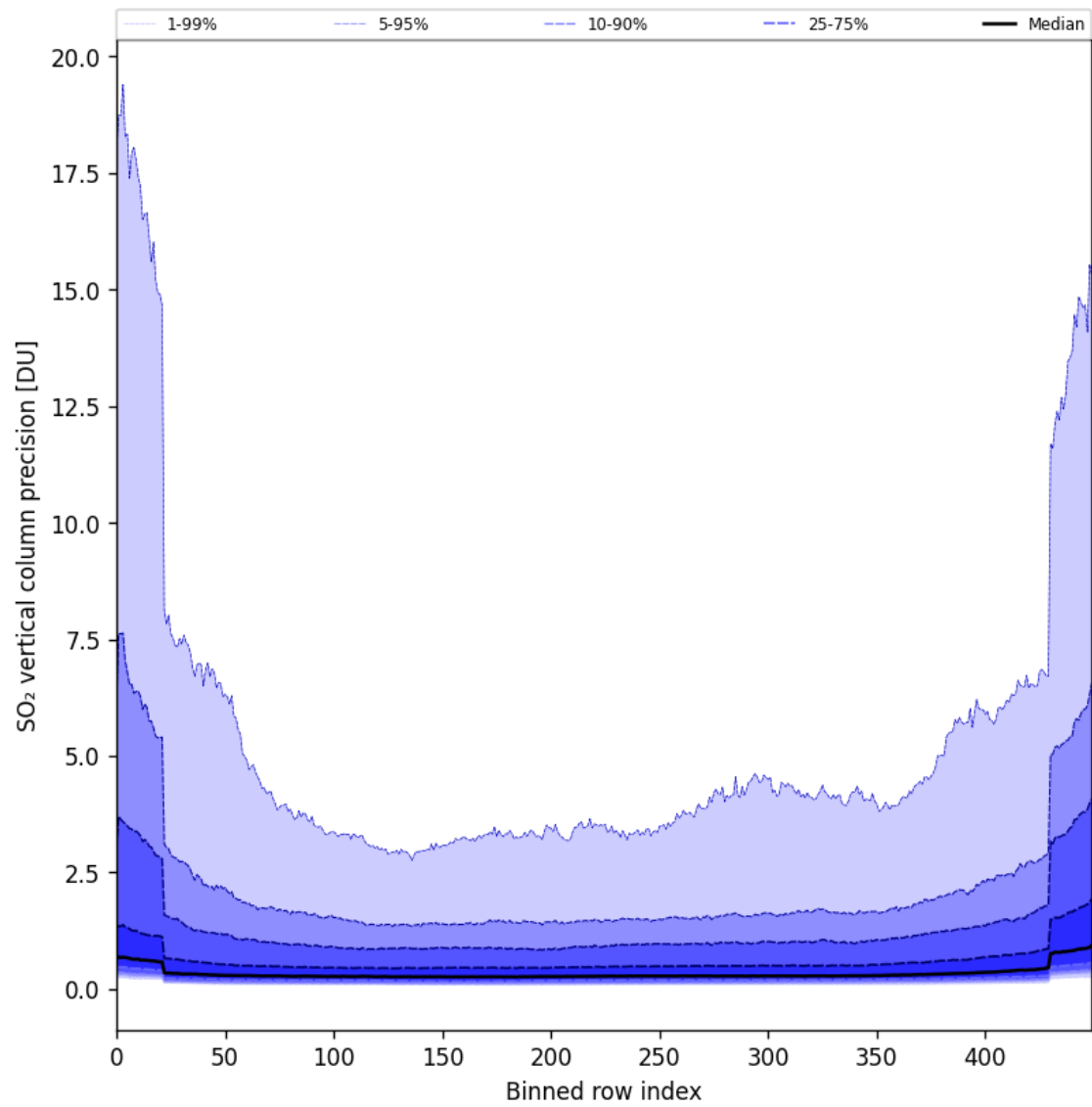
Figure 85: Along track statistics of “SO 2 vertical column precision” for 2025-02-06 to 2025-02-08
