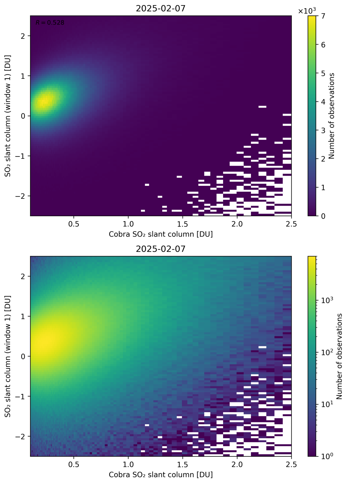
Figure 219: Scatter density plot of “Cobra SO 2 slant column” against “SO 2 slant column (window 1)” for 2025-02-06 to 2025-02-08.
