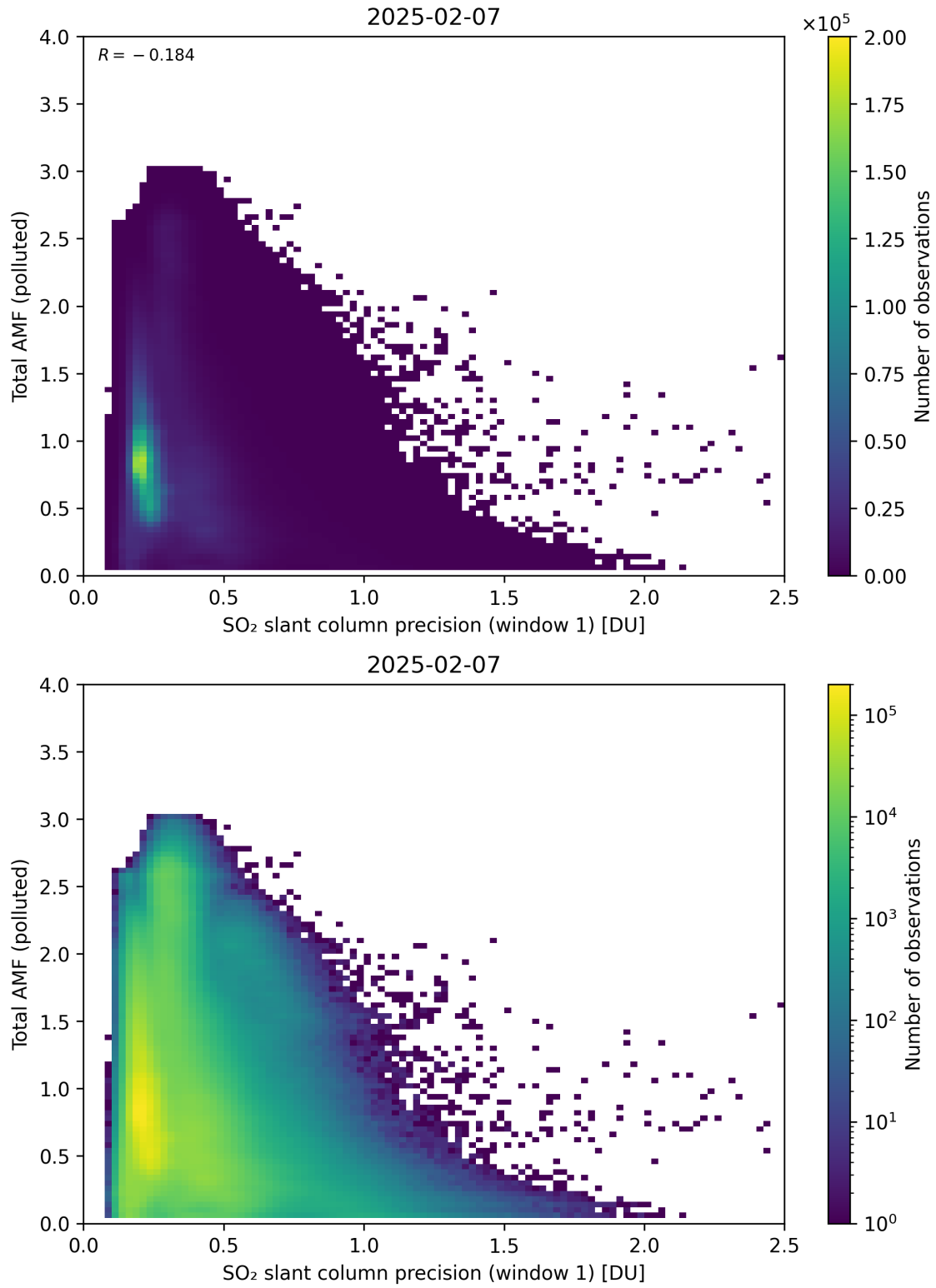
Figure 280: Scatter density plot of “SO 2 slant column precision (window 1)” against “Total AMF (polluted)” for 2025-02-06 to 2025-02-08.
