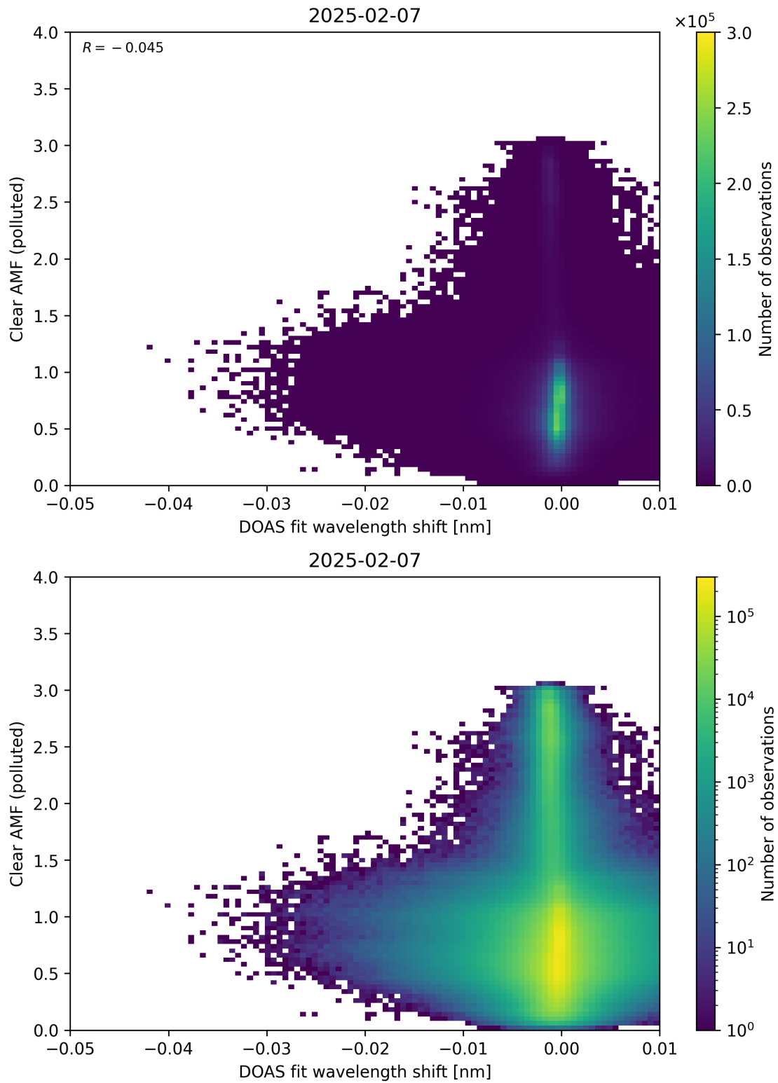
Figure 140: Scatter density plot of “DOAS fit wavelength shift” against “Clear AMF (polluted)” for 2025-02-06 to 2025-02-08.
