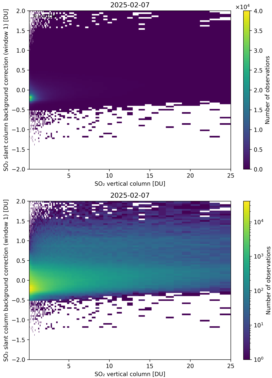
Figure 323: Scatter density plot of “SO 2 vertical column” against “SO 2 slant column background correction (window 1)” for 2025-02-06 to 2025-02-08.
