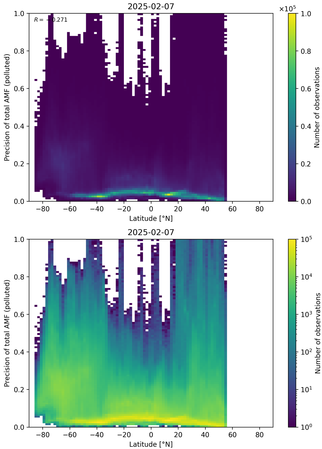
Figure 168: Scatter density plot of “Latitude” against “Precision of total AMF (polluted)” for 2025-02-06 to 2025-02-08.
