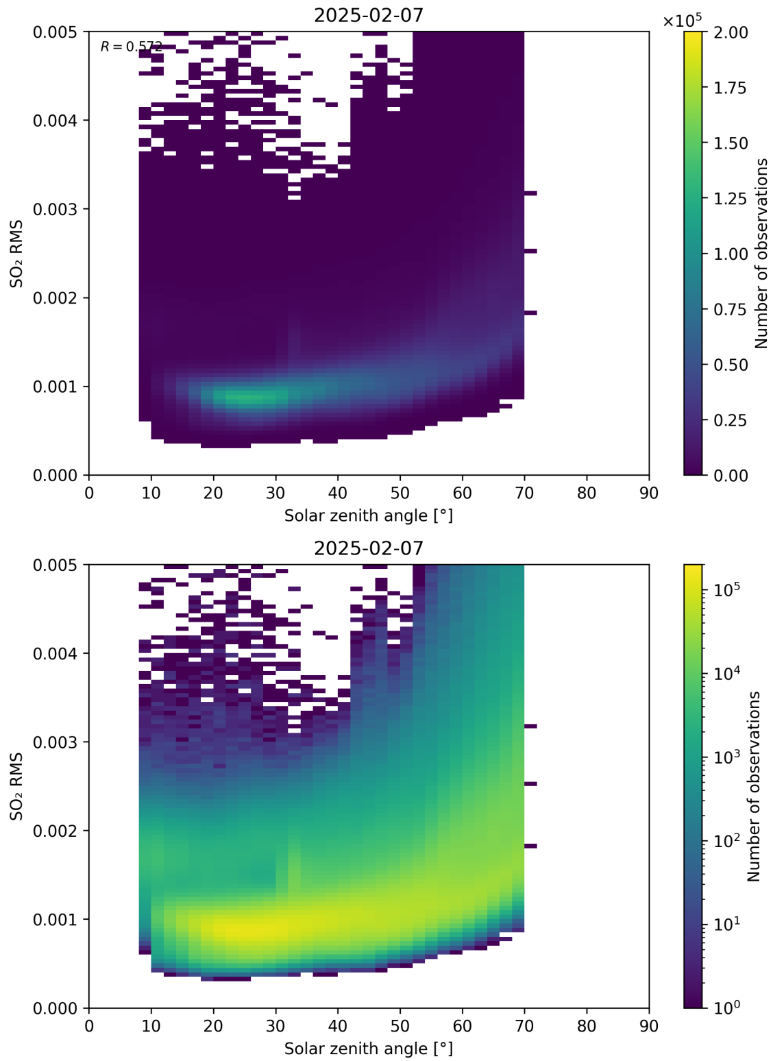
Figure 176: Scatter density plot of “Solar zenith angle” against “SO 2 RMS” for 2025-02-06 to 2025-02-08.
