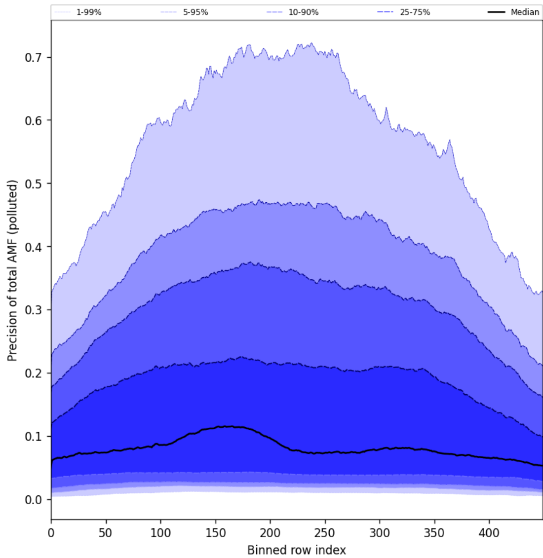
Figure 106: Along track statistics of “Precision of total AMF (polluted)” for 2025-02-06 to 2025-02-08
