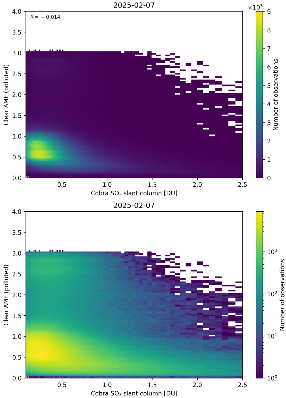
Figure 215: Scatter density plot of “Cobra SO 2 slant column” against “Clear AMF (polluted)” for 2025-02-06 to 2025-02-08.
