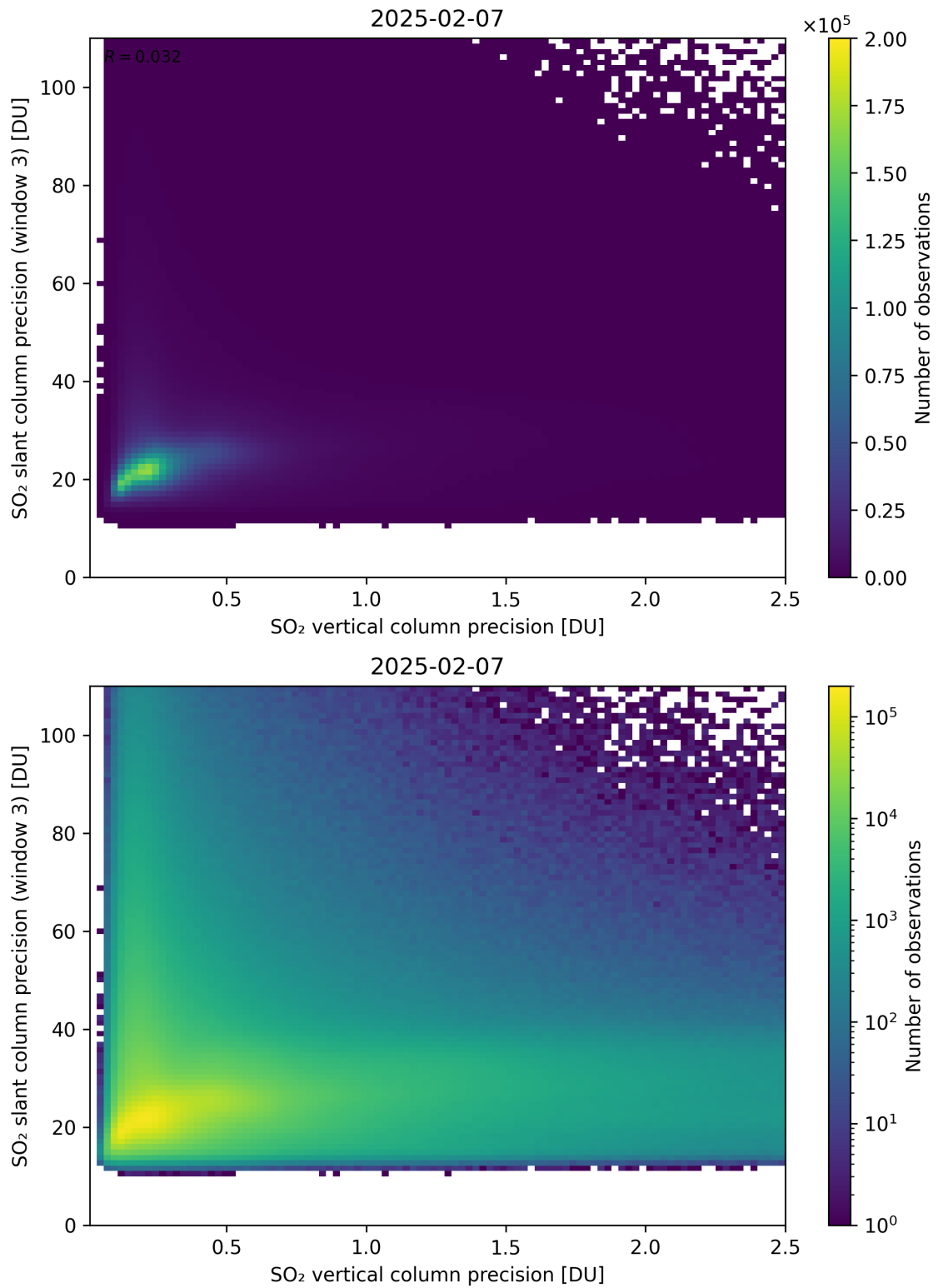
Figure 345: Scatter density plot of “SO 2 vertical column precision” against “SO 2 slant column precision (window 3)” for 2025-02-06 to 2025-02-08.
