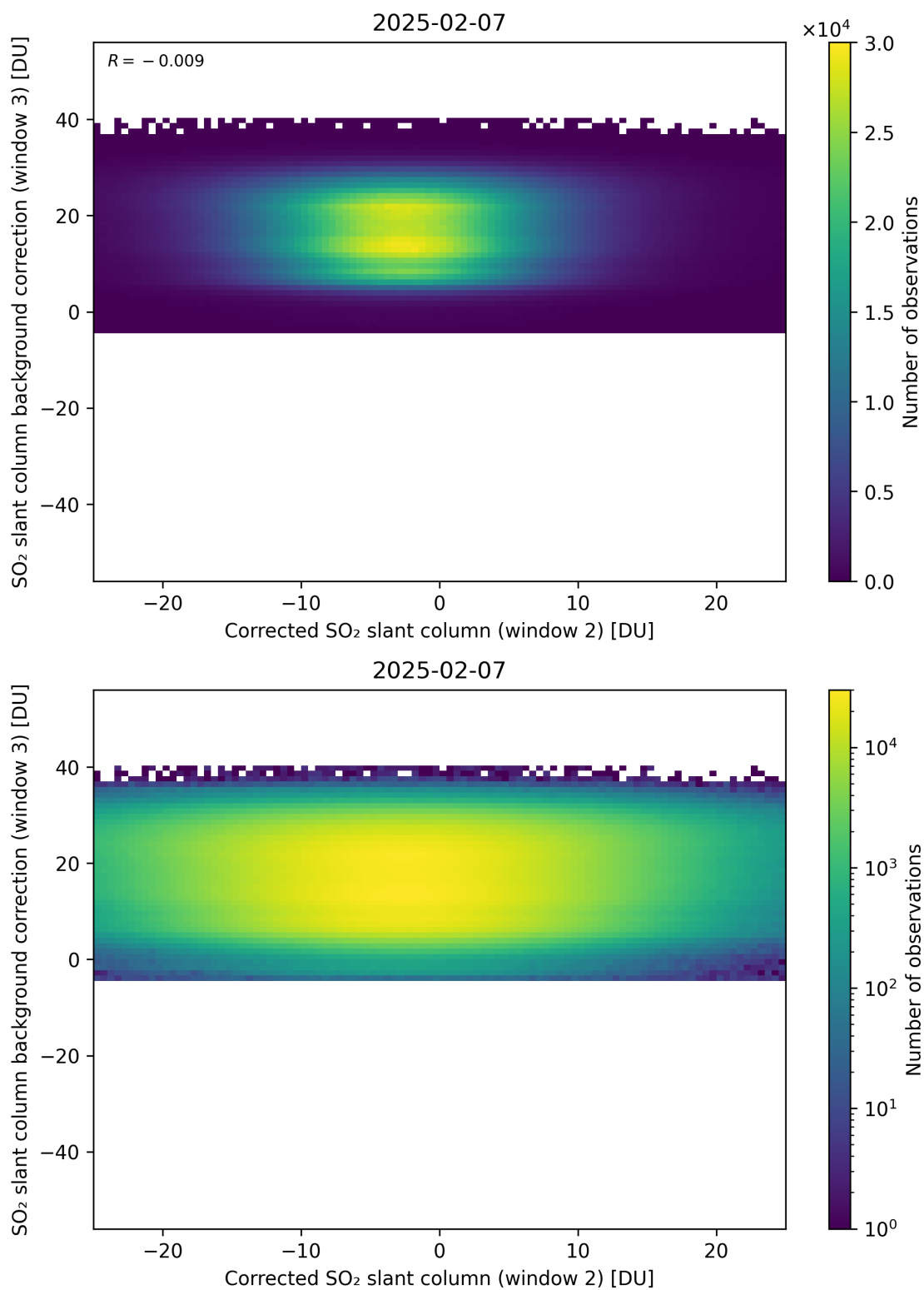
Figure 245: Scatter density plot of “Corrected SO 2 slant column (window 2)” against “SO 2 slant column background correction (window 3)” for 2025-02-06 to 2025-02-08.
