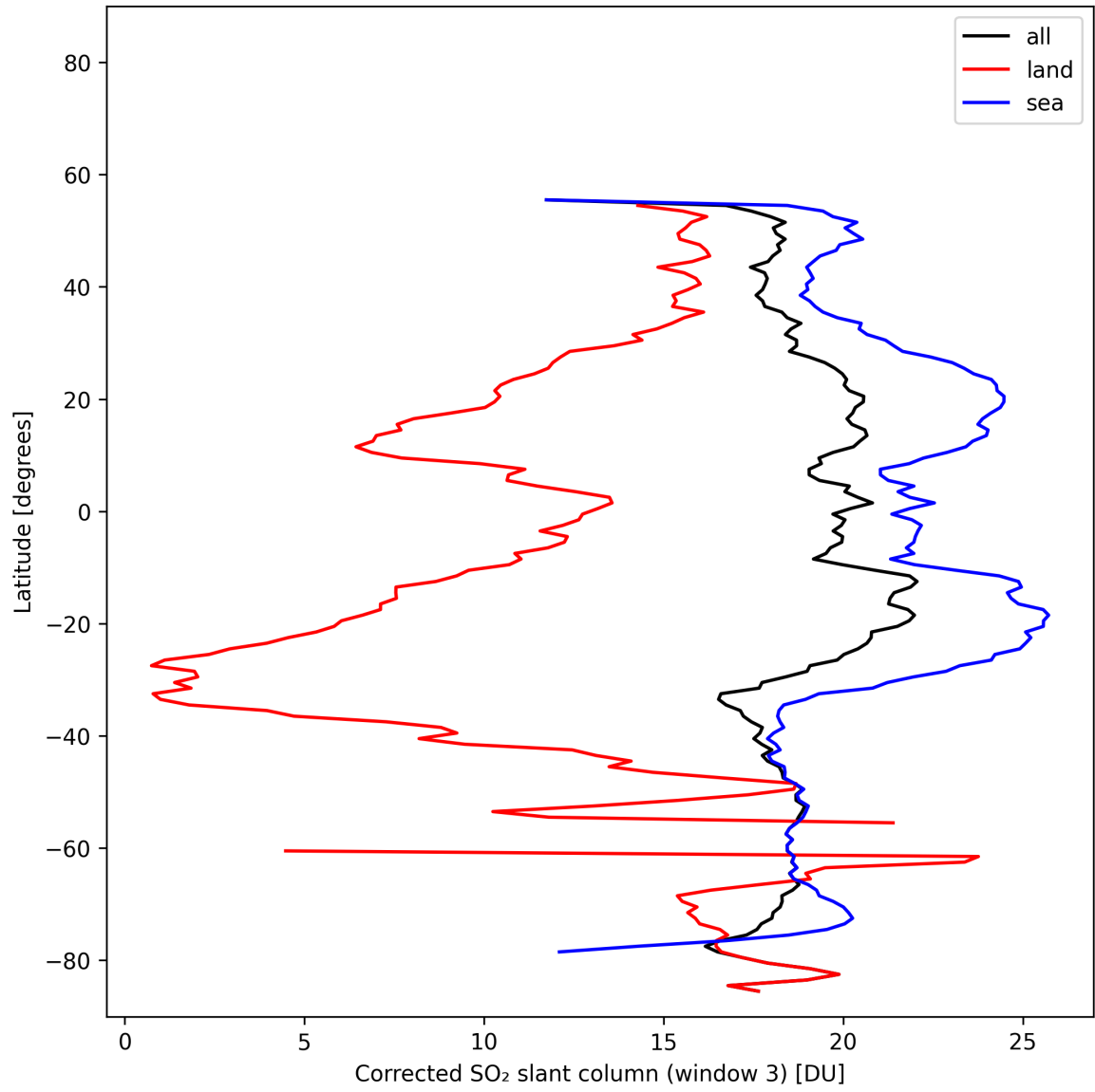
Figure 47: Zonal average of “Corrected SO 2 slant column (window 3)” for 2025-02-06 to 2025-02-08.
