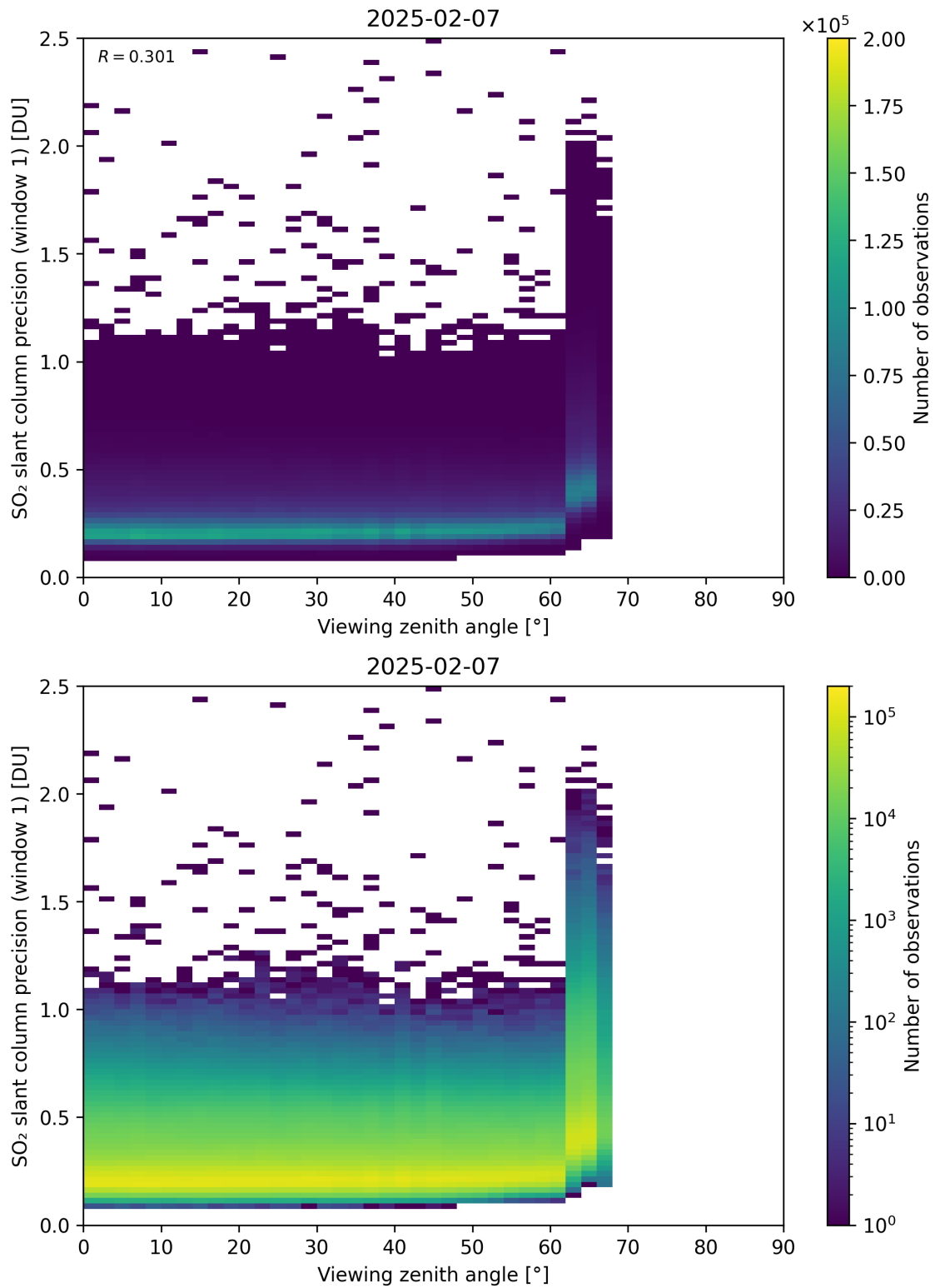
Figure 377: Scatter density plot of “Viewing zenith angle” against “SO 2 slant column precision (window 1)” for 2025-02-06 to 2025-02-08.
