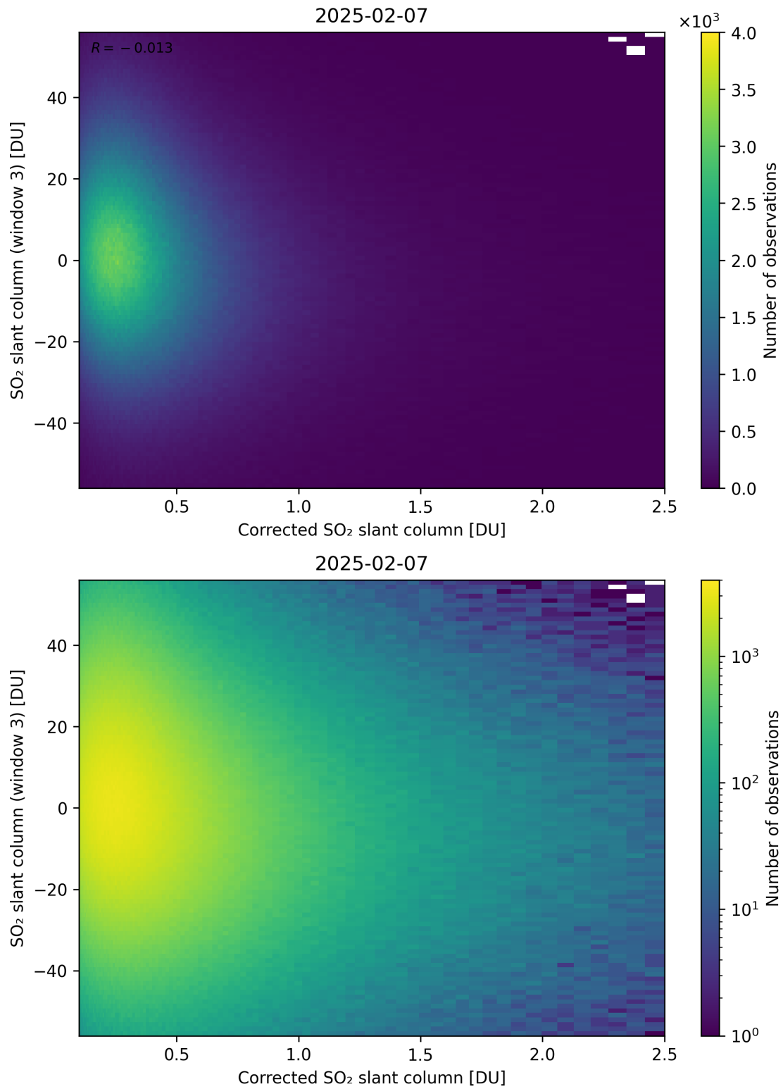
Figure 240: Scatter density plot of “Corrected SO 2 slant column” against “SO 2 slant column (window 3)” for 2025-02-06 to 2025-02-08.
