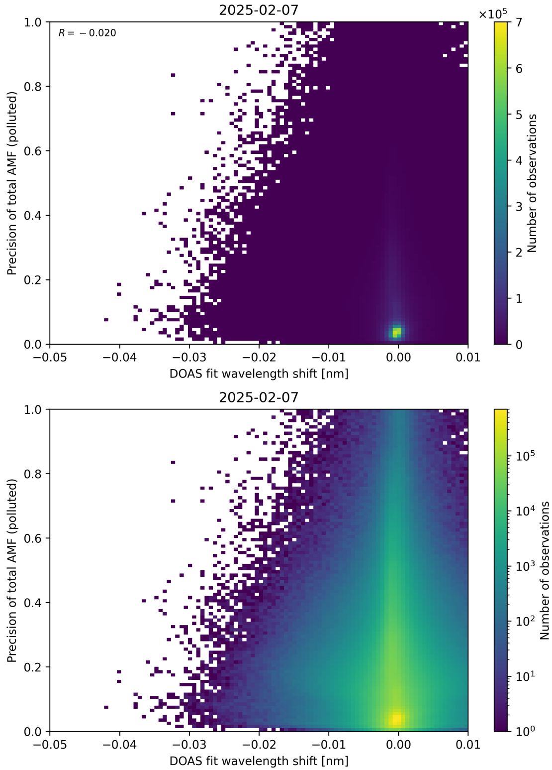
Figure 142: Scatter density plot of “DOAS fit wavelength shift” against “Precision of total AMF (polluted)” for 2025-02-06 to 2025-02-08.
