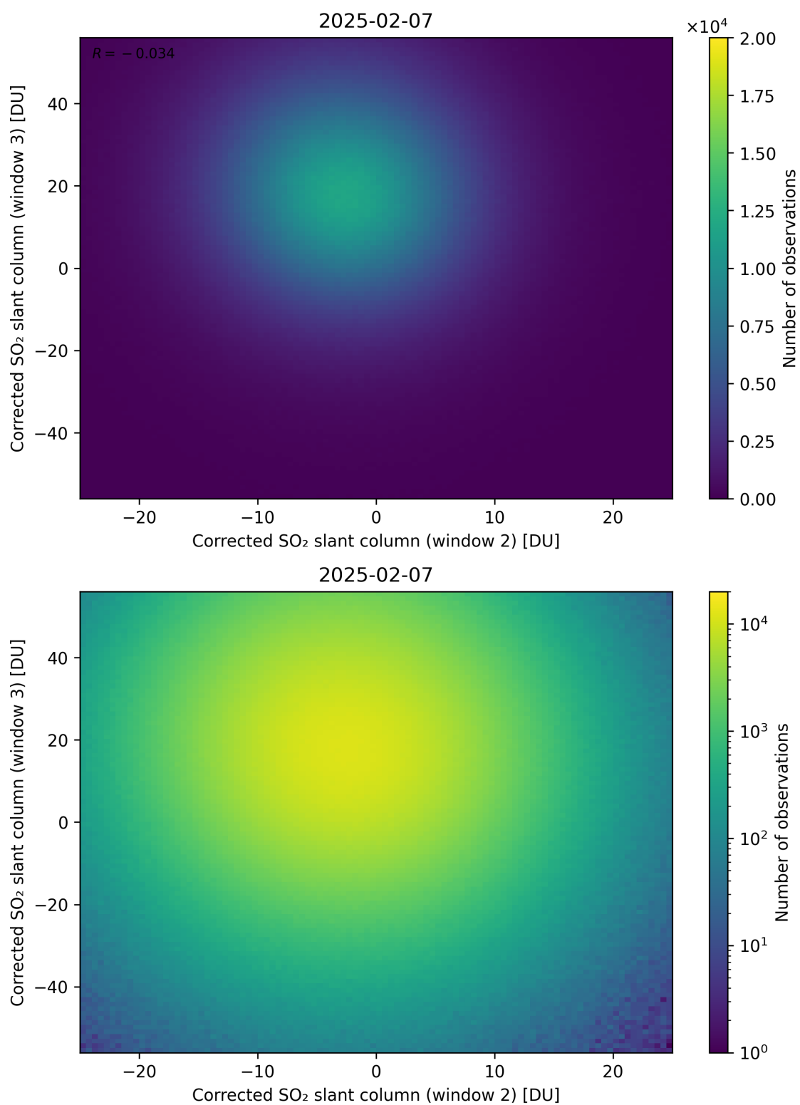
Figure 250: Scatter density plot of “Corrected SO 2 slant column (window 2)” against “Corrected SO 2 slant column (window 3)” for 2025-02-06 to 2025-02-08.
