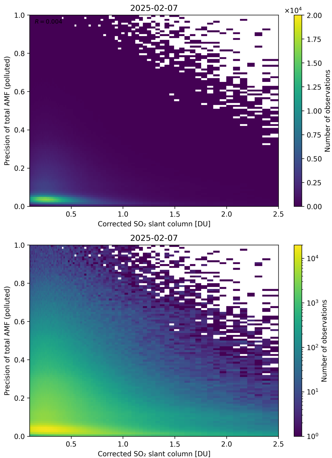
Figure 243: Scatter density plot of “Corrected SO 2 slant column” against “Precision of total AMF (polluted)” for 2025-02-06 to 2025-02-08.
