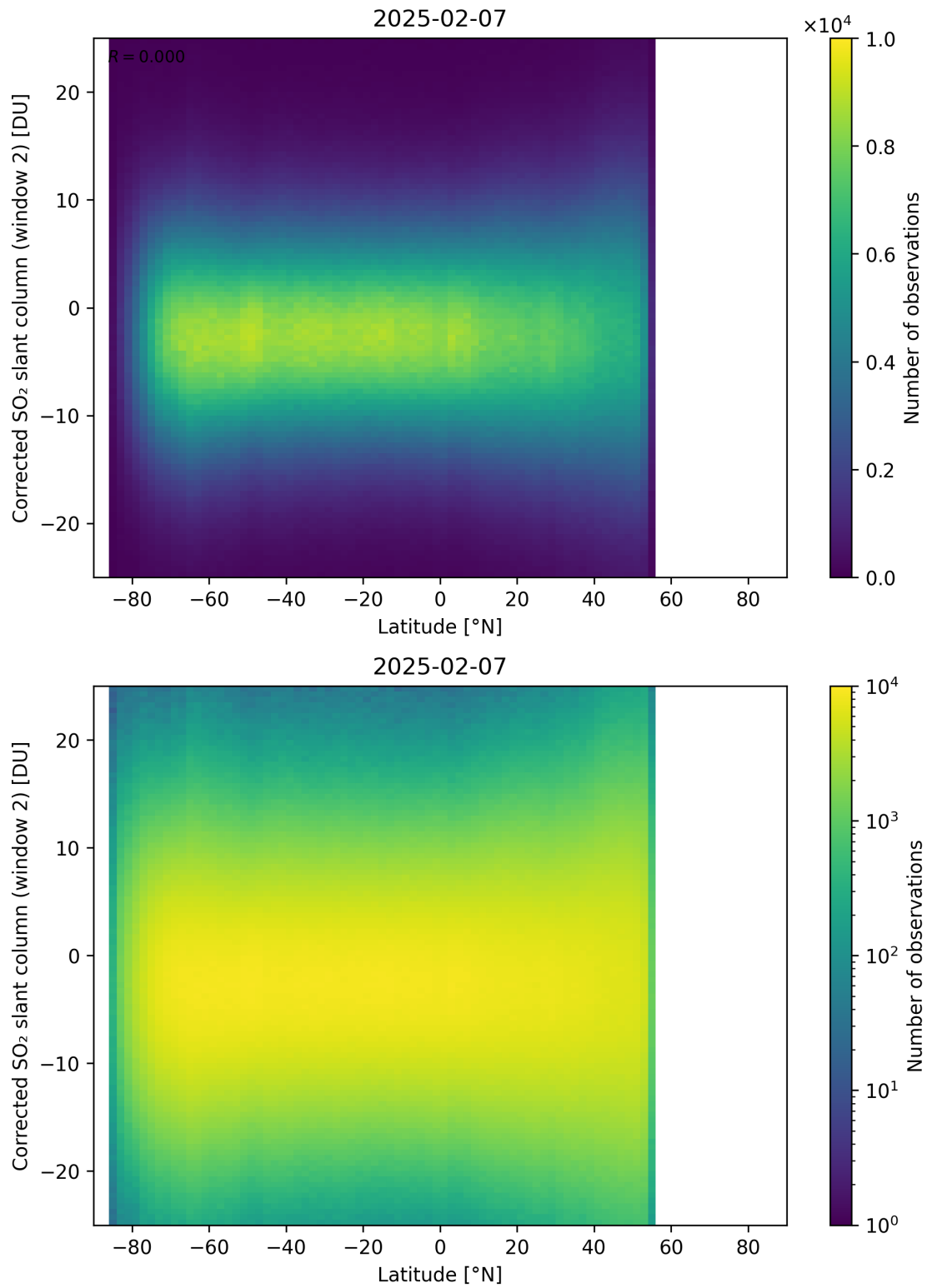
Figure 160: Scatter density plot of “Latitude” against “Corrected SO 2 slant column (window 2)” for 2025-02-06 to 2025-02-08.
