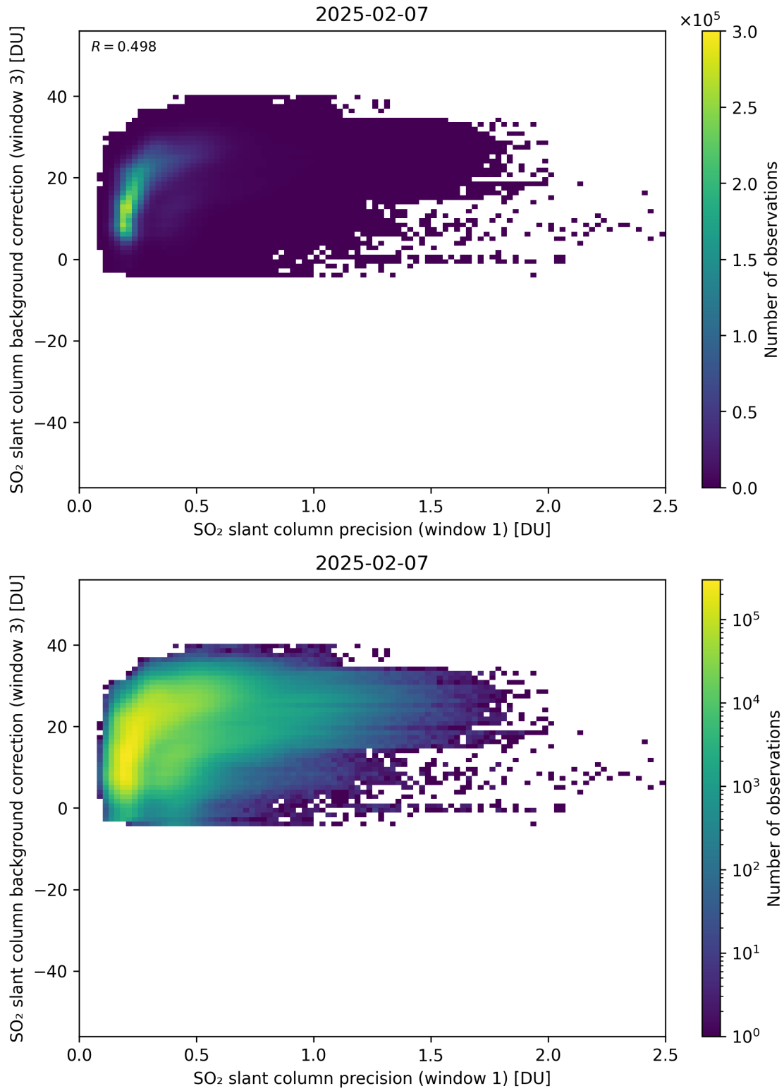
Figure 270: Scatter density plot of “SO 2 slant column precision (window 1)” against “SO 2 slant column background correction (window 3)” for 2025-02-06 to 2025-02-08.
