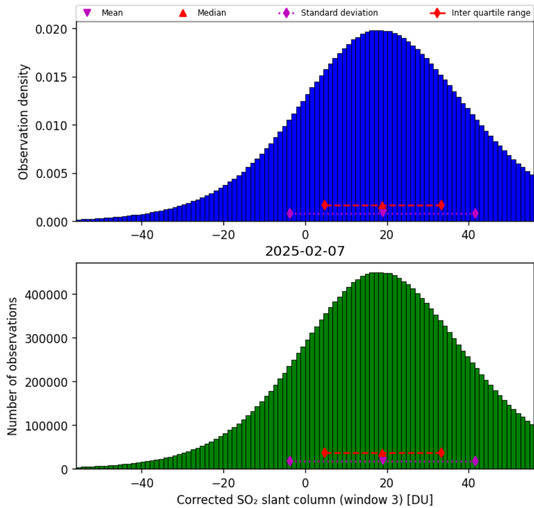
Figure 73: Histogram of “Corrected SO 2 slant column (window 3)” for 2025-02-06 to 2025-02-08
