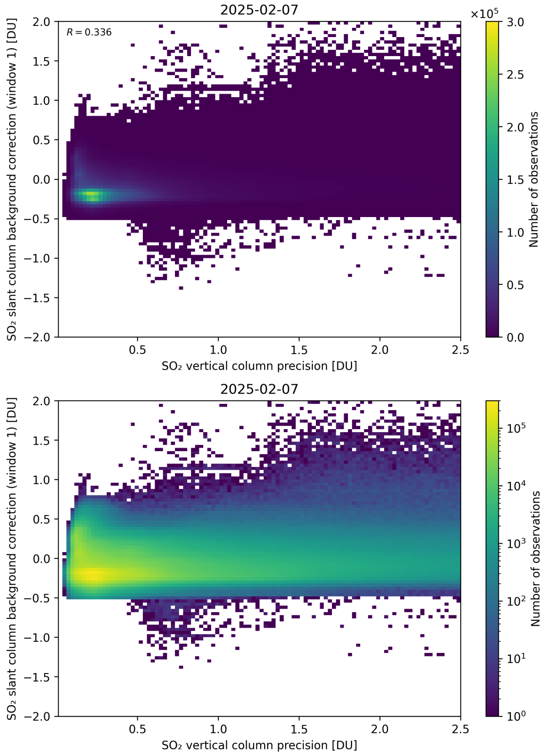
Figure 329: Scatter density plot of “SO 2 vertical column precision” against “SO 2 slant column background correction (window 1)” for 2025-02-06 to 2025-02-08.
