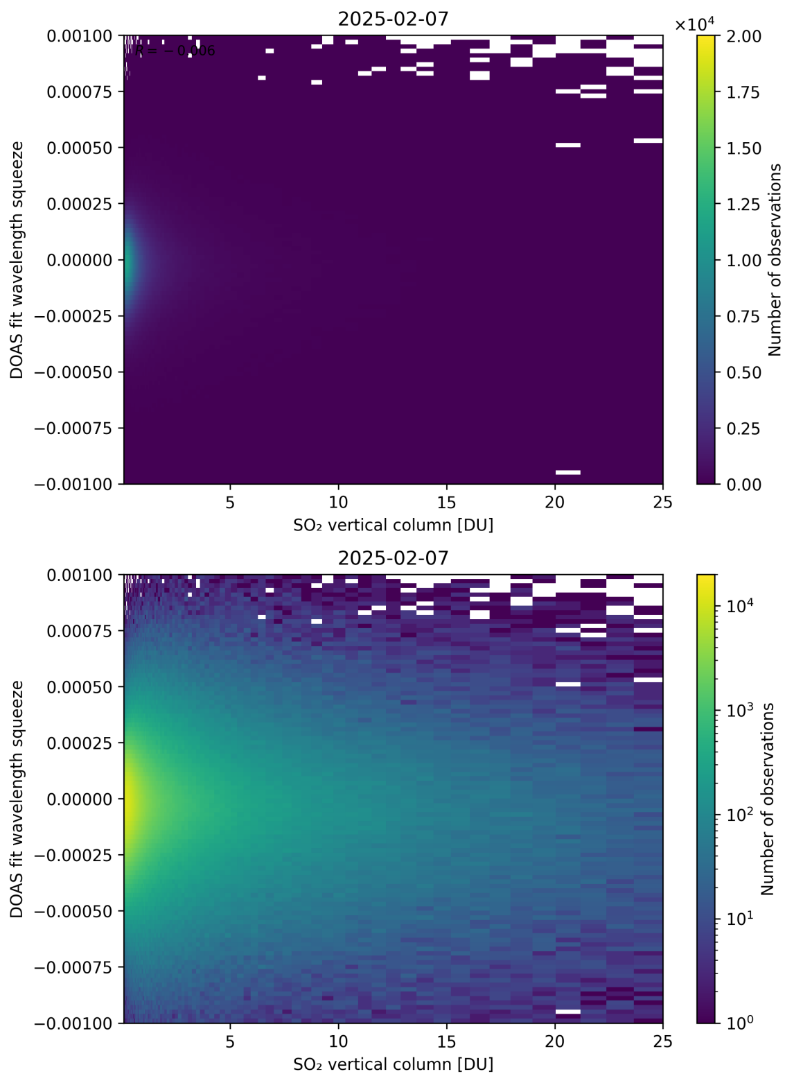
Figure 327: Scatter density plot of “SO 2 vertical column” against “DOAS fit wavelength squeeze” for 2025-02-06 to 2025-02-08.
