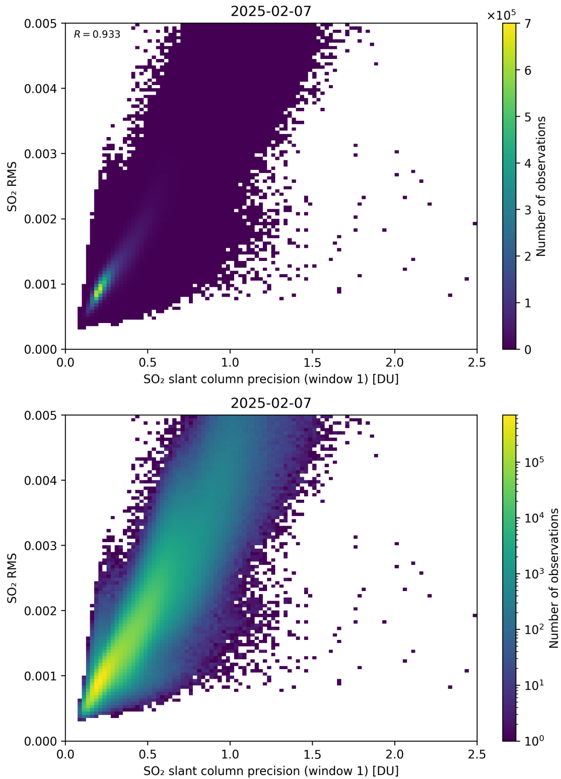
Figure 273: Scatter density plot of “SO 2 slant column precision (window 1)” against “SO 2 RMS” for 2025-02-06 to 2025-02-08.
