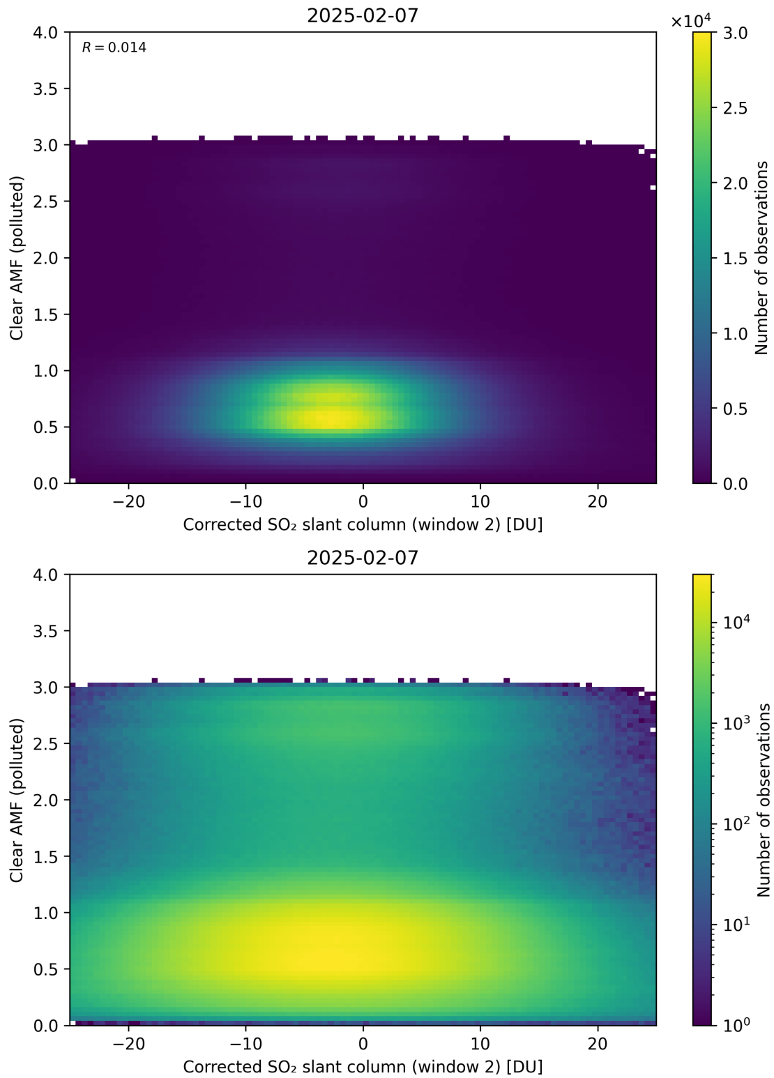
Figure 249: Scatter density plot of “Corrected SO 2 slant column (window 2)” against “Clear AMF (polluted)” for 2025-02-06 to 2025-02-08.
