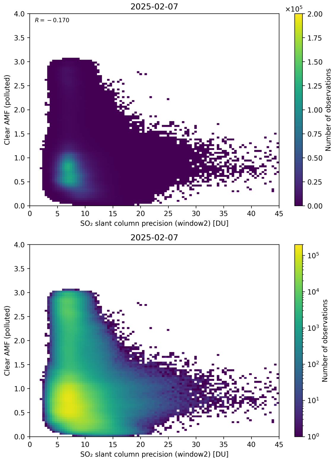
Figure 296: Scatter density plot of “SO 2 slant column precision (window2)” against “Clear AMF (polluted)” for 2025-02-06 to 2025-02-08.
