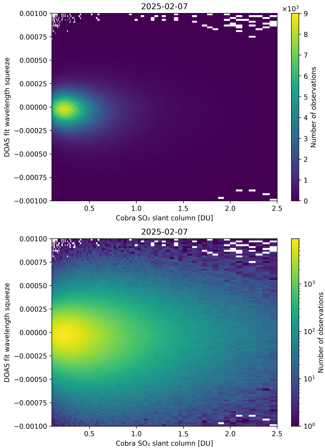
Figure 197: Scatter density plot of “Cobra SO 2 slant column” against “DOAS fit wavelength squeeze” for 2025-02-06 to 2025-02-08.
