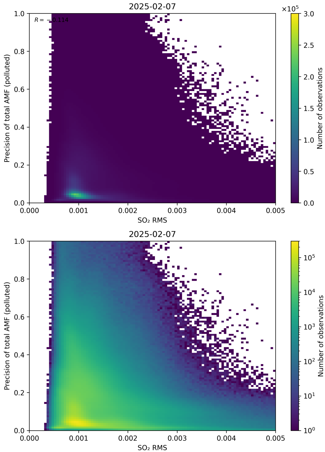
Figure 149: Scatter density plot of “SO 2 RMS” against “Precision of total AMF (polluted)” for 2025-02-06 to 2025-02-08.
