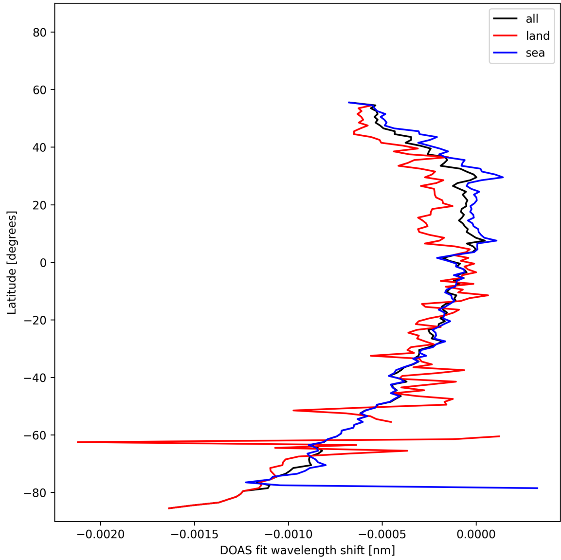
Figure 50: Zonal average of “DOAS fit wavelength shift” for 2025-02-06 to 2025-02-08.
