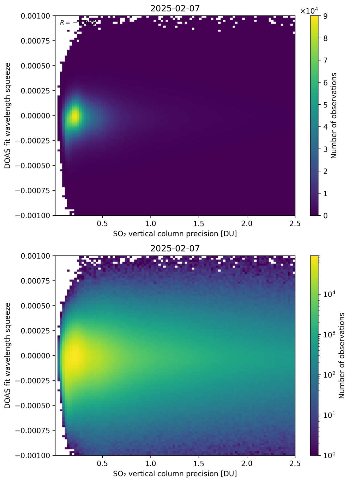
Figure 333: Scatter density plot of “SO 2 vertical column precision” against “DOAS fit wavelength squeeze” for 2025-02-06 to 2025-02-08.
