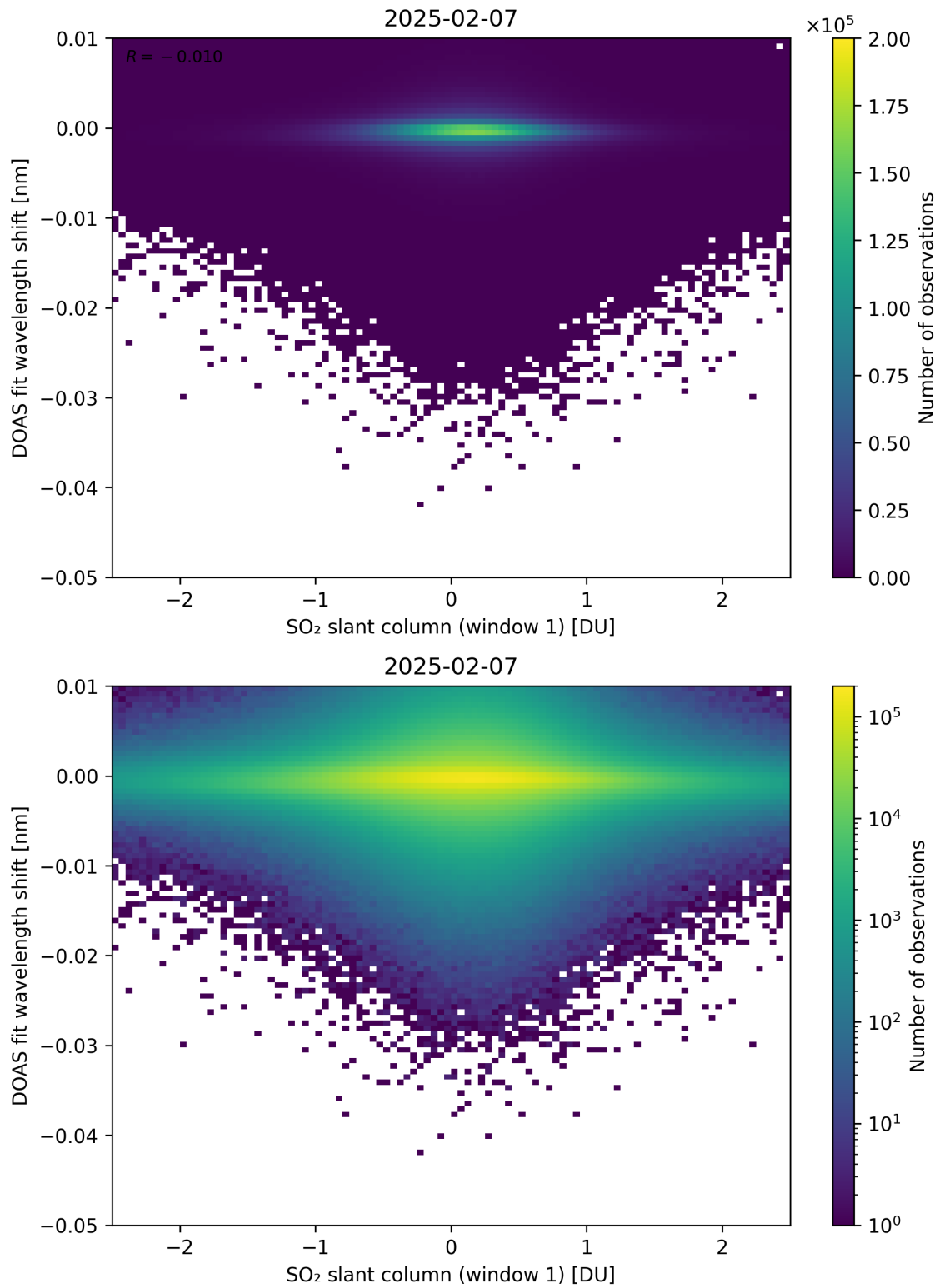
Figure 265: Scatter density plot of “SO 2 slant column (window 1)” against “DOAS fit wavelength shift” for 2025-02-06 to 2025-02-08.
