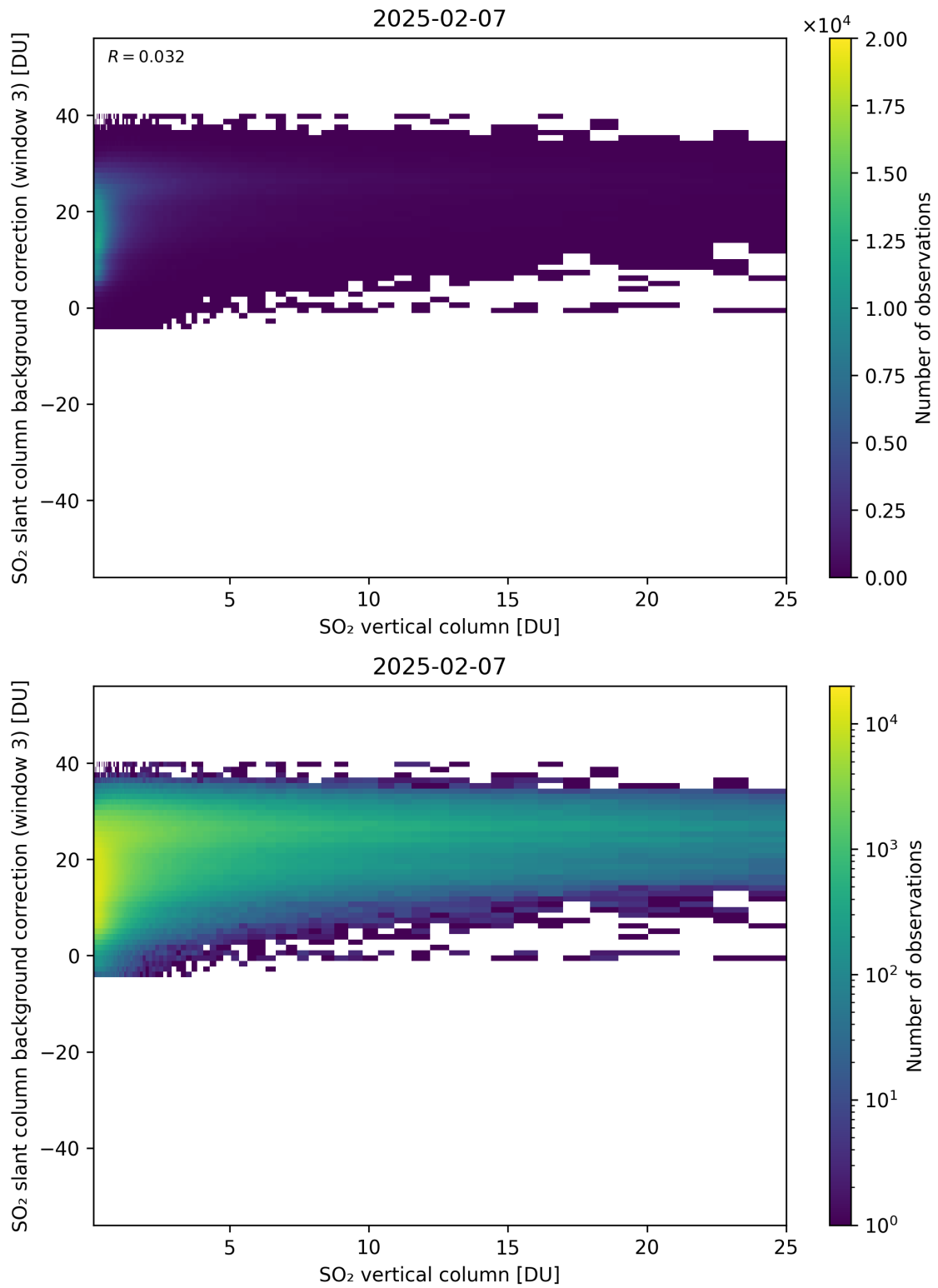
Figure 325: Scatter density plot of “SO 2 vertical column” against “SO 2 slant column background correction (window 3)” for 2025-02-06 to 2025-02-08.
