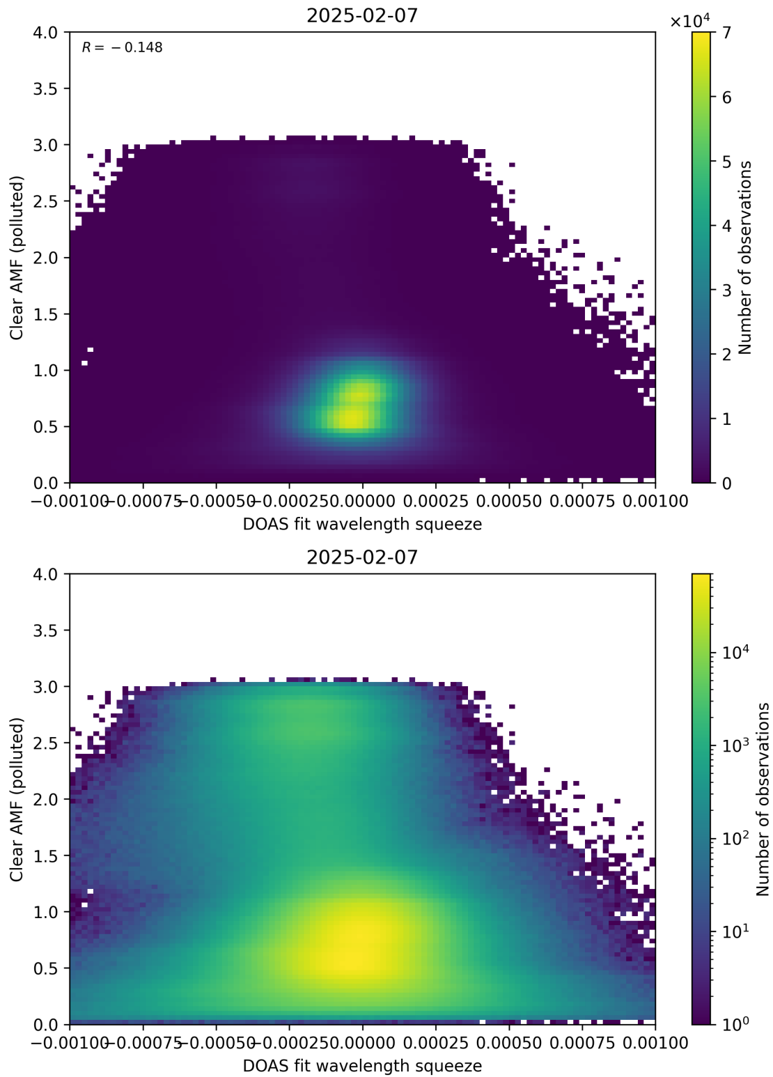
Figure 144: Scatter density plot of “DOAS fit wavelength squeeze” against “Clear AMF (polluted)” for 2025-02-06 to 2025-02-08.
