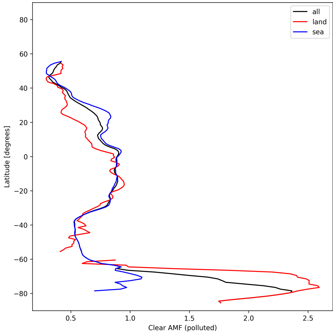
Figure 55: Zonal average of “Clear AMF (polluted)” for 2025-02-06 to 2025-02-08.
