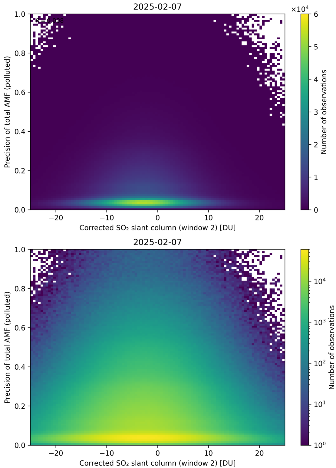
Figure 254: Scatter density plot of “Corrected SO 2 slant column (window 2)” against “Precision of total AMF (polluted)” for 2025-02-06 to 2025-02-08.
