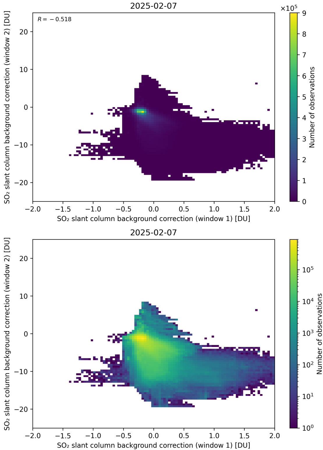
Figure 109: Scatter density plot of “SO 2 slant column background correction (window 1)” against “SO 2 slant column background correction (window 2)” for 2025-02-06 to 2025-02-08.
