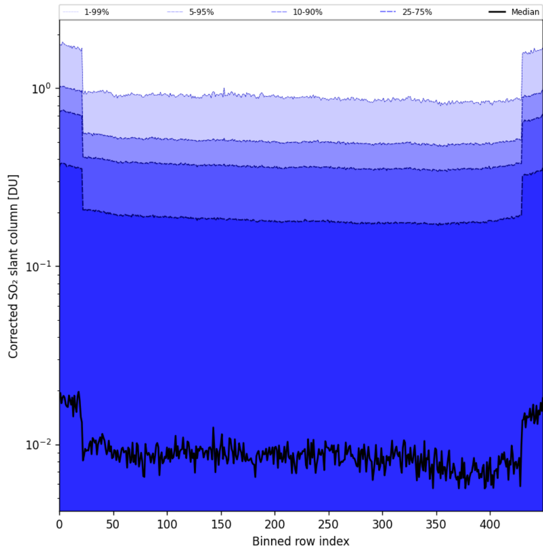
Figure 86: Along track statistics of “Corrected SO 2 slant column” for 2025-02-06 to 2025-02-08
