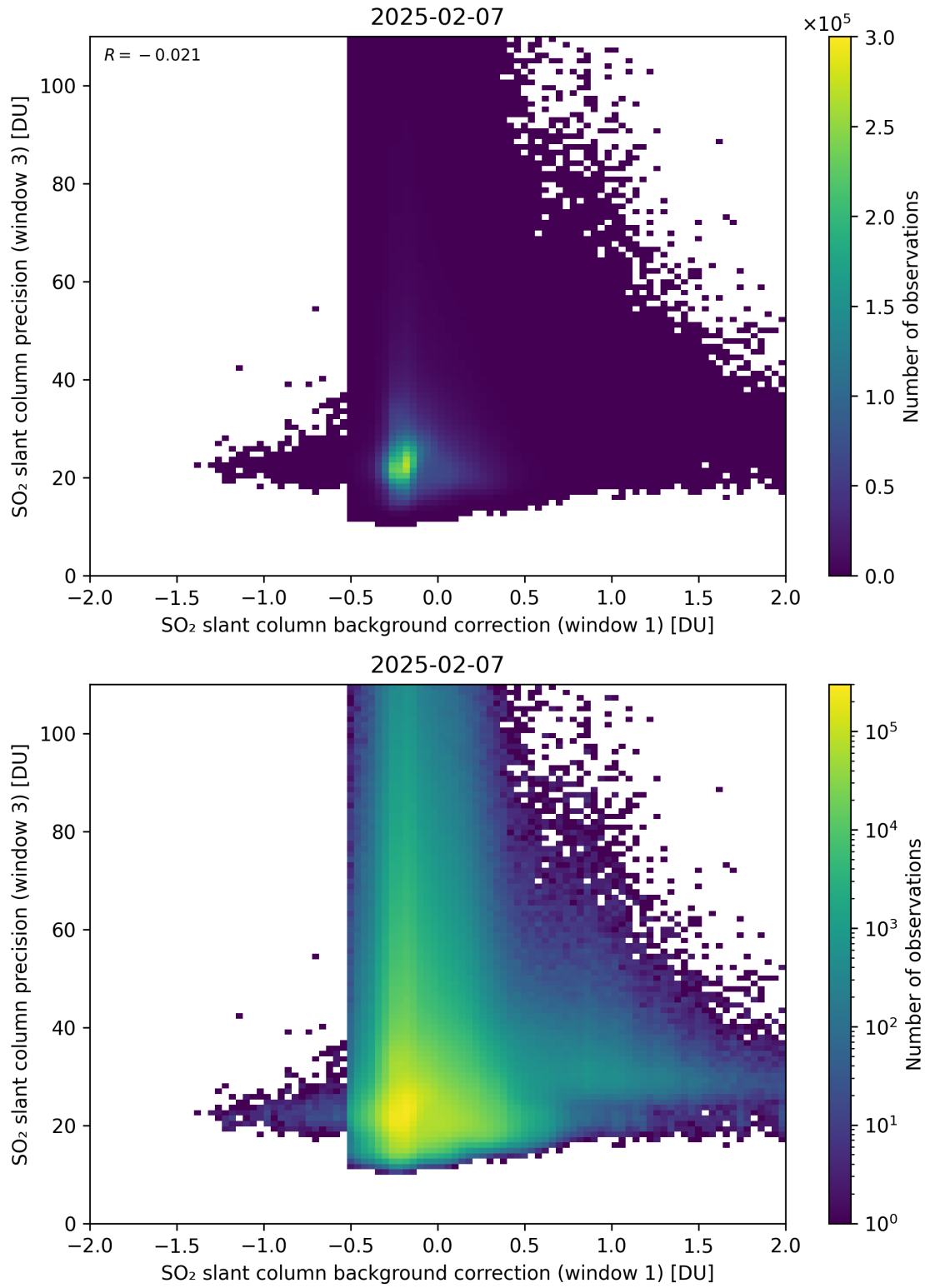
Figure 119: Scatter density plot of “SO 2 slant column background correction (window 1)” against “SO 2 slant column precision (window 3)” for 2025-02-06 to 2025-02-08.
