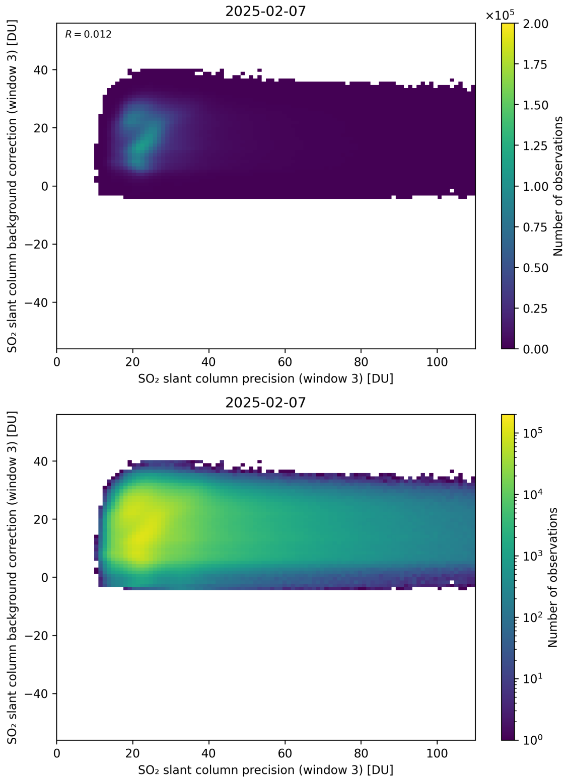
Figure 307: Scatter density plot of “SO 2 slant column precision (window 3)” against “SO 2 slant column background correction (window 3)” for 2025-02-06 to 2025-02-08.
