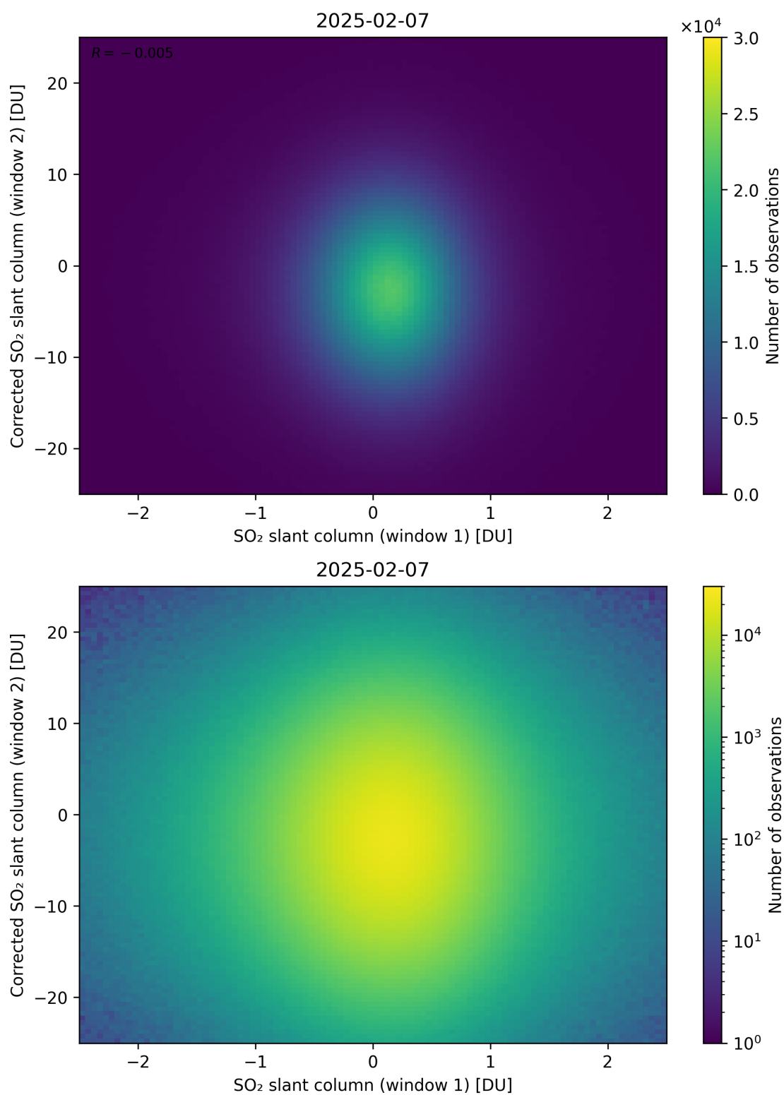
Figure 283: Scatter density plot of “SO 2 slant column (window 1)” against “Corrected SO 2 slant column (window 2)” for 2025-02-06 to 2025-02-08.
