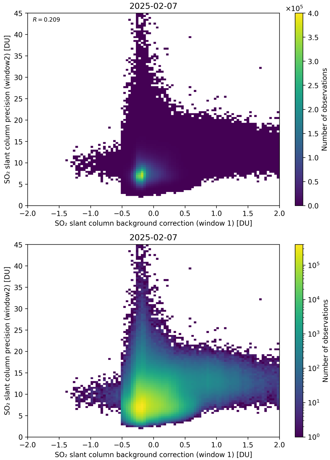
Figure 117: Scatter density plot of “SO 2 slant column background correction (window 1)” against “SO 2 slant column precision (window2)” for 2025-02-06 to 2025-02-08.
