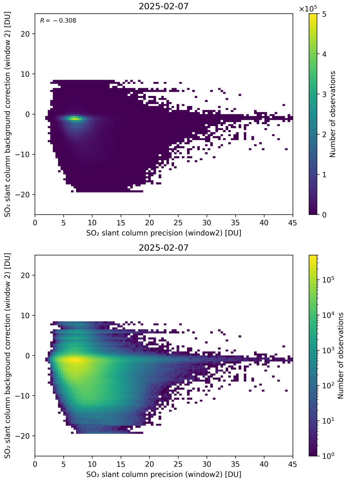
Figure 291: Scatter density plot of “SO 2 slant column precision (window2)” against “SO 2 slant column background correction (window 2)” for 2025-02-06 to 2025-02-08.
