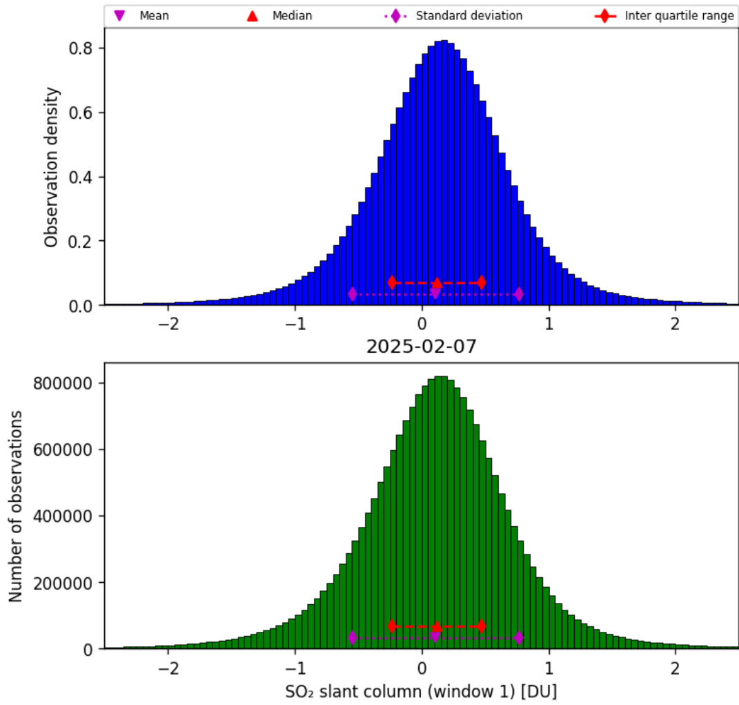
Figure 63: Histogram of “SO 2 slant column (window 1)” for 2025-02-06 to 2025-02-08
