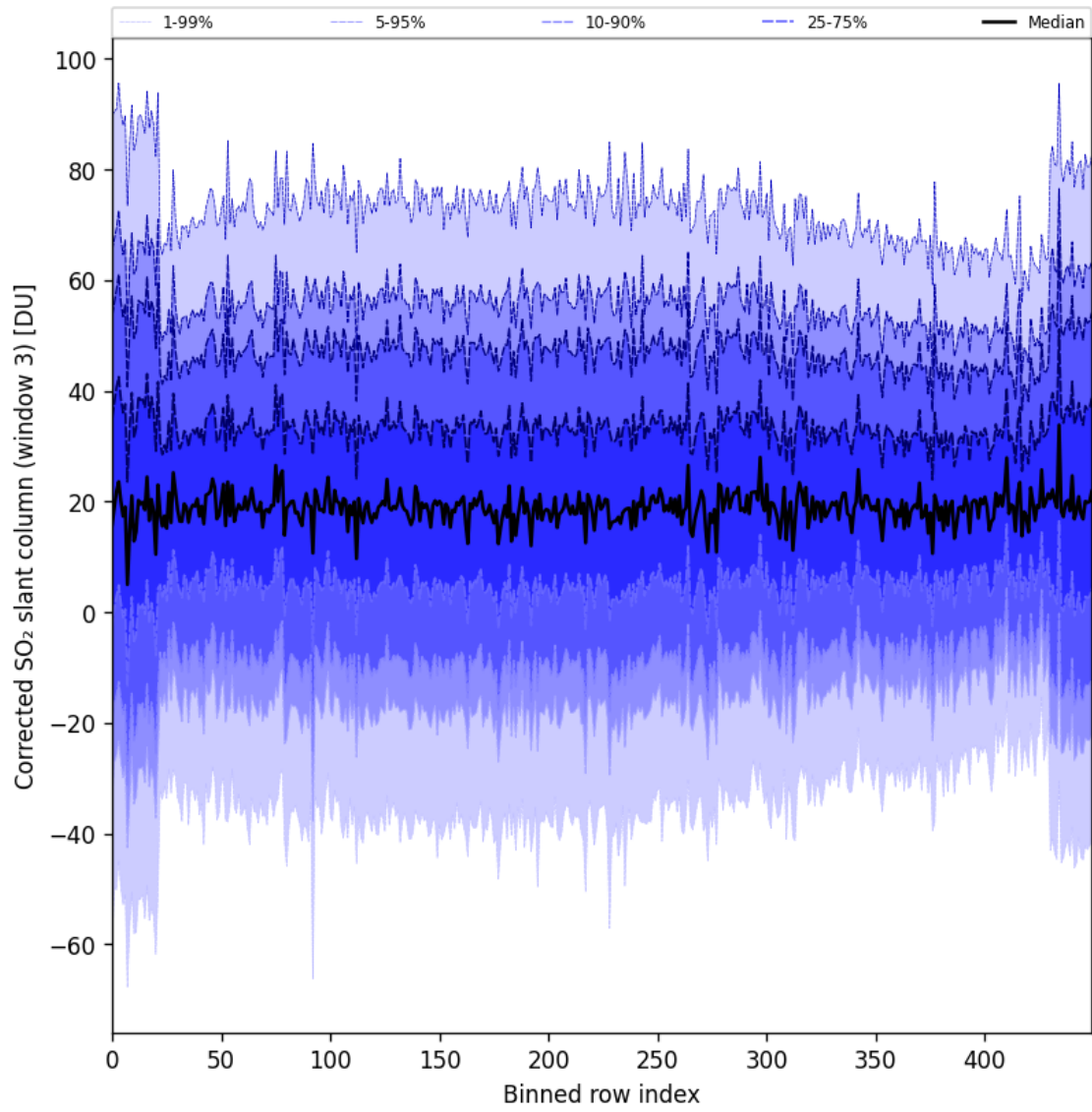
Figure 99: Along track statistics of “Corrected SO 2 slant column (window 3)” for 2025-02-06 to 2025-02-08
