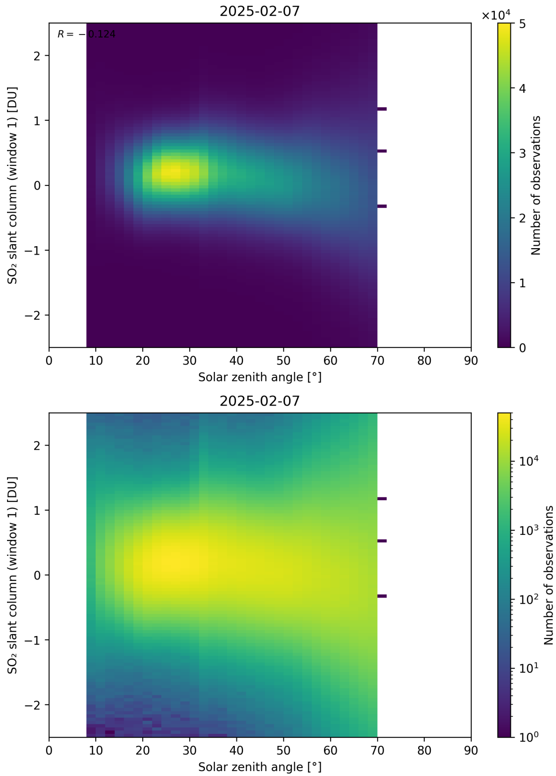
Figure 184: Scatter density plot of “Solar zenith angle” against “SO 2 slant column (window 1)” for 2025-02-06 to 2025-02-08.
