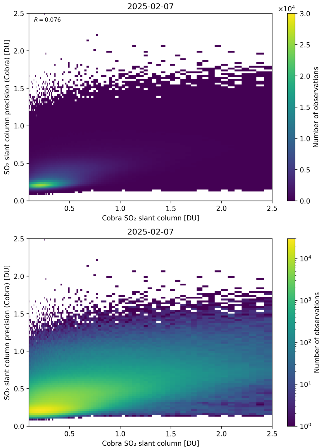
Figure 216: Scatter density plot of “Cobra SO 2 slant column” against “SO 2 slant column precision (Cobra)” for 2025-02-06 to 2025-02-08.
