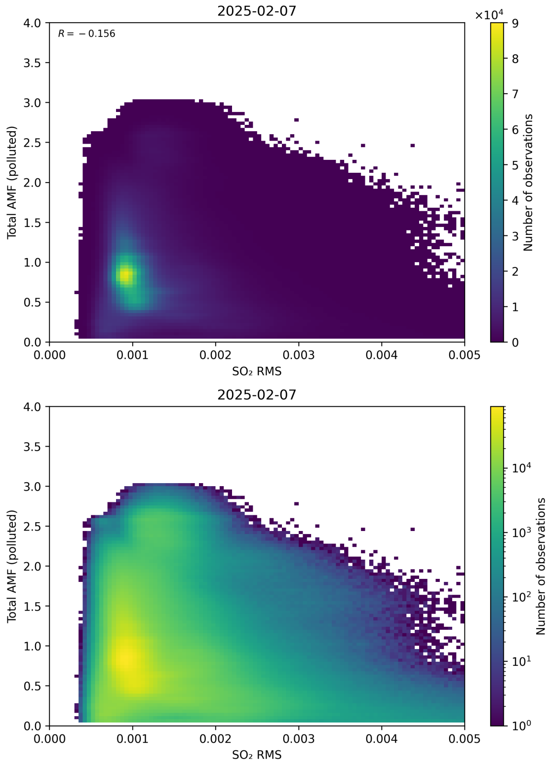
Figure 148: Scatter density plot of “SO 2 RMS” against “Total AMF (polluted)” for 2025-02-06 to 2025-02-08.
