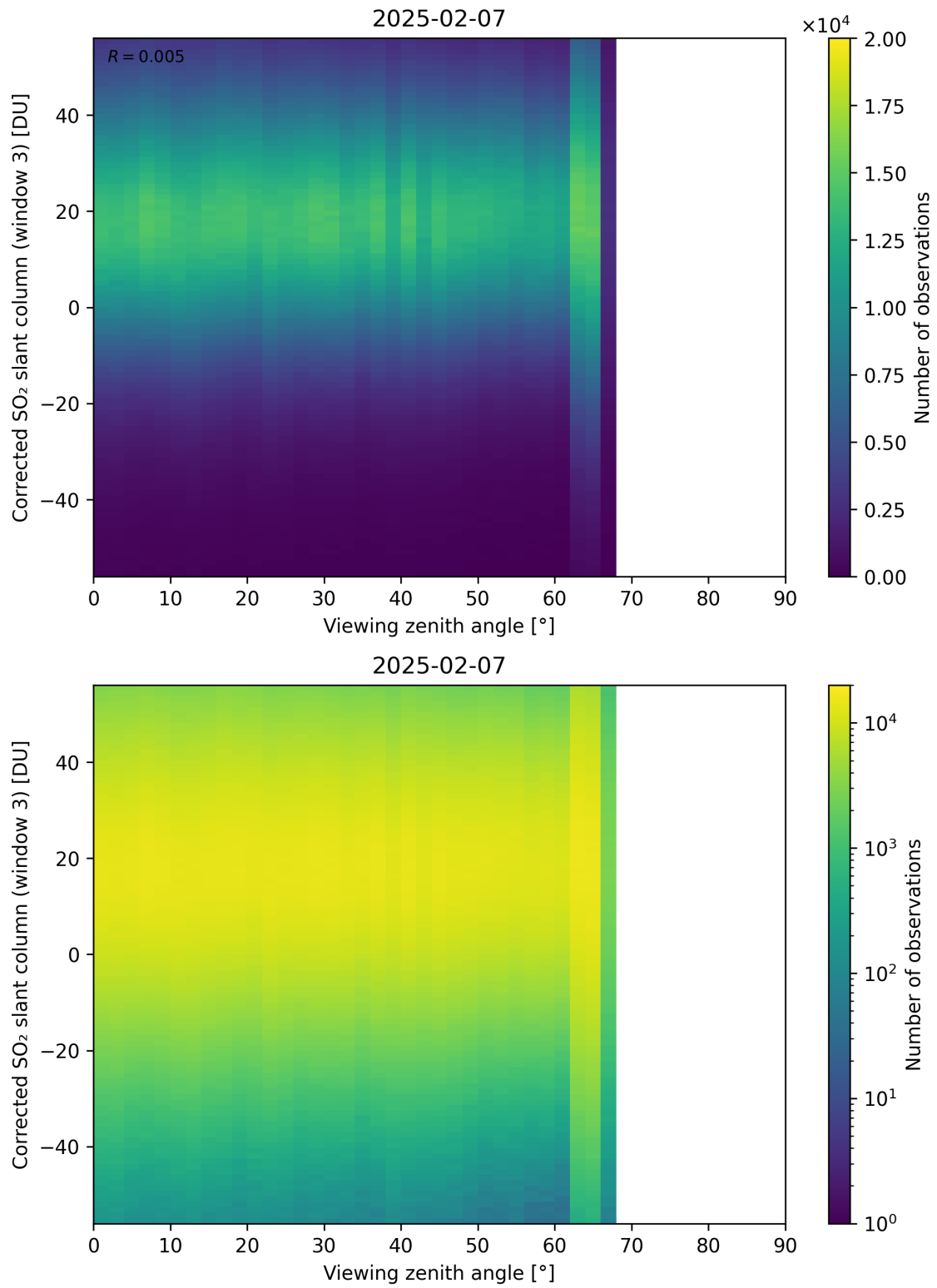
Figure 375: Scatter density plot of “Viewing zenith angle” against “Corrected SO 2 slant column (window 3)” for 2025-02-06 to 2025-02-08.
