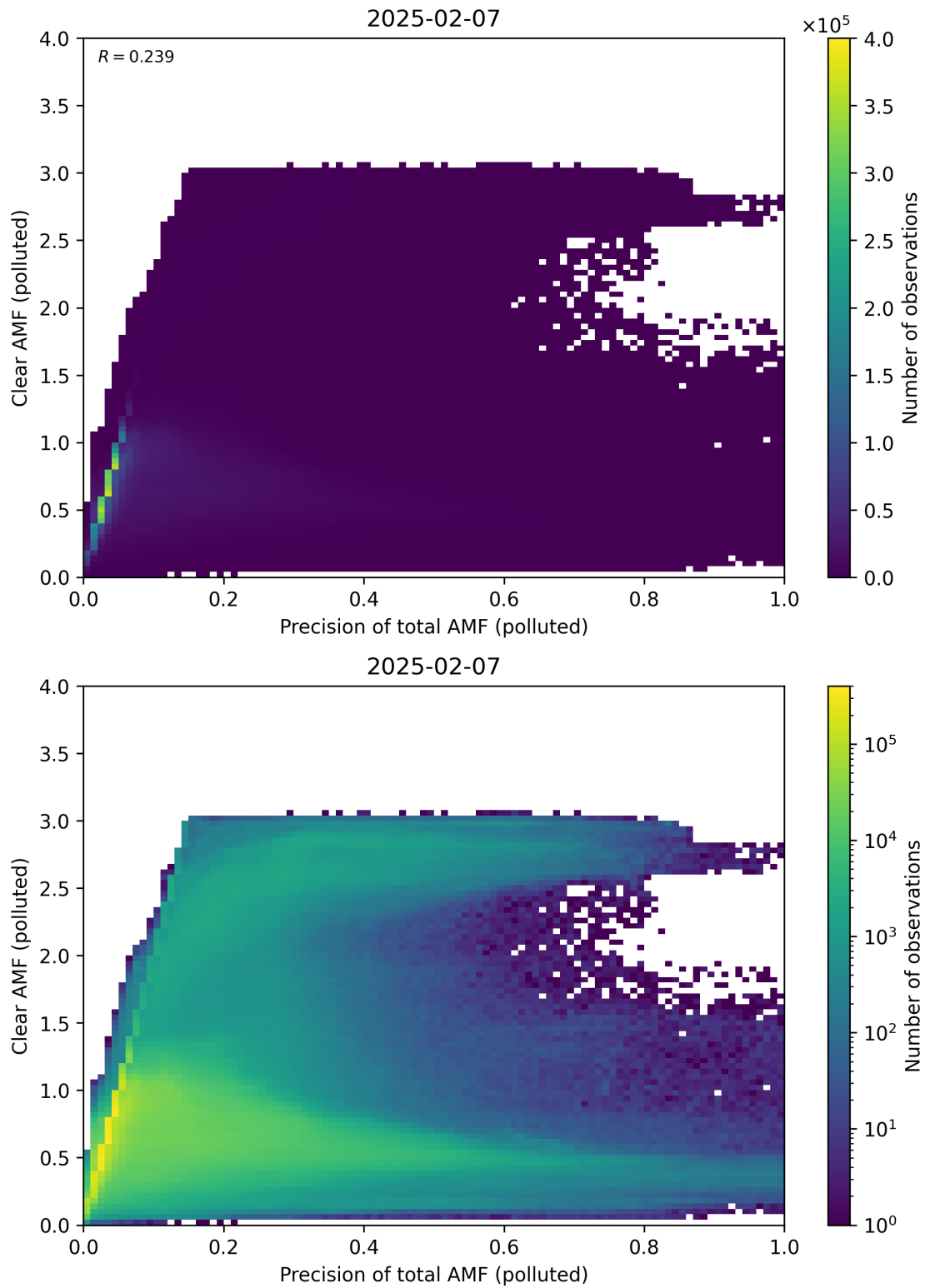
Figure 320: Scatter density plot of “Precision of total AMF (polluted)” against “Clear AMF (polluted)” for 2025-02-06 to 2025-02-08.
