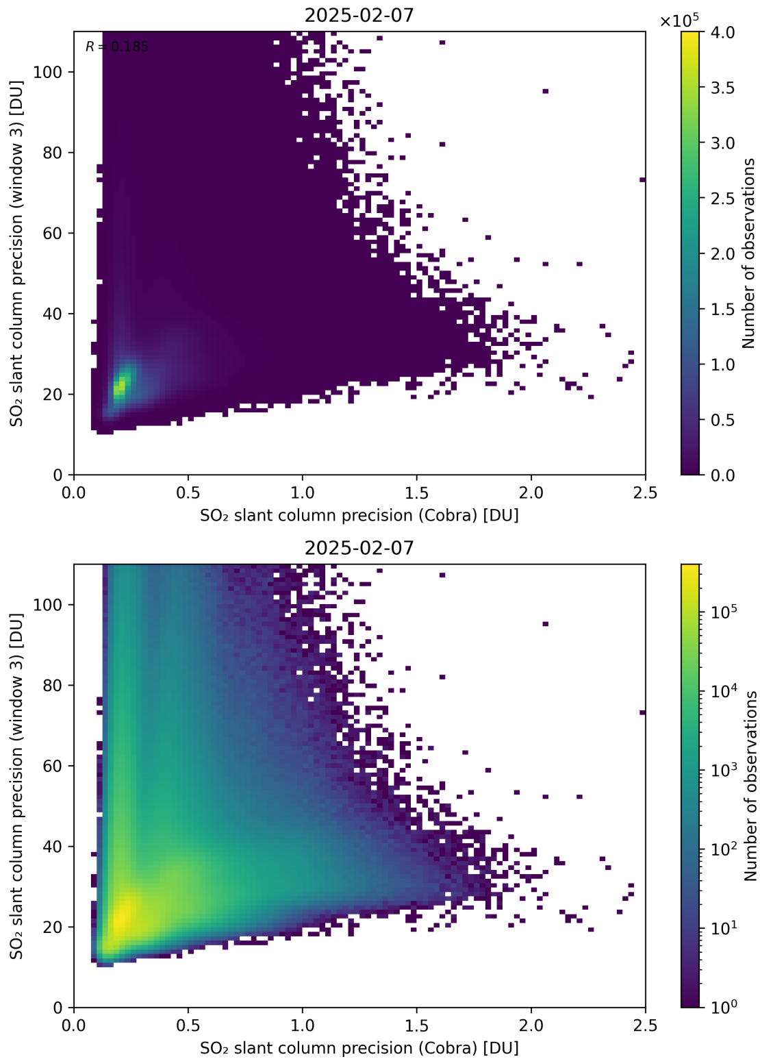
Figure 212: Scatter density plot of “SO 2 slant column precision (Cobra)” against “SO 2 slant column precision (window 3)” for 2025-02-06 to 2025-02-08.
