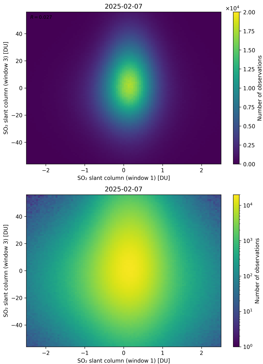
Figure 287: Scatter density plot of “SO 2 slant column (window 1)” against “SO 2 slant column (window 3)” for 2025-02-06 to 2025-02-08.
