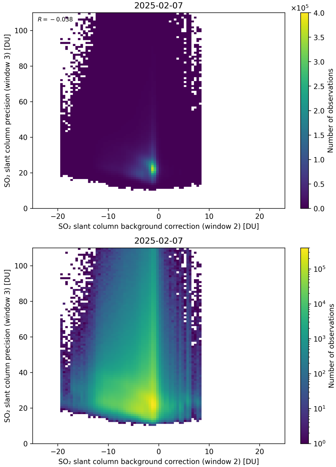
Figure 129: Scatter density plot of “SO 2 slant column background correction (window 2)” against “SO 2 slant column precision (window 3)” for 2025-02-06 to 2025-02-08.
