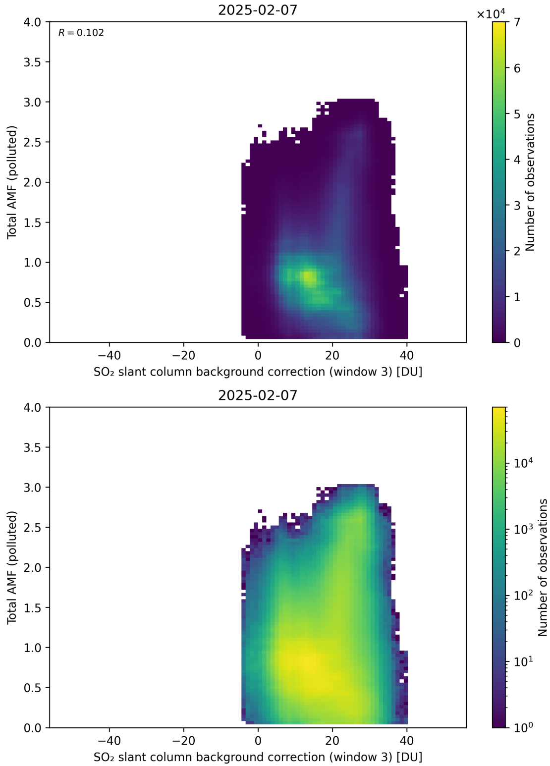
Figure 136: Scatter density plot of “SO 2 slant column background correction (window 3)” against “Total AMF (polluted)” for 2025-02-06 to 2025-02-08.
