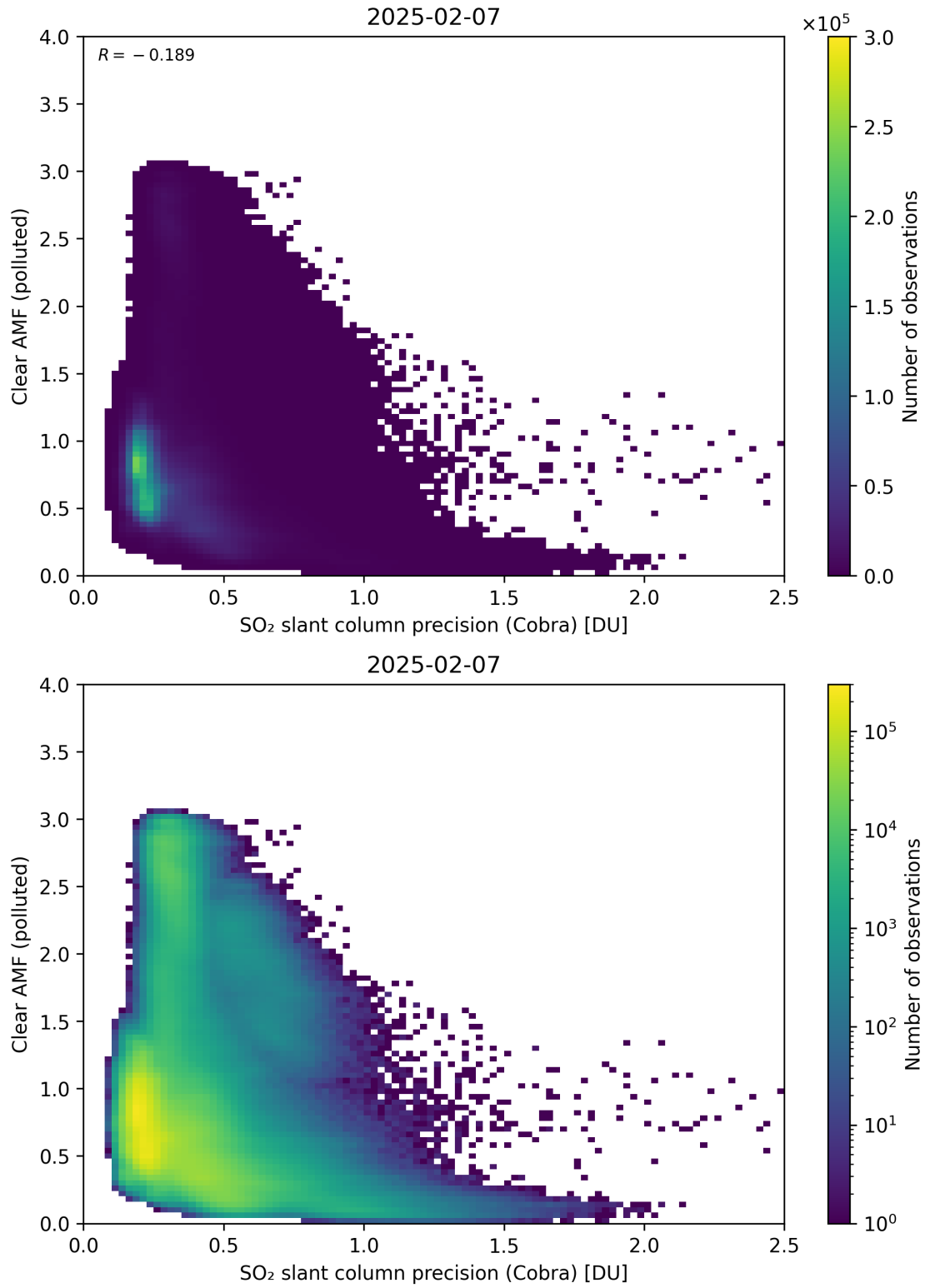
Figure 205: Scatter density plot of “SO 2 slant column precision (Cobra)” against “Clear AMF (polluted)” for 2025-02-06 to 2025-02-08.
