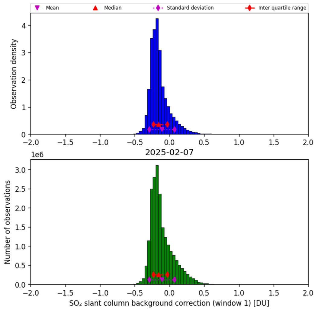
Figure 66: Histogram of “SO 2 slant column background correction (window 1)” for 2025-02-06 to 2025-02-08
