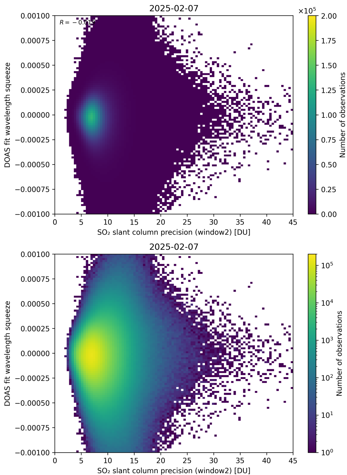
Figure 294: Scatter density plot of “SO 2 slant column precision (window2)” against “DOAS fit wavelength squeeze” for 2025-02-06 to 2025-02-08.
