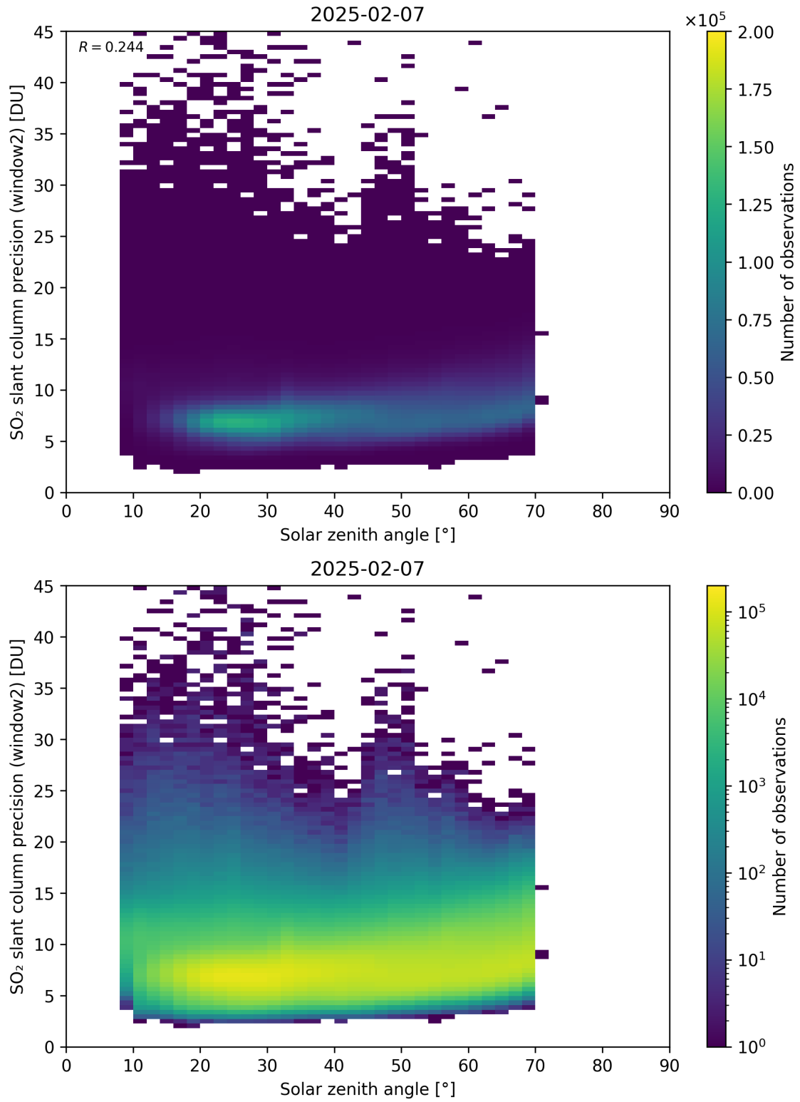
Figure 186: Scatter density plot of “Solar zenith angle” against “SO 2 slant column precision (window2)” for 2025-02-06 to 2025-02-08.
