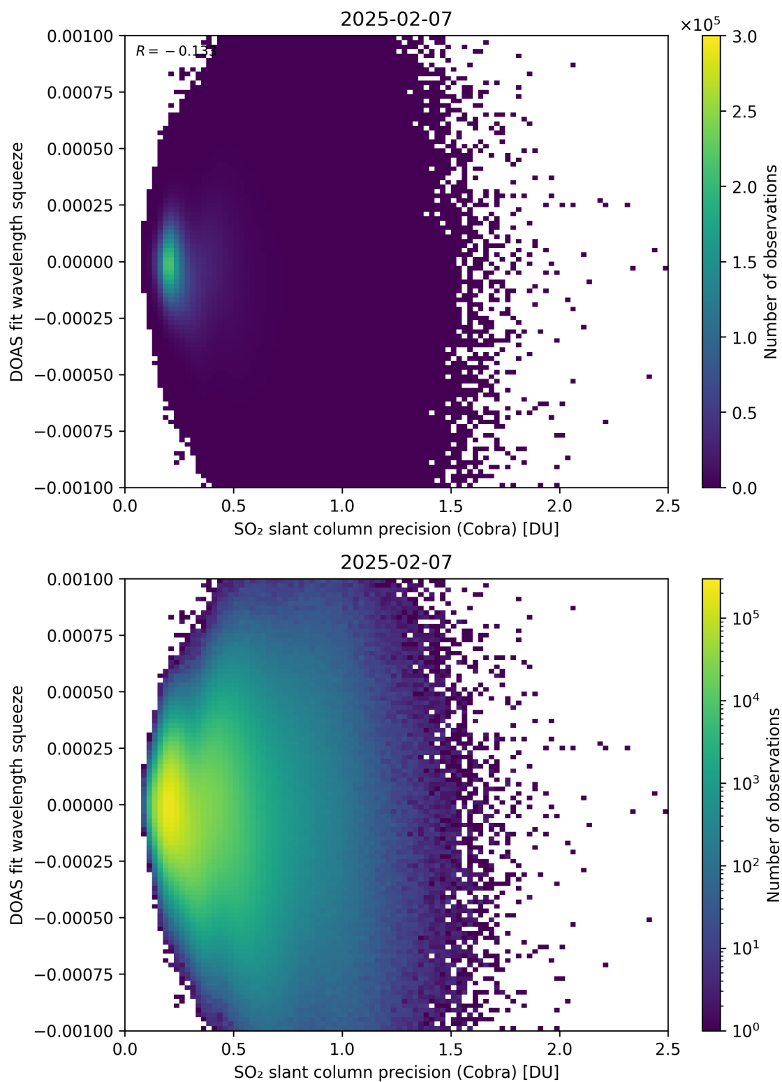
Figure 203: Scatter density plot of “SO 2 slant column precision (Cobra)” against “DOAS fit wavelength squeeze” for 2025-02-06 to 2025-02-08.
