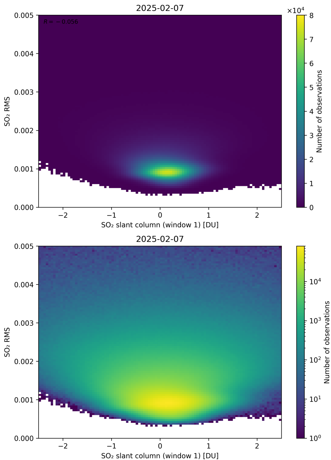
Figure 267: Scatter density plot of “SO 2 slant column (window 1)” against “SO 2 RMS” for 2025-02-06 to 2025-02-08.
