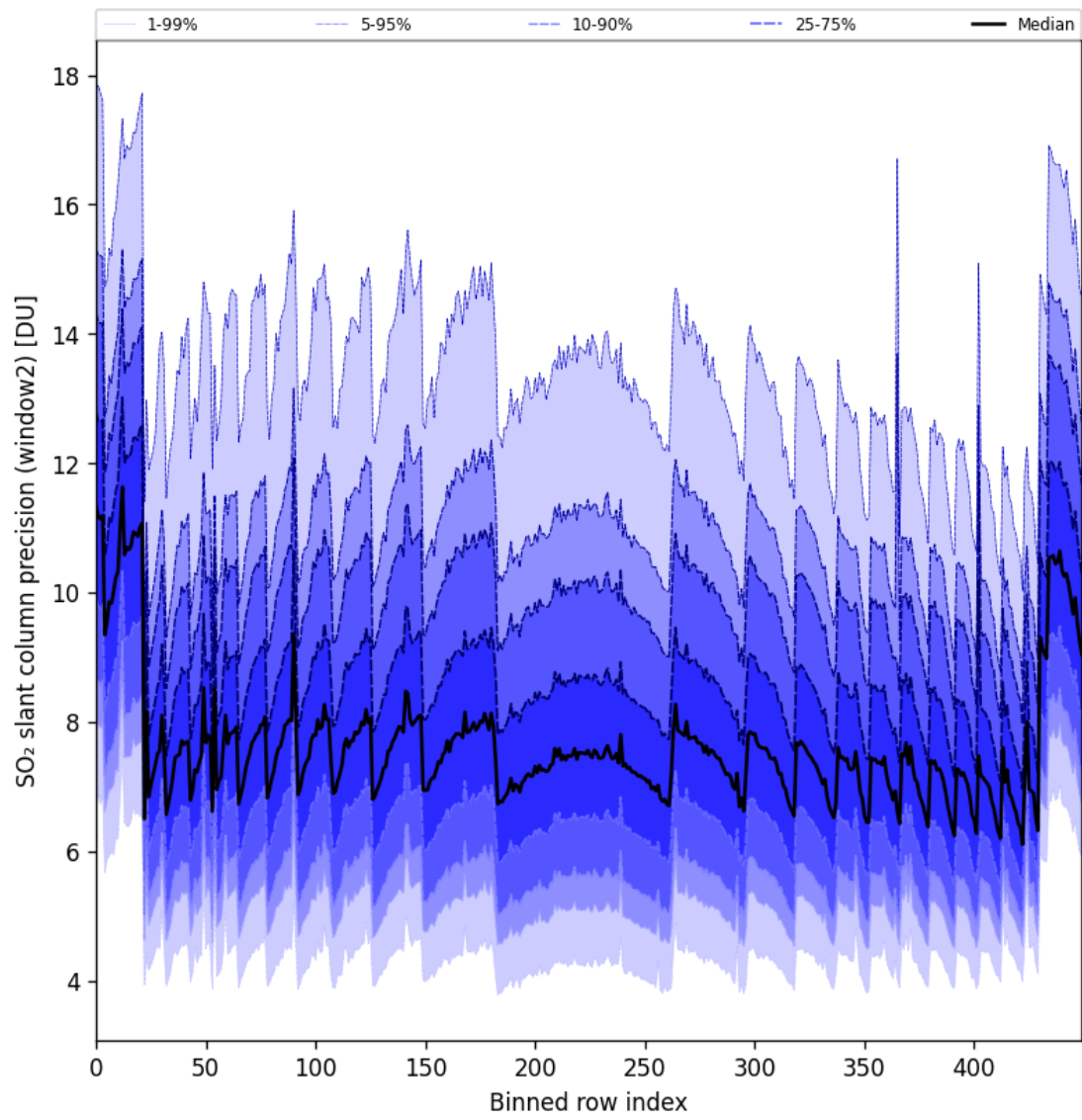
Figure 94: Along track statistics of “SO 2 slant column precision (window2)” for 2025-02-06 to 2025-02-08
