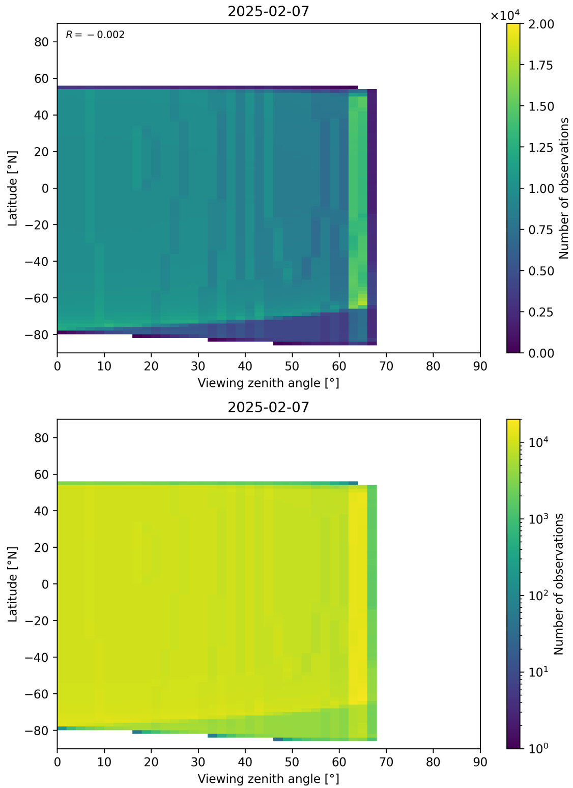
Figure 368: Scatter density plot of “Viewing zenith angle” against “Latitude” for 2025-02-06 to 2025-02-08.
