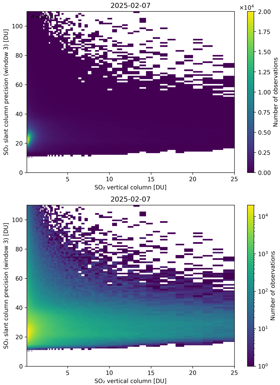
Figure 358: Scatter density plot of “SO 2 vertical column” against “SO 2 slant column precision (window 3)” for 2025-02-06 to 2025-02-08.
