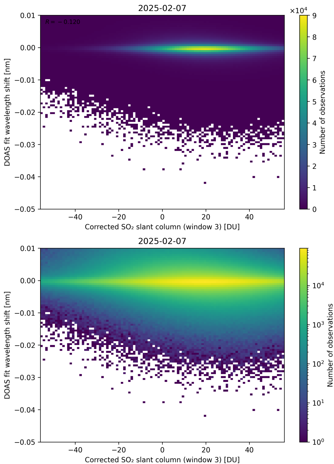
Figure 256: Scatter density plot of “Corrected SO 2 slant column (window 3)” against “DOAS fit wavelength shift” for 2025-02-06 to 2025-02-08.
