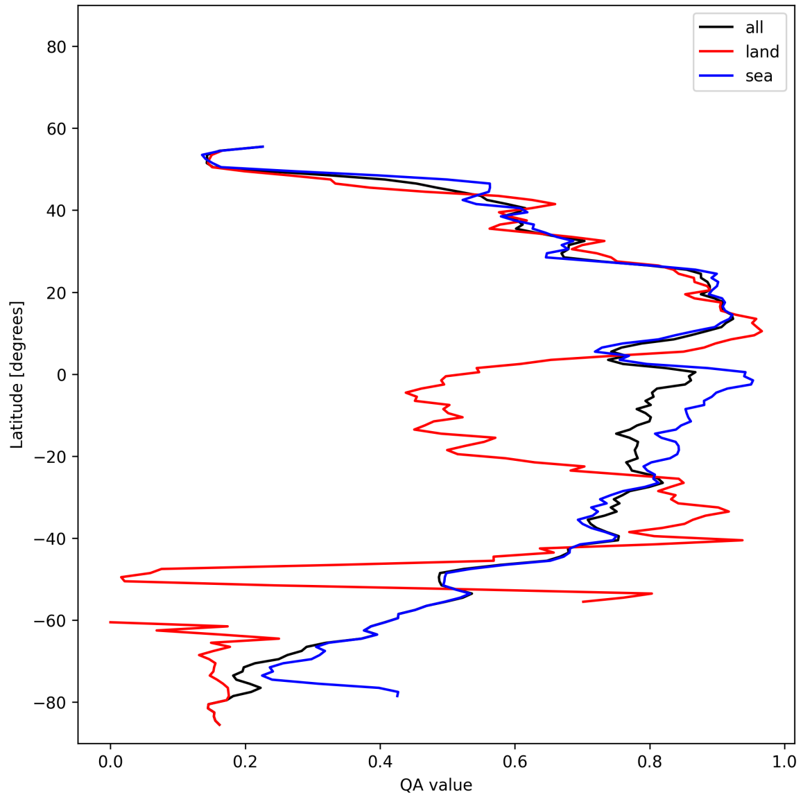
Figure 31: Zonal average of “QA value” for 2025-02-06 to 2025-02-08.
