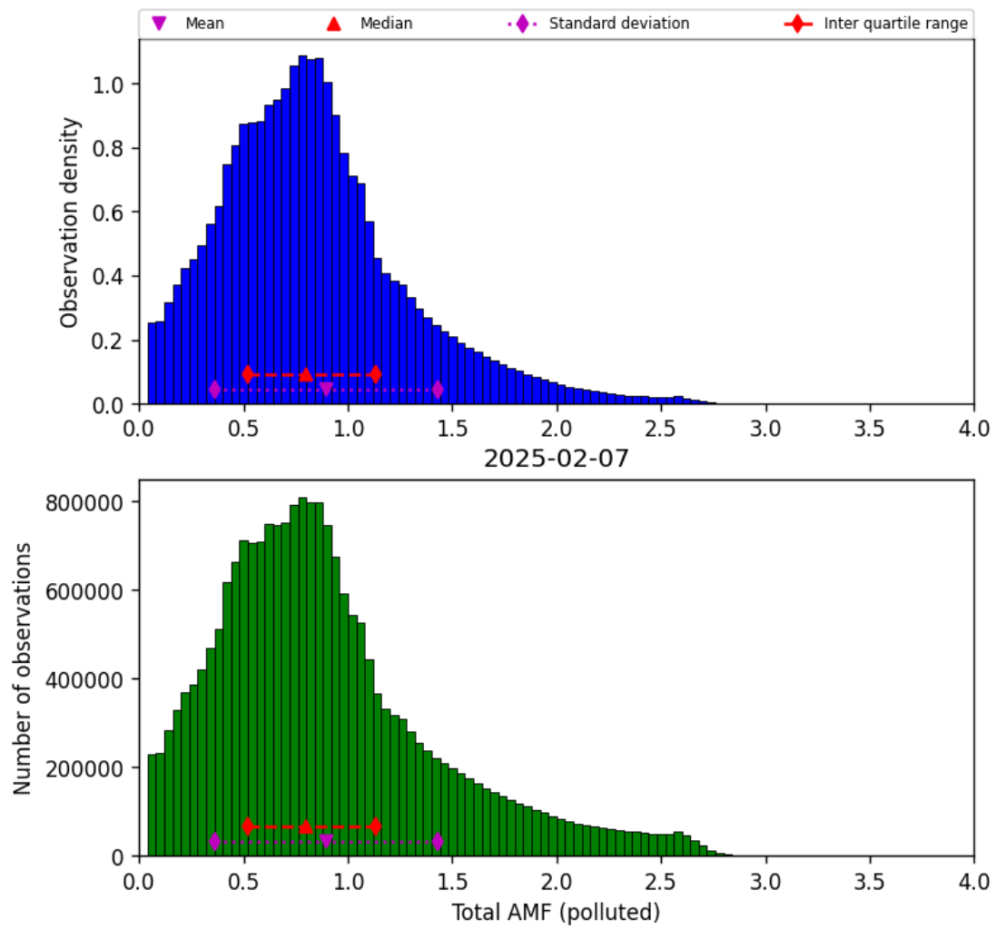
Figure 79: Histogram of “Total AMF (polluted)” for 2025-02-06 to 2025-02-08
