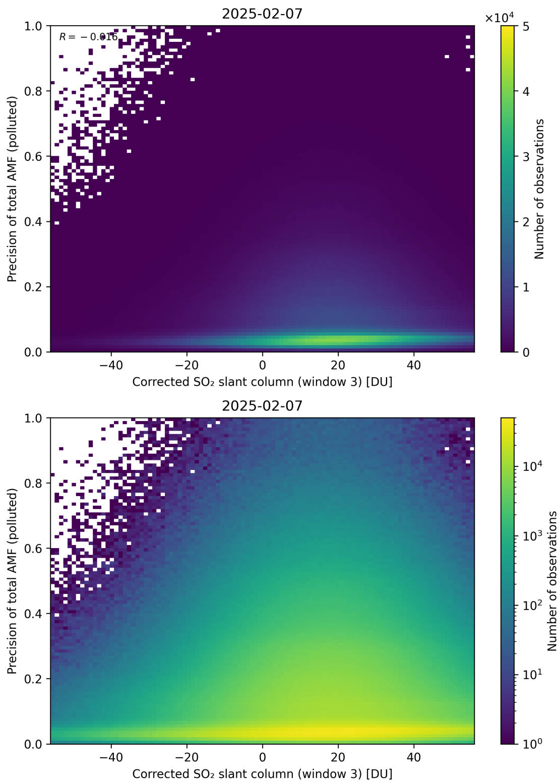
Figure 261: Scatter density plot of “Corrected SO 2 slant column (window 3)” against “Precision of total AMF (polluted)” for 2025-02-06 to 2025-02-08.
