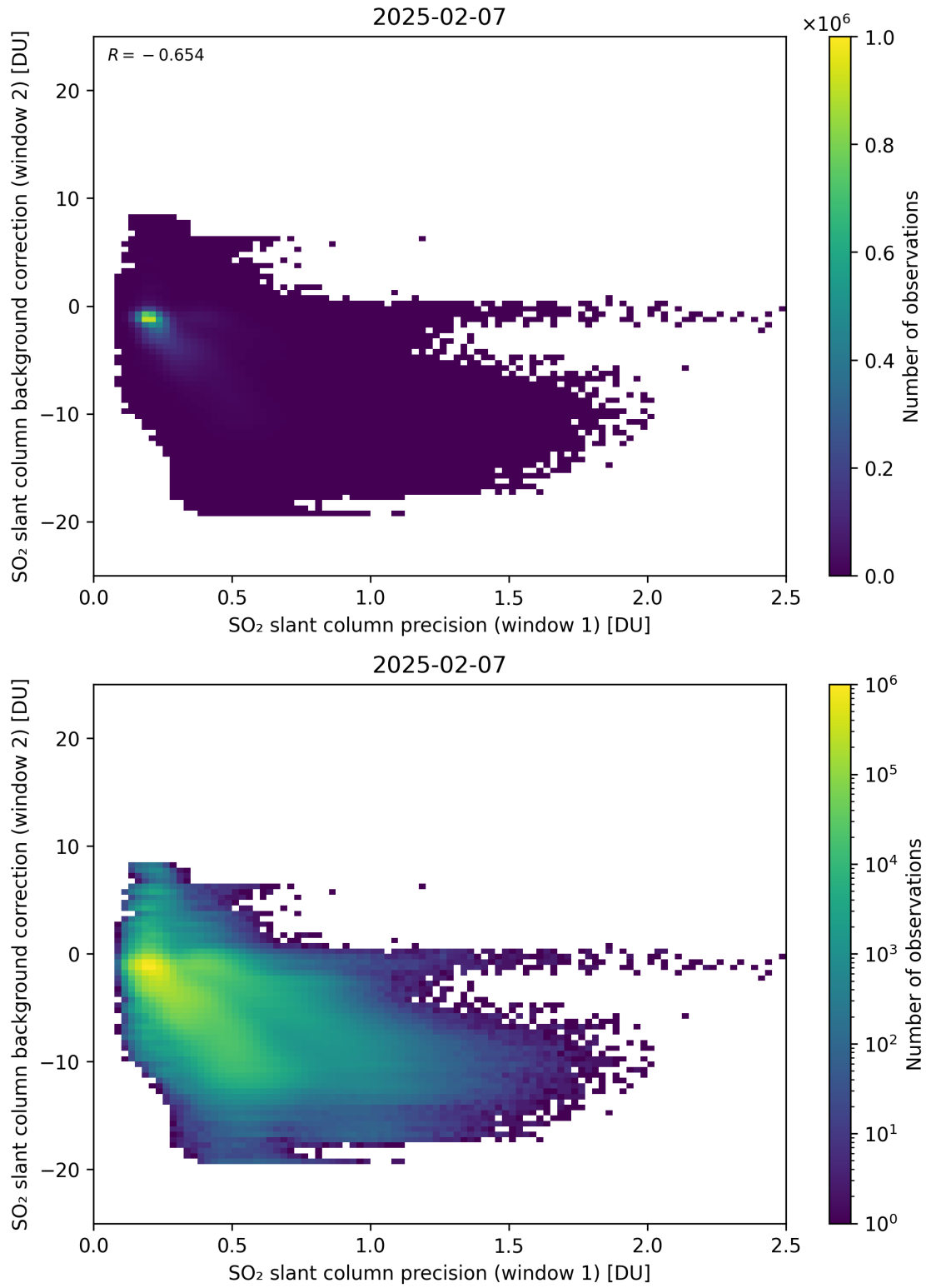
Figure 269: Scatter density plot of “SO 2 slant column precision (window 1)” against “SO 2 slant column background correction (window 2)” for 2025-02-06 to 2025-02-08.
