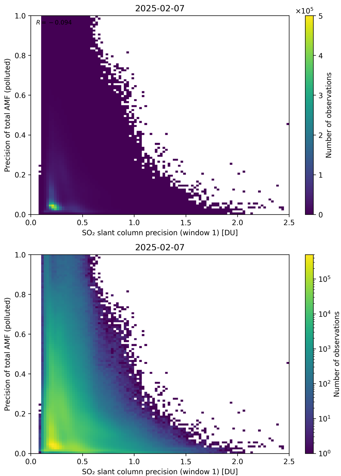
Figure 281: Scatter density plot of “SO 2 slant column precision (window 1)” against “Precision of total AMF (polluted)” for 2025-02-06 to 2025-02-08.
