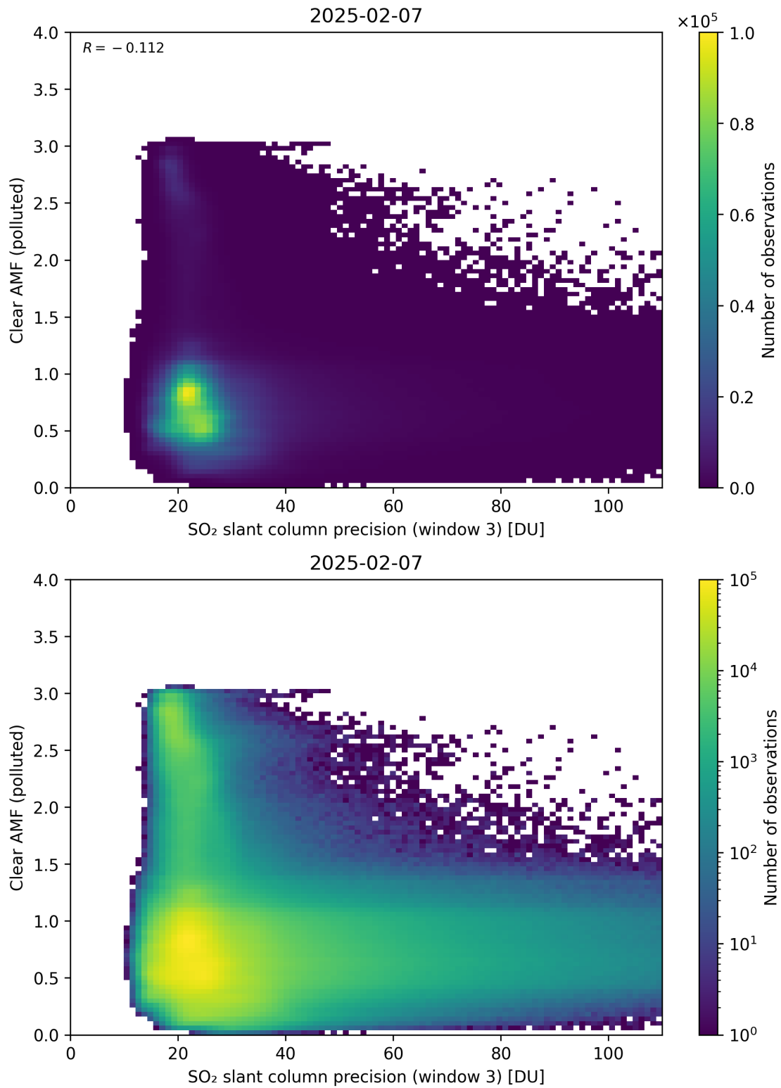
Figure 311: Scatter density plot of “SO 2 slant column precision (window 3)” against “Clear AMF (polluted)” for 2025-02-06 to 2025-02-08.
