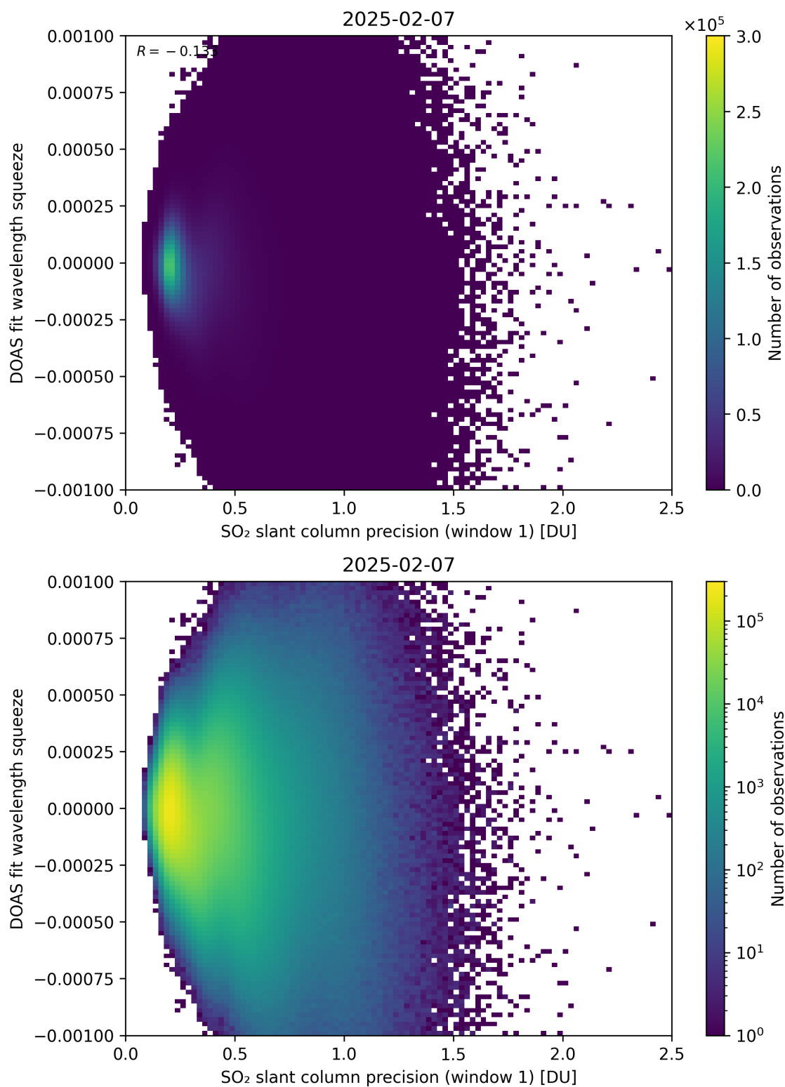
Figure 272: Scatter density plot of “SO 2 slant column precision (window 1)” against “DOAS fit wavelength squeeze” for 2025-02-06 to 2025-02-08.
