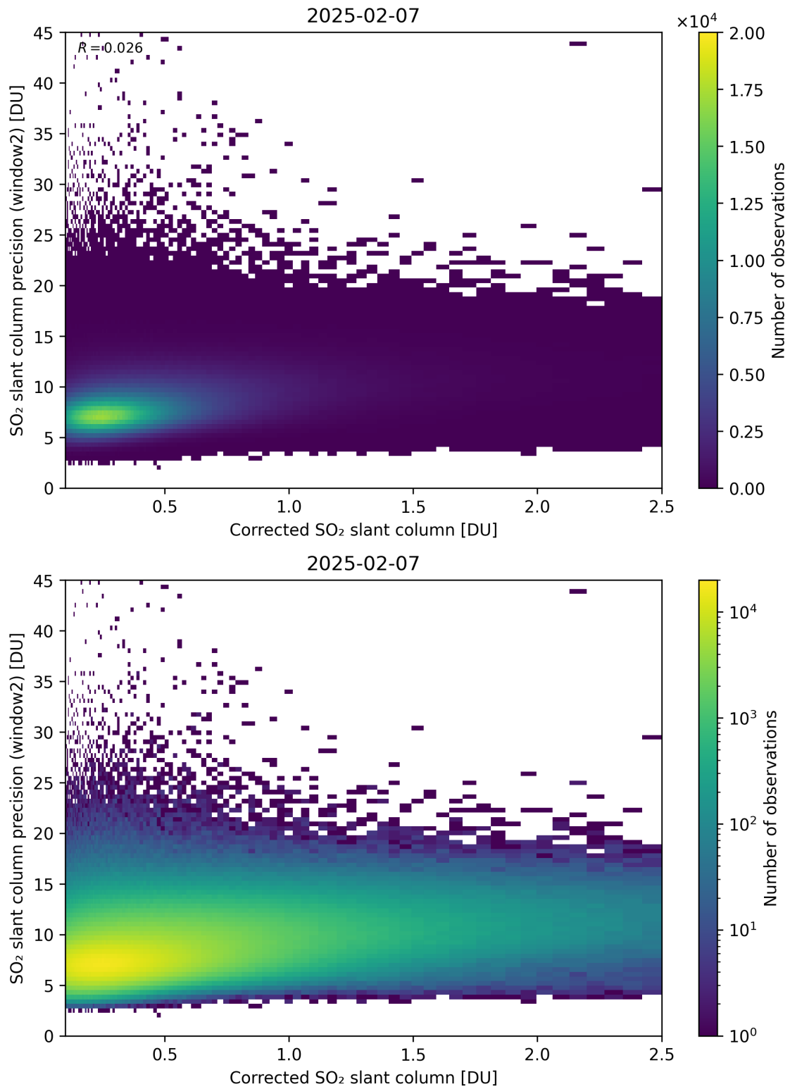
Figure 239: Scatter density plot of “Corrected SO 2 slant column” against “SO 2 slant column precision (window2)” for 2025-02-06 to 2025-02-08.
