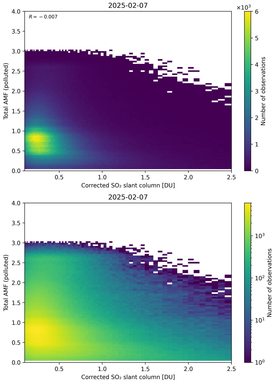
Figure 242: Scatter density plot of “Corrected SO 2 slant column” against “Total AMF (polluted)” for 2025-02-06 to 2025-02-08.
