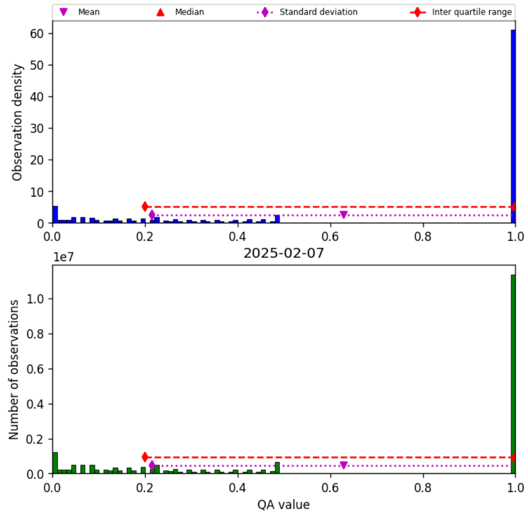
Figure 57: Histogram of “QA value” for 2025-02-06 to 2025-02-08
