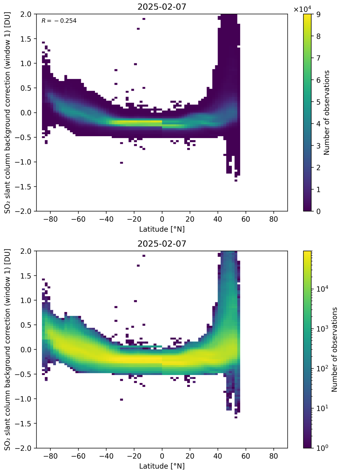
Figure 150: Scatter density plot of “Latitude” against “SO 2 slant column background correction (window 1)” for 2025-02-06 to 2025-02-08.
