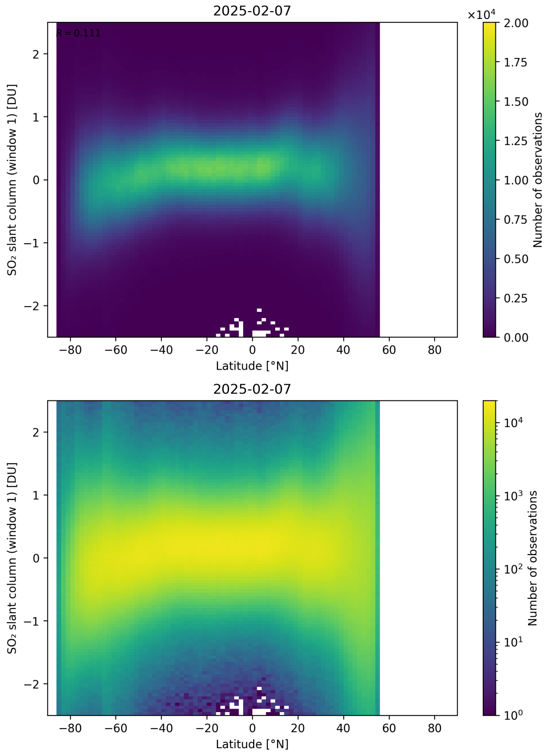
Figure 162: Scatter density plot of “Latitude” against “SO 2 slant column (window 1)” for 2025-02-06 to 2025-02-08.
