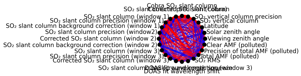
Figure 1: Map of correlation graph for 2025-02-06 to 2025-02-08.
