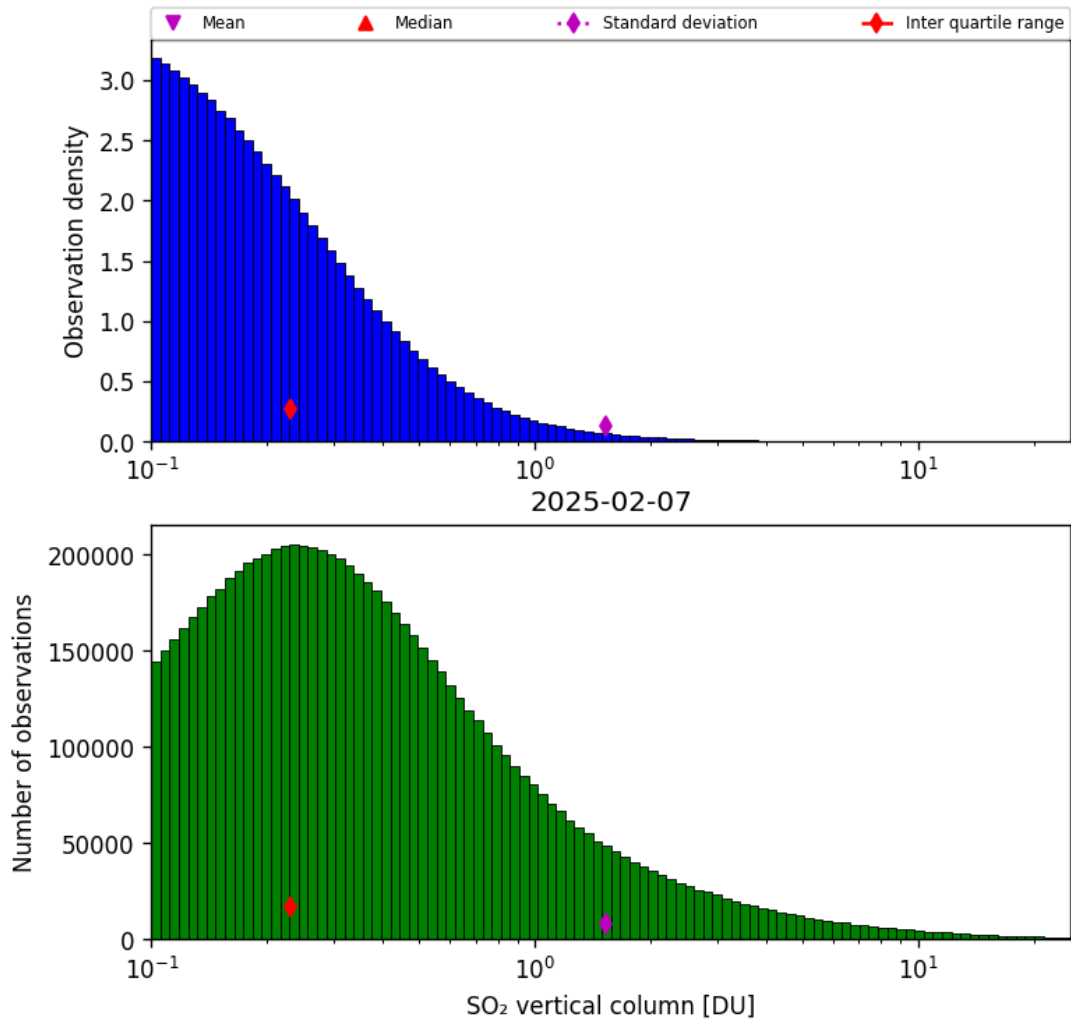
Figure 58: Histogram of “SO 2 vertical column” for 2025-02-06 to 2025-02-08
