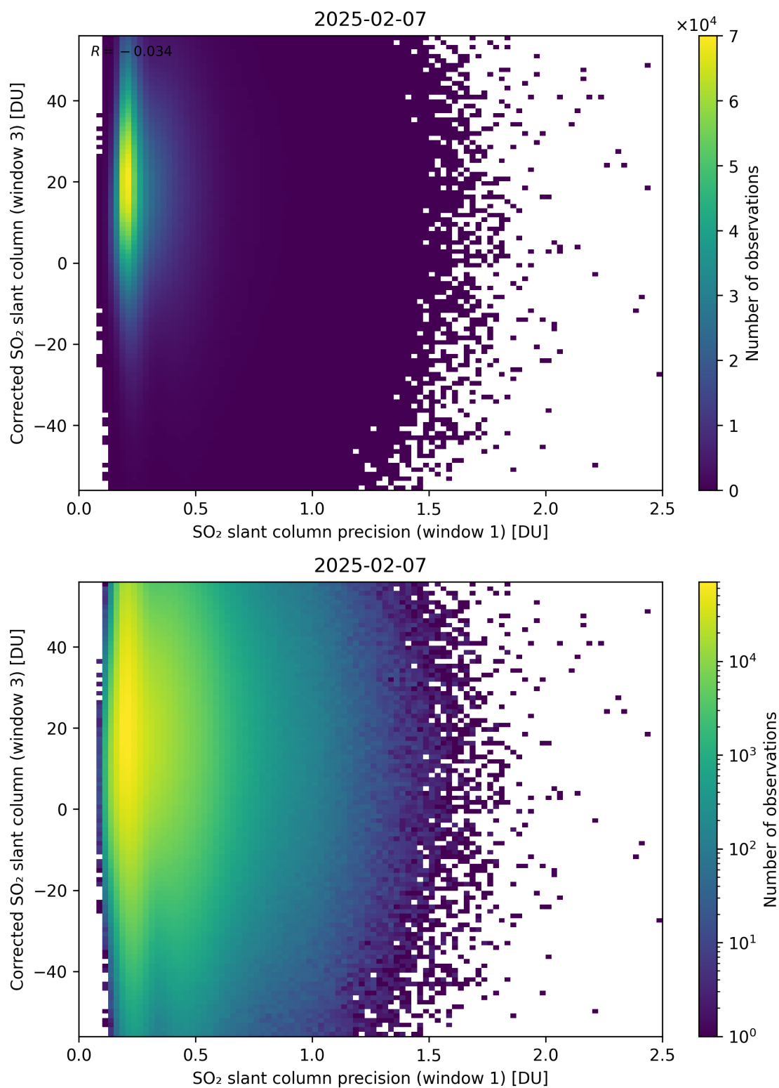
Figure 276: Scatter density plot of “SO 2 slant column precision (window 1)” against “Corrected SO 2 slant column (window 3)” for 2025-02-06 to 2025-02-08.
