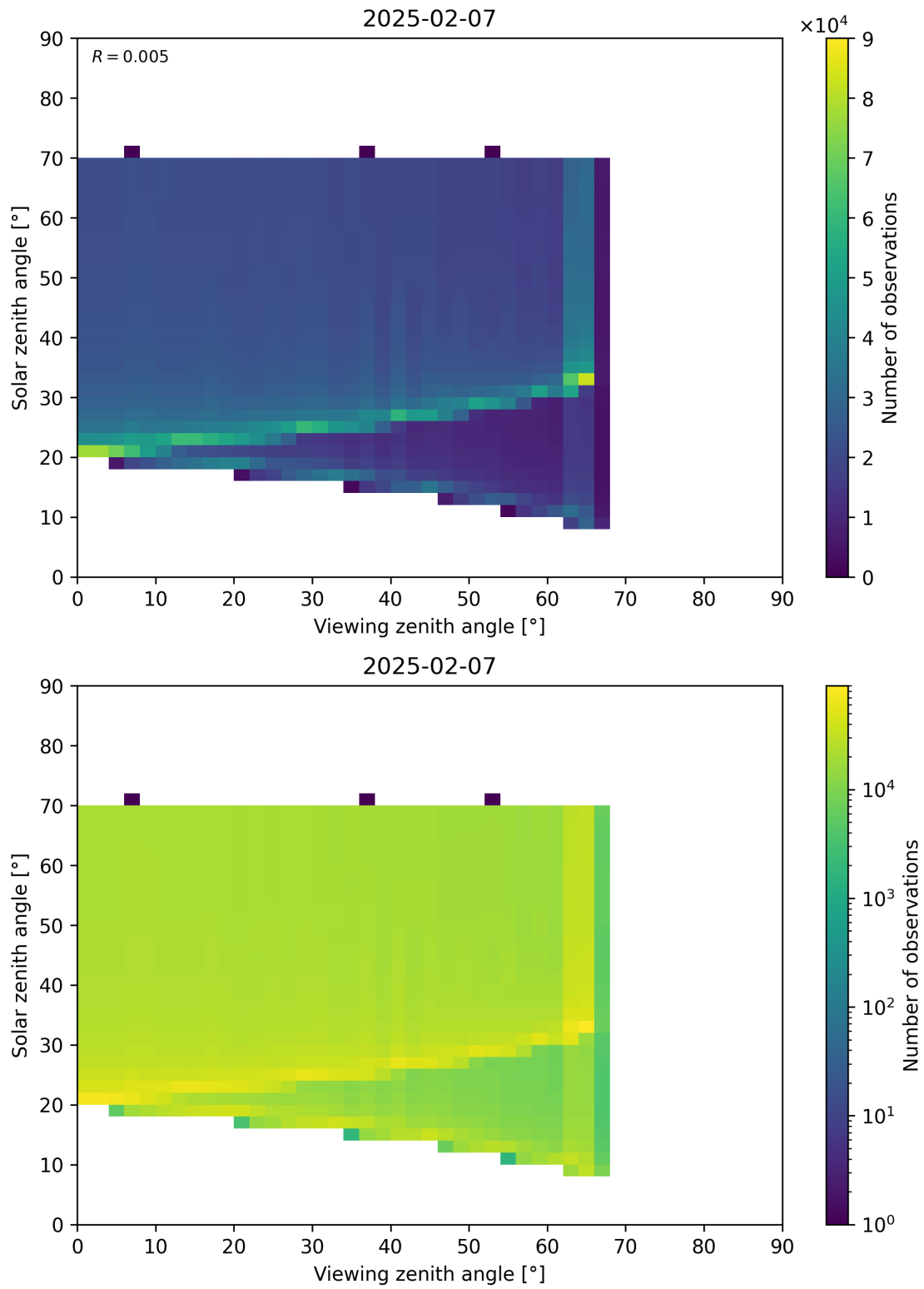
Figure 369: Scatter density plot of “Viewing zenith angle” against “Solar zenith angle” for 2025-02-06 to 2025-02-08.
