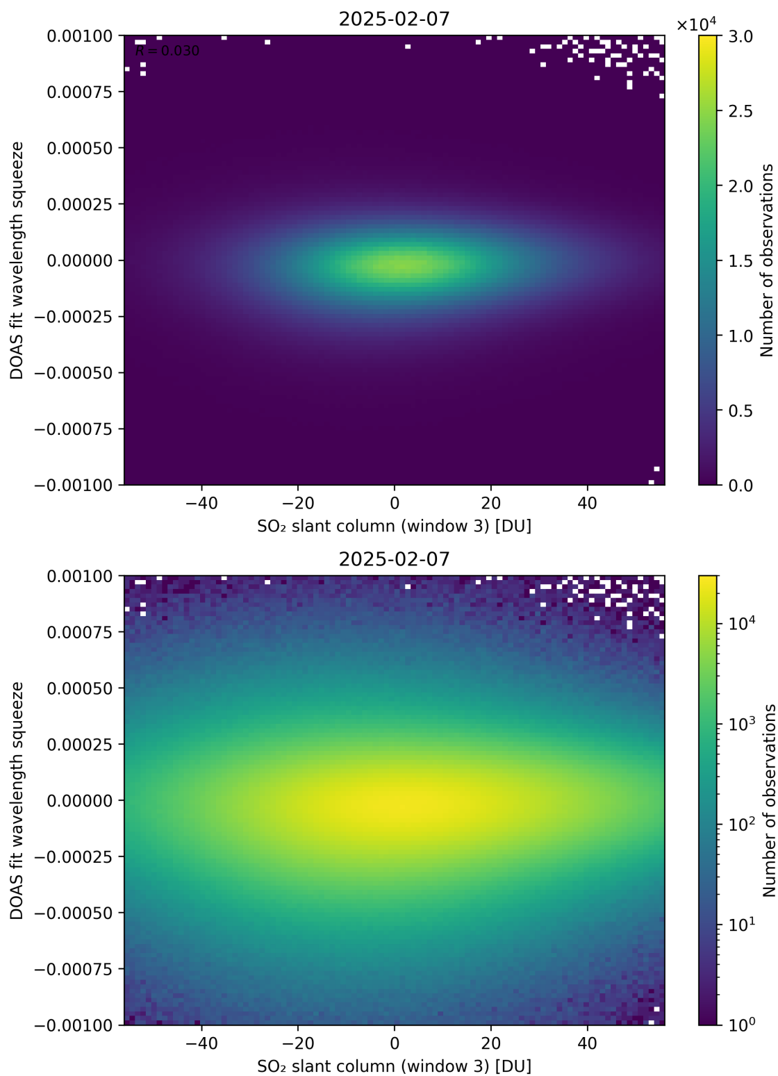
Figure 305: Scatter density plot of “SO 2 slant column (window 3)” against “DOAS fit wavelength squeeze” for 2025-02-06 to 2025-02-08.
