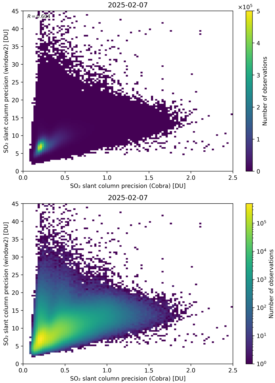
Figure 210: Scatter density plot of “SO 2 slant column precision (Cobra)” against “SO 2 slant column precision (window2)” for 2025-02-06 to 2025-02-08.
