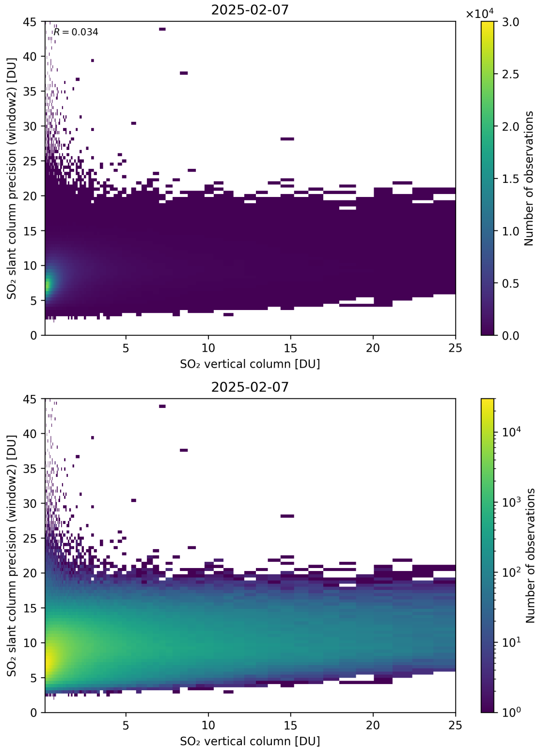
Figure 356: Scatter density plot of “SO 2 vertical column” against “SO 2 slant column precision (window2)” for 2025-02-06 to 2025-02-08.
