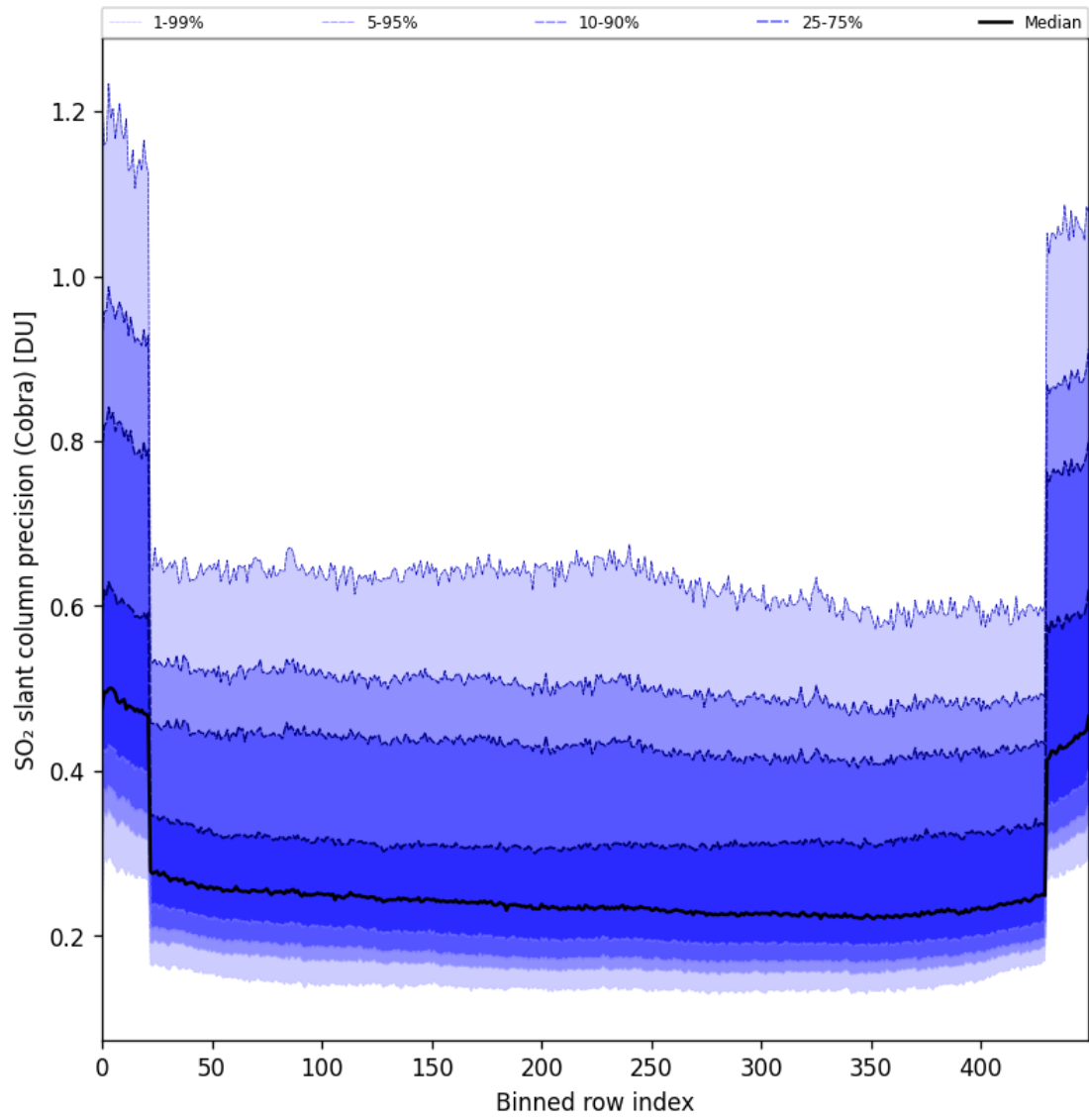
Figure 88: Along track statistics of “SO 2 slant column precision (Cobra)” for 2025-02-06 to 2025-02-08
