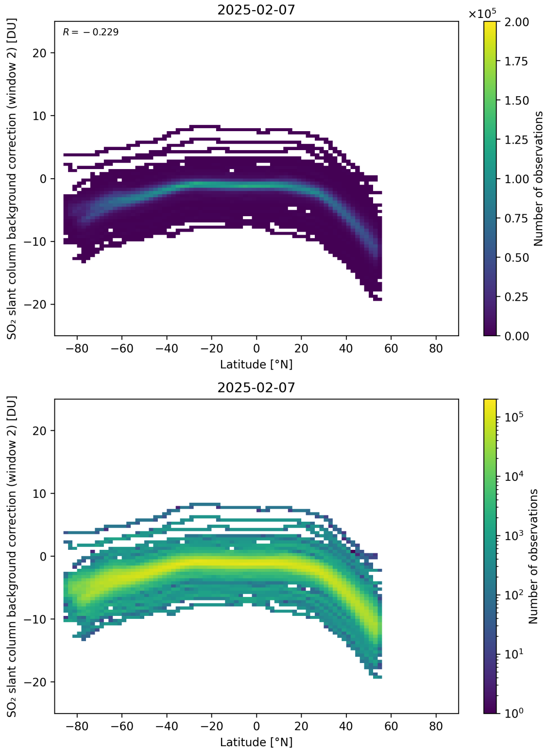
Figure 151: Scatter density plot of “Latitude” against “SO 2 slant column background correction (window 2)” for 2025-02-06 to 2025-02-08.
