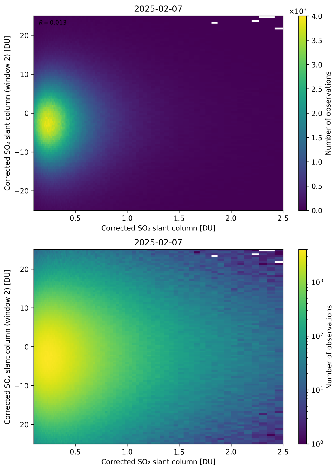
Figure 235: Scatter density plot of “Corrected SO 2 slant column” against “Corrected SO 2 slant column (window 2)” for 2025-02-06 to 2025-02-08.
