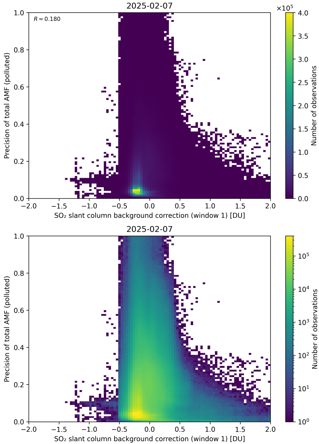
Figure 121: Scatter density plot of “SO 2 slant column background correction (window 1)” against “Precision of total AMF (polluted)” for 2025-02-06 to 2025-02-08.
