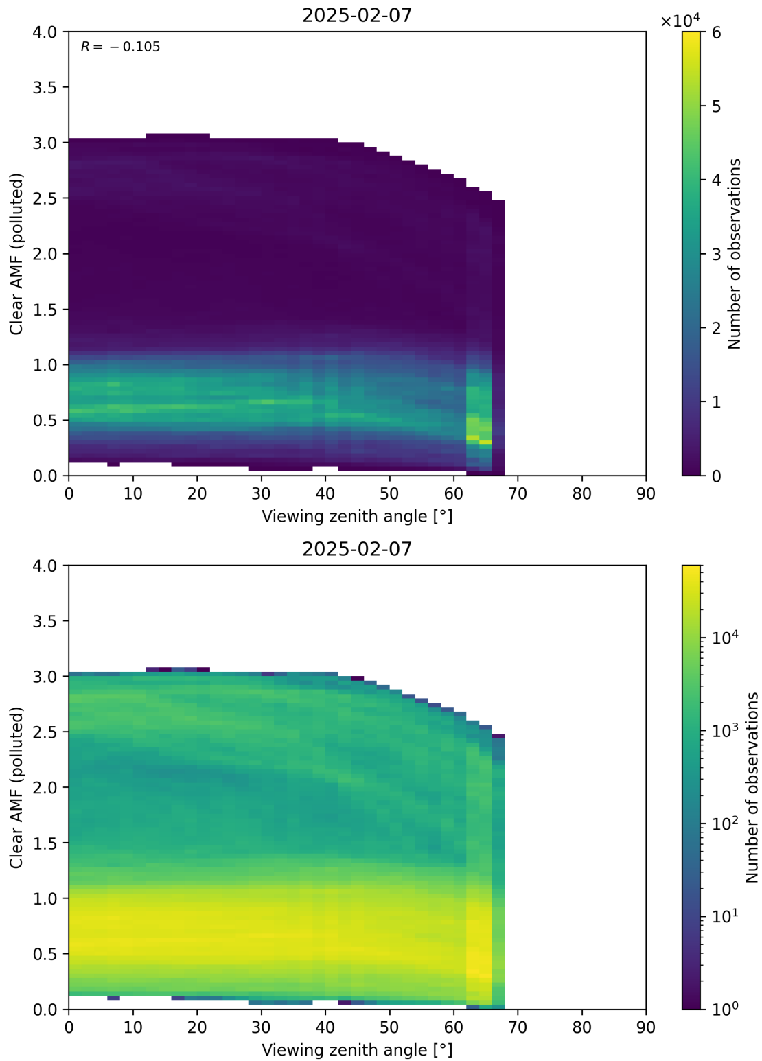
Figure 370: Scatter density plot of “Viewing zenith angle” against “Clear AMF (polluted)” for 2025-02-06 to 2025-02-08.
