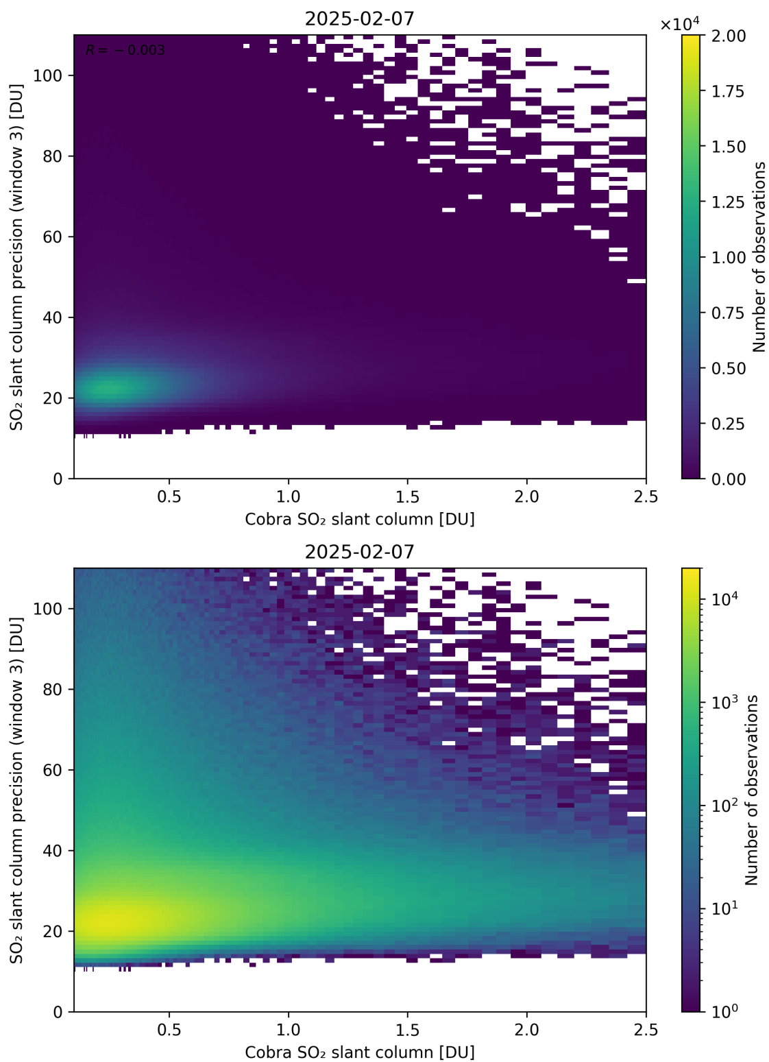
Figure 223: Scatter density plot of “Cobra SO 2 slant column” against “SO 2 slant column precision (window 3)” for 2025-02-06 to 2025-02-08.
