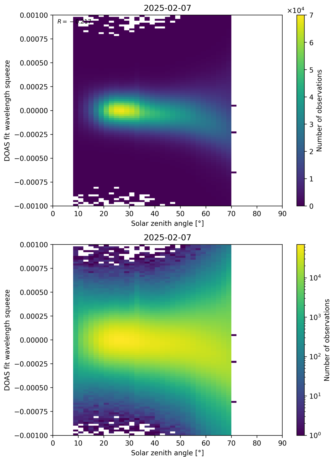
Figure 175: Scatter density plot of “Solar zenith angle” against “DOAS fit wavelength squeeze” for 2025-02-06 to 2025-02-08.
