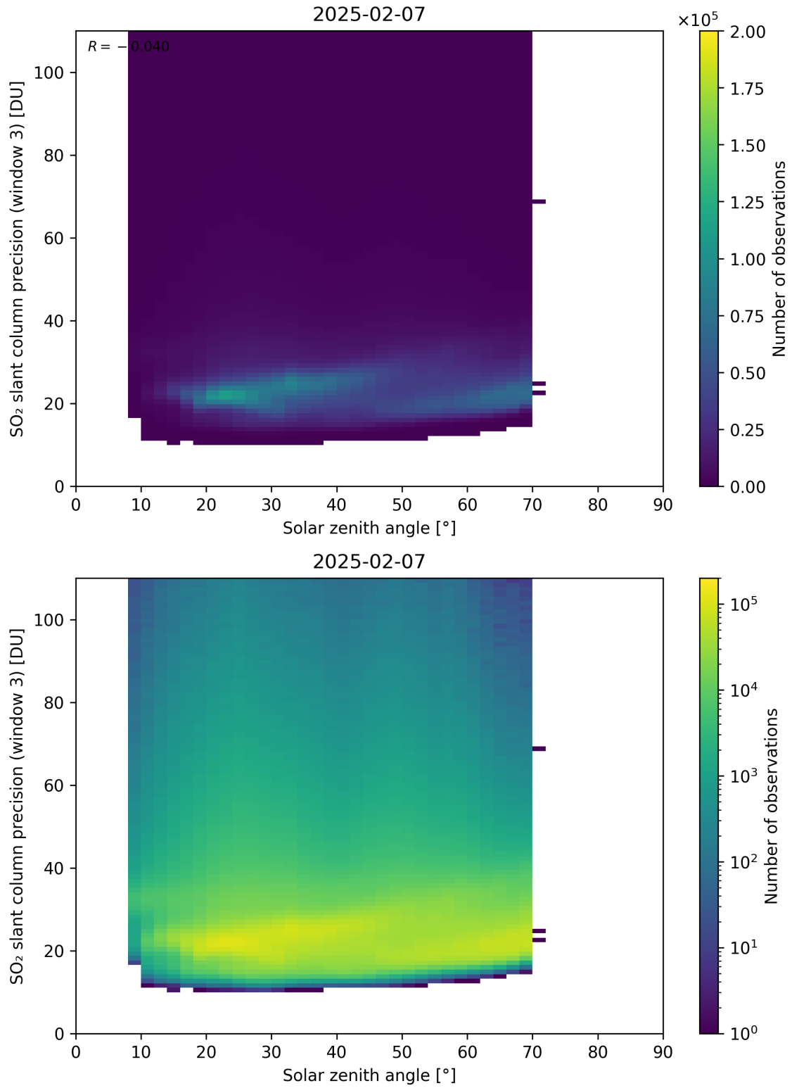
Figure 188: Scatter density plot of “Solar zenith angle” against “SO 2 slant column precision (window 3)” for 2025-02-06 to 2025-02-08.
