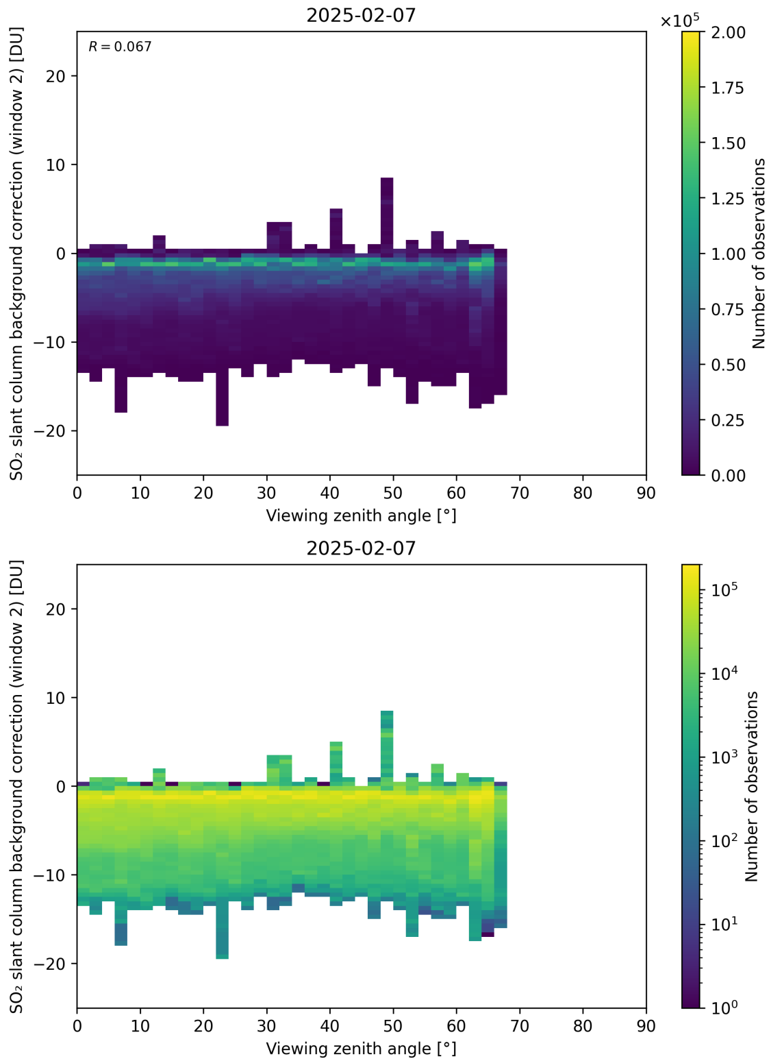
Figure 363: Scatter density plot of “Viewing zenith angle” against “SO 2 slant column background correction (window 2)” for 2025-02-06 to 2025-02-08.
