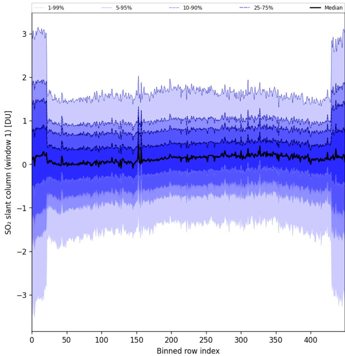
Figure 89: Along track statistics of “SO 2 slant column (window 1)” for 2025-02-06 to 2025-02-08
