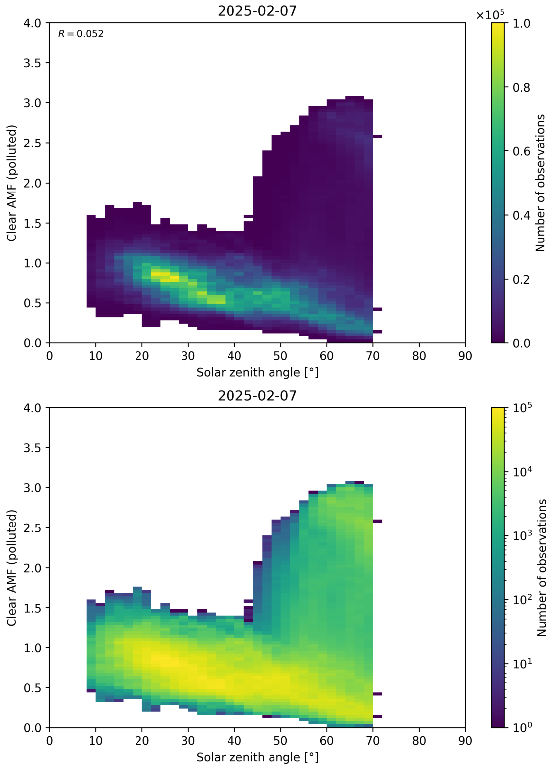
Figure 178: Scatter density plot of “Solar zenith angle” against “Clear AMF (polluted)” for 2025-02-06 to 2025-02-08.
