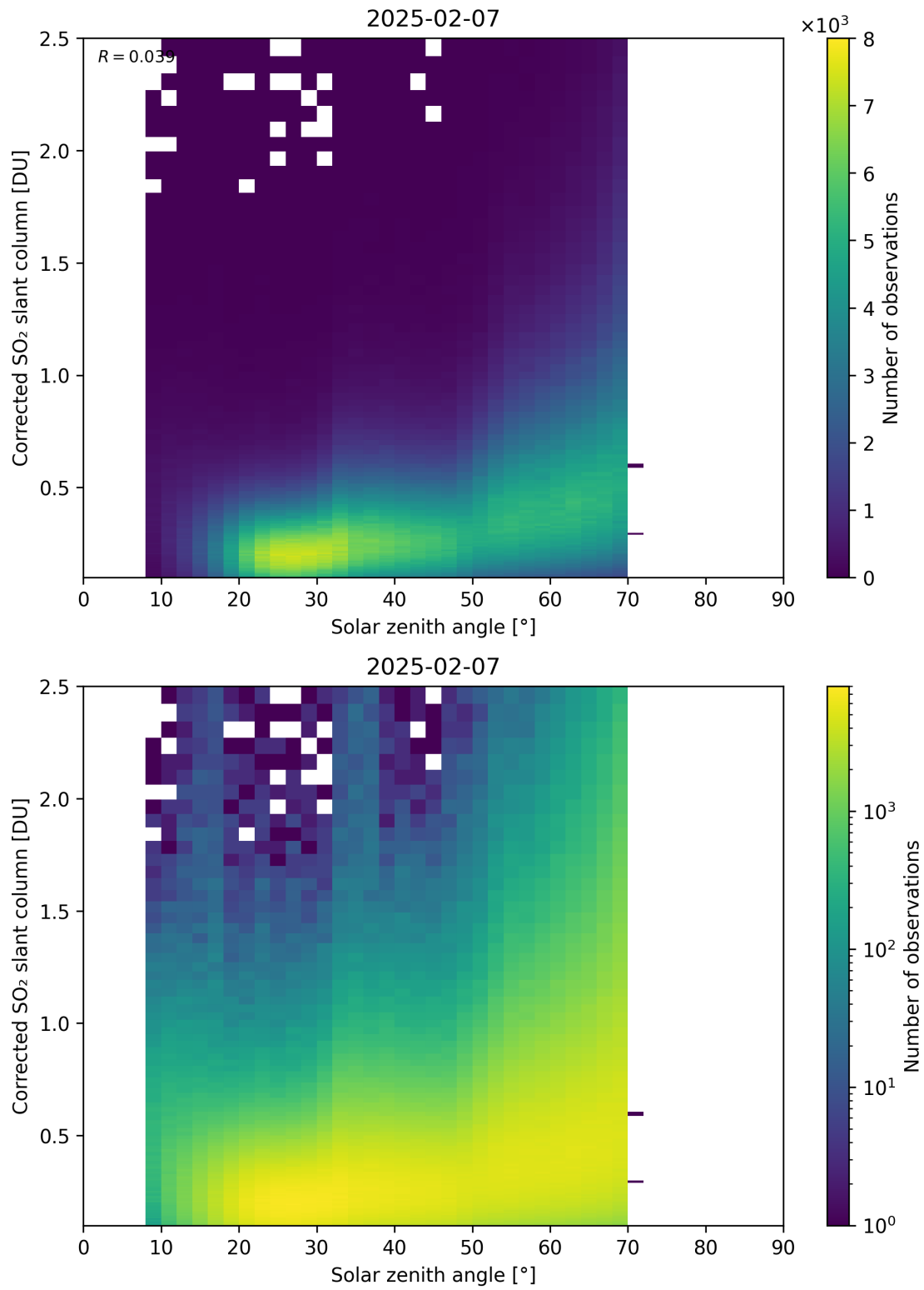
Figure 181: Scatter density plot of “Solar zenith angle” against “Corrected SO 2 slant column” for 2025-02-06 to 2025-02-08.
