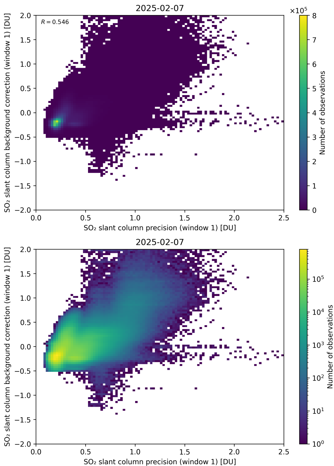
Figure 268: Scatter density plot of “SO 2 slant column precision (window 1)” against “SO 2 slant column background correction (window 1)” for 2025-02-06 to 2025-02-08.
