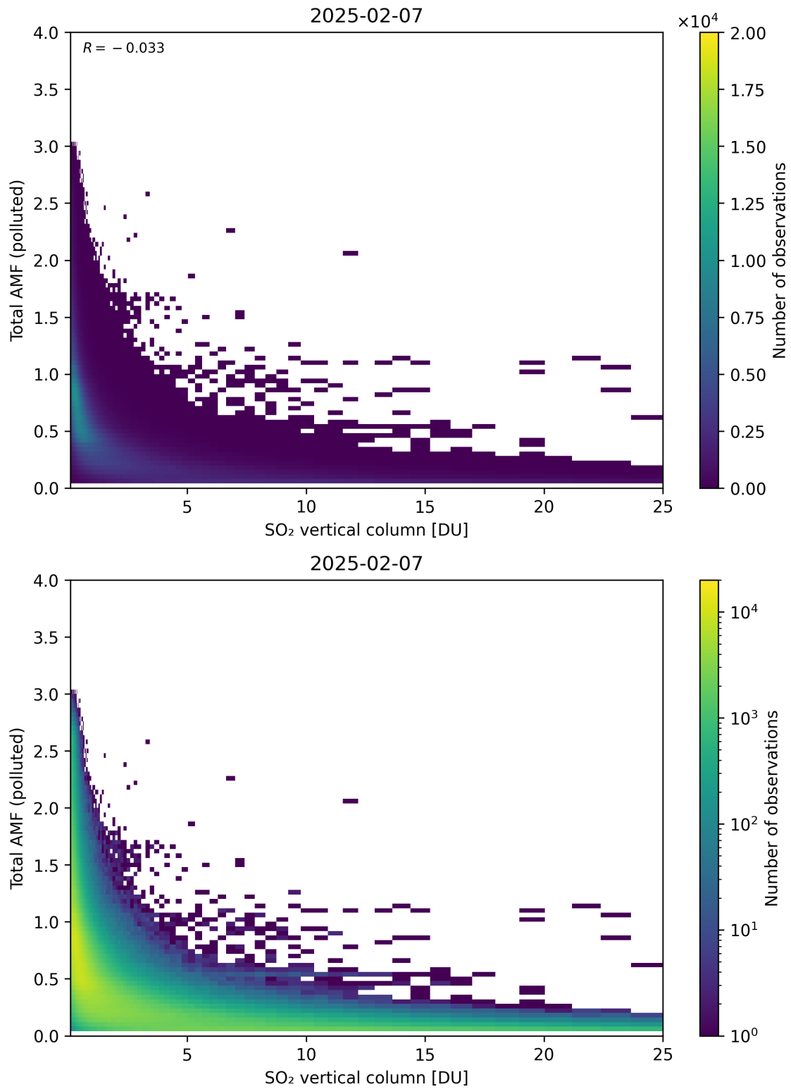
Figure 359: Scatter density plot of “SO 2 vertical column” against “Total AMF (polluted)” for 2025-02-06 to 2025-02-08.
