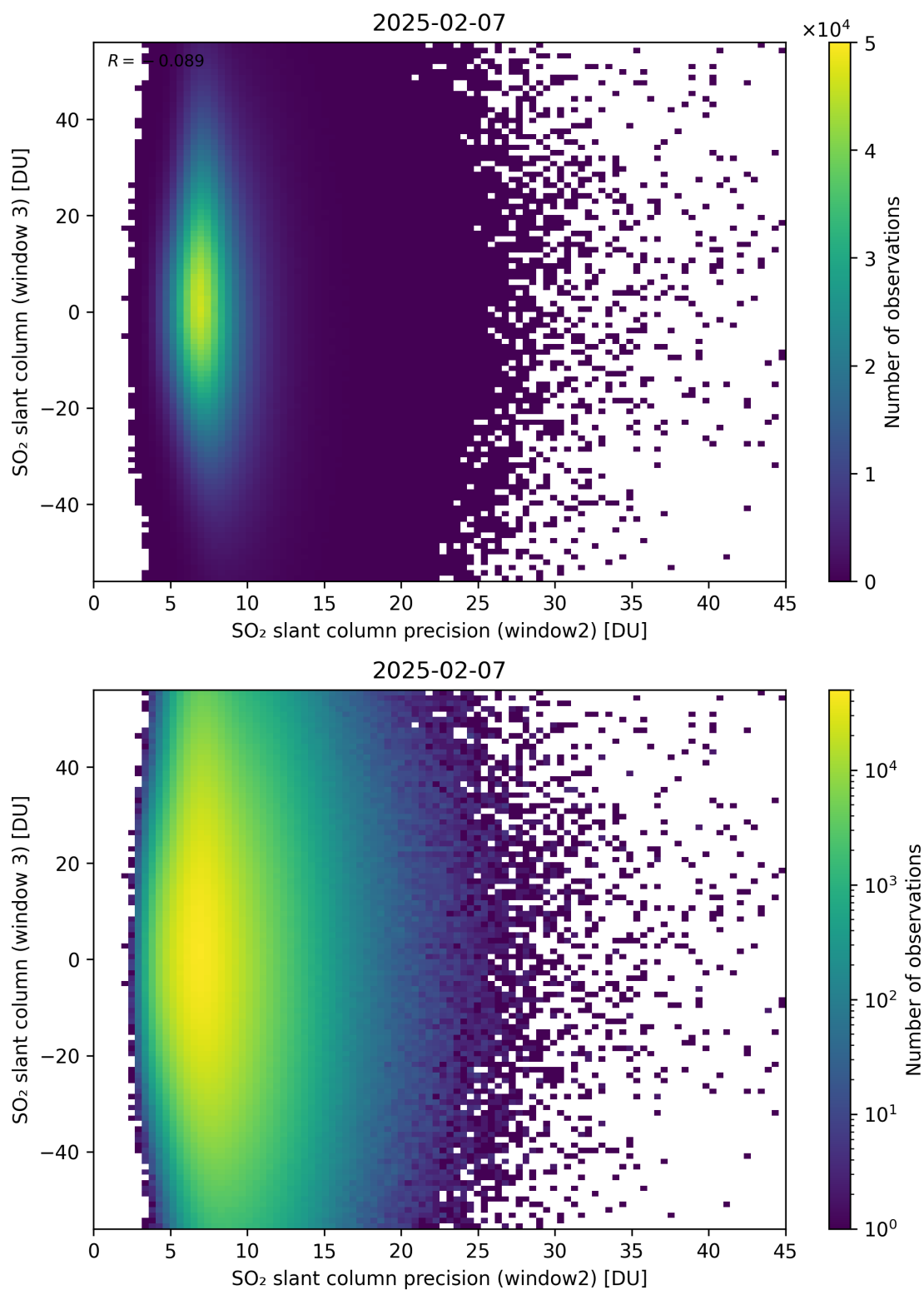
Figure 299: Scatter density plot of “SO 2 slant column precision (window2)” against “SO 2 slant column (window 3)” for 2025-02-06 to 2025-02-08.
