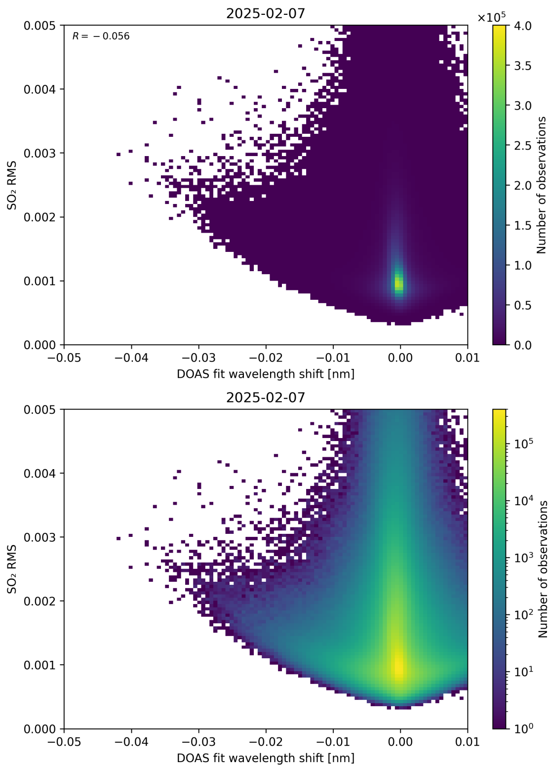
Figure 139: Scatter density plot of “DOAS fit wavelength shift” against “SO 2 RMS” for 2025-02-06 to 2025-02-08.
