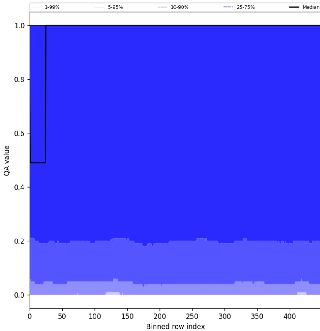
Figure 83: Along track statistics of “QA value” for 2025-02-06 to 2025-02-08
