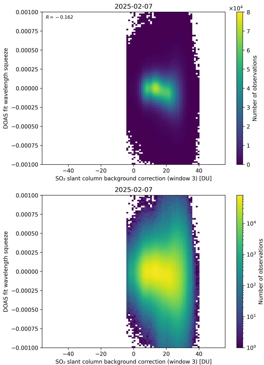
Figure 133: Scatter density plot of “SO 2 slant column background correction (window 3)” against “DOAS fit wavelength squeeze” for 2025-02-06 to 2025-02-08.
