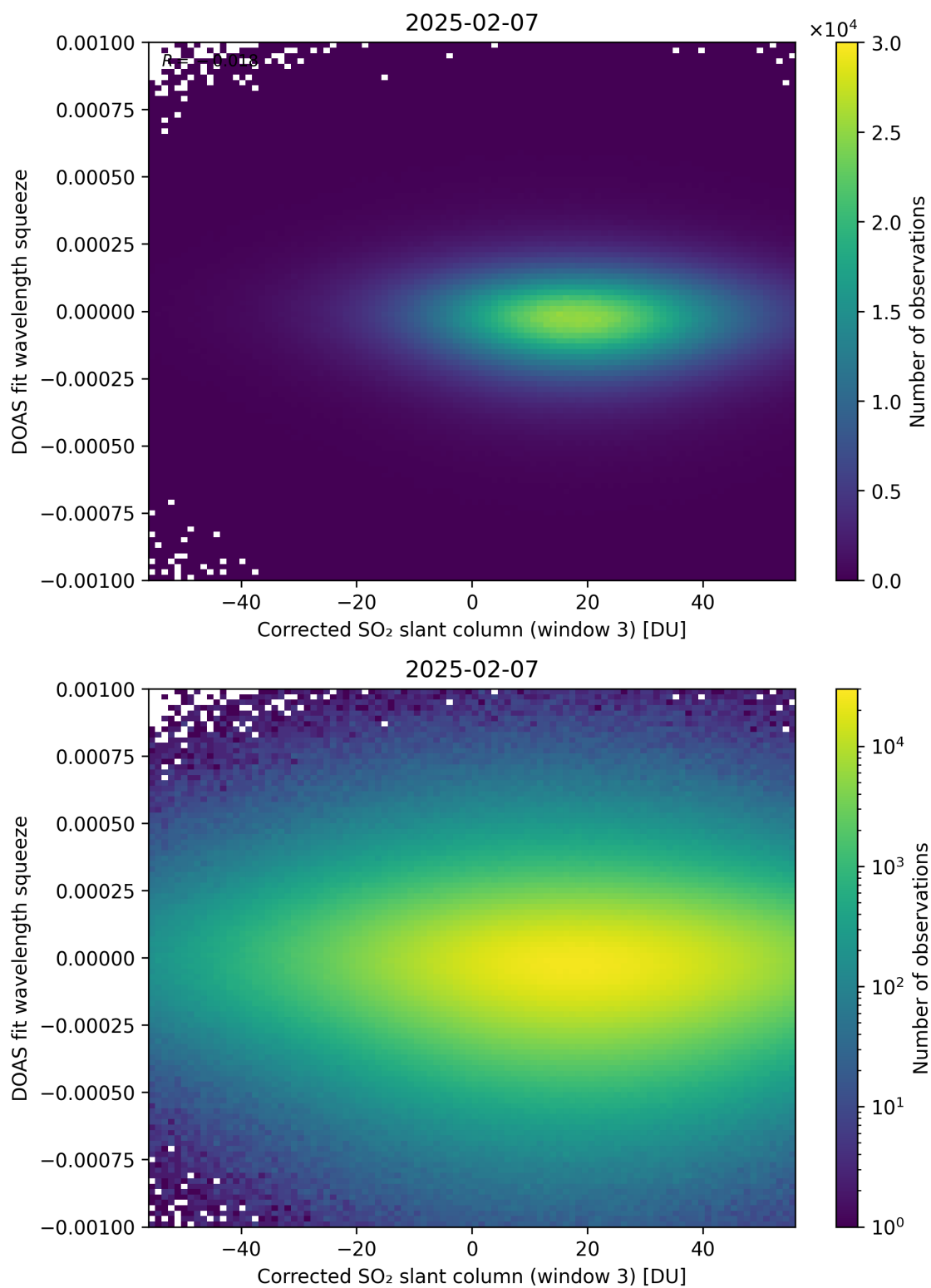
Figure 257: Scatter density plot of “Corrected SO 2 slant column (window 3)” against “DOAS fit wavelength squeeze” for 2025-02-06 to 2025-02-08.
