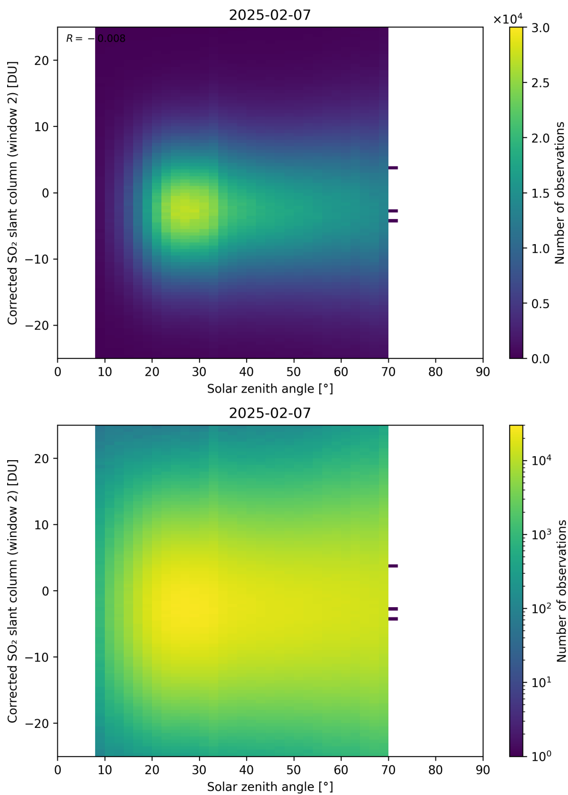
Figure 182: Scatter density plot of “Solar zenith angle” against “Corrected SO 2 slant column (window 2)” for 2025-02-06 to 2025-02-08.
