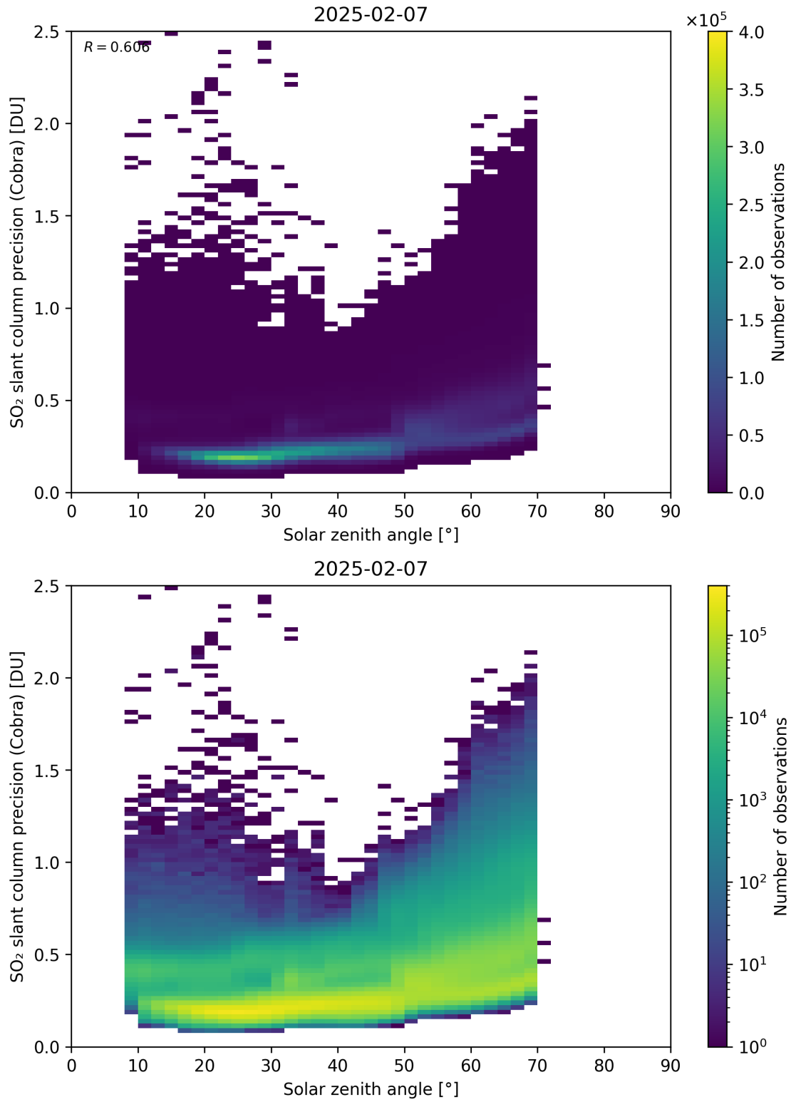
Figure 180: Scatter density plot of “Solar zenith angle” against “SO 2 slant column precision (Cobra)” for 2025-02-06 to 2025-02-08.
