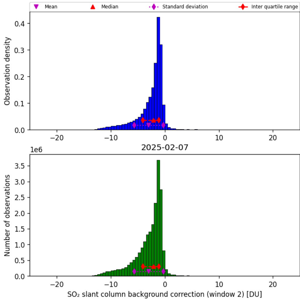
Figure 70: Histogram of “SO 2 slant column background correction (window 2)” for 2025-02-06 to 2025-02-08
