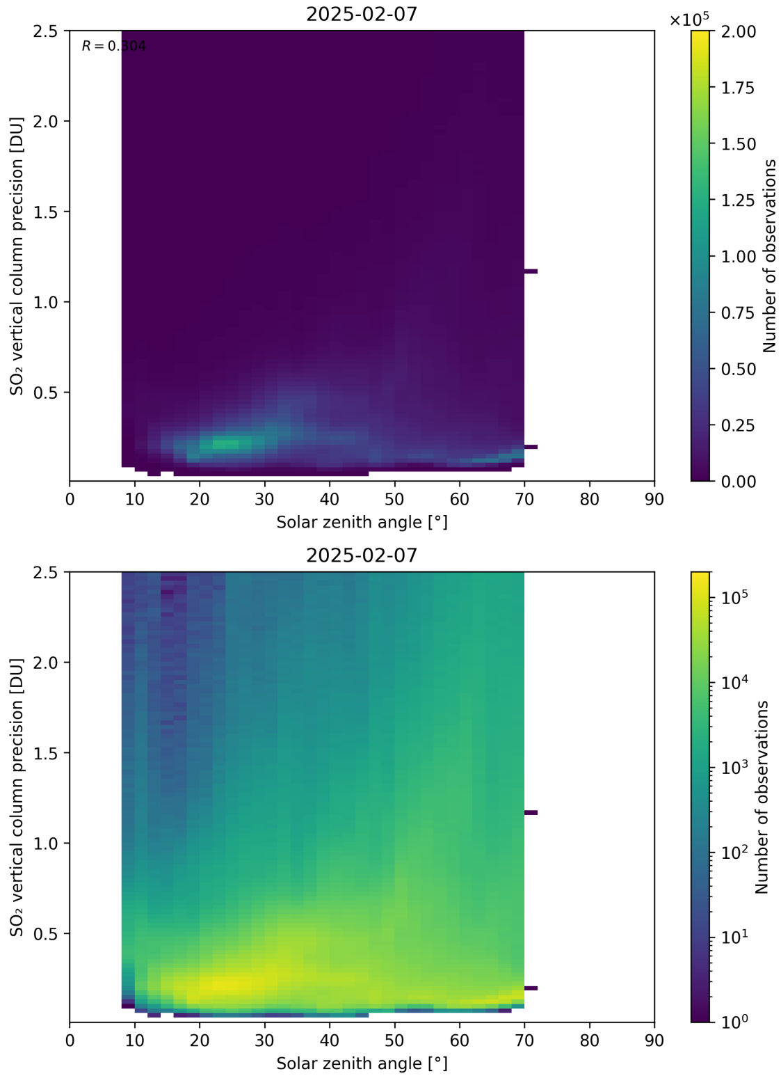
Figure 192: Scatter density plot of “Solar zenith angle” against “SO 2 vertical column precision” for 2025-02-06 to 2025-02-08.
