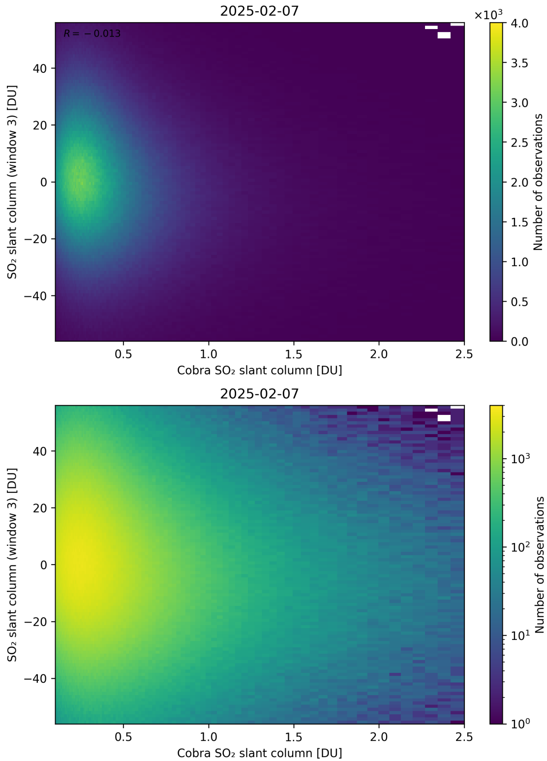
Figure 222: Scatter density plot of “Cobra SO 2 slant column” against “SO 2 slant column (window 3)” for 2025-02-06 to 2025-02-08.
