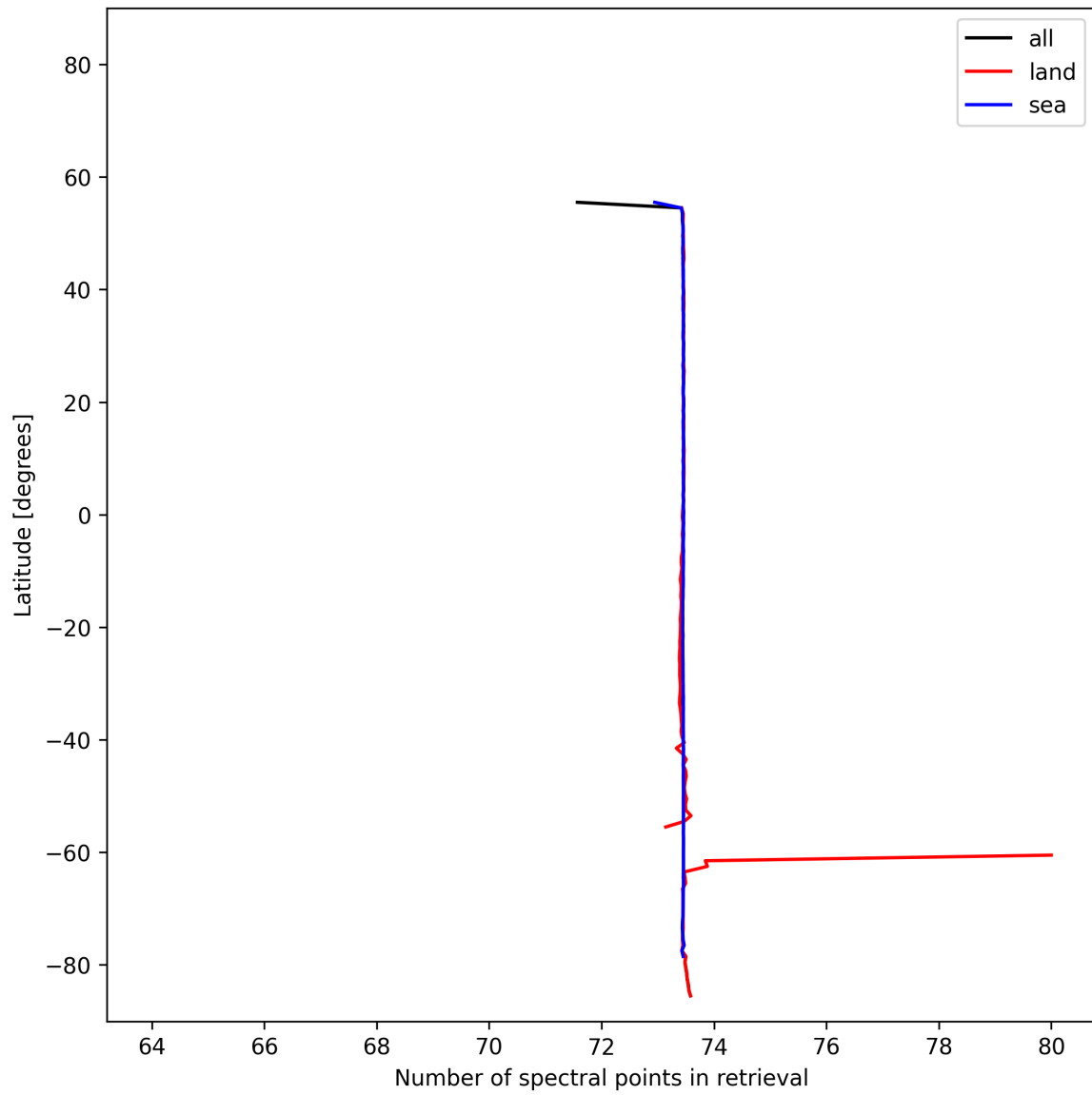
Figure 56: Zonal average of “Number of spectral points in retrieval” for 2025-02-06 to 2025-02-08.
