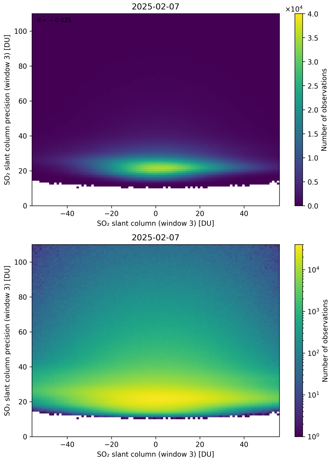
Figure 317: Scatter density plot of “SO 2 slant column (window 3)” against “SO 2 slant column precision (window 3)” for 2025-02-06 to 2025-02-08.
