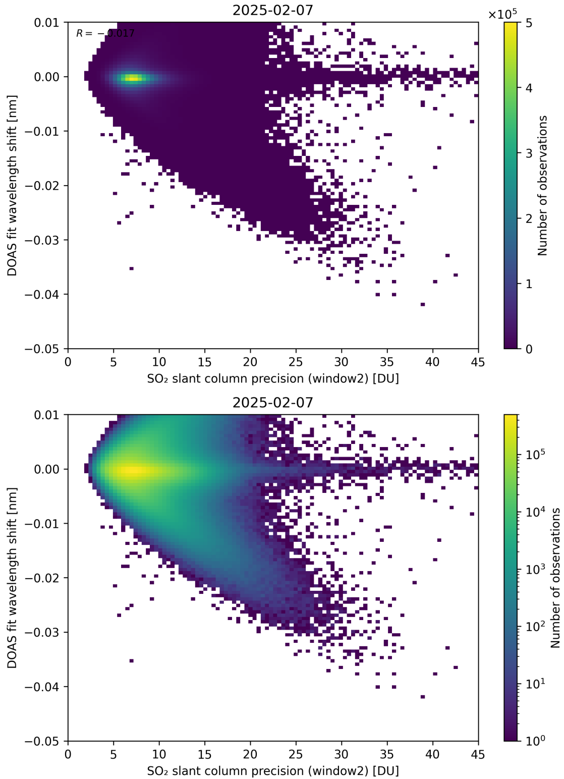
Figure 293: Scatter density plot of “SO 2 slant column precision (window2)” against “DOAS fit wavelength shift” for 2025-02-06 to 2025-02-08.
