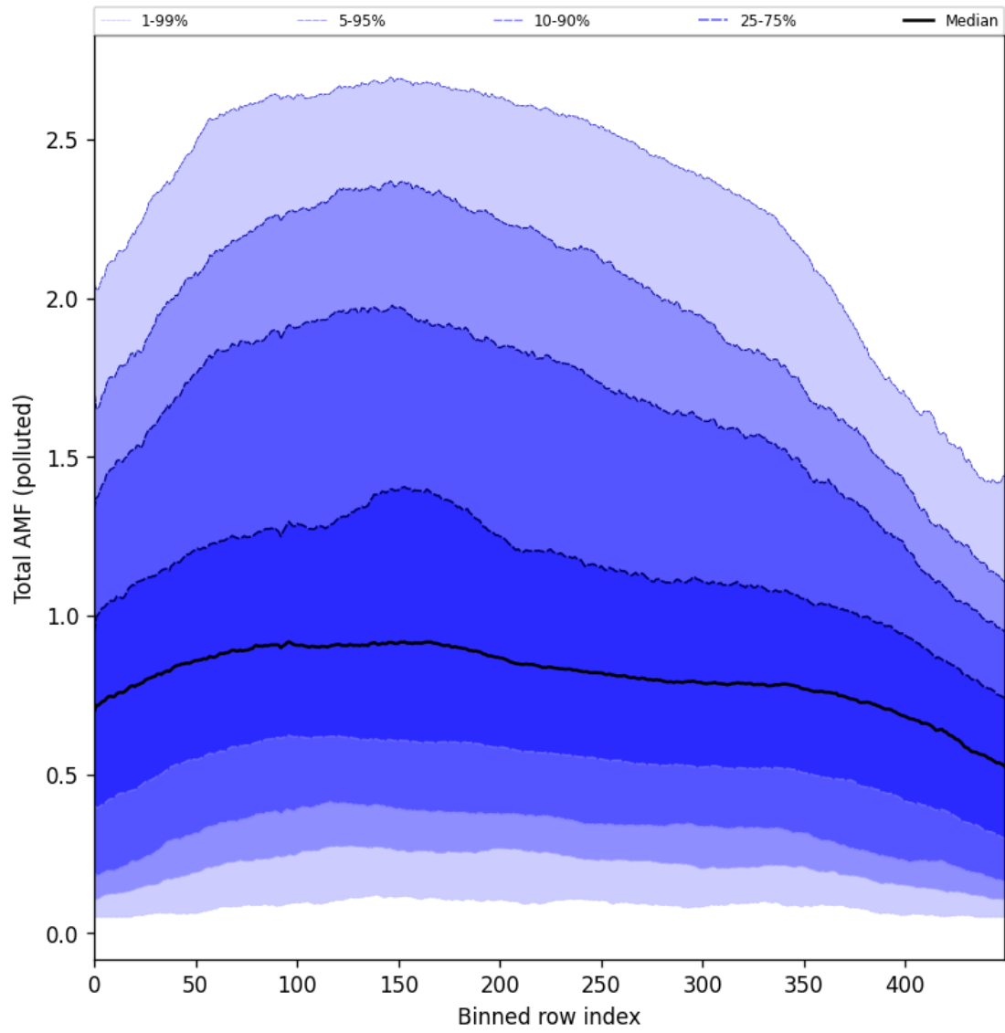
Figure 105: Along track statistics of “Total AMF (polluted)” for 2025-02-06 to 2025-02-08
