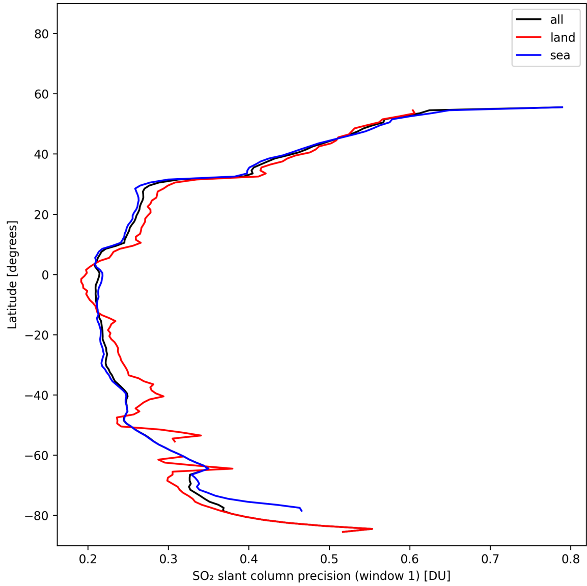
Figure 38: Zonal average of “SO 2 slant column precision (window 1)” for 2025-02-06 to 2025-02-08.
