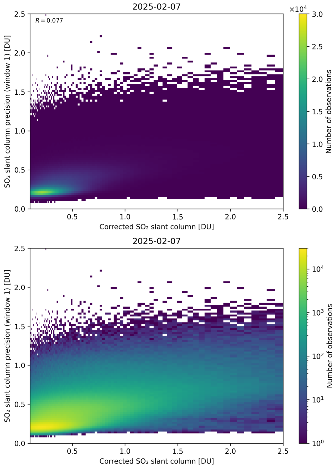
Figure 238: Scatter density plot of “Corrected SO 2 slant column” against “SO 2 slant column precision (window 1)” for 2025-02-06 to 2025-02-08.
