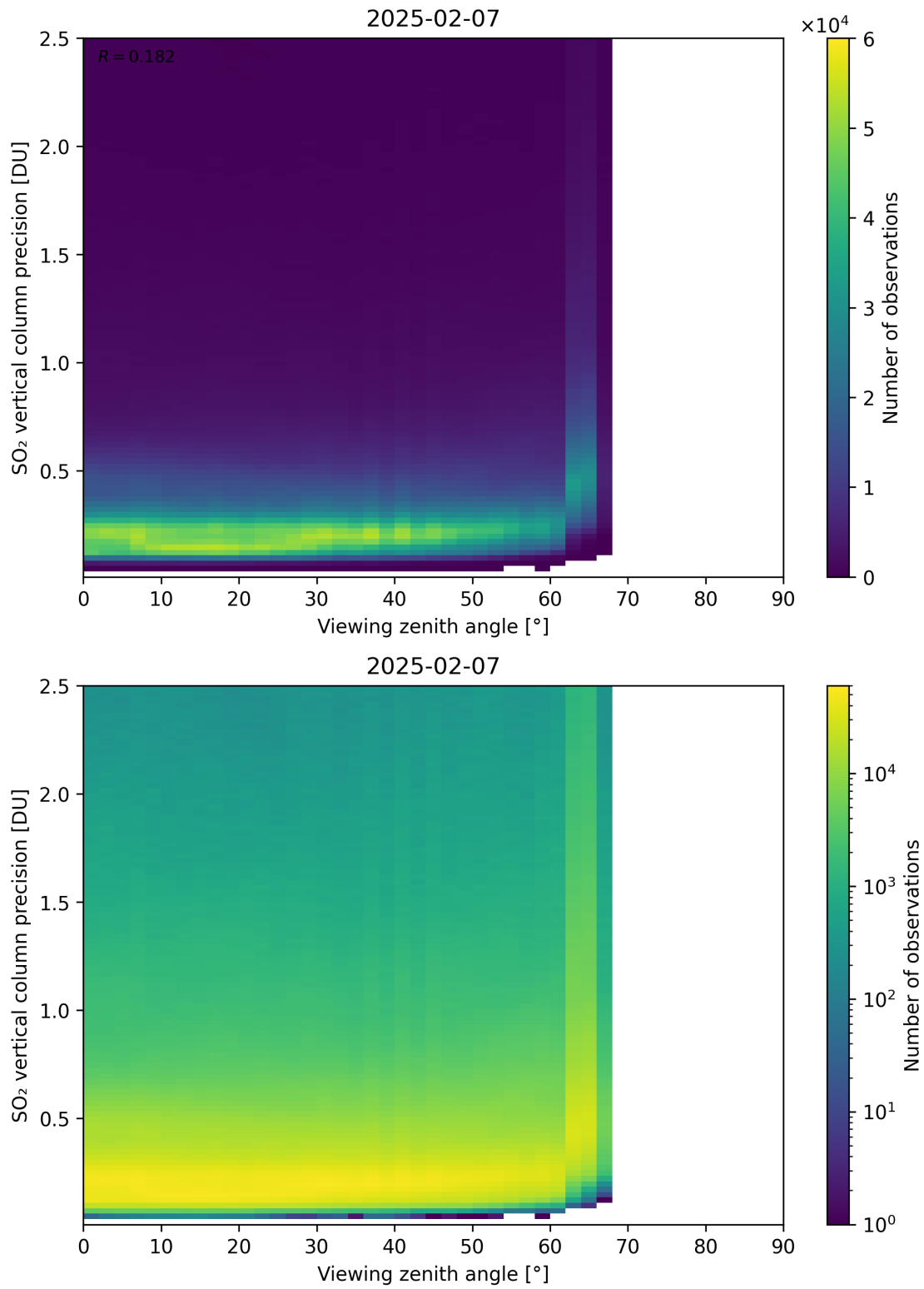
Figure 384: Scatter density plot of “Viewing zenith angle” against “SO 2 vertical column precision” for 2025-02-06 to 2025-02-08.
