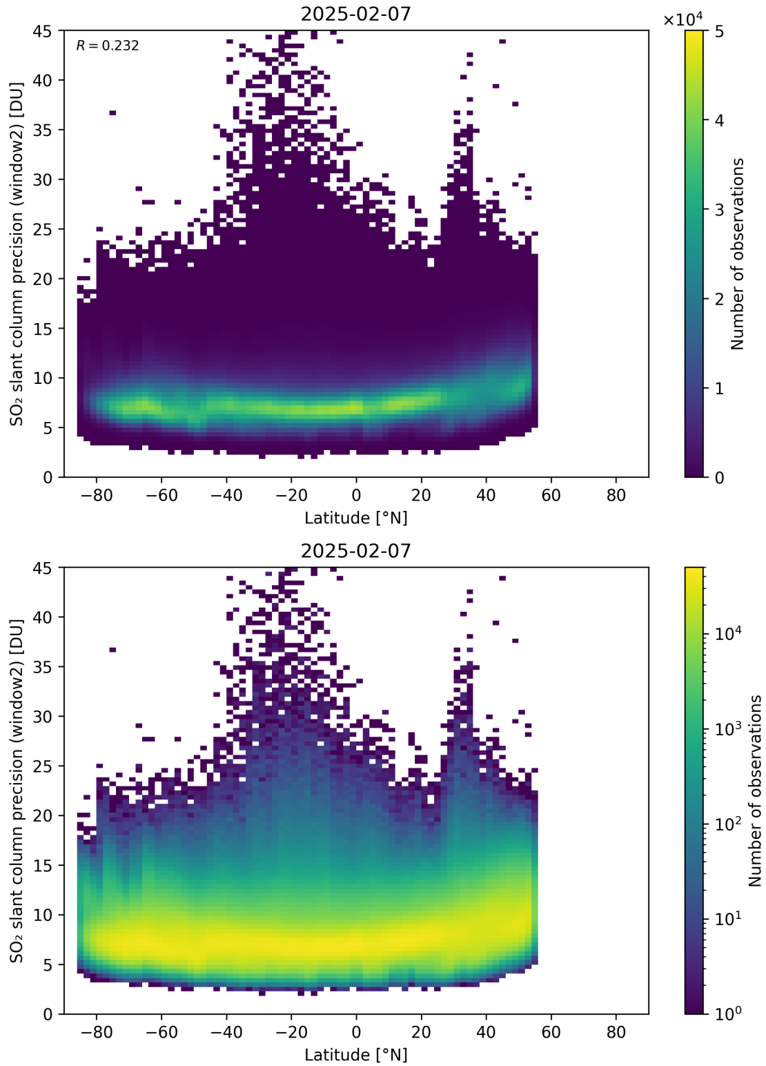
Figure 164: Scatter density plot of “Latitude” against “SO 2 slant column precision (window2)” for 2025-02-06 to 2025-02-08.
