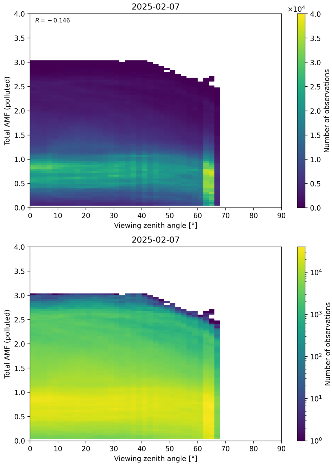
Figure 381: Scatter density plot of “Viewing zenith angle” against “Total AMF (polluted)” for 2025-02-06 to 2025-02-08.
