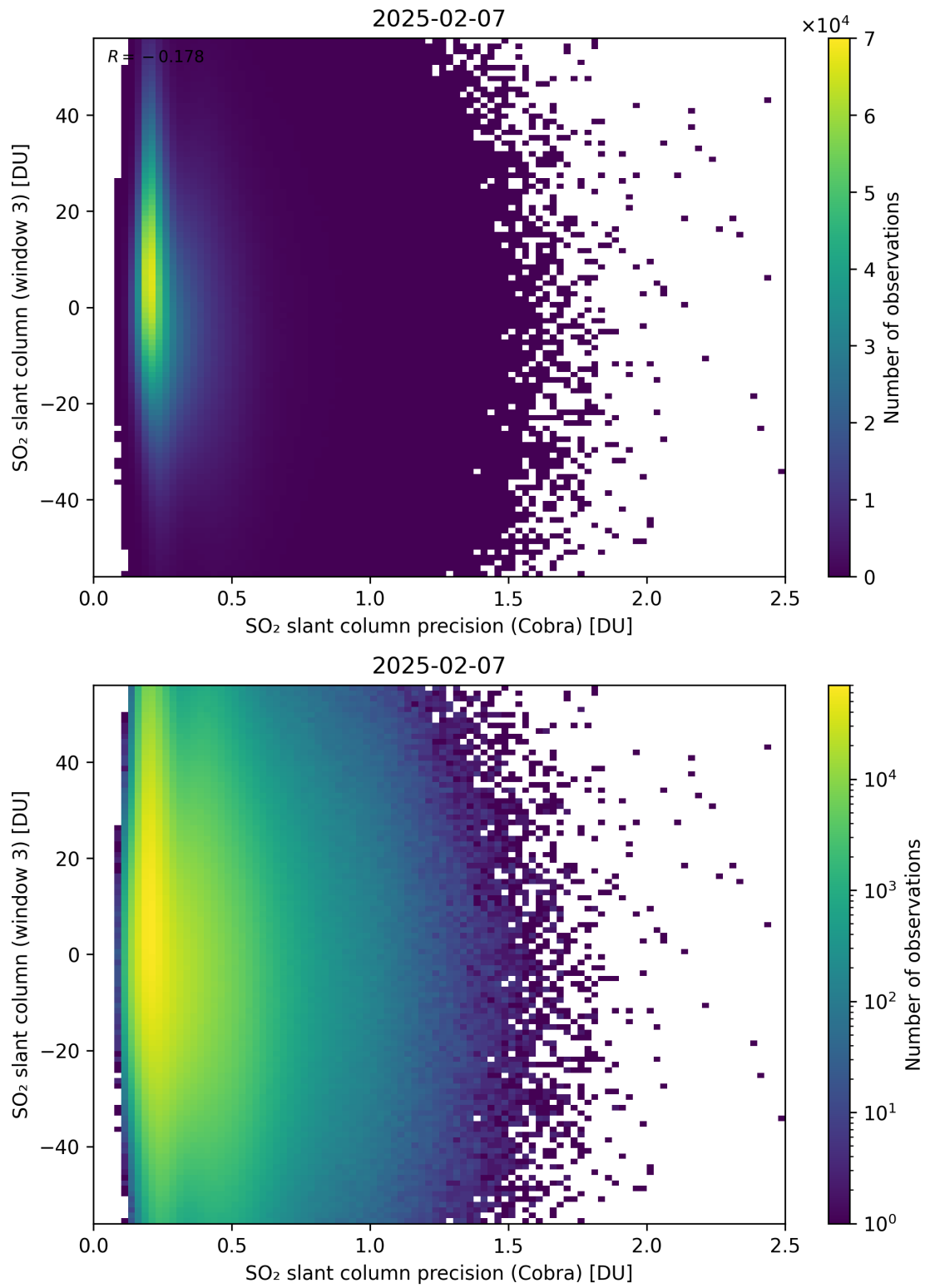
Figure 211: Scatter density plot of “SO 2 slant column precision (Cobra)” against “SO 2 slant column (window 3)” for 2025-02-06 to 2025-02-08.
