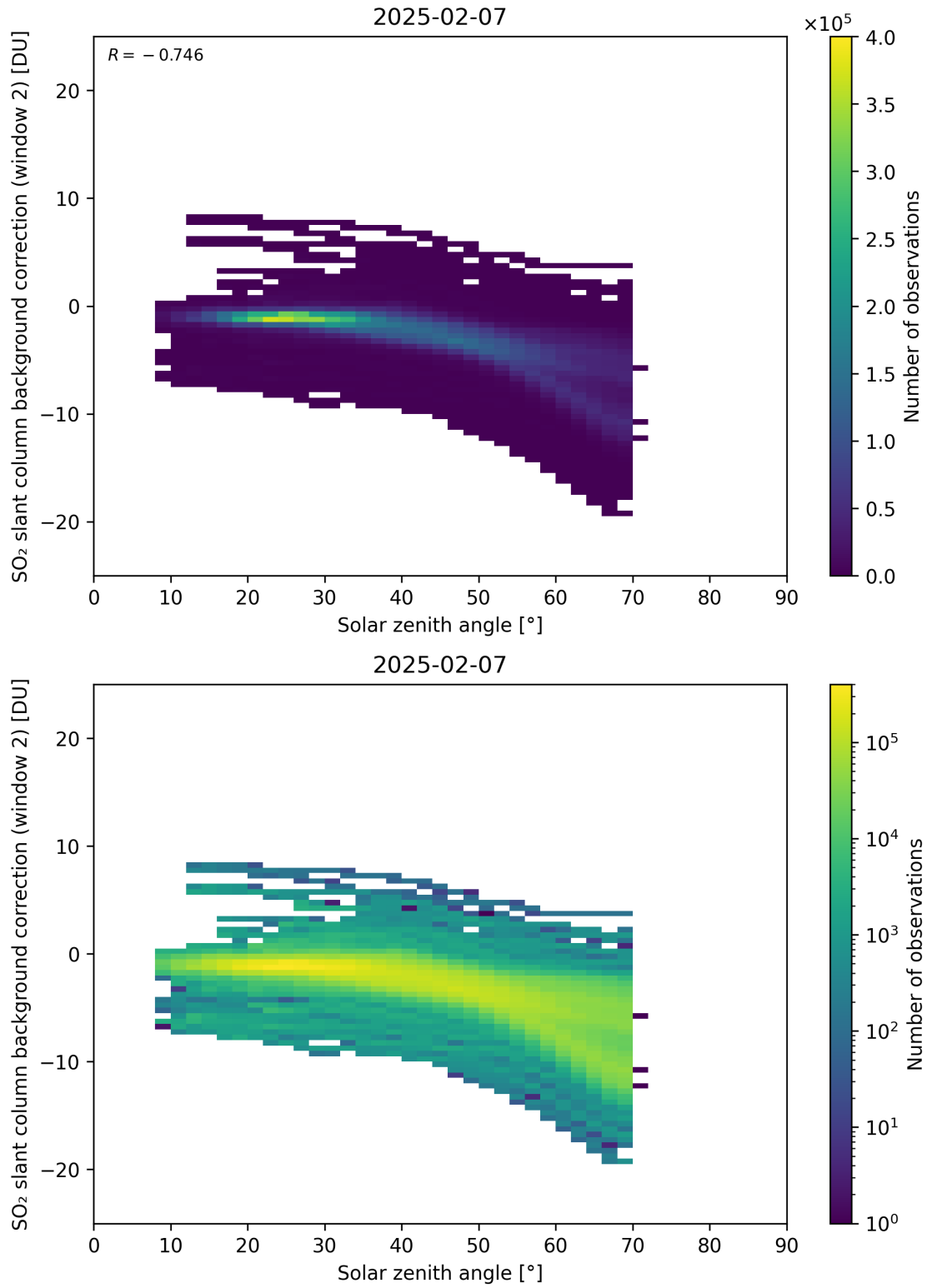
Figure 172: Scatter density plot of “Solar zenith angle” against “SO 2 slant column background correction (window 2)” for 2025-02-06 to 2025-02-08.
