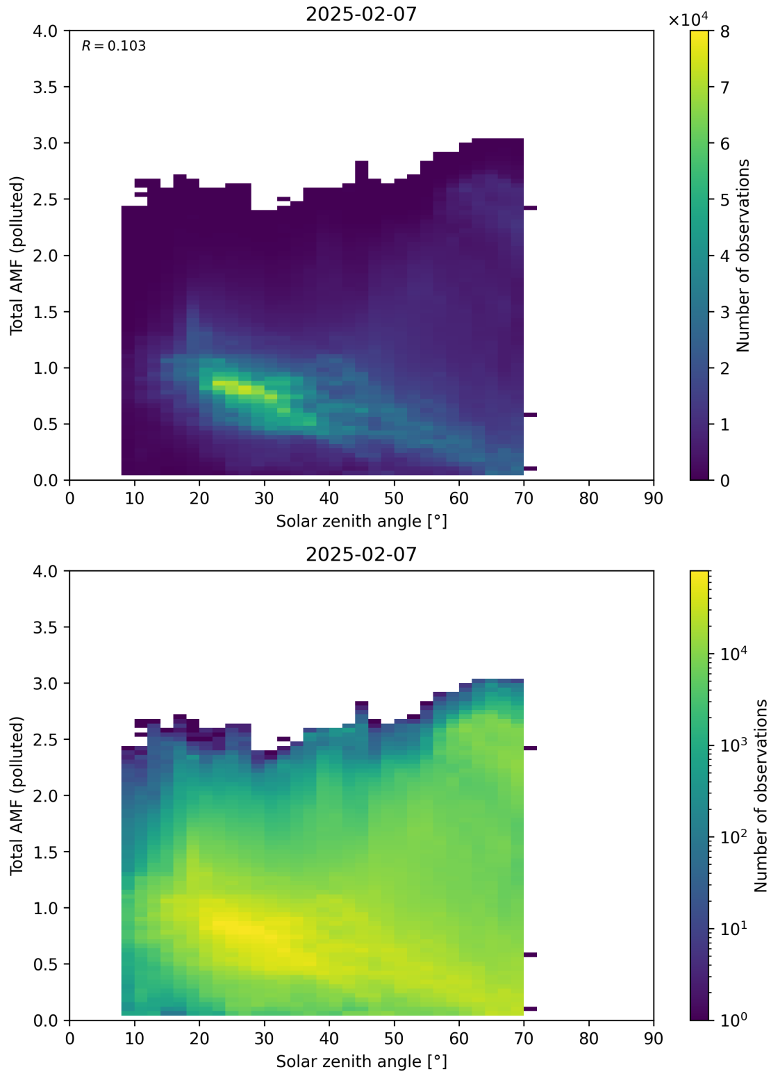
Figure 189: Scatter density plot of “Solar zenith angle” against “Total AMF (polluted)” for 2025-02-06 to 2025-02-08.
