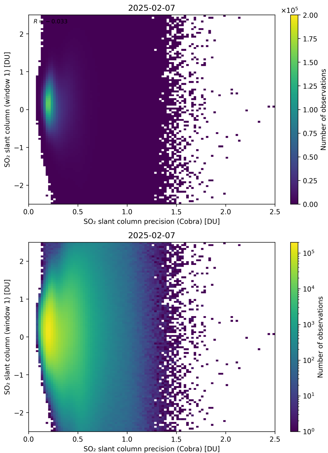
Figure 208: Scatter density plot of “SO 2 slant column precision (Cobra)” against “SO 2 slant column (window 1)” for 2025-02-06 to 2025-02-08.
