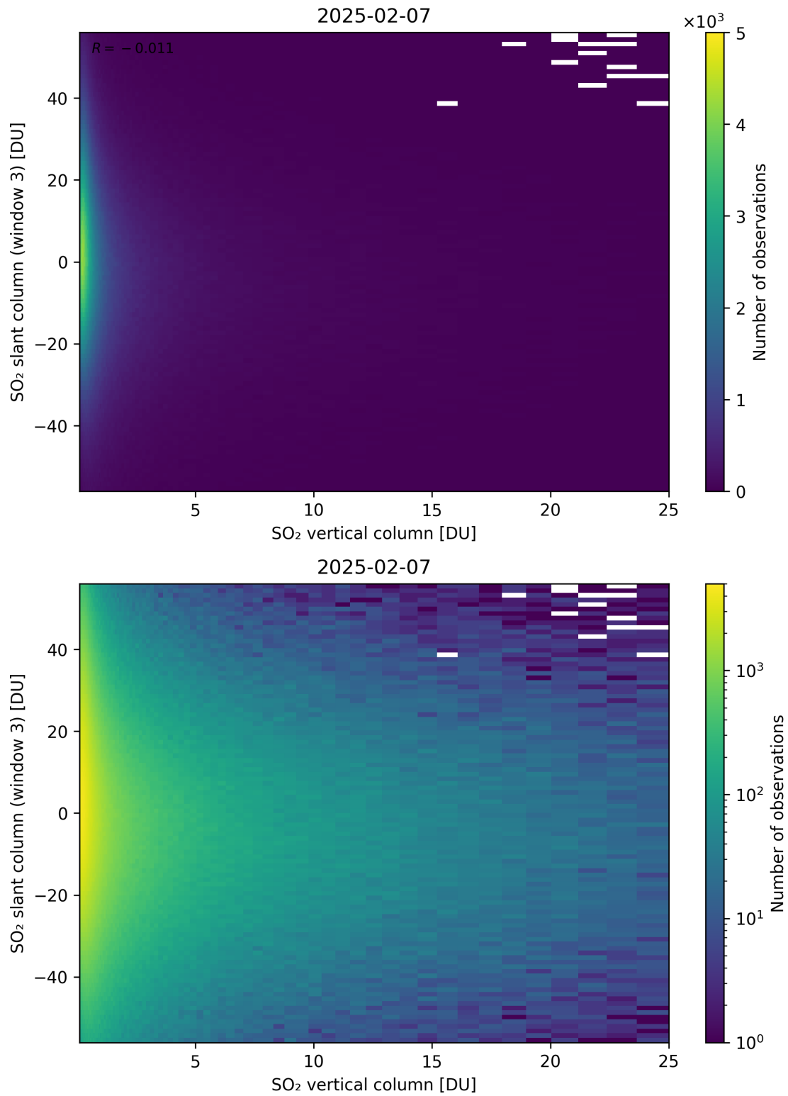
Figure 357: Scatter density plot of “SO 2 vertical column” against “SO 2 slant column (window 3)” for 2025-02-06 to 2025-02-08.
