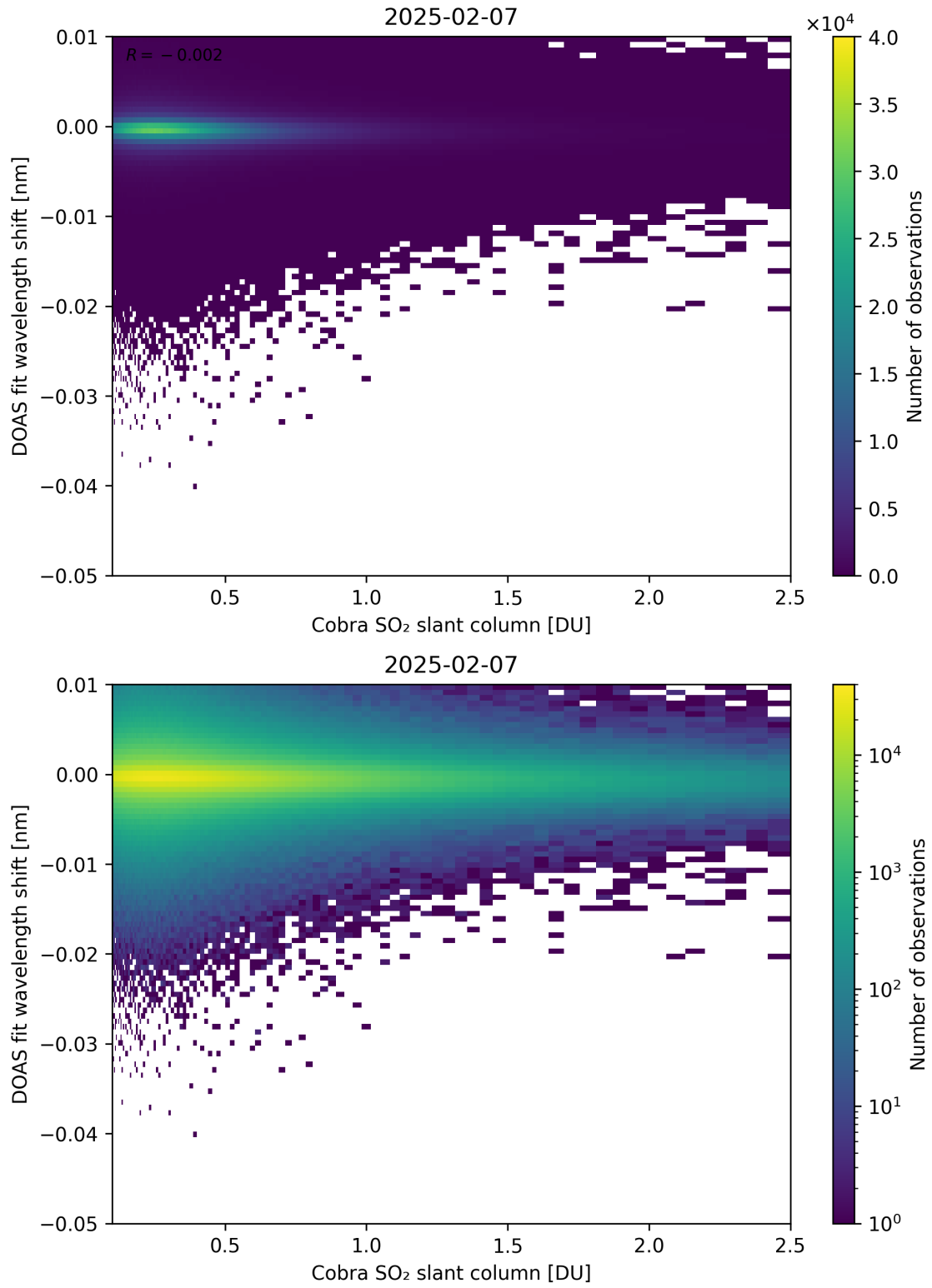
Figure 196: Scatter density plot of “Cobra SO 2 slant column” against “DOAS fit wavelength shift” for 2025-02-06 to 2025-02-08.
