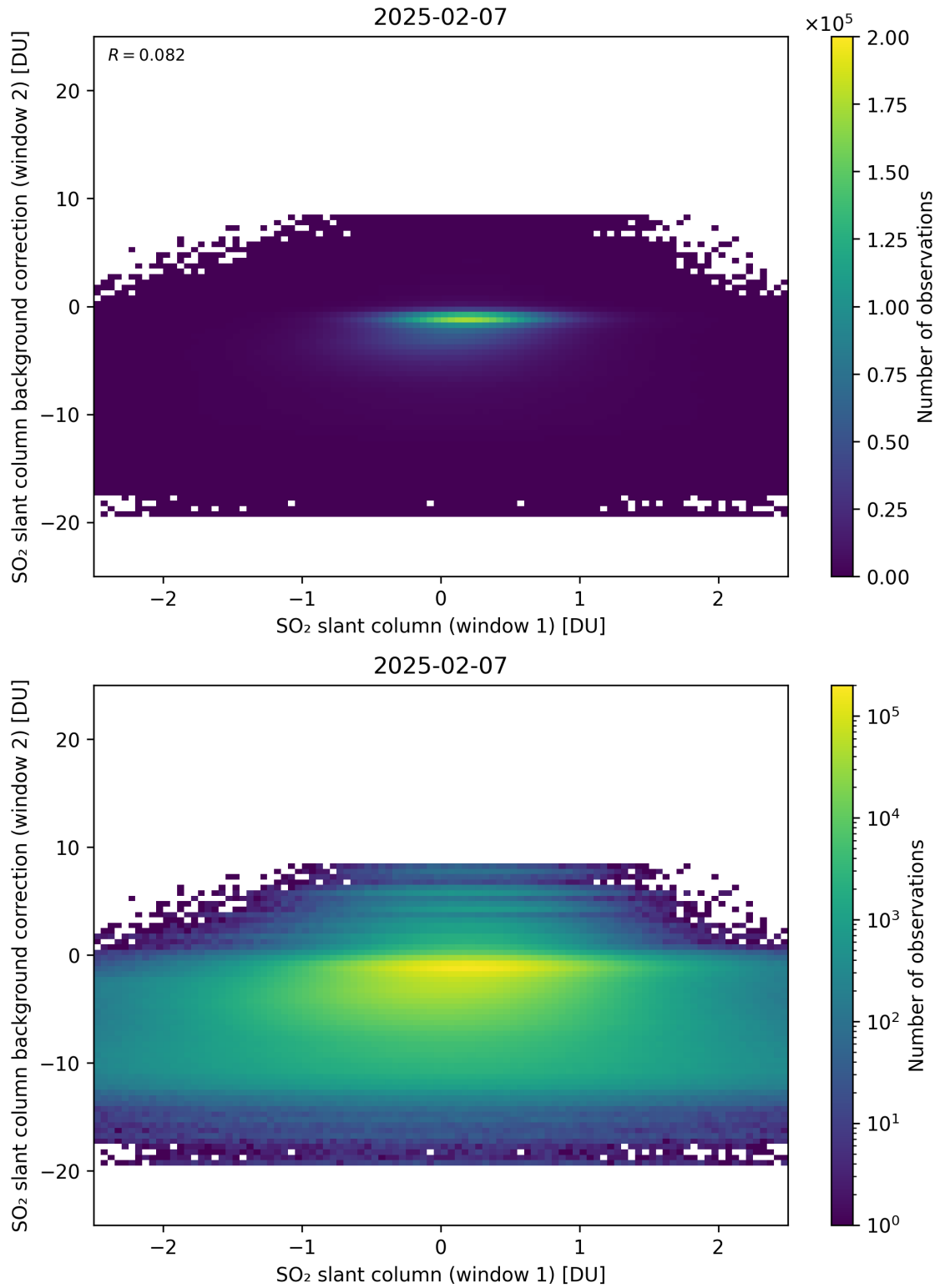
Figure 263: Scatter density plot of “SO 2 slant column (window 1)” against “SO 2 slant column background correction (window 2)” for 2025-02-06 to 2025-02-08.
