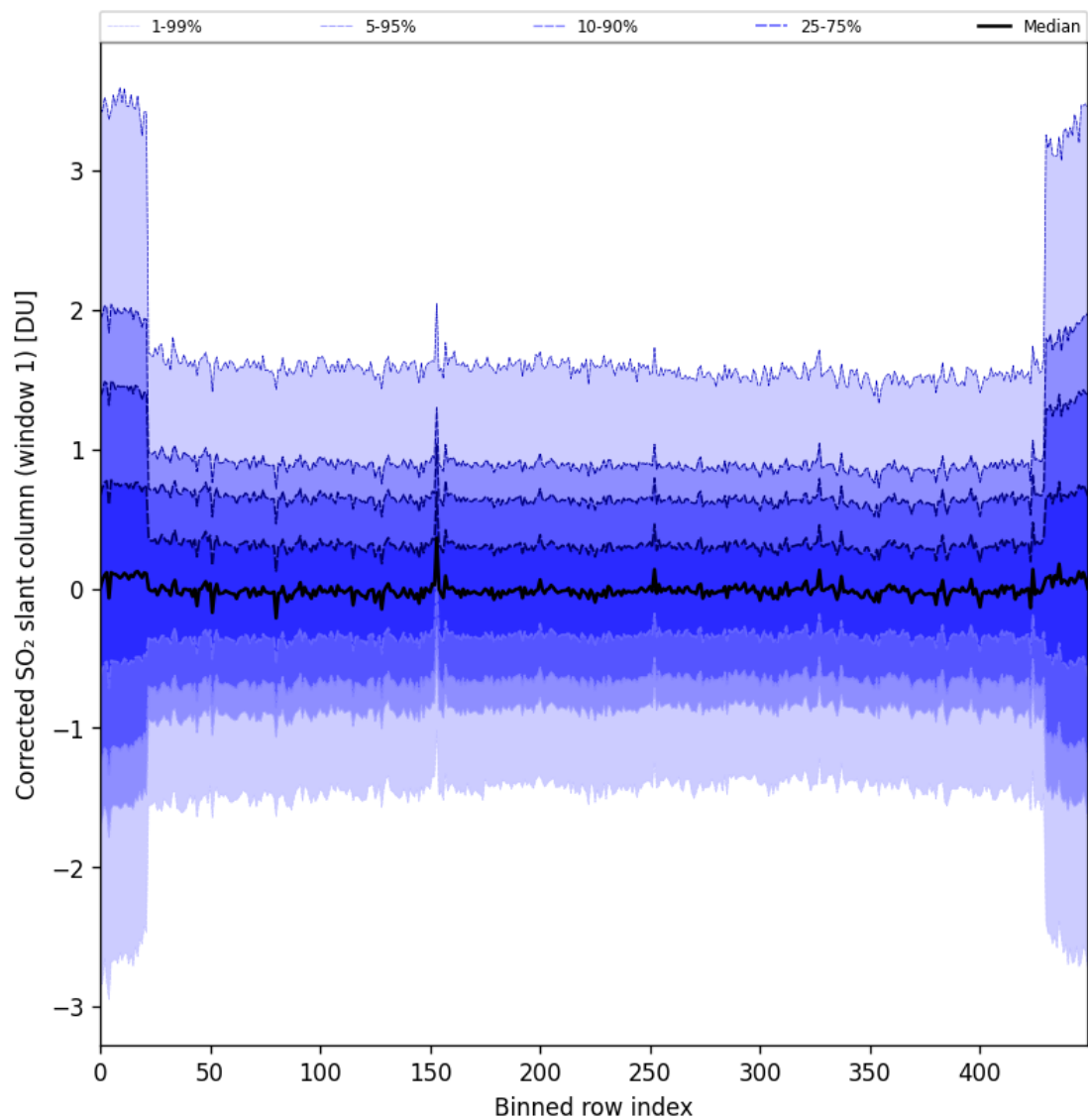
Figure 91: Along track statistics of “Corrected SO 2 slant column (window 1)” for 2025-02-06 to 2025-02-08
