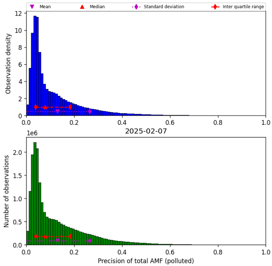
Figure 80: Histogram of “Precision of total AMF (polluted)” for 2025-02-06 to 2025-02-08
