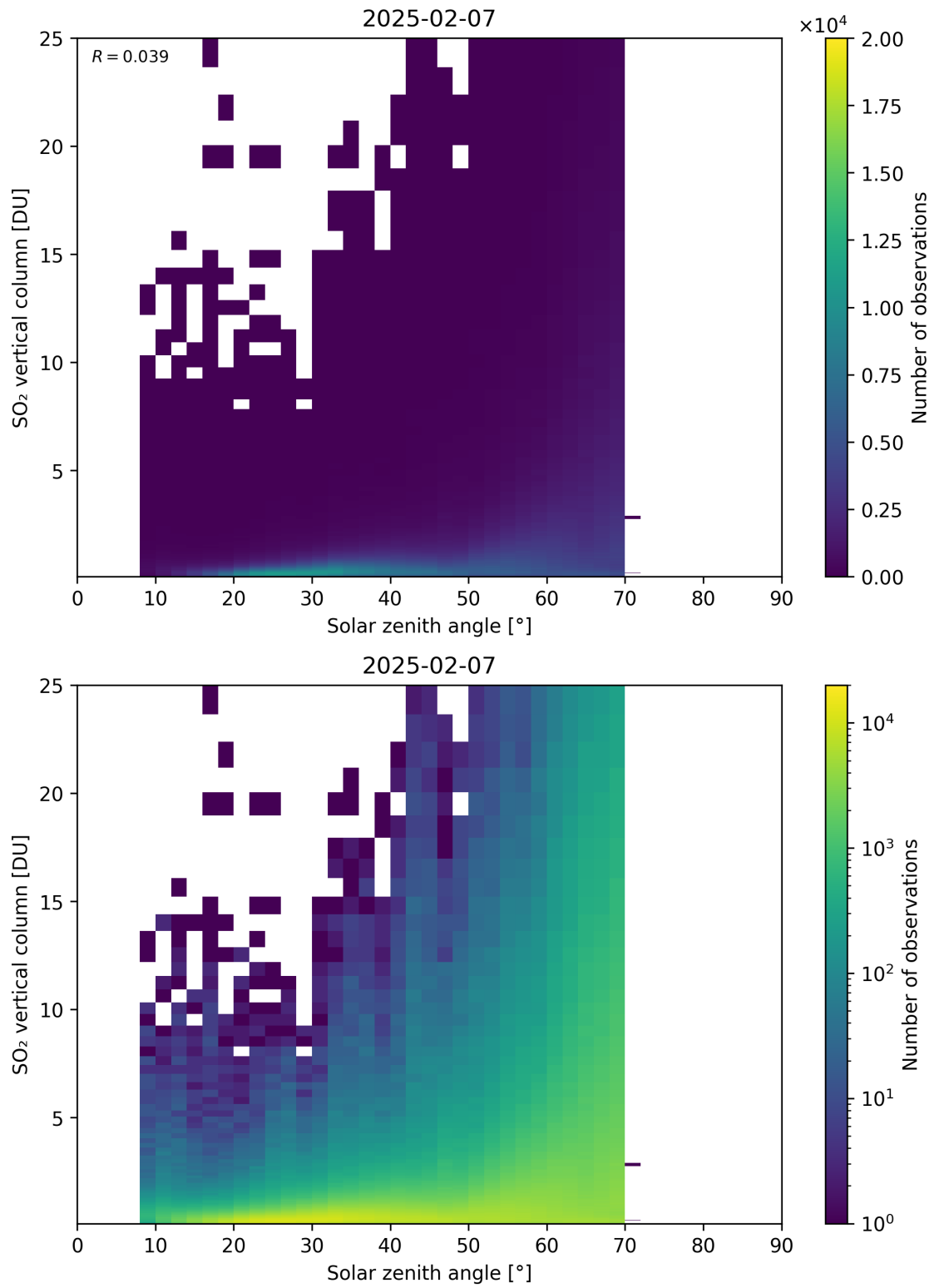
Figure 191: Scatter density plot of “Solar zenith angle” against “SO 2 vertical column” for 2025-02-06 to 2025-02-08.
