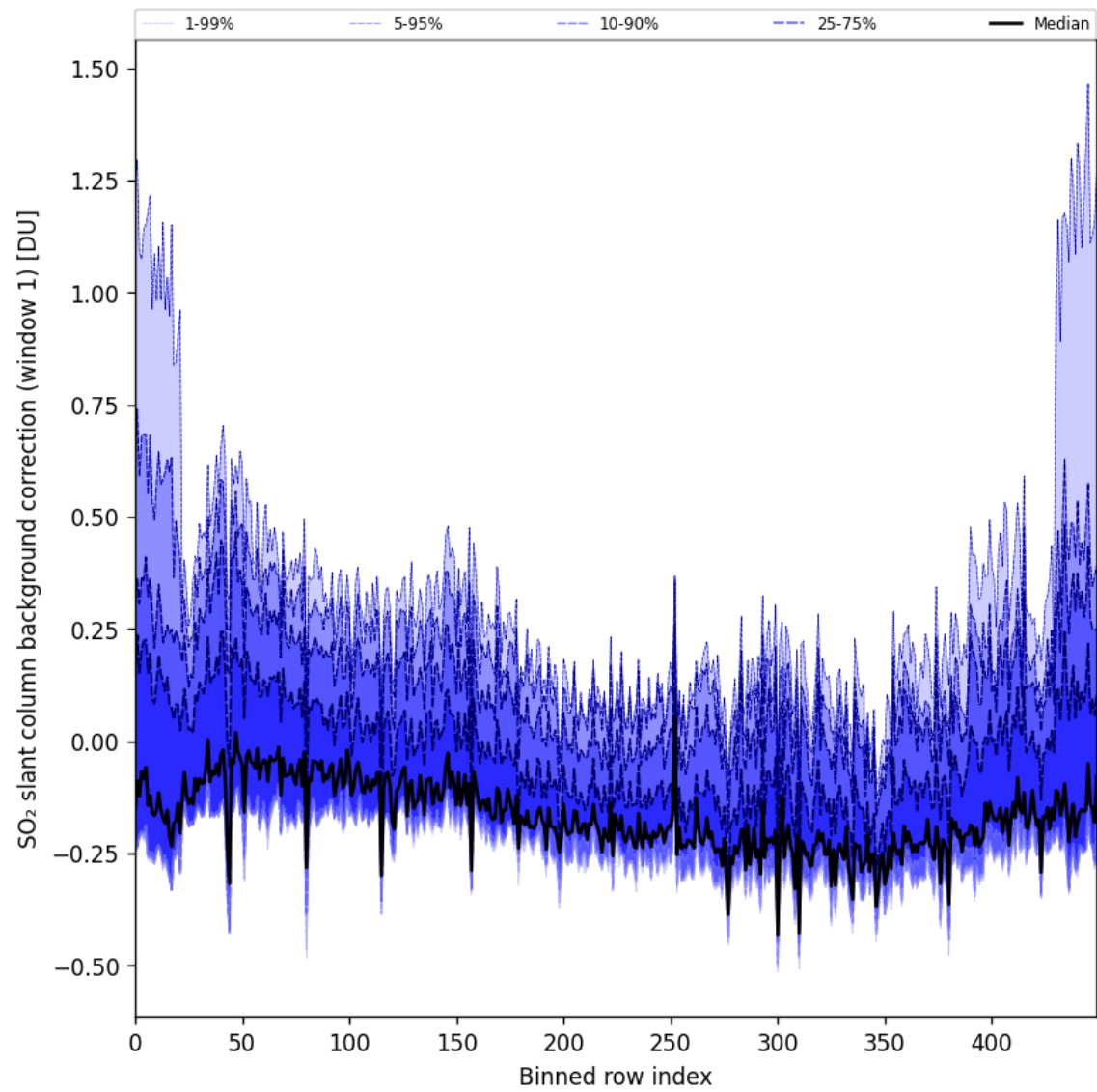
Figure 92: Along track statistics of “SO 2 slant column background correction (window 1)” for 2025-02-06 to 2025-02-08
