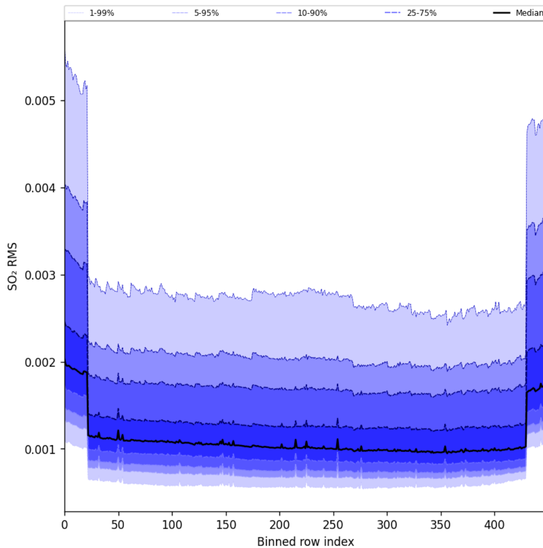
Figure 104: Along track statistics of “SO 2 RMS” for 2025-02-06 to 2025-02-08
