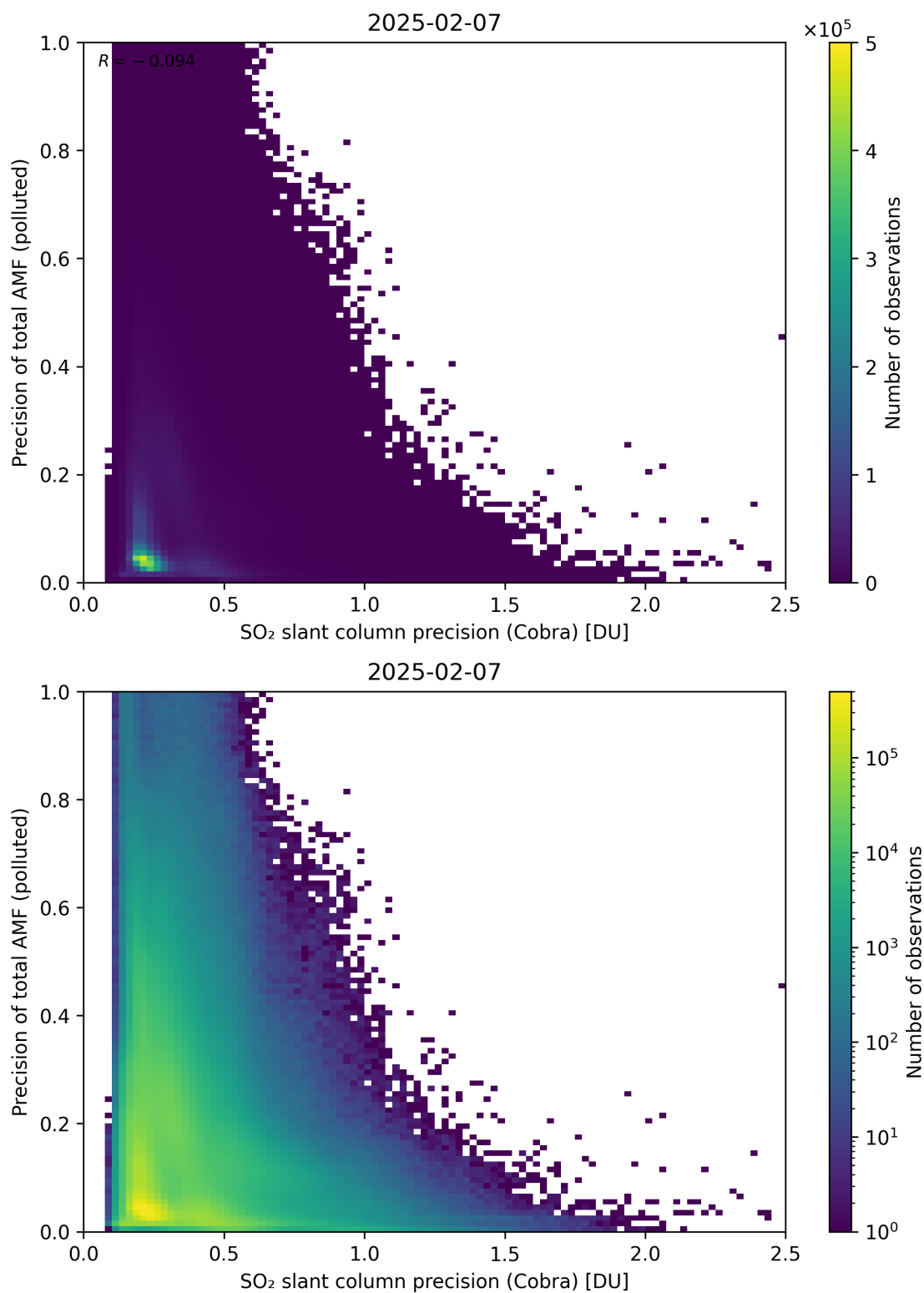
Figure 214: Scatter density plot of “SO 2 slant column precision (Cobra)” against “Precision of total AMF (polluted)” for 2025-02-06 to 2025-02-08.
