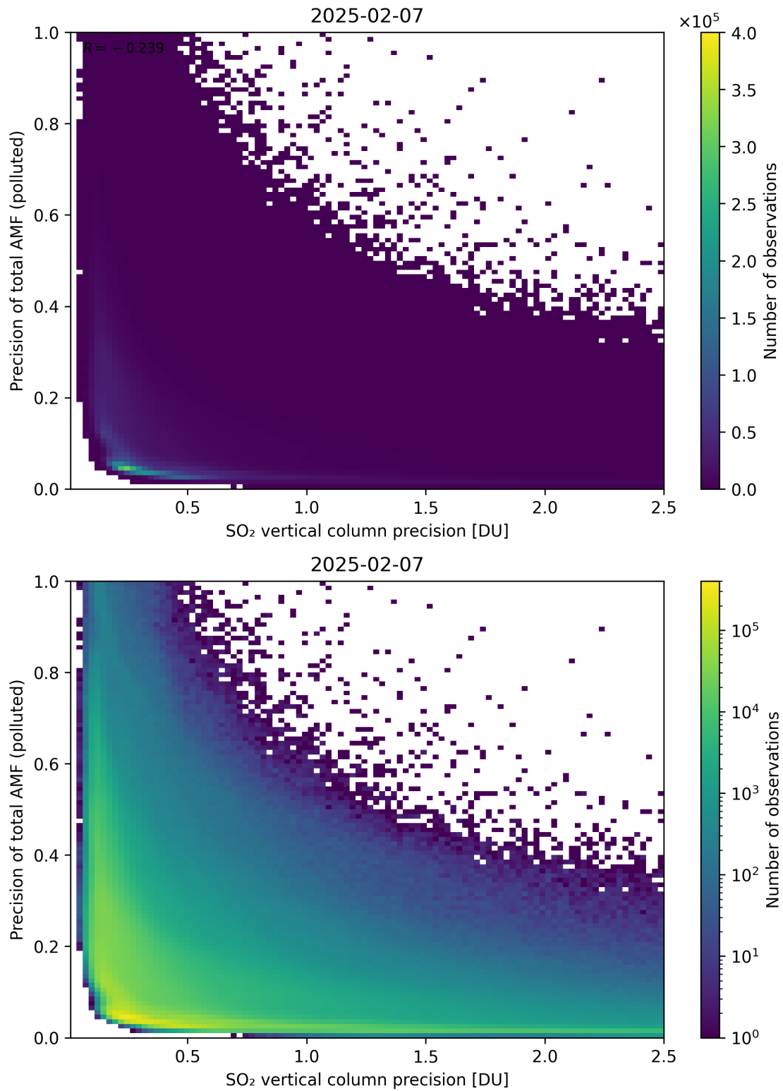
Figure 347: Scatter density plot of “SO 2 vertical column precision” against “Precision of total AMF (polluted)” for 2025-02-06 to 2025-02-08.
