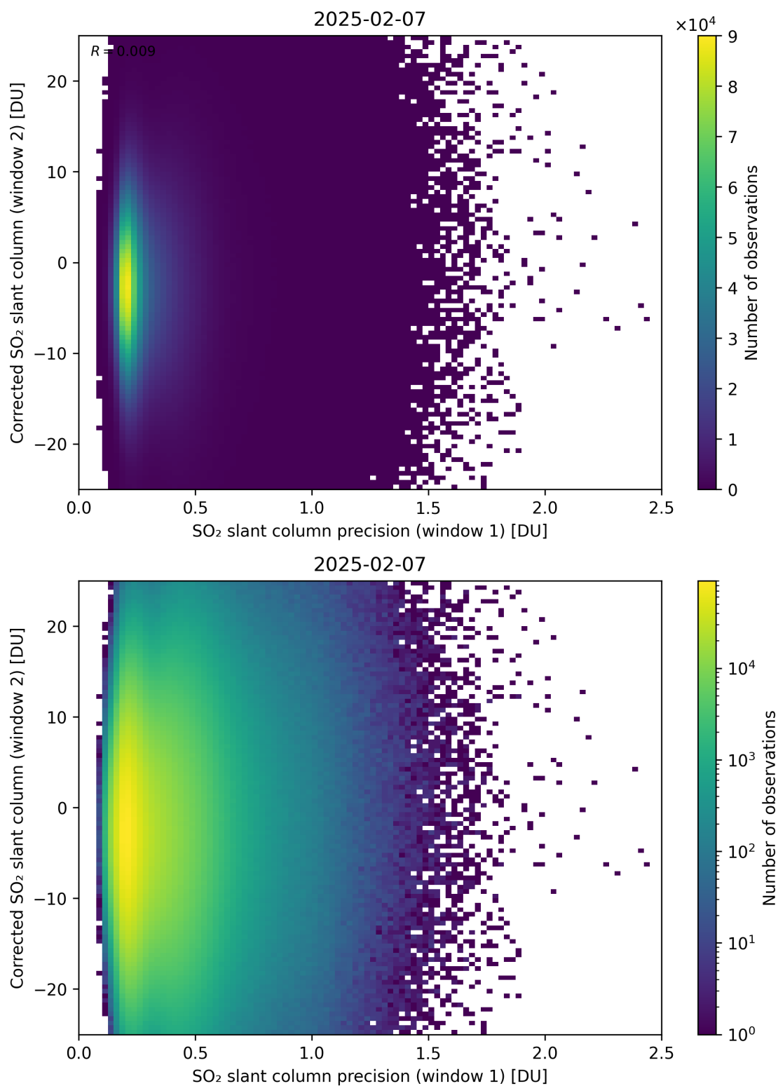
Figure 275: Scatter density plot of “SO 2 slant column precision (window 1)” against “Corrected SO 2 slant column (window 2)” for 2025-02-06 to 2025-02-08.
