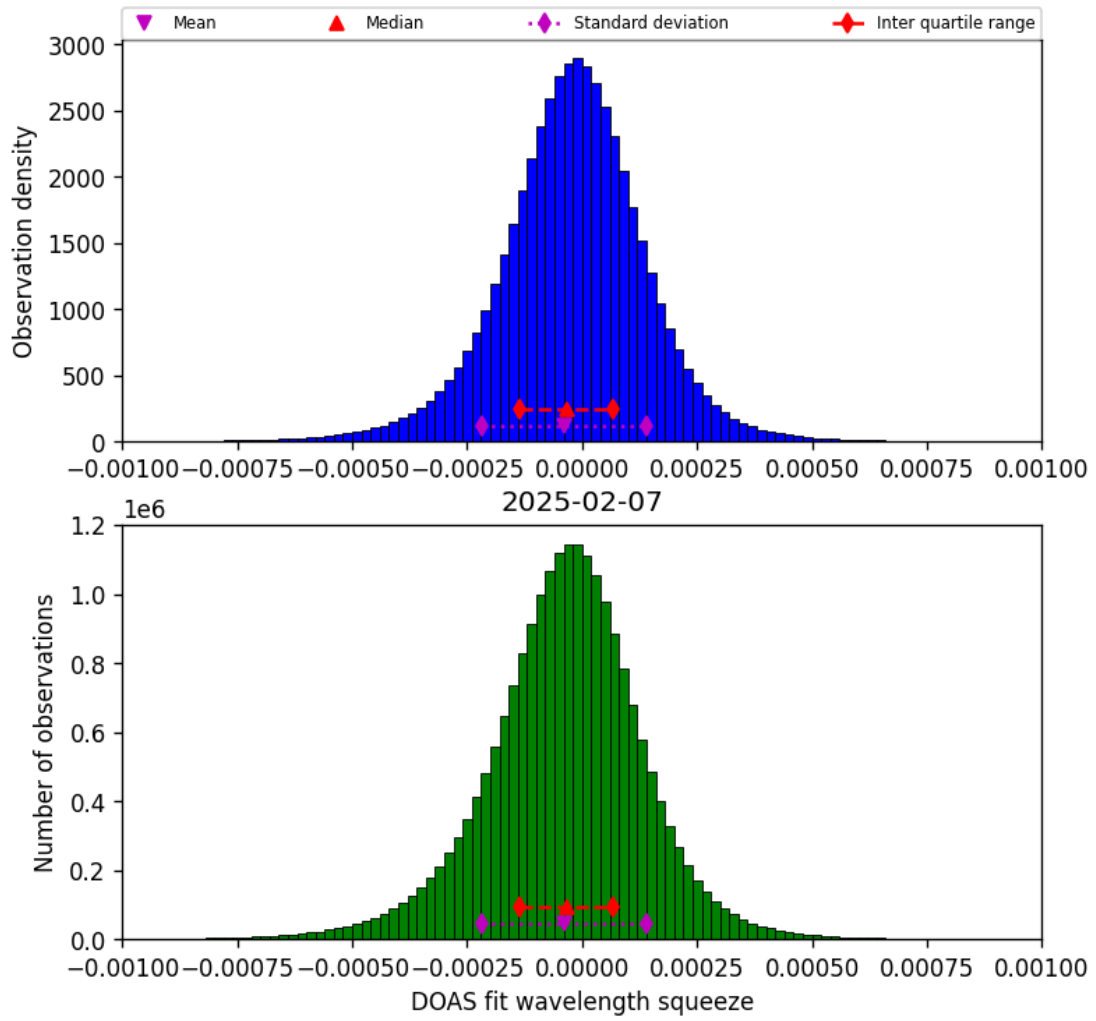
Figure 77: Histogram of “DOAS fit wavelength squeeze” for 2025-02-06 to 2025-02-08
