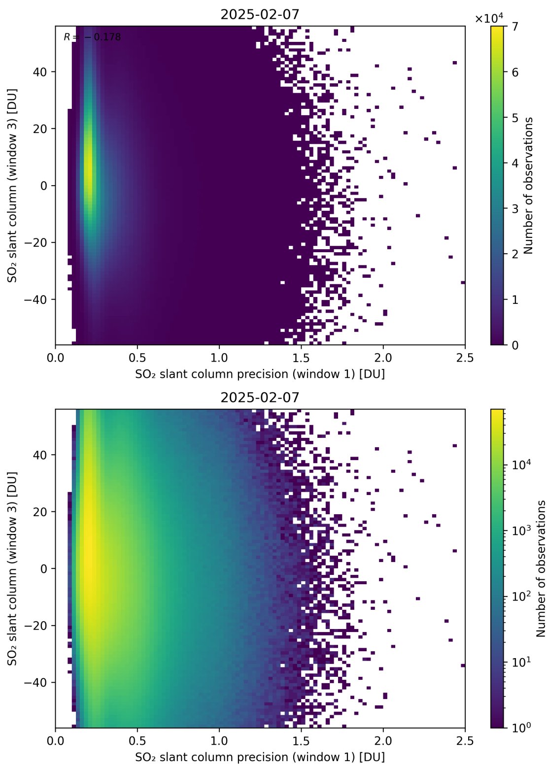
Figure 278: Scatter density plot of “SO 2 slant column precision (window 1)” against “SO 2 slant column (window 3)” for 2025-02-06 to 2025-02-08.
