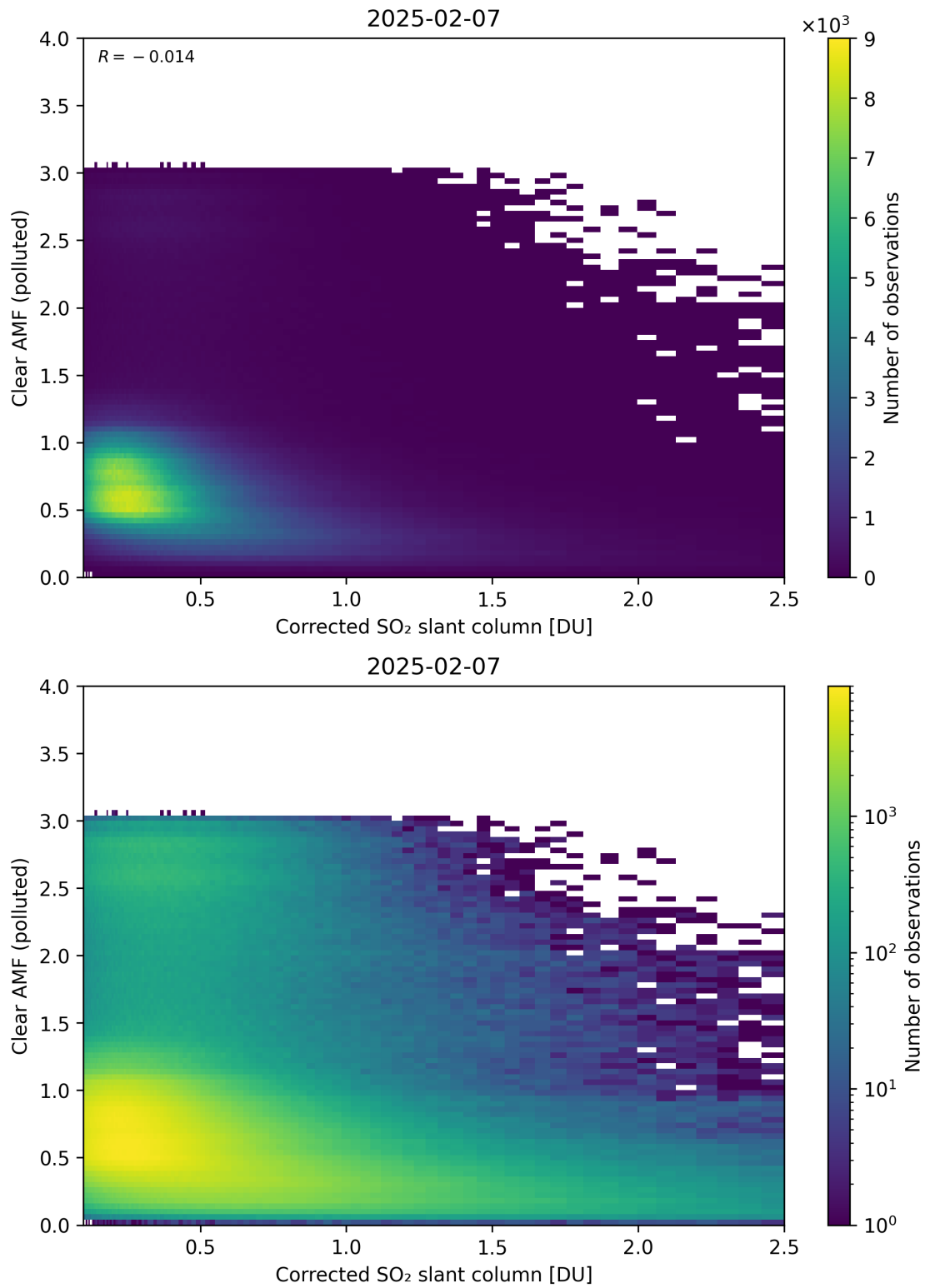
Figure 232: Scatter density plot of “Corrected SO 2 slant column” against “Clear AMF (polluted)” for 2025-02-06 to 2025-02-08.
