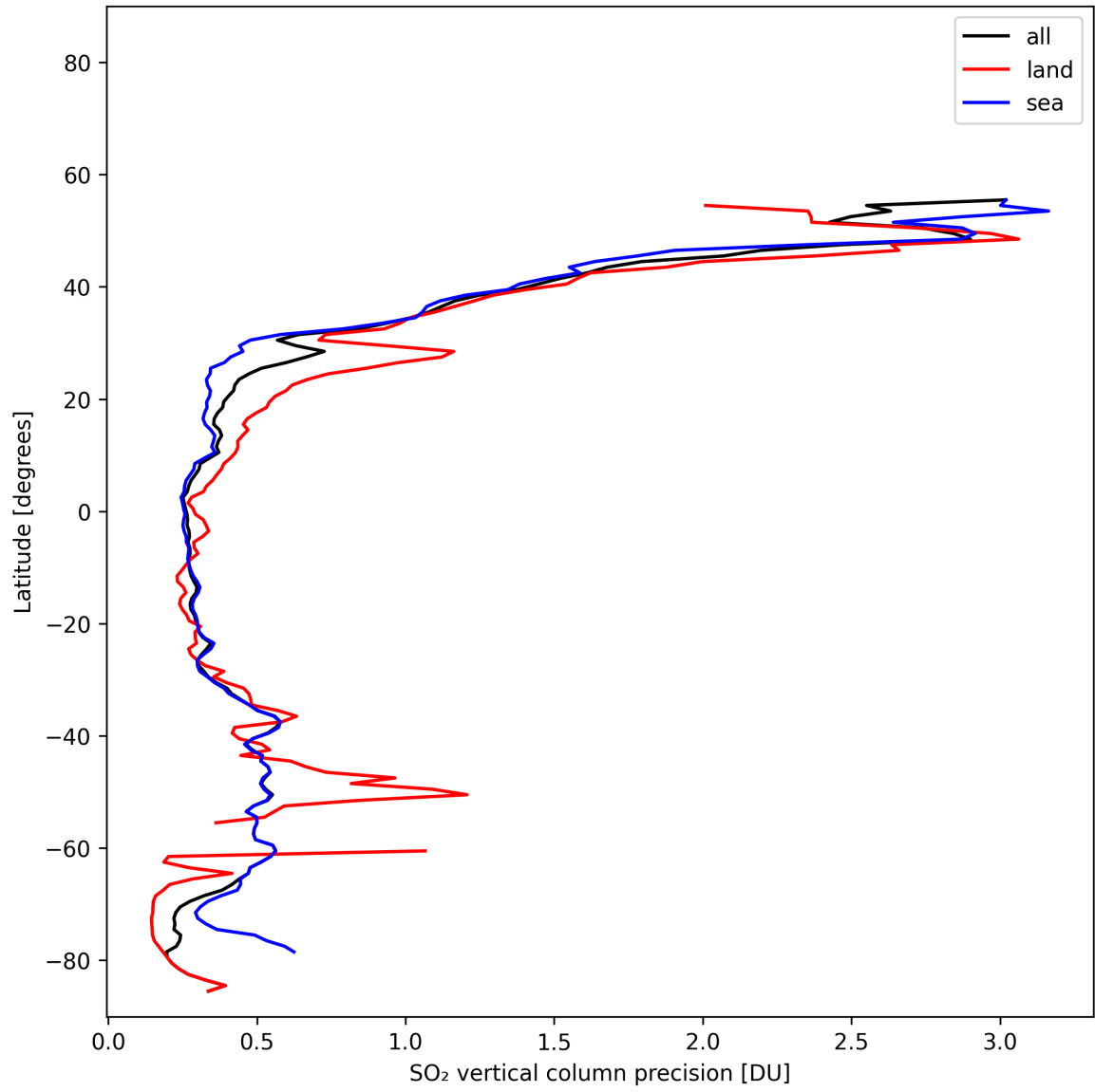
Figure 33: Zonal average of “SO 2 vertical column precision” for 2025-02-06 to 2025-02-08.
