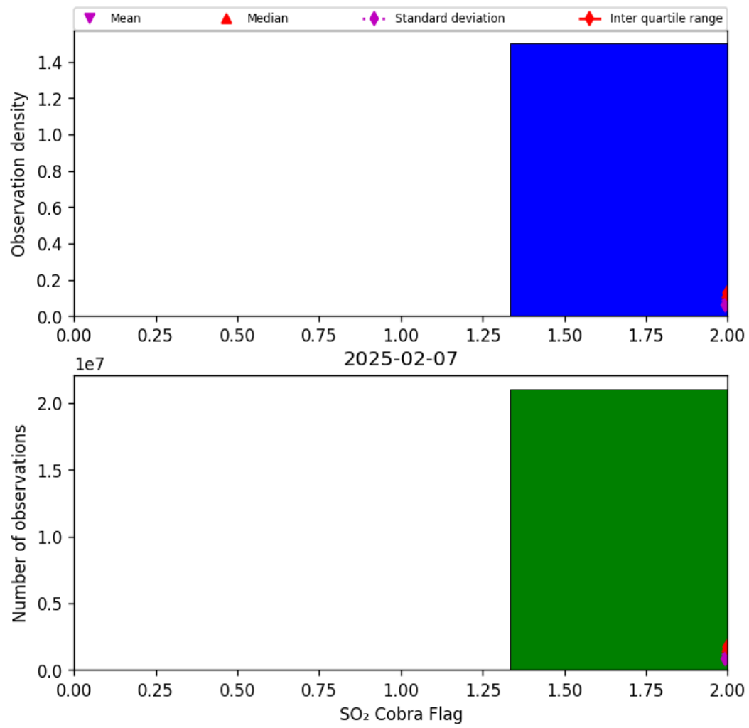
Figure 75: Histogram of “SO 2 Cobra Flag” for 2025-02-06 to 2025-02-08
