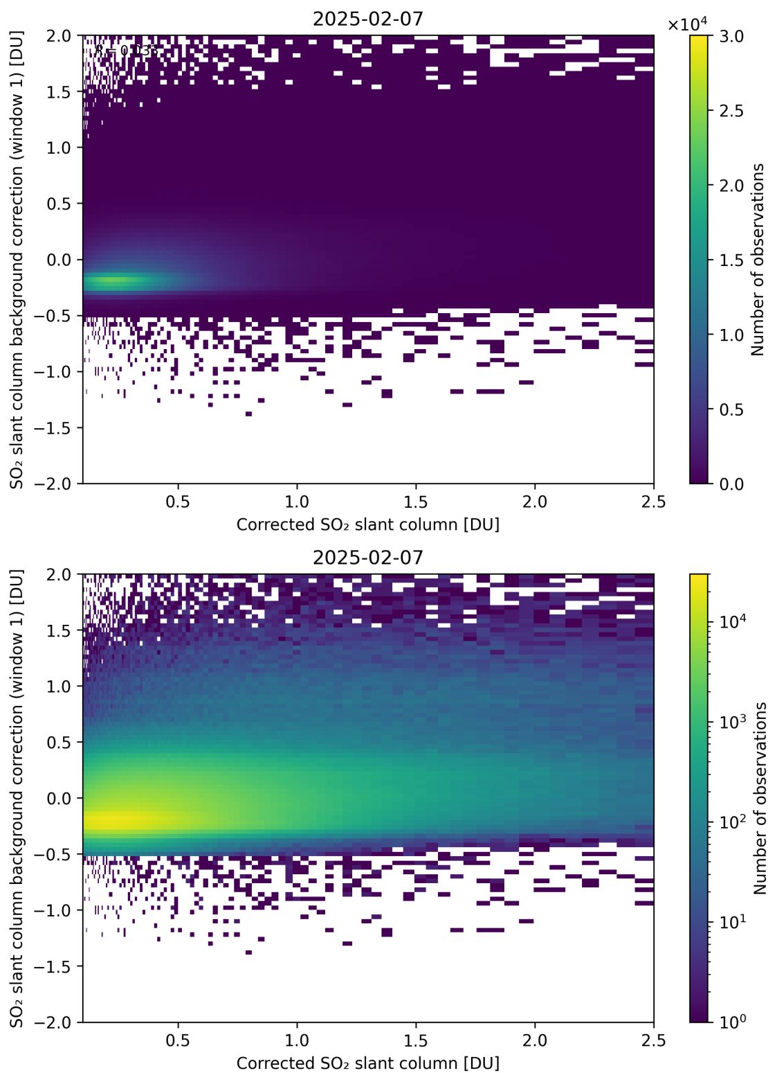
Figure 226: Scatter density plot of “Corrected SO 2 slant column” against “SO 2 slant column background correction (window 1)” for 2025-02-06 to 2025-02-08.
