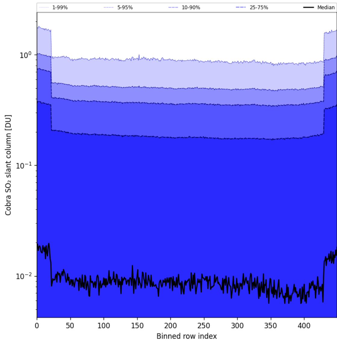
Figure 87: Along track statistics of “Cobra SO 2 slant column” for 2025-02-06 to 2025-02-08
