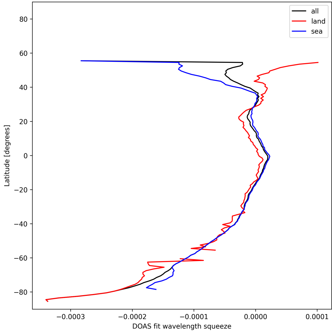
Figure 51: Zonal average of “DOAS fit wavelength squeeze” for 2025-02-06 to 2025-02-08.
