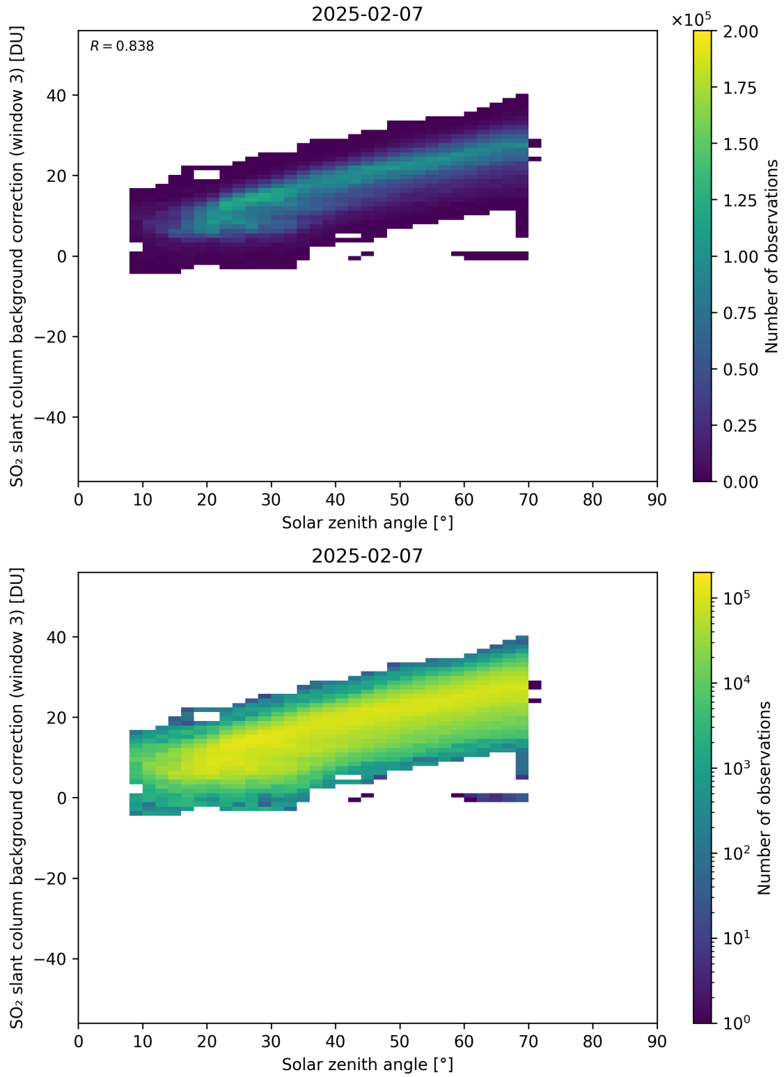
Figure 173: Scatter density plot of “Solar zenith angle” against “SO 2 slant column background correction (window 3)” for 2025-02-06 to 2025-02-08.
