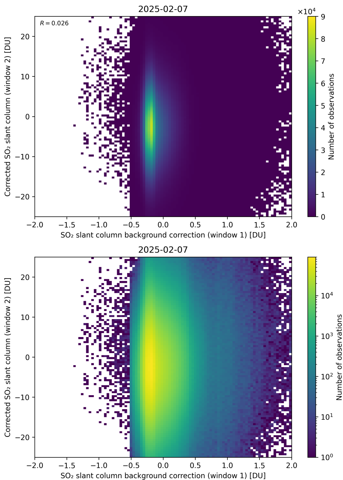
Figure 115: Scatter density plot of “SO 2 slant column background correction (window 1)” against “Corrected SO 2 slant column (window 2)” for 2025-02-06 to 2025-02-08.
