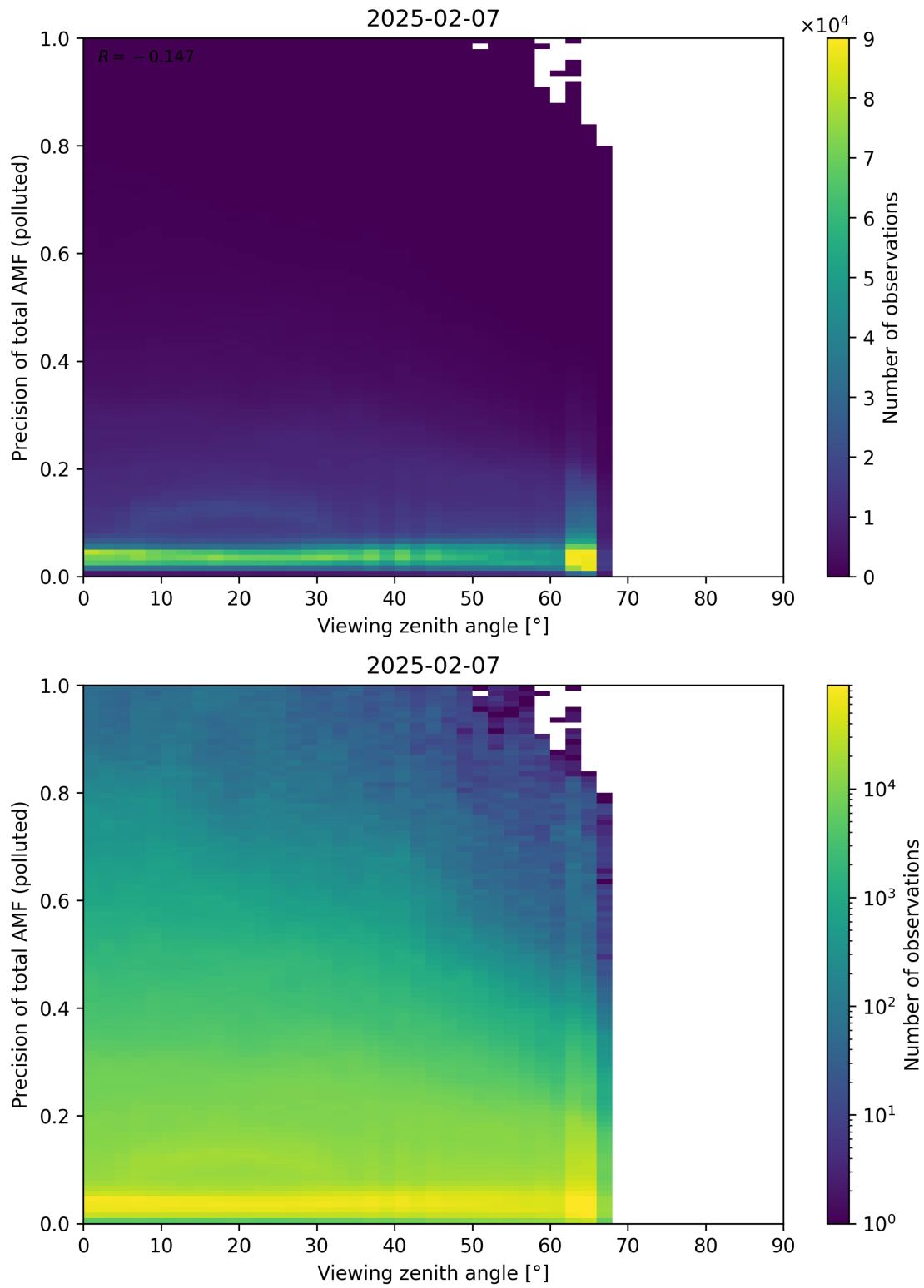
Figure 382: Scatter density plot of “Viewing zenith angle” against “Precision of total AMF (polluted)” for 2025-02-06 to 2025-02-08.
