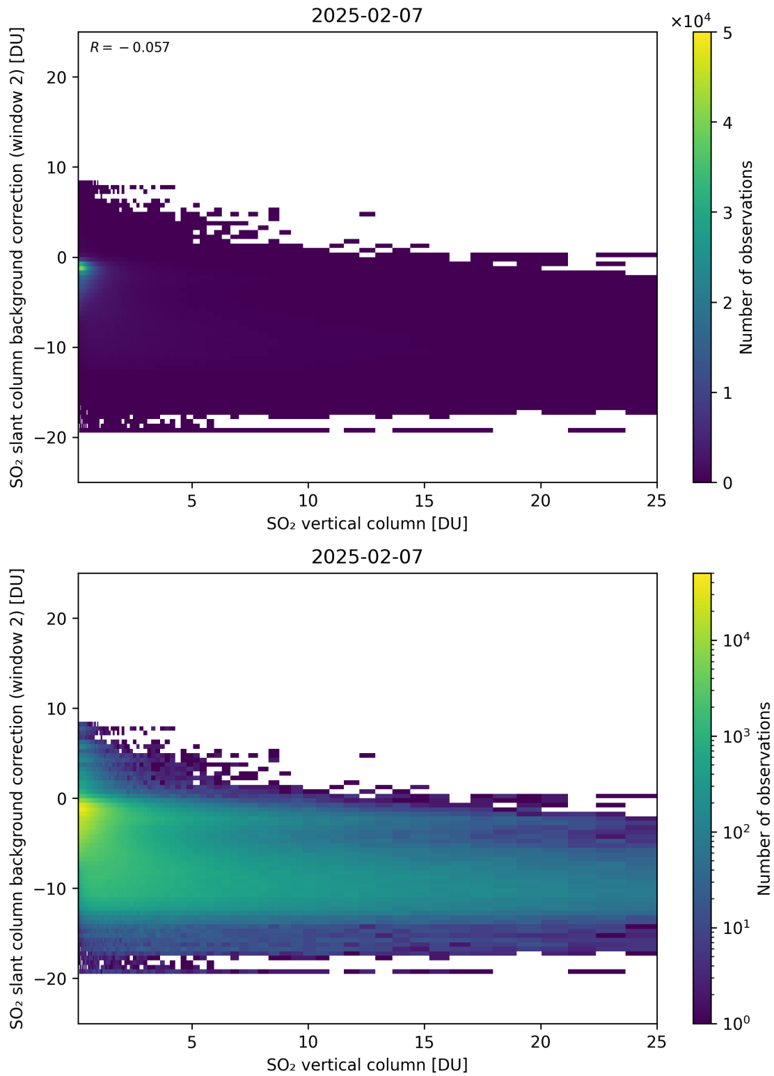
Figure 324: Scatter density plot of “SO 2 vertical column” against “SO 2 slant column background correction (window 2)” for 2025-02-06 to 2025-02-08.
