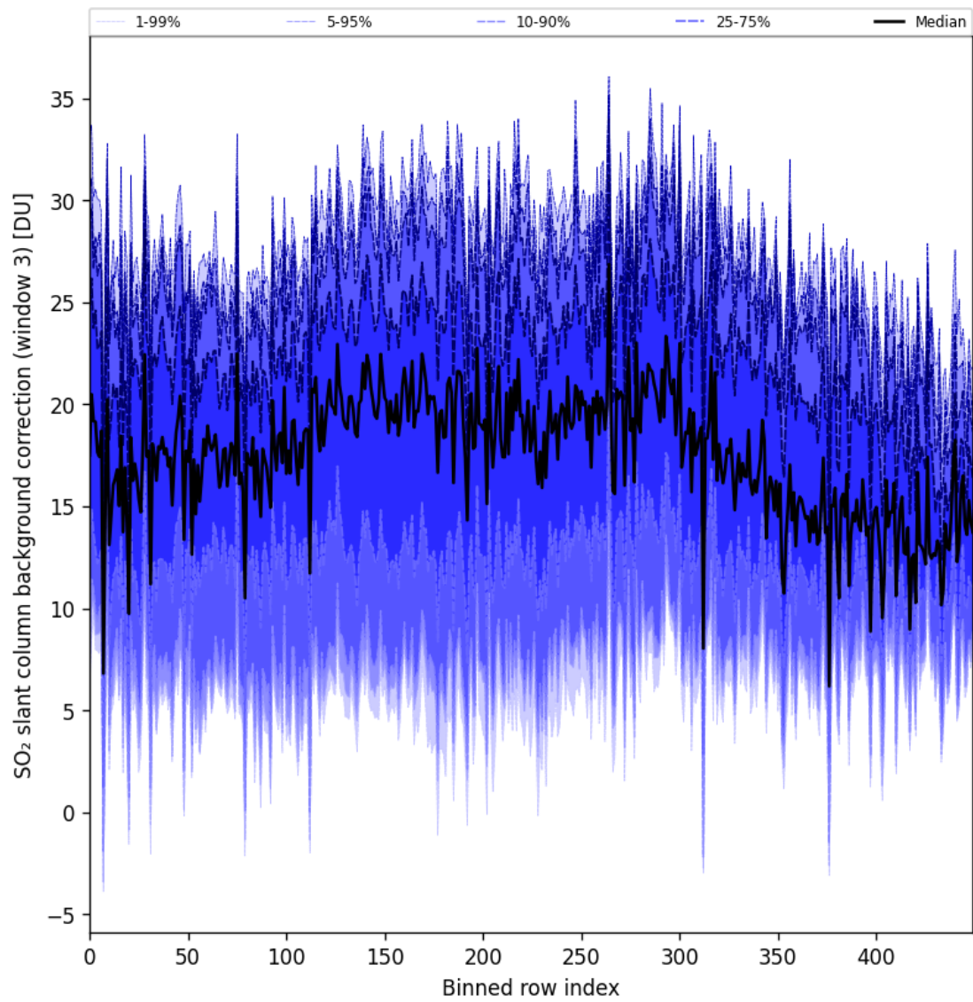
Figure 100: Along track statistics of “SO 2 slant column background correction (window 3)” for 2025-02-06 to 2025-02-08
