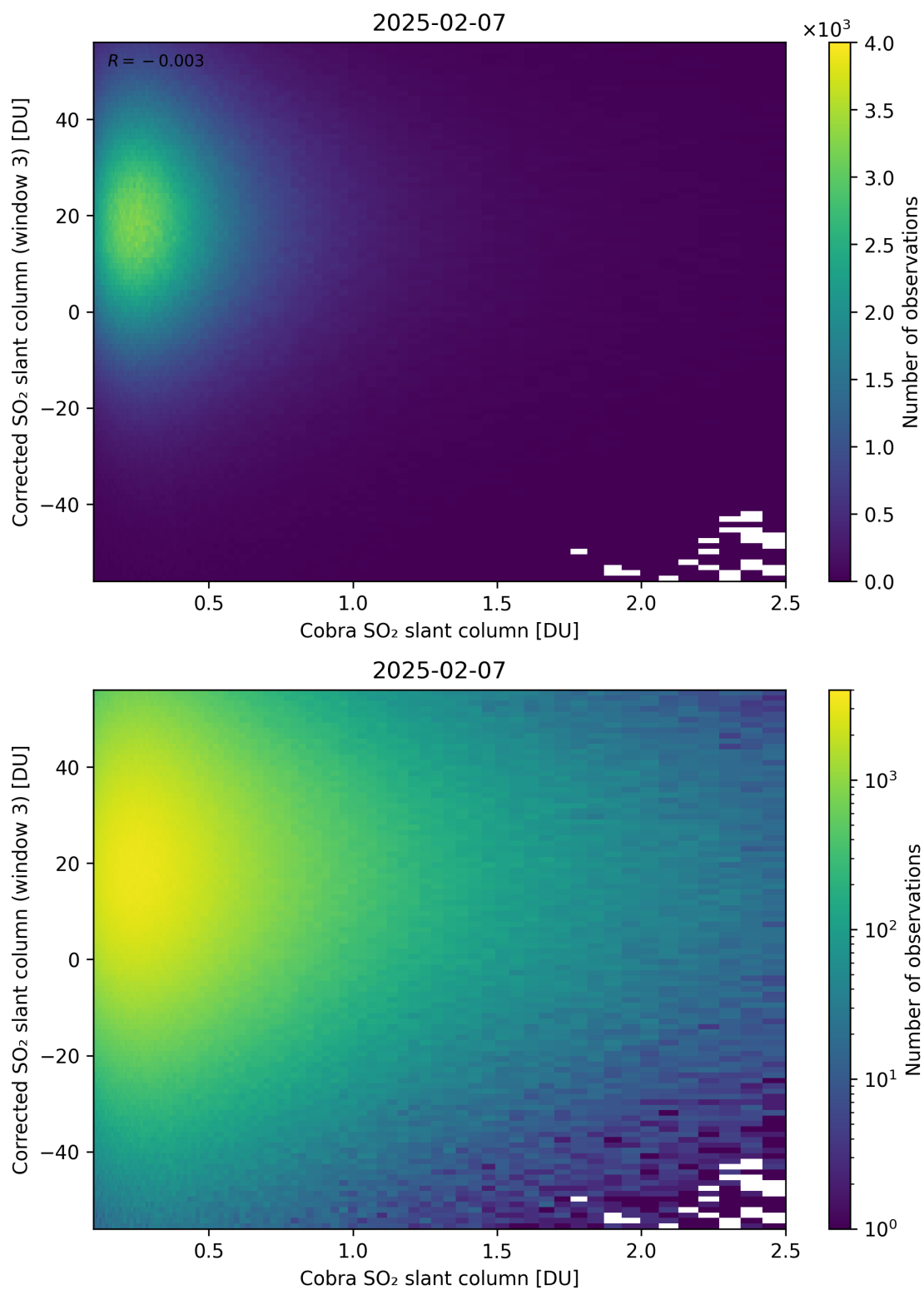
Figure 218: Scatter density plot of “Cobra SO 2 slant column” against “Corrected SO 2 slant column (window 3)” for 2025-02-06 to 2025-02-08.
