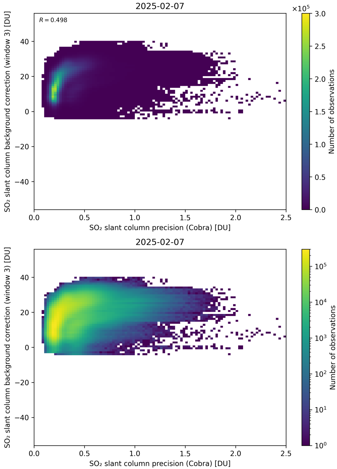
Figure 201: Scatter density plot of “SO 2 slant column precision (Cobra)” against “SO 2 slant column background correction (window 3)” for 2025-02-06 to 2025-02-08.
