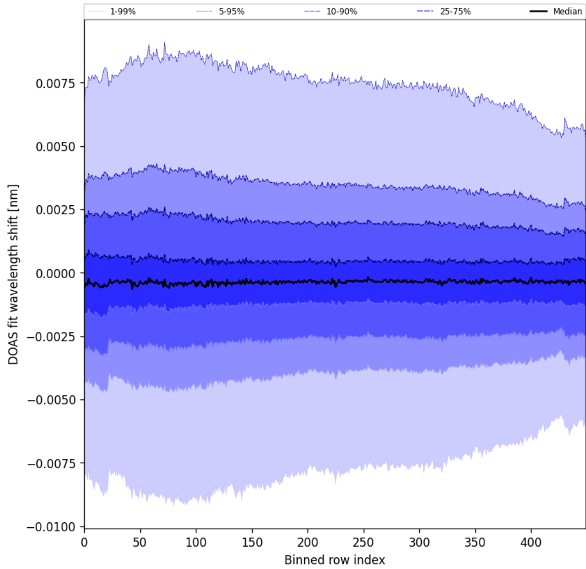
Figure 102: Along track statistics of “DOAS fit wavelength shift” for 2025-02-06 to 2025-02-08
