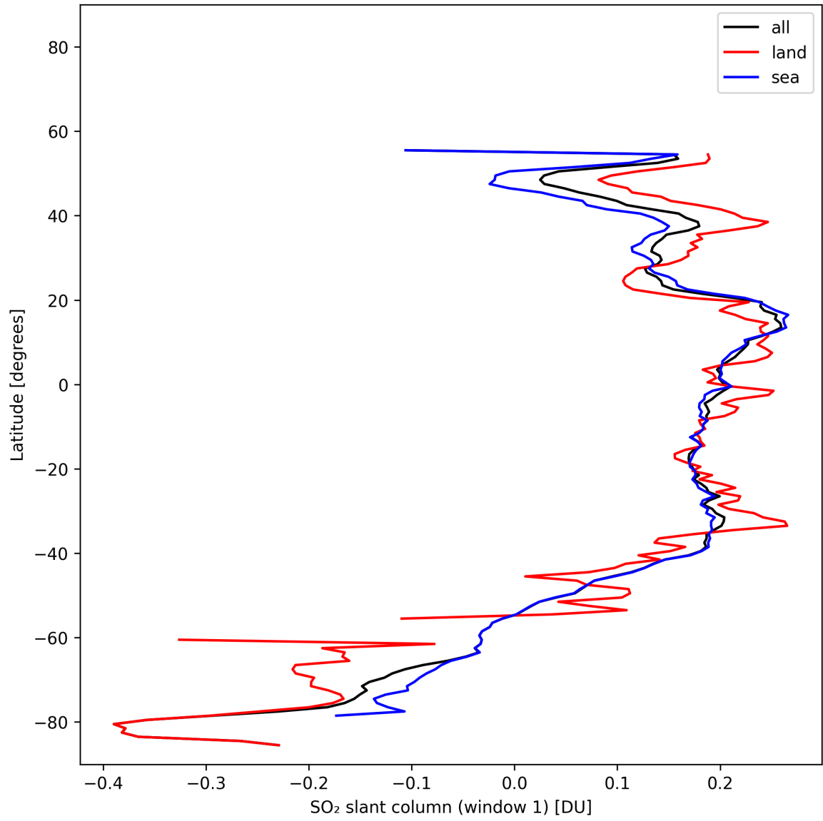
Figure 37: Zonal average of “SO 2 slant column (window 1)” for 2025-02-06 to 2025-02-08.
