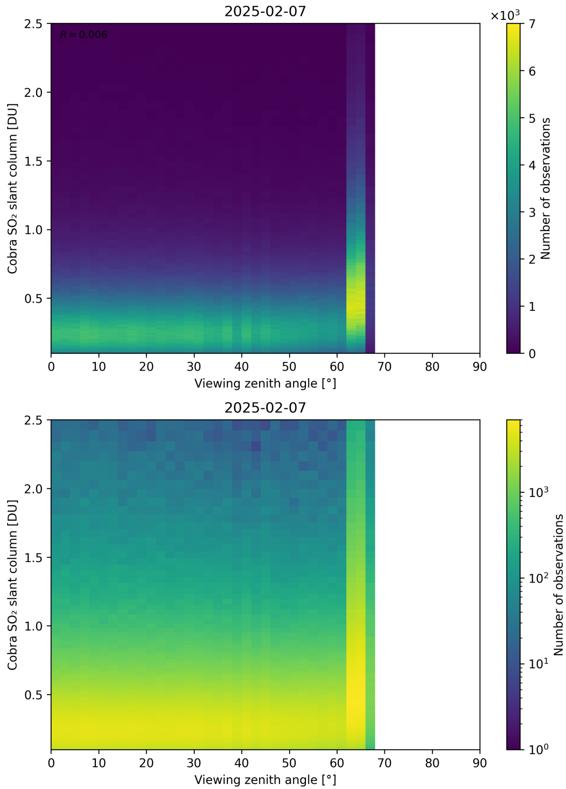
Figure 371: Scatter density plot of “Viewing zenith angle” against “Cobra SO 2 slant column” for 2025-02-06 to 2025-02-08.
