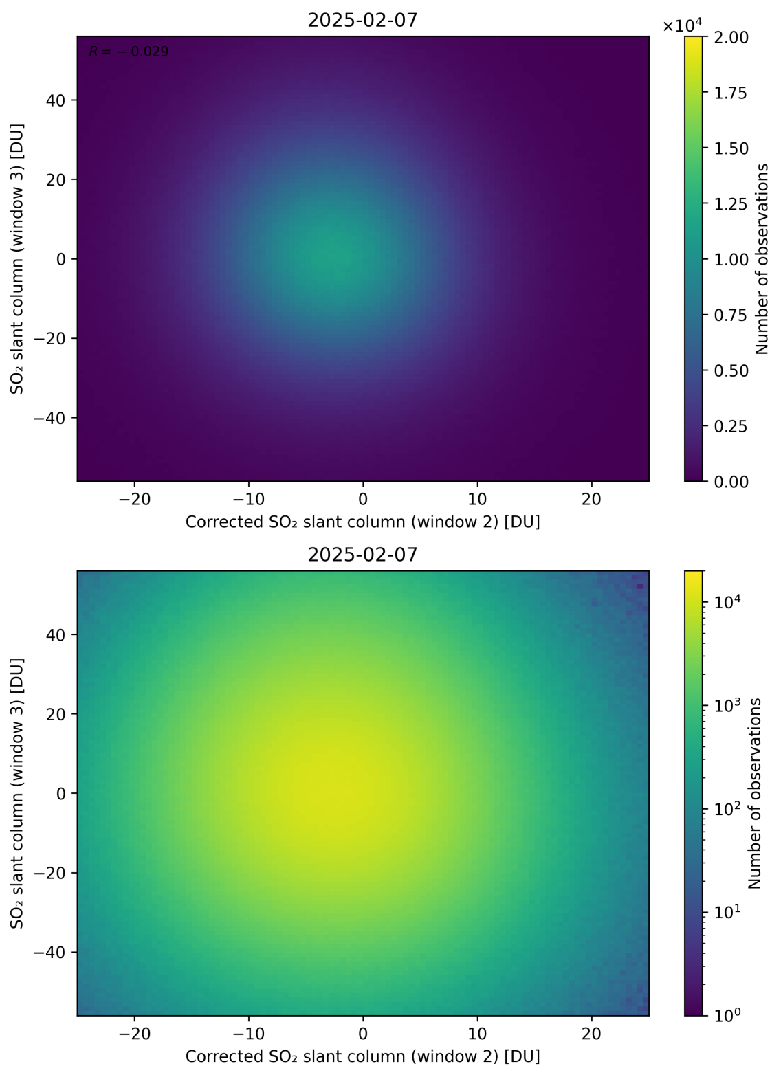
Figure 251: Scatter density plot of “Corrected SO 2 slant column (window 2)” against “SO 2 slant column (window 3)” for 2025-02-06 to 2025-02-08.
