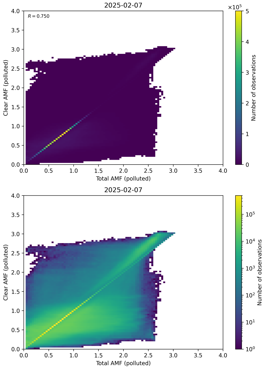
Figure 321: Scatter density plot of “Total AMF (polluted)” against “Clear AMF (polluted)” for 2025-02-06 to 2025-02-08.
