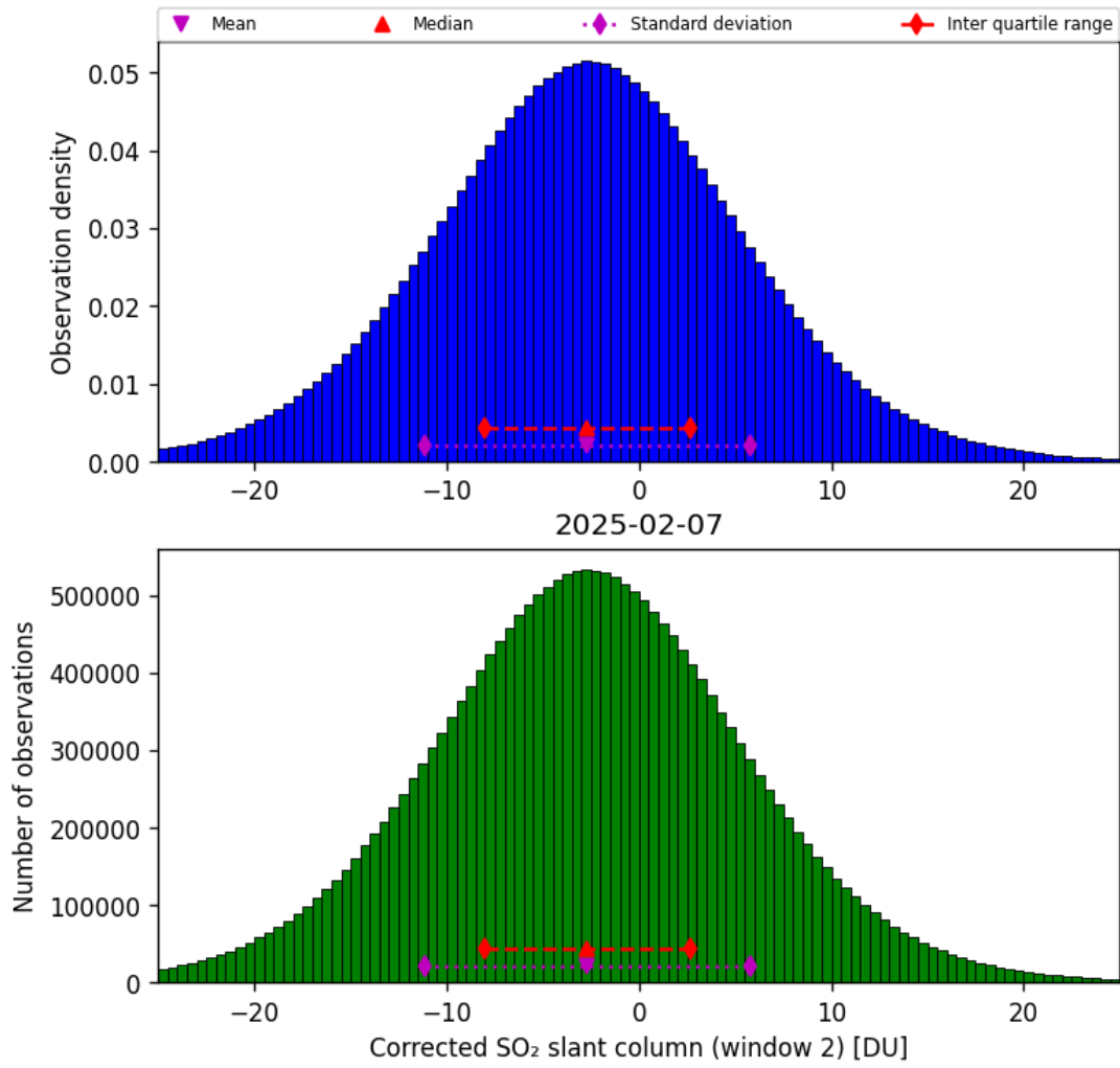
Figure 69: Histogram of “Corrected SO 2 slant column (window 2)” for 2025-02-06 to 2025-02-08
