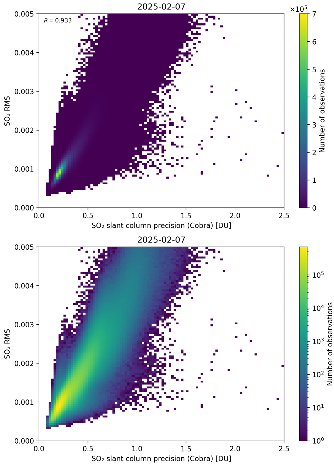
Figure 204: Scatter density plot of “SO 2 slant column precision (Cobra)” against “SO 2 RMS” for 2025-02-06 to 2025-02-08.
