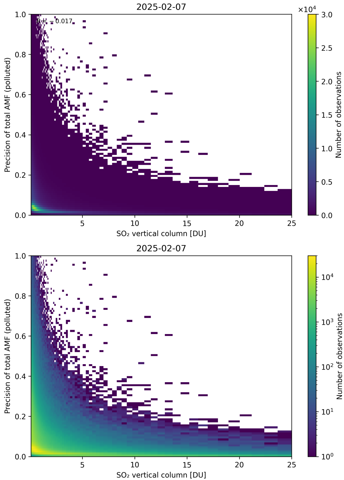
Figure 360: Scatter density plot of “SO 2 vertical column” against “Precision of total AMF (polluted)” for 2025-02-06 to 2025-02-08.
