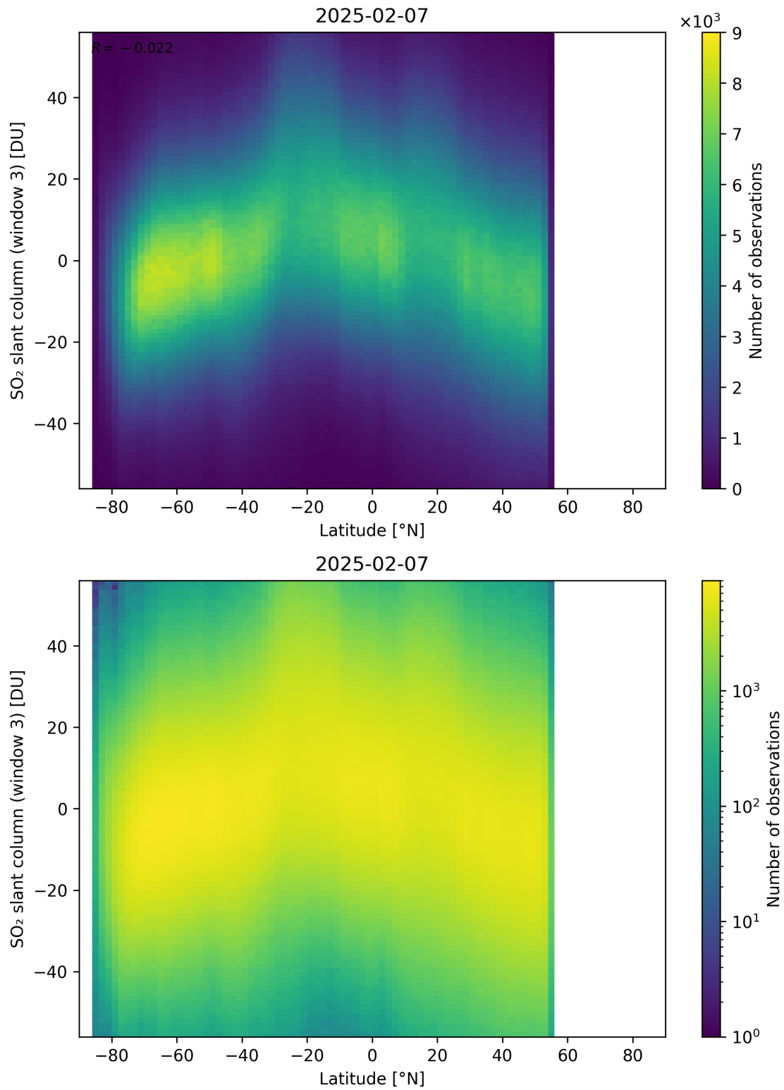
Figure 165: Scatter density plot of “Latitude” against “SO 2 slant column (window 3)” for 2025-02-06 to 2025-02-08.
