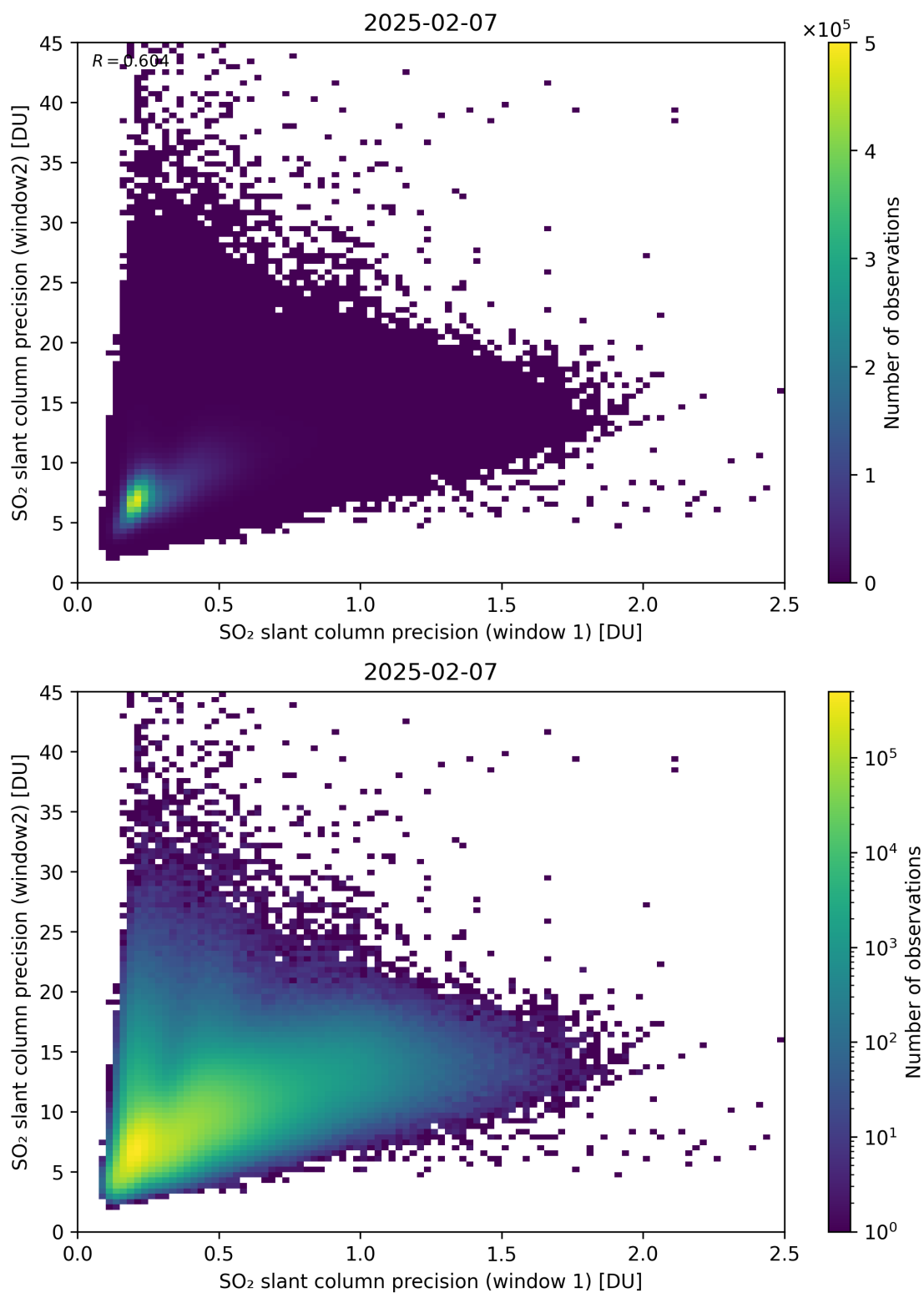
Figure 277: Scatter density plot of “SO 2 slant column precision (window 1)” against “SO 2 slant column precision (window2)” for 2025-02-06 to 2025-02-08.
