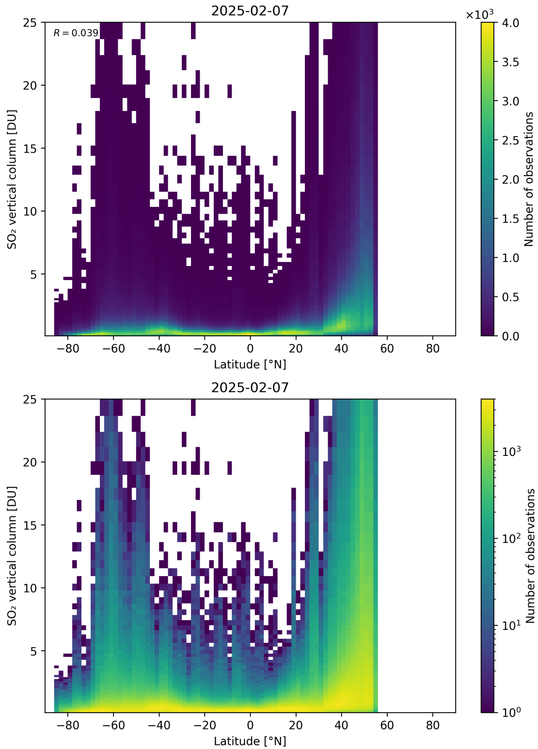
Figure 169: Scatter density plot of “Latitude” against “SO 2 vertical column” for 2025-02-06 to 2025-02-08.
