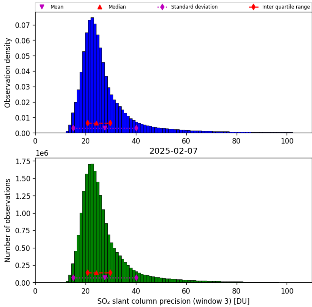
Figure 72: Histogram of “SO 2 slant column precision (window 3)” for 2025-02-06 to 2025-02-08
