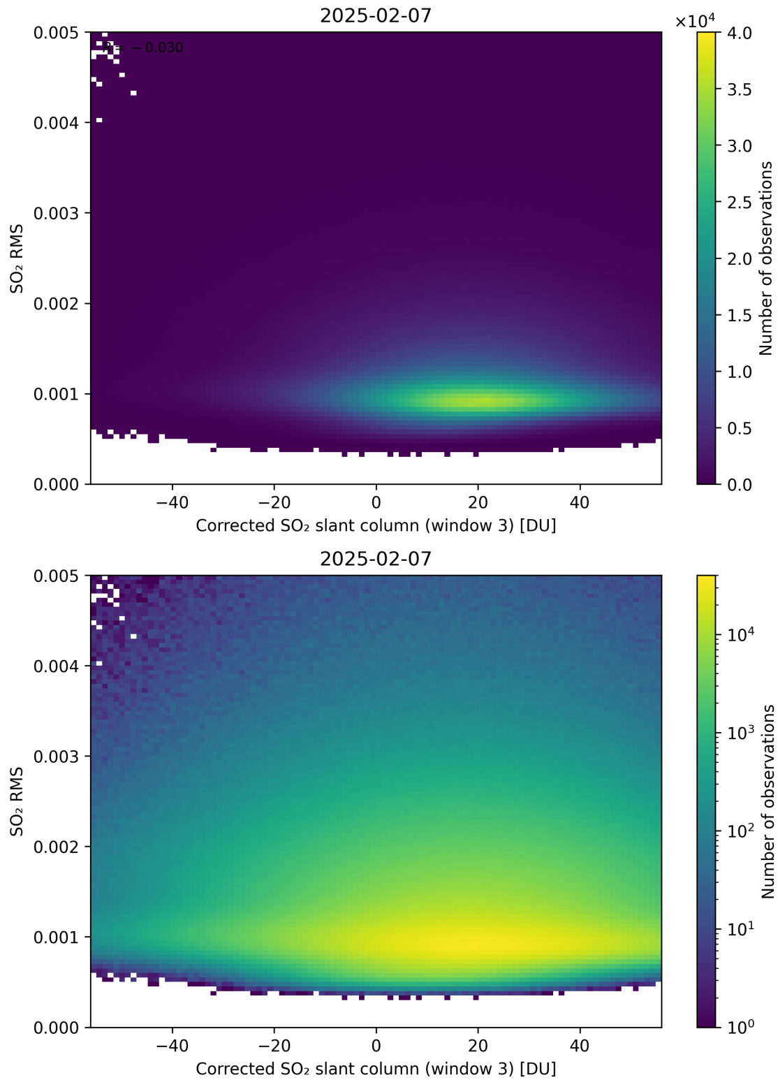
Figure 258: Scatter density plot of “Corrected SO 2 slant column (window 3)” against “SO 2 RMS” for 2025-02-06 to 2025-02-08.
