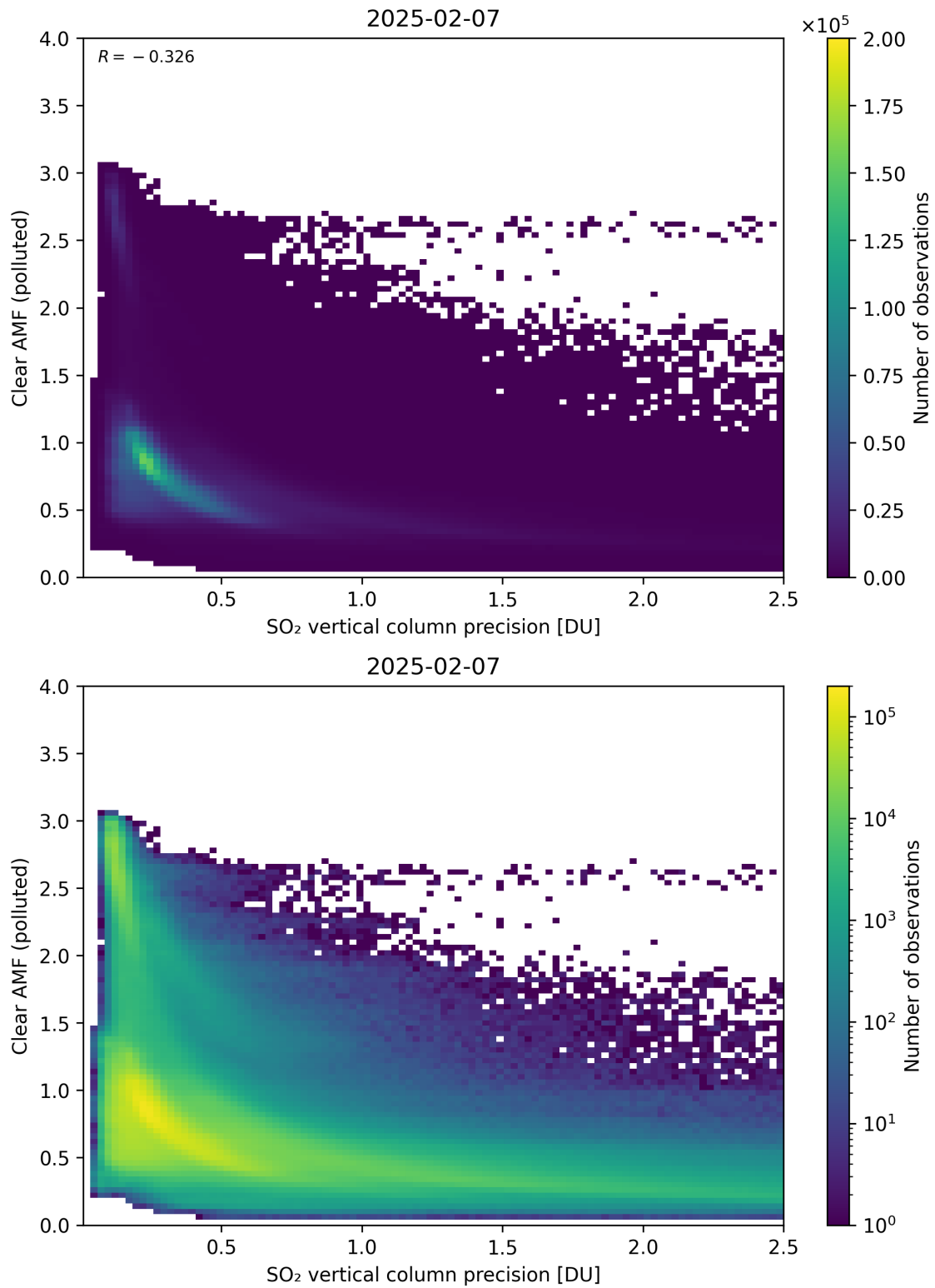
Figure 335: Scatter density plot of “SO 2 vertical column precision” against “Clear AMF (polluted)” for 2025-02-06 to 2025-02-08.
