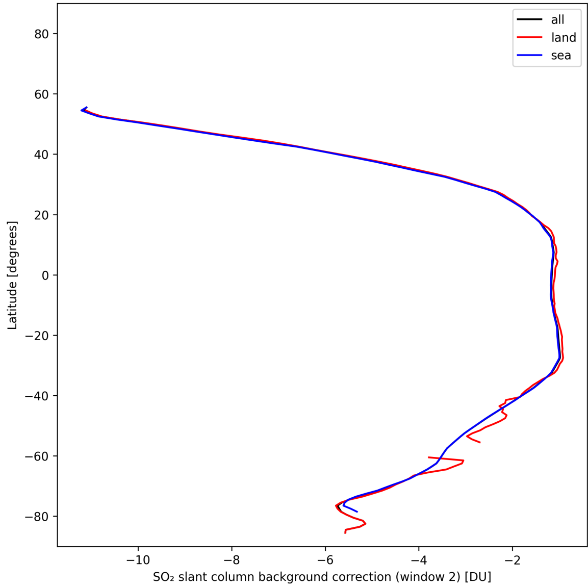
Figure 44: Zonal average of “SO 2 slant column background correction (window 2)” for 2025-02-06 to 2025-02-08.
