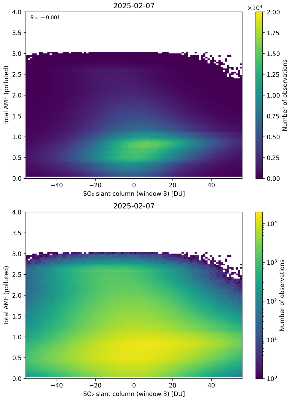
Figure 318: Scatter density plot of “SO 2 slant column (window 3)” against “Total AMF (polluted)” for 2025-02-06 to 2025-02-08.
