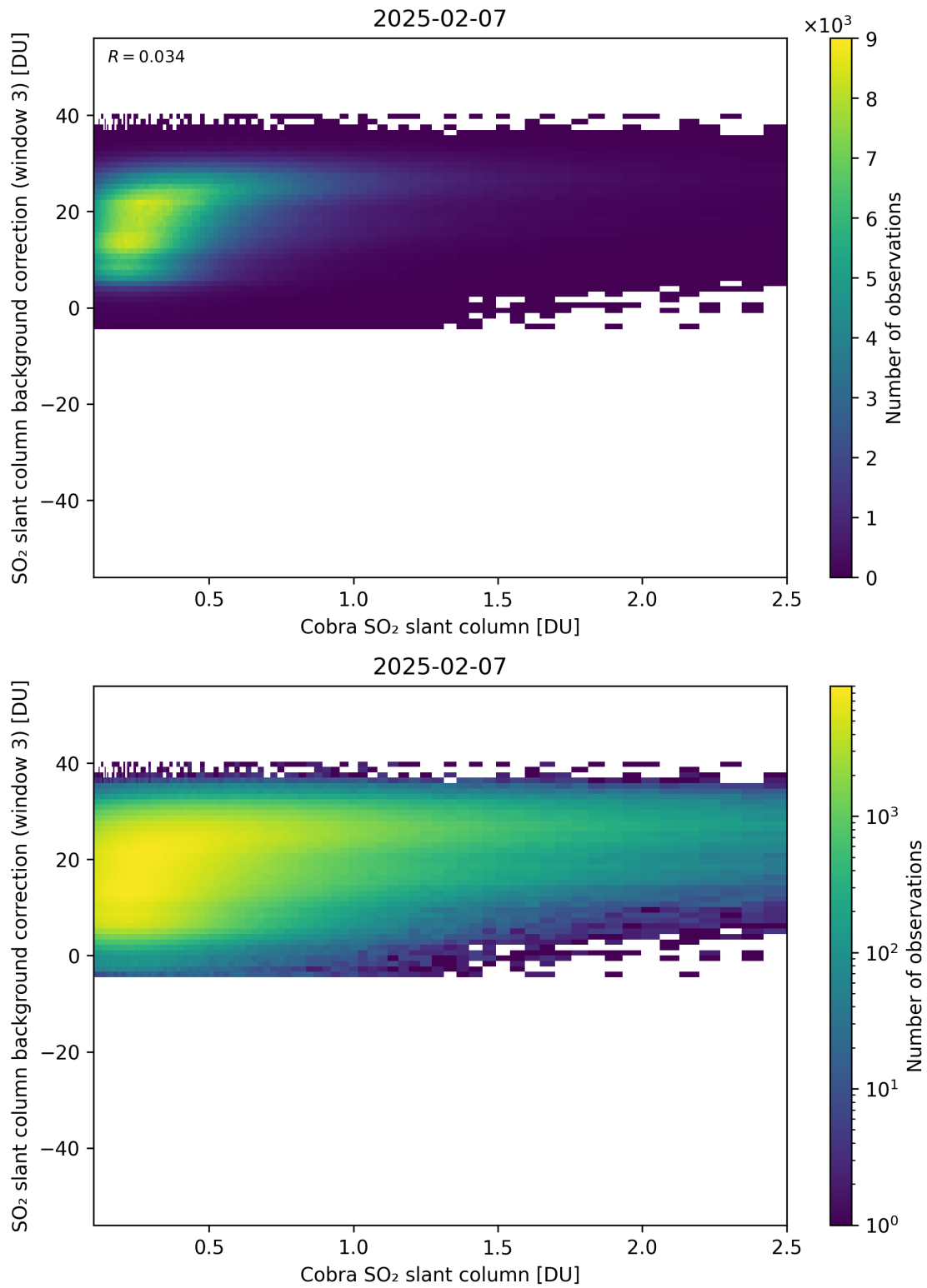
Figure 195: Scatter density plot of “Cobra SO 2 slant column” against “SO 2 slant column background correction (window 3)” for 2025-02-06 to 2025-02-08.
