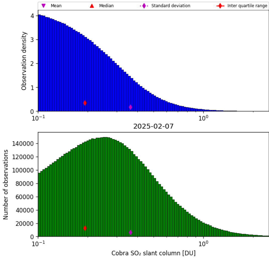
Figure 61: Histogram of “Cobra SO 2 slant column” for 2025-02-06 to 2025-02-08
