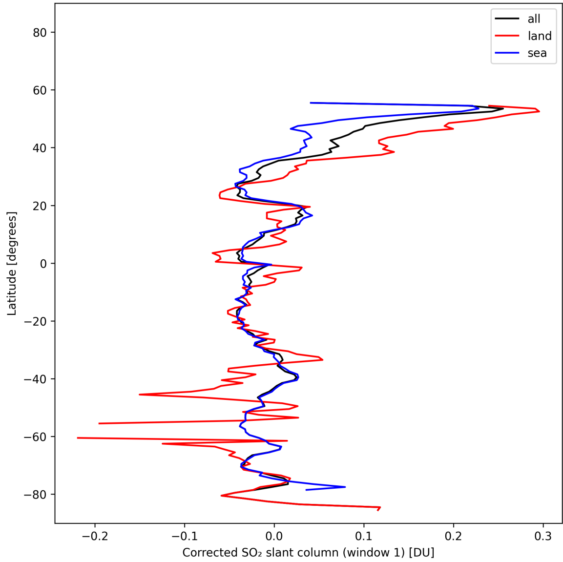
Figure 39: Zonal average of “Corrected SO 2 slant column (window 1)” for 2025-02-06 to 2025-02-08.
