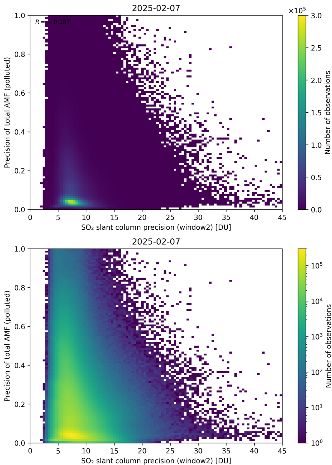
Figure 302: Scatter density plot of “SO 2 slant column precision (window2)” against “Precision of total AMF (polluted)” for 2025-02-06 to 2025-02-08.
