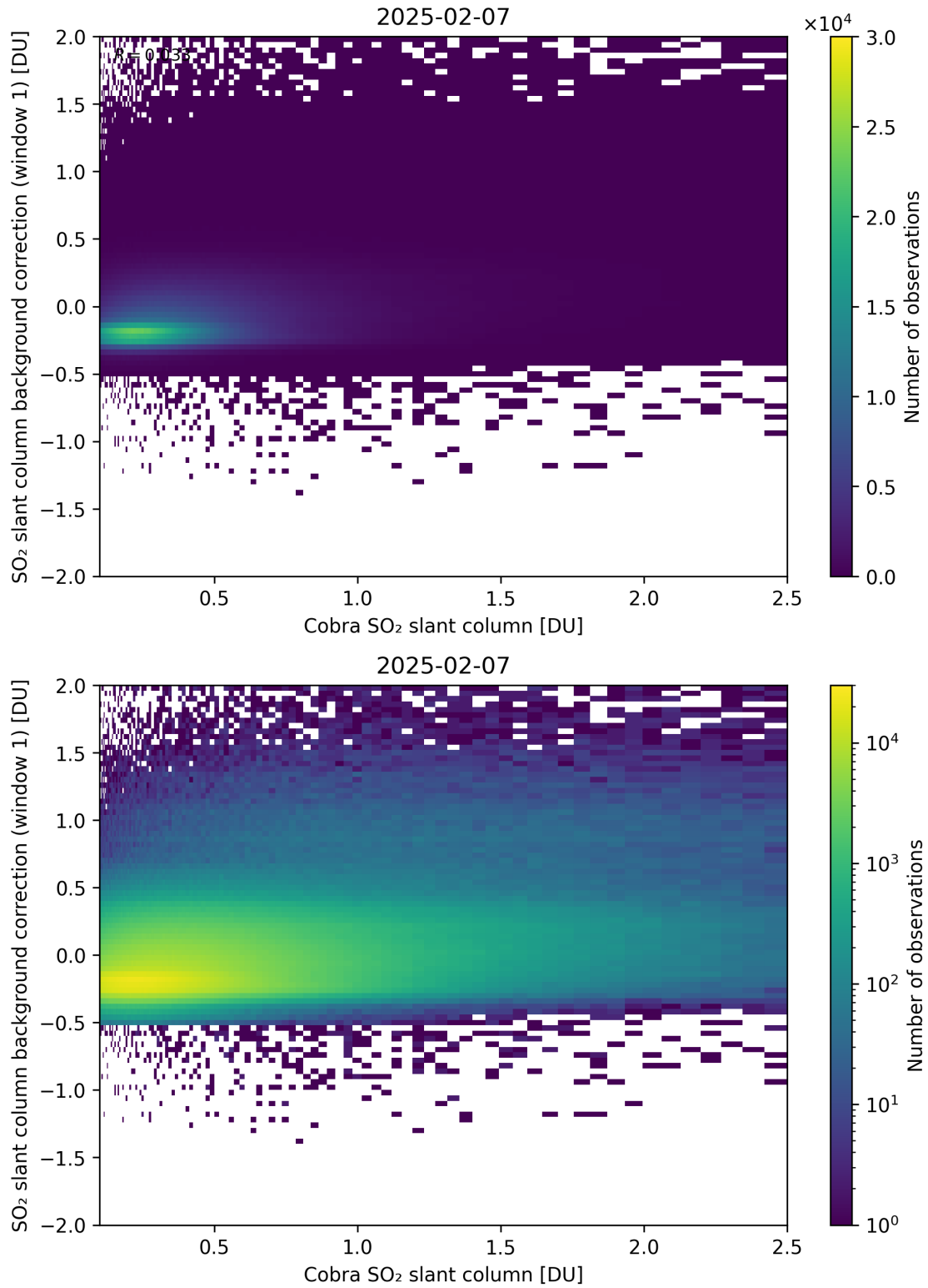
Figure 193: Scatter density plot of “Cobra SO 2 slant column” against “SO 2 slant column background correction (window 1)” for 2025-02-06 to 2025-02-08.
