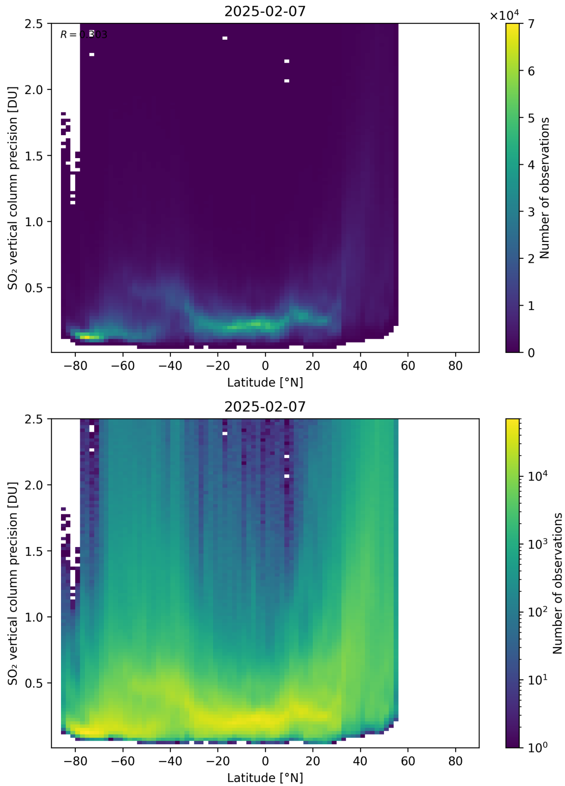
Figure 170: Scatter density plot of “Latitude” against “SO 2 vertical column precision” for 2025-02-06 to 2025-02-08.
