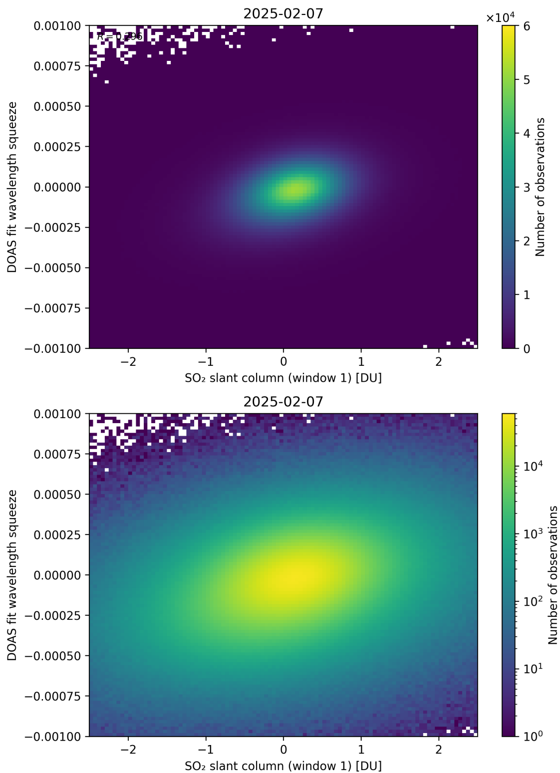
Figure 266: Scatter density plot of “SO 2 slant column (window 1)” against “DOAS fit wavelength squeeze” for 2025-02-06 to 2025-02-08.
