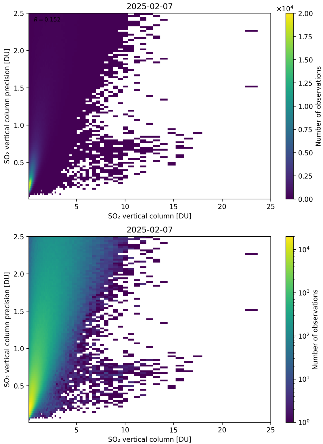
Figure 361: Scatter density plot of “SO 2 vertical column” against “SO 2 vertical column precision” for 2025-02-06 to 2025-02-08.
