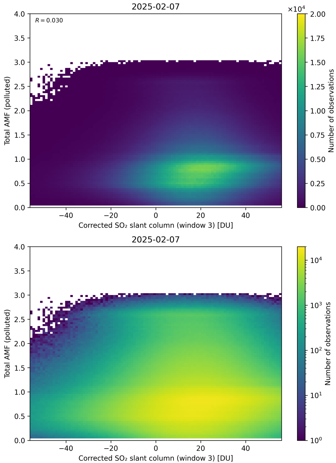
Figure 260: Scatter density plot of “Corrected SO 2 slant column (window 3)” against “Total AMF (polluted)” for 2025-02-06 to 2025-02-08.
