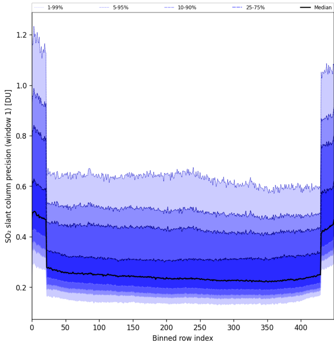
Figure 90: Along track statistics of “SO 2 slant column precision (window 1)” for 2025-02-06 to 2025-02-08
