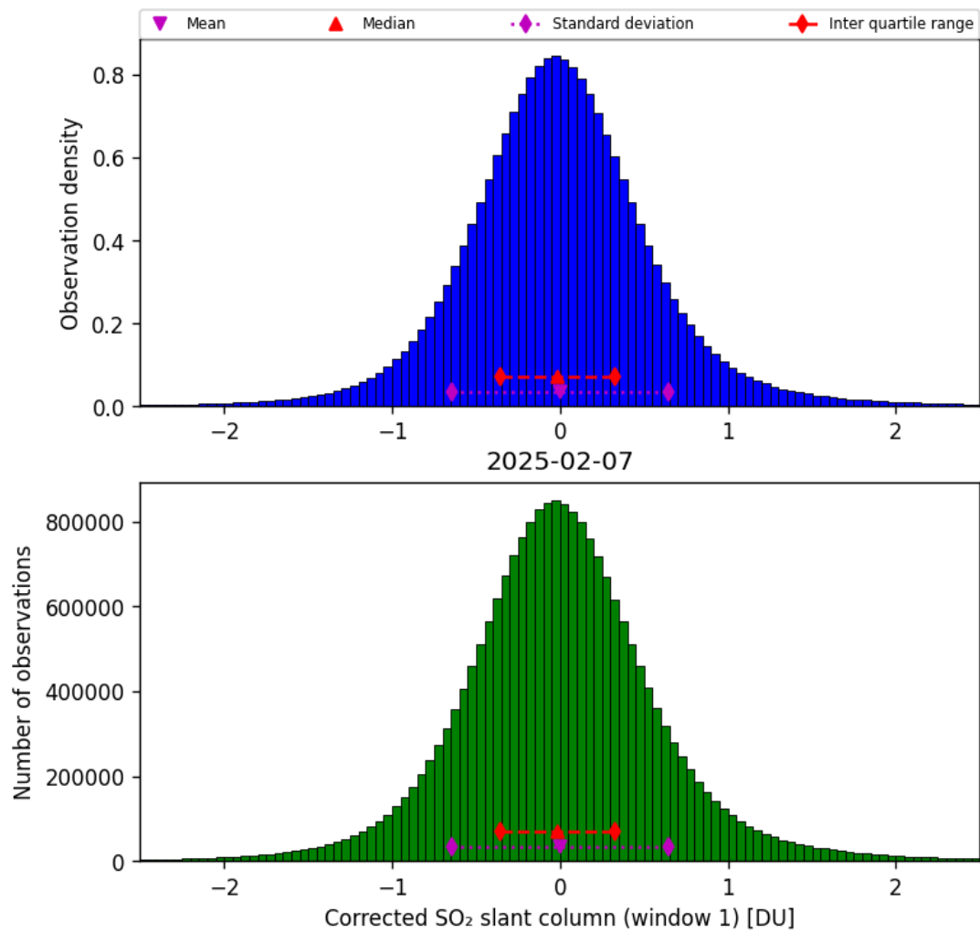
Figure 65: Histogram of “Corrected SO 2 slant column (window 1)” for 2025-02-06 to 2025-02-08
