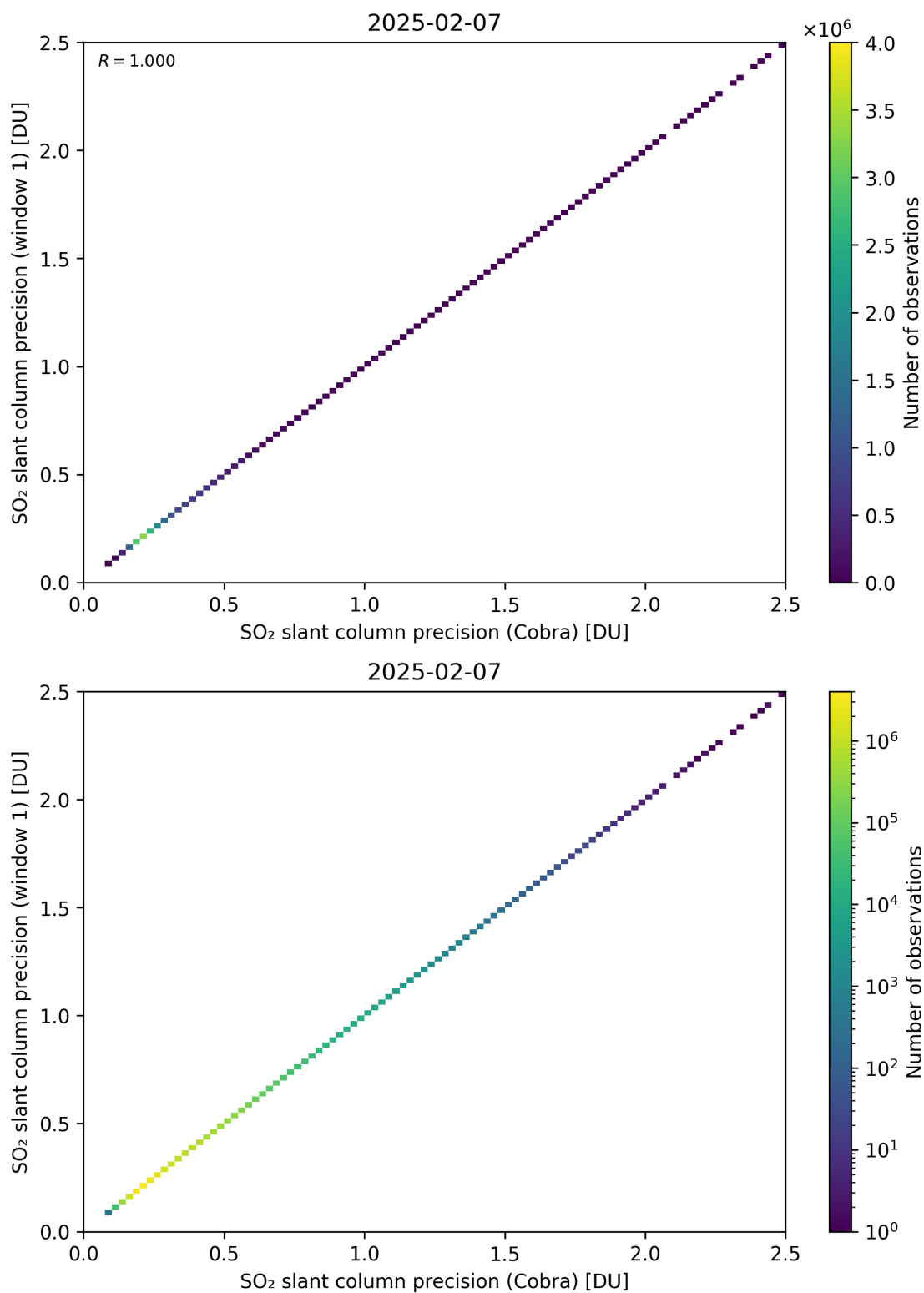
Figure 209: Scatter density plot of “SO 2 slant column precision (Cobra)” against “SO 2 slant column precision (window 1)” for 2025-02-06 to 2025-02-08.
