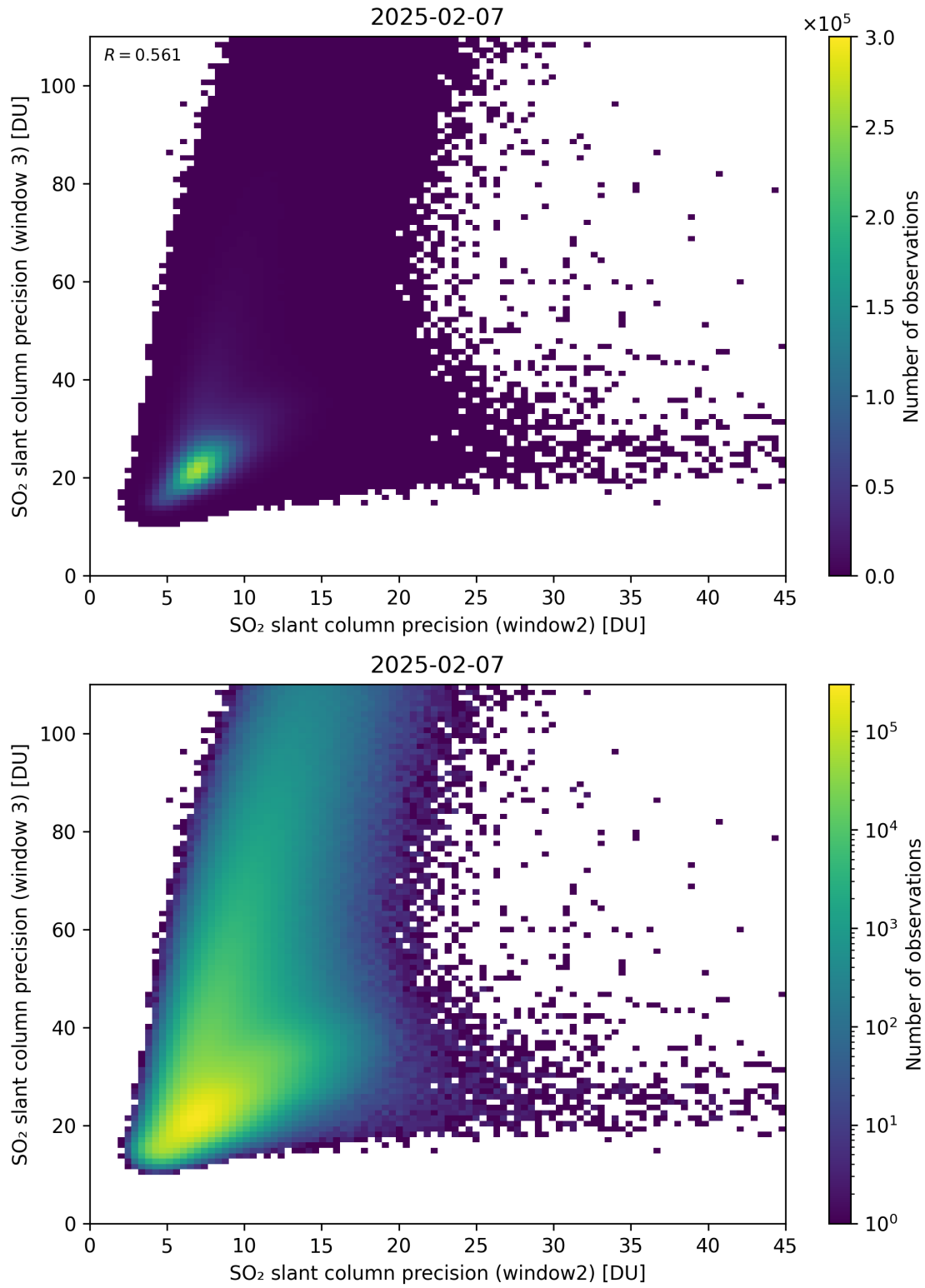
Figure 300: Scatter density plot of “SO 2 slant column precision (window2)” against “SO 2 slant column precision (window 3)” for 2025-02-06 to 2025-02-08.
