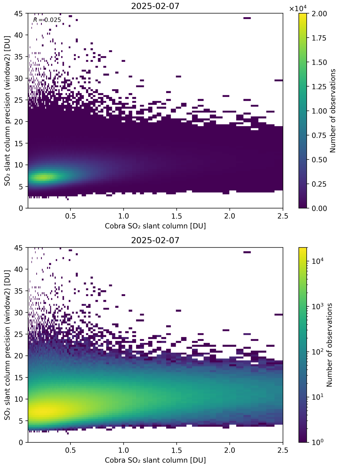
Figure 221: Scatter density plot of “Cobra SO 2 slant column” against “SO 2 slant column precision (window2)” for 2025-02-06 to 2025-02-08.
