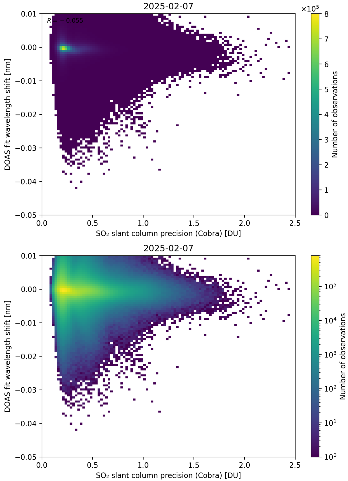
Figure 202: Scatter density plot of “SO 2 slant column precision (Cobra)” against “DOAS fit wavelength shift” for 2025-02-06 to 2025-02-08.
