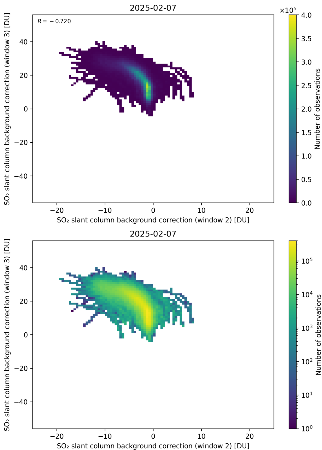
Figure 122: Scatter density plot of “SO 2 slant column background correction (window 2)” against “SO 2 slant column background correction (window 3)” for 2025-02-06 to 2025-02-08.
