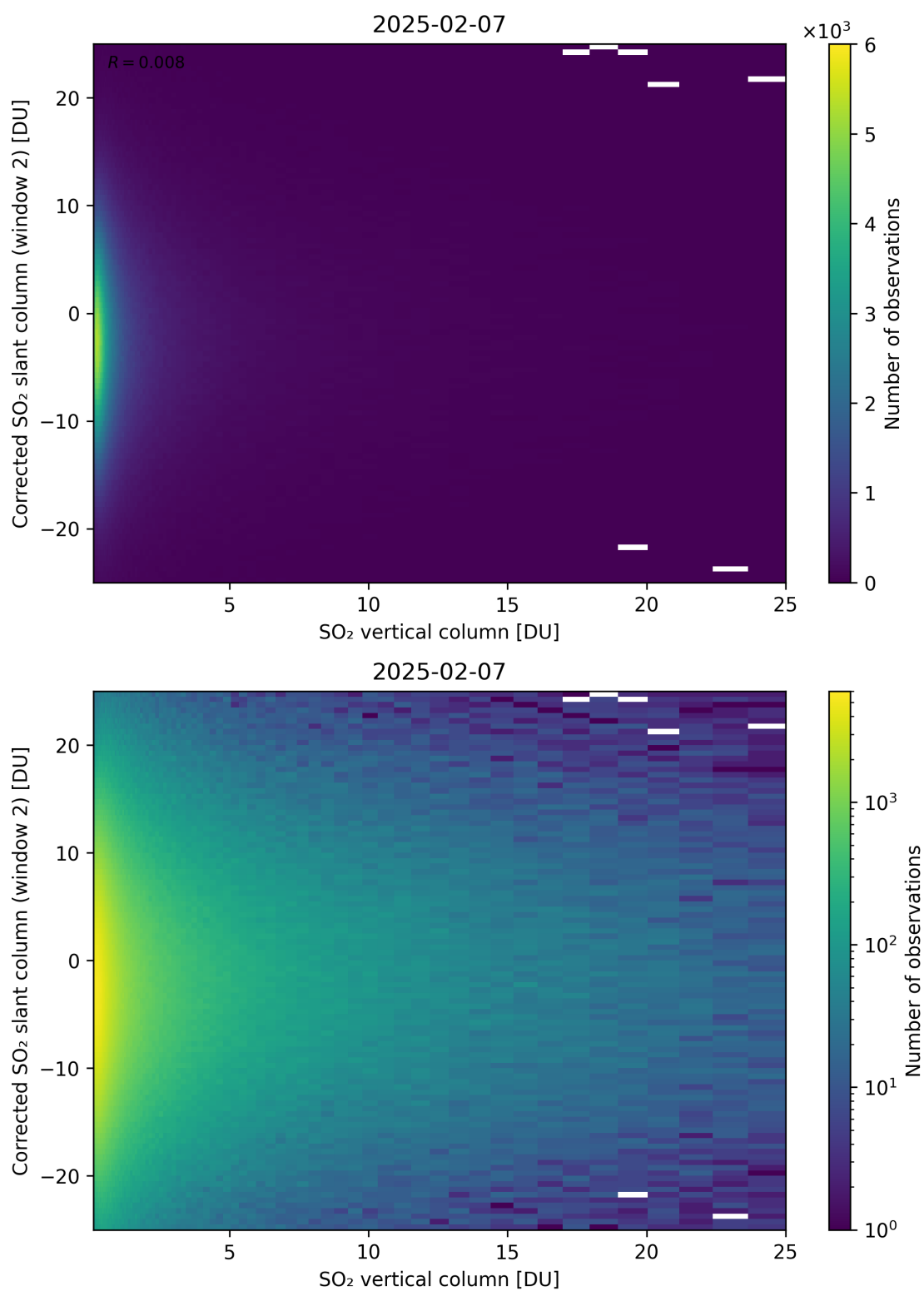
Figure 352: Scatter density plot of “SO 2 vertical column” against “Corrected SO 2 slant column (window 2)” for 2025-02-06 to 2025-02-08.
