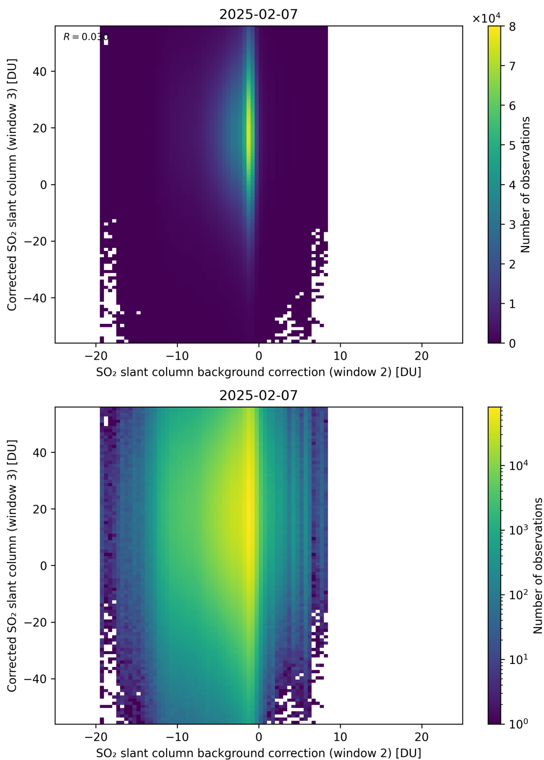
Figure 127: Scatter density plot of “SO 2 slant column background correction (window 2)” against “Corrected SO 2 slant column (window 3)” for 2025-02-06 to 2025-02-08.
