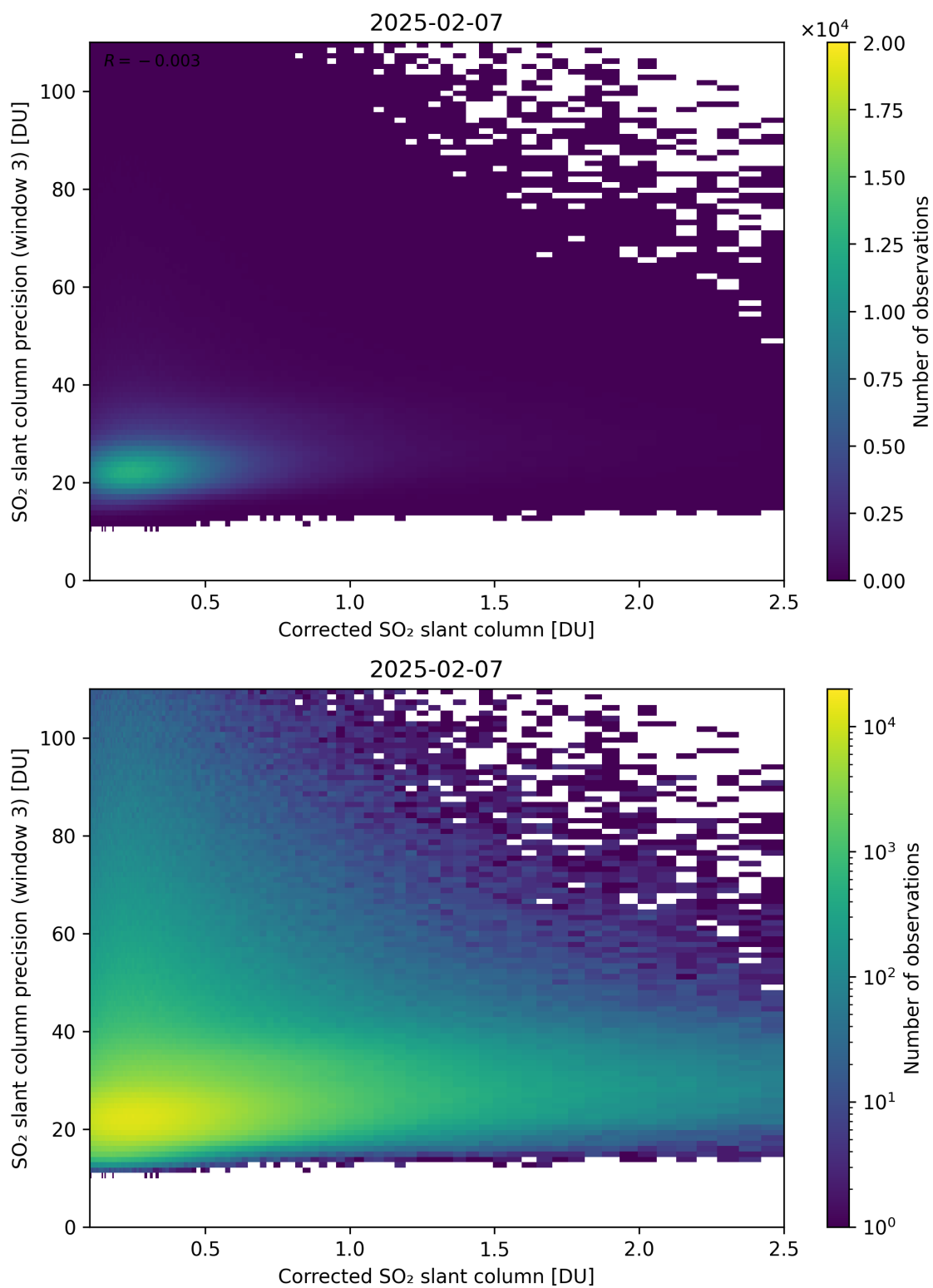
Figure 241: Scatter density plot of “Corrected SO 2 slant column” against “SO 2 slant column precision (window 3)” for 2025-02-06 to 2025-02-08.
