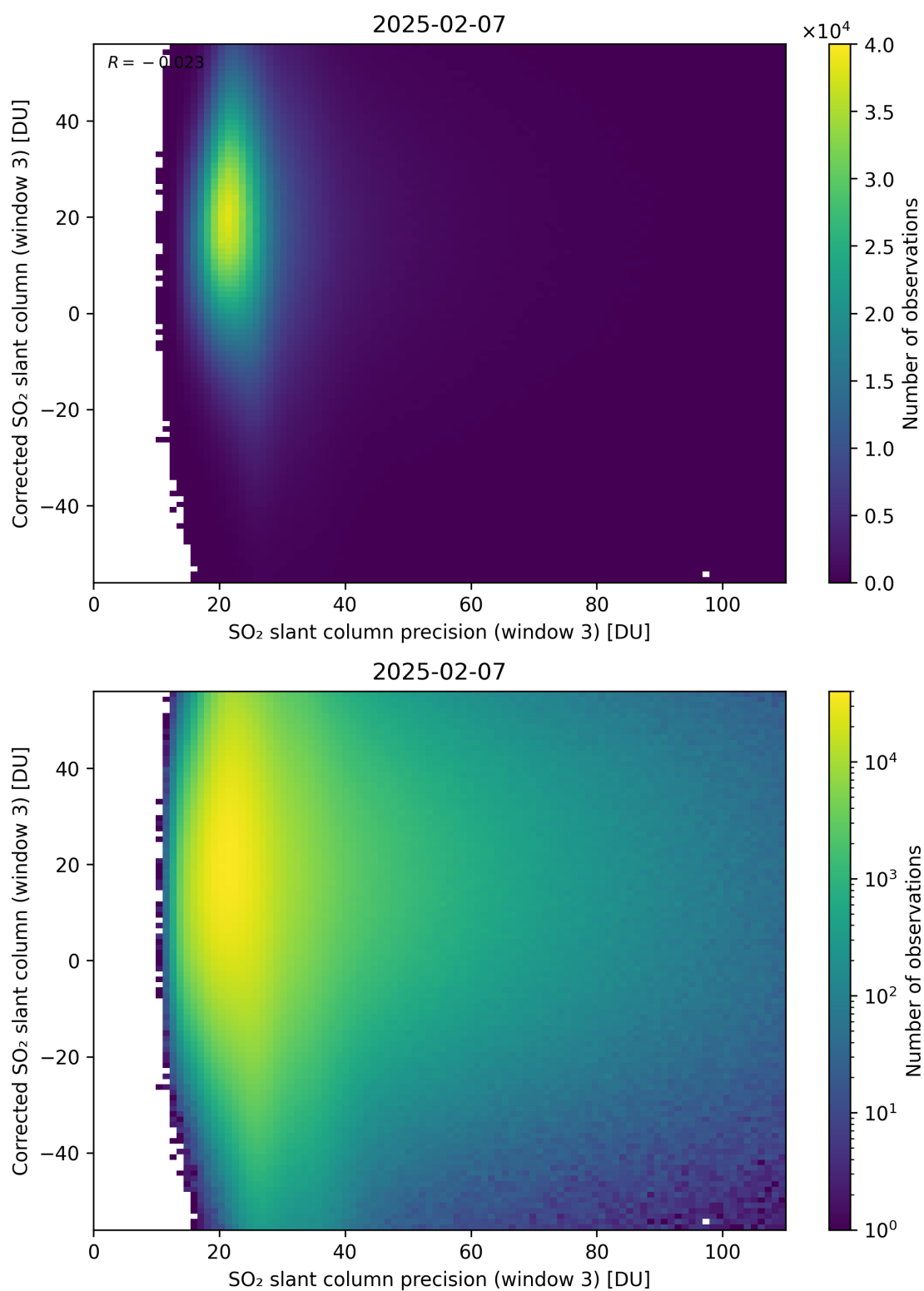
Figure 312: Scatter density plot of “SO 2 slant column precision (window 3)” against “Corrected SO 2 slant column (window 3)” for 2025-02-06 to 2025-02-08.
