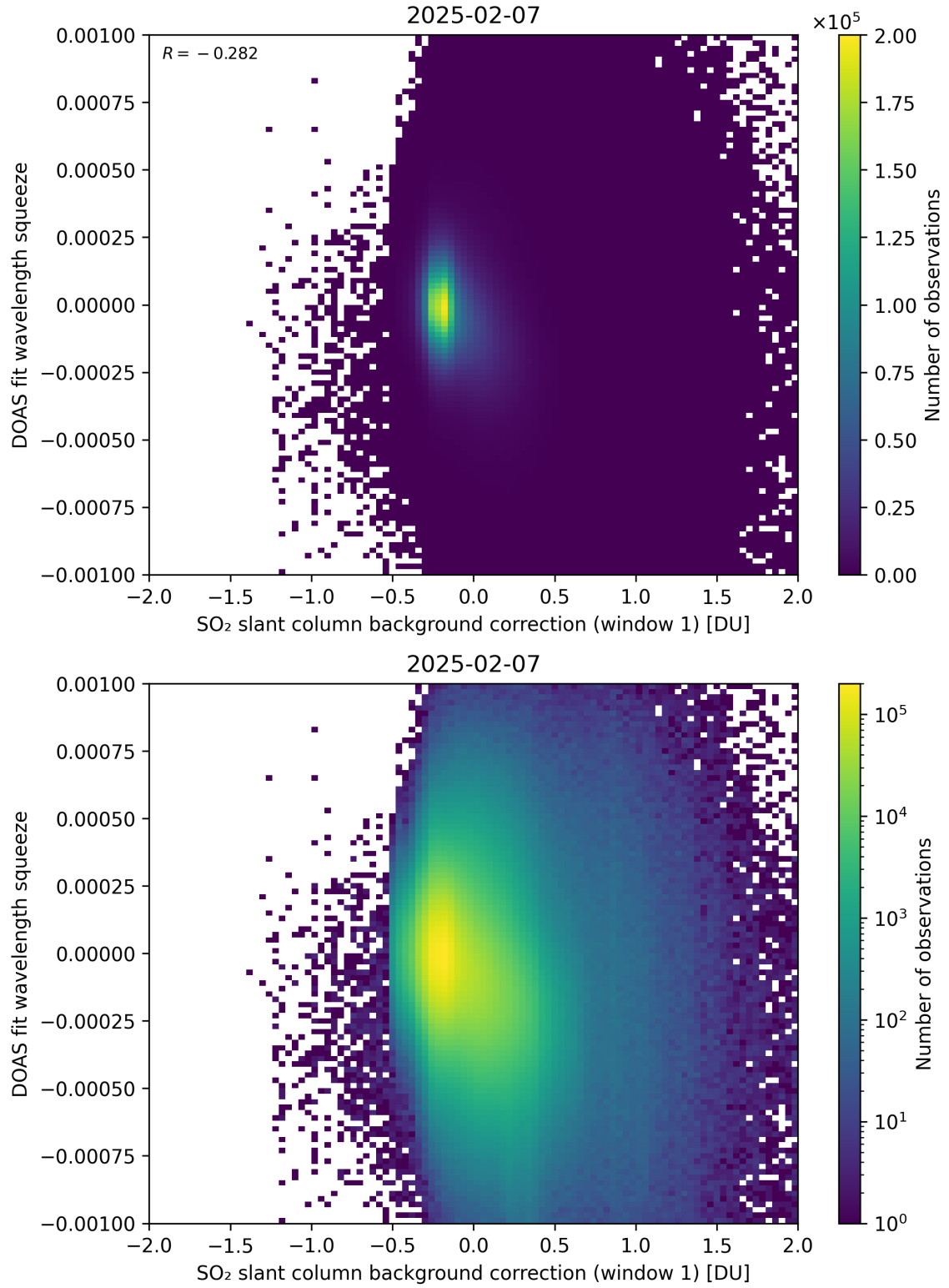
Figure 112: Scatter density plot of “SO 2 slant column background correction (window 1)” against “DOAS fit wavelength squeeze” for 2025-02-06 to 2025-02-08.
