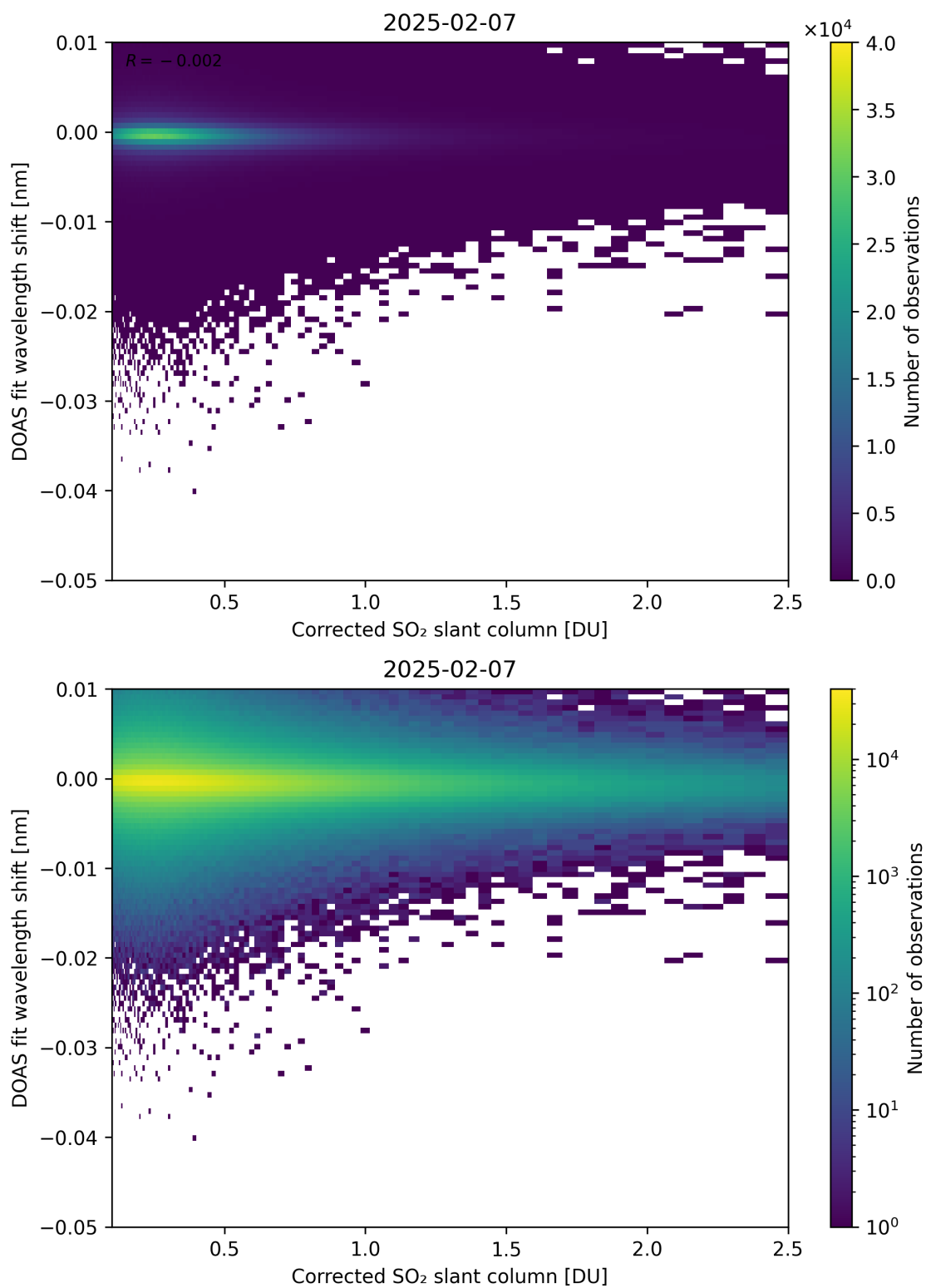
Figure 229: Scatter density plot of “Corrected SO 2 slant column” against “DOAS fit wavelength shift” for 2025-02-06 to 2025-02-08.
