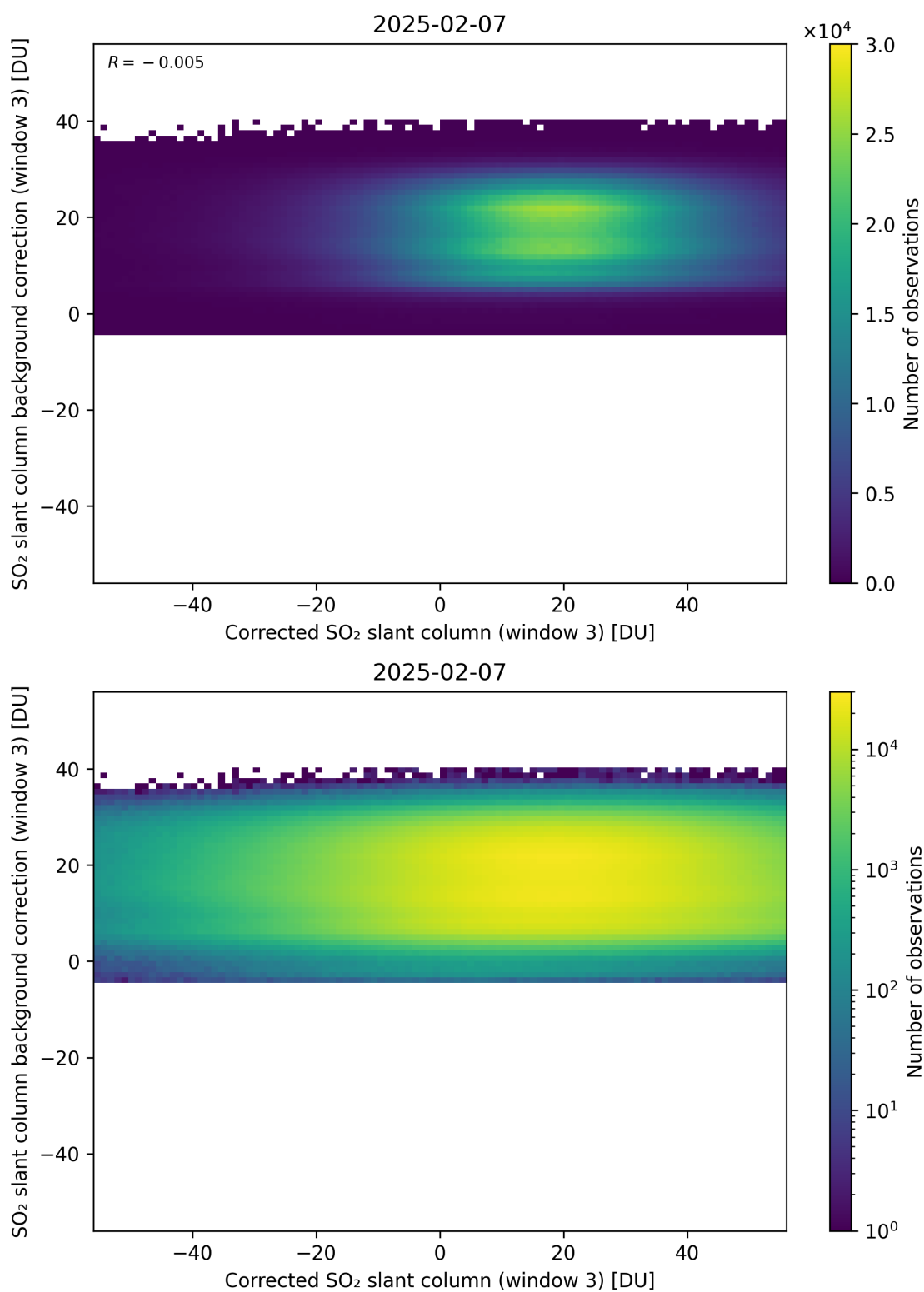
Figure 255: Scatter density plot of “Corrected SO 2 slant column (window 3)” against “SO 2 slant column background correction (window 3)” for 2025-02-06 to 2025-02-08.
