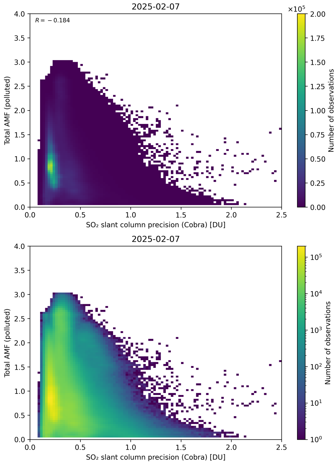
Figure 213: Scatter density plot of “SO 2 slant column precision (Cobra)” against “Total AMF (polluted)” for 2025-02-06 to 2025-02-08.
