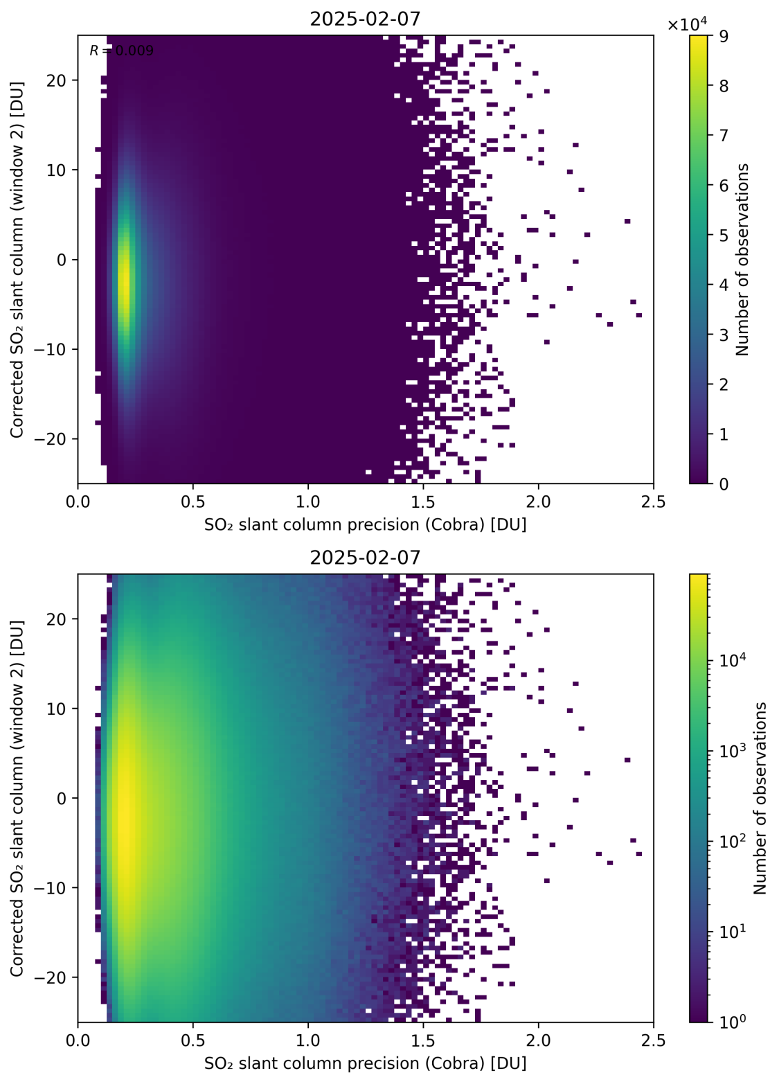
Figure 206: Scatter density plot of “SO 2 slant column precision (Cobra)” against “Corrected SO 2 slant column (window 2)” for 2025-02-06 to 2025-02-08.
