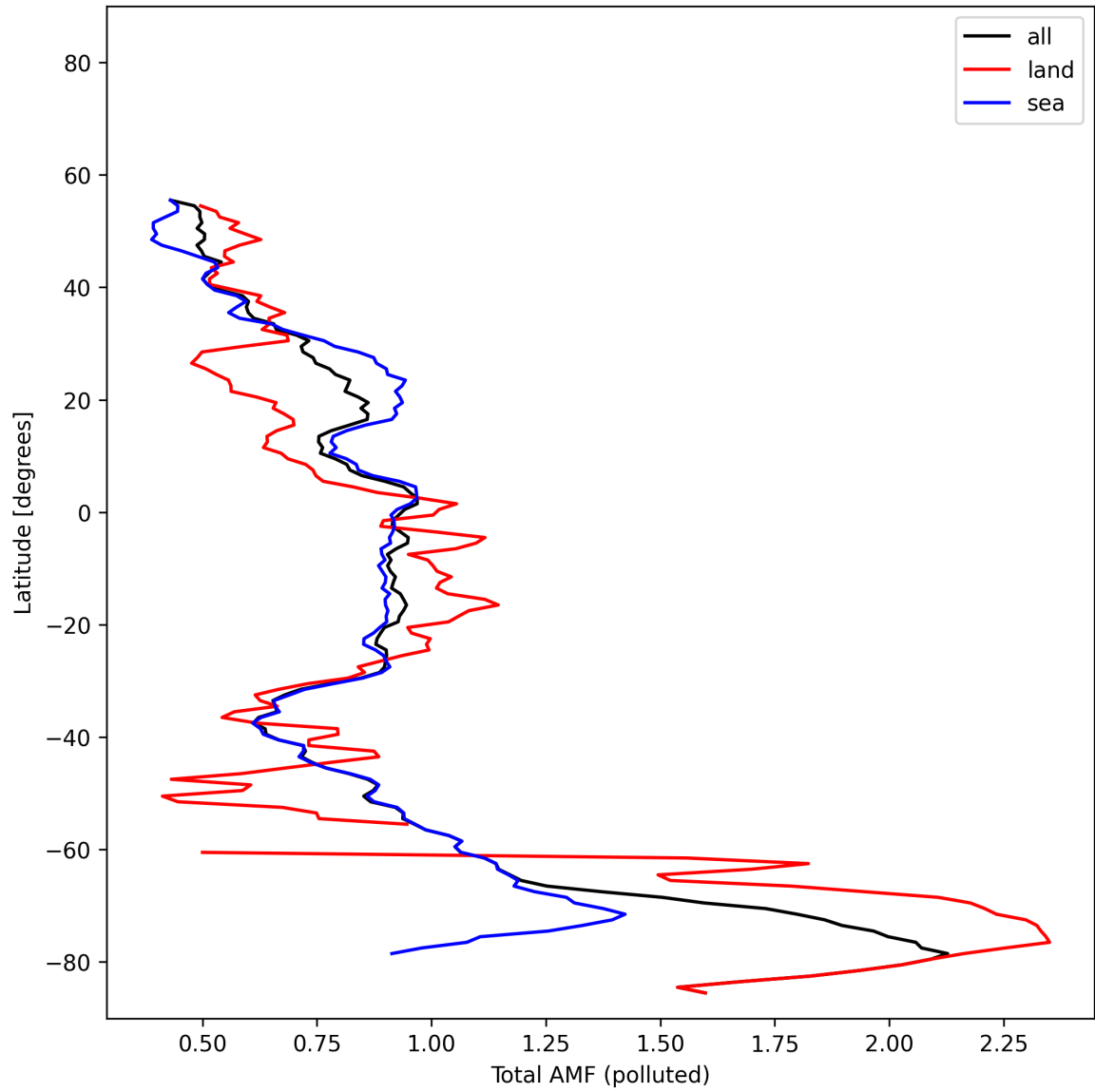
Figure 53: Zonal average of “Total AMF (polluted)” for 2025-02-06 to 2025-02-08.
