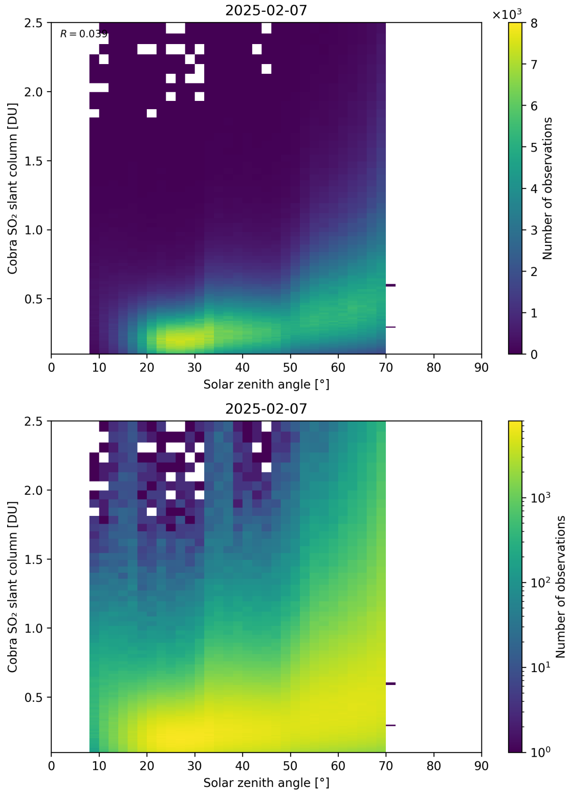
Figure 179: Scatter density plot of “Solar zenith angle” against “Cobra SO 2 slant column” for 2025-02-06 to 2025-02-08.
