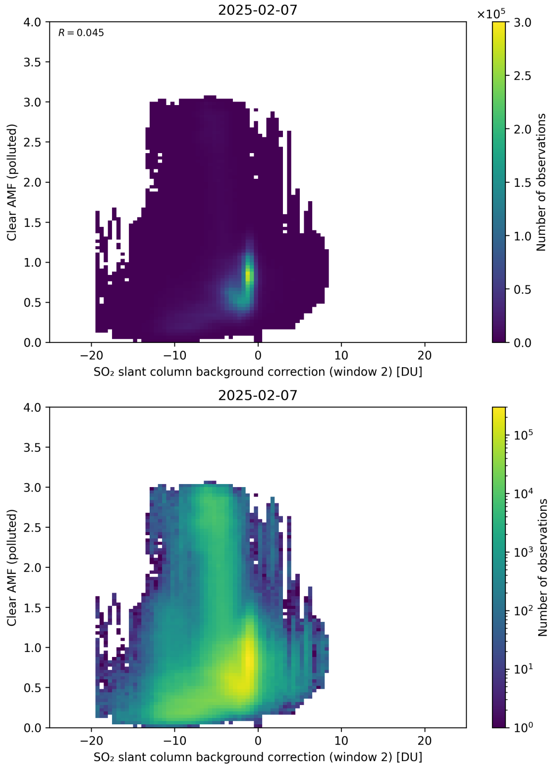
Figure 126: Scatter density plot of “SO 2 slant column background correction (window 2)” against “Clear AMF (polluted)” for 2025-02-06 to 2025-02-08.
