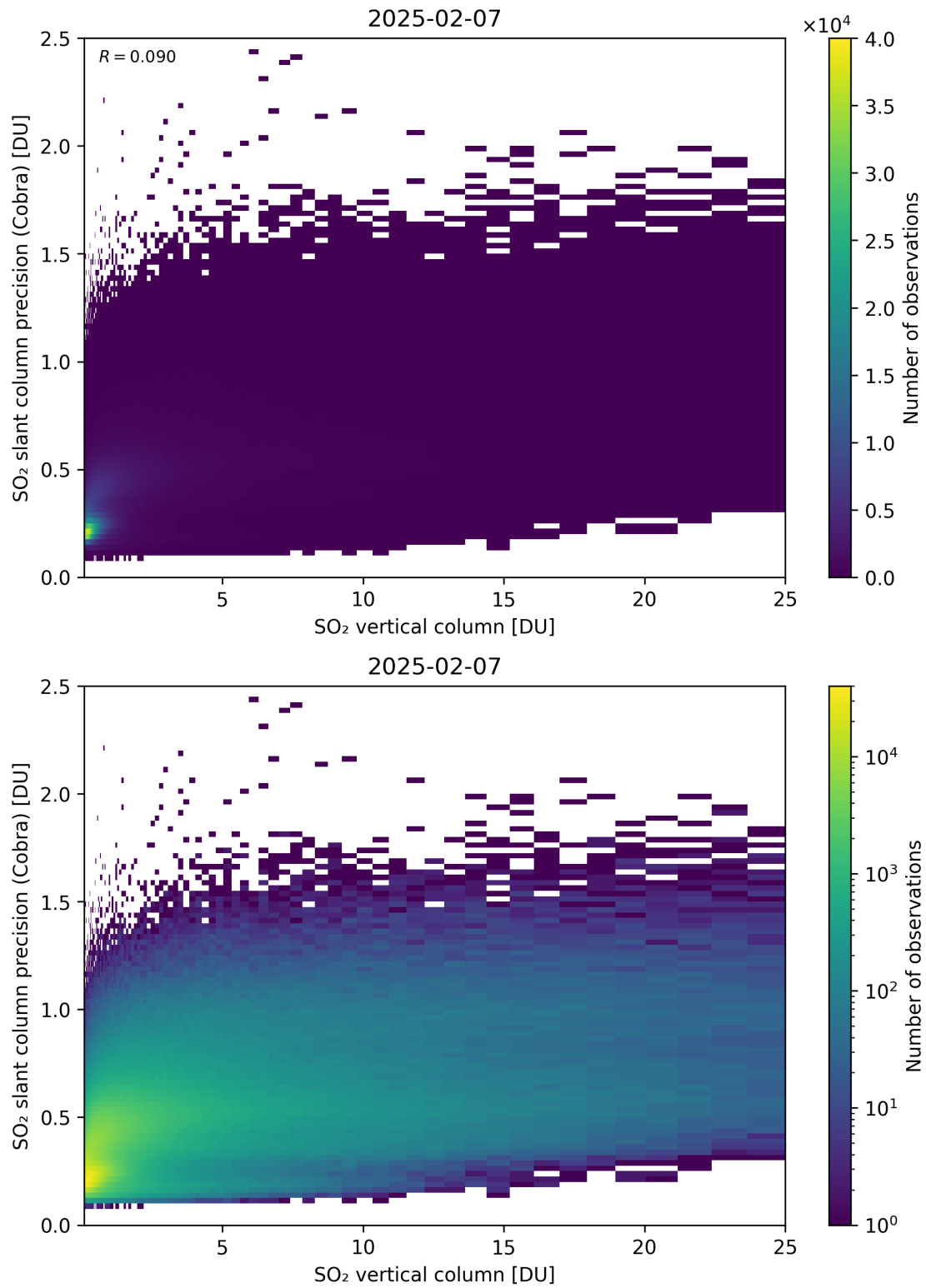
Figure 350: Scatter density plot of “SO 2 vertical column” against “SO 2 slant column precision (Cobra)” for 2025-02-06 to 2025-02-08.
