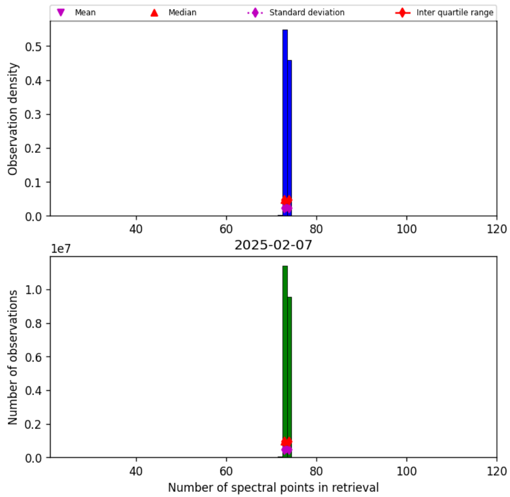
Figure 82: Histogram of “Number of spectral points in retrieval” for 2025-02-06 to 2025-02-08
