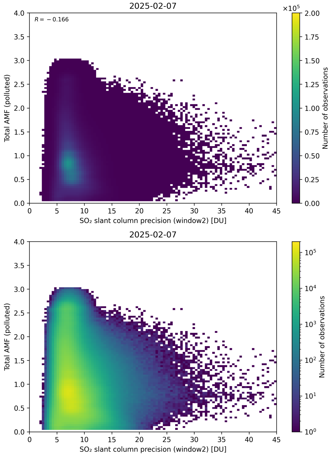
Figure 301: Scatter density plot of “SO 2 slant column precision (window2)” against “Total AMF (polluted)” for 2025-02-06 to 2025-02-08.
