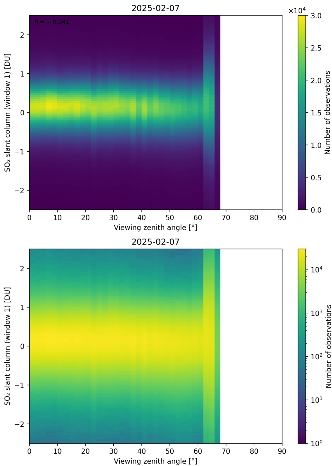
Figure 376: Scatter density plot of “Viewing zenith angle” against “SO 2 slant column (window 1)” for 2025-02-06 to 2025-02-08.
