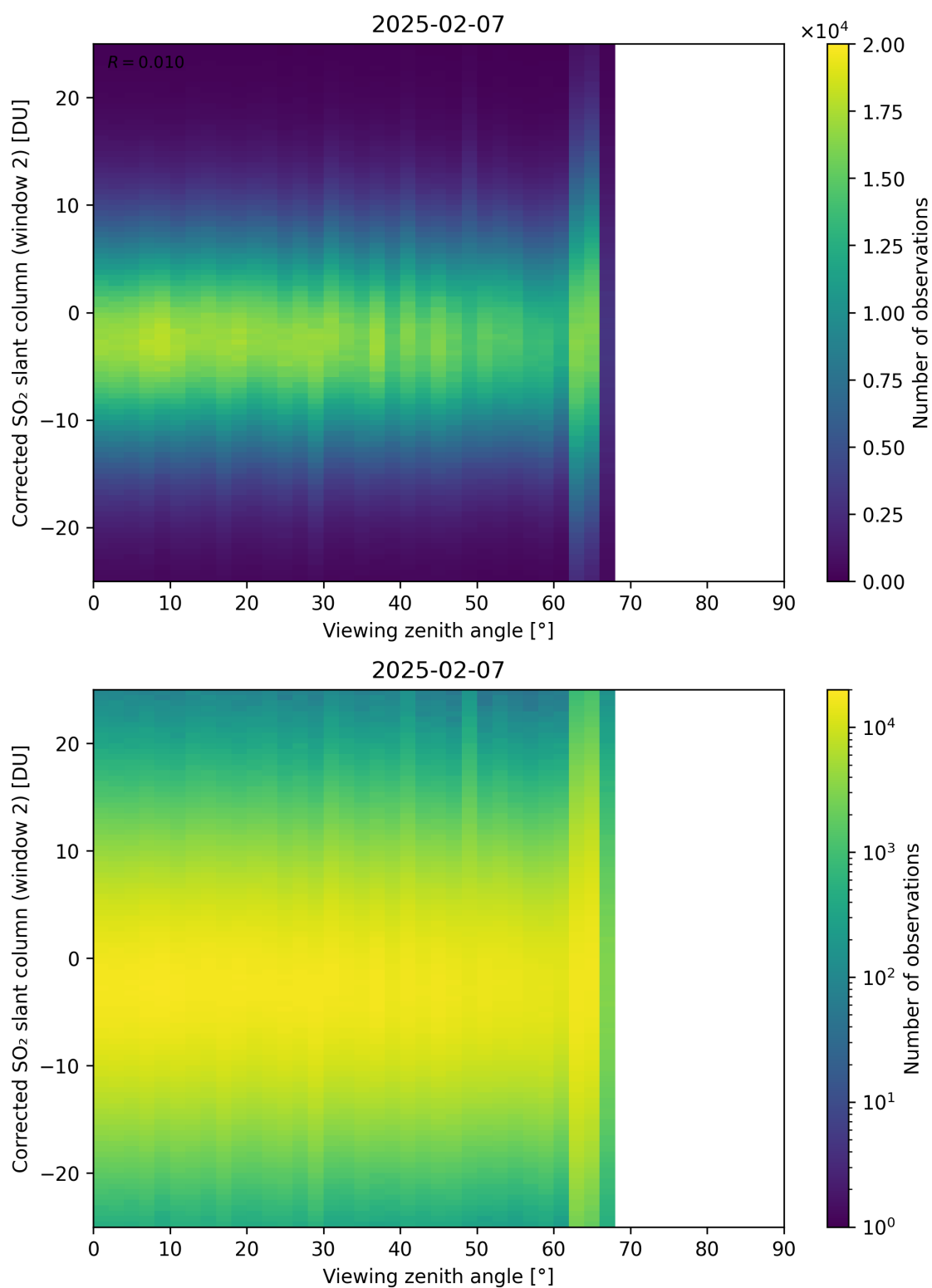
Figure 374: Scatter density plot of “Viewing zenith angle” against “Corrected SO 2 slant column (window 2)” for 2025-02-06 to 2025-02-08.
