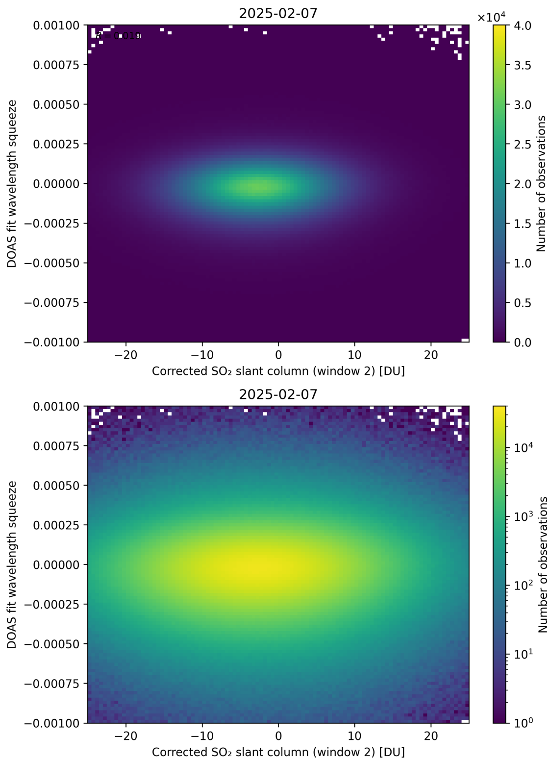
Figure 247: Scatter density plot of “Corrected SO 2 slant column (window 2)” against “DOAS fit wavelength squeeze” for 2025-02-06 to 2025-02-08.
