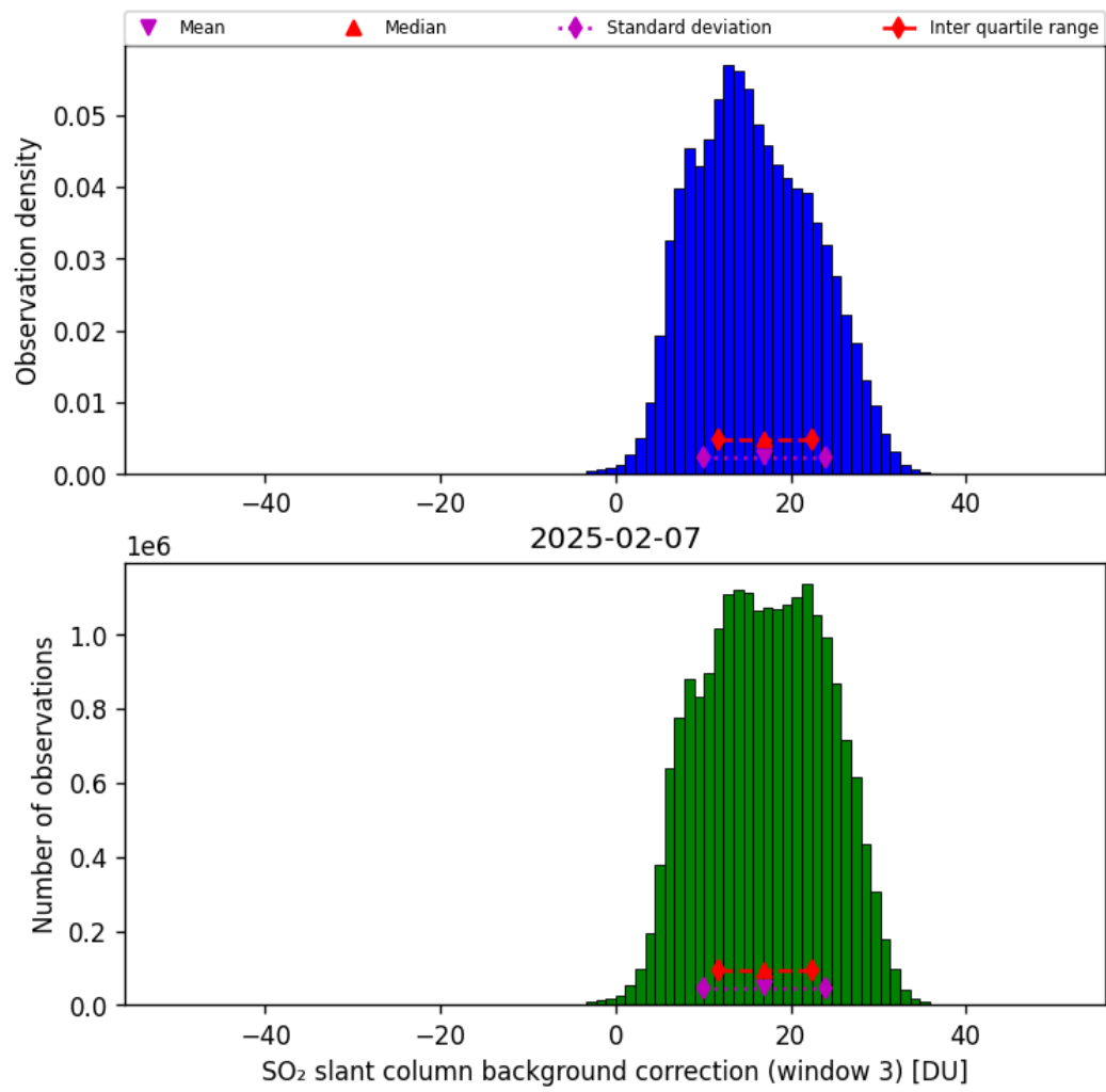
Figure 74: Histogram of “SO 2 slant column background correction (window 3)” for 2025-02-06 to 2025-02-08
