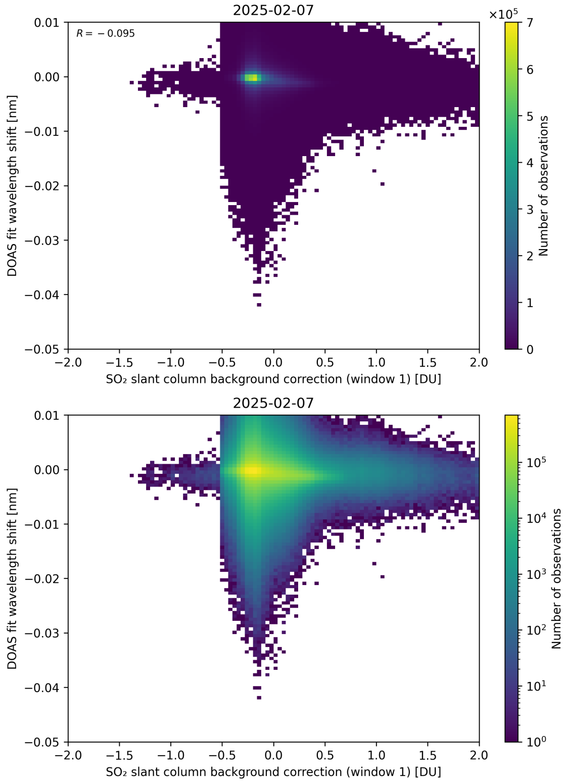
Figure 111: Scatter density plot of “SO 2 slant column background correction (window 1)” against “DOAS fit wavelength shift” for 2025-02-06 to 2025-02-08.
