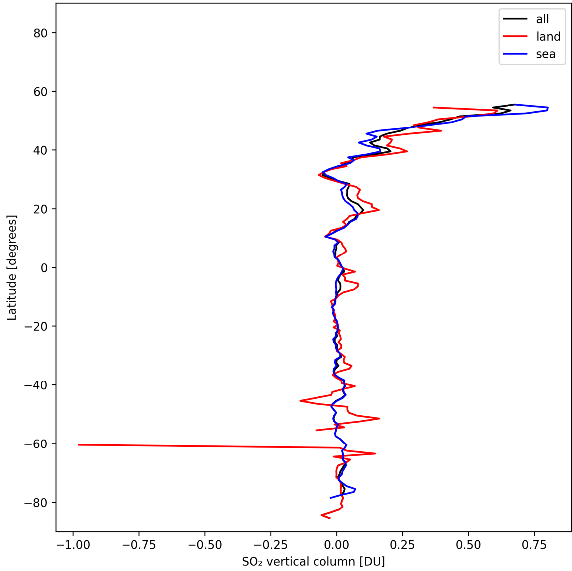
Figure 32: Zonal average of “SO 2 vertical column” for 2025-02-06 to 2025-02-08.
