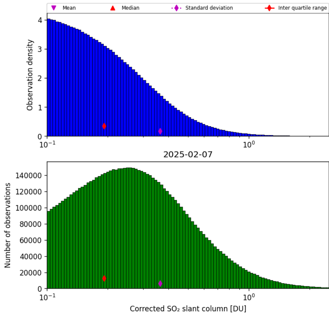
Figure 60: Histogram of “Corrected SO 2 slant column” for 2025-02-06 to 2025-02-08
