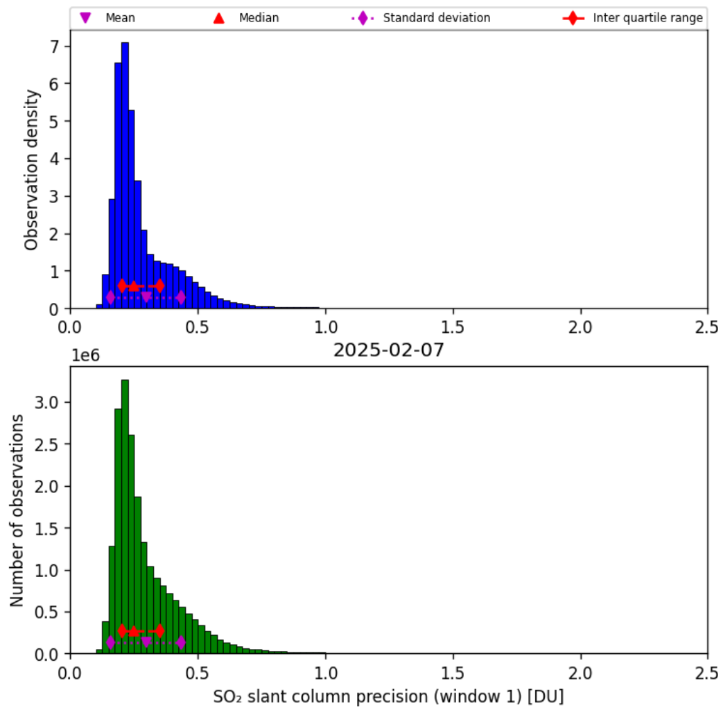
Figure 64: Histogram of “SO 2 slant column precision (window 1)” for 2025-02-06 to 2025-02-08
