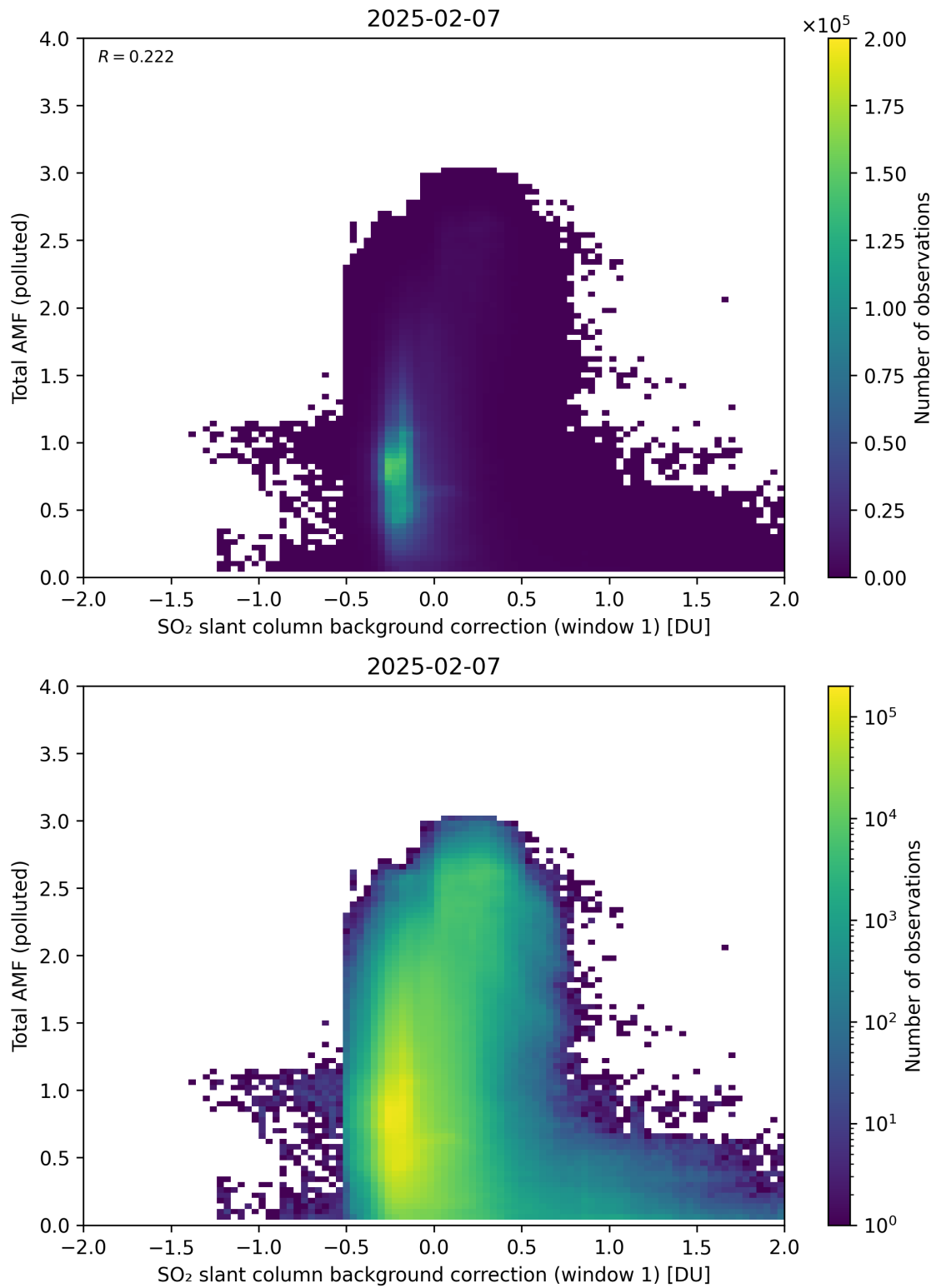
Figure 120: Scatter density plot of “SO 2 slant column background correction (window 1)” against “Total AMF (polluted)” for 2025-02-06 to 2025-02-08.
