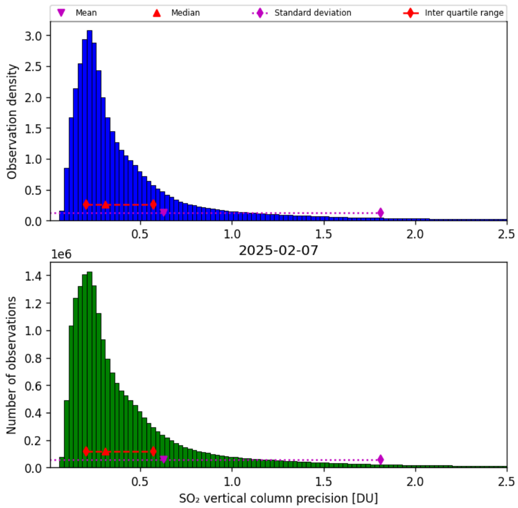
Figure 59: Histogram of “SO 2 vertical column precision” for 2025-02-06 to 2025-02-08
