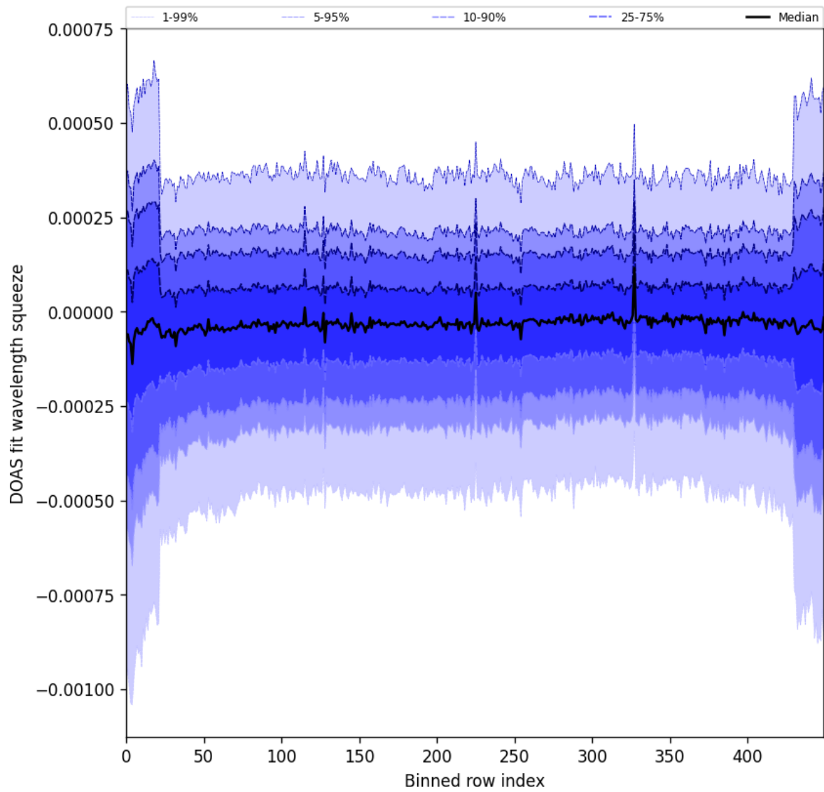
Figure 103: Along track statistics of “DOAS fit wavelength squeeze” for 2025-02-06 to 2025-02-08
