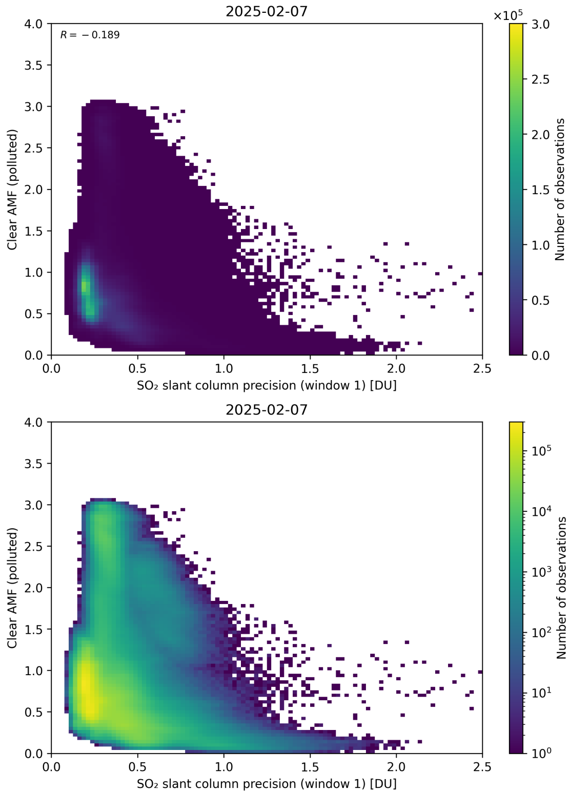
Figure 274: Scatter density plot of “SO 2 slant column precision (window 1)” against “Clear AMF (polluted)” for 2025-02-06 to 2025-02-08.
