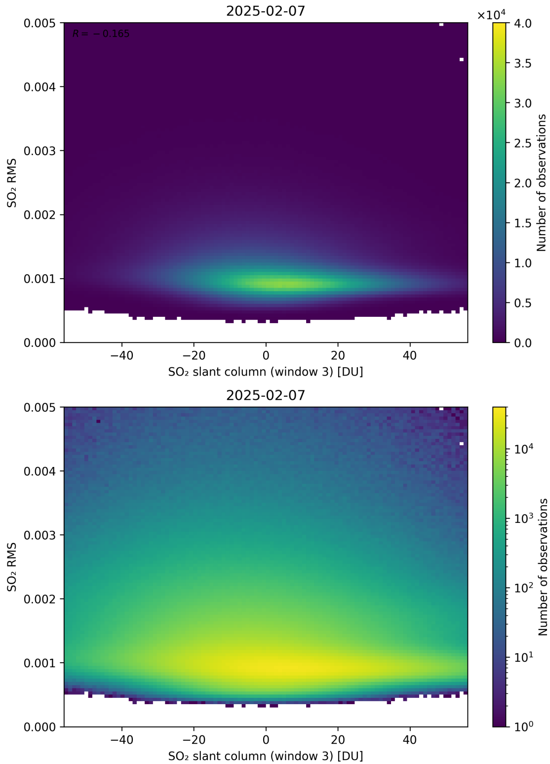
Figure 306: Scatter density plot of “SO 2 slant column (window 3)” against “SO 2 RMS” for 2025-02-06 to 2025-02-08.
