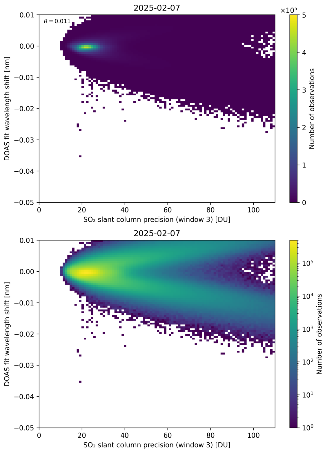
Figure 308: Scatter density plot of “SO 2 slant column precision (window 3)” against “DOAS fit wavelength shift” for 2025-02-06 to 2025-02-08.
