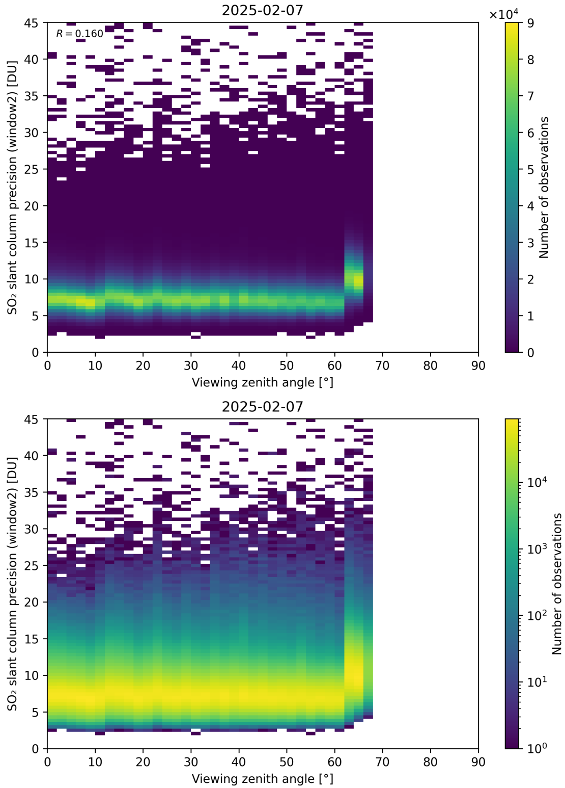
Figure 378: Scatter density plot of “Viewing zenith angle” against “SO 2 slant column precision (window2)” for 2025-02-06 to 2025-02-08.
