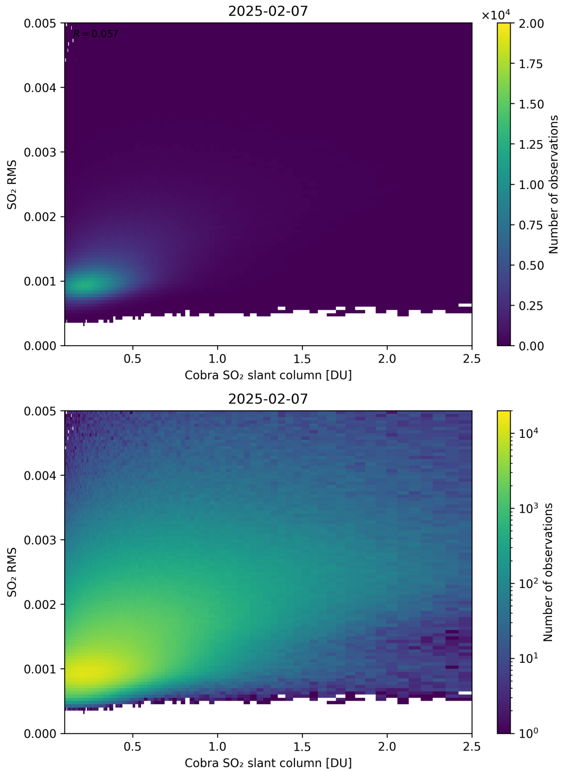
Figure 198: Scatter density plot of “Cobra SO 2 slant column” against “SO 2 RMS” for 2025-02-06 to 2025-02-08.
