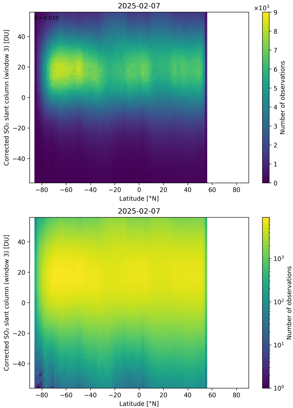
Figure 161: Scatter density plot of “Latitude” against “Corrected SO 2 slant column (window 3)” for 2025-02-06 to 2025-02-08.
