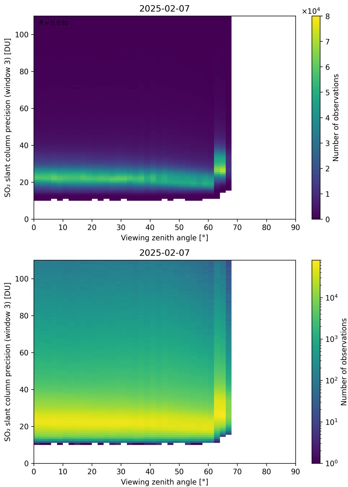
Figure 380: Scatter density plot of “Viewing zenith angle” against “SO 2 slant column precision (window 3)” for 2025-02-06 to 2025-02-08.
