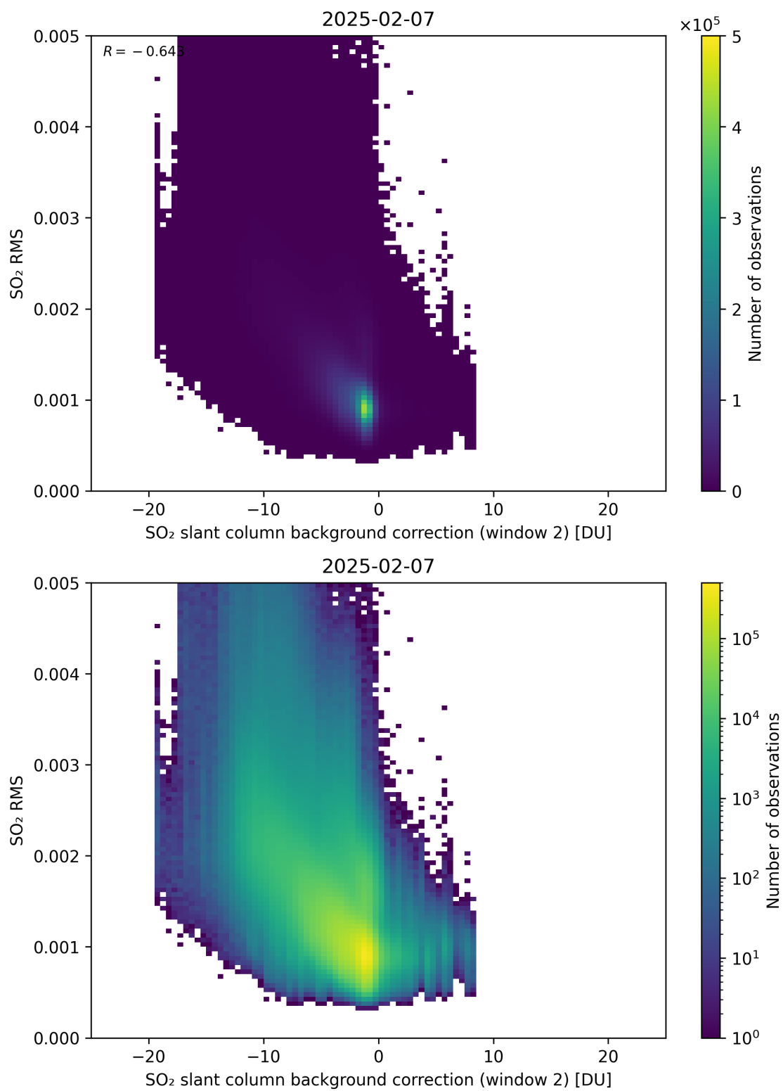
Figure 125: Scatter density plot of “SO 2 slant column background correction (window 2)” against “SO 2 RMS” for 2025-02-06 to 2025-02-08.
