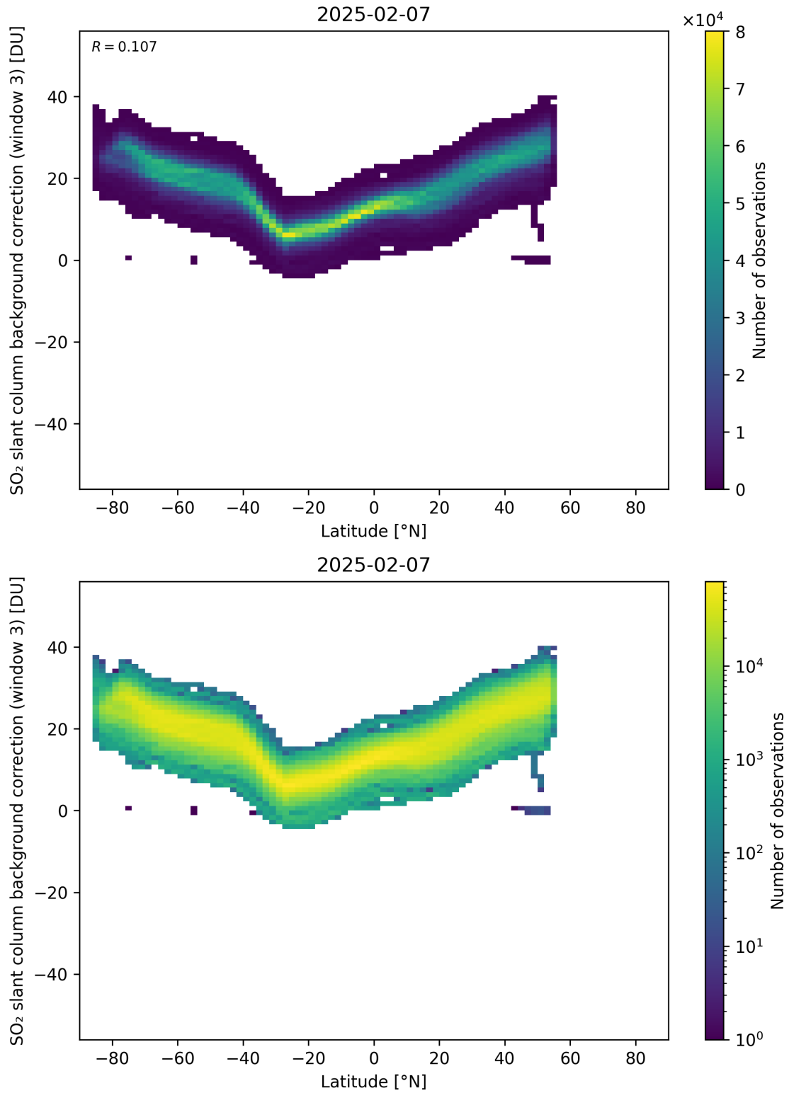
Figure 152: Scatter density plot of “Latitude” against “SO 2 slant column background correction (window 3)” for 2025-02-06 to 2025-02-08.
