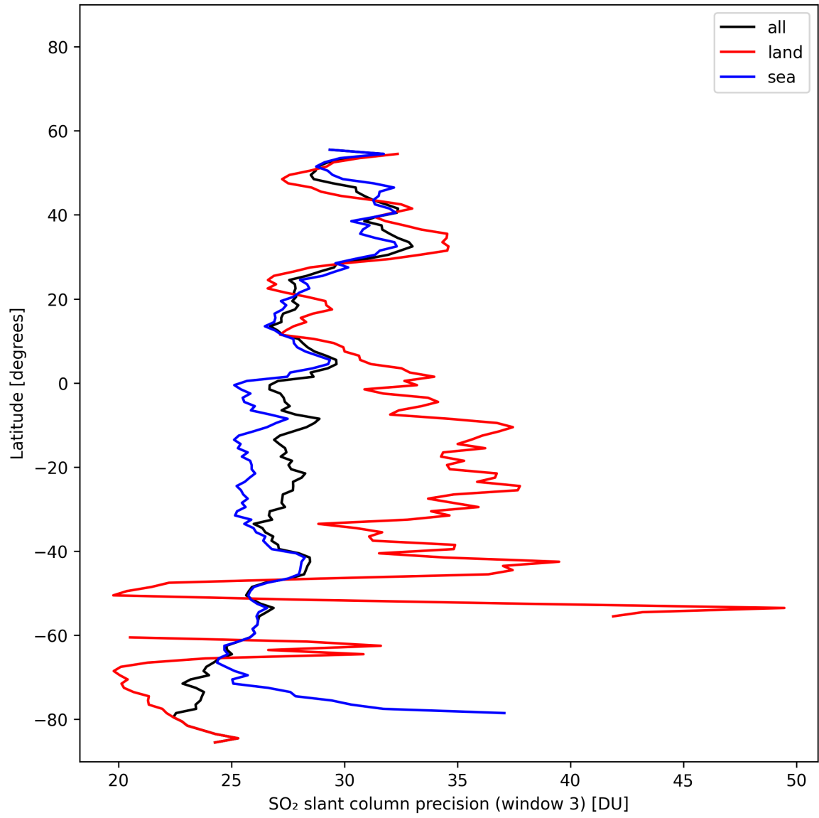
Figure 46: Zonal average of “SO 2 slant column precision (window 3)” for 2025-02-06 to 2025-02-08.
