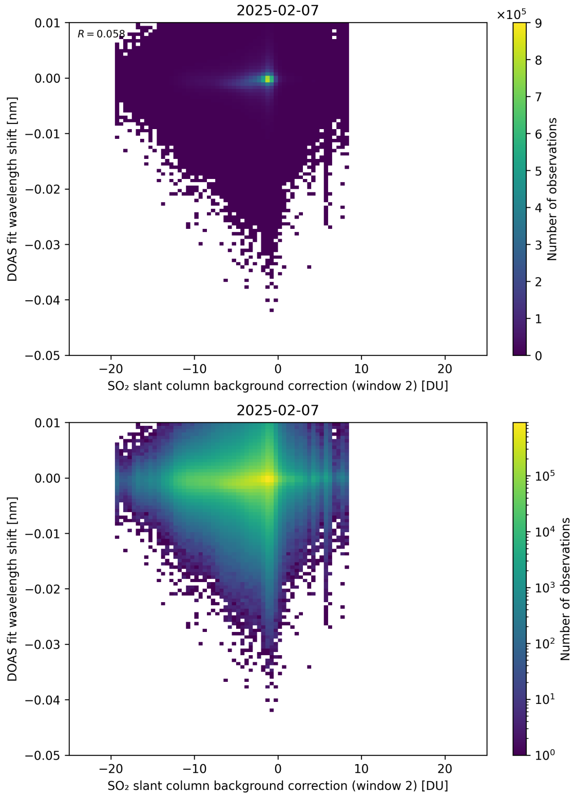
Figure 123: Scatter density plot of “SO 2 slant column background correction (window 2)” against “DOAS fit wavelength shift” for 2025-02-06 to 2025-02-08.
