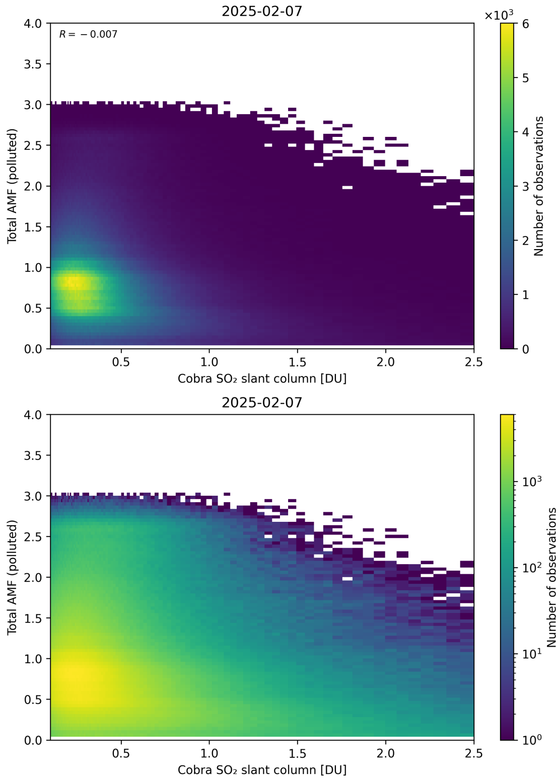
Figure 224: Scatter density plot of “Cobra SO 2 slant column” against “Total AMF (polluted)” for 2025-02-06 to 2025-02-08.
