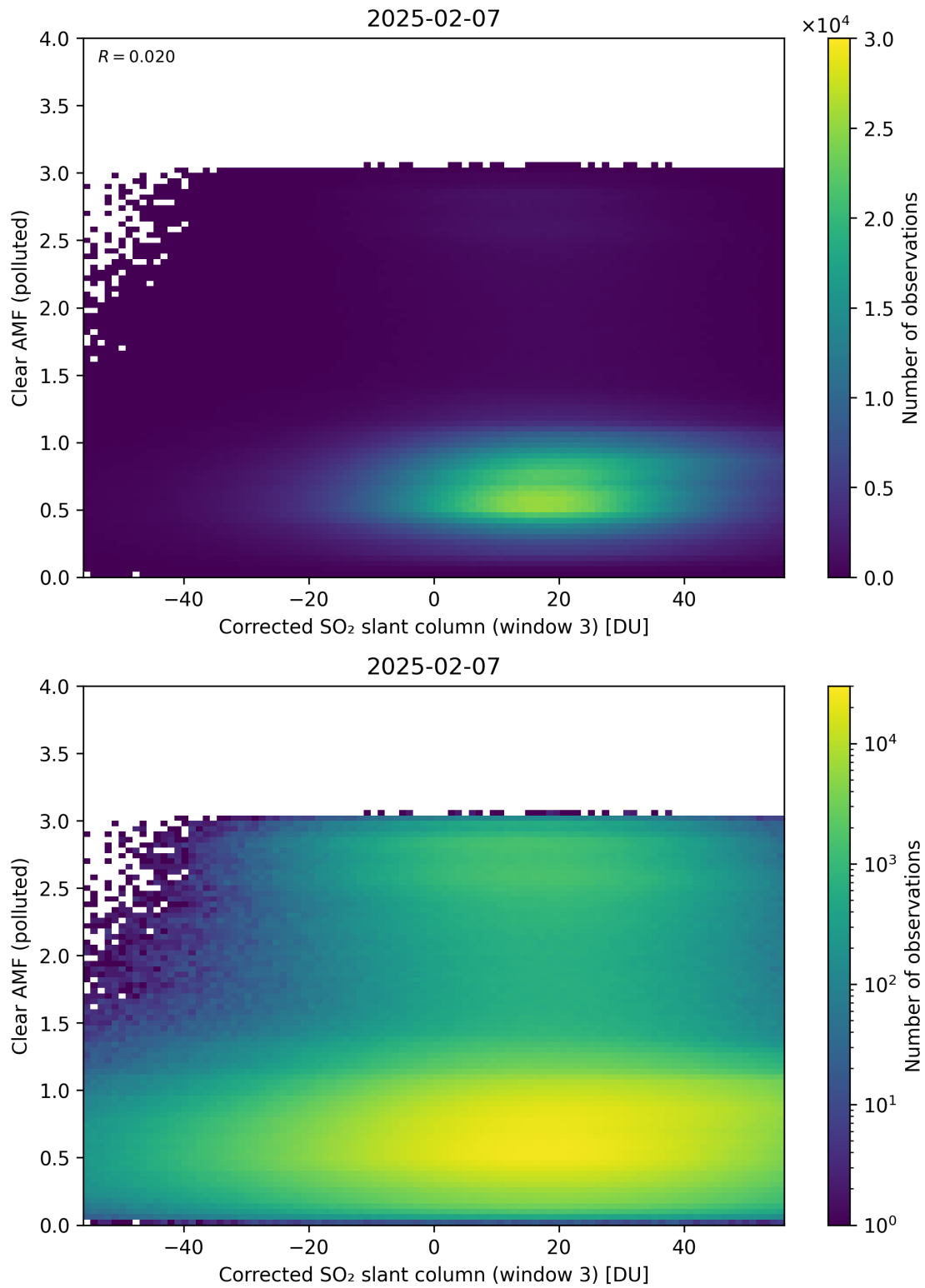
Figure 259: Scatter density plot of “Corrected SO 2 slant column (window 3)” against “Clear AMF (polluted)” for 2025-02-06 to 2025-02-08.
