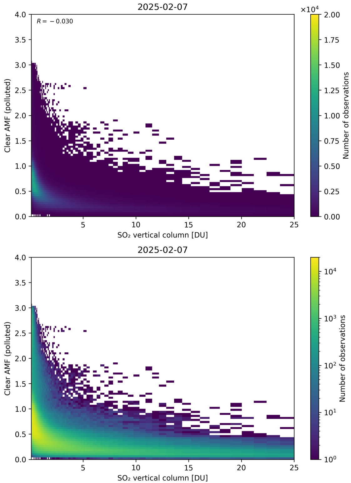
Figure 348: Scatter density plot of “SO 2 vertical column” against “Clear AMF (polluted)” for 2025-02-06 to 2025-02-08.
