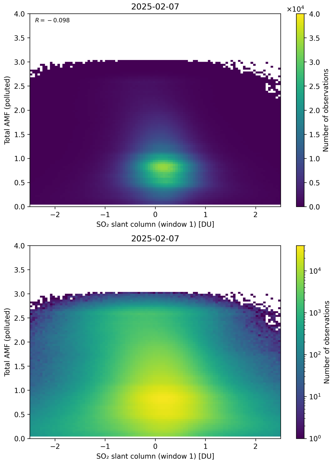
Figure 289: Scatter density plot of “SO 2 slant column (window 1)” against “Total AMF (polluted)” for 2025-02-06 to 2025-02-08.
