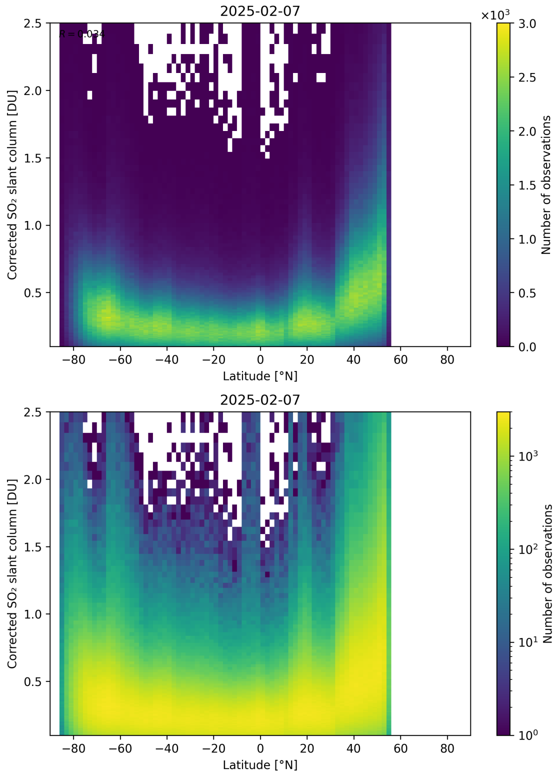
Figure 159: Scatter density plot of “Latitude” against “Corrected SO 2 slant column” for 2025-02-06 to 2025-02-08.
