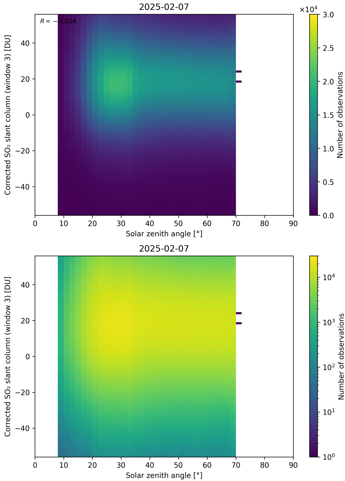
Figure 183: Scatter density plot of “Solar zenith angle” against “Corrected SO 2 slant column (window 3)” for 2025-02-06 to 2025-02-08.
