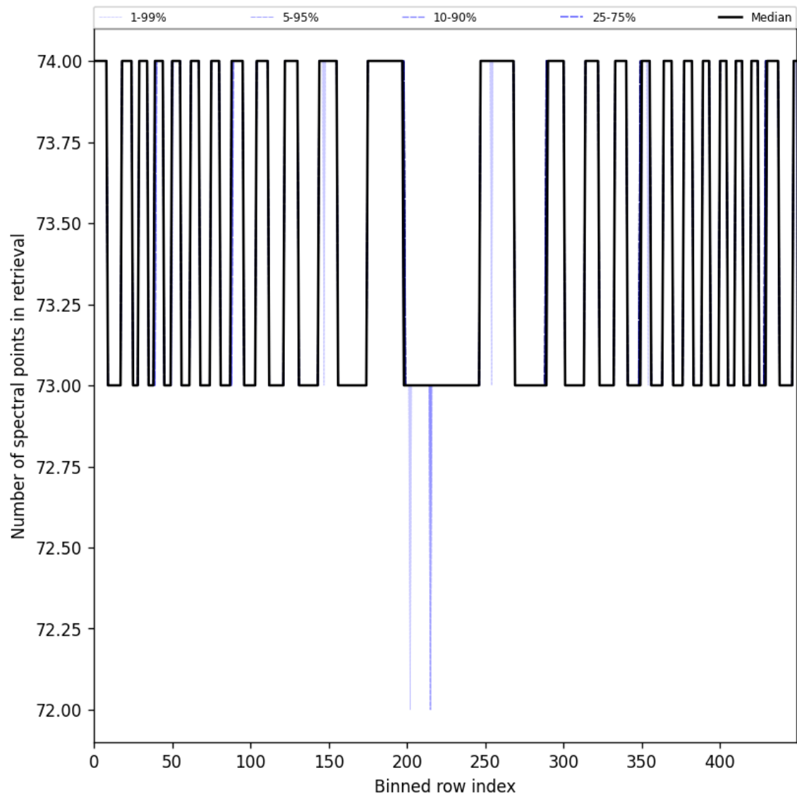
Figure 108: Along track statistics of “Number of spectral points in retrieval” for 2025-02-06 to 2025-02-08
