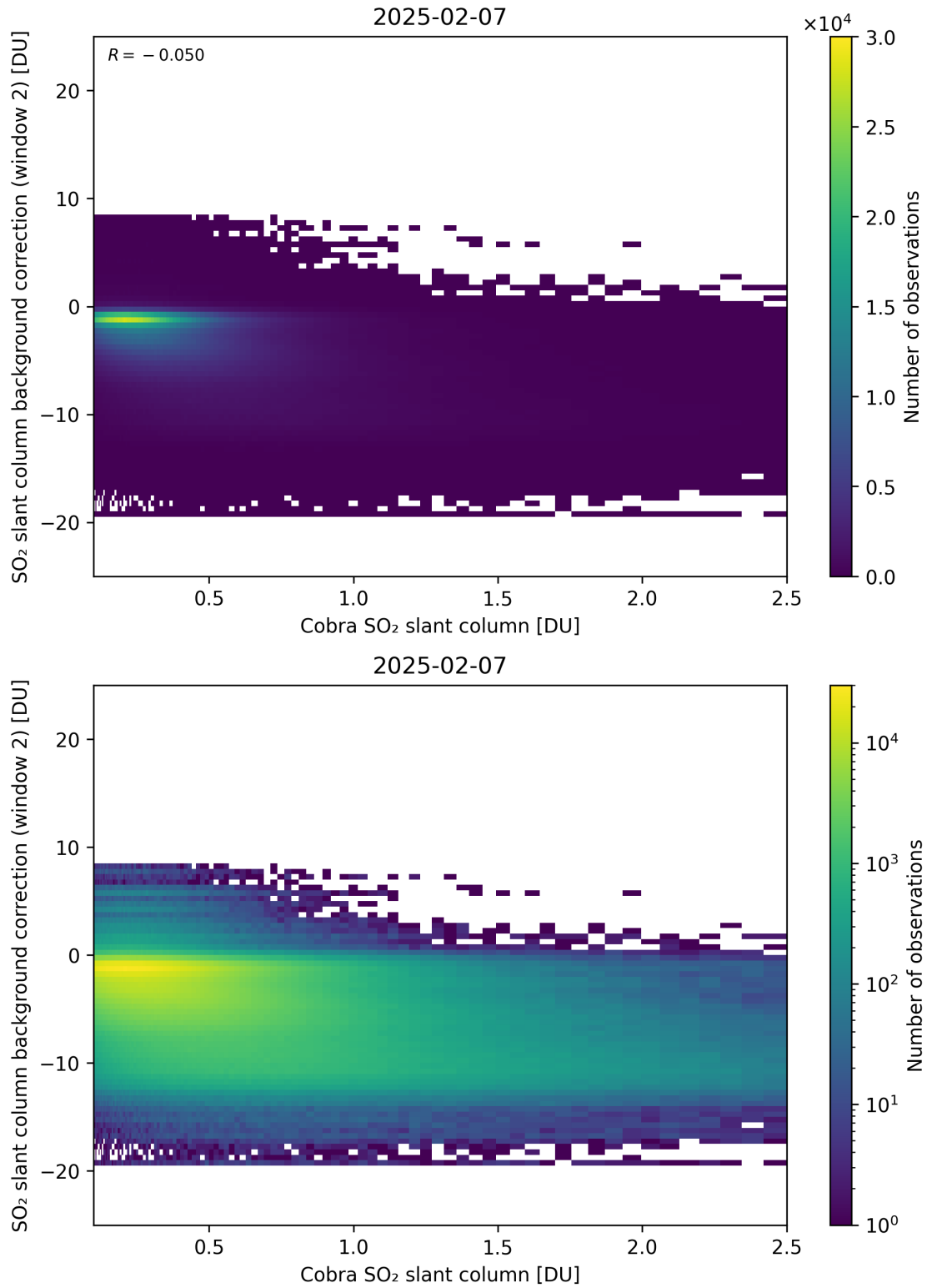
Figure 194: Scatter density plot of “Cobra SO 2 slant column” against “SO 2 slant column background correction (window 2)” for 2025-02-06 to 2025-02-08.
