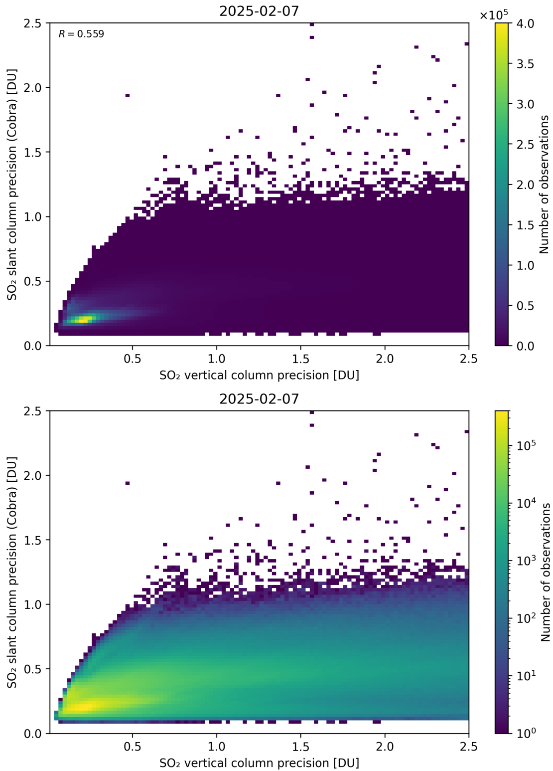
Figure 337: Scatter density plot of “SO 2 vertical column precision” against “SO 2 slant column precision (Cobra)” for 2025-02-06 to 2025-02-08.
