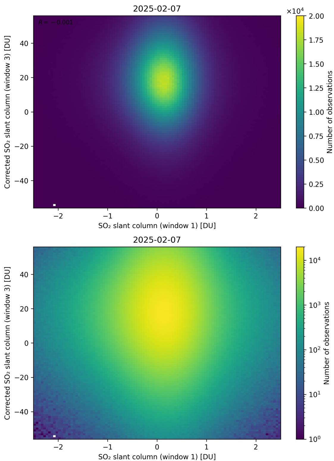
Figure 284: Scatter density plot of “SO 2 slant column (window 1)” against “Corrected SO 2 slant column (window 3)” for 2025-02-06 to 2025-02-08.
