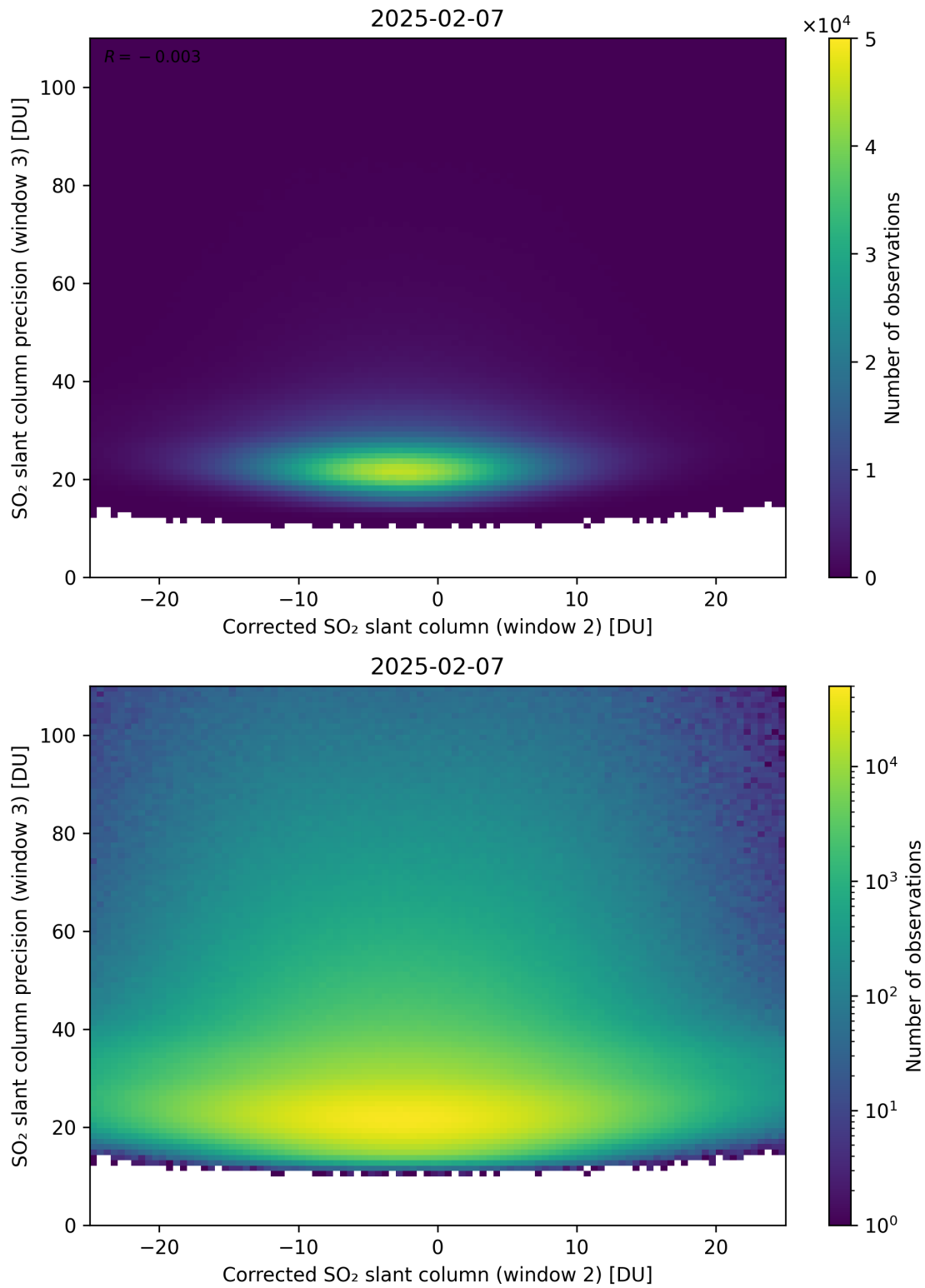
Figure 252: Scatter density plot of “Corrected SO 2 slant column (window 2)” against “SO 2 slant column precision (window 3)” for 2025-02-06 to 2025-02-08.
