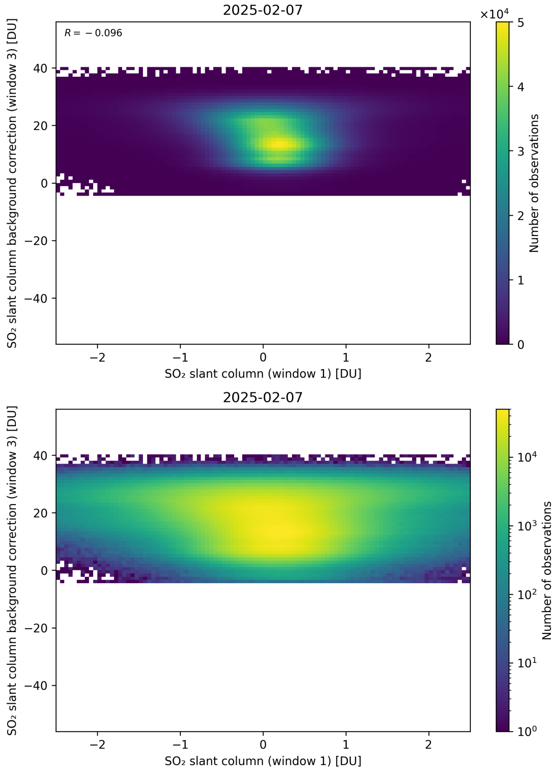
Figure 264: Scatter density plot of “SO 2 slant column (window 1)” against “SO 2 slant column background correction (window 3)” for 2025-02-06 to 2025-02-08.
