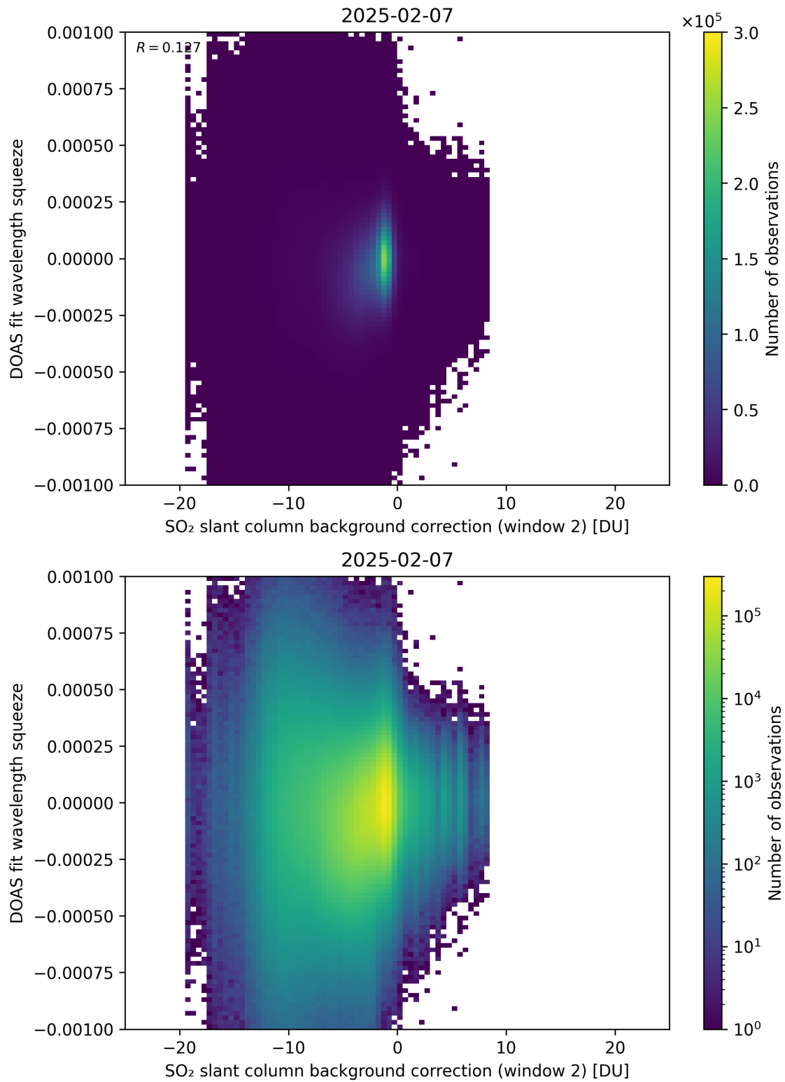
Figure 124: Scatter density plot of “SO 2 slant column background correction (window 2)” against “DOAS fit wavelength squeeze” for 2025-02-06 to 2025-02-08.
