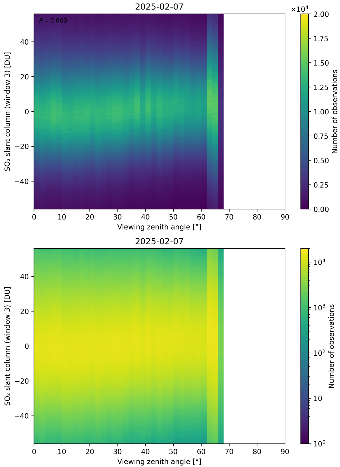
Figure 379: Scatter density plot of “Viewing zenith angle” against “SO 2 slant column (window 3)” for 2025-02-06 to 2025-02-08.
