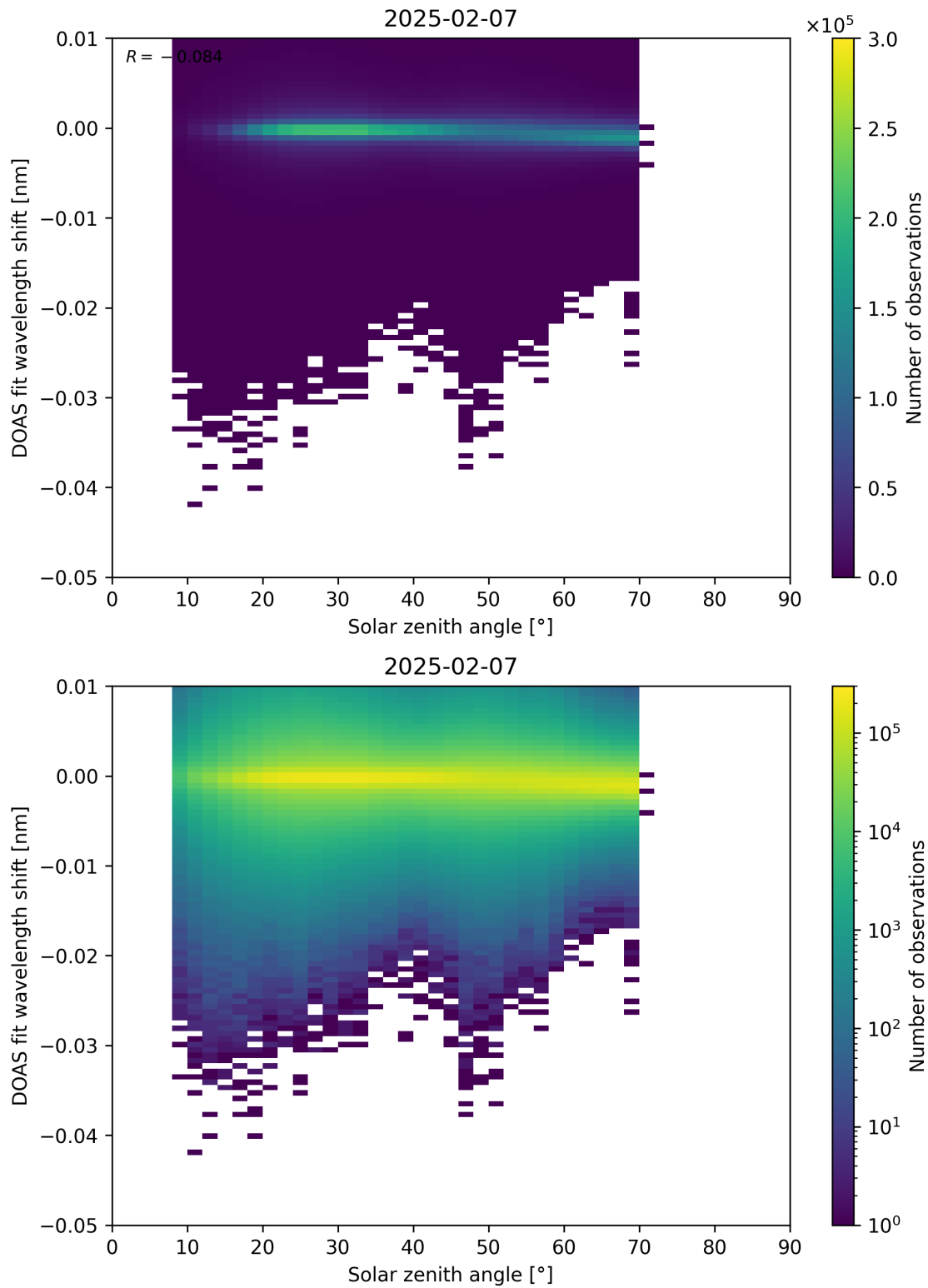
Figure 174: Scatter density plot of “Solar zenith angle” against “DOAS fit wavelength shift” for 2025-02-06 to 2025-02-08.
