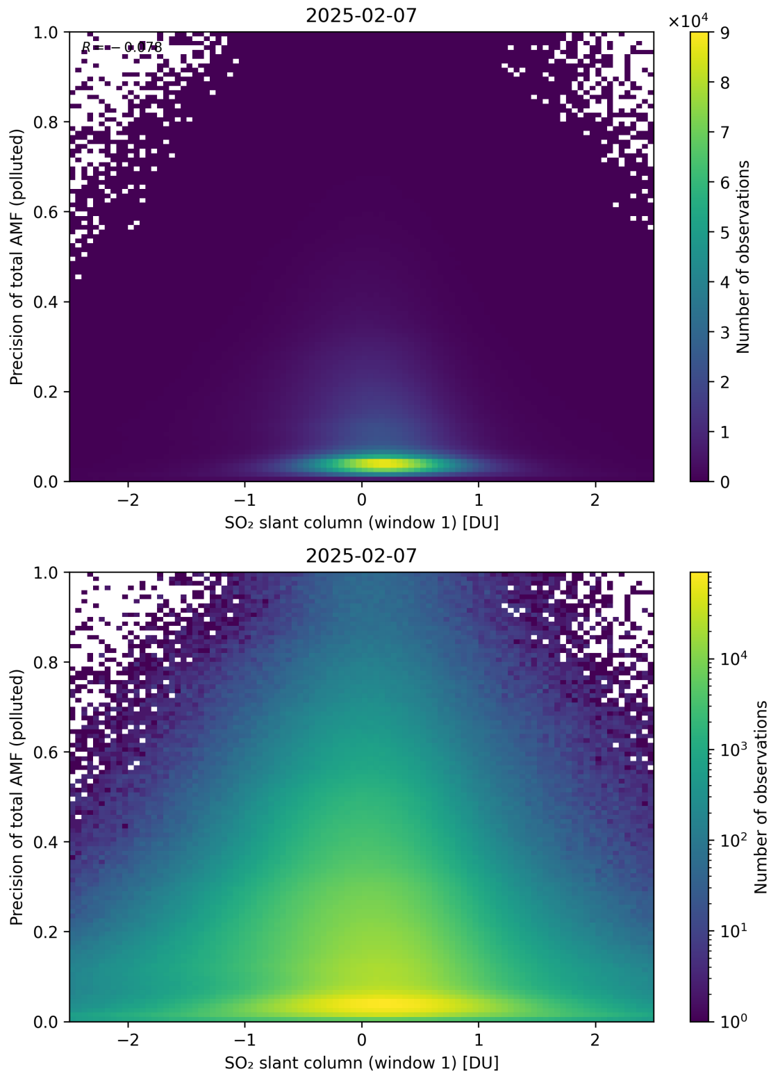
Figure 290: Scatter density plot of “SO 2 slant column (window 1)” against “Precision of total AMF (polluted)” for 2025-02-06 to 2025-02-08.
