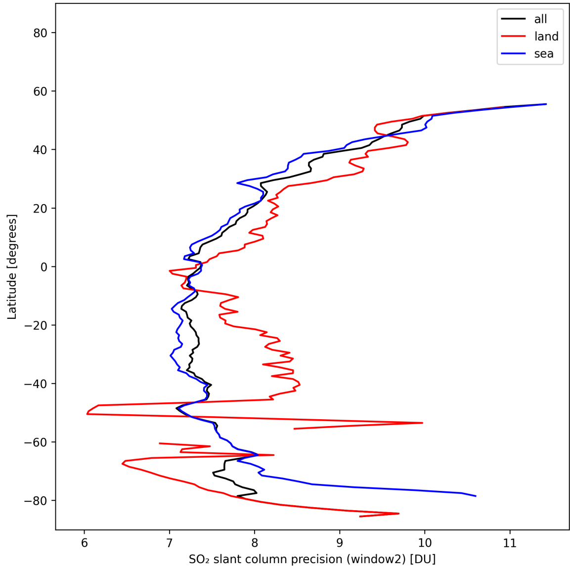
Figure 42: Zonal average of “SO 2 slant column precision (window2)” for 2025-02-06 to 2025-02-08.
