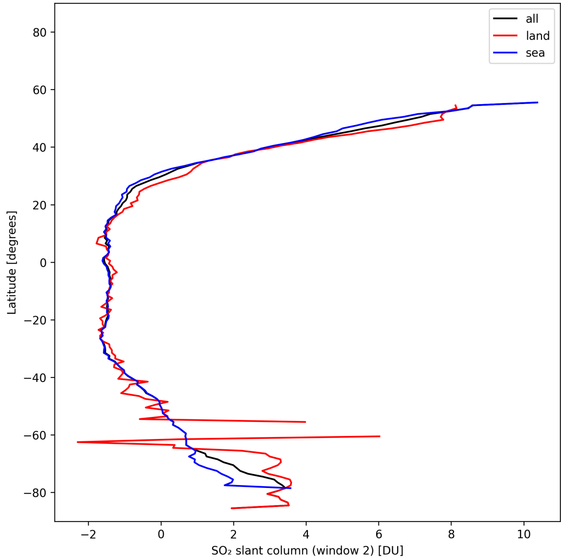
Figure 41: Zonal average of “SO 2 slant column (window 2)” for 2025-02-06 to 2025-02-08.
