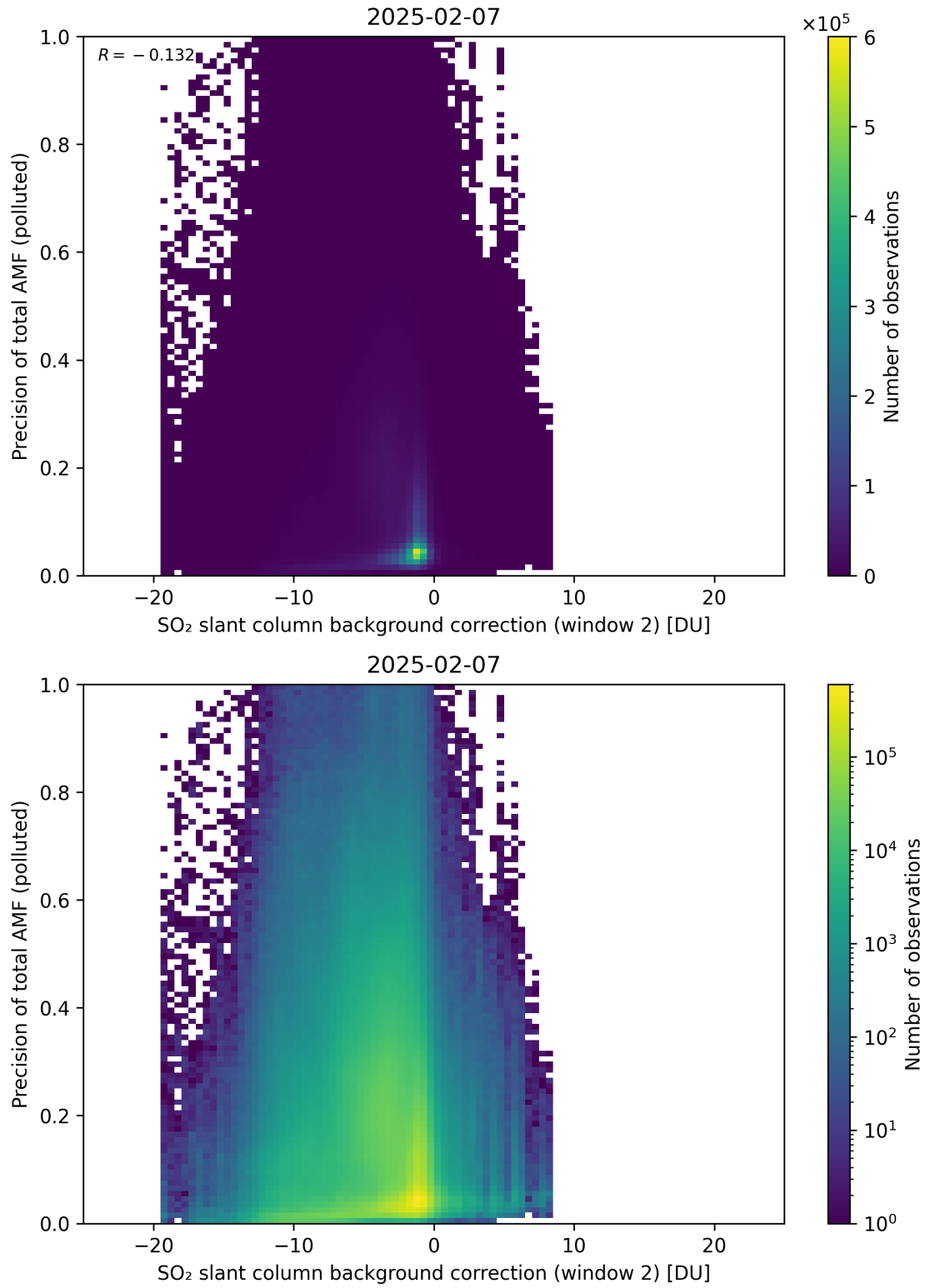
Figure 131: Scatter density plot of “SO 2 slant column background correction (window 2)” against “Precision of total AMF (polluted)” for 2025-02-06 to 2025-02-08.
