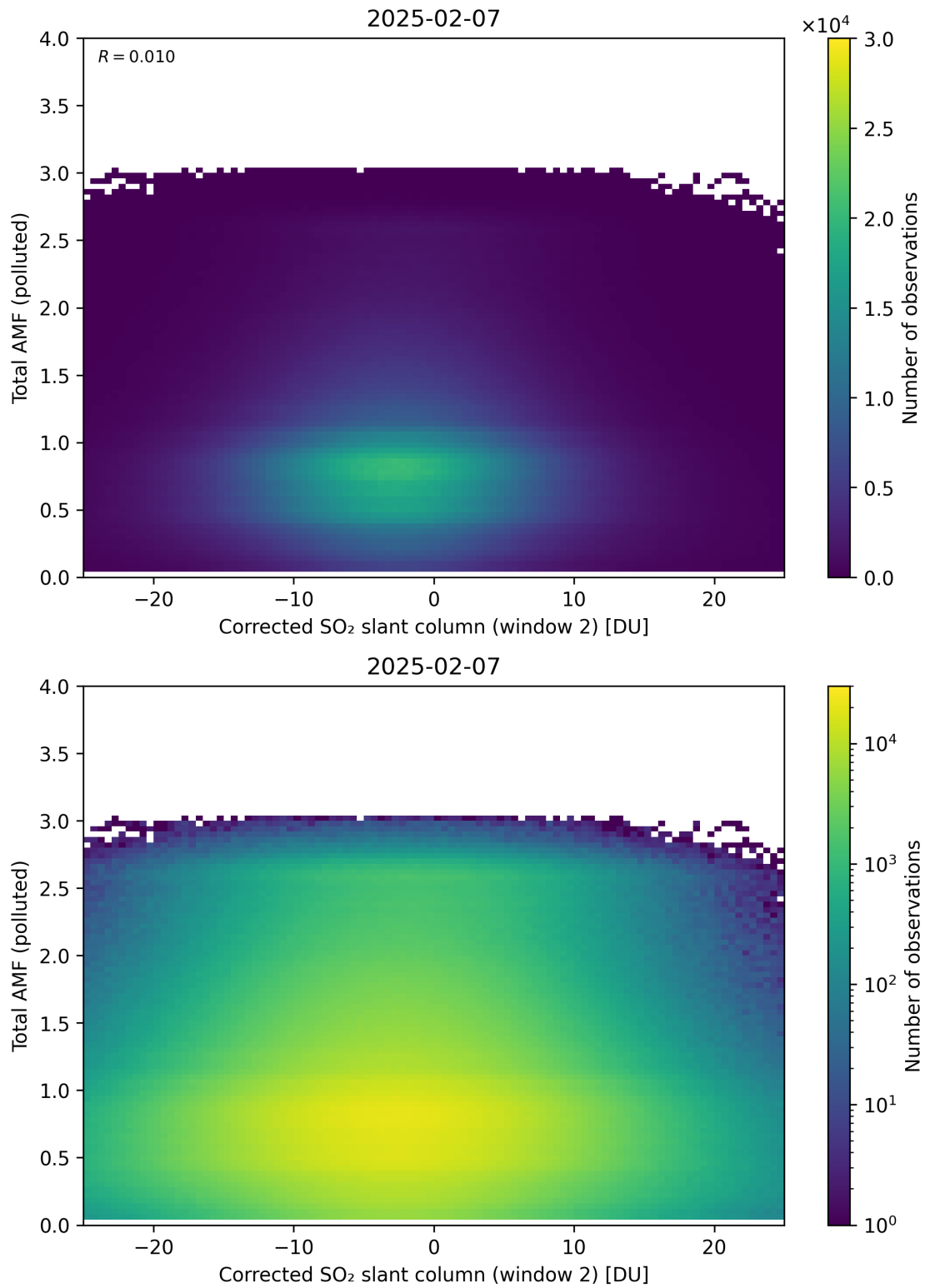
Figure 253: Scatter density plot of “Corrected SO 2 slant column (window 2)” against “Total AMF (polluted)” for 2025-02-06 to 2025-02-08.
