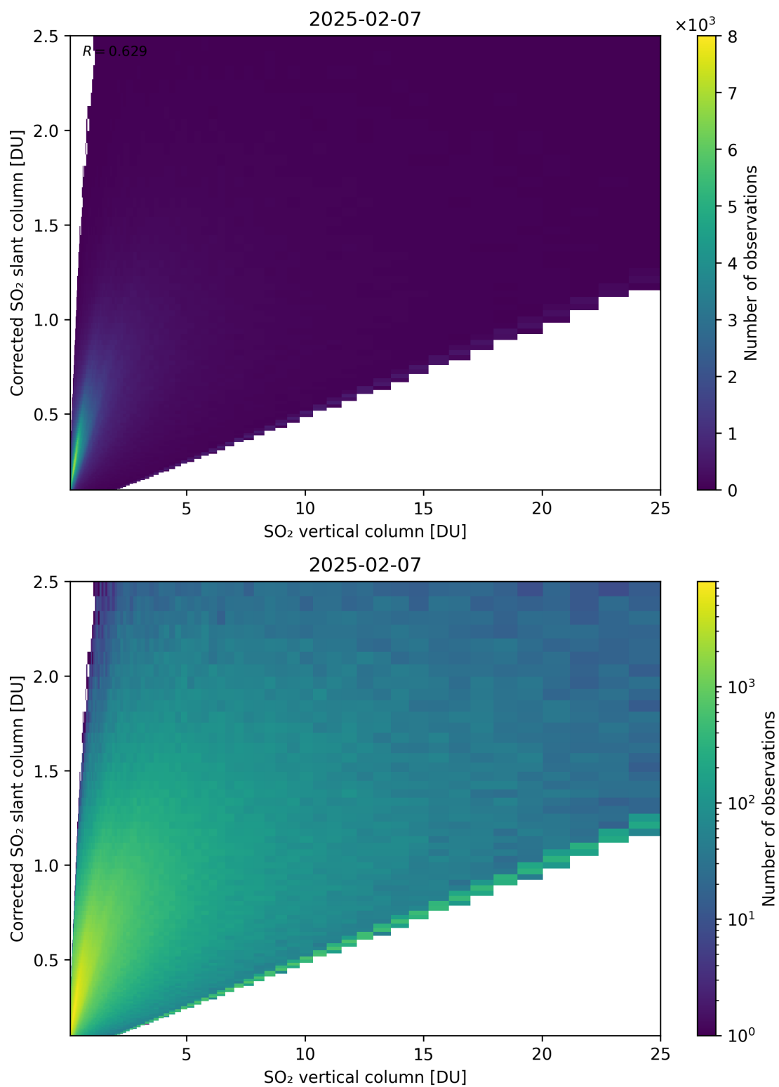
Figure 351: Scatter density plot of “SO 2 vertical column” against “Corrected SO 2 slant column” for 2025-02-06 to 2025-02-08.
