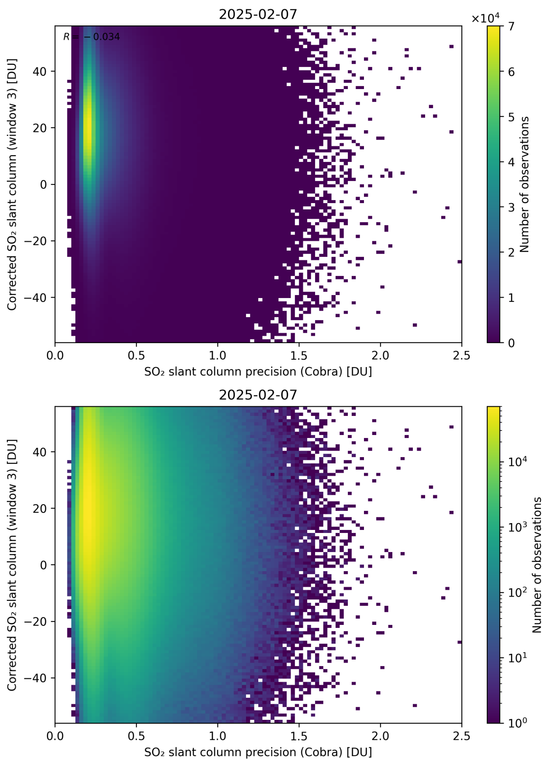
Figure 207: Scatter density plot of “SO 2 slant column precision (Cobra)” against “Corrected SO 2 slant column (window 3)” for 2025-02-06 to 2025-02-08.
