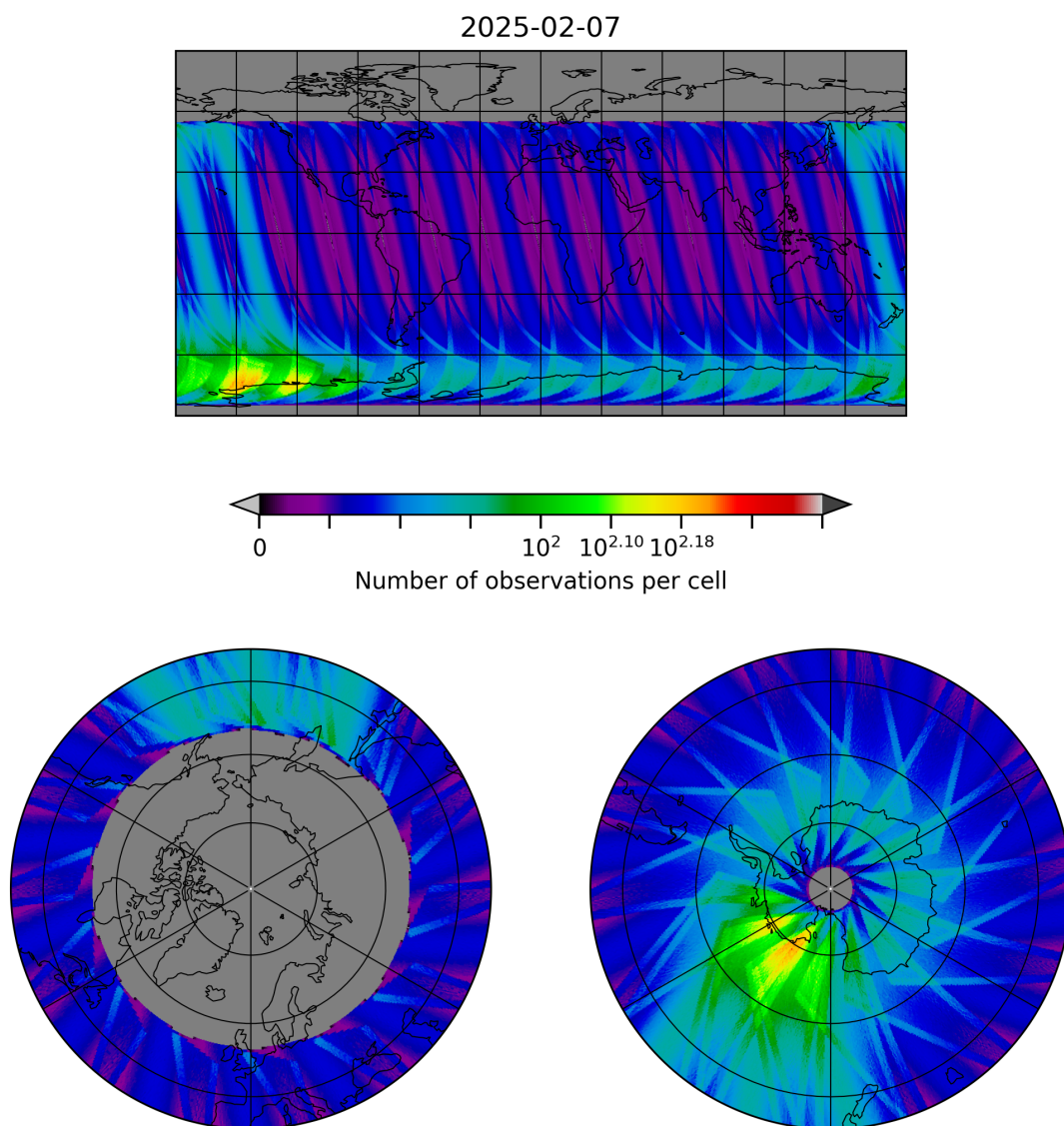
Figure 30: Map of the number of observations for 2025-02-06 to 2025-02-08
