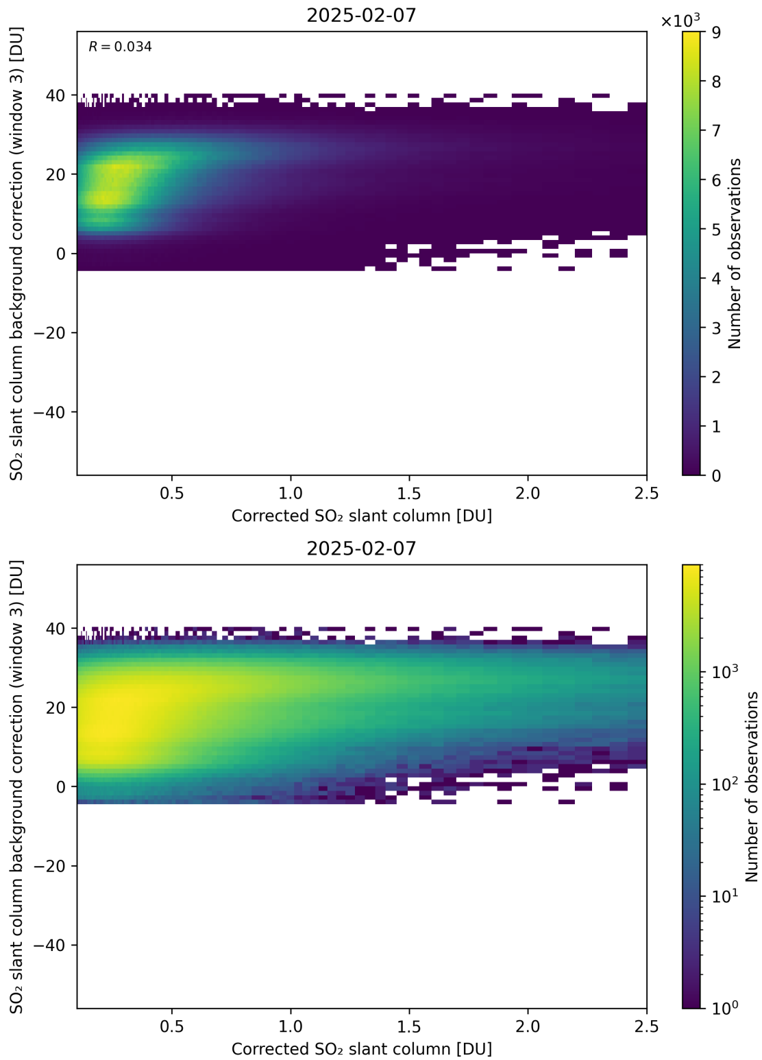
Figure 228: Scatter density plot of “Corrected SO 2 slant column” against “SO 2 slant column background correction (window 3)” for 2025-02-06 to 2025-02-08.
