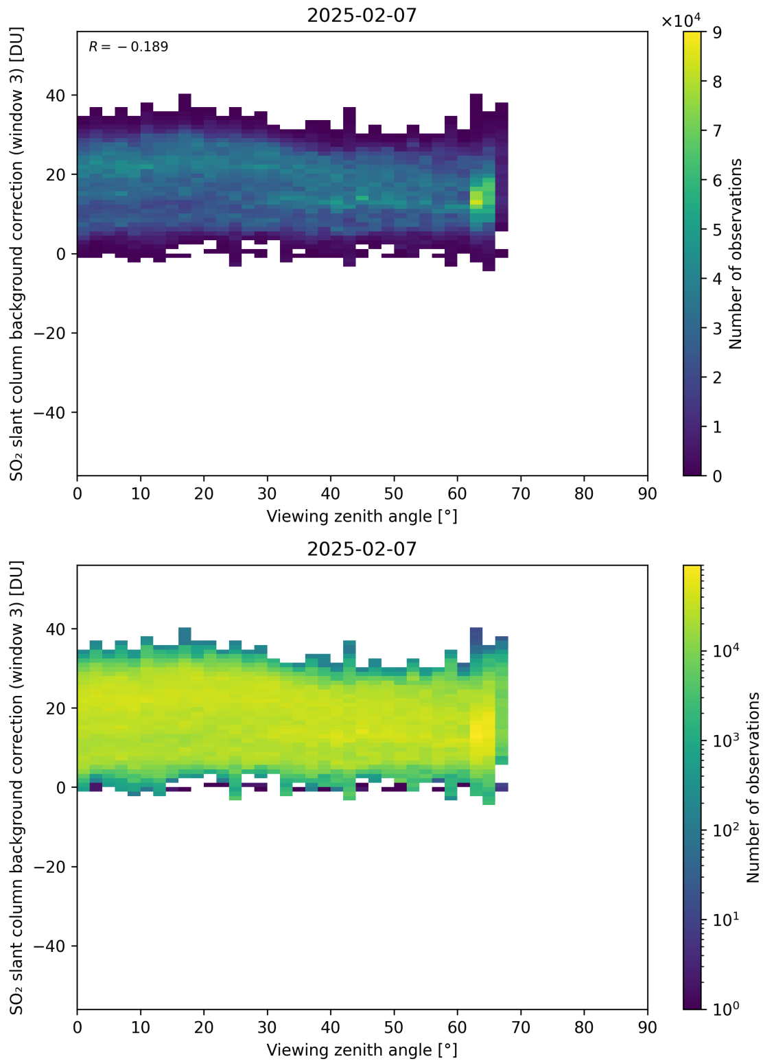
Figure 364: Scatter density plot of “Viewing zenith angle” against “SO 2 slant column background correction (window 3)” for 2025-02-06 to 2025-02-08.
