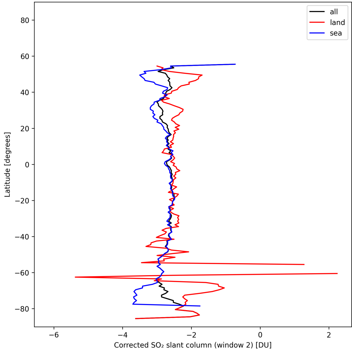
Figure 43: Zonal average of “Corrected SO 2 slant column (window 2)” for 2025-02-06 to 2025-02-08.
