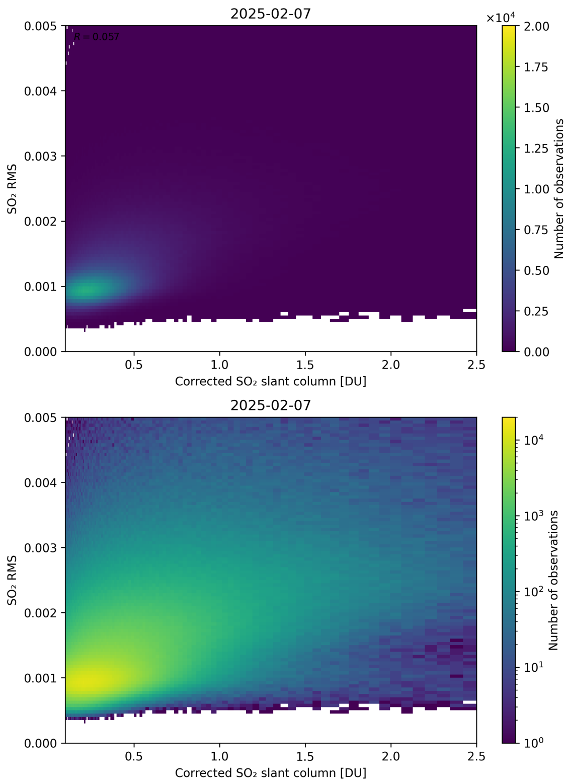
Figure 231: Scatter density plot of “Corrected SO 2 slant column” against “SO 2 RMS” for 2025-02-06 to 2025-02-08.
