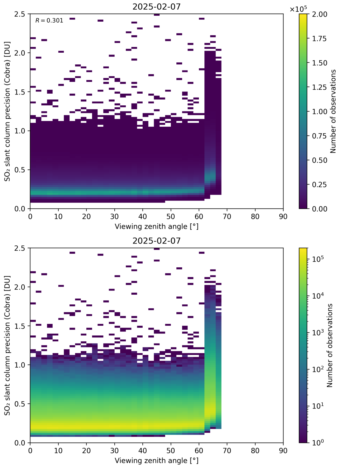
Figure 372: Scatter density plot of “Viewing zenith angle” against “SO 2 slant column precision (Cobra)” for 2025-02-06 to 2025-02-08.
