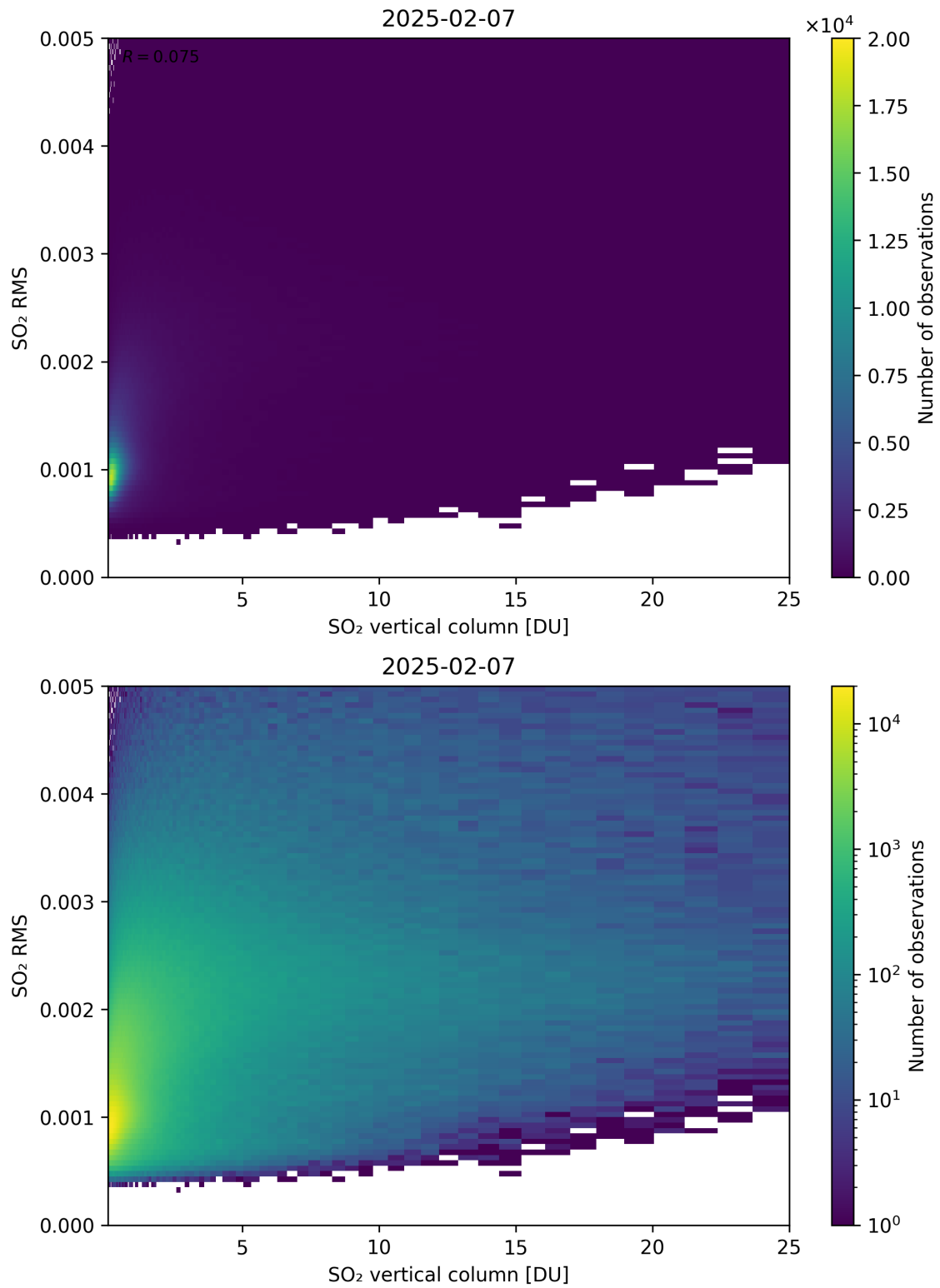
Figure 328: Scatter density plot of “SO 2 vertical column” against “SO 2 RMS” for 2025-02-06 to 2025-02-08.
