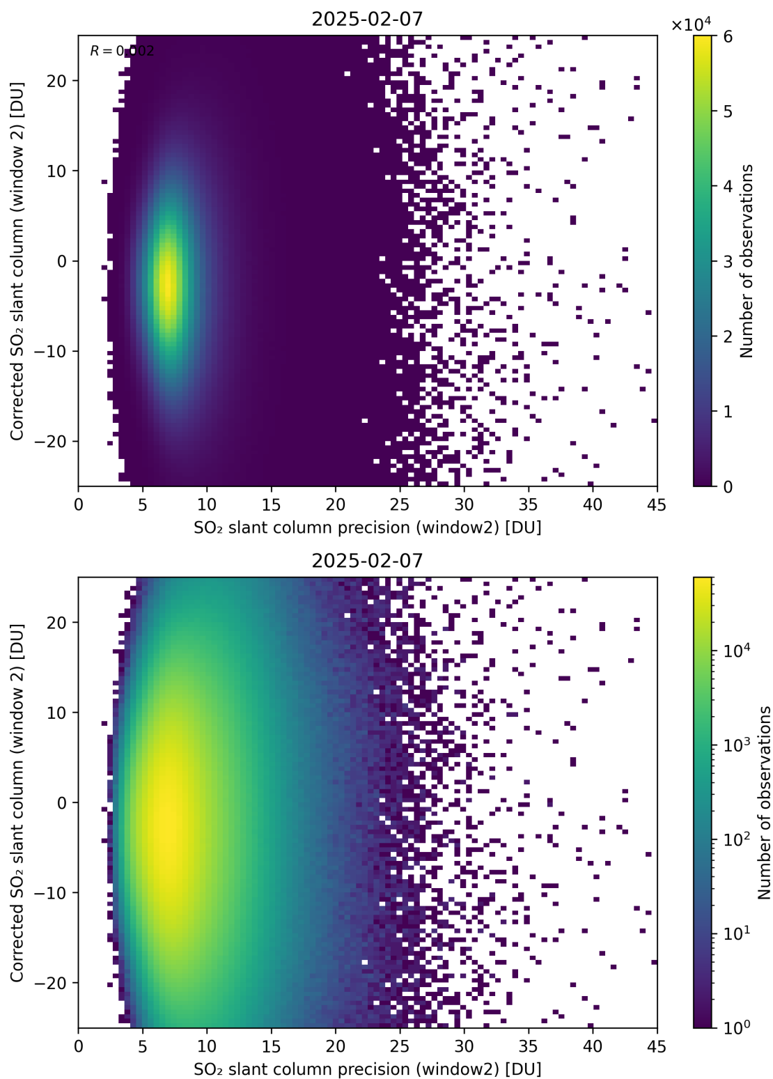
Figure 297: Scatter density plot of “SO 2 slant column precision (window2)” against “Corrected SO 2 slant column (window 2)” for 2025-02-06 to 2025-02-08.
