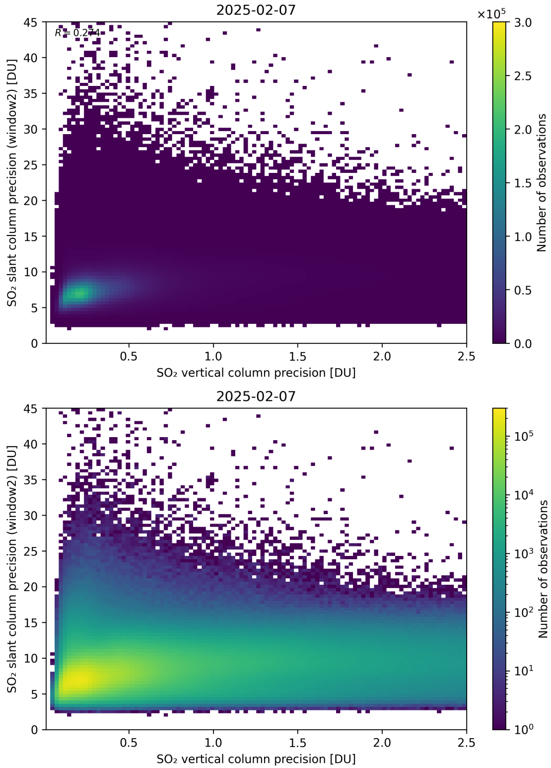
Figure 343: Scatter density plot of “SO 2 vertical column precision” against “SO 2 slant column precision (window2)” for 2025-02-06 to 2025-02-08.
