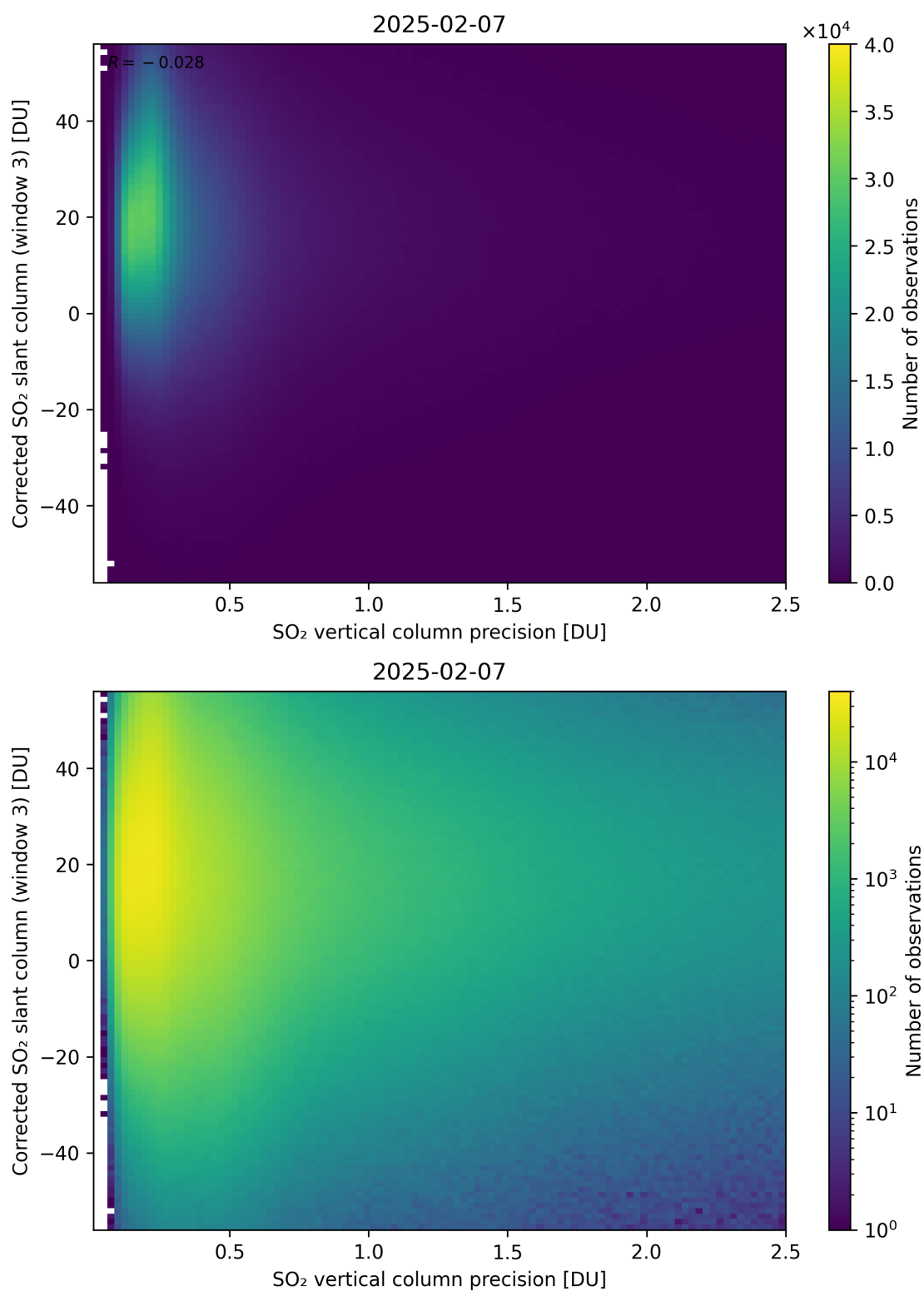
Figure 340: Scatter density plot of “SO 2 vertical column precision” against “Corrected SO 2 slant column (window 3)” for 2025-02-06 to 2025-02-08.
