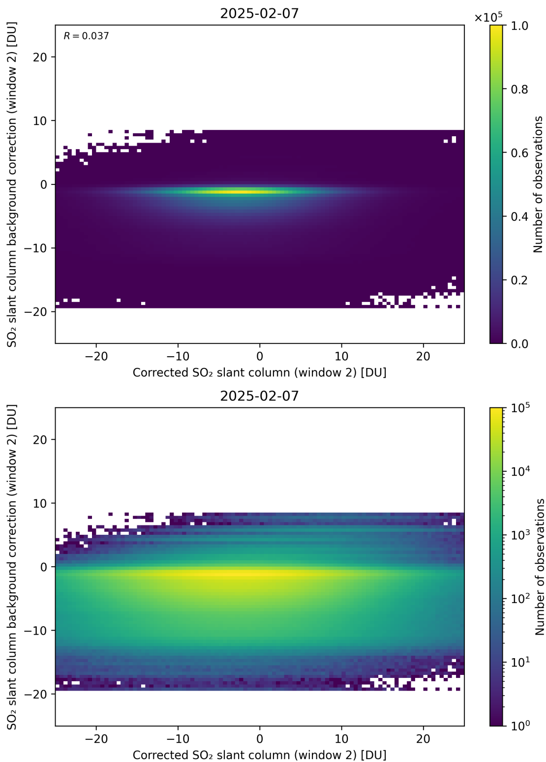
Figure 244: Scatter density plot of “Corrected SO 2 slant column (window 2)” against “SO 2 slant column background correction (window 2)” for 2025-02-06 to 2025-02-08.
