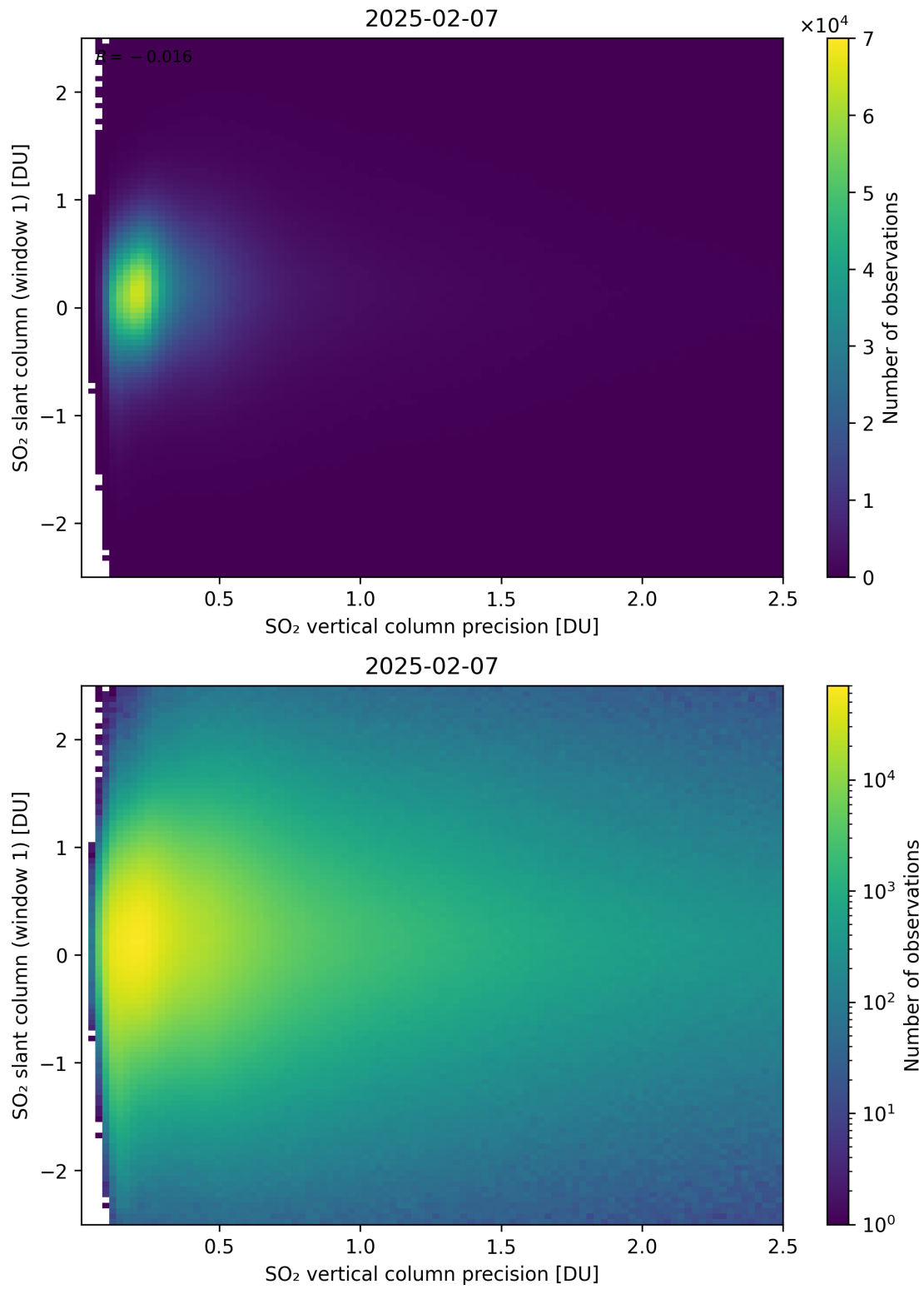
Figure 341: Scatter density plot of “SO 2 vertical column precision” against “SO 2 slant column (window 1)” for 2025-02-06 to 2025-02-08.
