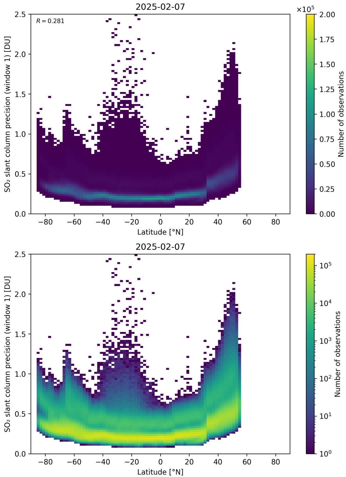
Figure 163: Scatter density plot of “Latitude” against “SO 2 slant column precision (window 1)” for 2025-02-06 to 2025-02-08.
