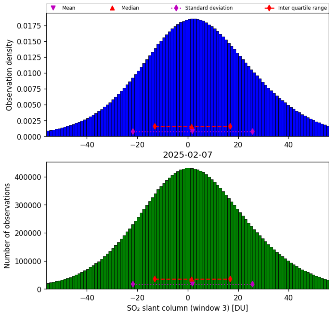
Figure 71: Histogram of “SO 2 slant column (window 3)” for 2025-02-06 to 2025-02-08
