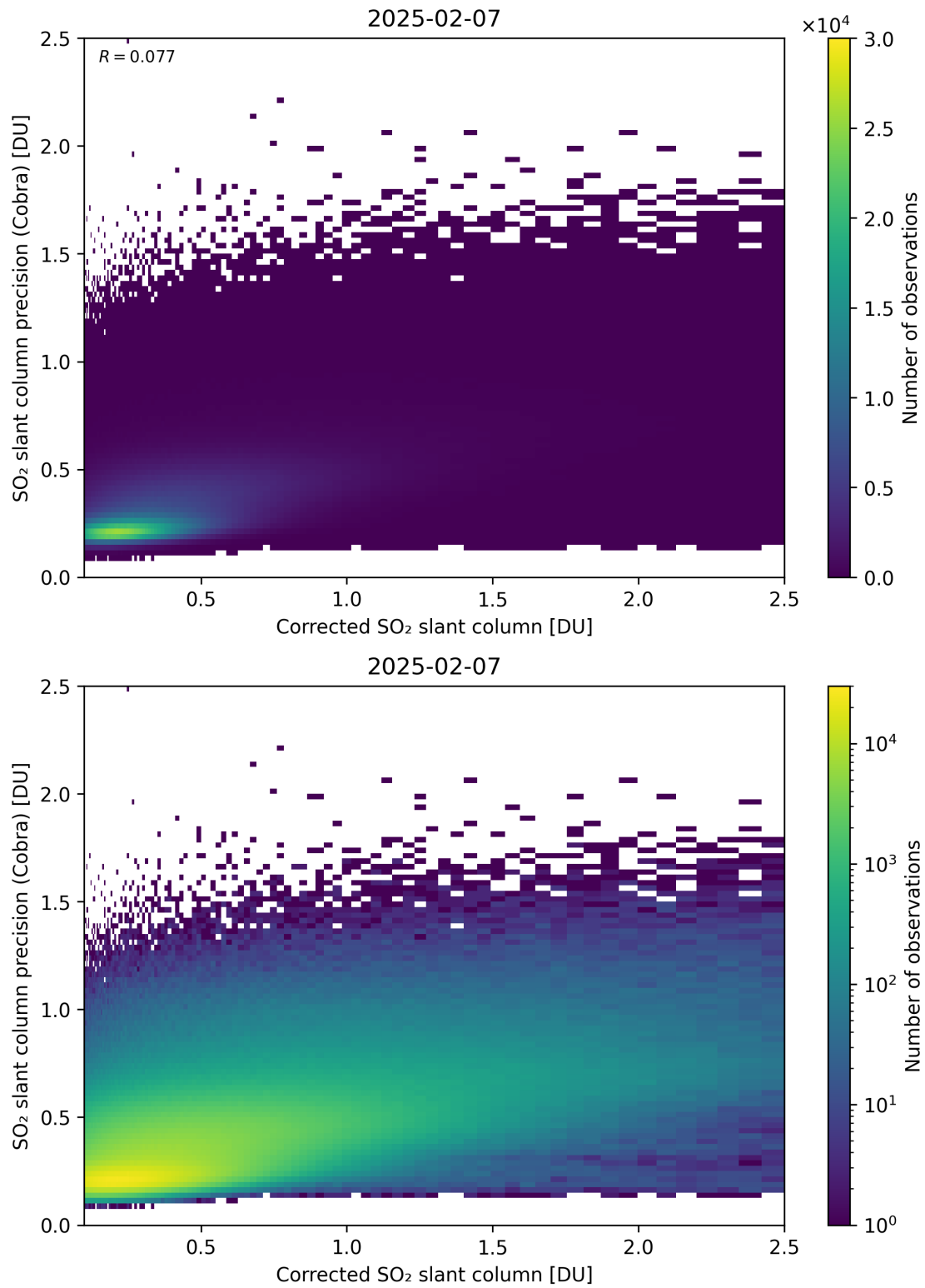
Figure 234: Scatter density plot of “Corrected SO 2 slant column” against “SO 2 slant column precision (Cobra)” for 2025-02-06 to 2025-02-08.
