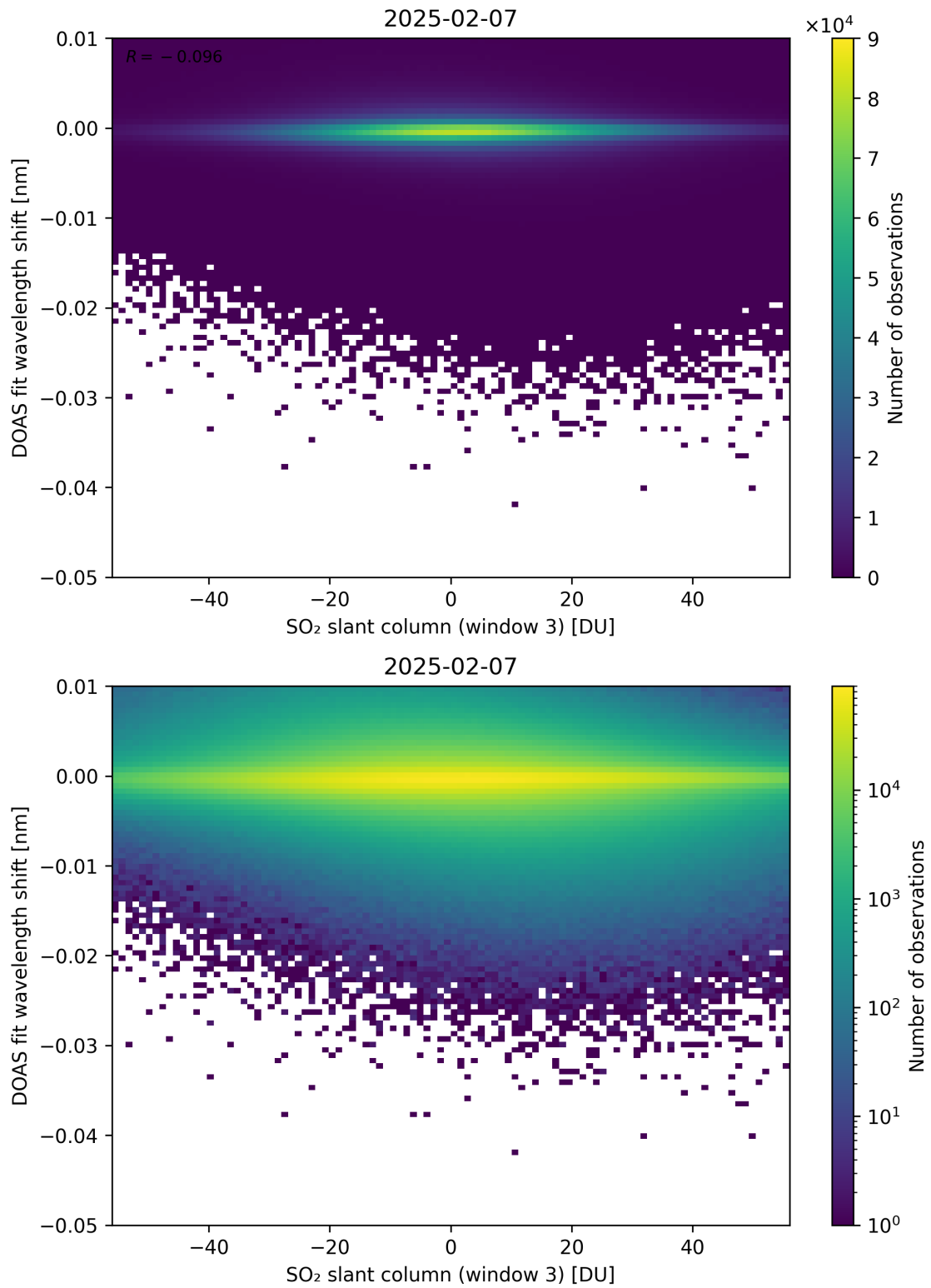
Figure 304: Scatter density plot of “SO 2 slant column (window 3)” against “DOAS fit wavelength shift” for 2025-02-06 to 2025-02-08.
