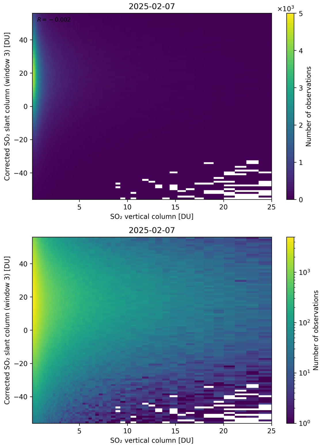
Figure 353: Scatter density plot of “SO 2 vertical column” against “Corrected SO 2 slant column (window 3)” for 2025-02-06 to 2025-02-08.
