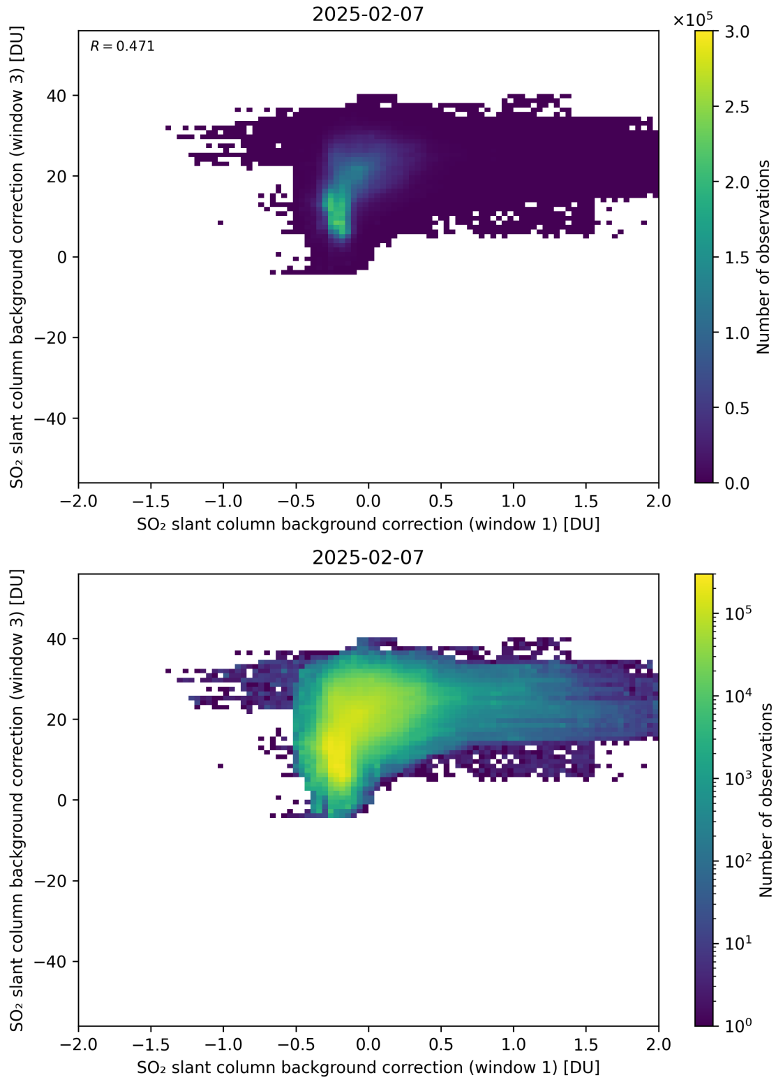
Figure 110: Scatter density plot of “SO 2 slant column background correction (window 1)” against “SO 2 slant column background correction (window 3)” for 2025-02-06 to 2025-02-08.
