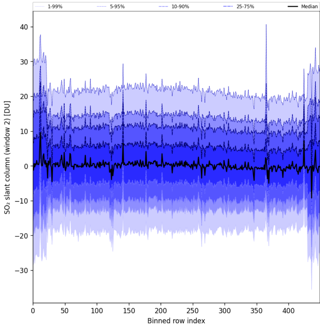
Figure 93: Along track statistics of “SO 2 slant column (window 2)” for 2025-02-06 to 2025-02-08
