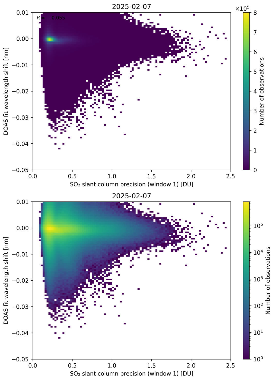
Figure 271: Scatter density plot of “SO 2 slant column precision (window 1)” against “DOAS fit wavelength shift” for 2025-02-06 to 2025-02-08.
