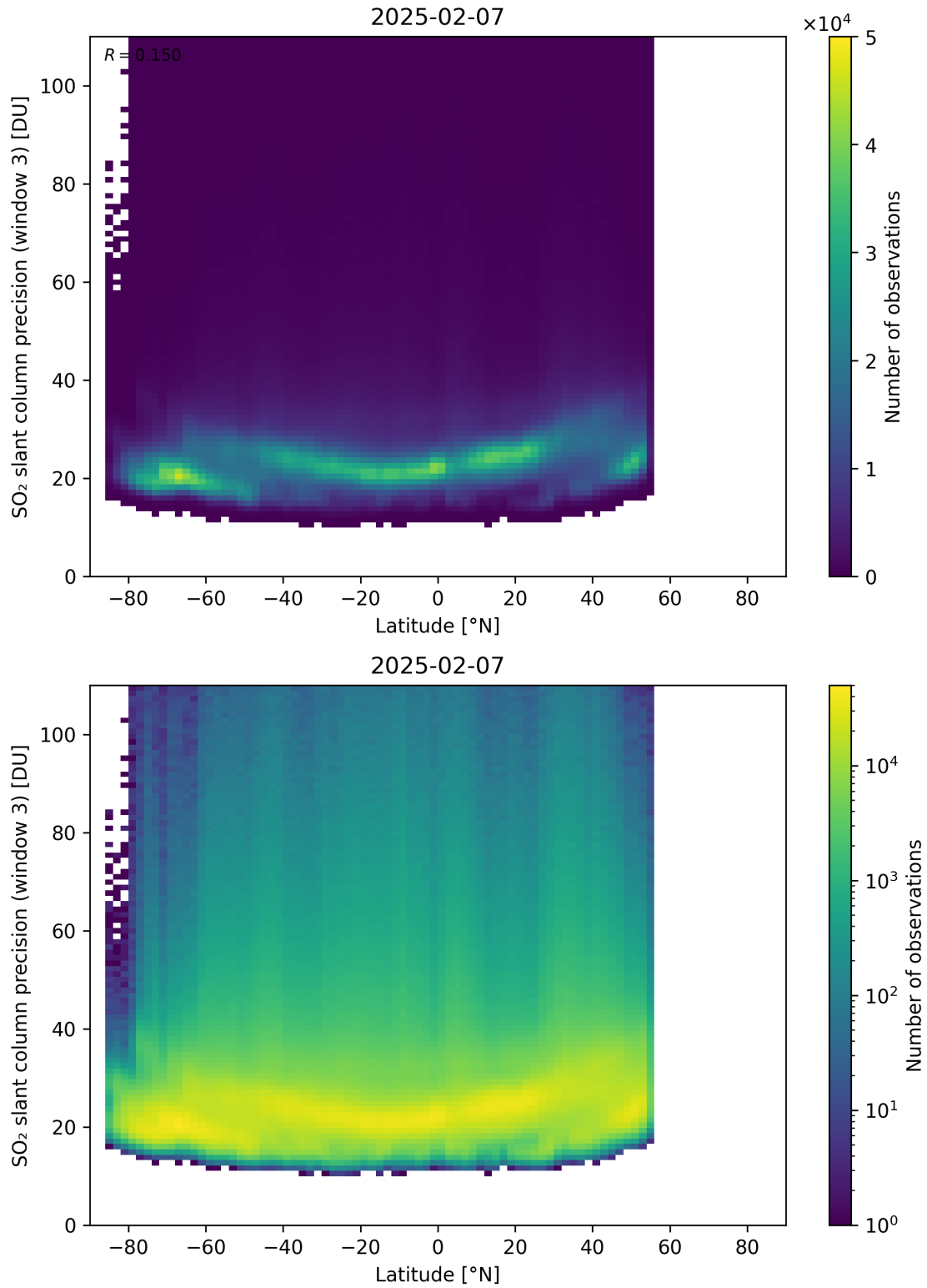
Figure 166: Scatter density plot of “Latitude” against “SO 2 slant column precision (window 3)” for 2025-02-06 to 2025-02-08.
