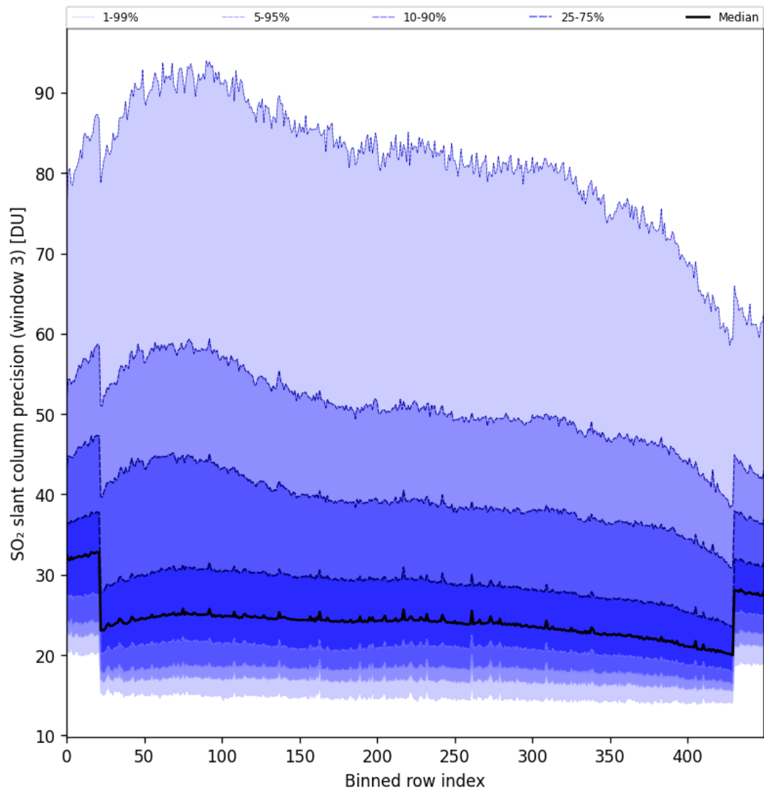
Figure 98: Along track statistics of “SO 2 slant column precision (window 3)” for 2025-02-06 to 2025-02-08
