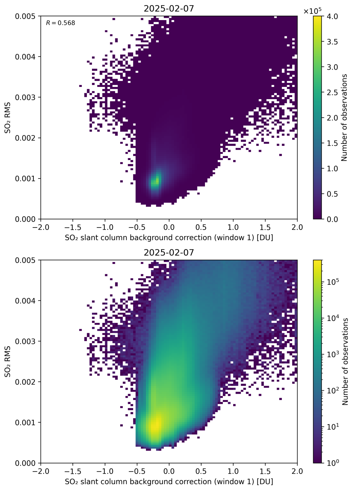
Figure 113: Scatter density plot of “SO 2 slant column background correction (window 1)” against “SO 2 RMS” for 2025-02-06 to 2025-02-08.
