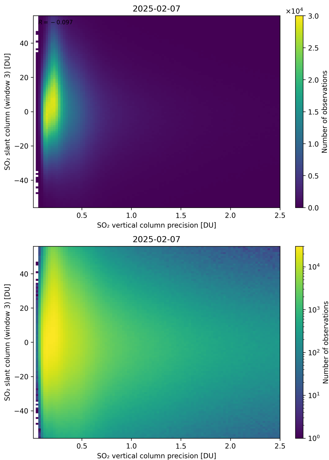
Figure 344: Scatter density plot of “SO 2 vertical column precision” against “SO 2 slant column (window 3)” for 2025-02-06 to 2025-02-08.
