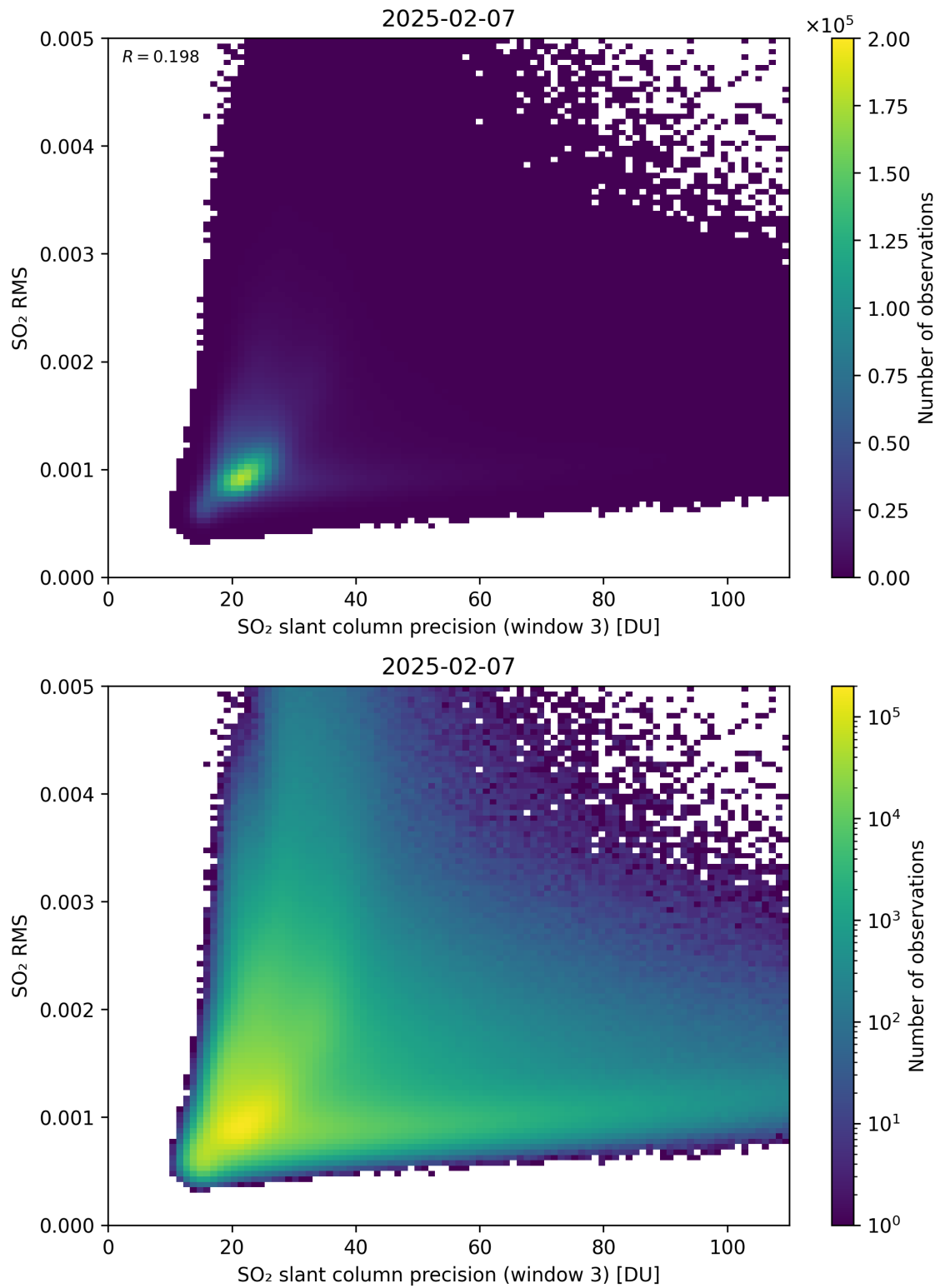
Figure 310: Scatter density plot of “SO 2 slant column precision (window 3)” against “SO 2 RMS” for 2025-02-06 to 2025-02-08.
