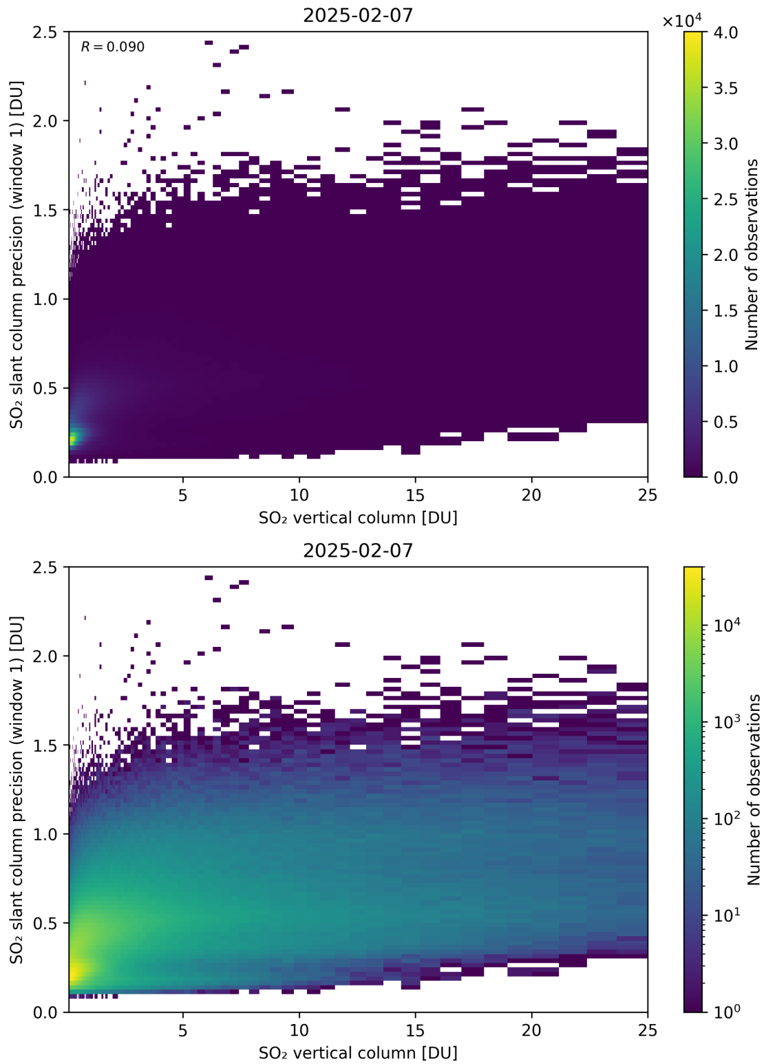
Figure 355: Scatter density plot of “SO 2 vertical column” against “SO 2 slant column precision (window 1)” for 2025-02-06 to 2025-02-08.
