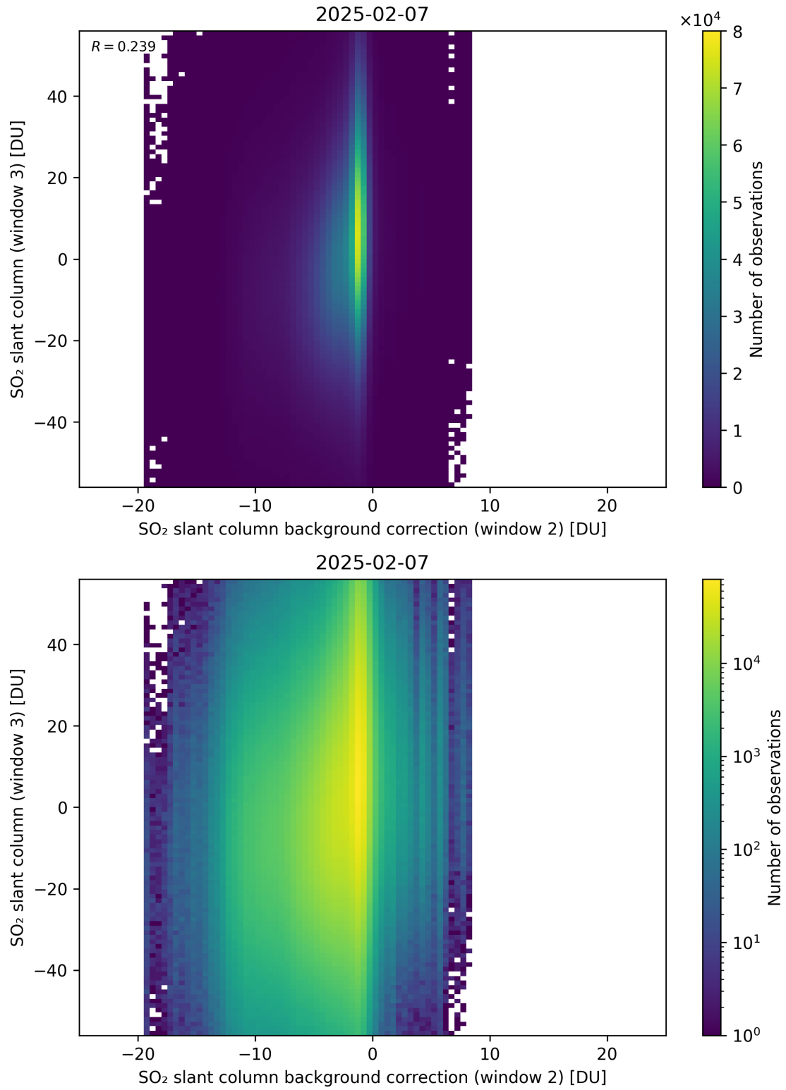
Figure 128: Scatter density plot of “SO 2 slant column background correction (window 2)” against “SO 2 slant column (window 3)” for 2025-02-06 to 2025-02-08.
