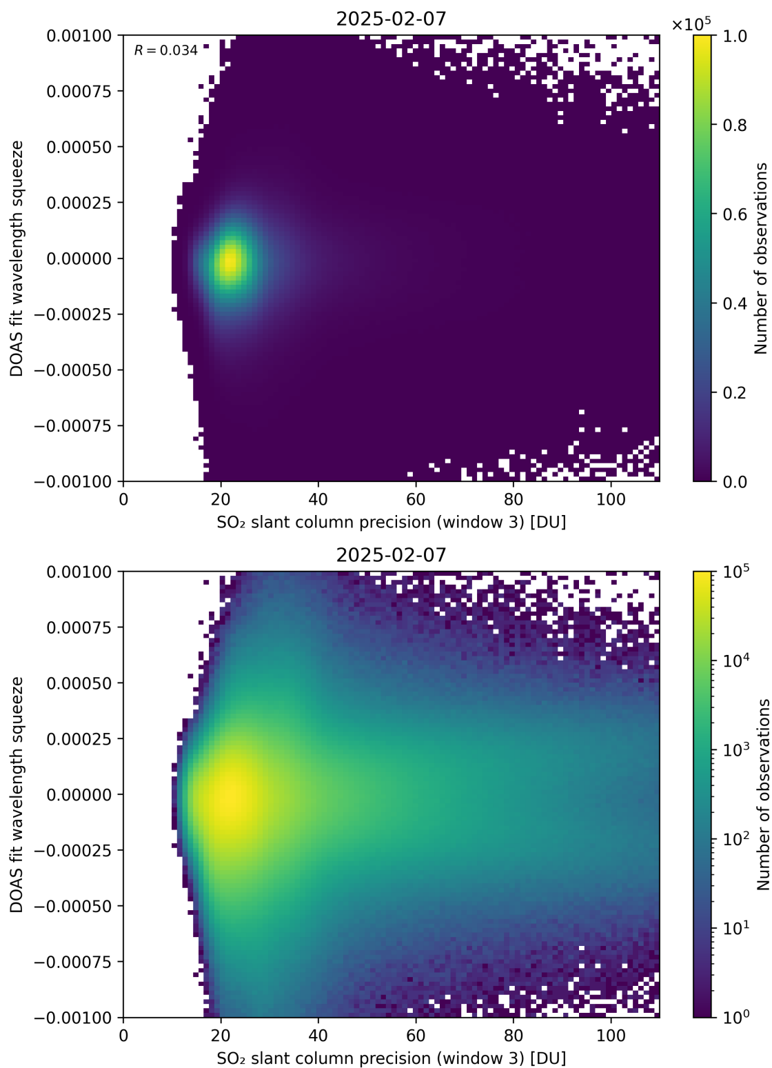
Figure 309: Scatter density plot of “SO 2 slant column precision (window 3)” against “DOAS fit wavelength squeeze” for 2025-02-06 to 2025-02-08.
