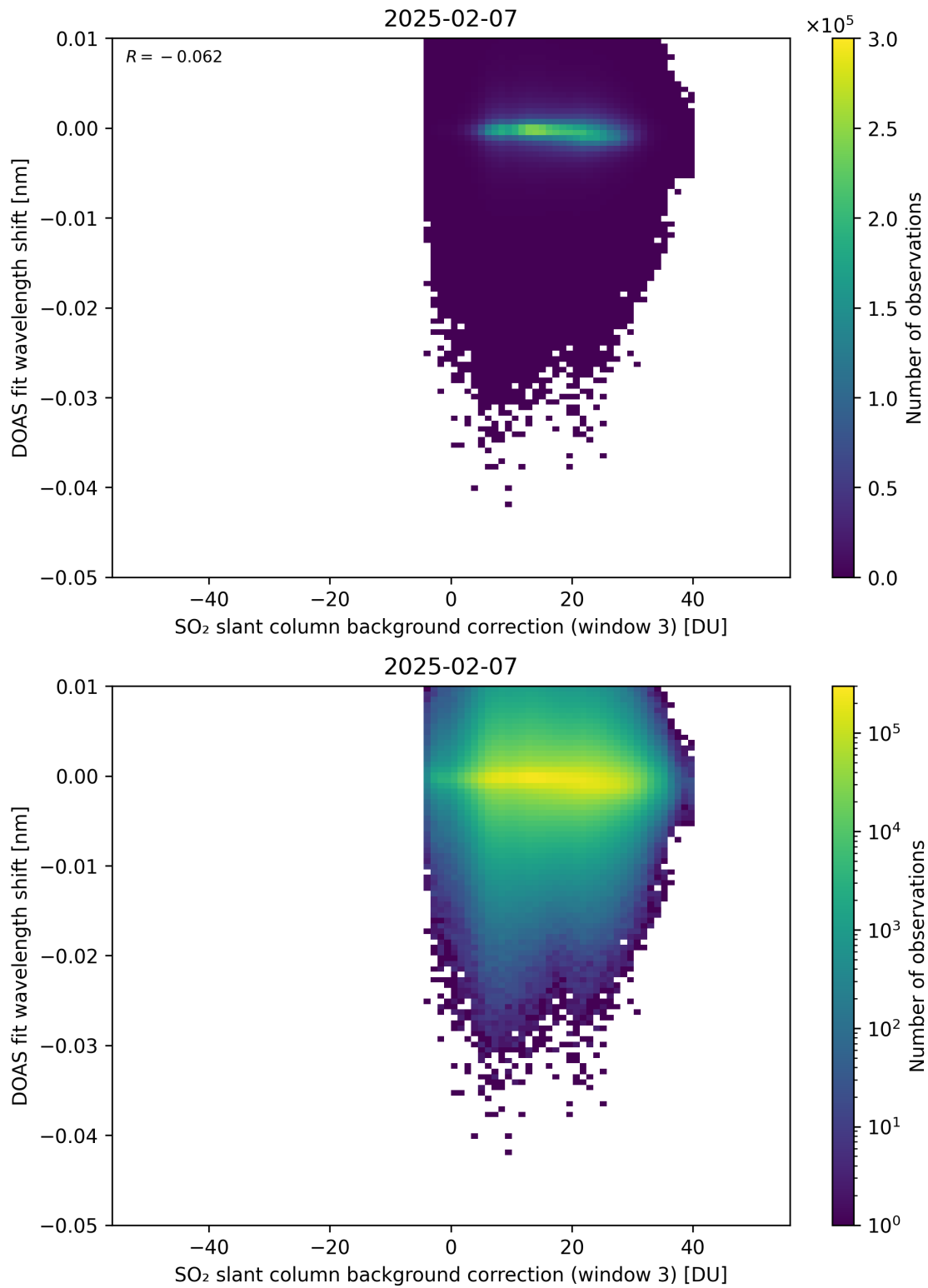
Figure 132: Scatter density plot of “SO 2 slant column background correction (window 3)” against “DOAS fit wavelength shift” for 2025-02-06 to 2025-02-08.
