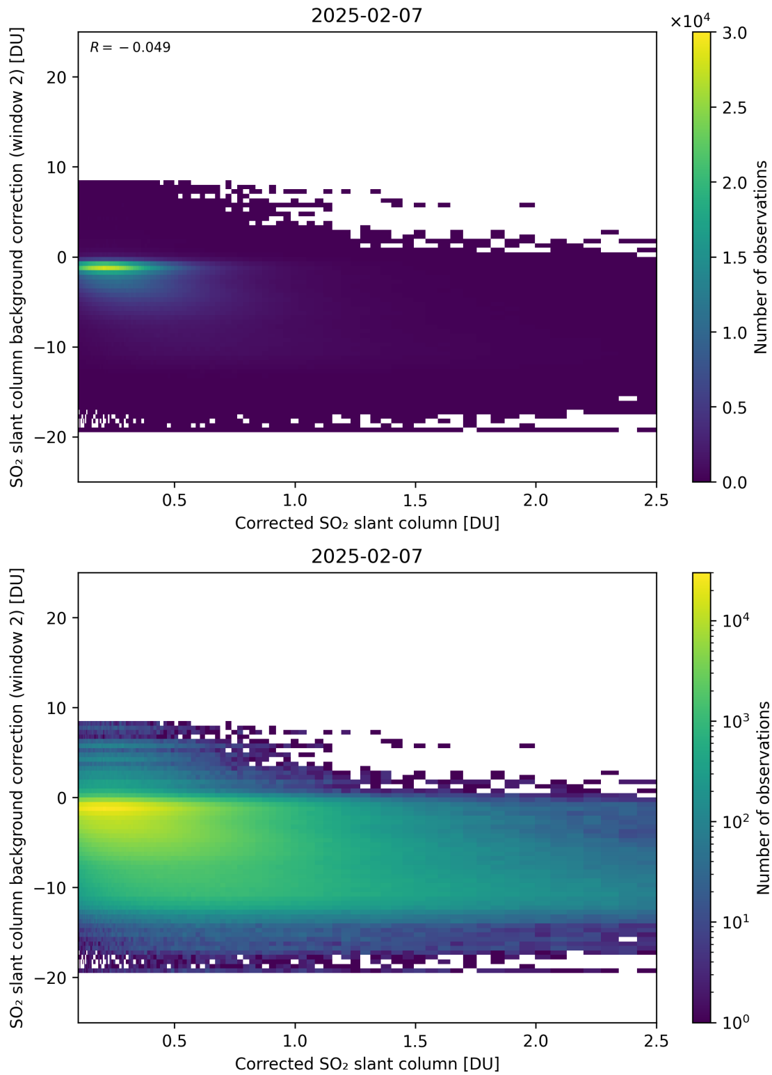
Figure 227: Scatter density plot of “Corrected SO 2 slant column” against “SO 2 slant column background correction (window 2)” for 2025-02-06 to 2025-02-08.
