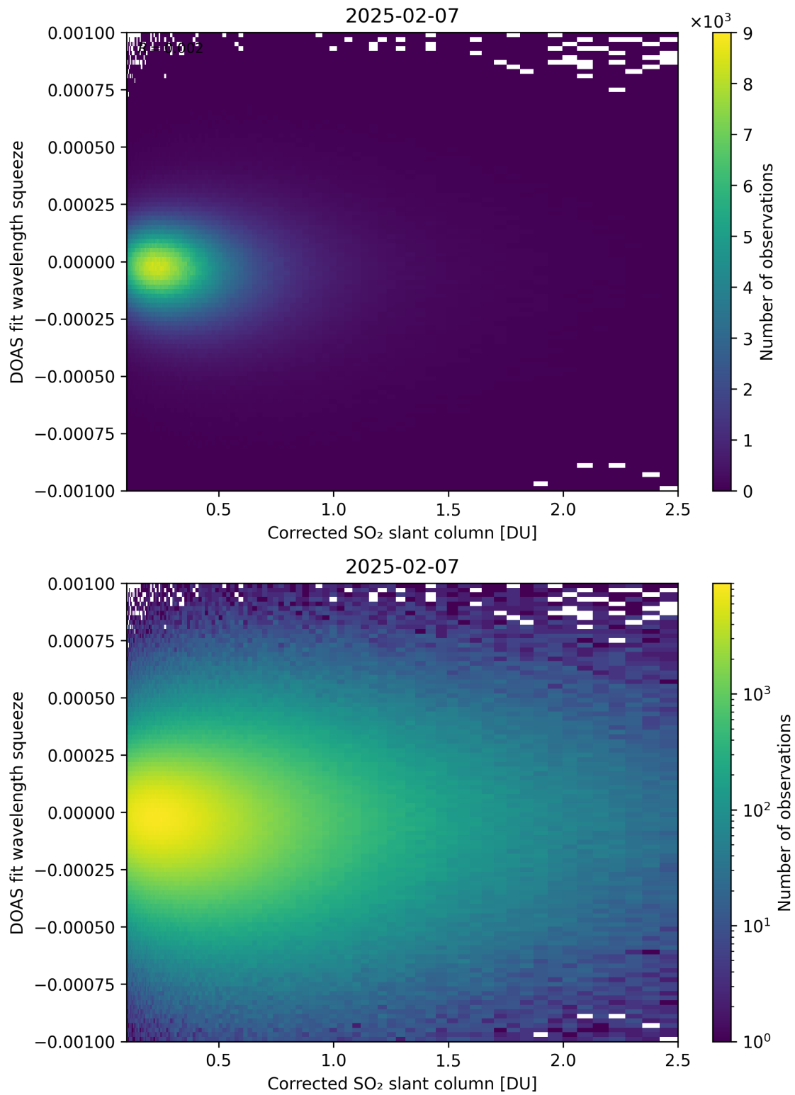
Figure 230: Scatter density plot of “Corrected SO 2 slant column” against “DOAS fit wavelength squeeze” for 2025-02-06 to 2025-02-08.
