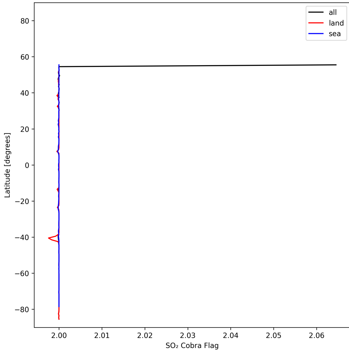
Figure 49: Zonal average of "SO 2 Cobra Flag" for 2025-02-06 to 2025-02-08.
