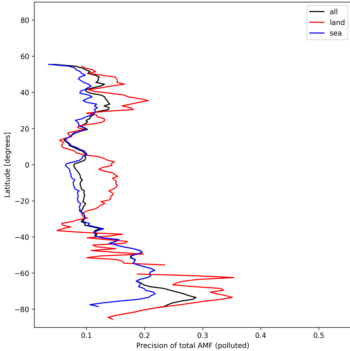
Figure 54: Zonal average of “Precision of total AMF (polluted)” for 2025-02-06 to 2025-02-08.
