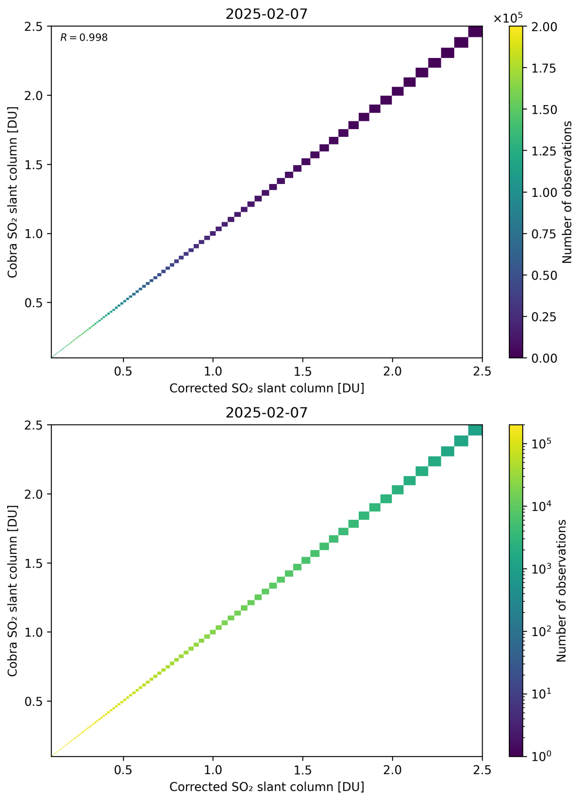
Figure 233: Scatter density plot of “Corrected SO 2 slant column” against “Cobra SO 2 slant column” for 2025-02-06 to 2025-02-08.
