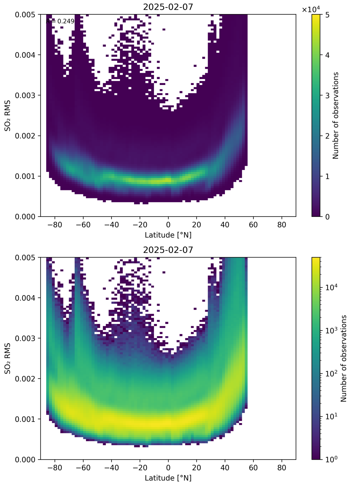
Figure 155: Scatter density plot of “Latitude” against “SO 2 RMS” for 2025-02-06 to 2025-02-08.
