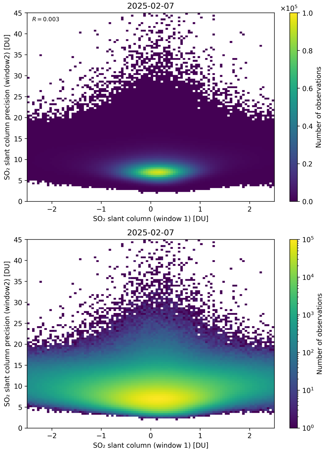
Figure 286: Scatter density plot of “SO 2 slant column (window 1)” against “SO 2 slant column precision (window2)” for 2025-02-06 to 2025-02-08.
