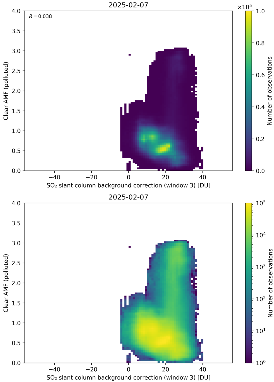
Figure 135: Scatter density plot of “SO 2 slant column background correction (window 3)” against “Clear AMF (polluted)” for 2025-02-06 to 2025-02-08.
