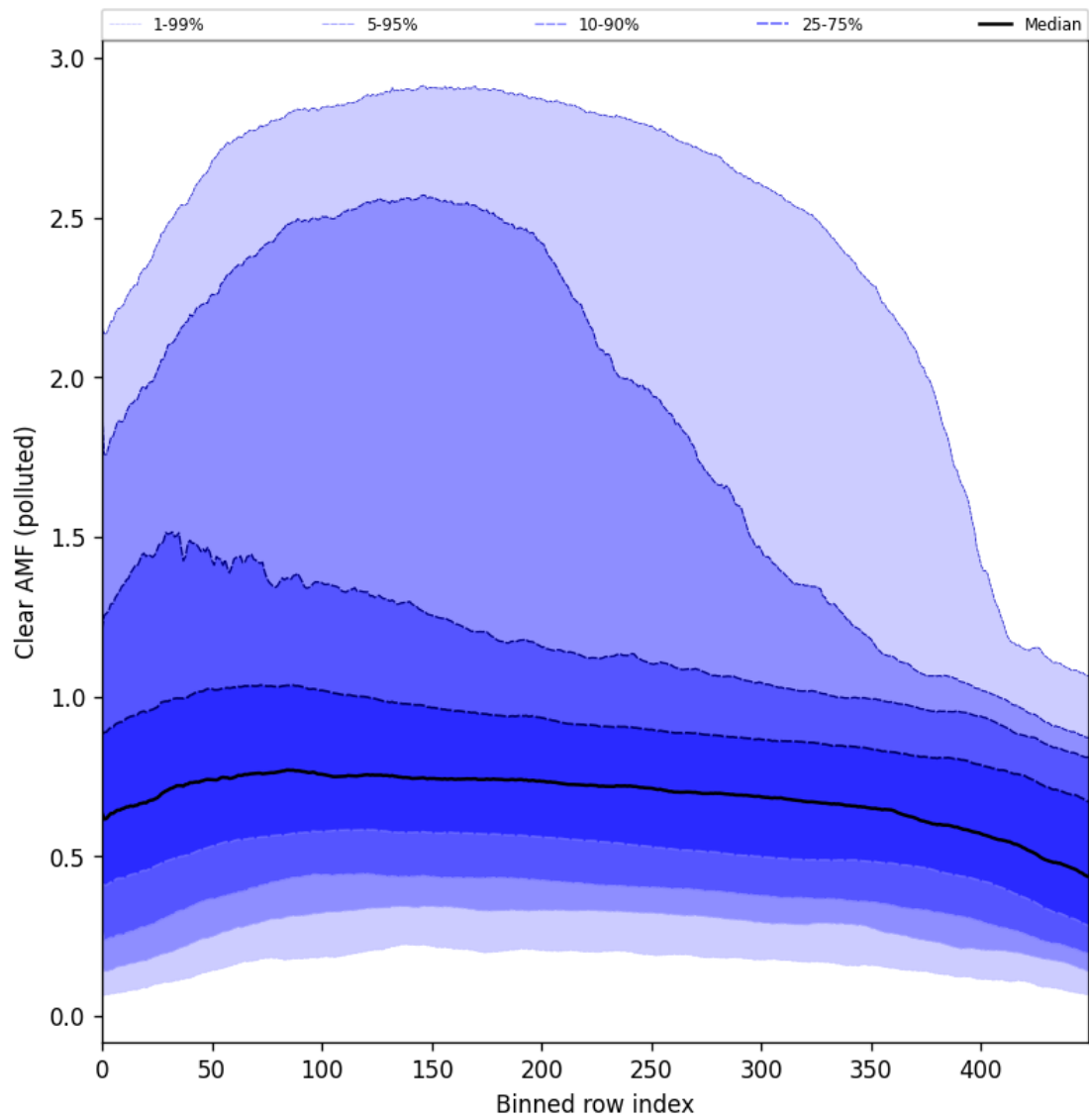
Figure 107: Along track statistics of “Clear AMF (polluted)” for 2025-02-06 to 2025-02-08
