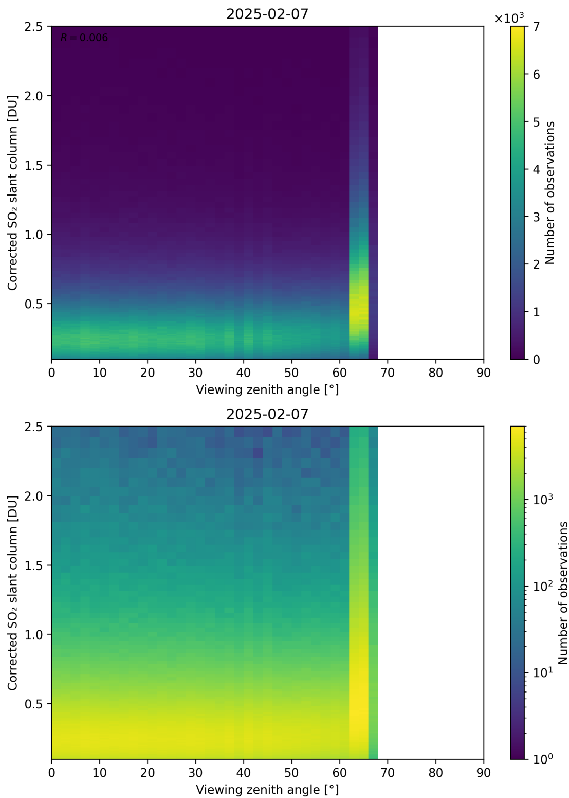
Figure 373: Scatter density plot of “Viewing zenith angle” against “Corrected SO 2 slant column” for 2025-02-06 to 2025-02-08.
