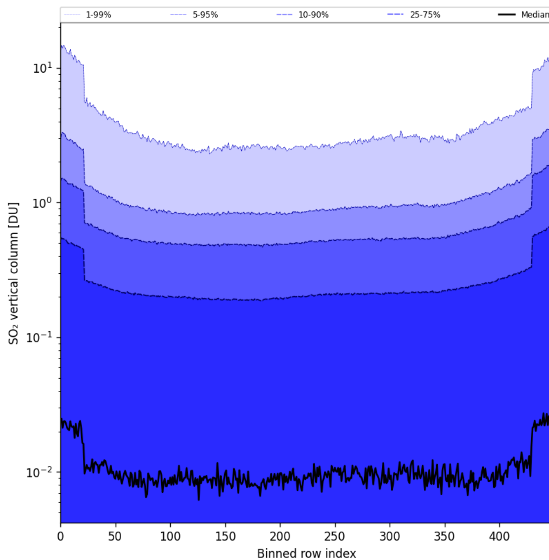
Figure 84: Along track statistics of “SO 2 vertical column” for 2025-02-06 to 2025-02-08
