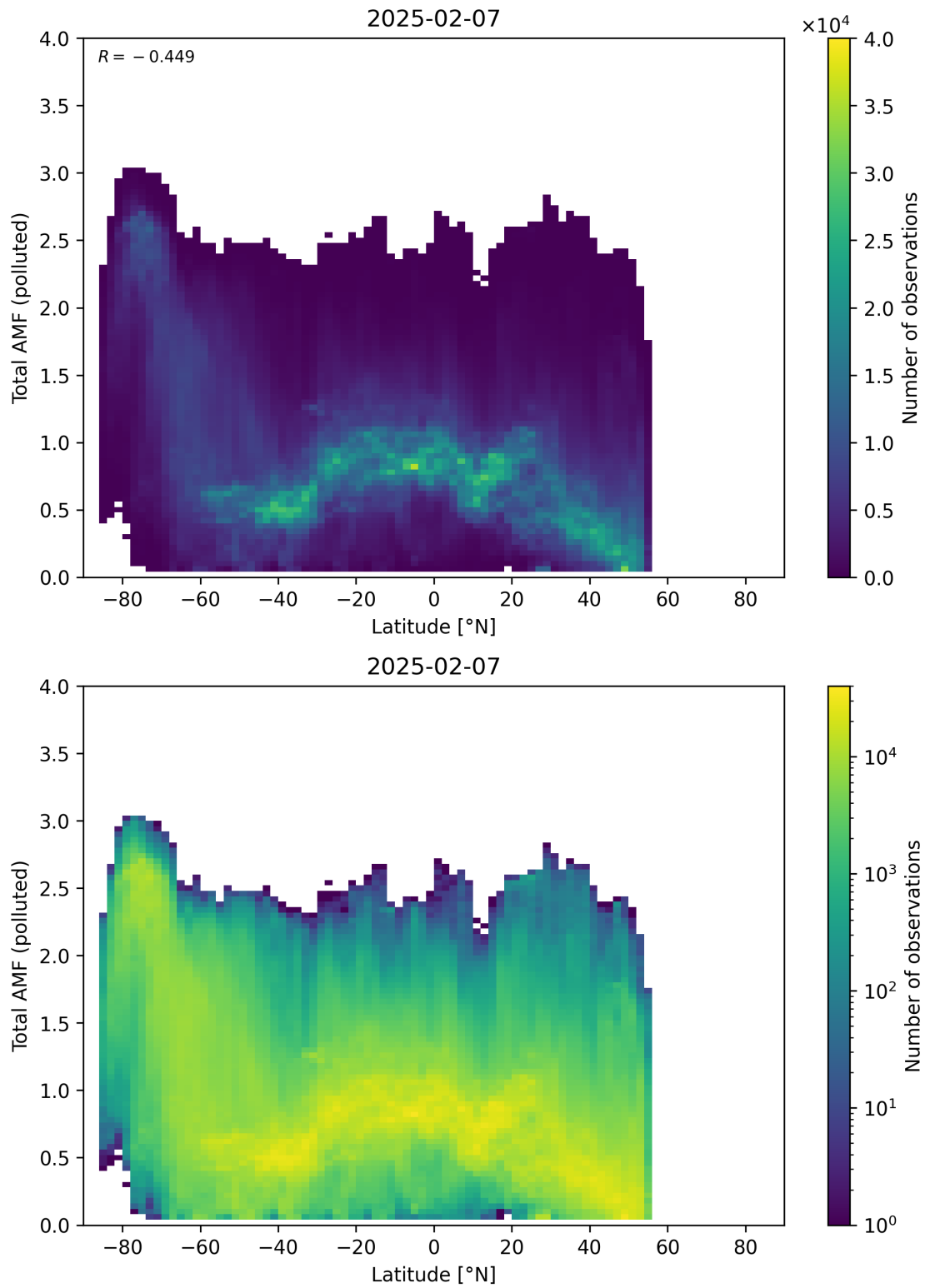
Figure 167: Scatter density plot of “Latitude” against “Total AMF (polluted)” for 2025-02-06 to 2025-02-08.
