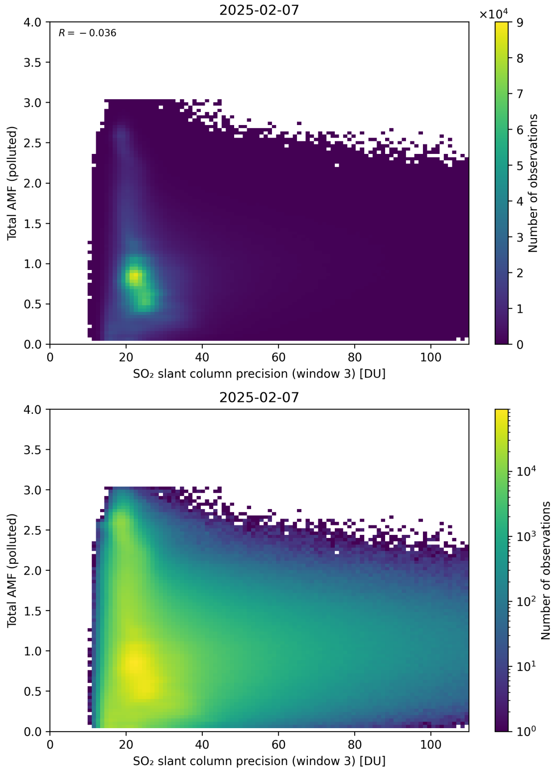
Figure 313: Scatter density plot of “SO 2 slant column precision (window 3)” against “Total AMF (polluted)” for 2025-02-06 to 2025-02-08.
