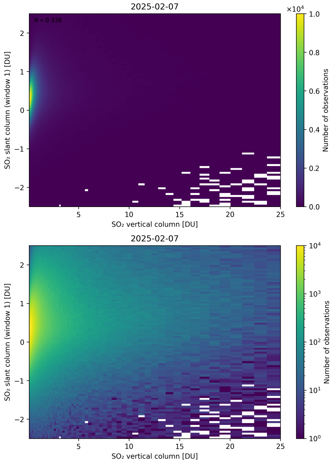
Figure 354: Scatter density plot of “SO 2 vertical column” against “SO 2 slant column (window 1)” for 2025-02-06 to 2025-02-08.
