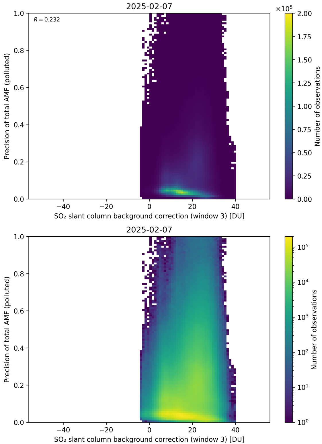
Figure 137: Scatter density plot of “SO 2 slant column background correction (window 3)” against “Precision of total AMF (polluted)” for 2025-02-06 to 2025-02-08.
