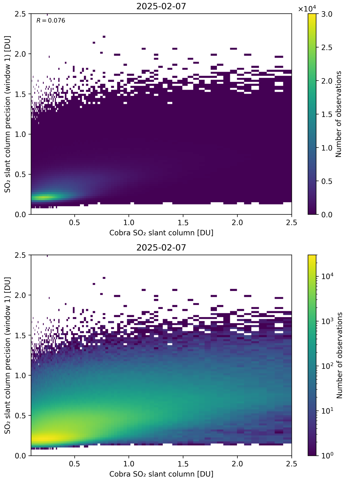
Figure 220: Scatter density plot of “Cobra SO 2 slant column” against “SO 2 slant column precision (window 1)” for 2025-02-06 to 2025-02-08.
