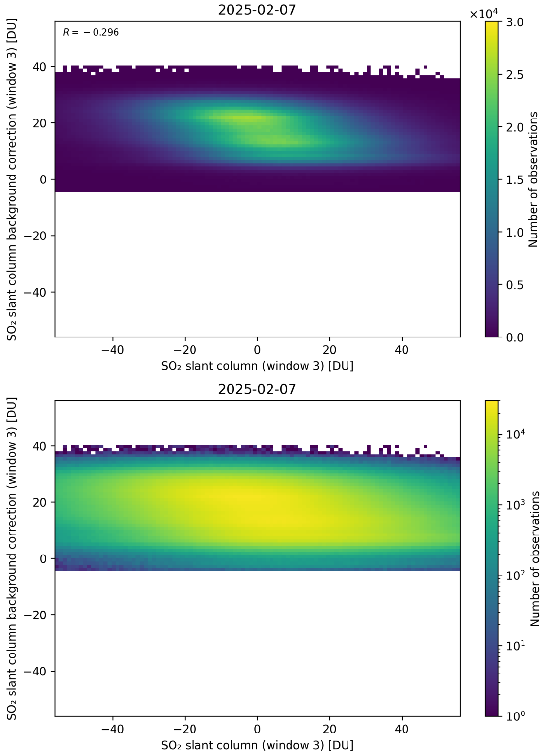
Figure 303: Scatter density plot of “SO 2 slant column (window 3)” against “SO 2 slant column background correction (window 3)” for 2025-02-06 to 2025-02-08.
