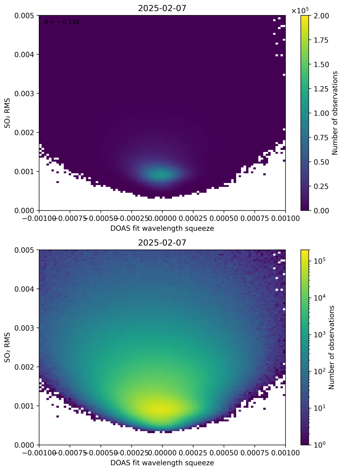
Figure 143: Scatter density plot of “DOAS fit wavelength squeeze” against “SO 2 RMS” for 2025-02-06 to 2025-02-08.
