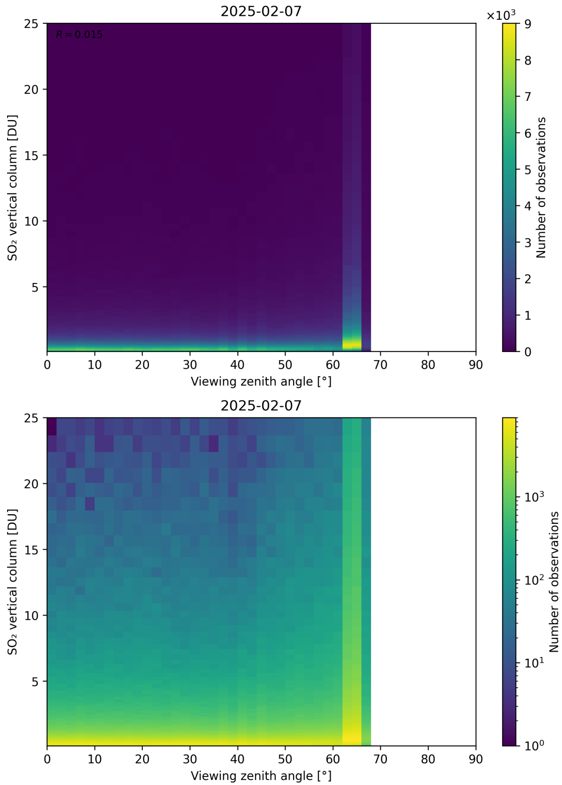
Figure 383: Scatter density plot of “Viewing zenith angle” against “SO 2 vertical column” for 2025-02-06 to 2025-02-08.
