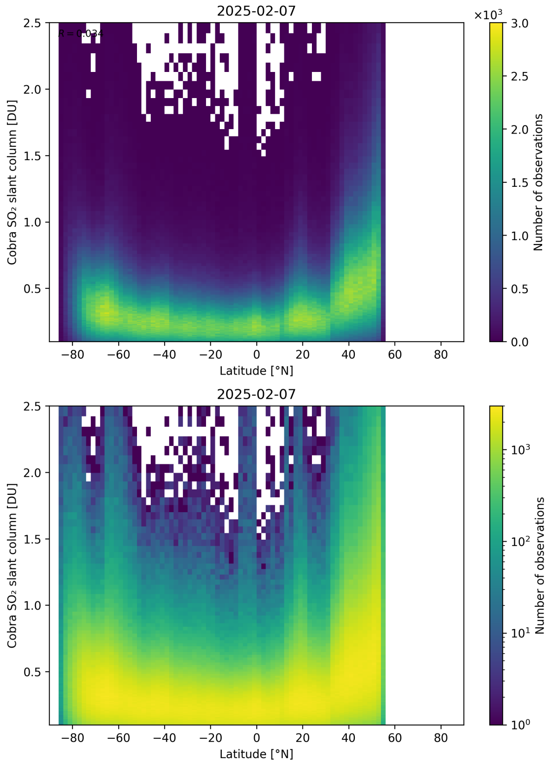
Figure 157: Scatter density plot of “Latitude” against “Cobra SO 2 slant column” for 2025-02-06 to 2025-02-08.
