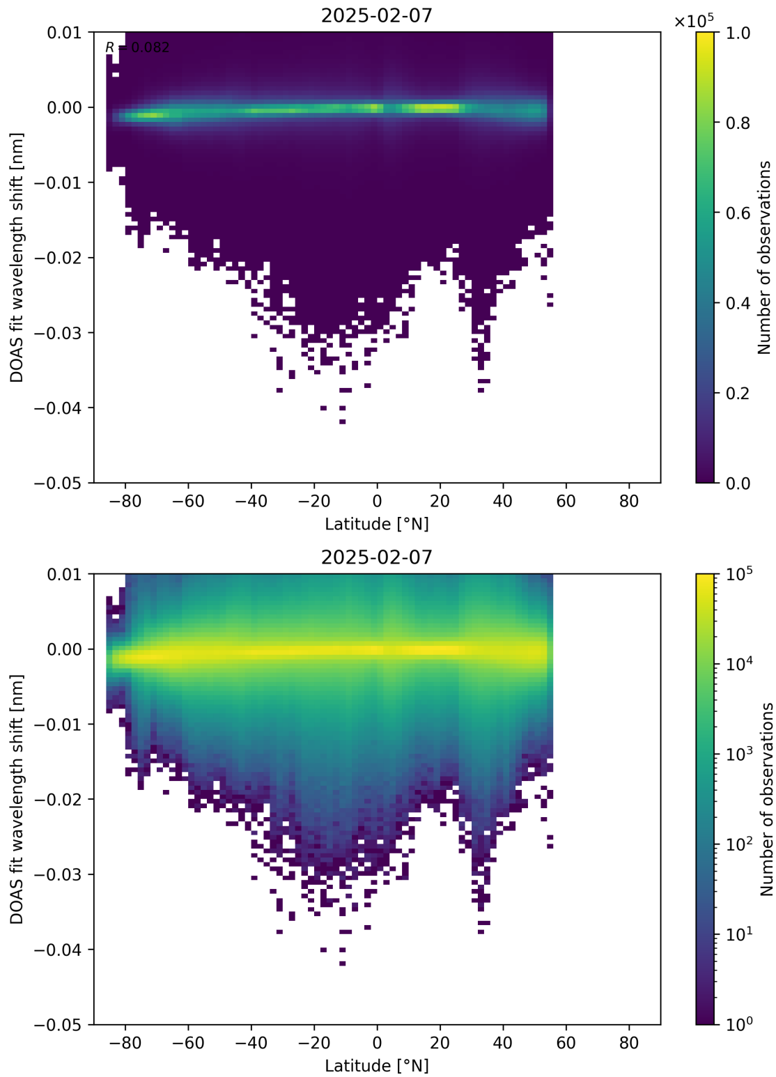
Figure 153: Scatter density plot of “Latitude” against “DOAS fit wavelength shift” for 2025-02-06 to 2025-02-08.
