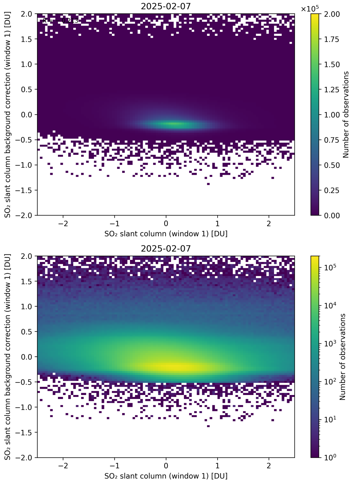
Figure 262: Scatter density plot of “SO 2 slant column (window 1)” against “SO 2 slant column background correction (window 1)” for 2025-02-06 to 2025-02-08.
