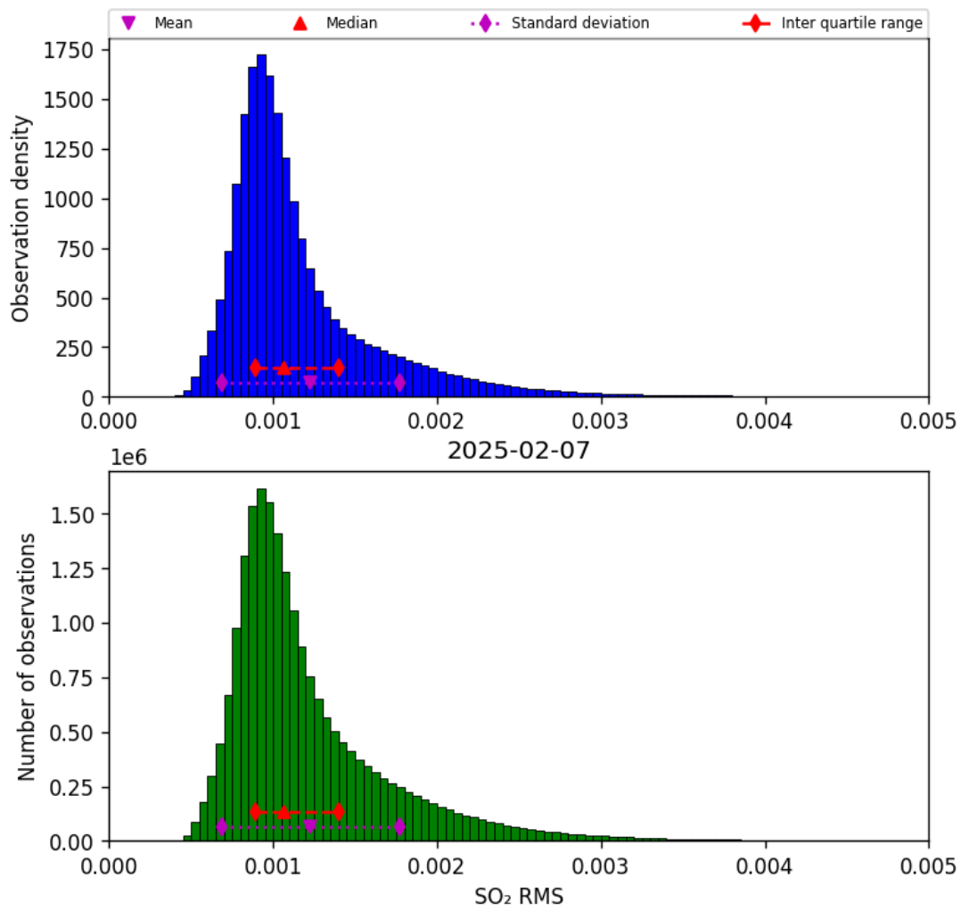
Figure 78: Histogram of “SO 2 RMS” for 2025-02-06 to 2025-02-08
