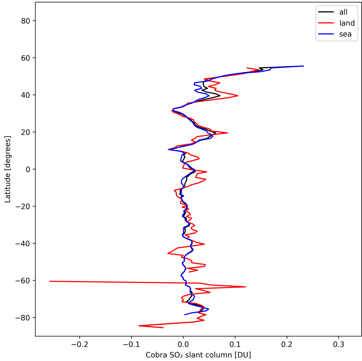
Figure 35: Zonal average of “Cobra SO 2 slant column” for 2025-02-06 to 2025-02-08.
