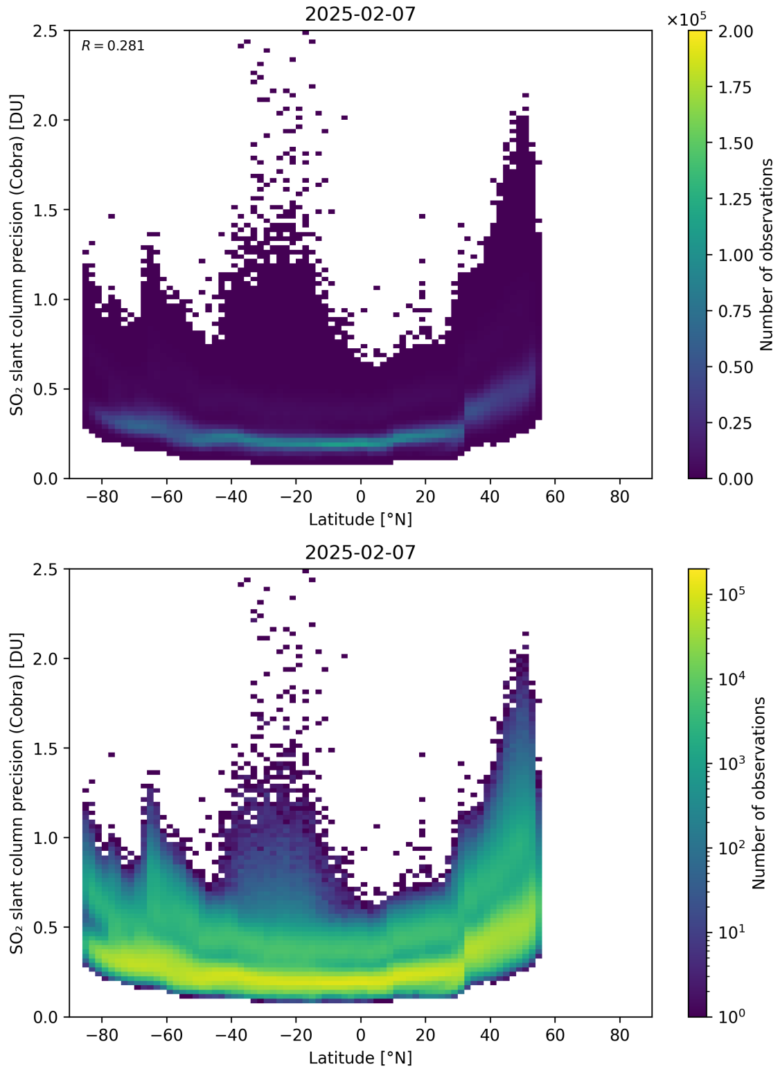
Figure 158: Scatter density plot of “Latitude” against “SO 2 slant column precision (Cobra)” for 2025-02-06 to 2025-02-08.
