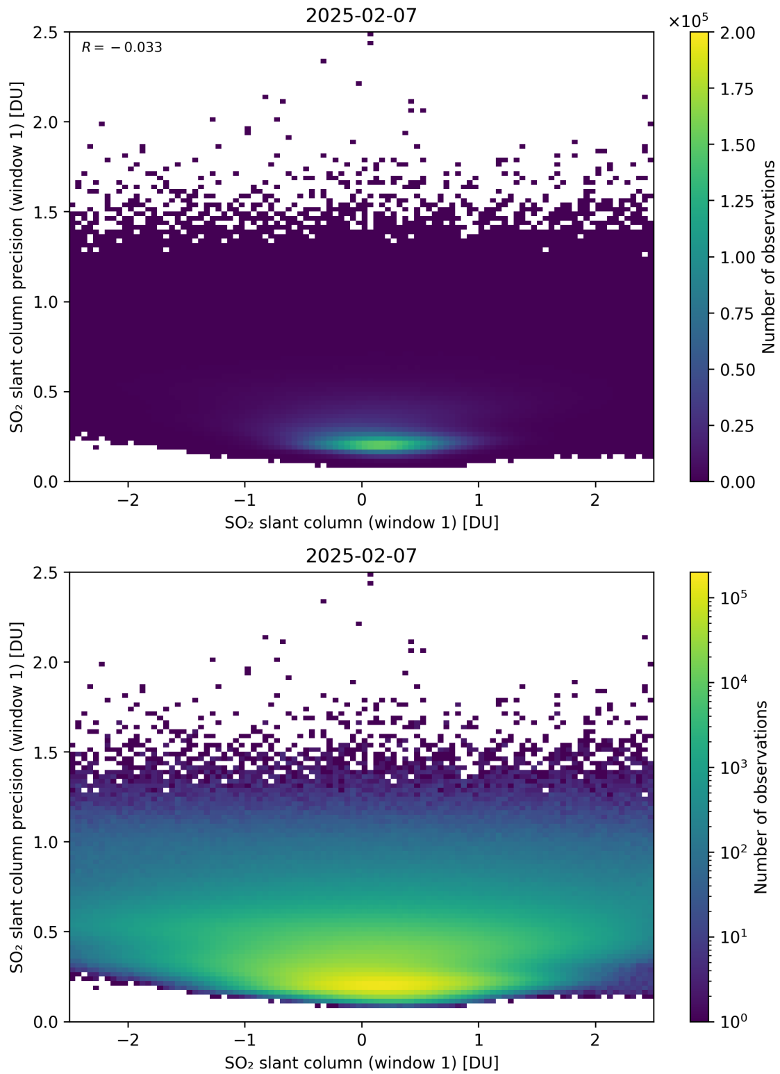
Figure 285: Scatter density plot of “SO 2 slant column (window 1)” against “SO 2 slant column precision (window 1)” for 2025-02-06 to 2025-02-08.
