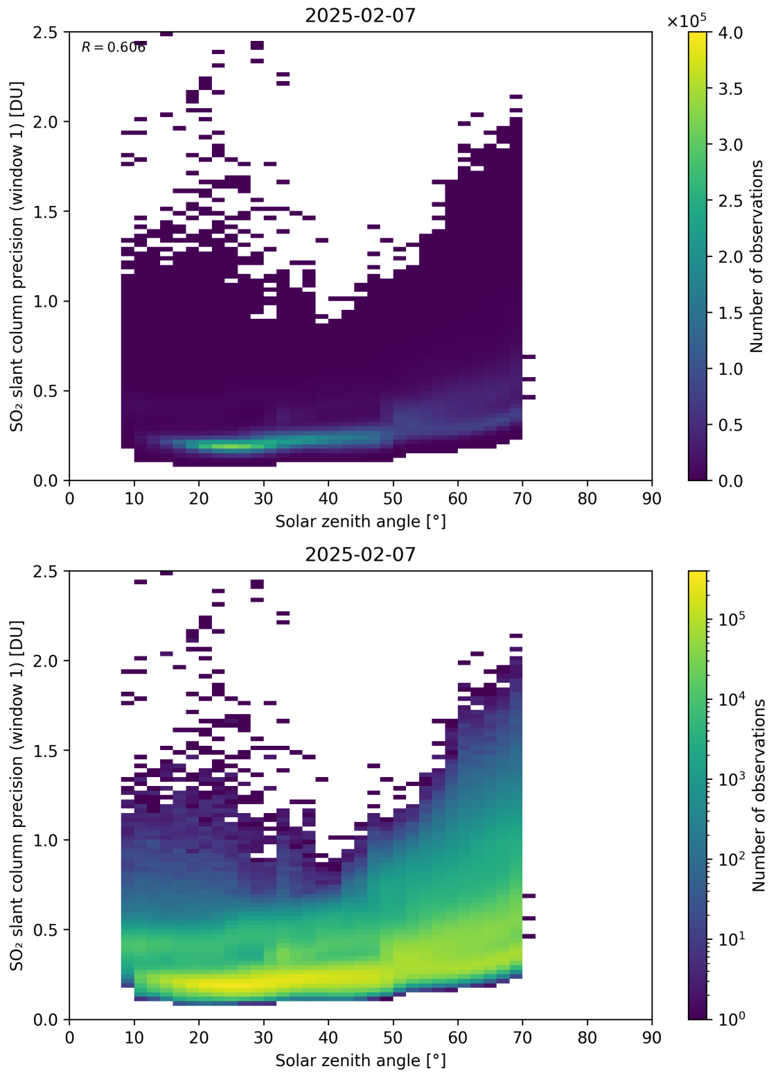
Figure 185: Scatter density plot of “Solar zenith angle” against “SO 2 slant column precision (window 1)” for 2025-02-06 to 2025-02-08.
