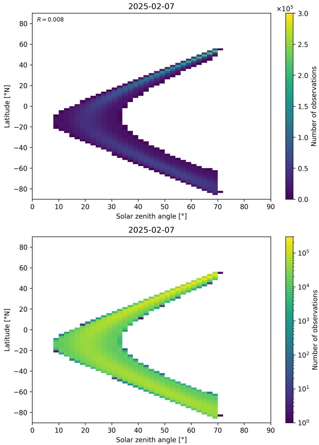
Figure 177: Scatter density plot of “Solar zenith angle” against “Latitude” for 2025-02-06 to 2025-02-08.
