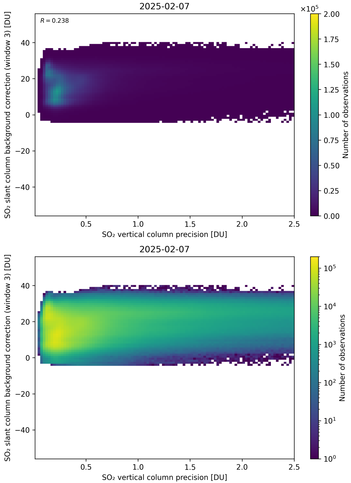
Figure 331: Scatter density plot of “SO 2 vertical column precision” against “SO 2 slant column background correction (window 3)” for 2025-02-06 to 2025-02-08.
