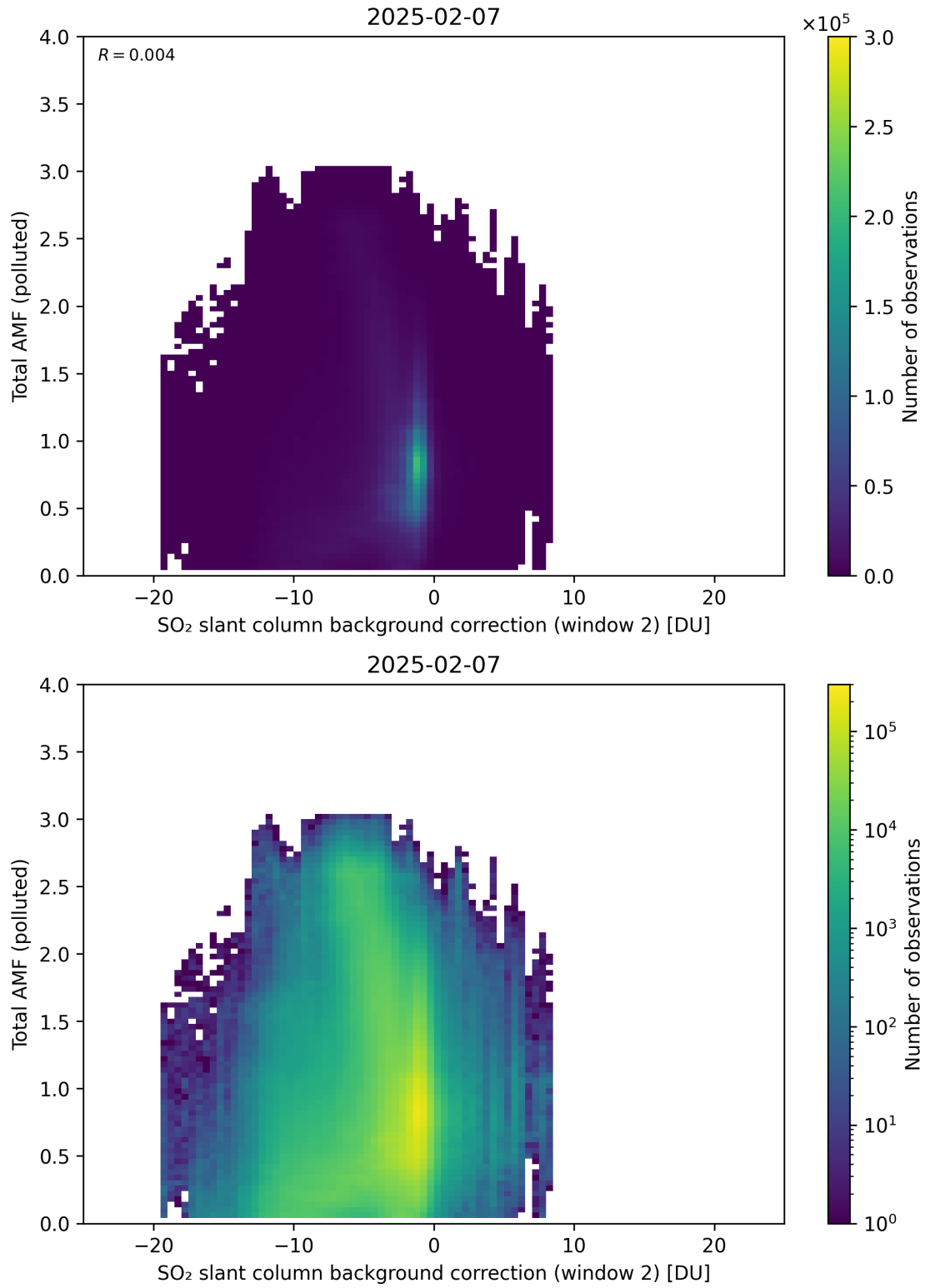
Figure 130: Scatter density plot of “SO 2 slant column background correction (window 2)” against “Total AMF (polluted)” for 2025-02-06 to 2025-02-08.
