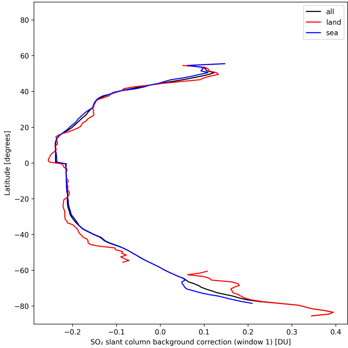
Figure 40: Zonal average of “SO 2 slant column background correction (window 1)” for 2025-02-06 to 2025-02-08.
