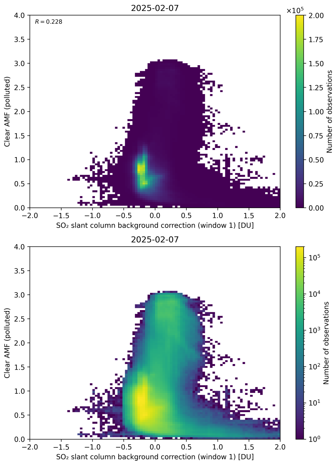
Figure 114: Scatter density plot of “SO 2 slant column background correction (window 1)” against “Clear AMF (polluted)” for 2025-02-06 to 2025-02-08.
