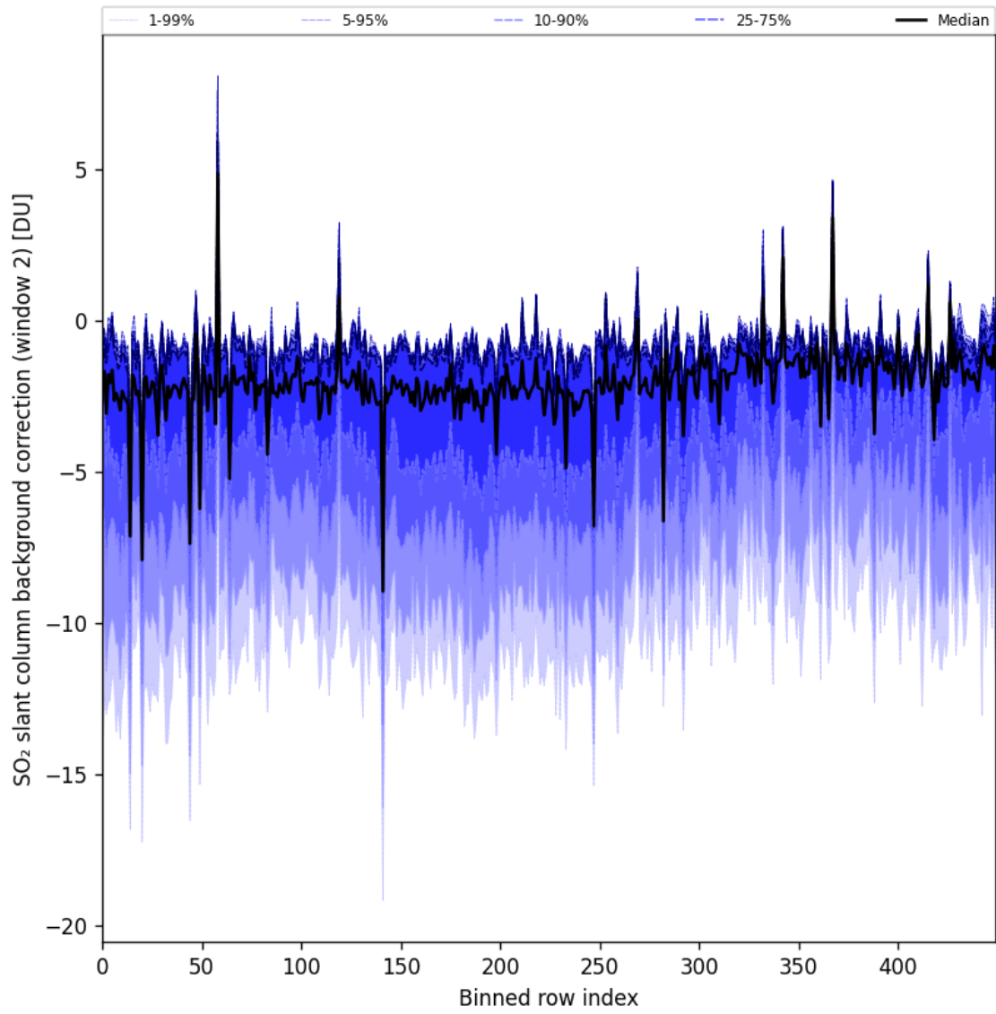
Figure 96: Along track statistics of “SO 2 slant column background correction (window 2)” for 2025-02-06 to 2025-02-08
