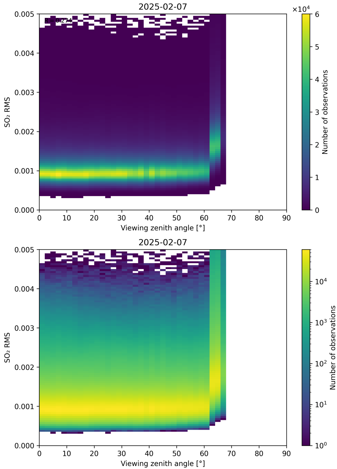
Figure 367: Scatter density plot of “Viewing zenith angle” against “SO 2 RMS” for 2025-02-06 to 2025-02-08.
