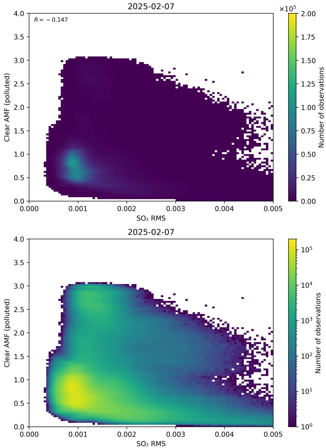
Figure 147: Scatter density plot of “SO 2 RMS” against “Clear AMF (polluted)” for 2025-02-06 to 2025-02-08.
