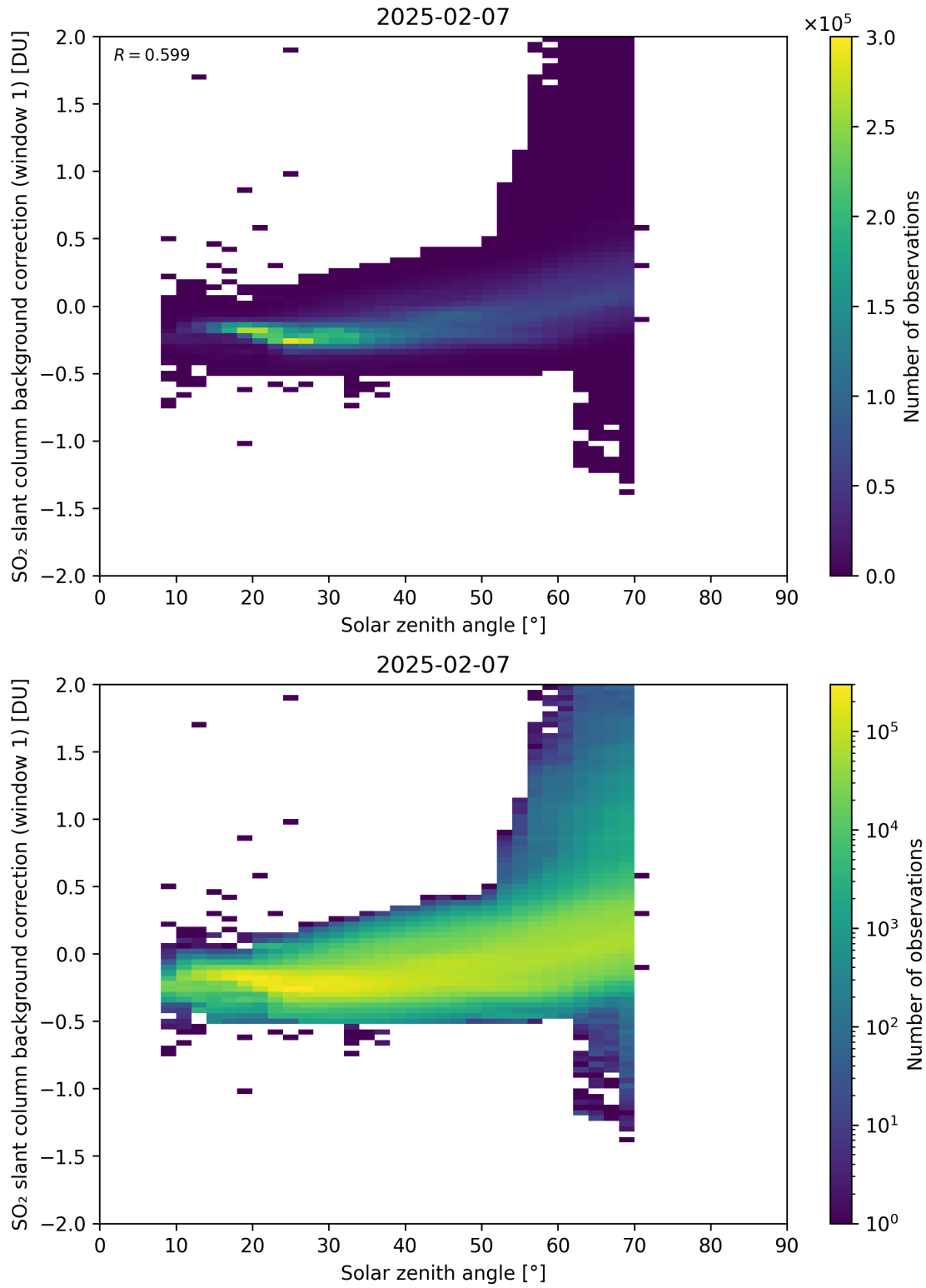
Figure 171: Scatter density plot of “Solar zenith angle” against “SO 2 slant column background correction (window 1)” for 2025-02-06 to 2025-02-08.
