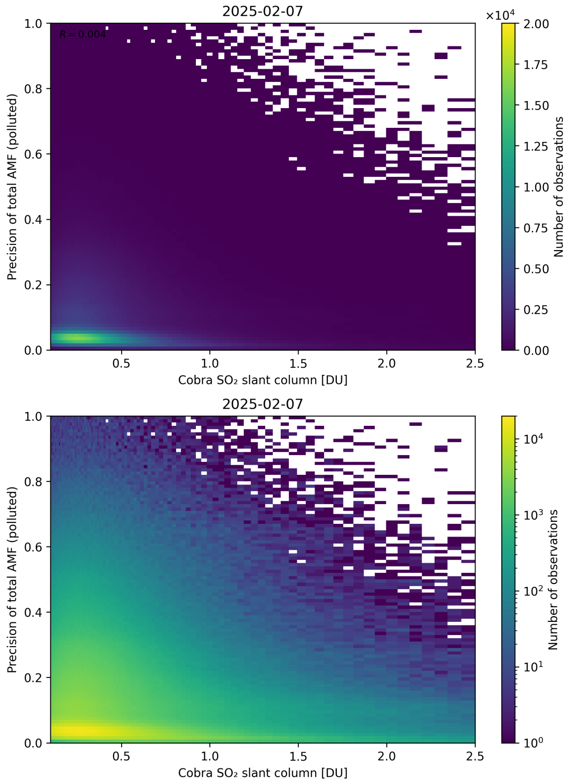
Figure 225: Scatter density plot of “Cobra SO 2 slant column” against “Precision of total AMF (polluted)” for 2025-02-06 to 2025-02-08.
