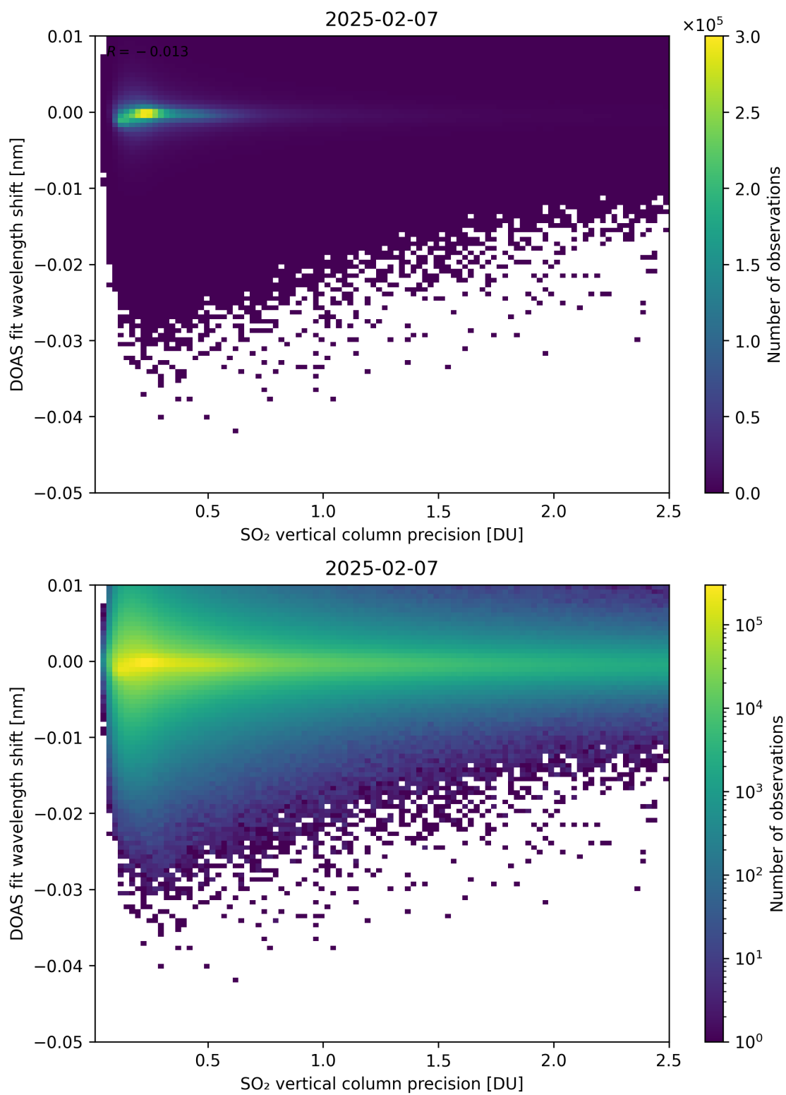
Figure 332: Scatter density plot of “SO 2 vertical column precision” against “DOAS fit wavelength shift” for 2025-02-06 to 2025-02-08.
