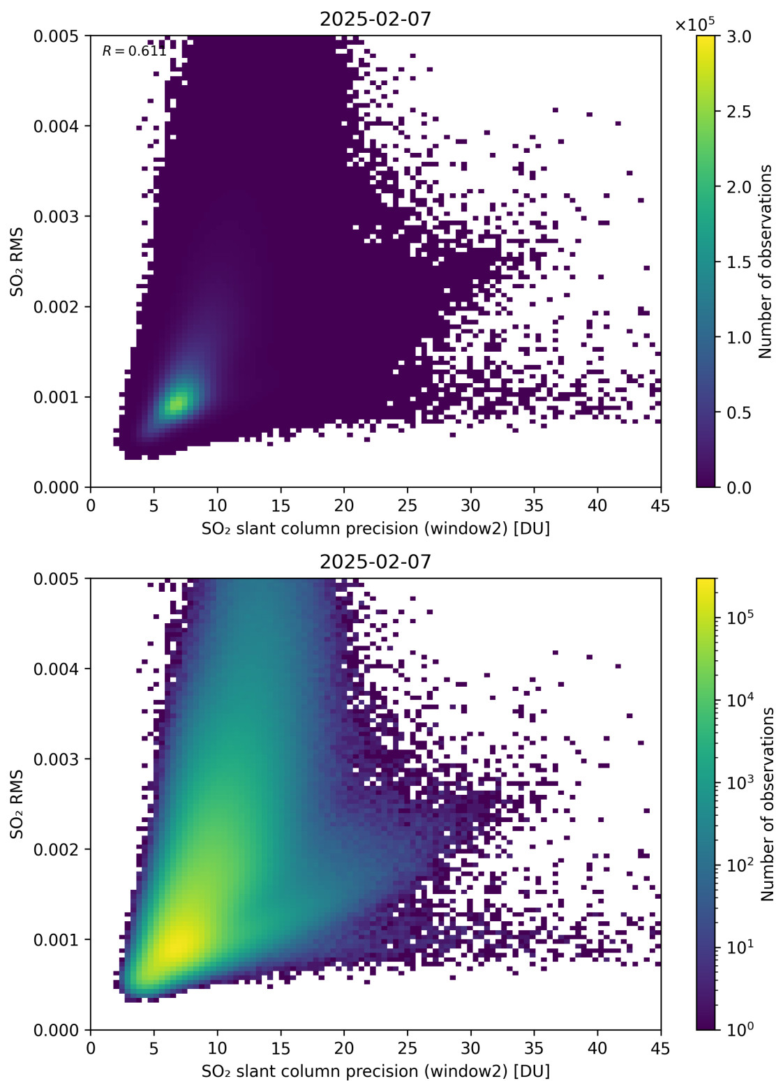
Figure 295: Scatter density plot of “SO 2 slant column precision (window2)” against “SO 2 RMS” for 2025-02-06 to 2025-02-08.
