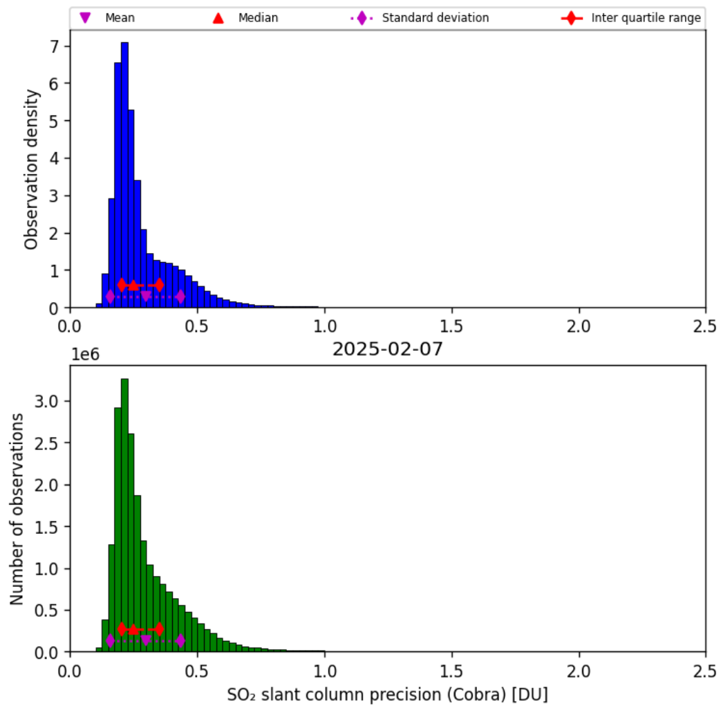
Figure 62: Histogram of “SO 2 slant column precision (Cobra)” for 2025-02-06 to 2025-02-08
