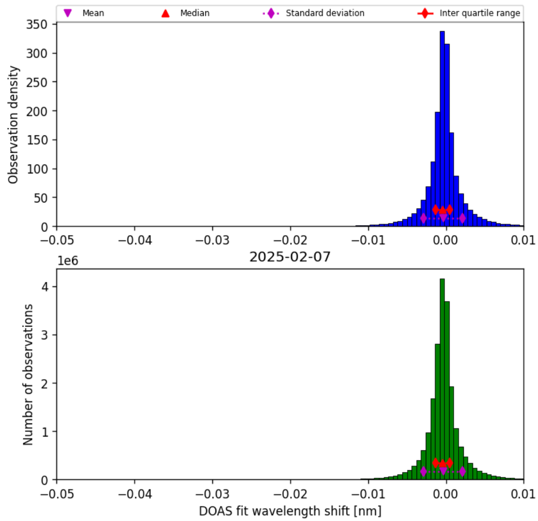
Figure 76: Histogram of “DOAS fit wavelength shift” for 2025-02-06 to 2025-02-08
