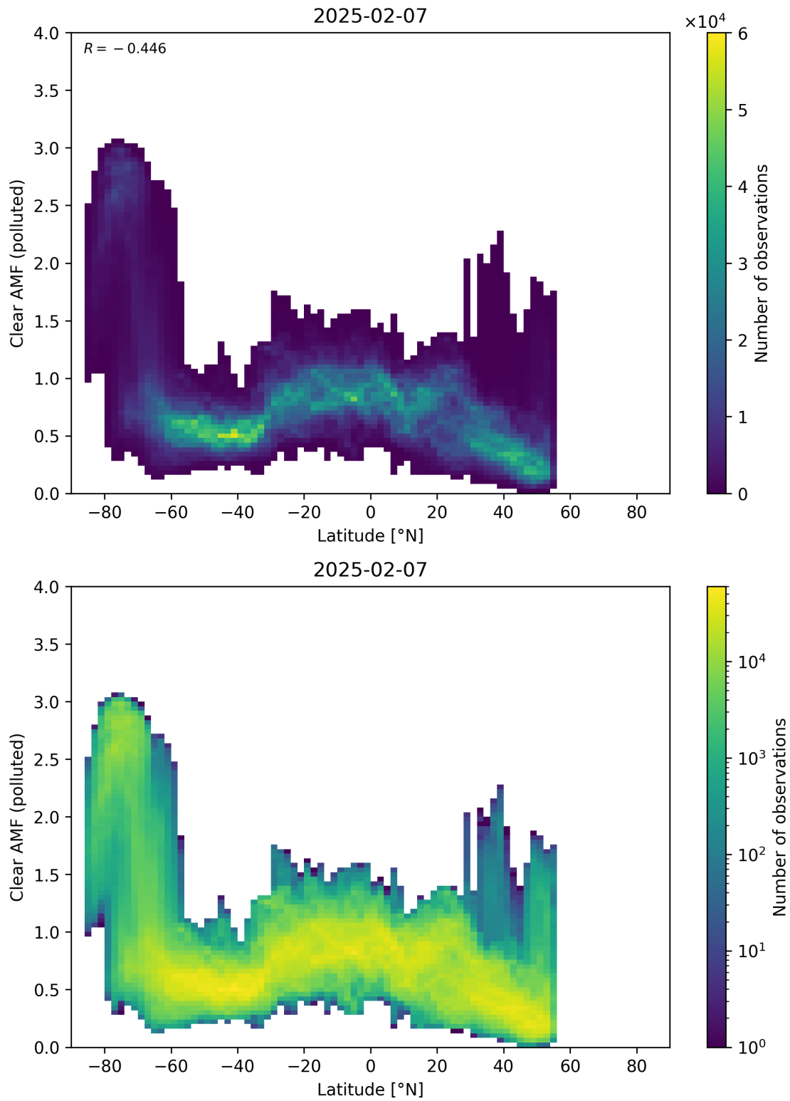
Figure 156: Scatter density plot of “Latitude” against “Clear AMF (polluted)” for 2025-02-06 to 2025-02-08.
