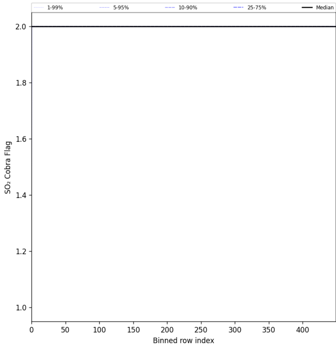
Figure 101: Along track statistics of “SO 2 Cobra Flag” for 2025-02-06 to 2025-02-08
