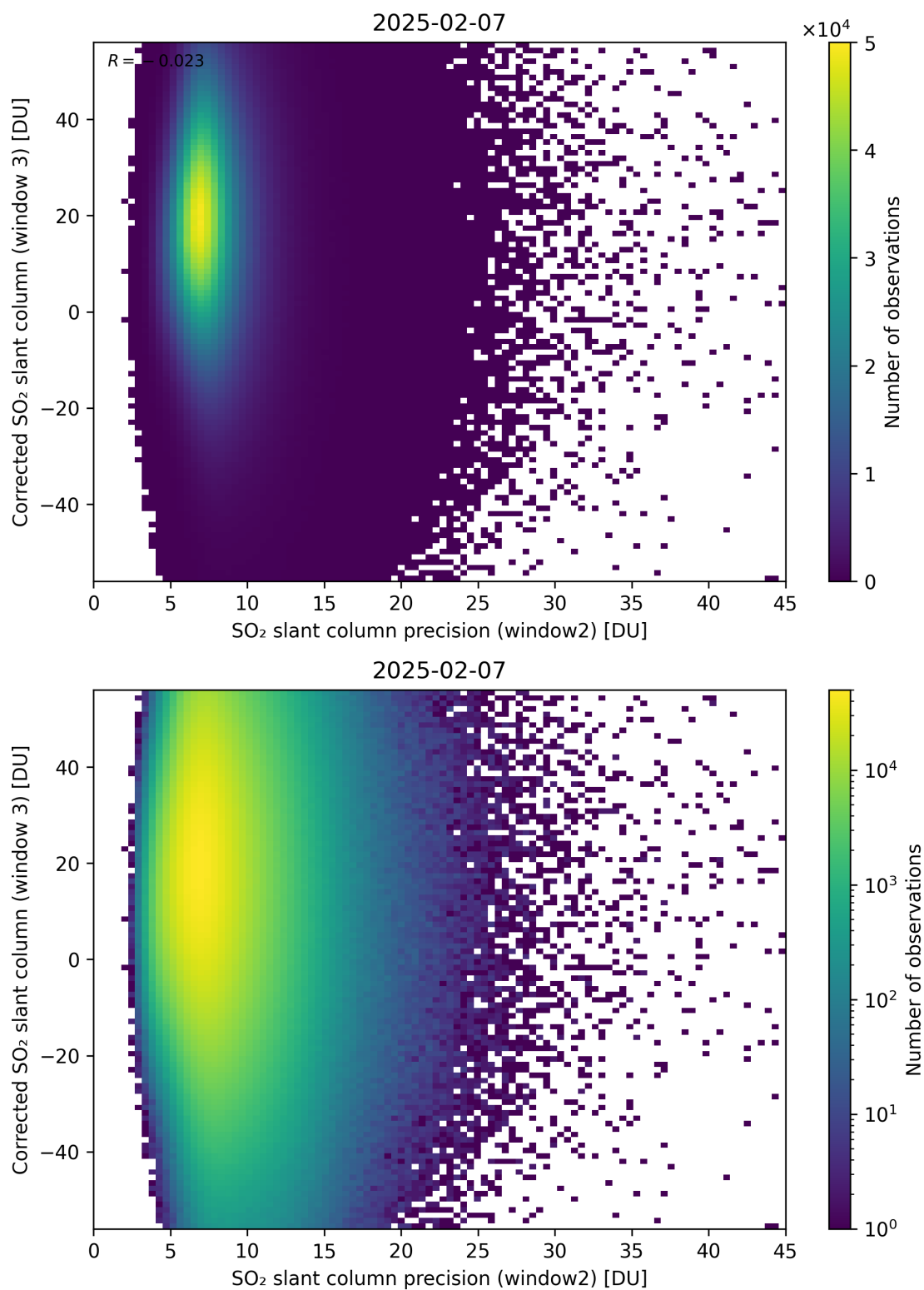
Figure 298: Scatter density plot of “SO 2 slant column precision (window2)” against “Corrected SO 2 slant column (window 3)” for 2025-02-06 to 2025-02-08.
