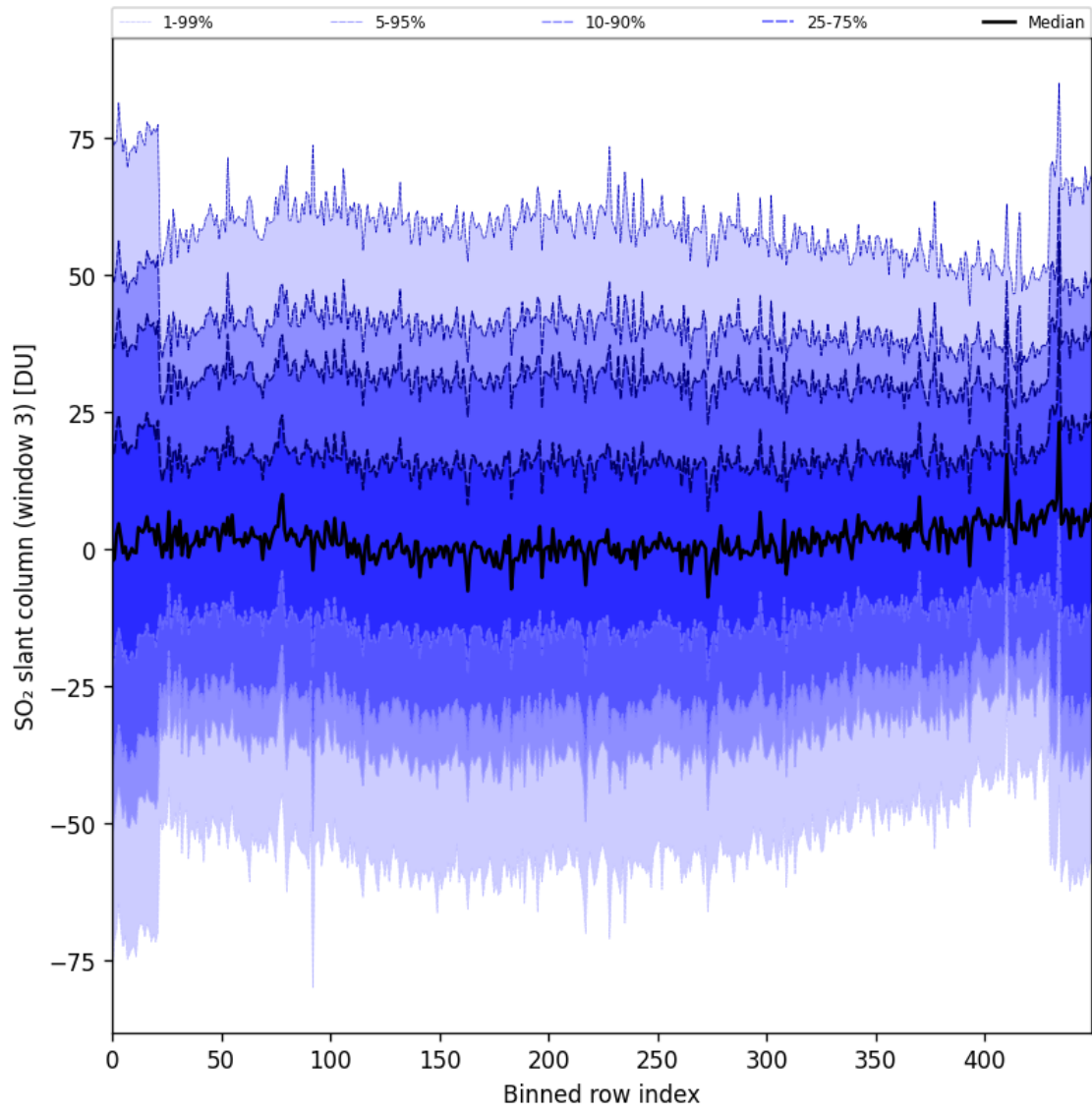
Figure 97: Along track statistics of “SO 2 slant column (window 3)” for 2025-02-06 to 2025-02-08
