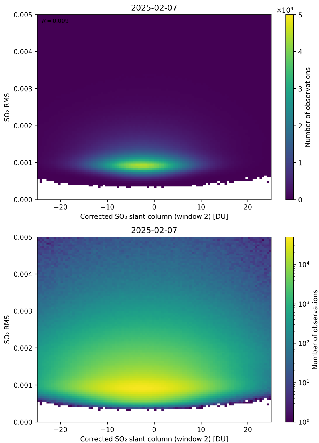
Figure 248: Scatter density plot of “Corrected SO 2 slant column (window 2)” against “SO 2 RMS” for 2025-02-06 to 2025-02-08.
