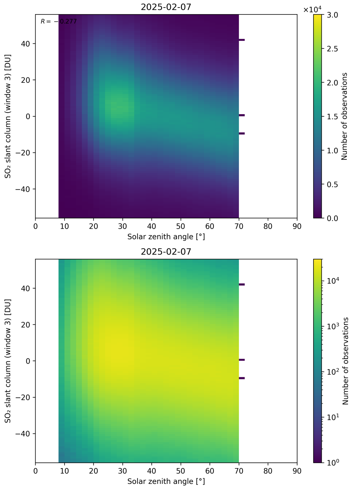
Figure 187: Scatter density plot of “Solar zenith angle” against “SO 2 slant column (window 3)” for 2025-02-06 to 2025-02-08.
