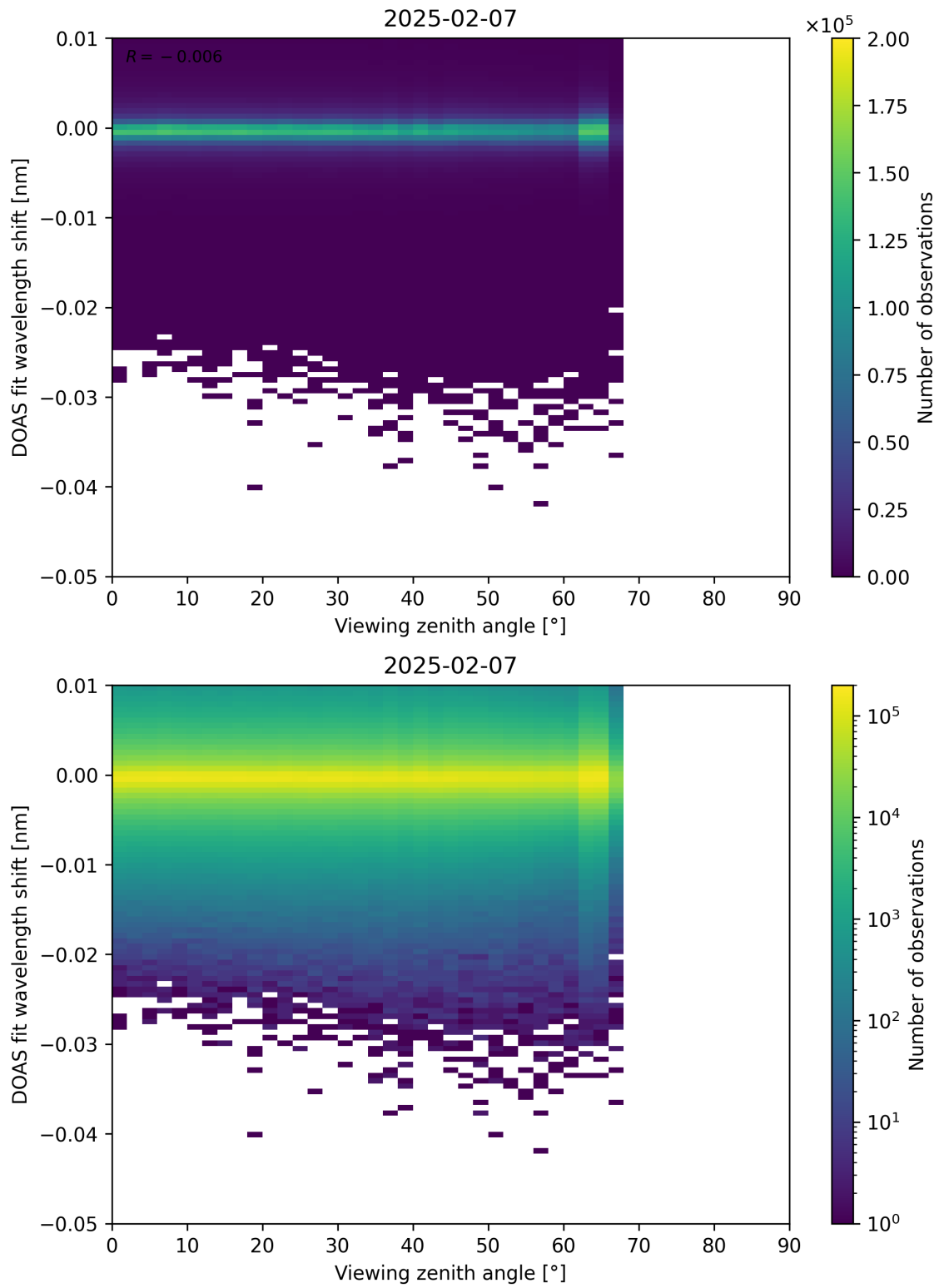
Figure 365: Scatter density plot of “Viewing zenith angle” against “DOAS fit wavelength shift” for 2025-02-06 to 2025-02-08.
