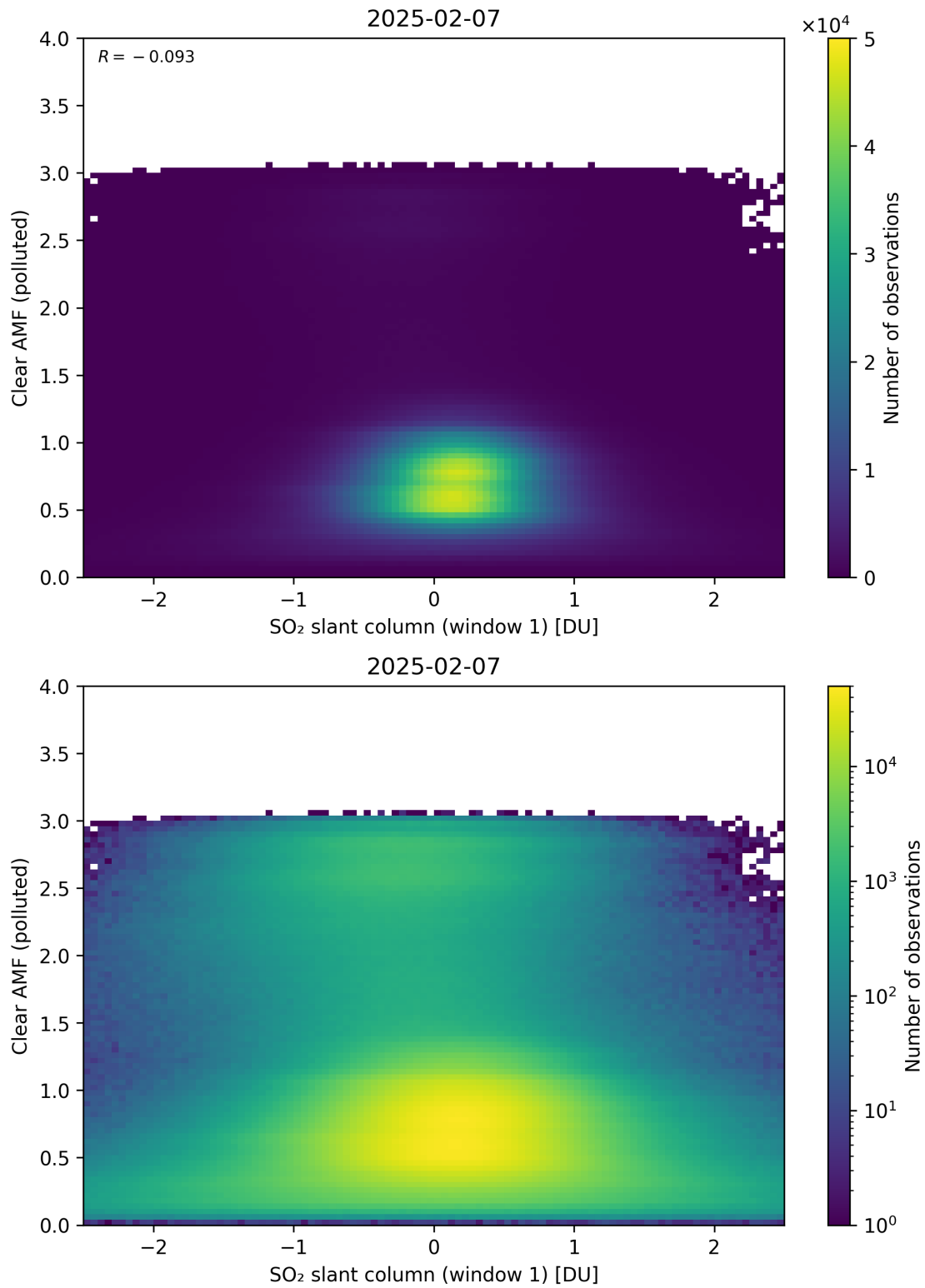
Figure 282: Scatter density plot of “SO 2 slant column (window 1)” against “Clear AMF (polluted)” for 2025-02-06 to 2025-02-08.
