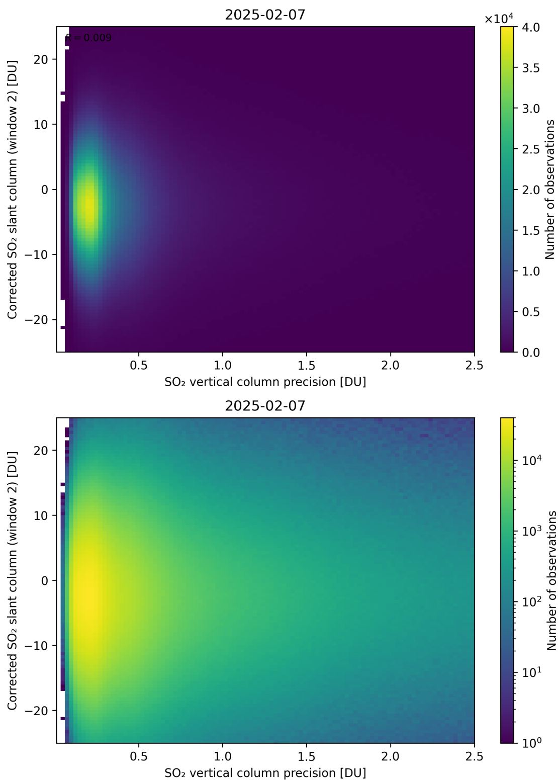
Figure 339: Scatter density plot of “SO 2 vertical column precision” against “Corrected SO 2 slant column (window 2)” for 2025-02-06 to 2025-02-08.
