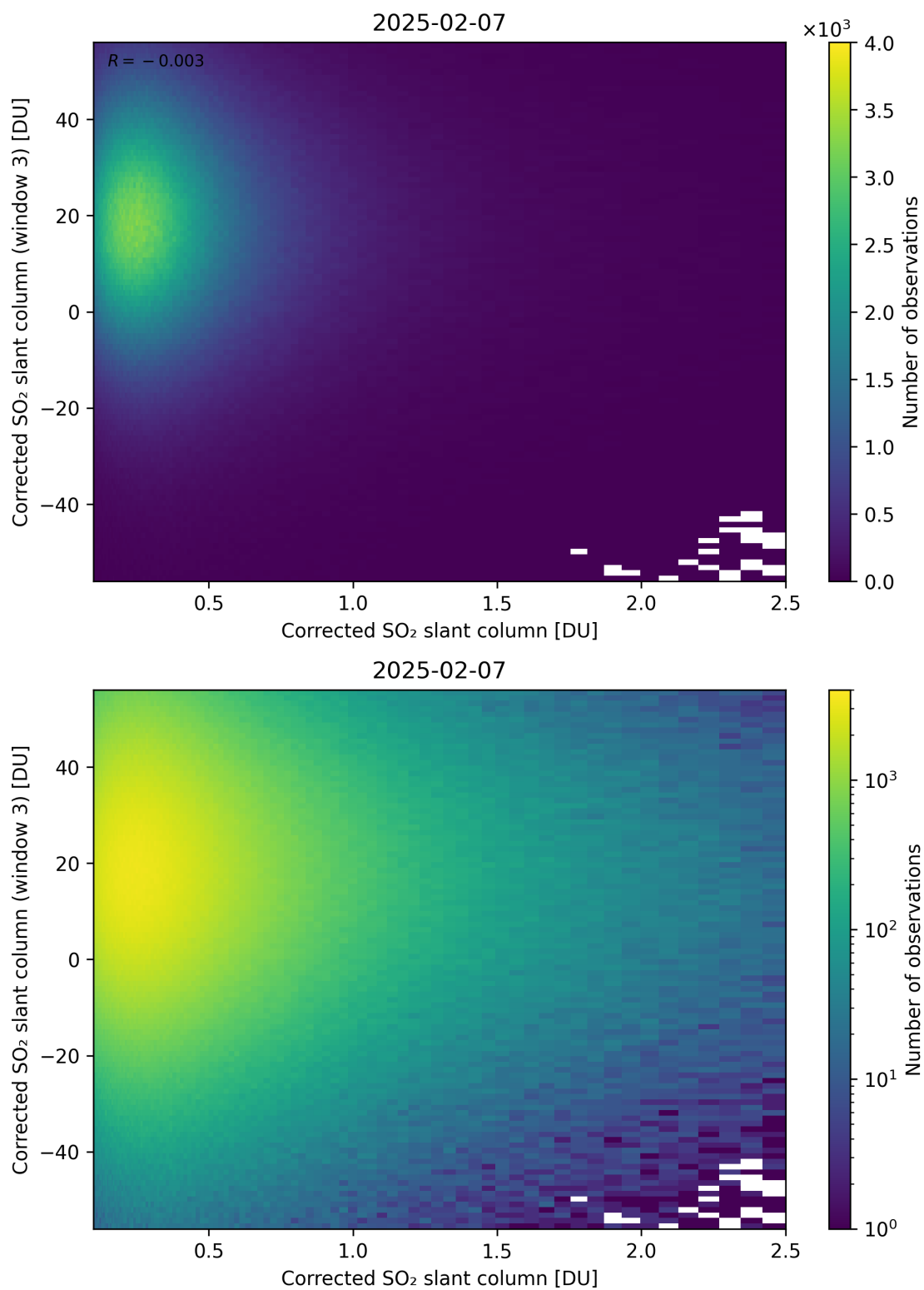
Figure 236: Scatter density plot of “Corrected SO 2 slant column” against “Corrected SO 2 slant column (window 3)” for 2025-02-06 to 2025-02-08.
