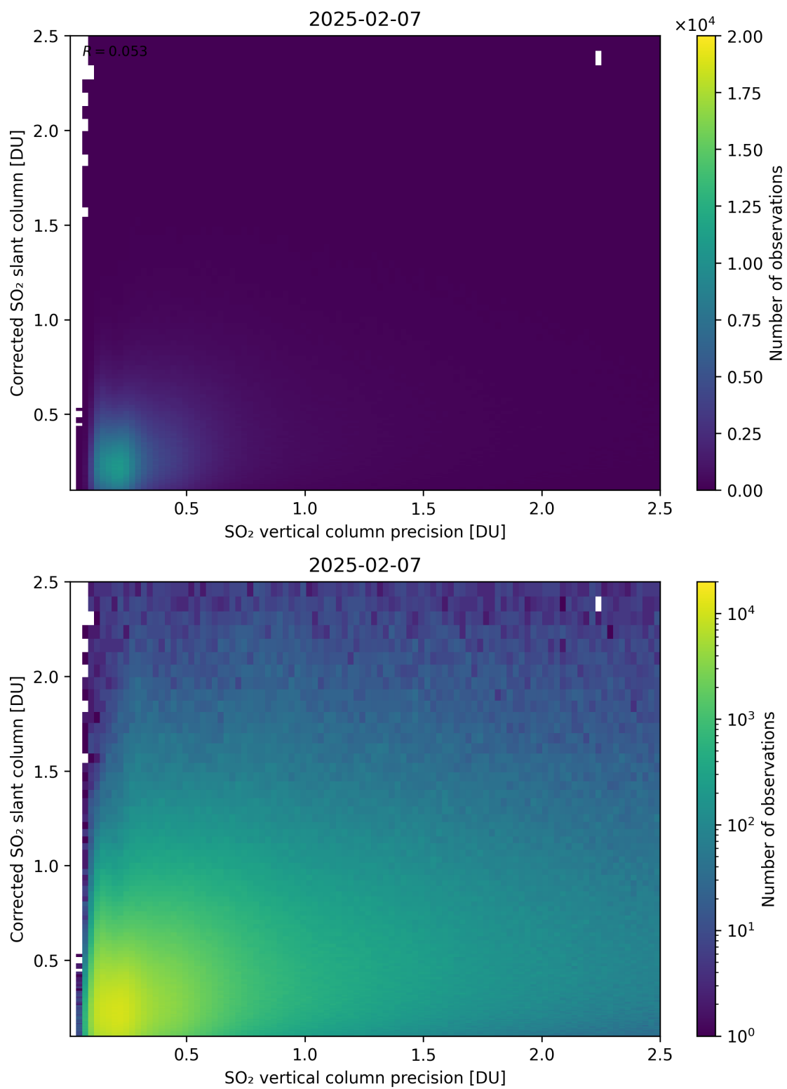
Figure 338: Scatter density plot of “SO 2 vertical column precision” against “Corrected SO 2 slant column” for 2025-02-06 to 2025-02-08.
