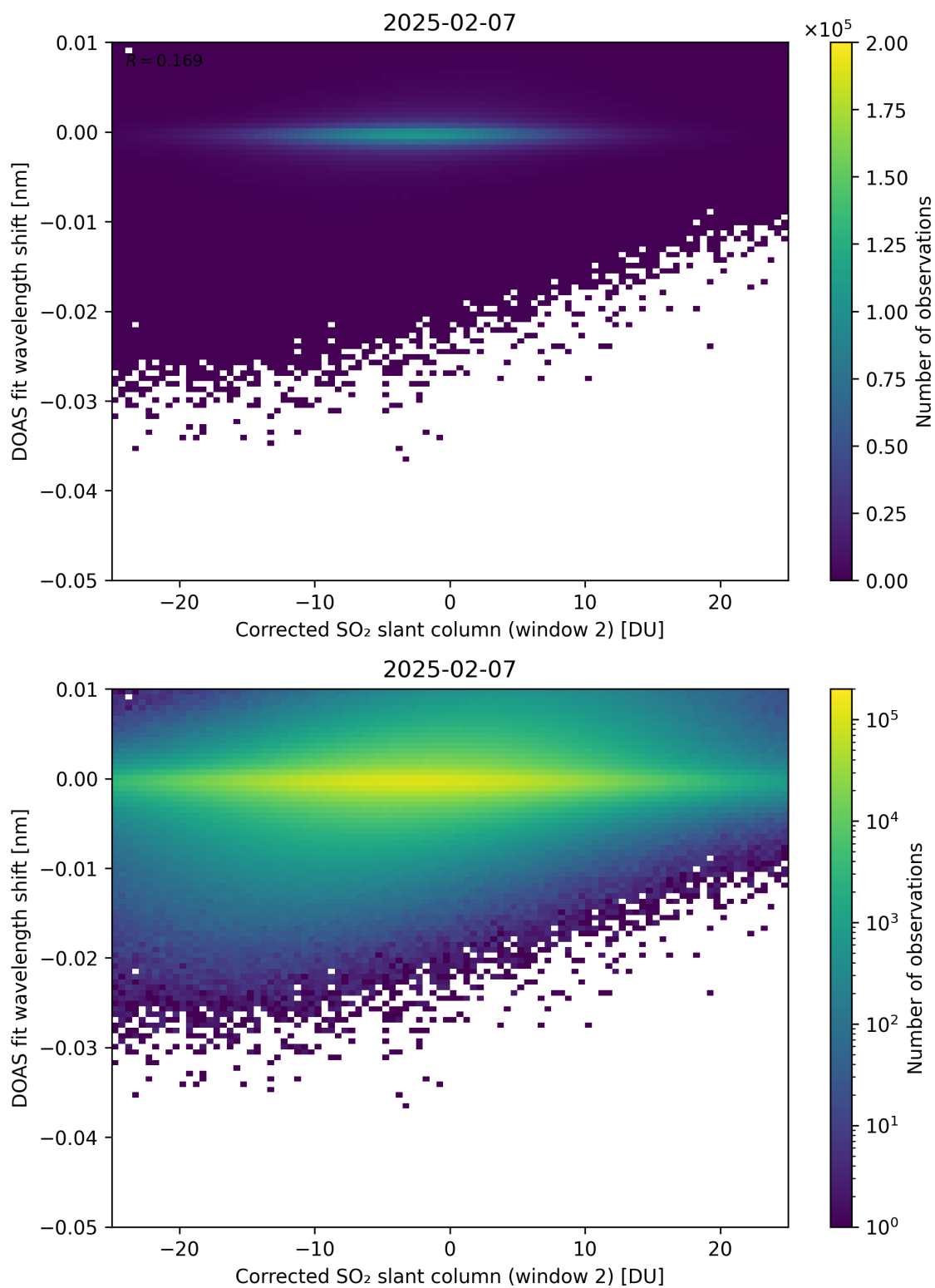
Figure 246: Scatter density plot of “Corrected SO 2 slant column (window 2)” against “DOAS fit wavelength shift” for 2025-02-06 to 2025-02-08.
