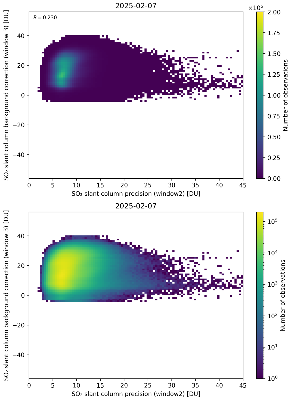
Figure 292: Scatter density plot of “SO 2 slant column precision (window2)” against “SO 2 slant column background correction (window 3)” for 2025-02-06 to 2025-02-08.
