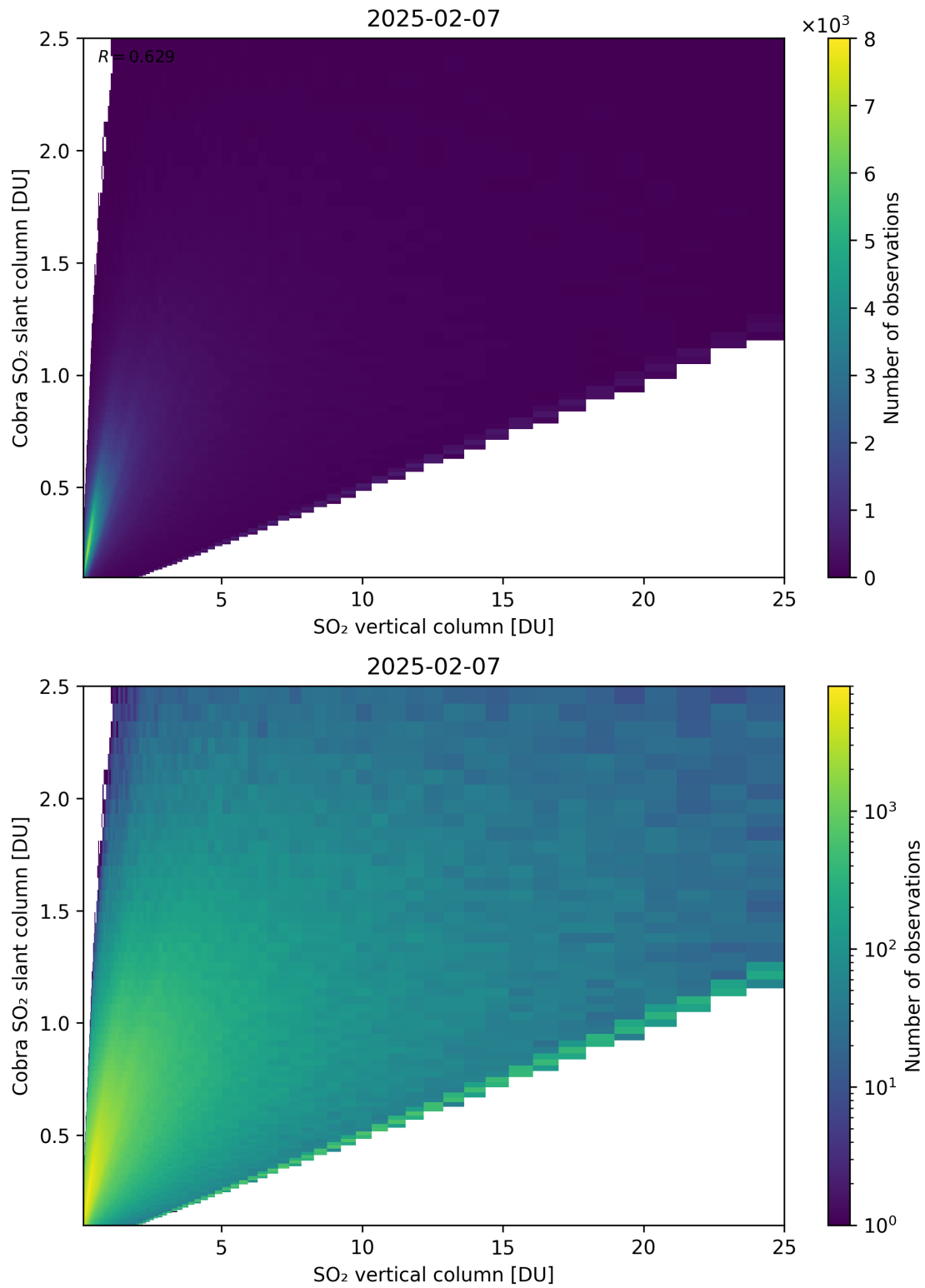
Figure 349: Scatter density plot of “SO 2 vertical column” against “Cobra SO 2 slant column” for 2025-02-06 to 2025-02-08.
