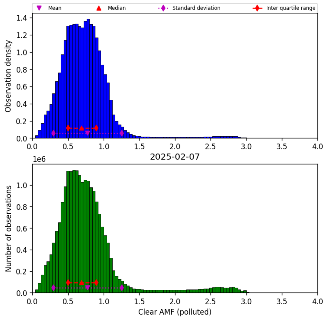
Figure 81: Histogram of “Clear AMF (polluted)” for 2025-02-06 to 2025-02-08
