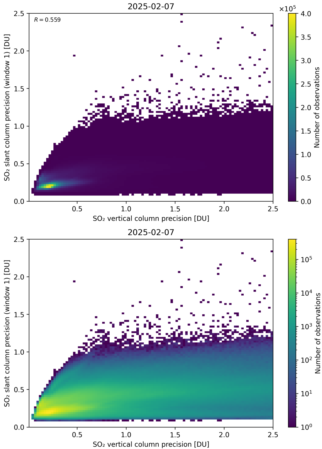
Figure 342: Scatter density plot of “SO 2 vertical column precision” against “SO 2 slant column precision (window 1)” for 2025-02-06 to 2025-02-08.
