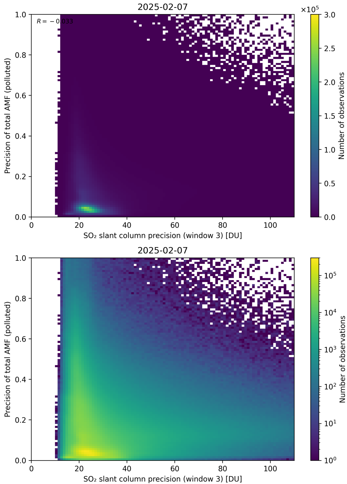
Figure 314: Scatter density plot of “SO 2 slant column precision (window 3)” against “Precision of total AMF (polluted)” for 2025-02-06 to 2025-02-08.
