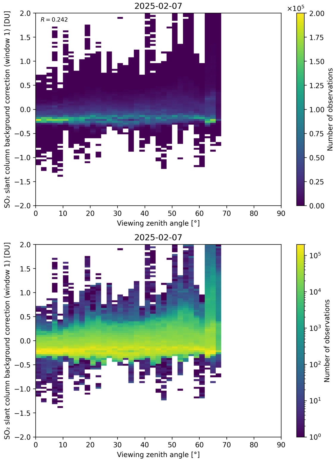
Figure 362: Scatter density plot of “Viewing zenith angle” against “SO 2 slant column background correction (window 1)” for 2025-02-06 to 2025-02-08.
