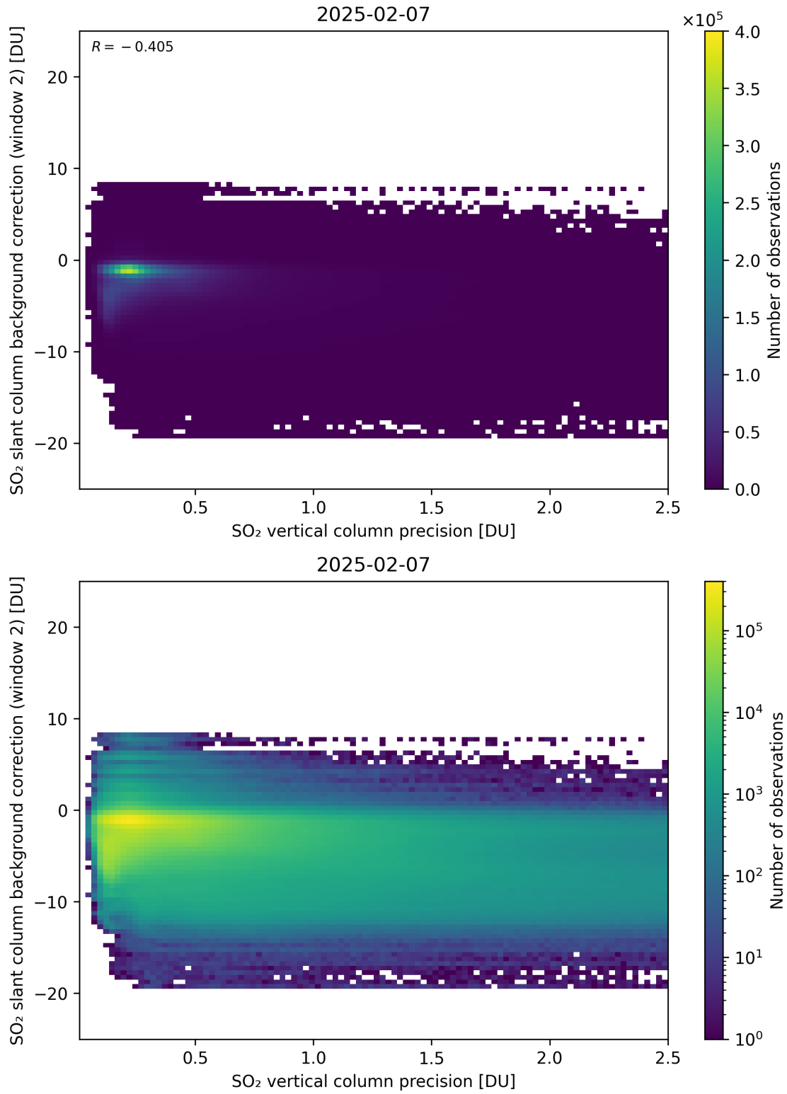
Figure 330: Scatter density plot of “SO 2 vertical column precision” against “SO 2 slant column background correction (window 2)” for 2025-02-06 to 2025-02-08.
