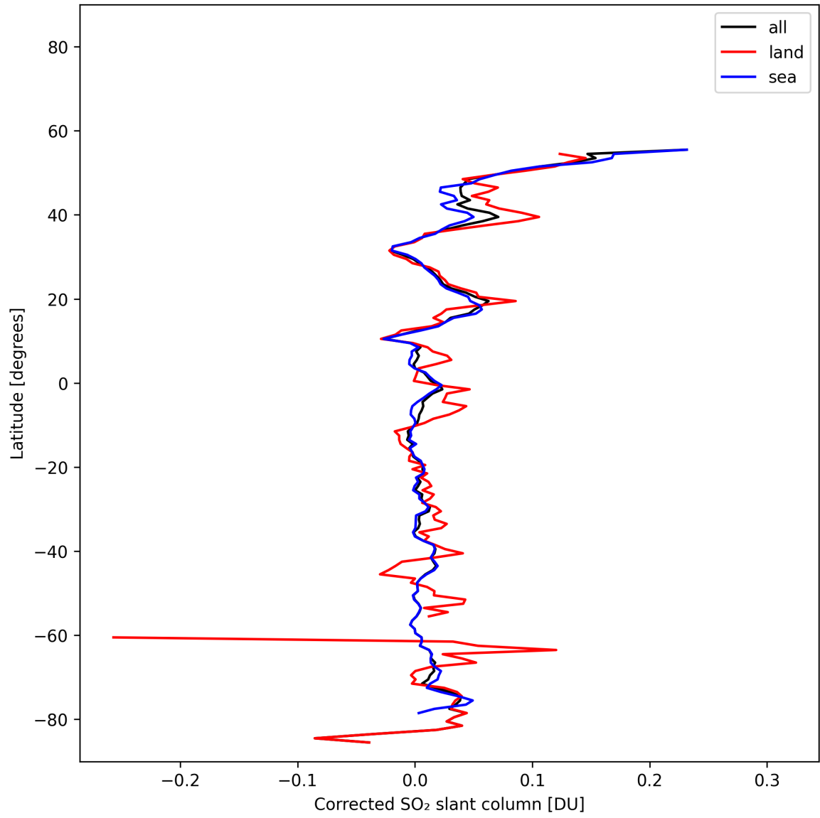
Figure 34: Zonal average of “Corrected SO 2 slant column” for 2025-02-06 to 2025-02-08.
