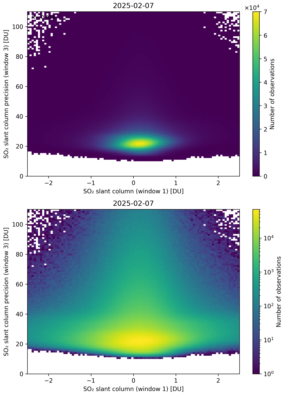
Figure 288: Scatter density plot of “SO 2 slant column (window 1)” against “SO 2 slant column precision (window 3)” for 2025-02-06 to 2025-02-08.
