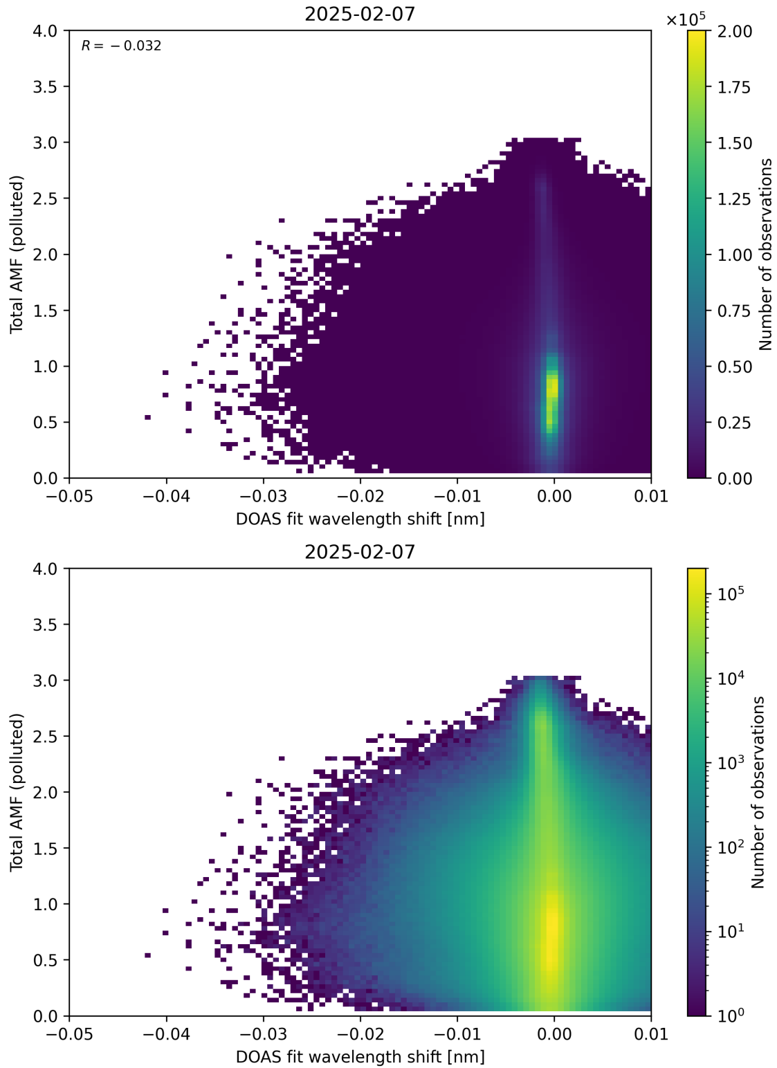
Figure 141: Scatter density plot of “DOAS fit wavelength shift” against “Total AMF (polluted)” for 2025-02-06 to 2025-02-08.
