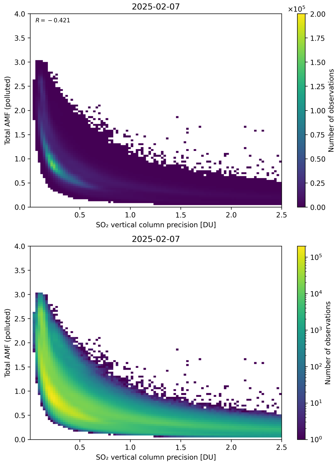
Figure 346: Scatter density plot of “SO 2 vertical column precision” against “Total AMF (polluted)” for 2025-02-06 to 2025-02-08.
