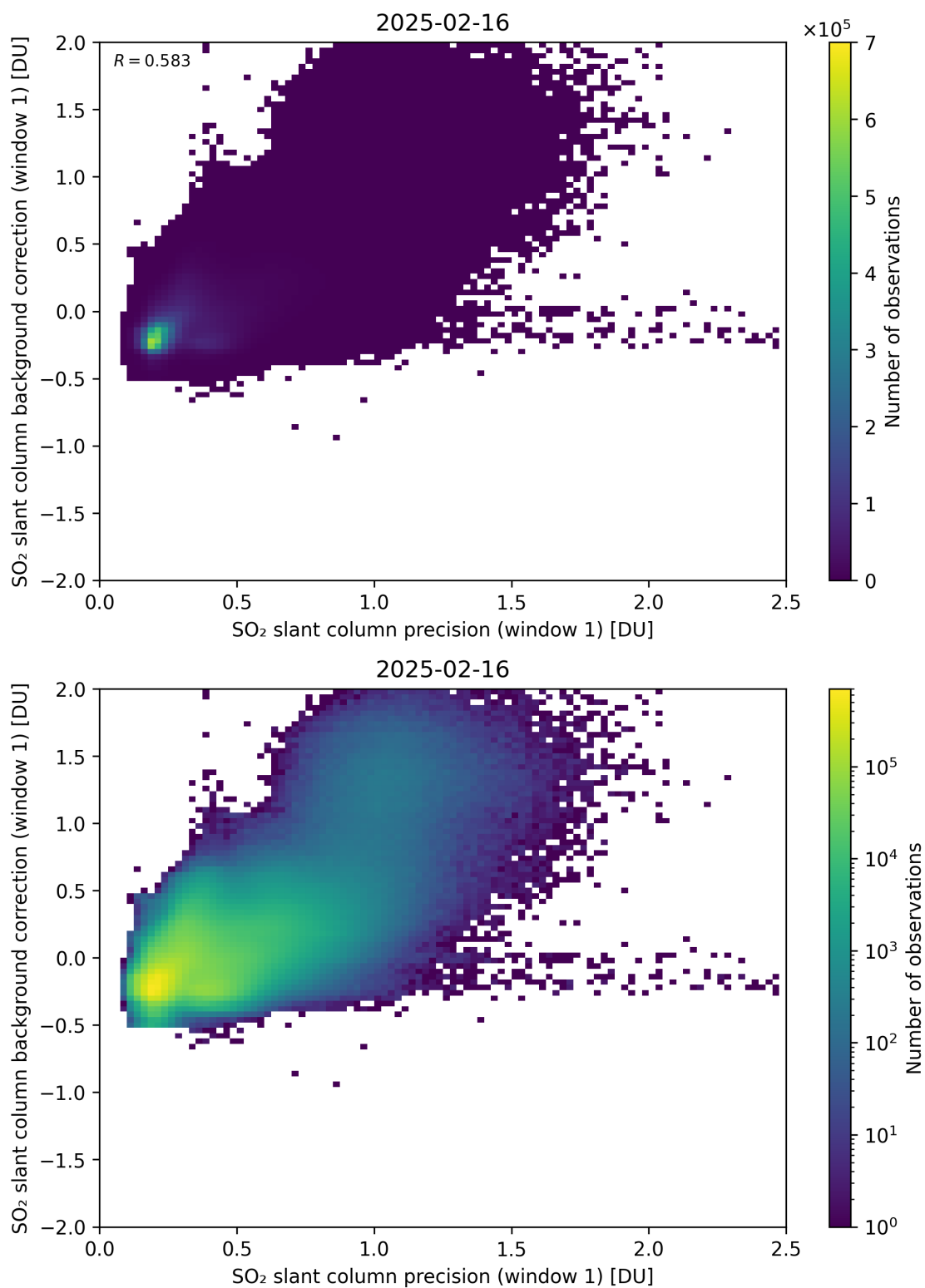
Figure 268: Scatter density plot of “SO 2 slant column precision (window 1)” against “SO 2 slant column background correction (window 1)” for 2025-02-15 to 2025-02-17.
