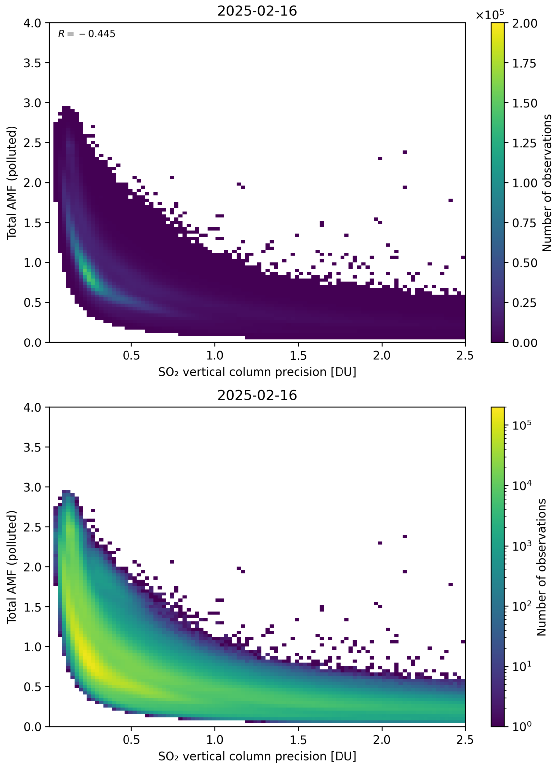
Figure 346: Scatter density plot of “SO 2 vertical column precision” against “Total AMF (polluted)” for 2025-02-15 to 2025-02-17.
