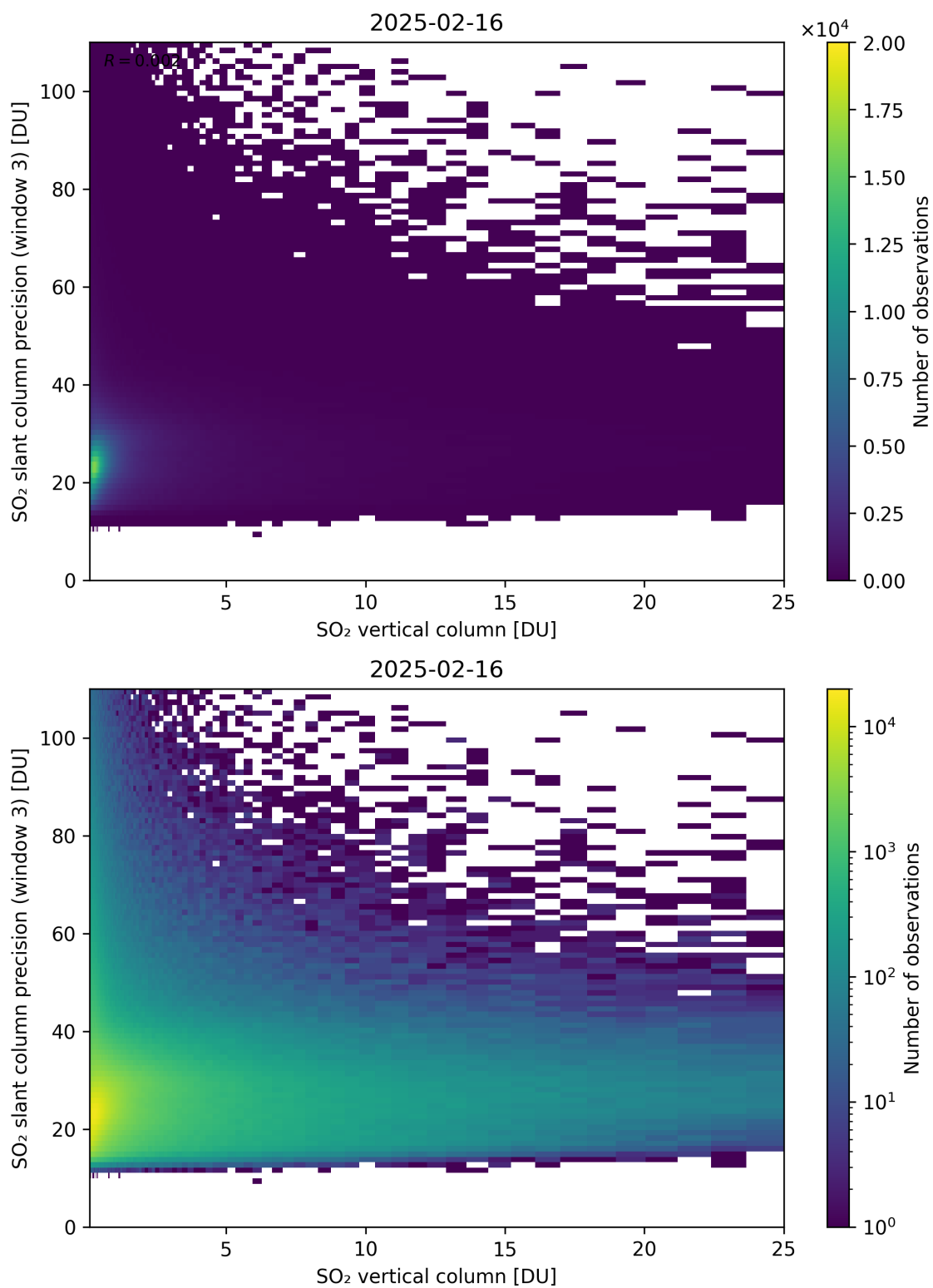
Figure 358: Scatter density plot of “SO 2 vertical column” against “SO 2 slant column precision (window 3)” for 2025-02-15 to 2025-02-17.
