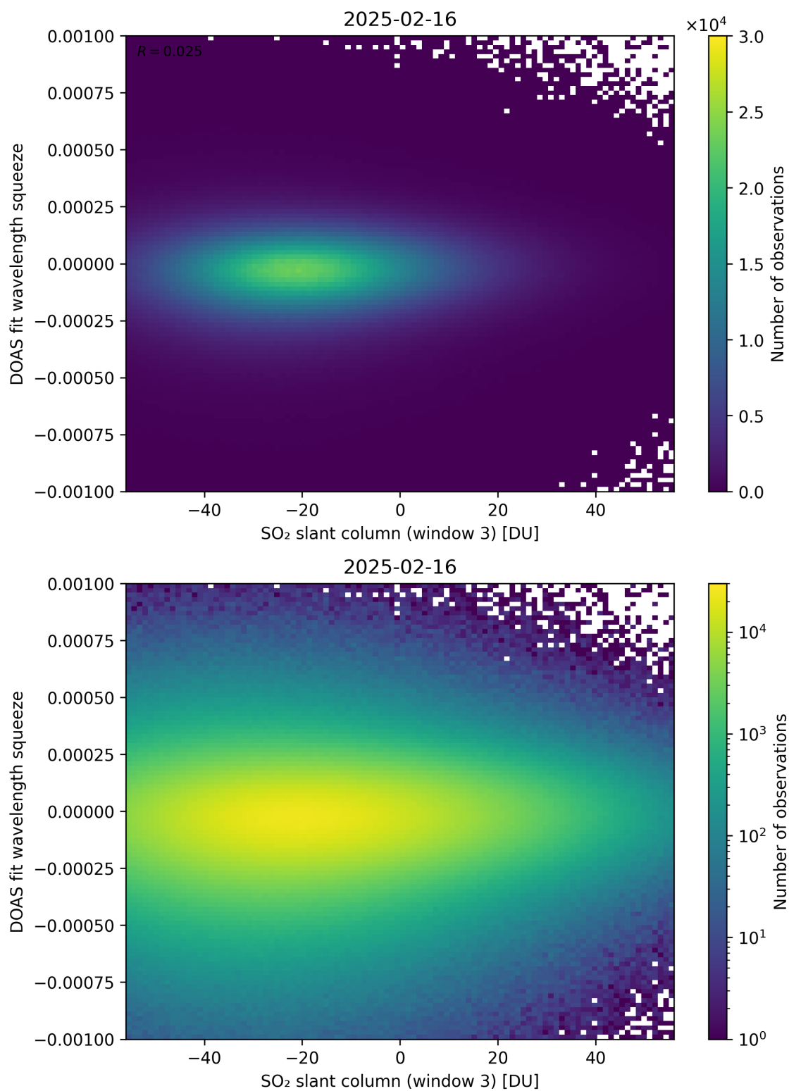
Figure 305: Scatter density plot of “SO 2 slant column (window 3)” against “DOAS fit wavelength squeeze” for 2025-02-15 to 2025-02-17.
