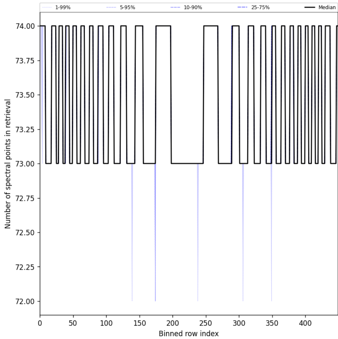
Figure 108: Along track statistics of “Number of spectral points in retrieval” for 2025-02-15 to 2025-02-17
