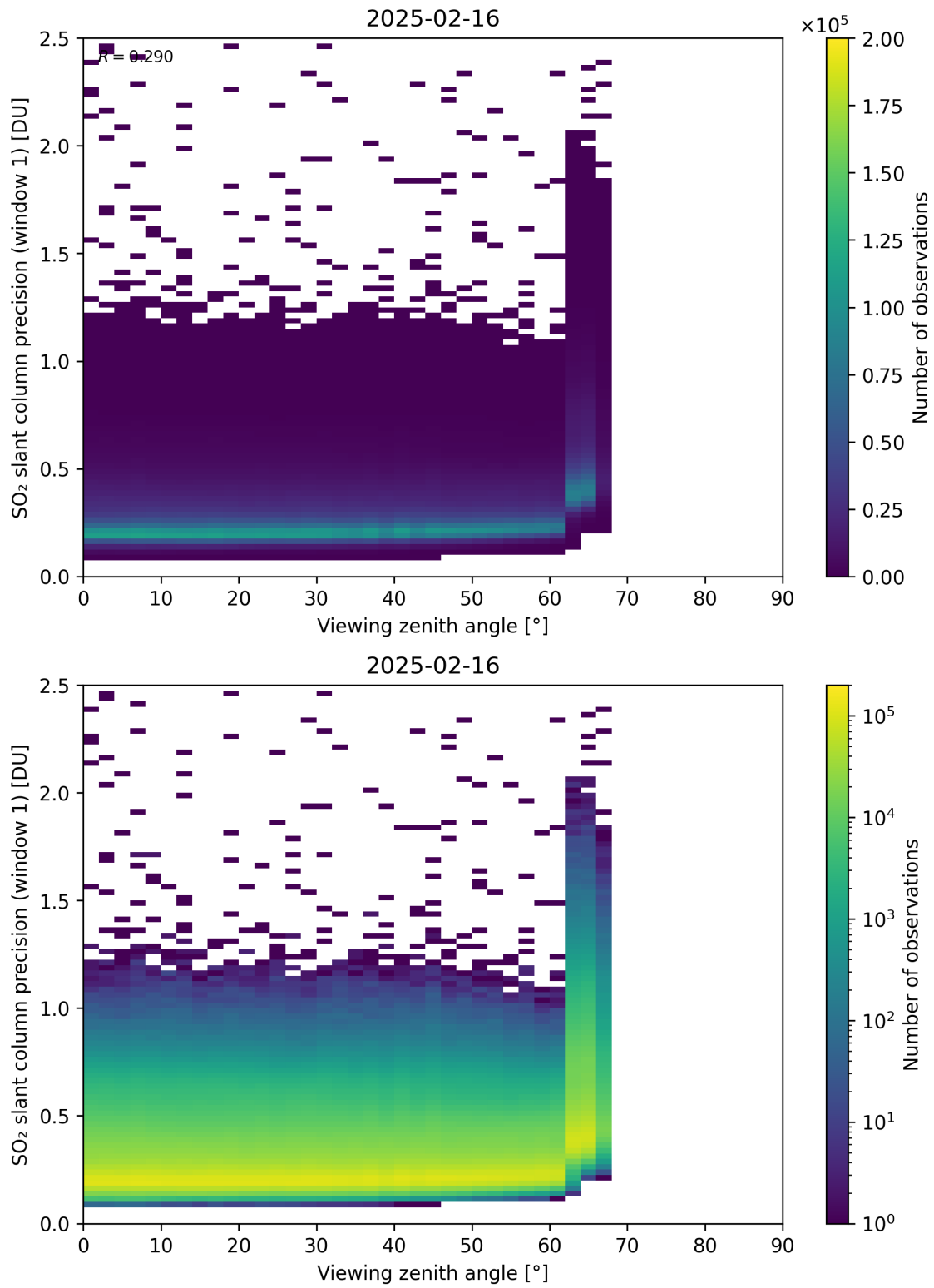
Figure 377: Scatter density plot of “Viewing zenith angle” against “SO 2 slant column precision (window 1)” for 2025-02-15 to 2025-02-17.
