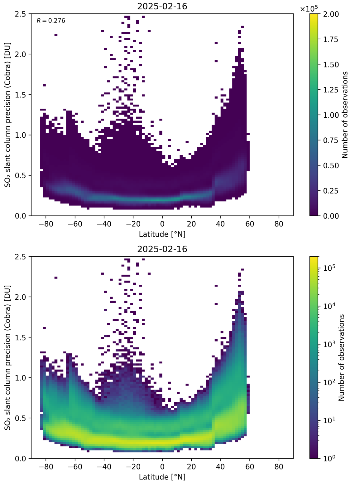
Figure 158: Scatter density plot of “Latitude” against “SO 2 slant column precision (Cobra)” for 2025-02-15 to 2025-02-17.
