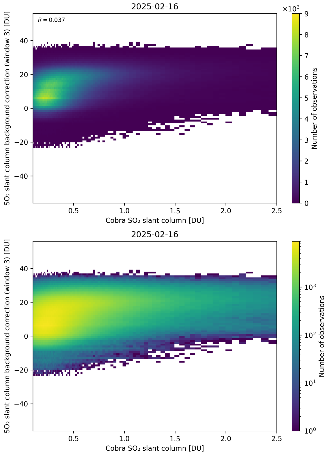
Figure 195: Scatter density plot of “Cobra SO 2 slant column” against “SO 2 slant column background correction (window 3)” for 2025-02-15 to 2025-02-17.
