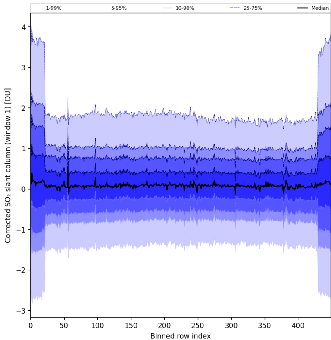
Figure 91: Along track statistics of “Corrected SO 2 slant column (window 1)” for 2025-02-15 to 2025-02-17
