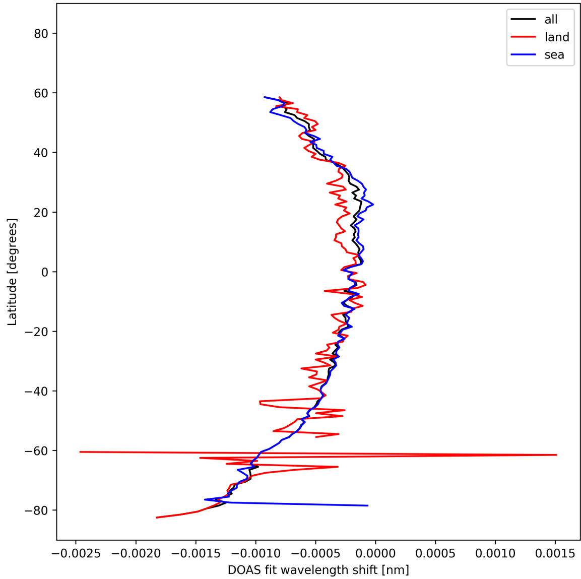
Figure 50: Zonal average of "DOAS fit wavelength shift" for 2025-02-15 to 2025-02-17.
