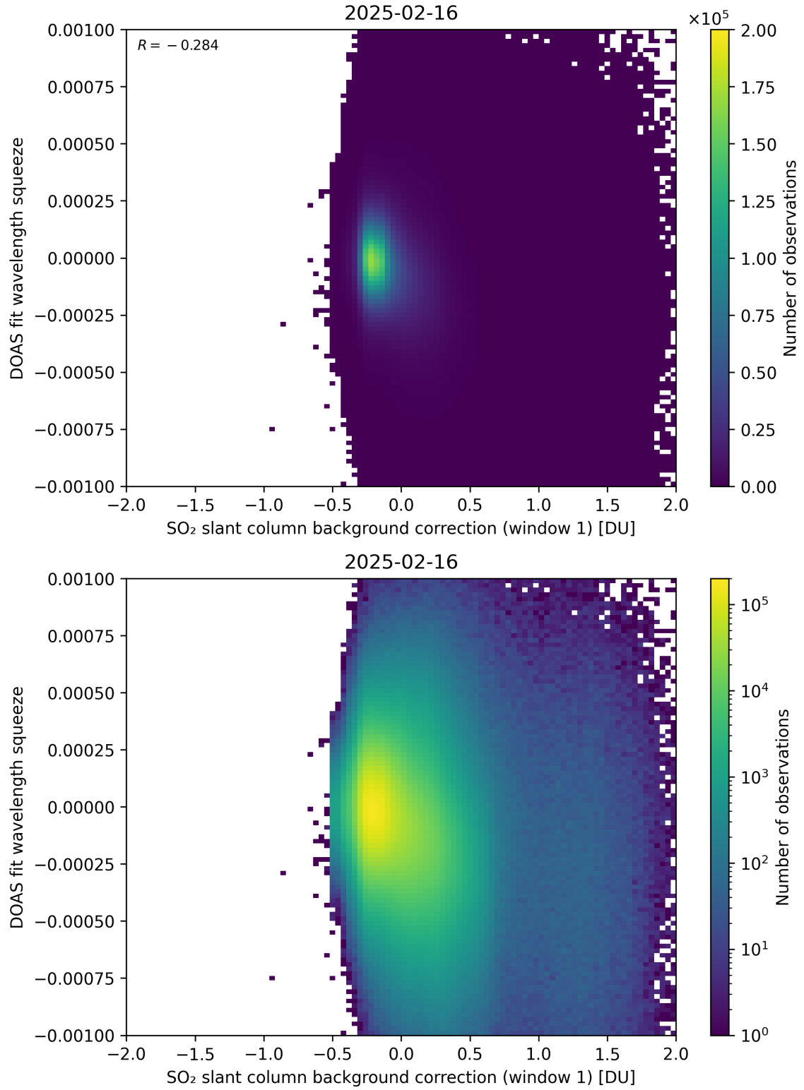
Figure 112: Scatter density plot of “SO 2 slant column background correction (window 1)” against “DOAS fit wavelength squeeze” for 2025-02-15 to 2025-02-17.
