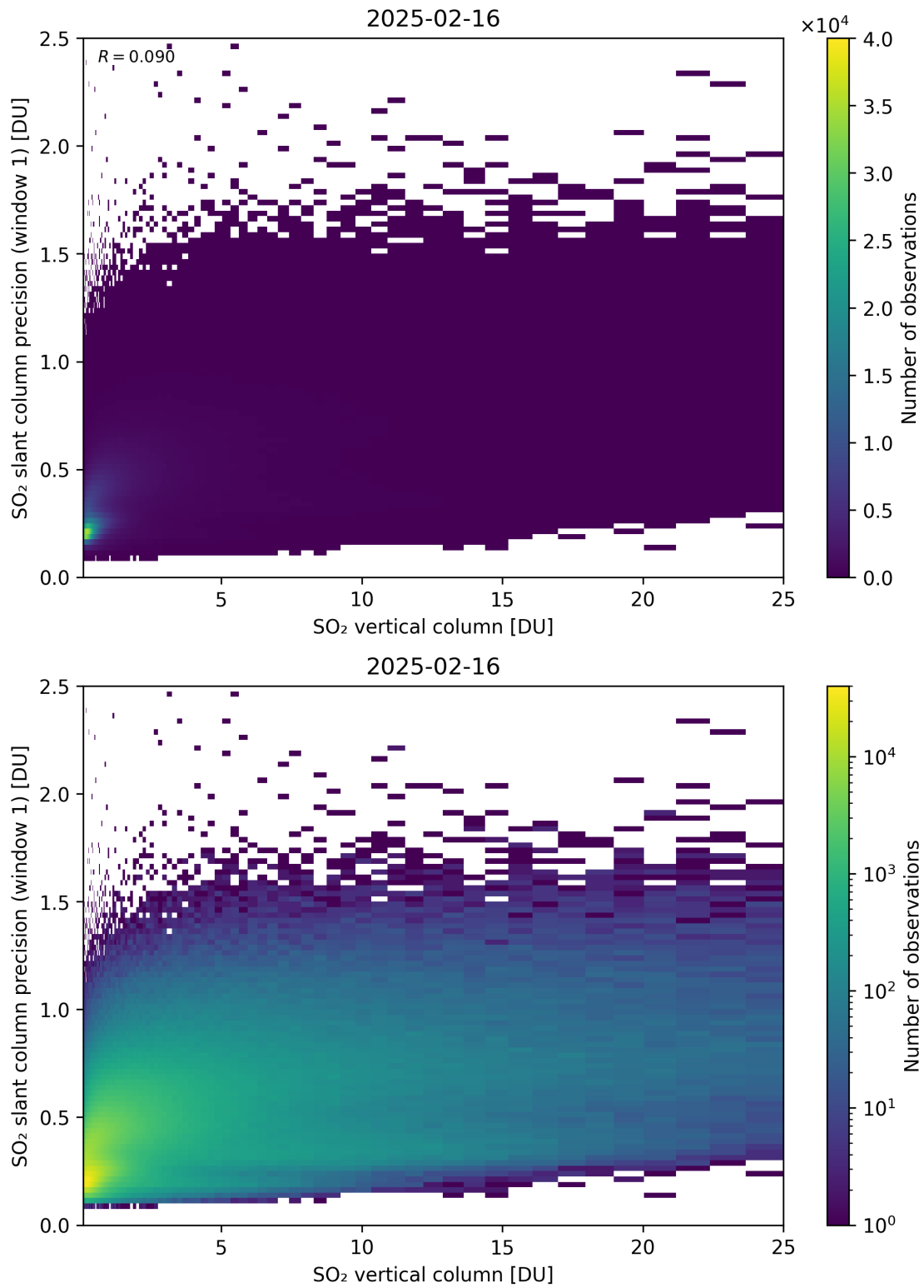
Figure 355: Scatter density plot of “SO 2 vertical column” against “SO 2 slant column precision (window 1)” for 2025-02-15 to 2025-02-17.
