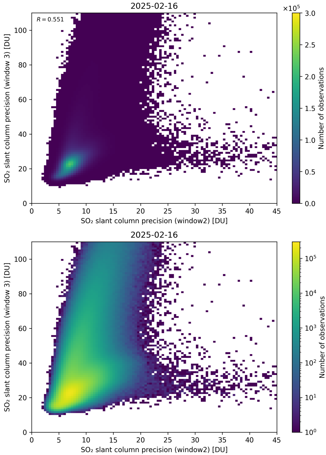
Figure 300: Scatter density plot of “SO 2 slant column precision (window2)” against “SO 2 slant column precision (window 3)” for 2025-02-15 to 2025-02-17.
