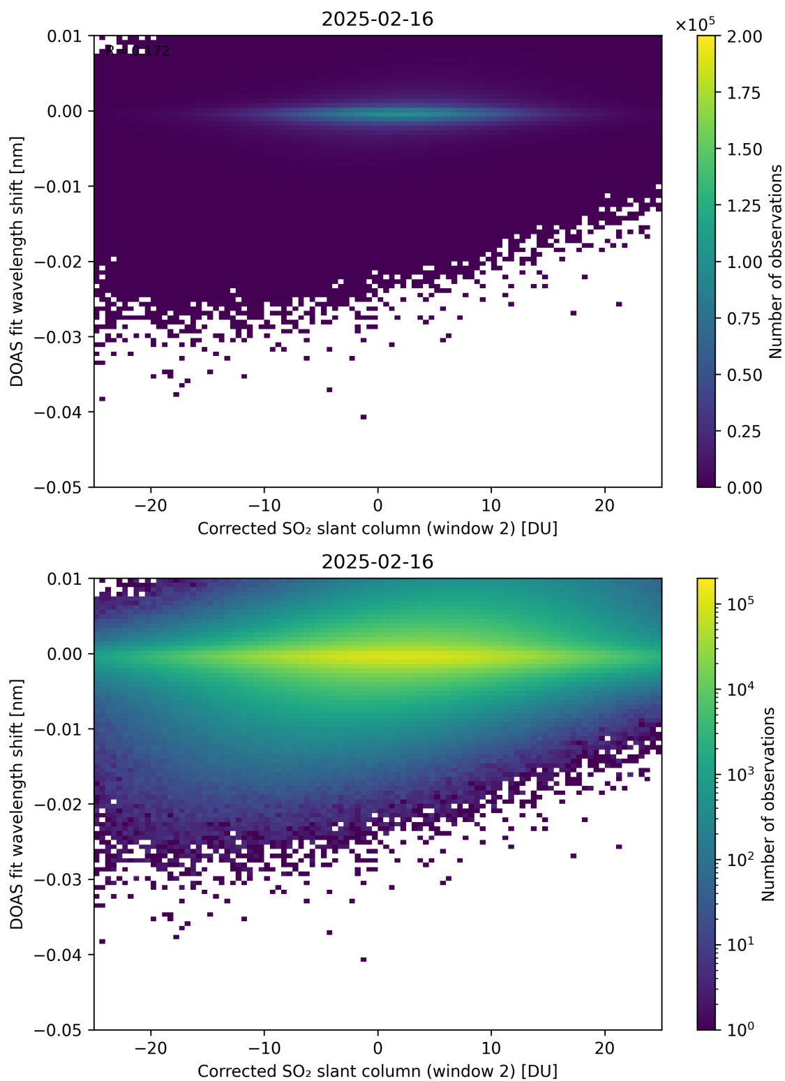
Figure 246: Scatter density plot of “Corrected SO 2 slant column (window 2)” against “DOAS fit wavelength shift” for 2025-02-15 to 2025-02-17.
