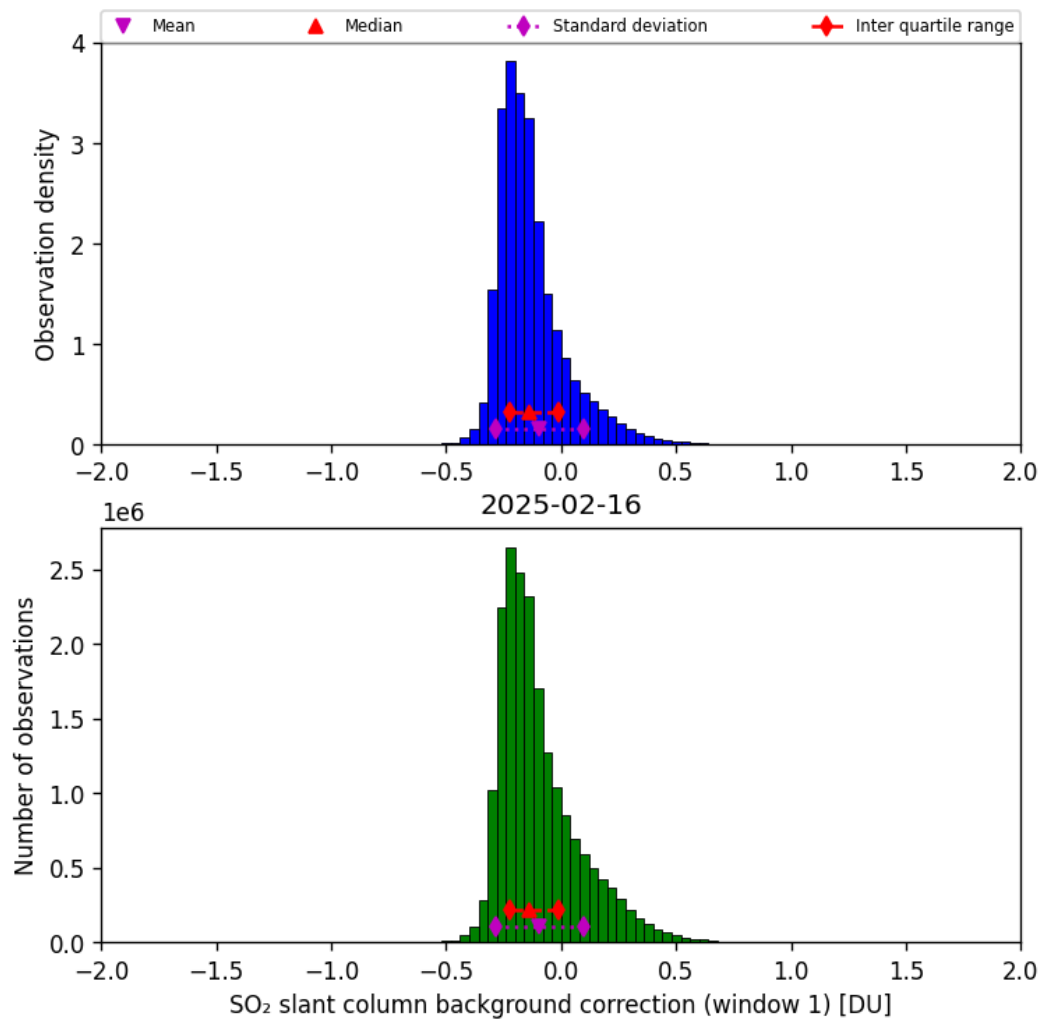
Figure 66: Histogram of “SO 2 slant column background correction (window 1)” for 2025-02-15 to 2025-02-17
