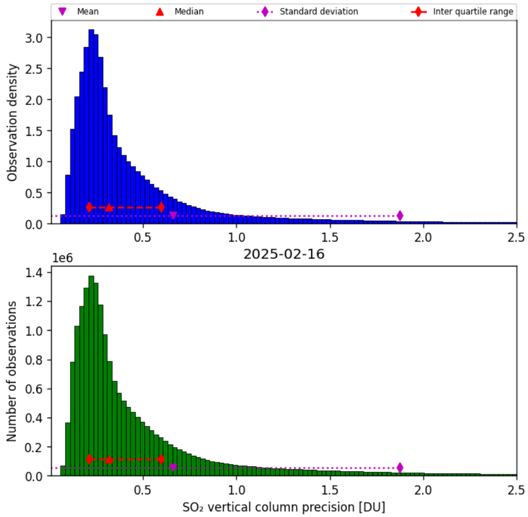
Figure 59: Histogram of “SO 2 vertical column precision” for 2025-02-15 to 2025-02-17
