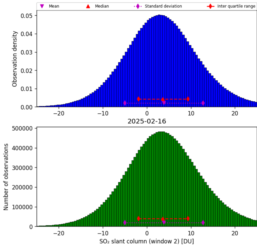
Figure 67: Histogram of “SO 2 slant column (window 2)” for 2025-02-15 to 2025-02-17
