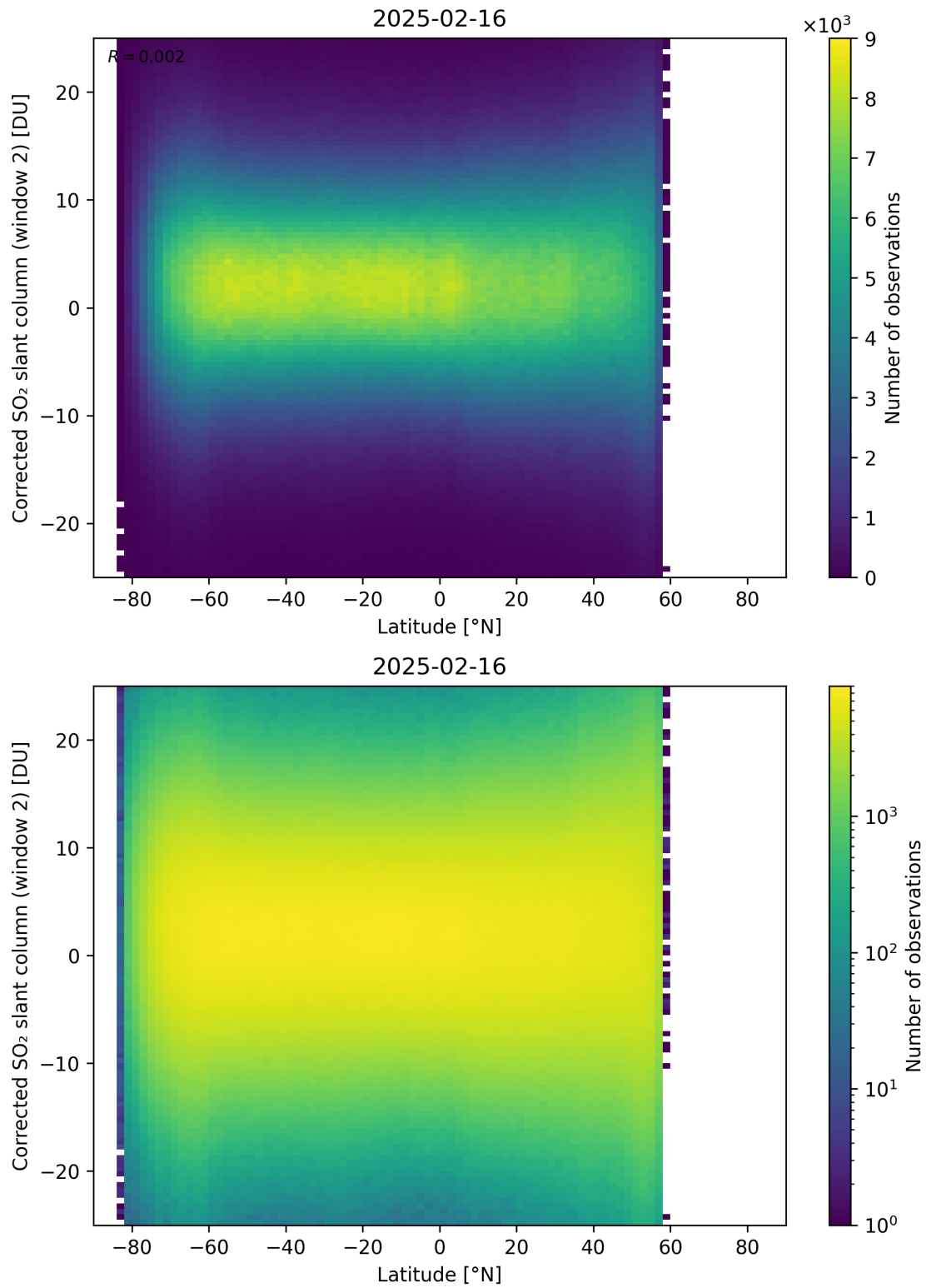
Figure 160: Scatter density plot of “Latitude” against “Corrected SO 2 slant column (window 2)” for 2025-02-15 to 2025-02-17.
