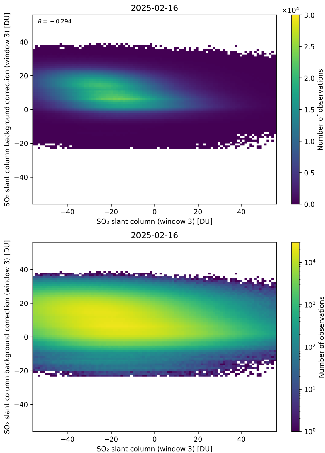
Figure 303: Scatter density plot of “SO 2 slant column (window 3)” against “SO 2 slant column background correction (window 3)” for 2025-02-15 to 2025-02-17.
