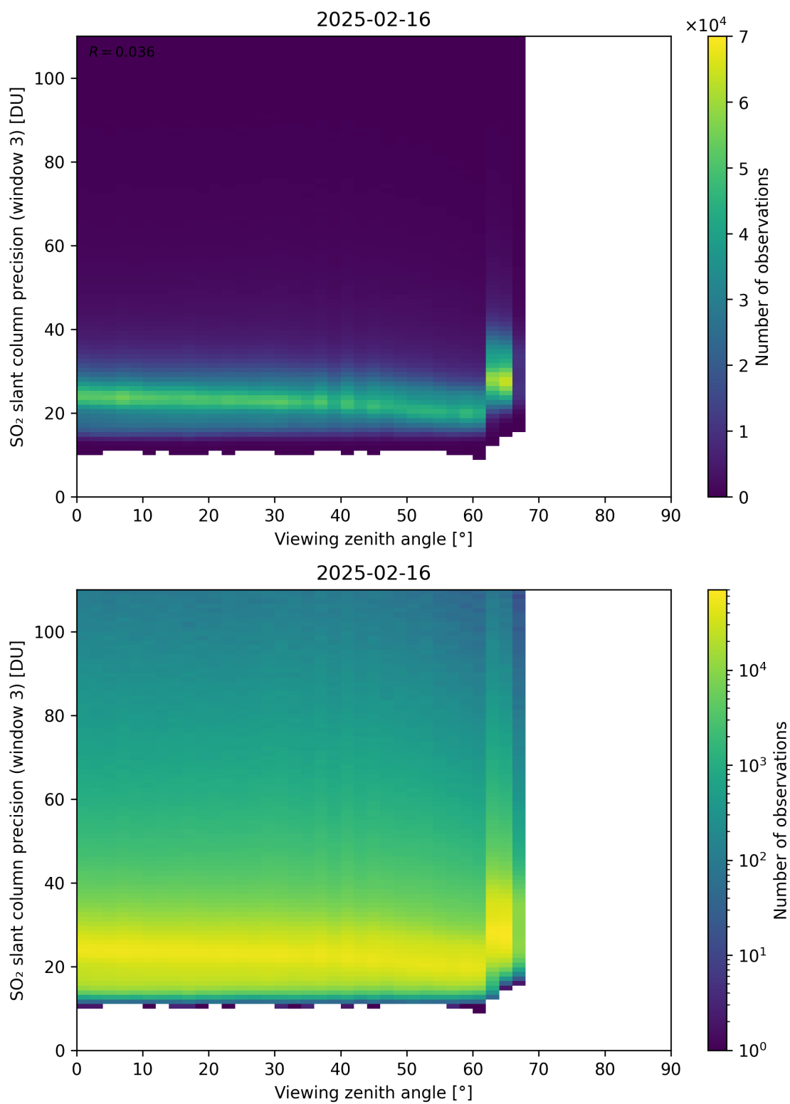
Figure 380: Scatter density plot of “Viewing zenith angle” against “SO 2 slant column precision (window 3)” for 2025-02-15 to 2025-02-17.
