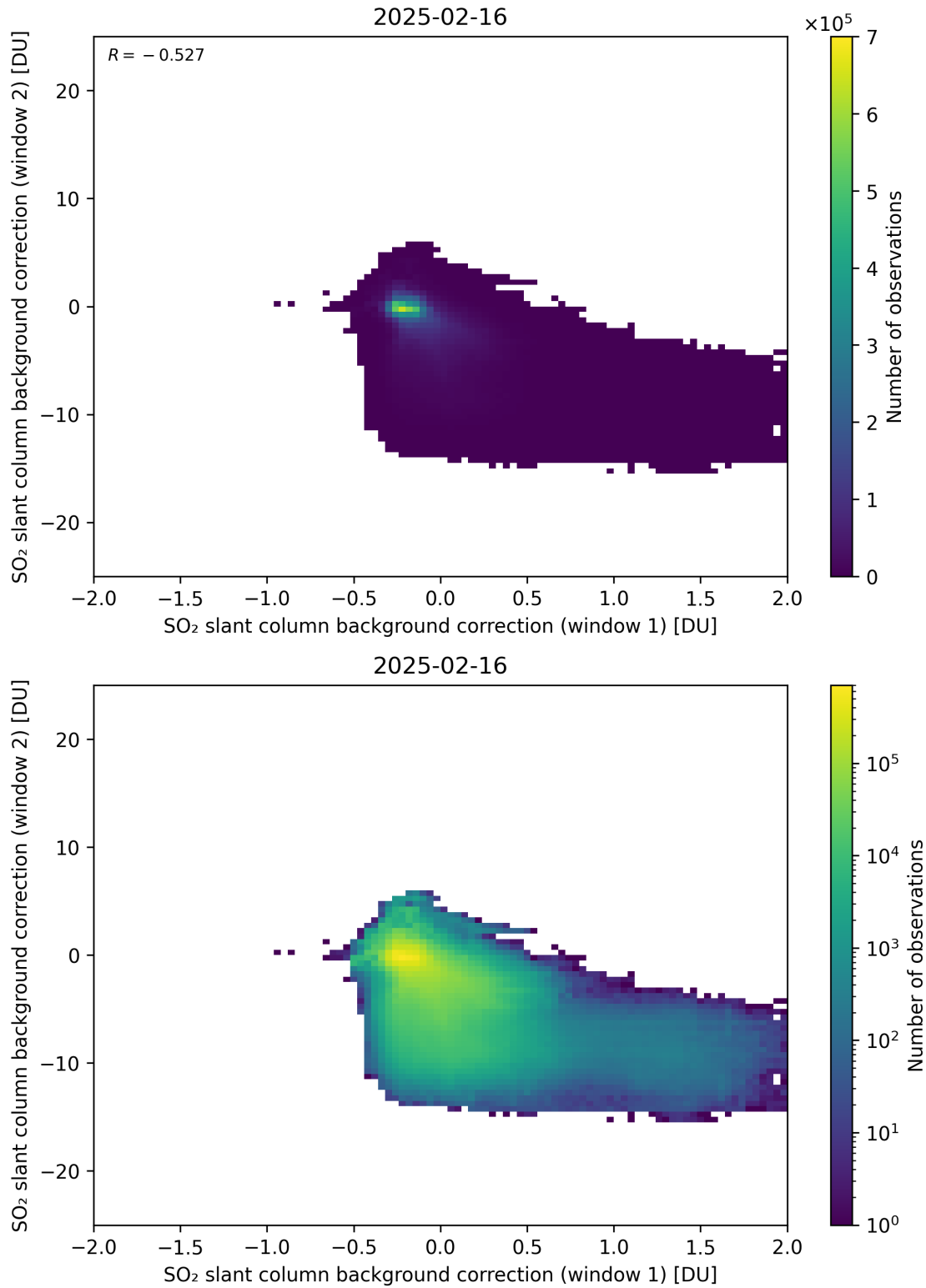
Figure 109: Scatter density plot of “SO 2 slant column background correction (window 1)” against “SO 2 slant column background correction (window 2)” for 2025-02-15 to 2025-02-17.
