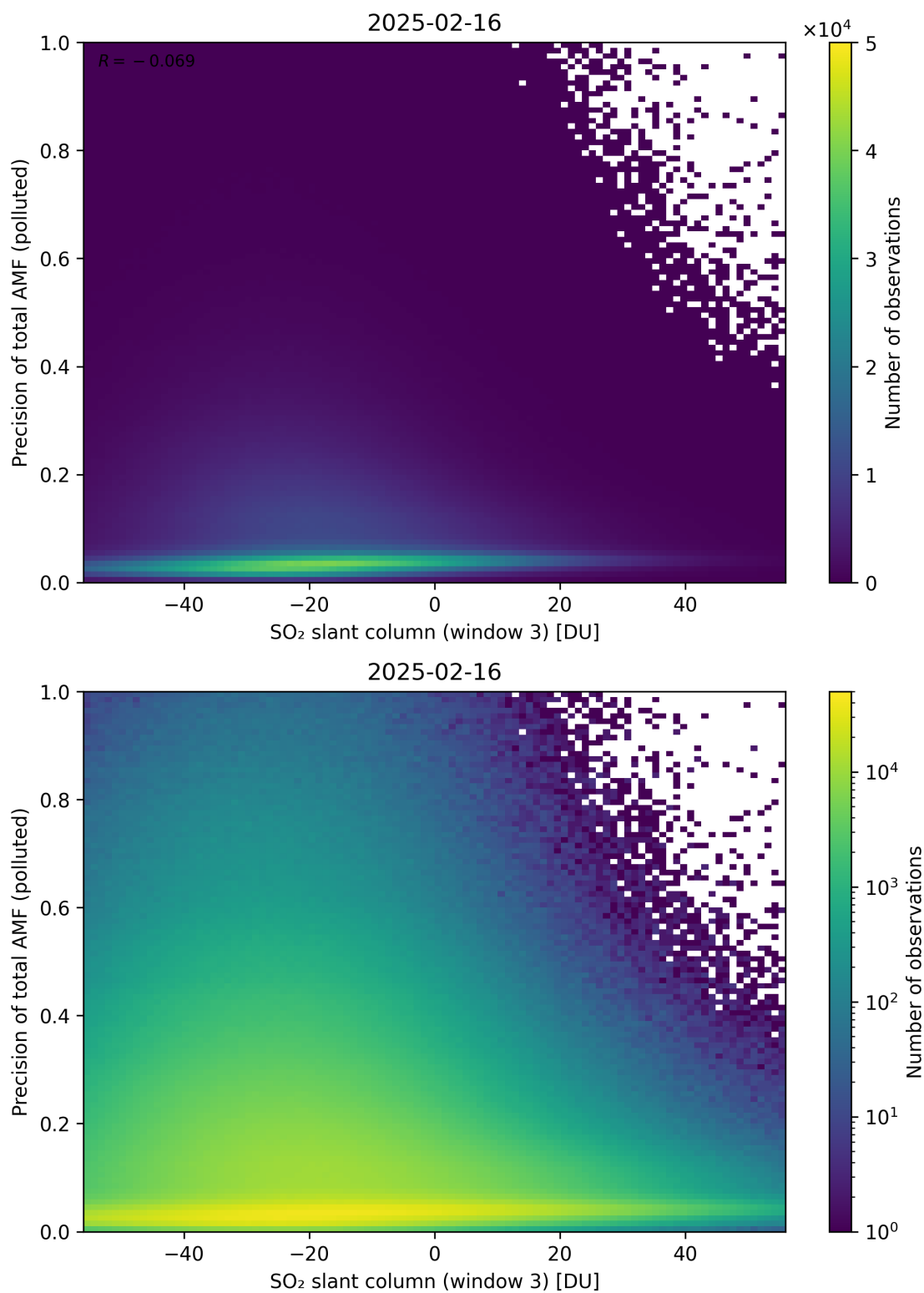
Figure 319: Scatter density plot of “SO 2 slant column (window 3)” against “Precision of total AMF (polluted)” for 2025-02-15 to 2025-02-17.
