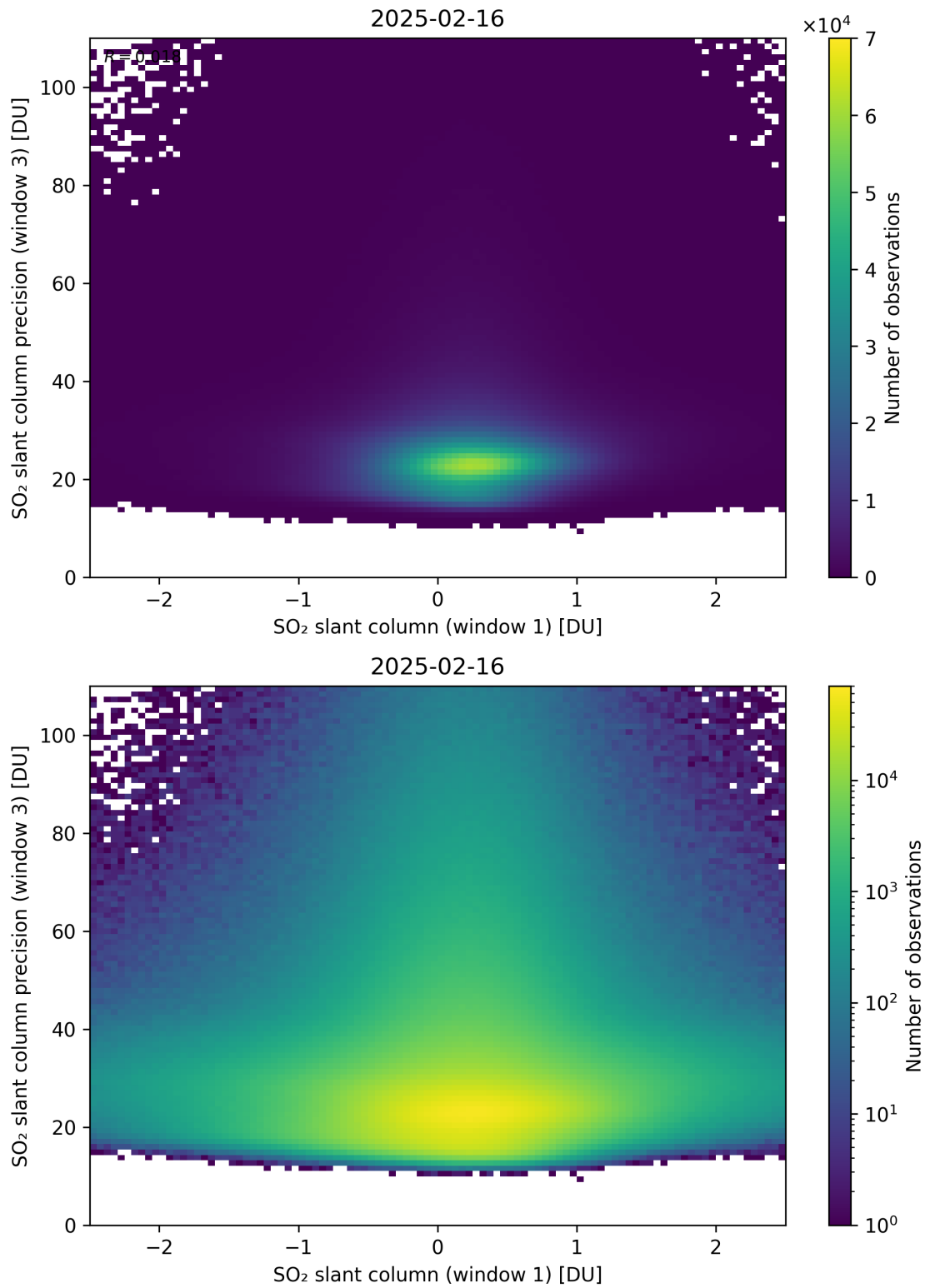
Figure 288: Scatter density plot of “SO 2 slant column (window 1)” against “SO 2 slant column precision (window 3)” for 2025-02-15 to 2025-02-17.
