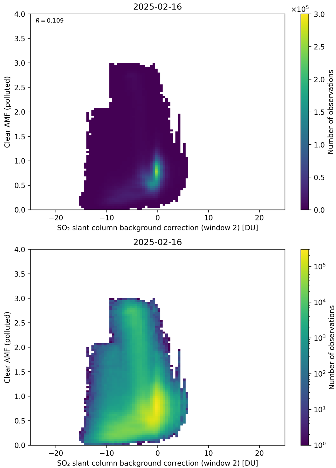
Figure 126: Scatter density plot of “SO 2 slant column background correction (window 2)” against “Clear AMF (polluted)” for 2025-02-15 to 2025-02-17.
