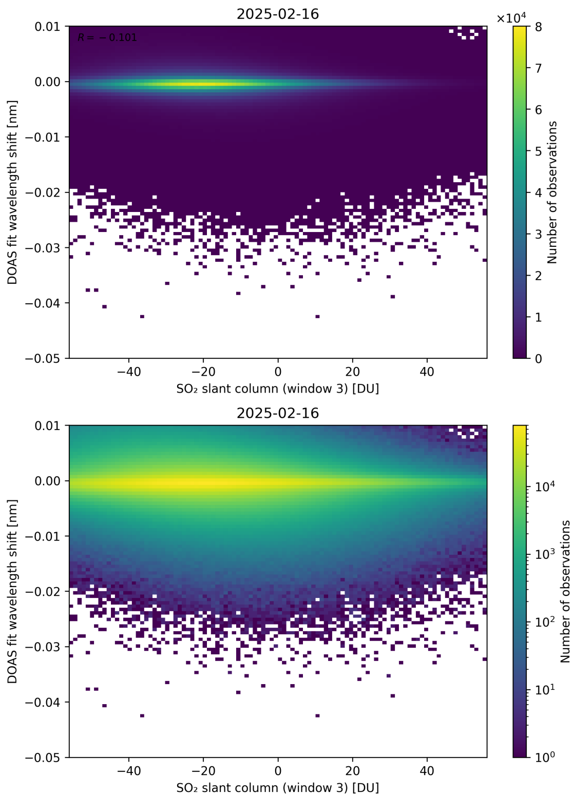
Figure 304: Scatter density plot of “SO 2 slant column (window 3)” against “DOAS fit wavelength shift” for 2025-02-15 to 2025-02-17.
