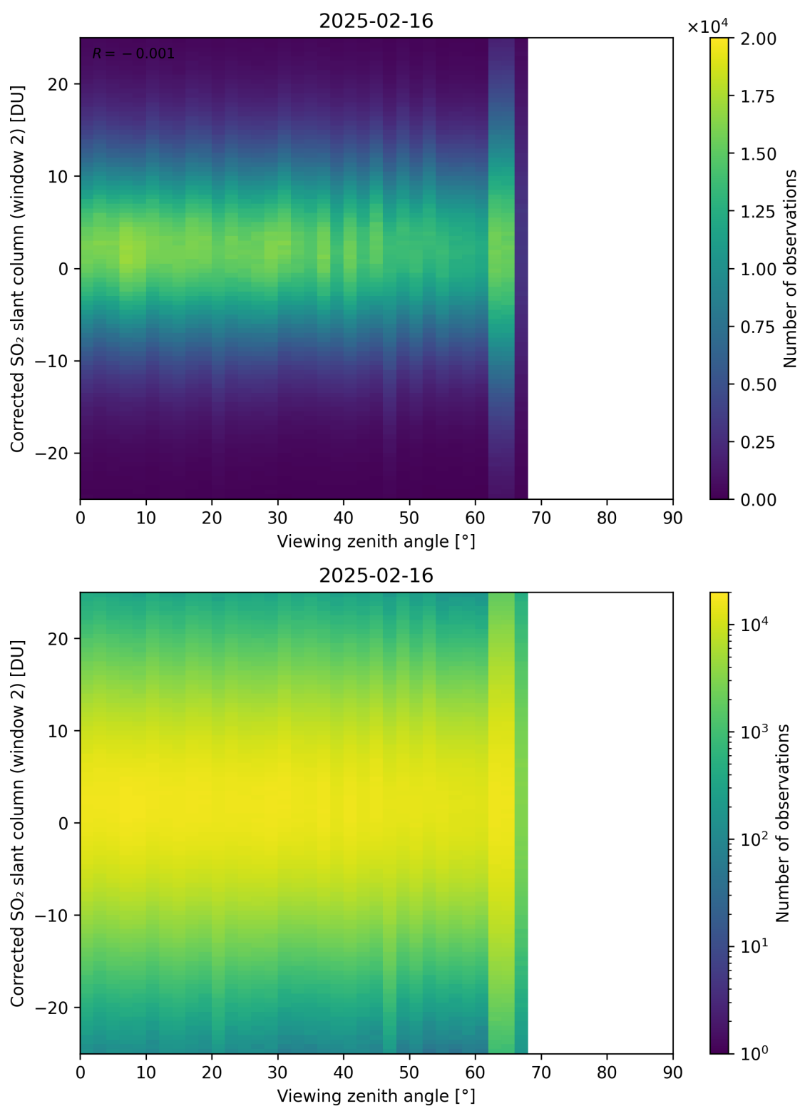
Figure 374: Scatter density plot of “Viewing zenith angle” against “Corrected SO 2 slant column (window 2)” for 2025-02-15 to 2025-02-17.
