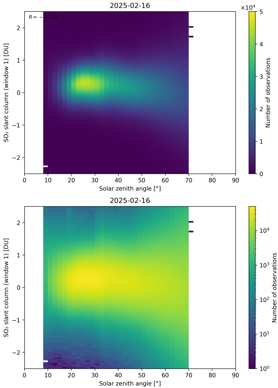
Figure 184: Scatter density plot of “Solar zenith angle” against “SO 2 slant column (window 1)” for 2025-02-15 to 2025-02-17.
