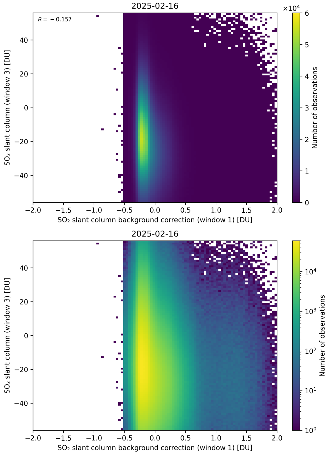
Figure 118: Scatter density plot of “SO 2 slant column background correction (window 1)” against “SO 2 slant column (window 3)” for 2025-02-15 to 2025-02-17.
