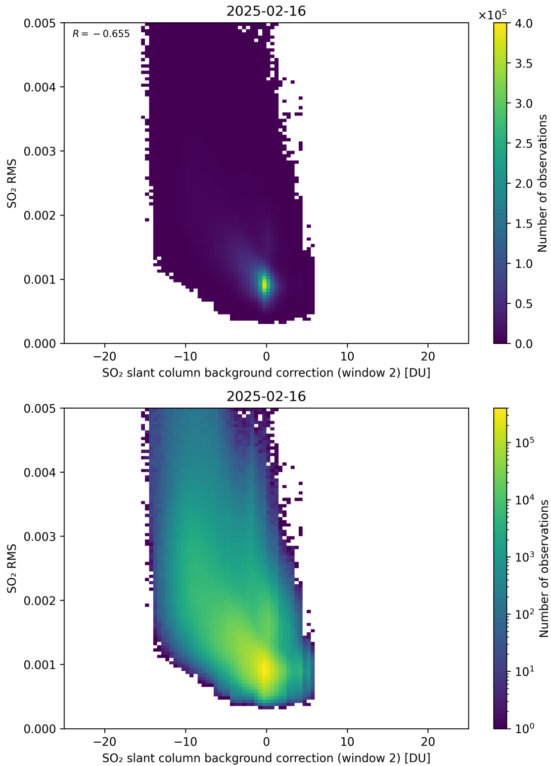
Figure 125: Scatter density plot of “SO 2 slant column background correction (window 2)” against “SO 2 RMS” for 2025-02-15 to 2025-02-17.
