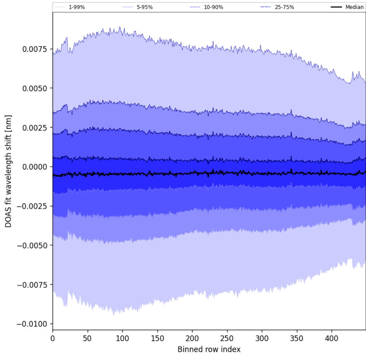
Figure 102: Along track statistics of “DOAS fit wavelength shift” for 2025-02-15 to 2025-02-17
