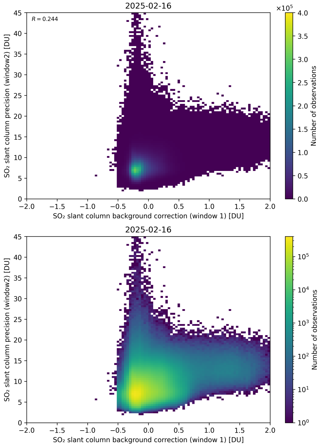
Figure 117: Scatter density plot of “SO 2 slant column background correction (window 1)” against “SO 2 slant column precision (window2)” for 2025-02-15 to 2025-02-17.
