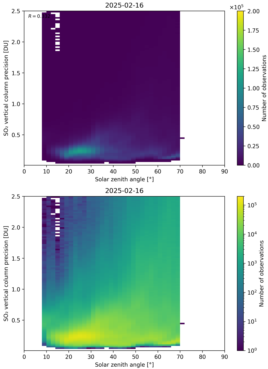
Figure 192: Scatter density plot of “Solar zenith angle” against “SO 2 vertical column precision” for 2025-02-15 to 2025-02-17.
