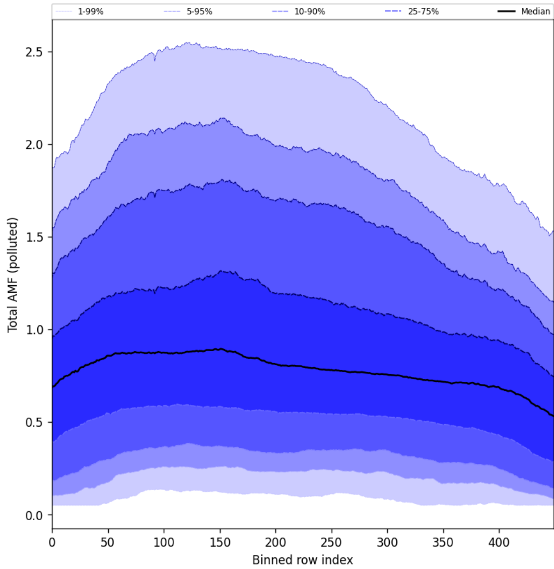
Figure 105: Along track statistics of “Total AMF (polluted)” for 2025-02-15 to 2025-02-17
