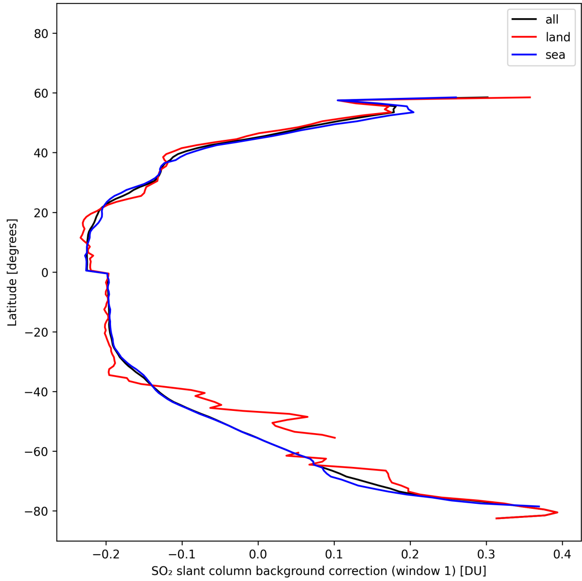
Figure 40: Zonal average of “SO 2 slant column background correction (window 1)” for 2025-02-15 to 2025-02-17.
