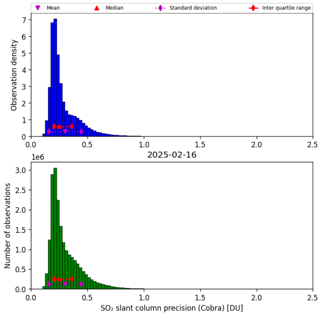
Figure 62: Histogram of “SO 2 slant column precision (Cobra)” for 2025-02-15 to 2025-02-17
