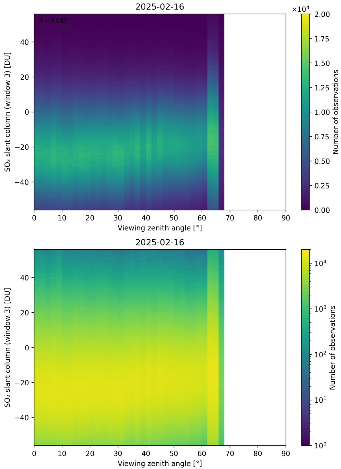
Figure 379: Scatter density plot of “Viewing zenith angle” against “SO 2 slant column (window 3)” for 2025-02-15 to 2025-02-17.
