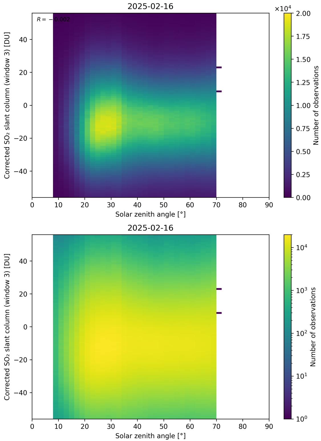
Figure 183: Scatter density plot of “Solar zenith angle” against “Corrected SO 2 slant column (window 3)” for 2025-02-15 to 2025-02-17.
