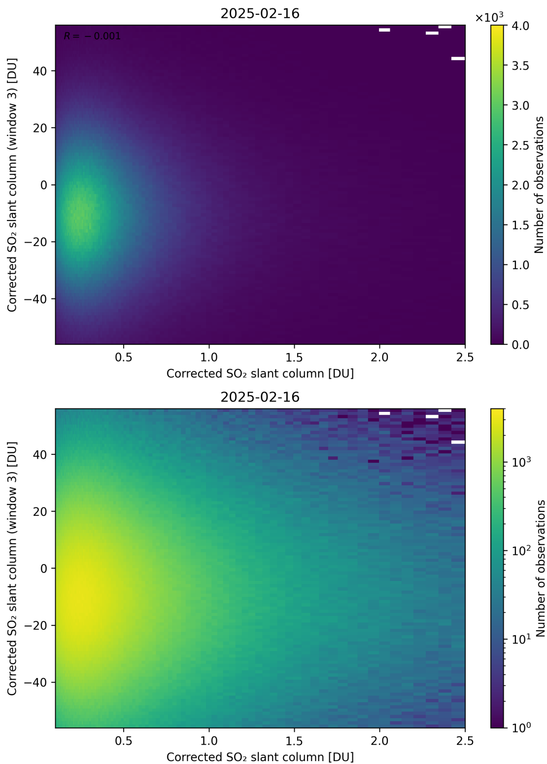
Figure 236: Scatter density plot of “Corrected SO 2 slant column” against “Corrected SO 2 slant column (window 3)” for 2025-02-15 to 2025-02-17.
