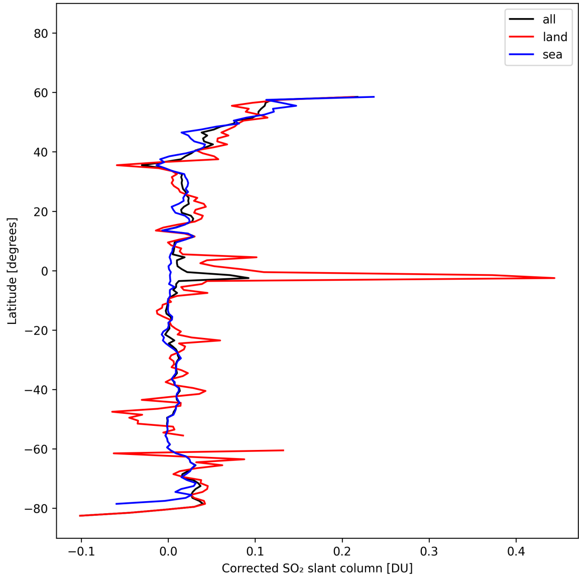
Figure 34: Zonal average of “Corrected SO 2 slant column” for 2025-02-15 to 2025-02-17.
