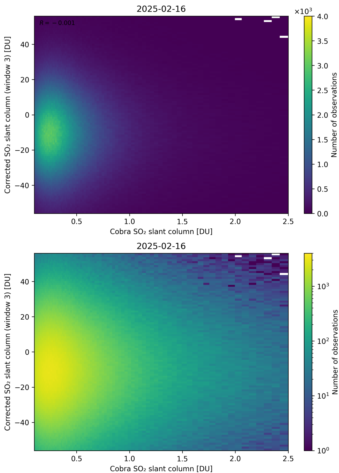
Figure 218: Scatter density plot of “Cobra SO 2 slant column” against “Corrected SO 2 slant column (window 3)” for 2025-02-15 to 2025-02-17.
