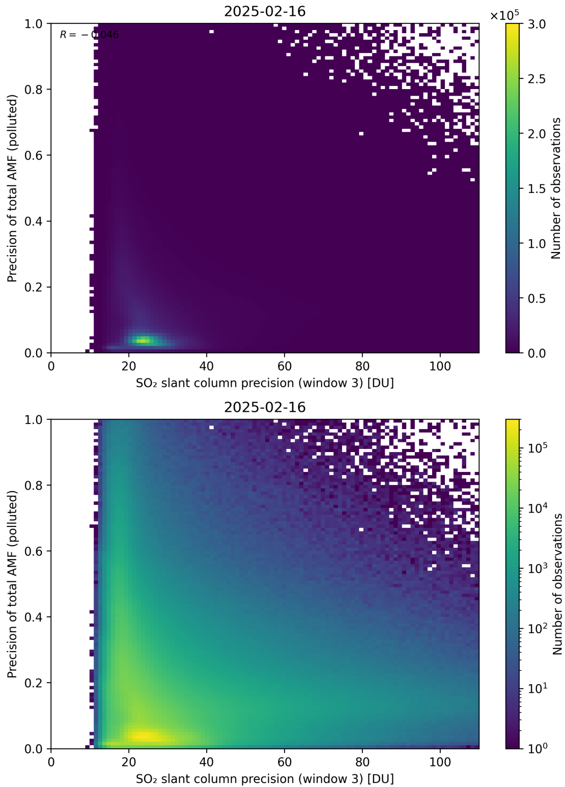
Figure 314: Scatter density plot of “SO 2 slant column precision (window 3)” against “Precision of total AMF (polluted)” for 2025-02-15 to 2025-02-17.
