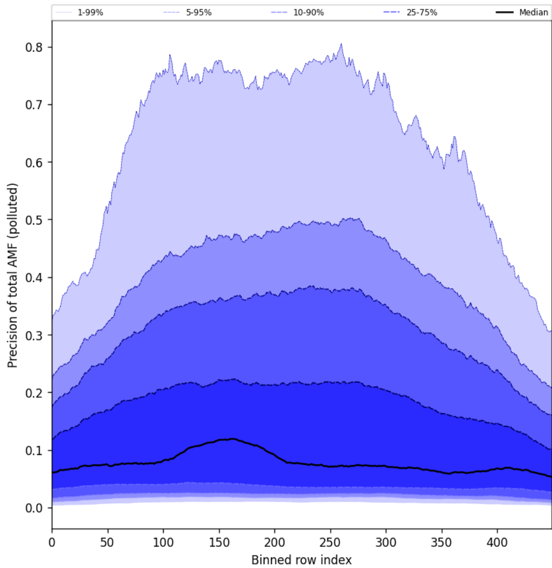
Figure 106: Along track statistics of “Precision of total AMF (polluted)” for 2025-02-15 to 2025-02-17
