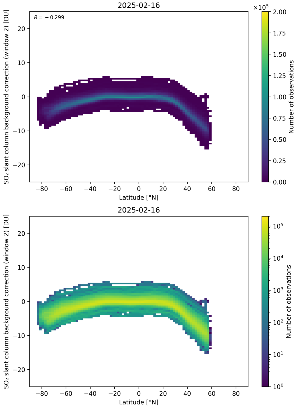
Figure 151: Scatter density plot of “Latitude” against “SO 2 slant column background correction (window 2)” for 2025-02-15 to 2025-02-17.
