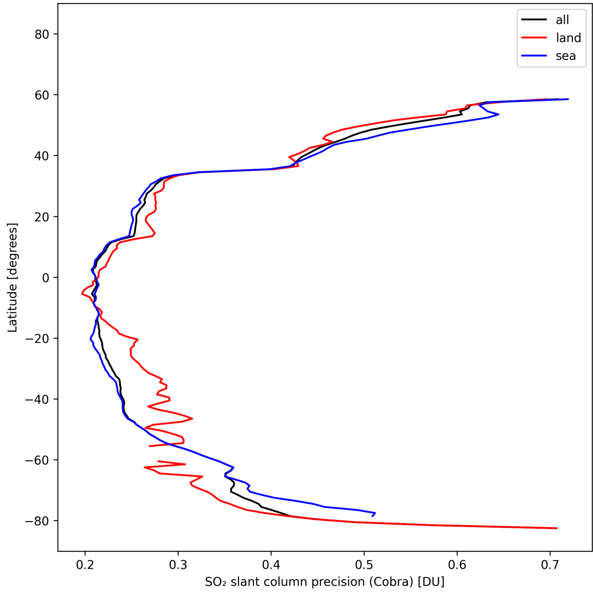
Figure 36: Zonal average of “SO 2 slant column precision (Cobra)” for 2025-02-15 to 2025-02-17.
