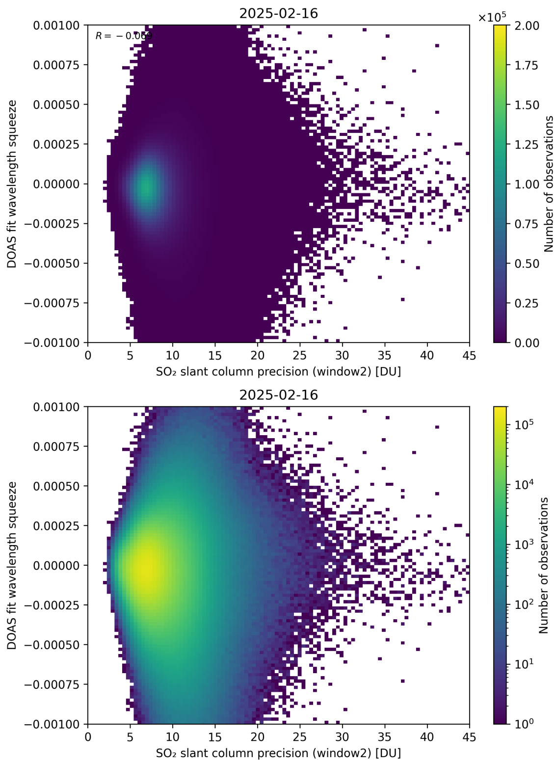
Figure 294: Scatter density plot of “SO 2 slant column precision (window2)” against “DOAS fit wavelength squeeze” for 2025-02-15 to 2025-02-17.
