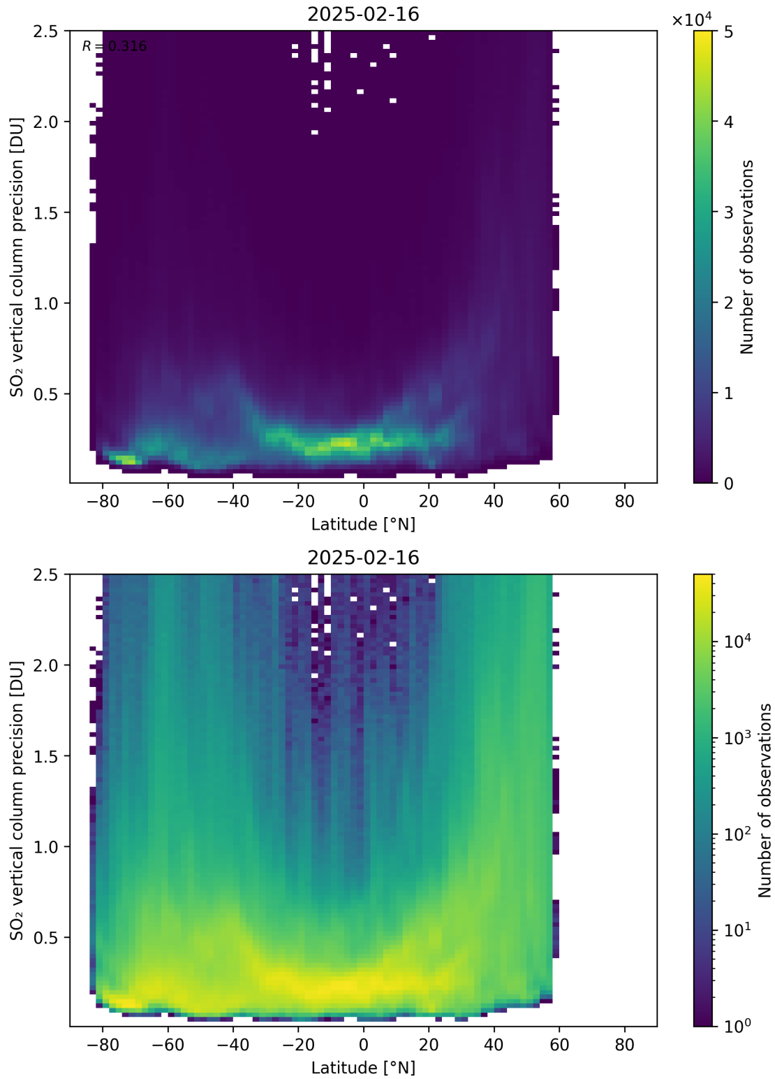
Figure 170: Scatter density plot of “Latitude” against “SO 2 vertical column precision” for 2025-02-15 to 2025-02-17.
