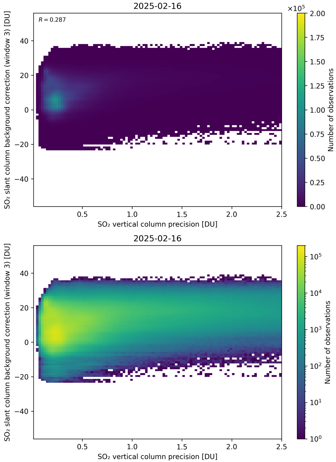
Figure 331: Scatter density plot of “SO 2 vertical column precision” against “SO 2 slant column background correction (window 3)” for 2025-02-15 to 2025-02-17.
