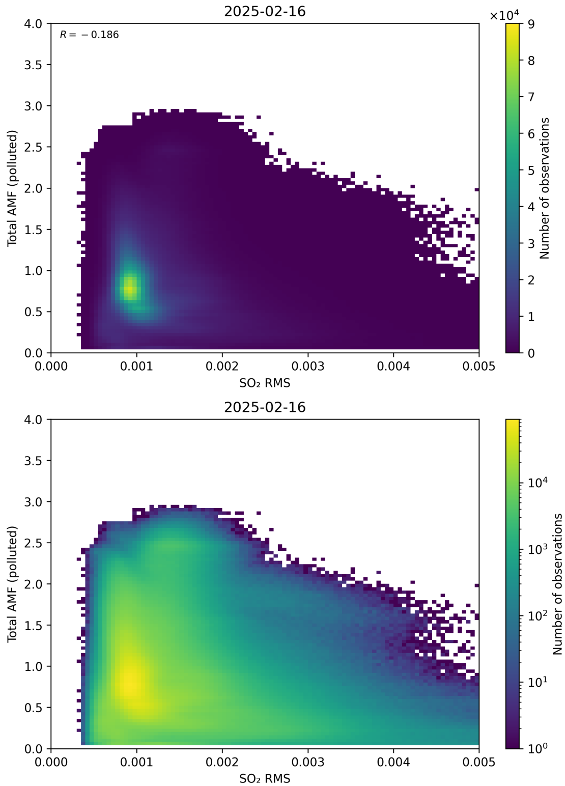
Figure 148: Scatter density plot of “SO 2 RMS” against “Total AMF (polluted)” for 2025-02-15 to 2025-02-17.
