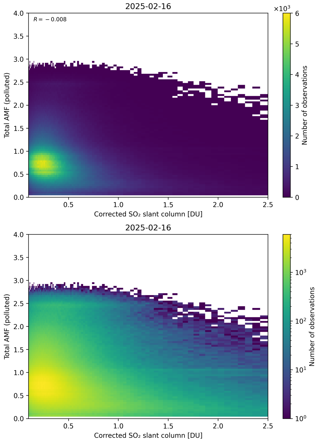
Figure 242: Scatter density plot of “Corrected SO 2 slant column” against “Total AMF (polluted)” for 2025-02-15 to 2025-02-17.
