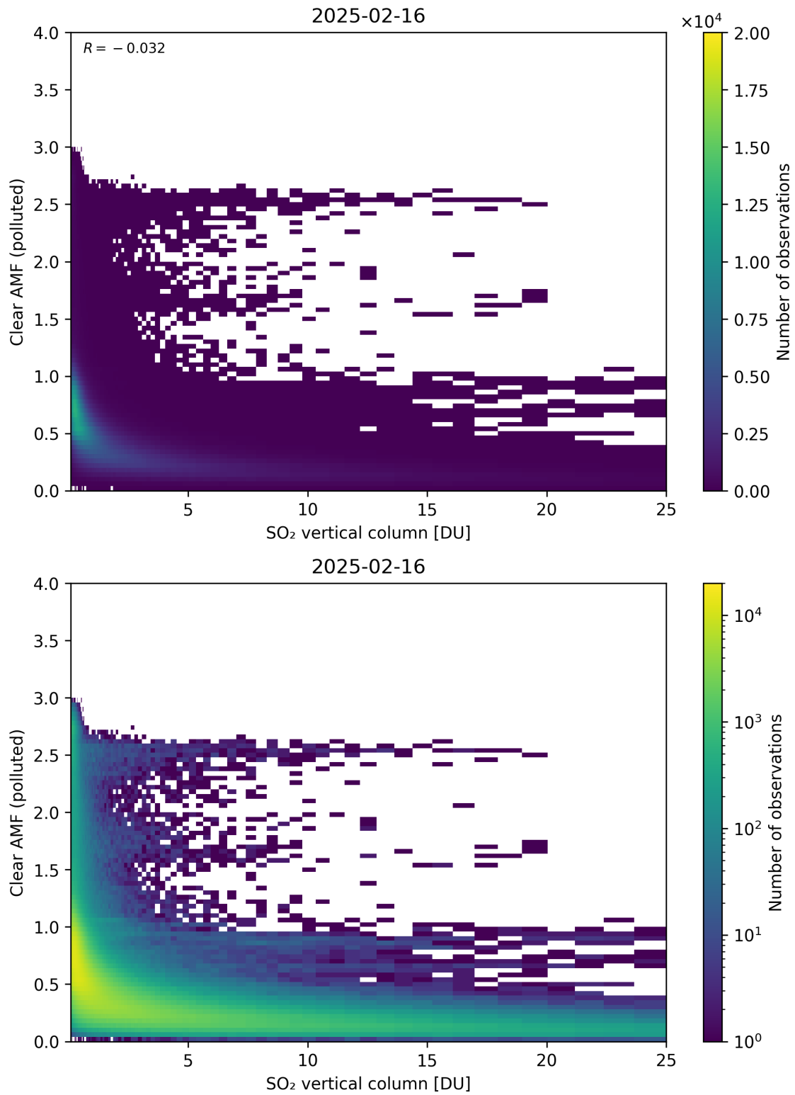
Figure 348: Scatter density plot of “SO 2 vertical column” against “Clear AMF (polluted)” for 2025-02-15 to 2025-02-17.
