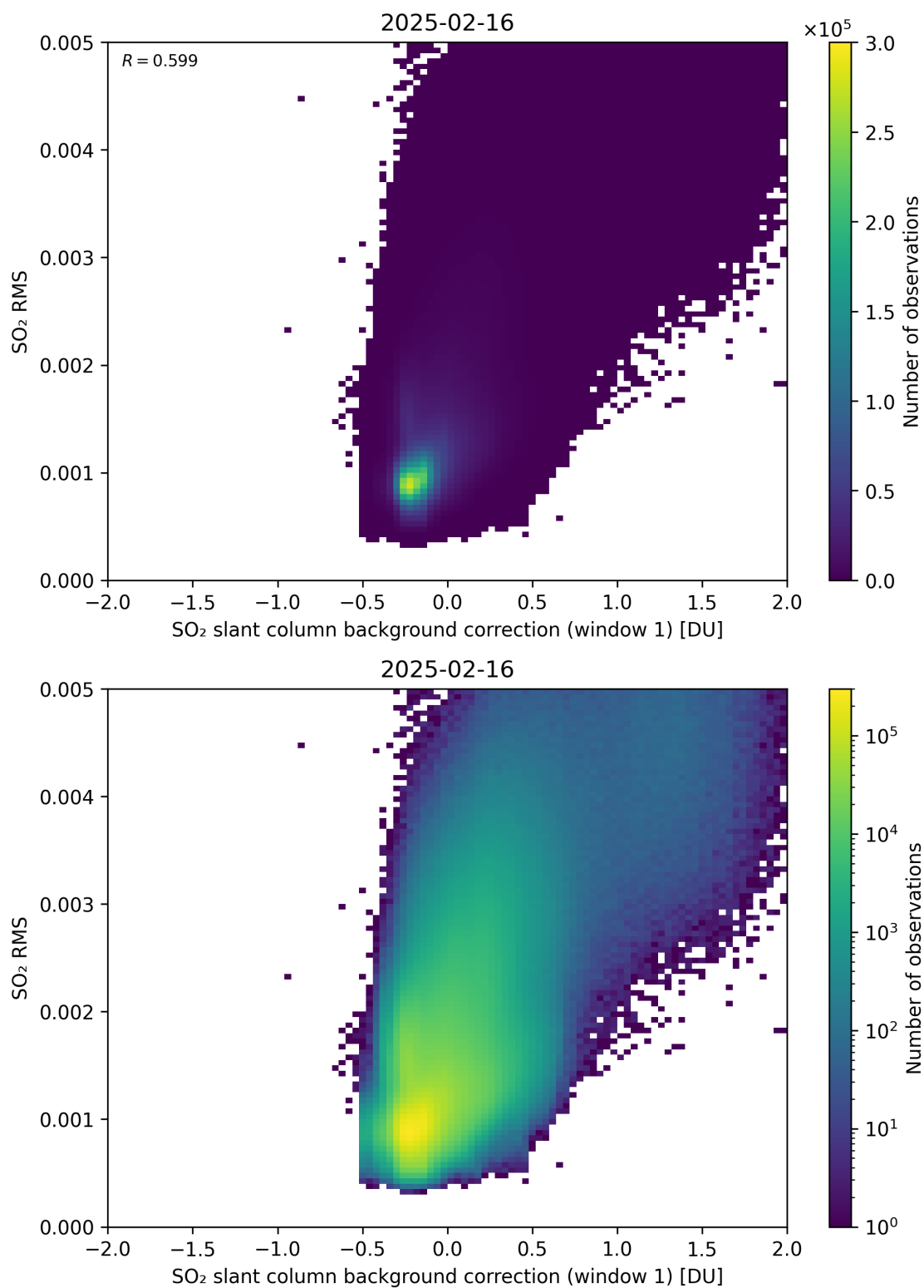
Figure 113: Scatter density plot of “SO 2 slant column background correction (window 1)” against “SO 2 RMS” for 2025-02-15 to 2025-02-17.
