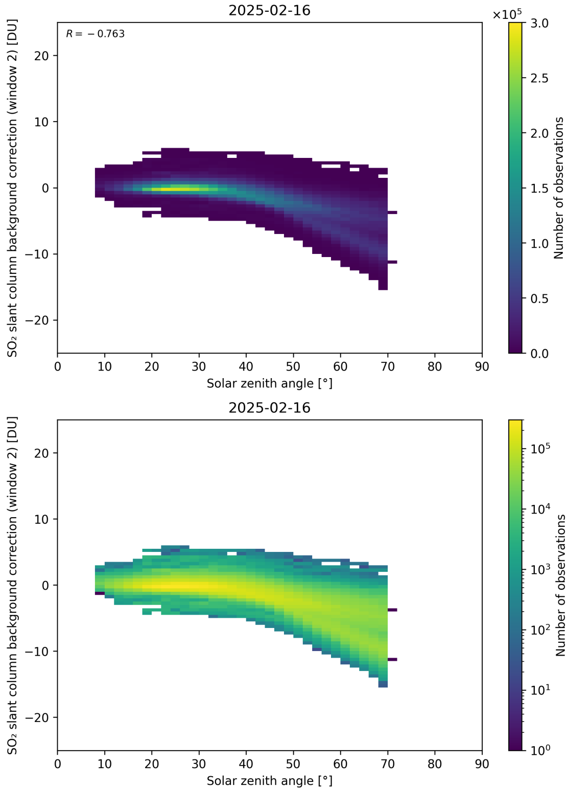
Figure 172: Scatter density plot of “Solar zenith angle” against “SO 2 slant column background correction (window 2)” for 2025-02-15 to 2025-02-17.
