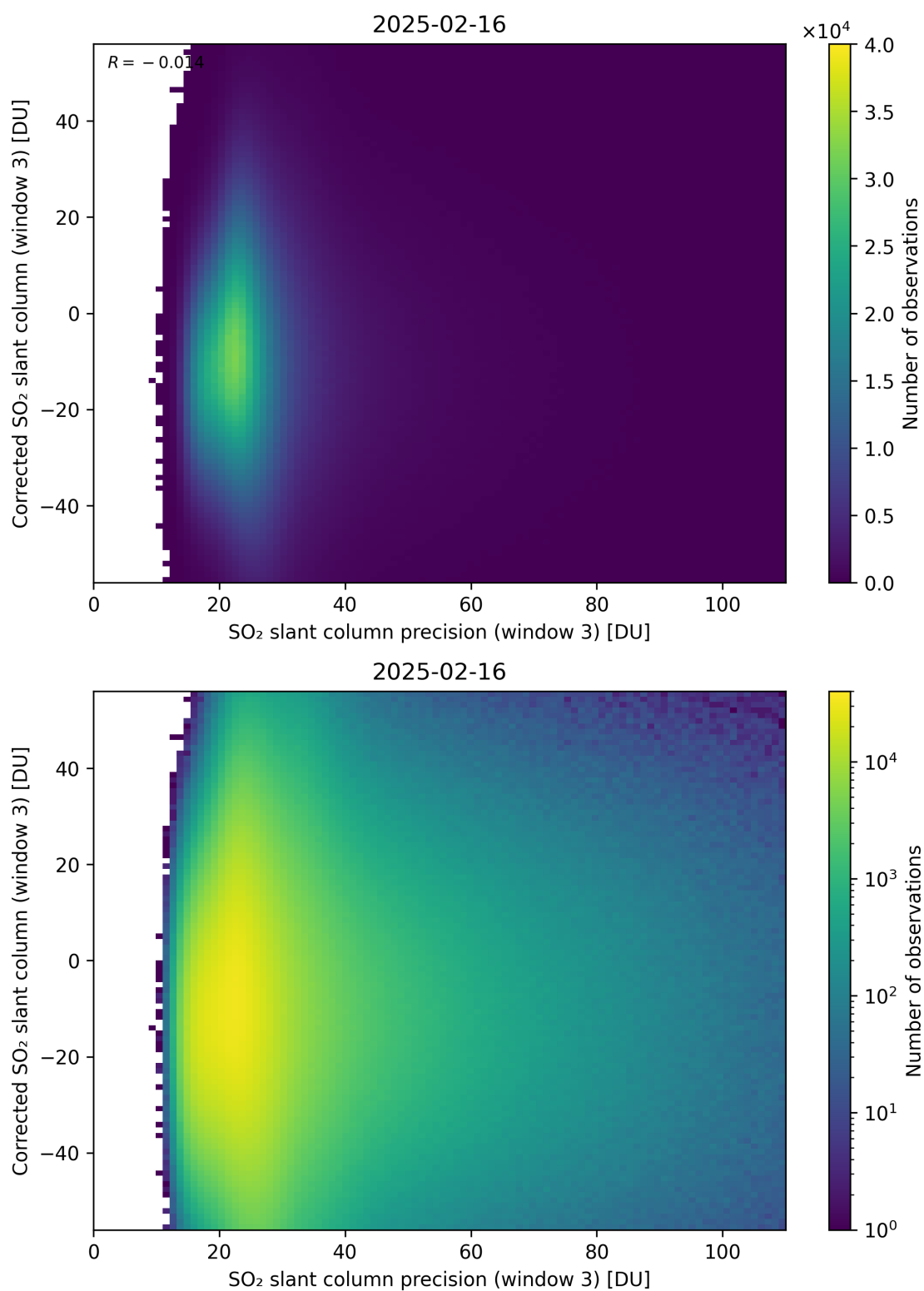
Figure 312: Scatter density plot of “SO 2 slant column precision (window 3)” against “Corrected SO 2 slant column (window 3)” for 2025-02-15 to 2025-02-17.
