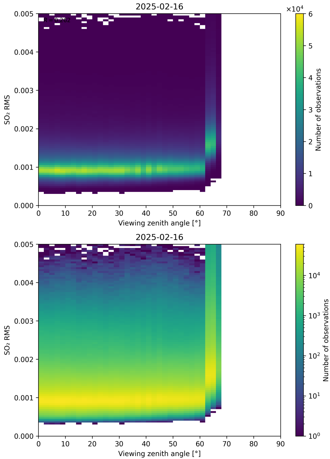
Figure 367: Scatter density plot of “Viewing zenith angle” against “SO 2 RMS” for 2025-02-15 to 2025-02-17.
