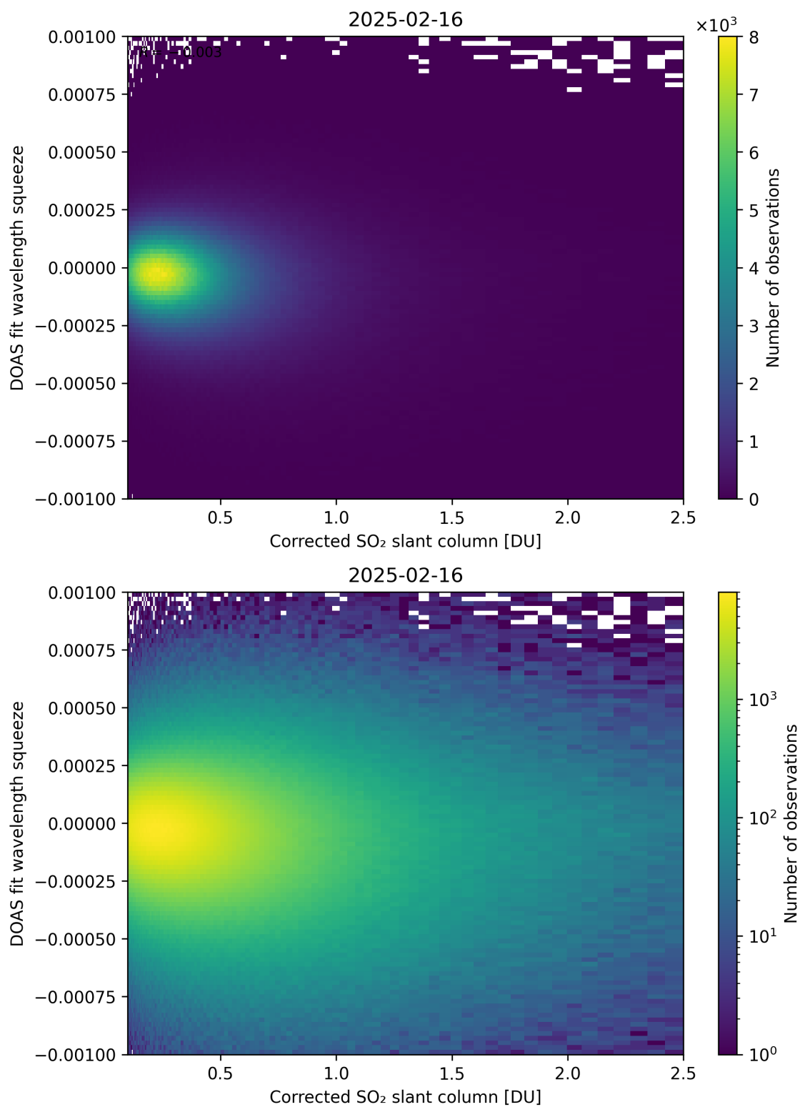
Figure 230: Scatter density plot of “Corrected SO 2 slant column” against “DOAS fit wavelength squeeze” for 2025-02-15 to 2025-02-17.
