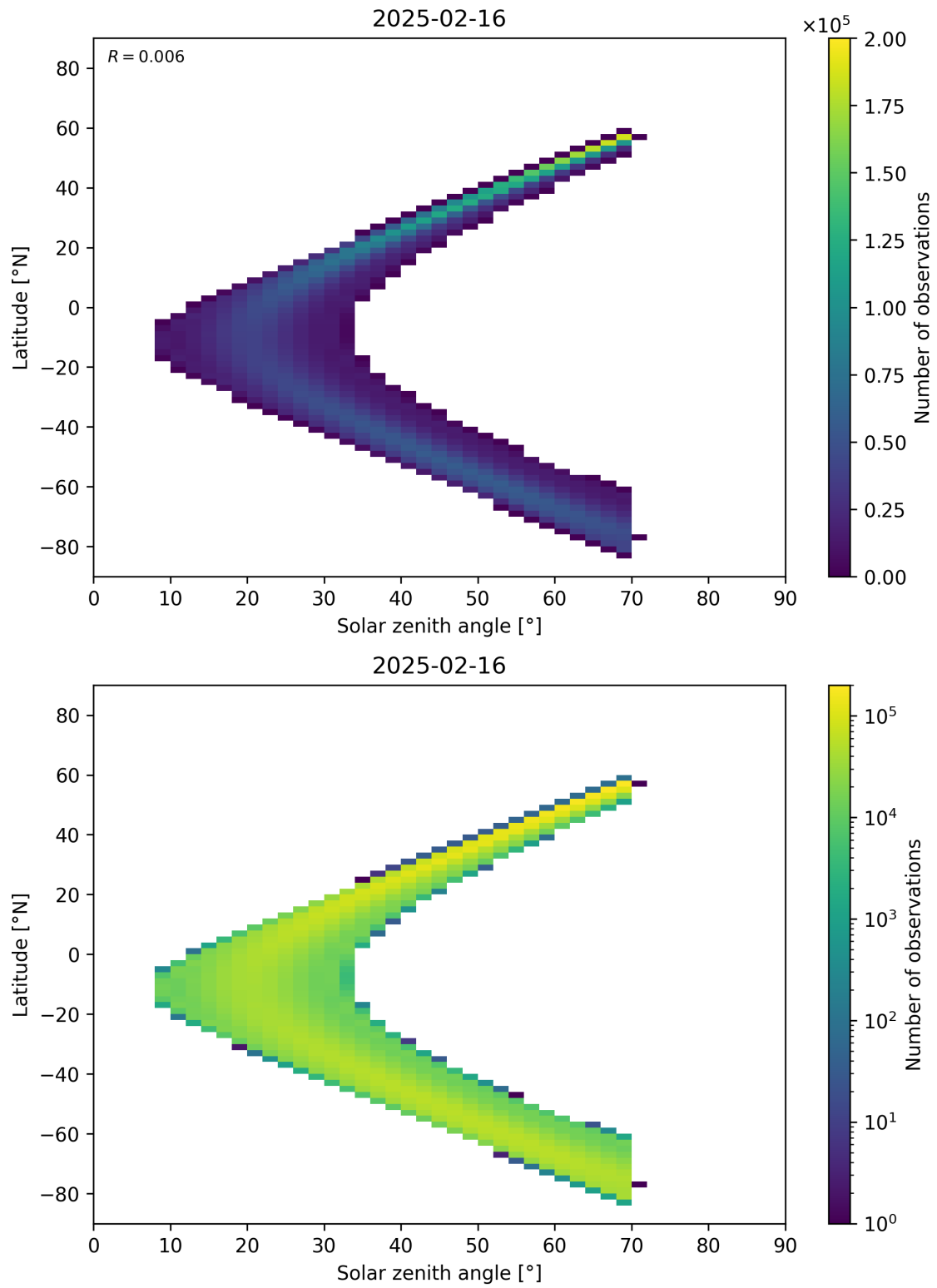
Figure 177: Scatter density plot of “Solar zenith angle” against “Latitude” for 2025-02-15 to 2025-02-17.
