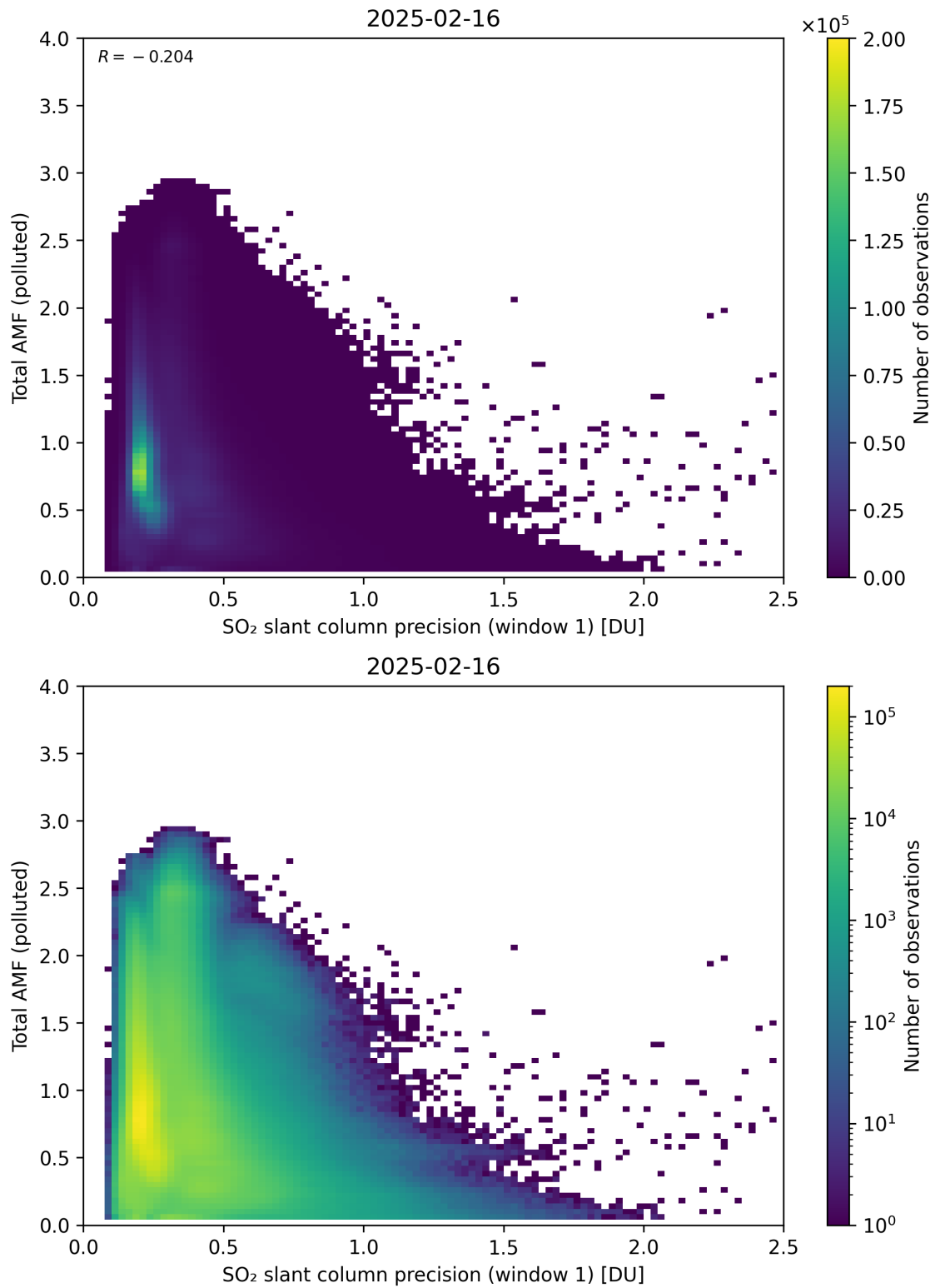
Figure 280: Scatter density plot of “SO 2 slant column precision (window 1)” against “Total AMF (polluted)” for 2025-02-15 to 2025-02-17.
