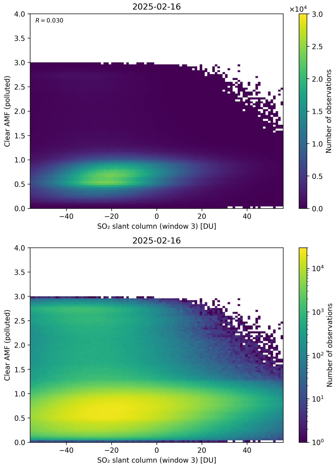
Figure 315: Scatter density plot of “SO 2 slant column (window 3)” against “Clear AMF (polluted)” for 2025-02-15 to 2025-02-17.
