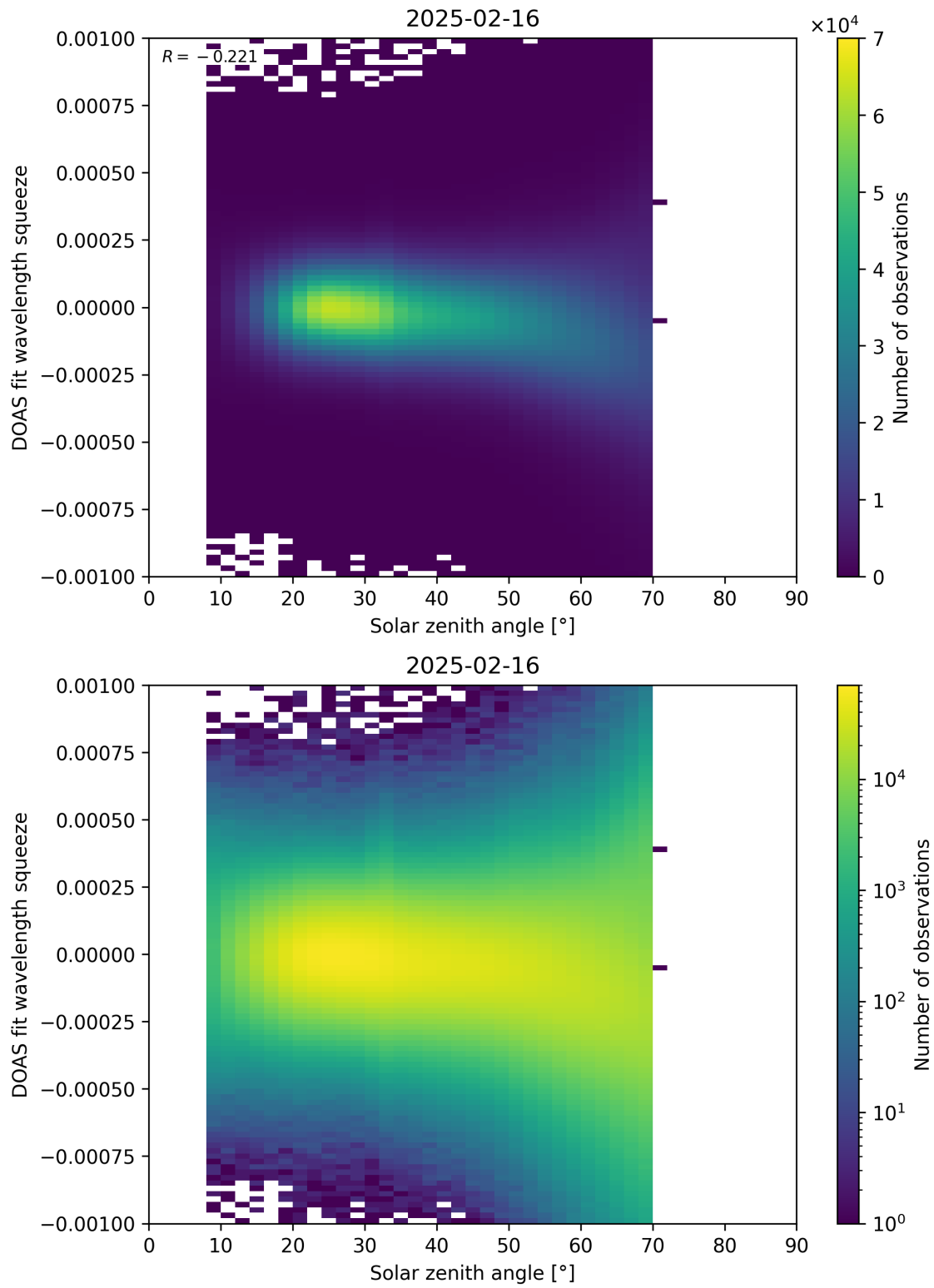
Figure 175: Scatter density plot of “Solar zenith angle” against “DOAS fit wavelength squeeze” for 2025-02-15 to 2025-02-17.
