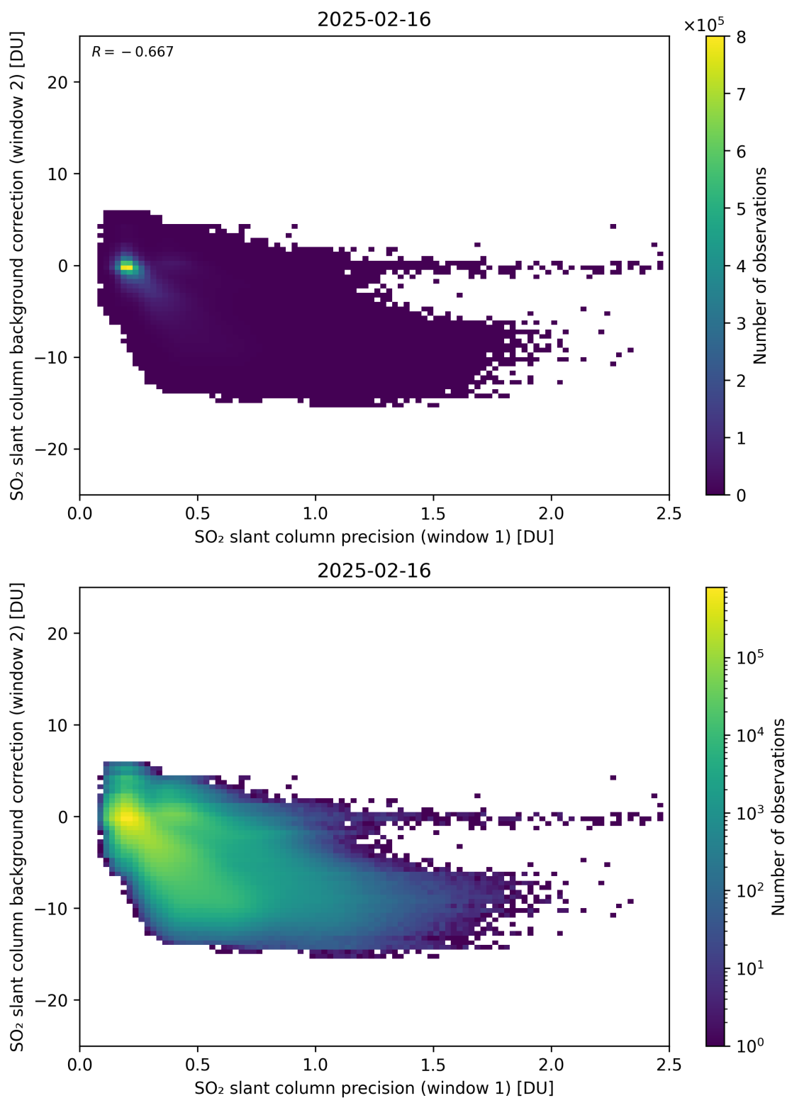
Figure 269: Scatter density plot of “SO 2 slant column precision (window 1)” against “SO 2 slant column background correction (window 2)” for 2025-02-15 to 2025-02-17.
