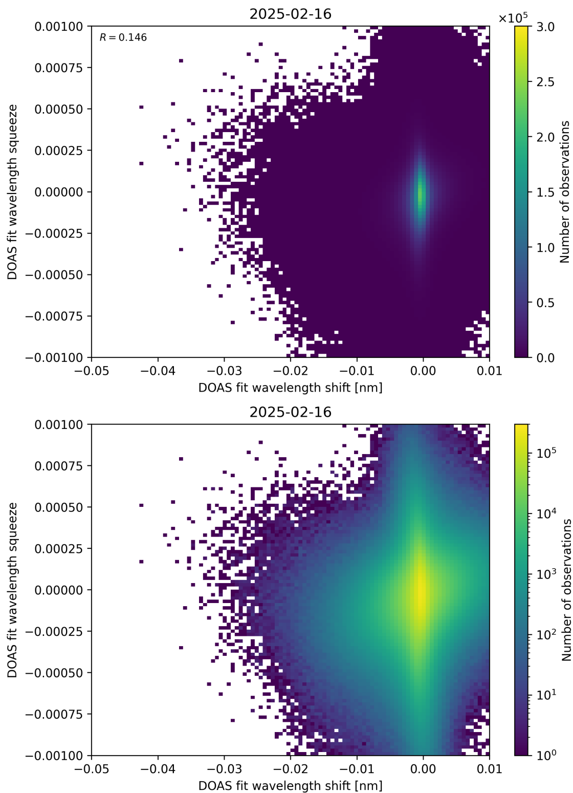
Figure 138: Scatter density plot of “DOAS fit wavelength shift” against “DOAS fit wavelength squeeze” for 2025-02-15 to 2025-02-17.
