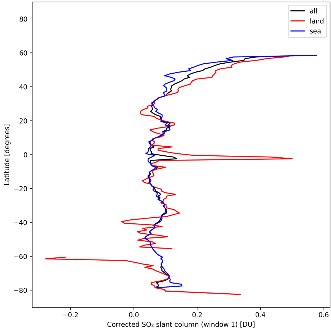
Figure 39: Zonal average of “Corrected SO 2 slant column (window 1)” for 2025-02-15 to 2025-02-17.
