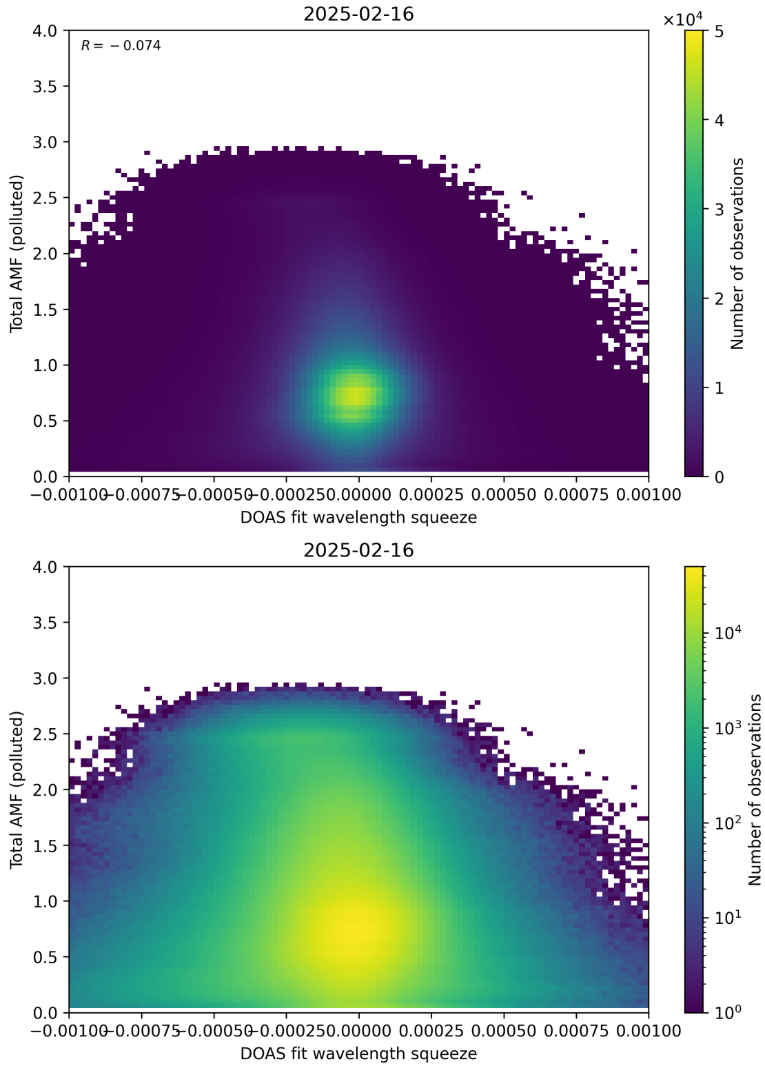
Figure 145: Scatter density plot of “DOAS fit wavelength squeeze” against “Total AMF (polluted)” for 2025-02-15 to 2025-02-17.
