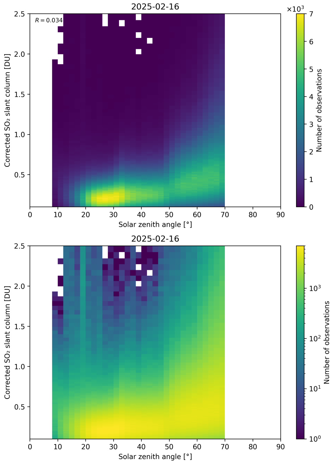
Figure 181: Scatter density plot of “Solar zenith angle” against “Corrected SO 2 slant column” for 2025-02-15 to 2025-02-17.
