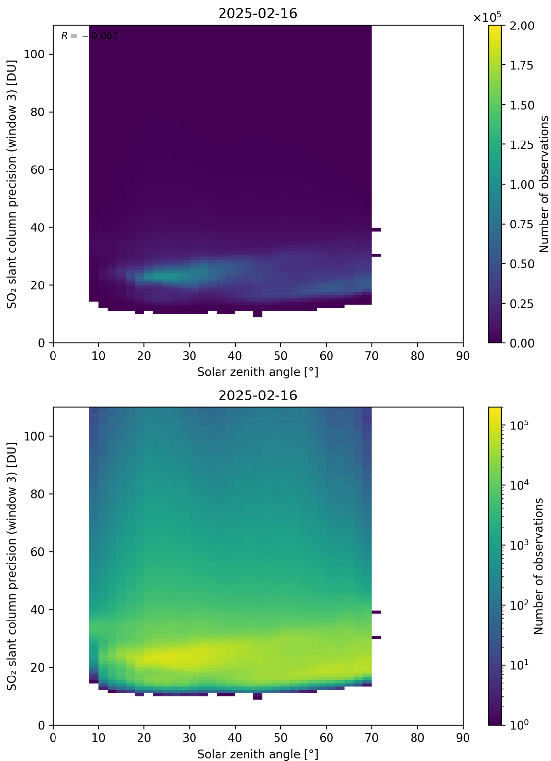
Figure 188: Scatter density plot of “Solar zenith angle” against “SO 2 slant column precision (window 3)” for 2025-02-15 to 2025-02-17.
