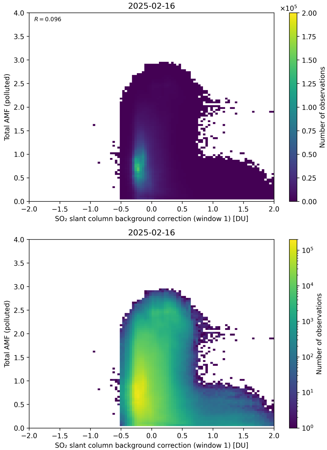
Figure 120: Scatter density plot of “SO 2 slant column background correction (window 1)” against “Total AMF (polluted)” for 2025-02-15 to 2025-02-17.
