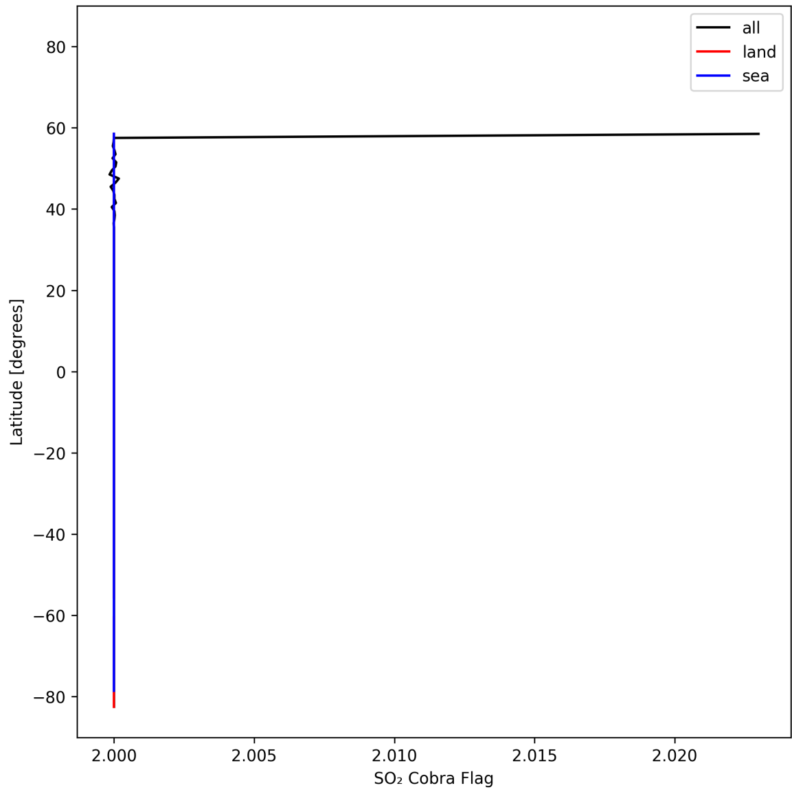
Figure 49: Zonal average of "SO 2 Cobra Flag" for 2025-02-15 to 2025-02-17.
