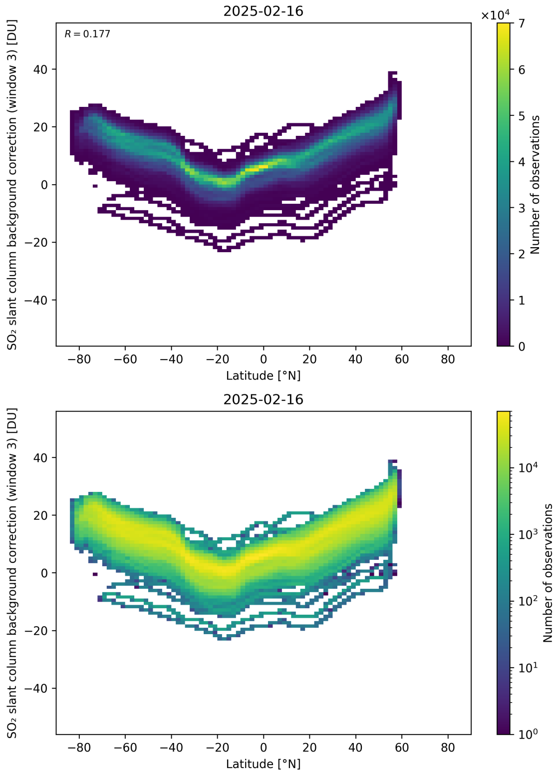
Figure 152: Scatter density plot of “Latitude” against “SO 2 slant column background correction (window 3)” for 2025-02-15 to 2025-02-17.
