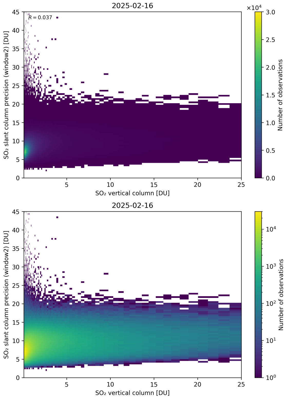
Figure 356: Scatter density plot of “SO 2 vertical column” against “SO 2 slant column precision (window2)” for 2025-02-15 to 2025-02-17.
