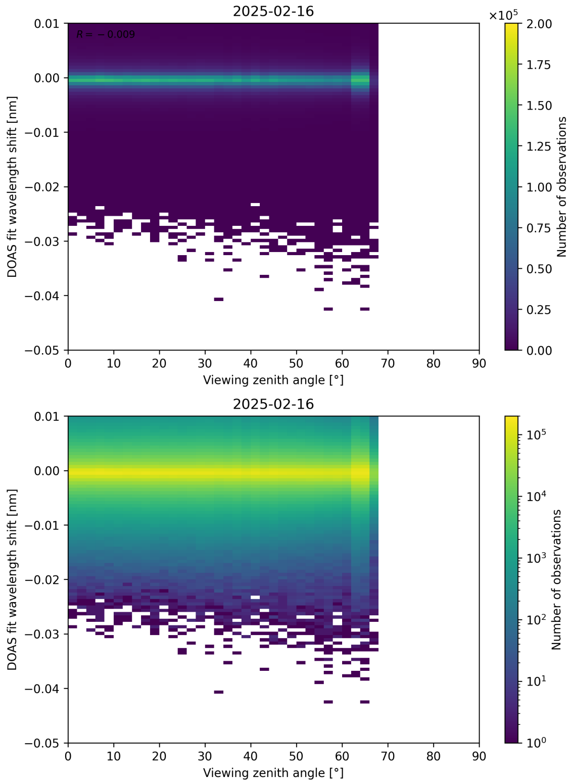
Figure 365: Scatter density plot of “Viewing zenith angle” against “DOAS fit wavelength shift” for 2025-02-15 to 2025-02-17.
