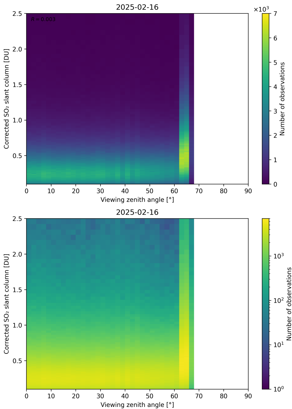
Figure 373: Scatter density plot of “Viewing zenith angle” against “Corrected SO 2 slant column” for 2025-02-15 to 2025-02-17.
