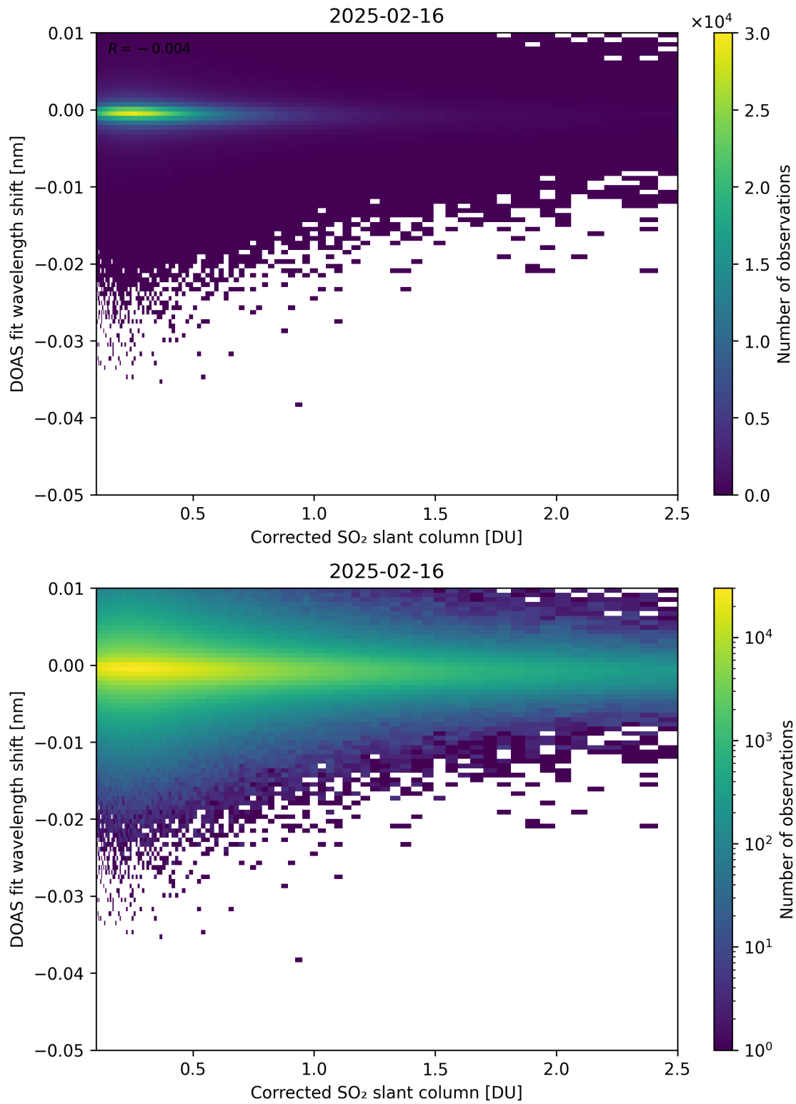
Figure 229: Scatter density plot of “Corrected SO 2 slant column” against “DOAS fit wavelength shift” for 2025-02-15 to 2025-02-17.
