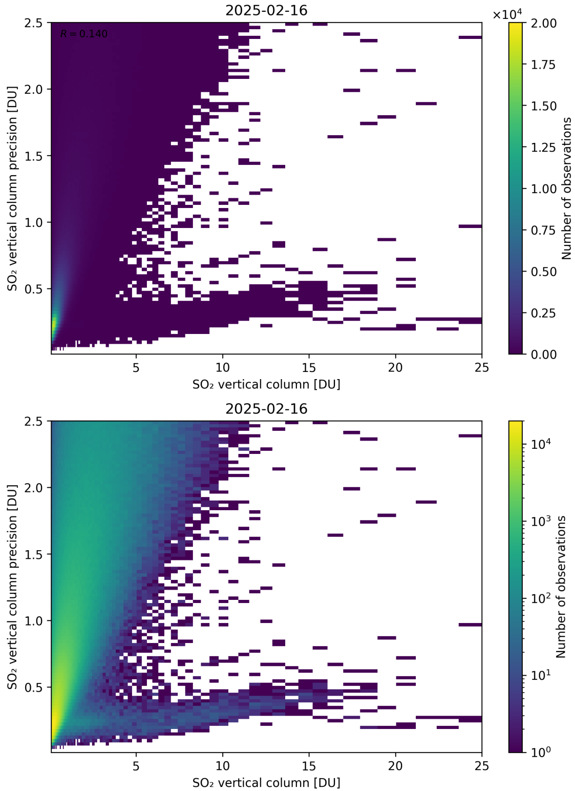
Figure 361: Scatter density plot of “SO 2 vertical column” against “SO 2 vertical column precision” for 2025-02-15 to 2025-02-17.
