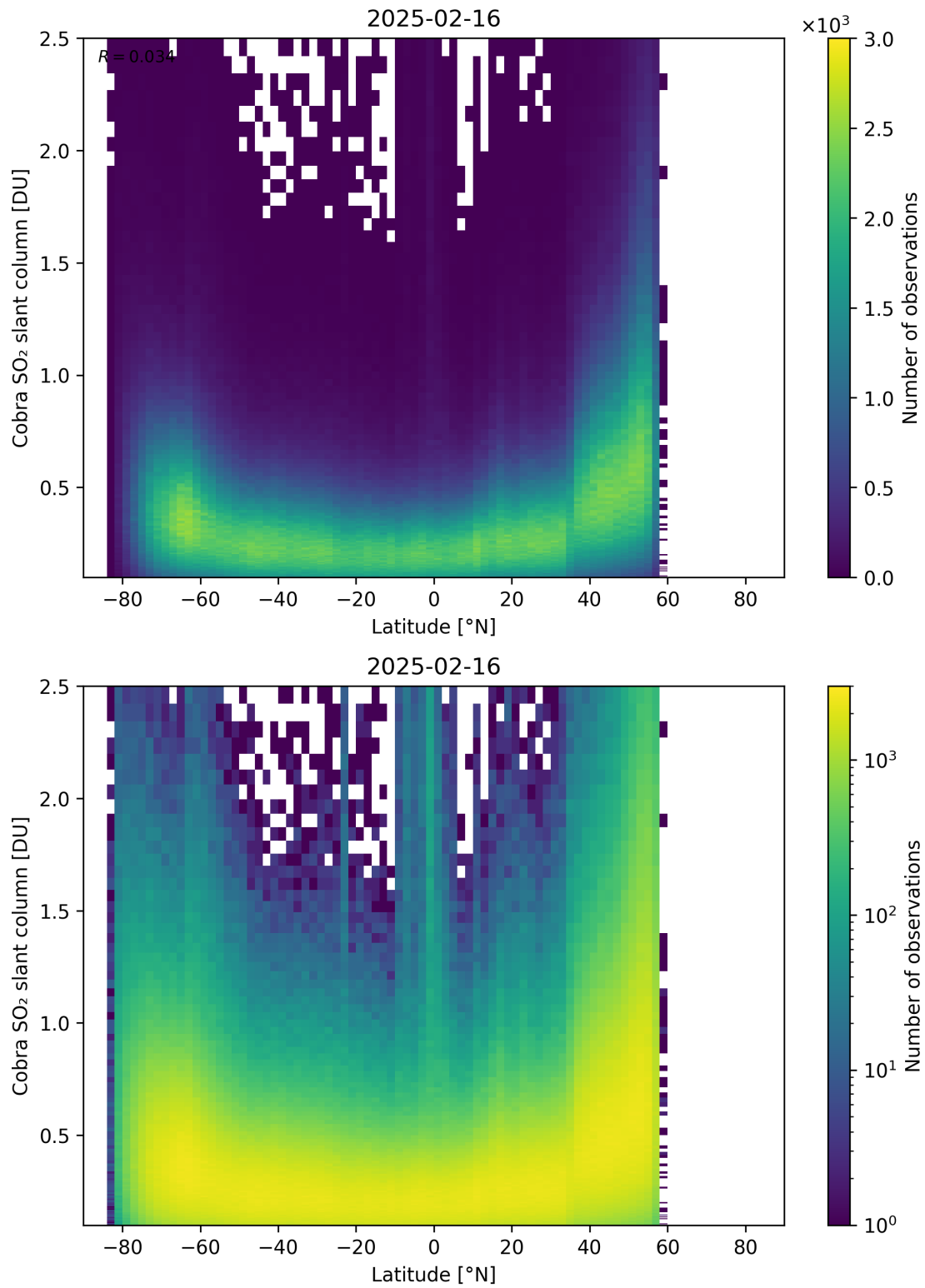
Figure 157: Scatter density plot of “Latitude” against “Cobra SO 2 slant column” for 2025-02-15 to 2025-02-17.
