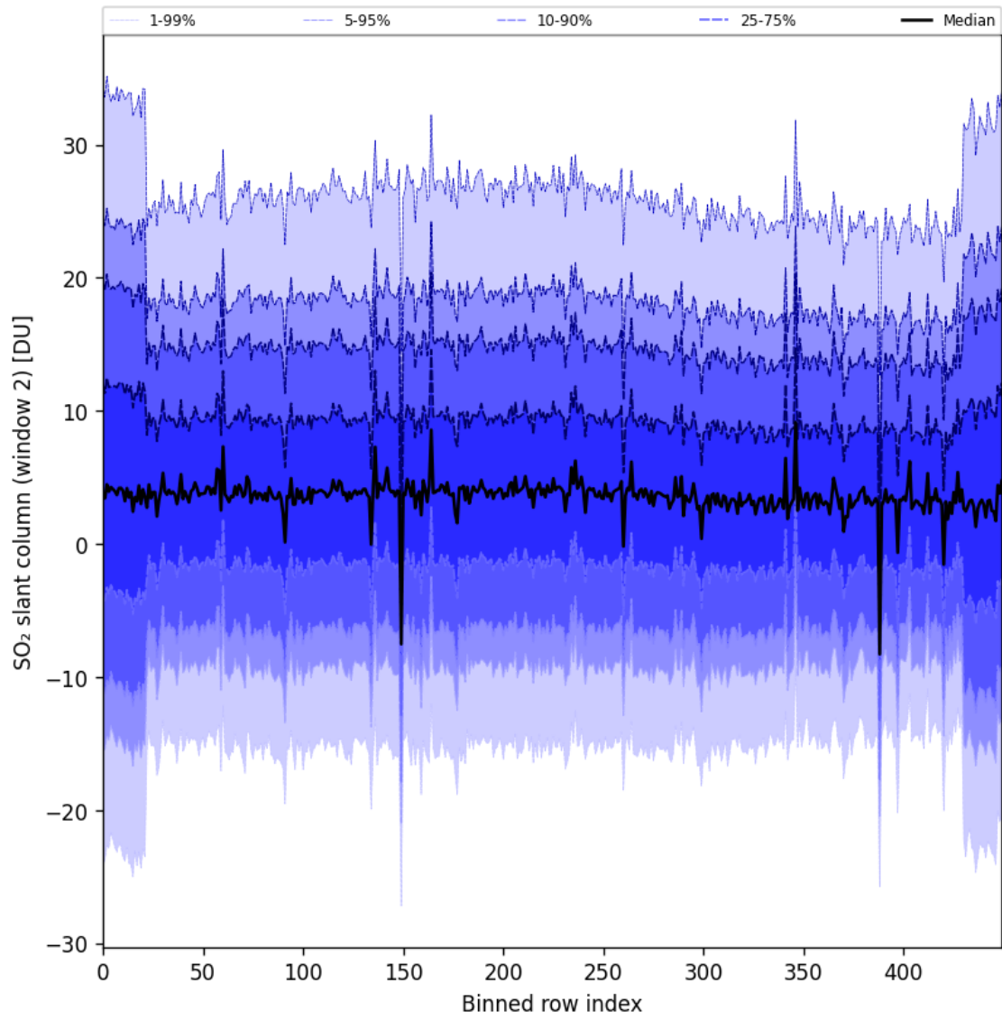
Figure 93: Along track statistics of “SO 2 slant column (window 2)” for 2025-02-15 to 2025-02-17
