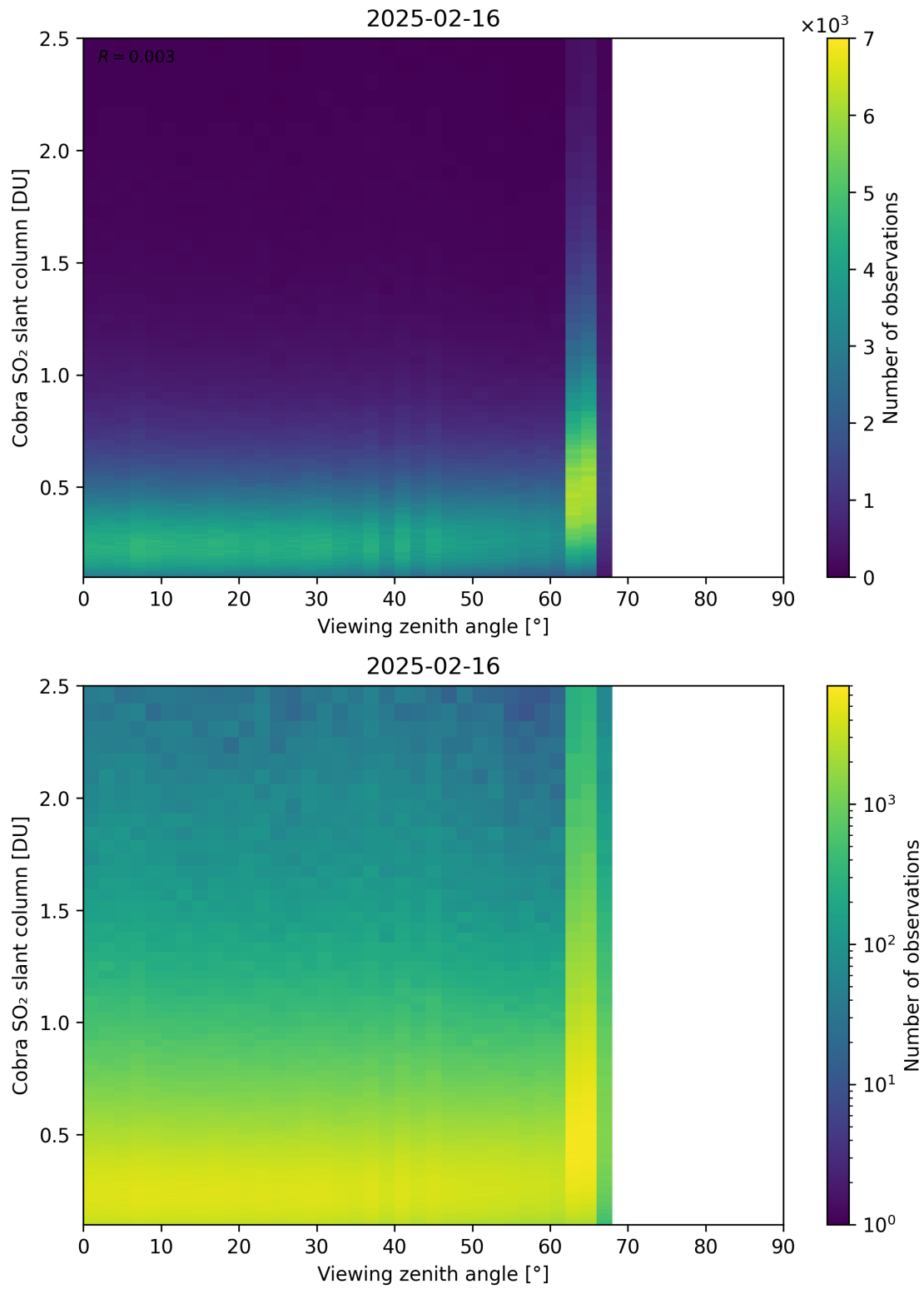
Figure 371: Scatter density plot of “Viewing zenith angle” against “Cobra SO 2 slant column” for 2025-02-15 to 2025-02-17.
