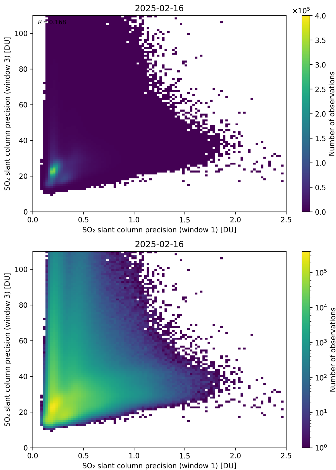
Figure 279: Scatter density plot of “SO 2 slant column precision (window 1)” against “SO 2 slant column precision (window 3)” for 2025-02-15 to 2025-02-17.
