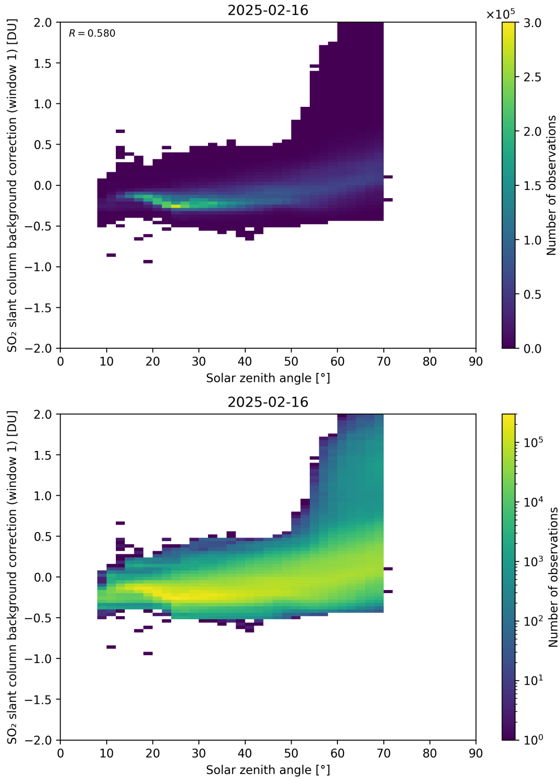
Figure 171: Scatter density plot of “Solar zenith angle” against “SO 2 slant column background correction (window 1)” for 2025-02-15 to 2025-02-17.
