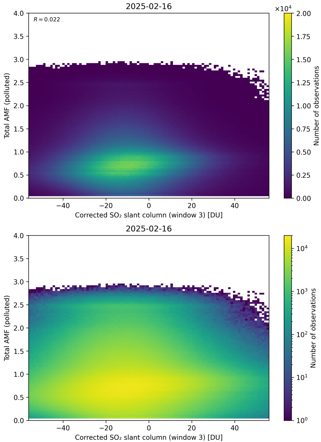
Figure 260: Scatter density plot of “Corrected SO 2 slant column (window 3)” against “Total AMF (polluted)” for 2025-02-15 to 2025-02-17.
