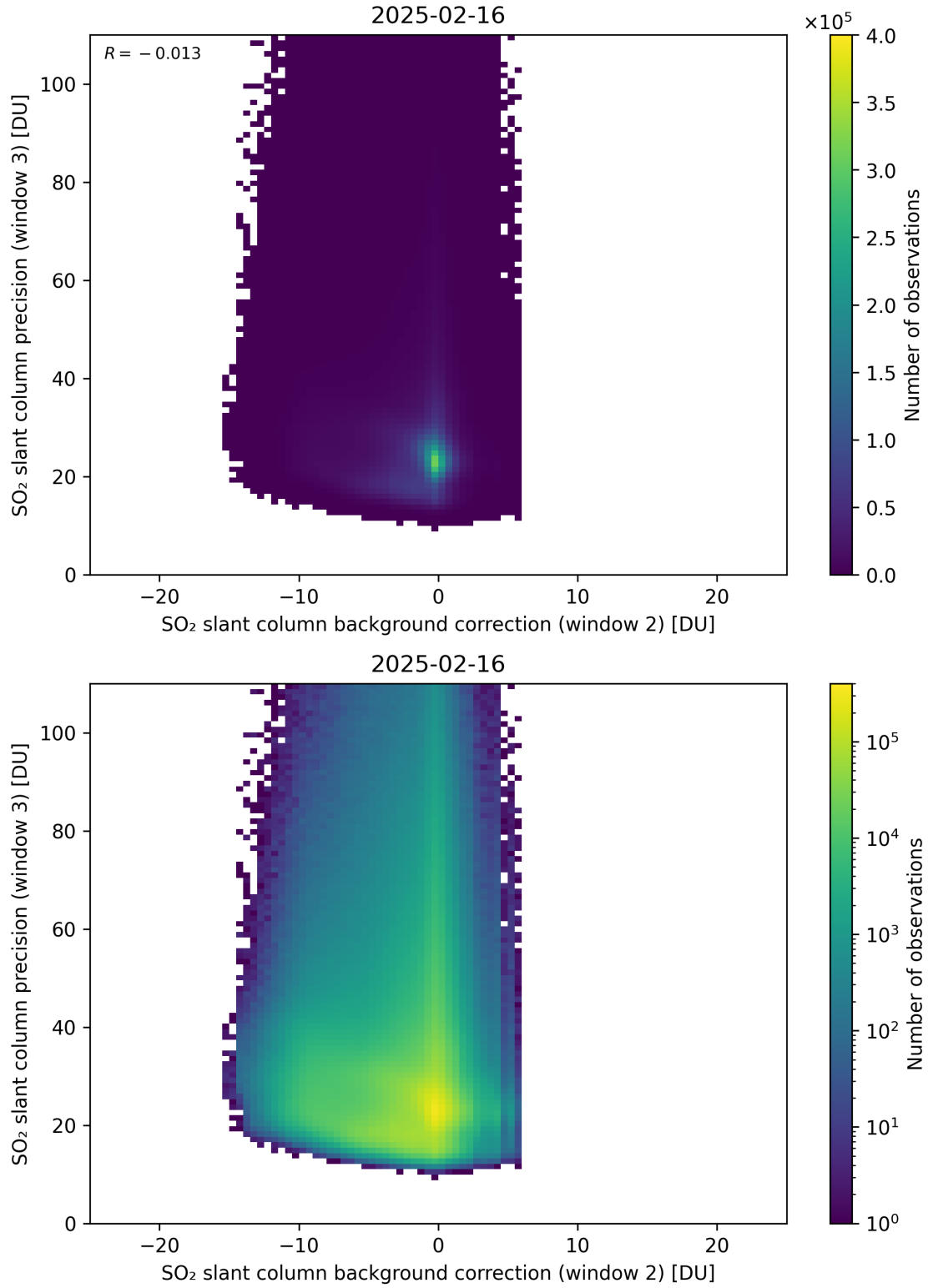
Figure 129: Scatter density plot of “SO 2 slant column background correction (window 2)” against “SO 2 slant column precision (window 3)” for 2025-02-15 to 2025-02-17.
