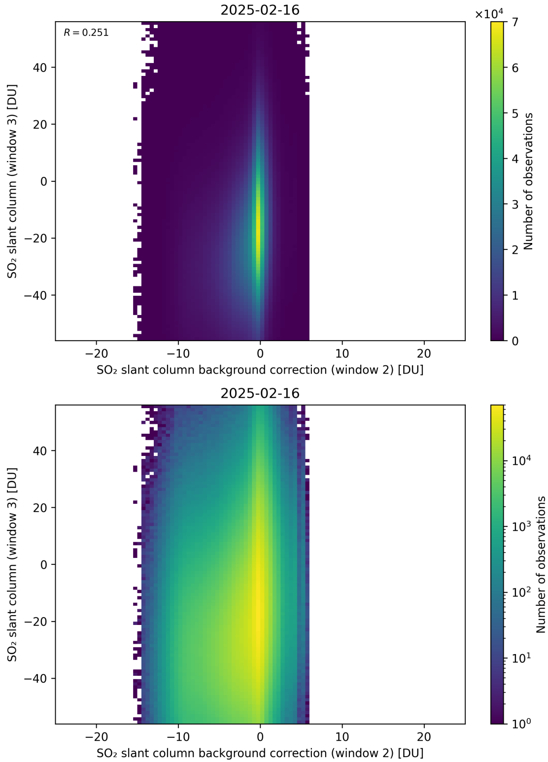
Figure 128: Scatter density plot of “SO 2 slant column background correction (window 2)” against “SO 2 slant column (window 3)” for 2025-02-15 to 2025-02-17.
