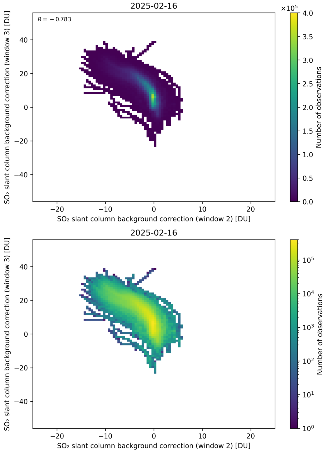
Figure 122: Scatter density plot of “SO 2 slant column background correction (window 2)” against “SO 2 slant column background correction (window 3)” for 2025-02-15 to 2025-02-17.
