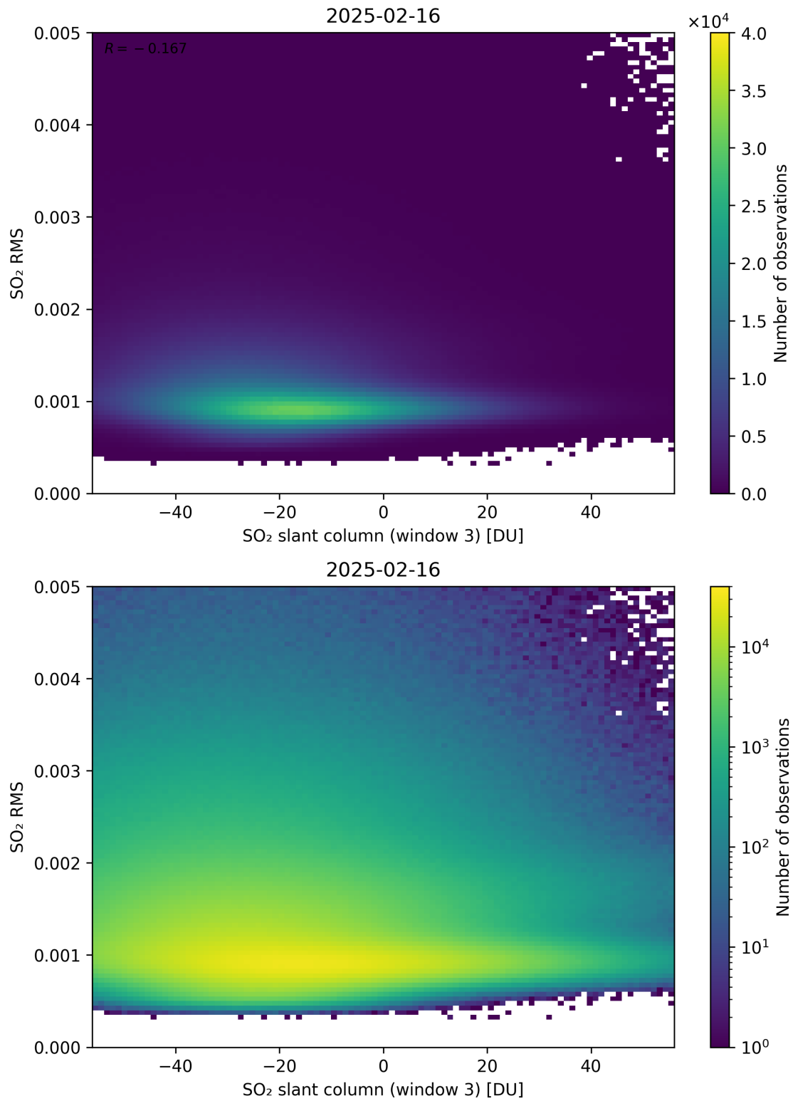
Figure 306: Scatter density plot of “SO 2 slant column (window 3)” against “SO 2 RMS” for 2025-02-15 to 2025-02-17.
