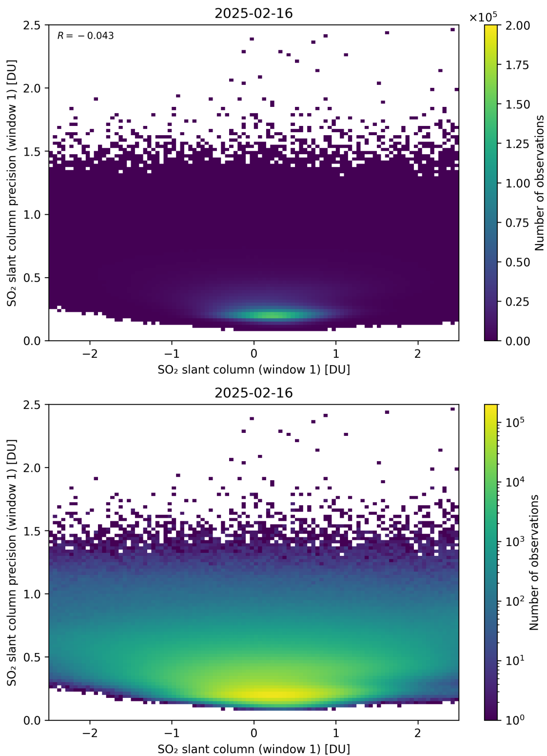
Figure 285: Scatter density plot of “SO 2 slant column (window 1)” against “SO 2 slant column precision (window 1)” for 2025-02-15 to 2025-02-17.
