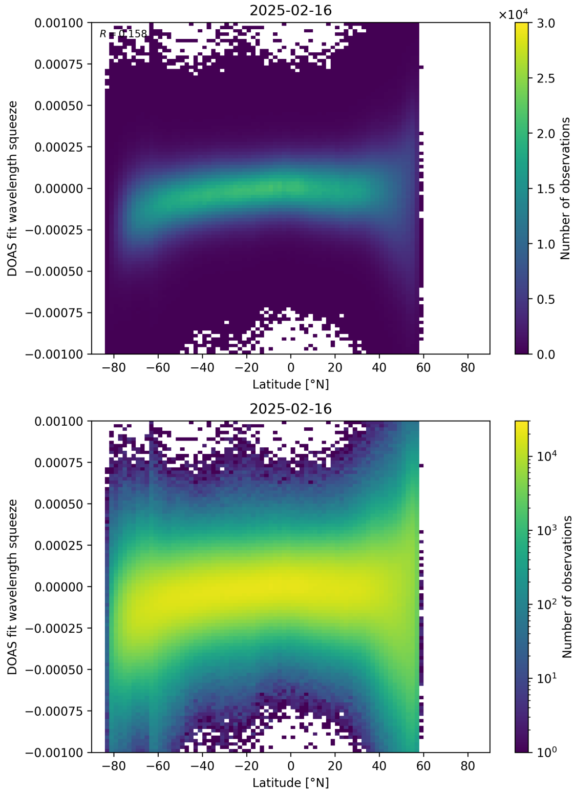
Figure 154: Scatter density plot of “Latitude” against “DOAS fit wavelength squeeze” for 2025-02-15 to 2025-02-17.
