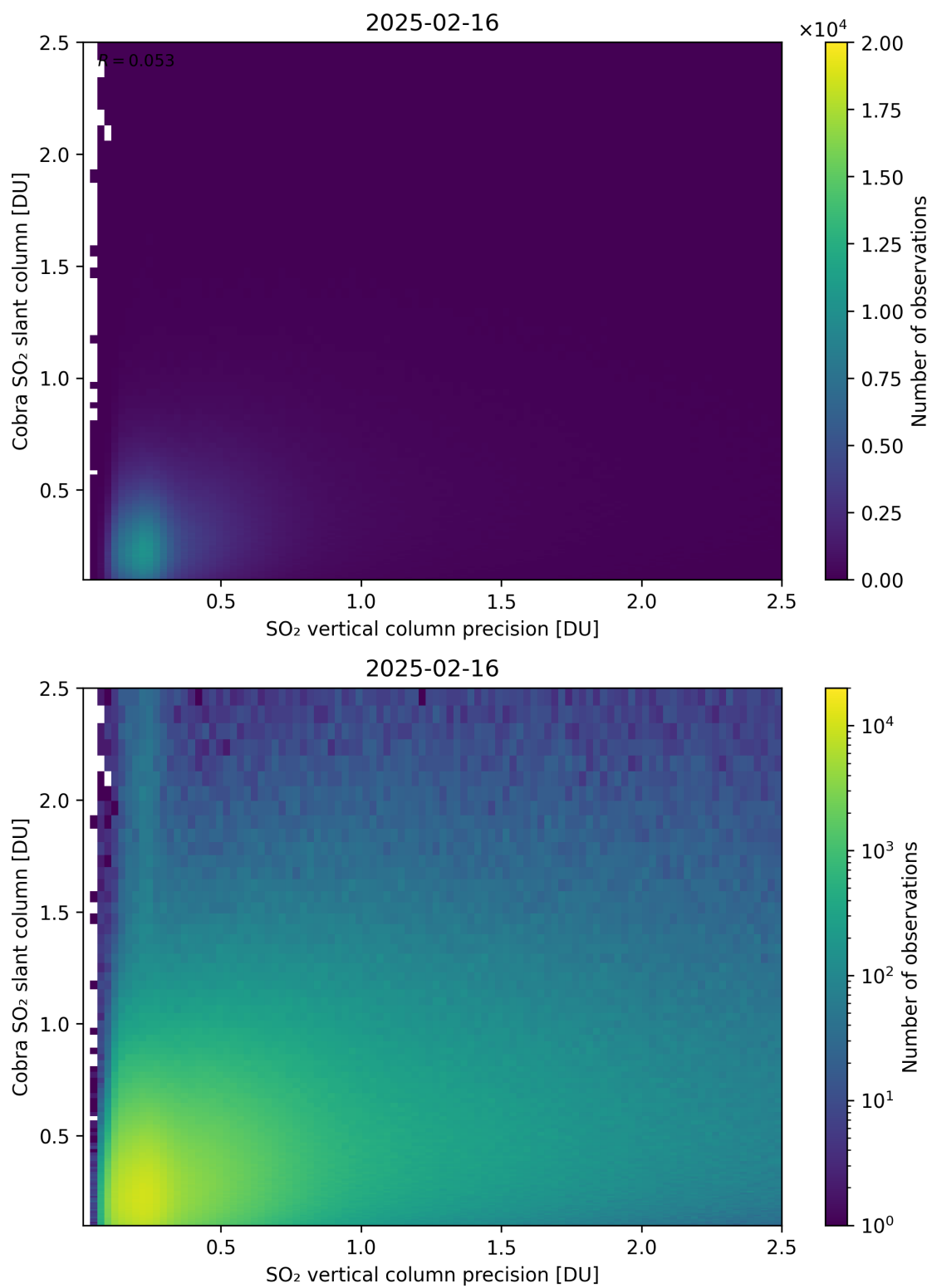
Figure 336: Scatter density plot of “SO 2 vertical column precision” against “Cobra SO 2 slant column” for 2025-02-15 to 2025-02-17.
