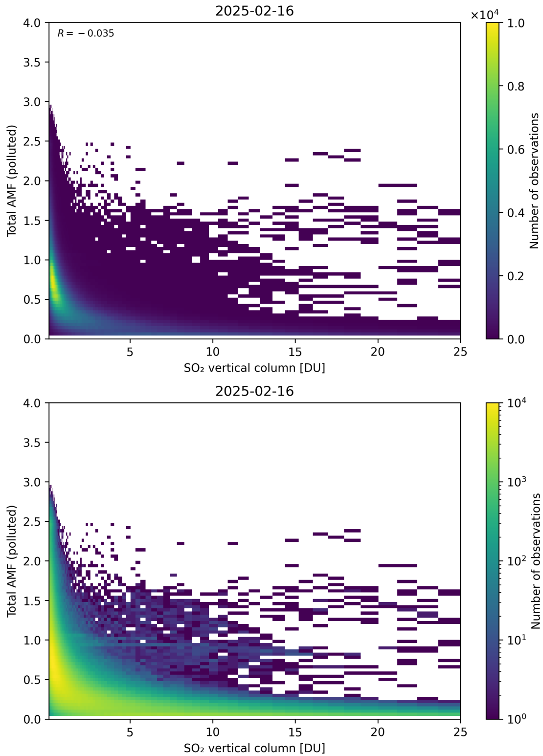
Figure 359: Scatter density plot of “SO 2 vertical column” against “Total AMF (polluted)” for 2025-02-15 to 2025-02-17.
