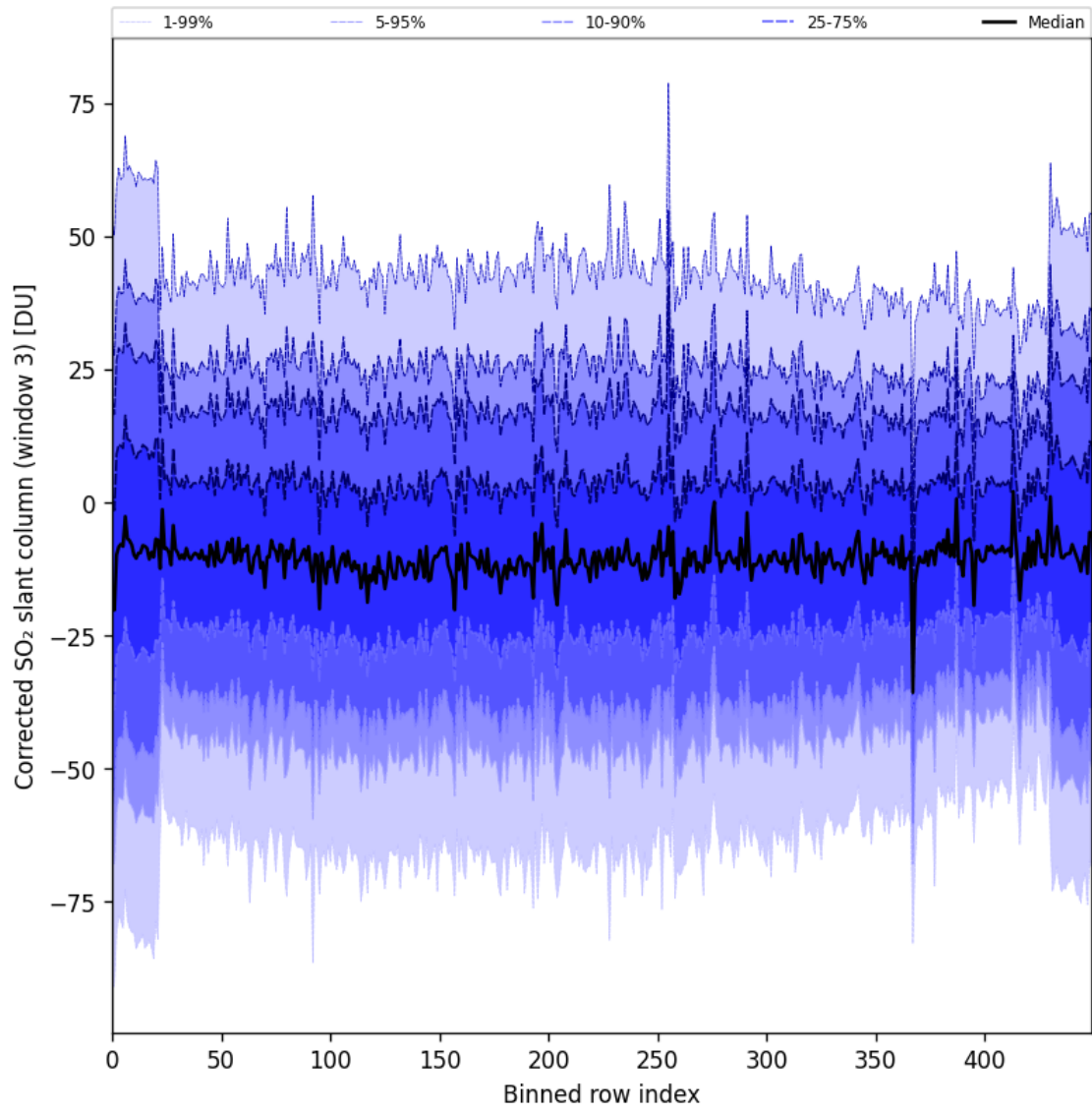
Figure 99: Along track statistics of “Corrected SO 2 slant column (window 3)” for 2025-02-15 to 2025-02-17
