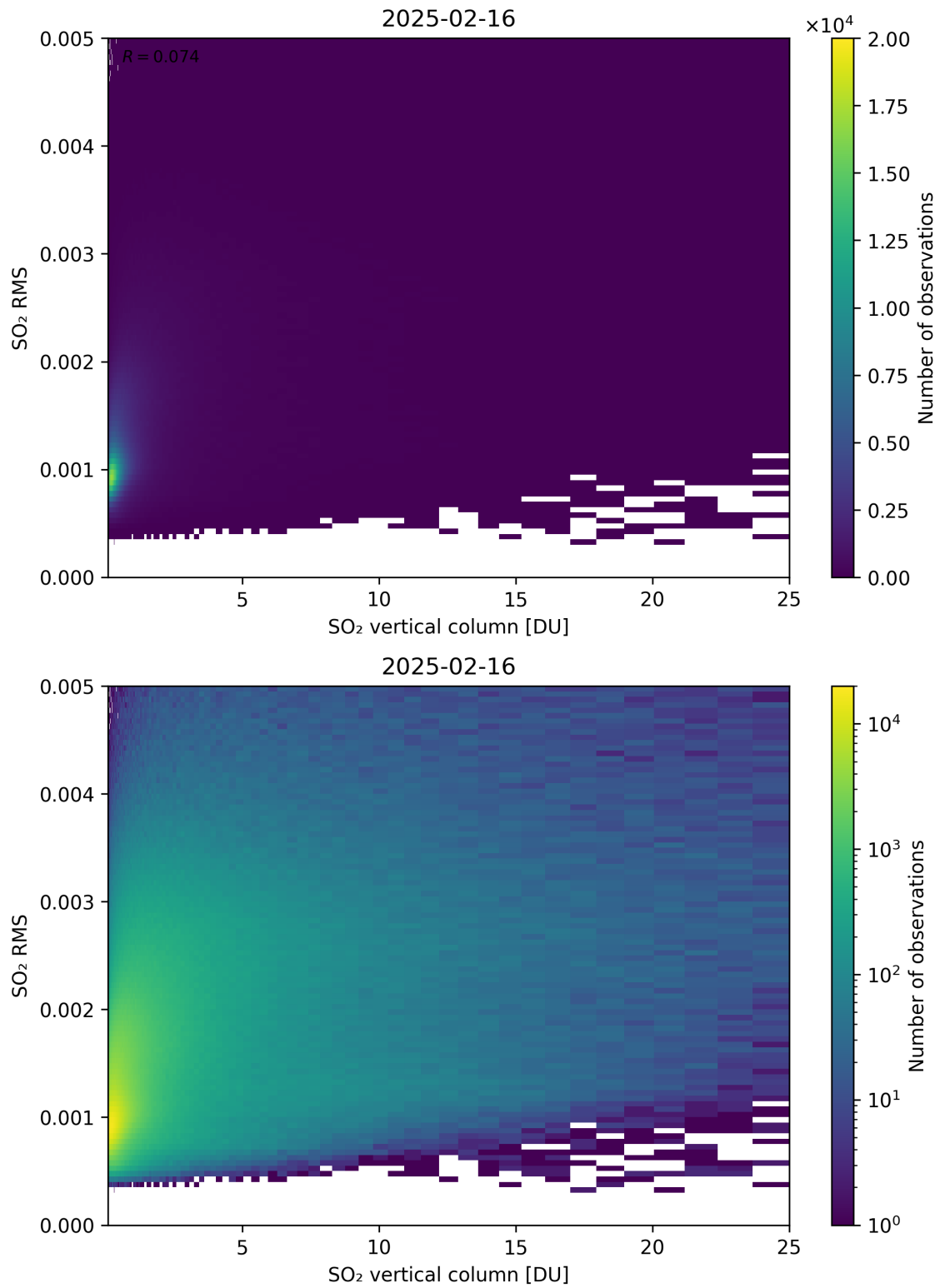
Figure 328: Scatter density plot of “SO 2 vertical column” against “SO 2 RMS” for 2025-02-15 to 2025-02-17.
