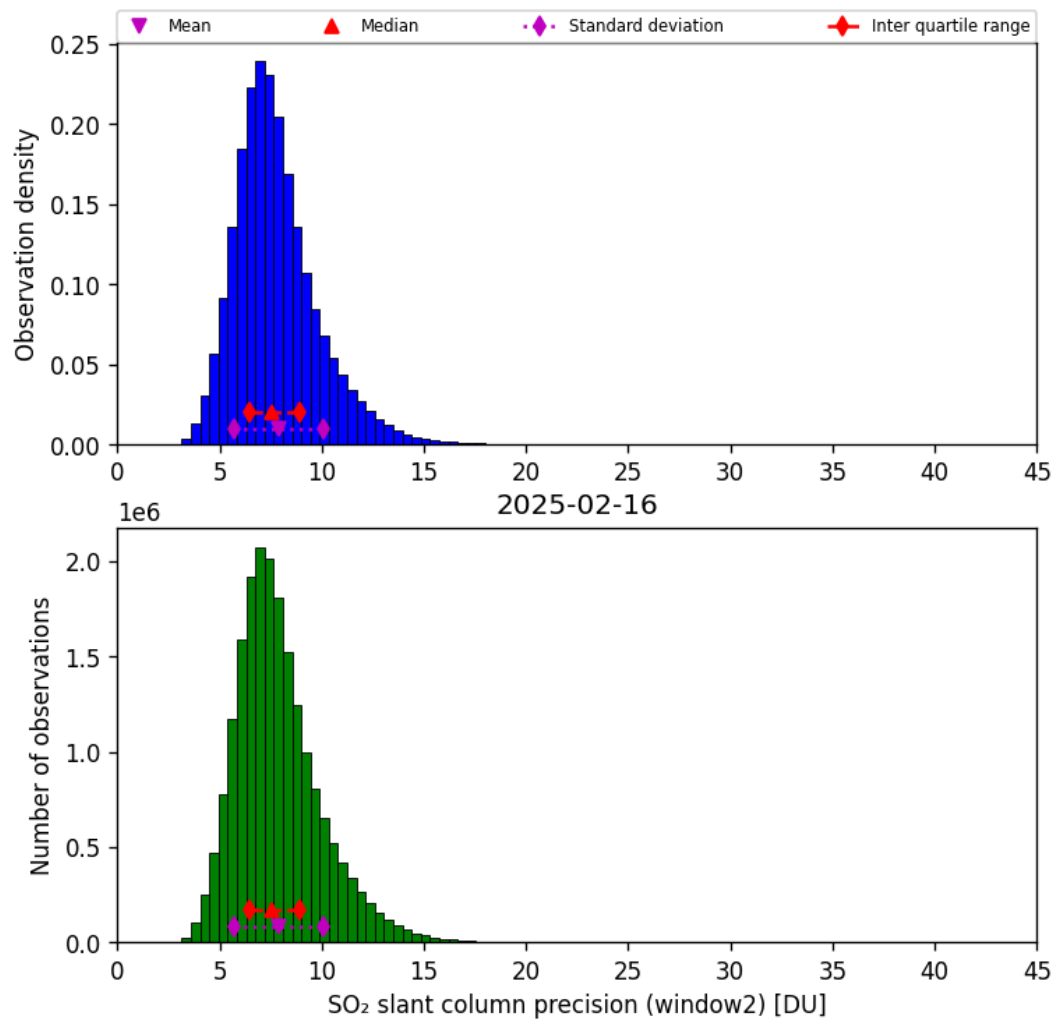
Figure 68: Histogram of “SO 2 slant column precision (window2)” for 2025-02-15 to 2025-02-17
