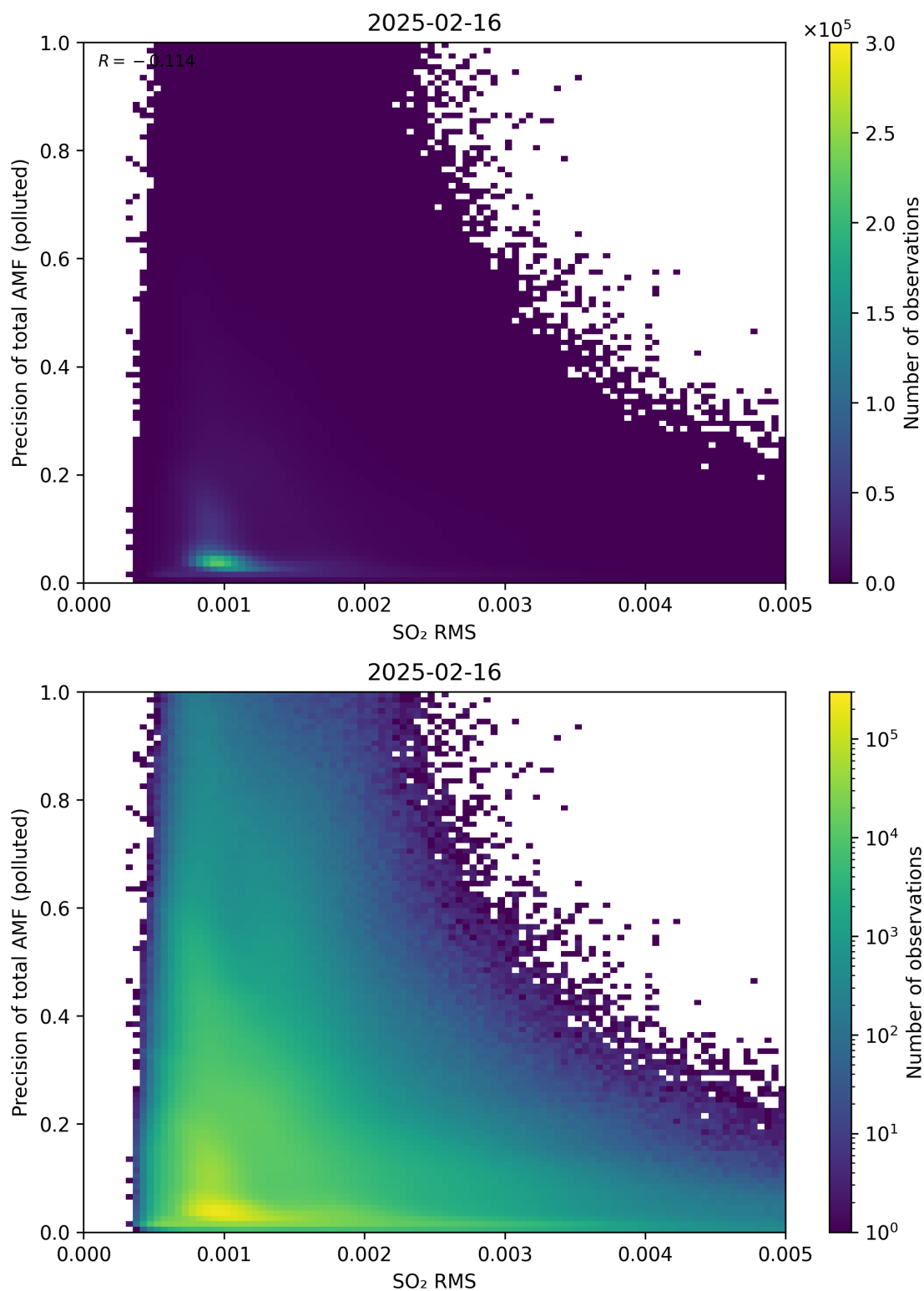
Figure 149: Scatter density plot of “SO 2 RMS” against “Precision of total AMF (polluted)” for 2025-02-15 to 2025-02-17.
