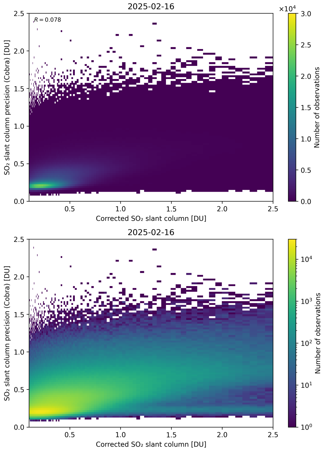
Figure 234: Scatter density plot of “Corrected SO 2 slant column” against “SO 2 slant column precision (Cobra)” for 2025-02-15 to 2025-02-17.
