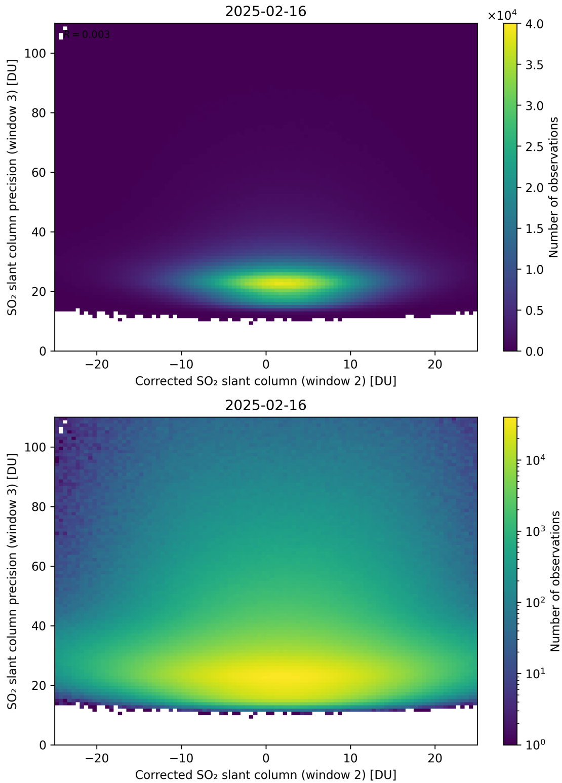
Figure 252: Scatter density plot of “Corrected SO 2 slant column (window 2)” against “SO 2 slant column precision (window 3)” for 2025-02-15 to 2025-02-17.
