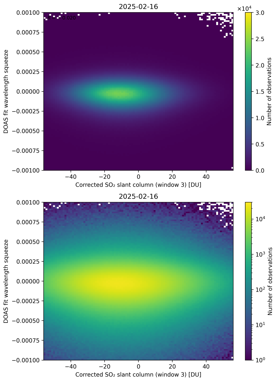
Figure 257: Scatter density plot of “Corrected SO 2 slant column (window 3)” against “DOAS fit wavelength squeeze” for 2025-02-15 to 2025-02-17.
