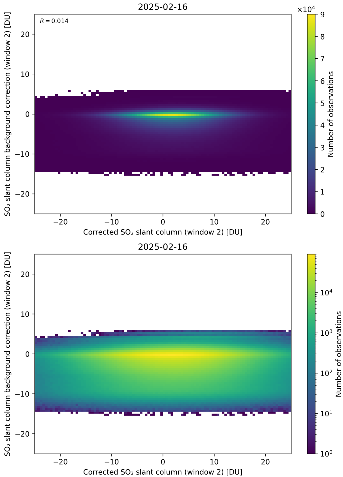
Figure 244: Scatter density plot of “Corrected SO 2 slant column (window 2)” against “SO 2 slant column background correction (window 2)” for 2025-02-15 to 2025-02-17.
