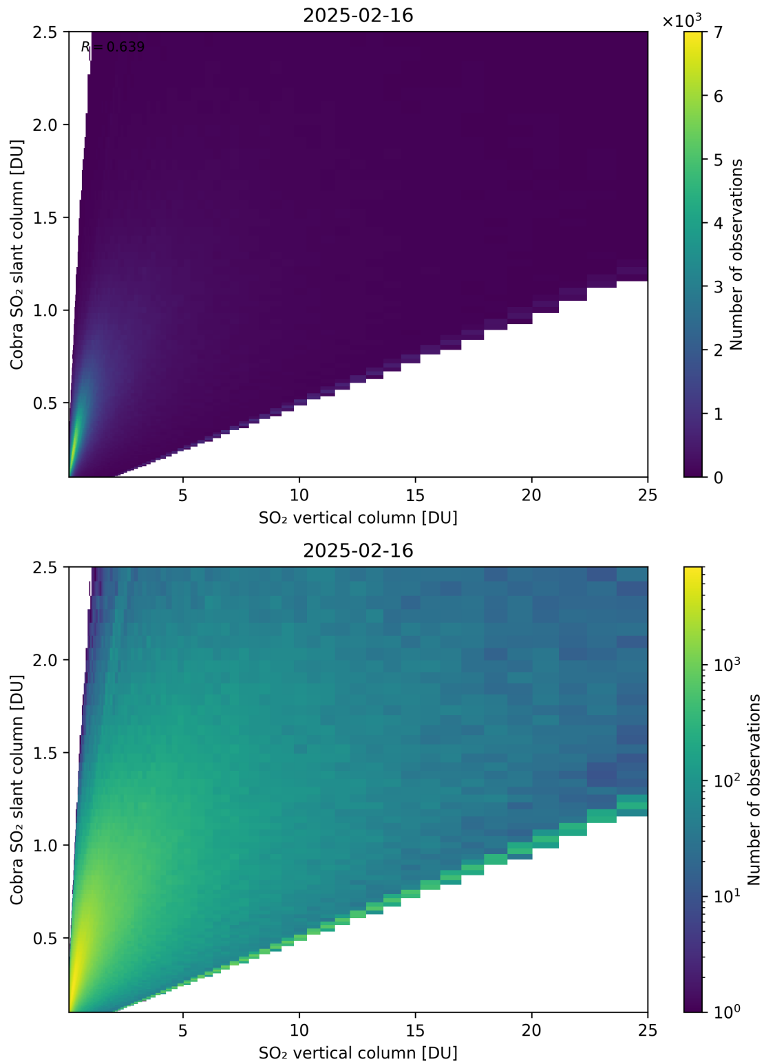
Figure 349: Scatter density plot of “SO 2 vertical column” against “Cobra SO 2 slant column” for 2025-02-15 to 2025-02-17.
