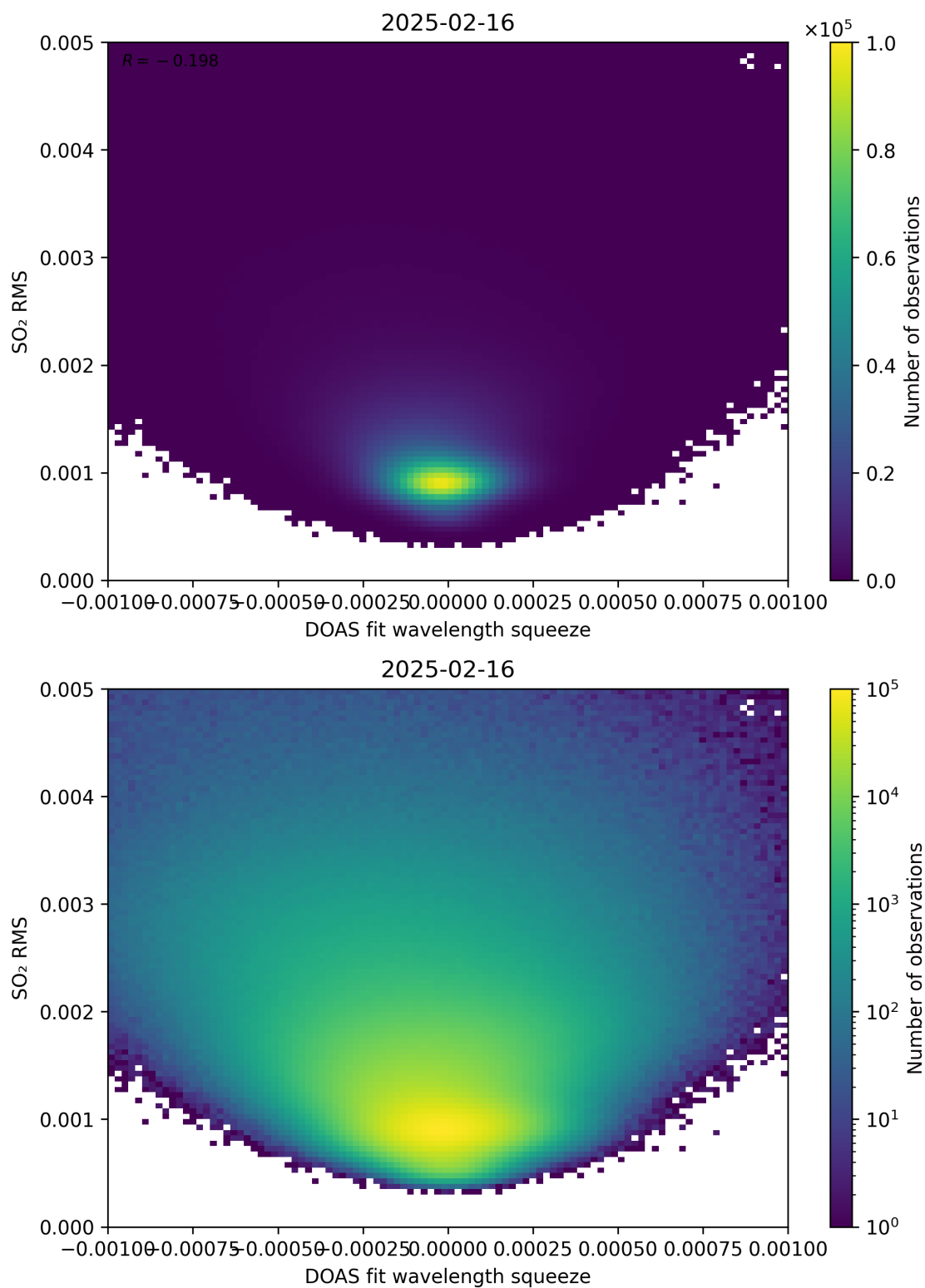
Figure 143: Scatter density plot of “DOAS fit wavelength squeeze” against “SO 2 RMS” for 2025-02-15 to 2025-02-17.
