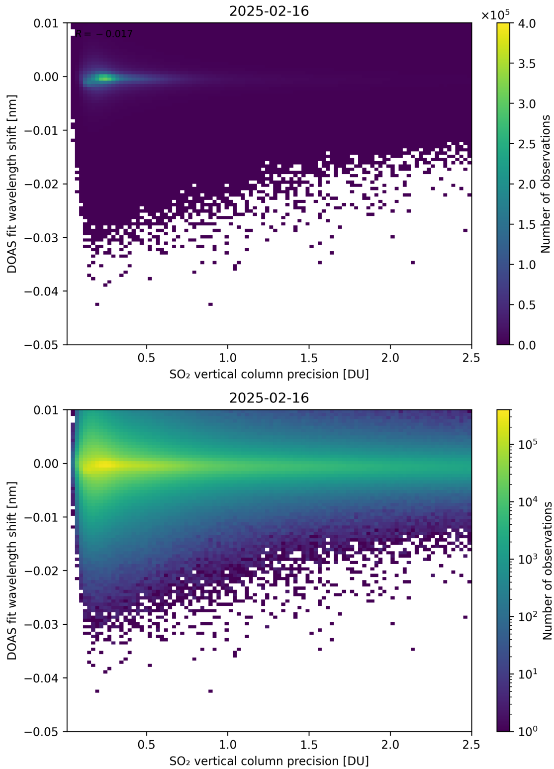
Figure 332: Scatter density plot of “SO 2 vertical column precision” against “DOAS fit wavelength shift” for 2025-02-15 to 2025-02-17.
