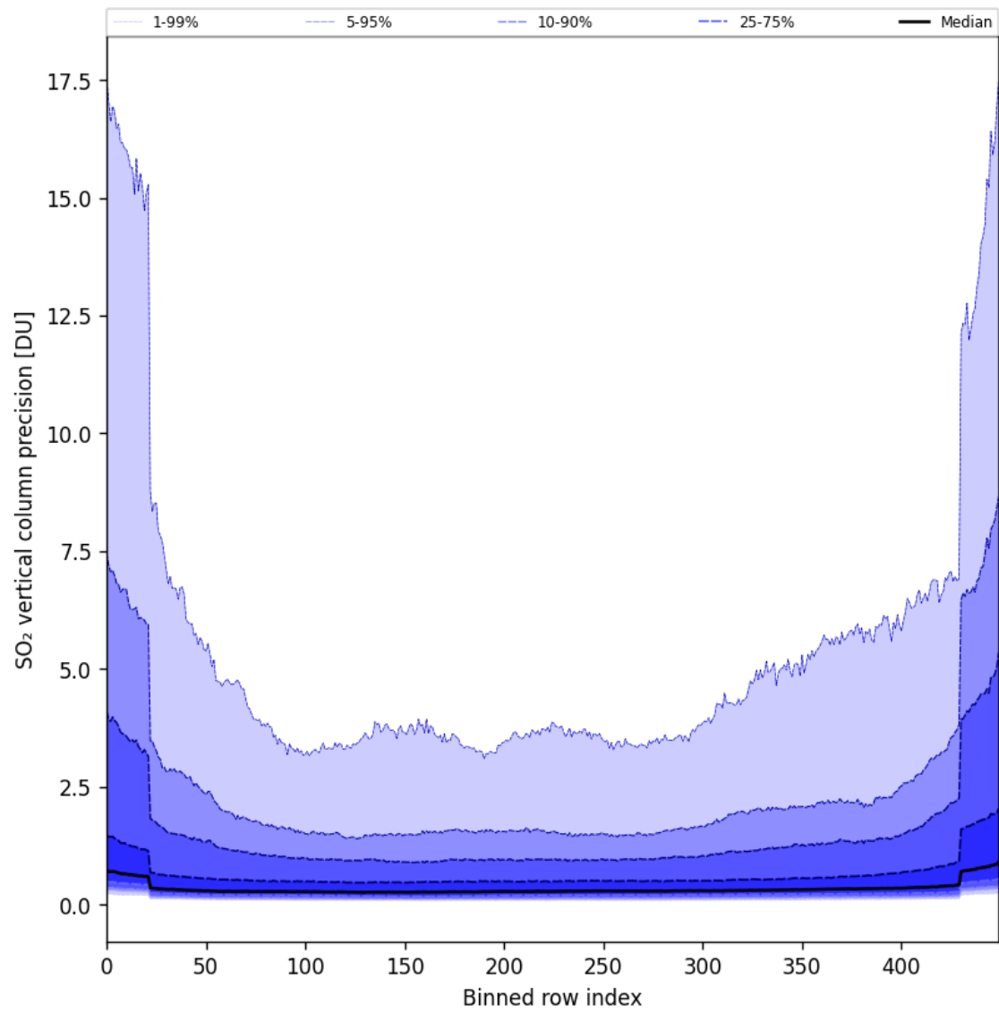
Figure 85: Along track statistics of “SO 2 vertical column precision” for 2025-02-15 to 2025-02-17
