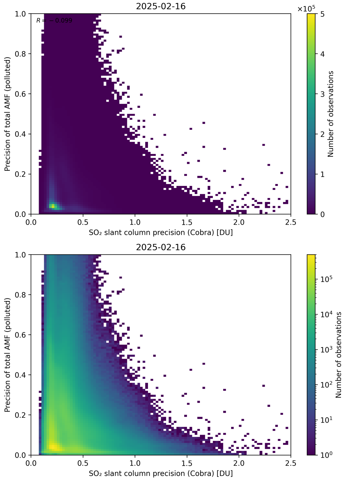
Figure 214: Scatter density plot of “SO 2 slant column precision (Cobra)” against “Precision of total AMF (polluted)” for 2025-02-15 to 2025-02-17.
