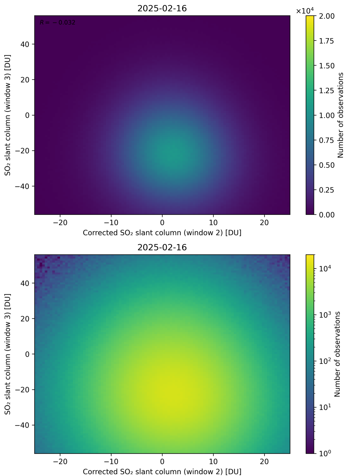
Figure 251: Scatter density plot of “Corrected SO 2 slant column (window 2)” against “SO 2 slant column (window 3)” for 2025-02-15 to 2025-02-17.
