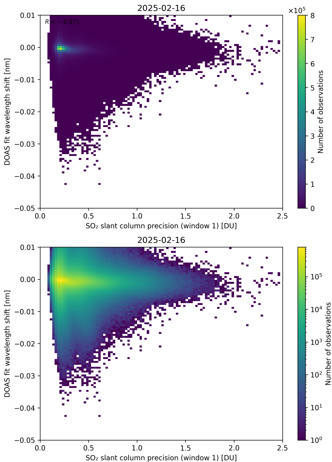
Figure 271: Scatter density plot of “SO 2 slant column precision (window 1)” against “DOAS fit wavelength shift” for 2025-02-15 to 2025-02-17.
