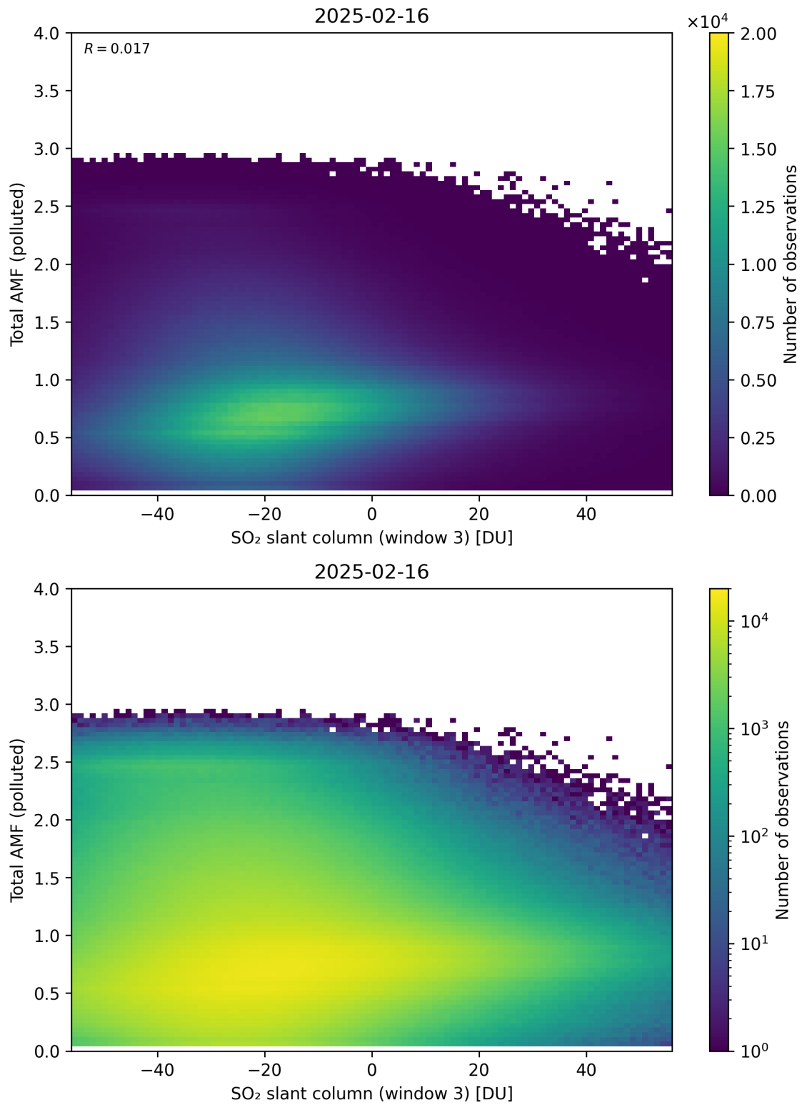
Figure 318: Scatter density plot of “SO 2 slant column (window 3)” against “Total AMF (polluted)” for 2025-02-15 to 2025-02-17.
