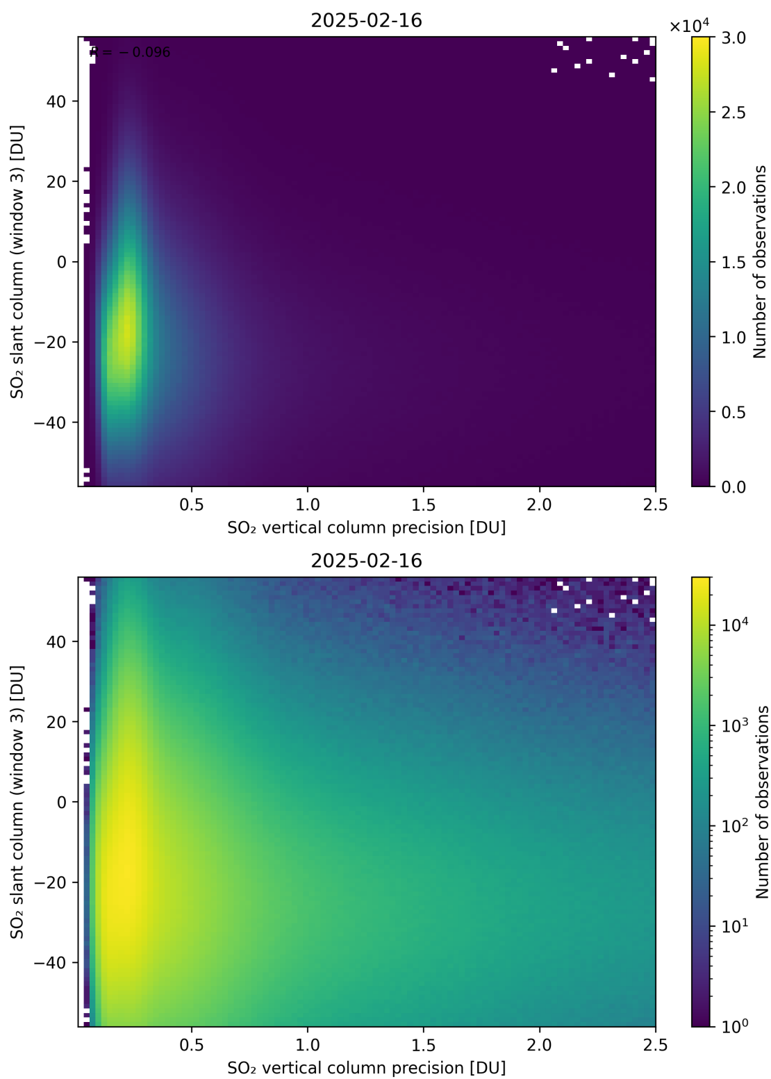
Figure 344: Scatter density plot of “SO 2 vertical column precision” against “SO 2 slant column (window 3)” for 2025-02-15 to 2025-02-17.
