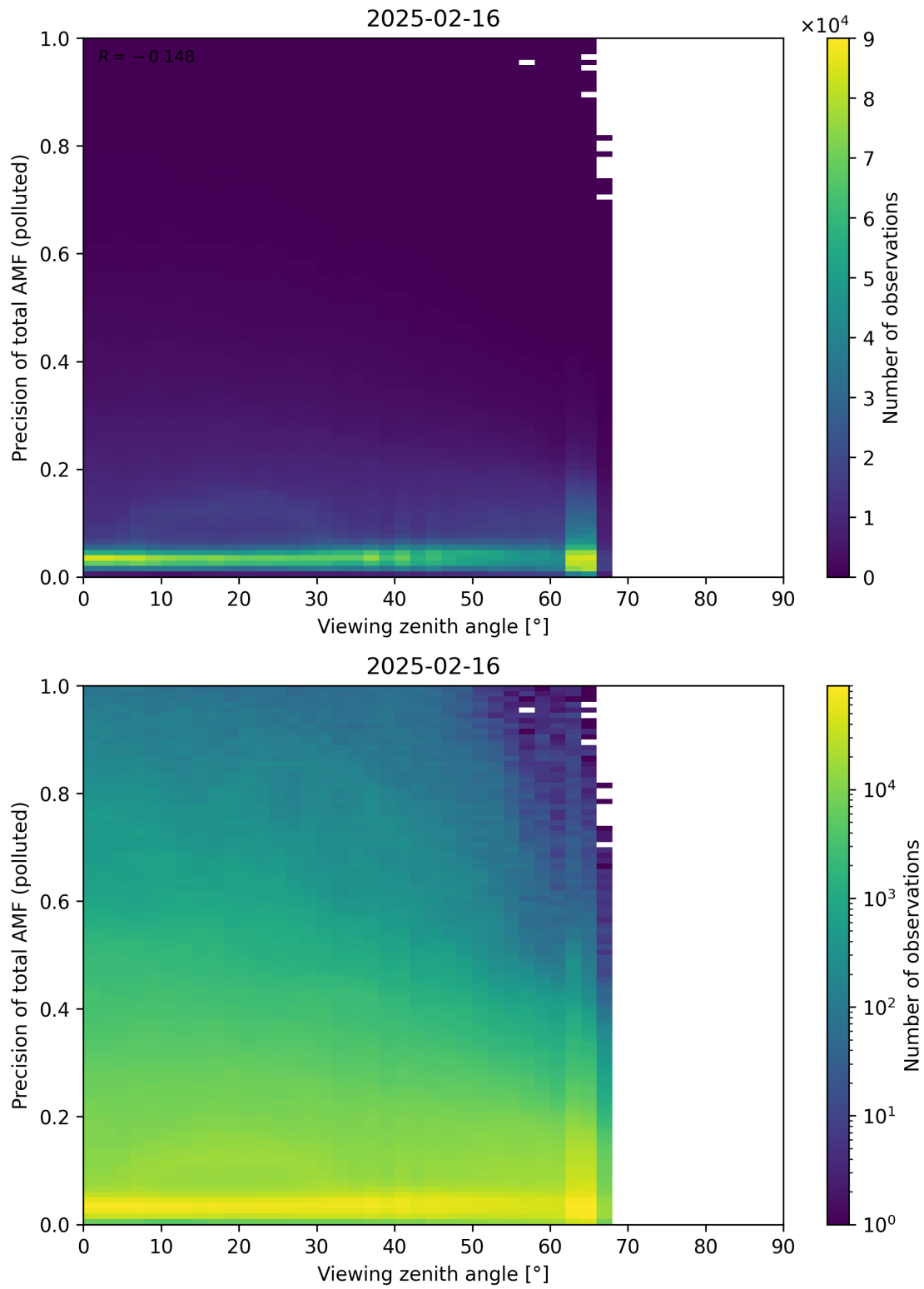
Figure 382: Scatter density plot of “Viewing zenith angle” against “Precision of total AMF (polluted)” for 2025-02-15 to 2025-02-17.
