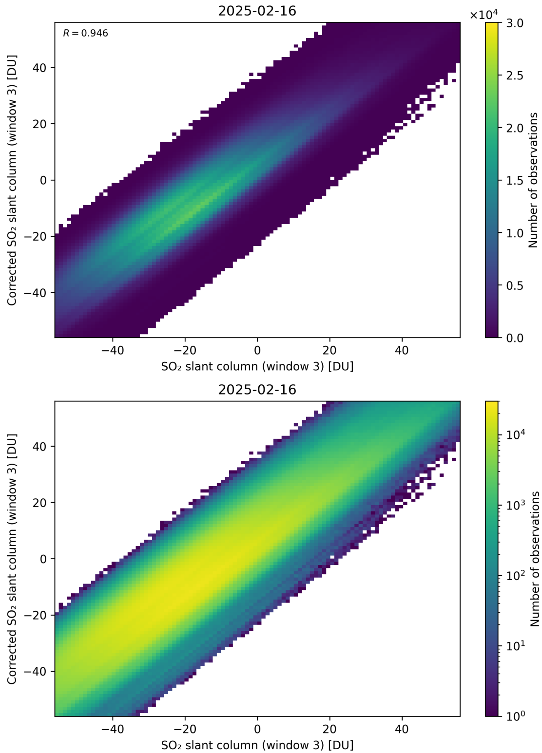
Figure 316: Scatter density plot of “SO 2 slant column (window 3)” against “Corrected SO 2 slant column (window 3)” for 2025-02-15 to 2025-02-17.
