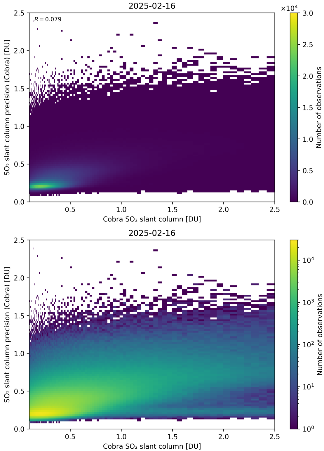
Figure 216: Scatter density plot of “Cobra SO 2 slant column” against “SO 2 slant column precision (Cobra)” for 2025-02-15 to 2025-02-17.
