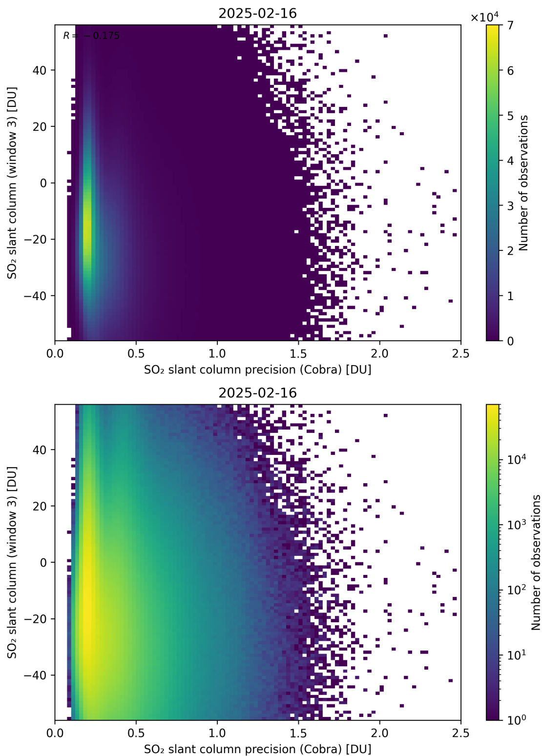
Figure 211: Scatter density plot of “SO 2 slant column precision (Cobra)” against “SO 2 slant column (window 3)” for 2025-02-15 to 2025-02-17.
