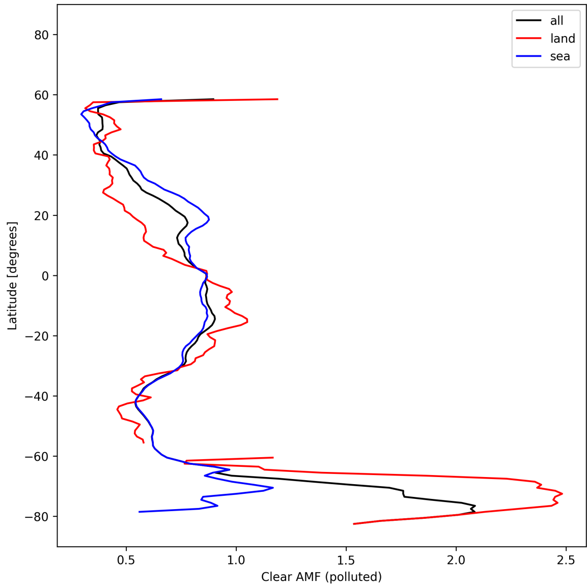
Figure 55: Zonal average of “Clear AMF (polluted)” for 2025-02-15 to 2025-02-17.
