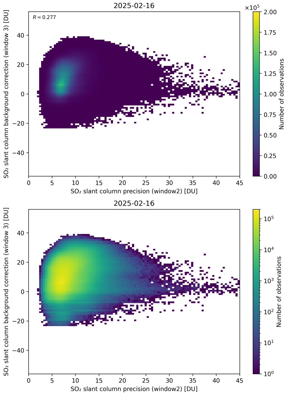
Figure 292: Scatter density plot of “SO 2 slant column precision (window2)” against “SO 2 slant column background correction (window 3)” for 2025-02-15 to 2025-02-17.
