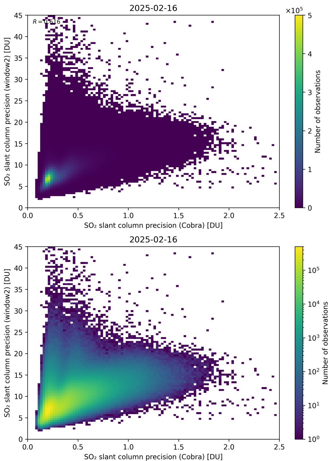
Figure 210: Scatter density plot of “SO 2 slant column precision (Cobra)” against “SO 2 slant column precision (window2)” for 2025-02-15 to 2025-02-17.
