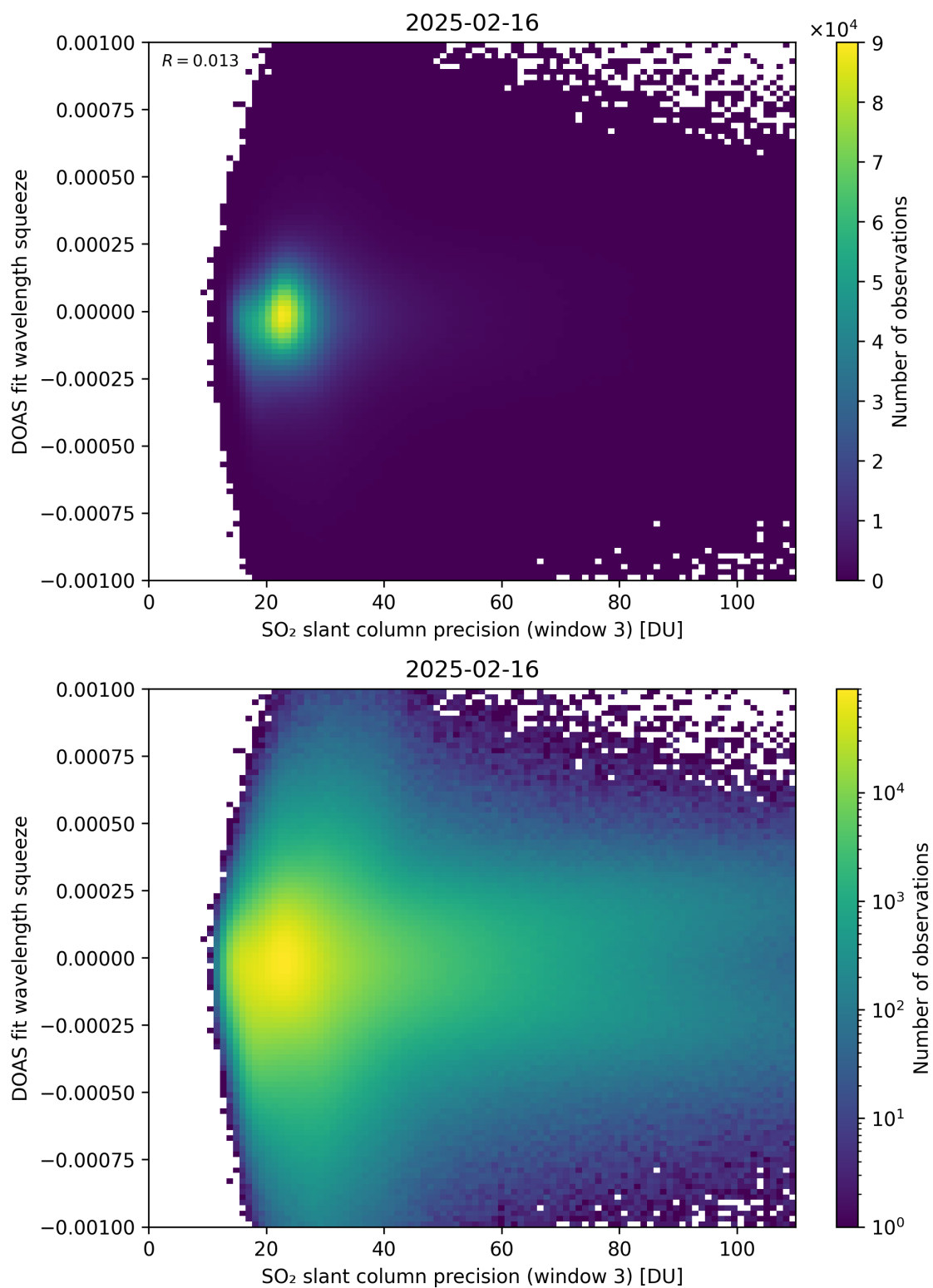
Figure 309: Scatter density plot of “SO 2 slant column precision (window 3)” against “DOAS fit wavelength squeeze” for 2025-02-15 to 2025-02-17.
