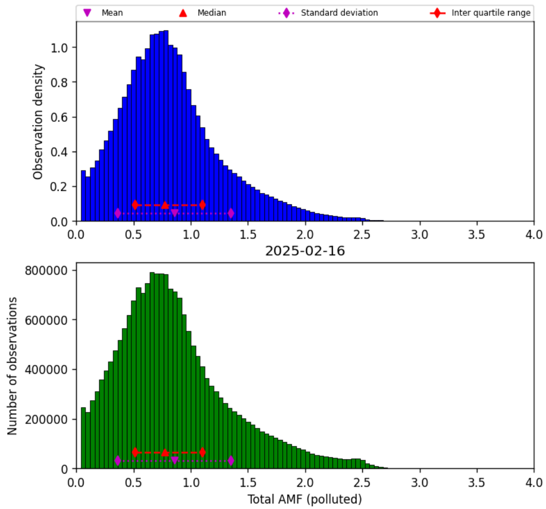
Figure 79: Histogram of “Total AMF (polluted)” for 2025-02-15 to 2025-02-17
