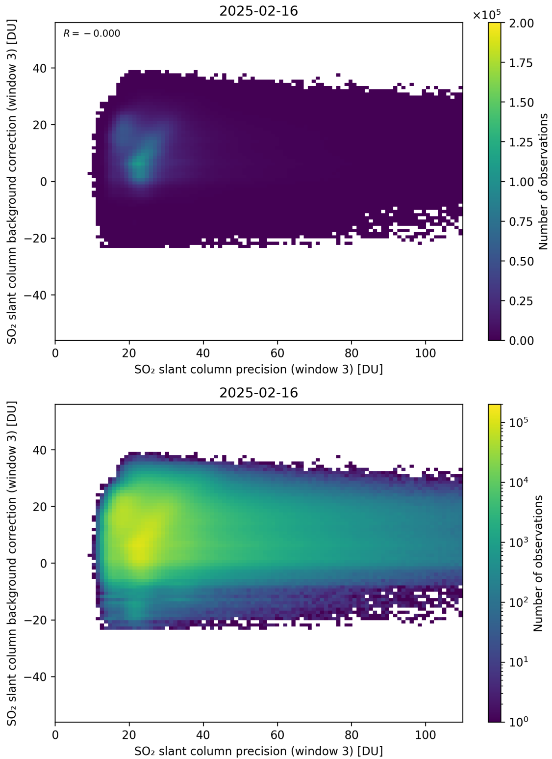
Figure 307: Scatter density plot of “SO 2 slant column precision (window 3)” against “SO 2 slant column background correction (window 3)” for 2025-02-15 to 2025-02-17.
