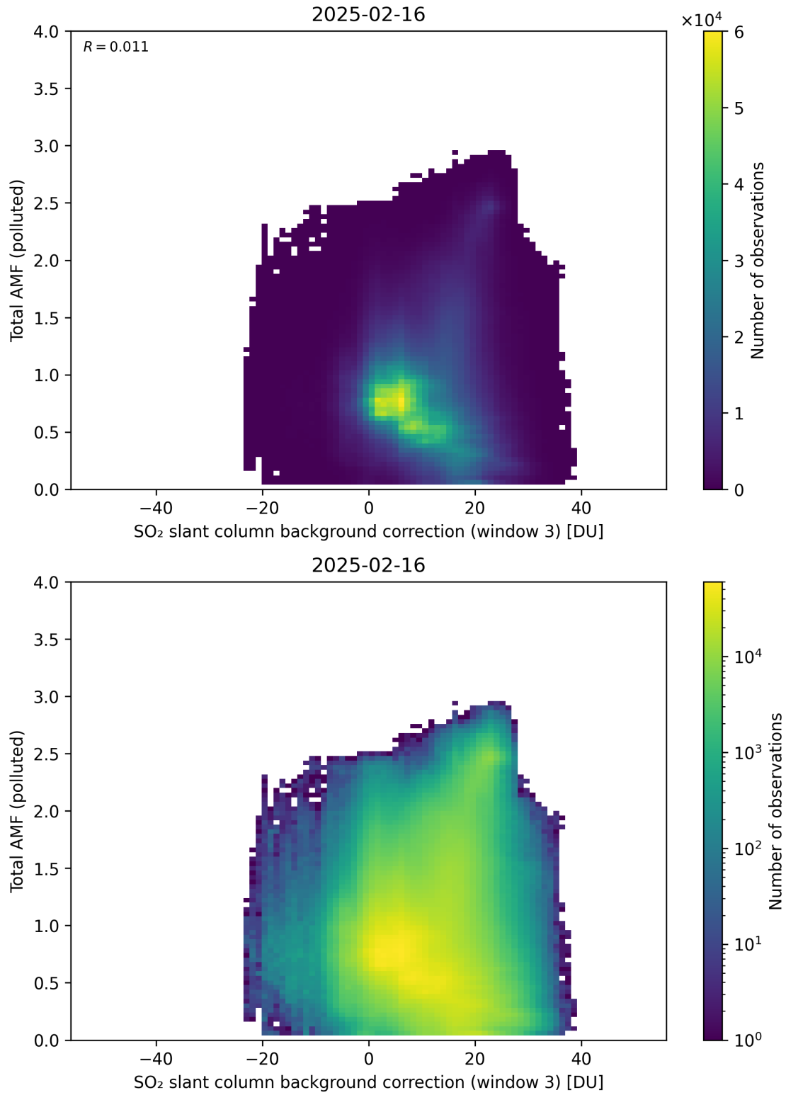
Figure 136: Scatter density plot of “SO 2 slant column background correction (window 3)” against “Total AMF (polluted)” for 2025-02-15 to 2025-02-17.
