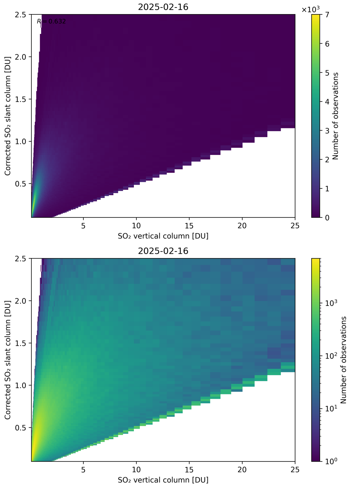
Figure 351: Scatter density plot of “SO 2 vertical column” against “Corrected SO 2 slant column” for 2025-02-15 to 2025-02-17.
