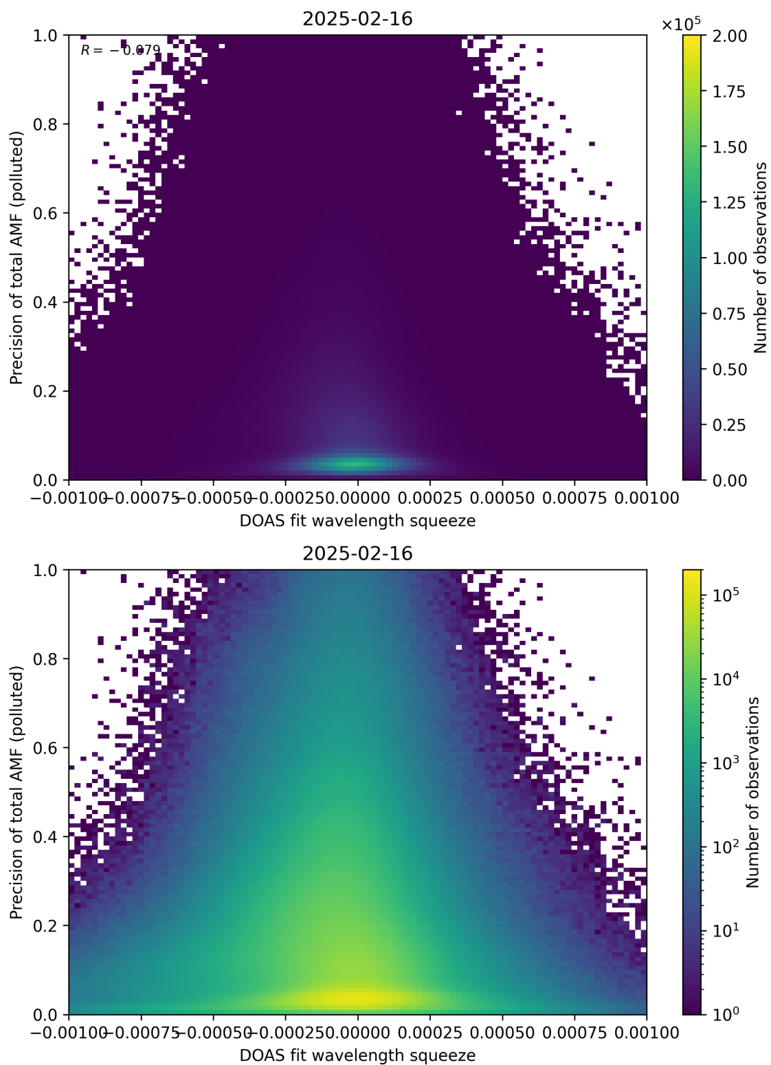
Figure 146: Scatter density plot of “DOAS fit wavelength squeeze” against “Precision of total AMF (polluted)” for 2025-02-15 to 2025-02-17.
