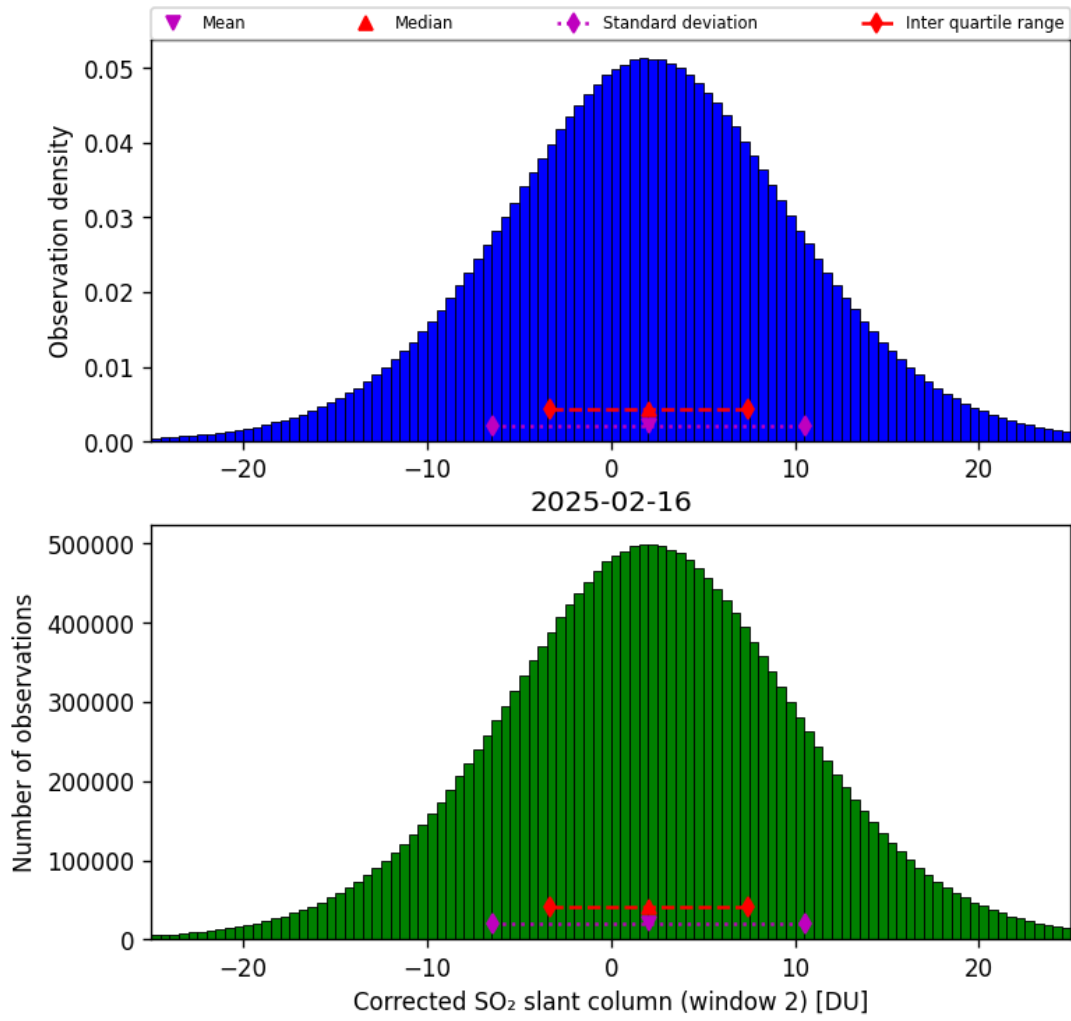
Figure 69: Histogram of “Corrected SO 2 slant column (window 2)” for 2025-02-15 to 2025-02-17
