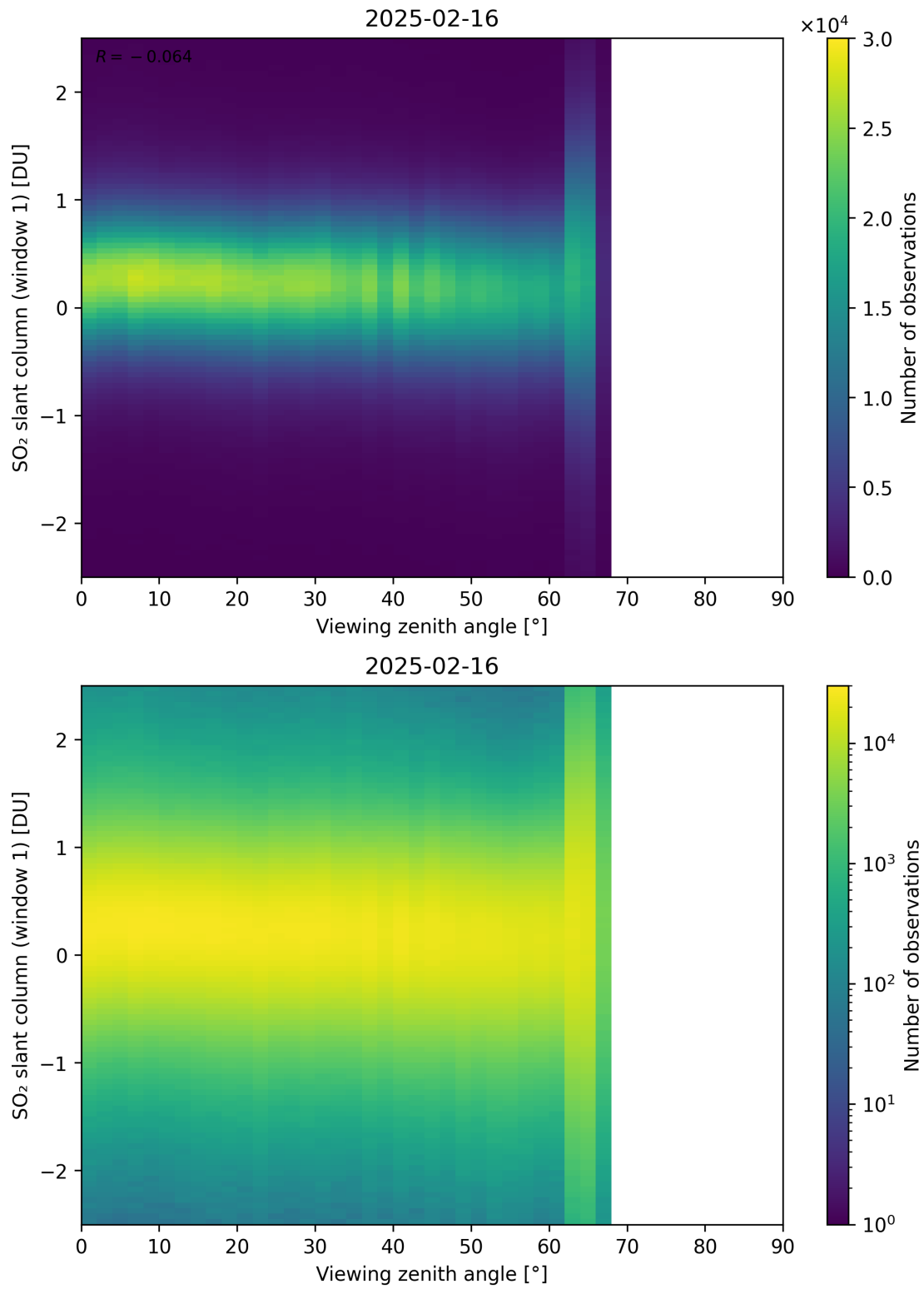
Figure 376: Scatter density plot of “Viewing zenith angle” against “SO 2 slant column (window 1)” for 2025-02-15 to 2025-02-17.
