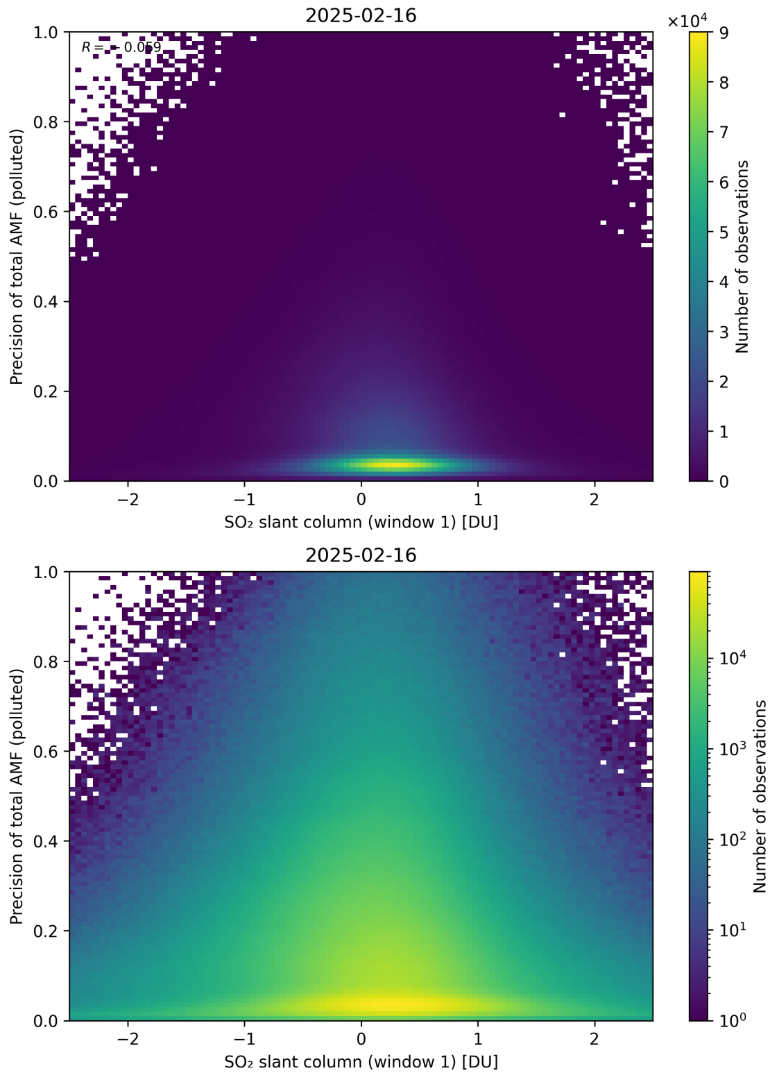
Figure 290: Scatter density plot of “SO 2 slant column (window 1)” against “Precision of total AMF (polluted)” for 2025-02-15 to 2025-02-17.
