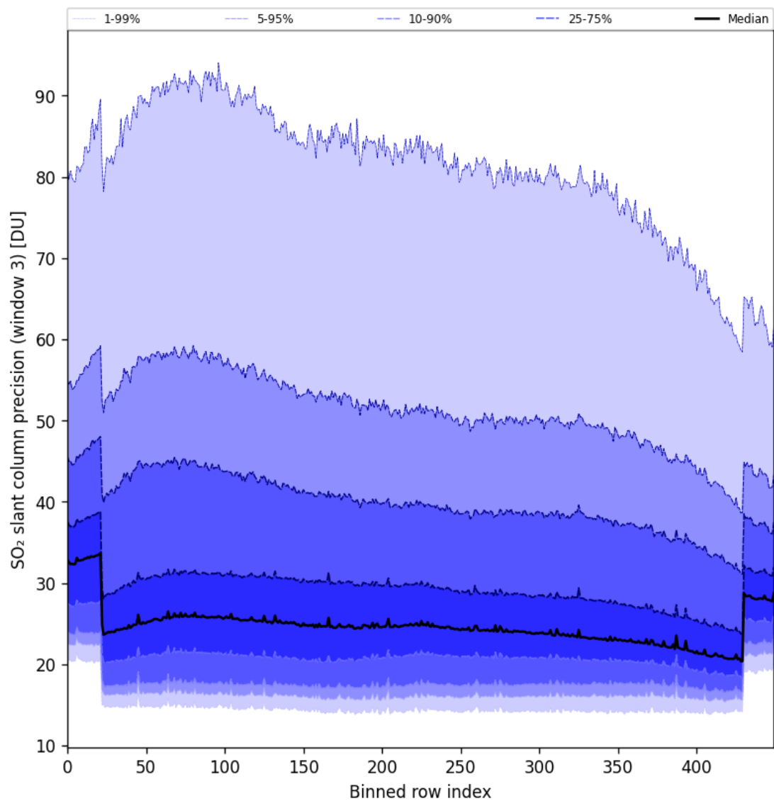
Figure 98: Along track statistics of “SO 2 slant column precision (window 3)” for 2025-02-15 to 2025-02-17
