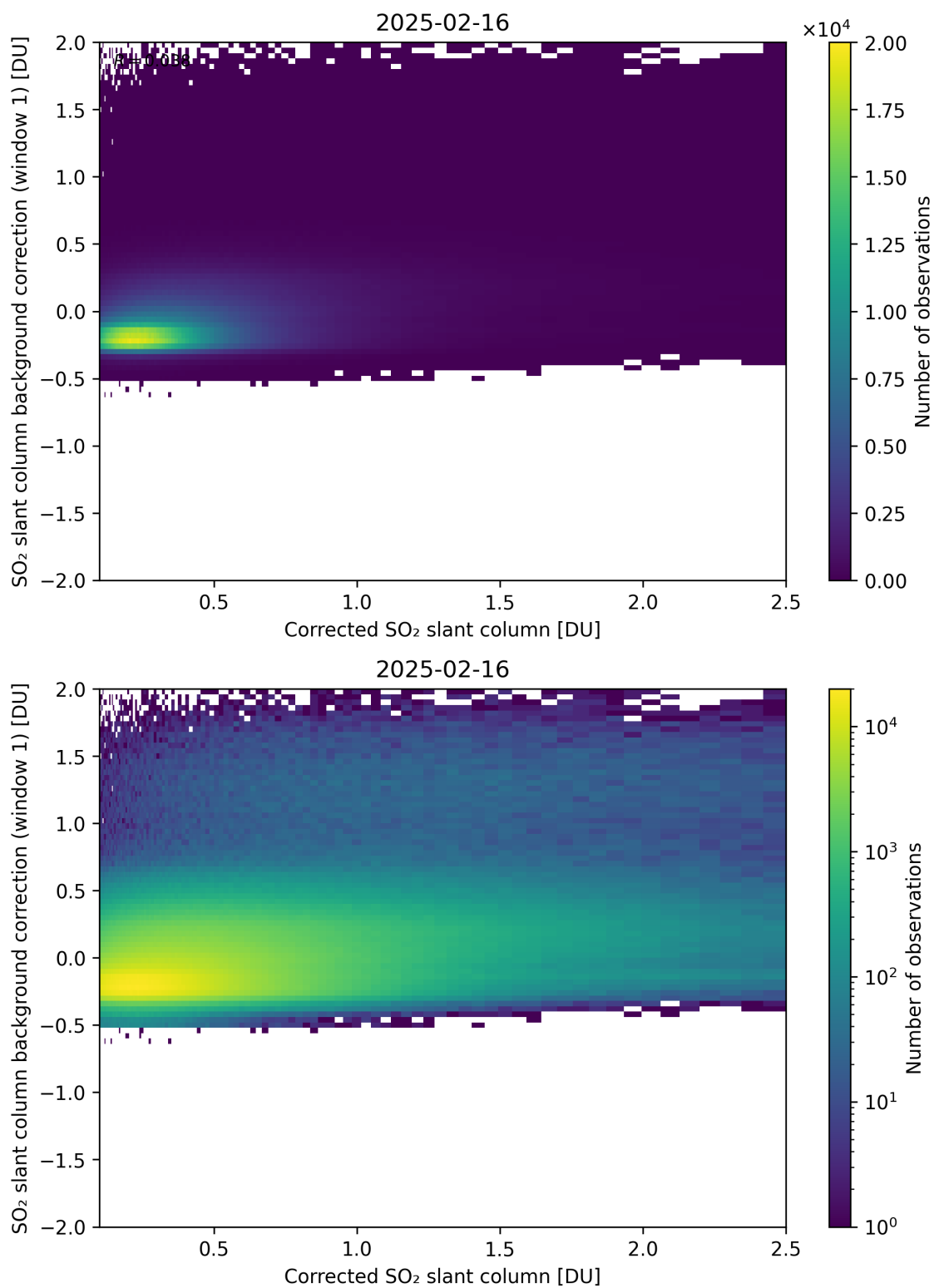
Figure 226: Scatter density plot of “Corrected SO 2 slant column” against “SO 2 slant column background correction (window 1)” for 2025-02-15 to 2025-02-17.
