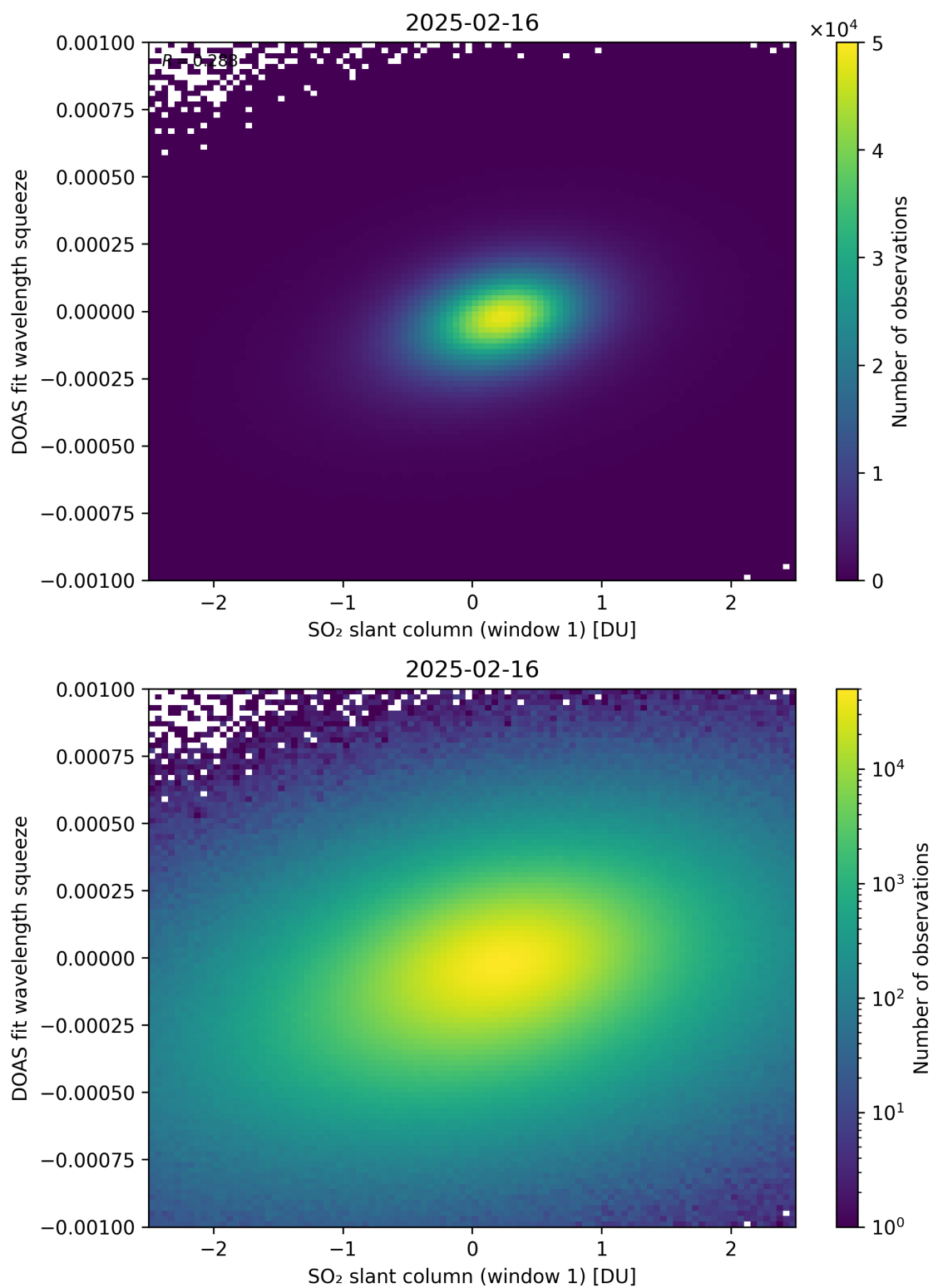
Figure 266: Scatter density plot of “SO 2 slant column (window 1)” against “DOAS fit wavelength squeeze” for 2025-02-15 to 2025-02-17.
