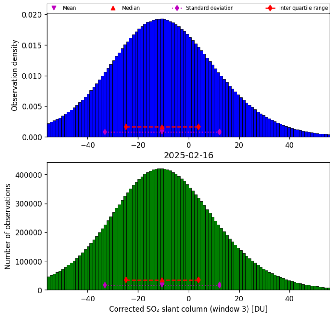
Figure 73: Histogram of “Corrected SO 2 slant column (window 3)” for 2025-02-15 to 2025-02-17
