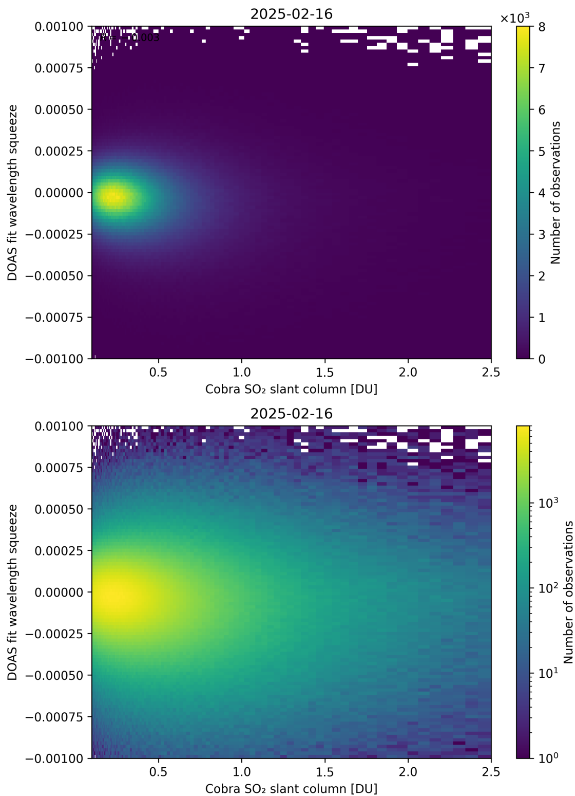
Figure 197: Scatter density plot of “Cobra SO 2 slant column” against “DOAS fit wavelength squeeze” for 2025-02-15 to 2025-02-17.
