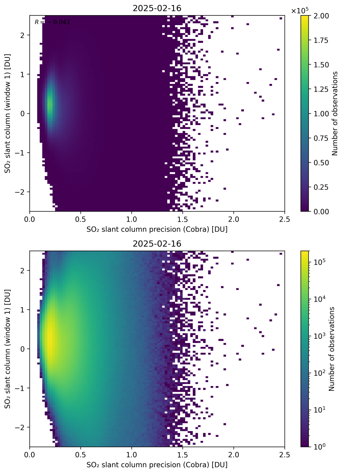
Figure 208: Scatter density plot of “SO 2 slant column precision (Cobra)” against “SO 2 slant column (window 1)” for 2025-02-15 to 2025-02-17.
