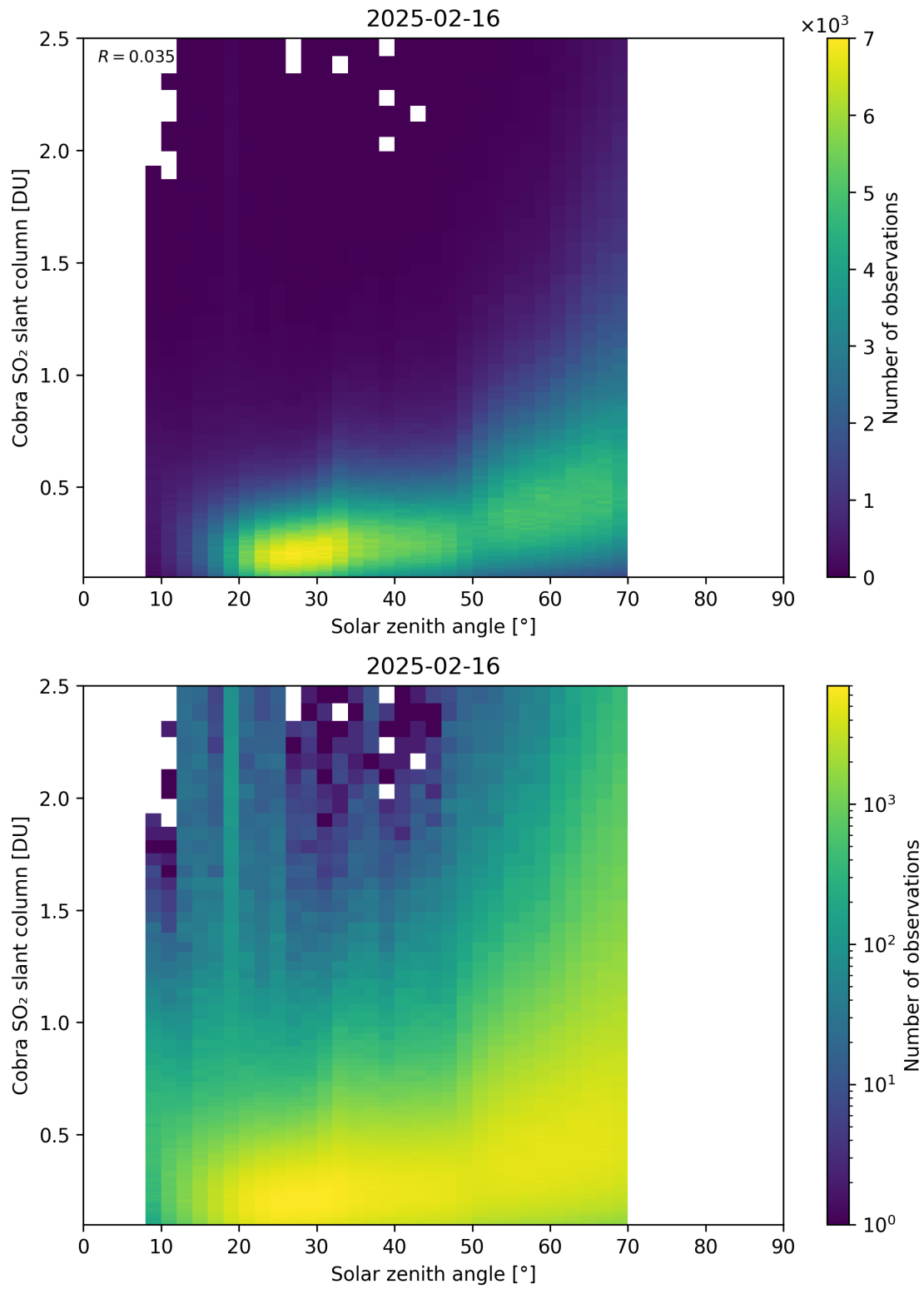
Figure 179: Scatter density plot of “Solar zenith angle” against “Cobra SO 2 slant column” for 2025-02-15 to 2025-02-17.
