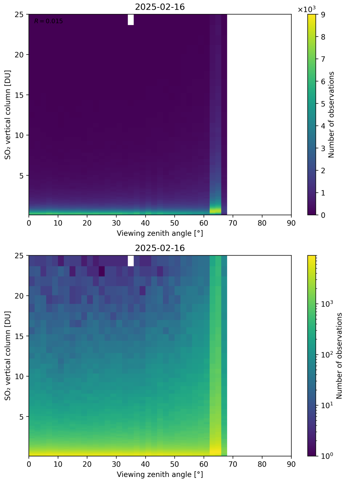
Figure 383: Scatter density plot of “Viewing zenith angle” against “SO 2 vertical column” for 2025-02-15 to 2025-02-17.
