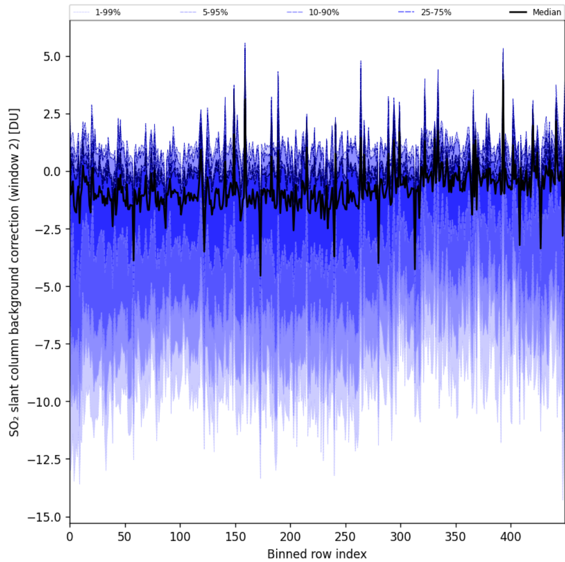
Figure 96: Along track statistics of “SO 2 slant column background correction (window 2)” for 2025-02-15 to 2025-02-17
