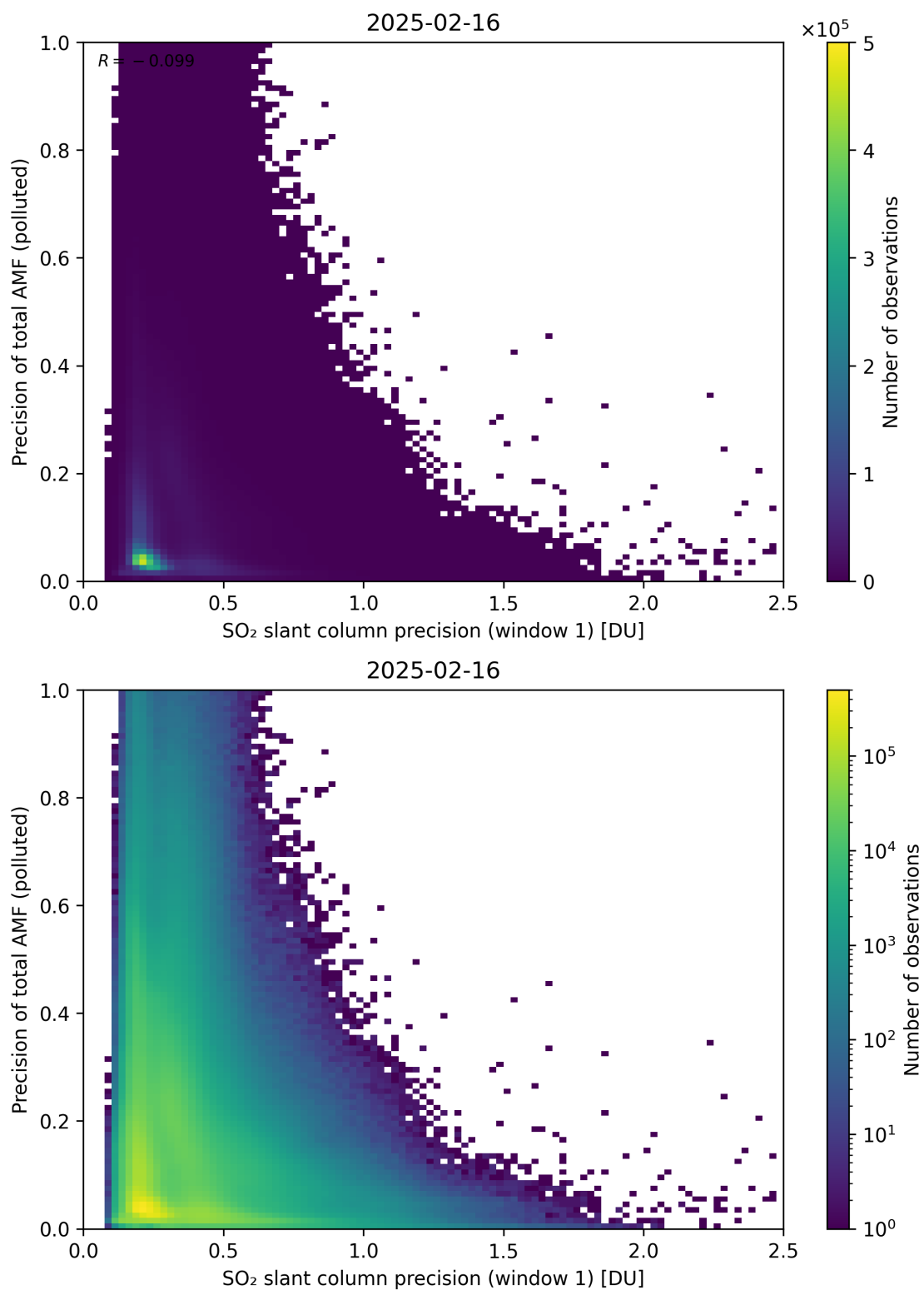
Figure 281: Scatter density plot of “SO 2 slant column precision (window 1)” against “Precision of total AMF (polluted)” for 2025-02-15 to 2025-02-17.
