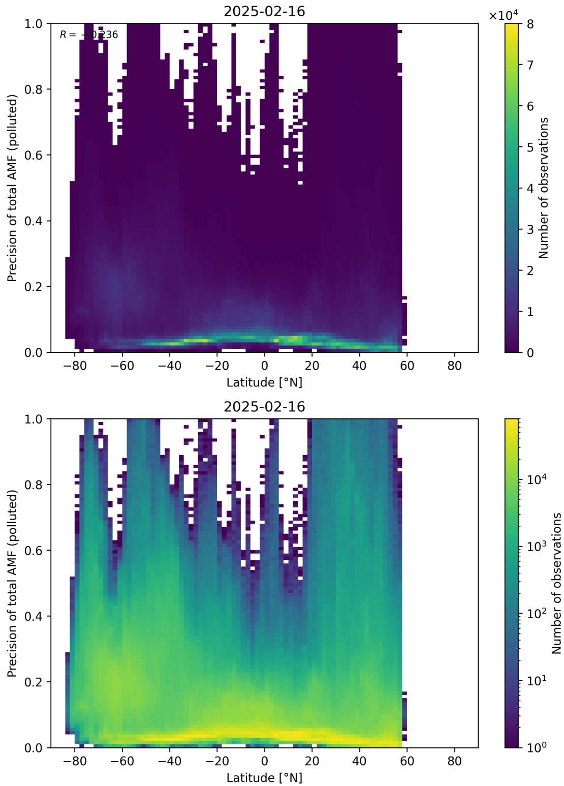
Figure 168: Scatter density plot of “Latitude” against “Precision of total AMF (polluted)” for 2025-02-15 to 2025-02-17.
