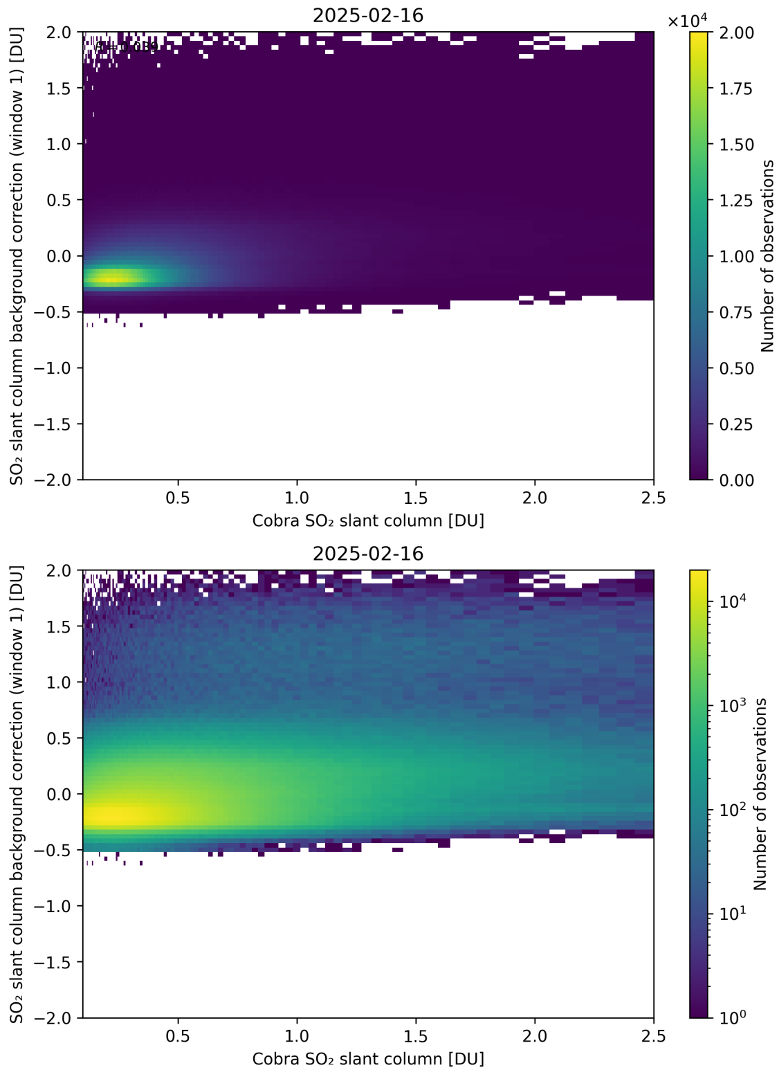
Figure 193: Scatter density plot of “Cobra SO 2 slant column” against “SO 2 slant column background correction (window 1)” for 2025-02-15 to 2025-02-17.
