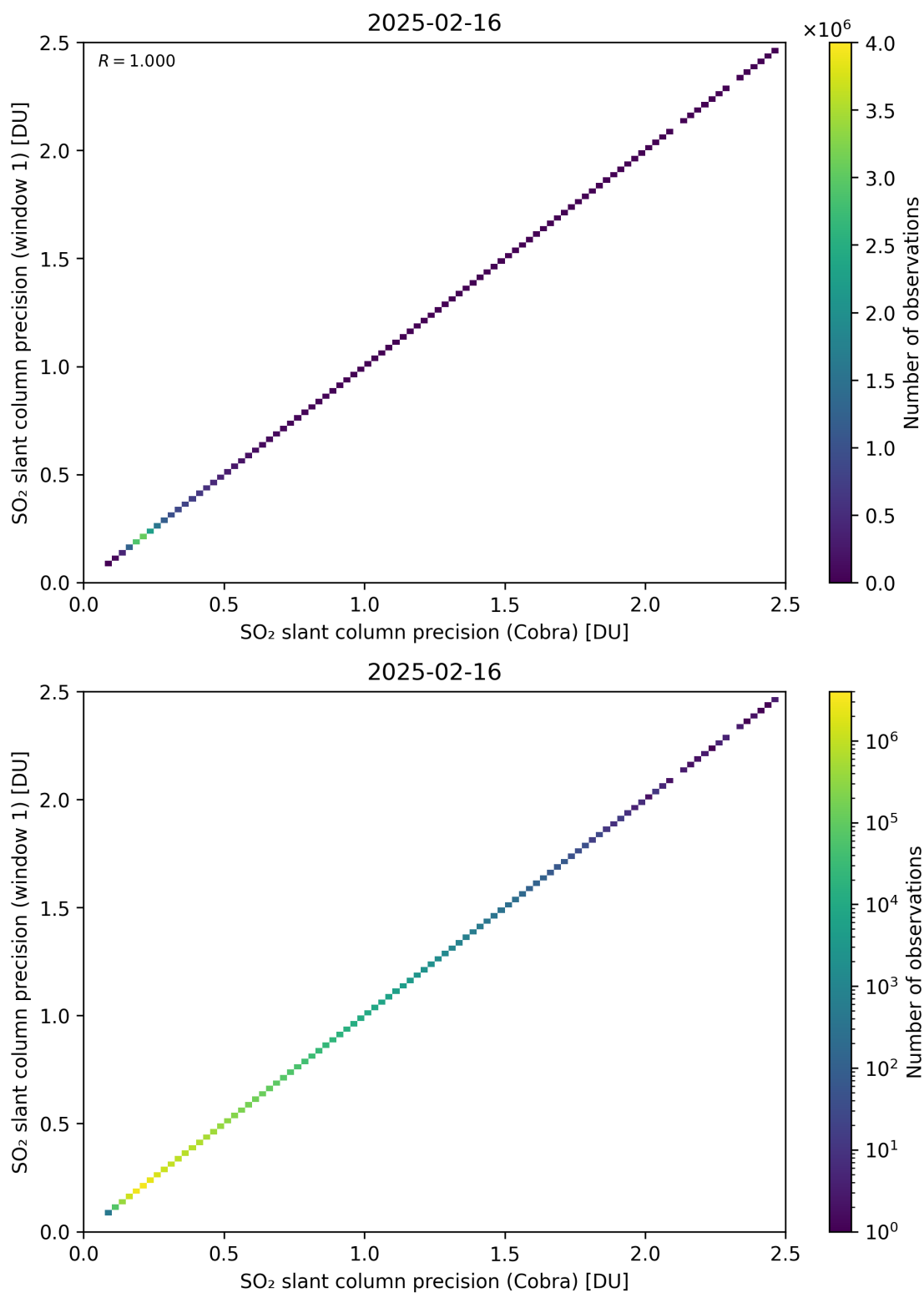
Figure 209: Scatter density plot of “SO 2 slant column precision (Cobra)” against “SO 2 slant column precision (window 1)” for 2025-02-15 to 2025-02-17.
