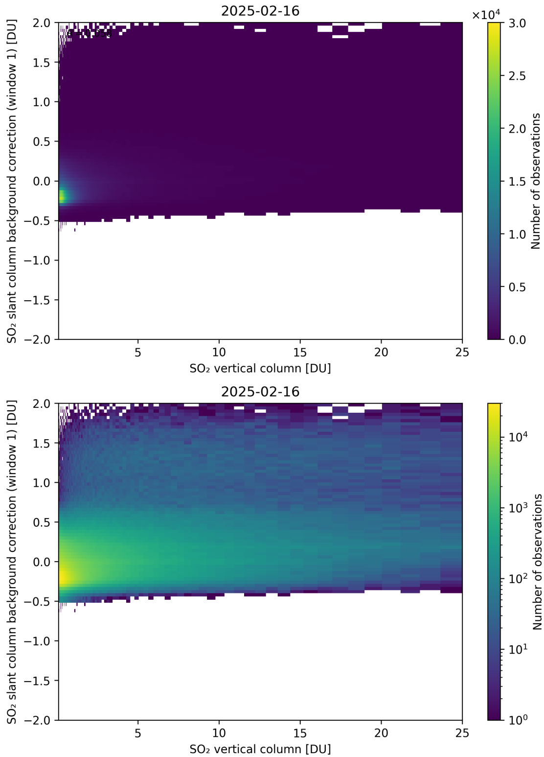
Figure 323: Scatter density plot of “SO 2 vertical column” against “SO 2 slant column background correction (window 1)” for 2025-02-15 to 2025-02-17.
