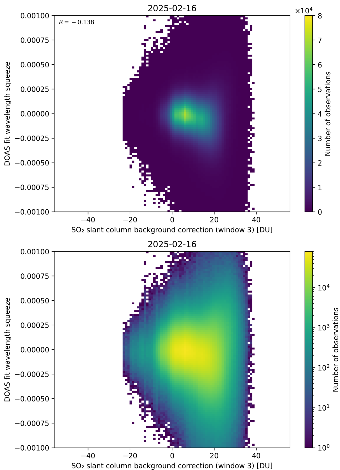
Figure 133: Scatter density plot of “SO 2 slant column background correction (window 3)” against “DOAS fit wavelength squeeze” for 2025-02-15 to 2025-02-17.
