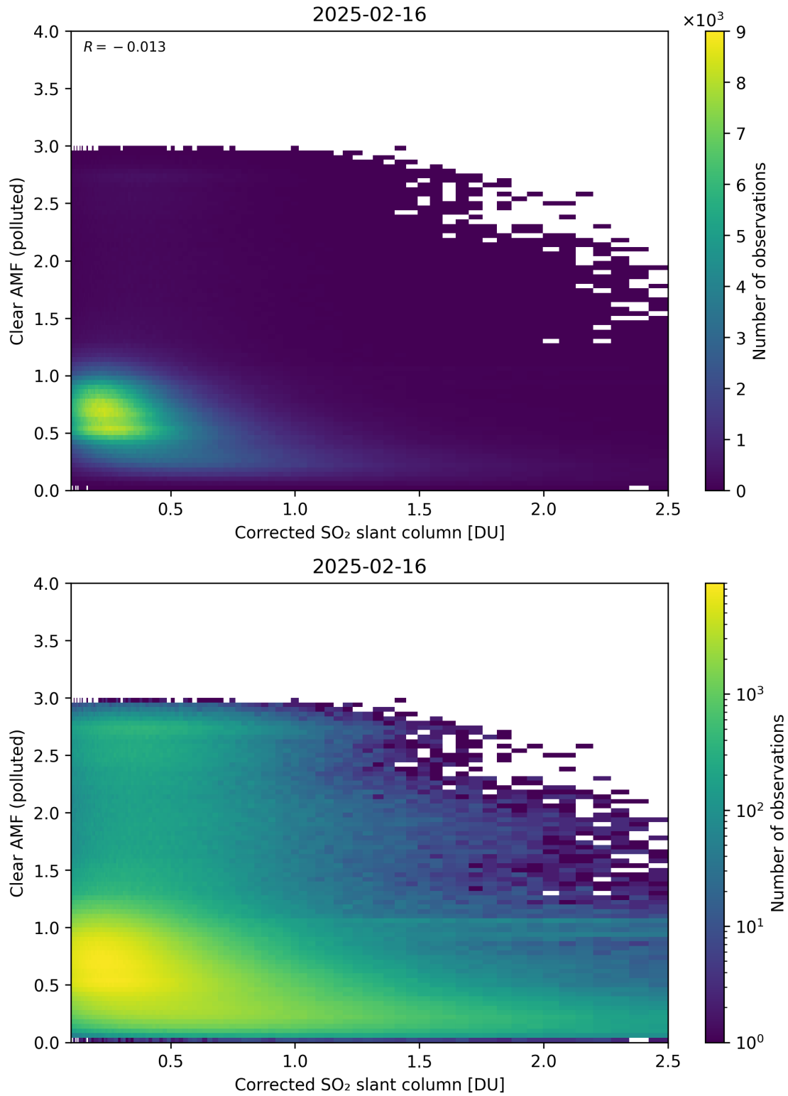
Figure 232: Scatter density plot of “Corrected SO 2 slant column” against “Clear AMF (polluted)” for 2025-02-15 to 2025-02-17.
