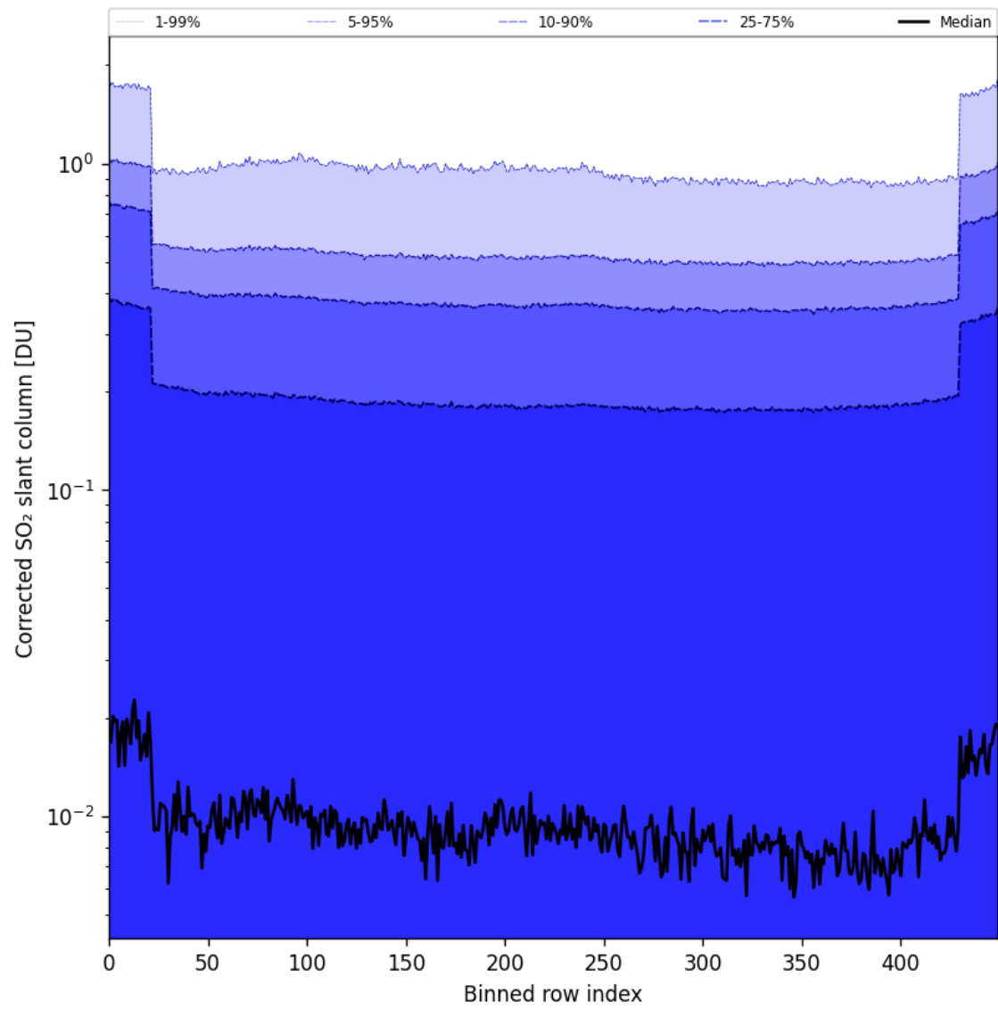
Figure 86: Along track statistics of “Corrected SO 2 slant column” for 2025-02-15 to 2025-02-17
