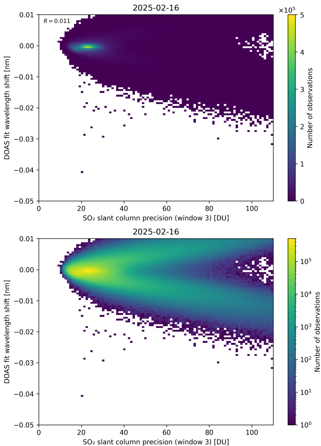
Figure 308: Scatter density plot of “SO 2 slant column precision (window 3)” against “DOAS fit wavelength shift” for 2025-02-15 to 2025-02-17.
