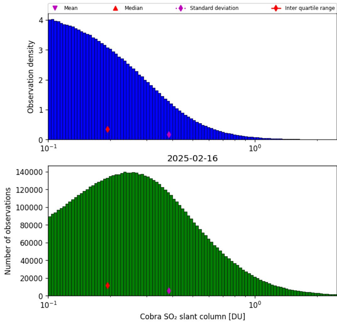
Figure 61: Histogram of “Cobra SO 2 slant column” for 2025-02-15 to 2025-02-17
