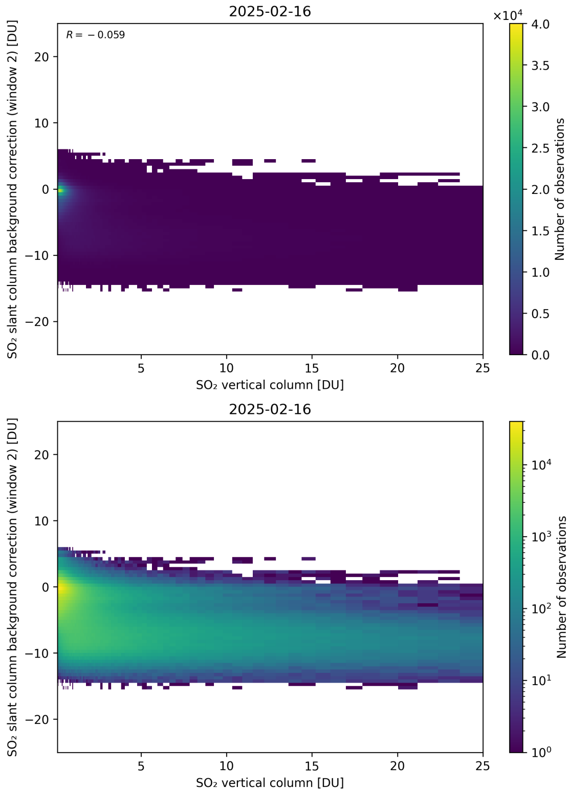
Figure 324: Scatter density plot of “SO 2 vertical column” against “SO 2 slant column background correction (window 2)” for 2025-02-15 to 2025-02-17.
