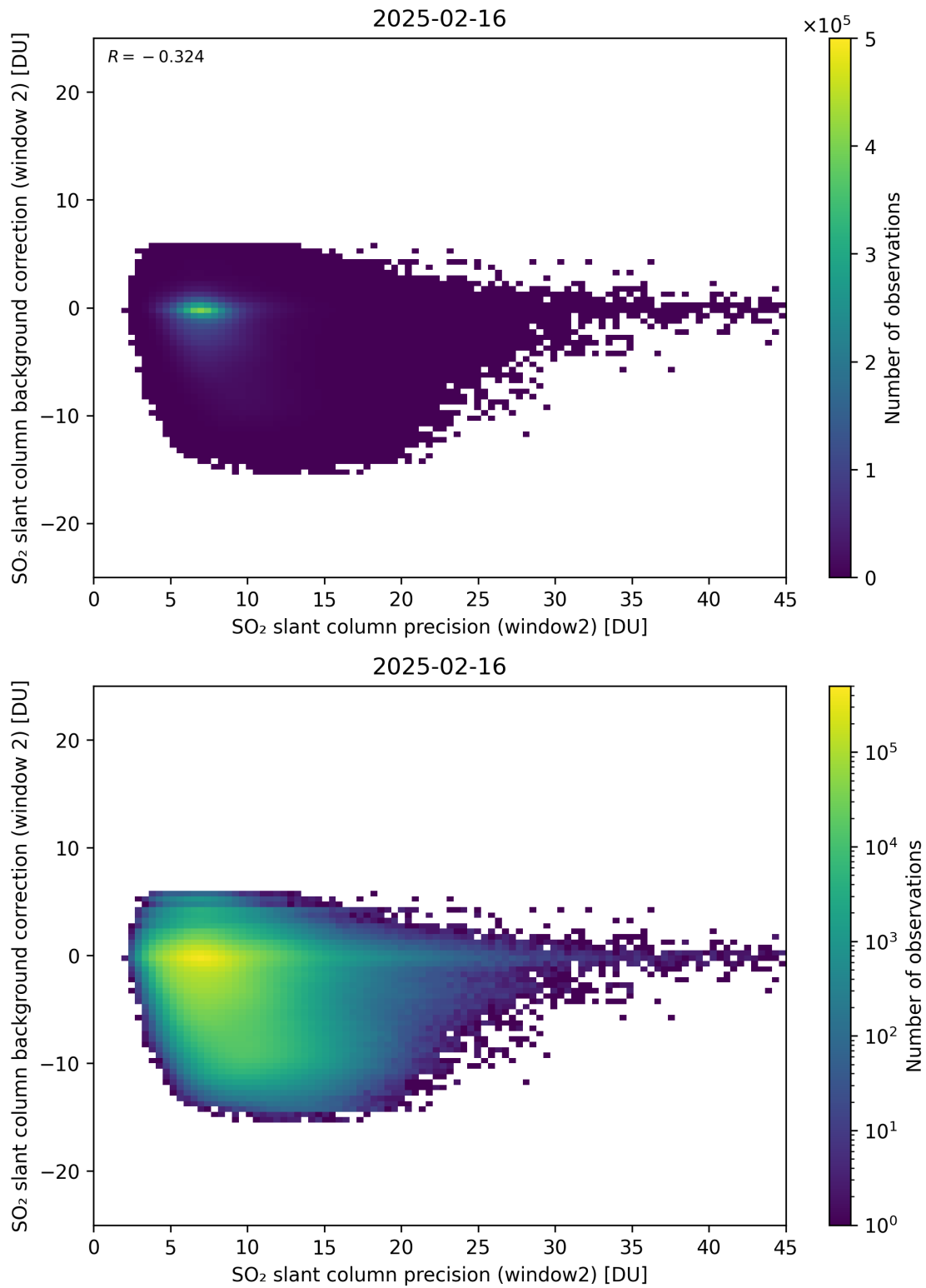
Figure 291: Scatter density plot of “SO 2 slant column precision (window2)” against “SO 2 slant column background correction (window 2)” for 2025-02-15 to 2025-02-17.
