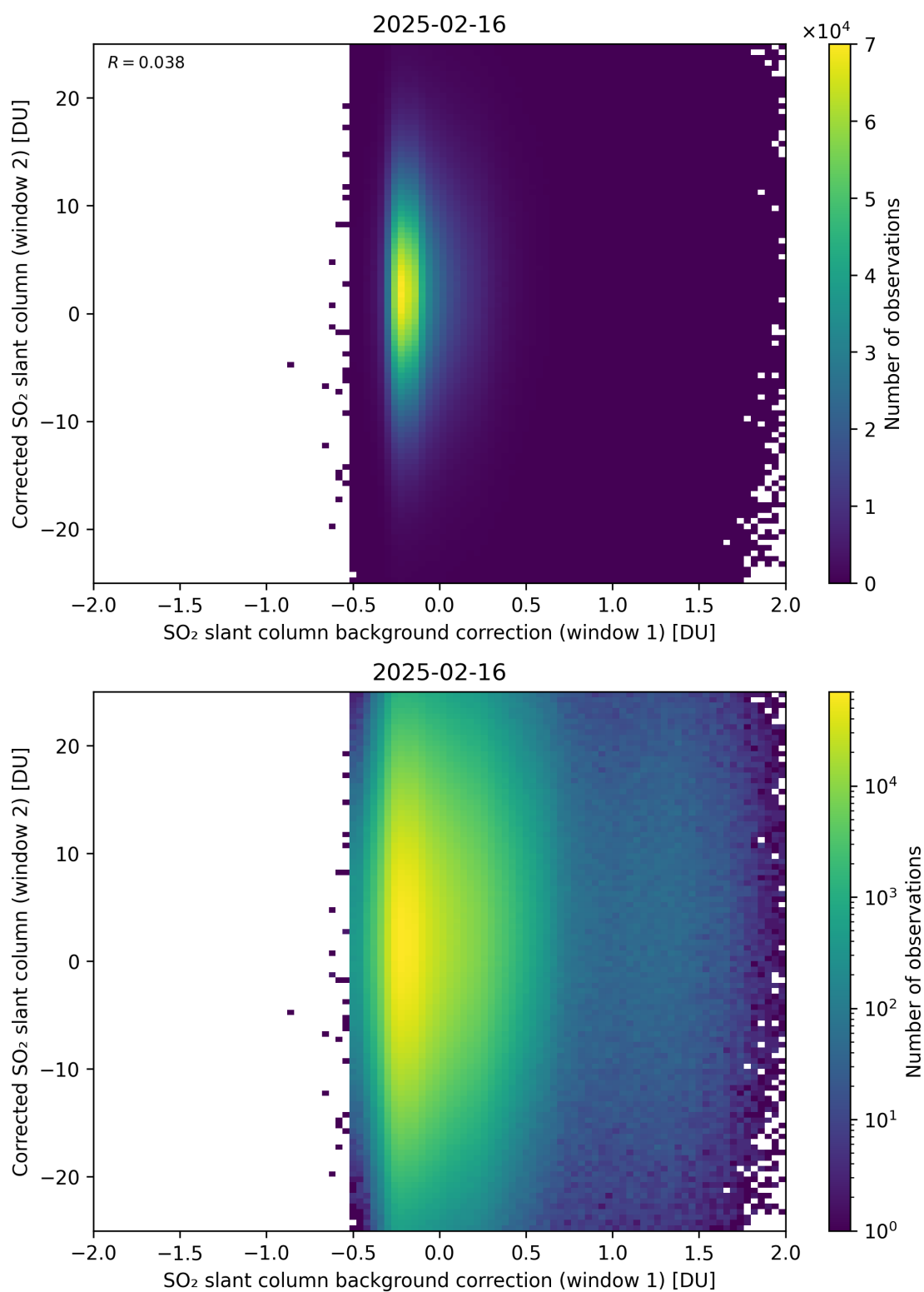
Figure 115: Scatter density plot of “SO 2 slant column background correction (window 1)” against “Corrected SO 2 slant column (window 2)” for 2025-02-15 to 2025-02-17.
