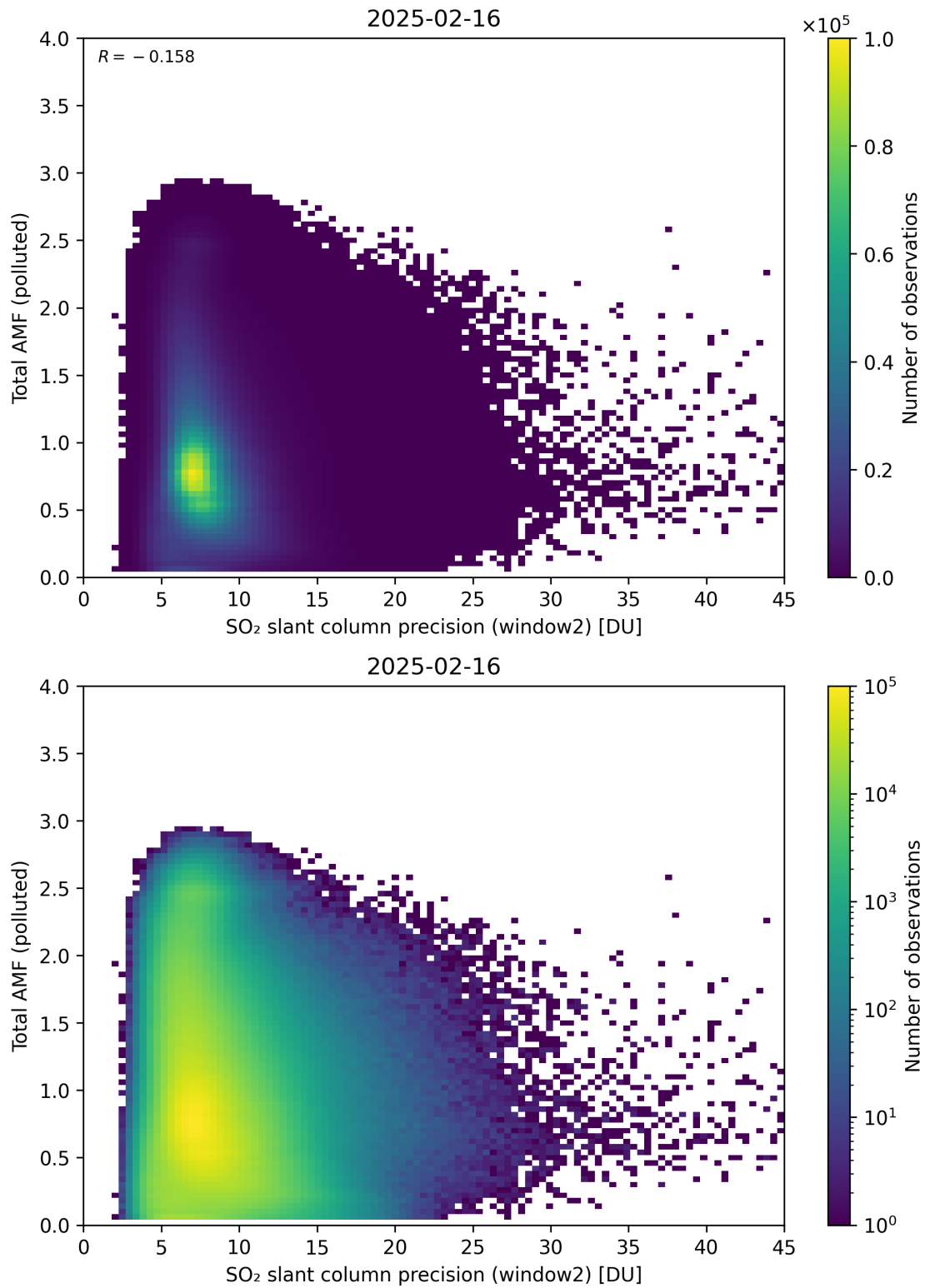
Figure 301: Scatter density plot of “SO 2 slant column precision (window2)” against “Total AMF (polluted)” for 2025-02-15 to 2025-02-17.
