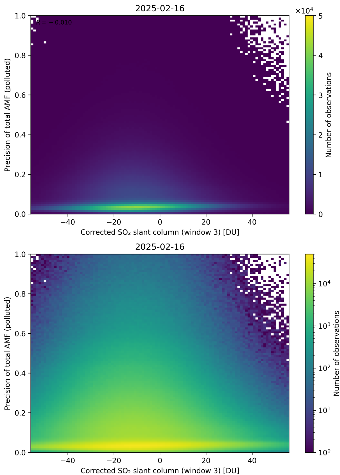
Figure 261: Scatter density plot of “Corrected SO 2 slant column (window 3)” against “Precision of total AMF (polluted)” for 2025-02-15 to 2025-02-17.
