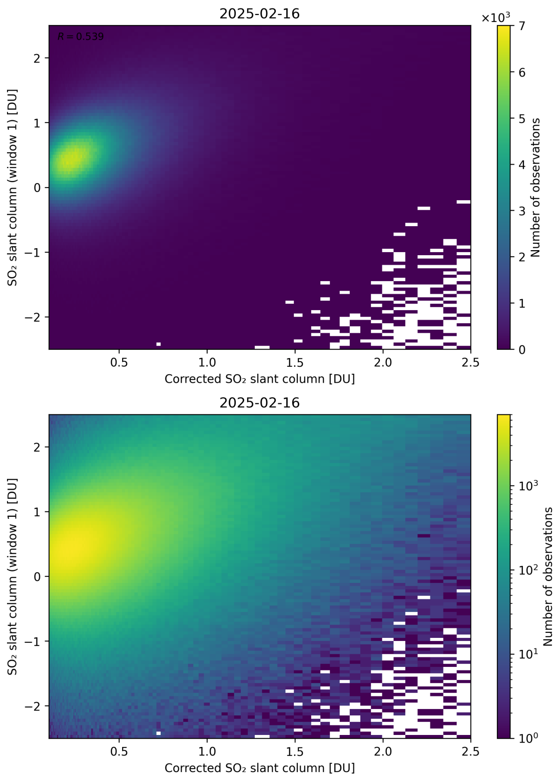
Figure 237: Scatter density plot of “Corrected SO 2 slant column” against “SO 2 slant column (window 1)” for 2025-02-15 to 2025-02-17.
