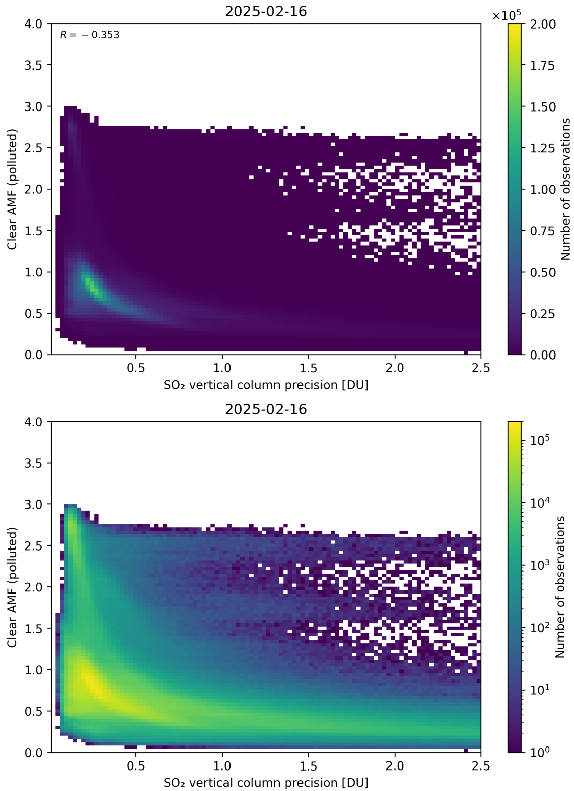
Figure 335: Scatter density plot of “SO 2 vertical column precision” against “Clear AMF (polluted)” for 2025-02-15 to 2025-02-17.
