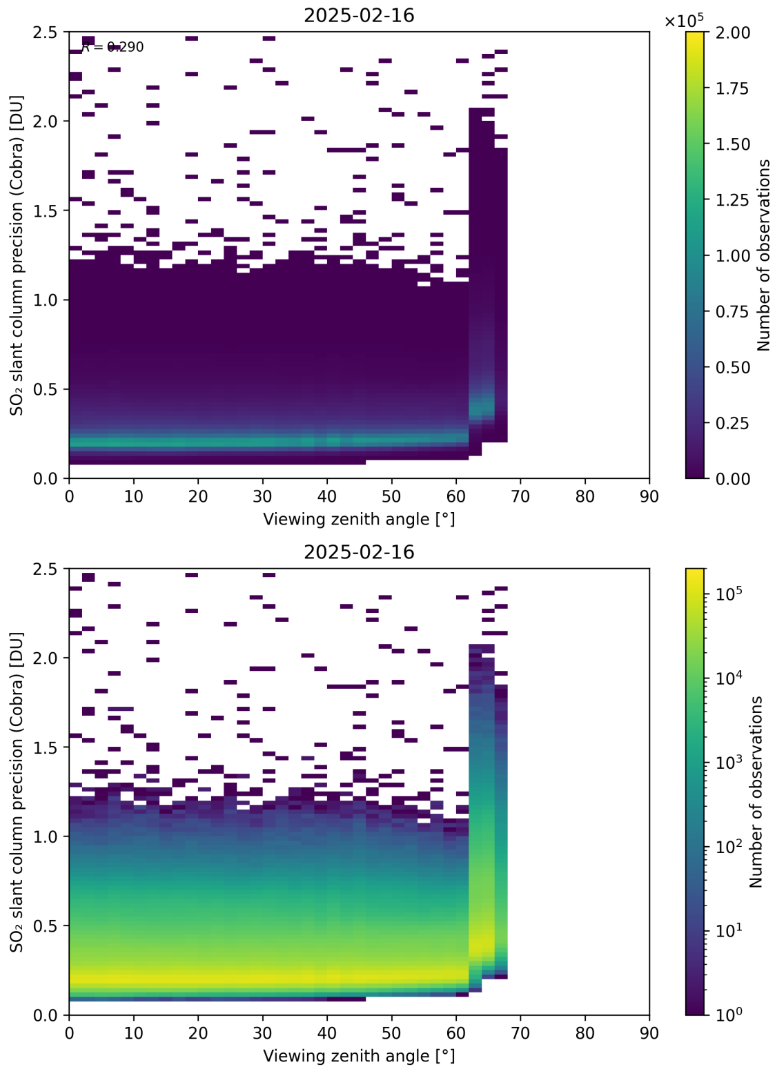
Figure 372: Scatter density plot of “Viewing zenith angle” against “SO 2 slant column precision (Cobra)” for 2025-02-15 to 2025-02-17.
