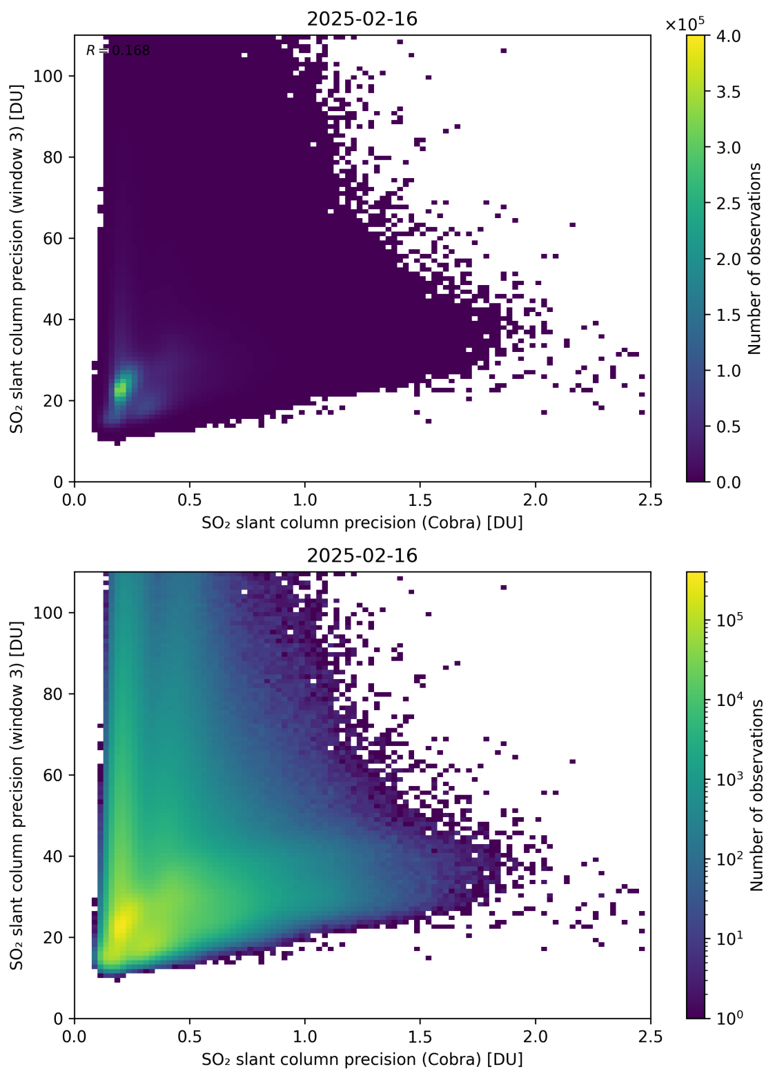
Figure 212: Scatter density plot of “SO 2 slant column precision (Cobra)” against “SO 2 slant column precision (window 3)” for 2025-02-15 to 2025-02-17.
