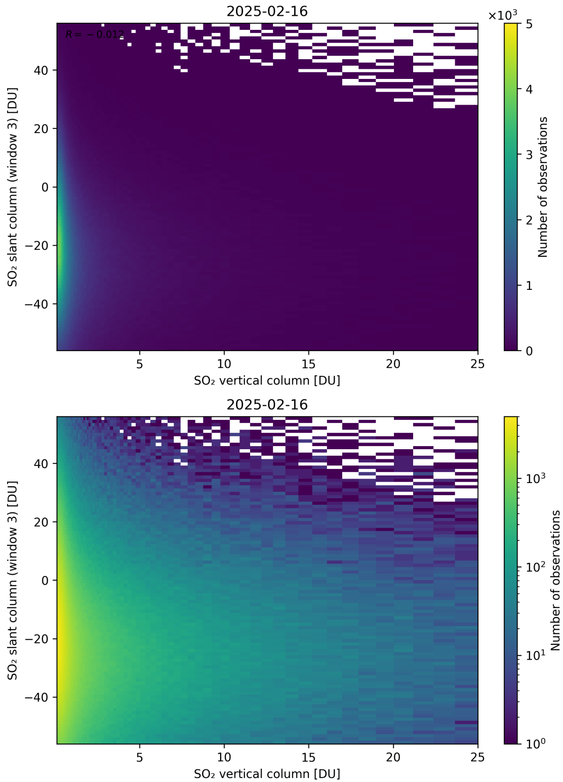
Figure 357: Scatter density plot of “SO 2 vertical column” against “SO 2 slant column (window 3)” for 2025-02-15 to 2025-02-17.
