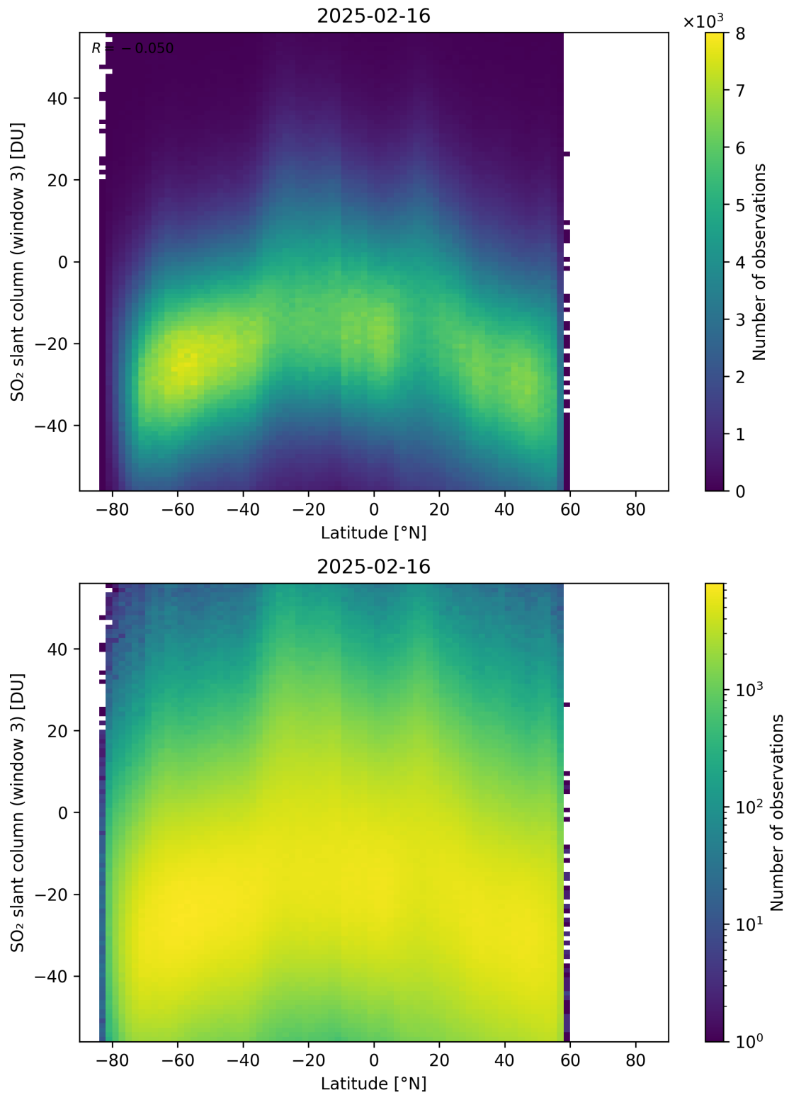
Figure 165: Scatter density plot of “Latitude” against “SO 2 slant column (window 3)” for 2025-02-15 to 2025-02-17.
