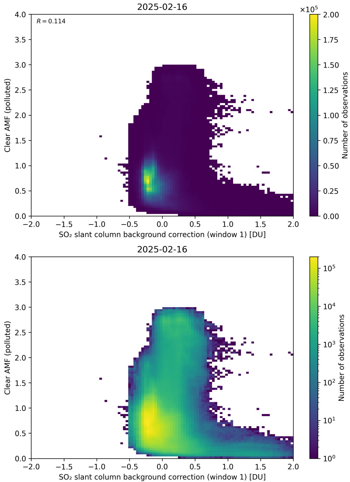
Figure 114: Scatter density plot of “SO 2 slant column background correction (window 1)” against “Clear AMF (polluted)” for 2025-02-15 to 2025-02-17.
