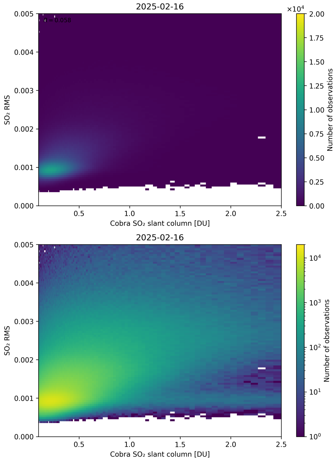
Figure 198: Scatter density plot of “Cobra SO 2 slant column” against “SO 2 RMS” for 2025-02-15 to 2025-02-17.
