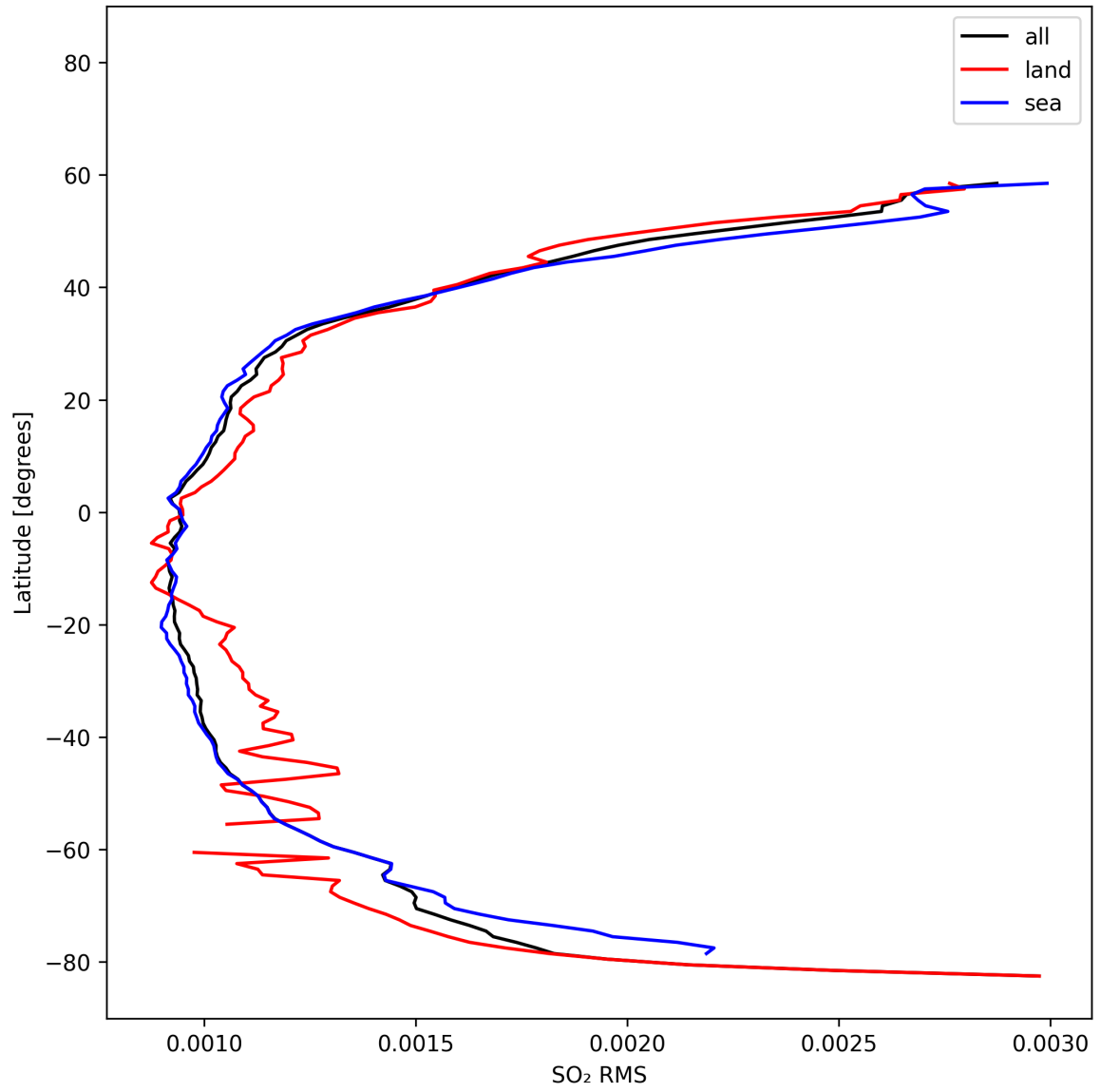
Figure 52: Zonal average of “SO 2 RMS” for 2025-02-15 to 2025-02-17.
