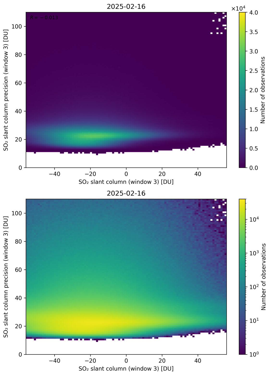
Figure 317: Scatter density plot of “SO 2 slant column (window 3)” against “SO 2 slant column precision (window 3)” for 2025-02-15 to 2025-02-17.
