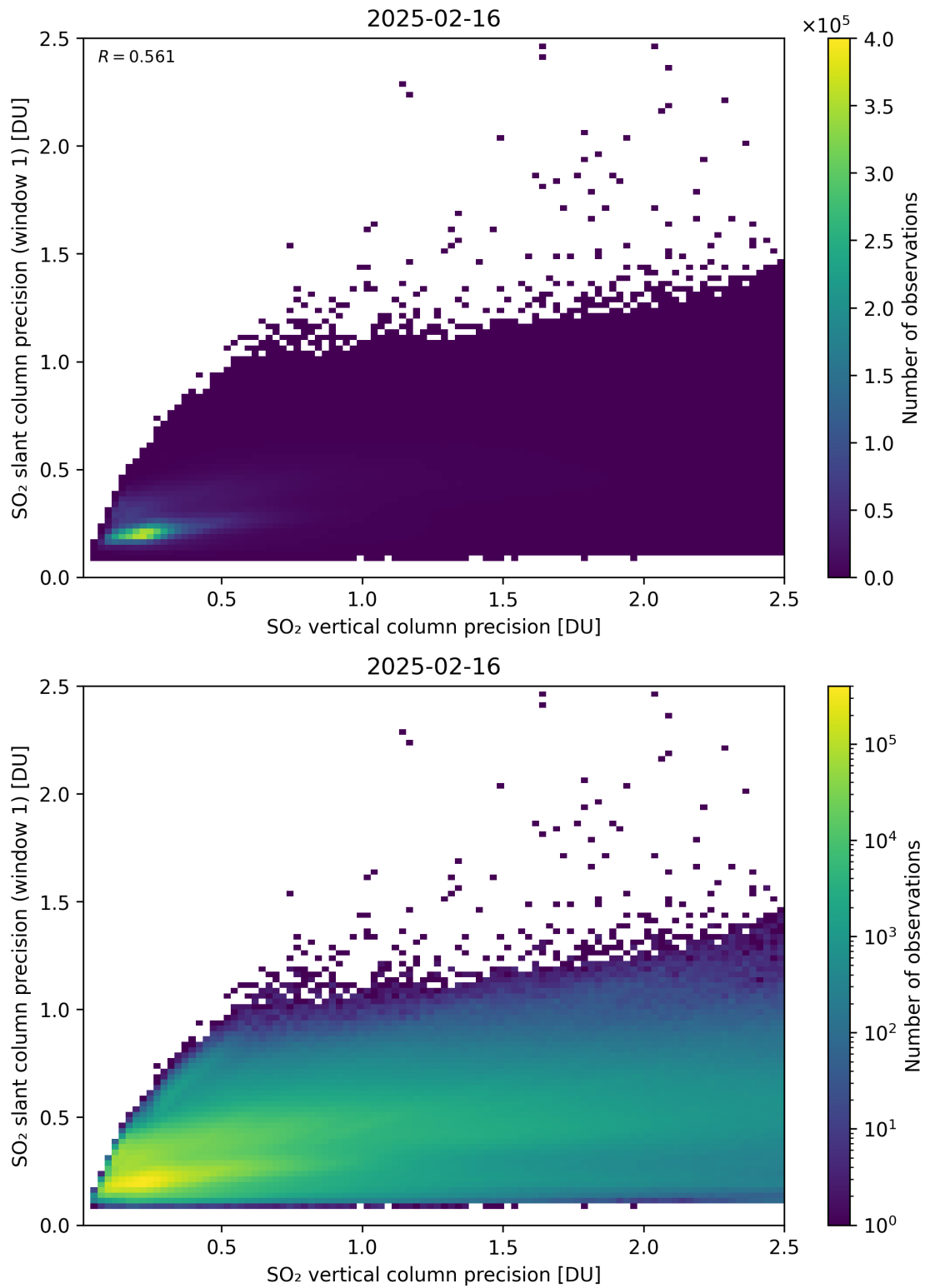
Figure 342: Scatter density plot of “SO 2 vertical column precision” against “SO 2 slant column precision (window 1)” for 2025-02-15 to 2025-02-17.
