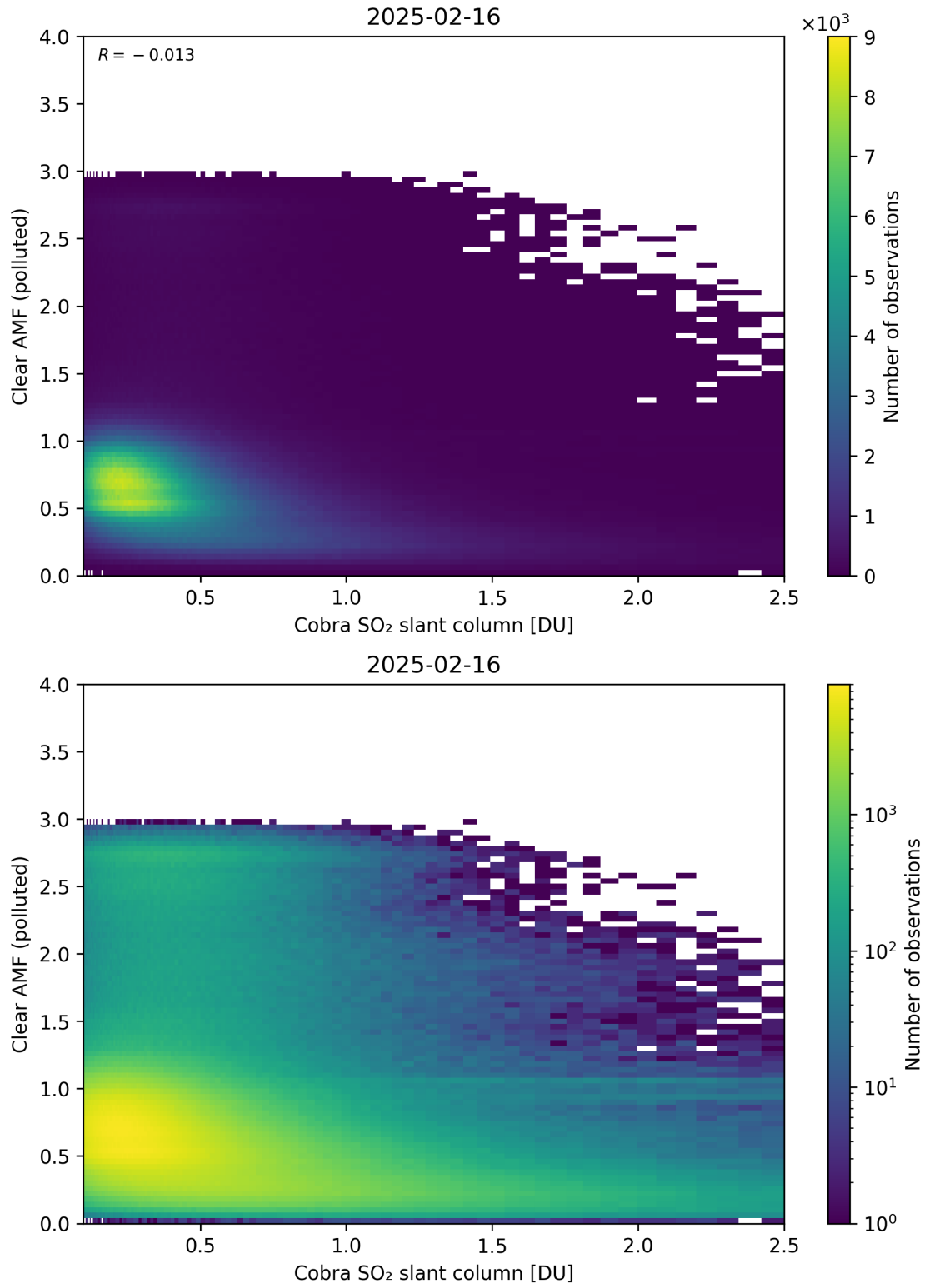
Figure 215: Scatter density plot of “Cobra SO 2 slant column” against “Clear AMF (polluted)” for 2025-02-15 to 2025-02-17.
