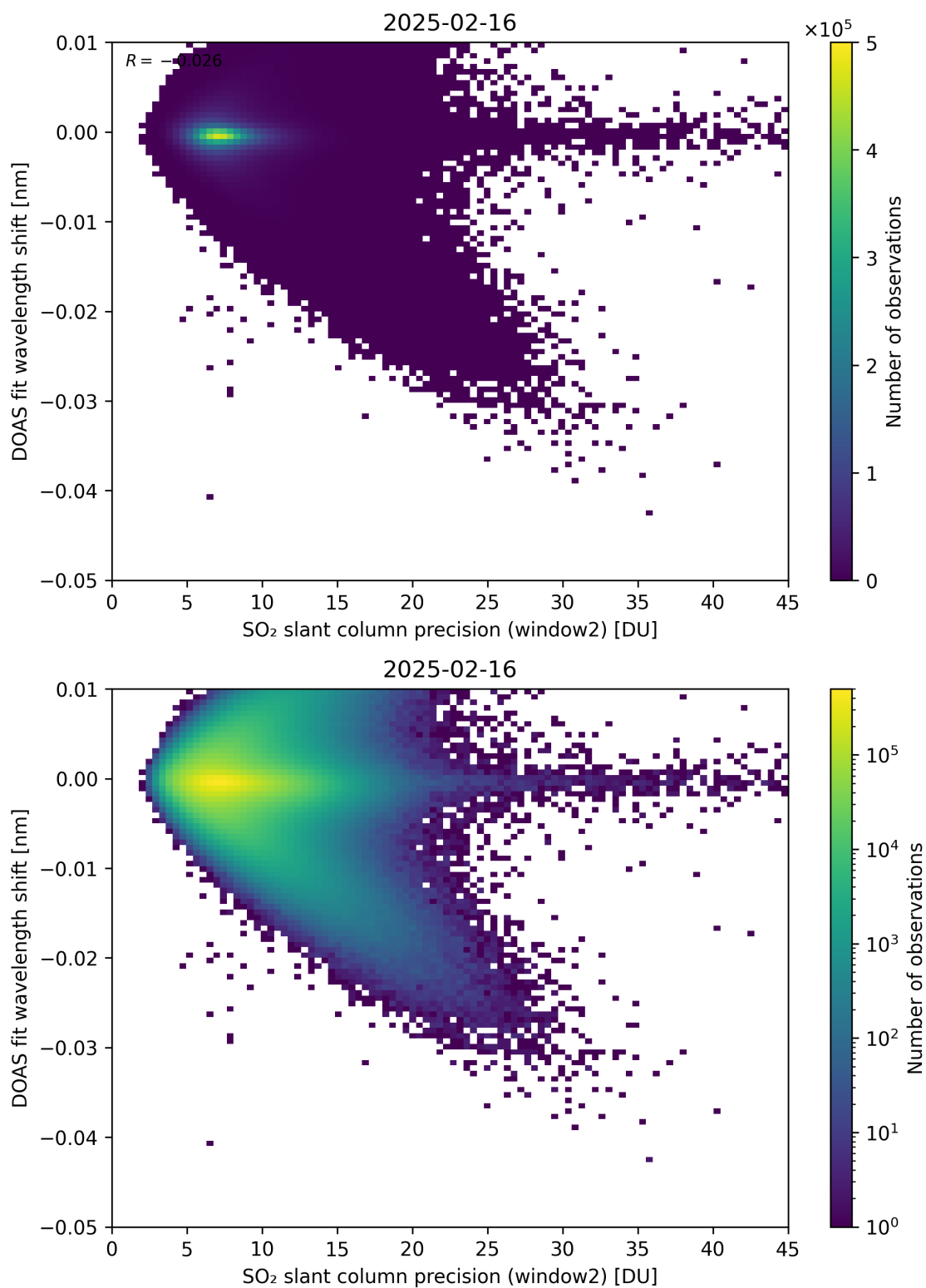
Figure 293: Scatter density plot of “SO 2 slant column precision (window2)” against “DOAS fit wavelength shift” for 2025-02-15 to 2025-02-17.
