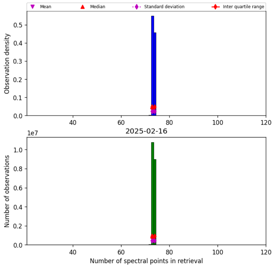
Figure 82: Histogram of “Number of spectral points in retrieval” for 2025-02-15 to 2025-02-17
