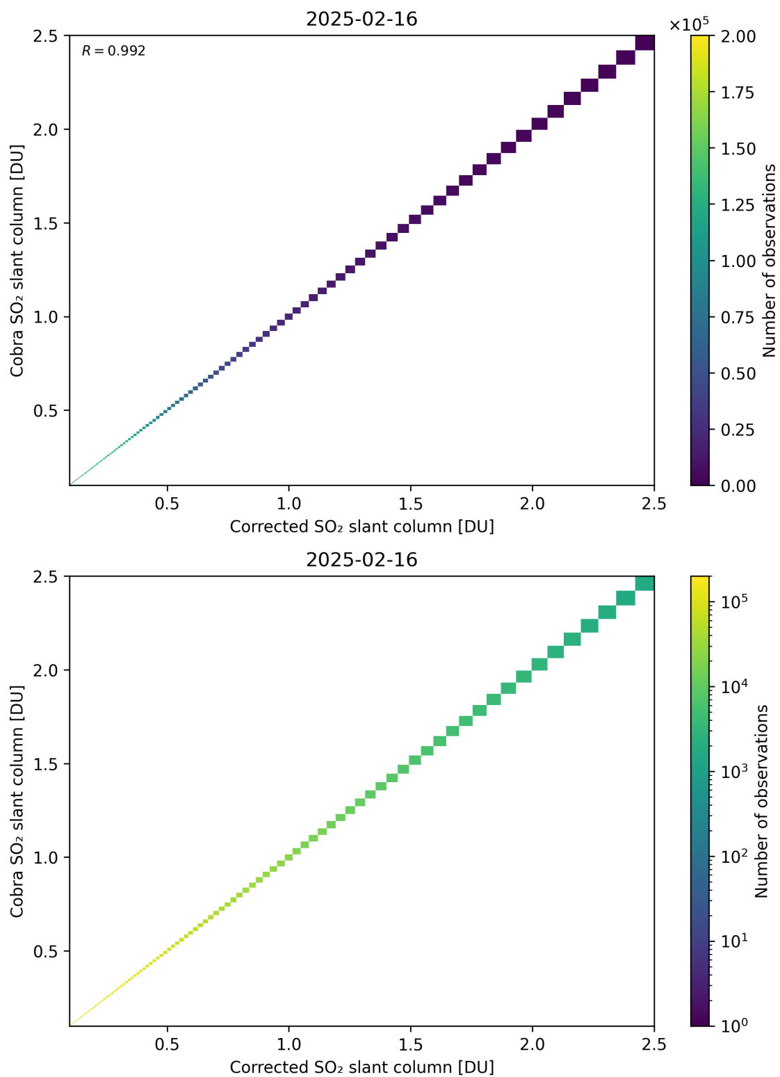
Figure 233: Scatter density plot of “Corrected SO 2 slant column” against “Cobra SO 2 slant column” for 2025-02-15 to 2025-02-17.
