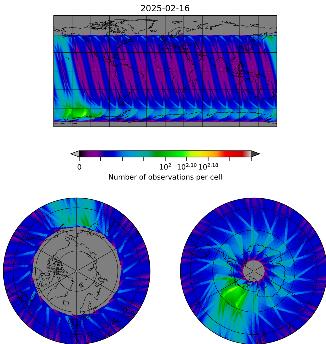
Figure 30: Map of the number of observations for 2025-02-15 to 2025-02-17
