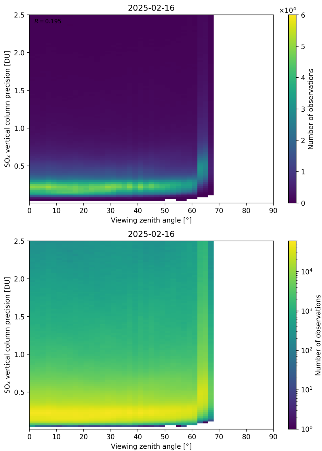
Figure 384: Scatter density plot of “Viewing zenith angle” against “SO 2 vertical column precision” for 2025-02-15 to 2025-02-17.
