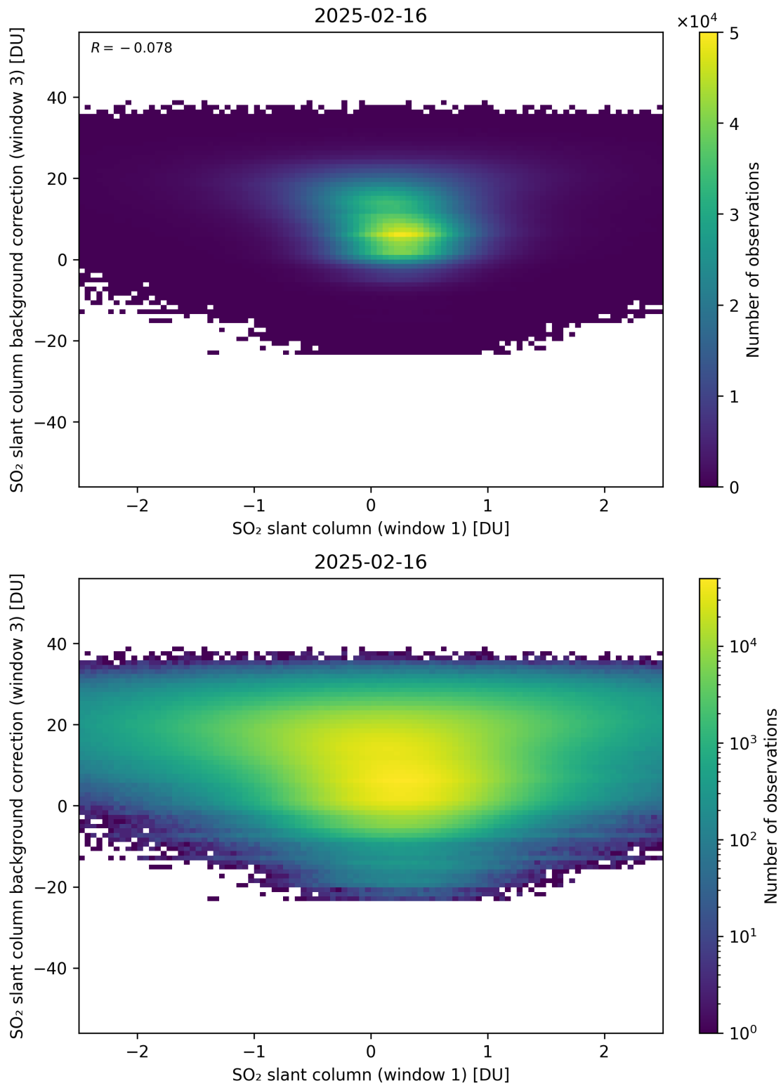
Figure 264: Scatter density plot of “SO 2 slant column (window 1)” against “SO 2 slant column background correction (window 3)” for 2025-02-15 to 2025-02-17.
