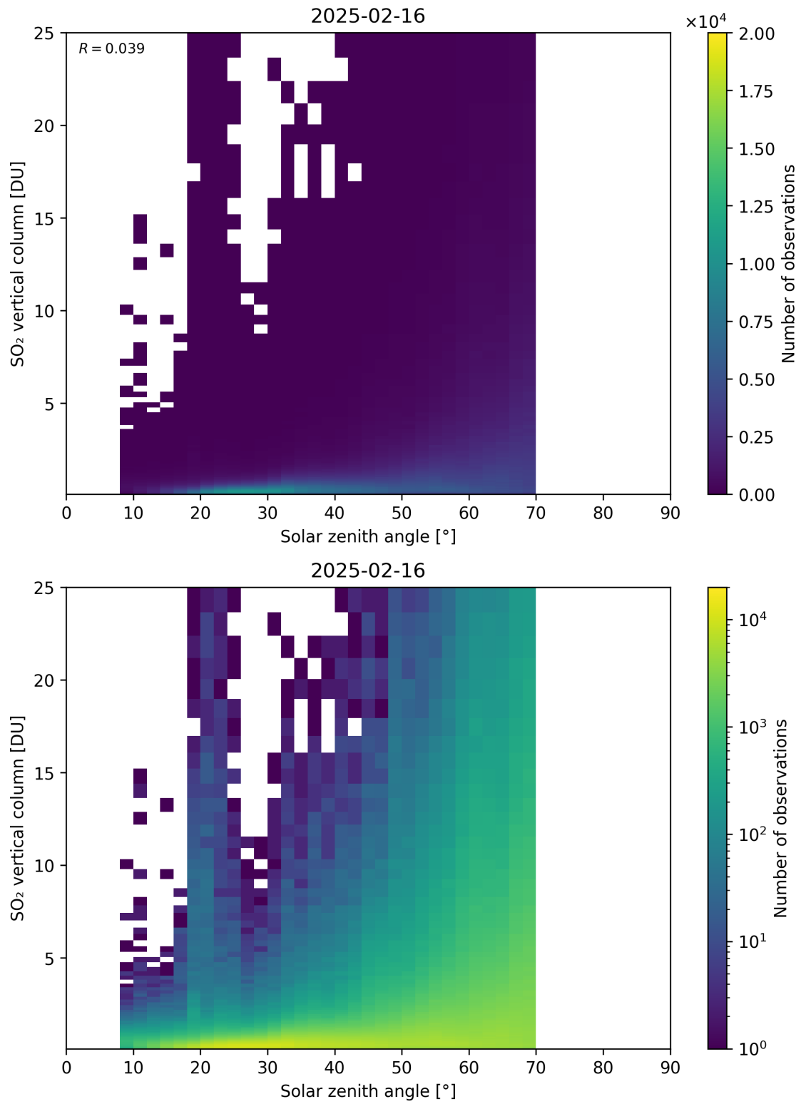
Figure 191: Scatter density plot of “Solar zenith angle” against “SO 2 vertical column” for 2025-02-15 to 2025-02-17.
