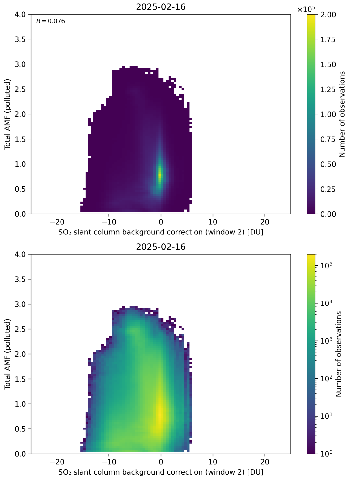
Figure 130: Scatter density plot of “SO 2 slant column background correction (window 2)” against “Total AMF (polluted)” for 2025-02-15 to 2025-02-17.
