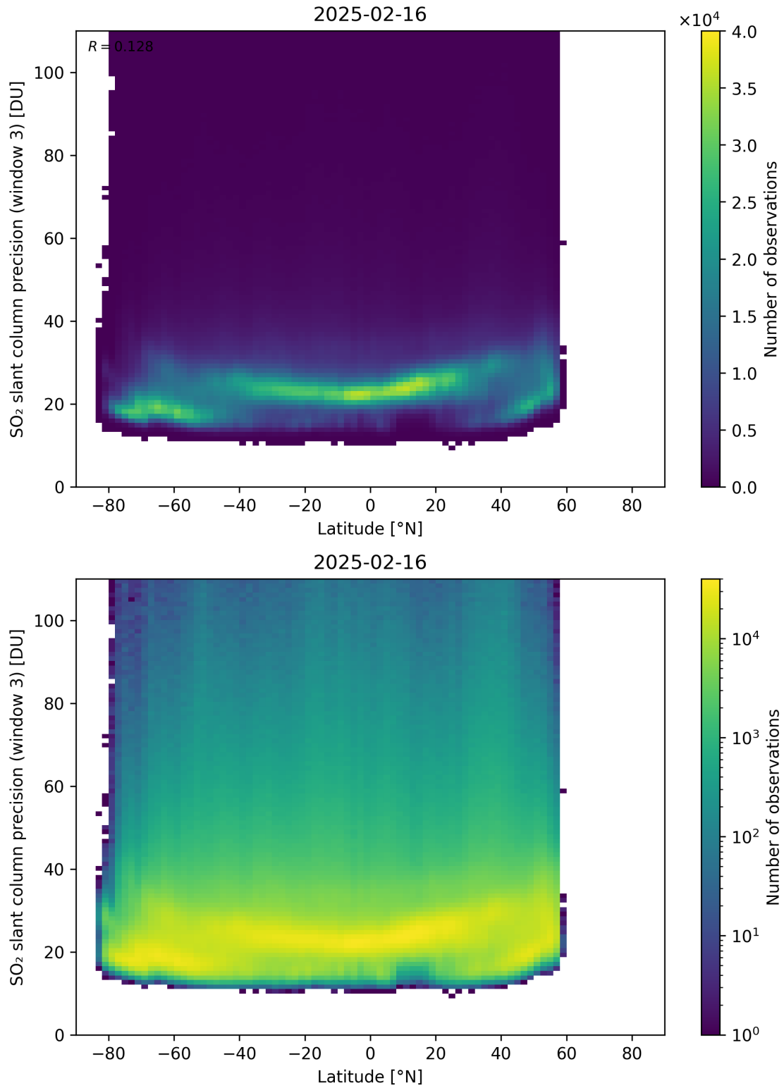
Figure 166: Scatter density plot of “Latitude” against “SO 2 slant column precision (window 3)” for 2025-02-15 to 2025-02-17.
