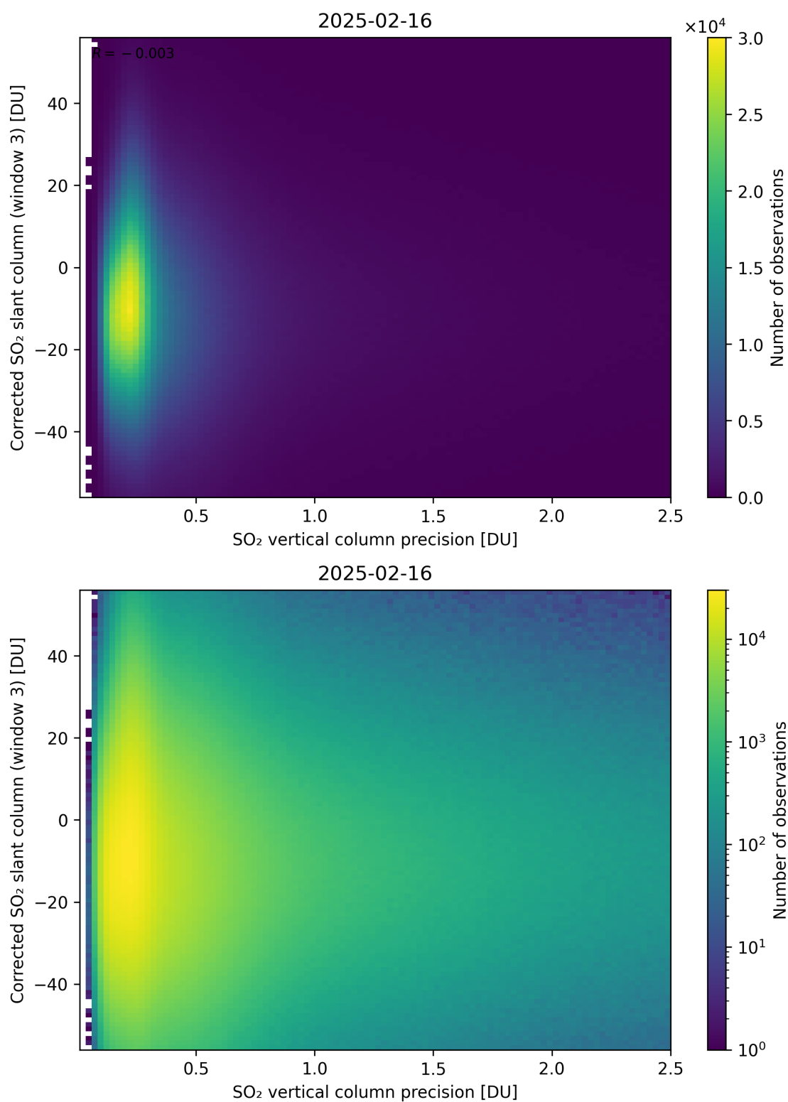
Figure 340: Scatter density plot of “SO 2 vertical column precision” against “Corrected SO 2 slant column (window 3)” for 2025-02-15 to 2025-02-17.
