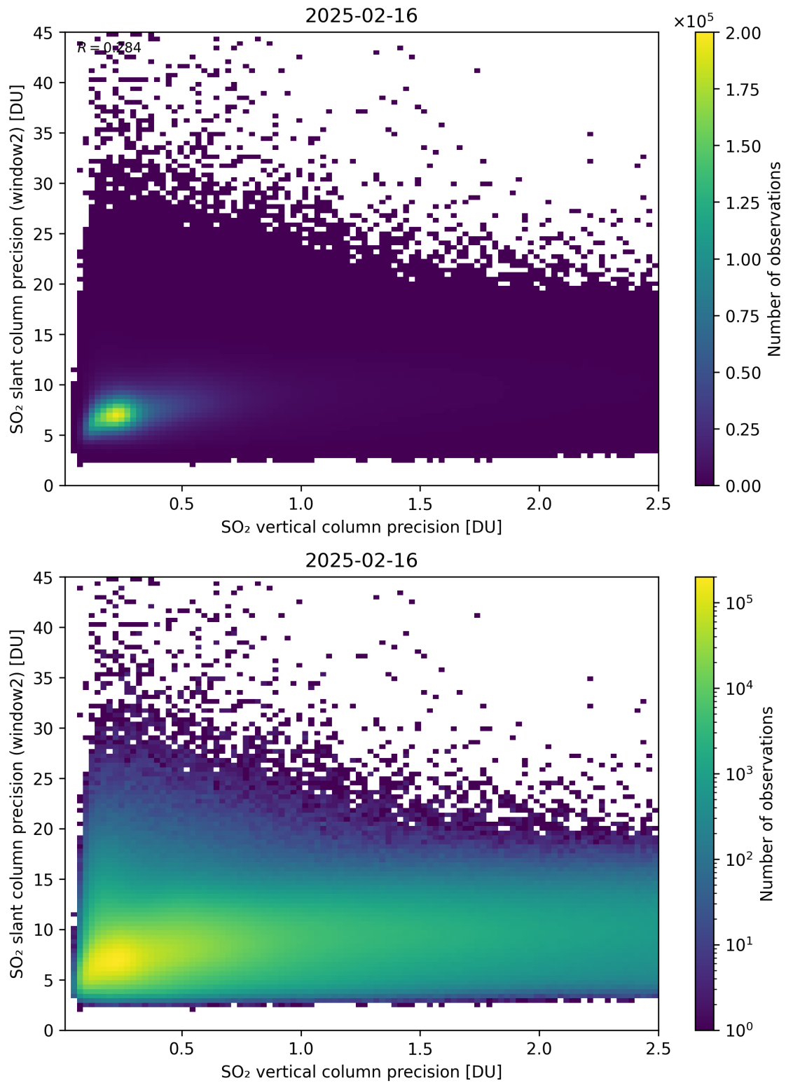
Figure 343: Scatter density plot of “SO 2 vertical column precision” against “SO 2 slant column precision (window2)” for 2025-02-15 to 2025-02-17.
