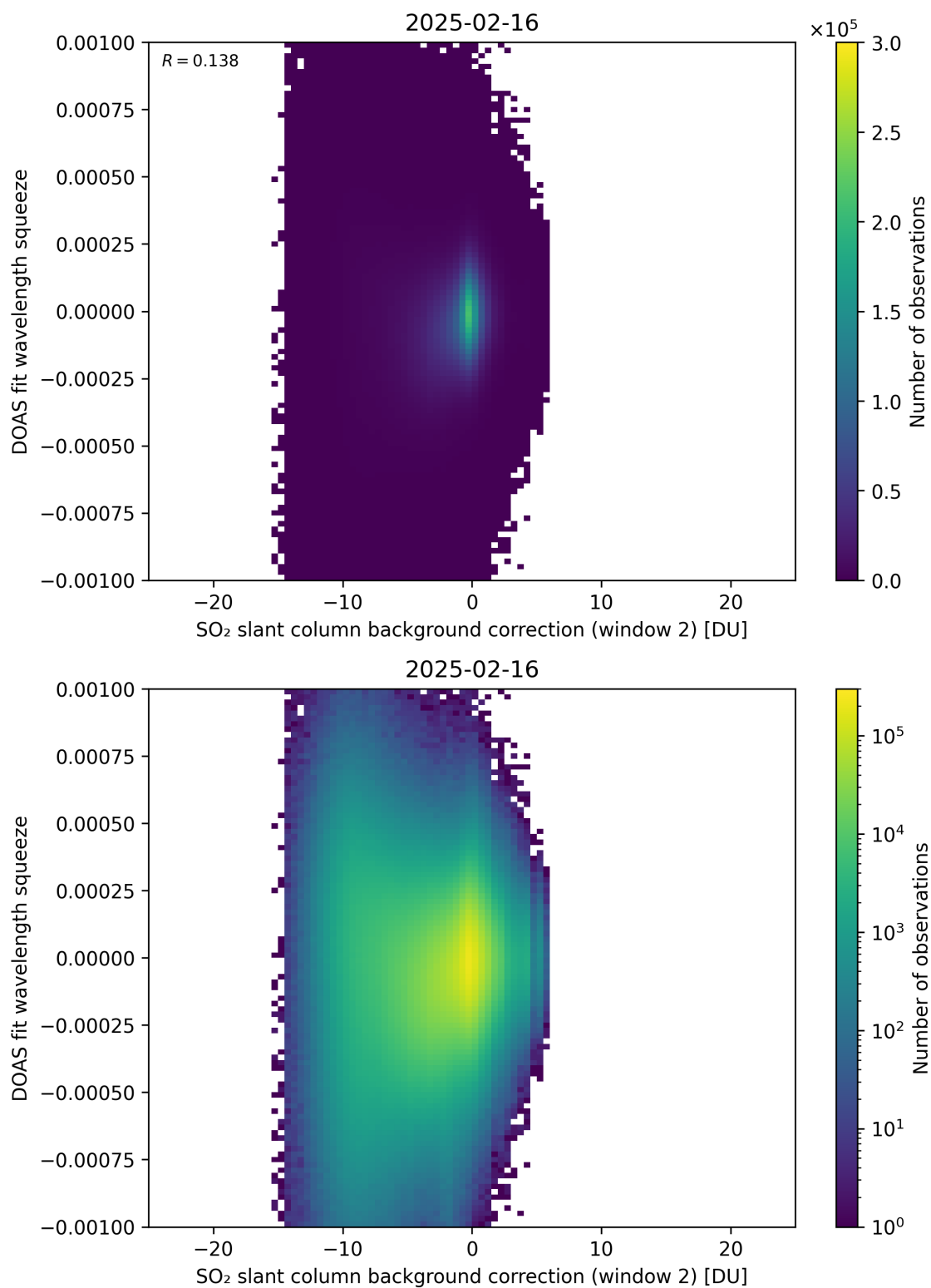
Figure 124: Scatter density plot of “SO 2 slant column background correction (window 2)” against “DOAS fit wavelength squeeze” for 2025-02-15 to 2025-02-17.
