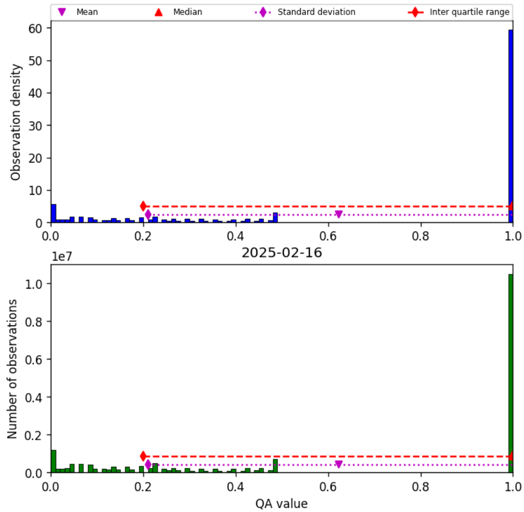
Figure 57: Histogram of “QA value” for 2025-02-15 to 2025-02-17
