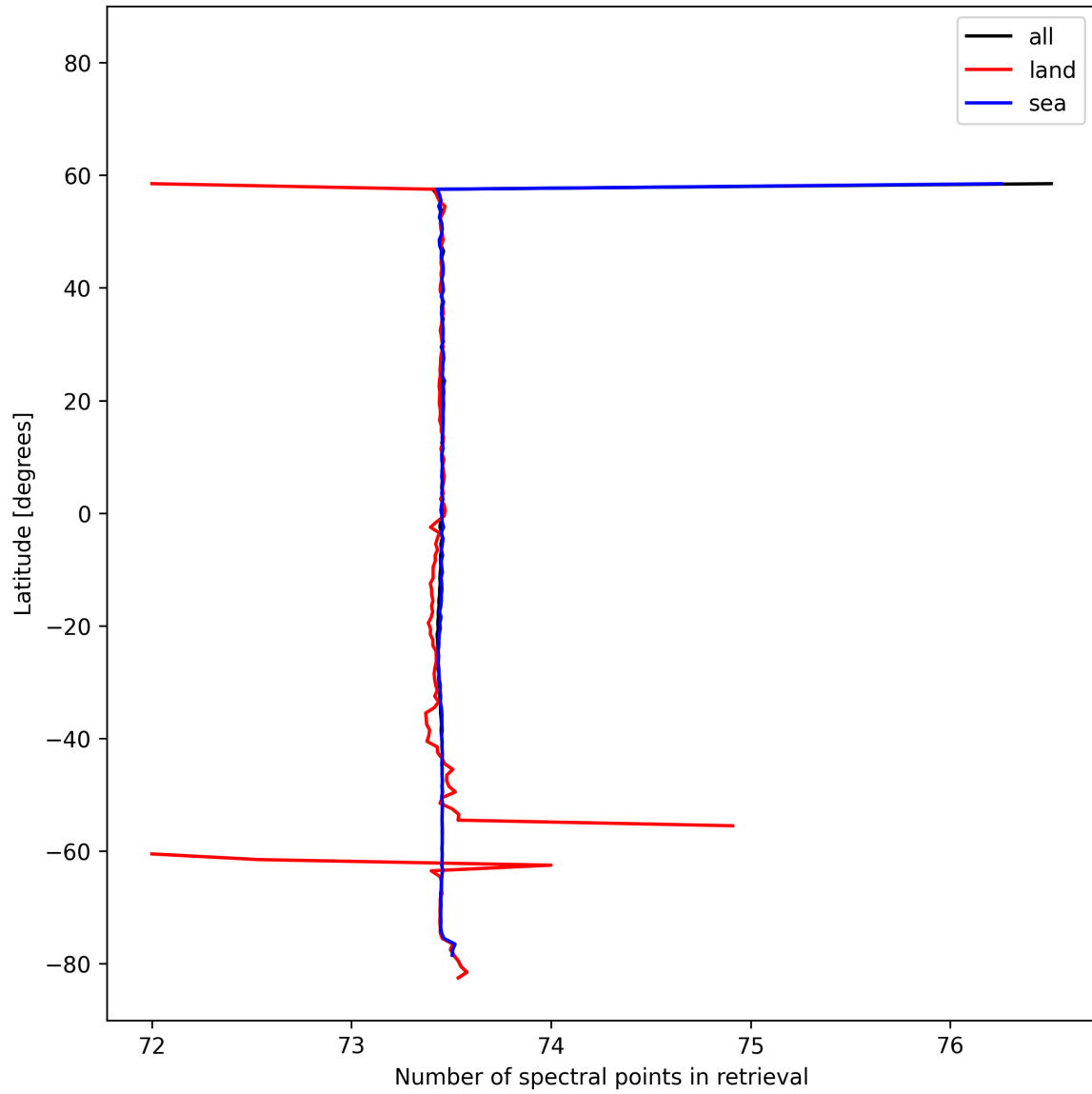
Figure 56: Zonal average of “Number of spectral points in retrieval” for 2025-02-15 to 2025-02-17.
