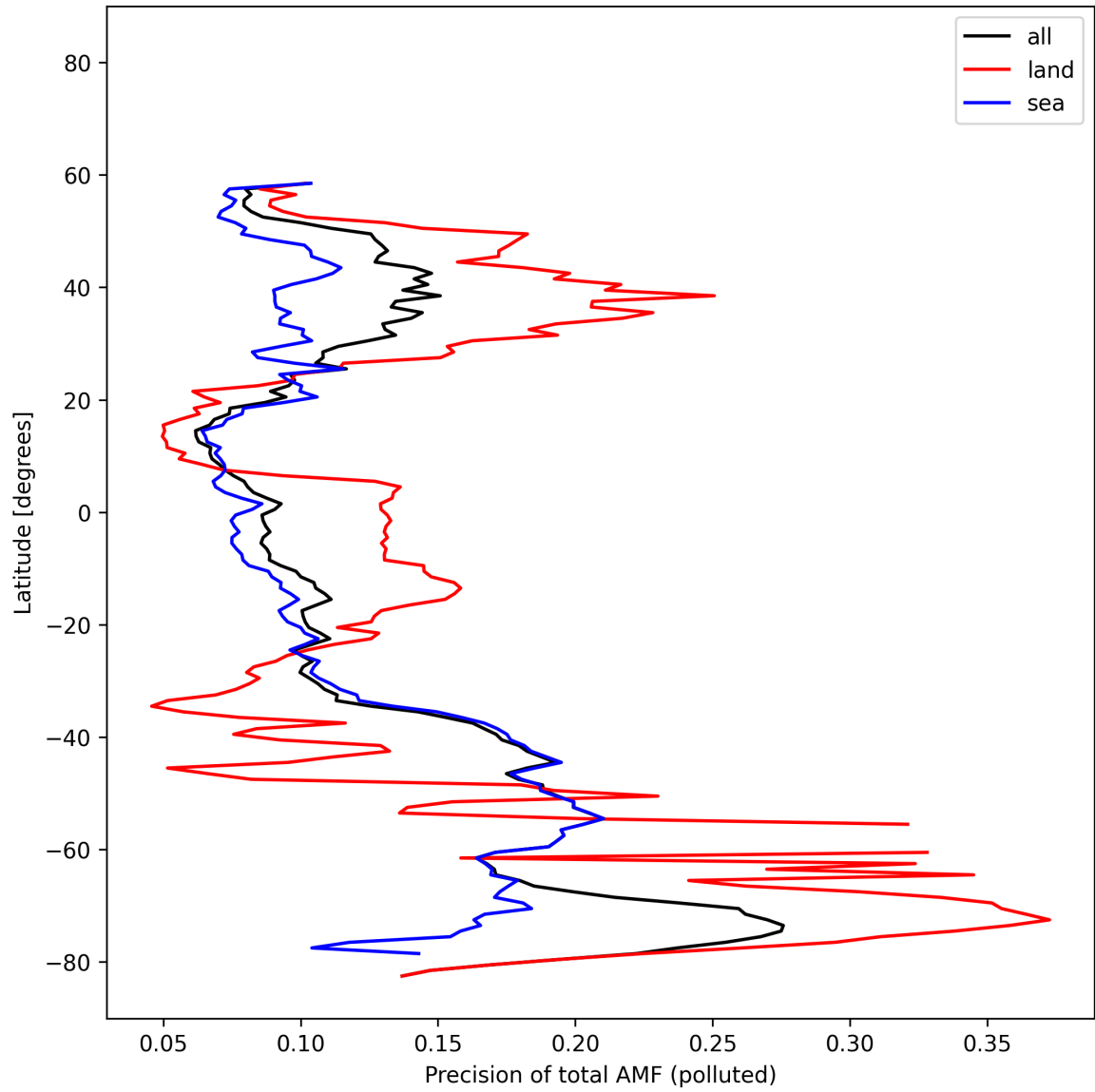
Figure 54: Zonal average of “Precision of total AMF (polluted)” for 2025-02-15 to 2025-02-17.
