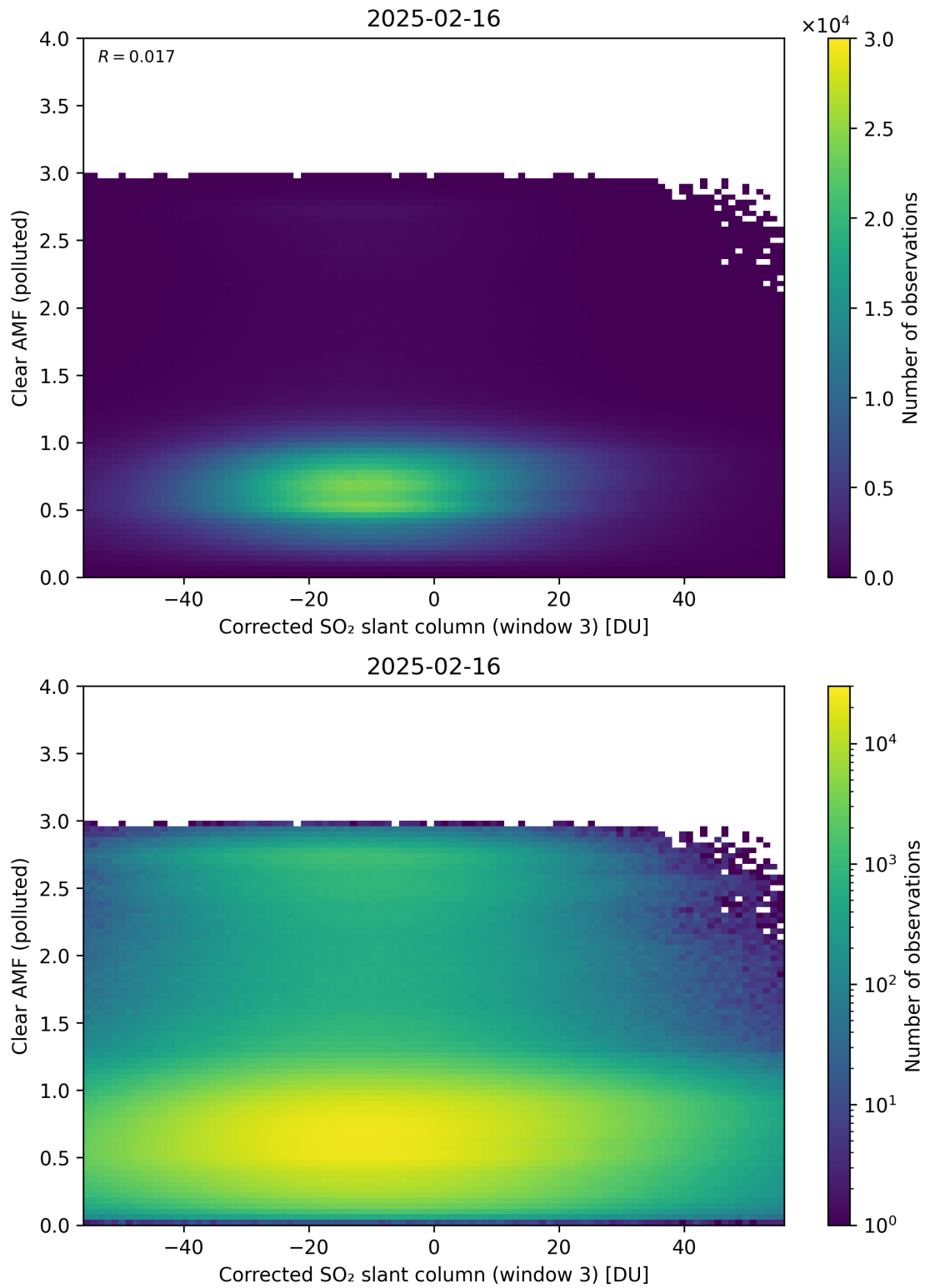
Figure 259: Scatter density plot of “Corrected SO 2 slant column (window 3)” against “Clear AMF (polluted)” for 2025-02-15 to 2025-02-17.
