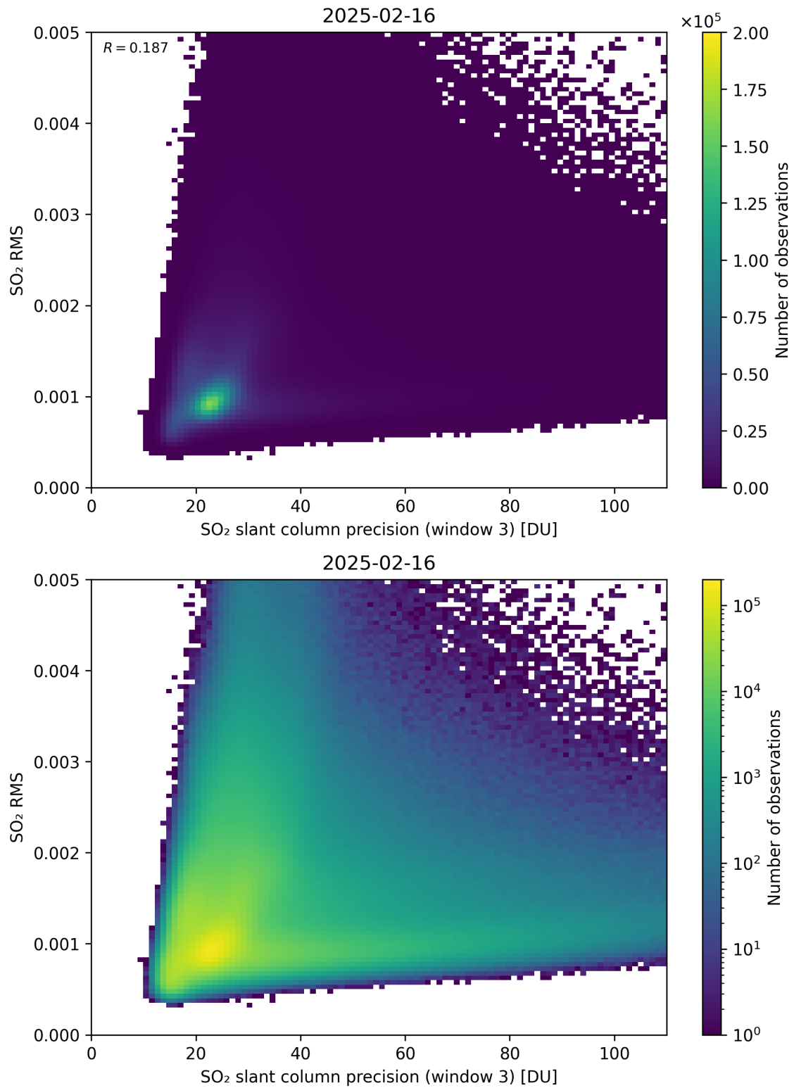
Figure 310: Scatter density plot of “SO 2 slant column precision (window 3)” against “SO 2 RMS” for 2025-02-15 to 2025-02-17.
