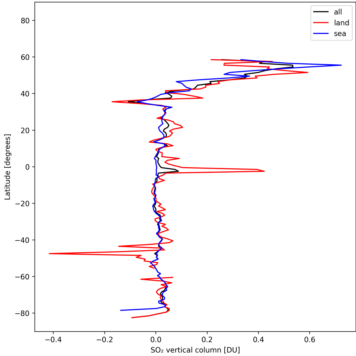
Figure 32: Zonal average of “SO 2 vertical column” for 2025-02-15 to 2025-02-17.
