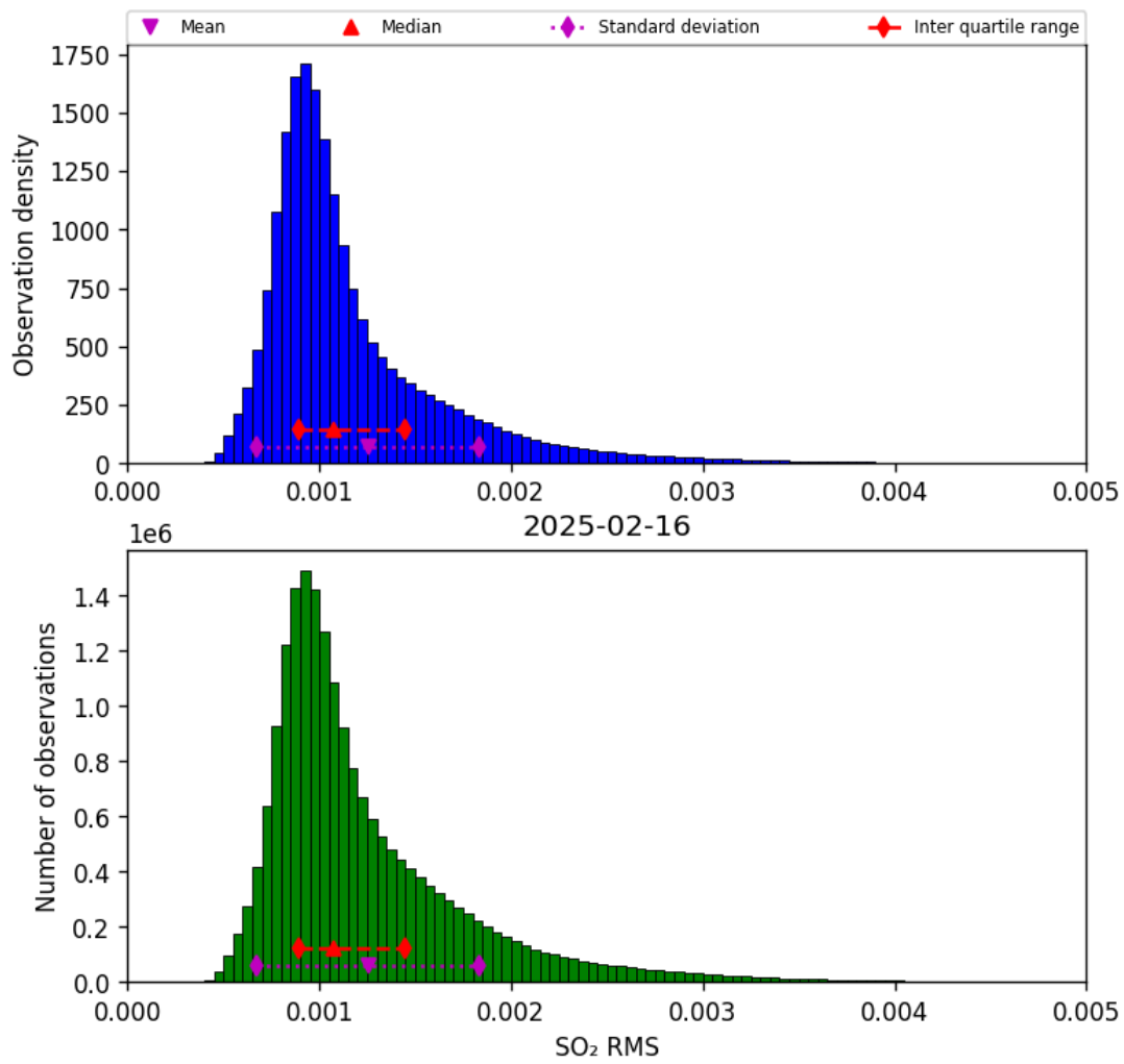
Figure 78: Histogram of “SO 2 RMS” for 2025-02-15 to 2025-02-17
