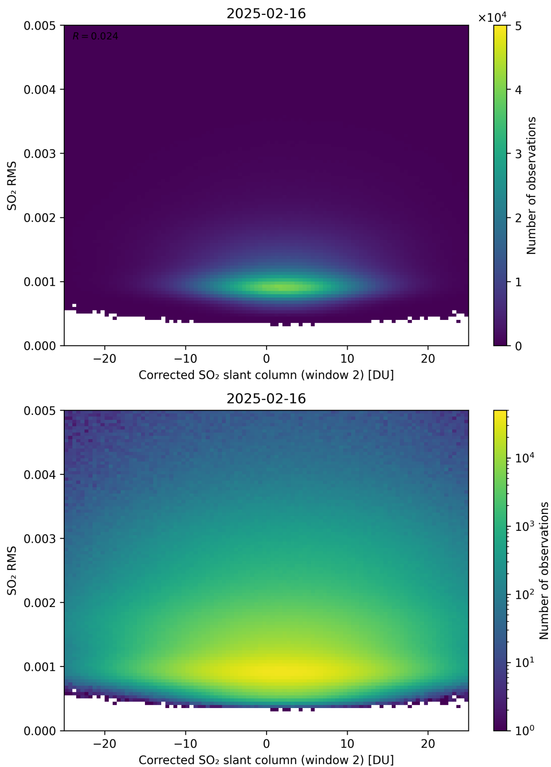
Figure 248: Scatter density plot of “Corrected SO 2 slant column (window 2)” against “SO 2 RMS” for 2025-02-15 to 2025-02-17.
