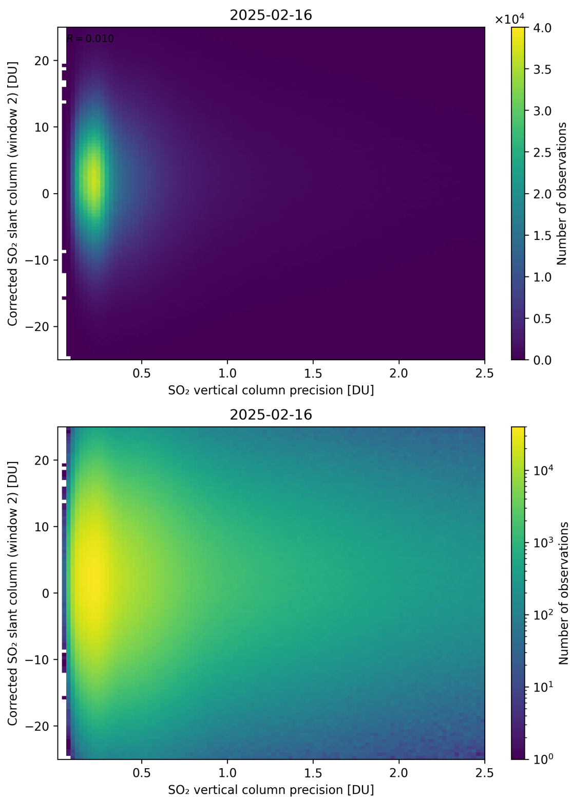
Figure 339: Scatter density plot of “SO 2 vertical column precision” against “Corrected SO 2 slant column (window 2)” for 2025-02-15 to 2025-02-17.
