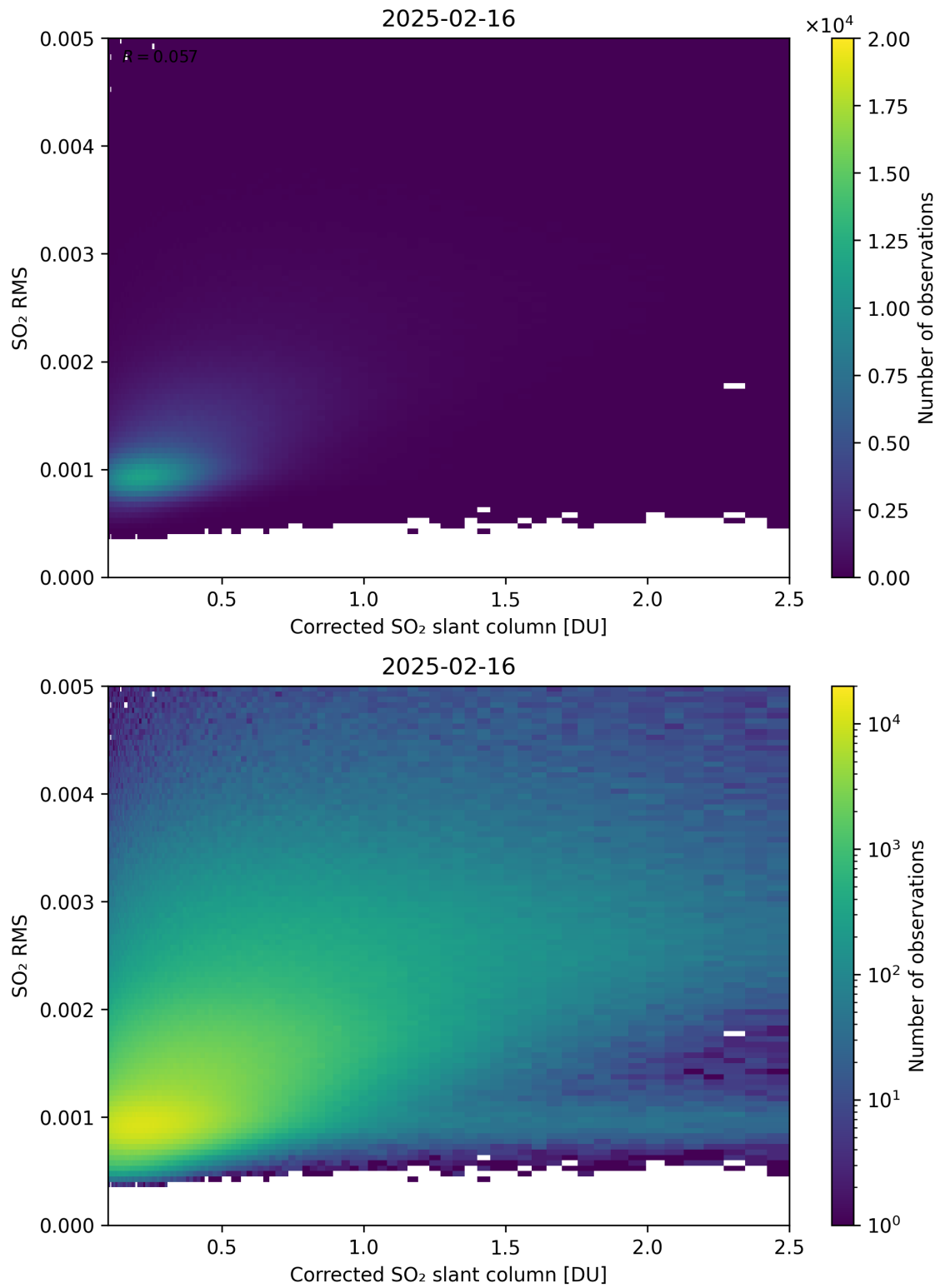
Figure 231: Scatter density plot of “Corrected SO 2 slant column” against “SO 2 RMS” for 2025-02-15 to 2025-02-17.
