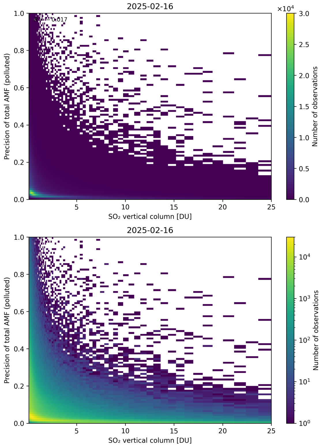
Figure 360: Scatter density plot of “SO 2 vertical column” against “Precision of total AMF (polluted)” for 2025-02-15 to 2025-02-17.
