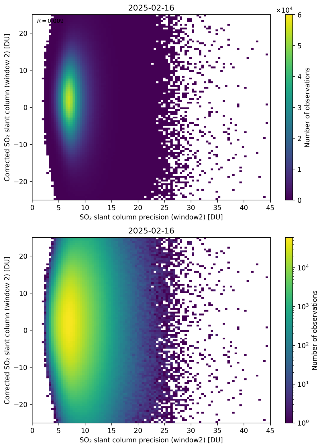
Figure 297: Scatter density plot of “SO 2 slant column precision (window2)” against “Corrected SO 2 slant column (window 2)” for 2025-02-15 to 2025-02-17.
