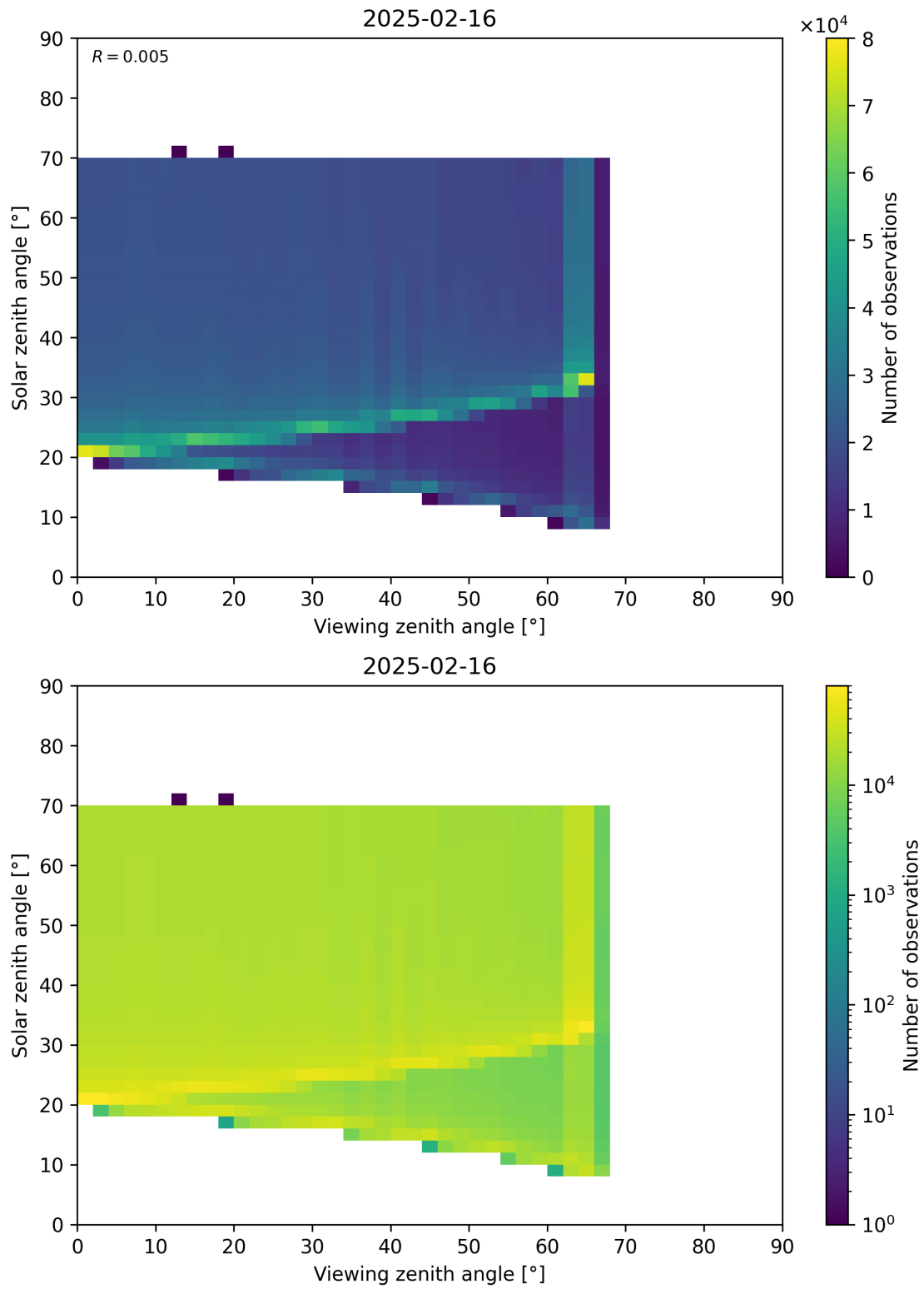
Figure 369: Scatter density plot of “Viewing zenith angle” against “Solar zenith angle” for 2025-02-15 to 2025-02-17.
