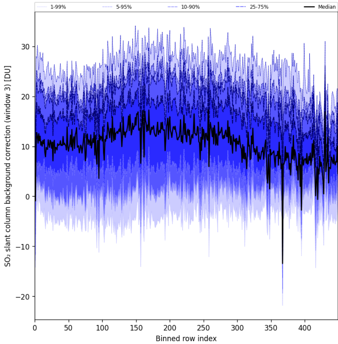
Figure 100: Along track statistics of “SO 2 slant column background correction (window 3)” for 2025-02-15 to 2025-02-17
