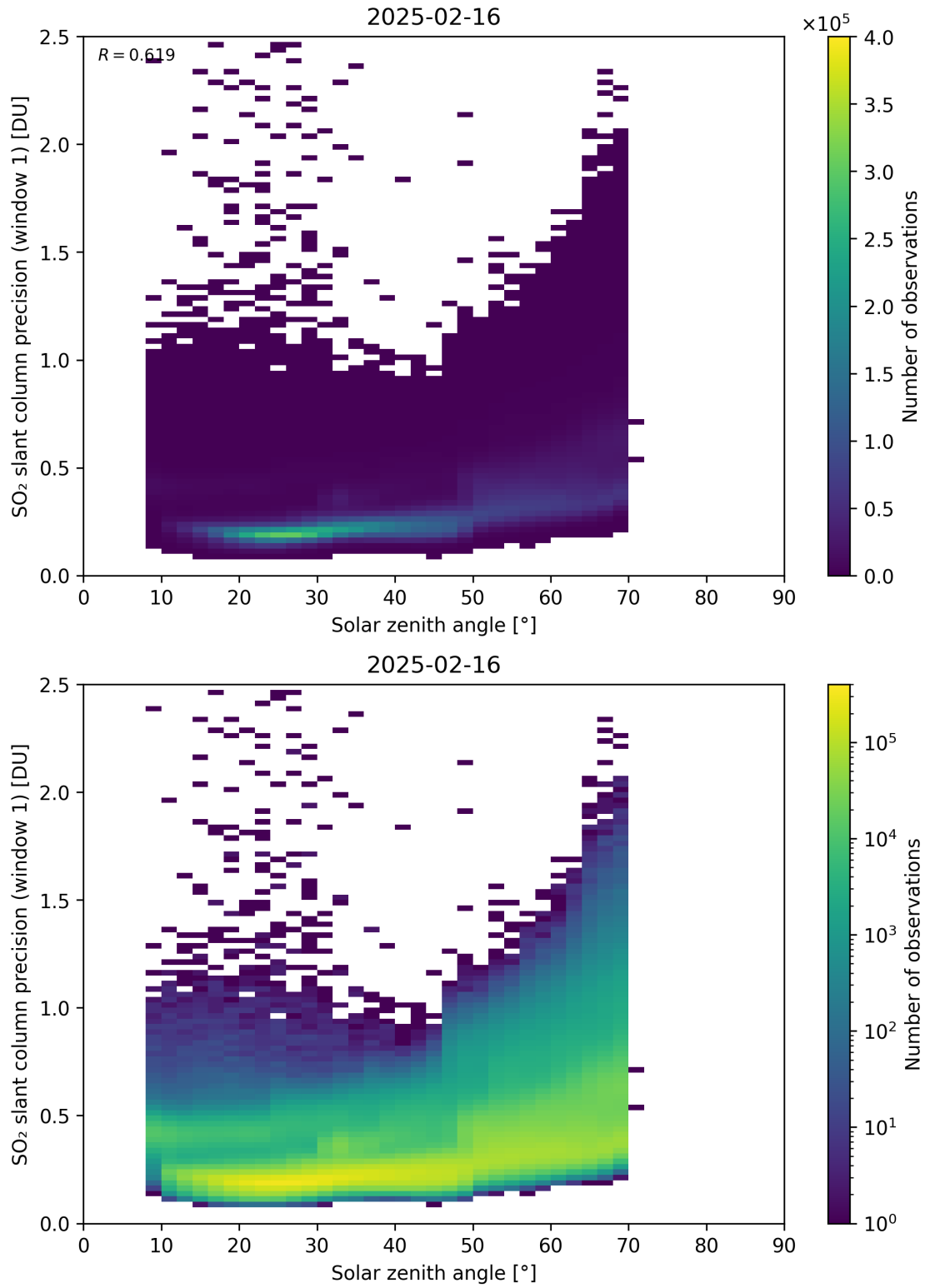
Figure 185: Scatter density plot of “Solar zenith angle” against “SO 2 slant column precision (window 1)” for 2025-02-15 to 2025-02-17.
