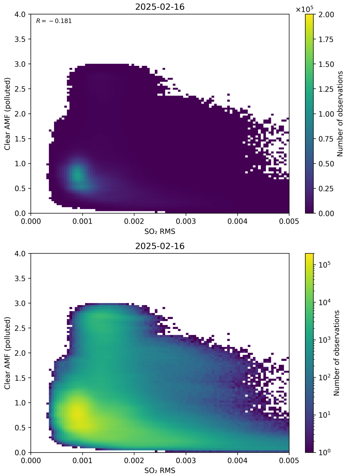
Figure 147: Scatter density plot of “SO 2 RMS” against “Clear AMF (polluted)” for 2025-02-15 to 2025-02-17.
