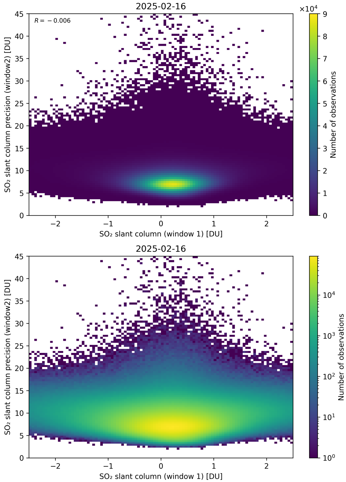
Figure 286: Scatter density plot of “SO 2 slant column (window 1)” against “SO 2 slant column precision (window2)” for 2025-02-15 to 2025-02-17.
