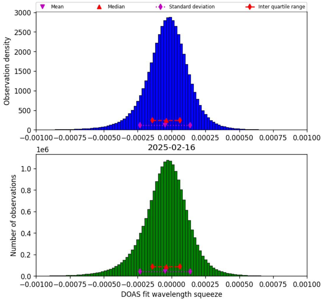
Figure 77: Histogram of “DOAS fit wavelength squeeze” for 2025-02-15 to 2025-02-17
