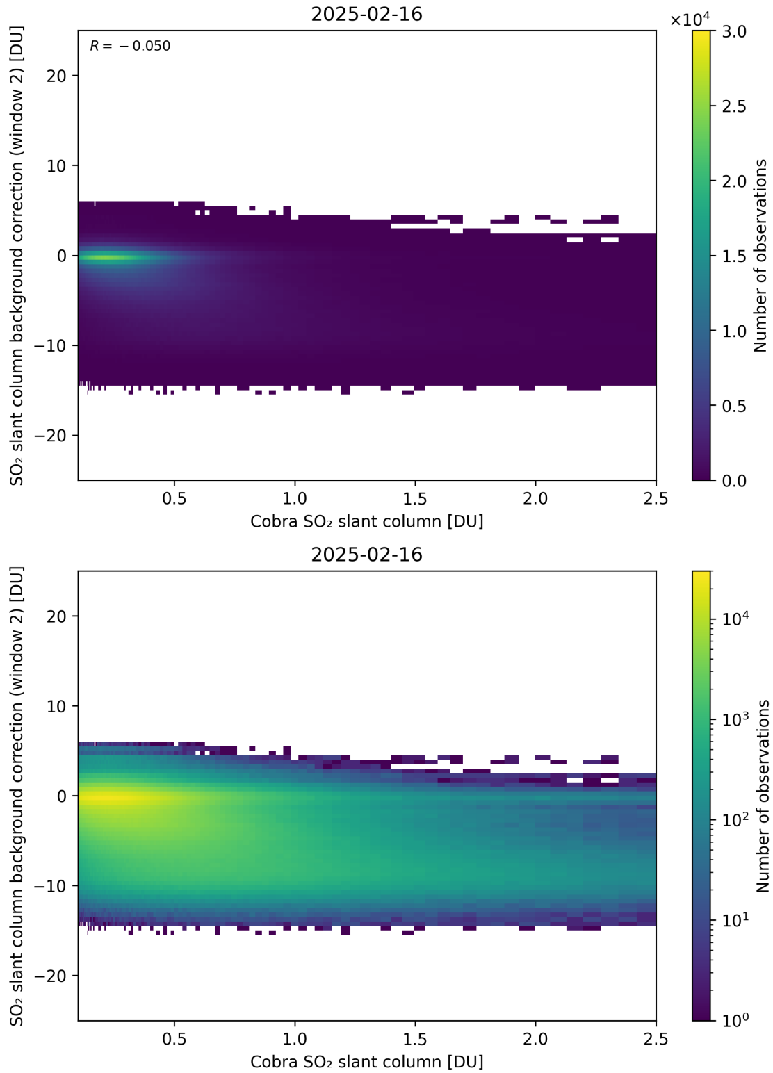
Figure 194: Scatter density plot of “Cobra SO 2 slant column” against “SO 2 slant column background correction (window 2)” for 2025-02-15 to 2025-02-17.
