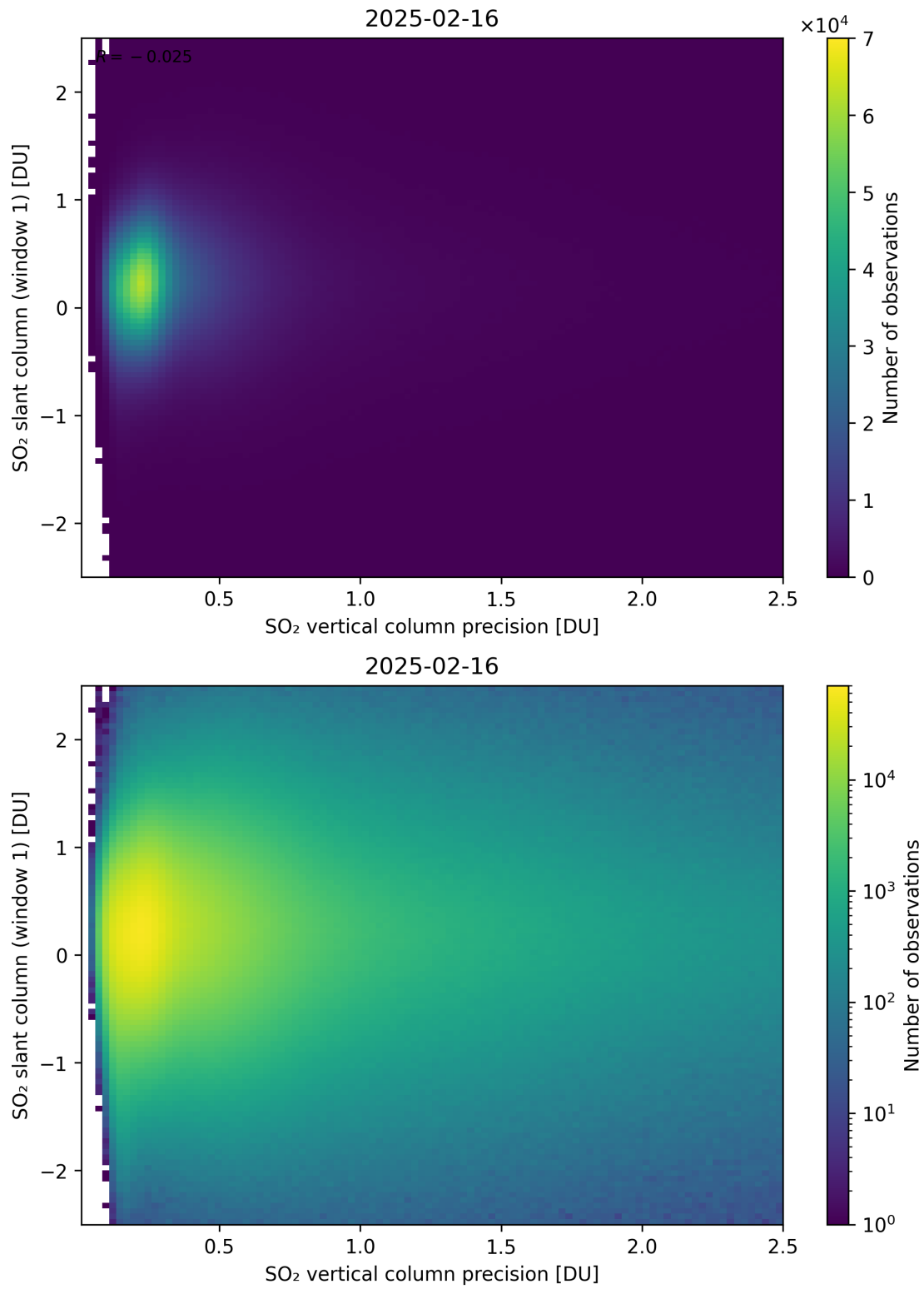
Figure 341: Scatter density plot of “SO 2 vertical column precision” against “SO 2 slant column (window 1)” for 2025-02-15 to 2025-02-17.
