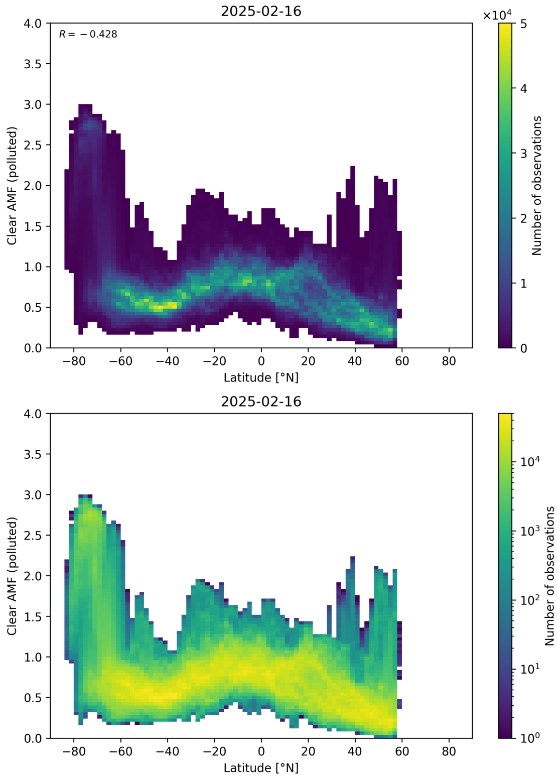
Figure 156: Scatter density plot of “Latitude” against “Clear AMF (polluted)” for 2025-02-15 to 2025-02-17.
