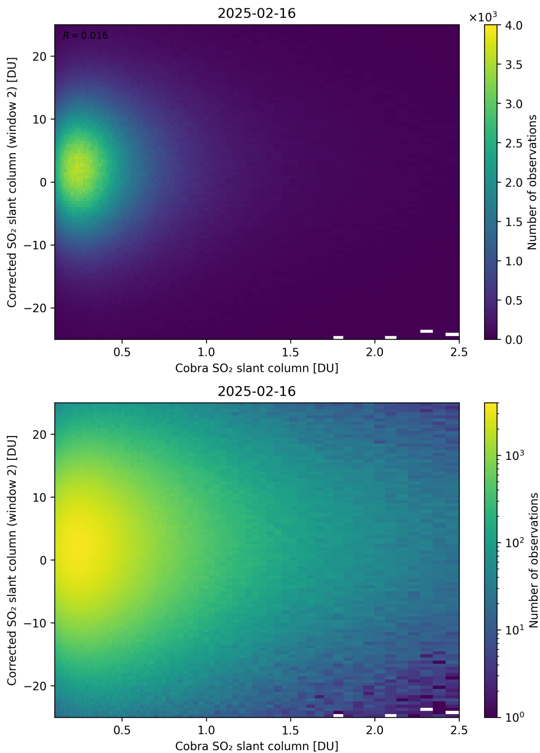
Figure 217: Scatter density plot of “Cobra SO 2 slant column” against “Corrected SO 2 slant column (window 2)” for 2025-02-15 to 2025-02-17.
