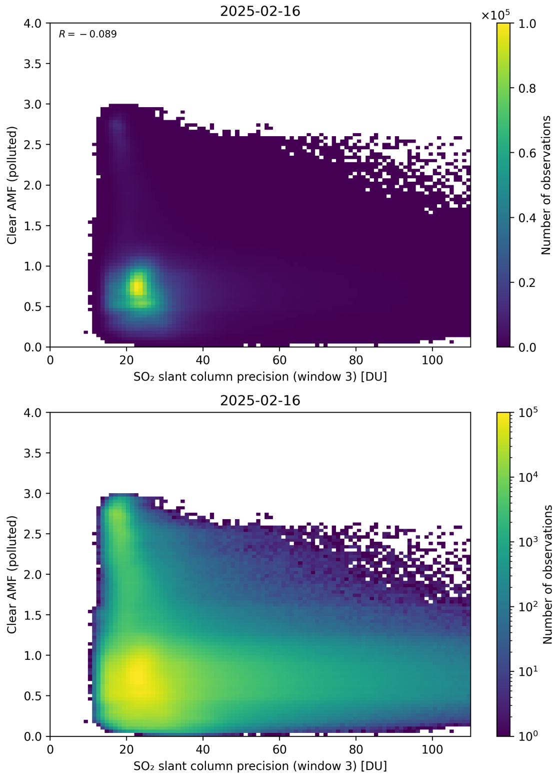
Figure 311: Scatter density plot of “SO 2 slant column precision (window 3)” against “Clear AMF (polluted)” for 2025-02-15 to 2025-02-17.
