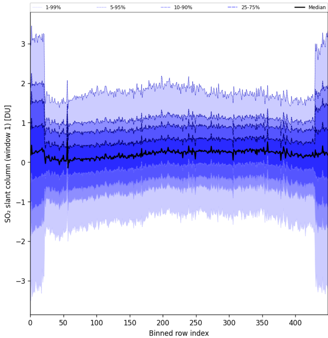
Figure 89: Along track statistics of “SO 2 slant column (window 1)” for 2025-02-15 to 2025-02-17
