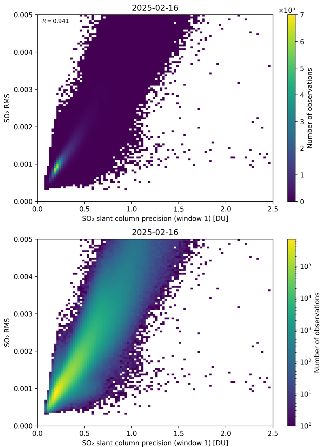
Figure 273: Scatter density plot of “SO 2 slant column precision (window 1)” against “SO 2 RMS” for 2025-02-15 to 2025-02-17.
