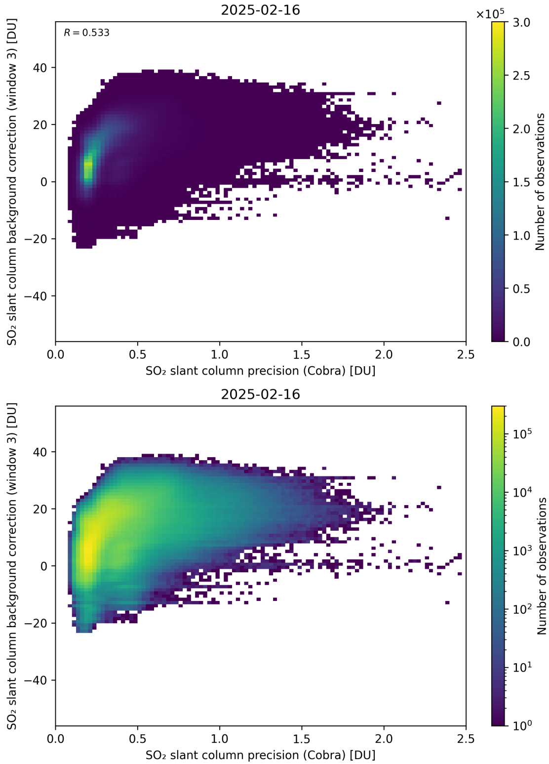
Figure 201: Scatter density plot of “SO 2 slant column precision (Cobra)” against “SO 2 slant column background correction (window 3)” for 2025-02-15 to 2025-02-17.
