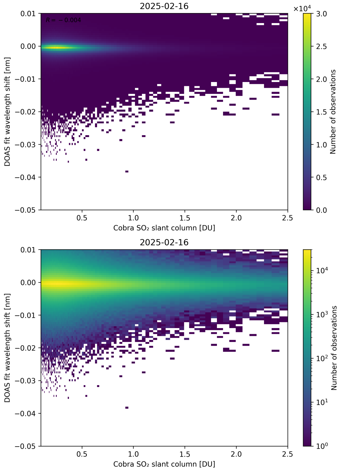
Figure 196: Scatter density plot of “Cobra SO 2 slant column” against “DOAS fit wavelength shift” for 2025-02-15 to 2025-02-17.
