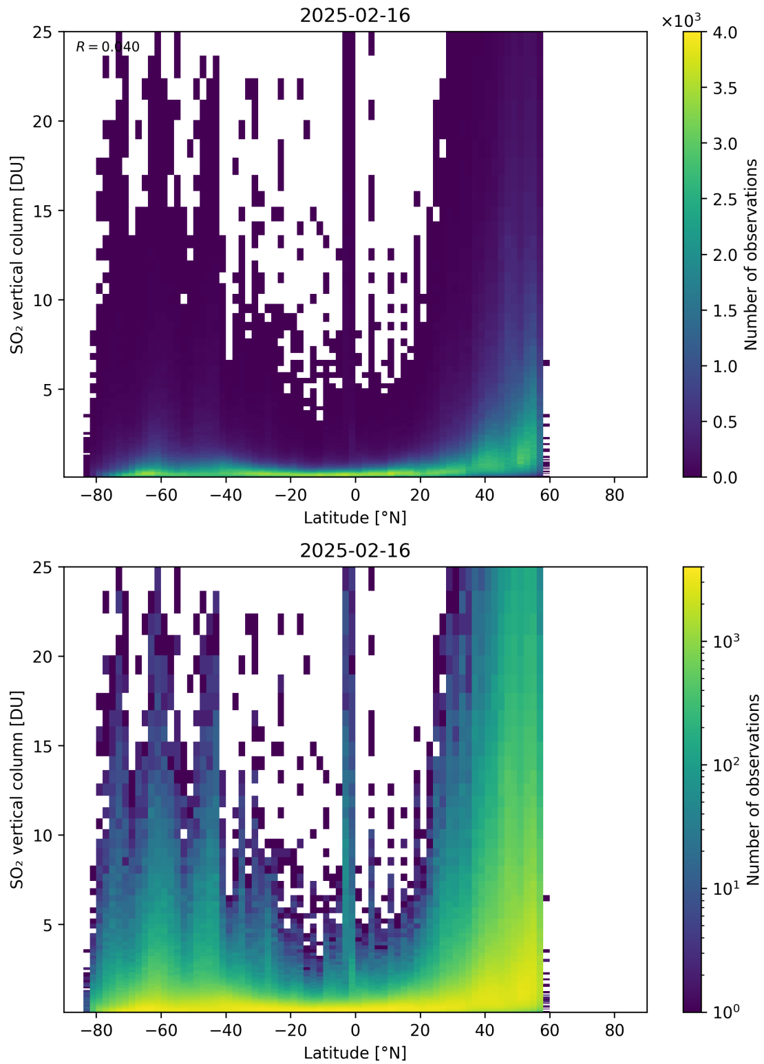
Figure 169: Scatter density plot of “Latitude” against “SO 2 vertical column” for 2025-02-15 to 2025-02-17.
