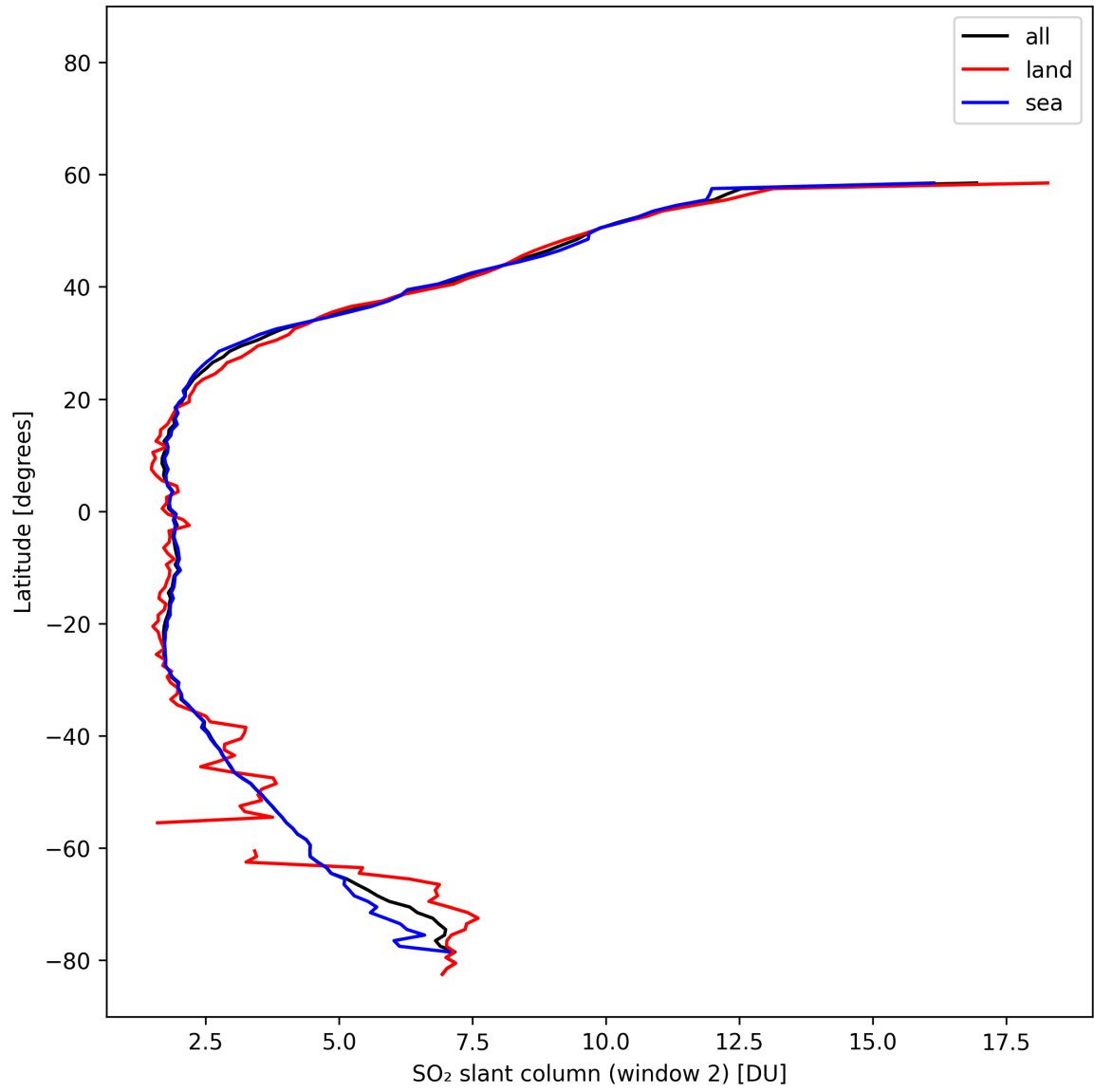
Figure 41: Zonal average of “SO 2 slant column (window 2)” for 2025-02-15 to 2025-02-17.
