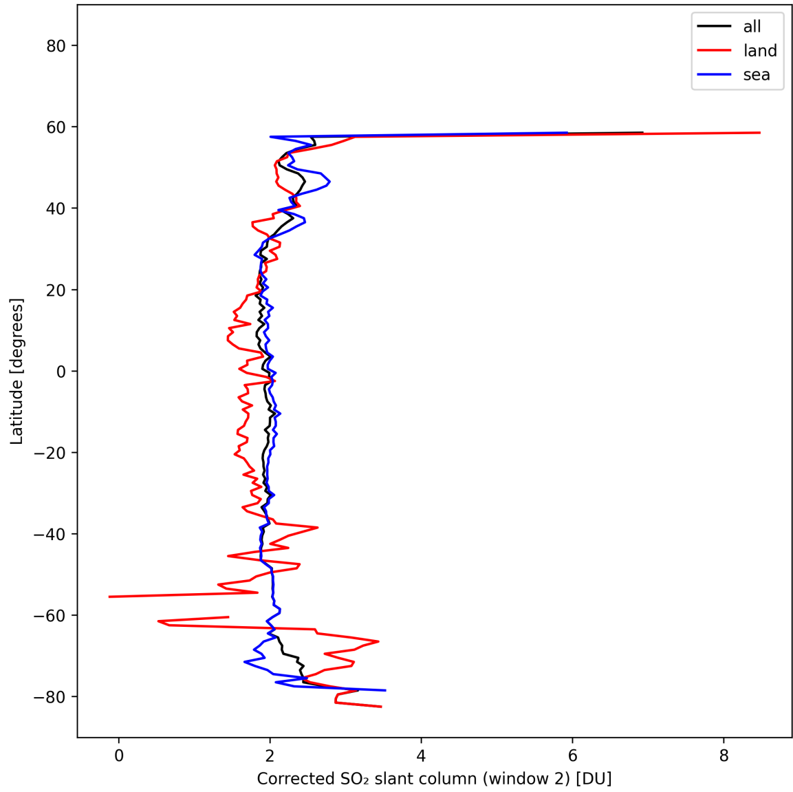
Figure 43: Zonal average of “Corrected SO 2 slant column (window 2)” for 2025-02-15 to 2025-02-17.
