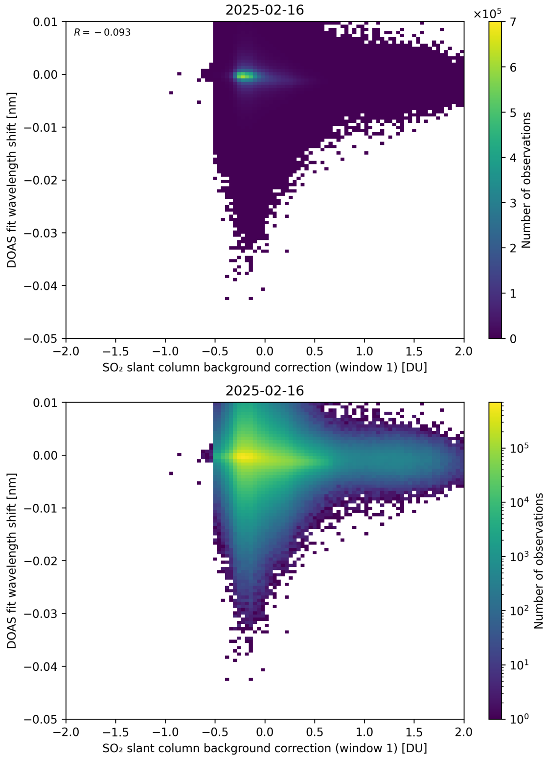
Figure 111: Scatter density plot of “SO 2 slant column background correction (window 1)” against “DOAS fit wavelength shift” for 2025-02-15 to 2025-02-17.
