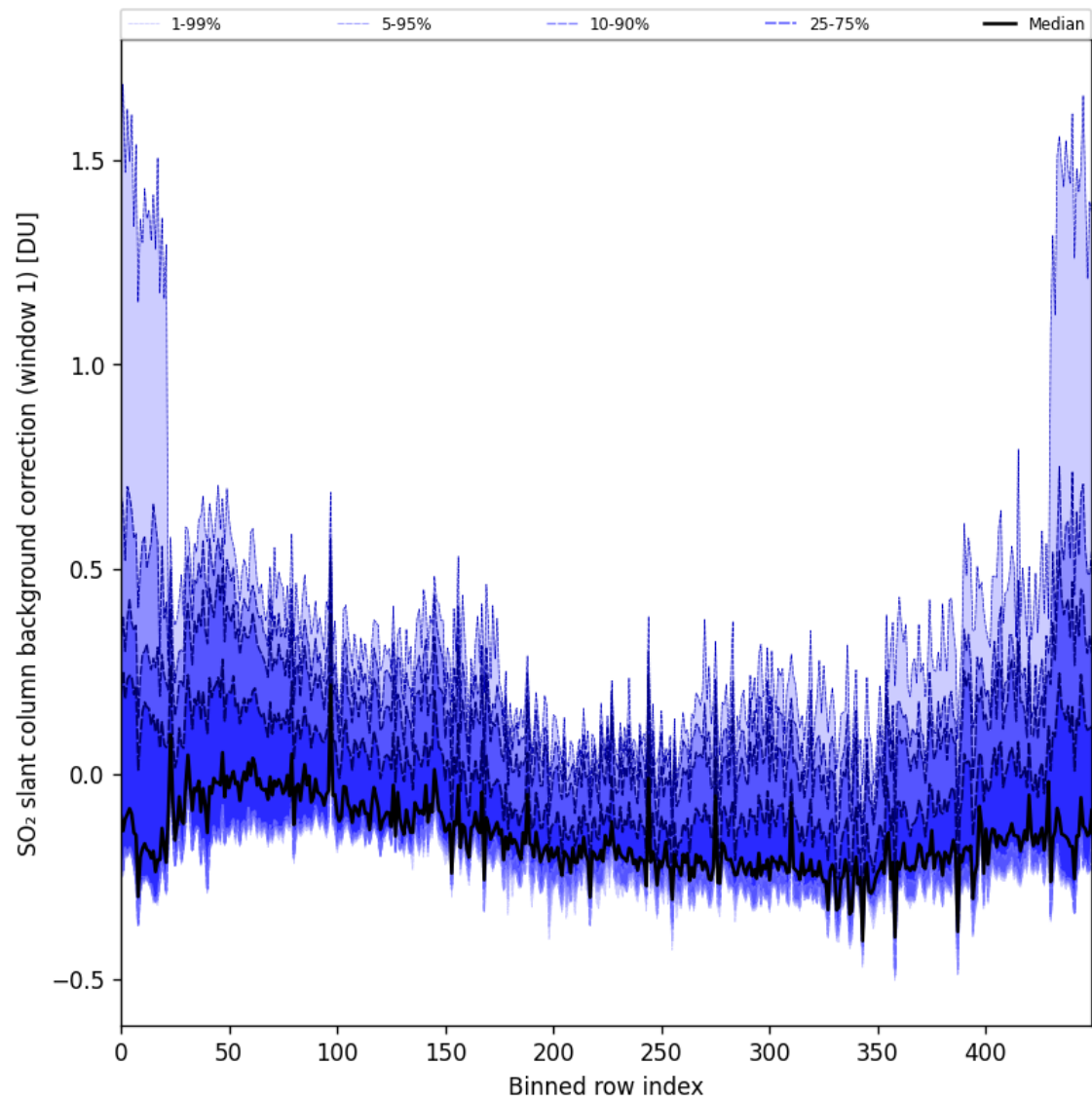
Figure 92: Along track statistics of “SO 2 slant column background correction (window 1)” for 2025-02-15 to 2025-02-17
