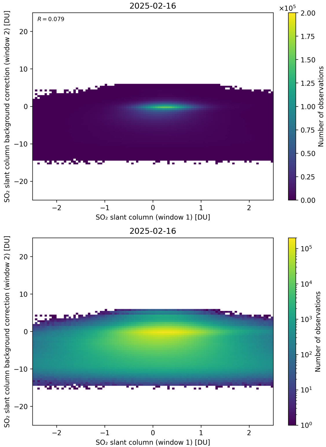
Figure 263: Scatter density plot of “SO 2 slant column (window 1)” against “SO 2 slant column background correction (window 2)” for 2025-02-15 to 2025-02-17.
