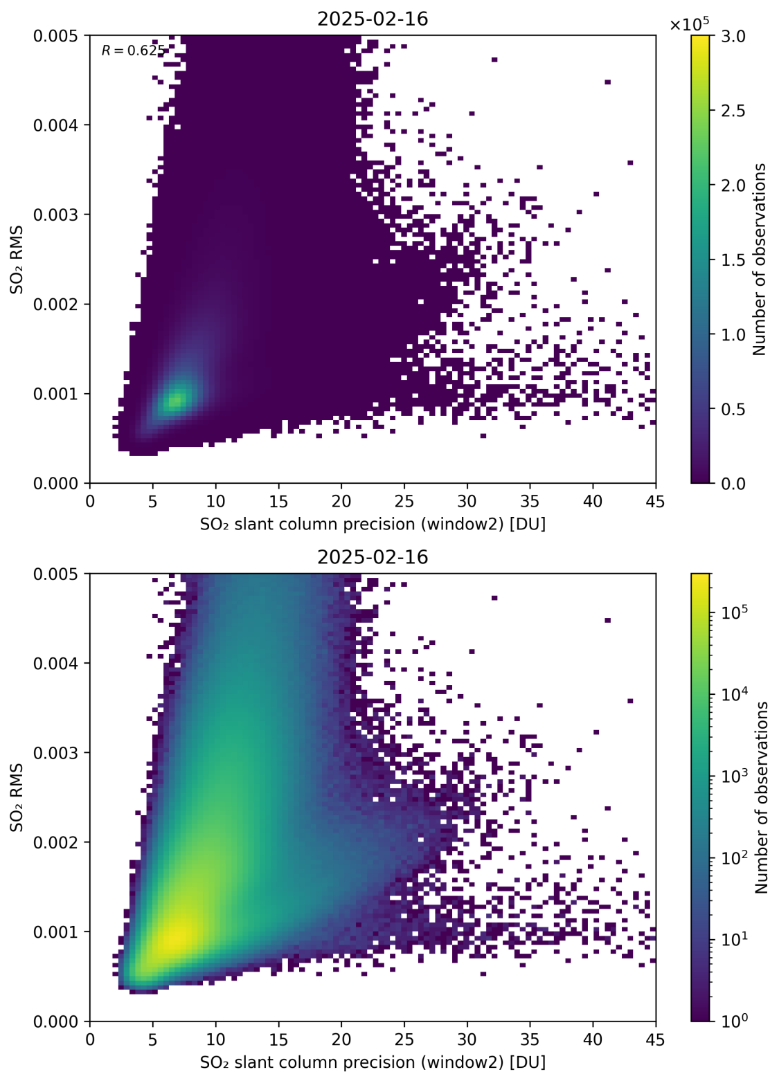
Figure 295: Scatter density plot of “SO 2 slant column precision (window2)” against “SO 2 RMS” for 2025-02-15 to 2025-02-17.
