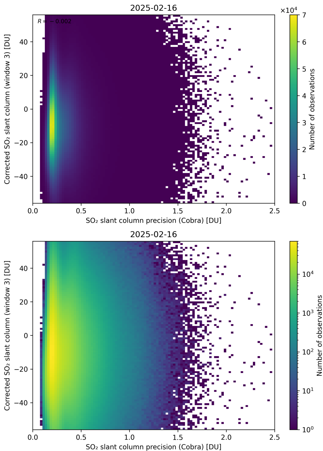
Figure 207: Scatter density plot of “SO 2 slant column precision (Cobra)” against “Corrected SO 2 slant column (window 3)” for 2025-02-15 to 2025-02-17.
