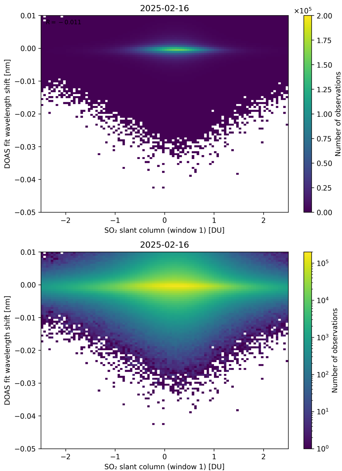
Figure 265: Scatter density plot of “SO 2 slant column (window 1)” against “DOAS fit wavelength shift” for 2025-02-15 to 2025-02-17.
