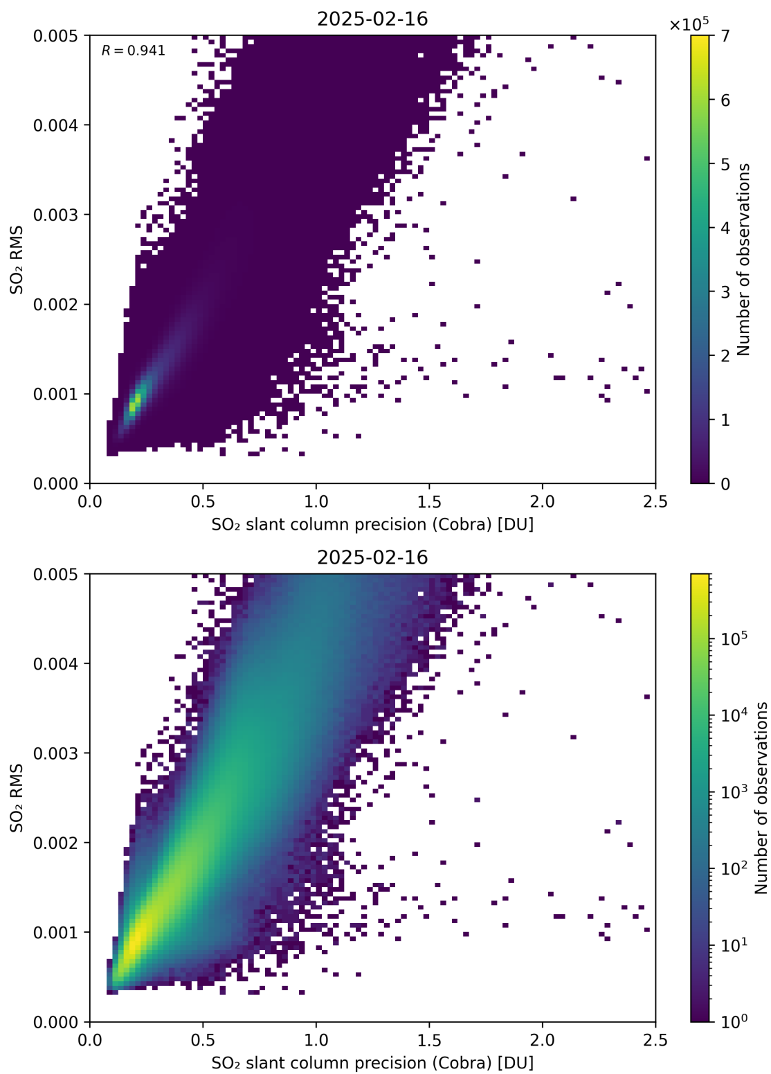
Figure 204: Scatter density plot of “SO 2 slant column precision (Cobra)” against “SO 2 RMS” for 2025-02-15 to 2025-02-17.
