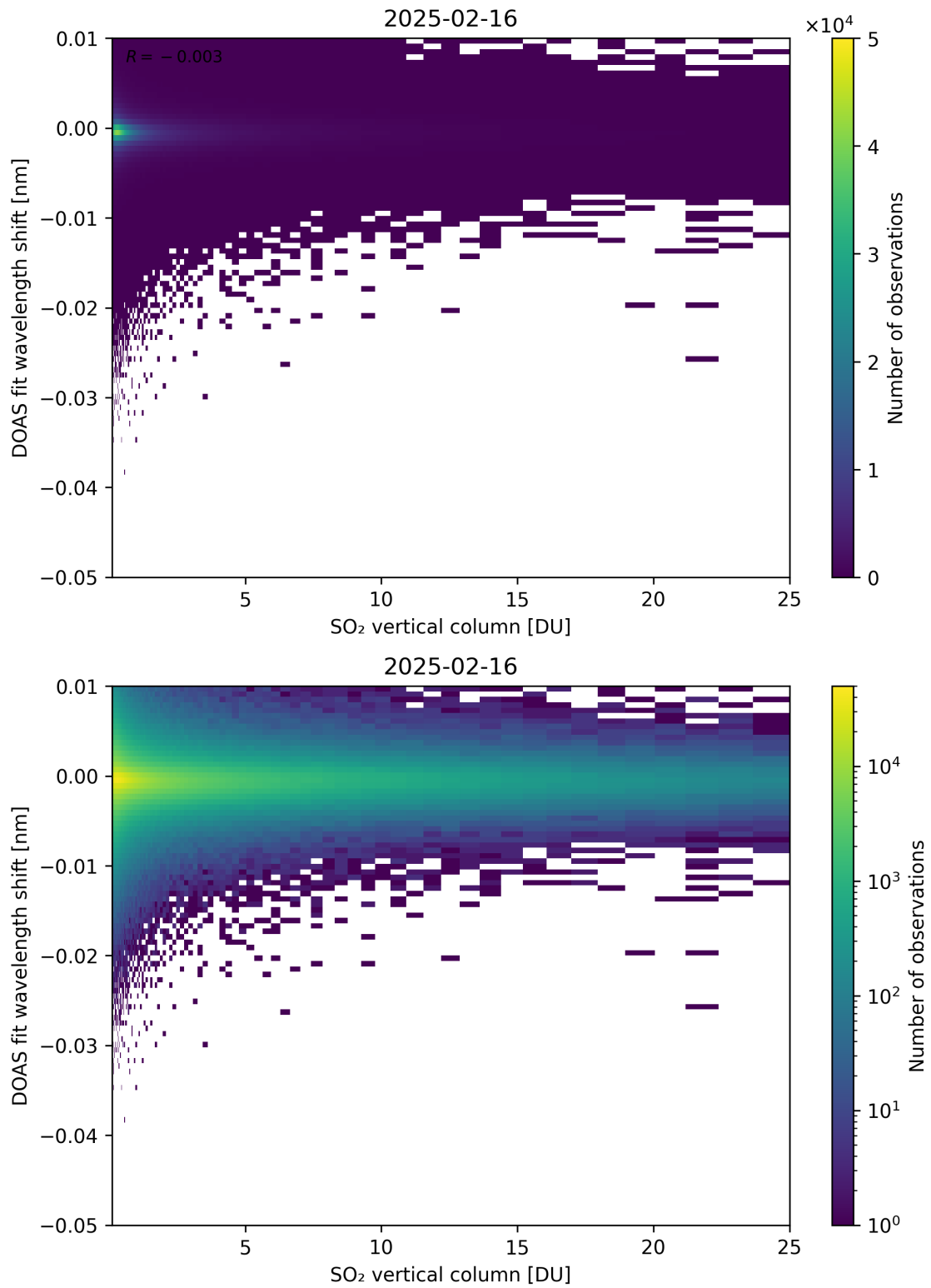
Figure 326: Scatter density plot of “SO 2 vertical column” against “DOAS fit wavelength shift” for 2025-02-15 to 2025-02-17.
