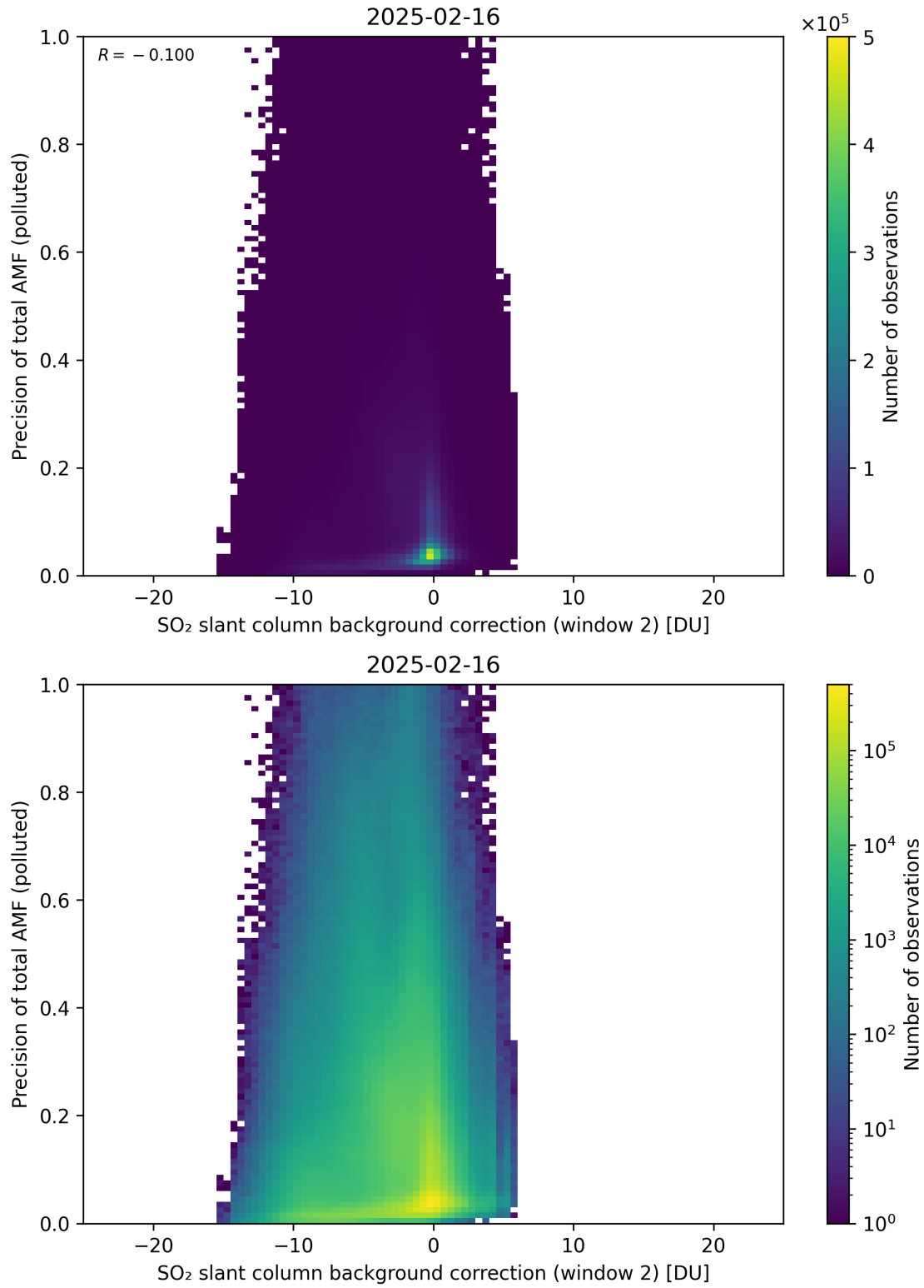
Figure 131: Scatter density plot of “SO 2 slant column background correction (window 2)” against “Precision of total AMF (polluted)” for 2025-02-15 to 2025-02-17.
