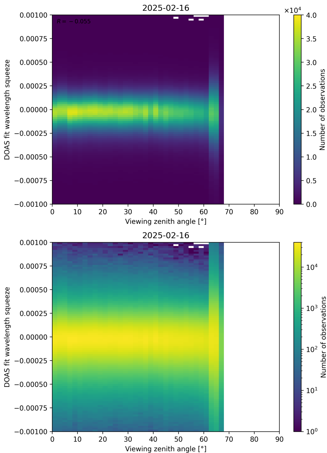
Figure 366: Scatter density plot of “Viewing zenith angle” against “DOAS fit wavelength squeeze” for 2025-02-15 to 2025-02-17.
