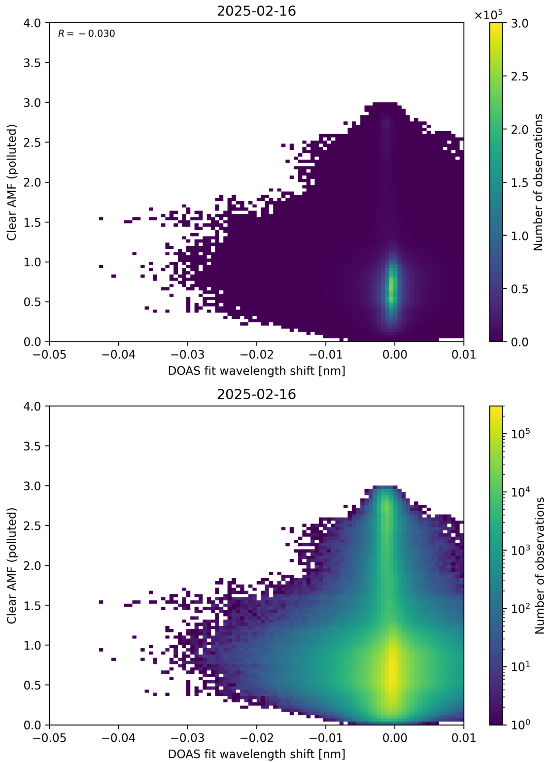
Figure 140: Scatter density plot of “DOAS fit wavelength shift” against “Clear AMF (polluted)” for 2025-02-15 to 2025-02-17.
