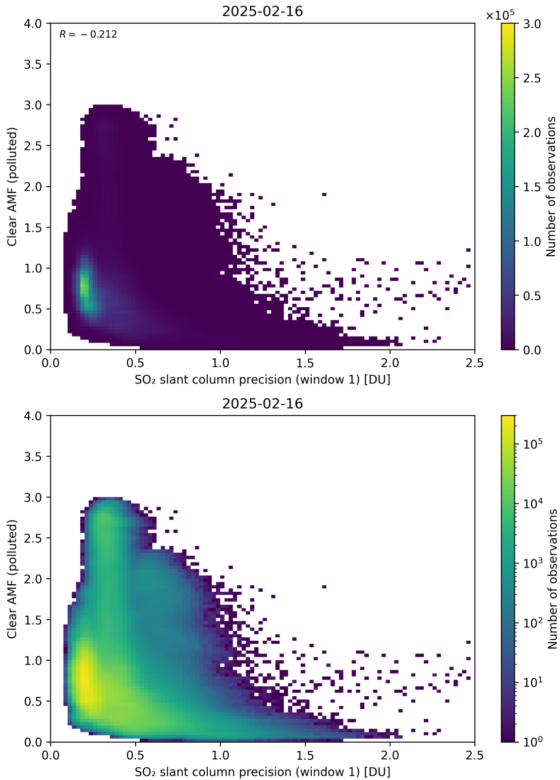
Figure 274: Scatter density plot of “SO 2 slant column precision (window 1)” against “Clear AMF (polluted)” for 2025-02-15 to 2025-02-17.
