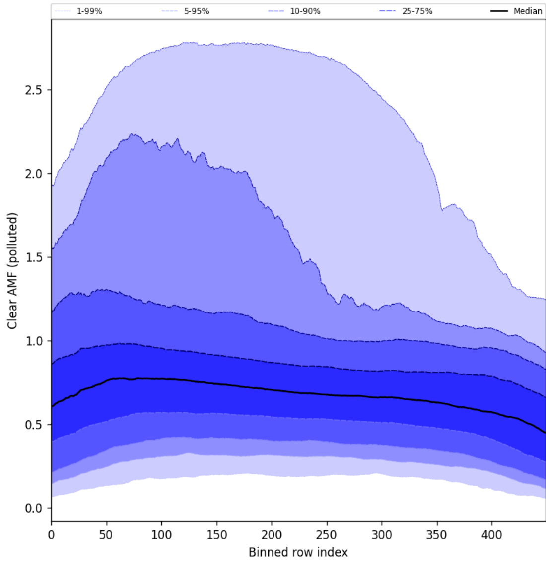
Figure 107: Along track statistics of “Clear AMF (polluted)” for 2025-02-15 to 2025-02-17
