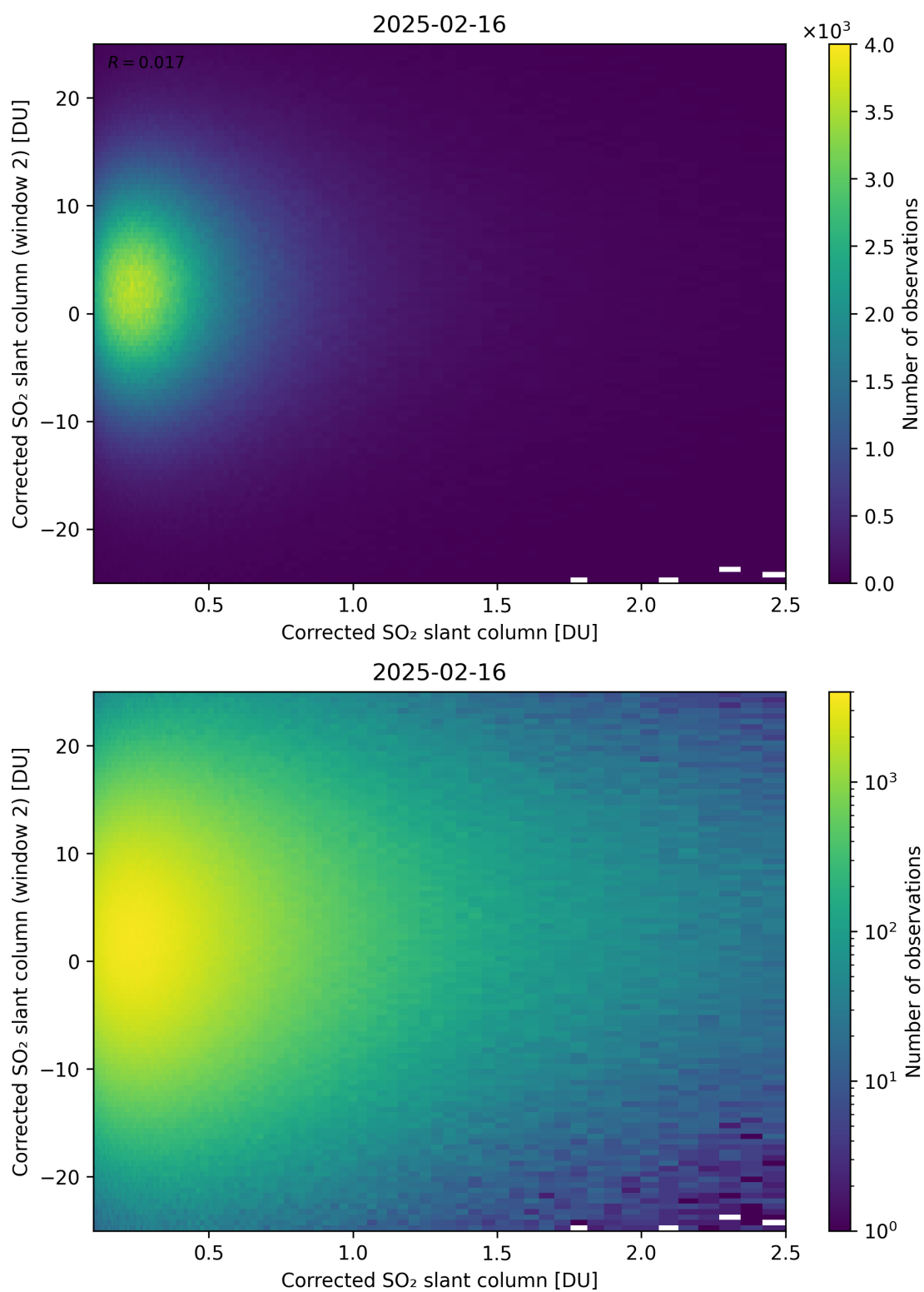
Figure 235: Scatter density plot of “Corrected SO 2 slant column” against “Corrected SO 2 slant column (window 2)” for 2025-02-15 to 2025-02-17.
