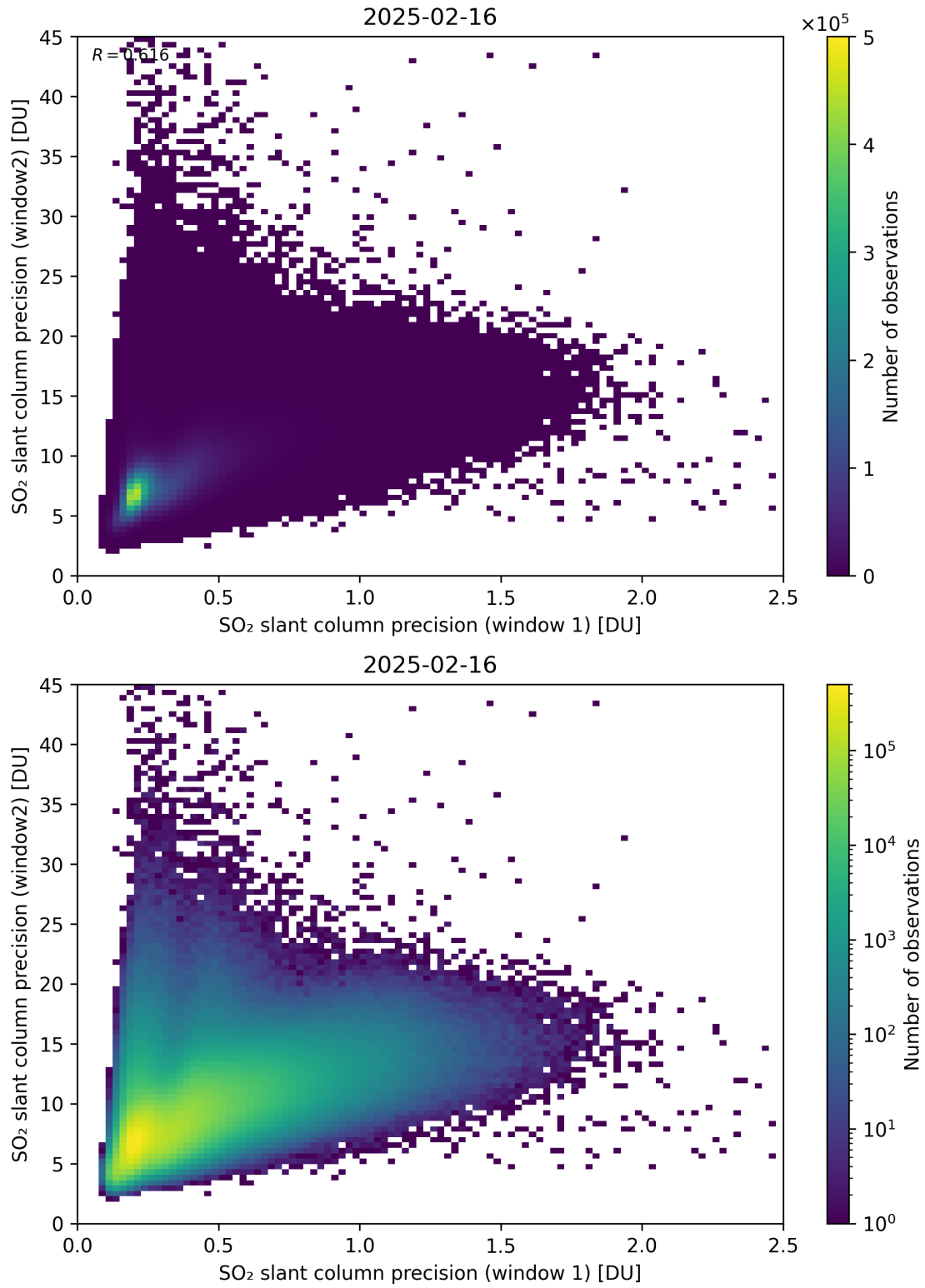
Figure 277: Scatter density plot of “SO 2 slant column precision (window 1)” against “SO 2 slant column precision (window2)” for 2025-02-15 to 2025-02-17.
