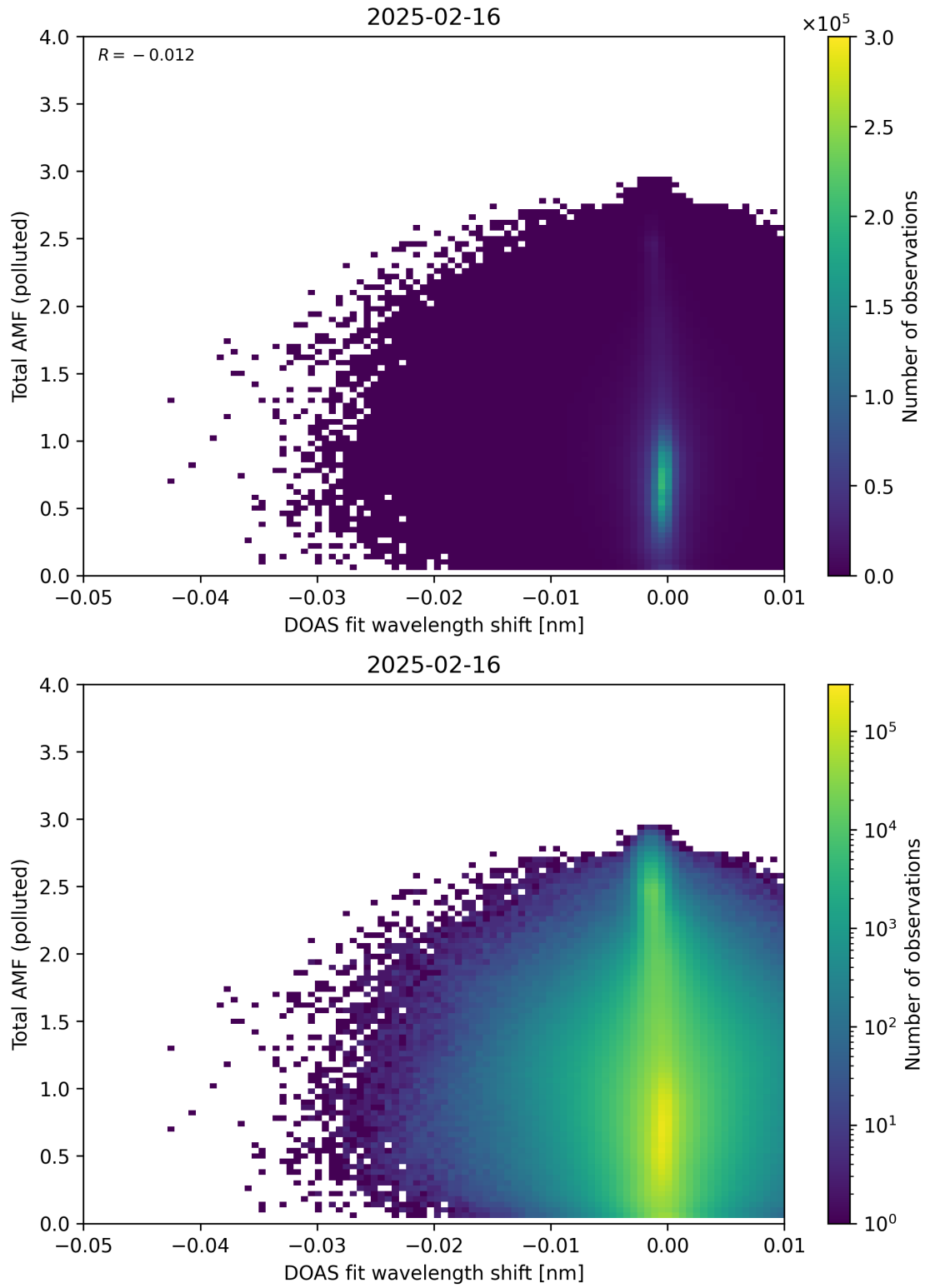
Figure 141: Scatter density plot of “DOAS fit wavelength shift” against “Total AMF (polluted)” for 2025-02-15 to 2025-02-17.
