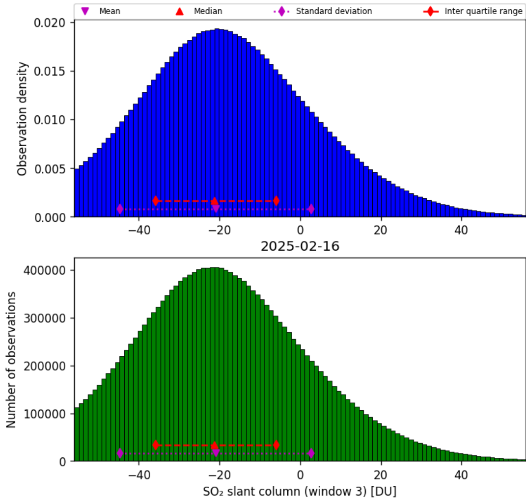
Figure 71: Histogram of “SO 2 slant column (window 3)” for 2025-02-15 to 2025-02-17
