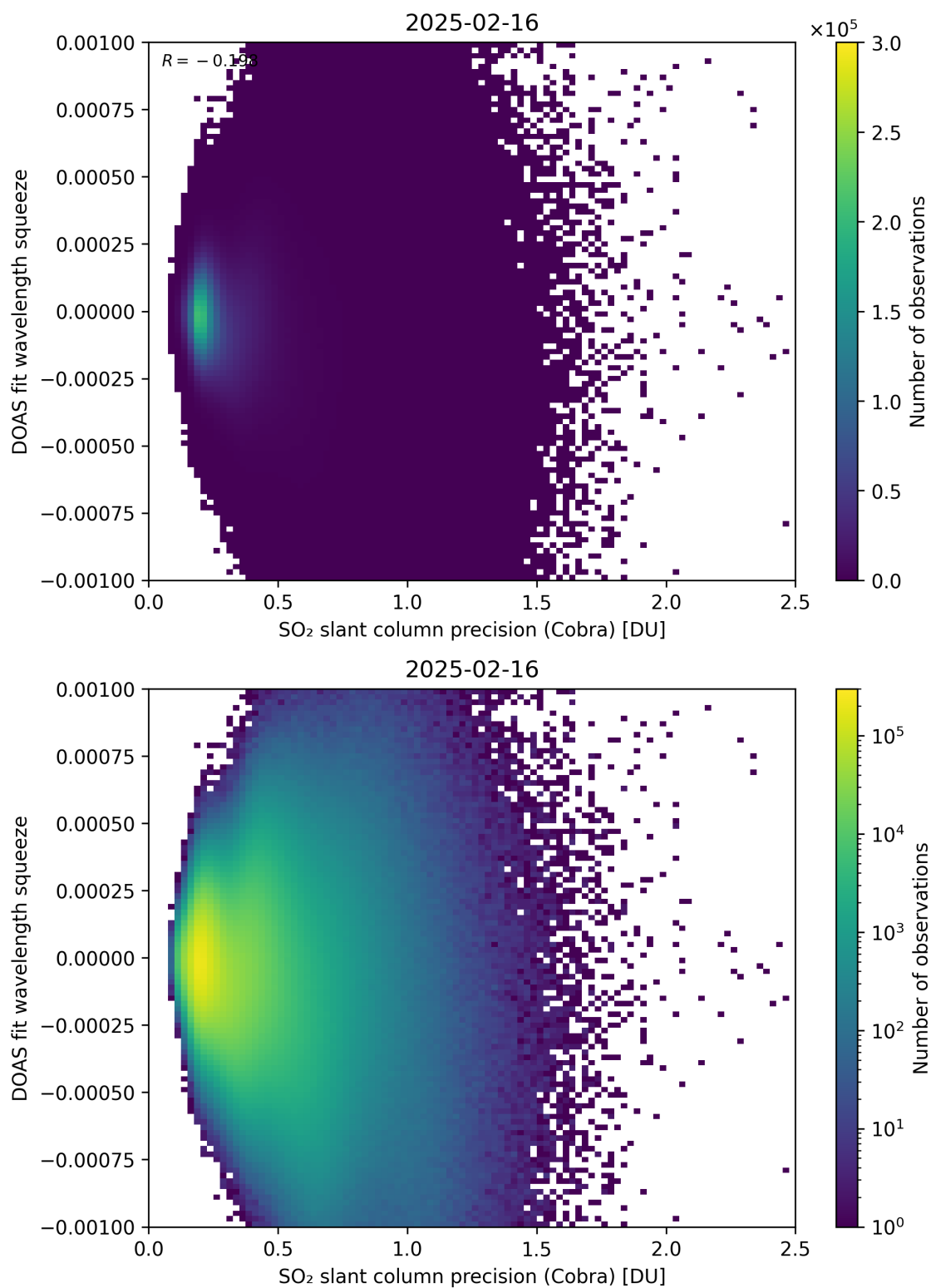
Figure 203: Scatter density plot of “SO 2 slant column precision (Cobra)” against “DOAS fit wavelength squeeze” for 2025-02-15 to 2025-02-17.
