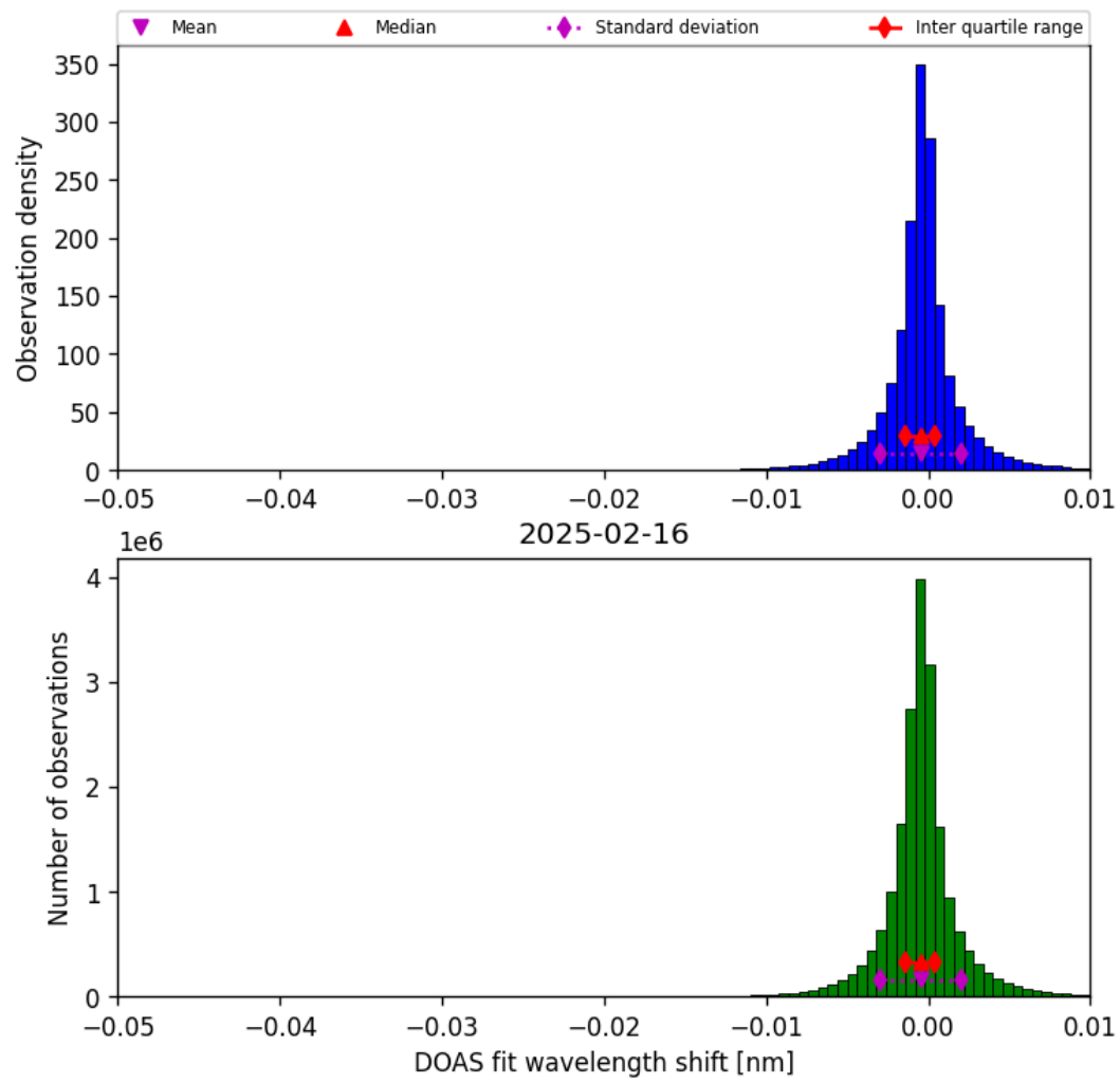
Figure 76: Histogram of “DOAS fit wavelength shift” for 2025-02-15 to 2025-02-17
