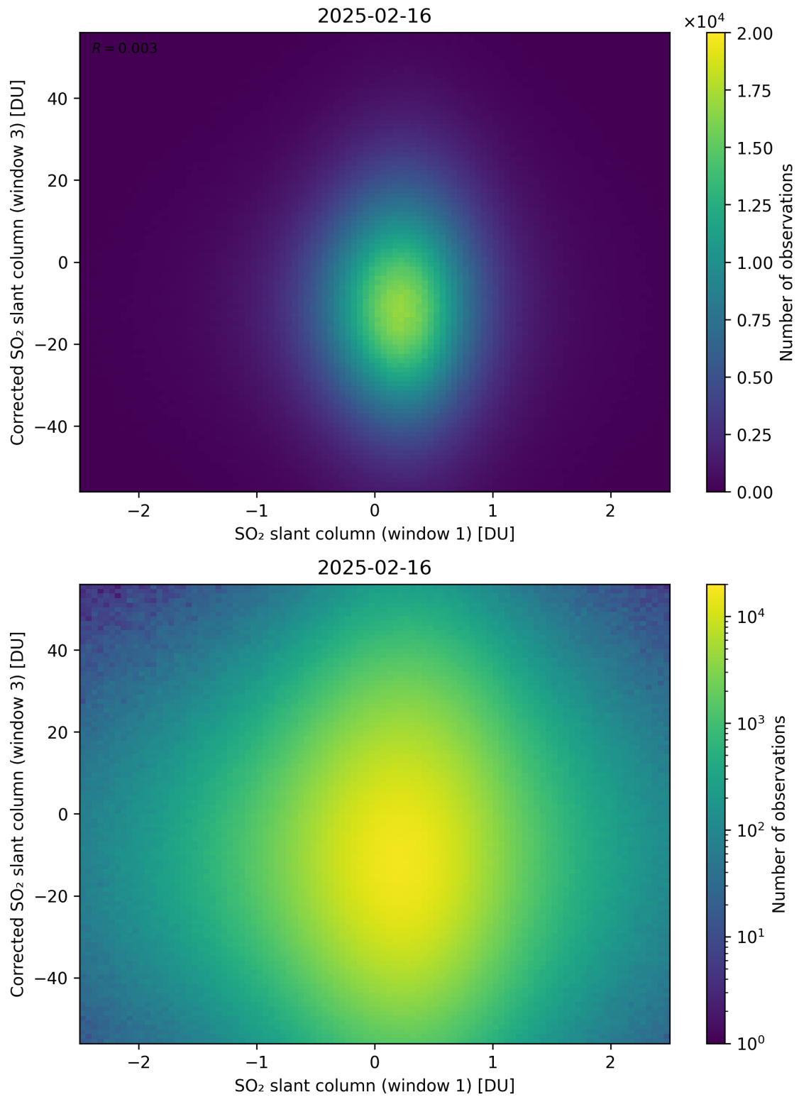
Figure 284: Scatter density plot of “SO 2 slant column (window 1)” against “Corrected SO 2 slant column (window 3)” for 2025-02-15 to 2025-02-17.
