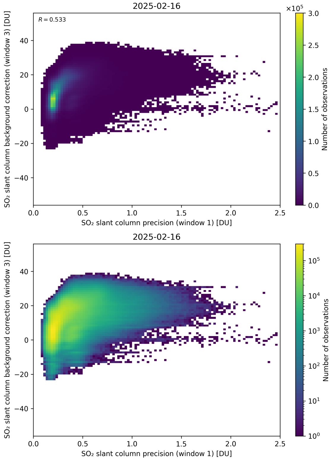
Figure 270: Scatter density plot of “SO 2 slant column precision (window 1)” against “SO 2 slant column background correction (window 3)” for 2025-02-15 to 2025-02-17.
