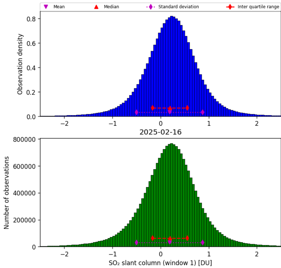
Figure 63: Histogram of “SO 2 slant column (window 1)” for 2025-02-15 to 2025-02-17
