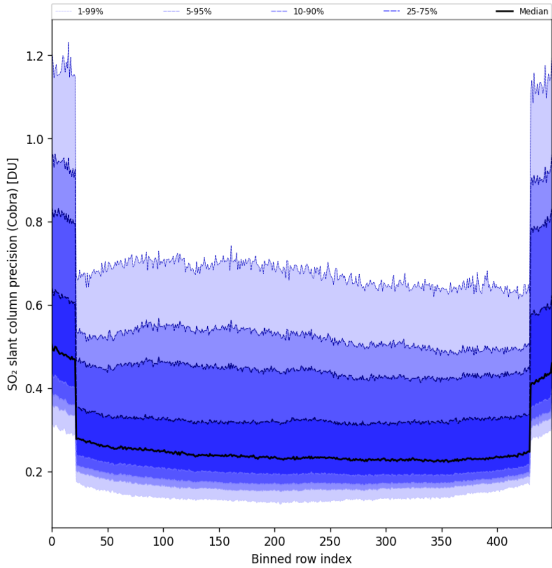
Figure 88: Along track statistics of “SO 2 slant column precision (Cobra)” for 2025-02-15 to 2025-02-17
