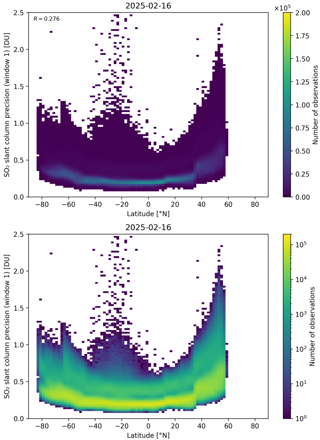
Figure 163: Scatter density plot of “Latitude” against “SO 2 slant column precision (window 1)” for 2025-02-15 to 2025-02-17.
