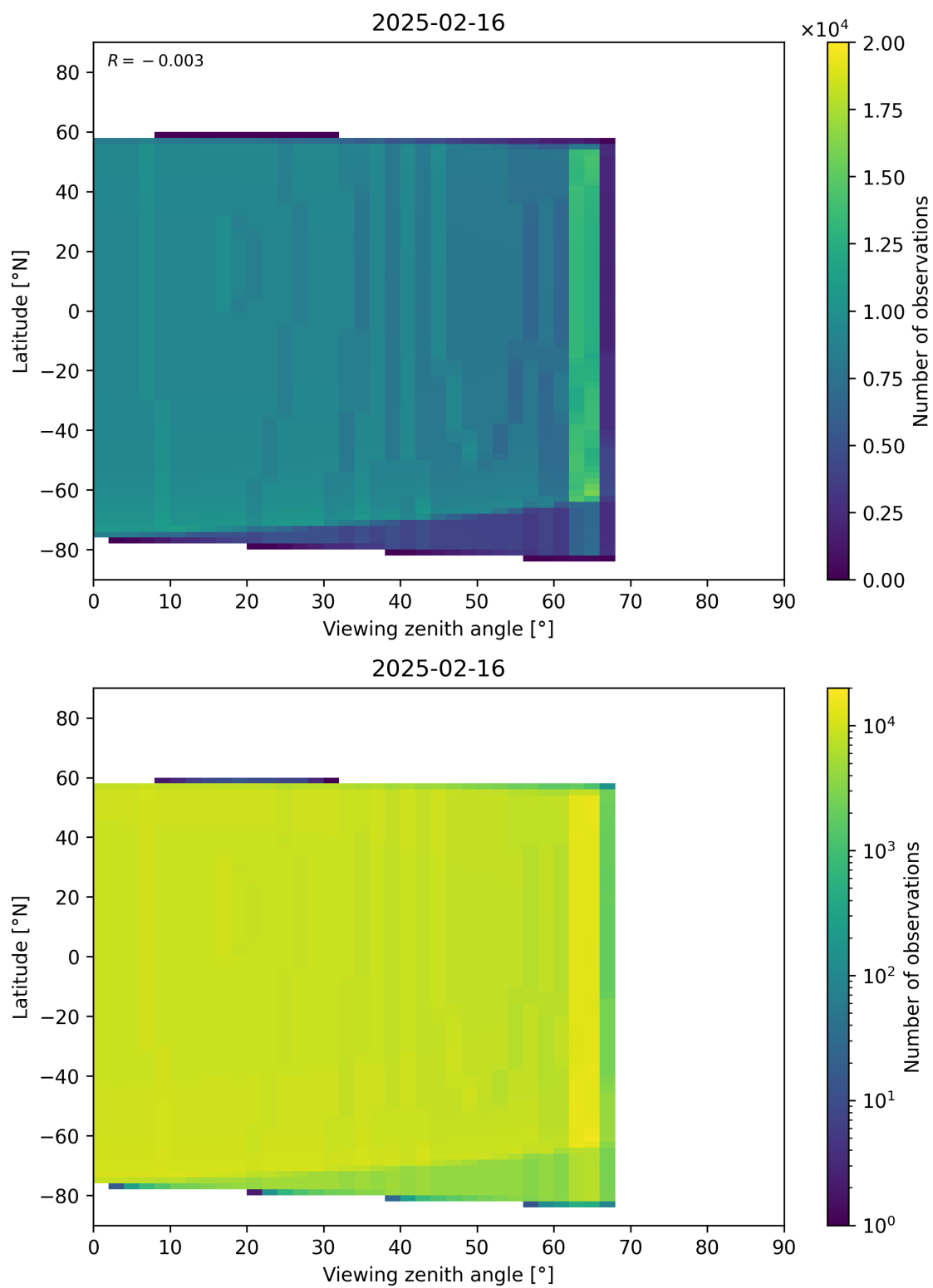
Figure 368: Scatter density plot of “Viewing zenith angle” against “Latitude” for 2025-02-15 to 2025-02-17.
