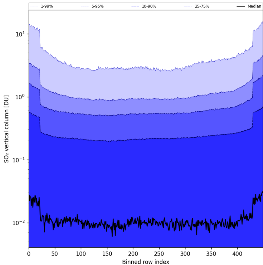
Figure 84: Along track statistics of “SO 2 vertical column” for 2025-02-15 to 2025-02-17
