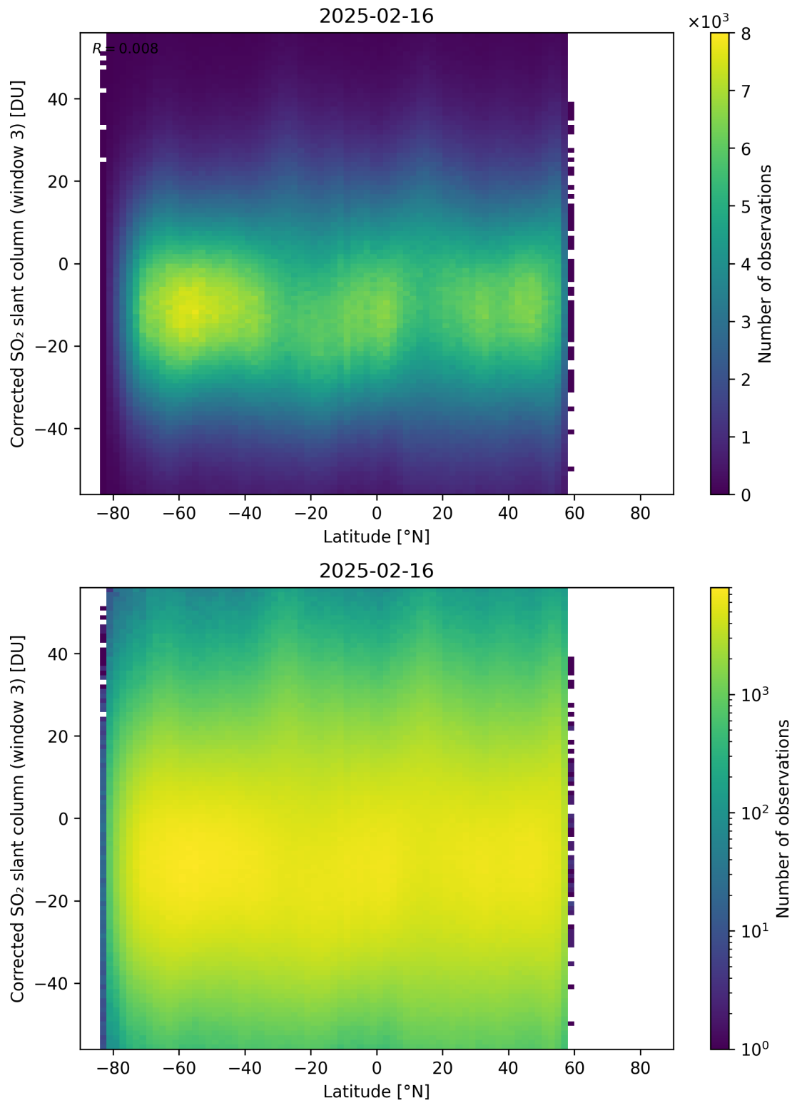
Figure 161: Scatter density plot of “Latitude” against “Corrected SO 2 slant column (window 3)” for 2025-02-15 to 2025-02-17.
