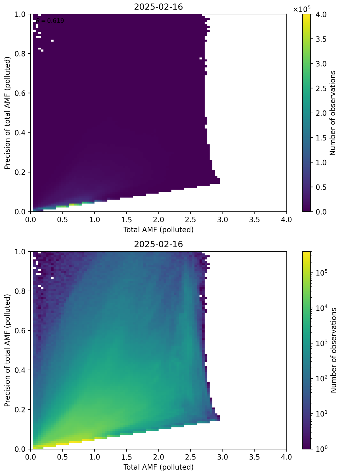
Figure 322: Scatter density plot of “Total AMF (polluted)” against “Precision of total AMF (polluted)” for 2025-02-15 to 2025-02-17.
