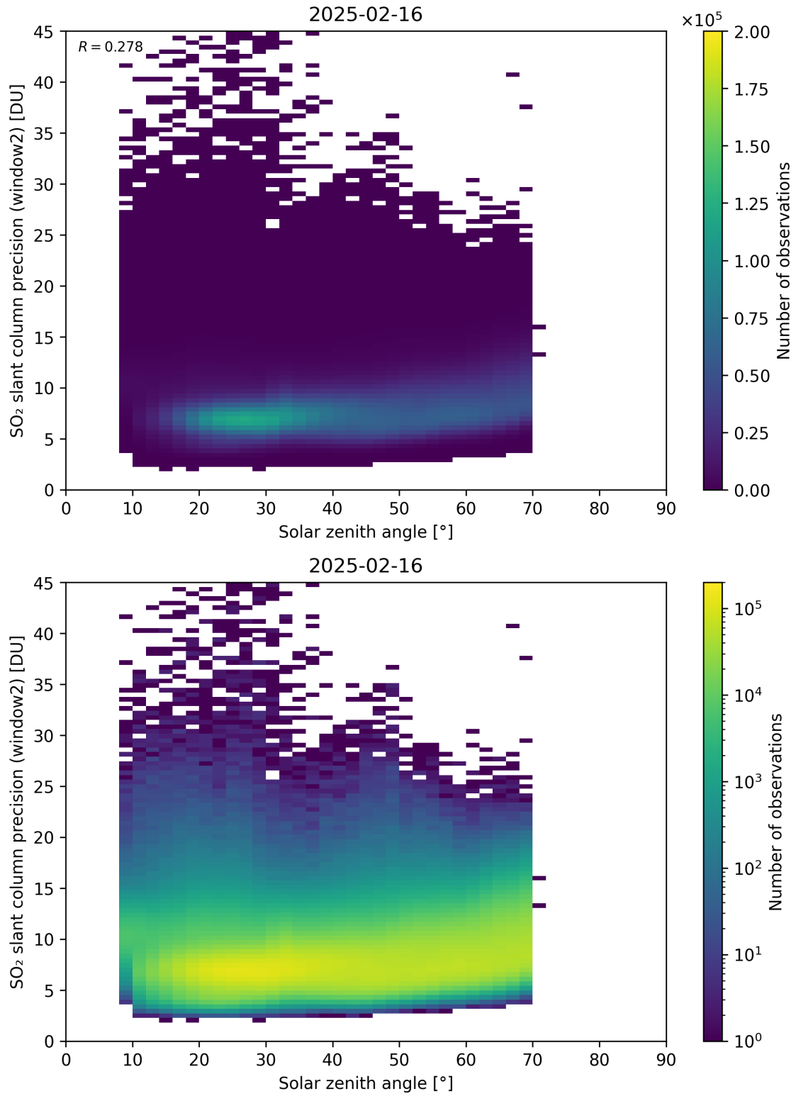
Figure 186: Scatter density plot of “Solar zenith angle” against “SO 2 slant column precision (window2)” for 2025-02-15 to 2025-02-17.
