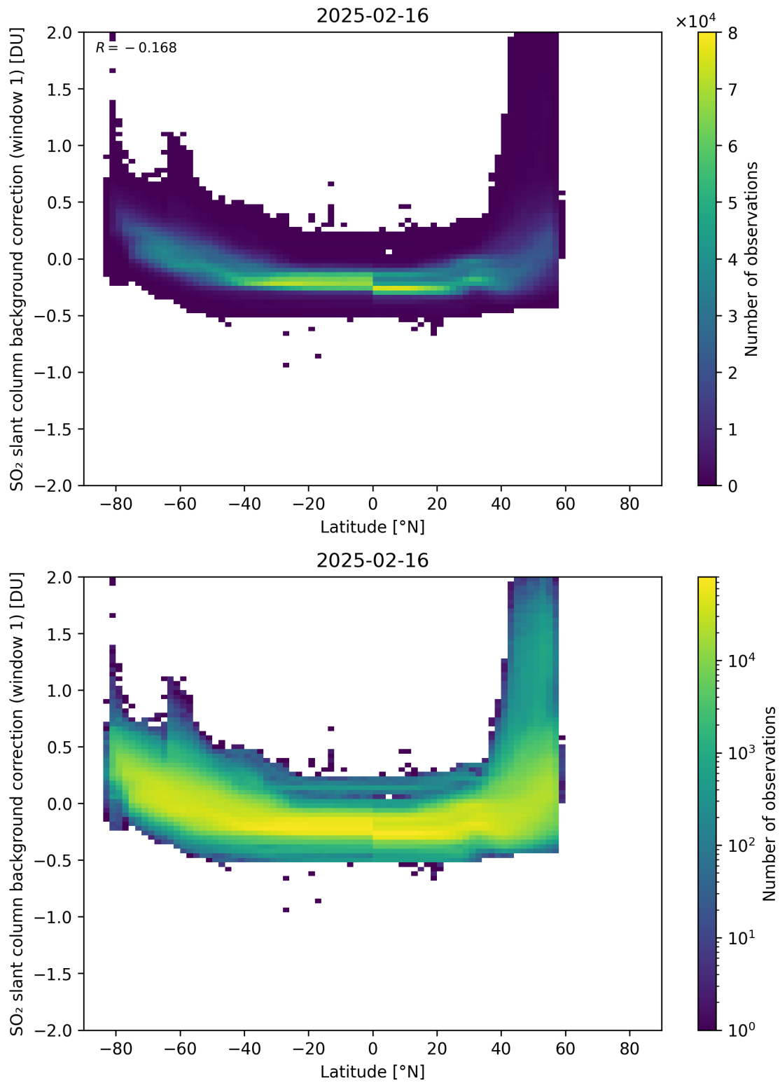
Figure 150: Scatter density plot of “Latitude” against “SO 2 slant column background correction (window 1)” for 2025-02-15 to 2025-02-17.
