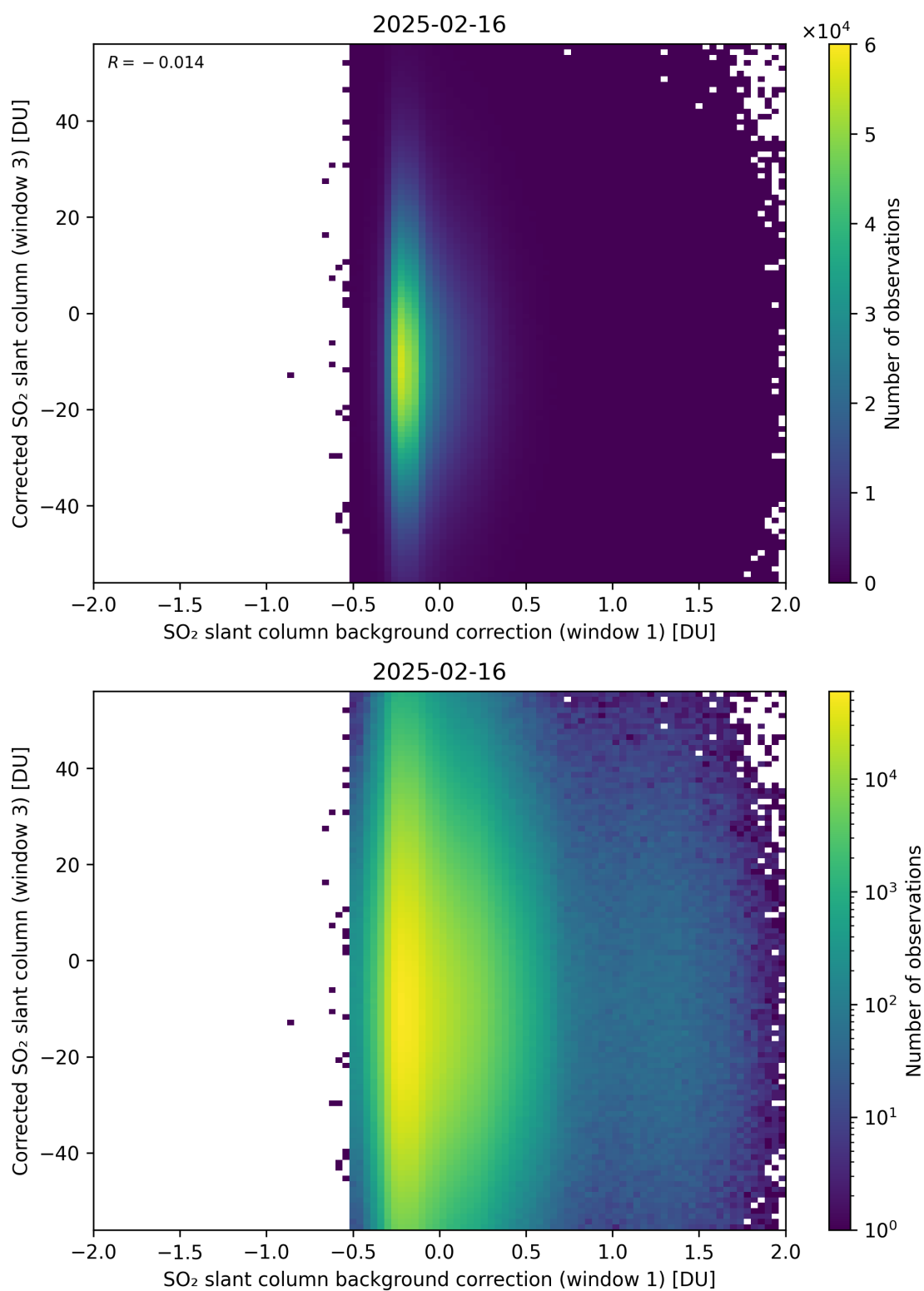
Figure 116: Scatter density plot of “SO 2 slant column background correction (window 1)” against “Corrected SO 2 slant column (window 3)” for 2025-02-15 to 2025-02-17.
