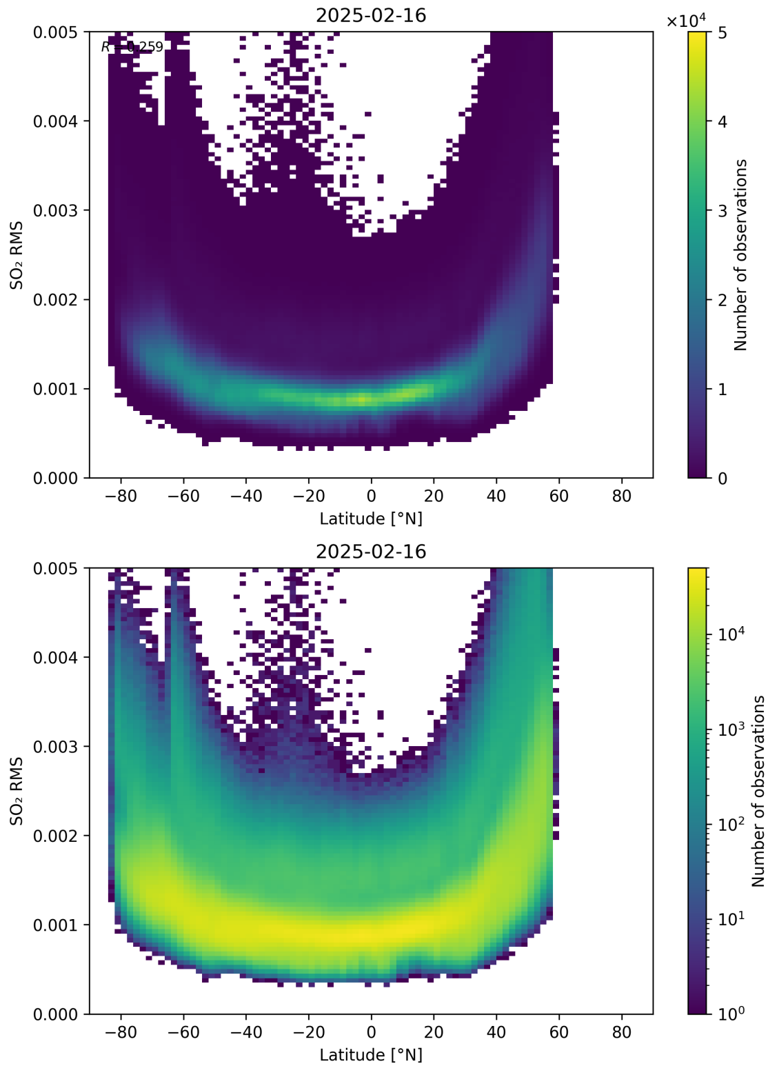
Figure 155: Scatter density plot of “Latitude” against “SO 2 RMS” for 2025-02-15 to 2025-02-17.
