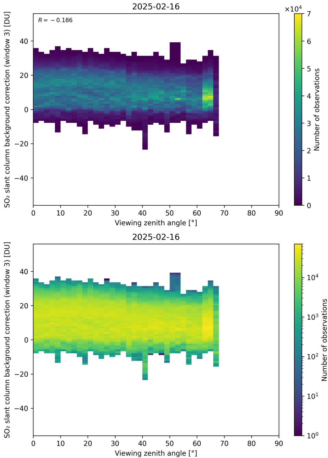
Figure 364: Scatter density plot of “Viewing zenith angle” against “SO 2 slant column background correction (window 3)” for 2025-02-15 to 2025-02-17.
