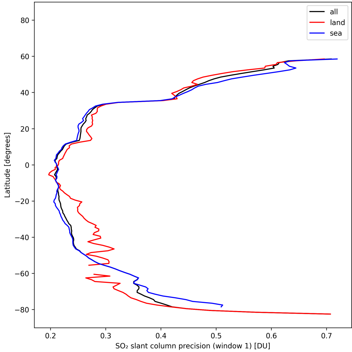
Figure 38: Zonal average of “SO 2 slant column precision (window 1)” for 2025-02-15 to 2025-02-17.
