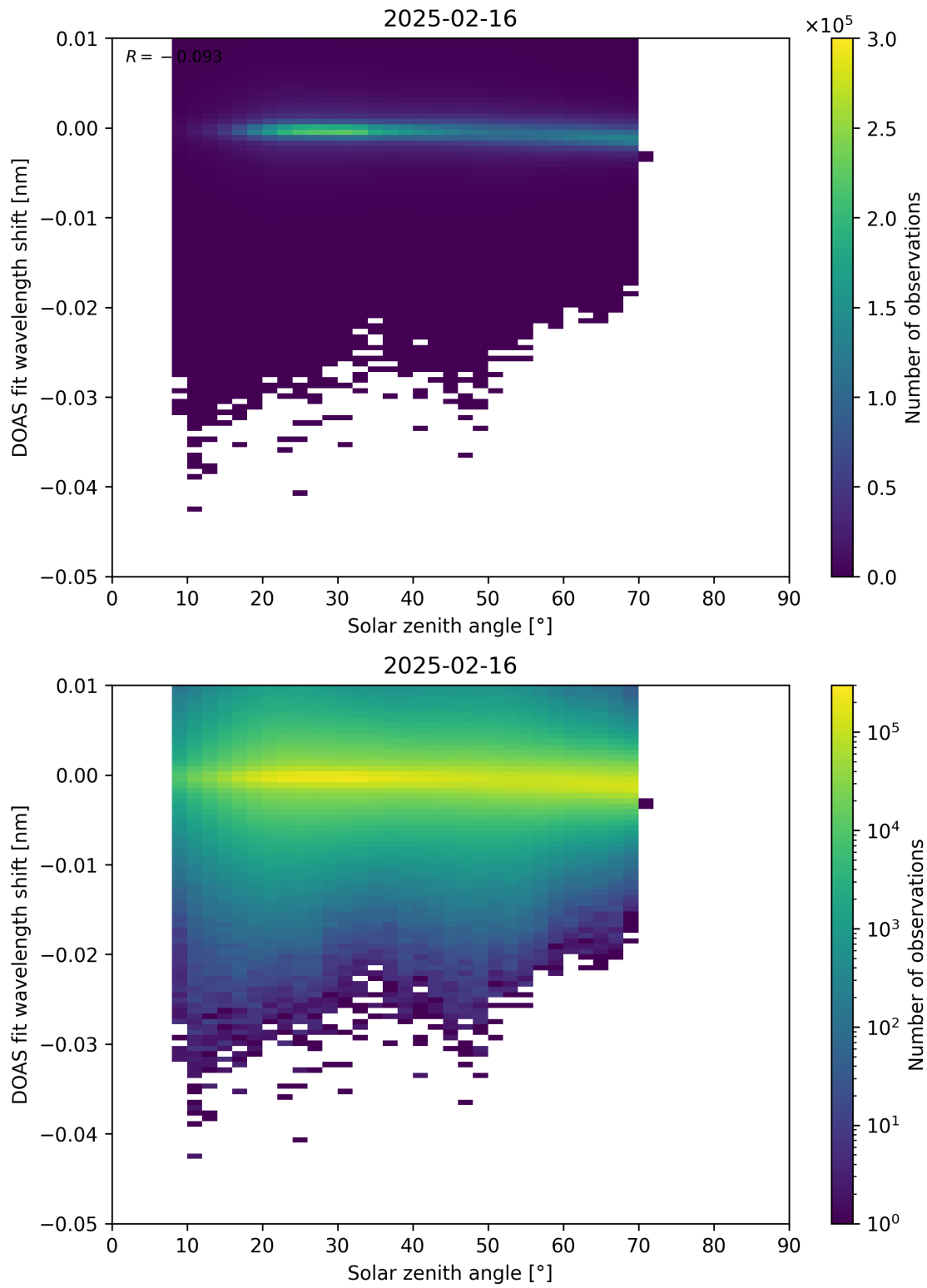
Figure 174: Scatter density plot of “Solar zenith angle” against “DOAS fit wavelength shift” for 2025-02-15 to 2025-02-17.
