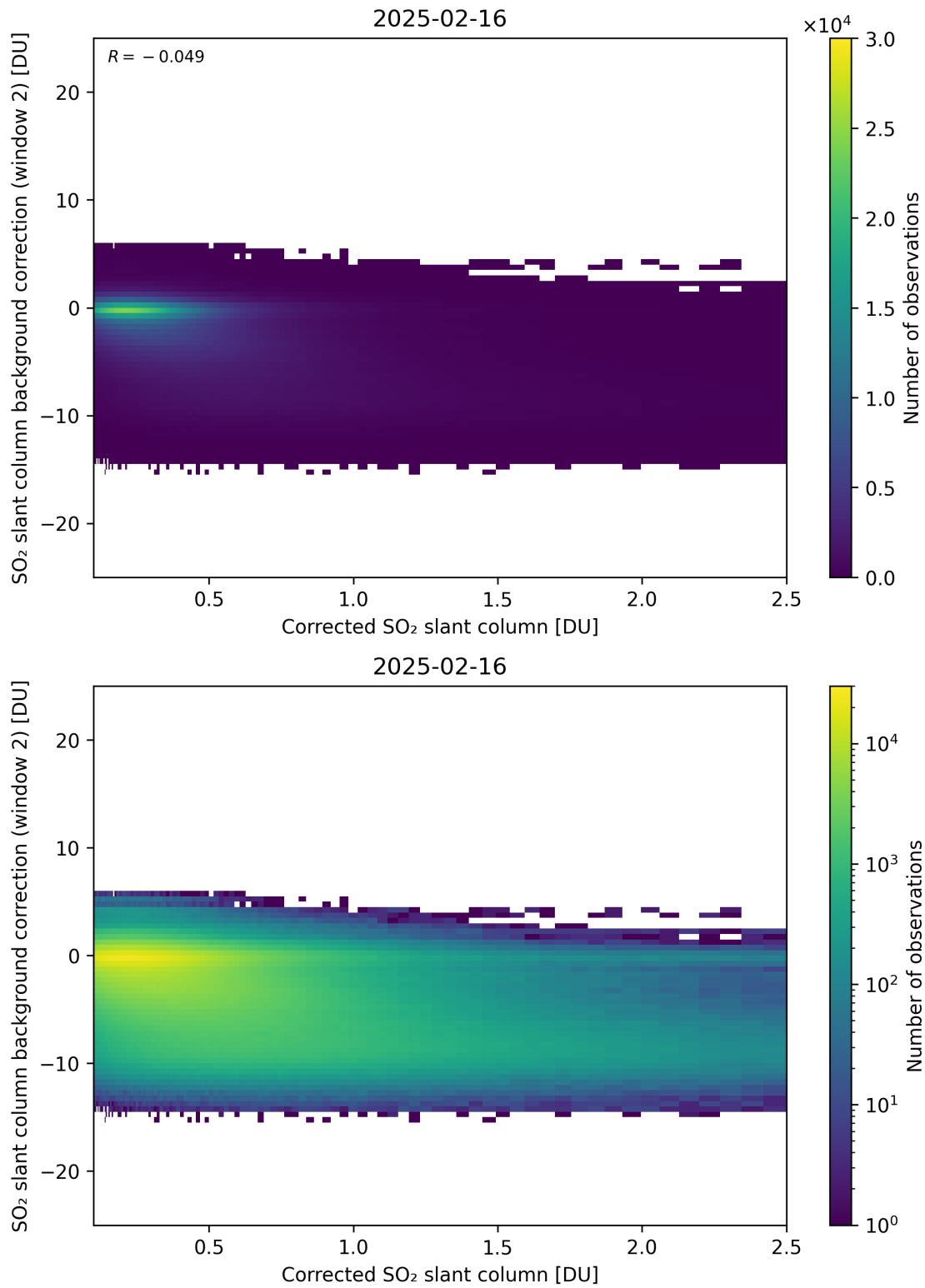
Figure 227: Scatter density plot of “Corrected SO 2 slant column” against “SO 2 slant column background correction (window 2)” for 2025-02-15 to 2025-02-17.
