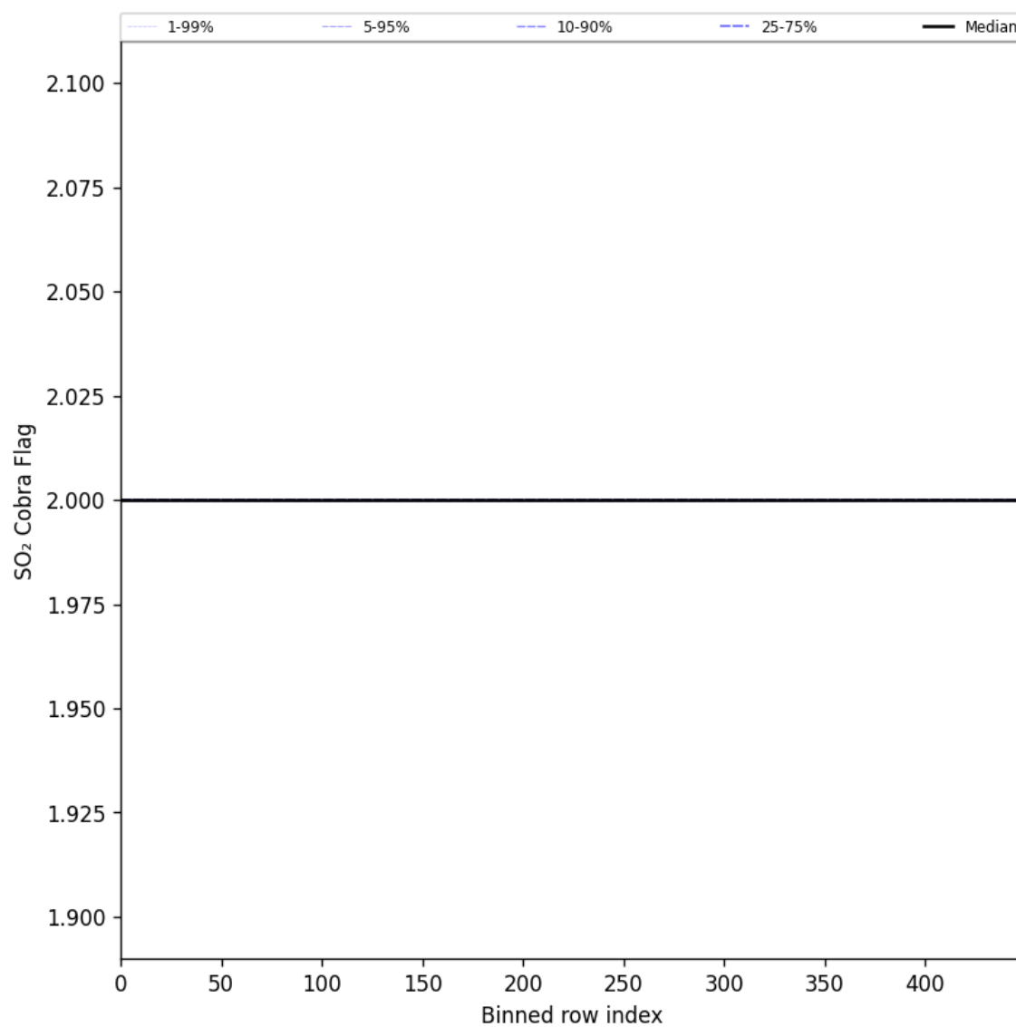
Figure 101: Along track statistics of “SO 2 Cobra Flag” for 2025-02-15 to 2025-02-17
