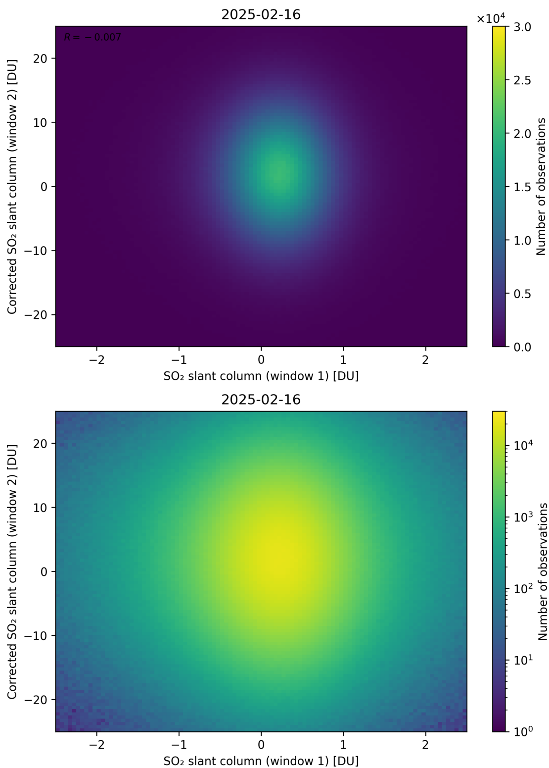
Figure 283: Scatter density plot of “SO 2 slant column (window 1)” against “Corrected SO 2 slant column (window 2)” for 2025-02-15 to 2025-02-17.
