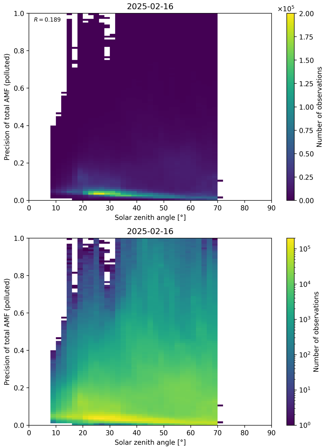
Figure 190: Scatter density plot of “Solar zenith angle” against “Precision of total AMF (polluted)” for 2025-02-15 to 2025-02-17.
