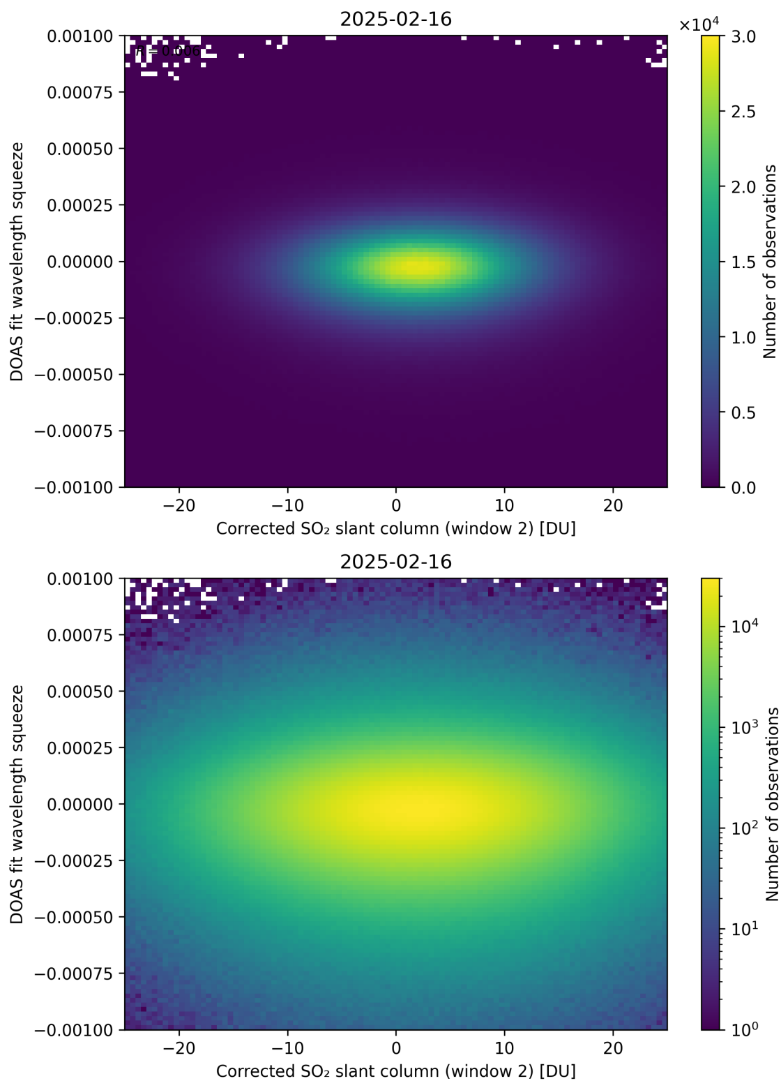
Figure 247: Scatter density plot of “Corrected SO 2 slant column (window 2)” against “DOAS fit wavelength squeeze” for 2025-02-15 to 2025-02-17.
