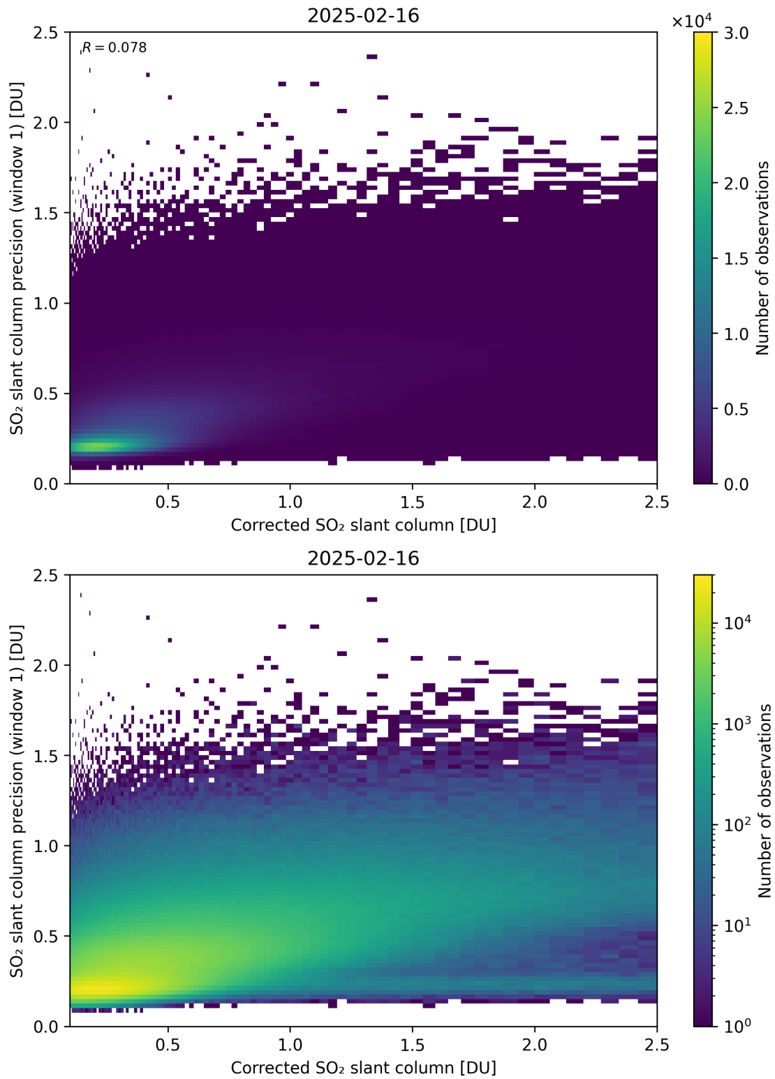
Figure 238: Scatter density plot of “Corrected SO 2 slant column” against “SO 2 slant column precision (window 1)” for 2025-02-15 to 2025-02-17.
