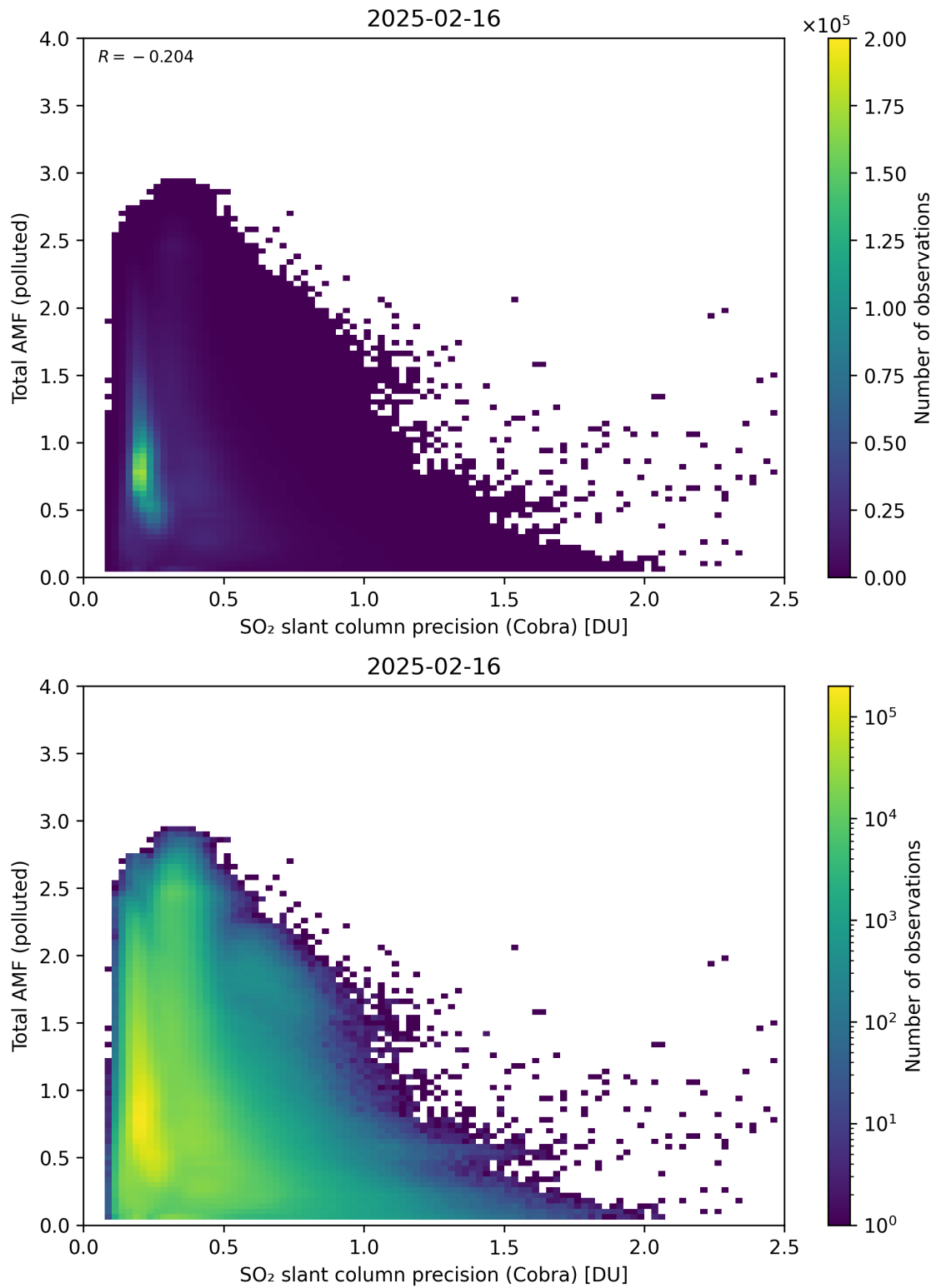
Figure 213: Scatter density plot of “SO 2 slant column precision (Cobra)” against “Total AMF (polluted)” for 2025-02-15 to 2025-02-17.
