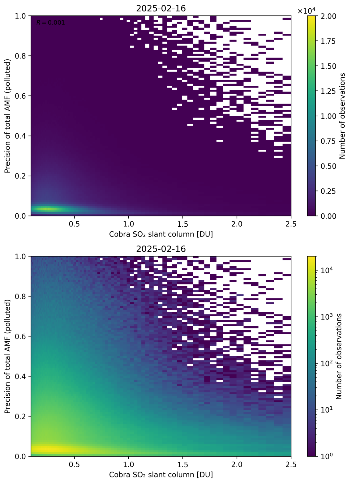
Figure 225: Scatter density plot of “Cobra SO 2 slant column” against “Precision of total AMF (polluted)” for 2025-02-15 to 2025-02-17.
