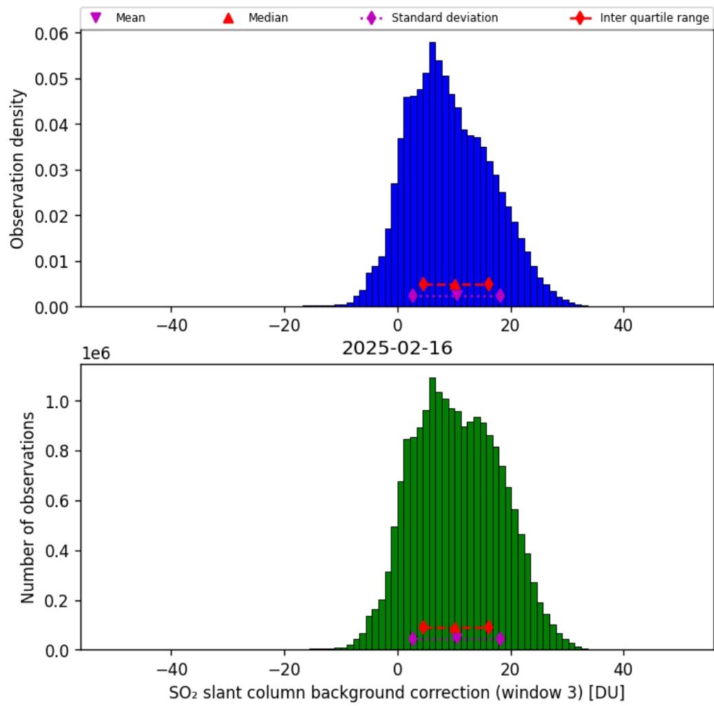
Figure 74: Histogram of “SO 2 slant column background correction (window 3)” for 2025-02-15 to 2025-02-17
