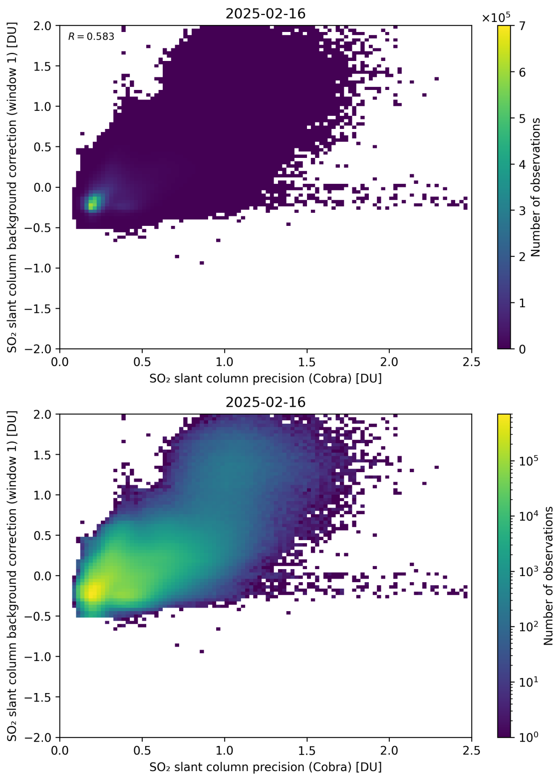
Figure 199: Scatter density plot of “SO 2 slant column precision (Cobra)” against “SO 2 slant column background correction (window 1)” for 2025-02-15 to 2025-02-17.
