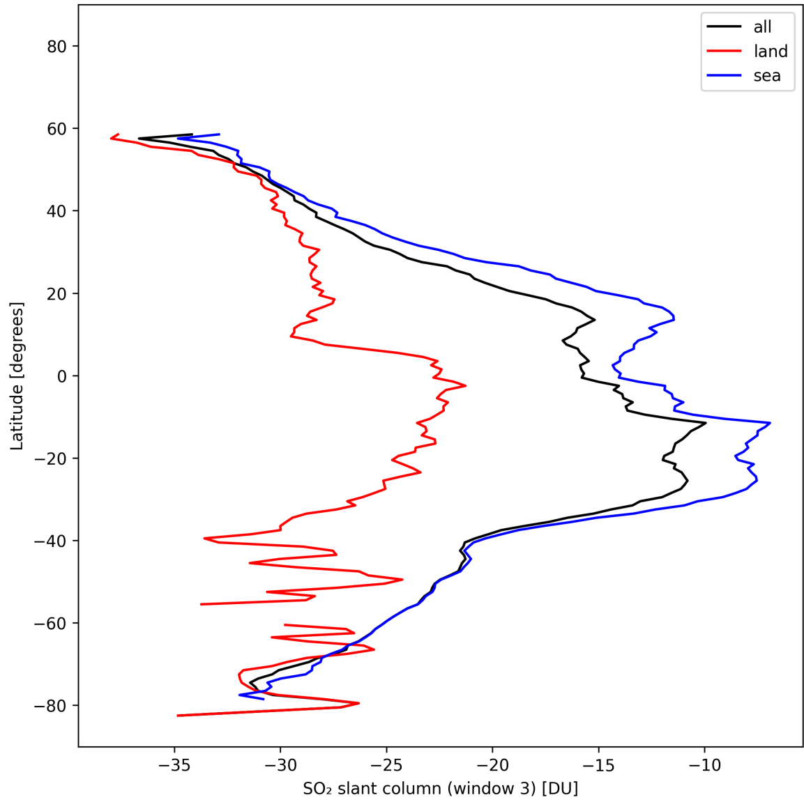
Figure 45: Zonal average of “SO 2 slant column (window 3)” for 2025-02-15 to 2025-02-17.
