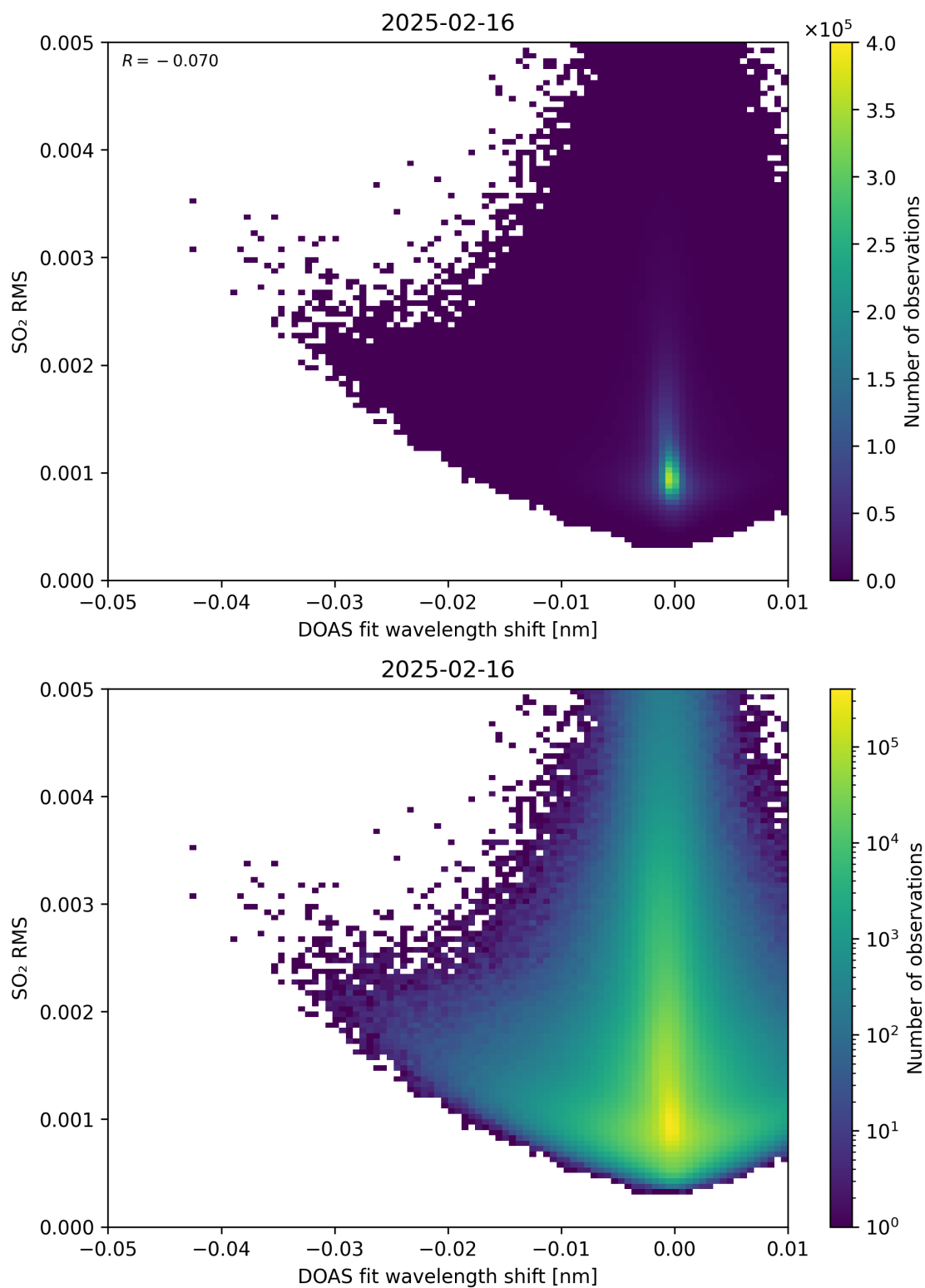
Figure 139: Scatter density plot of “DOAS fit wavelength shift” against “SO 2 RMS” for 2025-02-15 to 2025-02-17.
