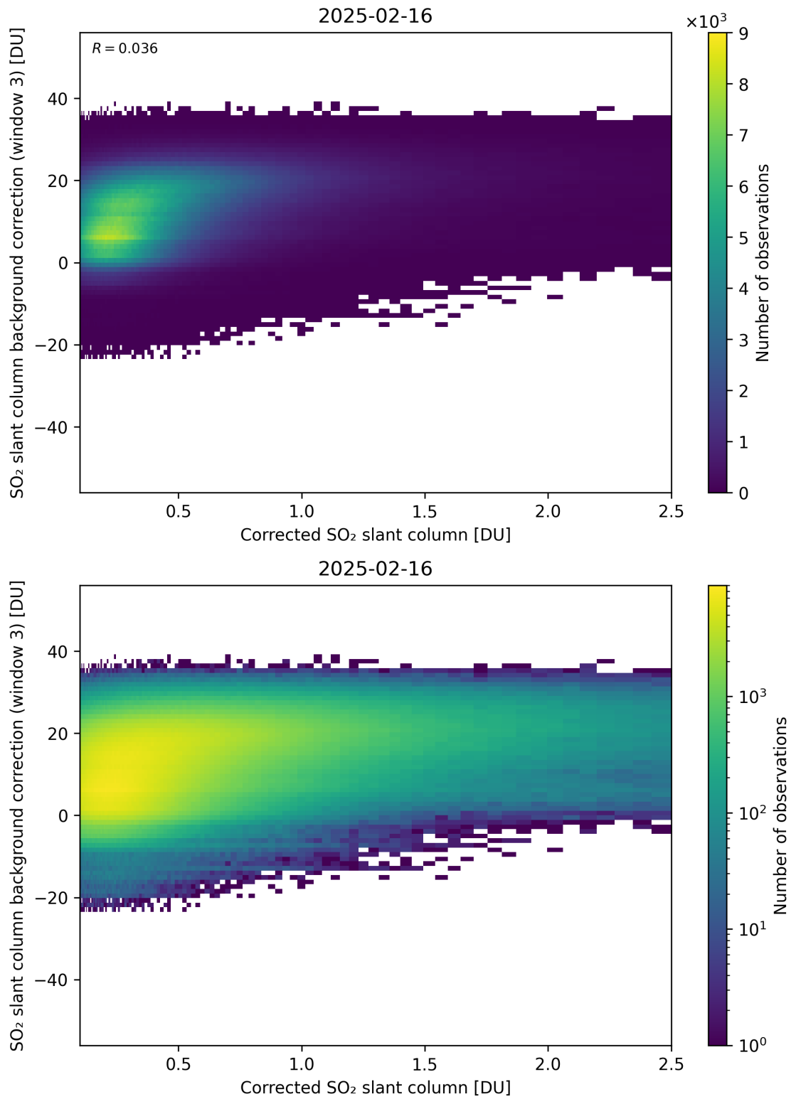
Figure 228: Scatter density plot of “Corrected SO 2 slant column” against “SO 2 slant column background correction (window 3)” for 2025-02-15 to 2025-02-17.
