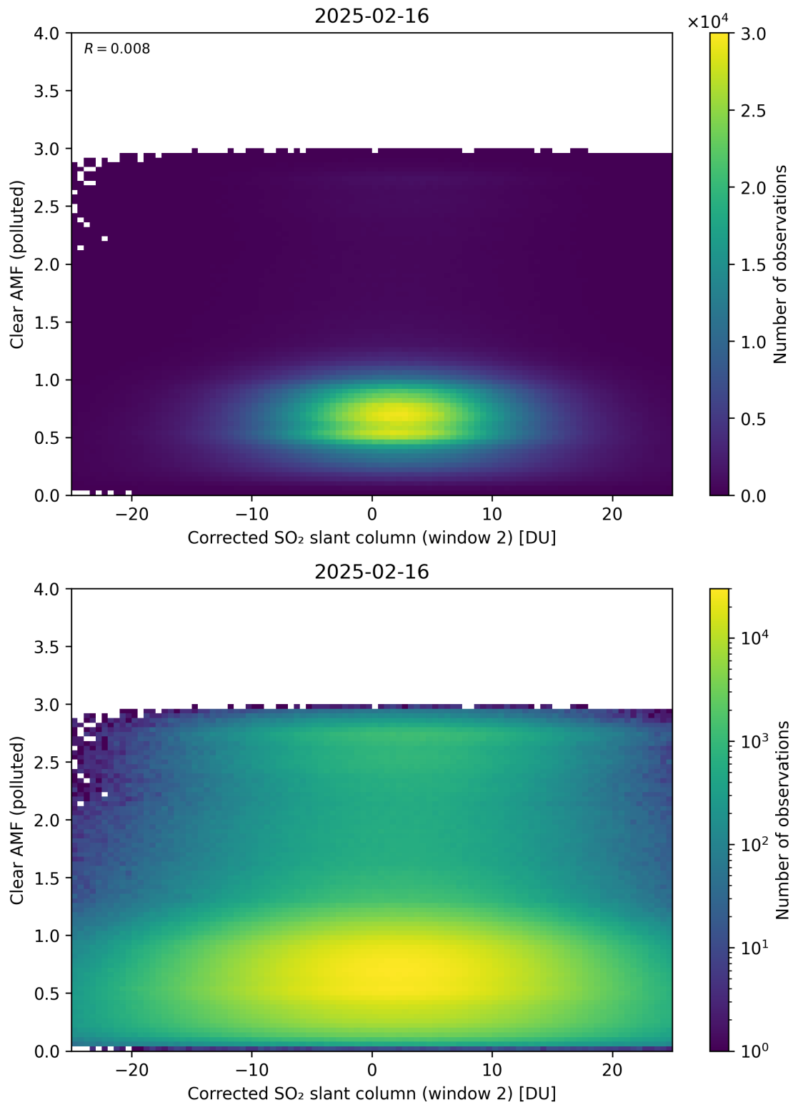
Figure 249: Scatter density plot of “Corrected SO 2 slant column (window 2)” against “Clear AMF (polluted)” for 2025-02-15 to 2025-02-17.
