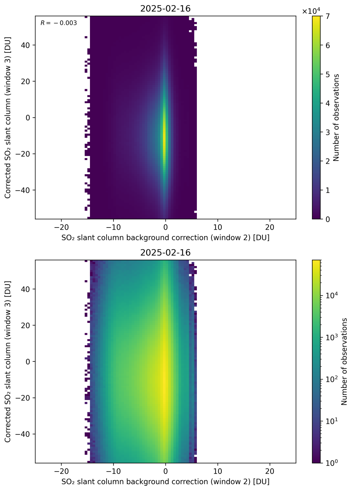
Figure 127: Scatter density plot of “SO 2 slant column background correction (window 2)” against “Corrected SO 2 slant column (window 3)” for 2025-02-15 to 2025-02-17.
