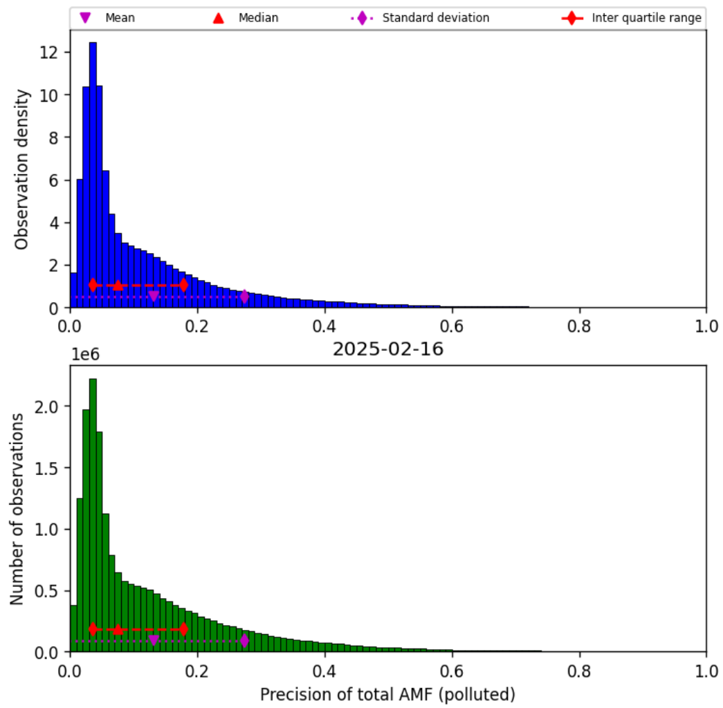
Figure 80: Histogram of “Precision of total AMF (polluted)” for 2025-02-15 to 2025-02-17
