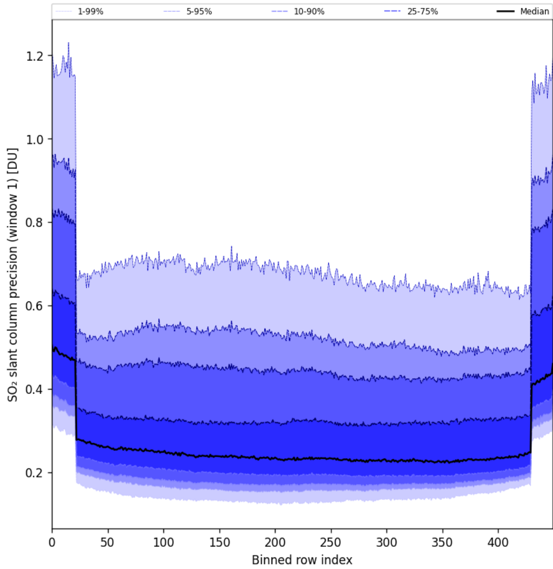
Figure 90: Along track statistics of “SO 2 slant column precision (window 1)” for 2025-02-15 to 2025-02-17
