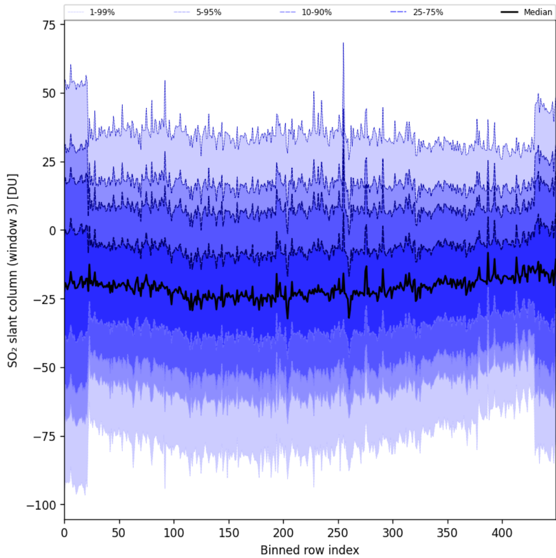
Figure 97: Along track statistics of “SO 2 slant column (window 3)” for 2025-02-15 to 2025-02-17
