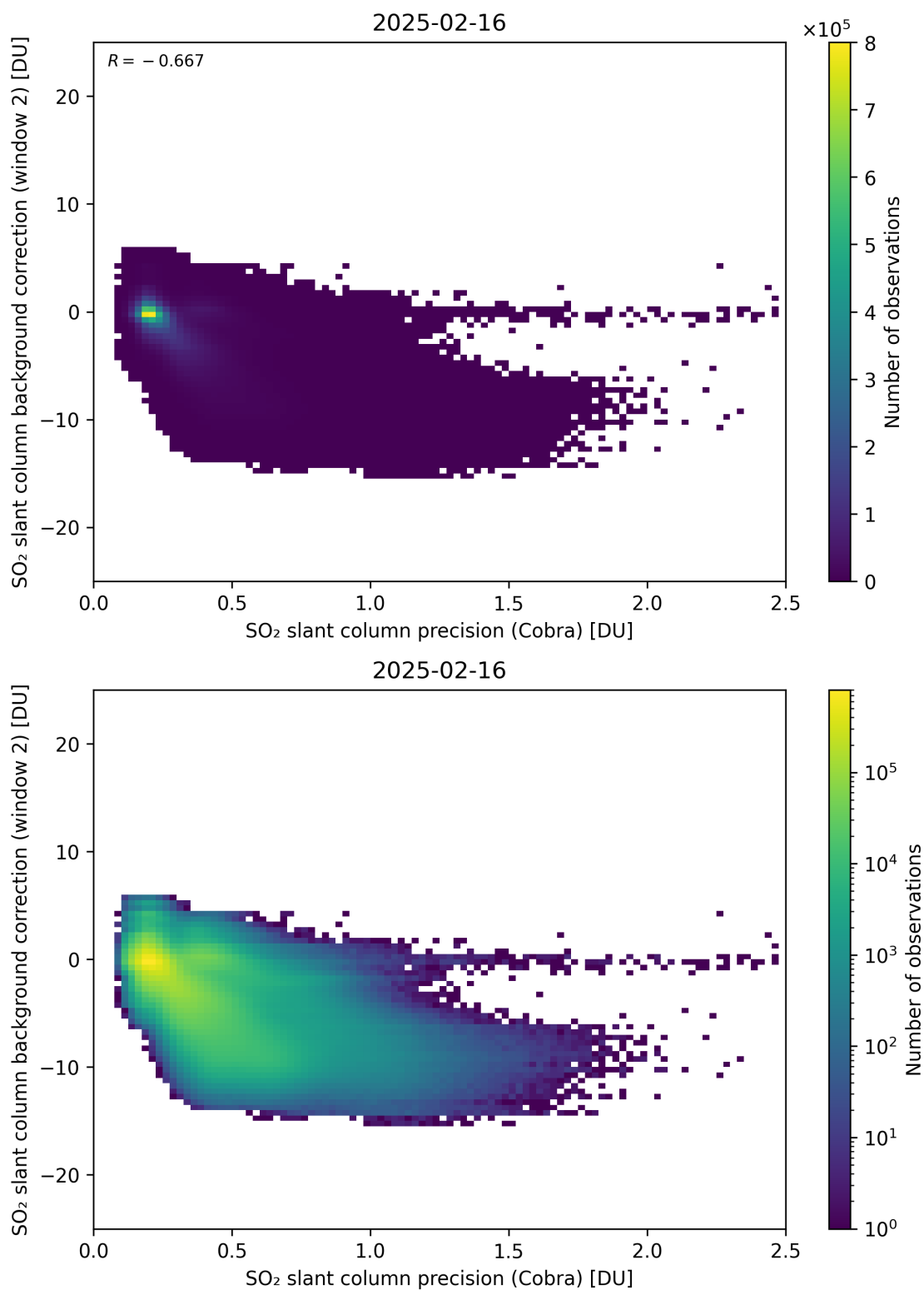
Figure 200: Scatter density plot of “SO 2 slant column precision (Cobra)” against “SO 2 slant column background correction (window 2)” for 2025-02-15 to 2025-02-17.
