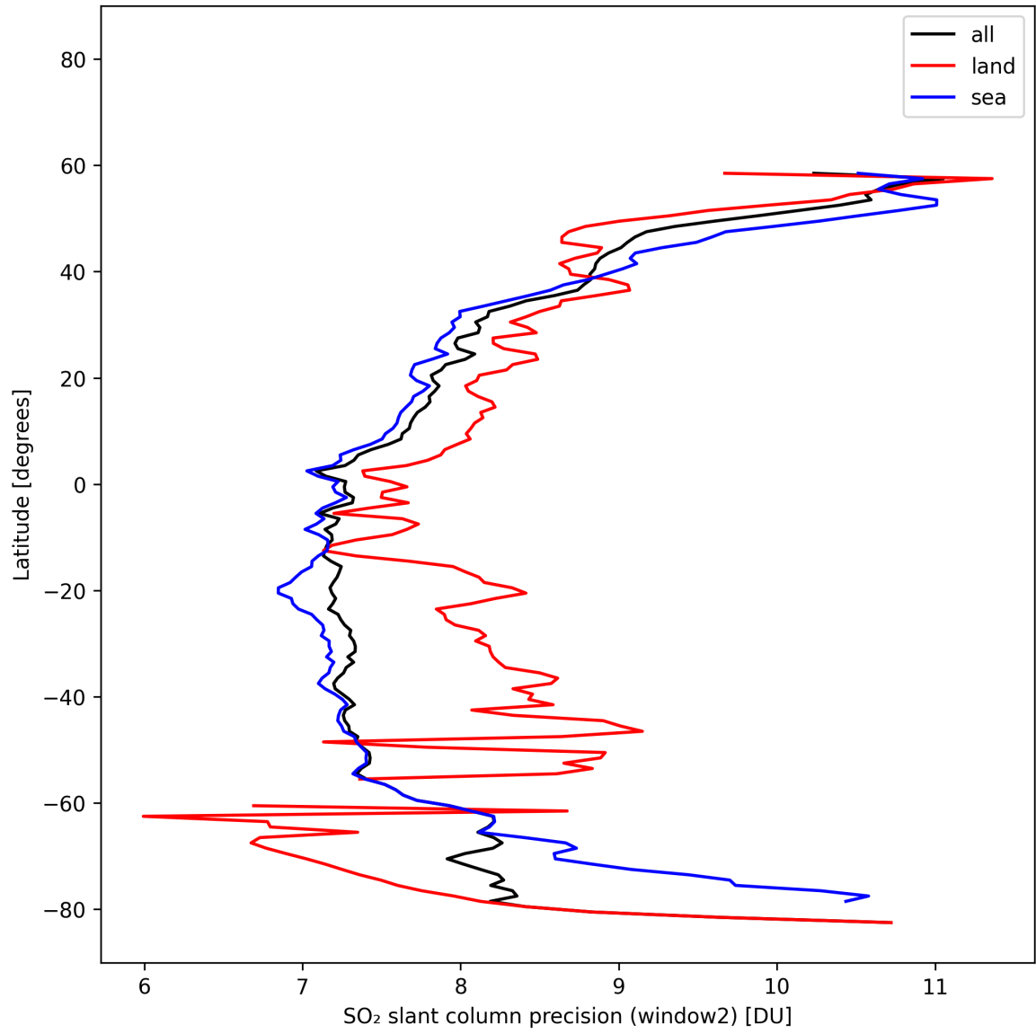
Figure 42: Zonal average of “SO 2 slant column precision (window2)” for 2025-02-15 to 2025-02-17.
