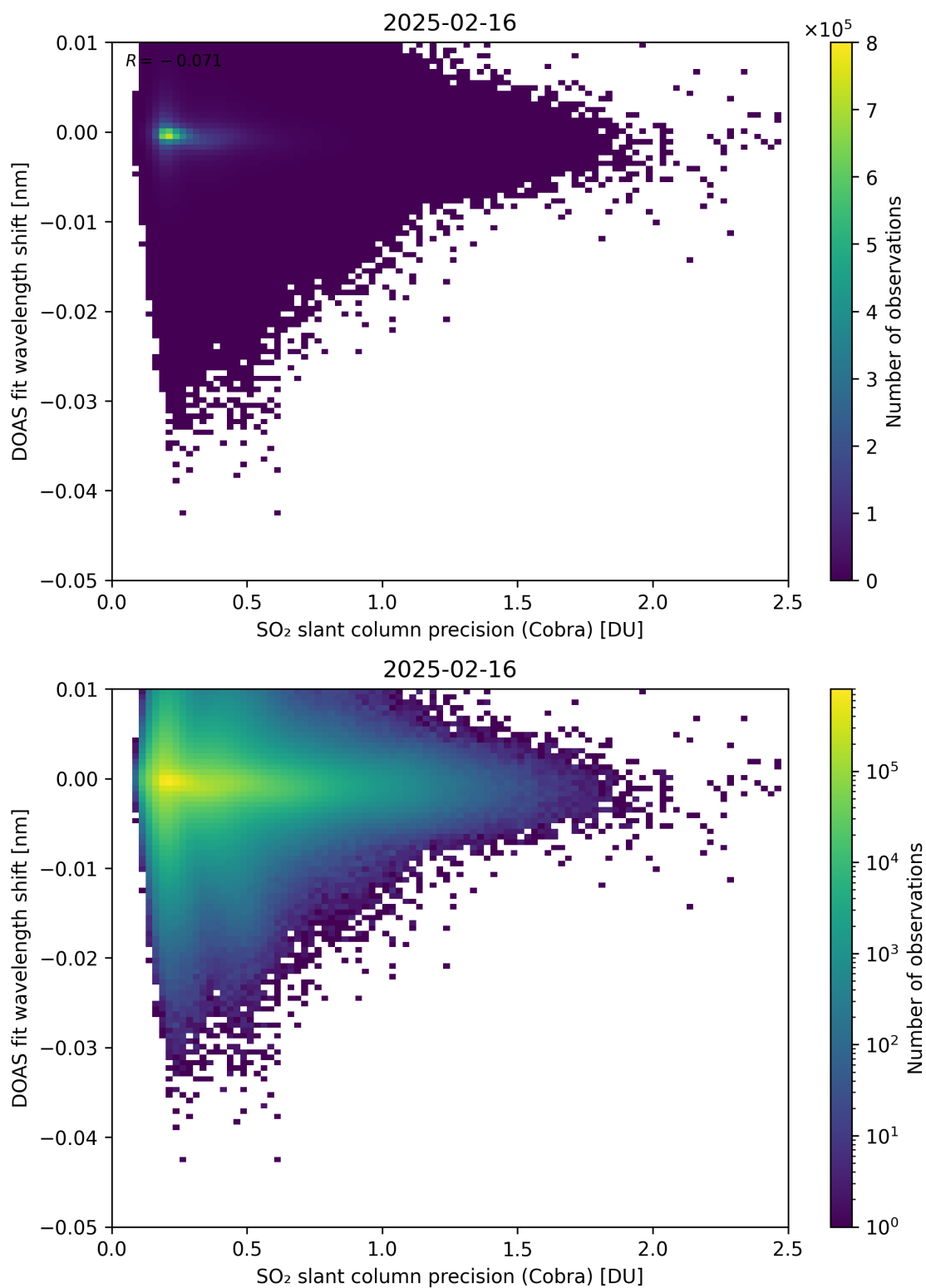
Figure 202: Scatter density plot of “SO 2 slant column precision (Cobra)” against “DOAS fit wavelength shift” for 2025-02-15 to 2025-02-17.
