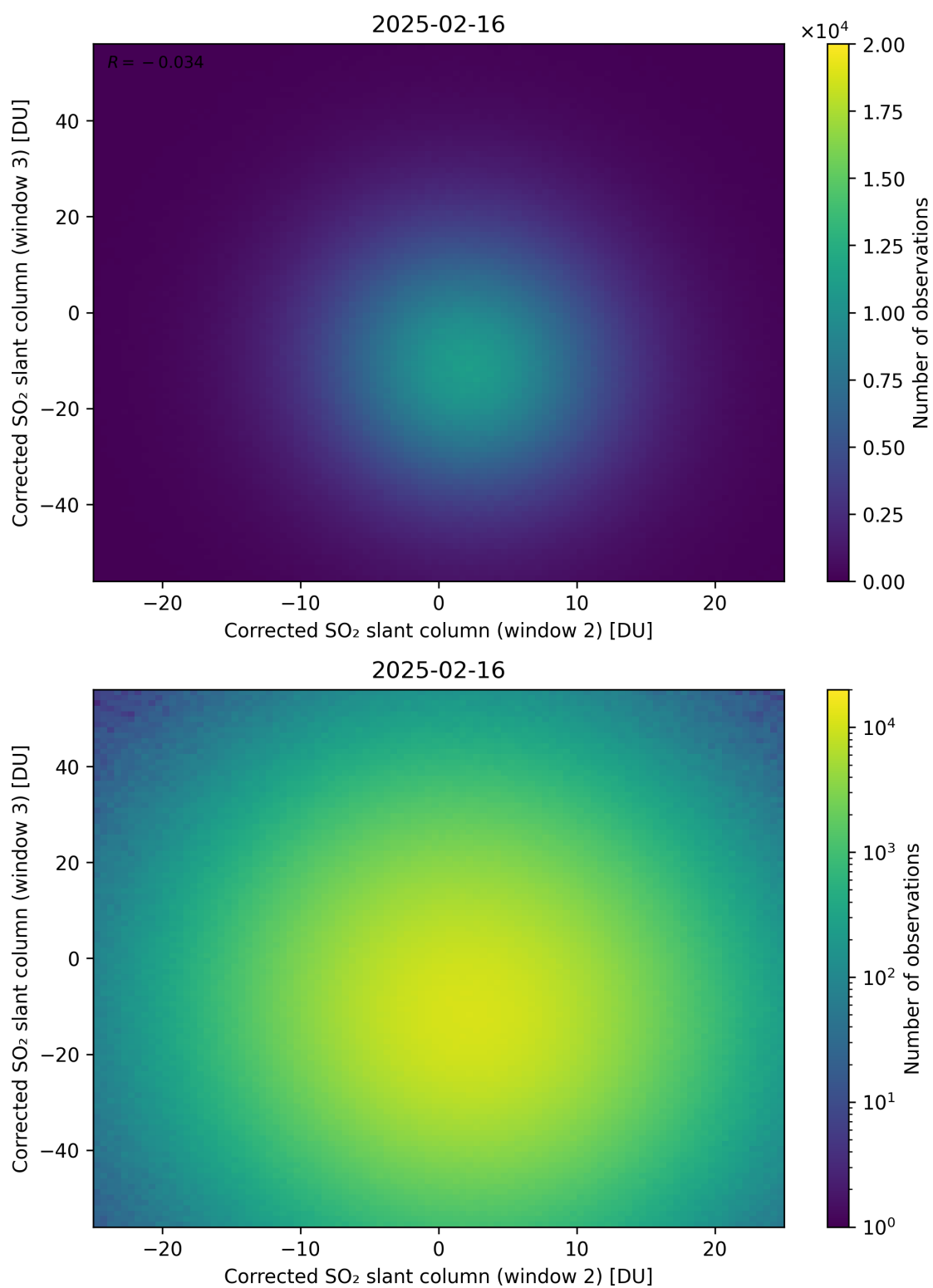
Figure 250: Scatter density plot of “Corrected SO 2 slant column (window 2)” against “Corrected SO 2 slant column (window 3)” for 2025-02-15 to 2025-02-17.
