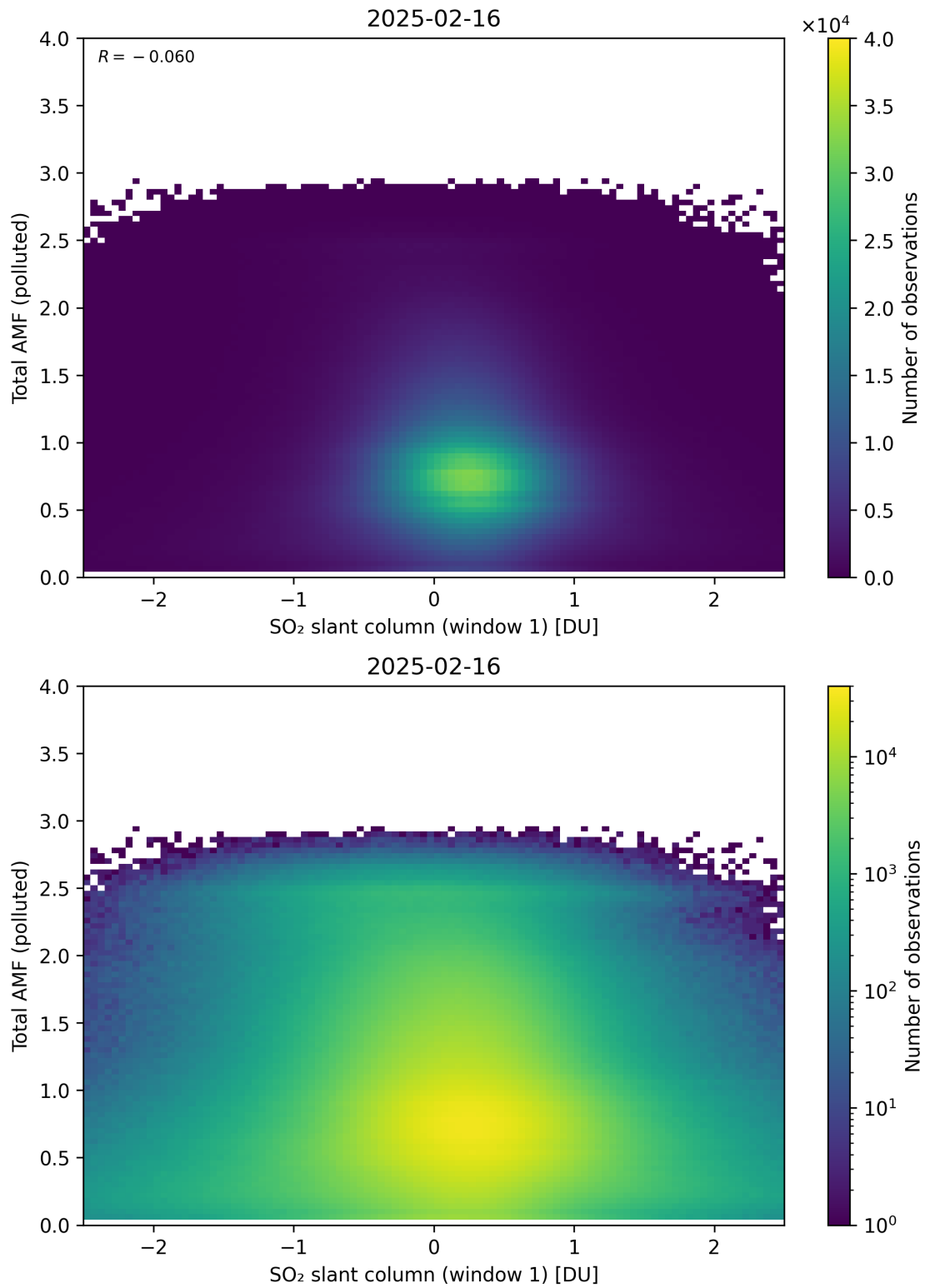
Figure 289: Scatter density plot of “SO 2 slant column (window 1)” against “Total AMF (polluted)” for 2025-02-15 to 2025-02-17.
