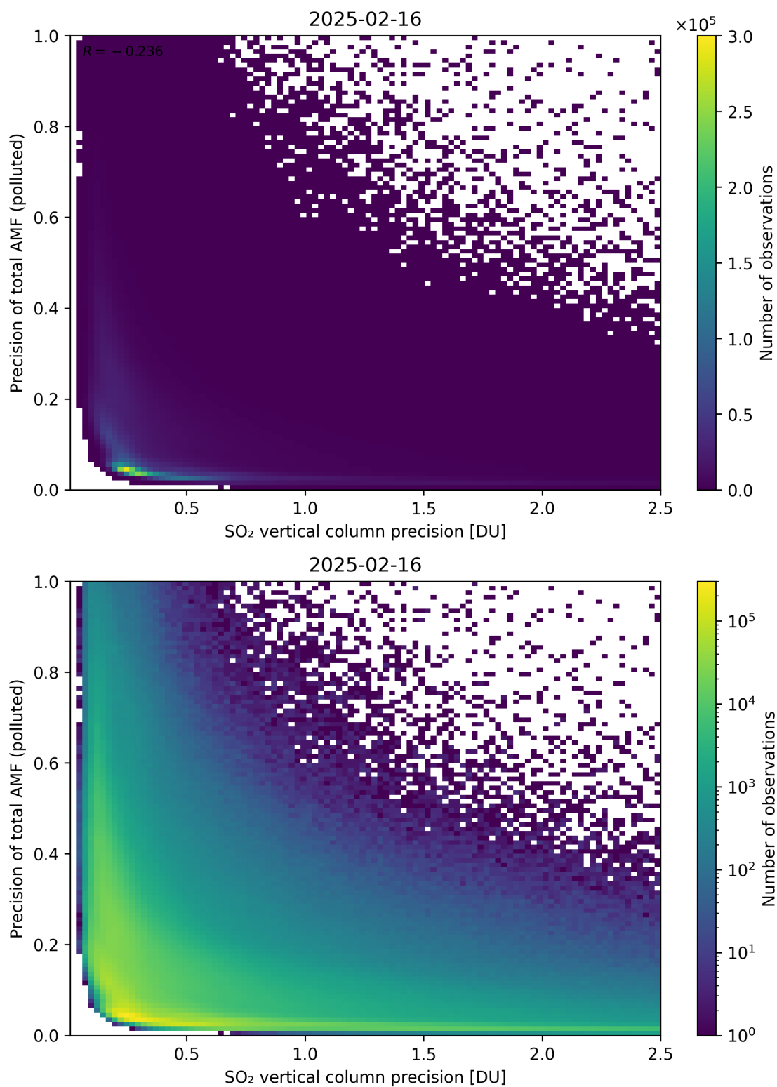
Figure 347: Scatter density plot of “SO 2 vertical column precision” against “Precision of total AMF (polluted)” for 2025-02-15 to 2025-02-17.
