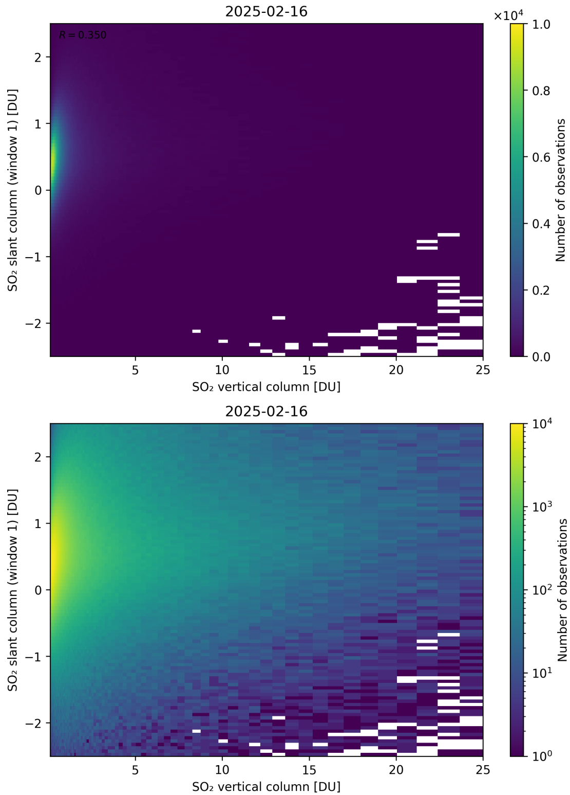
Figure 354: Scatter density plot of “SO 2 vertical column” against “SO 2 slant column (window 1)” for 2025-02-15 to 2025-02-17.
