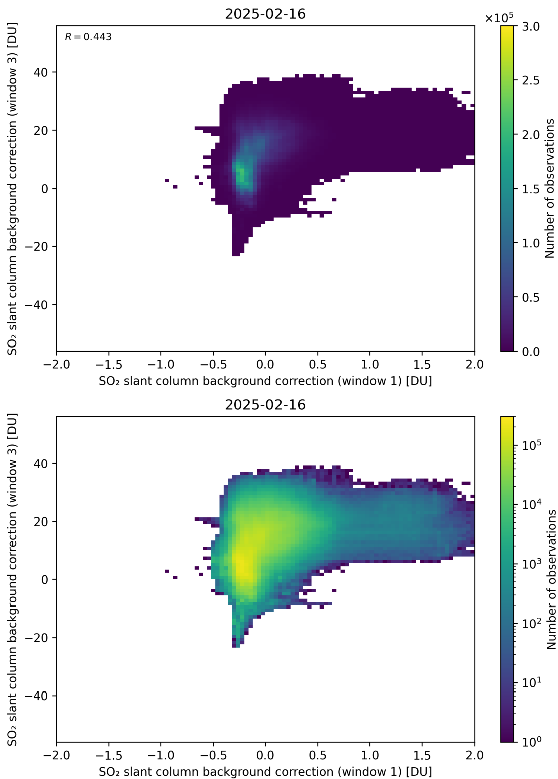
Figure 110: Scatter density plot of “SO 2 slant column background correction (window 1)” against “SO 2 slant column background correction (window 3)” for 2025-02-15 to 2025-02-17.
