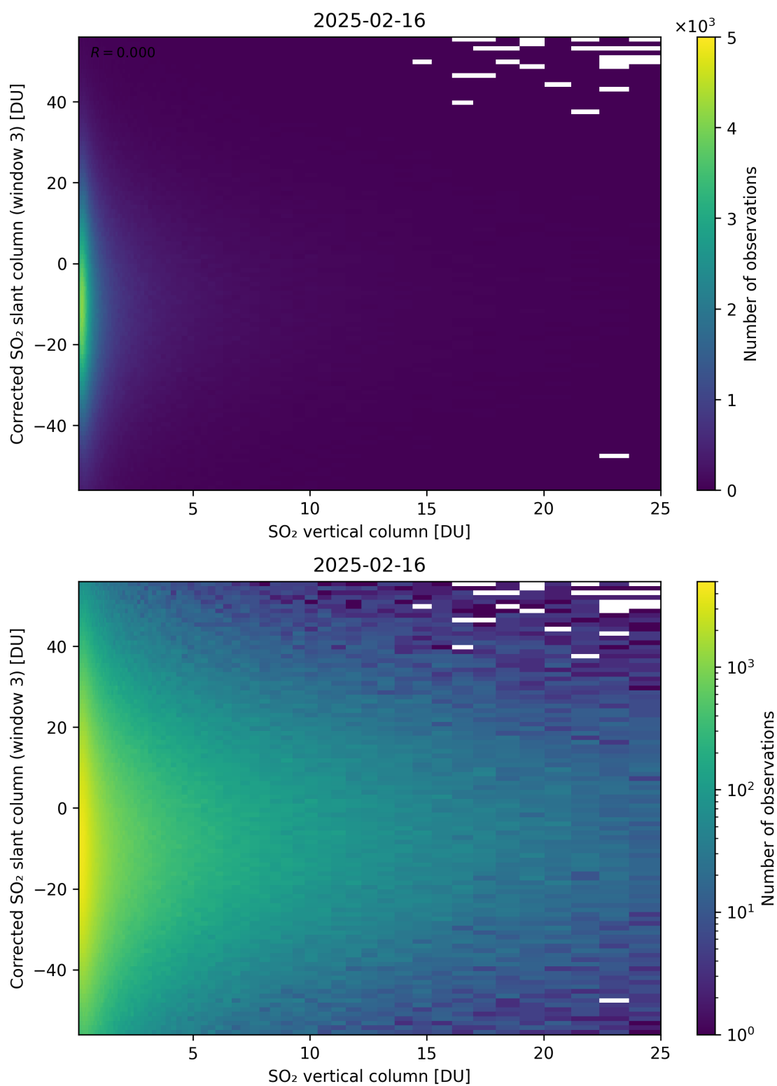
Figure 353: Scatter density plot of “SO 2 vertical column” against “Corrected SO 2 slant column (window 3)” for 2025-02-15 to 2025-02-17.
