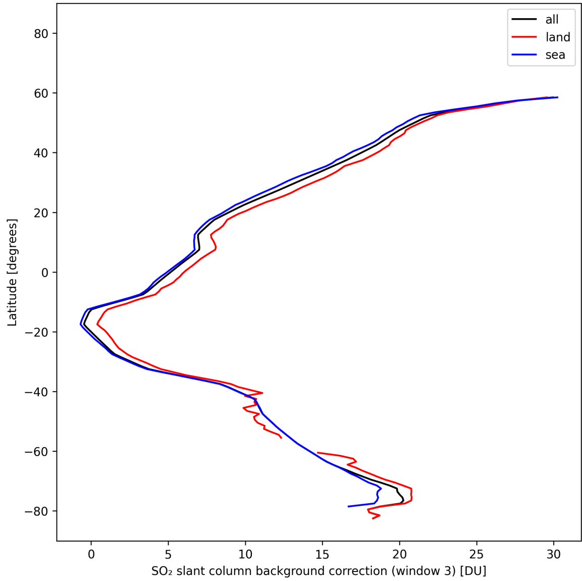
Figure 48: Zonal average of “SO 2 slant column background correction (window 3)” for 2025-02-15 to 2025-02-17.
