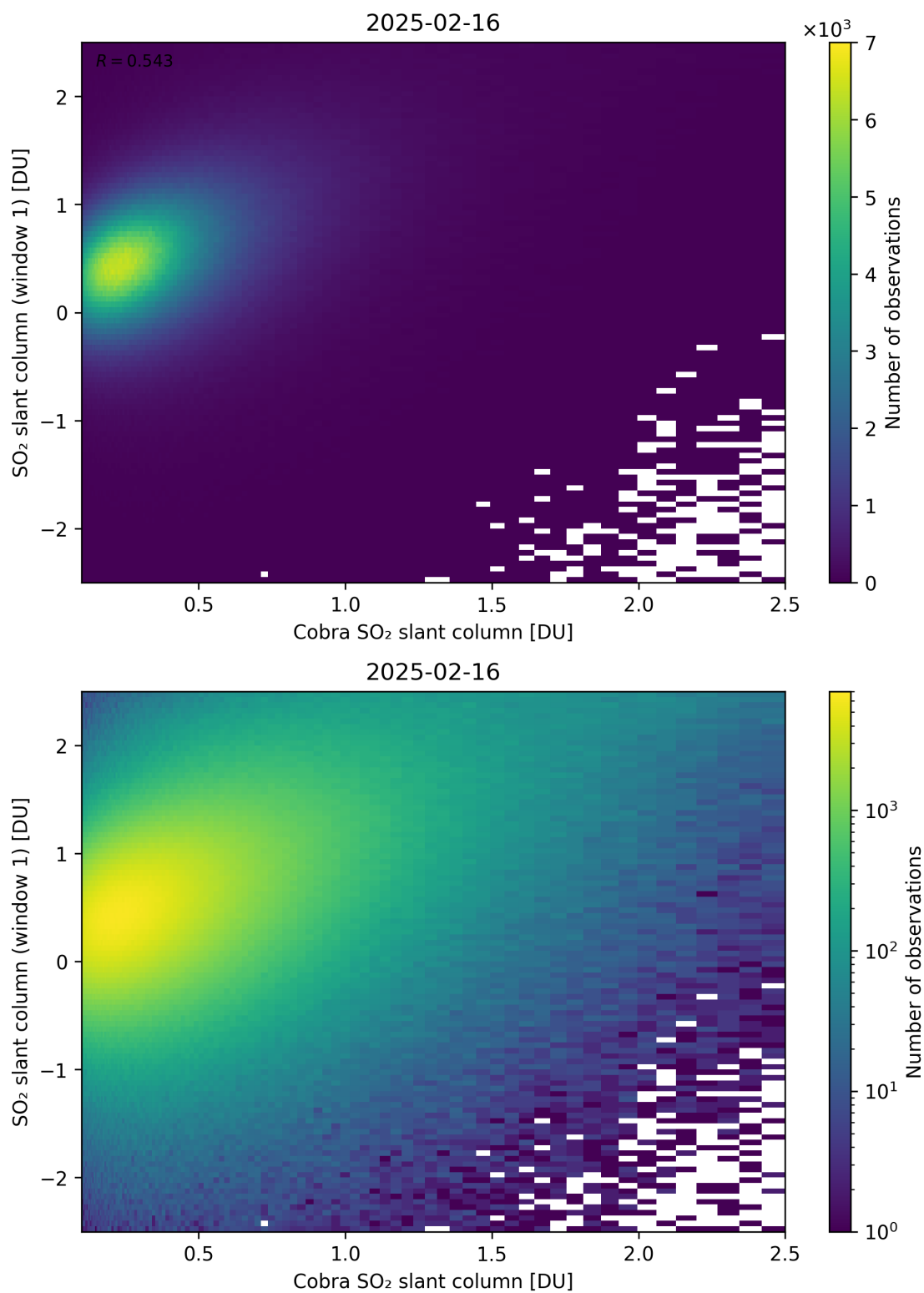
Figure 219: Scatter density plot of “Cobra SO 2 slant column” against “SO 2 slant column (window 1)” for 2025-02-15 to 2025-02-17.
