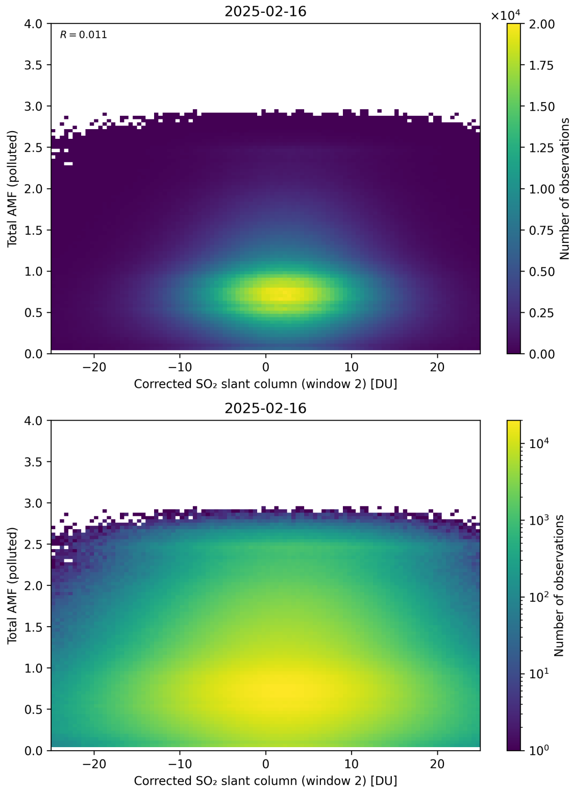
Figure 253: Scatter density plot of “Corrected SO 2 slant column (window 2)” against “Total AMF (polluted)” for 2025-02-15 to 2025-02-17.
