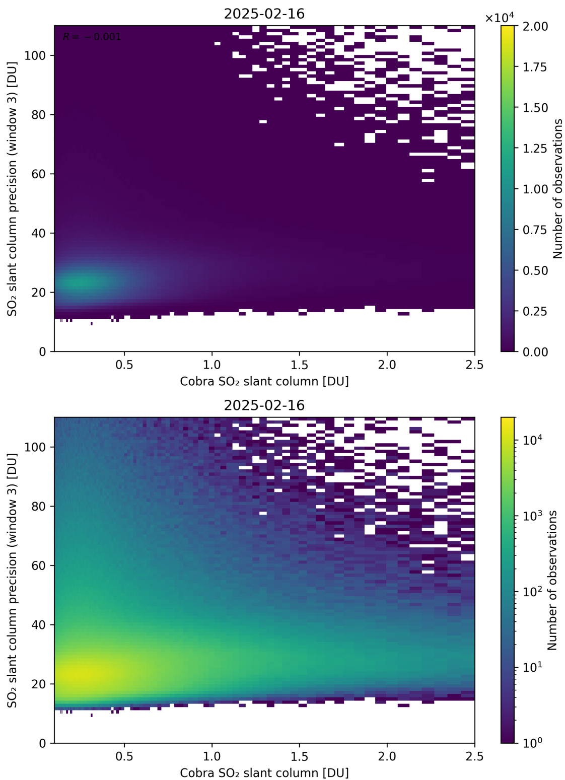
Figure 223: Scatter density plot of “Cobra SO 2 slant column” against “SO 2 slant column precision (window 3)” for 2025-02-15 to 2025-02-17.
