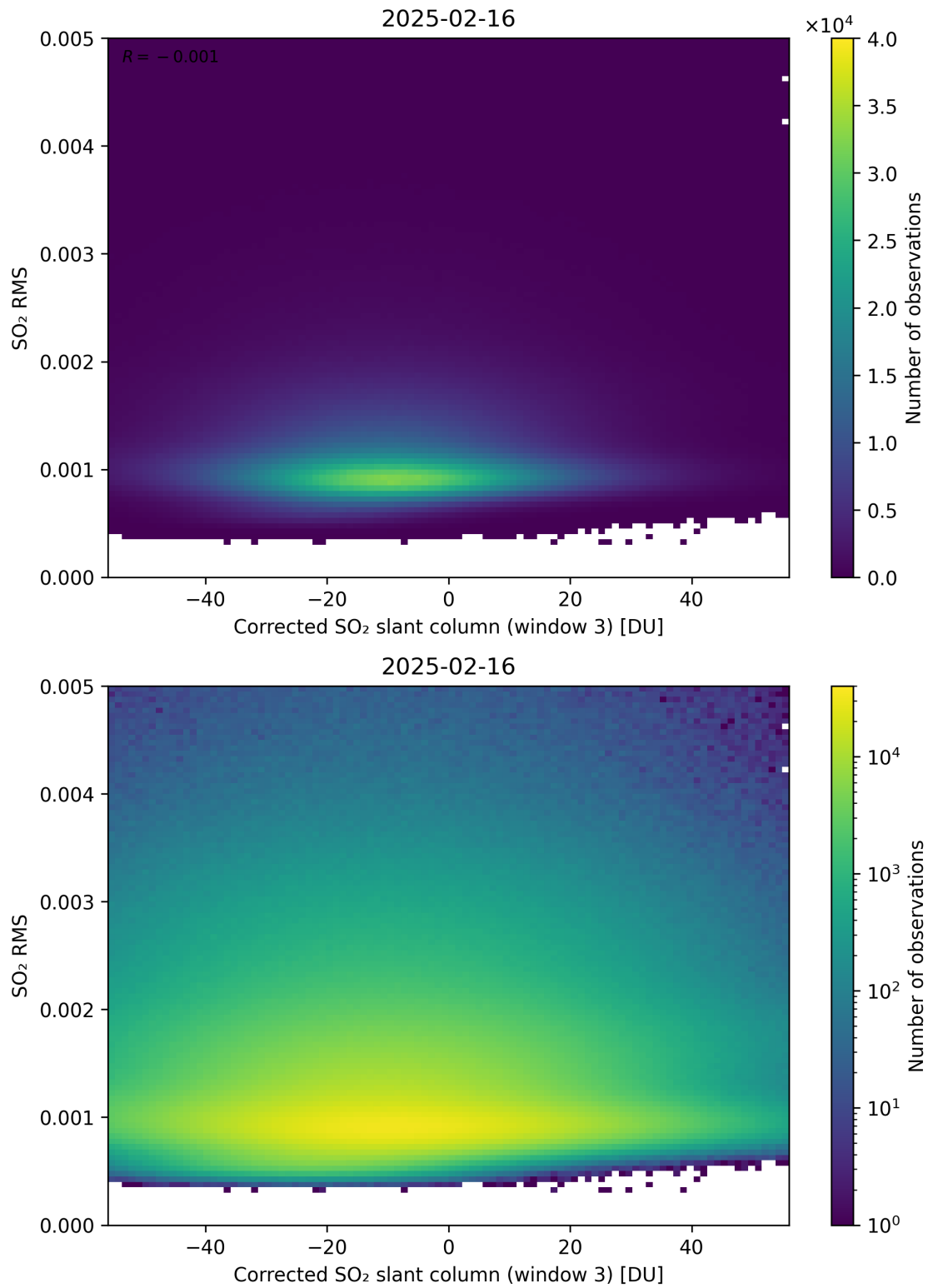
Figure 258: Scatter density plot of “Corrected SO 2 slant column (window 3)” against “SO 2 RMS” for 2025-02-15 to 2025-02-17.
