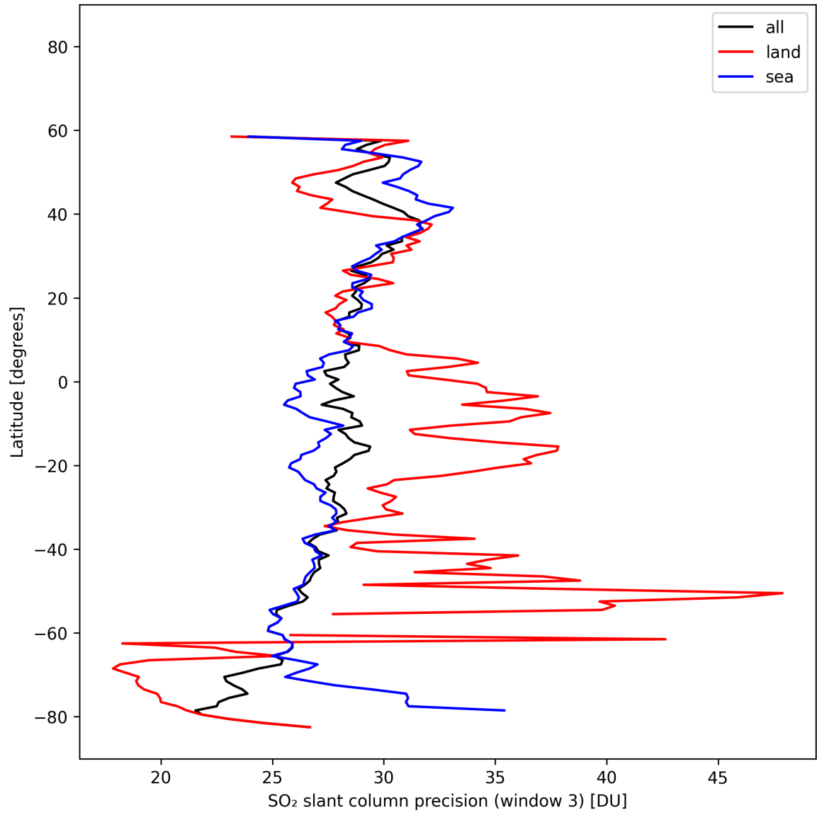
Figure 46: Zonal average of “SO 2 slant column precision (window 3)” for 2025-02-15 to 2025-02-17.
