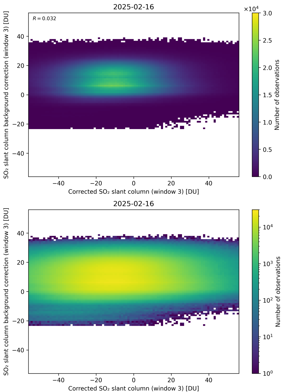
Figure 255: Scatter density plot of “Corrected SO 2 slant column (window 3)” against “SO 2 slant column background correction (window 3)” for 2025-02-15 to 2025-02-17.
