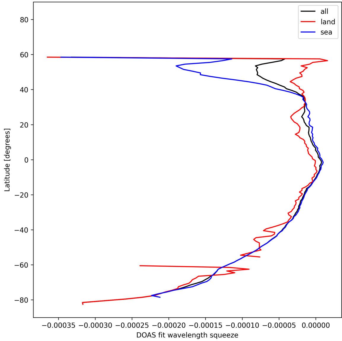
Figure 51: Zonal average of “DOAS fit wavelength squeeze” for 2025-02-15 to 2025-02-17.
