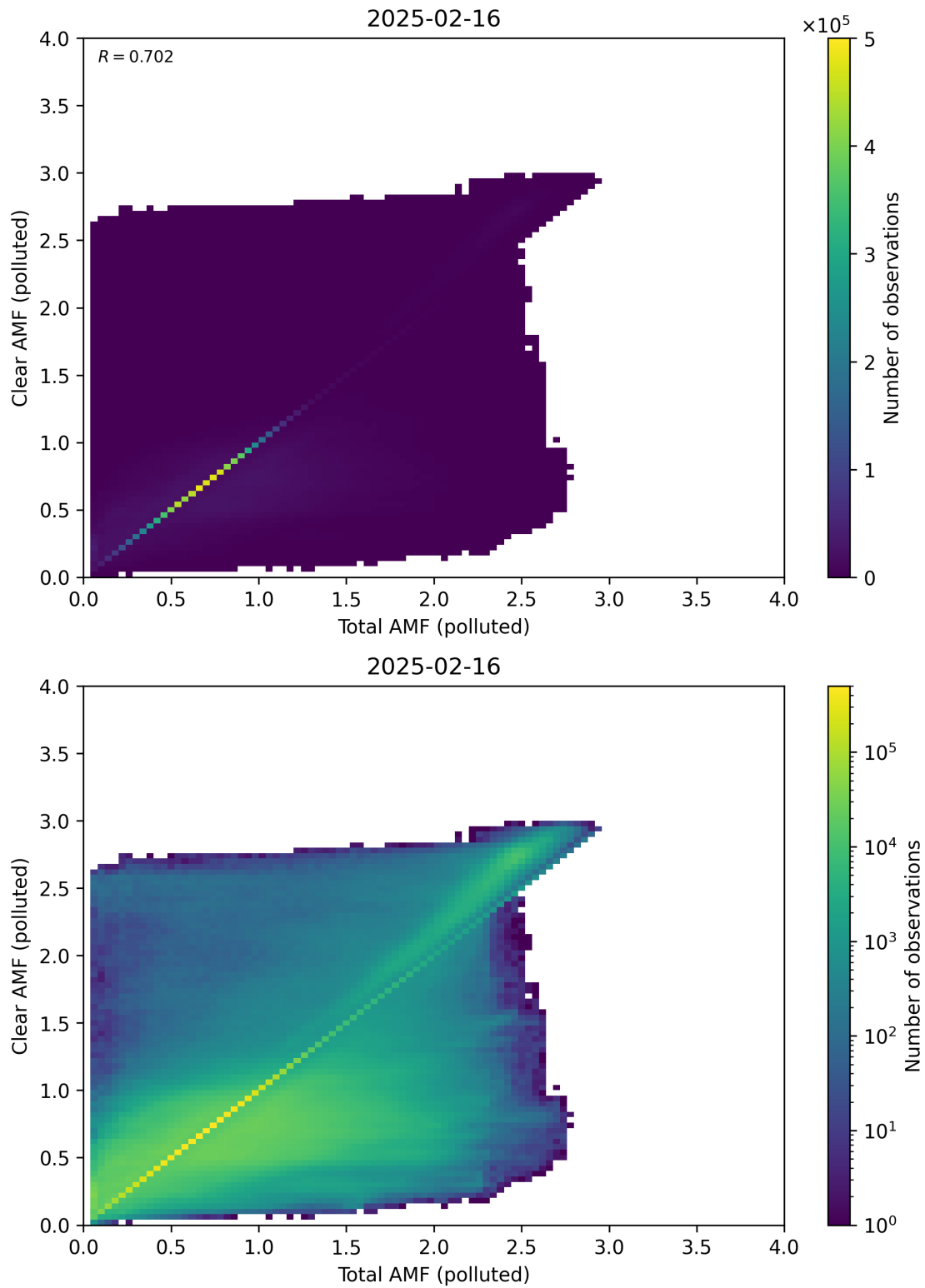
Figure 321: Scatter density plot of “Total AMF (polluted)” against “Clear AMF (polluted)” for 2025-02-15 to 2025-02-17.
