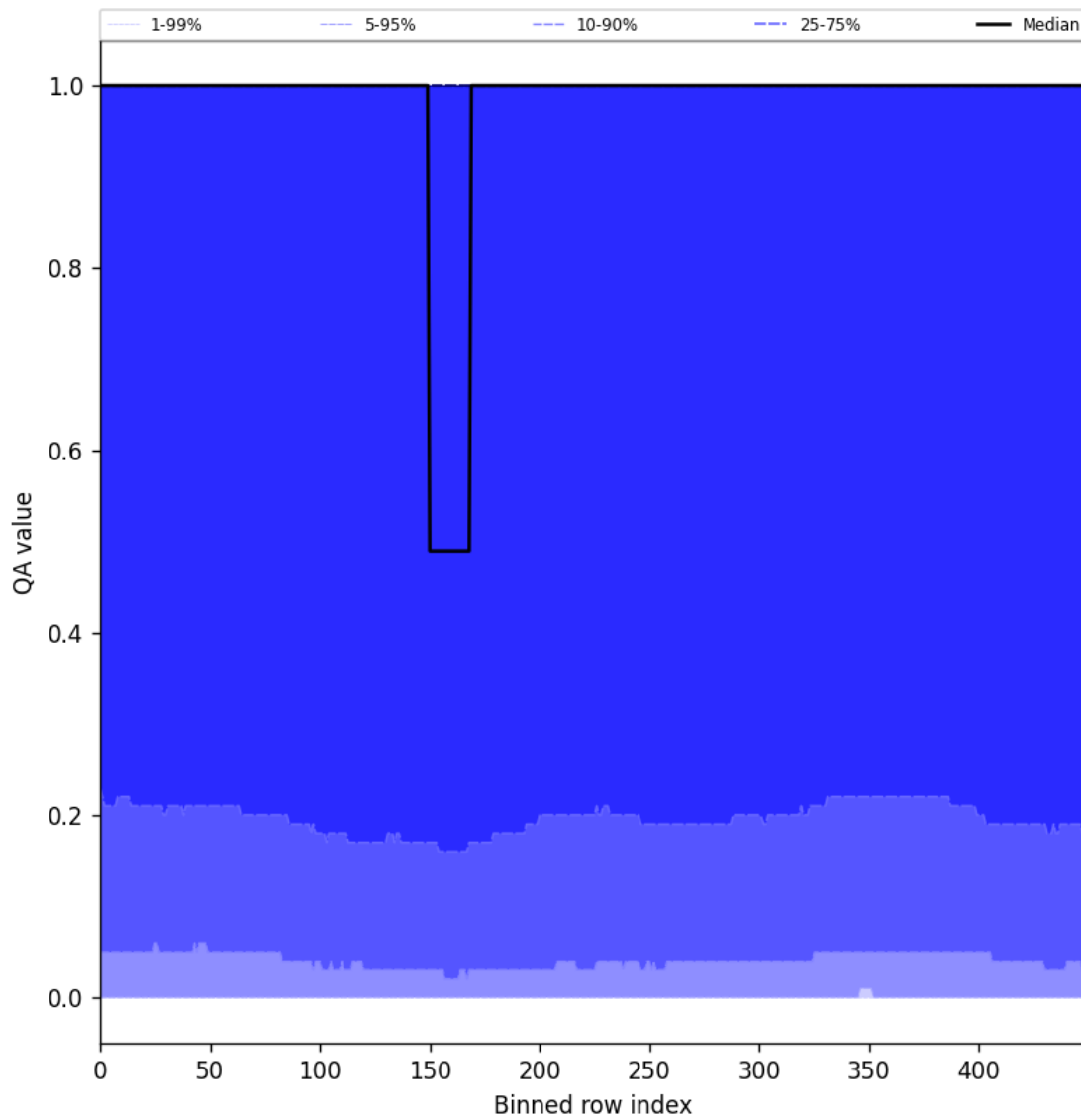
Figure 83: Along track statistics of “QA value” for 2025-02-15 to 2025-02-17
