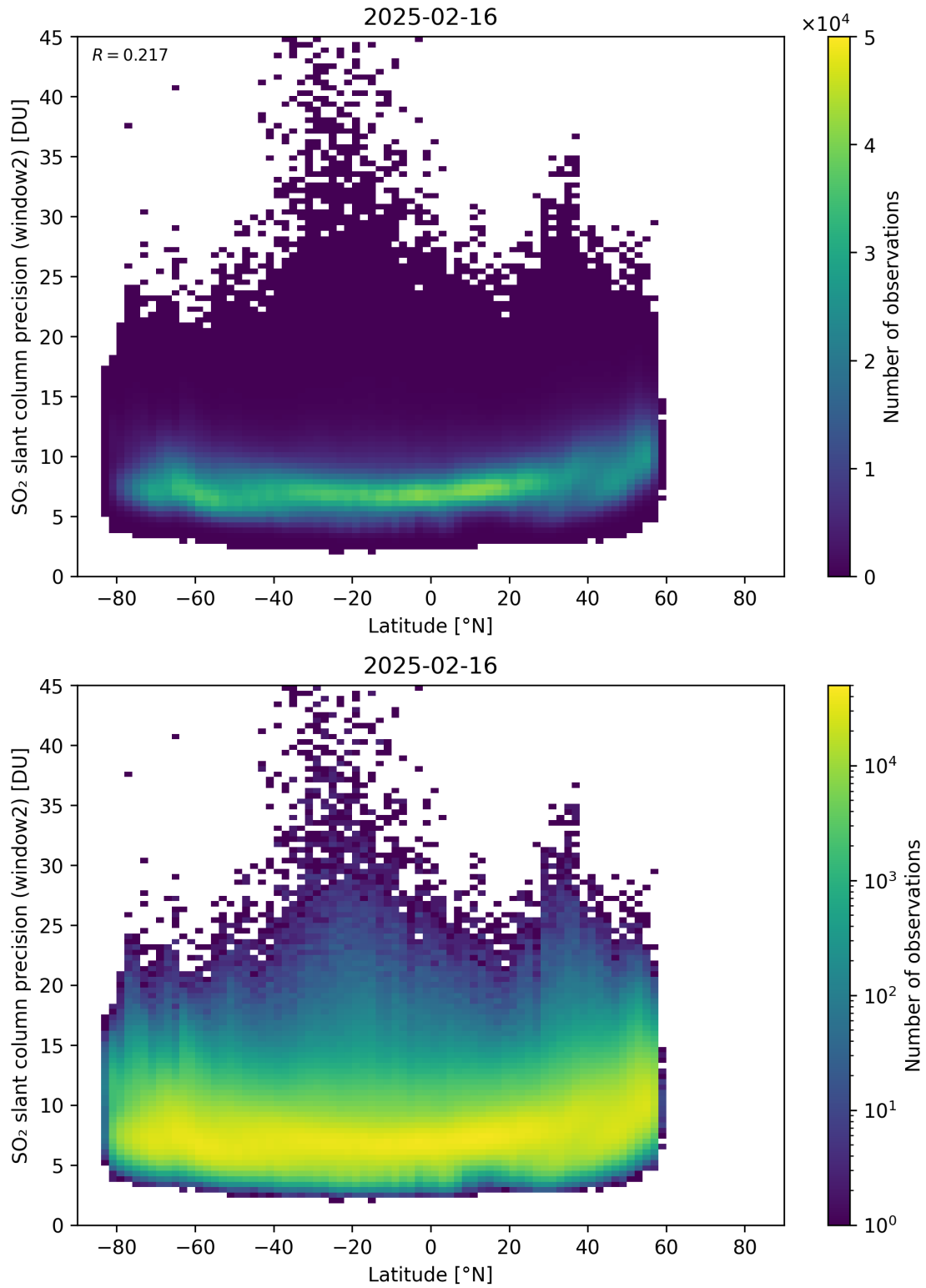
Figure 164: Scatter density plot of “Latitude” against “SO 2 slant column precision (window2)” for 2025-02-15 to 2025-02-17.
