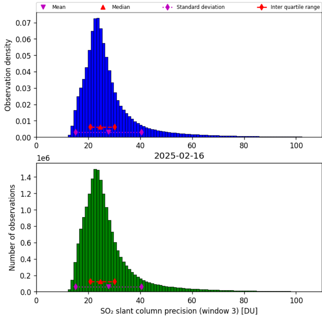
Figure 72: Histogram of “SO 2 slant column precision (window 3)” for 2025-02-15 to 2025-02-17
