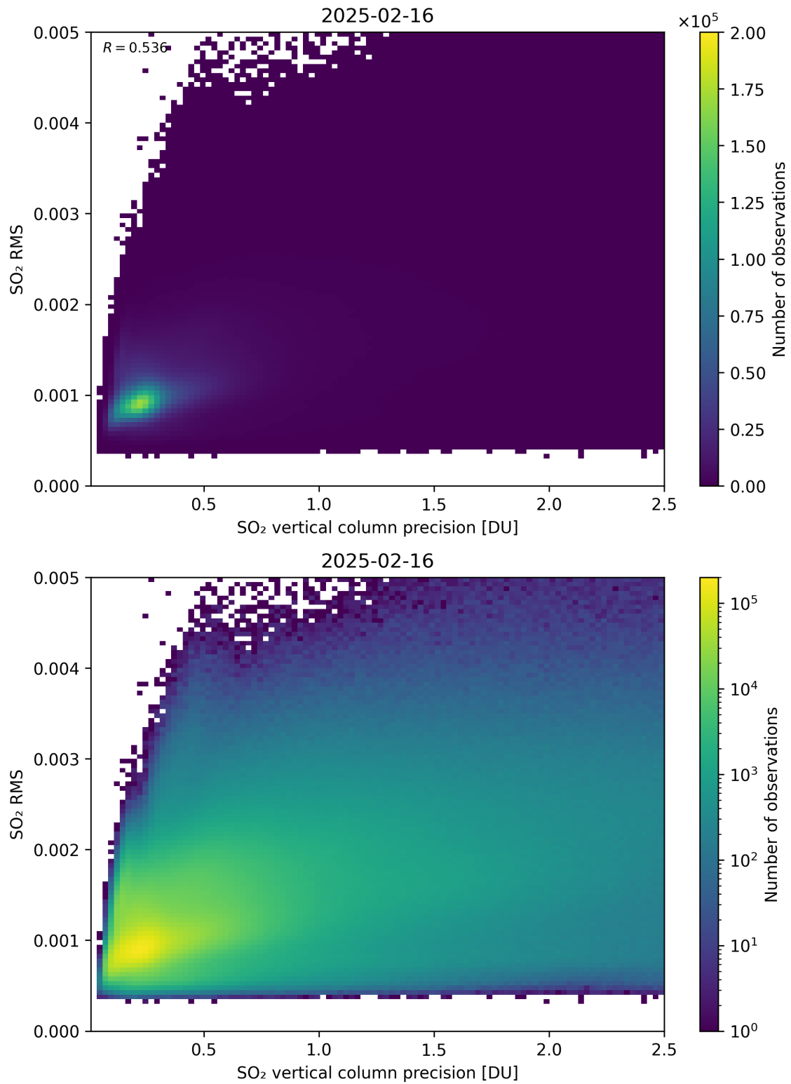
Figure 334: Scatter density plot of “SO 2 vertical column precision” against “SO 2 RMS” for 2025-02-15 to 2025-02-17.
