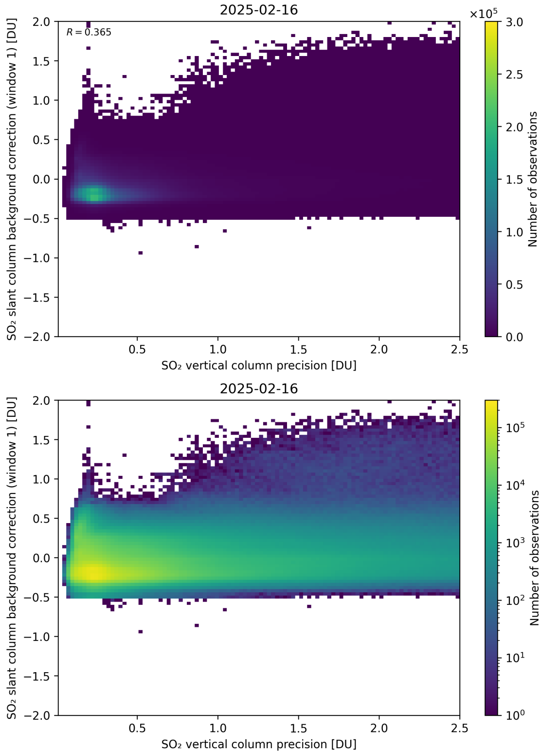
Figure 329: Scatter density plot of “SO 2 vertical column precision” against “SO 2 slant column background correction (window 1)” for 2025-02-15 to 2025-02-17.
