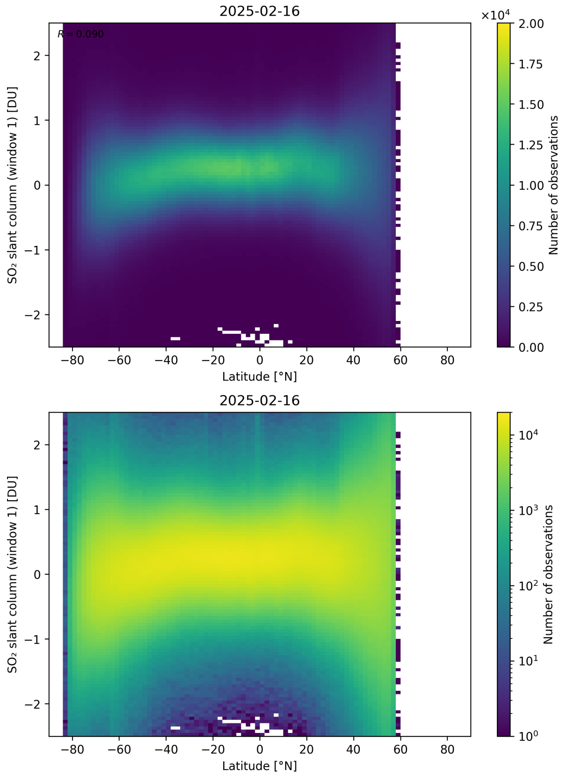
Figure 162: Scatter density plot of “Latitude” against “SO 2 slant column (window 1)” for 2025-02-15 to 2025-02-17.
