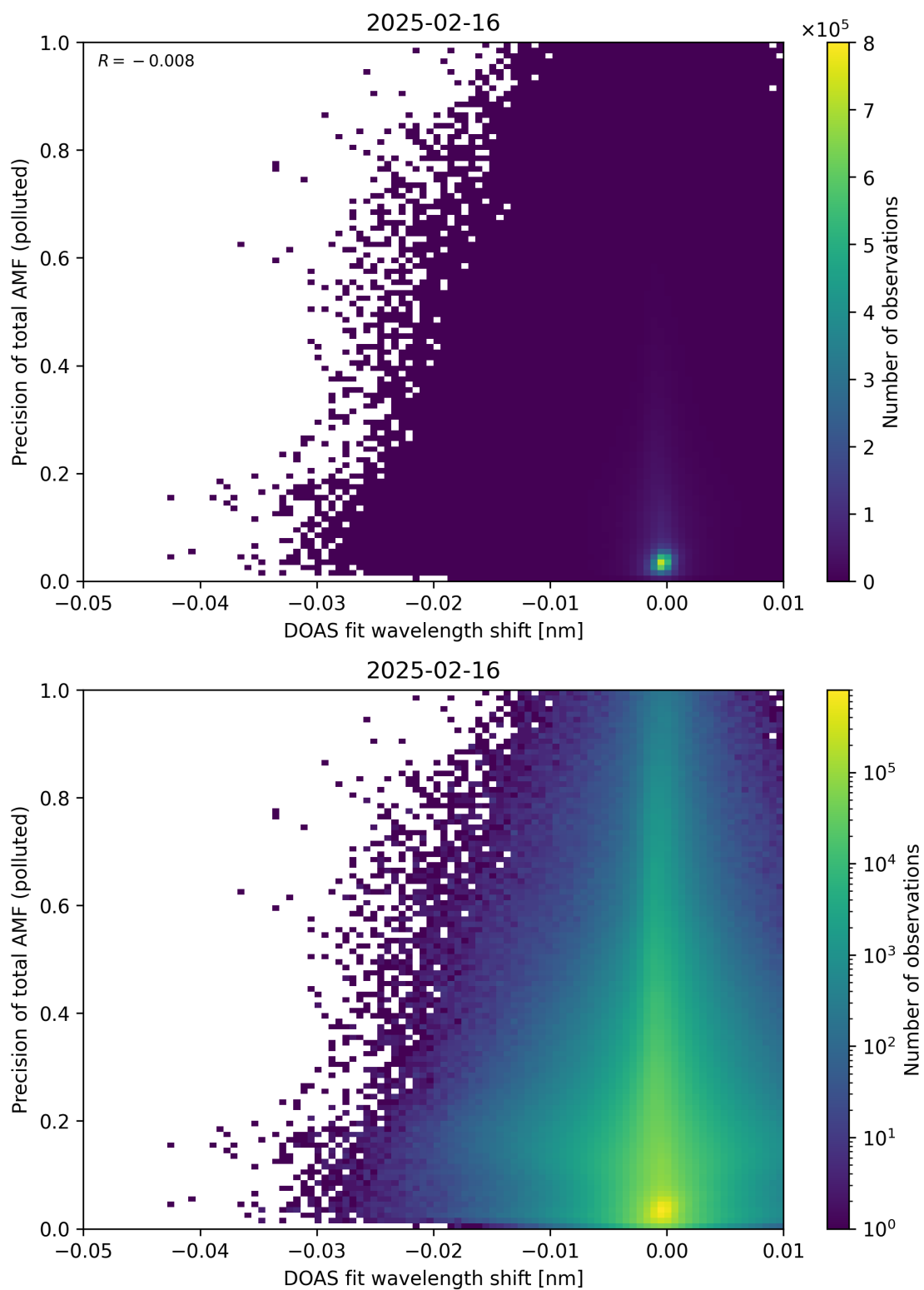
Figure 142: Scatter density plot of “DOAS fit wavelength shift” against “Precision of total AMF (polluted)” for 2025-02-15 to 2025-02-17.
