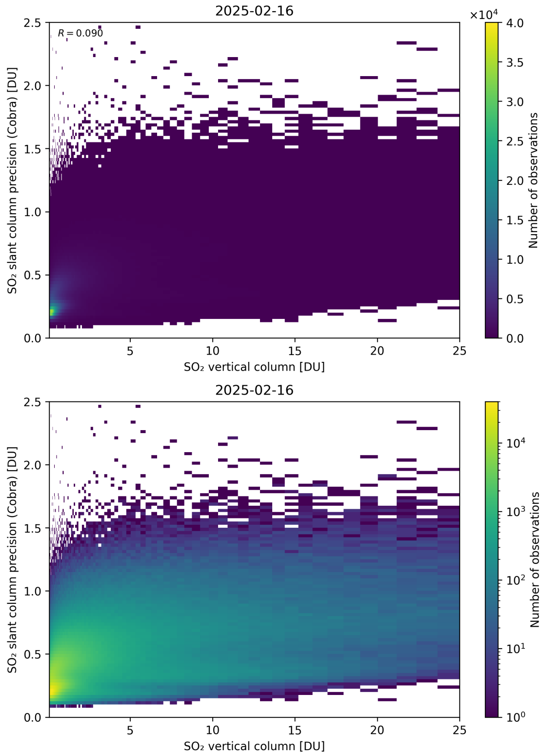
Figure 350: Scatter density plot of “SO 2 vertical column” against “SO 2 slant column precision (Cobra)” for 2025-02-15 to 2025-02-17.
