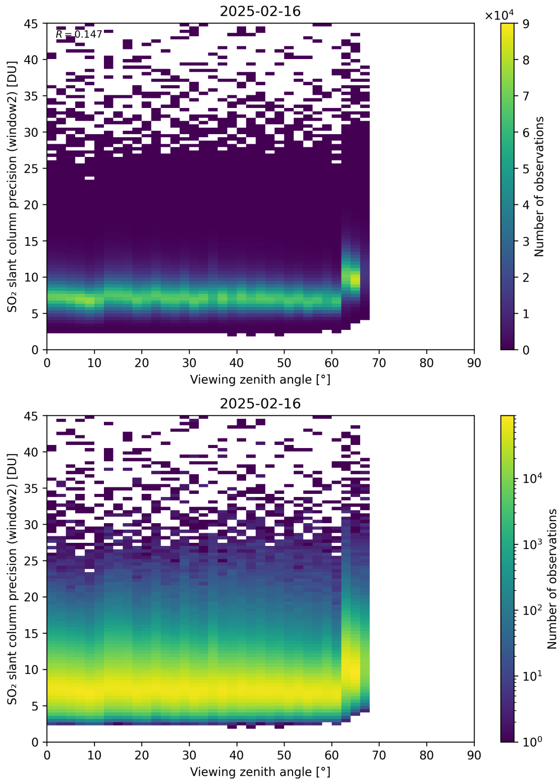
Figure 378: Scatter density plot of “Viewing zenith angle” against “SO 2 slant column precision (window2)” for 2025-02-15 to 2025-02-17.
