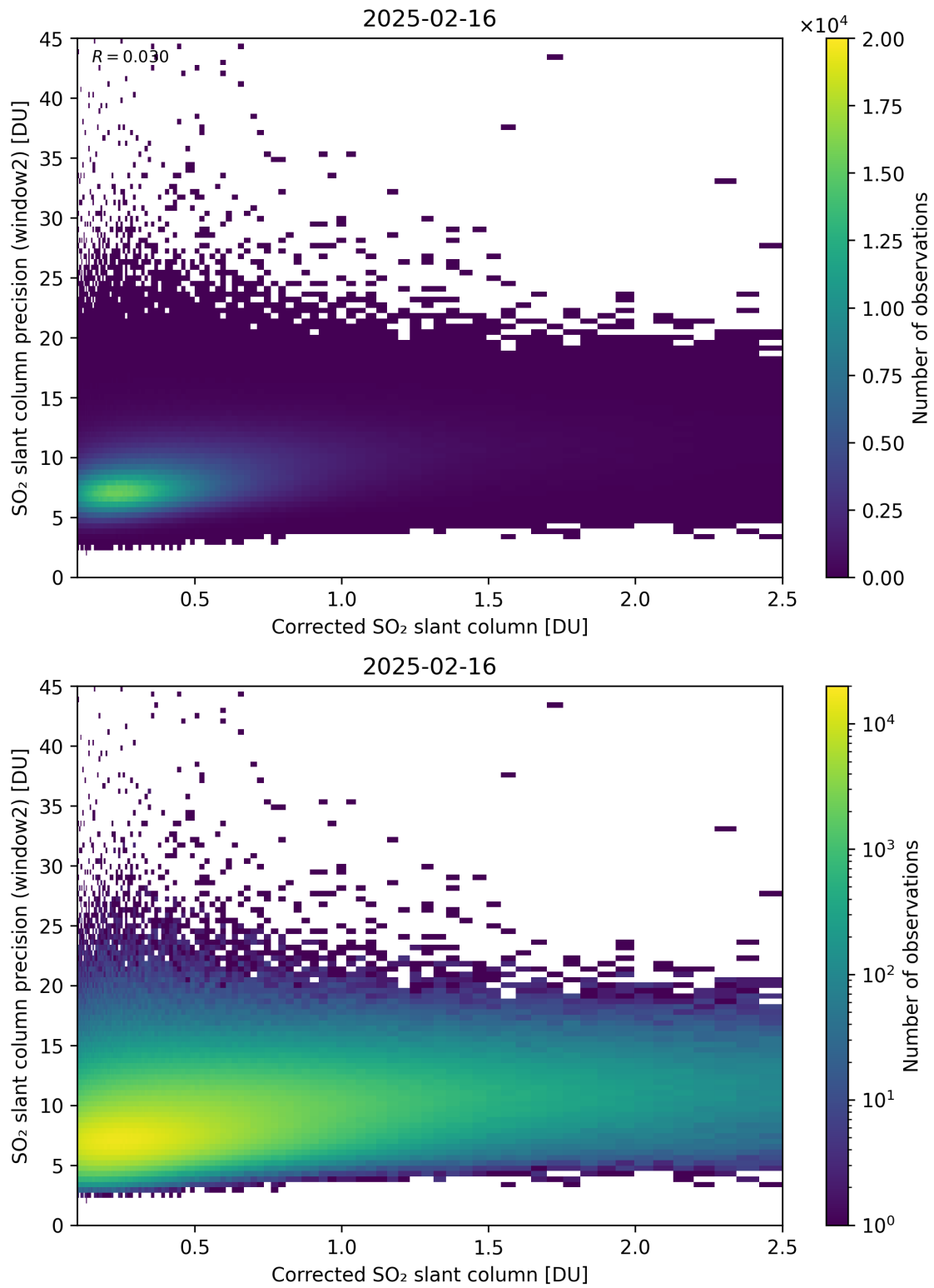
Figure 239: Scatter density plot of “Corrected SO 2 slant column” against “SO 2 slant column precision (window2)” for 2025-02-15 to 2025-02-17.
