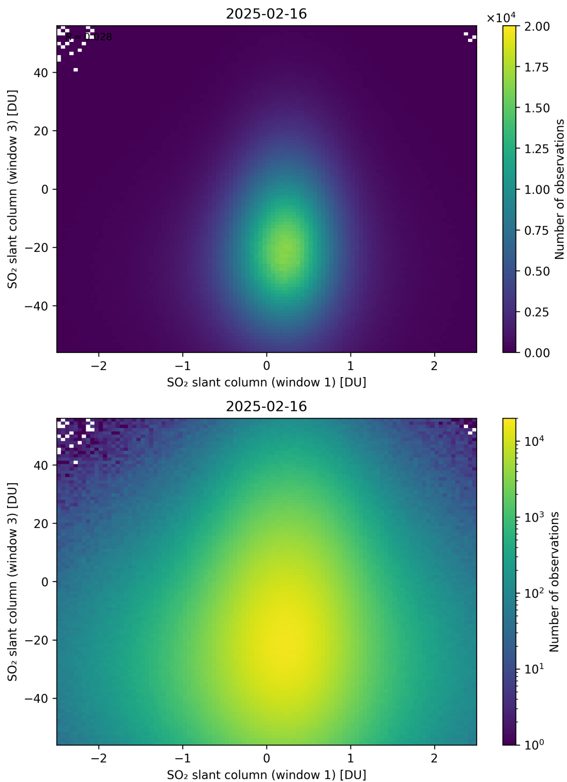
Figure 287: Scatter density plot of “SO 2 slant column (window 1)” against “SO 2 slant column (window 3)” for 2025-02-15 to 2025-02-17.
