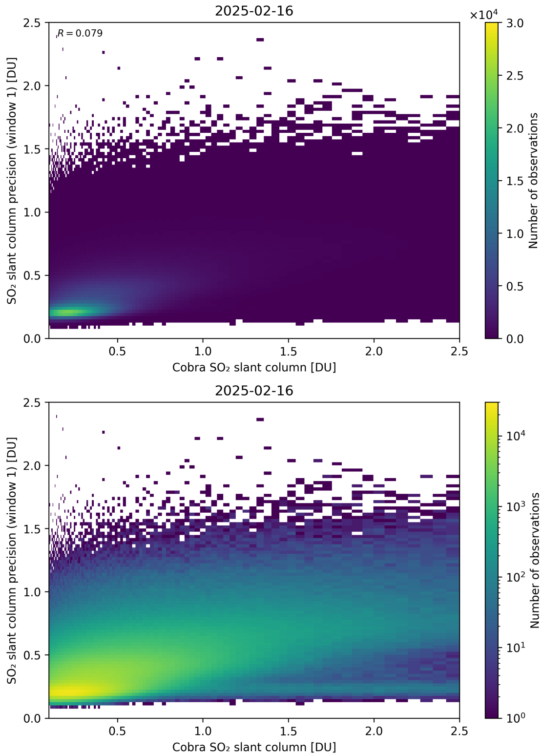
Figure 220: Scatter density plot of “Cobra SO 2 slant column” against “SO 2 slant column precision (window 1)” for 2025-02-15 to 2025-02-17.
