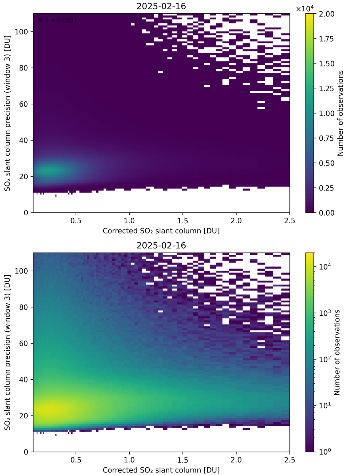
Figure 241: Scatter density plot of “Corrected SO 2 slant column” against “SO 2 slant column precision (window 3)” for 2025-02-15 to 2025-02-17.
