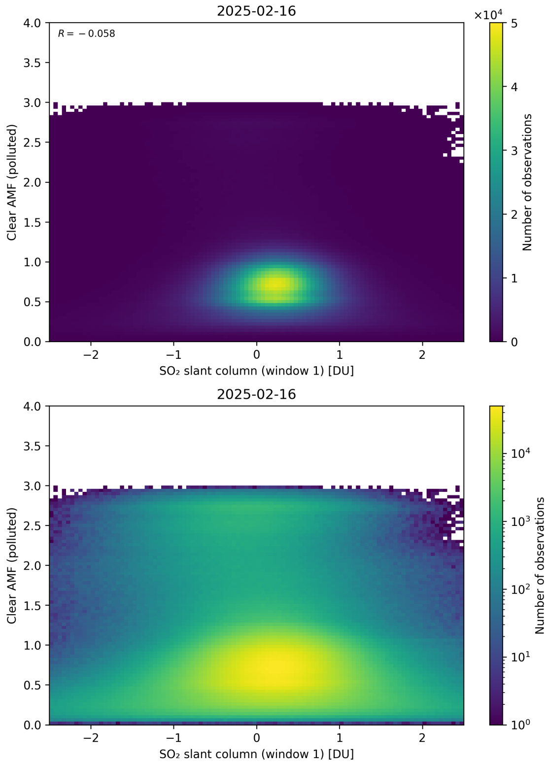
Figure 282: Scatter density plot of “SO 2 slant column (window 1)” against “Clear AMF (polluted)” for 2025-02-15 to 2025-02-17.
