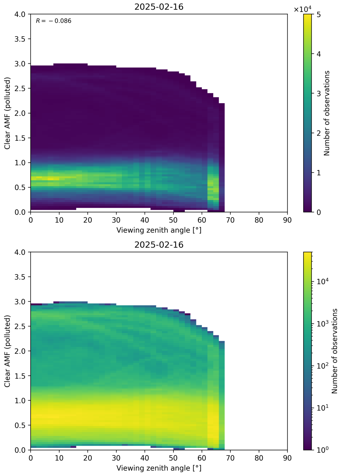
Figure 370: Scatter density plot of “Viewing zenith angle” against “Clear AMF (polluted)” for 2025-02-15 to 2025-02-17.
