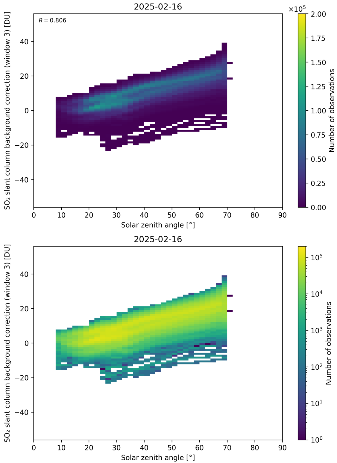
Figure 173: Scatter density plot of “Solar zenith angle” against “SO 2 slant column background correction (window 3)” for 2025-02-15 to 2025-02-17.
