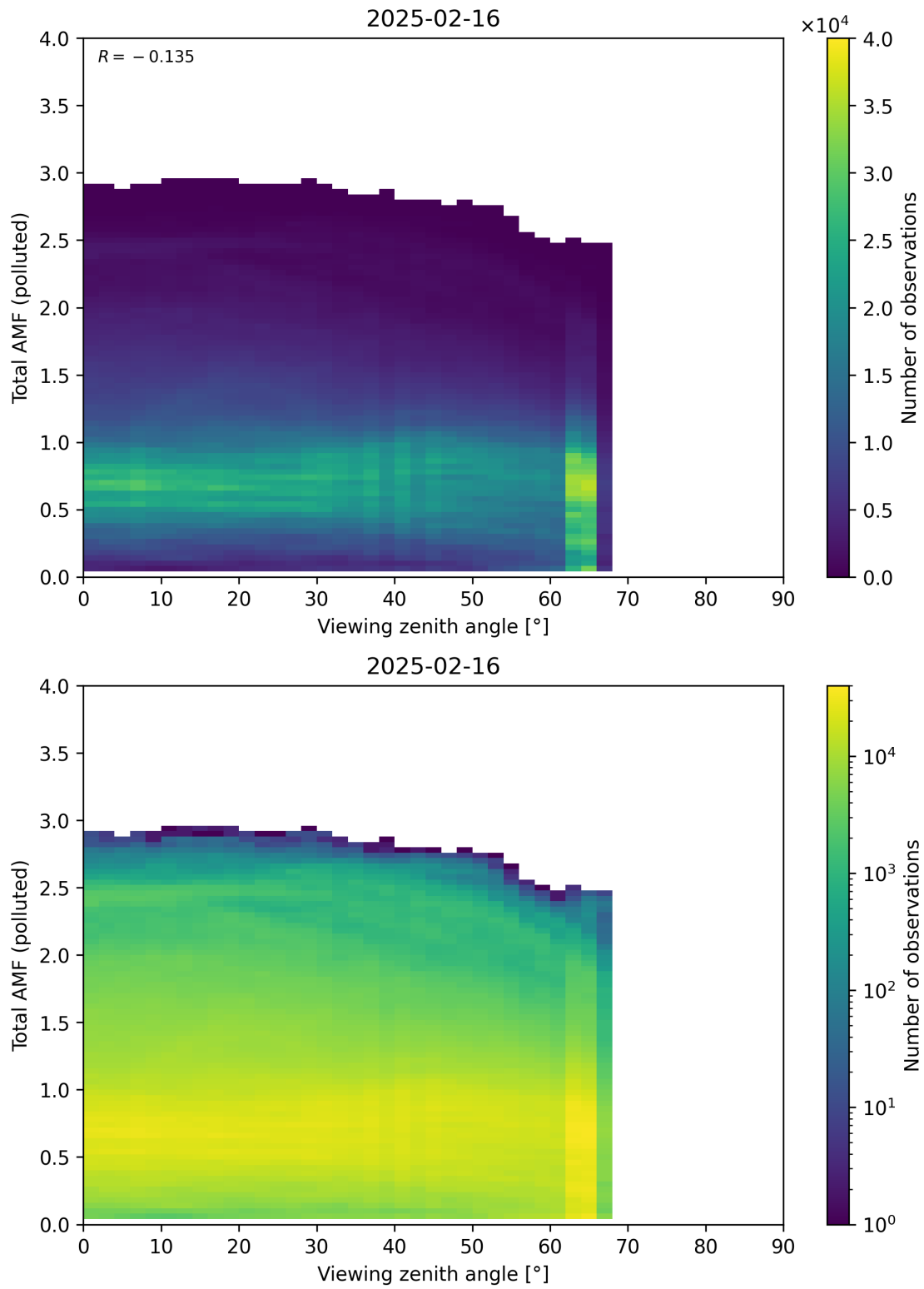
Figure 381: Scatter density plot of “Viewing zenith angle” against “Total AMF (polluted)” for 2025-02-15 to 2025-02-17.
