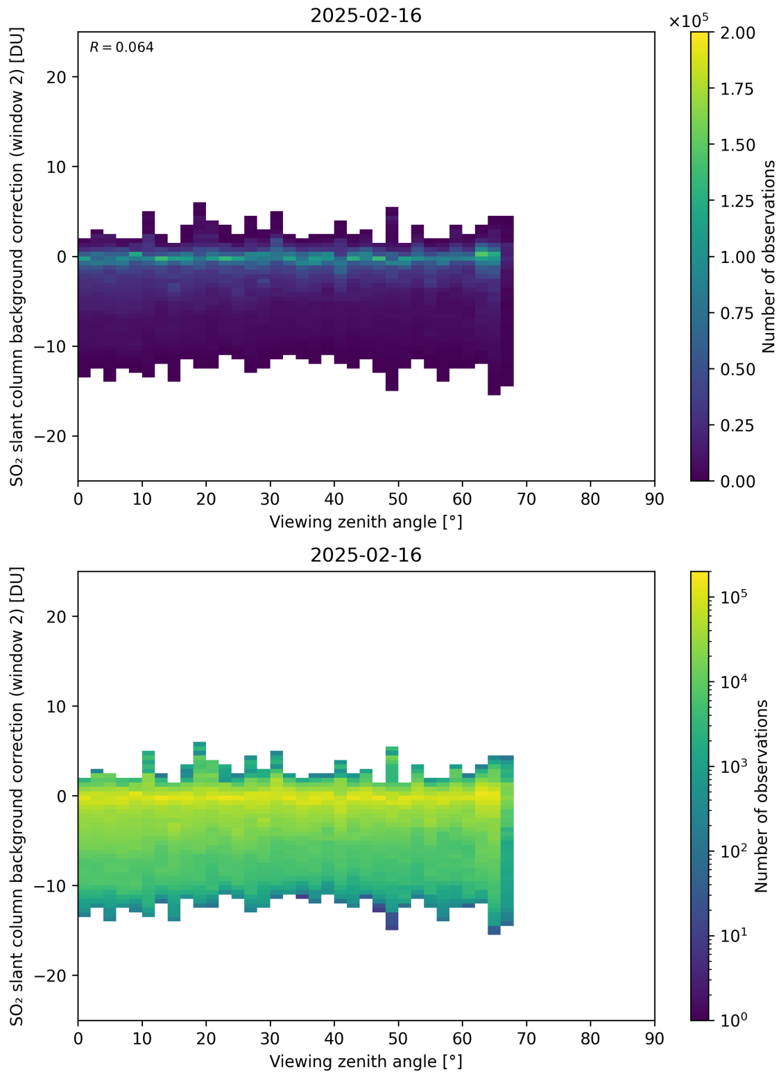
Figure 363: Scatter density plot of “Viewing zenith angle” against “SO 2 slant column background correction (window 2)” for 2025-02-15 to 2025-02-17.
