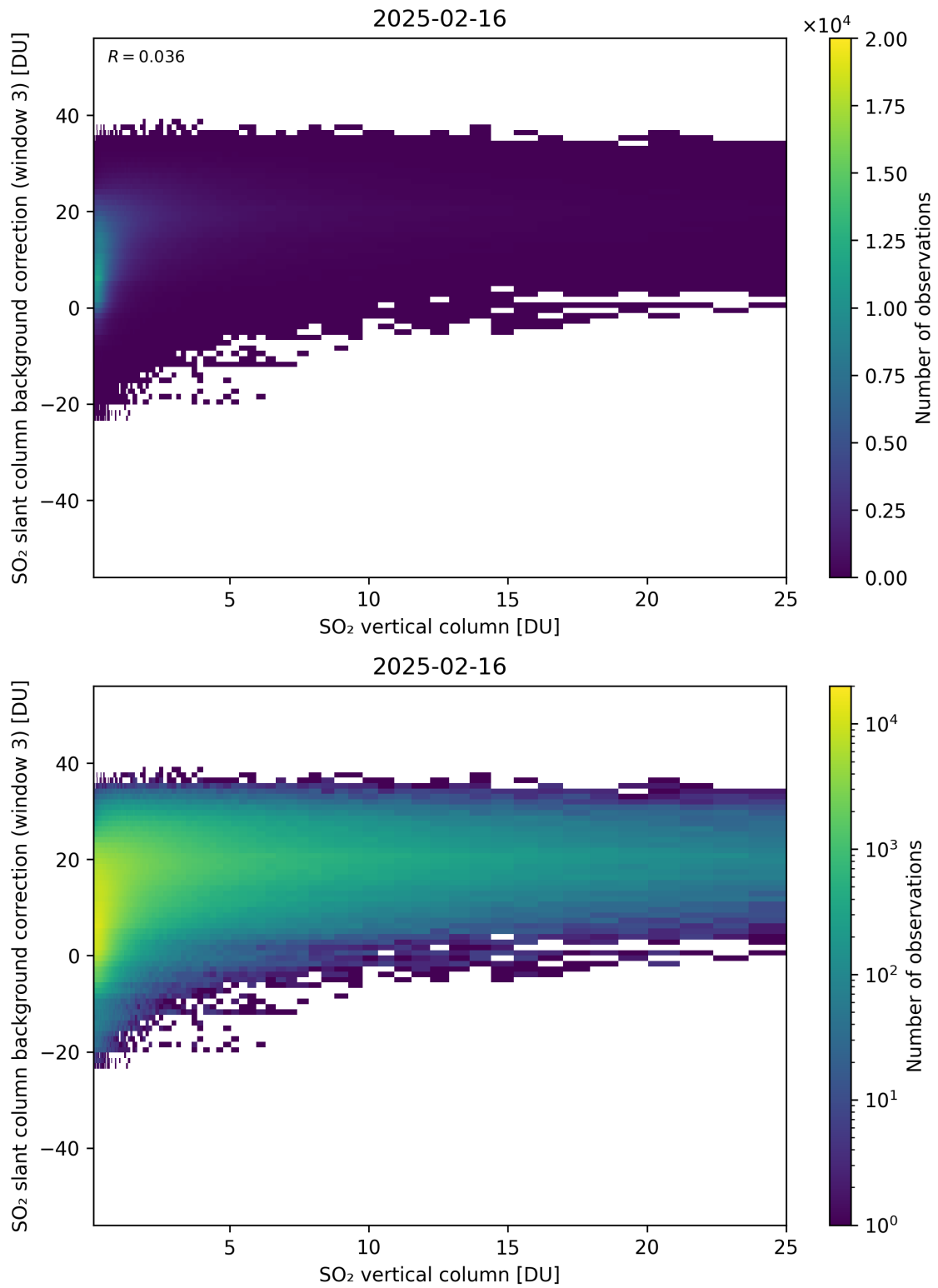
Figure 325: Scatter density plot of “SO 2 vertical column” against “SO 2 slant column background correction (window 3)” for 2025-02-15 to 2025-02-17.
