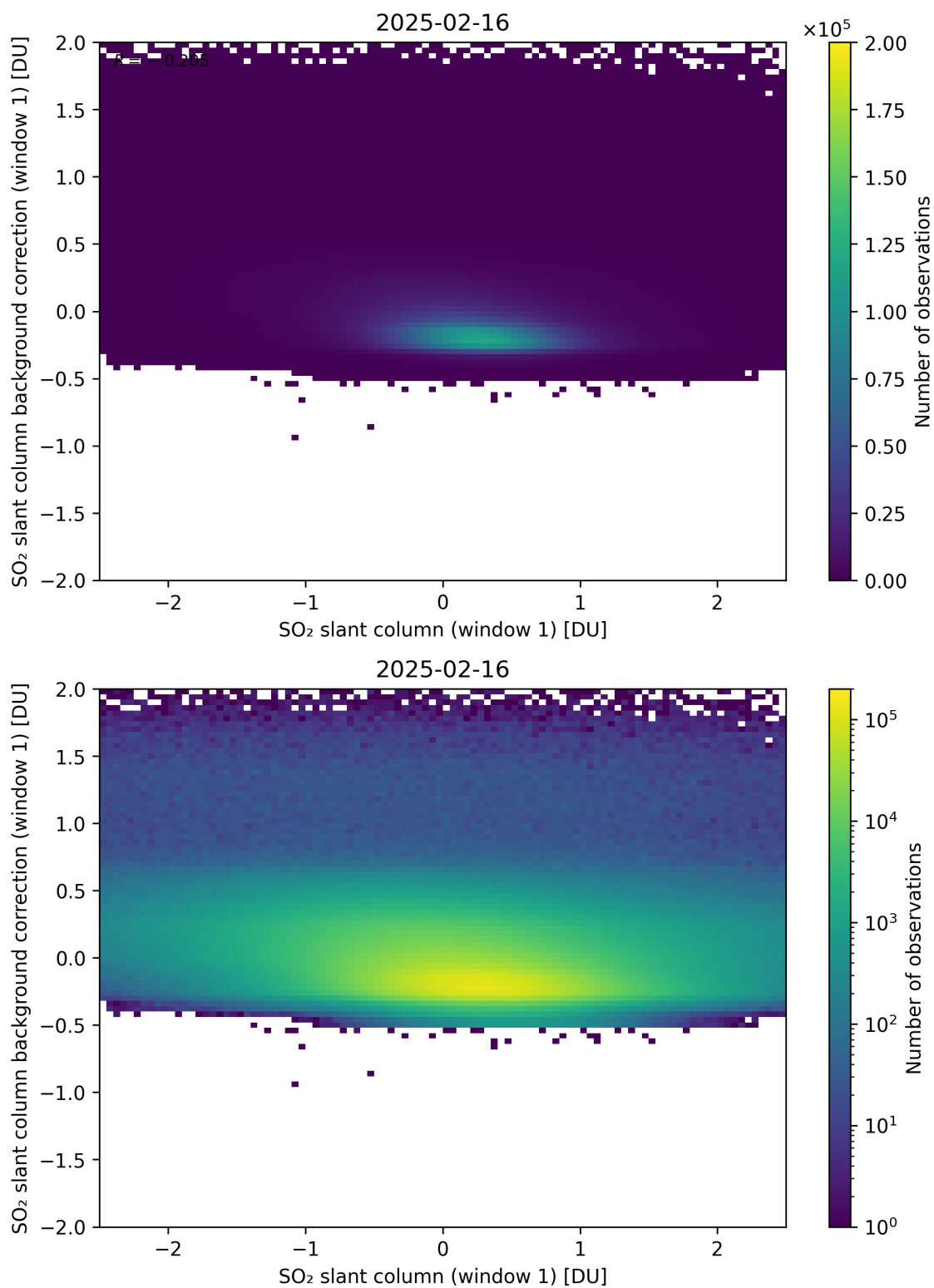
Figure 262: Scatter density plot of "SO 2 slant column (window 1)" against "SO 2 slant column background correction (window 1)" for 2025-02-15 to 2025-02-17.
