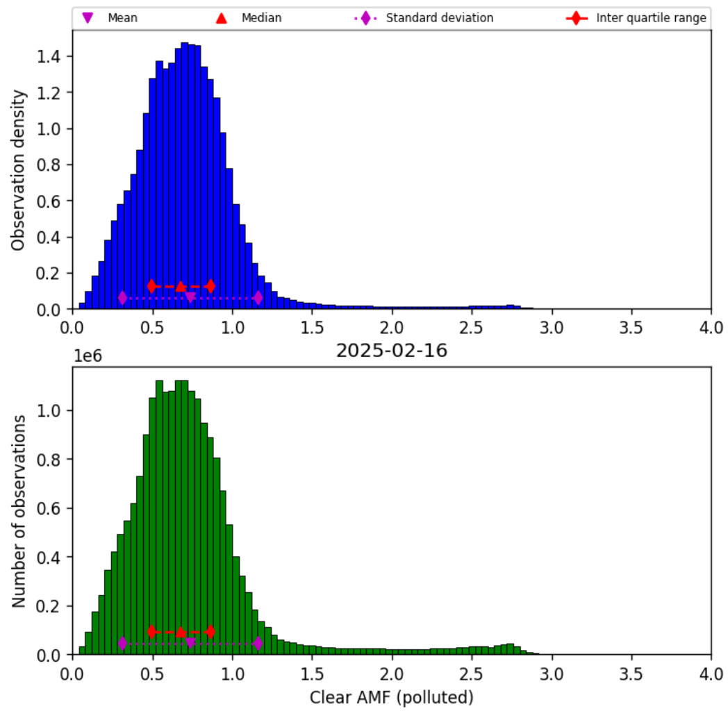
Figure 81: Histogram of “Clear AMF (polluted)” for 2025-02-15 to 2025-02-17
