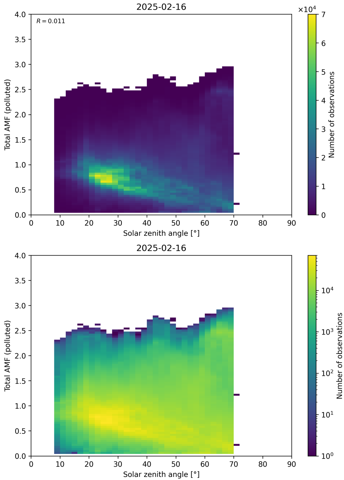
Figure 189: Scatter density plot of “Solar zenith angle” against “Total AMF (polluted)” for 2025-02-15 to 2025-02-17.
