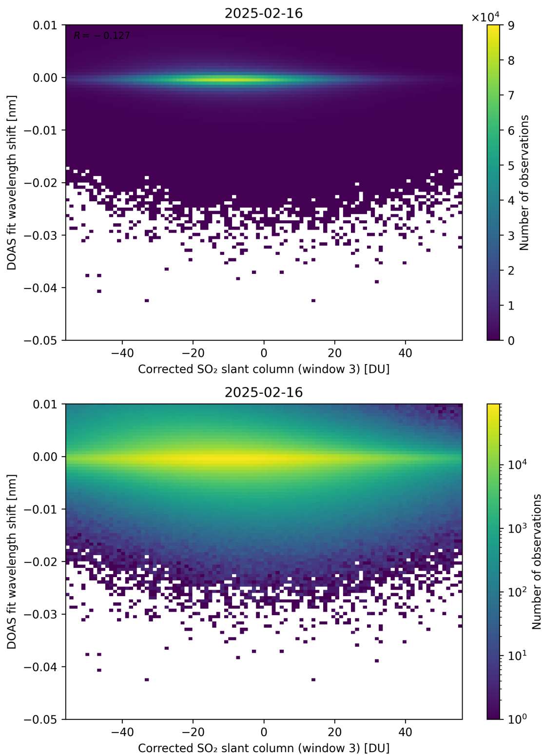
Figure 256: Scatter density plot of “Corrected SO 2 slant column (window 3)” against “DOAS fit wavelength shift” for 2025-02-15 to 2025-02-17.
