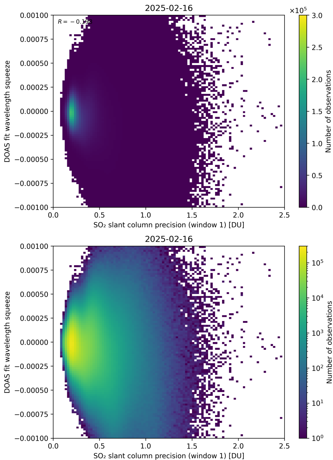
Figure 272: Scatter density plot of “SO 2 slant column precision (window 1)” against “DOAS fit wavelength squeeze” for 2025-02-15 to 2025-02-17.
