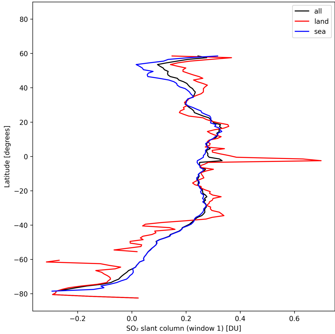
Figure 37: Zonal average of “SO 2 slant column (window 1)” for 2025-02-15 to 2025-02-17.
