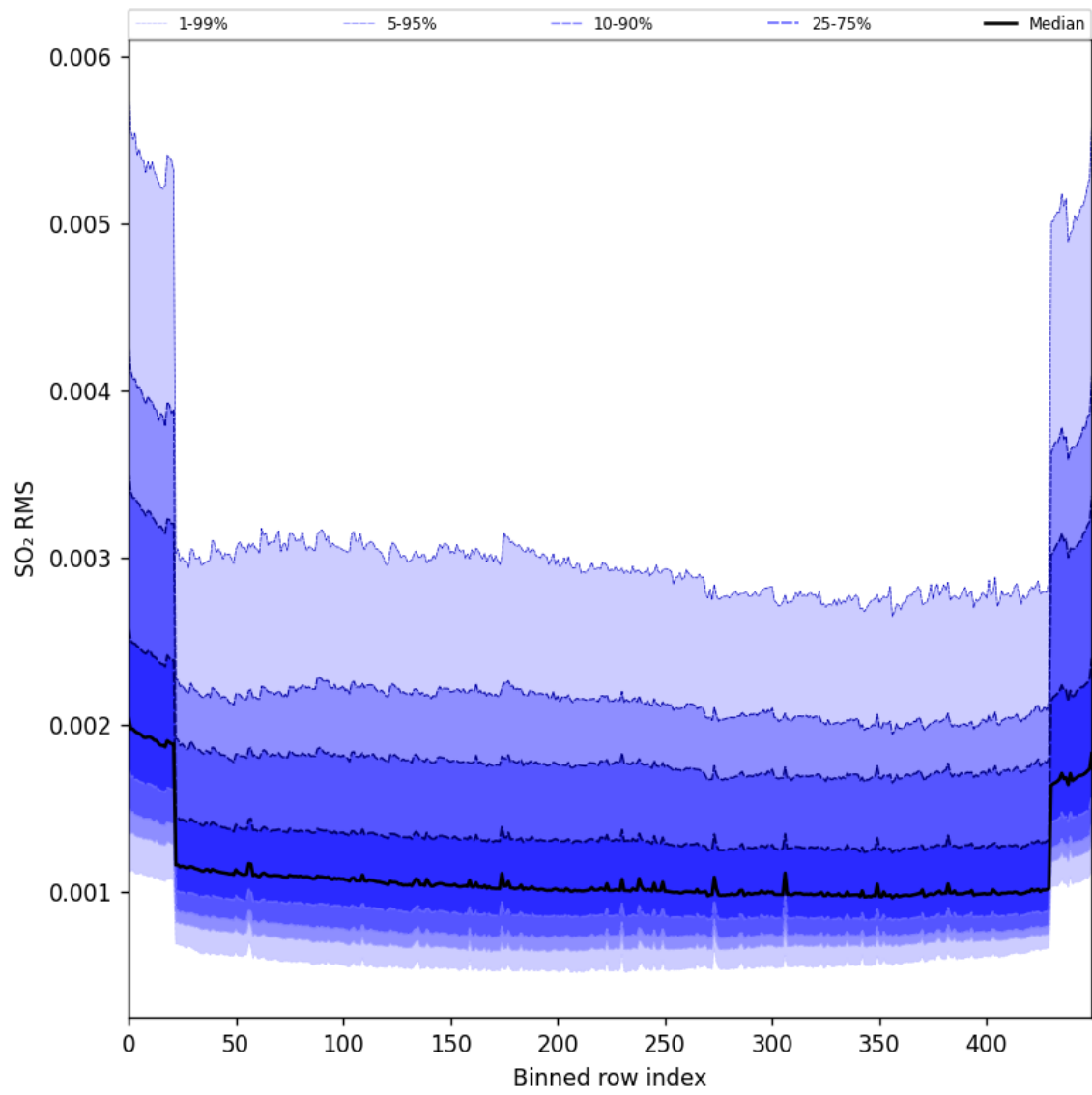
Figure 104: Along track statistics of “SO 2 RMS” for 2025-02-15 to 2025-02-17
