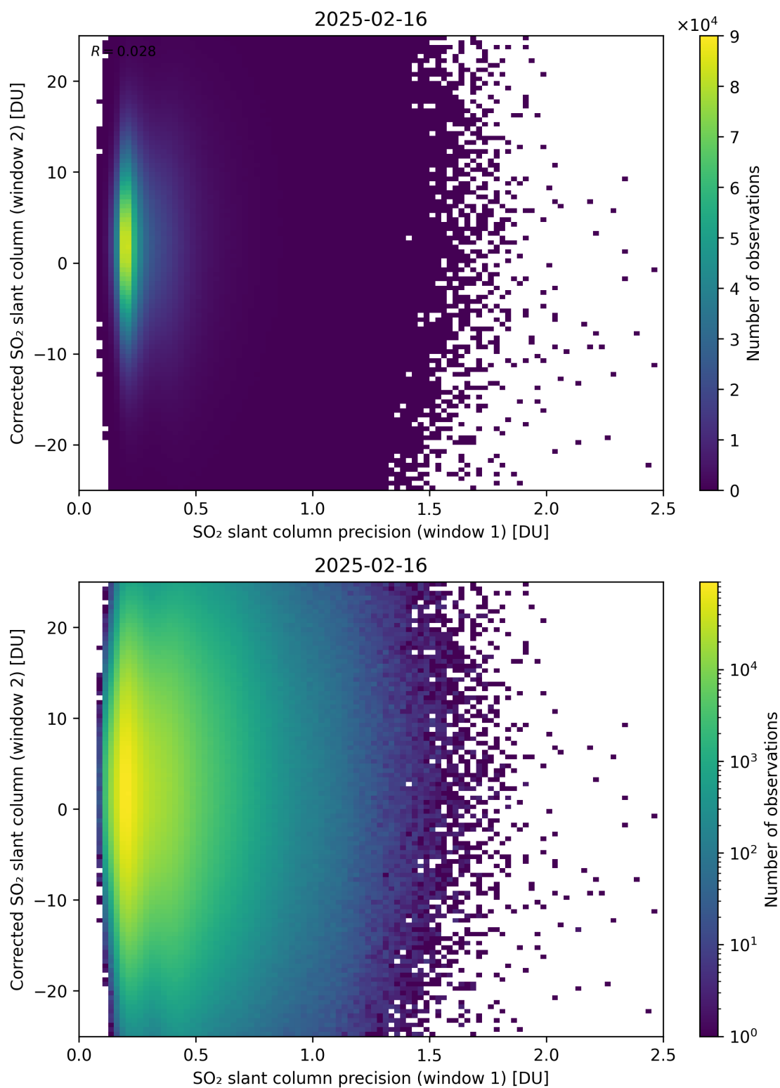
Figure 275: Scatter density plot of “SO 2 slant column precision (window 1)” against “Corrected SO 2 slant column (window 2)” for 2025-02-15 to 2025-02-17.
