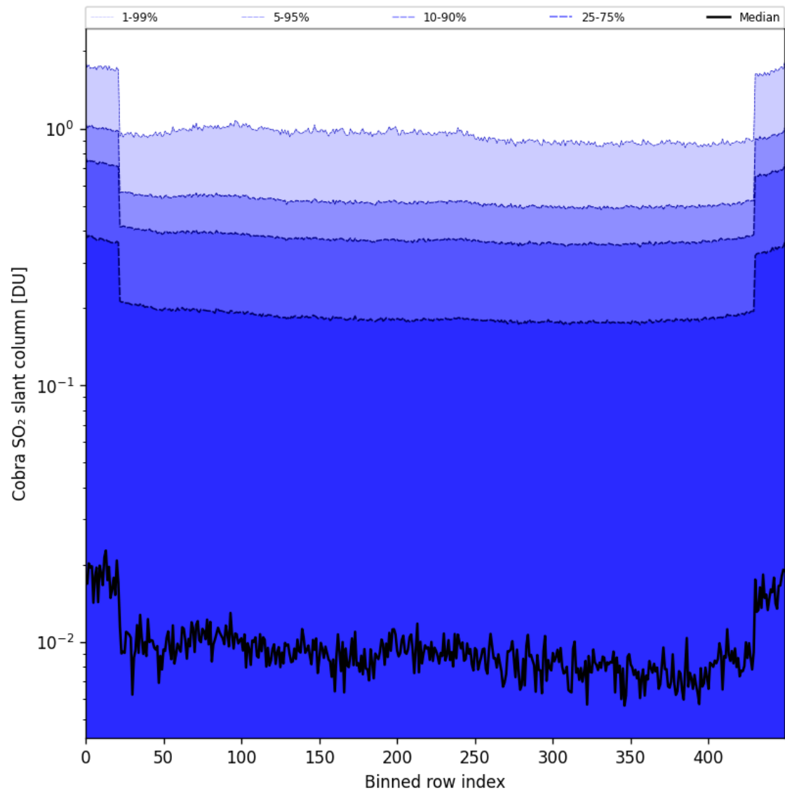
Figure 87: Along track statistics of “Cobra SO 2 slant column” for 2025-02-15 to 2025-02-17
