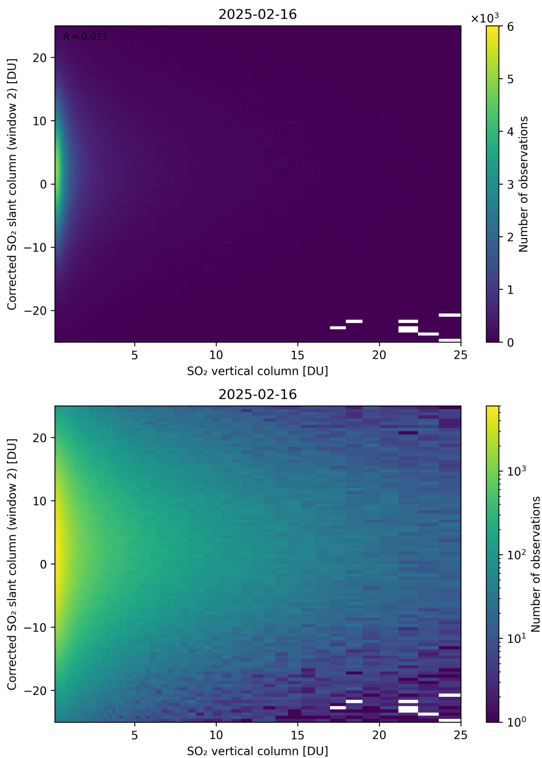
Figure 352: Scatter density plot of “SO 2 vertical column” against “Corrected SO 2 slant column (window 2)” for 2025-02-15 to 2025-02-17.
