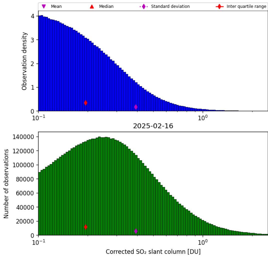
Figure 60: Histogram of "Corrected SO 2 slant column" for 2025-02-15 to 2025-02-17
