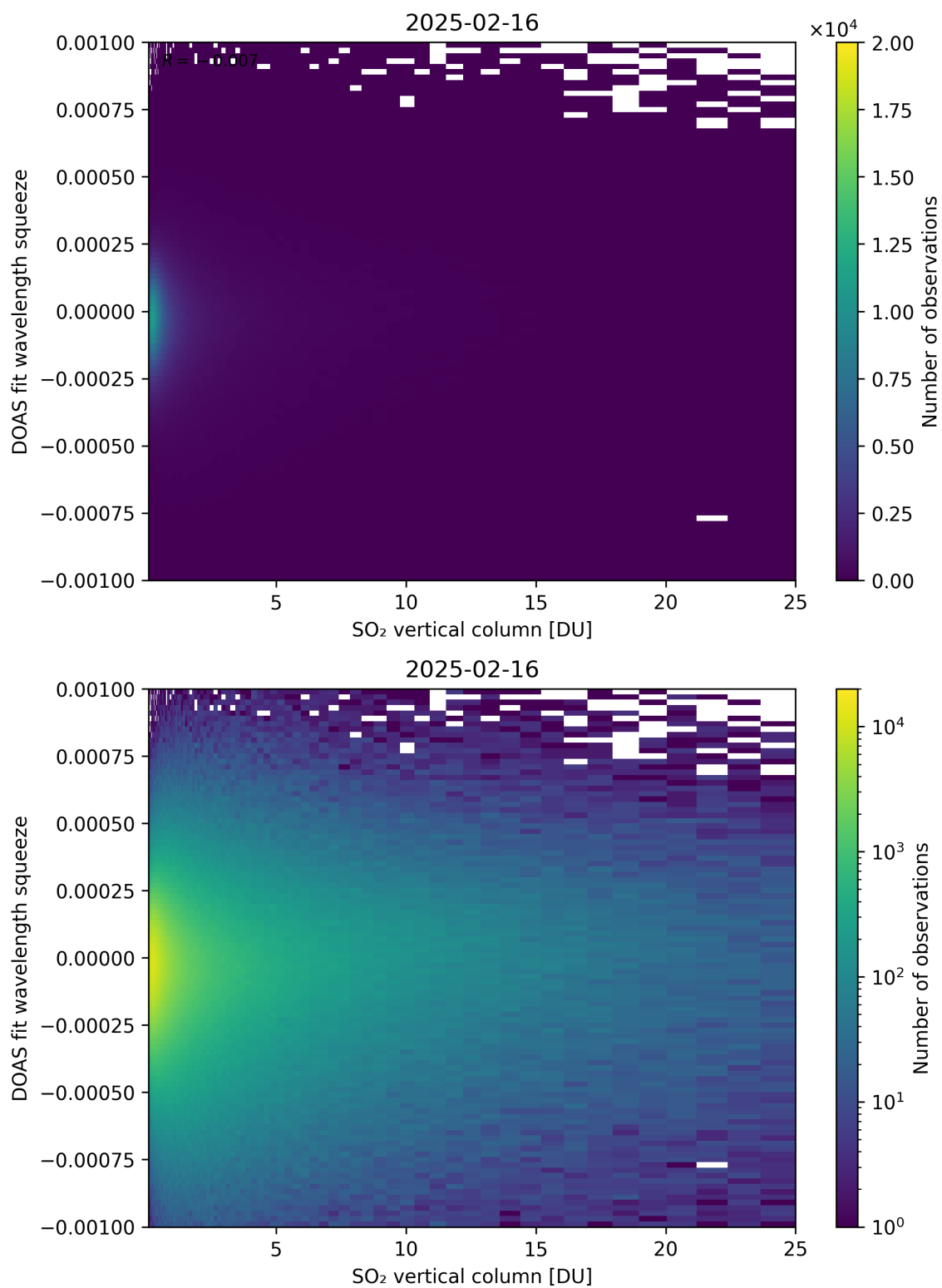
Figure 327: Scatter density plot of “SO 2 vertical column” against “DOAS fit wavelength squeeze” for 2025-02-15 to 2025-02-17.
