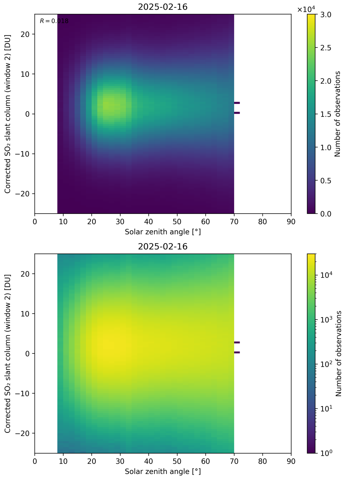
Figure 182: Scatter density plot of “Solar zenith angle” against “Corrected SO 2 slant column (window 2)” for 2025-02-15 to 2025-02-17.
