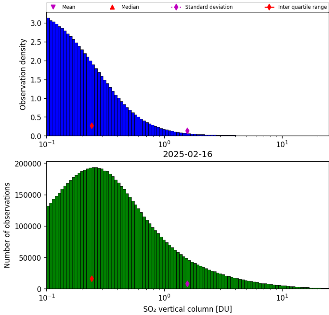
Figure 58: Histogram of “SO 2 vertical column” for 2025-02-15 to 2025-02-17
