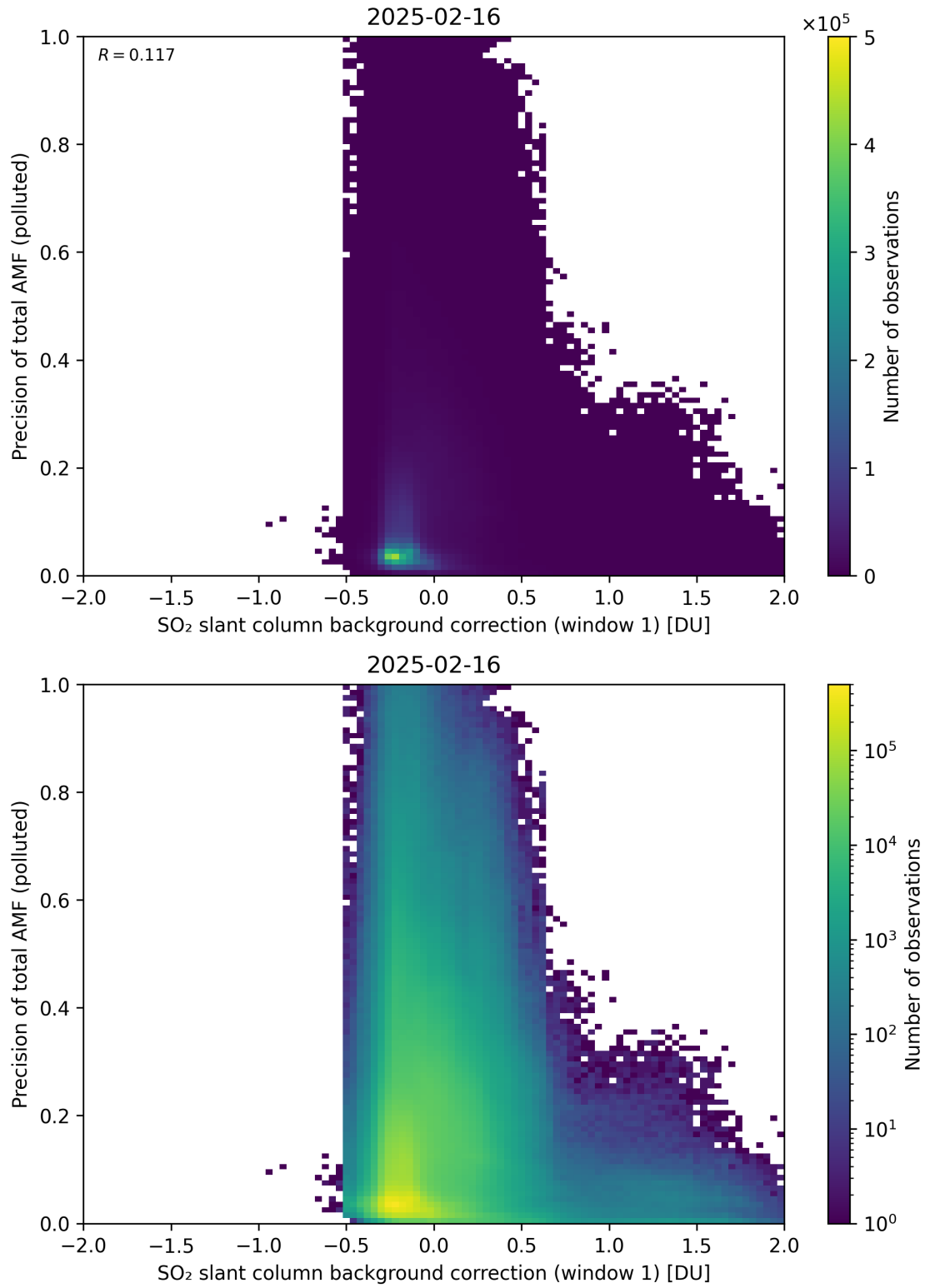
Figure 121: Scatter density plot of “SO 2 slant column background correction (window 1)” against “Precision of total AMF (polluted)” for 2025-02-15 to 2025-02-17.
