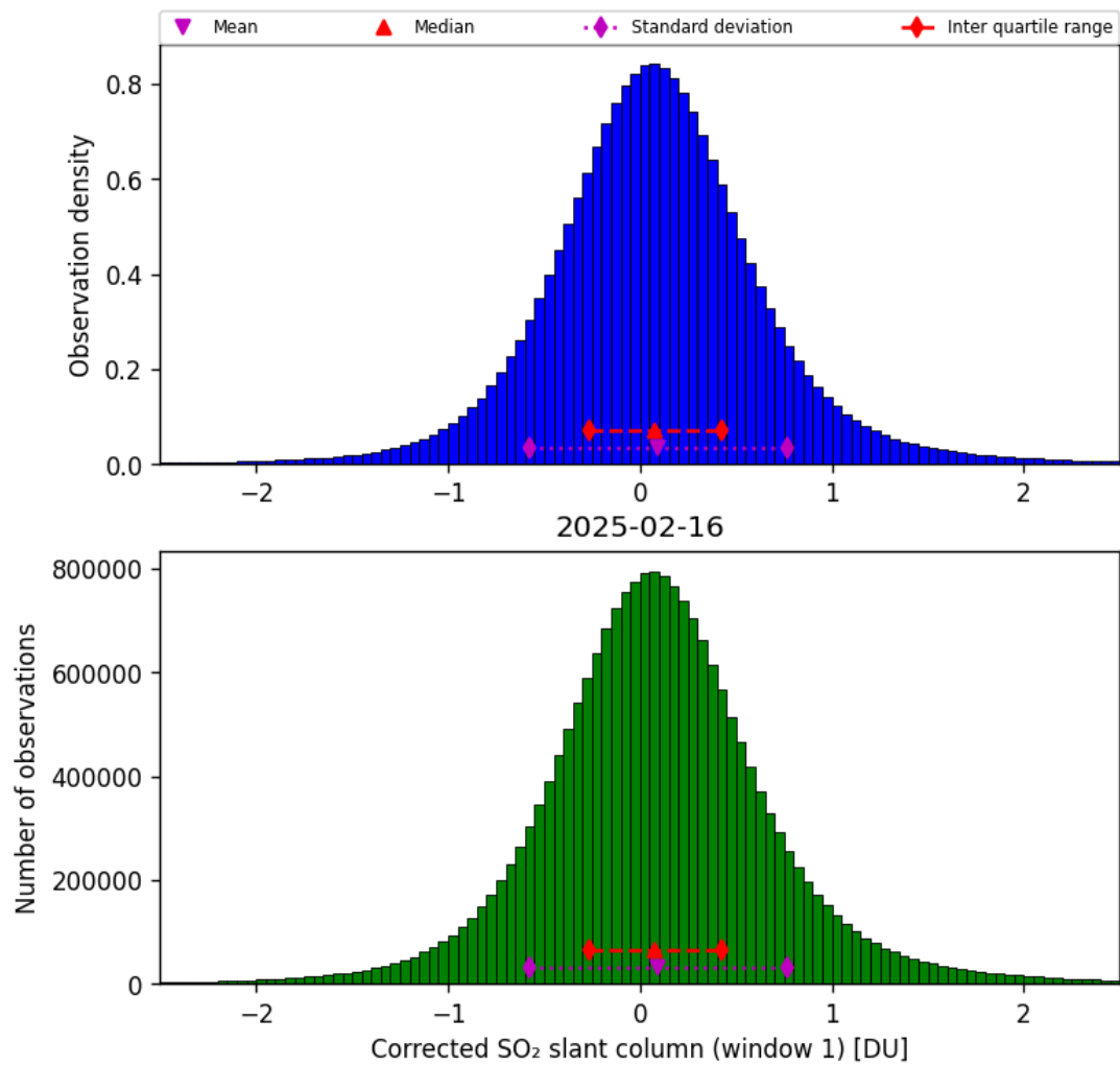
Figure 65: Histogram of “Corrected SO 2 slant column (window 1)” for 2025-02-15 to 2025-02-17
