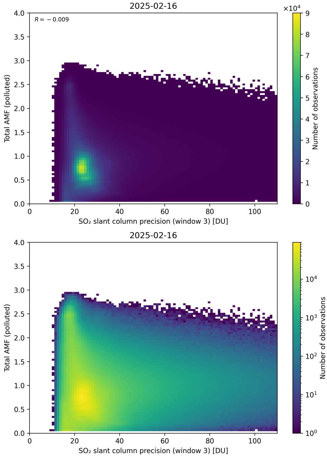
Figure 313: Scatter density plot of “SO 2 slant column precision (window 3)” against “Total AMF (polluted)” for 2025-02-15 to 2025-02-17.
