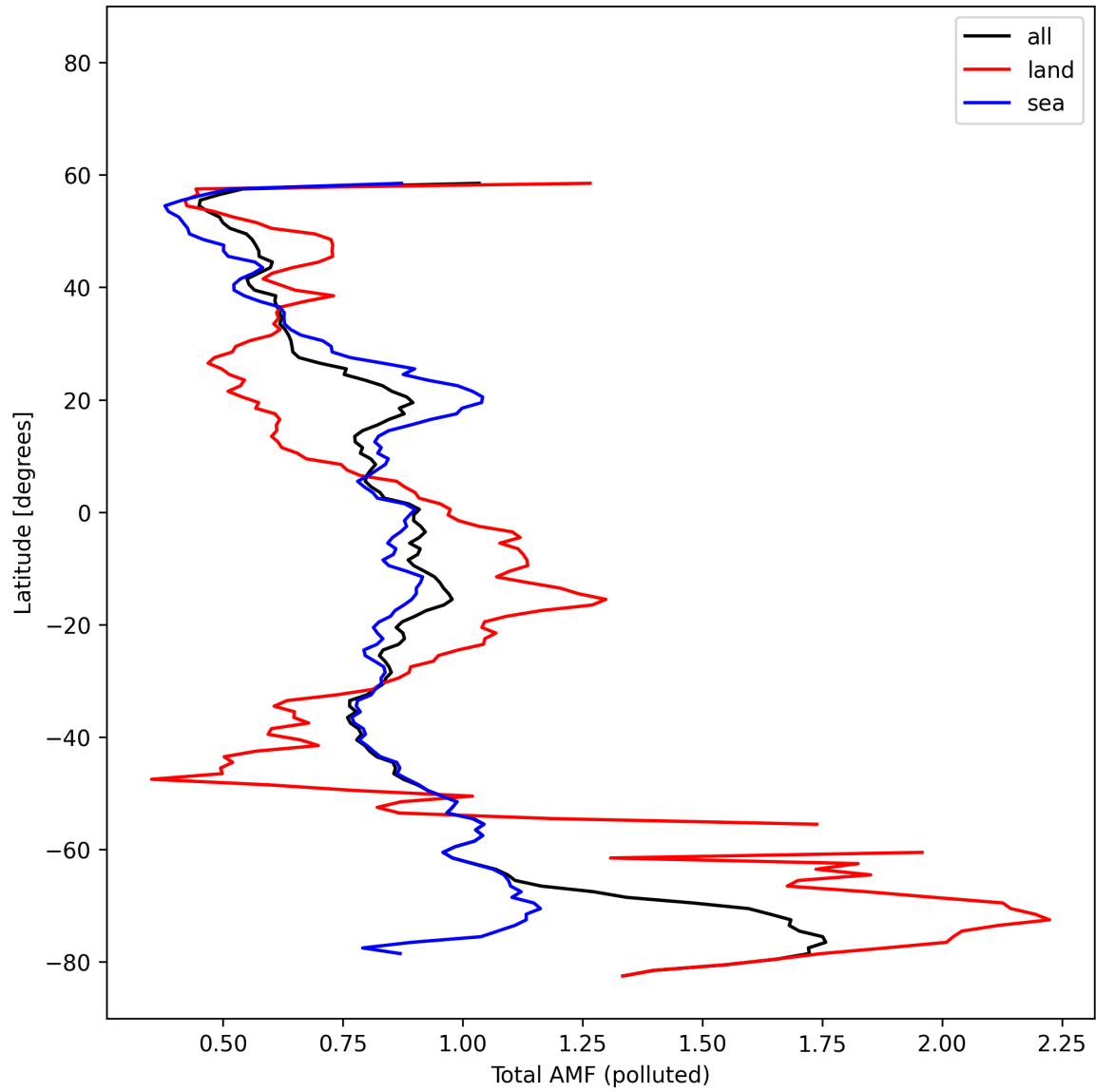
Figure 53: Zonal average of “Total AMF (polluted)” for 2025-02-15 to 2025-02-17.
