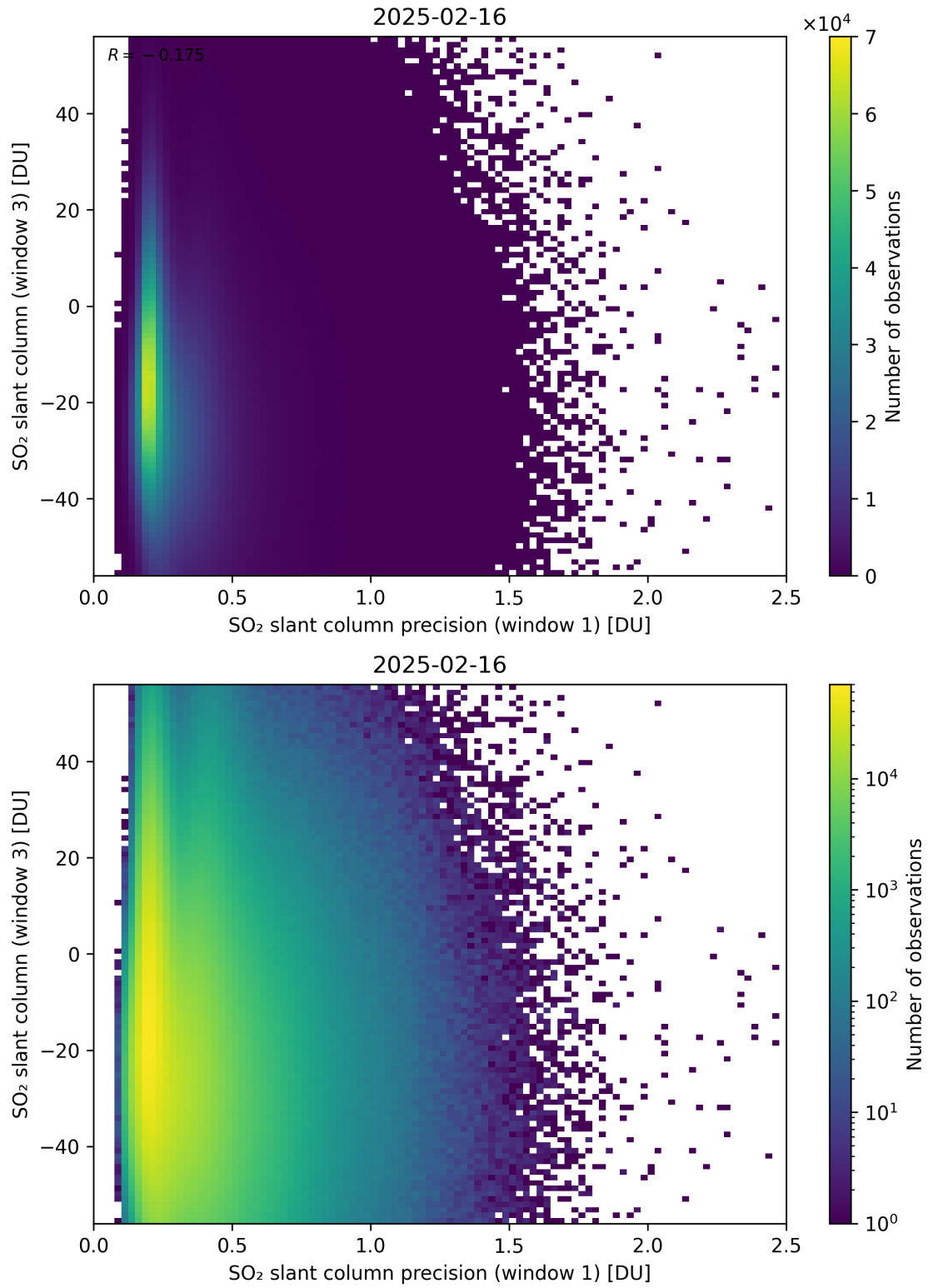
Figure 278: Scatter density plot of “SO 2 slant column precision (window 1)” against “SO 2 slant column (window 3)” for 2025-02-15 to 2025-02-17.
