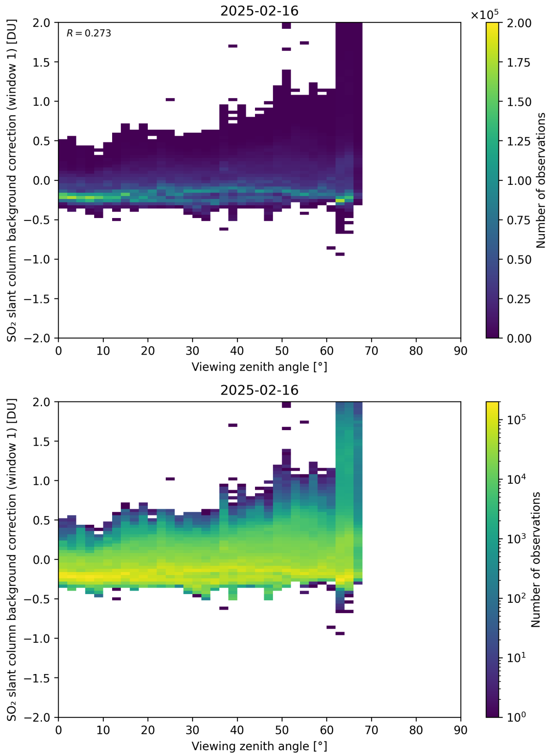
Figure 362: Scatter density plot of “Viewing zenith angle” against “SO 2 slant column background correction (window 1)” for 2025-02-15 to 2025-02-17.
