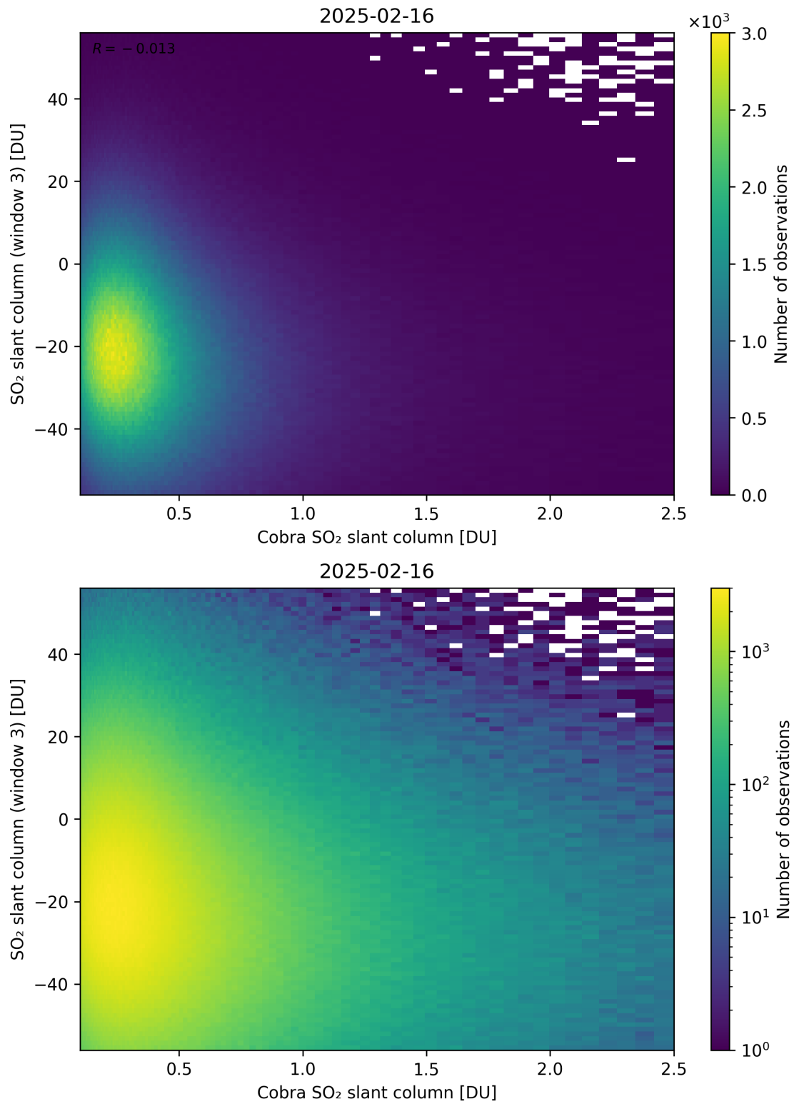
Figure 222: Scatter density plot of “Cobra SO 2 slant column” against “SO 2 slant column (window 3)” for 2025-02-15 to 2025-02-17.
