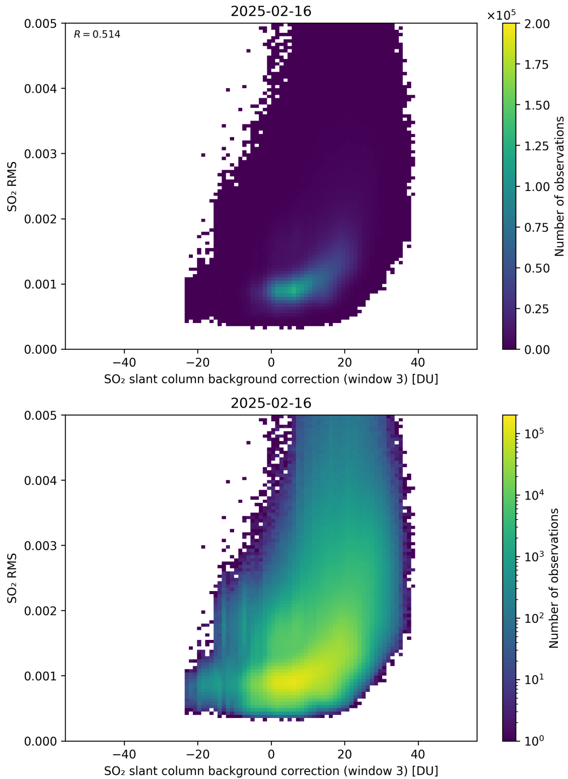
Figure 134: Scatter density plot of “SO 2 slant column background correction (window 3)” against “SO 2 RMS” for 2025-02-15 to 2025-02-17.
