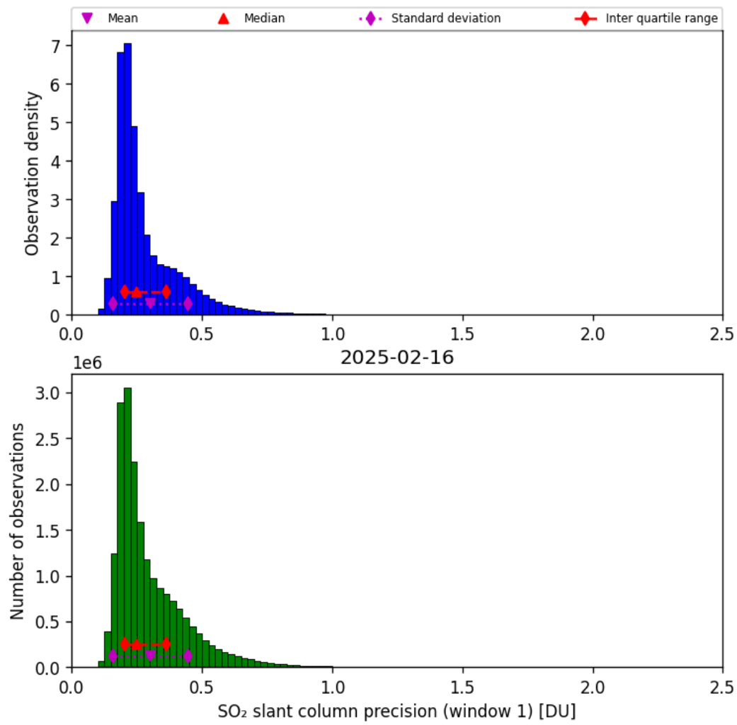
Figure 64: Histogram of “SO 2 slant column precision (window 1)” for 2025-02-15 to 2025-02-17
