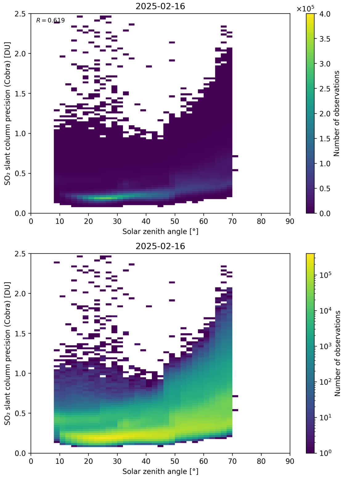
Figure 180: Scatter density plot of “Solar zenith angle” against “SO 2 slant column precision (Cobra)” for 2025-02-15 to 2025-02-17.
