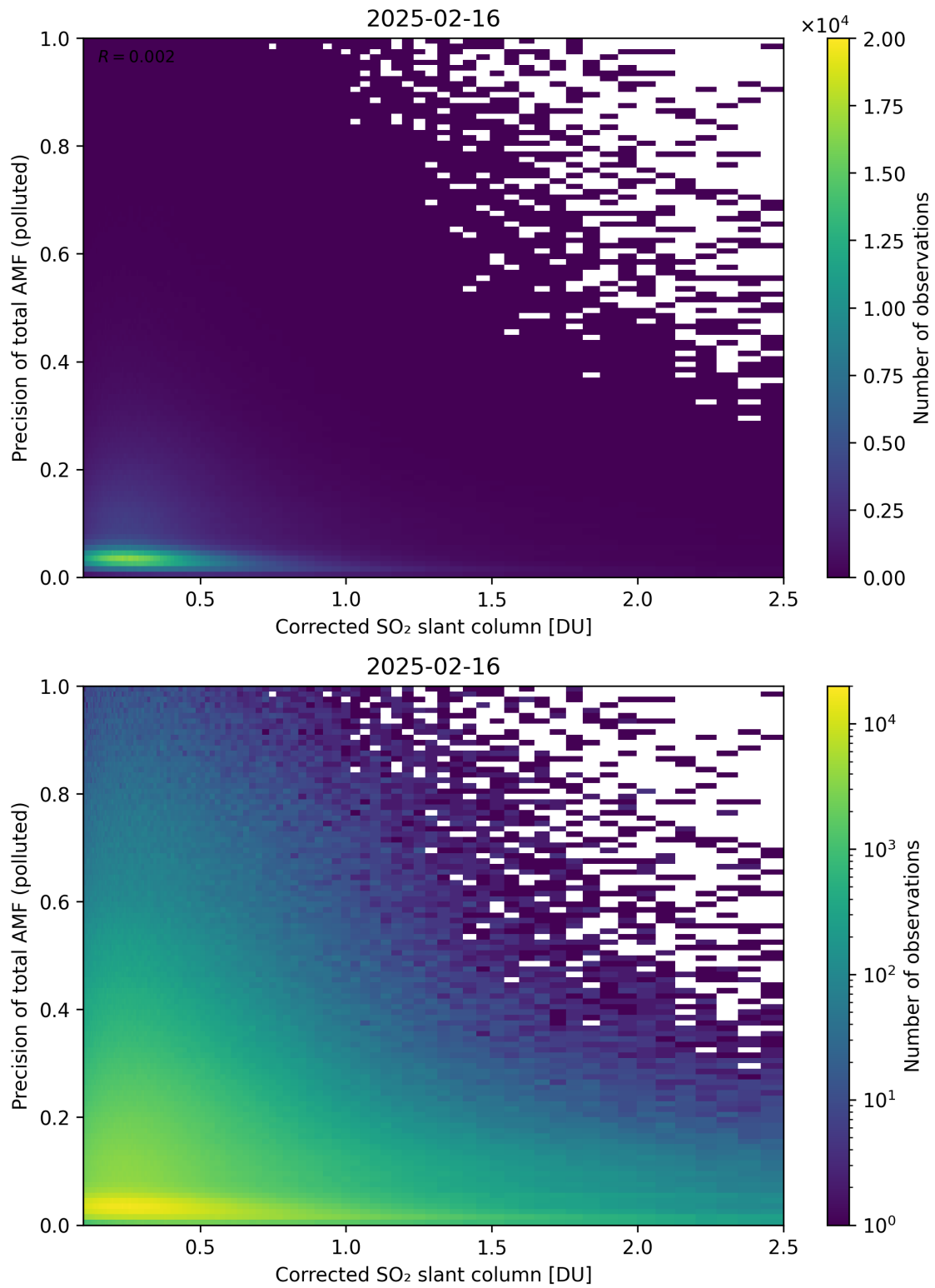
Figure 243: Scatter density plot of “Corrected SO 2 slant column” against “Precision of total AMF (polluted)” for 2025-02-15 to 2025-02-17.
