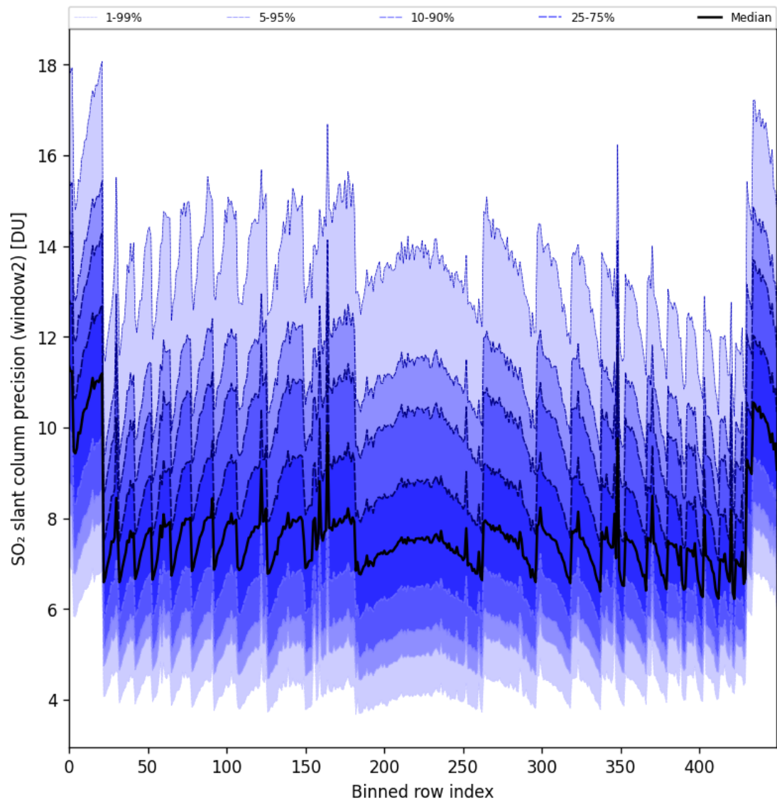
Figure 94: Along track statistics of “SO 2 slant column precision (window2)” for 2025-02-15 to 2025-02-17
