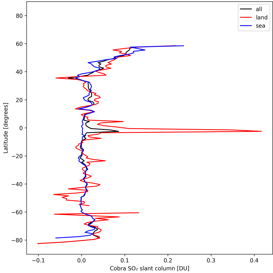
Figure 35: Zonal average of “Cobra SO 2 slant column” for 2025-02-15 to 2025-02-17.
