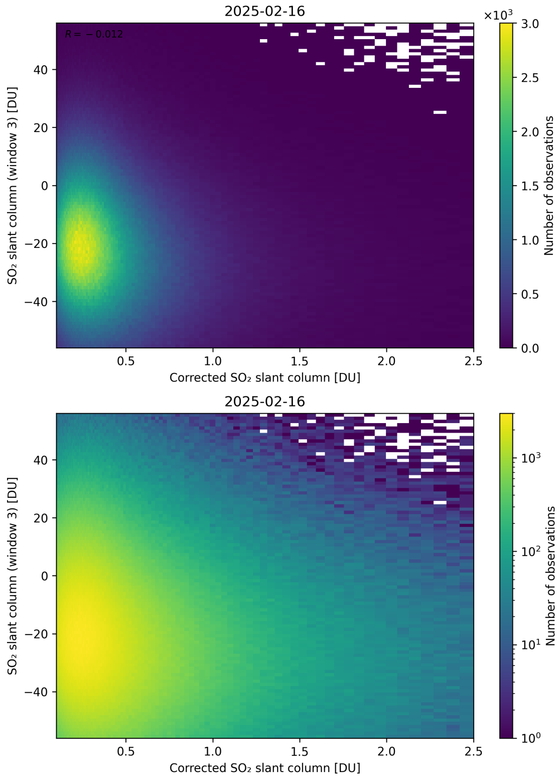
Figure 240: Scatter density plot of “Corrected SO 2 slant column” against “SO 2 slant column (window 3)” for 2025-02-15 to 2025-02-17.
