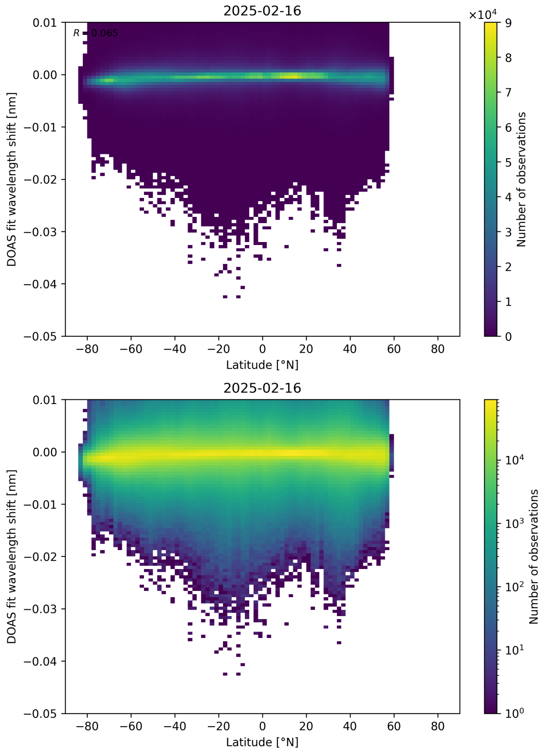
Figure 153: Scatter density plot of “Latitude” against “DOAS fit wavelength shift” for 2025-02-15 to 2025-02-17.
