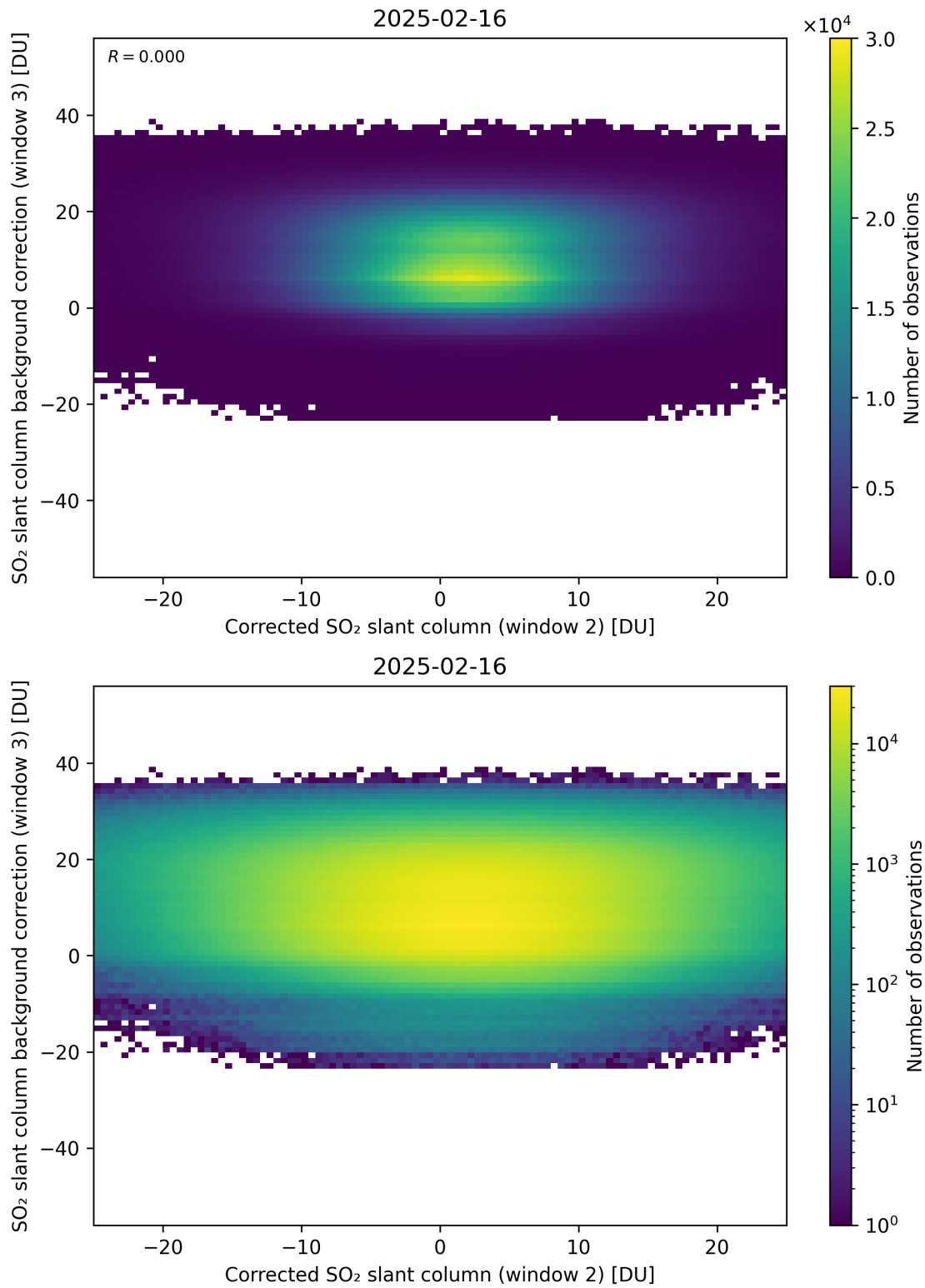
Figure 245: Scatter density plot of “Corrected SO 2 slant column (window 2)” against “SO 2 slant column background correction (window 3)” for 2025-02-15 to 2025-02-17.
