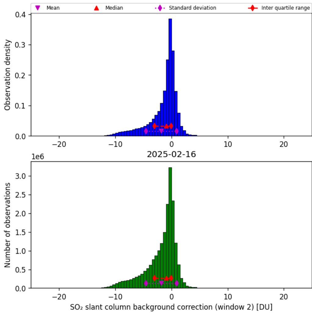
Figure 70: Histogram of “SO 2 slant column background correction (window 2)” for 2025-02-15 to 2025-02-17
