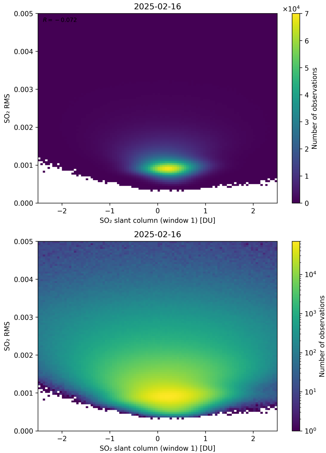
Figure 267: Scatter density plot of “SO 2 slant column (window 1)” against “SO 2 RMS” for 2025-02-15 to 2025-02-17.
