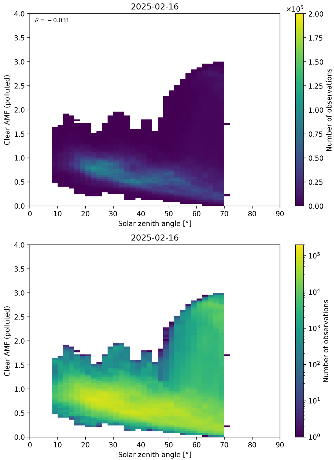
Figure 178: Scatter density plot of “Solar zenith angle” against “Clear AMF (polluted)” for 2025-02-15 to 2025-02-17.
