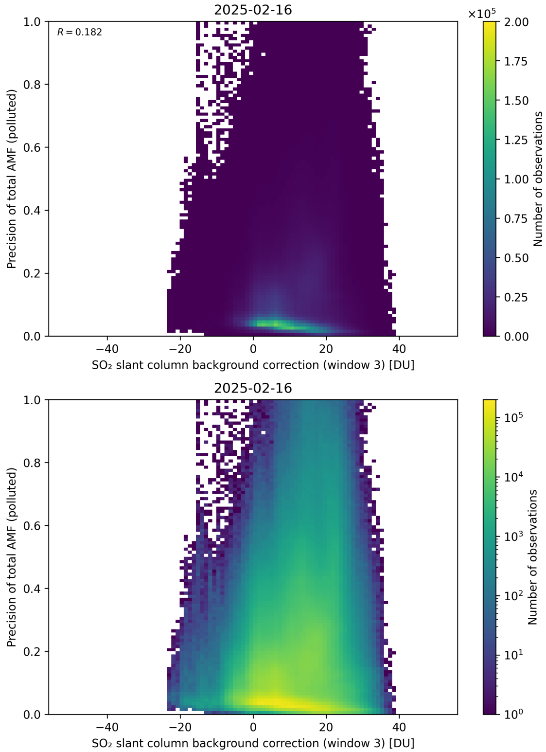
Figure 137: Scatter density plot of “SO 2 slant column background correction (window 3)” against “Precision of total AMF (polluted)” for 2025-02-15 to 2025-02-17.
