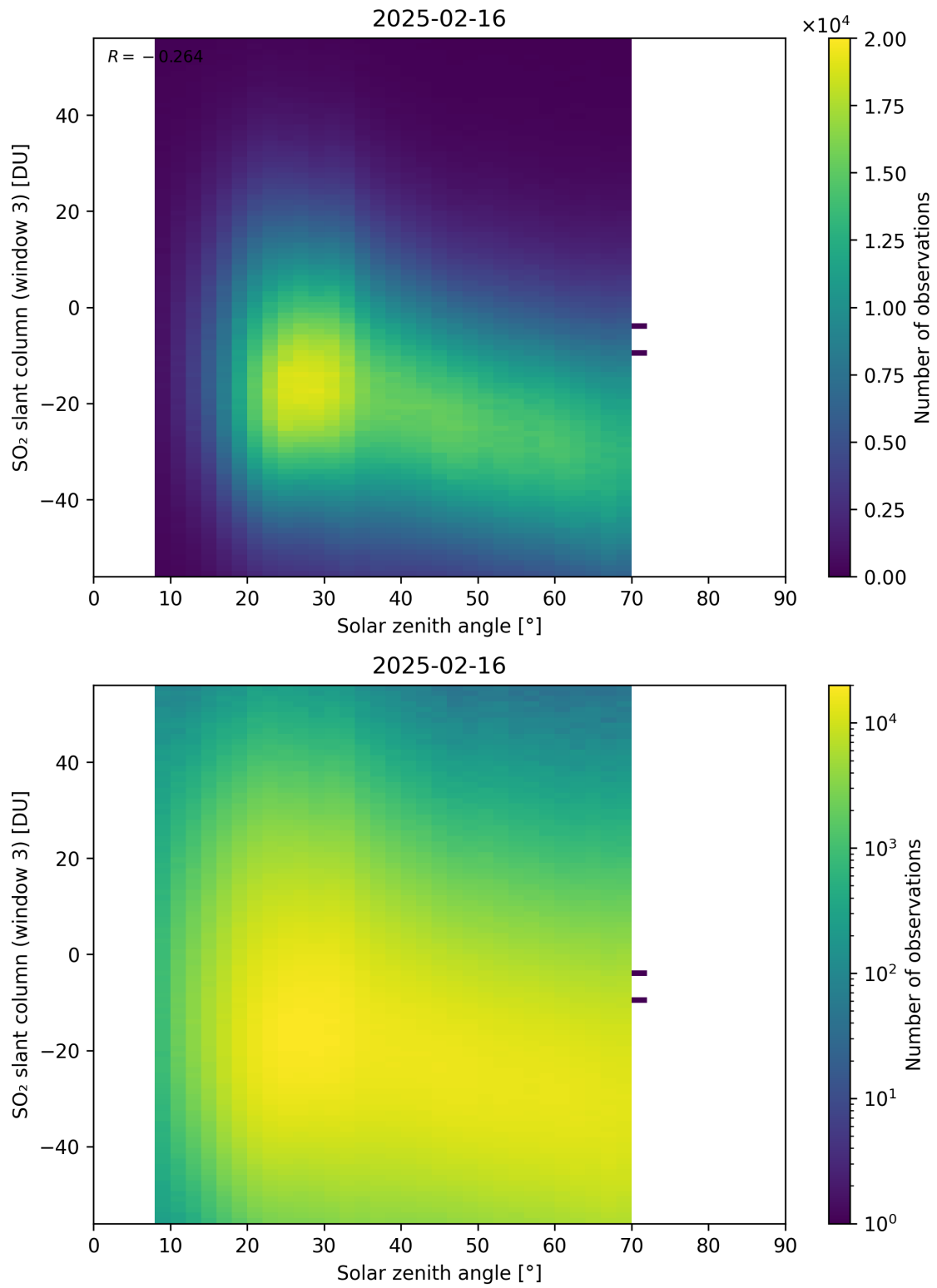
Figure 187: Scatter density plot of “Solar zenith angle” against “SO 2 slant column (window 3)” for 2025-02-15 to 2025-02-17.
