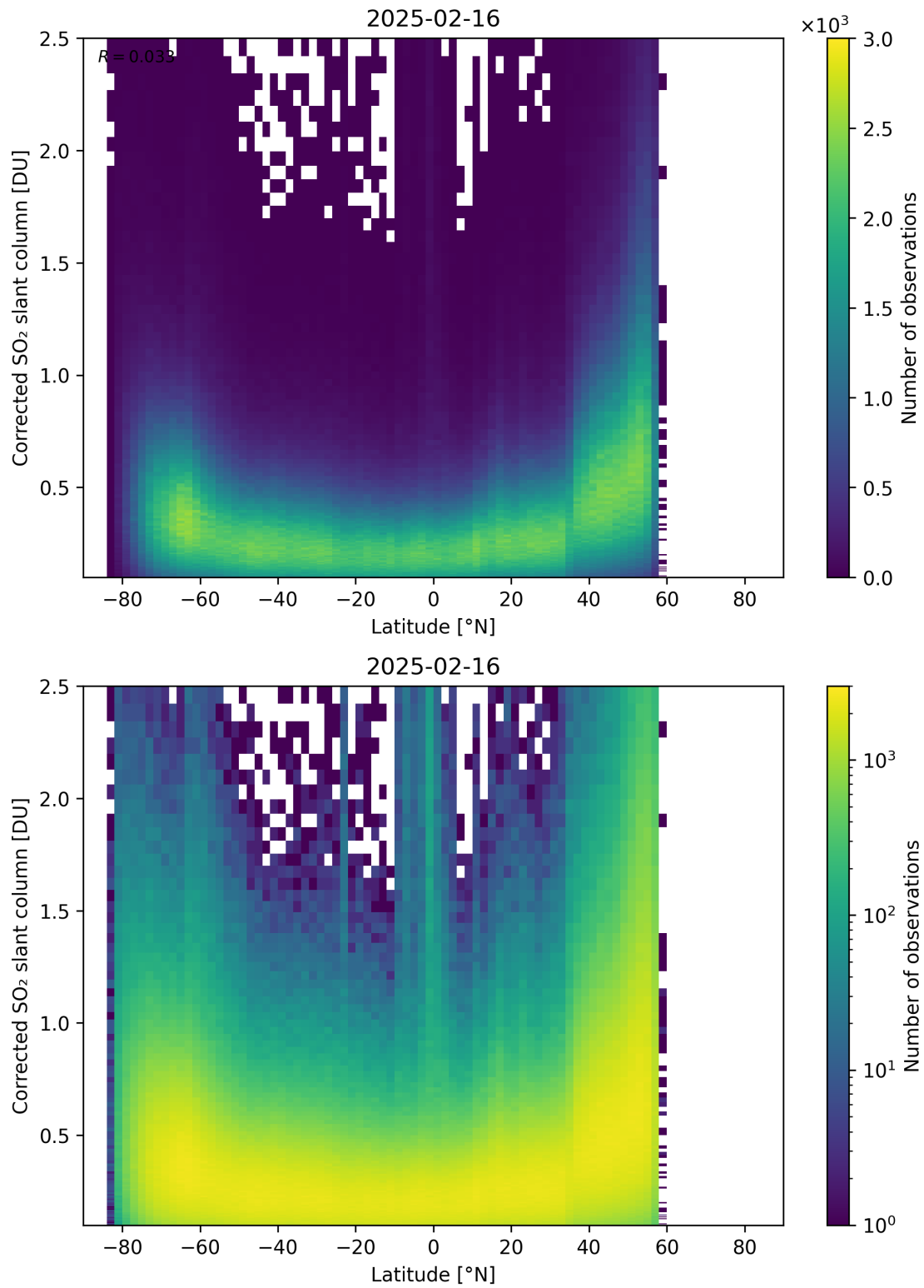
Figure 159: Scatter density plot of “Latitude” against “Corrected SO 2 slant column” for 2025-02-15 to 2025-02-17.
