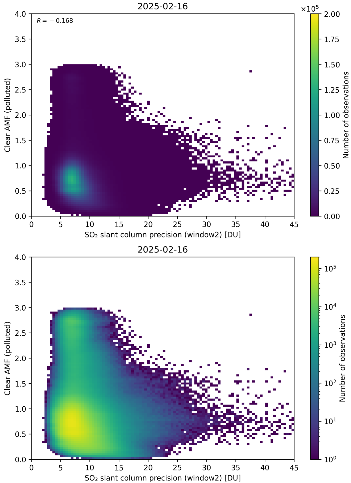
Figure 296: Scatter density plot of “SO 2 slant column precision (window2)” against “Clear AMF (polluted)” for 2025-02-15 to 2025-02-17.
