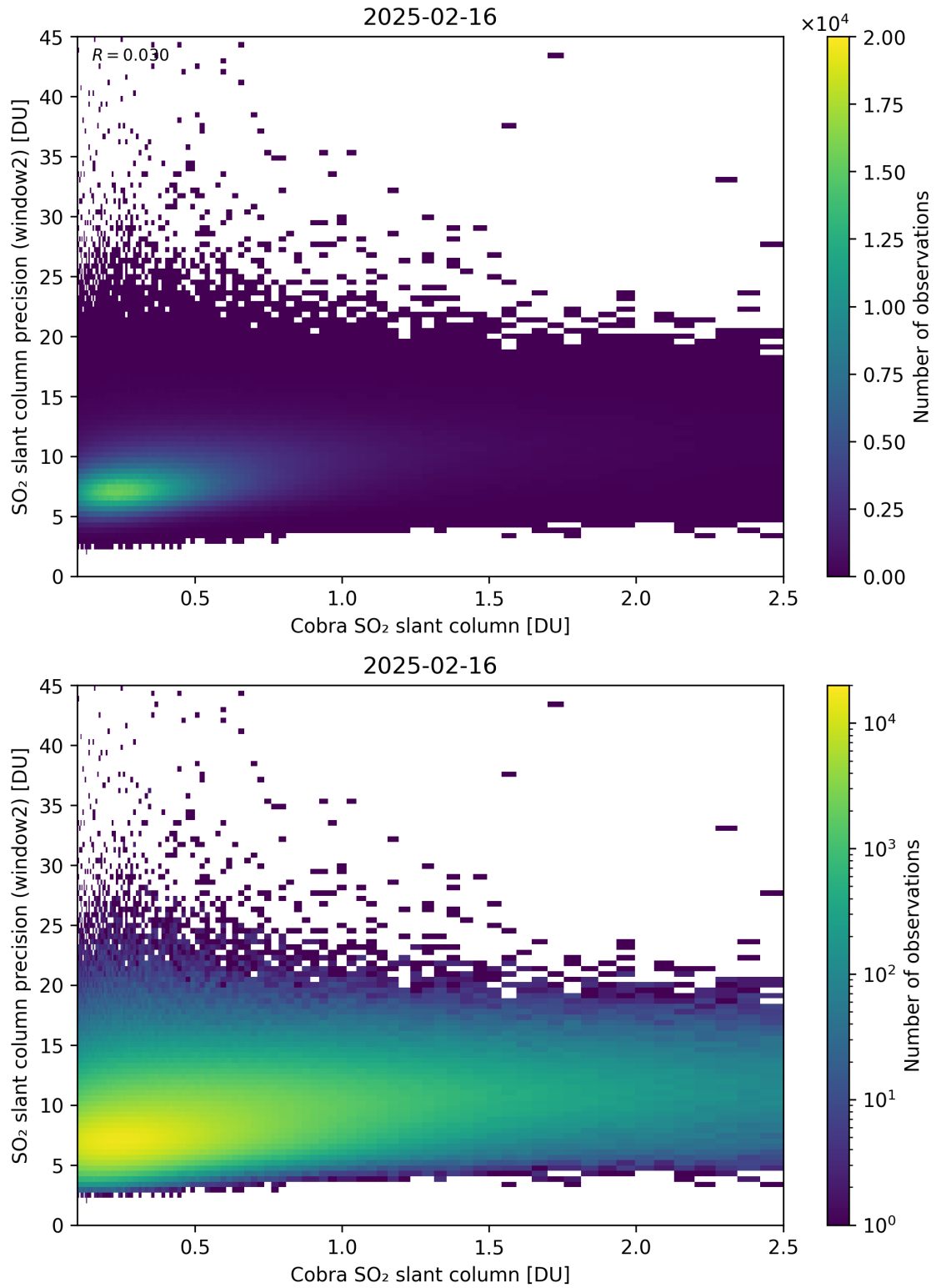
Figure 221: Scatter density plot of “Cobra SO 2 slant column” against “SO 2 slant column precision (window2)” for 2025-02-15 to 2025-02-17.
