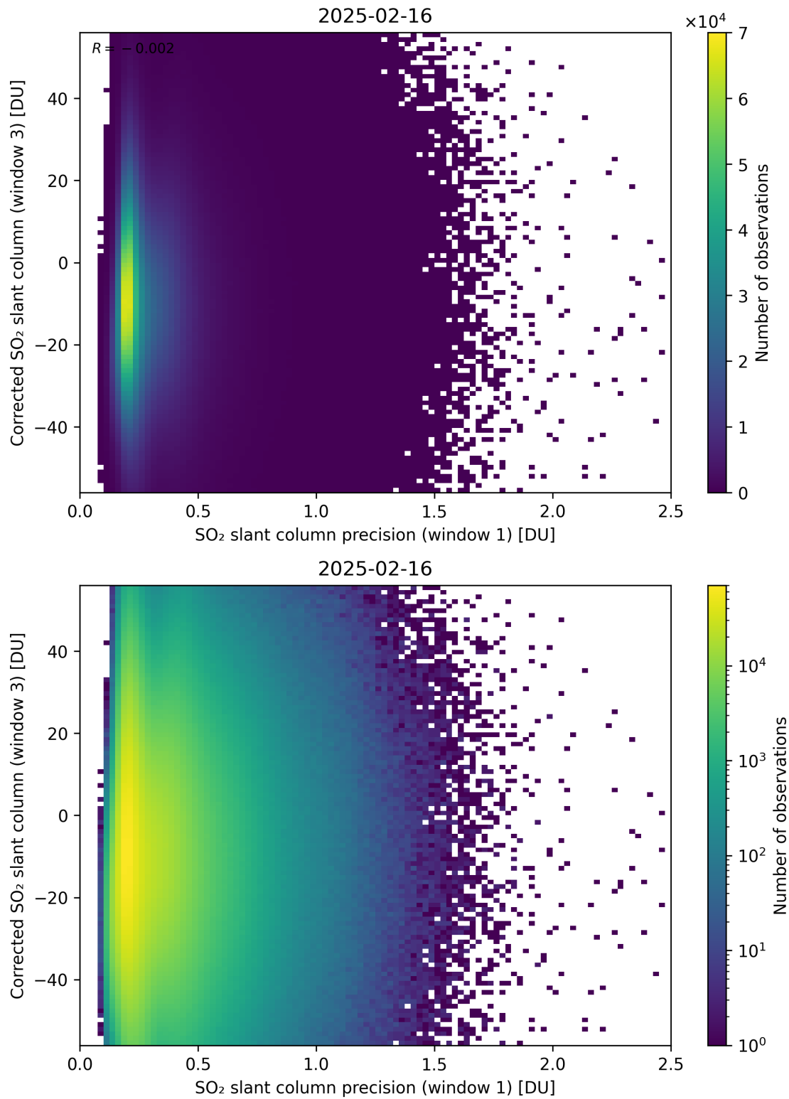
Figure 276: Scatter density plot of “SO 2 slant column precision (window 1)” against “Corrected SO 2 slant column (window 3)” for 2025-02-15 to 2025-02-17.
