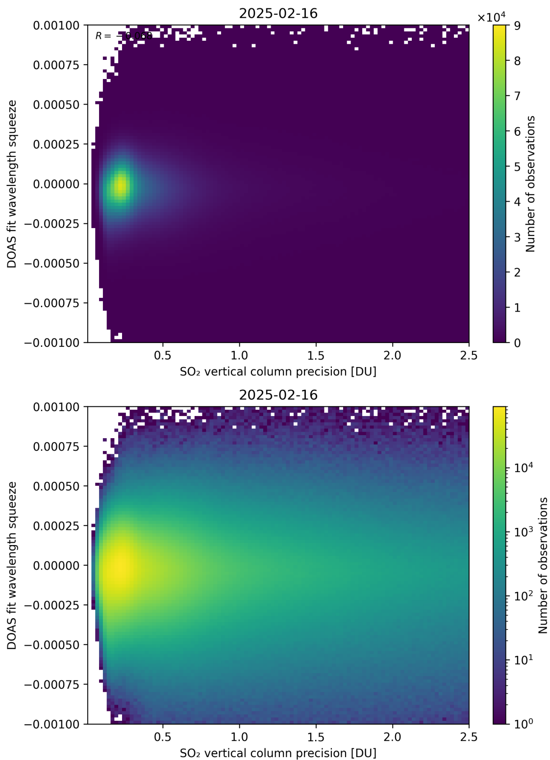
Figure 333: Scatter density plot of “SO 2 vertical column precision” against “DOAS fit wavelength squeeze” for 2025-02-15 to 2025-02-17.
