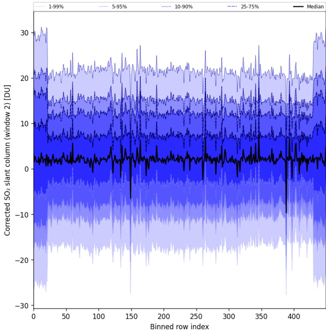
Figure 95: Along track statistics of “Corrected SO 2 slant column (window 2)” for 2025-02-15 to 2025-02-17
