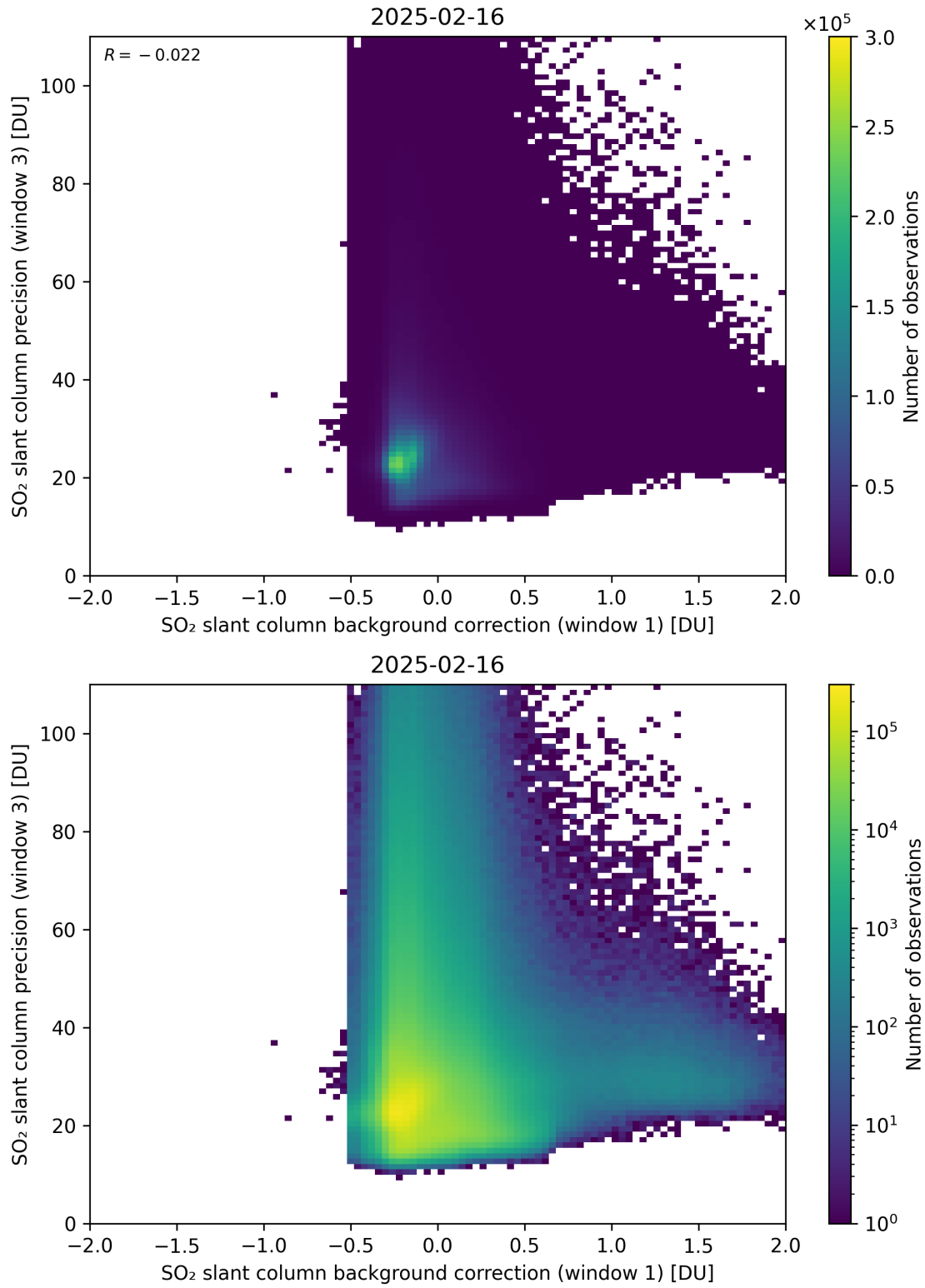
Figure 119: Scatter density plot of “SO 2 slant column background correction (window 1)” against “SO 2 slant column precision (window 3)” for 2025-02-15 to 2025-02-17.
