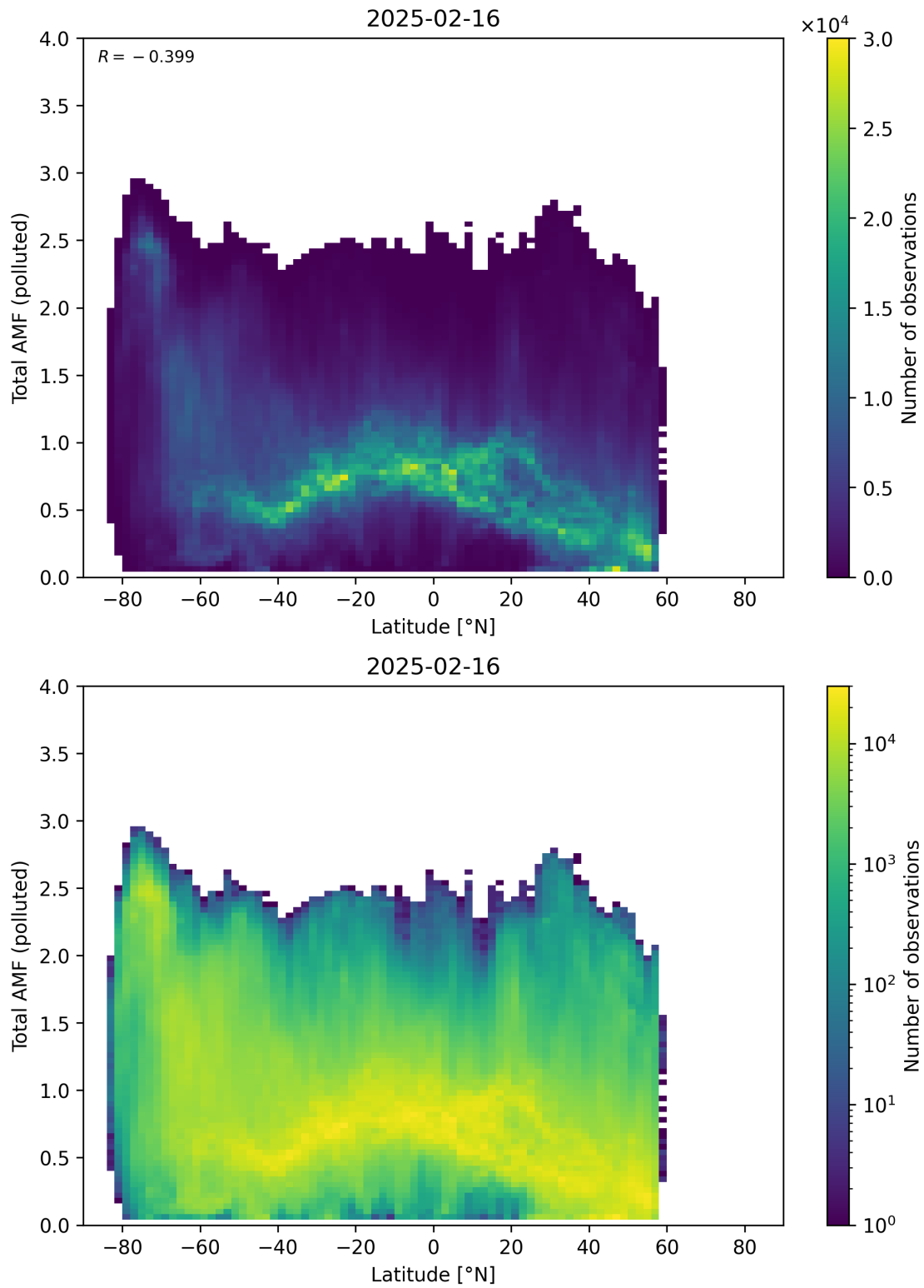
Figure 167: Scatter density plot of “Latitude” against “Total AMF (polluted)” for 2025-02-15 to 2025-02-17.
