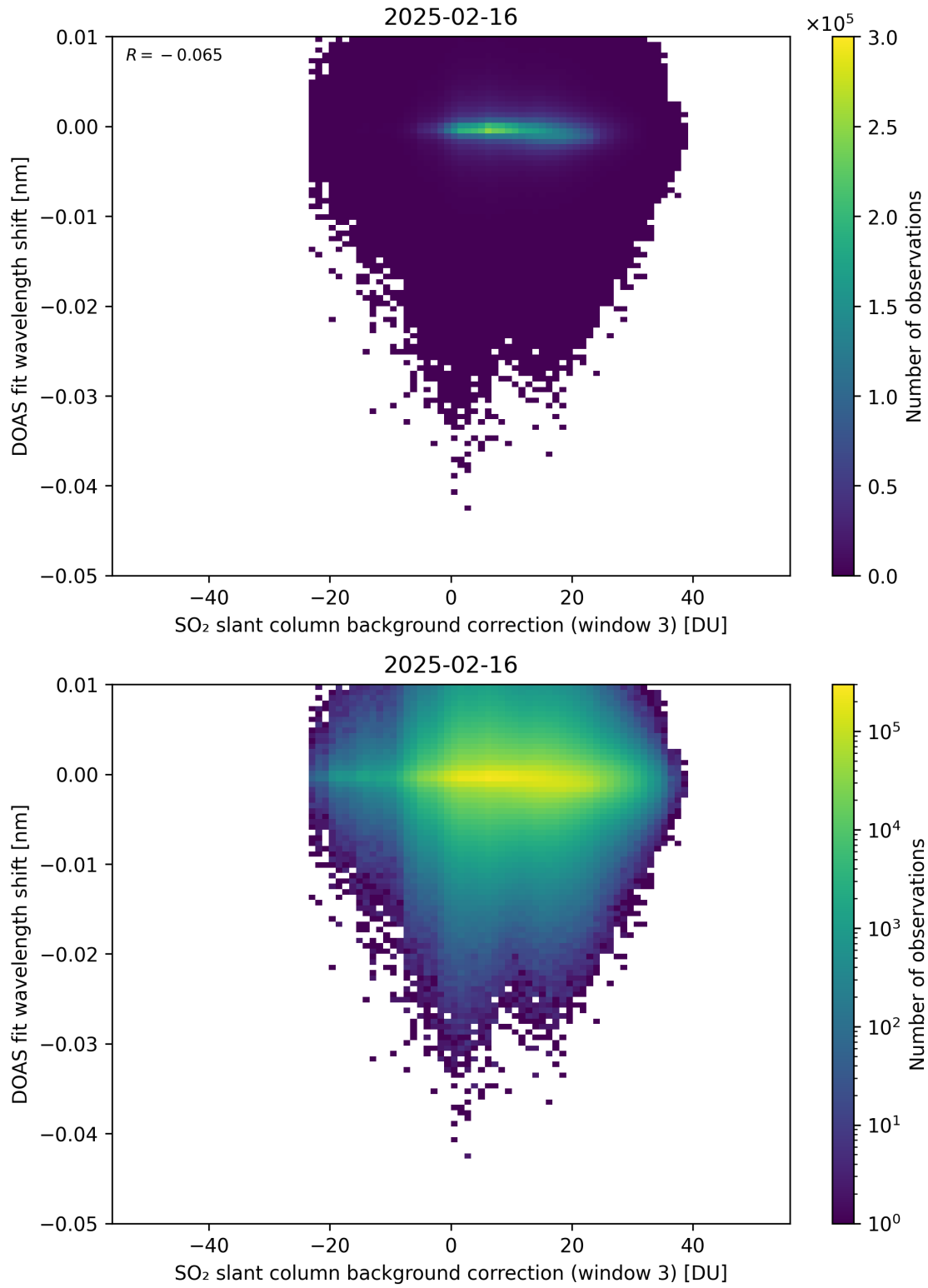
Figure 132: Scatter density plot of “SO 2 slant column background correction (window 3)” against “DOAS fit wavelength shift” for 2025-02-15 to 2025-02-17.
