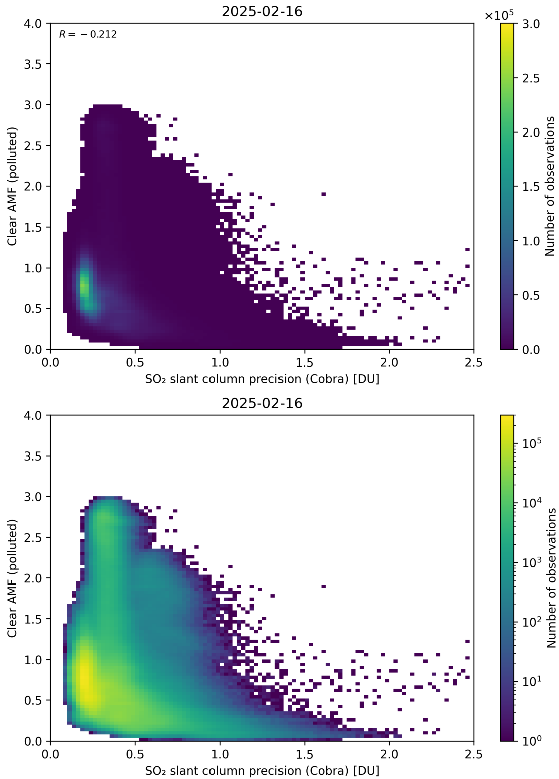
Figure 205: Scatter density plot of “SO 2 slant column precision (Cobra)” against “Clear AMF (polluted)” for 2025-02-15 to 2025-02-17.
