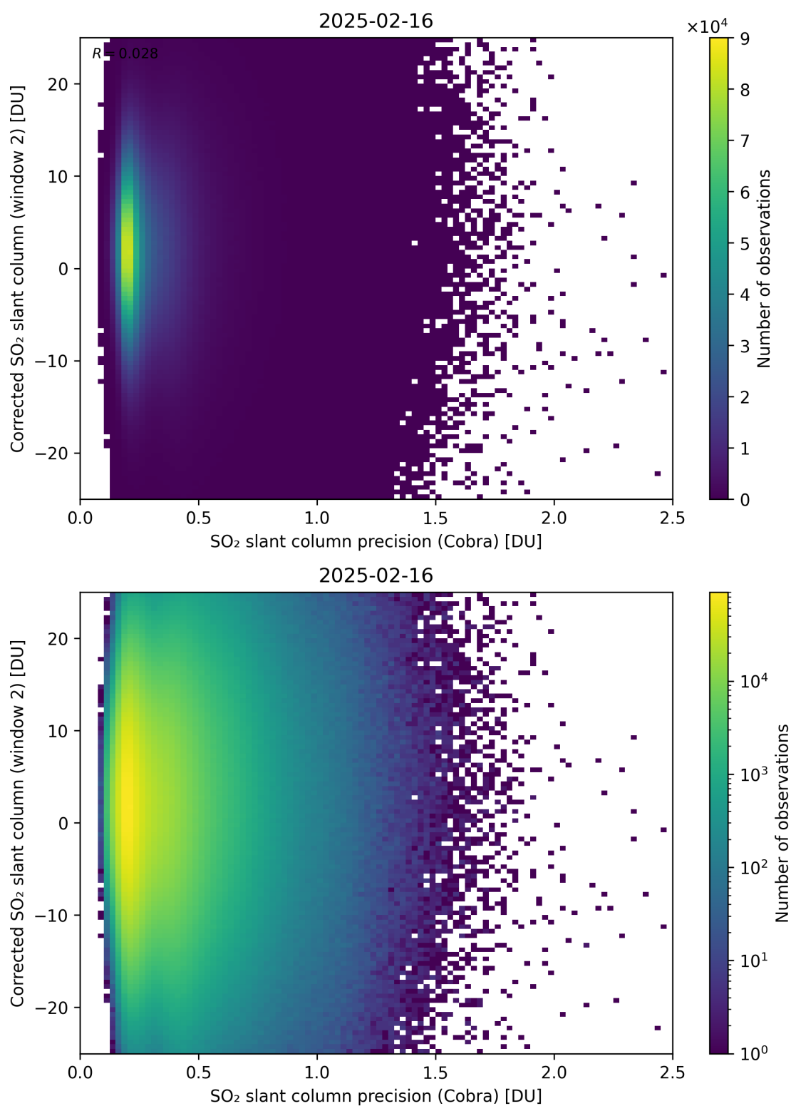
Figure 206: Scatter density plot of “SO 2 slant column precision (Cobra)” against “Corrected SO 2 slant column (window 2)” for 2025-02-15 to 2025-02-17.
