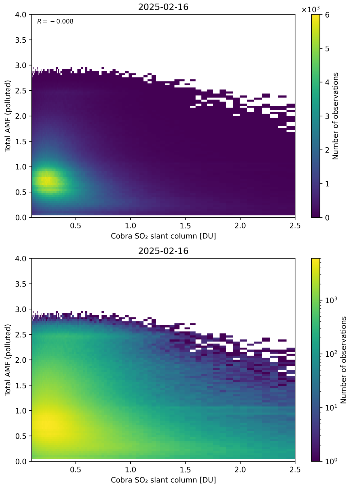
Figure 224: Scatter density plot of “Cobra SO 2 slant column” against “Total AMF (polluted)” for 2025-02-15 to 2025-02-17.
