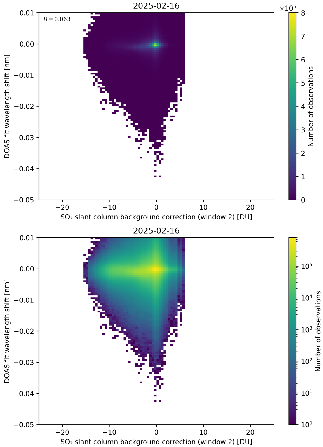
Figure 123: Scatter density plot of “SO 2 slant column background correction (window 2)” against “DOAS fit wavelength shift” for 2025-02-15 to 2025-02-17.
