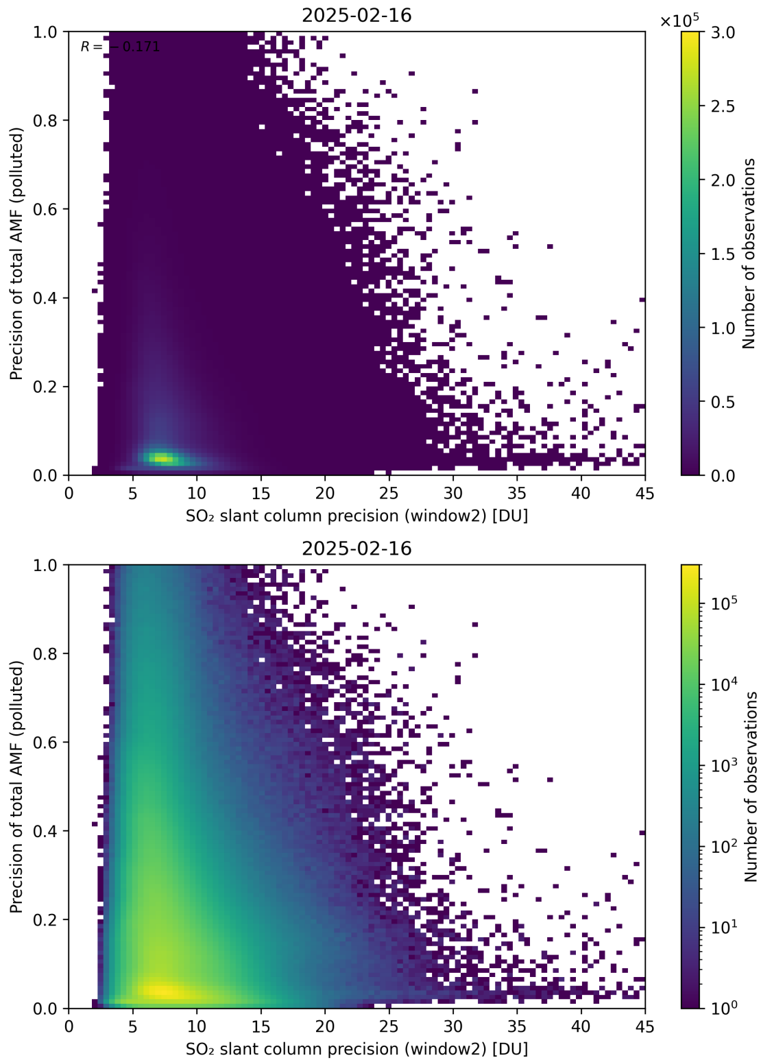
Figure 302: Scatter density plot of “SO 2 slant column precision (window2)” against “Precision of total AMF (polluted)” for 2025-02-15 to 2025-02-17.
