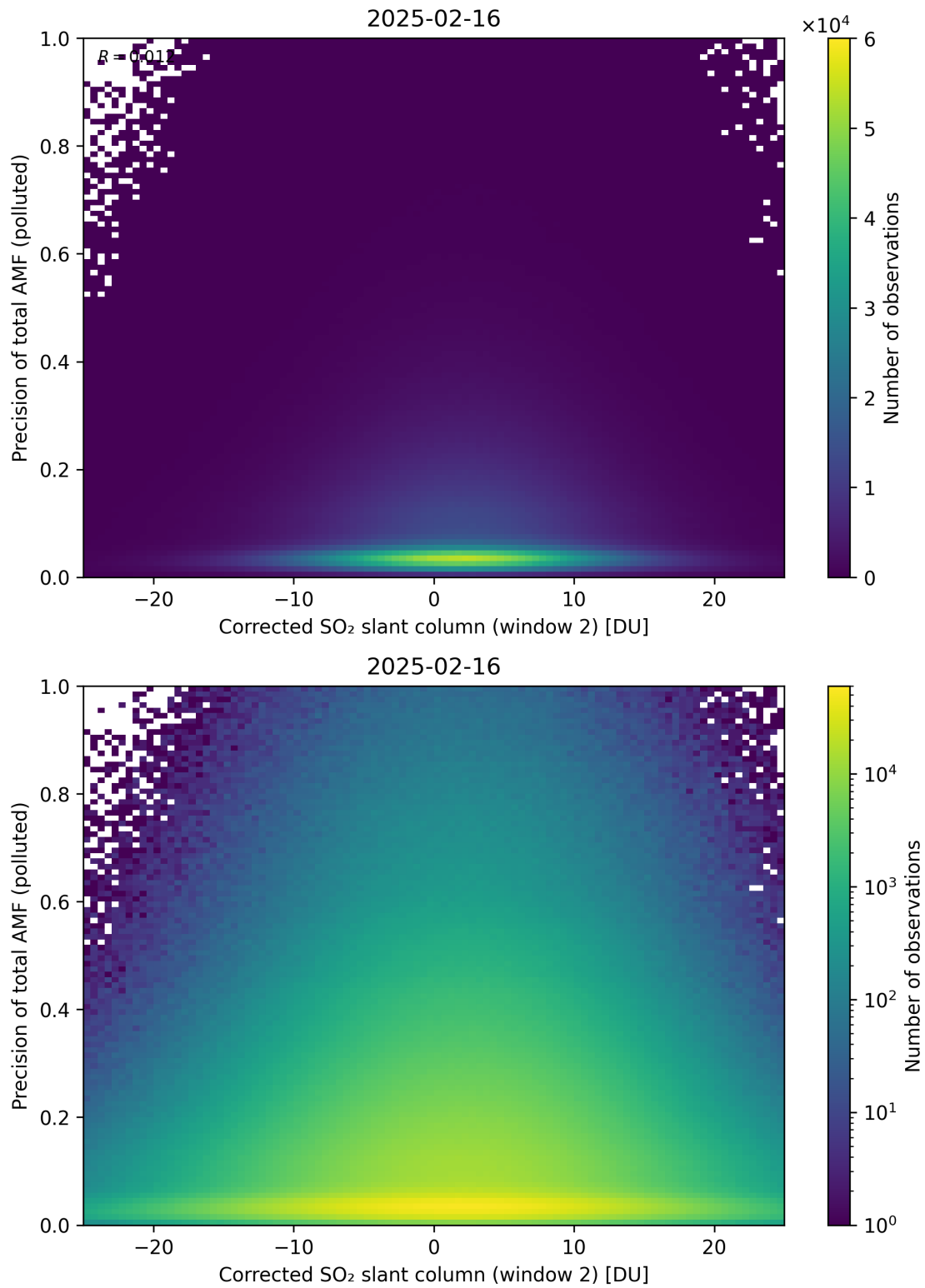
Figure 254: Scatter density plot of “Corrected SO 2 slant column (window 2)” against “Precision of total AMF (polluted)” for 2025-02-15 to 2025-02-17.
