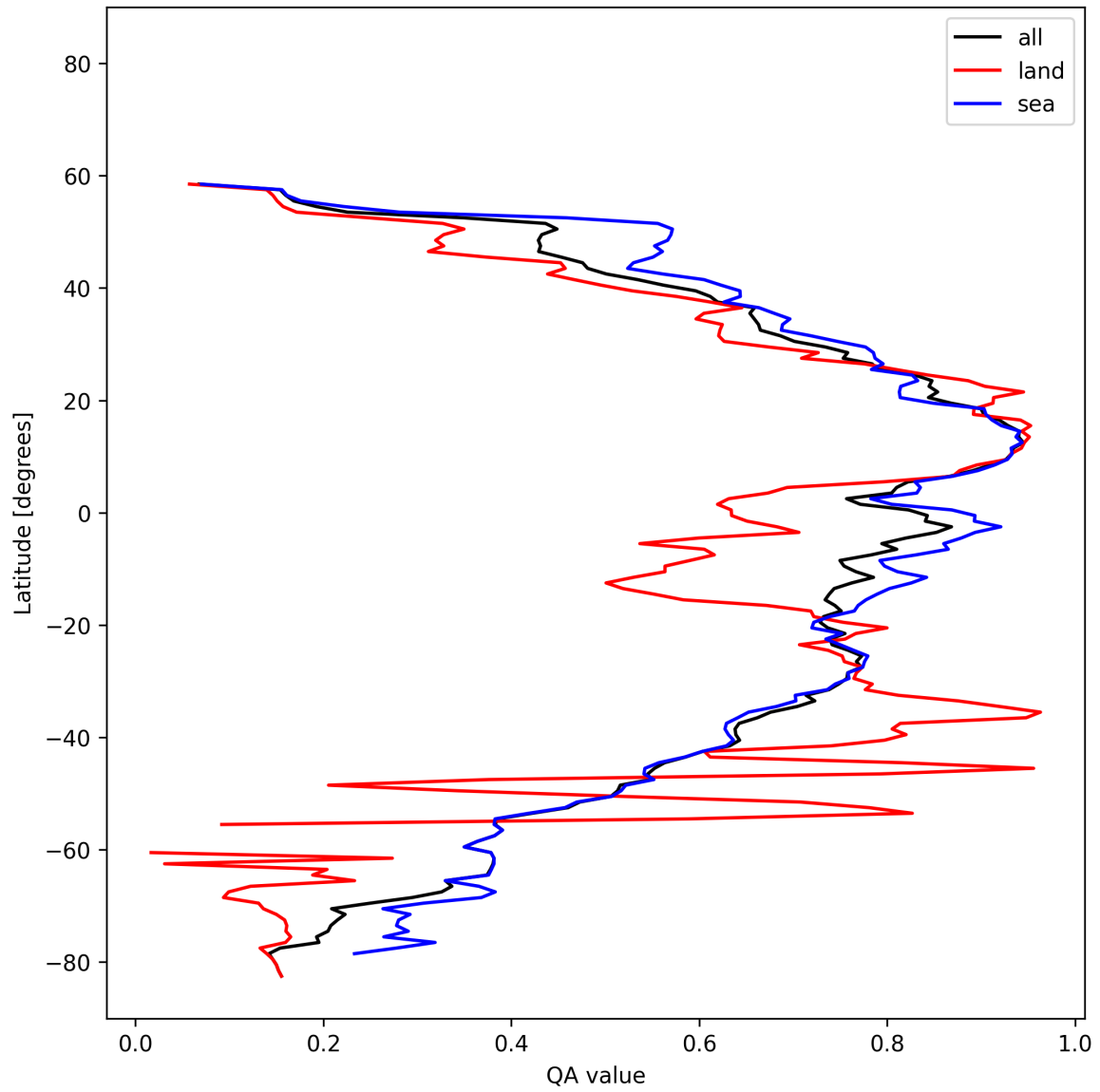
Figure 31: Zonal average of “QA value” for 2025-02-15 to 2025-02-17.
