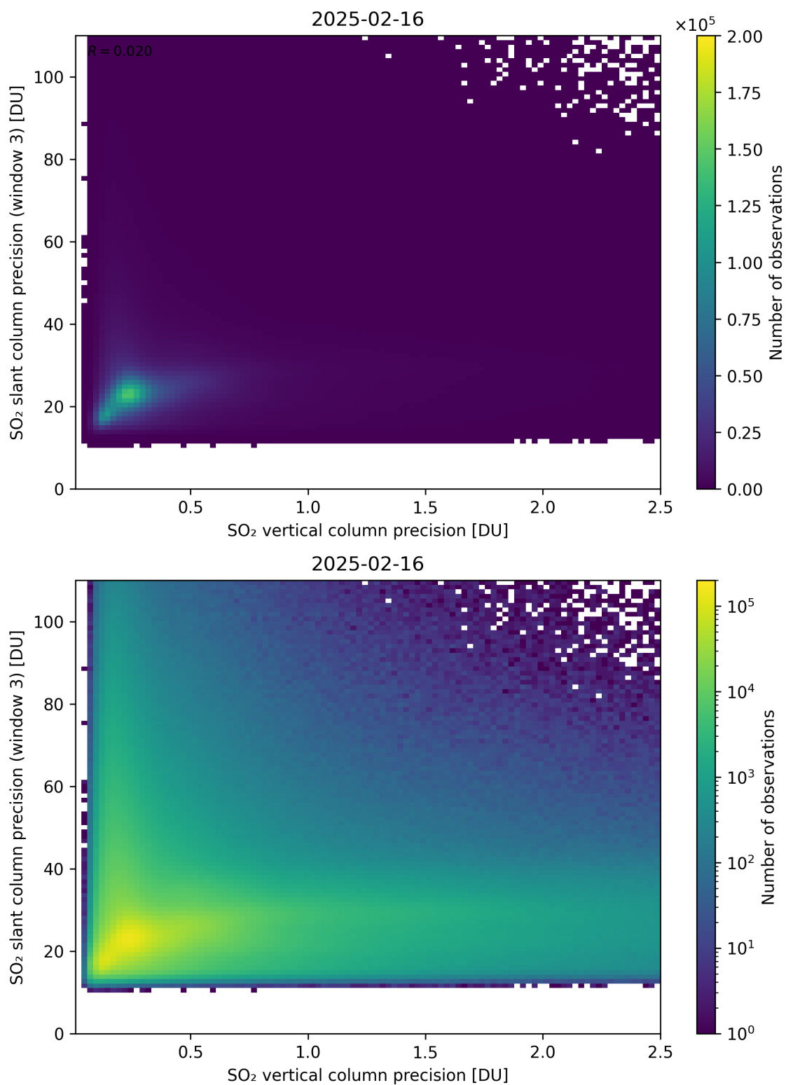
Figure 345: Scatter density plot of “SO 2 vertical column precision” against “SO 2 slant column precision (window 3)” for 2025-02-15 to 2025-02-17.
