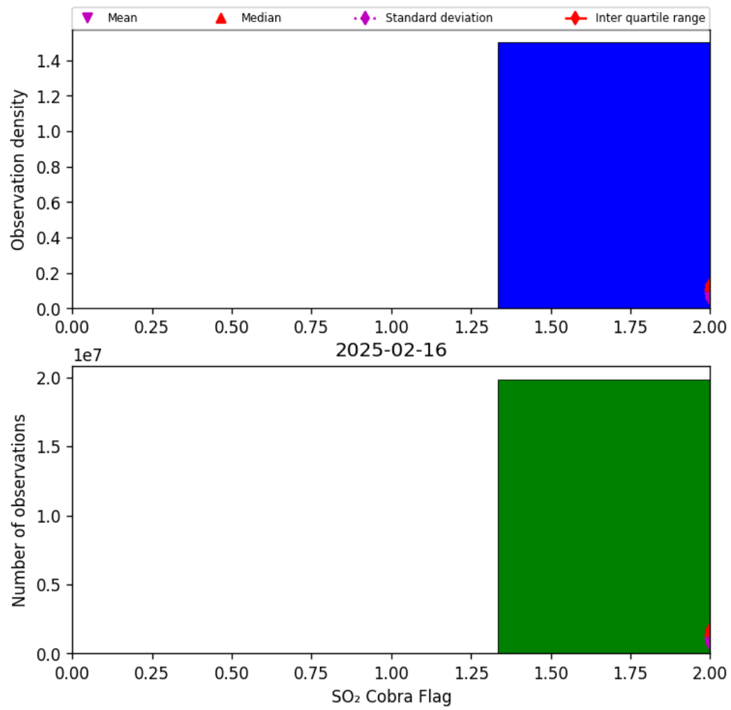
Figure 75: Histogram of “SO 2 Cobra Flag” for 2025-02-15 to 2025-02-17
