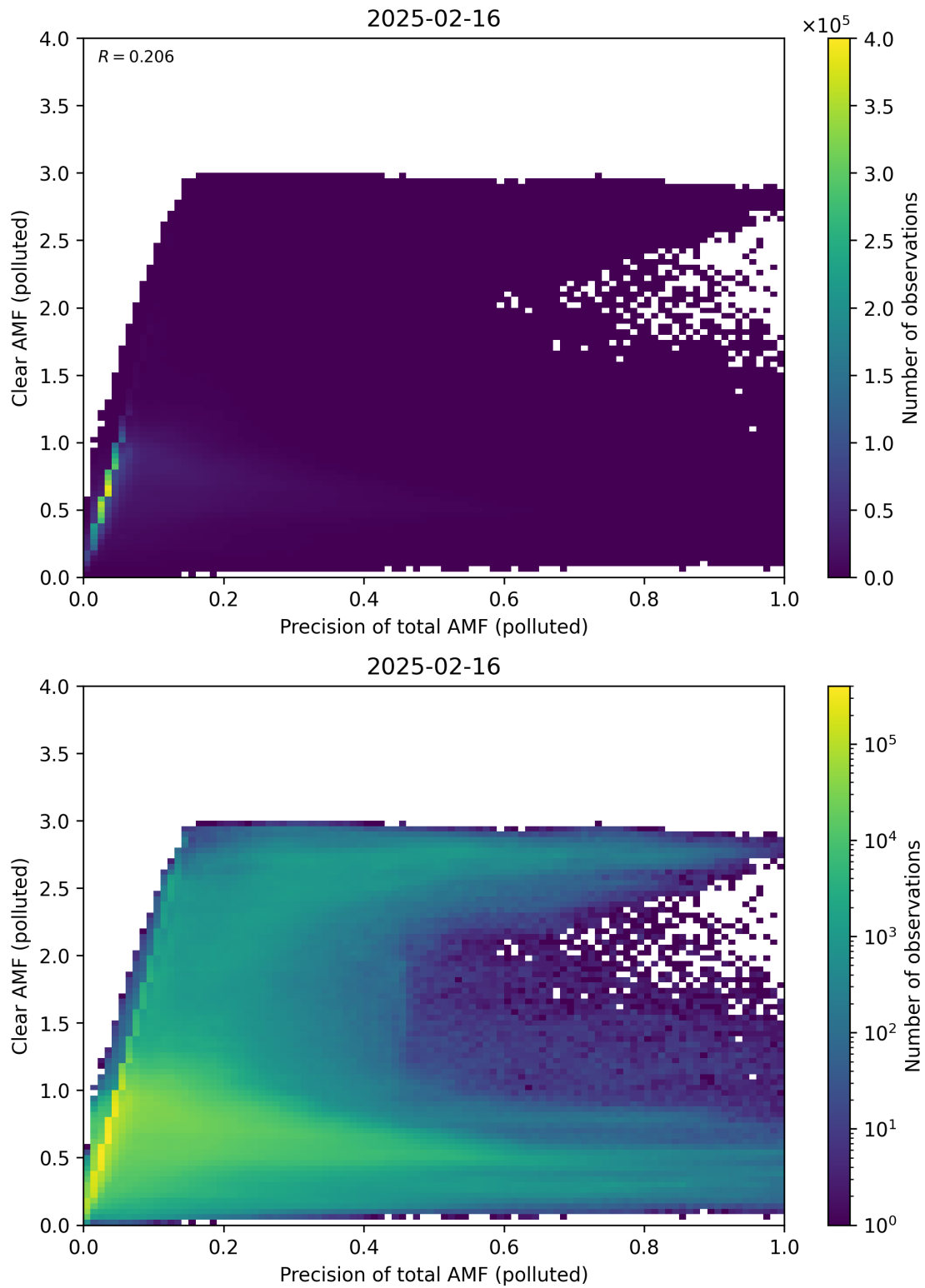
Figure 320: Scatter density plot of “Precision of total AMF (polluted)” against “Clear AMF (polluted)” for 2025-02-15 to 2025-02-17.
