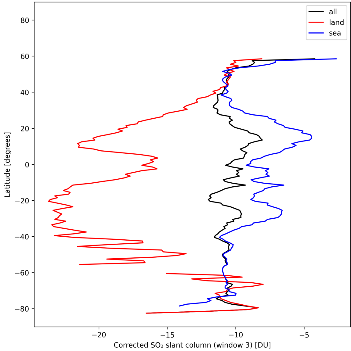
Figure 47: Zonal average of “Corrected SO 2 slant column (window 3)” for 2025-02-15 to 2025-02-17.
