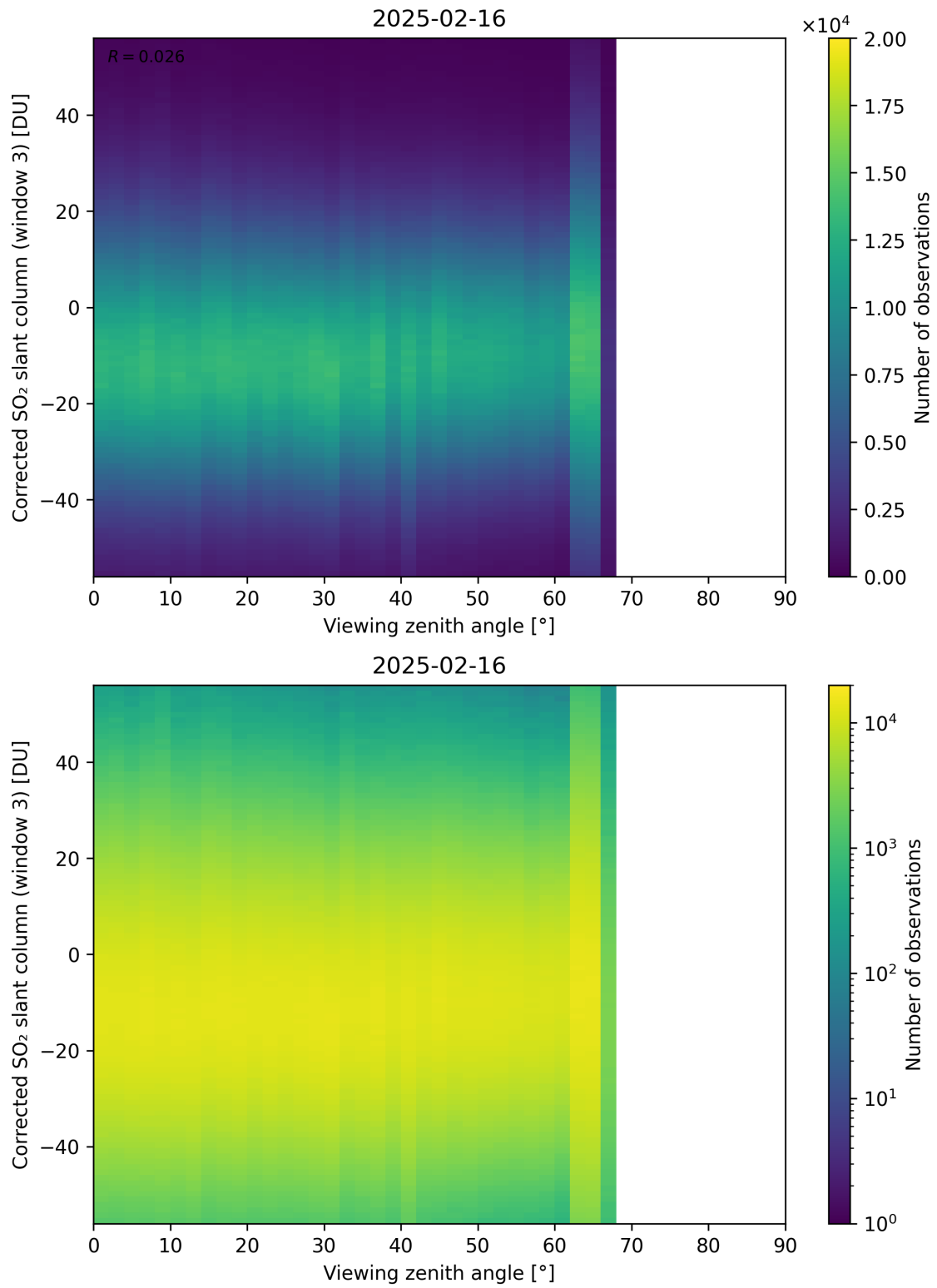
Figure 375: Scatter density plot of “Viewing zenith angle” against “Corrected SO 2 slant column (window 3)” for 2025-02-15 to 2025-02-17.
