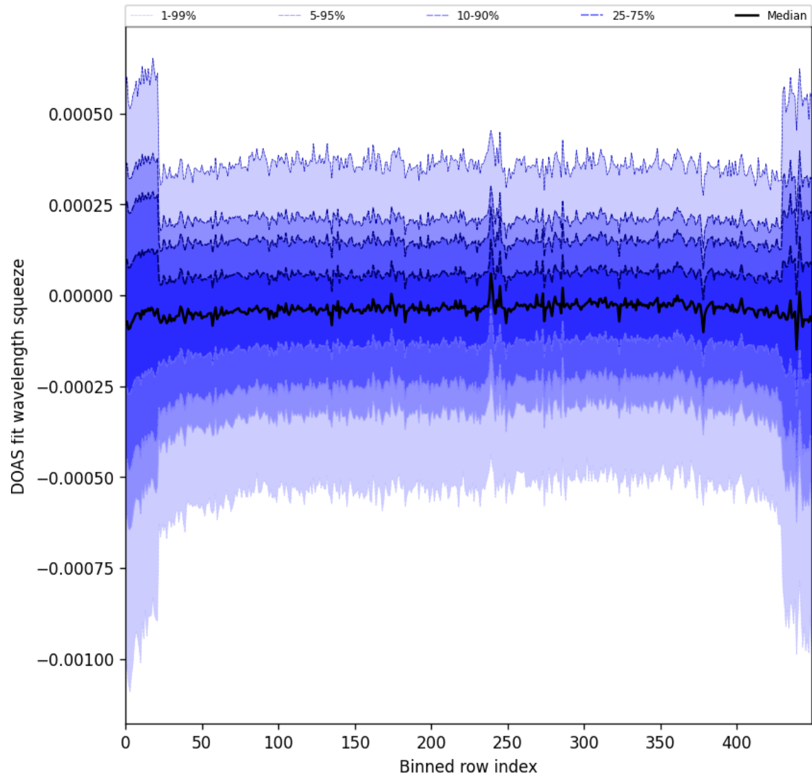
Figure 103: Along track statistics of “DOAS fit wavelength squeeze” for 2025-02-15 to 2025-02-17
