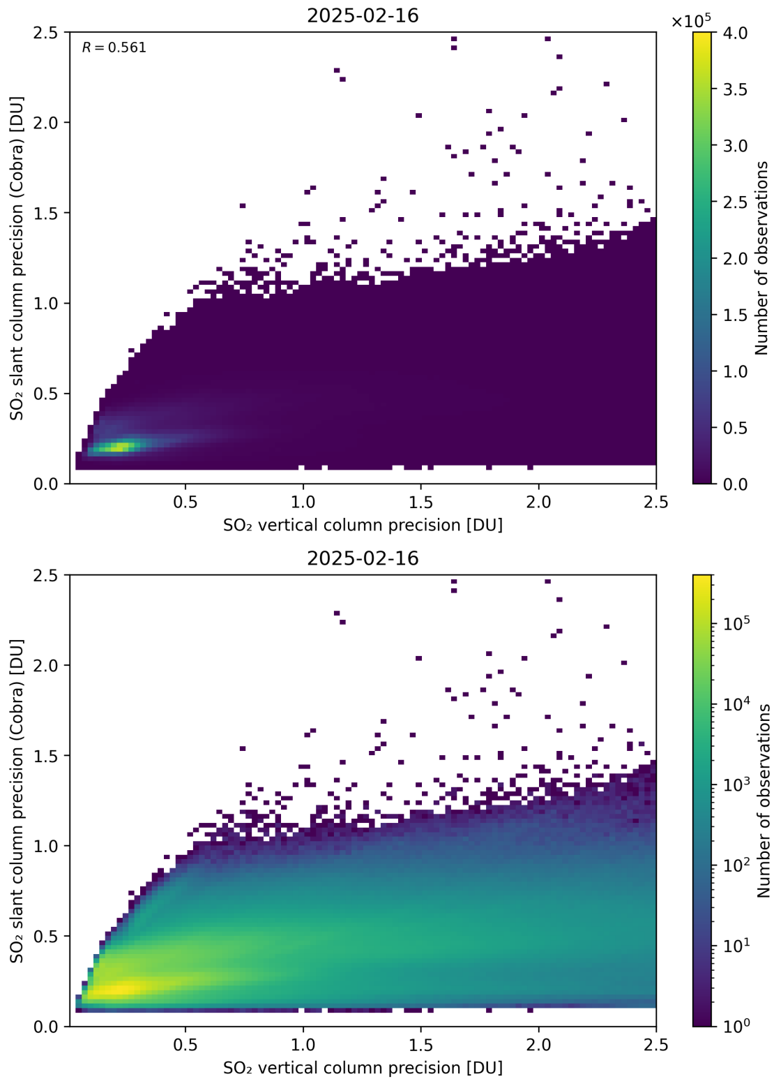
Figure 337: Scatter density plot of “SO 2 vertical column precision” against “SO 2 slant column precision (Cobra)” for 2025-02-15 to 2025-02-17.
