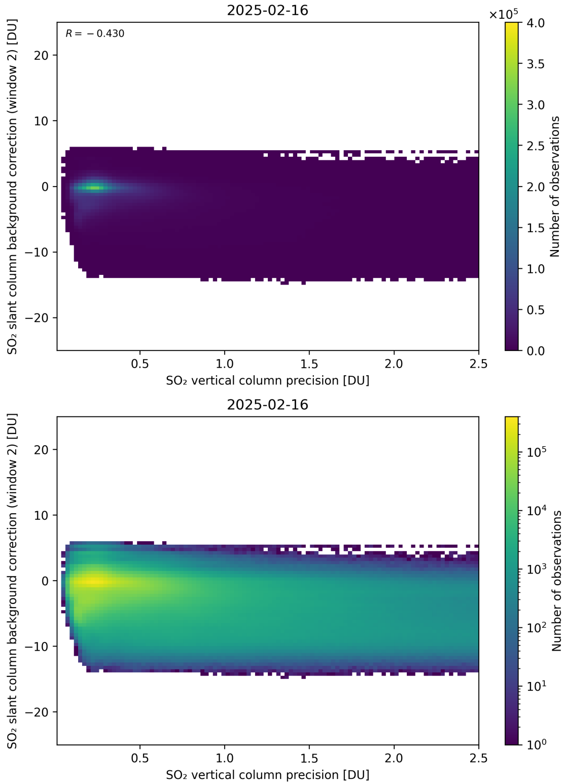
Figure 330: Scatter density plot of “SO 2 vertical column precision” against “SO 2 slant column background correction (window 2)” for 2025-02-15 to 2025-02-17.
