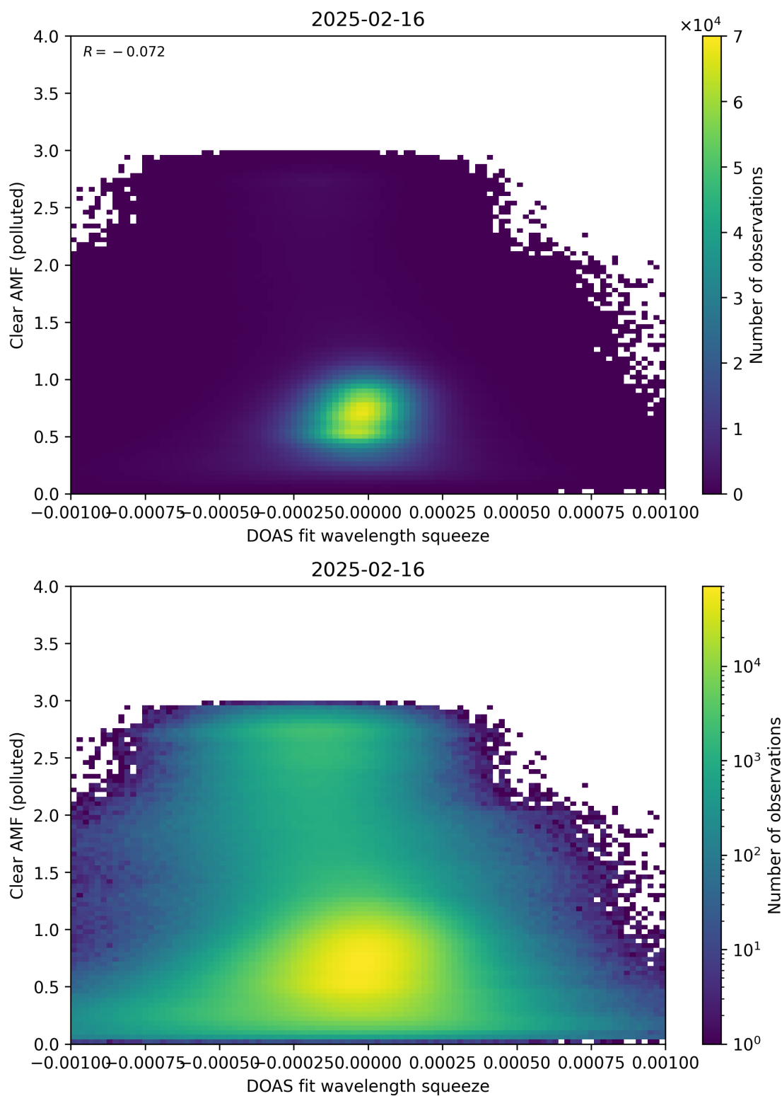
Figure 144: Scatter density plot of “DOAS fit wavelength squeeze” against “Clear AMF (polluted)” for 2025-02-15 to 2025-02-17.
