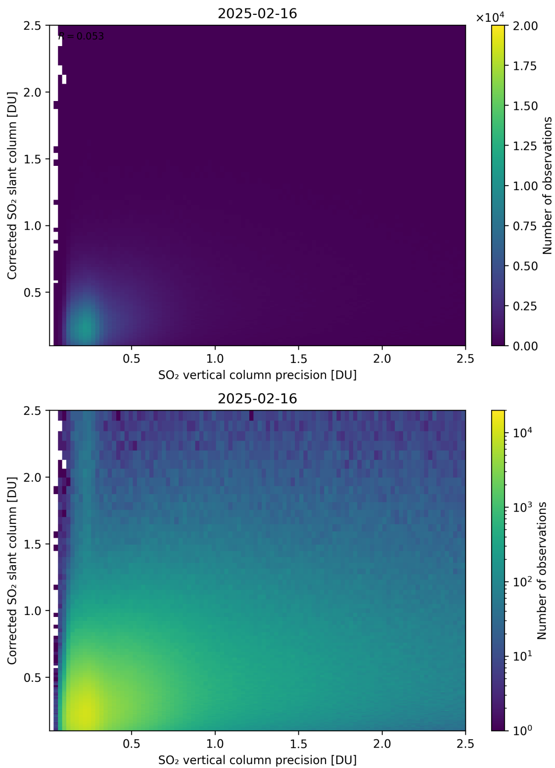
Figure 338: Scatter density plot of “SO 2 vertical column precision” against “Corrected SO 2 slant column” for 2025-02-15 to 2025-02-17.
