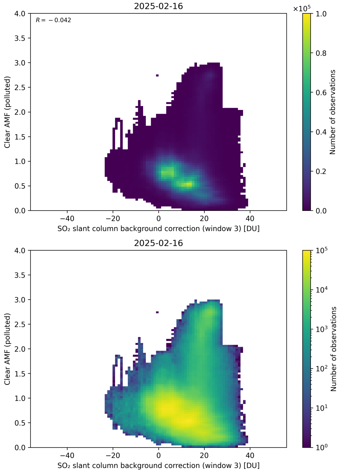
Figure 135: Scatter density plot of “SO 2 slant column background correction (window 3)” against “Clear AMF (polluted)” for 2025-02-15 to 2025-02-17.
