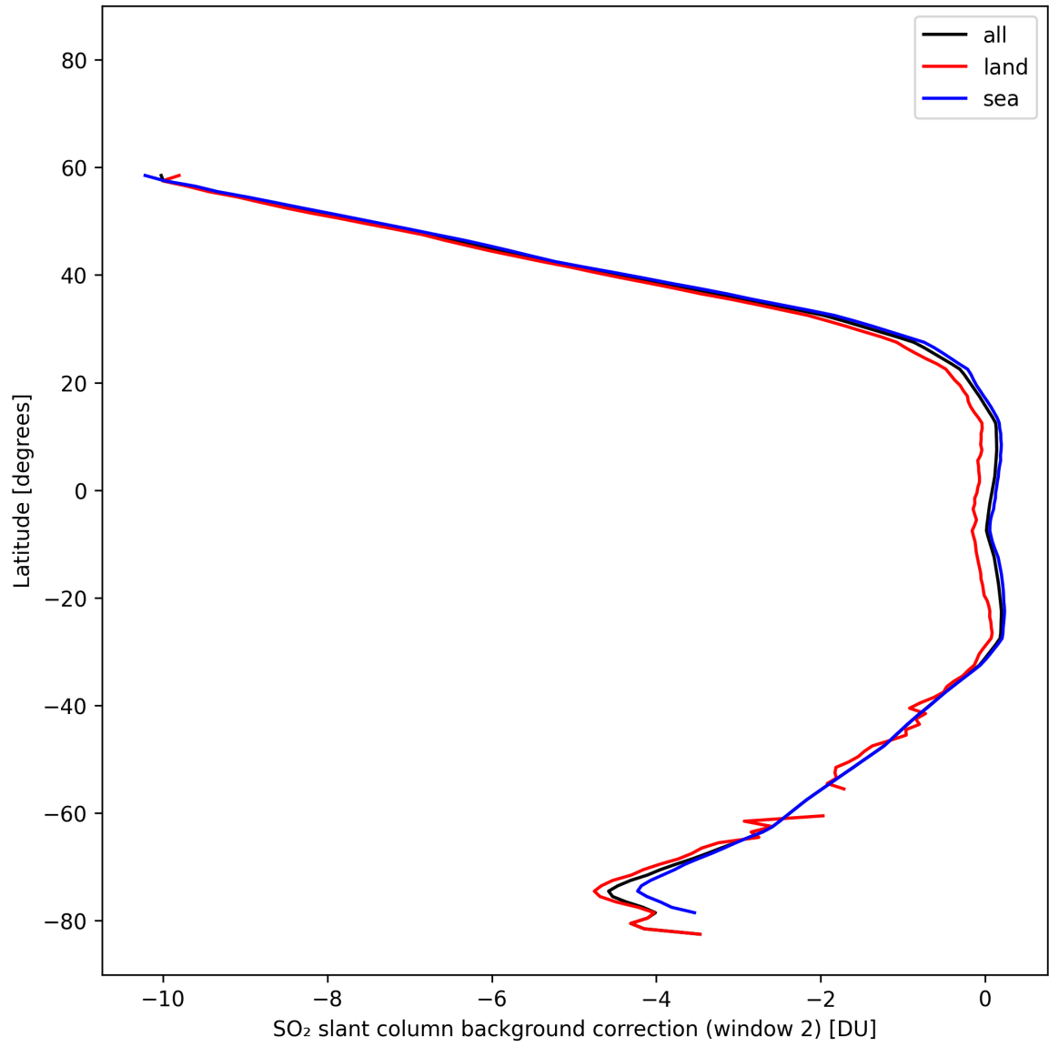
Figure 44: Zonal average of “SO 2 slant column background correction (window 2)” for 2025-02-15 to 2025-02-17.
