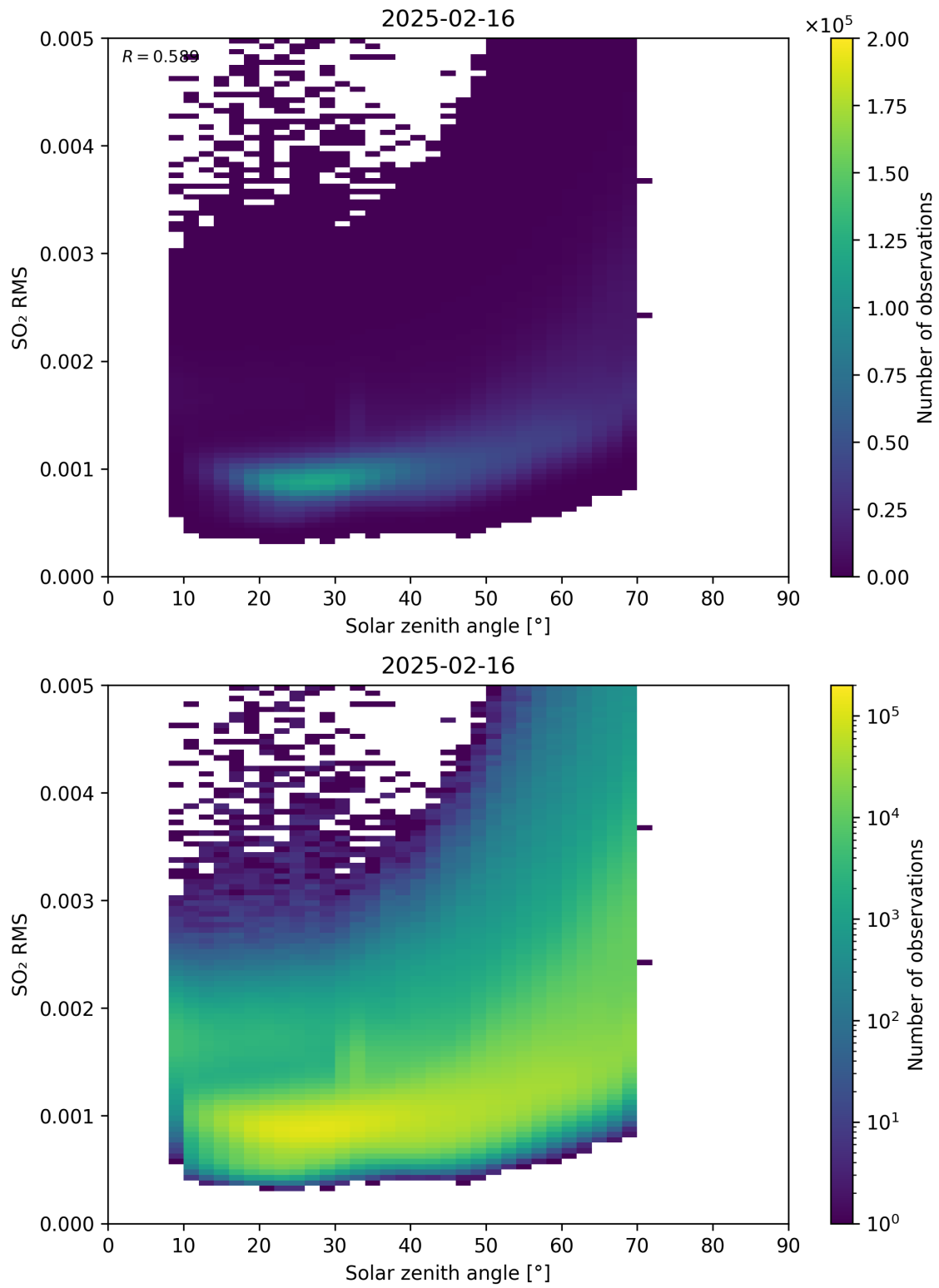
Figure 176: Scatter density plot of “Solar zenith angle” against “SO 2 RMS” for 2025-02-15 to 2025-02-17.
