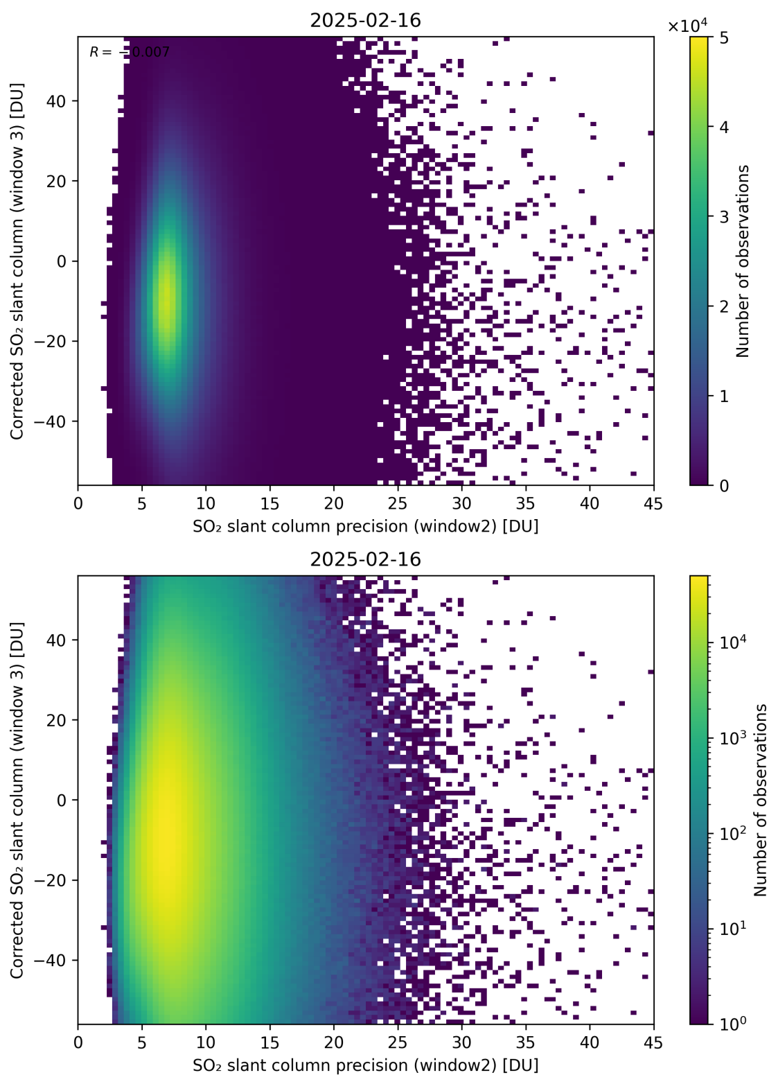
Figure 298: Scatter density plot of “SO 2 slant column precision (window2)” against “Corrected SO 2 slant column (window 3)” for 2025-02-15 to 2025-02-17.
