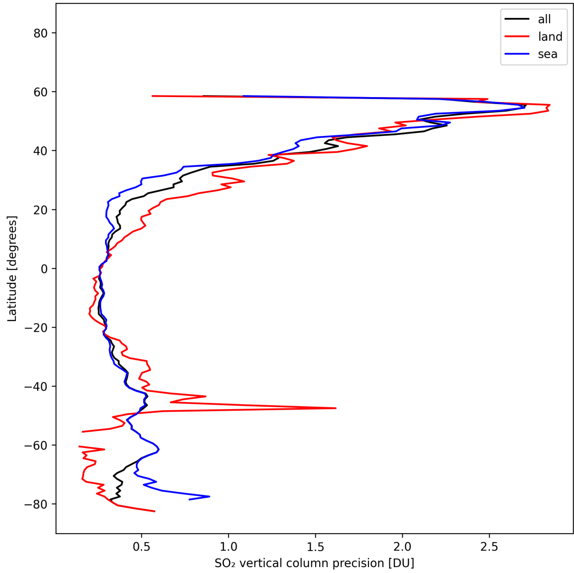
Figure 33: Zonal average of “SO 2 vertical column precision” for 2025-02-15 to 2025-02-17.
