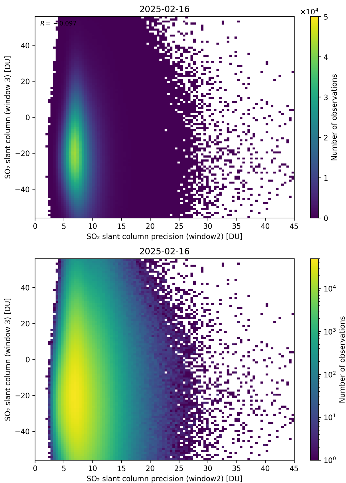
Figure 299: Scatter density plot of “SO 2 slant column precision (window2)” against “SO 2 slant column (window 3)” for 2025-02-15 to 2025-02-17.
