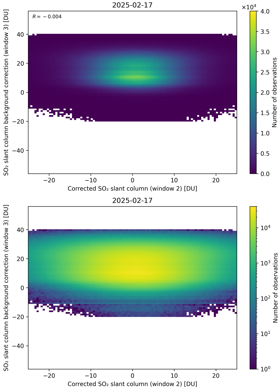
Figure 245: Scatter density plot of “Corrected SO 2 slant column (window 2)” against “SO 2 slant column background correction (window 3)” for 2025-02-16 to 2025-02-18.
