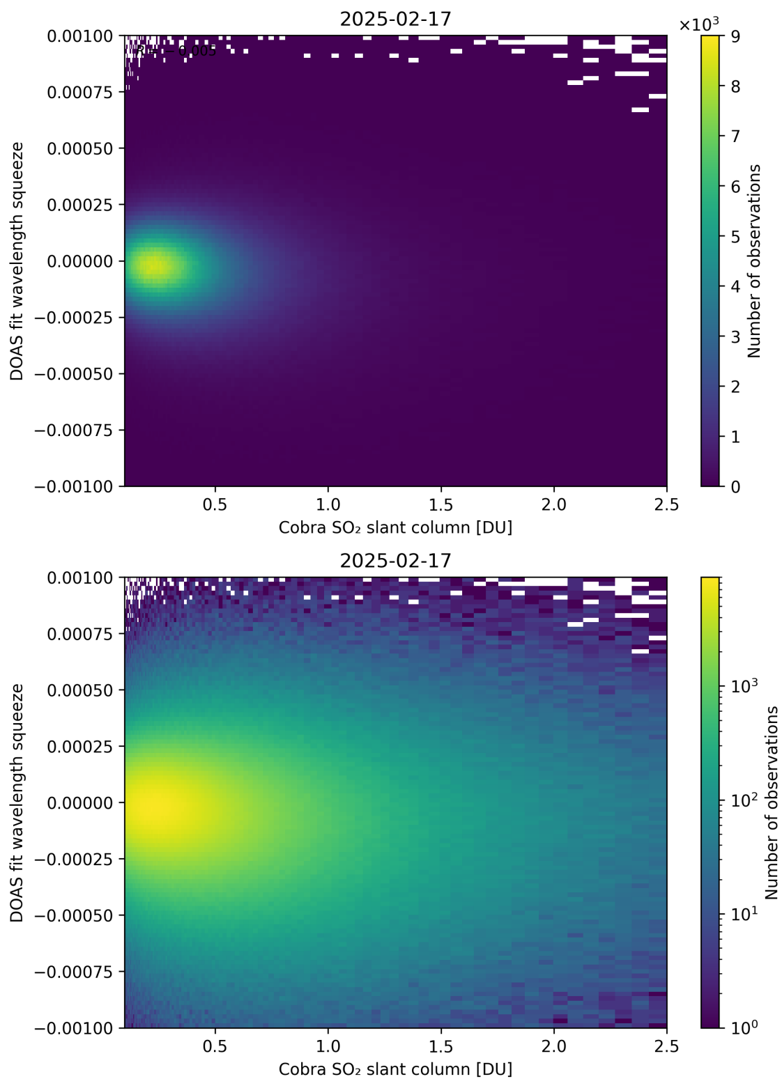
Figure 197: Scatter density plot of “Cobra SO 2 slant column” against “DOAS fit wavelength squeeze” for 2025-02-16 to 2025-02-18.
