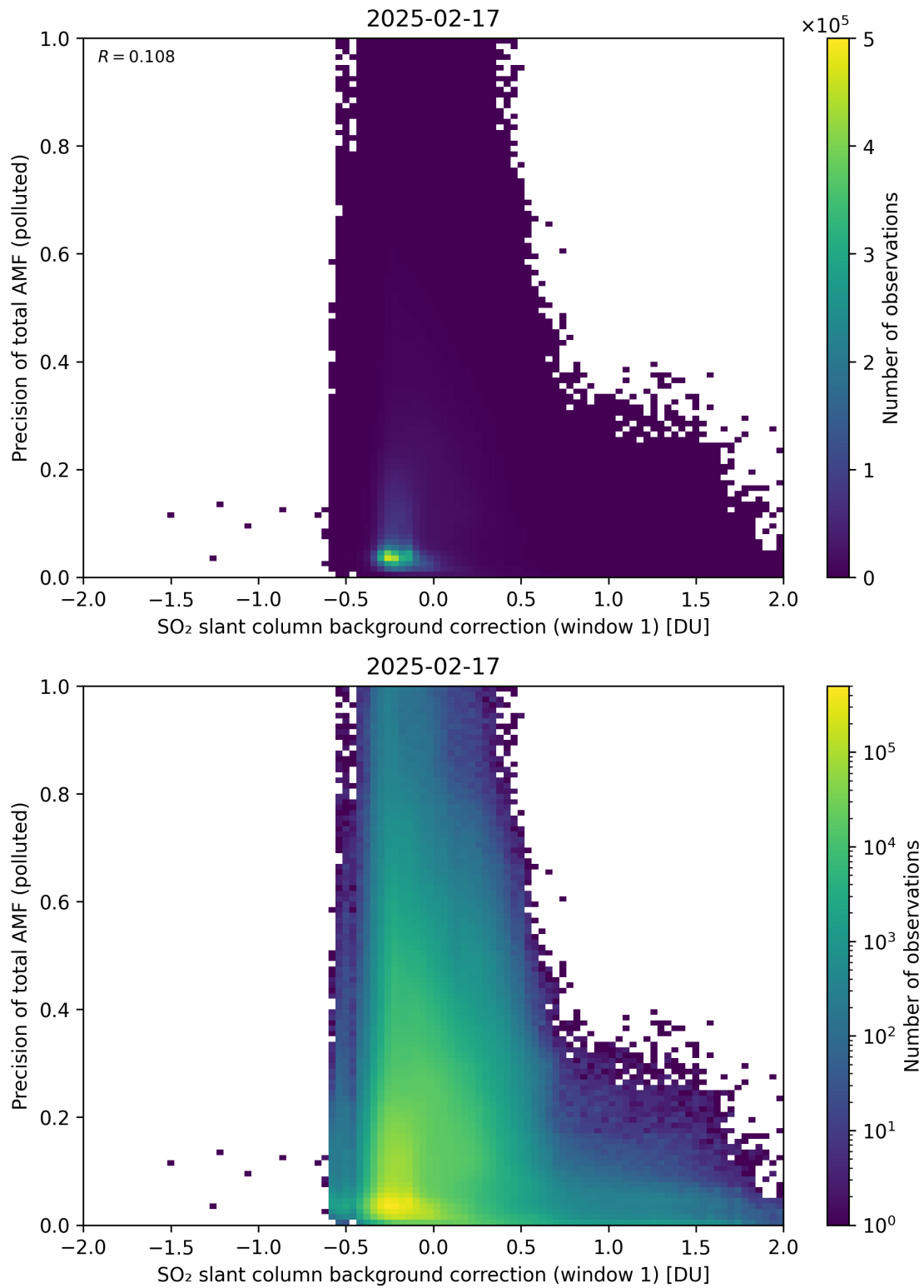
Figure 121: Scatter density plot of “SO 2 slant column background correction (window 1)” against “Precision of total AMF (polluted)” for 2025-02-16 to 2025-02-18.
