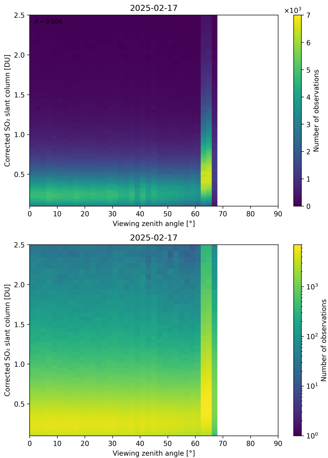
Figure 373: Scatter density plot of “Viewing zenith angle” against “Corrected SO 2 slant column” for 2025-02-16 to 2025-02-18.
