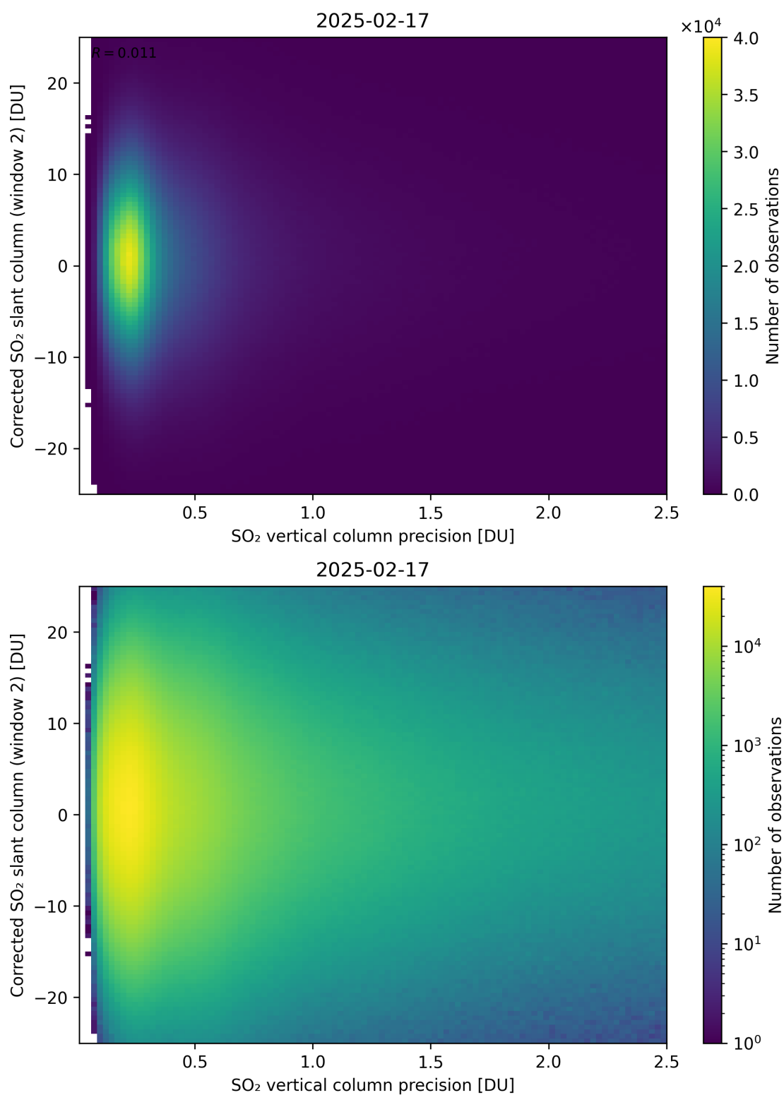
Figure 339: Scatter density plot of “SO 2 vertical column precision” against “Corrected SO 2 slant column (window 2)” for 2025-02-16 to 2025-02-18.
