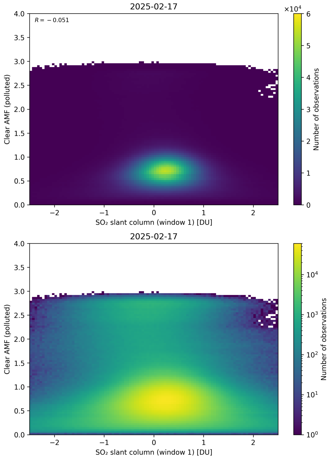
Figure 282: Scatter density plot of “SO 2 slant column (window 1)” against “Clear AMF (polluted)” for 2025-02-16 to 2025-02-18.
