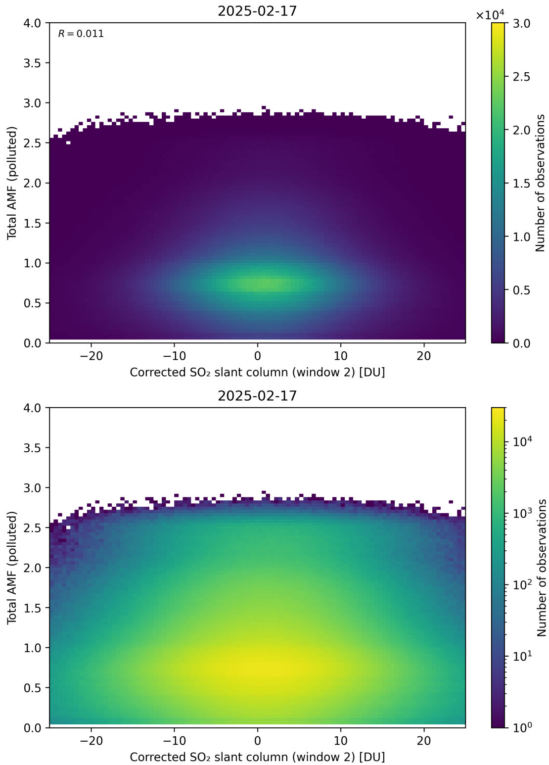
Figure 253: Scatter density plot of “Corrected SO 2 slant column (window 2)” against “Total AMF (polluted)” for 2025-02-16 to 2025-02-18.
