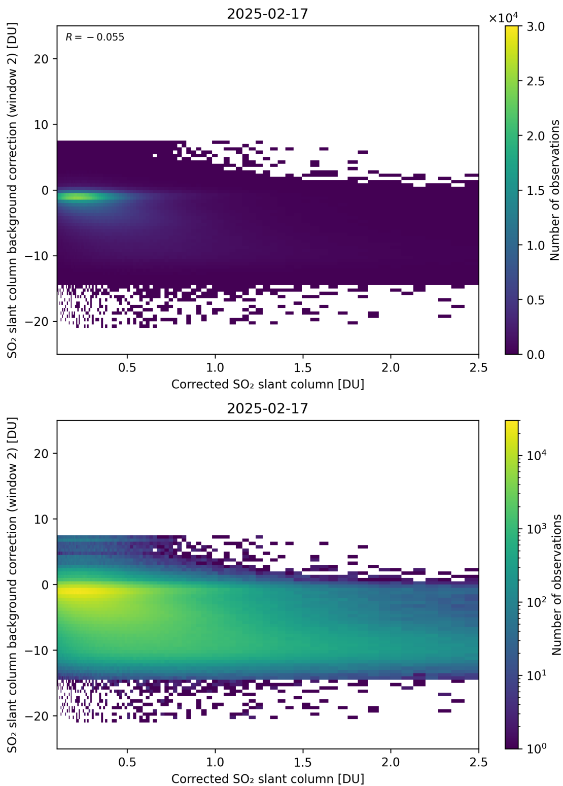
Figure 227: Scatter density plot of “Corrected SO 2 slant column” against “SO 2 slant column background correction (window 2)” for 2025-02-16 to 2025-02-18.
