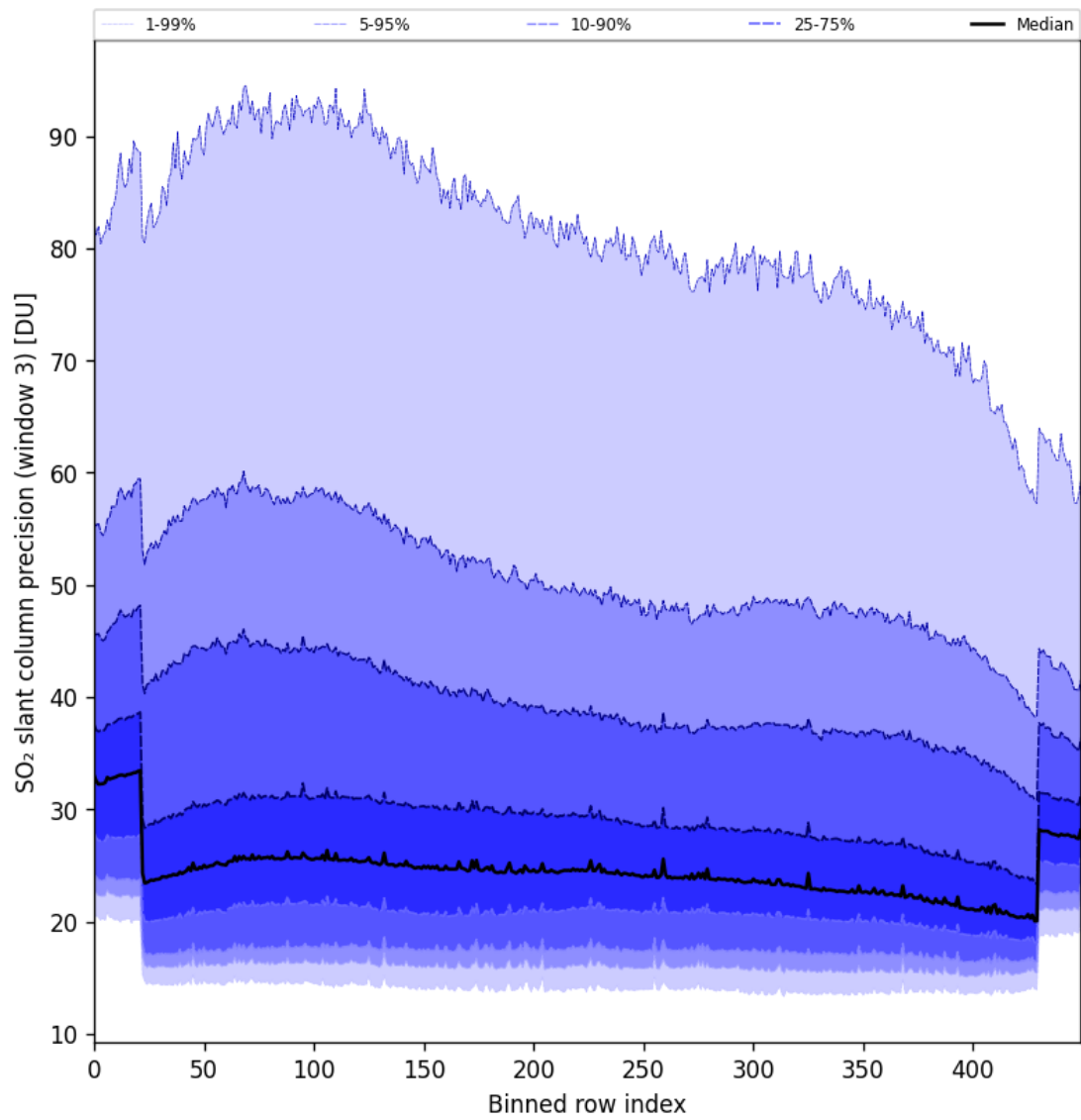
Figure 98: Along track statistics of “SO 2 slant column precision (window 3)” for 2025-02-16 to 2025-02-18
