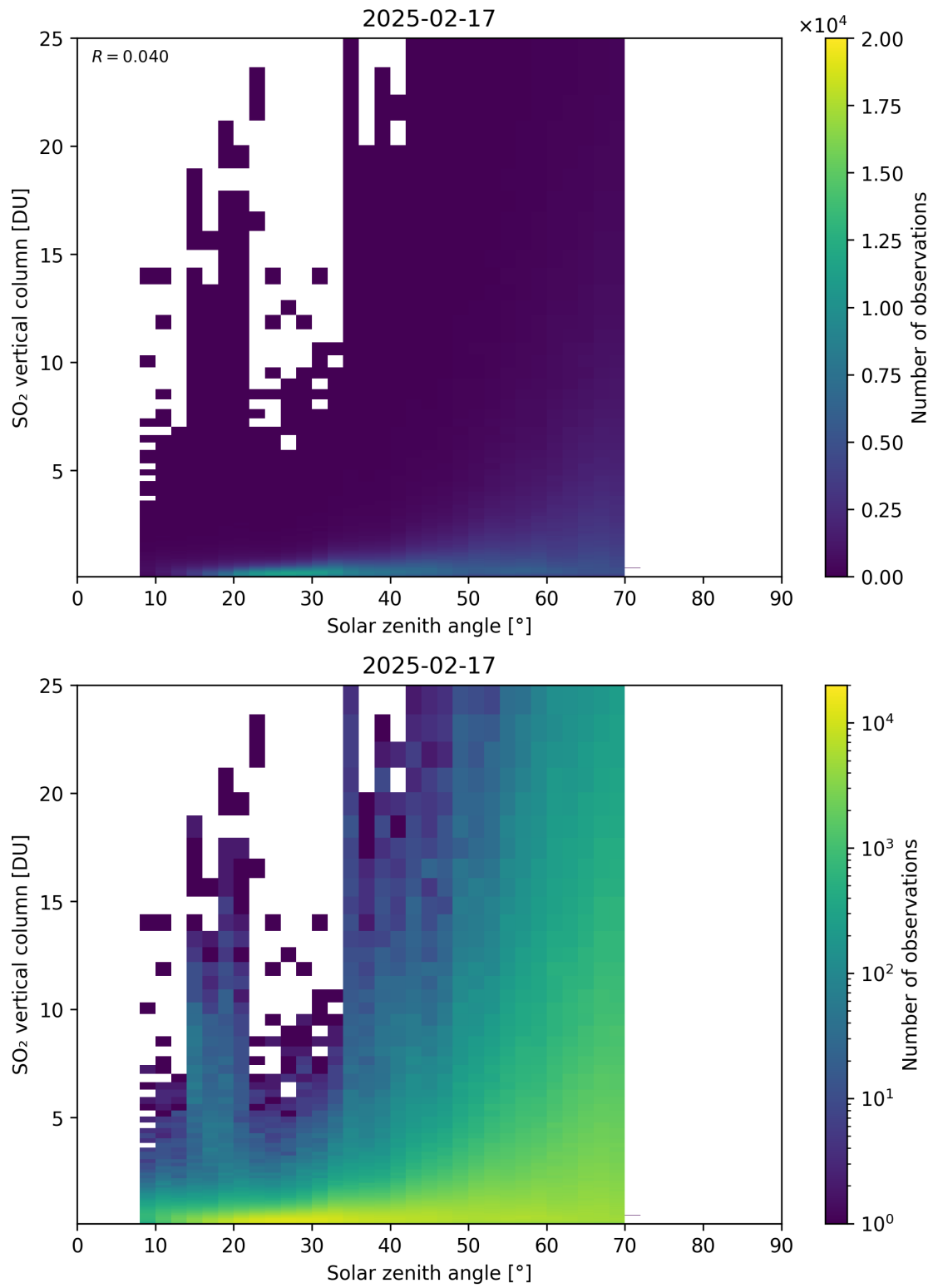
Figure 191: Scatter density plot of “Solar zenith angle” against “SO 2 vertical column” for 2025-02-16 to 2025-02-18.
