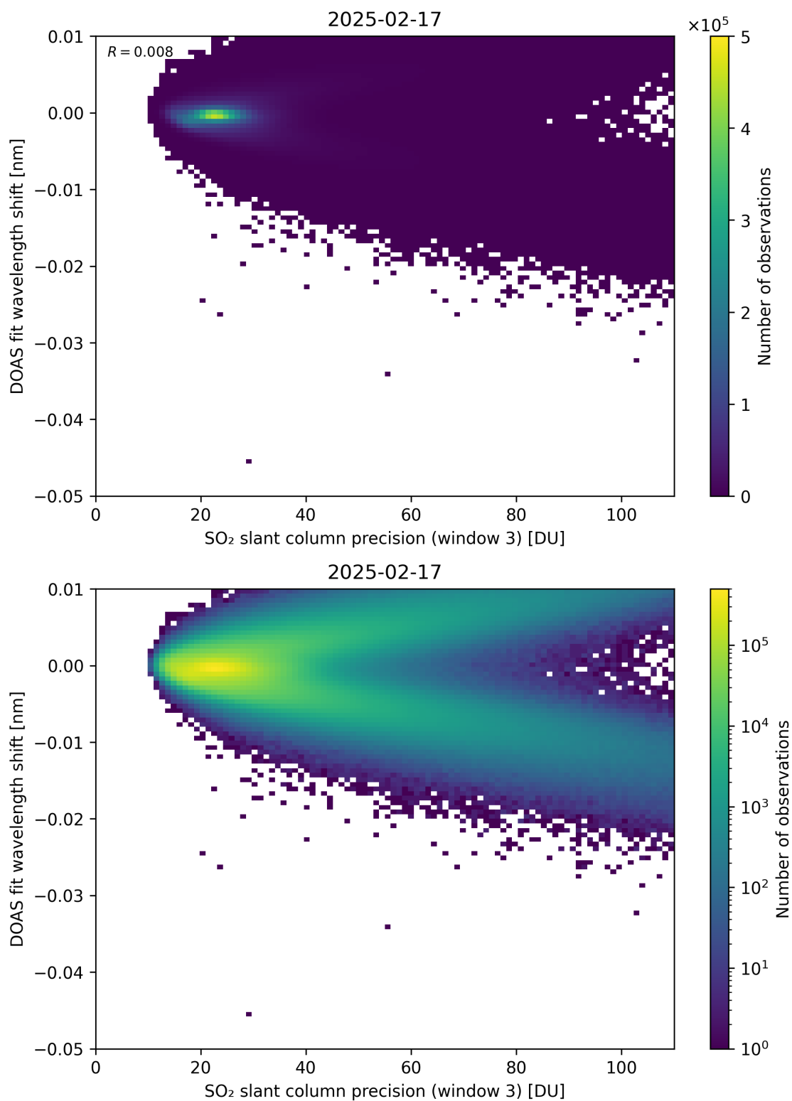
Figure 308: Scatter density plot of “SO 2 slant column precision (window 3)” against “DOAS fit wavelength shift” for 2025-02-16 to 2025-02-18.
