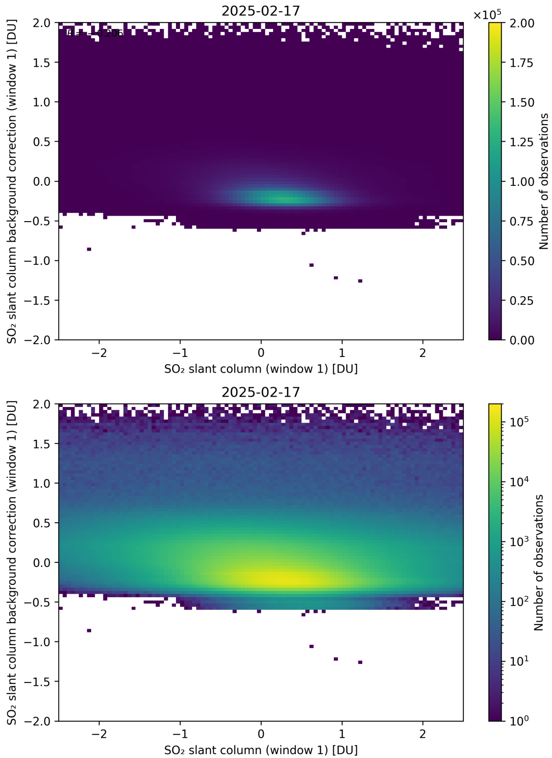
Figure 262: Scatter density plot of “SO 2 slant column (window 1)” against “SO 2 slant column background correction (window 1)” for 2025-02-16 to 2025-02-18.
