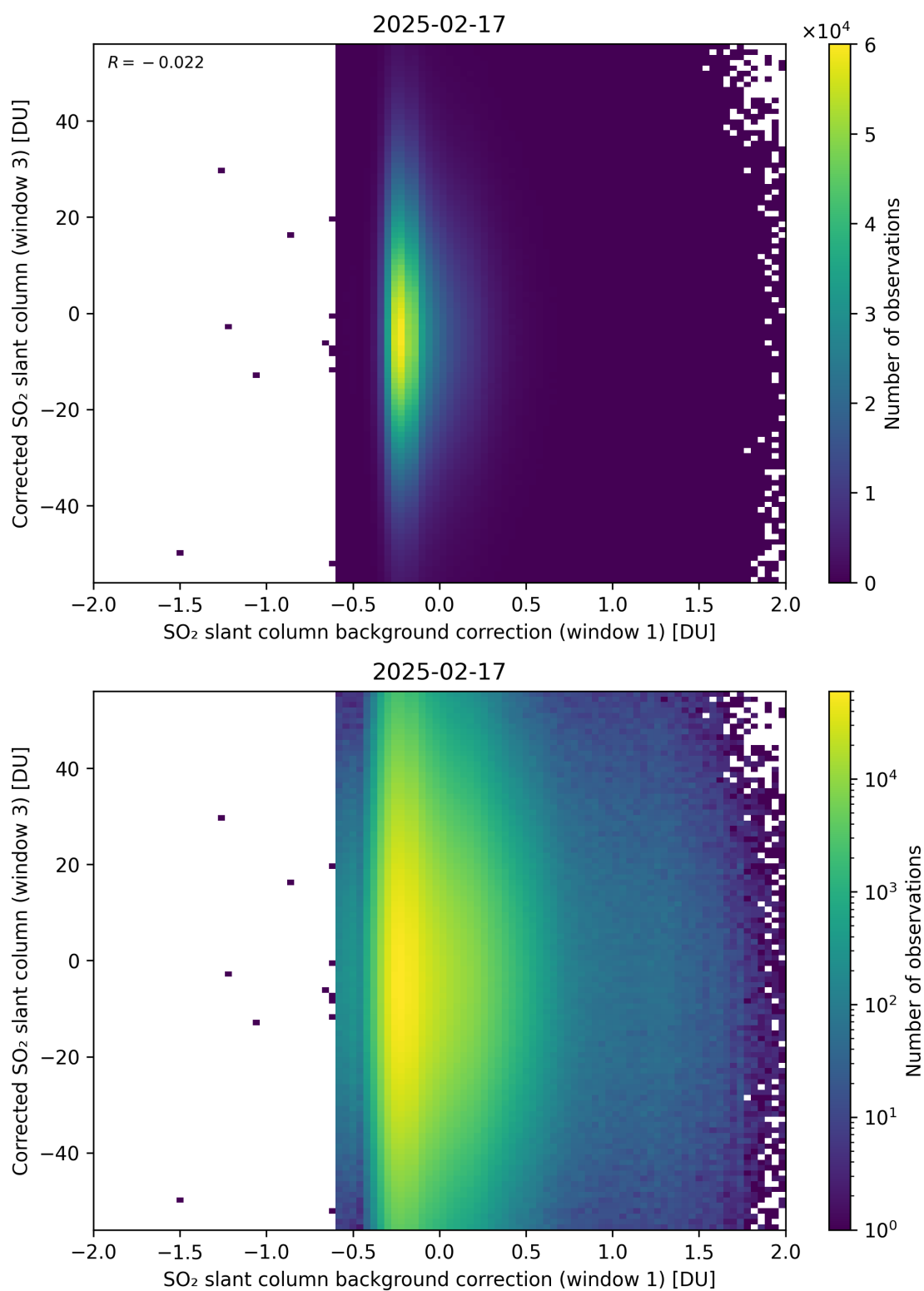
Figure 116: Scatter density plot of “SO 2 slant column background correction (window 1)” against “Corrected SO 2 slant column (window 3)” for 2025-02-16 to 2025-02-18.
