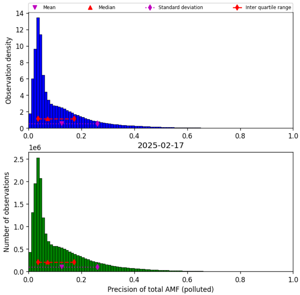
Figure 80: Histogram of “Precision of total AMF (polluted)” for 2025-02-16 to 2025-02-18
