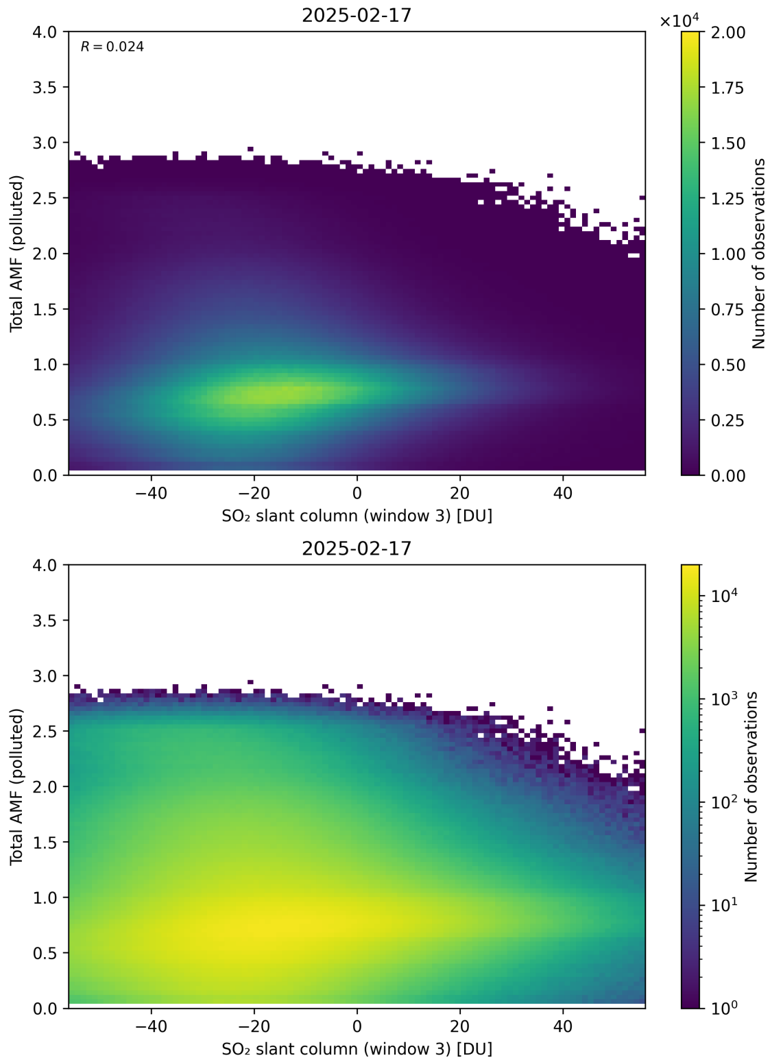
Figure 318: Scatter density plot of “SO 2 slant column (window 3)” against “Total AMF (polluted)” for 2025-02-16 to 2025-02-18.
