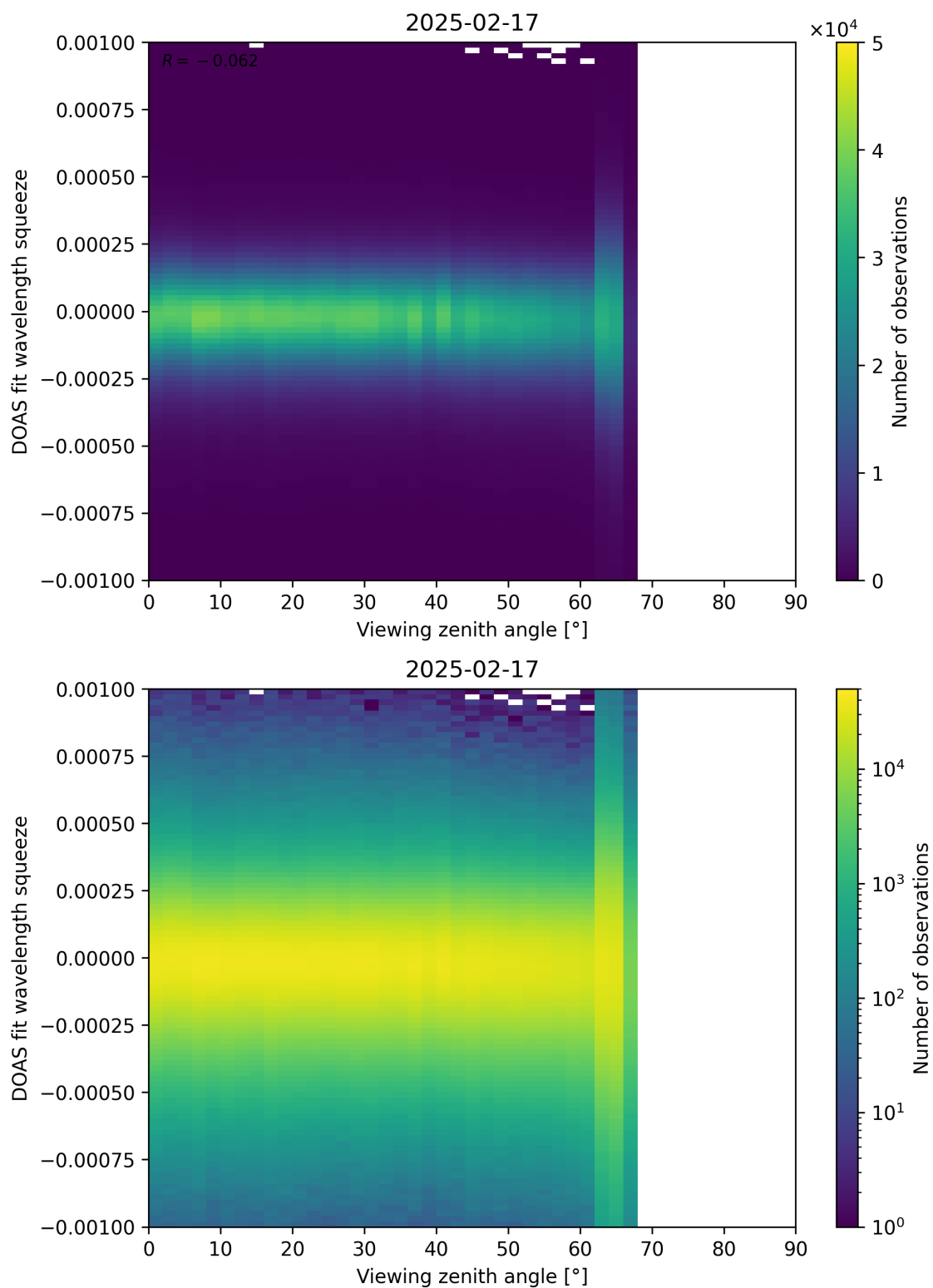
Figure 366: Scatter density plot of “Viewing zenith angle” against “DOAS fit wavelength squeeze” for 2025-02-16 to 2025-02-18.
