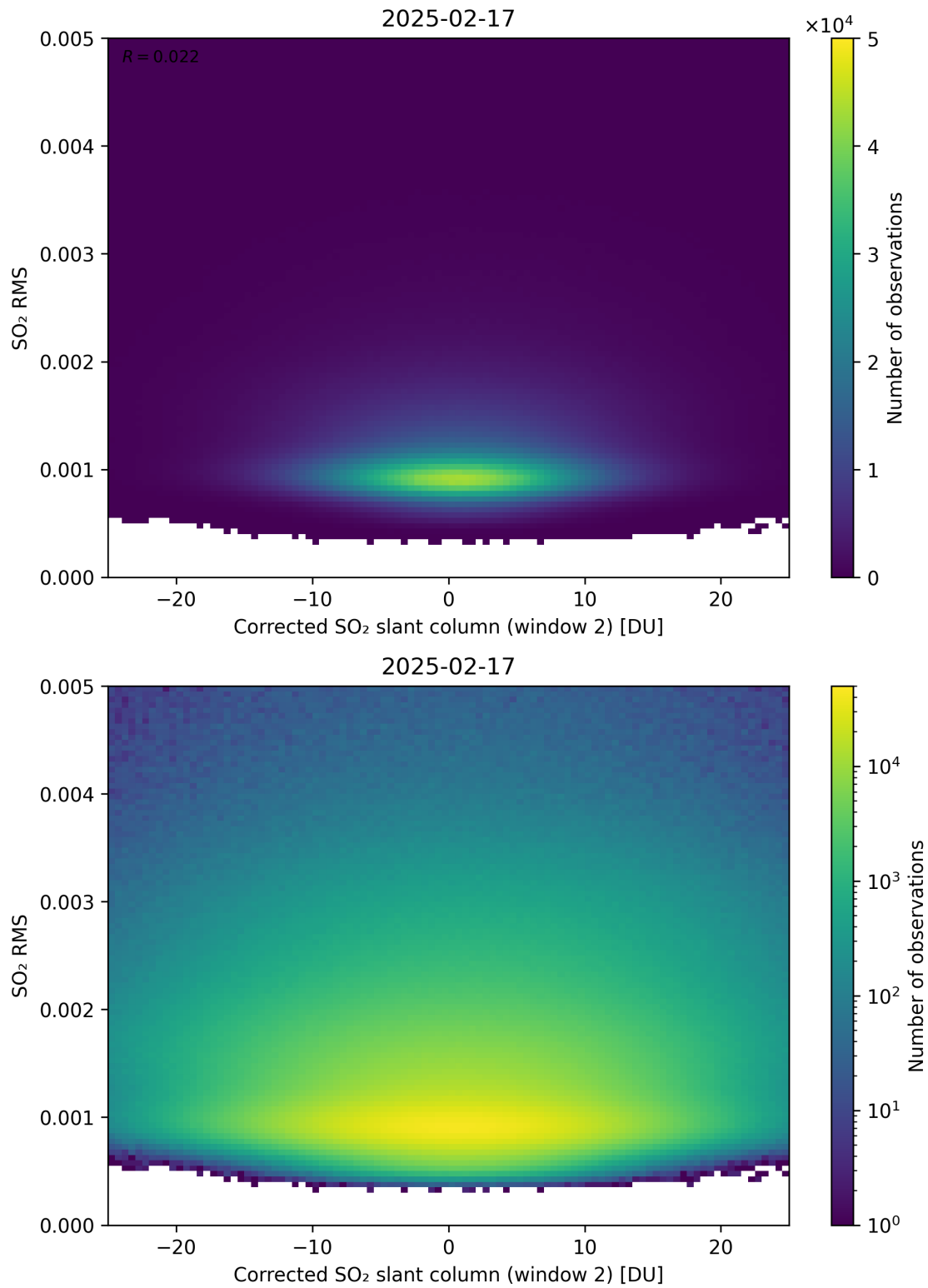
Figure 248: Scatter density plot of “Corrected SO 2 slant column (window 2)” against “SO 2 RMS” for 2025-02-16 to 2025-02-18.
