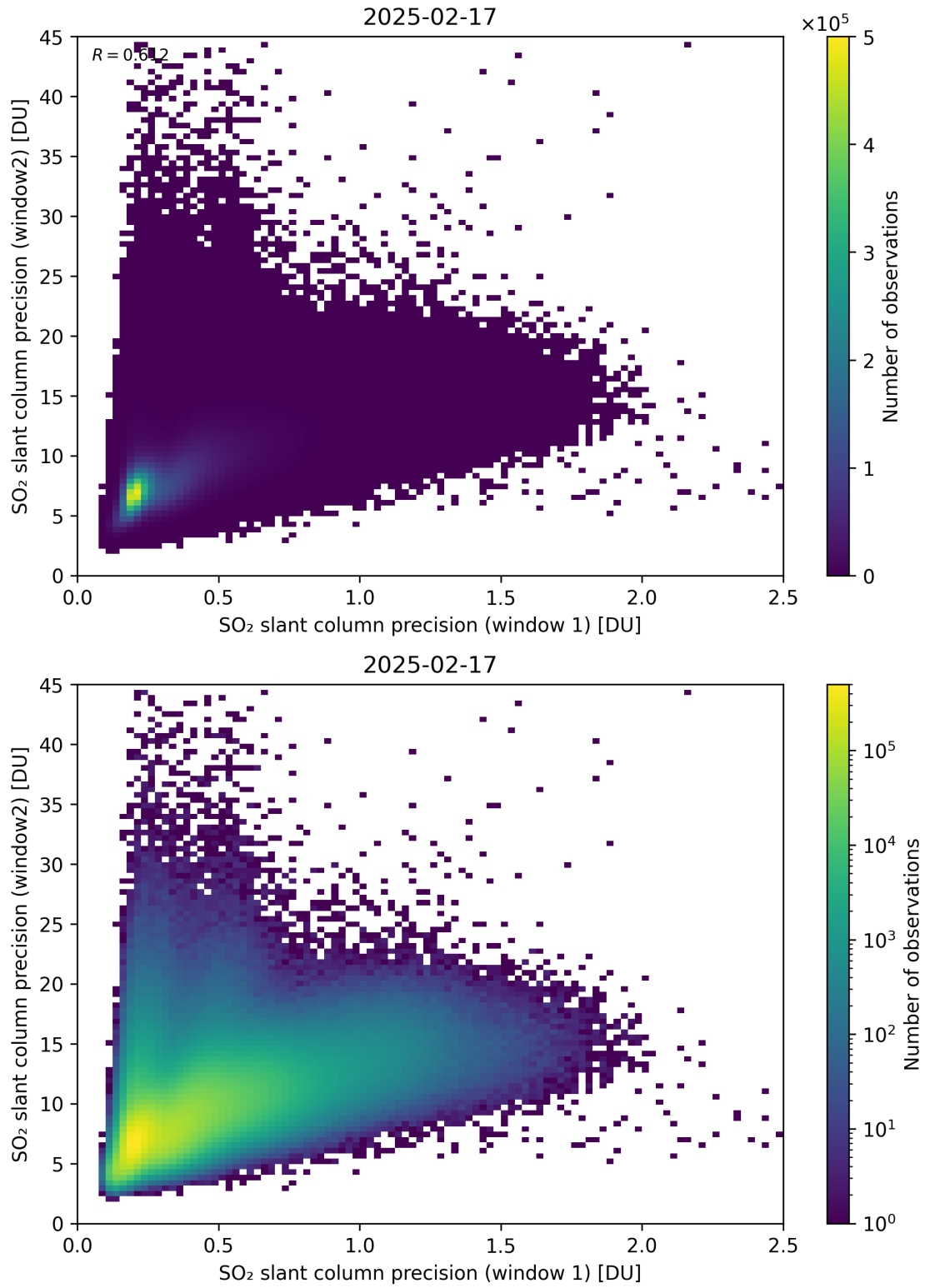
Figure 277: Scatter density plot of “SO 2 slant column precision (window 1)” against “SO 2 slant column precision (window2)” for 2025-02-16 to 2025-02-18.
