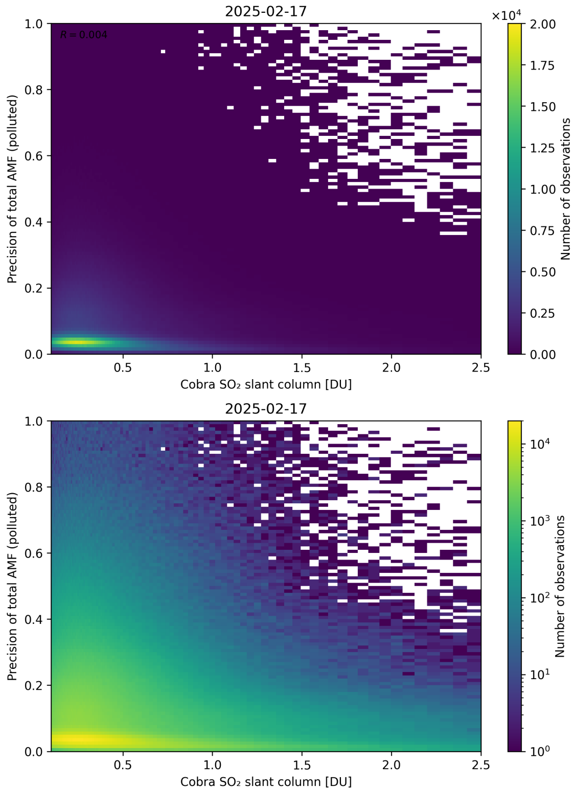
Figure 225: Scatter density plot of “Cobra SO 2 slant column” against “Precision of total AMF (polluted)” for 2025-02-16 to 2025-02-18.
