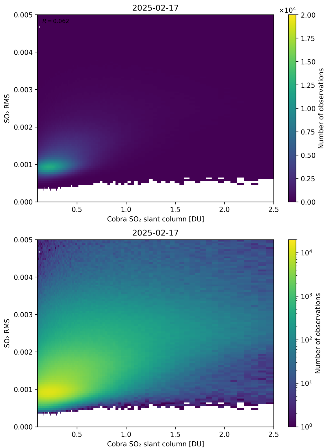
Figure 198: Scatter density plot of “Cobra SO 2 slant column” against “SO 2 RMS” for 2025-02-16 to 2025-02-18.
