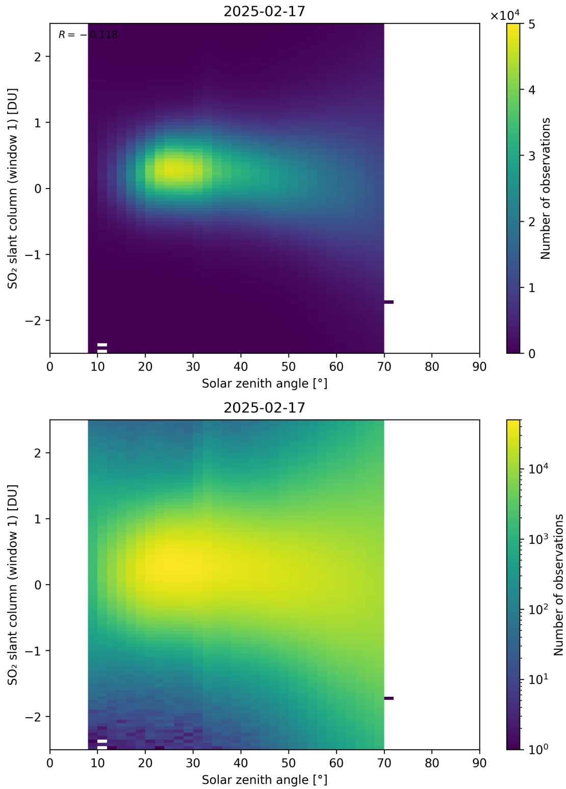
Figure 184: Scatter density plot of “Solar zenith angle” against “SO 2 slant column (window 1)” for 2025-02-16 to 2025-02-18.
