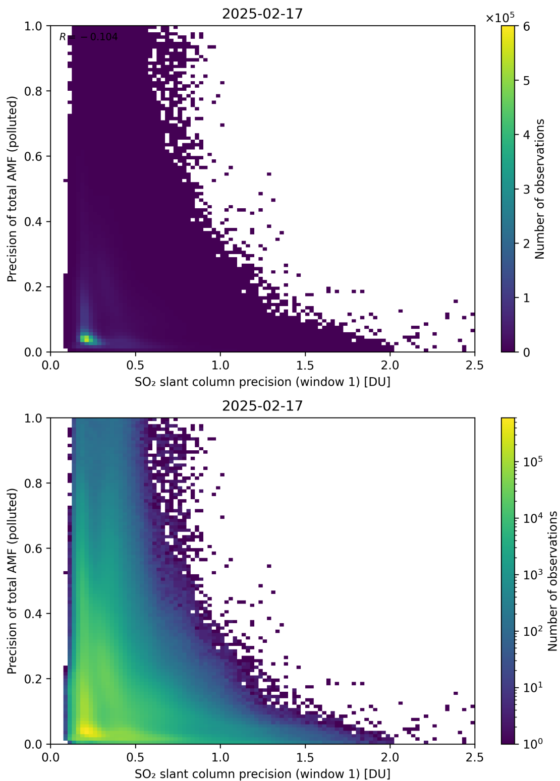
Figure 281: Scatter density plot of “SO 2 slant column precision (window 1)” against “Precision of total AMF (polluted)” for 2025-02-16 to 2025-02-18.
