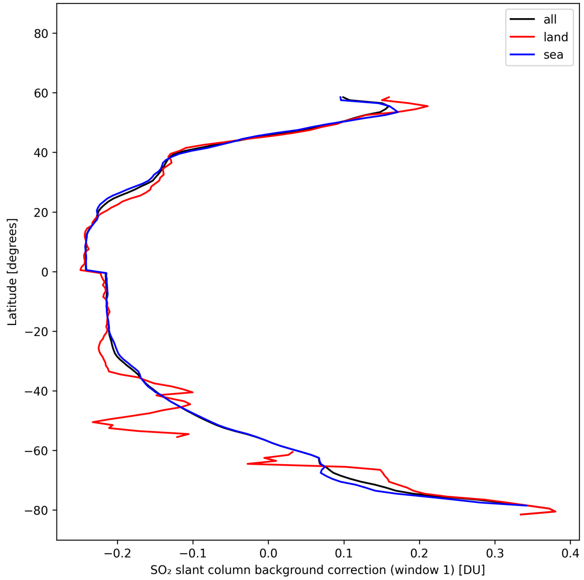
Figure 40: Zonal average of “SO 2 slant column background correction (window 1)” for 2025-02-16 to 2025-02-18.
