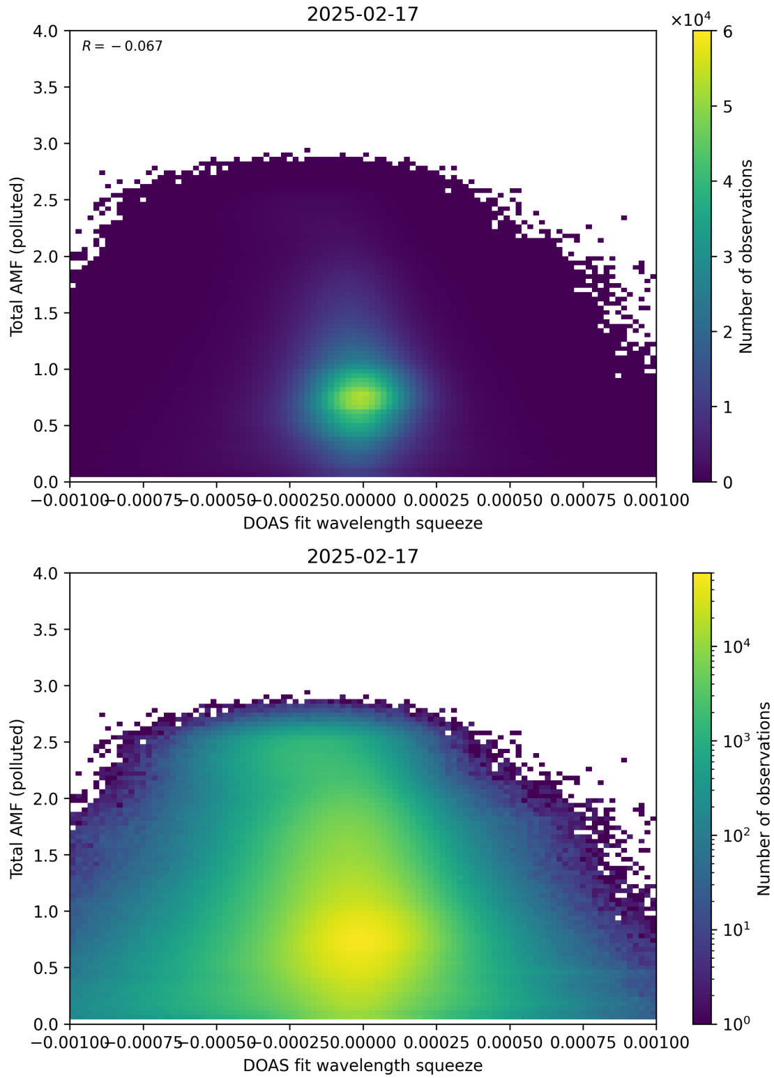
Figure 145: Scatter density plot of “DOAS fit wavelength squeeze” against “Total AMF (polluted)” for 2025-02-16 to 2025-02-18.
