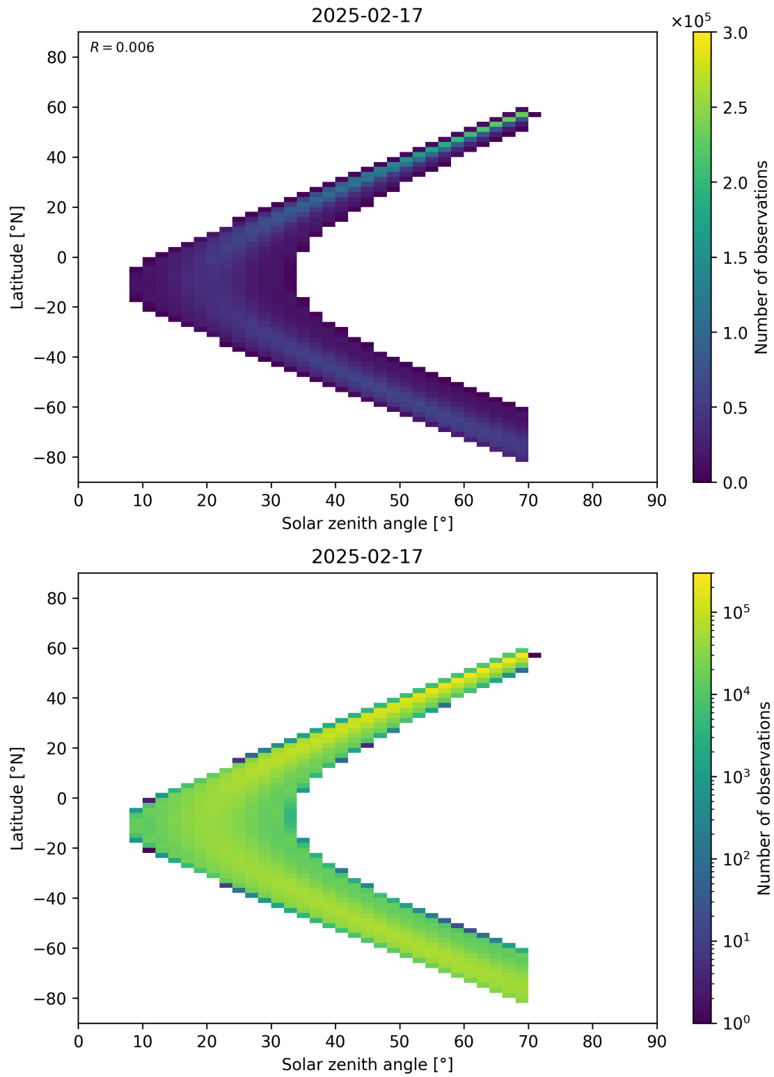
Figure 177: Scatter density plot of “Solar zenith angle” against “Latitude” for 2025-02-16 to 2025-02-18.
