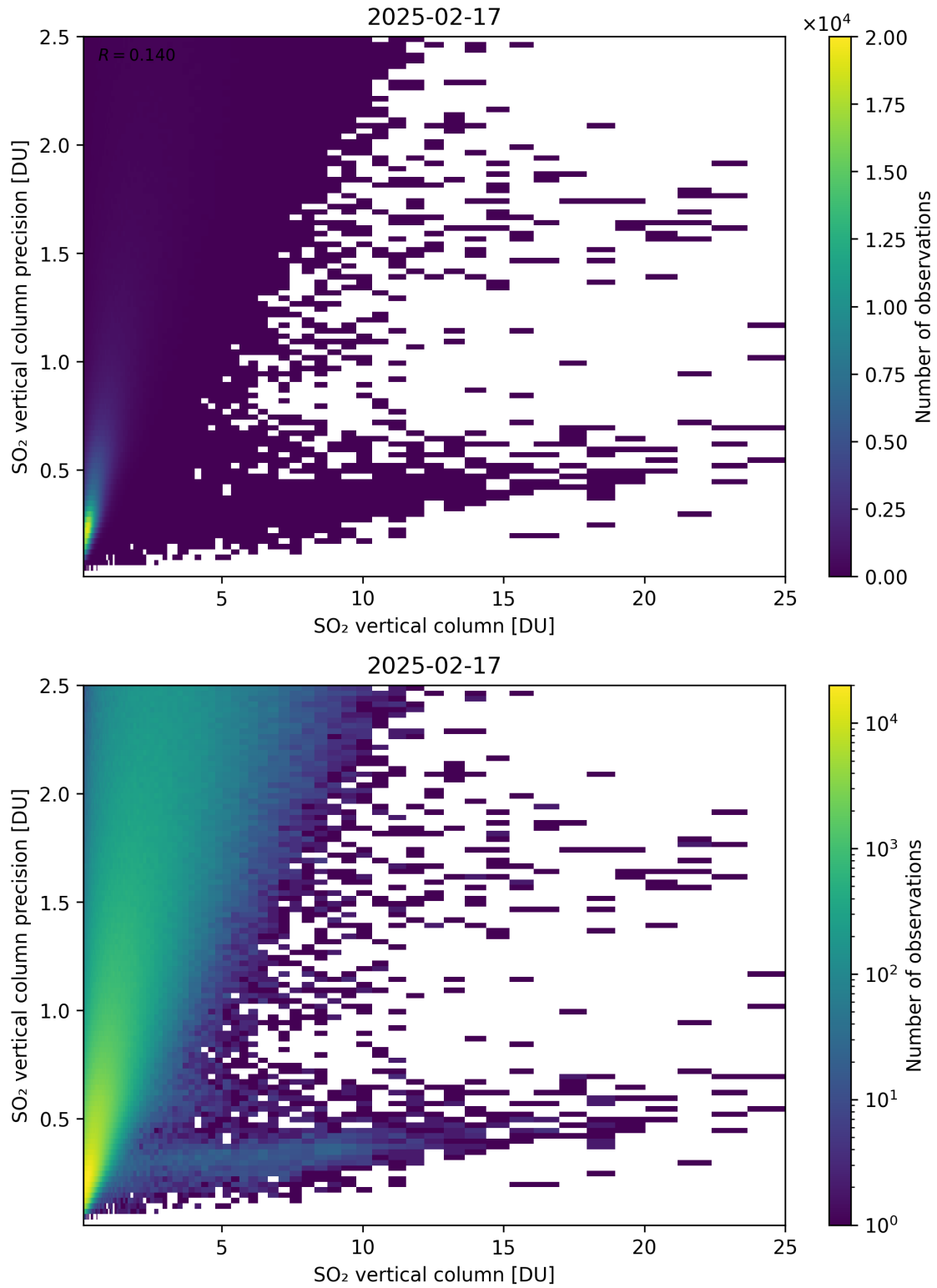
Figure 361: Scatter density plot of “SO 2 vertical column” against “SO 2 vertical column precision” for 2025-02-16 to 2025-02-18.
