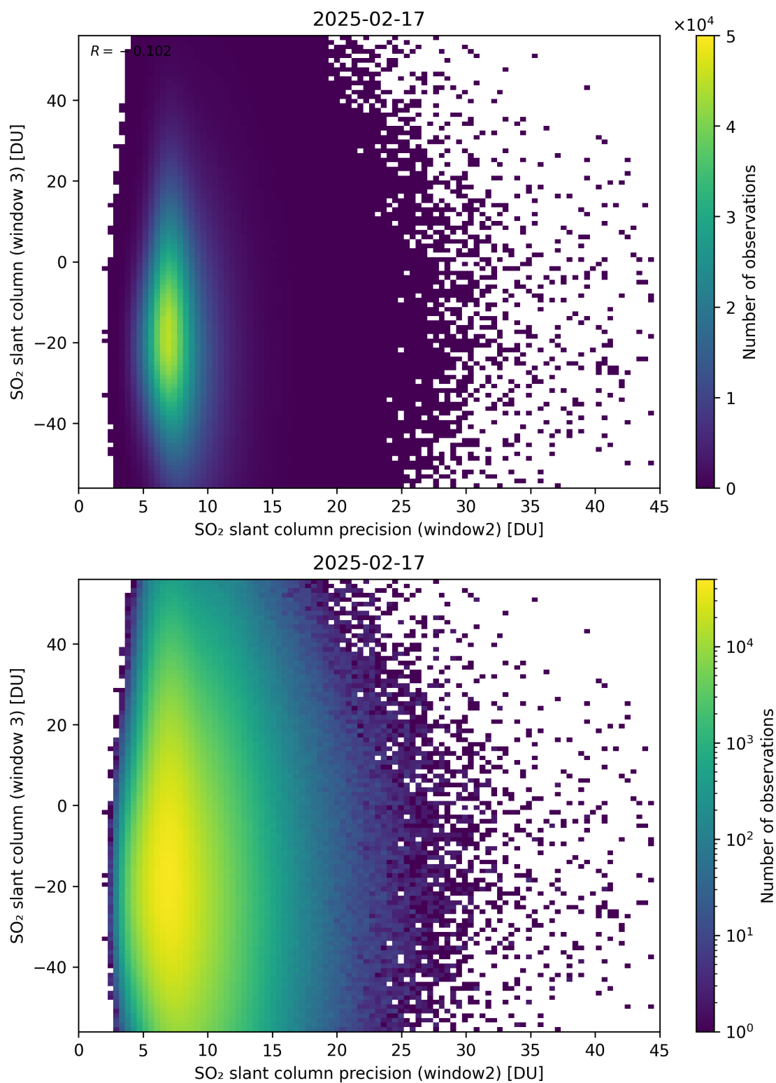
Figure 299: Scatter density plot of “SO 2 slant column precision (window2)” against “SO 2 slant column (window 3)” for 2025-02-16 to 2025-02-18.
