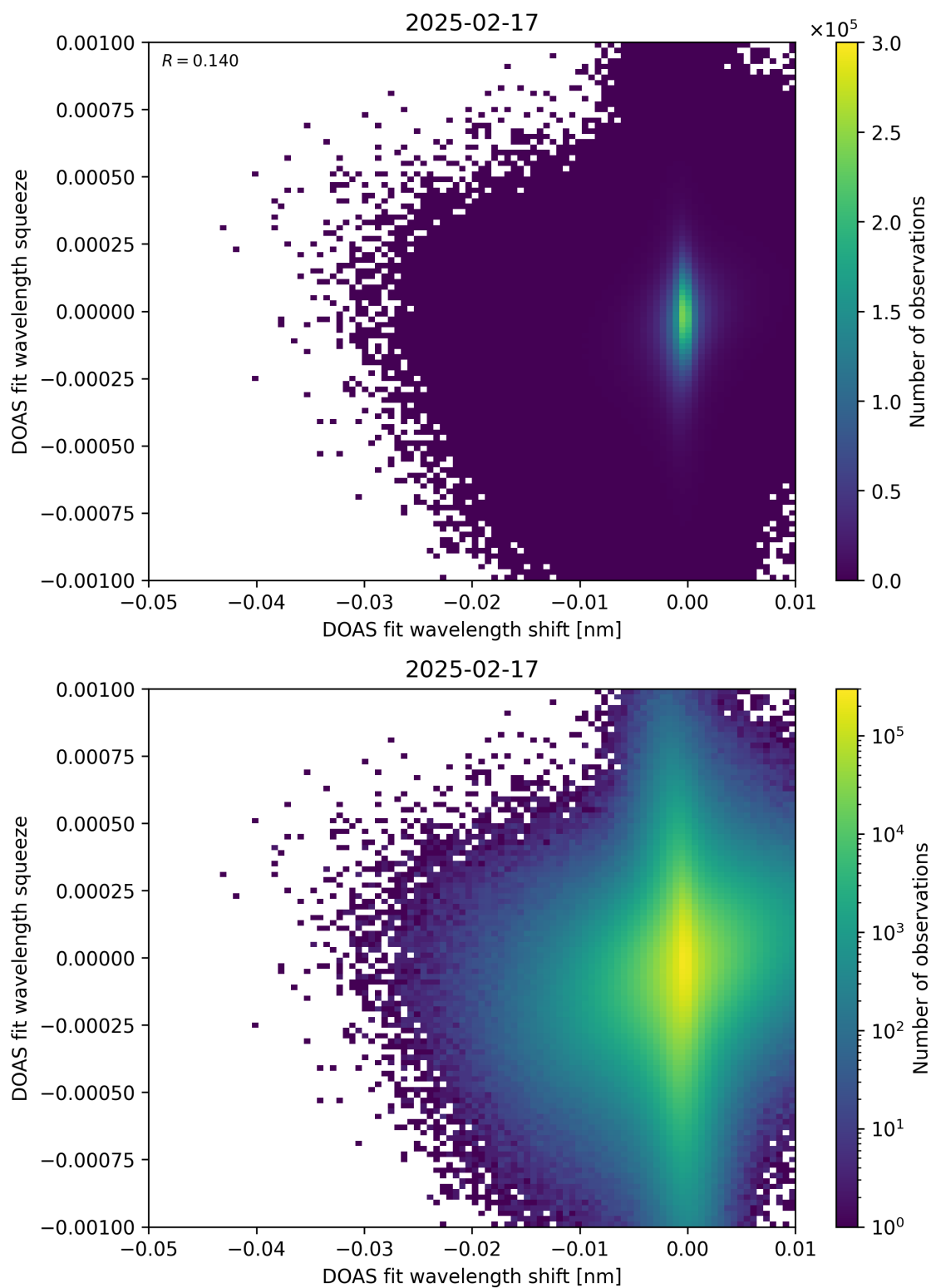
Figure 138: Scatter density plot of “DOAS fit wavelength shift” against “DOAS fit wavelength squeeze” for 2025-02-16 to 2025-02-18.
