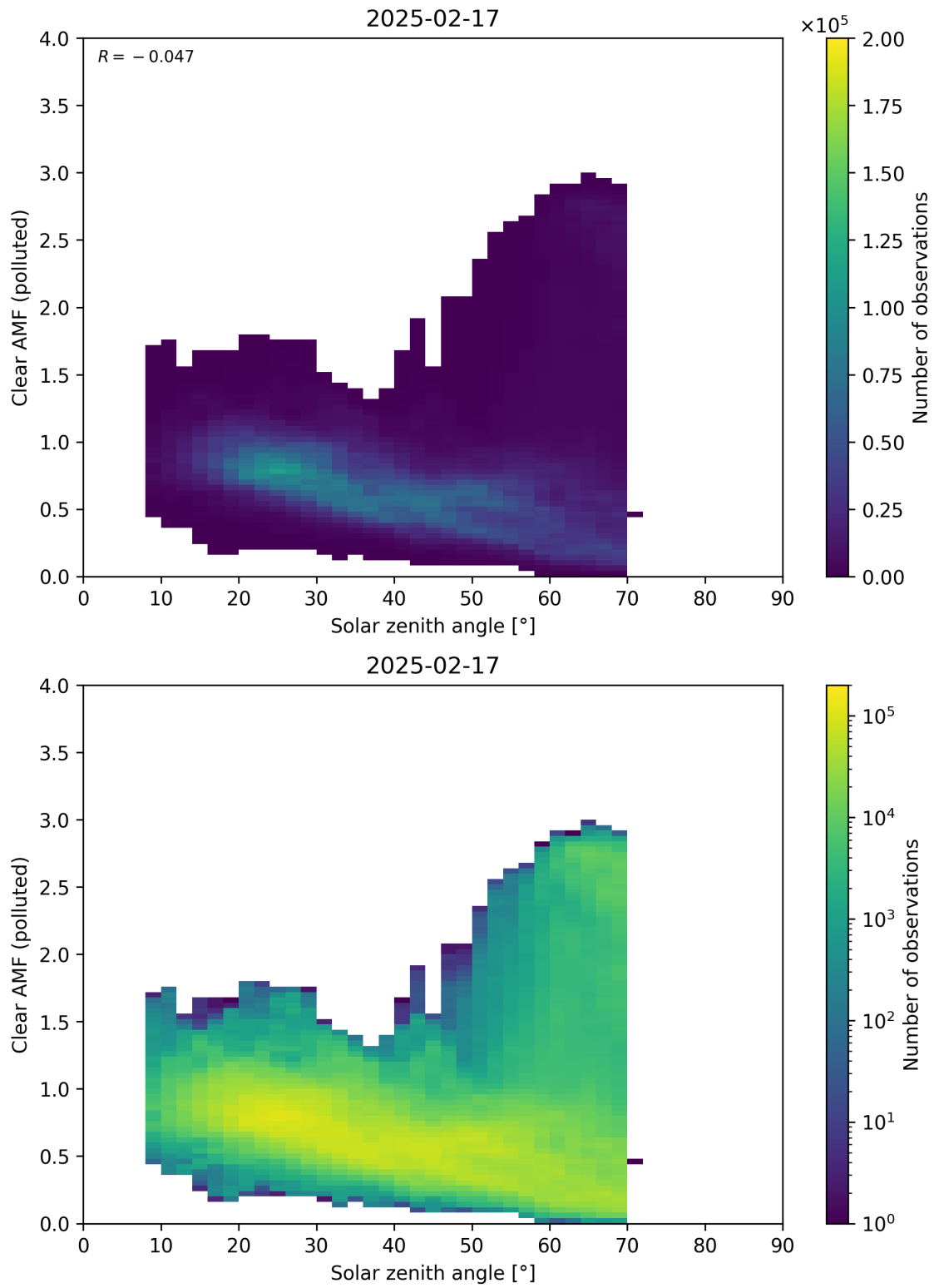
Figure 178: Scatter density plot of “Solar zenith angle” against “Clear AMF (polluted)” for 2025-02-16 to 2025-02-18.
