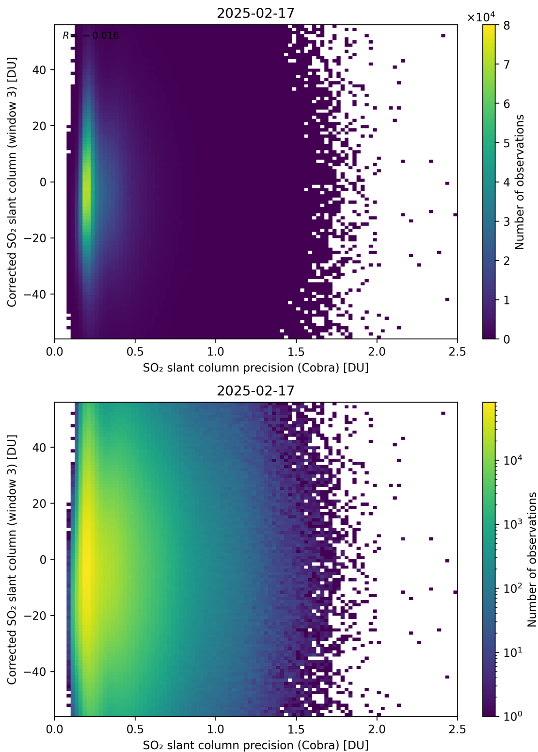
Figure 207: Scatter density plot of “SO 2 slant column precision (Cobra)” against “Corrected SO 2 slant column (window 3)” for 2025-02-16 to 2025-02-18.
