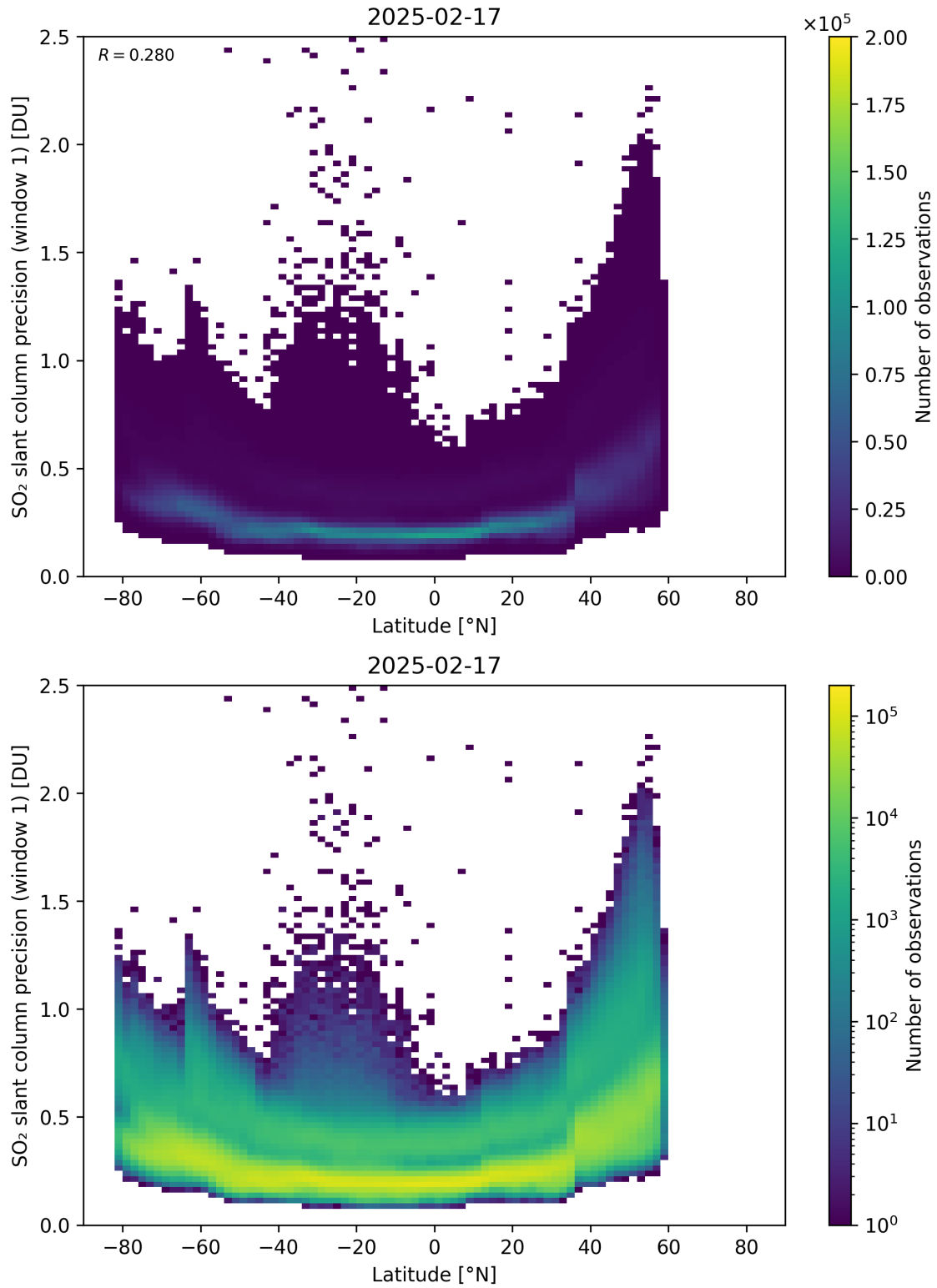
Figure 163: Scatter density plot of “Latitude” against “SO 2 slant column precision (window 1)” for 2025-02-16 to 2025-02-18.
