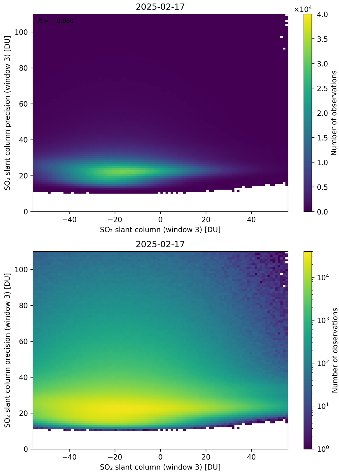
Figure 317: Scatter density plot of “SO 2 slant column (window 3)” against “SO 2 slant column precision (window 3)” for 2025-02-16 to 2025-02-18.
