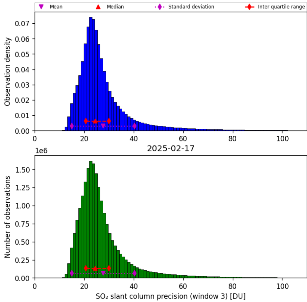
Figure 72: Histogram of “SO 2 slant column precision (window 3)” for 2025-02-16 to 2025-02-18
