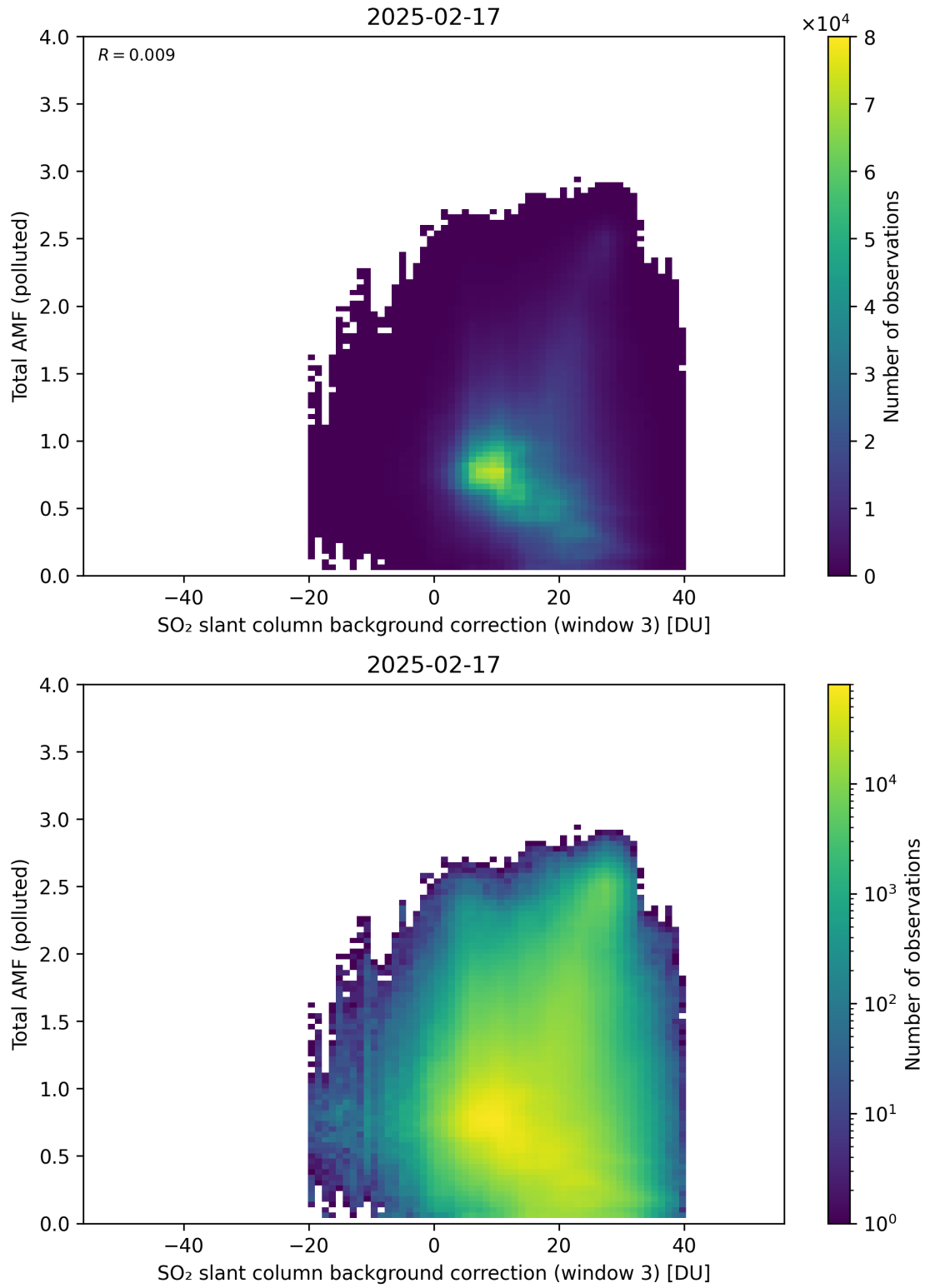
Figure 136: Scatter density plot of “SO 2 slant column background correction (window 3)” against “Total AMF (polluted)” for 2025-02-16 to 2025-02-18.
