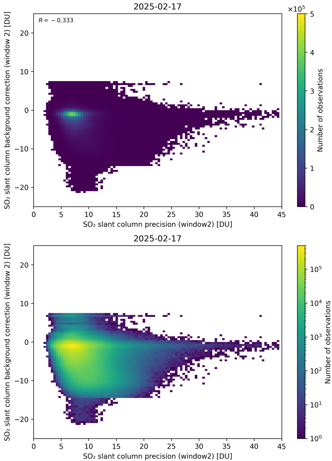
Figure 291: Scatter density plot of “SO 2 slant column precision (window2)” against “SO 2 slant column background correction (window 2)” for 2025-02-16 to 2025-02-18.
