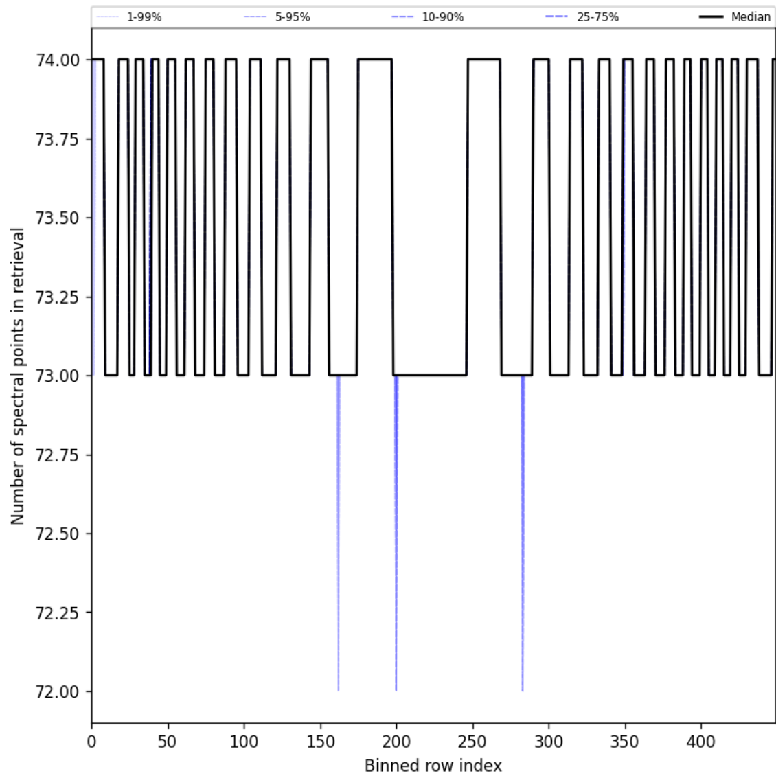
Figure 108: Along track statistics of “Number of spectral points in retrieval” for 2025-02-16 to 2025-02-18
