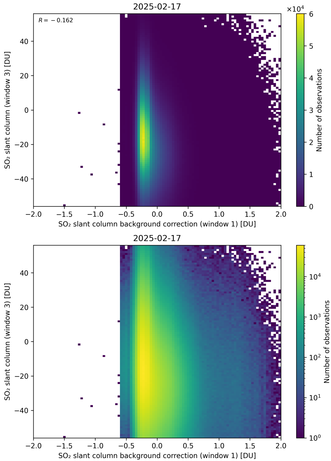
Figure 118: Scatter density plot of “SO 2 slant column background correction (window 1)” against “SO 2 slant column (window 3)” for 2025-02-16 to 2025-02-18.
