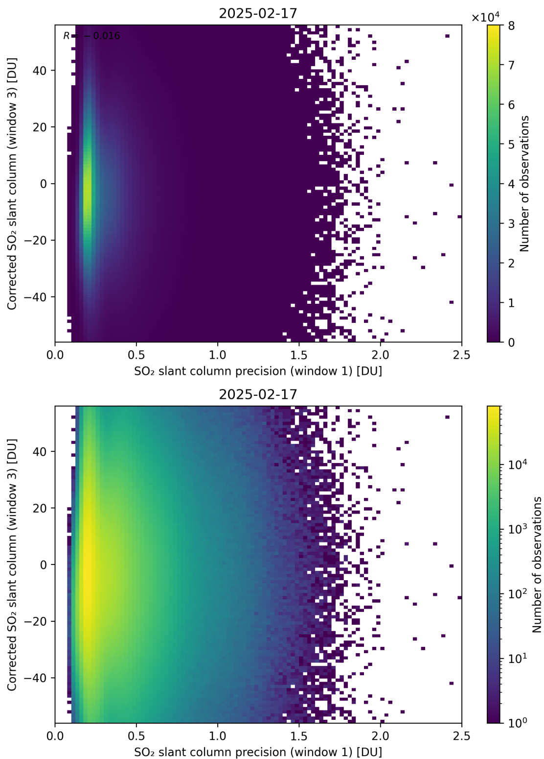
Figure 276: Scatter density plot of “SO 2 slant column precision (window 1)” against “Corrected SO 2 slant column (window 3)” for 2025-02-16 to 2025-02-18.
