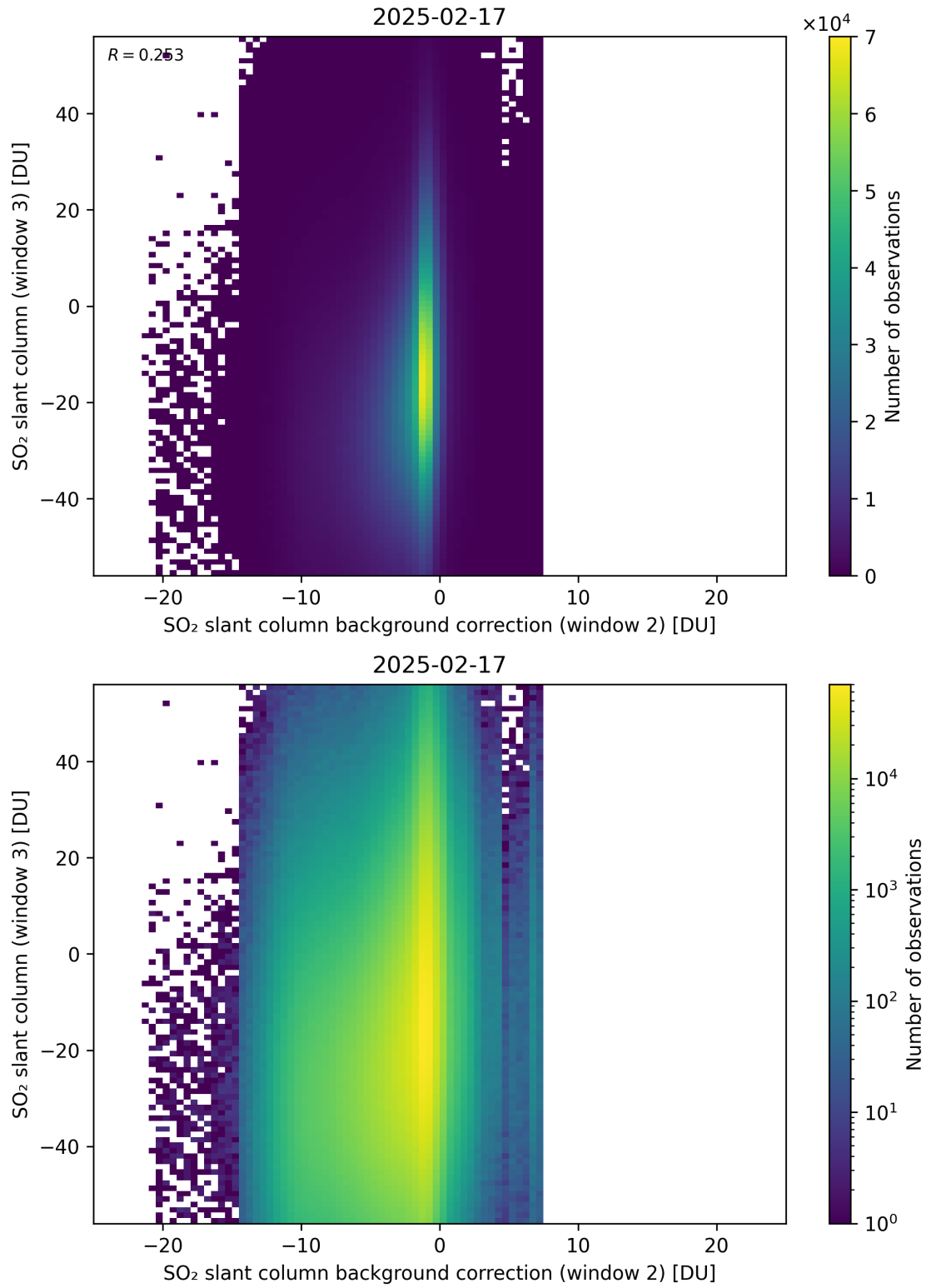
Figure 128: Scatter density plot of “SO 2 slant column background correction (window 2)” against “SO 2 slant column (window 3)” for 2025-02-16 to 2025-02-18.
