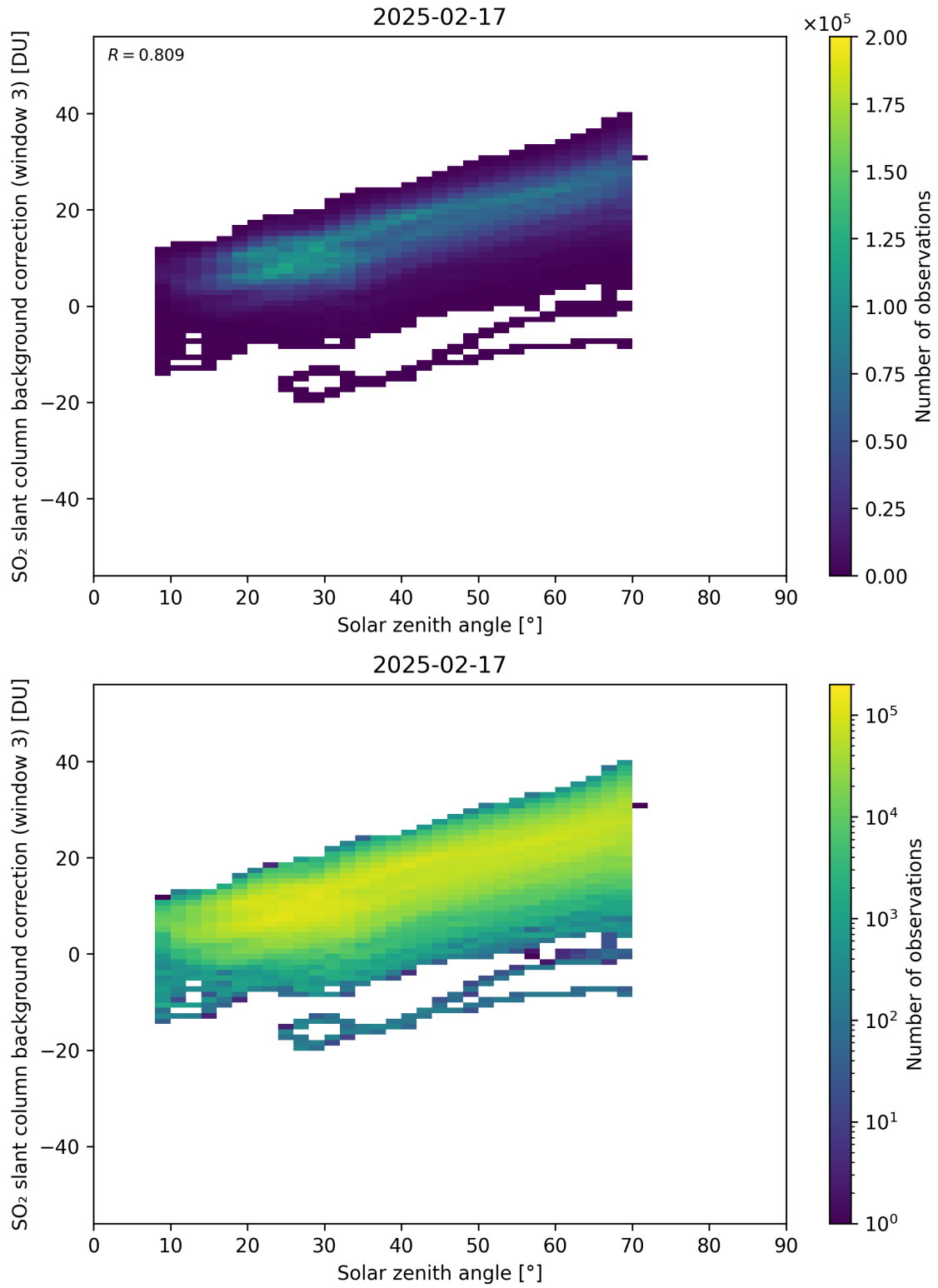
Figure 173: Scatter density plot of “Solar zenith angle” against “SO 2 slant column background correction (window 3)” for 2025-02-16 to 2025-02-18.
