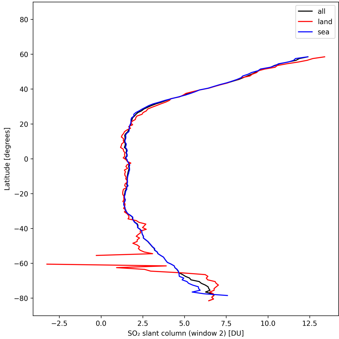
Figure 41: Zonal average of “SO 2 slant column (window 2)” for 2025-02-16 to 2025-02-18.
