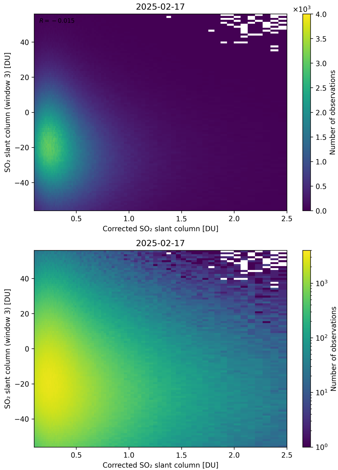
Figure 240: Scatter density plot of “Corrected SO 2 slant column” against “SO 2 slant column (window 3)” for 2025-02-16 to 2025-02-18.
