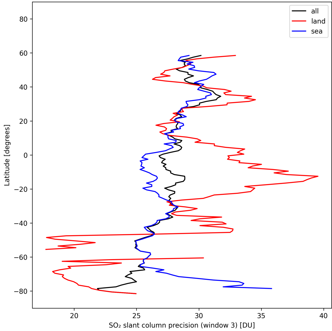
Figure 46: Zonal average of “SO 2 slant column precision (window 3)” for 2025-02-16 to 2025-02-18.
