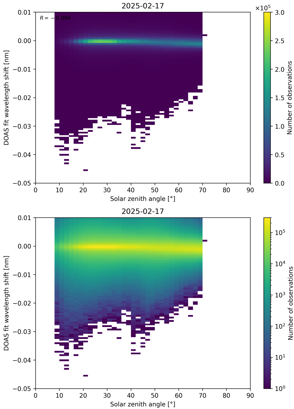
Figure 174: Scatter density plot of “Solar zenith angle” against “DOAS fit wavelength shift” for 2025-02-16 to 2025-02-18.
