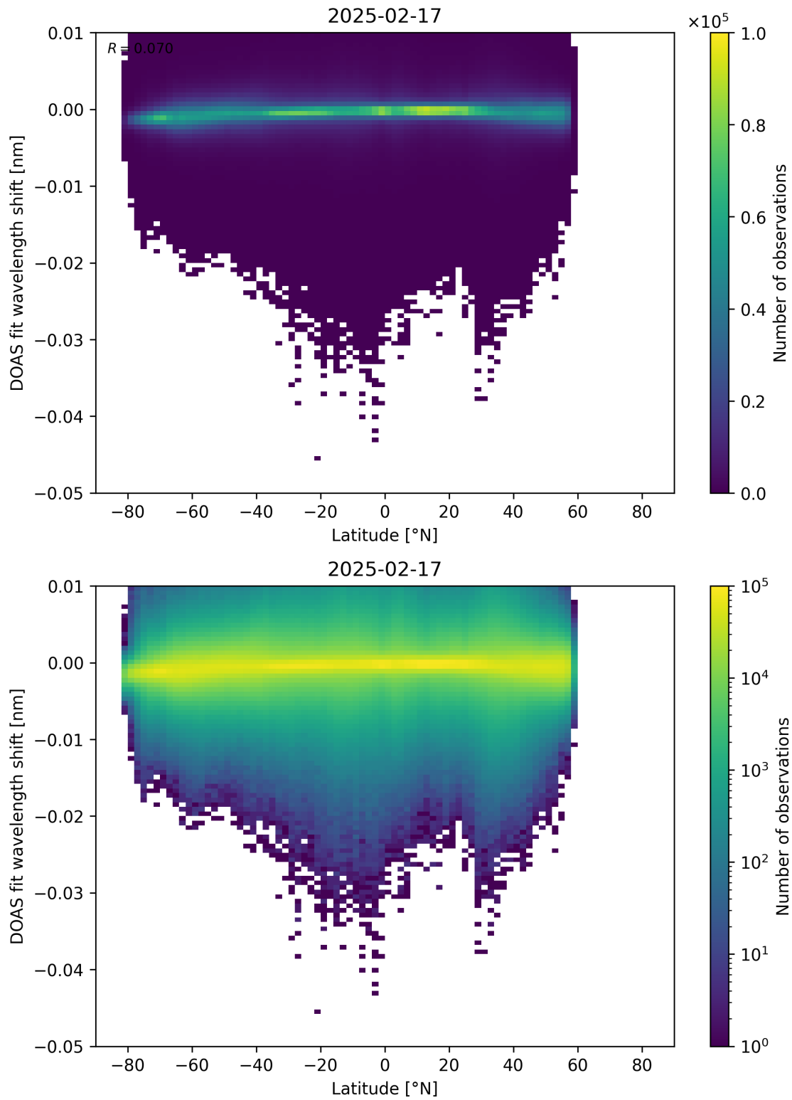
Figure 153: Scatter density plot of “Latitude” against “DOAS fit wavelength shift” for 2025-02-16 to 2025-02-18.
