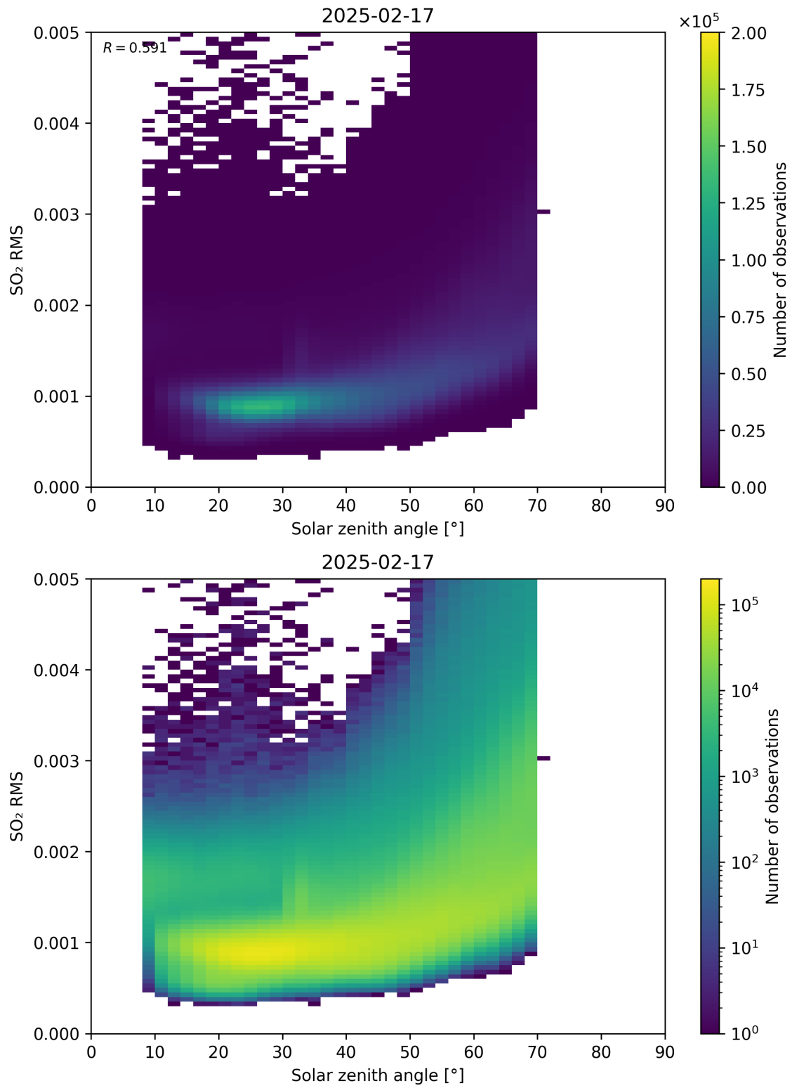
Figure 176: Scatter density plot of “Solar zenith angle” against “SO 2 RMS” for 2025-02-16 to 2025-02-18.
