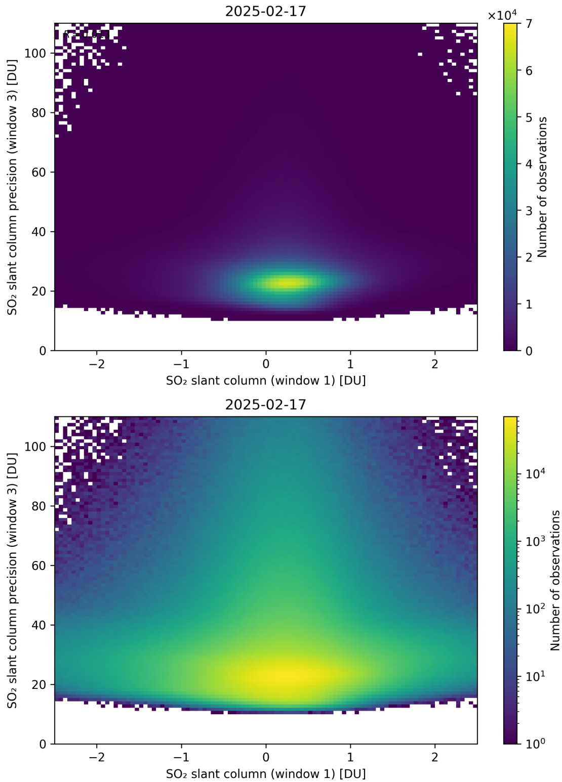
Figure 288: Scatter density plot of “SO 2 slant column (window 1)” against “SO 2 slant column precision (window 3)” for 2025-02-16 to 2025-02-18.
