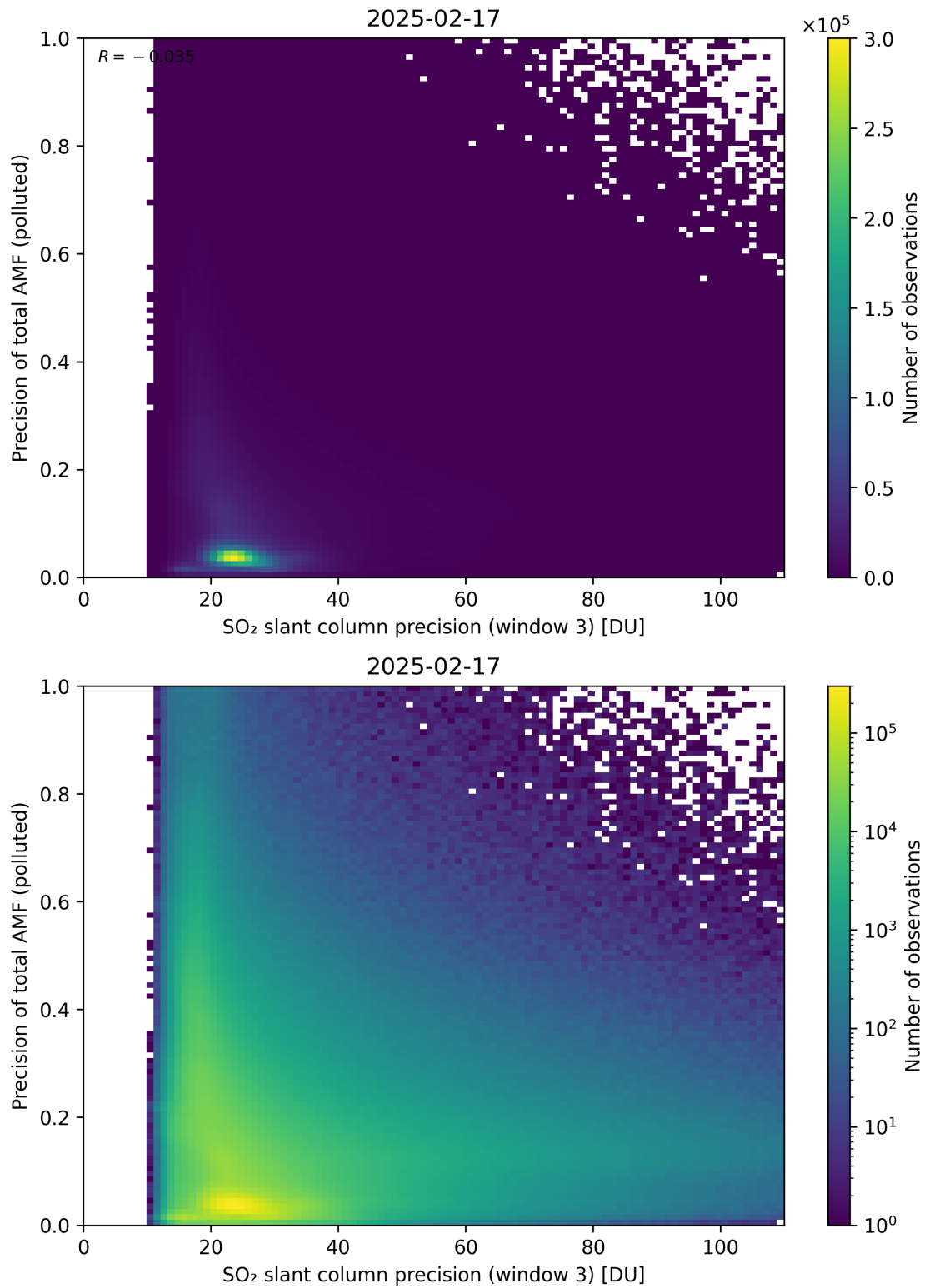
Figure 314: Scatter density plot of “SO 2 slant column precision (window 3)” against “Precision of total AMF (polluted)” for 2025-02-16 to 2025-02-18.
