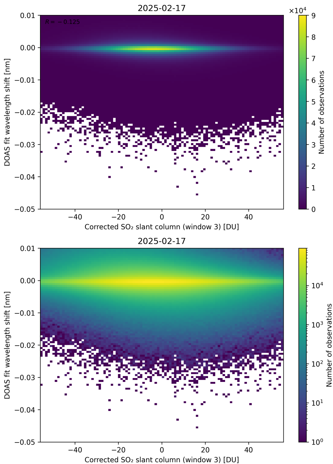
Figure 256: Scatter density plot of “Corrected SO 2 slant column (window 3)” against “DOAS fit wavelength shift” for 2025-02-16 to 2025-02-18.
