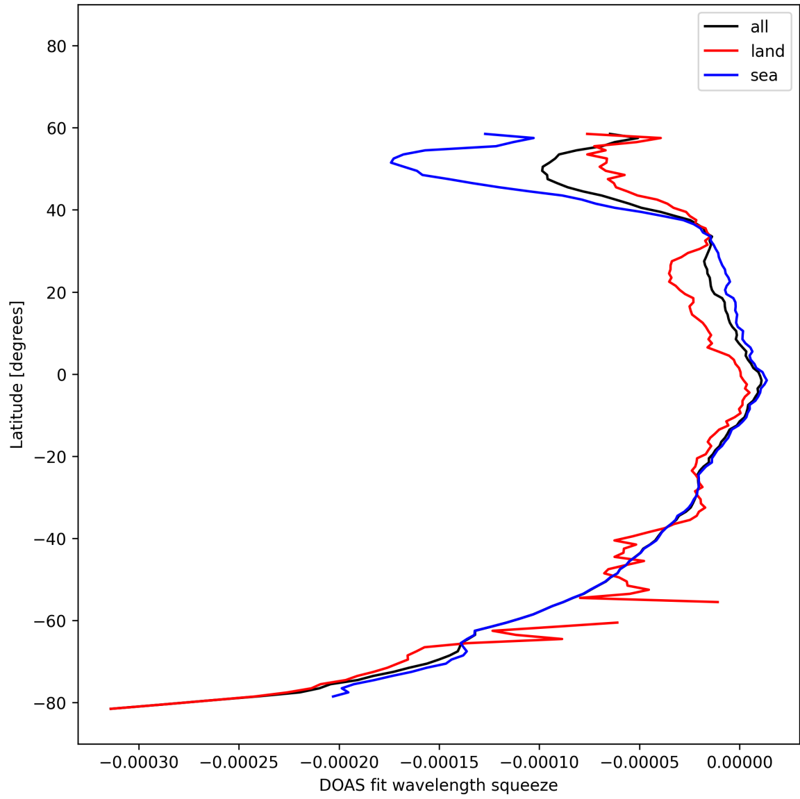
Figure 51: Zonal average of “DOAS fit wavelength squeeze” for 2025-02-16 to 2025-02-18.
