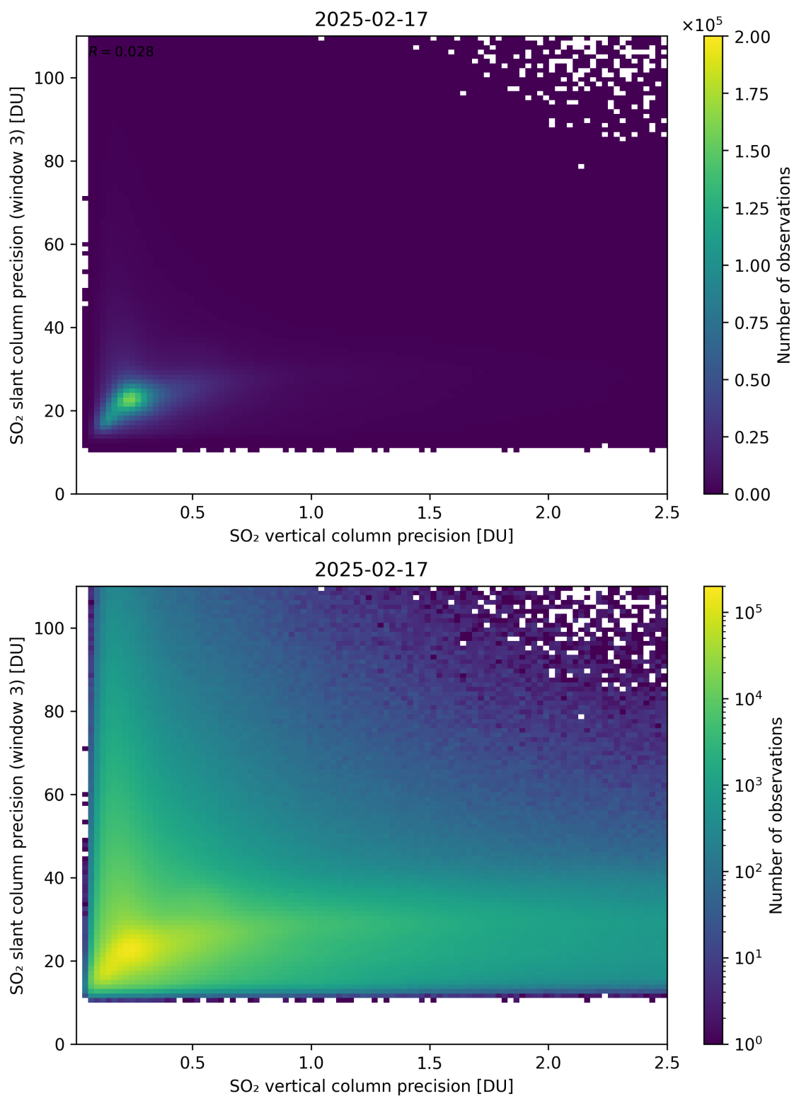
Figure 345: Scatter density plot of “SO 2 vertical column precision” against “SO 2 slant column precision (window 3)” for 2025-02-16 to 2025-02-18.
