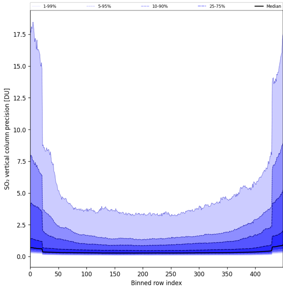
Figure 85: Along track statistics of “SO 2 vertical column precision” for 2025-02-16 to 2025-02-18
