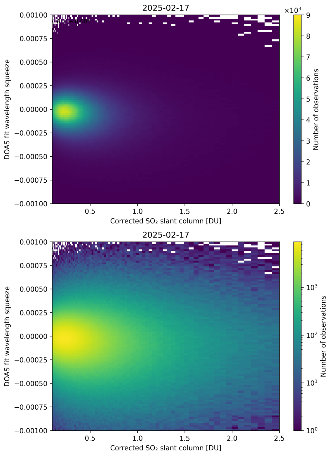
Figure 230: Scatter density plot of “Corrected SO 2 slant column” against “DOAS fit wavelength squeeze” for 2025-02-16 to 2025-02-18.
