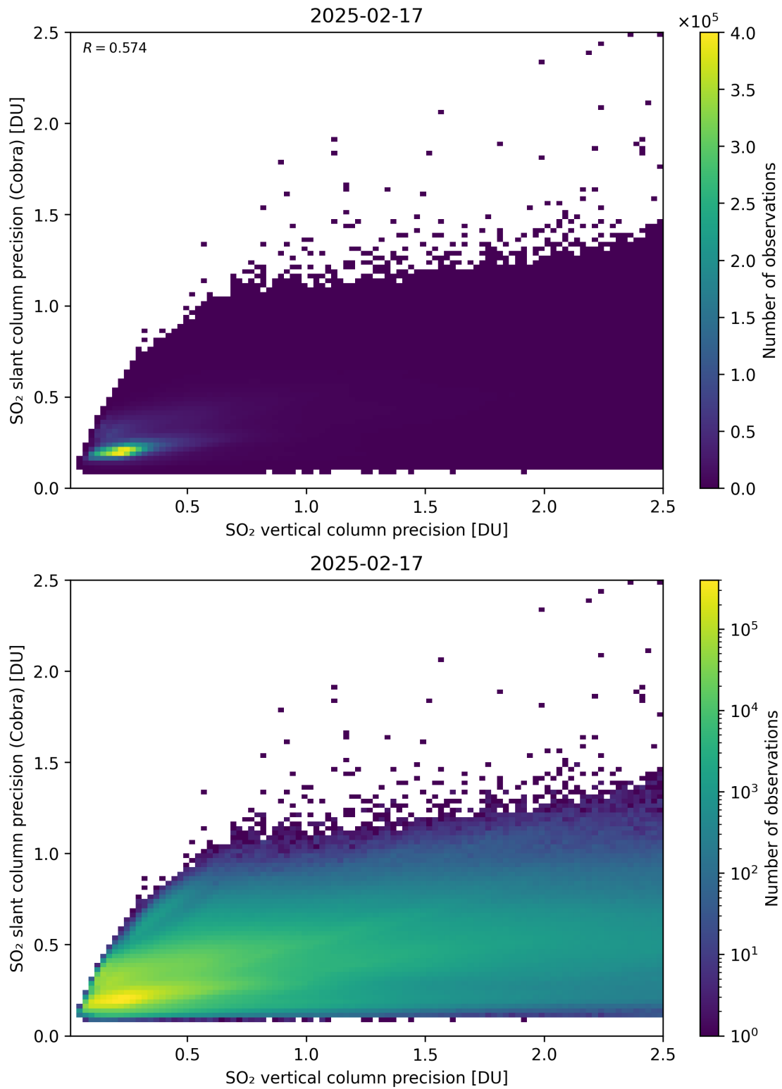
Figure 337: Scatter density plot of “SO 2 vertical column precision” against “SO 2 slant column precision (Cobra)” for 2025-02-16 to 2025-02-18.
