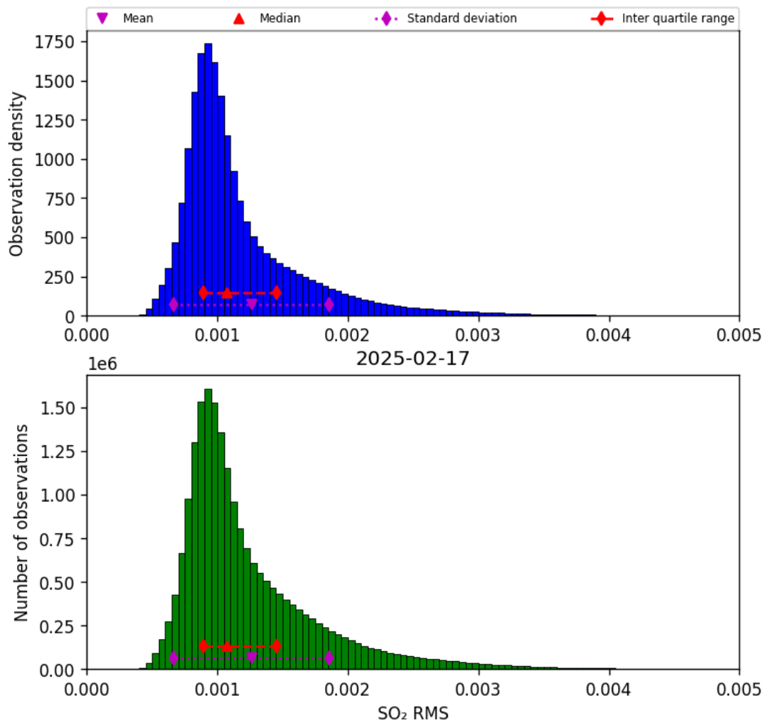
Figure 78: Histogram of “SO 2 RMS” for 2025-02-16 to 2025-02-18
