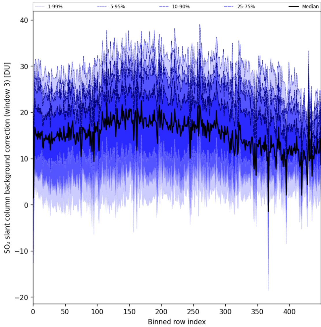
Figure 100: Along track statistics of “SO 2 slant column background correction (window 3)” for 2025-02-16 to 2025-02-18
