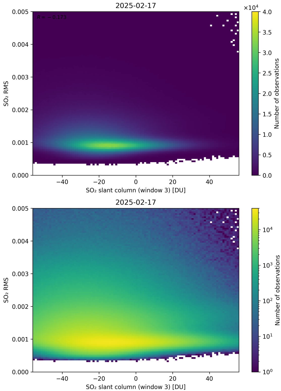
Figure 306: Scatter density plot of “SO 2 slant column (window 3)” against “SO 2 RMS” for 2025-02-16 to 2025-02-18.
