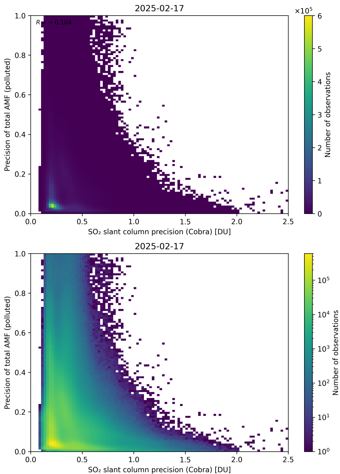
Figure 214: Scatter density plot of “SO 2 slant column precision (Cobra)” against “Precision of total AMF (polluted)” for 2025-02-16 to 2025-02-18.
