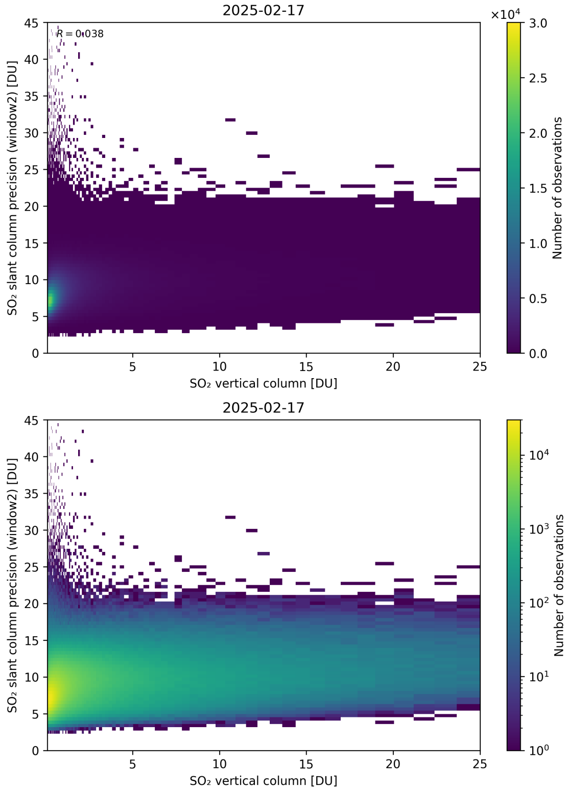
Figure 356: Scatter density plot of “SO 2 vertical column” against “SO 2 slant column precision (window2)” for 2025-02-16 to 2025-02-18.
