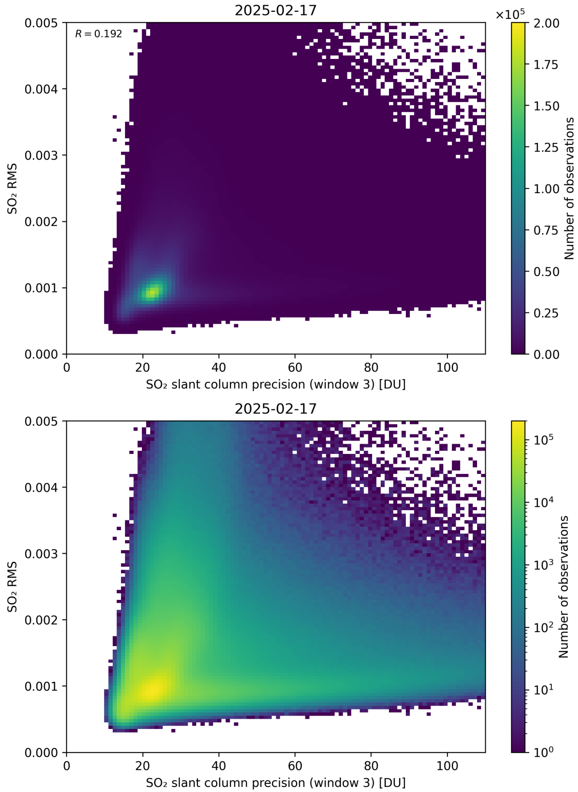
Figure 310: Scatter density plot of “SO 2 slant column precision (window 3)” against “SO 2 RMS” for 2025-02-16 to 2025-02-18.
