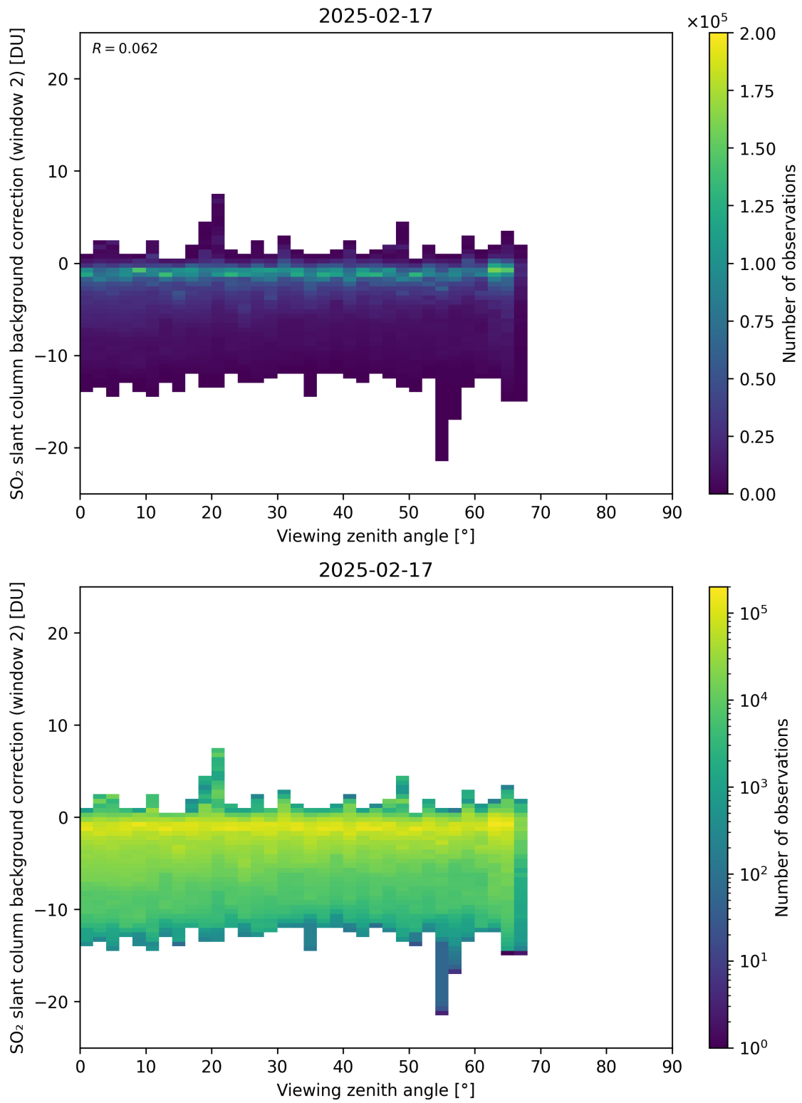
Figure 363: Scatter density plot of “Viewing zenith angle” against “SO 2 slant column background correction (window 2)” for 2025-02-16 to 2025-02-18.
