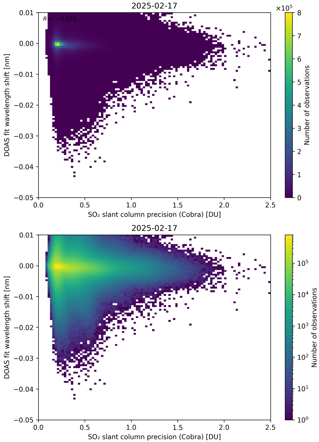
Figure 202: Scatter density plot of “SO 2 slant column precision (Cobra)” against “DOAS fit wavelength shift” for 2025-02-16 to 2025-02-18.
