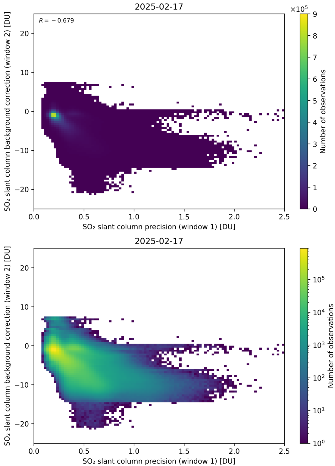
Figure 269: Scatter density plot of “SO 2 slant column precision (window 1)” against “SO 2 slant column background correction (window 2)” for 2025-02-16 to 2025-02-18.
