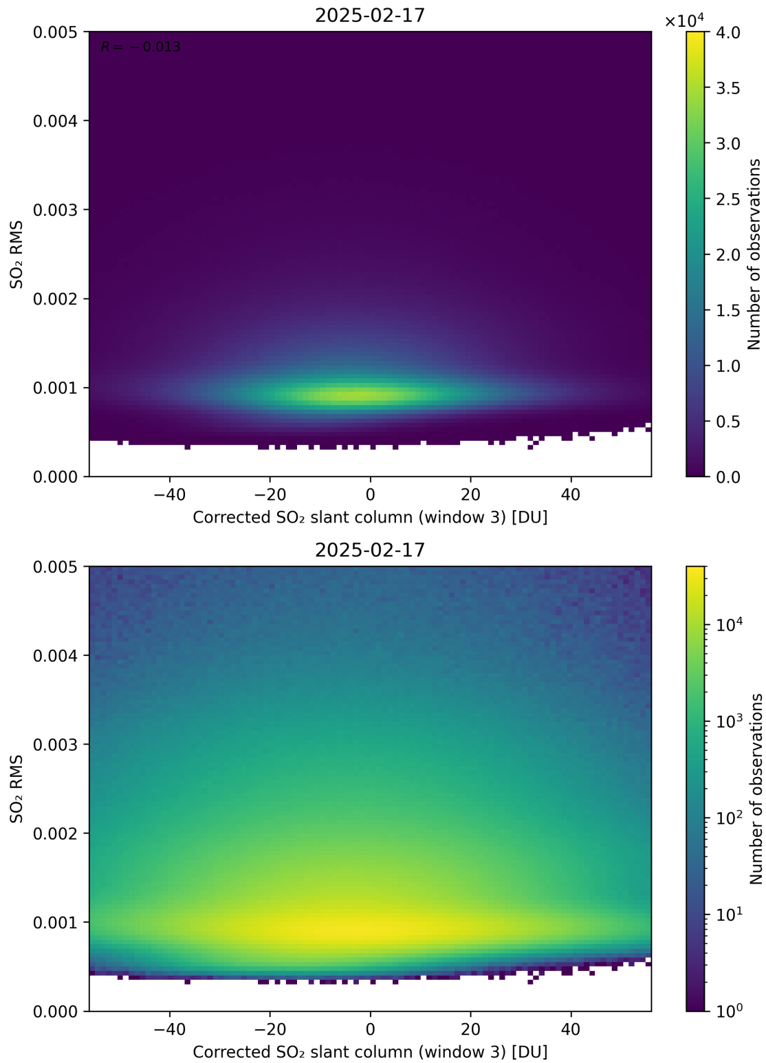
Figure 258: Scatter density plot of “Corrected SO 2 slant column (window 3)” against “SO 2 RMS” for 2025-02-16 to 2025-02-18.
