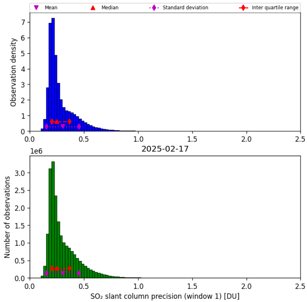
Figure 64: Histogram of “SO 2 slant column precision (window 1)” for 2025-02-16 to 2025-02-18
