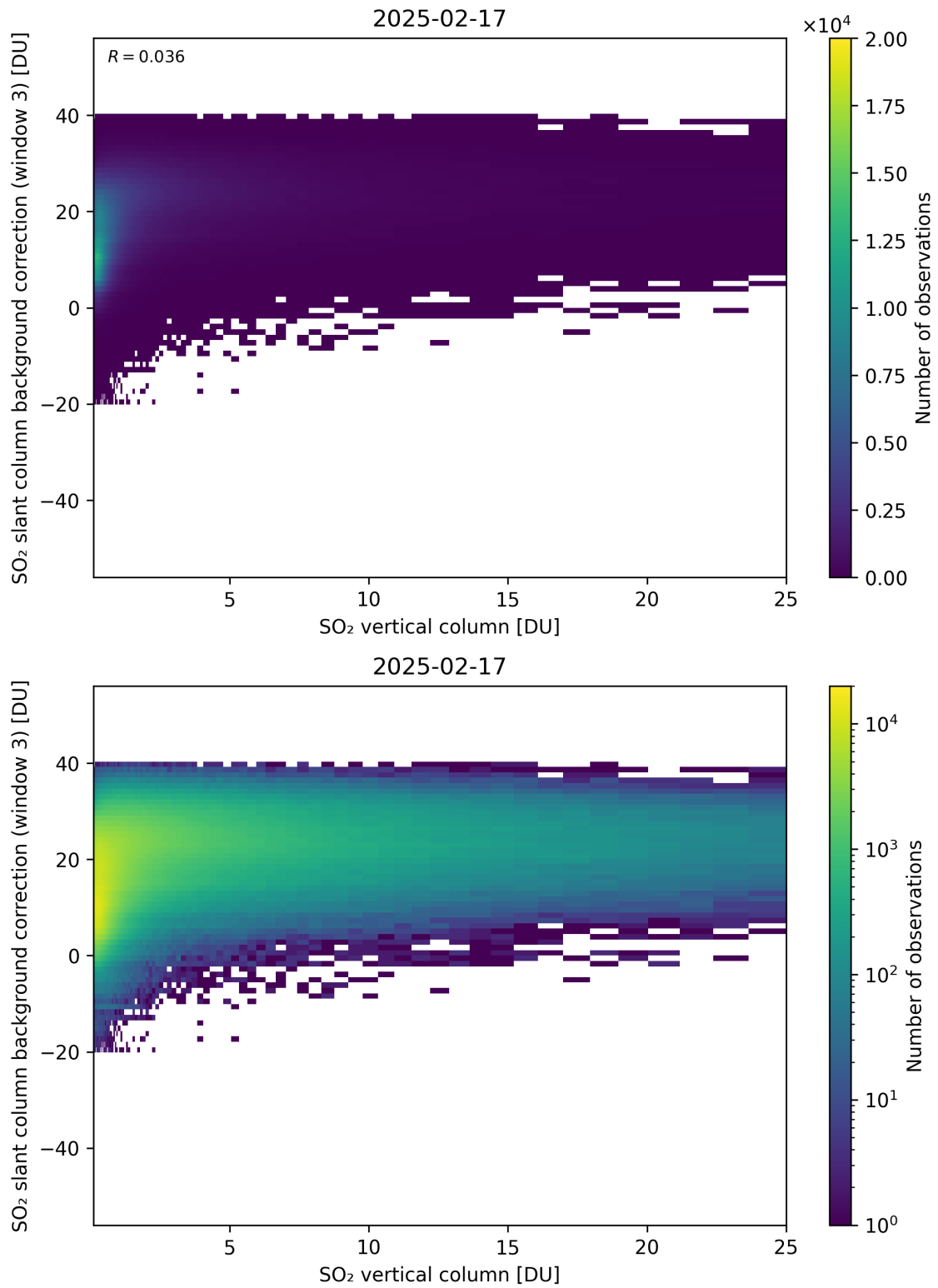
Figure 325: Scatter density plot of “SO 2 vertical column” against “SO 2 slant column background correction (window 3)” for 2025-02-16 to 2025-02-18.
