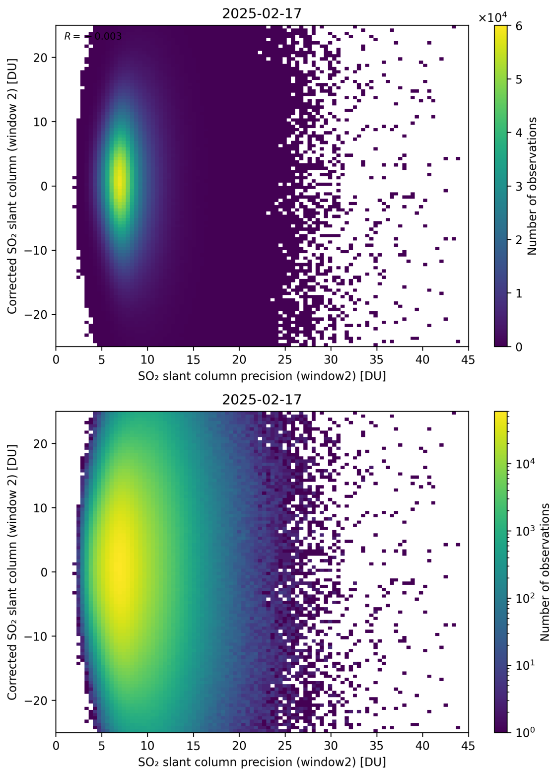
Figure 297: Scatter density plot of “SO 2 slant column precision (window2)” against “Corrected SO 2 slant column (window 2)” for 2025-02-16 to 2025-02-18.
