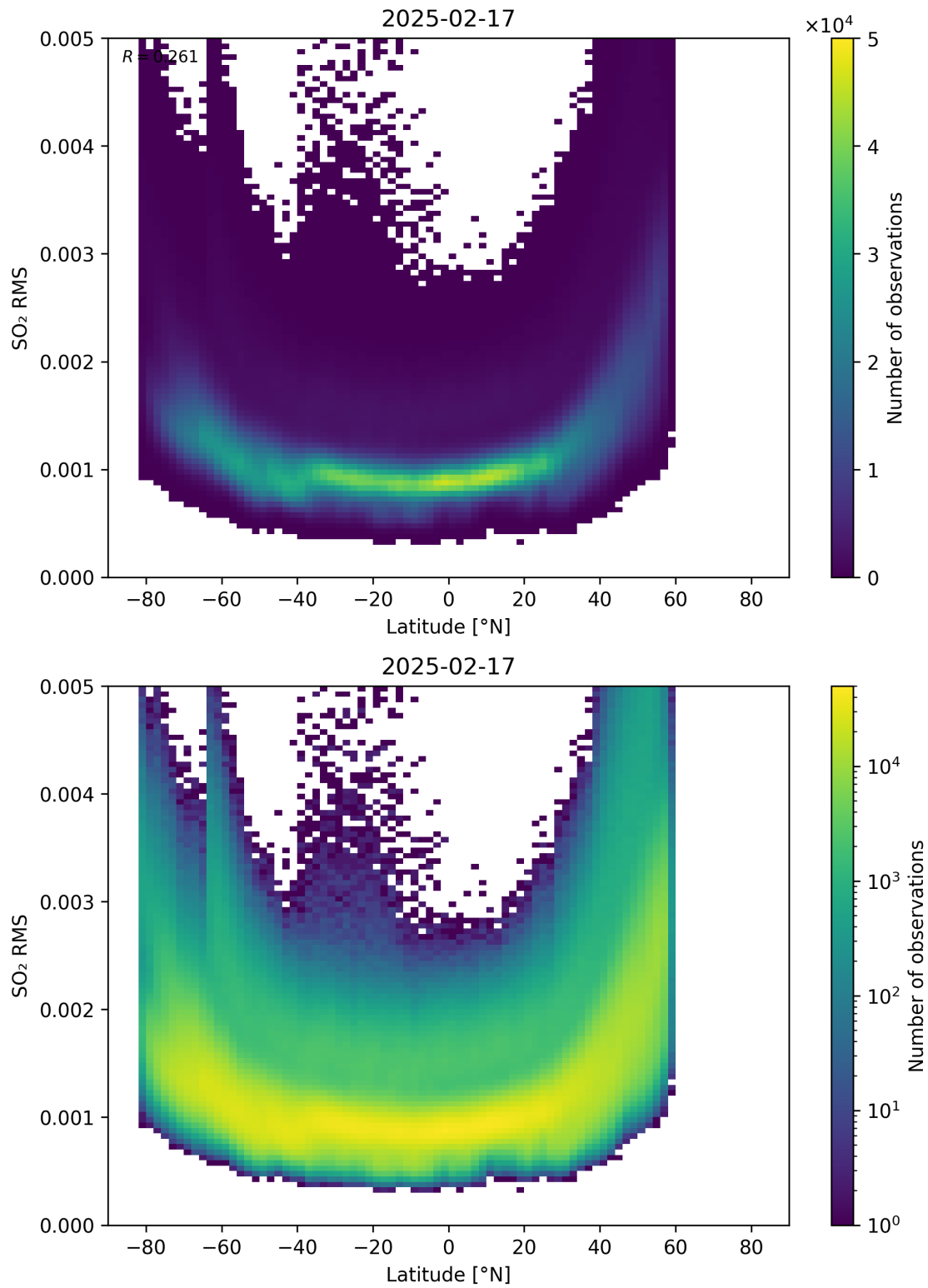
Figure 155: Scatter density plot of “Latitude” against “SO 2 RMS” for 2025-02-16 to 2025-02-18.
