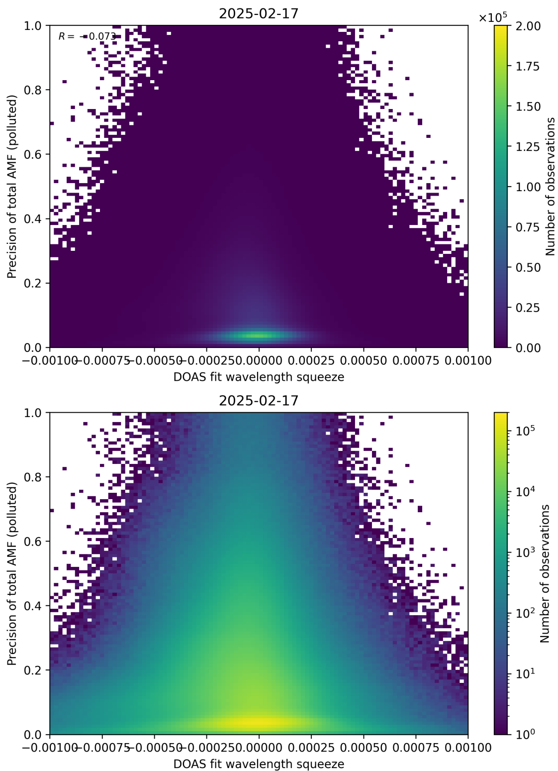
Figure 146: Scatter density plot of “DOAS fit wavelength squeeze” against “Precision of total AMF (polluted)” for 2025-02-16 to 2025-02-18.
