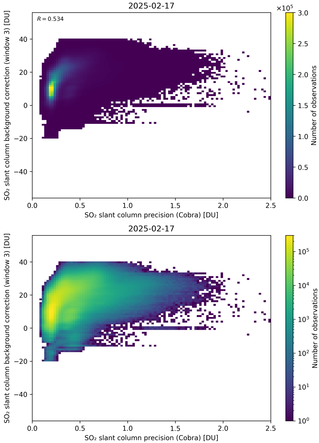
Figure 201: Scatter density plot of “SO 2 slant column precision (Cobra)” against “SO 2 slant column background correction (window 3)” for 2025-02-16 to 2025-02-18.
