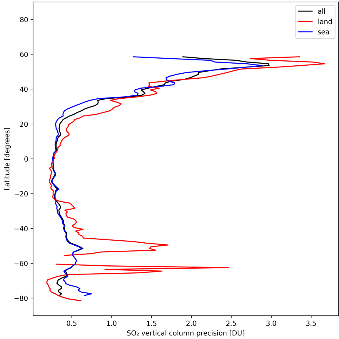
Figure 33: Zonal average of “SO 2 vertical column precision” for 2025-02-16 to 2025-02-18.
