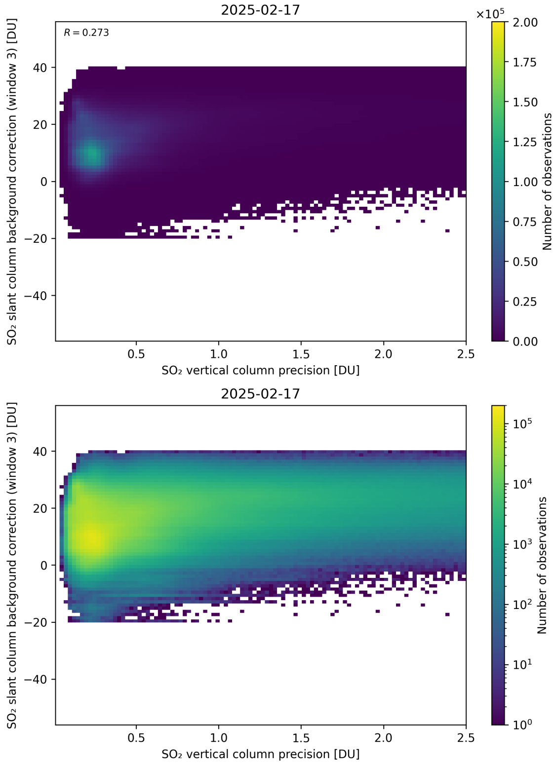
Figure 331: Scatter density plot of “SO 2 vertical column precision” against “SO 2 slant column background correction (window 3)” for 2025-02-16 to 2025-02-18.
