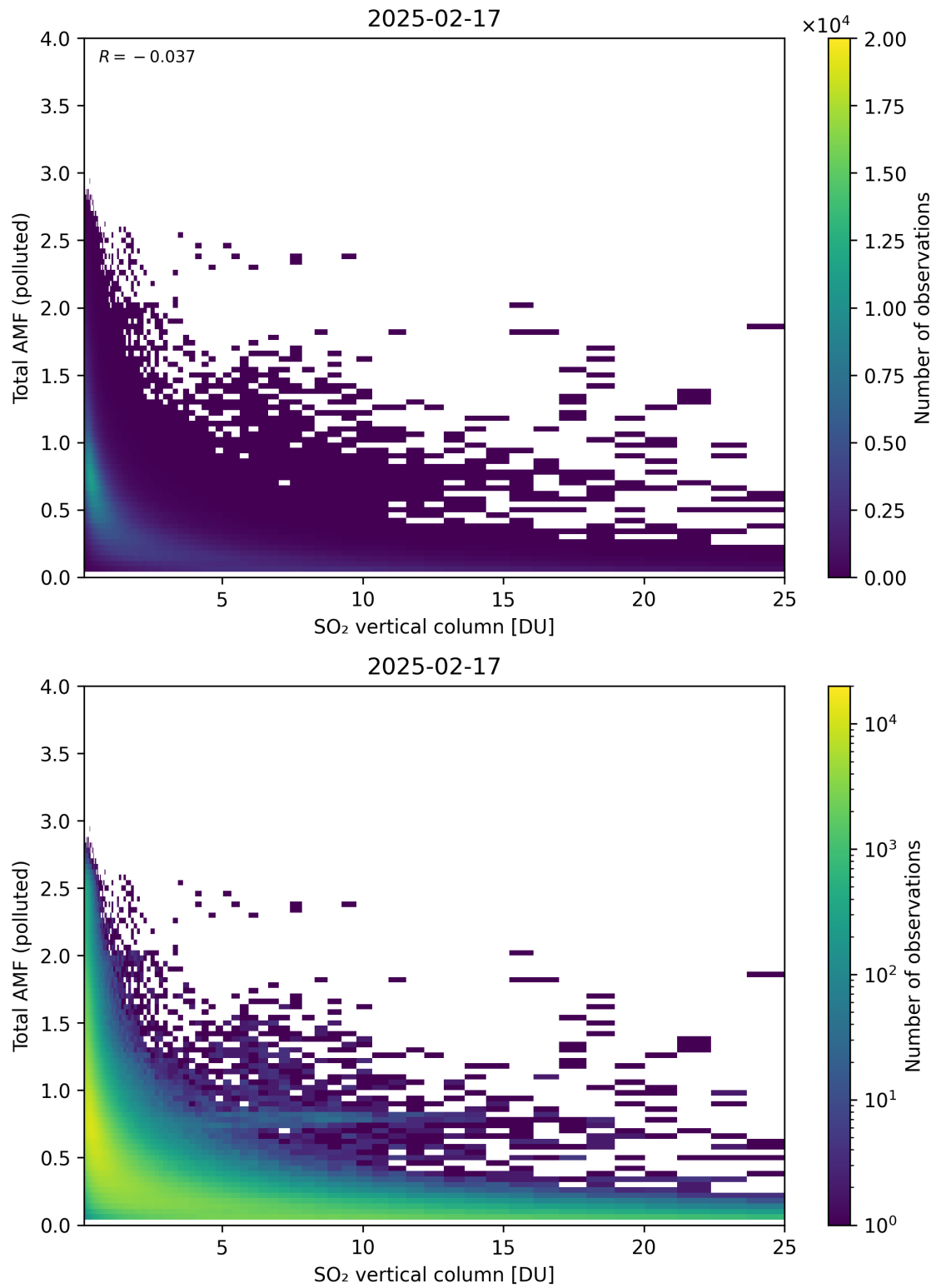
Figure 359: Scatter density plot of “SO 2 vertical column” against “Total AMF (polluted)” for 2025-02-16 to 2025-02-18.
