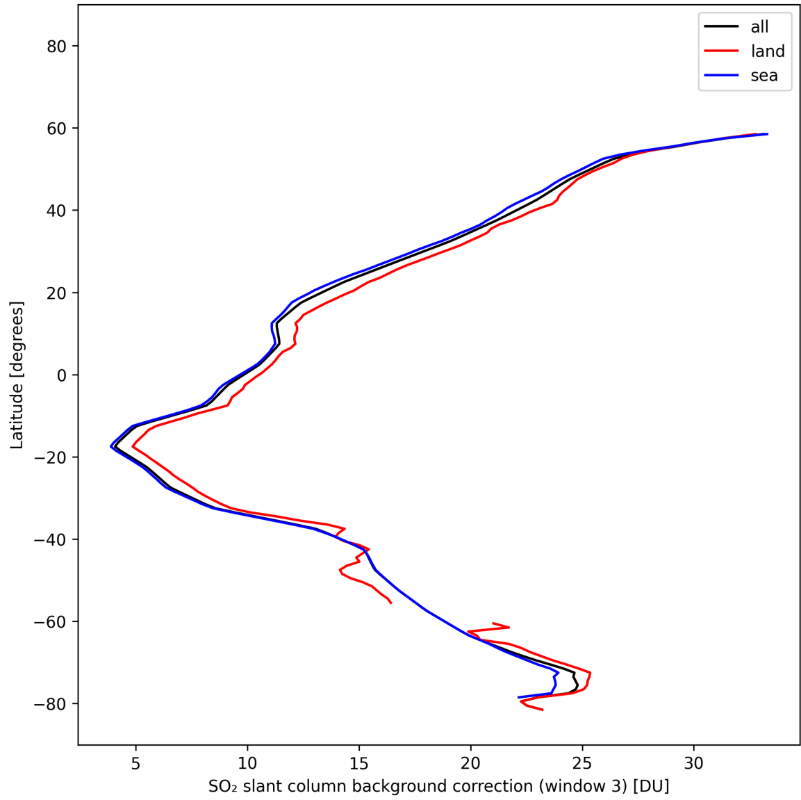
Figure 48: Zonal average of “SO 2 slant column background correction (window 3)” for 2025-02-16 to 2025-02-18.
