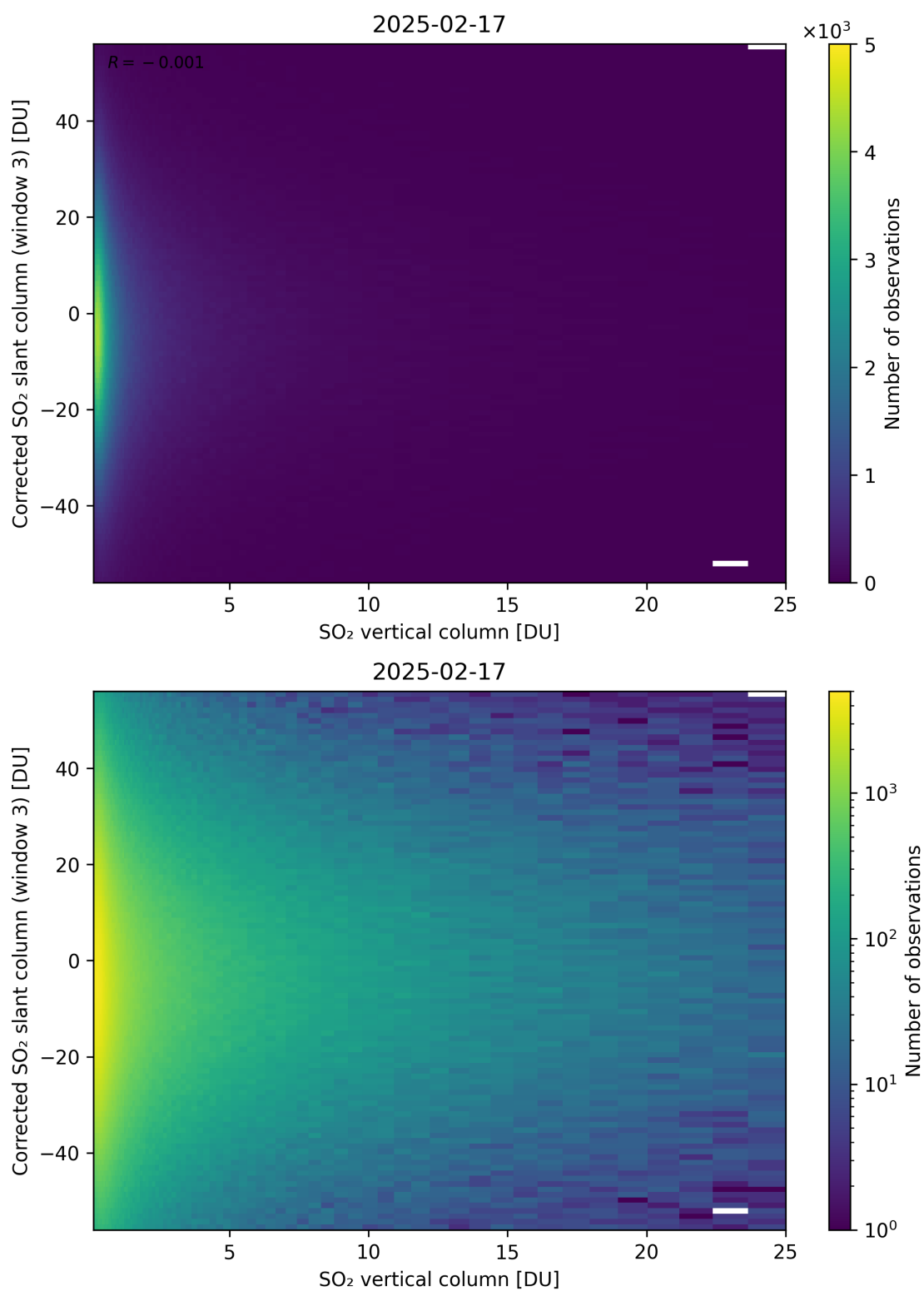
Figure 353: Scatter density plot of “SO 2 vertical column” against “Corrected SO 2 slant column (window 3)” for 2025-02-16 to 2025-02-18.
