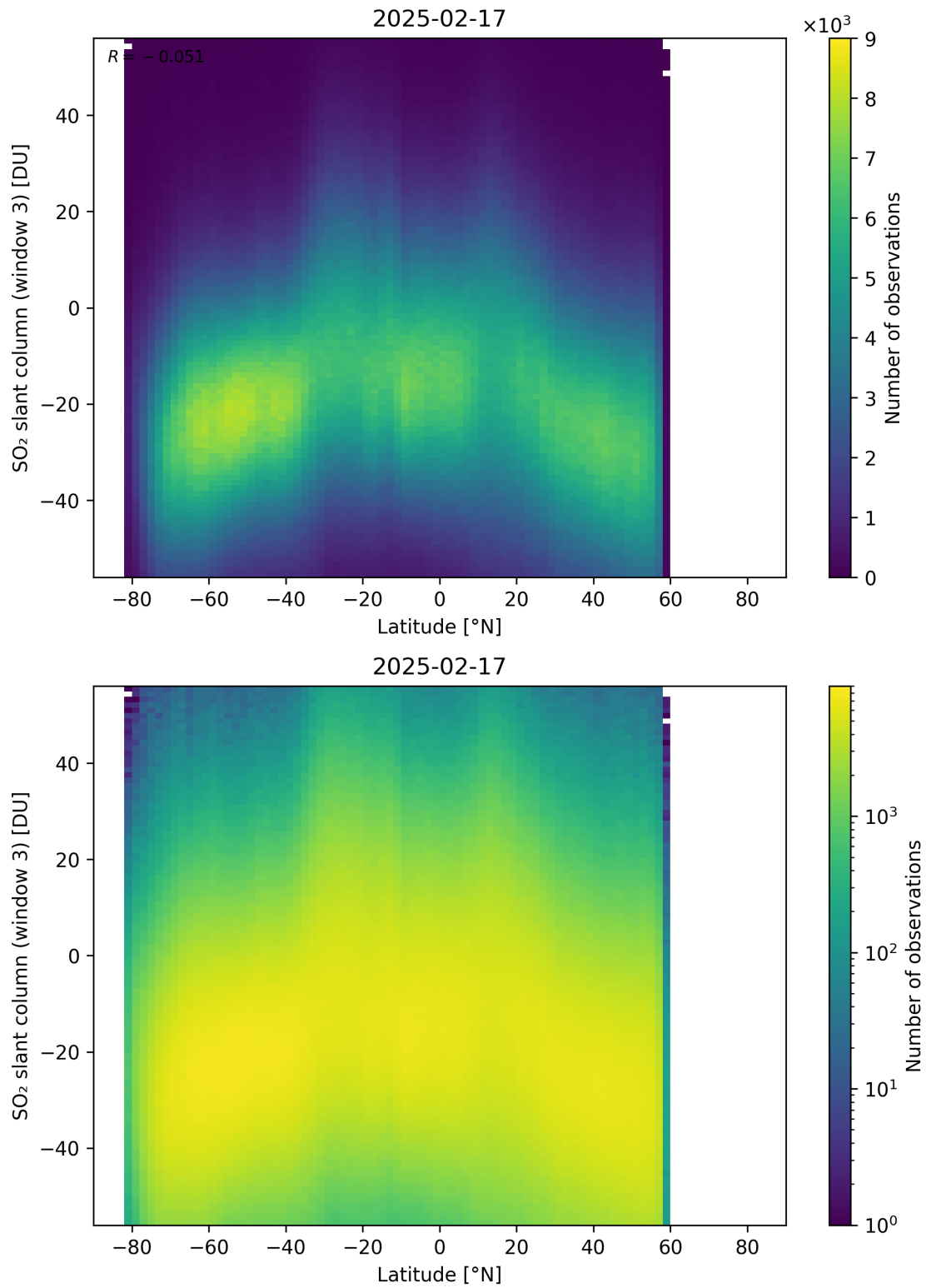
Figure 165: Scatter density plot of “Latitude” against “SO 2 slant column (window 3)” for 2025-02-16 to 2025-02-18.
