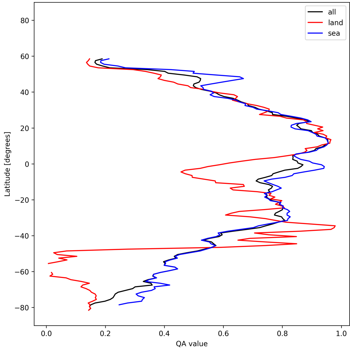
Figure 31: Zonal average of “QA value” for 2025-02-16 to 2025-02-18.
