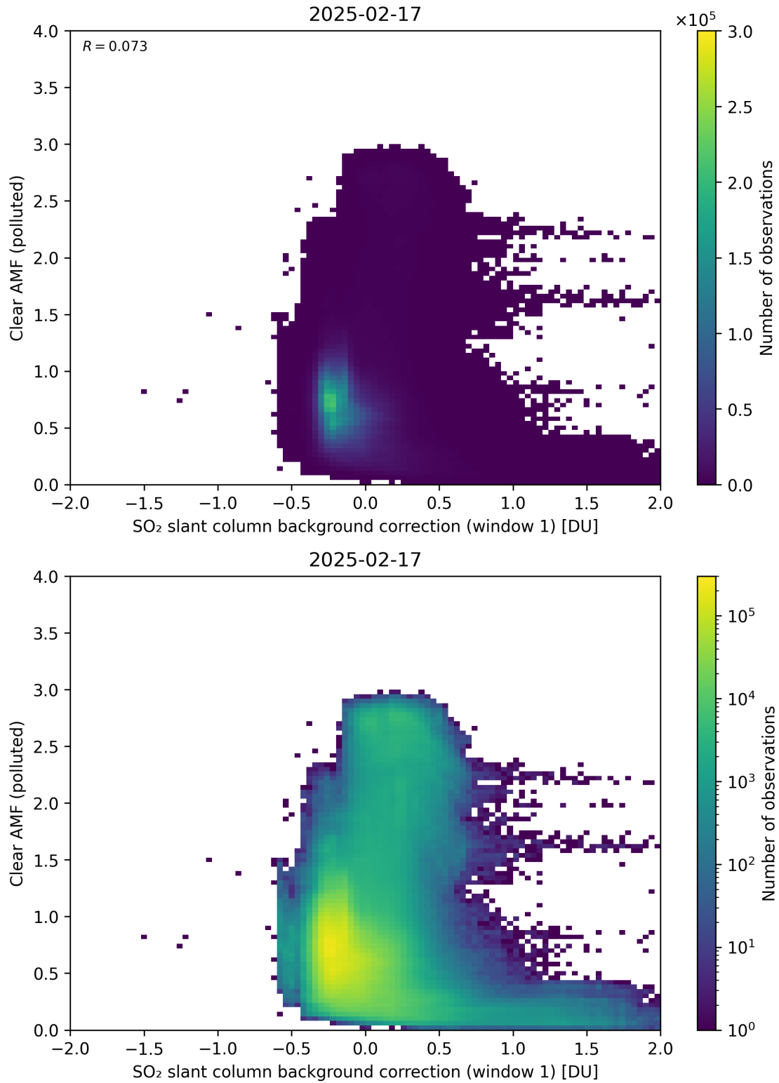
Figure 114: Scatter density plot of “SO 2 slant column background correction (window 1)” against “Clear AMF (polluted)” for 2025-02-16 to 2025-02-18.
