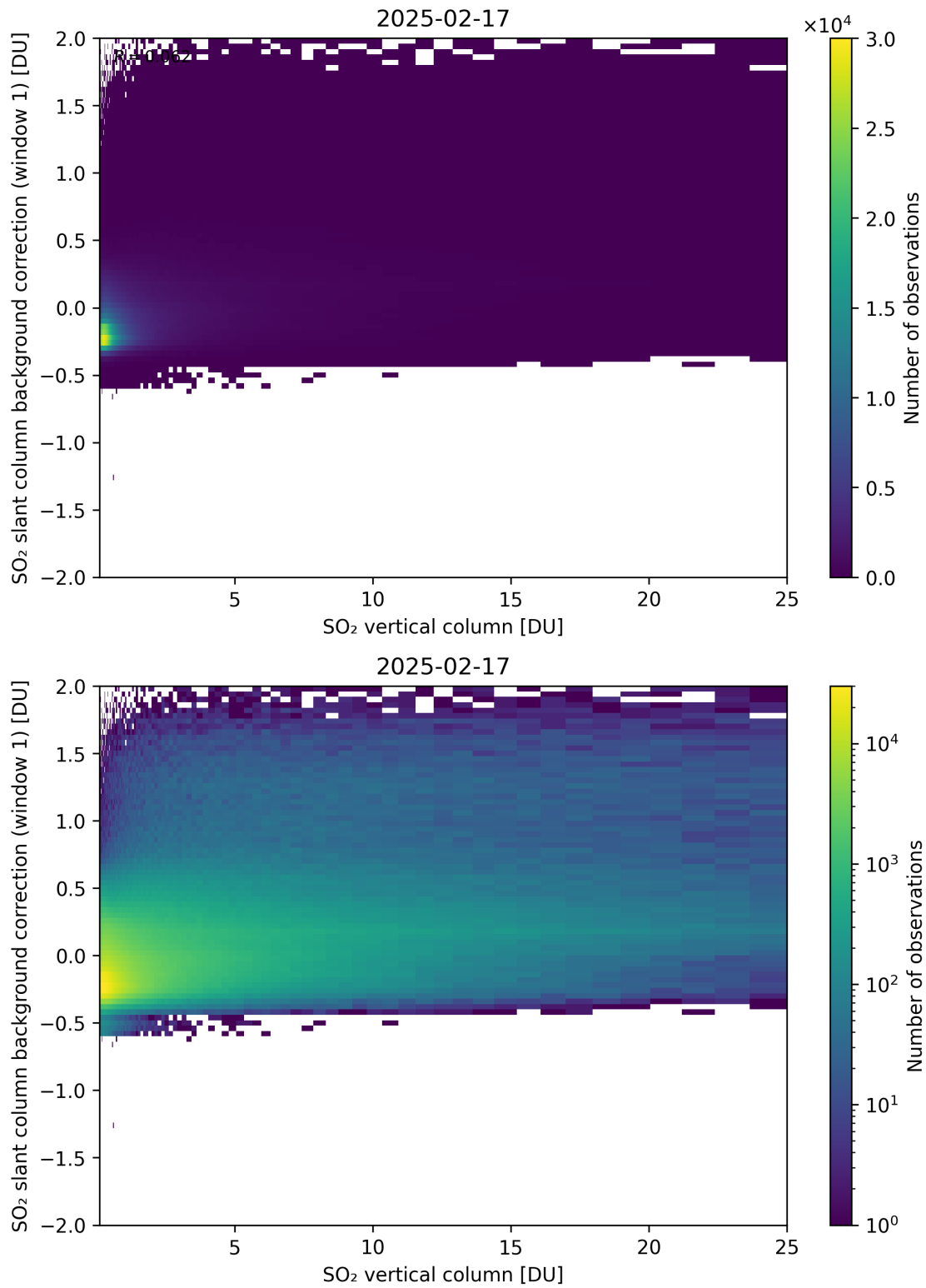
Figure 323: Scatter density plot of “SO 2 vertical column” against “SO 2 slant column background correction (window 1)” for 2025-02-16 to 2025-02-18.
