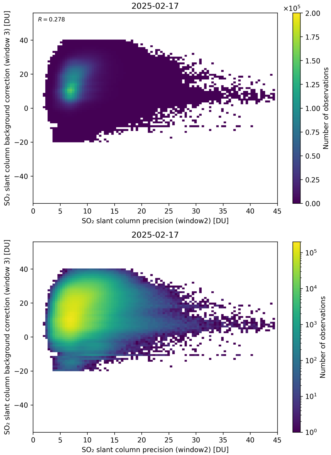
Figure 292: Scatter density plot of “SO 2 slant column precision (window2)” against “SO 2 slant column background correction (window 3)” for 2025-02-16 to 2025-02-18.
