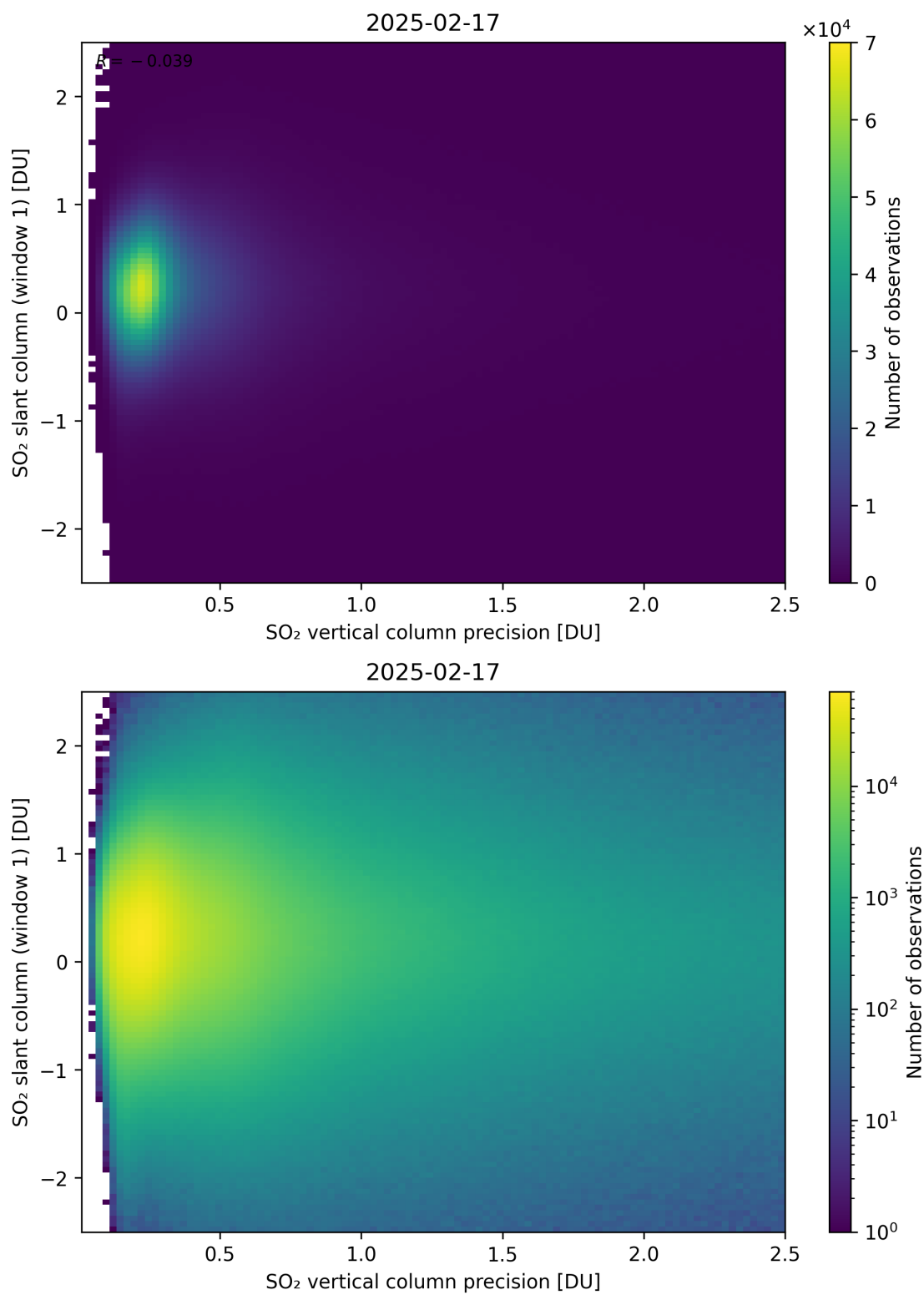
Figure 341: Scatter density plot of “SO 2 vertical column precision” against “SO 2 slant column (window 1)” for 2025-02-16 to 2025-02-18.
