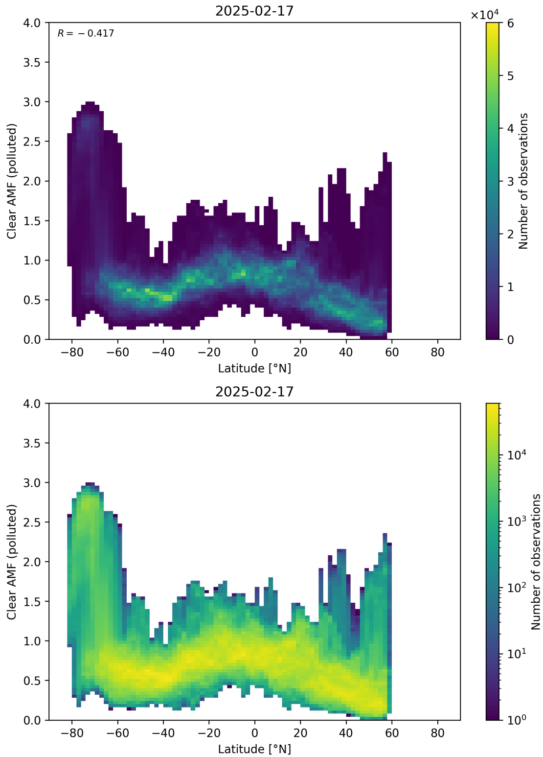
Figure 156: Scatter density plot of “Latitude” against “Clear AMF (polluted)” for 2025-02-16 to 2025-02-18.
