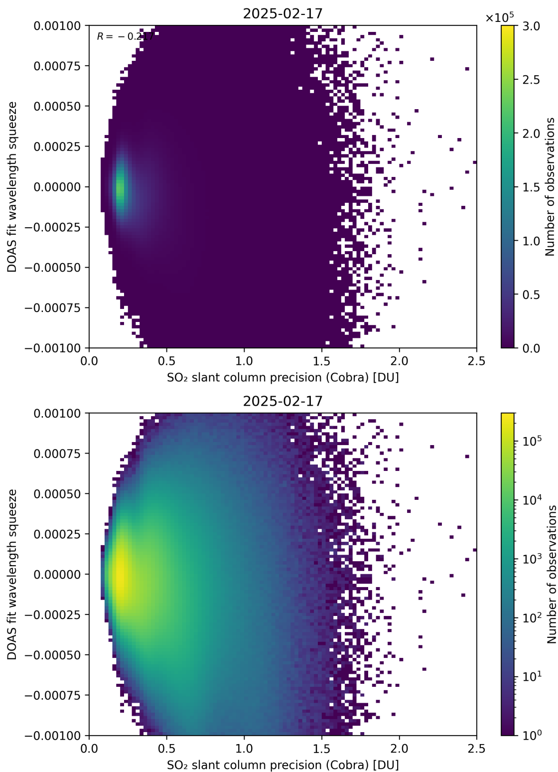
Figure 203: Scatter density plot of “SO 2 slant column precision (Cobra)” against “DOAS fit wavelength squeeze” for 2025-02-16 to 2025-02-18.
