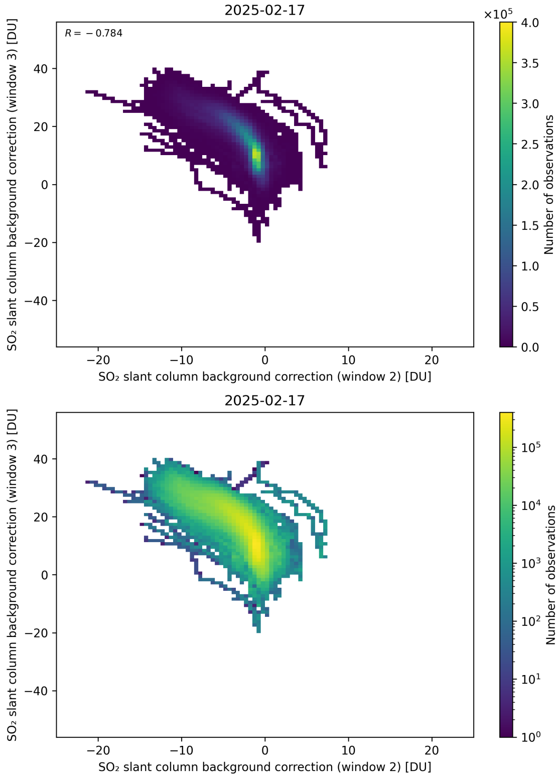
Figure 122: Scatter density plot of “SO 2 slant column background correction (window 2)” against “SO 2 slant column background correction (window 3)” for 2025-02-16 to 2025-02-18.
