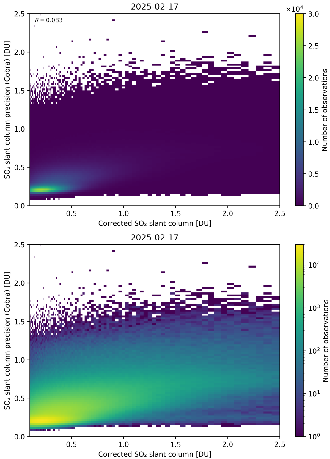
Figure 234: Scatter density plot of “Corrected SO 2 slant column” against “SO 2 slant column precision (Cobra)” for 2025-02-16 to 2025-02-18.
