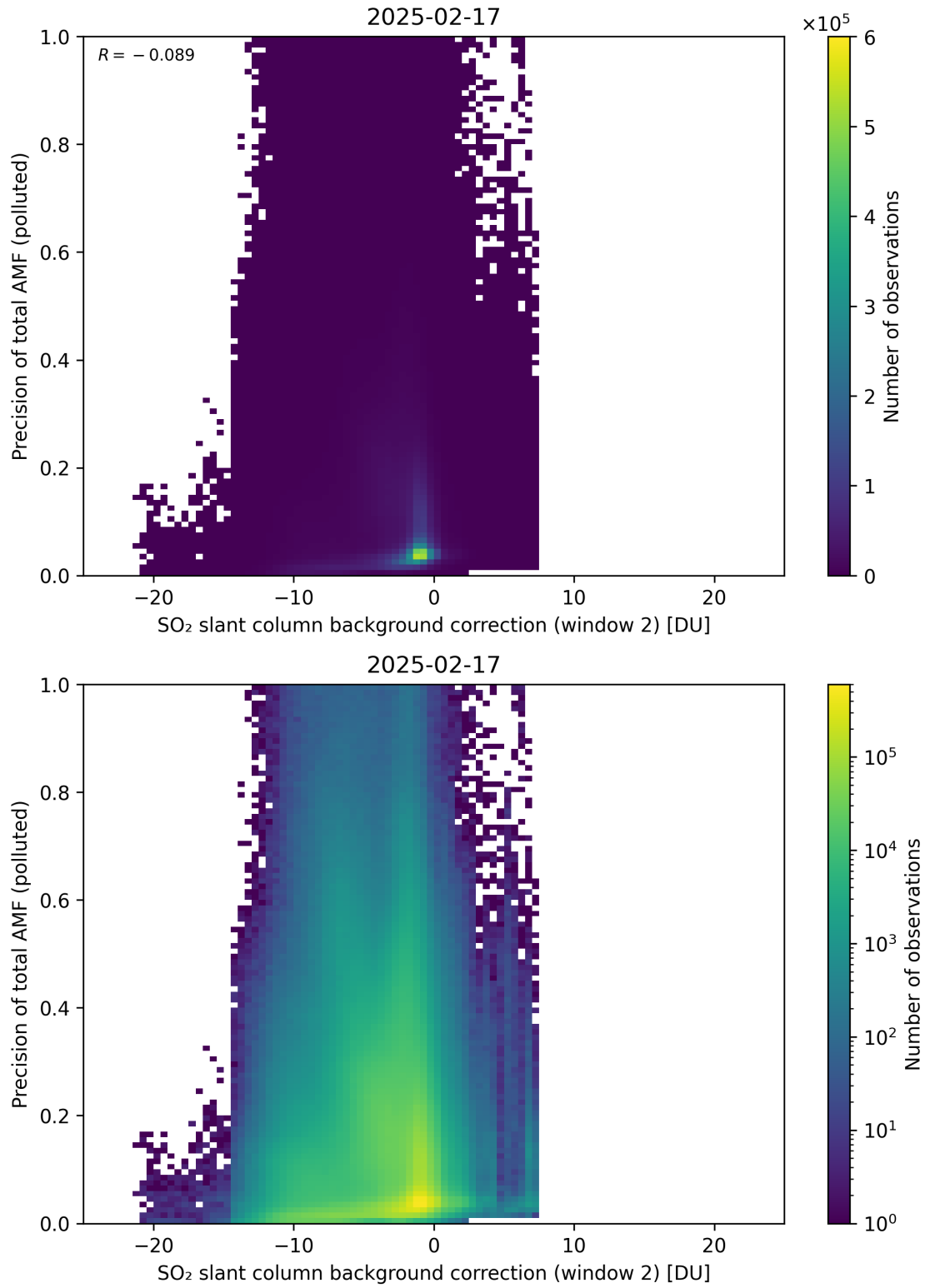
Figure 131: Scatter density plot of “SO 2 slant column background correction (window 2)” against “Precision of total AMF (polluted)” for 2025-02-16 to 2025-02-18.
