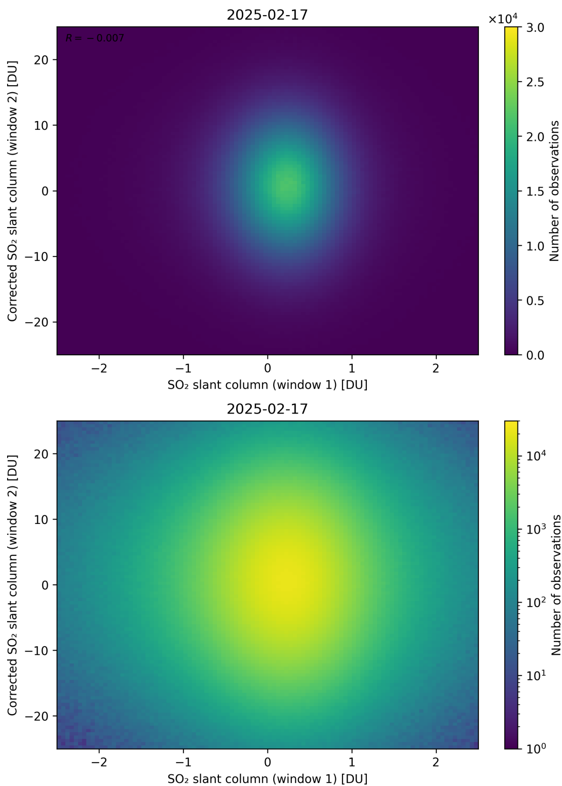
Figure 283: Scatter density plot of “SO 2 slant column (window 1)” against “Corrected SO 2 slant column (window 2)” for 2025-02-16 to 2025-02-18.
