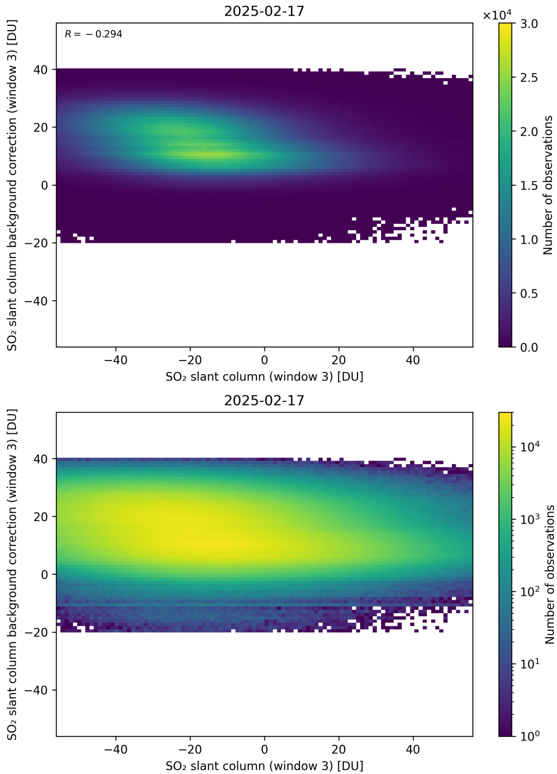
Figure 303: Scatter density plot of “SO 2 slant column (window 3)” against “SO 2 slant column background correction (window 3)” for 2025-02-16 to 2025-02-18.
