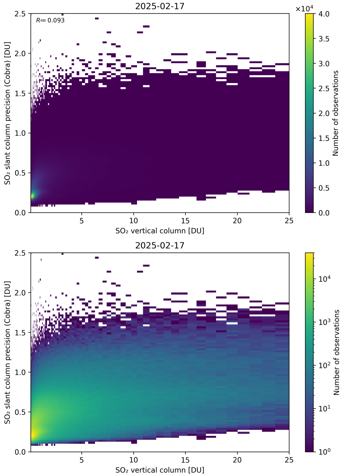
Figure 350: Scatter density plot of “SO 2 vertical column” against “SO 2 slant column precision (Cobra)” for 2025-02-16 to 2025-02-18.
