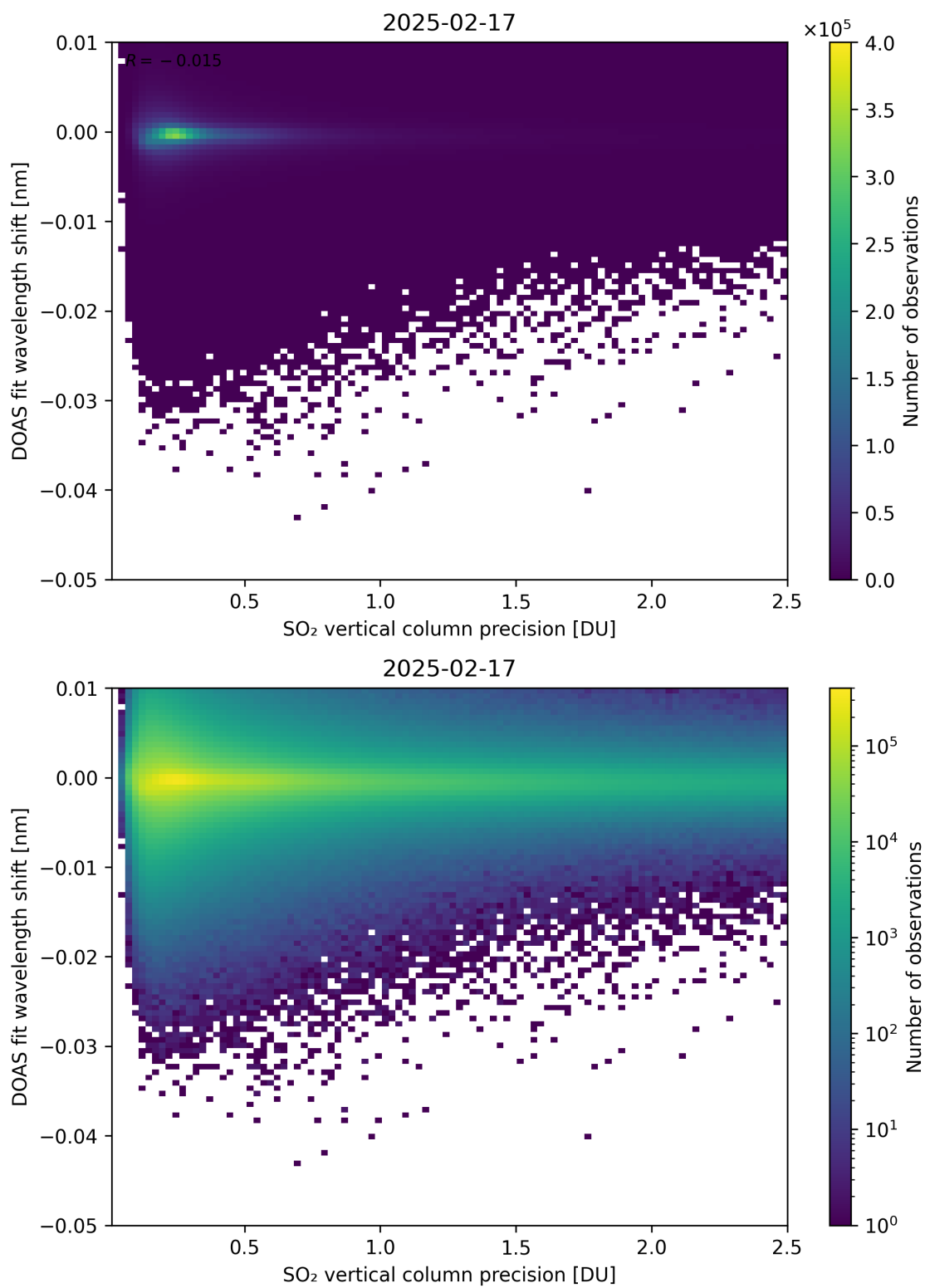
Figure 332: Scatter density plot of “SO 2 vertical column precision” against “DOAS fit wavelength shift” for 2025-02-16 to 2025-02-18.
