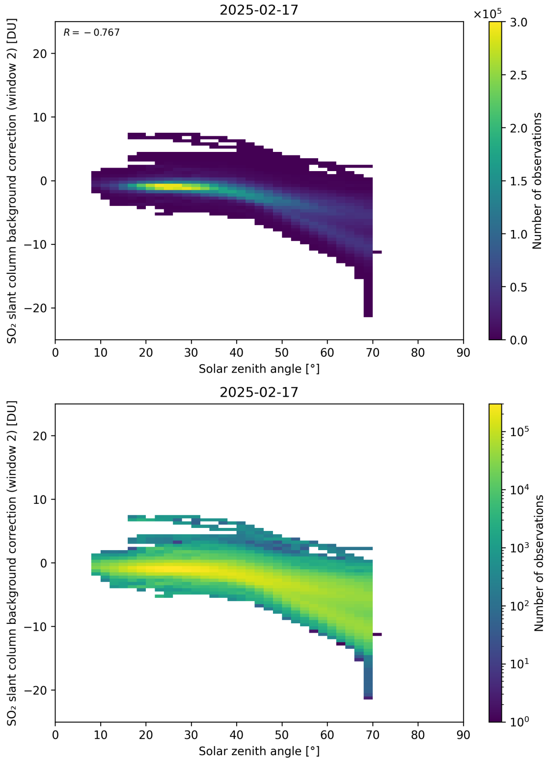
Figure 172: Scatter density plot of “Solar zenith angle” against “SO 2 slant column background correction (window 2)” for 2025-02-16 to 2025-02-18.
