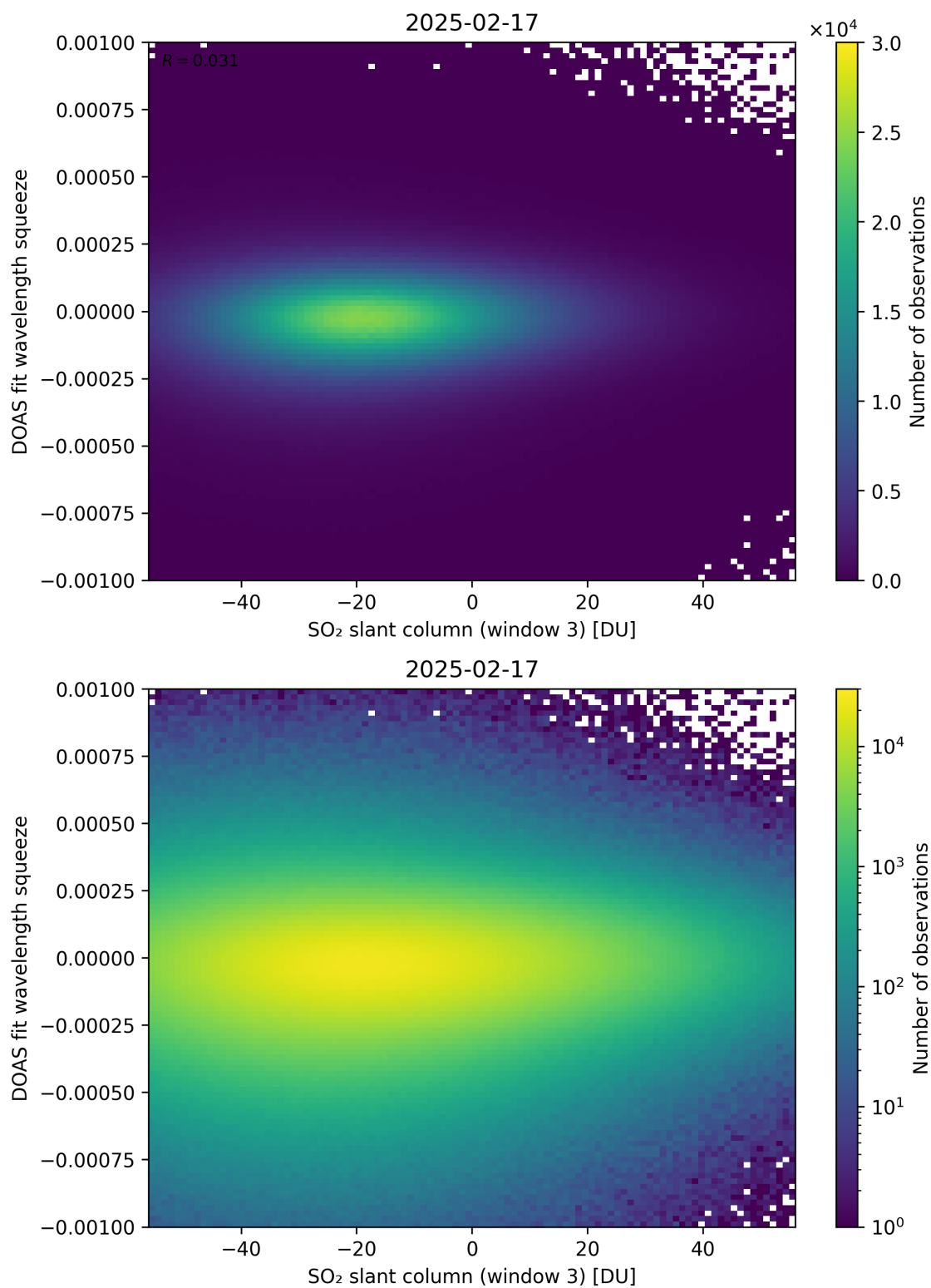
Figure 305: Scatter density plot of “SO 2 slant column (window 3)” against “DOAS fit wavelength squeeze” for 2025-02-16 to 2025-02-18.
