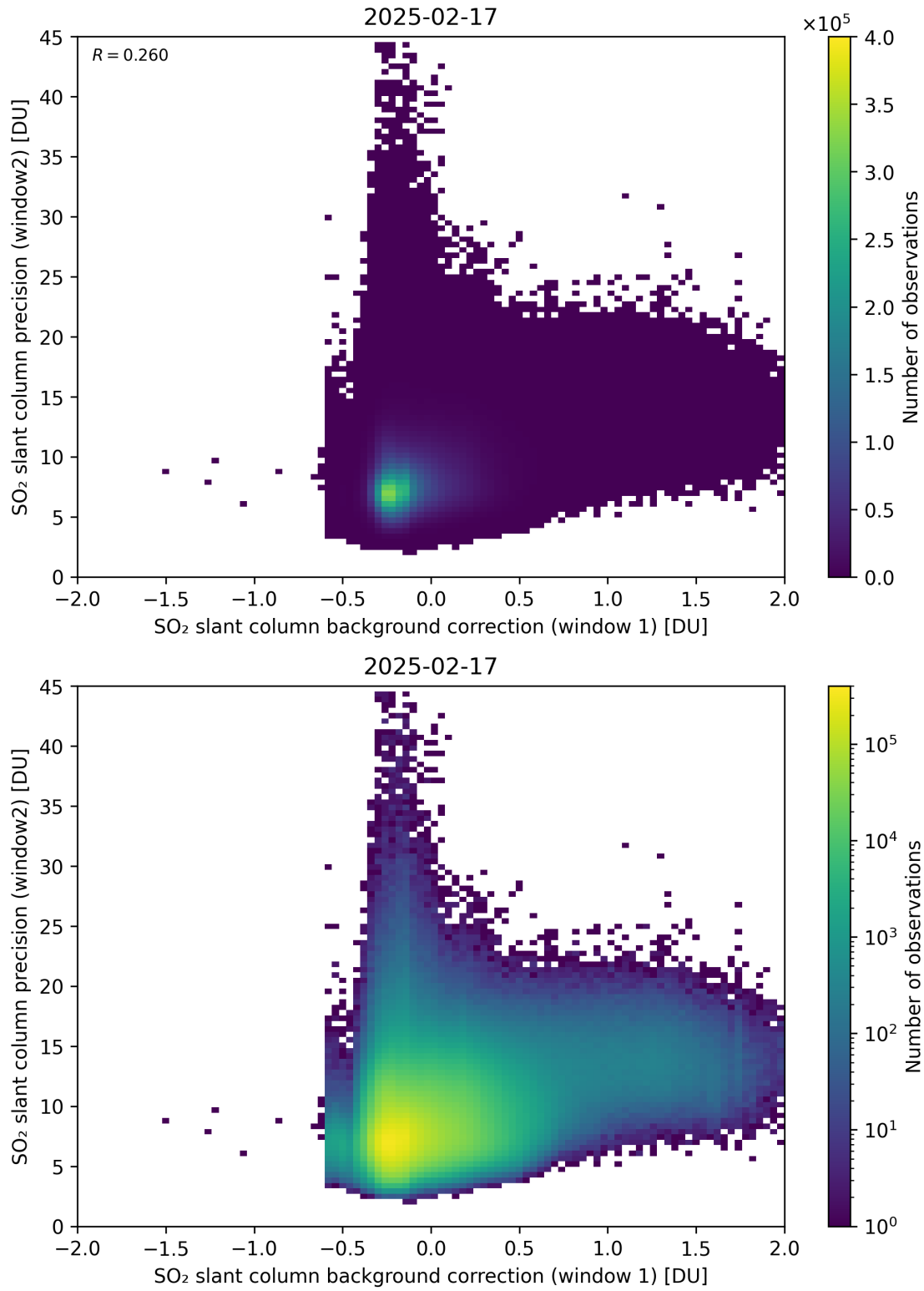
Figure 117: Scatter density plot of “SO 2 slant column background correction (window 1)” against “SO 2 slant column precision (window2)” for 2025-02-16 to 2025-02-18.
