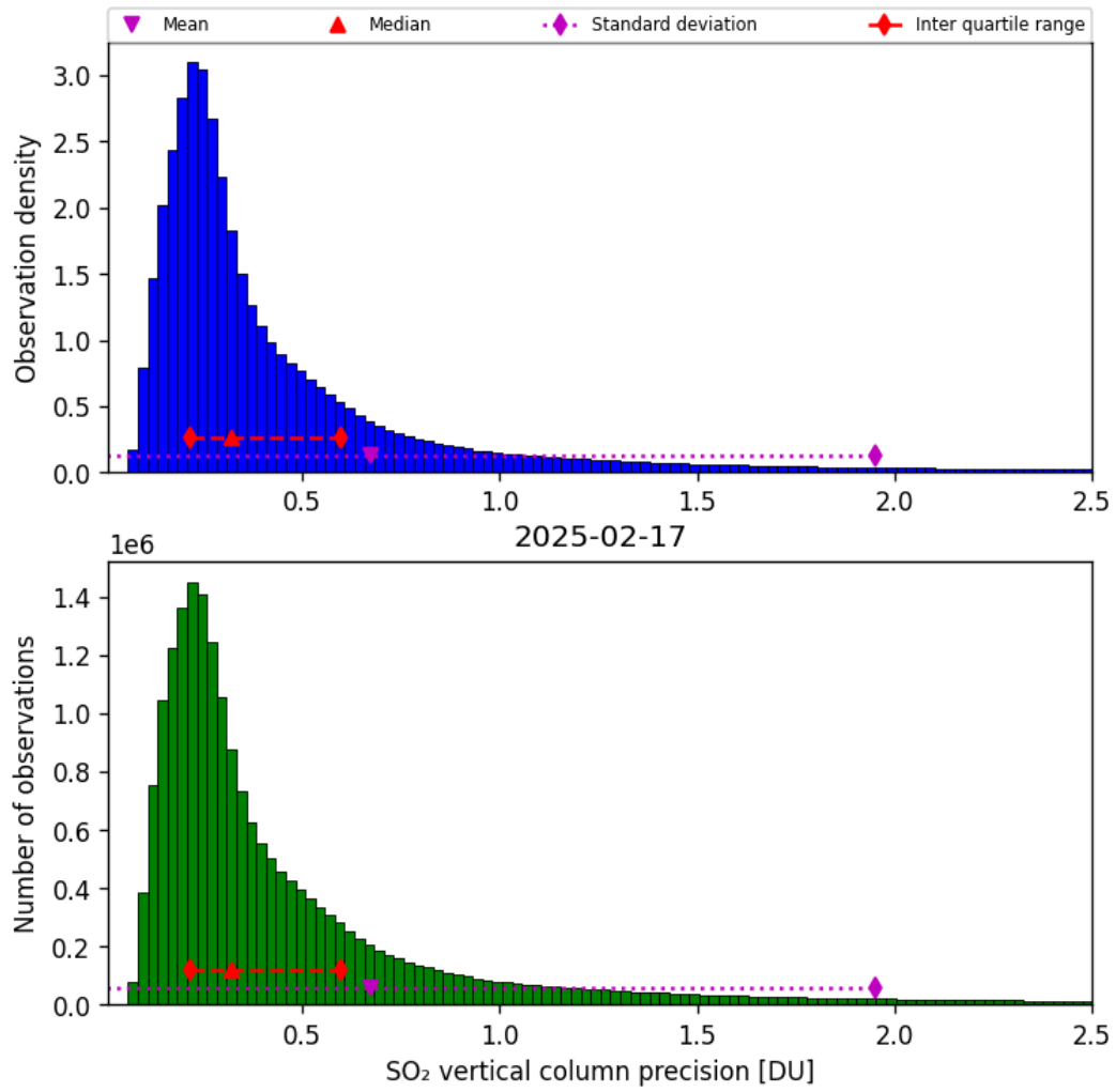
Figure 59: Histogram of “SO 2 vertical column precision” for 2025-02-16 to 2025-02-18
