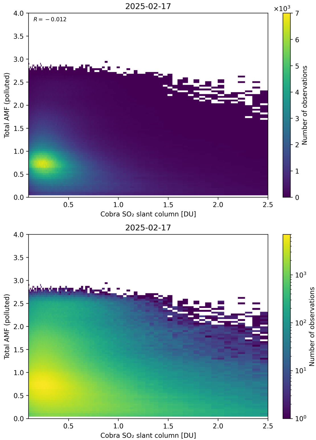
Figure 224: Scatter density plot of “Cobra SO 2 slant column” against “Total AMF (polluted)” for 2025-02-16 to 2025-02-18.
