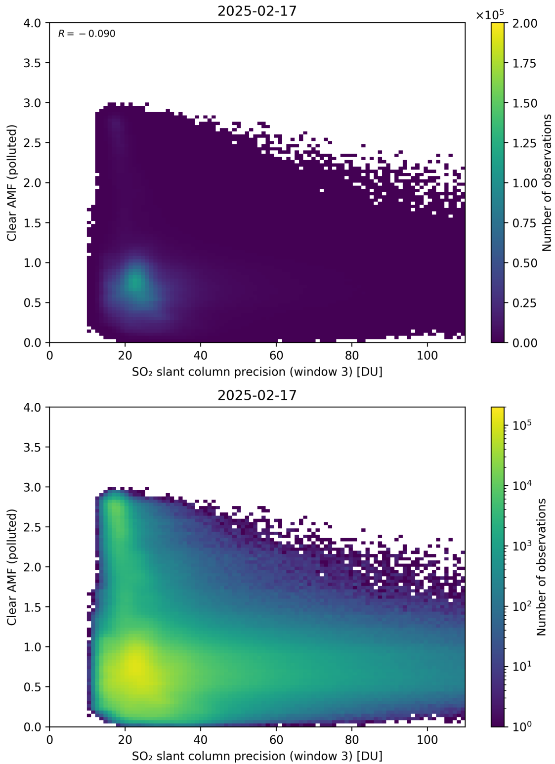
Figure 311: Scatter density plot of “SO 2 slant column precision (window 3)” against “Clear AMF (polluted)” for 2025-02-16 to 2025-02-18.
