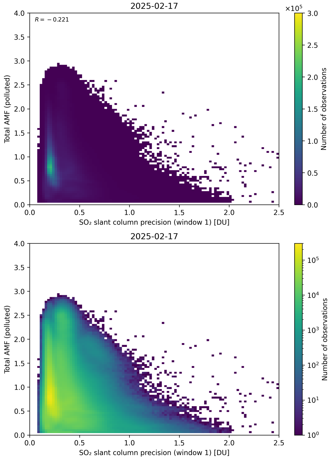
Figure 280: Scatter density plot of “SO 2 slant column precision (window 1)” against “Total AMF (polluted)” for 2025-02-16 to 2025-02-18.
