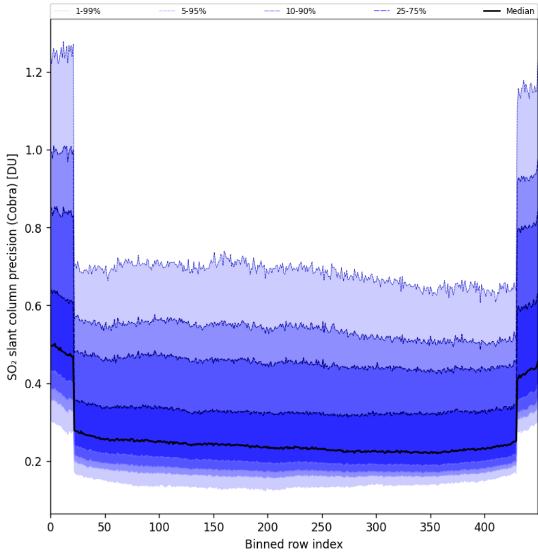
Figure 88: Along track statistics of “SO 2 slant column precision (Cobra)” for 2025-02-16 to 2025-02-18
