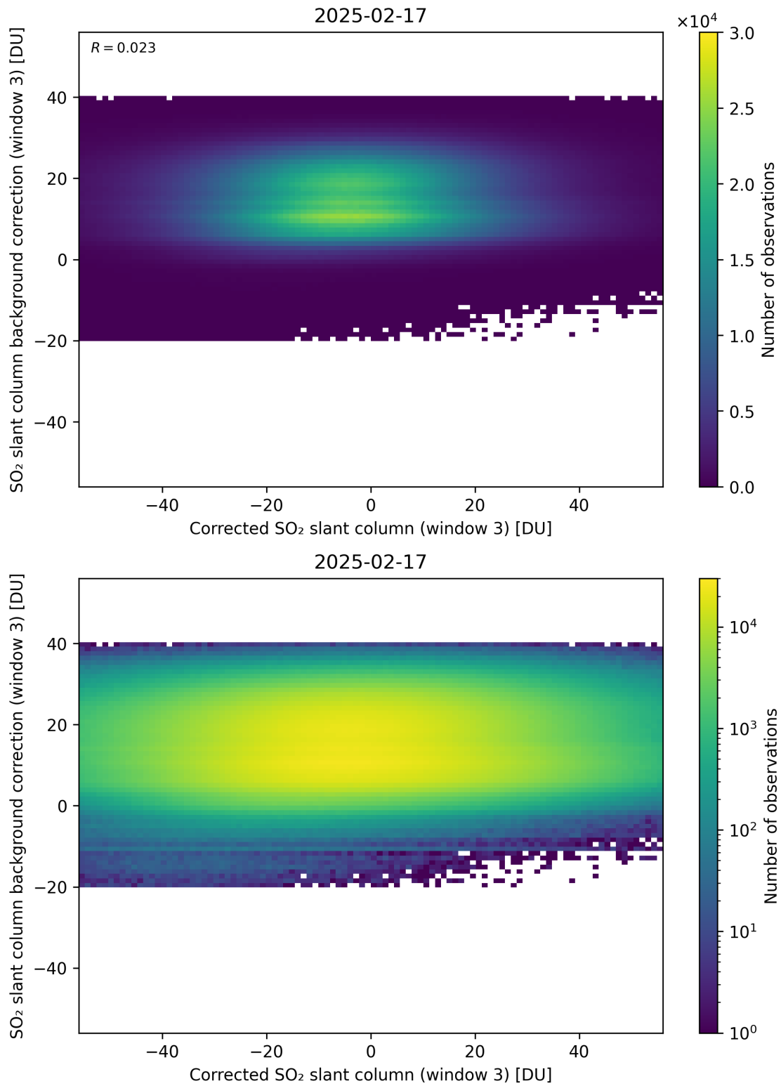
Figure 255: Scatter density plot of “Corrected SO 2 slant column (window 3)” against “SO 2 slant column background correction (window 3)” for 2025-02-16 to 2025-02-18.
