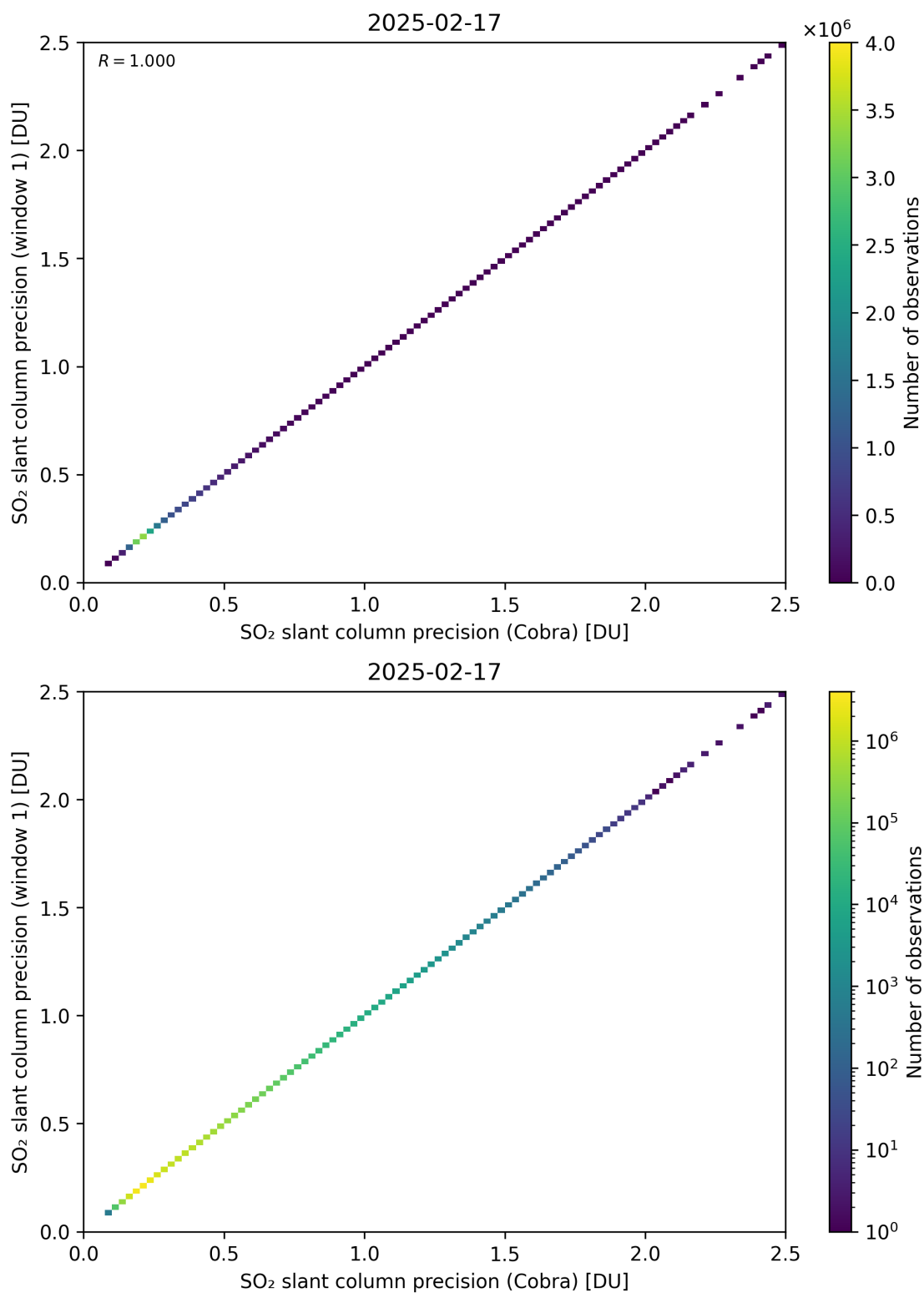
Figure 209: Scatter density plot of “SO 2 slant column precision (Cobra)” against “SO 2 slant column precision (window 1)” for 2025-02-16 to 2025-02-18.
