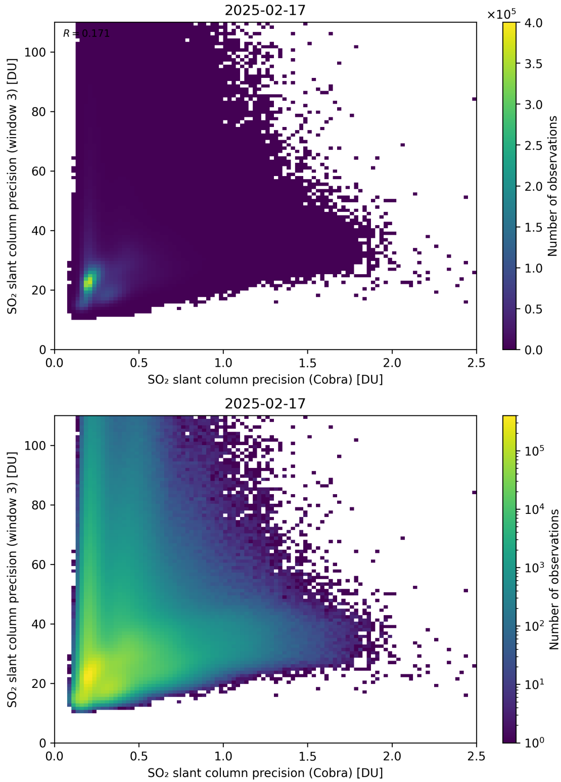
Figure 212: Scatter density plot of “SO 2 slant column precision (Cobra)” against “SO 2 slant column precision (window 3)” for 2025-02-16 to 2025-02-18.
