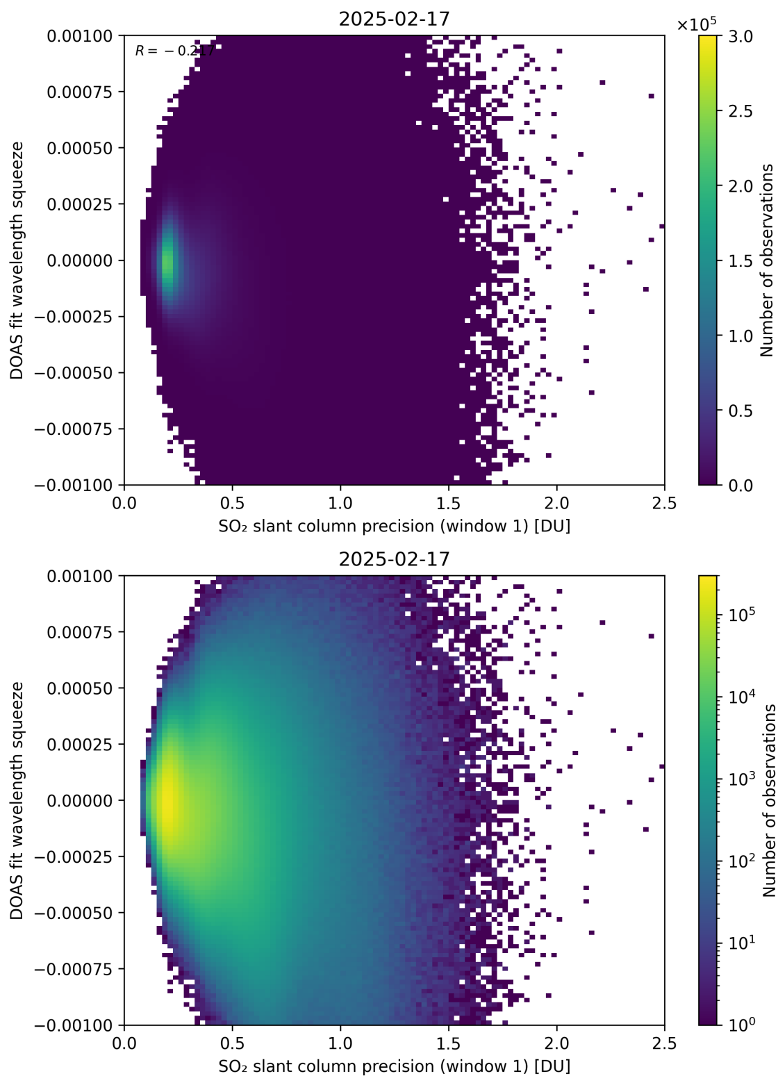
Figure 272: Scatter density plot of “SO 2 slant column precision (window 1)” against “DOAS fit wavelength squeeze” for 2025-02-16 to 2025-02-18.
