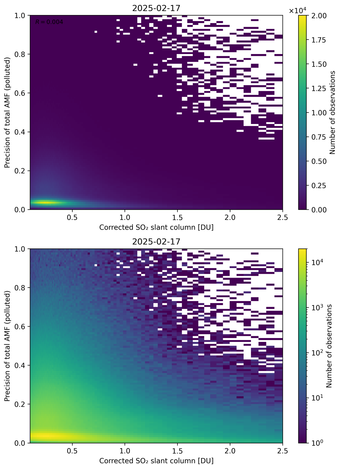
Figure 243: Scatter density plot of “Corrected SO 2 slant column” against “Precision of total AMF (polluted)” for 2025-02-16 to 2025-02-18.
