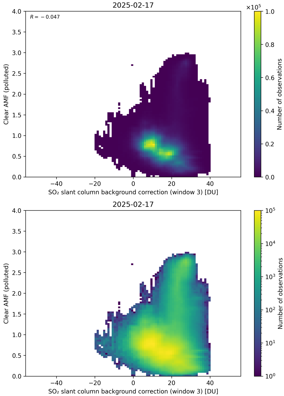
Figure 135: Scatter density plot of “SO 2 slant column background correction (window 3)” against “Clear AMF (polluted)” for 2025-02-16 to 2025-02-18.
