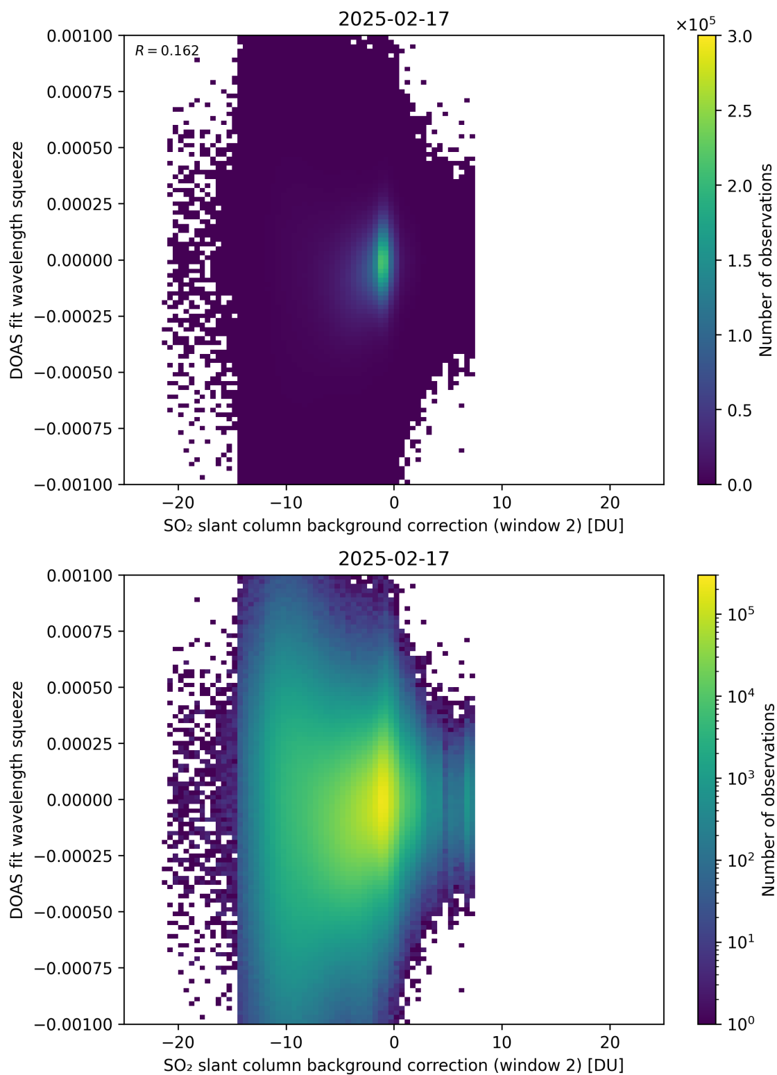
Figure 124: Scatter density plot of “SO 2 slant column background correction (window 2)” against “DOAS fit wavelength squeeze” for 2025-02-16 to 2025-02-18.
