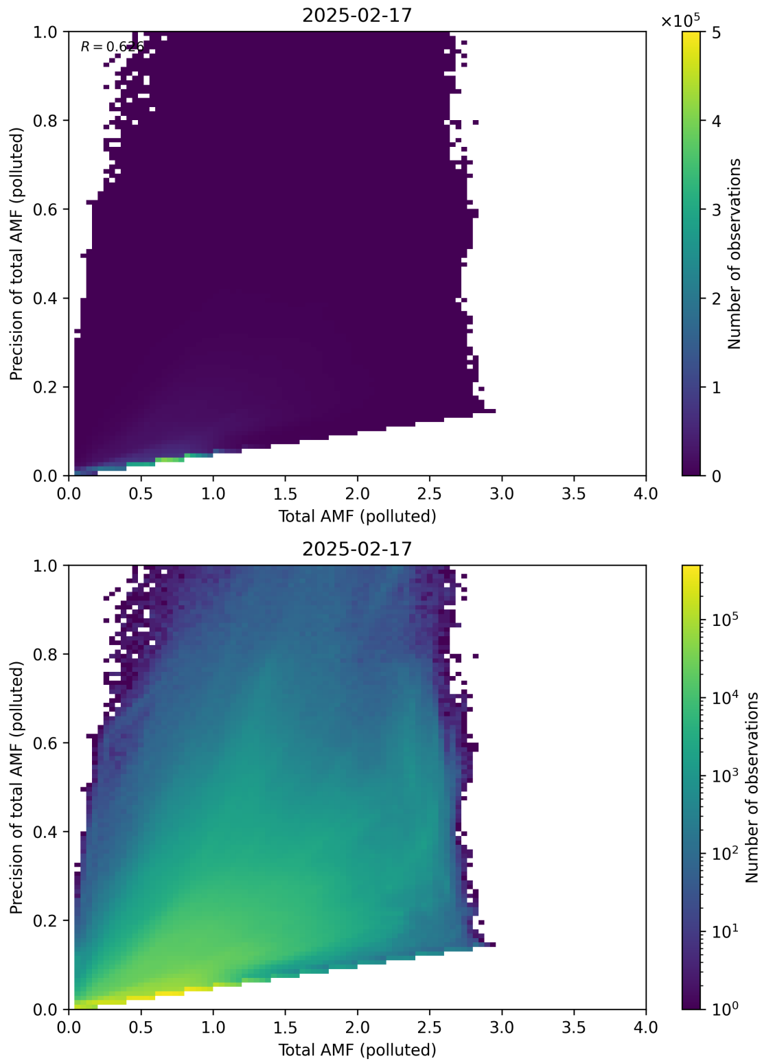
Figure 322: Scatter density plot of “Total AMF (polluted)” against “Precision of total AMF (polluted)” for 2025-02-16 to 2025-02-18.
