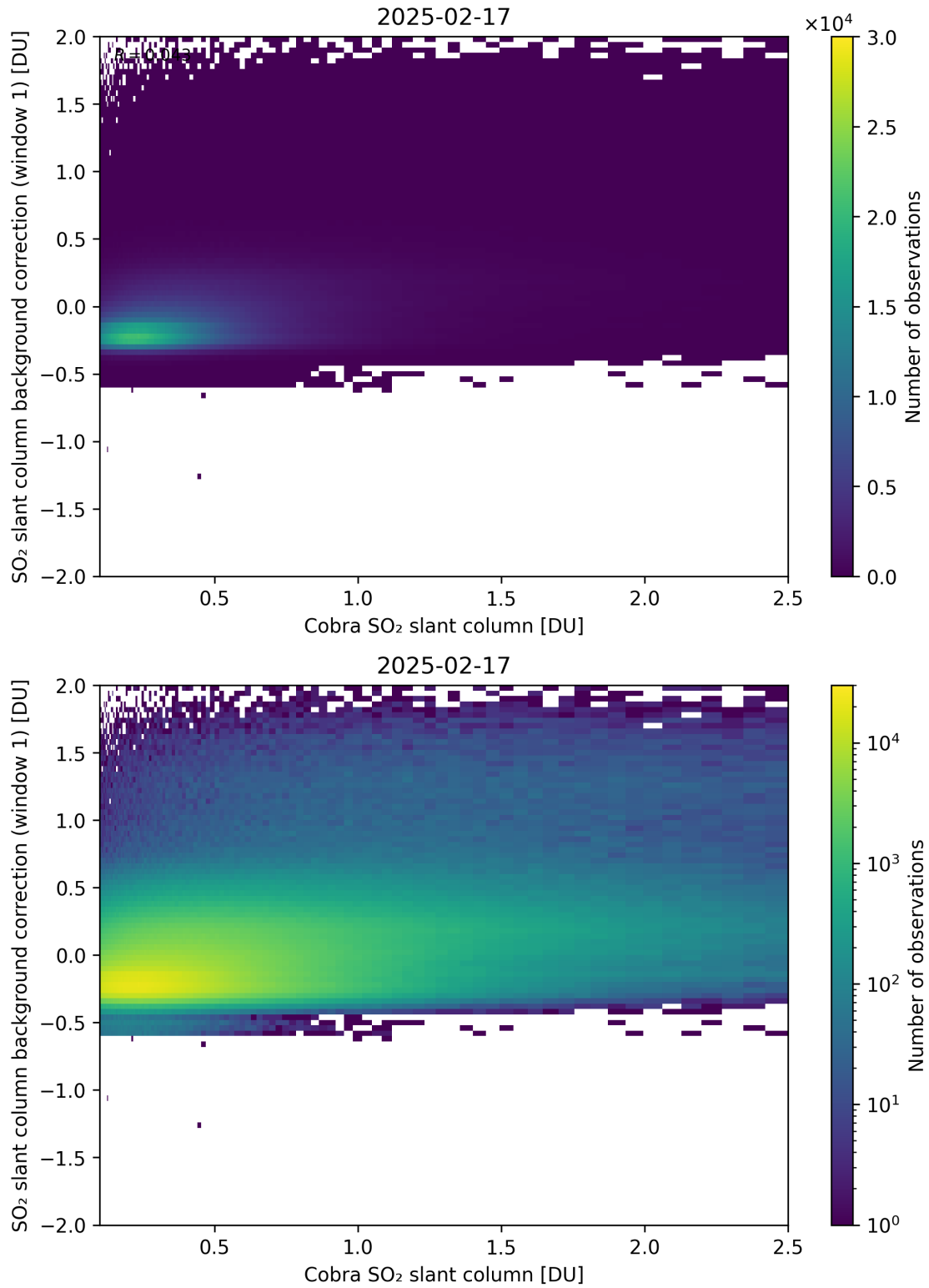
Figure 193: Scatter density plot of “Cobra SO 2 slant column” against “SO 2 slant column background correction (window 1)” for 2025-02-16 to 2025-02-18.
