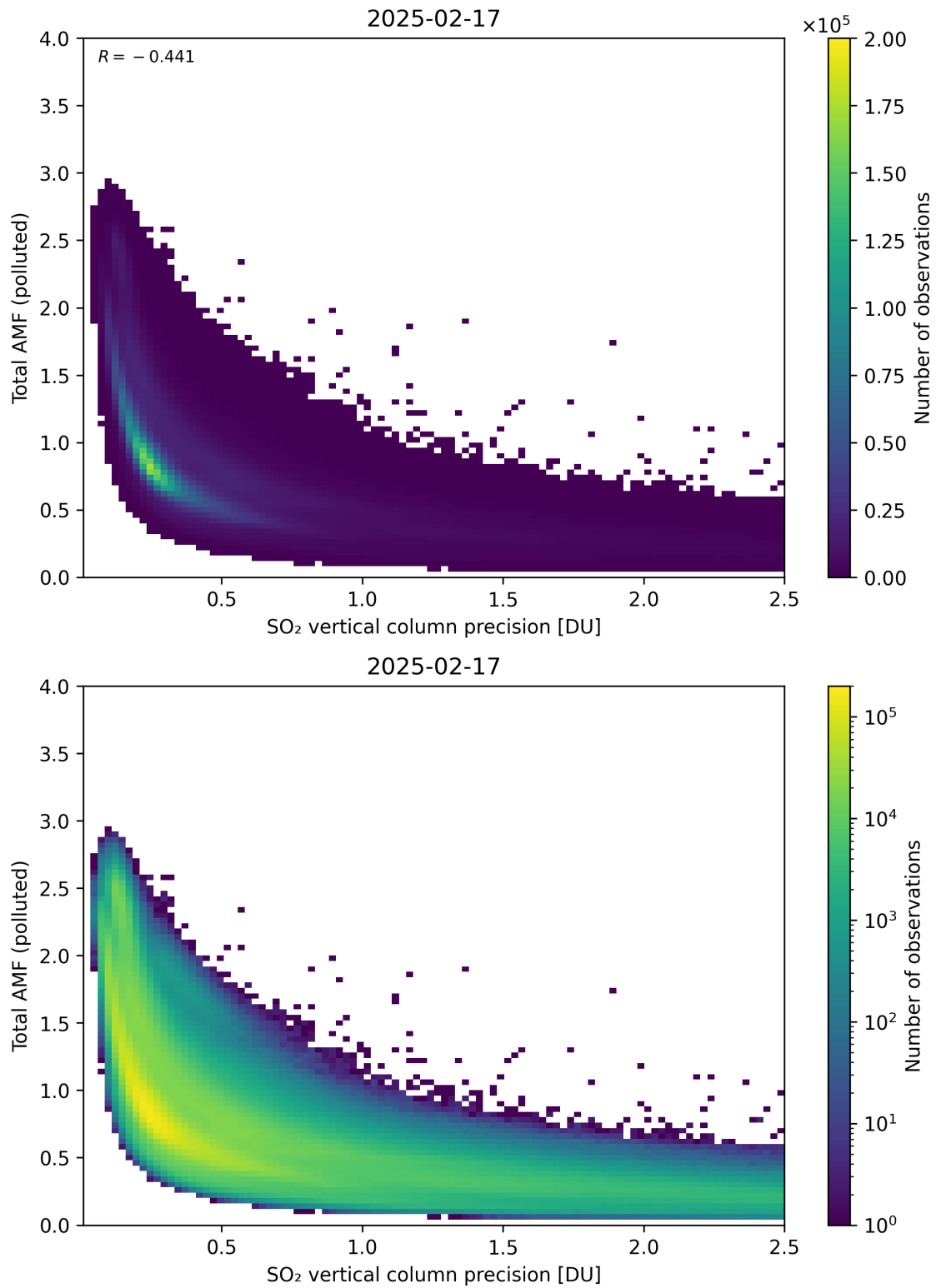
Figure 346: Scatter density plot of “SO 2 vertical column precision” against “Total AMF (polluted)” for 2025-02-16 to 2025-02-18.
