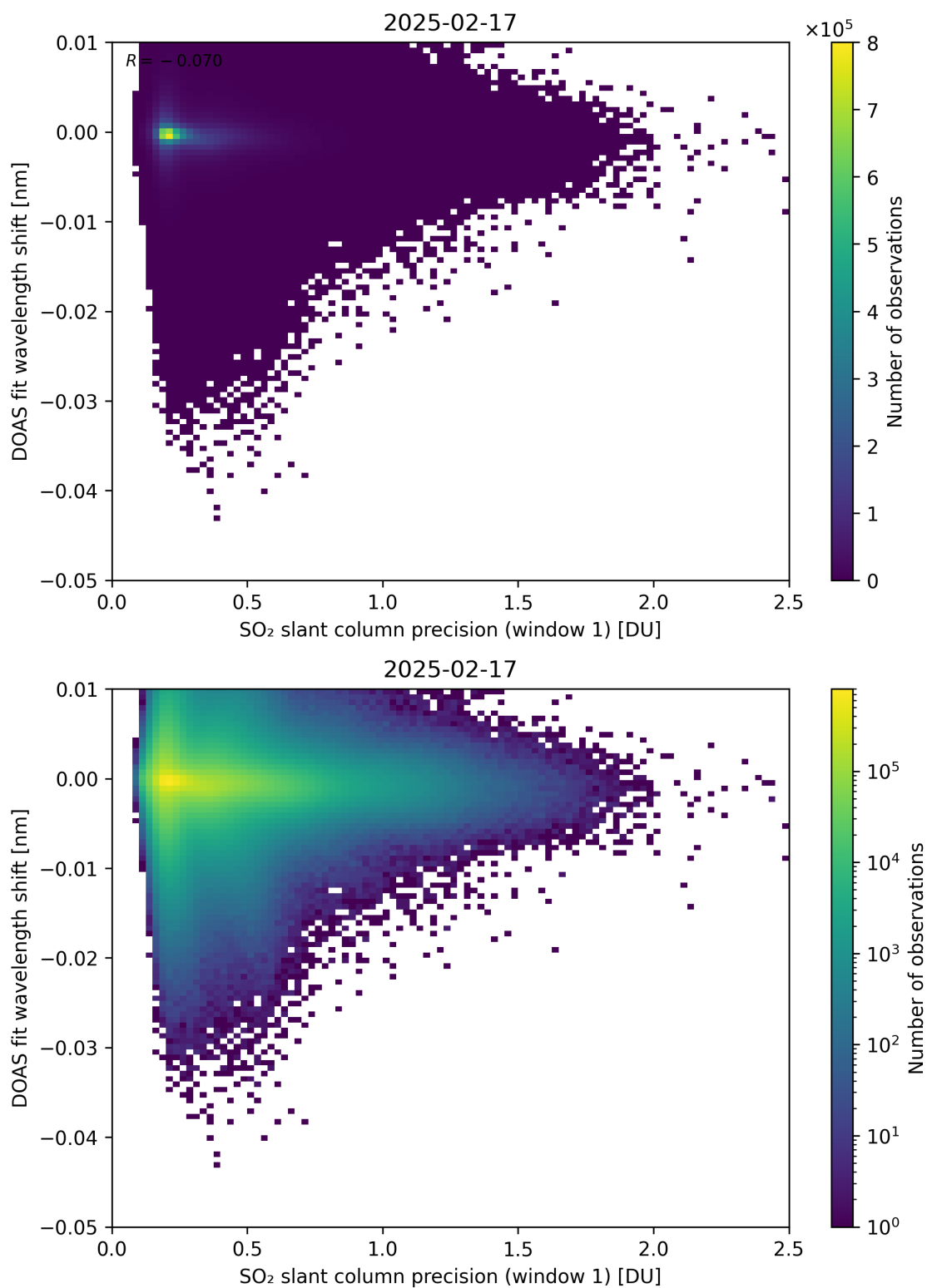
Figure 271: Scatter density plot of “SO 2 slant column precision (window 1)” against “DOAS fit wavelength shift” for 2025-02-16 to 2025-02-18.
