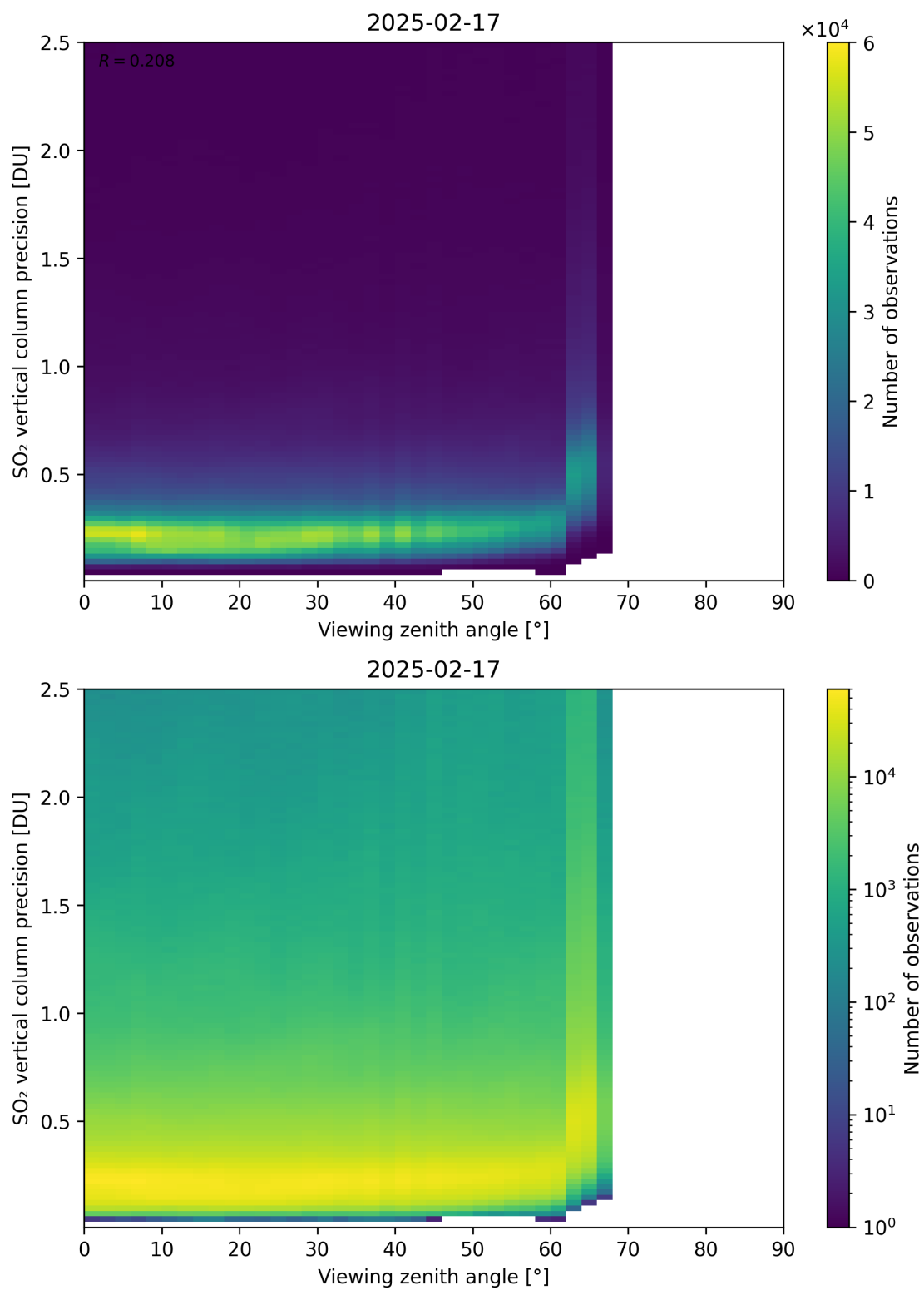
Figure 384: Scatter density plot of “Viewing zenith angle” against “SO 2 vertical column precision” for 2025-02-16 to 2025-02-18.
