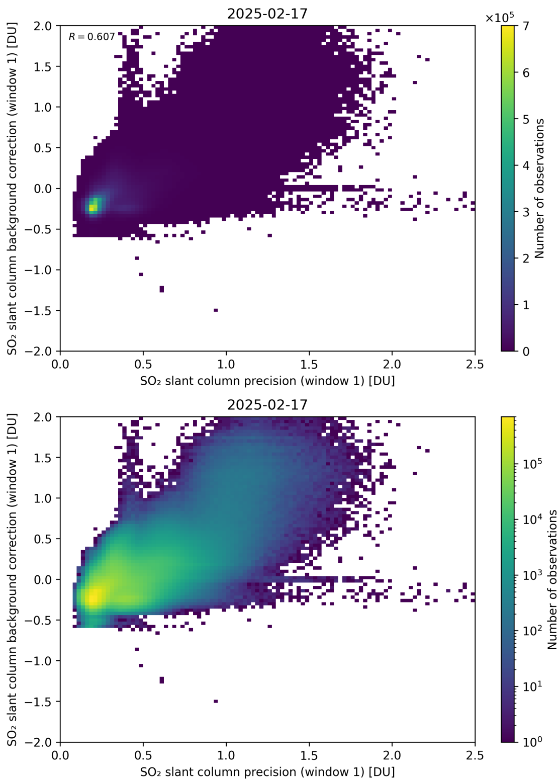
Figure 268: Scatter density plot of “SO 2 slant column precision (window 1)” against “SO 2 slant column background correction (window 1)” for 2025-02-16 to 2025-02-18.
