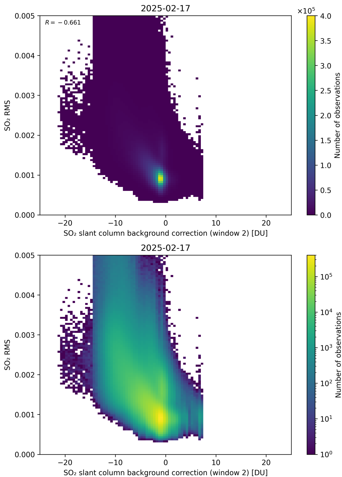
Figure 125: Scatter density plot of “SO 2 slant column background correction (window 2)” against “SO 2 RMS” for 2025-02-16 to 2025-02-18.
