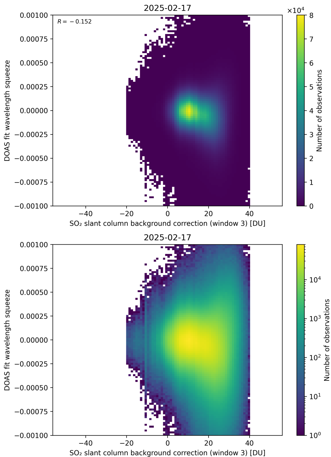
Figure 133: Scatter density plot of “SO 2 slant column background correction (window 3)” against “DOAS fit wavelength squeeze” for 2025-02-16 to 2025-02-18.
