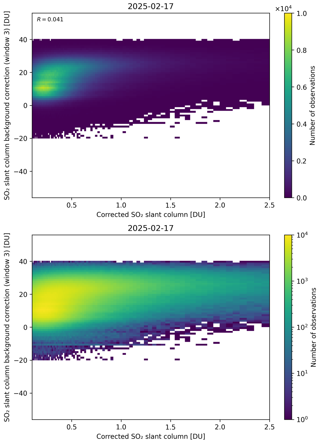
Figure 228: Scatter density plot of “Corrected SO 2 slant column” against “SO 2 slant column background correction (window 3)” for 2025-02-16 to 2025-02-18.
