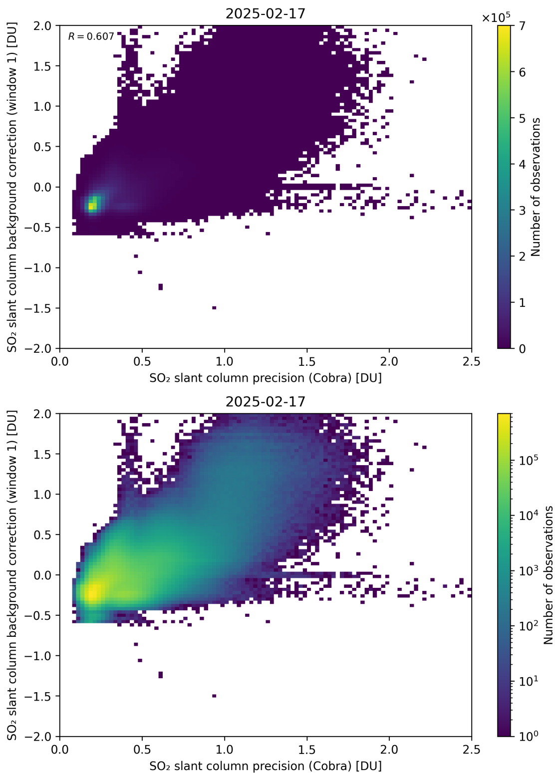
Figure 199: Scatter density plot of “SO 2 slant column precision (Cobra)” against “SO 2 slant column background correction (window 1)” for 2025-02-16 to 2025-02-18.
