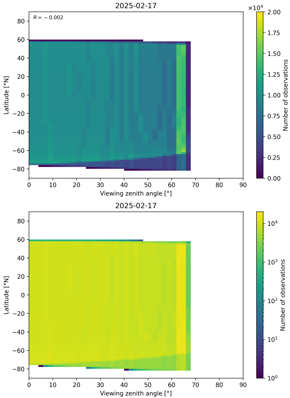
Figure 368: Scatter density plot of “Viewing zenith angle” against “Latitude” for 2025-02-16 to 2025-02-18.
