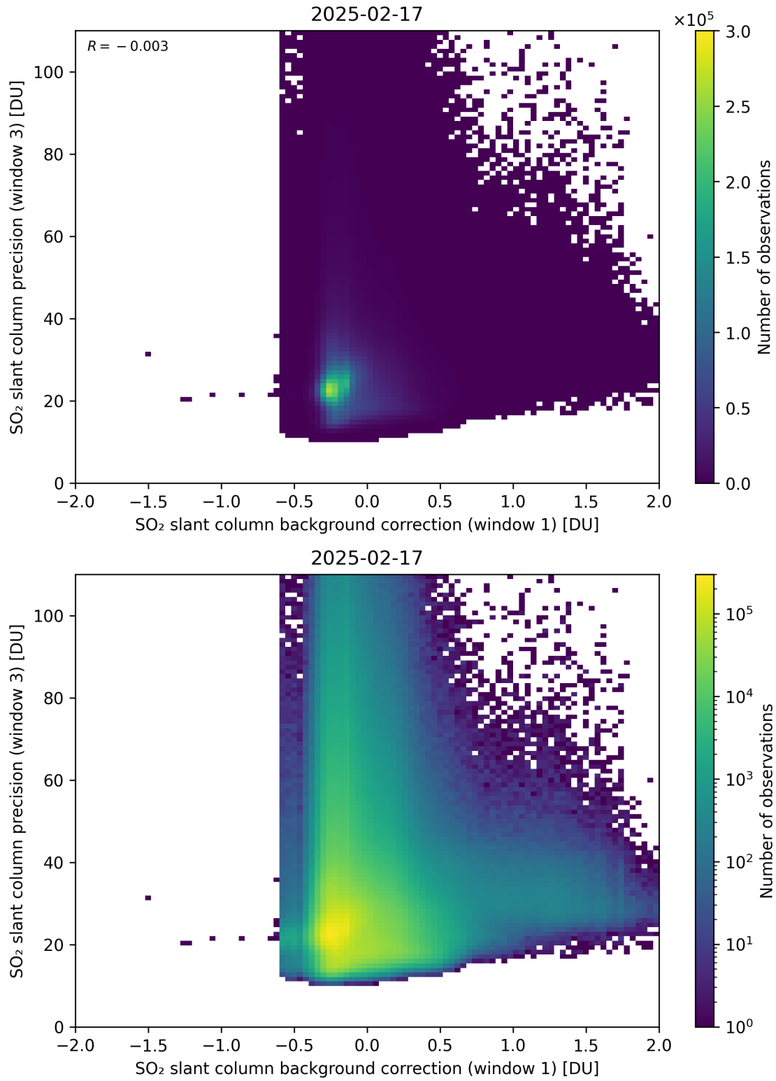
Figure 119: Scatter density plot of “SO 2 slant column background correction (window 1)” against “SO 2 slant column precision (window 3)” for 2025-02-16 to 2025-02-18.
