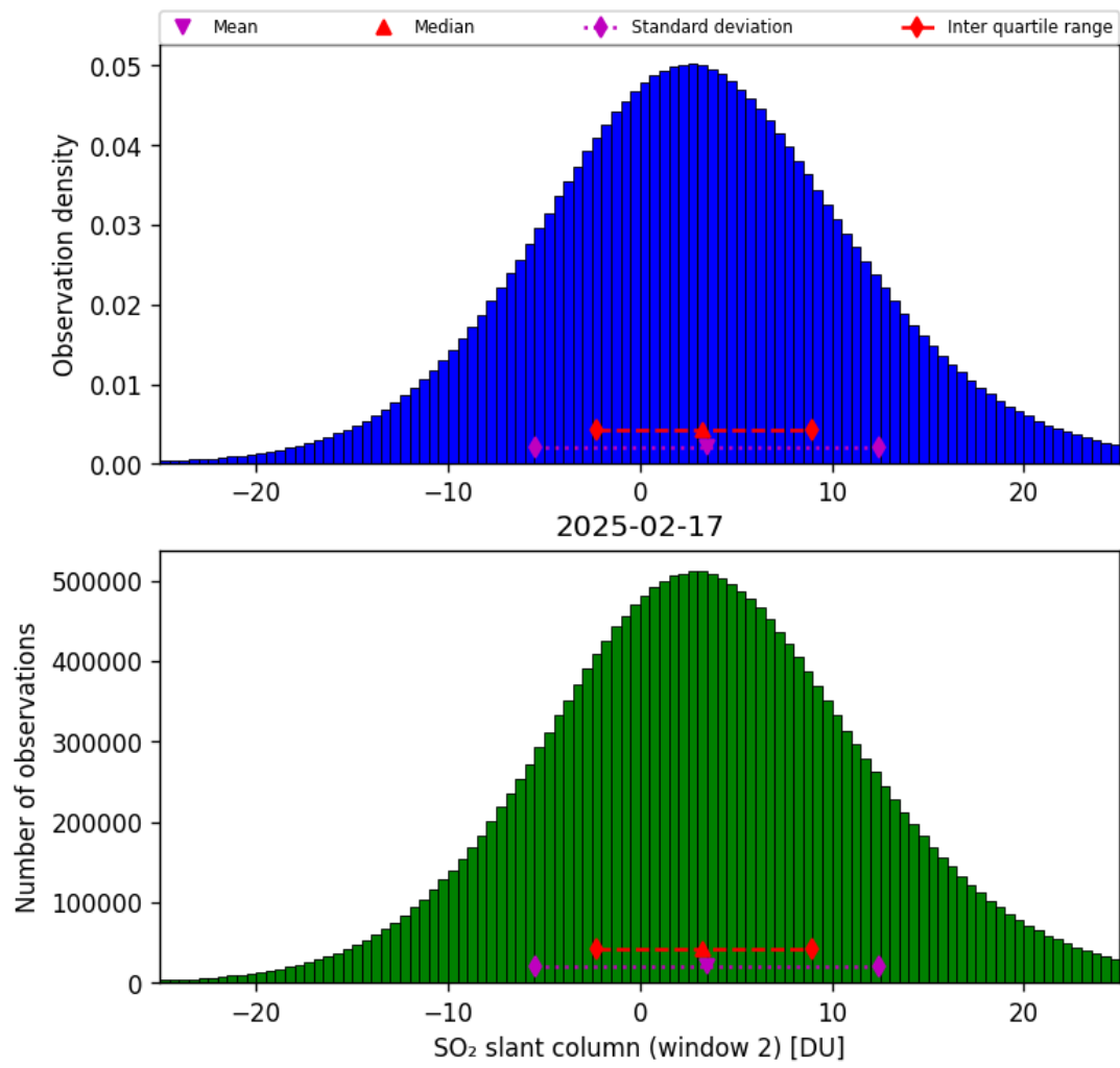
Figure 67: Histogram of “SO 2 slant column (window 2)” for 2025-02-16 to 2025-02-18
