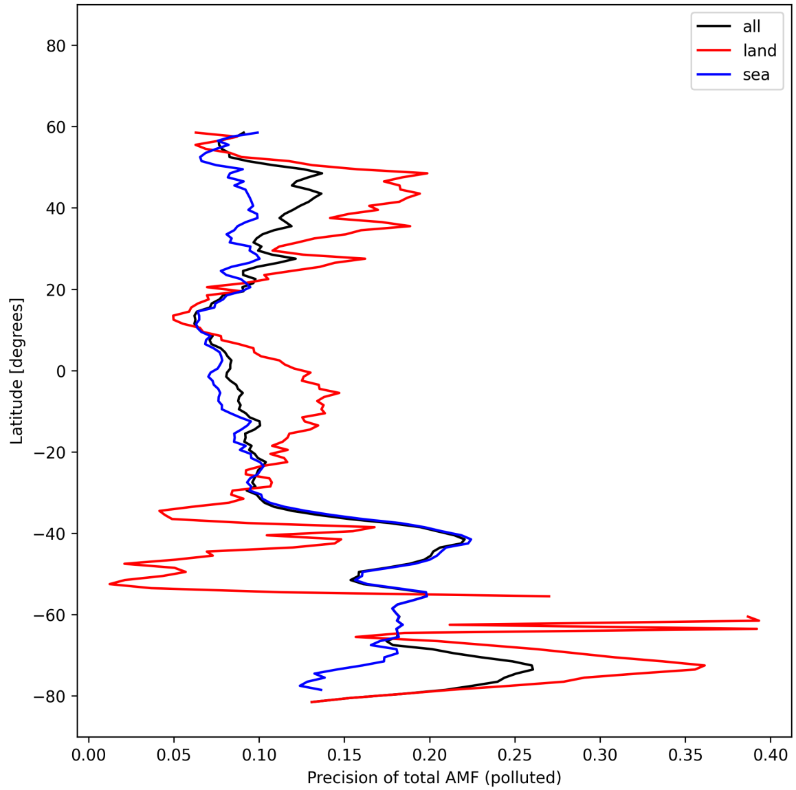
Figure 54: Zonal average of “Precision of total AMF (polluted)” for 2025-02-16 to 2025-02-18.
