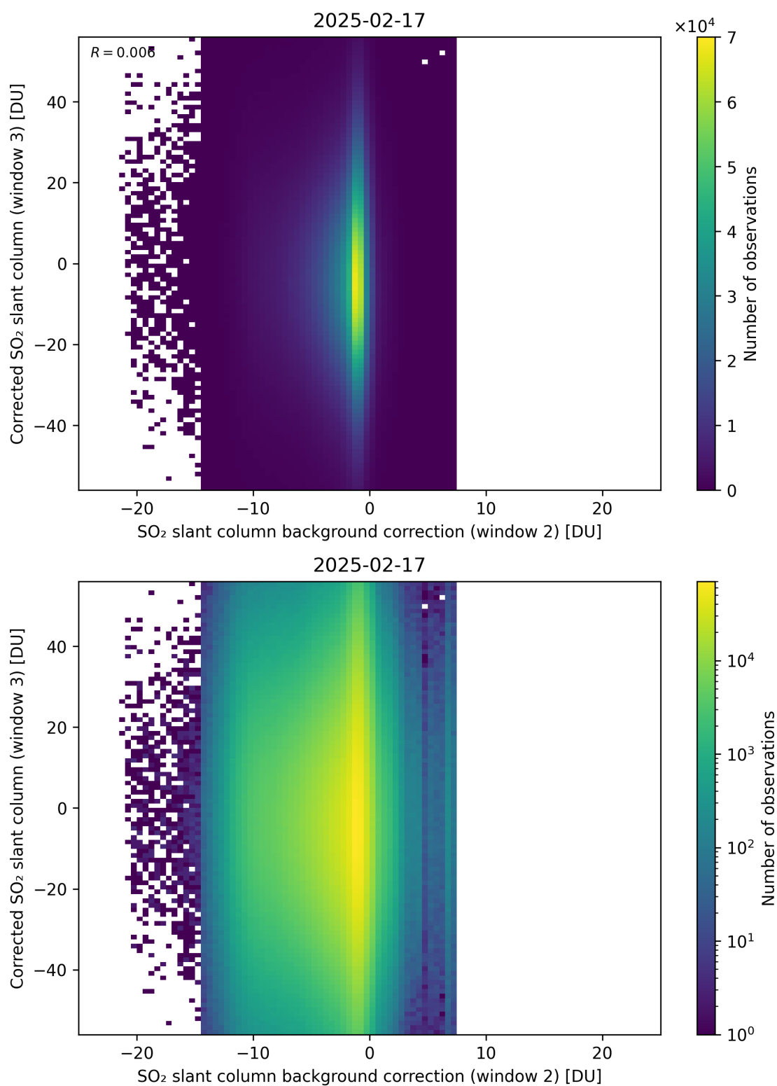
Figure 127: Scatter density plot of “SO 2 slant column background correction (window 2)” against “Corrected SO 2 slant column (window 3)” for 2025-02-16 to 2025-02-18.
