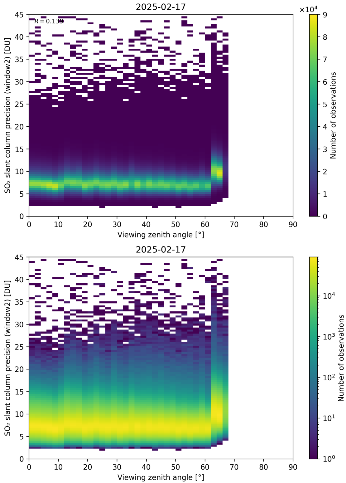
Figure 378: Scatter density plot of “Viewing zenith angle” against “SO 2 slant column precision (window2)” for 2025-02-16 to 2025-02-18.
