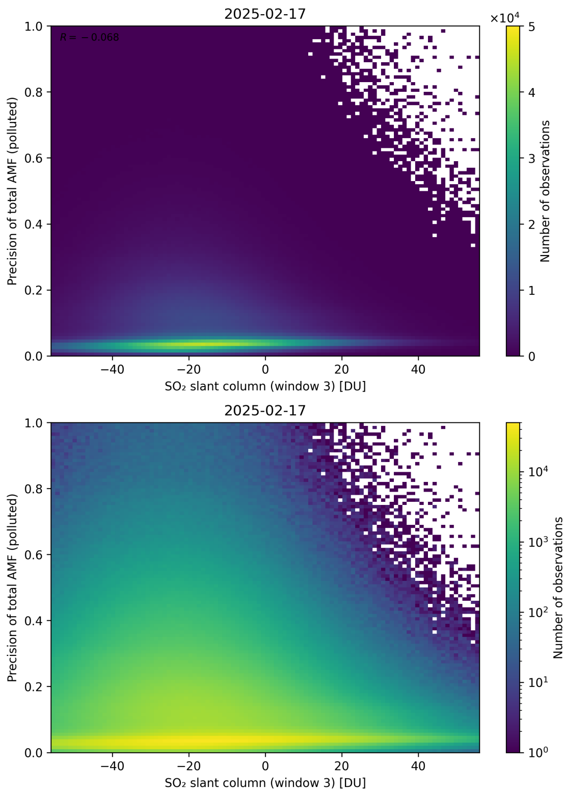
Figure 319: Scatter density plot of “SO 2 slant column (window 3)” against “Precision of total AMF (polluted)” for 2025-02-16 to 2025-02-18.
