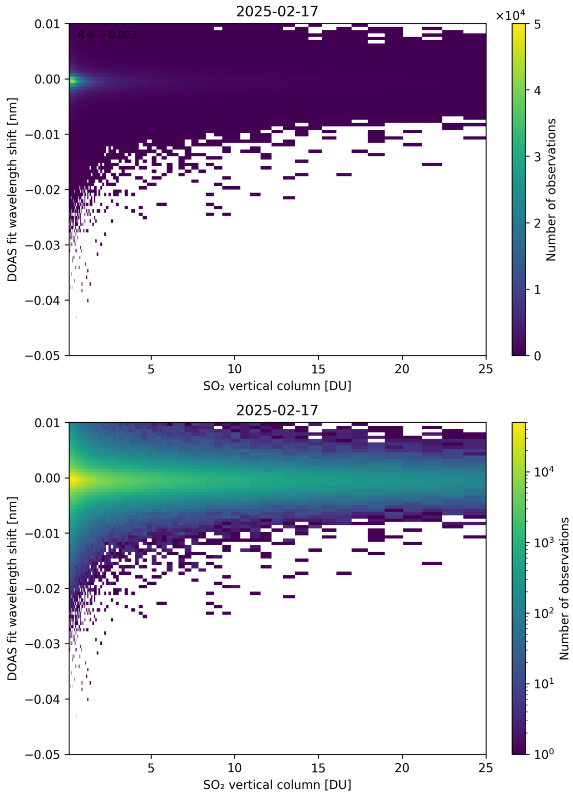
Figure 326: Scatter density plot of “SO 2 vertical column” against “DOAS fit wavelength shift” for 2025-02-16 to 2025-02-18.
