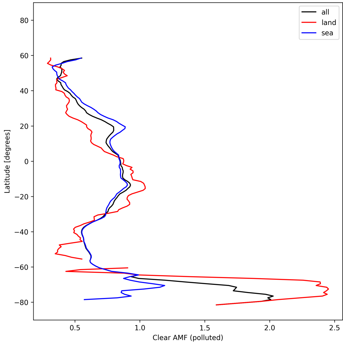
Figure 55: Zonal average of “Clear AMF (polluted)” for 2025-02-16 to 2025-02-18.
