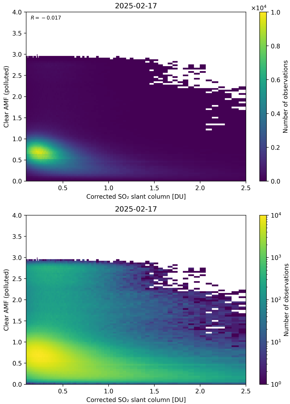
Figure 232: Scatter density plot of “Corrected SO 2 slant column” against “Clear AMF (polluted)” for 2025-02-16 to 2025-02-18.
