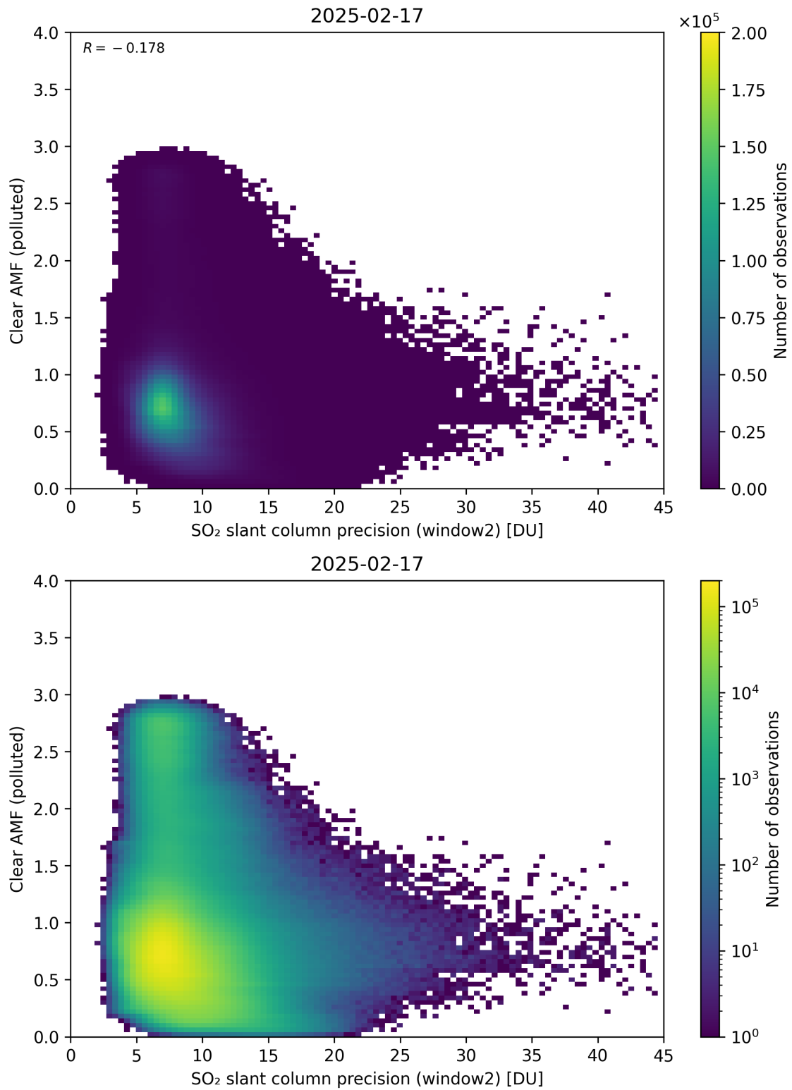
Figure 296: Scatter density plot of “SO 2 slant column precision (window2)” against “Clear AMF (polluted)” for 2025-02-16 to 2025-02-18.
