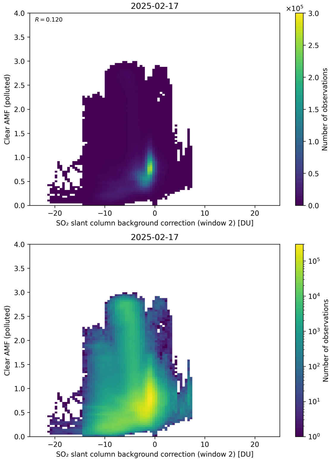
Figure 126: Scatter density plot of “SO 2 slant column background correction (window 2)” against “Clear AMF (polluted)” for 2025-02-16 to 2025-02-18.
