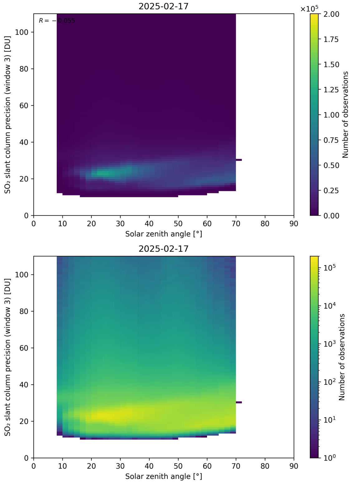
Figure 188: Scatter density plot of “Solar zenith angle” against “SO 2 slant column precision (window 3)” for 2025-02-16 to 2025-02-18.
