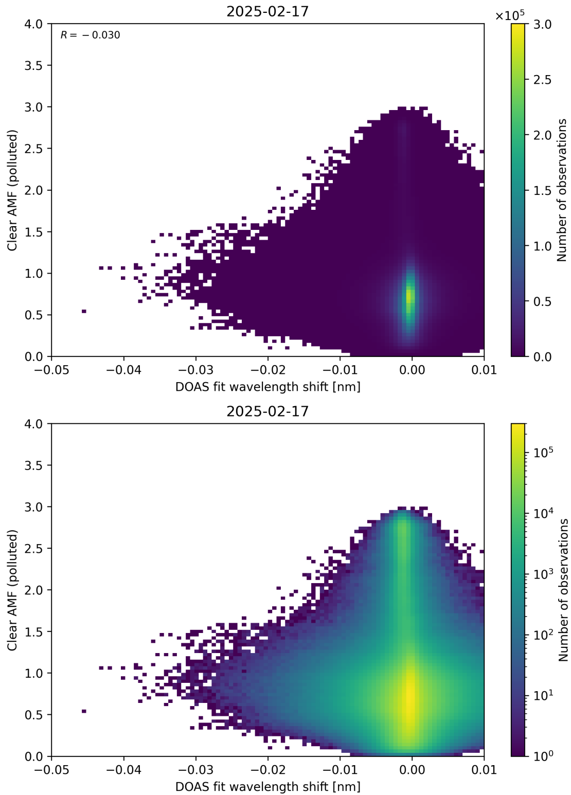
Figure 140: Scatter density plot of “DOAS fit wavelength shift” against “Clear AMF (polluted)” for 2025-02-16 to 2025-02-18.
