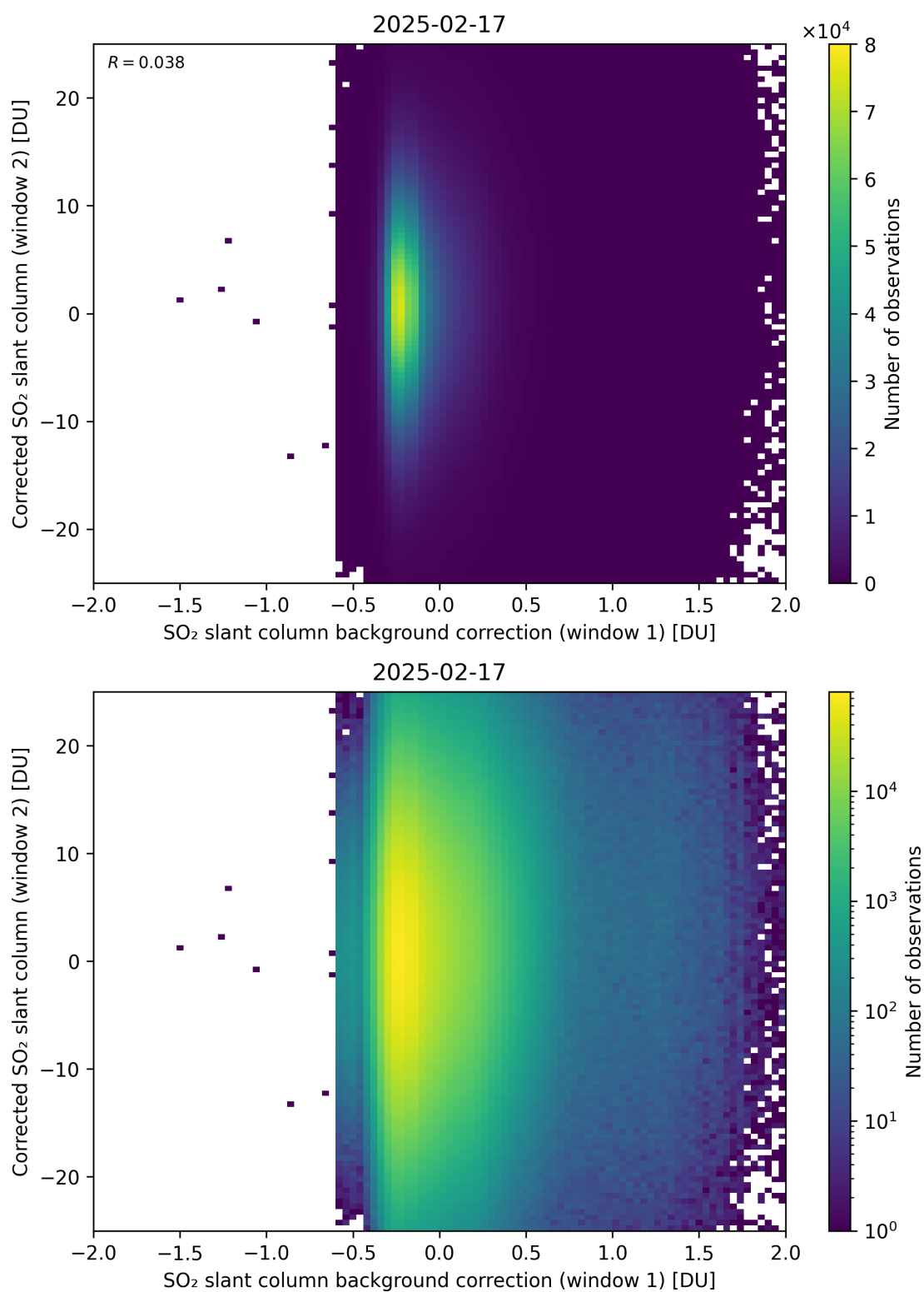
Figure 115: Scatter density plot of “SO 2 slant column background correction (window 1)” against “Corrected SO 2 slant column (window 2)” for 2025-02-16 to 2025-02-18.
