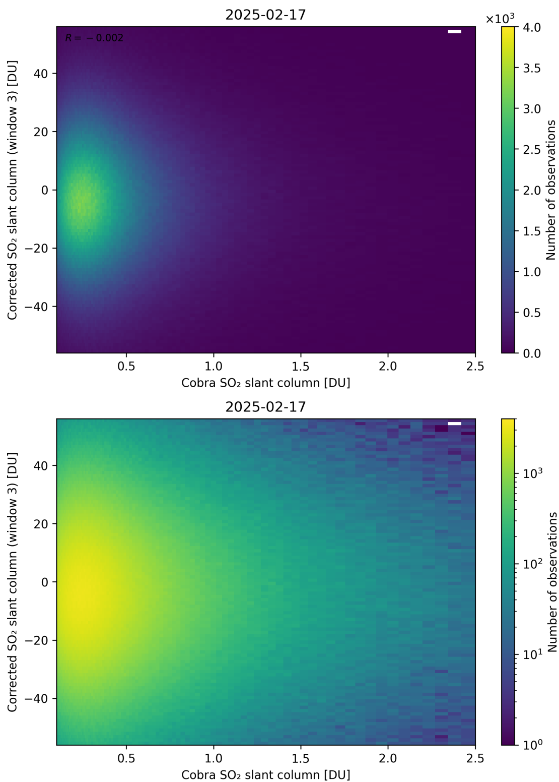
Figure 218: Scatter density plot of “Cobra SO 2 slant column” against “Corrected SO 2 slant column (window 3)” for 2025-02-16 to 2025-02-18.
