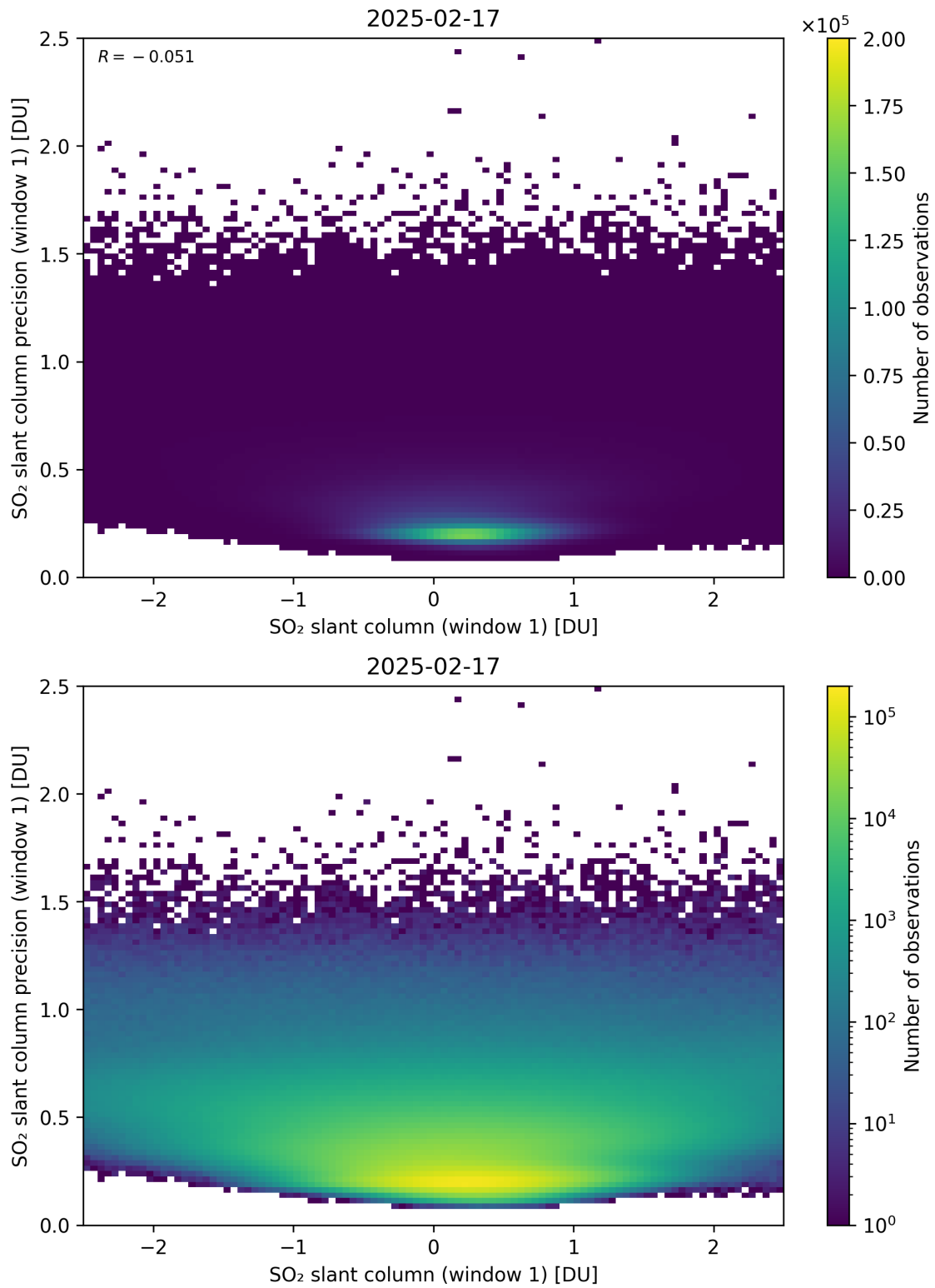
Figure 285: Scatter density plot of “SO 2 slant column (window 1)” against “SO 2 slant column precision (window 1)” for 2025-02-16 to 2025-02-18.
