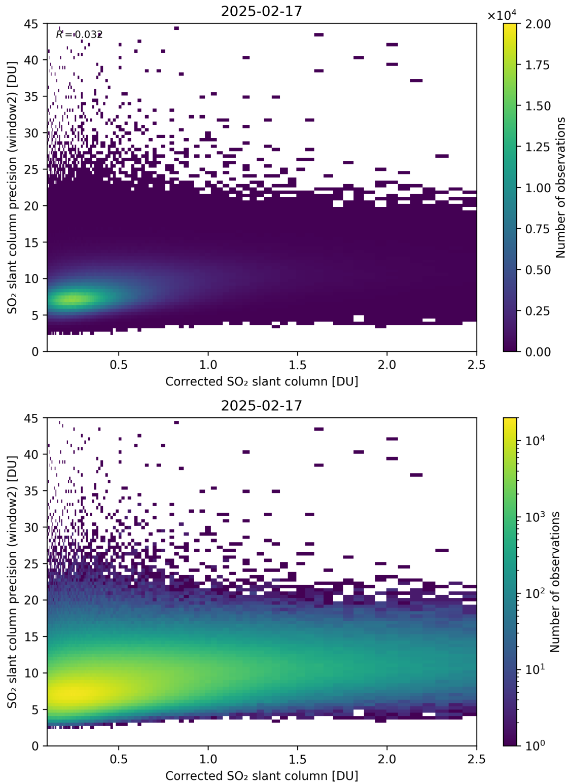
Figure 239: Scatter density plot of “Corrected SO 2 slant column” against “SO 2 slant column precision (window2)” for 2025-02-16 to 2025-02-18.
