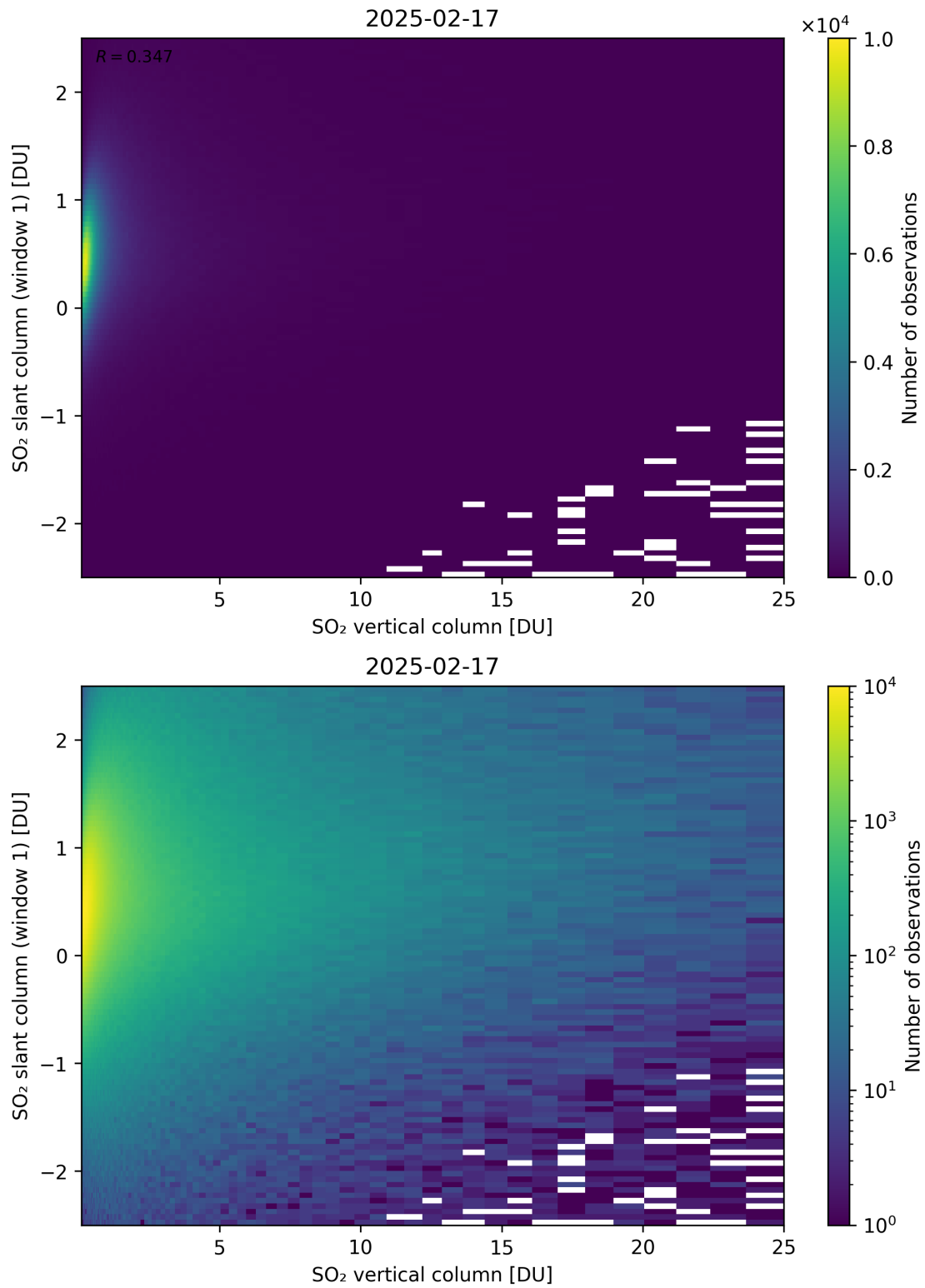
Figure 354: Scatter density plot of “SO 2 vertical column” against “SO 2 slant column (window 1)” for 2025-02-16 to 2025-02-18.
