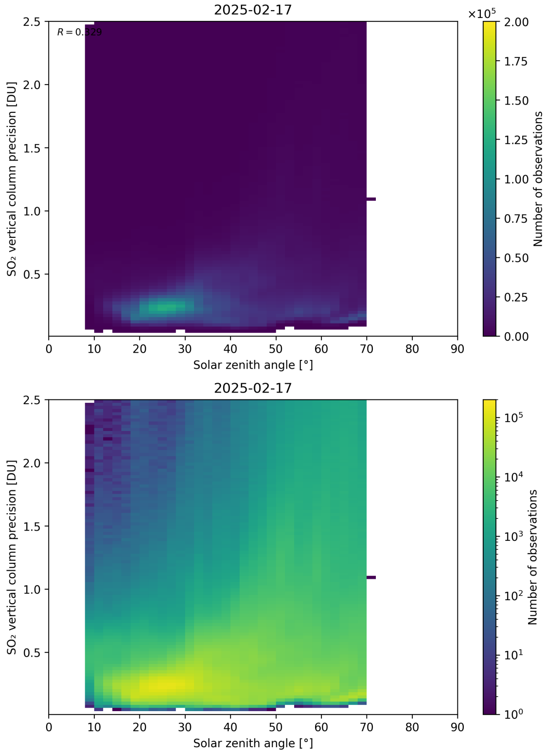
Figure 192: Scatter density plot of “Solar zenith angle” against “SO 2 vertical column precision” for 2025-02-16 to 2025-02-18.
