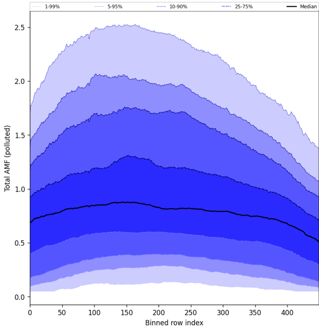
Figure 105: Along track statistics of “Total AMF (polluted)” for 2025-02-16 to 2025-02-18
