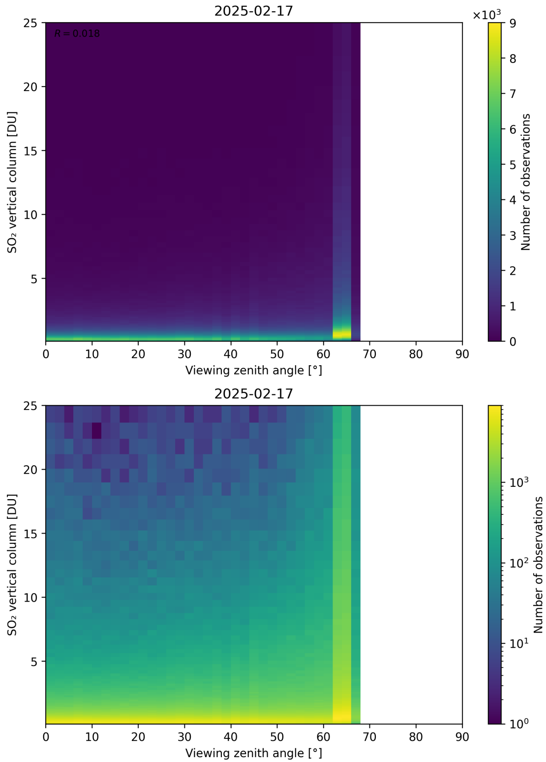
Figure 383: Scatter density plot of “Viewing zenith angle” against “SO 2 vertical column” for 2025-02-16 to 2025-02-18.
