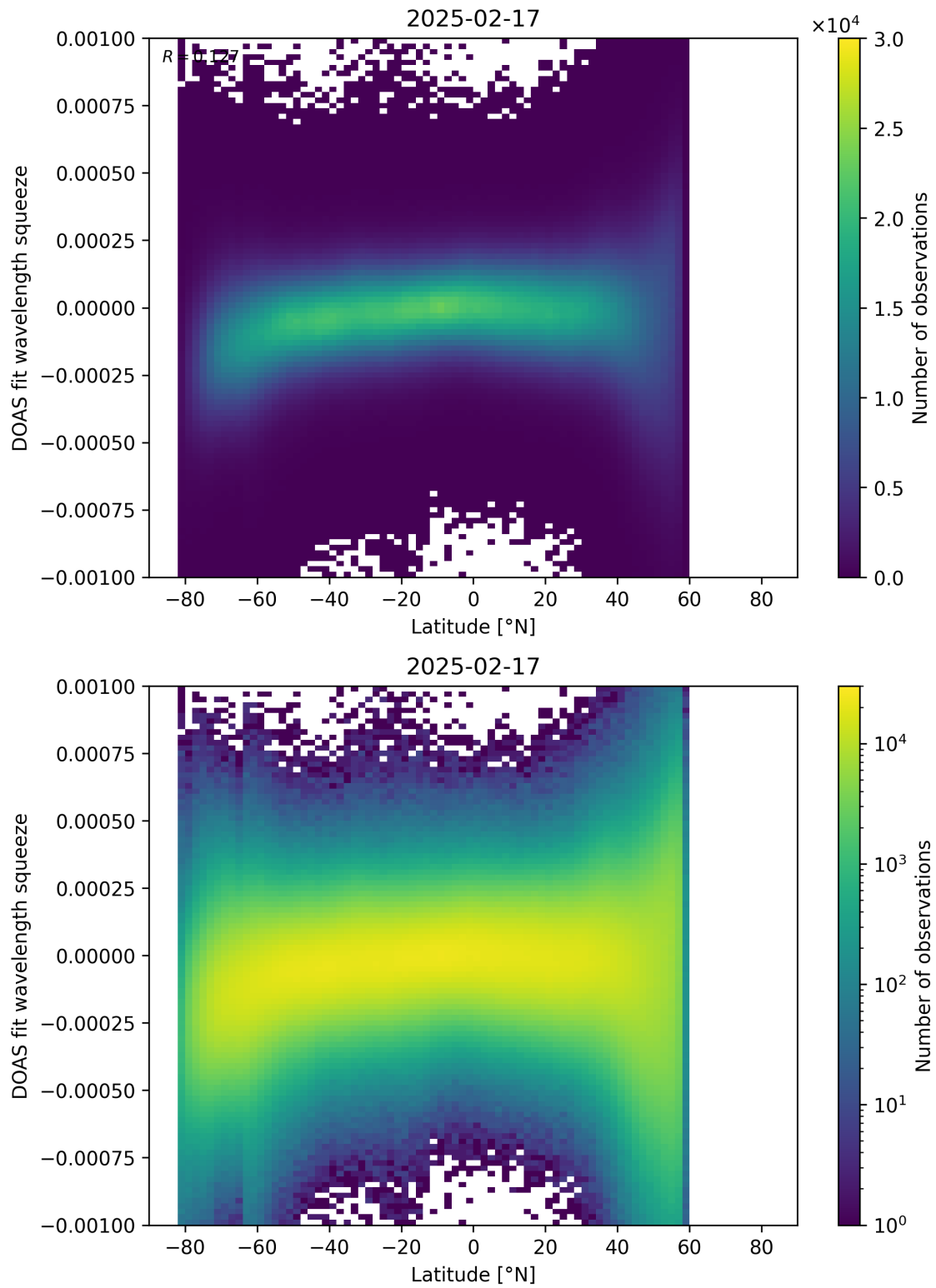
Figure 154: Scatter density plot of “Latitude” against “DOAS fit wavelength squeeze” for 2025-02-16 to 2025-02-18.
