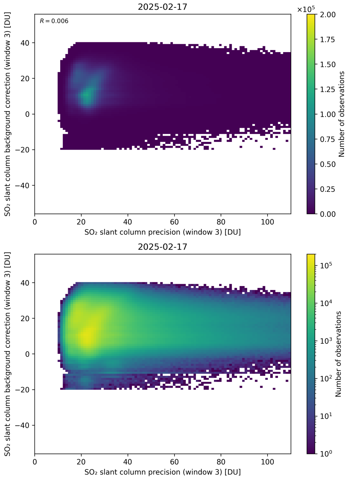
Figure 307: Scatter density plot of “SO 2 slant column precision (window 3)” against “SO 2 slant column background correction (window 3)” for 2025-02-16 to 2025-02-18.
