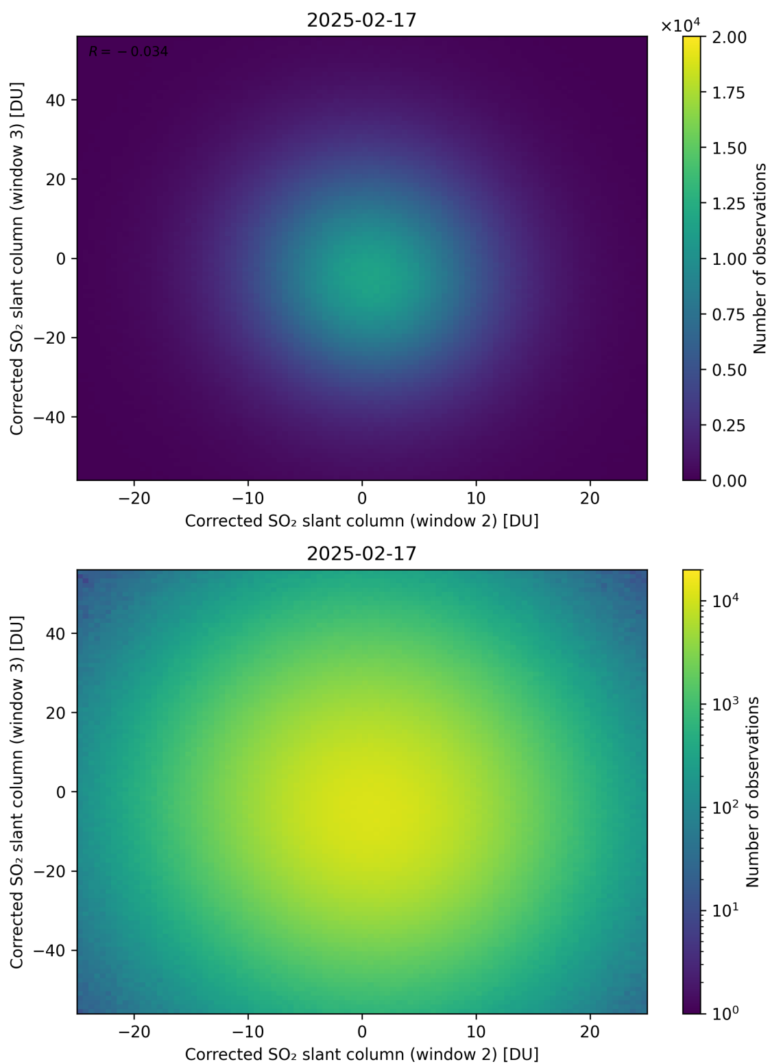
Figure 250: Scatter density plot of “Corrected SO 2 slant column (window 2)” against “Corrected SO 2 slant column (window 3)” for 2025-02-16 to 2025-02-18.
