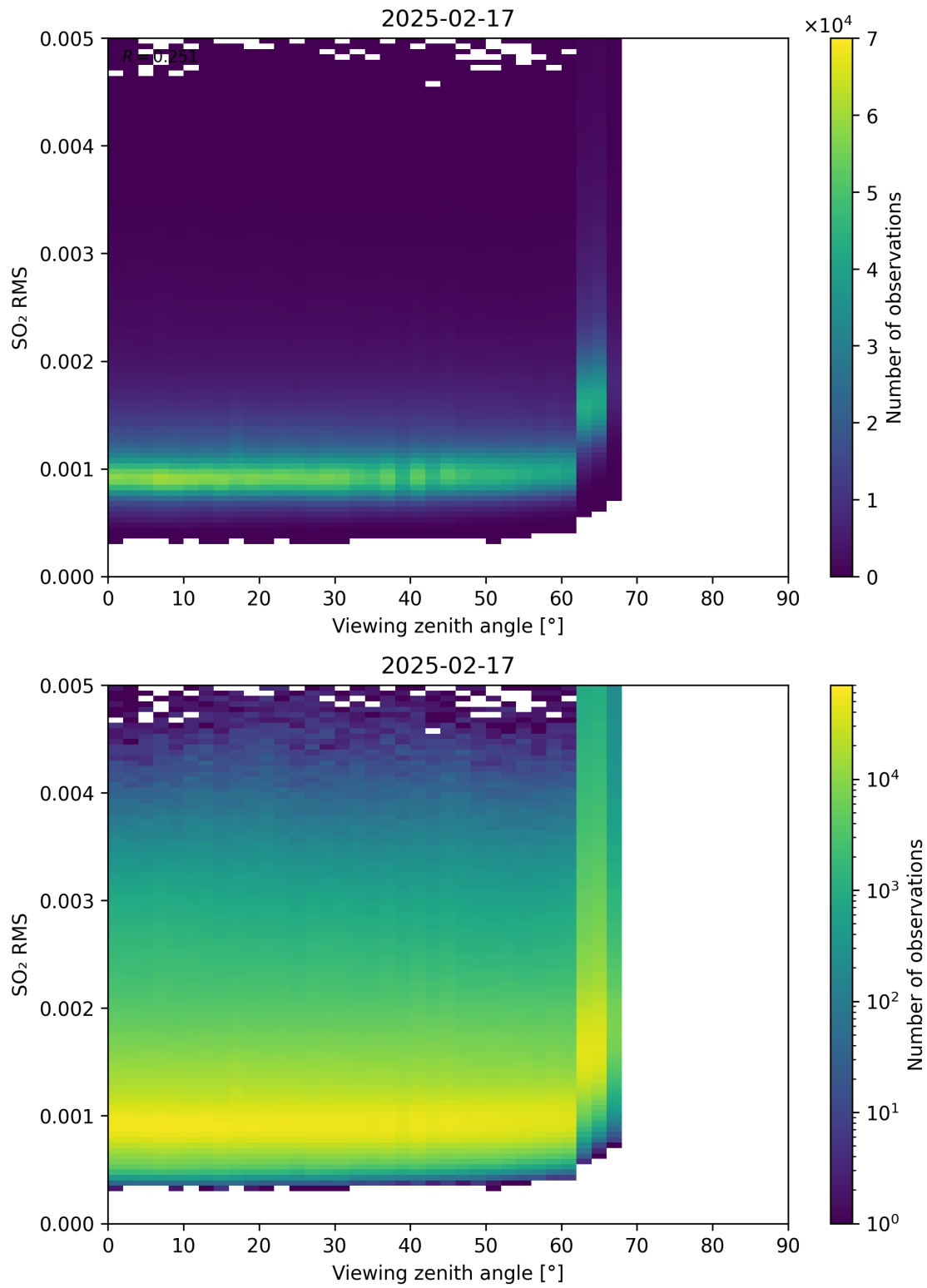
Figure 367: Scatter density plot of “Viewing zenith angle” against “SO 2 RMS” for 2025-02-16 to 2025-02-18.
