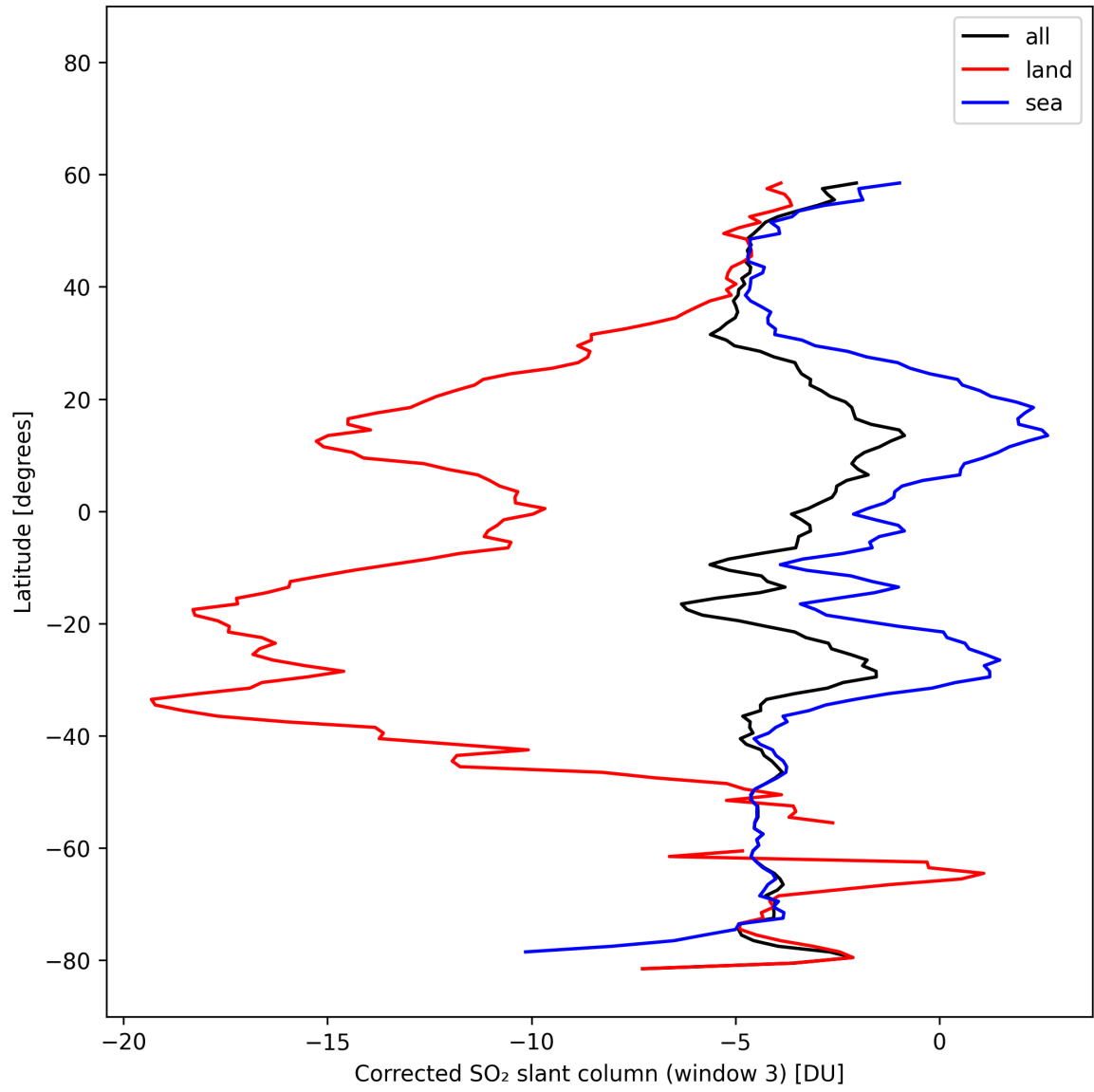
Figure 47: Zonal average of “Corrected SO 2 slant column (window 3)” for 2025-02-16 to 2025-02-18.
