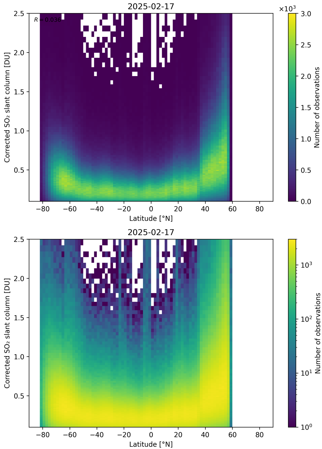
Figure 159: Scatter density plot of “Latitude” against “Corrected SO 2 slant column” for 2025-02-16 to 2025-02-18.
