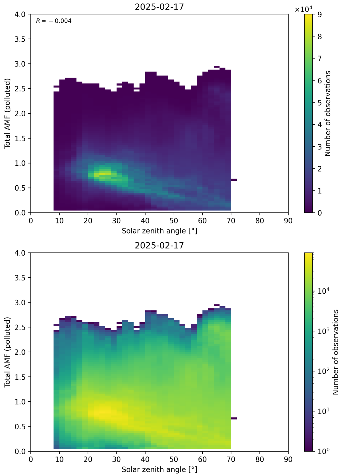
Figure 189: Scatter density plot of “Solar zenith angle” against “Total AMF (polluted)” for 2025-02-16 to 2025-02-18.
