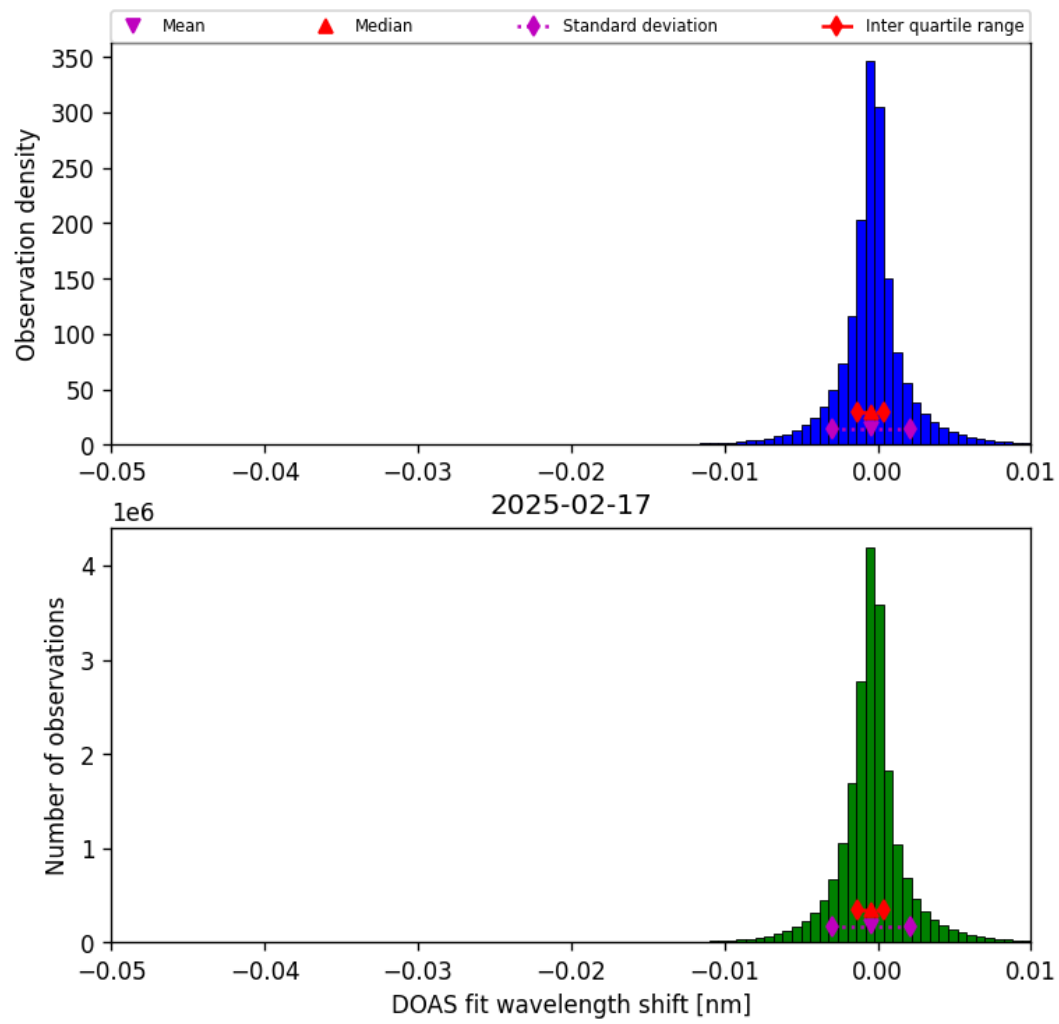
Figure 76: Histogram of “DOAS fit wavelength shift” for 2025-02-16 to 2025-02-18
