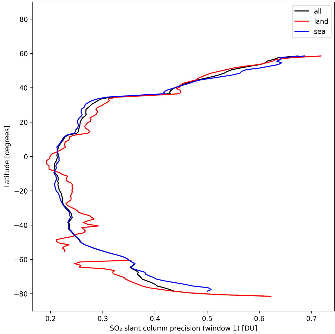
Figure 38: Zonal average of “SO 2 slant column precision (window 1)” for 2025-02-16 to 2025-02-18.
