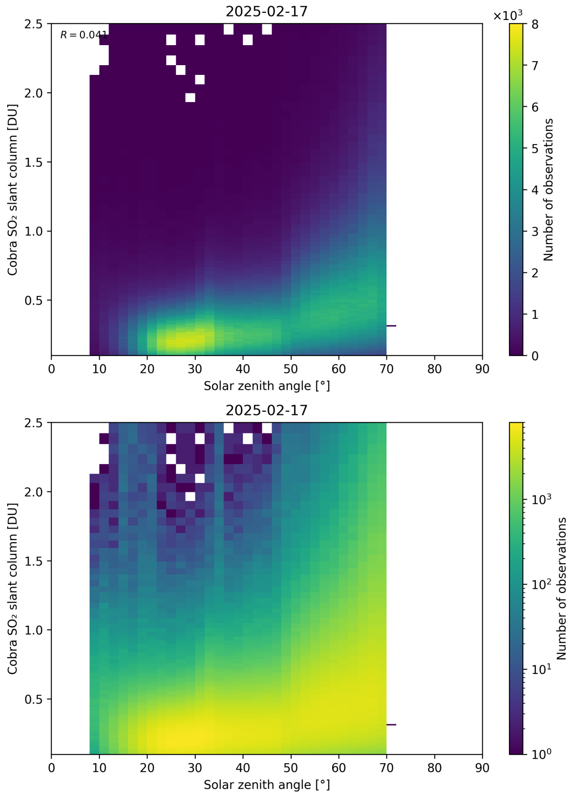
Figure 179: Scatter density plot of “Solar zenith angle” against “Cobra SO 2 slant column” for 2025-02-16 to 2025-02-18.
