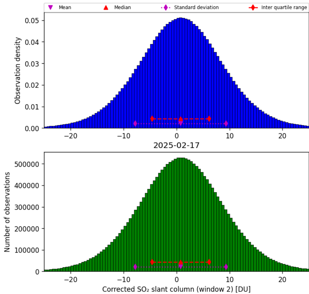
Figure 69: Histogram of “Corrected SO 2 slant column (window 2)” for 2025-02-16 to 2025-02-18
