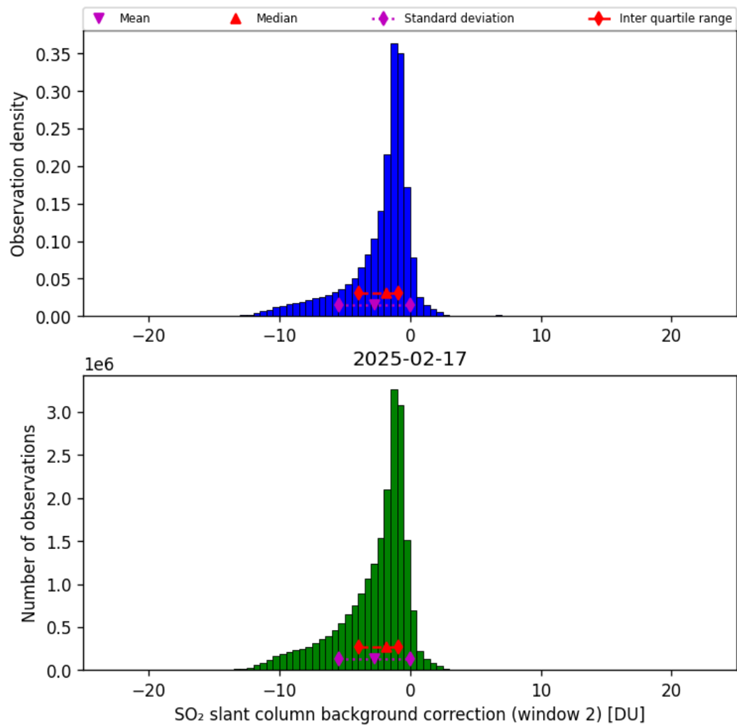
Figure 70: Histogram of “SO 2 slant column background correction (window 2)” for 2025-02-16 to 2025-02-18
