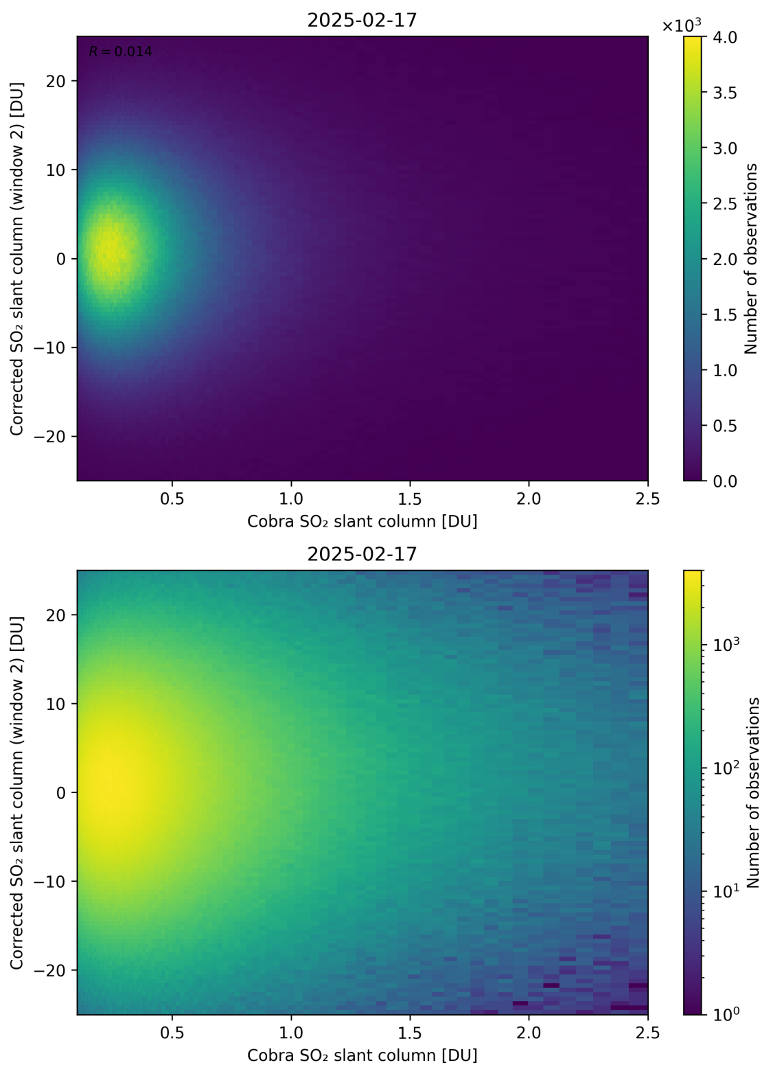
Figure 217: Scatter density plot of “Cobra SO 2 slant column” against “Corrected SO 2 slant column (window 2)” for 2025-02-16 to 2025-02-18.
