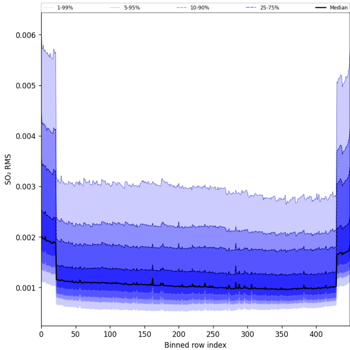
Figure 104: Along track statistics of “SO 2 RMS” for 2025-02-16 to 2025-02-18
