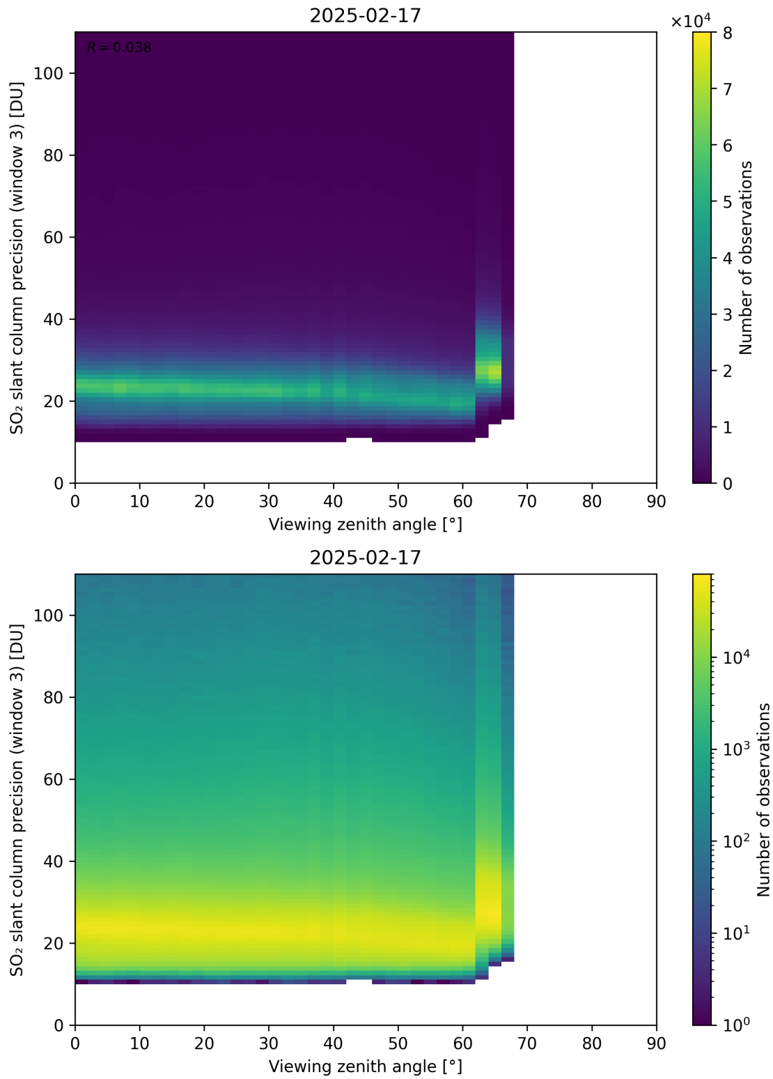
Figure 380: Scatter density plot of “Viewing zenith angle” against “SO 2 slant column precision (window 3)” for 2025-02-16 to 2025-02-18.
