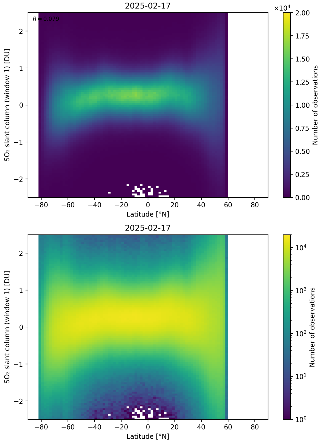
Figure 162: Scatter density plot of “Latitude” against “SO 2 slant column (window 1)” for 2025-02-16 to 2025-02-18.
