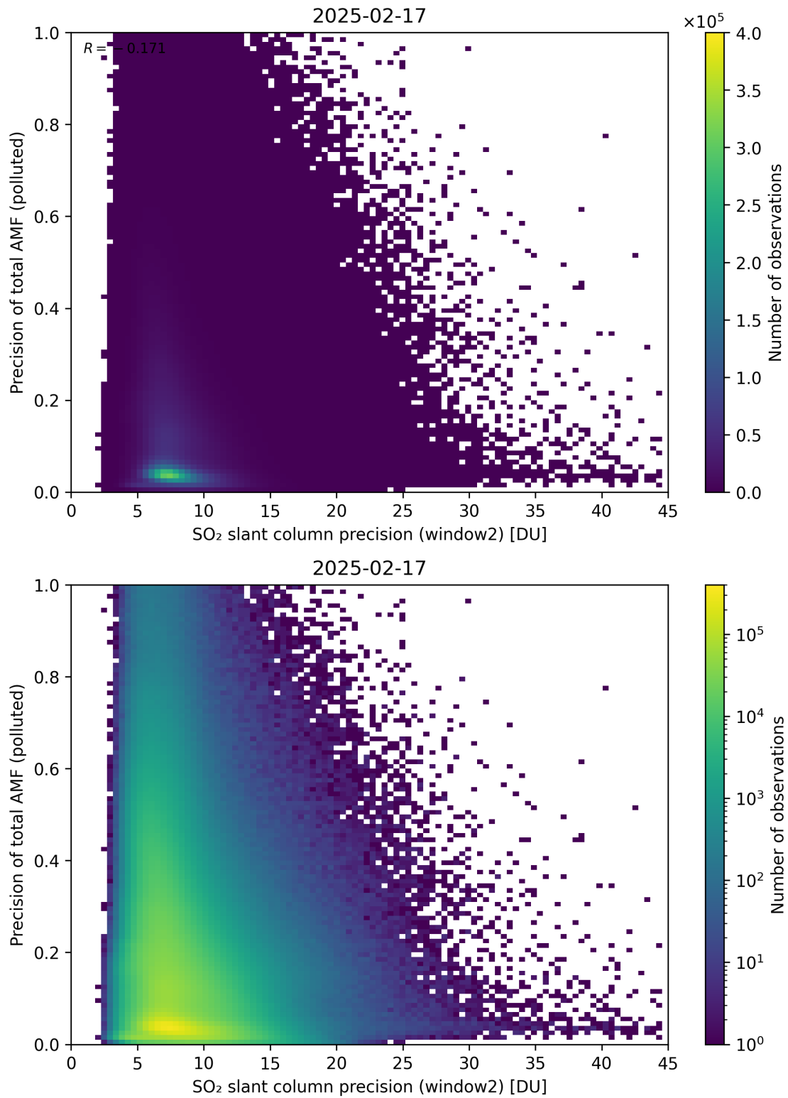
Figure 302: Scatter density plot of “SO 2 slant column precision (window2)” against “Precision of total AMF (polluted)” for 2025-02-16 to 2025-02-18.
