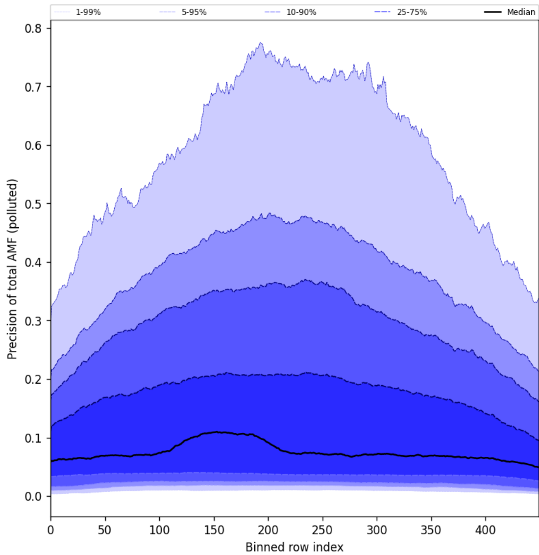
Figure 106: Along track statistics of “Precision of total AMF (polluted)” for 2025-02-16 to 2025-02-18
