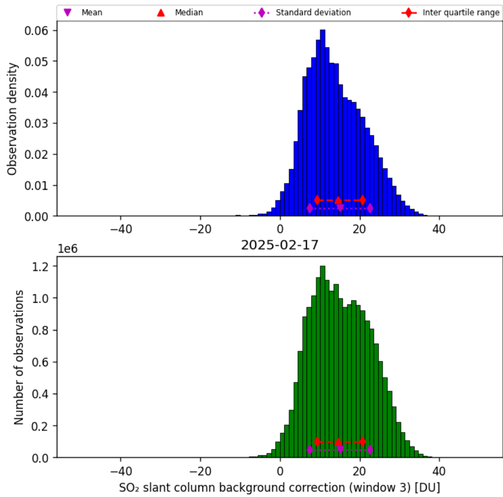
Figure 74: Histogram of “SO 2 slant column background correction (window 3)” for 2025-02-16 to 2025-02-18
