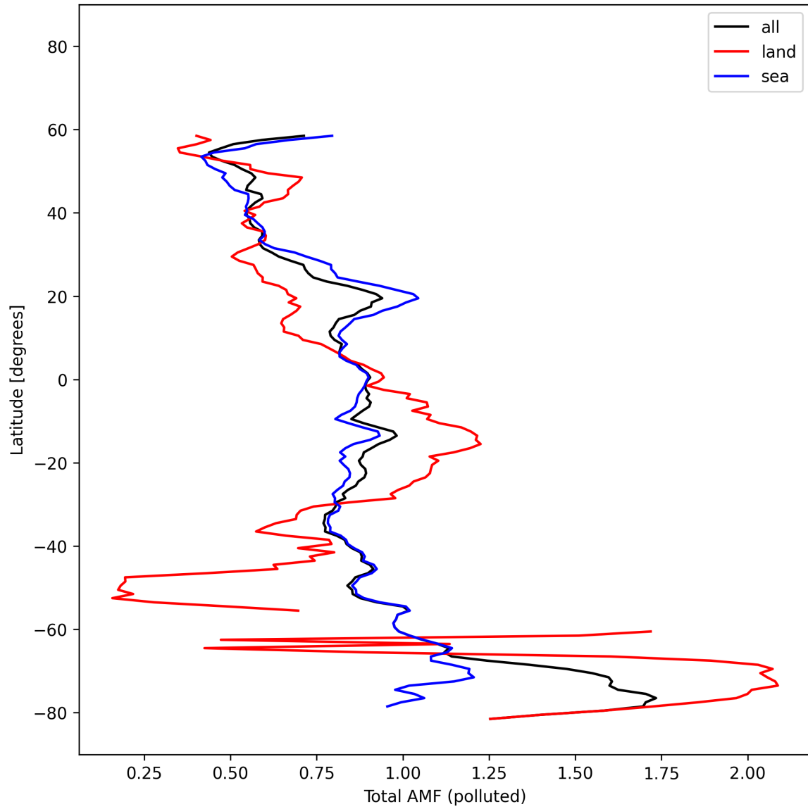
Figure 53: Zonal average of “Total AMF (polluted)” for 2025-02-16 to 2025-02-18.
