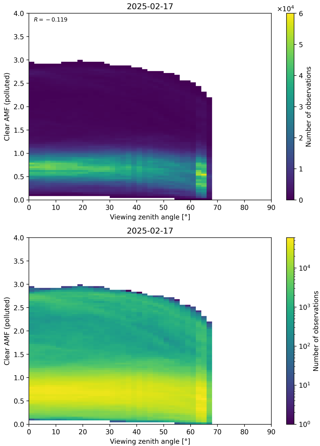
Figure 370: Scatter density plot of “Viewing zenith angle” against “Clear AMF (polluted)” for 2025-02-16 to 2025-02-18.
