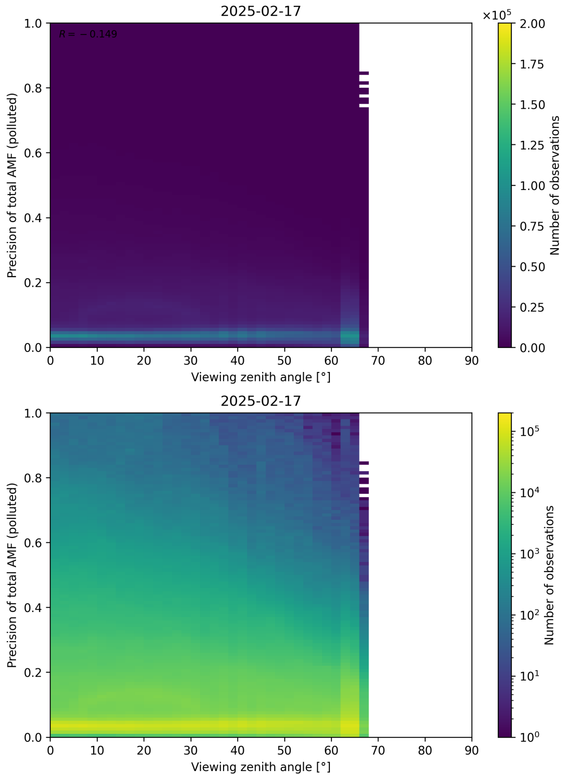
Figure 382: Scatter density plot of “Viewing zenith angle” against “Precision of total AMF (polluted)” for 2025-02-16 to 2025-02-18.
