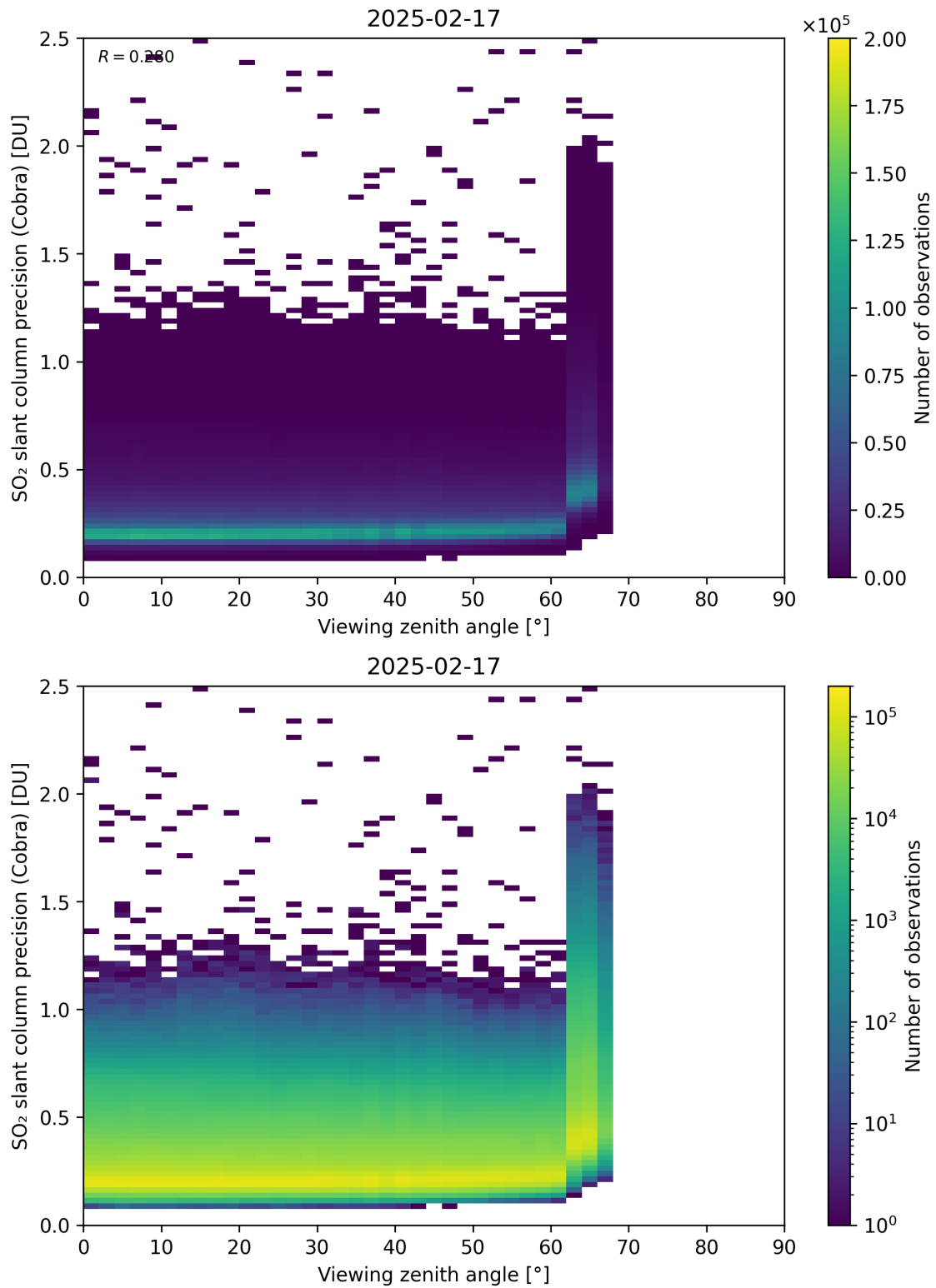
Figure 372: Scatter density plot of “Viewing zenith angle” against “SO 2 slant column precision (Cobra)” for 2025-02-16 to 2025-02-18.
