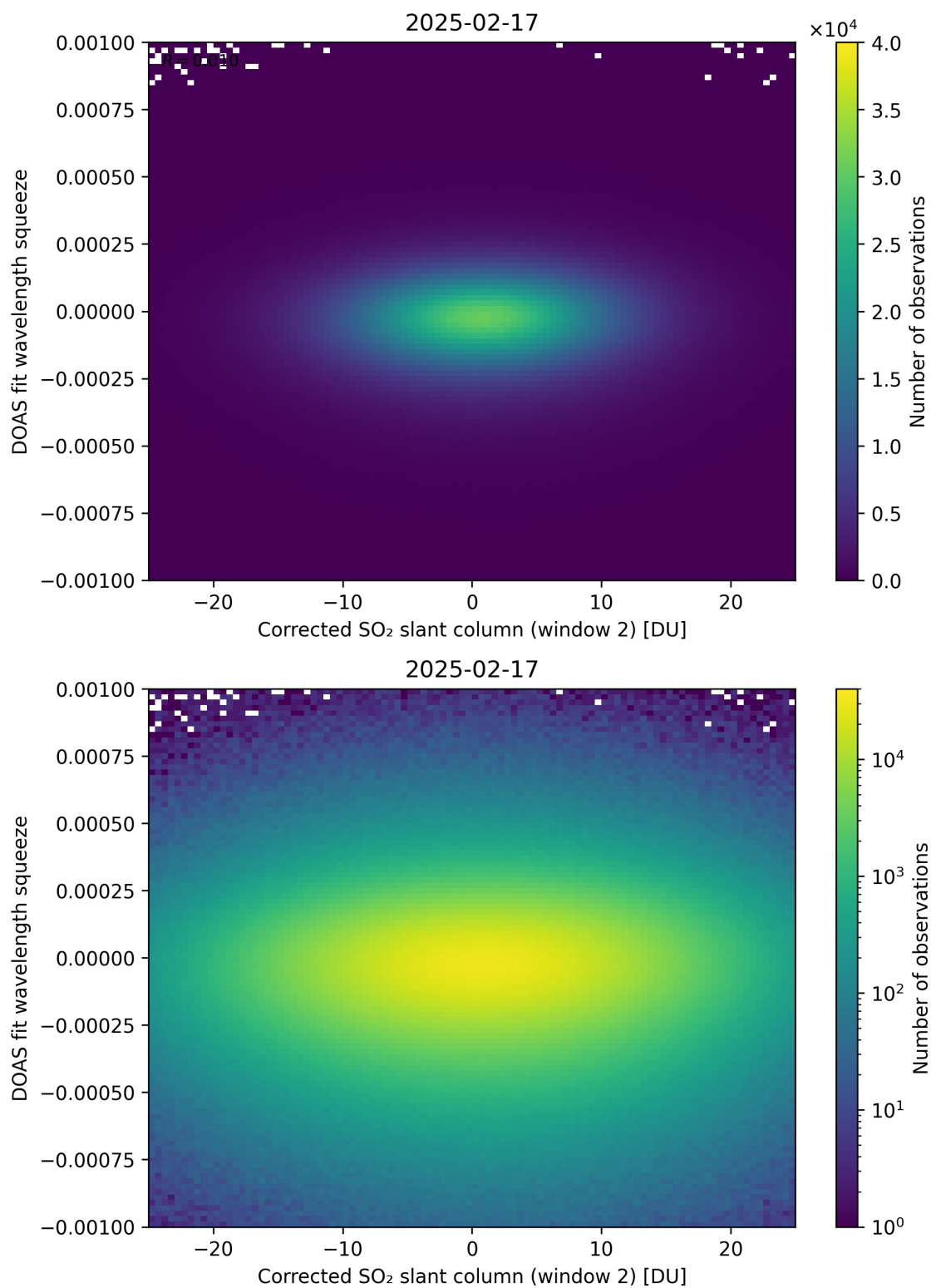
Figure 247: Scatter density plot of “Corrected SO 2 slant column (window 2)” against “DOAS fit wavelength squeeze” for 2025-02-16 to 2025-02-18.
