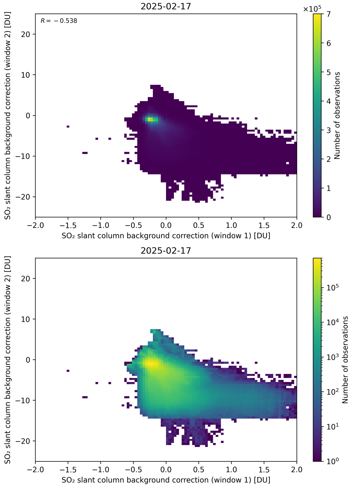
Figure 109: Scatter density plot of “SO 2 slant column background correction (window 1)” against “SO 2 slant column background correction (window 2)” for 2025-02-16 to 2025-02-18.
