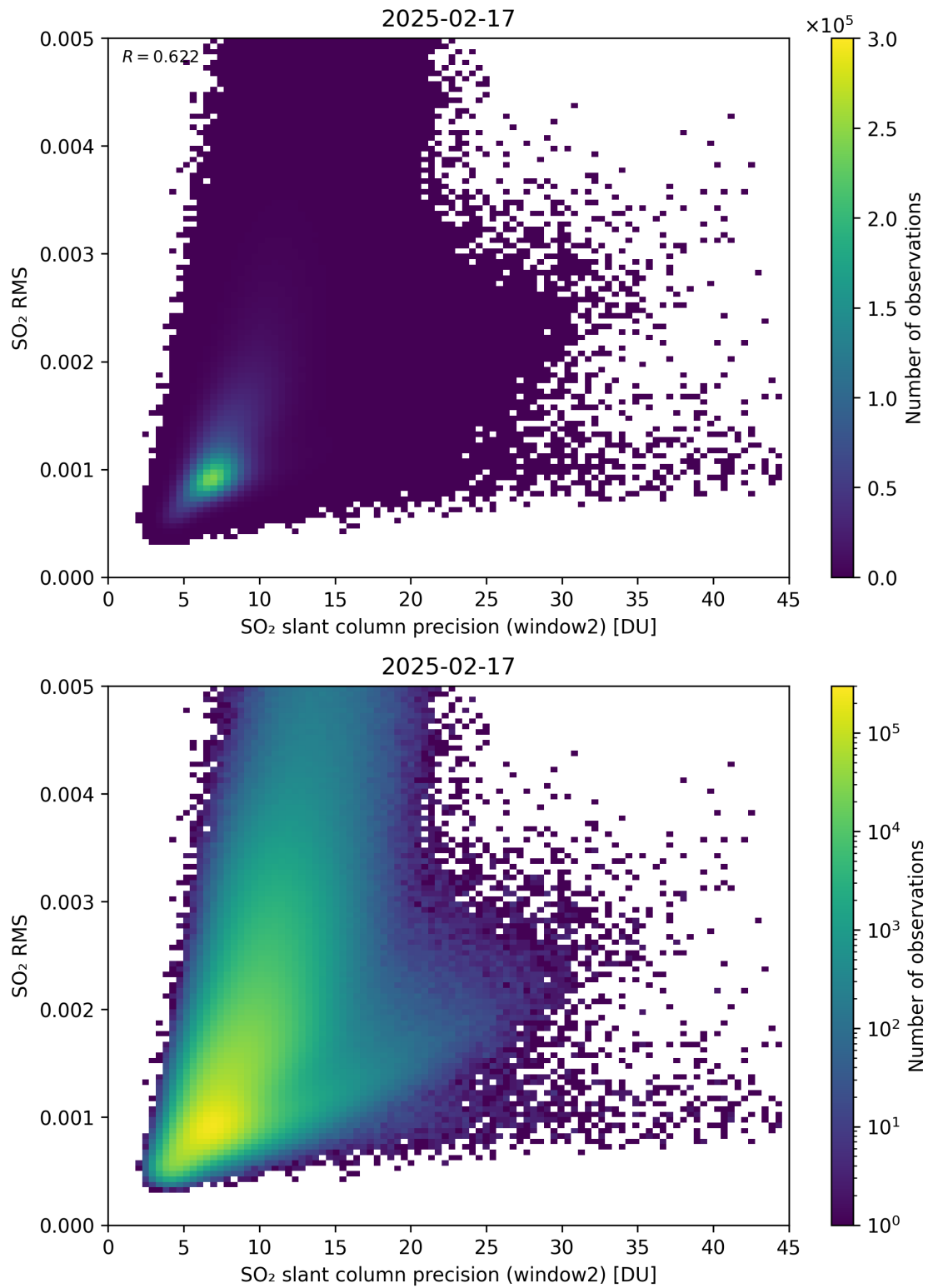
Figure 295: Scatter density plot of “SO 2 slant column precision (window2)” against “SO 2 RMS” for 2025-02-16 to 2025-02-18.
