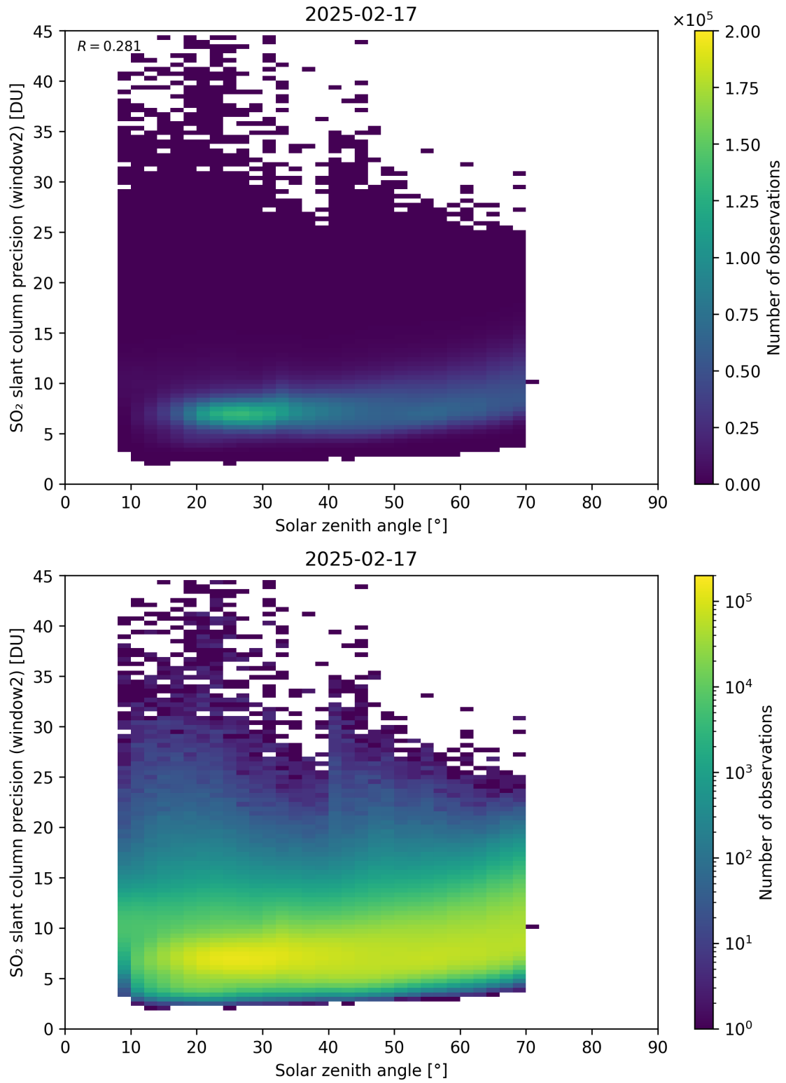
Figure 186: Scatter density plot of “Solar zenith angle” against “SO 2 slant column precision (window2)” for 2025-02-16 to 2025-02-18.
