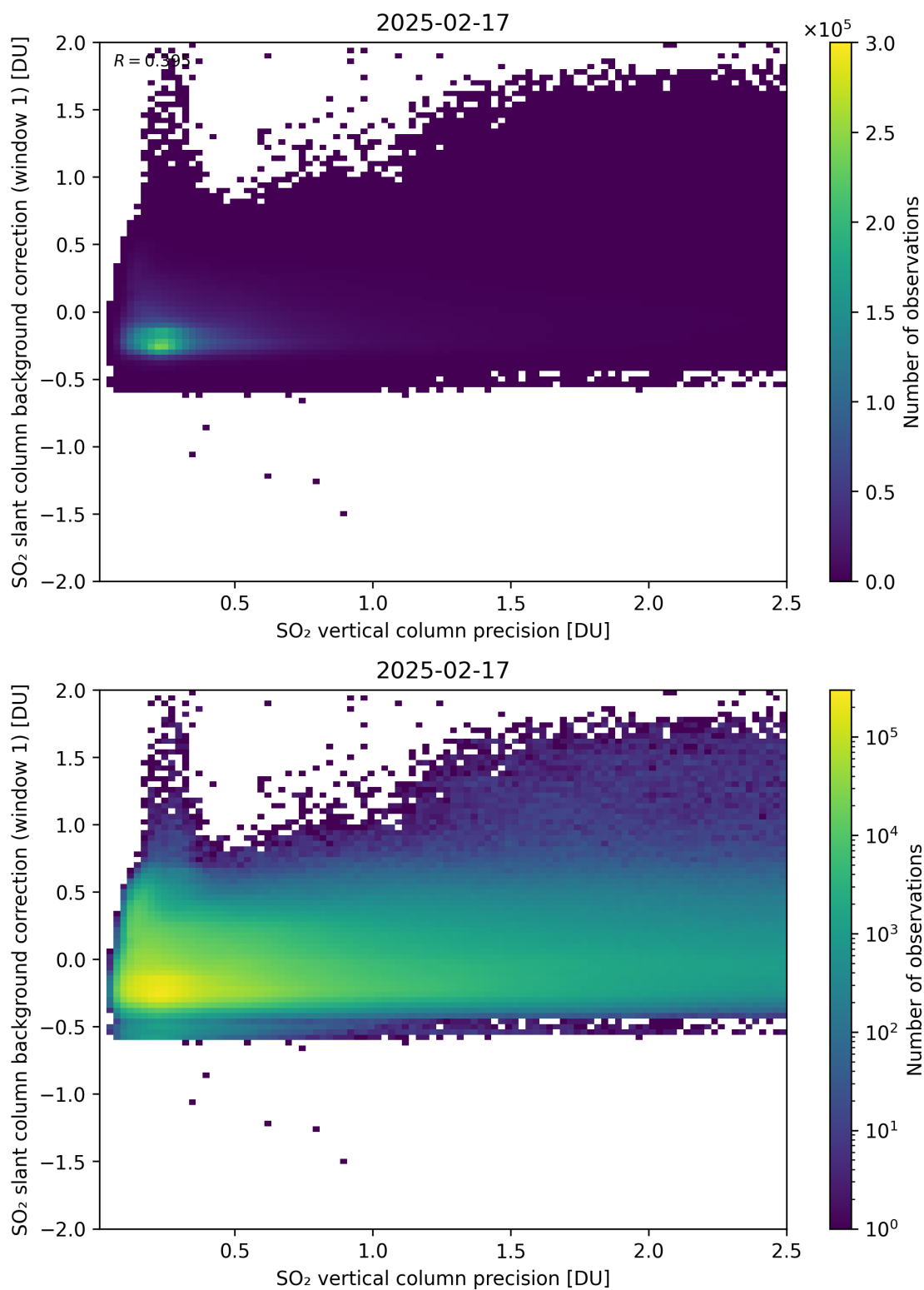
Figure 329: Scatter density plot of “SO 2 vertical column precision” against “SO 2 slant column background correction (window 1)” for 2025-02-16 to 2025-02-18.
