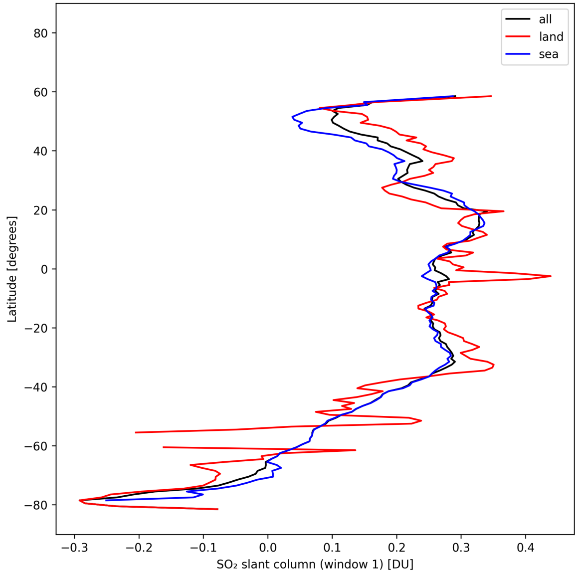
Figure 37: Zonal average of “SO 2 slant column (window 1)” for 2025-02-16 to 2025-02-18.
