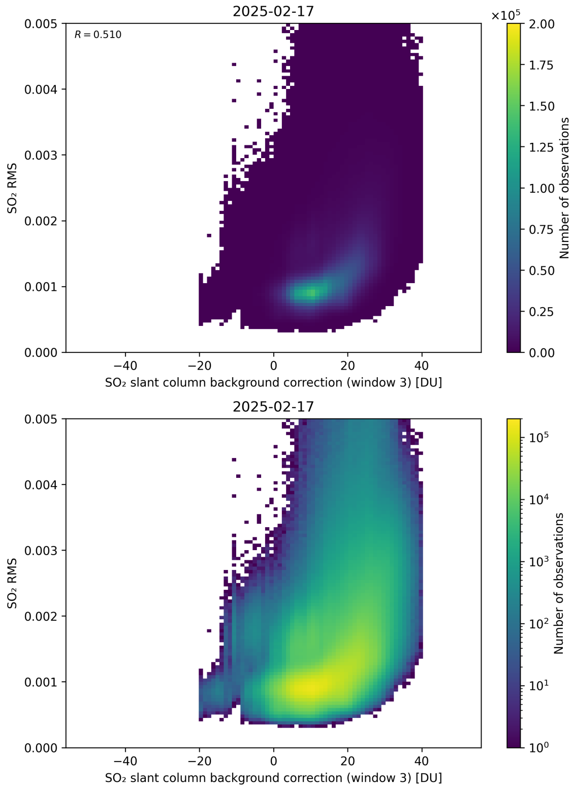
Figure 134: Scatter density plot of “SO 2 slant column background correction (window 3)” against “SO 2 RMS” for 2025-02-16 to 2025-02-18.
