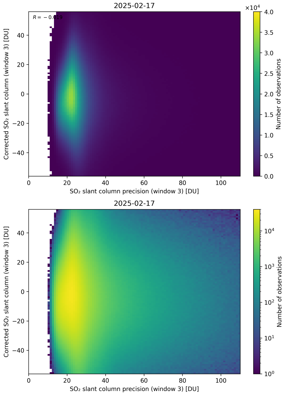
Figure 312: Scatter density plot of “SO 2 slant column precision (window 3)” against “Corrected SO 2 slant column (window 3)” for 2025-02-16 to 2025-02-18.
