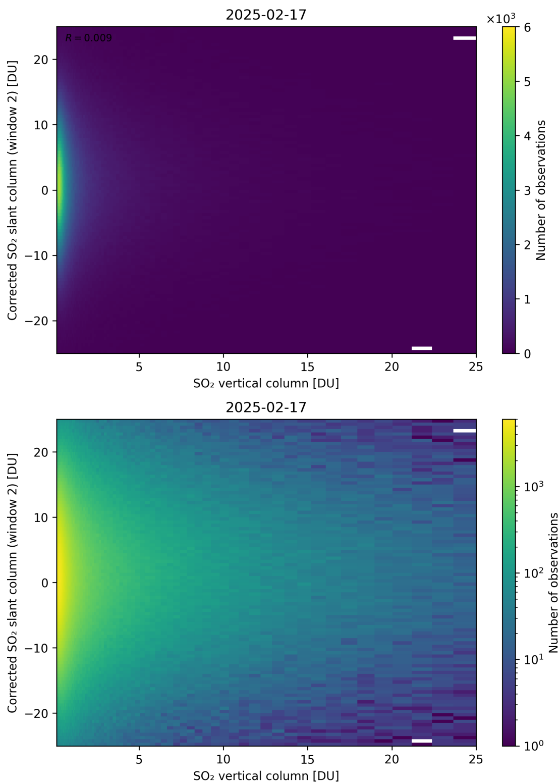
Figure 352: Scatter density plot of “SO 2 vertical column” against “Corrected SO 2 slant column (window 2)” for 2025-02-16 to 2025-02-18.
