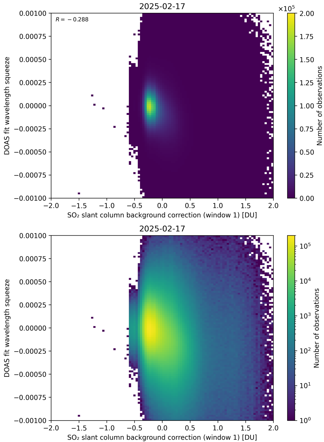
Figure 112: Scatter density plot of “SO 2 slant column background correction (window 1)” against “DOAS fit wavelength squeeze” for 2025-02-16 to 2025-02-18.
