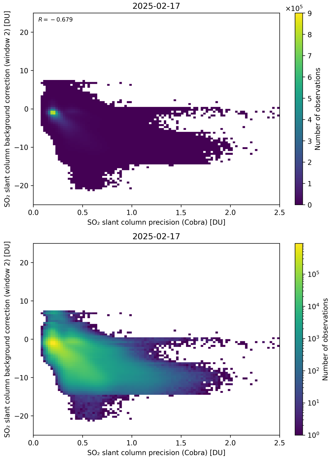
Figure 200: Scatter density plot of “SO 2 slant column precision (Cobra)” against “SO 2 slant column background correction (window 2)” for 2025-02-16 to 2025-02-18.
