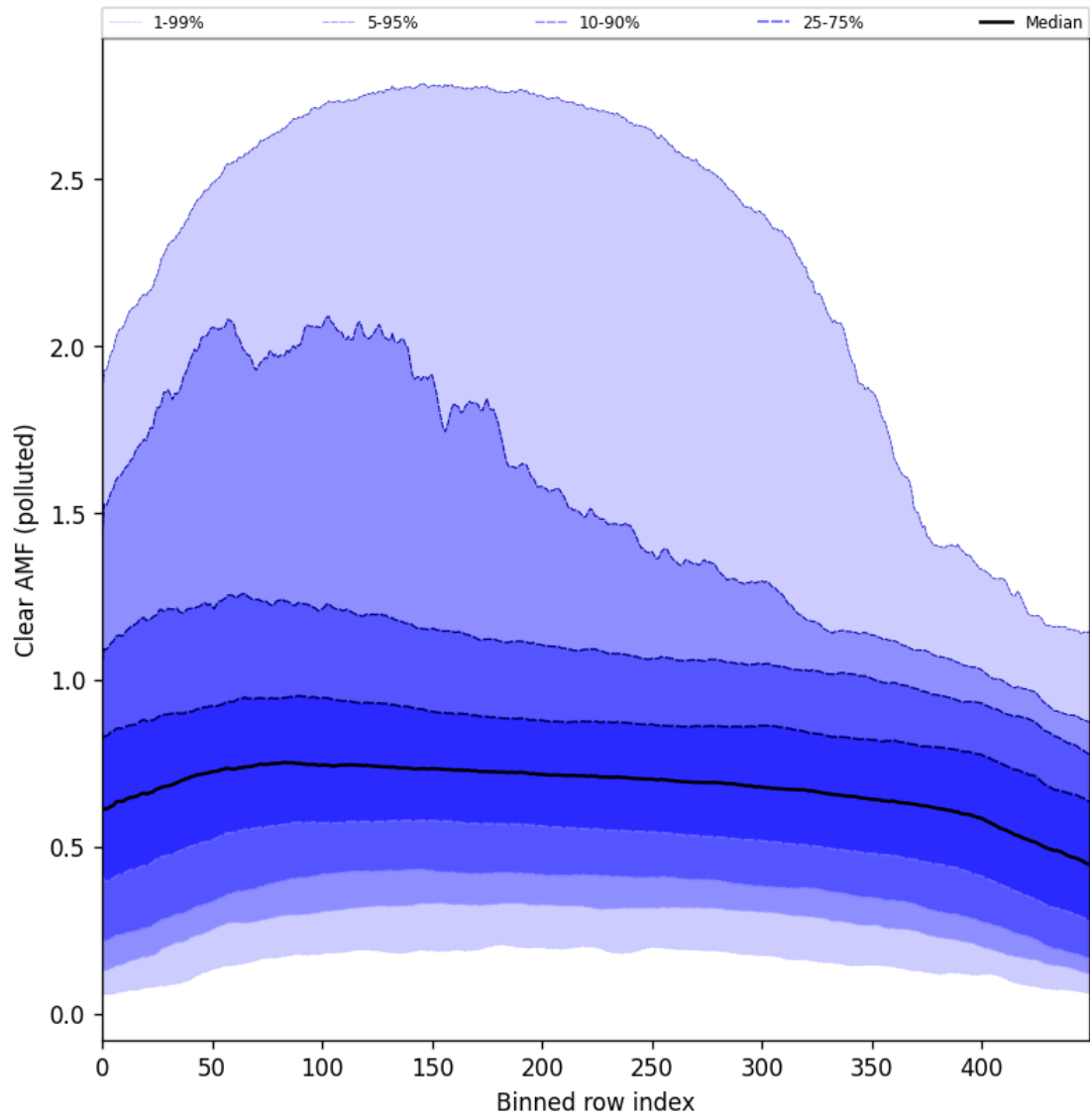
Figure 107: Along track statistics of “Clear AMF (polluted)” for 2025-02-16 to 2025-02-18
