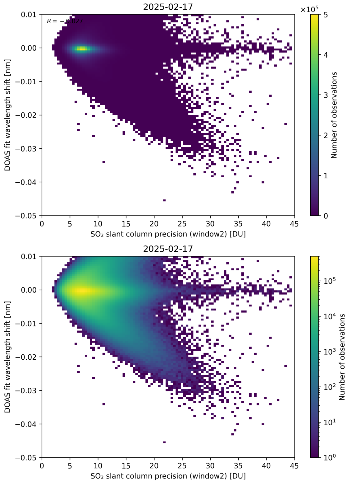
Figure 293: Scatter density plot of “SO 2 slant column precision (window2)” against “DOAS fit wavelength shift” for 2025-02-16 to 2025-02-18.
