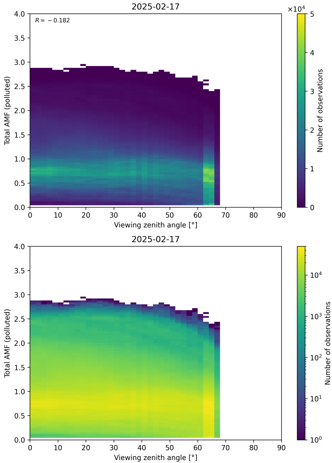
Figure 381: Scatter density plot of “Viewing zenith angle” against “Total AMF (polluted)” for 2025-02-16 to 2025-02-18.
