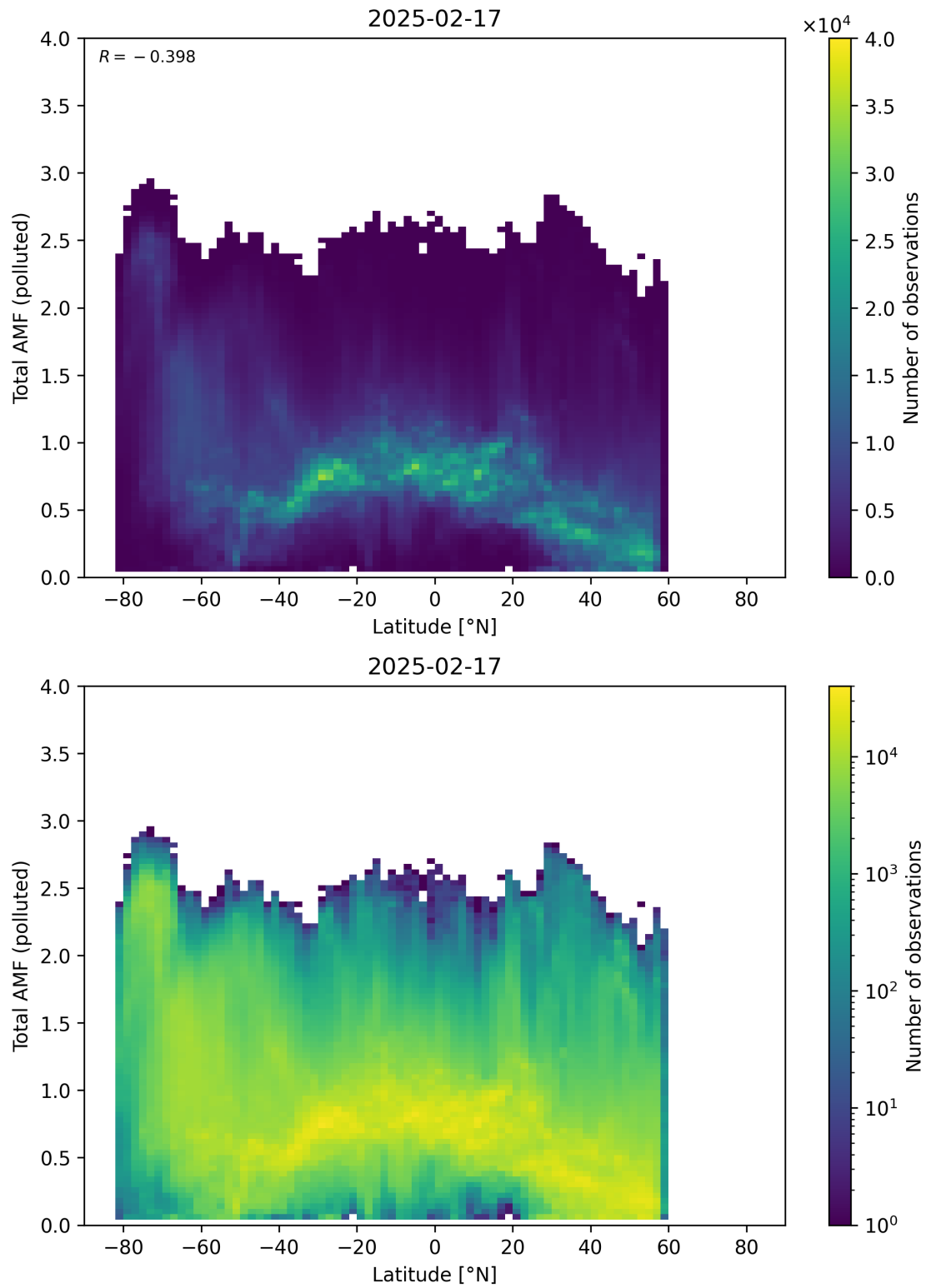
Figure 167: Scatter density plot of “Latitude” against “Total AMF (polluted)” for 2025-02-16 to 2025-02-18.
