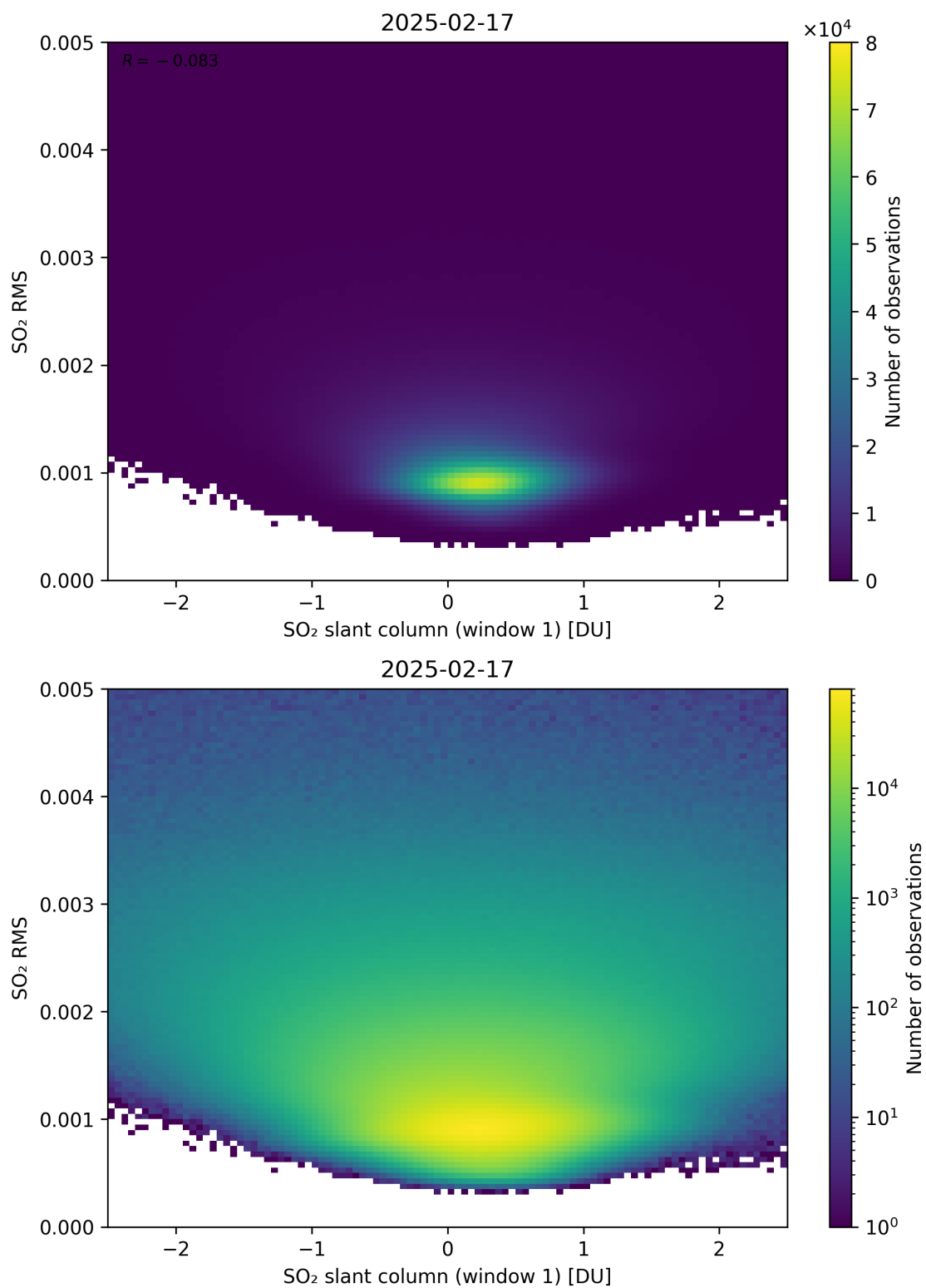
Figure 267: Scatter density plot of “SO 2 slant column (window 1)” against “SO 2 RMS” for 2025-02-16 to 2025-02-18.
