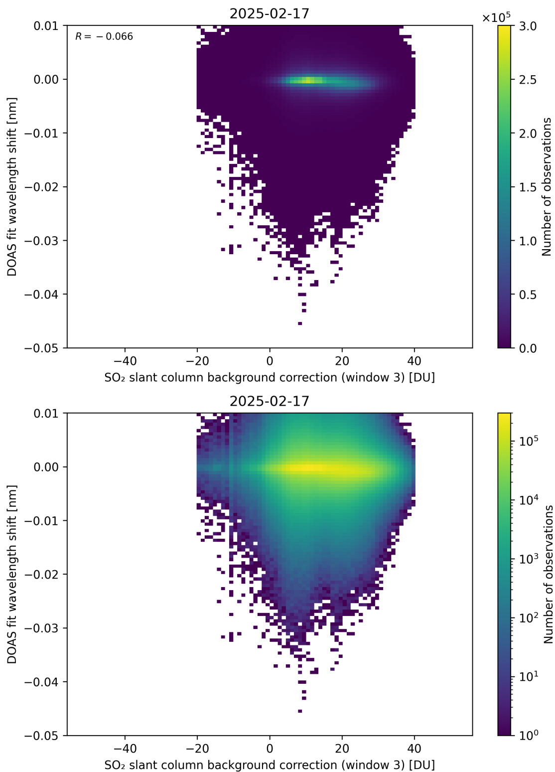
Figure 132: Scatter density plot of “SO 2 slant column background correction (window 3)” against “DOAS fit wavelength shift” for 2025-02-16 to 2025-02-18.
