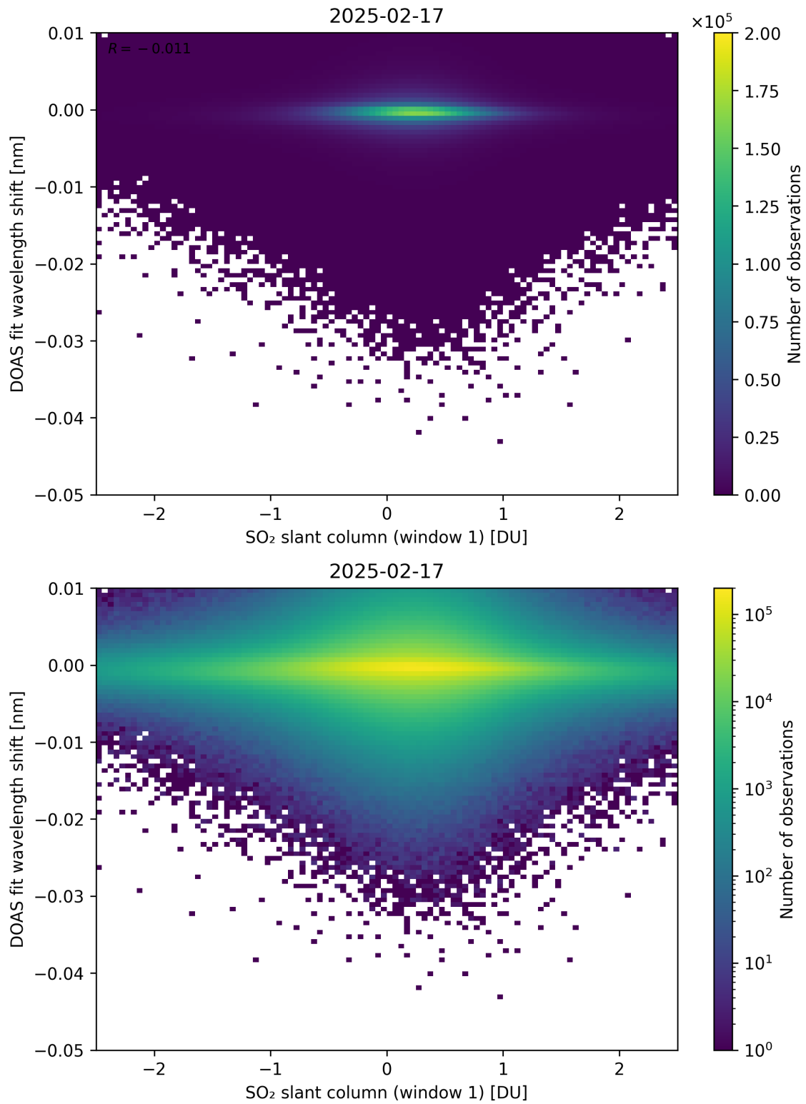
Figure 265: Scatter density plot of “SO 2 slant column (window 1)” against “DOAS fit wavelength shift” for 2025-02-16 to 2025-02-18.
