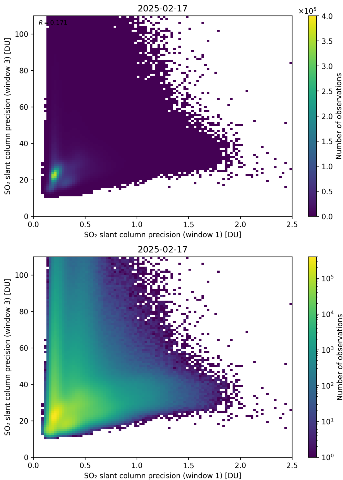
Figure 279: Scatter density plot of “SO 2 slant column precision (window 1)” against “SO 2 slant column precision (window 3)” for 2025-02-16 to 2025-02-18.
