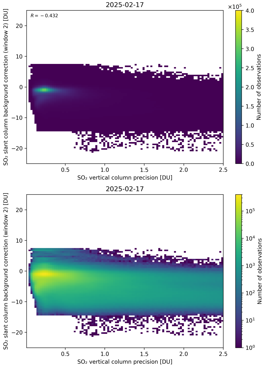
Figure 330: Scatter density plot of “SO 2 vertical column precision” against “SO 2 slant column background correction (window 2)” for 2025-02-16 to 2025-02-18.
