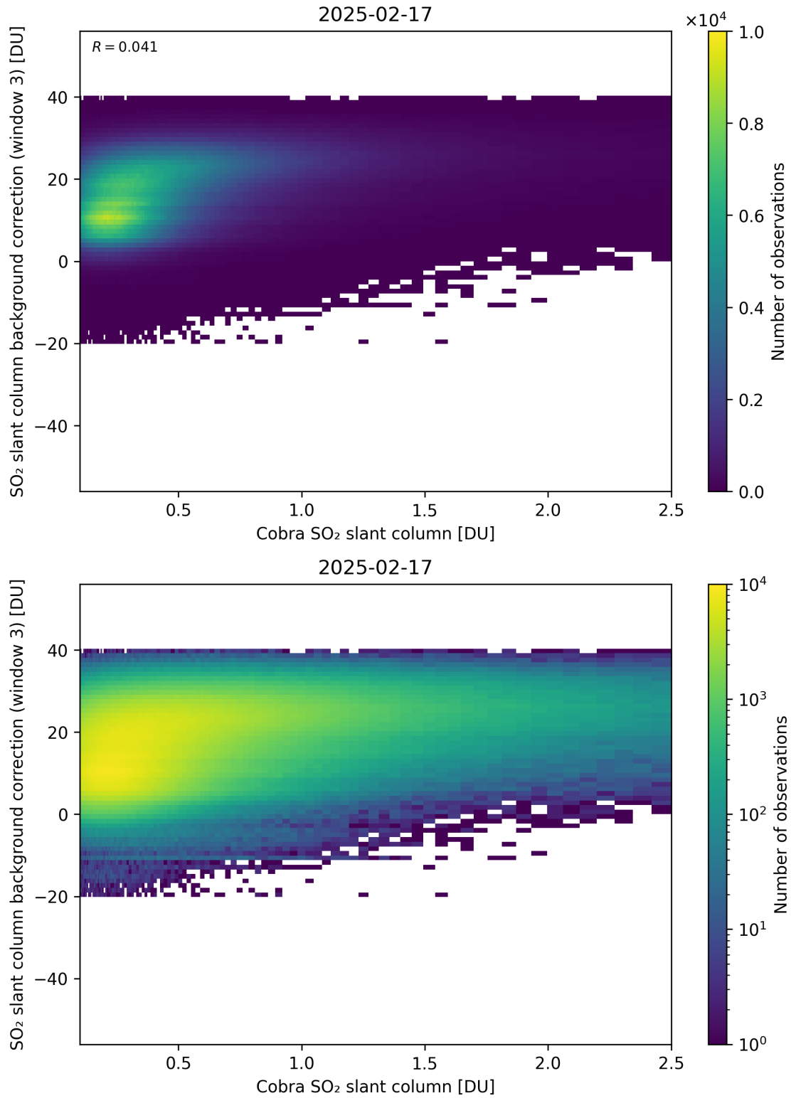
Figure 195: Scatter density plot of “Cobra SO 2 slant column” against “SO 2 slant column background correction (window 3)” for 2025-02-16 to 2025-02-18.
