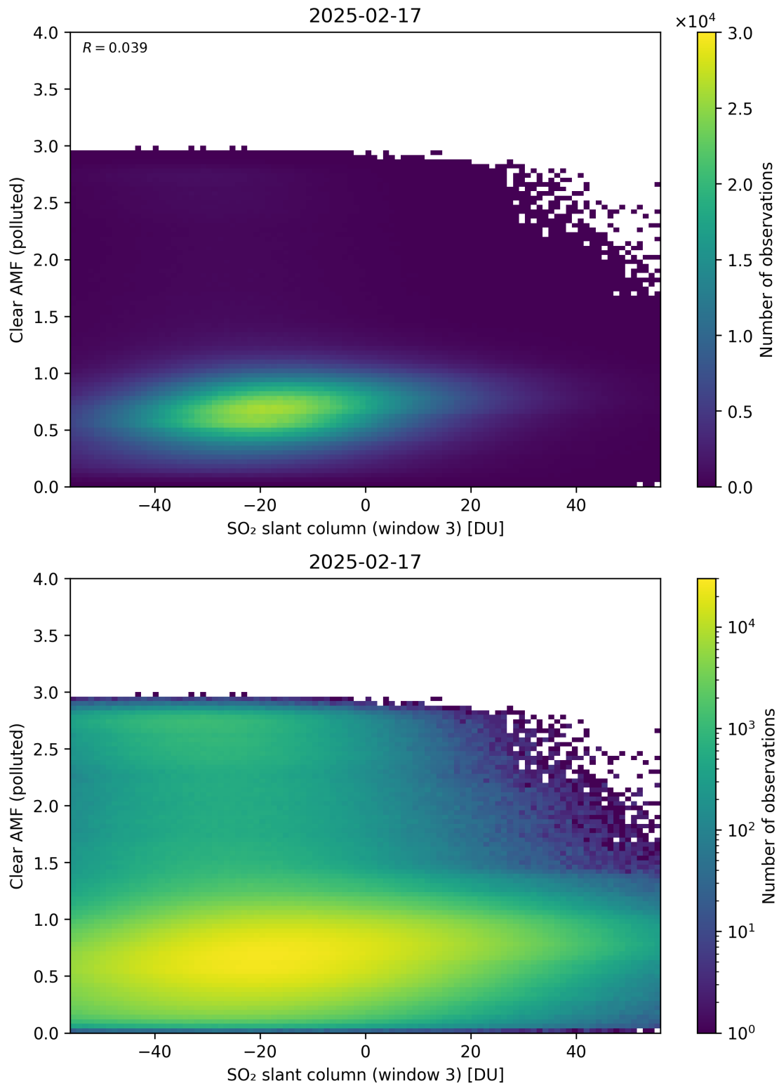
Figure 315: Scatter density plot of “SO 2 slant column (window 3)” against “Clear AMF (polluted)” for 2025-02-16 to 2025-02-18.
