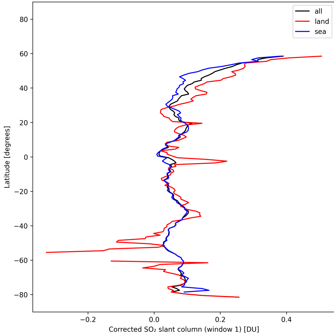
Figure 39: Zonal average of “Corrected SO 2 slant column (window 1)” for 2025-02-16 to 2025-02-18.
