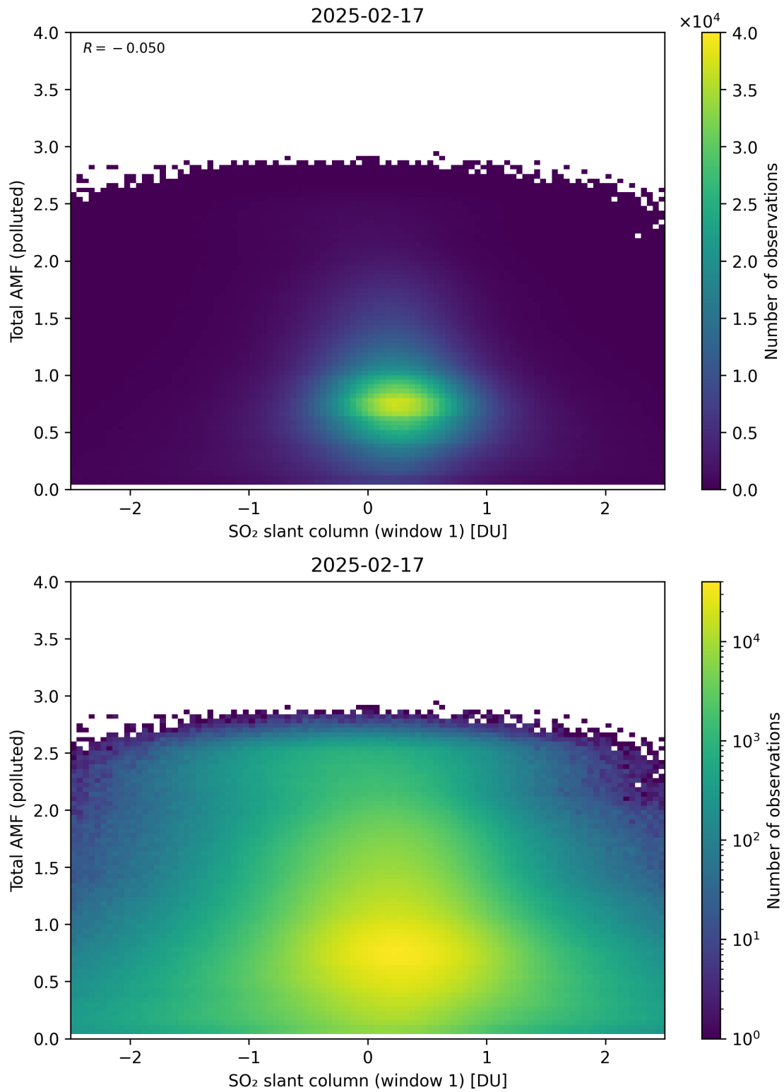
Figure 289: Scatter density plot of “SO 2 slant column (window 1)” against “Total AMF (polluted)” for 2025-02-16 to 2025-02-18.
