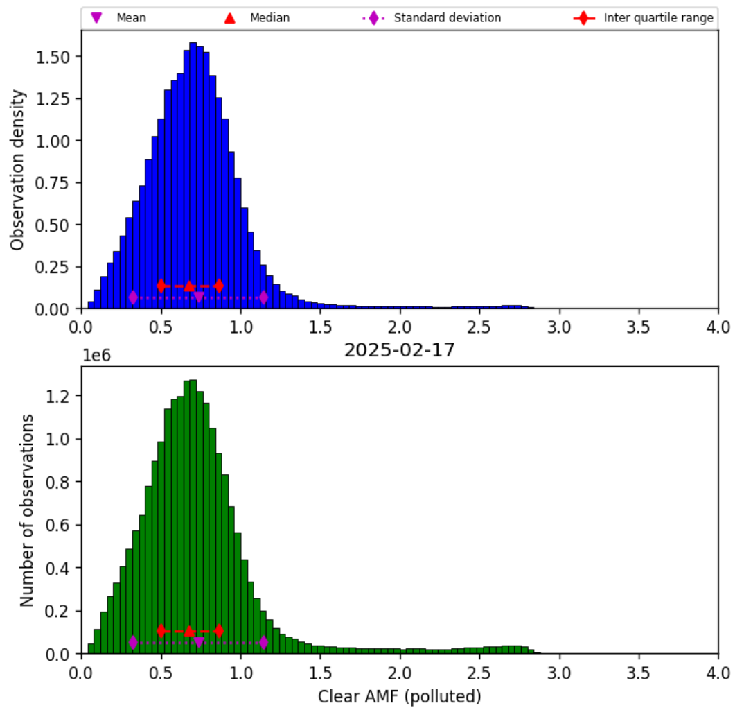
Figure 81: Histogram of “Clear AMF (polluted)” for 2025-02-16 to 2025-02-18
