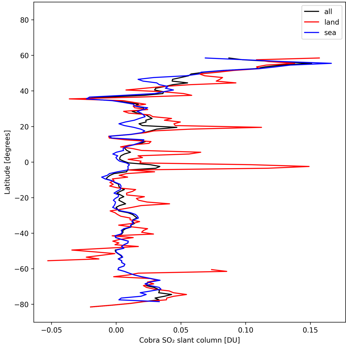
Figure 35: Zonal average of “Cobra SO 2 slant column” for 2025-02-16 to 2025-02-18.
