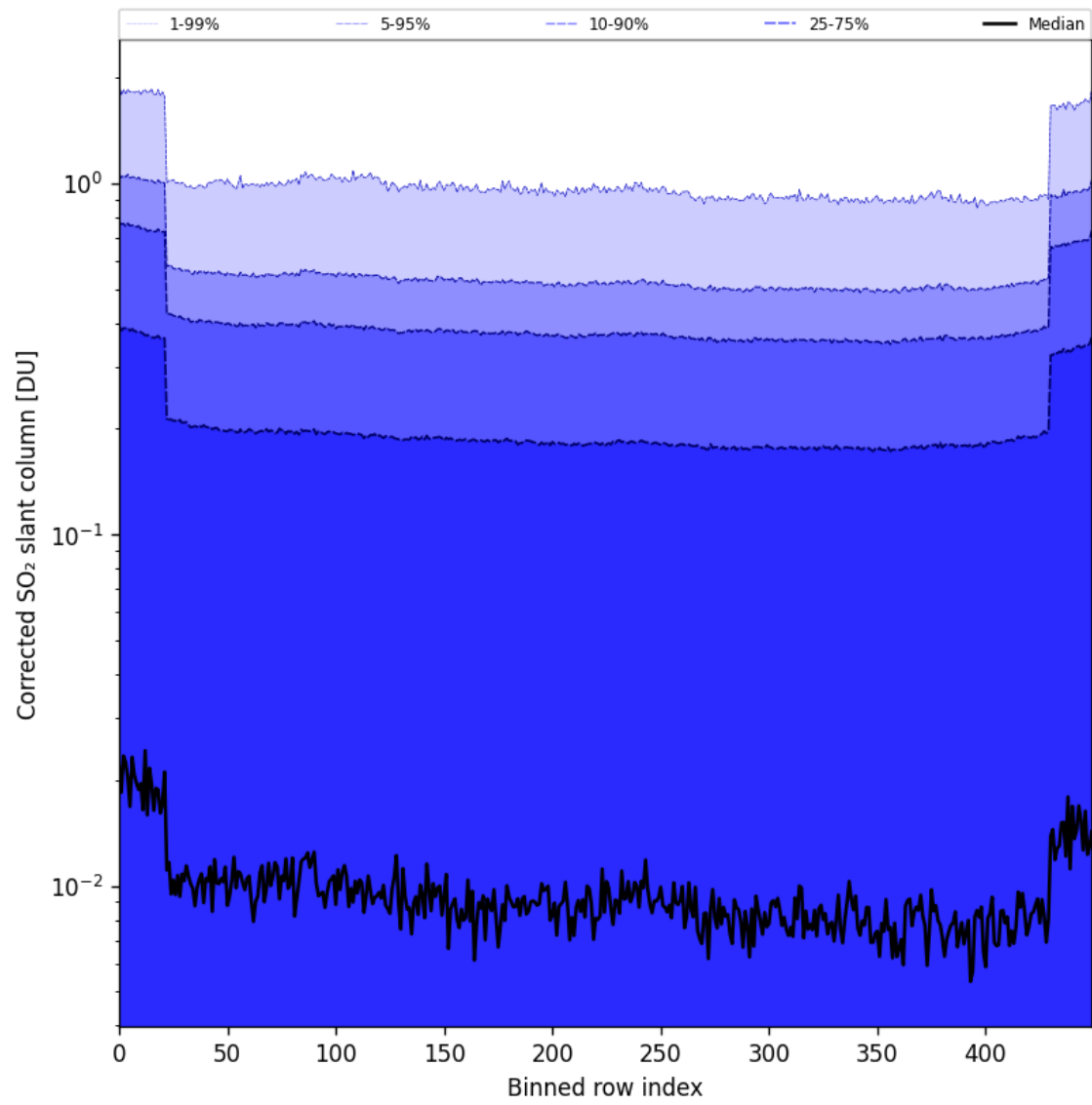
Figure 86: Along track statistics of “Corrected SO 2 slant column” for 2025-02-16 to 2025-02-18
