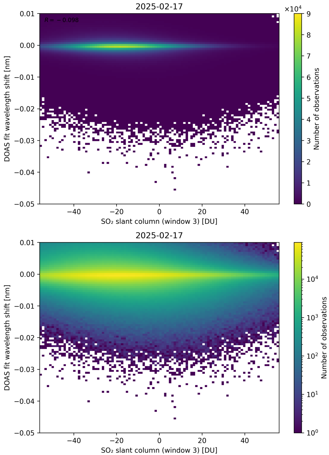
Figure 304: Scatter density plot of “SO 2 slant column (window 3)” against “DOAS fit wavelength shift” for 2025-02-16 to 2025-02-18.
