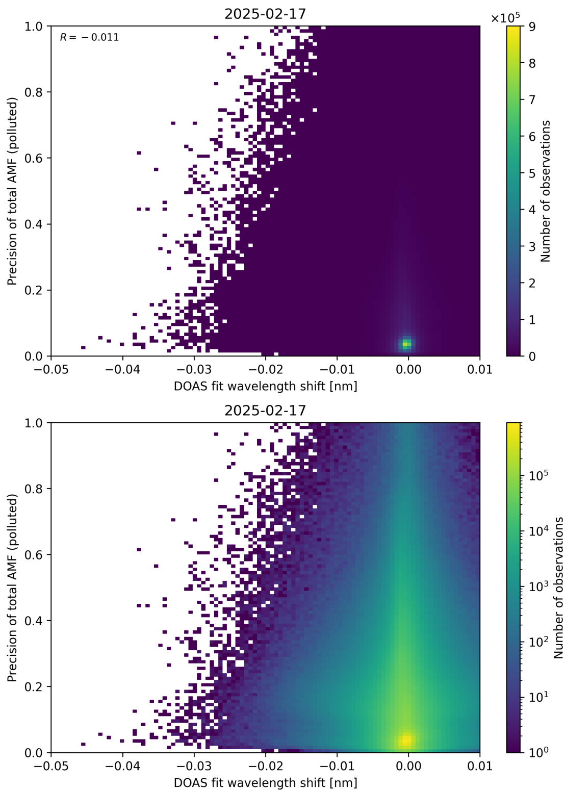
Figure 142: Scatter density plot of “DOAS fit wavelength shift” against “Precision of total AMF (polluted)” for 2025-02-16 to 2025-02-18.
