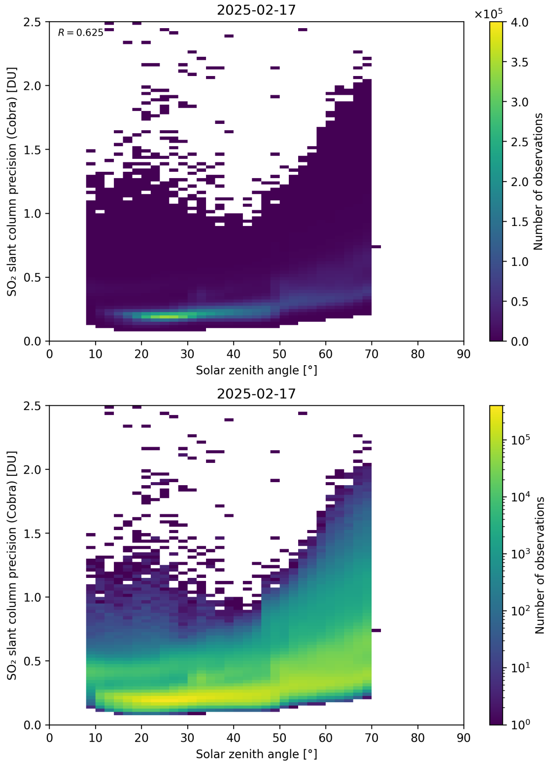
Figure 180: Scatter density plot of “Solar zenith angle” against “SO 2 slant column precision (Cobra)” for 2025-02-16 to 2025-02-18.
