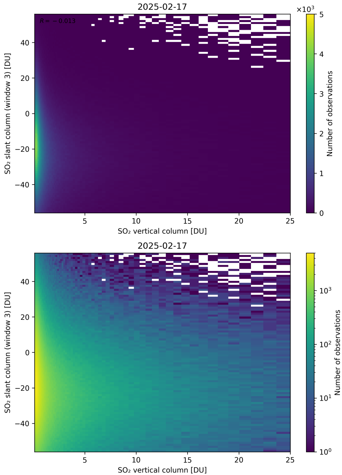
Figure 357: Scatter density plot of “SO 2 vertical column” against “SO 2 slant column (window 3)” for 2025-02-16 to 2025-02-18.
