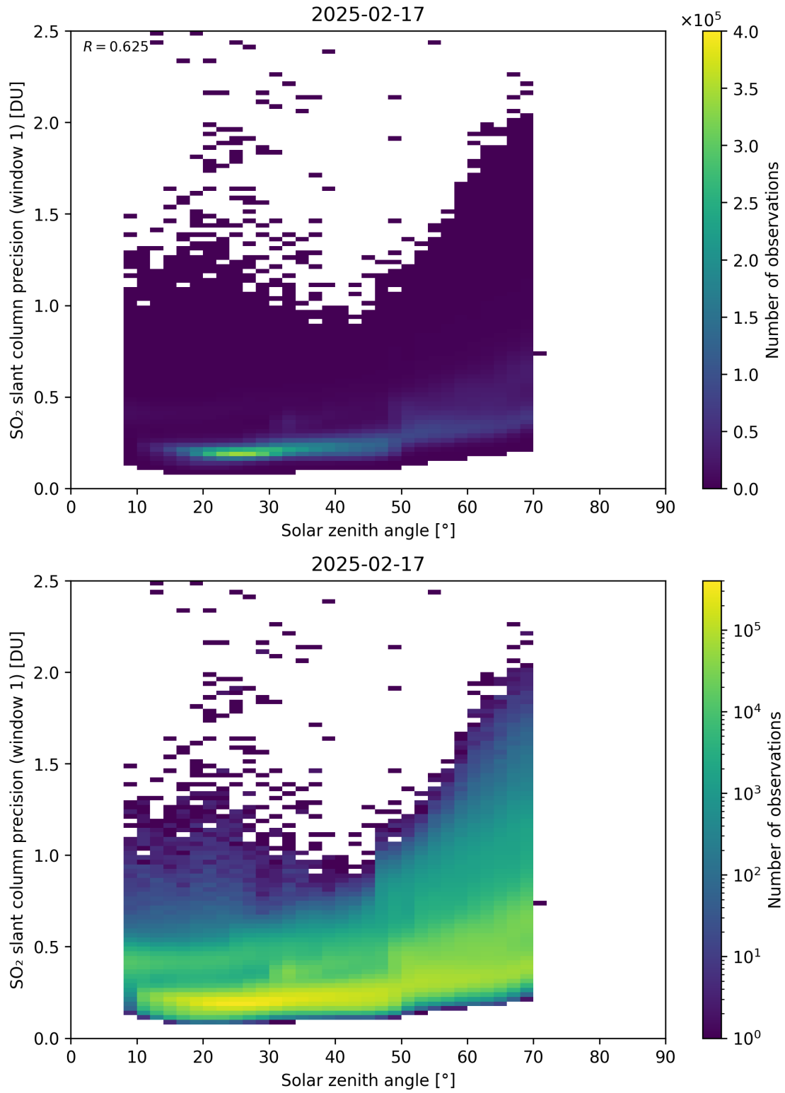
Figure 185: Scatter density plot of “Solar zenith angle” against “SO 2 slant column precision (window 1)” for 2025-02-16 to 2025-02-18.
