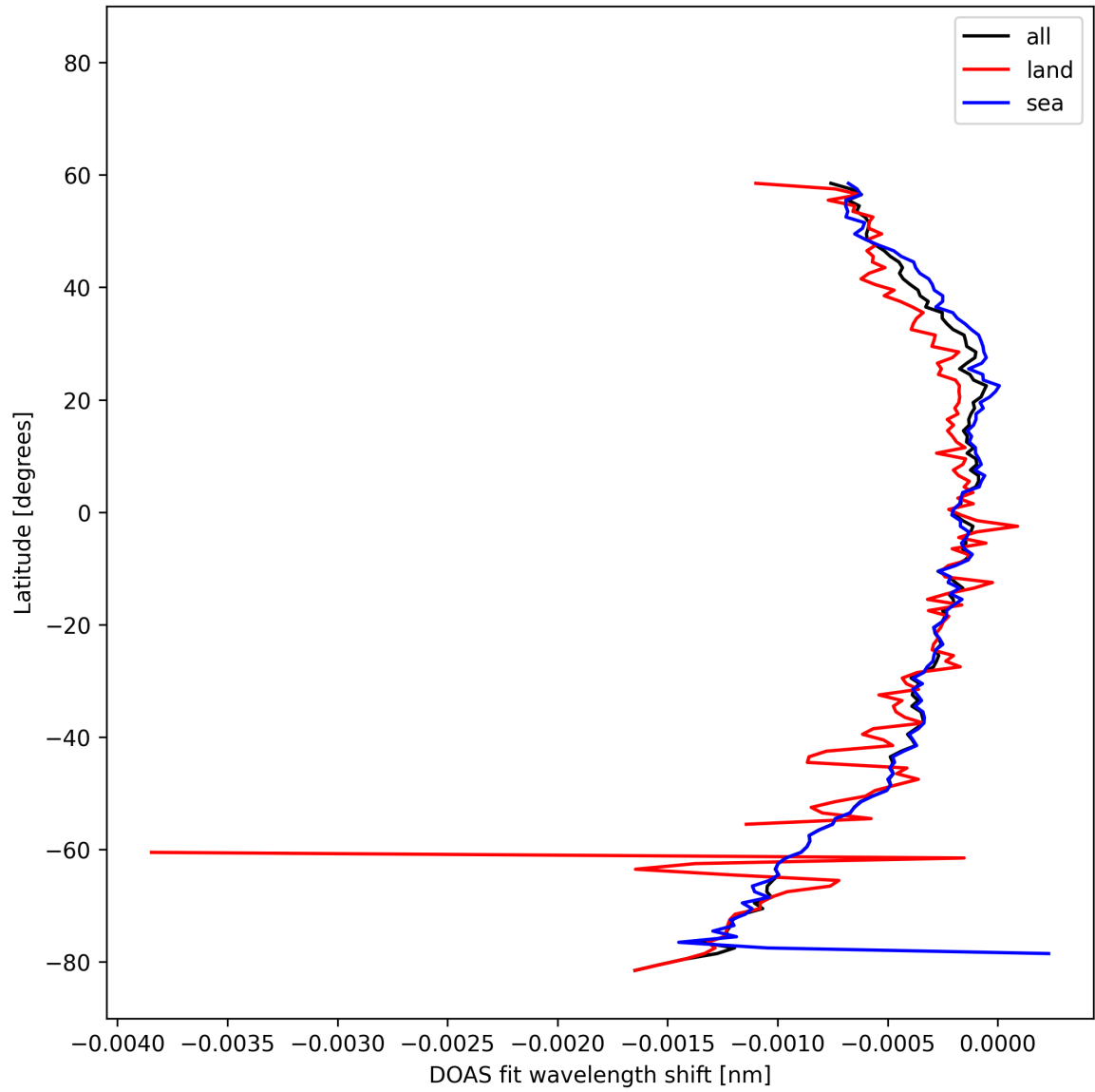
Figure 50: Zonal average of “DOAS fit wavelength shift” for 2025-02-16 to 2025-02-18.
