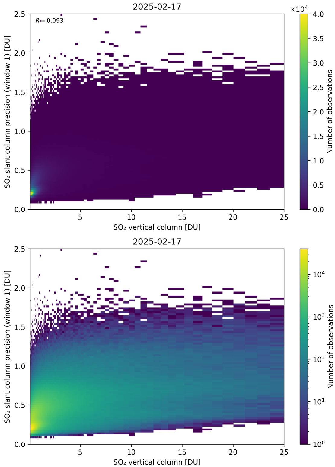
Figure 355: Scatter density plot of “SO 2 vertical column” against “SO 2 slant column precision (window 1)” for 2025-02-16 to 2025-02-18.
