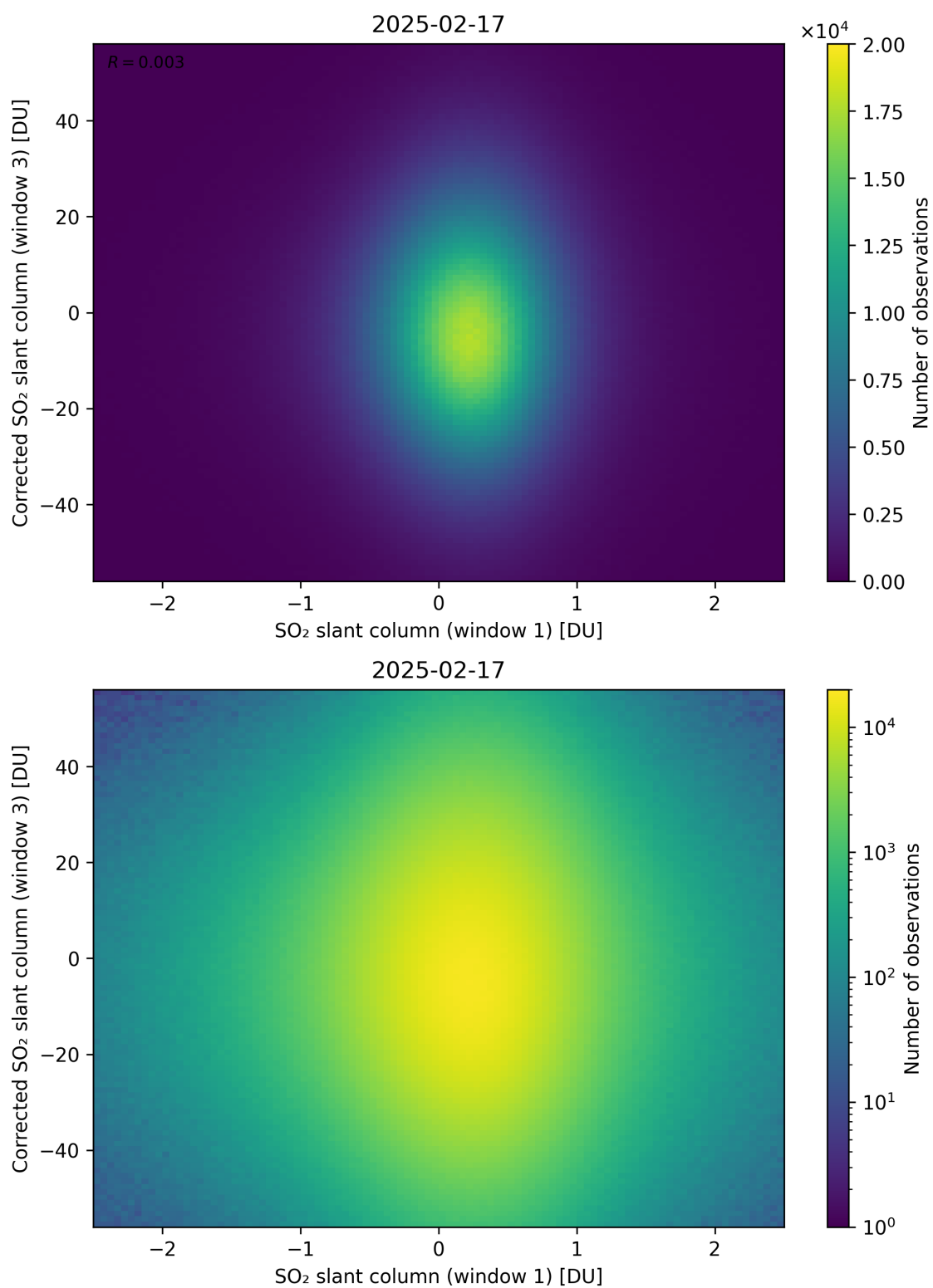
Figure 284: Scatter density plot of “SO 2 slant column (window 1)” against “Corrected SO 2 slant column (window 3)” for 2025-02-16 to 2025-02-18.
