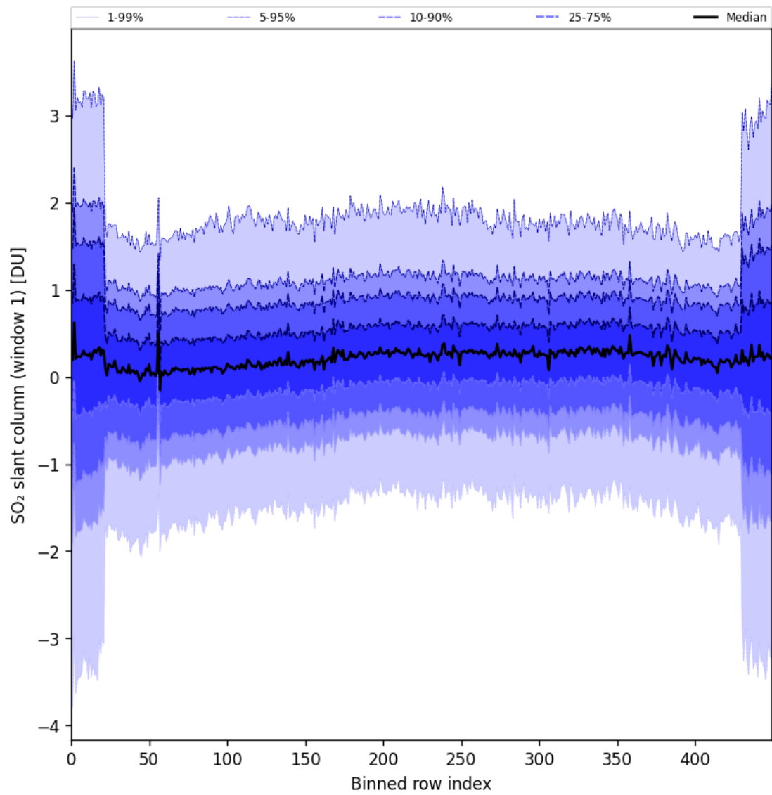
Figure 89: Along track statistics of “SO 2 slant column (window 1)” for 2025-02-16 to 2025-02-18
