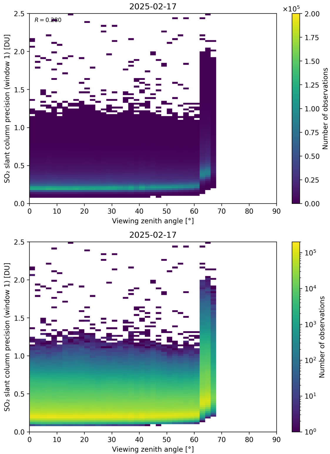
Figure 377: Scatter density plot of “Viewing zenith angle” against “SO 2 slant column precision (window 1)” for 2025-02-16 to 2025-02-18.
