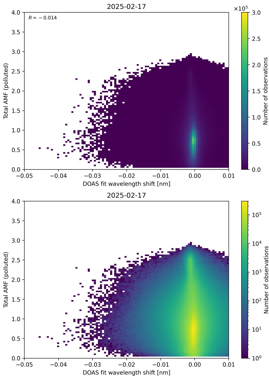
Figure 141: Scatter density plot of “DOAS fit wavelength shift” against “Total AMF (polluted)” for 2025-02-16 to 2025-02-18.
