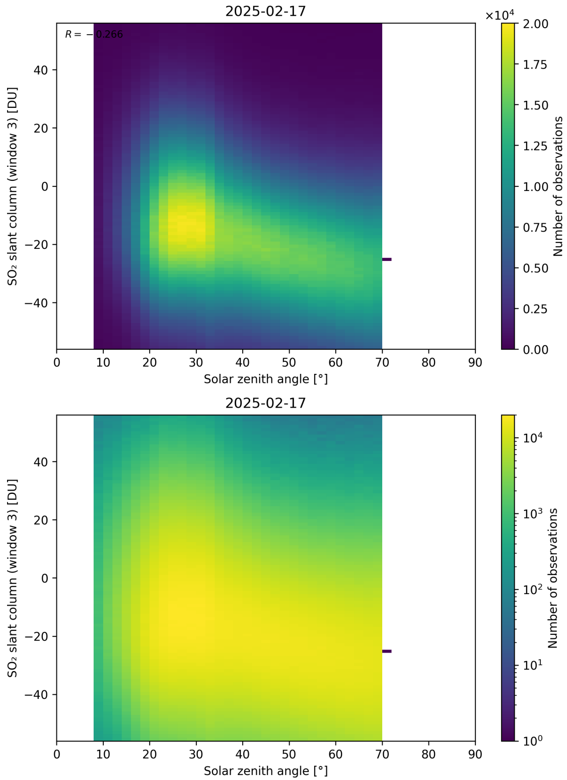
Figure 187: Scatter density plot of “Solar zenith angle” against “SO 2 slant column (window 3)” for 2025-02-16 to 2025-02-18.
