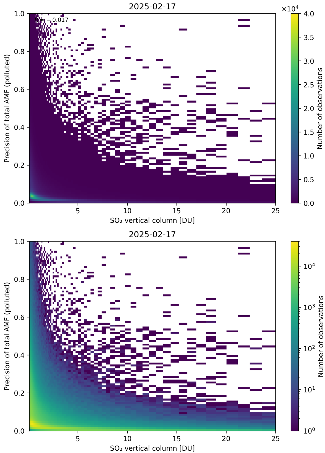
Figure 360: Scatter density plot of “SO 2 vertical column” against “Precision of total AMF (polluted)” for 2025-02-16 to 2025-02-18.
