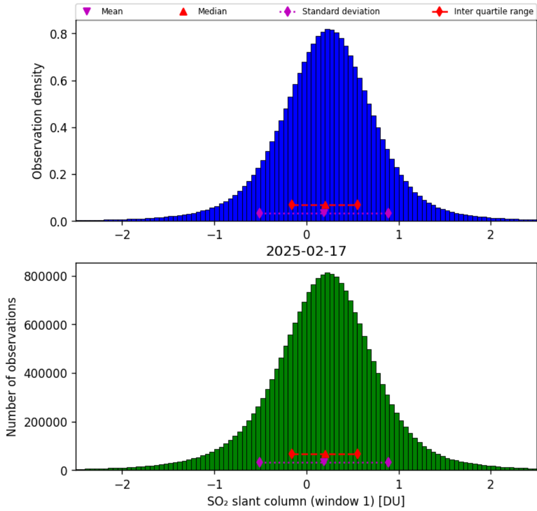
Figure 63: Histogram of “SO 2 slant column (window 1)” for 2025-02-16 to 2025-02-18
