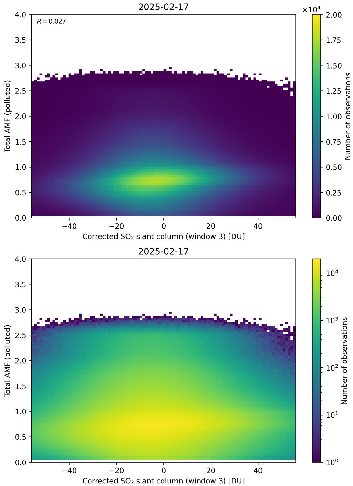
Figure 260: Scatter density plot of “Corrected SO 2 slant column (window 3)” against “Total AMF (polluted)” for 2025-02-16 to 2025-02-18.
