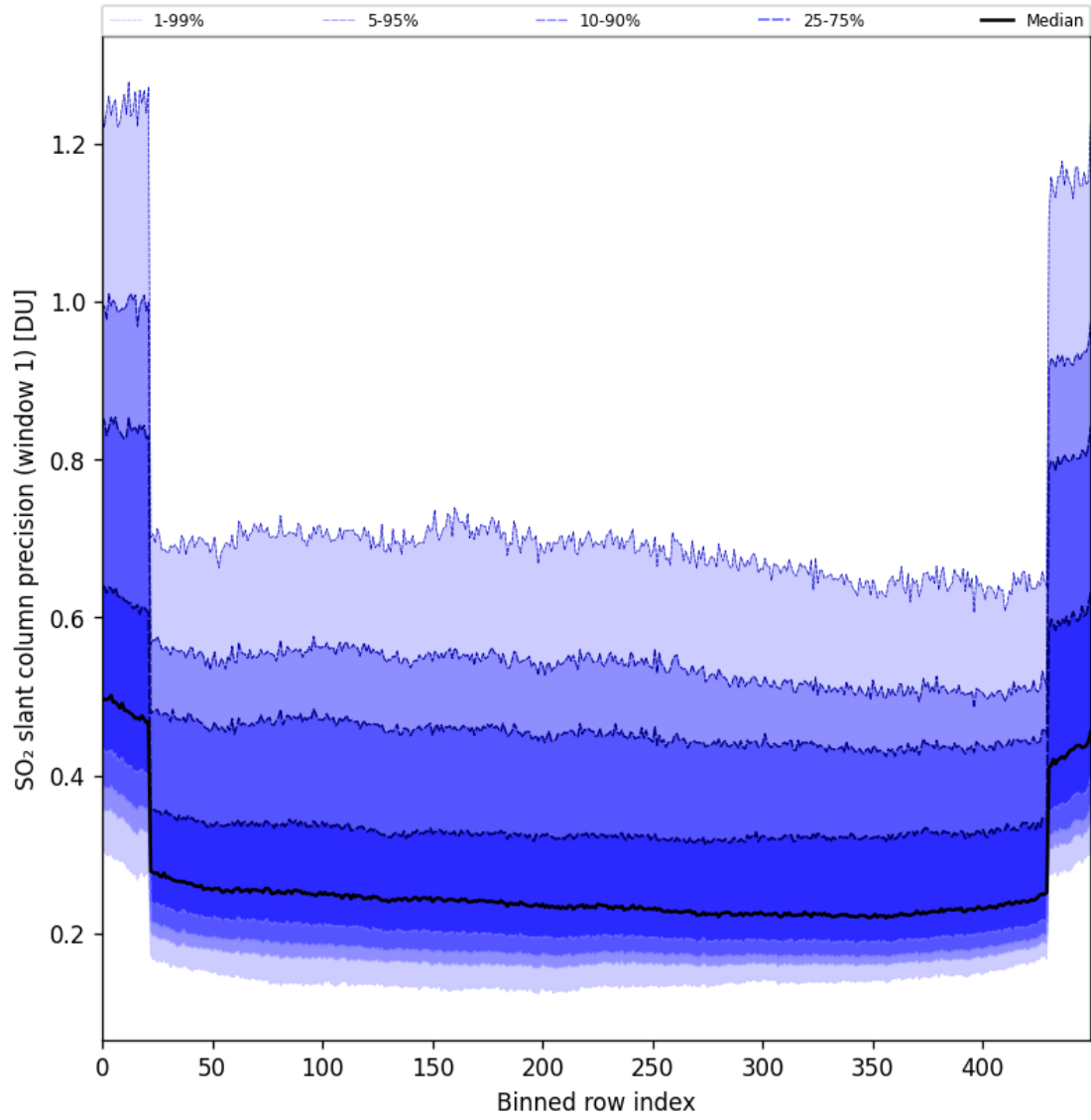
Figure 90: Along track statistics of “SO 2 slant column precision (window 1)” for 2025-02-16 to 2025-02-18
