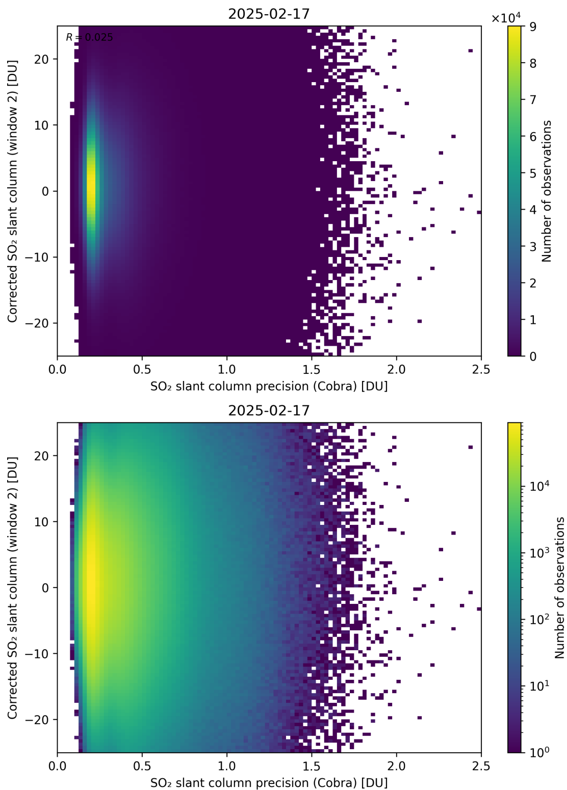
Figure 206: Scatter density plot of “SO 2 slant column precision (Cobra)” against “Corrected SO 2 slant column (window 2)” for 2025-02-16 to 2025-02-18.
