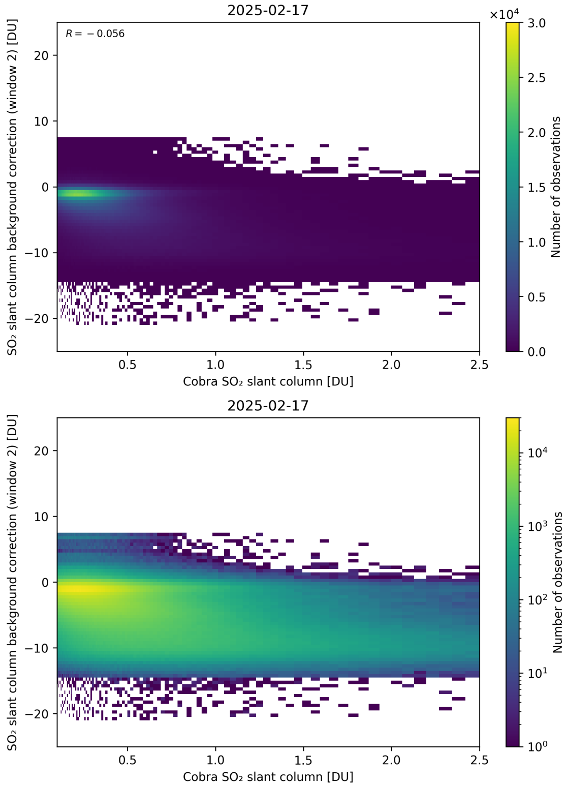
Figure 194: Scatter density plot of “Cobra SO 2 slant column” against “SO 2 slant column background correction (window 2)” for 2025-02-16 to 2025-02-18.
