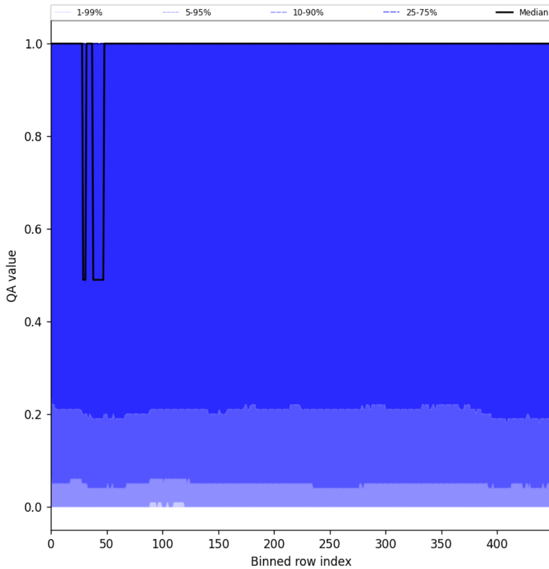
Figure 83: Along track statistics of “QA value” for 2025-02-16 to 2025-02-18
