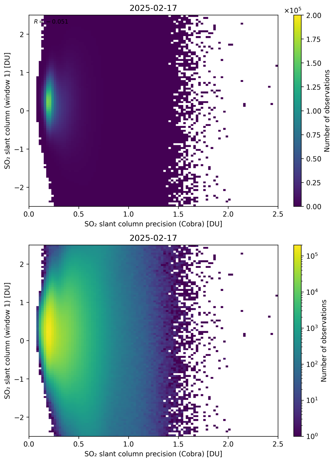
Figure 208: Scatter density plot of “SO 2 slant column precision (Cobra)” against “SO 2 slant column (window 1)” for 2025-02-16 to 2025-02-18.
