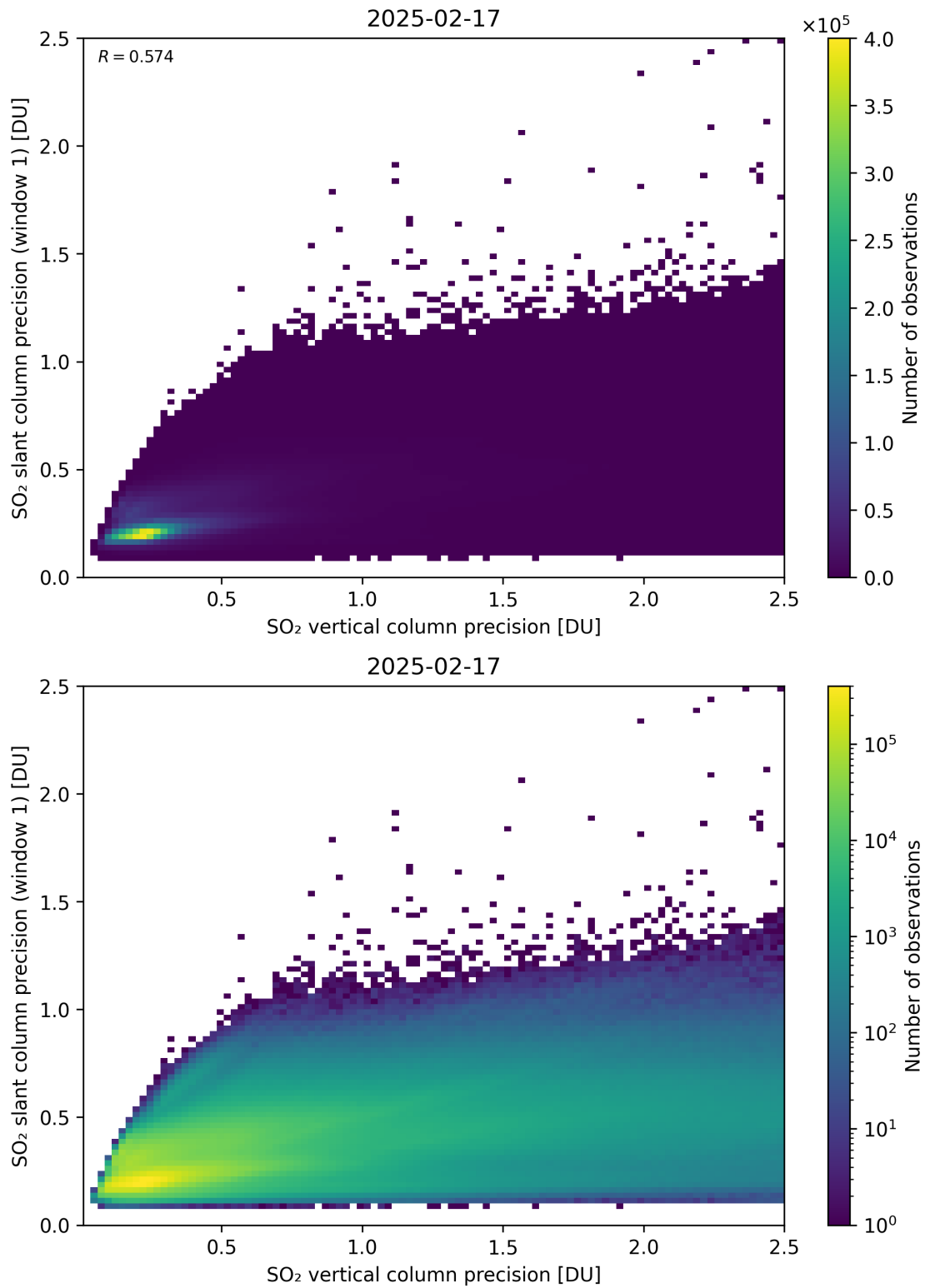
Figure 342: Scatter density plot of “SO 2 vertical column precision” against “SO 2 slant column precision (window 1)” for 2025-02-16 to 2025-02-18.
