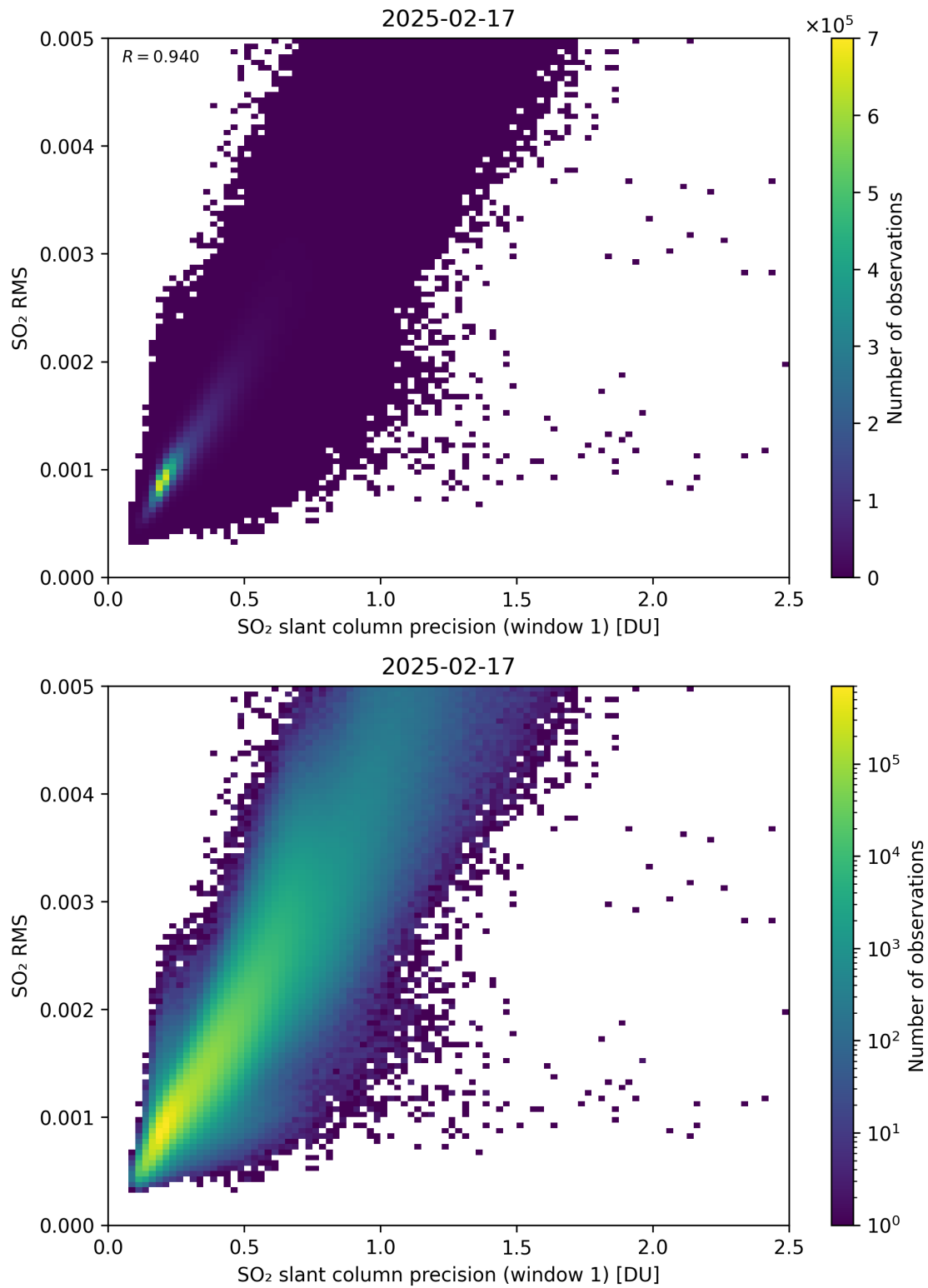
Figure 273: Scatter density plot of “SO 2 slant column precision (window 1)” against “SO 2 RMS” for 2025-02-16 to 2025-02-18.
