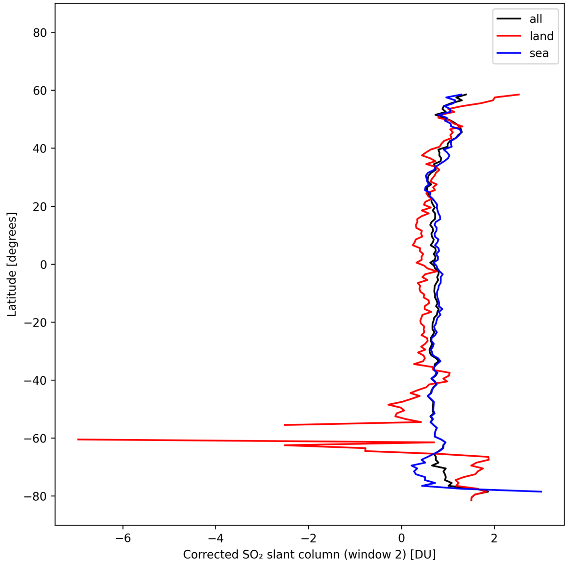
Figure 43: Zonal average of “Corrected SO 2 slant column (window 2)” for 2025-02-16 to 2025-02-18.
