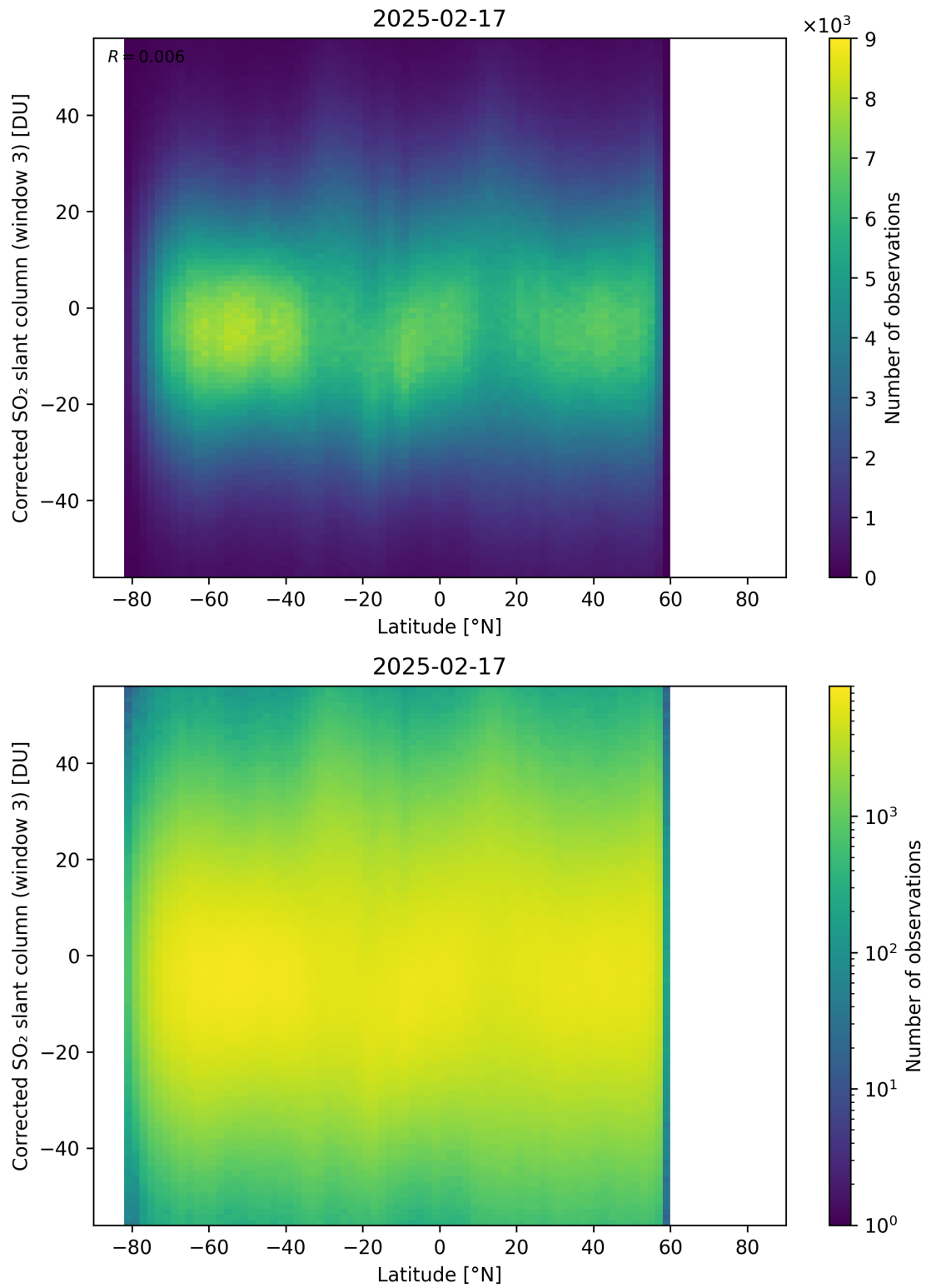
Figure 161: Scatter density plot of “Latitude” against “Corrected SO 2 slant column (window 3)” for 2025-02-16 to 2025-02-18.
