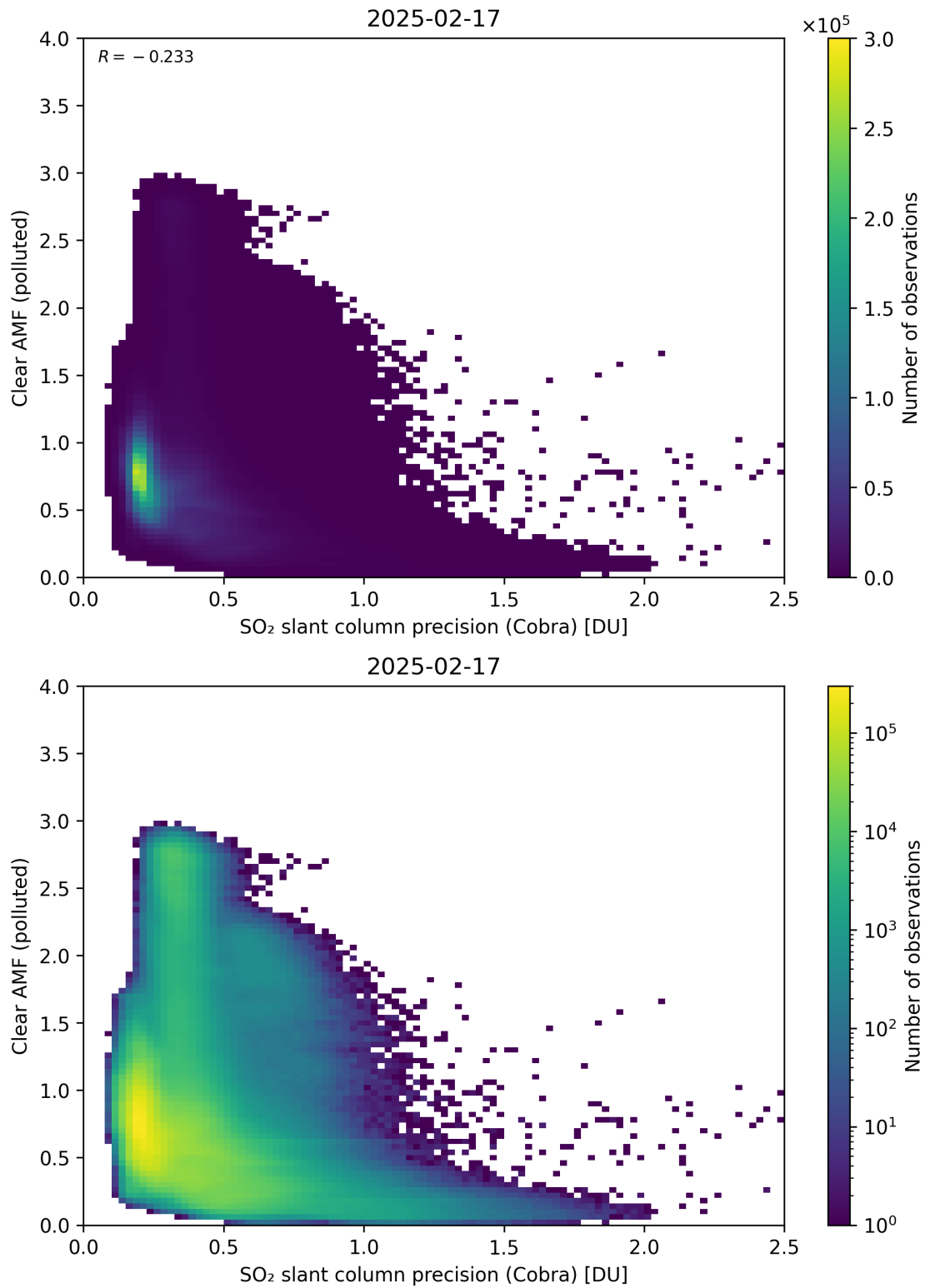
Figure 205: Scatter density plot of “SO 2 slant column precision (Cobra)” against “Clear AMF (polluted)” for 2025-02-16 to 2025-02-18.
