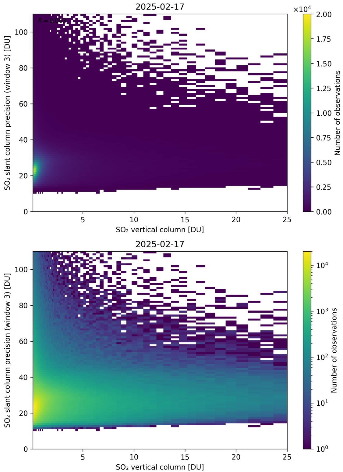
Figure 358: Scatter density plot of “SO 2 vertical column” against “SO 2 slant column precision (window 3)” for 2025-02-16 to 2025-02-18.
