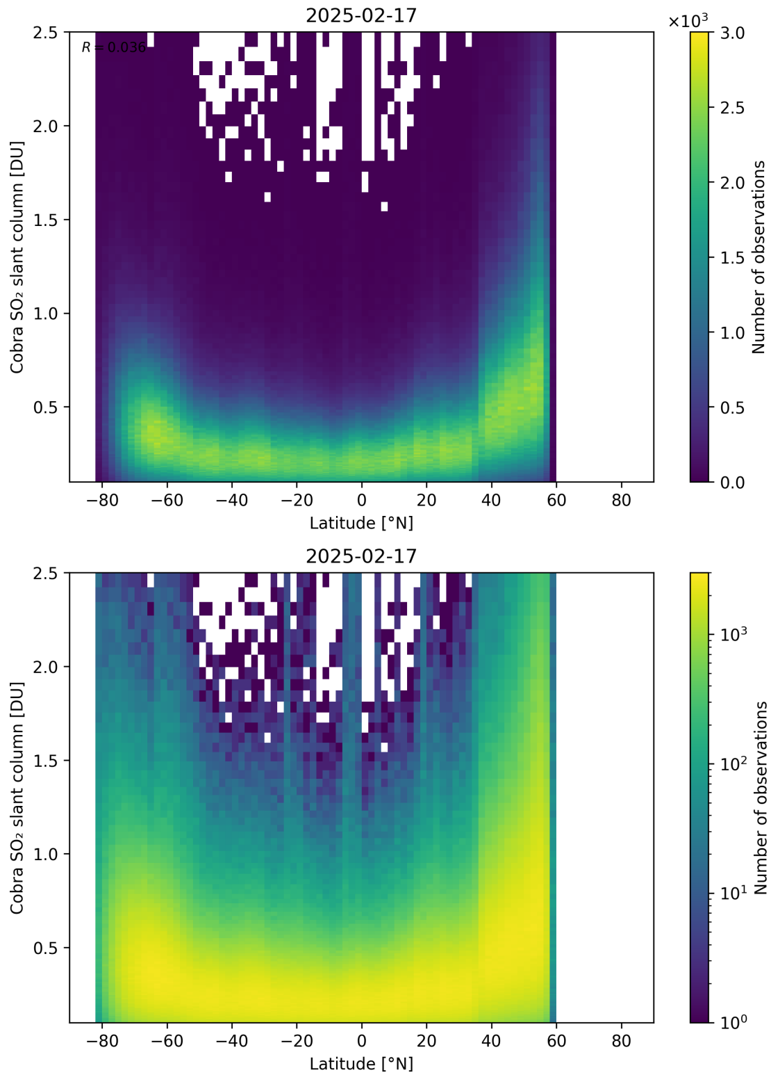
Figure 157: Scatter density plot of “Latitude” against “Cobra SO 2 slant column” for 2025-02-16 to 2025-02-18.
