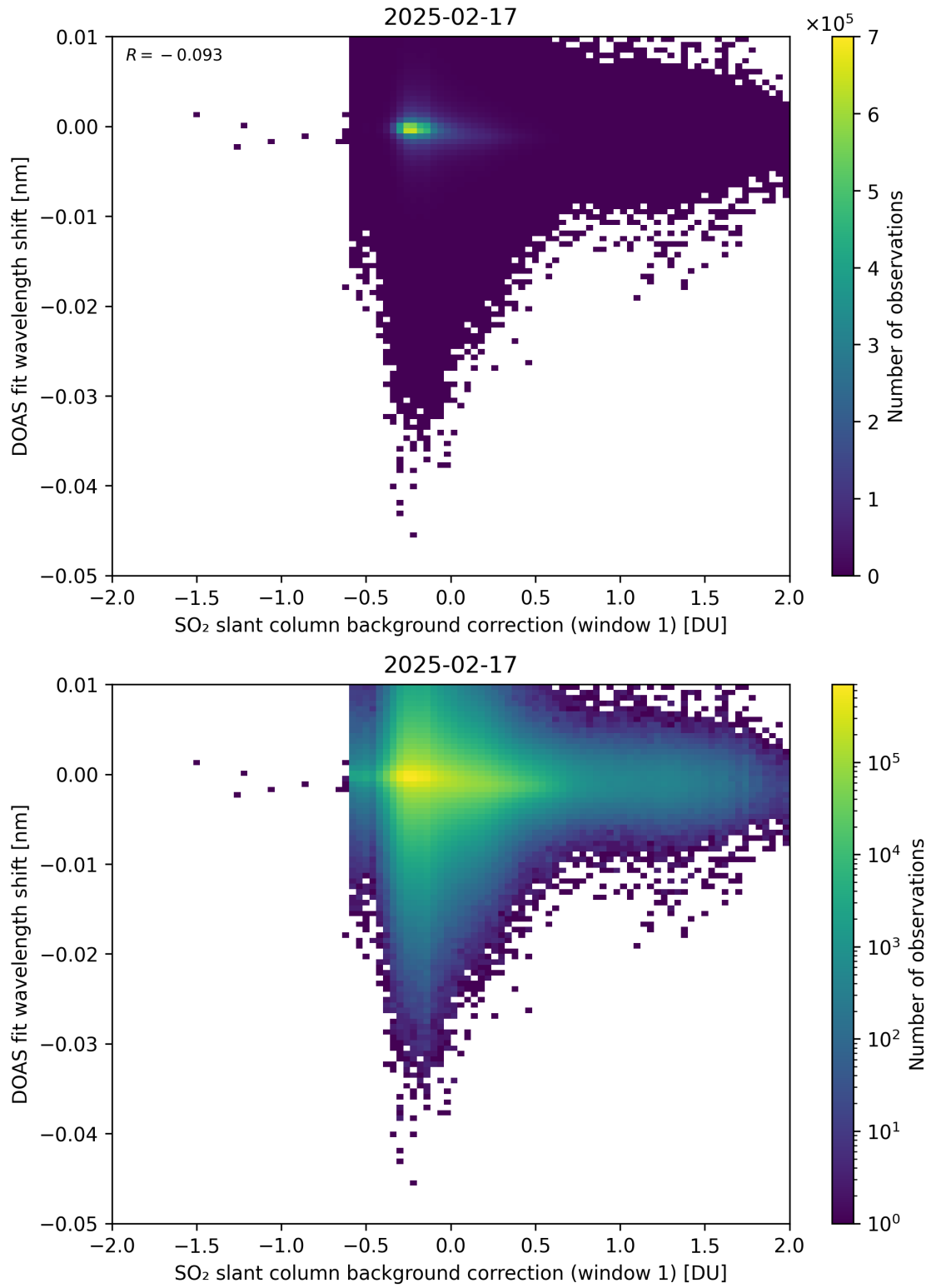
Figure 111: Scatter density plot of “SO 2 slant column background correction (window 1)” against “DOAS fit wavelength shift” for 2025-02-16 to 2025-02-18.
