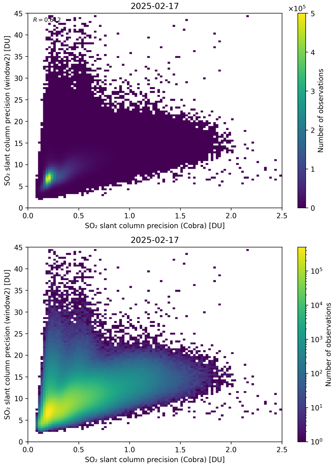
Figure 210: Scatter density plot of “SO 2 slant column precision (Cobra)” against “SO 2 slant column precision (window2)” for 2025-02-16 to 2025-02-18.
