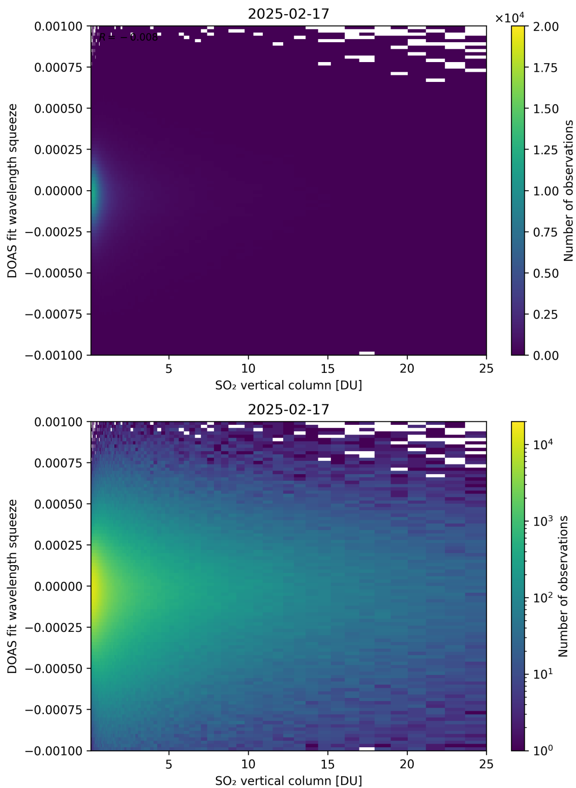
Figure 327: Scatter density plot of “SO 2 vertical column” against “DOAS fit wavelength squeeze” for 2025-02-16 to 2025-02-18.
