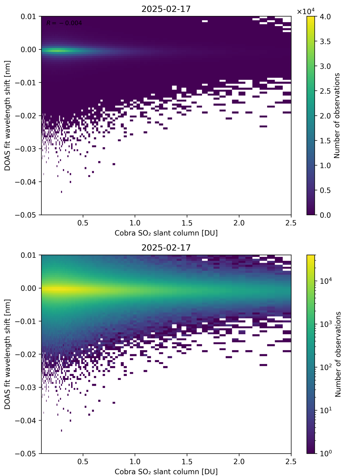
Figure 196: Scatter density plot of “Cobra SO 2 slant column” against “DOAS fit wavelength shift” for 2025-02-16 to 2025-02-18.
