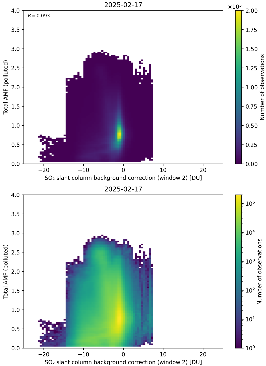
Figure 130: Scatter density plot of “SO 2 slant column background correction (window 2)” against “Total AMF (polluted)” for 2025-02-16 to 2025-02-18.
