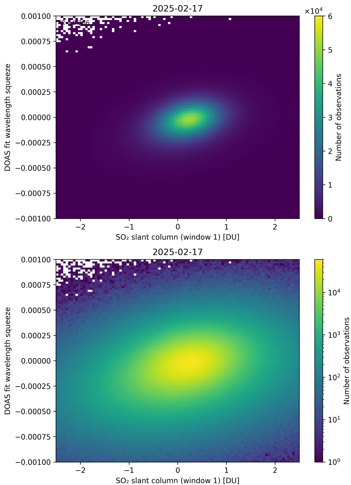
Figure 266: Scatter density plot of “SO 2 slant column (window 1)” against “DOAS fit wavelength squeeze” for 2025-02-16 to 2025-02-18.
