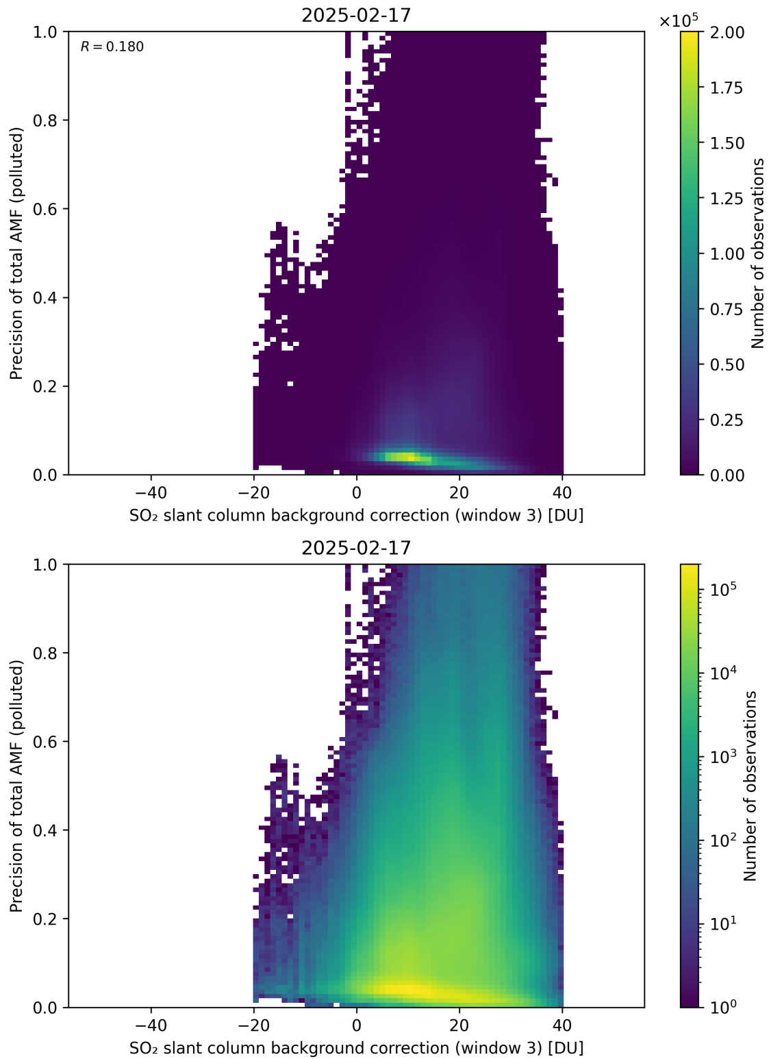
Figure 137: Scatter density plot of “SO 2 slant column background correction (window 3)” against “Precision of total AMF (polluted)” for 2025-02-16 to 2025-02-18.
