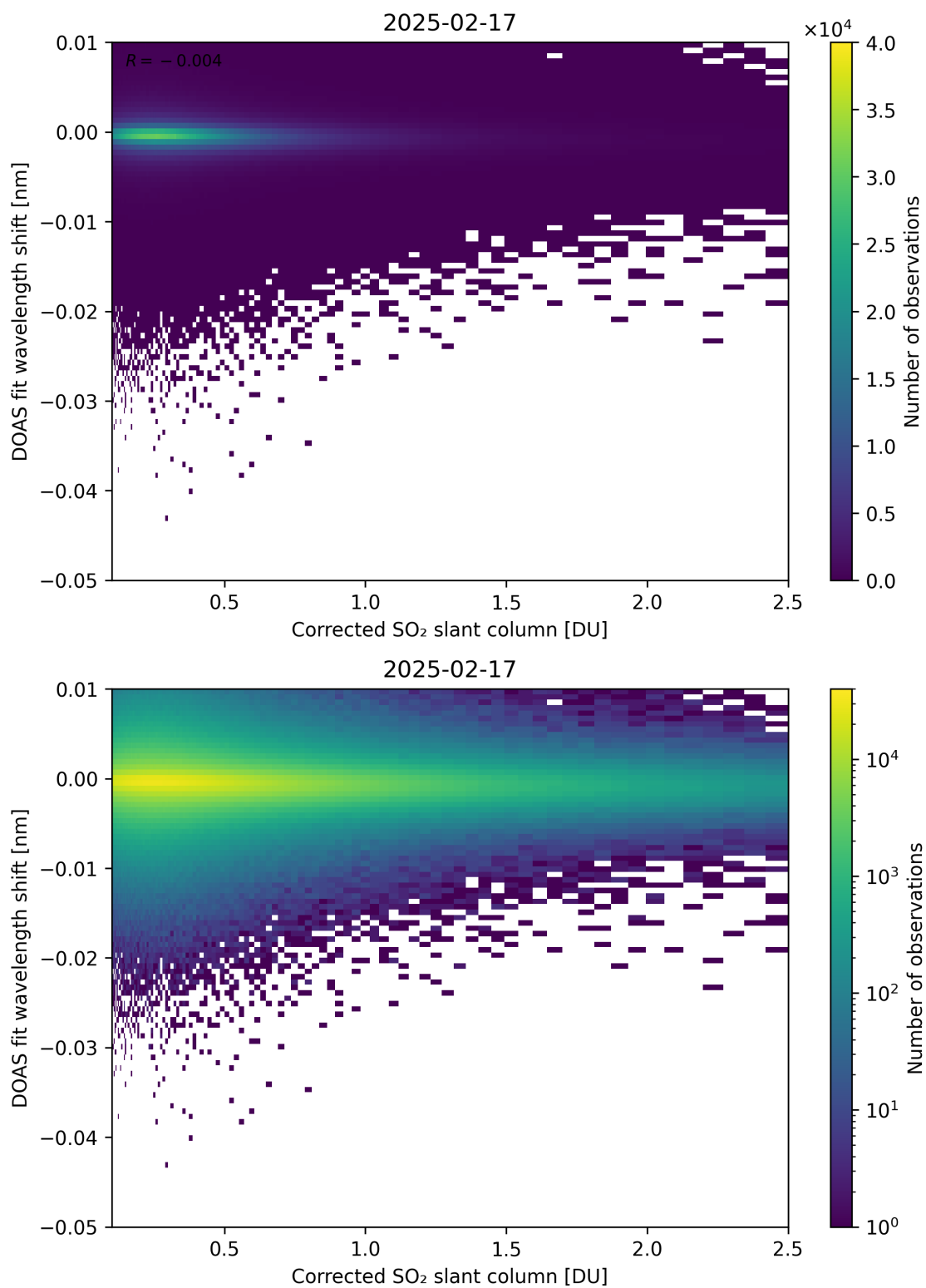
Figure 229: Scatter density plot of “Corrected SO 2 slant column” against “DOAS fit wavelength shift” for 2025-02-16 to 2025-02-18.
