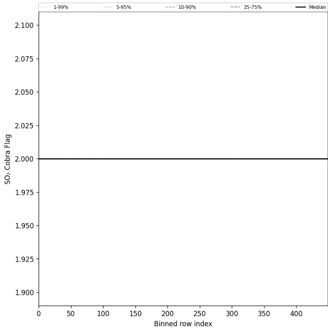
Figure 101: Along track statistics of “SO 2 Cobra Flag” for 2025-02-16 to 2025-02-18
