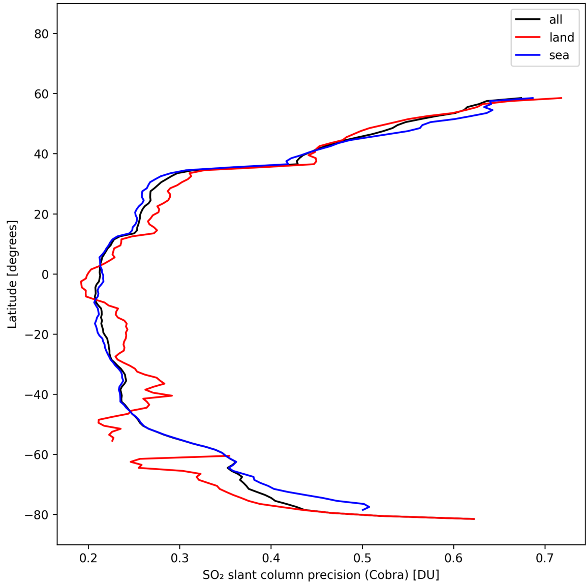
Figure 36: Zonal average of "SO 2 slant column precision (Cobra)" for 2025-02-16 to 2025-02-18.
