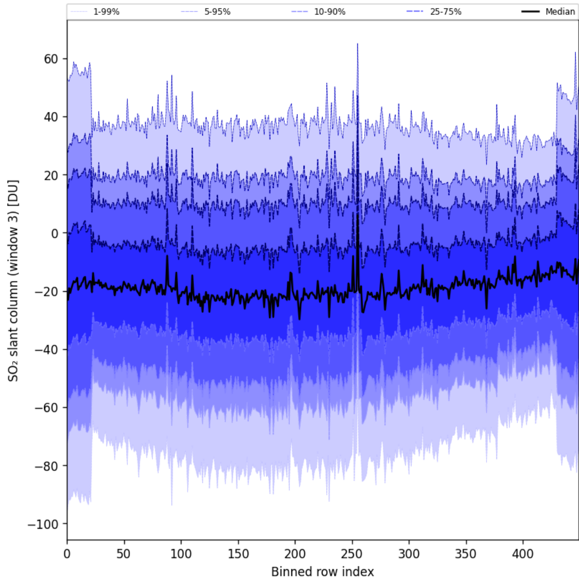
Figure 97: Along track statistics of “SO 2 slant column (window 3)” for 2025-02-16 to 2025-02-18
