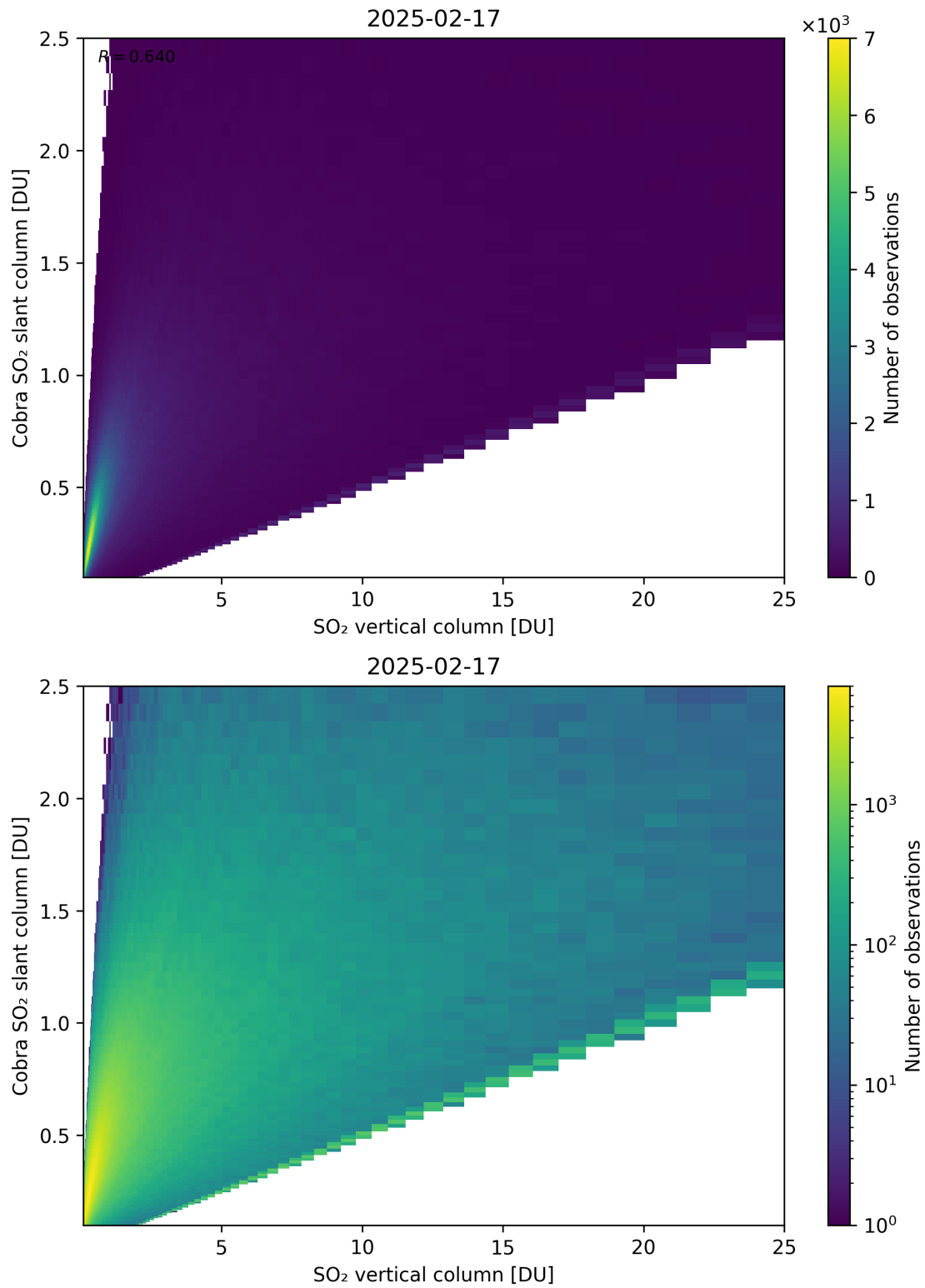
Figure 349: Scatter density plot of “SO 2 vertical column” against “Cobra SO 2 slant column” for 2025-02-16 to 2025-02-18.
