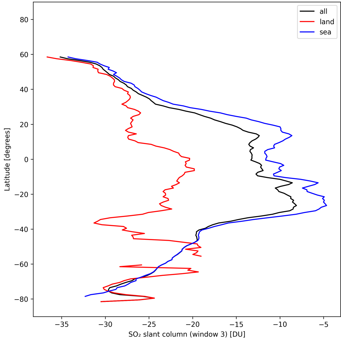
Figure 45: Zonal average of “SO 2 slant column (window 3)” for 2025-02-16 to 2025-02-18.
