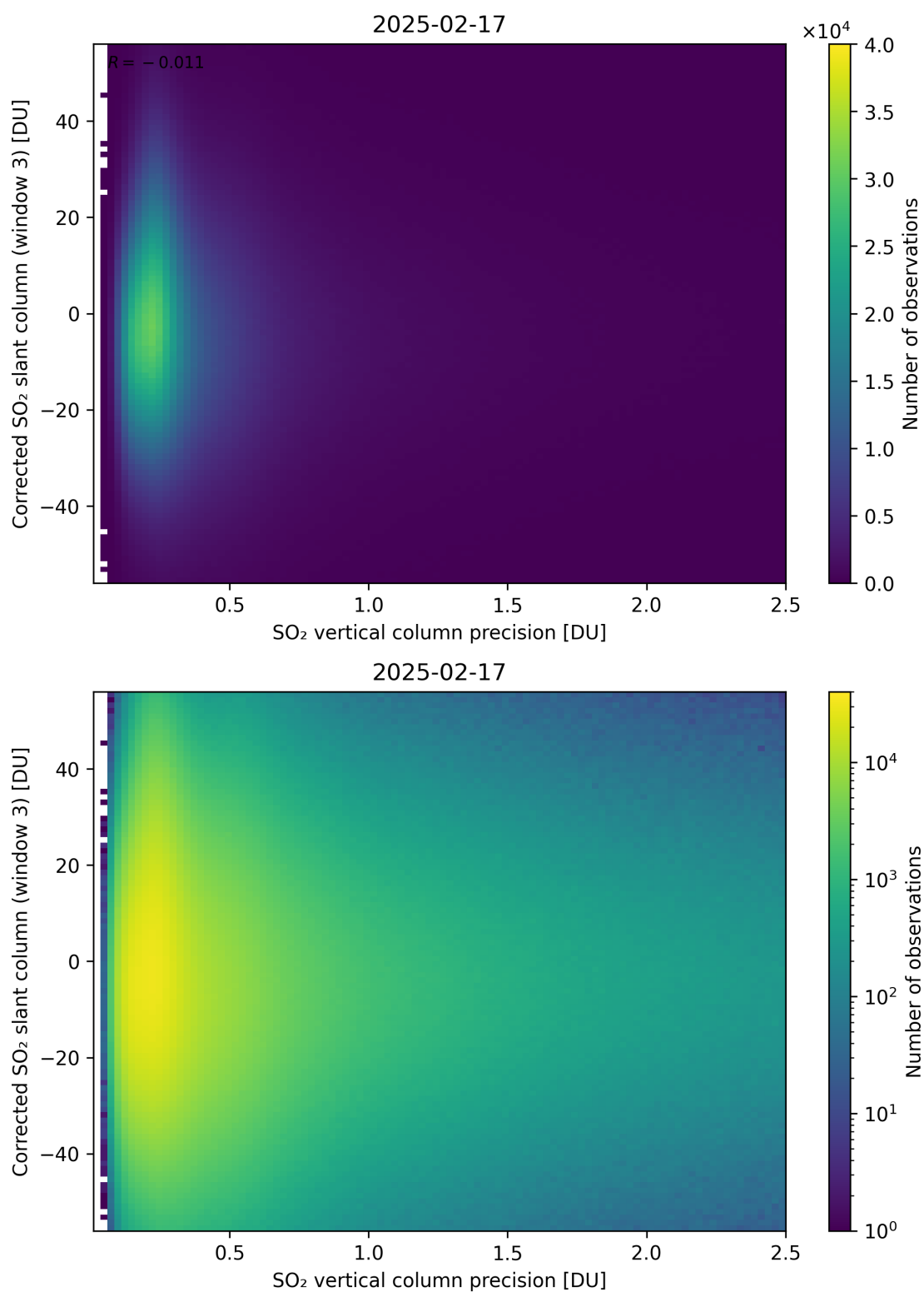
Figure 340: Scatter density plot of “SO 2 vertical column precision” against “Corrected SO 2 slant column (window 3)” for 2025-02-16 to 2025-02-18.
