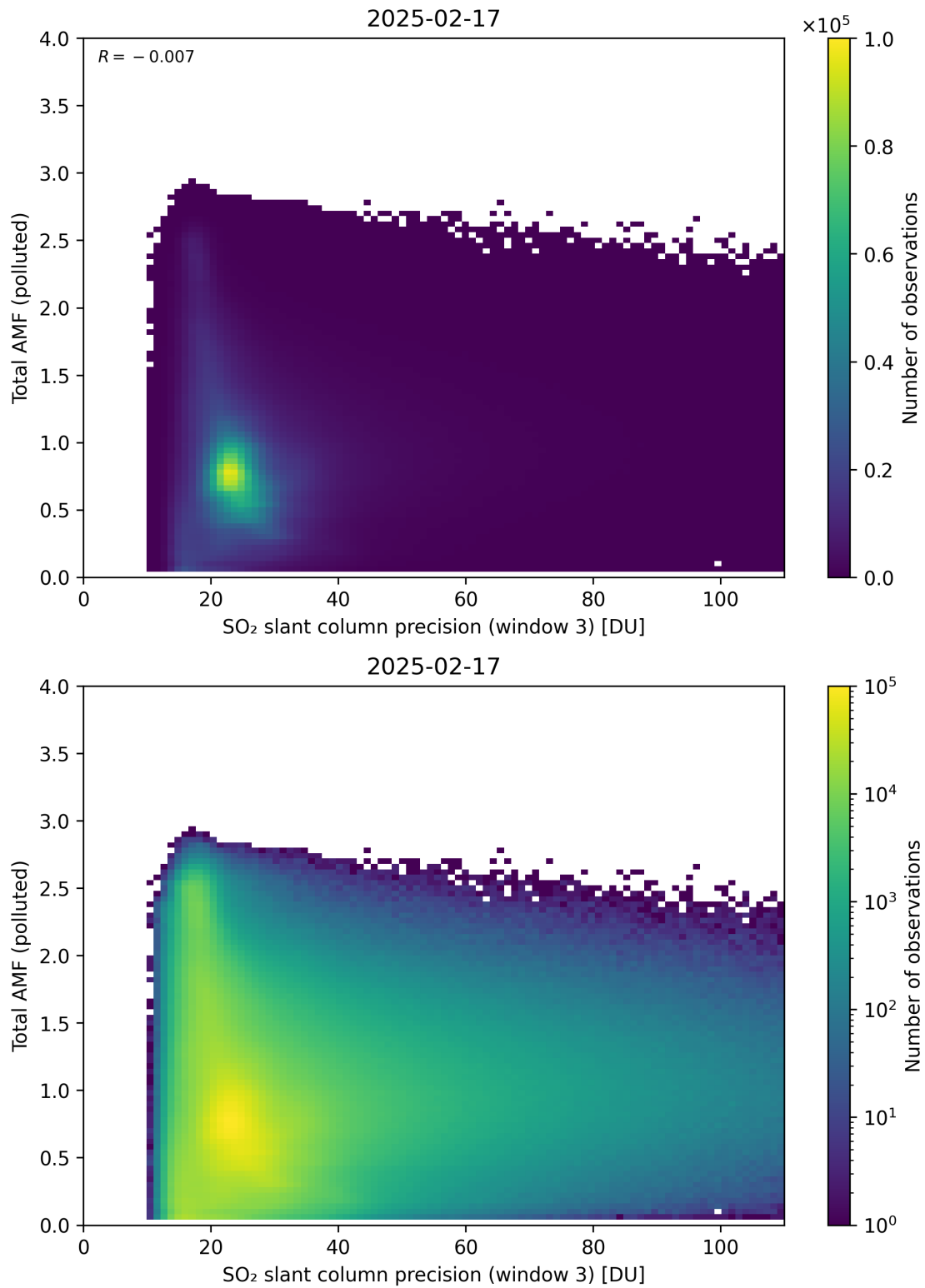
Figure 313: Scatter density plot of “SO 2 slant column precision (window 3)” against “Total AMF (polluted)” for 2025-02-16 to 2025-02-18.
