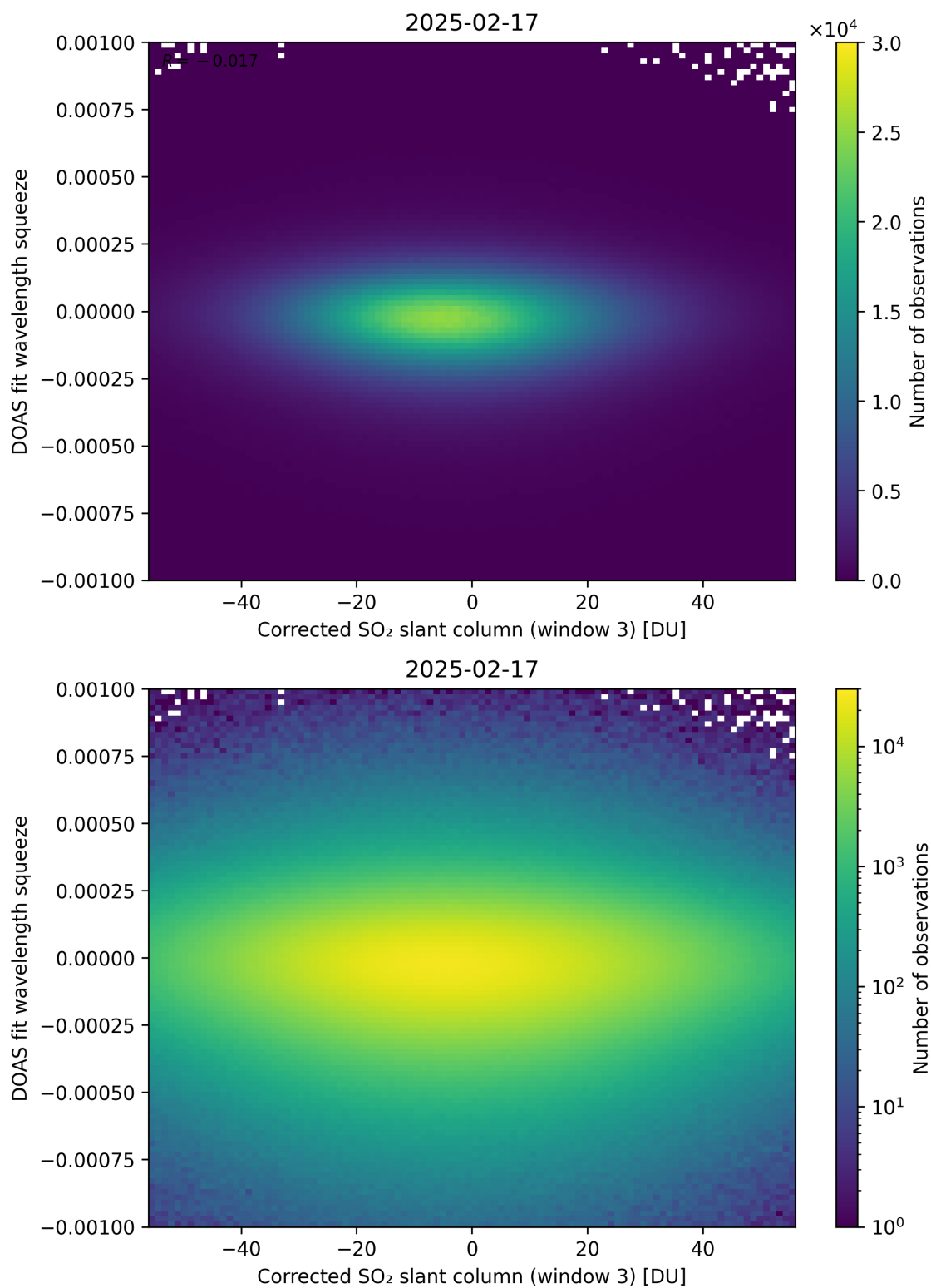
Figure 257: Scatter density plot of “Corrected SO 2 slant column (window 3)” against “DOAS fit wavelength squeeze” for 2025-02-16 to 2025-02-18.
