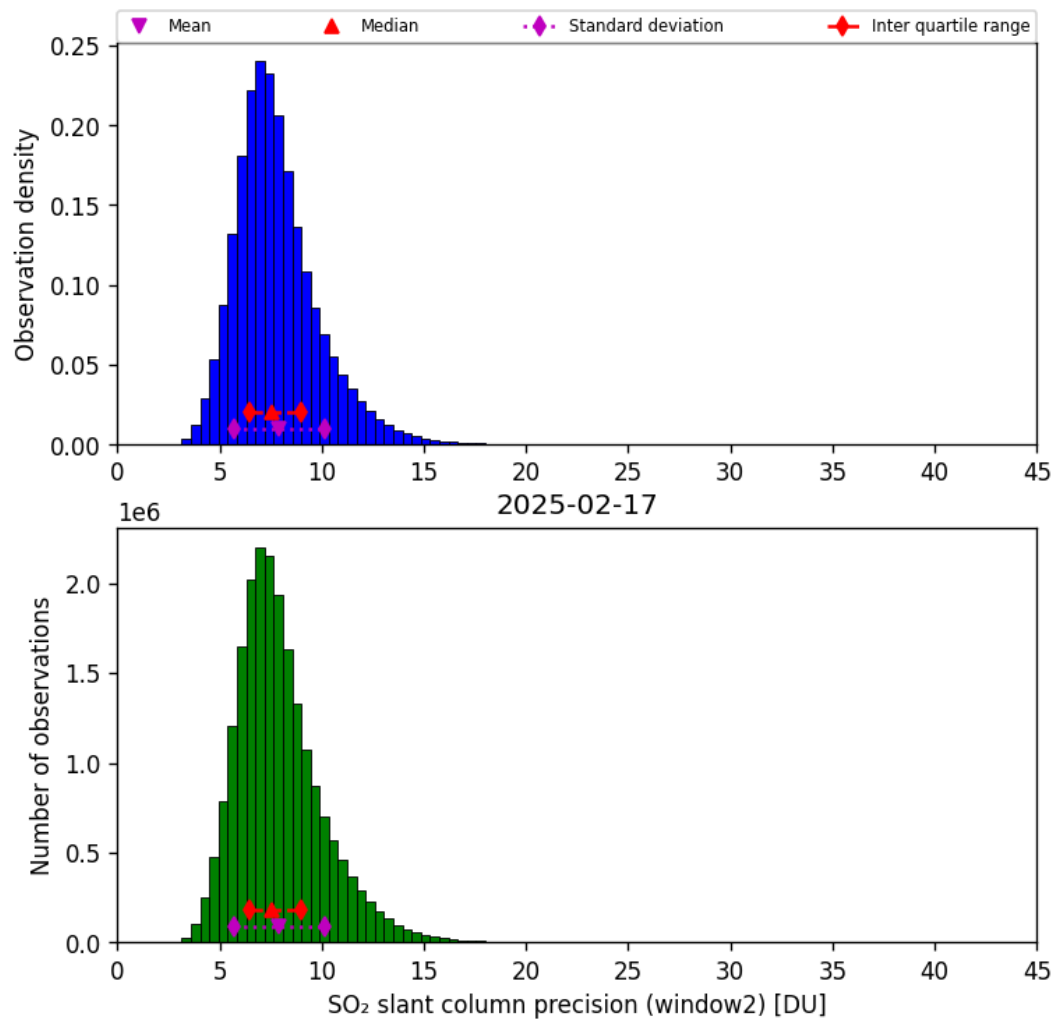
Figure 68: Histogram of “SO 2 slant column precision (window2)” for 2025-02-16 to 2025-02-18
