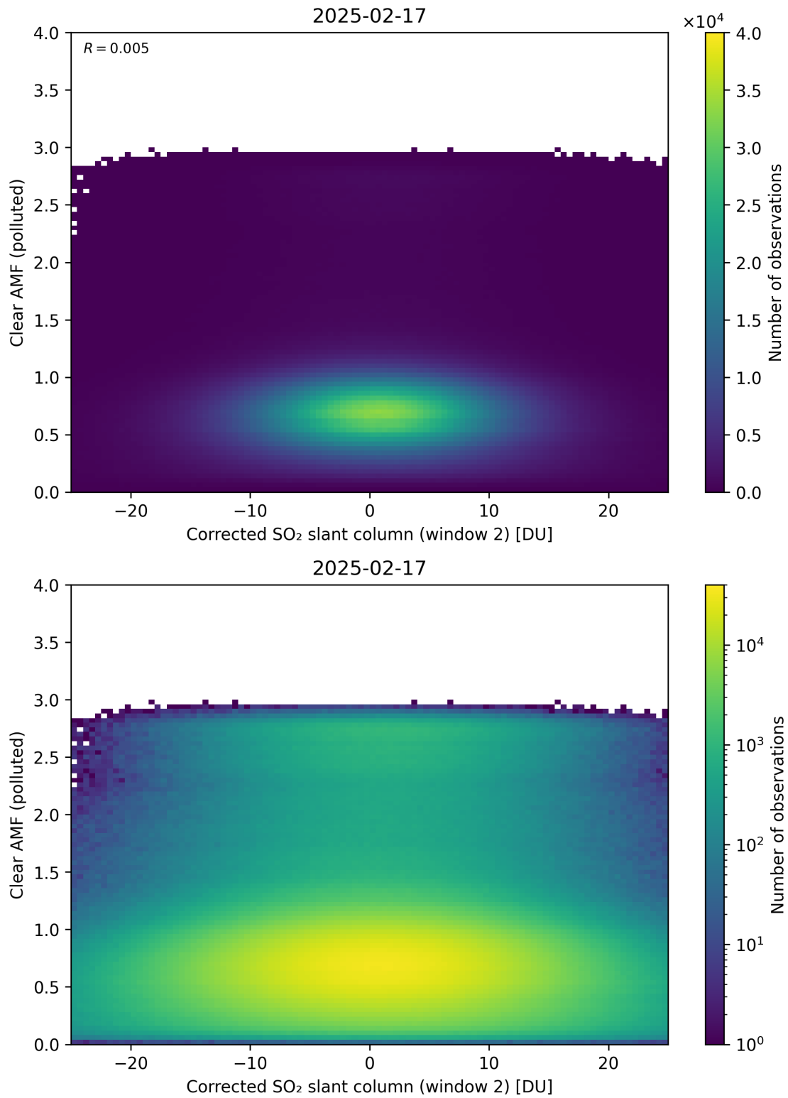
Figure 249: Scatter density plot of “Corrected SO 2 slant column (window 2)” against “Clear AMF (polluted)” for 2025-02-16 to 2025-02-18.
