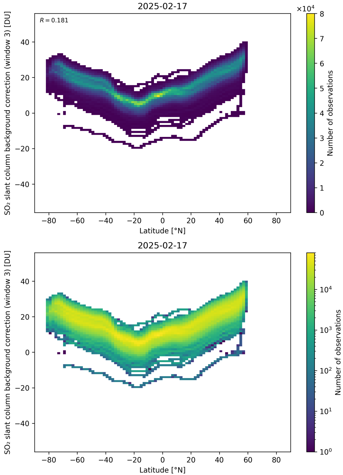
Figure 152: Scatter density plot of “Latitude” against “SO 2 slant column background correction (window 3)” for 2025-02-16 to 2025-02-18.
