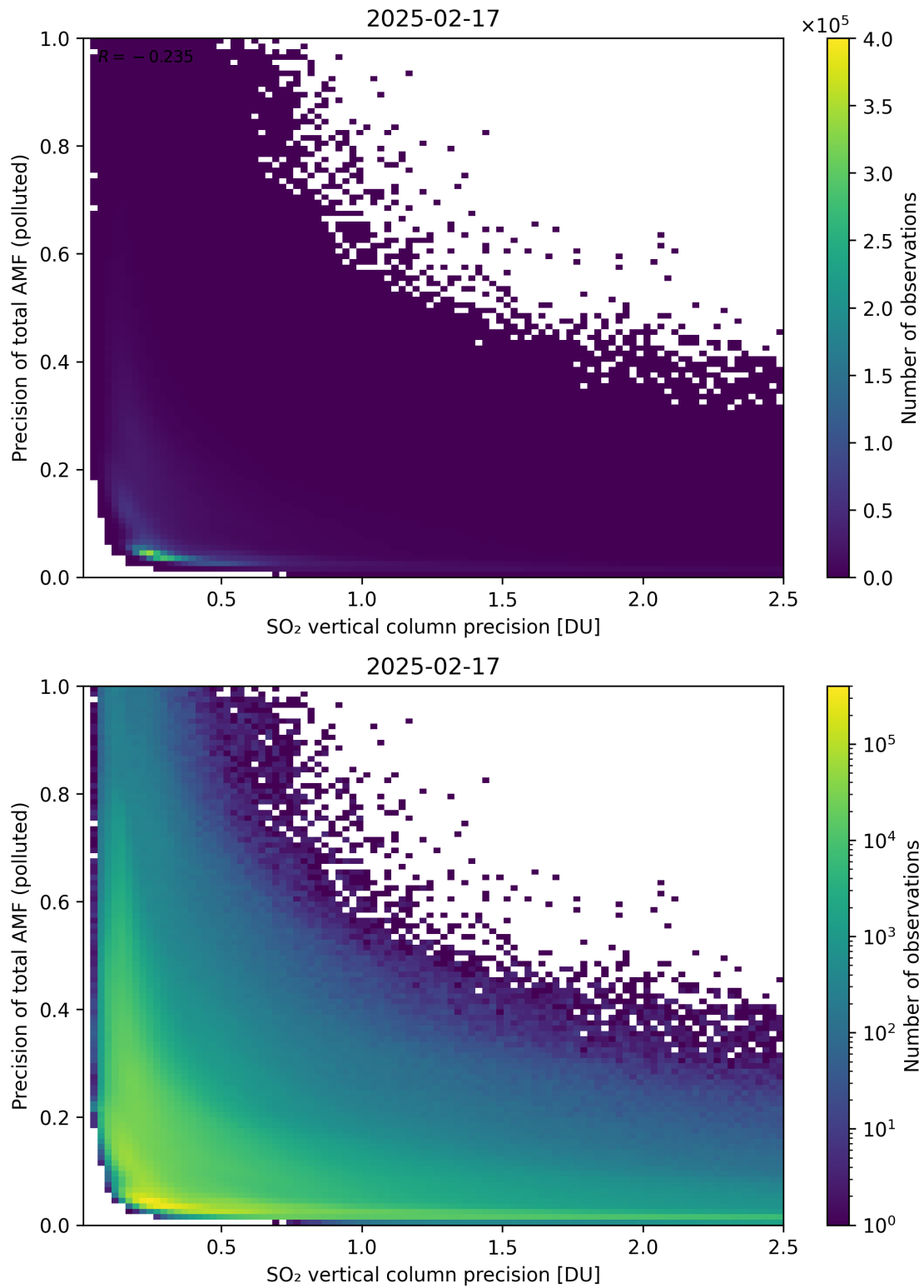
Figure 347: Scatter density plot of “SO 2 vertical column precision” against “Precision of total AMF (polluted)” for 2025-02-16 to 2025-02-18.
