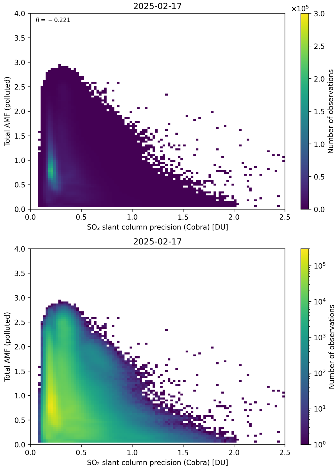
Figure 213: Scatter density plot of “SO 2 slant column precision (Cobra)” against “Total AMF (polluted)” for 2025-02-16 to 2025-02-18.
