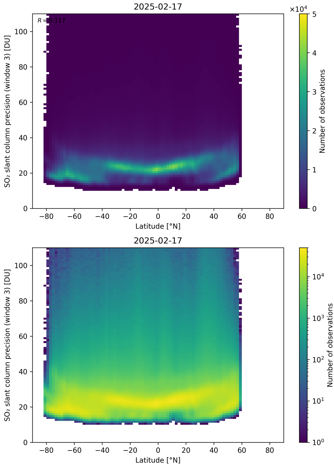
Figure 166: Scatter density plot of “Latitude” against “SO 2 slant column precision (window 3)” for 2025-02-16 to 2025-02-18.
