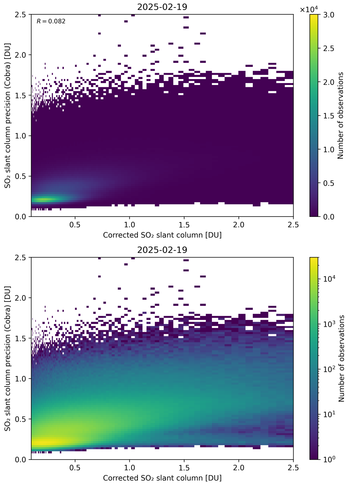
Figure 234: Scatter density plot of “Corrected SO 2 slant column” against “SO 2 slant column precision (Cobra)” for 2025-02-19 to 2025-02-20.
