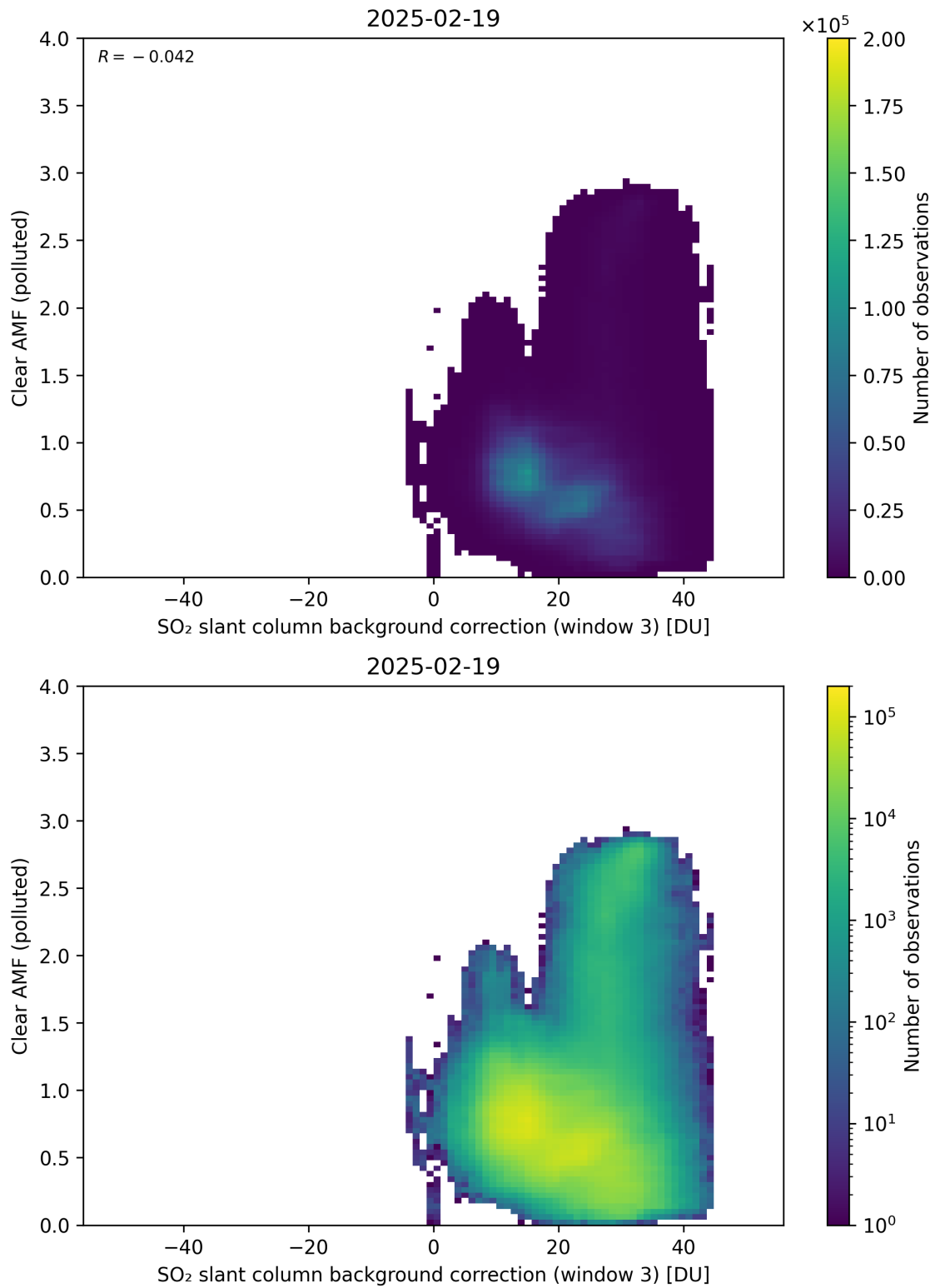
Figure 135: Scatter density plot of “SO 2 slant column background correction (window 3)” against “Clear AMF (polluted)” for 2025-02-19 to 2025-02-20.
