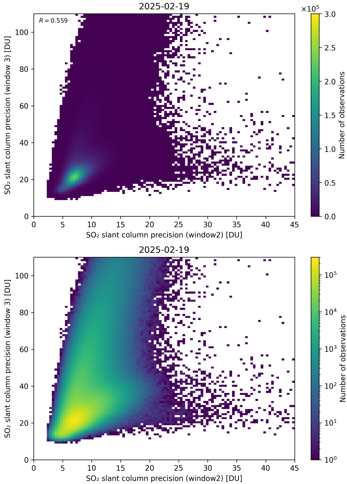
Figure 300: Scatter density plot of “SO 2 slant column precision (window2)” against “SO 2 slant column precision (window 3)” for 2025-02-19 to 2025-02-20.
