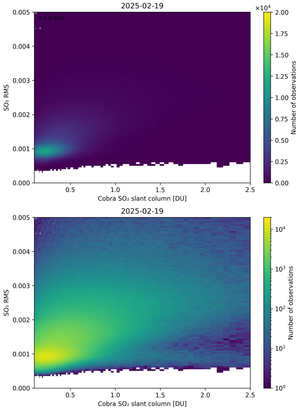
Figure 198: Scatter density plot of “Cobra SO 2 slant column” against “SO 2 RMS” for 2025-02-19 to 2025-02-20.
