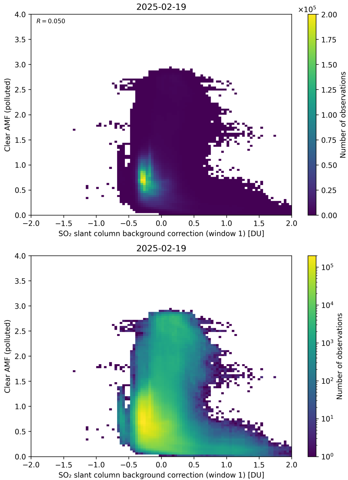
Figure 114: Scatter density plot of “SO 2 slant column background correction (window 1)” against “Clear AMF (polluted)” for 2025-02-19 to 2025-02-20.
