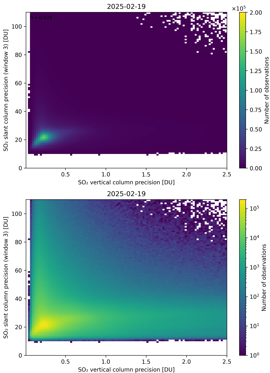
Figure 345: Scatter density plot of “SO 2 vertical column precision” against “SO 2 slant column precision (window 3)” for 2025-02-19 to 2025-02-20.
