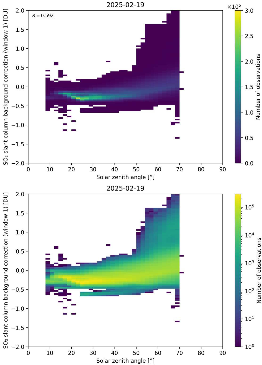
Figure 171: Scatter density plot of “Solar zenith angle” against “SO 2 slant column background correction (window 1)” for 2025-02-19 to 2025-02-20.
