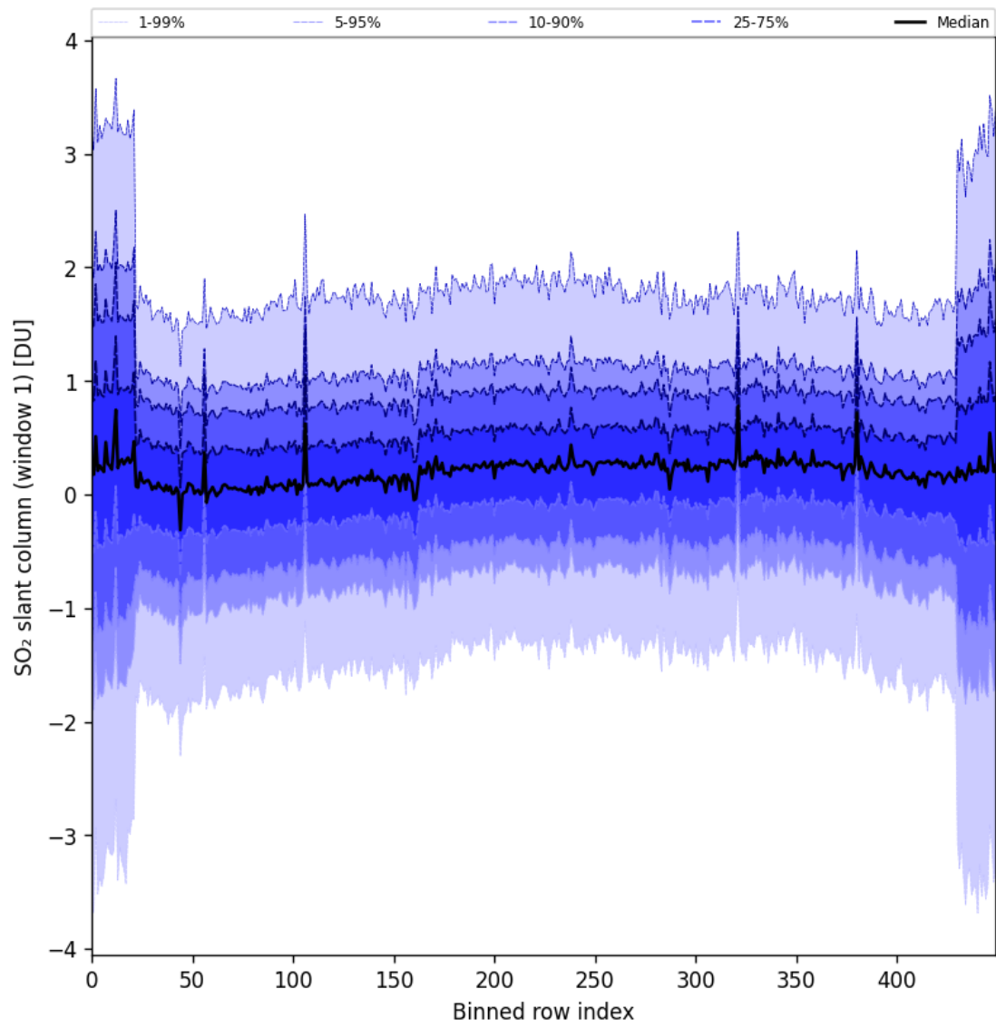
Figure 89: Along track statistics of “SO 2 slant column (window 1)” for 2025-02-19 to 2025-02-20
