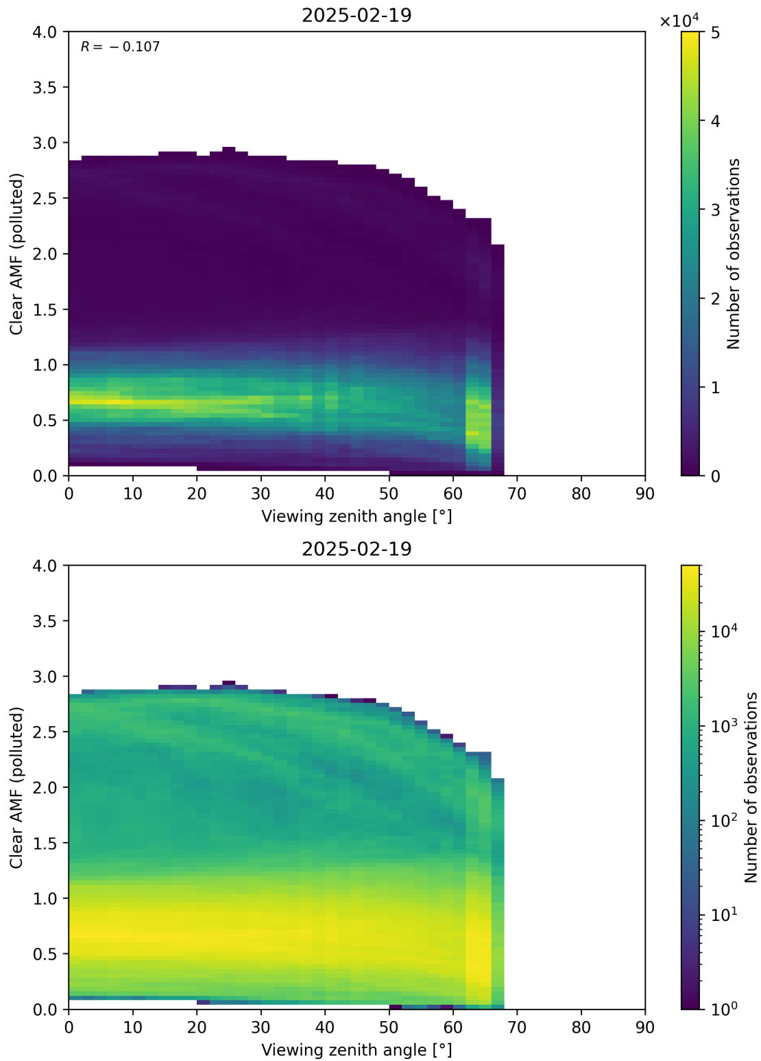
Figure 370: Scatter density plot of “Viewing zenith angle” against “Clear AMF (polluted)” for 2025-02-19 to 2025-02-20.
