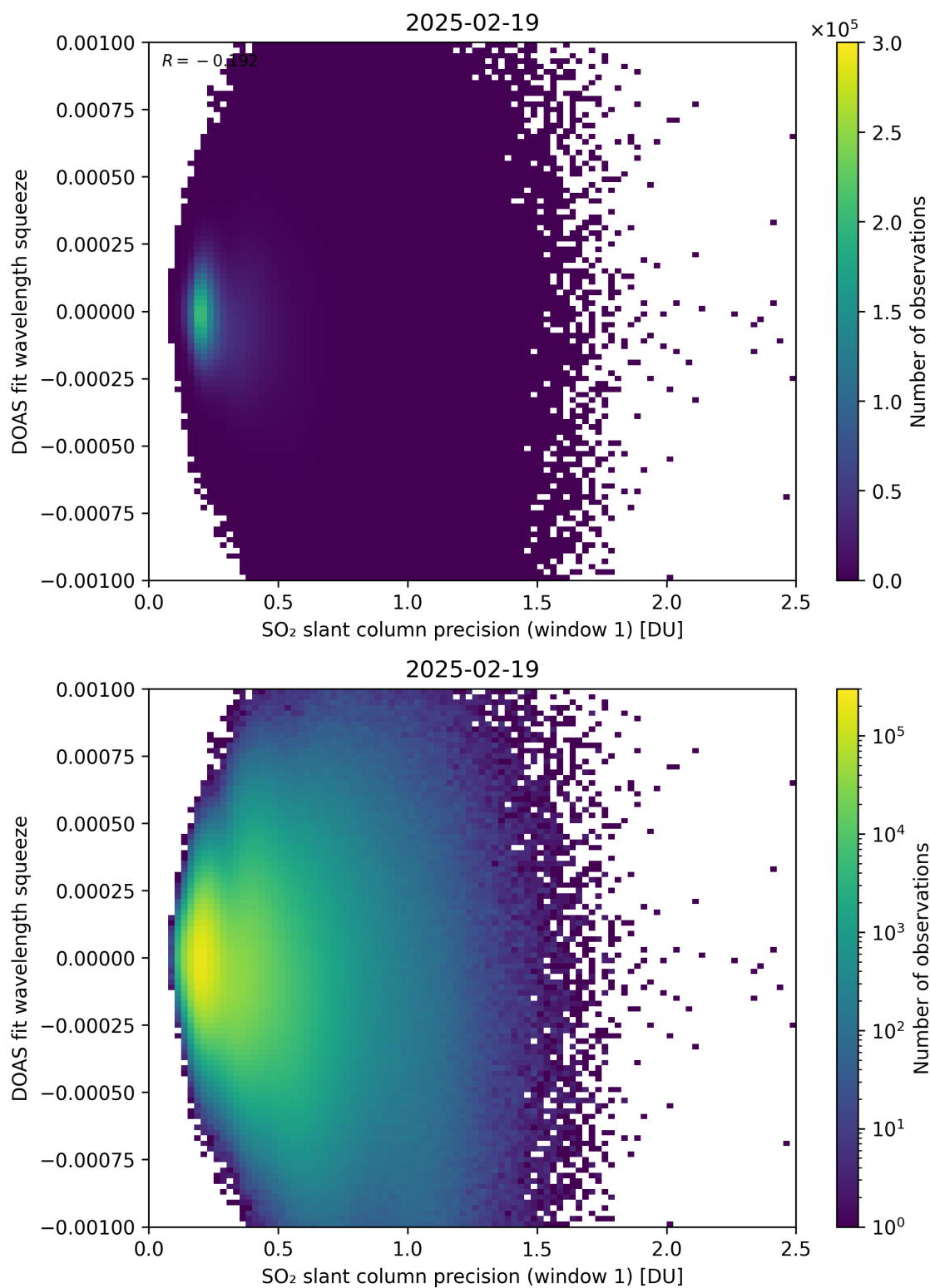
Figure 272: Scatter density plot of “SO 2 slant column precision (window 1)” against “DOAS fit wavelength squeeze” for 2025-02-19 to 2025-02-20.
