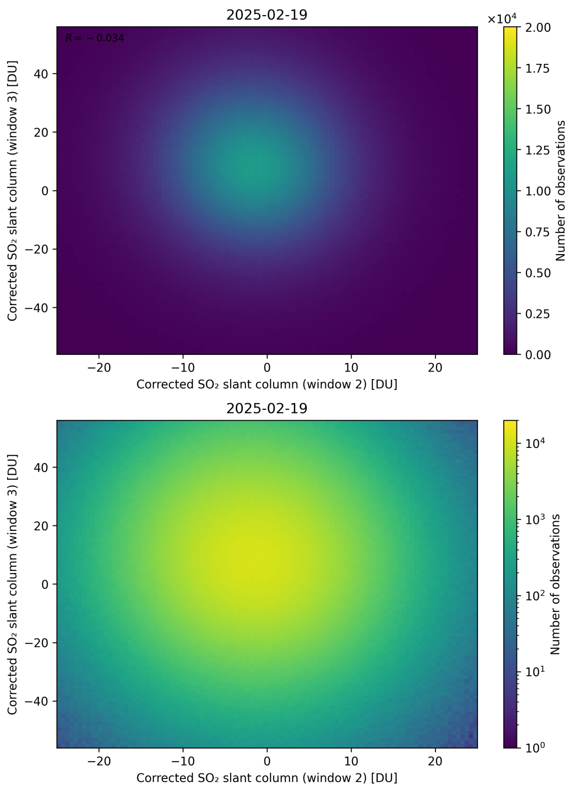
Figure 250: Scatter density plot of “Corrected SO 2 slant column (window 2)” against “Corrected SO 2 slant column (window 3)” for 2025-02-19 to 2025-02-20.
