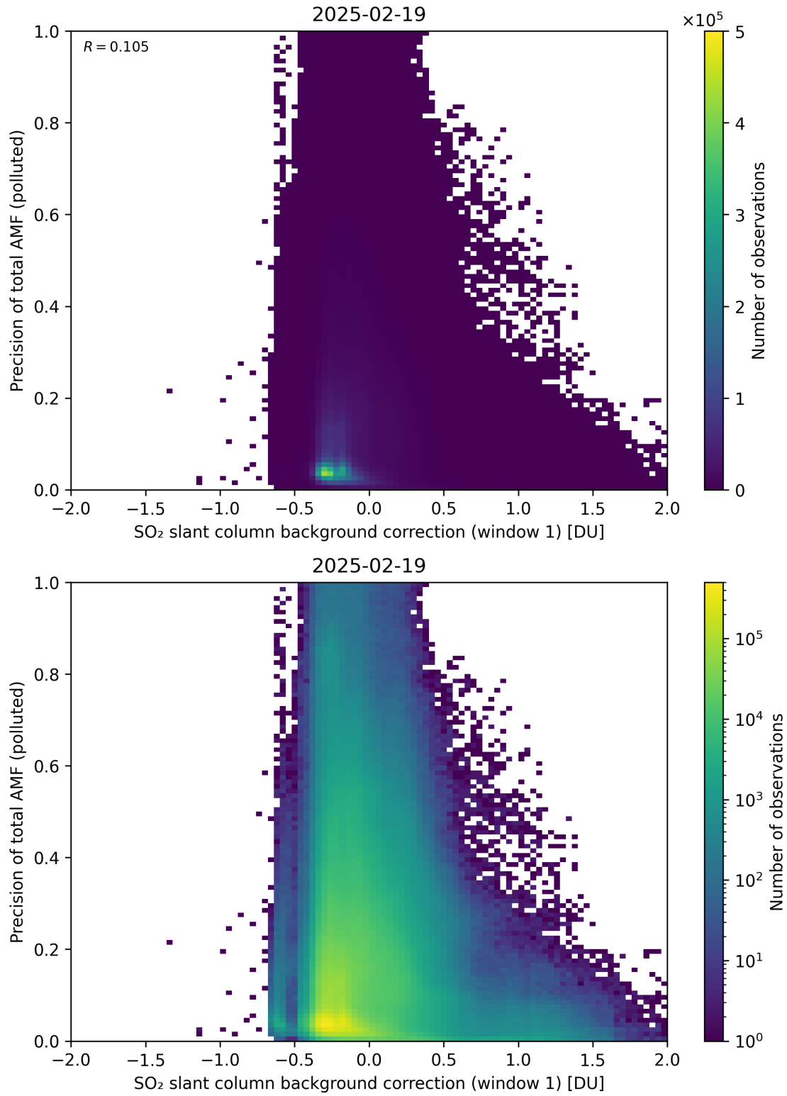
Figure 121: Scatter density plot of “SO 2 slant column background correction (window 1)” against “Precision of total AMF (polluted)” for 2025-02-19 to 2025-02-20.
