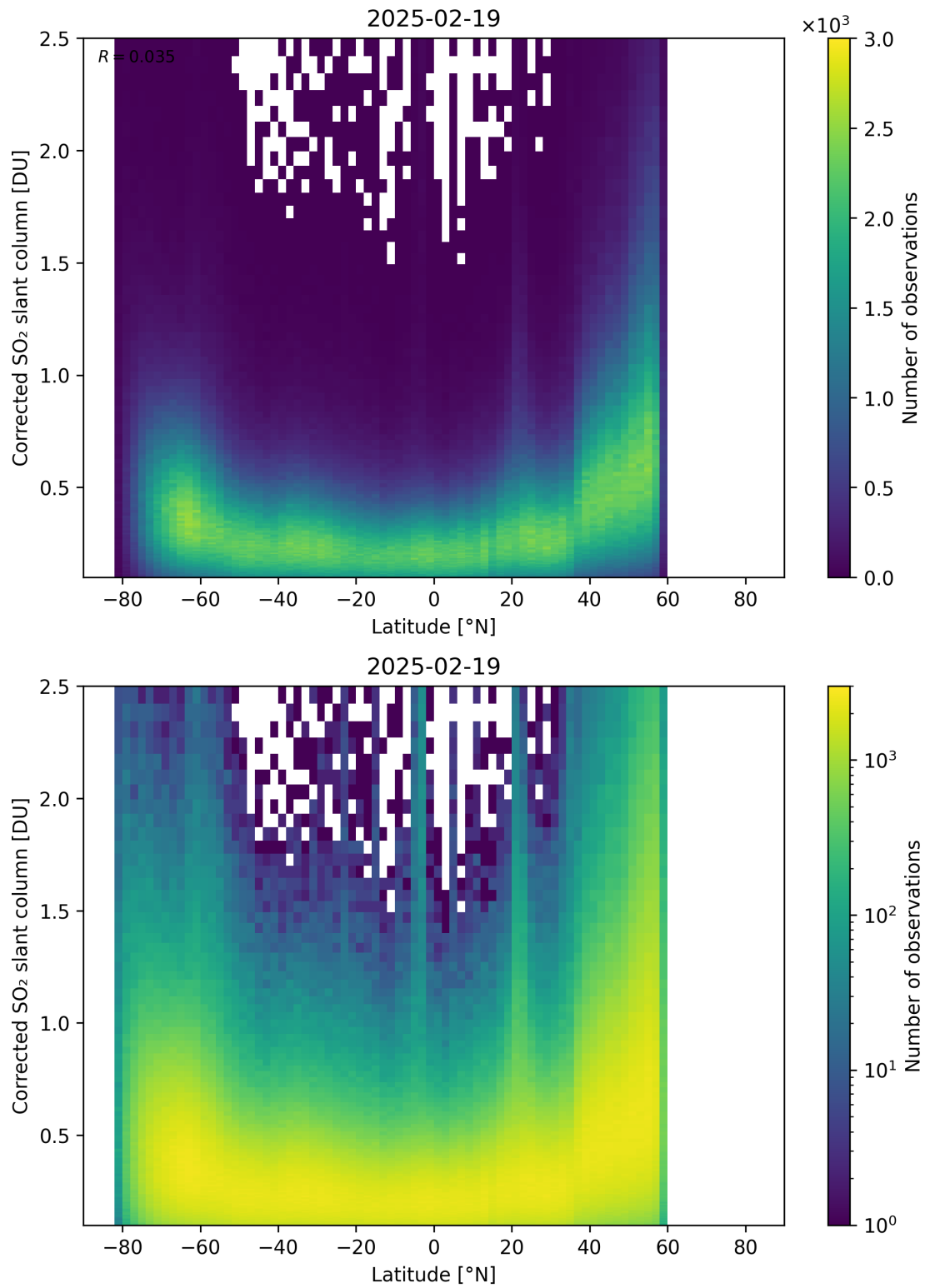
Figure 159: Scatter density plot of “Latitude” against “Corrected SO 2 slant column” for 2025-02-19 to 2025-02-20.
