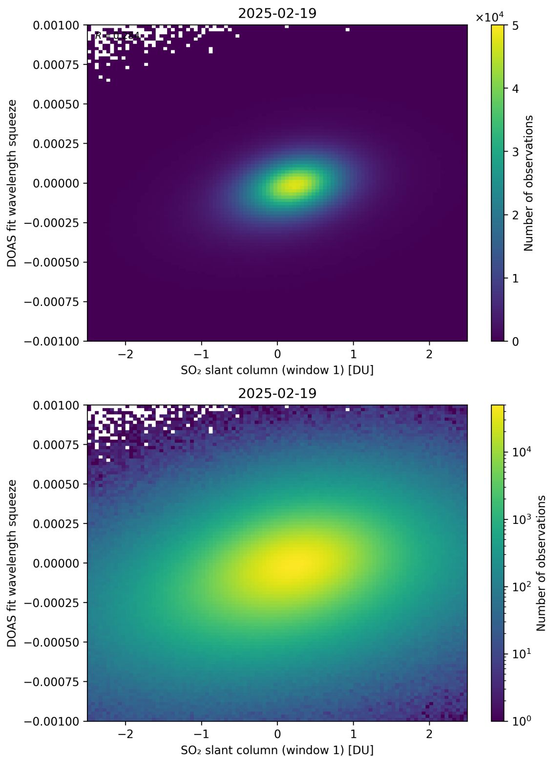
Figure 266: Scatter density plot of “SO 2 slant column (window 1)” against “DOAS fit wavelength squeeze” for 2025-02-19 to 2025-02-20.
