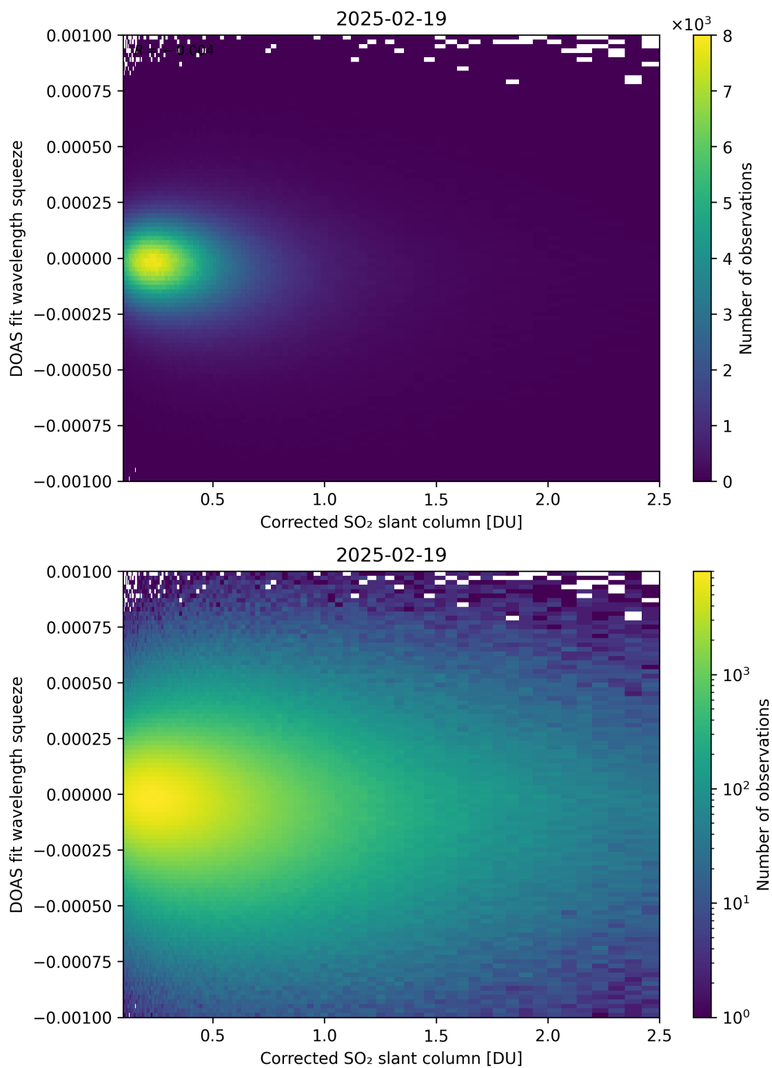
Figure 230: Scatter density plot of “Corrected SO 2 slant column” against “DOAS fit wavelength squeeze” for 2025-02-19 to 2025-02-20.
