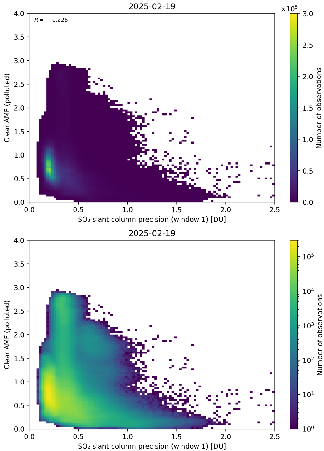
Figure 274: Scatter density plot of “SO 2 slant column precision (window 1)” against “Clear AMF (polluted)” for 2025-02-19 to 2025-02-20.
