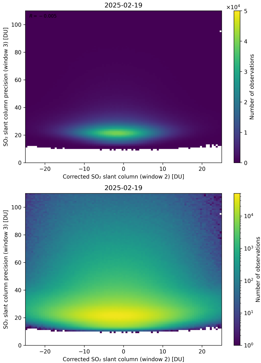
Figure 252: Scatter density plot of “Corrected SO 2 slant column (window 2)” against “SO 2 slant column precision (window 3)” for 2025-02-19 to 2025-02-20.
