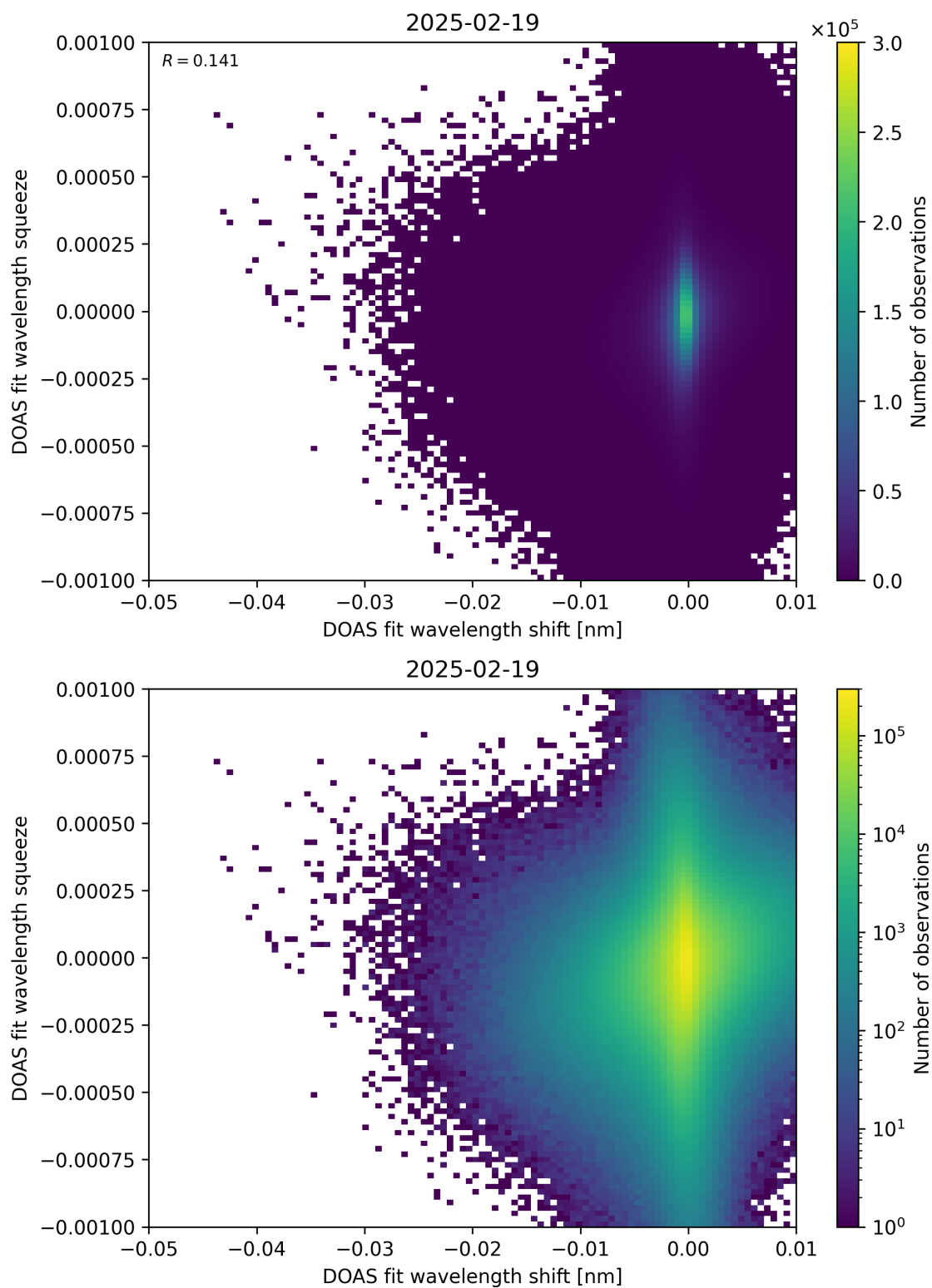
Figure 138: Scatter density plot of “DOAS fit wavelength shift” against “DOAS fit wavelength squeeze” for 2025-02-19 to 2025-02-20.
