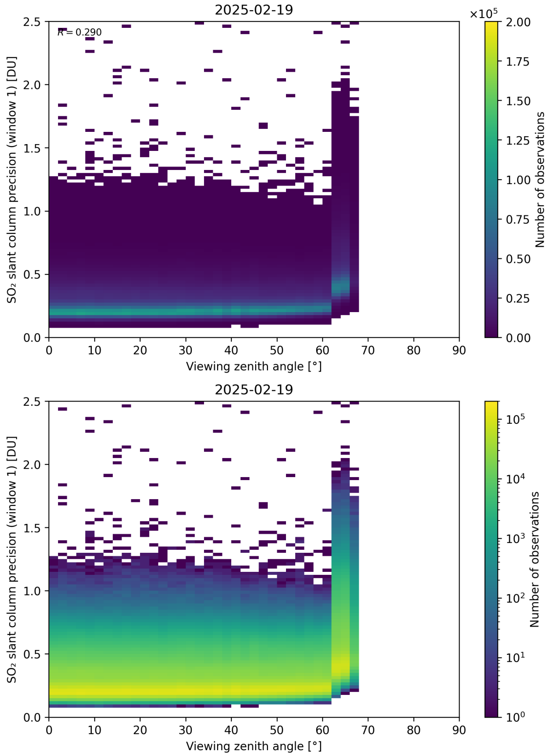
Figure 377: Scatter density plot of “Viewing zenith angle” against “SO 2 slant column precision (window 1)” for 2025-02-19 to 2025-02-20.
