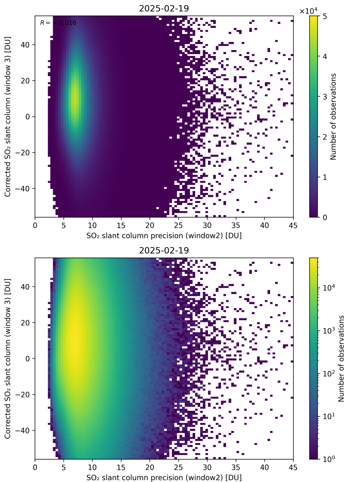
Figure 298: Scatter density plot of “SO 2 slant column precision (window2)” against “Corrected SO 2 slant column (window 3)” for 2025-02-19 to 2025-02-20.
