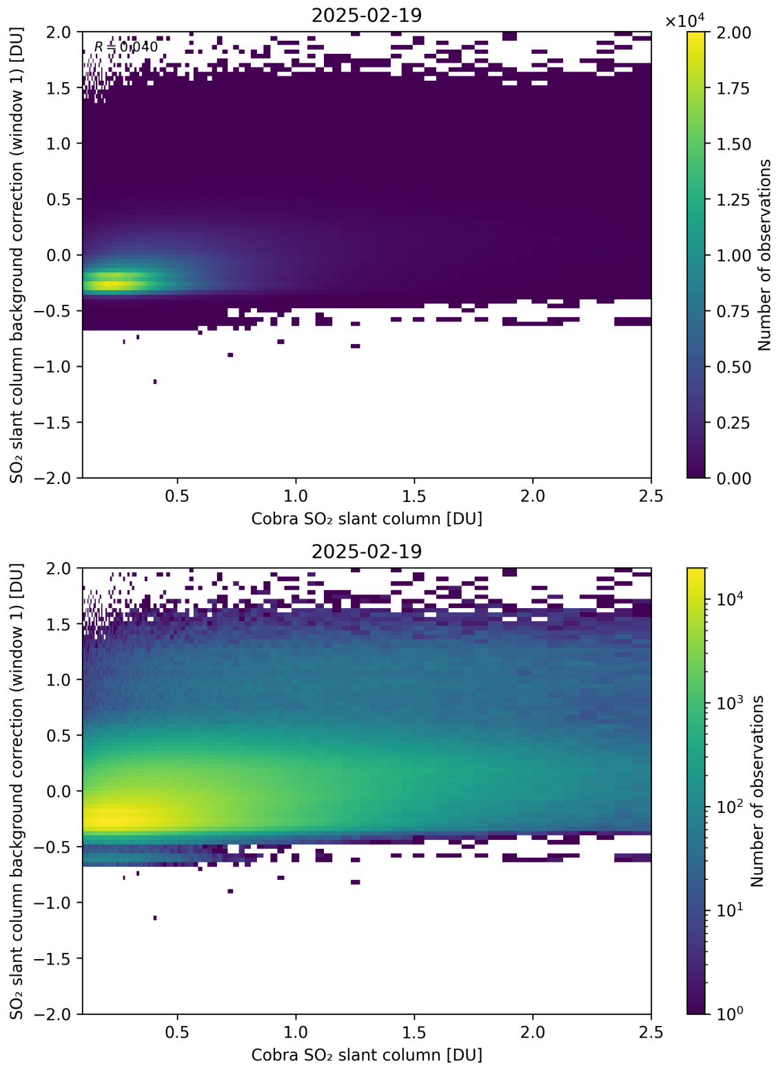
Figure 193: Scatter density plot of “Cobra SO 2 slant column” against “SO 2 slant column background correction (window 1)” for 2025-02-19 to 2025-02-20.
