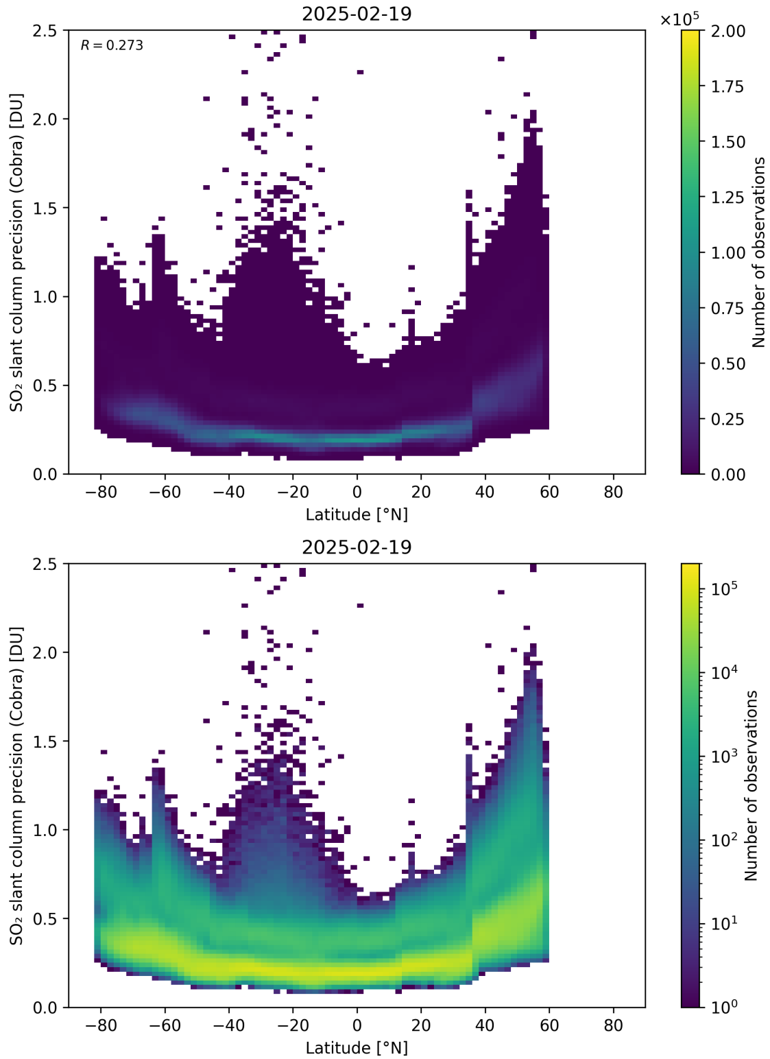
Figure 158: Scatter density plot of “Latitude” against “SO 2 slant column precision (Cobra)” for 2025-02-19 to 2025-02-20.
