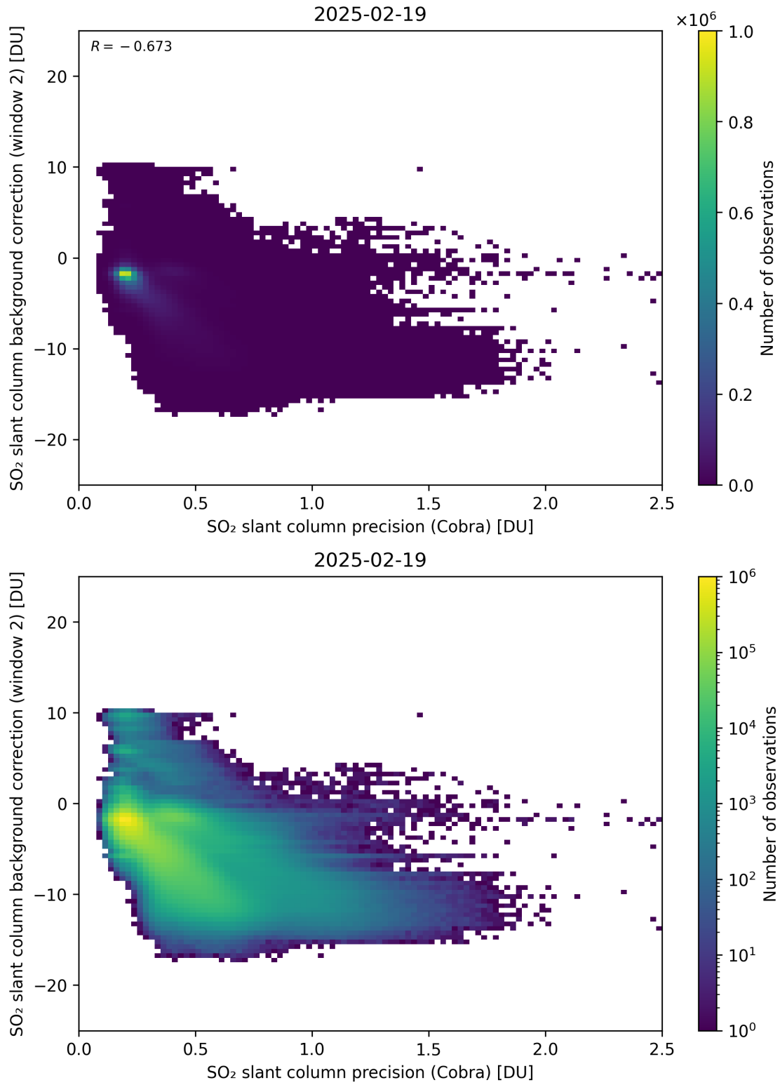
Figure 200: Scatter density plot of “SO 2 slant column precision (Cobra)” against “SO 2 slant column background correction (window 2)” for 2025-02-19 to 2025-02-20.
