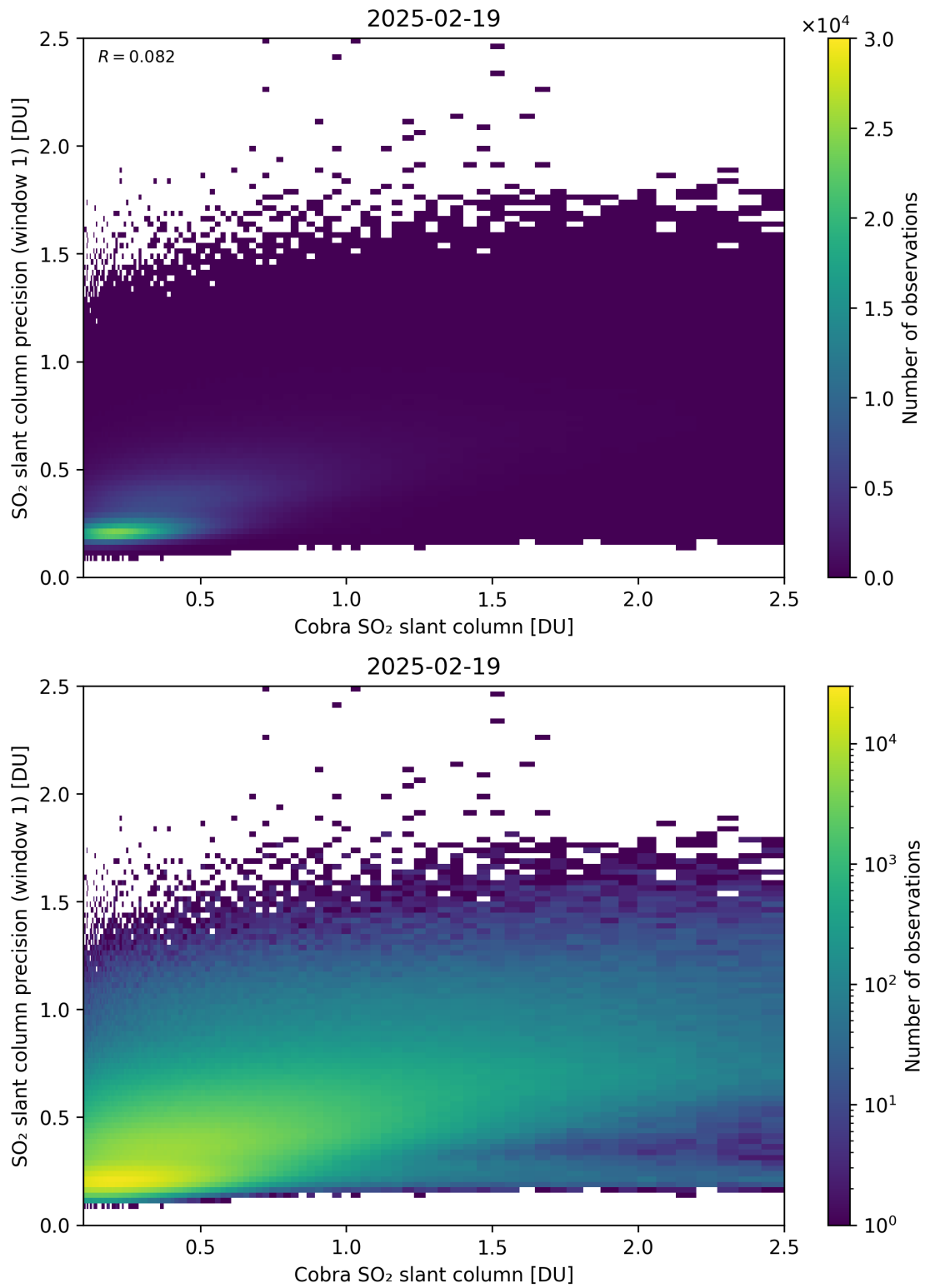
Figure 220: Scatter density plot of “Cobra SO 2 slant column” against “SO 2 slant column precision (window 1)” for 2025-02-19 to 2025-02-20.
