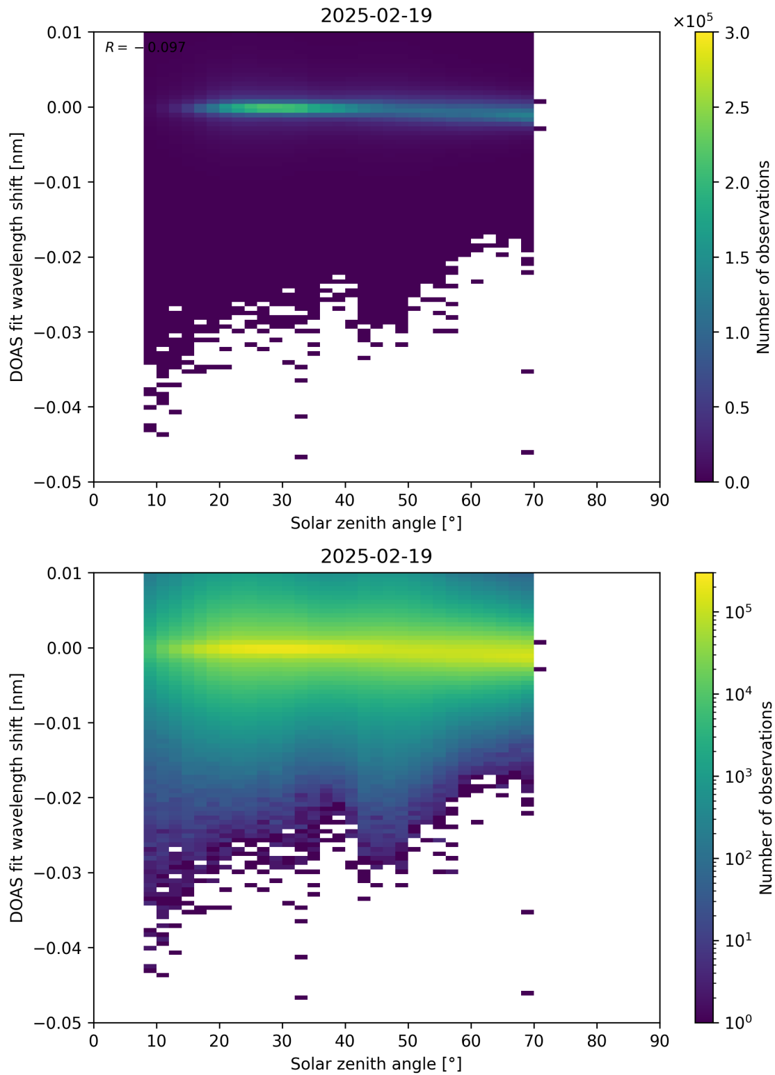
Figure 174: Scatter density plot of “Solar zenith angle” against “DOAS fit wavelength shift” for 2025-02-19 to 2025-02-20.
