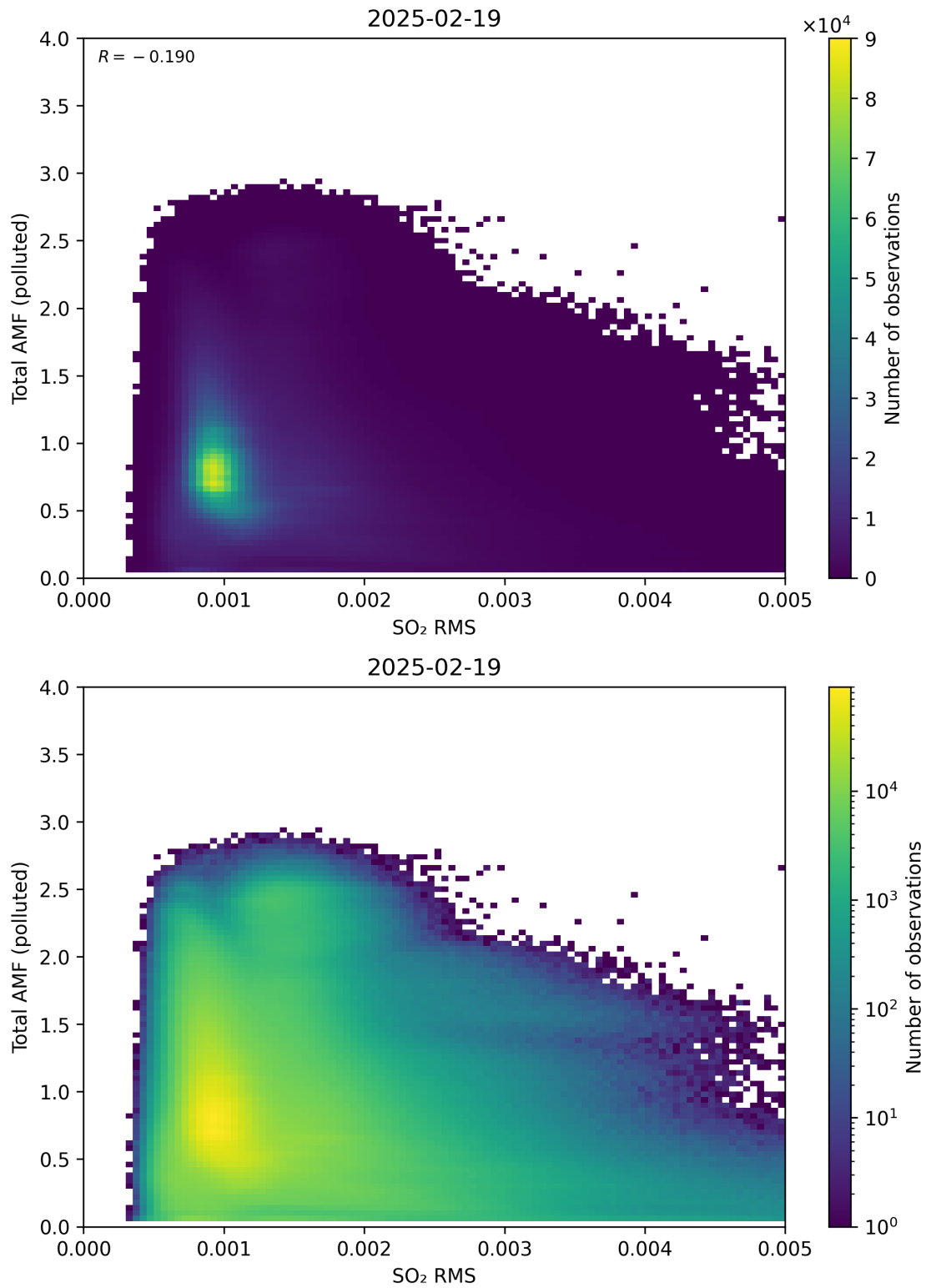
Figure 148: Scatter density plot of “SO 2 RMS” against “Total AMF (polluted)” for 2025-02-19 to 2025-02-20.
