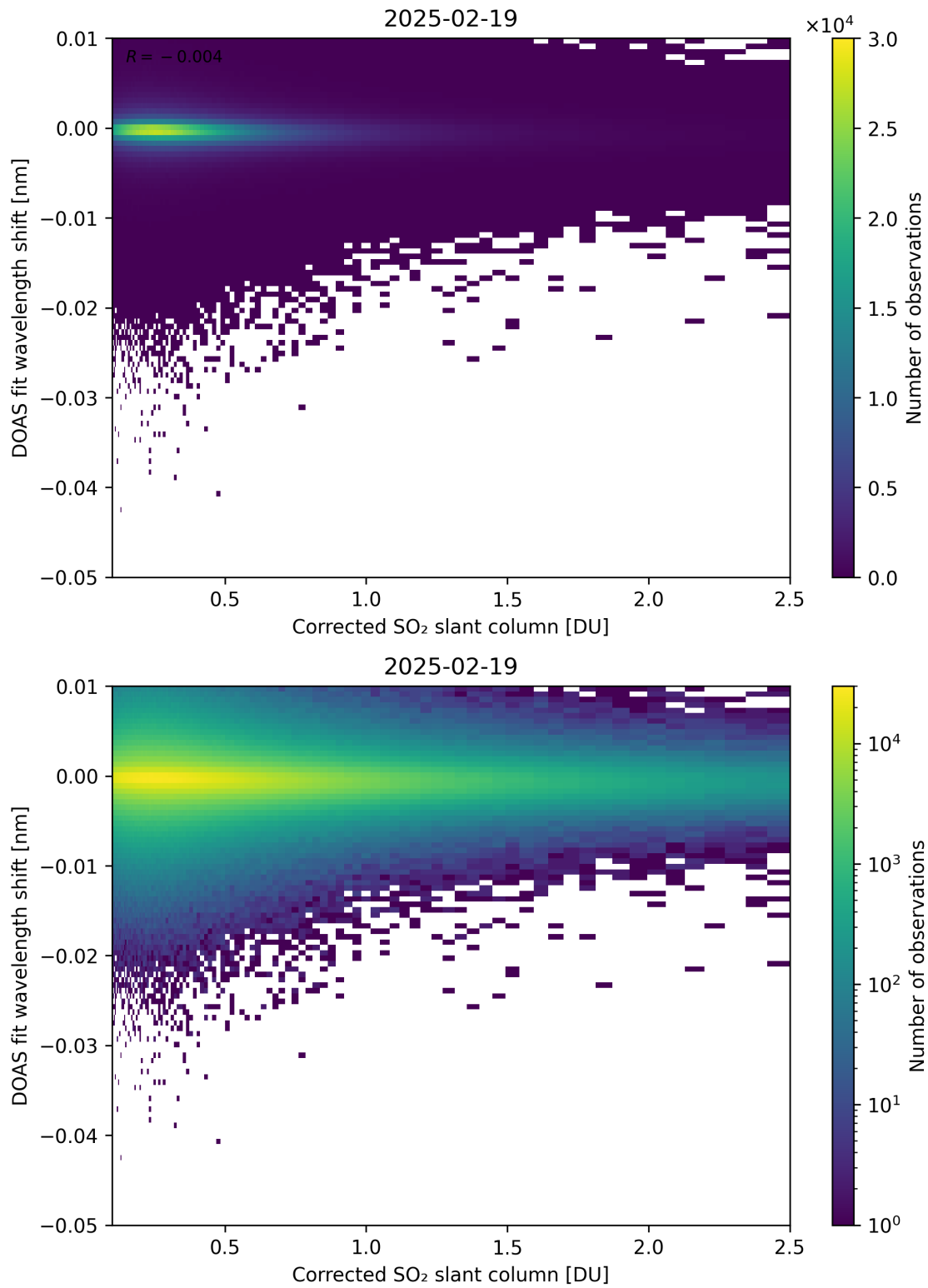
Figure 229: Scatter density plot of “Corrected SO 2 slant column” against “DOAS fit wavelength shift” for 2025-02-19 to 2025-02-20.
