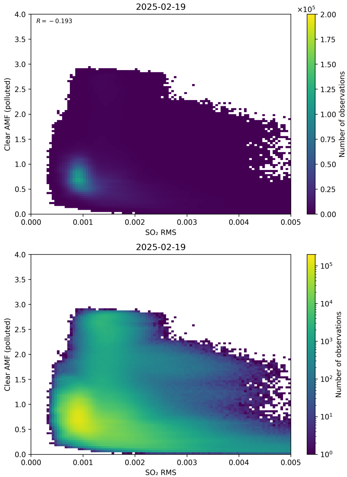
Figure 147: Scatter density plot of “SO 2 RMS” against “Clear AMF (polluted)” for 2025-02-19 to 2025-02-20.
