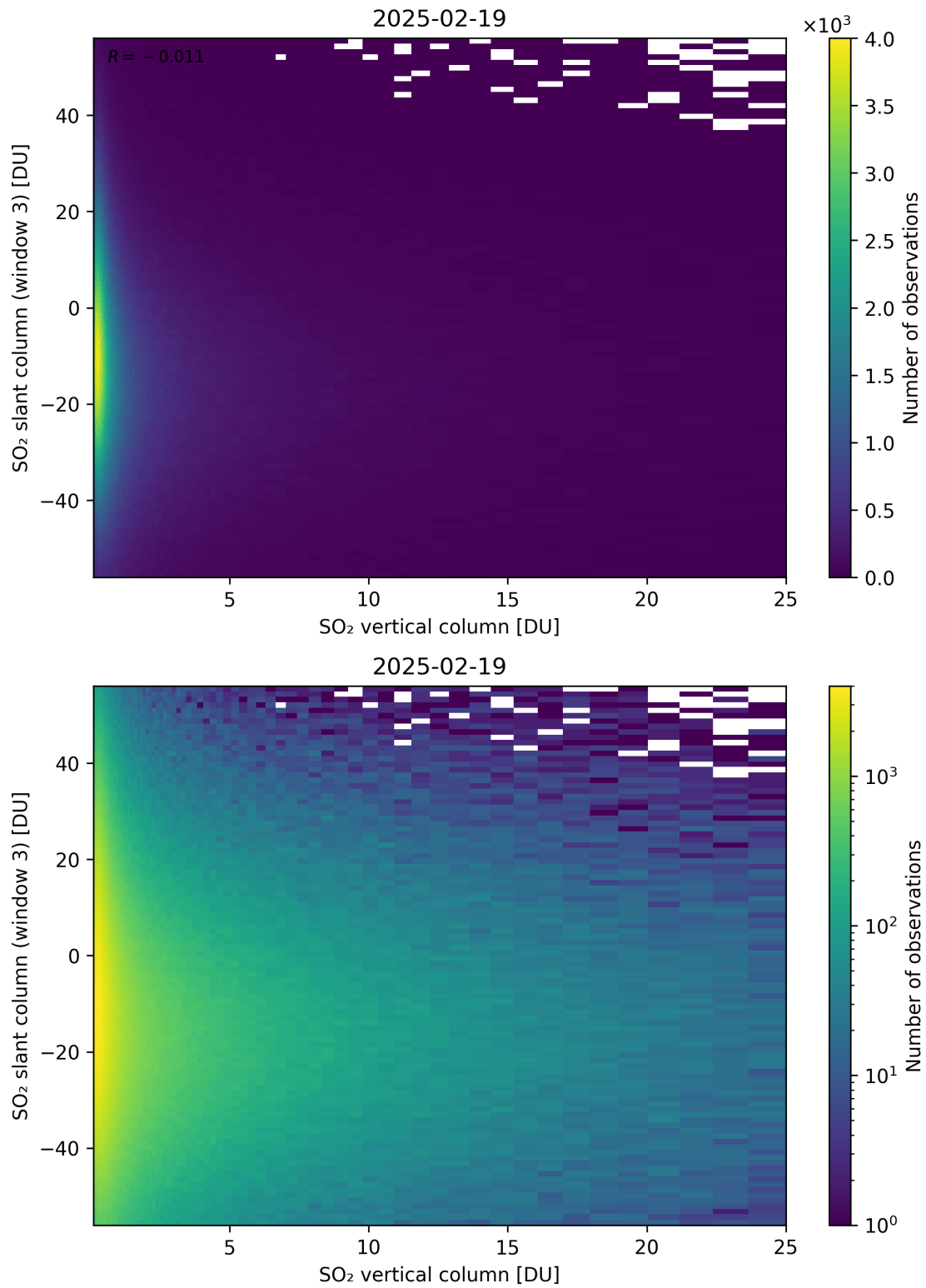
Figure 357: Scatter density plot of “SO 2 vertical column” against “SO 2 slant column (window 3)” for 2025-02-19 to 2025-02-20.
