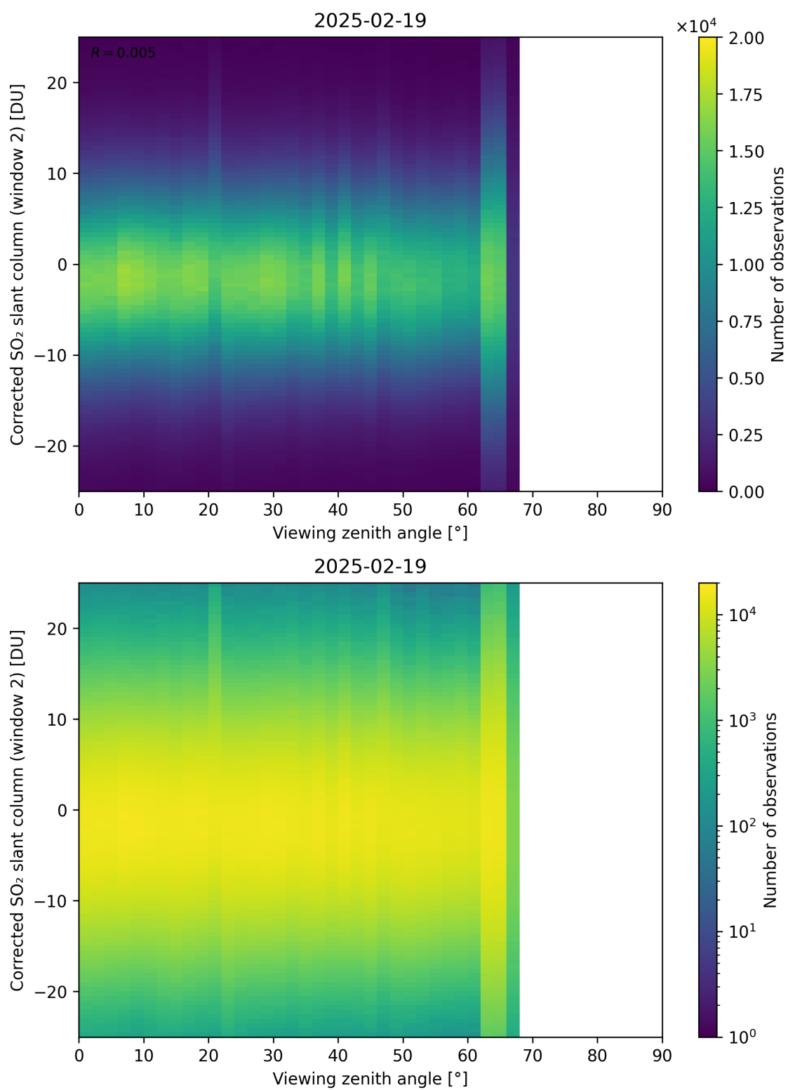
Figure 374: Scatter density plot of “Viewing zenith angle” against “Corrected SO 2 slant column (window 2)” for 2025-02-19 to 2025-02-20.
