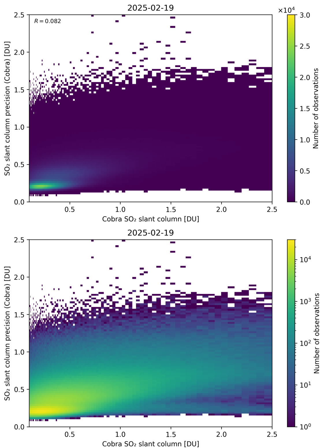
Figure 216: Scatter density plot of “Cobra SO 2 slant column” against “SO 2 slant column precision (Cobra)” for 2025-02-19 to 2025-02-20.
