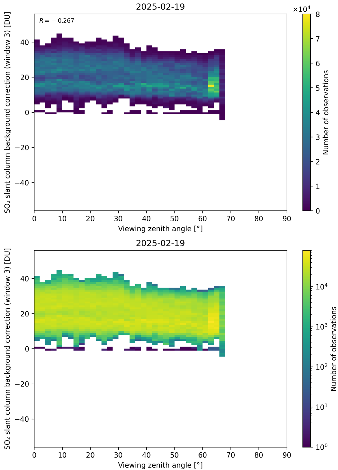
Figure 364: Scatter density plot of “Viewing zenith angle” against “SO 2 slant column background correction (window 3)” for 2025-02-19 to 2025-02-20.
