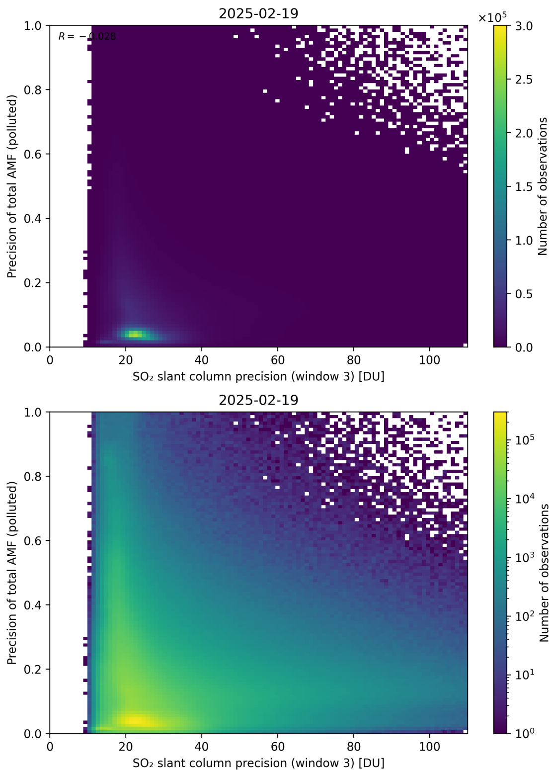
Figure 314: Scatter density plot of “SO 2 slant column precision (window 3)” against “Precision of total AMF (polluted)” for 2025-02-19 to 2025-02-20.
