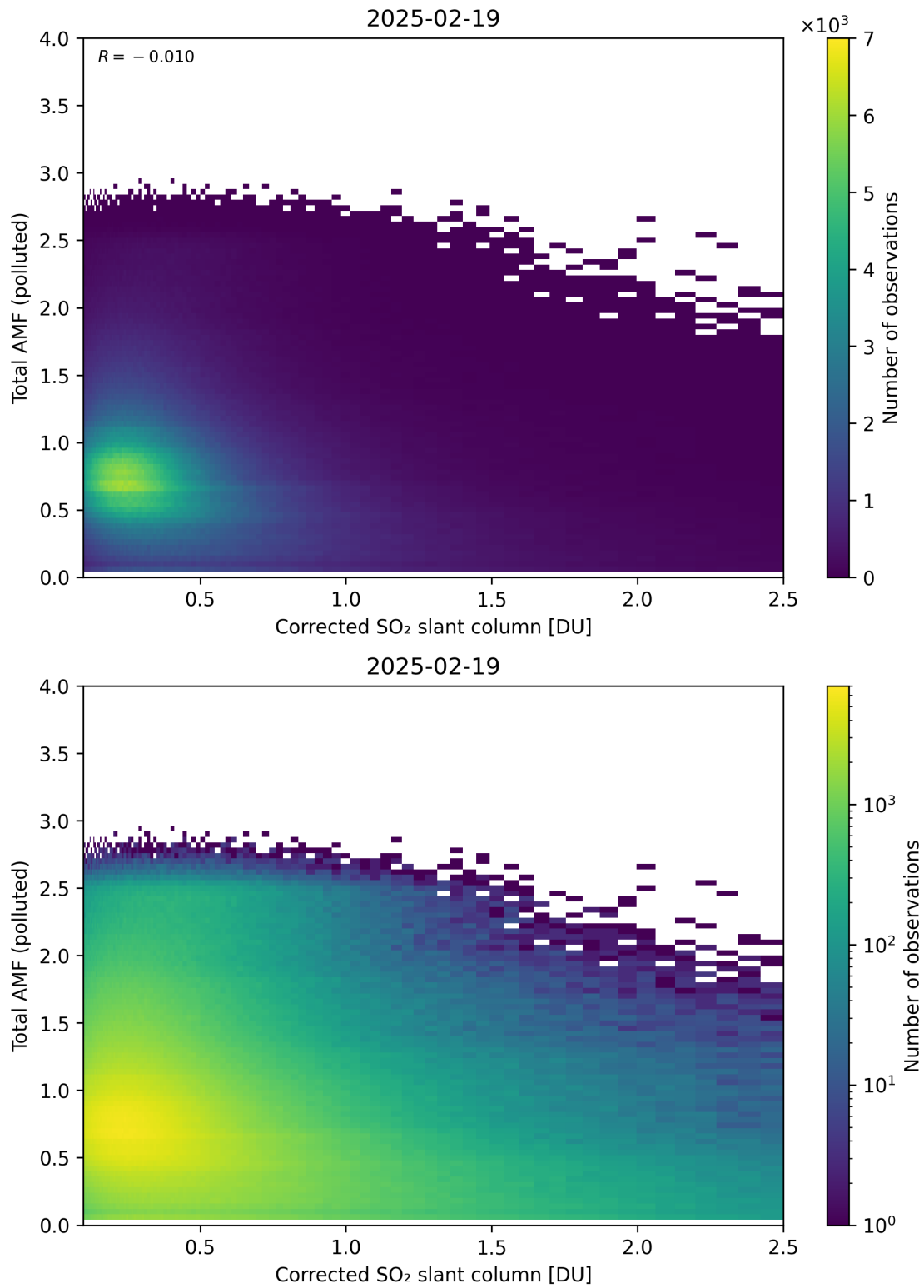
Figure 242: Scatter density plot of “Corrected SO 2 slant column” against “Total AMF (polluted)” for 2025-02-19 to 2025-02-20.
