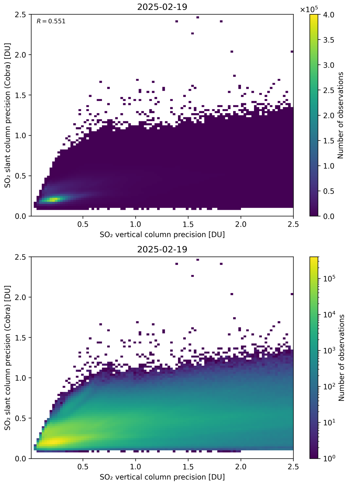
Figure 337: Scatter density plot of “SO 2 vertical column precision” against “SO 2 slant column precision (Cobra)” for 2025-02-19 to 2025-02-20.
