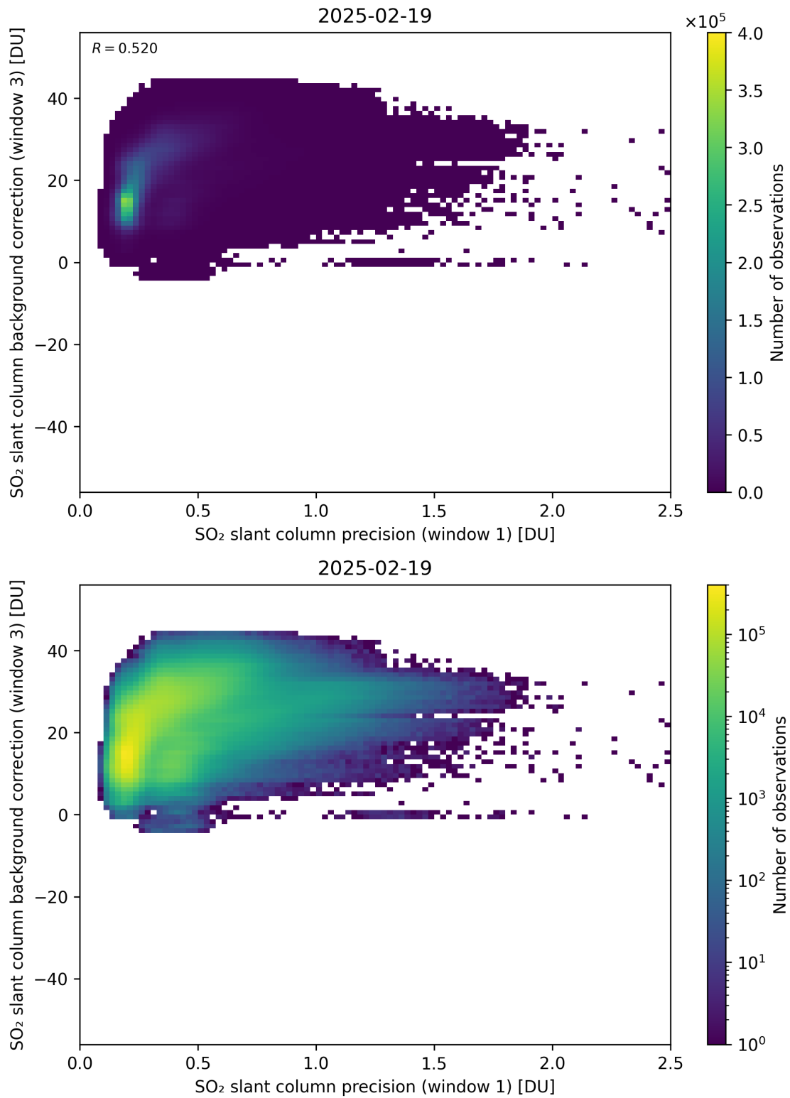
Figure 270: Scatter density plot of “SO 2 slant column precision (window 1)” against “SO 2 slant column background correction (window 3)” for 2025-02-19 to 2025-02-20.
