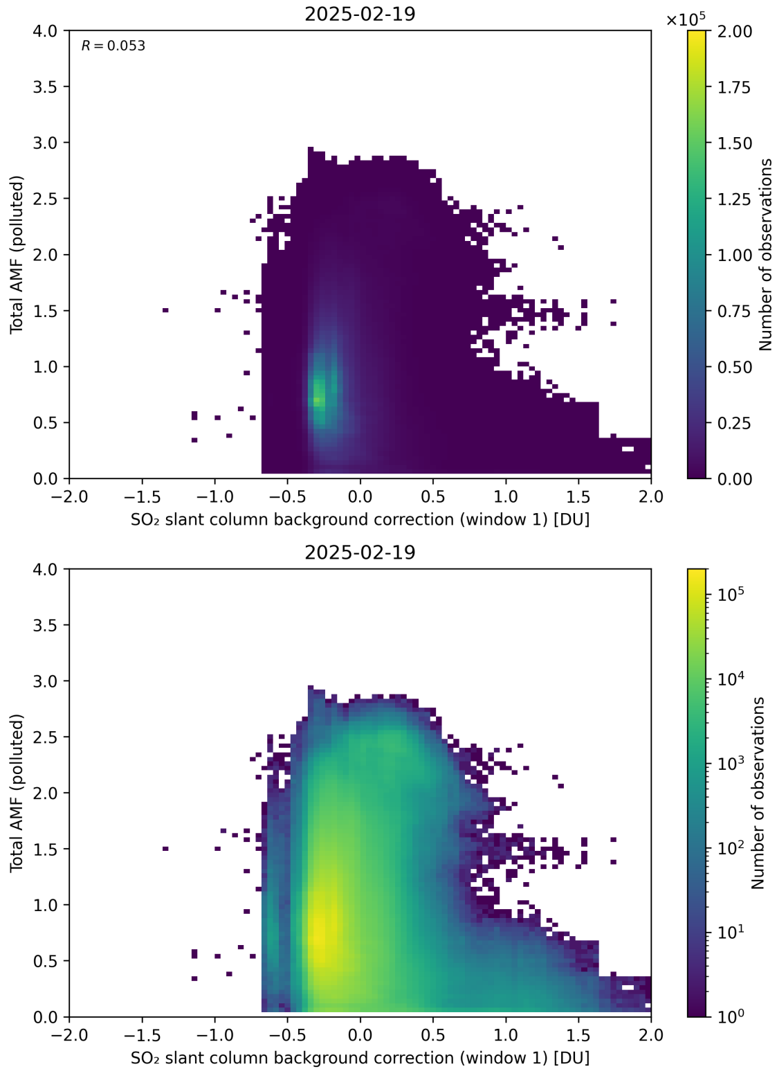
Figure 120: Scatter density plot of “SO 2 slant column background correction (window 1)” against “Total AMF (polluted)” for 2025-02-19 to 2025-02-20.
