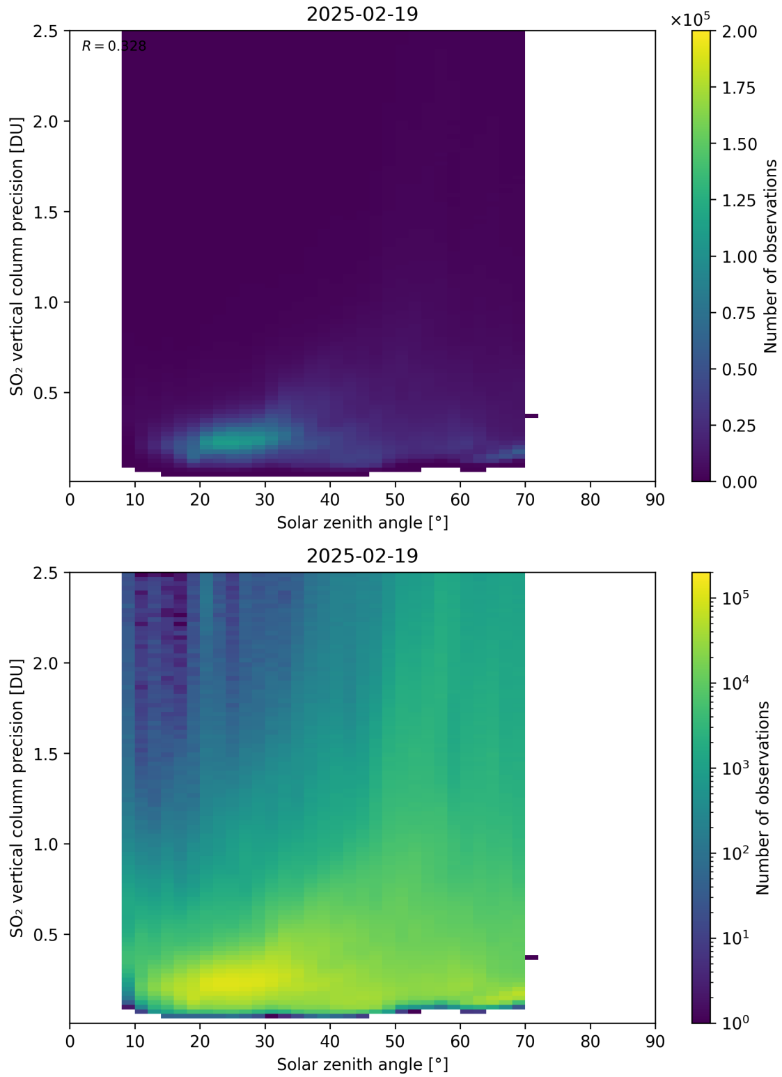
Figure 192: Scatter density plot of “Solar zenith angle” against “SO 2 vertical column precision” for 2025-02-19 to 2025-02-20.
