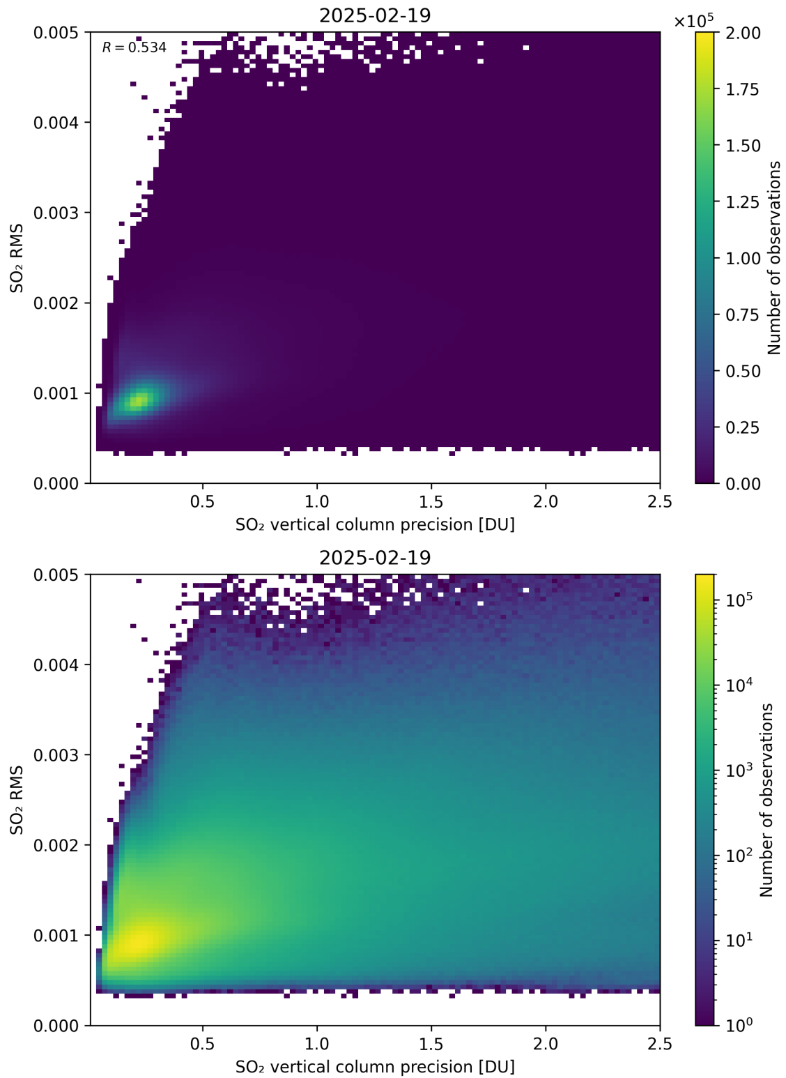
Figure 334: Scatter density plot of “SO 2 vertical column precision” against “SO 2 RMS” for 2025-02-19 to 2025-02-20.
