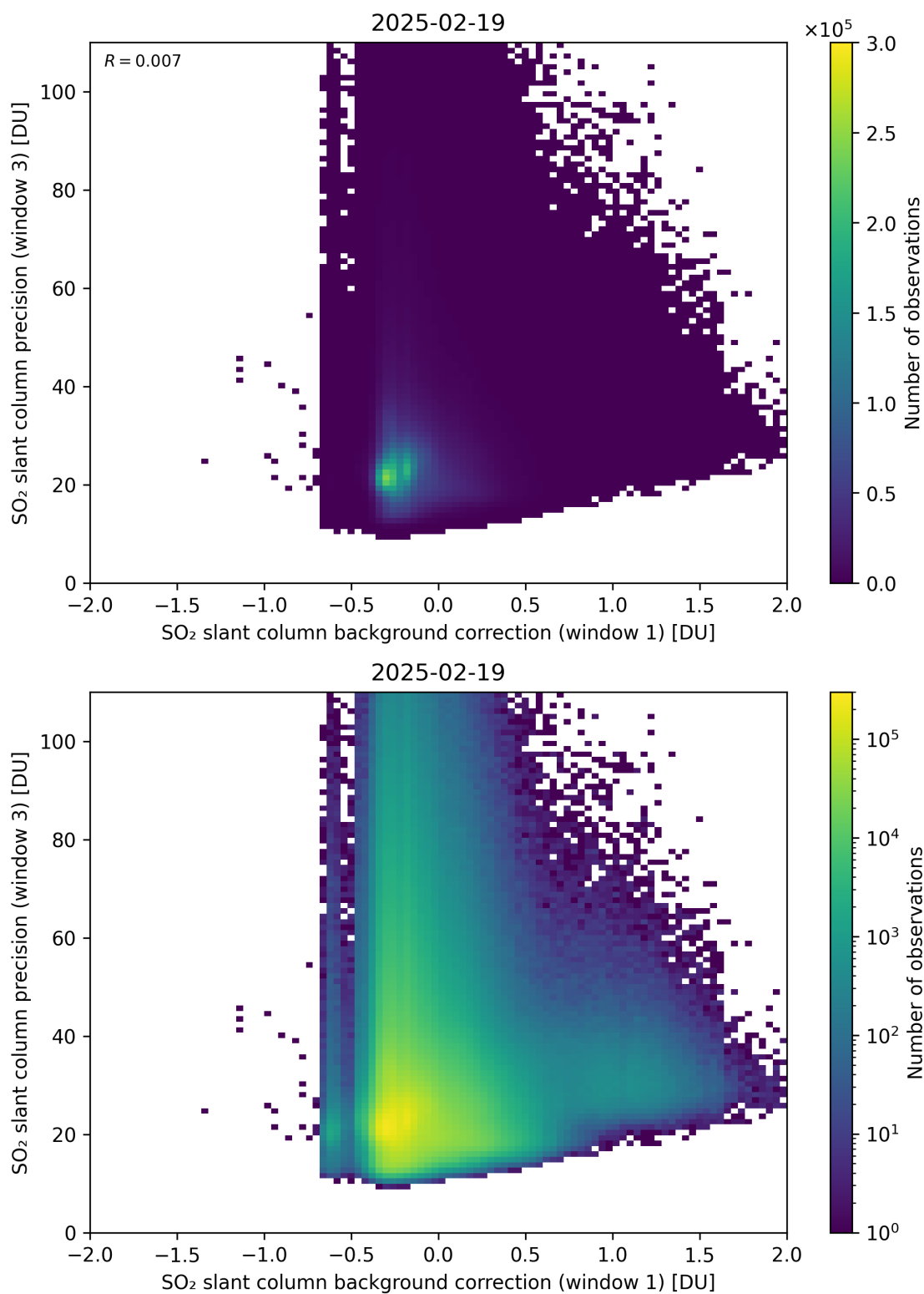
Figure 119: Scatter density plot of “SO 2 slant column background correction (window 1)” against “SO 2 slant column precision (window 3)” for 2025-02-19 to 2025-02-20.
