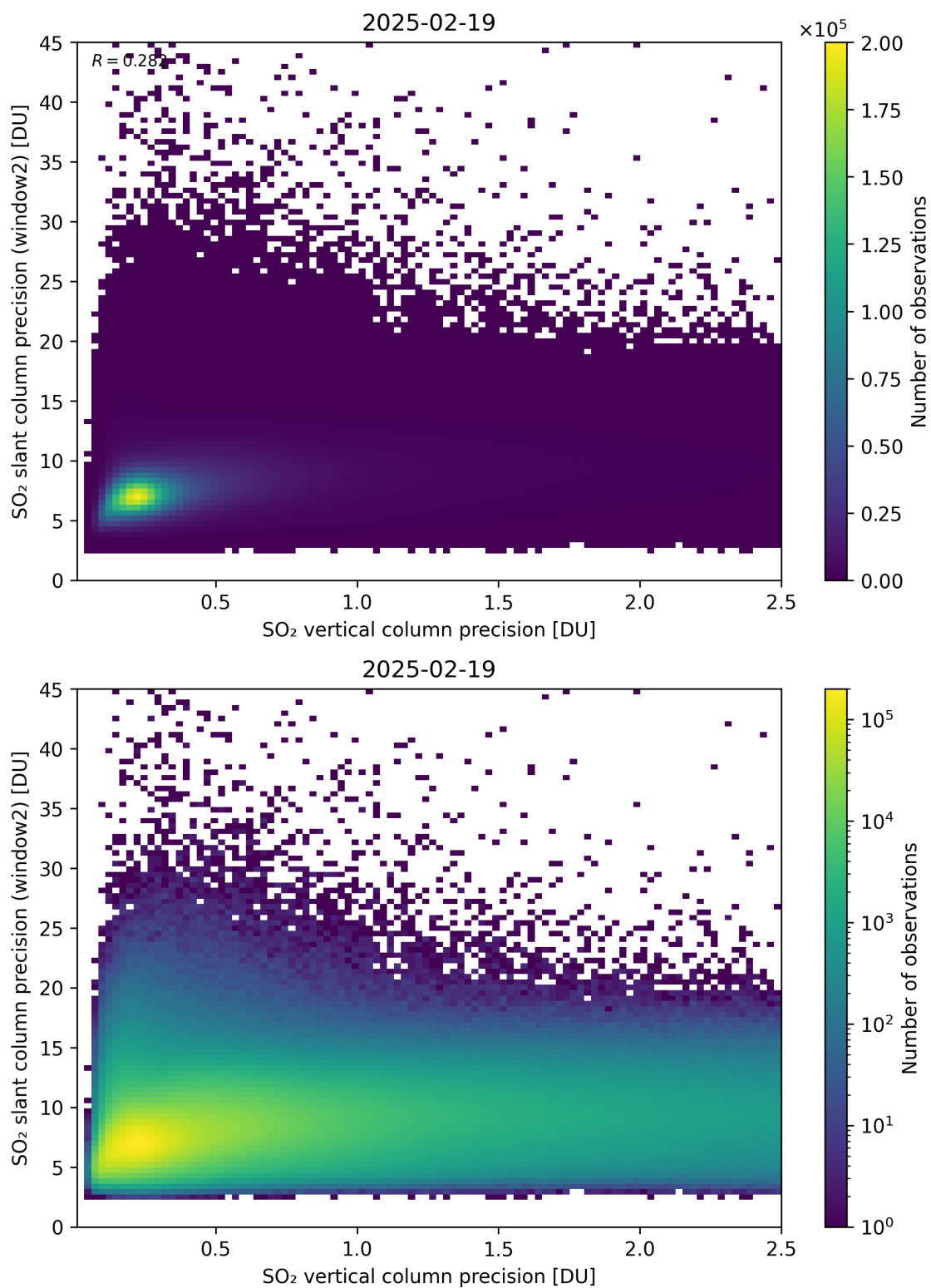
Figure 343: Scatter density plot of “SO 2 vertical column precision” against “SO 2 slant column precision (window2)” for 2025-02-19 to 2025-02-20.
