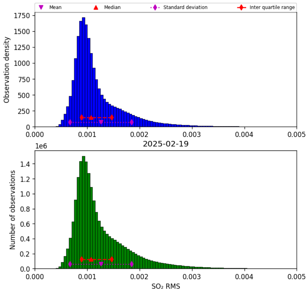
Figure 78: Histogram of “SO 2 RMS” for 2025-02-19 to 2025-02-20
