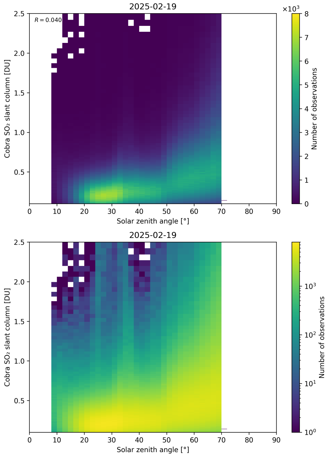
Figure 179: Scatter density plot of “Solar zenith angle” against “Cobra SO 2 slant column” for 2025-02-19 to 2025-02-20.
