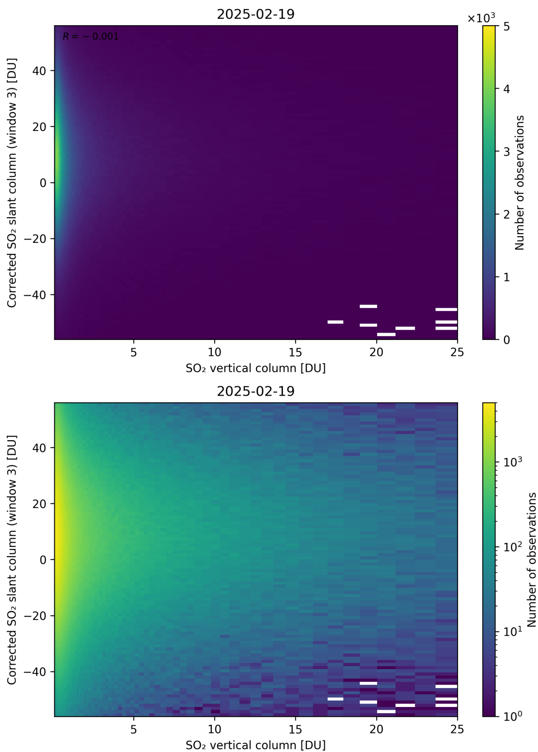
Figure 353: Scatter density plot of “SO 2 vertical column” against “Corrected SO 2 slant column (window 3)” for 2025-02-19 to 2025-02-20.
