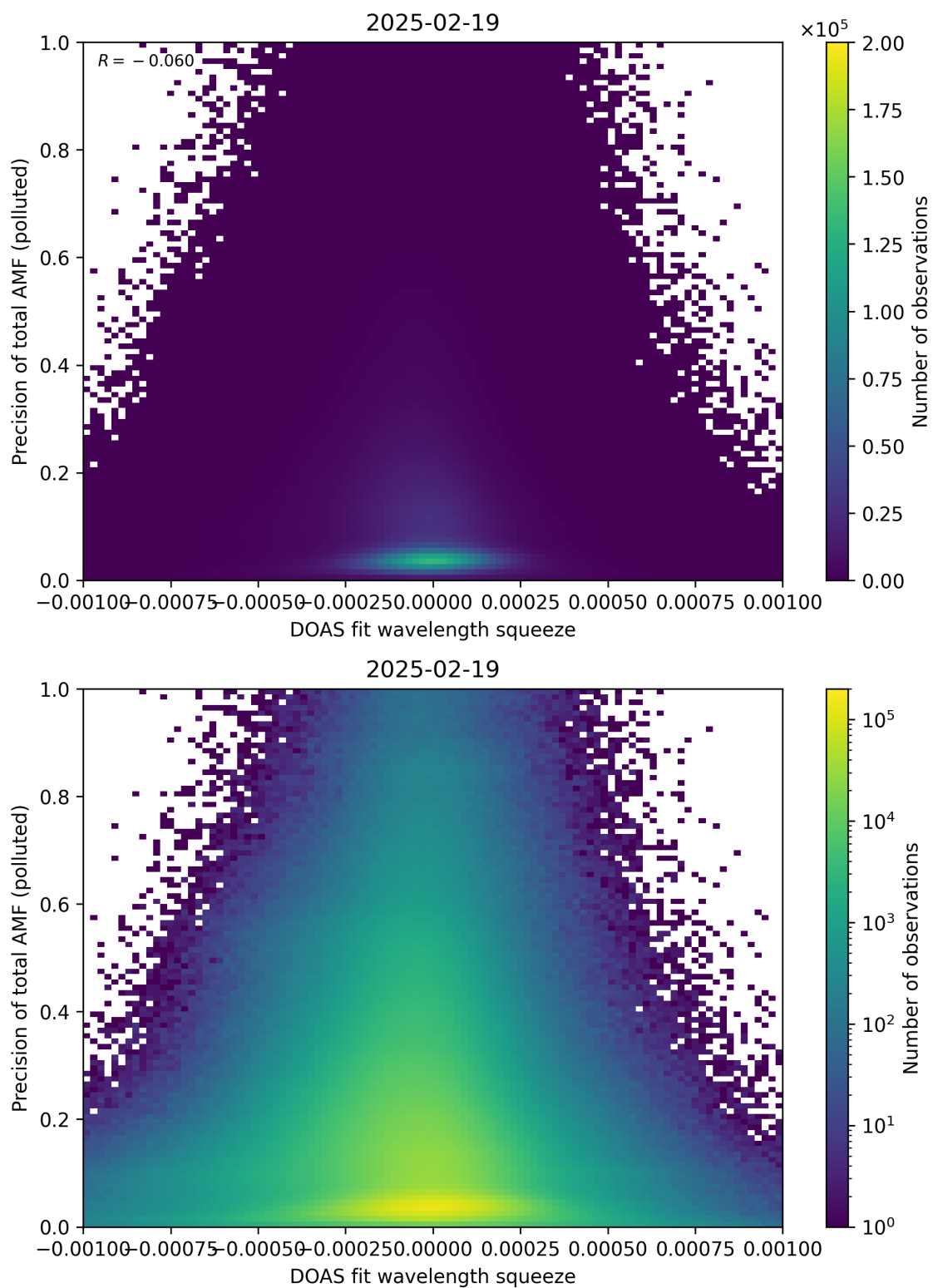
Figure 146: Scatter density plot of “DOAS fit wavelength squeeze” against “Precision of total AMF (polluted)” for 2025-02-19 to 2025-02-20.
