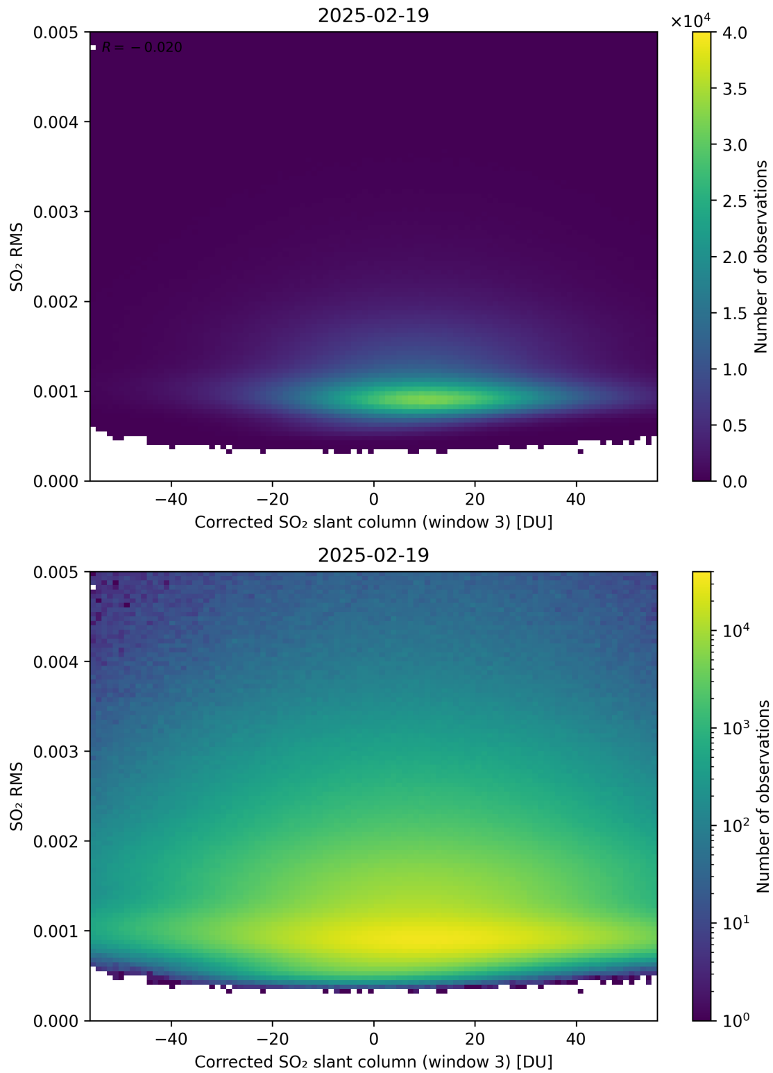
Figure 258: Scatter density plot of “Corrected SO 2 slant column (window 3)” against “SO 2 RMS” for 2025-02-19 to 2025-02-20.
