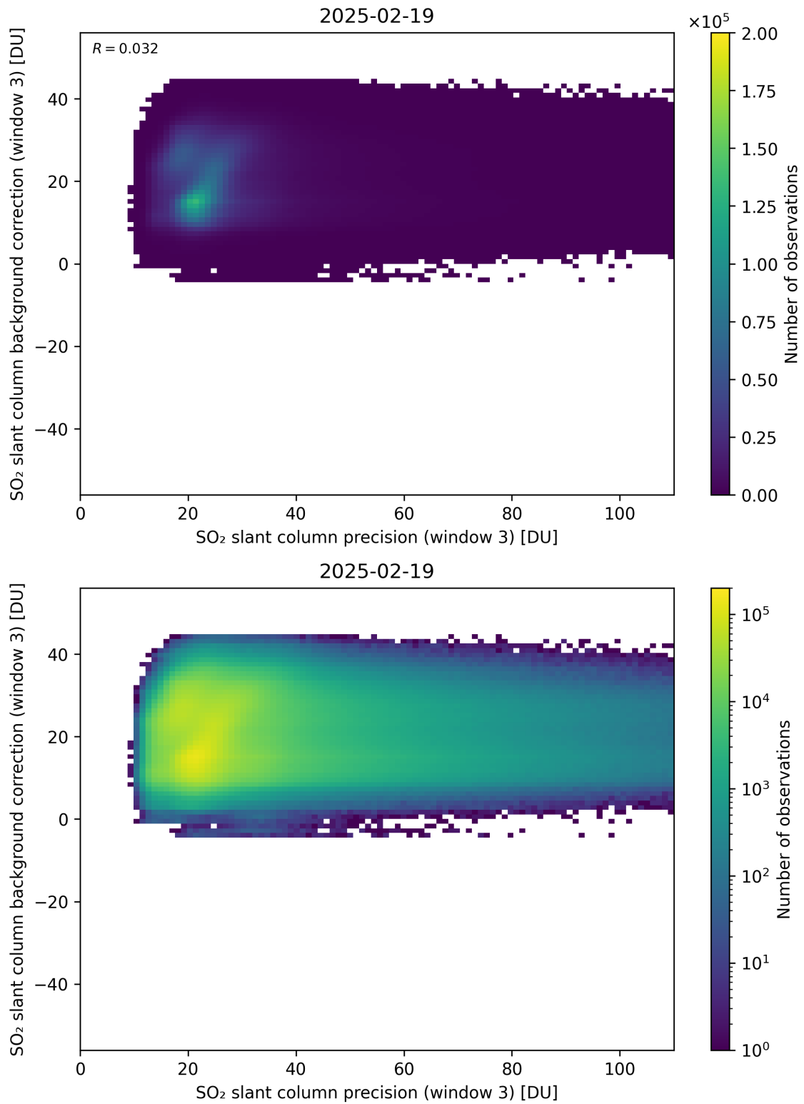
Figure 307: Scatter density plot of “SO 2 slant column precision (window 3)” against “SO 2 slant column background correction (window 3)” for 2025-02-19 to 2025-02-20.
