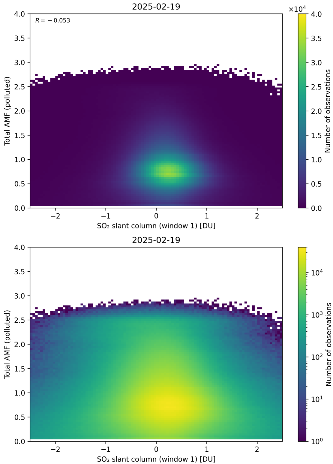
Figure 289: Scatter density plot of “SO 2 slant column (window 1)” against “Total AMF (polluted)” for 2025-02-19 to 2025-02-20.
