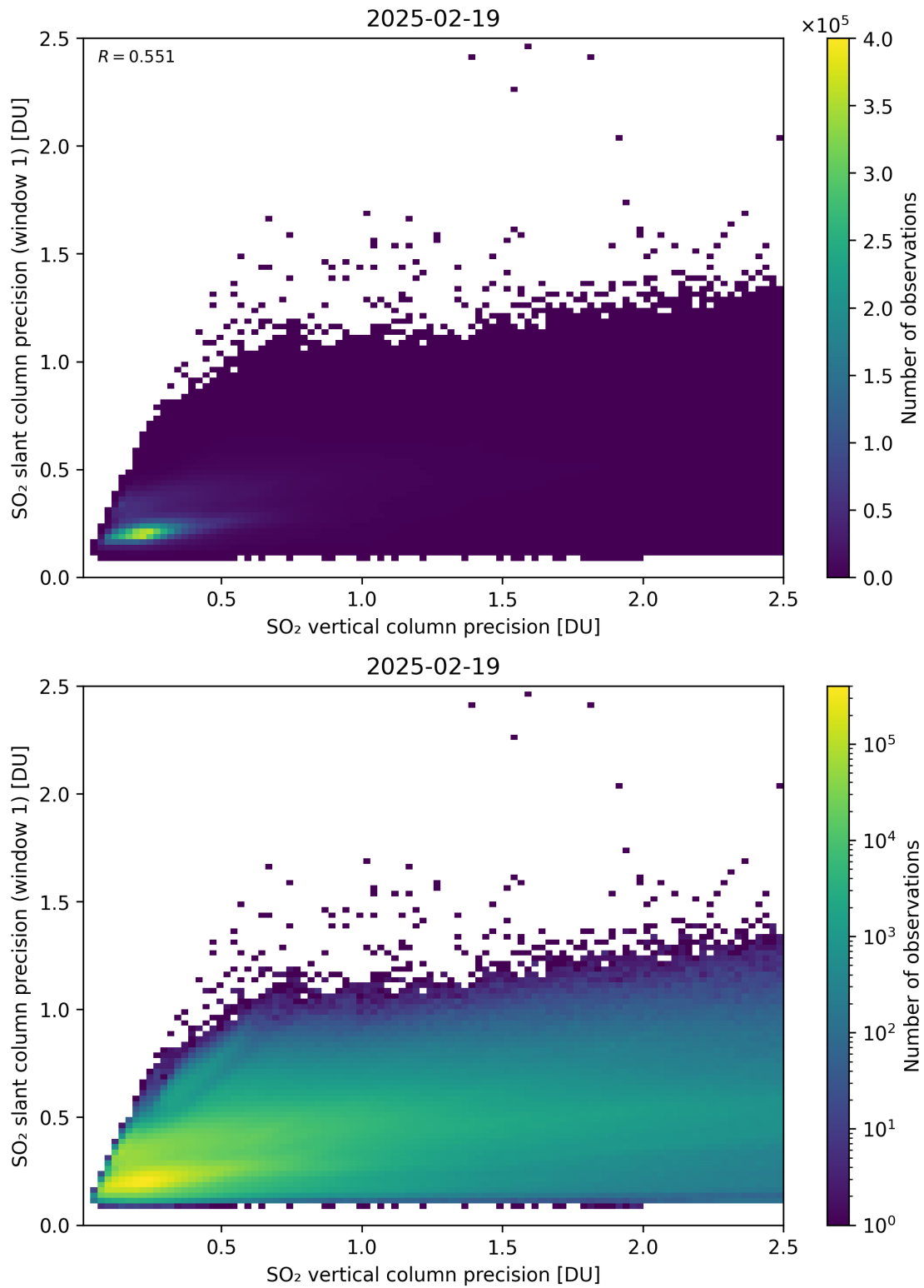
Figure 342: Scatter density plot of “SO 2 vertical column precision” against “SO 2 slant column precision (window 1)” for 2025-02-19 to 2025-02-20.
