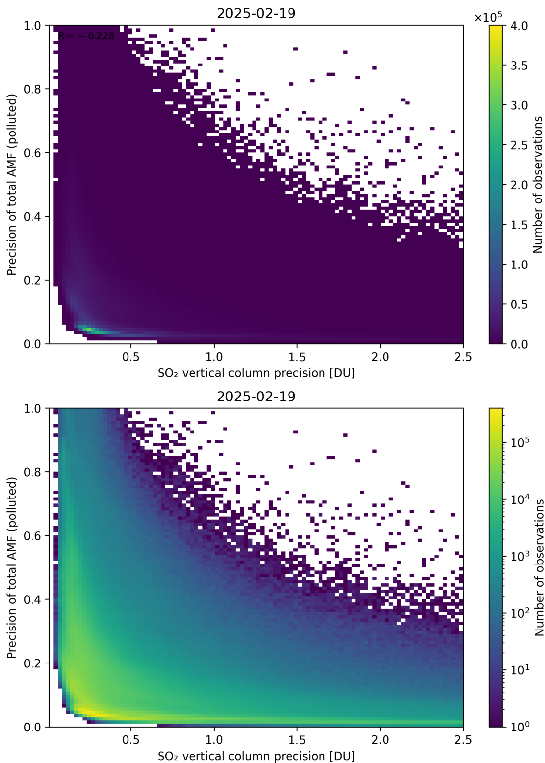
Figure 347: Scatter density plot of “SO 2 vertical column precision” against “Precision of total AMF (polluted)” for 2025-02-19 to 2025-02-20.
