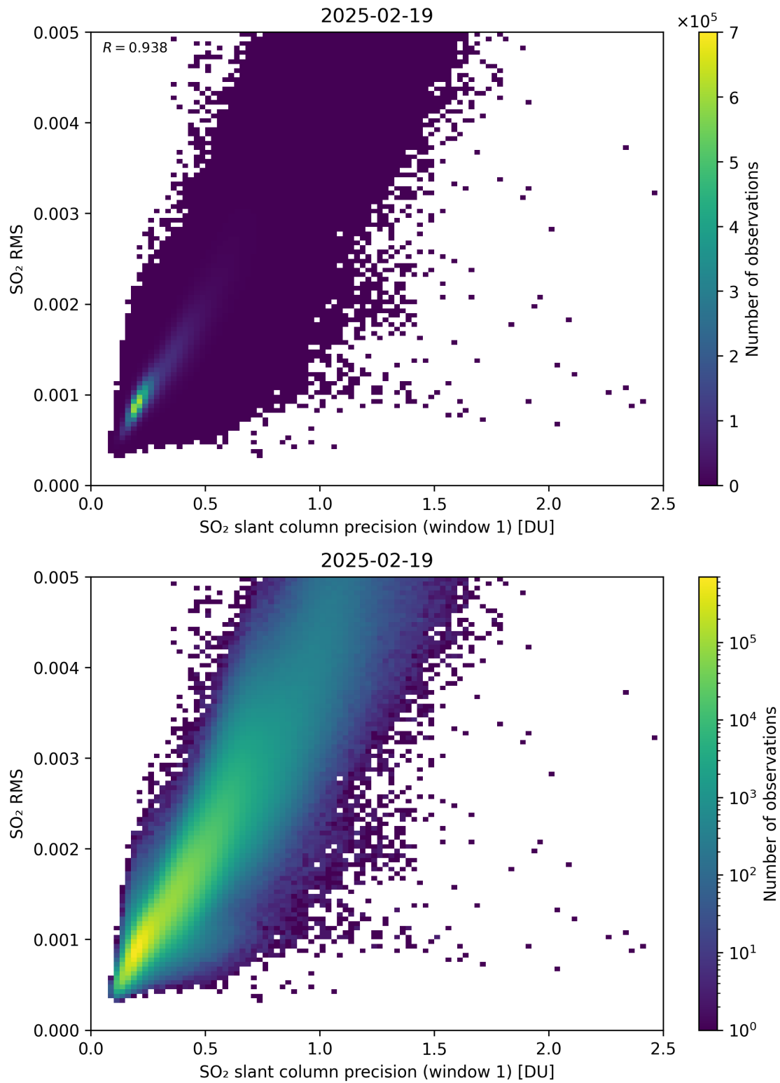
Figure 273: Scatter density plot of “SO 2 slant column precision (window 1)” against “SO 2 RMS” for 2025-02-19 to 2025-02-20.
