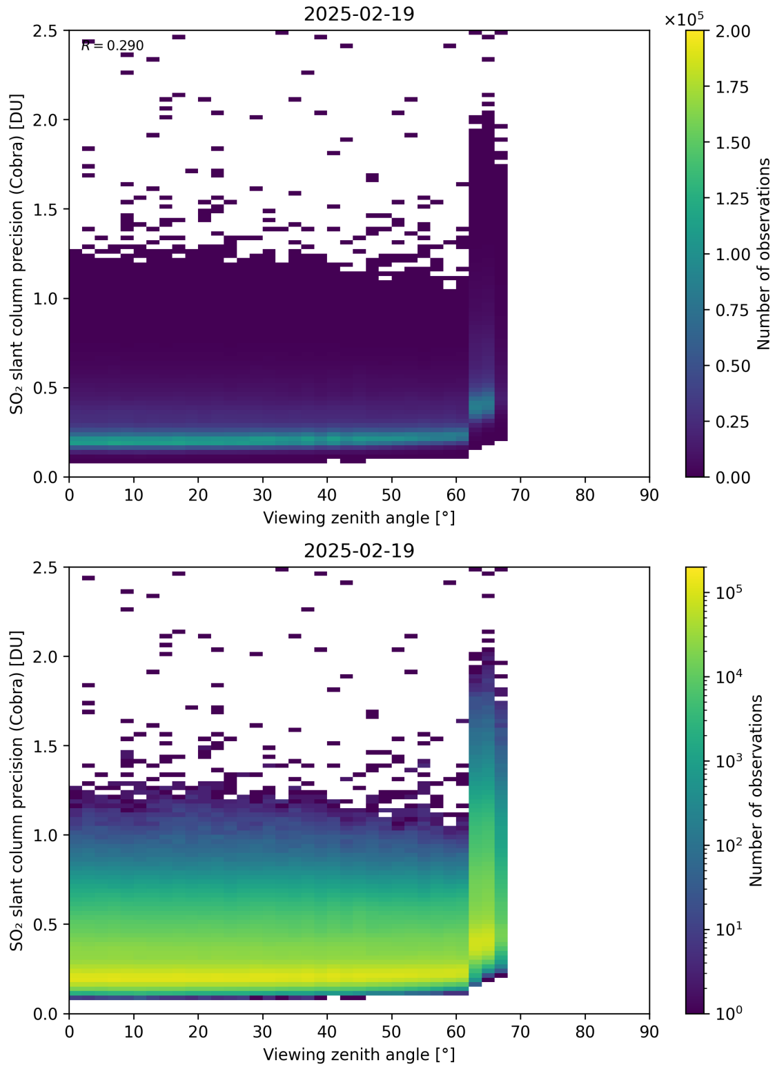
Figure 372: Scatter density plot of “Viewing zenith angle” against “SO 2 slant column precision (Cobra)” for 2025-02-19 to 2025-02-20.
