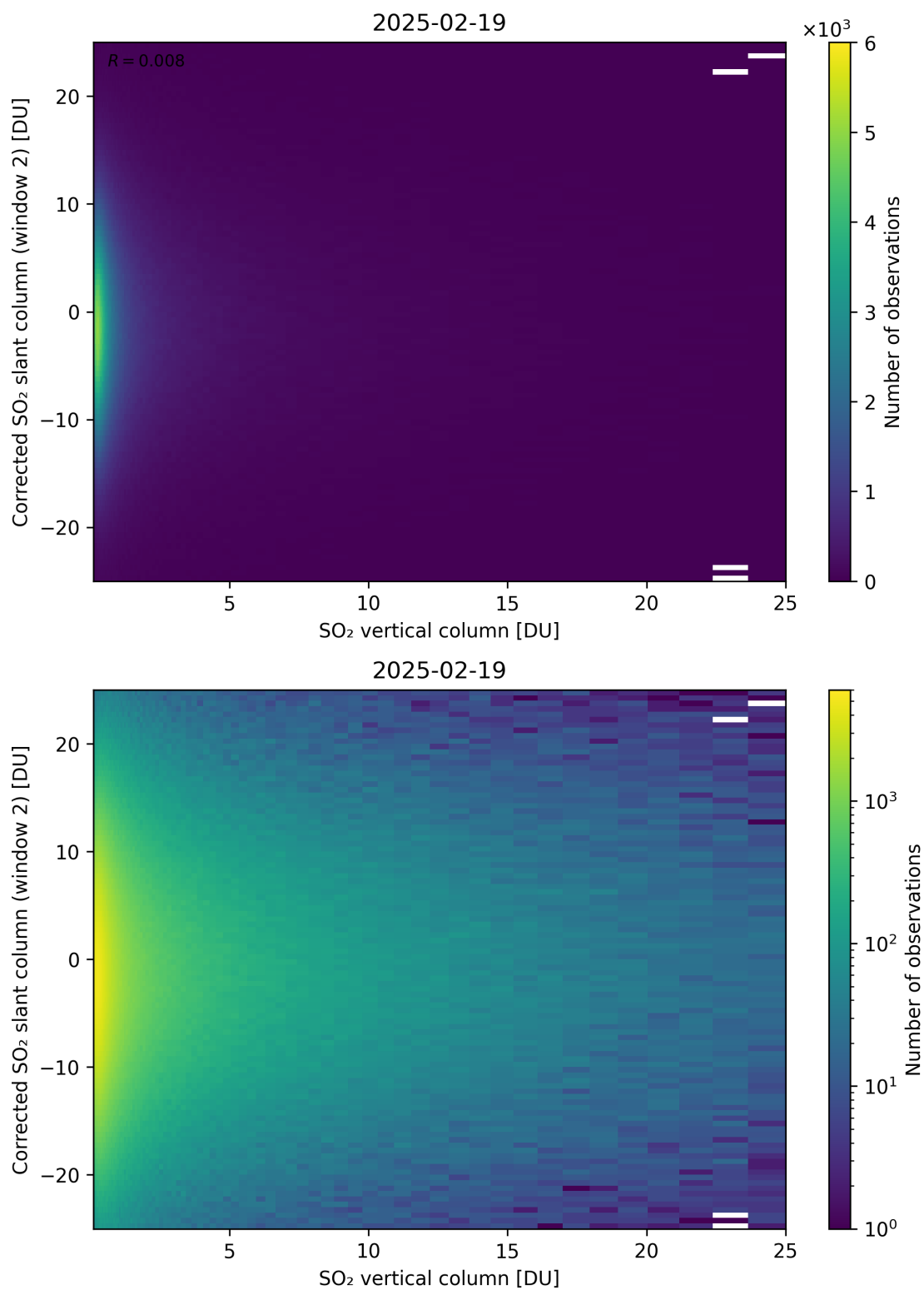
Figure 352: Scatter density plot of “SO 2 vertical column” against “Corrected SO 2 slant column (window 2)” for 2025-02-19 to 2025-02-20.
