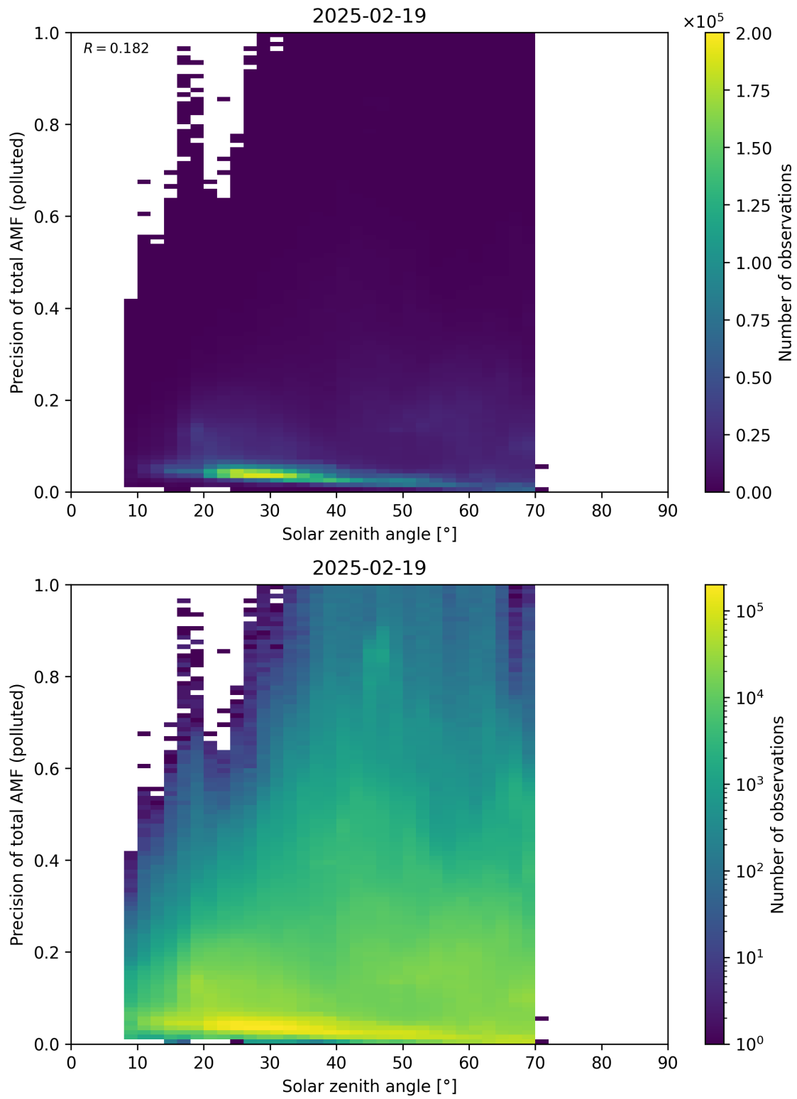
Figure 190: Scatter density plot of “Solar zenith angle” against “Precision of total AMF (polluted)” for 2025-02-19 to 2025-02-20.
