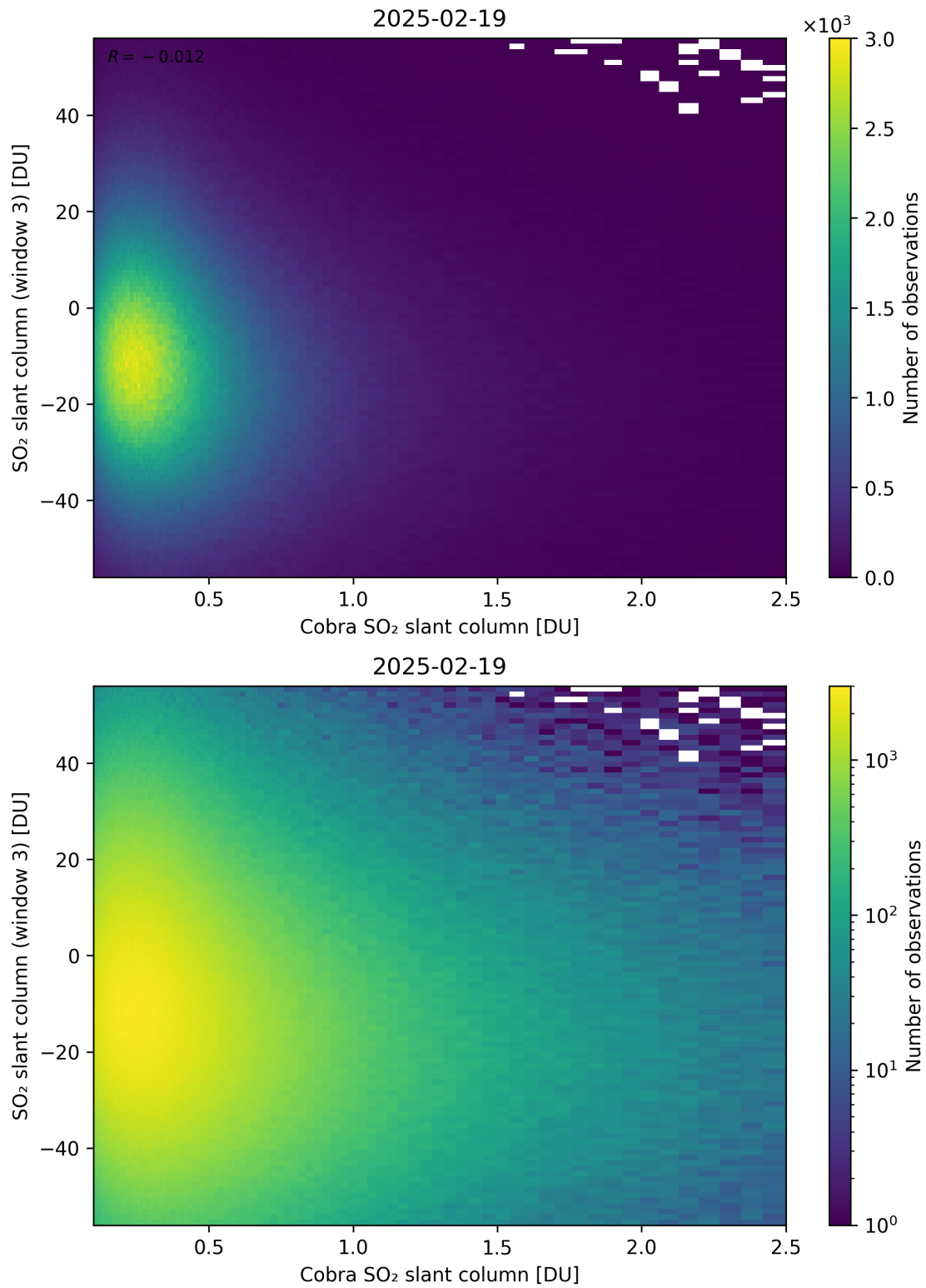
Figure 222: Scatter density plot of “Cobra SO 2 slant column” against “SO 2 slant column (window 3)” for 2025-02-19 to 2025-02-20.
