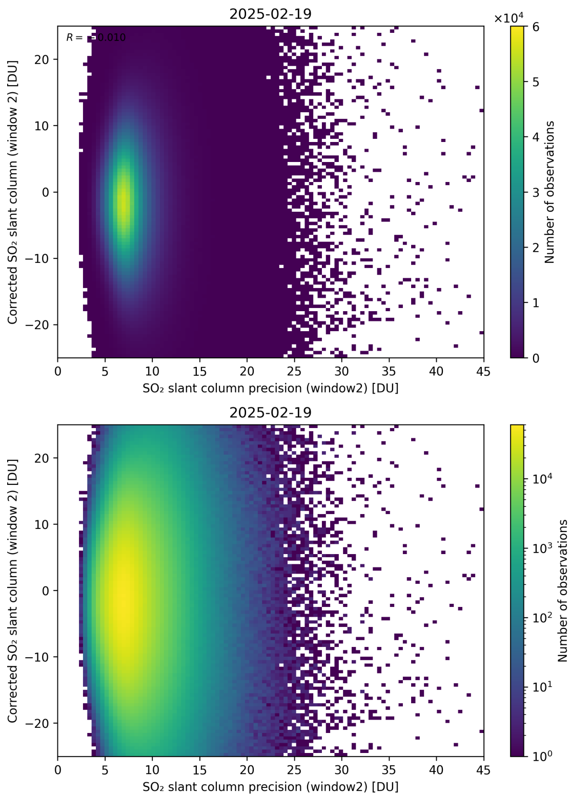
Figure 297: Scatter density plot of “SO 2 slant column precision (window2)” against “Corrected SO 2 slant column (window 2)” for 2025-02-19 to 2025-02-20.
