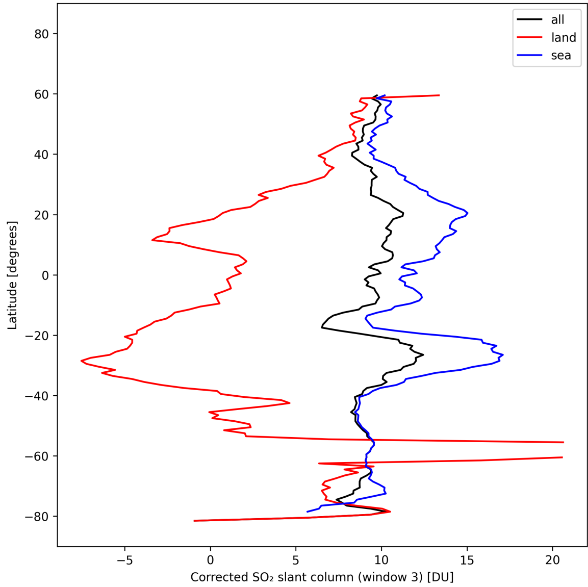
Figure 47: Zonal average of “Corrected SO 2 slant column (window 3)” for 2025-02-19 to 2025-02-20.
