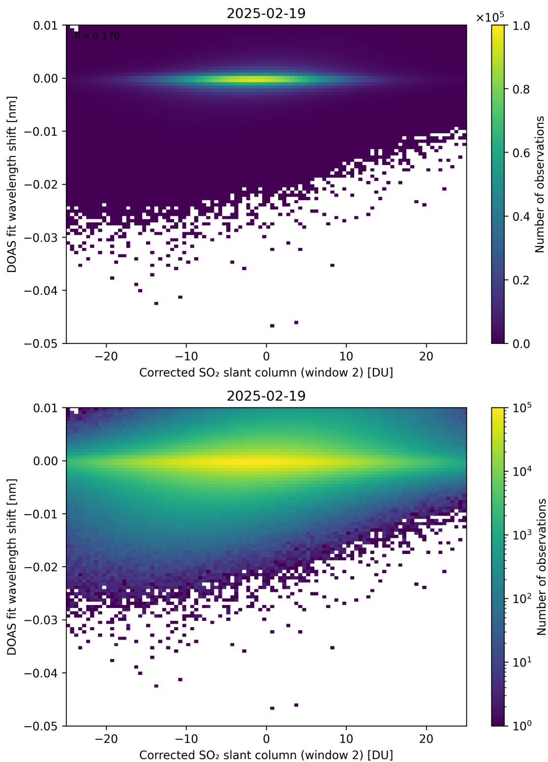
Figure 246: Scatter density plot of “Corrected SO 2 slant column (window 2)” against “DOAS fit wavelength shift” for 2025-02-19 to 2025-02-20.
