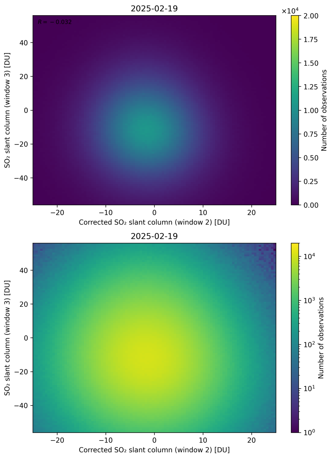
Figure 251: Scatter density plot of “Corrected SO 2 slant column (window 2)” against “SO 2 slant column (window 3)” for 2025-02-19 to 2025-02-20.
