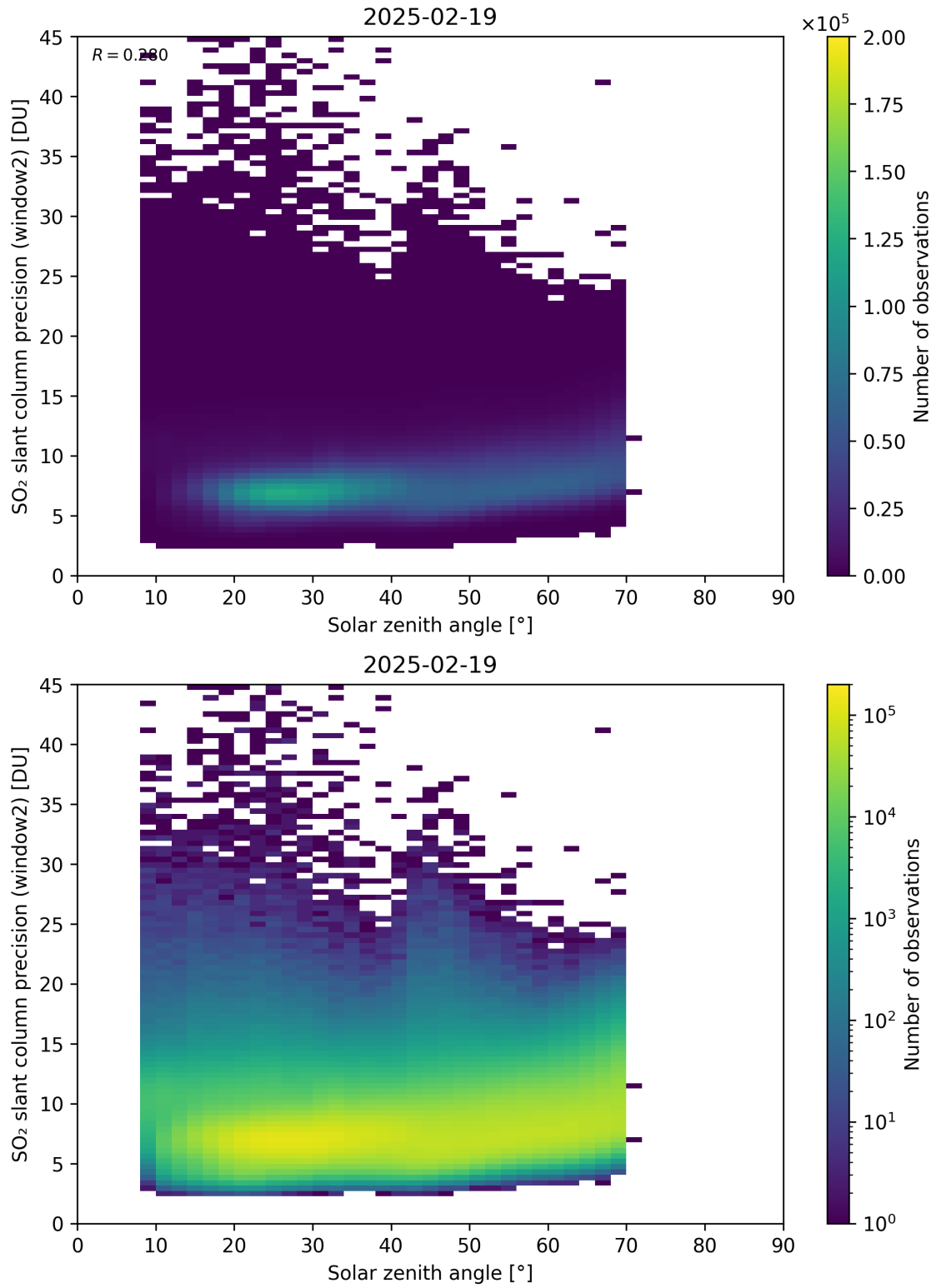
Figure 186: Scatter density plot of “Solar zenith angle” against “SO 2 slant column precision (window2)” for 2025-02-19 to 2025-02-20.
