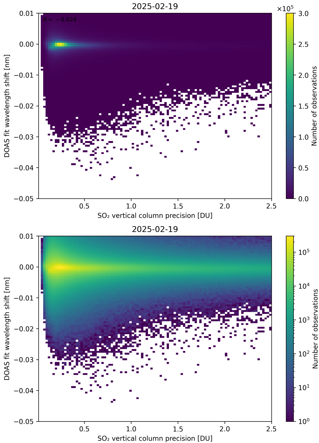
Figure 332: Scatter density plot of “SO 2 vertical column precision” against “DOAS fit wavelength shift” for 2025-02-19 to 2025-02-20.
