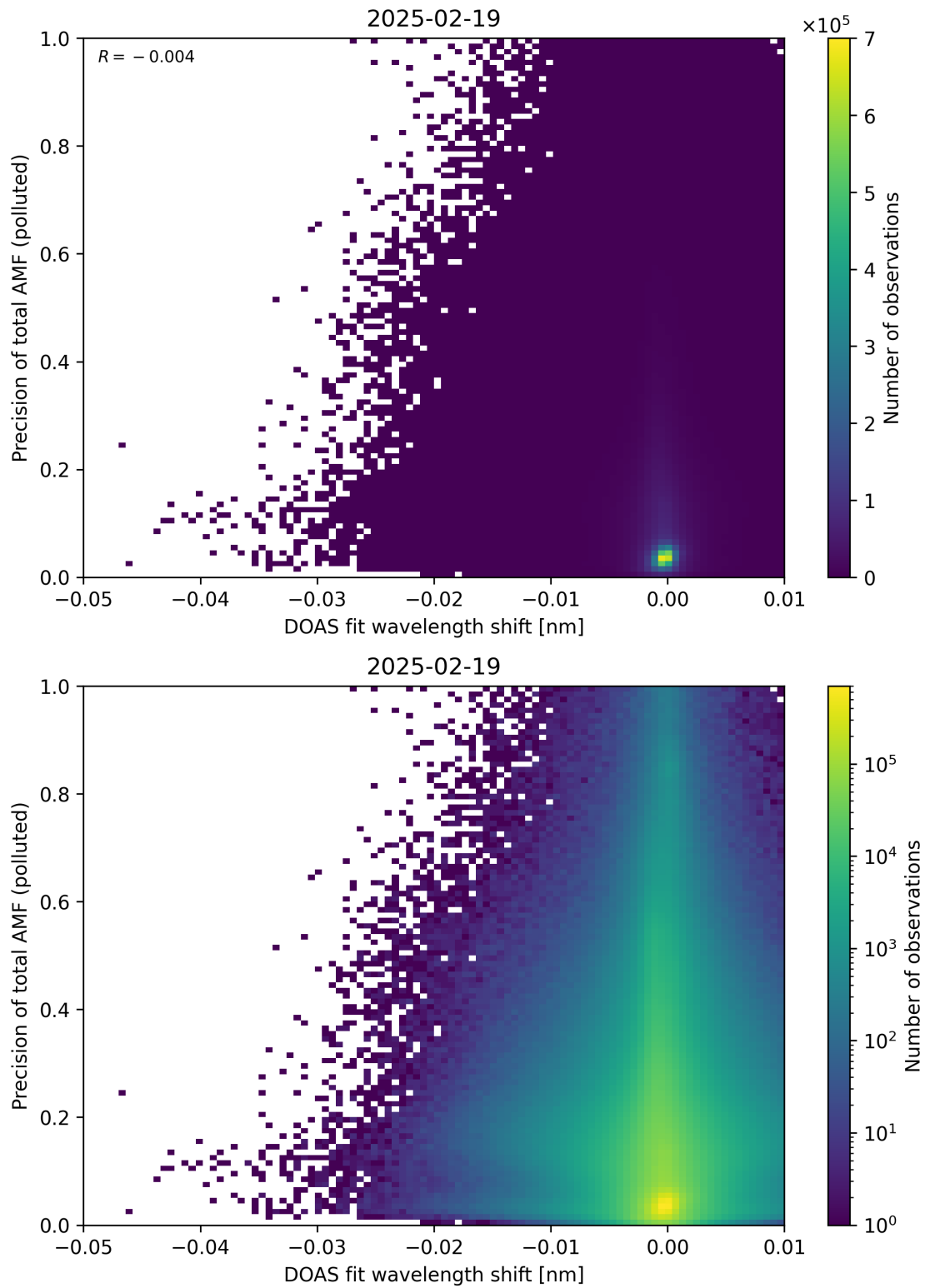
Figure 142: Scatter density plot of “DOAS fit wavelength shift” against “Precision of total AMF (polluted)” for 2025-02-19 to 2025-02-20.
