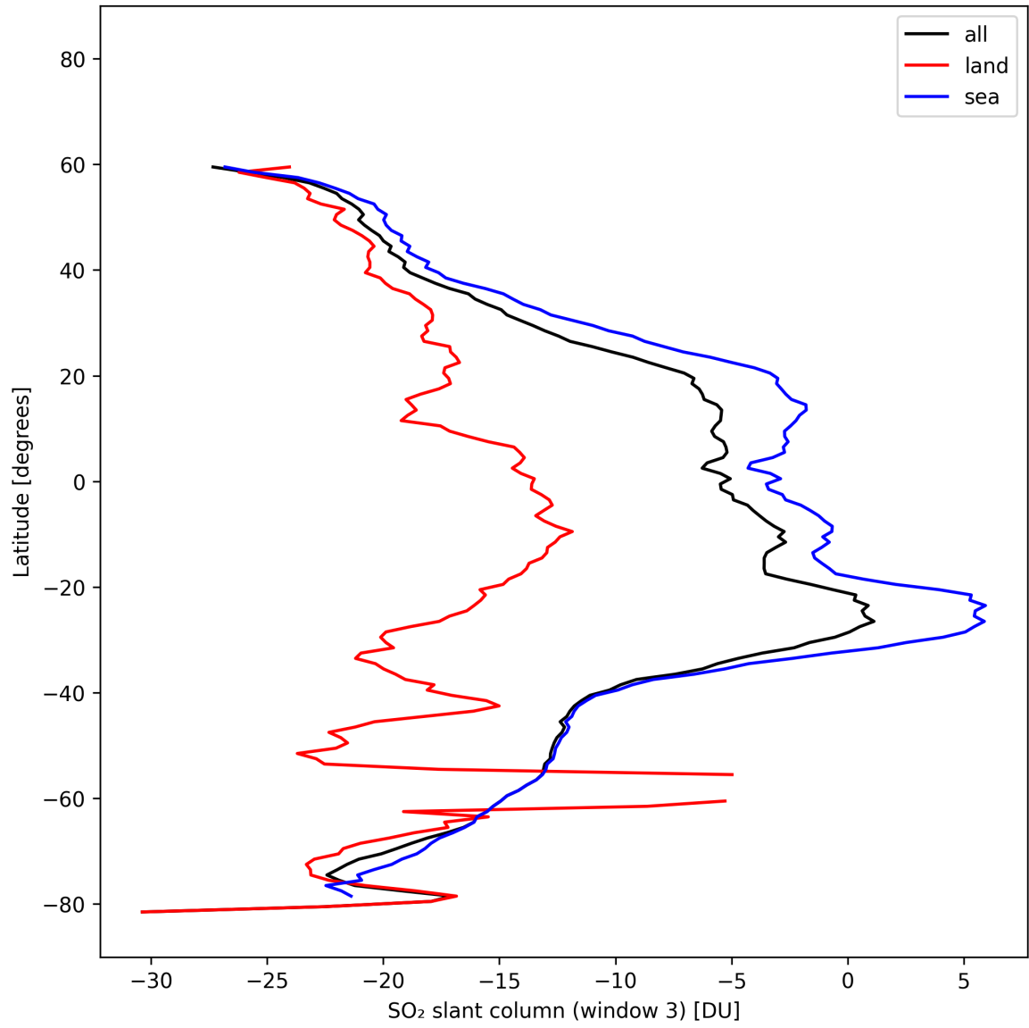
Figure 45: Zonal average of “SO 2 slant column (window 3)” for 2025-02-19 to 2025-02-20.
