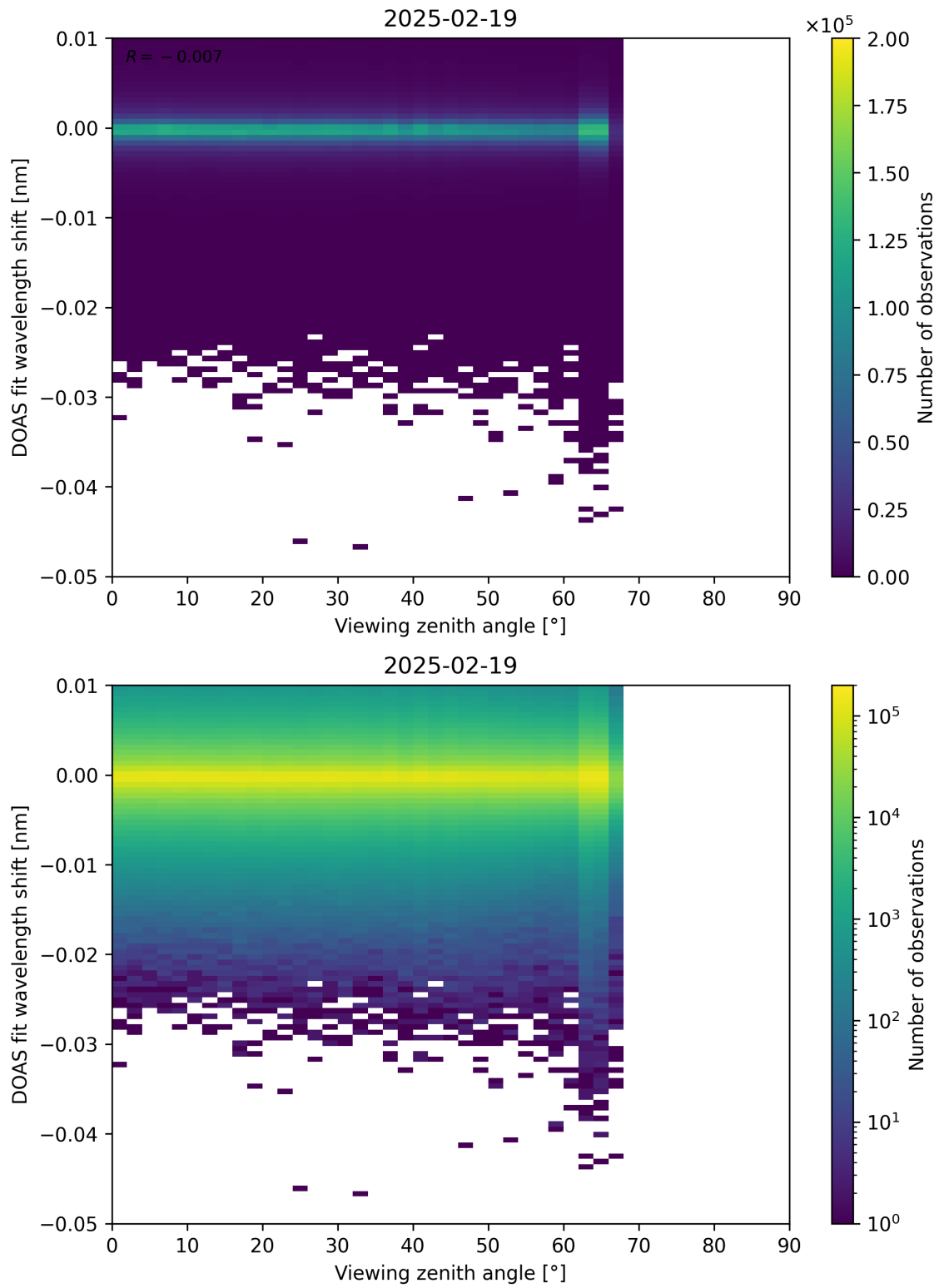
Figure 365: Scatter density plot of “Viewing zenith angle” against “DOAS fit wavelength shift” for 2025-02-19 to 2025-02-20.
