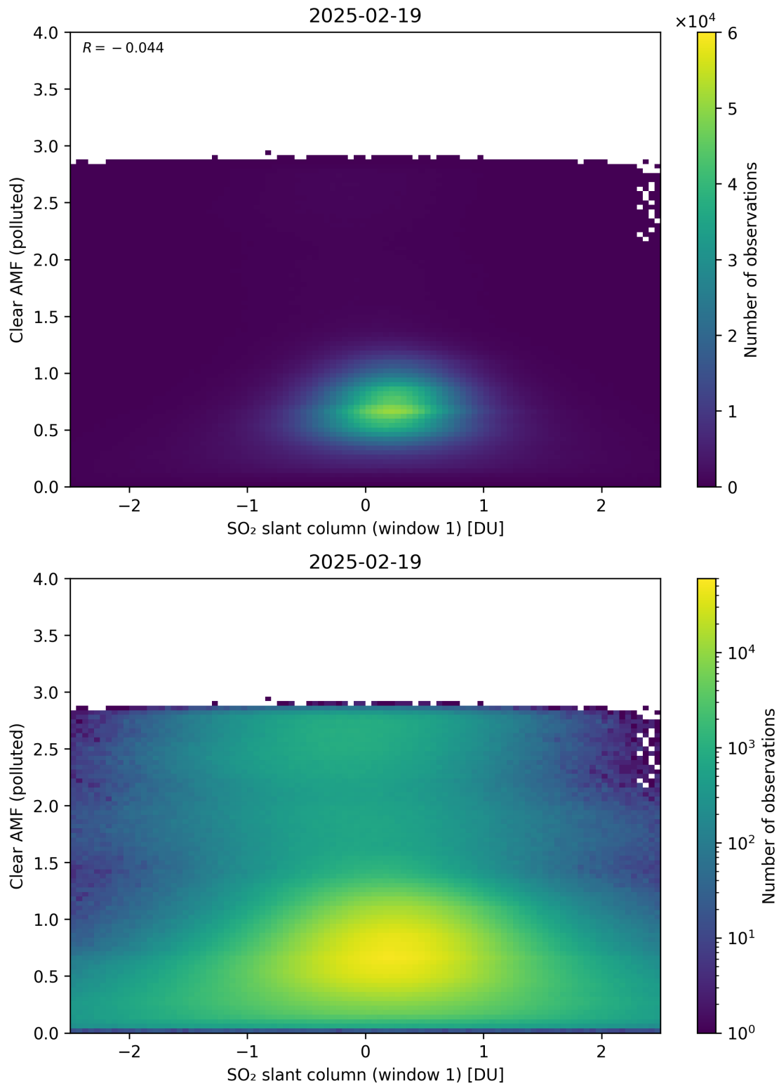
Figure 282: Scatter density plot of “SO 2 slant column (window 1)” against “Clear AMF (polluted)” for 2025-02-19 to 2025-02-20.
