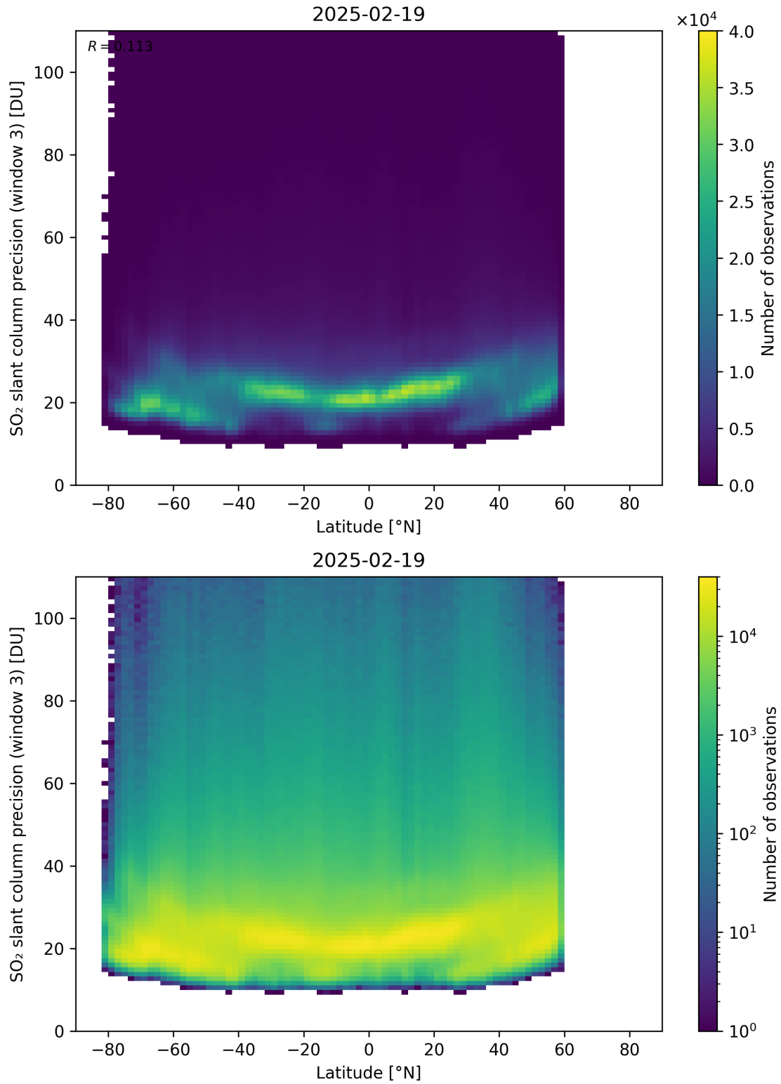
Figure 166: Scatter density plot of “Latitude” against “SO 2 slant column precision (window 3)” for 2025-02-19 to 2025-02-20.
