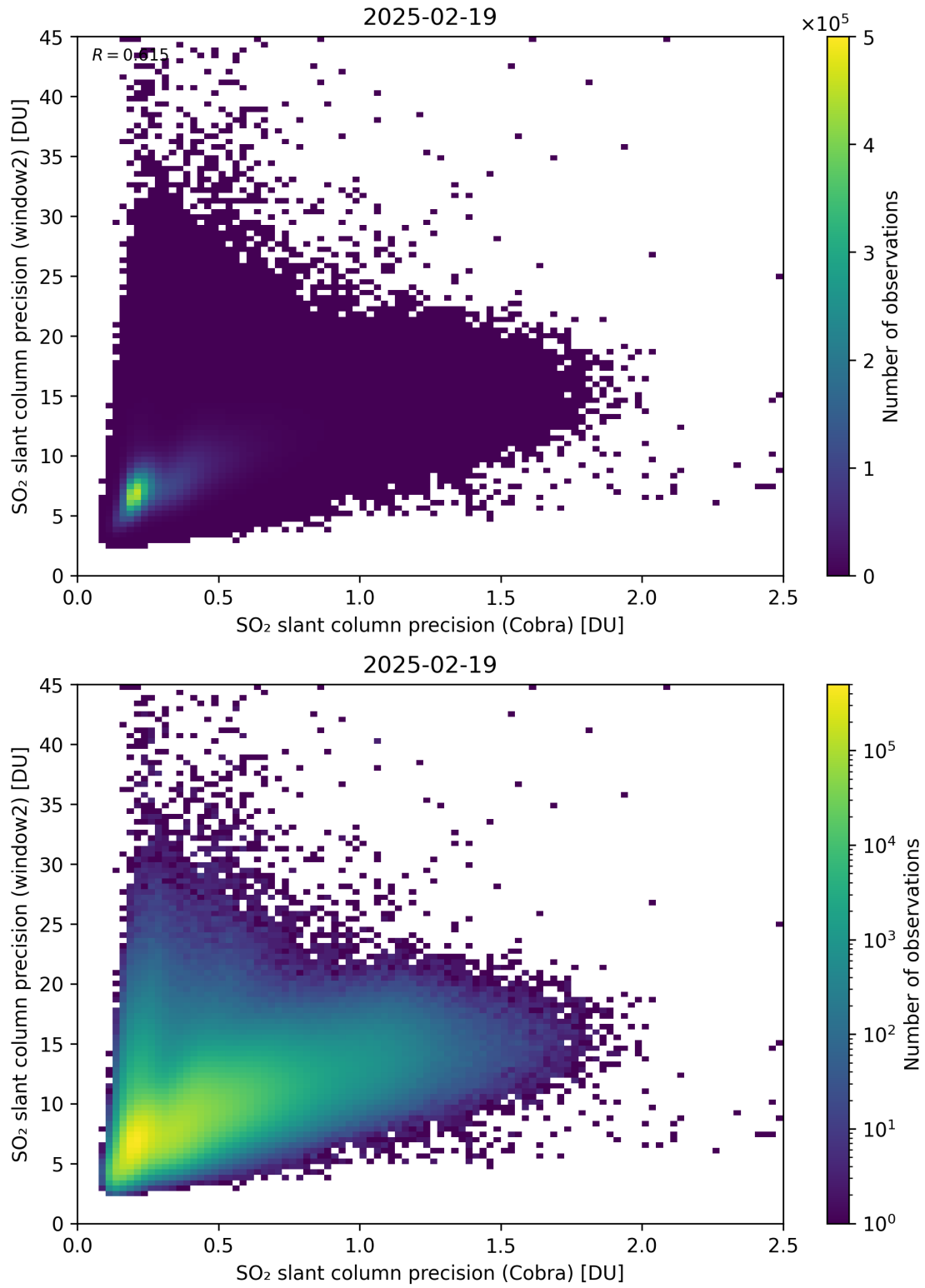
Figure 210: Scatter density plot of “SO 2 slant column precision (Cobra)” against “SO 2 slant column precision (window2)” for 2025-02-19 to 2025-02-20.
