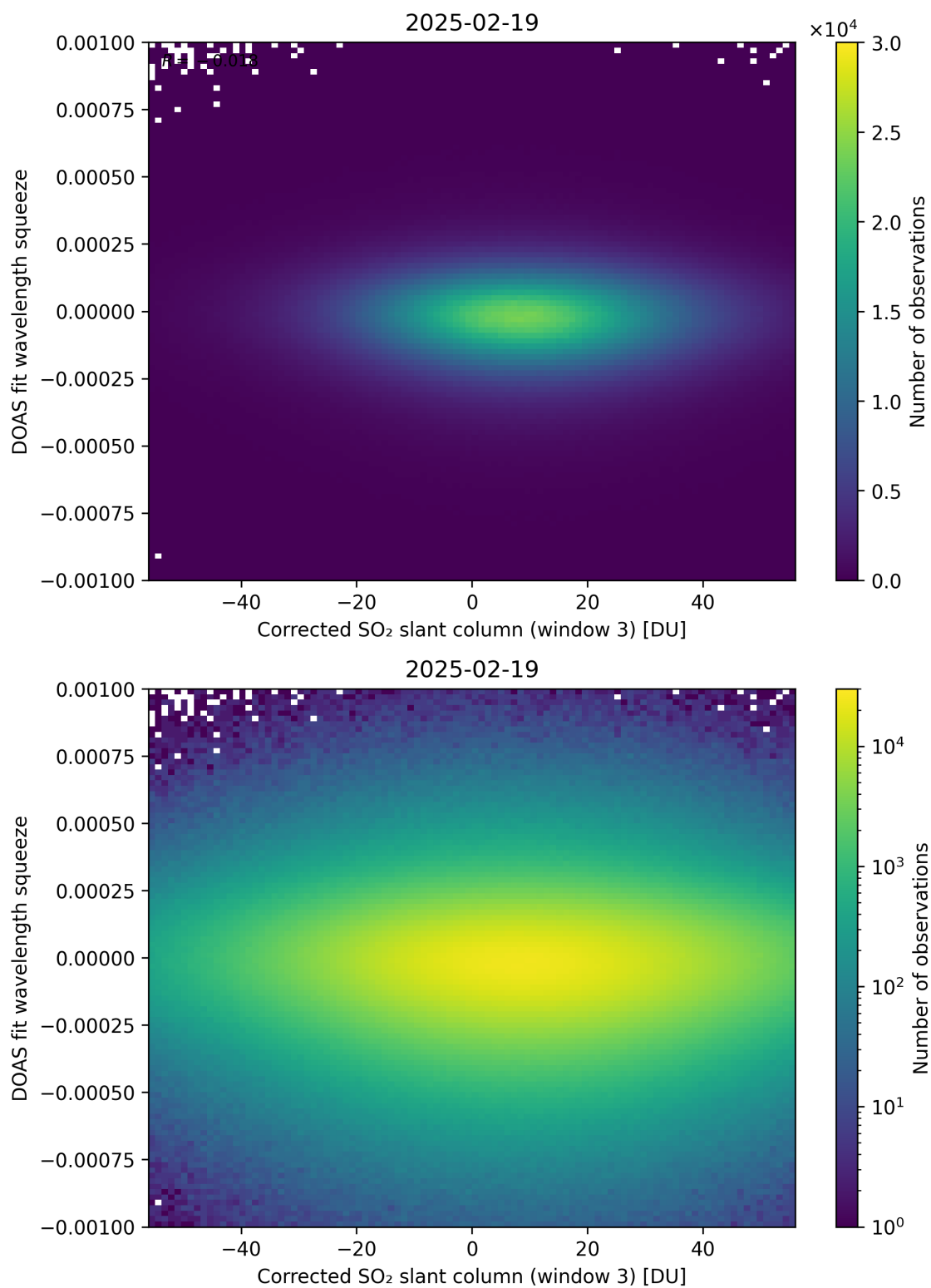
Figure 257: Scatter density plot of “Corrected SO 2 slant column (window 3)” against “DOAS fit wavelength squeeze” for 2025-02-19 to 2025-02-20.
