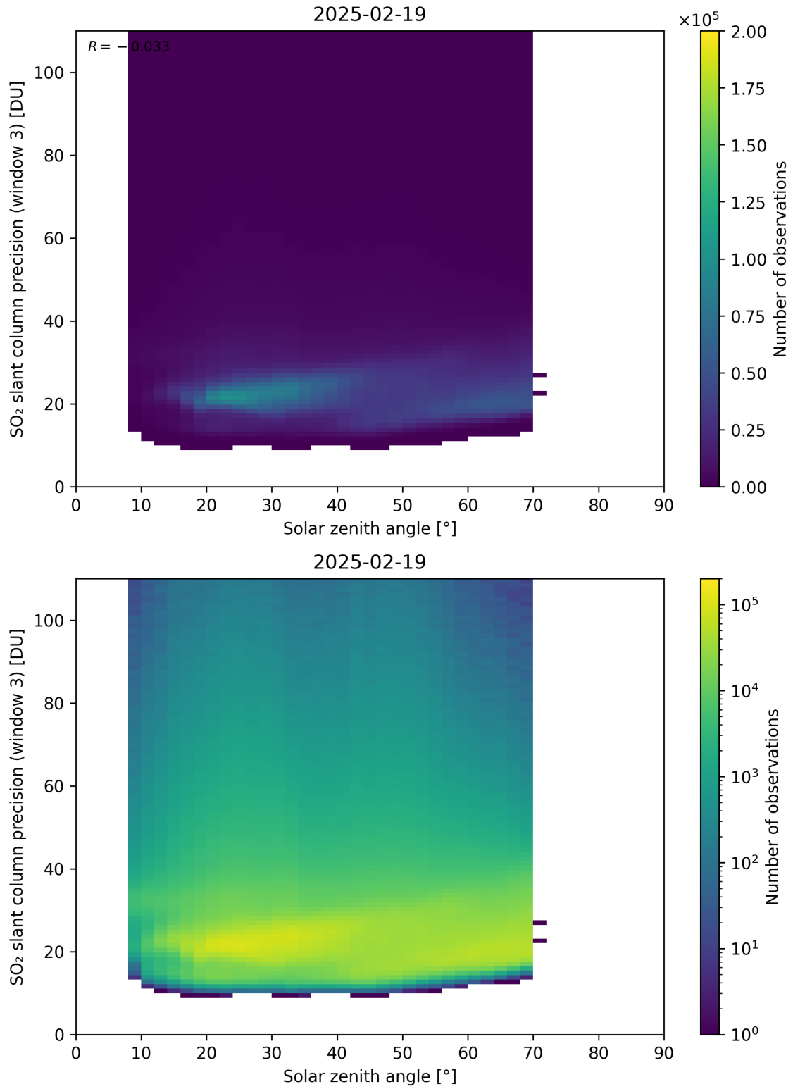
Figure 188: Scatter density plot of “Solar zenith angle” against “SO 2 slant column precision (window 3)” for 2025-02-19 to 2025-02-20.
