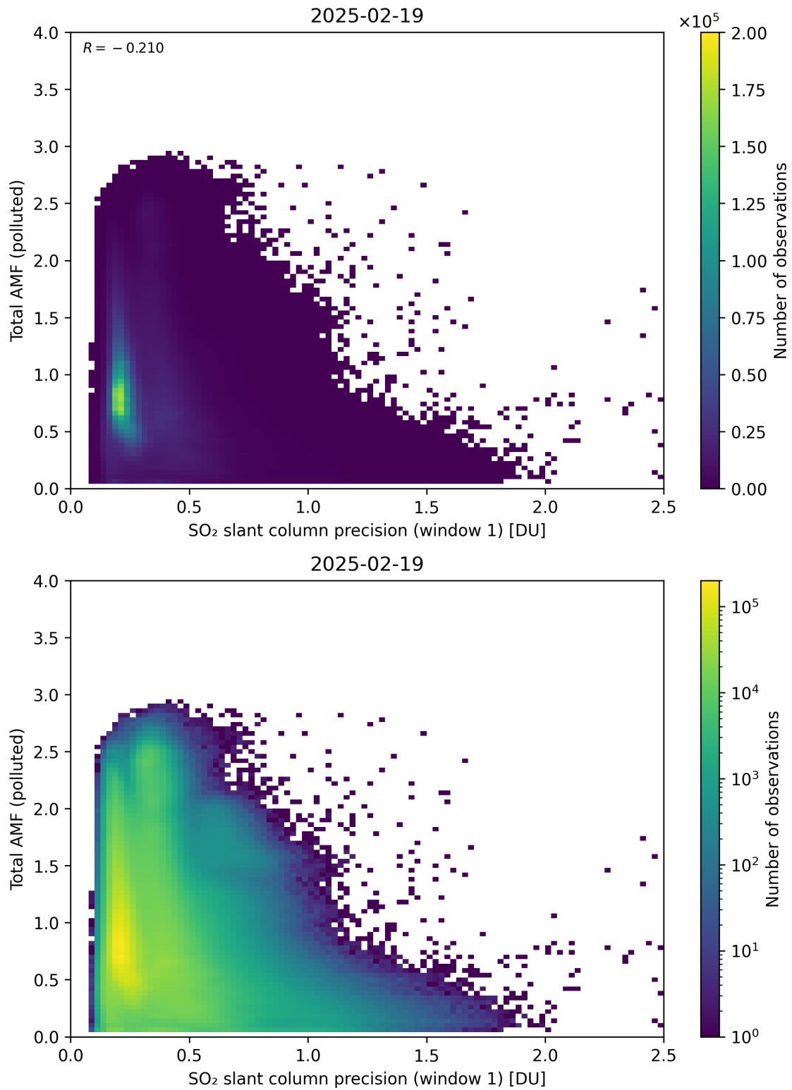
Figure 280: Scatter density plot of “SO 2 slant column precision (window 1)” against “Total AMF (polluted)” for 2025-02-19 to 2025-02-20.
