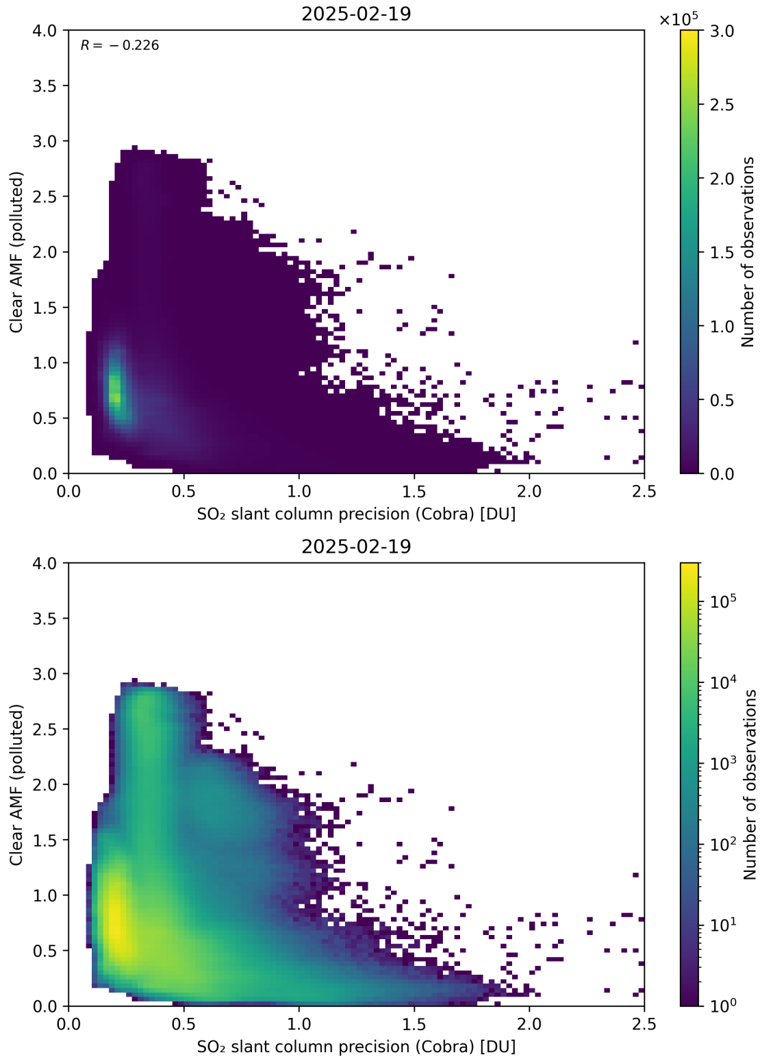
Figure 205: Scatter density plot of “SO 2 slant column precision (Cobra)” against “Clear AMF (polluted)” for 2025-02-19 to 2025-02-20.
