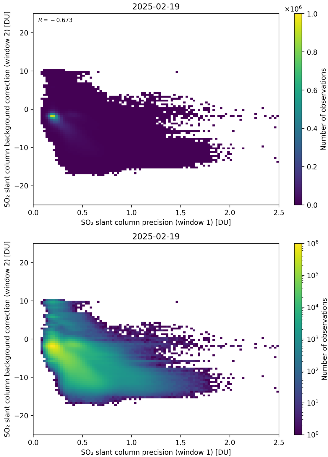
Figure 269: Scatter density plot of “SO 2 slant column precision (window 1)” against “SO 2 slant column background correction (window 2)” for 2025-02-19 to 2025-02-20.
