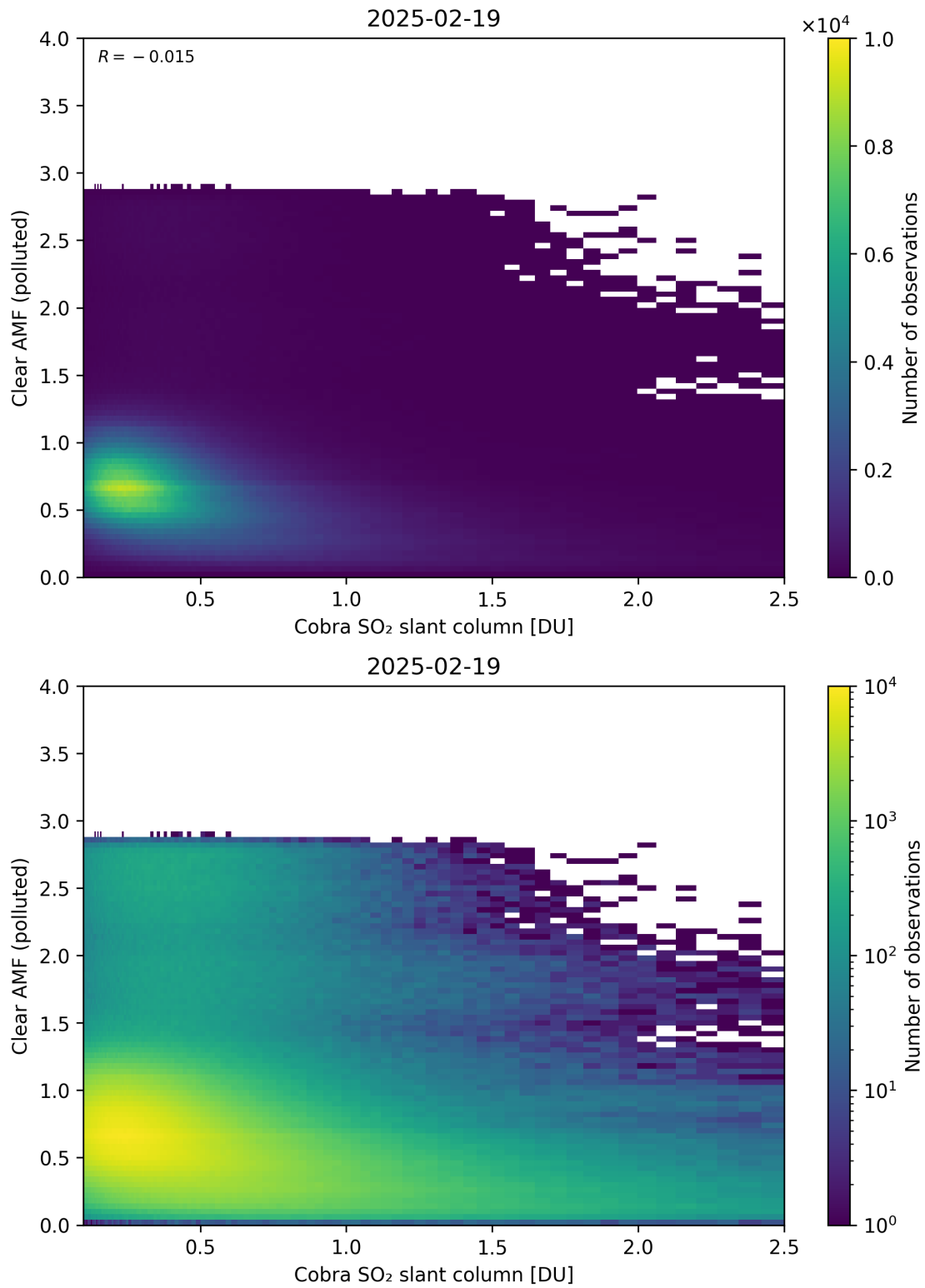
Figure 215: Scatter density plot of “Cobra SO 2 slant column” against “Clear AMF (polluted)” for 2025-02-19 to 2025-02-20.
