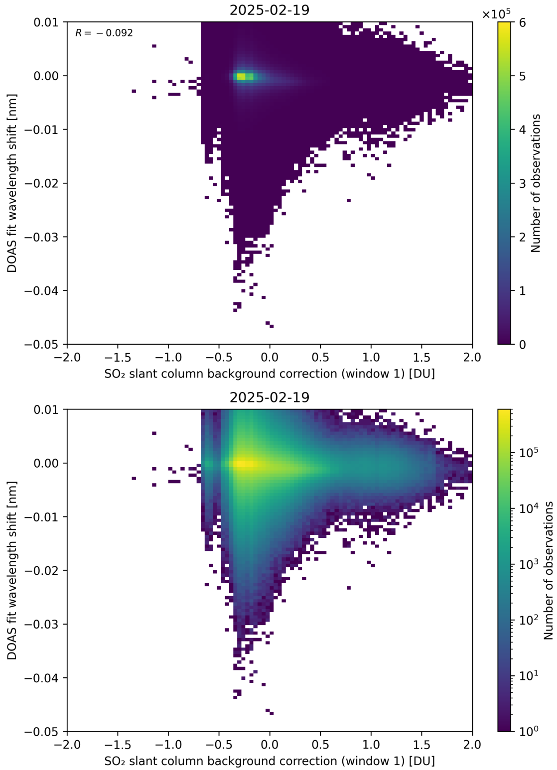
Figure 111: Scatter density plot of “SO 2 slant column background correction (window 1)” against “DOAS fit wavelength shift” for 2025-02-19 to 2025-02-20.
