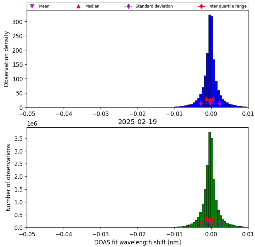
Figure 76: Histogram of “DOAS fit wavelength shift” for 2025-02-19 to 2025-02-20
