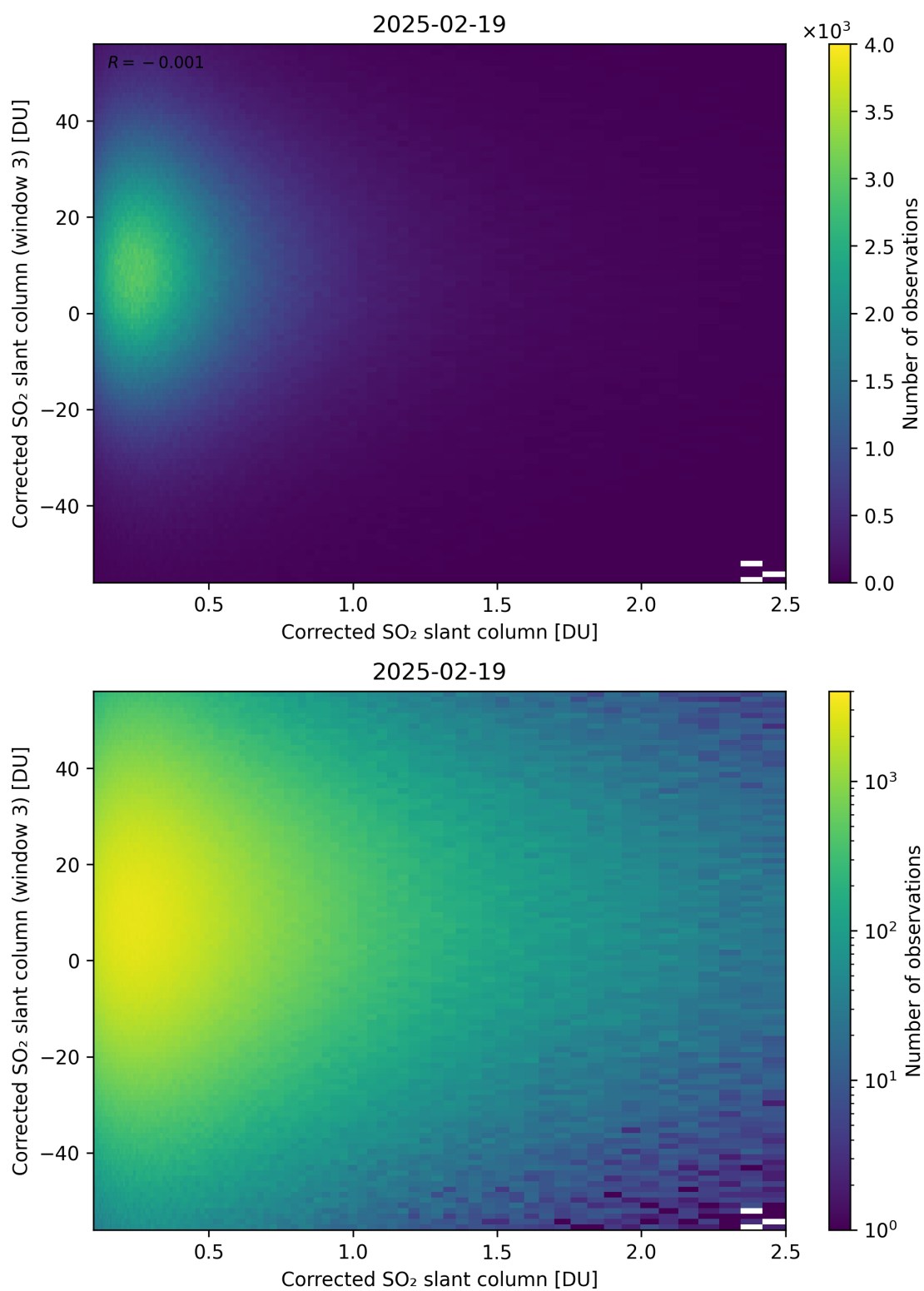
Figure 236: Scatter density plot of “Corrected SO 2 slant column” against “Corrected SO 2 slant column (window 3)” for 2025-02-19 to 2025-02-20.
