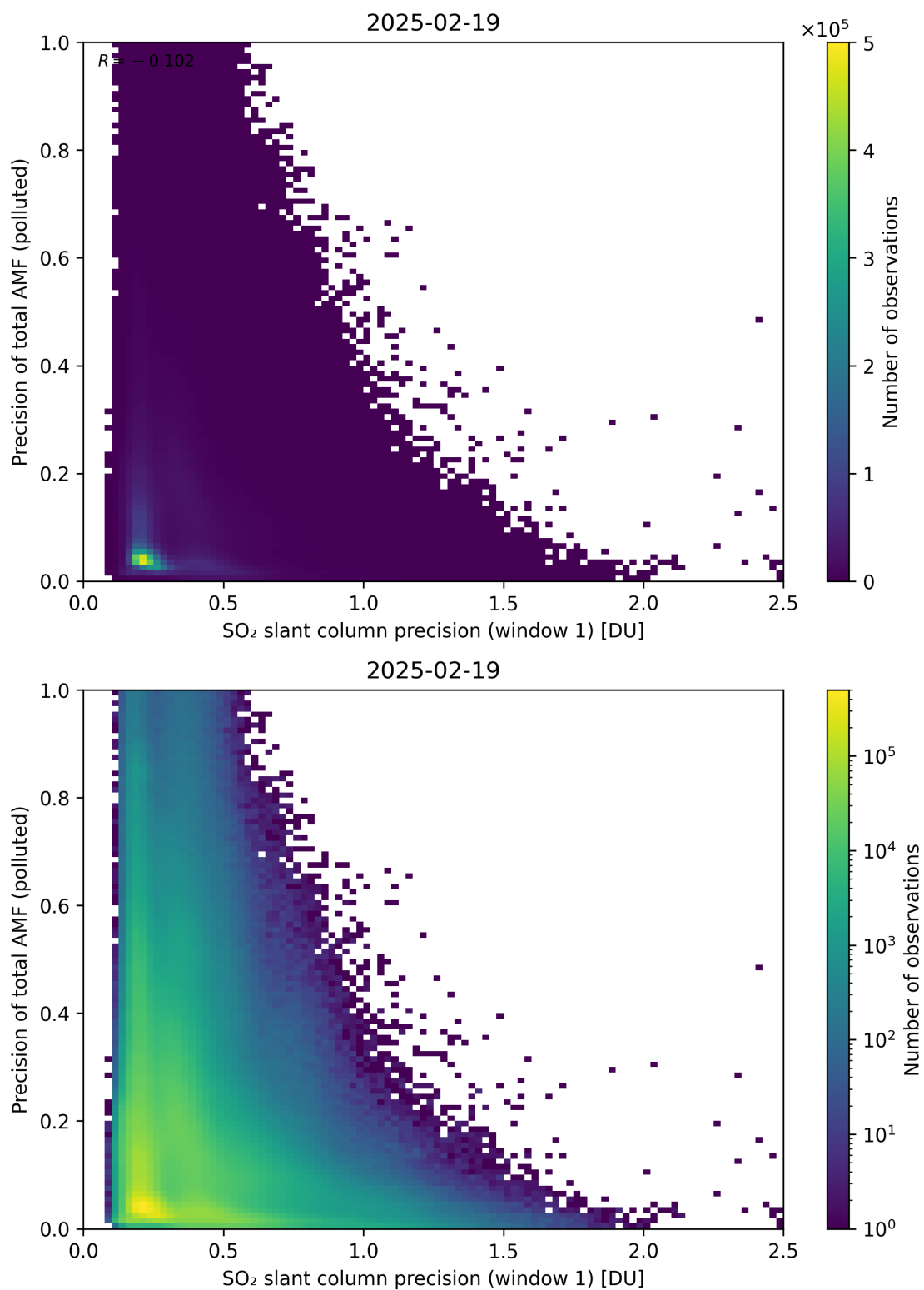
Figure 281: Scatter density plot of “SO 2 slant column precision (window 1)” against “Precision of total AMF (polluted)” for 2025-02-19 to 2025-02-20.
