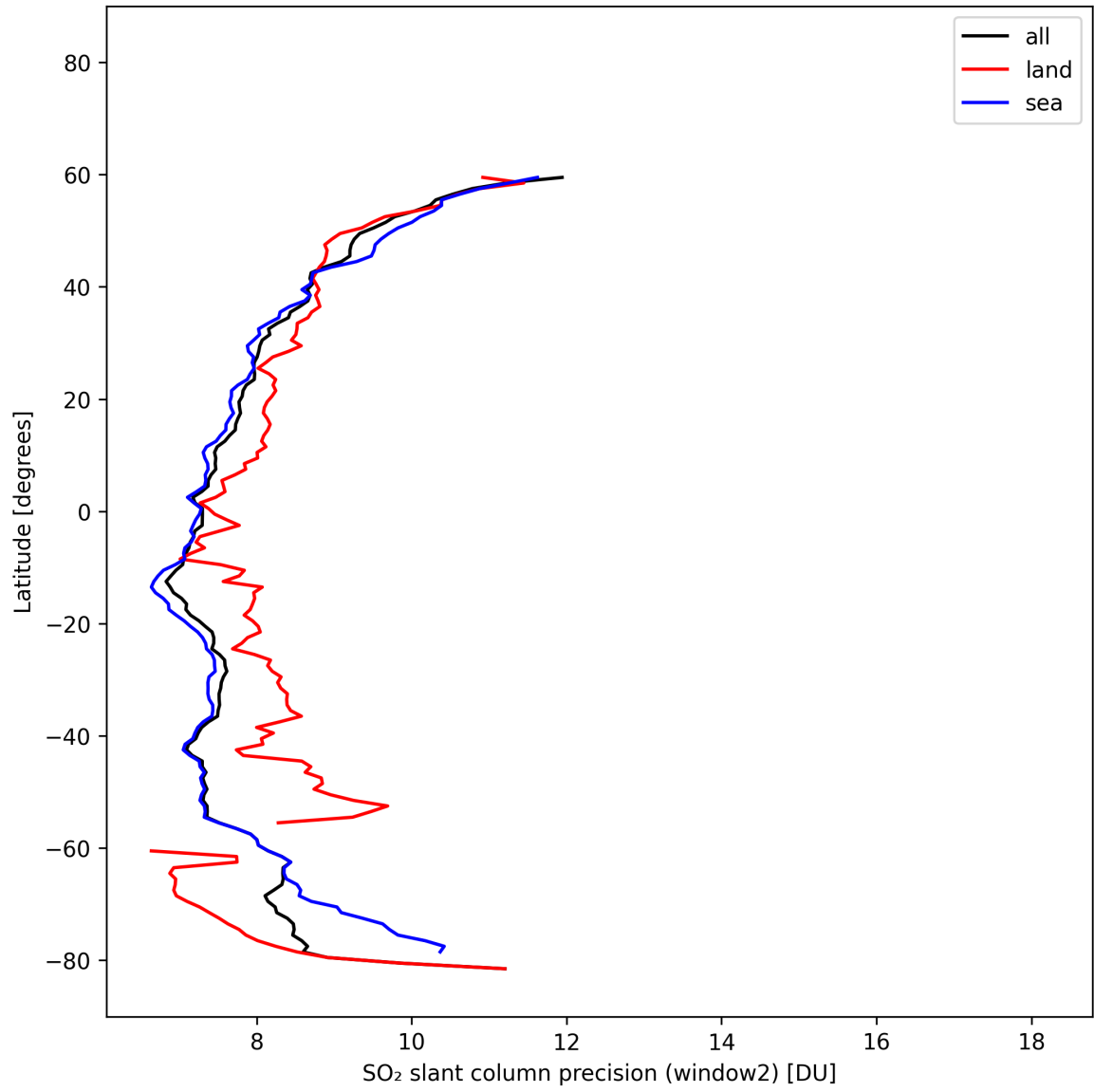
Figure 42: Zonal average of “SO 2 slant column precision (window2)” for 2025-02-19 to 2025-02-20.
