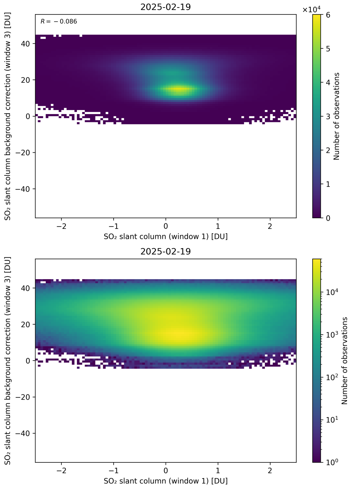
Figure 264: Scatter density plot of “SO 2 slant column (window 1)” against “SO 2 slant column background correction (window 3)” for 2025-02-19 to 2025-02-20.
