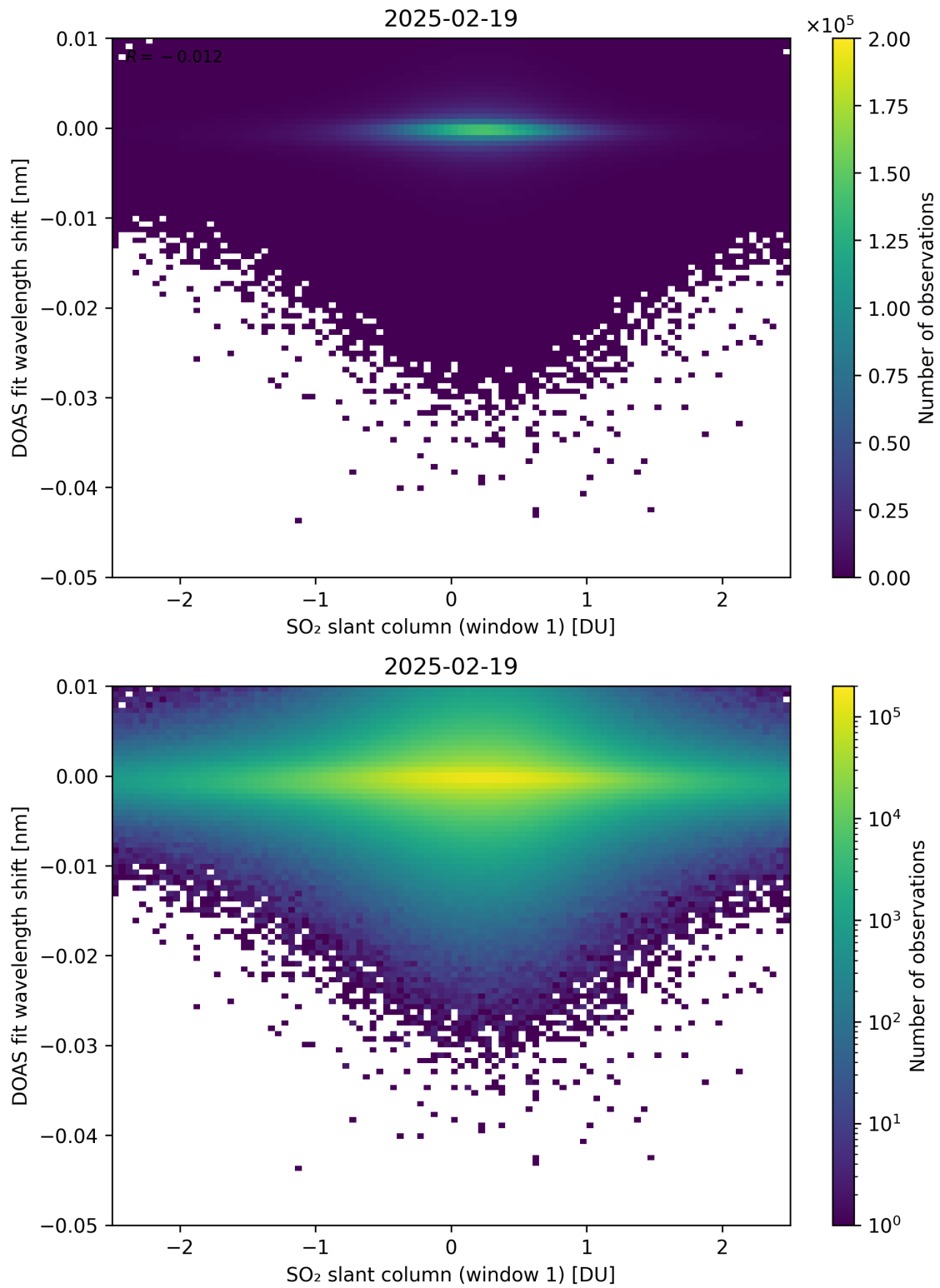
Figure 265: Scatter density plot of “SO 2 slant column (window 1)” against “DOAS fit wavelength shift” for 2025-02-19 to 2025-02-20.
