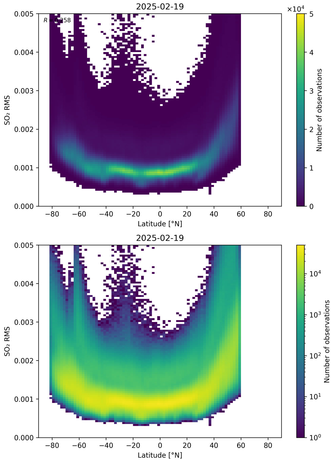
Figure 155: Scatter density plot of “Latitude” against “SO 2 RMS” for 2025-02-19 to 2025-02-20.
