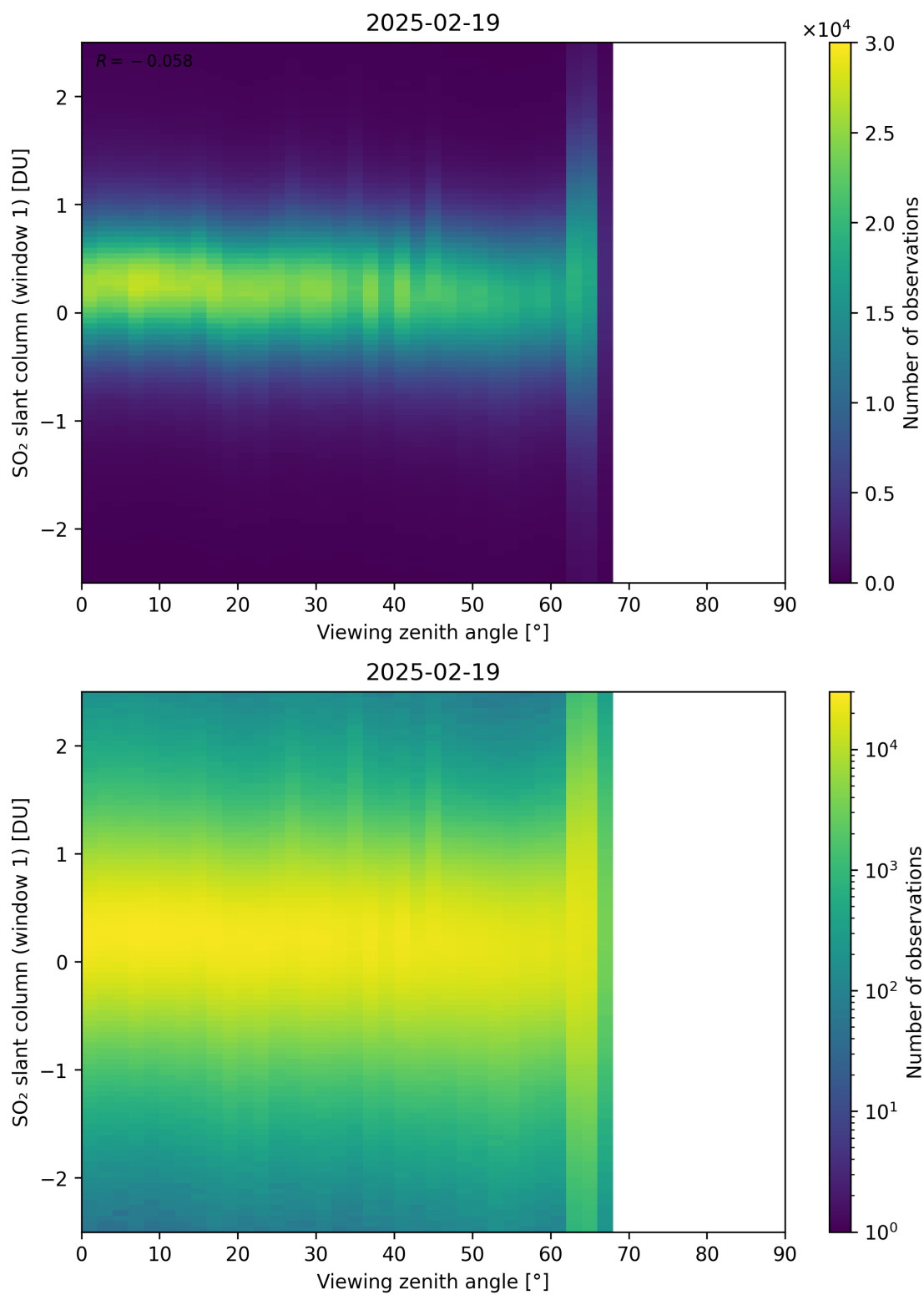
Figure 376: Scatter density plot of “Viewing zenith angle” against “SO 2 slant column (window 1)” for 2025-02-19 to 2025-02-20.
