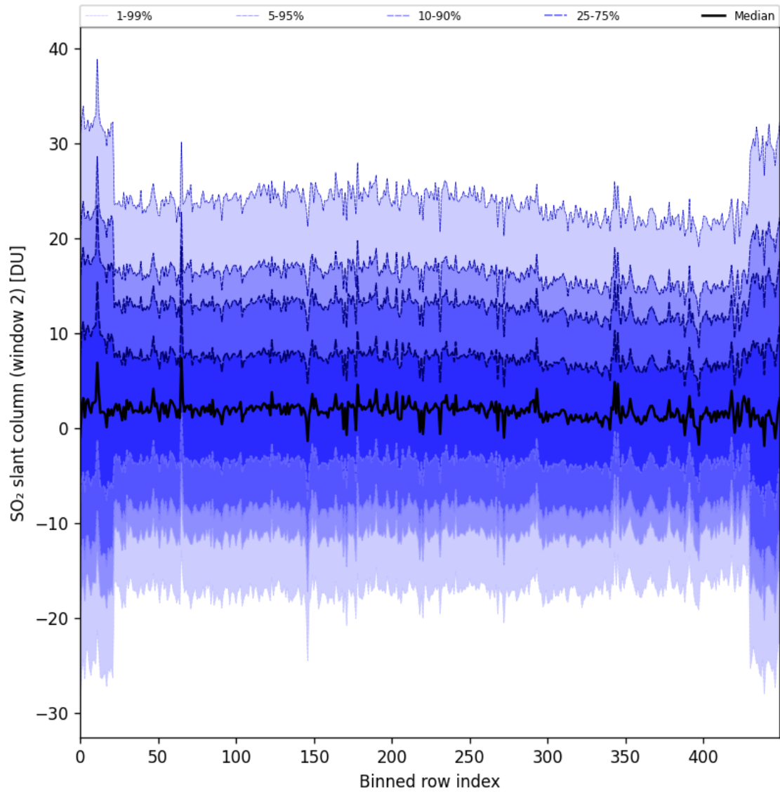
Figure 93: Along track statistics of “SO 2 slant column (window 2)” for 2025-02-19 to 2025-02-20
