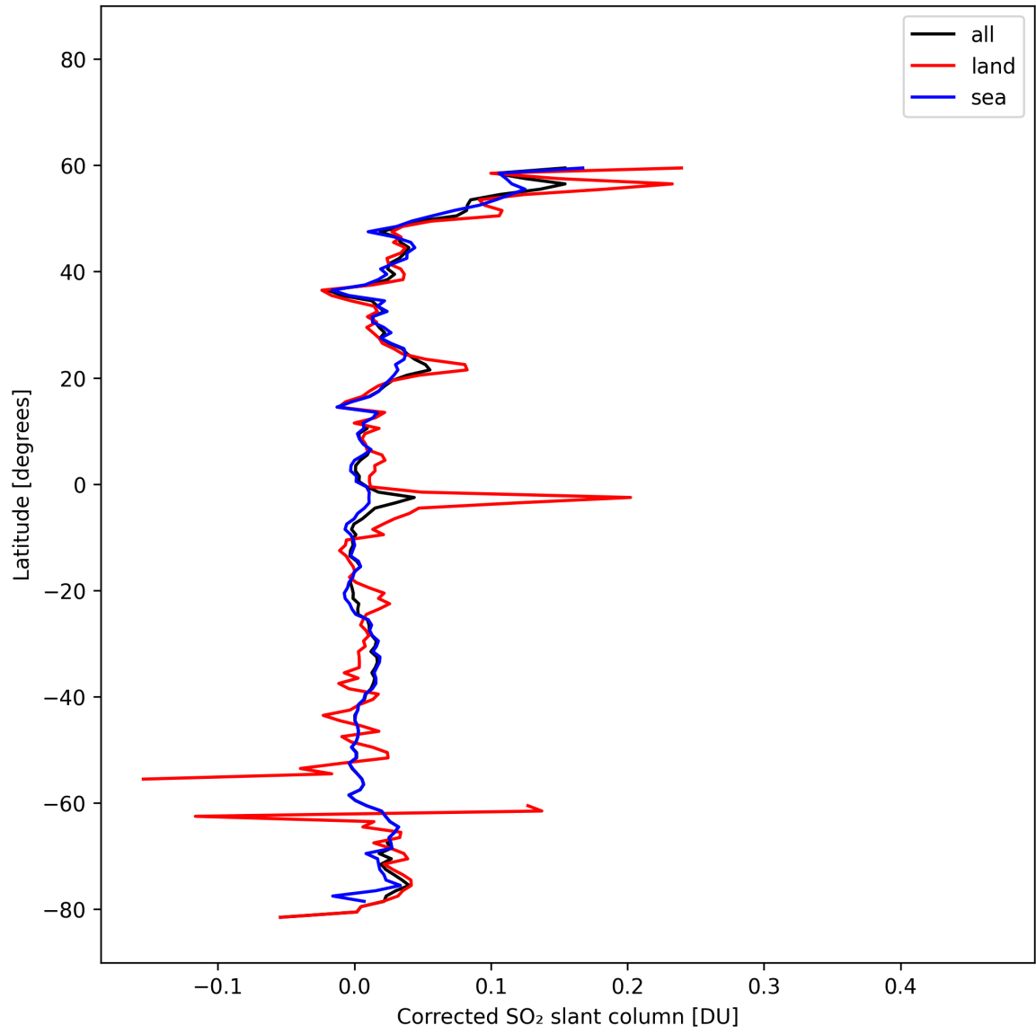
Figure 34: Zonal average of "Corrected SO 2 slant column" for 2025-02-19 to 2025-02-20.
