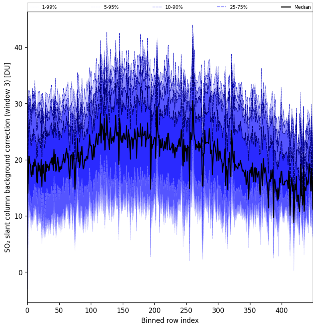
Figure 100: Along track statistics of “SO 2 slant column background correction (window 3)” for 2025-02-19 to 2025-02-20
