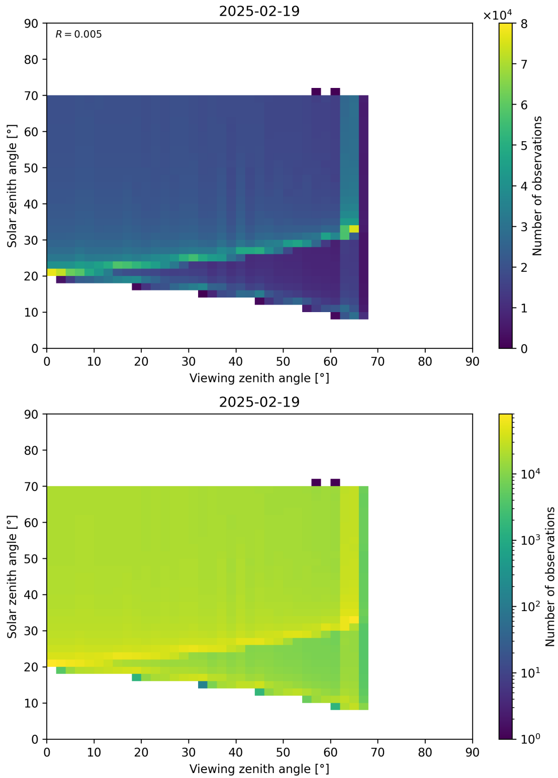
Figure 369: Scatter density plot of “Viewing zenith angle” against “Solar zenith angle” for 2025-02-19 to 2025-02-20.
