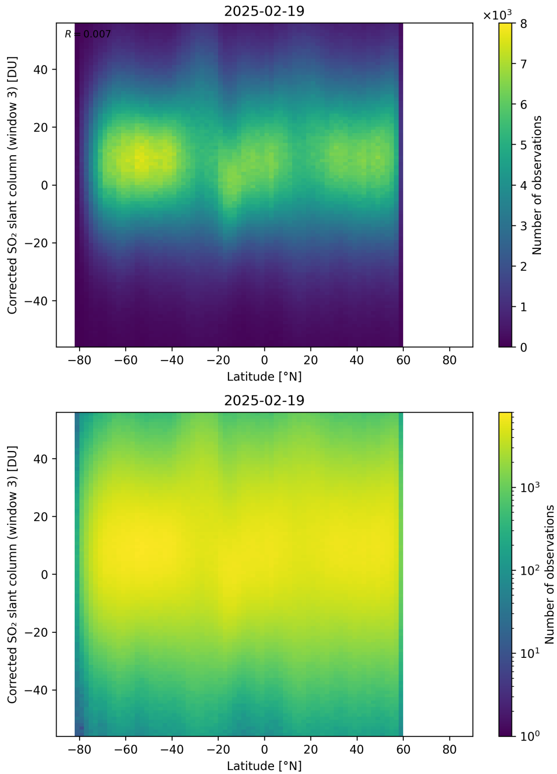
Figure 161: Scatter density plot of “Latitude” against “Corrected SO 2 slant column (window 3)” for 2025-02-19 to 2025-02-20.
