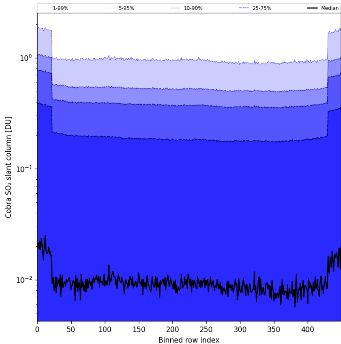
Figure 87: Along track statistics of “Cobra SO 2 slant column” for 2025-02-19 to 2025-02-20
