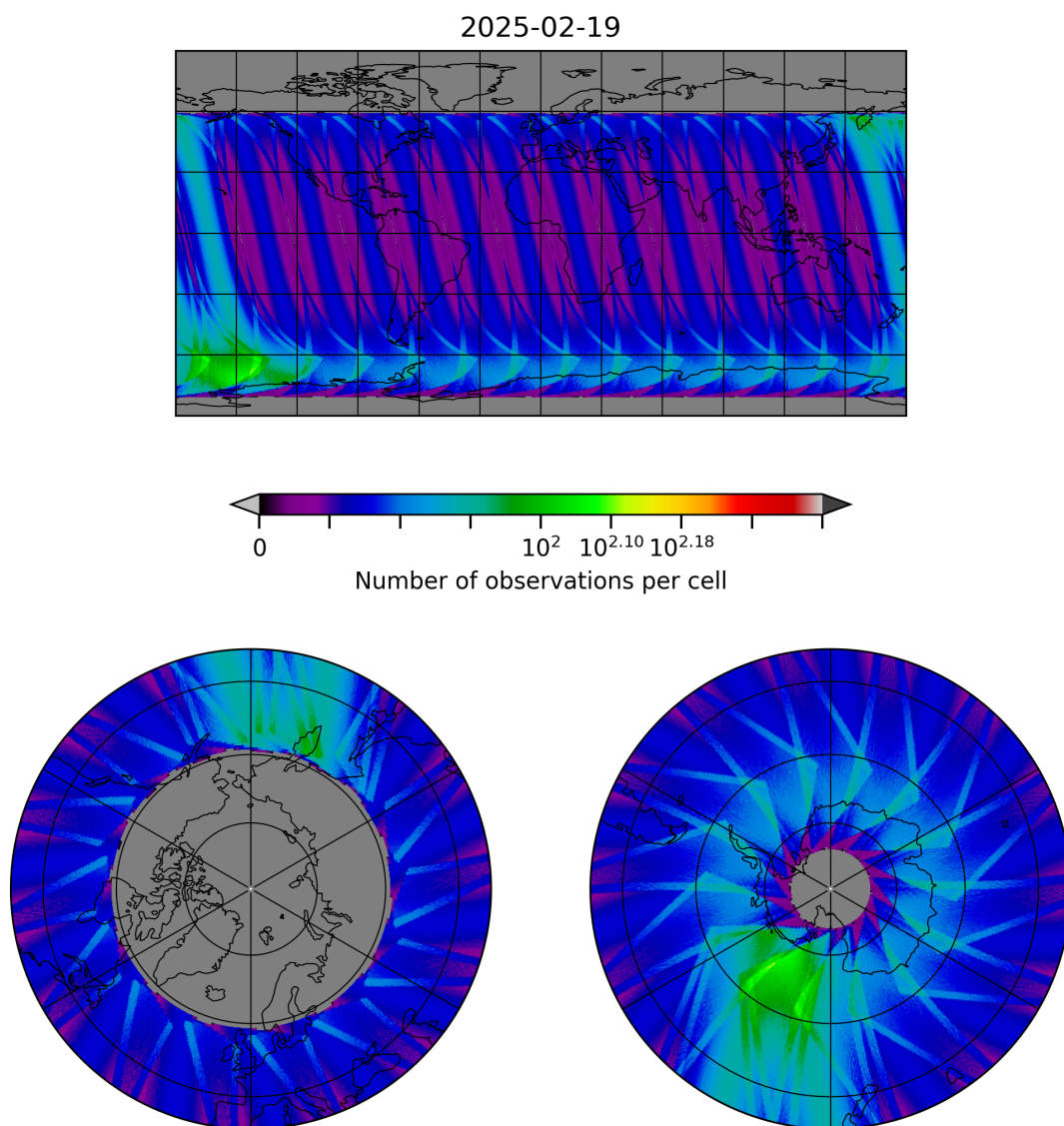
Figure 30: Map of the number of observations for 2025-02-19 to 2025-02-20
