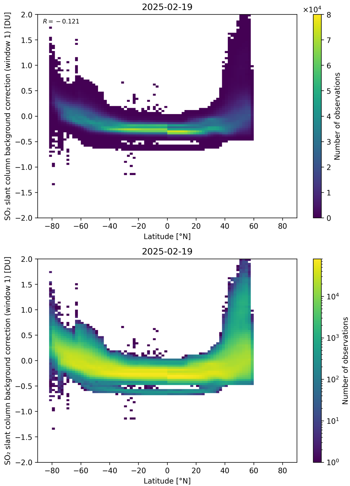
Figure 150: Scatter density plot of “Latitude” against “SO 2 slant column background correction (window 1)” for 2025-02-19 to 2025-02-20.
