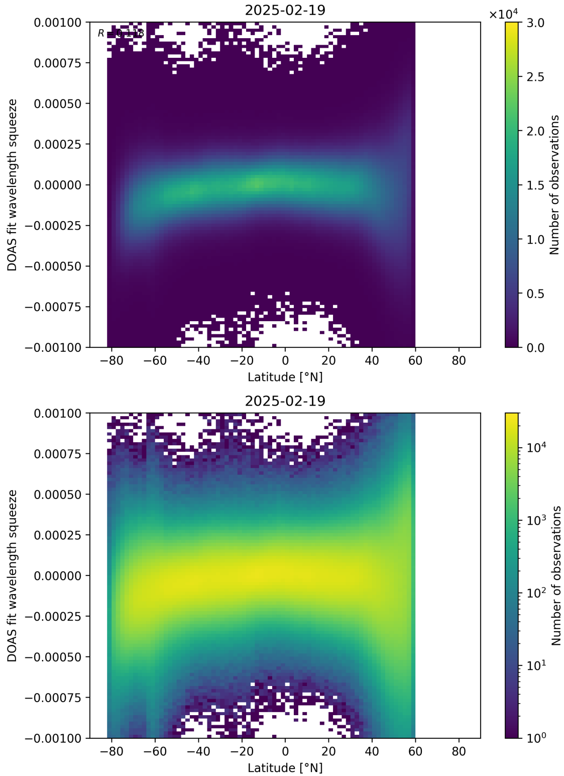
Figure 154: Scatter density plot of "Latitude" against "DOAS fit wavelength squeeze" for 2025-02-19 to 2025-02-20.
