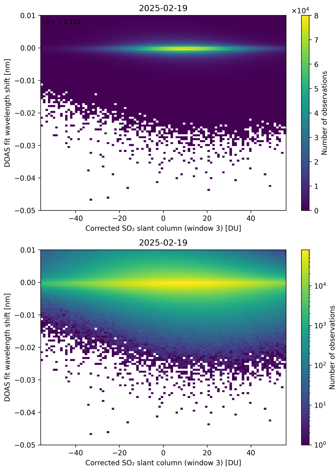
Figure 256: Scatter density plot of “Corrected SO 2 slant column (window 3)” against “DOAS fit wavelength shift” for 2025-02-19 to 2025-02-20.
