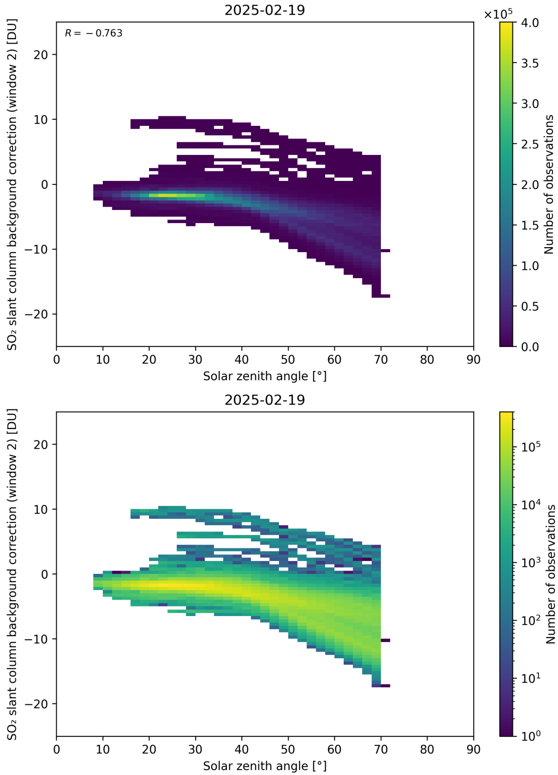
Figure 172: Scatter density plot of “Solar zenith angle” against “SO 2 slant column background correction (window 2)” for 2025-02-19 to 2025-02-20.
