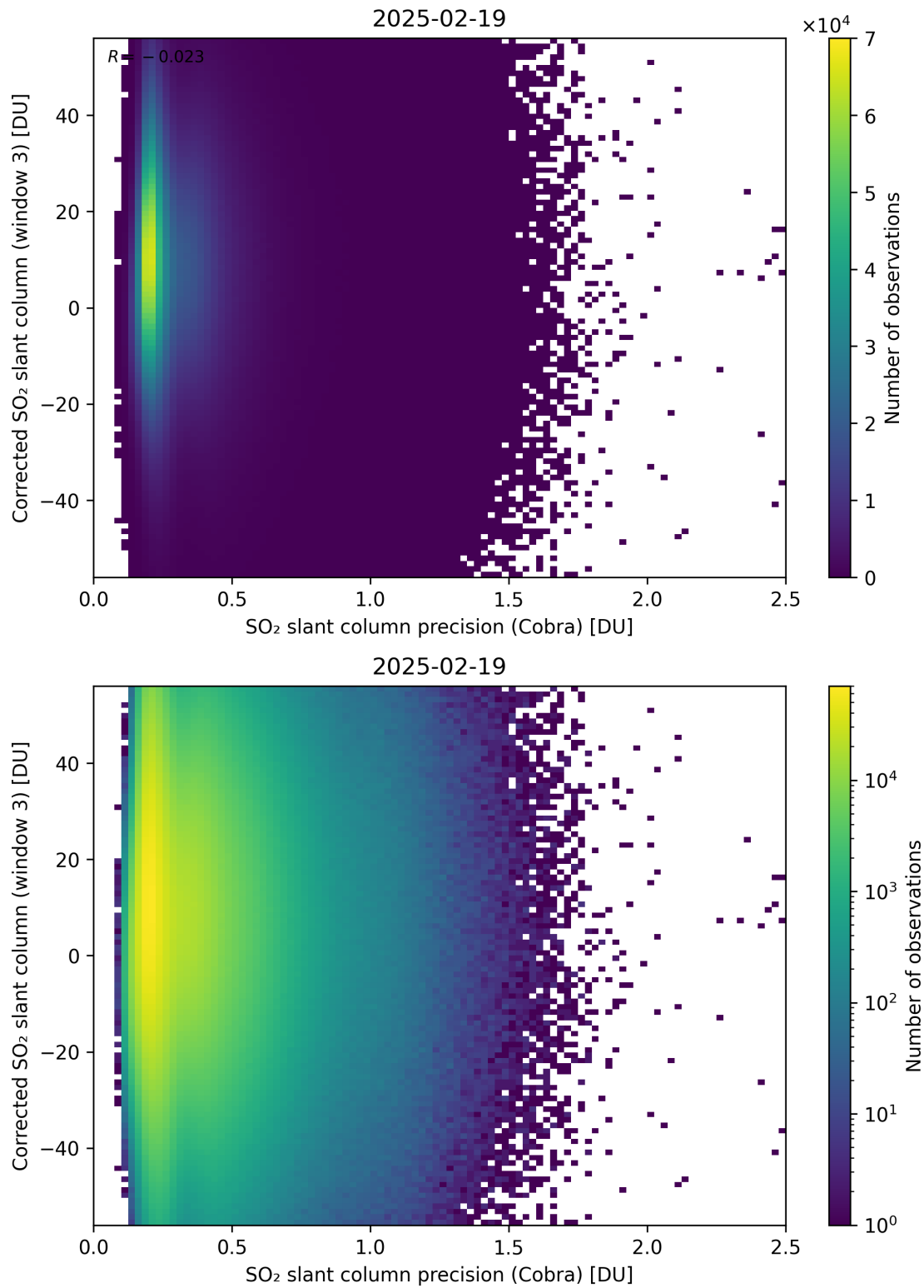
Figure 207: Scatter density plot of “SO 2 slant column precision (Cobra)” against “Corrected SO 2 slant column (window 3)” for 2025-02-19 to 2025-02-20.
