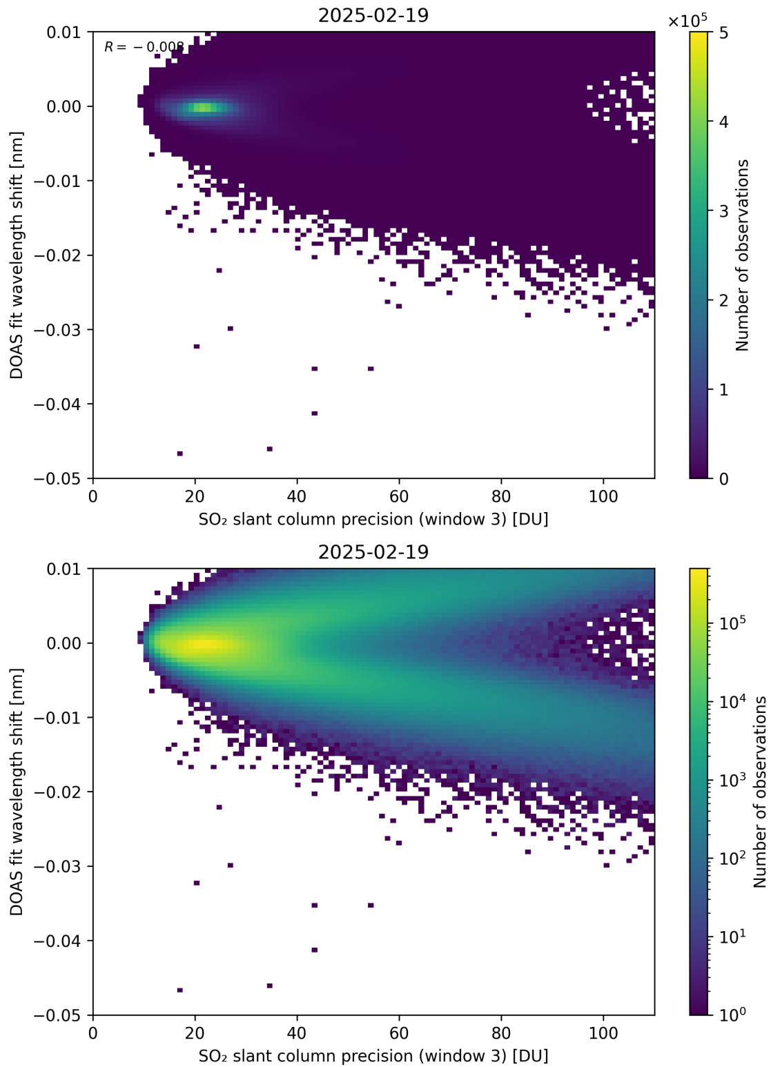
Figure 308: Scatter density plot of “SO 2 slant column precision (window 3)” against “DOAS fit wavelength shift” for 2025-02-19 to 2025-02-20.
