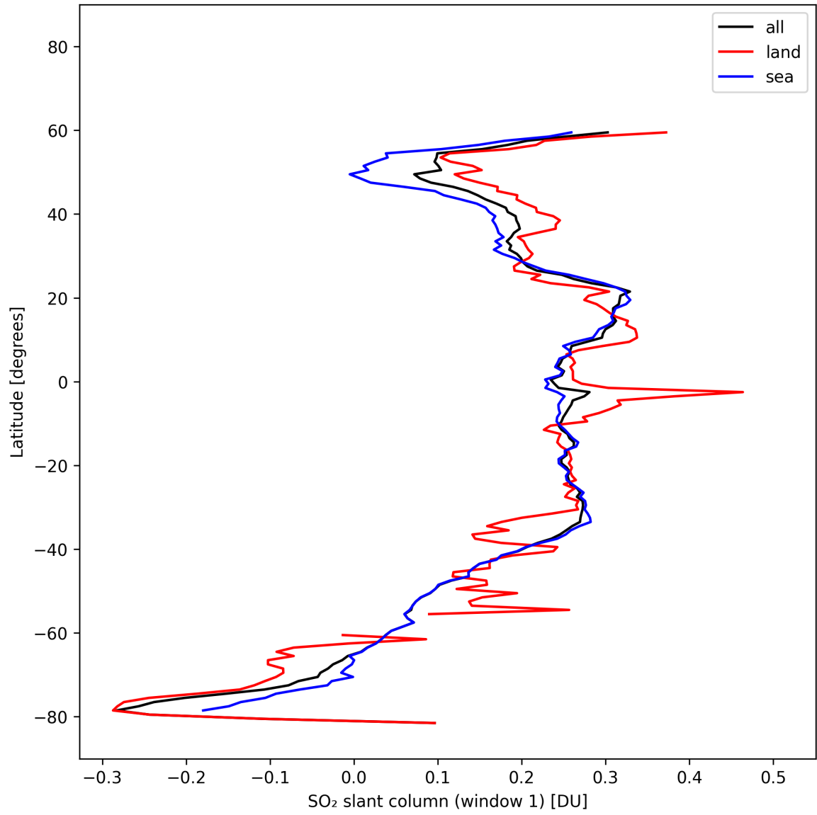
Figure 37: Zonal average of “SO 2 slant column (window 1)” for 2025-02-19 to 2025-02-20.
