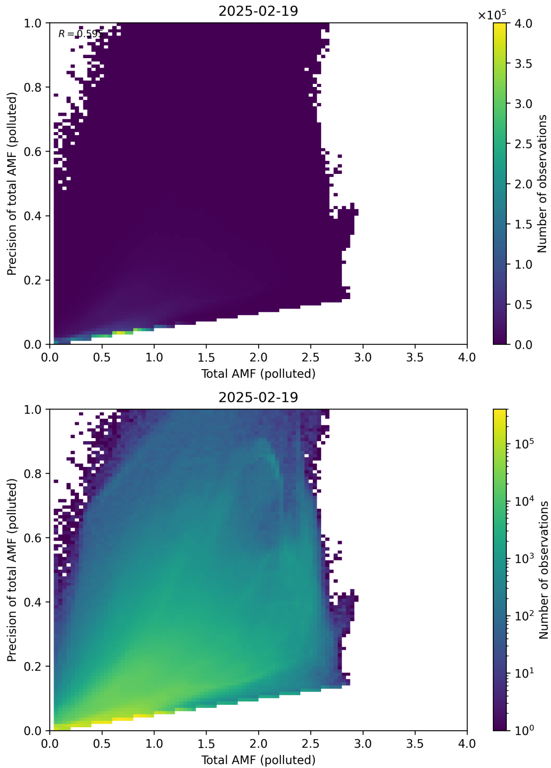
Figure 322: Scatter density plot of “Total AMF (polluted)” against “Precision of total AMF (polluted)” for 2025-02-19 to 2025-02-20.
