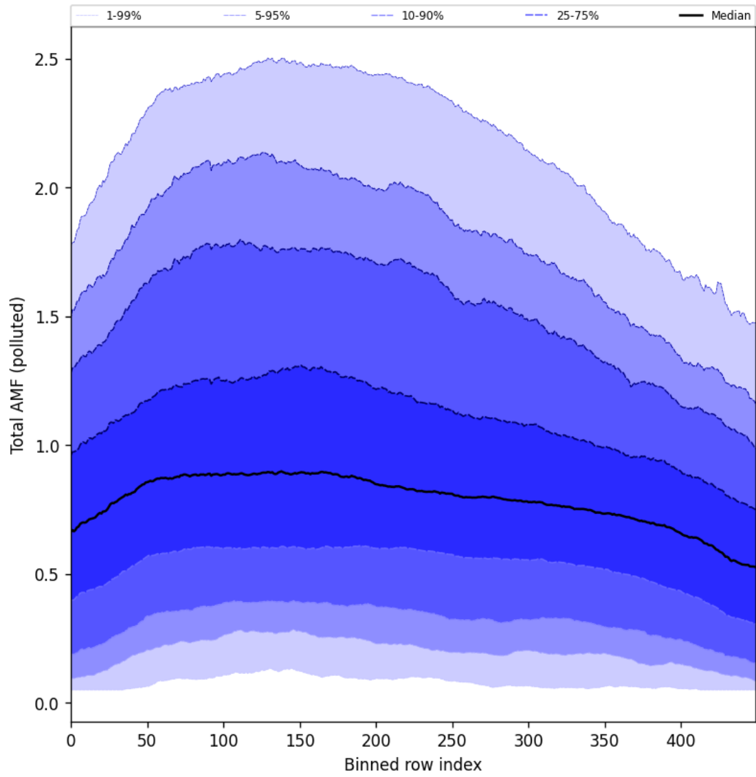
Figure 105: Along track statistics of “Total AMF (polluted)” for 2025-02-19 to 2025-02-20
