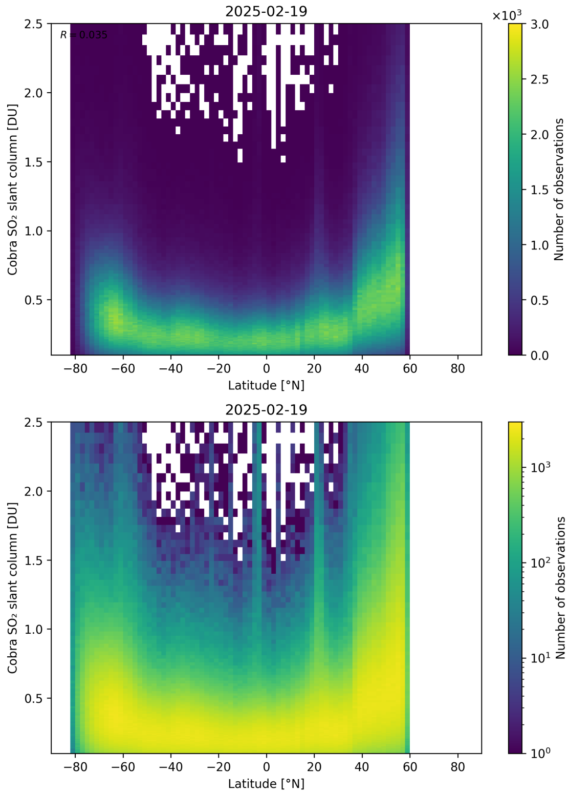
Figure 157: Scatter density plot of “Latitude” against “Cobra SO 2 slant column” for 2025-02-19 to 2025-02-20.
