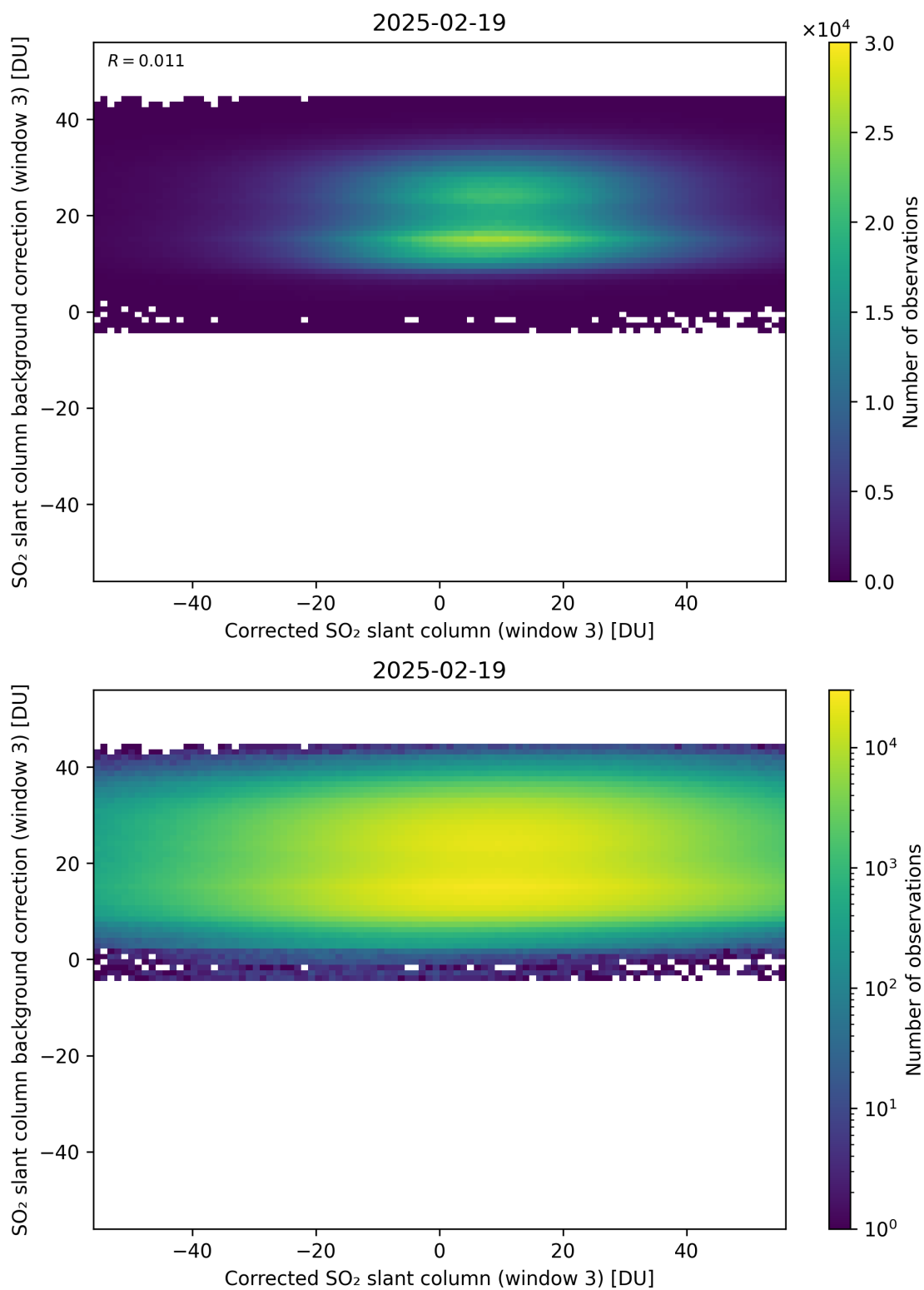
Figure 255: Scatter density plot of “Corrected SO 2 slant column (window 3)” against “SO 2 slant column background correction (window 3)” for 2025-02-19 to 2025-02-20.
