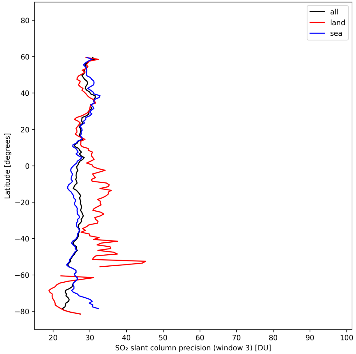
Figure 46: Zonal average of “SO 2 slant column precision (window 3)” for 2025-02-19 to 2025-02-20.
