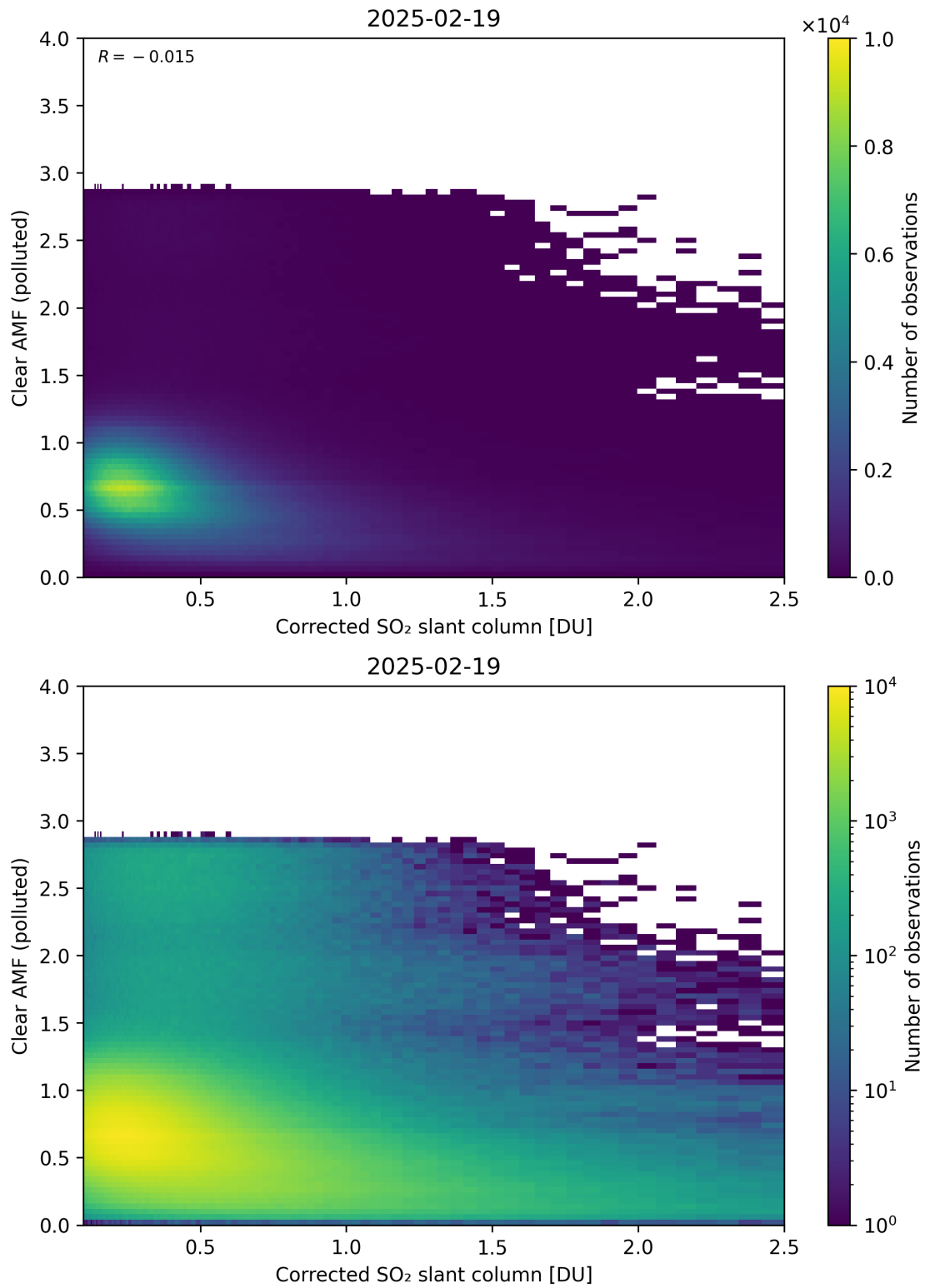
Figure 232: Scatter density plot of “Corrected SO 2 slant column” against “Clear AMF (polluted)” for 2025-02-19 to 2025-02-20.
