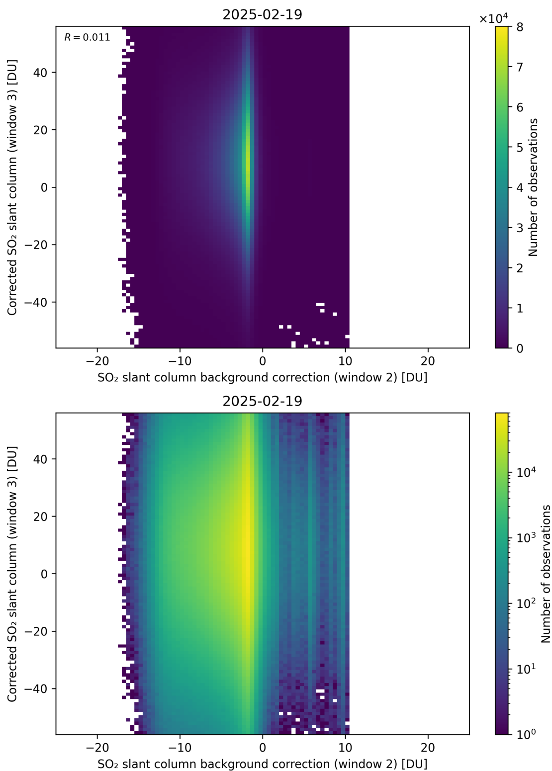
Figure 127: Scatter density plot of “SO 2 slant column background correction (window 2)” against “Corrected SO 2 slant column (window 3)” for 2025-02-19 to 2025-02-20.
