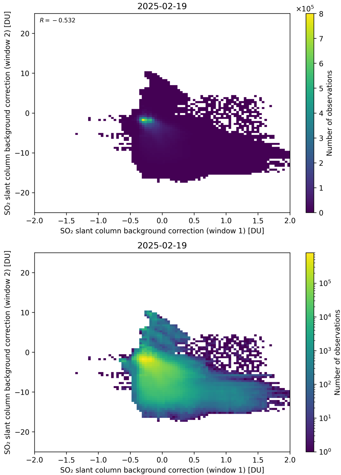
Figure 109: Scatter density plot of “SO 2 slant column background correction (window 1)” against “SO 2 slant column background correction (window 2)” for 2025-02-19 to 2025-02-20.
