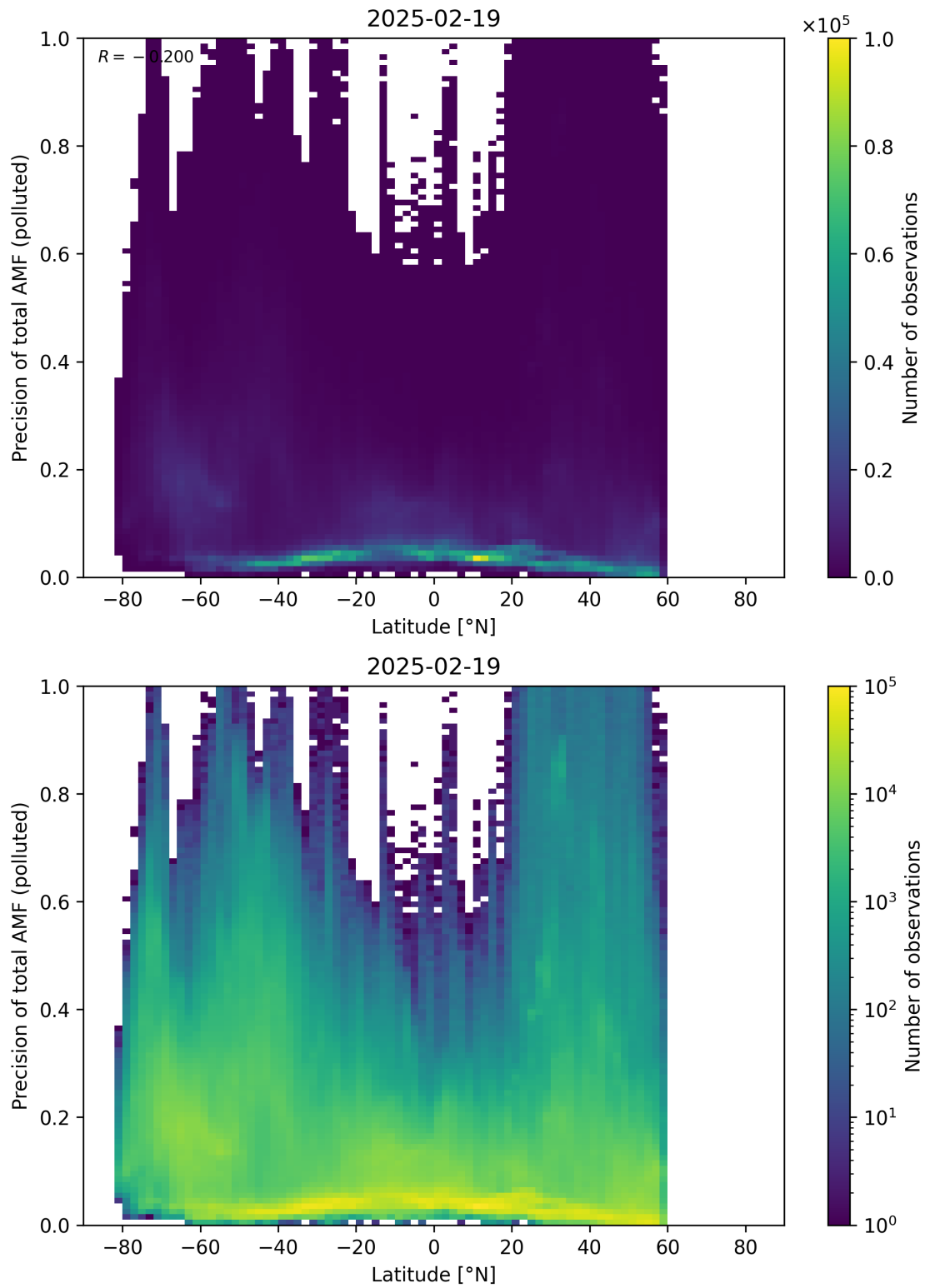
Figure 168: Scatter density plot of “Latitude” against “Precision of total AMF (polluted)” for 2025-02-19 to 2025-02-20.
