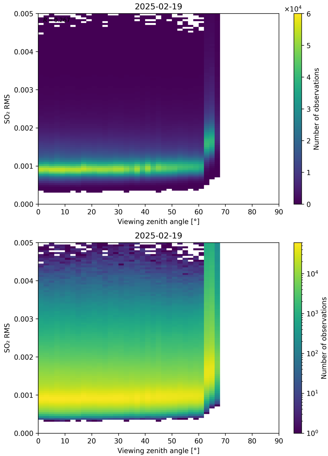
Figure 367: Scatter density plot of “Viewing zenith angle” against “SO 2 RMS” for 2025-02-19 to 2025-02-20.
