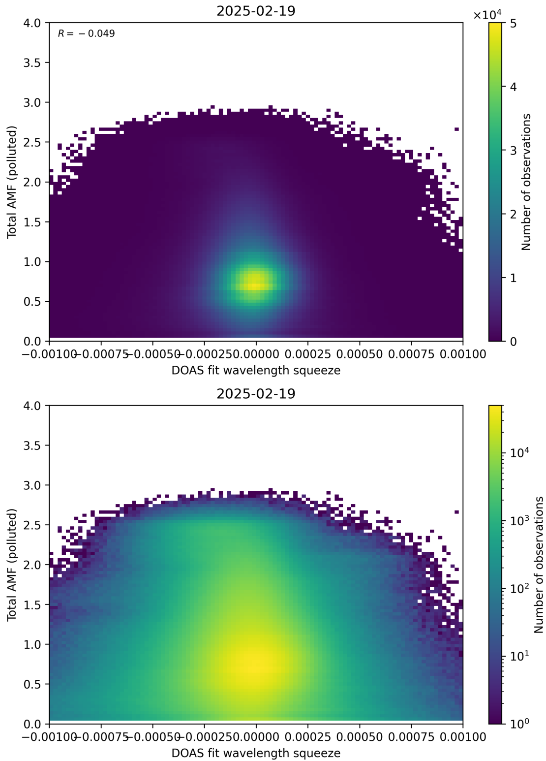
Figure 145: Scatter density plot of “DOAS fit wavelength squeeze” against “Total AMF (polluted)” for 2025-02-19 to 2025-02-20.
