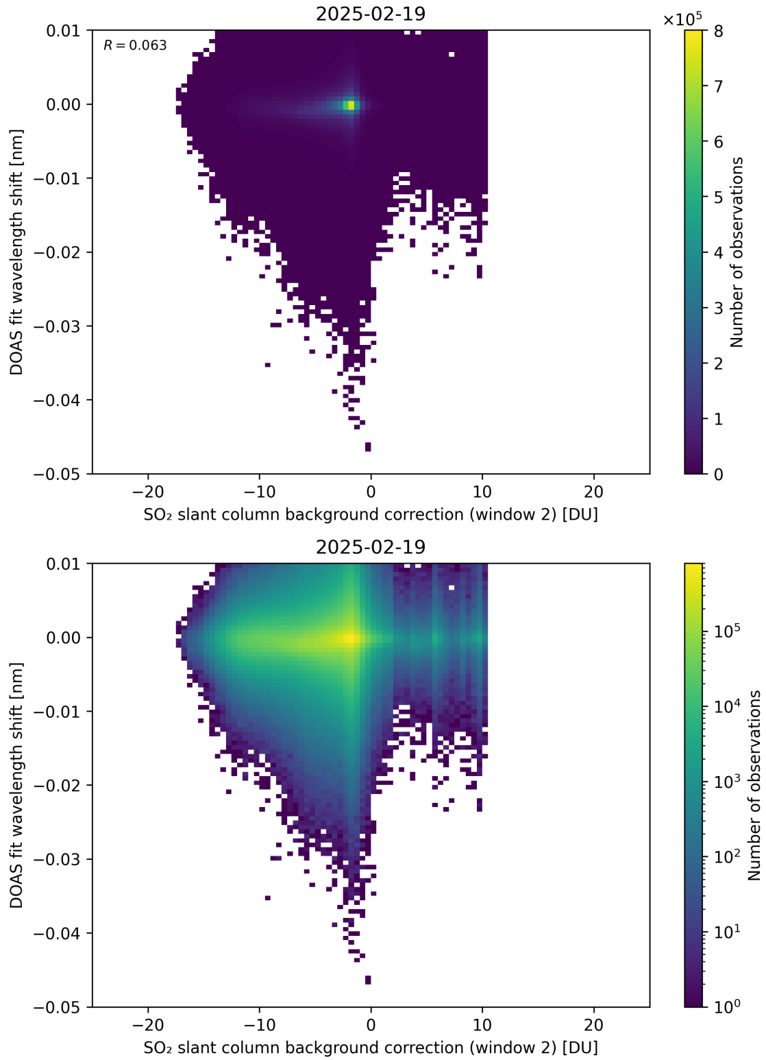
Figure 123: Scatter density plot of “SO 2 slant column background correction (window 2)” against “DOAS fit wavelength shift” for 2025-02-19 to 2025-02-20.
