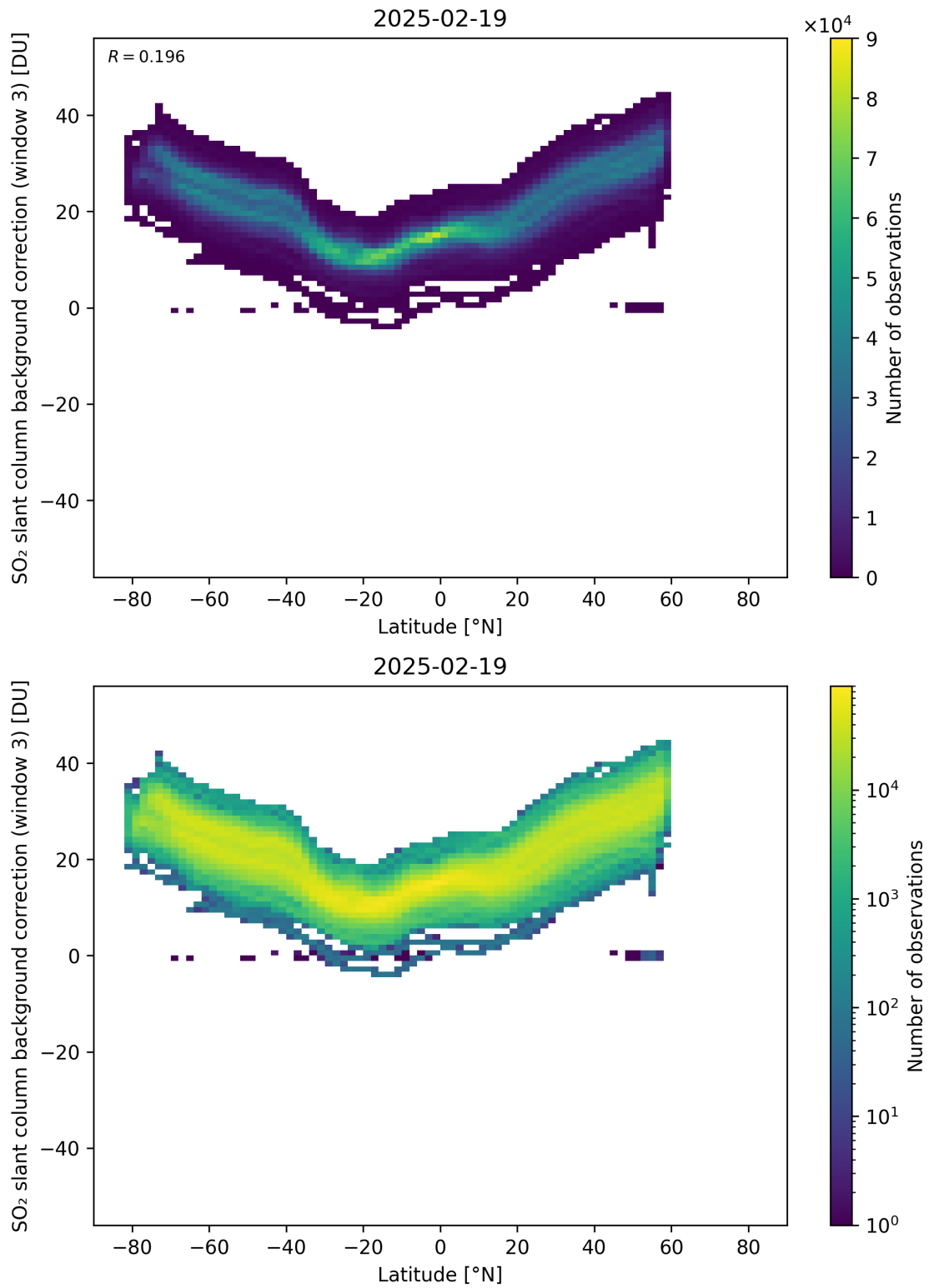
Figure 152: Scatter density plot of “Latitude” against “SO 2 slant column background correction (window 3)” for 2025-02-19 to 2025-02-20.
