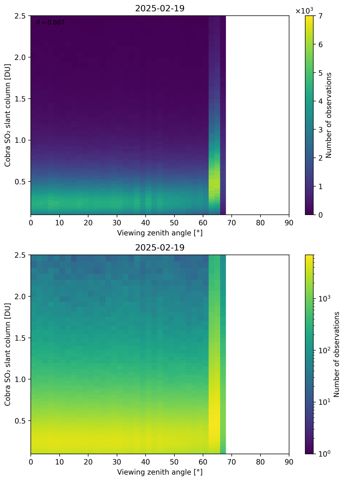
Figure 371: Scatter density plot of “Viewing zenith angle” against “Cobra SO 2 slant column” for 2025-02-19 to 2025-02-20.
