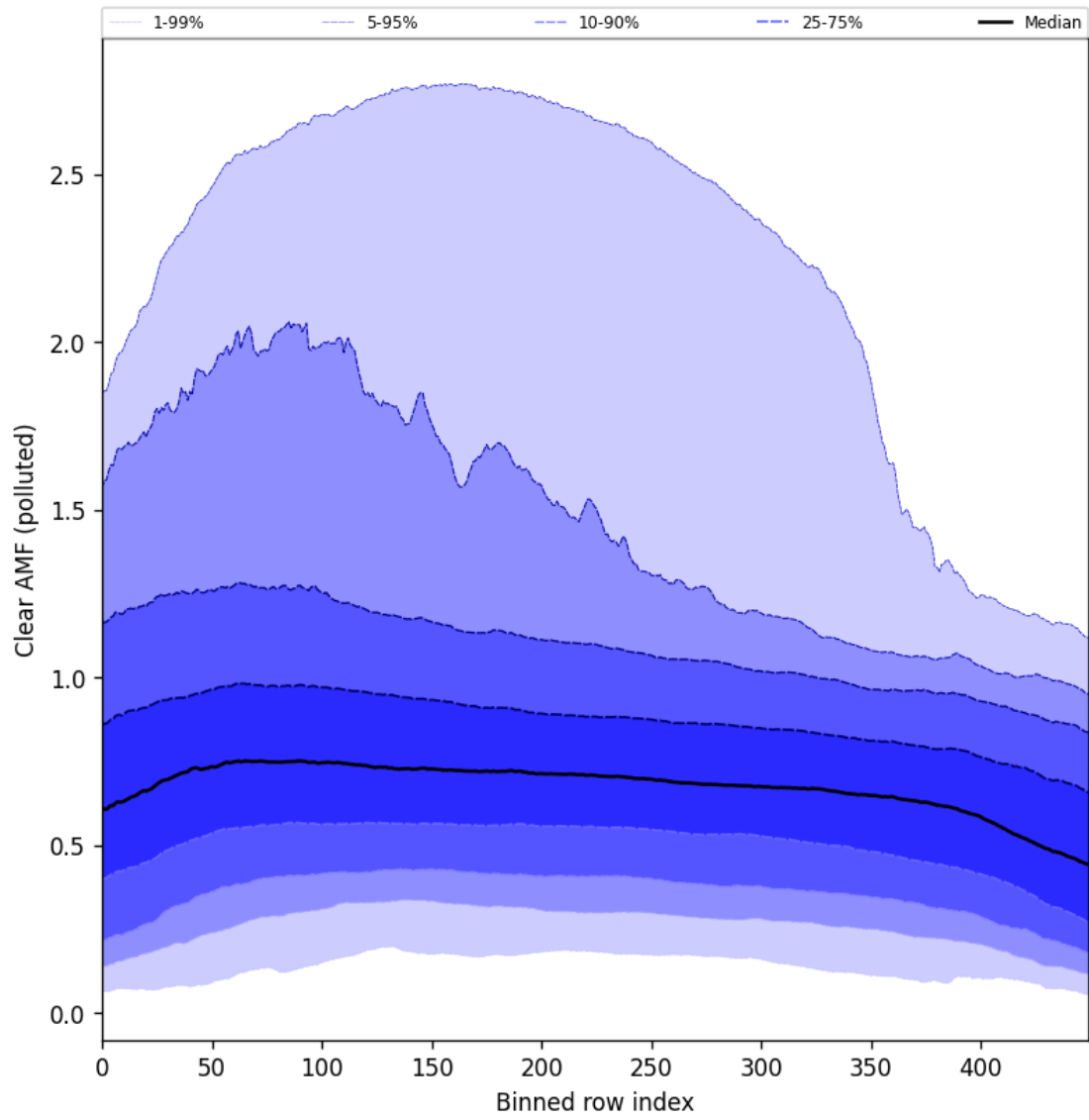
Figure 107: Along track statistics of “Clear AMF (polluted)” for 2025-02-19 to 2025-02-20
