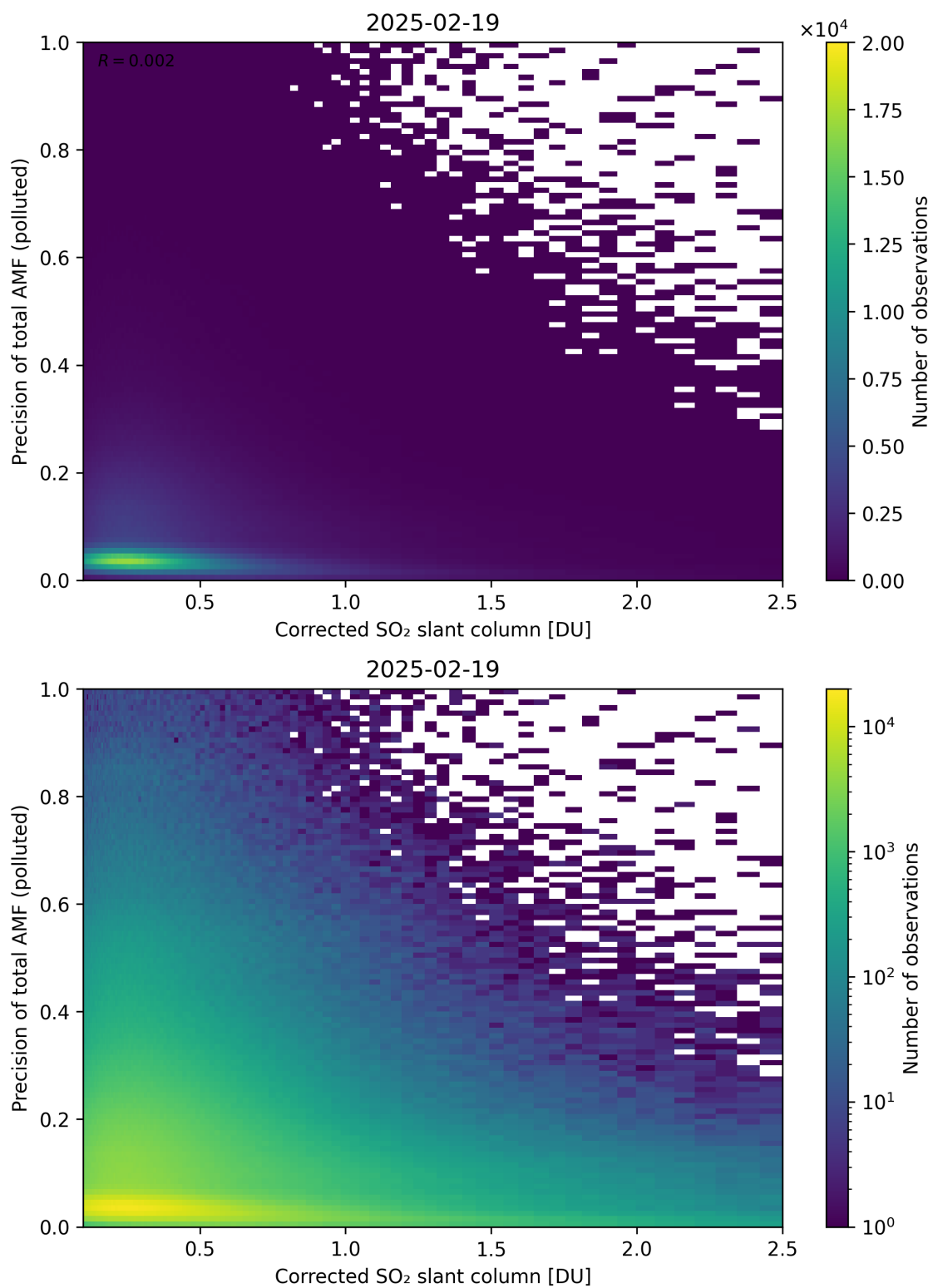
Figure 243: Scatter density plot of “Corrected SO 2 slant column” against “Precision of total AMF (polluted)” for 2025-02-19 to 2025-02-20.
