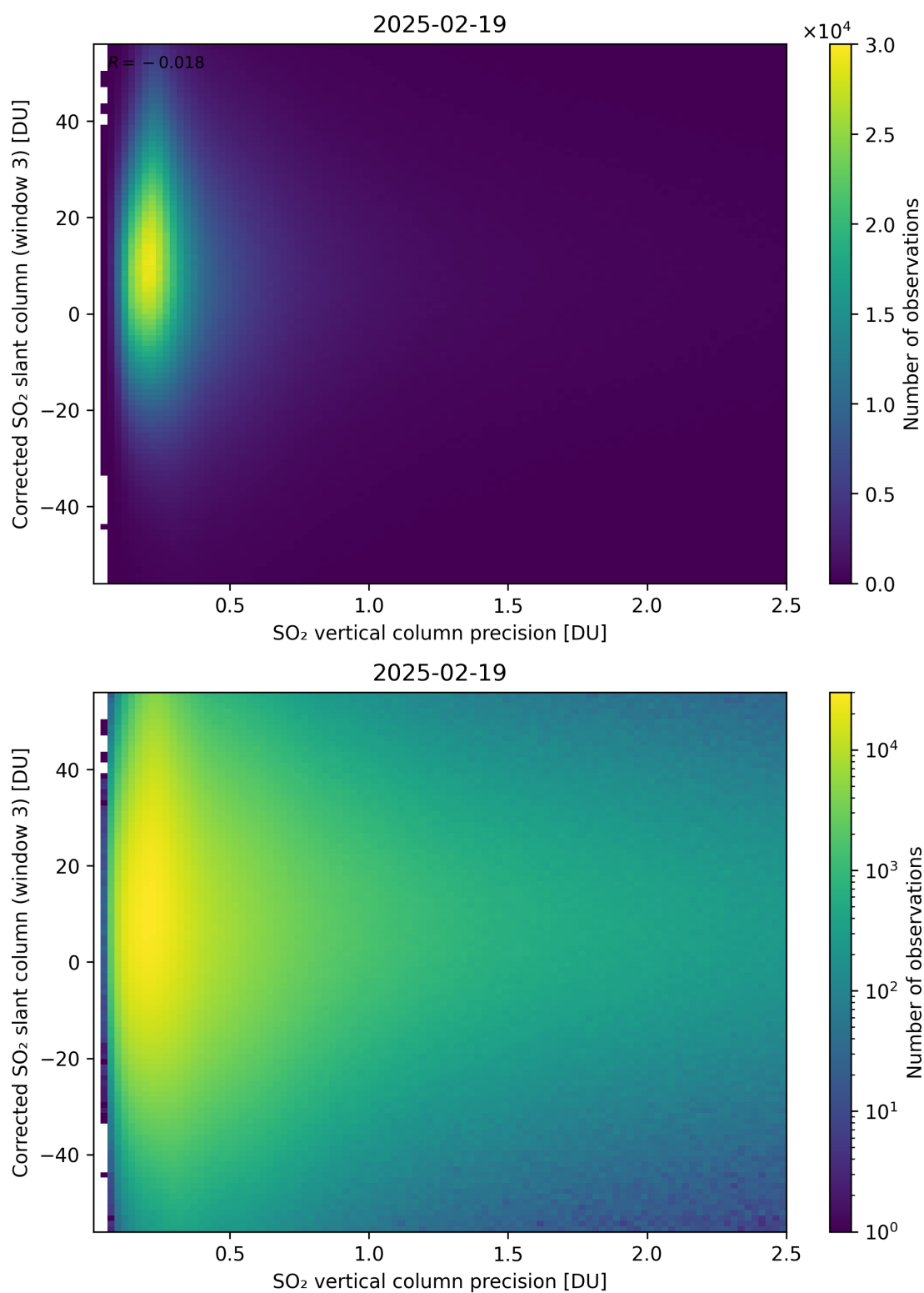
Figure 340: Scatter density plot of “SO 2 vertical column precision” against “Corrected SO 2 slant column (window 3)” for 2025-02-19 to 2025-02-20.
