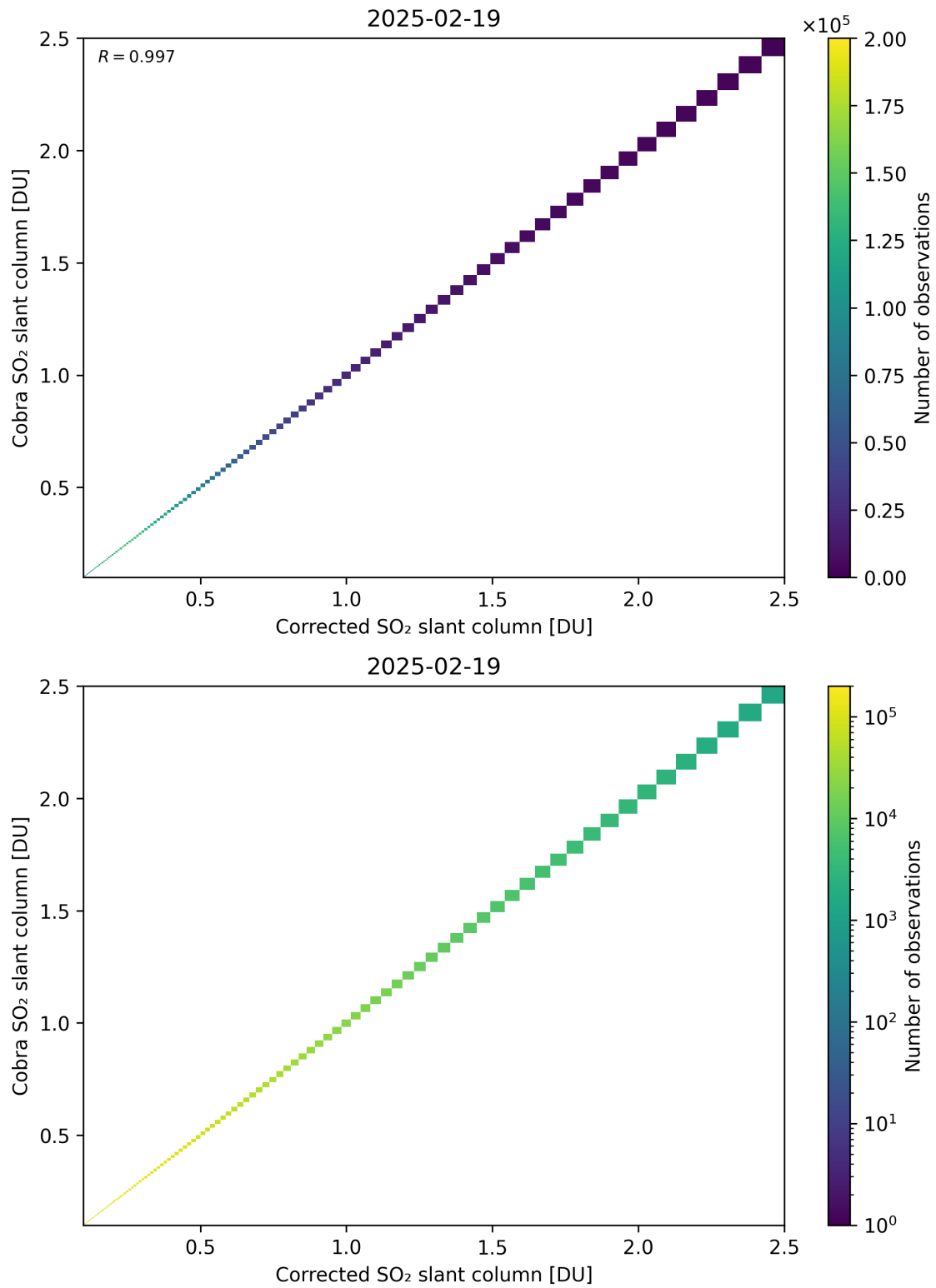
Figure 233: Scatter density plot of “Corrected SO 2 slant column” against “Cobra SO 2 slant column” for 2025-02-19 to 2025-02-20.
