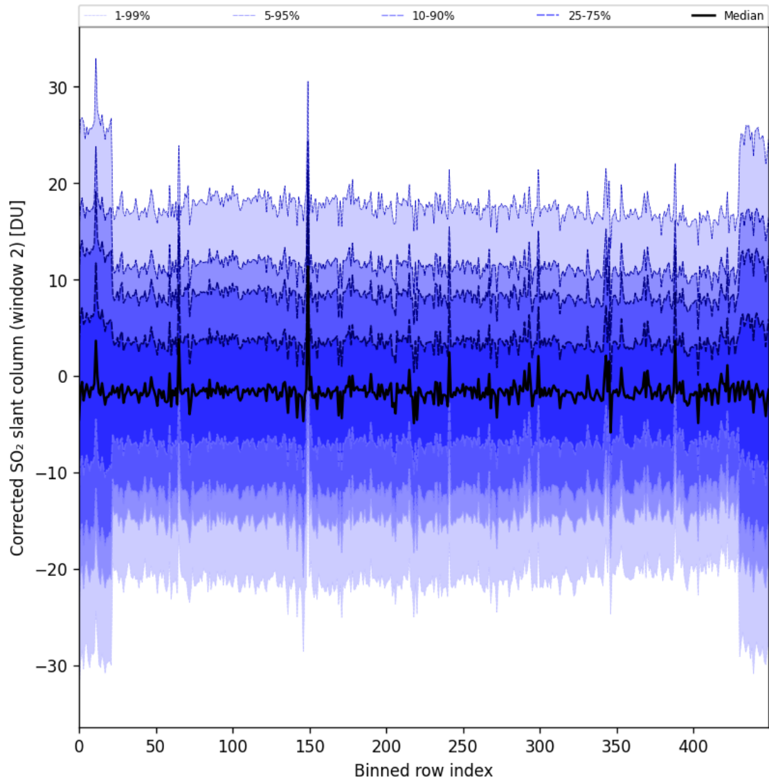
Figure 95: Along track statistics of “Corrected SO 2 slant column (window 2)” for 2025-02-19 to 2025-02-20
