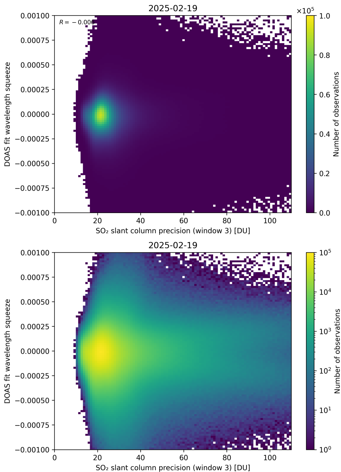
Figure 309: Scatter density plot of “SO 2 slant column precision (window 3)” against “DOAS fit wavelength squeeze” for 2025-02-19 to 2025-02-20.
