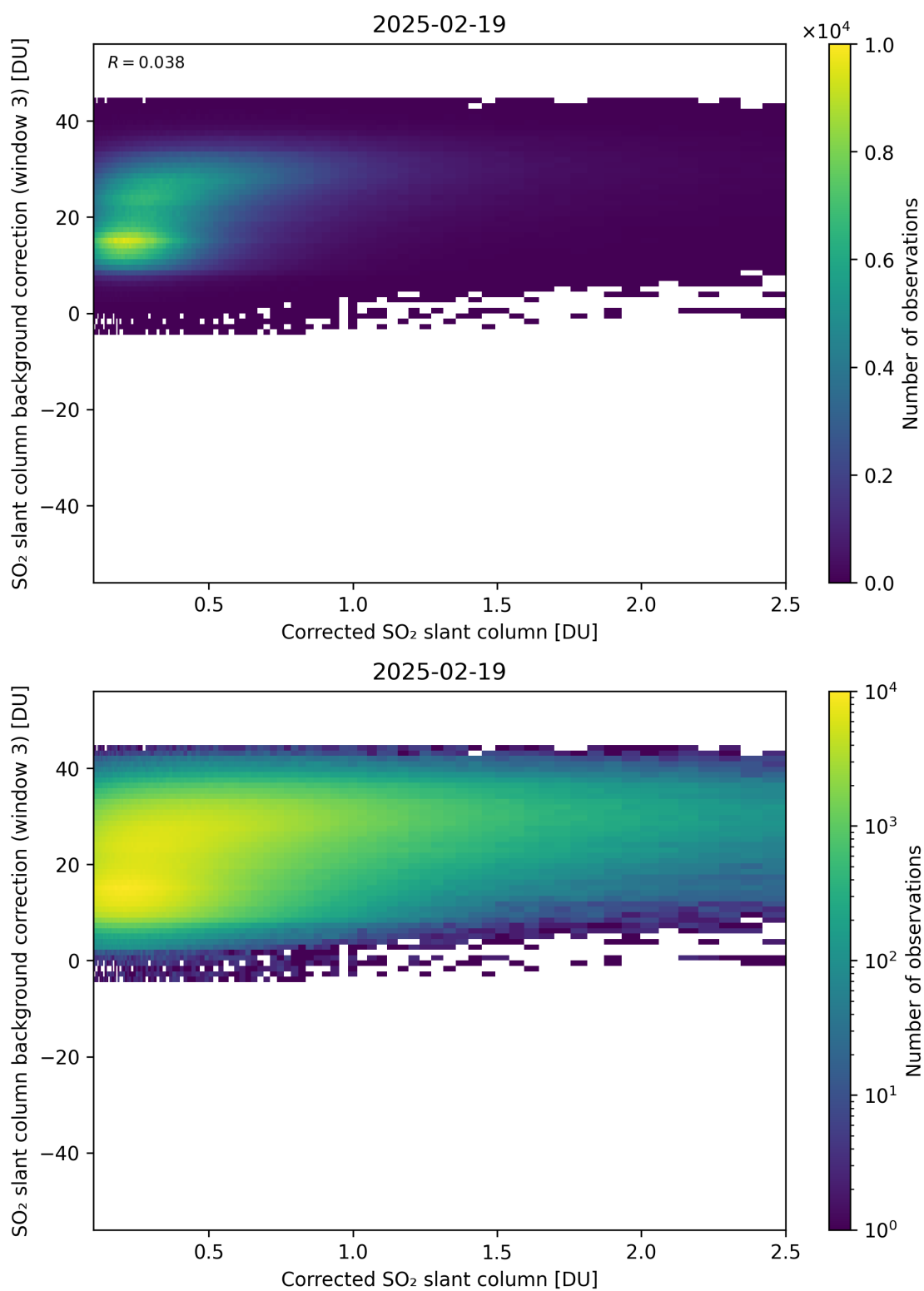
Figure 228: Scatter density plot of “Corrected SO 2 slant column” against “SO 2 slant column background correction (window 3)” for 2025-02-19 to 2025-02-20.
