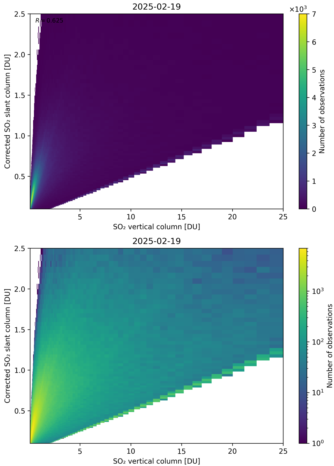
Figure 351: Scatter density plot of “SO 2 vertical column” against “Corrected SO 2 slant column” for 2025-02-19 to 2025-02-20.
