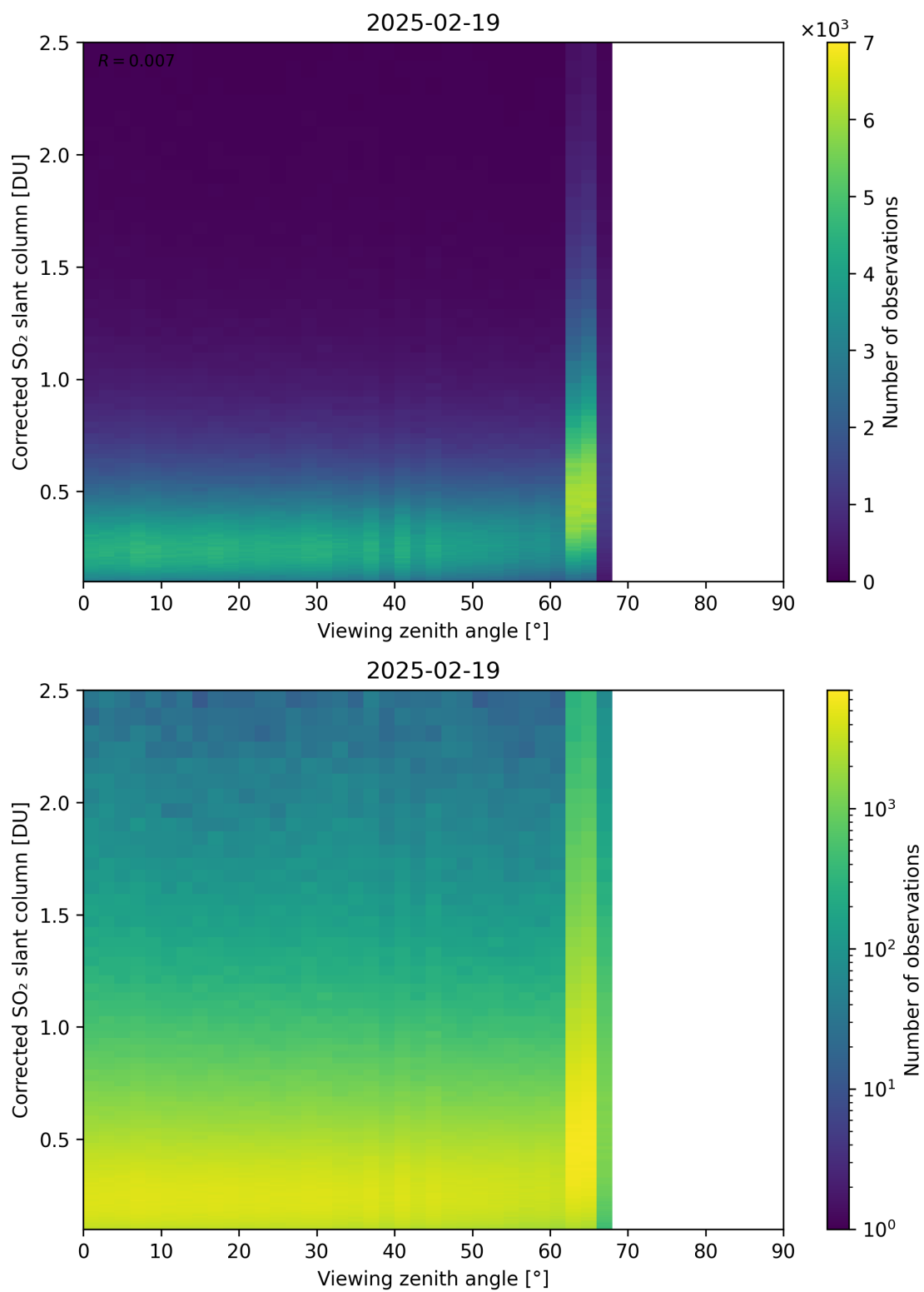
Figure 373: Scatter density plot of “Viewing zenith angle” against “Corrected SO 2 slant column” for 2025-02-19 to 2025-02-20.
