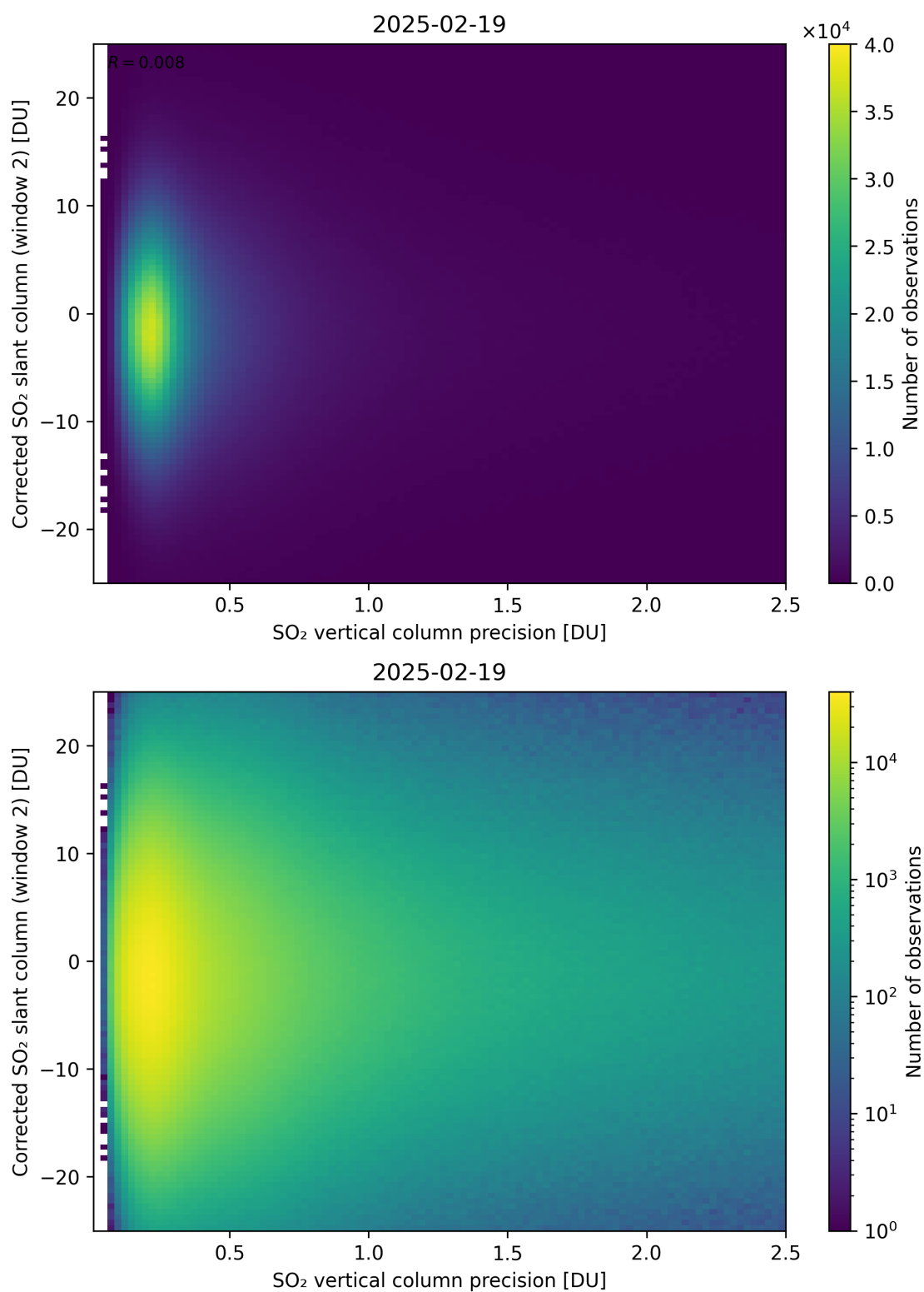
Figure 339: Scatter density plot of “SO 2 vertical column precision” against “Corrected SO 2 slant column (window 2)” for 2025-02-19 to 2025-02-20.
