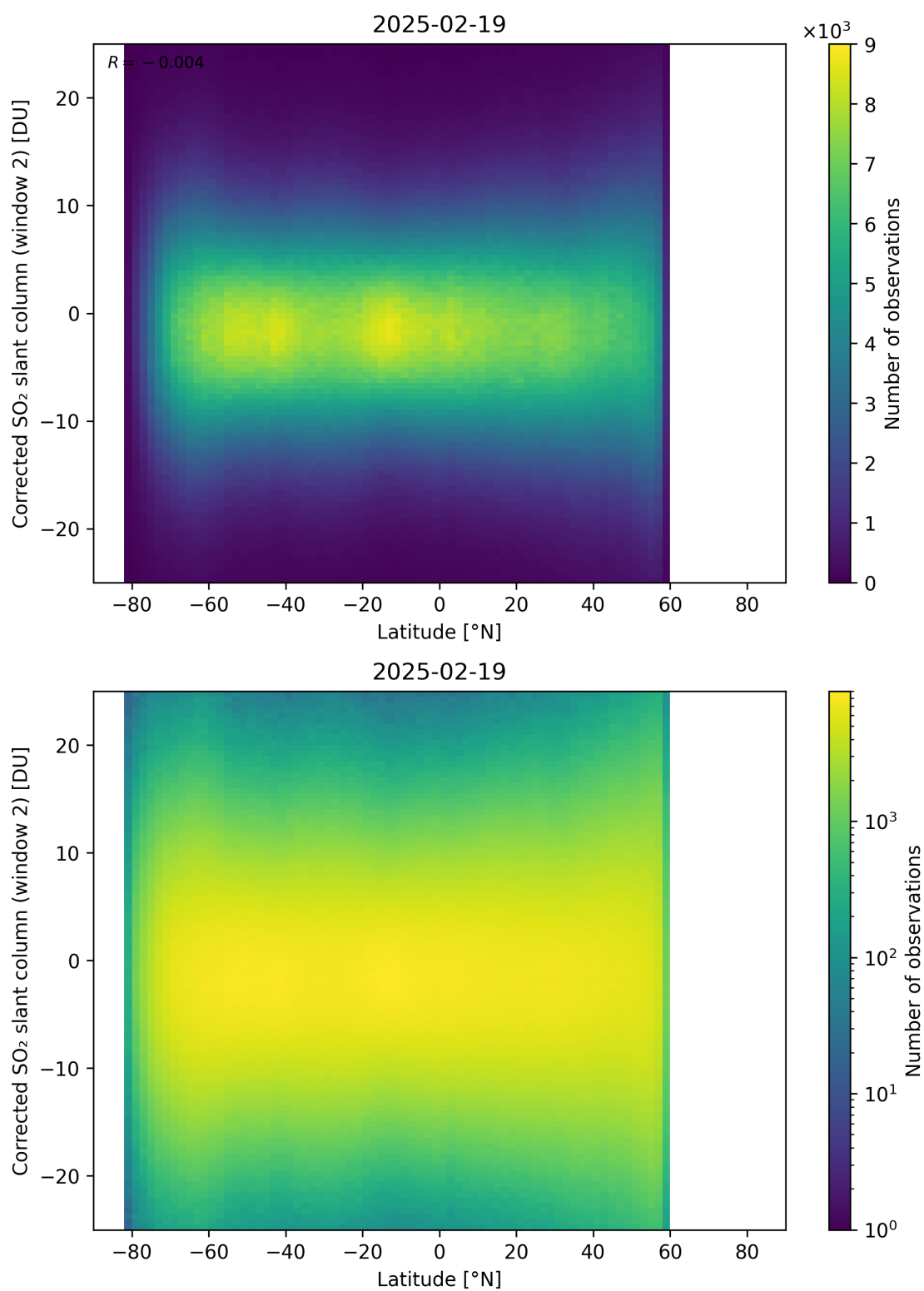
Figure 160: Scatter density plot of “Latitude” against “Corrected SO 2 slant column (window 2)” for 2025-02-19 to 2025-02-20.
