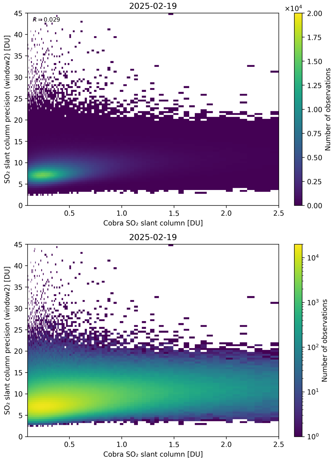
Figure 221: Scatter density plot of “Cobra SO 2 slant column” against “SO 2 slant column precision (window2)” for 2025-02-19 to 2025-02-20.
