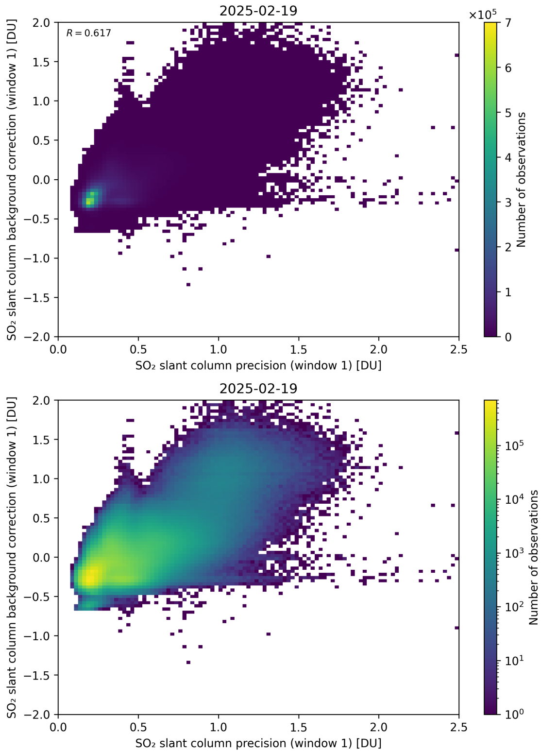
Figure 268: Scatter density plot of “SO 2 slant column precision (window 1)” against “SO 2 slant column background correction (window 1)” for 2025-02-19 to 2025-02-20.
