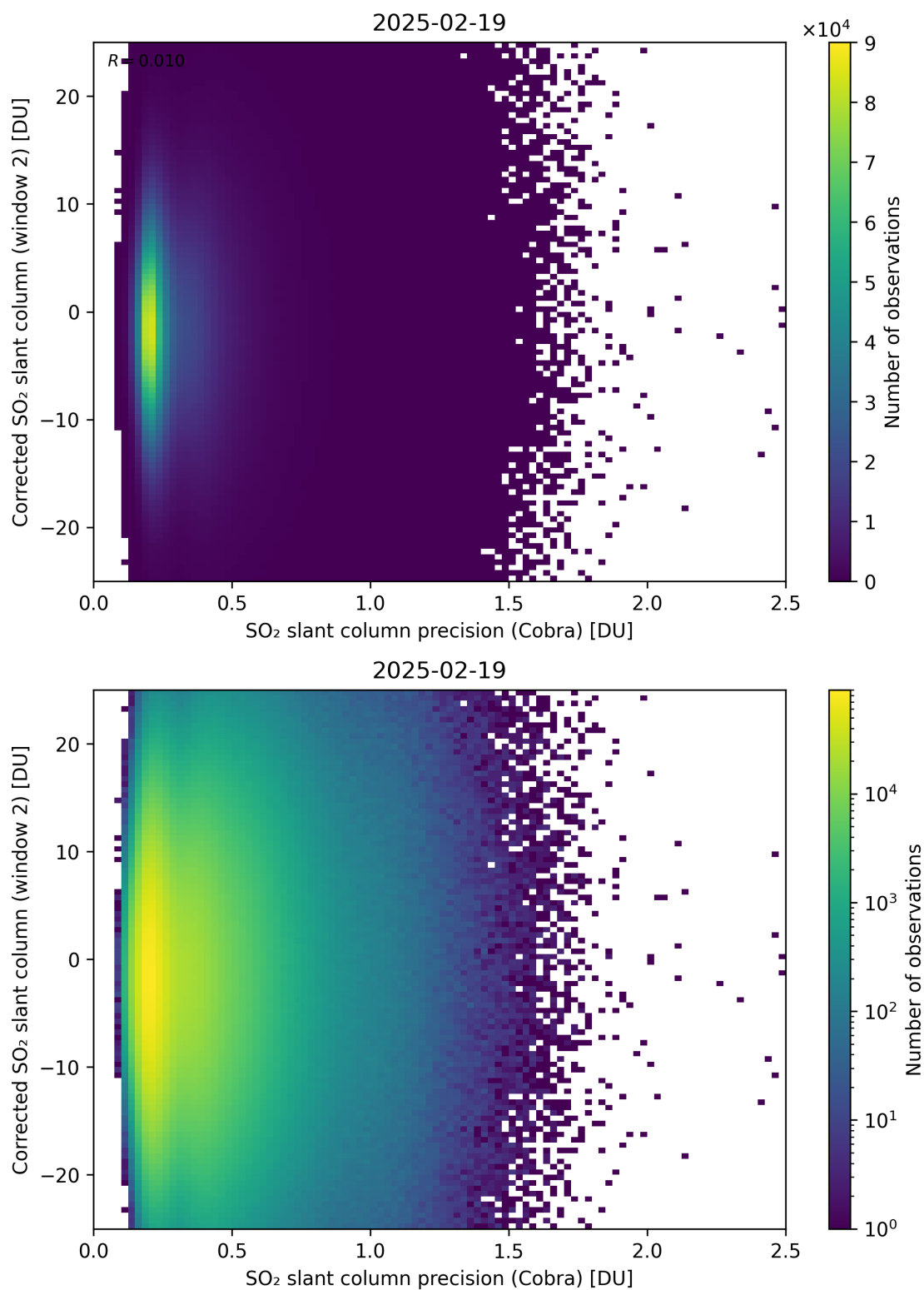
Figure 206: Scatter density plot of “SO 2 slant column precision (Cobra)” against “Corrected SO 2 slant column (window 2)” for 2025-02-19 to 2025-02-20.
