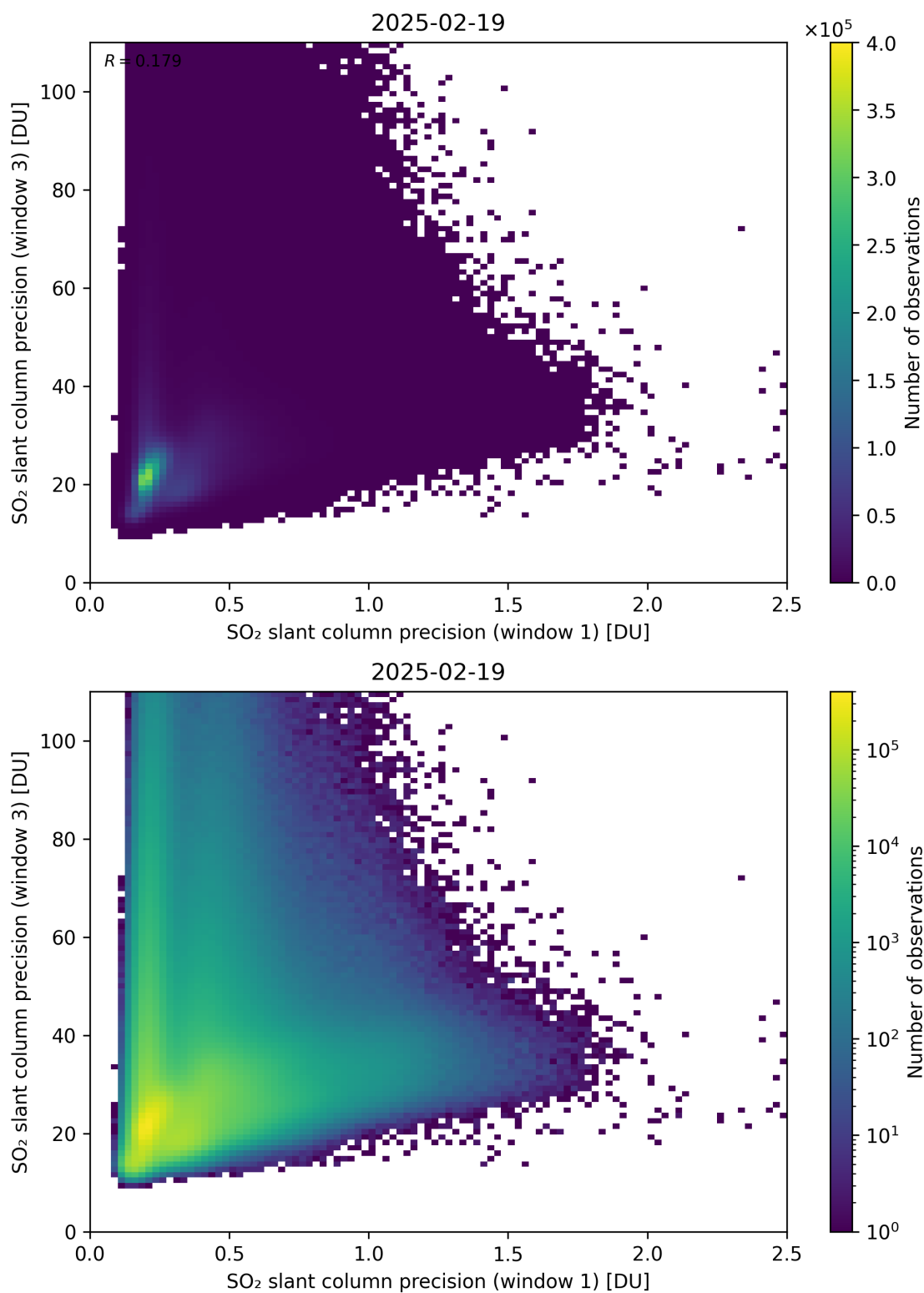
Figure 279: Scatter density plot of “SO 2 slant column precision (window 1)” against “SO 2 slant column precision (window 3)” for 2025-02-19 to 2025-02-20.
