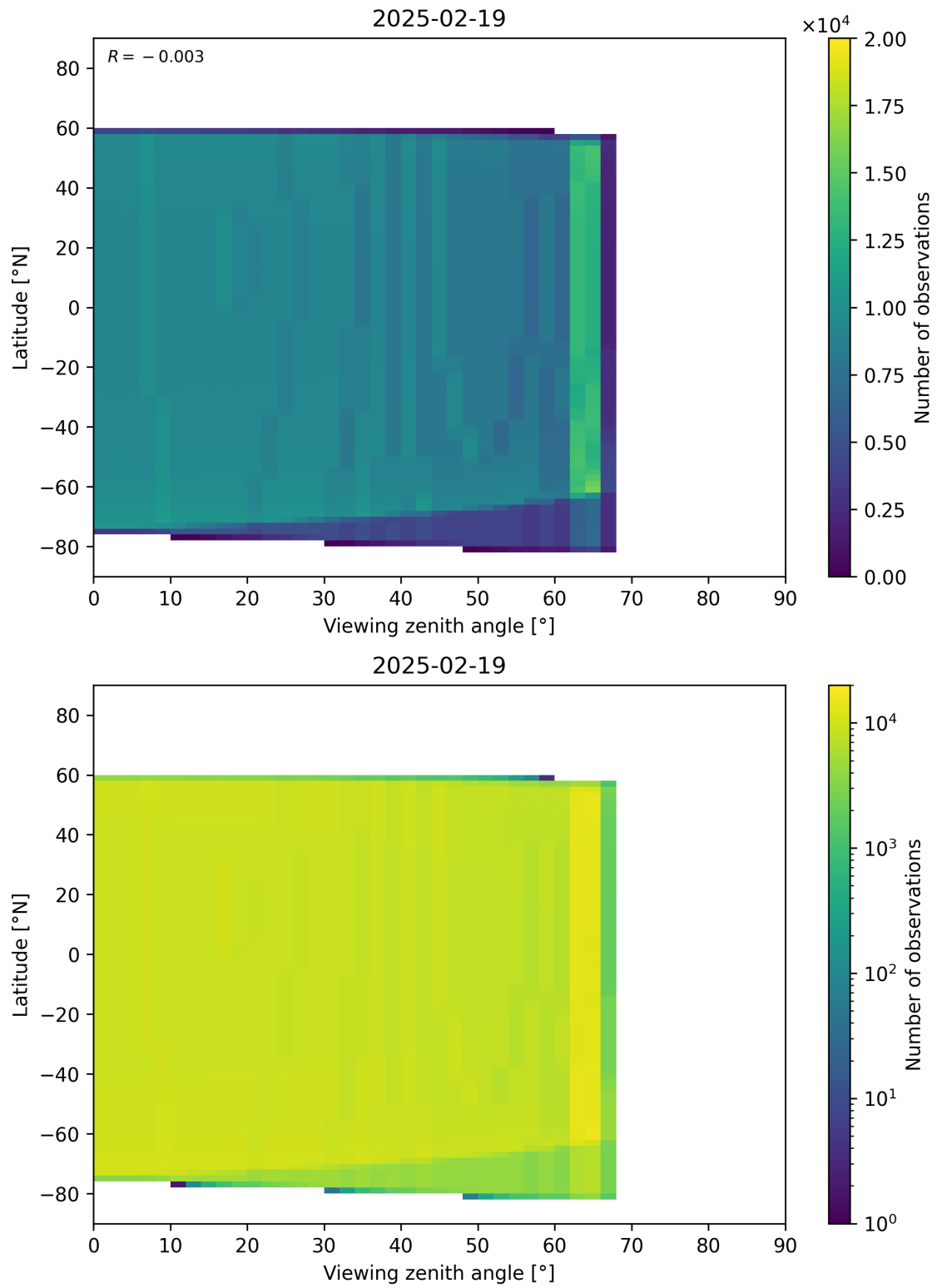
Figure 368: Scatter density plot of “Viewing zenith angle” against “Latitude” for 2025-02-19 to 2025-02-20.
