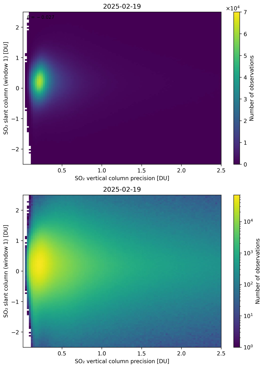
Figure 341: Scatter density plot of “SO 2 vertical column precision” against “SO 2 slant column (window 1)” for 2025-02-19 to 2025-02-20.
