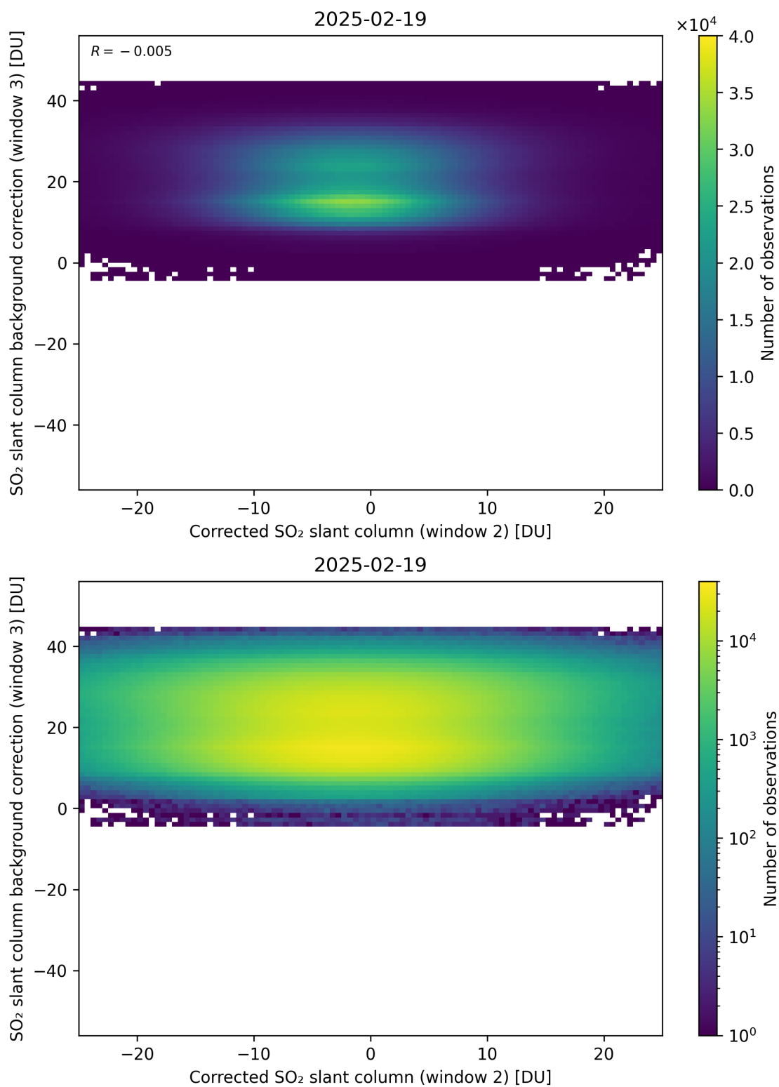
Figure 245: Scatter density plot of “Corrected SO 2 slant column (window 2)” against “SO 2 slant column background correction (window 3)” for 2025-02-19 to 2025-02-20.
