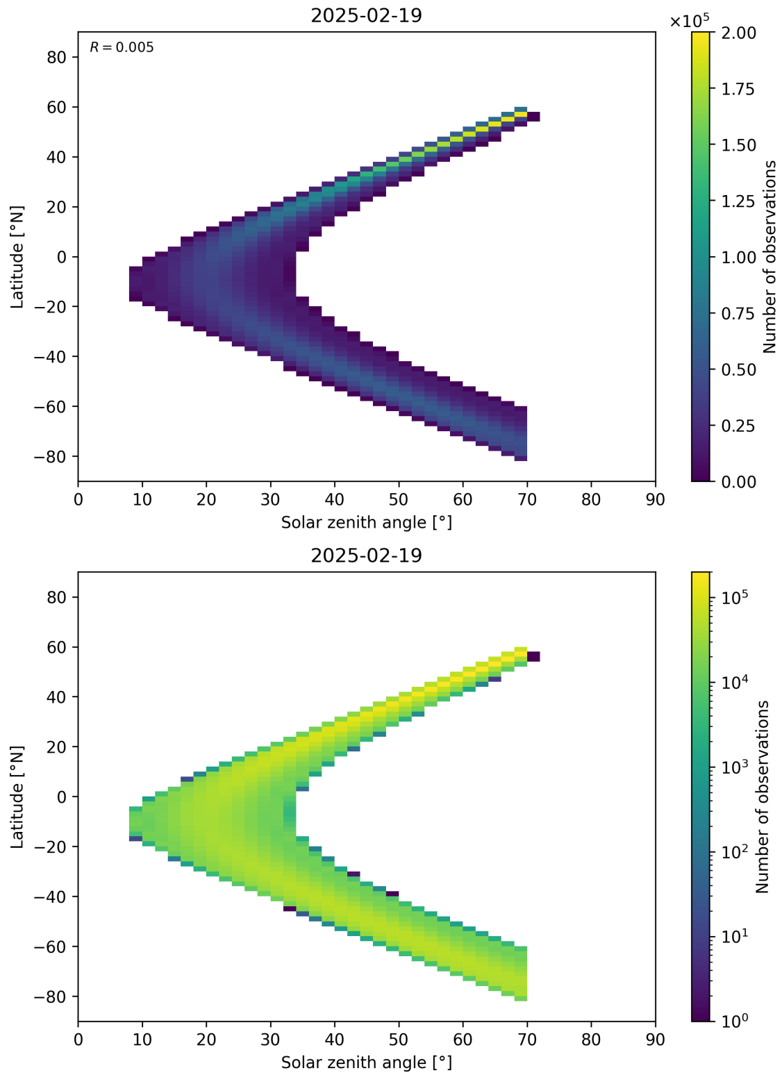
Figure 177: Scatter density plot of “Solar zenith angle” against “Latitude” for 2025-02-19 to 2025-02-20.
