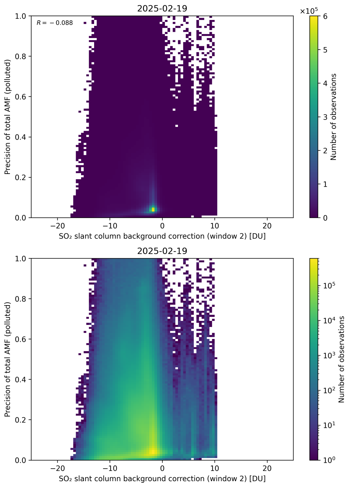
Figure 131: Scatter density plot of “SO 2 slant column background correction (window 2)” against “Precision of total AMF (polluted)” for 2025-02-19 to 2025-02-20.
