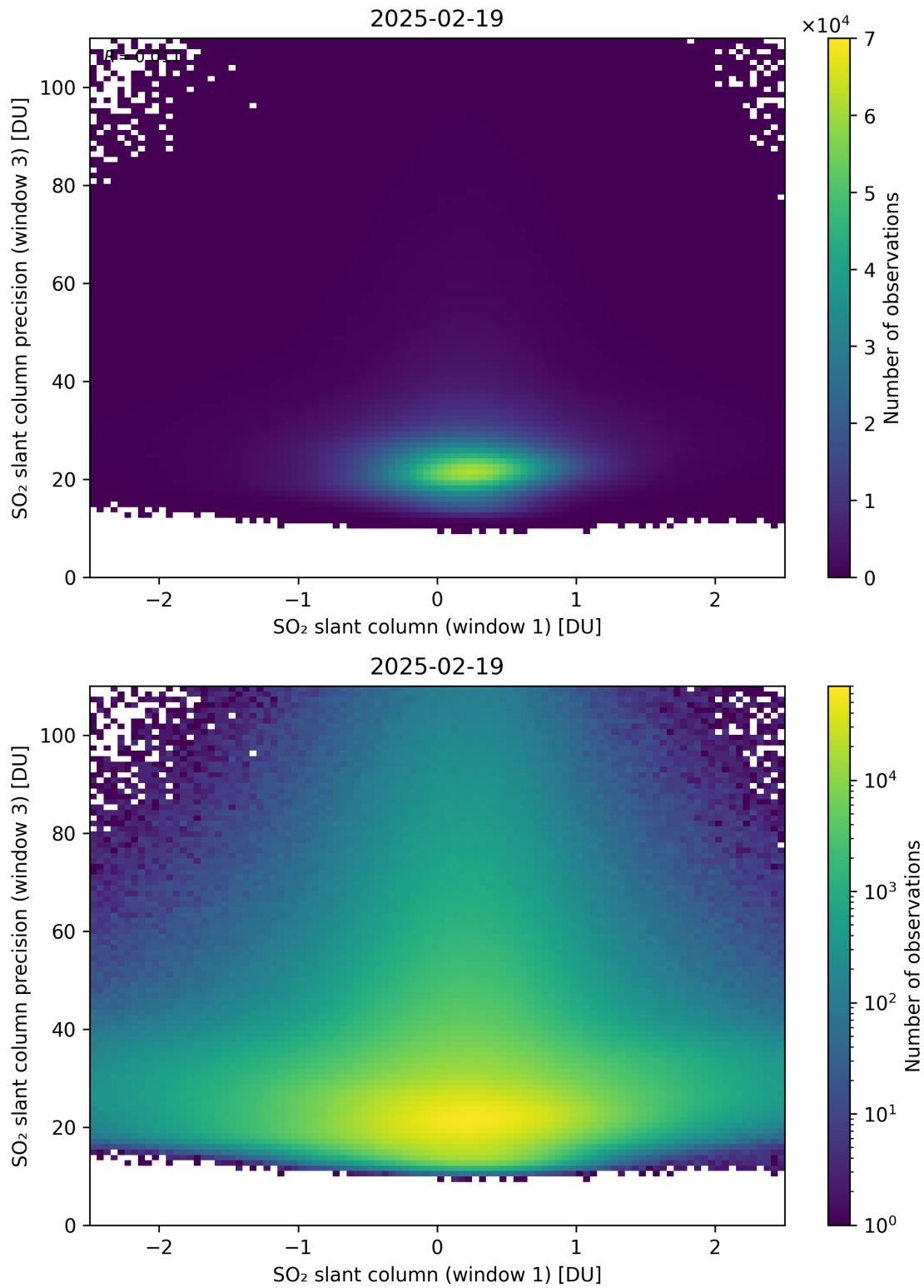
Figure 288: Scatter density plot of “SO 2 slant column (window 1)” against “SO 2 slant column precision (window 3)” for 2025-02-19 to 2025-02-20.
