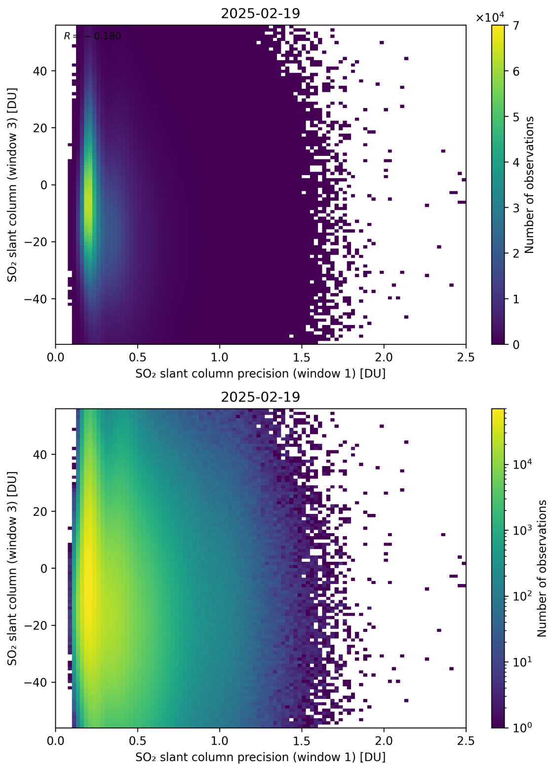
Figure 278: Scatter density plot of “SO 2 slant column precision (window 1)” against “SO 2 slant column (window 3)” for 2025-02-19 to 2025-02-20.
