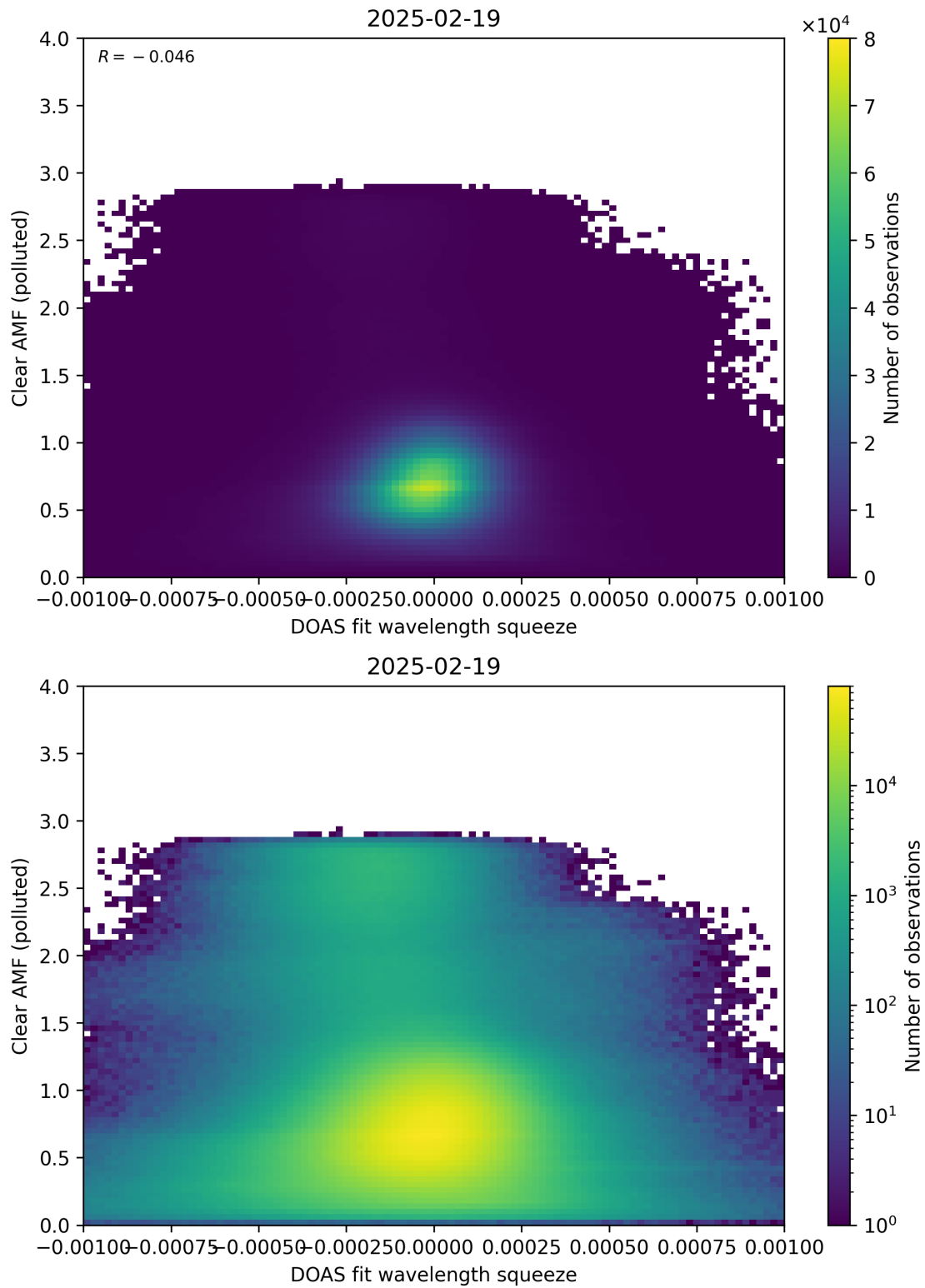
Figure 144: Scatter density plot of “DOAS fit wavelength squeeze” against “Clear AMF (polluted)” for 2025-02-19 to 2025-02-20.
