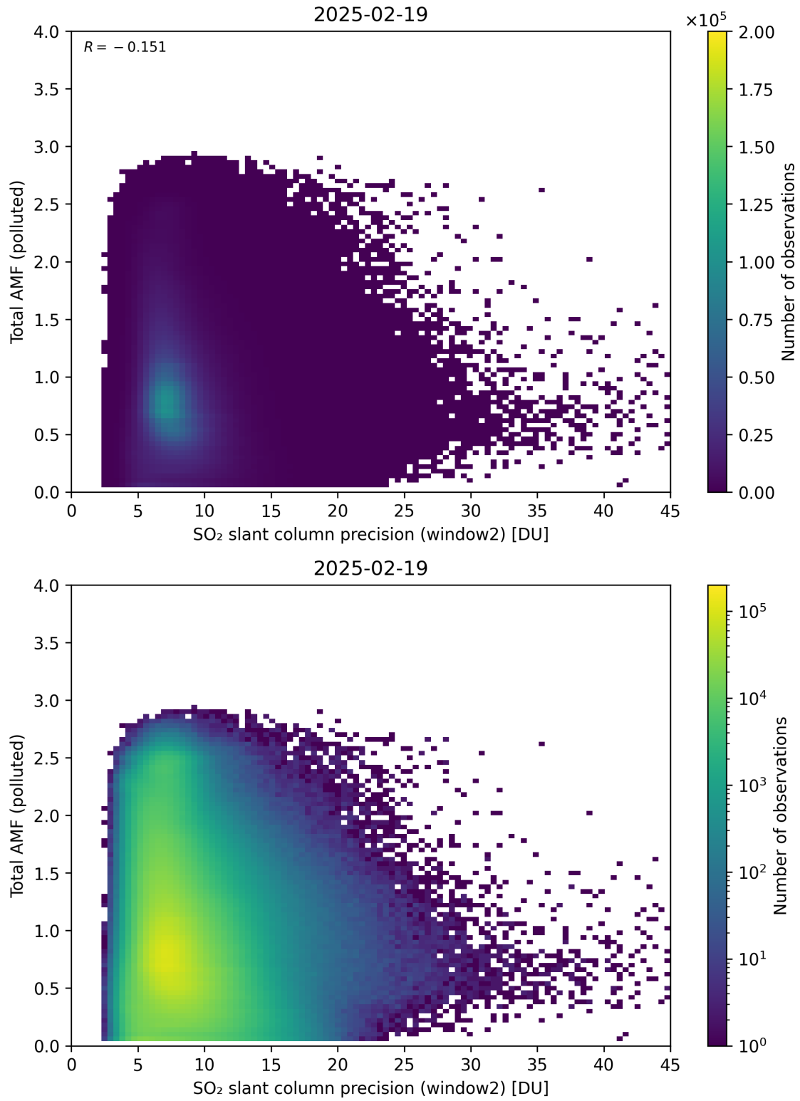
Figure 301: Scatter density plot of “SO 2 slant column precision (window2)” against “Total AMF (polluted)” for 2025-02-19 to 2025-02-20.
