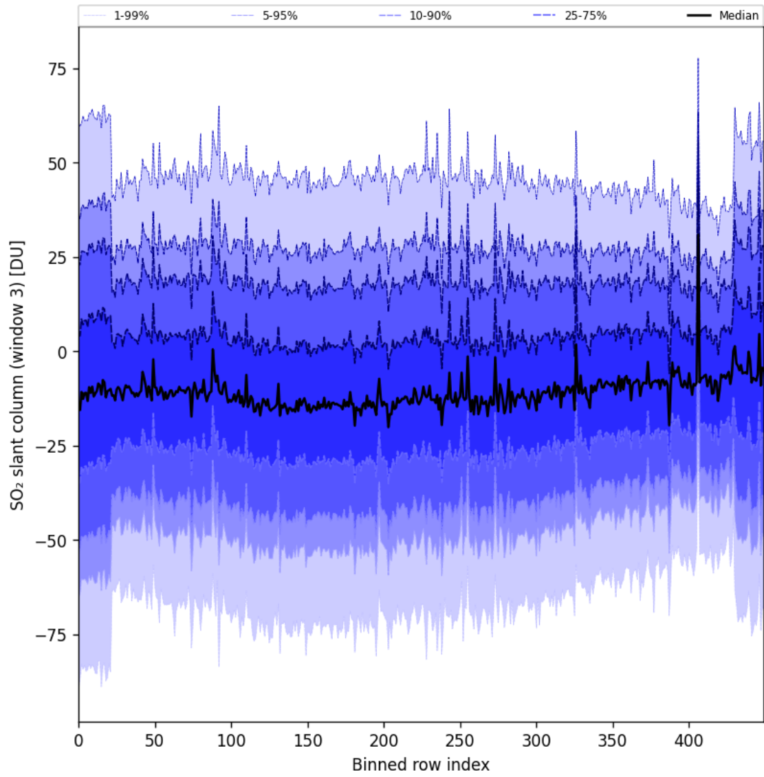
Figure 97: Along track statistics of “SO 2 slant column (window 3)” for 2025-02-19 to 2025-02-20
