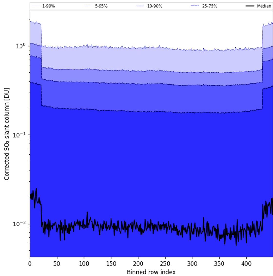
Figure 86: Along track statistics of “Corrected SO 2 slant column” for 2025-02-19 to 2025-02-20
