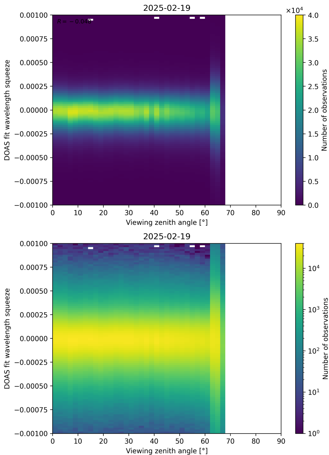
Figure 366: Scatter density plot of “Viewing zenith angle” against “DOAS fit wavelength squeeze” for 2025-02-19 to 2025-02-20.
