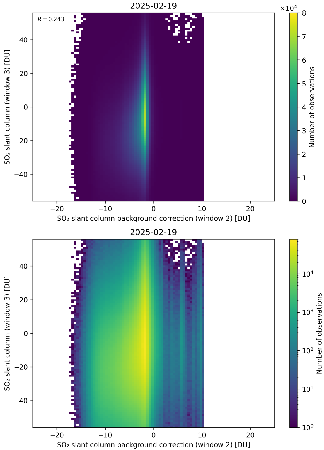
Figure 128: Scatter density plot of “SO 2 slant column background correction (window 2)” against “SO 2 slant column (window 3)” for 2025-02-19 to 2025-02-20.
