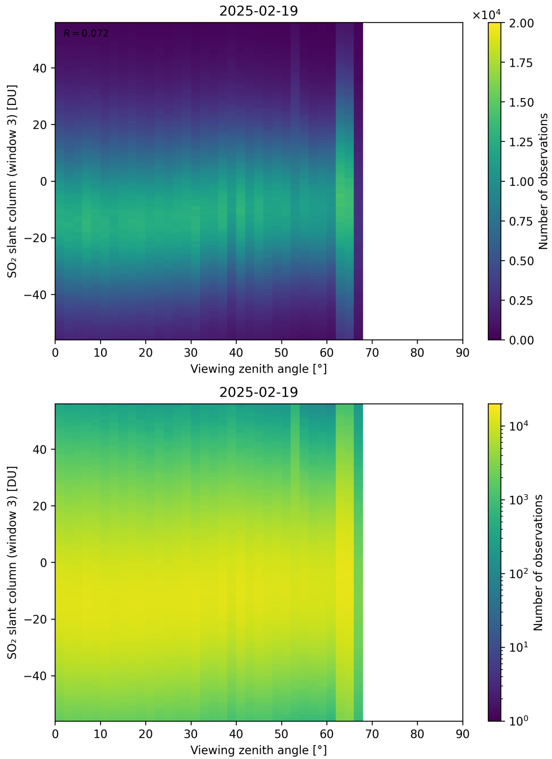
Figure 379: Scatter density plot of “Viewing zenith angle” against “SO 2 slant column (window 3)” for 2025-02-19 to 2025-02-20.
