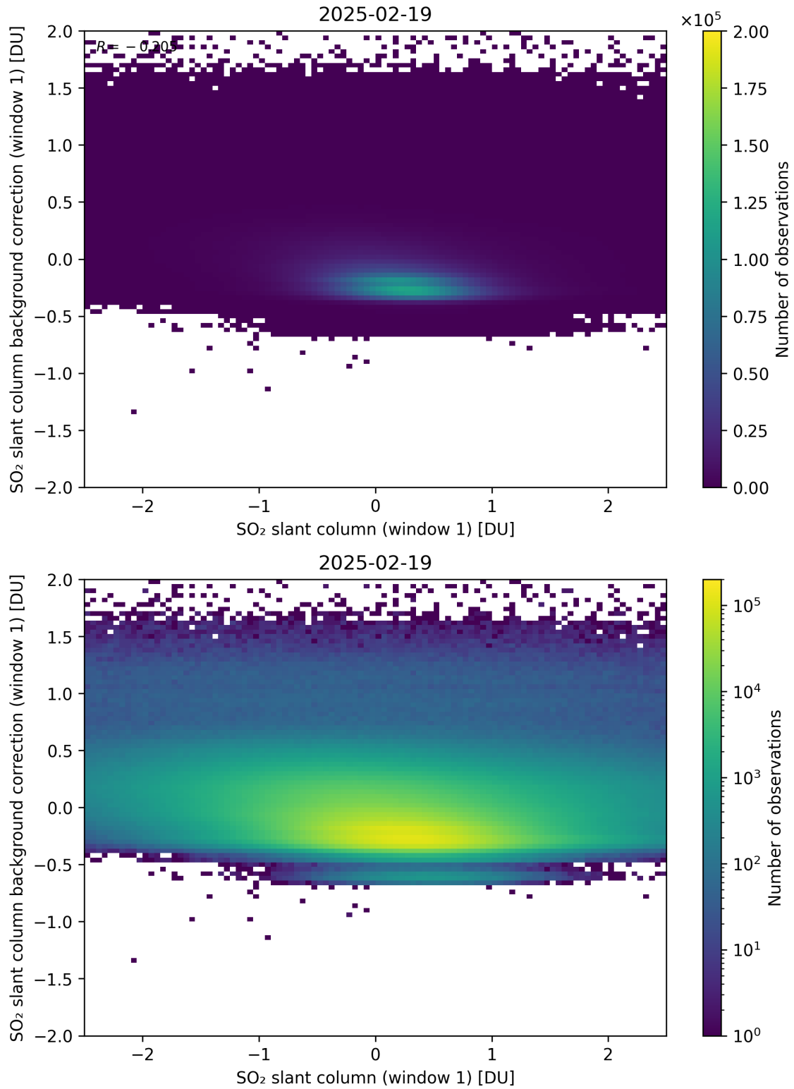
Figure 262: Scatter density plot of “SO 2 slant column (window 1)” against “SO 2 slant column background correction (window 1)” for 2025-02-19 to 2025-02-20.
