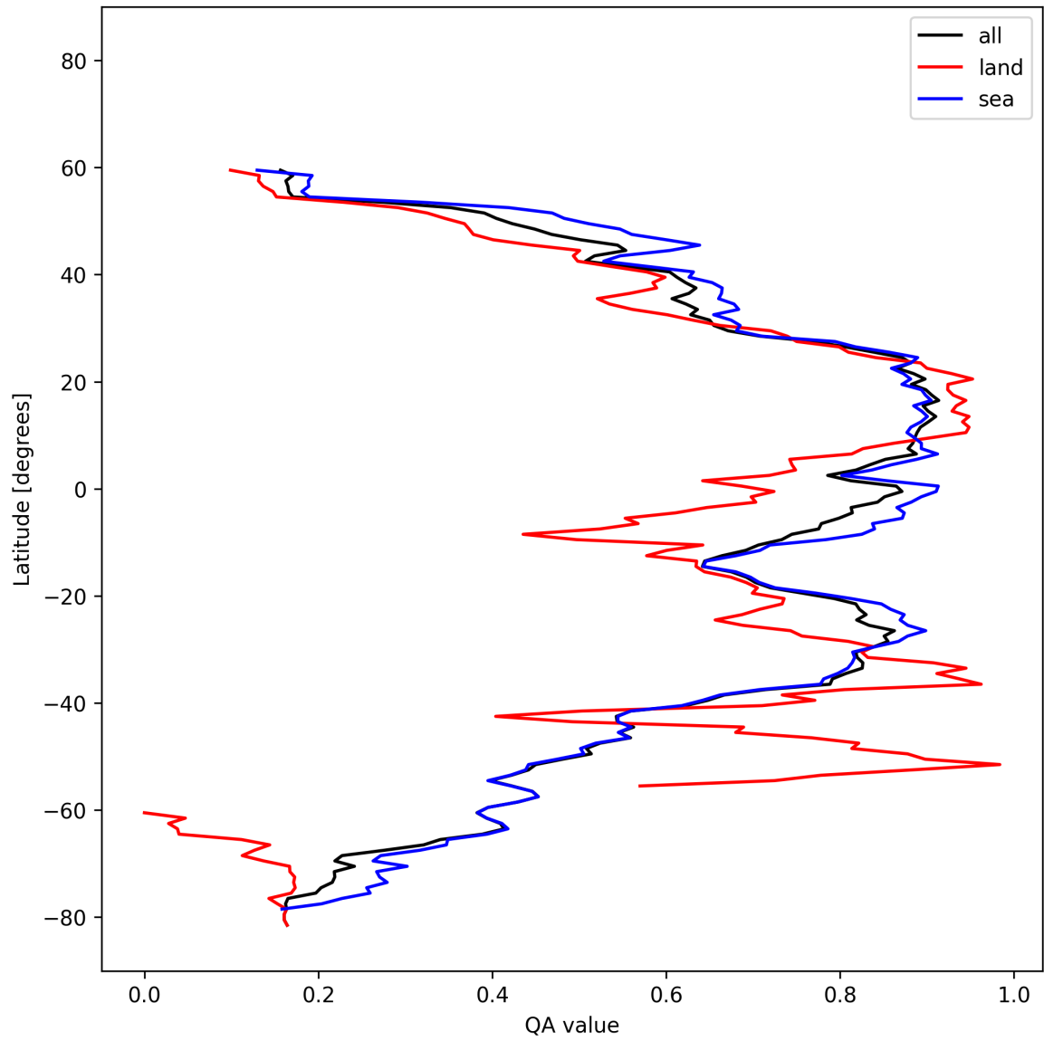
Figure 31: Zonal average of “QA value” for 2025-02-19 to 2025-02-20.
