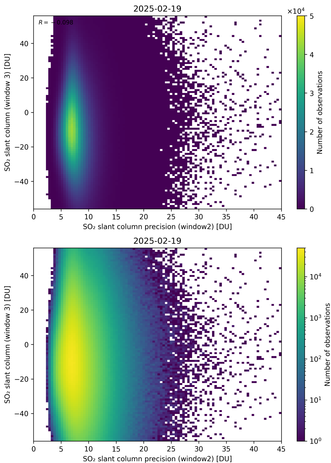
Figure 299: Scatter density plot of “SO 2 slant column precision (window2)” against “SO 2 slant column (window 3)” for 2025-02-19 to 2025-02-20.
