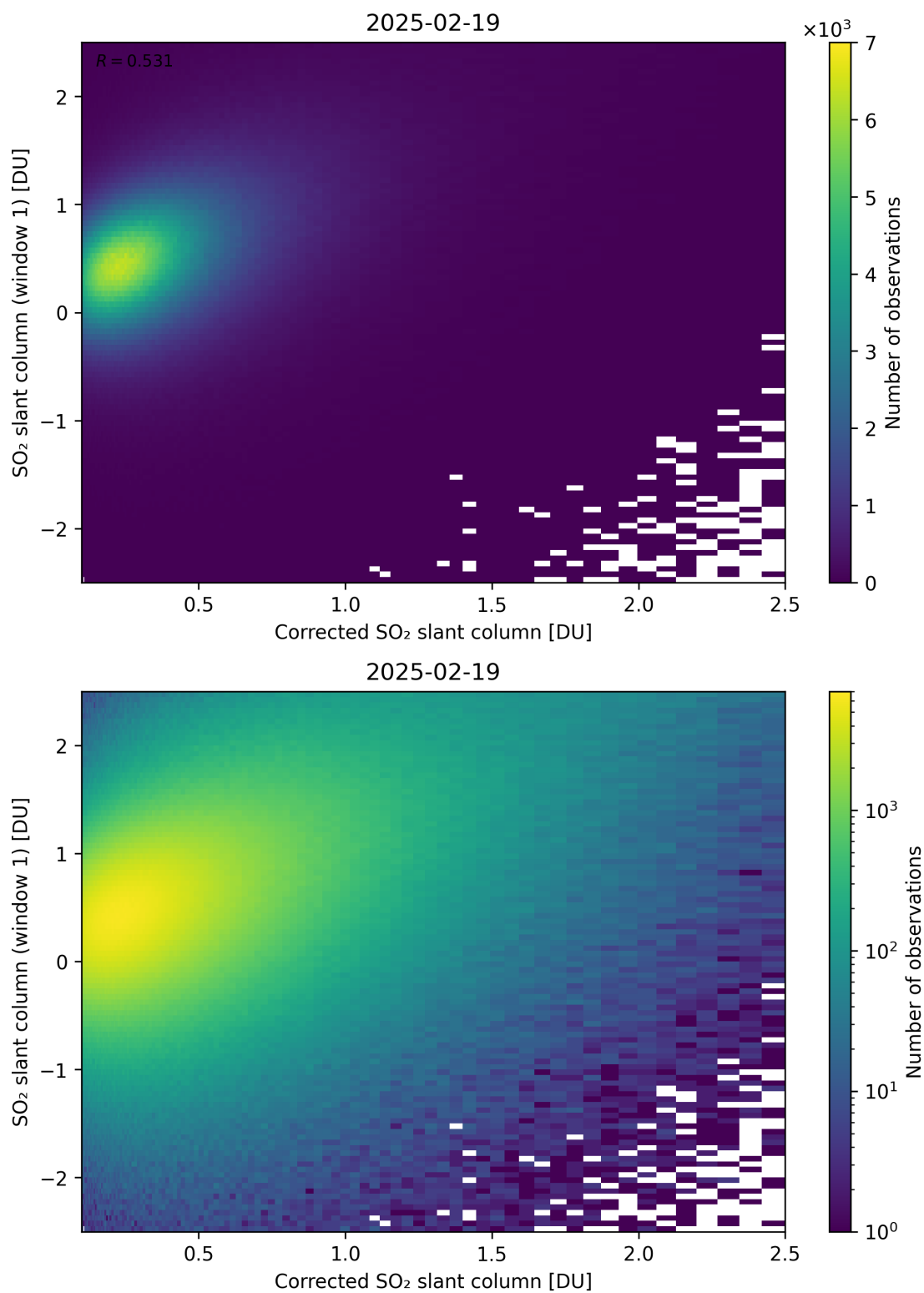
Figure 237: Scatter density plot of “Corrected SO 2 slant column” against “SO 2 slant column (window 1)” for 2025-02-19 to 2025-02-20.
