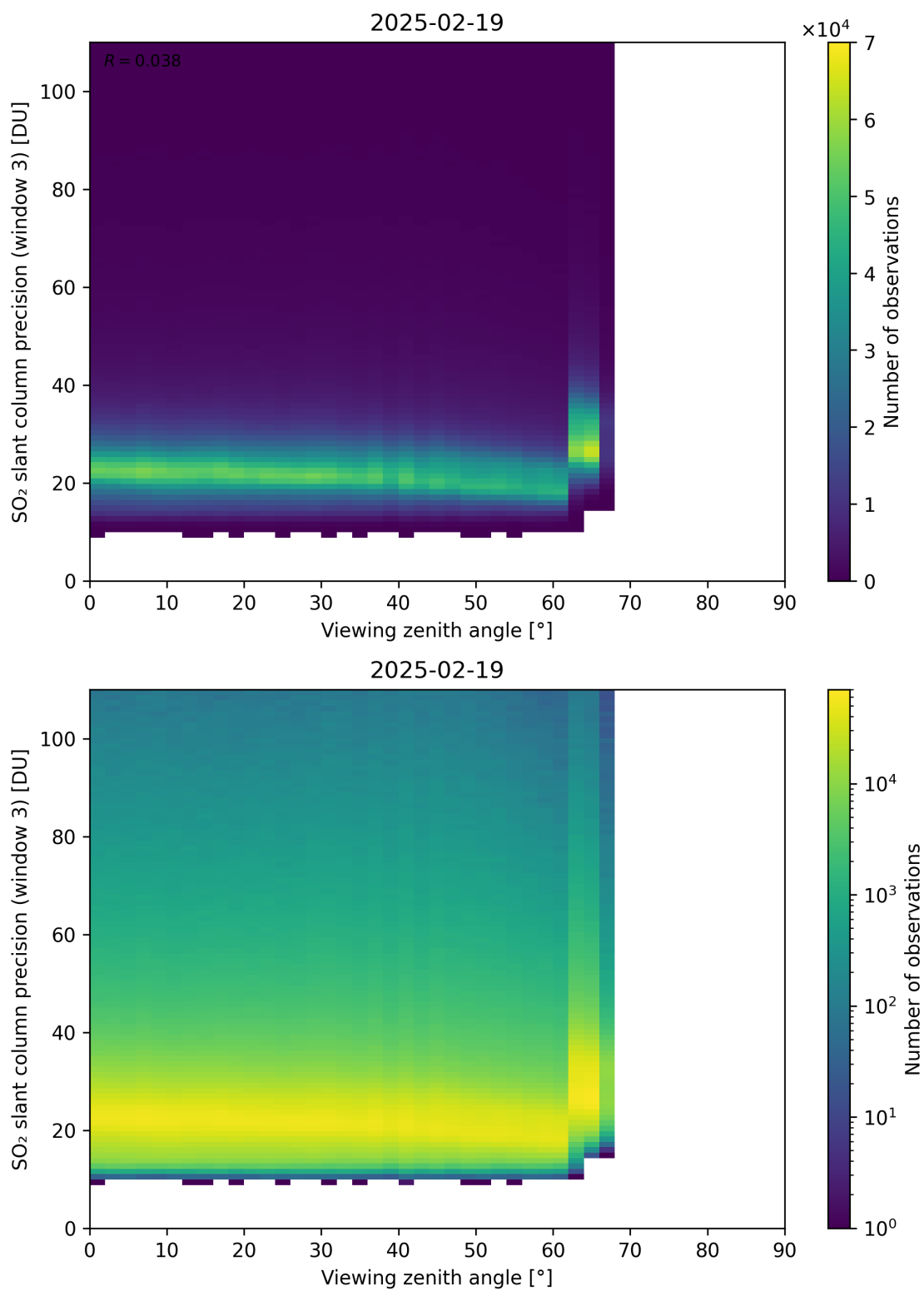
Figure 380: Scatter density plot of “Viewing zenith angle” against “SO 2 slant column precision (window 3)” for 2025-02-19 to 2025-02-20.
