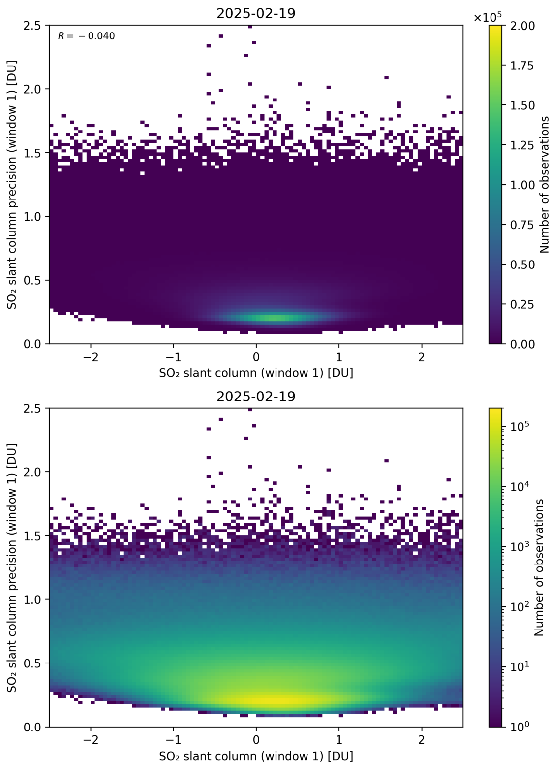
Figure 285: Scatter density plot of “SO 2 slant column (window 1)” against “SO 2 slant column precision (window 1)” for 2025-02-19 to 2025-02-20.
