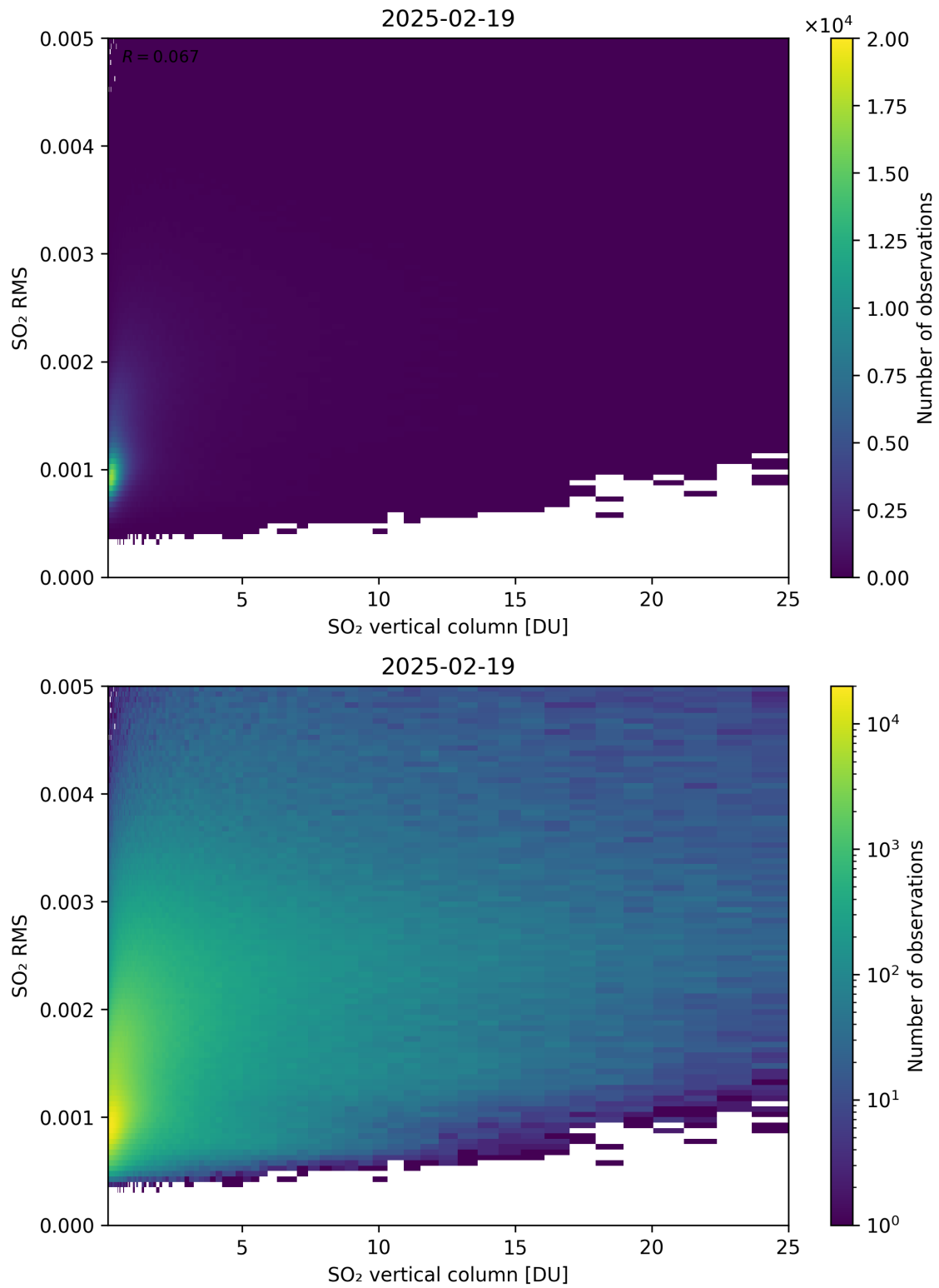
Figure 328: Scatter density plot of “SO 2 vertical column” against “SO 2 RMS” for 2025-02-19 to 2025-02-20.
