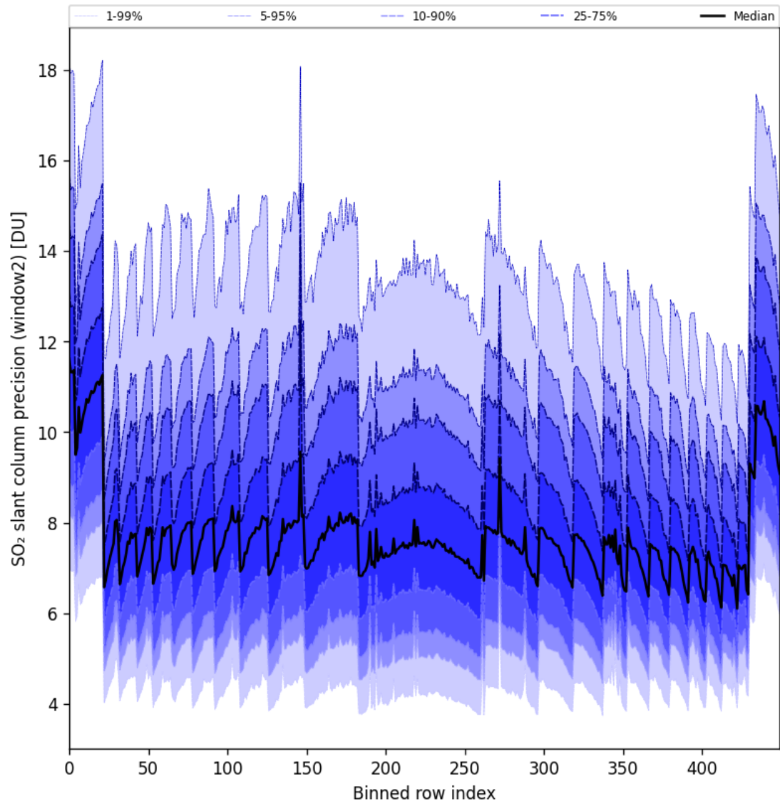
Figure 94: Along track statistics of “SO 2 slant column precision (window2)” for 2025-02-19 to 2025-02-20
