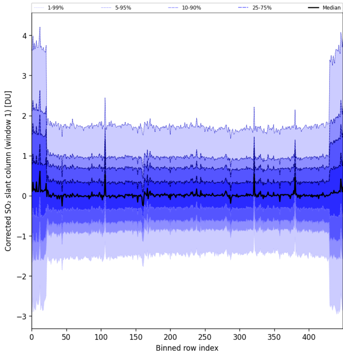
Figure 91: Along track statistics of “Corrected SO 2 slant column (window 1)” for 2025-02-19 to 2025-02-20
