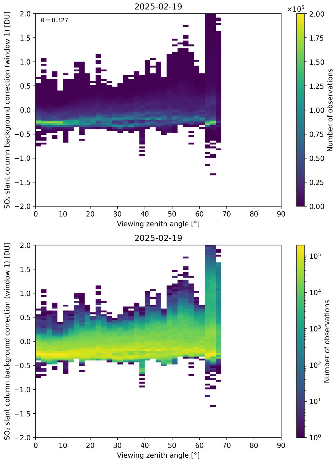
Figure 362: Scatter density plot of “Viewing zenith angle” against “SO 2 slant column background correction (window 1)” for 2025-02-19 to 2025-02-20.
