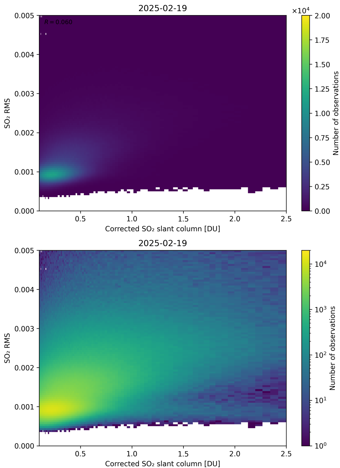
Figure 231: Scatter density plot of “Corrected SO 2 slant column” against “SO 2 RMS” for 2025-02-19 to 2025-02-20.
