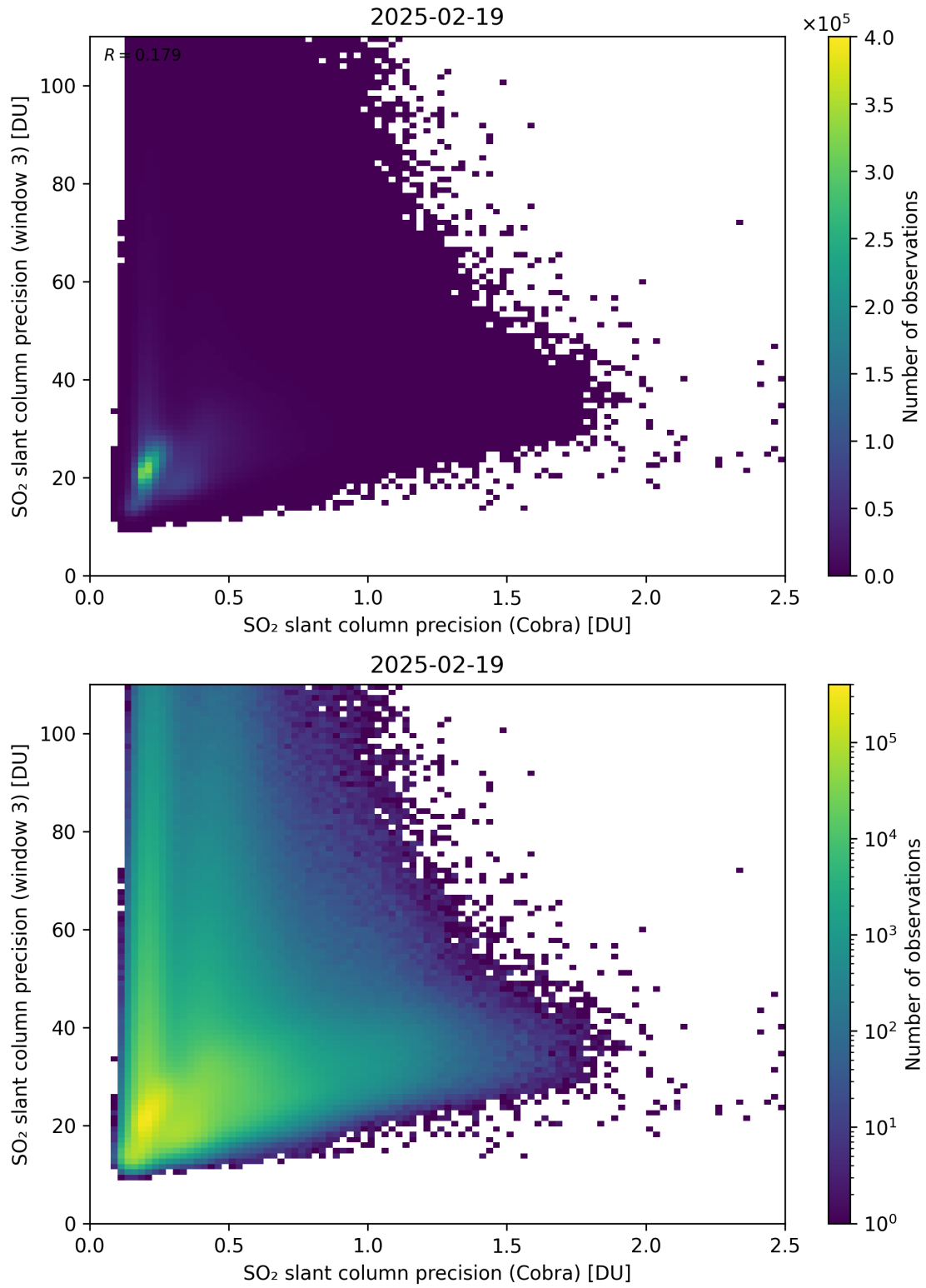
Figure 212: Scatter density plot of “SO 2 slant column precision (Cobra)” against “SO 2 slant column precision (window 3)” for 2025-02-19 to 2025-02-20.
