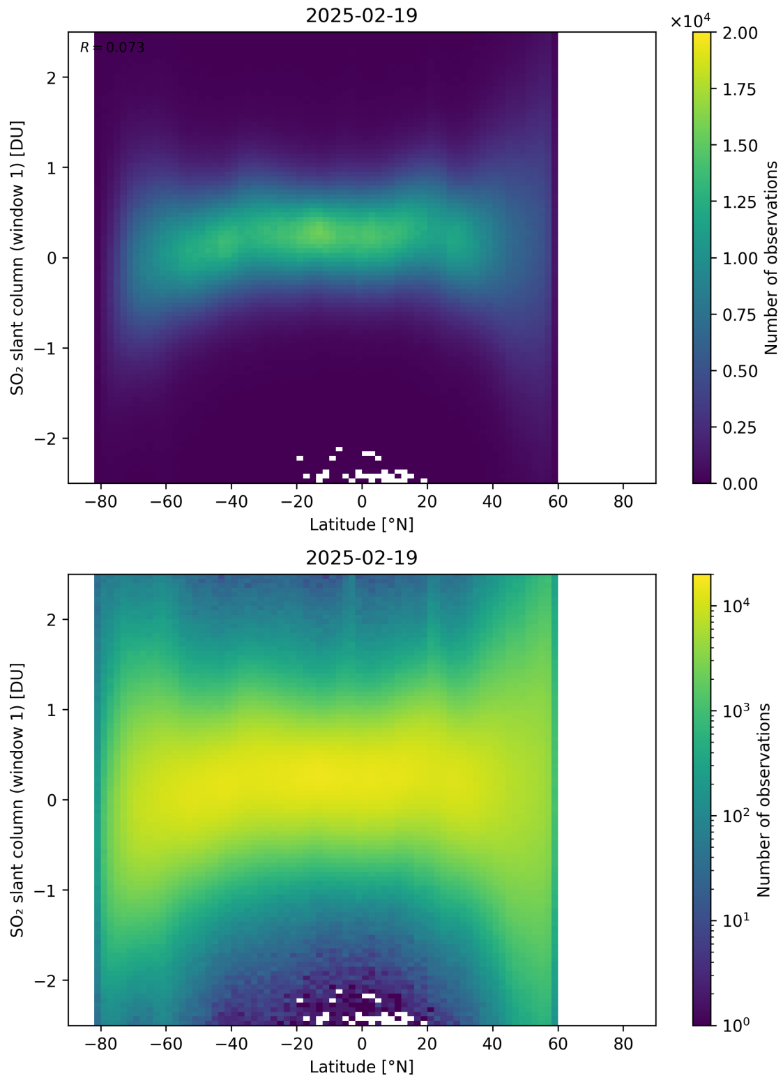
Figure 162: Scatter density plot of “Latitude” against “SO 2 slant column (window 1)” for 2025-02-19 to 2025-02-20.
