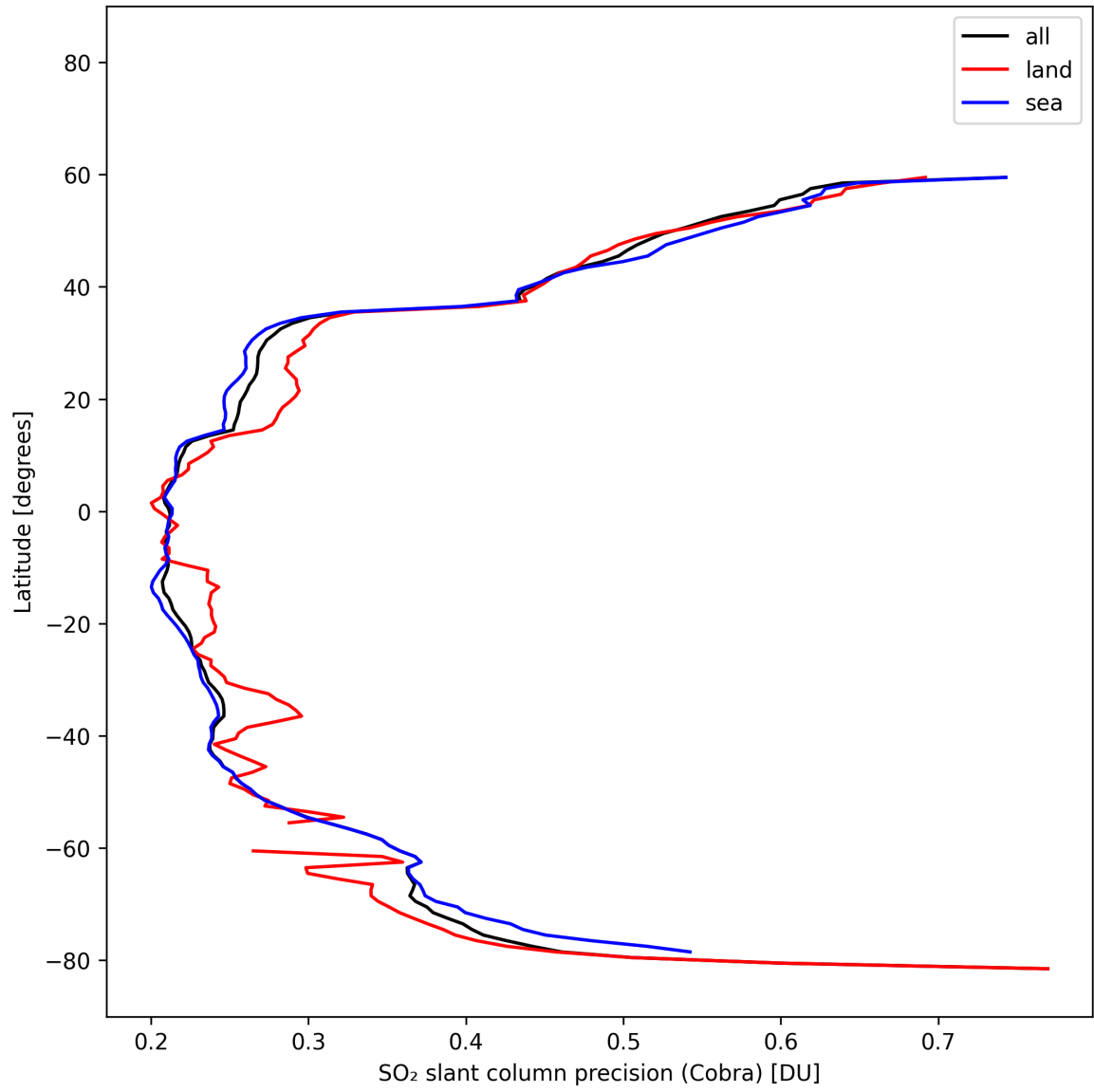
Figure 36: Zonal average of “SO 2 slant column precision (Cobra)” for 2025-02-19 to 2025-02-20.
