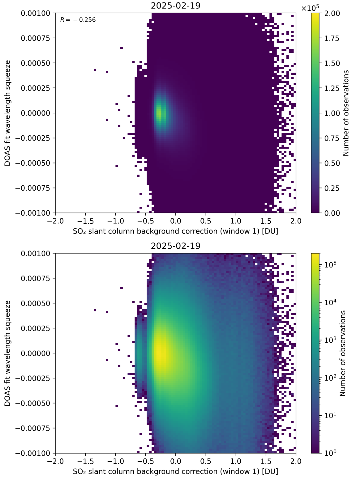
Figure 112: Scatter density plot of “SO 2 slant column background correction (window 1)” against “DOAS fit wavelength squeeze” for 2025-02-19 to 2025-02-20.
