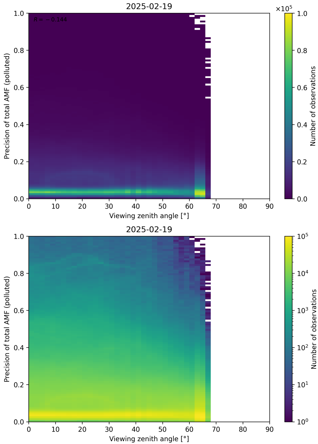
Figure 382: Scatter density plot of “Viewing zenith angle” against “Precision of total AMF (polluted)” for 2025-02-19 to 2025-02-20.
