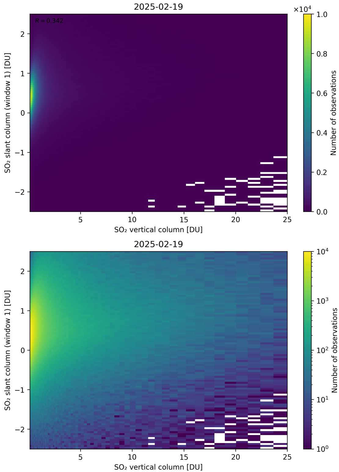
Figure 354: Scatter density plot of “SO 2 vertical column” against “SO 2 slant column (window 1)” for 2025-02-19 to 2025-02-20.
