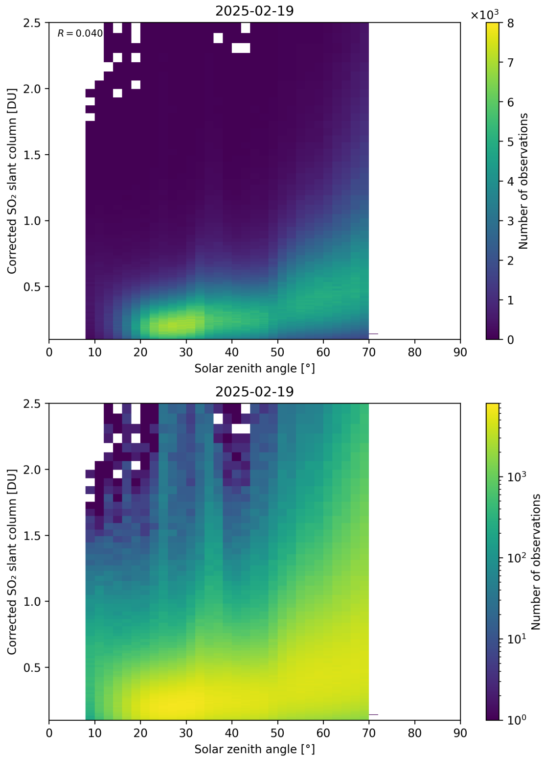
Figure 181: Scatter density plot of “Solar zenith angle” against “Corrected SO 2 slant column” for 2025-02-19 to 2025-02-20.
