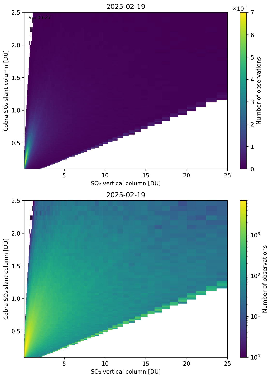
Figure 349: Scatter density plot of “SO 2 vertical column” against “Cobra SO 2 slant column” for 2025-02-19 to 2025-02-20.
