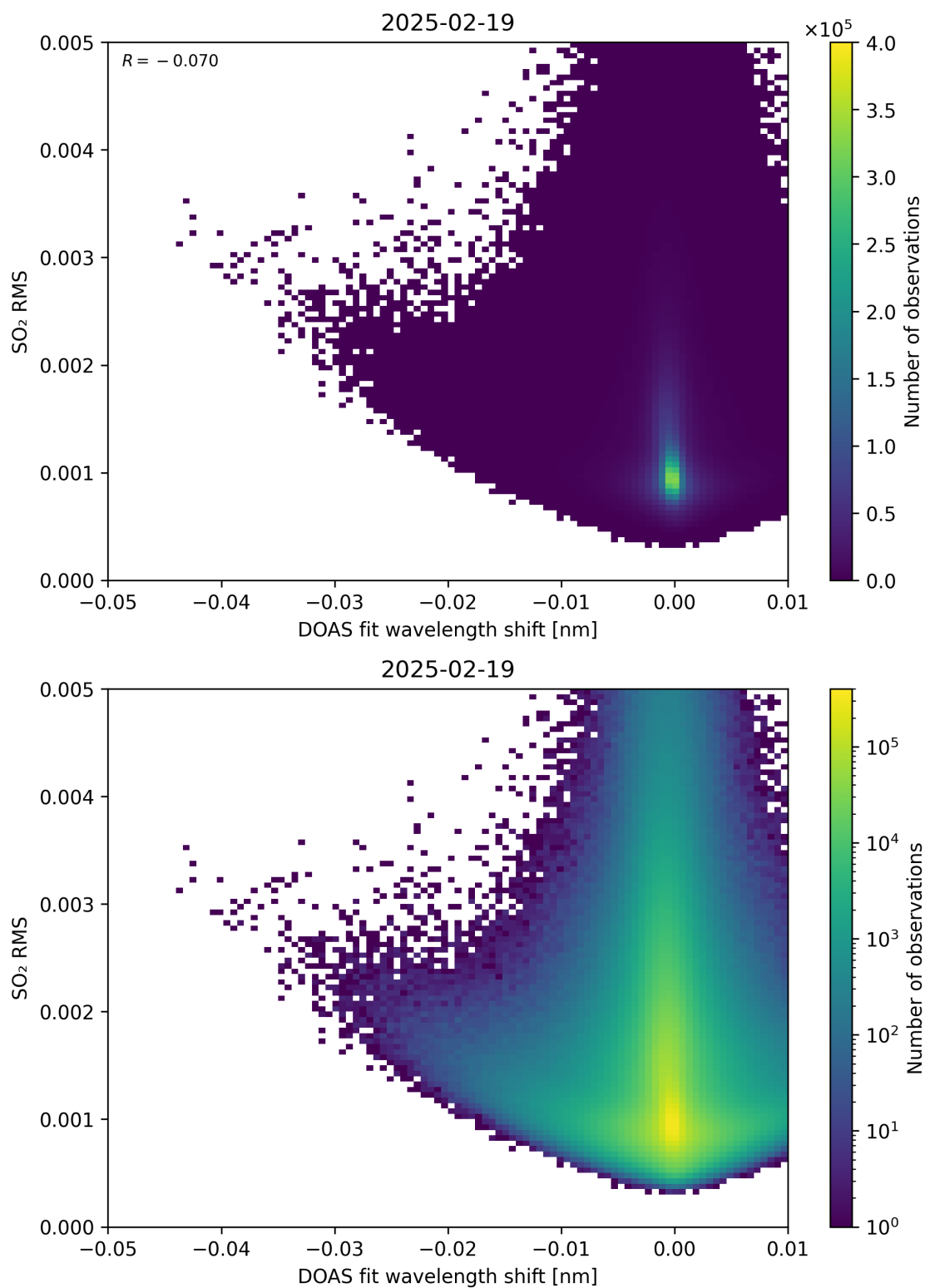
Figure 139: Scatter density plot of “DOAS fit wavelength shift” against “SO 2 RMS” for 2025-02-19 to 2025-02-20.
