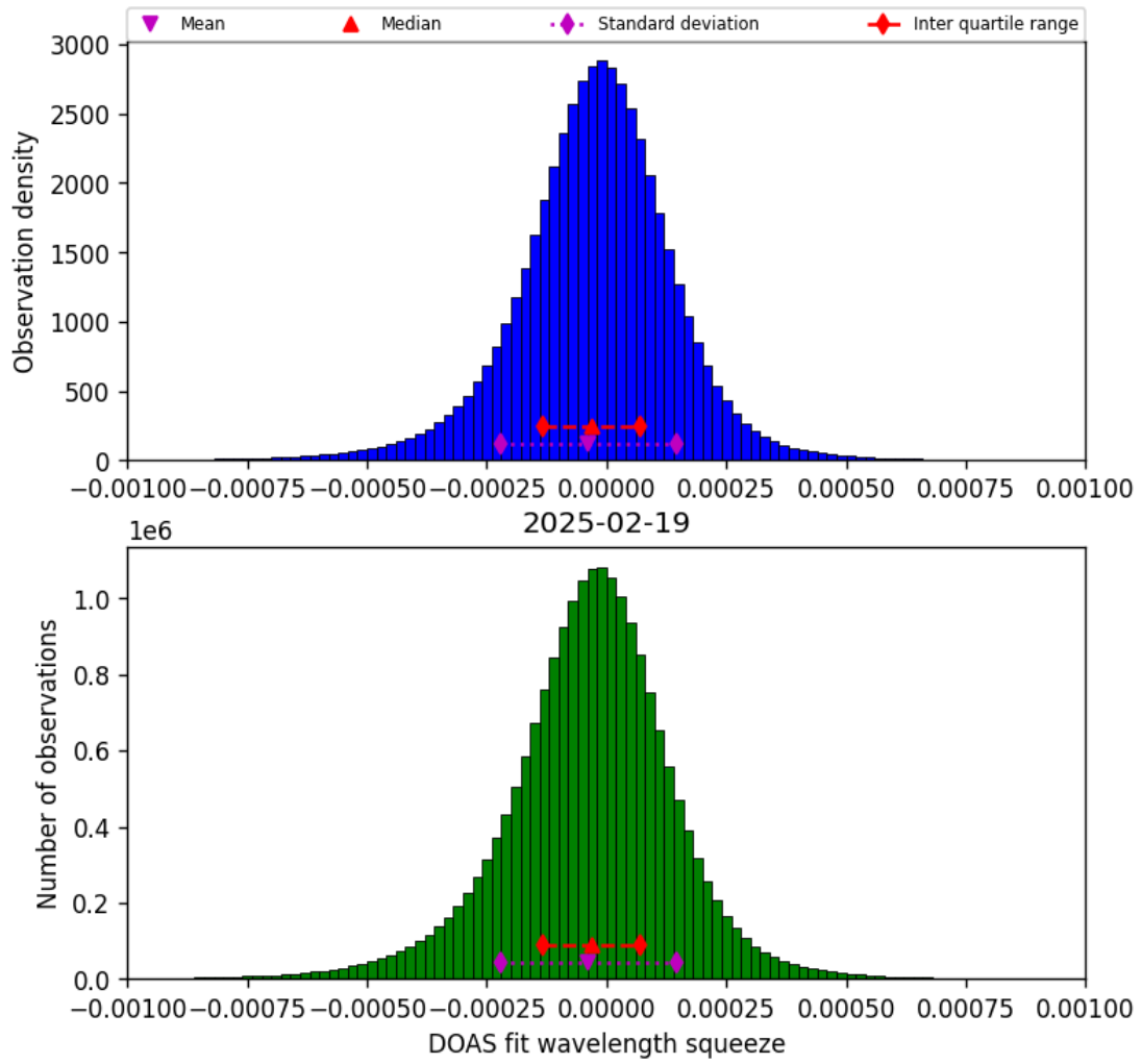
Figure 77: Histogram of “DOAS fit wavelength squeeze” for 2025-02-19 to 2025-02-20
