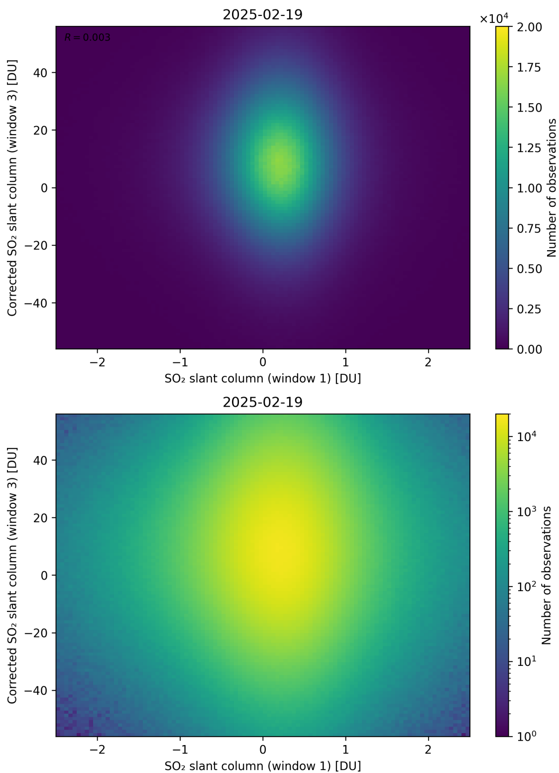
Figure 284: Scatter density plot of “SO 2 slant column (window 1)” against “Corrected SO 2 slant column (window 3)” for 2025-02-19 to 2025-02-20.
