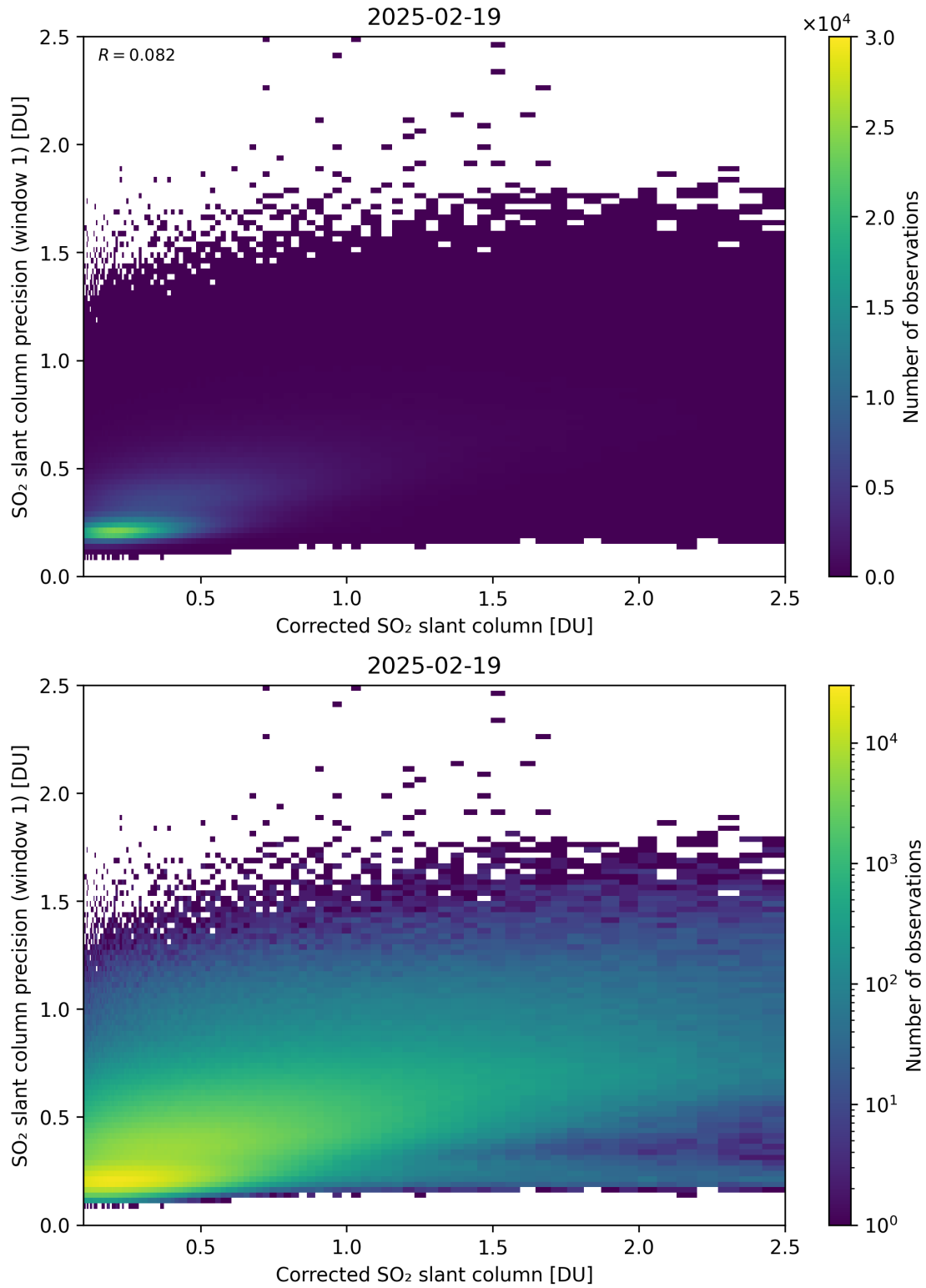
Figure 238: Scatter density plot of “Corrected SO 2 slant column” against “SO 2 slant column precision (window 1)” for 2025-02-19 to 2025-02-20.
