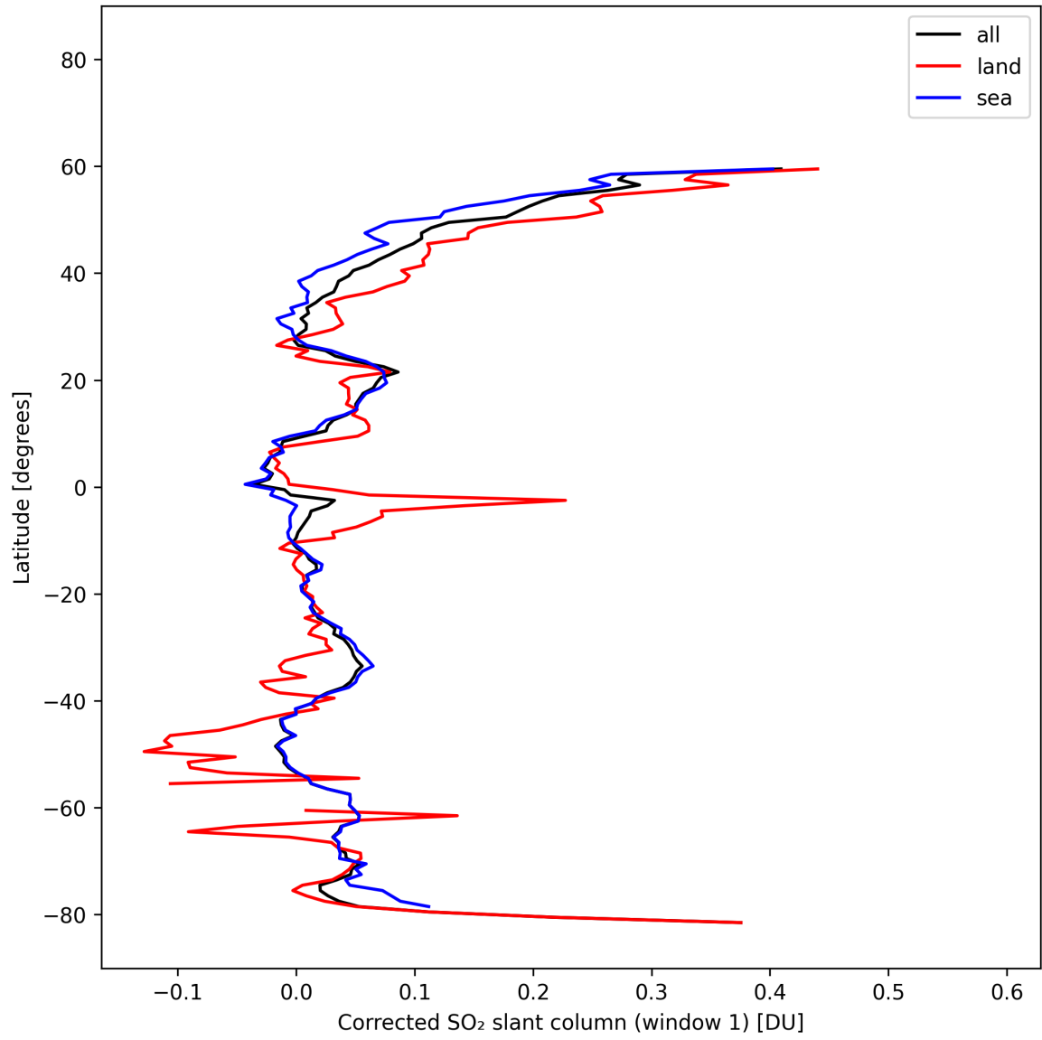
Figure 39: Zonal average of “Corrected SO 2 slant column (window 1)” for 2025-02-19 to 2025-02-20.
