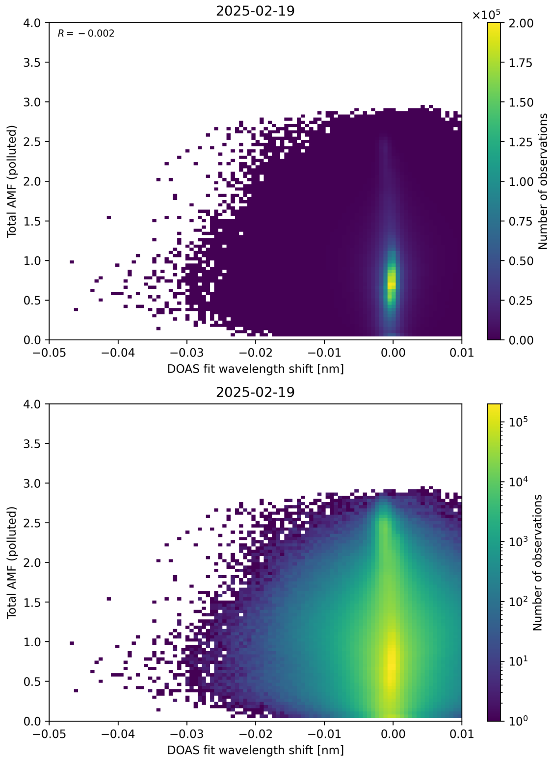
Figure 141: Scatter density plot of “DOAS fit wavelength shift” against “Total AMF (polluted)” for 2025-02-19 to 2025-02-20.
