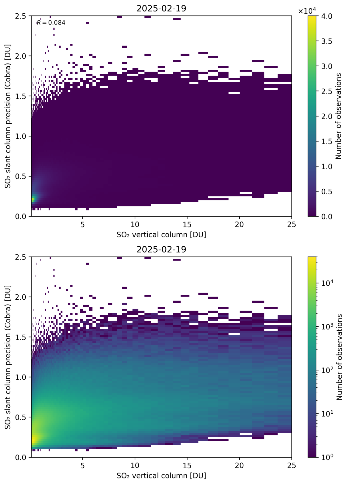
Figure 350: Scatter density plot of “SO 2 vertical column” against “SO 2 slant column precision (Cobra)” for 2025-02-19 to 2025-02-20.
