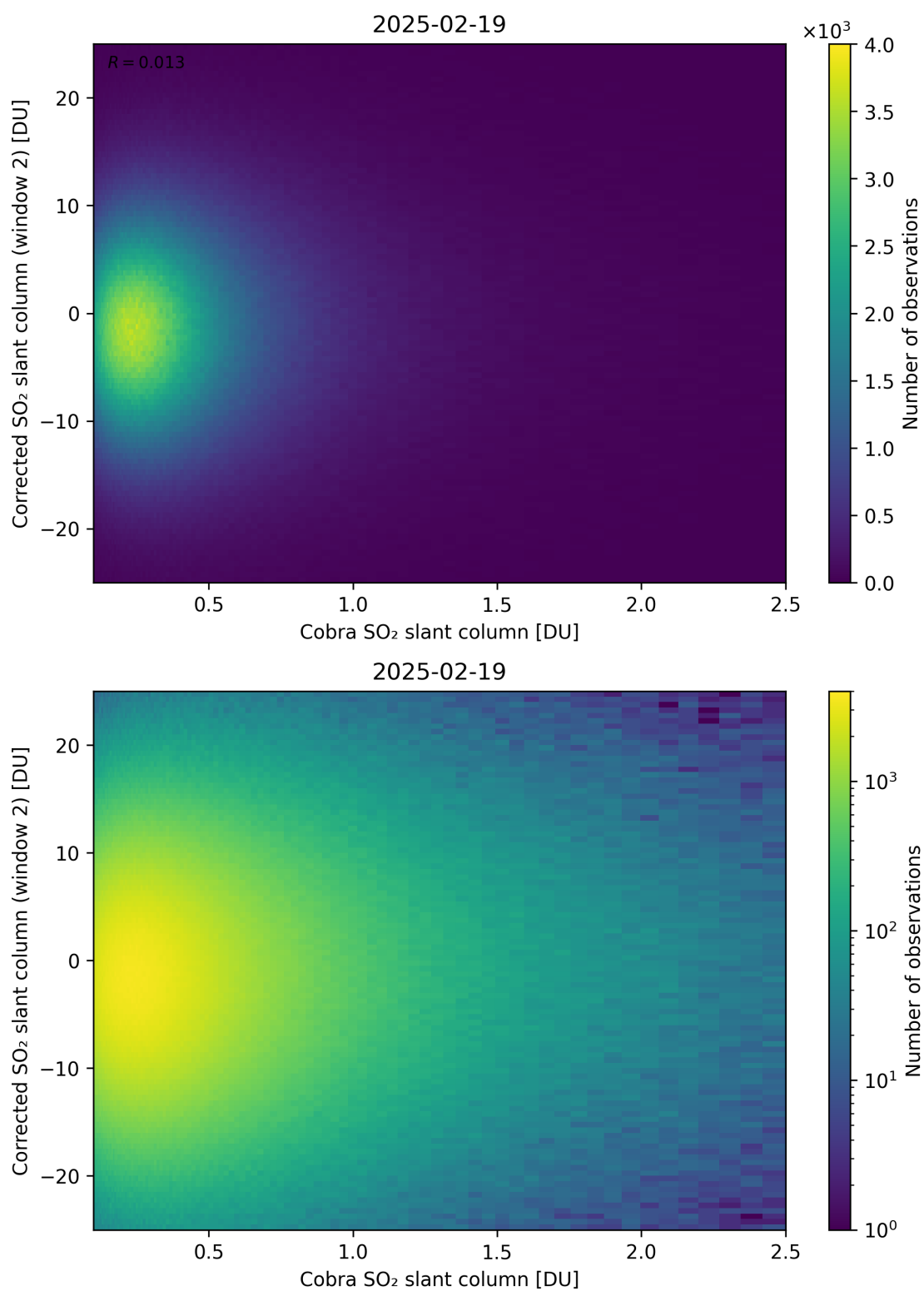
Figure 217: Scatter density plot of “Cobra SO 2 slant column” against “Corrected SO 2 slant column (window 2)” for 2025-02-19 to 2025-02-20.
