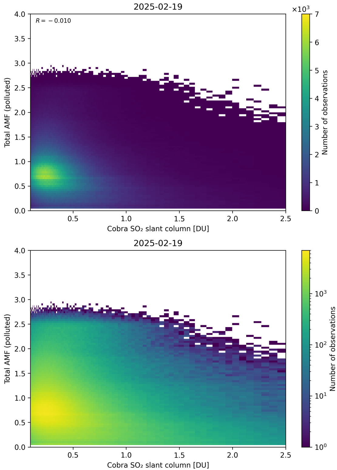
Figure 224: Scatter density plot of “Cobra SO 2 slant column” against “Total AMF (polluted)” for 2025-02-19 to 2025-02-20.
