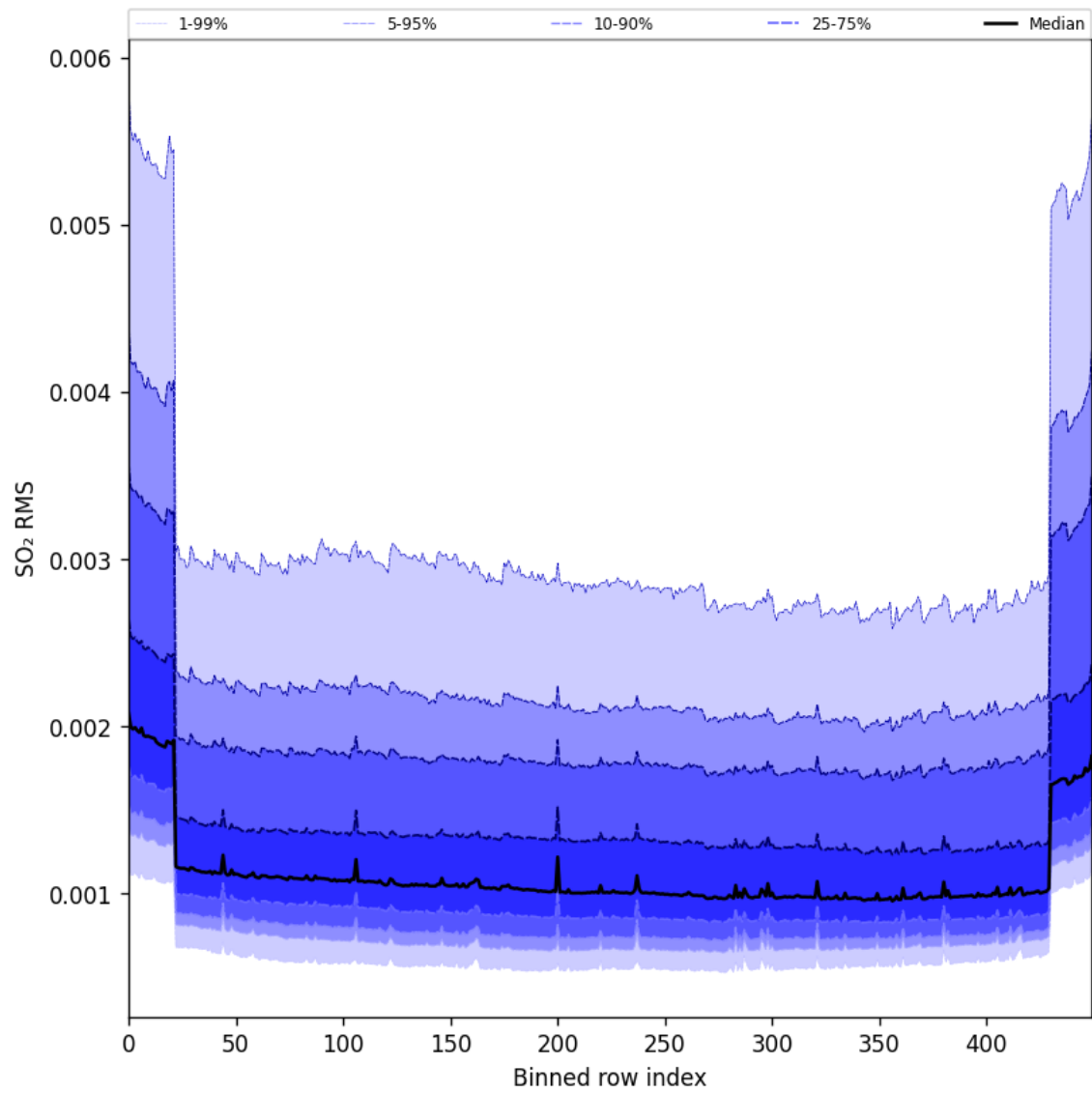
Figure 104: Along track statistics of “SO 2 RMS” for 2025-02-19 to 2025-02-20
