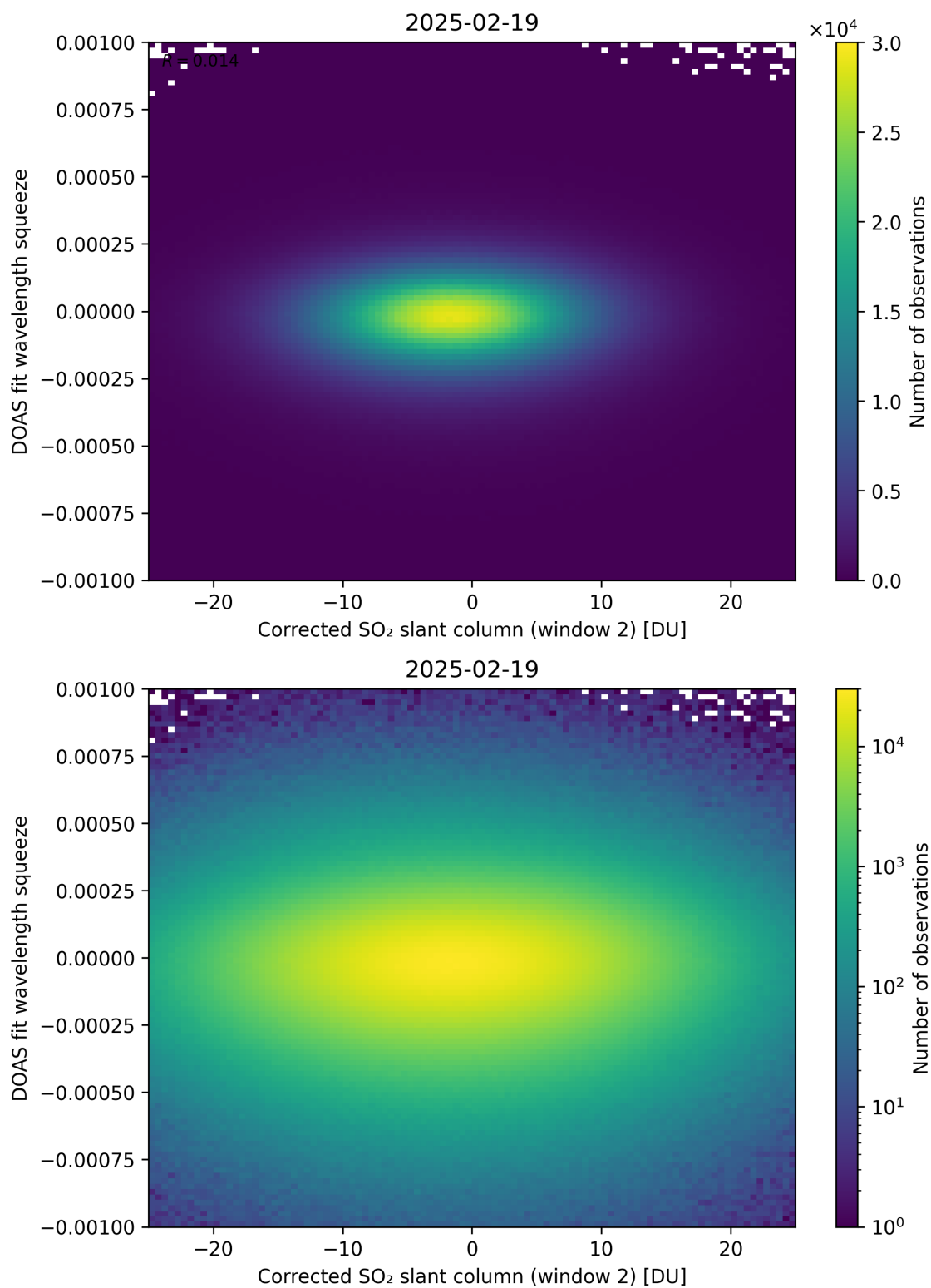
Figure 247: Scatter density plot of “Corrected SO 2 slant column (window 2)” against “DOAS fit wavelength squeeze” for 2025-02-19 to 2025-02-20.
