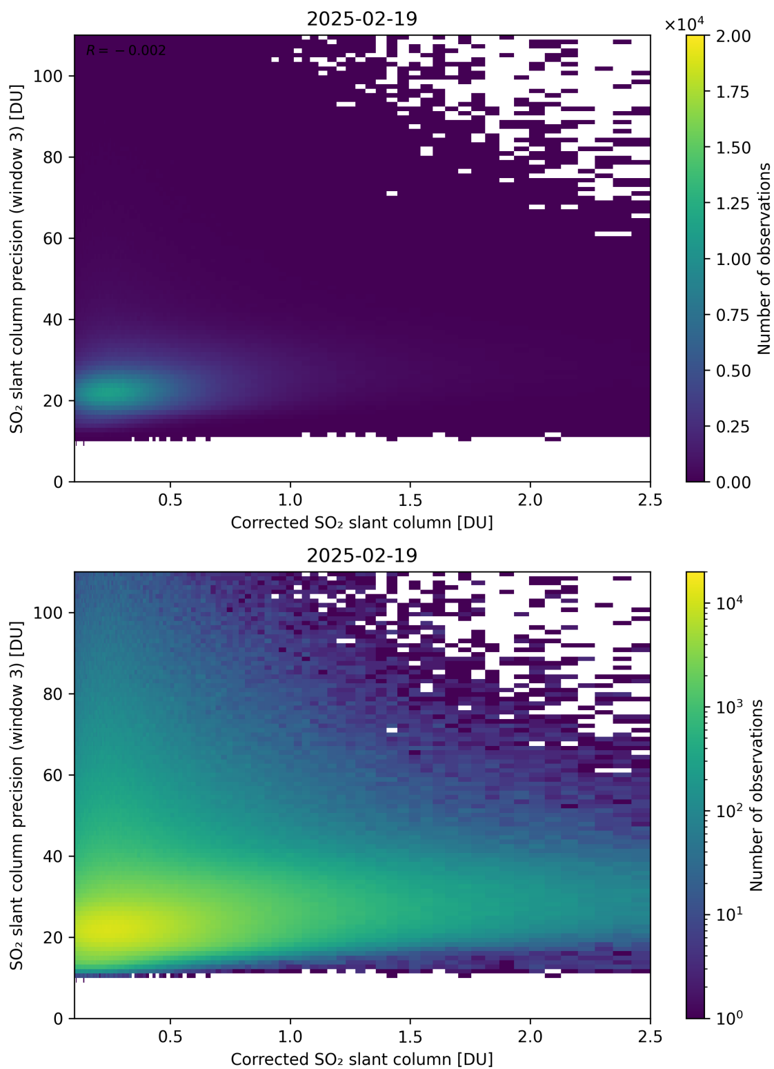
Figure 241: Scatter density plot of “Corrected SO 2 slant column” against “SO 2 slant column precision (window 3)” for 2025-02-19 to 2025-02-20.
