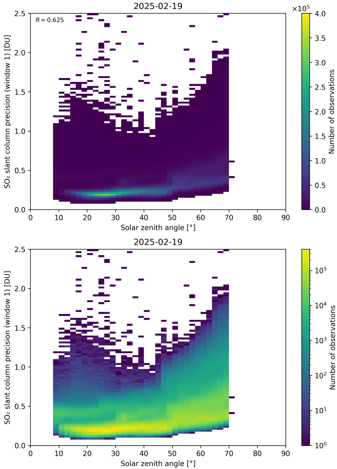
Figure 185: Scatter density plot of “Solar zenith angle” against “SO 2 slant column precision (window 1)” for 2025-02-19 to 2025-02-20.
