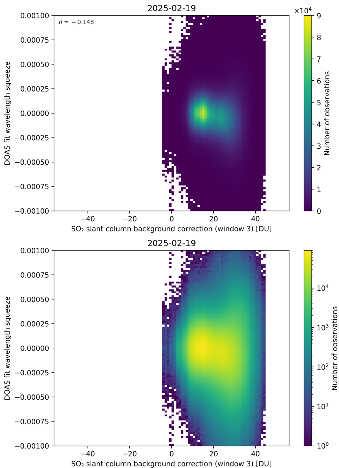
Figure 133: Scatter density plot of “SO 2 slant column background correction (window 3)” against “DOAS fit wavelength squeeze” for 2025-02-19 to 2025-02-20.
