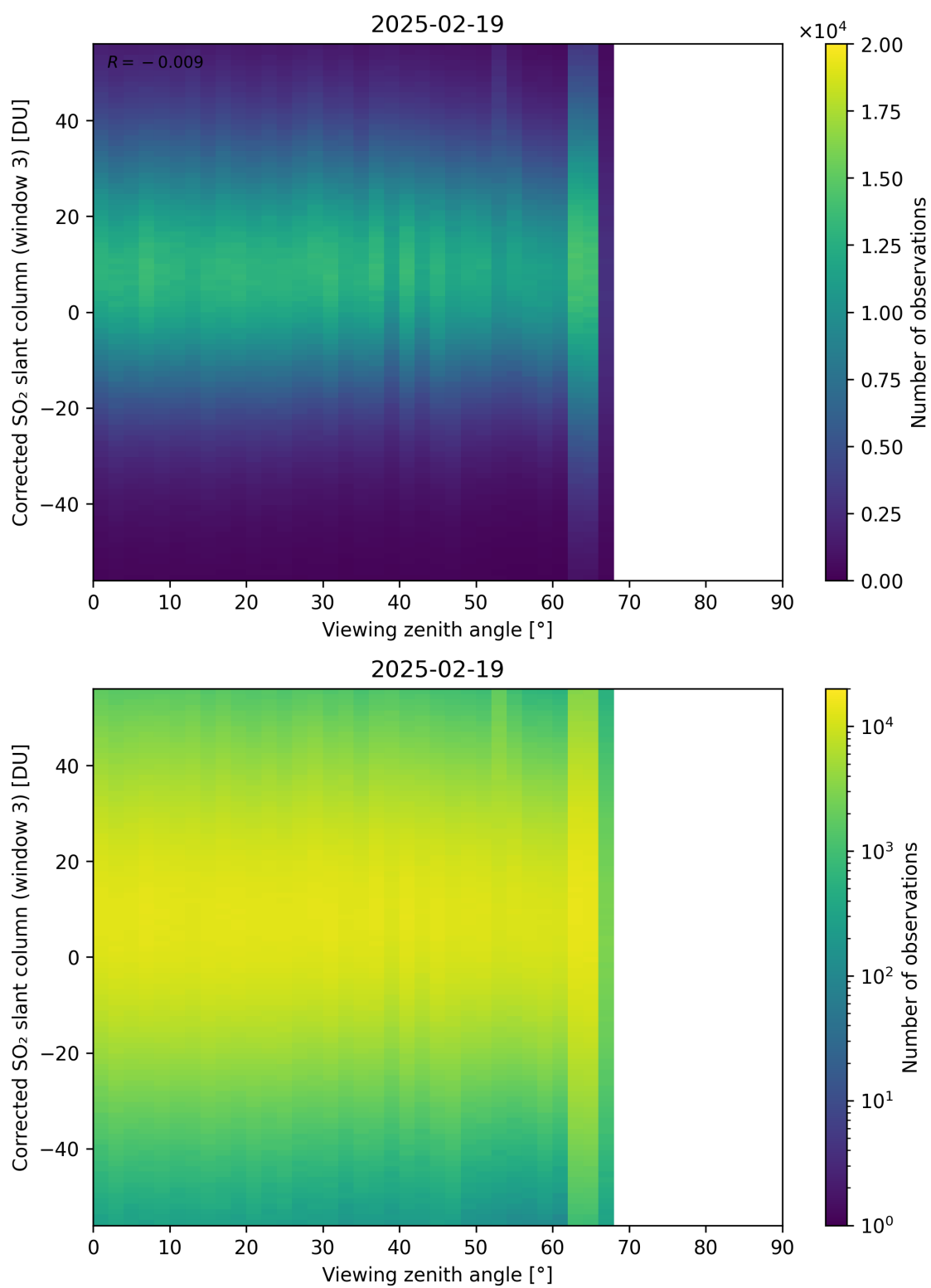
Figure 375: Scatter density plot of “Viewing zenith angle” against “Corrected SO 2 slant column (window 3)” for 2025-02-19 to 2025-02-20.
