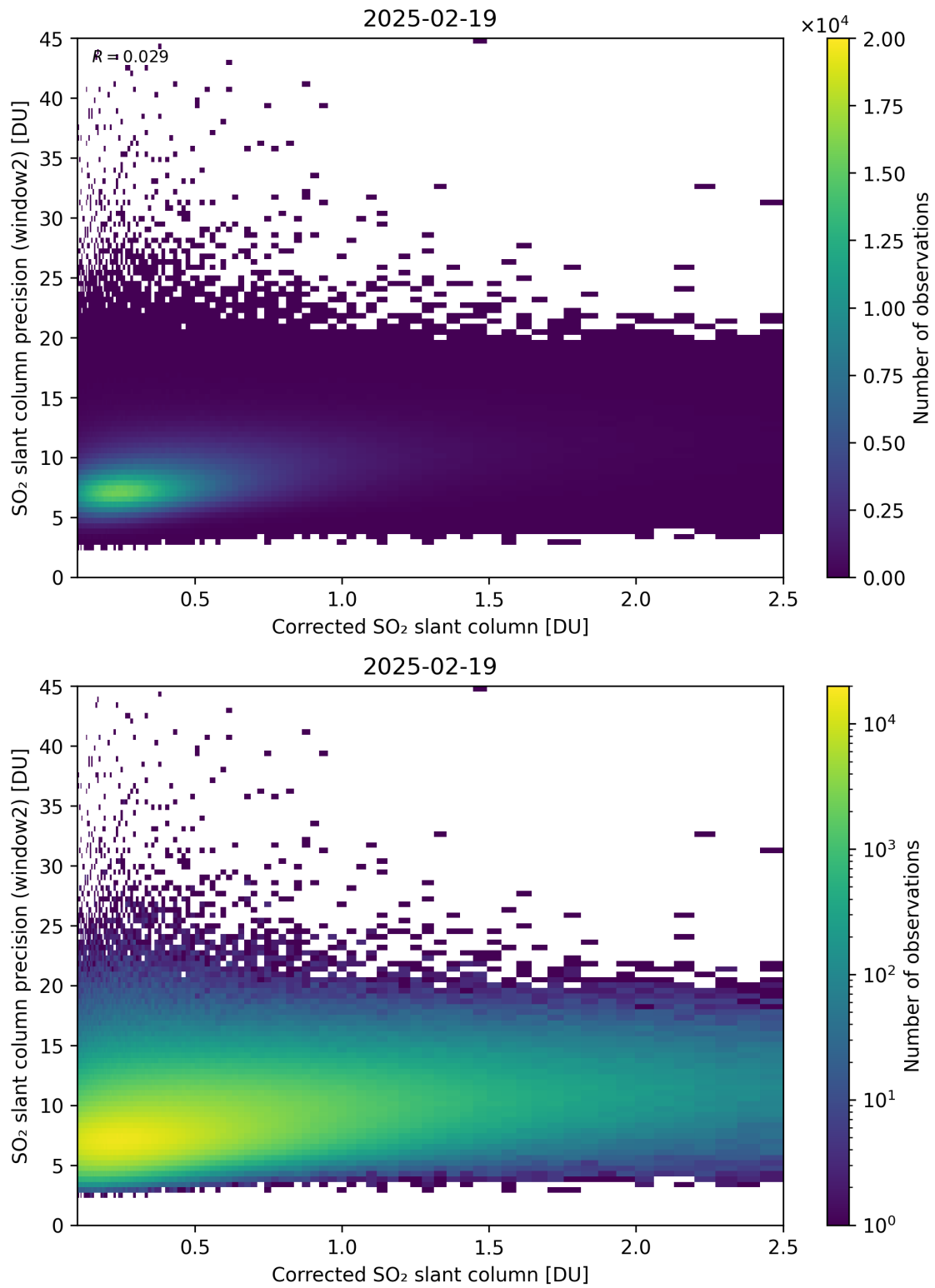
Figure 239: Scatter density plot of “Corrected SO 2 slant column” against “SO 2 slant column precision (window2)” for 2025-02-19 to 2025-02-20.
