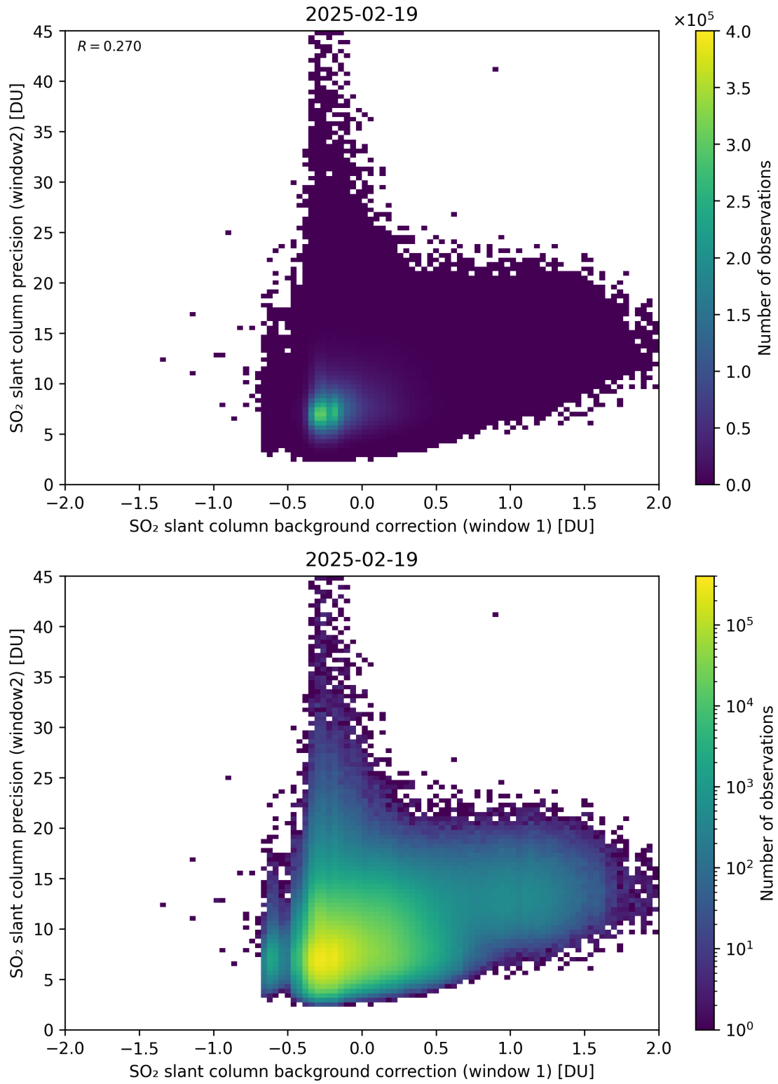
Figure 117: Scatter density plot of “SO 2 slant column background correction (window 1)” against “SO 2 slant column precision (window2)” for 2025-02-19 to 2025-02-20.
