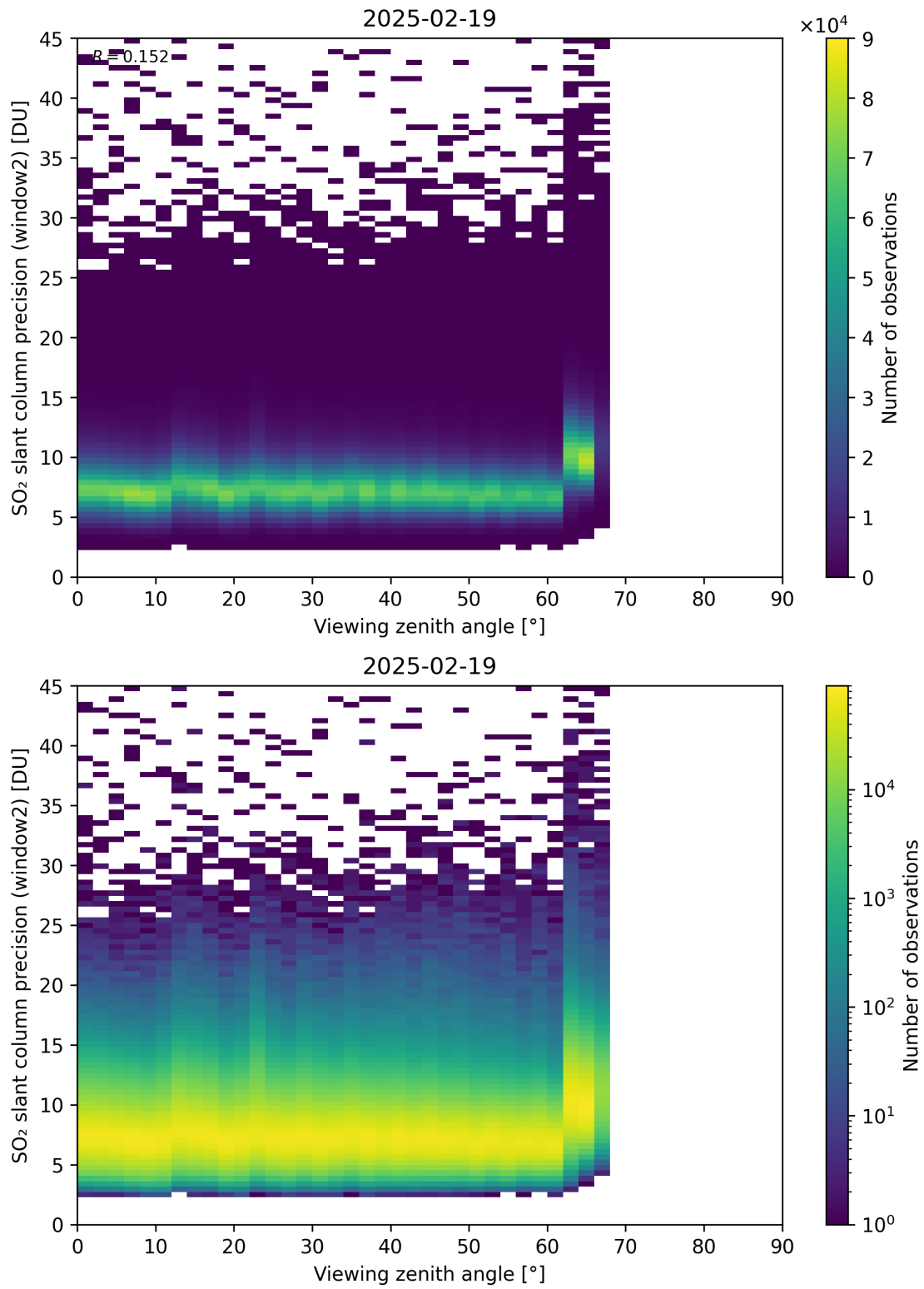
Figure 378: Scatter density plot of “Viewing zenith angle” against “SO 2 slant column precision (window2)” for 2025-02-19 to 2025-02-20.
