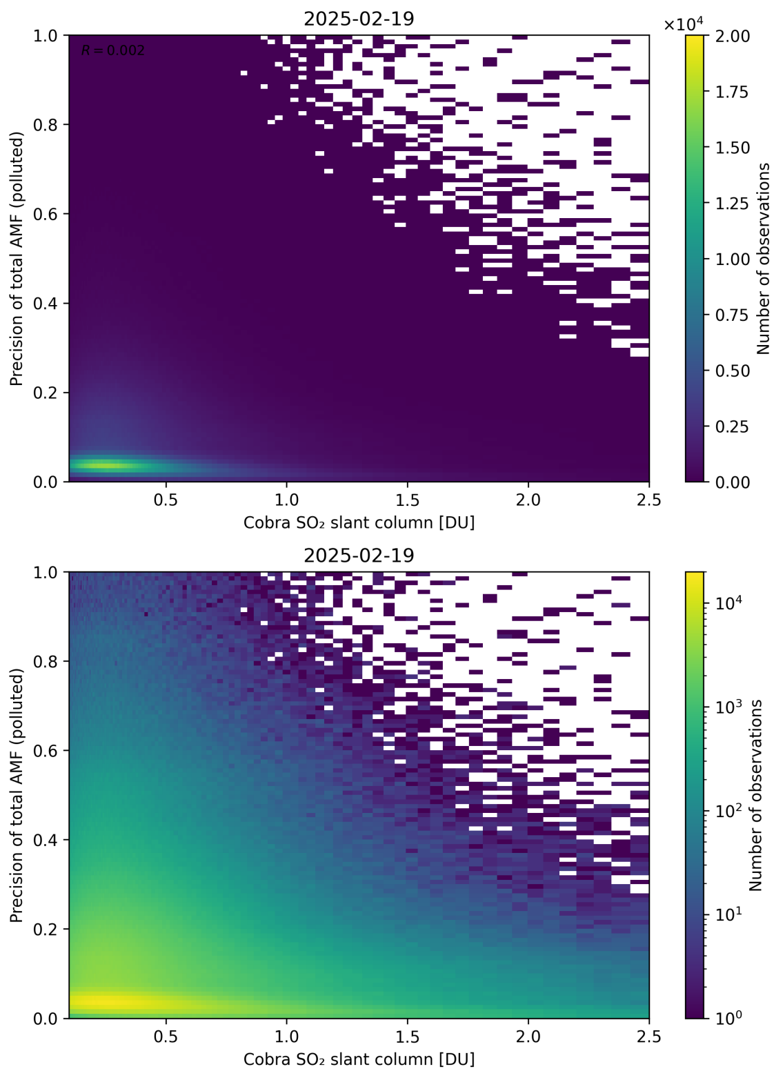
Figure 225: Scatter density plot of “Cobra SO 2 slant column” against “Precision of total AMF (polluted)” for 2025-02-19 to 2025-02-20.
