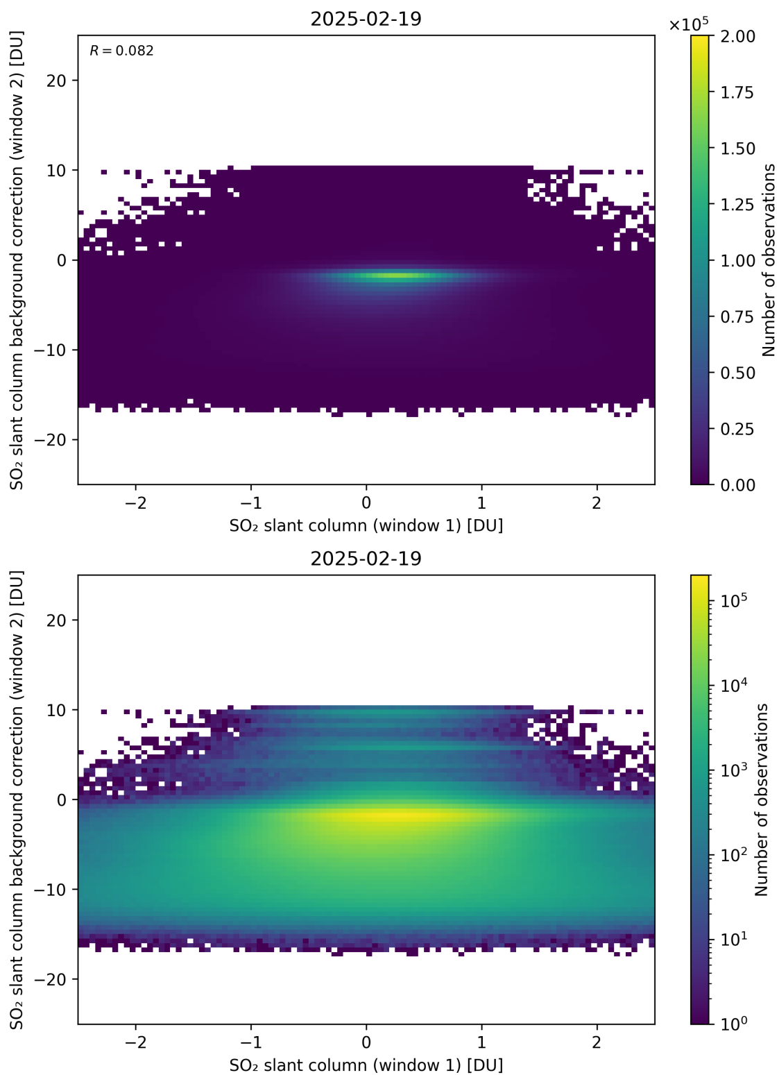
Figure 263: Scatter density plot of “SO 2 slant column (window 1)” against “SO 2 slant column background correction (window 2)” for 2025-02-19 to 2025-02-20.
