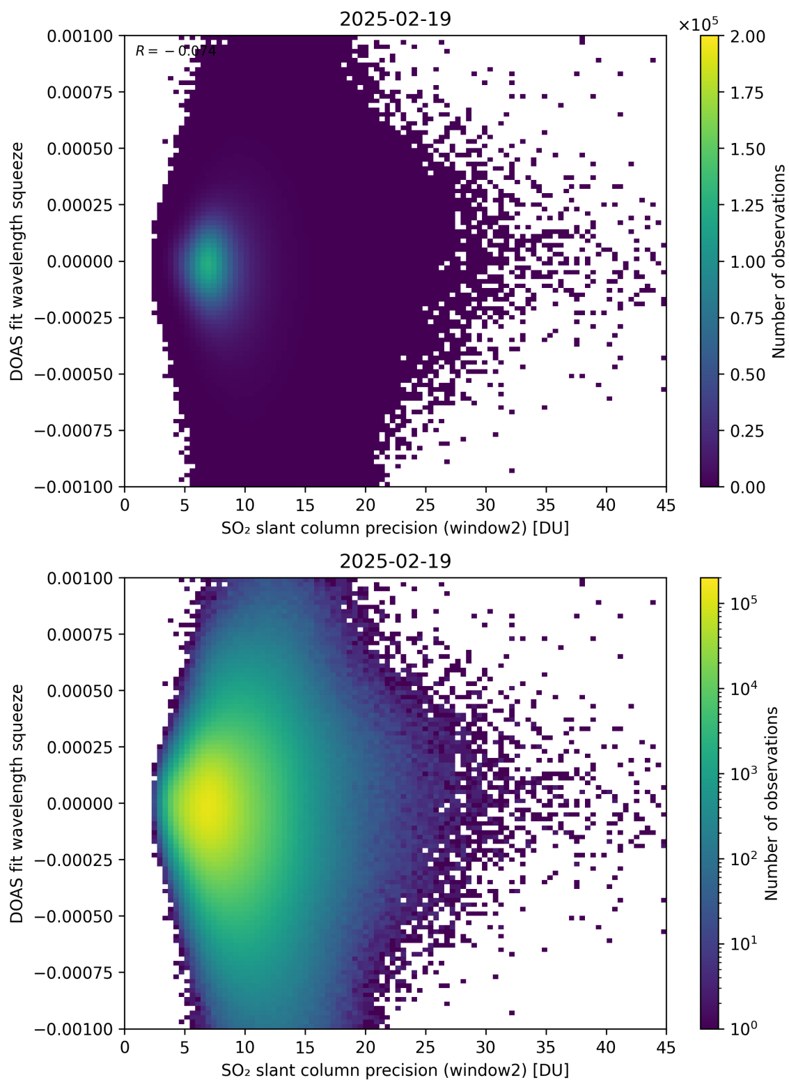
Figure 294: Scatter density plot of “SO 2 slant column precision (window2)” against “DOAS fit wavelength squeeze” for 2025-02-19 to 2025-02-20.
