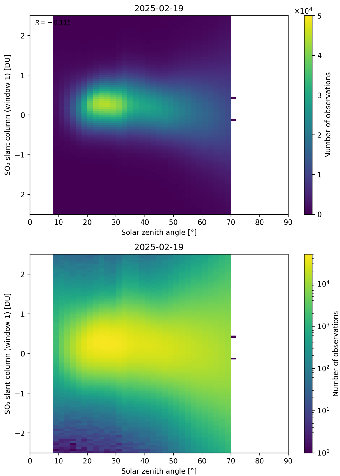
Figure 184: Scatter density plot of “Solar zenith angle” against “SO 2 slant column (window 1)” for 2025-02-19 to 2025-02-20.
