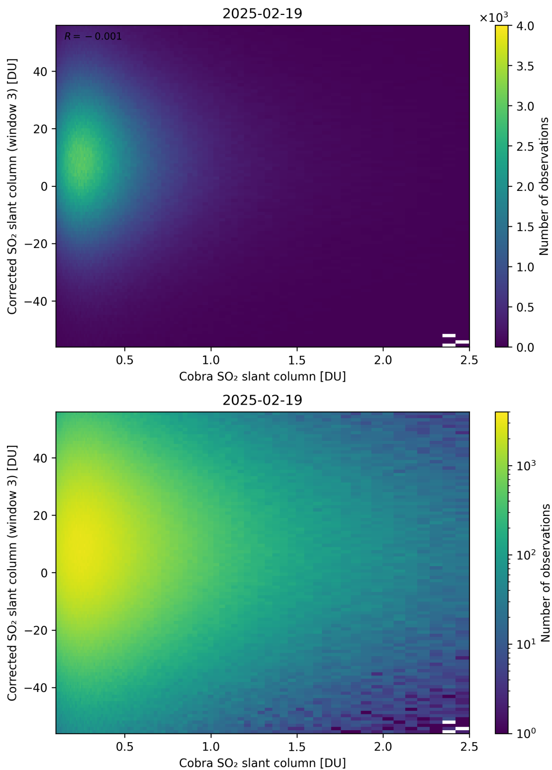
Figure 218: Scatter density plot of “Cobra SO 2 slant column” against “Corrected SO 2 slant column (window 3)” for 2025-02-19 to 2025-02-20.
