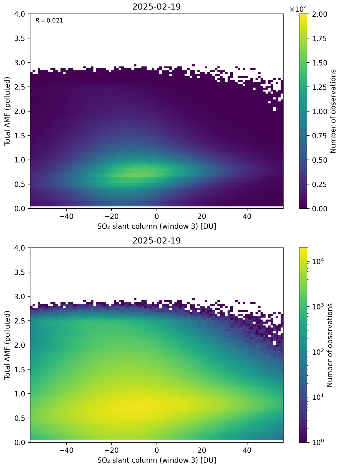
Figure 318: Scatter density plot of “SO 2 slant column (window 3)” against “Total AMF (polluted)” for 2025-02-19 to 2025-02-20.
