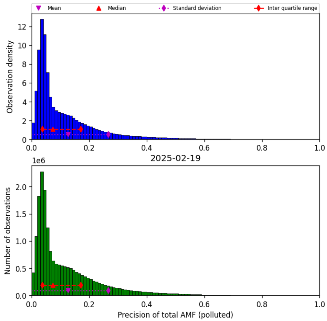
Figure 80: Histogram of “Precision of total AMF (polluted)” for 2025-02-19 to 2025-02-20
