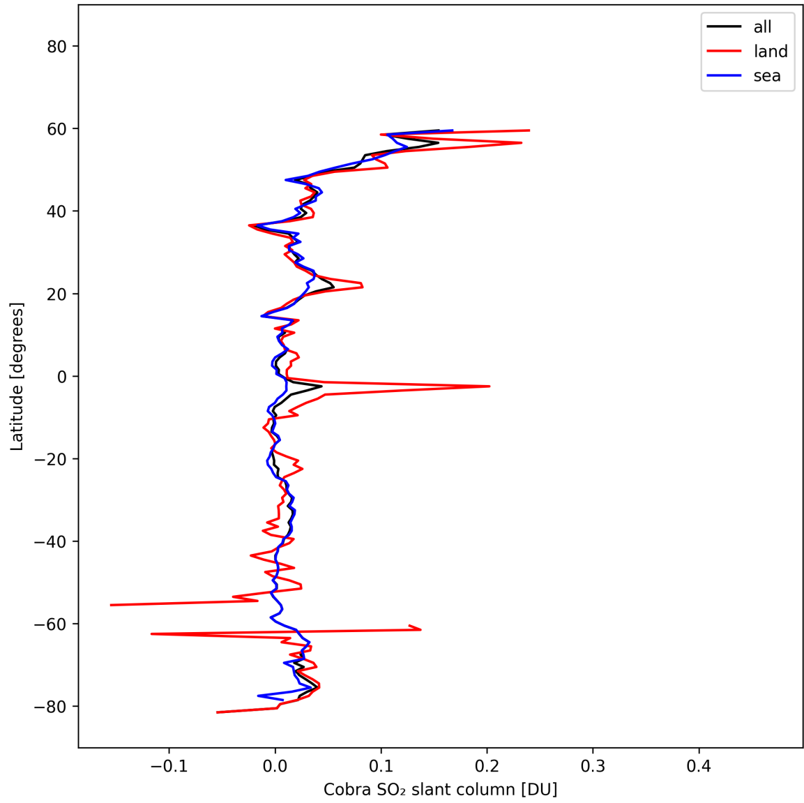
Figure 35: Zonal average of “Cobra SO 2 slant column” for 2025-02-19 to 2025-02-20.
