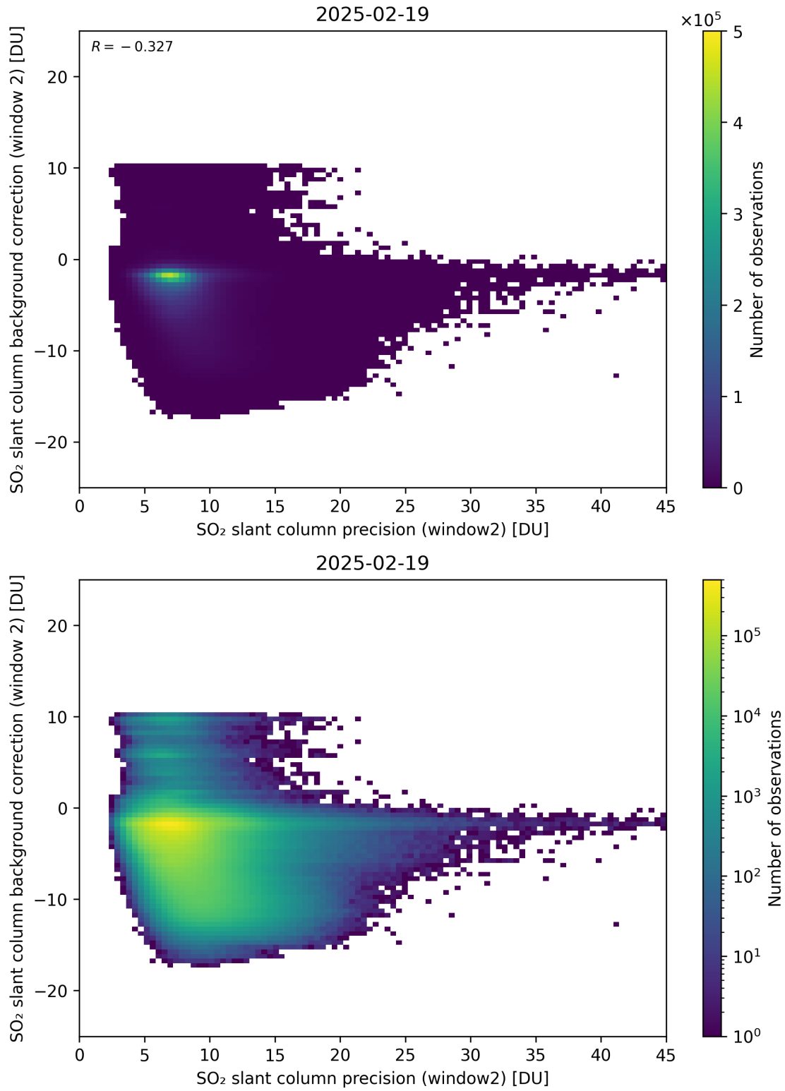
Figure 291: Scatter density plot of “SO 2 slant column precision (window2)” against “SO 2 slant column background correction (window 2)” for 2025-02-19 to 2025-02-20.
