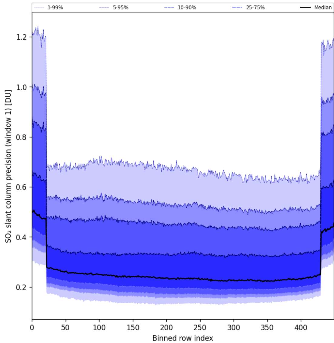
Figure 90: Along track statistics of “SO 2 slant column precision (window 1)” for 2025-02-19 to 2025-02-20
