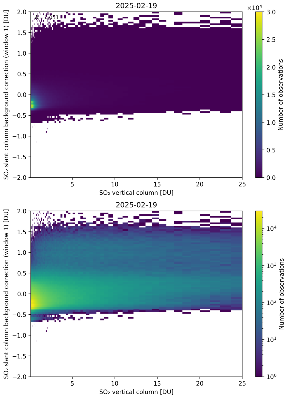
Figure 323: Scatter density plot of “SO 2 vertical column” against “SO 2 slant column background correction (window 1)” for 2025-02-19 to 2025-02-20.
