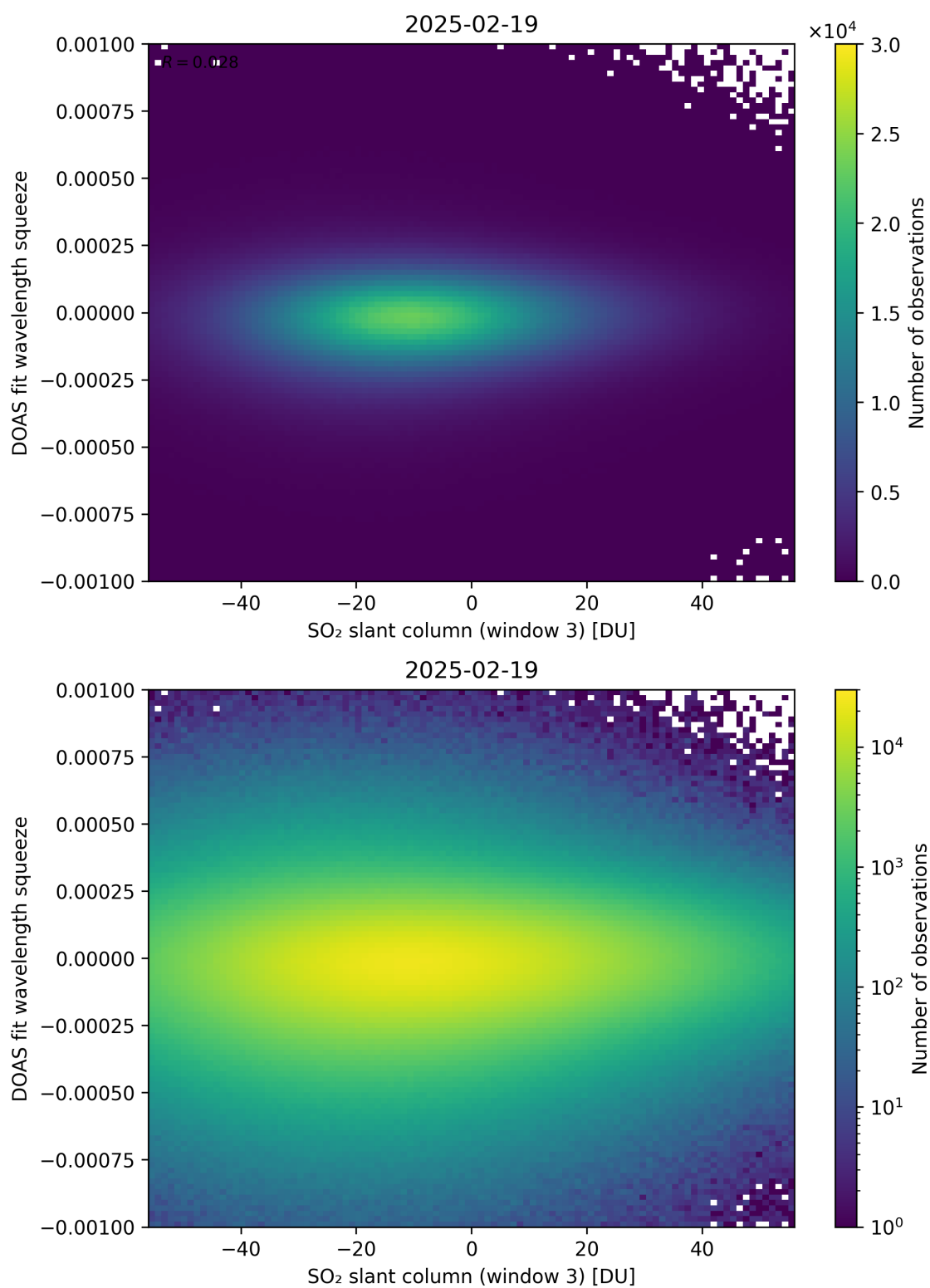
Figure 305: Scatter density plot of “SO 2 slant column (window 3)” against “DOAS fit wavelength squeeze” for 2025-02-19 to 2025-02-20.
