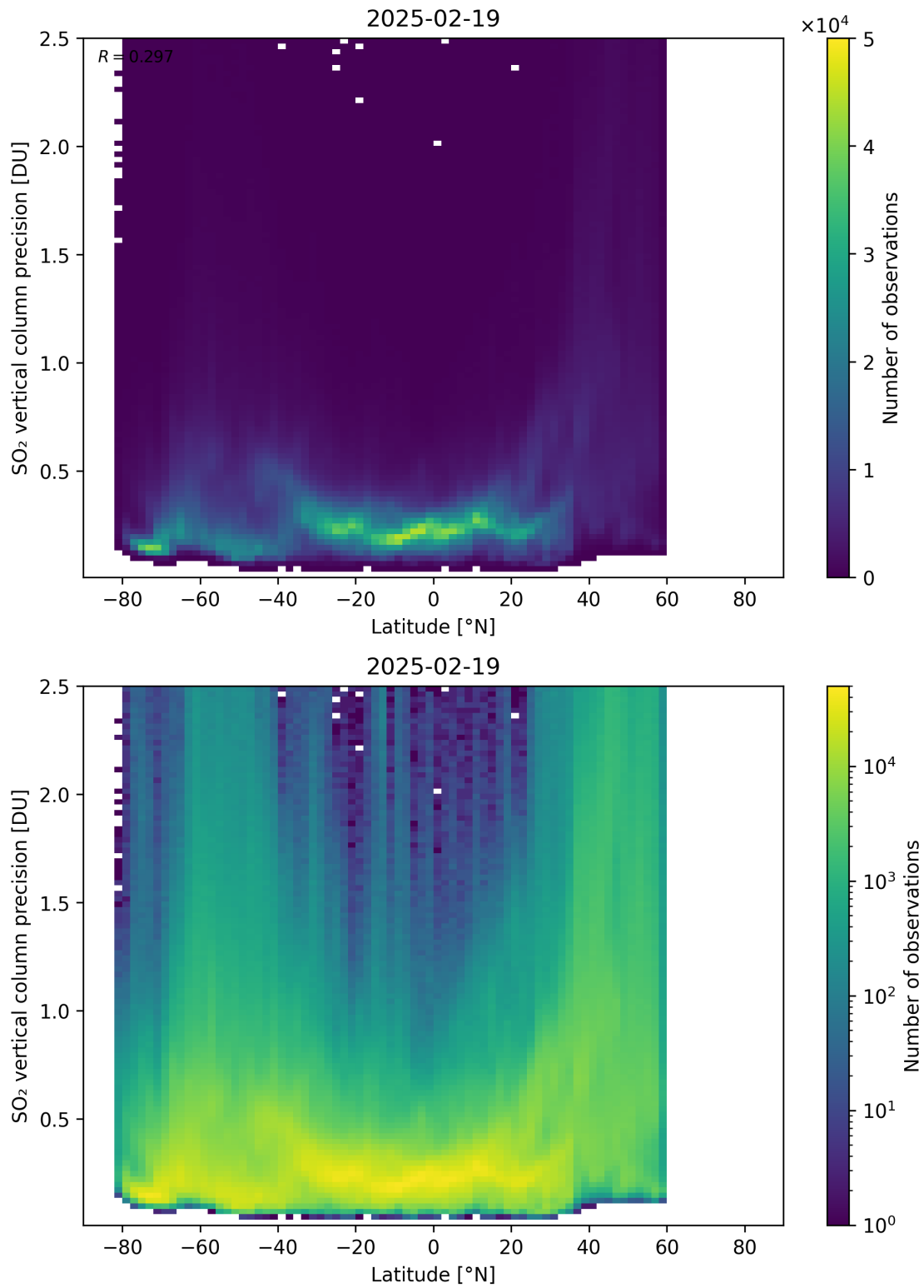
Figure 170: Scatter density plot of “Latitude” against “SO 2 vertical column precision” for 2025-02-19 to 2025-02-20.
