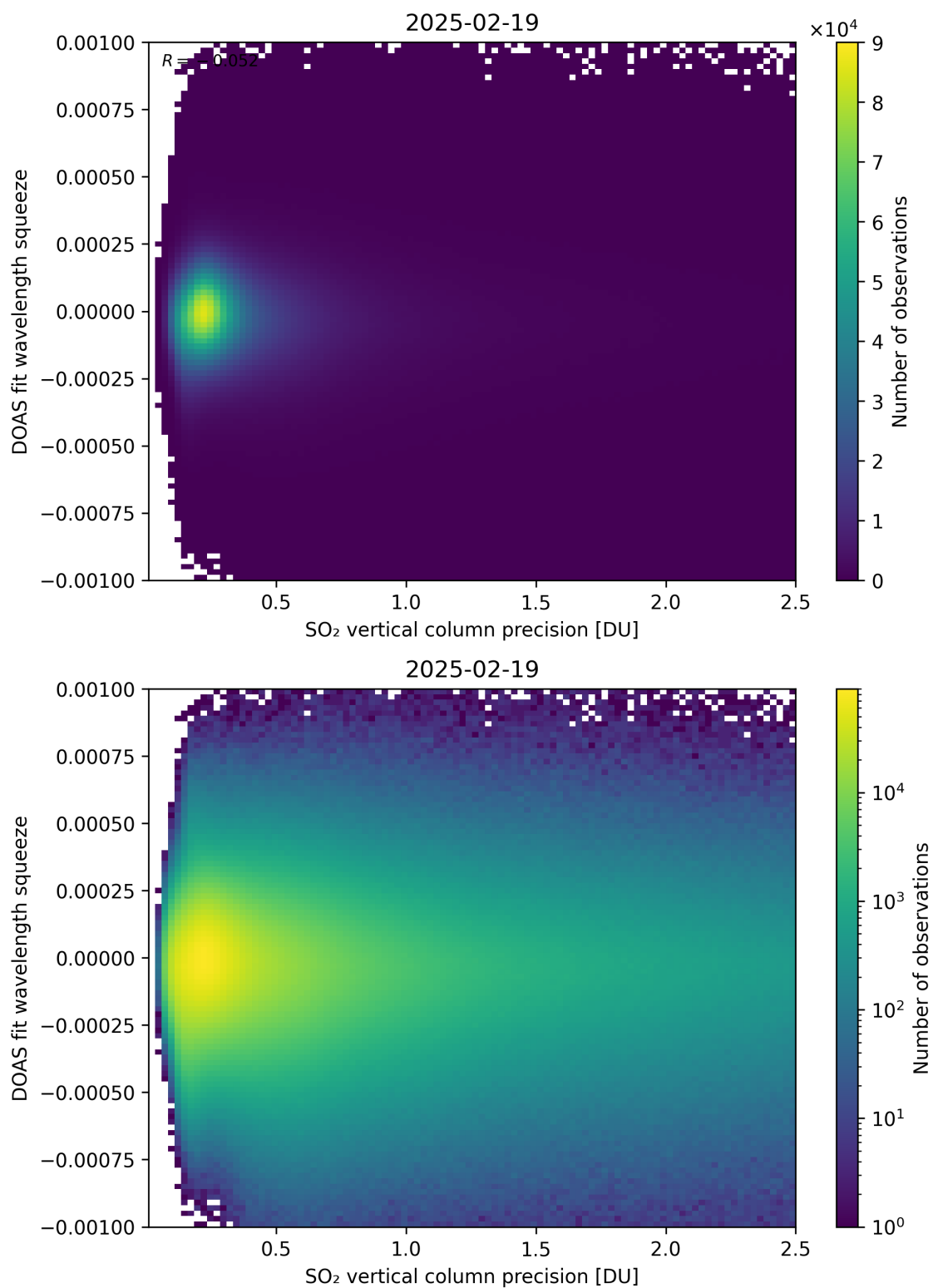
Figure 333: Scatter density plot of “SO 2 vertical column precision” against “DOAS fit wavelength squeeze” for 2025-02-19 to 2025-02-20.
