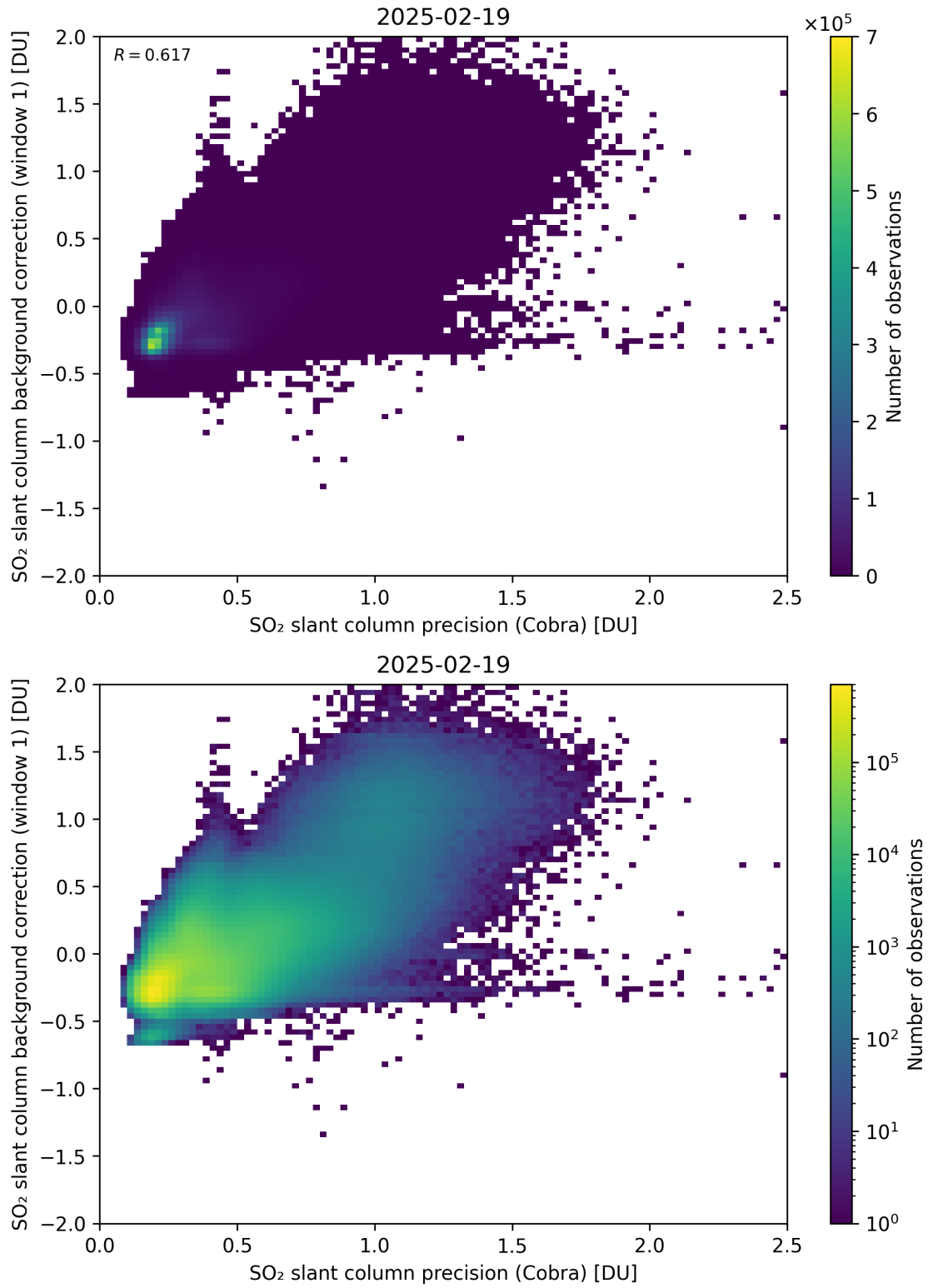
Figure 199: Scatter density plot of “SO 2 slant column precision (Cobra)” against “SO 2 slant column background correction (window 1)” for 2025-02-19 to 2025-02-20.
