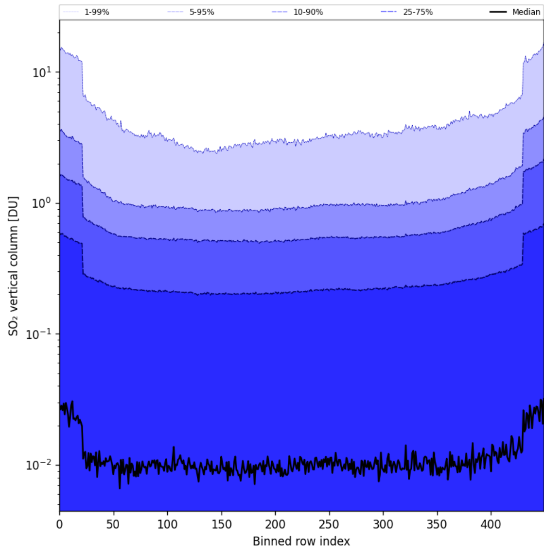
Figure 84: Along track statistics of “SO 2 vertical column” for 2025-02-19 to 2025-02-20
