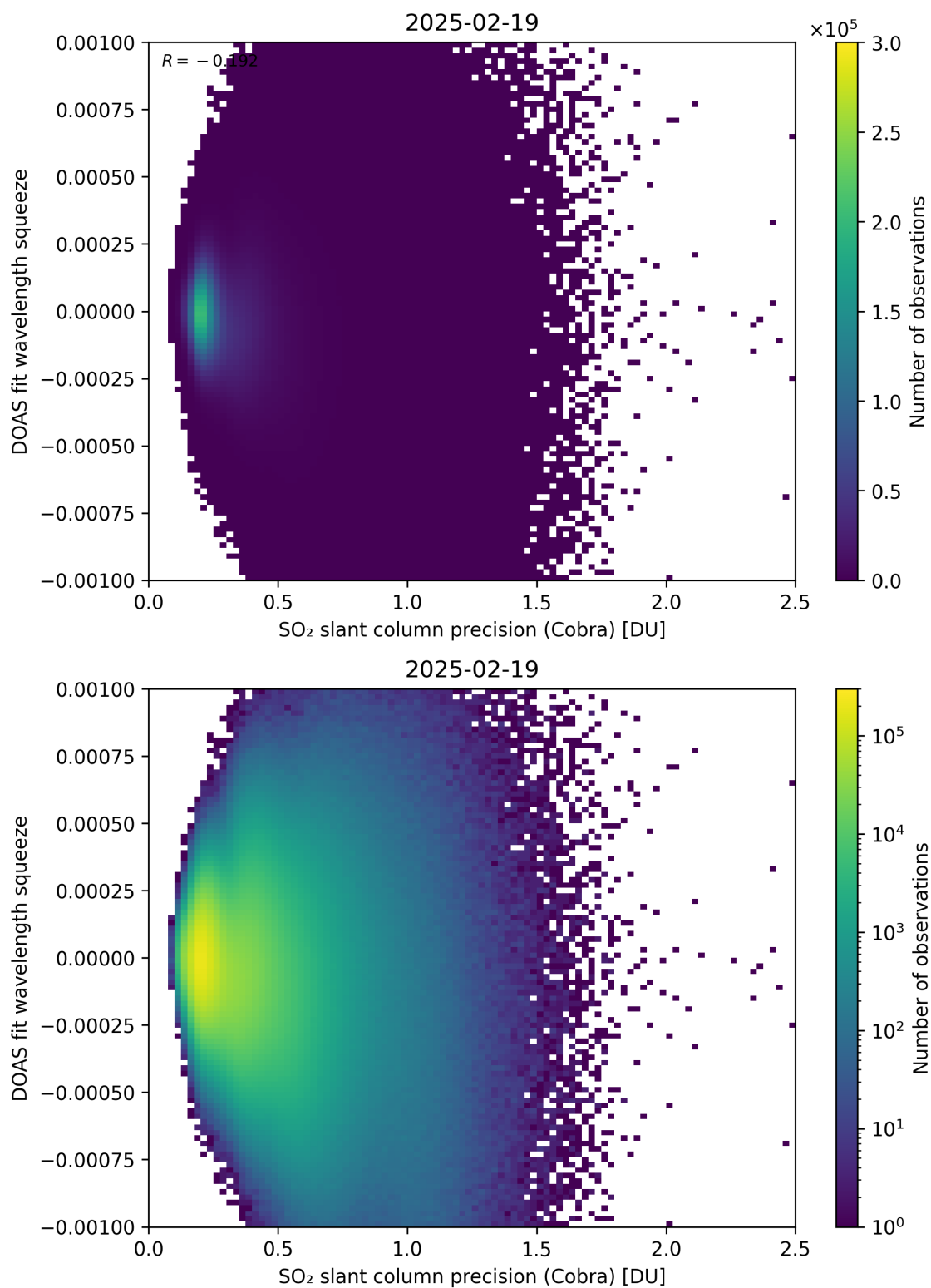
Figure 203: Scatter density plot of “SO 2 slant column precision (Cobra)” against “DOAS fit wavelength squeeze” for 2025-02-19 to 2025-02-20.
