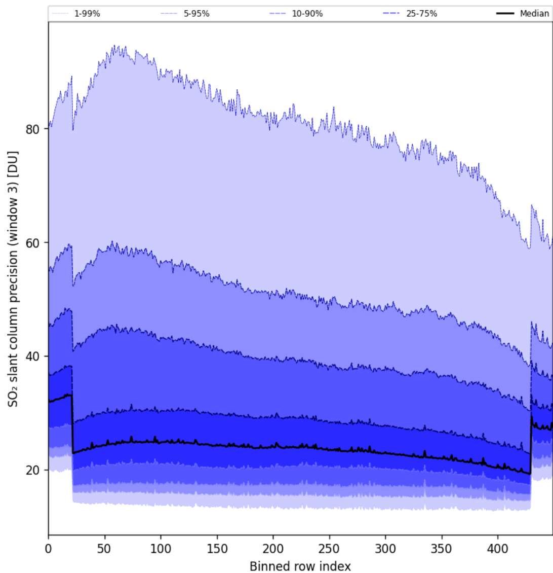
Figure 98: Along track statistics of “SO 2 slant column precision (window 3)” for 2025-02-19 to 2025-02-20
