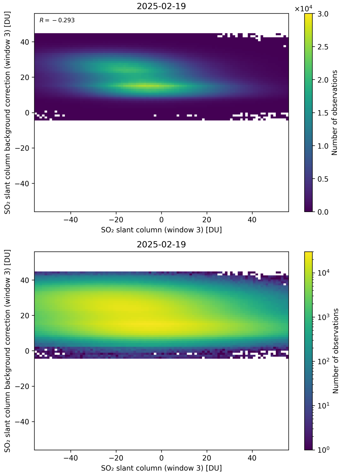
Figure 303: Scatter density plot of “SO 2 slant column (window 3)” against “SO 2 slant column background correction (window 3)” for 2025-02-19 to 2025-02-20.
