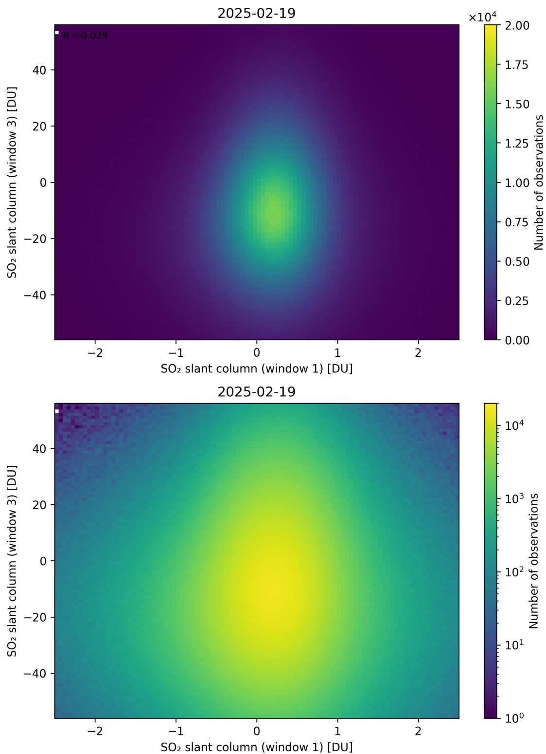
Figure 287: Scatter density plot of “SO 2 slant column (window 1)” against “SO 2 slant column (window 3)” for 2025-02-19 to 2025-02-20.
