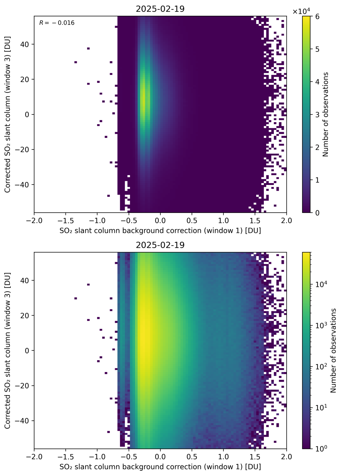
Figure 116: Scatter density plot of “SO 2 slant column background correction (window 1)” against “Corrected SO 2 slant column (window 3)” for 2025-02-19 to 2025-02-20.
