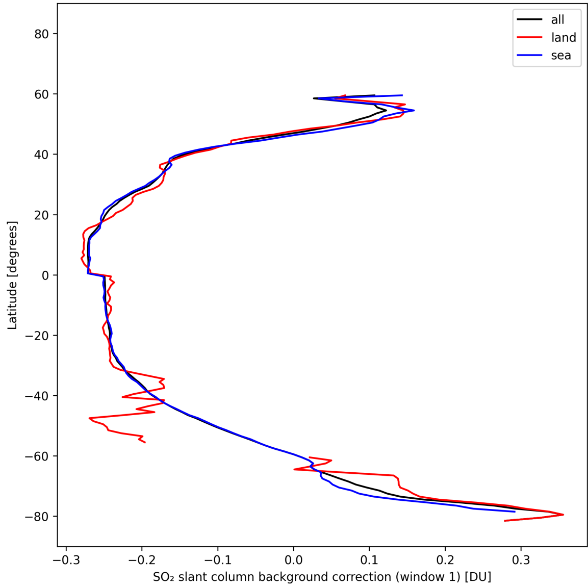
Figure 40: Zonal average of “SO 2 slant column background correction (window 1)” for 2025-02-19 to 2025-02-20.
