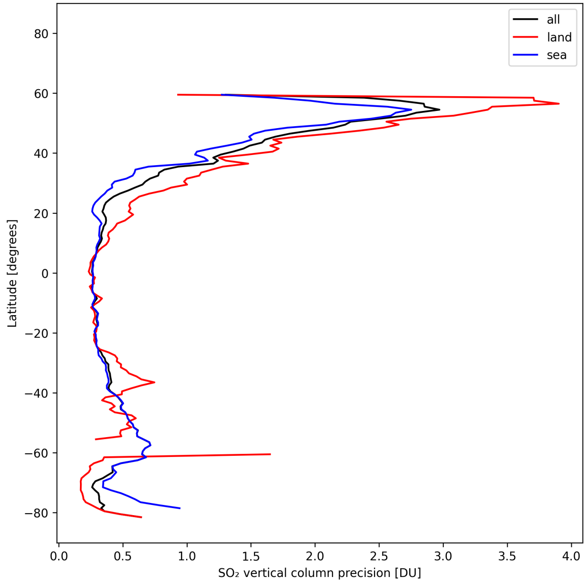
Figure 33: Zonal average of “SO 2 vertical column precision” for 2025-02-19 to 2025-02-20.
