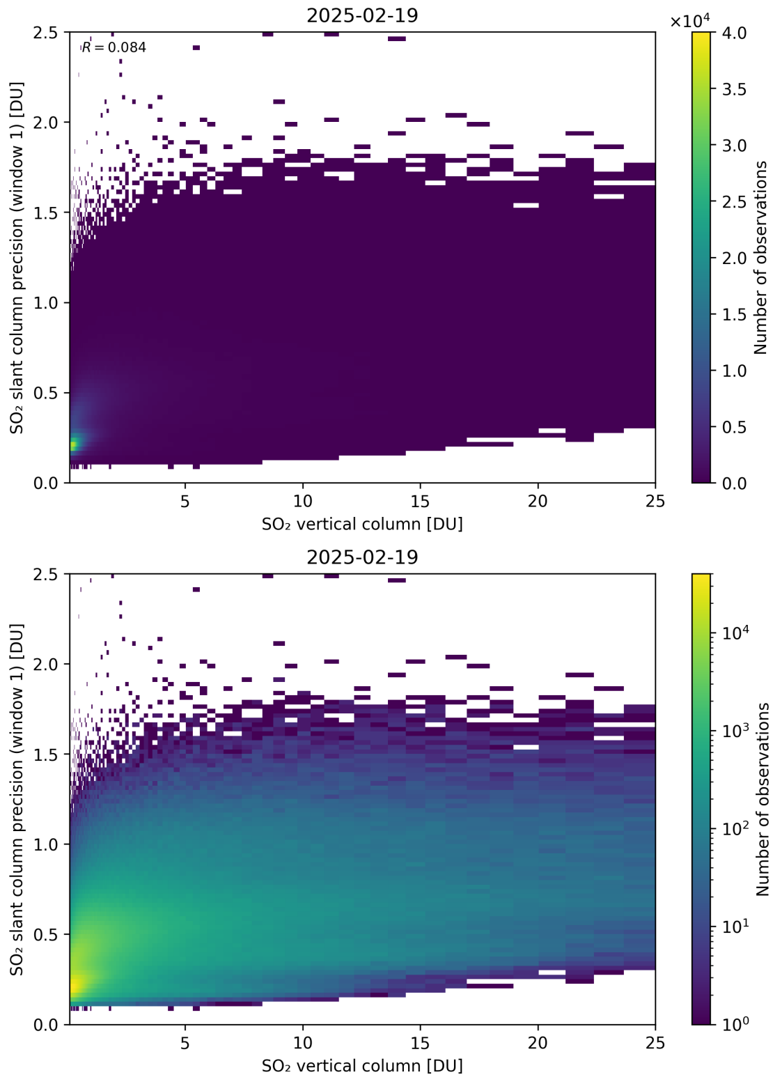
Figure 355: Scatter density plot of “SO 2 vertical column” against “SO 2 slant column precision (window 1)” for 2025-02-19 to 2025-02-20.
