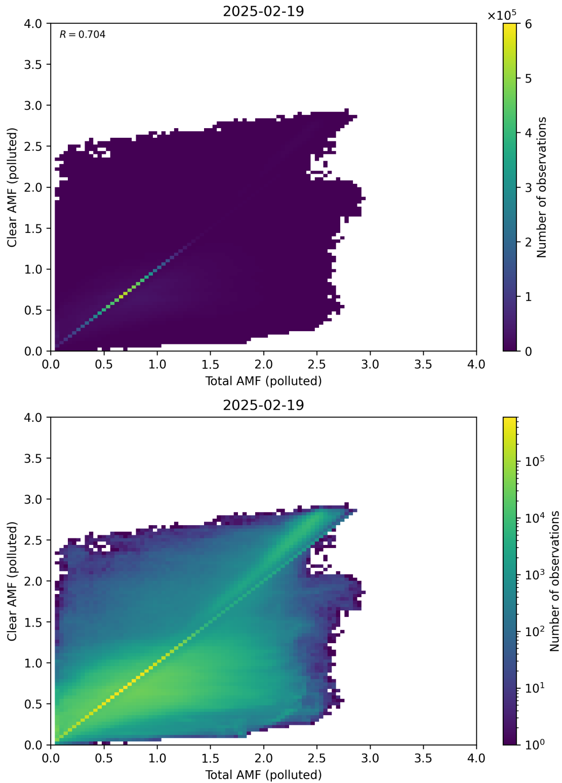
Figure 321: Scatter density plot of “Total AMF (polluted)” against “Clear AMF (polluted)” for 2025-02-19 to 2025-02-20.
