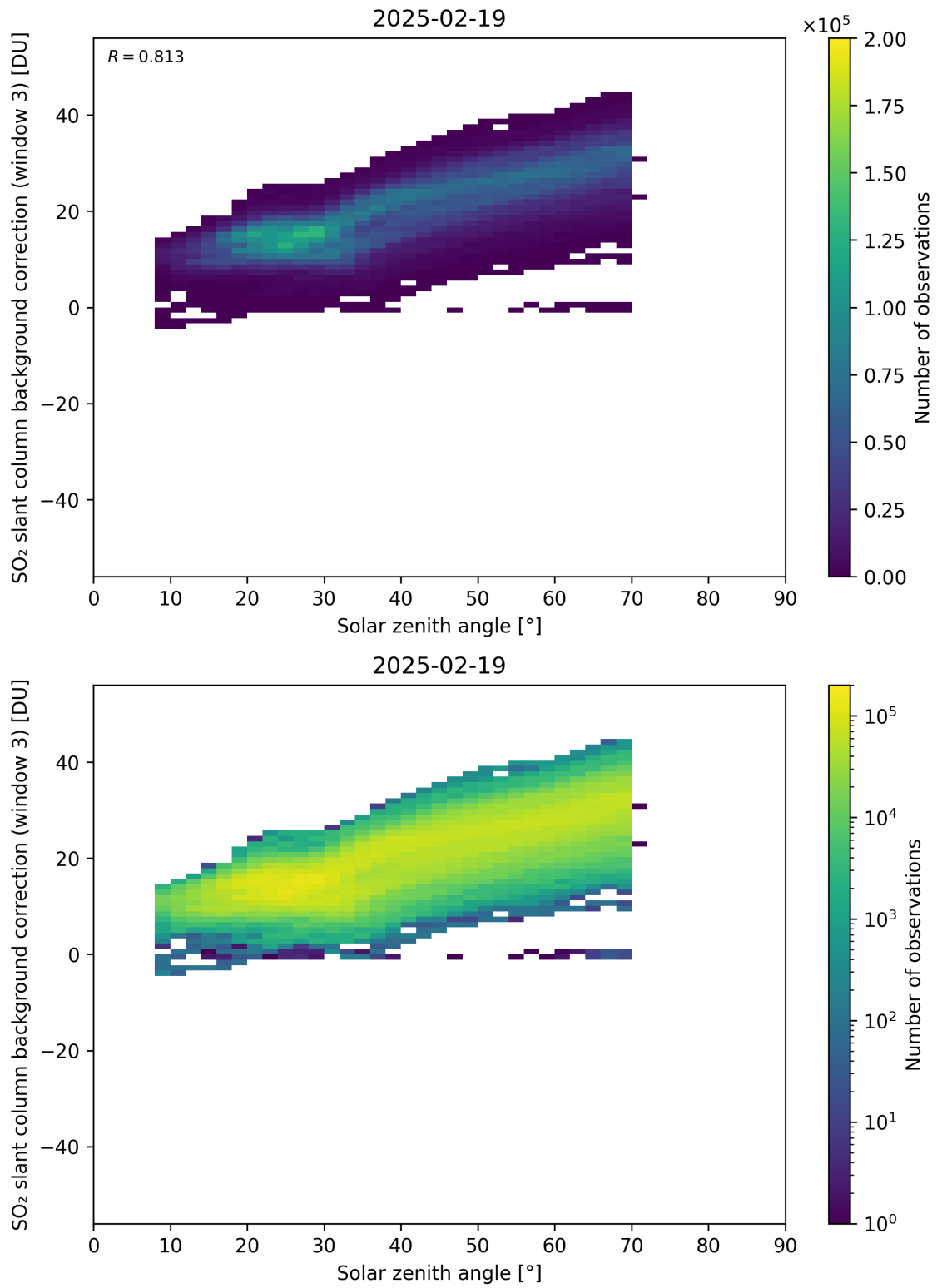
Figure 173: Scatter density plot of “Solar zenith angle” against “SO 2 slant column background correction (window 3)” for 2025-02-19 to 2025-02-20.
