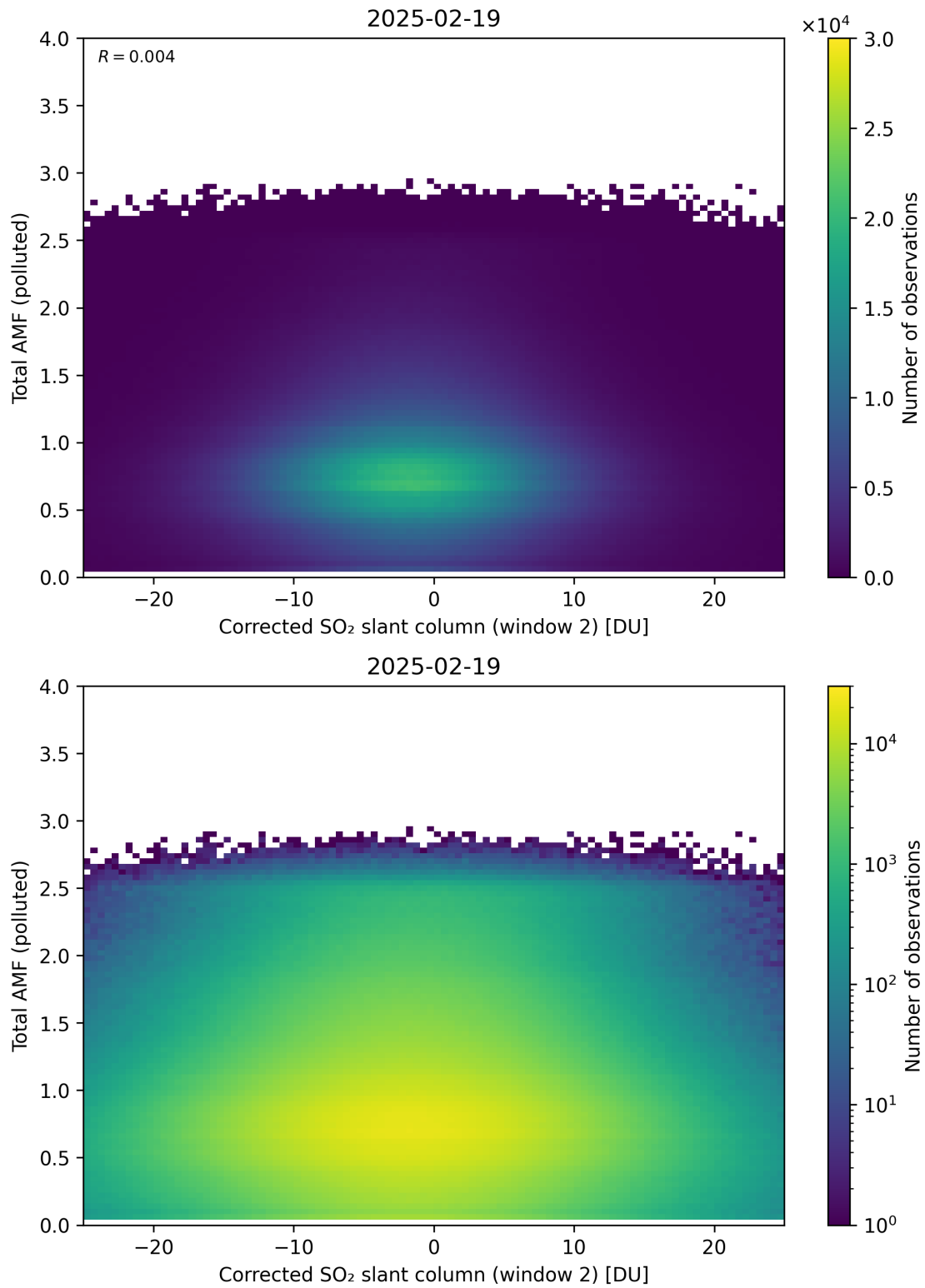
Figure 253: Scatter density plot of “Corrected SO 2 slant column (window 2)” against “Total AMF (polluted)” for 2025-02-19 to 2025-02-20.
