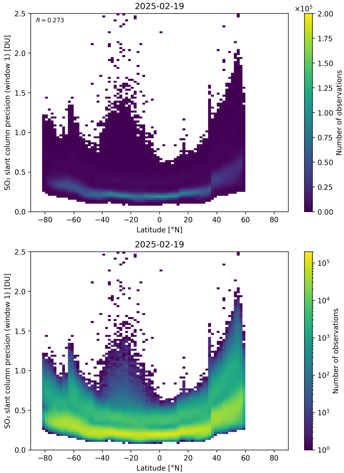
Figure 163: Scatter density plot of “Latitude” against “SO 2 slant column precision (window 1)” for 2025-02-19 to 2025-02-20.
