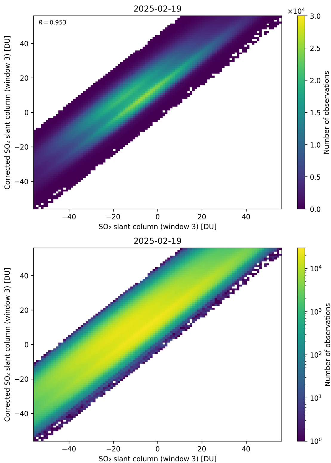
Figure 316: Scatter density plot of “SO 2 slant column (window 3)” against “Corrected SO 2 slant column (window 3)” for 2025-02-19 to 2025-02-20.
