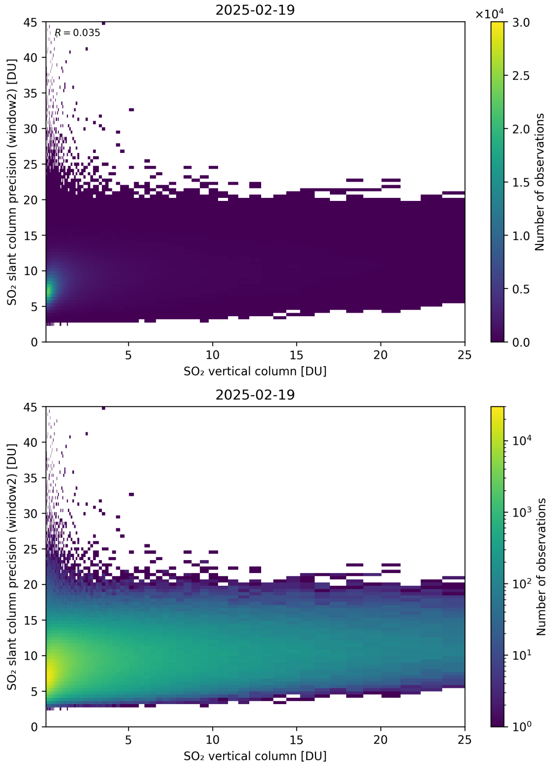
Figure 356: Scatter density plot of “SO 2 vertical column” against “SO 2 slant column precision (window2)” for 2025-02-19 to 2025-02-20.
