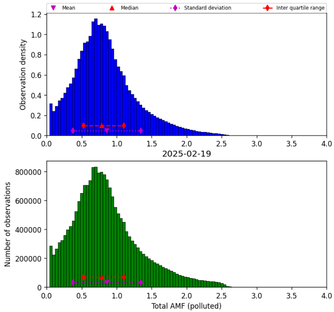
Figure 79: Histogram of “Total AMF (polluted)” for 2025-02-19 to 2025-02-20
