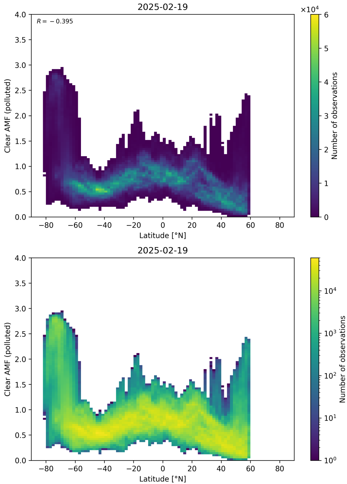
Figure 156: Scatter density plot of “Latitude” against “Clear AMF (polluted)” for 2025-02-19 to 2025-02-20.
