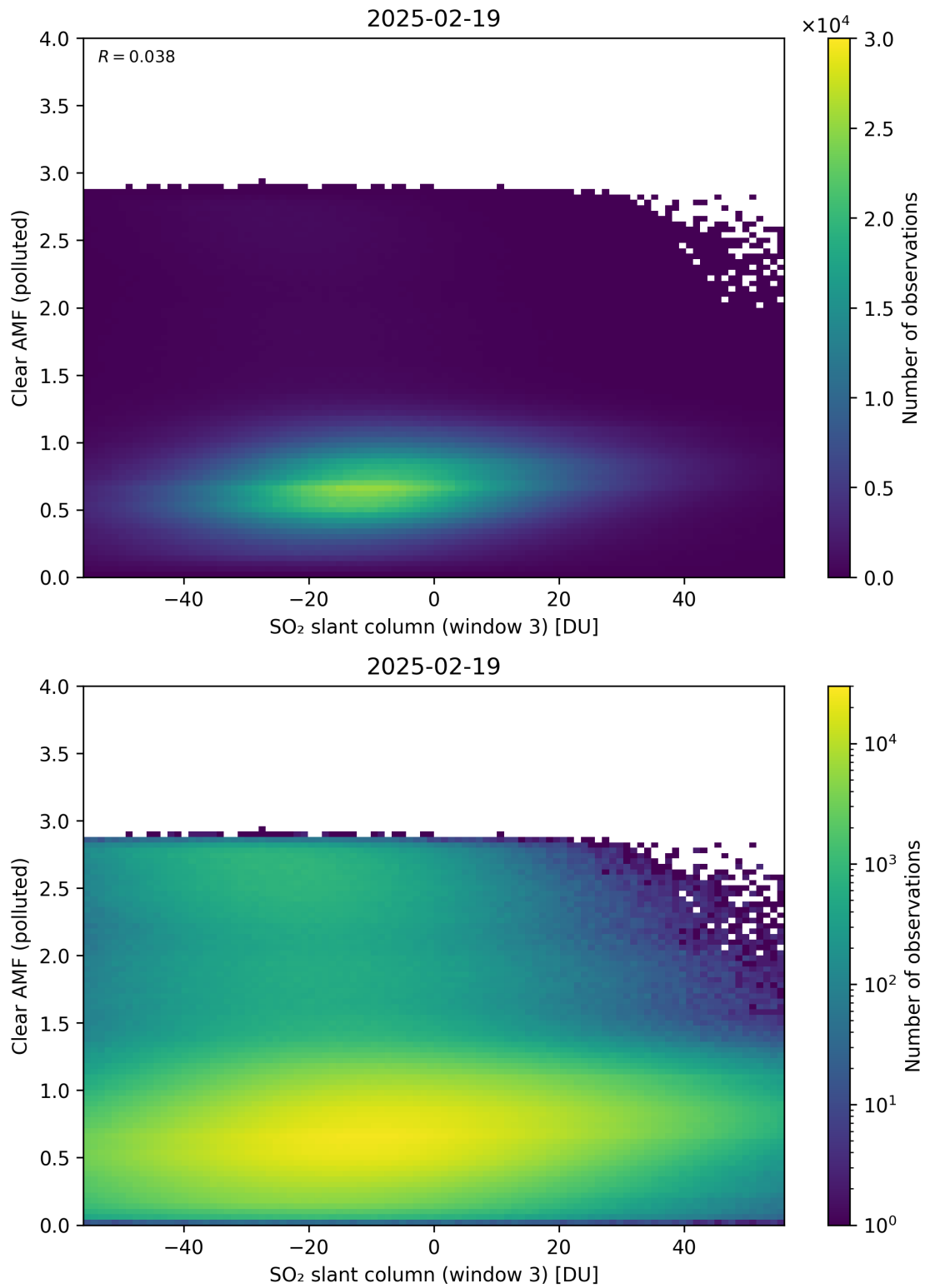
Figure 315: Scatter density plot of “SO 2 slant column (window 3)” against “Clear AMF (polluted)” for 2025-02-19 to 2025-02-20.
