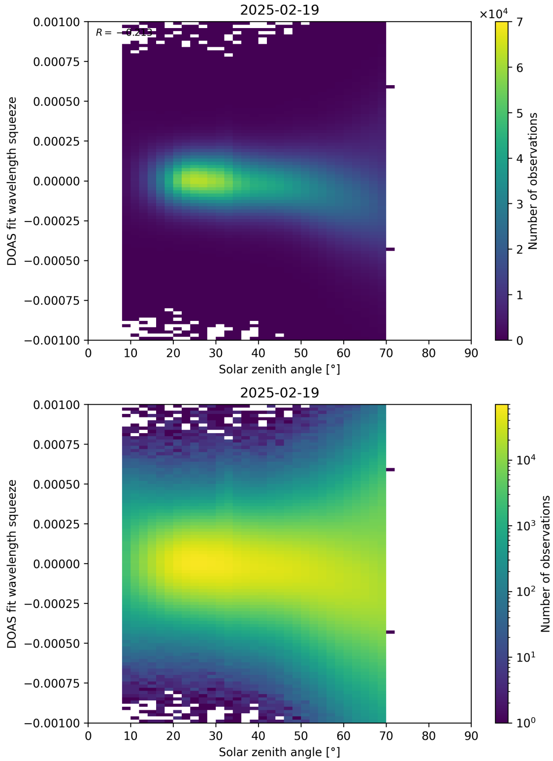
Figure 175: Scatter density plot of “Solar zenith angle” against “DOAS fit wavelength squeeze” for 2025-02-19 to 2025-02-20.
