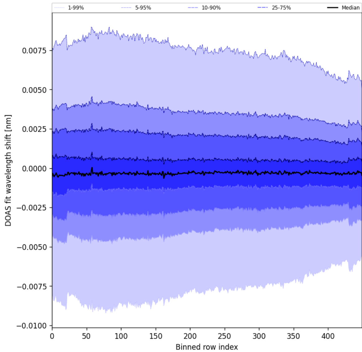
Figure 102: Along track statistics of “DOAS fit wavelength shift” for 2025-02-19 to 2025-02-20
