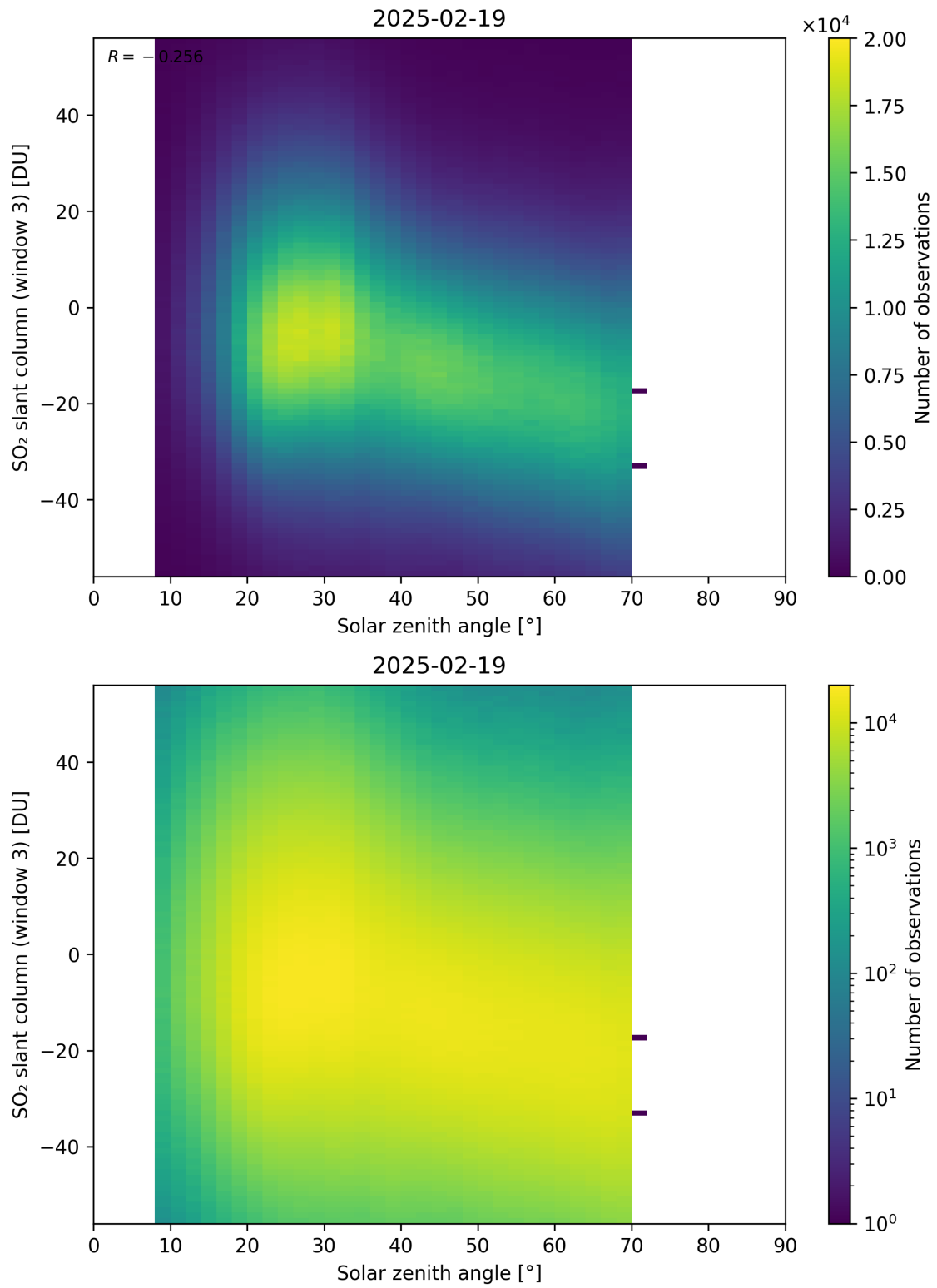
Figure 187: Scatter density plot of “Solar zenith angle” against “SO 2 slant column (window 3)” for 2025-02-19 to 2025-02-20.
