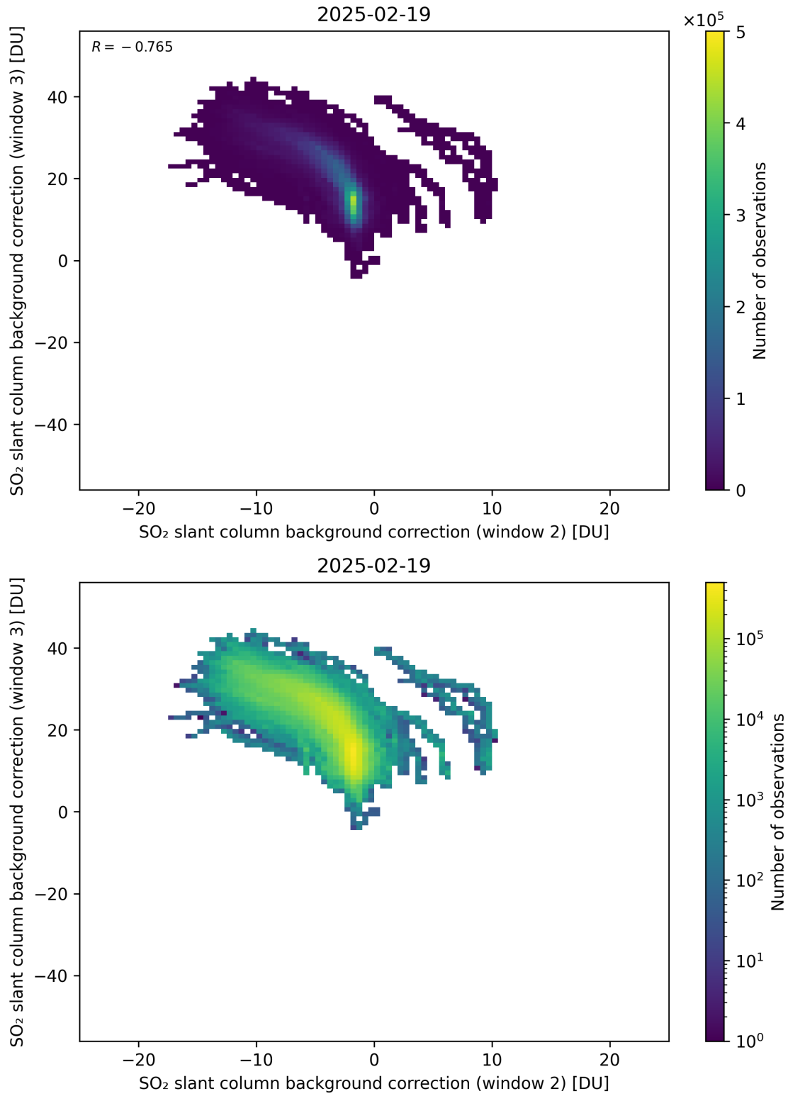
Figure 122: Scatter density plot of “SO 2 slant column background correction (window 2)” against “SO 2 slant column background correction (window 3)” for 2025-02-19 to 2025-02-20.
