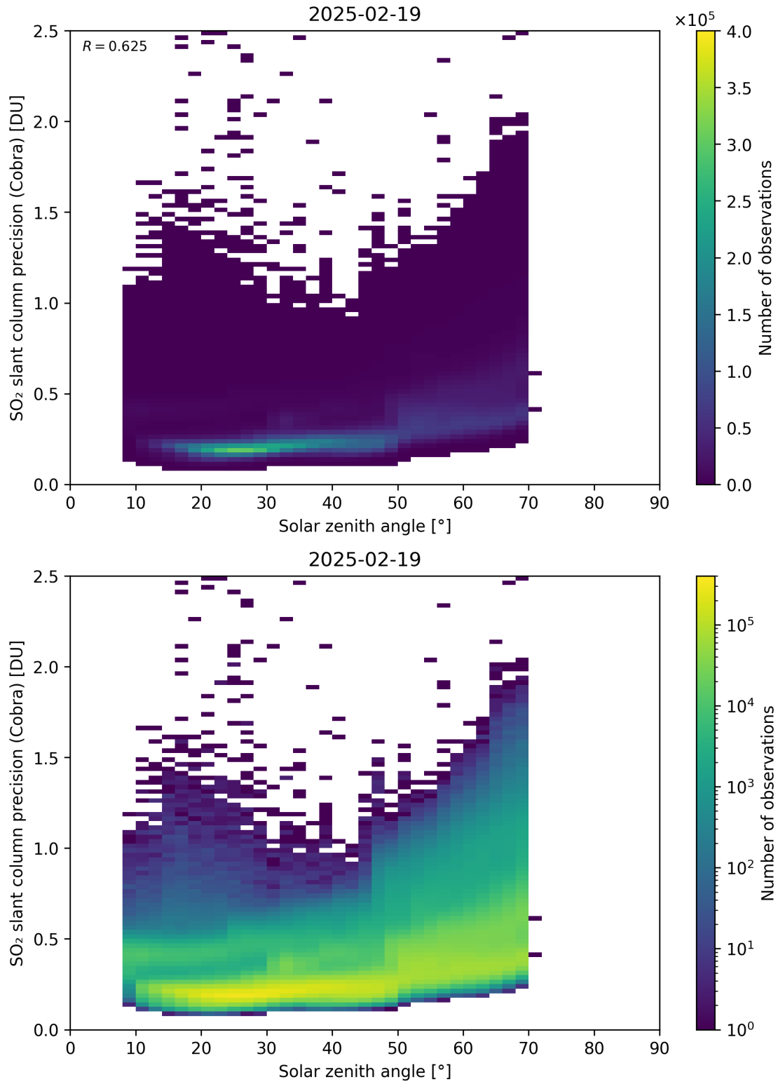
Figure 180: Scatter density plot of “Solar zenith angle” against “SO 2 slant column precision (Cobra)” for 2025-02-19 to 2025-02-20.
