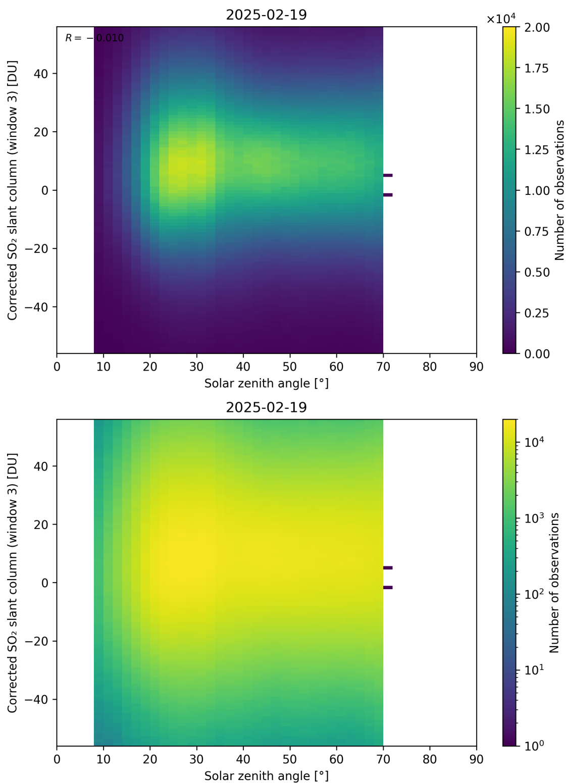
Figure 183: Scatter density plot of “Solar zenith angle” against “Corrected SO 2 slant column (window 3)” for 2025-02-19 to 2025-02-20.
