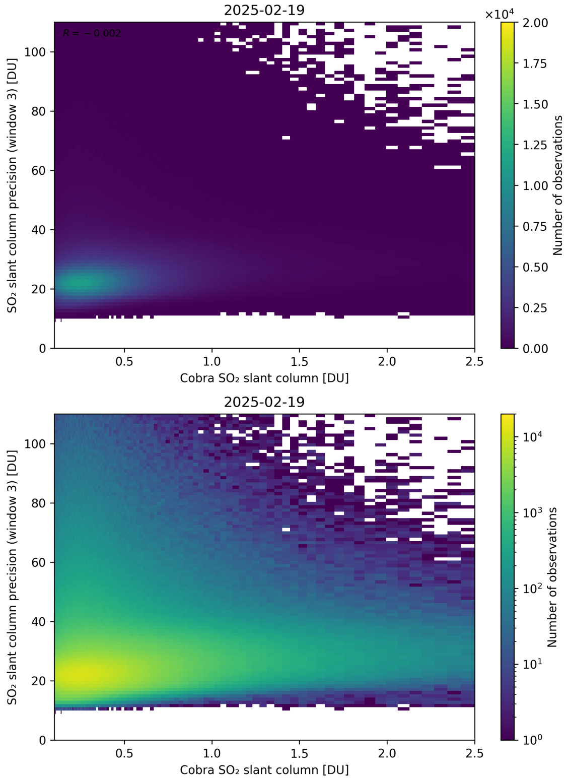
Figure 223: Scatter density plot of “Cobra SO 2 slant column” against “SO 2 slant column precision (window 3)” for 2025-02-19 to 2025-02-20.
