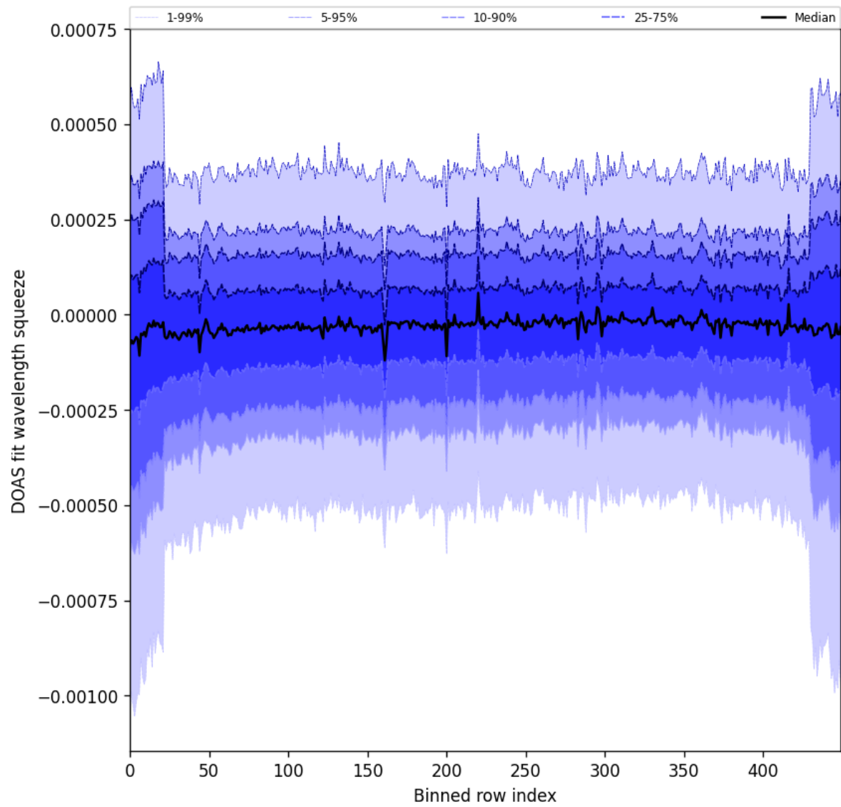
Figure 103: Along track statistics of “DOAS fit wavelength squeeze” for 2025-02-19 to 2025-02-20
