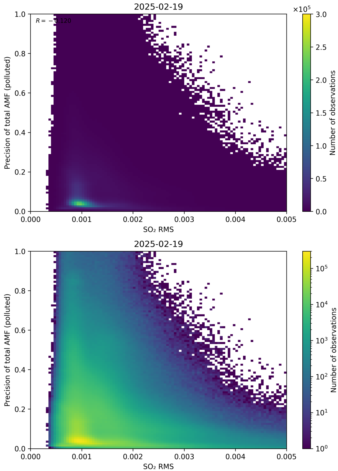
Figure 149: Scatter density plot of “SO 2 RMS” against “Precision of total AMF (polluted)” for 2025-02-19 to 2025-02-20.
