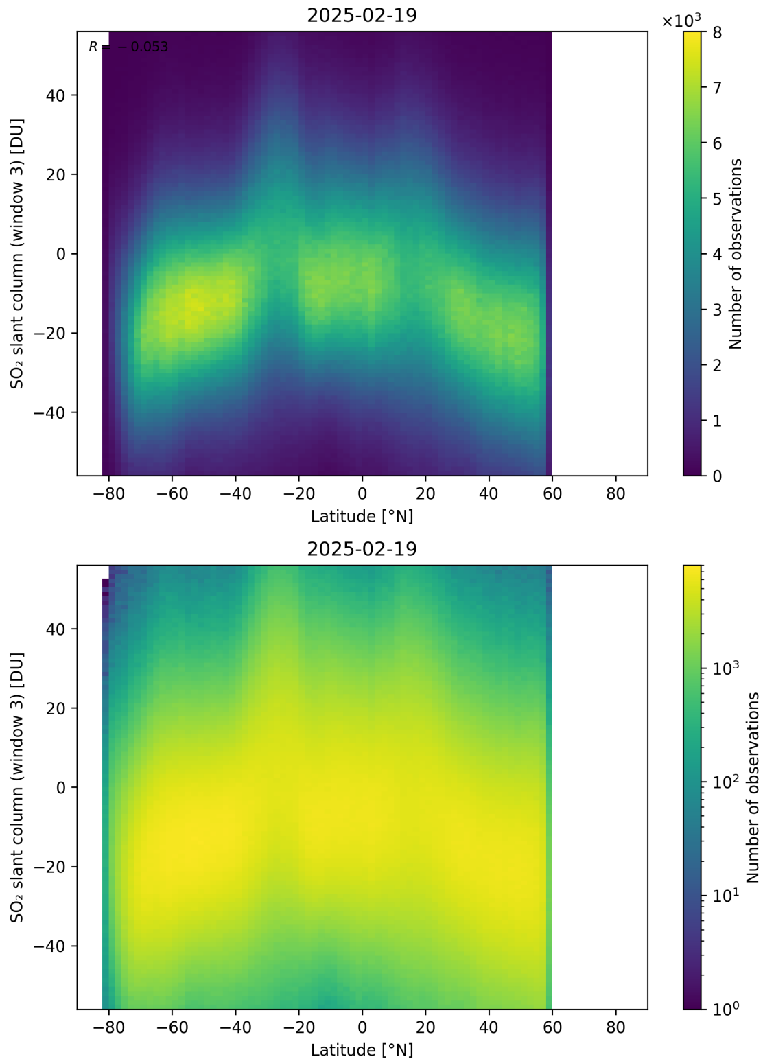
Figure 165: Scatter density plot of “Latitude” against “SO 2 slant column (window 3)” for 2025-02-19 to 2025-02-20.
