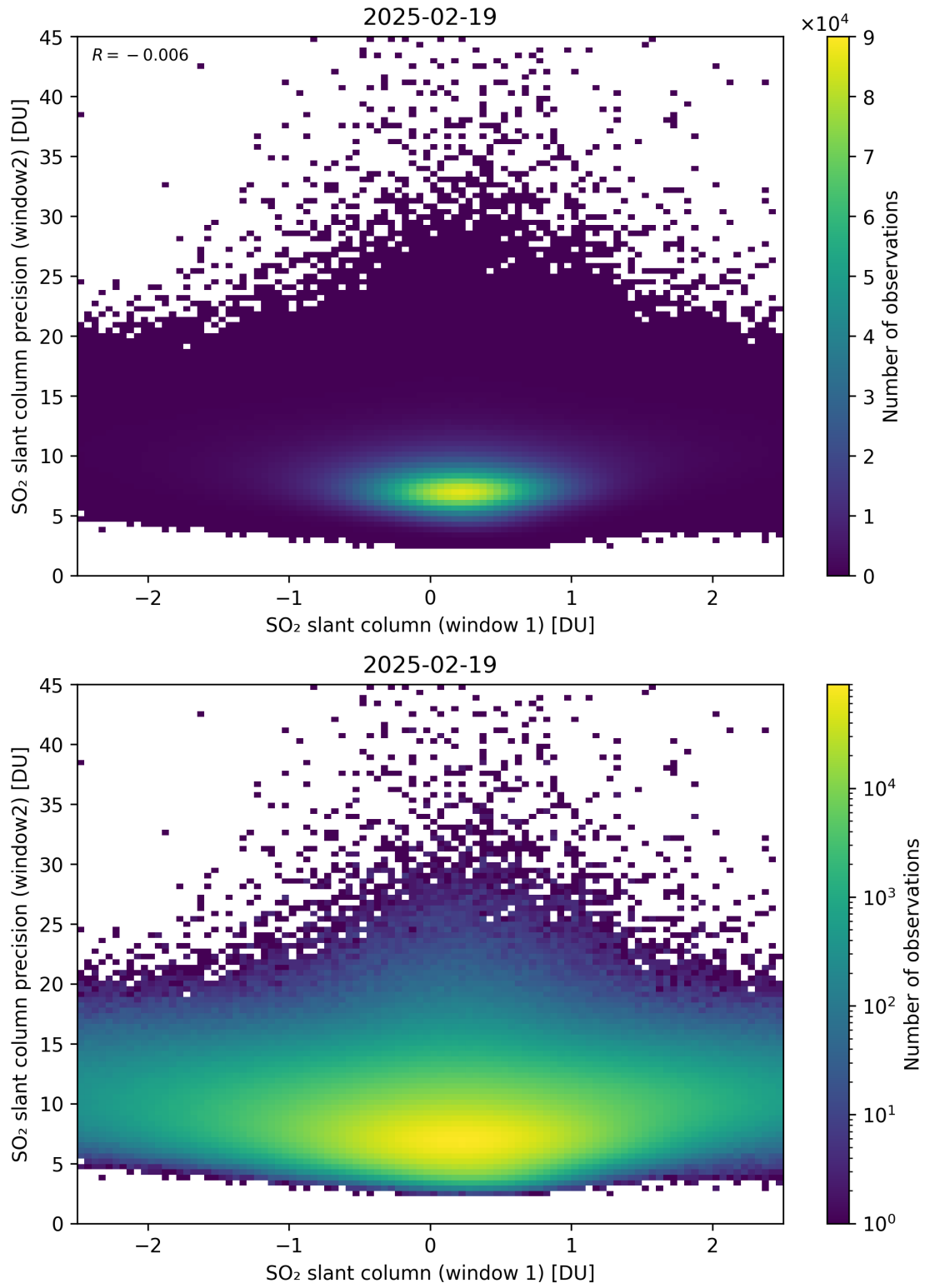
Figure 286: Scatter density plot of “SO 2 slant column (window 1)” against “SO 2 slant column precision (window2)” for 2025-02-19 to 2025-02-20.
