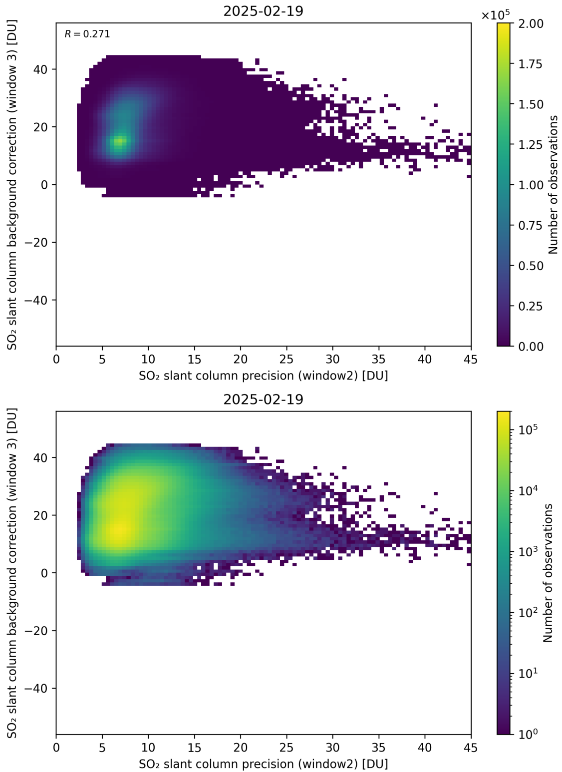
Figure 292: Scatter density plot of “SO 2 slant column precision (window2)” against “SO 2 slant column background correction (window 3)” for 2025-02-19 to 2025-02-20.
