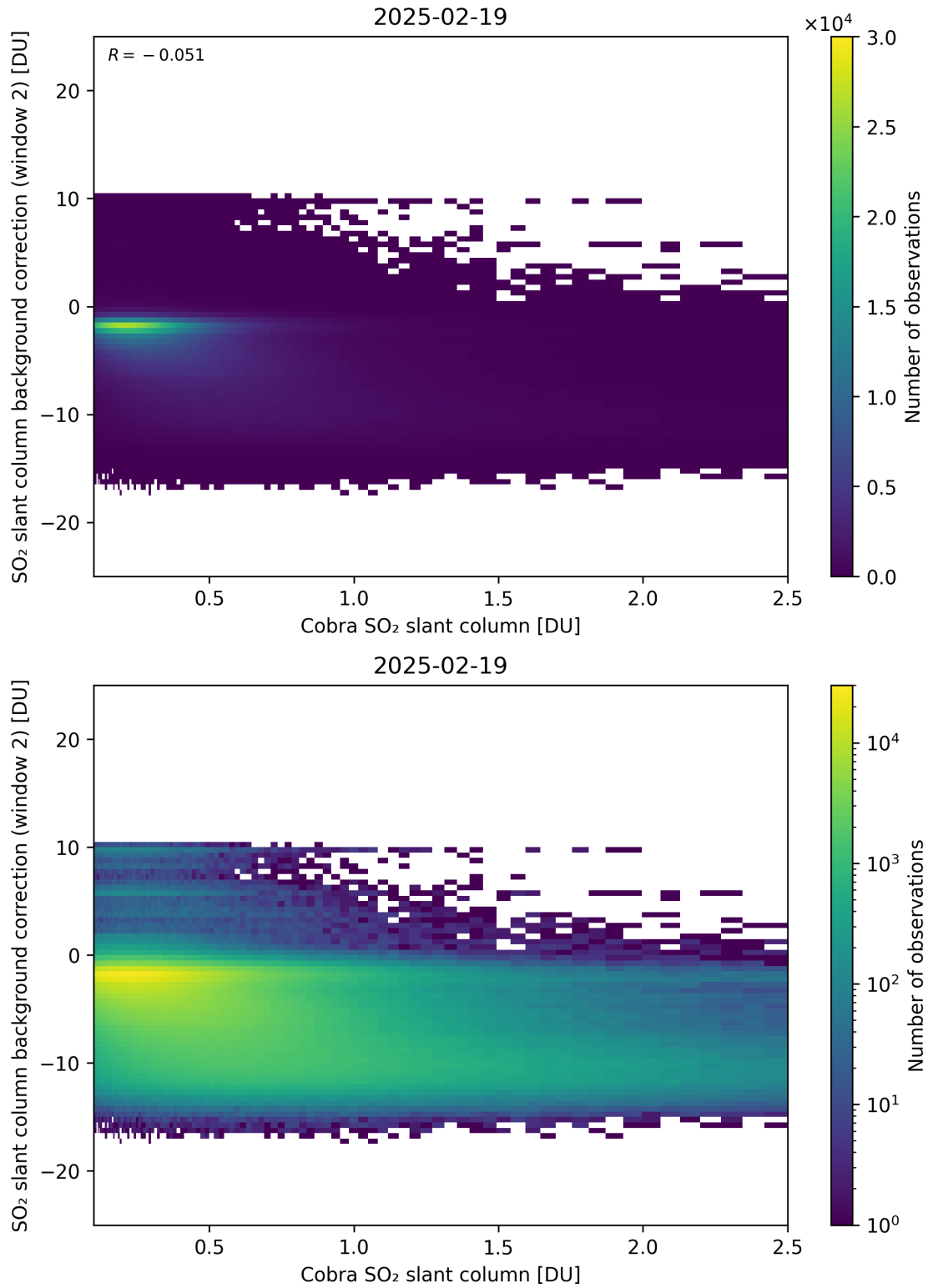
Figure 194: Scatter density plot of “Cobra SO 2 slant column” against “SO 2 slant column background correction (window 2)” for 2025-02-19 to 2025-02-20.
