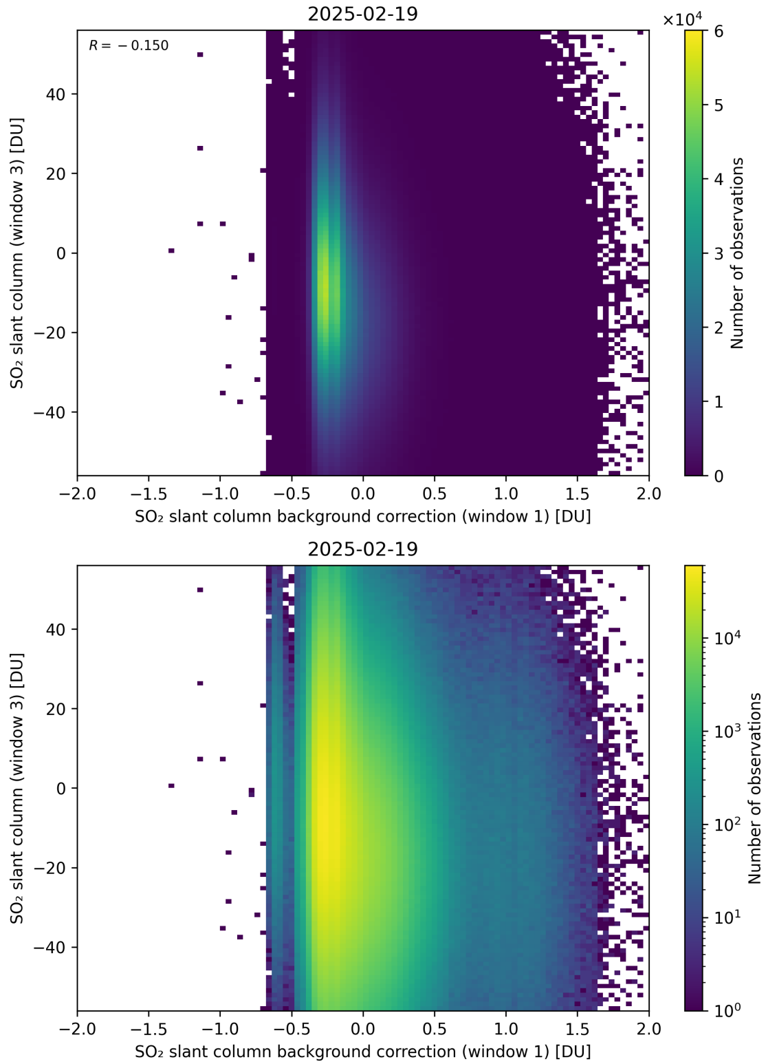
Figure 118: Scatter density plot of “SO 2 slant column background correction (window 1)” against “SO 2 slant column (window 3)” for 2025-02-19 to 2025-02-20.
