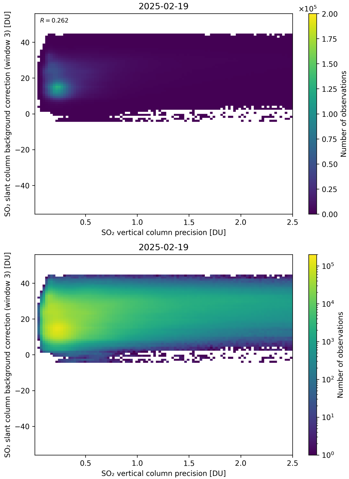
Figure 331: Scatter density plot of “SO 2 vertical column precision” against “SO 2 slant column background correction (window 3)” for 2025-02-19 to 2025-02-20.
