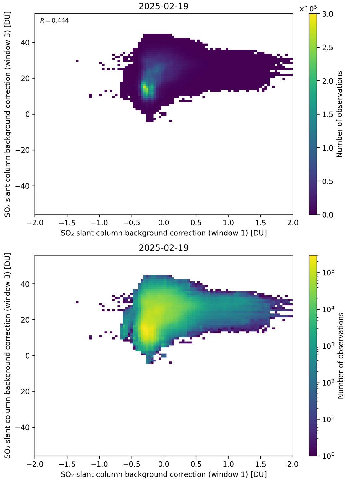
Figure 110: Scatter density plot of “SO 2 slant column background correction (window 1)” against “SO 2 slant column background correction (window 3)” for 2025-02-19 to 2025-02-20.
