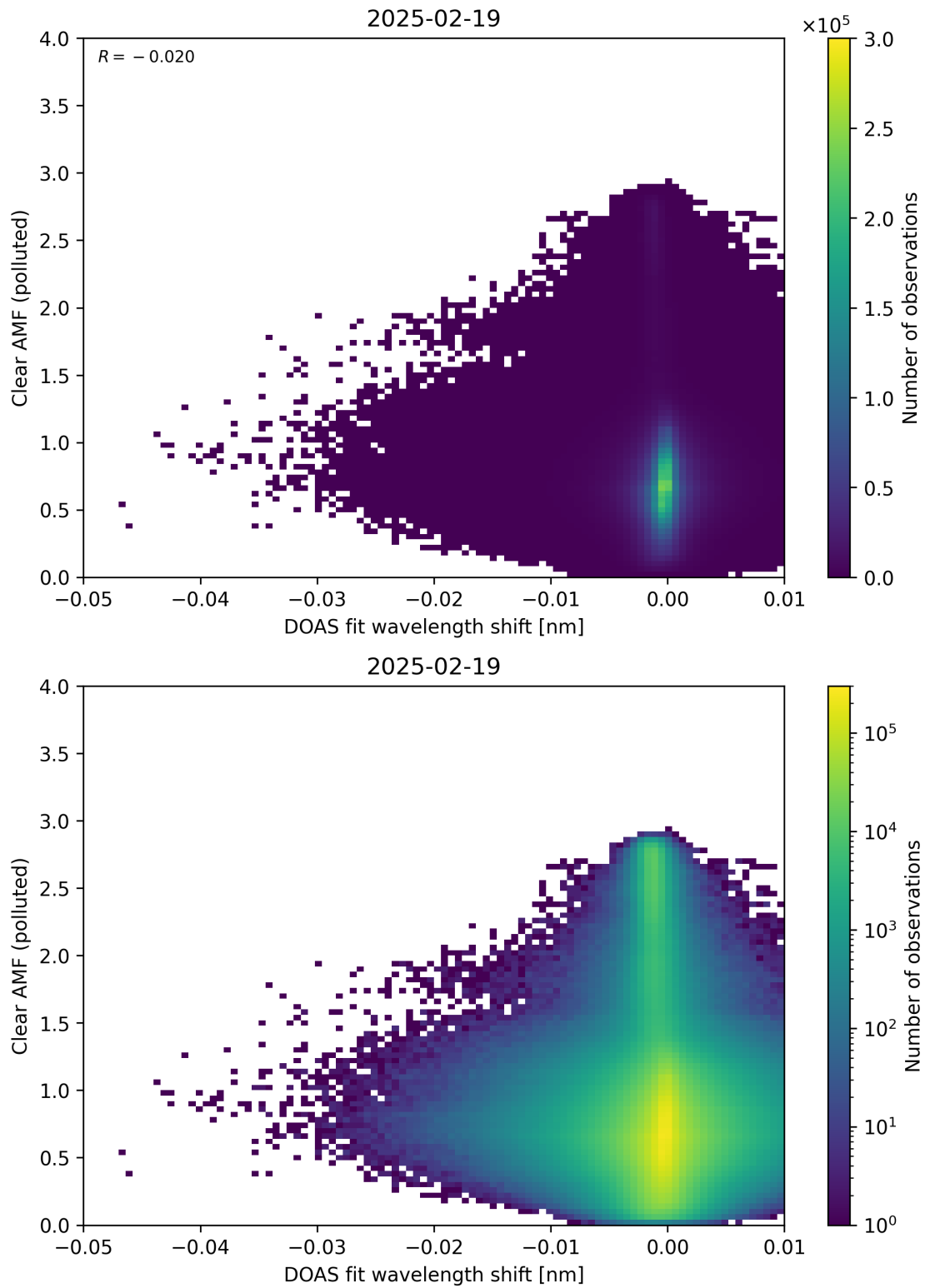
Figure 140: Scatter density plot of “DOAS fit wavelength shift” against “Clear AMF (polluted)” for 2025-02-19 to 2025-02-20.
