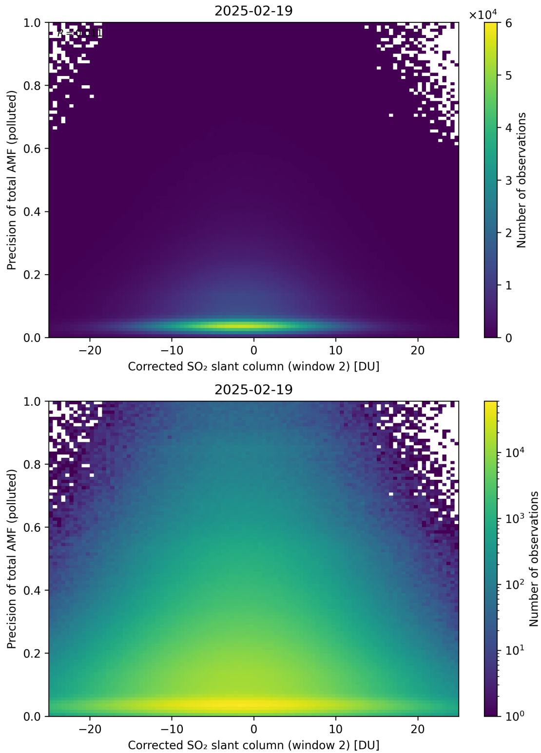
Figure 254: Scatter density plot of “Corrected SO 2 slant column (window 2)” against “Precision of total AMF (polluted)” for 2025-02-19 to 2025-02-20.
