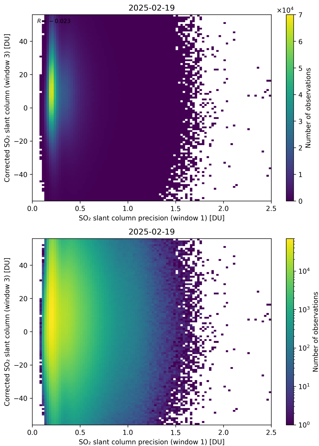
Figure 276: Scatter density plot of “SO 2 slant column precision (window 1)” against “Corrected SO 2 slant column (window 3)” for 2025-02-19 to 2025-02-20.
