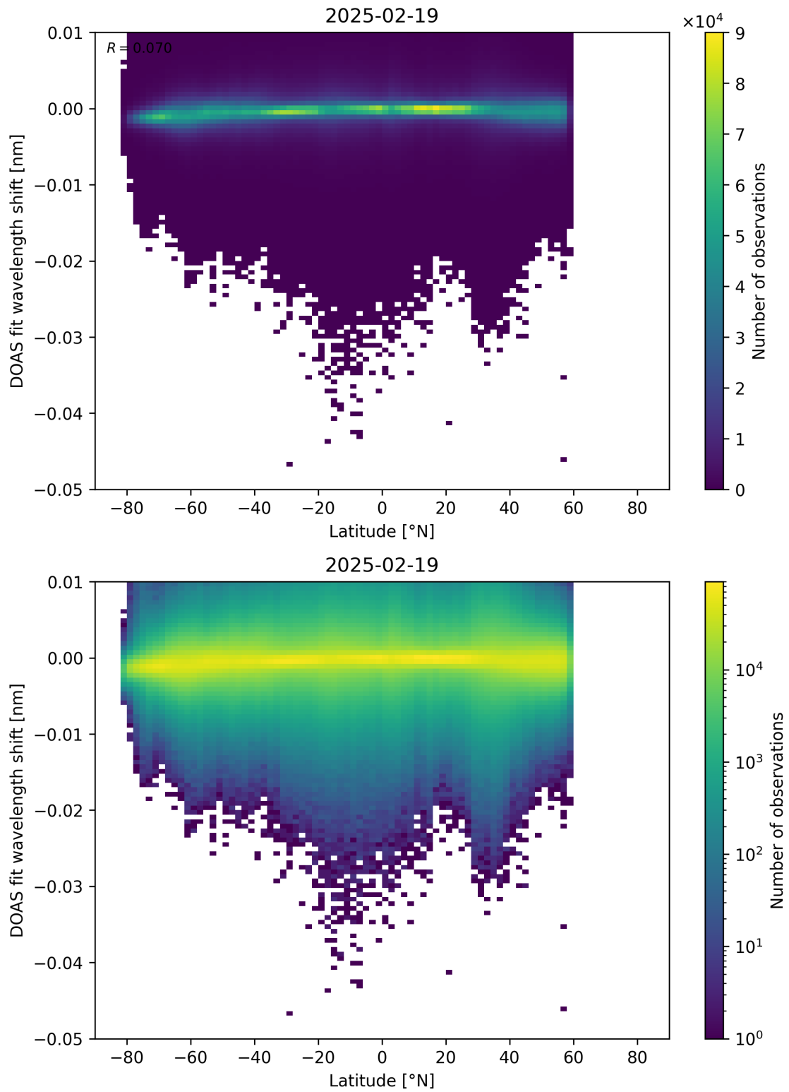
Figure 153: Scatter density plot of “Latitude” against “DOAS fit wavelength shift” for 2025-02-19 to 2025-02-20.
