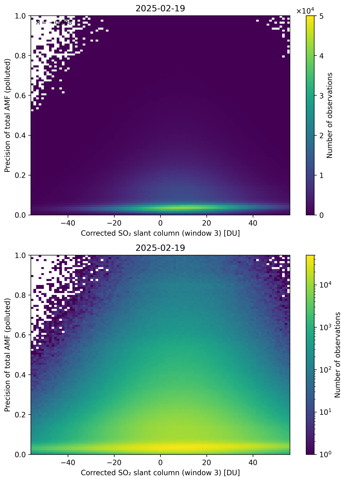
Figure 261: Scatter density plot of “Corrected SO 2 slant column (window 3)” against “Precision of total AMF (polluted)” for 2025-02-19 to 2025-02-20.
