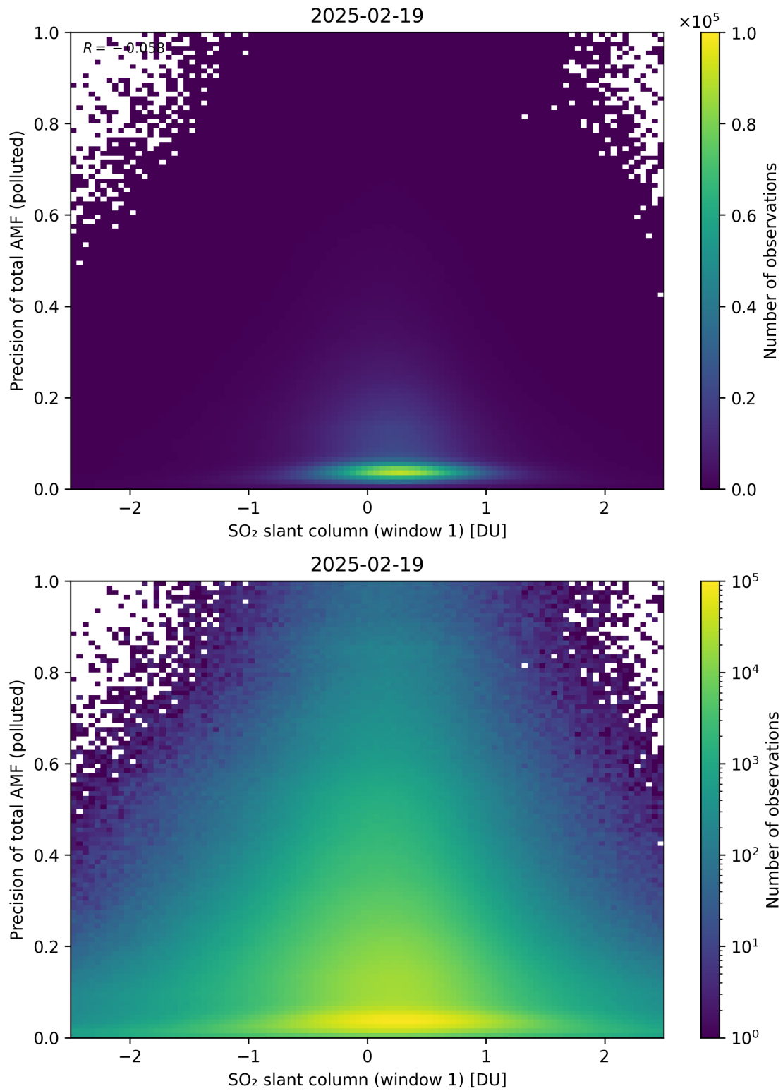
Figure 290: Scatter density plot of “SO 2 slant column (window 1)” against “Precision of total AMF (polluted)” for 2025-02-19 to 2025-02-20.
