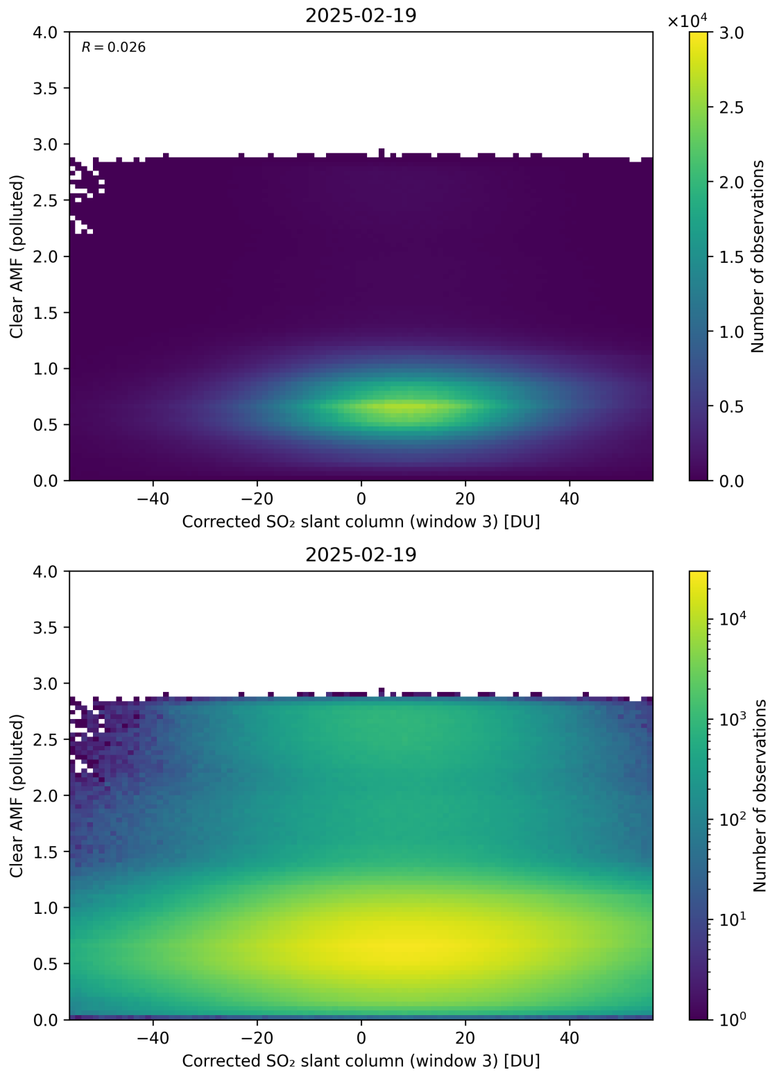
Figure 259: Scatter density plot of “Corrected SO 2 slant column (window 3)” against “Clear AMF (polluted)” for 2025-02-19 to 2025-02-20.
