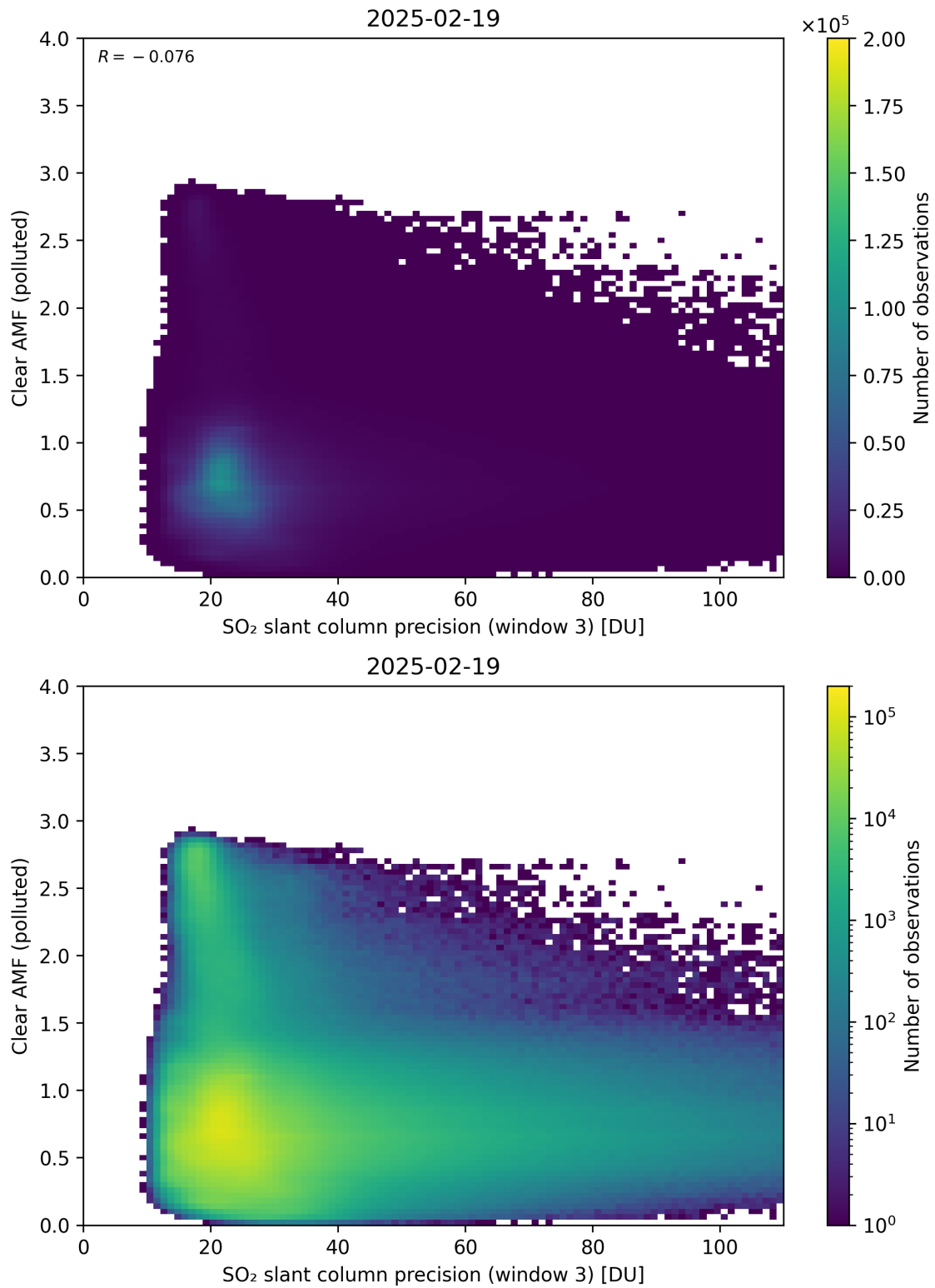
Figure 311: Scatter density plot of “SO 2 slant column precision (window 3)” against “Clear AMF (polluted)” for 2025-02-19 to 2025-02-20.
