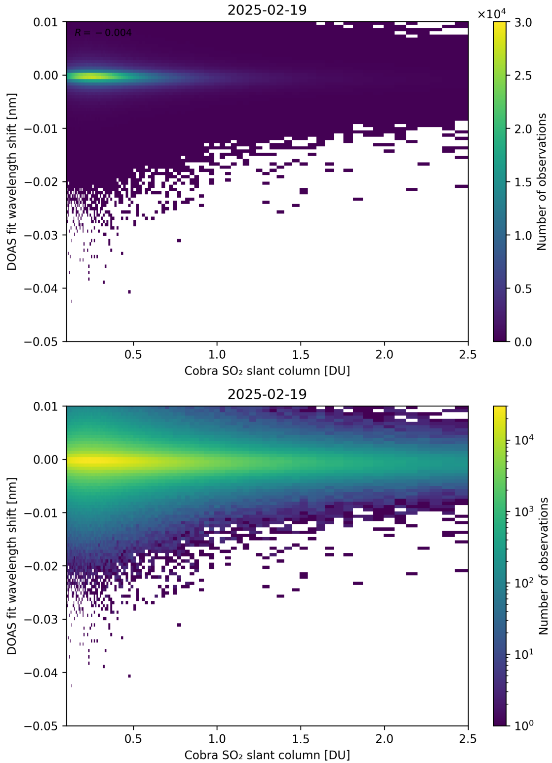
Figure 196: Scatter density plot of “Cobra SO 2 slant column” against “DOAS fit wavelength shift” for 2025-02-19 to 2025-02-20.
