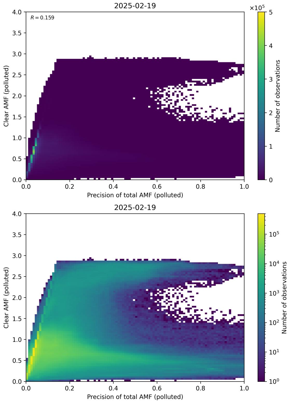
Figure 320: Scatter density plot of “Precision of total AMF (polluted)” against “Clear AMF (polluted)” for 2025-02-19 to 2025-02-20.
