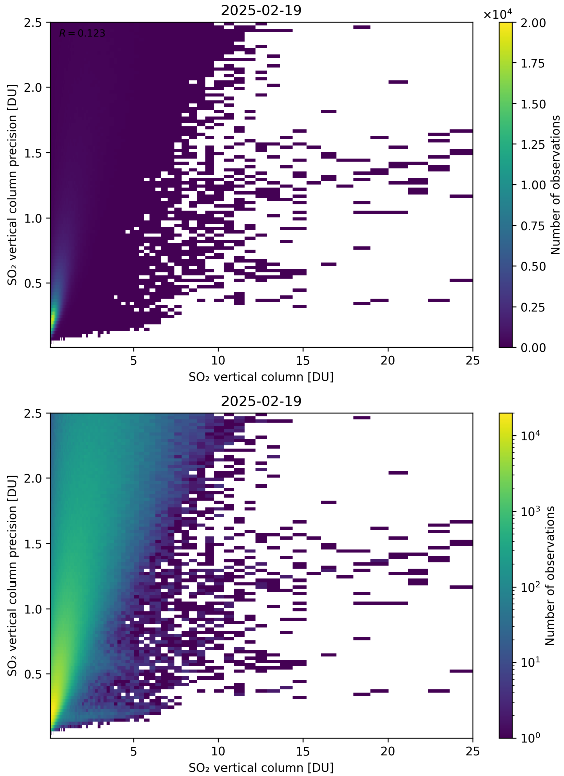
Figure 361: Scatter density plot of “SO 2 vertical column” against “SO 2 vertical column precision” for 2025-02-19 to 2025-02-20.
