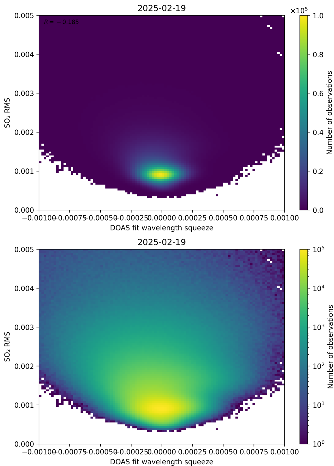
Figure 143: Scatter density plot of “DOAS fit wavelength squeeze” against “SO 2 RMS” for 2025-02-19 to 2025-02-20.
