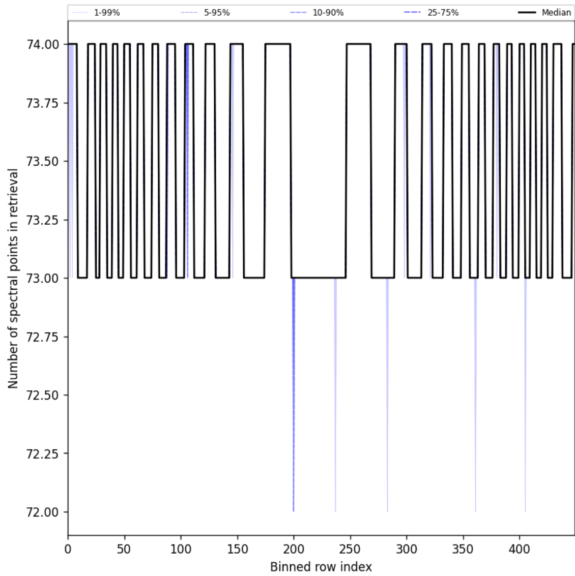
Figure 108: Along track statistics of “Number of spectral points in retrieval” for 2025-02-19 to 2025-02-20
