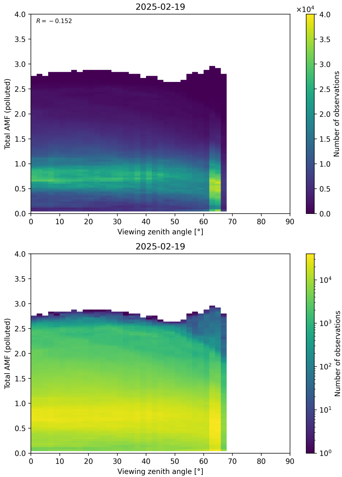
Figure 381: Scatter density plot of “Viewing zenith angle” against “Total AMF (polluted)” for 2025-02-19 to 2025-02-20.
