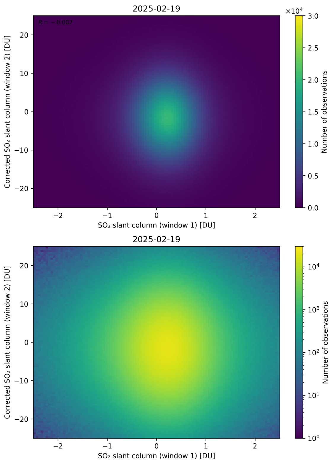
Figure 283: Scatter density plot of “SO 2 slant column (window 1)” against “Corrected SO 2 slant column (window 2)” for 2025-02-19 to 2025-02-20.
