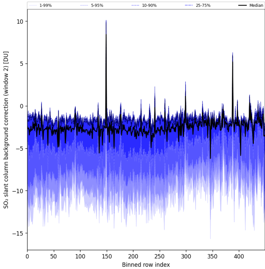
Figure 96: Along track statistics of “SO 2 slant column background correction (window 2)” for 2025-02-19 to 2025-02-20
