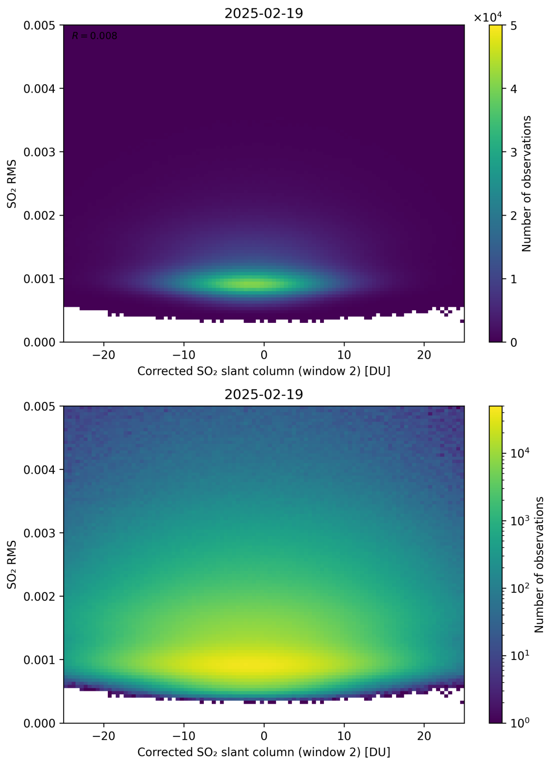
Figure 248: Scatter density plot of “Corrected SO 2 slant column (window 2)” against “SO 2 RMS” for 2025-02-19 to 2025-02-20.
