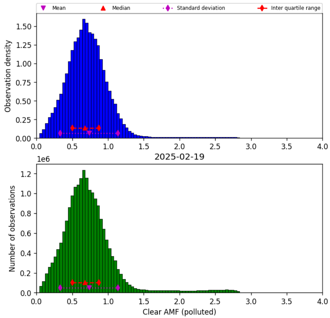
Figure 81: Histogram of “Clear AMF (polluted)” for 2025-02-19 to 2025-02-20
