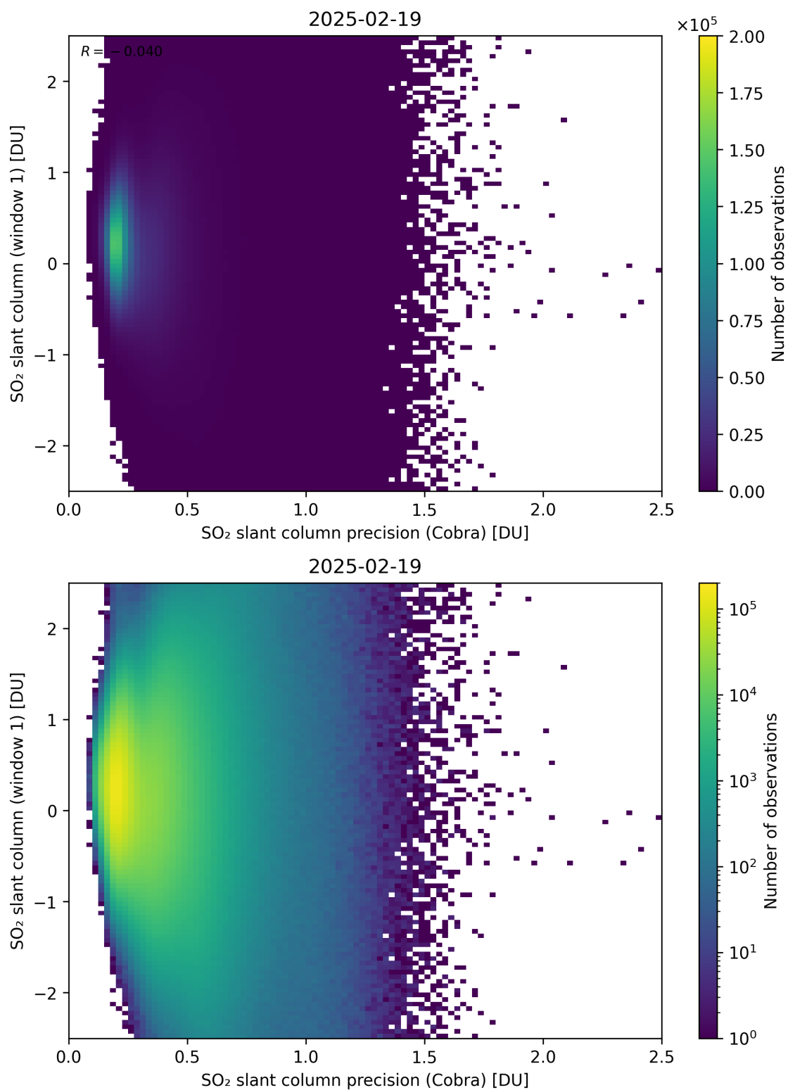
Figure 208: Scatter density plot of “SO 2 slant column precision (Cobra)” against “SO 2 slant column (window 1)” for 2025-02-19 to 2025-02-20.
