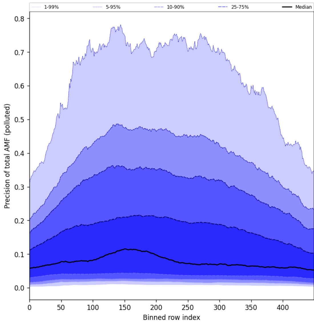
Figure 106: Along track statistics of “Precision of total AMF (polluted)” for 2025-02-19 to 2025-02-20
