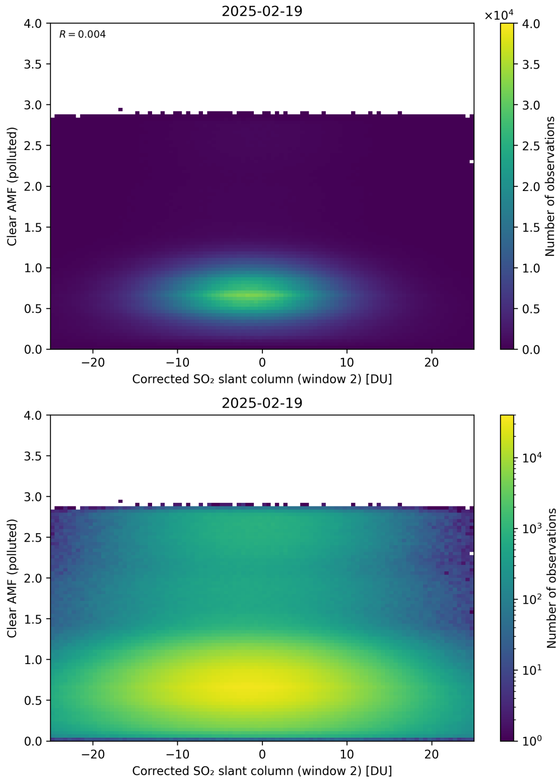
Figure 249: Scatter density plot of “Corrected SO 2 slant column (window 2)” against “Clear AMF (polluted)” for 2025-02-19 to 2025-02-20.
