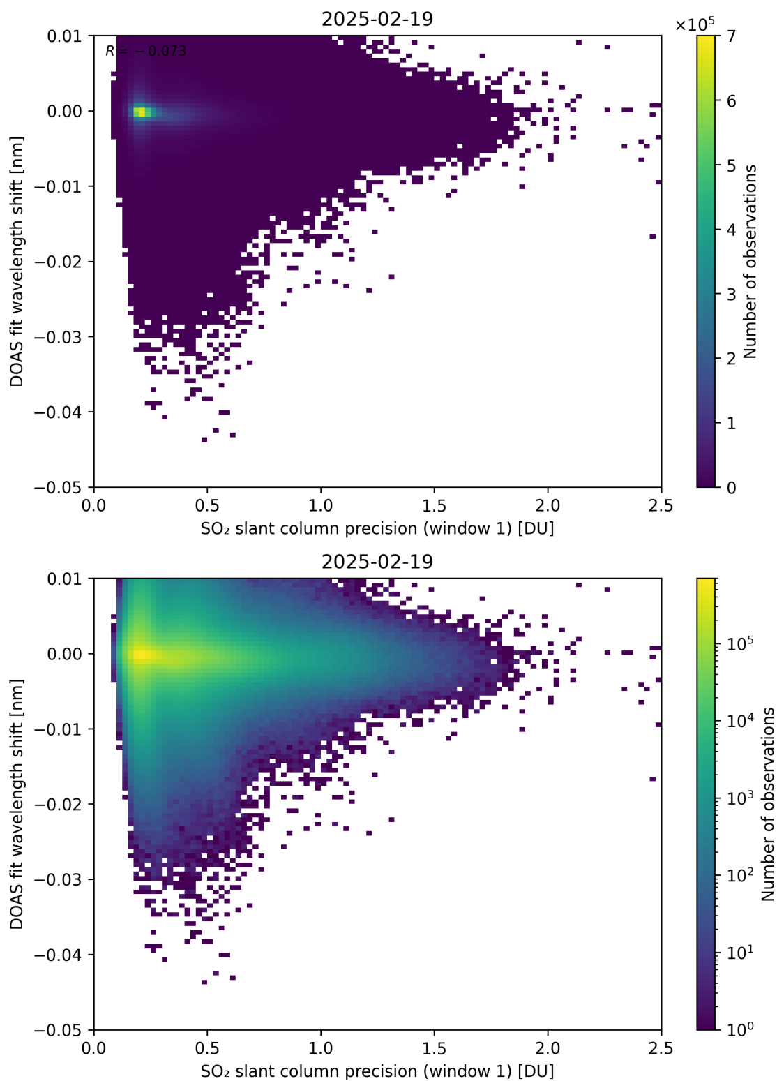
Figure 271: Scatter density plot of “SO 2 slant column precision (window 1)” against “DOAS fit wavelength shift” for 2025-02-19 to 2025-02-20.
