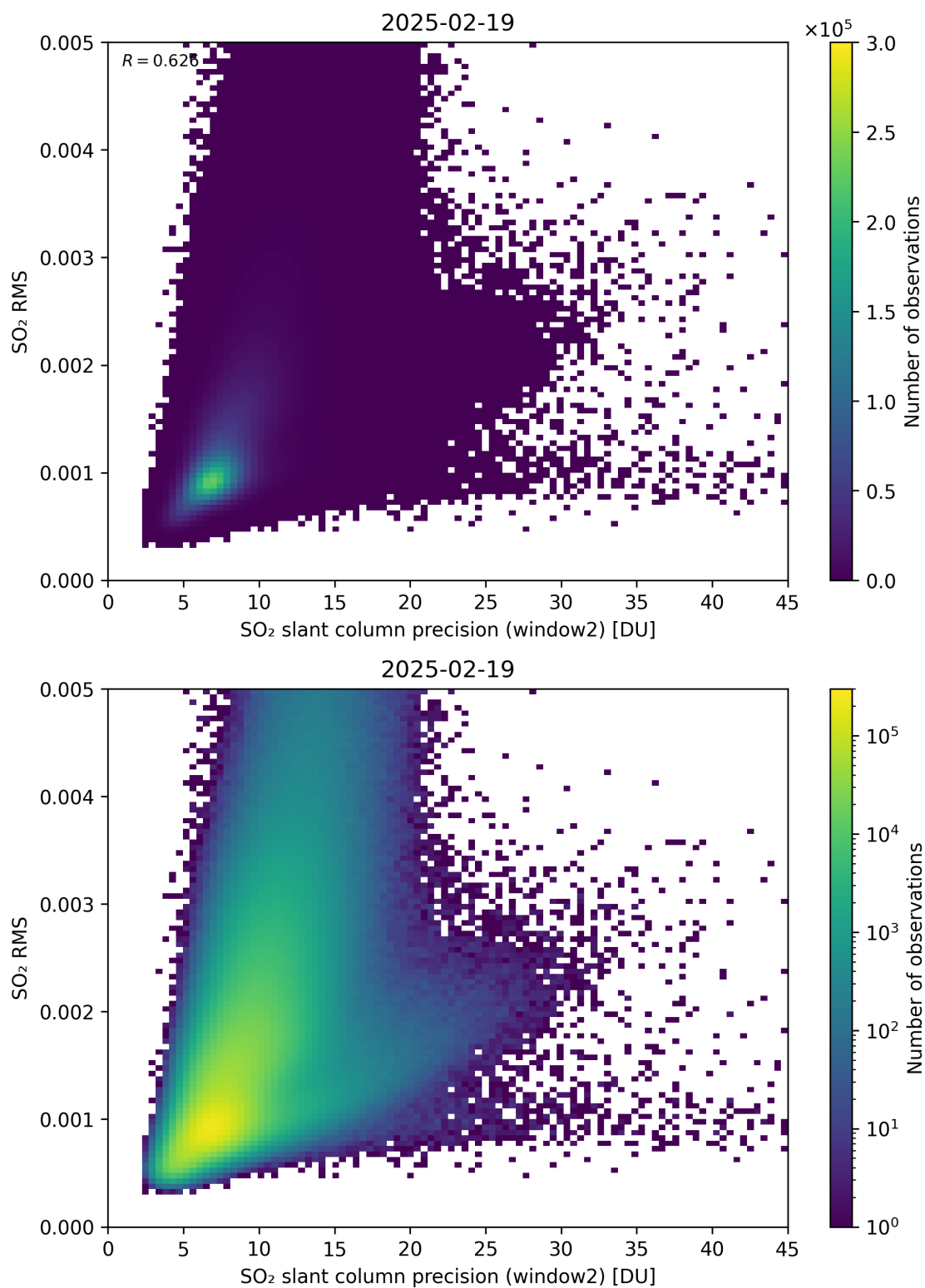
Figure 295: Scatter density plot of “SO 2 slant column precision (window2)” against “SO 2 RMS” for 2025-02-19 to 2025-02-20.
