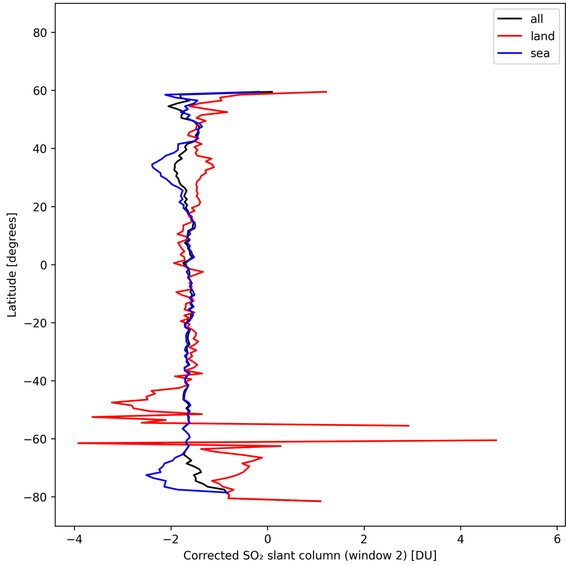
Figure 43: Zonal average of “Corrected SO 2 slant column (window 2)” for 2025-02-19 to 2025-02-20.
