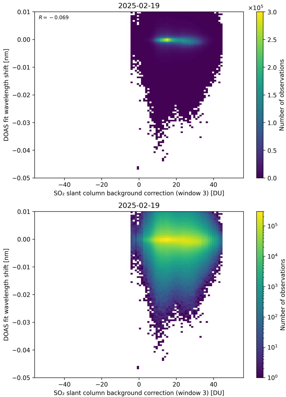
Figure 132: Scatter density plot of “SO 2 slant column background correction (window 3)” against “DOAS fit wavelength shift” for 2025-02-19 to 2025-02-20.
