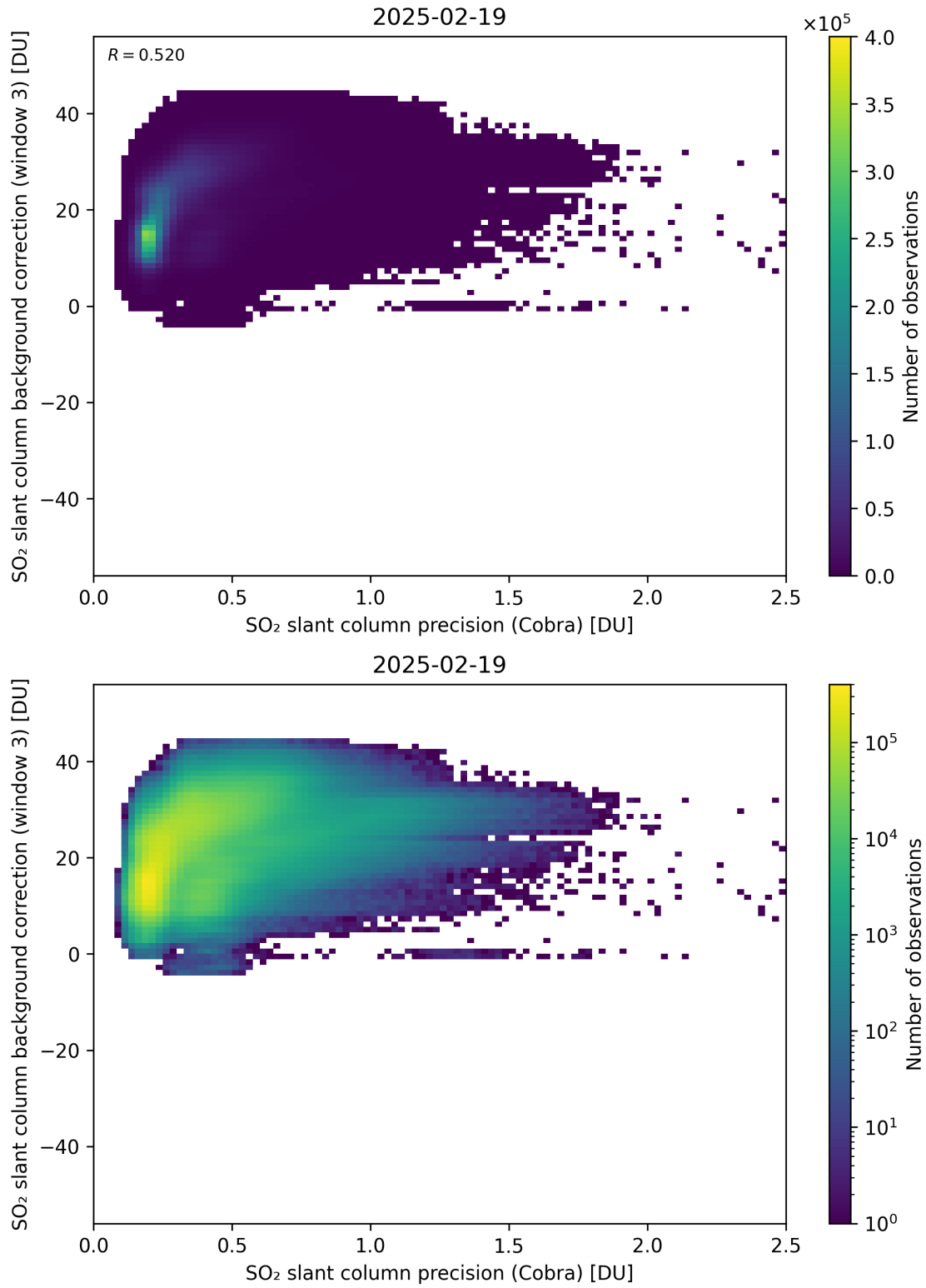
Figure 201: Scatter density plot of “SO 2 slant column precision (Cobra)” against “SO 2 slant column background correction (window 3)” for 2025-02-19 to 2025-02-20.
