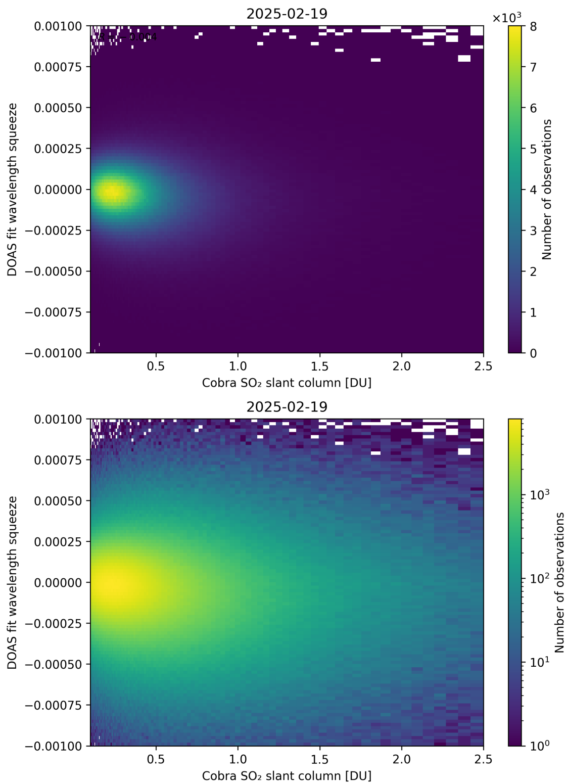
Figure 197: Scatter density plot of “Cobra SO 2 slant column” against “DOAS fit wavelength squeeze” for 2025-02-19 to 2025-02-20.
