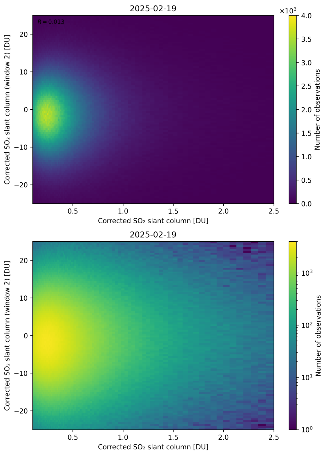
Figure 235: Scatter density plot of “Corrected SO 2 slant column” against “Corrected SO 2 slant column (window 2)” for 2025-02-19 to 2025-02-20.
