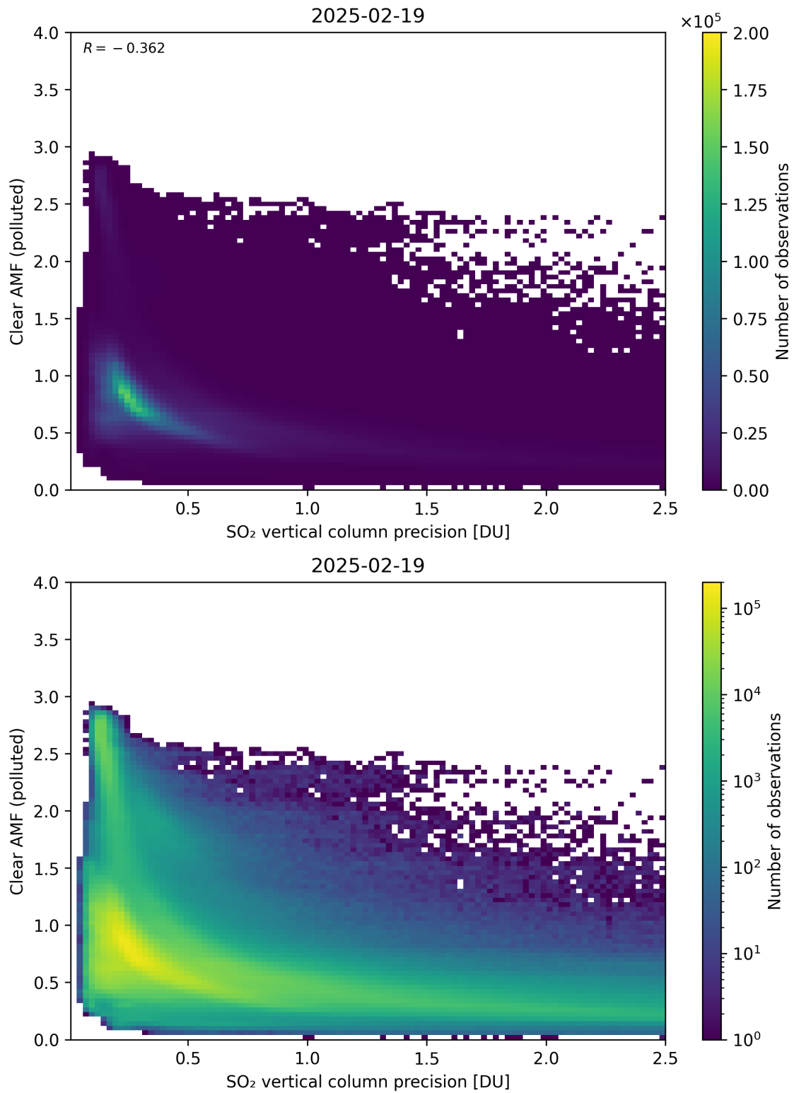
Figure 335: Scatter density plot of “SO 2 vertical column precision” against “Clear AMF (polluted)” for 2025-02-19 to 2025-02-20.
