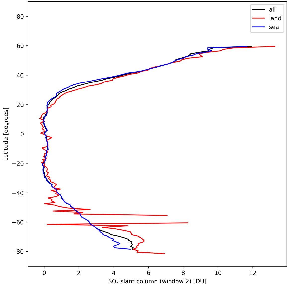
Figure 41: Zonal average of “SO 2 slant column (window 2)” for 2025-02-19 to 2025-02-20.
