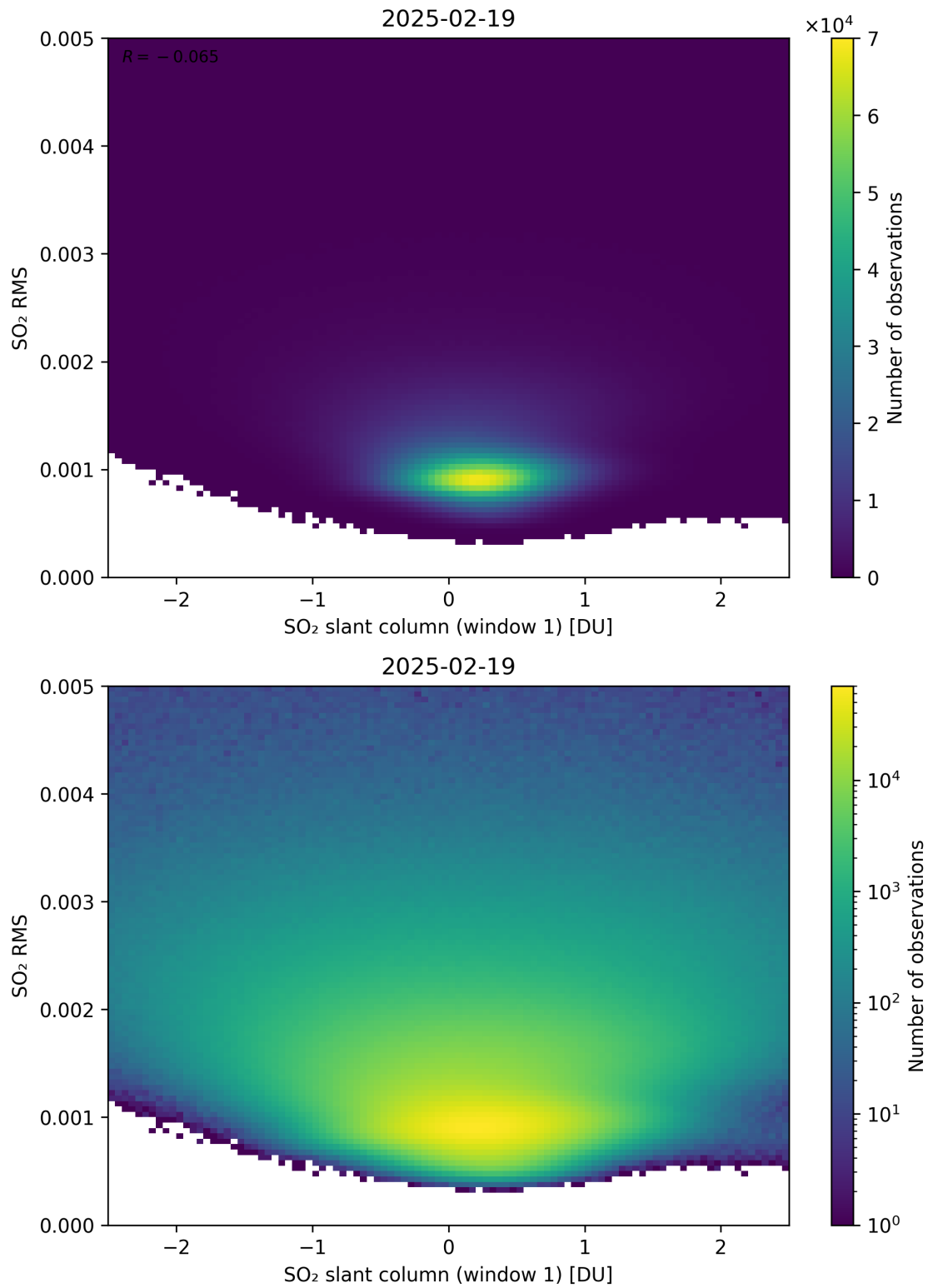
Figure 267: Scatter density plot of “SO 2 slant column (window 1)” against “SO 2 RMS” for 2025-02-19 to 2025-02-20.
