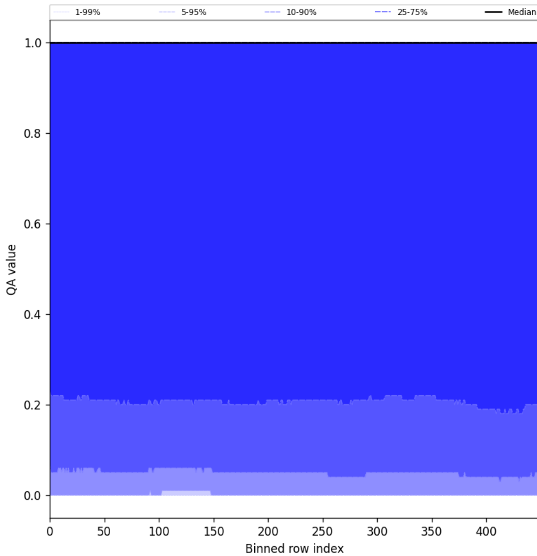
Figure 83: Along track statistics of “QA value” for 2025-02-19 to 2025-02-20
