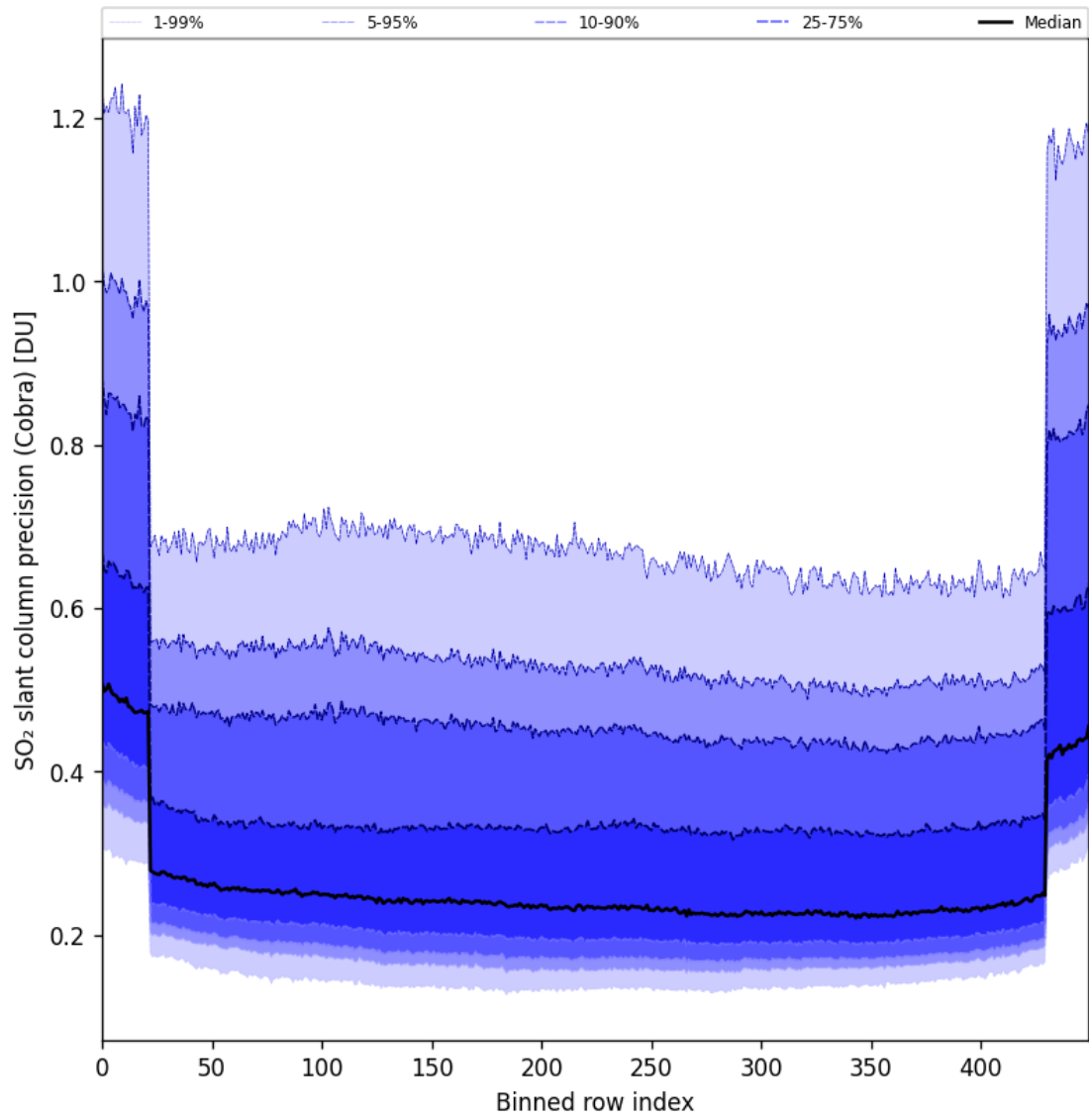
Figure 88: Along track statistics of “SO 2 slant column precision (Cobra)” for 2025-02-19 to 2025-02-20
