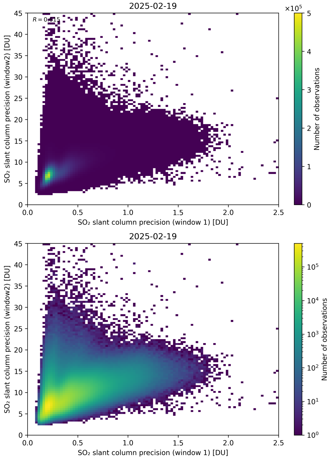
Figure 277: Scatter density plot of “SO 2 slant column precision (window 1)” against “SO 2 slant column precision (window2)” for 2025-02-19 to 2025-02-20.
