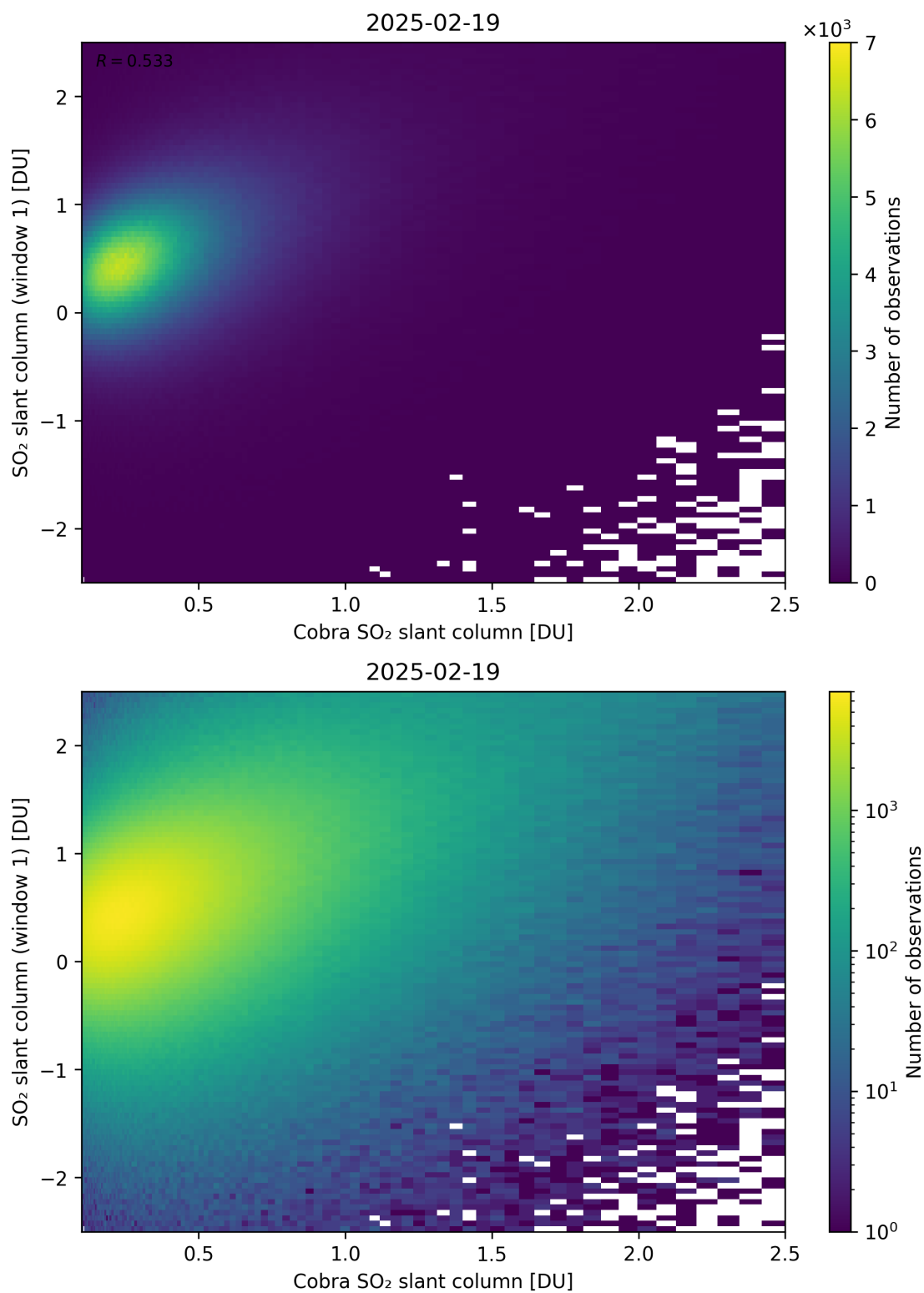
Figure 219: Scatter density plot of “Cobra SO 2 slant column” against “SO 2 slant column (window 1)” for 2025-02-19 to 2025-02-20.
