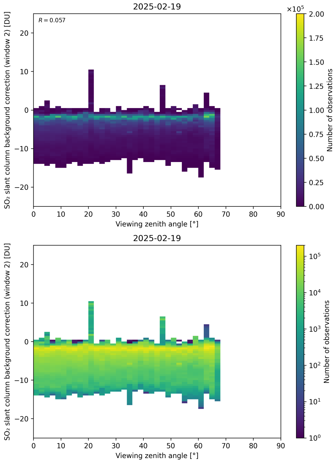
Figure 363: Scatter density plot of “Viewing zenith angle” against “SO 2 slant column background correction (window 2)” for 2025-02-19 to 2025-02-20.
