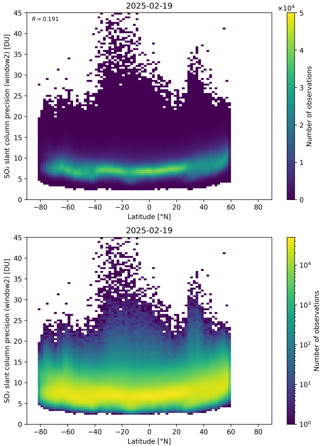
Figure 164: Scatter density plot of “Latitude” against “SO 2 slant column precision (window2)” for 2025-02-19 to 2025-02-20.
