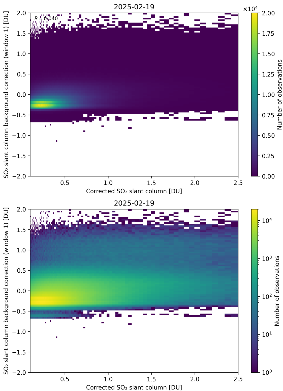
Figure 226: Scatter density plot of “Corrected SO 2 slant column” against “SO 2 slant column background correction (window 1)” for 2025-02-19 to 2025-02-20.
