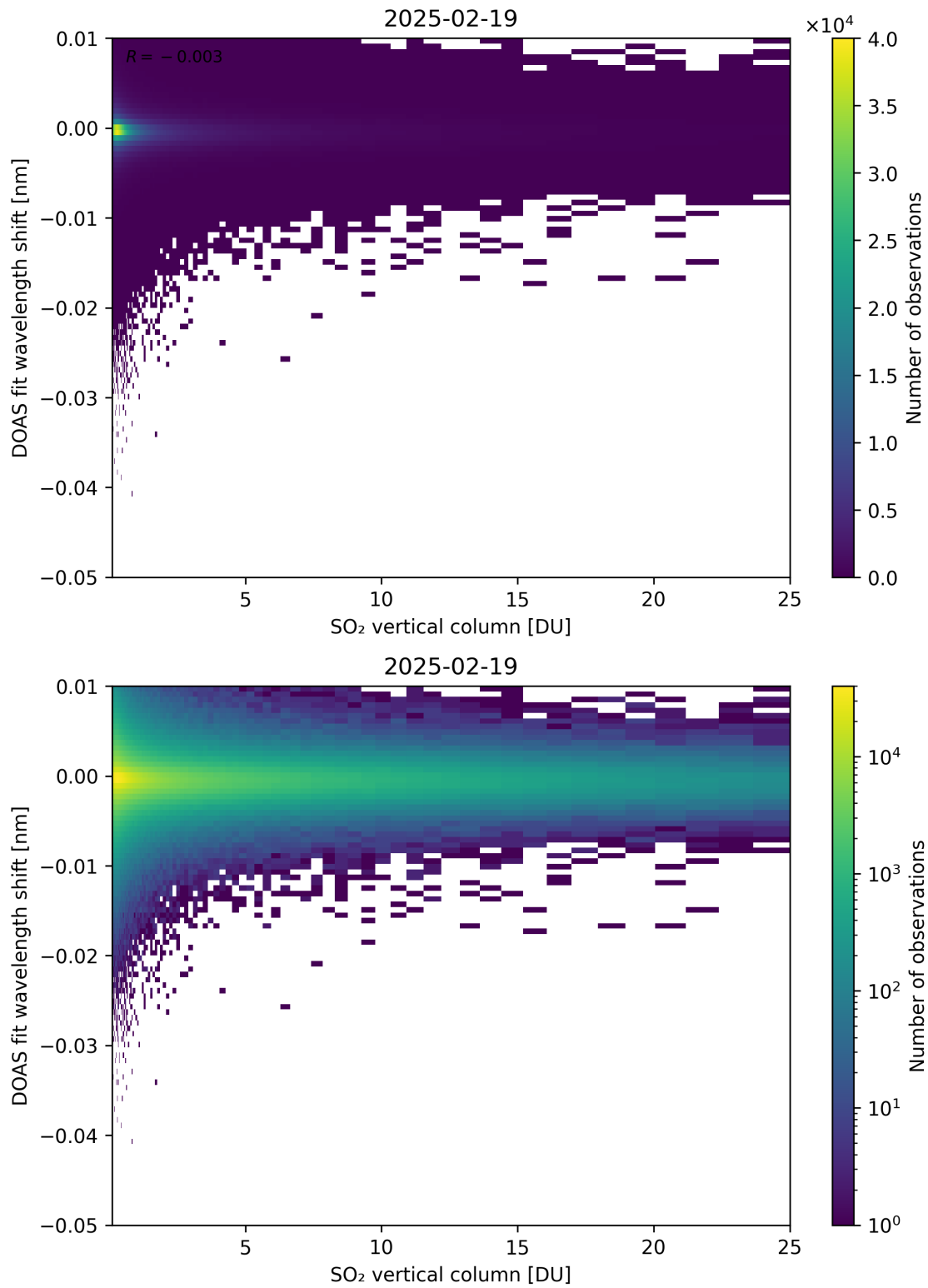
Figure 326: Scatter density plot of “SO 2 vertical column” against “DOAS fit wavelength shift” for 2025-02-19 to 2025-02-20.
