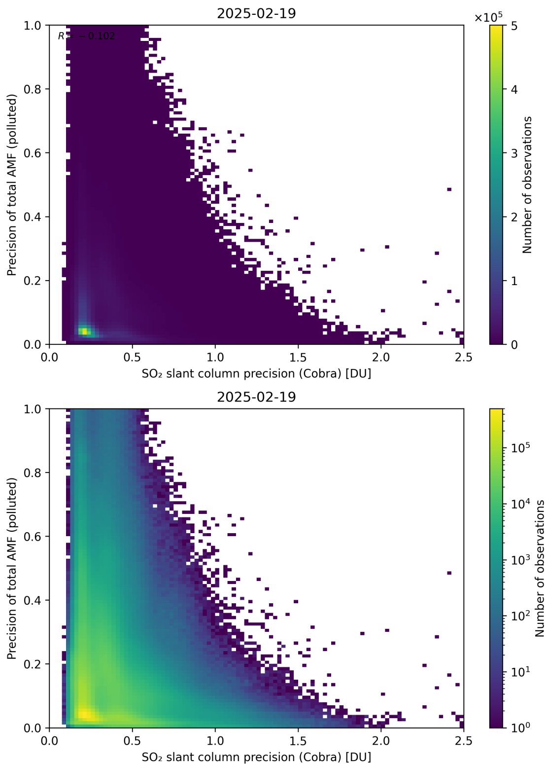
Figure 214: Scatter density plot of “SO 2 slant column precision (Cobra)” against “Precision of total AMF (polluted)” for 2025-02-19 to 2025-02-20.
