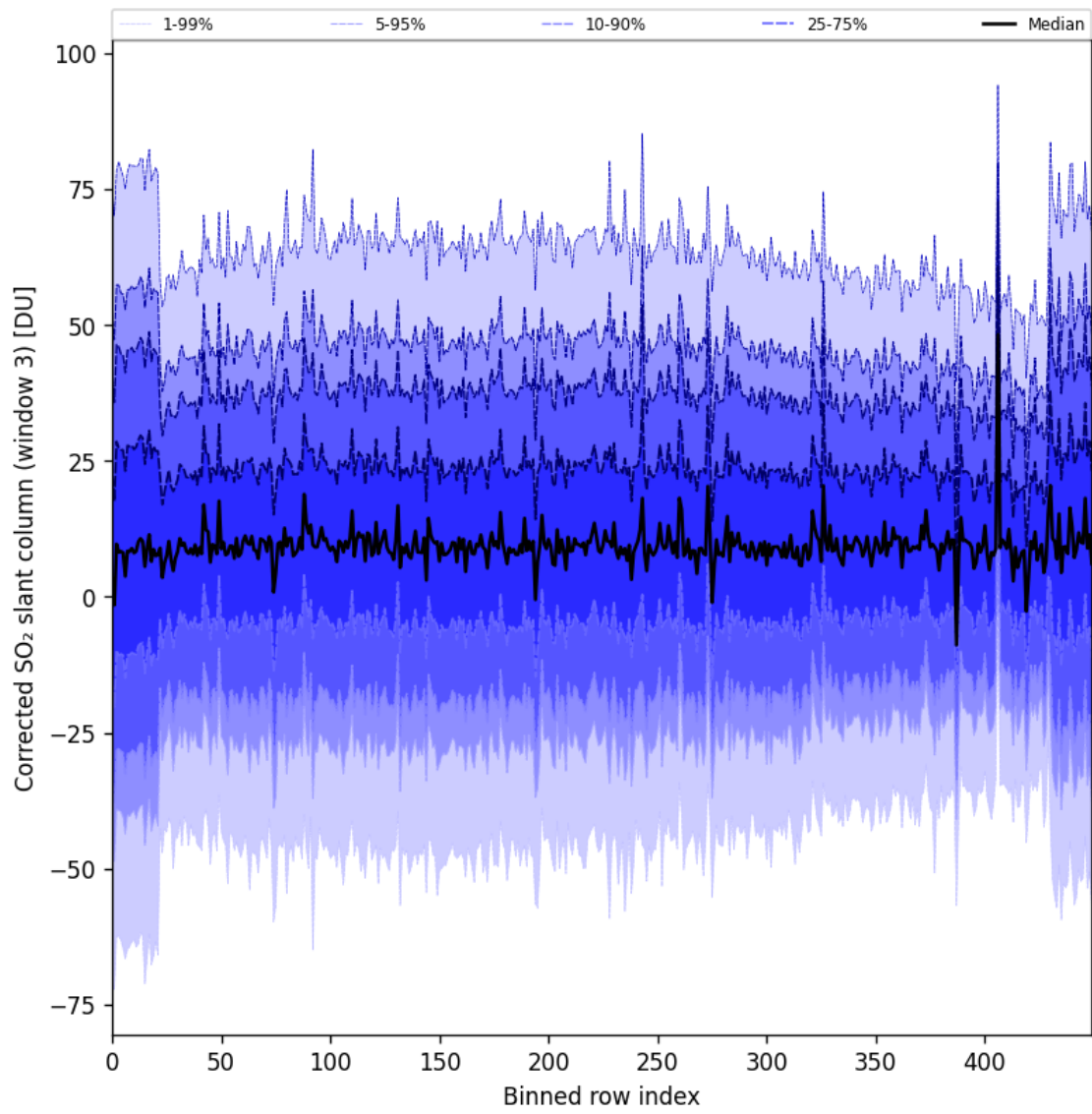
Figure 99: Along track statistics of “Corrected SO 2 slant column (window 3)” for 2025-02-19 to 2025-02-20
