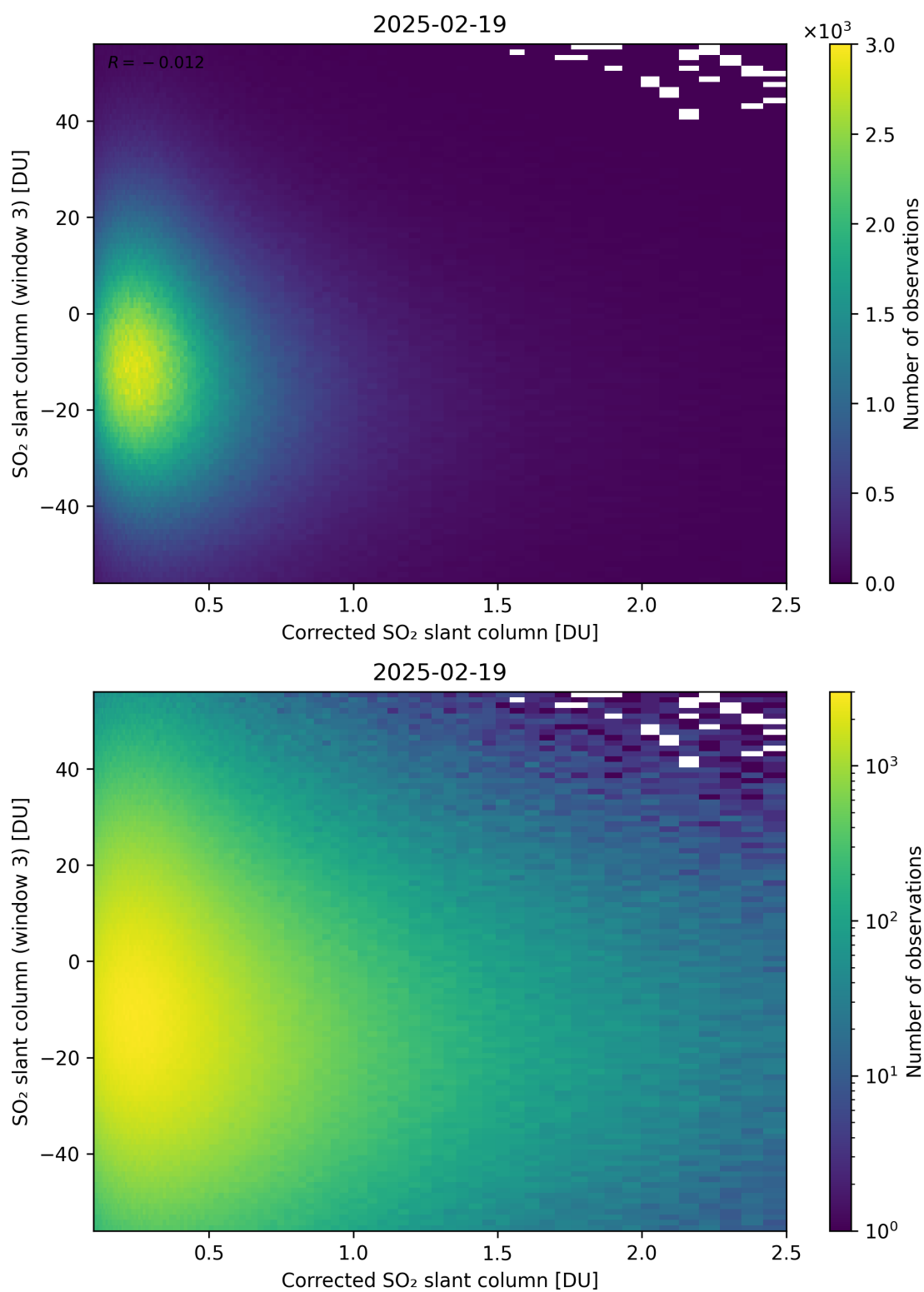
Figure 240: Scatter density plot of “Corrected SO 2 slant column” against “SO 2 slant column (window 3)” for 2025-02-19 to 2025-02-20.
