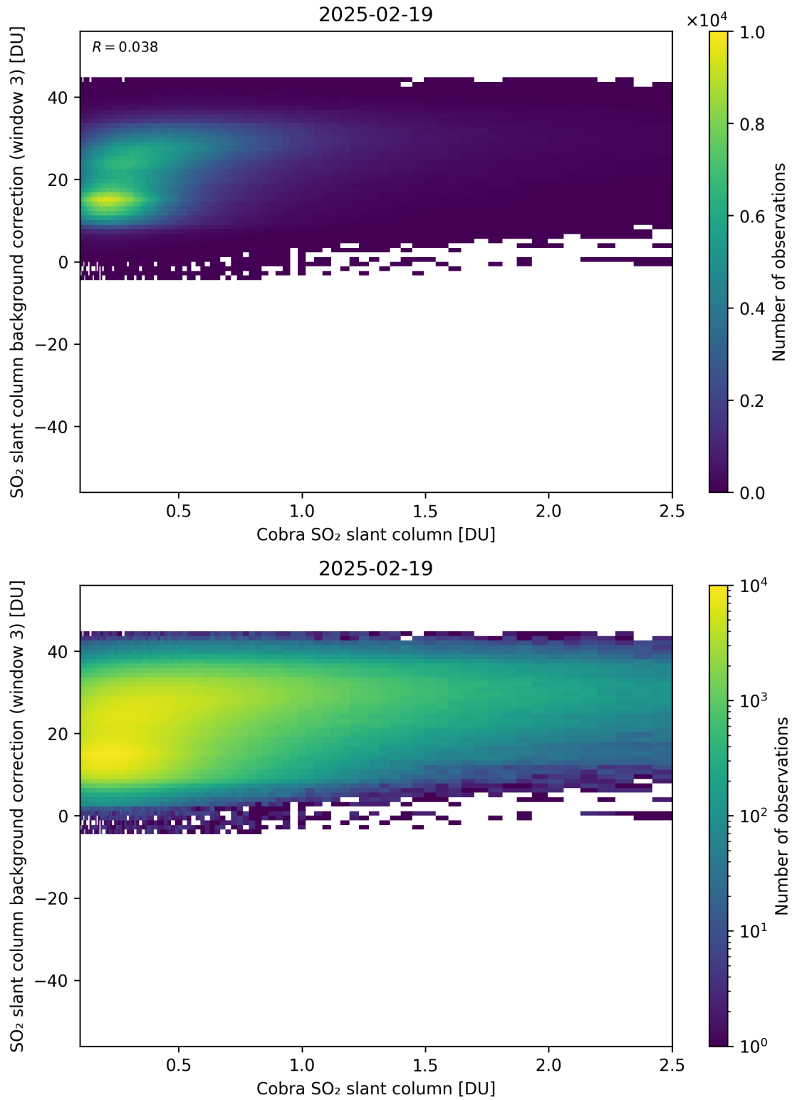
Figure 195: Scatter density plot of “Cobra SO 2 slant column” against “SO 2 slant column background correction (window 3)” for 2025-02-19 to 2025-02-20.
