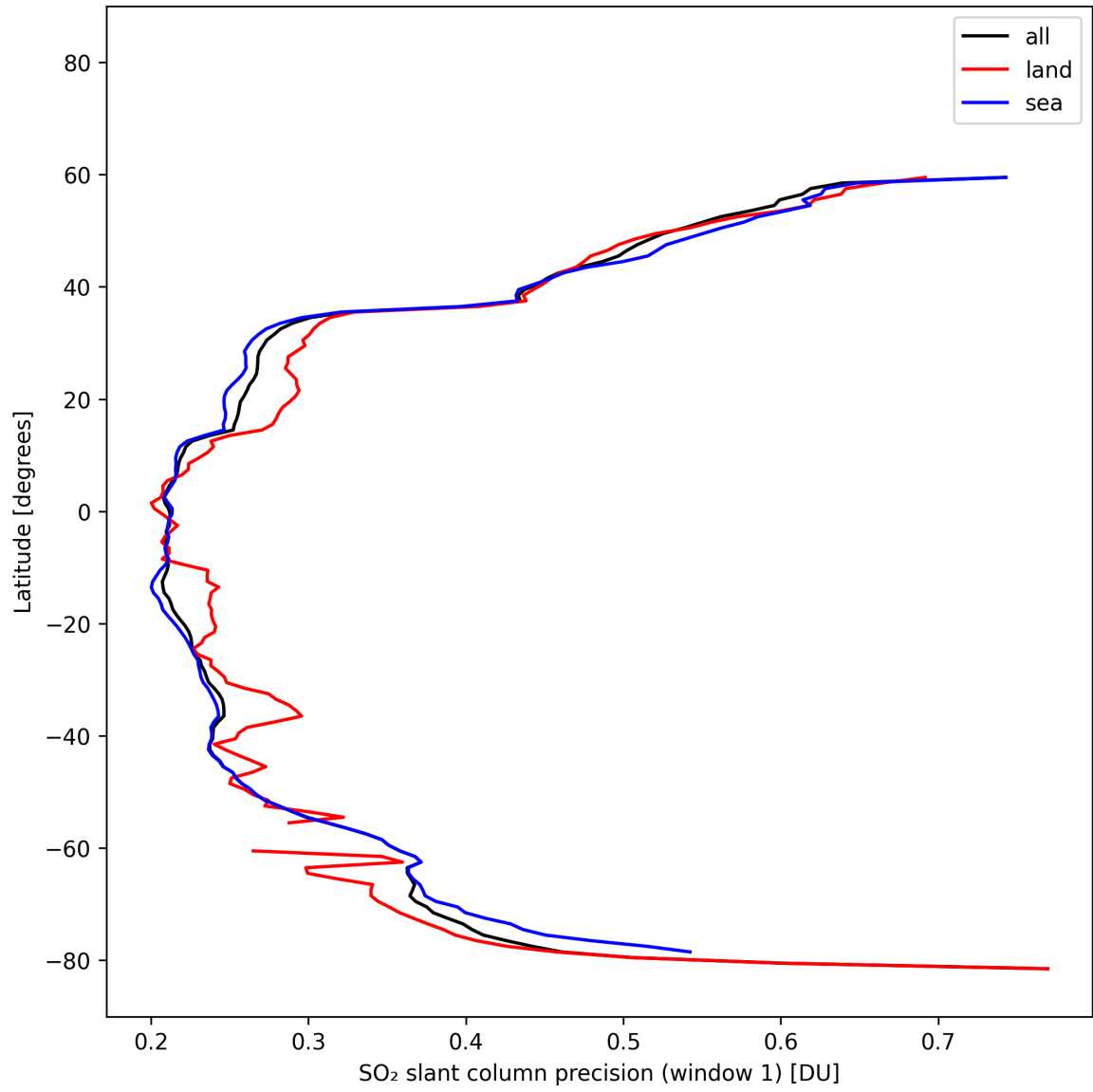
Figure 38: Zonal average of “SO 2 slant column precision (window 1)” for 2025-02-19 to 2025-02-20.
