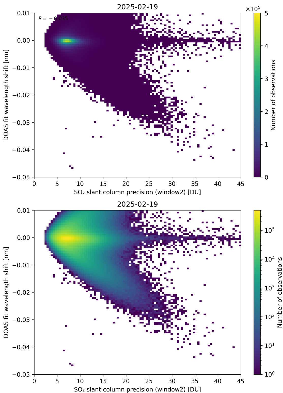
Figure 293: Scatter density plot of “SO 2 slant column precision (window2)” against “DOAS fit wavelength shift” for 2025-02-19 to 2025-02-20.
