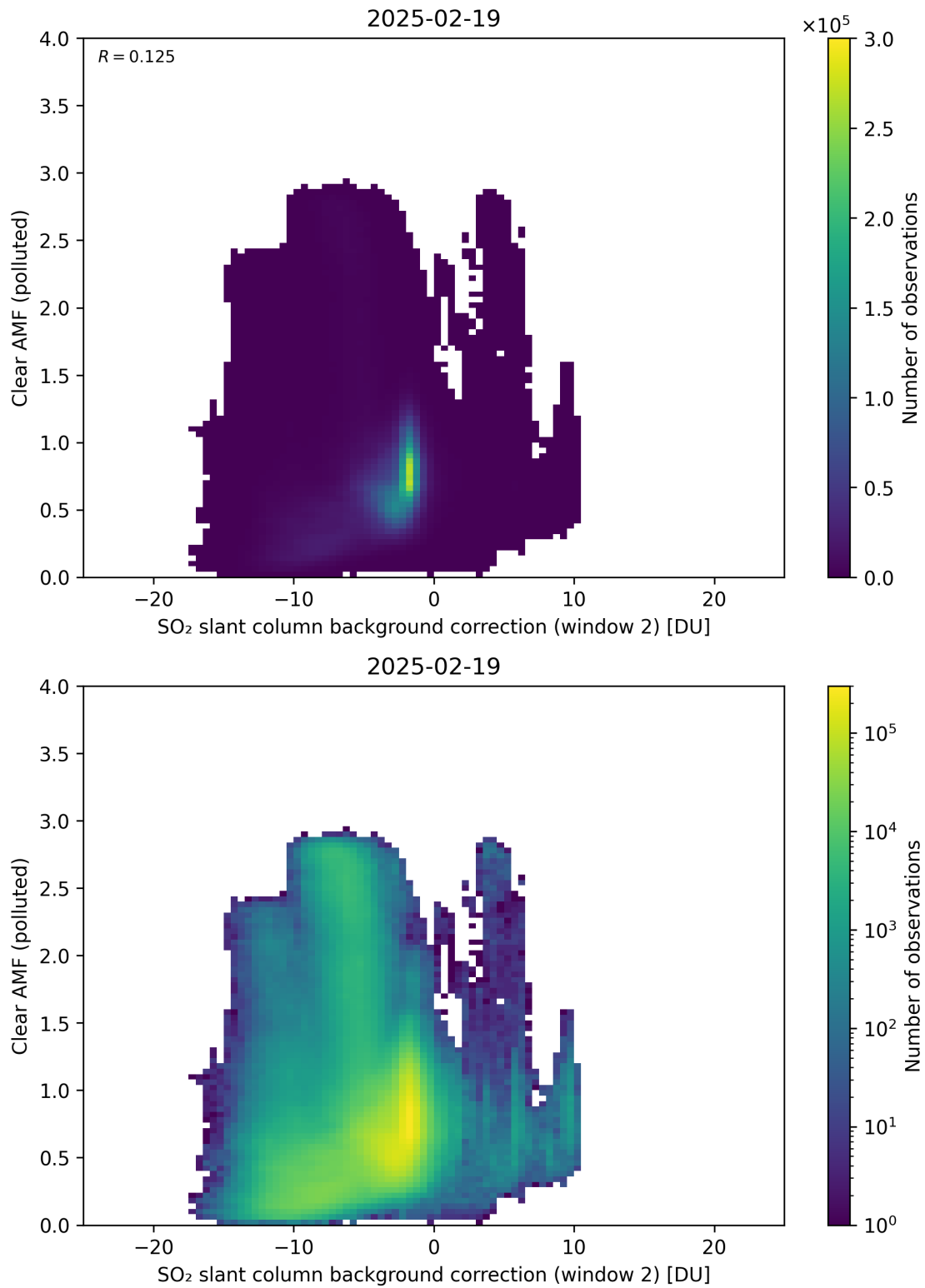
Figure 126: Scatter density plot of “SO 2 slant column background correction (window 2)” against “Clear AMF (polluted)” for 2025-02-19 to 2025-02-20.
