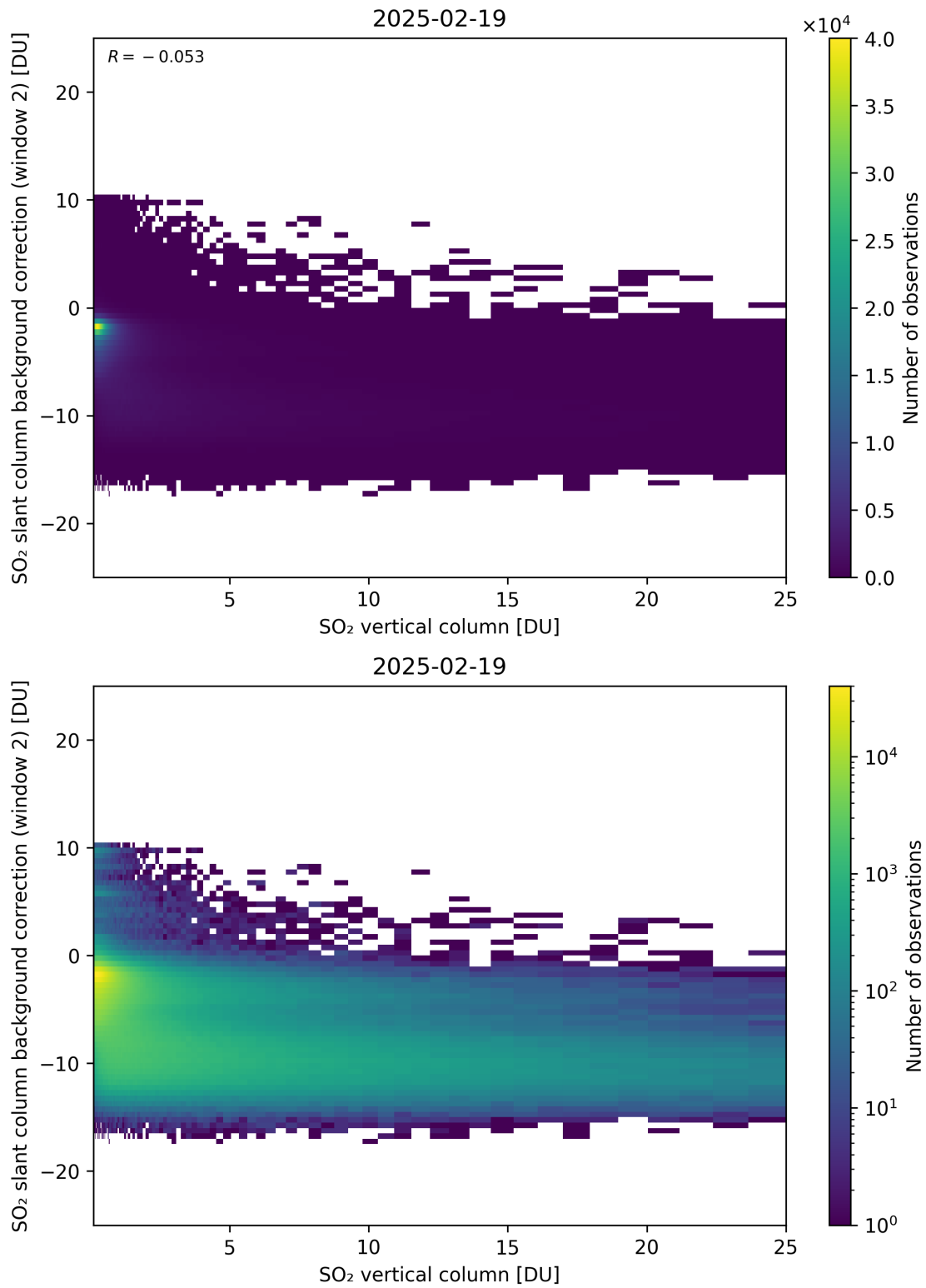
Figure 324: Scatter density plot of “SO 2 vertical column” against “SO 2 slant column background correction (window 2)” for 2025-02-19 to 2025-02-20.
