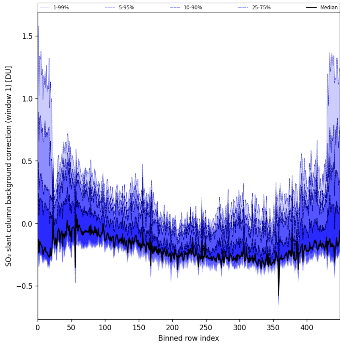
Figure 92: Along track statistics of “SO 2 slant column background correction (window 1)” for 2025-02-19 to 2025-02-20
