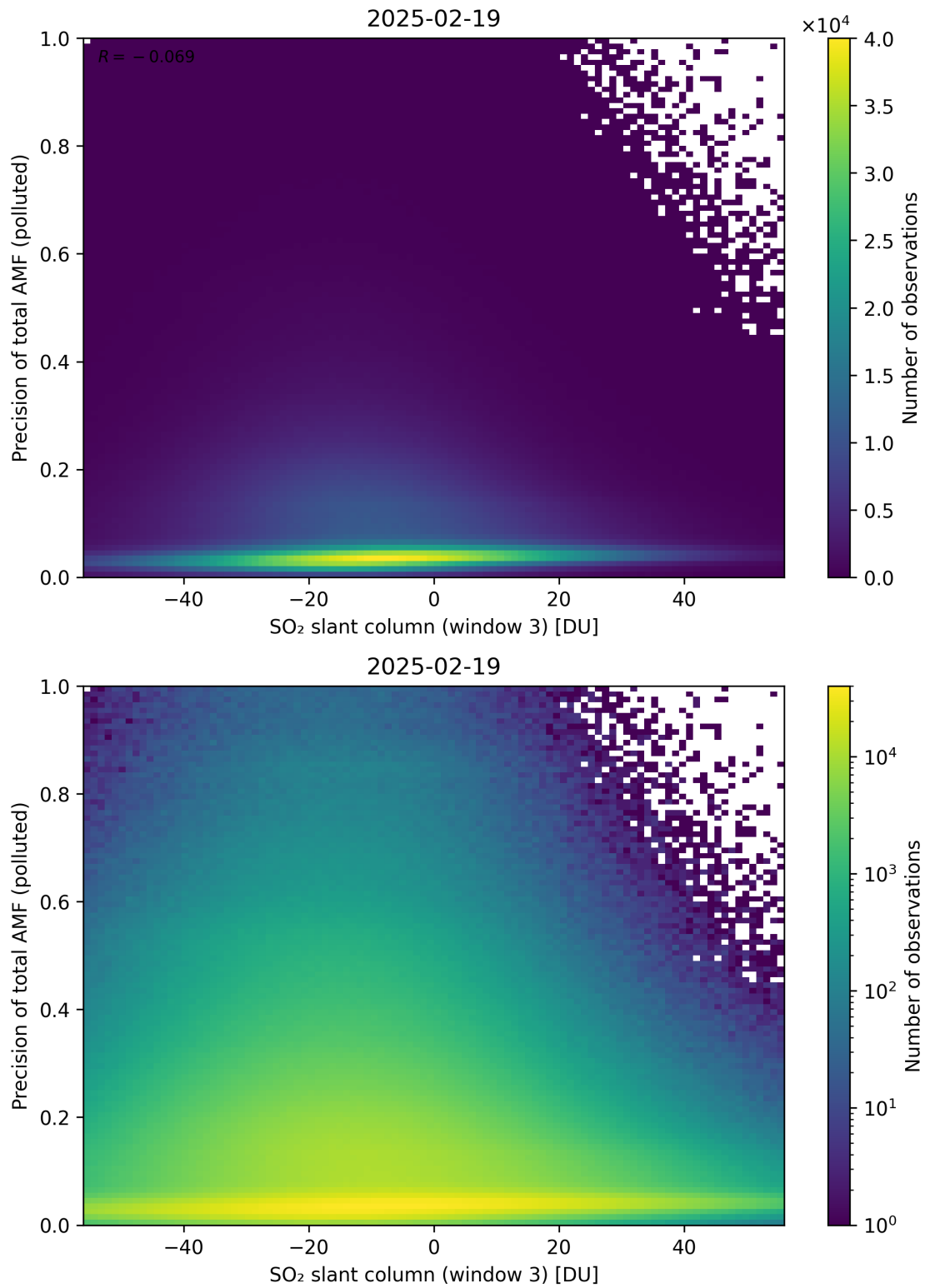
Figure 319: Scatter density plot of “SO 2 slant column (window 3)” against “Precision of total AMF (polluted)” for 2025-02-19 to 2025-02-20.
