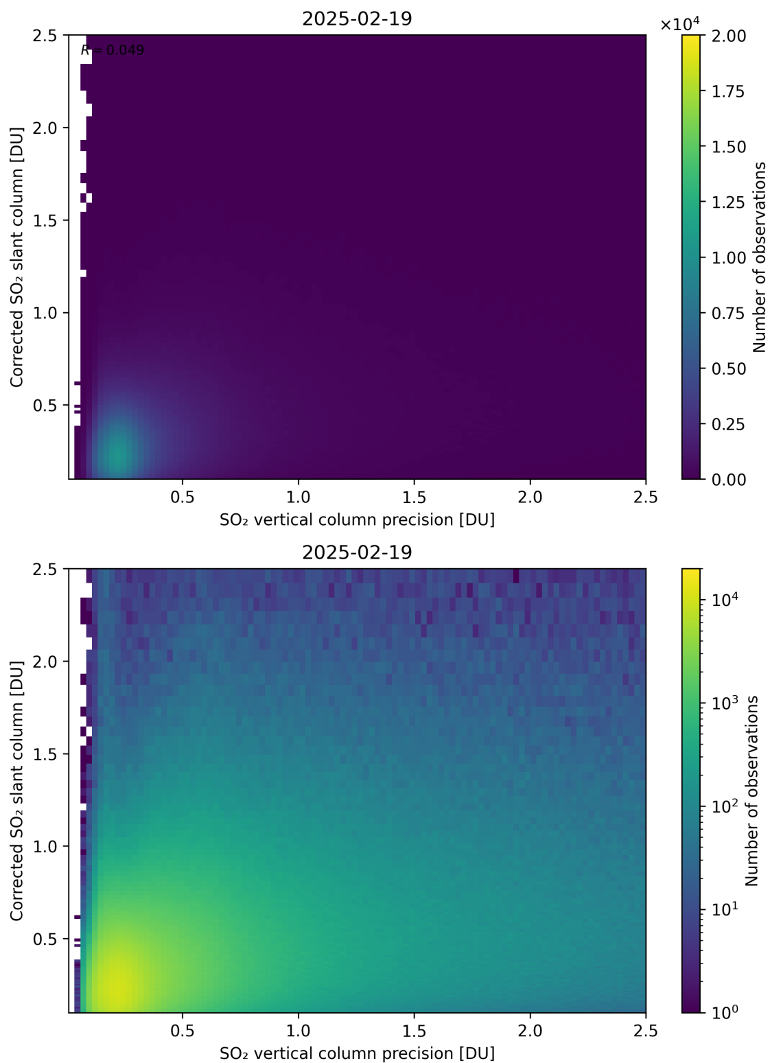
Figure 338: Scatter density plot of “SO 2 vertical column precision” against “Corrected SO 2 slant column” for 2025-02-19 to 2025-02-20.
