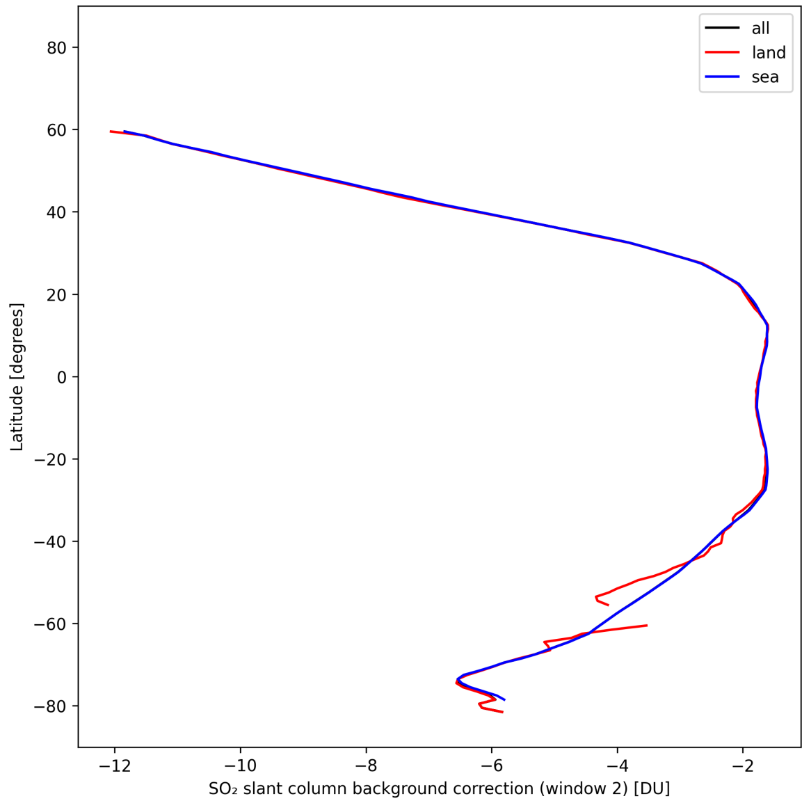
Figure 44: Zonal average of “SO 2 slant column background correction (window 2)” for 2025-02-19 to 2025-02-20.
