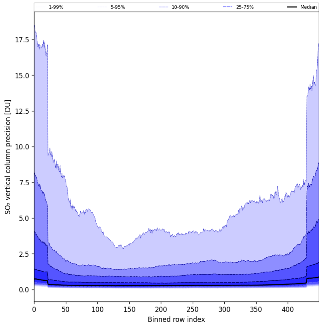
Figure 85: Along track statistics of “SO 2 vertical column precision” for 2025-02-19 to 2025-02-20
