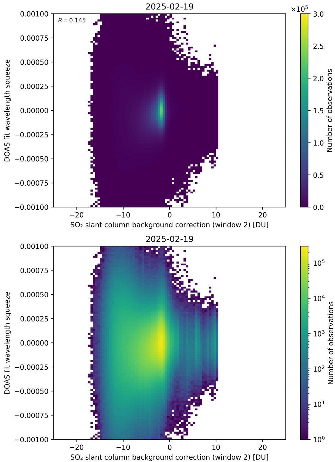
Figure 124: Scatter density plot of “SO 2 slant column background correction (window 2)” against “DOAS fit wavelength squeeze” for 2025-02-19 to 2025-02-20.
