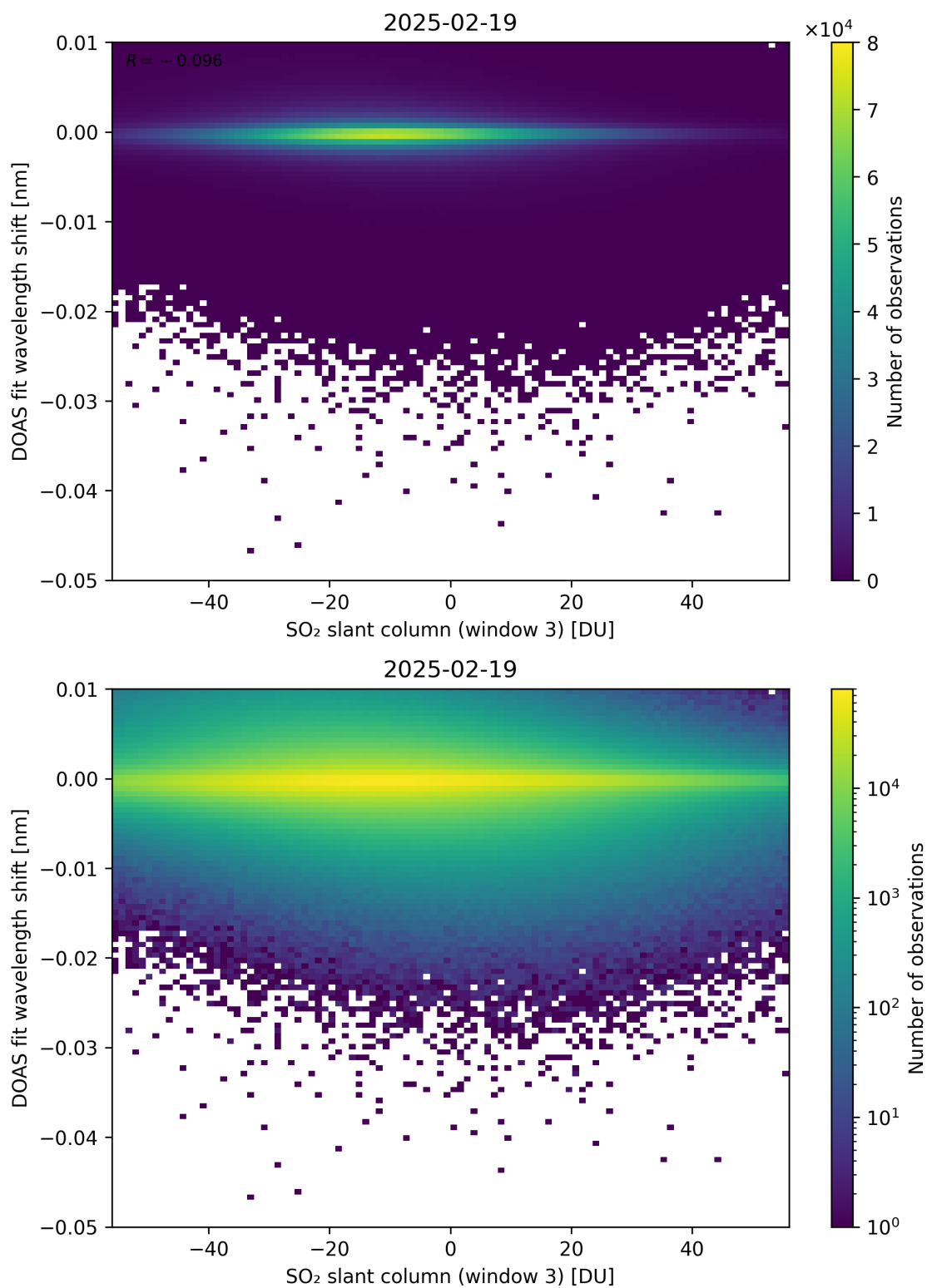
Figure 304: Scatter density plot of “SO 2 slant column (window 3)” against “DOAS fit wavelength shift” for 2025-02-19 to 2025-02-20.
