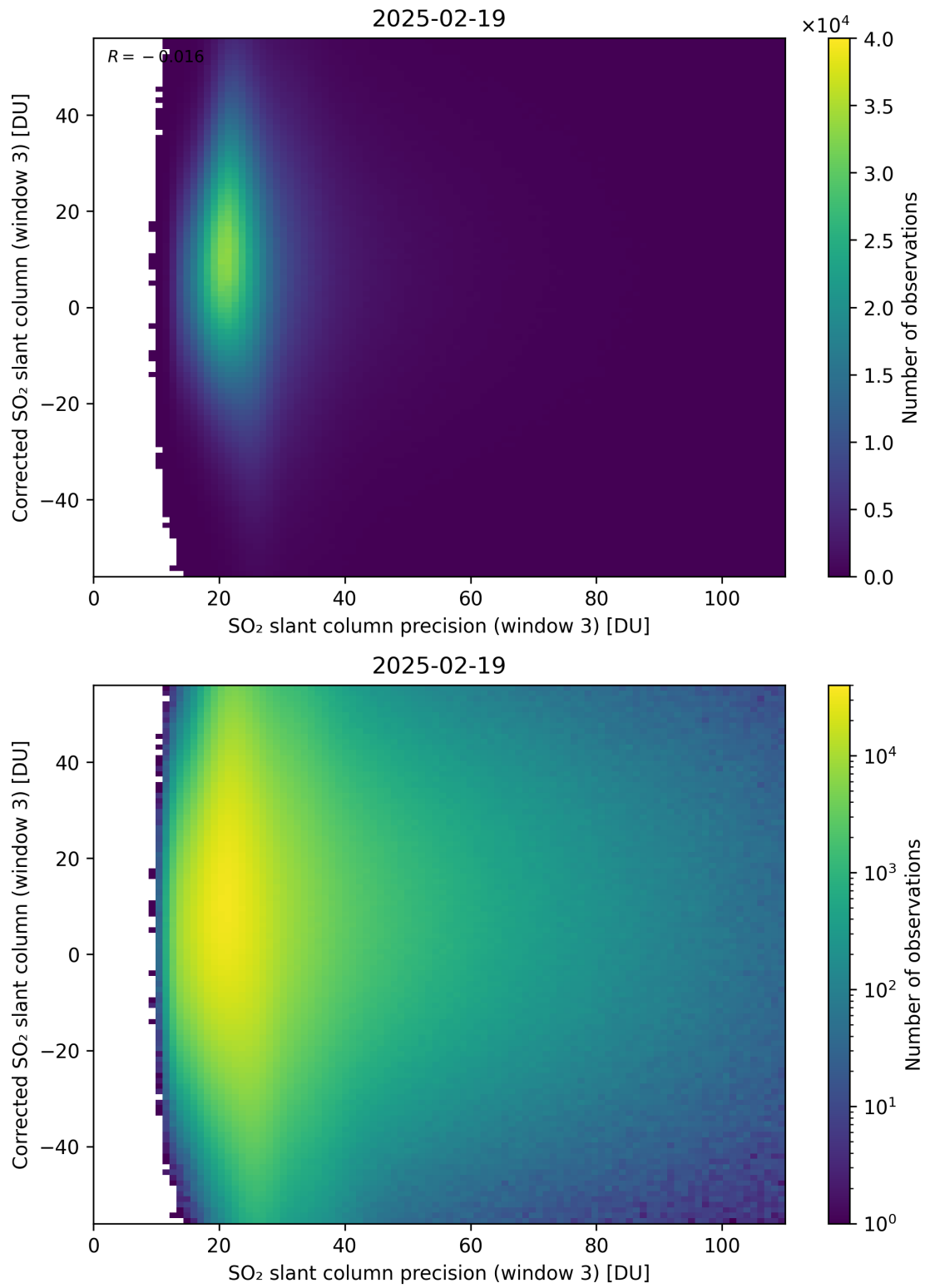
Figure 312: Scatter density plot of “SO 2 slant column precision (window 3)” against “Corrected SO 2 slant column (window 3)” for 2025-02-19 to 2025-02-20.
