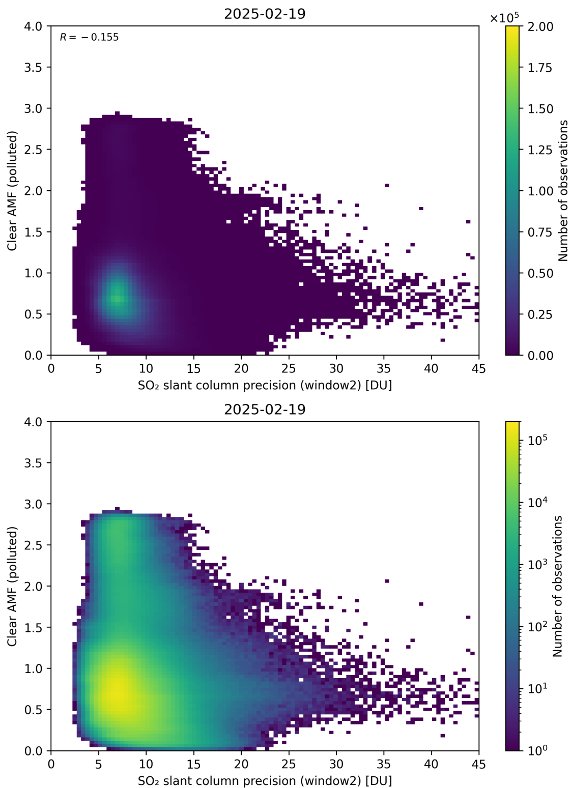
Figure 296: Scatter density plot of “SO 2 slant column precision (window2)” against “Clear AMF (polluted)” for 2025-02-19 to 2025-02-20.
