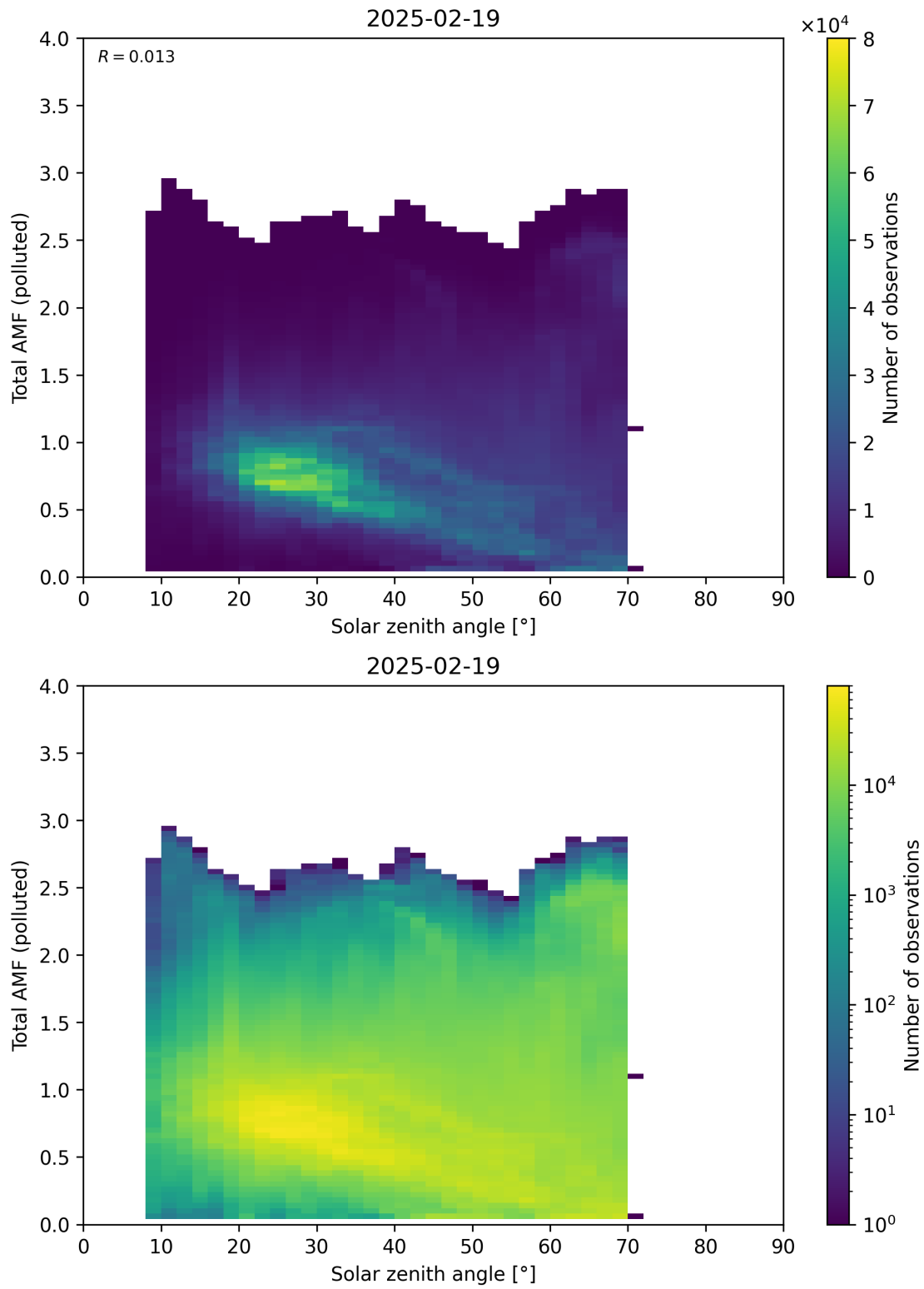
Figure 189: Scatter density plot of “Solar zenith angle” against “Total AMF (polluted)” for 2025-02-19 to 2025-02-20.
