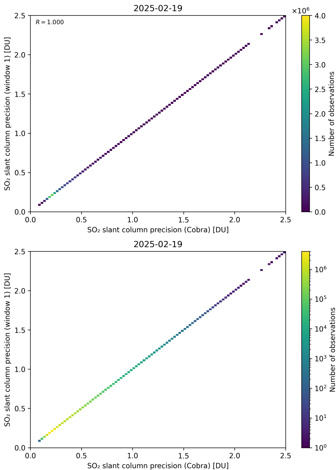
Figure 209: Scatter density plot of “SO 2 slant column precision (Cobra)” against “SO 2 slant column precision (window 1)” for 2025-02-19 to 2025-02-20.
