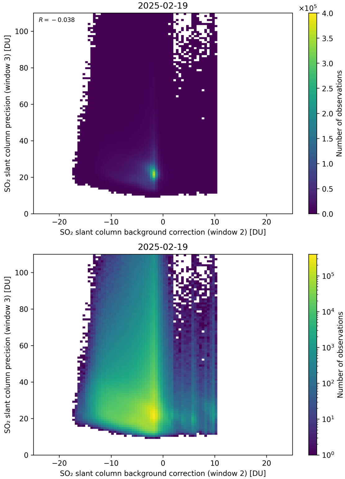
Figure 129: Scatter density plot of “SO 2 slant column background correction (window 2)” against “SO 2 slant column precision (window 3)” for 2025-02-19 to 2025-02-20.
