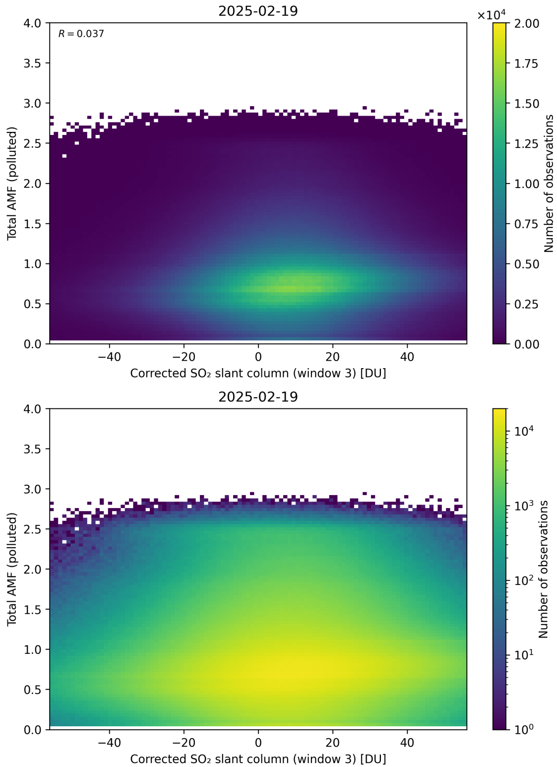
Figure 260: Scatter density plot of “Corrected SO 2 slant column (window 3)” against “Total AMF (polluted)” for 2025-02-19 to 2025-02-20.
