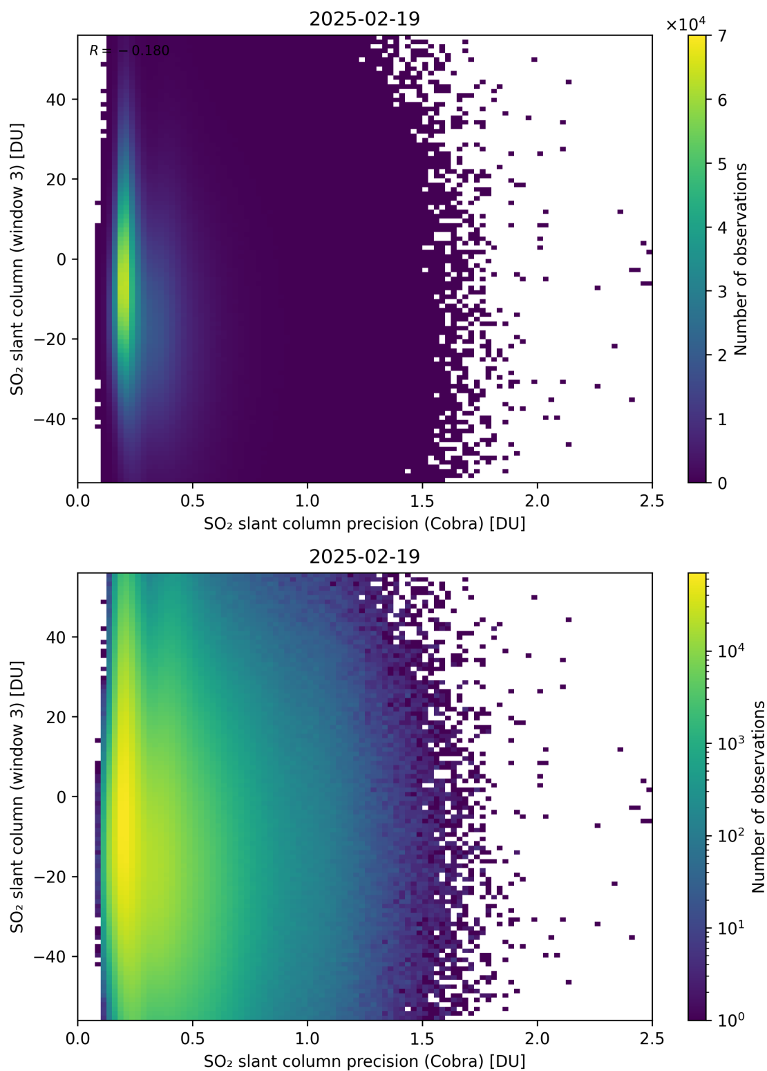
Figure 211: Scatter density plot of “SO 2 slant column precision (Cobra)” against “SO 2 slant column (window 3)” for 2025-02-19 to 2025-02-20.
