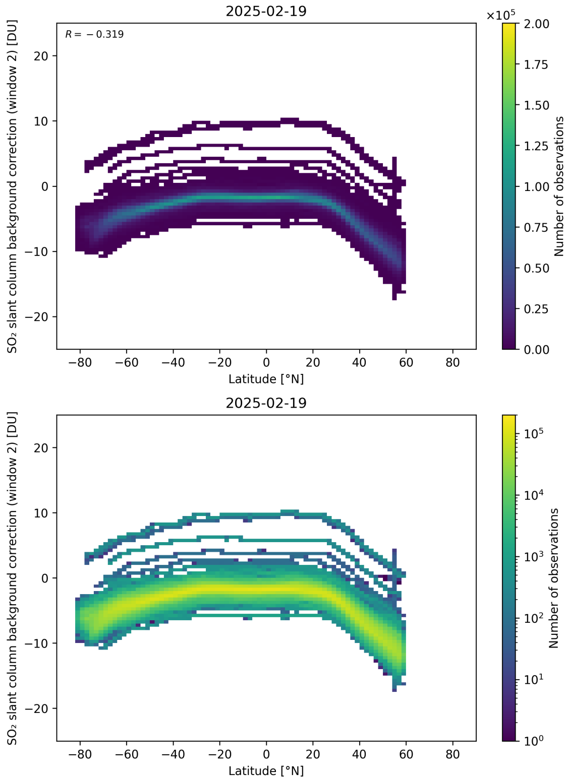
Figure 151: Scatter density plot of “Latitude” against “SO 2 slant column background correction (window 2)” for 2025-02-19 to 2025-02-20.
