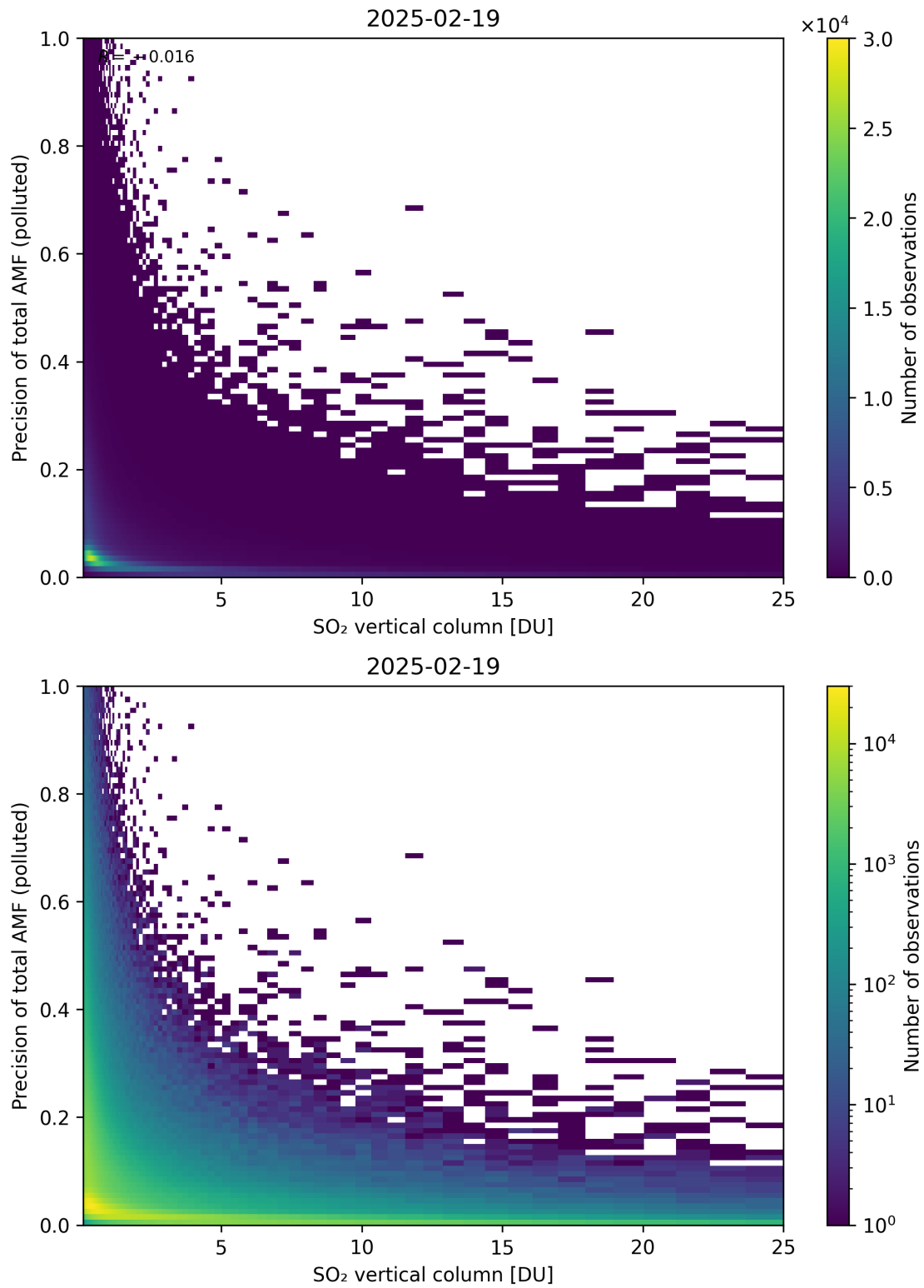
Figure 360: Scatter density plot of “SO 2 vertical column” against “Precision of total AMF (polluted)” for 2025-02-19 to 2025-02-20.
