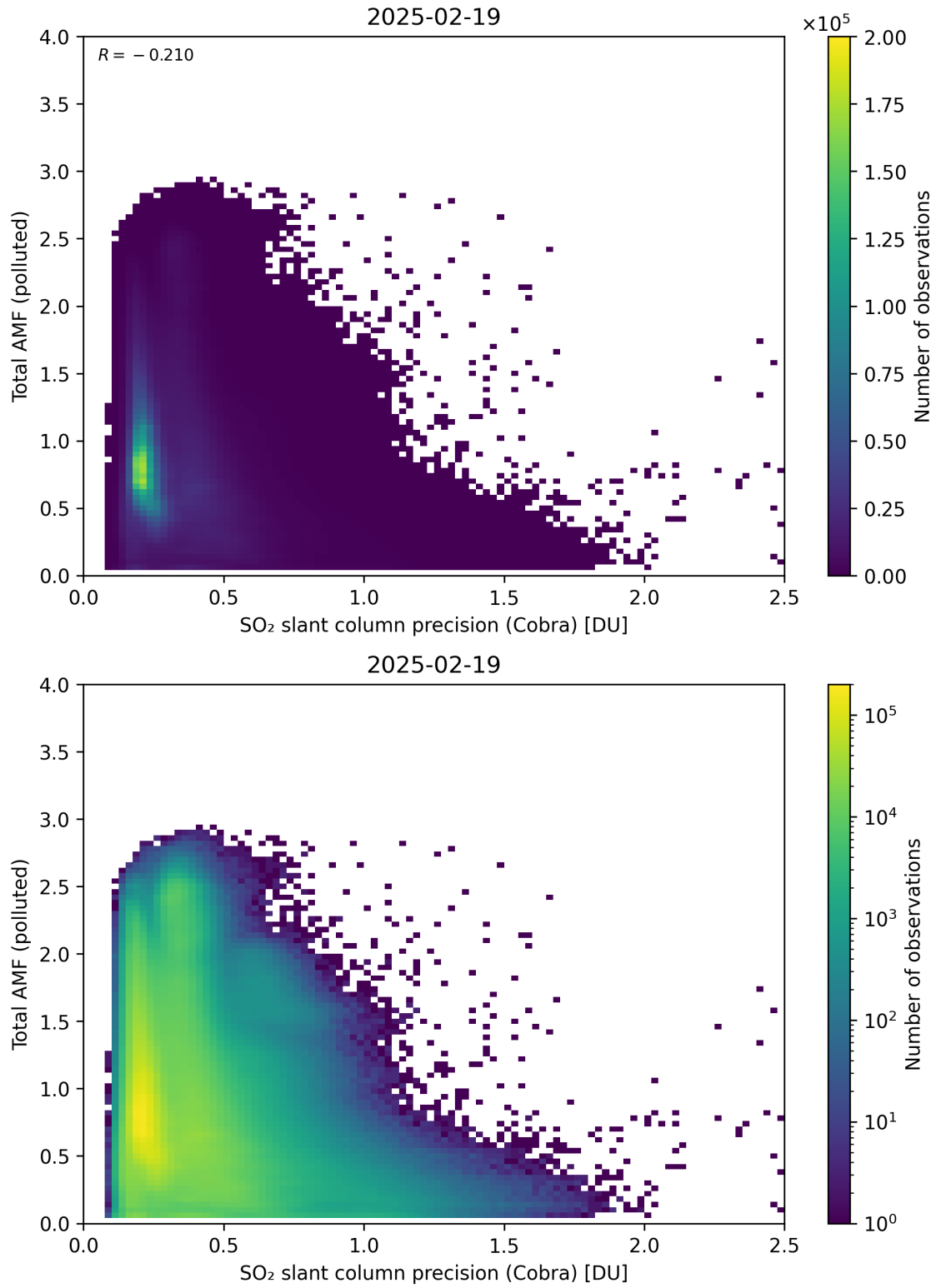
Figure 213: Scatter density plot of “SO 2 slant column precision (Cobra)” against “Total AMF (polluted)” for 2025-02-19 to 2025-02-20.
