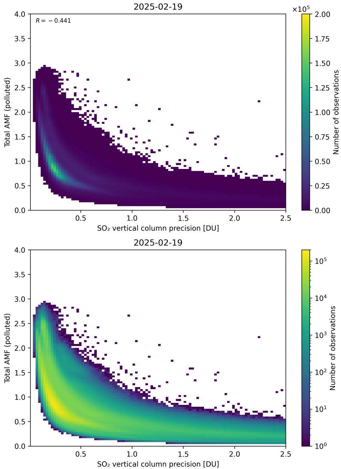
Figure 346: Scatter density plot of “SO 2 vertical column precision” against “Total AMF (polluted)” for 2025-02-19 to 2025-02-20.
