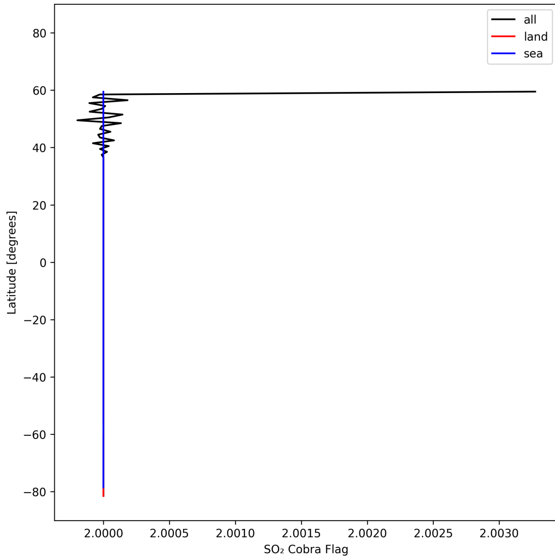
Figure 49: Zonal average of "SO 2 Cobra Flag" for 2025-02-19 to 2025-02-20.
