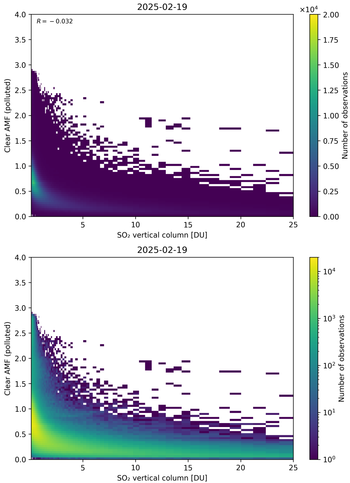
Figure 348: Scatter density plot of “SO 2 vertical column” against “Clear AMF (polluted)” for 2025-02-19 to 2025-02-20.
