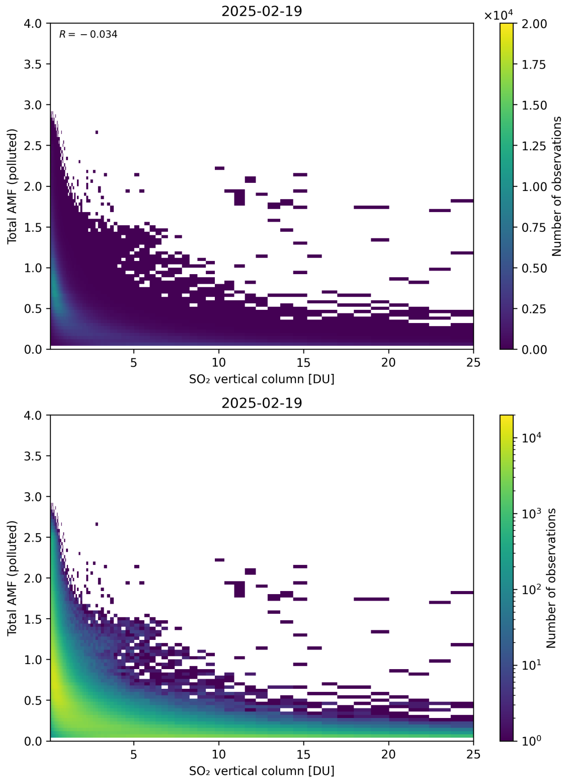
Figure 359: Scatter density plot of “SO 2 vertical column” against “Total AMF (polluted)” for 2025-02-19 to 2025-02-20.
