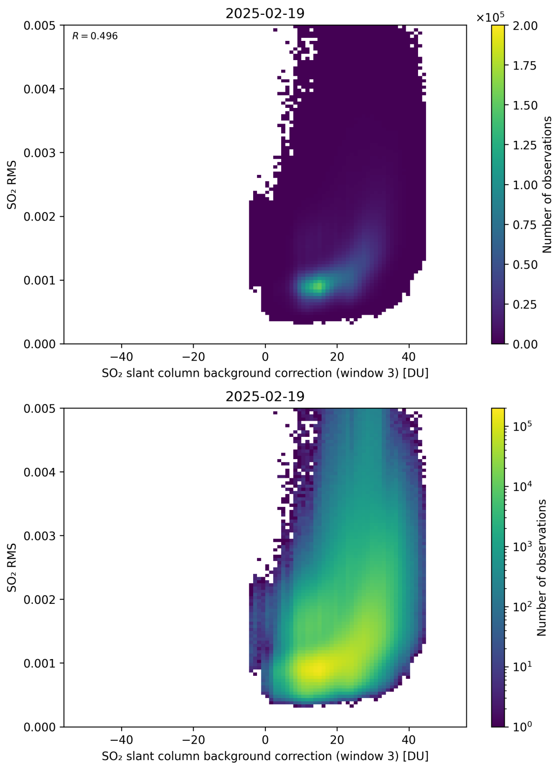
Figure 134: Scatter density plot of “SO 2 slant column background correction (window 3)” against “SO 2 RMS” for 2025-02-19 to 2025-02-20.
