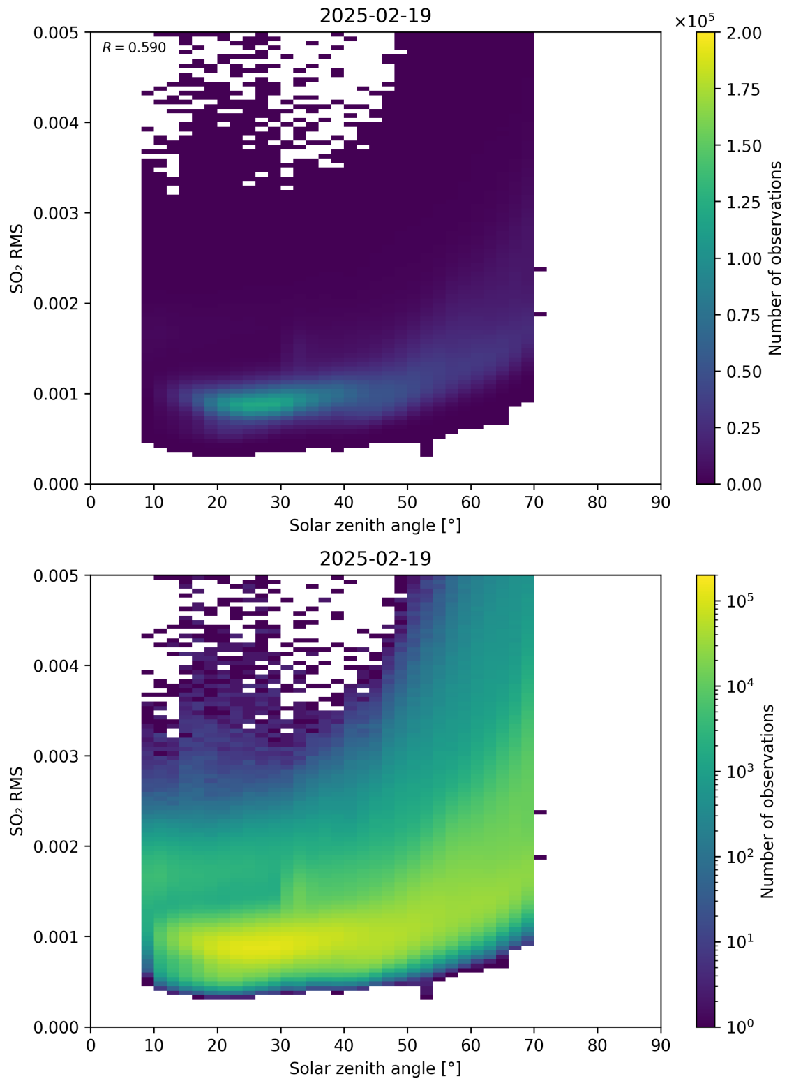
Figure 176: Scatter density plot of “Solar zenith angle” against “SO 2 RMS” for 2025-02-19 to 2025-02-20.
