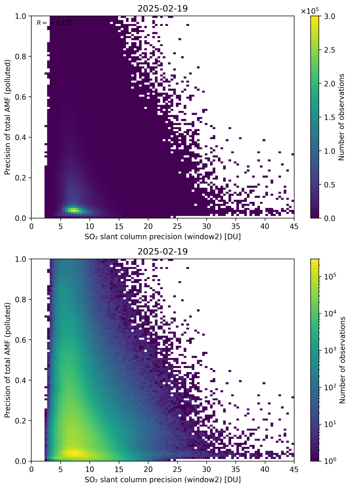
Figure 302: Scatter density plot of “SO 2 slant column precision (window2)” against “Precision of total AMF (polluted)” for 2025-02-19 to 2025-02-20.
