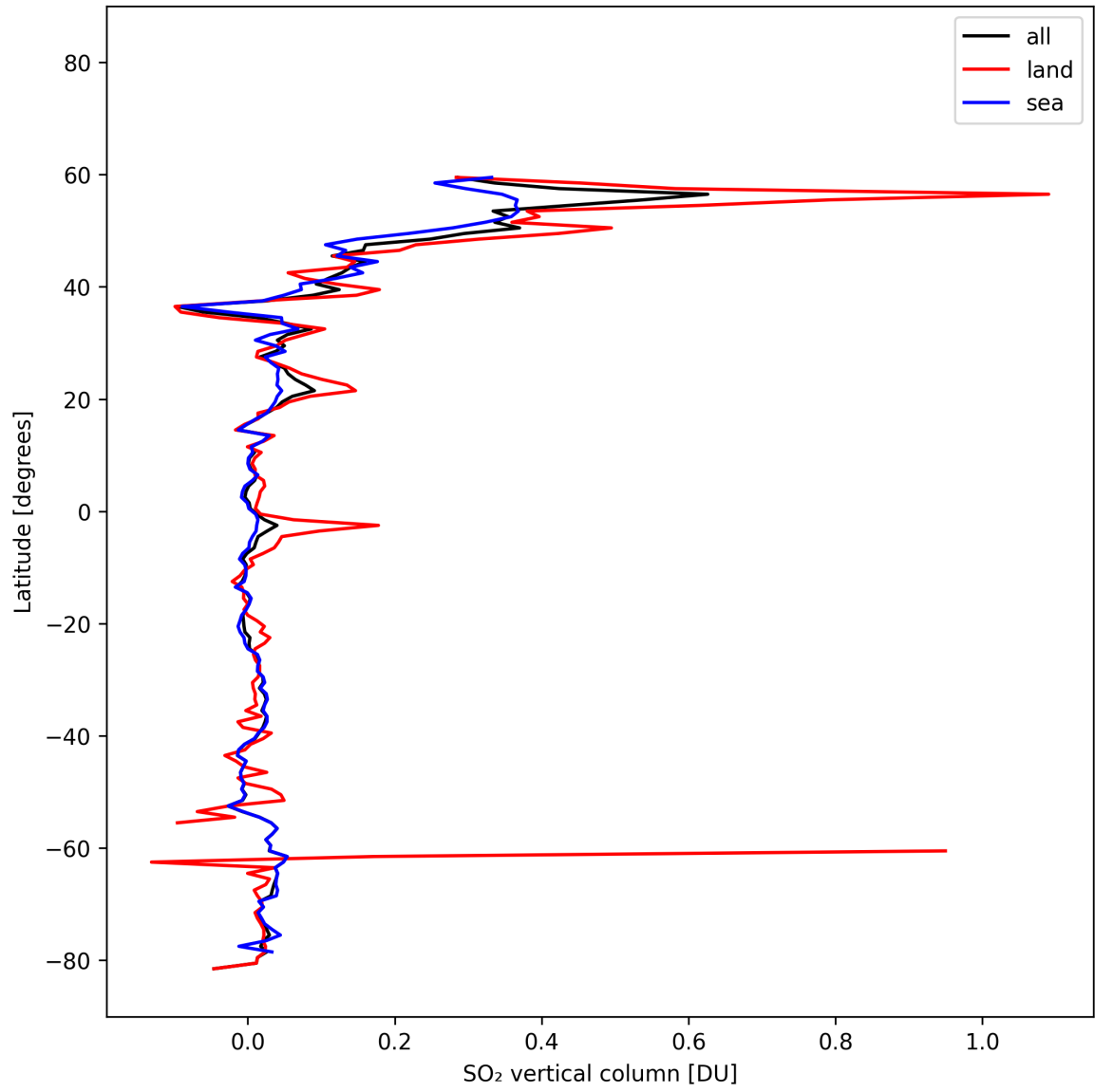
Figure 32: Zonal average of “SO 2 vertical column” for 2025-02-19 to 2025-02-20.
