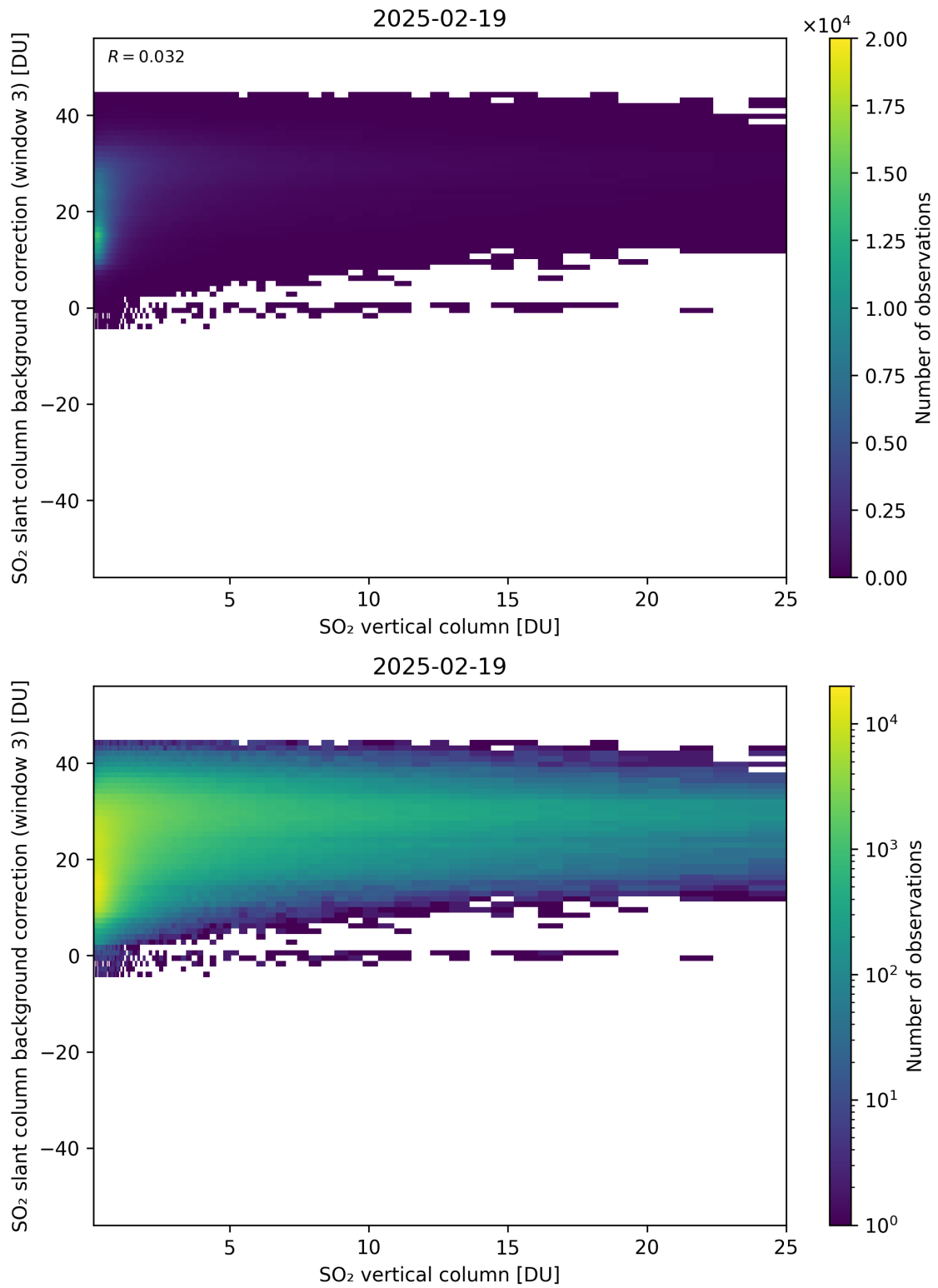
Figure 325: Scatter density plot of “SO 2 vertical column” against “SO 2 slant column background correction (window 3)” for 2025-02-19 to 2025-02-20.
