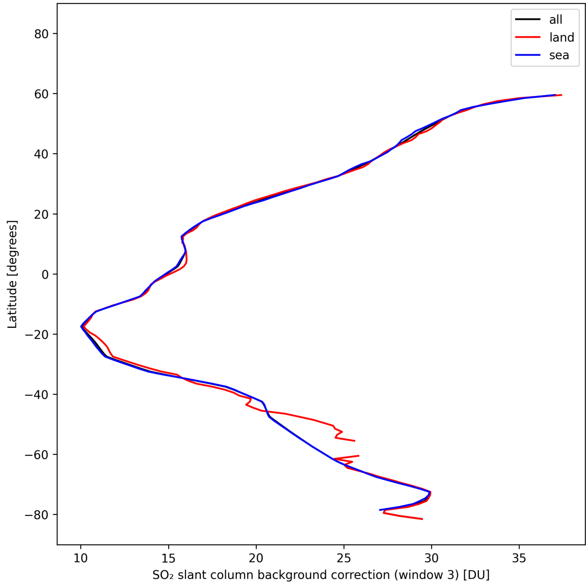
Figure 48: Zonal average of “SO 2 slant column background correction (window 3)” for 2025-02-19 to 2025-02-20.
