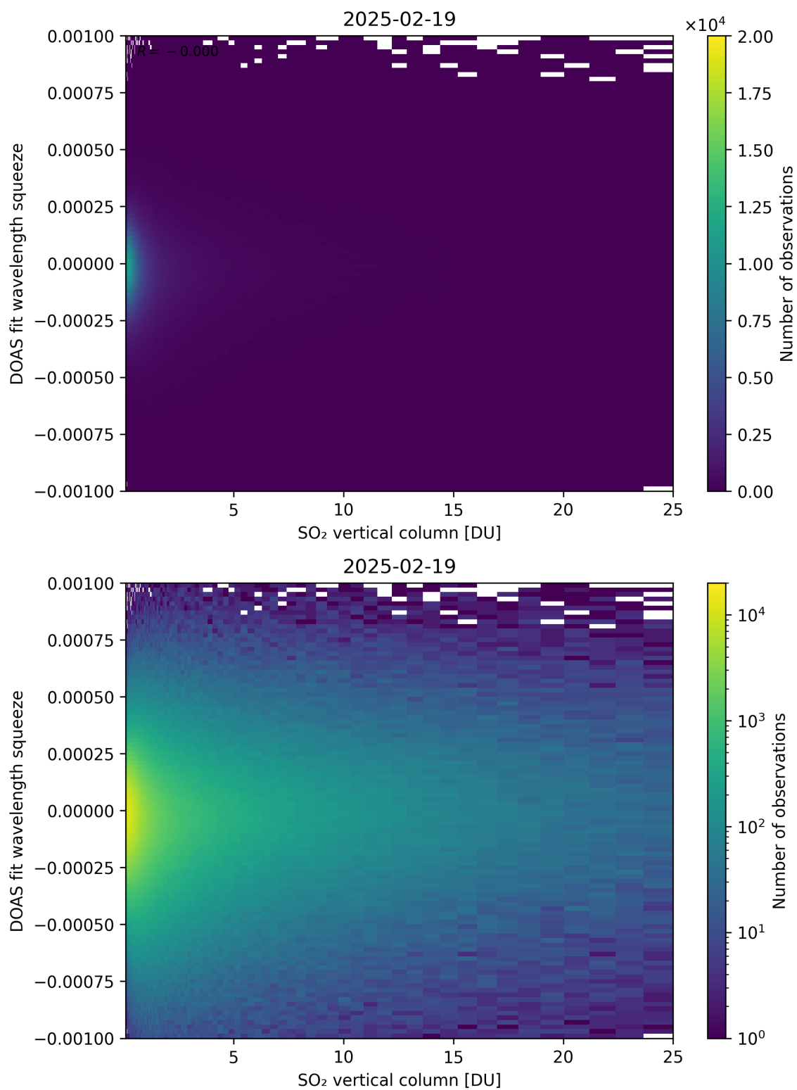
Figure 327: Scatter density plot of “SO 2 vertical column” against “DOAS fit wavelength squeeze” for 2025-02-19 to 2025-02-20.
