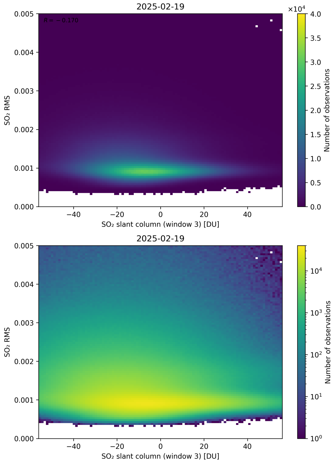
Figure 306: Scatter density plot of “SO 2 slant column (window 3)” against “SO 2 RMS” for 2025-02-19 to 2025-02-20.
