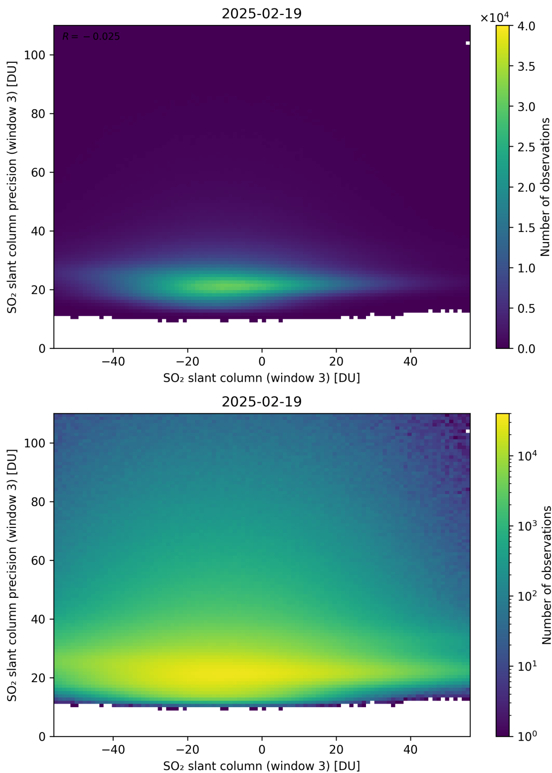
Figure 317: Scatter density plot of “SO 2 slant column (window 3)” against “SO 2 slant column precision (window 3)” for 2025-02-19 to 2025-02-20.
