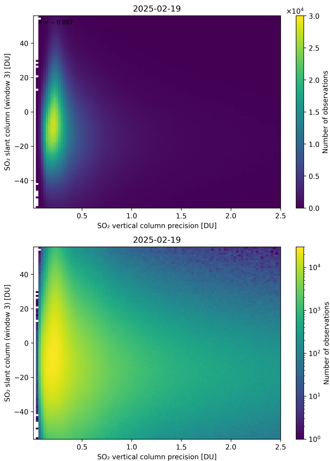
Figure 344: Scatter density plot of “SO 2 vertical column precision” against “SO 2 slant column (window 3)” for 2025-02-19 to 2025-02-20.
