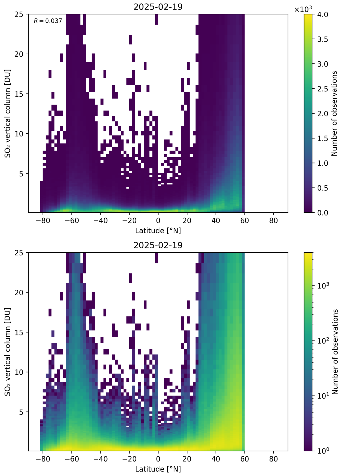
Figure 169: Scatter density plot of “Latitude” against “SO 2 vertical column” for 2025-02-19 to 2025-02-20.
