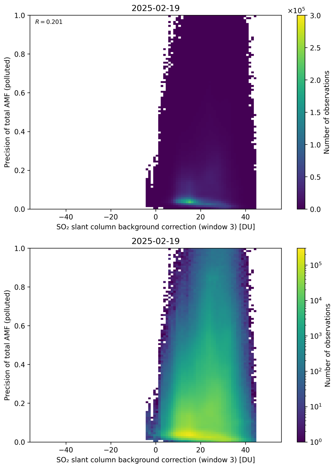
Figure 137: Scatter density plot of “SO 2 slant column background correction (window 3)” against “Precision of total AMF (polluted)” for 2025-02-19 to 2025-02-20.
