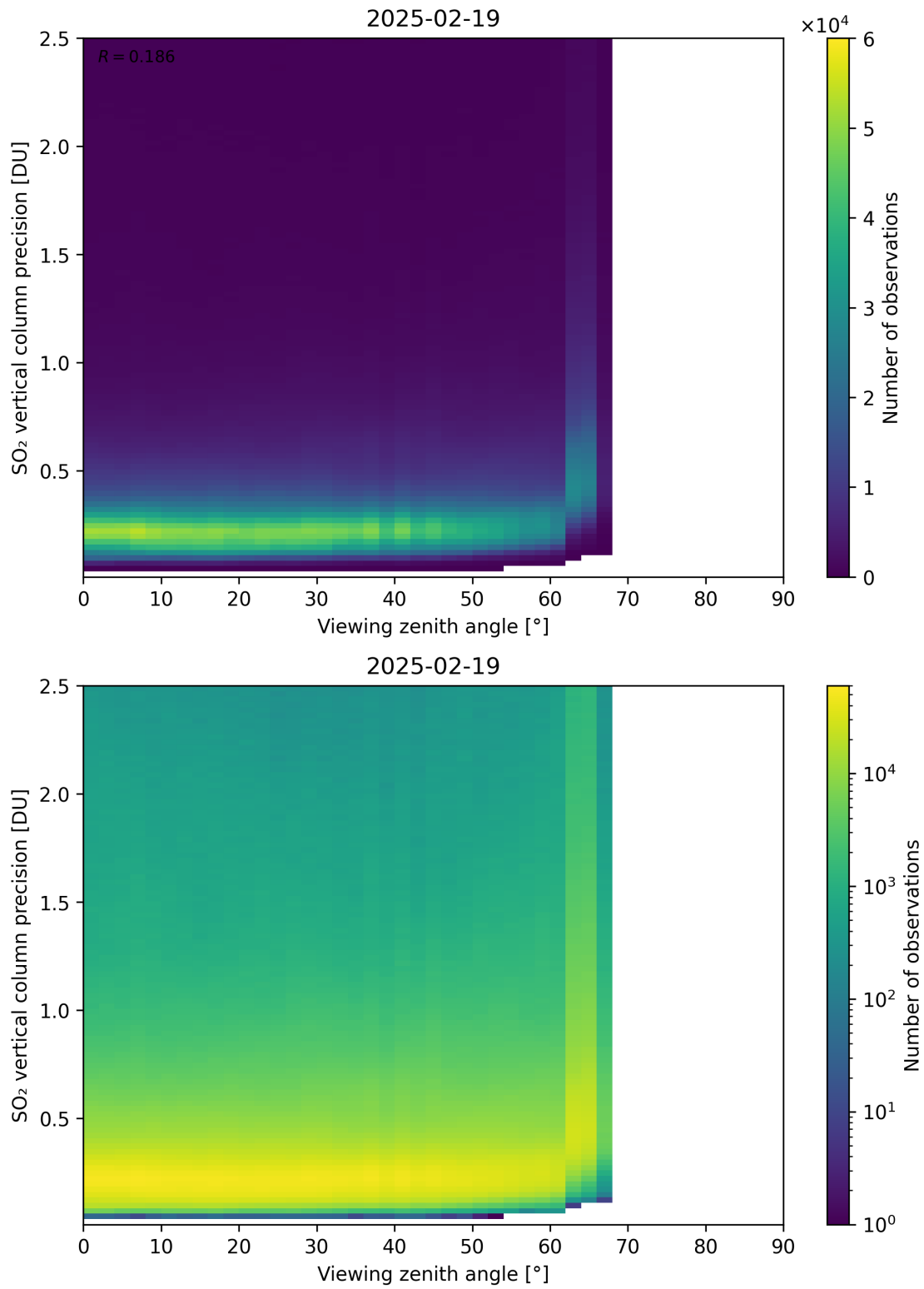
Figure 384: Scatter density plot of “Viewing zenith angle” against “SO 2 vertical column precision” for 2025-02-19 to 2025-02-20.
