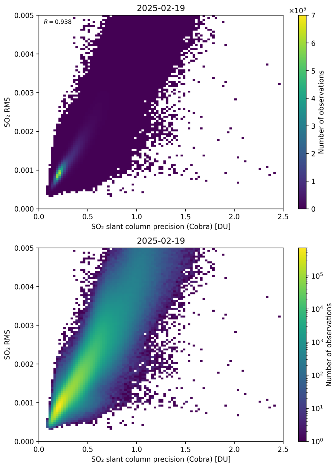
Figure 204: Scatter density plot of “SO 2 slant column precision (Cobra)” against “SO 2 RMS” for 2025-02-19 to 2025-02-20.
