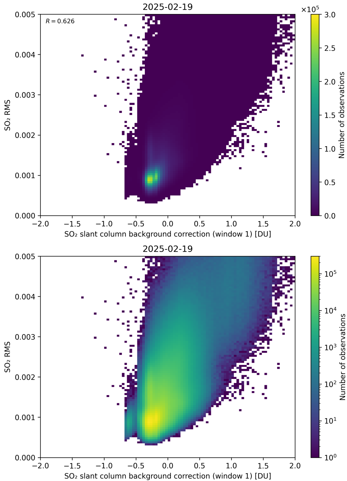
Figure 113: Scatter density plot of “SO 2 slant column background correction (window 1)” against “SO 2 RMS” for 2025-02-19 to 2025-02-20.
