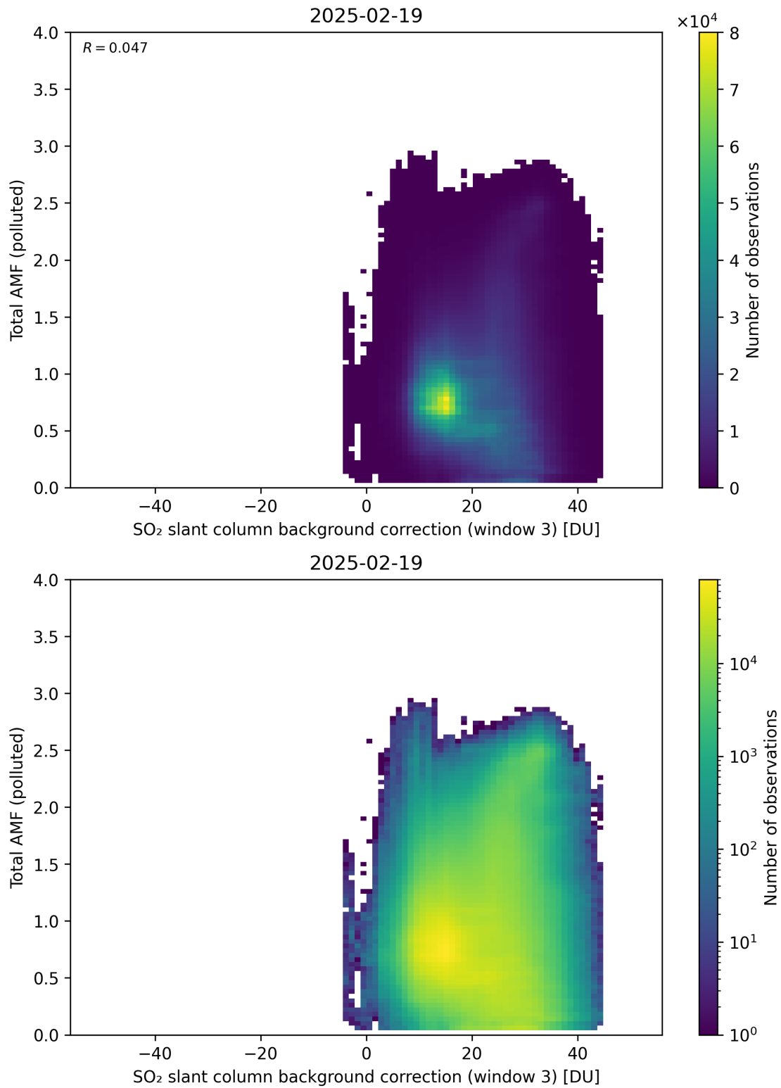
Figure 136: Scatter density plot of “SO 2 slant column background correction (window 3)” against “Total AMF (polluted)” for 2025-02-19 to 2025-02-20.
