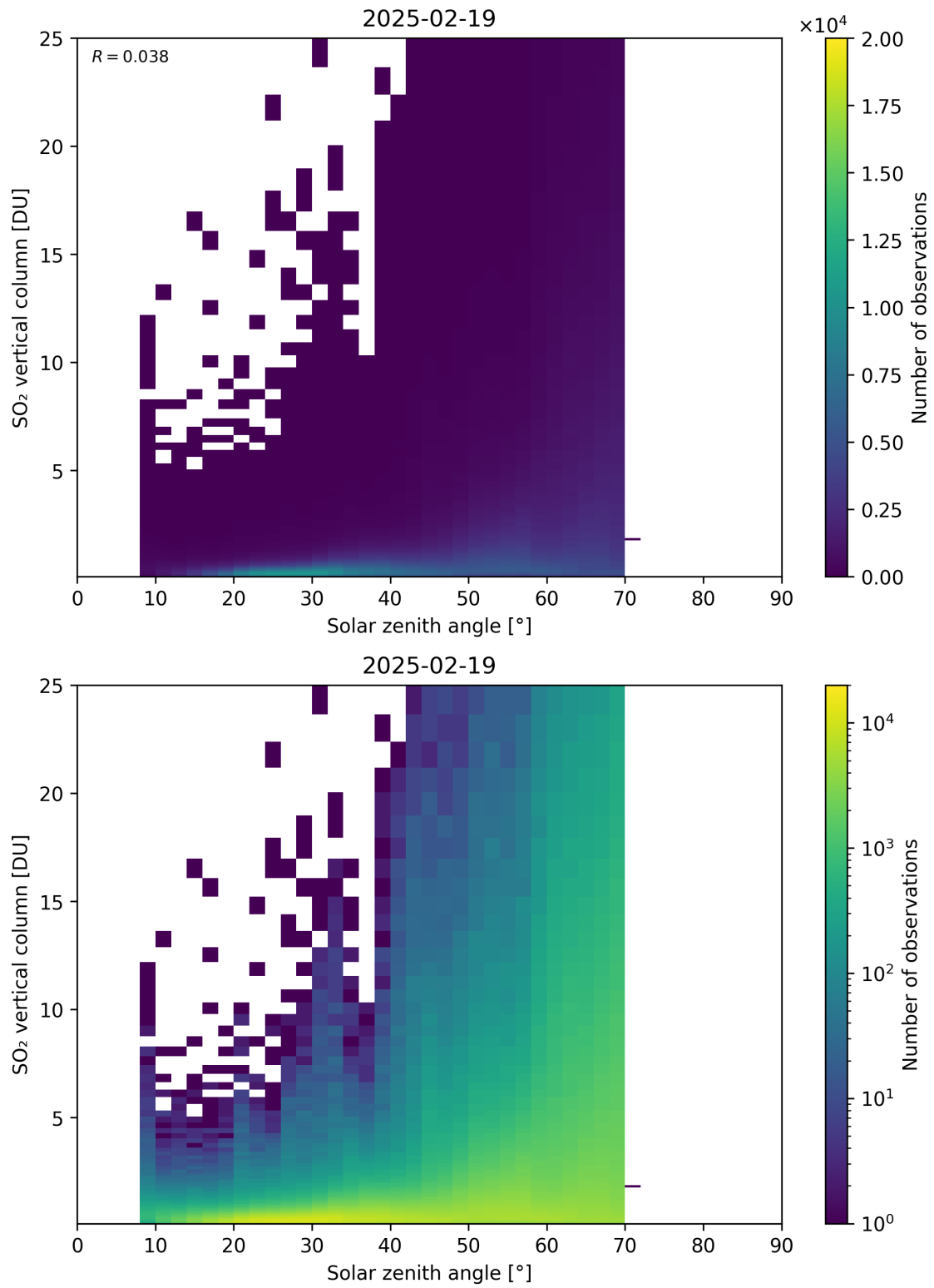
Figure 191: Scatter density plot of “Solar zenith angle” against “SO 2 vertical column” for 2025-02-19 to 2025-02-20.
