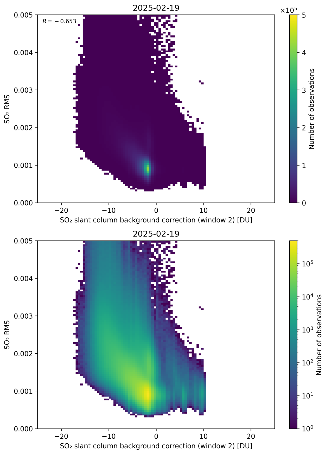
Figure 125: Scatter density plot of “SO 2 slant column background correction (window 2)” against “SO 2 RMS” for 2025-02-19 to 2025-02-20.
