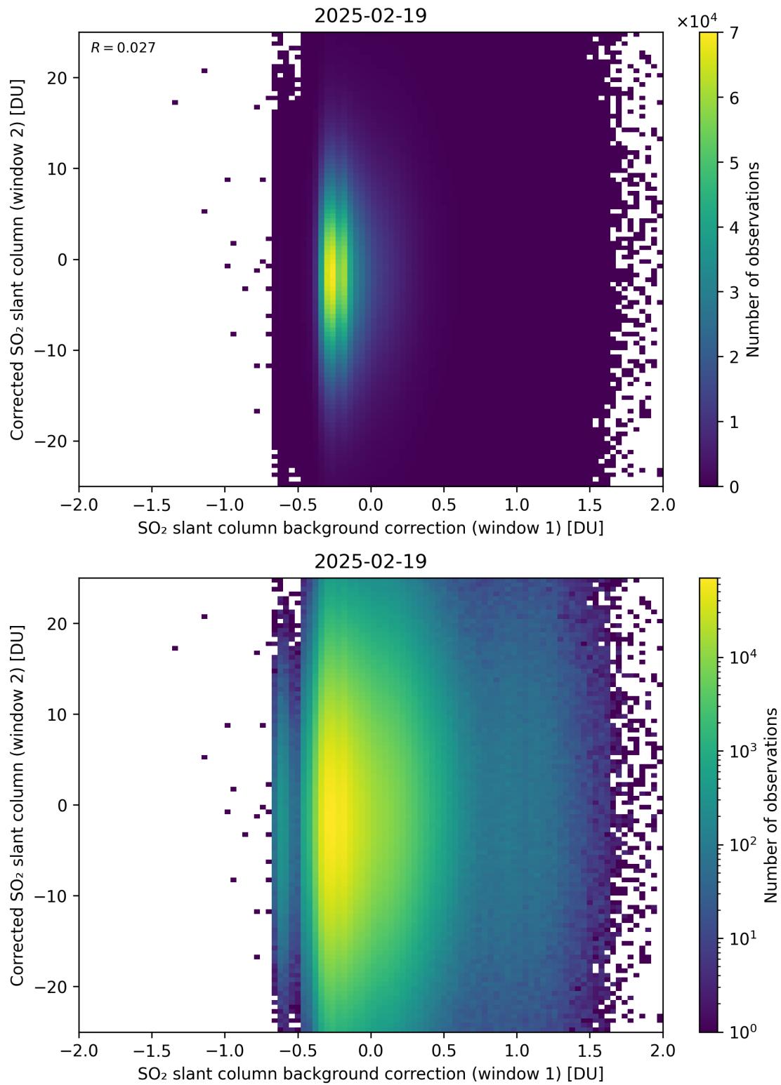
Figure 115: Scatter density plot of “SO 2 slant column background correction (window 1)” against “Corrected SO 2 slant column (window 2)” for 2025-02-19 to 2025-02-20.
