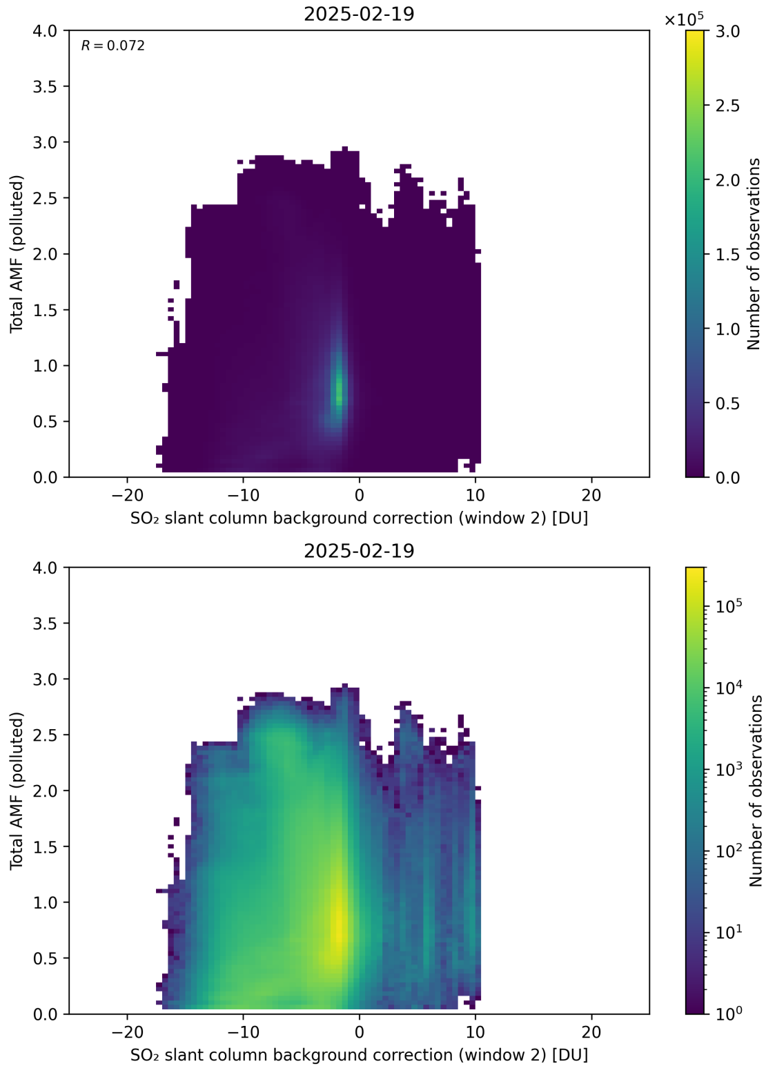
Figure 130: Scatter density plot of “SO 2 slant column background correction (window 2)” against “Total AMF (polluted)” for 2025-02-19 to 2025-02-20.
