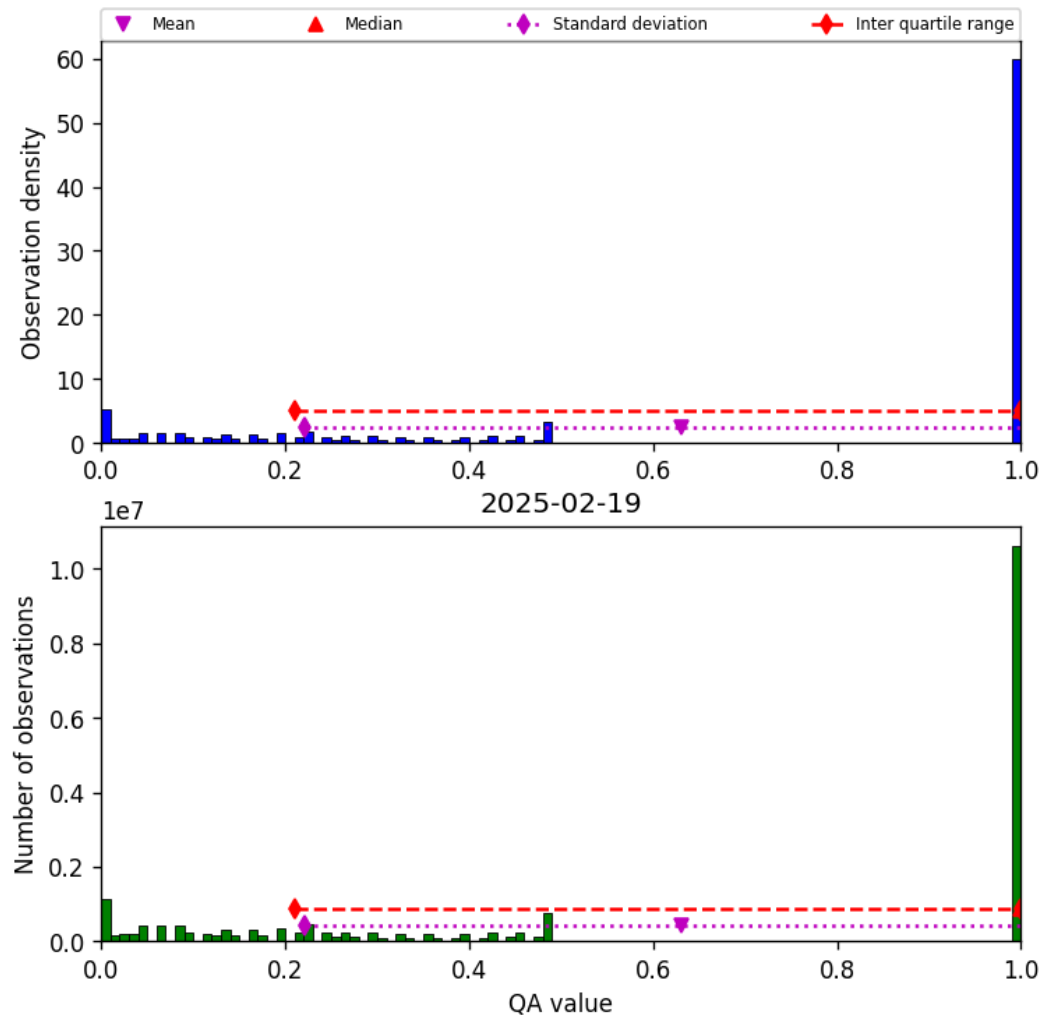
Figure 57: Histogram of “QA value” for 2025-02-19 to 2025-02-20
