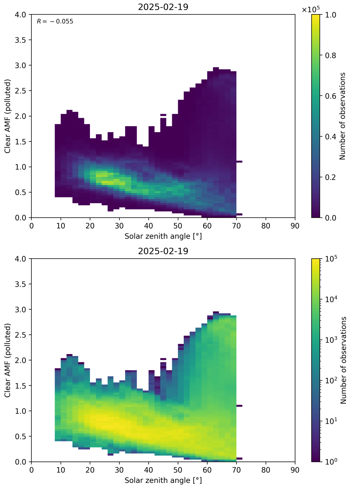
Figure 178: Scatter density plot of “Solar zenith angle” against “Clear AMF (polluted)” for 2025-02-19 to 2025-02-20.
