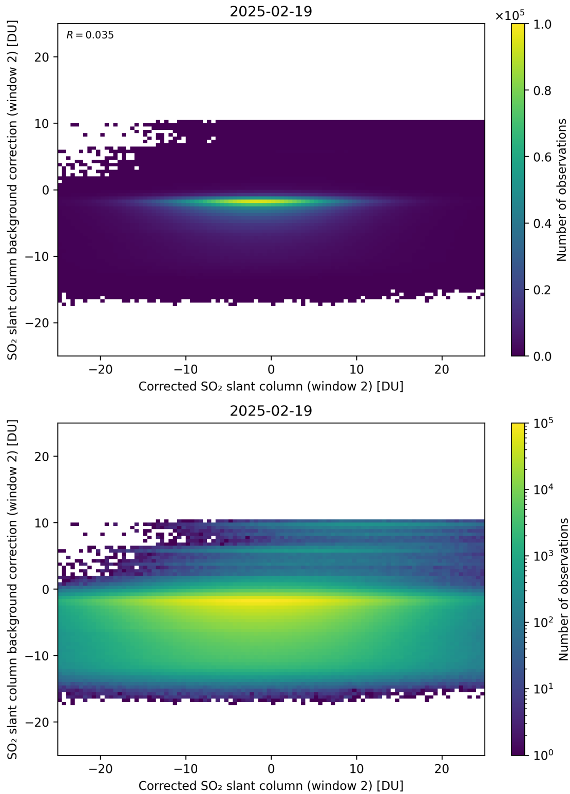
Figure 244: Scatter density plot of “Corrected SO 2 slant column (window 2)” against “SO 2 slant column background correction (window 2)” for 2025-02-19 to 2025-02-20.
