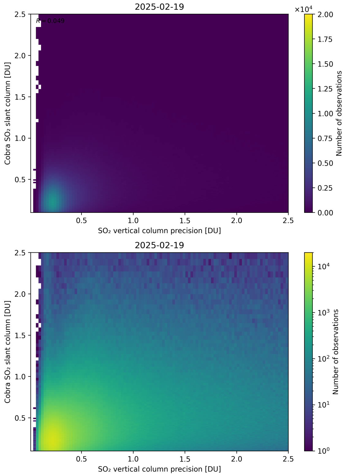
Figure 336: Scatter density plot of “SO 2 vertical column precision” against “Cobra SO 2 slant column” for 2025-02-19 to 2025-02-20.
