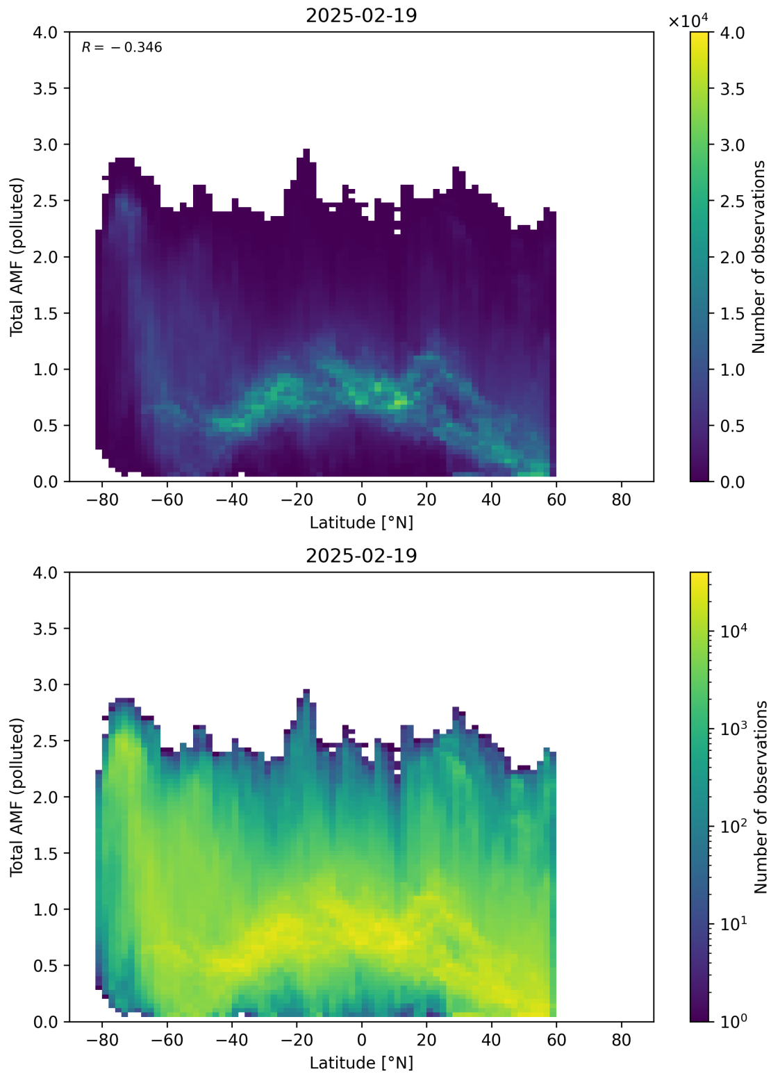
Figure 167: Scatter density plot of “Latitude” against “Total AMF (polluted)” for 2025-02-19 to 2025-02-20.
