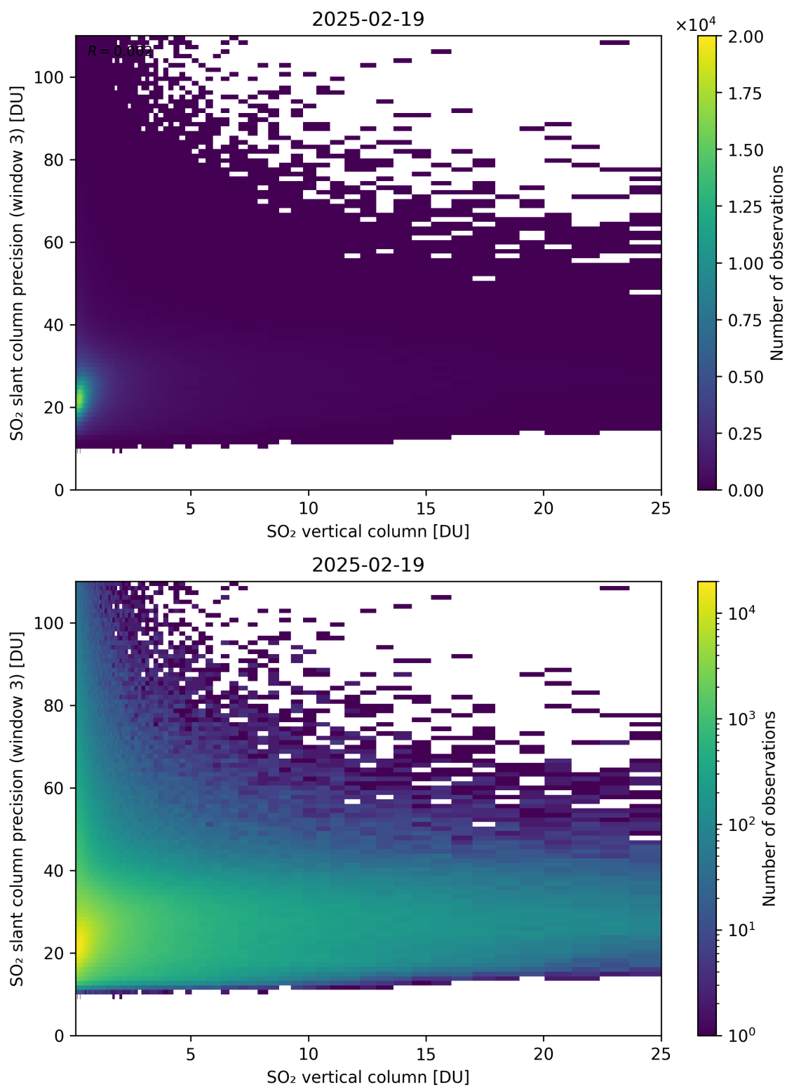
Figure 358: Scatter density plot of “SO 2 vertical column” against “SO 2 slant column precision (window 3)” for 2025-02-19 to 2025-02-20.
