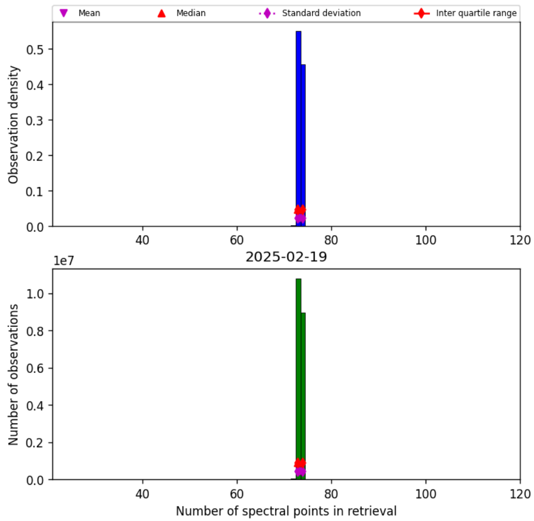
Figure 82: Histogram of “Number of spectral points in retrieval” for 2025-02-19 to 2025-02-20
