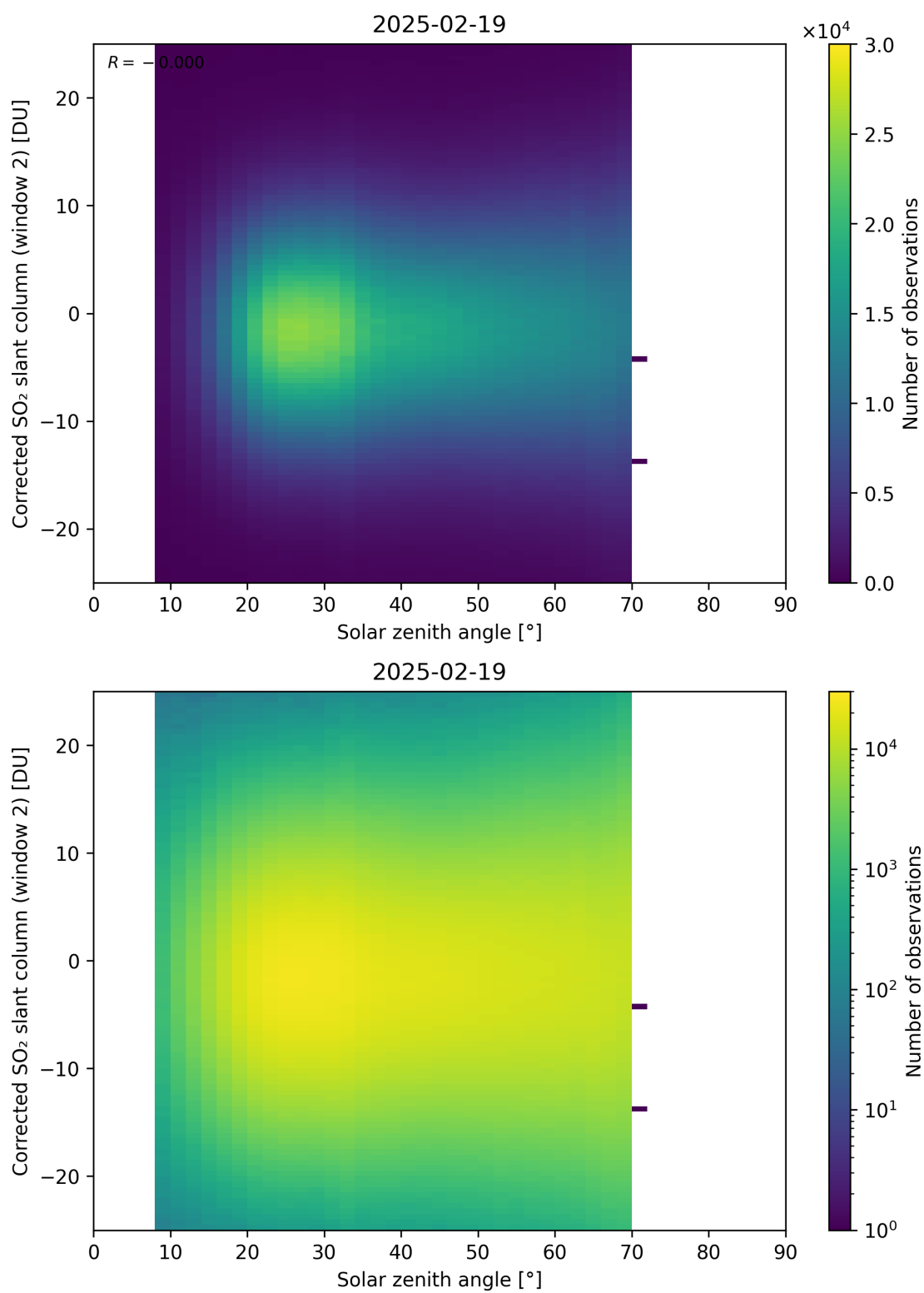
Figure 182: Scatter density plot of “Solar zenith angle” against “Corrected SO 2 slant column (window 2)” for 2025-02-19 to 2025-02-20.
