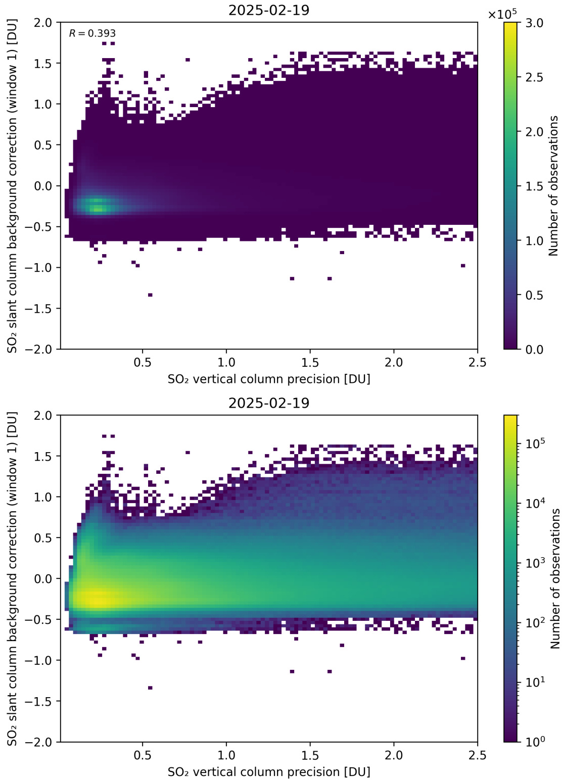
Figure 329: Scatter density plot of “SO 2 vertical column precision” against “SO 2 slant column background correction (window 1)” for 2025-02-19 to 2025-02-20.
