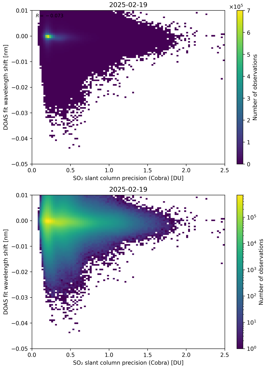
Figure 202: Scatter density plot of “SO 2 slant column precision (Cobra)” against “DOAS fit wavelength shift” for 2025-02-19 to 2025-02-20.
