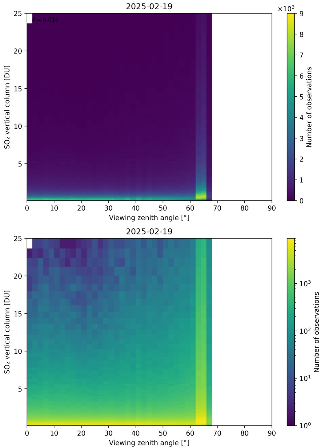
Figure 383: Scatter density plot of “Viewing zenith angle” against “SO 2 vertical column” for 2025-02-19 to 2025-02-20.
