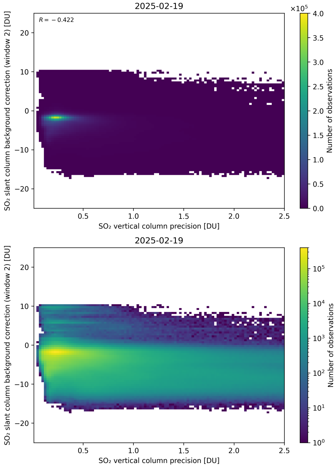
Figure 330: Scatter density plot of “SO 2 vertical column precision” against “SO 2 slant column background correction (window 2)” for 2025-02-19 to 2025-02-20.
