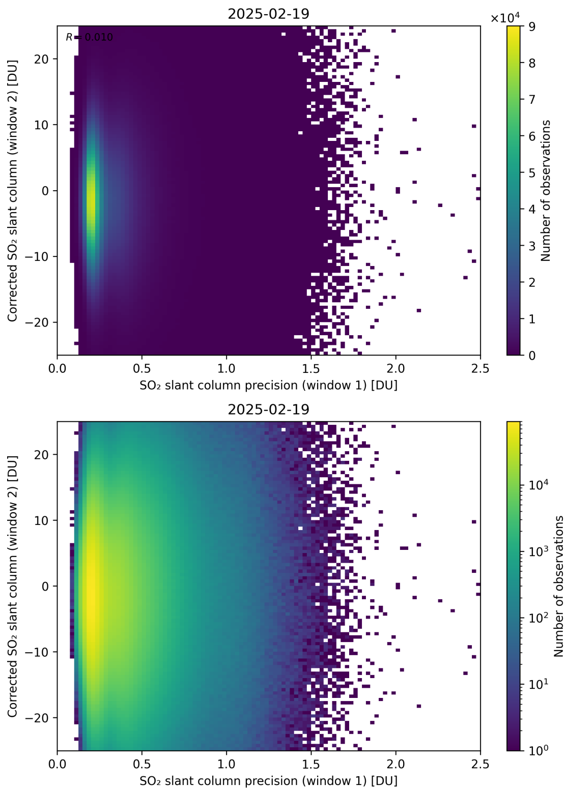
Figure 275: Scatter density plot of “SO 2 slant column precision (window 1)” against “Corrected SO 2 slant column (window 2)” for 2025-02-19 to 2025-02-20.
