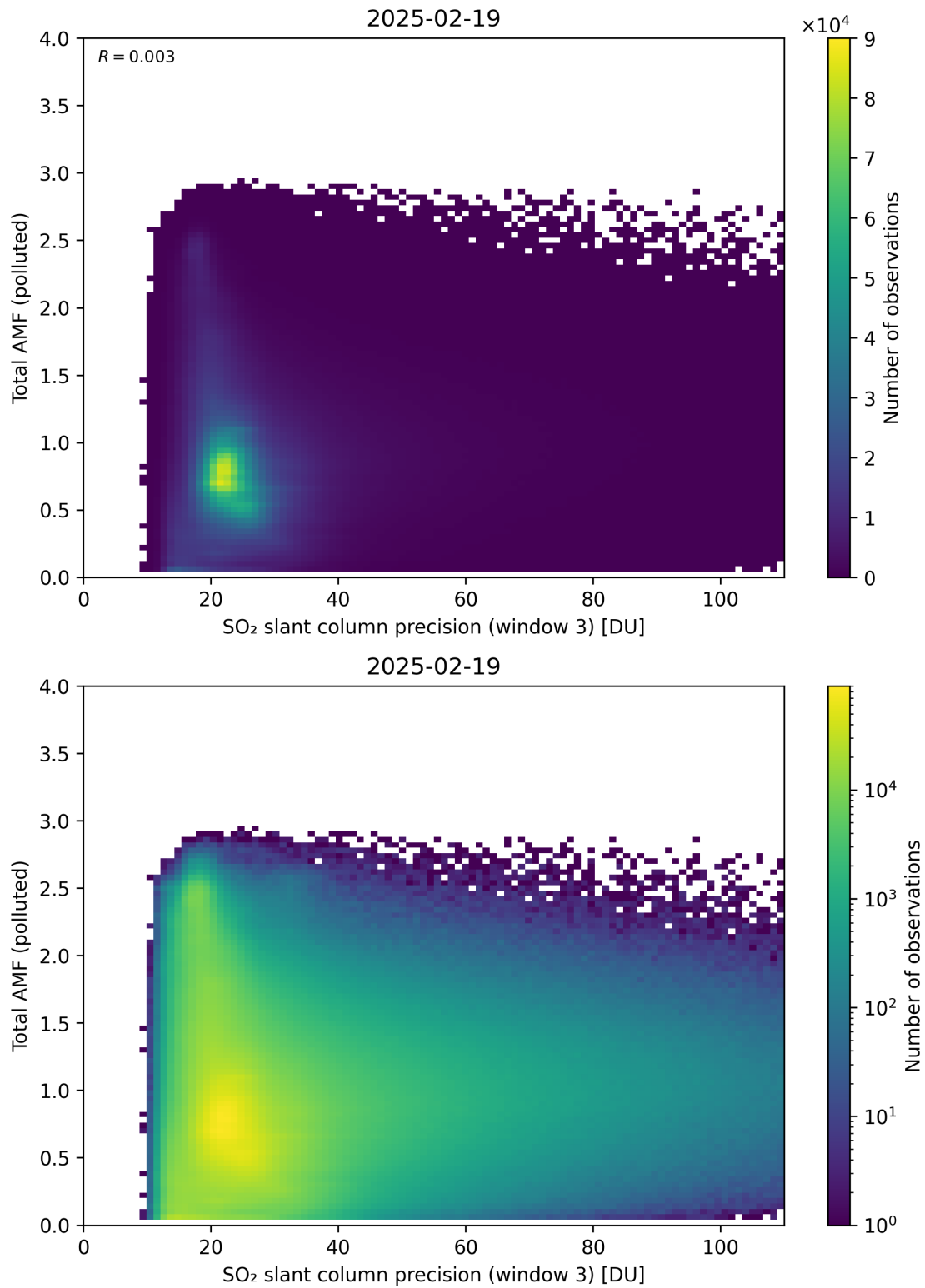
Figure 313: Scatter density plot of “SO 2 slant column precision (window 3)” against “Total AMF (polluted)” for 2025-02-19 to 2025-02-20.
