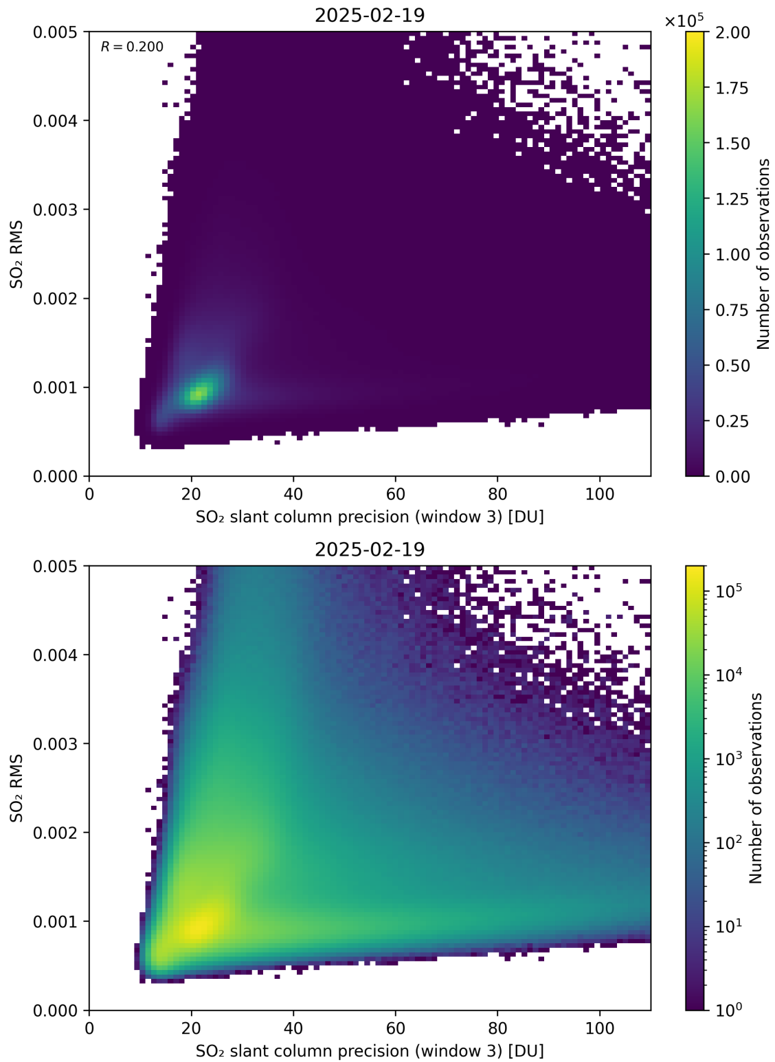
Figure 310: Scatter density plot of “SO 2 slant column precision (window 3)” against “SO 2 RMS” for 2025-02-19 to 2025-02-20.
