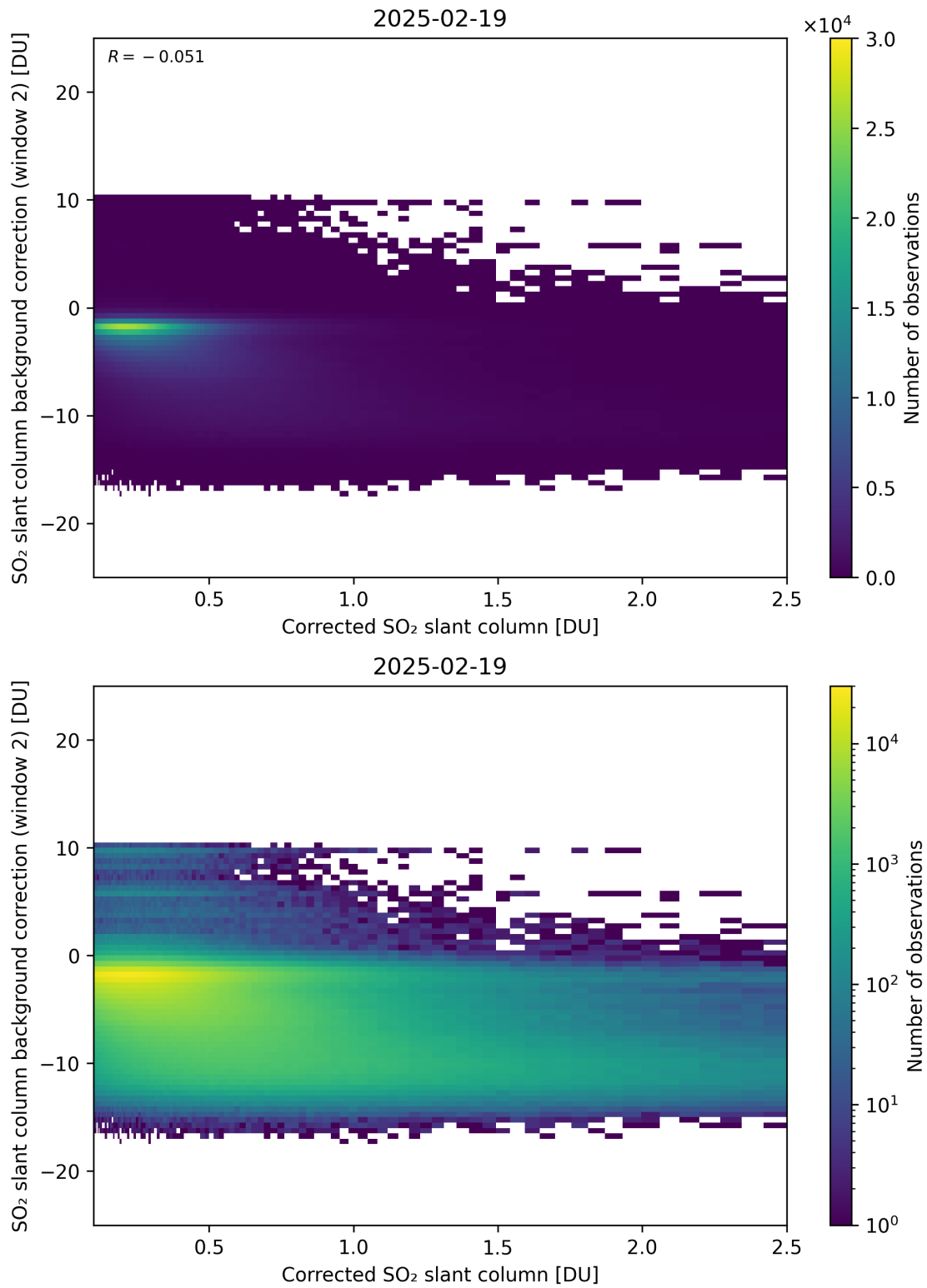
Figure 227: Scatter density plot of “Corrected SO 2 slant column” against “SO 2 slant column background correction (window 2)” for 2025-02-19 to 2025-02-20.
