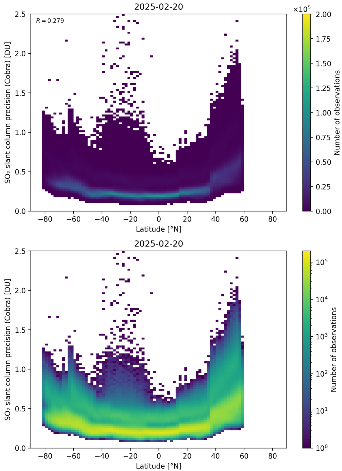
Figure 158: Scatter density plot of “Latitude” against “SO 2 slant column precision (Cobra)” for 2025-02-19 to 2025-02-21.
