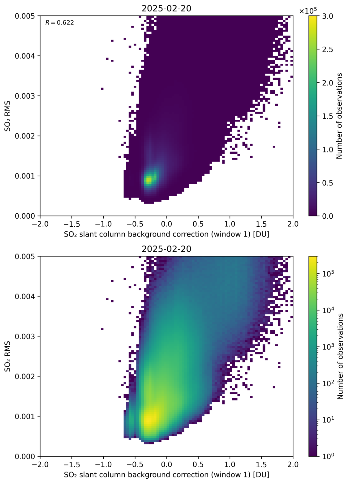
Figure 113: Scatter density plot of “SO 2 slant column background correction (window 1)” against “SO 2 RMS” for 2025-02-19 to 2025-02-21.
