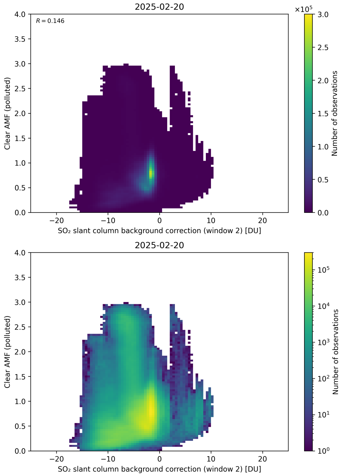
Figure 126: Scatter density plot of “SO 2 slant column background correction (window 2)” against “Clear AMF (polluted)” for 2025-02-19 to 2025-02-21.
