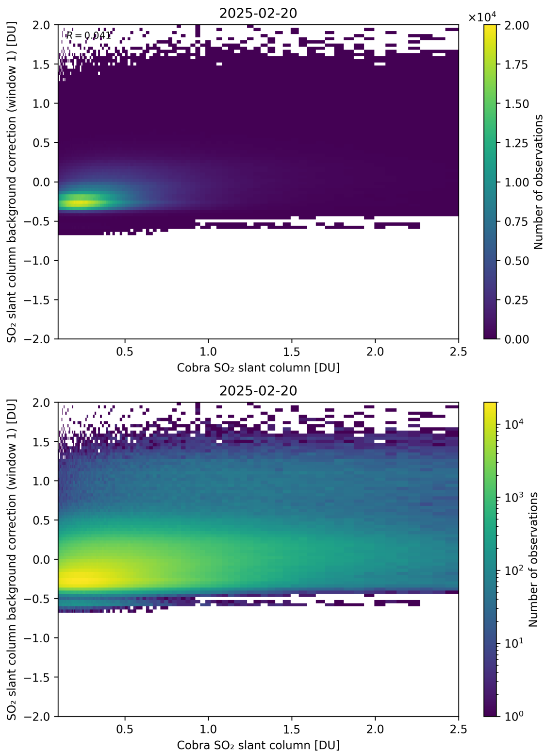
Figure 193: Scatter density plot of “Cobra SO 2 slant column” against “SO 2 slant column background correction (window 1)” for 2025-02-19 to 2025-02-21.
