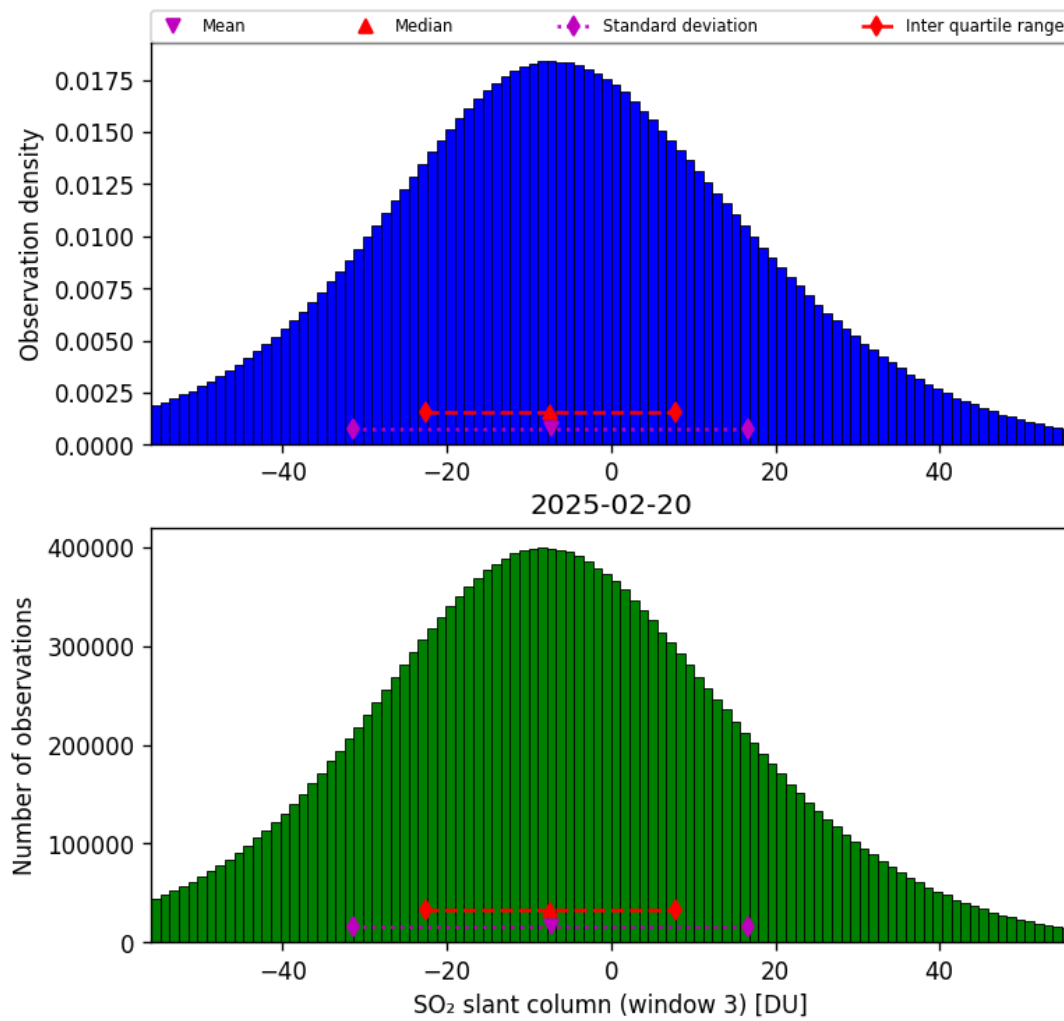
Figure 71: Histogram of “SO 2 slant column (window 3)” for 2025-02-19 to 2025-02-21
