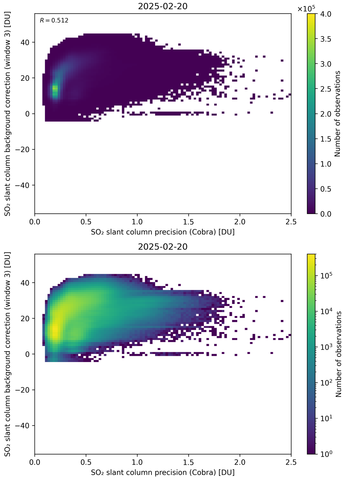
Figure 201: Scatter density plot of “SO 2 slant column precision (Cobra)” against “SO 2 slant column background correction (window 3)” for 2025-02-19 to 2025-02-21.
