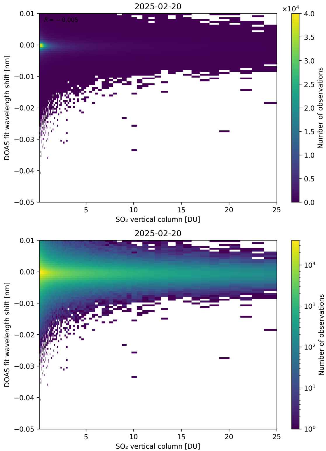
Figure 326: Scatter density plot of “SO 2 vertical column” against “DOAS fit wavelength shift” for 2025-02-19 to 2025-02-21.
