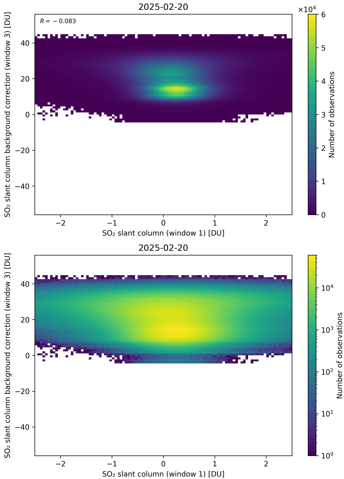
Figure 264: Scatter density plot of “SO 2 slant column (window 1)” against “SO 2 slant column background correction (window 3)” for 2025-02-19 to 2025-02-21.
