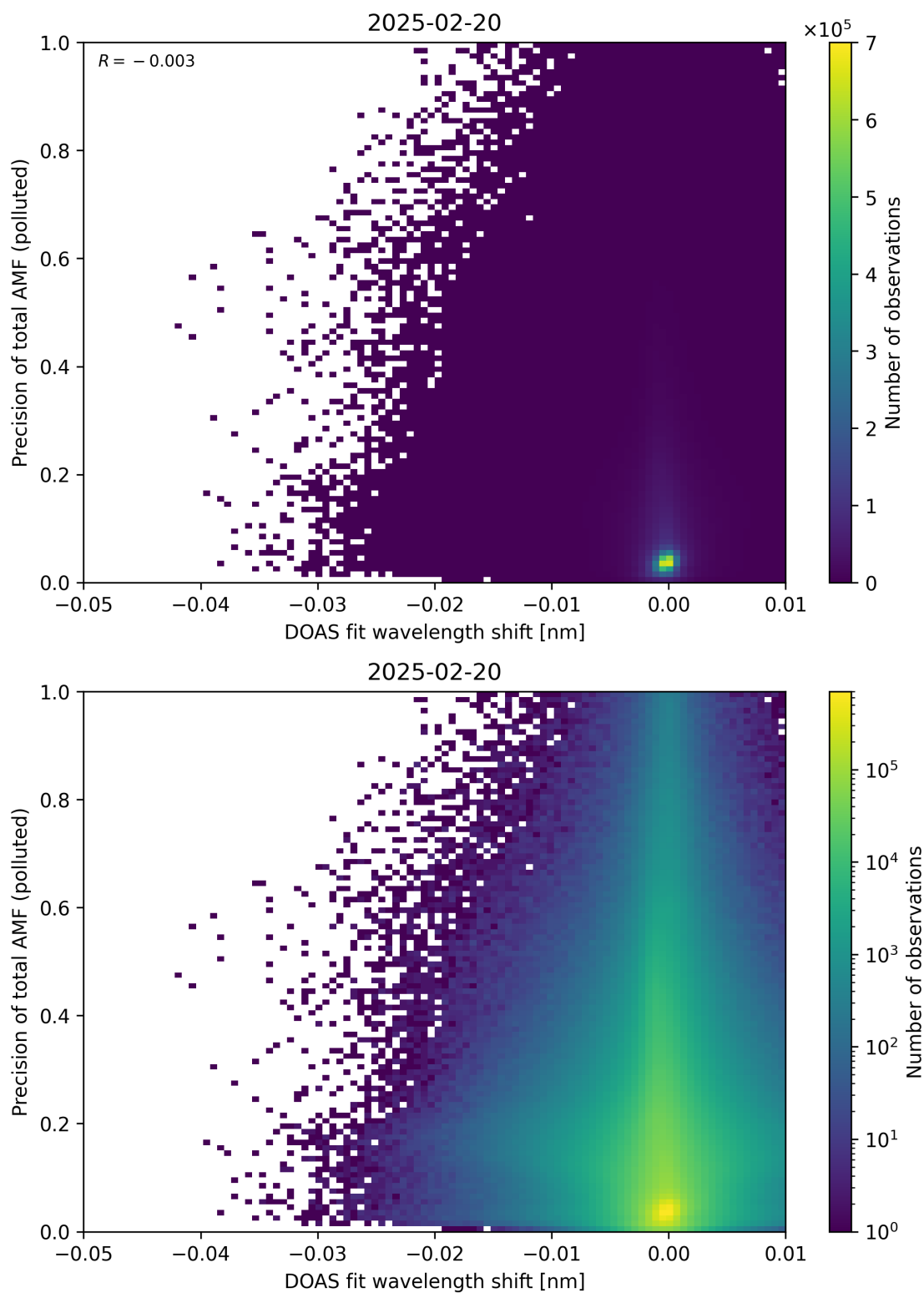
Figure 142: Scatter density plot of “DOAS fit wavelength shift” against “Precision of total AMF (polluted)” for 2025-02-19 to 2025-02-21.
