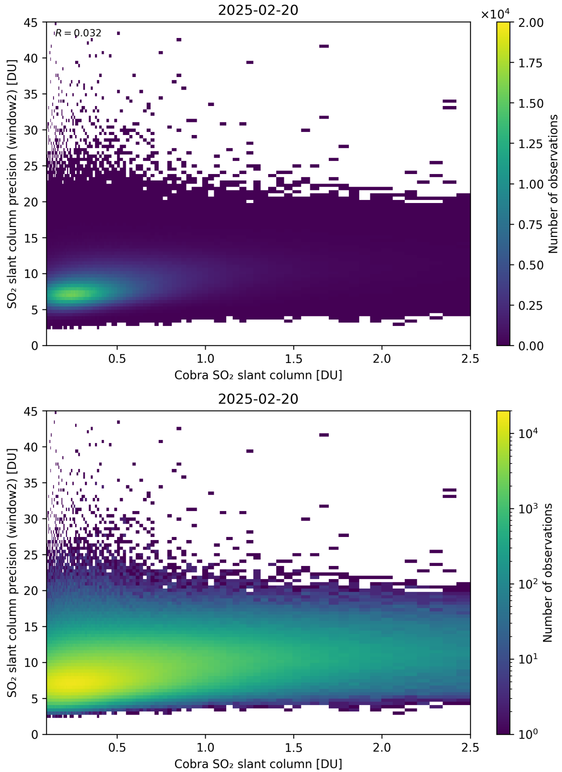
Figure 221: Scatter density plot of “Cobra SO 2 slant column” against “SO 2 slant column precision (window2)” for 2025-02-19 to 2025-02-21.
