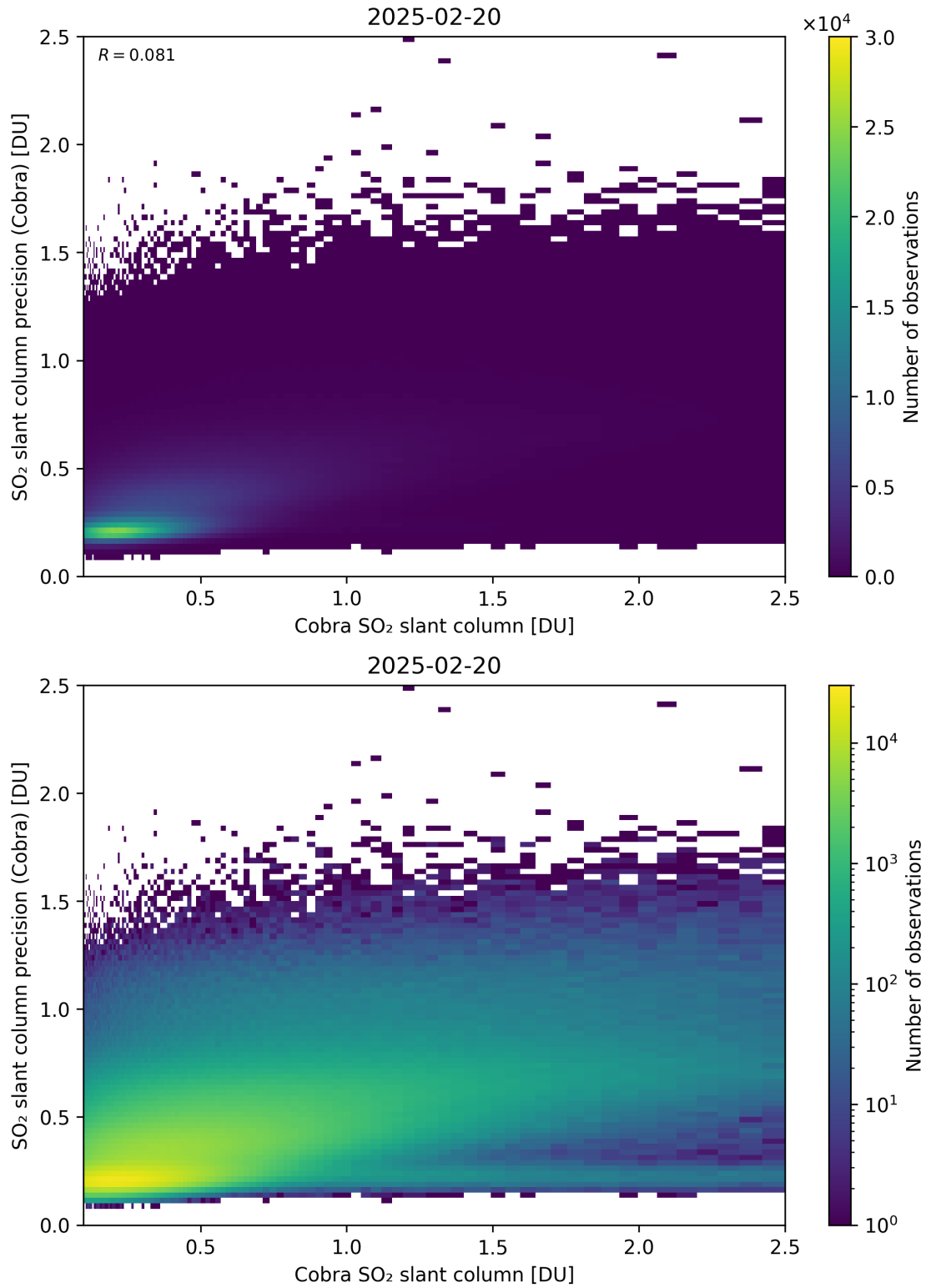
Figure 216: Scatter density plot of “Cobra SO 2 slant column” against “SO 2 slant column precision (Cobra)” for 2025-02-19 to 2025-02-21.
