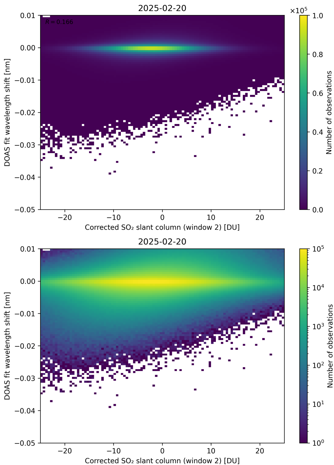
Figure 246: Scatter density plot of “Corrected SO 2 slant column (window 2)” against “DOAS fit wavelength shift” for 2025-02-19 to 2025-02-21.
