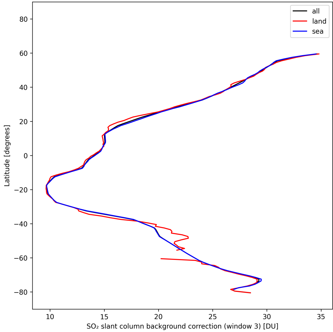
Figure 48: Zonal average of “SO 2 slant column background correction (window 3)” for 2025-02-19 to 2025-02-21.
