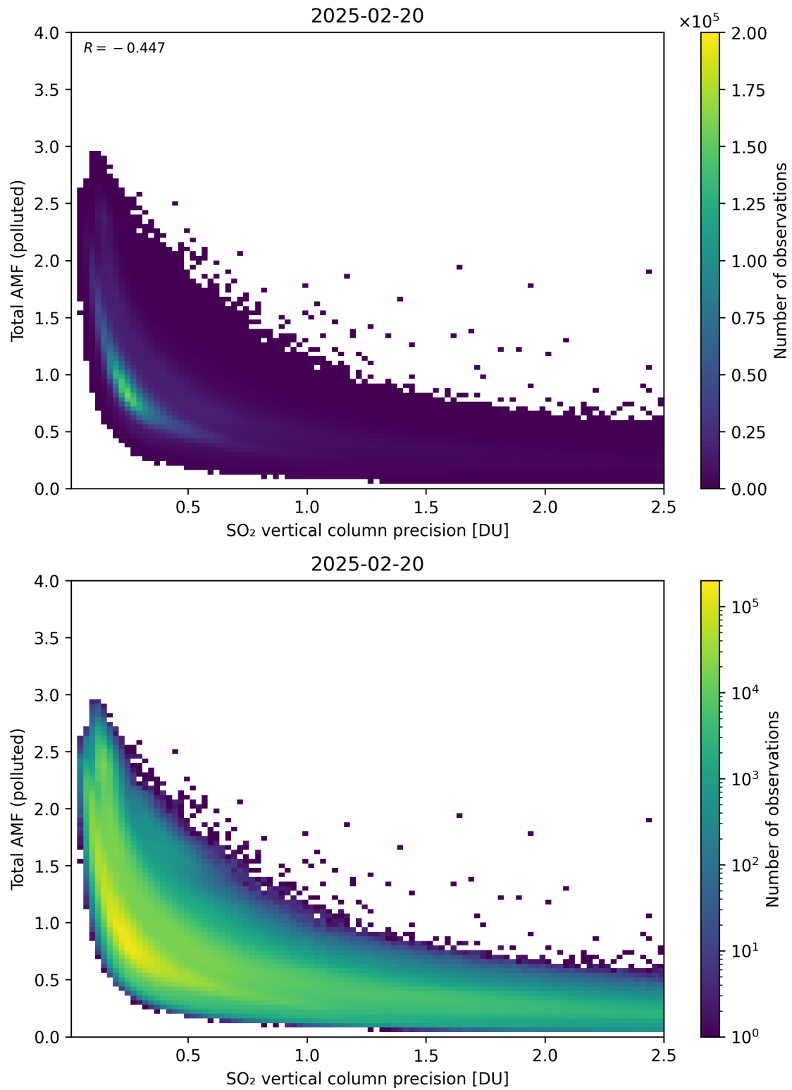
Figure 346: Scatter density plot of “SO 2 vertical column precision” against “Total AMF (polluted)” for 2025-02-19 to 2025-02-21.
