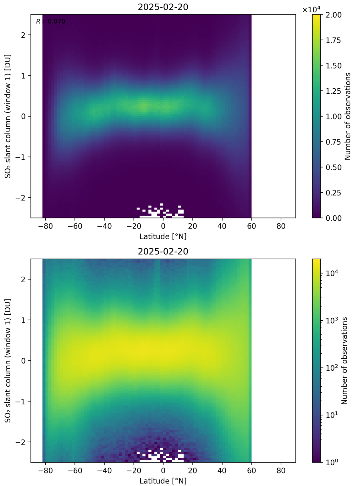
Figure 162: Scatter density plot of “Latitude” against “SO 2 slant column (window 1)” for 2025-02-19 to 2025-02-21.
