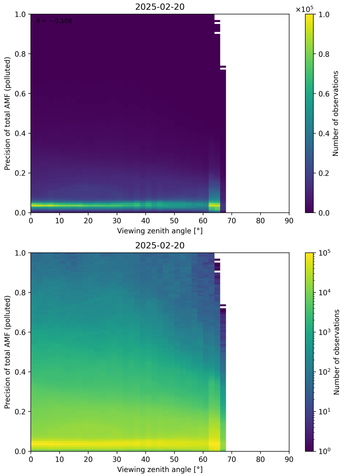
Figure 382: Scatter density plot of “Viewing zenith angle” against “Precision of total AMF (polluted)” for 2025-02-19 to 2025-02-21.
