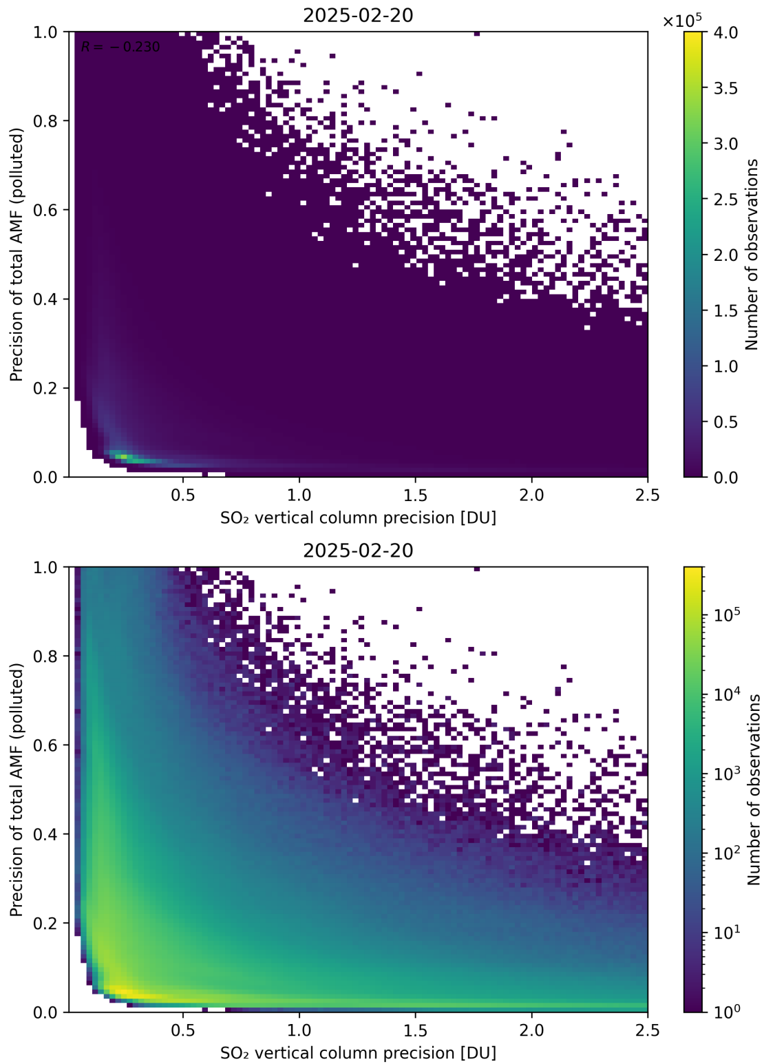
Figure 347: Scatter density plot of “SO 2 vertical column precision” against “Precision of total AMF (polluted)” for 2025-02-19 to 2025-02-21.
