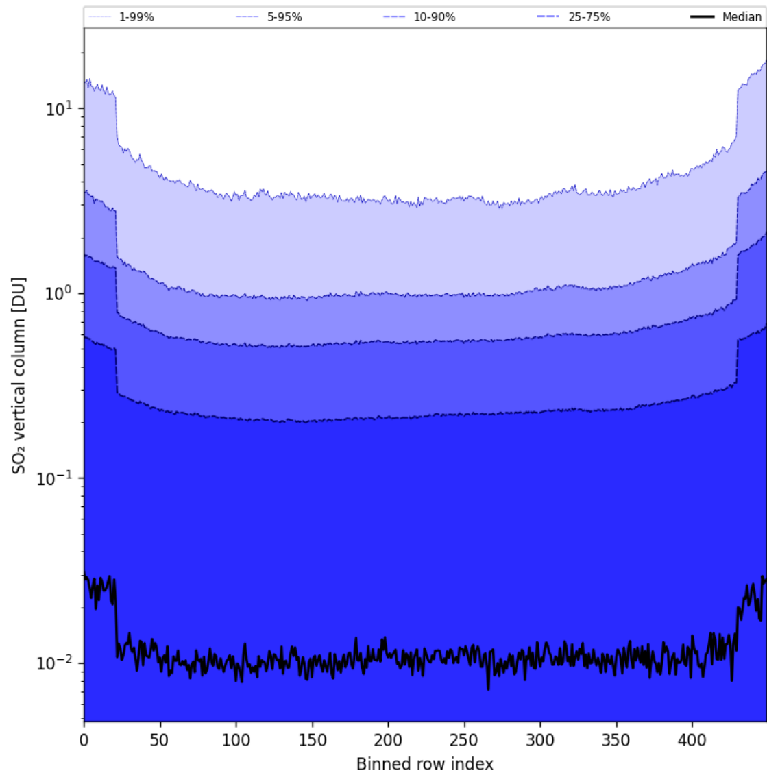
Figure 84: Along track statistics of “SO 2 vertical column” for 2025-02-19 to 2025-02-21
