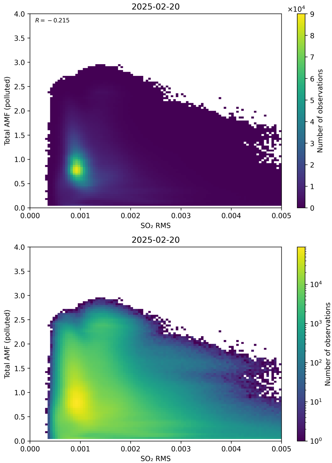
Figure 148: Scatter density plot of “SO 2 RMS” against “Total AMF (polluted)” for 2025-02-19 to 2025-02-21.
