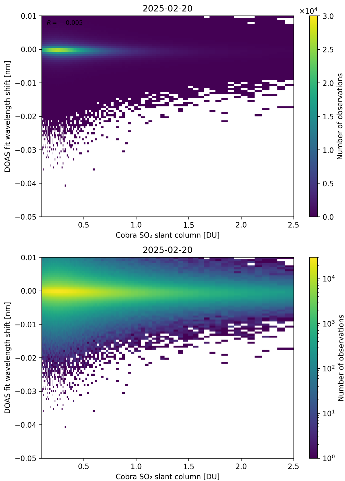
Figure 196: Scatter density plot of “Cobra SO 2 slant column” against “DOAS fit wavelength shift” for 2025-02-19 to 2025-02-21.
