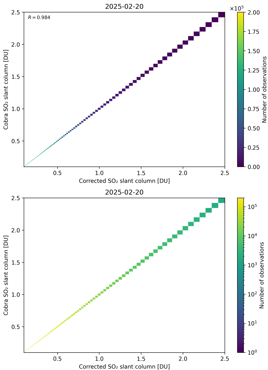
Figure 233: Scatter density plot of “Corrected SO 2 slant column” against “Cobra SO 2 slant column” for 2025-02-19 to 2025-02-21.
