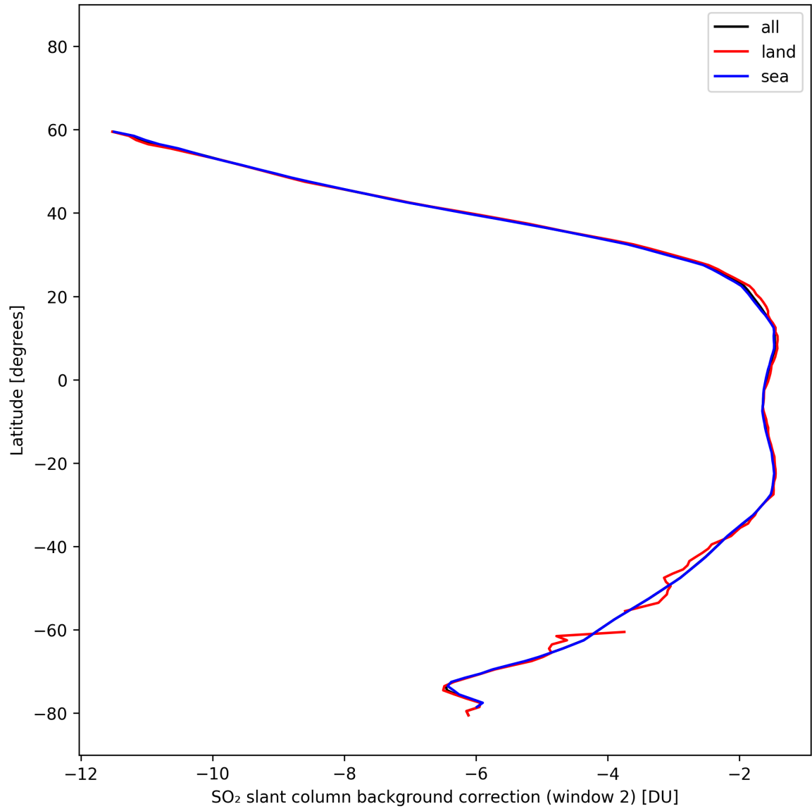
Figure 44: Zonal average of “SO 2 slant column background correction (window 2)” for 2025-02-19 to 2025-02-21.
