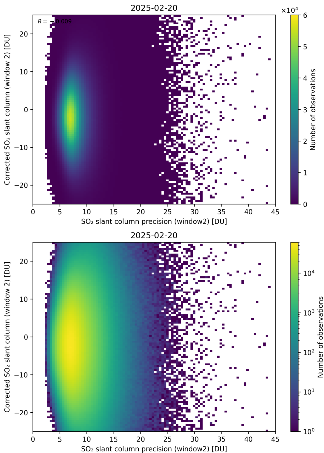
Figure 297: Scatter density plot of “SO 2 slant column precision (window2)” against “Corrected SO 2 slant column (window 2)” for 2025-02-19 to 2025-02-21.
