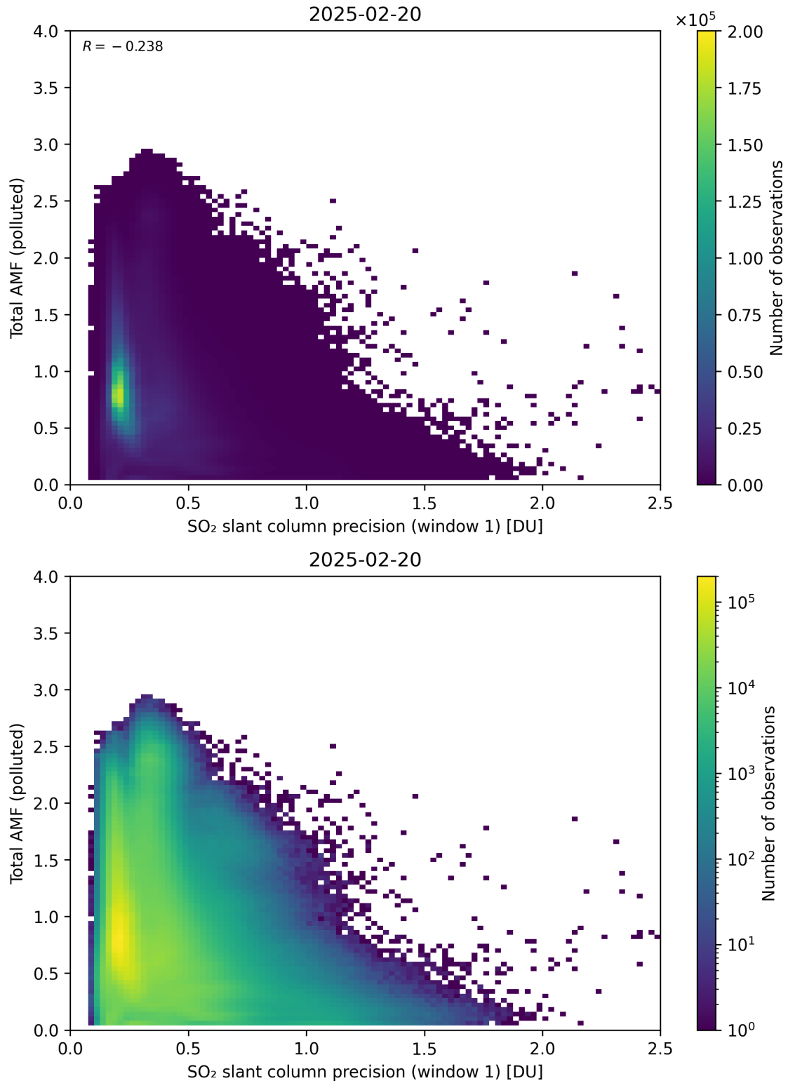
Figure 280: Scatter density plot of “SO 2 slant column precision (window 1)” against “Total AMF (polluted)” for 2025-02-19 to 2025-02-21.
