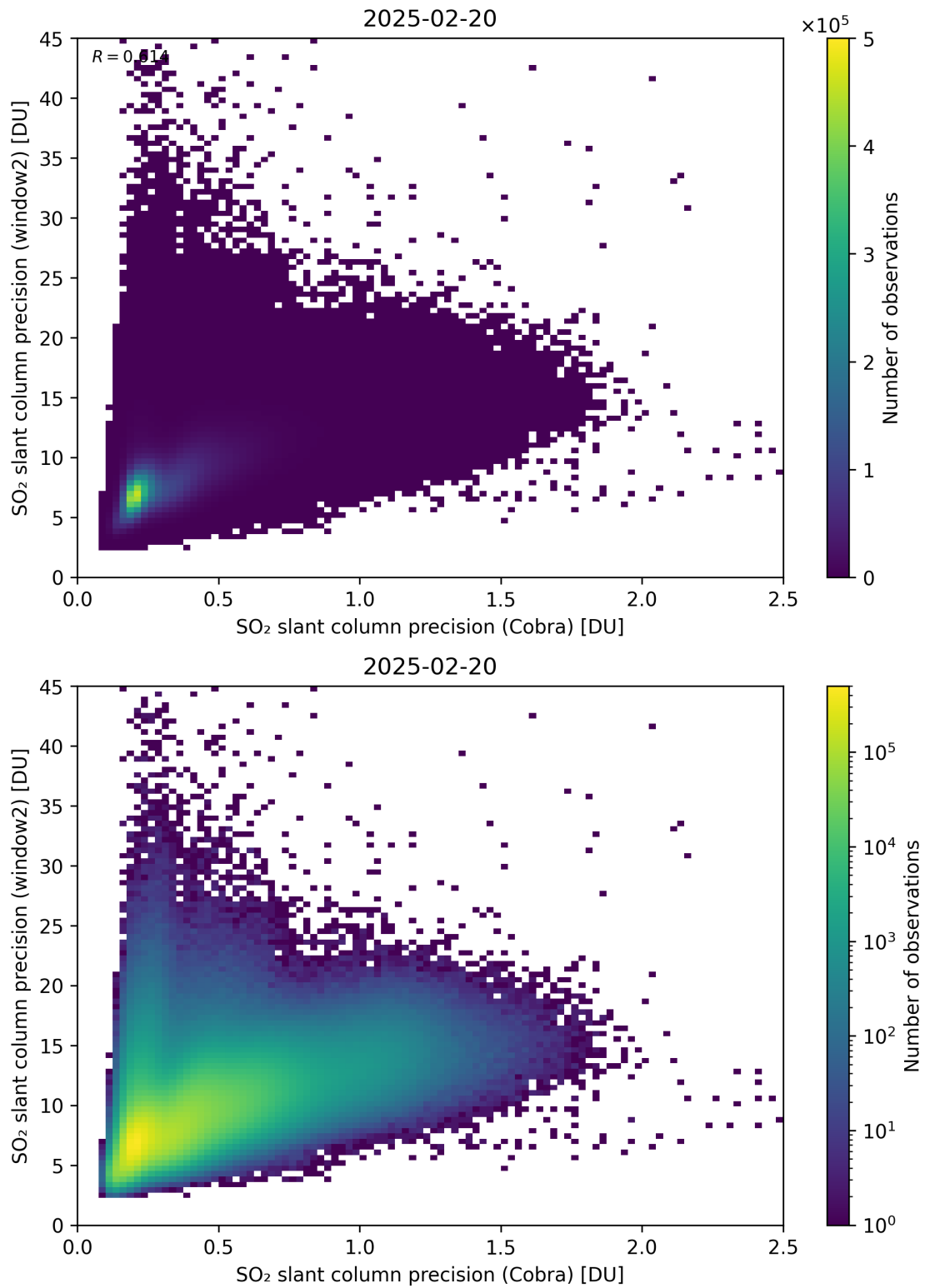
Figure 210: Scatter density plot of “SO 2 slant column precision (Cobra)” against “SO 2 slant column precision (window2)” for 2025-02-19 to 2025-02-21.
