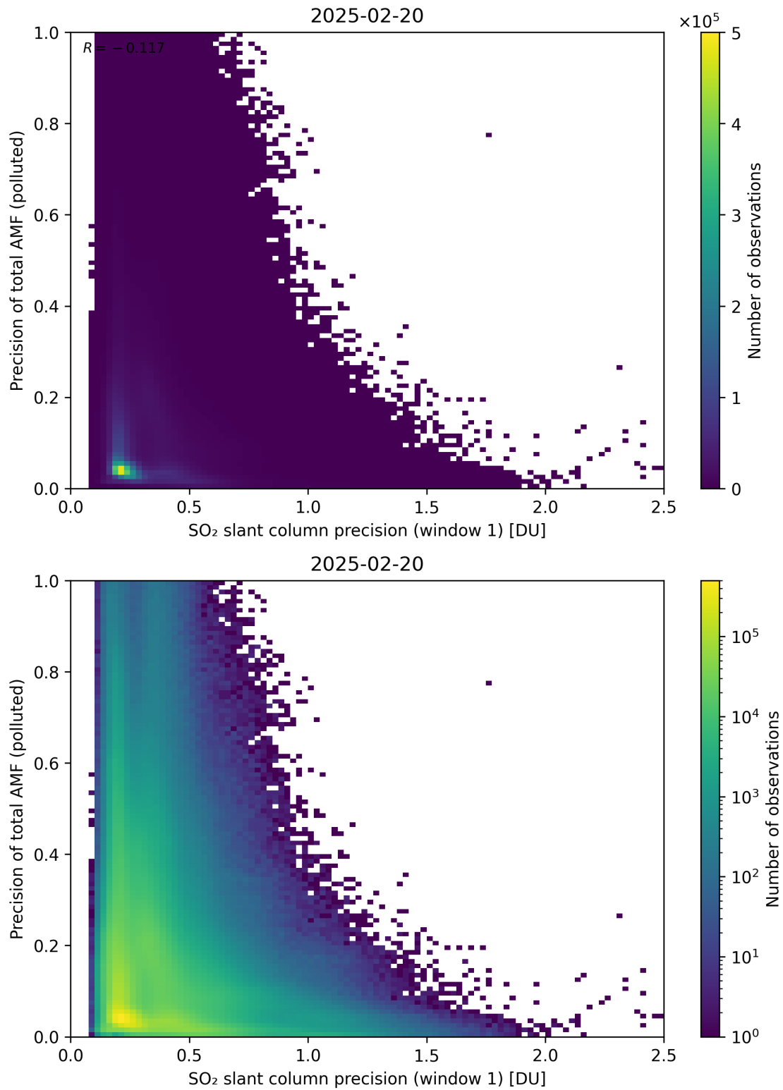
Figure 281: Scatter density plot of “SO 2 slant column precision (window 1)” against “Precision of total AMF (polluted)” for 2025-02-19 to 2025-02-21.
