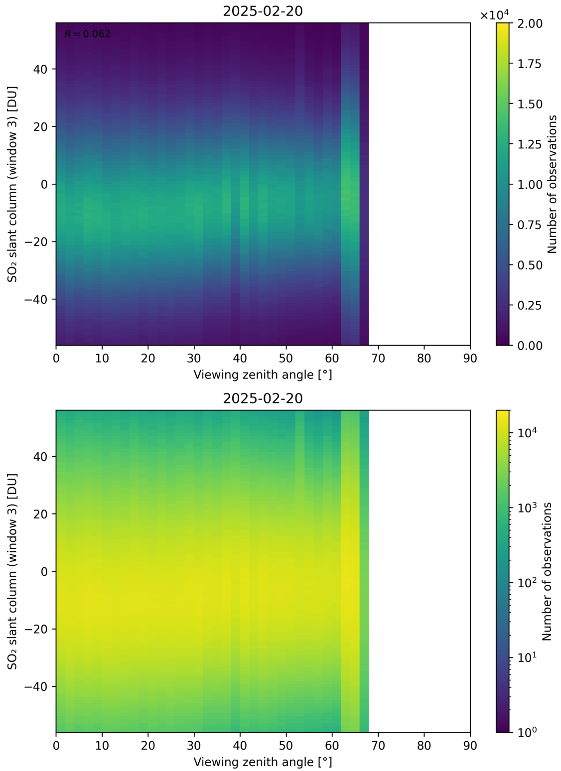
Figure 379: Scatter density plot of “Viewing zenith angle” against “SO 2 slant column (window 3)” for 2025-02-19 to 2025-02-21.
