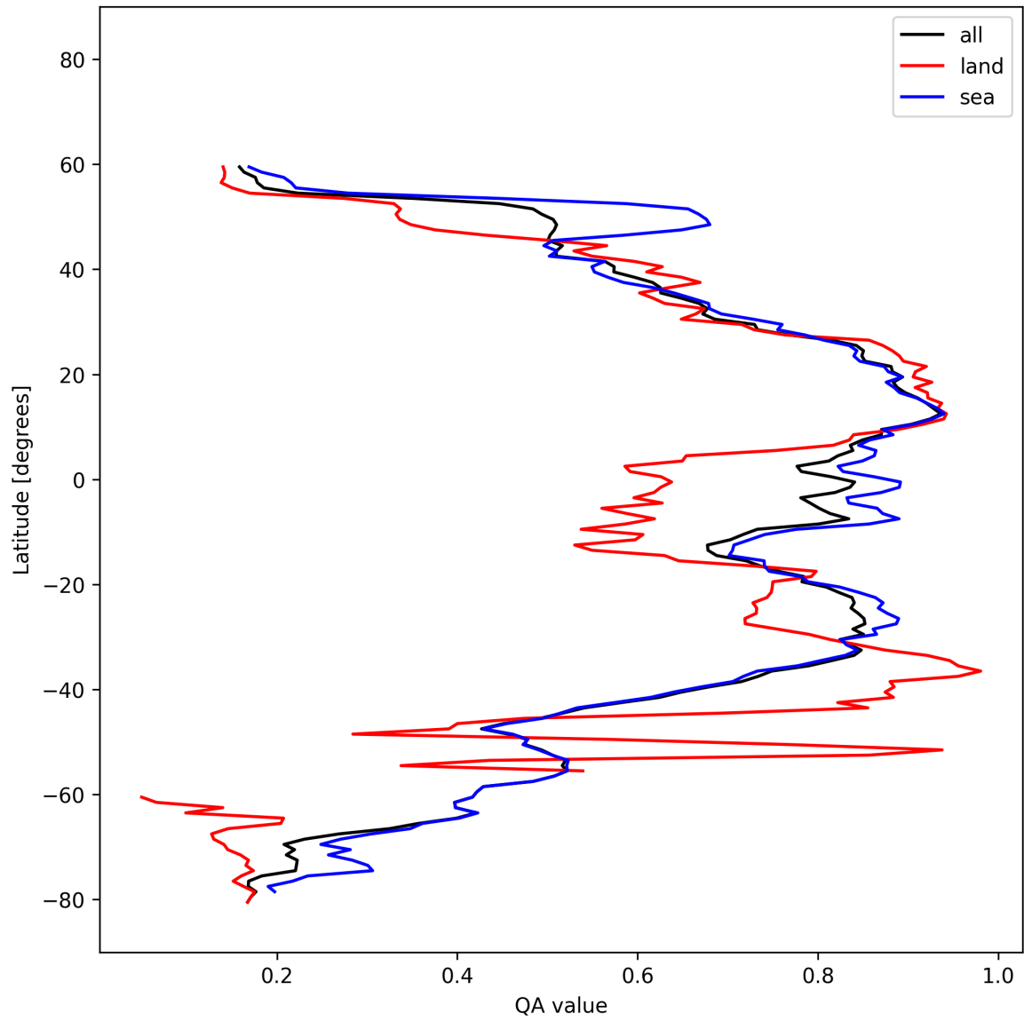
Figure 31: Zonal average of “QA value” for 2025-02-19 to 2025-02-21.
