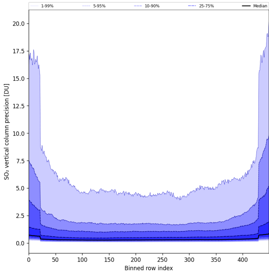
Figure 85: Along track statistics of “SO 2 vertical column precision” for 2025-02-19 to 2025-02-21
