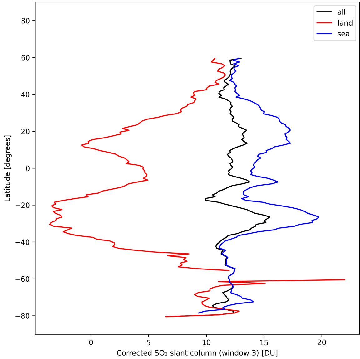
Figure 47: Zonal average of “Corrected SO 2 slant column (window 3)” for 2025-02-19 to 2025-02-21.
