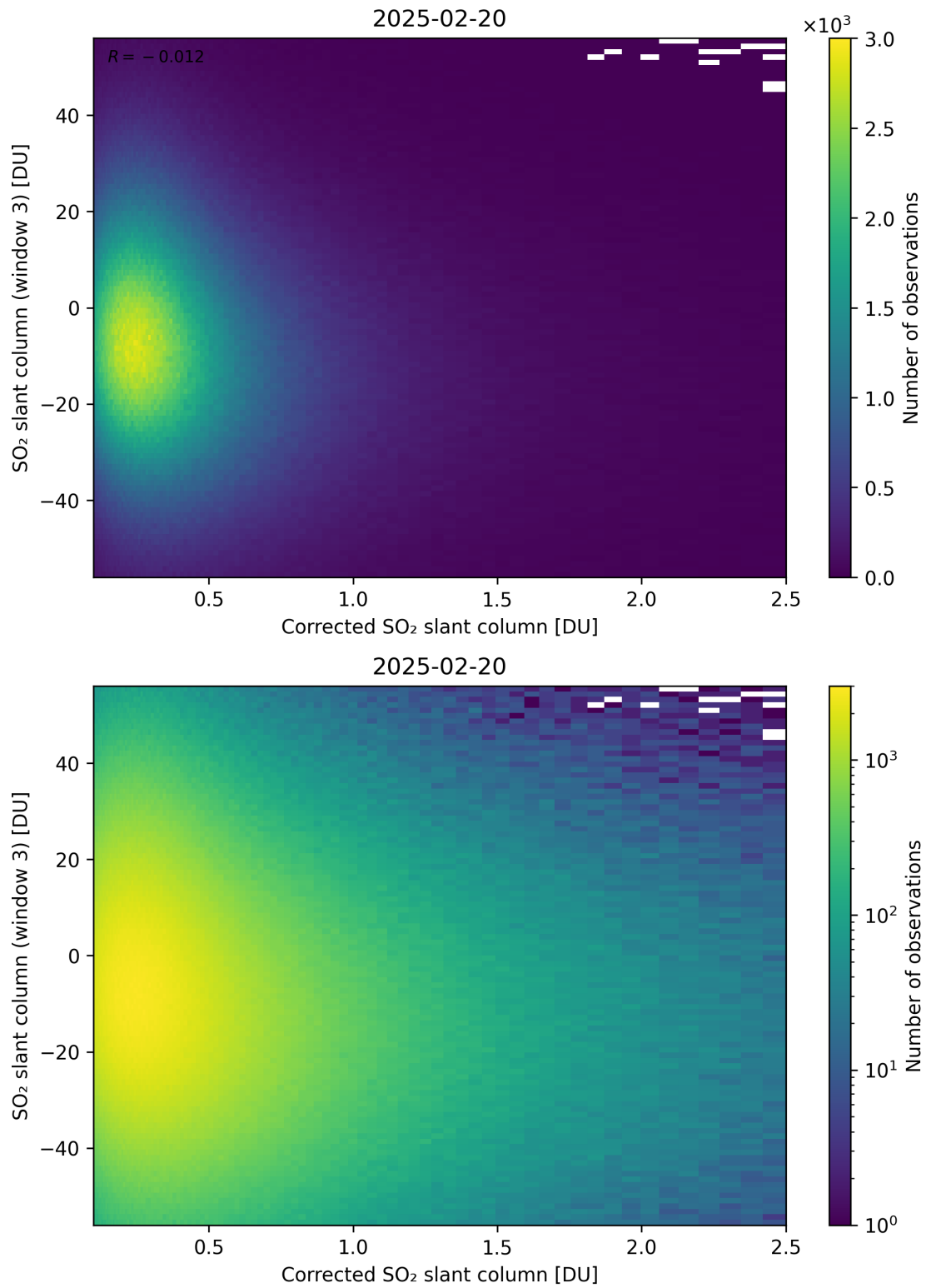
Figure 240: Scatter density plot of “Corrected SO 2 slant column” against “SO 2 slant column (window 3)” for 2025-02-19 to 2025-02-21.
