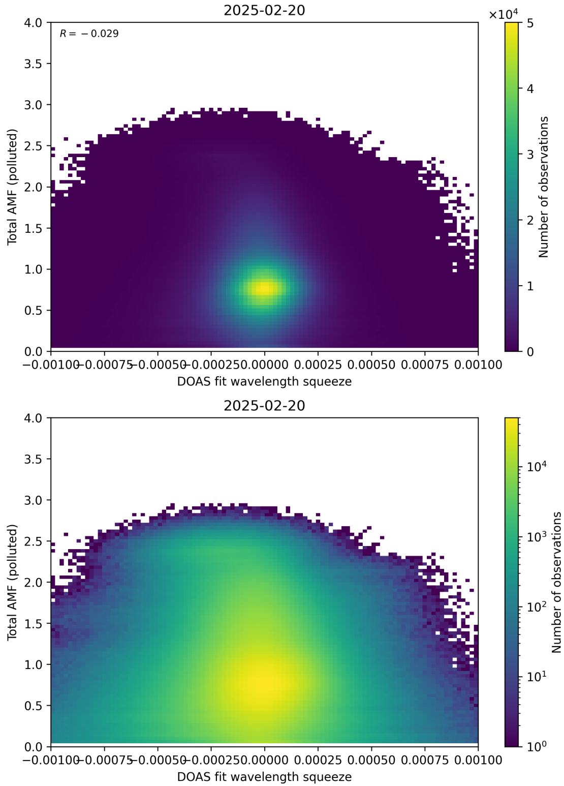
Figure 145: Scatter density plot of “DOAS fit wavelength squeeze” against “Total AMF (polluted)” for 2025-02-19 to 2025-02-21.
