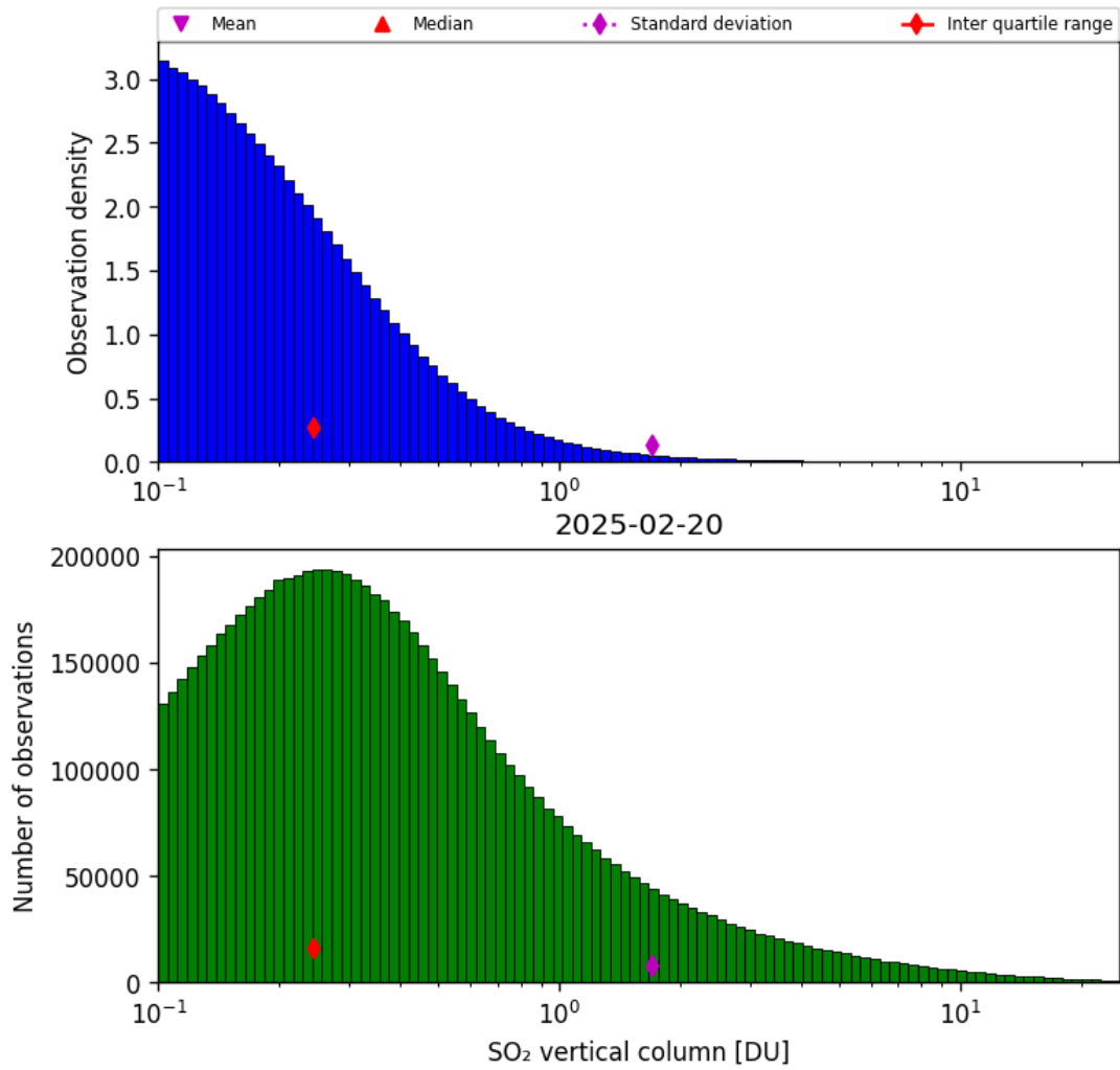
Figure 58: Histogram of “SO 2 vertical column” for 2025-02-19 to 2025-02-21
