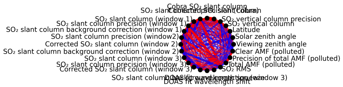
Figure 1: Map of correlation graph for 2025-02-19 to 2025-02-21.
