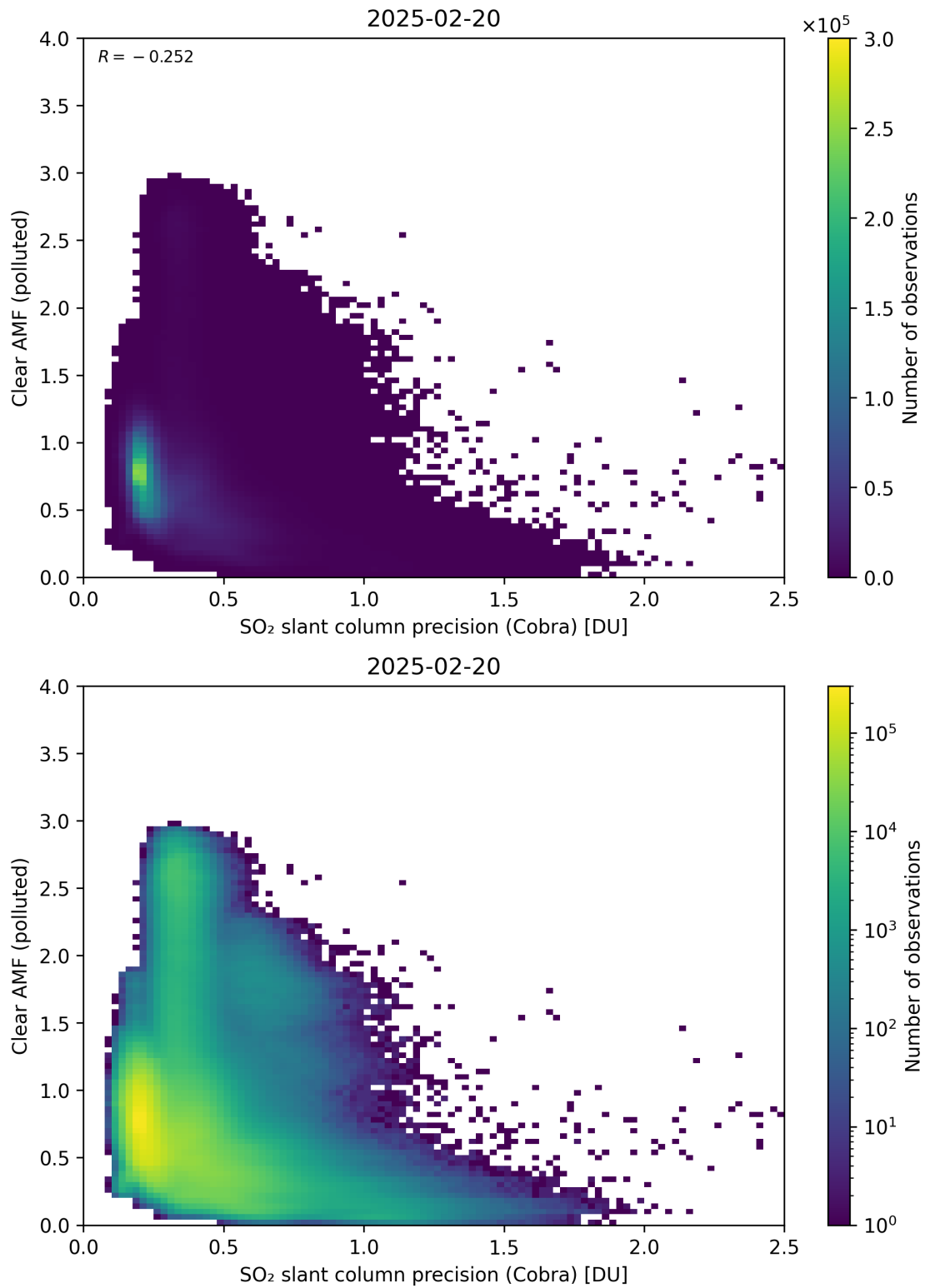
Figure 205: Scatter density plot of “SO 2 slant column precision (Cobra)” against “Clear AMF (polluted)” for 2025-02-19 to 2025-02-21.
