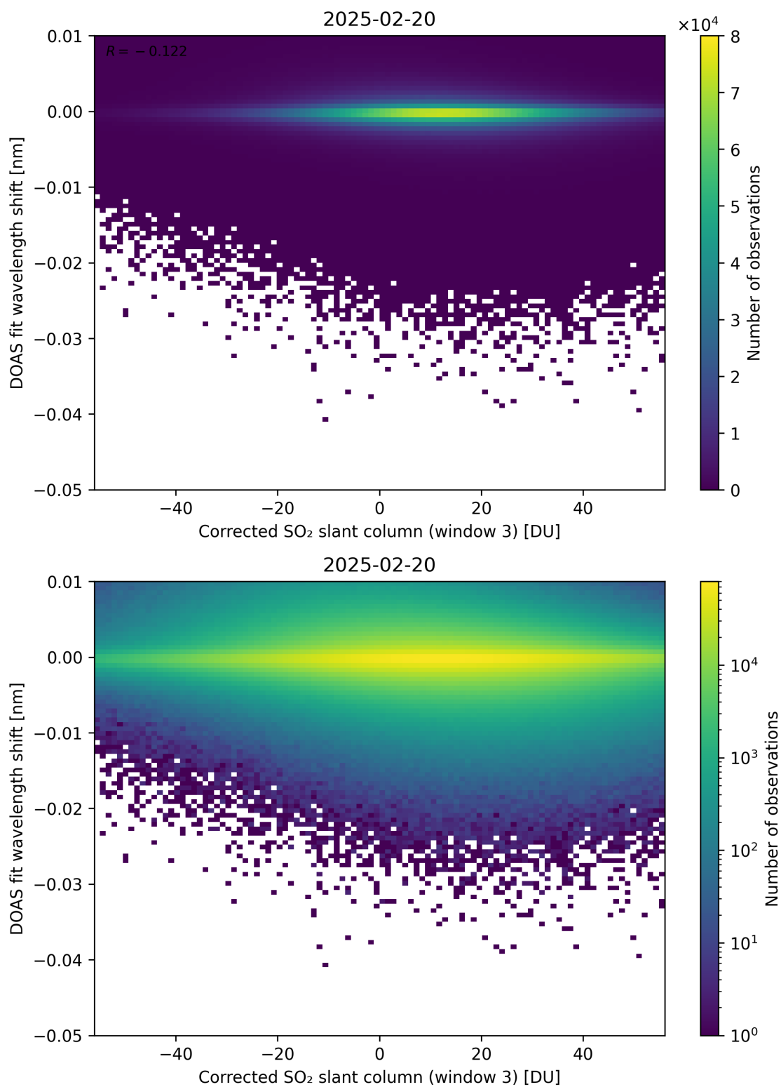
Figure 256: Scatter density plot of “Corrected SO 2 slant column (window 3)” against “DOAS fit wavelength shift” for 2025-02-19 to 2025-02-21.
