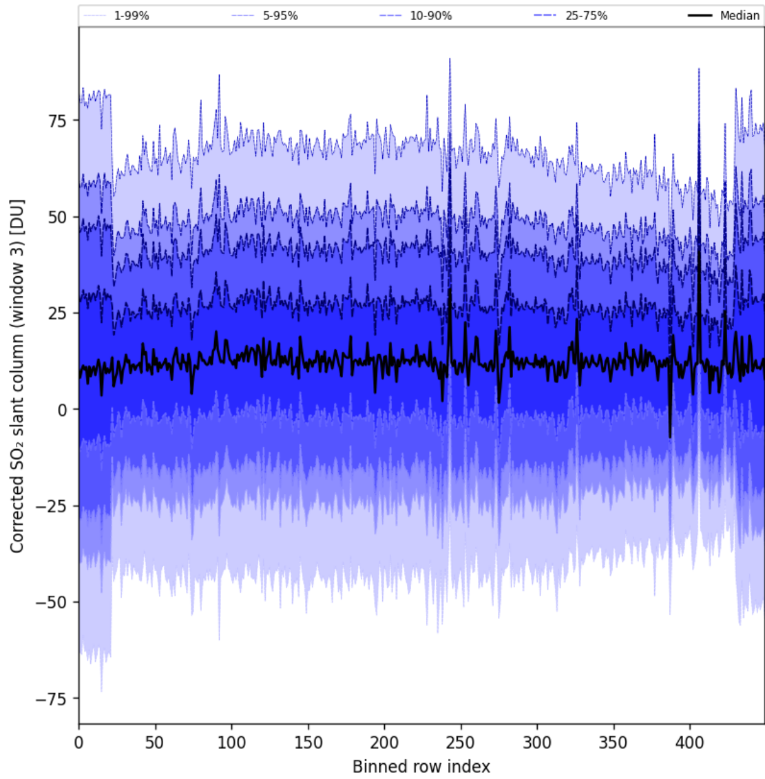
Figure 99: Along track statistics of “Corrected SO 2 slant column (window 3)” for 2025-02-19 to 2025-02-21
