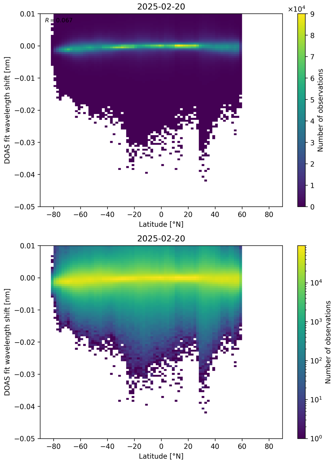
Figure 153: Scatter density plot of “Latitude” against “DOAS fit wavelength shift” for 2025-02-19 to 2025-02-21.
