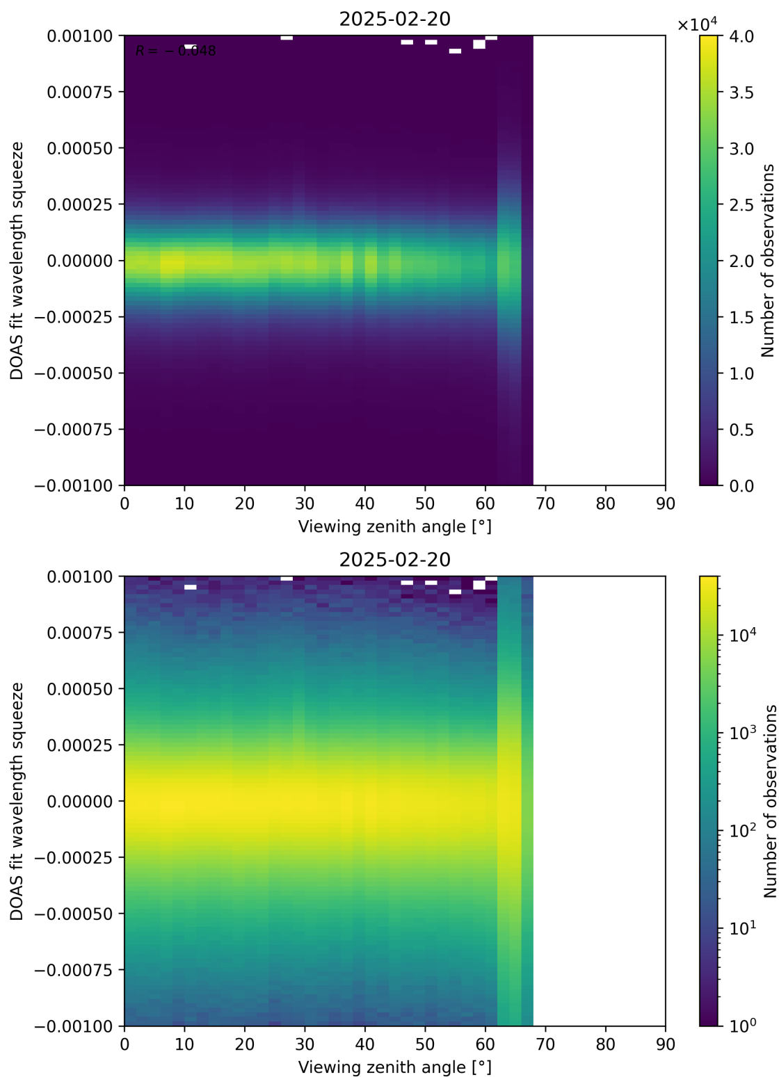
Figure 366: Scatter density plot of “Viewing zenith angle” against “DOAS fit wavelength squeeze” for 2025-02-19 to 2025-02-21.
