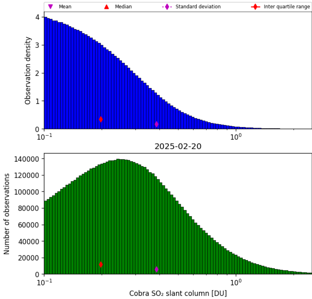
Figure 61: Histogram of “Cobra SO 2 slant column” for 2025-02-19 to 2025-02-21
