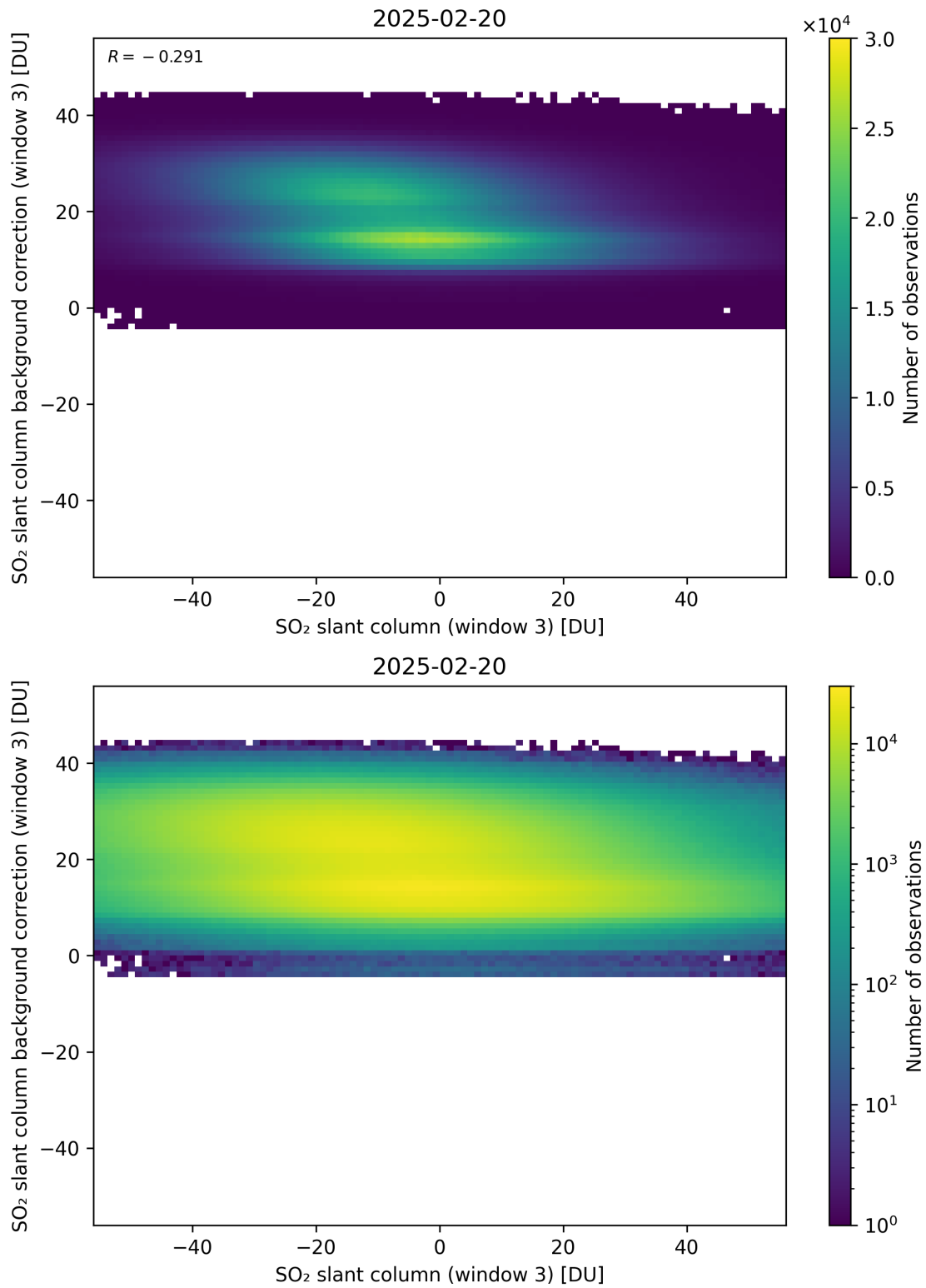
Figure 303: Scatter density plot of “SO 2 slant column (window 3)” against “SO 2 slant column background correction (window 3)” for 2025-02-19 to 2025-02-21.
