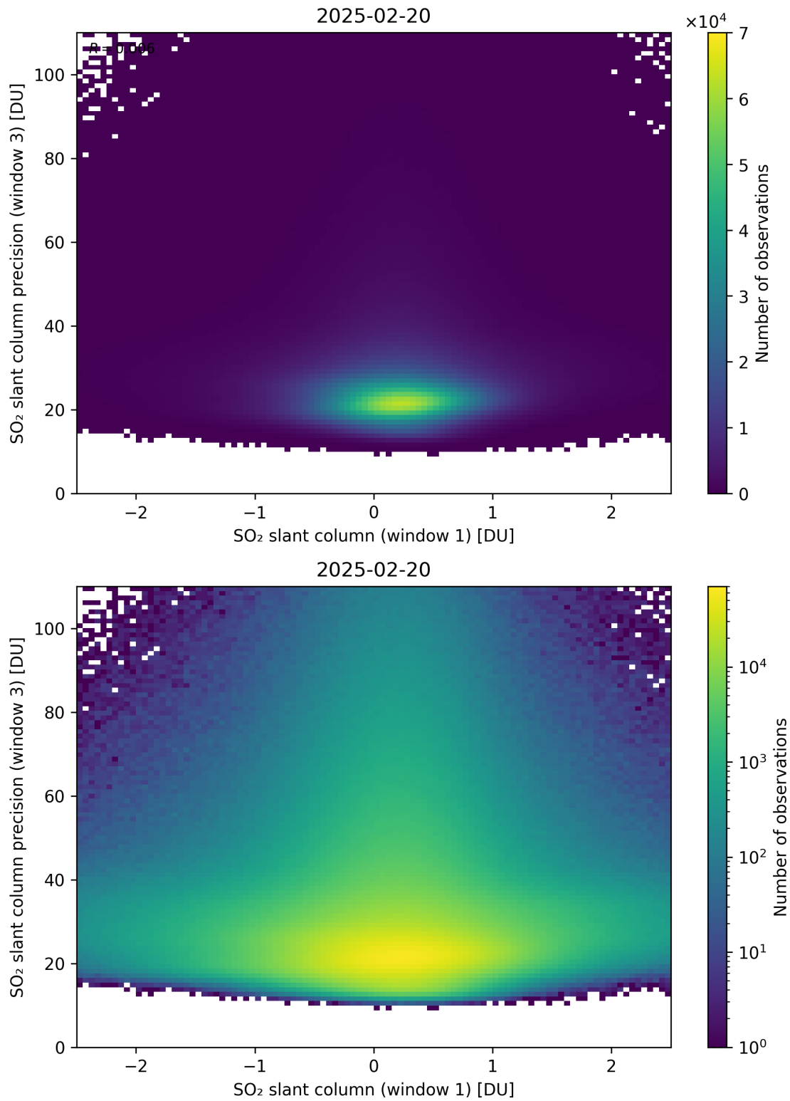
Figure 288: Scatter density plot of “SO 2 slant column (window 1)” against “SO 2 slant column precision (window 3)” for 2025-02-19 to 2025-02-21.
