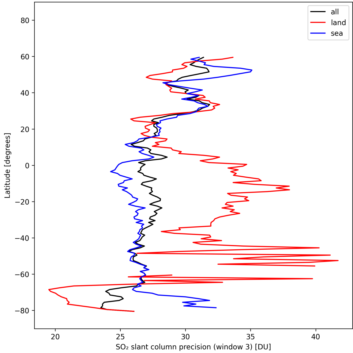
Figure 46: Zonal average of “SO 2 slant column precision (window 3)” for 2025-02-19 to 2025-02-21.
