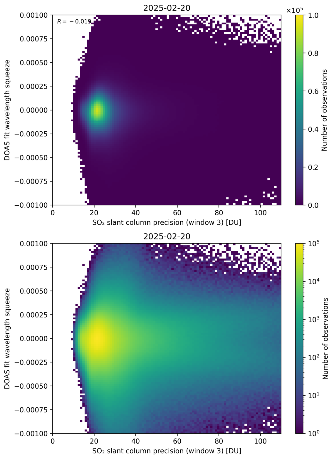
Figure 309: Scatter density plot of “SO 2 slant column precision (window 3)” against “DOAS fit wavelength squeeze” for 2025-02-19 to 2025-02-21.
