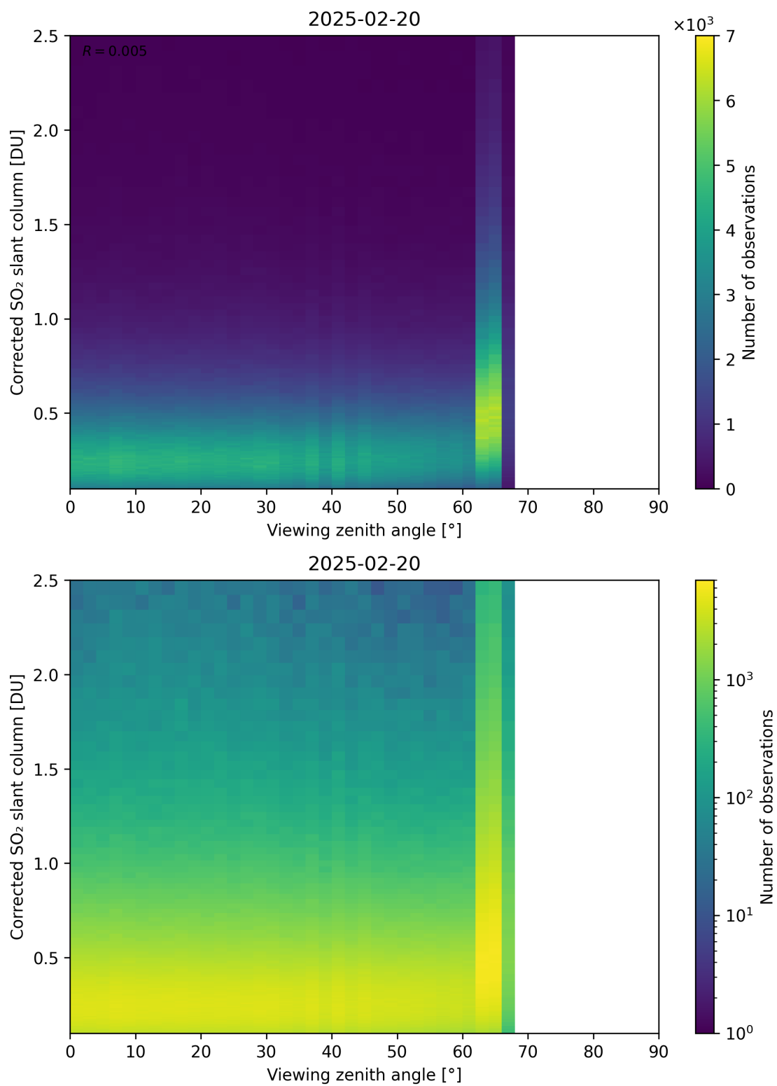
Figure 373: Scatter density plot of “Viewing zenith angle” against “Corrected SO 2 slant column” for 2025-02-19 to 2025-02-21.
