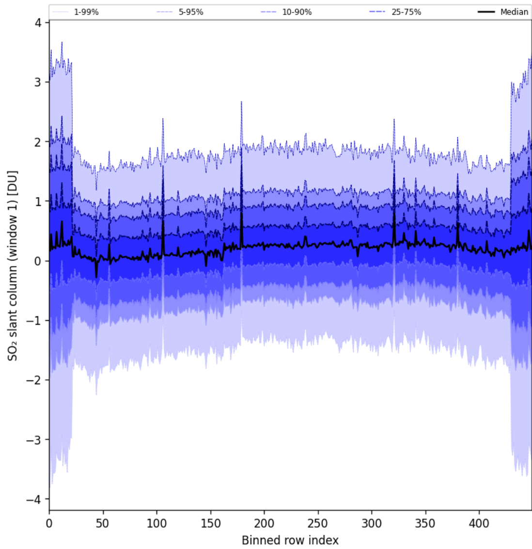
Figure 89: Along track statistics of “SO 2 slant column (window 1)” for 2025-02-19 to 2025-02-21
