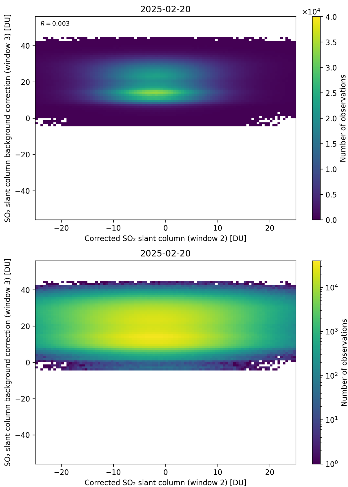
Figure 245: Scatter density plot of “Corrected SO 2 slant column (window 2)” against “SO 2 slant column background correction (window 3)” for 2025-02-19 to 2025-02-21.
