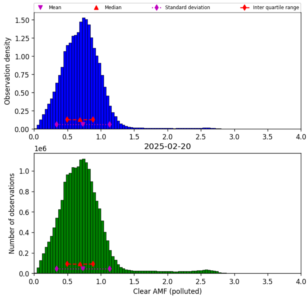
Figure 81: Histogram of “Clear AMF (polluted)” for 2025-02-19 to 2025-02-21
