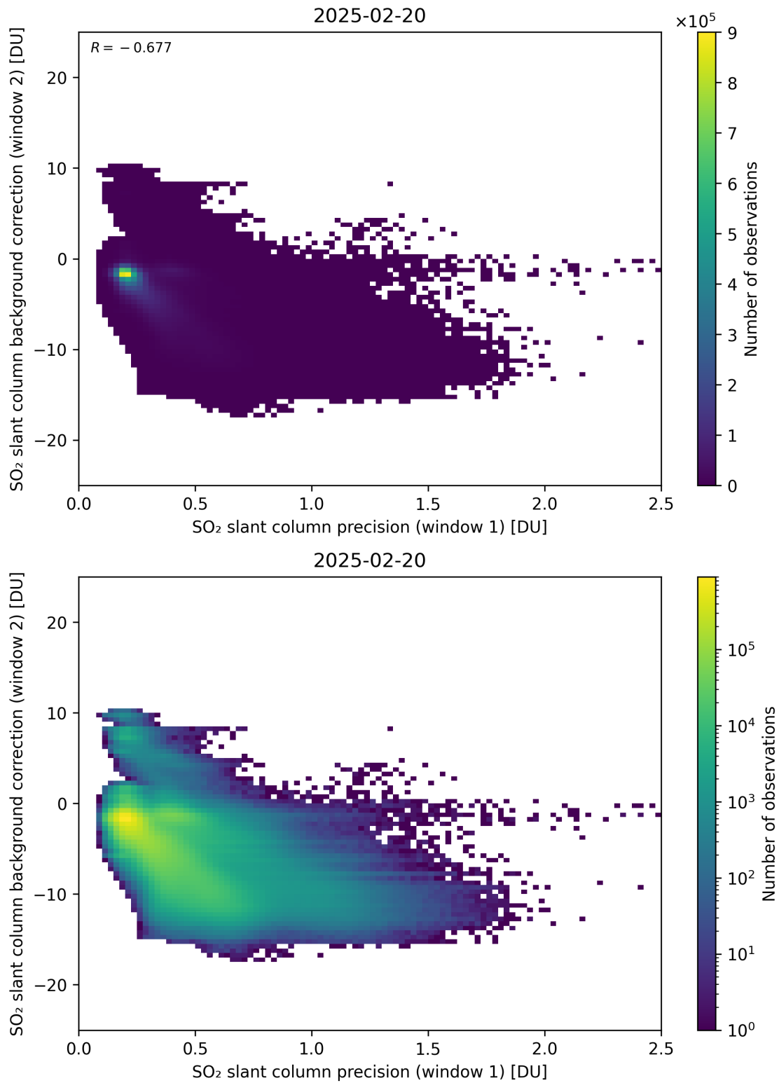
Figure 269: Scatter density plot of “SO 2 slant column precision (window 1)” against “SO 2 slant column background correction (window 2)” for 2025-02-19 to 2025-02-21.
