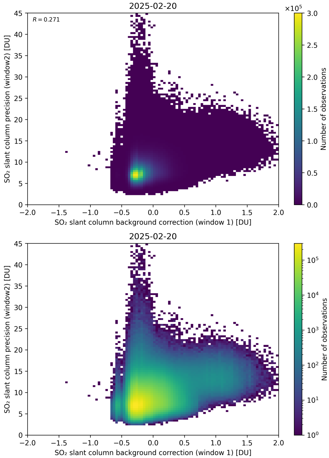
Figure 117: Scatter density plot of “SO 2 slant column background correction (window 1)” against “SO 2 slant column precision (window2)” for 2025-02-19 to 2025-02-21.
