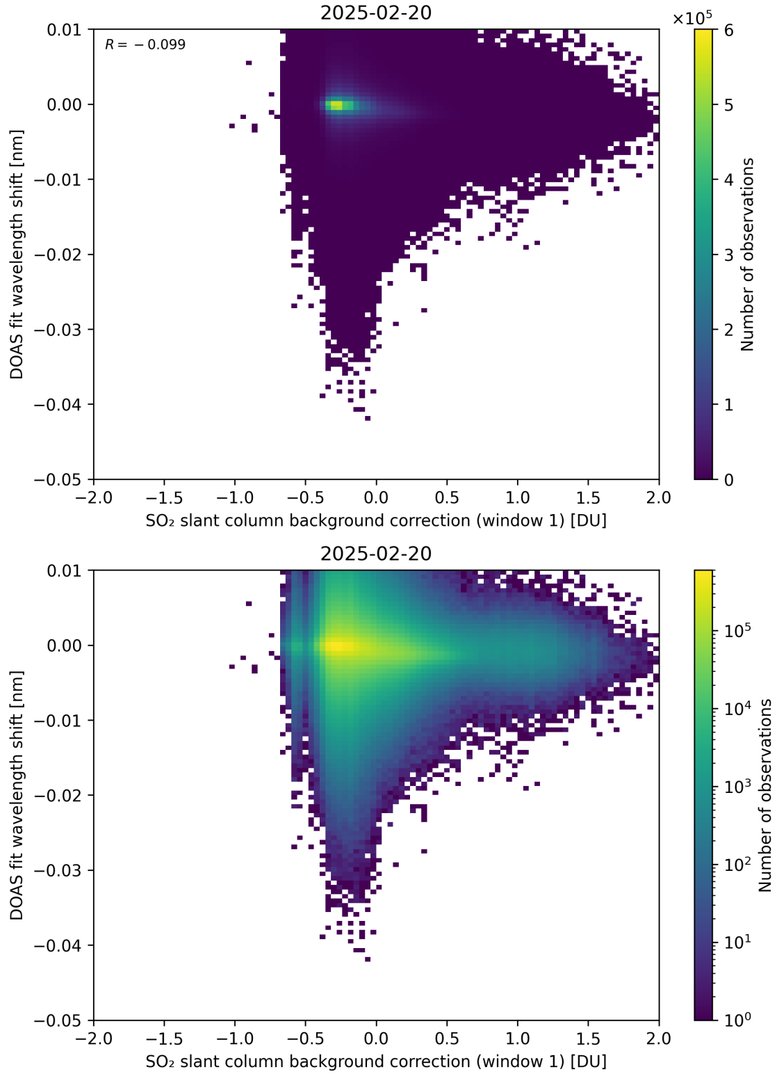
Figure 111: Scatter density plot of “SO 2 slant column background correction (window 1)” against “DOAS fit wavelength shift” for 2025-02-19 to 2025-02-21.
