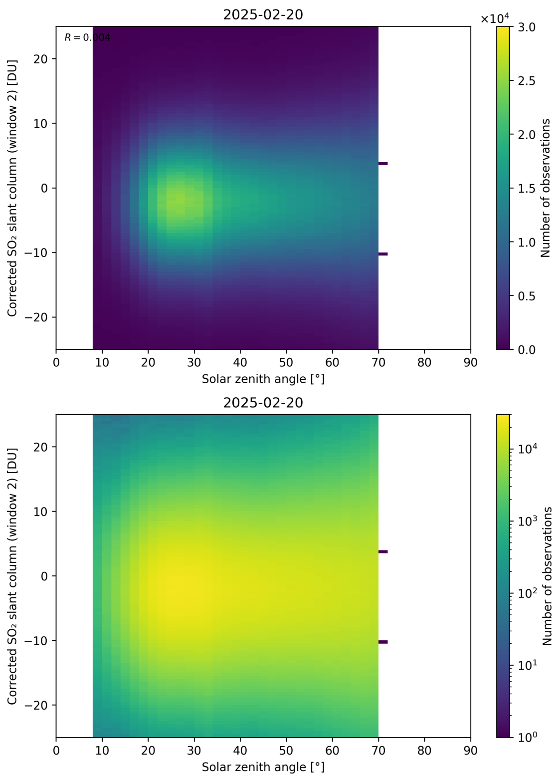
Figure 182: Scatter density plot of “Solar zenith angle” against “Corrected SO 2 slant column (window 2)” for 2025-02-19 to 2025-02-21.
