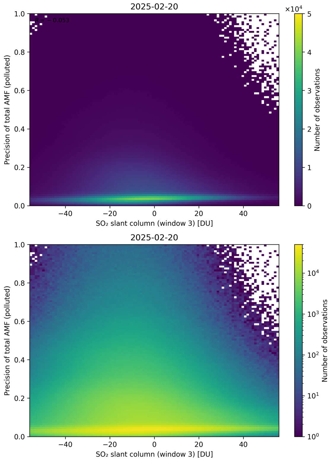
Figure 319: Scatter density plot of “SO 2 slant column (window 3)” against “Precision of total AMF (polluted)” for 2025-02-19 to 2025-02-21.
