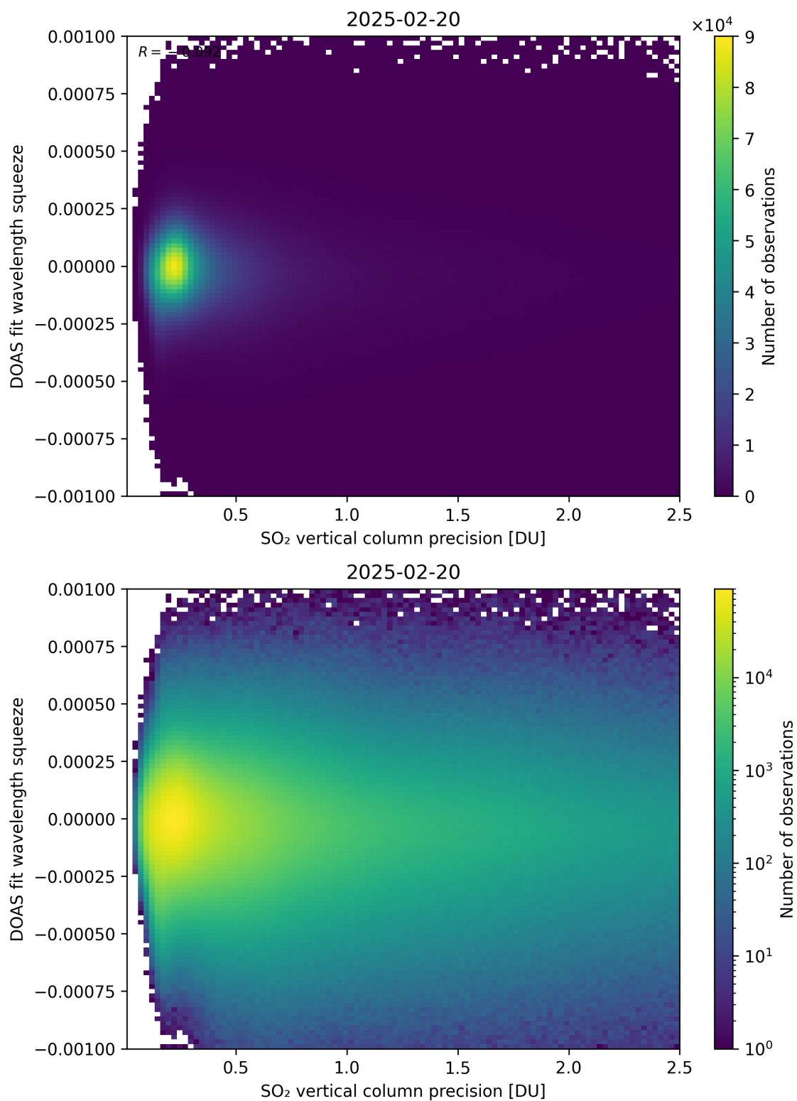
Figure 333: Scatter density plot of “SO 2 vertical column precision” against “DOAS fit wavelength squeeze” for 2025-02-19 to 2025-02-21.
