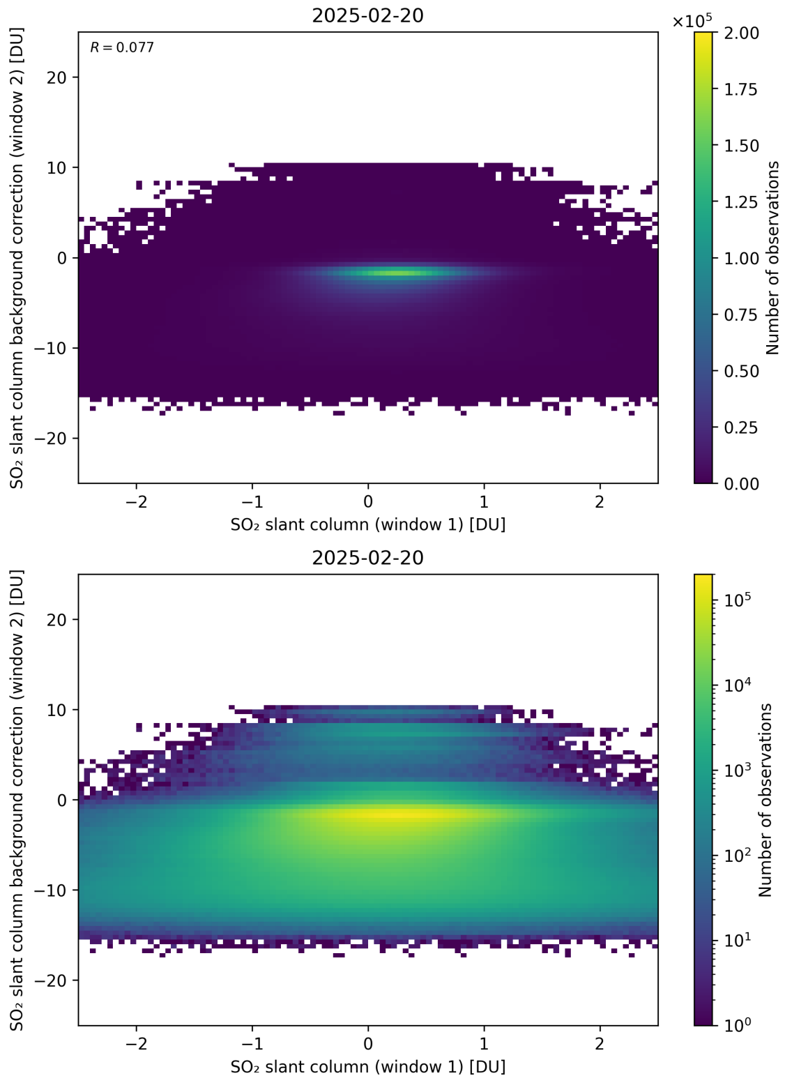
Figure 263: Scatter density plot of “SO 2 slant column (window 1)” against “SO 2 slant column background correction (window 2)” for 2025-02-19 to 2025-02-21.
