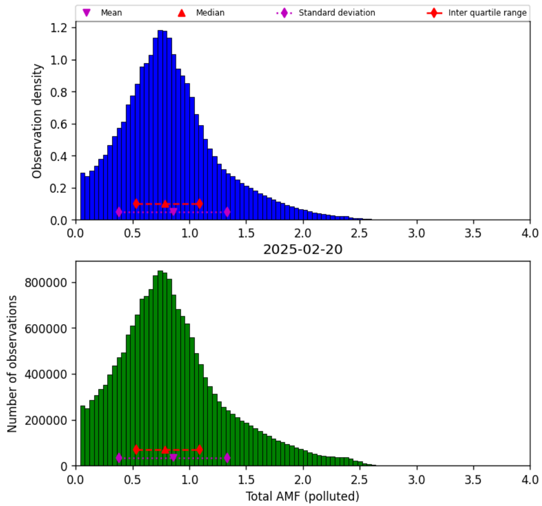
Figure 79: Histogram of “Total AMF (polluted)” for 2025-02-19 to 2025-02-21
