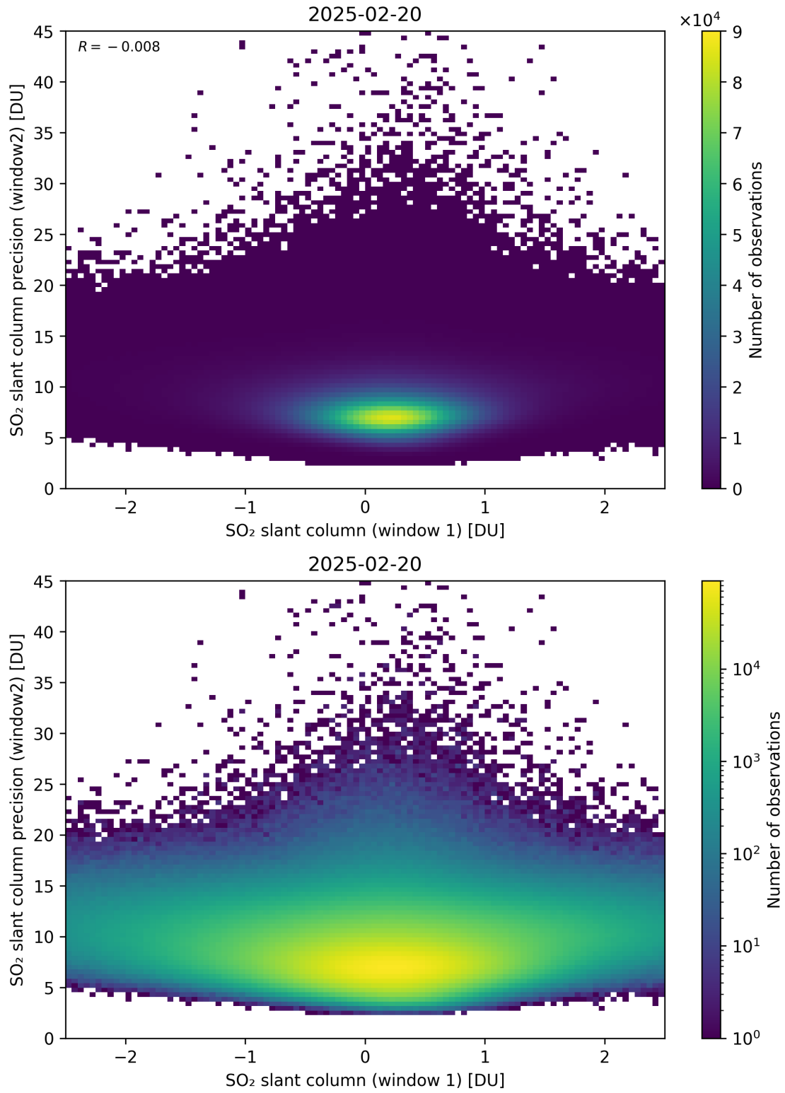
Figure 286: Scatter density plot of “SO 2 slant column (window 1)” against “SO 2 slant column precision (window2)” for 2025-02-19 to 2025-02-21.
