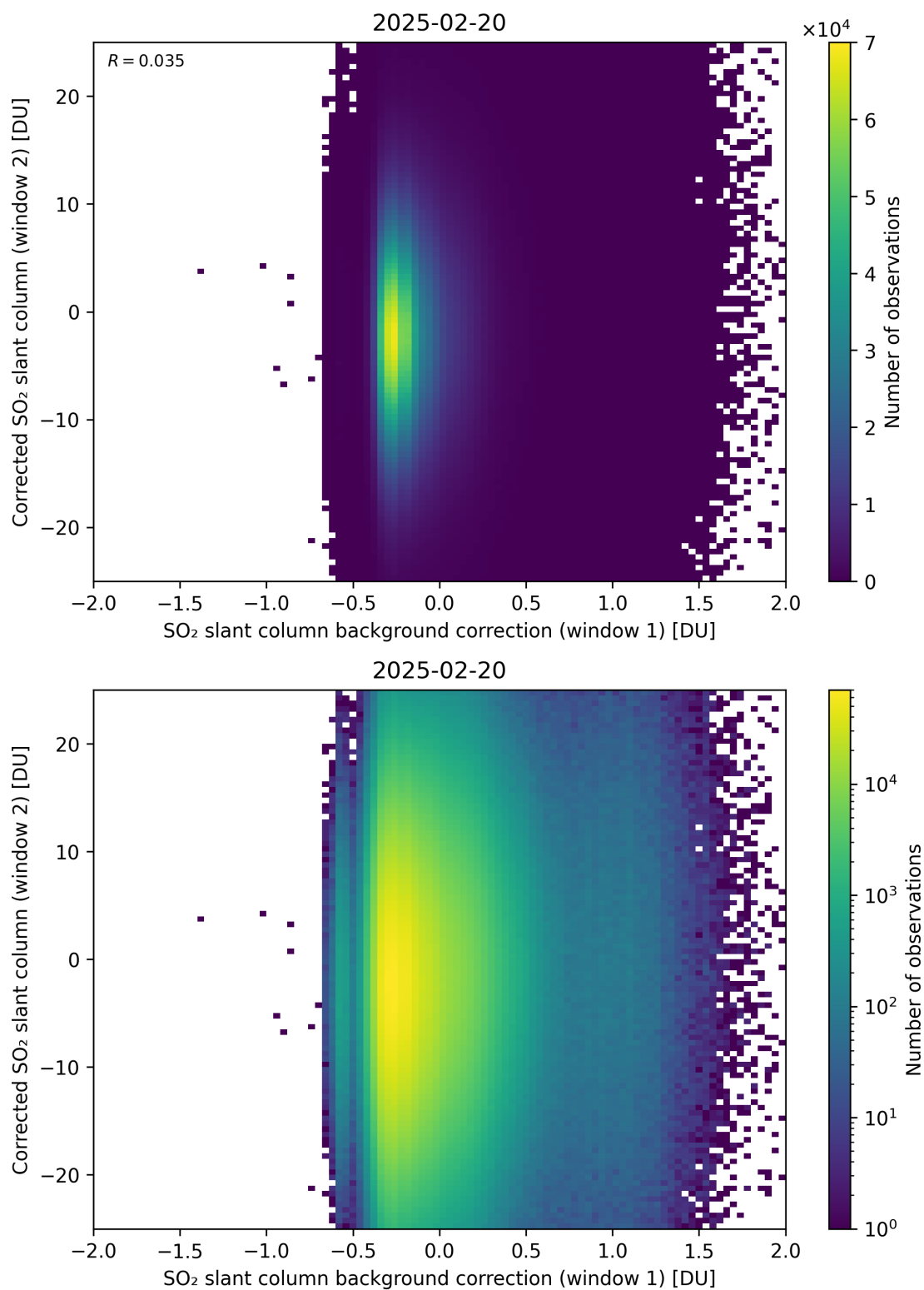
Figure 115: Scatter density plot of “SO 2 slant column background correction (window 1)” against “Corrected SO 2 slant column (window 2)” for 2025-02-19 to 2025-02-21.
