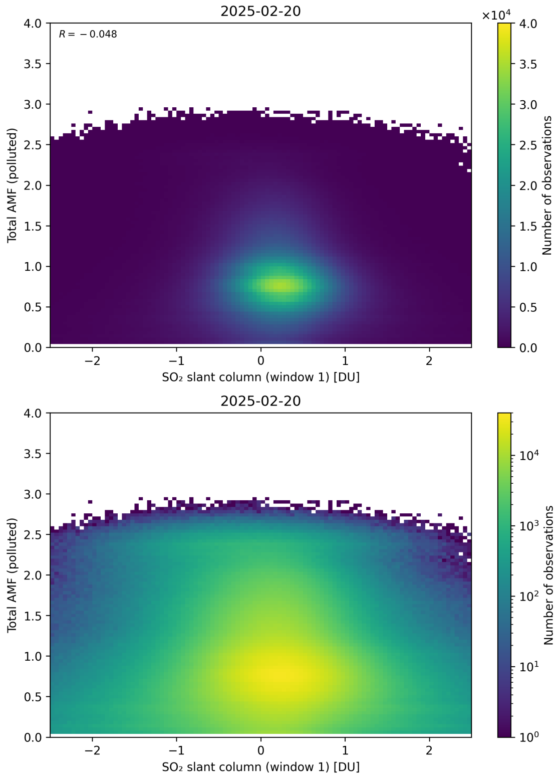
Figure 289: Scatter density plot of “SO 2 slant column (window 1)” against “Total AMF (polluted)” for 2025-02-19 to 2025-02-21.
