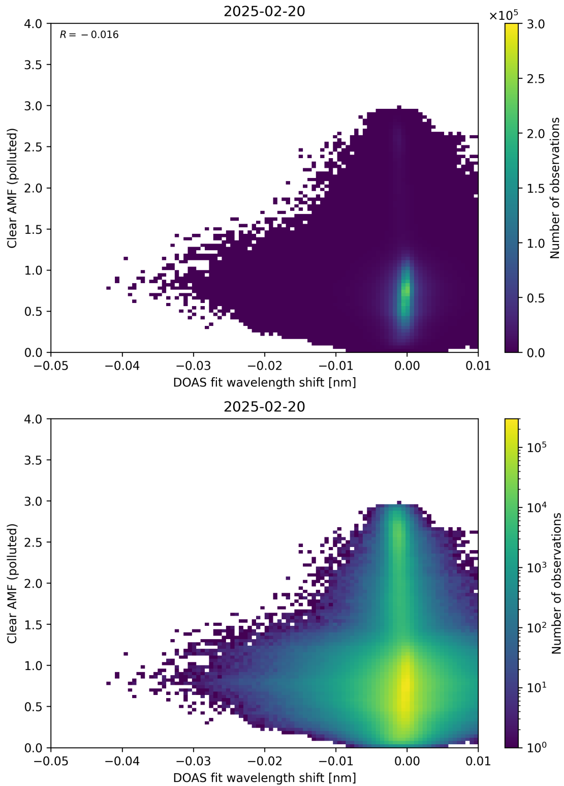
Figure 140: Scatter density plot of “DOAS fit wavelength shift” against “Clear AMF (polluted)” for 2025-02-19 to 2025-02-21.
