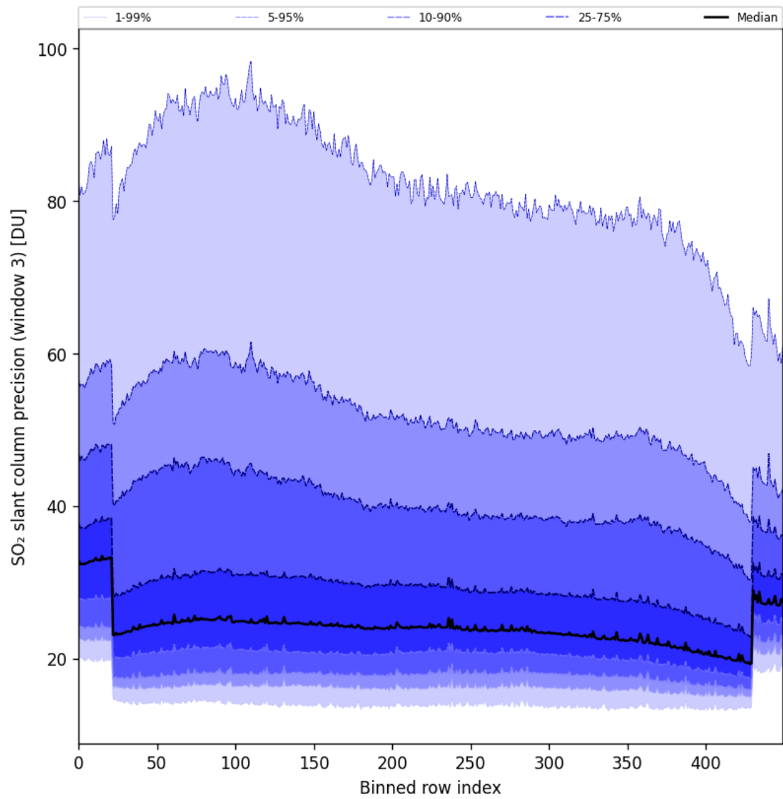
Figure 98: Along track statistics of “SO 2 slant column precision (window 3)” for 2025-02-19 to 2025-02-21
