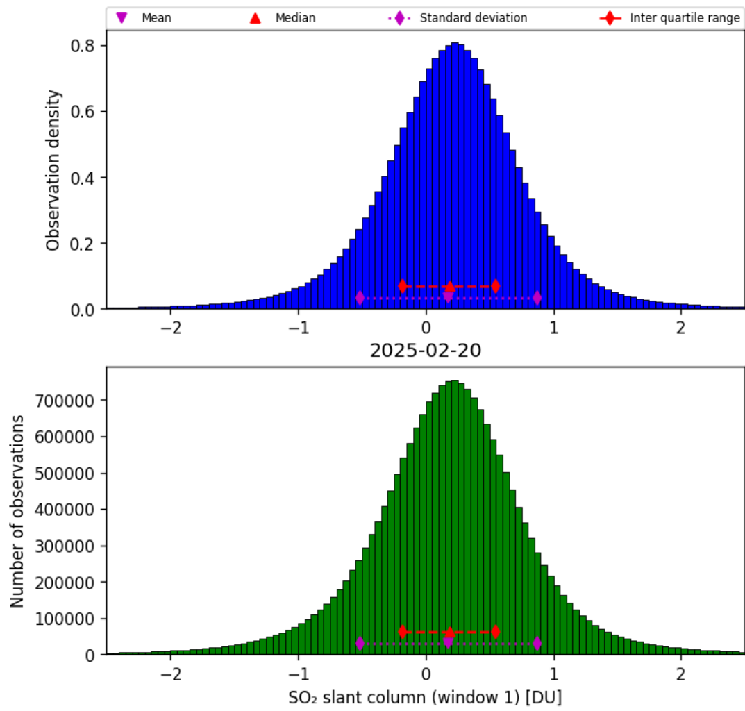
Figure 63: Histogram of “SO 2 slant column (window 1)” for 2025-02-19 to 2025-02-21
