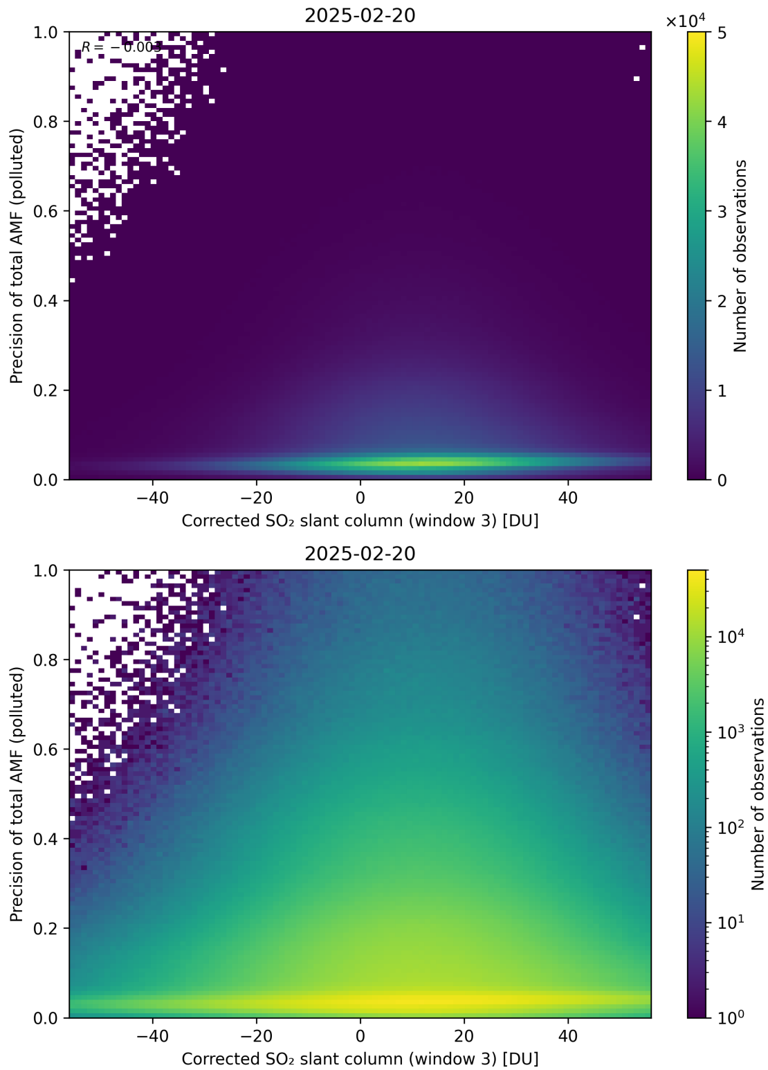
Figure 261: Scatter density plot of “Corrected SO 2 slant column (window 3)” against “Precision of total AMF (polluted)” for 2025-02-19 to 2025-02-21.
