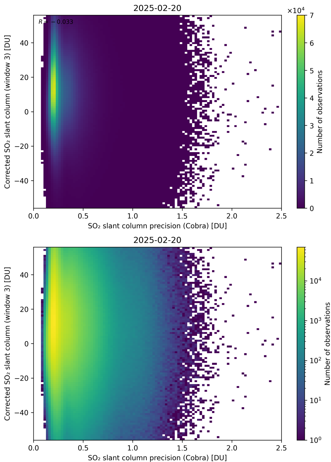
Figure 207: Scatter density plot of “SO 2 slant column precision (Cobra)” against “Corrected SO 2 slant column (window 3)” for 2025-02-19 to 2025-02-21.
