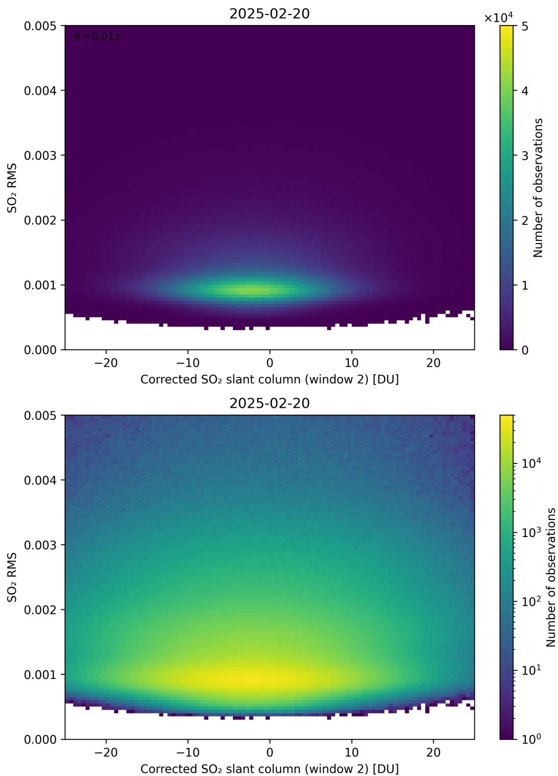
Figure 248: Scatter density plot of “Corrected SO 2 slant column (window 2)” against “SO 2 RMS” for 2025-02-19 to 2025-02-21.
