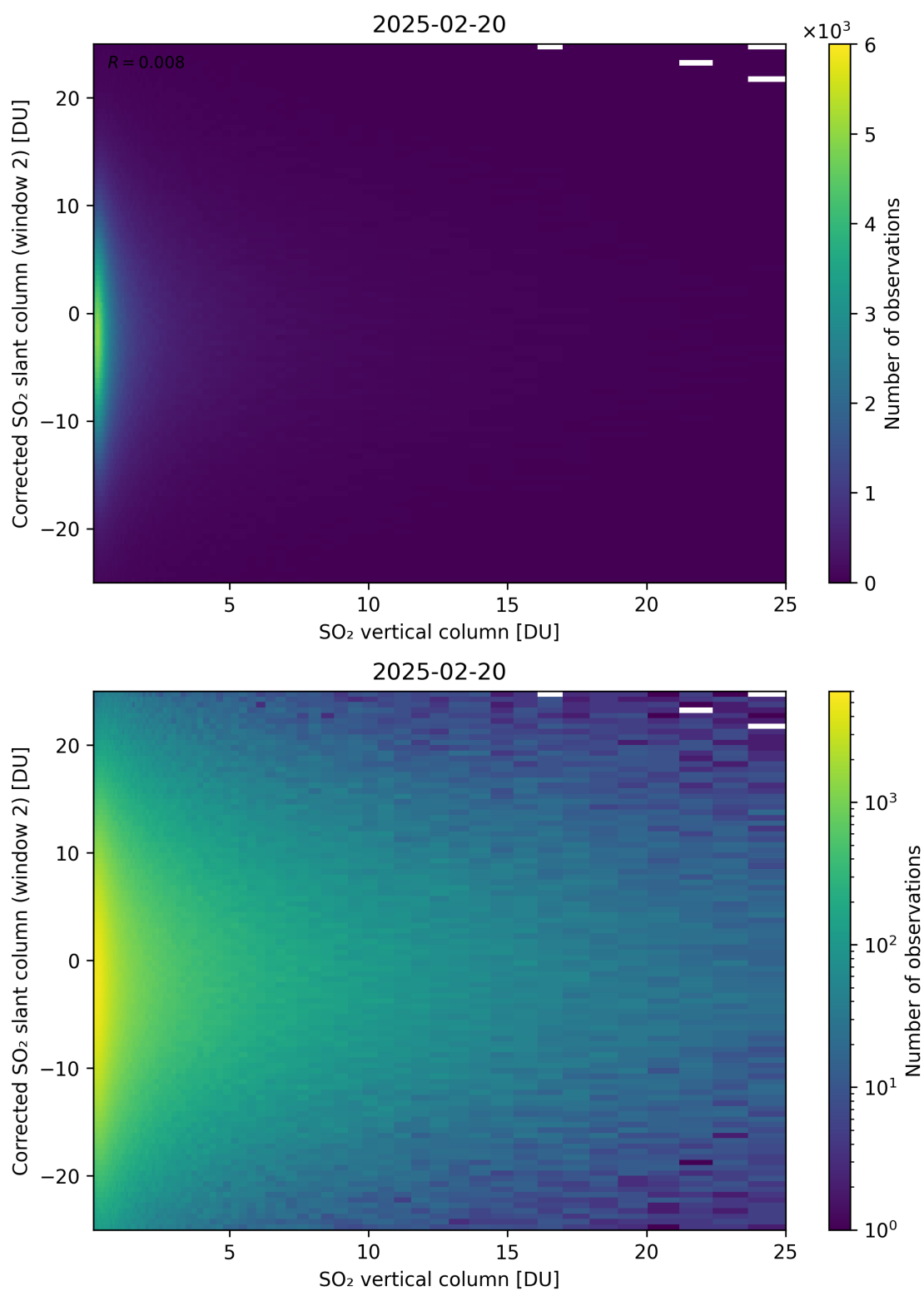
Figure 352: Scatter density plot of “SO 2 vertical column” against “Corrected SO 2 slant column (window 2)” for 2025-02-19 to 2025-02-21.
