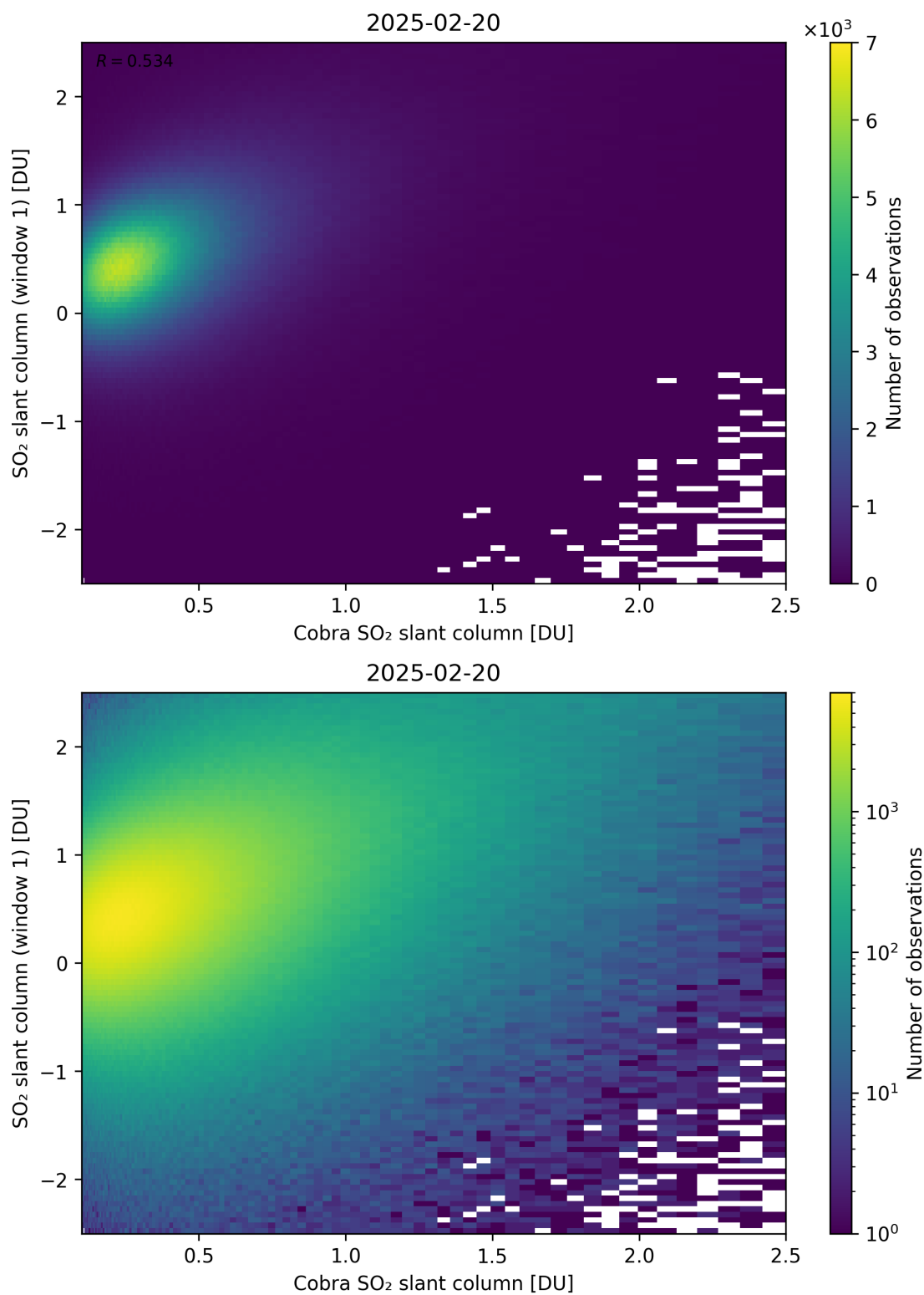
Figure 219: Scatter density plot of “Cobra SO 2 slant column” against “SO 2 slant column (window 1)” for 2025-02-19 to 2025-02-21.
