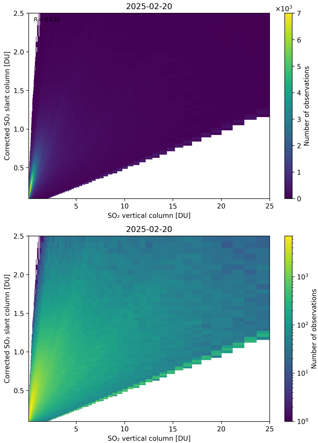
Figure 351: Scatter density plot of “SO 2 vertical column” against “Corrected SO 2 slant column” for 2025-02-19 to 2025-02-21.
