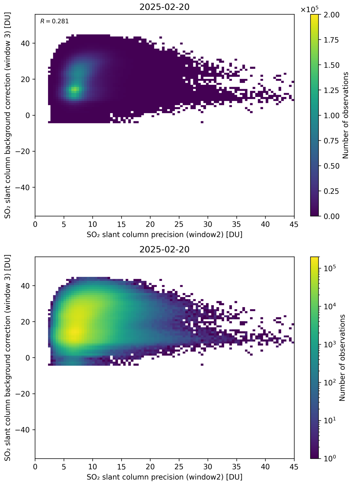
Figure 292: Scatter density plot of “SO 2 slant column precision (window2)” against “SO 2 slant column background correction (window 3)” for 2025-02-19 to 2025-02-21.
