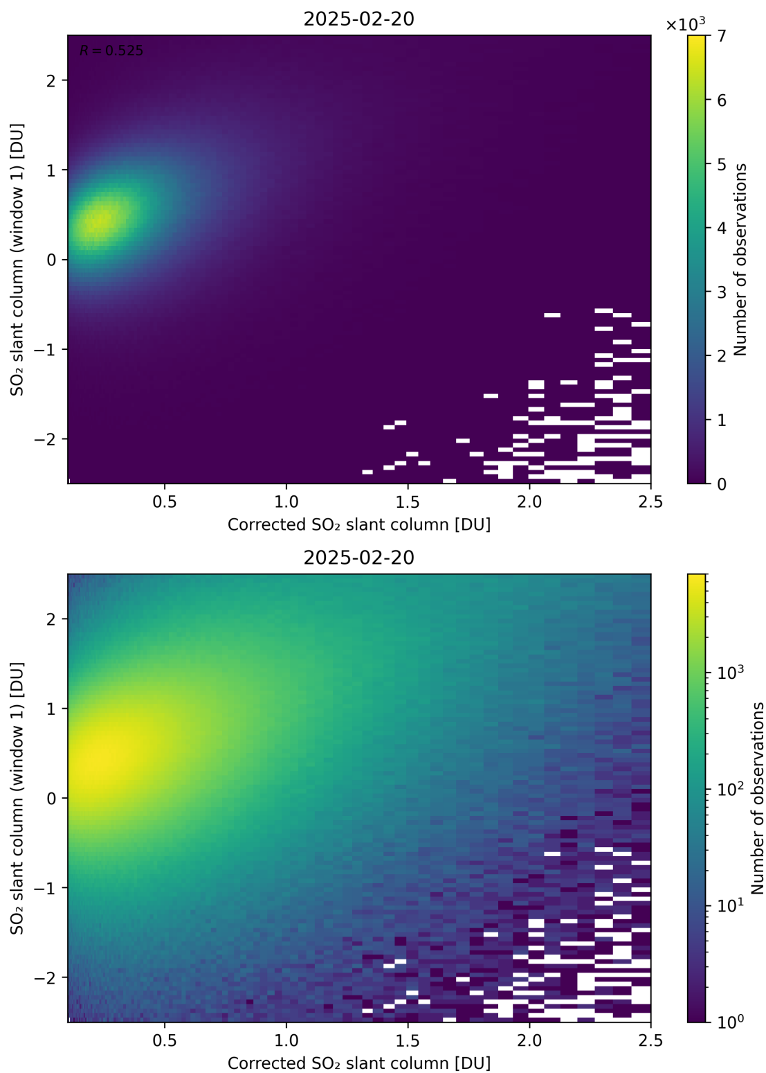
Figure 237: Scatter density plot of “Corrected SO 2 slant column” against “SO 2 slant column (window 1)” for 2025-02-19 to 2025-02-21.
