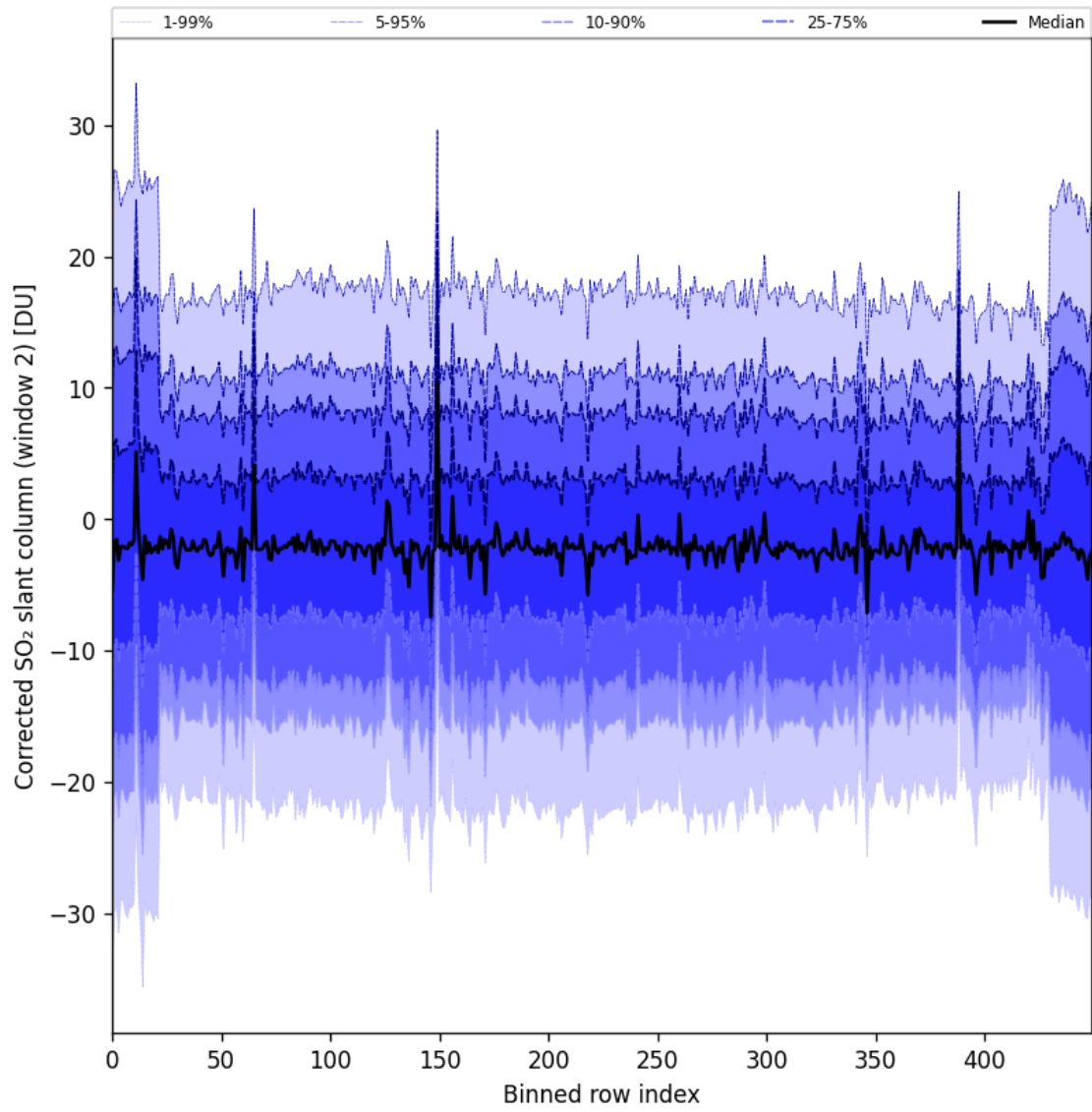
Figure 95: Along track statistics of “Corrected SO 2 slant column (window 2)” for 2025-02-19 to 2025-02-21
