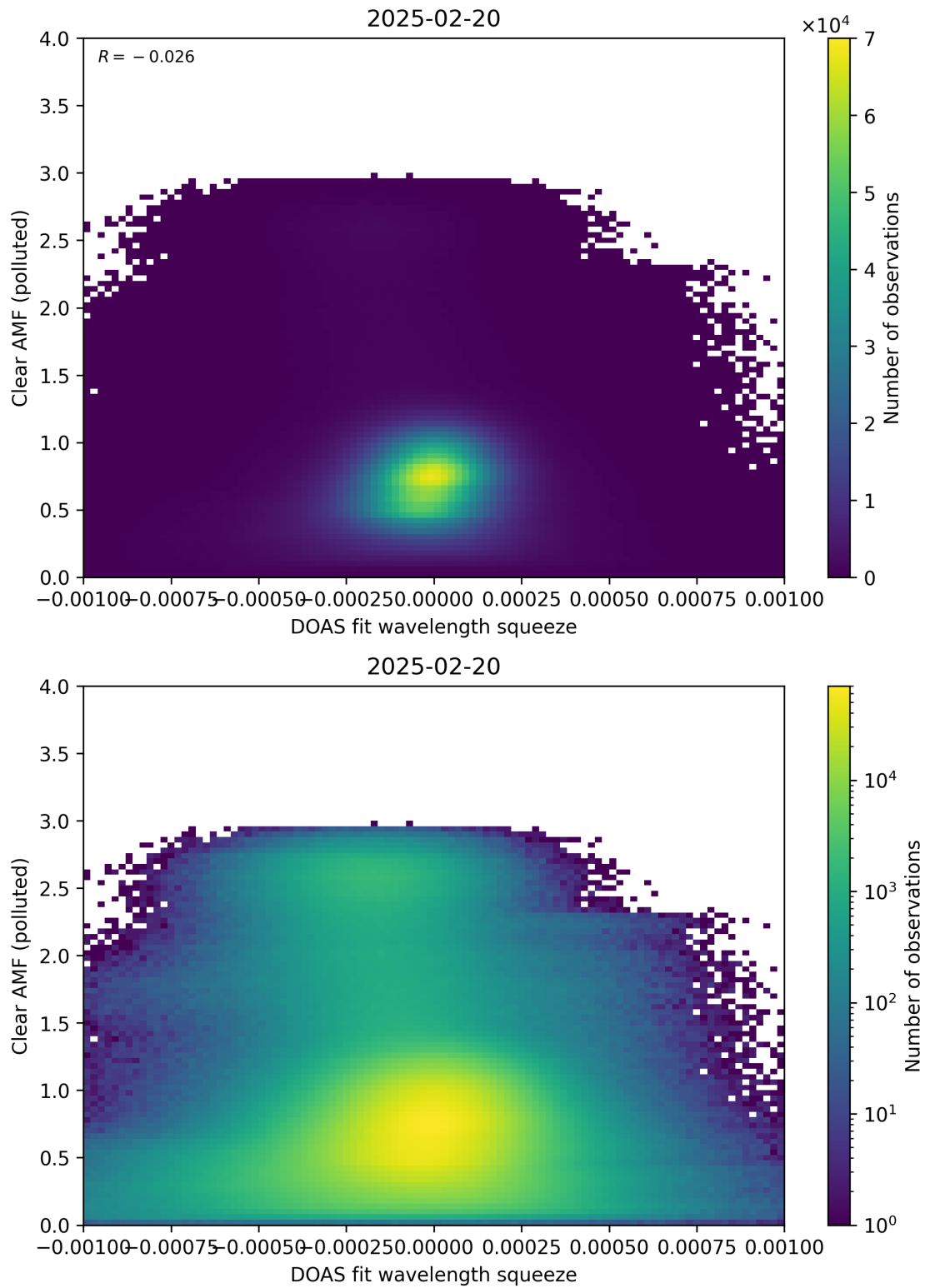
Figure 144: Scatter density plot of “DOAS fit wavelength squeeze” against “Clear AMF (polluted)” for 2025-02-19 to 2025-02-21.
