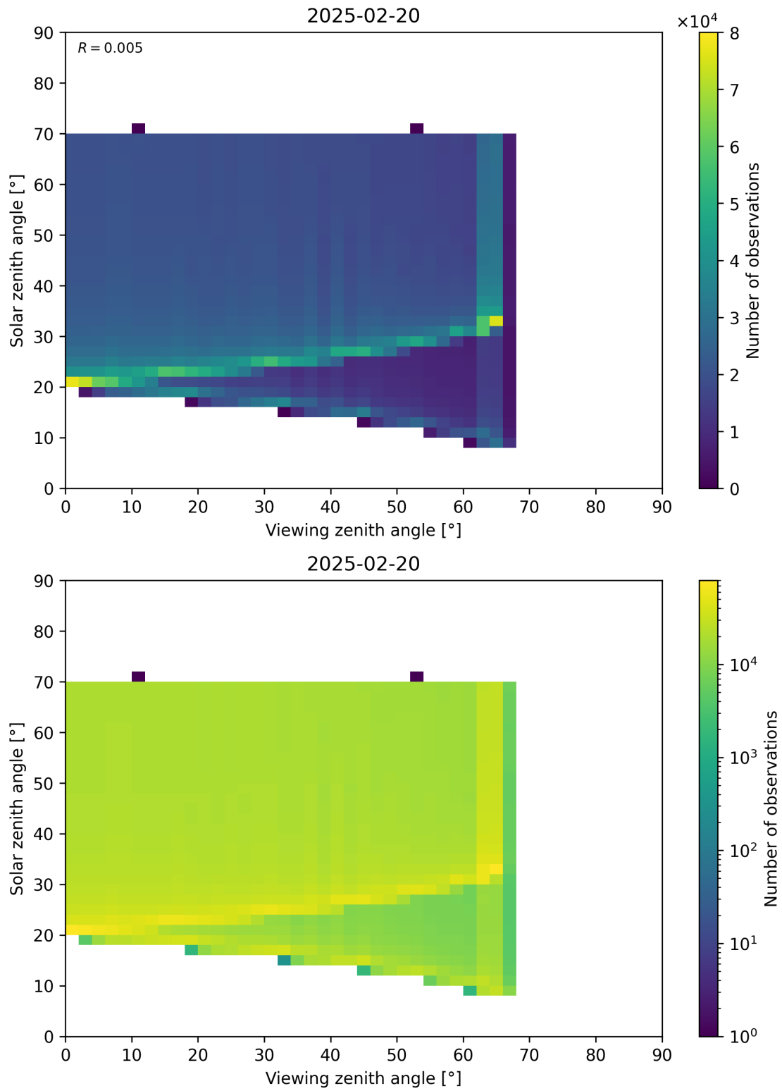
Figure 369: Scatter density plot of “Viewing zenith angle” against “Solar zenith angle” for 2025-02-19 to 2025-02-21.
