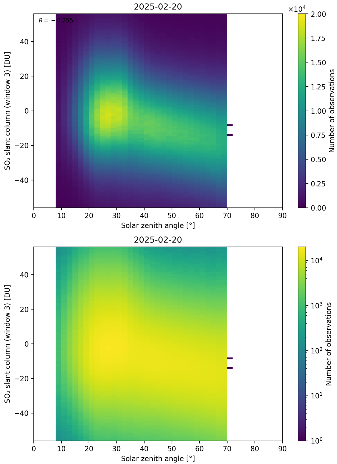
Figure 187: Scatter density plot of “Solar zenith angle” against “SO 2 slant column (window 3)” for 2025-02-19 to 2025-02-21.
