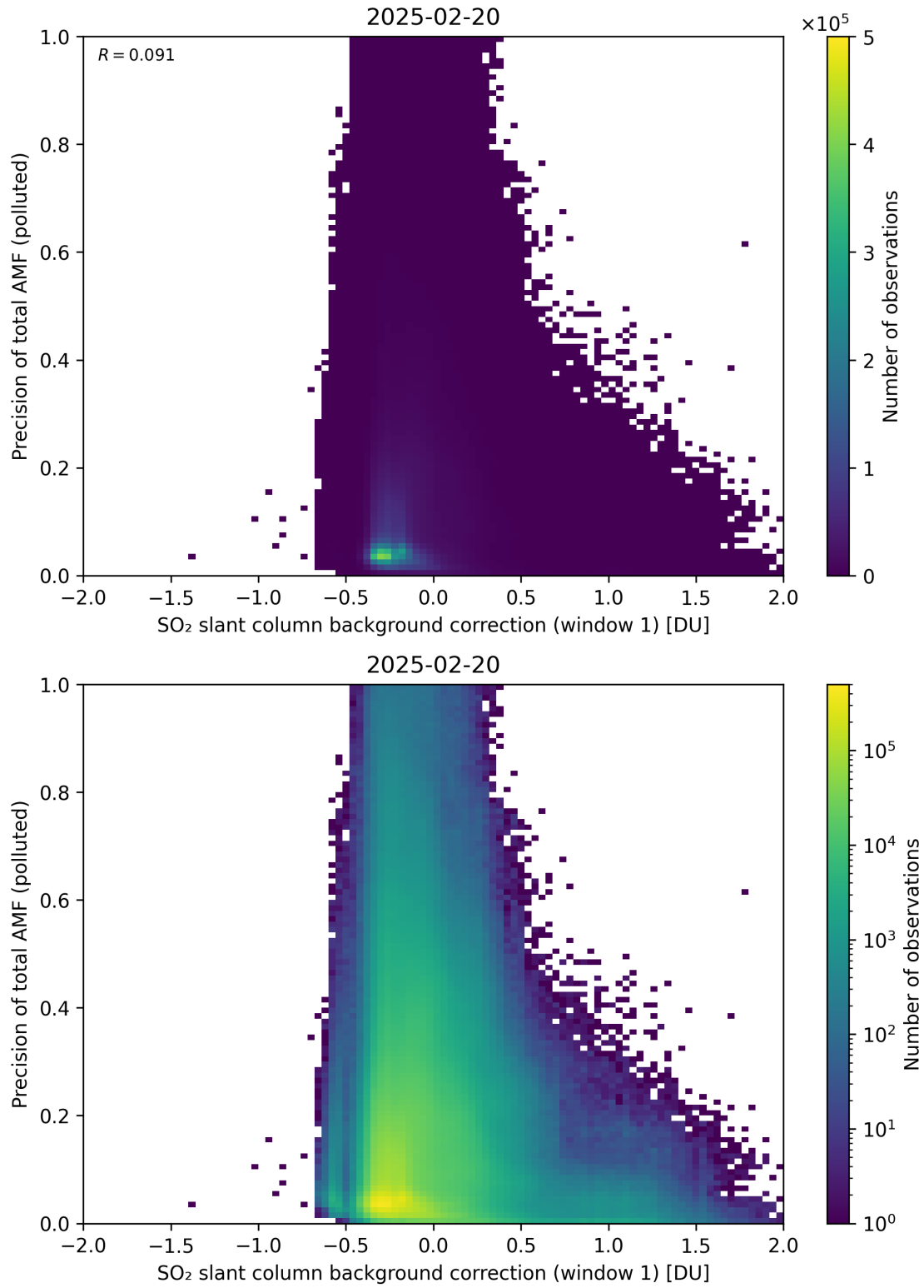
Figure 121: Scatter density plot of “SO 2 slant column background correction (window 1)” against “Precision of total AMF (polluted)” for 2025-02-19 to 2025-02-21.
