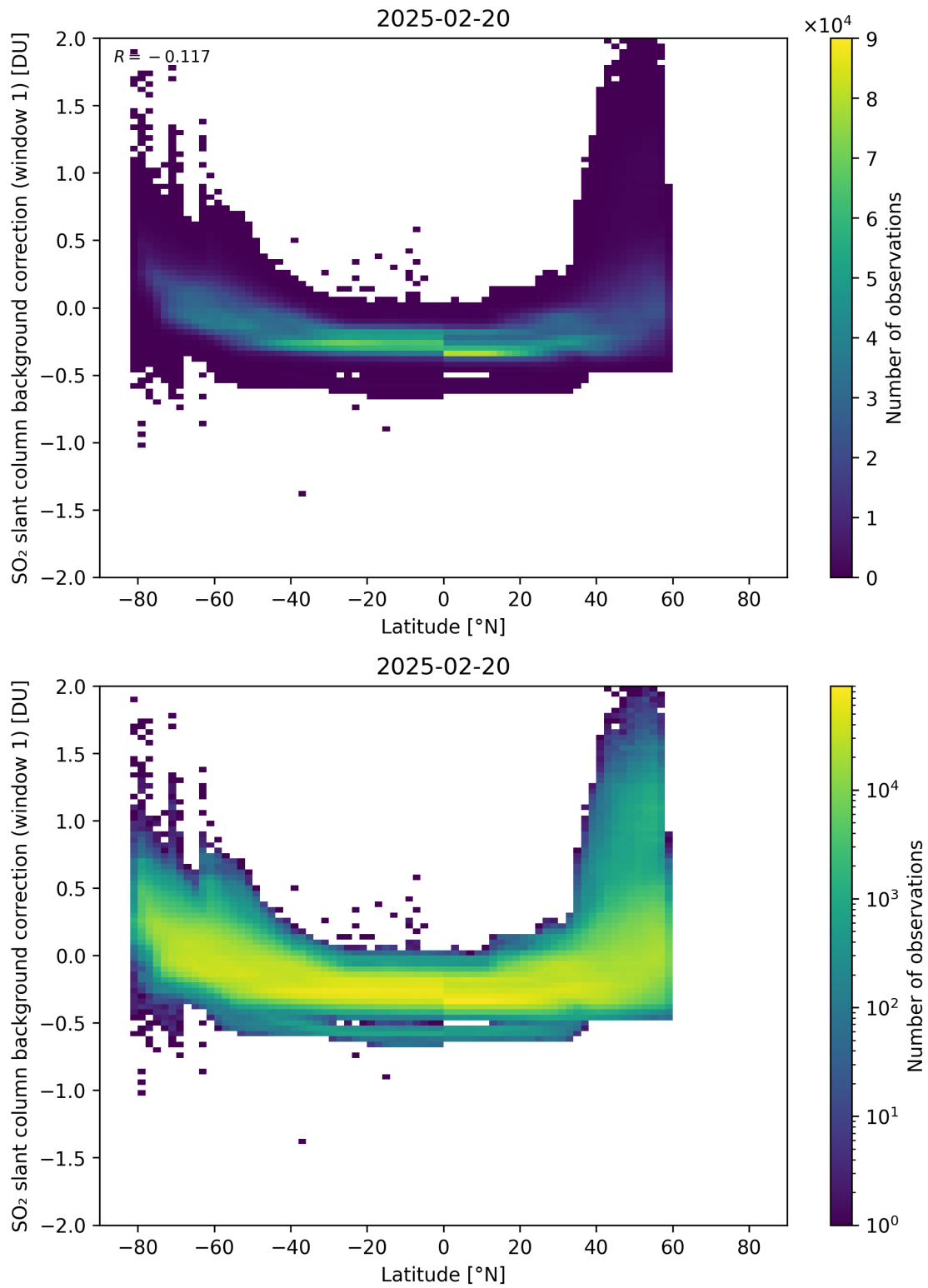
Figure 150: Scatter density plot of “Latitude” against “SO 2 slant column background correction (window 1)” for 2025-02-19 to 2025-02-21.
