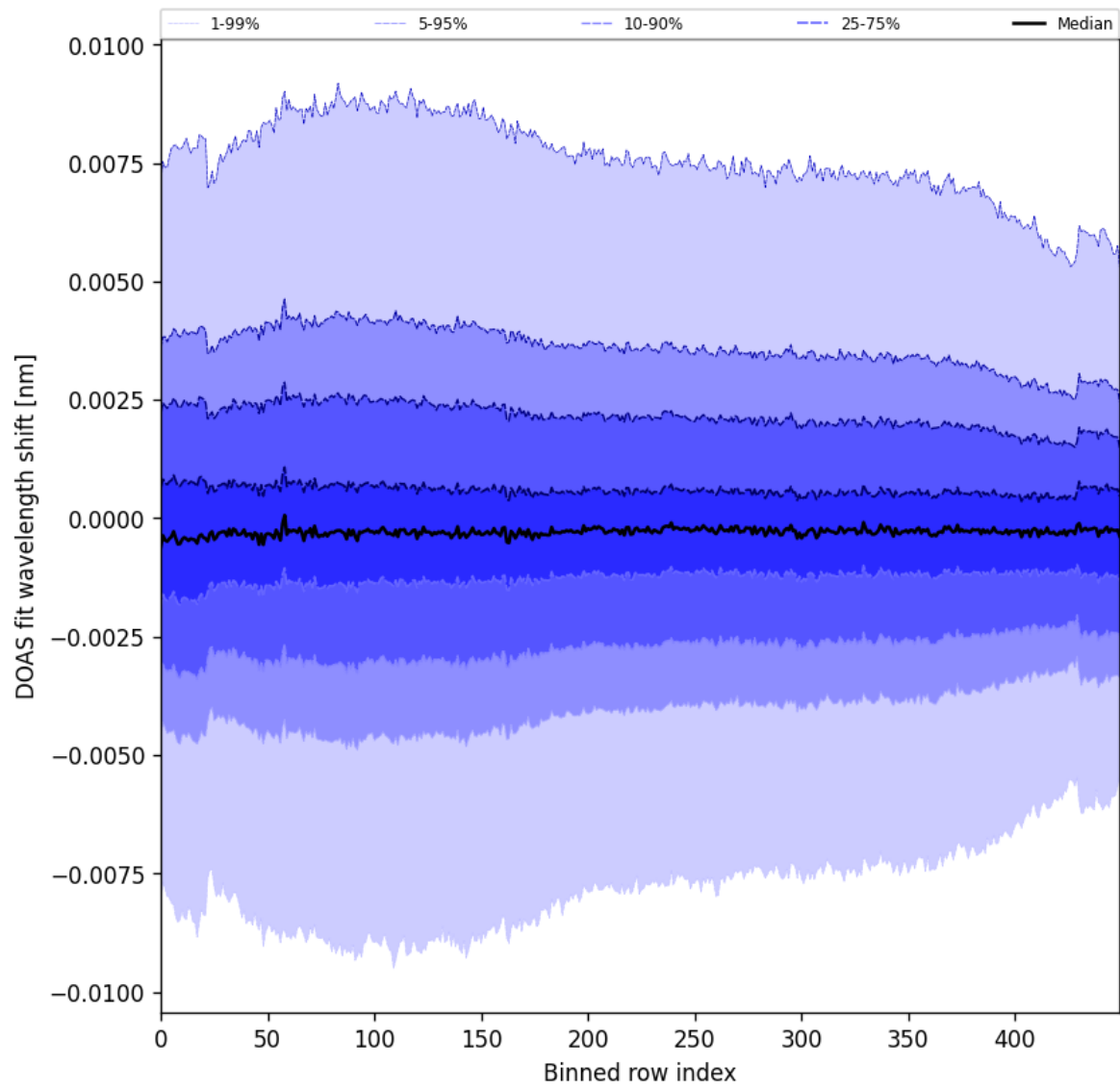
Figure 102: Along track statistics of “DOAS fit wavelength shift” for 2025-02-19 to 2025-02-21
