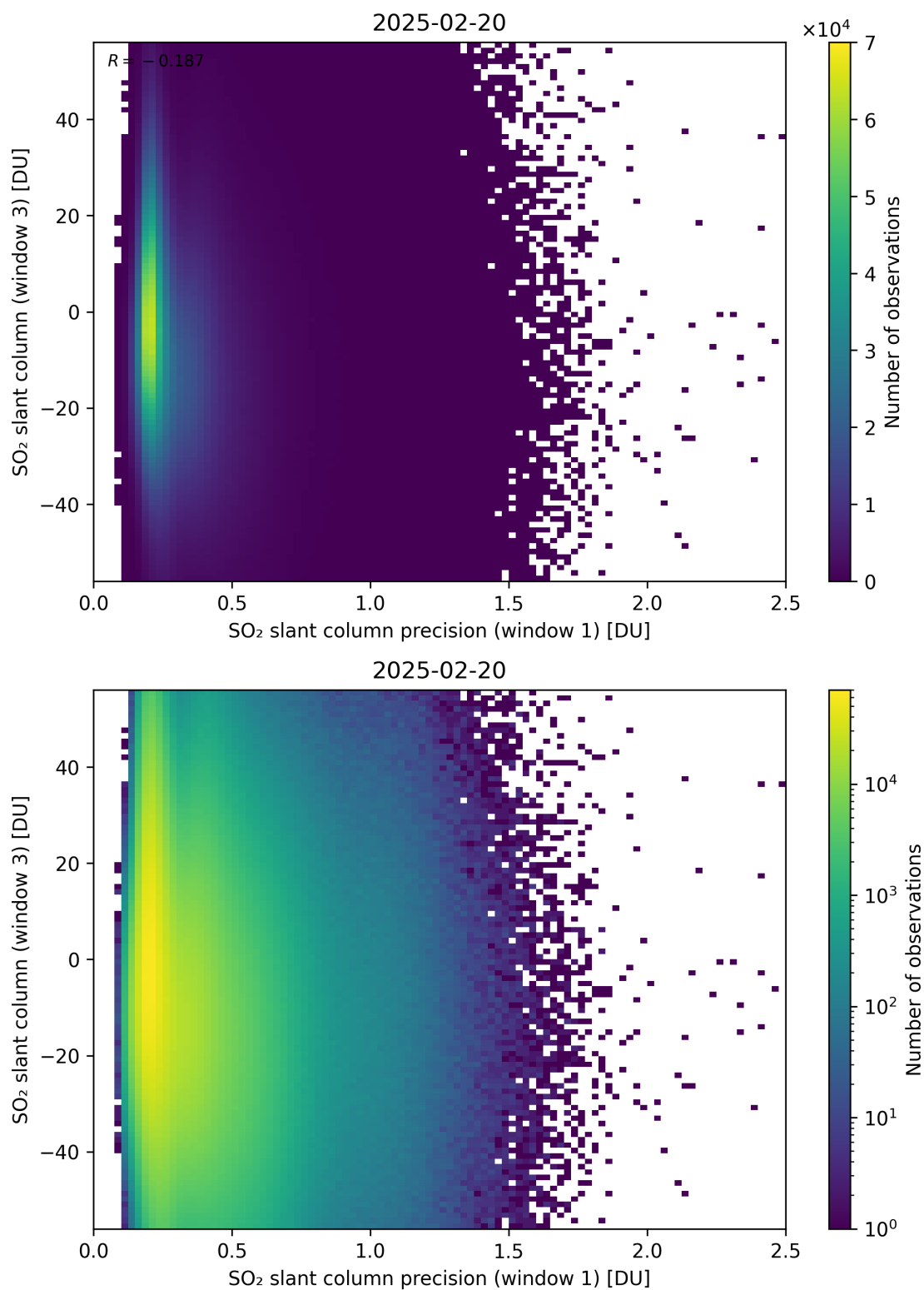
Figure 278: Scatter density plot of “SO 2 slant column precision (window 1)” against “SO 2 slant column (window 3)” for 2025-02-19 to 2025-02-21.
