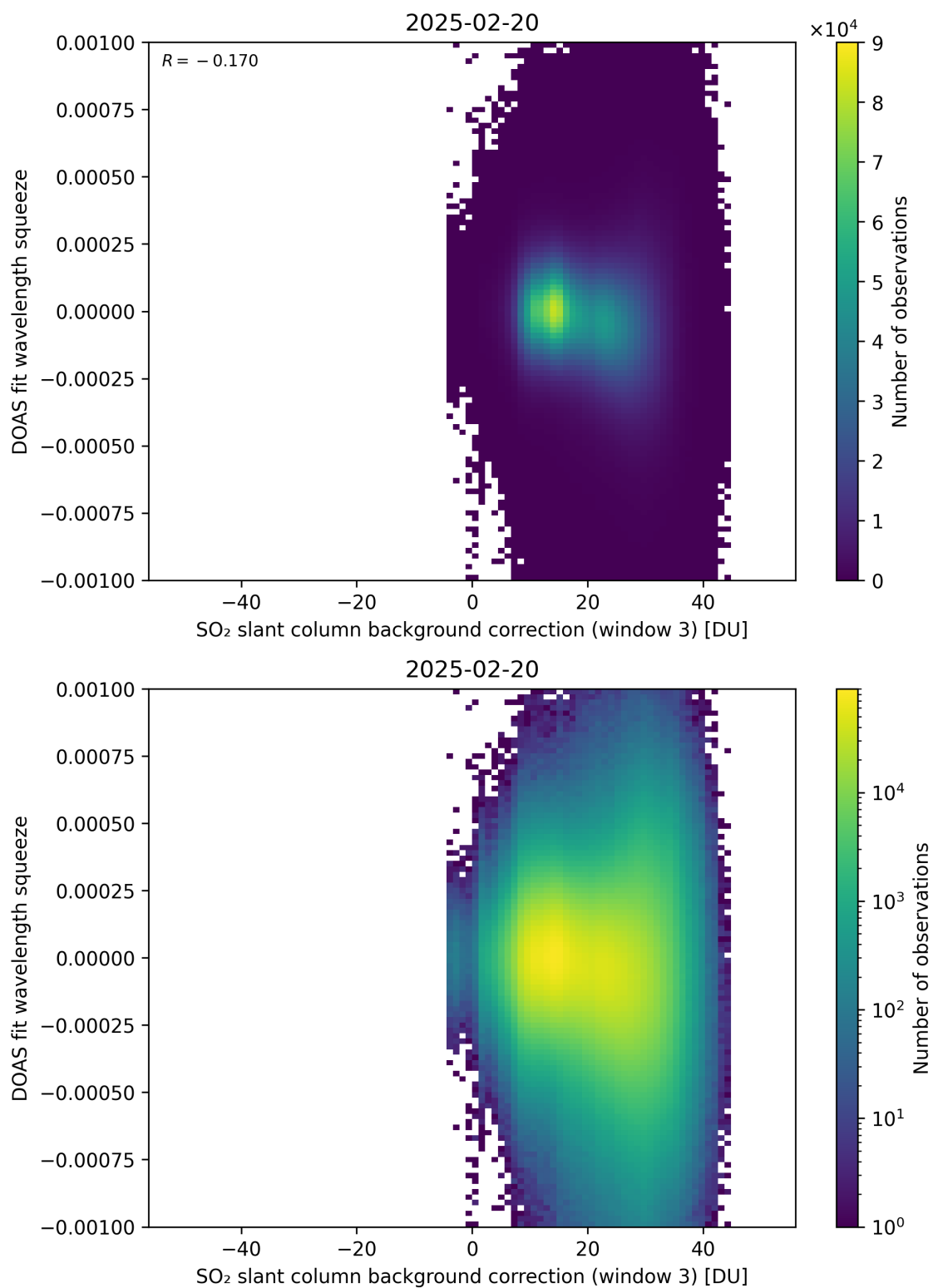
Figure 133: Scatter density plot of “SO 2 slant column background correction (window 3)” against “DOAS fit wavelength squeeze” for 2025-02-19 to 2025-02-21.
