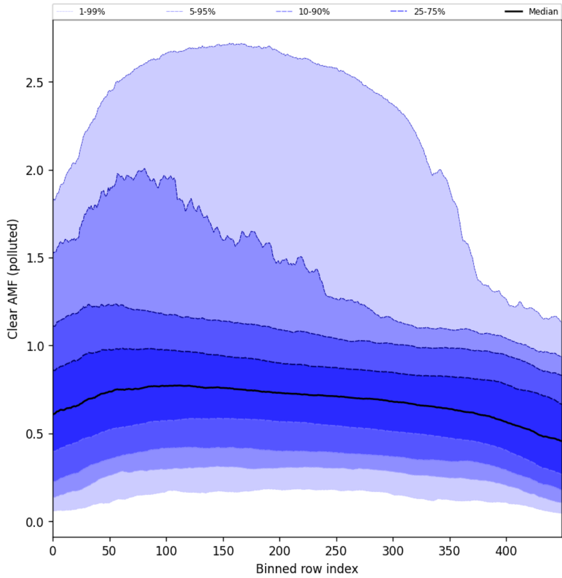
Figure 107: Along track statistics of “Clear AMF (polluted)” for 2025-02-19 to 2025-02-21
