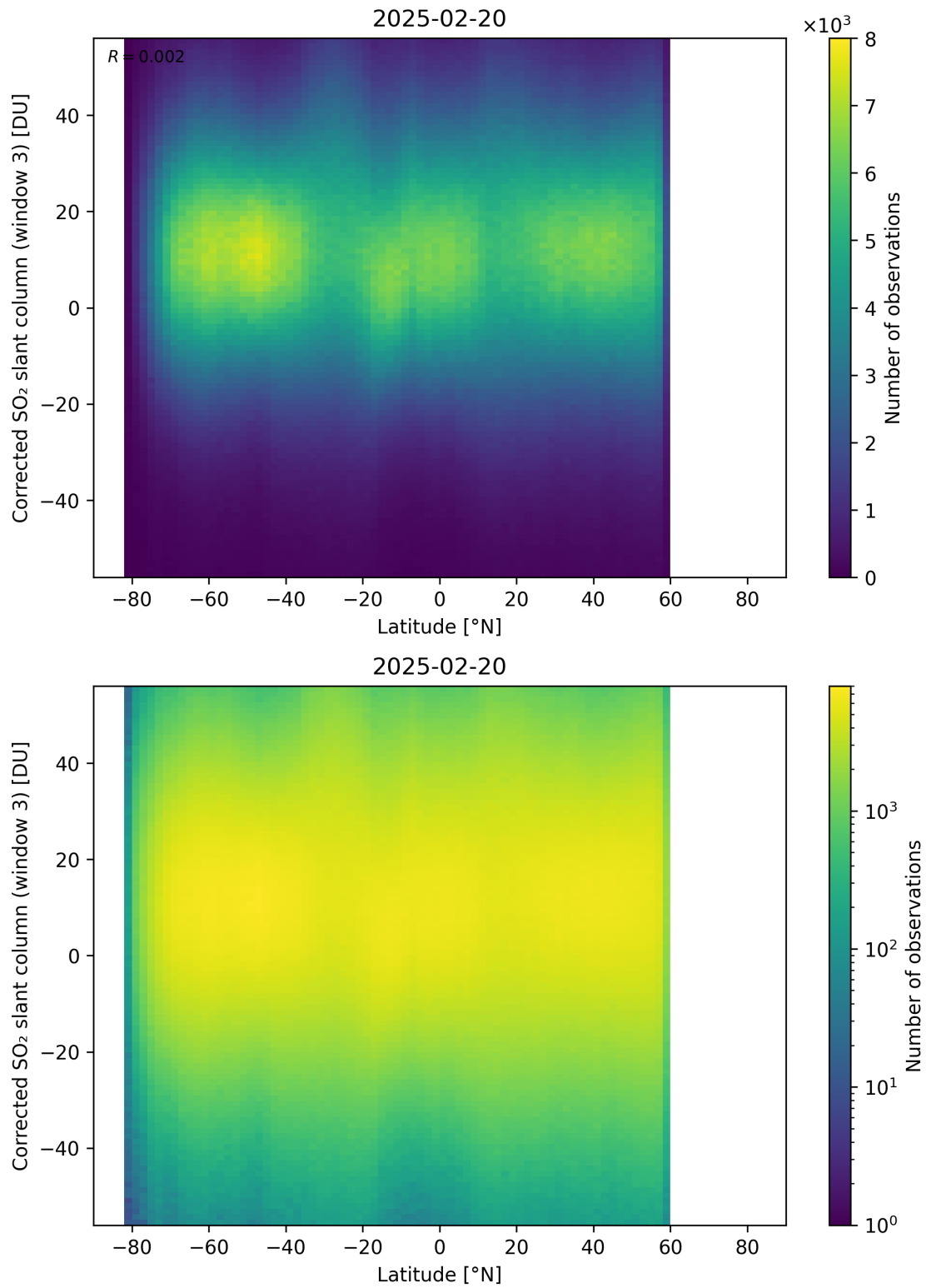
Figure 161: Scatter density plot of “Latitude” against “Corrected SO 2 slant column (window 3)” for 2025-02-19 to 2025-02-21.
