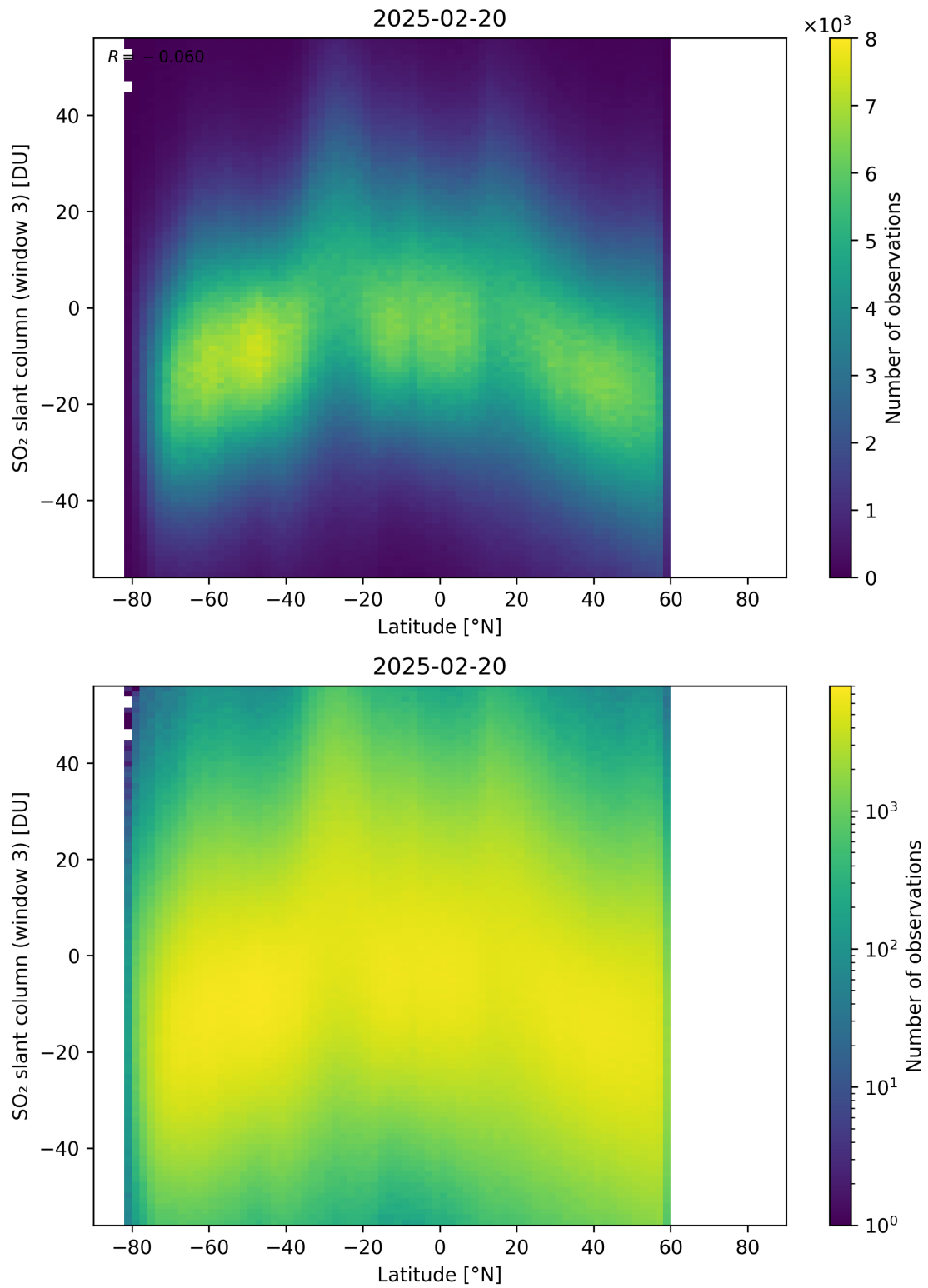
Figure 165: Scatter density plot of “Latitude” against “SO 2 slant column (window 3)” for 2025-02-19 to 2025-02-21.
