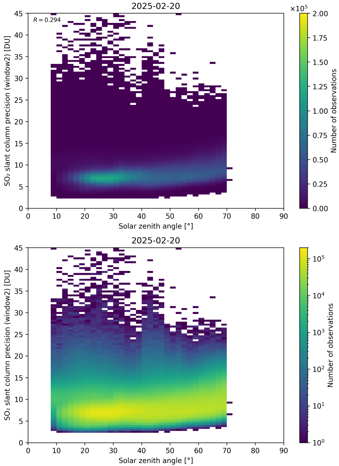
Figure 186: Scatter density plot of “Solar zenith angle” against “SO 2 slant column precision (window2)” for 2025-02-19 to 2025-02-21.
