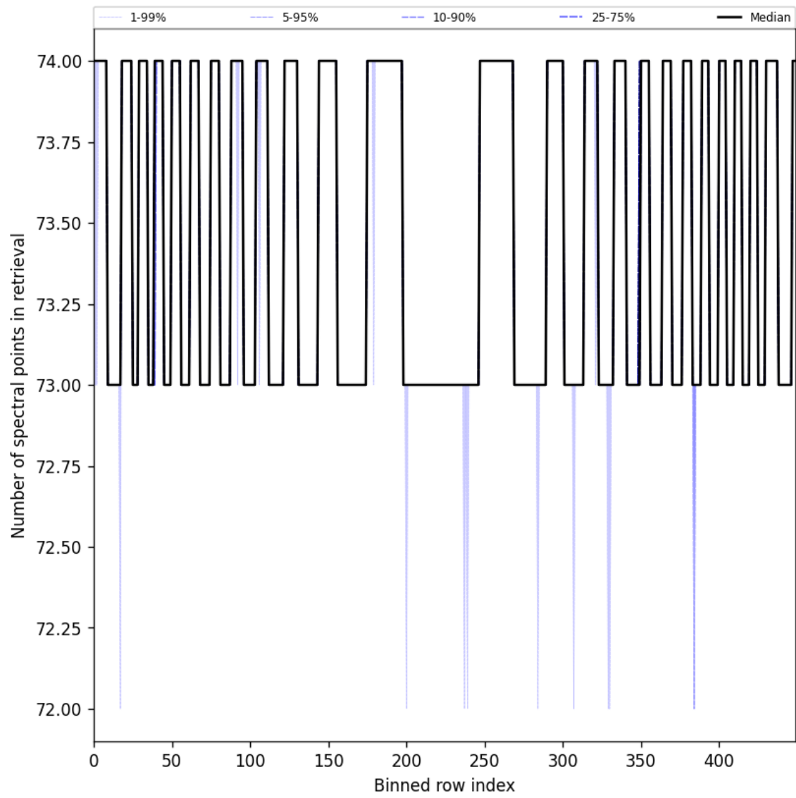
Figure 108: Along track statistics of “Number of spectral points in retrieval” for 2025-02-19 to 2025-02-21
