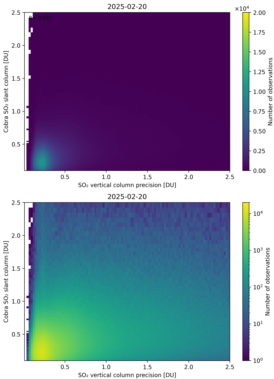
Figure 336: Scatter density plot of “SO 2 vertical column precision” against “Cobra SO 2 slant column” for 2025-02-19 to 2025-02-21.
