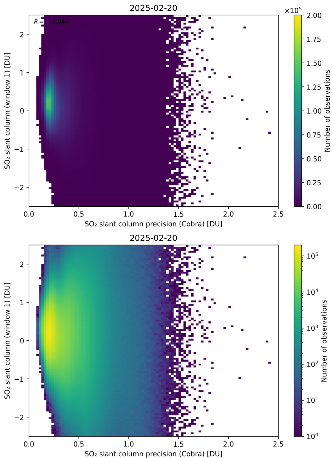
Figure 208: Scatter density plot of “SO 2 slant column precision (Cobra)” against “SO 2 slant column (window 1)” for 2025-02-19 to 2025-02-21.
