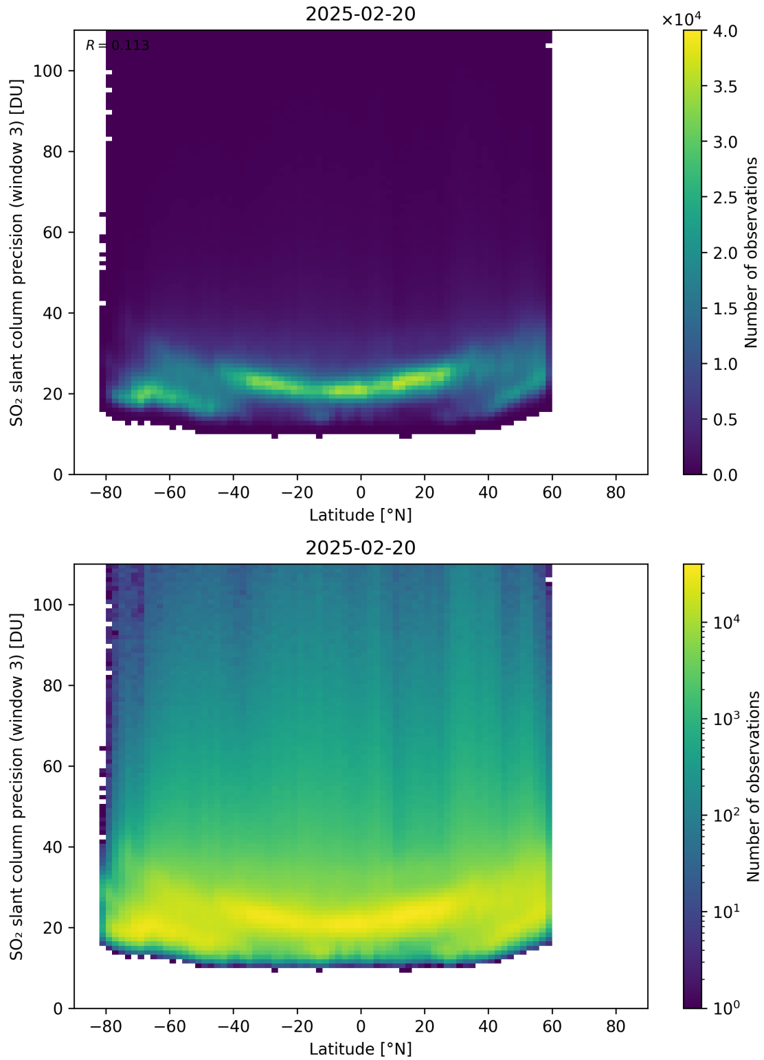
Figure 166: Scatter density plot of “Latitude” against “SO 2 slant column precision (window 3)” for 2025-02-19 to 2025-02-21.
