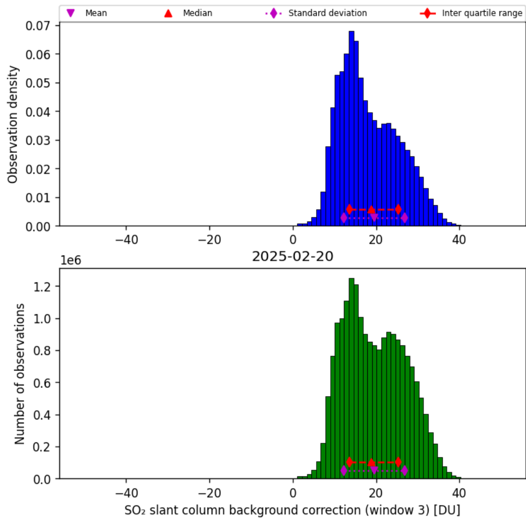
Figure 74: Histogram of “SO 2 slant column background correction (window 3)” for 2025-02-19 to 2025-02-21
