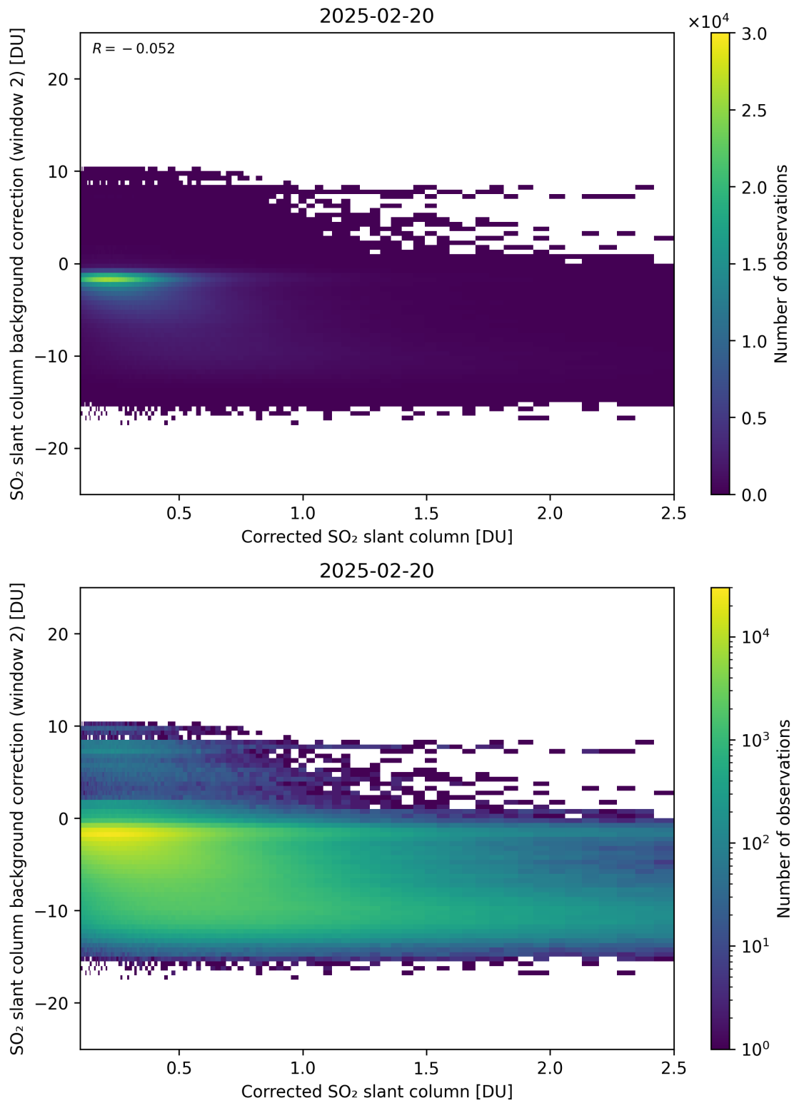
Figure 227: Scatter density plot of “Corrected SO 2 slant column” against “SO 2 slant column background correction (window 2)” for 2025-02-19 to 2025-02-21.
