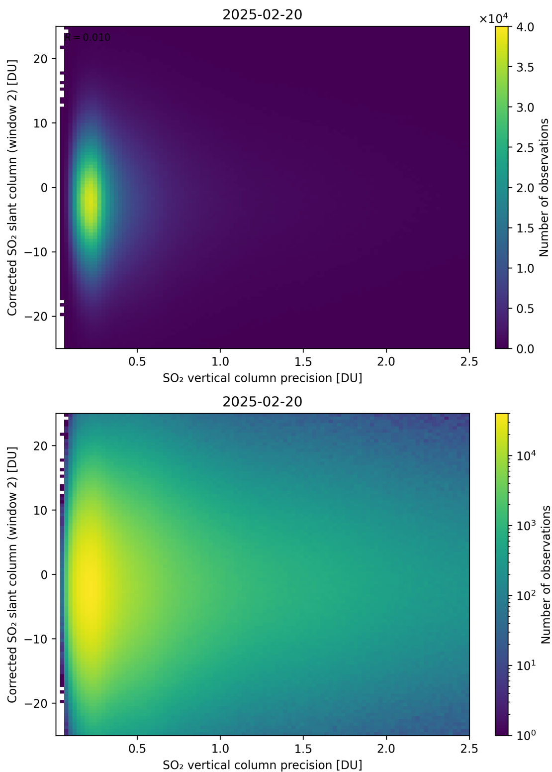
Figure 339: Scatter density plot of “SO 2 vertical column precision” against “Corrected SO 2 slant column (window 2)” for 2025-02-19 to 2025-02-21.
