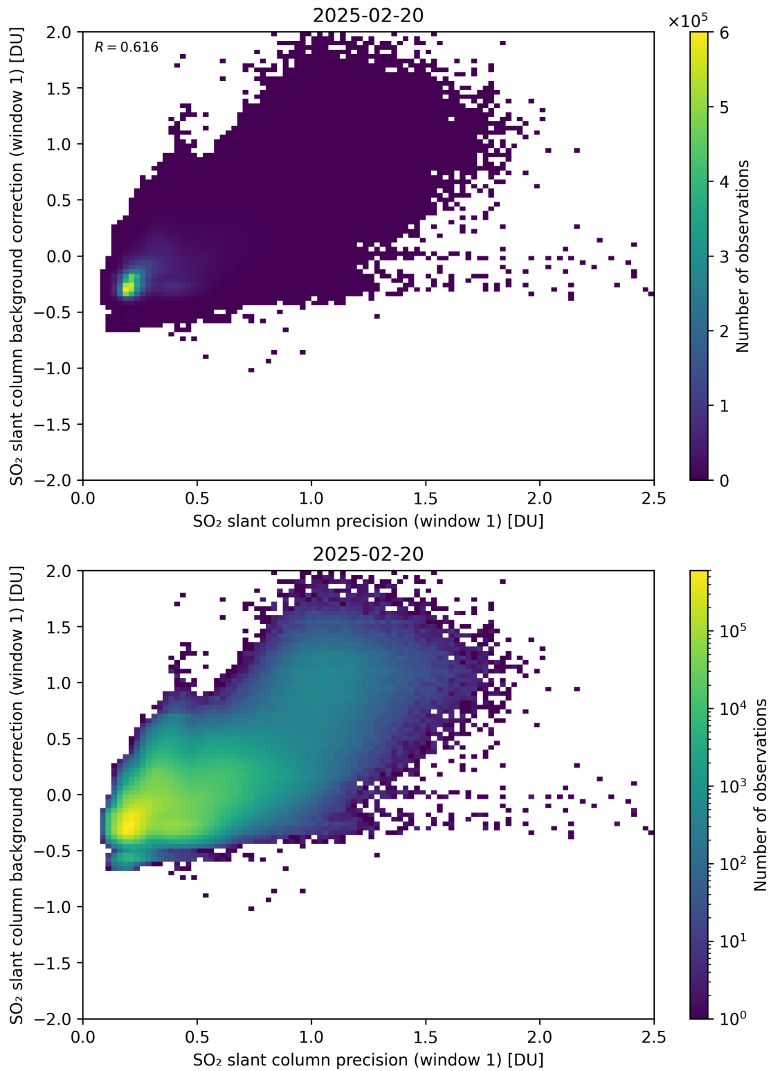
Figure 268: Scatter density plot of “SO 2 slant column precision (window 1)” against “SO 2 slant column background correction (window 1)” for 2025-02-19 to 2025-02-21.
