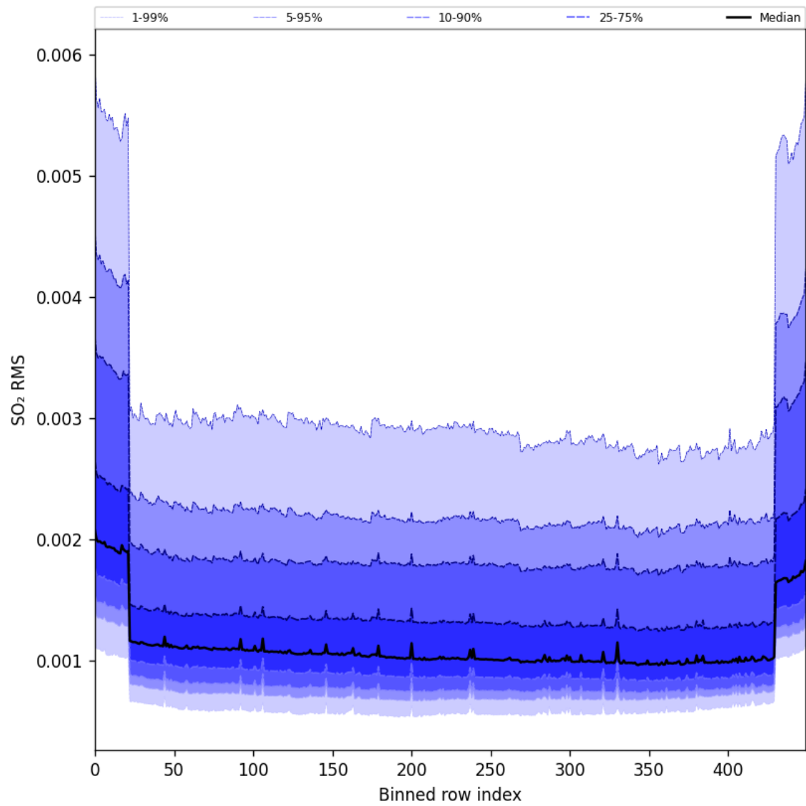
Figure 104: Along track statistics of “SO 2 RMS” for 2025-02-19 to 2025-02-21
