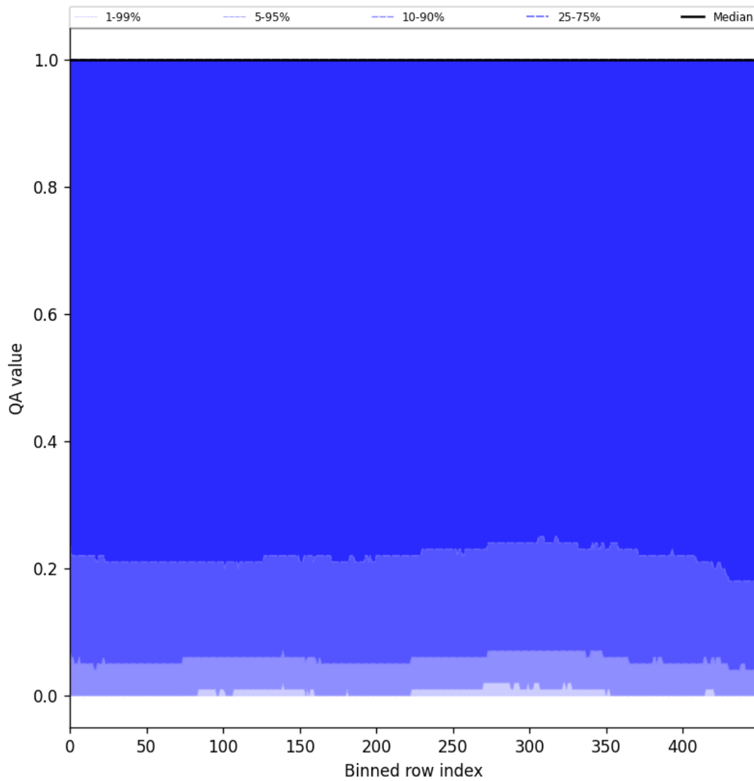
Figure 83: Along track statistics of “QA value” for 2025-02-19 to 2025-02-21
