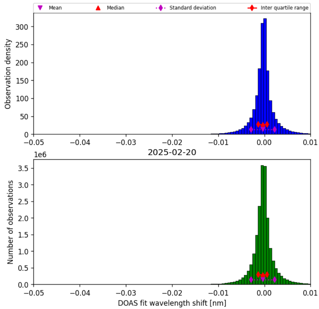
Figure 76: Histogram of “DOAS fit wavelength shift” for 2025-02-19 to 2025-02-21
