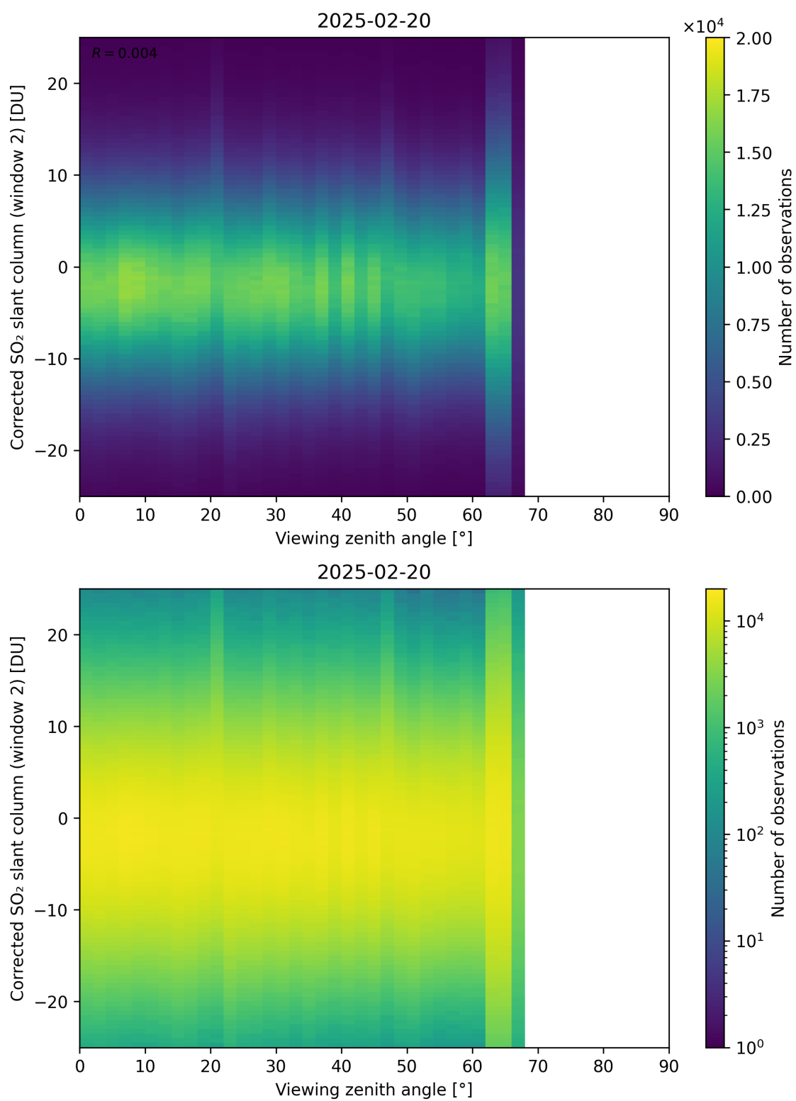
Figure 374: Scatter density plot of “Viewing zenith angle” against “Corrected SO 2 slant column (window 2)” for 2025-02-19 to 2025-02-21.
