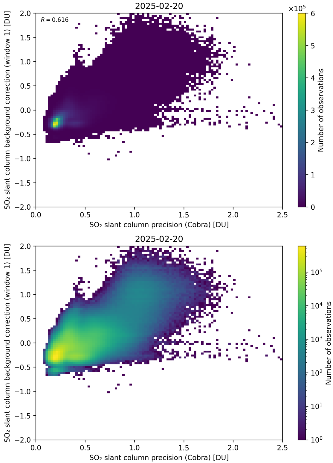
Figure 199: Scatter density plot of “SO 2 slant column precision (Cobra)” against “SO 2 slant column background correction (window 1)” for 2025-02-19 to 2025-02-21.
