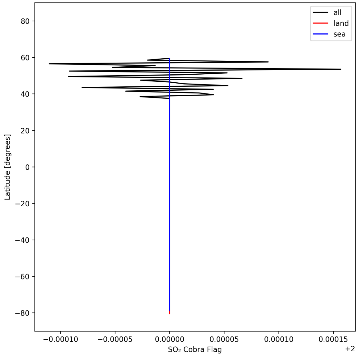
Figure 49: Zonal average of "SO 2 Cobra Flag" for 2025-02-19 to 2025-02-21.
