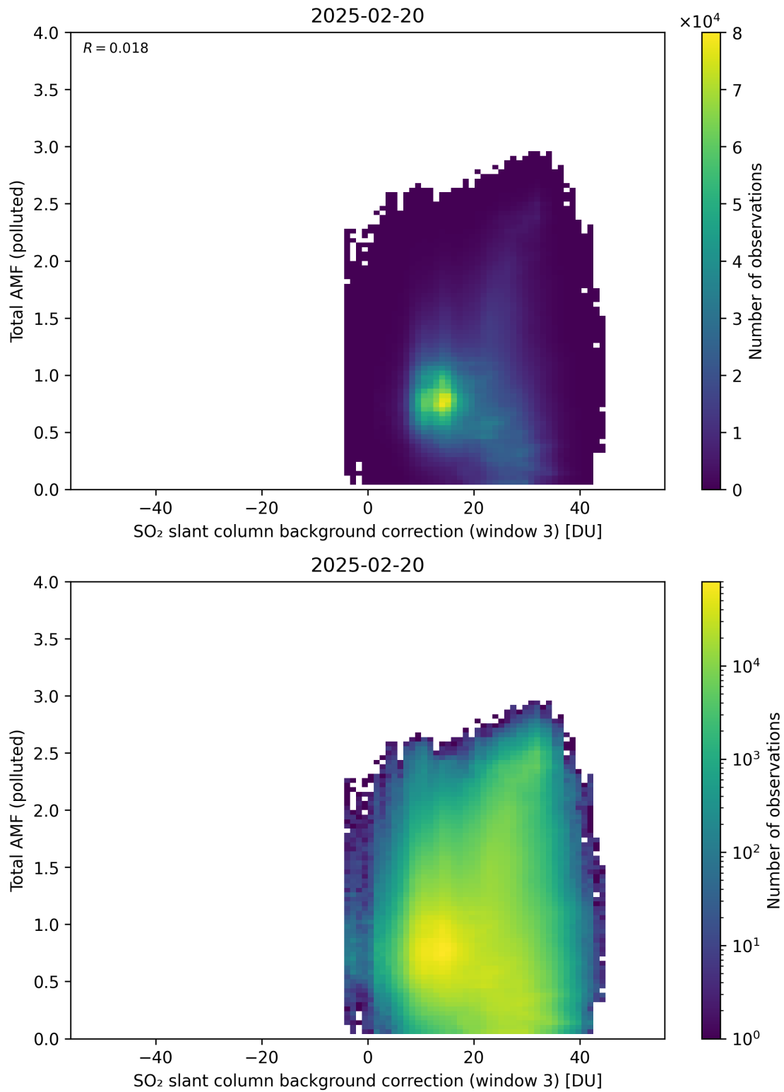
Figure 136: Scatter density plot of “SO 2 slant column background correction (window 3)” against “Total AMF (polluted)” for 2025-02-19 to 2025-02-21.
