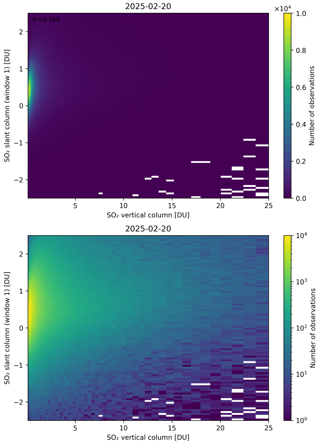
Figure 354: Scatter density plot of “SO 2 vertical column” against “SO 2 slant column (window 1)” for 2025-02-19 to 2025-02-21.
