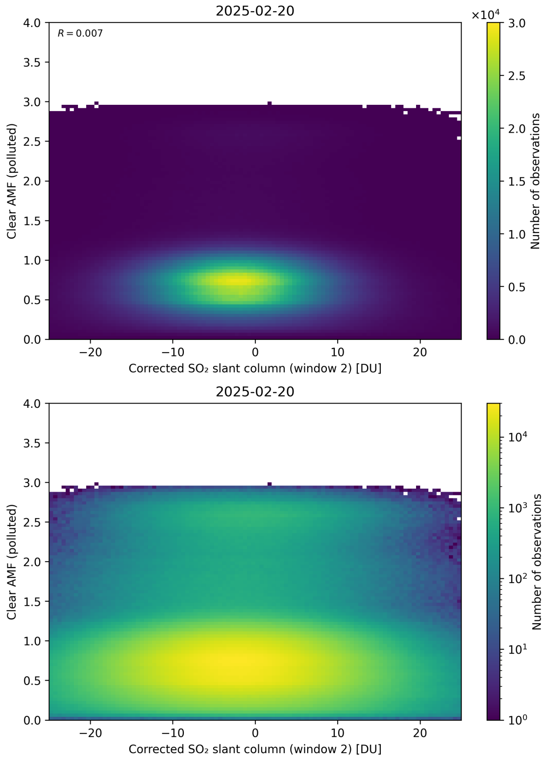
Figure 249: Scatter density plot of “Corrected SO 2 slant column (window 2)” against “Clear AMF (polluted)” for 2025-02-19 to 2025-02-21.
