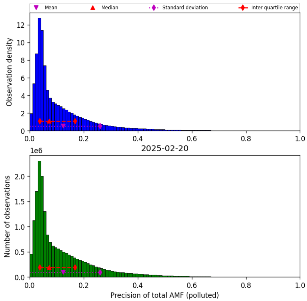
Figure 80: Histogram of “Precision of total AMF (polluted)” for 2025-02-19 to 2025-02-21
