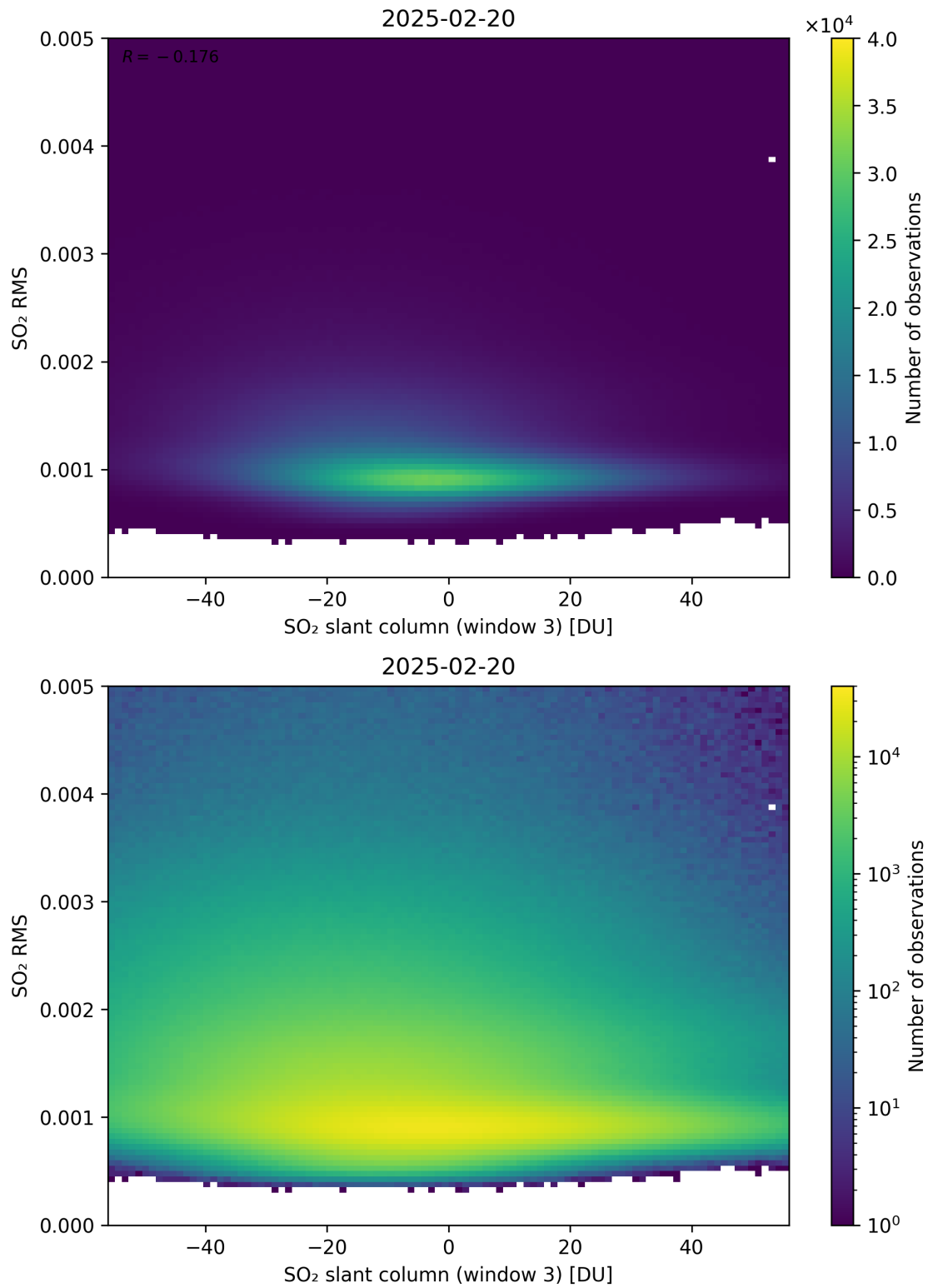
Figure 306: Scatter density plot of “SO 2 slant column (window 3)” against “SO 2 RMS” for 2025-02-19 to 2025-02-21.
