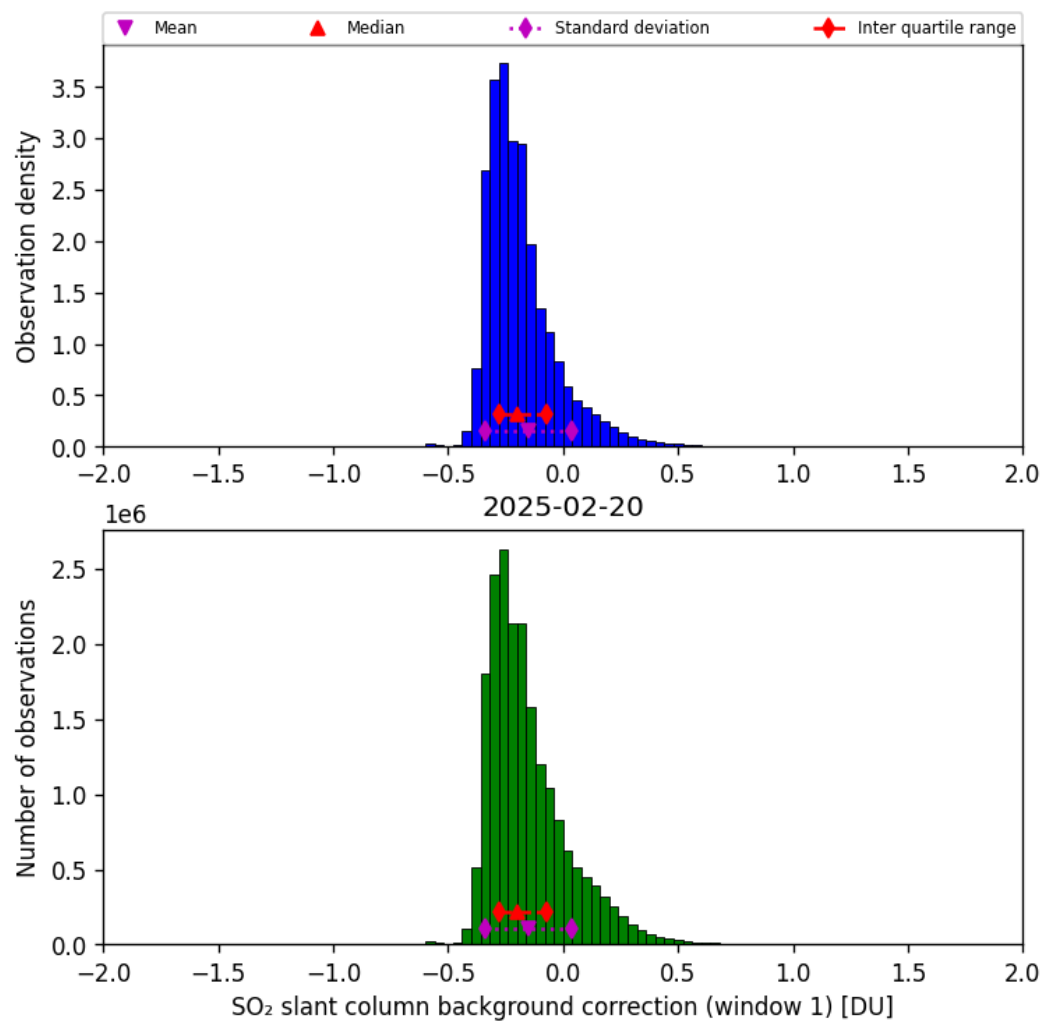
Figure 66: Histogram of “SO 2 slant column background correction (window 1)” for 2025-02-19 to 2025-02-21
