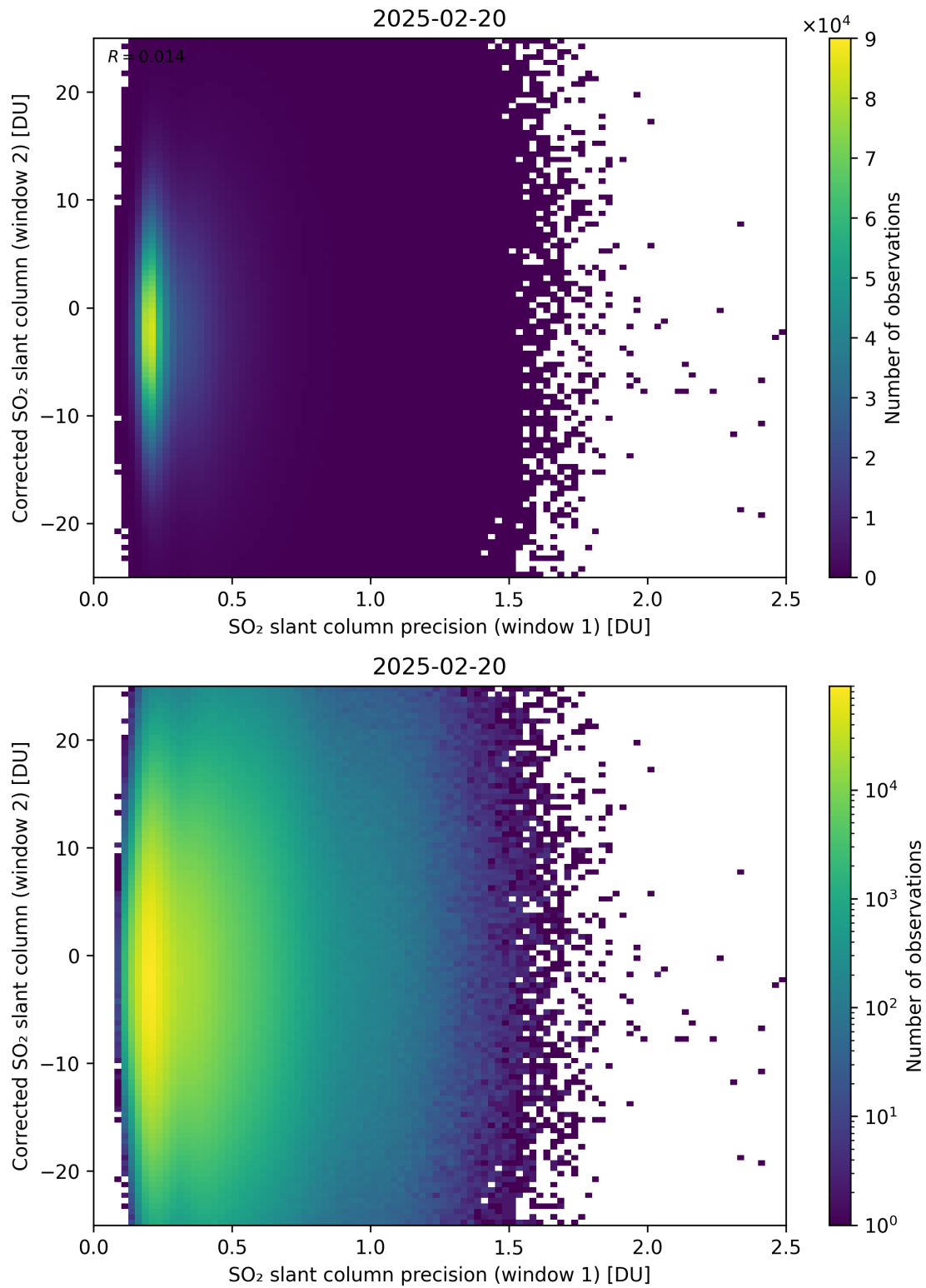
Figure 275: Scatter density plot of “SO 2 slant column precision (window 1)” against “Corrected SO 2 slant column (window 2)” for 2025-02-19 to 2025-02-21.
