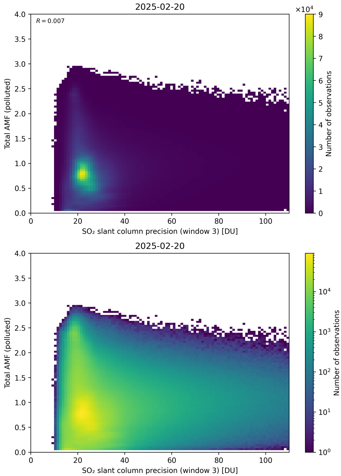
Figure 313: Scatter density plot of “SO 2 slant column precision (window 3)” against “Total AMF (polluted)” for 2025-02-19 to 2025-02-21.
