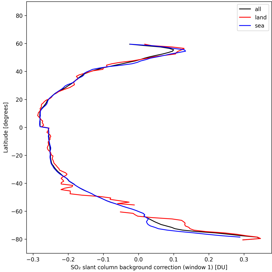
Figure 40: Zonal average of “SO 2 slant column background correction (window 1)” for 2025-02-19 to 2025-02-21.
