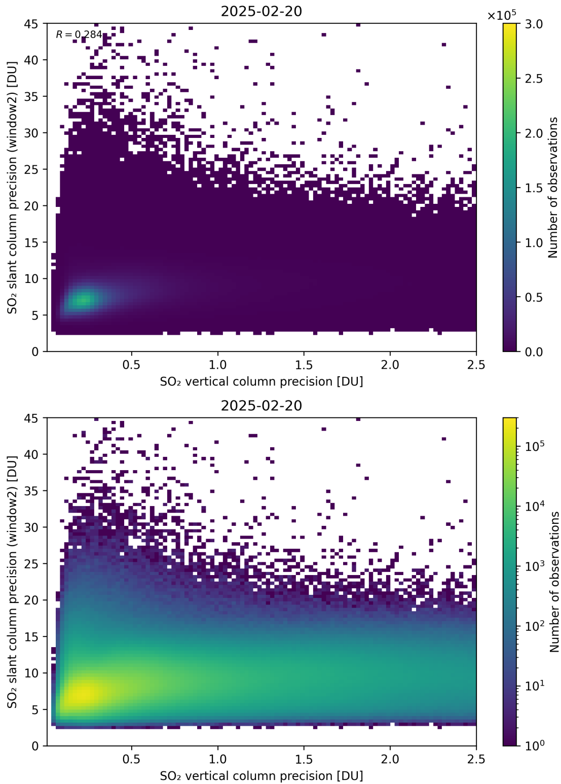
Figure 343: Scatter density plot of “SO 2 vertical column precision” against “SO 2 slant column precision (window2)” for 2025-02-19 to 2025-02-21.
