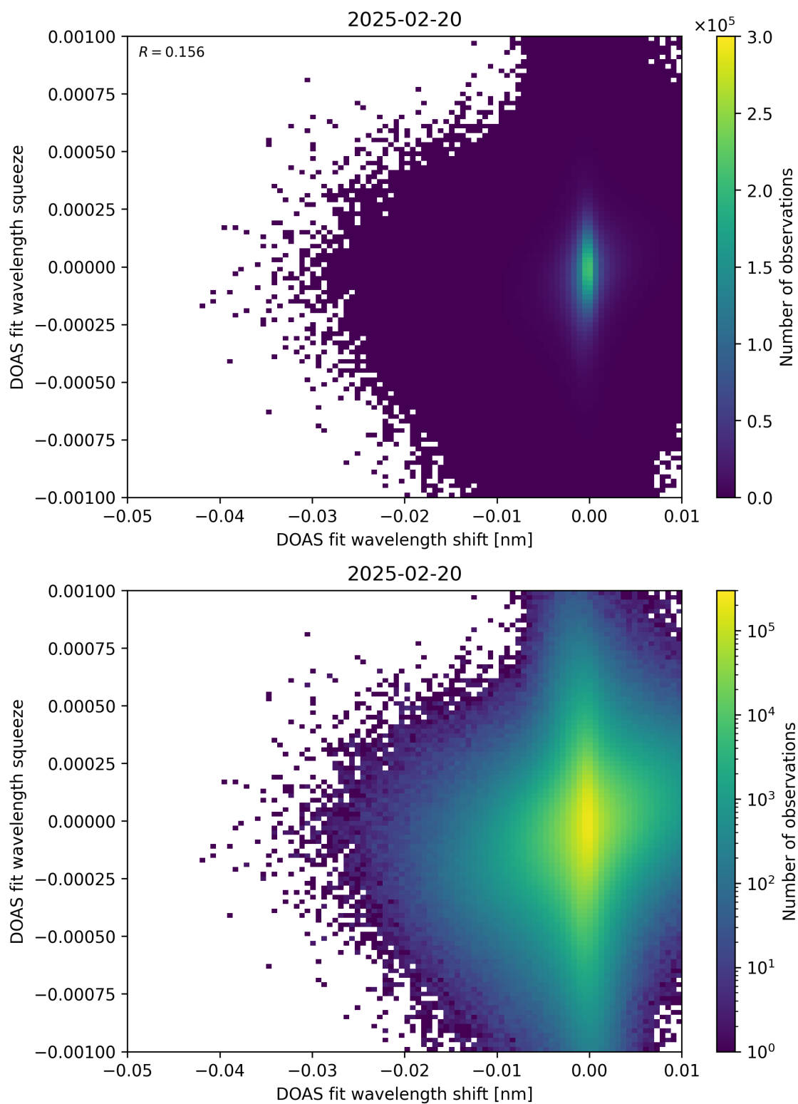
Figure 138: Scatter density plot of “DOAS fit wavelength shift” against “DOAS fit wavelength squeeze” for 2025-02-19 to 2025-02-21.
