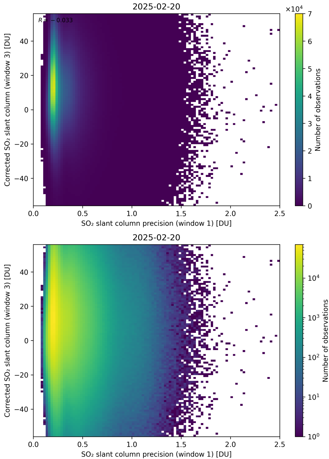
Figure 276: Scatter density plot of “SO 2 slant column precision (window 1)” against “Corrected SO 2 slant column (window 3)” for 2025-02-19 to 2025-02-21.
