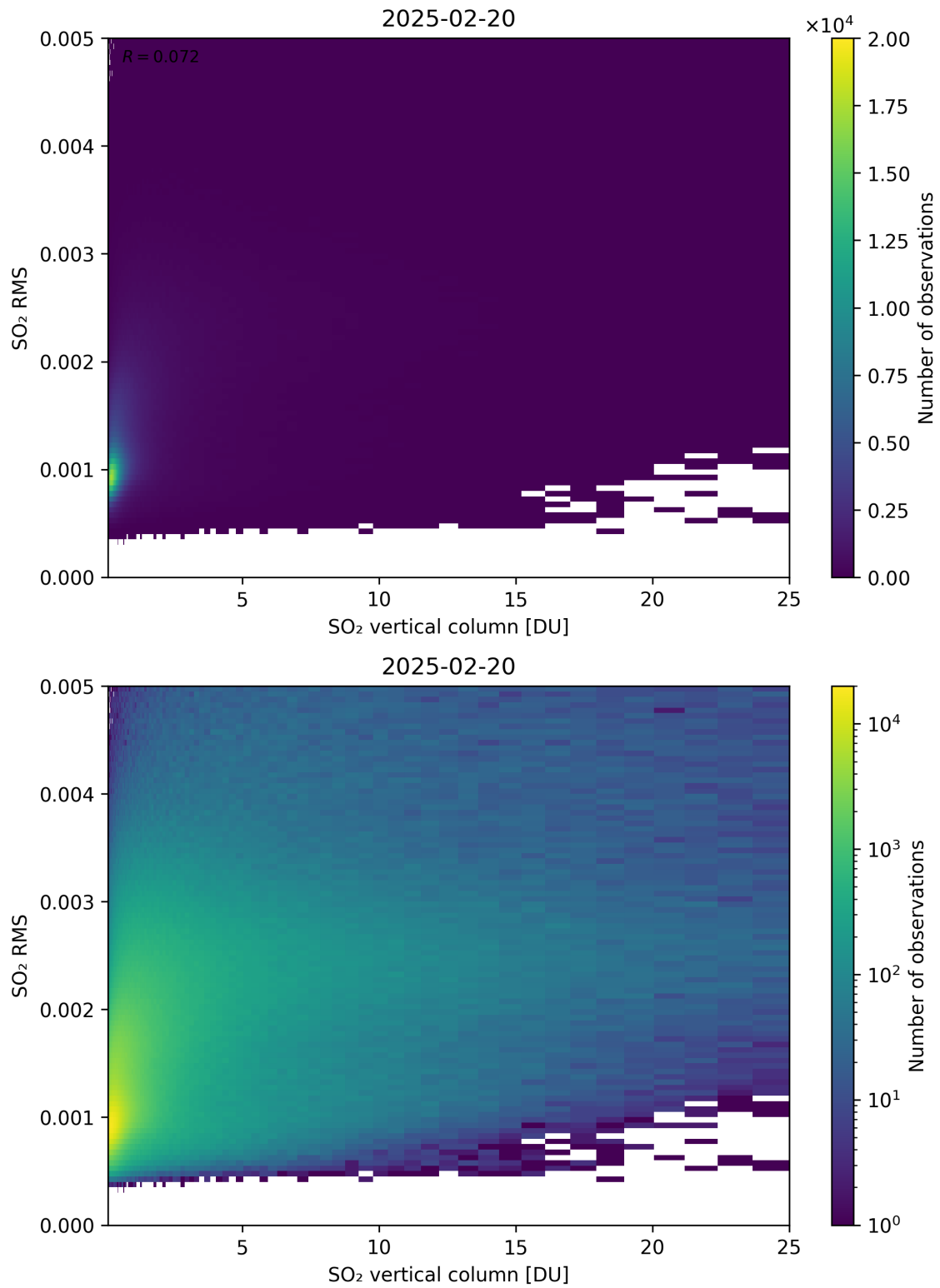
Figure 328: Scatter density plot of “SO 2 vertical column” against “SO 2 RMS” for 2025-02-19 to 2025-02-21.
