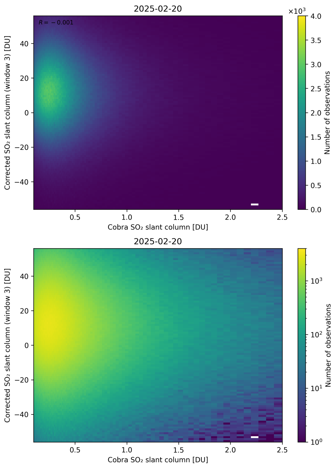
Figure 218: Scatter density plot of “Cobra SO 2 slant column” against “Corrected SO 2 slant column (window 3)” for 2025-02-19 to 2025-02-21.
