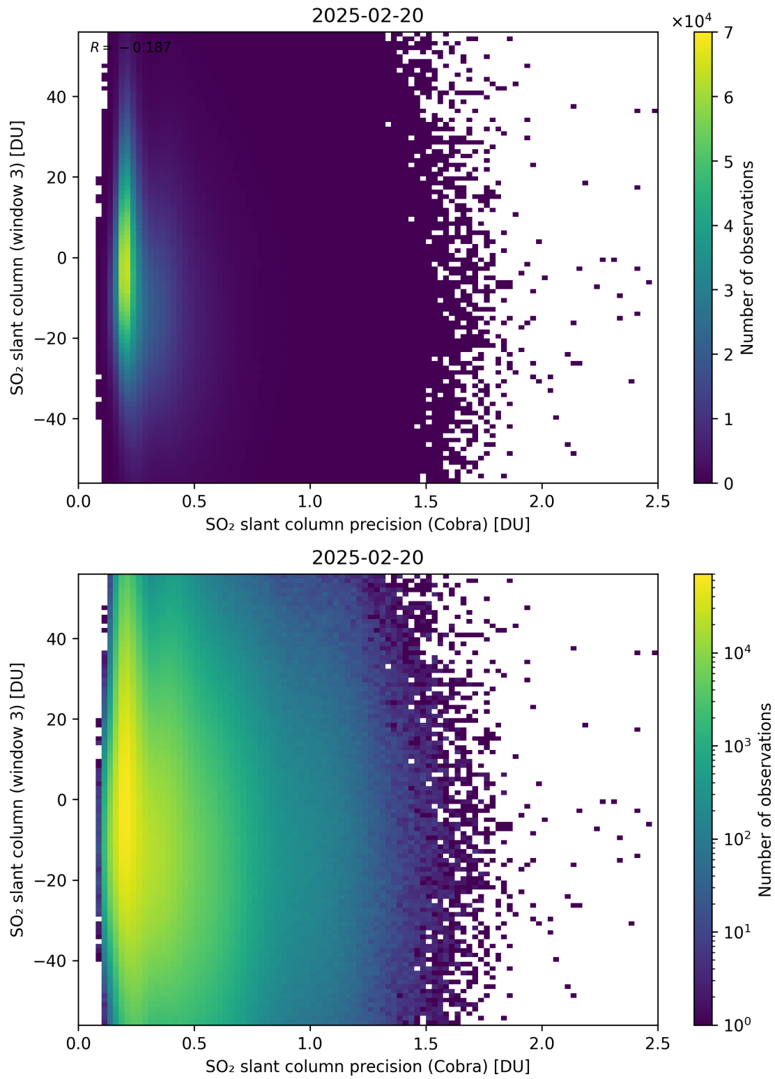
Figure 211: Scatter density plot of “SO 2 slant column precision (Cobra)” against “SO 2 slant column (window 3)” for 2025-02-19 to 2025-02-21.
