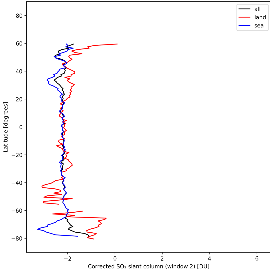
Figure 43: Zonal average of “Corrected SO 2 slant column (window 2)” for 2025-02-19 to 2025-02-21.
