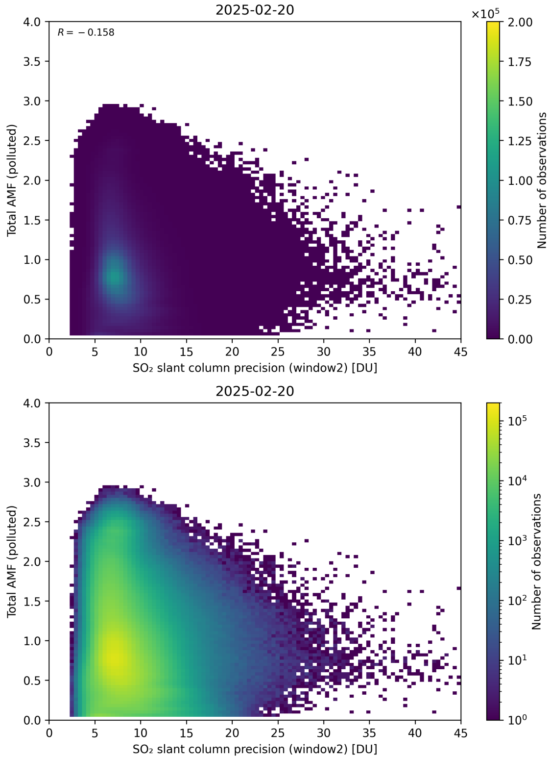
Figure 301: Scatter density plot of “SO 2 slant column precision (window2)” against “Total AMF (polluted)” for 2025-02-19 to 2025-02-21.
