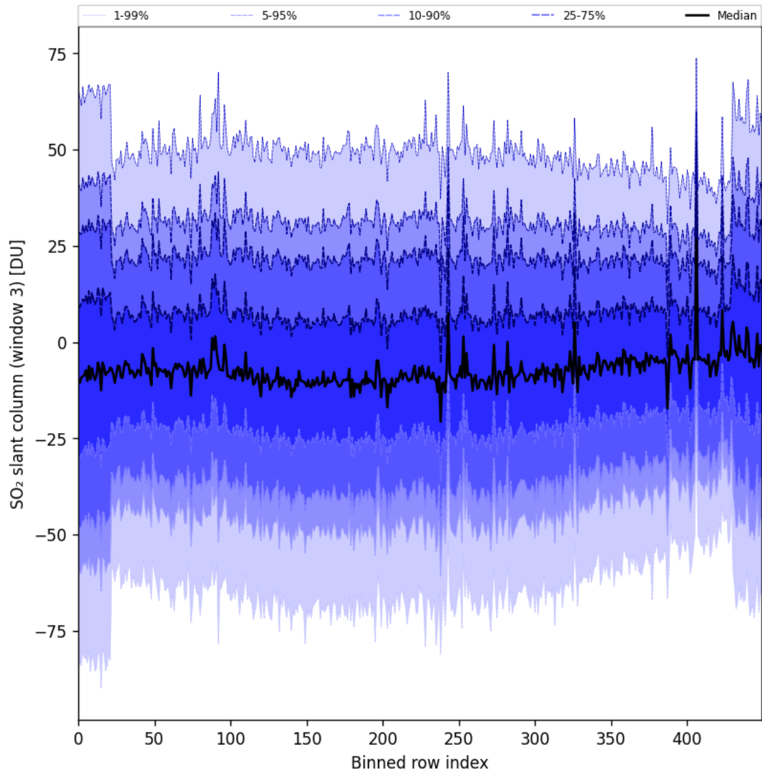
Figure 97: Along track statistics of “SO 2 slant column (window 3)” for 2025-02-19 to 2025-02-21
