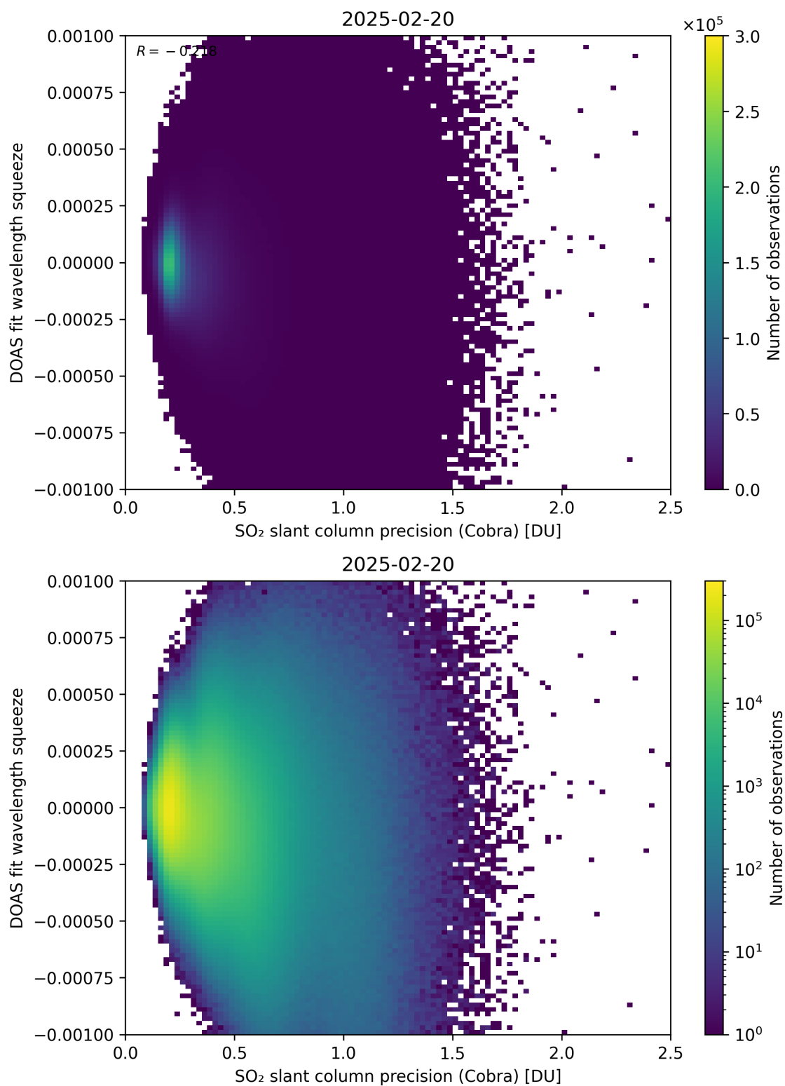
Figure 203: Scatter density plot of “SO 2 slant column precision (Cobra)” against “DOAS fit wavelength squeeze” for 2025-02-19 to 2025-02-21.
