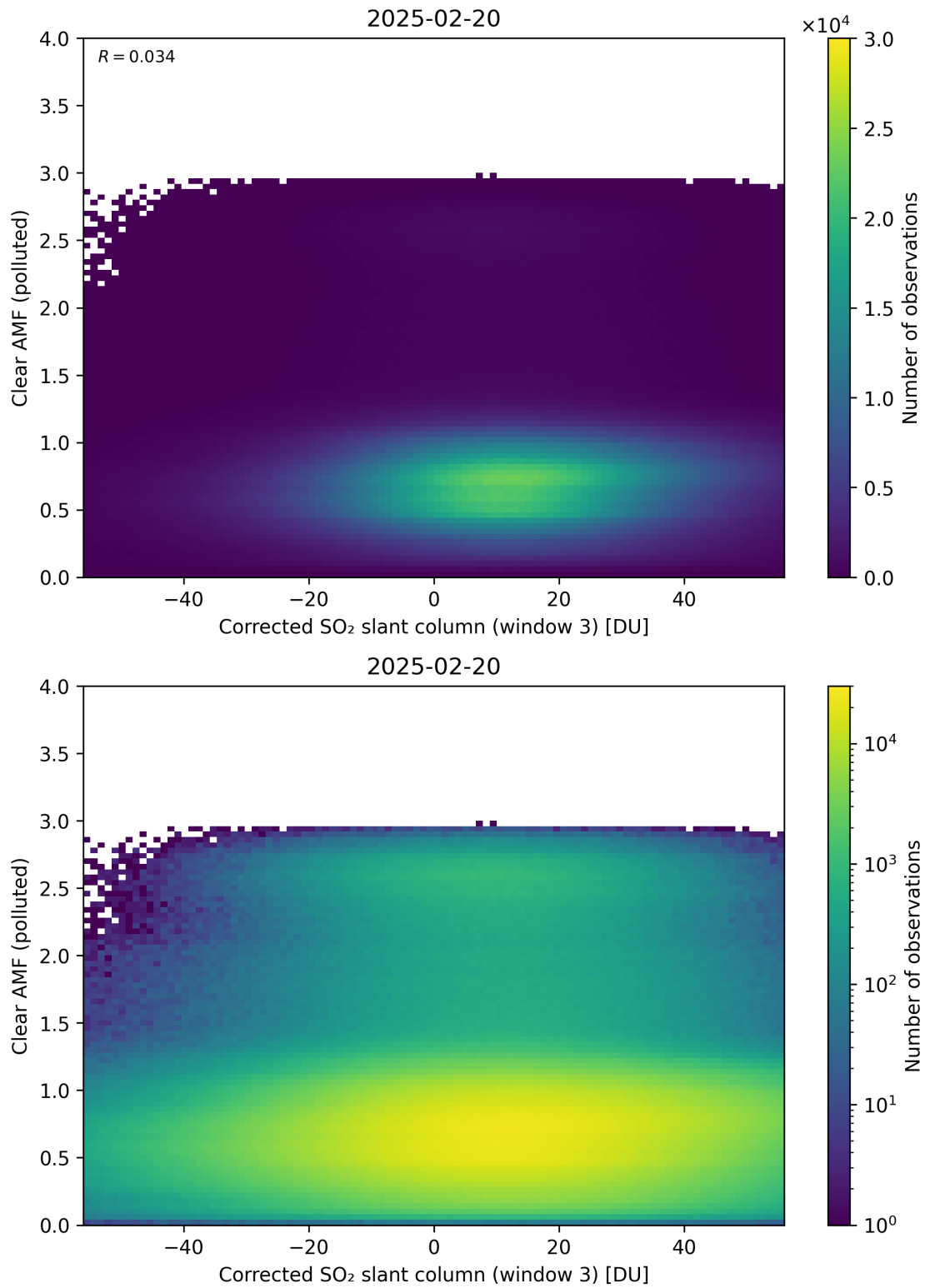
Figure 259: Scatter density plot of “Corrected SO 2 slant column (window 3)” against “Clear AMF (polluted)” for 2025-02-19 to 2025-02-21.
