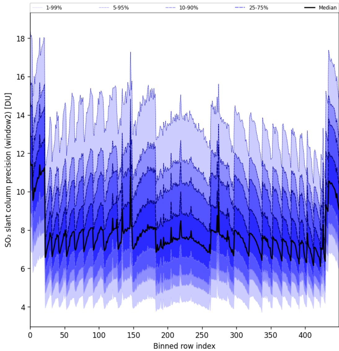
Figure 94: Along track statistics of “SO 2 slant column precision (window2)” for 2025-02-19 to 2025-02-21
