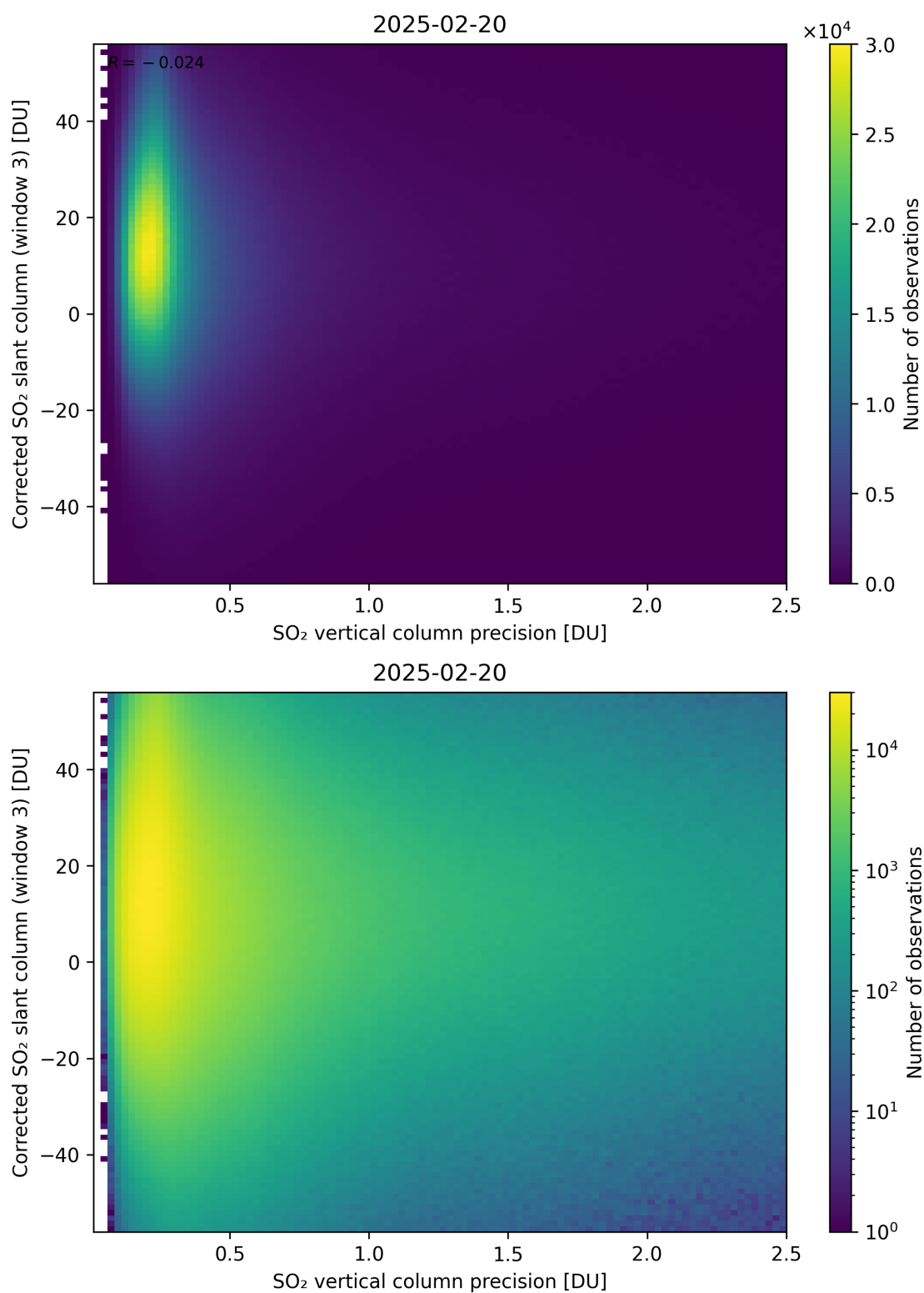
Figure 340: Scatter density plot of “SO 2 vertical column precision” against “Corrected SO 2 slant column (window 3)” for 2025-02-19 to 2025-02-21.
