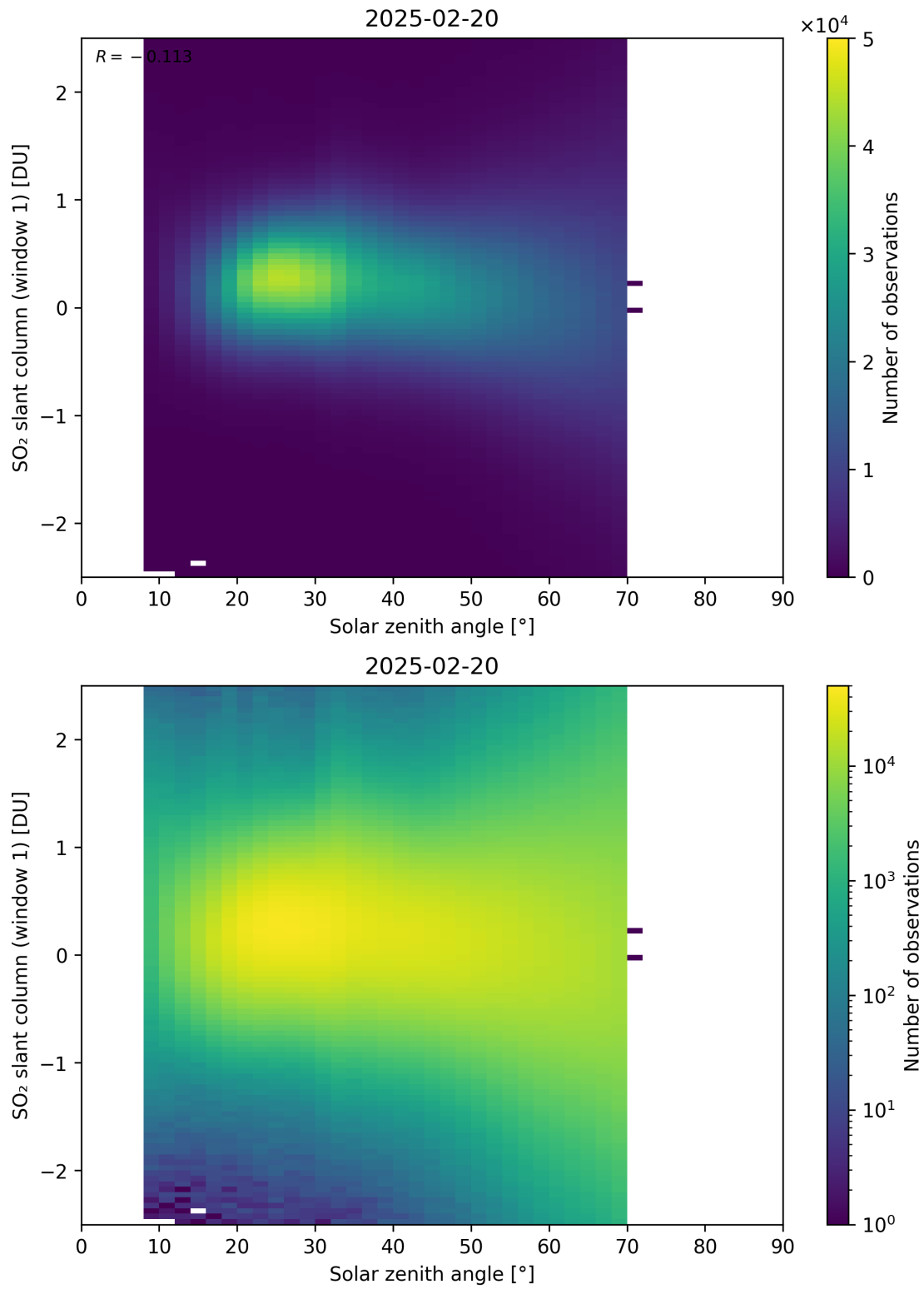
Figure 184: Scatter density plot of “Solar zenith angle” against “SO 2 slant column (window 1)” for 2025-02-19 to 2025-02-21.
