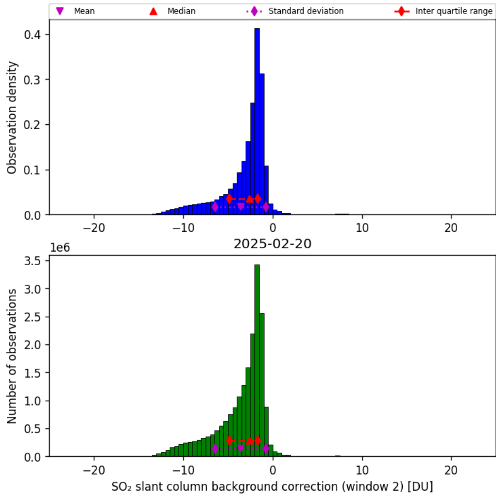
Figure 70: Histogram of “SO 2 slant column background correction (window 2)” for 2025-02-19 to 2025-02-21
