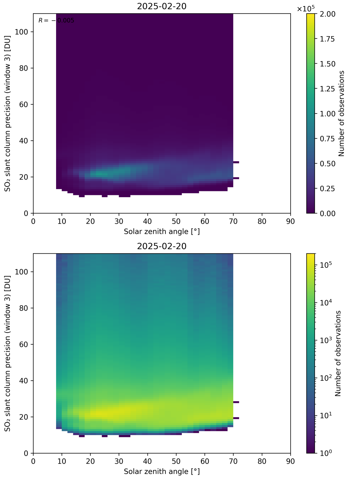
Figure 188: Scatter density plot of “Solar zenith angle” against “SO 2 slant column precision (window 3)” for 2025-02-19 to 2025-02-21.
