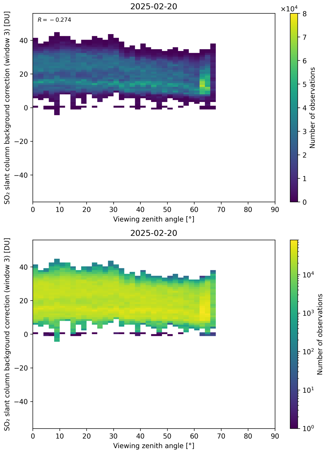
Figure 364: Scatter density plot of “Viewing zenith angle” against “SO 2 slant column background correction (window 3)” for 2025-02-19 to 2025-02-21.
