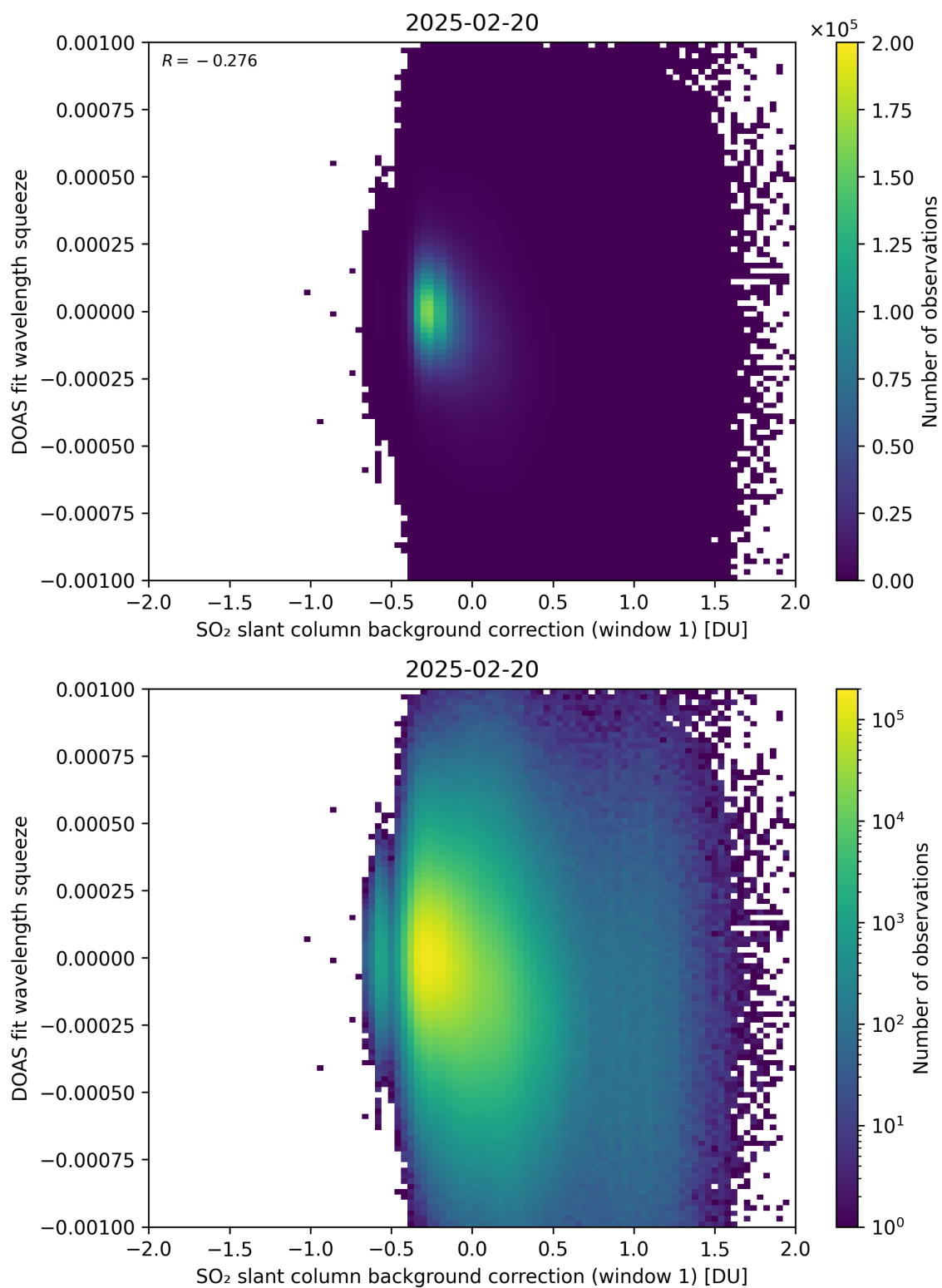
Figure 112: Scatter density plot of “SO 2 slant column background correction (window 1)” against “DOAS fit wavelength squeeze” for 2025-02-19 to 2025-02-21.
