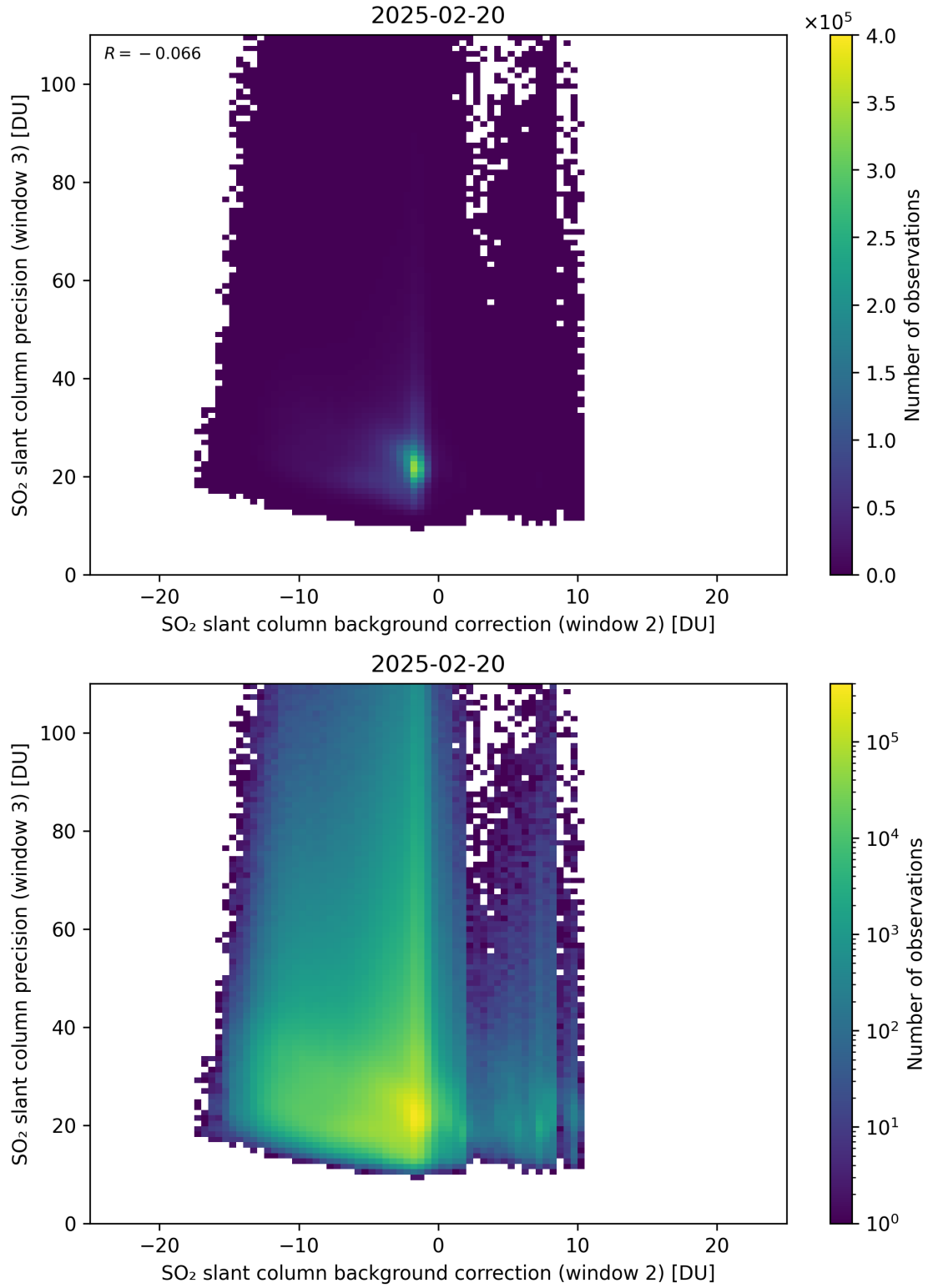
Figure 129: Scatter density plot of “SO 2 slant column background correction (window 2)” against “SO 2 slant column precision (window 3)” for 2025-02-19 to 2025-02-21.
