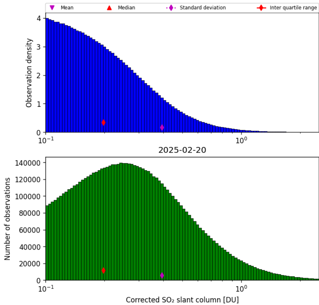
Figure 60: Histogram of “Corrected SO 2 slant column” for 2025-02-19 to 2025-02-21
