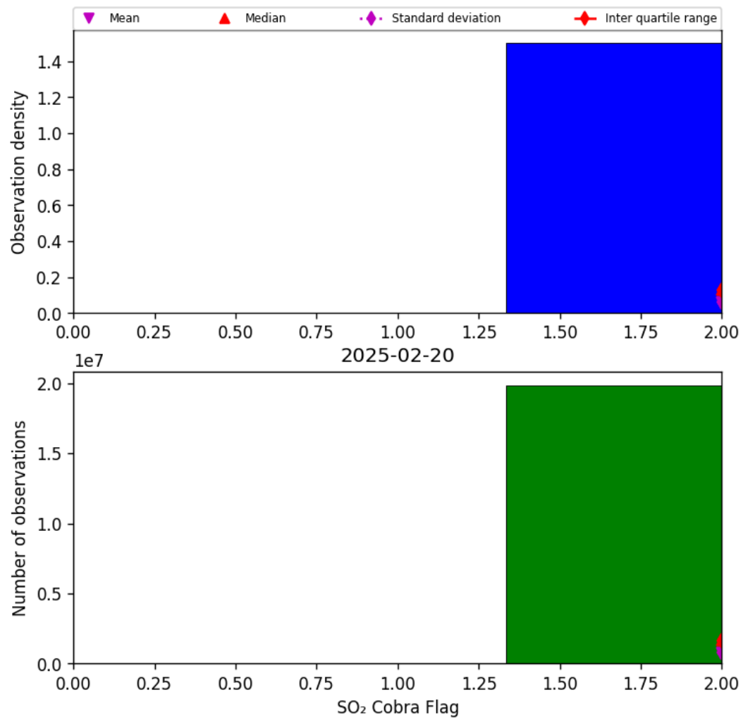
Figure 75: Histogram of “SO 2 Cobra Flag” for 2025-02-19 to 2025-02-21
