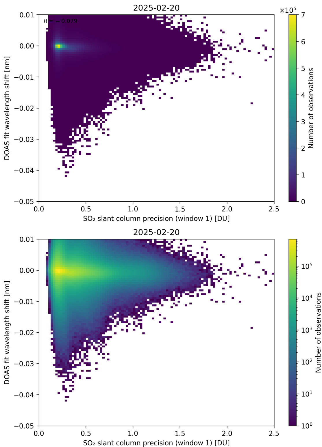
Figure 271: Scatter density plot of “SO 2 slant column precision (window 1)” against “DOAS fit wavelength shift” for 2025-02-19 to 2025-02-21.
