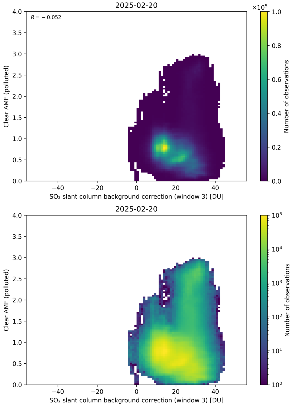
Figure 135: Scatter density plot of “SO 2 slant column background correction (window 3)” against “Clear AMF (polluted)” for 2025-02-19 to 2025-02-21.
