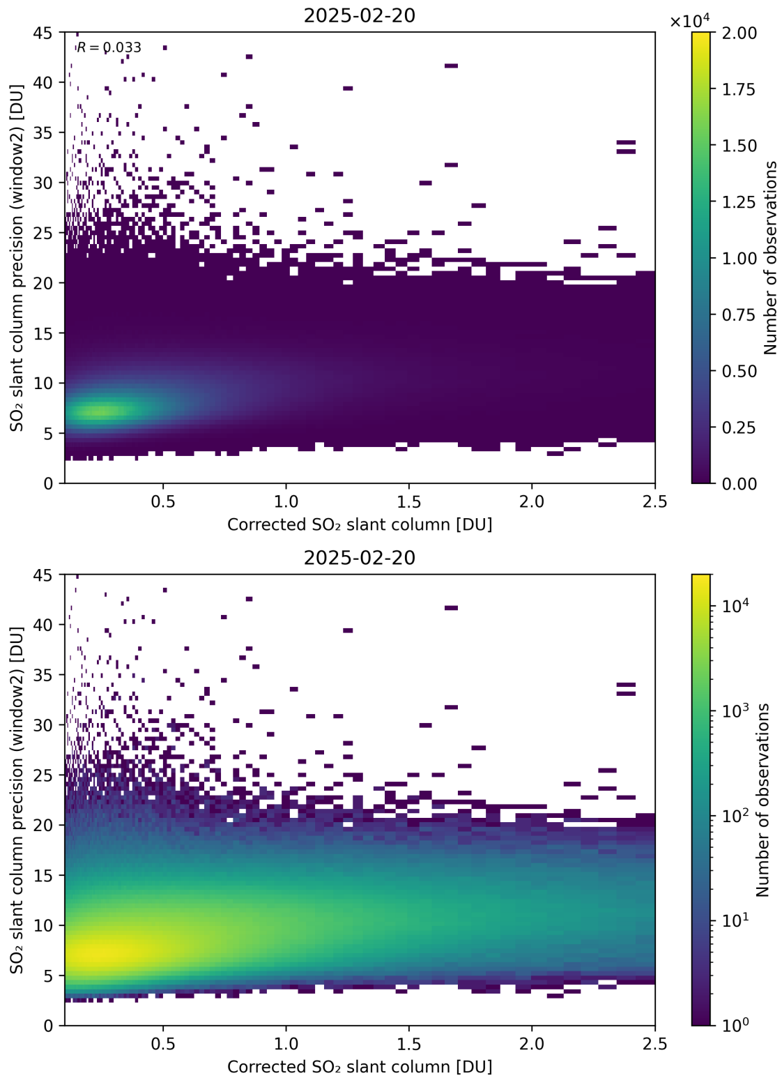
Figure 239: Scatter density plot of “Corrected SO 2 slant column” against “SO 2 slant column precision (window2)” for 2025-02-19 to 2025-02-21.
