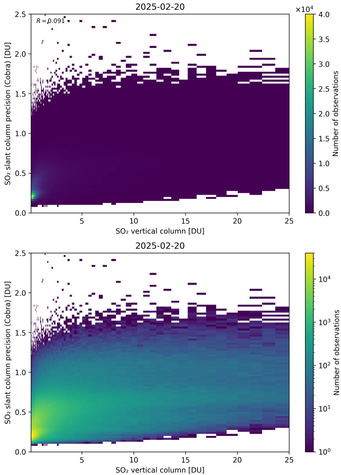
Figure 350: Scatter density plot of “SO 2 vertical column” against “SO 2 slant column precision (Cobra)” for 2025-02-19 to 2025-02-21.
