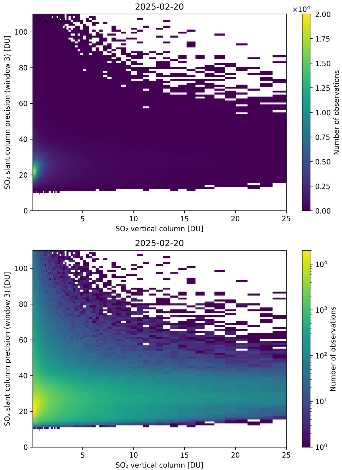
Figure 358: Scatter density plot of “SO 2 vertical column” against “SO 2 slant column precision (window 3)” for 2025-02-19 to 2025-02-21.
