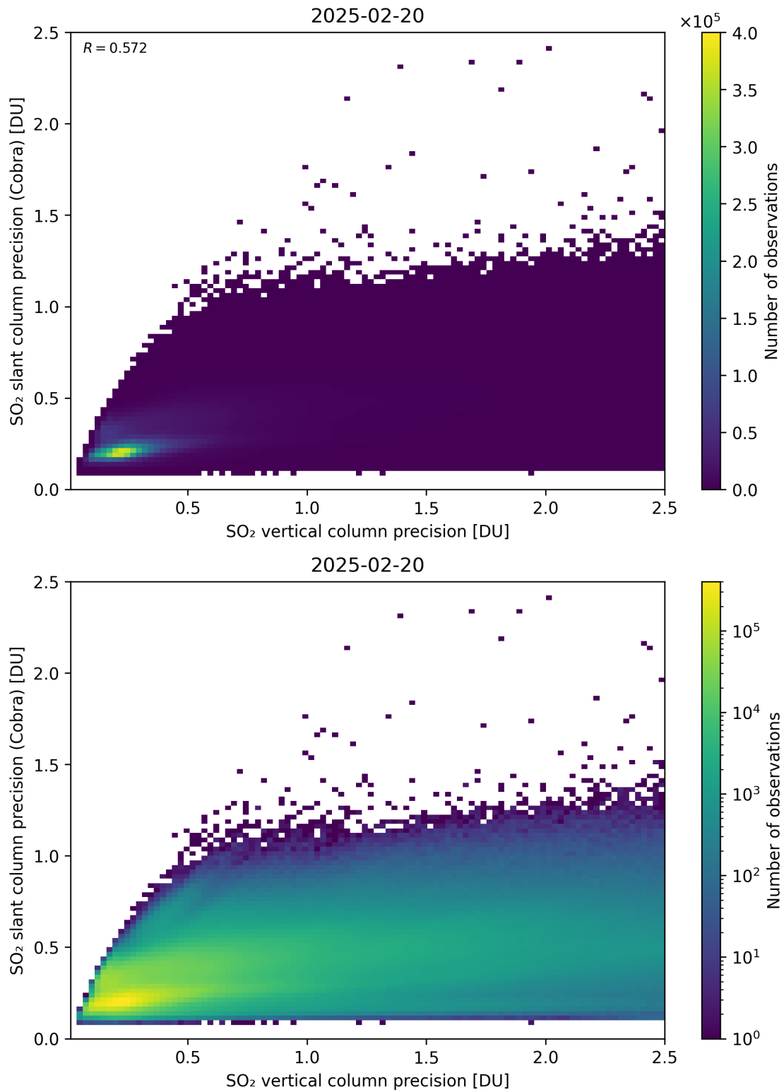
Figure 337: Scatter density plot of “SO 2 vertical column precision” against “SO 2 slant column precision (Cobra)” for 2025-02-19 to 2025-02-21.
