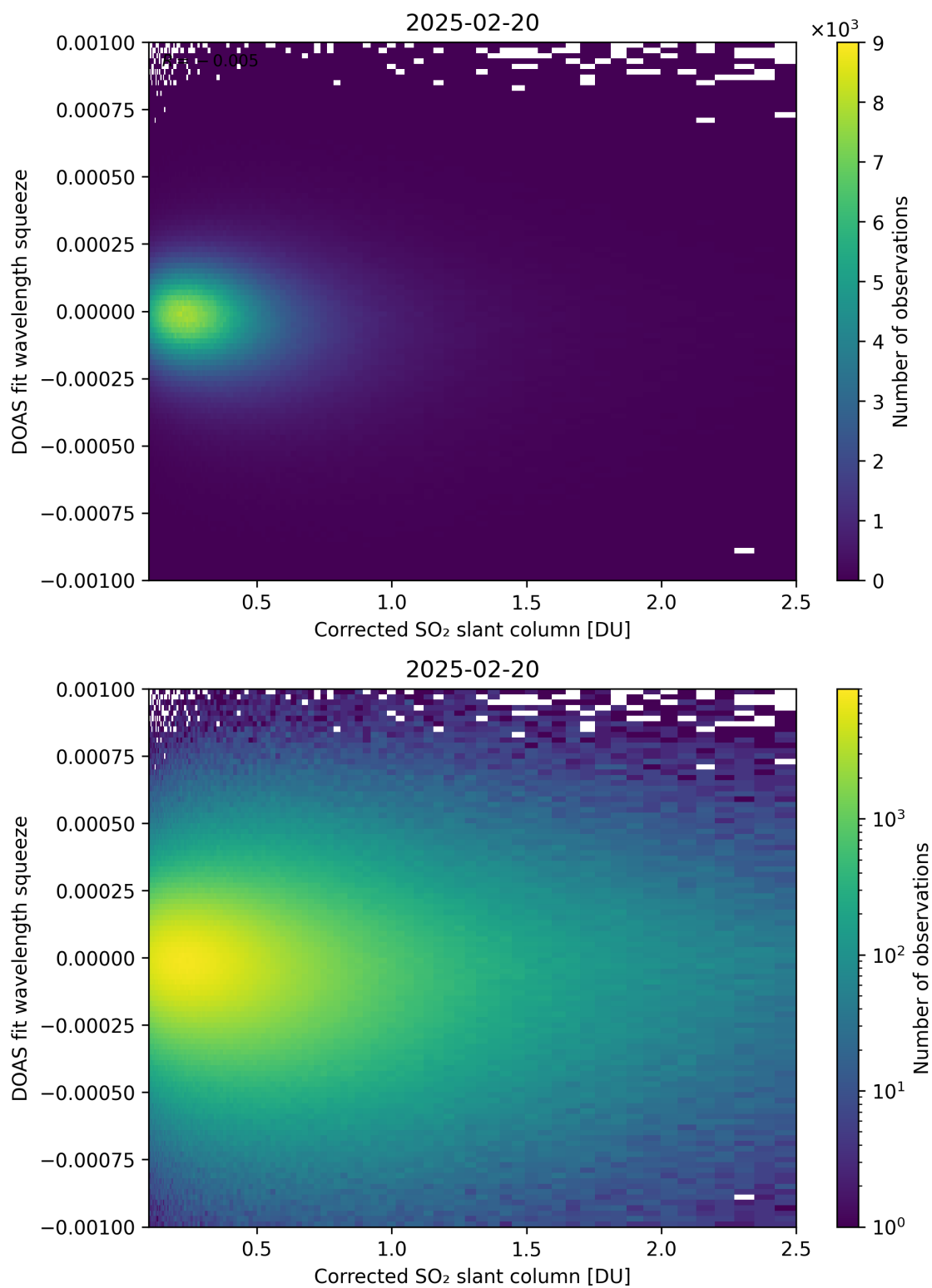
Figure 230: Scatter density plot of “Corrected SO 2 slant column” against “DOAS fit wavelength squeeze” for 2025-02-19 to 2025-02-21.
