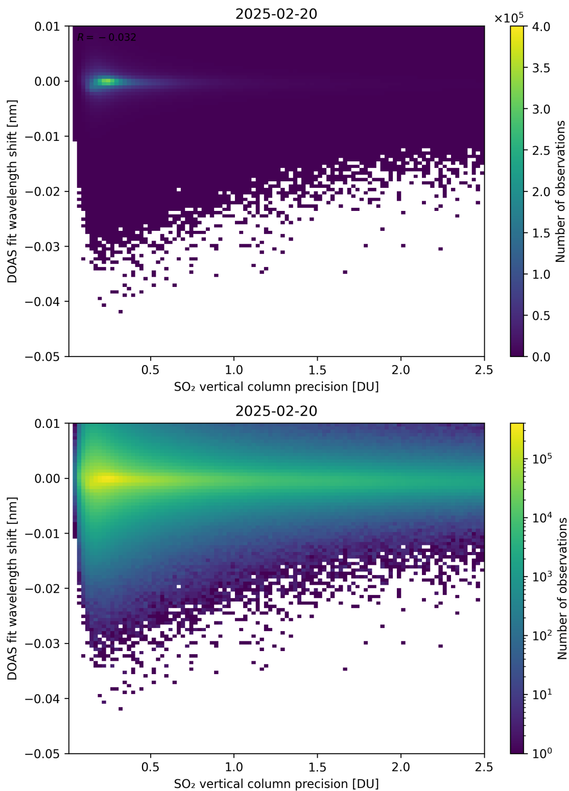
Figure 332: Scatter density plot of “SO 2 vertical column precision” against “DOAS fit wavelength shift” for 2025-02-19 to 2025-02-21.
