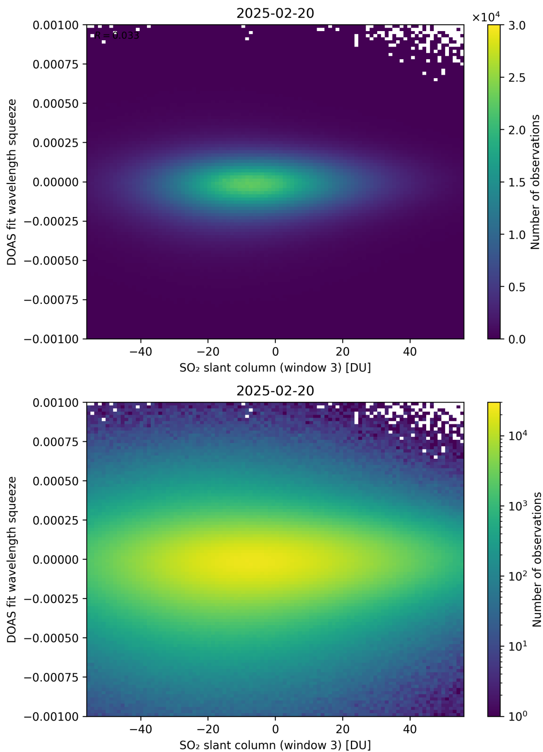
Figure 305: Scatter density plot of “SO 2 slant column (window 3)” against “DOAS fit wavelength squeeze” for 2025-02-19 to 2025-02-21.
