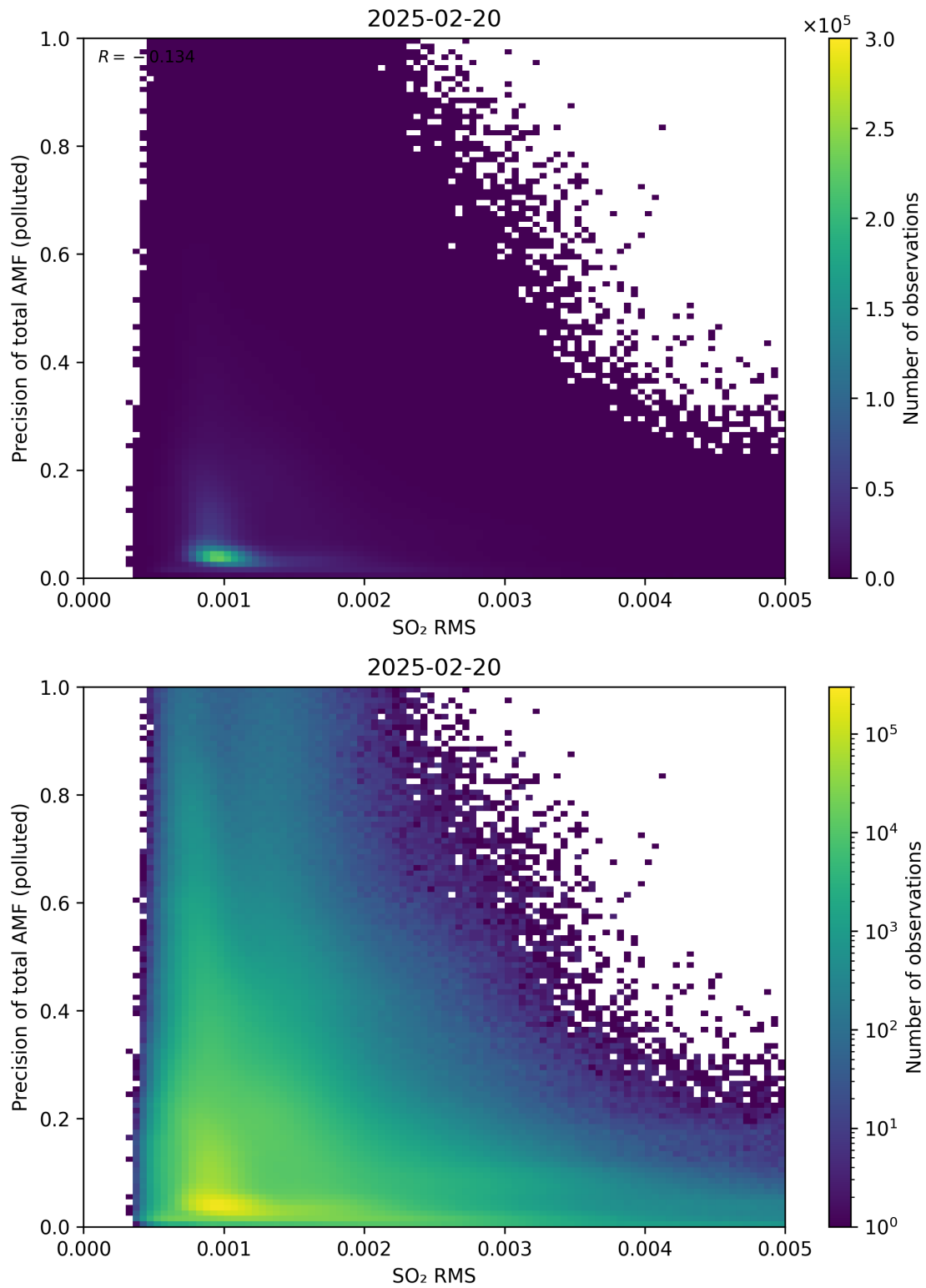
Figure 149: Scatter density plot of “SO 2 RMS” against “Precision of total AMF (polluted)” for 2025-02-19 to 2025-02-21.
