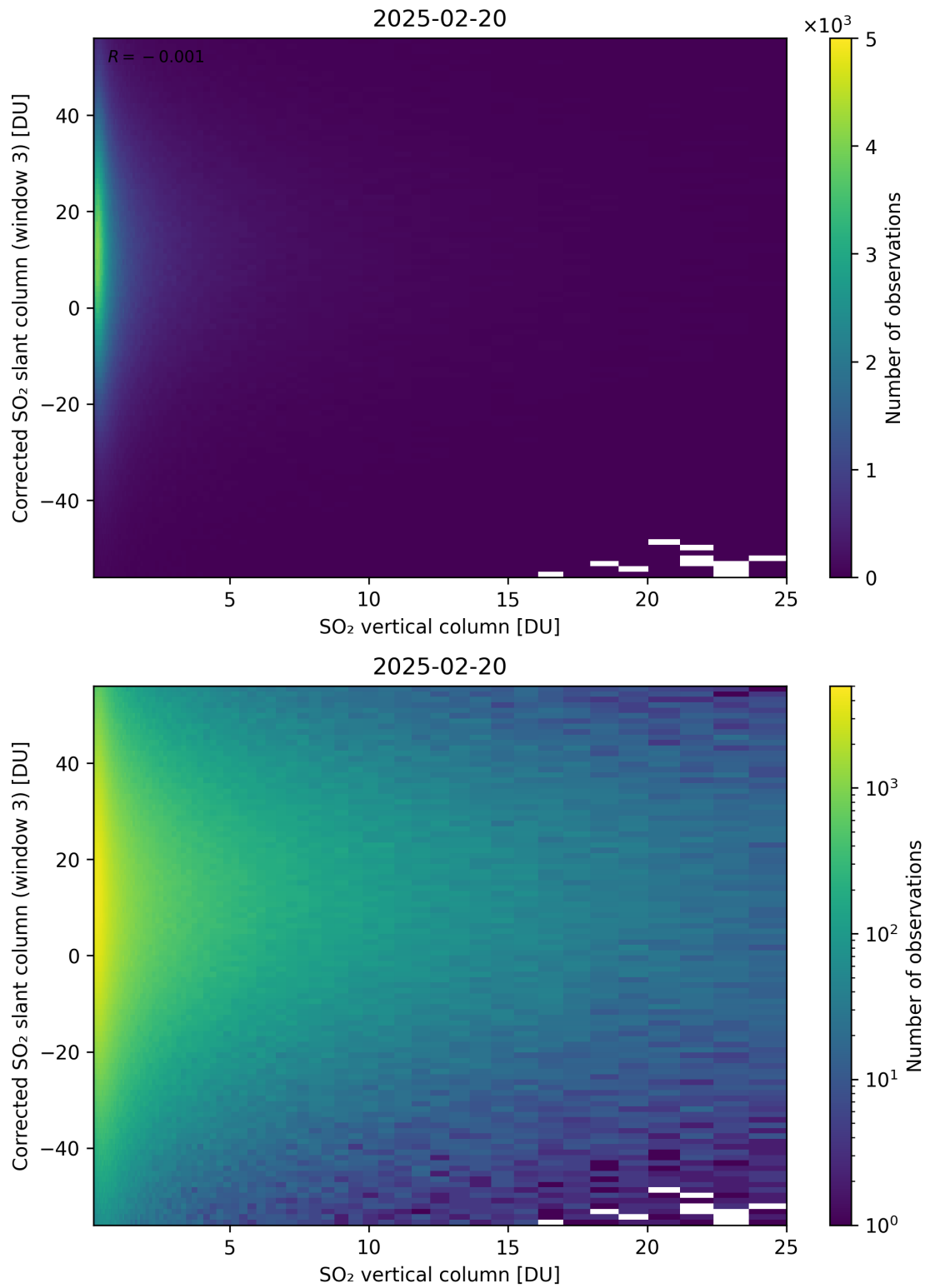
Figure 353: Scatter density plot of “SO 2 vertical column” against “Corrected SO 2 slant column (window 3)” for 2025-02-19 to 2025-02-21.
