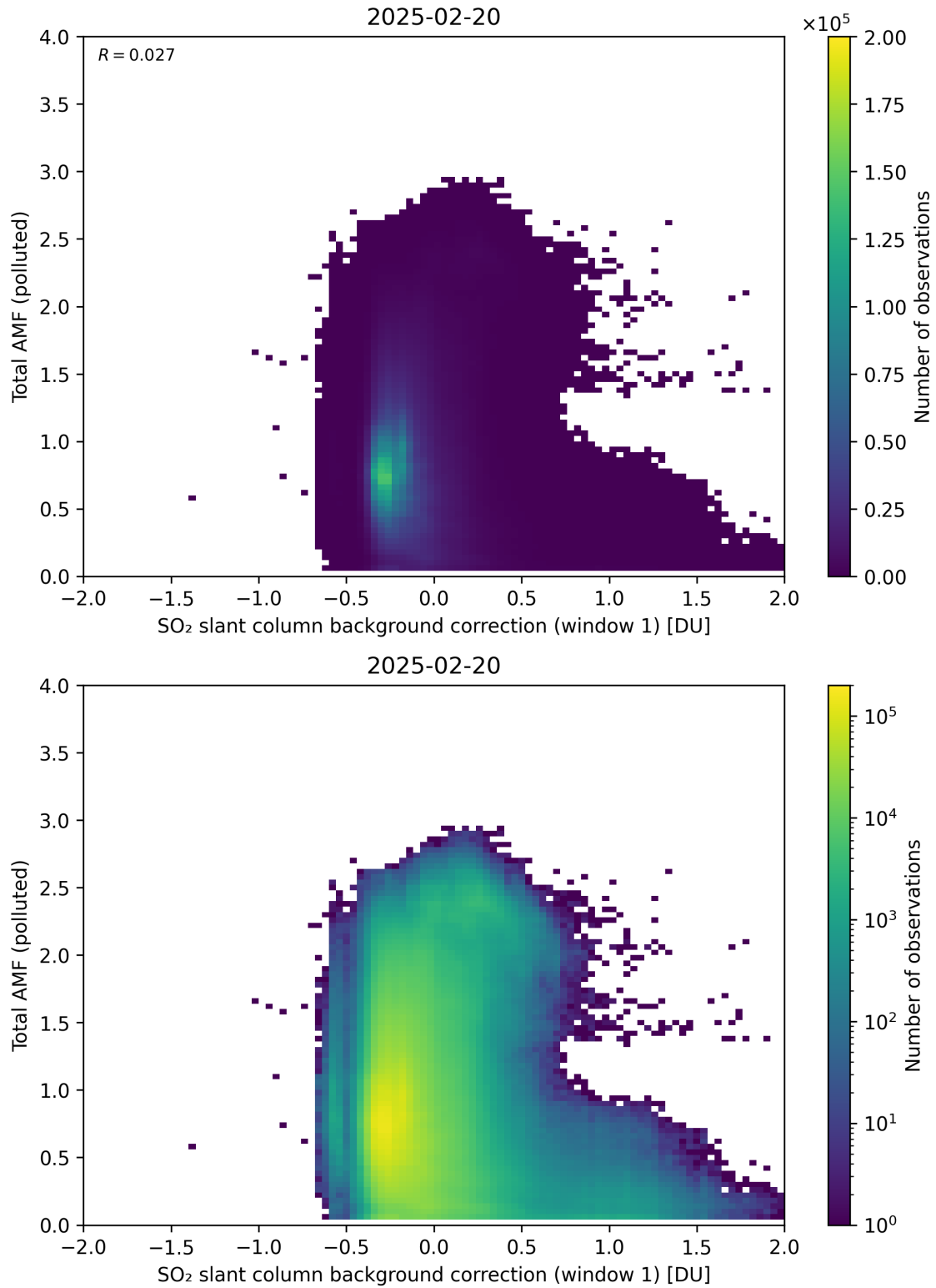
Figure 120: Scatter density plot of “SO 2 slant column background correction (window 1)” against “Total AMF (polluted)” for 2025-02-19 to 2025-02-21.
