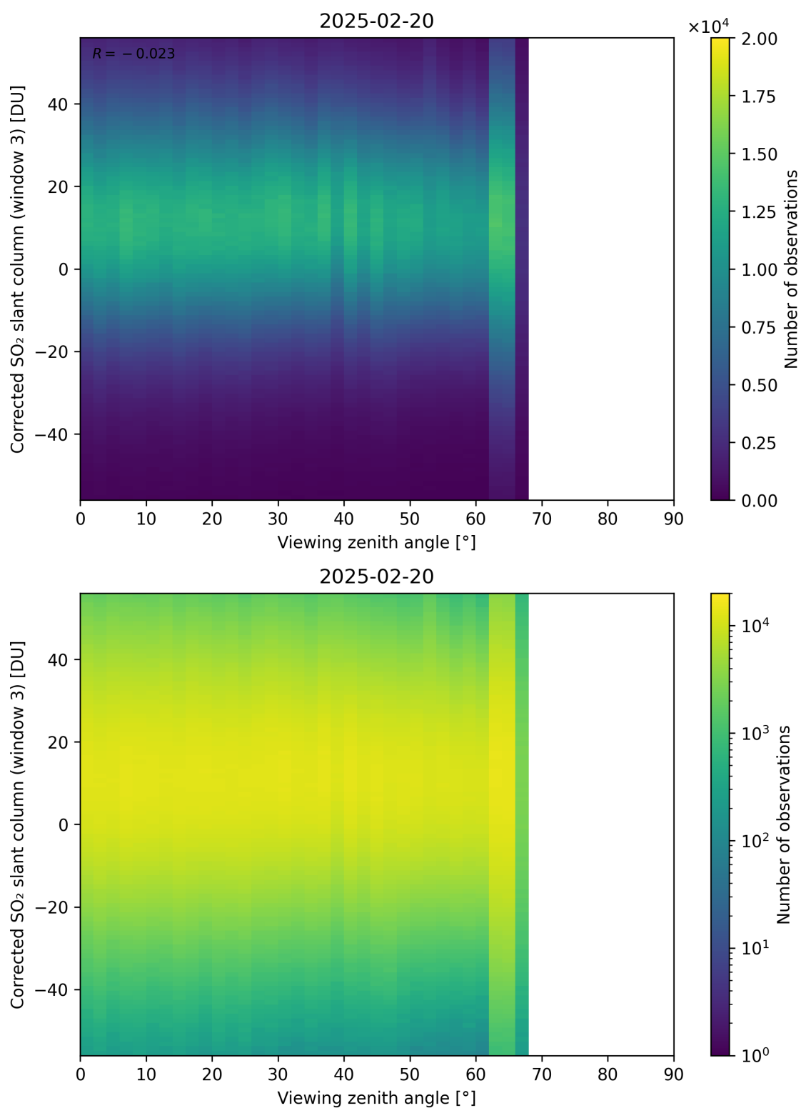
Figure 375: Scatter density plot of “Viewing zenith angle” against “Corrected SO 2 slant column (window 3)” for 2025-02-19 to 2025-02-21.
