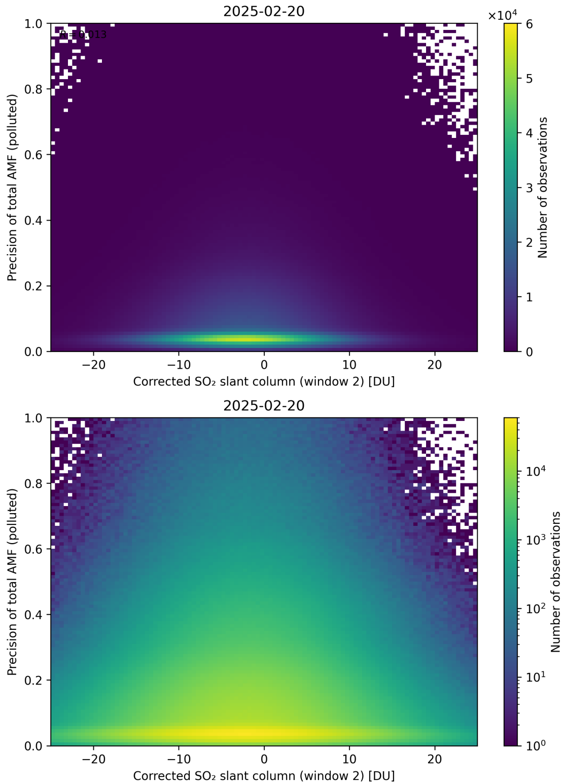
Figure 254: Scatter density plot of “Corrected SO 2 slant column (window 2)” against “Precision of total AMF (polluted)” for 2025-02-19 to 2025-02-21.
