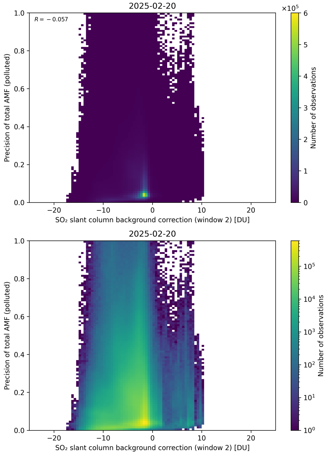
Figure 131: Scatter density plot of “SO 2 slant column background correction (window 2)” against “Precision of total AMF (polluted)” for 2025-02-19 to 2025-02-21.
