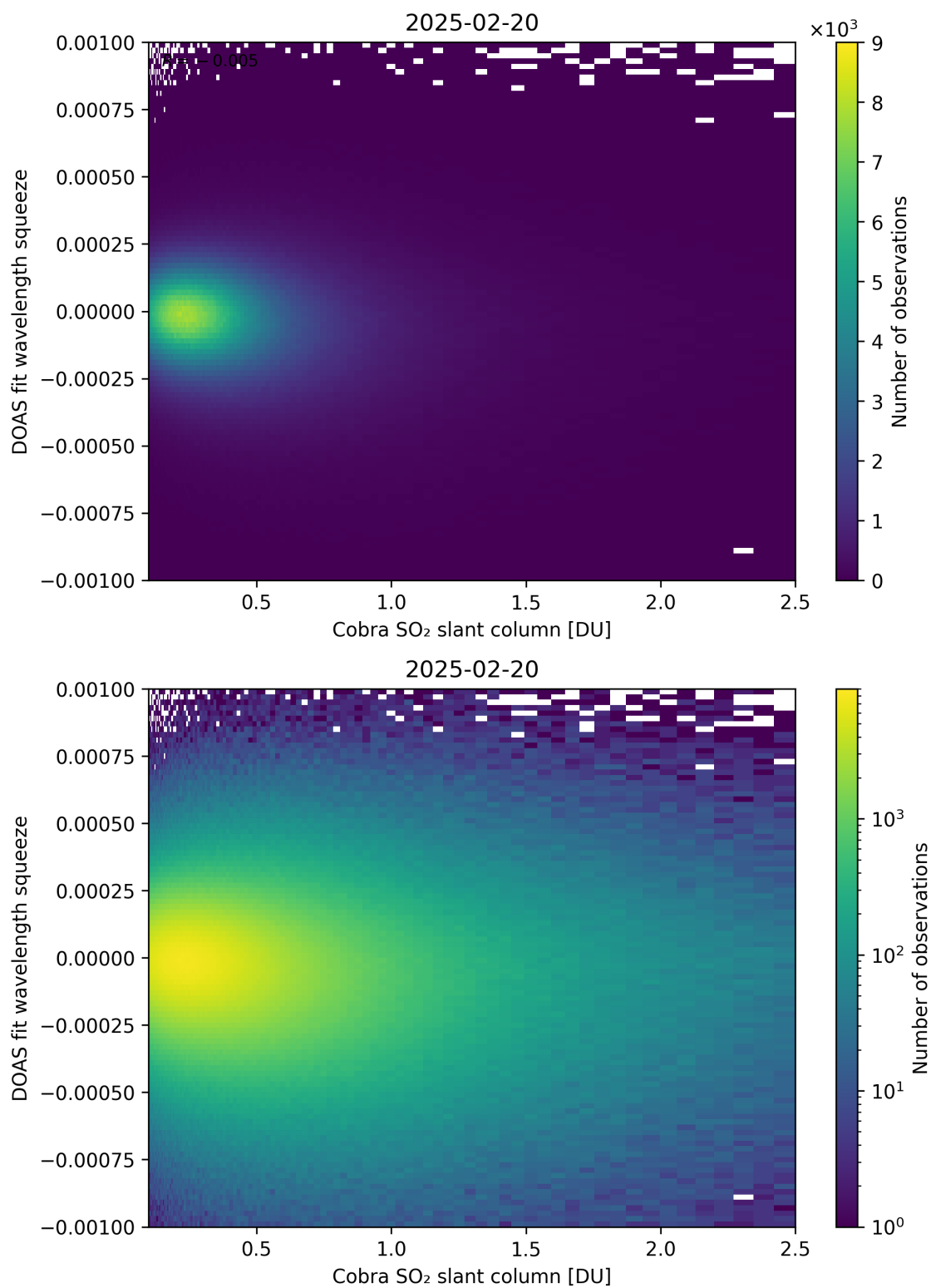
Figure 197: Scatter density plot of “Cobra SO 2 slant column” against “DOAS fit wavelength squeeze” for 2025-02-19 to 2025-02-21.
