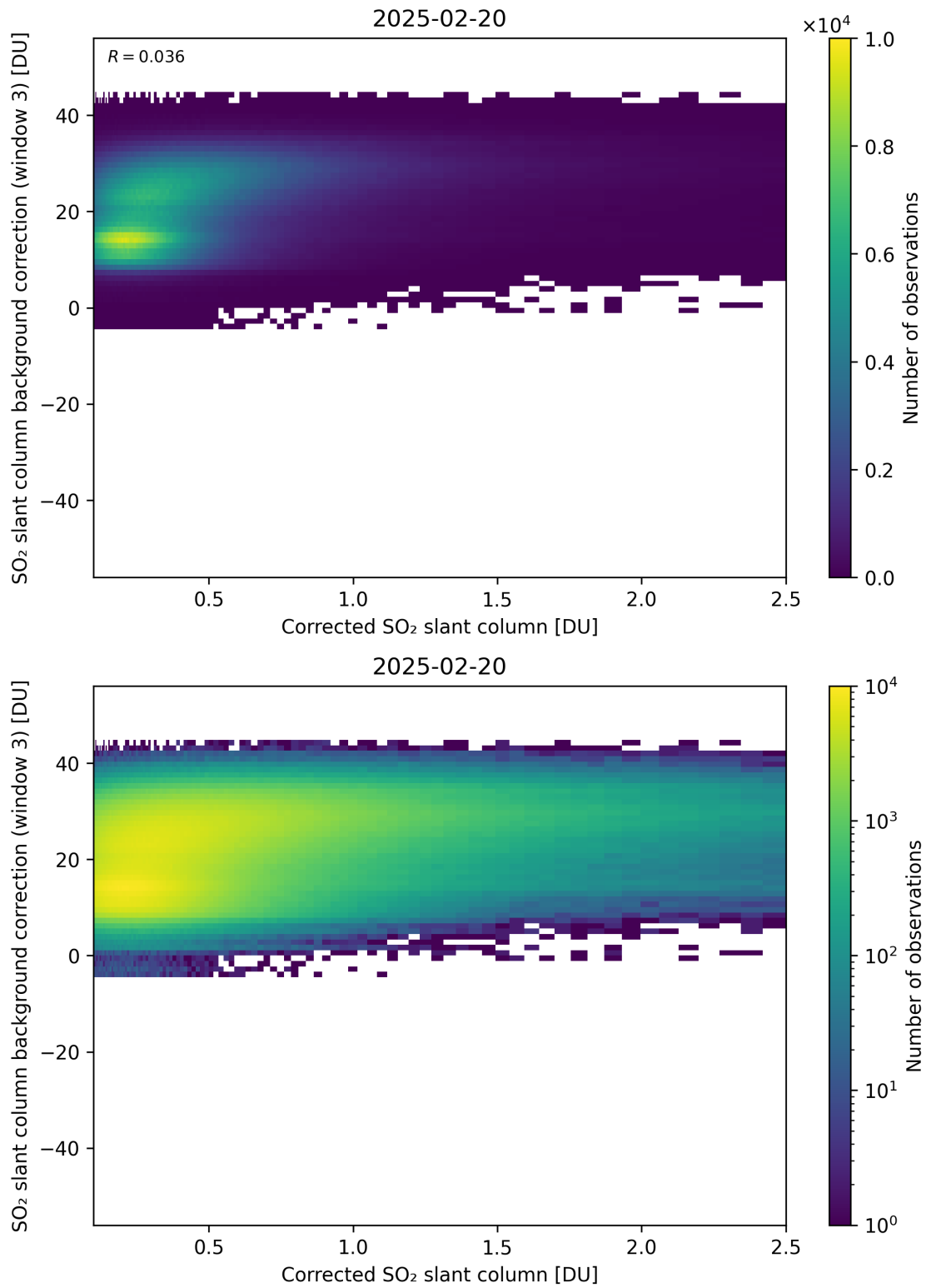
Figure 228: Scatter density plot of “Corrected SO 2 slant column” against “SO 2 slant column background correction (window 3)” for 2025-02-19 to 2025-02-21.
