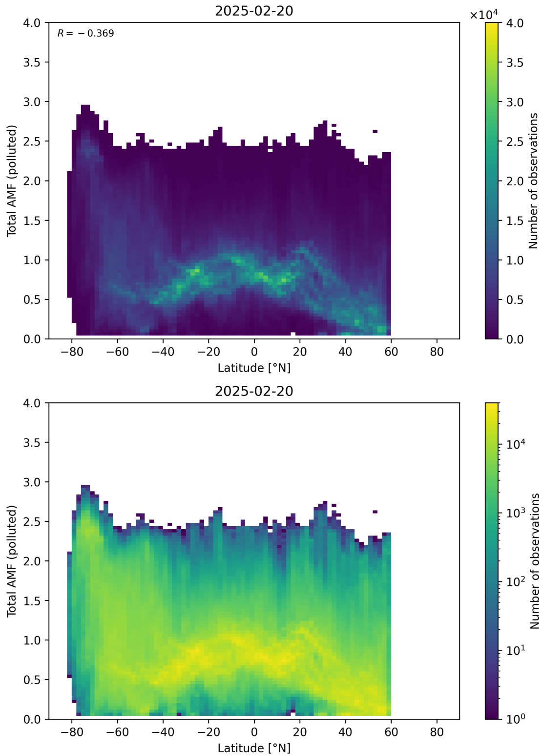
Figure 167: Scatter density plot of “Latitude” against “Total AMF (polluted)” for 2025-02-19 to 2025-02-21.
