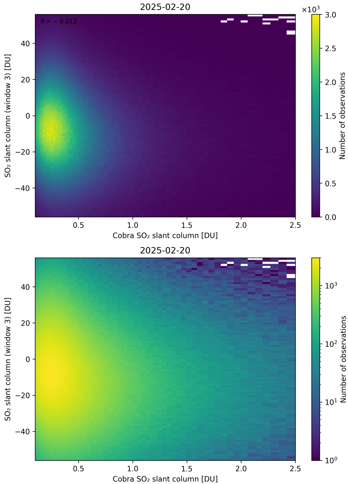
Figure 222: Scatter density plot of “Cobra SO 2 slant column” against “SO 2 slant column (window 3)” for 2025-02-19 to 2025-02-21.
