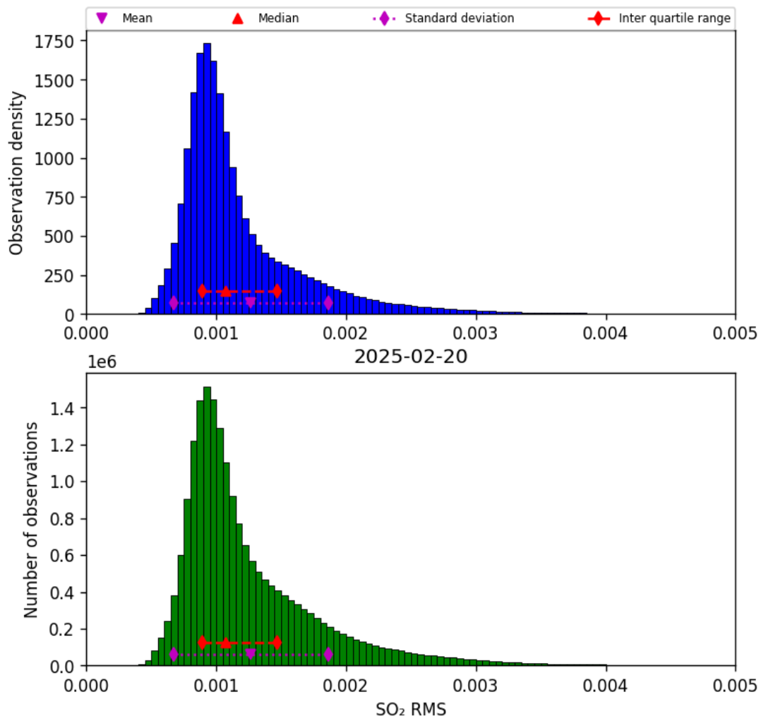
Figure 78: Histogram of “SO 2 RMS” for 2025-02-19 to 2025-02-21
