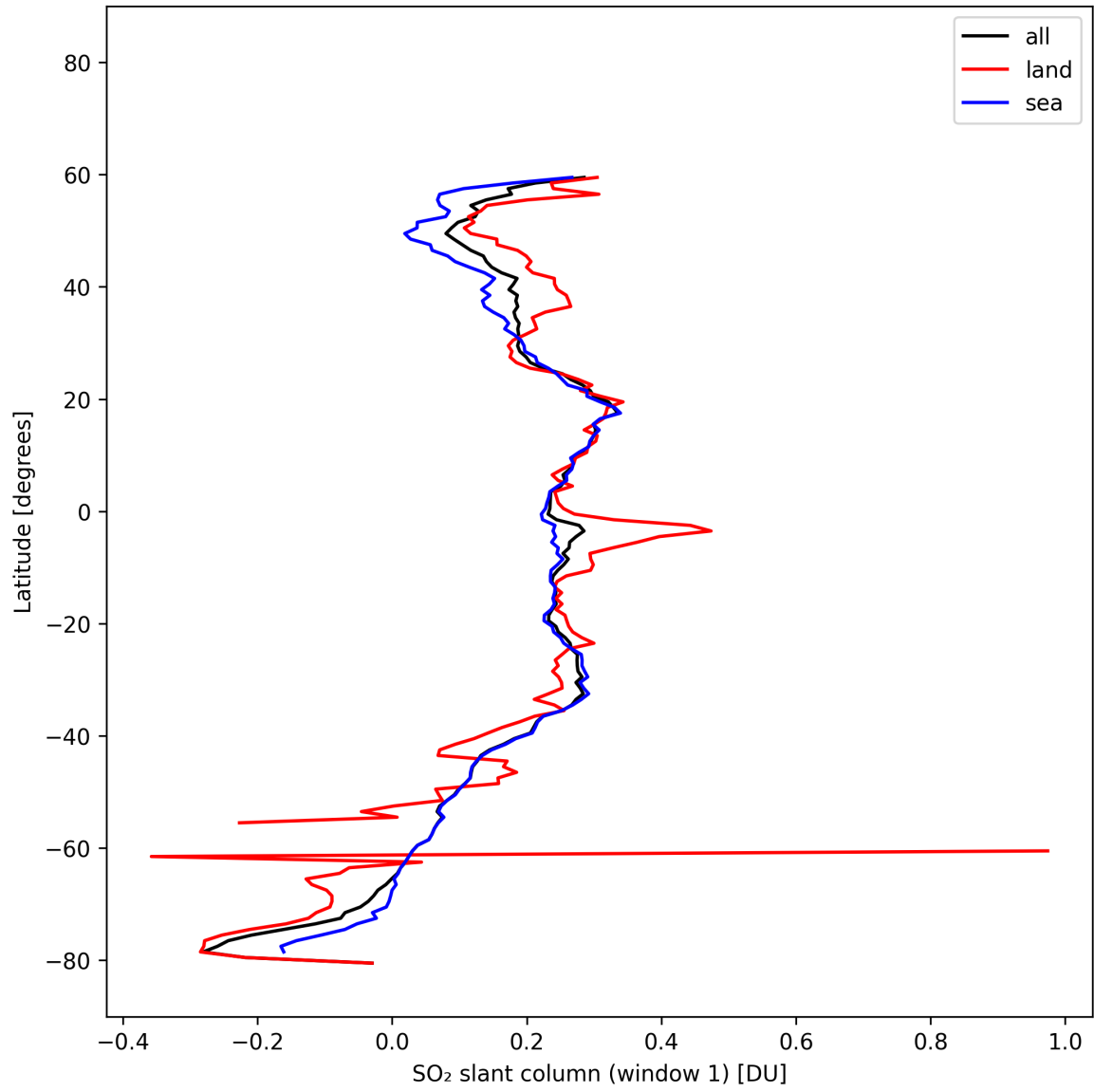
Figure 37: Zonal average of “SO 2 slant column (window 1)” for 2025-02-19 to 2025-02-21.
