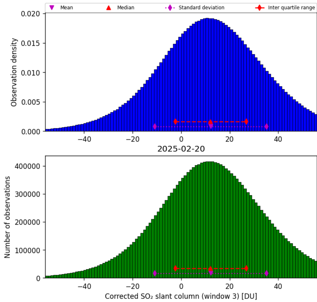
Figure 73: Histogram of “Corrected SO 2 slant column (window 3)” for 2025-02-19 to 2025-02-21
