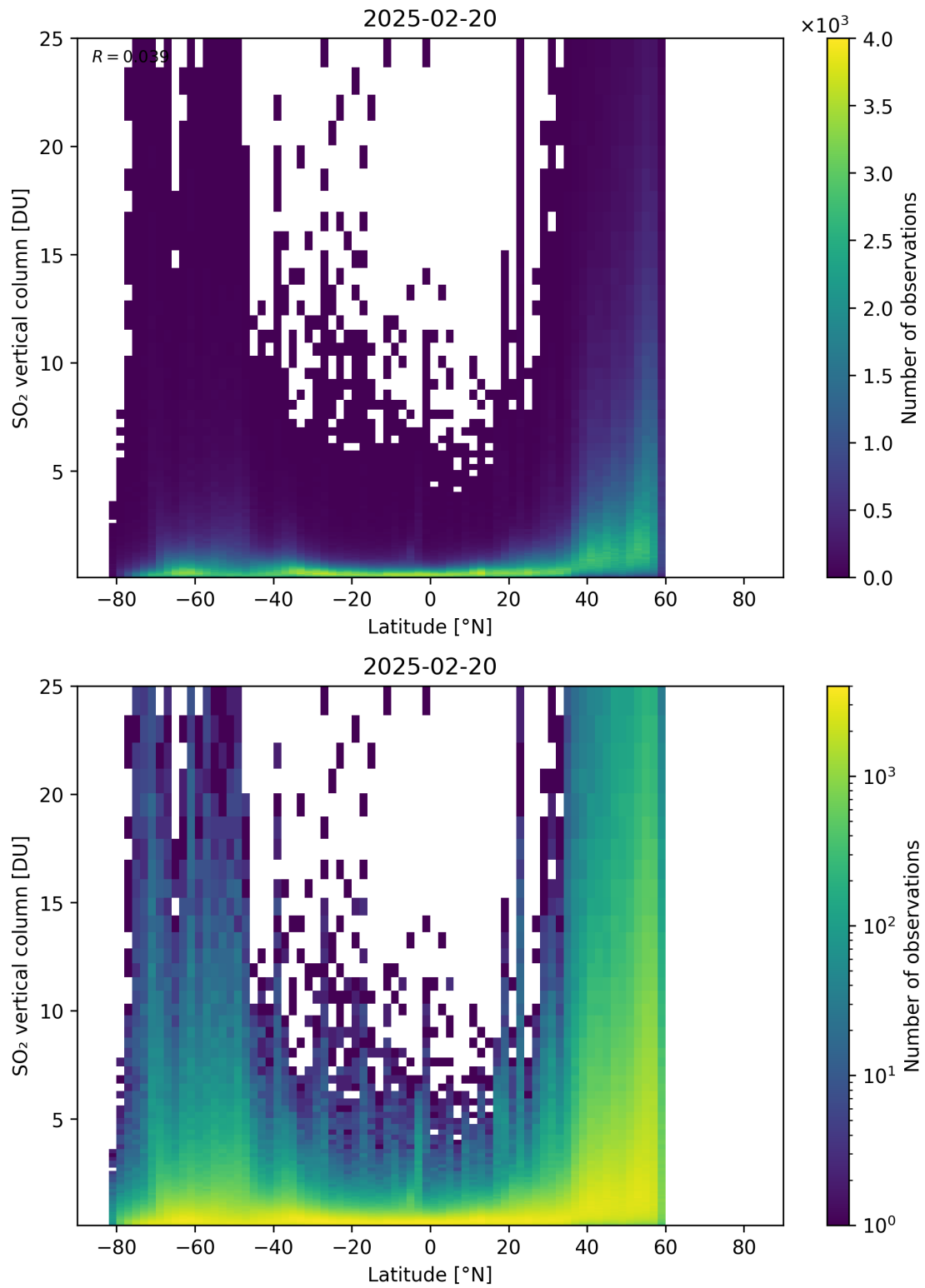
Figure 169: Scatter density plot of “Latitude” against “SO 2 vertical column” for 2025-02-19 to 2025-02-21.
