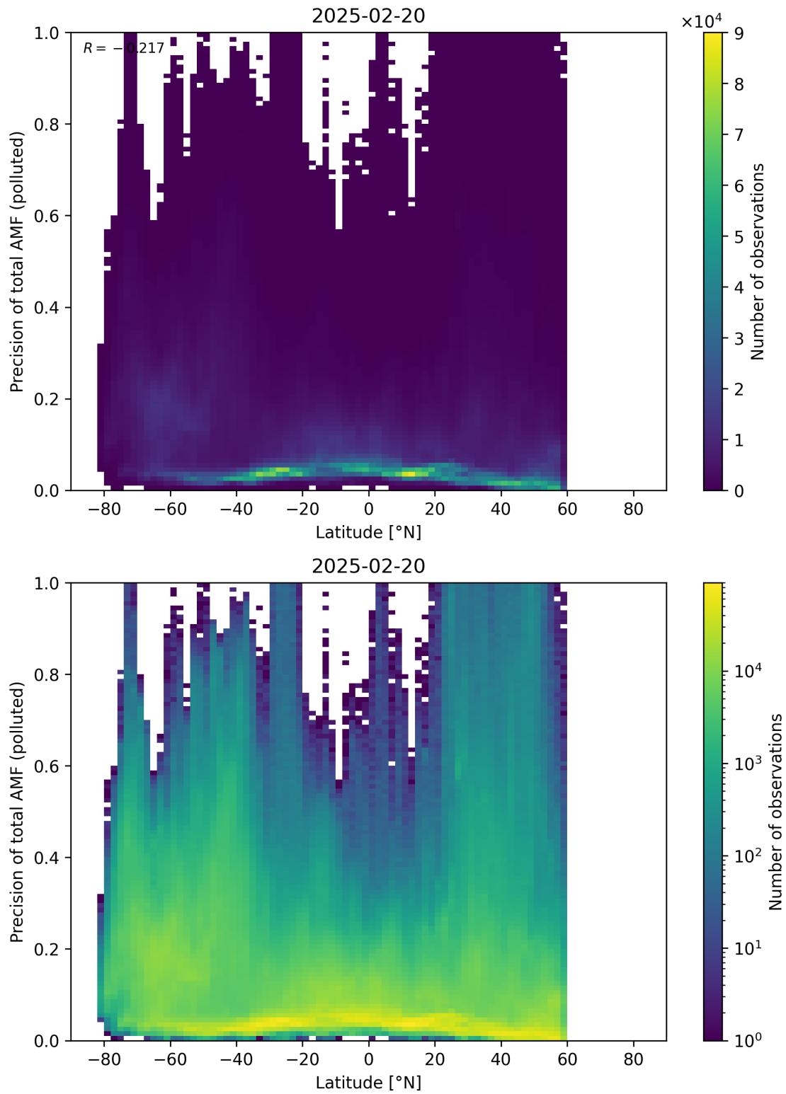
Figure 168: Scatter density plot of “Latitude” against “Precision of total AMF (polluted)” for 2025-02-19 to 2025-02-21.
