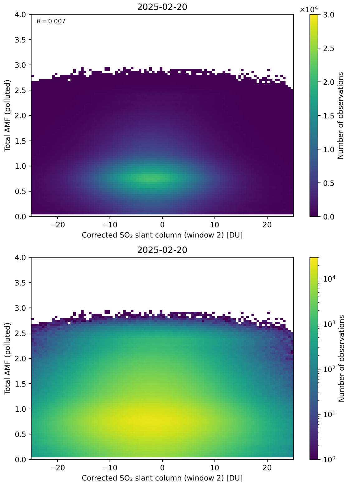
Figure 253: Scatter density plot of “Corrected SO 2 slant column (window 2)” against “Total AMF (polluted)” for 2025-02-19 to 2025-02-21.
