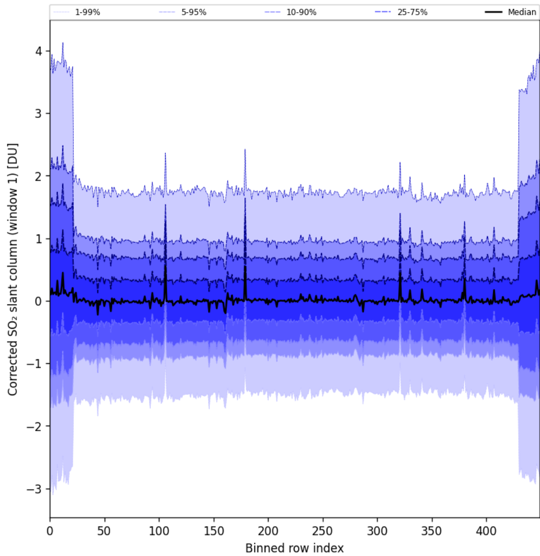
Figure 91: Along track statistics of “Corrected SO 2 slant column (window 1)” for 2025-02-19 to 2025-02-21
