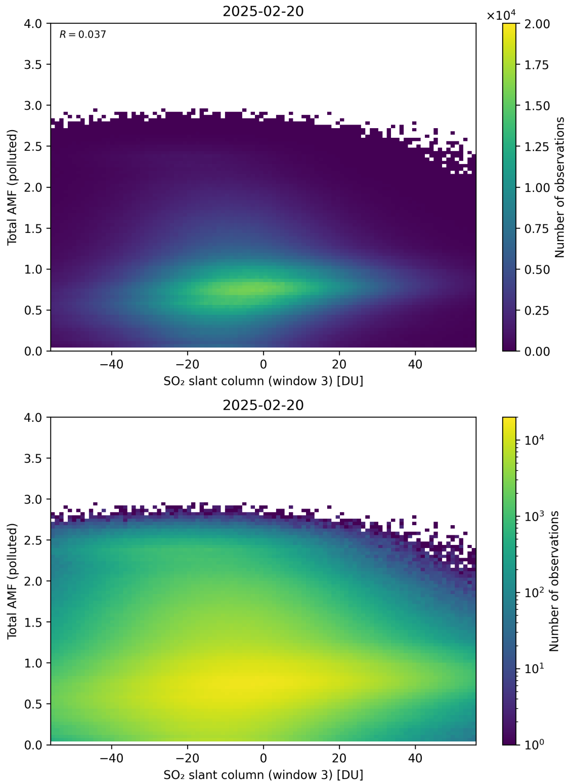
Figure 318: Scatter density plot of “SO 2 slant column (window 3)” against “Total AMF (polluted)” for 2025-02-19 to 2025-02-21.
