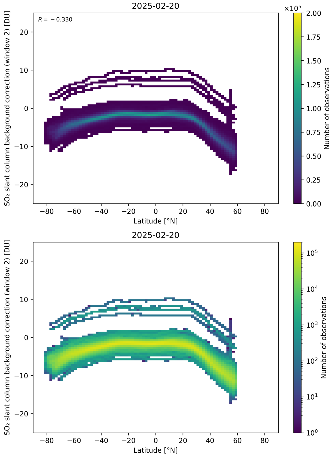
Figure 151: Scatter density plot of “Latitude” against “SO 2 slant column background correction (window 2)” for 2025-02-19 to 2025-02-21.
