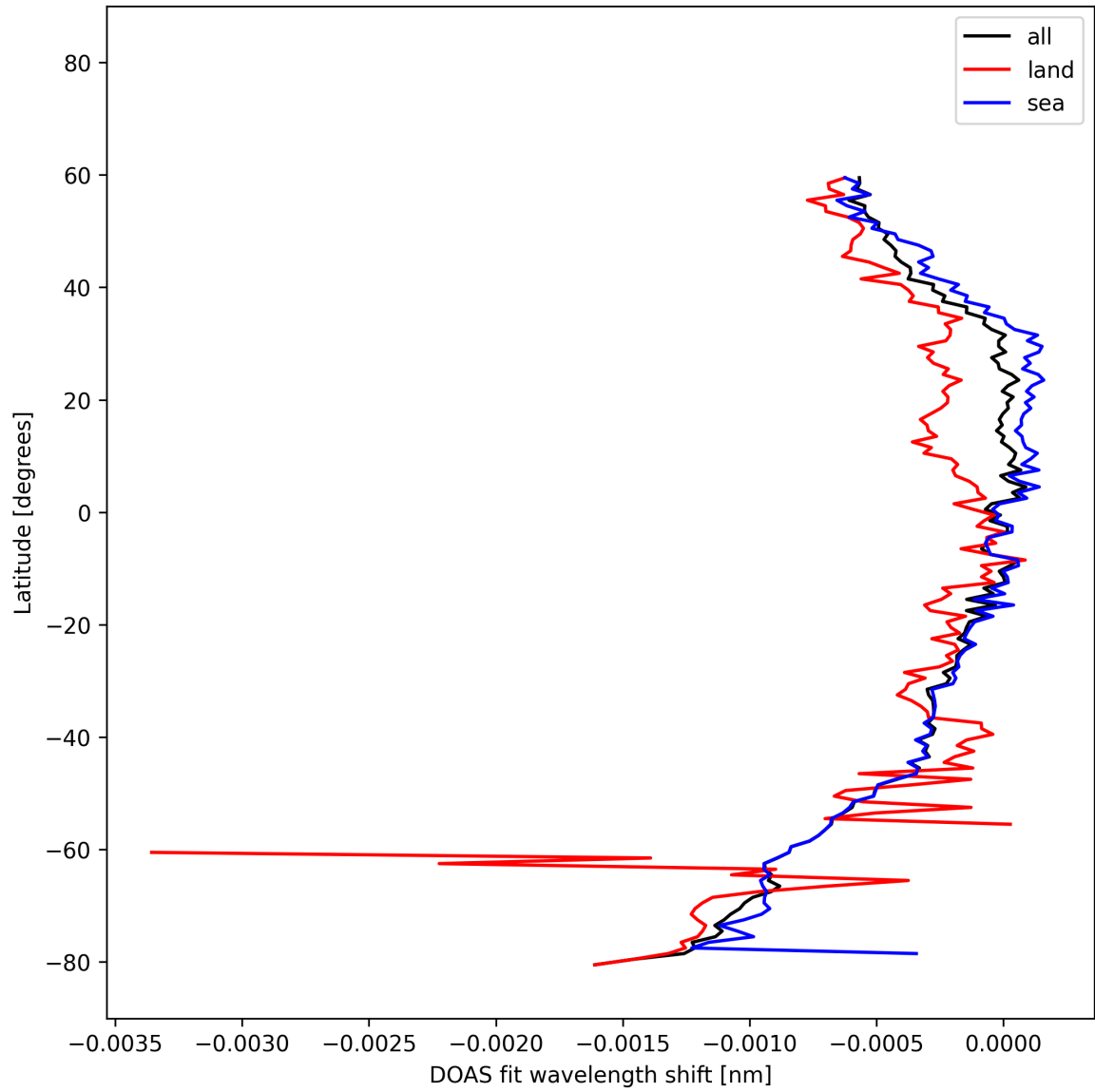
Figure 50: Zonal average of “DOAS fit wavelength shift” for 2025-02-19 to 2025-02-21.
