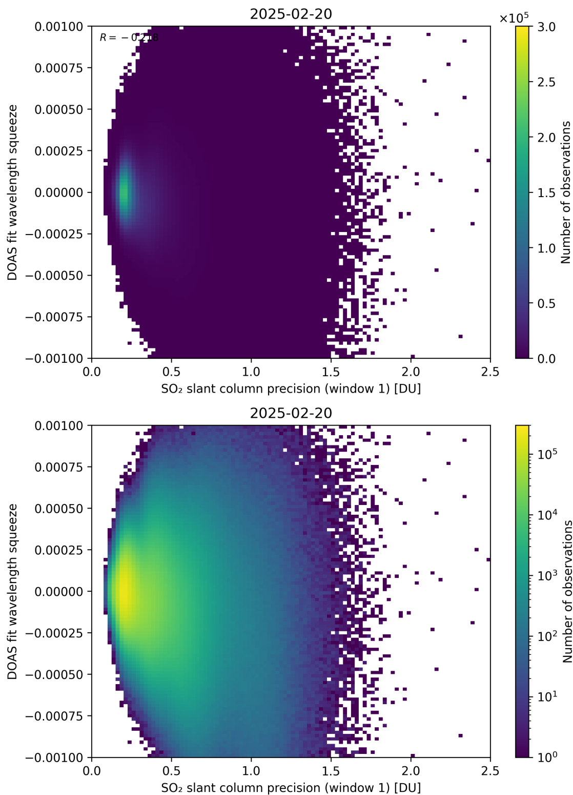
Figure 272: Scatter density plot of “SO 2 slant column precision (window 1)” against “DOAS fit wavelength squeeze” for 2025-02-19 to 2025-02-21.
