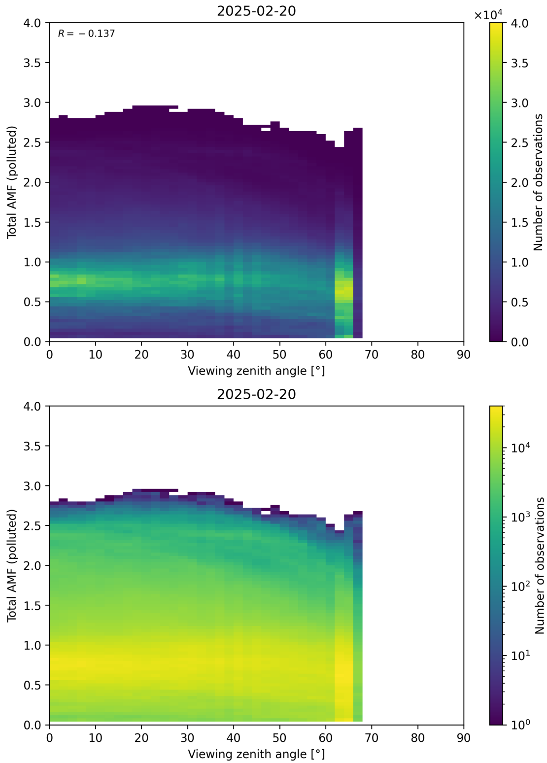
Figure 381: Scatter density plot of “Viewing zenith angle” against “Total AMF (polluted)” for 2025-02-19 to 2025-02-21.
