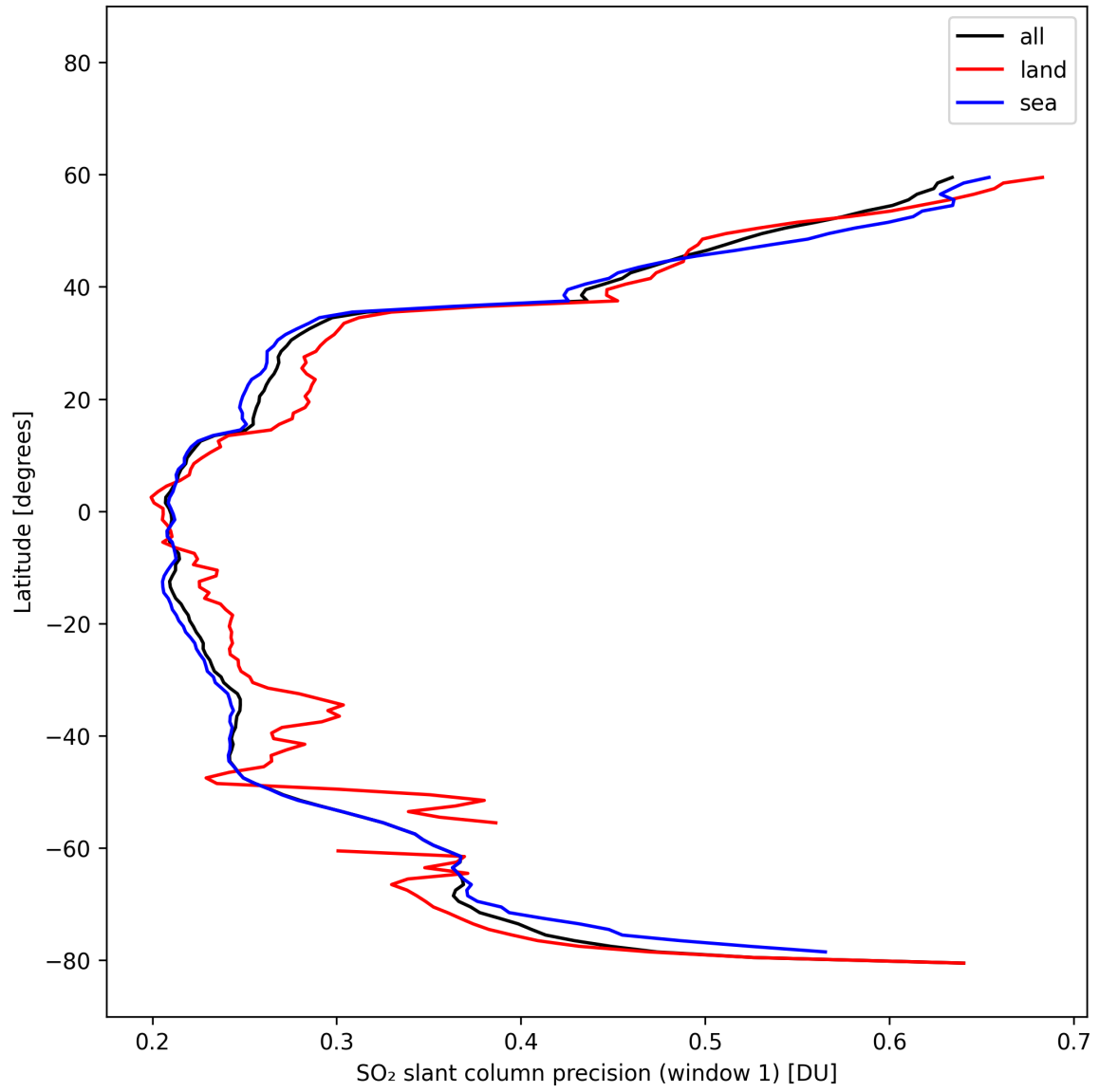
Figure 38: Zonal average of “SO 2 slant column precision (window 1)” for 2025-02-19 to 2025-02-21.
