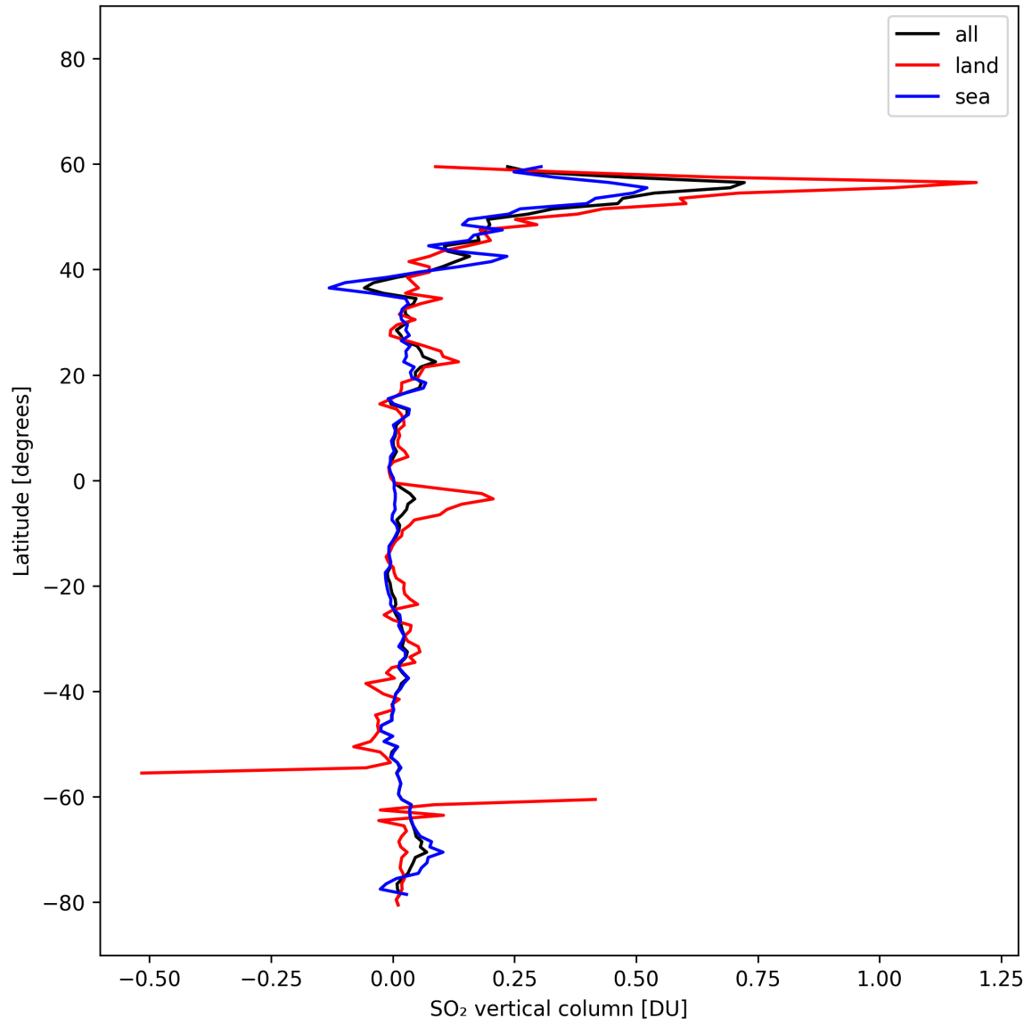
Figure 32: Zonal average of “SO 2 vertical column” for 2025-02-19 to 2025-02-21.
