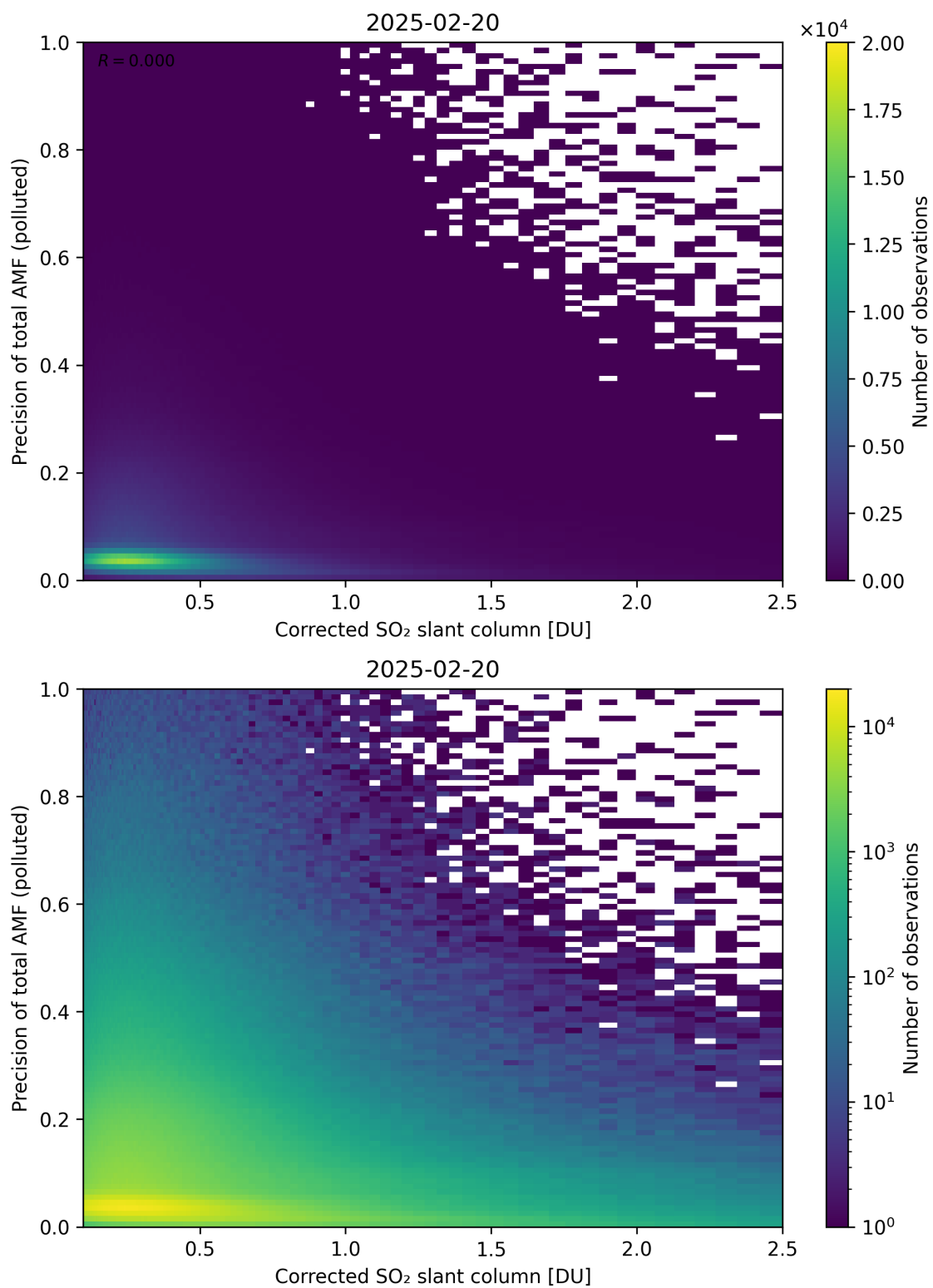
Figure 243: Scatter density plot of “Corrected SO 2 slant column” against “Precision of total AMF (polluted)” for 2025-02-19 to 2025-02-21.
