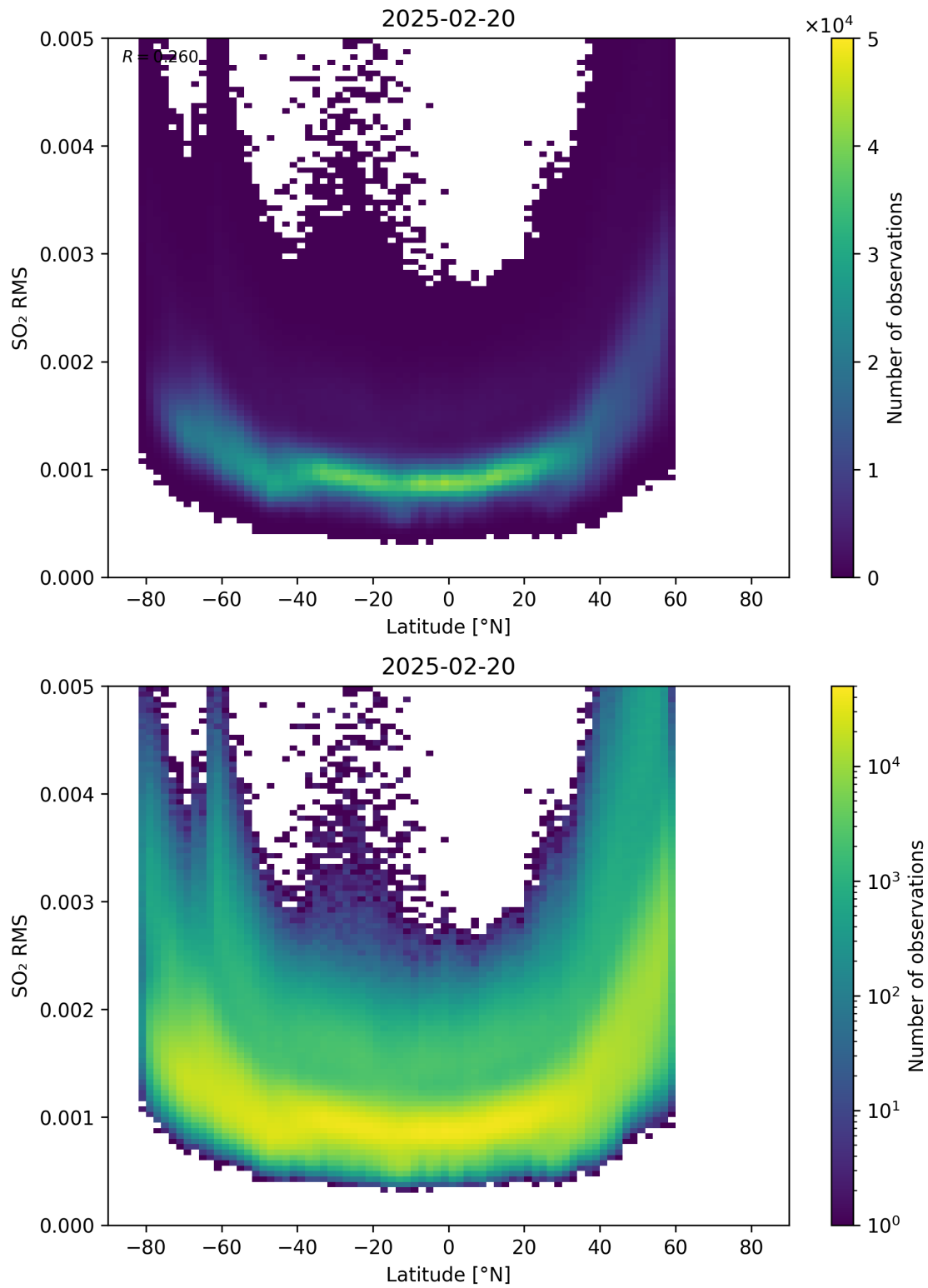
Figure 155: Scatter density plot of “Latitude” against “SO 2 RMS” for 2025-02-19 to 2025-02-21.
