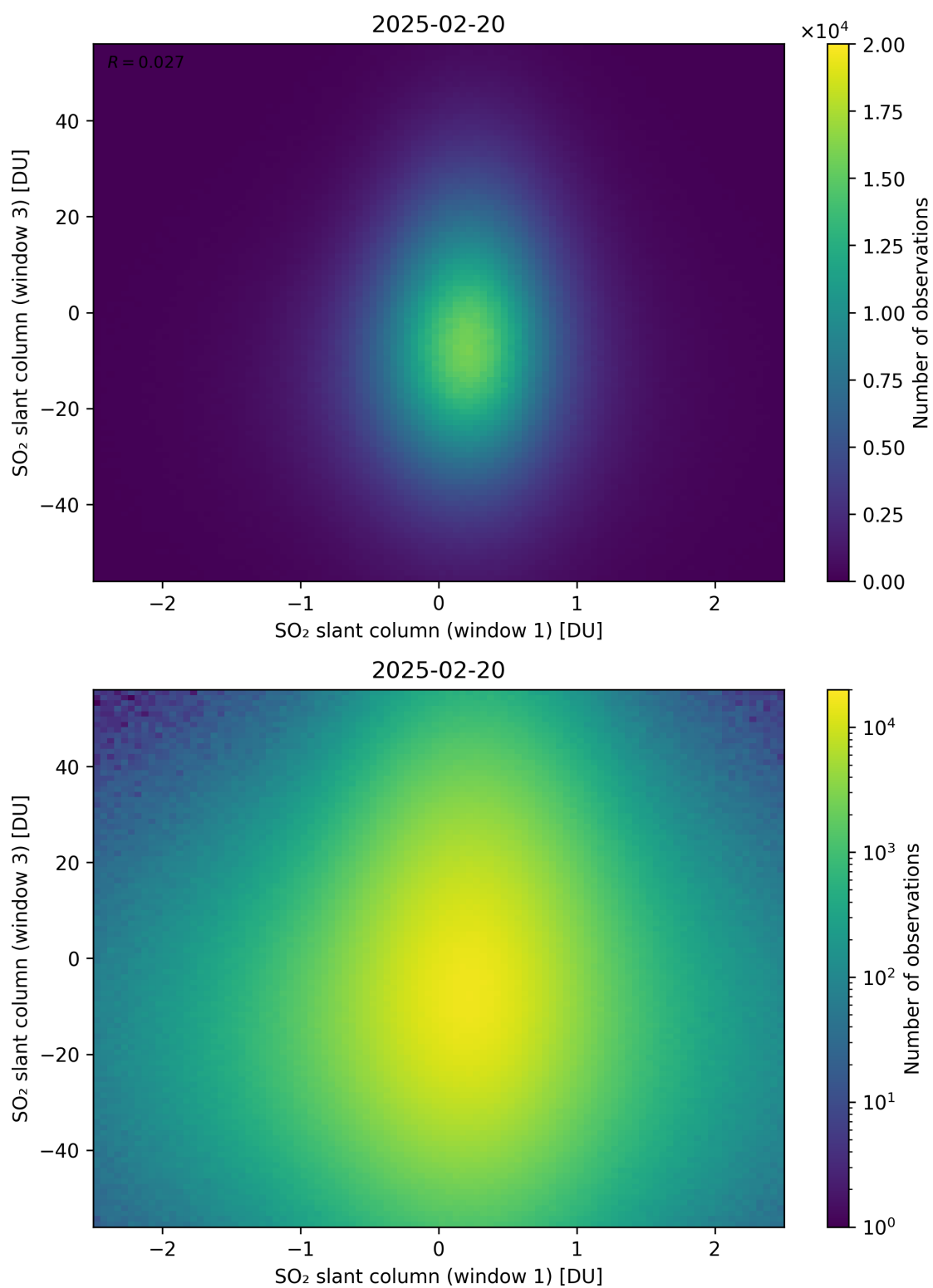
Figure 287: Scatter density plot of “SO 2 slant column (window 1)” against “SO 2 slant column (window 3)” for 2025-02-19 to 2025-02-21.
