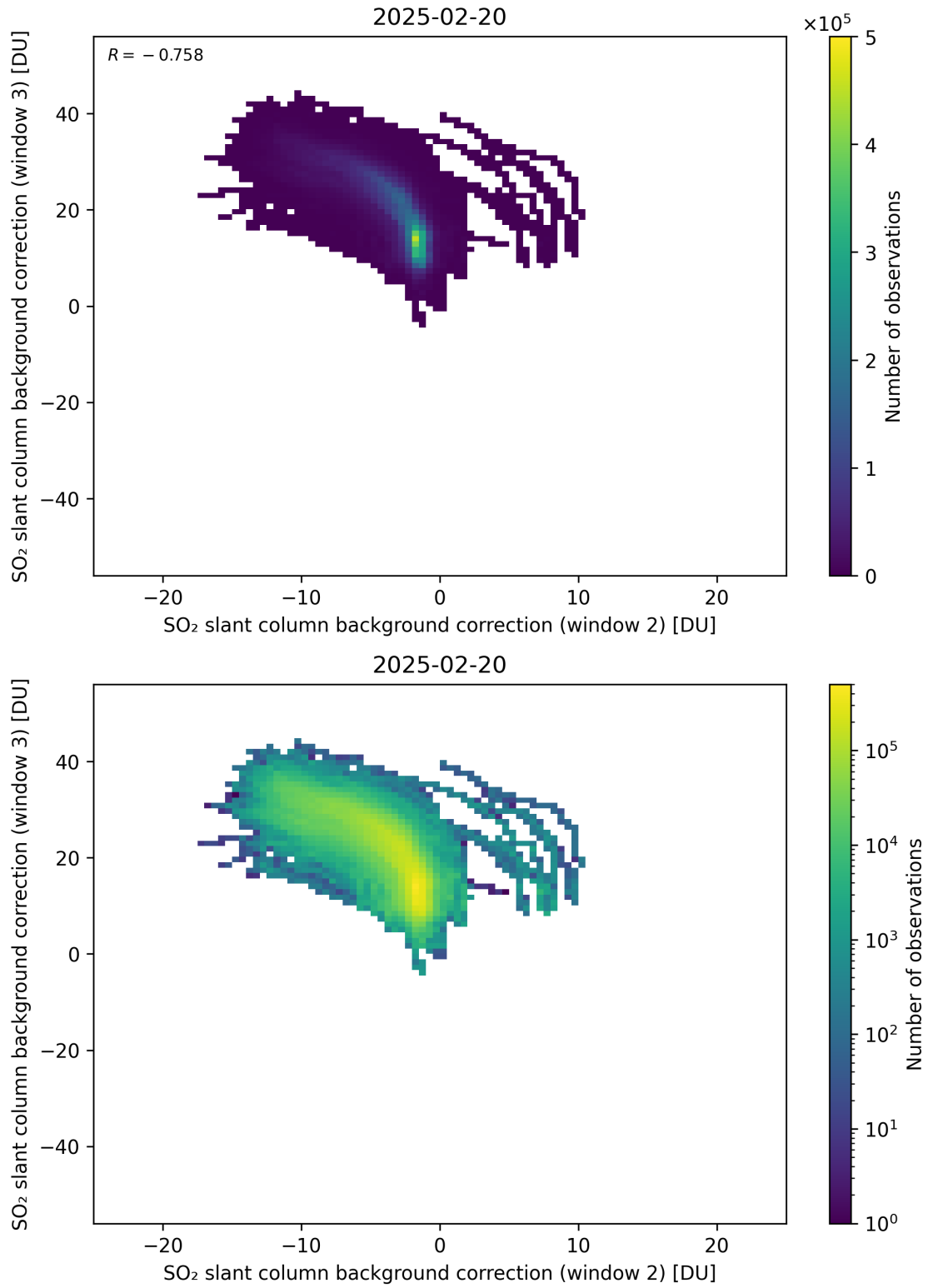
Figure 122: Scatter density plot of “SO 2 slant column background correction (window 2)” against “SO 2 slant column background correction (window 3)” for 2025-02-19 to 2025-02-21.
