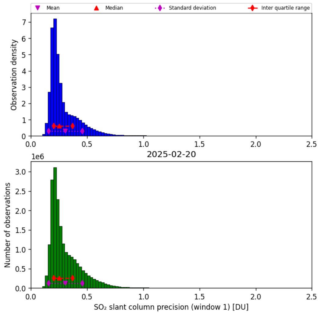
Figure 64: Histogram of “SO 2 slant column precision (window 1)” for 2025-02-19 to 2025-02-21
