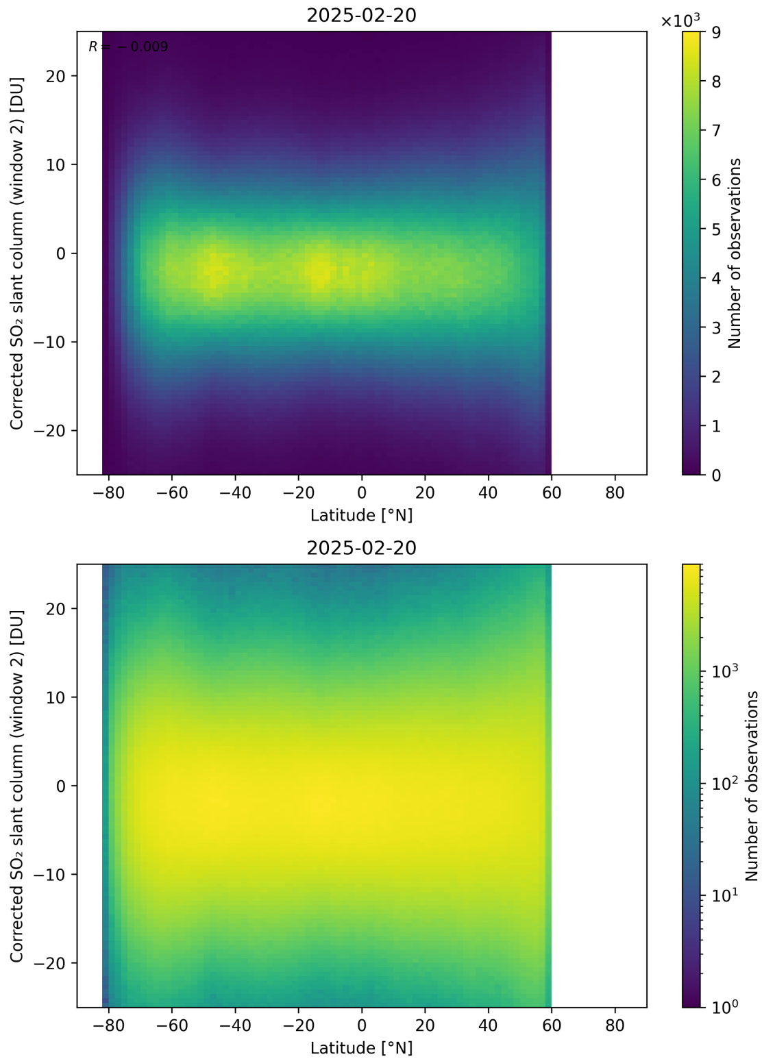
Figure 160: Scatter density plot of “Latitude” against “Corrected SO 2 slant column (window 2)” for 2025-02-19 to 2025-02-21.
