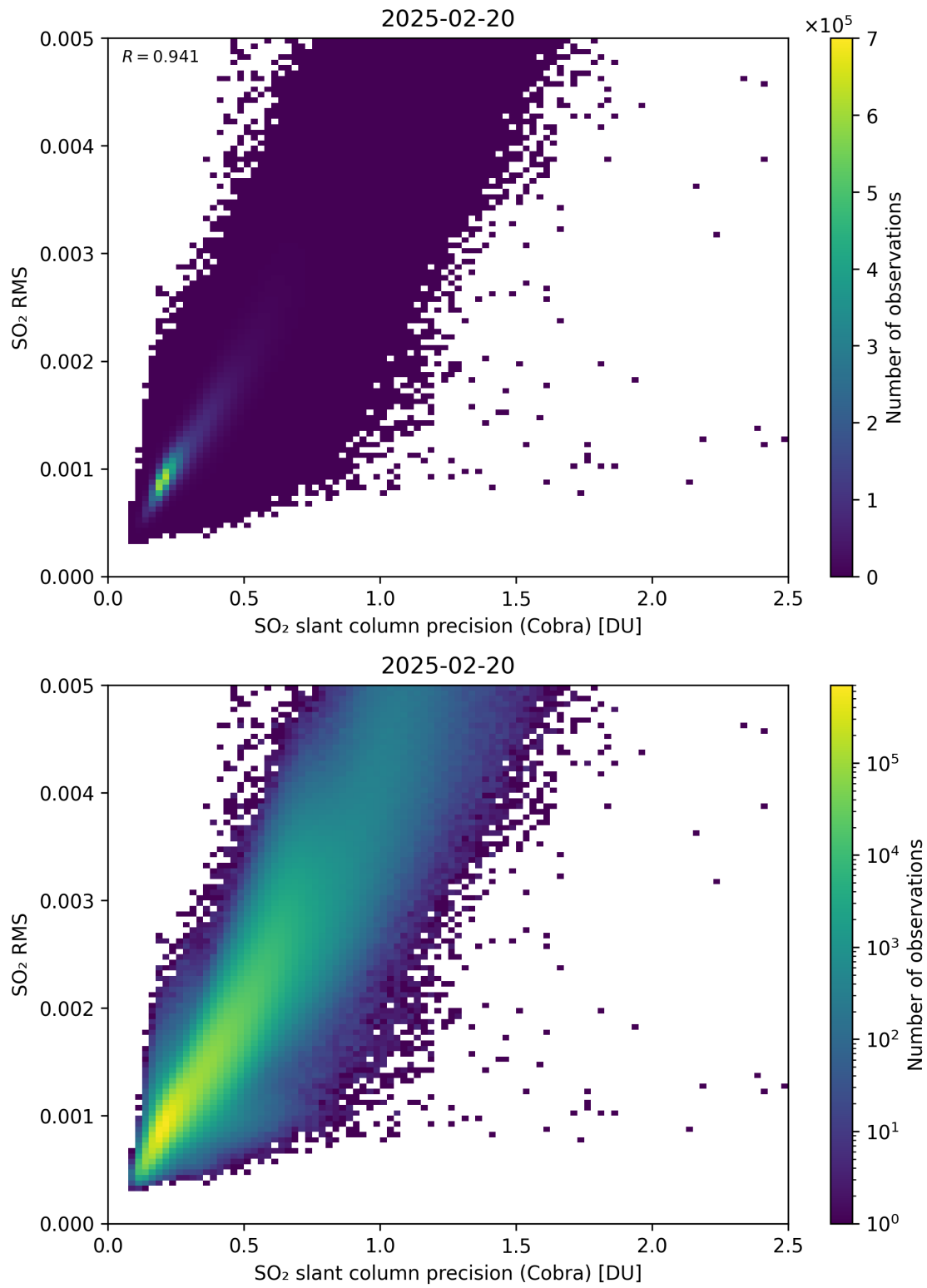
Figure 204: Scatter density plot of “SO 2 slant column precision (Cobra)” against “SO 2 RMS” for 2025-02-19 to 2025-02-21.
