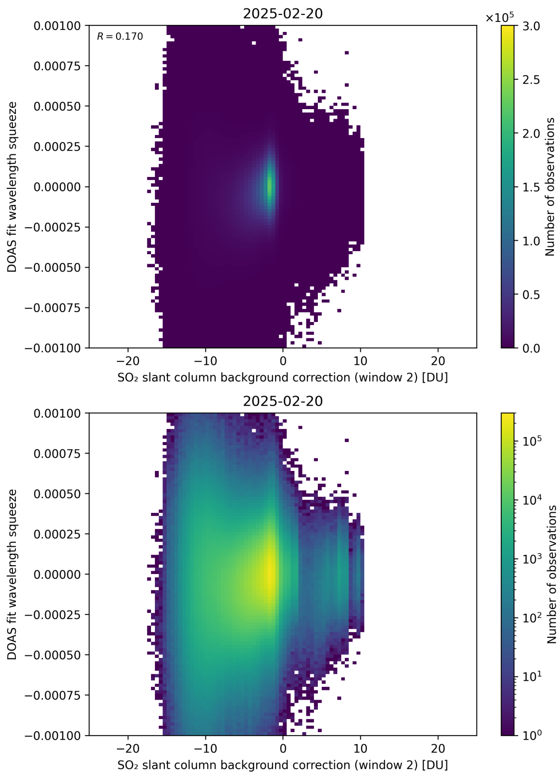
Figure 124: Scatter density plot of “SO 2 slant column background correction (window 2)” against “DOAS fit wavelength squeeze” for 2025-02-19 to 2025-02-21.
