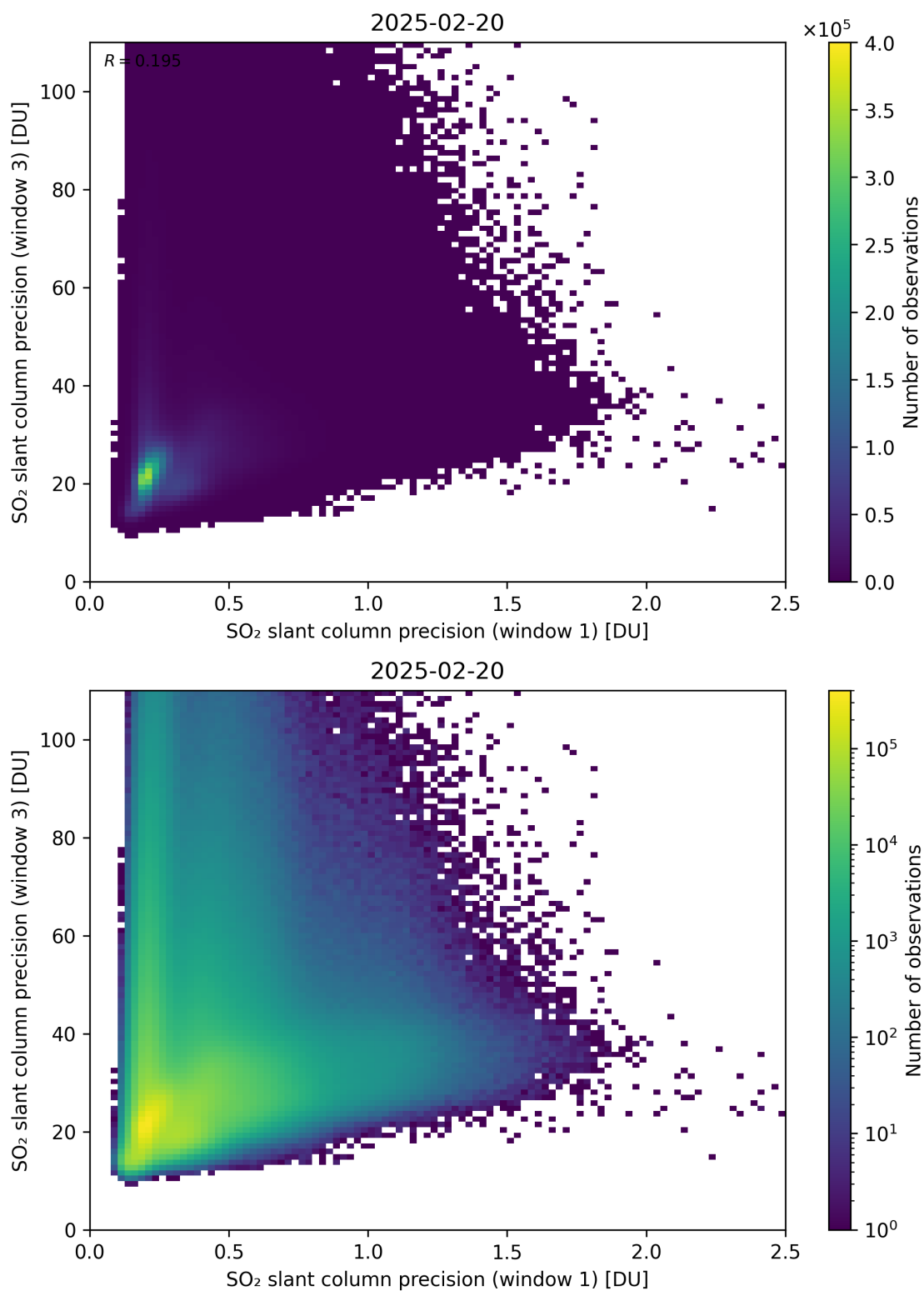
Figure 279: Scatter density plot of “SO 2 slant column precision (window 1)” against “SO 2 slant column precision (window 3)” for 2025-02-19 to 2025-02-21.
