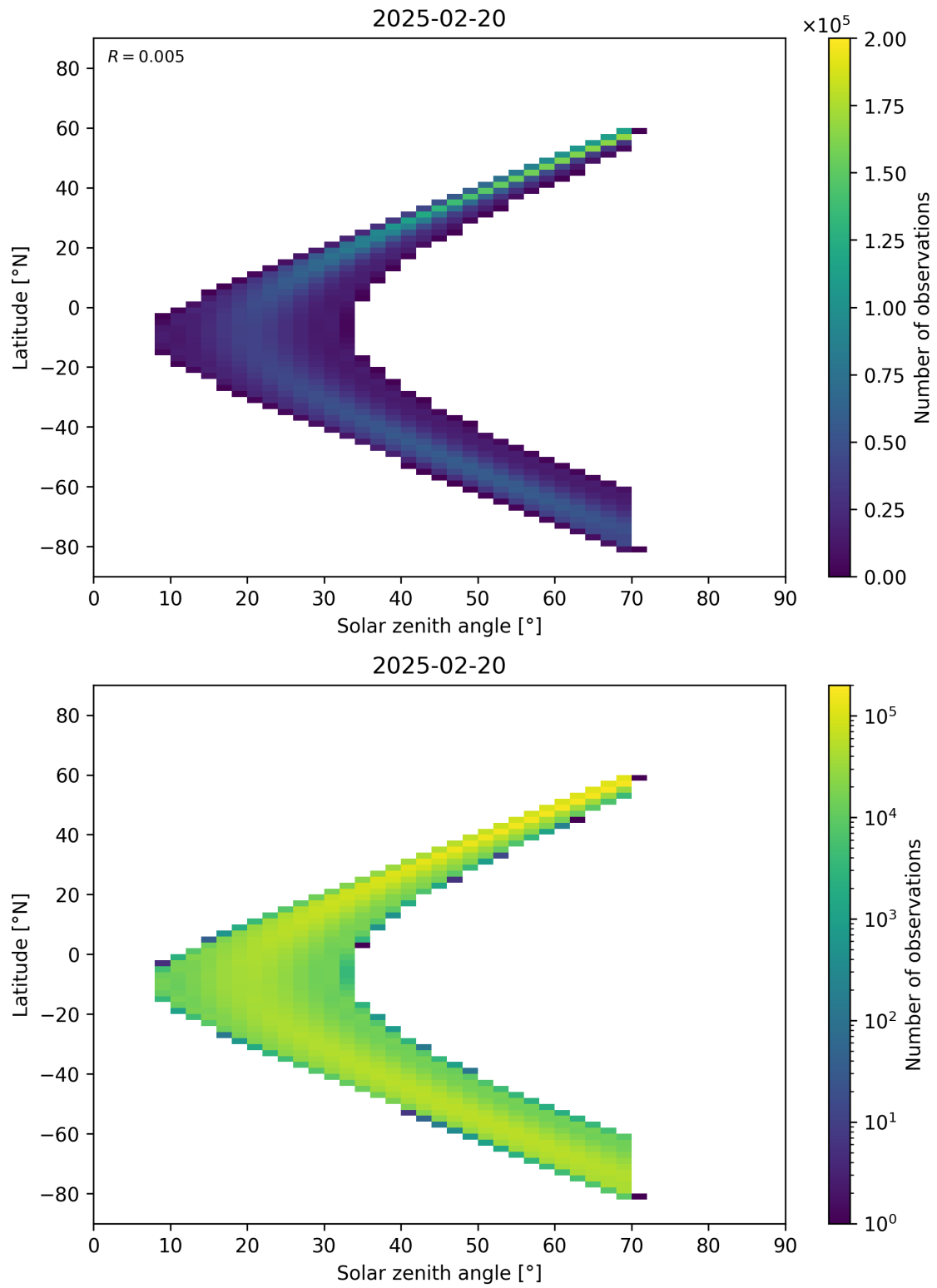
Figure 177: Scatter density plot of “Solar zenith angle” against “Latitude” for 2025-02-19 to 2025-02-21.
