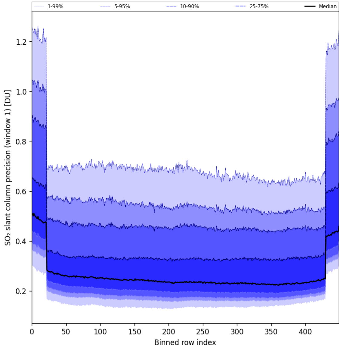
Figure 90: Along track statistics of “SO 2 slant column precision (window 1)” for 2025-02-19 to 2025-02-21
