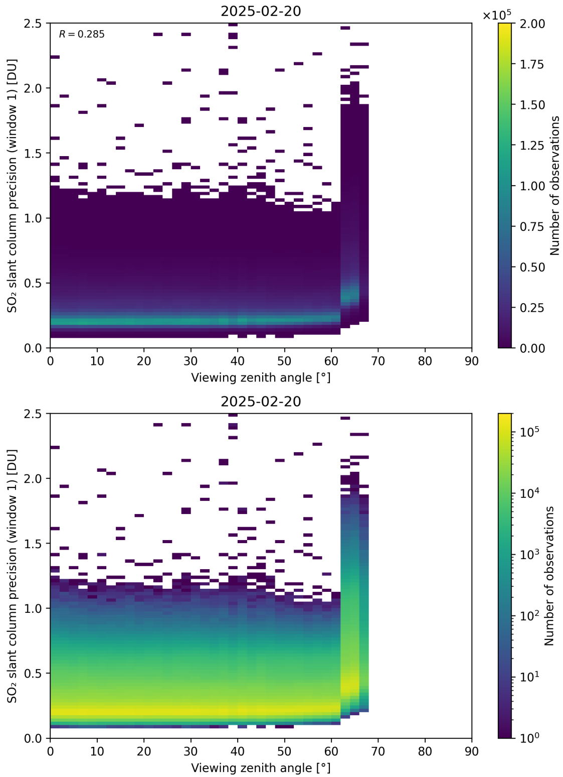
Figure 377: Scatter density plot of “Viewing zenith angle” against “SO 2 slant column precision (window 1)” for 2025-02-19 to 2025-02-21.
