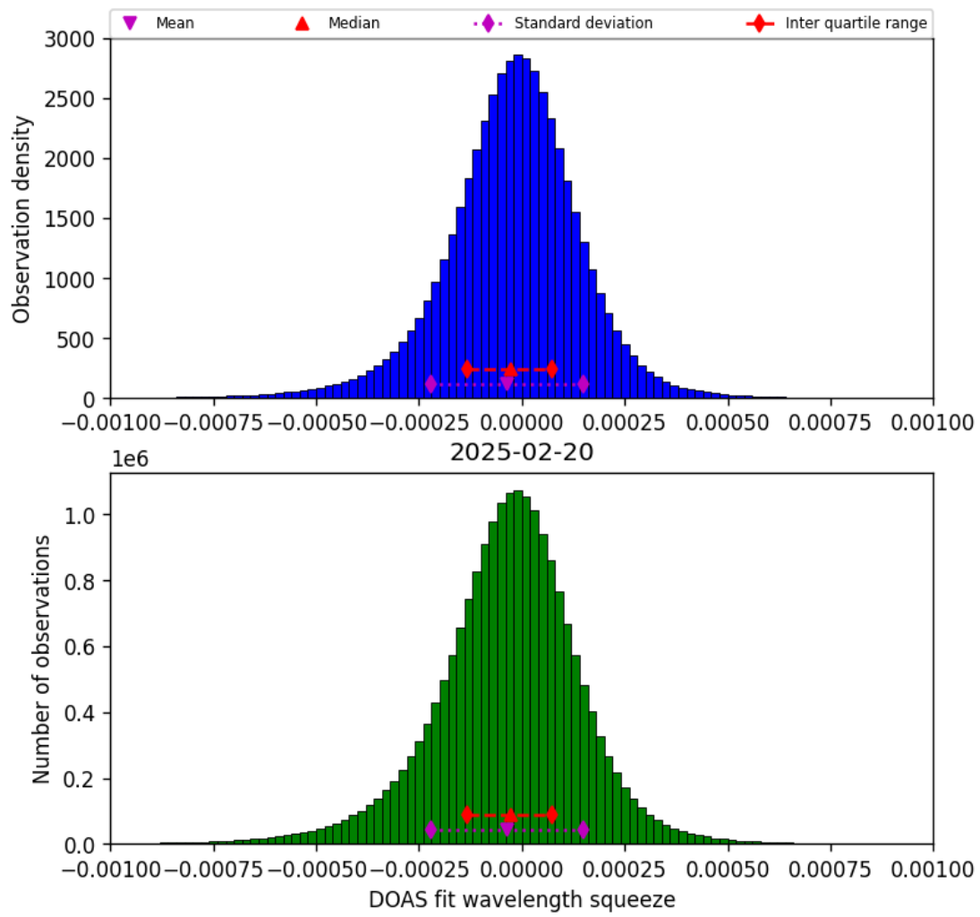
Figure 77: Histogram of “DOAS fit wavelength squeeze” for 2025-02-19 to 2025-02-21
