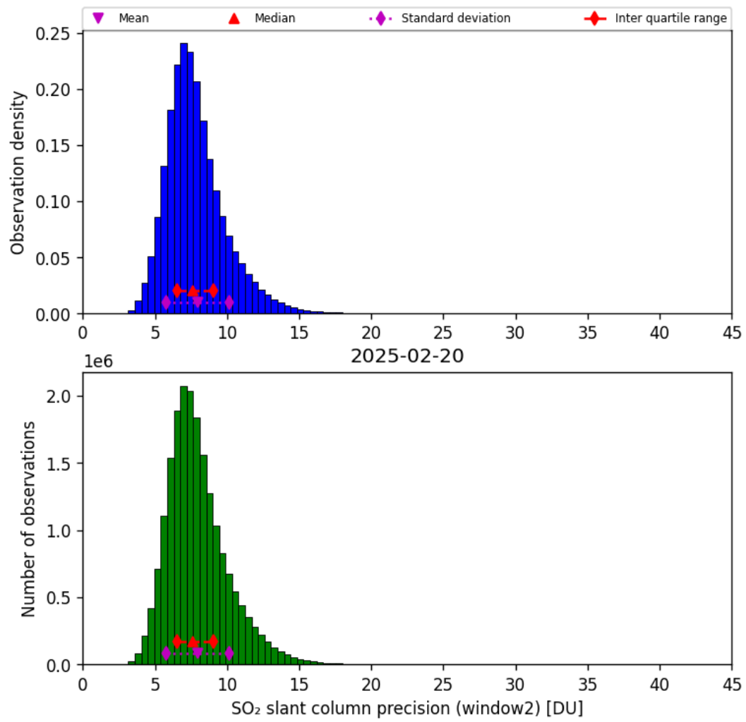
Figure 68: Histogram of “SO 2 slant column precision (window2)” for 2025-02-19 to 2025-02-21
