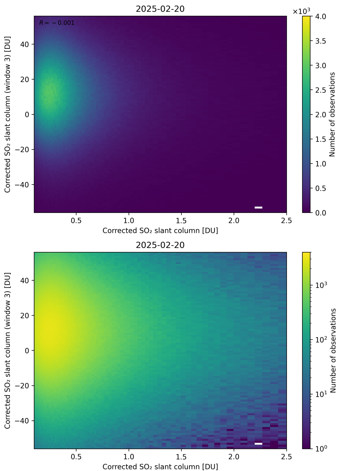
Figure 236: Scatter density plot of “Corrected SO 2 slant column” against “Corrected SO 2 slant column (window 3)” for 2025-02-19 to 2025-02-21.
