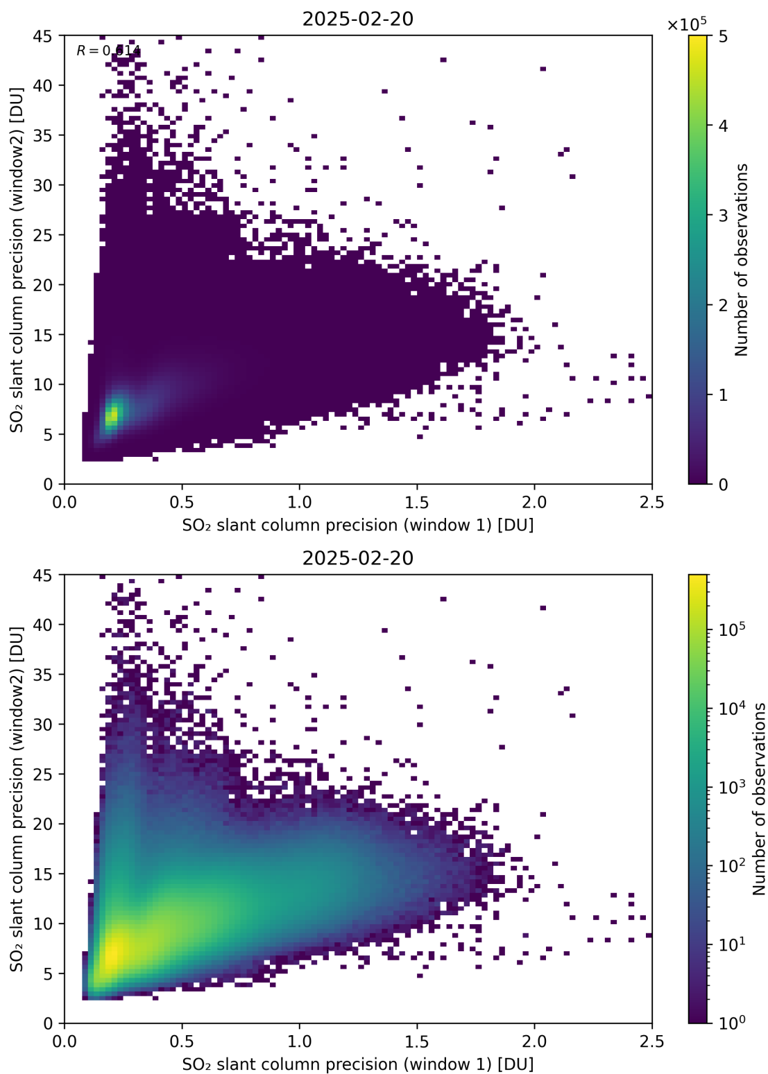
Figure 277: Scatter density plot of “SO 2 slant column precision (window 1)” against “SO 2 slant column precision (window2)” for 2025-02-19 to 2025-02-21.
