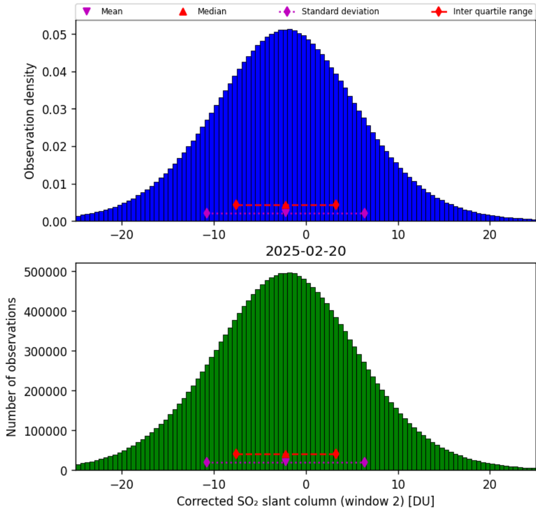
Figure 69: Histogram of “Corrected SO 2 slant column (window 2)” for 2025-02-19 to 2025-02-21
