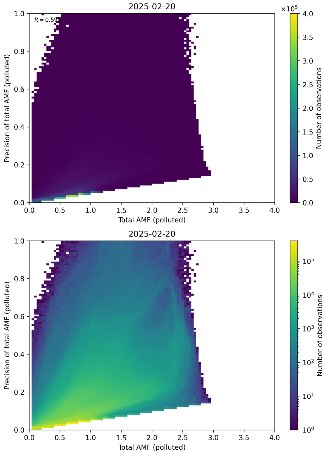
Figure 322: Scatter density plot of “Total AMF (polluted)” against “Precision of total AMF (polluted)” for 2025-02-19 to 2025-02-21.
