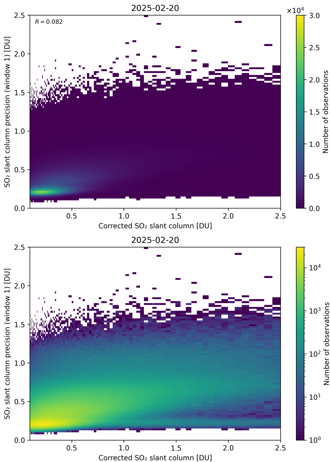
Figure 238: Scatter density plot of “Corrected SO 2 slant column” against “SO 2 slant column precision (window 1)” for 2025-02-19 to 2025-02-21.
