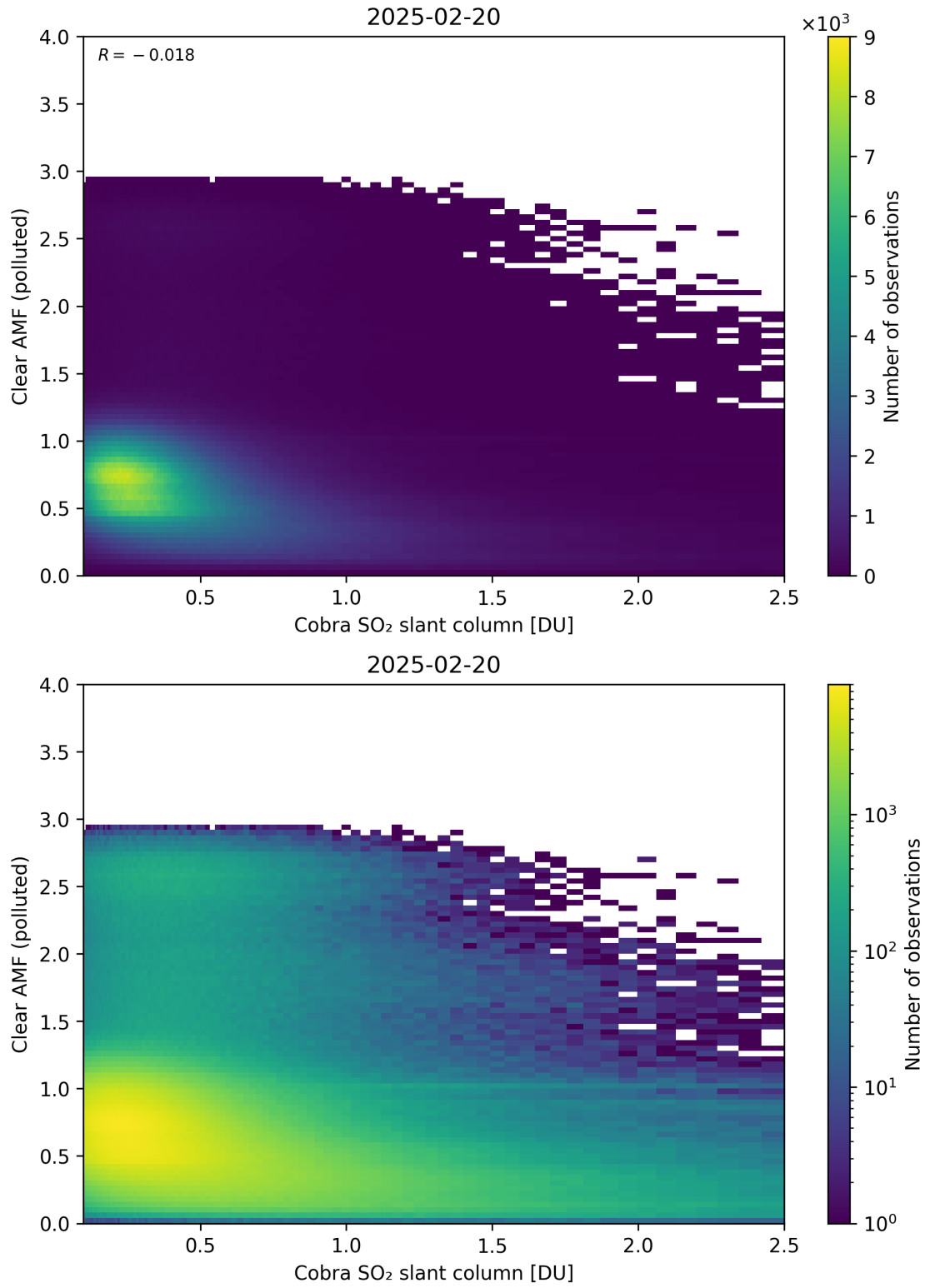
Figure 215: Scatter density plot of “Cobra SO 2 slant column” against “Clear AMF (polluted)” for 2025-02-19 to 2025-02-21.
