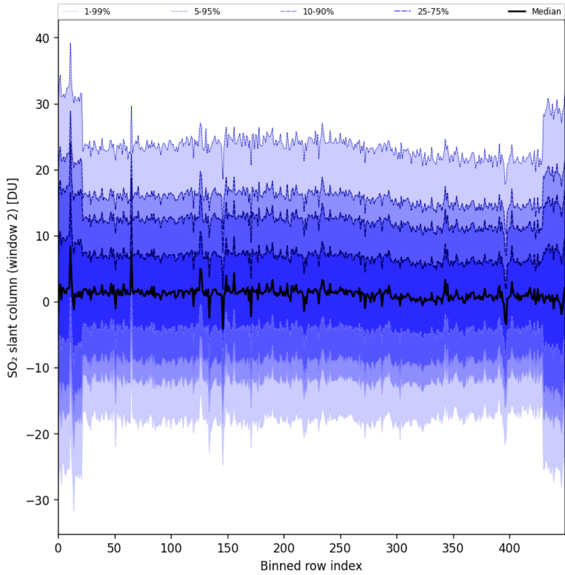
Figure 93: Along track statistics of “SO 2 slant column (window 2)” for 2025-02-19 to 2025-02-21
