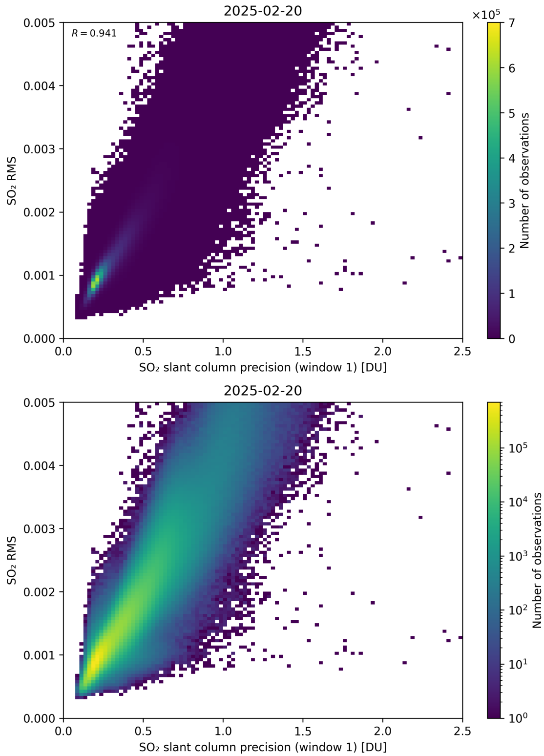
Figure 273: Scatter density plot of “SO 2 slant column precision (window 1)” against “SO 2 RMS” for 2025-02-19 to 2025-02-21.
