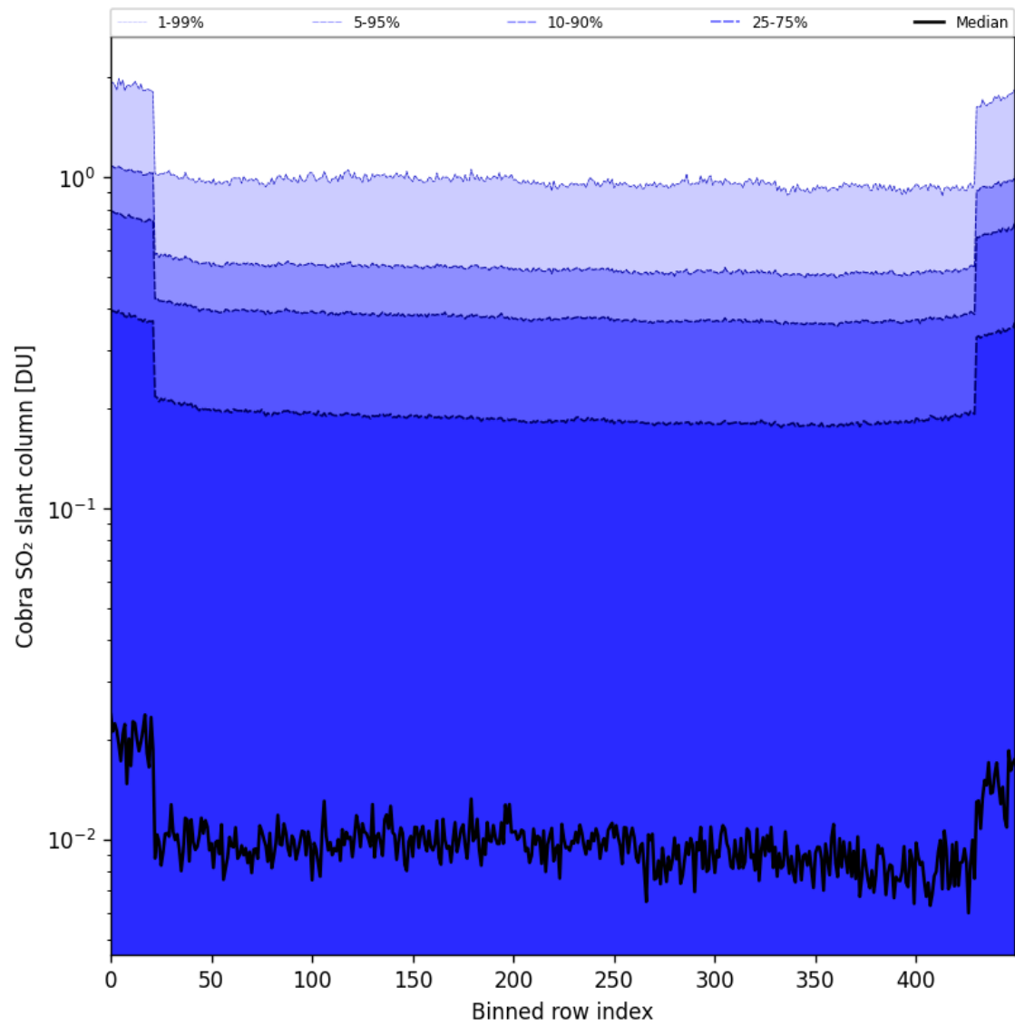
Figure 87: Along track statistics of “Cobra SO 2 slant column” for 2025-02-19 to 2025-02-21
