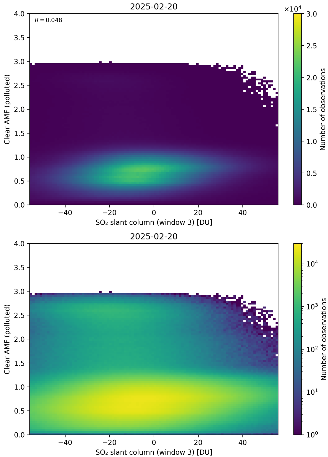
Figure 315: Scatter density plot of “SO 2 slant column (window 3)” against “Clear AMF (polluted)” for 2025-02-19 to 2025-02-21.
