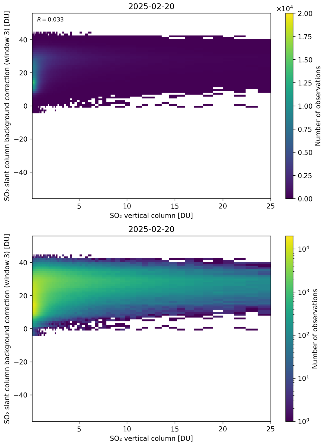
Figure 325: Scatter density plot of “SO 2 vertical column” against “SO 2 slant column background correction (window 3)” for 2025-02-19 to 2025-02-21.
