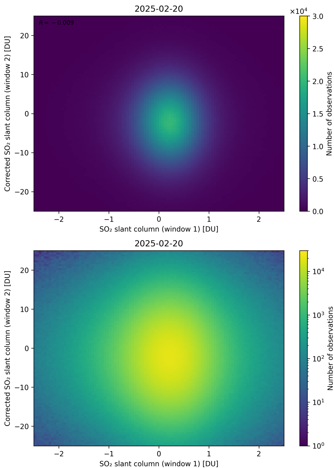
Figure 283: Scatter density plot of “SO 2 slant column (window 1)” against “Corrected SO 2 slant column (window 2)” for 2025-02-19 to 2025-02-21.
