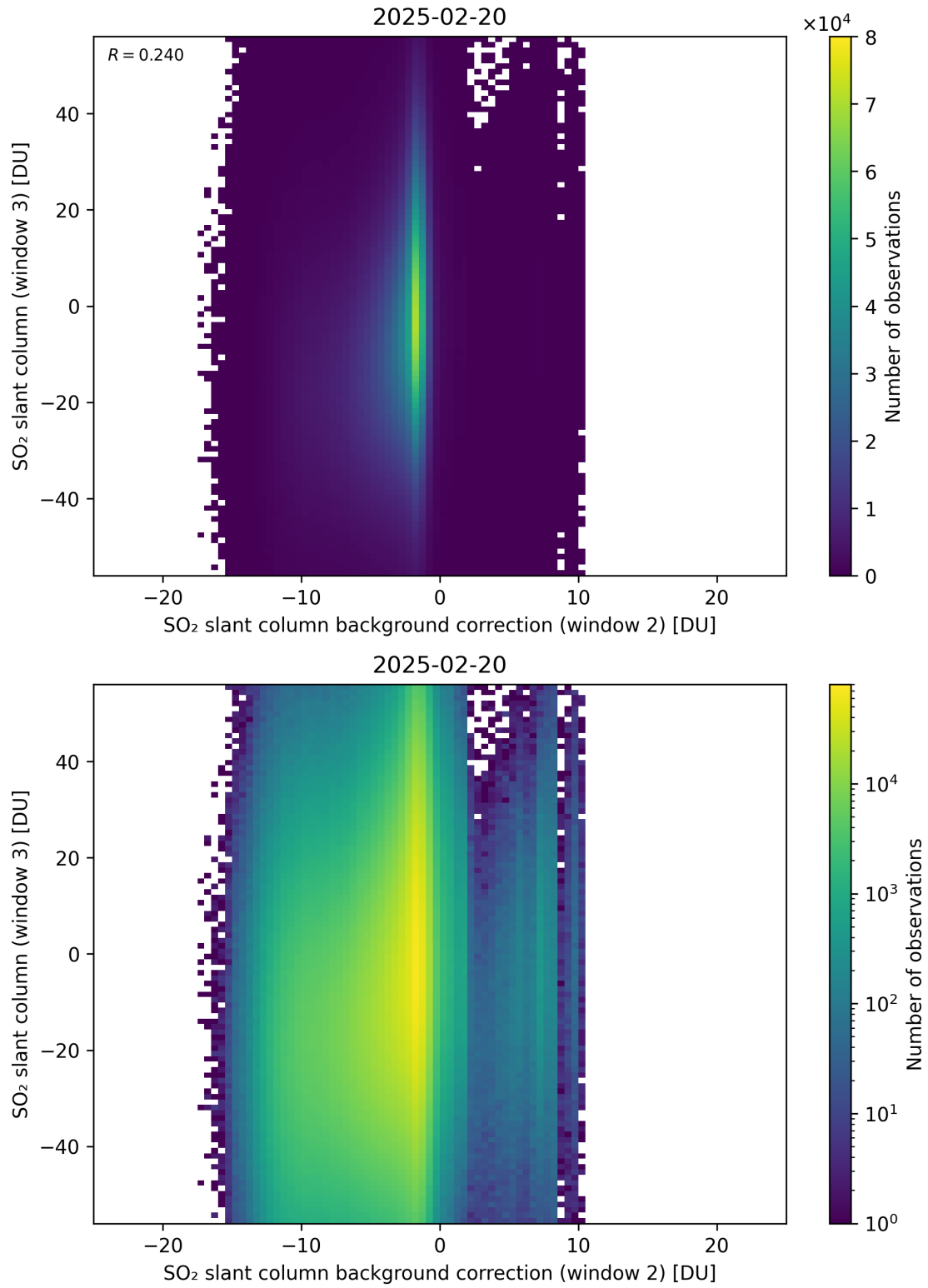
Figure 128: Scatter density plot of “SO 2 slant column background correction (window 2)” against “SO 2 slant column (window 3)” for 2025-02-19 to 2025-02-21.
