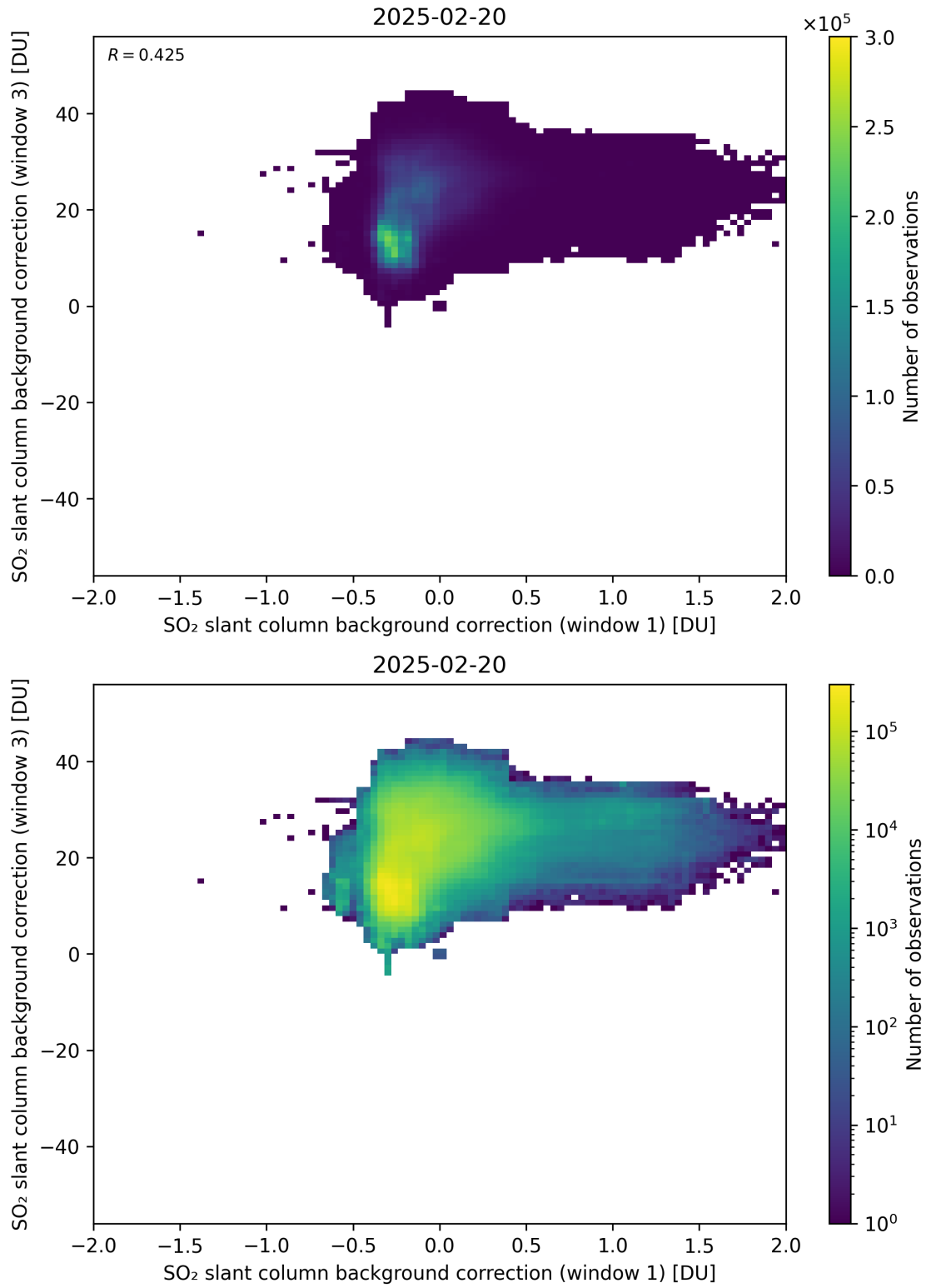
Figure 110: Scatter density plot of “SO 2 slant column background correction (window 1)” against “SO 2 slant column background correction (window 3)” for 2025-02-19 to 2025-02-21.
