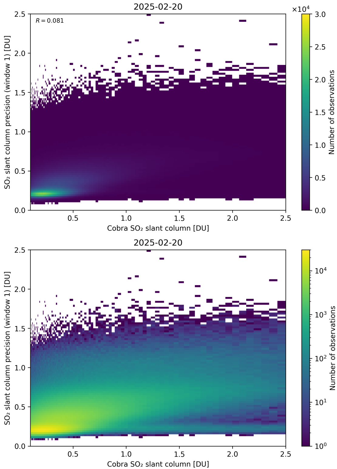
Figure 220: Scatter density plot of “Cobra SO 2 slant column” against “SO 2 slant column precision (window 1)” for 2025-02-19 to 2025-02-21.
