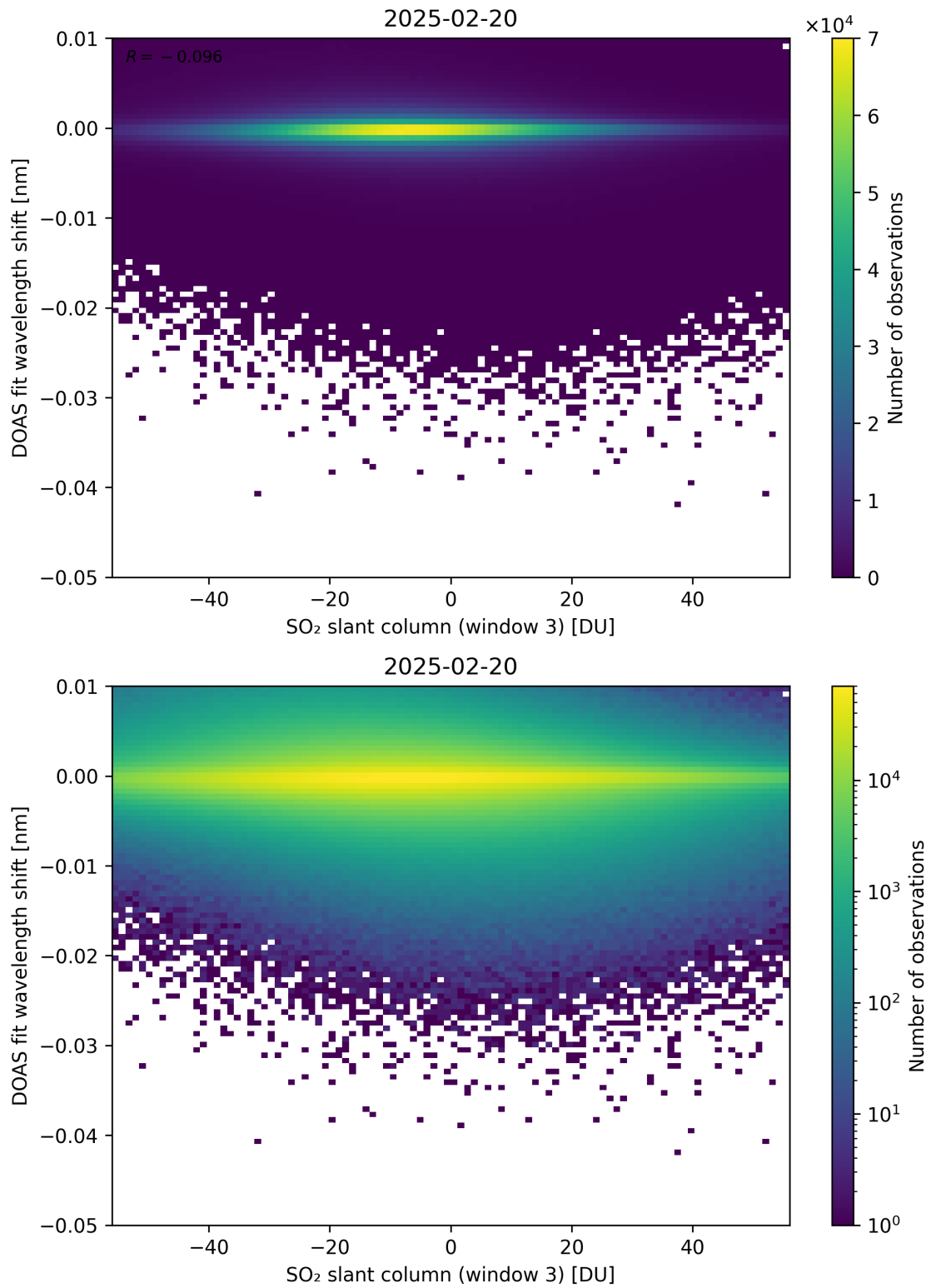
Figure 304: Scatter density plot of “SO 2 slant column (window 3)” against “DOAS fit wavelength shift” for 2025-02-19 to 2025-02-21.
