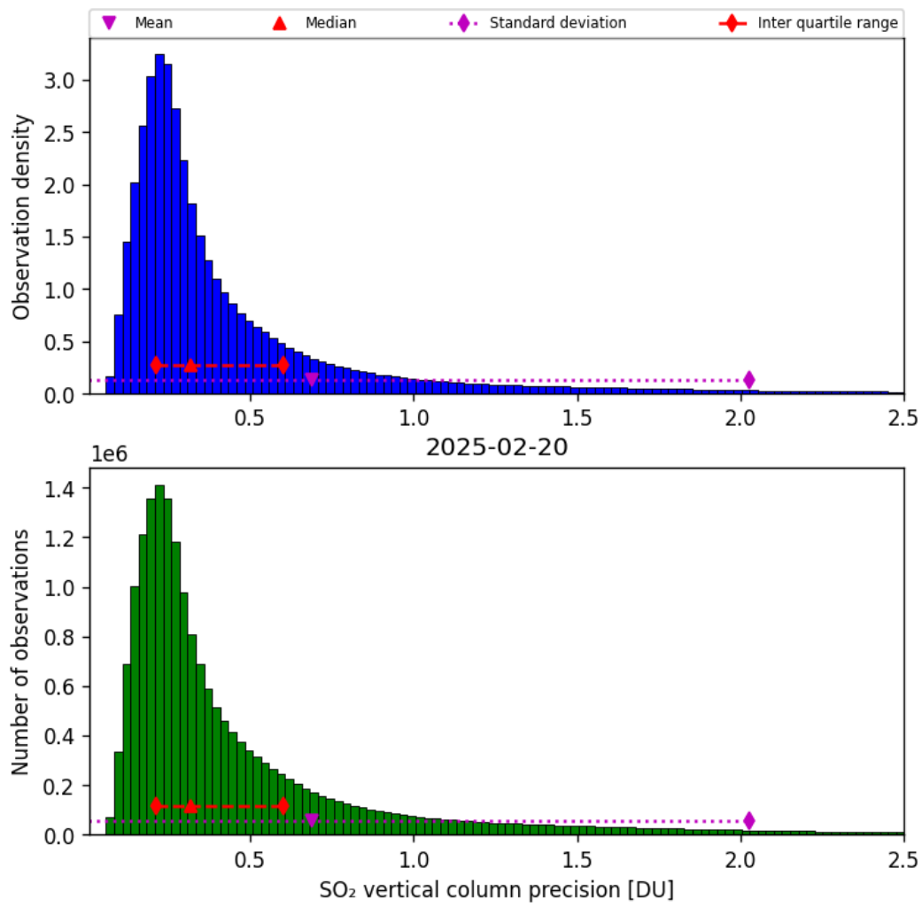
Figure 59: Histogram of “SO 2 vertical column precision” for 2025-02-19 to 2025-02-21
