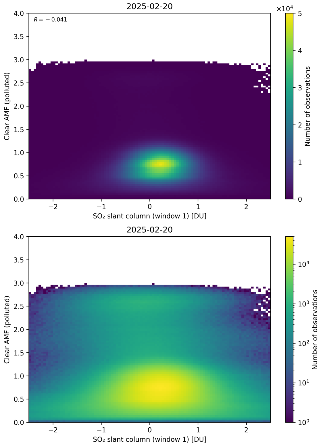
Figure 282: Scatter density plot of “SO 2 slant column (window 1)” against “Clear AMF (polluted)” for 2025-02-19 to 2025-02-21.
