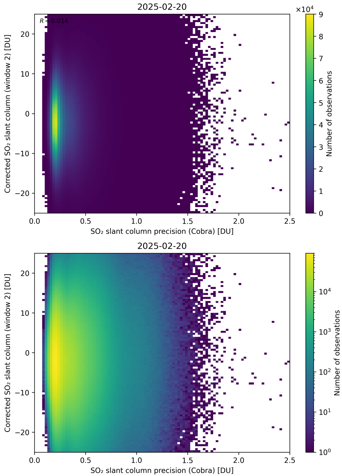
Figure 206: Scatter density plot of “SO 2 slant column precision (Cobra)” against “Corrected SO 2 slant column (window 2)” for 2025-02-19 to 2025-02-21.
