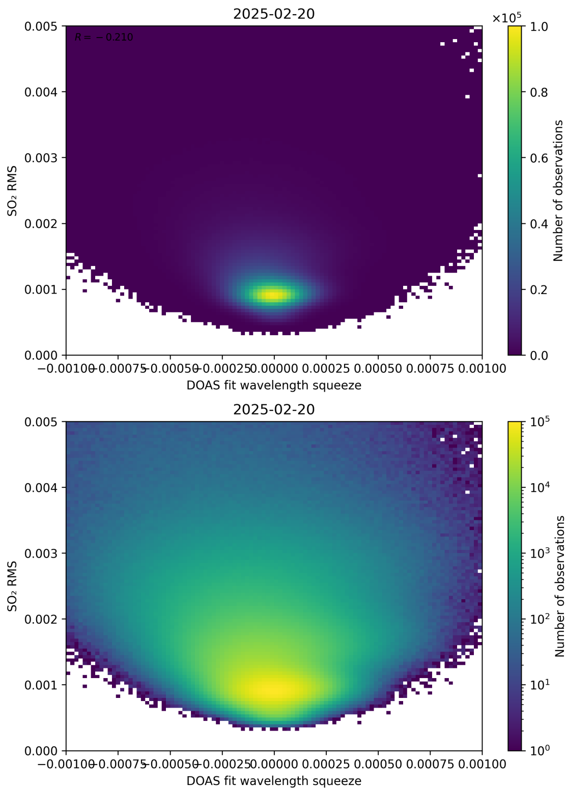
Figure 143: Scatter density plot of “DOAS fit wavelength squeeze” against “SO 2 RMS” for 2025-02-19 to 2025-02-21.
