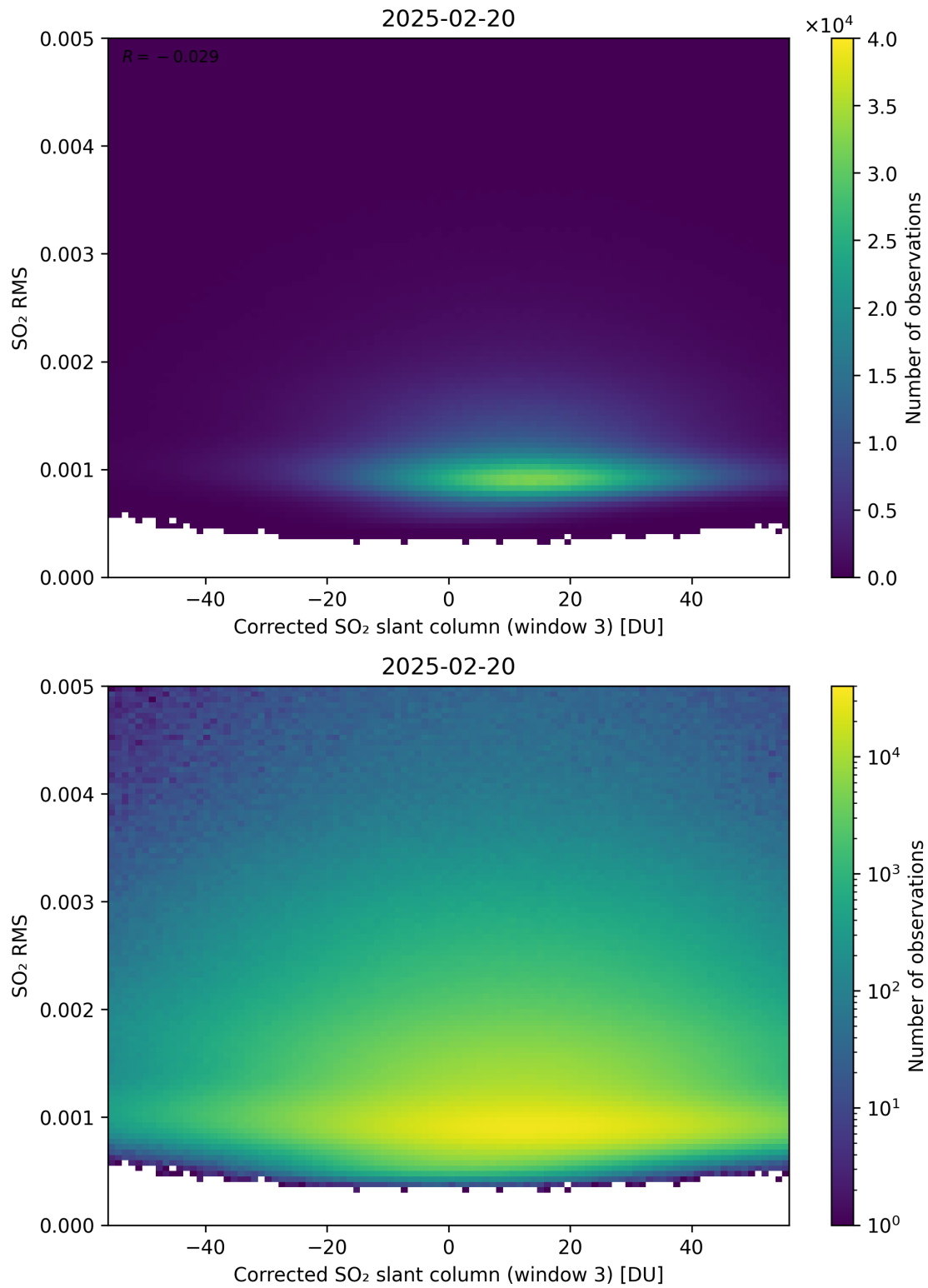
Figure 258: Scatter density plot of “Corrected SO 2 slant column (window 3)” against “SO 2 RMS” for 2025-02-19 to 2025-02-21.
