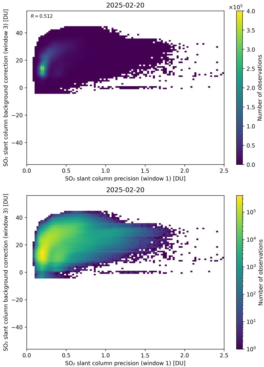
Figure 270: Scatter density plot of “SO 2 slant column precision (window 1)” against “SO 2 slant column background correction (window 3)” for 2025-02-19 to 2025-02-21.
