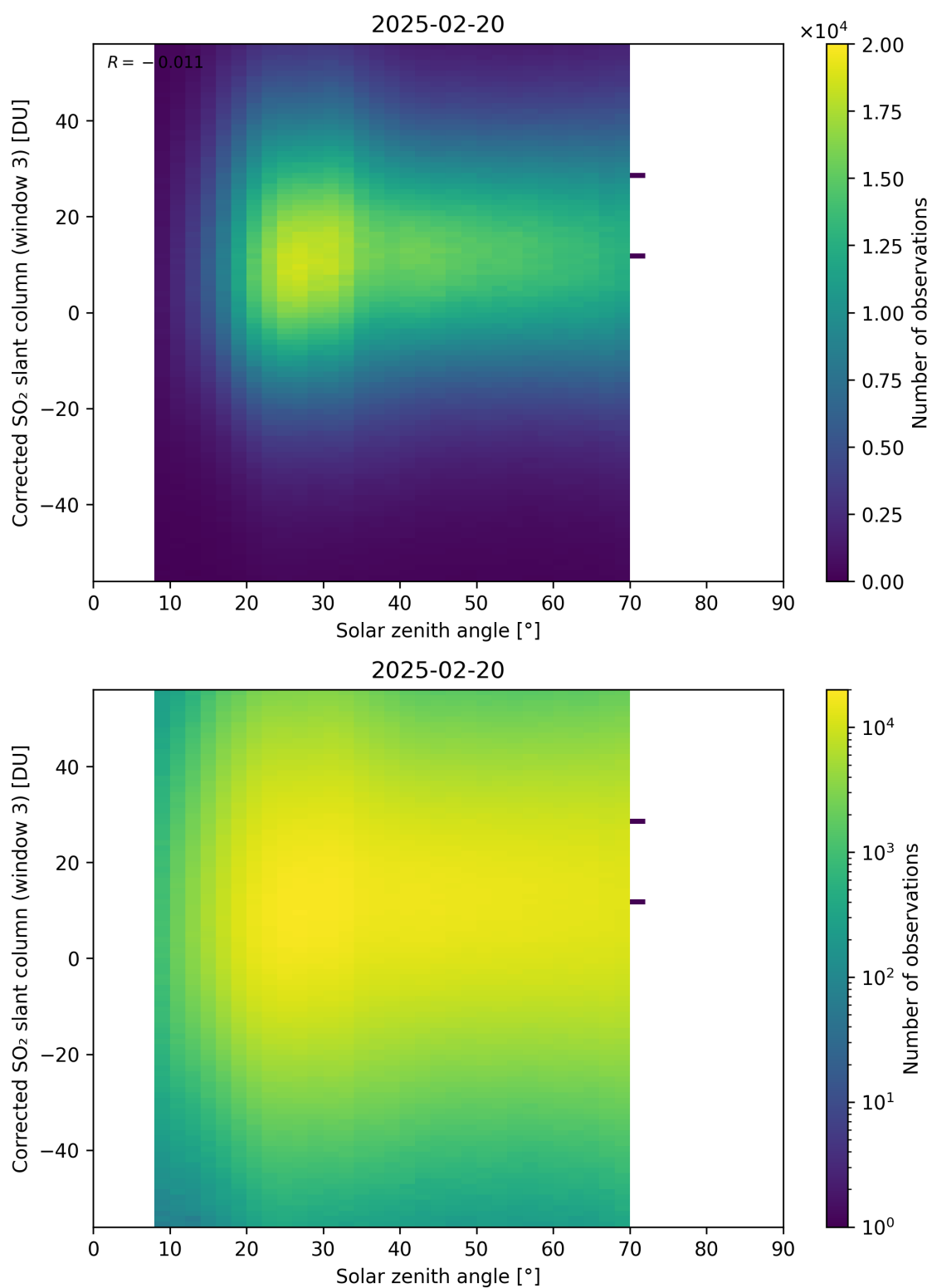
Figure 183: Scatter density plot of “Solar zenith angle” against “Corrected SO 2 slant column (window 3)” for 2025-02-19 to 2025-02-21.
