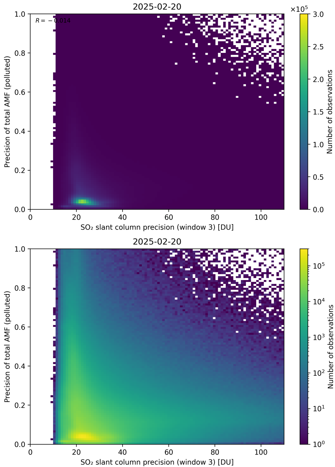
Figure 314: Scatter density plot of “SO 2 slant column precision (window 3)” against “Precision of total AMF (polluted)” for 2025-02-19 to 2025-02-21.
