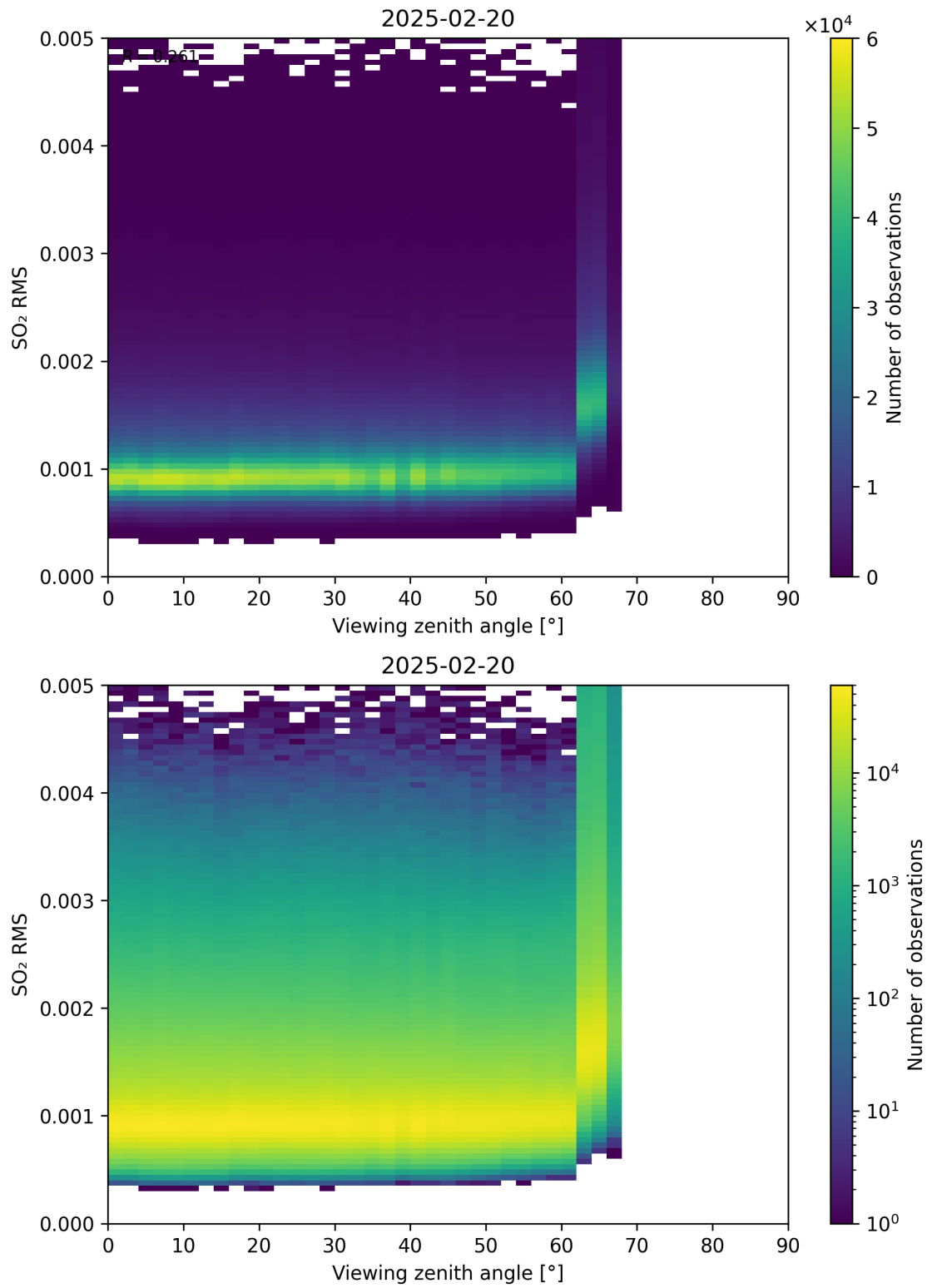
Figure 367: Scatter density plot of “Viewing zenith angle” against “SO 2 RMS” for 2025-02-19 to 2025-02-21.
