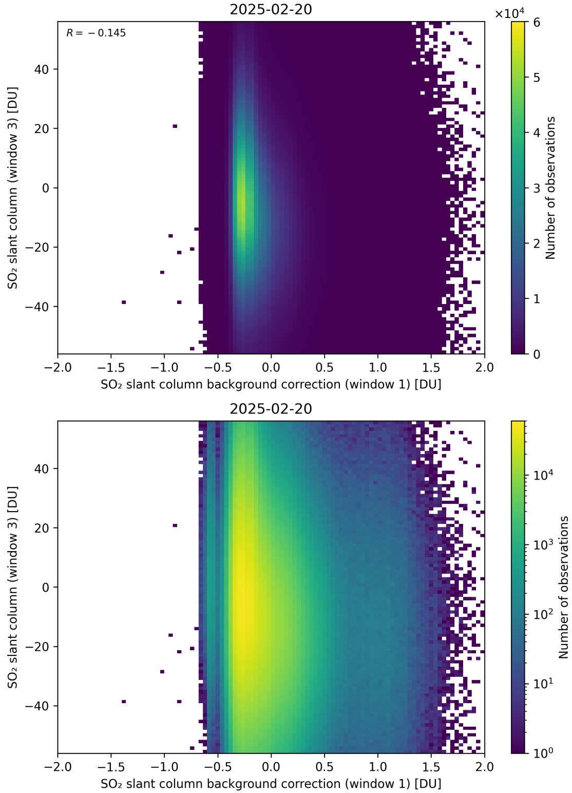
Figure 118: Scatter density plot of “SO 2 slant column background correction (window 1)” against “SO 2 slant column (window 3)” for 2025-02-19 to 2025-02-21.
