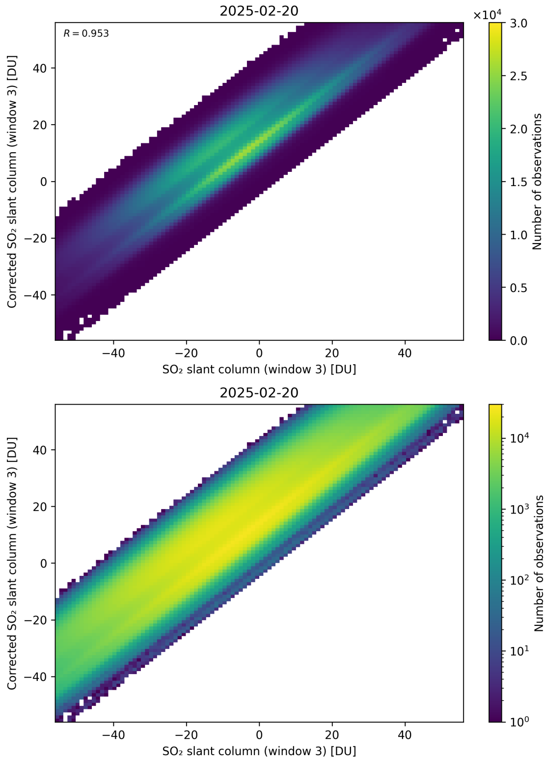
Figure 316: Scatter density plot of “SO 2 slant column (window 3)” against “Corrected SO 2 slant column (window 3)” for 2025-02-19 to 2025-02-21.
