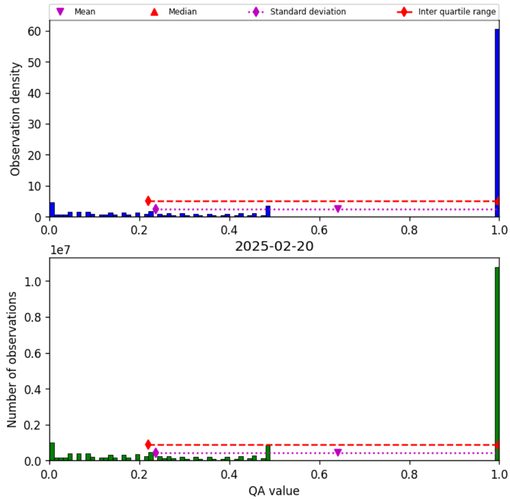
Figure 57: Histogram of “QA value” for 2025-02-19 to 2025-02-21
