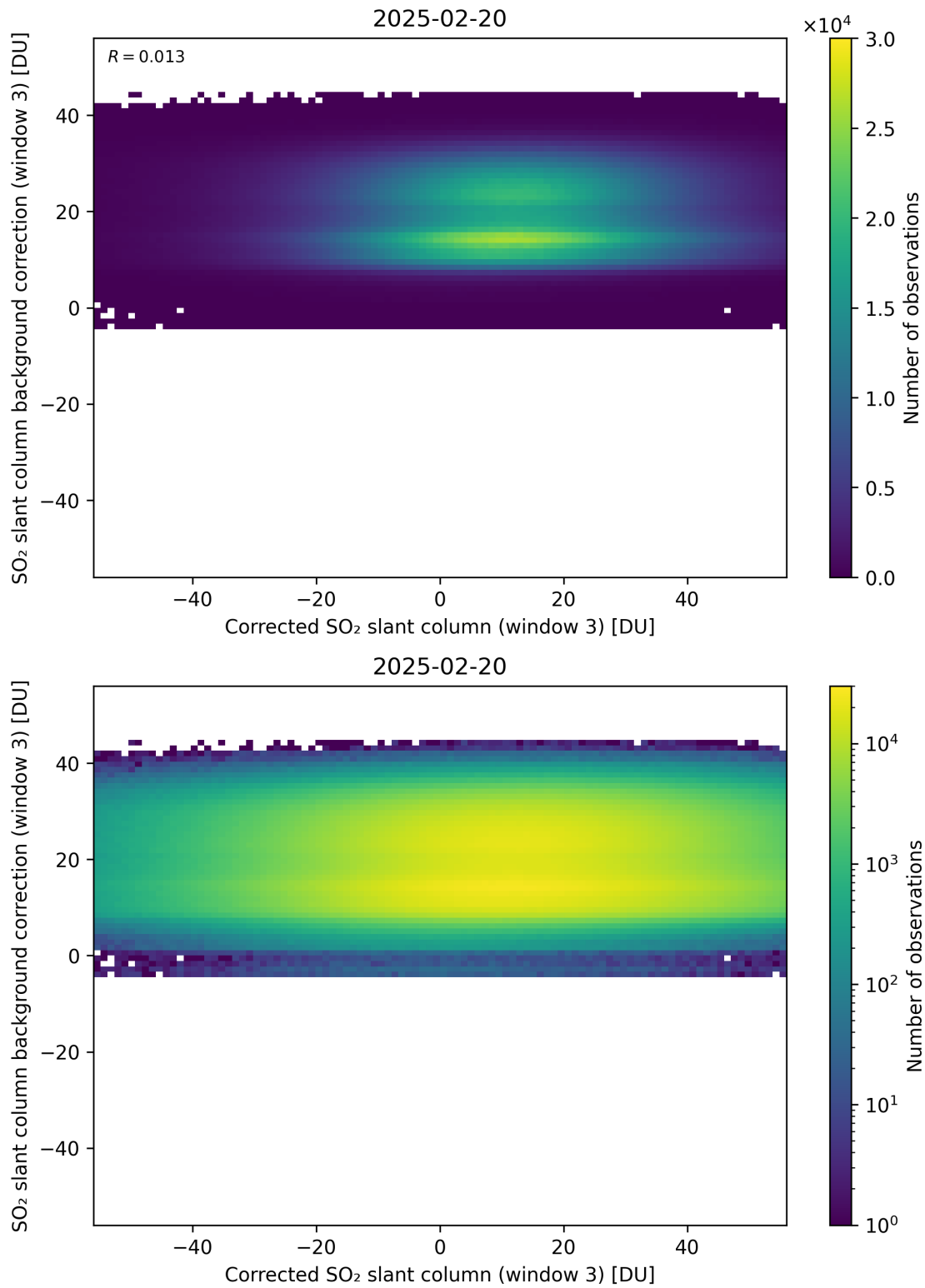
Figure 255: Scatter density plot of “Corrected SO 2 slant column (window 3)” against “SO 2 slant column background correction (window 3)” for 2025-02-19 to 2025-02-21.
