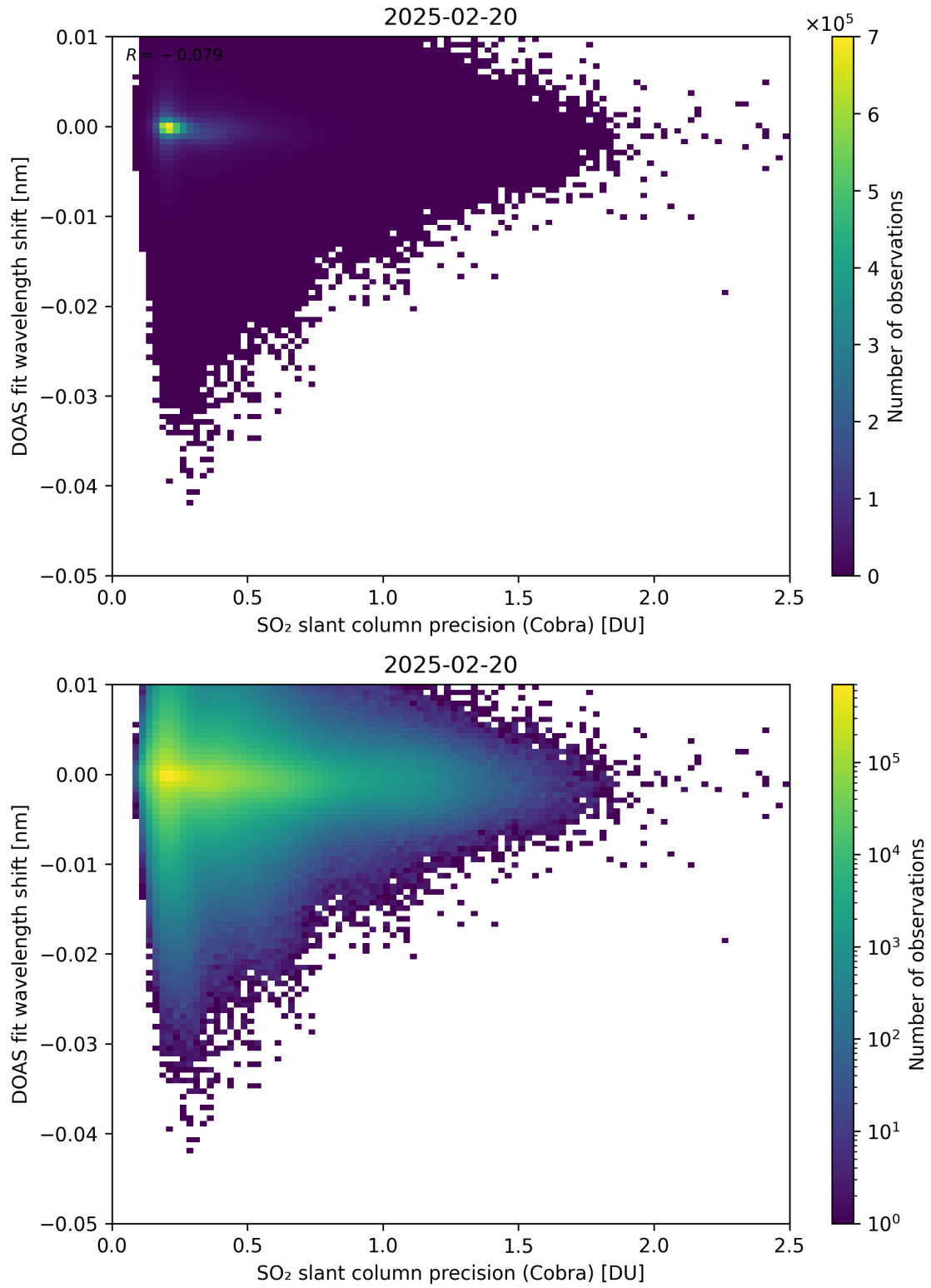
Figure 202: Scatter density plot of “SO 2 slant column precision (Cobra)” against “DOAS fit wavelength shift” for 2025-02-19 to 2025-02-21.
