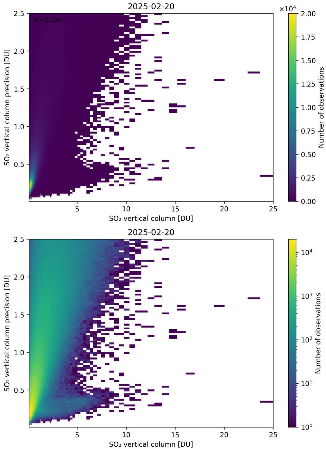
Figure 361: Scatter density plot of “SO 2 vertical column” against “SO 2 vertical column precision” for 2025-02-19 to 2025-02-21.
