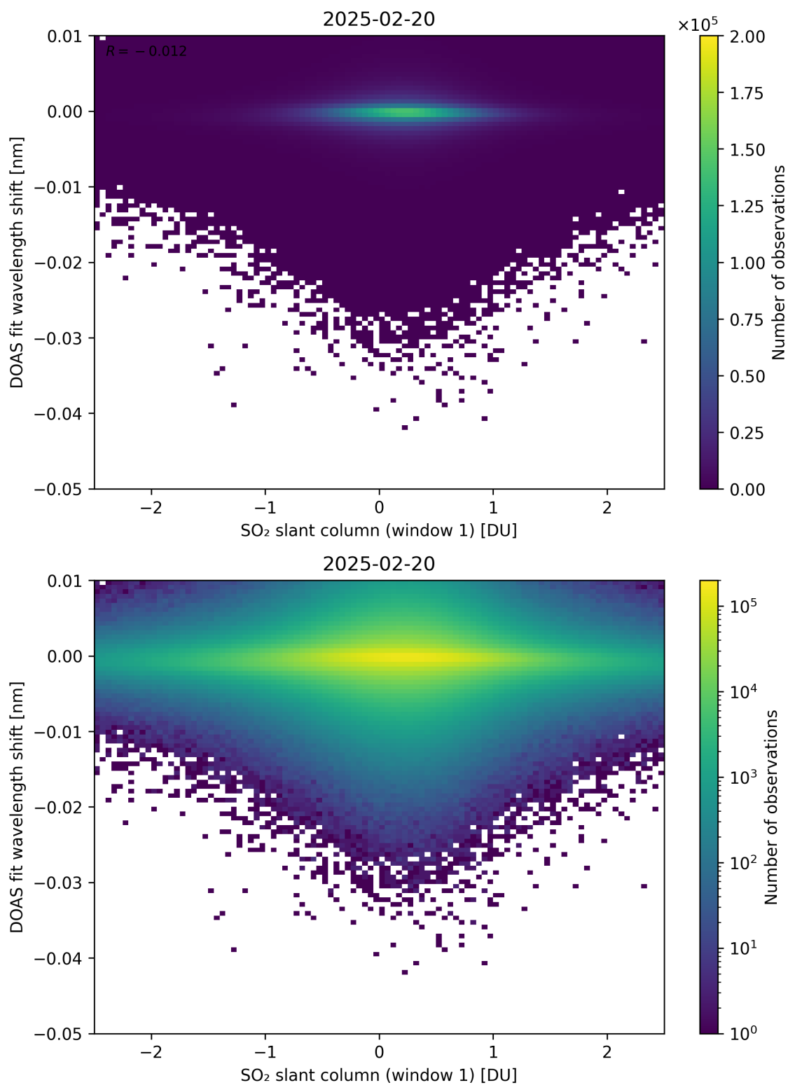
Figure 265: Scatter density plot of “SO 2 slant column (window 1)” against “DOAS fit wavelength shift” for 2025-02-19 to 2025-02-21.
