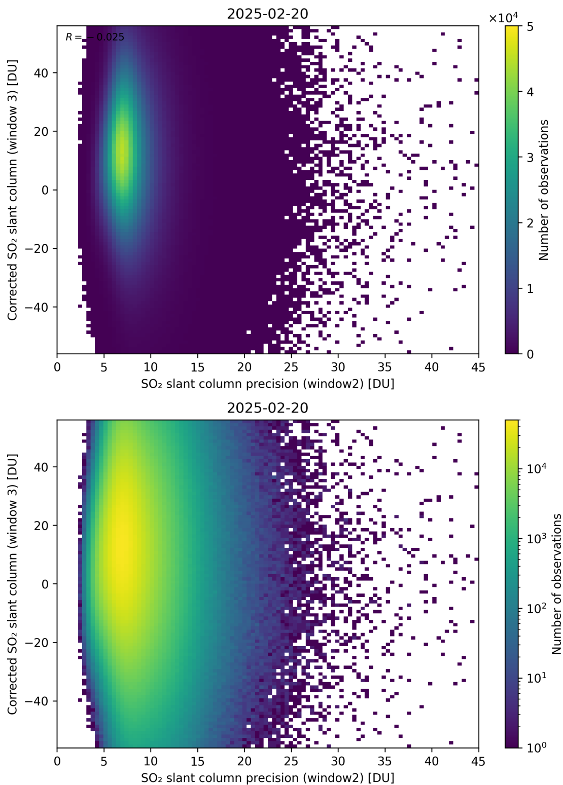
Figure 298: Scatter density plot of “SO 2 slant column precision (window2)” against “Corrected SO 2 slant column (window 3)” for 2025-02-19 to 2025-02-21.
