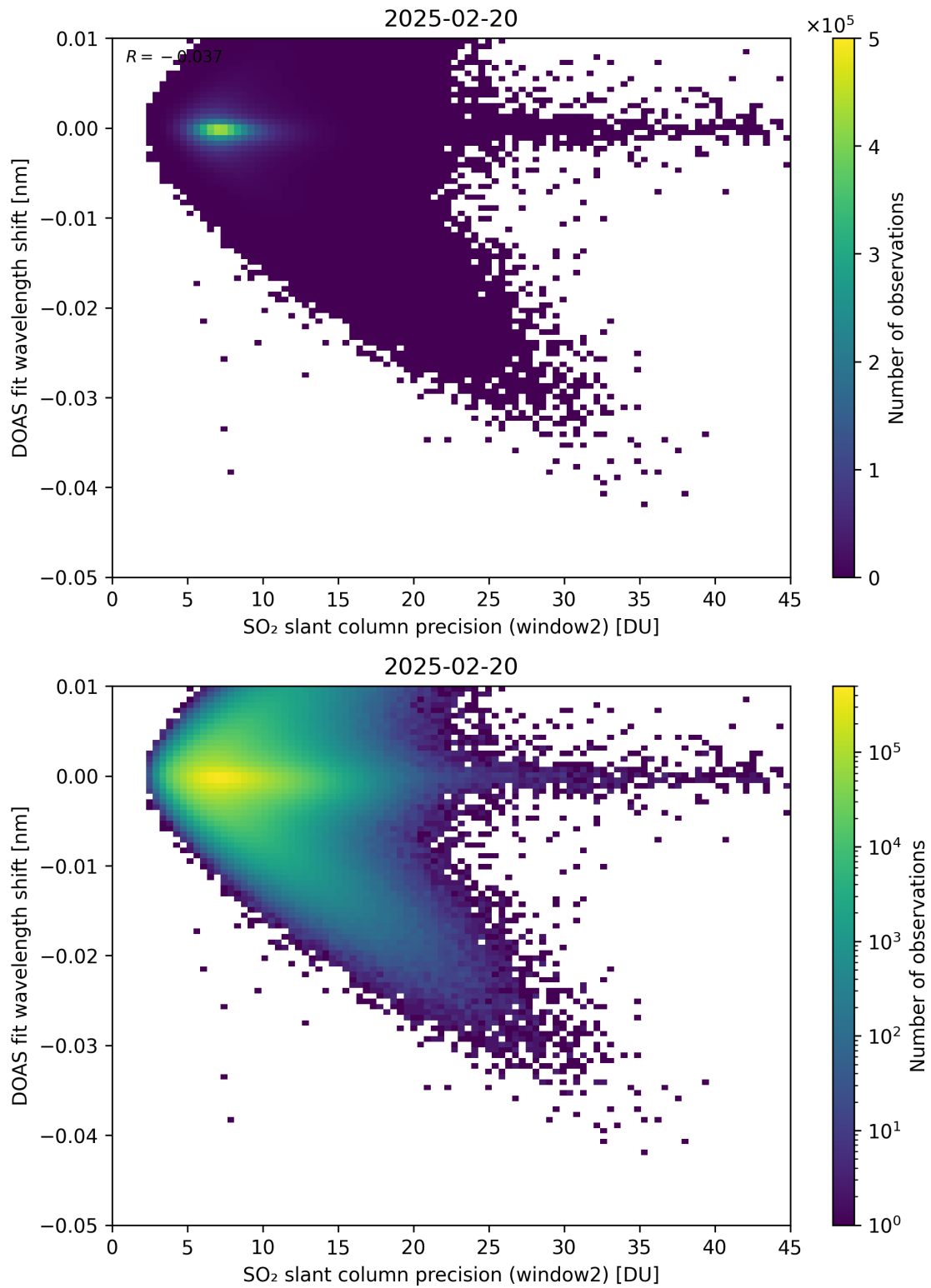
Figure 293: Scatter density plot of “SO 2 slant column precision (window2)” against “DOAS fit wavelength shift” for 2025-02-19 to 2025-02-21.
