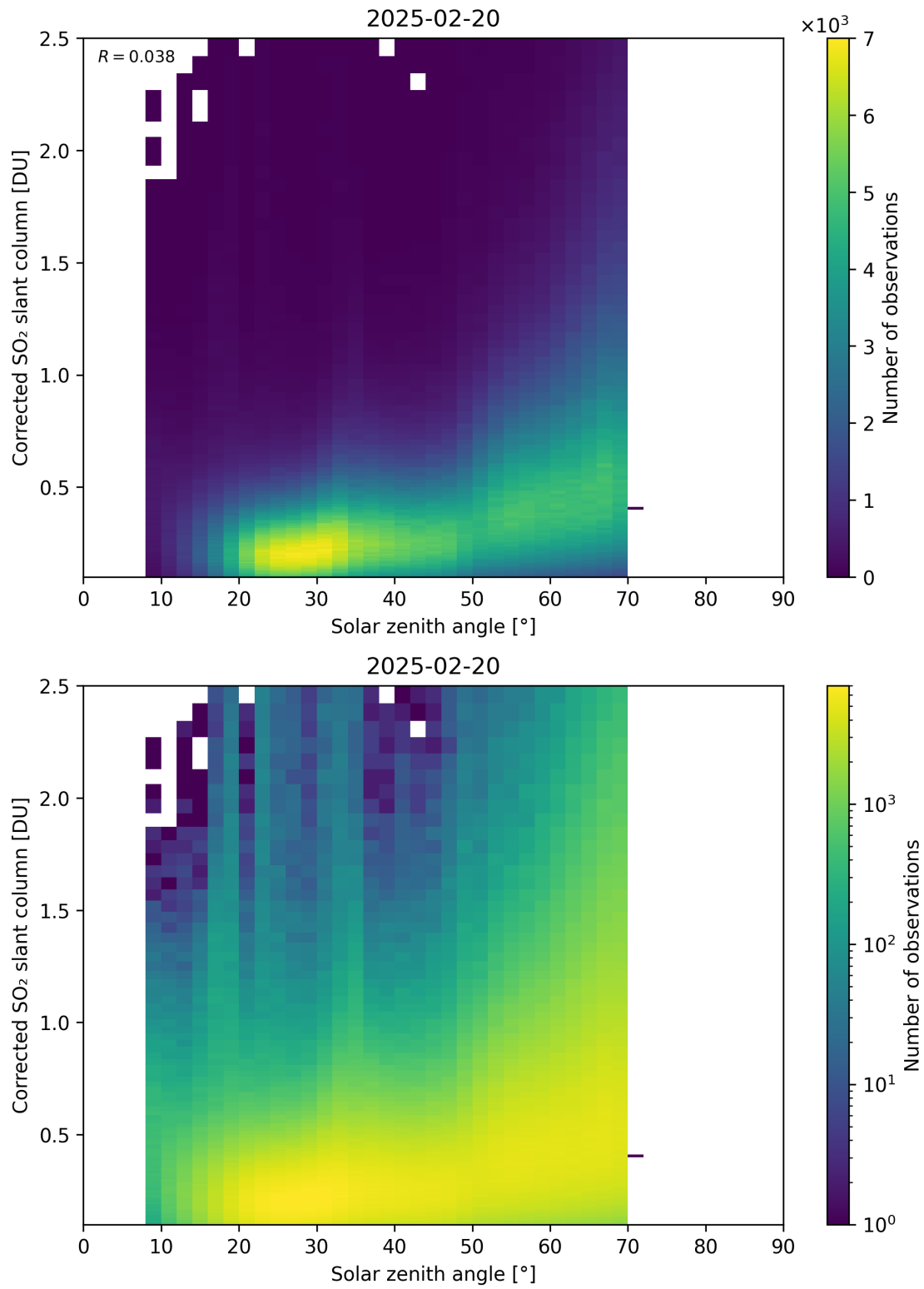
Figure 181: Scatter density plot of “Solar zenith angle” against “Corrected SO 2 slant column” for 2025-02-19 to 2025-02-21.
