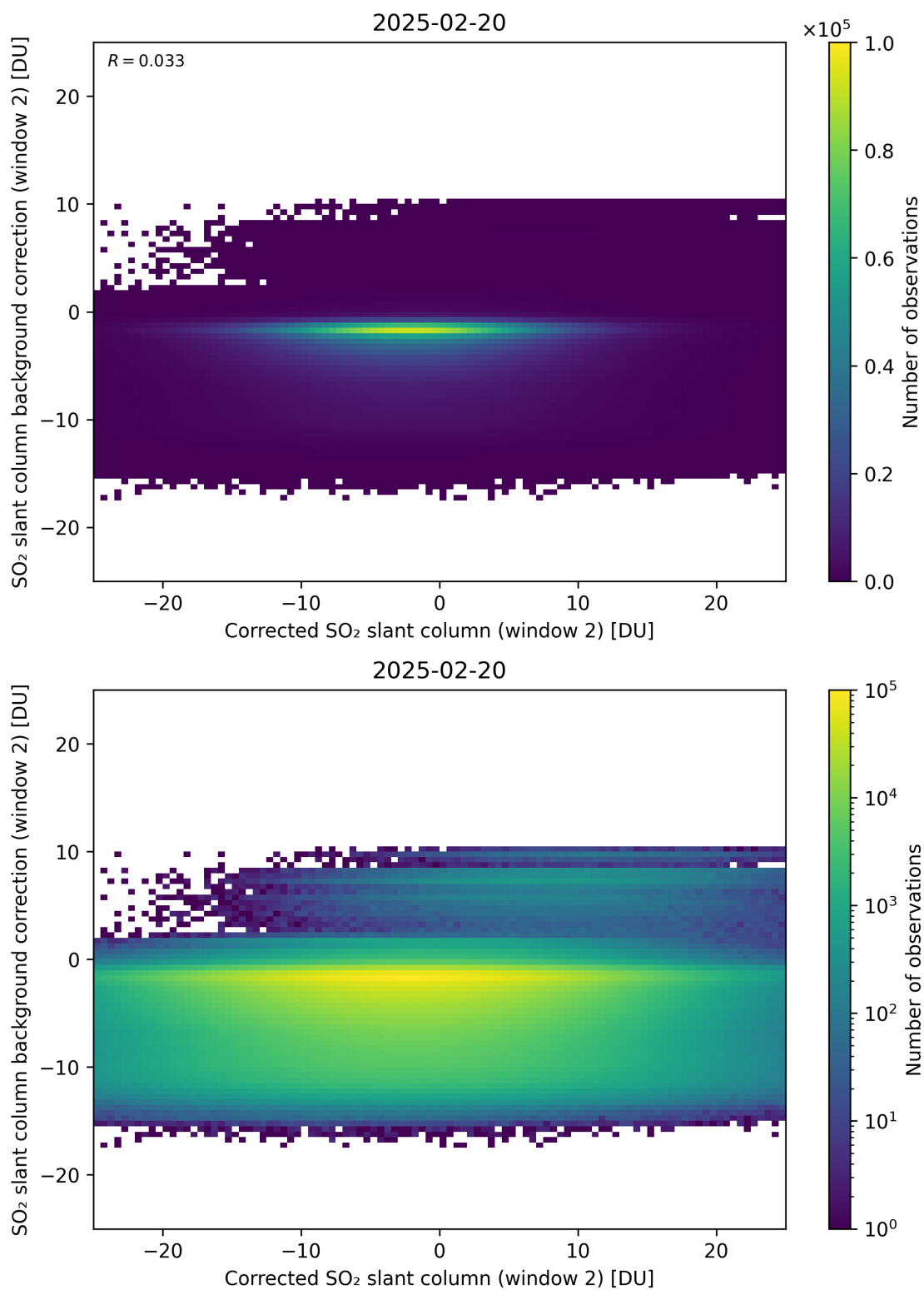
Figure 244: Scatter density plot of “Corrected SO 2 slant column (window 2)” against “SO 2 slant column background correction (window 2)” for 2025-02-19 to 2025-02-21.
