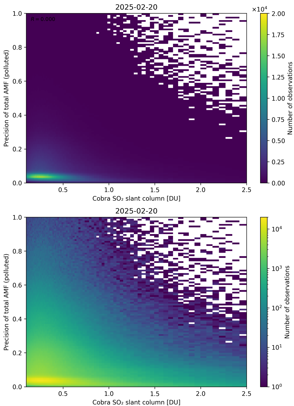
Figure 225: Scatter density plot of “Cobra SO 2 slant column” against “Precision of total AMF (polluted)” for 2025-02-19 to 2025-02-21.
