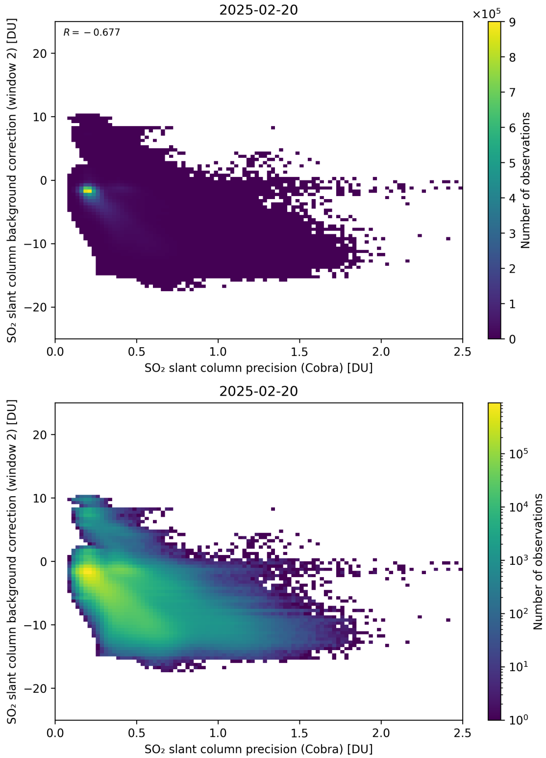
Figure 200: Scatter density plot of “SO 2 slant column precision (Cobra)” against “SO 2 slant column background correction (window 2)” for 2025-02-19 to 2025-02-21.
