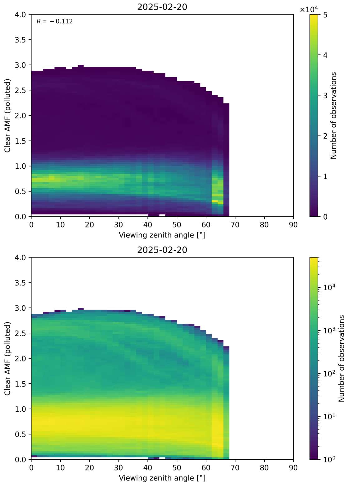
Figure 370: Scatter density plot of “Viewing zenith angle” against “Clear AMF (polluted)” for 2025-02-19 to 2025-02-21.
