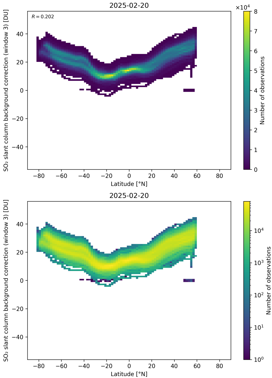
Figure 152: Scatter density plot of “Latitude” against “SO 2 slant column background correction (window 3)” for 2025-02-19 to 2025-02-21.
