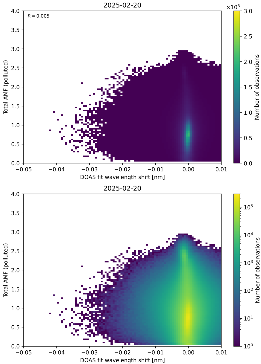
Figure 141: Scatter density plot of “DOAS fit wavelength shift” against “Total AMF (polluted)” for 2025-02-19 to 2025-02-21.
