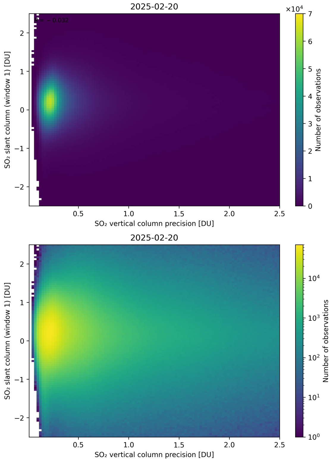
Figure 341: Scatter density plot of “SO 2 vertical column precision” against “SO 2 slant column (window 1)” for 2025-02-19 to 2025-02-21.
