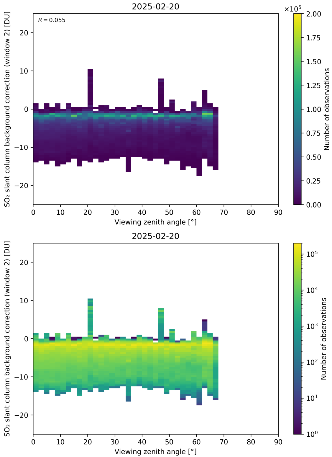
Figure 363: Scatter density plot of “Viewing zenith angle” against “SO 2 slant column background correction (window 2)” for 2025-02-19 to 2025-02-21.
