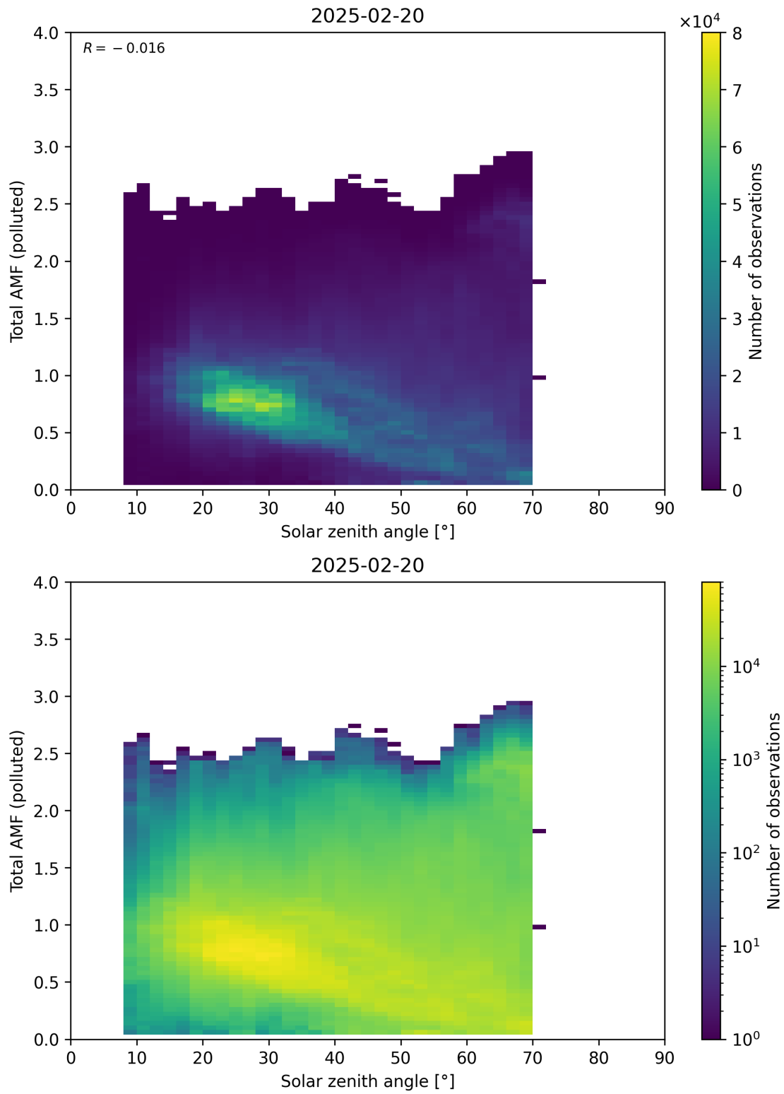
Figure 189: Scatter density plot of “Solar zenith angle” against “Total AMF (polluted)” for 2025-02-19 to 2025-02-21.
