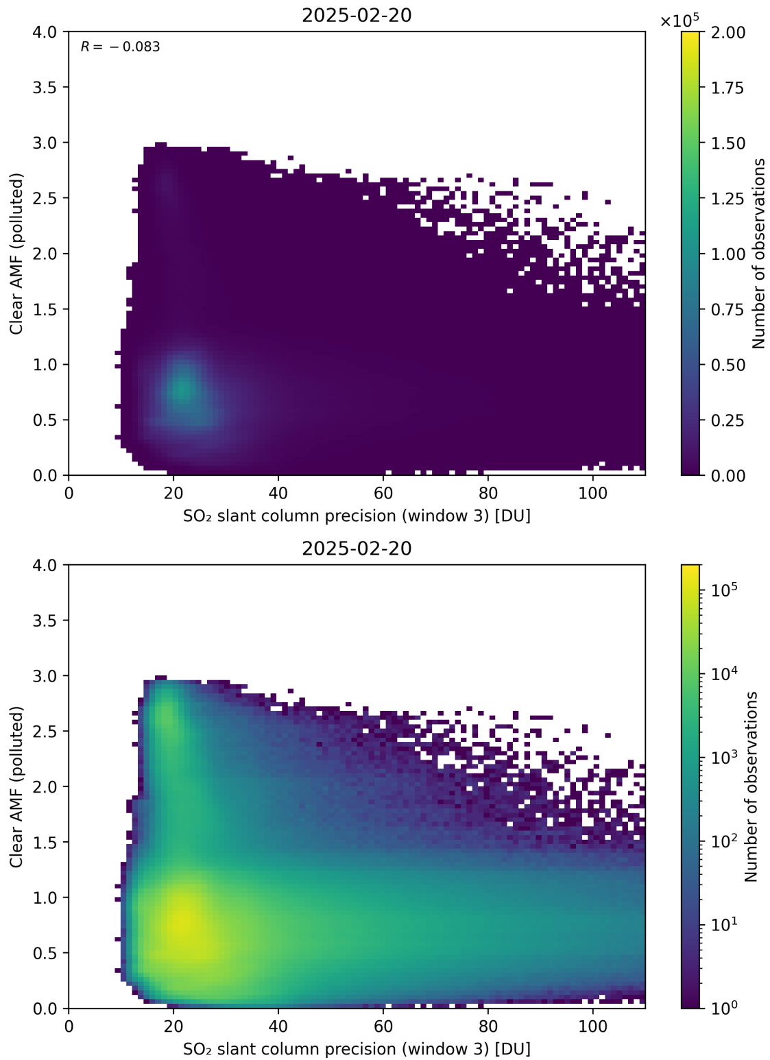
Figure 311: Scatter density plot of “SO 2 slant column precision (window 3)” against “Clear AMF (polluted)” for 2025-02-19 to 2025-02-21.
