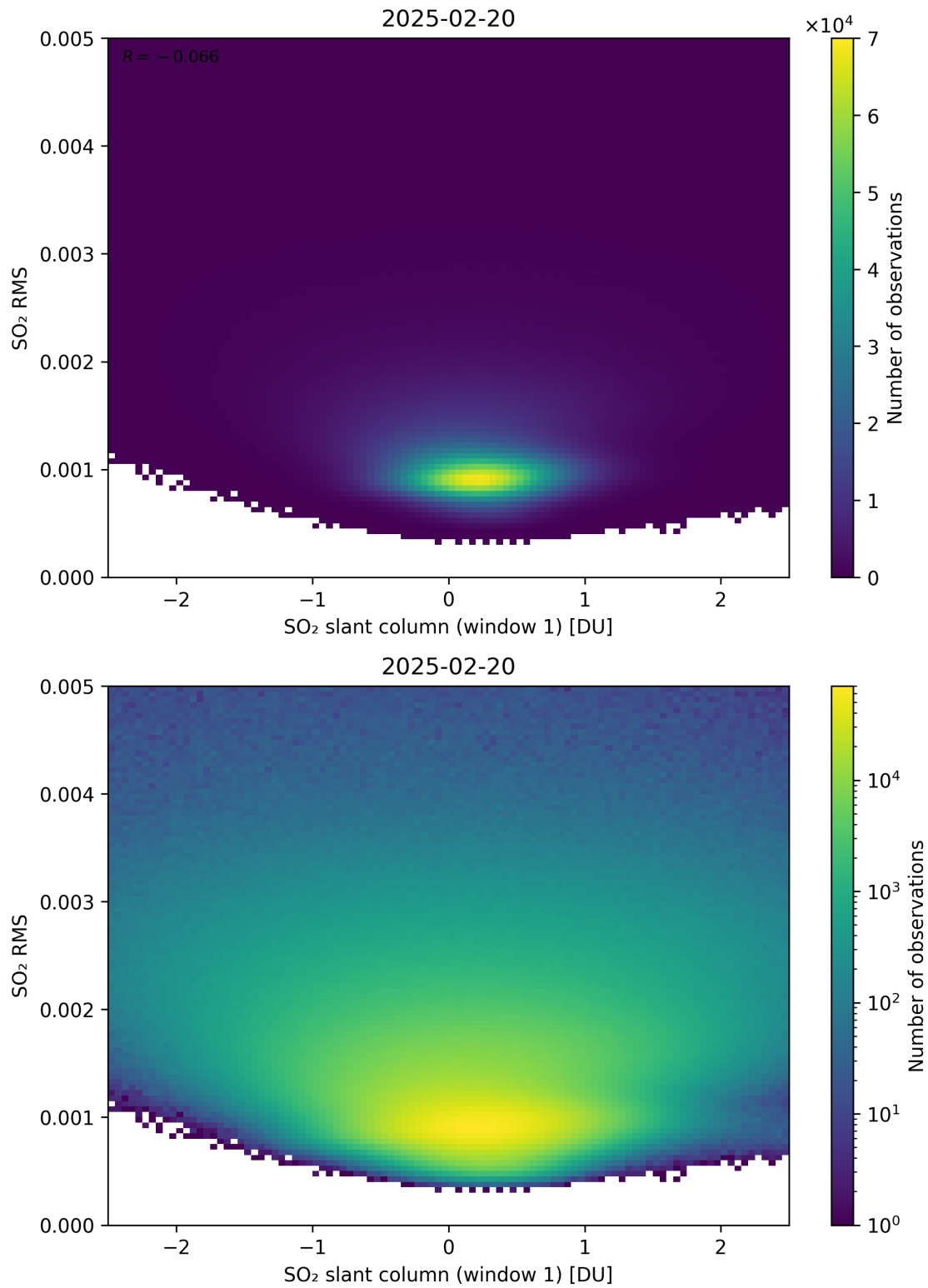
Figure 267: Scatter density plot of “SO 2 slant column (window 1)” against “SO 2 RMS” for 2025-02-19 to 2025-02-21.
