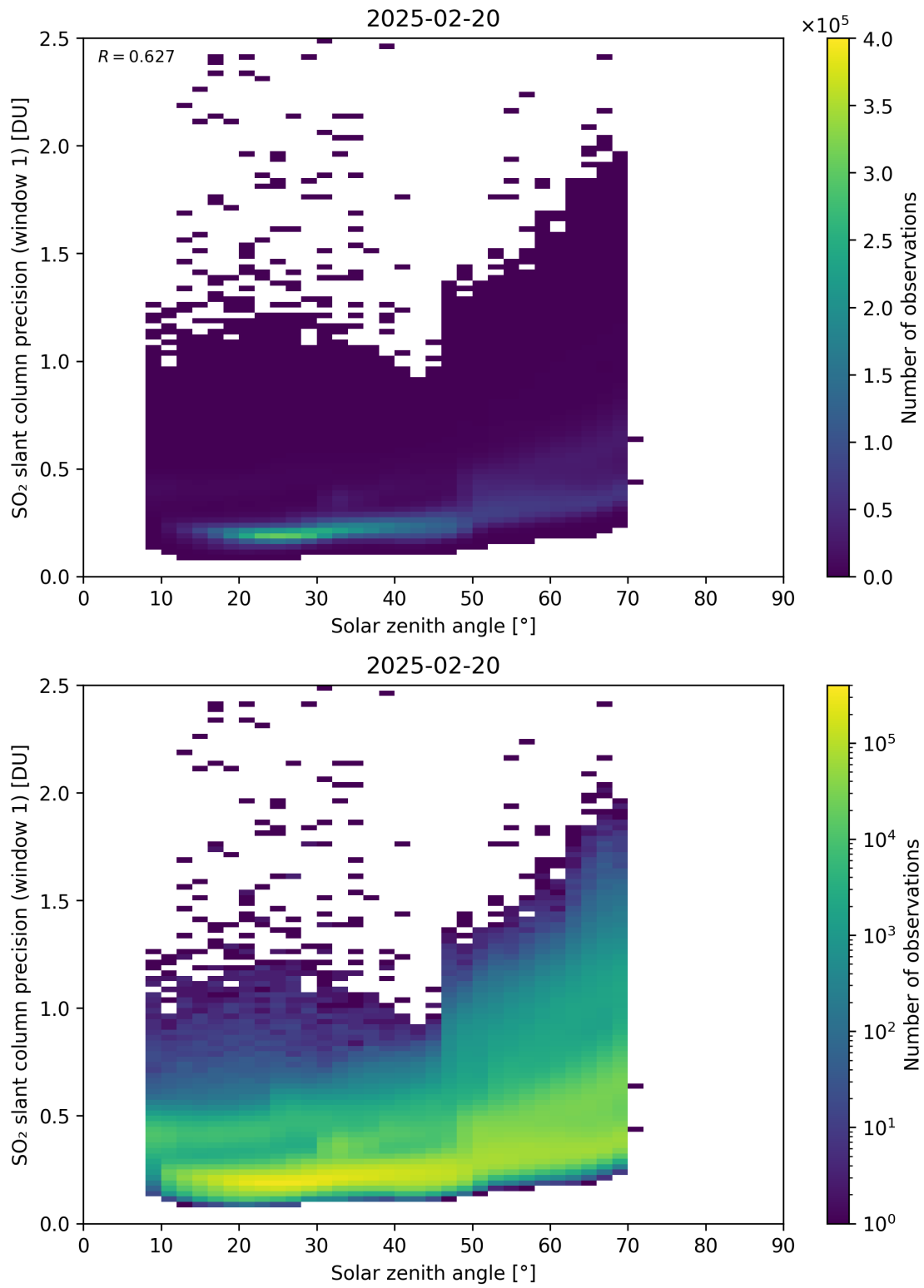
Figure 185: Scatter density plot of “Solar zenith angle” against “SO 2 slant column precision (window 1)” for 2025-02-19 to 2025-02-21.
