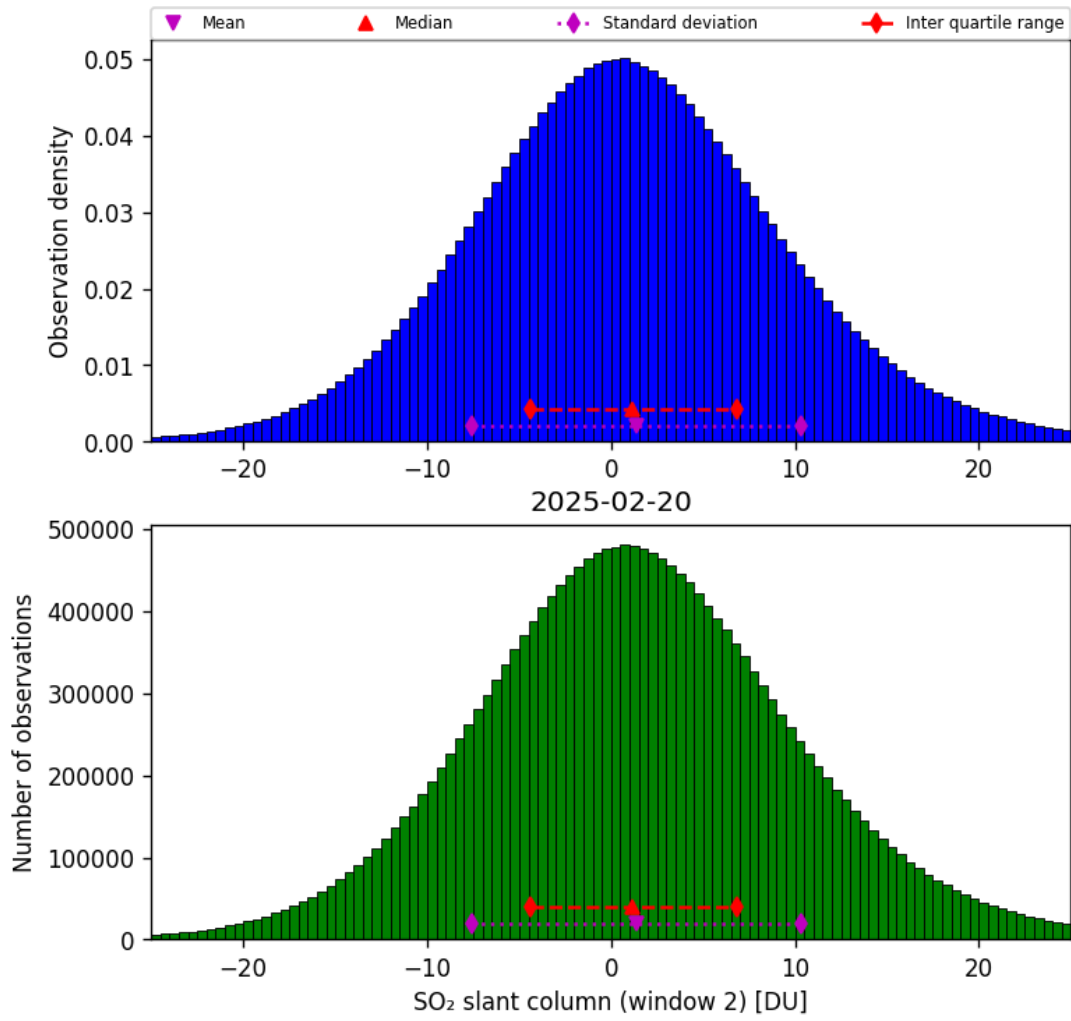
Figure 67: Histogram of “SO 2 slant column (window 2)” for 2025-02-19 to 2025-02-21
