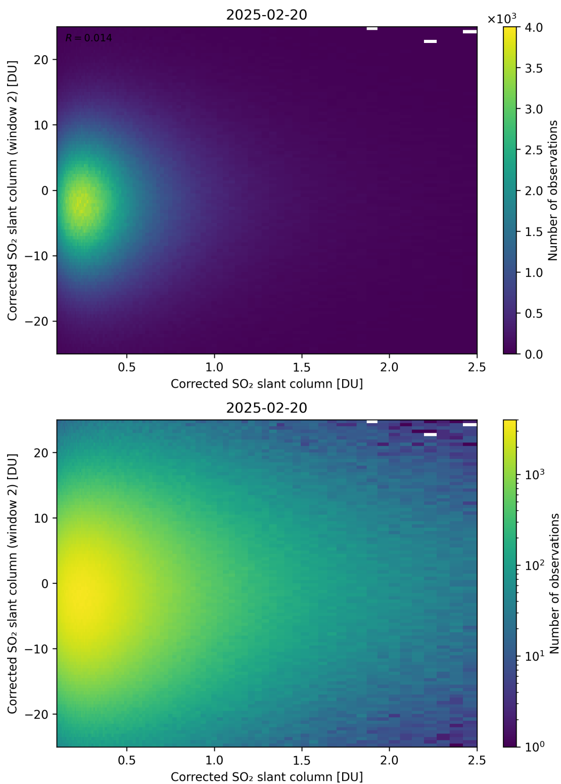
Figure 235: Scatter density plot of “Corrected SO 2 slant column” against “Corrected SO 2 slant column (window 2)” for 2025-02-19 to 2025-02-21.
