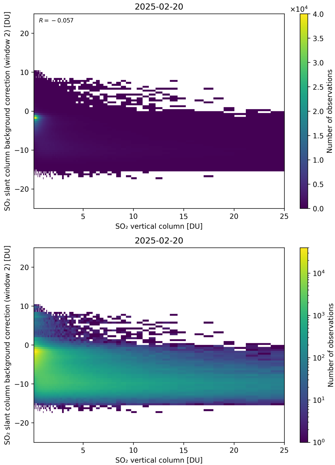
Figure 324: Scatter density plot of “SO 2 vertical column” against “SO 2 slant column background correction (window 2)” for 2025-02-19 to 2025-02-21.
