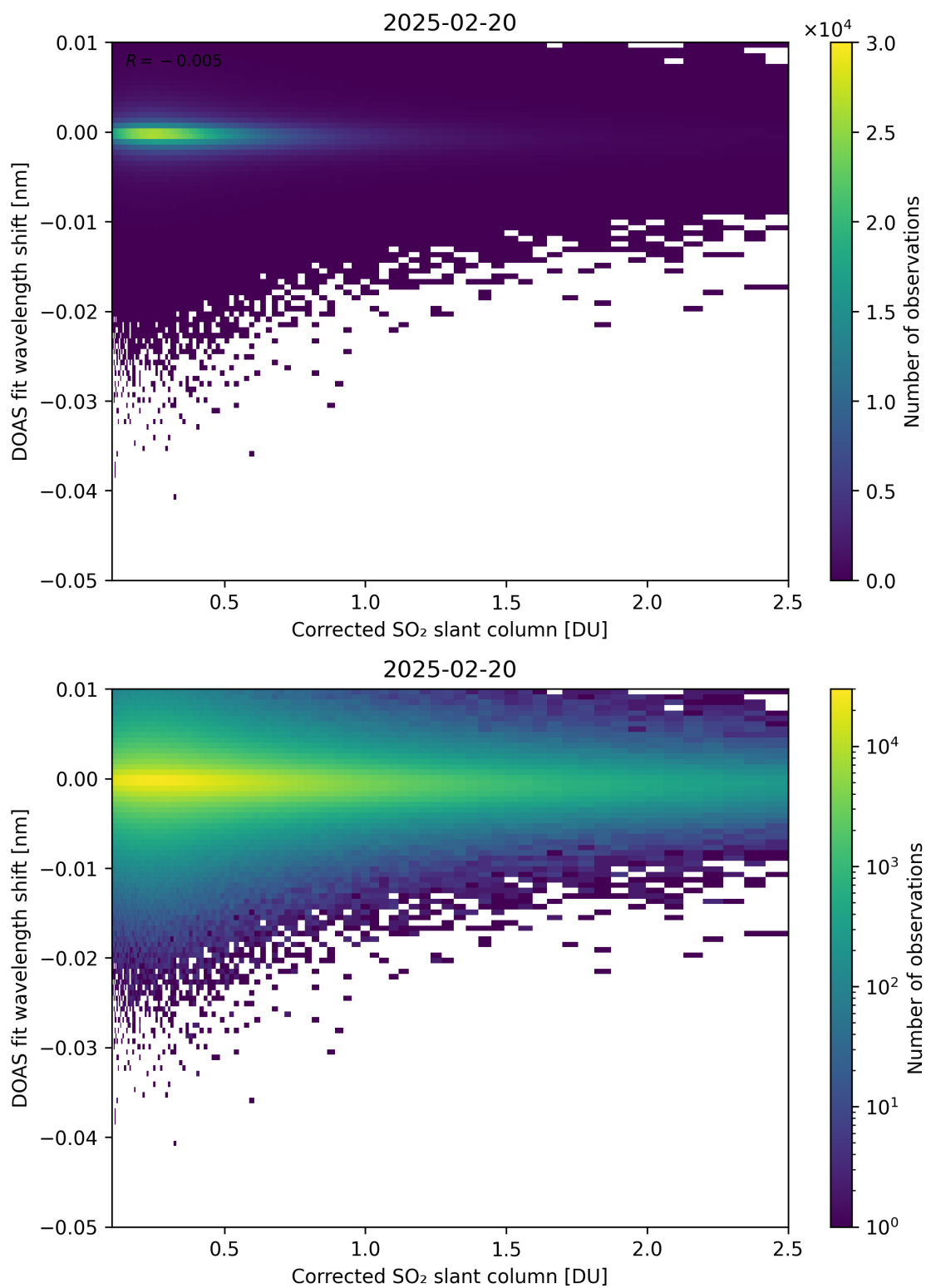
Figure 229: Scatter density plot of “Corrected SO 2 slant column” against “DOAS fit wavelength shift” for 2025-02-19 to 2025-02-21.
