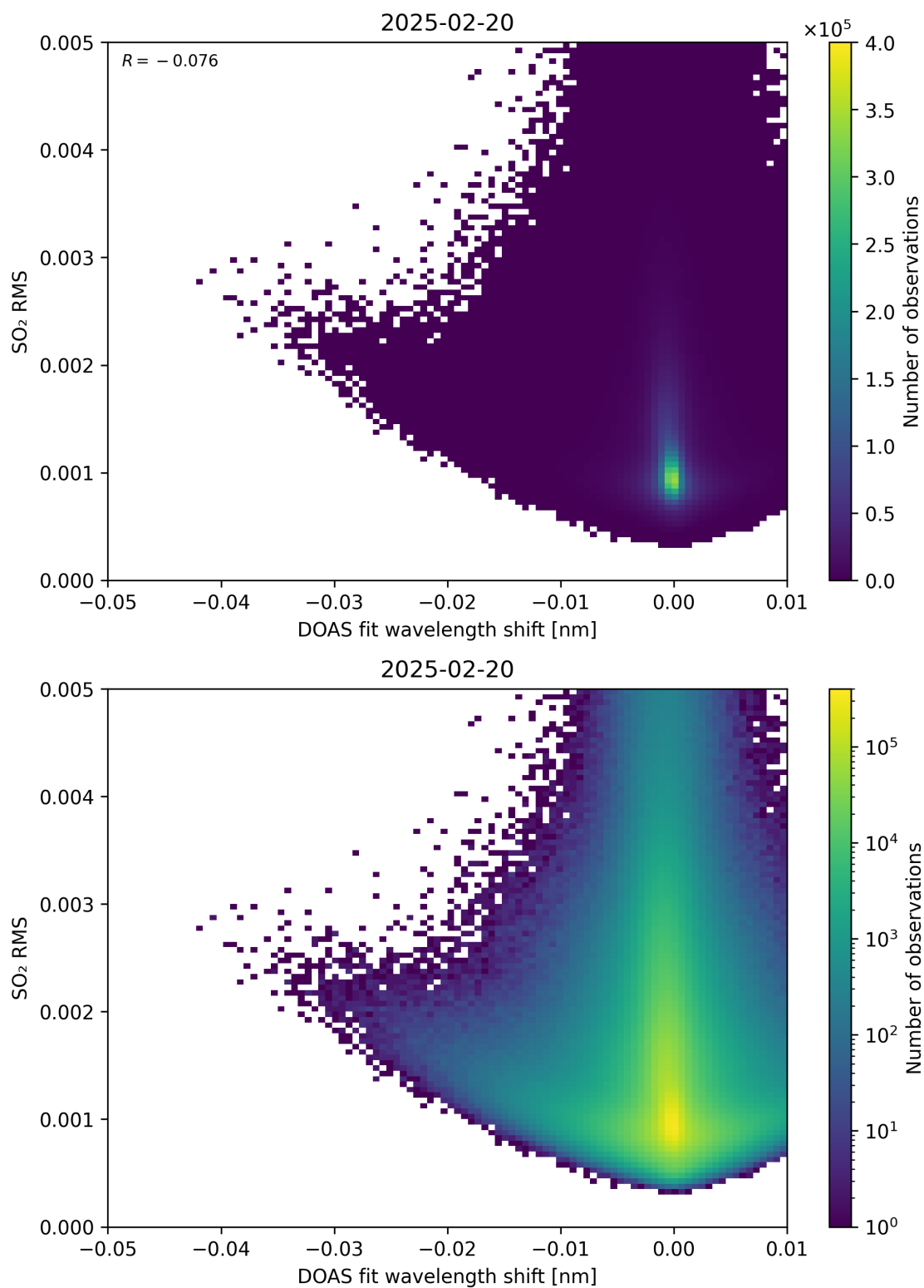
Figure 139: Scatter density plot of “DOAS fit wavelength shift” against “SO 2 RMS” for 2025-02-19 to 2025-02-21.
