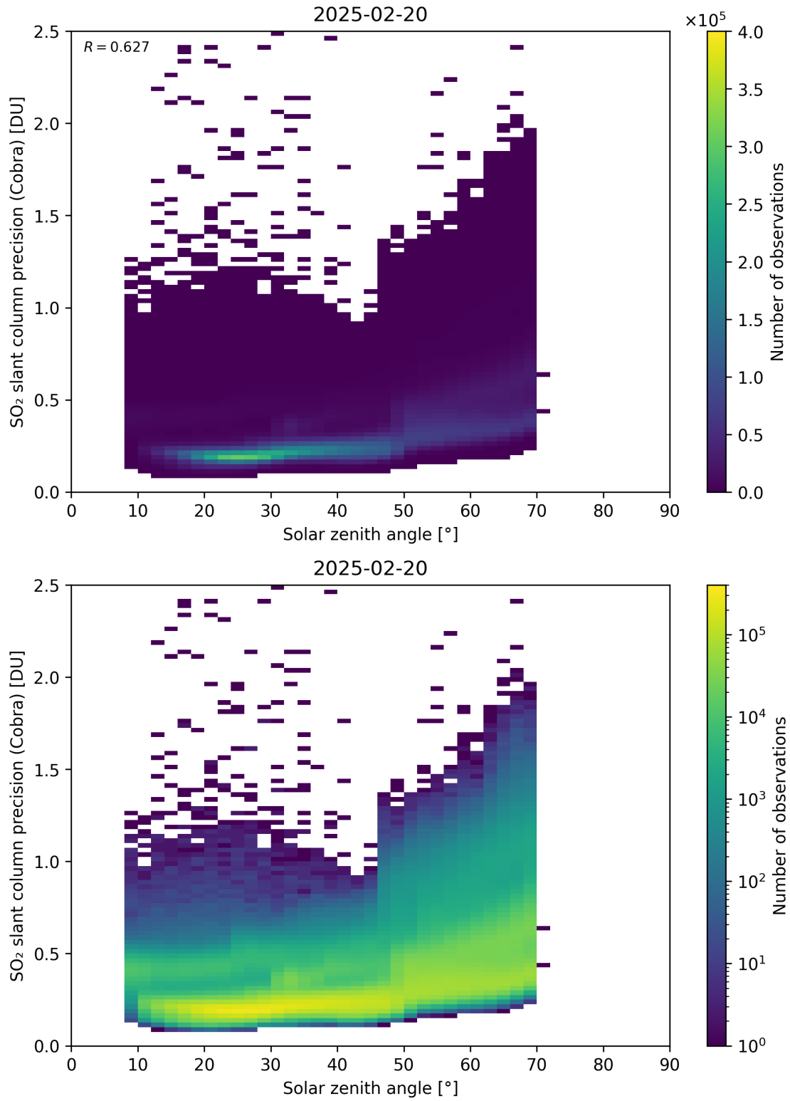
Figure 180: Scatter density plot of “Solar zenith angle” against “SO 2 slant column precision (Cobra)” for 2025-02-19 to 2025-02-21.
