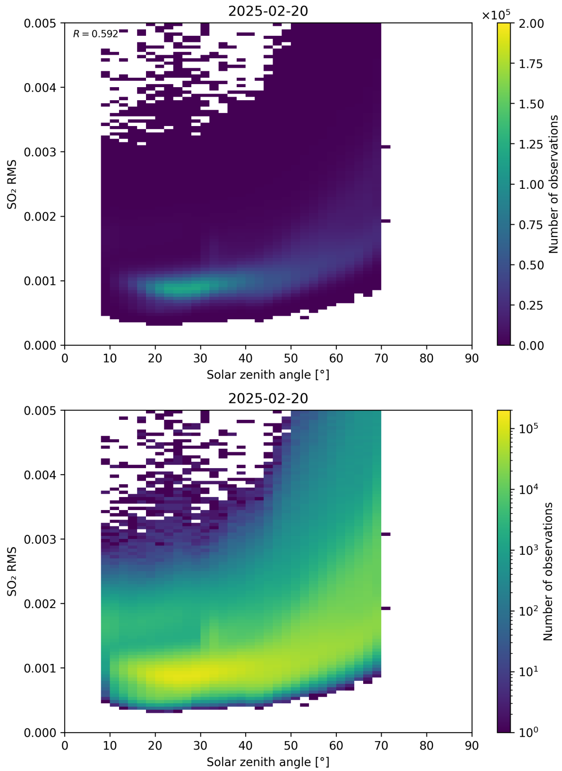
Figure 176: Scatter density plot of “Solar zenith angle” against “SO 2 RMS” for 2025-02-19 to 2025-02-21.
