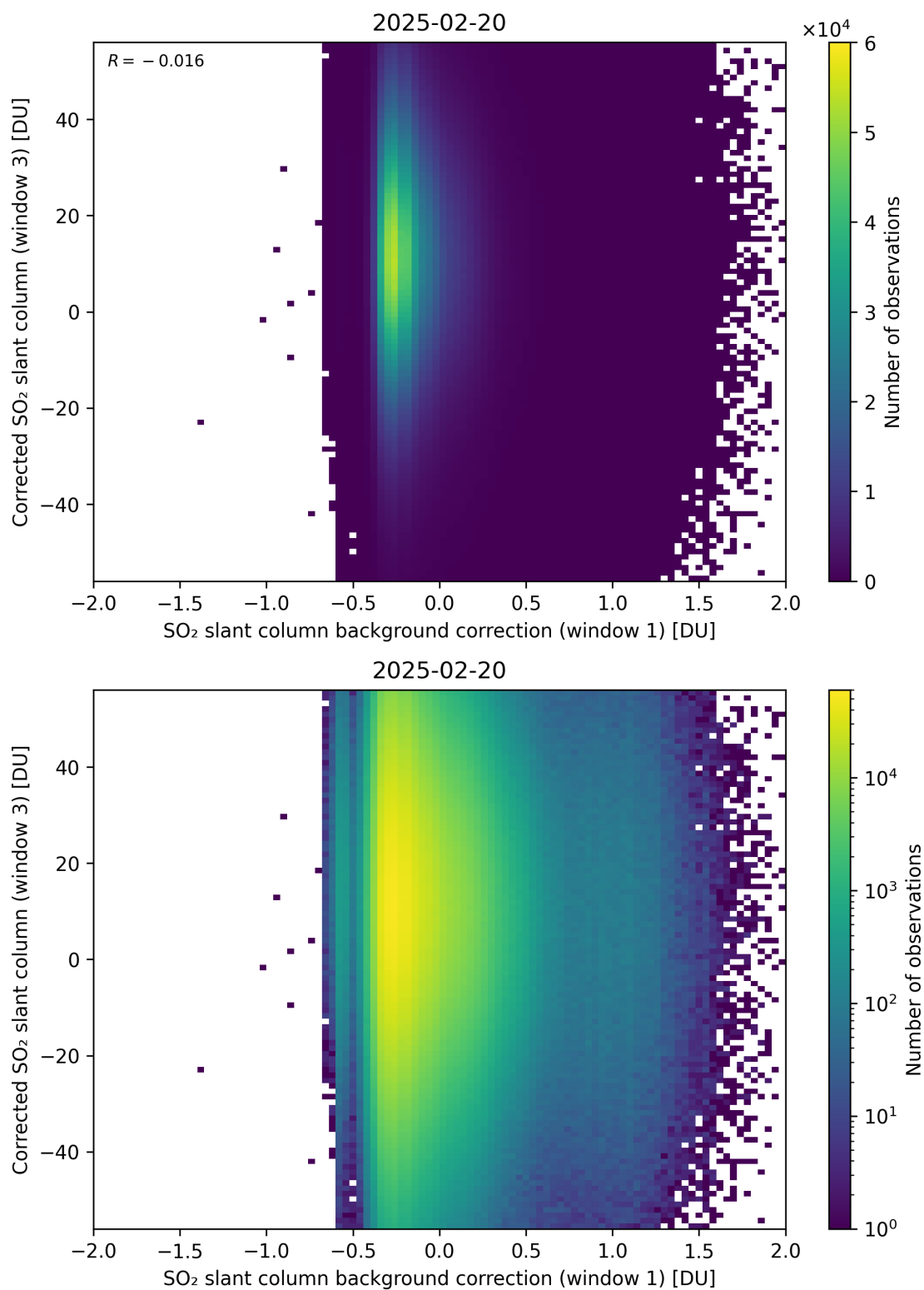
Figure 116: Scatter density plot of “SO 2 slant column background correction (window 1)” against “Corrected SO 2 slant column (window 3)” for 2025-02-19 to 2025-02-21.
