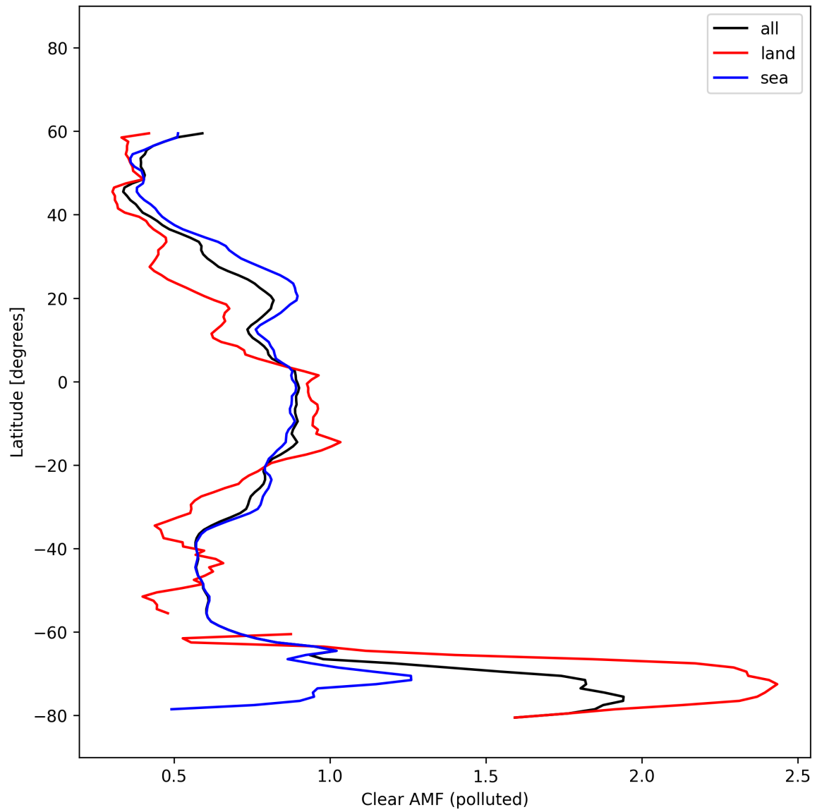
Figure 55: Zonal average of “Clear AMF (polluted)” for 2025-02-19 to 2025-02-21.
