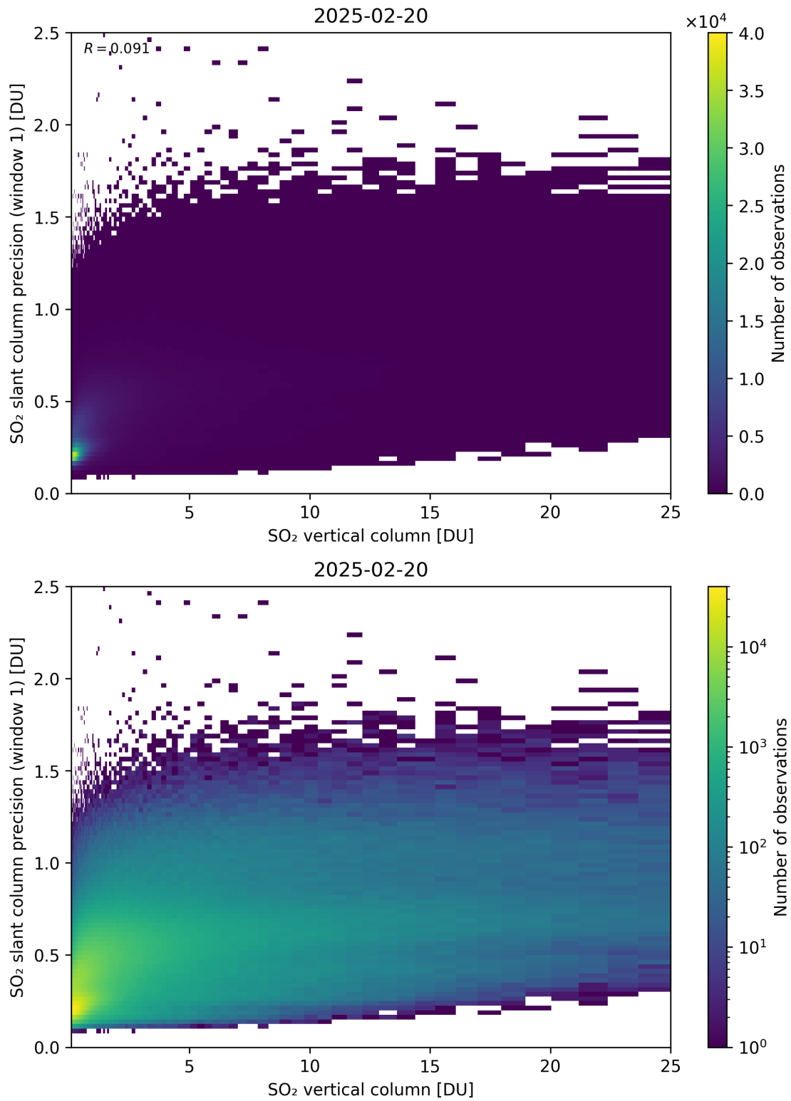
Figure 355: Scatter density plot of “SO 2 vertical column” against “SO 2 slant column precision (window 1)” for 2025-02-19 to 2025-02-21.
