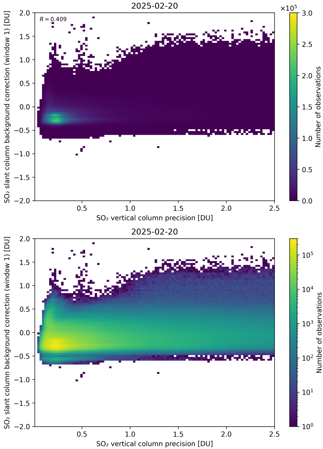
Figure 329: Scatter density plot of “SO 2 vertical column precision” against “SO 2 slant column background correction (window 1)” for 2025-02-19 to 2025-02-21.
