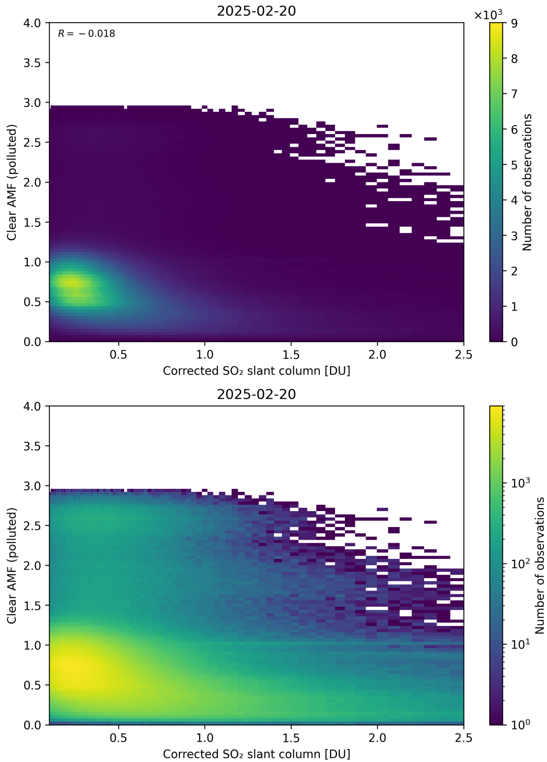
Figure 232: Scatter density plot of “Corrected SO 2 slant column” against “Clear AMF (polluted)” for 2025-02-19 to 2025-02-21.
