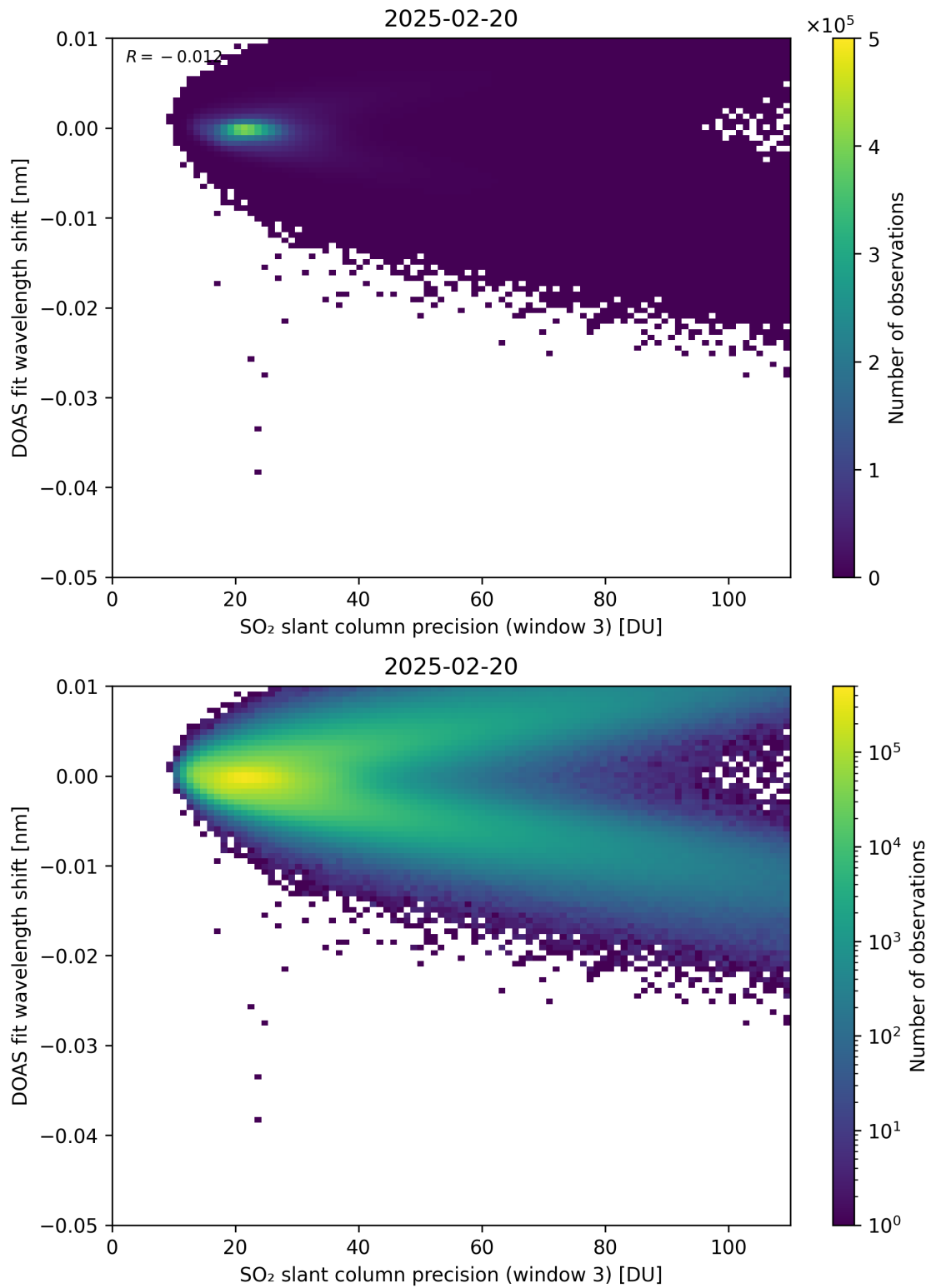
Figure 308: Scatter density plot of “SO 2 slant column precision (window 3)” against “DOAS fit wavelength shift” for 2025-02-19 to 2025-02-21.
