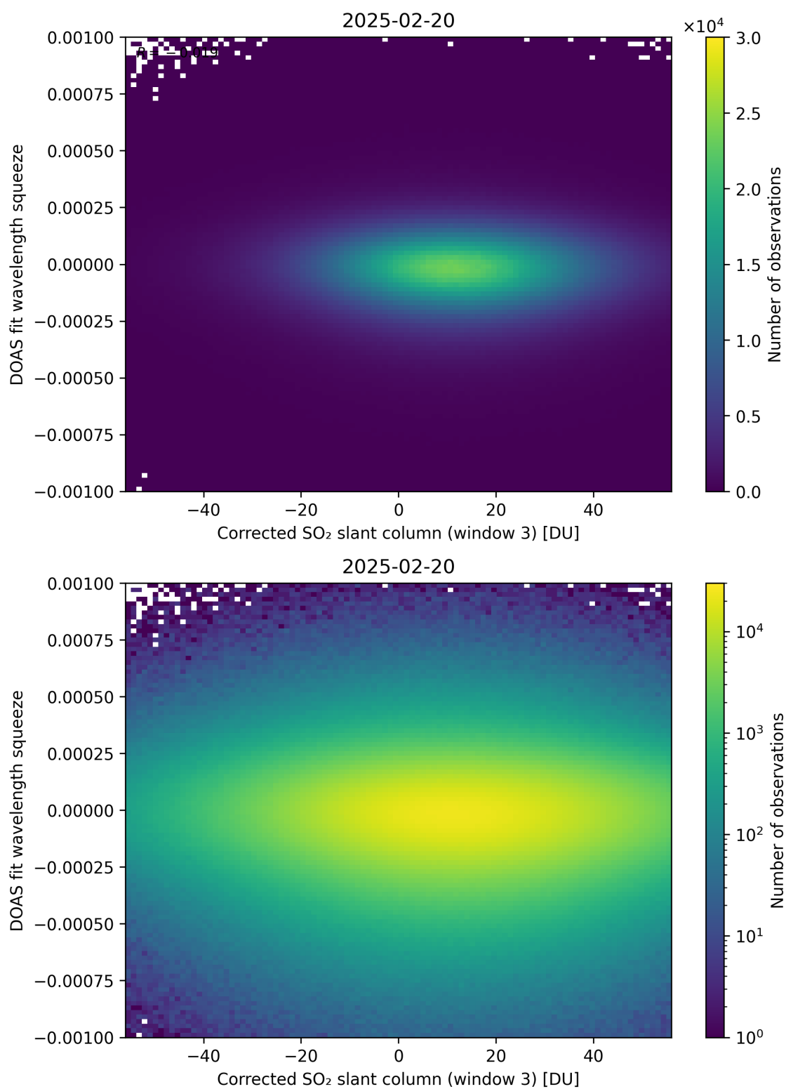
Figure 257: Scatter density plot of “Corrected SO 2 slant column (window 3)” against “DOAS fit wavelength squeeze” for 2025-02-19 to 2025-02-21.
