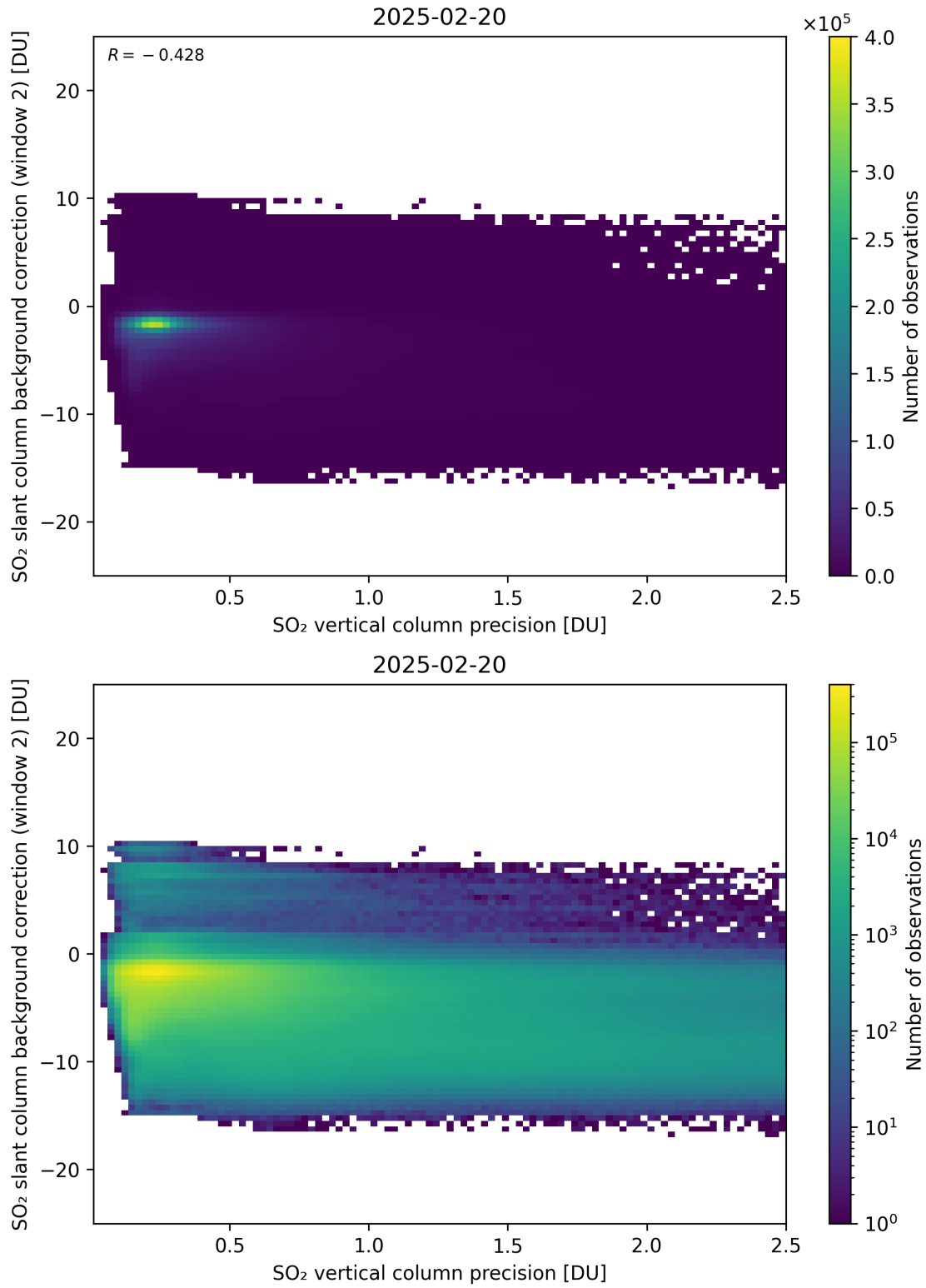
Figure 330: Scatter density plot of “SO 2 vertical column precision” against “SO 2 slant column background correction (window 2)” for 2025-02-19 to 2025-02-21.
