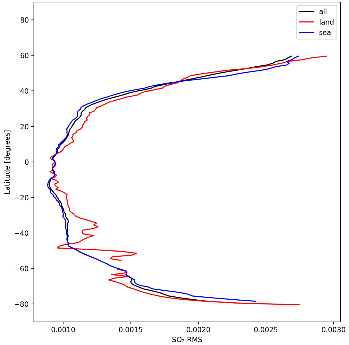
Figure 52: Zonal average of “SO 2 RMS” for 2025-02-19 to 2025-02-21.
