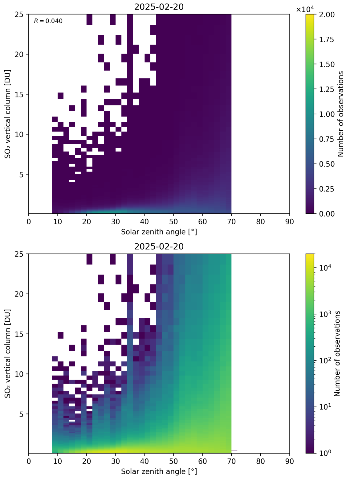
Figure 191: Scatter density plot of “Solar zenith angle” against “SO 2 vertical column” for 2025-02-19 to 2025-02-21.
