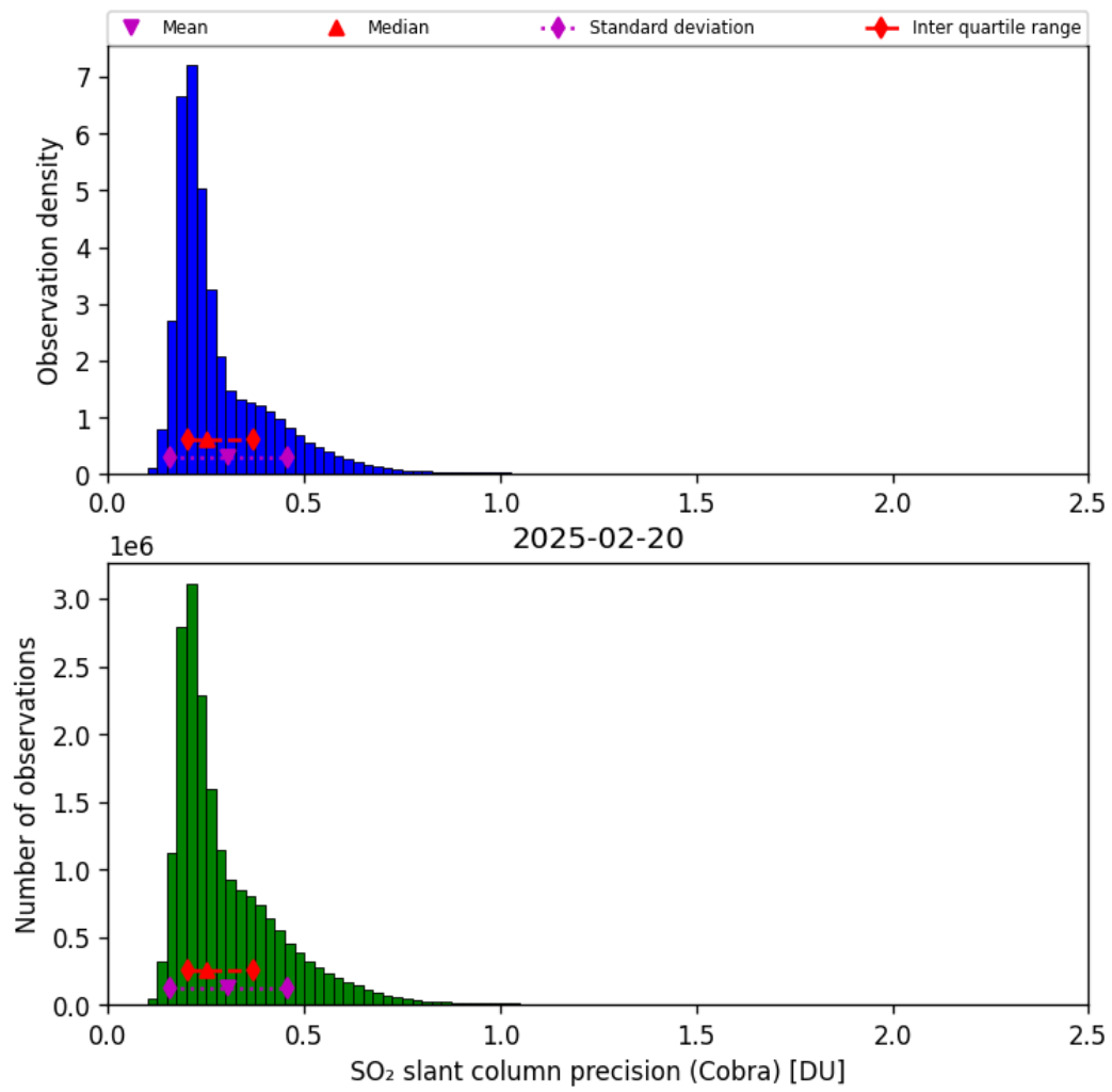
Figure 62: Histogram of “SO 2 slant column precision (Cobra)” for 2025-02-19 to 2025-02-21
