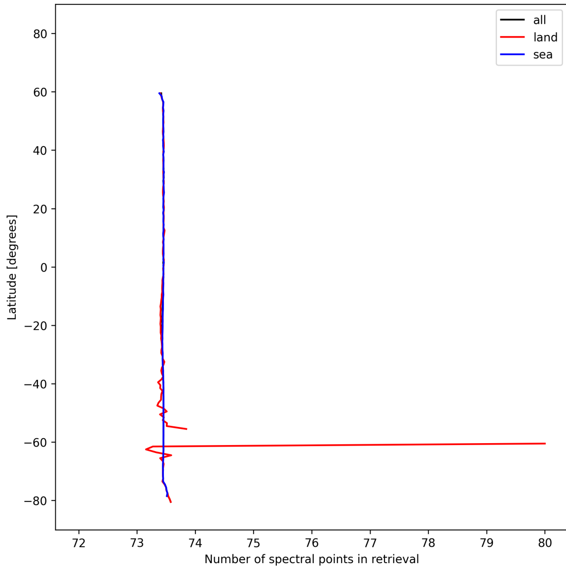
Figure 56: Zonal average of “Number of spectral points in retrieval” for 2025-02-19 to 2025-02-21.
