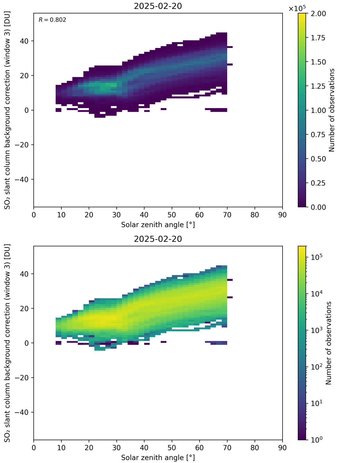
Figure 173: Scatter density plot of “Solar zenith angle” against “SO 2 slant column background correction (window 3)” for 2025-02-19 to 2025-02-21.
