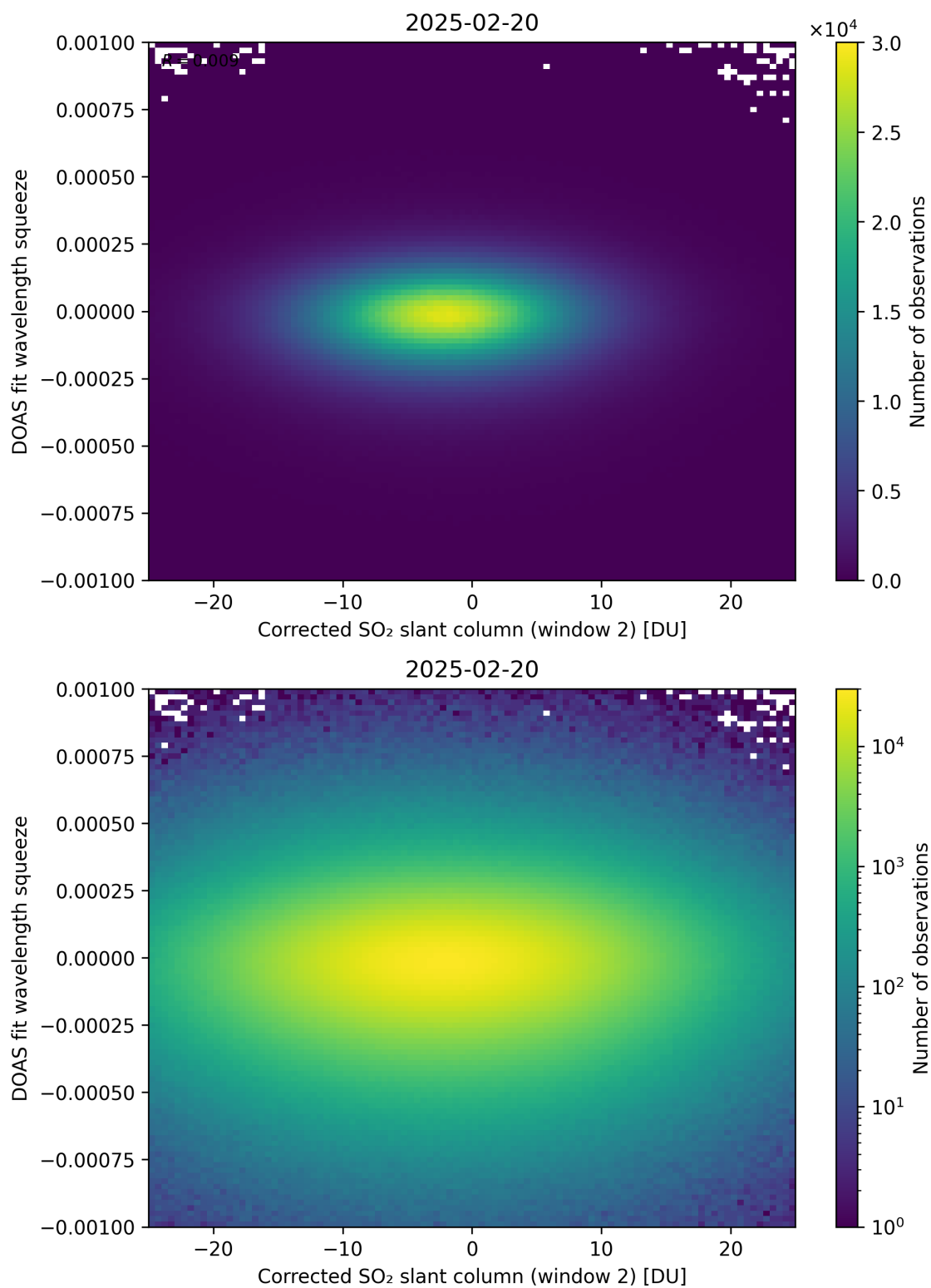
Figure 247: Scatter density plot of “Corrected SO 2 slant column (window 2)” against “DOAS fit wavelength squeeze” for 2025-02-19 to 2025-02-21.
