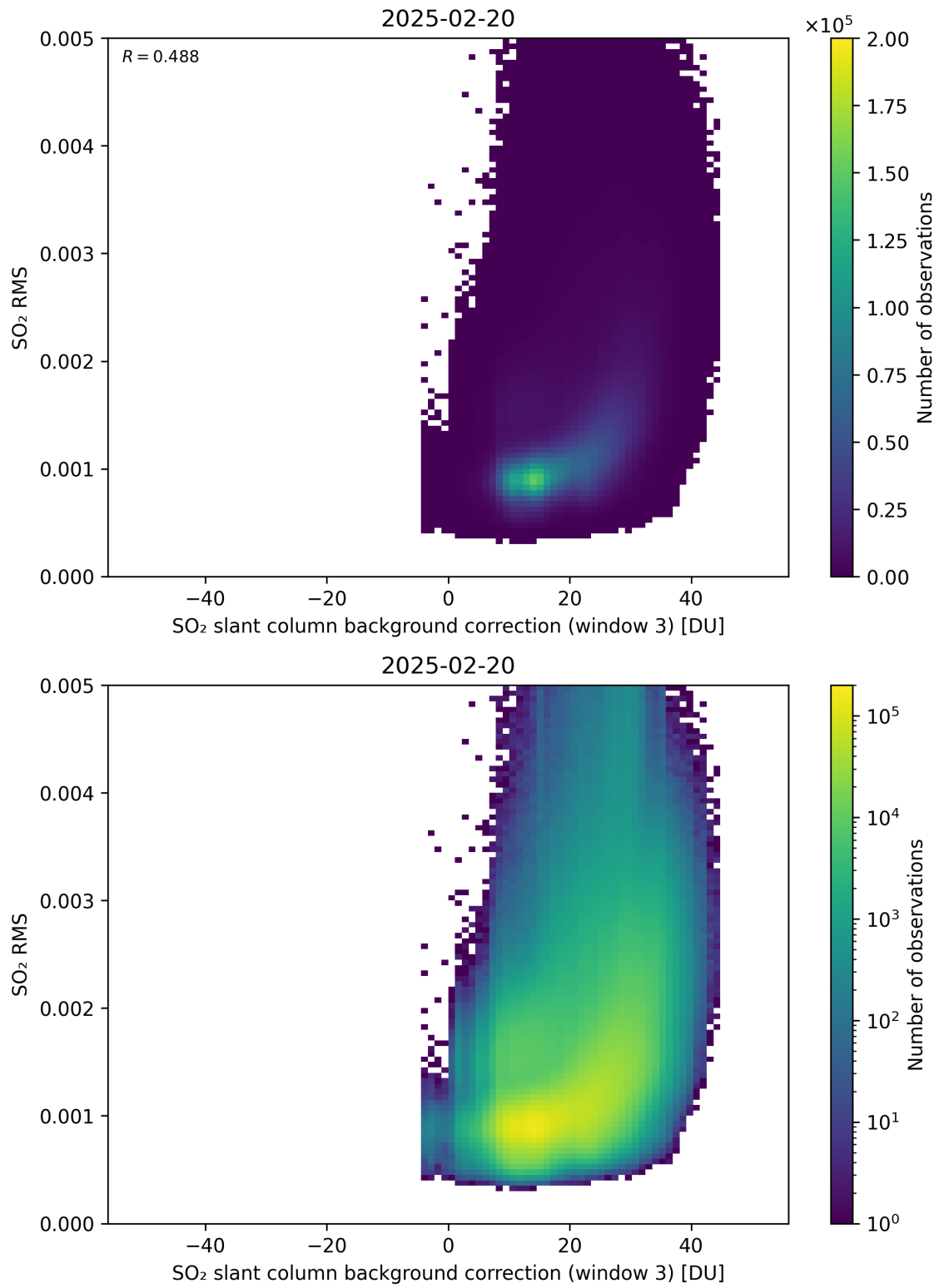
Figure 134: Scatter density plot of “SO 2 slant column background correction (window 3)” against “SO 2 RMS” for 2025-02-19 to 2025-02-21.
