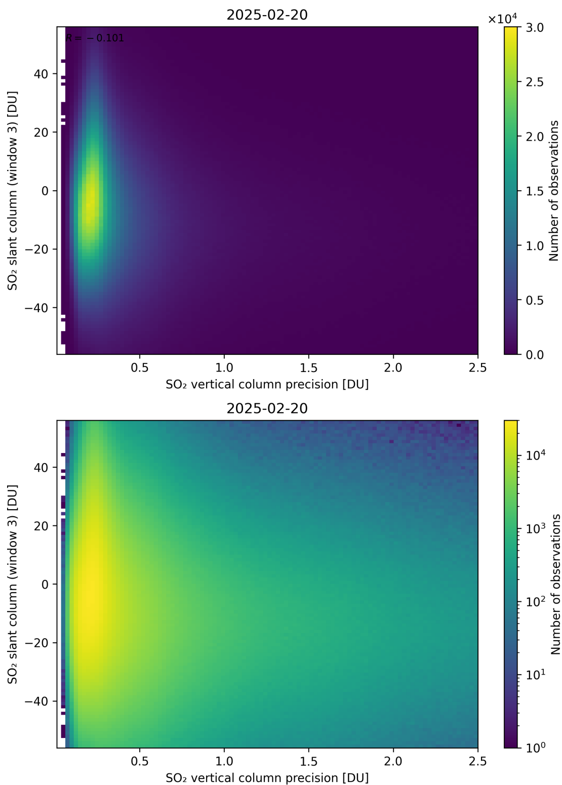
Figure 344: Scatter density plot of “SO 2 vertical column precision” against “SO 2 slant column (window 3)” for 2025-02-19 to 2025-02-21.
