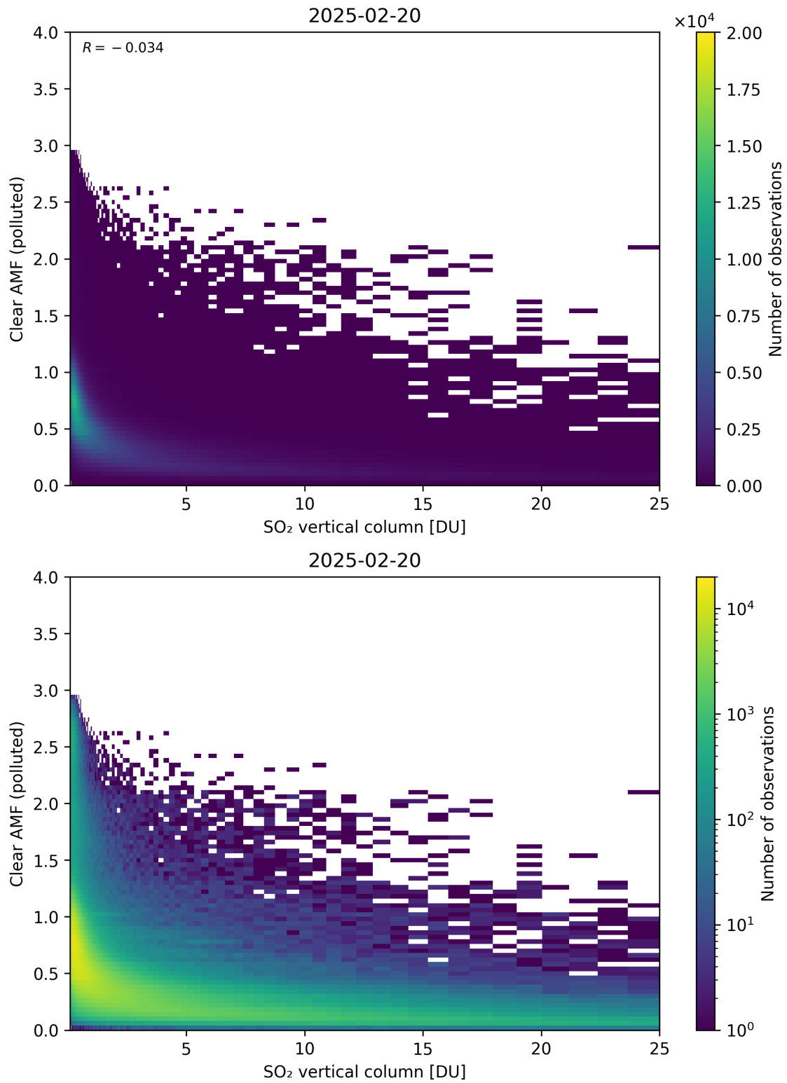
Figure 348: Scatter density plot of “SO 2 vertical column” against “Clear AMF (polluted)” for 2025-02-19 to 2025-02-21.
