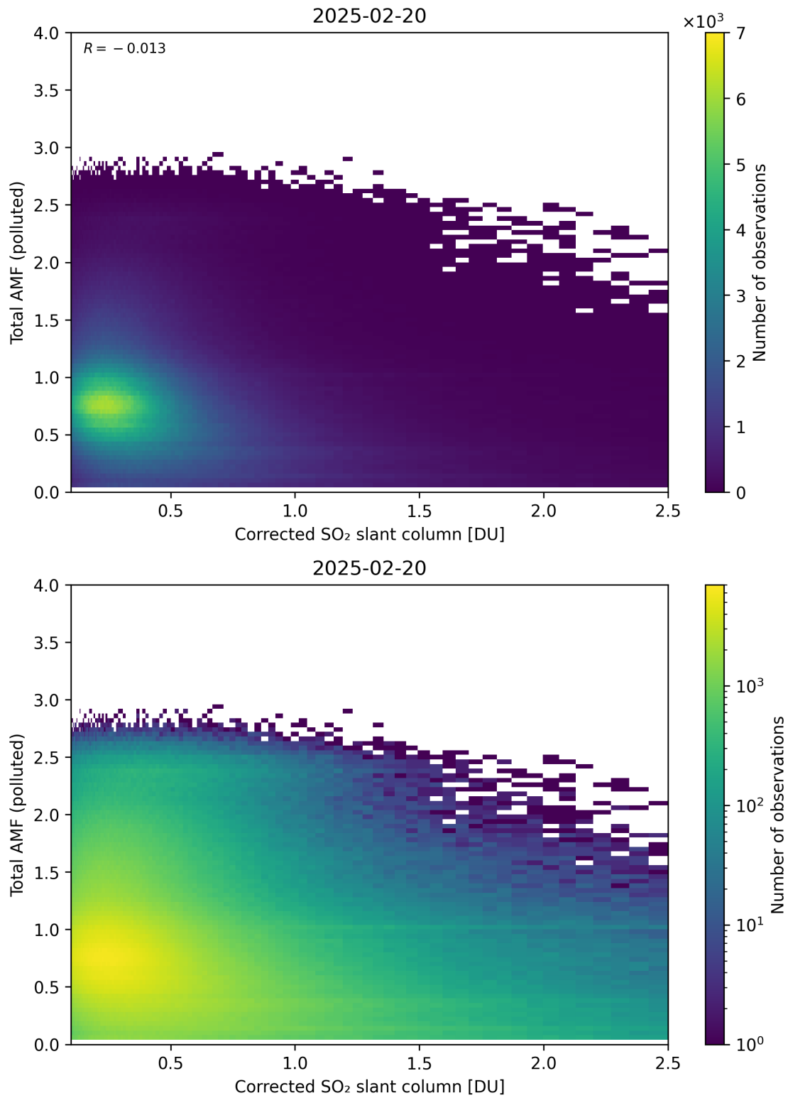
Figure 242: Scatter density plot of “Corrected SO 2 slant column” against “Total AMF (polluted)” for 2025-02-19 to 2025-02-21.
