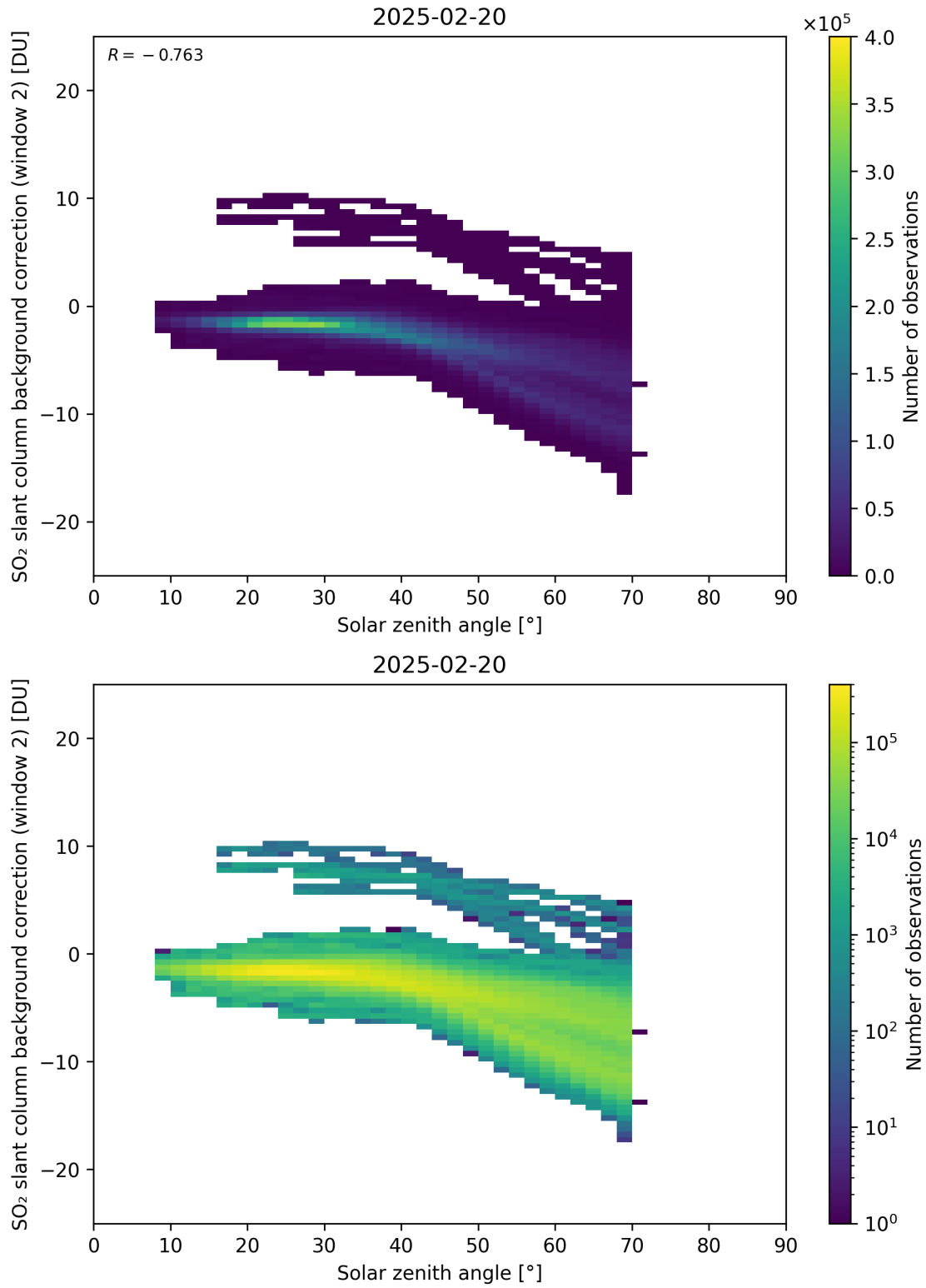
Figure 172: Scatter density plot of “Solar zenith angle” against “SO 2 slant column background correction (window 2)” for 2025-02-19 to 2025-02-21.
