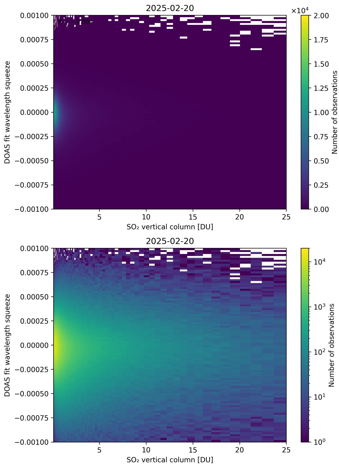
Figure 327: Scatter density plot of “SO 2 vertical column” against “DOAS fit wavelength squeeze” for 2025-02-19 to 2025-02-21.
