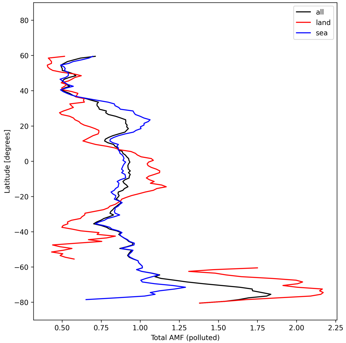
Figure 53: Zonal average of “Total AMF (polluted)” for 2025-02-19 to 2025-02-21.
