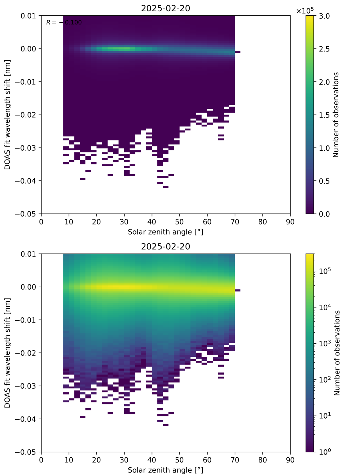
Figure 174: Scatter density plot of “Solar zenith angle” against “DOAS fit wavelength shift” for 2025-02-19 to 2025-02-21.
