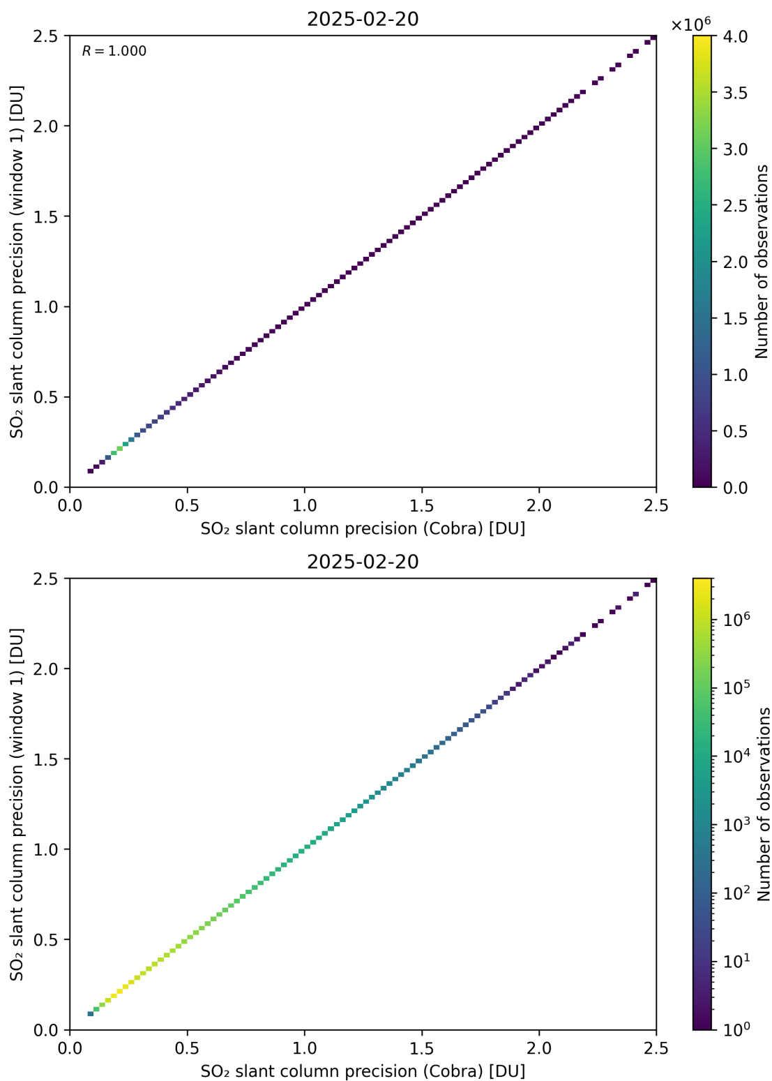
Figure 209: Scatter density plot of “SO 2 slant column precision (Cobra)” against “SO 2 slant column precision (window 1)” for 2025-02-19 to 2025-02-21.
