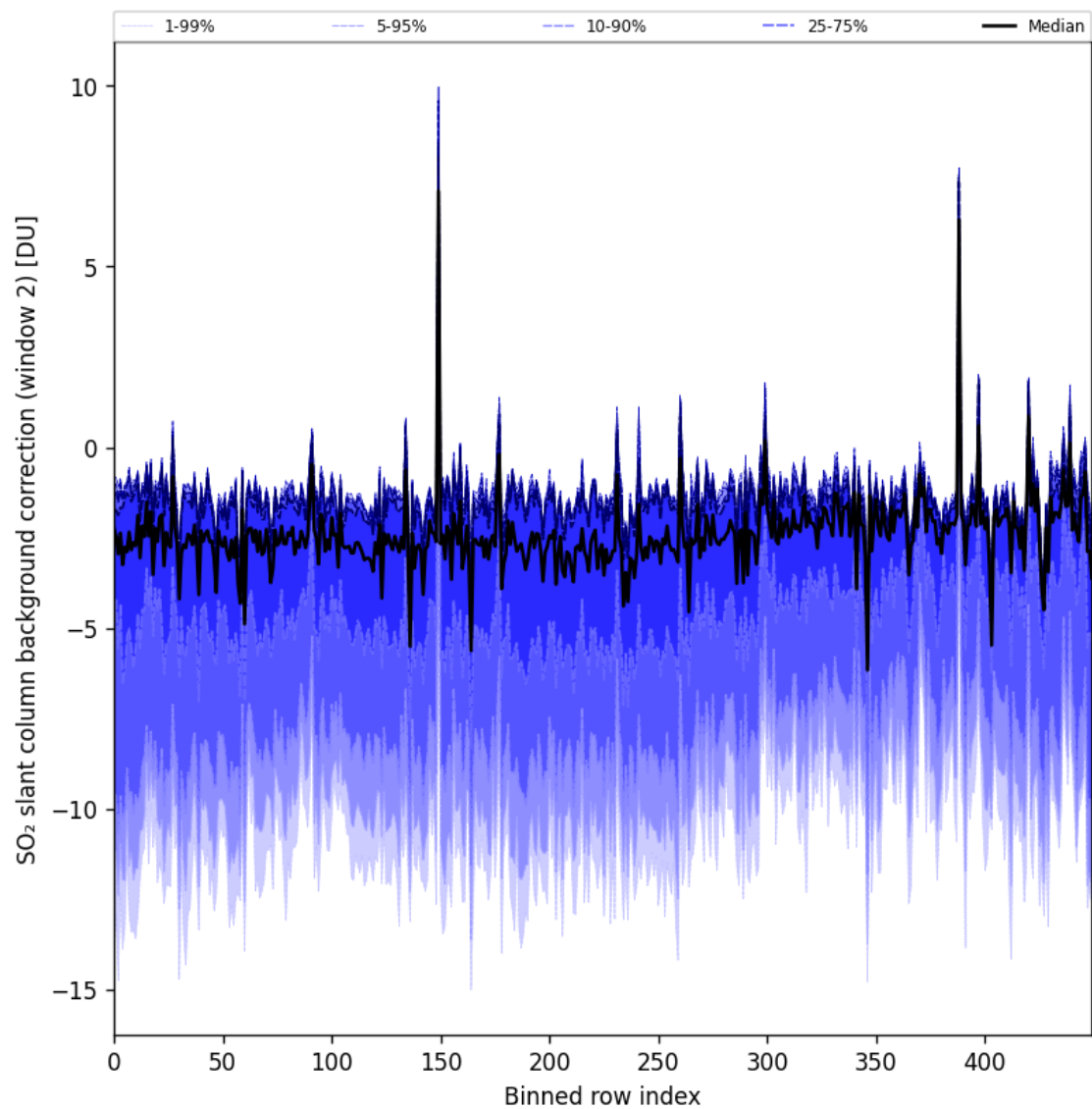
Figure 96: Along track statistics of “SO 2 slant column background correction (window 2)” for 2025-02-19 to 2025-02-21
