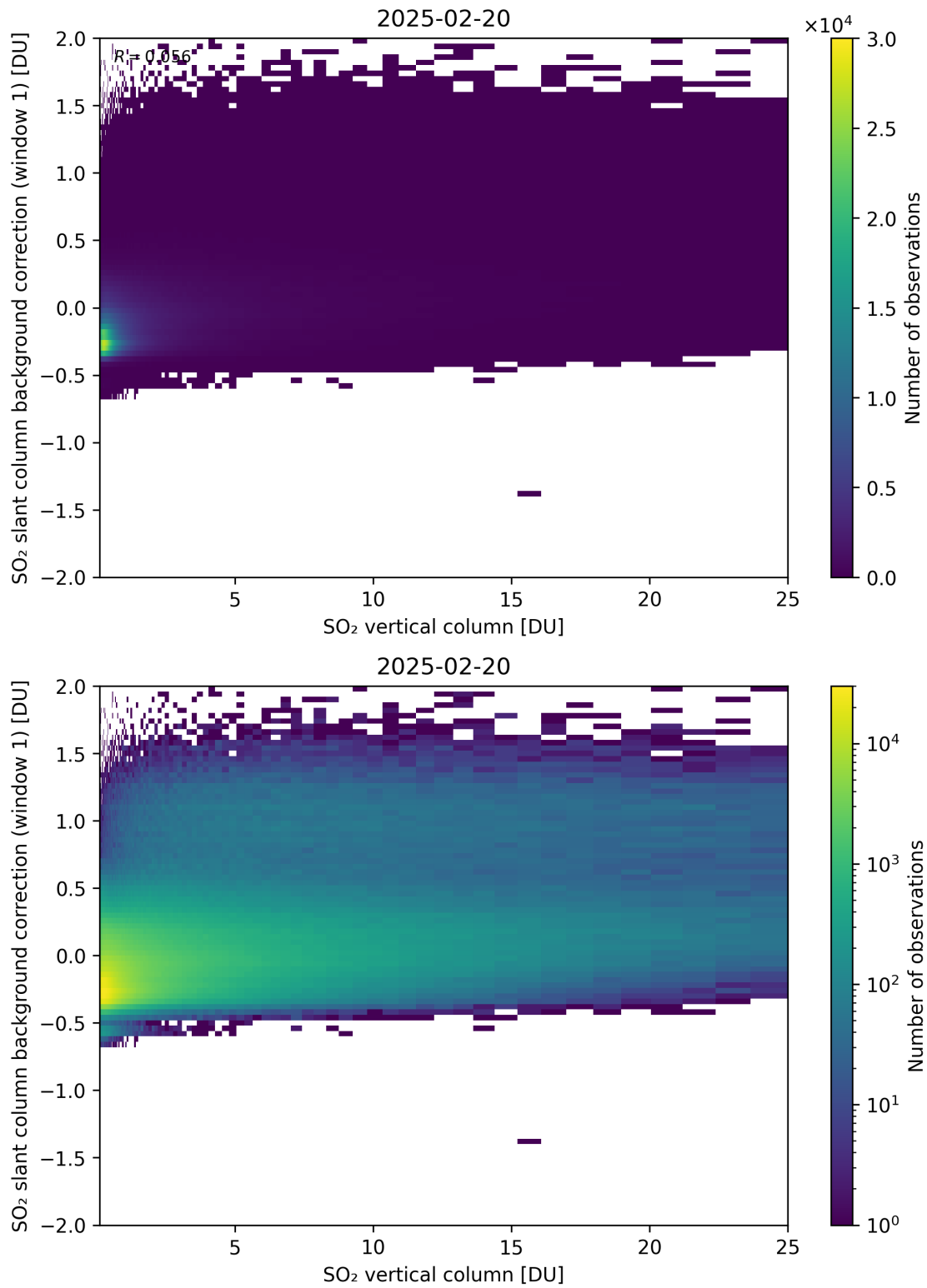
Figure 323: Scatter density plot of “SO 2 vertical column” against “SO 2 slant column background correction (window 1)” for 2025-02-19 to 2025-02-21.
