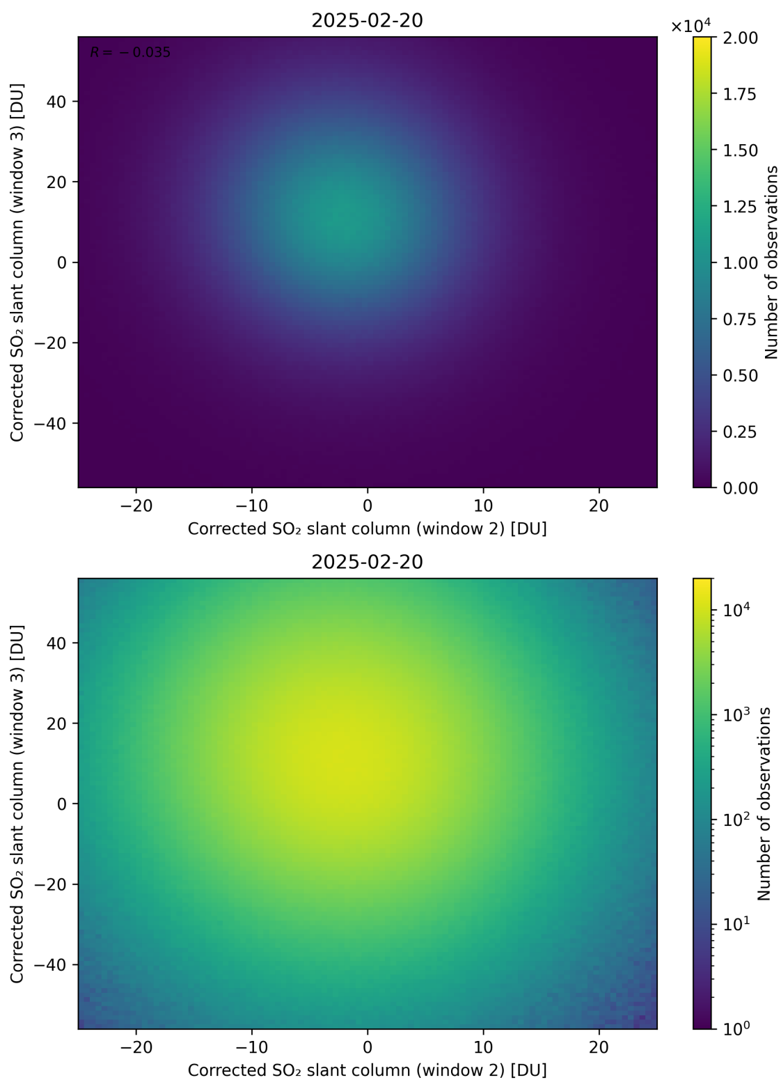
Figure 250: Scatter density plot of “Corrected SO 2 slant column (window 2)” against “Corrected SO 2 slant column (window 3)” for 2025-02-19 to 2025-02-21.
