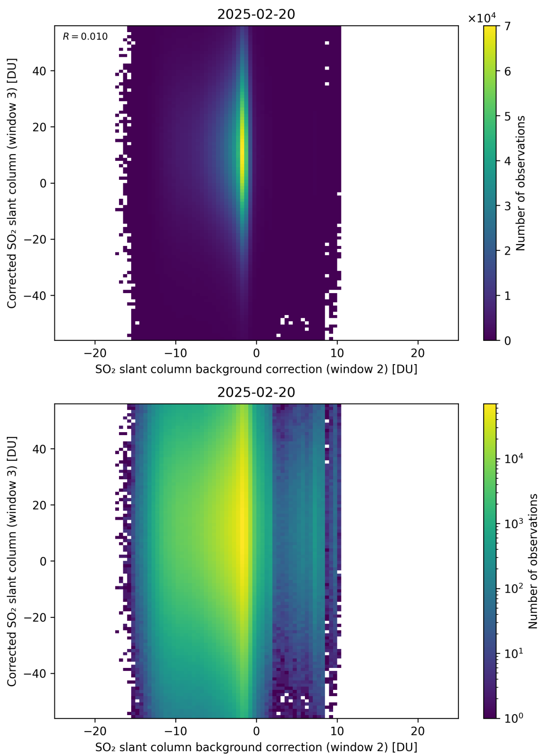
Figure 127: Scatter density plot of “SO 2 slant column background correction (window 2)” against “Corrected SO 2 slant column (window 3)” for 2025-02-19 to 2025-02-21.
