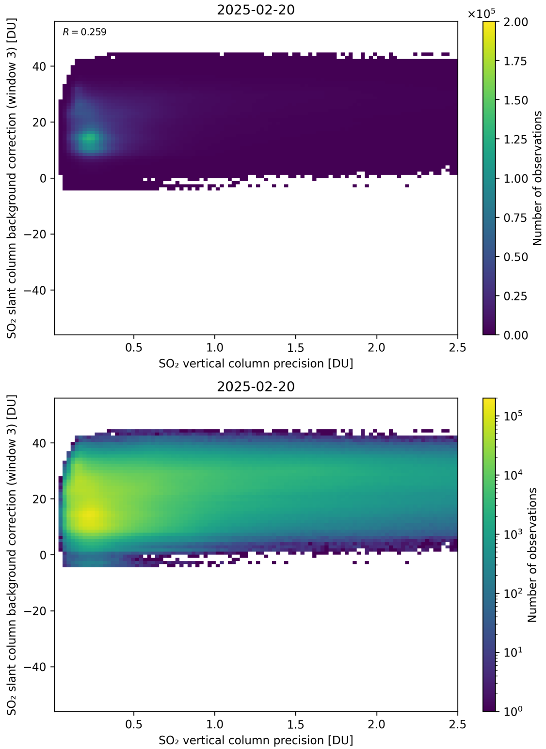
Figure 331: Scatter density plot of “SO 2 vertical column precision” against “SO 2 slant column background correction (window 3)” for 2025-02-19 to 2025-02-21.
