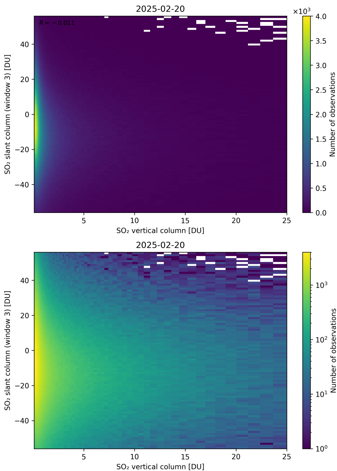
Figure 357: Scatter density plot of “SO 2 vertical column” against “SO 2 slant column (window 3)” for 2025-02-19 to 2025-02-21.
