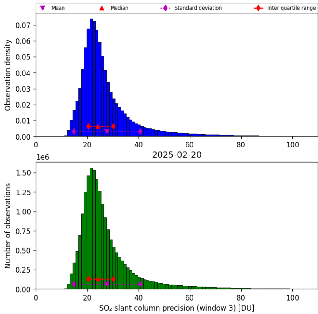
Figure 72: Histogram of “SO 2 slant column precision (window 3)” for 2025-02-19 to 2025-02-21
