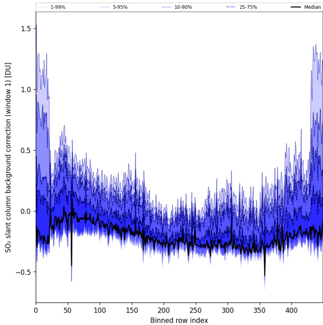
Figure 92: Along track statistics of “SO 2 slant column background correction (window 1)” for 2025-02-19 to 2025-02-21
