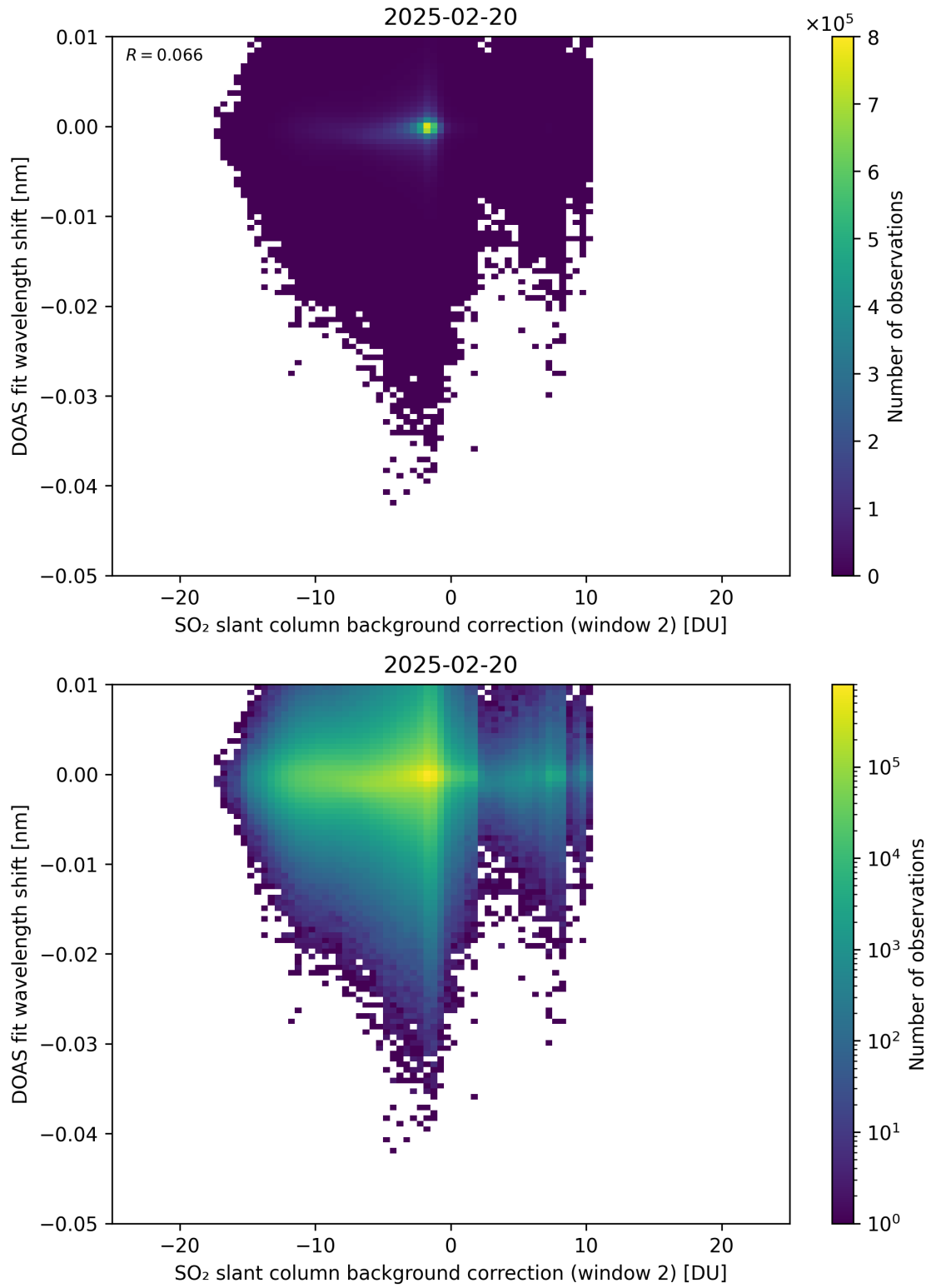
Figure 123: Scatter density plot of “SO 2 slant column background correction (window 2)” against “DOAS fit wavelength shift” for 2025-02-19 to 2025-02-21.
