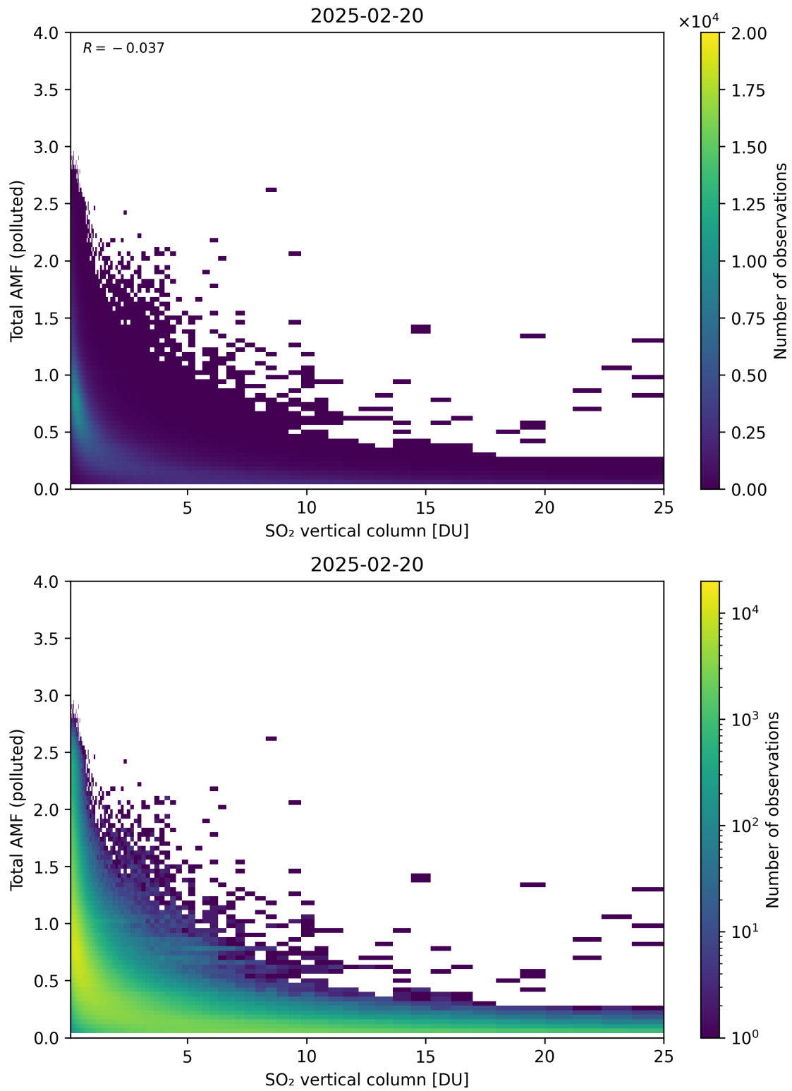
Figure 359: Scatter density plot of “SO 2 vertical column” against “Total AMF (polluted)” for 2025-02-19 to 2025-02-21.
