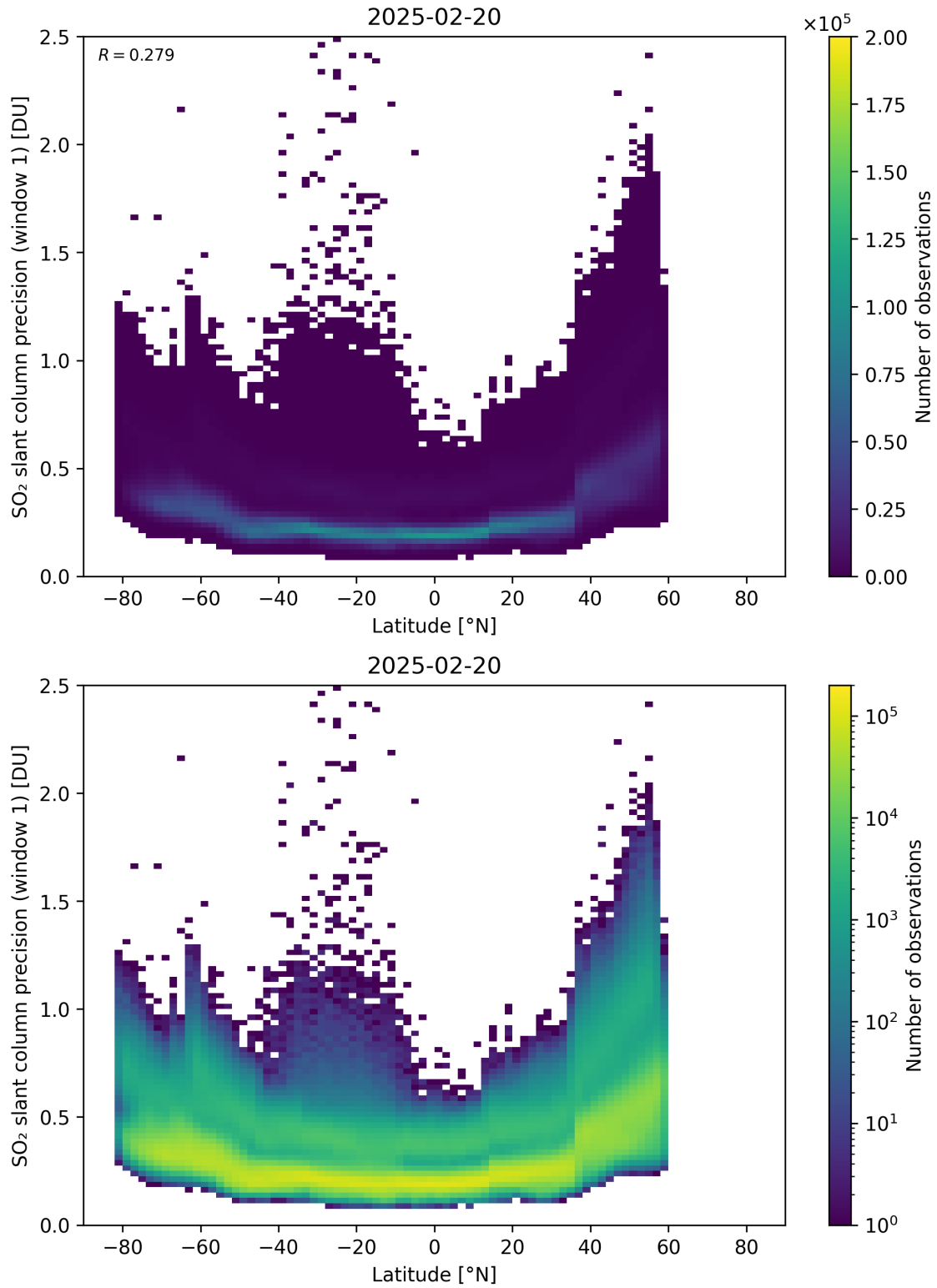
Figure 163: Scatter density plot of “Latitude” against “SO 2 slant column precision (window 1)” for 2025-02-19 to 2025-02-21.
