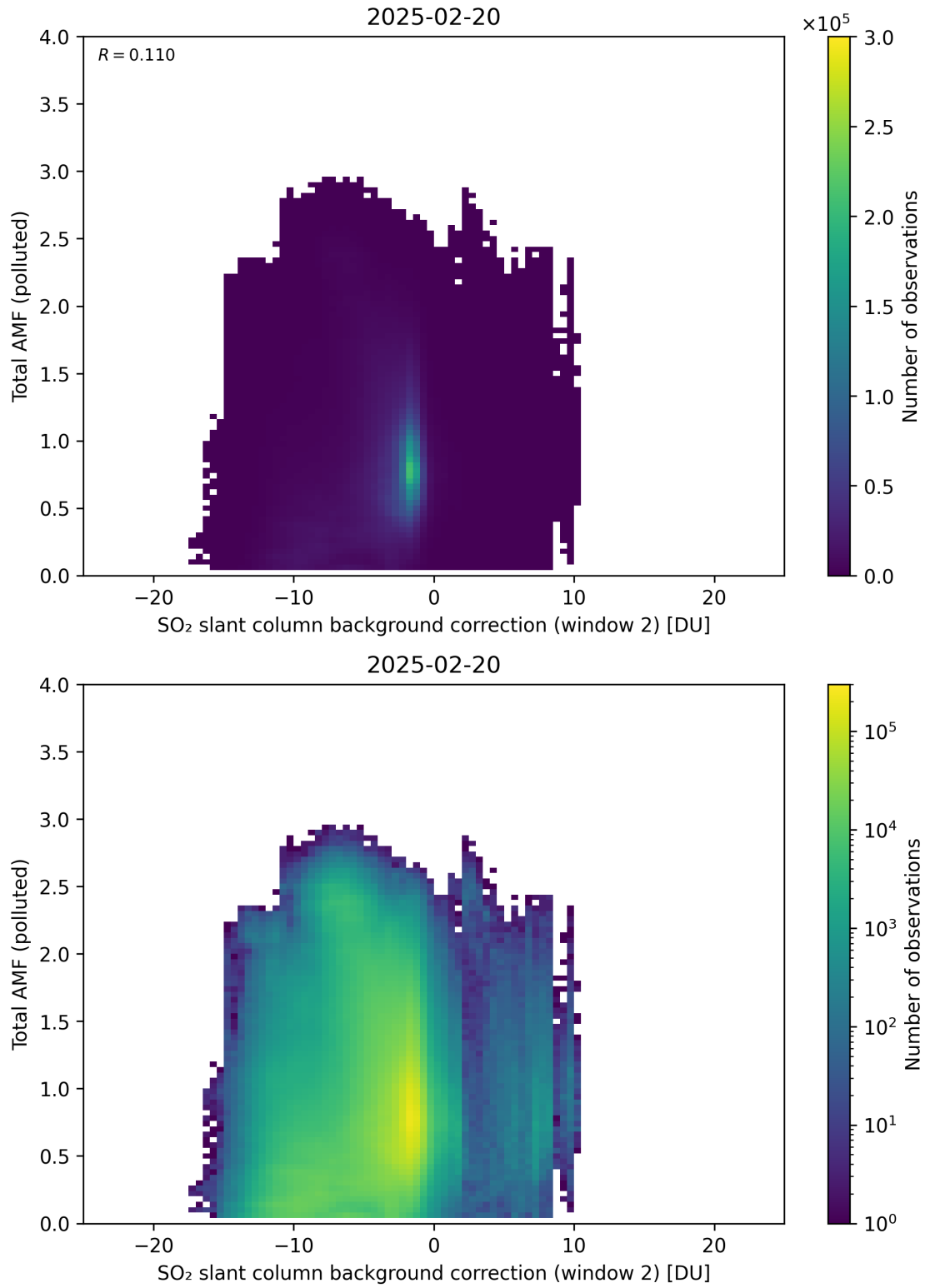
Figure 130: Scatter density plot of “SO 2 slant column background correction (window 2)” against “Total AMF (polluted)” for 2025-02-19 to 2025-02-21.
