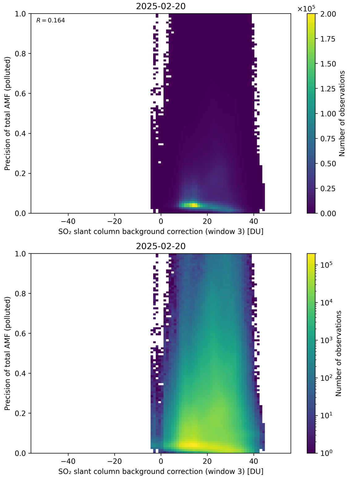
Figure 137: Scatter density plot of “SO 2 slant column background correction (window 3)” against “Precision of total AMF (polluted)” for 2025-02-19 to 2025-02-21.
