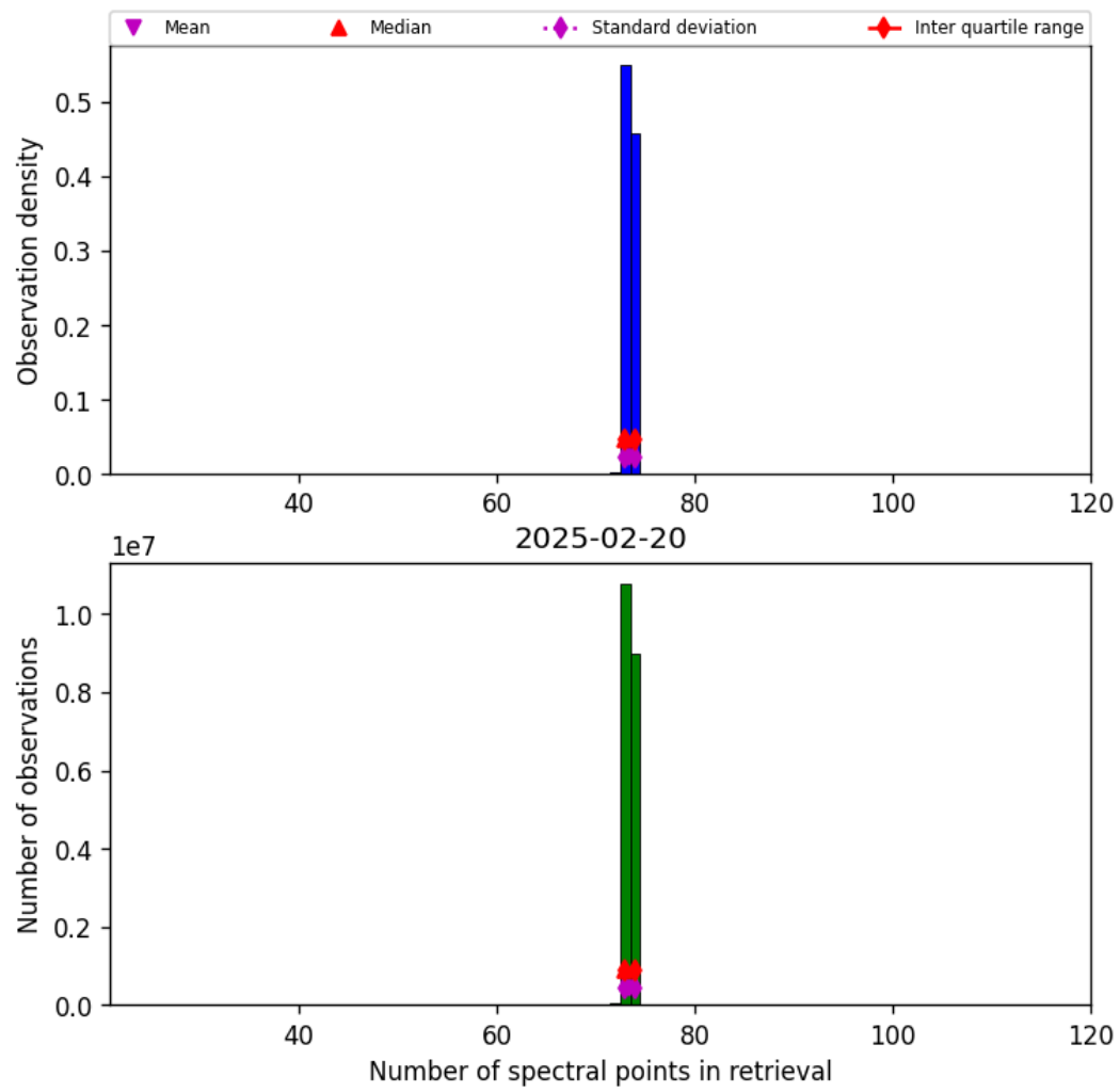
Figure 82: Histogram of “Number of spectral points in retrieval” for 2025-02-19 to 2025-02-21
