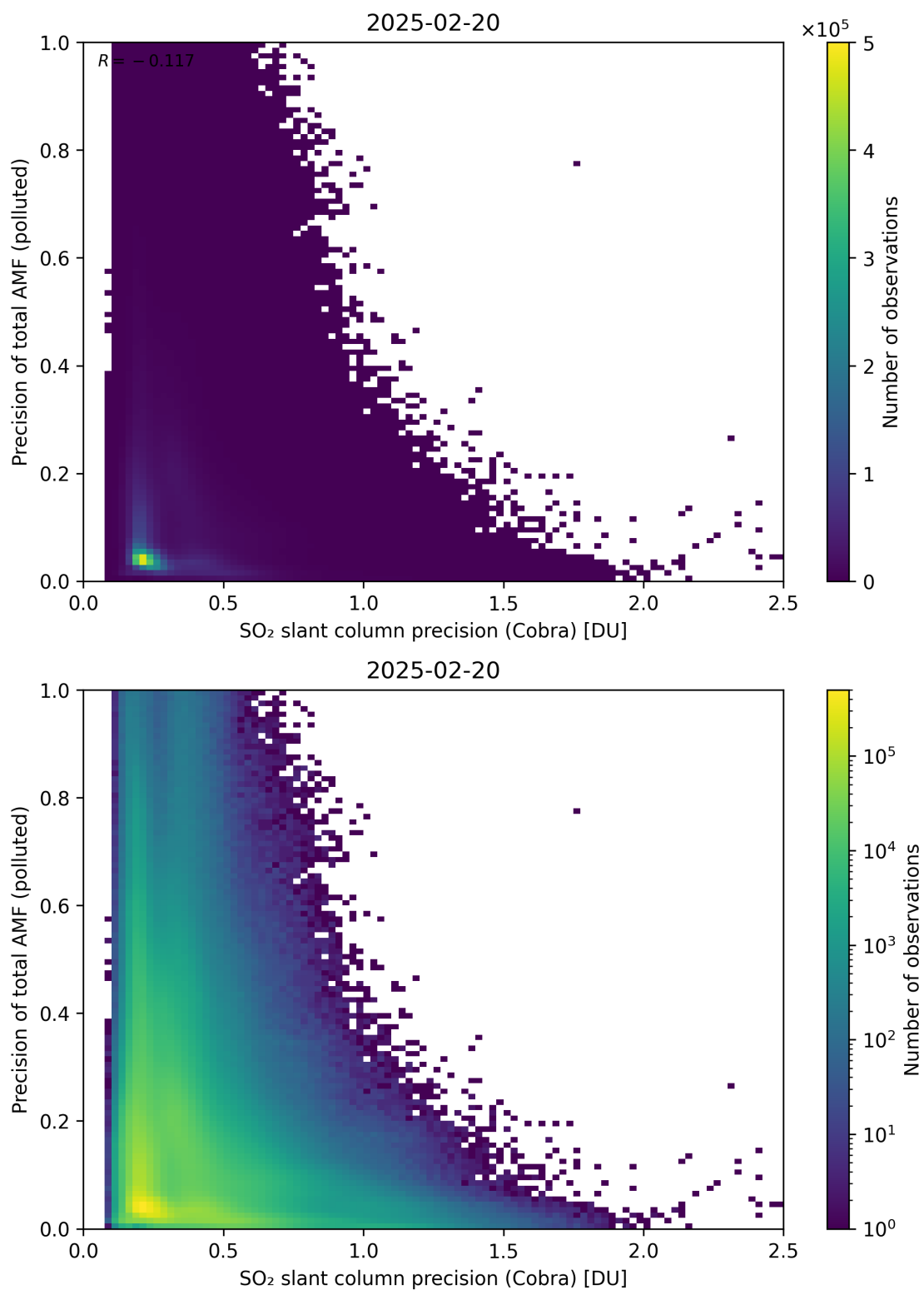
Figure 214: Scatter density plot of “SO 2 slant column precision (Cobra)” against “Precision of total AMF (polluted)” for 2025-02-19 to 2025-02-21.
