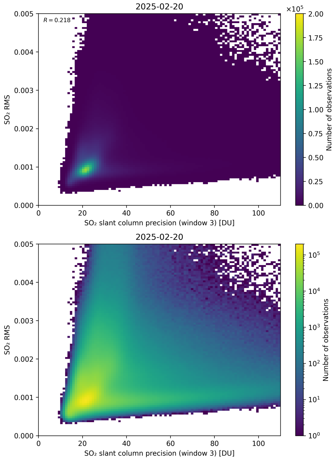
Figure 310: Scatter density plot of “SO 2 slant column precision (window 3)” against “SO 2 RMS” for 2025-02-19 to 2025-02-21.
