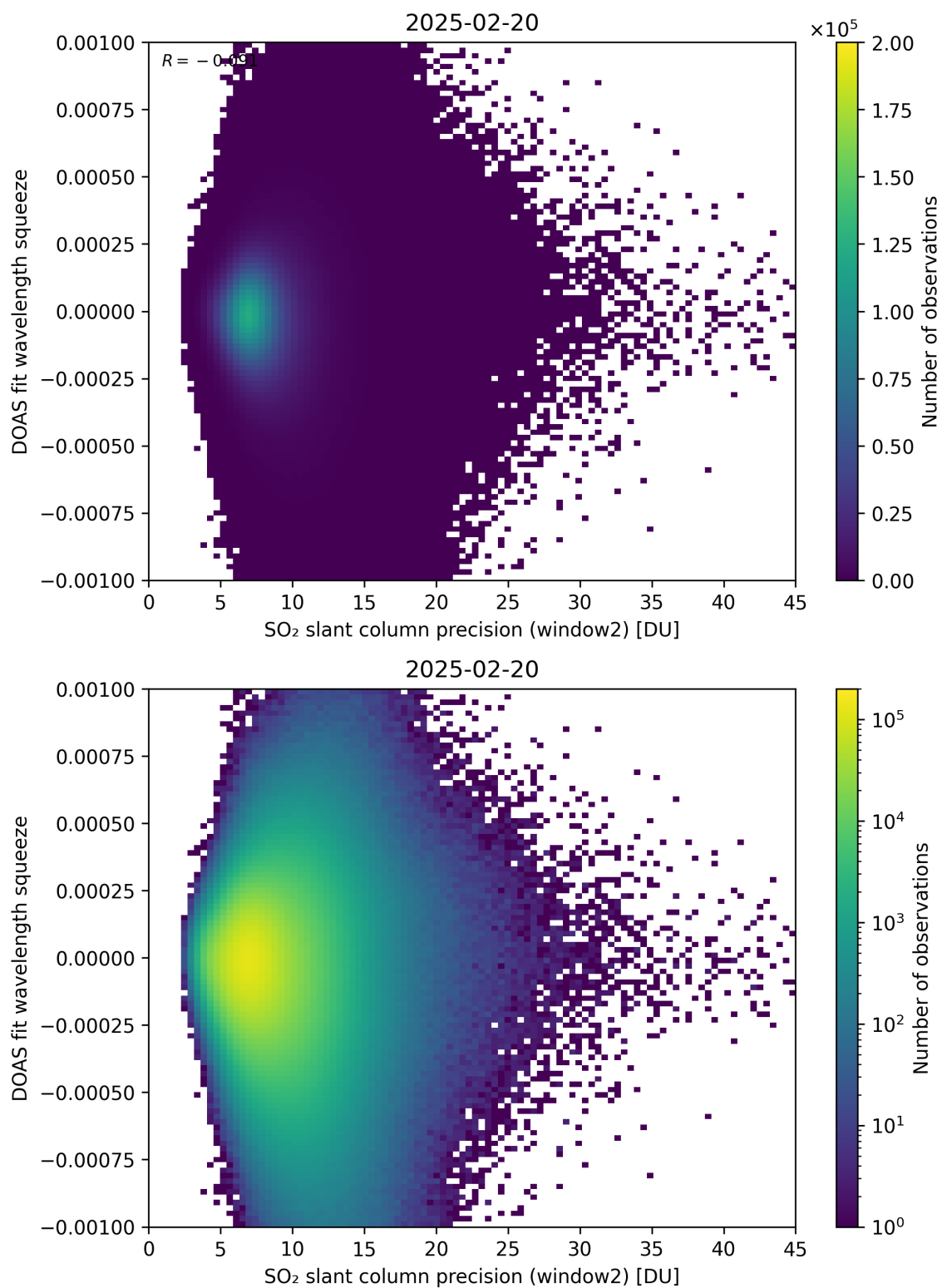
Figure 294: Scatter density plot of “SO 2 slant column precision (window2)” against “DOAS fit wavelength squeeze” for 2025-02-19 to 2025-02-21.
