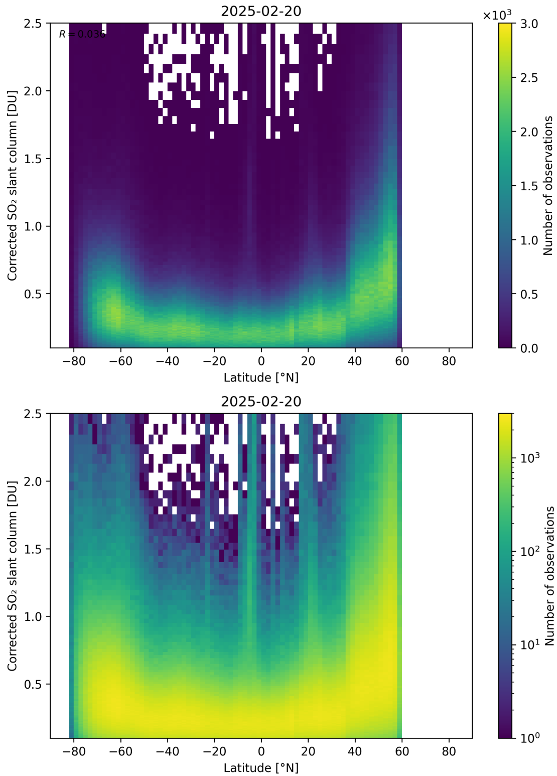
Figure 159: Scatter density plot of “Latitude” against “Corrected SO 2 slant column” for 2025-02-19 to 2025-02-21.
