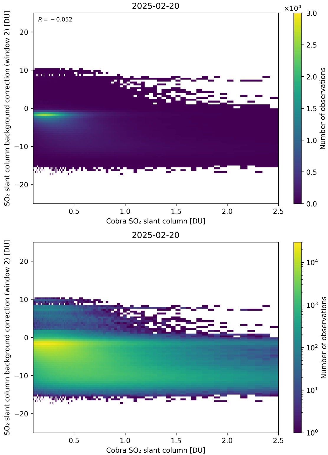
Figure 194: Scatter density plot of “Cobra SO 2 slant column” against “SO 2 slant column background correction (window 2)” for 2025-02-19 to 2025-02-21.
