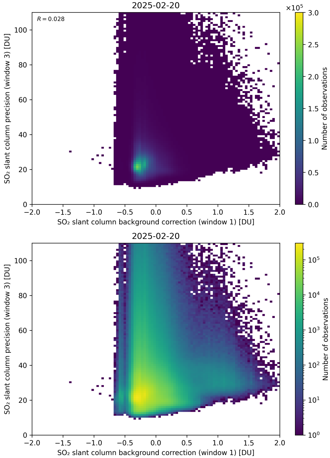
Figure 119: Scatter density plot of “SO 2 slant column background correction (window 1)” against “SO 2 slant column precision (window 3)” for 2025-02-19 to 2025-02-21.
