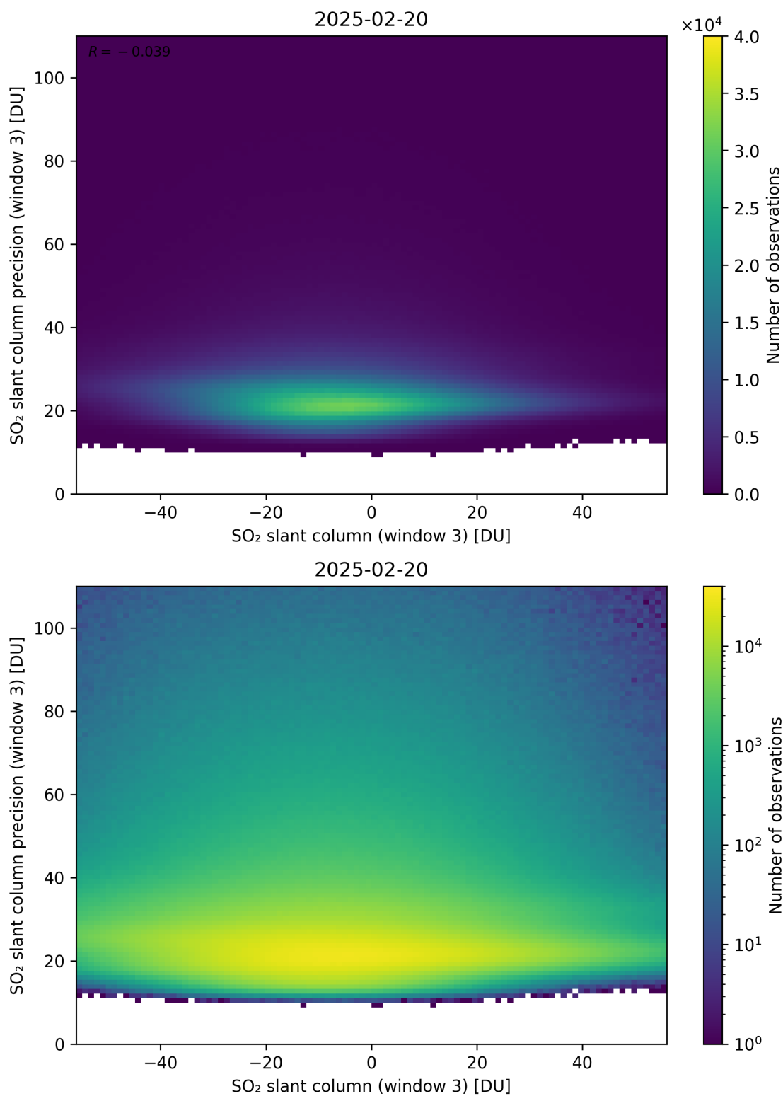
Figure 317: Scatter density plot of “SO 2 slant column (window 3)” against “SO 2 slant column precision (window 3)” for 2025-02-19 to 2025-02-21.
