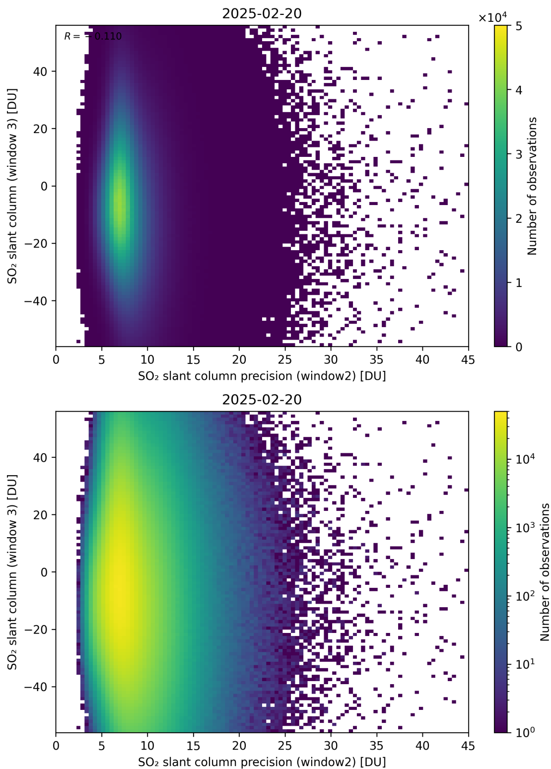
Figure 299: Scatter density plot of “SO 2 slant column precision (window2)” against “SO 2 slant column (window 3)” for 2025-02-19 to 2025-02-21.
