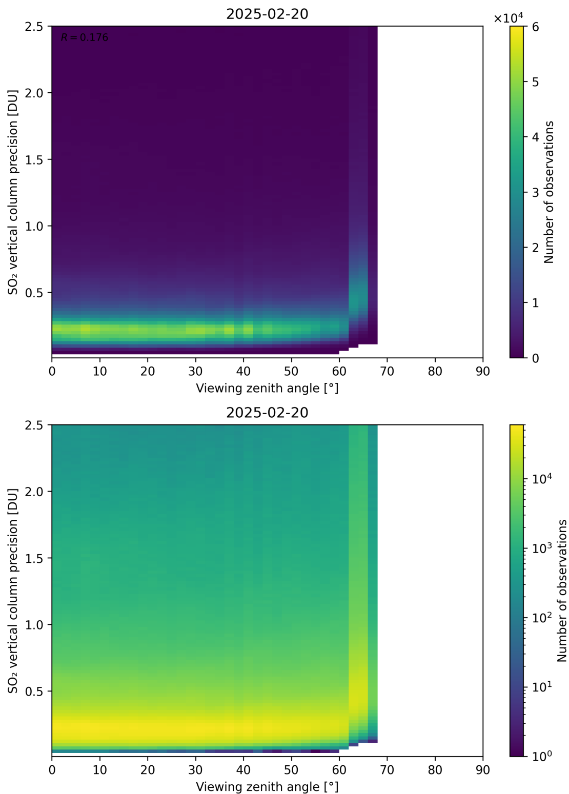
Figure 384: Scatter density plot of “Viewing zenith angle” against “SO 2 vertical column precision” for 2025-02-19 to 2025-02-21.
