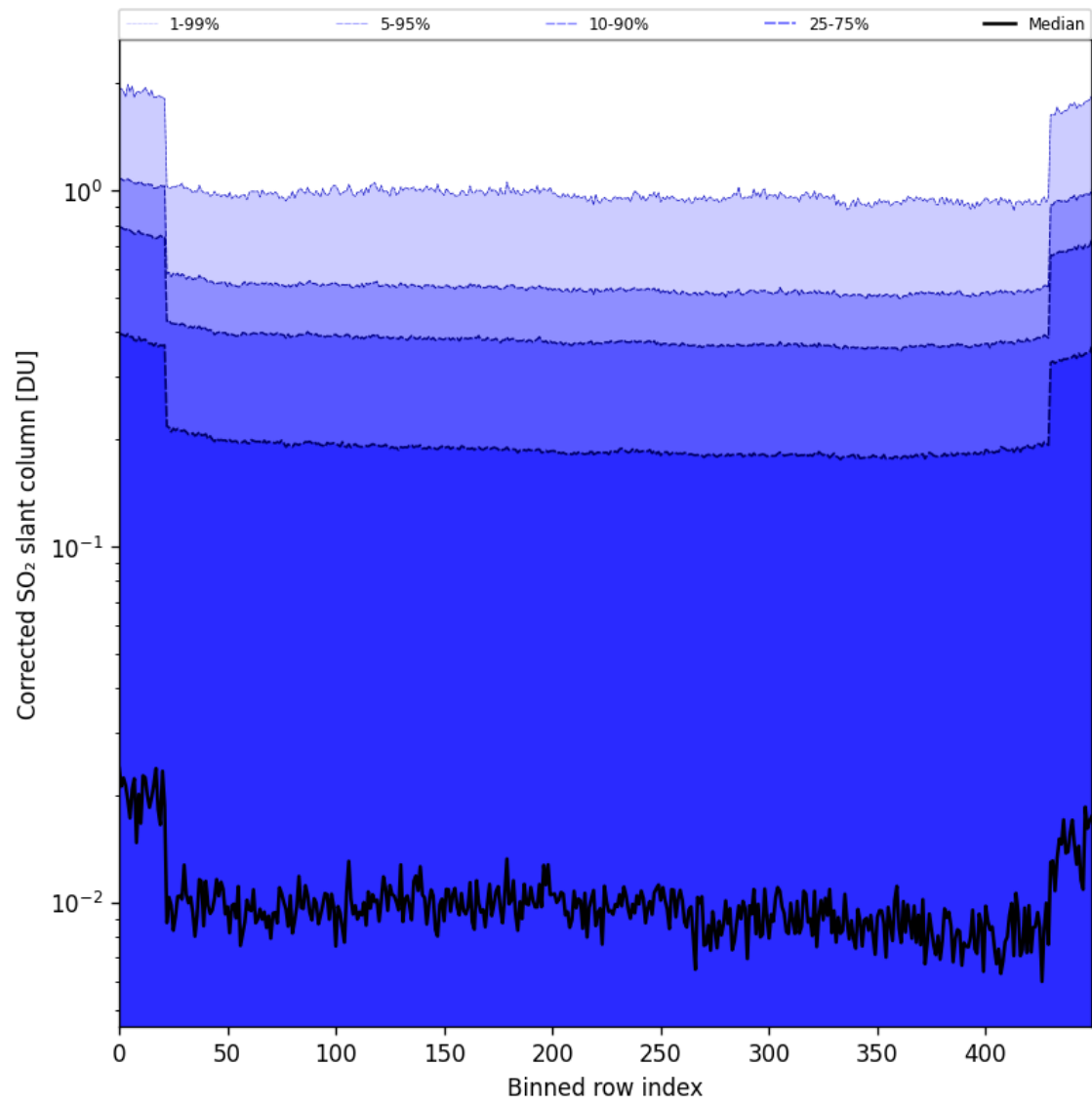
Figure 86: Along track statistics of “Corrected SO 2 slant column” for 2025-02-19 to 2025-02-21
