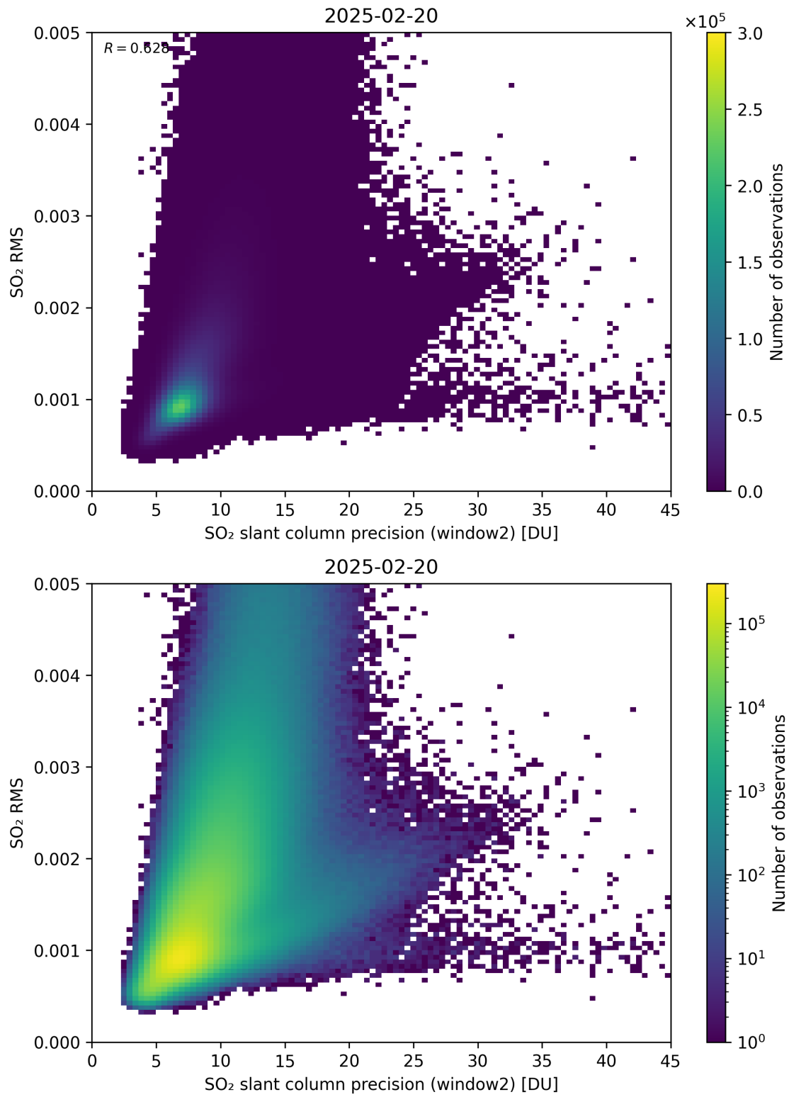
Figure 295: Scatter density plot of “SO 2 slant column precision (window2)” against “SO 2 RMS” for 2025-02-19 to 2025-02-21.
