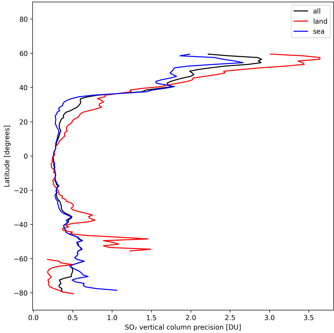
Figure 33: Zonal average of “SO 2 vertical column precision” for 2025-02-19 to 2025-02-21.
