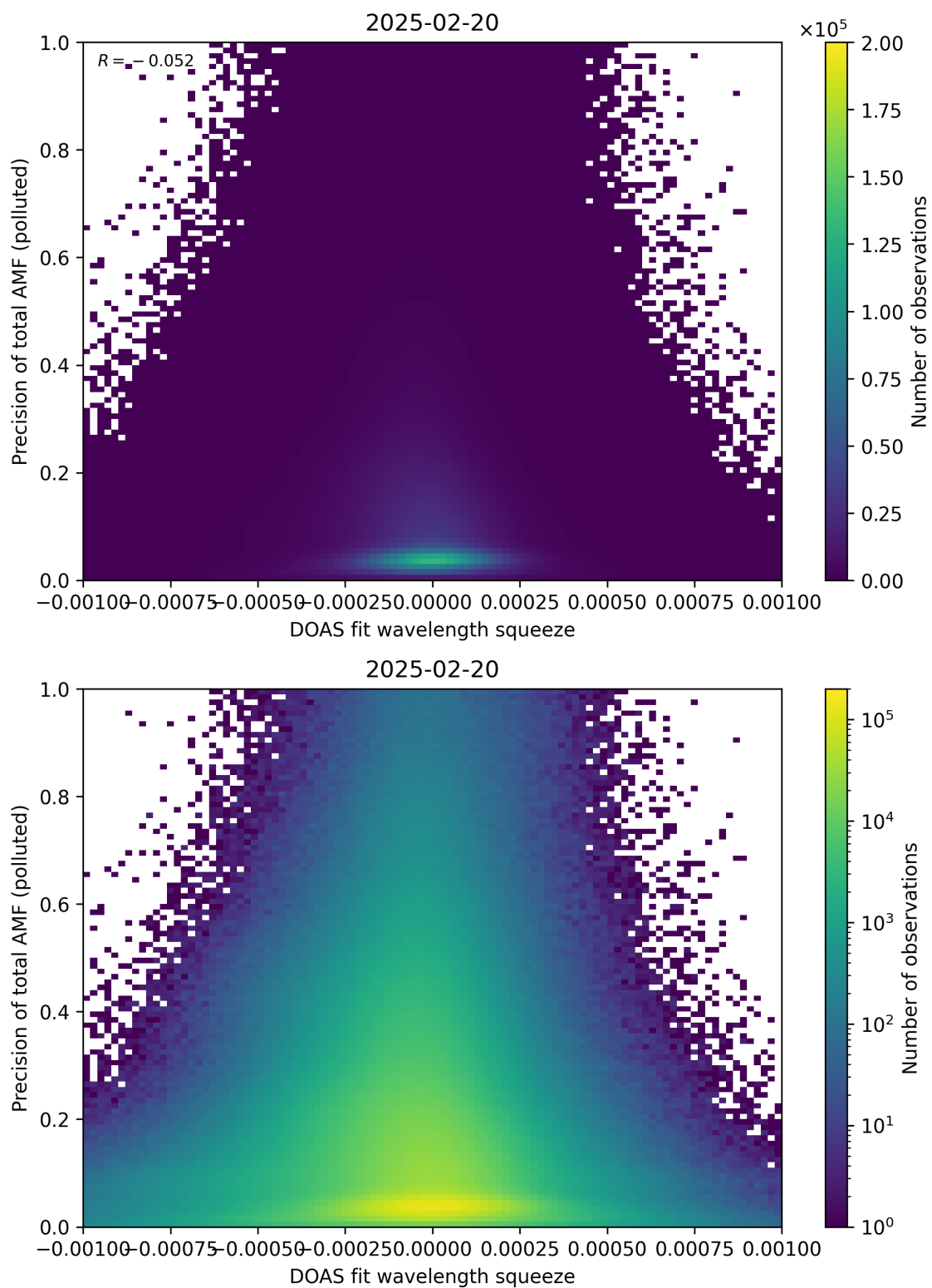
Figure 146: Scatter density plot of “DOAS fit wavelength squeeze” against “Precision of total AMF (polluted)” for 2025-02-19 to 2025-02-21.
