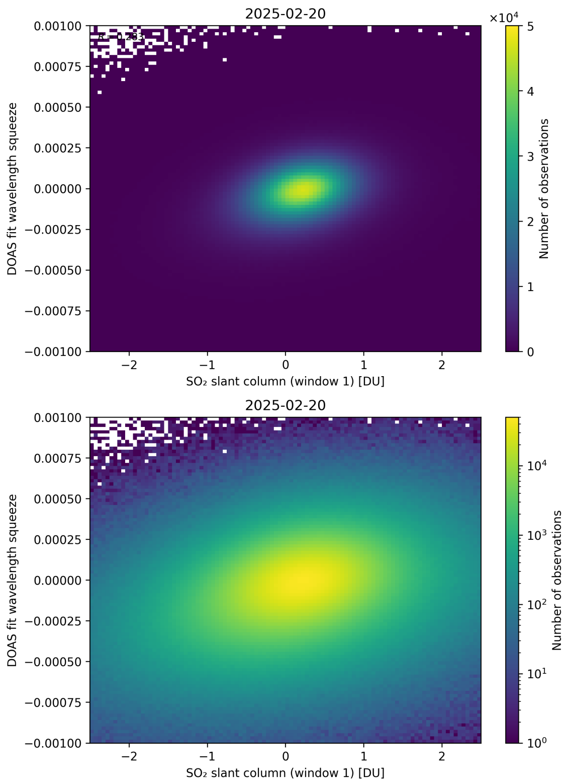
Figure 266: Scatter density plot of “SO 2 slant column (window 1)” against “DOAS fit wavelength squeeze” for 2025-02-19 to 2025-02-21.
