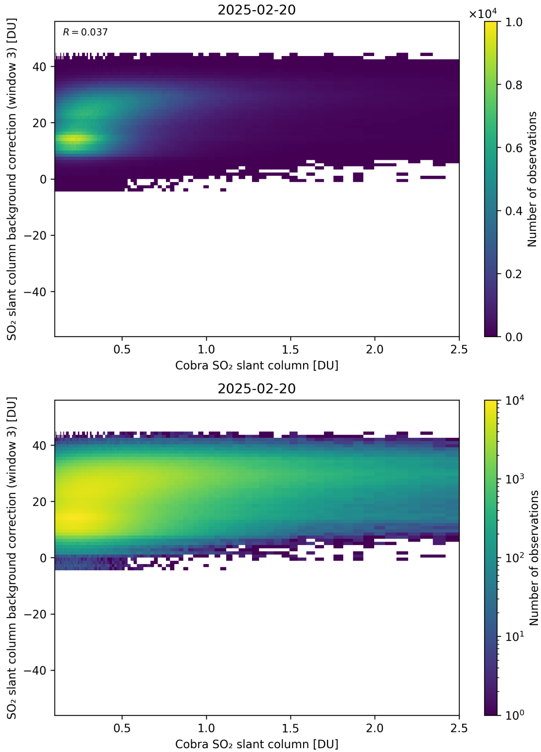
Figure 195: Scatter density plot of “Cobra SO 2 slant column” against “SO 2 slant column background correction (window 3)” for 2025-02-19 to 2025-02-21.
