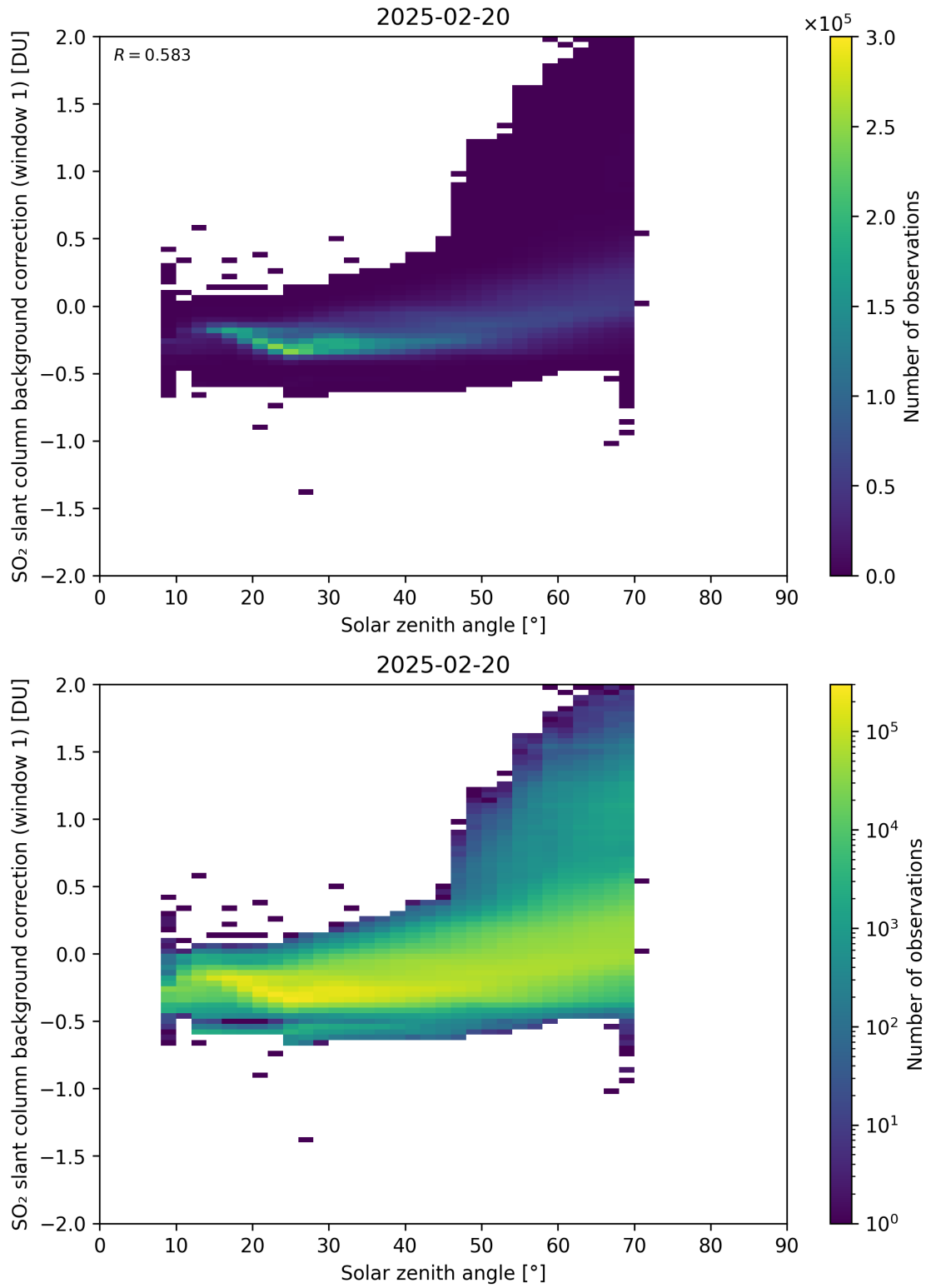
Figure 171: Scatter density plot of “Solar zenith angle” against “SO 2 slant column background correction (window 1)” for 2025-02-19 to 2025-02-21.
