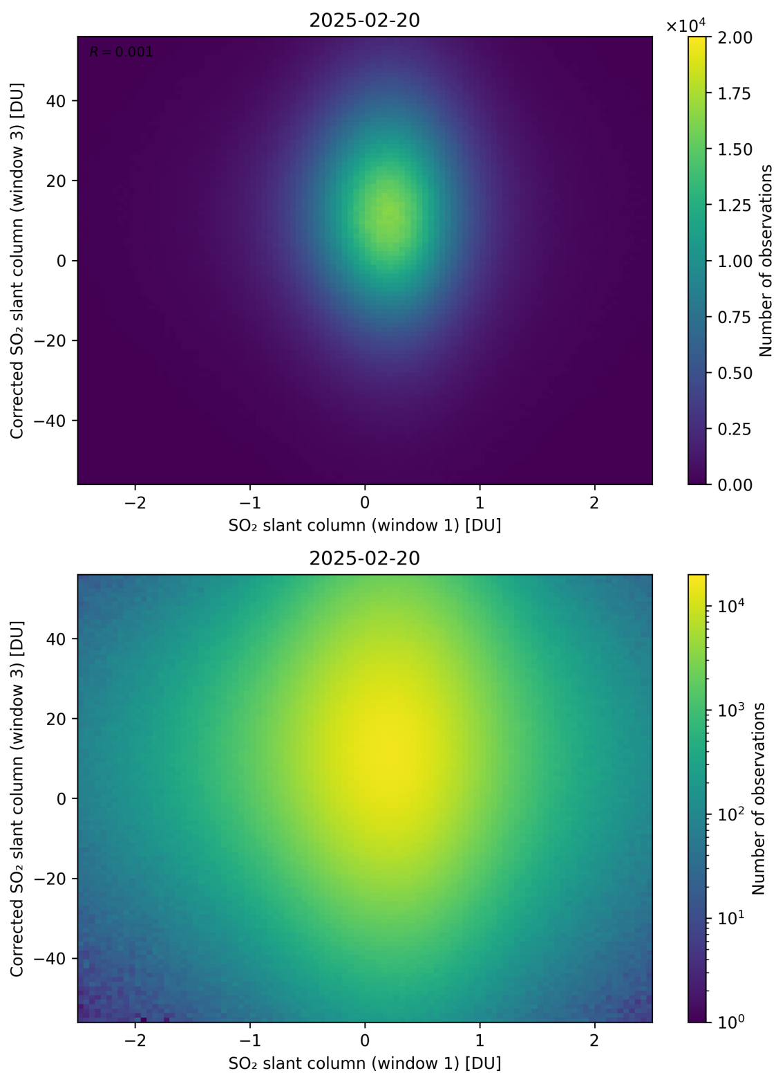
Figure 284: Scatter density plot of “SO 2 slant column (window 1)” against “Corrected SO 2 slant column (window 3)” for 2025-02-19 to 2025-02-21.
