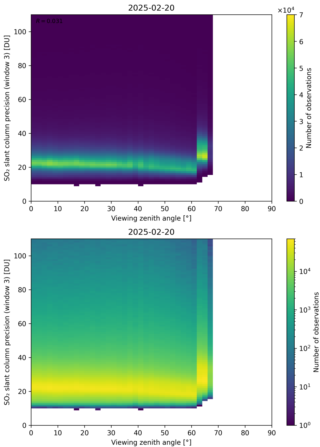
Figure 380: Scatter density plot of “Viewing zenith angle” against “SO 2 slant column precision (window 3)” for 2025-02-19 to 2025-02-21.
