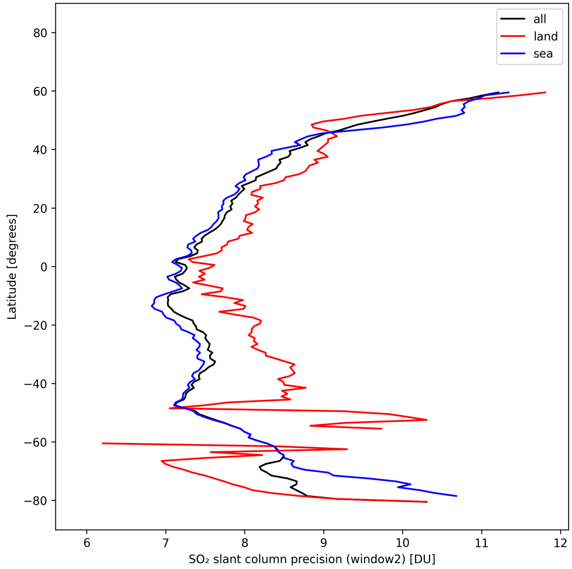
Figure 42: Zonal average of “SO 2 slant column precision (window2)” for 2025-02-19 to 2025-02-21.
