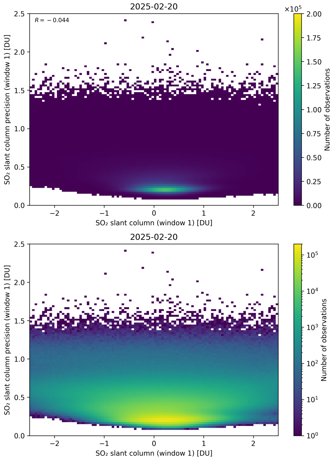
Figure 285: Scatter density plot of “SO 2 slant column (window 1)” against “SO 2 slant column precision (window 1)” for 2025-02-19 to 2025-02-21.
