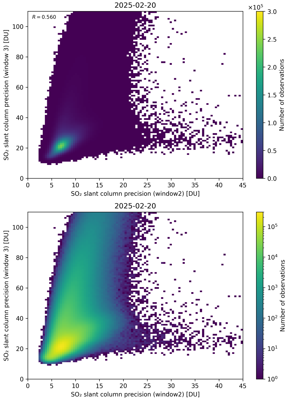
Figure 300: Scatter density plot of “SO 2 slant column precision (window2)” against “SO 2 slant column precision (window 3)” for 2025-02-19 to 2025-02-21.
