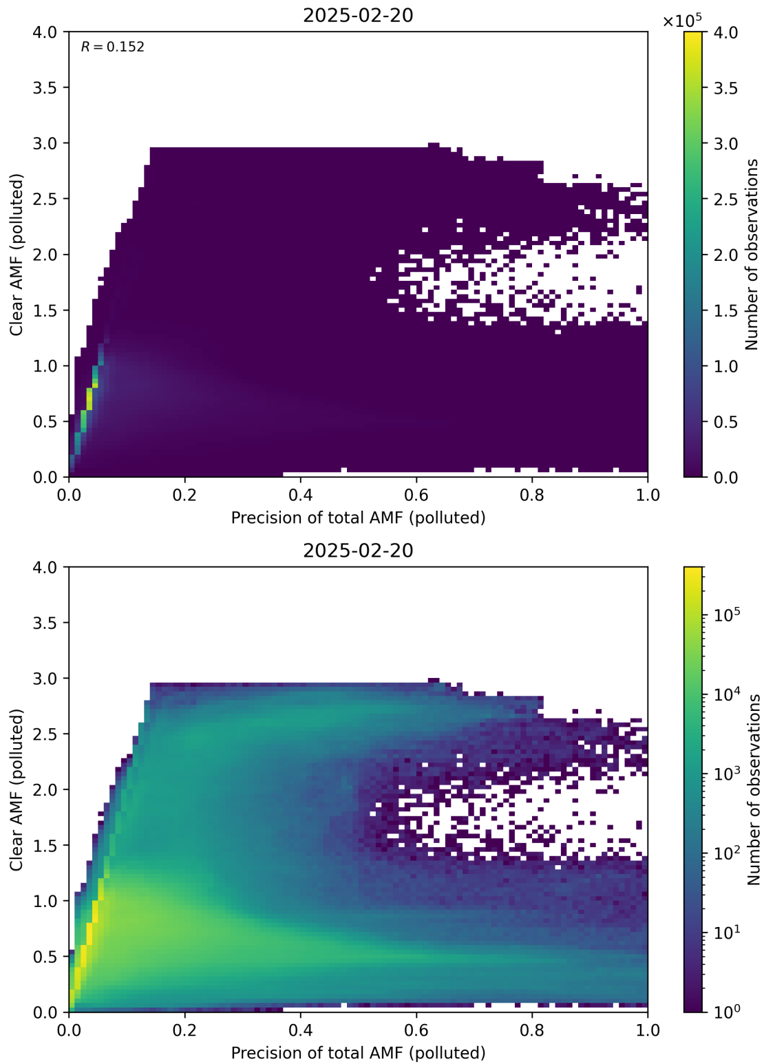
Figure 320: Scatter density plot of “Precision of total AMF (polluted)” against “Clear AMF (polluted)” for 2025-02-19 to 2025-02-21.
