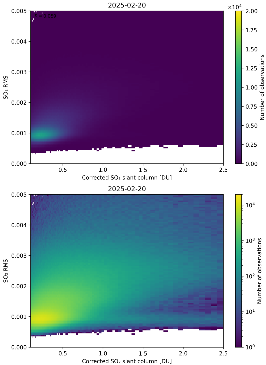
Figure 231: Scatter density plot of “Corrected SO 2 slant column” against “SO 2 RMS” for 2025-02-19 to 2025-02-21.
