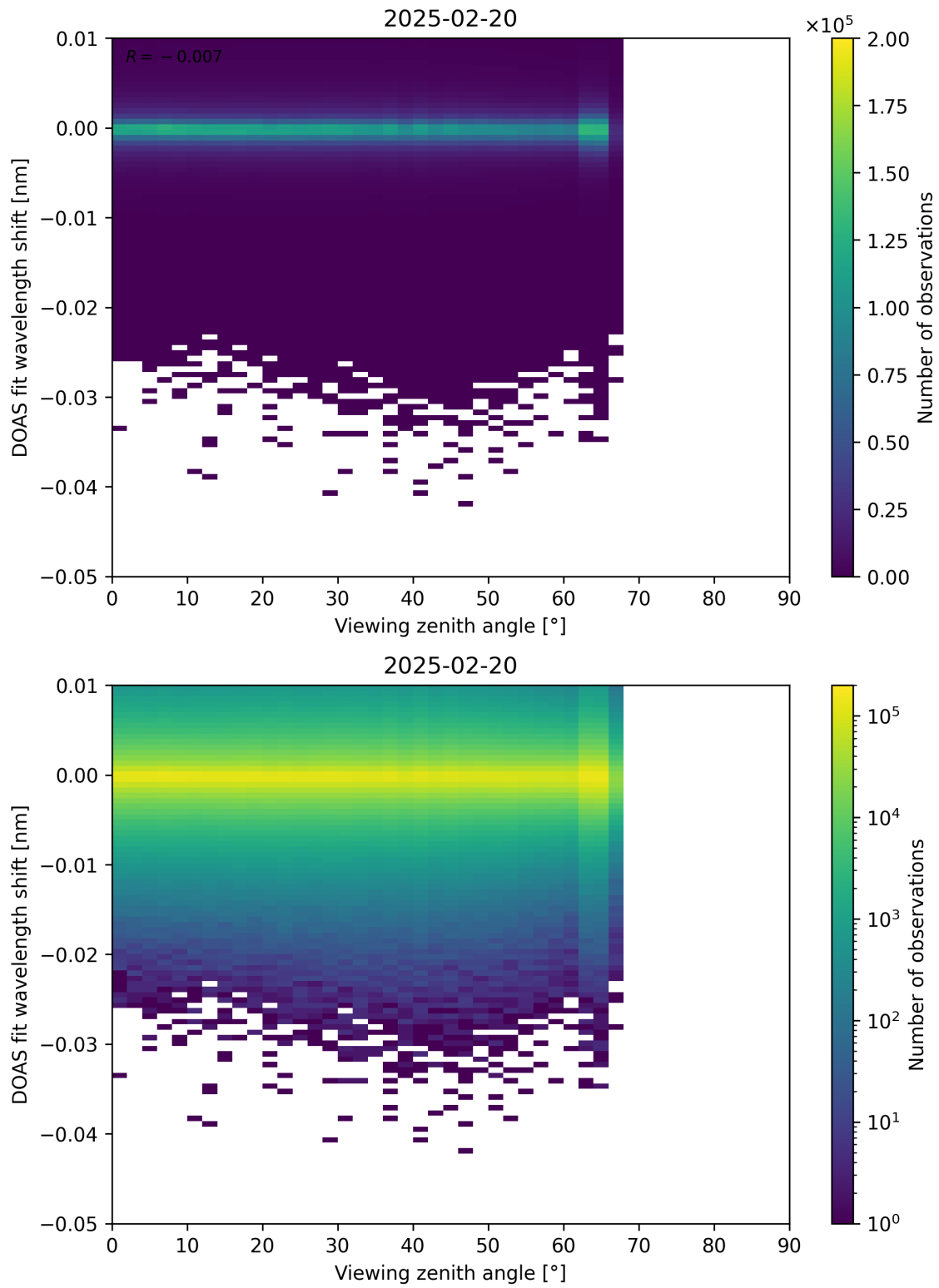
Figure 365: Scatter density plot of “Viewing zenith angle” against “DOAS fit wavelength shift” for 2025-02-19 to 2025-02-21.
