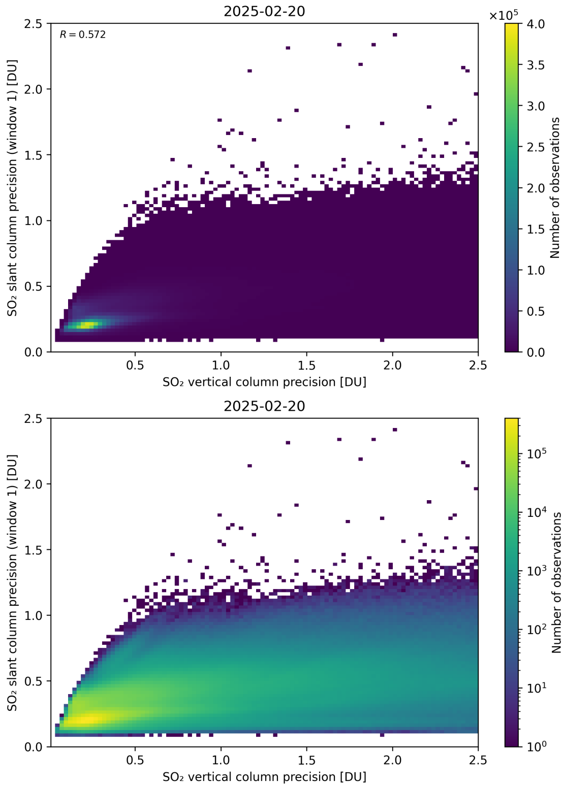
Figure 342: Scatter density plot of “SO 2 vertical column precision” against “SO 2 slant column precision (window 1)” for 2025-02-19 to 2025-02-21.
