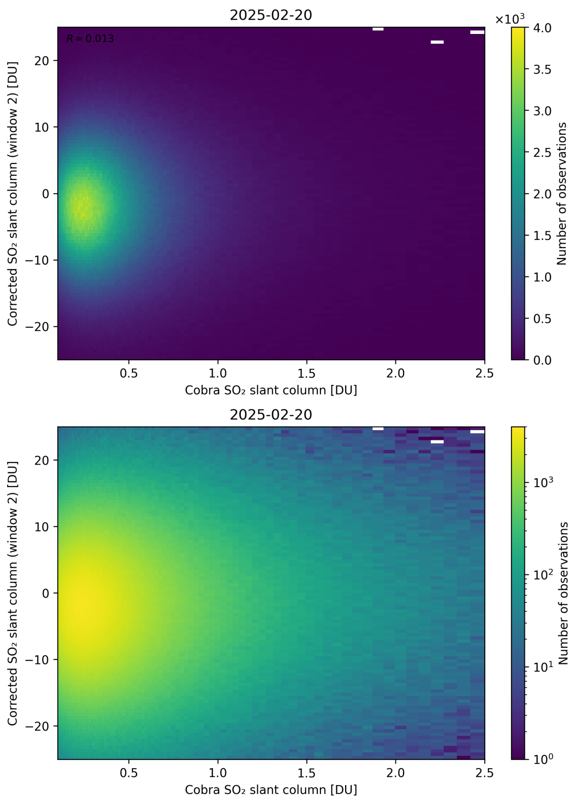
Figure 217: Scatter density plot of “Cobra SO 2 slant column” against “Corrected SO 2 slant column (window 2)” for 2025-02-19 to 2025-02-21.
