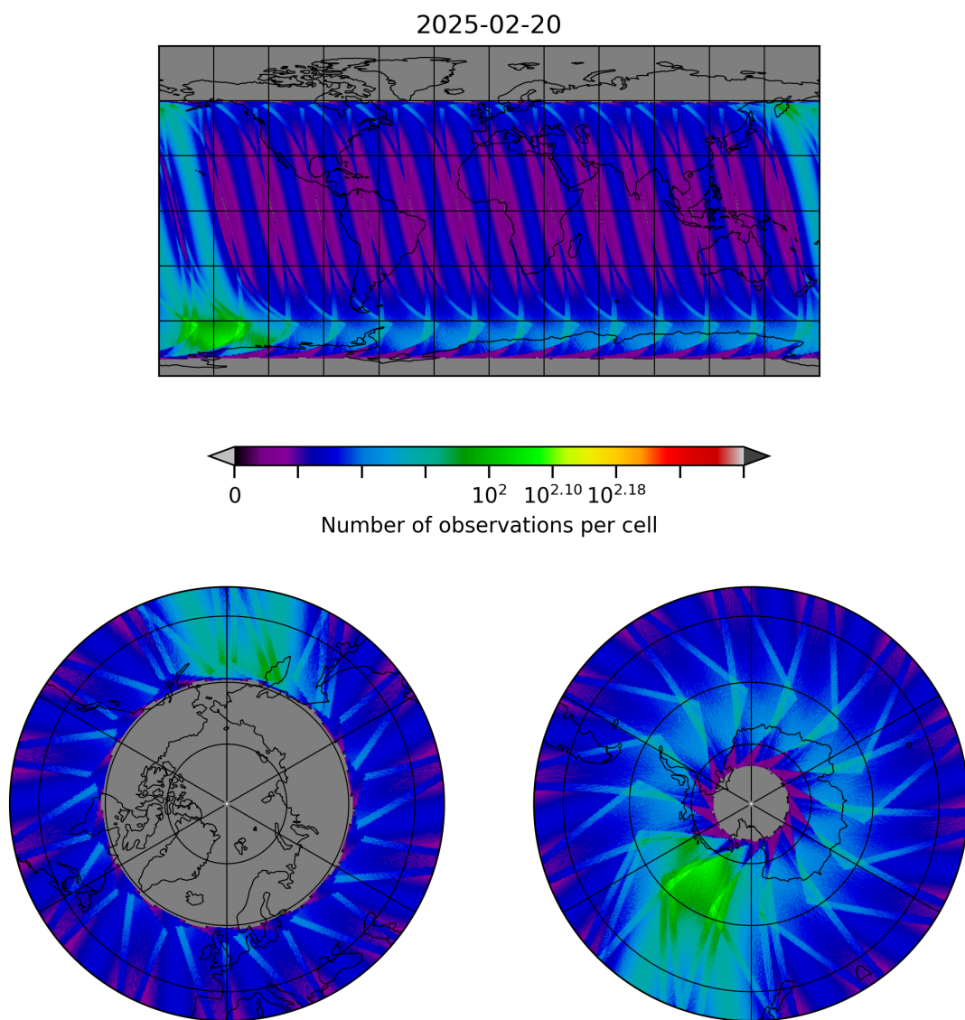
Figure 30: Map of the number of observations for 2025-02-19 to 2025-02-21
