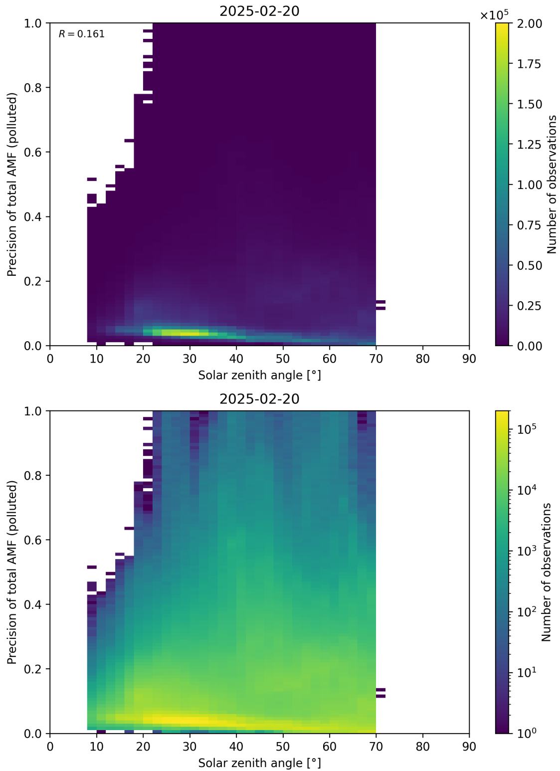
Figure 190: Scatter density plot of “Solar zenith angle” against “Precision of total AMF (polluted)” for 2025-02-19 to 2025-02-21.
