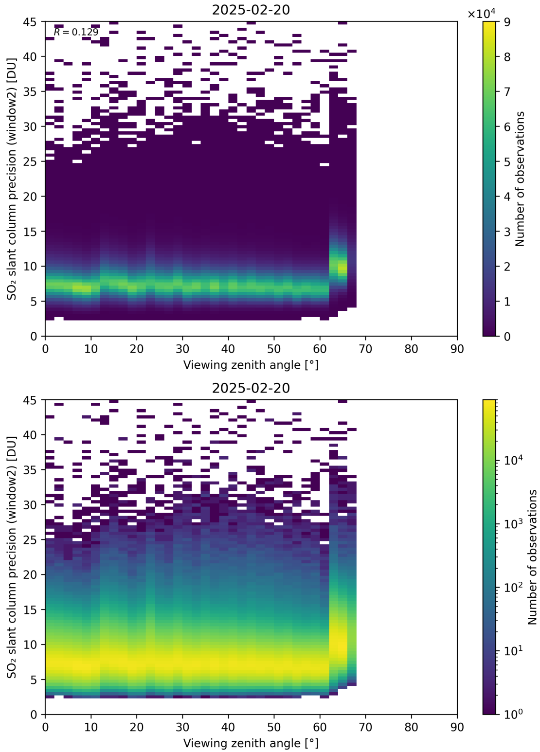
Figure 378: Scatter density plot of “Viewing zenith angle” against “SO 2 slant column precision (window2)” for 2025-02-19 to 2025-02-21.
