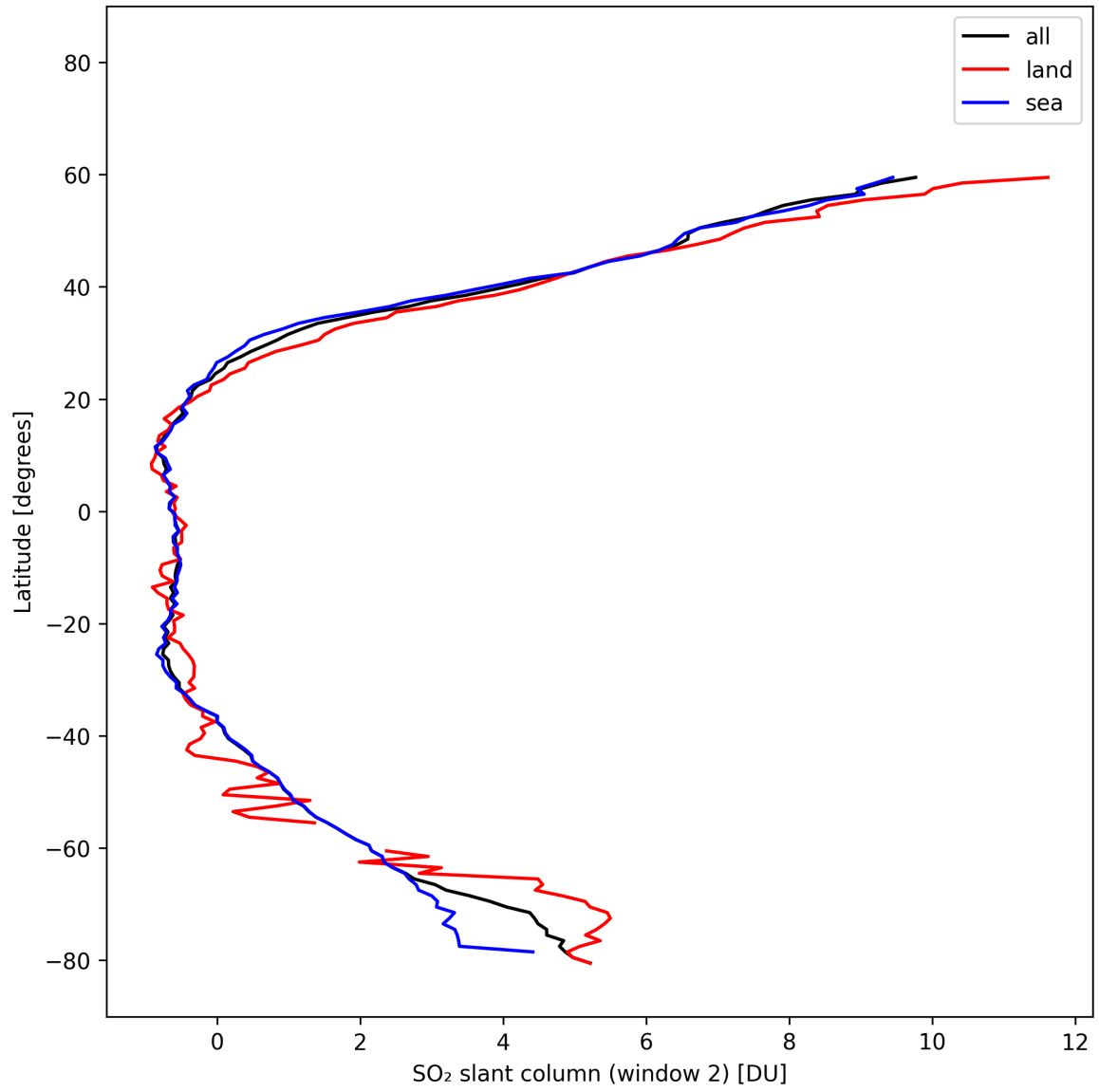
Figure 41: Zonal average of “SO 2 slant column (window 2)” for 2025-02-19 to 2025-02-21.
