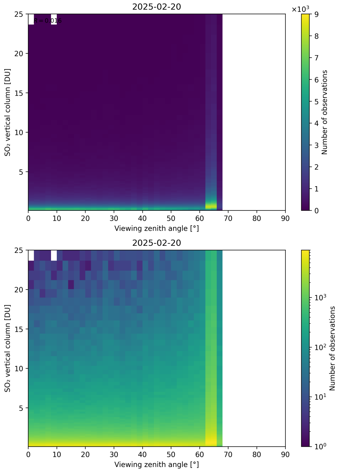
Figure 383: Scatter density plot of “Viewing zenith angle” against “SO 2 vertical column” for 2025-02-19 to 2025-02-21.
