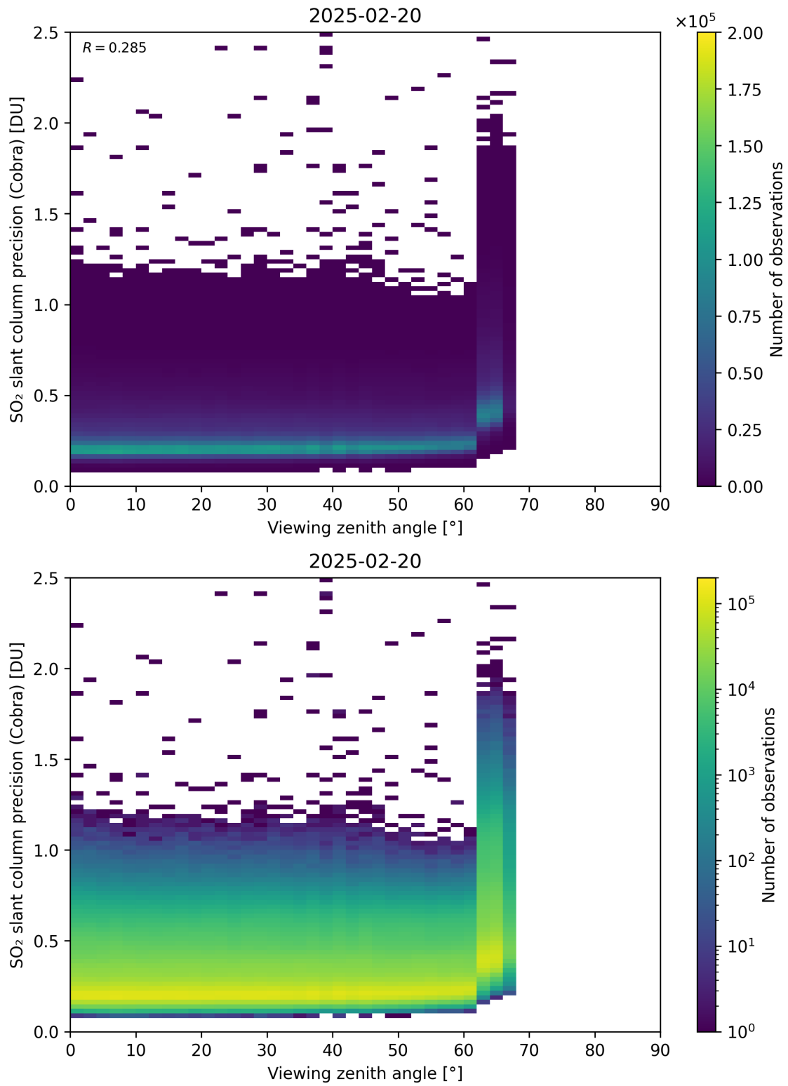
Figure 372: Scatter density plot of “Viewing zenith angle” against “SO 2 slant column precision (Cobra)” for 2025-02-19 to 2025-02-21.
