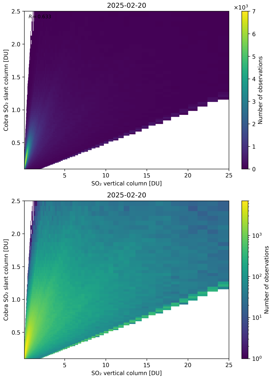
Figure 349: Scatter density plot of “SO 2 vertical column” against “Cobra SO 2 slant column” for 2025-02-19 to 2025-02-21.
