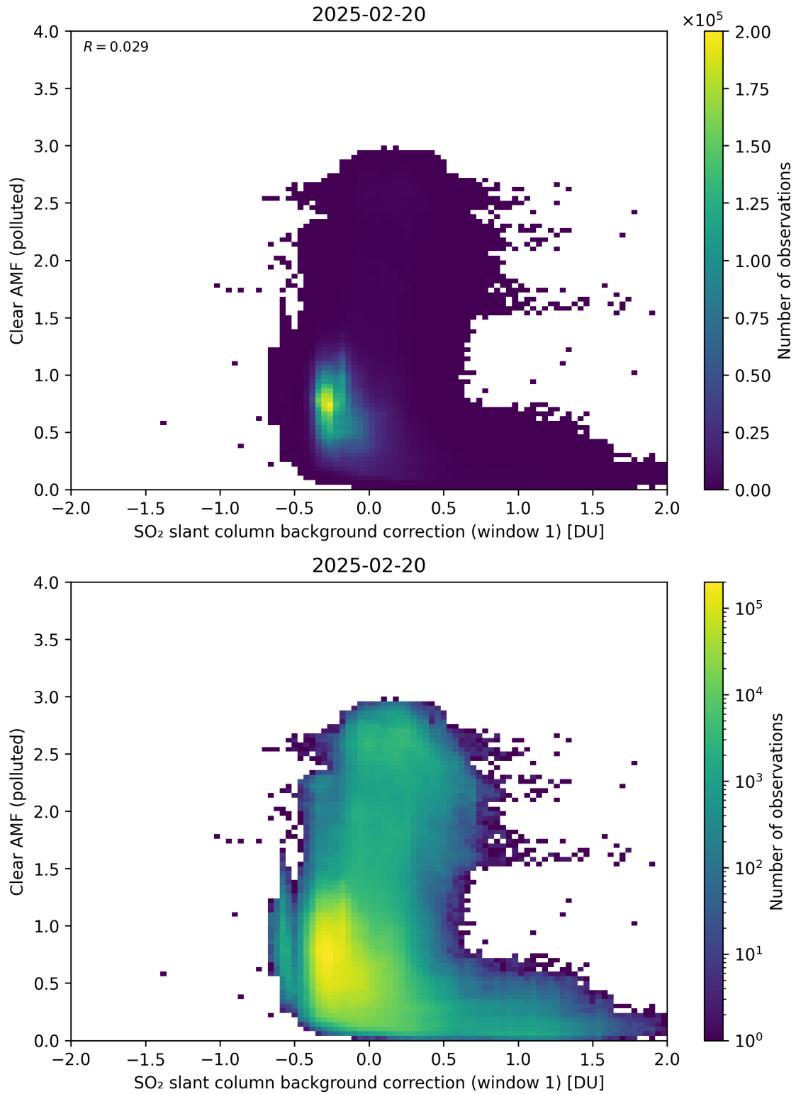
Figure 114: Scatter density plot of “SO 2 slant column background correction (window 1)” against “Clear AMF (polluted)” for 2025-02-19 to 2025-02-21.
