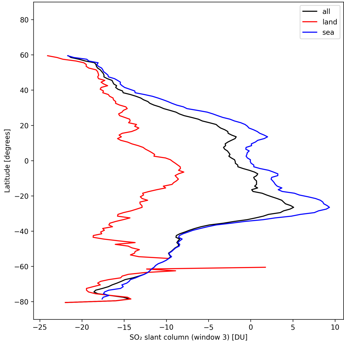
Figure 45: Zonal average of “SO 2 slant column (window 3)” for 2025-02-19 to 2025-02-21.
