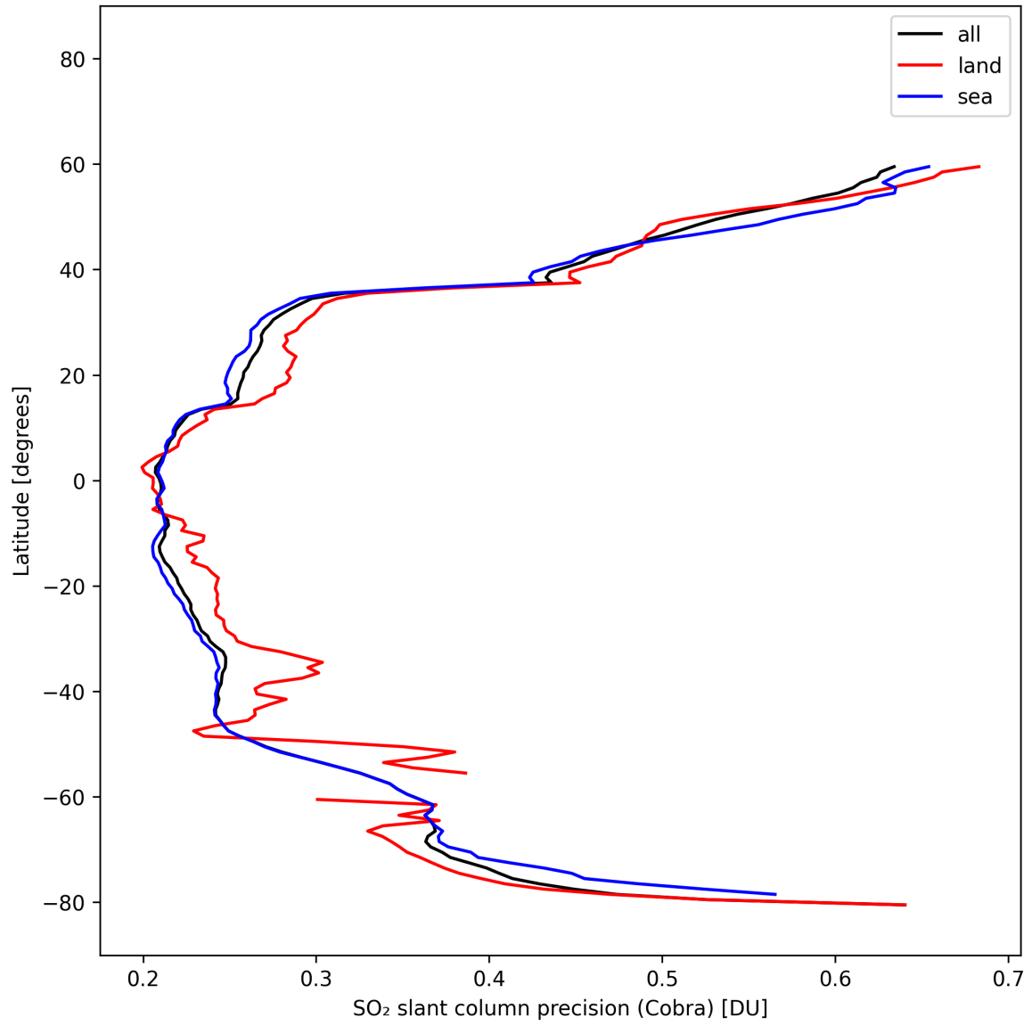
Figure 36: Zonal average of “SO 2 slant column precision (Cobra)” for 2025-02-19 to 2025-02-21.
