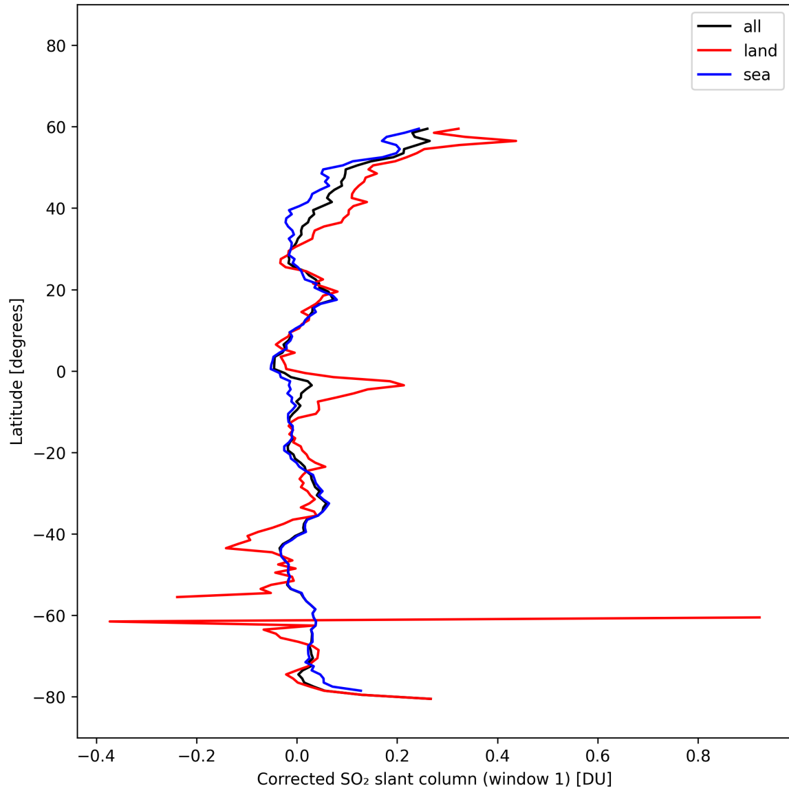
Figure 39: Zonal average of “Corrected SO 2 slant column (window 1)” for 2025-02-19 to 2025-02-21.
