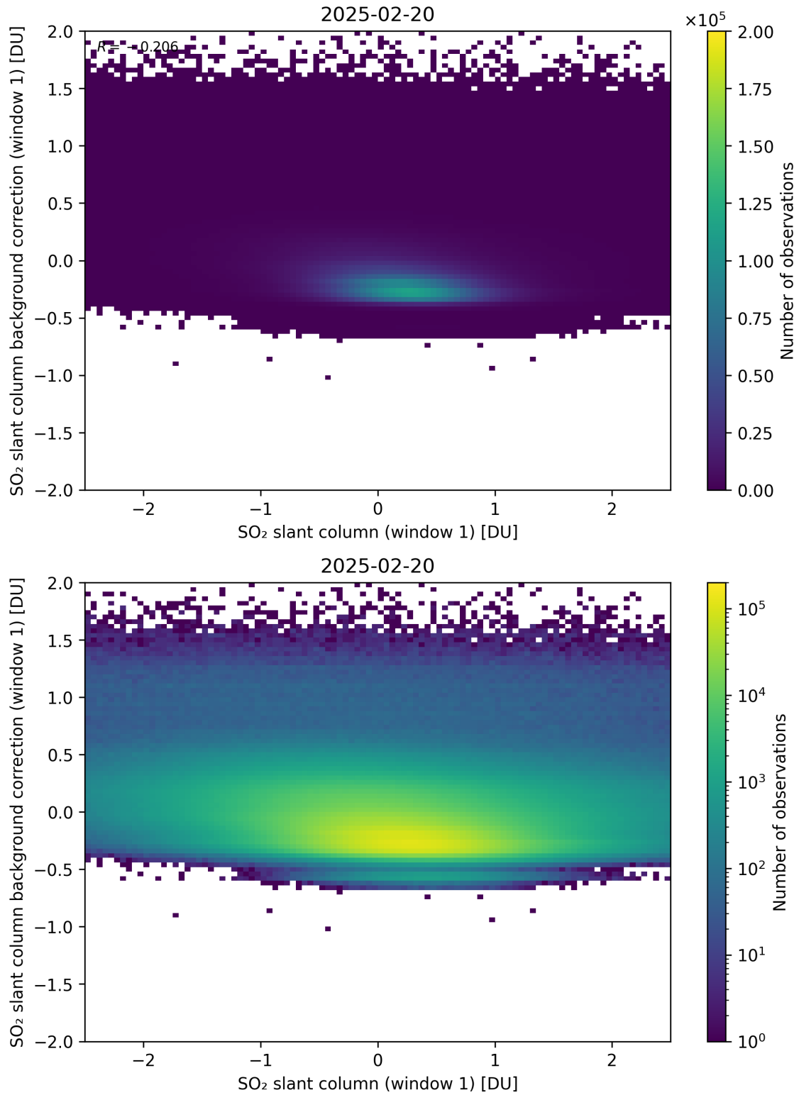
Figure 262: Scatter density plot of “SO 2 slant column (window 1)” against “SO 2 slant column background correction (window 1)” for 2025-02-19 to 2025-02-21.
