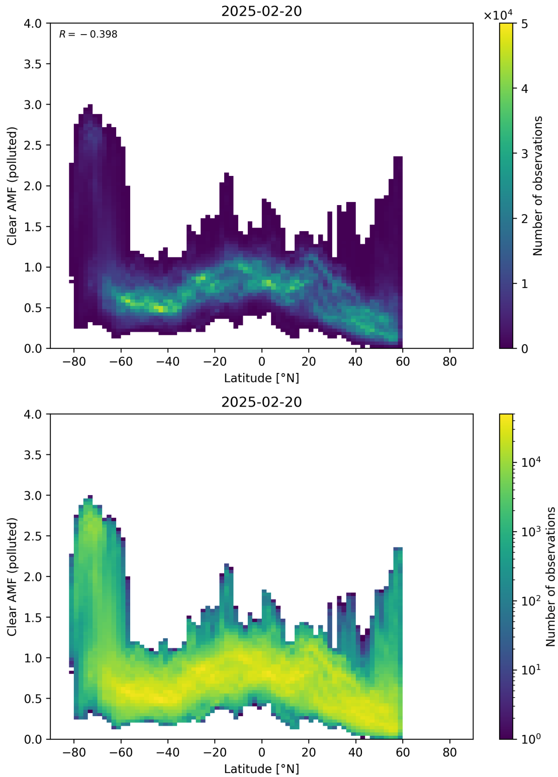
Figure 156: Scatter density plot of “Latitude” against “Clear AMF (polluted)” for 2025-02-19 to 2025-02-21.
