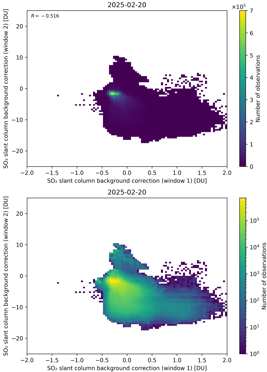
Figure 109: Scatter density plot of “SO 2 slant column background correction (window 1)” against “SO 2 slant column background correction (window 2)” for 2025-02-19 to 2025-02-21.
