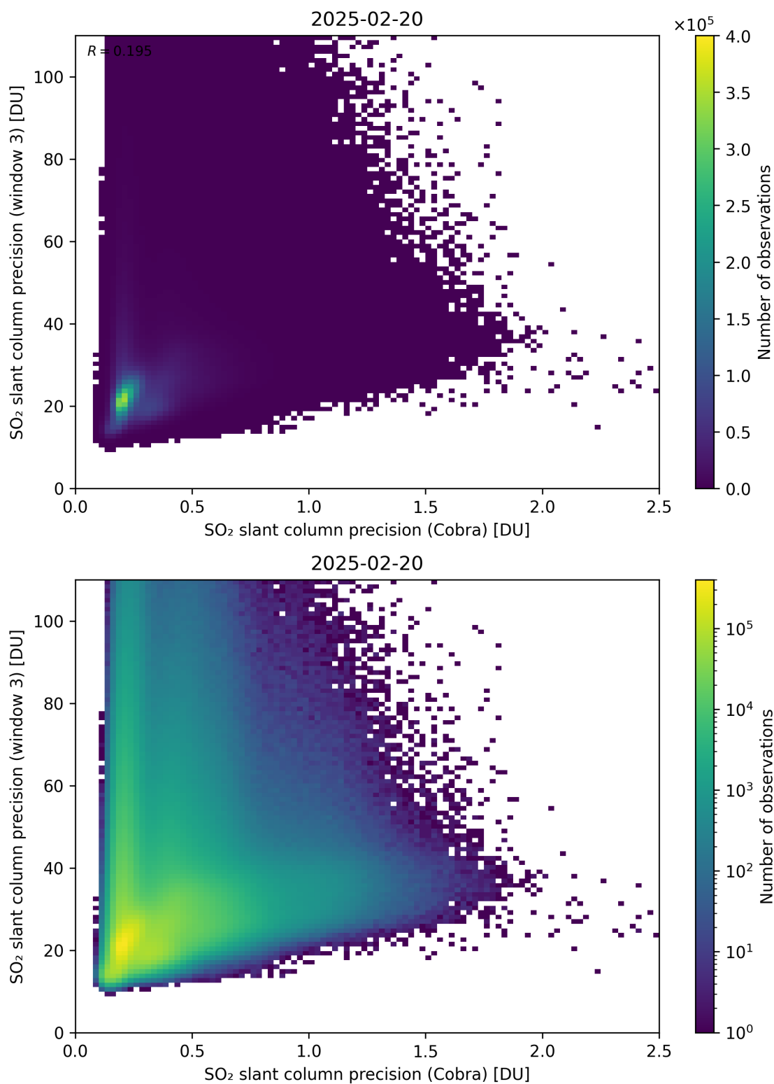
Figure 212: Scatter density plot of “SO 2 slant column precision (Cobra)” against “SO 2 slant column precision (window 3)” for 2025-02-19 to 2025-02-21.
