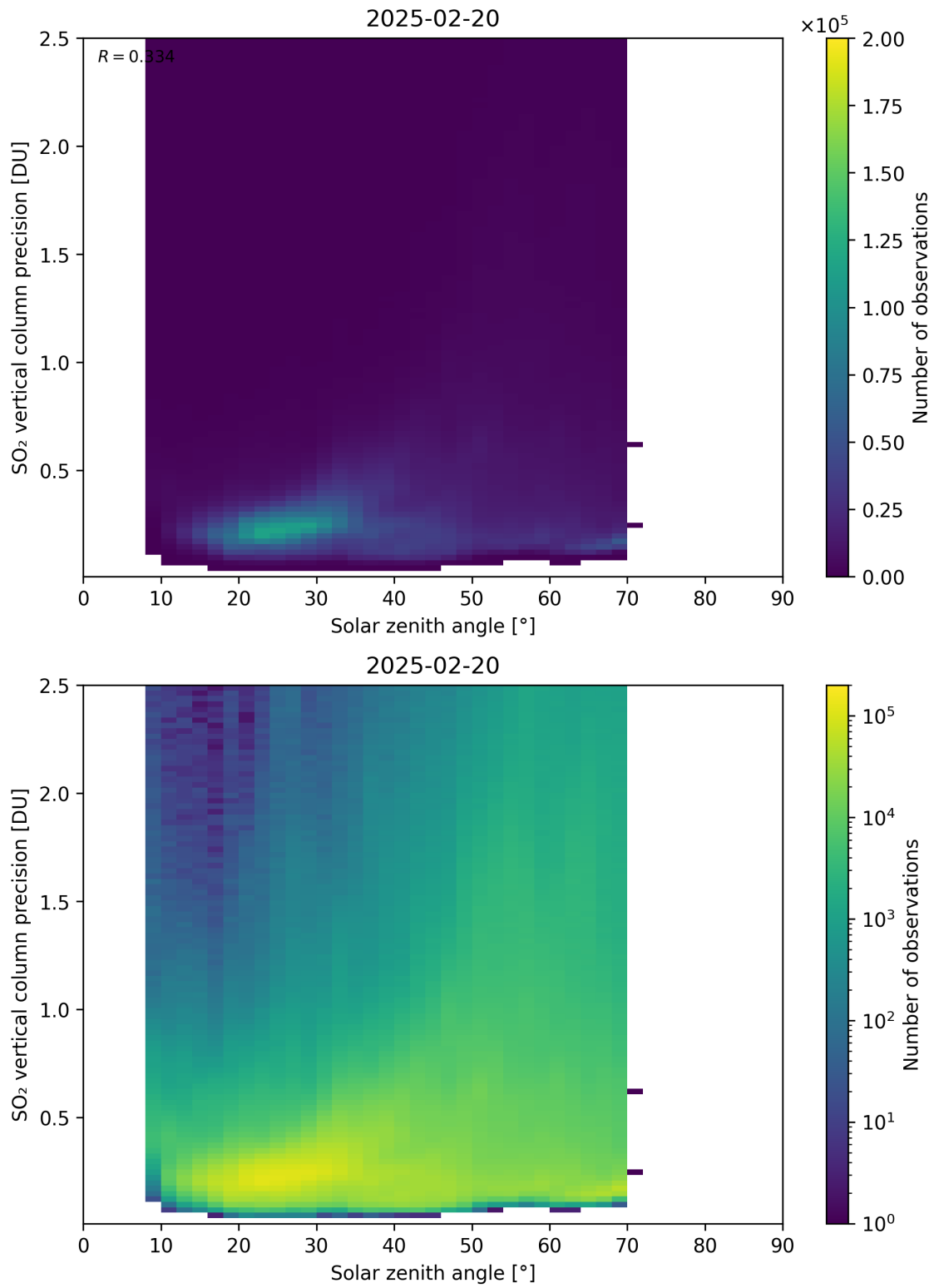
Figure 192: Scatter density plot of “Solar zenith angle” against “SO 2 vertical column precision” for 2025-02-19 to 2025-02-21.
