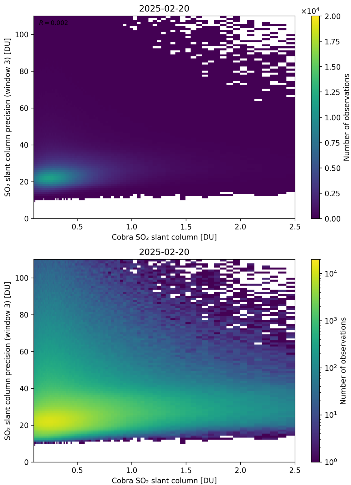
Figure 223: Scatter density plot of “Cobra SO 2 slant column” against “SO 2 slant column precision (window 3)” for 2025-02-19 to 2025-02-21.
