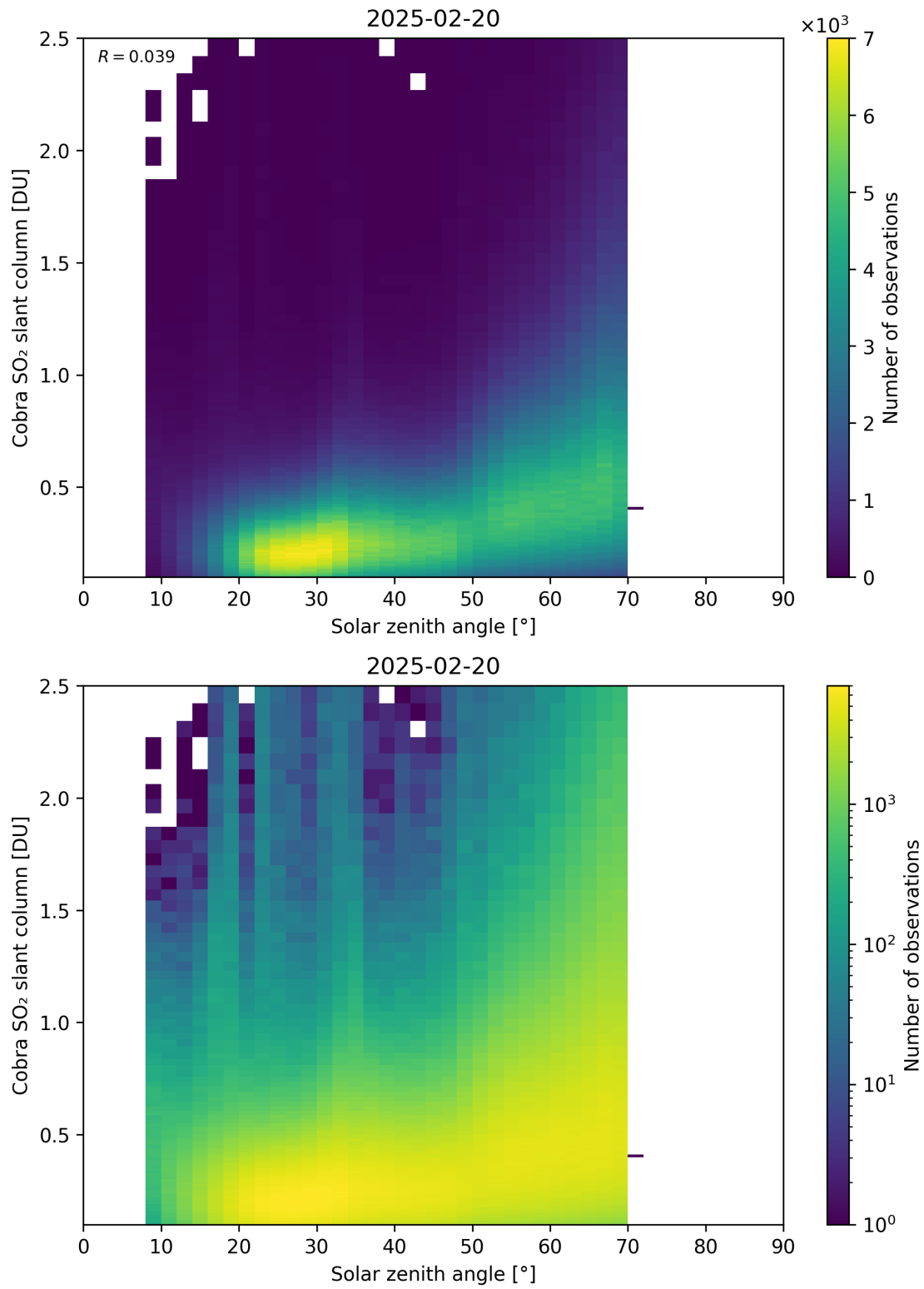
Figure 179: Scatter density plot of “Solar zenith angle” against “Cobra SO 2 slant column” for 2025-02-19 to 2025-02-21.
