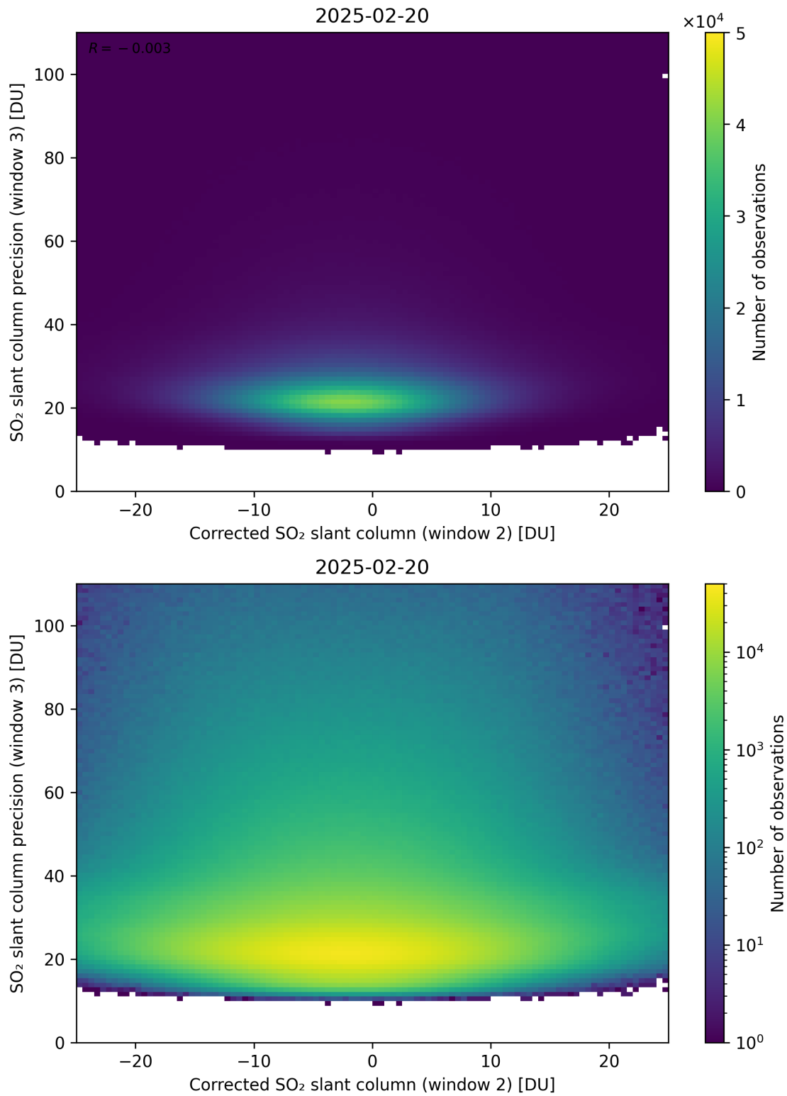
Figure 252: Scatter density plot of “Corrected SO 2 slant column (window 2)” against “SO 2 slant column precision (window 3)” for 2025-02-19 to 2025-02-21.
