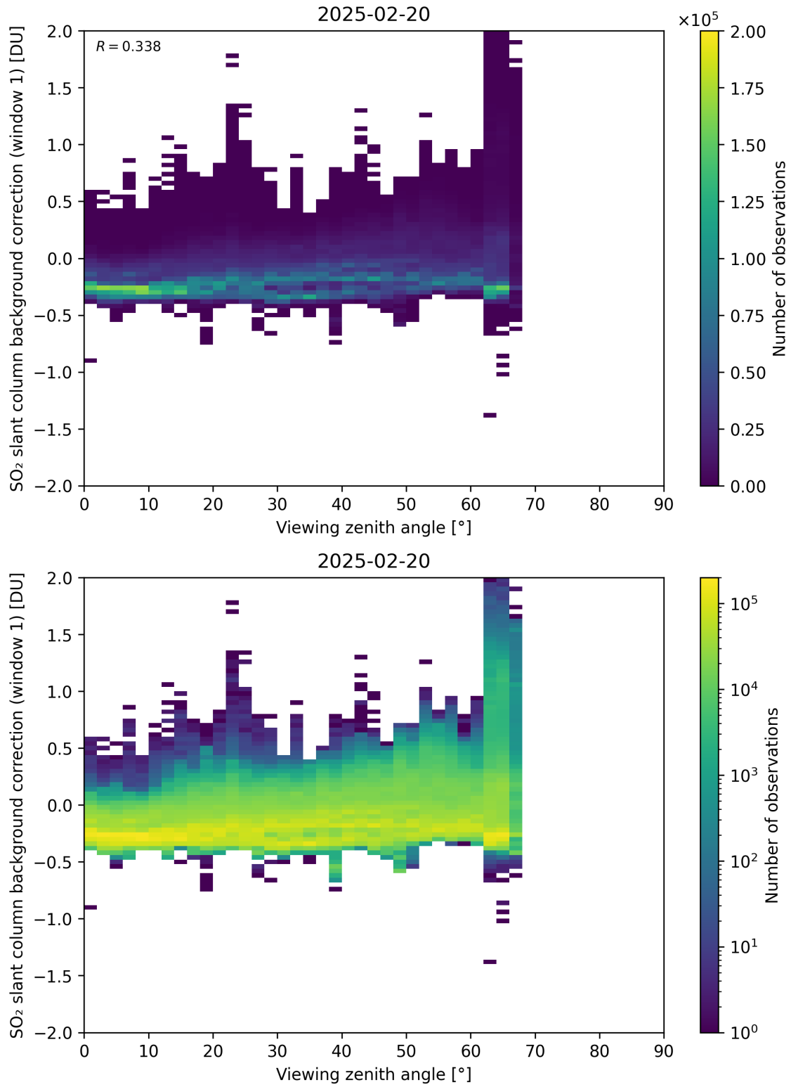
Figure 362: Scatter density plot of “Viewing zenith angle” against “SO 2 slant column background correction (window 1)” for 2025-02-19 to 2025-02-21.
