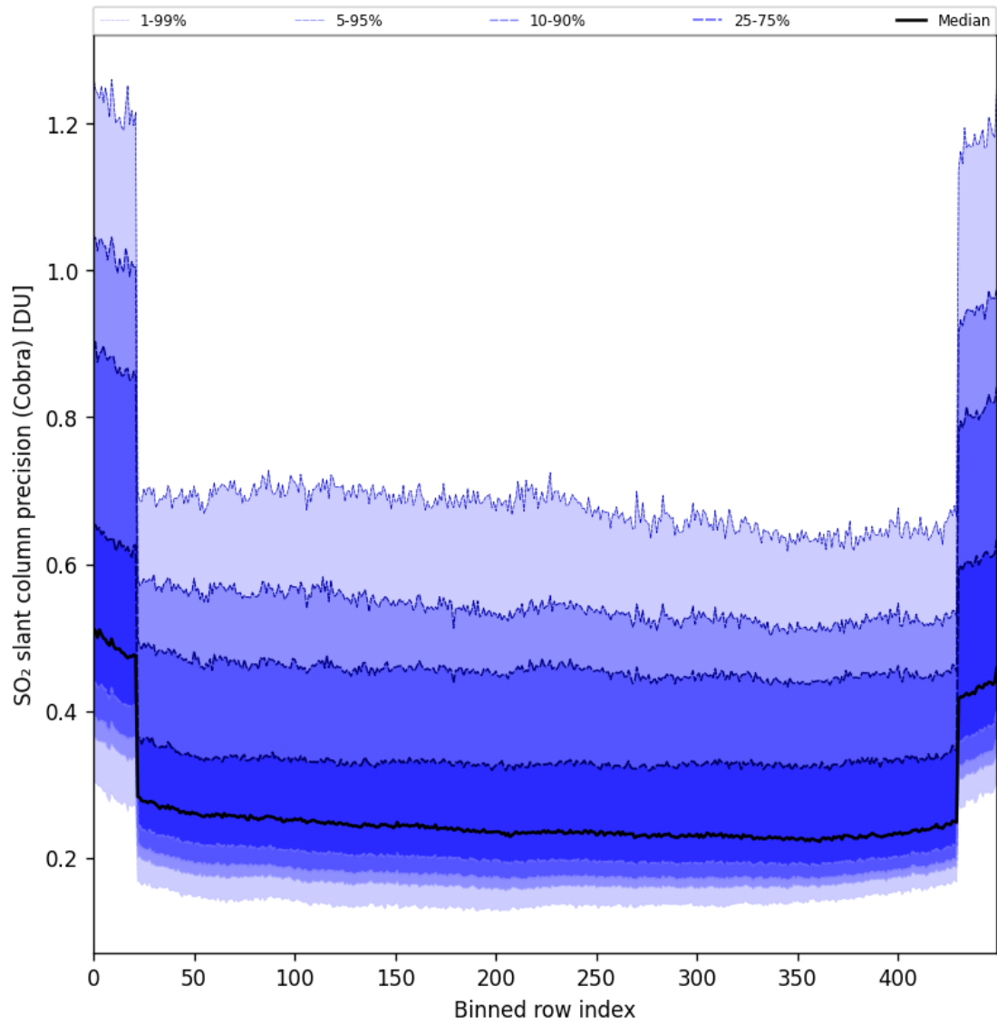
Figure 88: Along track statistics of "SO 2 slant column precision (Cobra)" for 2025-02-19 to 2025-02-21
