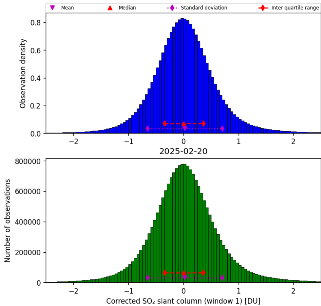
Figure 65: Histogram of “Corrected SO 2 slant column (window 1)” for 2025-02-19 to 2025-02-21
