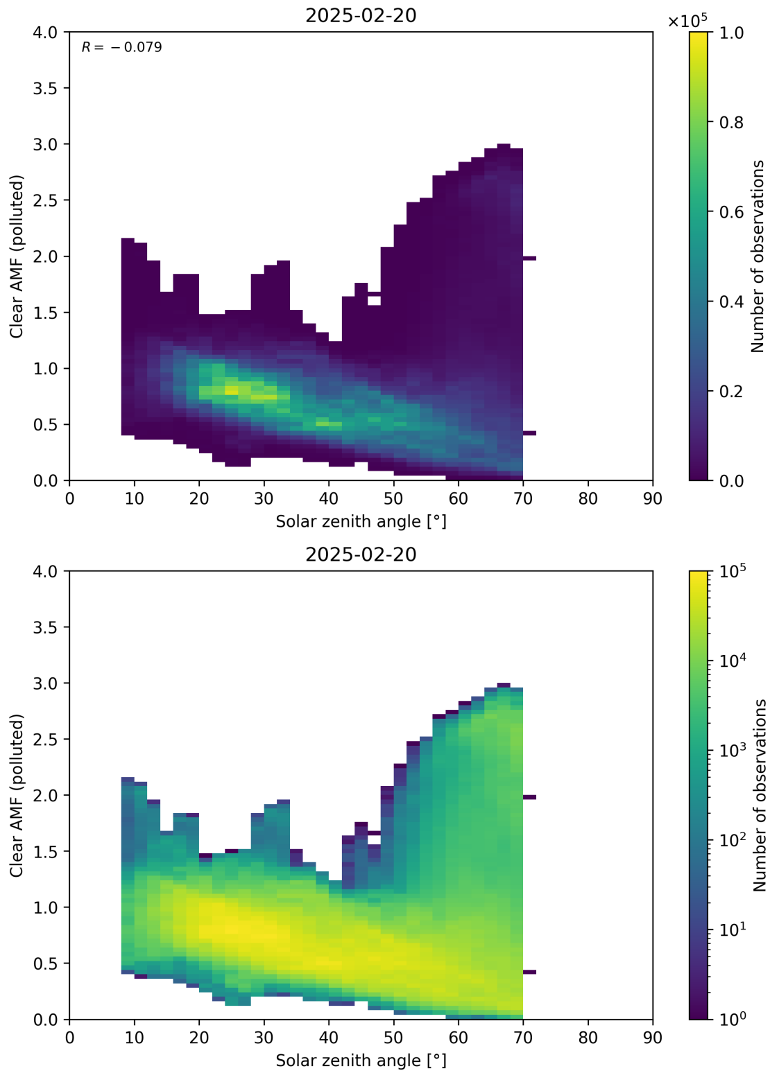
Figure 178: Scatter density plot of “Solar zenith angle” against “Clear AMF (polluted)” for 2025-02-19 to 2025-02-21.
