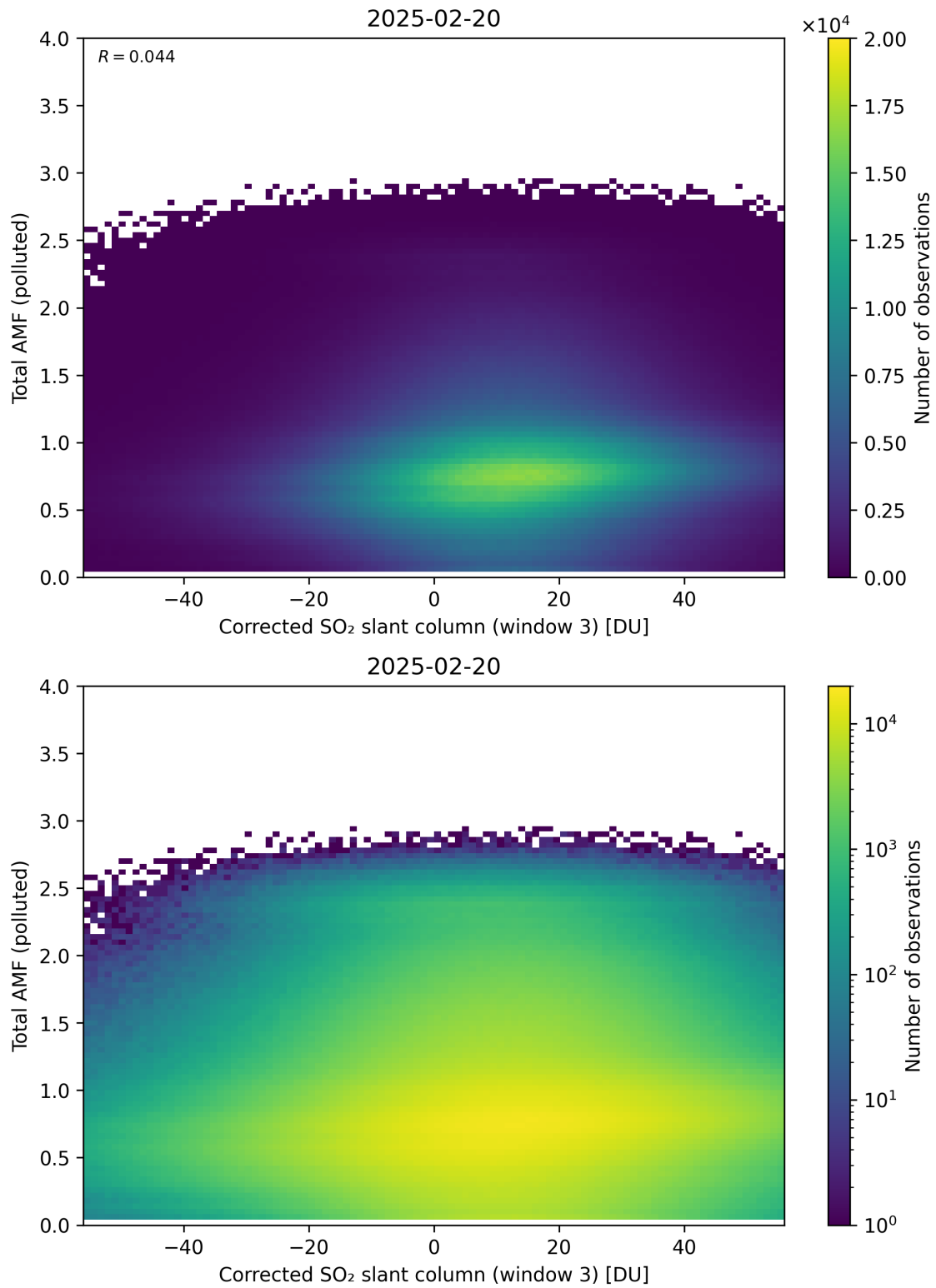
Figure 260: Scatter density plot of “Corrected SO 2 slant column (window 3)” against “Total AMF (polluted)” for 2025-02-19 to 2025-02-21.
