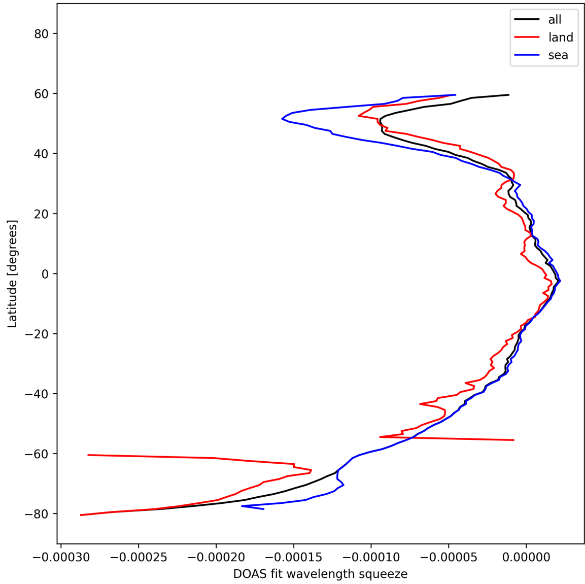
Figure 51: Zonal average of “DOAS fit wavelength squeeze” for 2025-02-19 to 2025-02-21.
