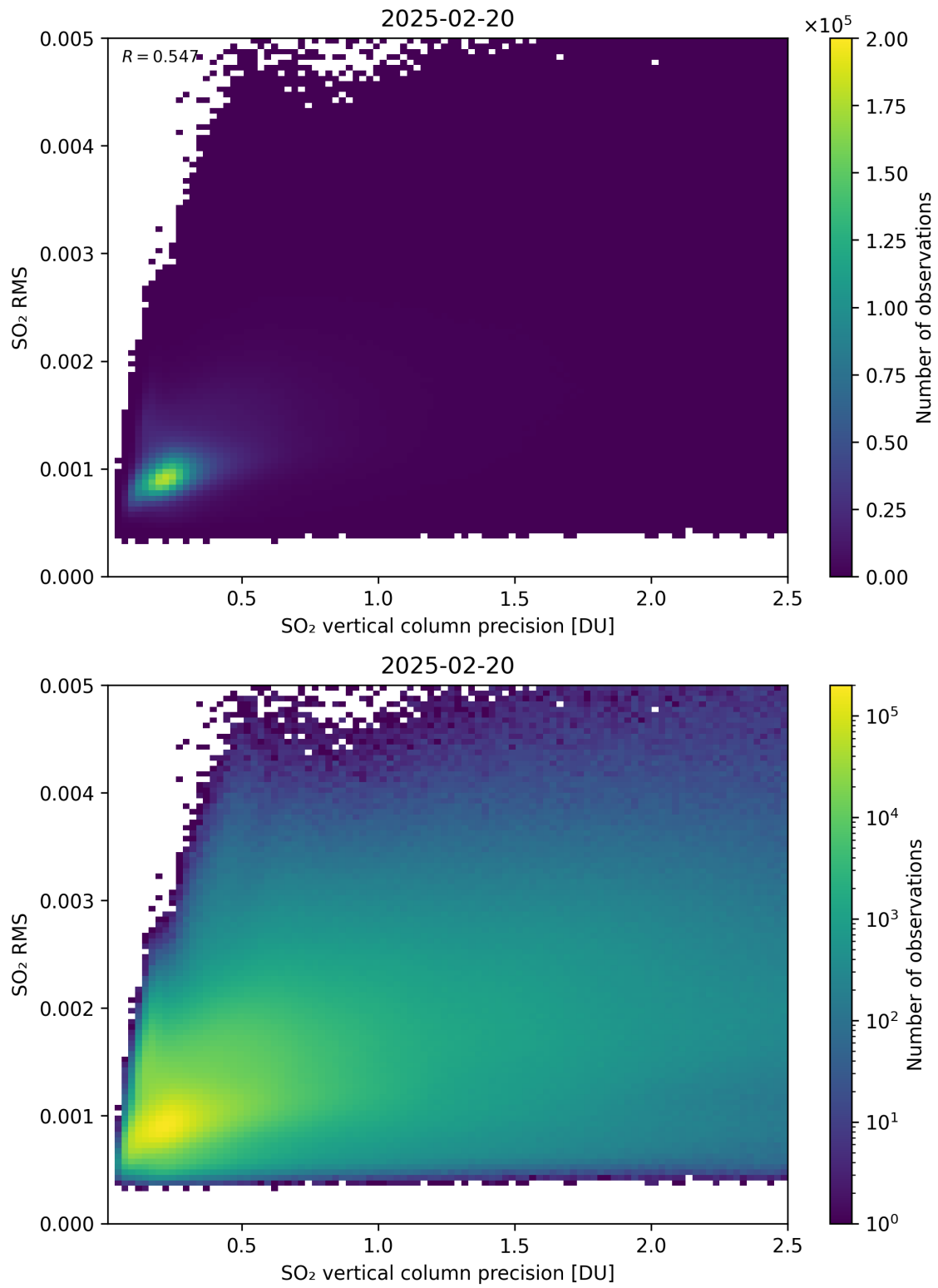
Figure 334: Scatter density plot of “SO 2 vertical column precision” against “SO 2 RMS” for 2025-02-19 to 2025-02-21.
