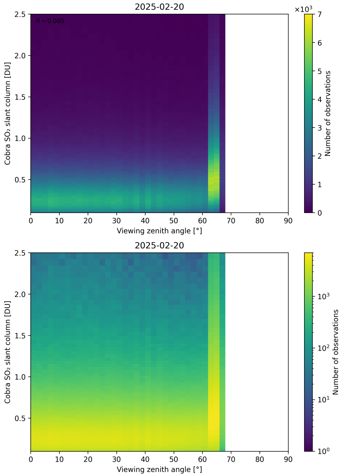
Figure 371: Scatter density plot of “Viewing zenith angle” against “Cobra SO 2 slant column” for 2025-02-19 to 2025-02-21.
