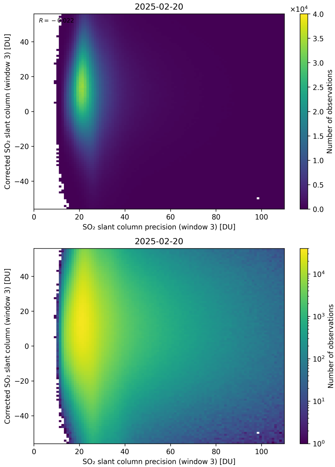
Figure 312: Scatter density plot of “SO 2 slant column precision (window 3)” against “Corrected SO 2 slant column (window 3)” for 2025-02-19 to 2025-02-21.
