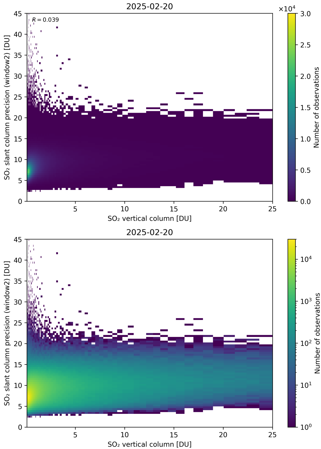
Figure 356: Scatter density plot of “SO 2 vertical column” against “SO 2 slant column precision (window2)” for 2025-02-19 to 2025-02-21.
