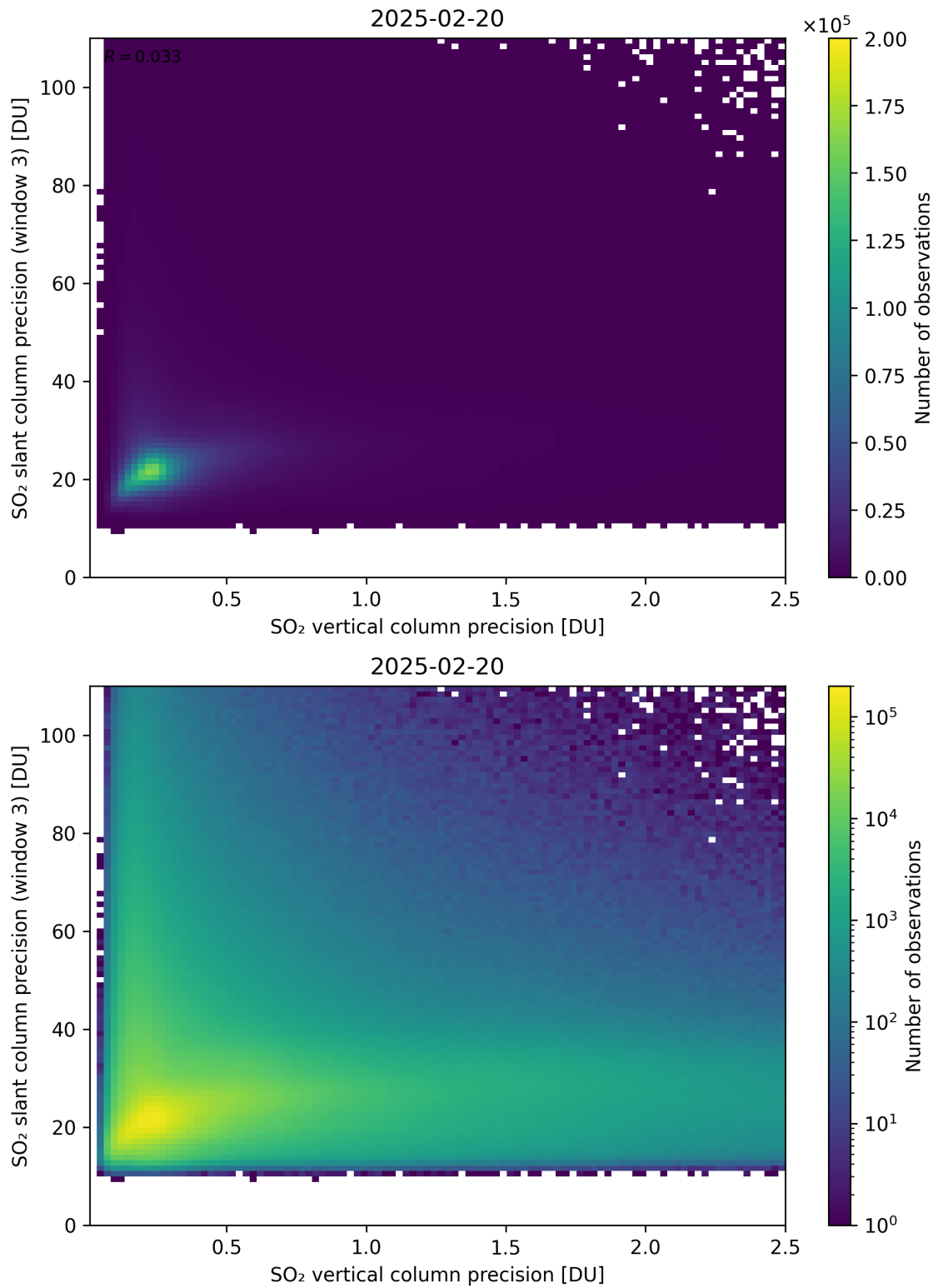
Figure 345: Scatter density plot of “SO 2 vertical column precision” against “SO 2 slant column precision (window 3)” for 2025-02-19 to 2025-02-21.
