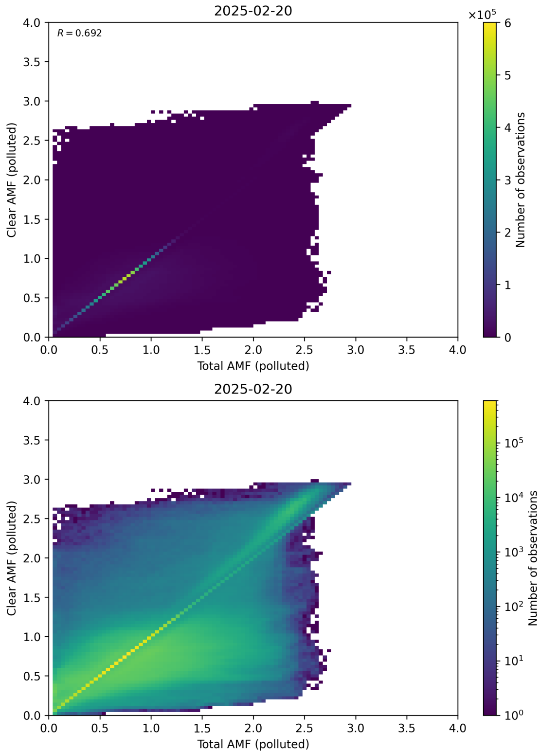
Figure 321: Scatter density plot of “Total AMF (polluted)” against “Clear AMF (polluted)” for 2025-02-19 to 2025-02-21.
