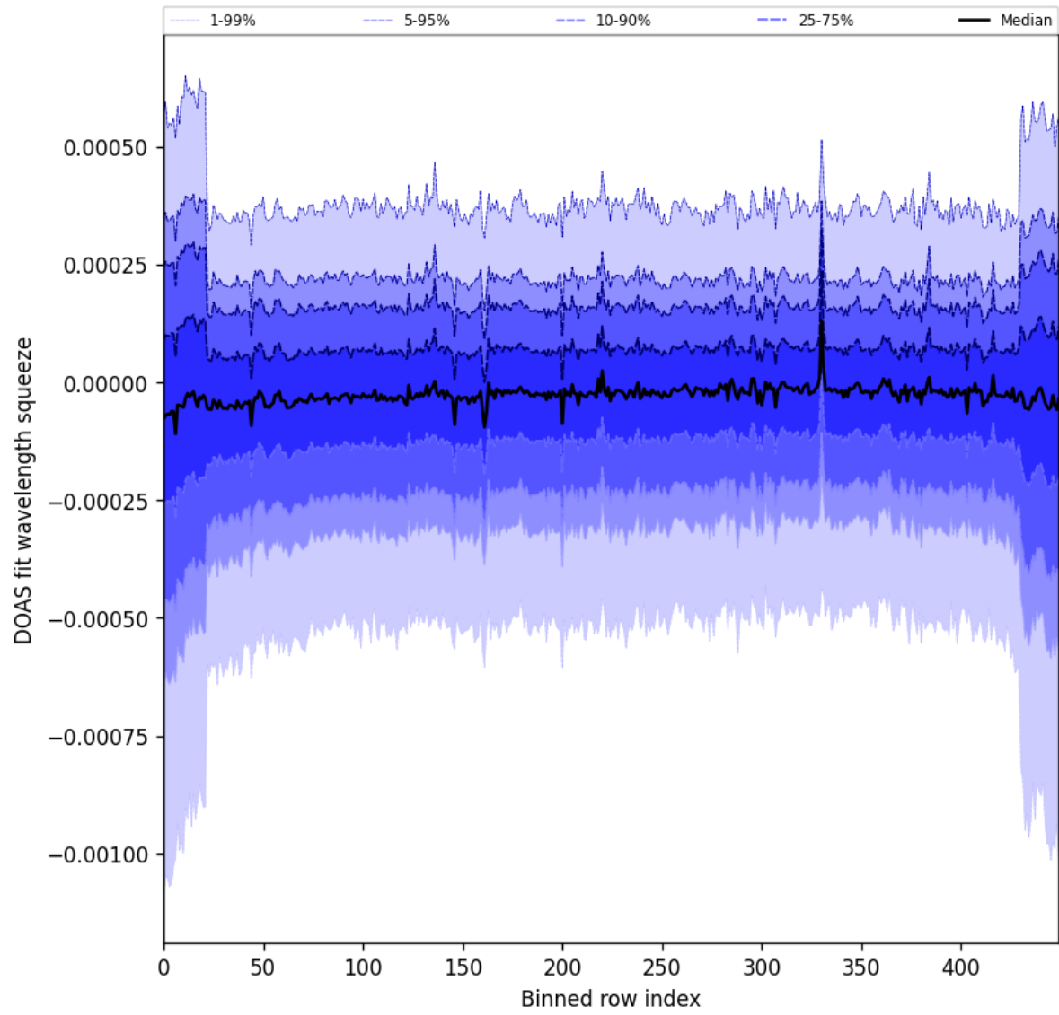
Figure 103: Along track statistics of “DOAS fit wavelength squeeze” for 2025-02-19 to 2025-02-21
