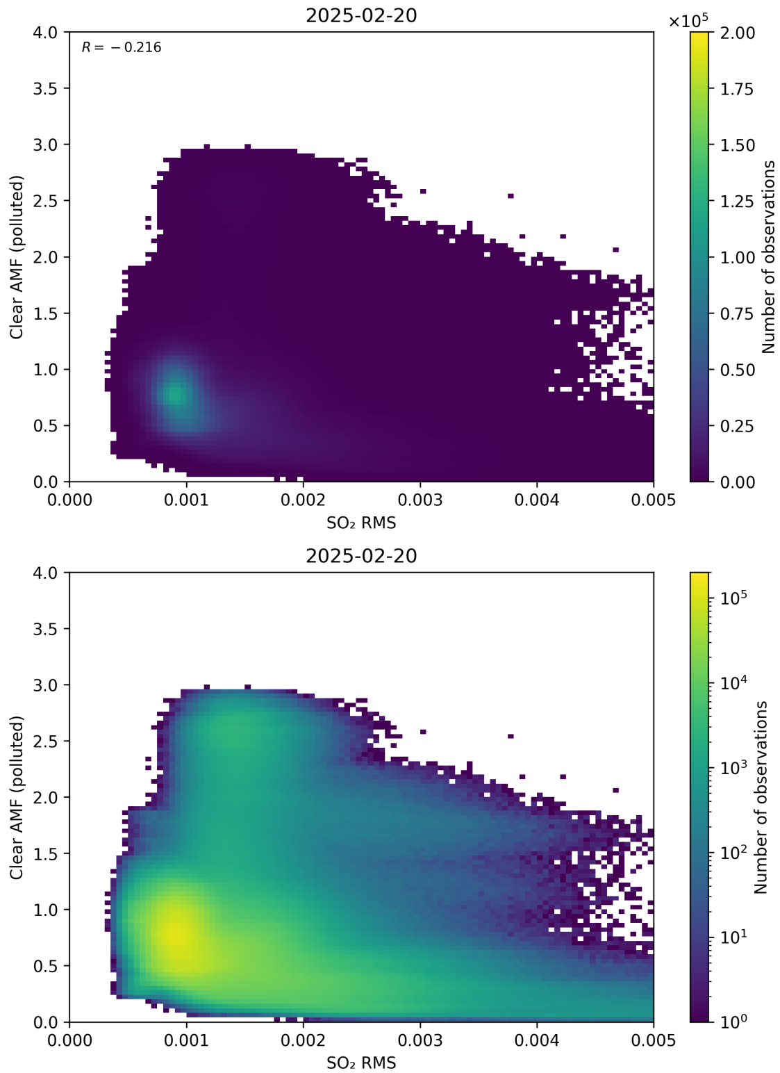
Figure 147: Scatter density plot of “SO 2 RMS” against “Clear AMF (polluted)” for 2025-02-19 to 2025-02-21.
