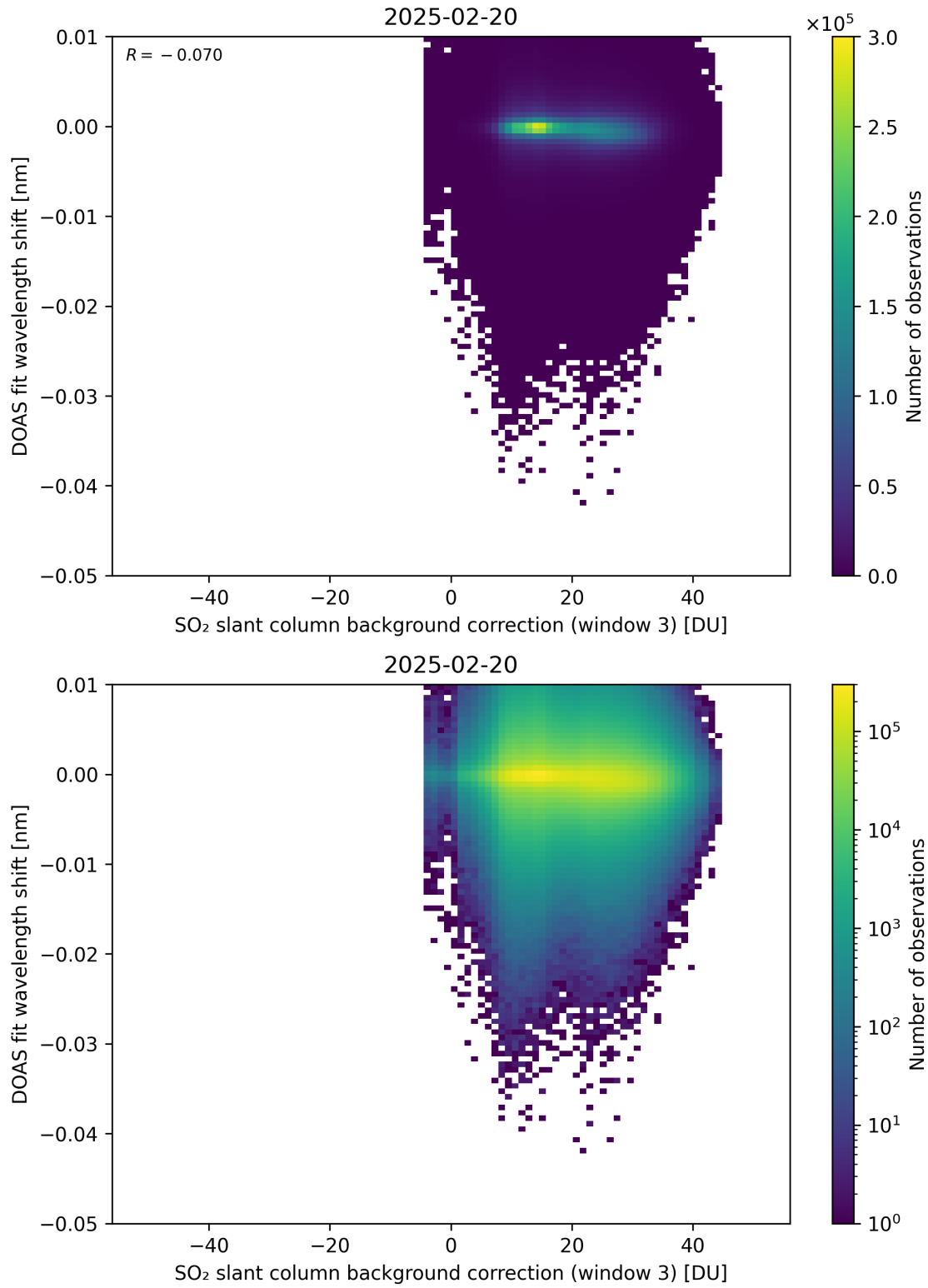
Figure 132: Scatter density plot of “SO 2 slant column background correction (window 3)” against “DOAS fit wavelength shift” for 2025-02-19 to 2025-02-21.
