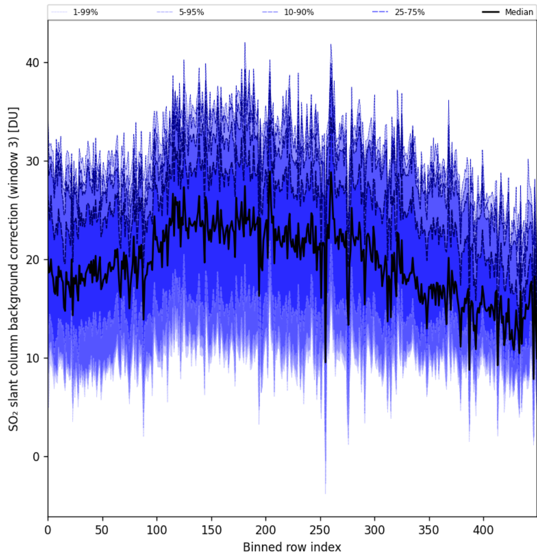
Figure 100: Along track statistics of “SO 2 slant column background correction (window 3)” for 2025-02-19 to 2025-02-21
