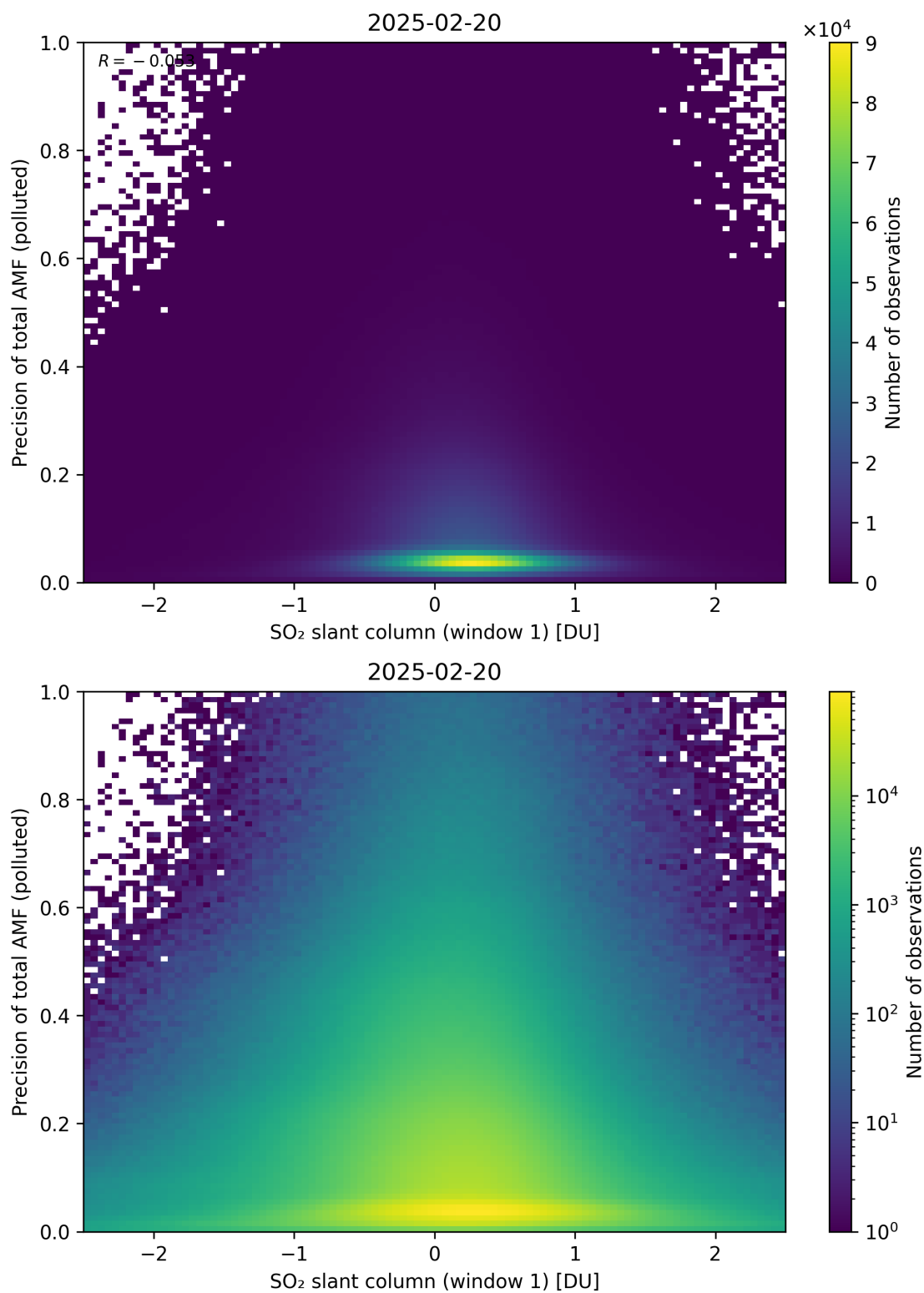
Figure 290: Scatter density plot of “SO 2 slant column (window 1)” against “Precision of total AMF (polluted)” for 2025-02-19 to 2025-02-21.
