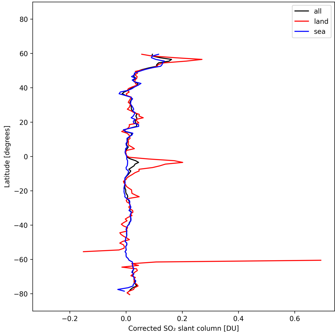
Figure 34: Zonal average of “Corrected SO 2 slant column” for 2025-02-19 to 2025-02-21.
