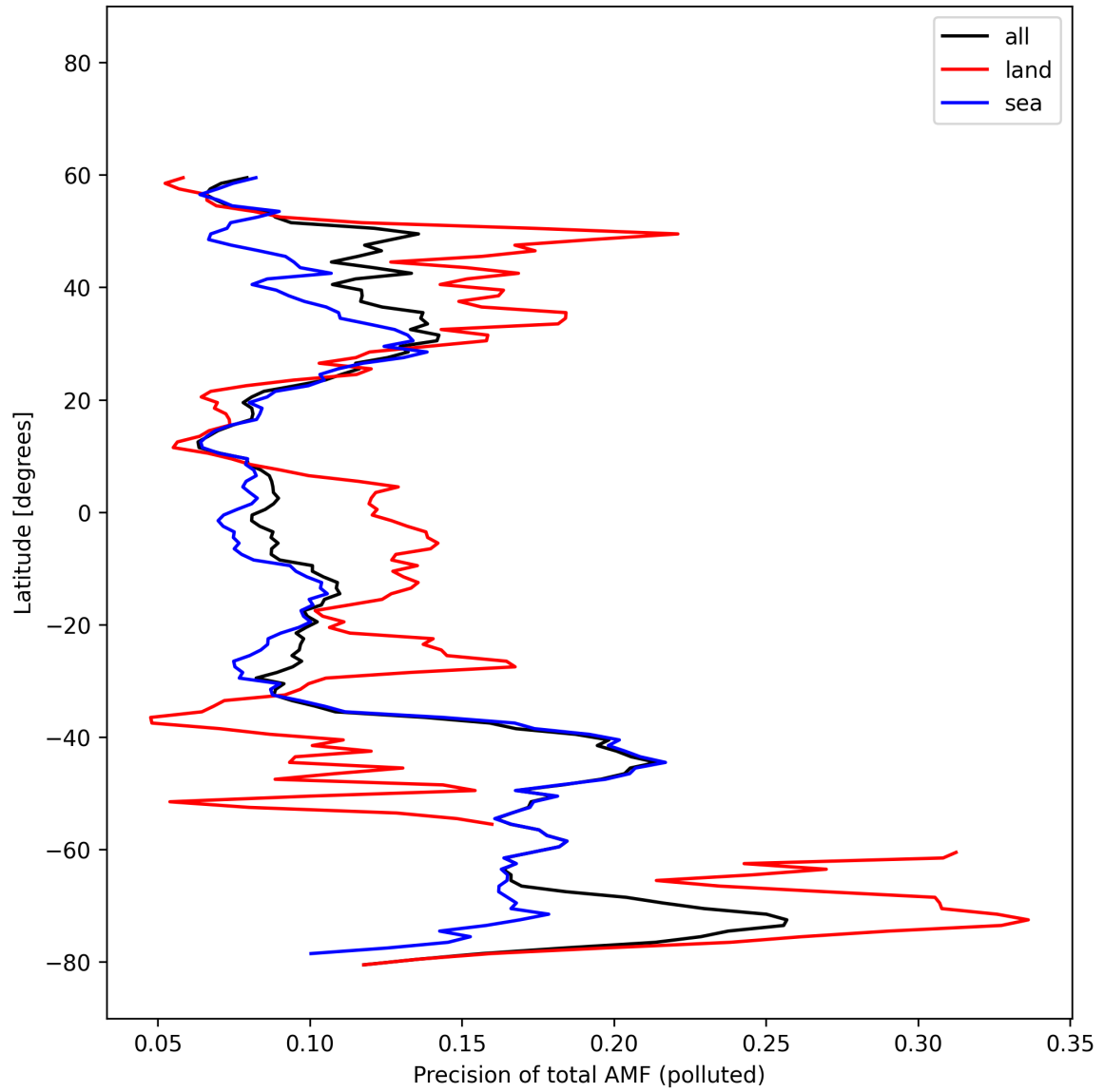
Figure 54: Zonal average of “Precision of total AMF (polluted)” for 2025-02-19 to 2025-02-21.
