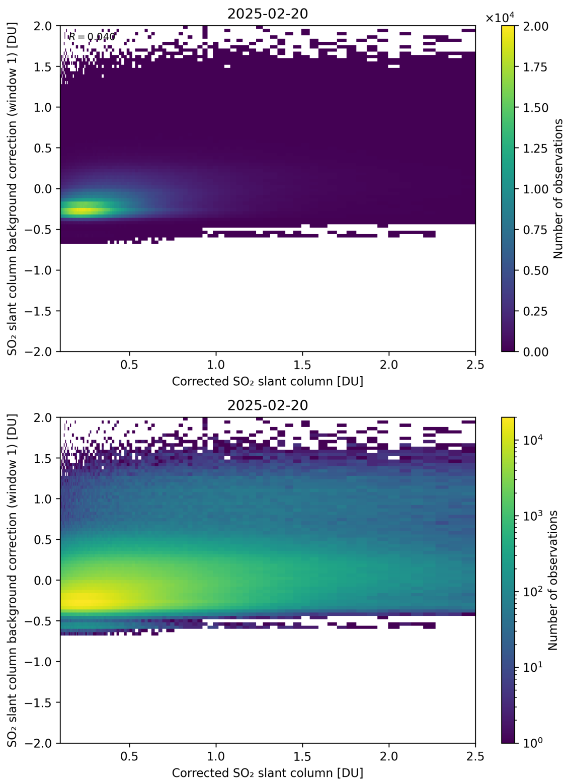
Figure 226: Scatter density plot of “Corrected SO 2 slant column” against “SO 2 slant column background correction (window 1)” for 2025-02-19 to 2025-02-21.
