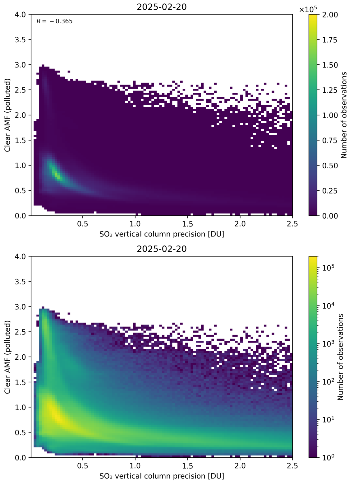
Figure 335: Scatter density plot of “SO 2 vertical column precision” against “Clear AMF (polluted)” for 2025-02-19 to 2025-02-21.
