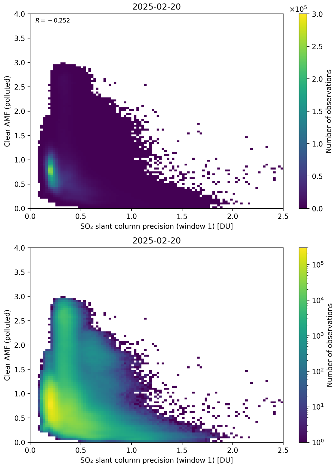
Figure 274: Scatter density plot of “SO 2 slant column precision (window 1)” against “Clear AMF (polluted)” for 2025-02-19 to 2025-02-21.
