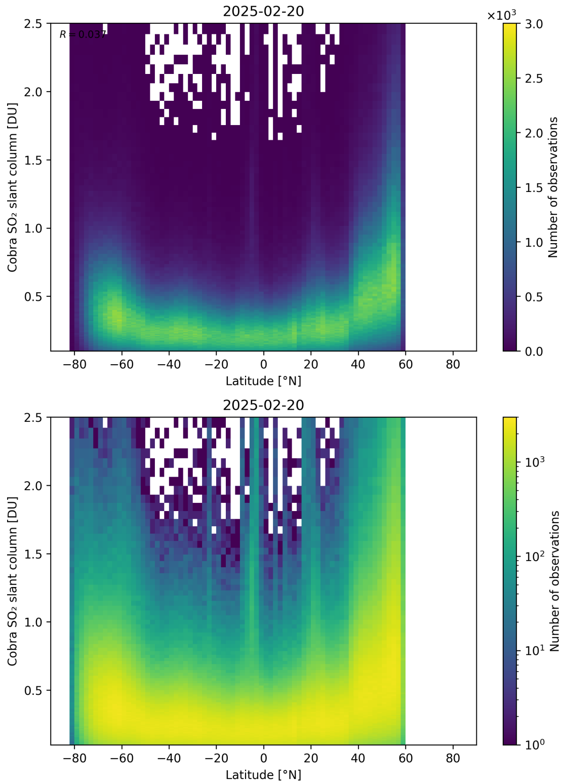
Figure 157: Scatter density plot of “Latitude” against “Cobra SO 2 slant column” for 2025-02-19 to 2025-02-21.
