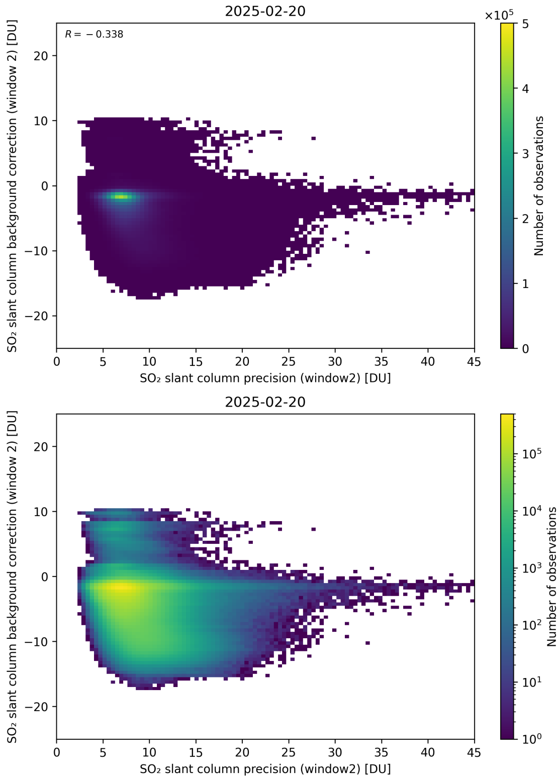
Figure 291: Scatter density plot of “SO 2 slant column precision (window2)” against “SO 2 slant column background correction (window 2)” for 2025-02-19 to 2025-02-21.
