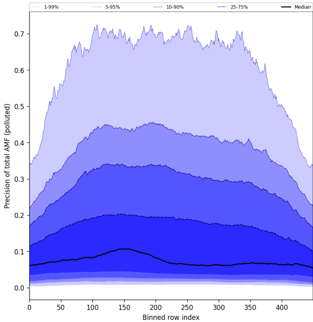
Figure 106: Along track statistics of “Precision of total AMF (polluted)” for 2025-02-19 to 2025-02-21
