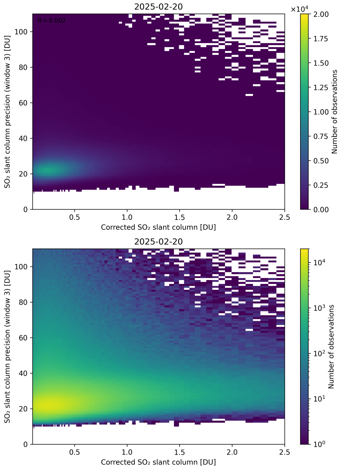
Figure 241: Scatter density plot of “Corrected SO 2 slant column” against “SO 2 slant column precision (window 3)” for 2025-02-19 to 2025-02-21.
