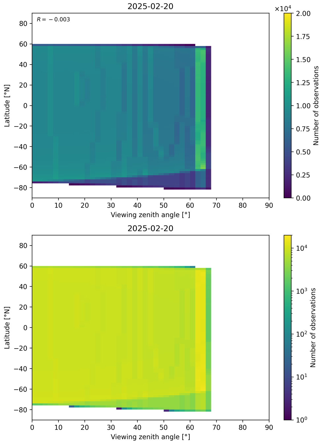
Figure 368: Scatter density plot of “Viewing zenith angle” against “Latitude” for 2025-02-19 to 2025-02-21.
