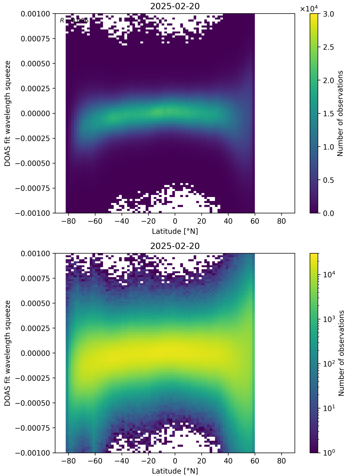
Figure 154: Scatter density plot of “Latitude” against “DOAS fit wavelength squeeze” for 2025-02-19 to 2025-02-21.
