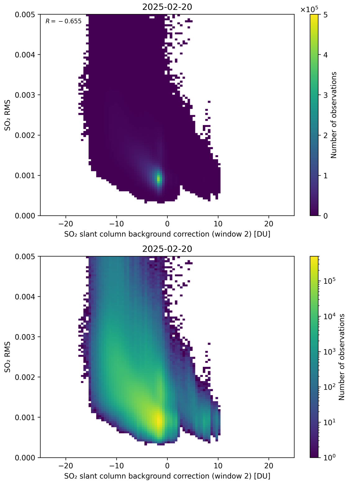
Figure 125: Scatter density plot of “SO 2 slant column background correction (window 2)” against “SO 2 RMS” for 2025-02-19 to 2025-02-21.
