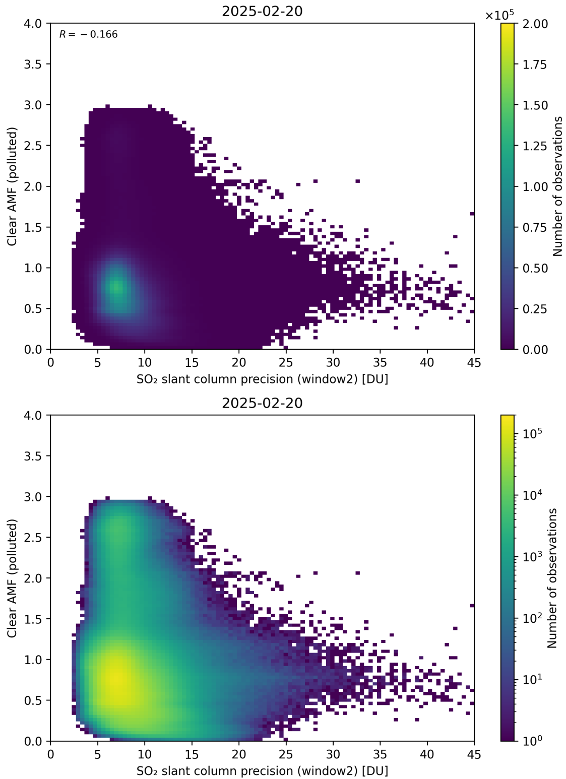
Figure 296: Scatter density plot of “SO 2 slant column precision (window2)” against “Clear AMF (polluted)” for 2025-02-19 to 2025-02-21.
