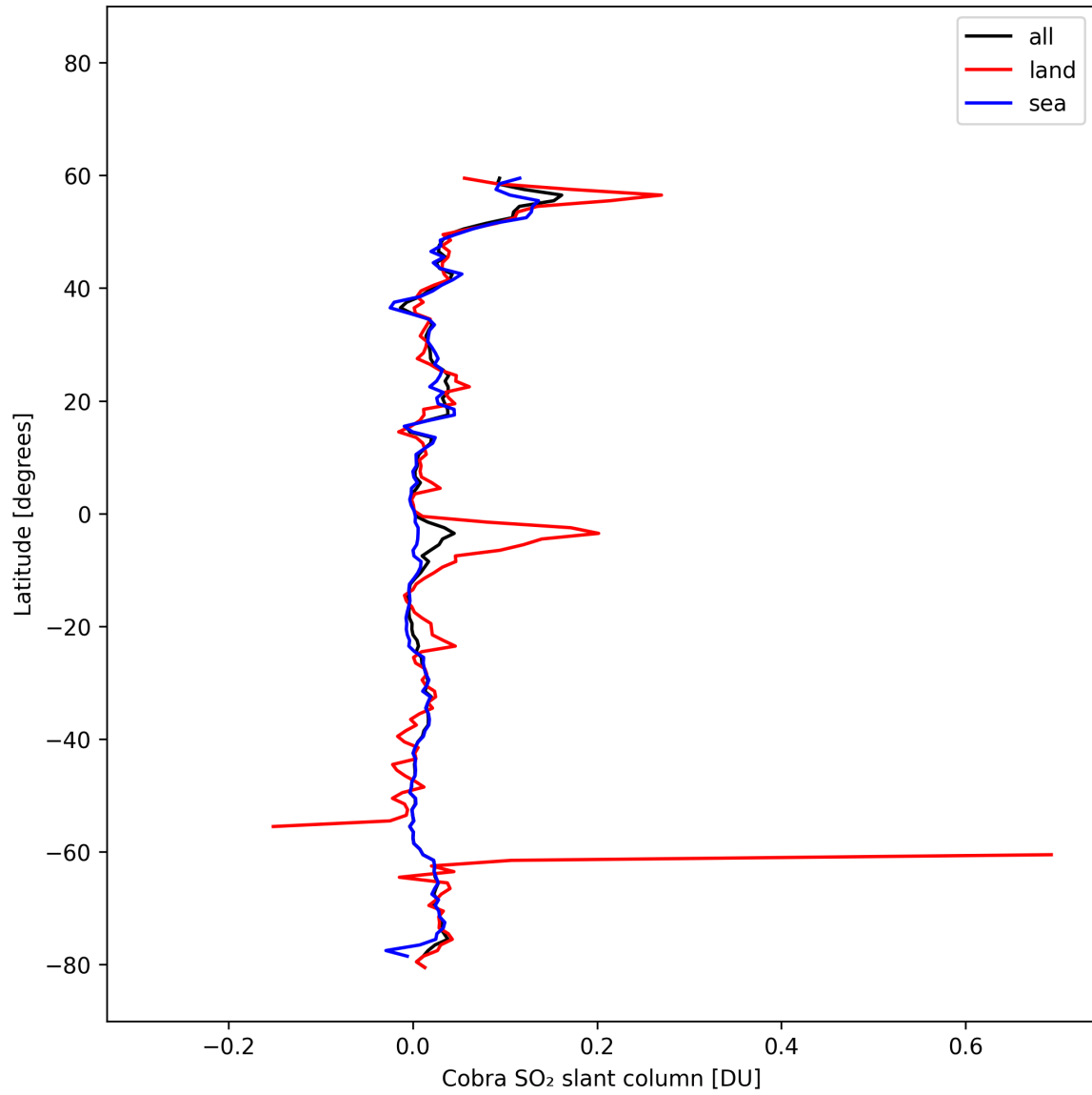
Figure 35: Zonal average of “Cobra SO 2 slant column” for 2025-02-19 to 2025-02-21.
