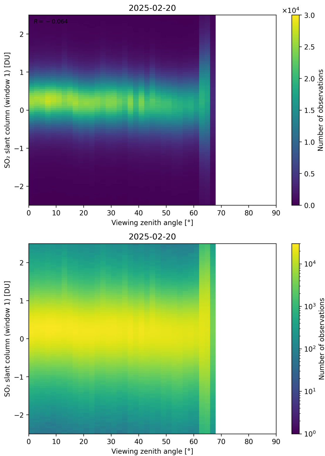
Figure 376: Scatter density plot of “Viewing zenith angle” against “SO 2 slant column (window 1)” for 2025-02-19 to 2025-02-21.
