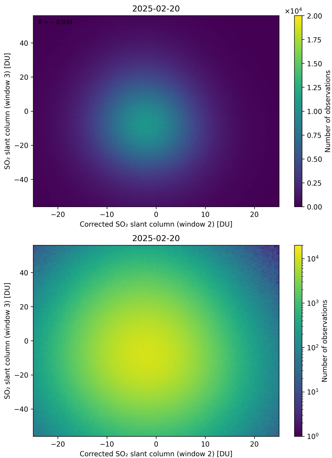
Figure 251: Scatter density plot of “Corrected SO 2 slant column (window 2)” against “SO 2 slant column (window 3)” for 2025-02-19 to 2025-02-21.
