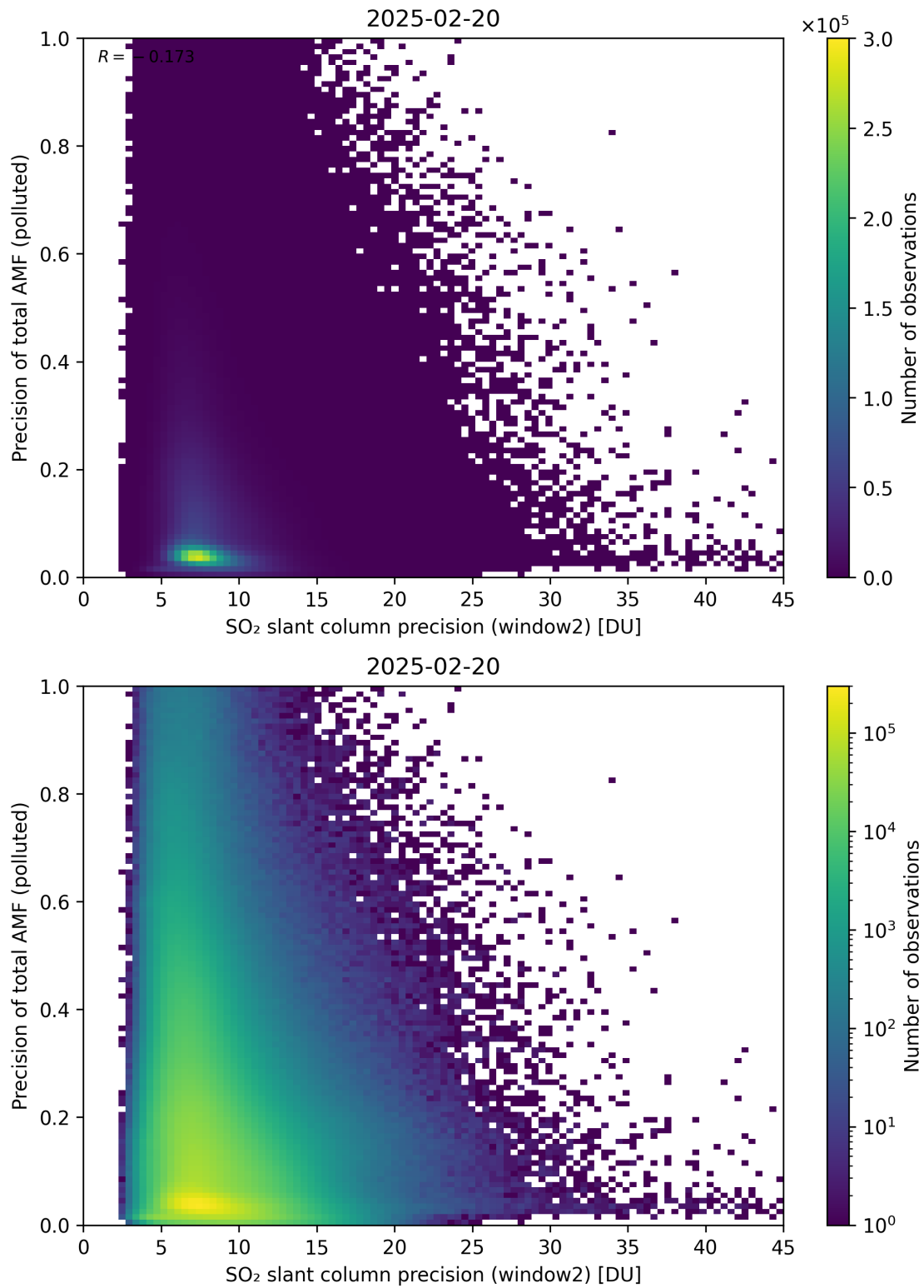
Figure 302: Scatter density plot of “SO 2 slant column precision (window2)” against “Precision of total AMF (polluted)” for 2025-02-19 to 2025-02-21.
