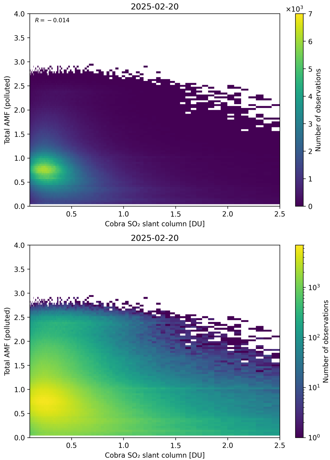
Figure 224: Scatter density plot of “Cobra SO 2 slant column” against “Total AMF (polluted)” for 2025-02-19 to 2025-02-21.
