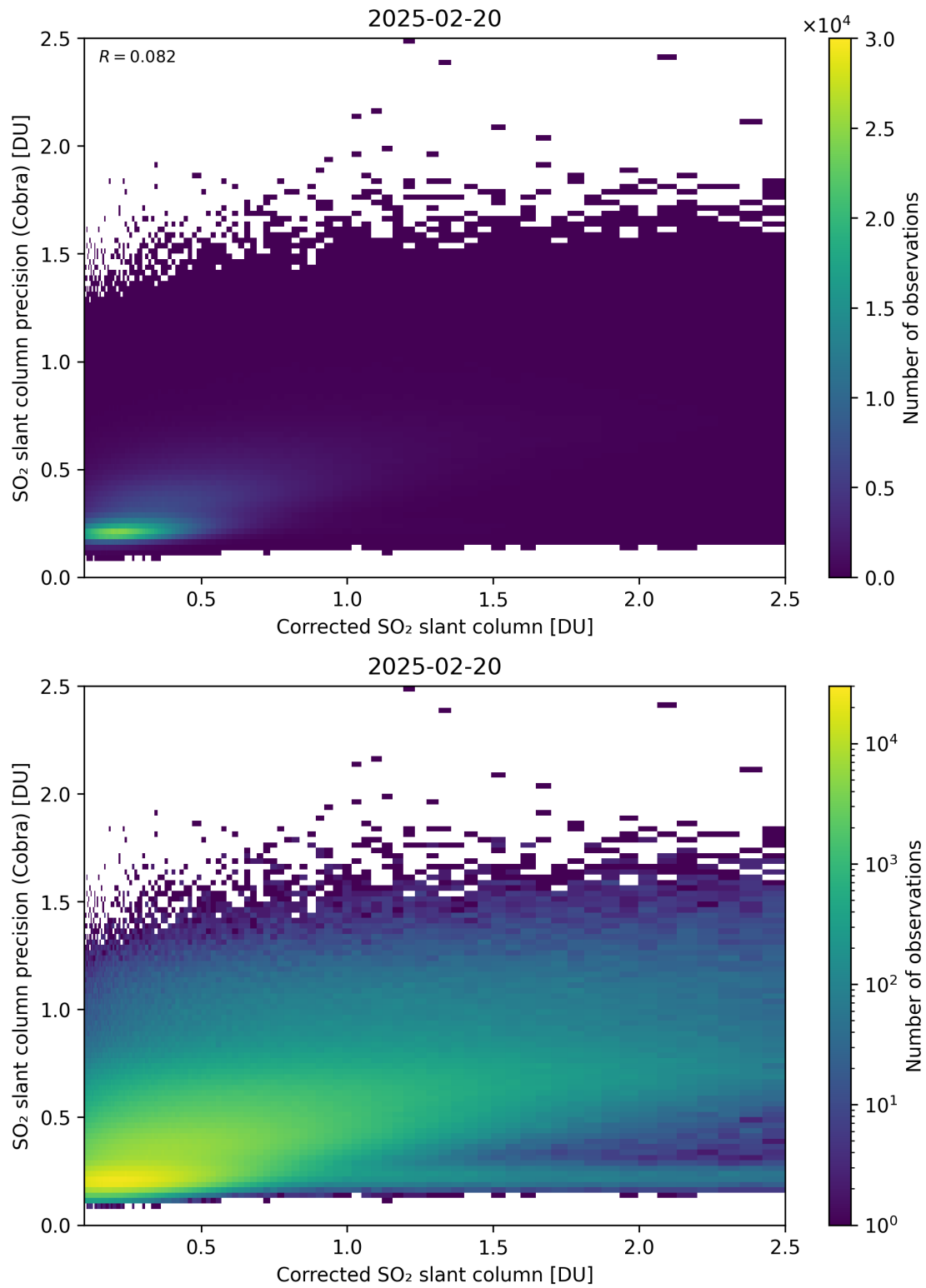
Figure 234: Scatter density plot of “Corrected SO 2 slant column” against “SO 2 slant column precision (Cobra)” for 2025-02-19 to 2025-02-21.
