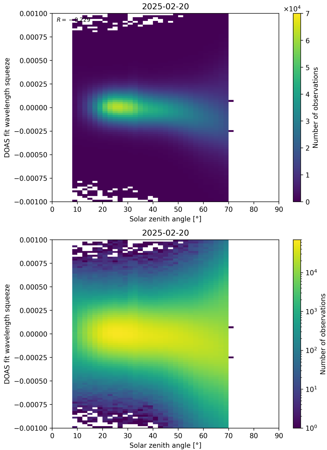
Figure 175: Scatter density plot of “Solar zenith angle” against “DOAS fit wavelength squeeze” for 2025-02-19 to 2025-02-21.
