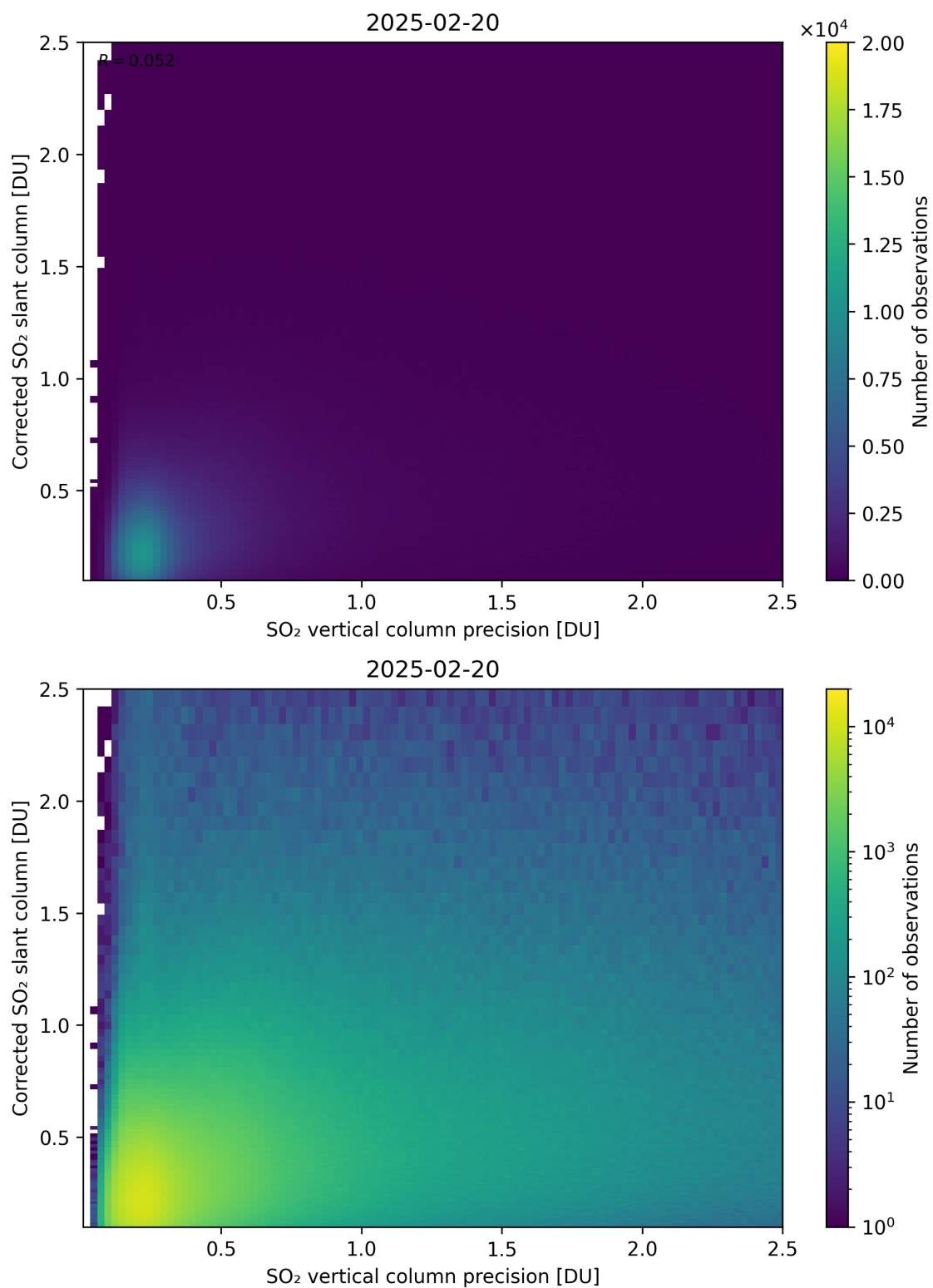
Figure 338: Scatter density plot of “SO 2 vertical column precision” against “Corrected SO 2 slant column” for 2025-02-19 to 2025-02-21.
