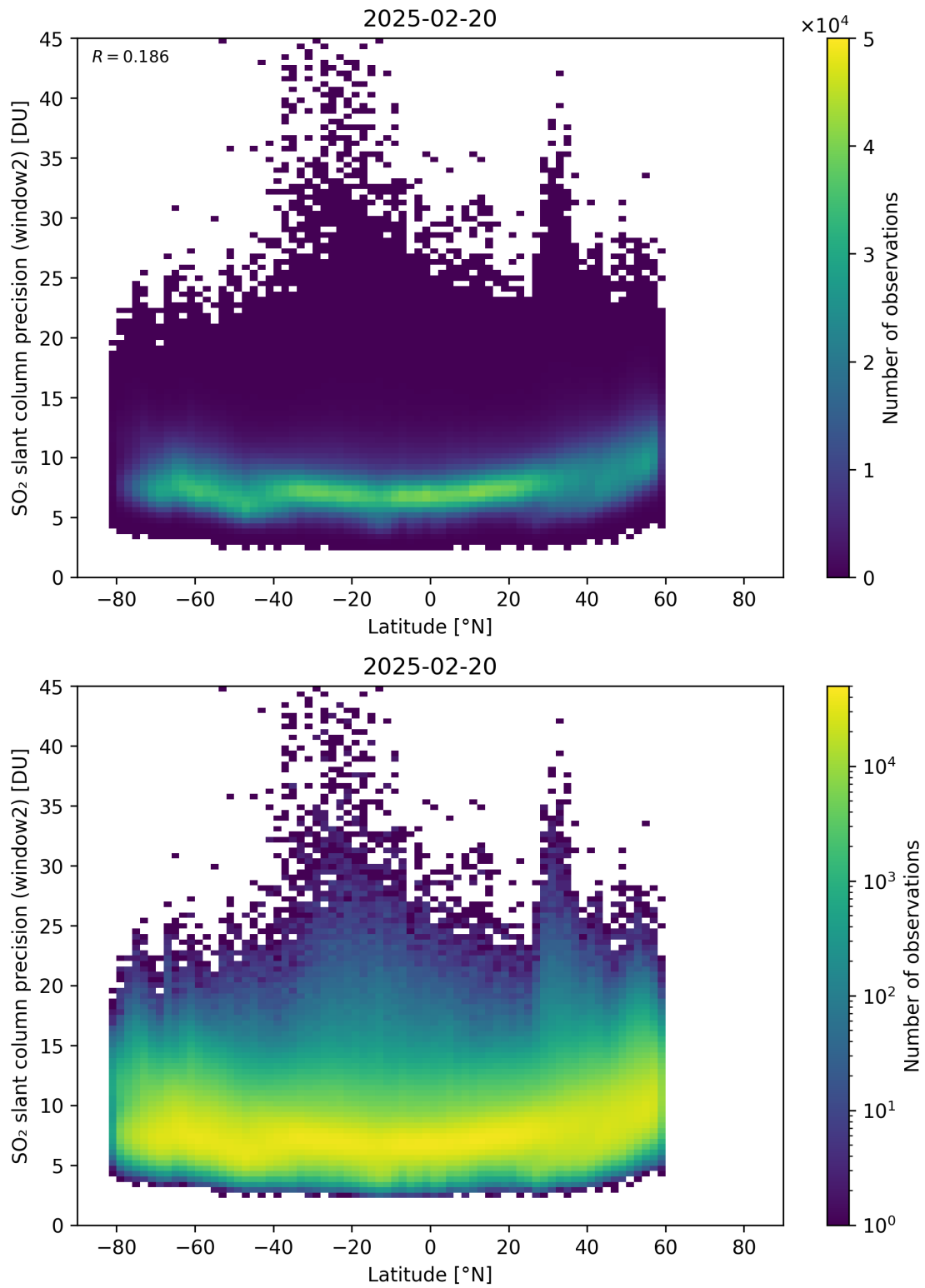
Figure 164: Scatter density plot of “Latitude” against “SO 2 slant column precision (window2)” for 2025-02-19 to 2025-02-21.
