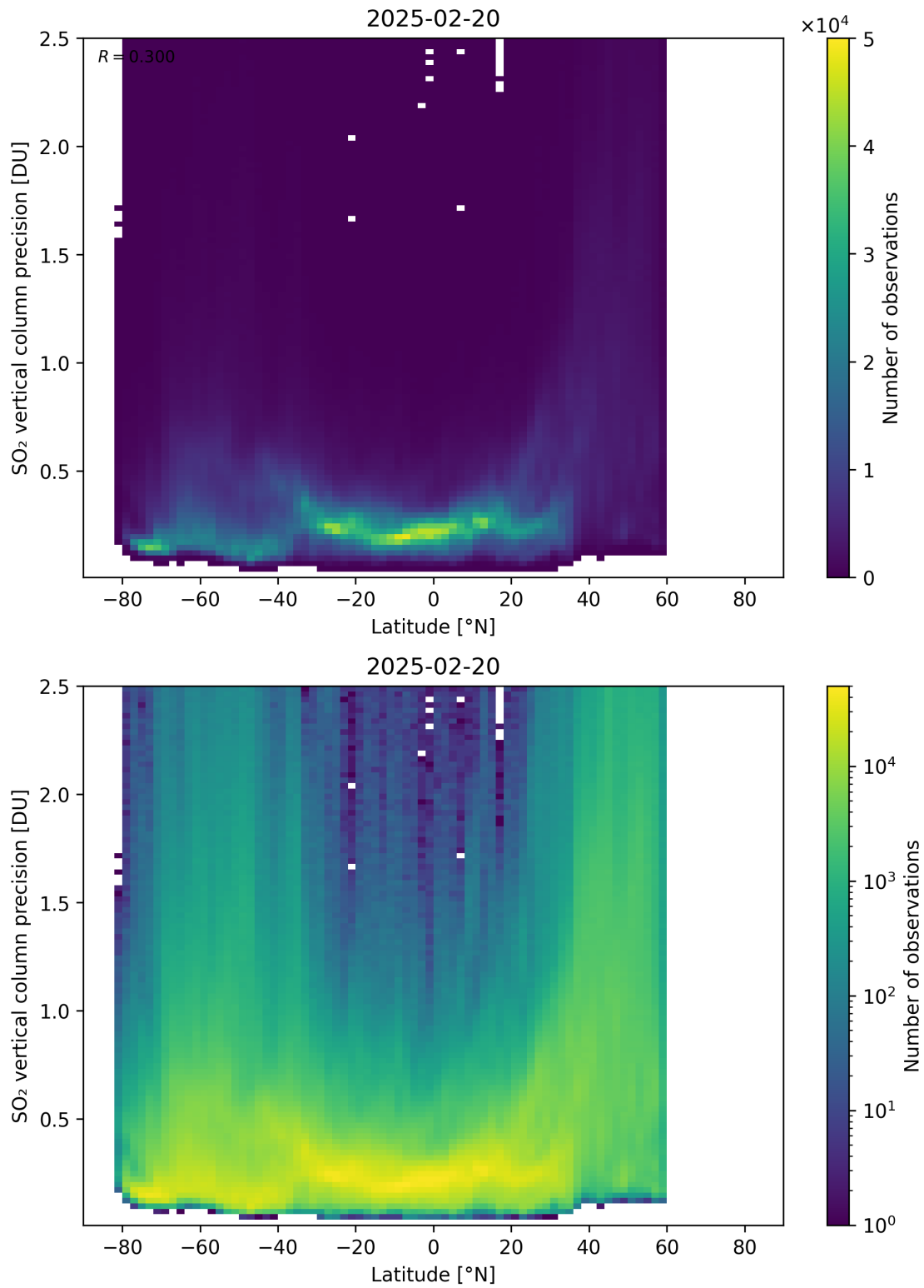
Figure 170: Scatter density plot of “Latitude” against “SO 2 vertical column precision” for 2025-02-19 to 2025-02-21.
