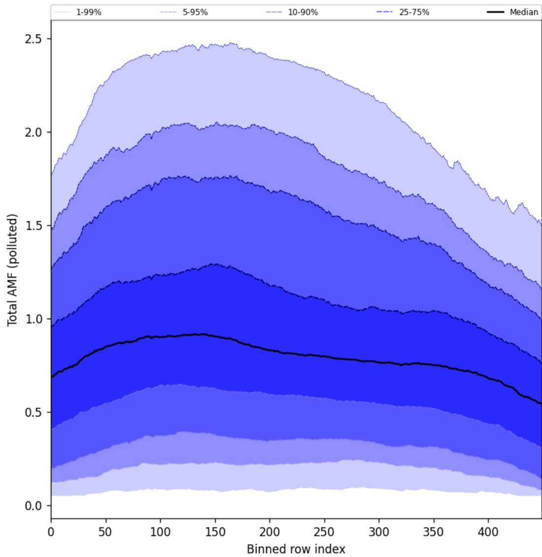
Figure 105: Along track statistics of “Total AMF (polluted)” for 2025-02-19 to 2025-02-21
