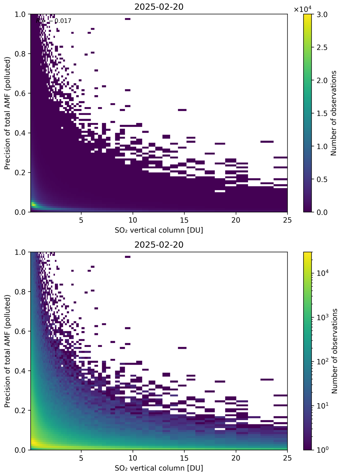
Figure 360: Scatter density plot of “SO 2 vertical column” against “Precision of total AMF (polluted)” for 2025-02-19 to 2025-02-21.
