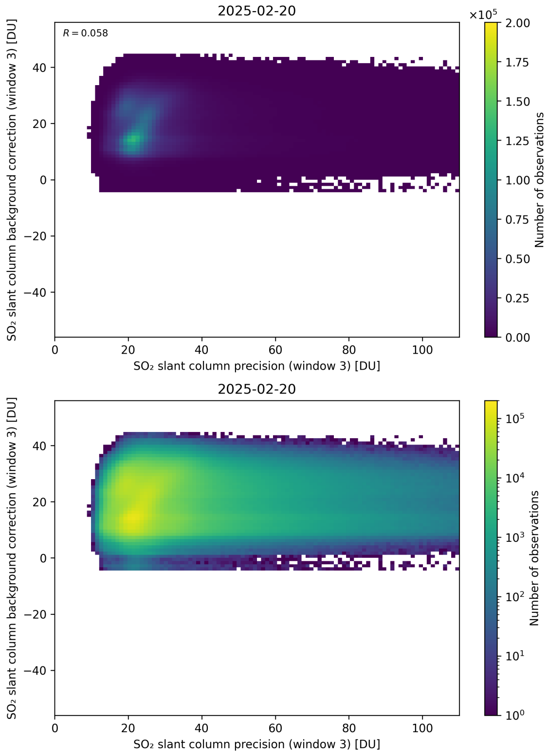
Figure 307: Scatter density plot of “SO 2 slant column precision (window 3)” against “SO 2 slant column background correction (window 3)” for 2025-02-19 to 2025-02-21.
