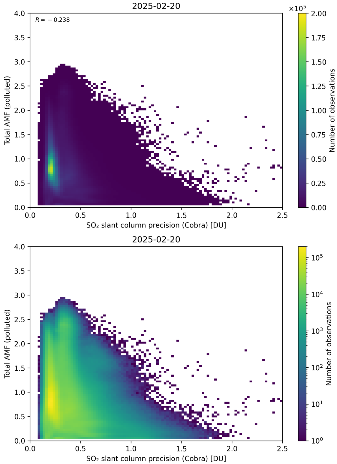
Figure 213: Scatter density plot of “SO 2 slant column precision (Cobra)” against “Total AMF (polluted)” for 2025-02-19 to 2025-02-21.
