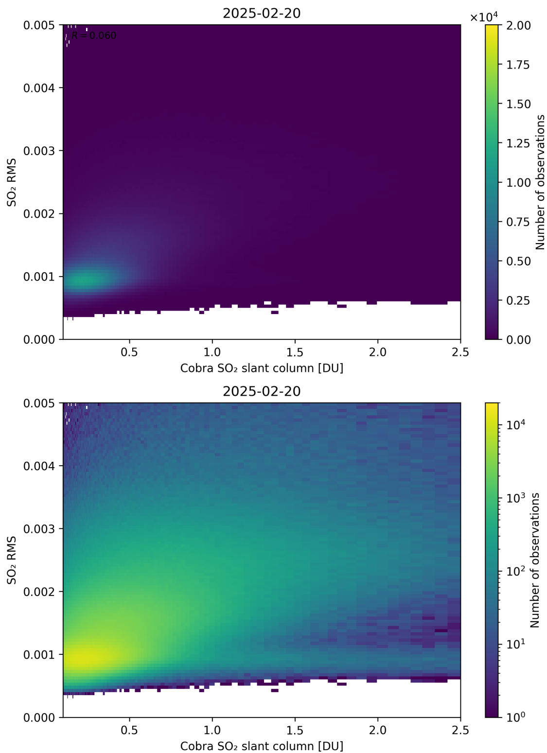
Figure 198: Scatter density plot of “Cobra SO 2 slant column” against “SO 2 RMS” for 2025-02-19 to 2025-02-21.
