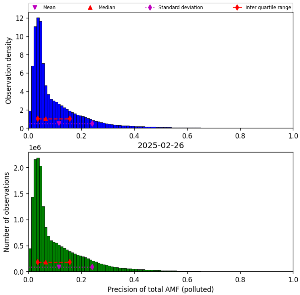
Figure 80: Histogram of “Precision of total AMF (polluted)” for 2025-02-25 to 2025-02-27
