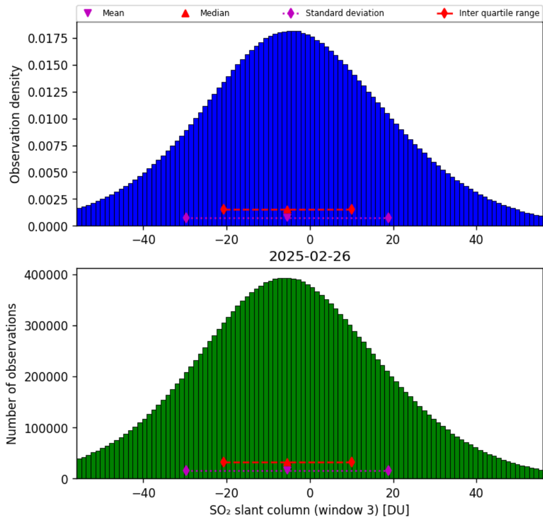
Figure 71: Histogram of “SO 2 slant column (window 3)” for 2025-02-25 to 2025-02-27
