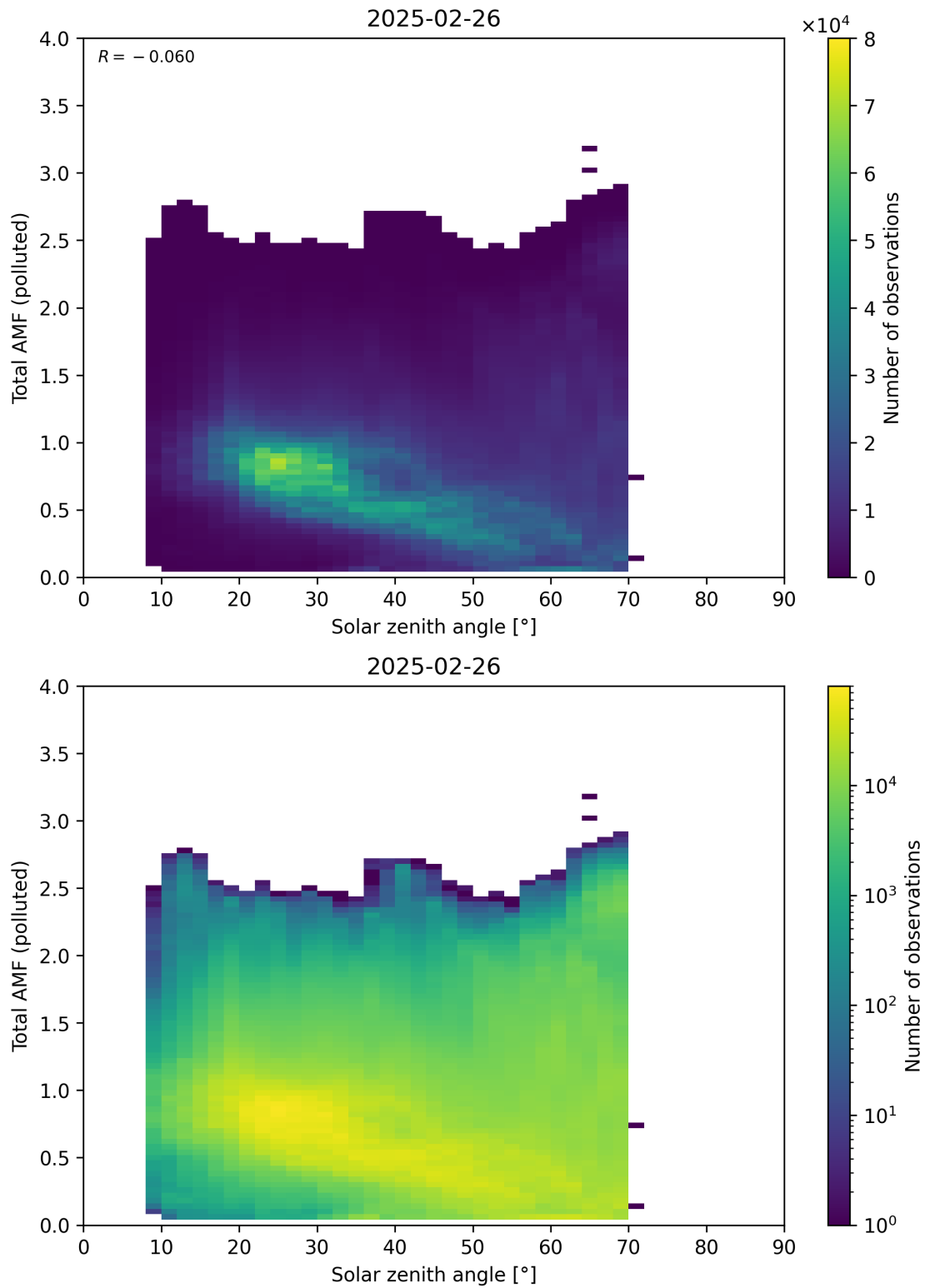
Figure 189: Scatter density plot of “Solar zenith angle” against “Total AMF (polluted)” for 2025-02-25 to 2025-02-27.
