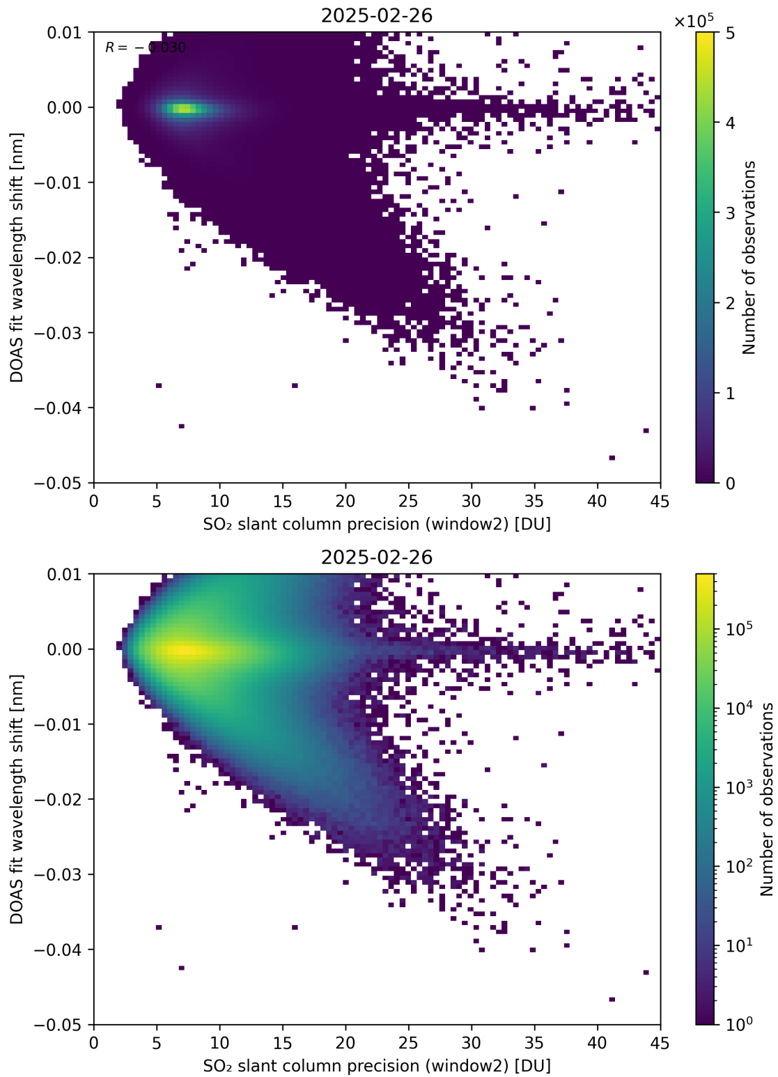
Figure 293: Scatter density plot of “SO 2 slant column precision (window2)” against “DOAS fit wavelength shift” for 2025-02-25 to 2025-02-27.
