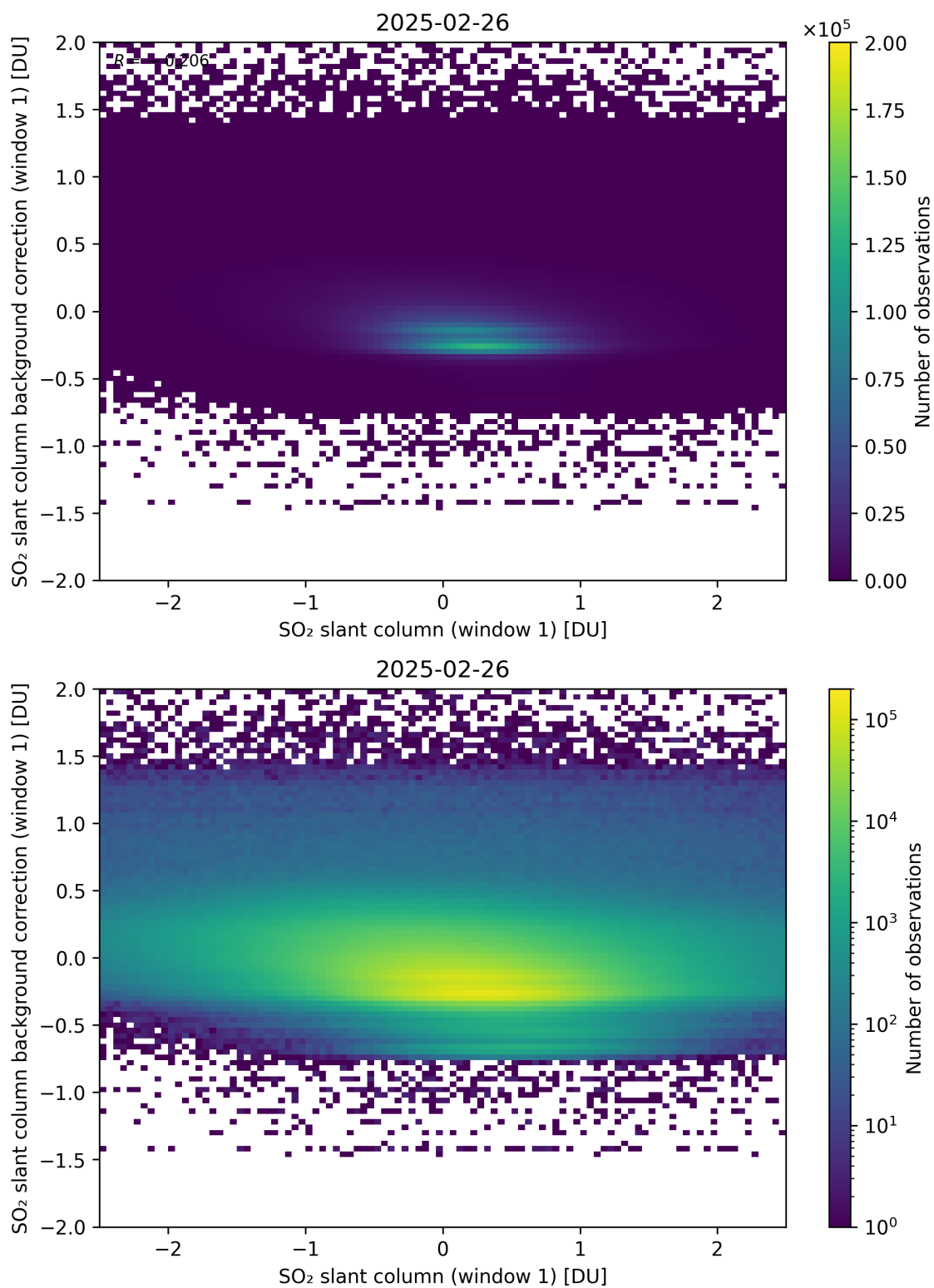
Figure 262: Scatter density plot of “SO 2 slant column (window 1)” against “SO 2 slant column background correction (window 1)” for 2025-02-25 to 2025-02-27.
