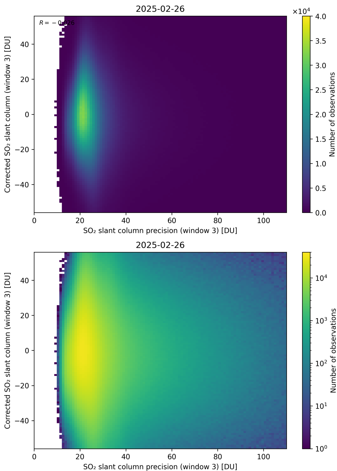
Figure 312: Scatter density plot of “SO 2 slant column precision (window 3)” against “Corrected SO 2 slant column (window 3)” for 2025-02-25 to 2025-02-27.
