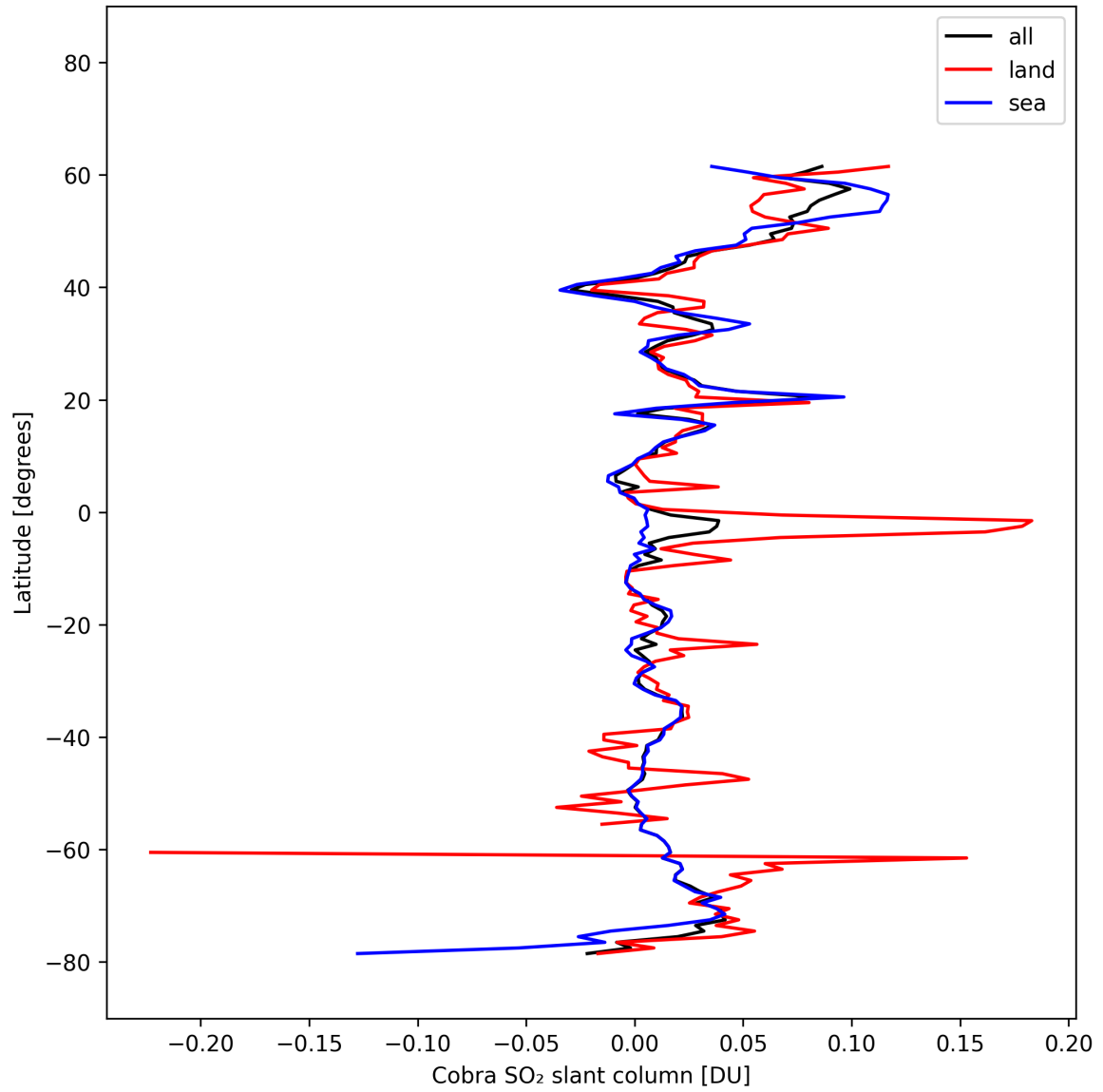
Figure 35: Zonal average of “Cobra SO 2 slant column” for 2025-02-25 to 2025-02-27.
