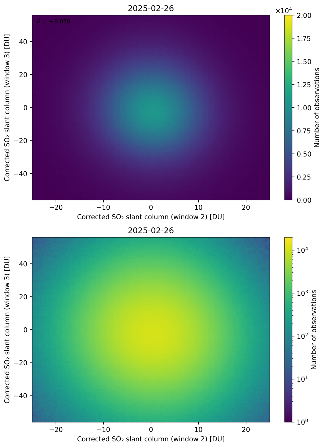
Figure 250: Scatter density plot of “Corrected SO 2 slant column (window 2)” against “Corrected SO 2 slant column (window 3)” for 2025-02-25 to 2025-02-27.
