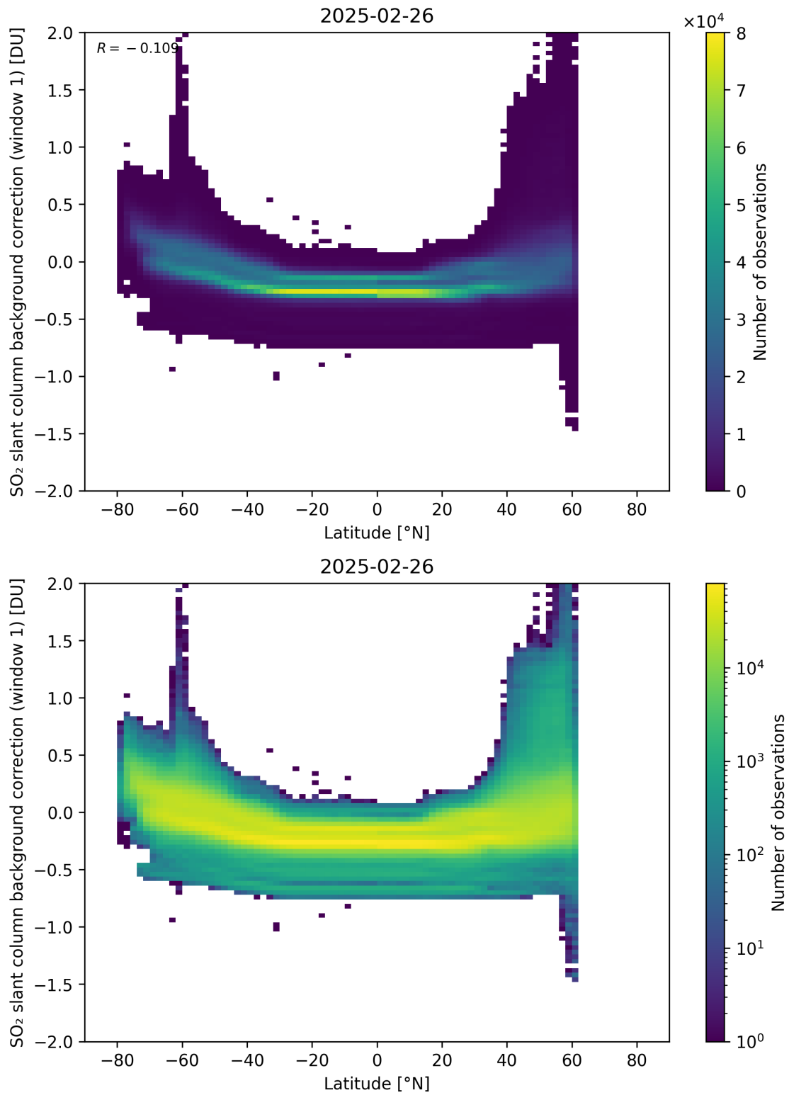
Figure 150: Scatter density plot of “Latitude” against “SO 2 slant column background correction (window 1)” for 2025-02-25 to 2025-02-27.
