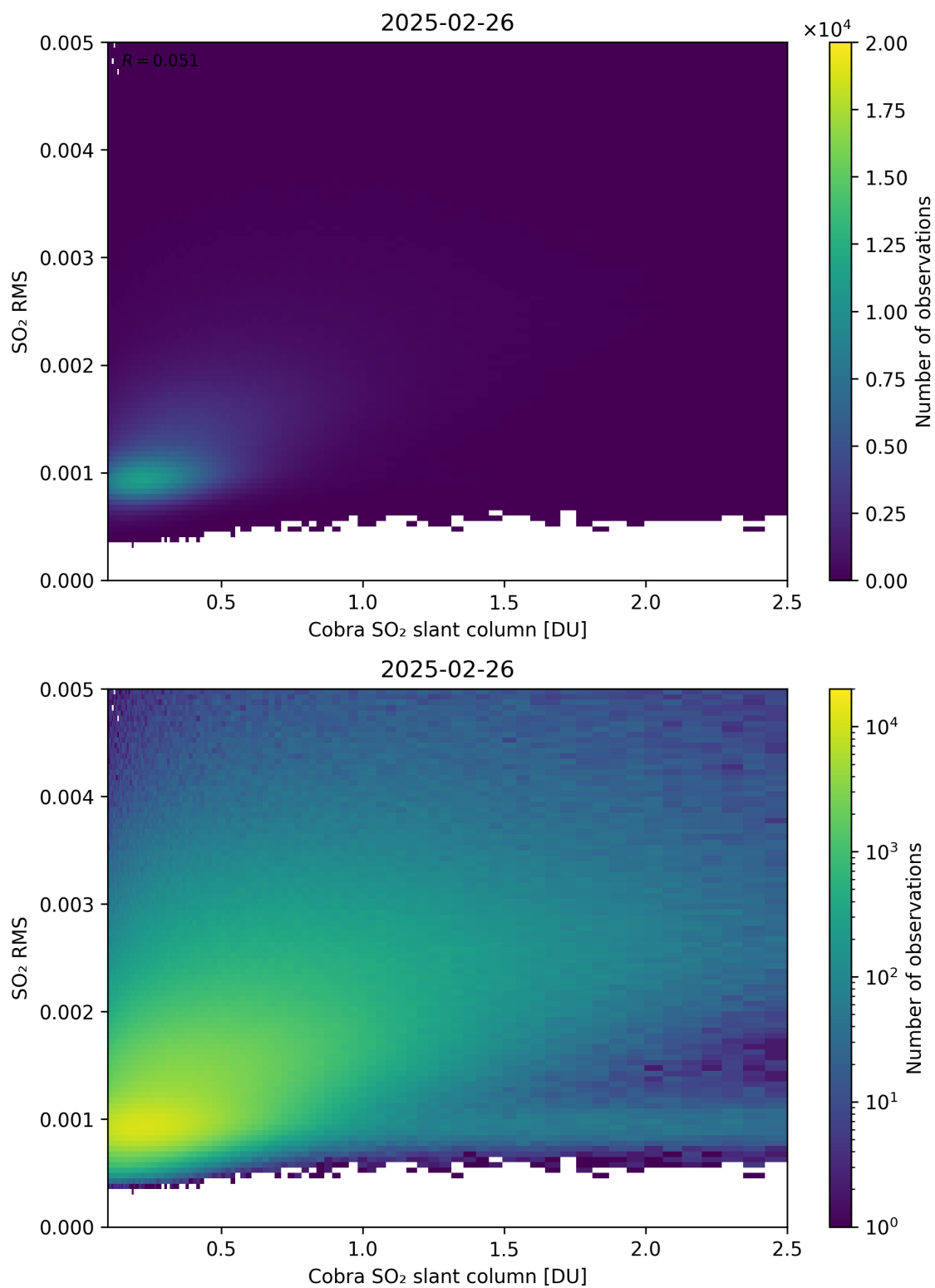
Figure 198: Scatter density plot of “Cobra SO 2 slant column” against “SO 2 RMS” for 2025-02-25 to 2025-02-27.
