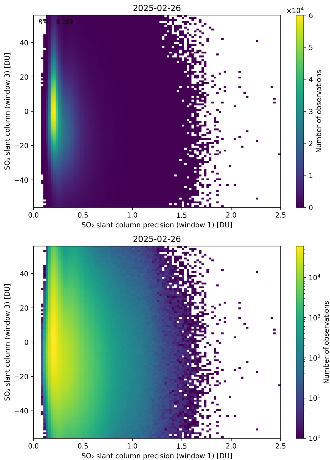
Figure 278: Scatter density plot of “SO 2 slant column precision (window 1)” against “SO 2 slant column (window 3)” for 2025-02-25 to 2025-02-27.
