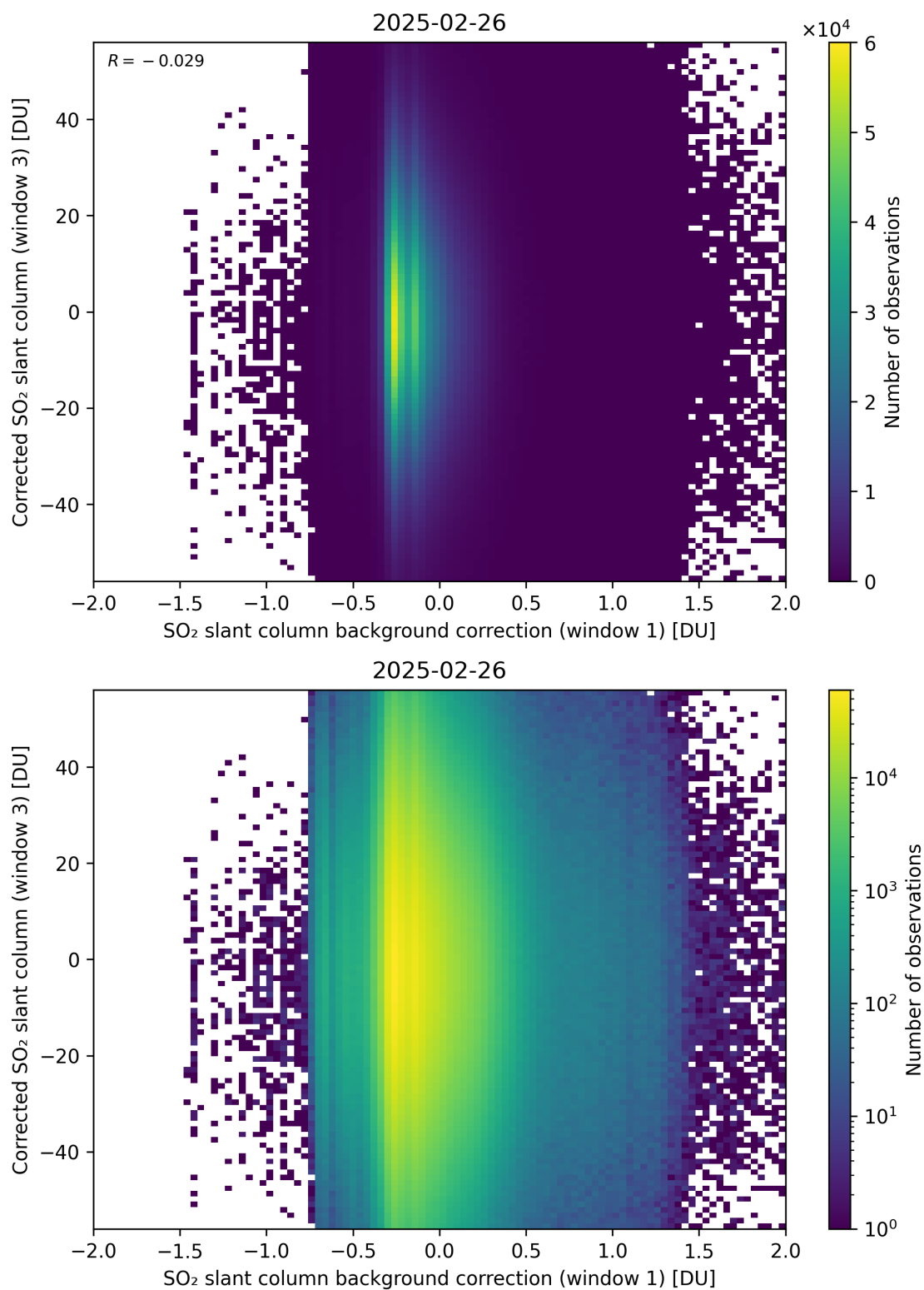
Figure 116: Scatter density plot of “SO 2 slant column background correction (window 1)” against “Corrected SO 2 slant column (window 3)” for 2025-02-25 to 2025-02-27.
