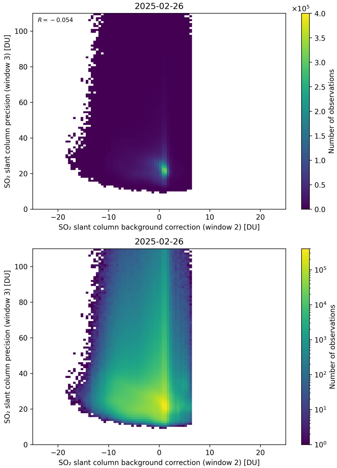
Figure 129: Scatter density plot of “SO 2 slant column background correction (window 2)” against “SO 2 slant column precision (window 3)” for 2025-02-25 to 2025-02-27.
