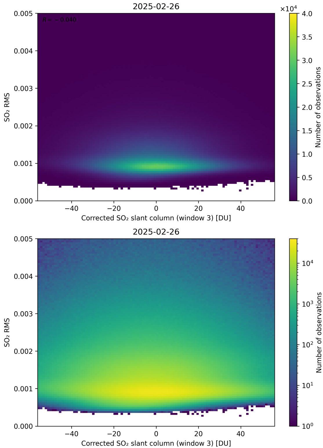
Figure 258: Scatter density plot of “Corrected SO 2 slant column (window 3)” against “SO 2 RMS” for 2025-02-25 to 2025-02-27.
