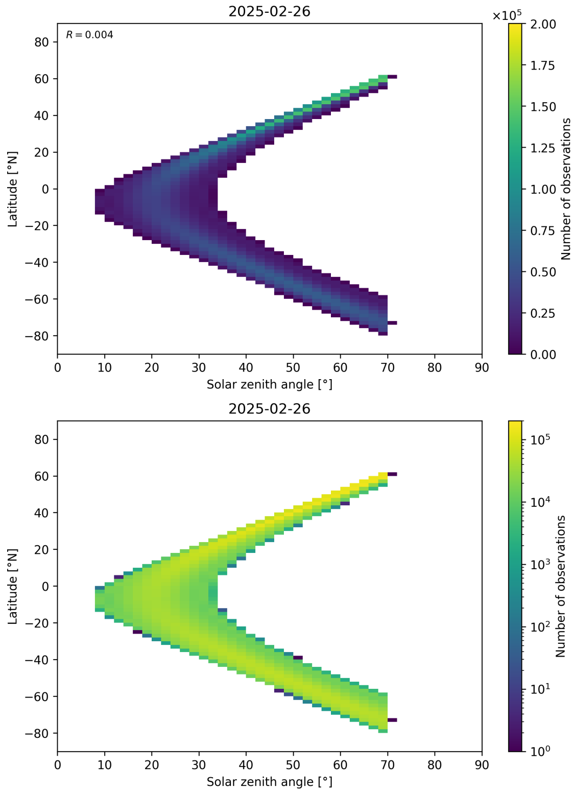
Figure 177: Scatter density plot of “Solar zenith angle” against “Latitude” for 2025-02-25 to 2025-02-27.
