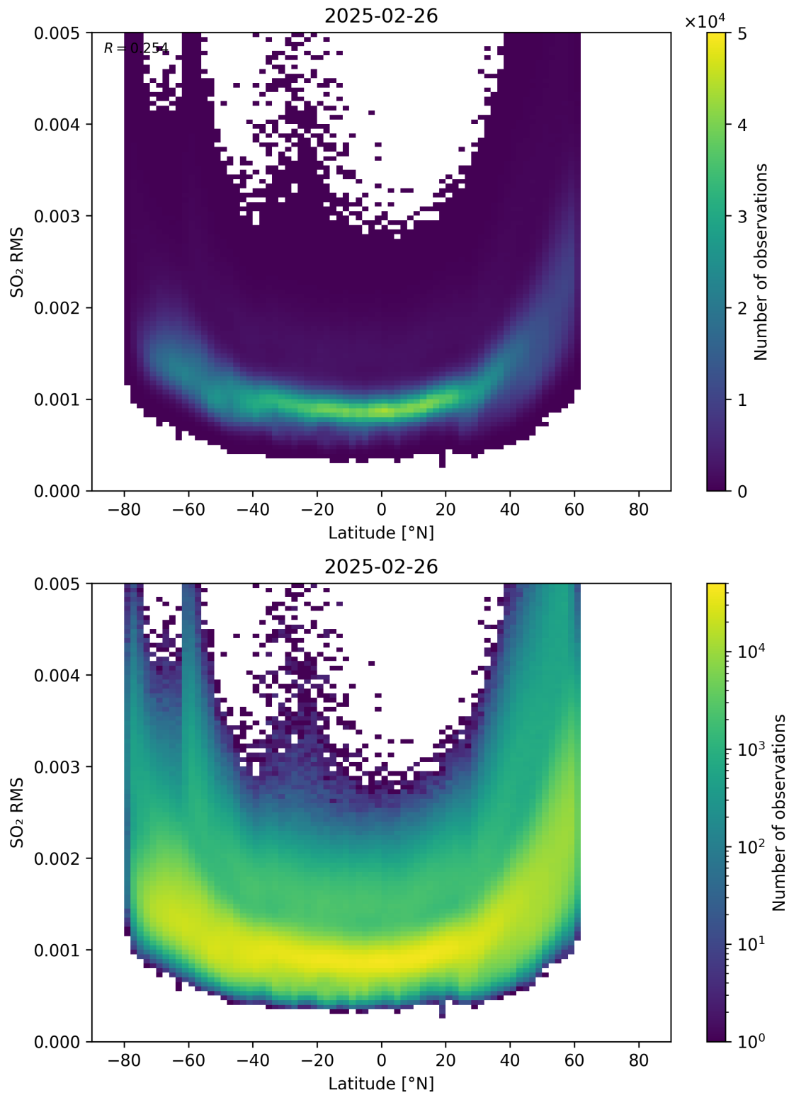
Figure 155: Scatter density plot of “Latitude” against “SO 2 RMS” for 2025-02-25 to 2025-02-27.
