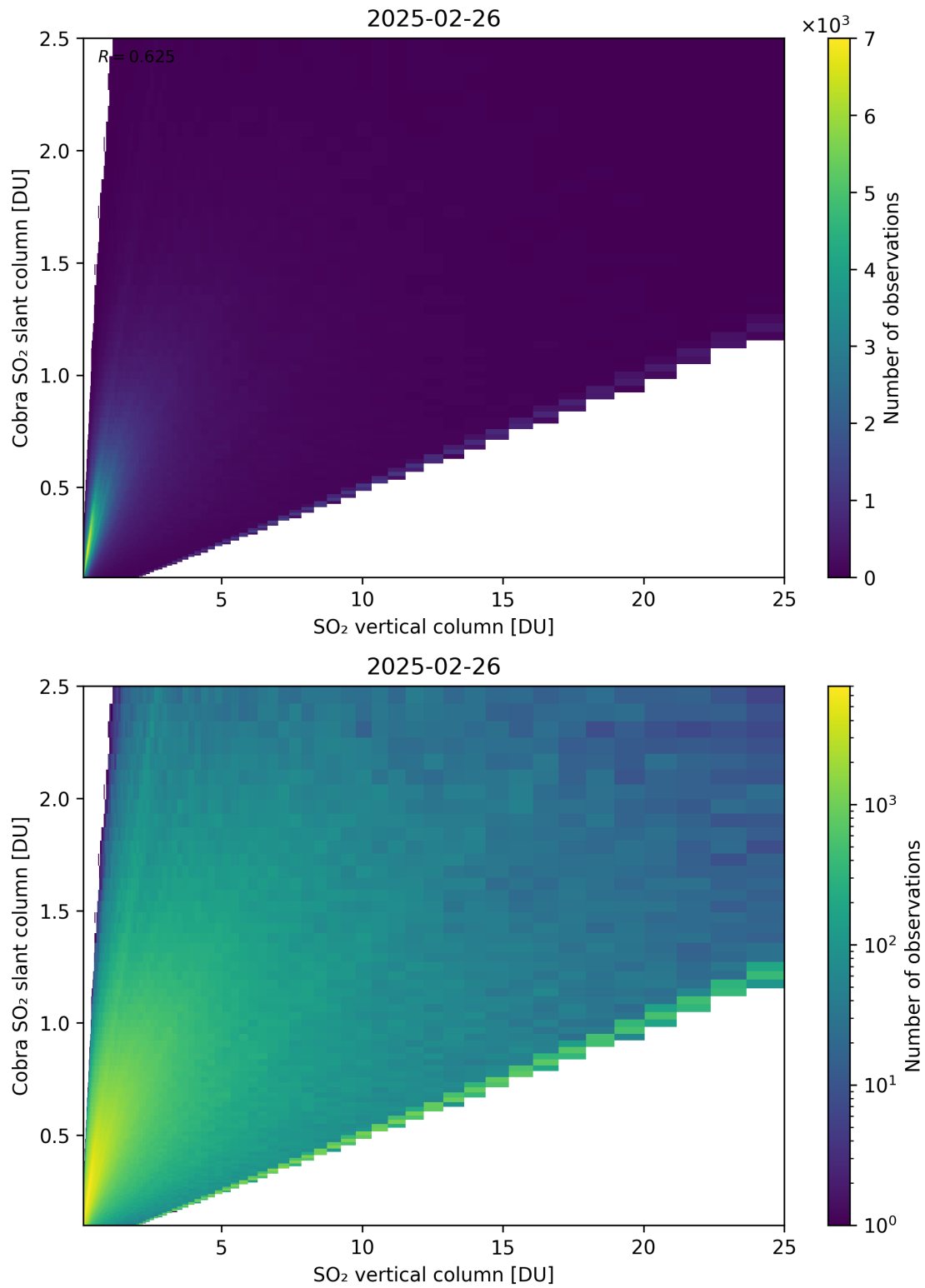
Figure 349: Scatter density plot of “SO 2 vertical column” against “Cobra SO 2 slant column” for 2025-02-25 to 2025-02-27.
