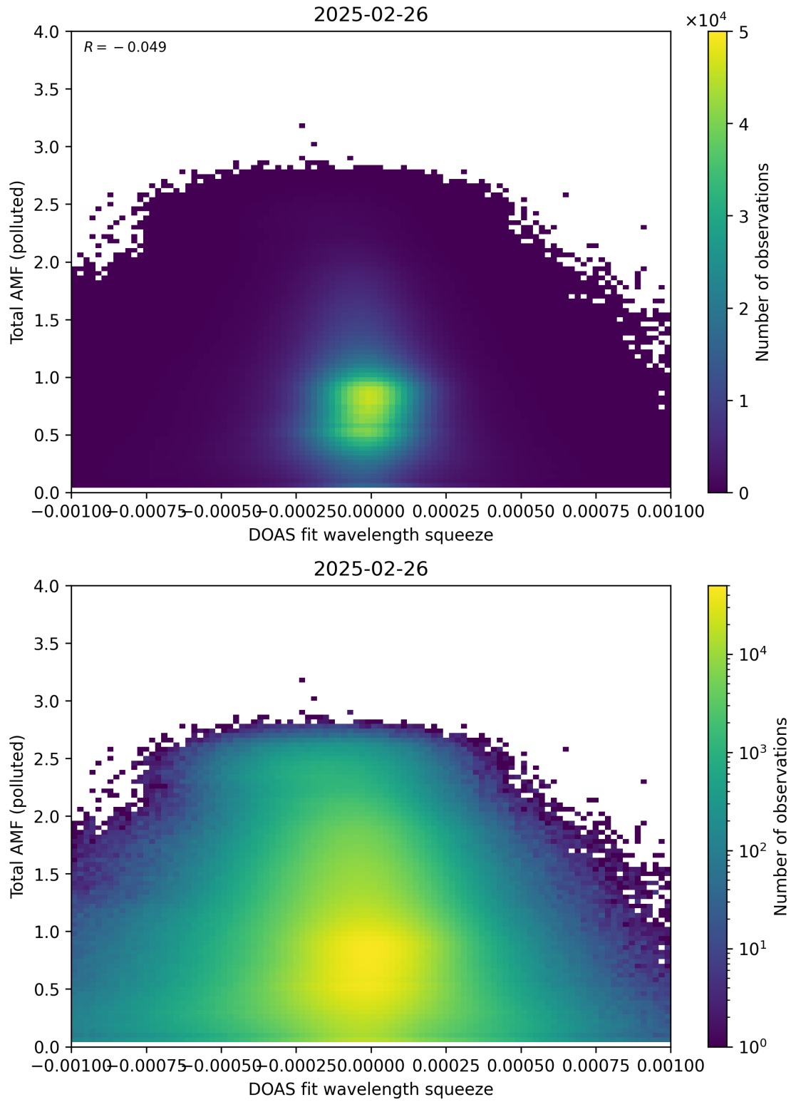
Figure 145: Scatter density plot of “DOAS fit wavelength squeeze” against “Total AMF (polluted)” for 2025-02-25 to 2025-02-27.
