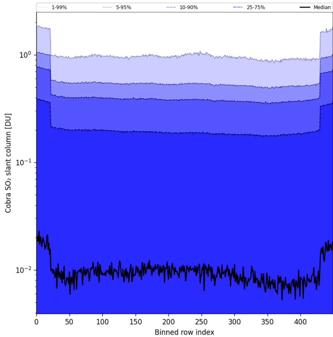
Figure 87: Along track statistics of “Cobra SO 2 slant column” for 2025-02-25 to 2025-02-27
