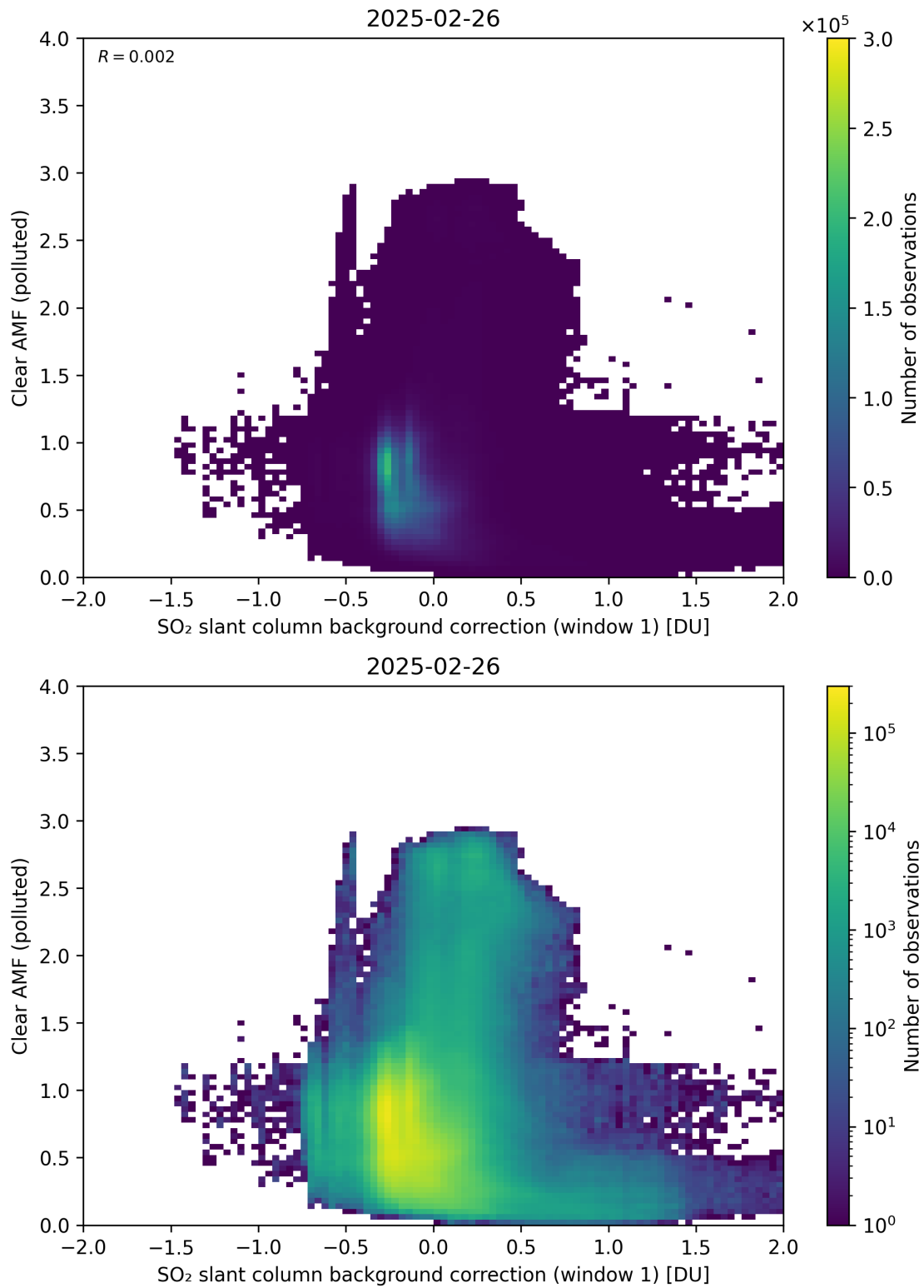
Figure 114: Scatter density plot of “SO 2 slant column background correction (window 1)” against “Clear AMF (polluted)” for 2025-02-25 to 2025-02-27.
