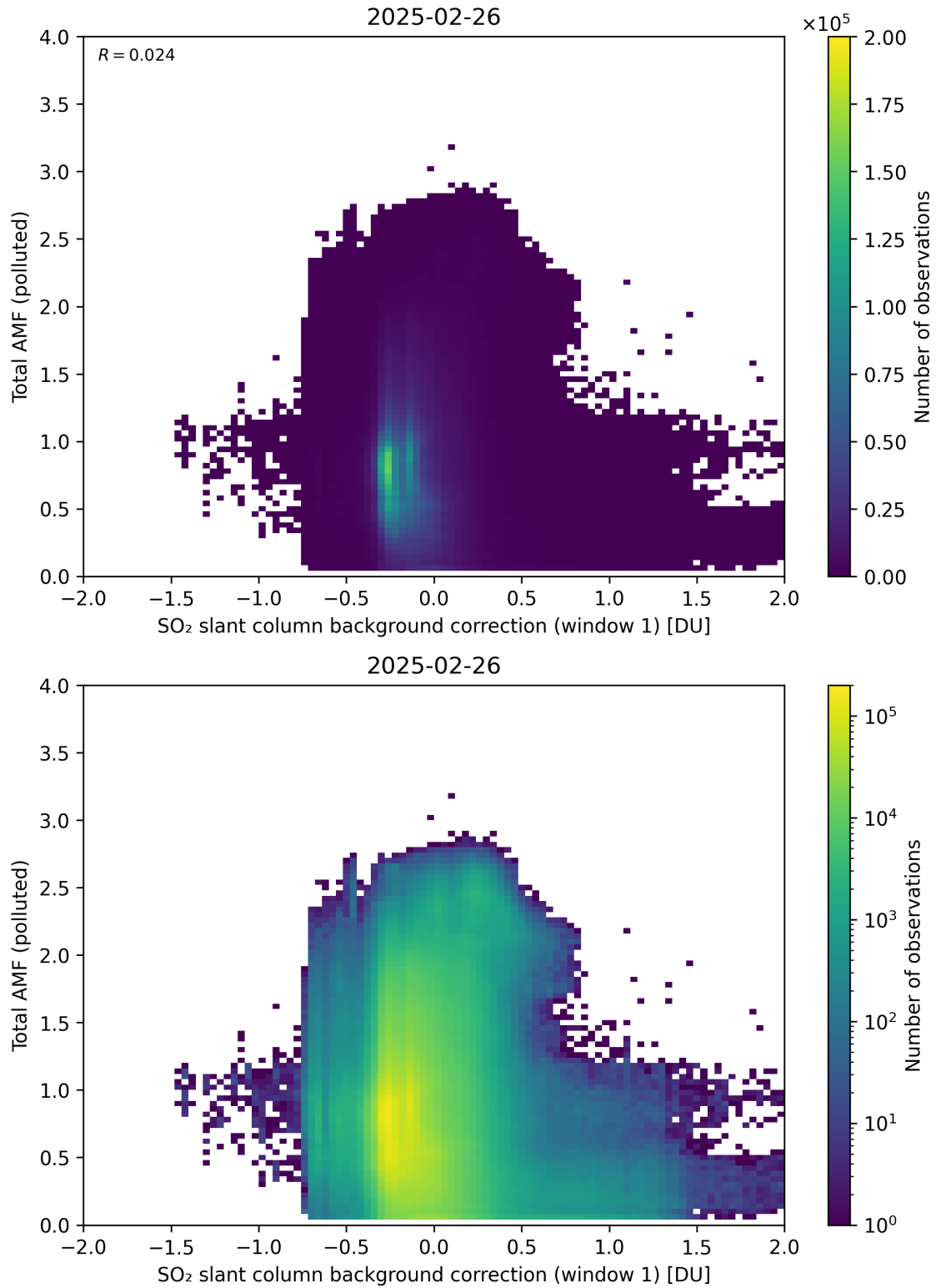
Figure 120: Scatter density plot of “SO 2 slant column background correction (window 1)” against “Total AMF (polluted)” for 2025-02-25 to 2025-02-27.
