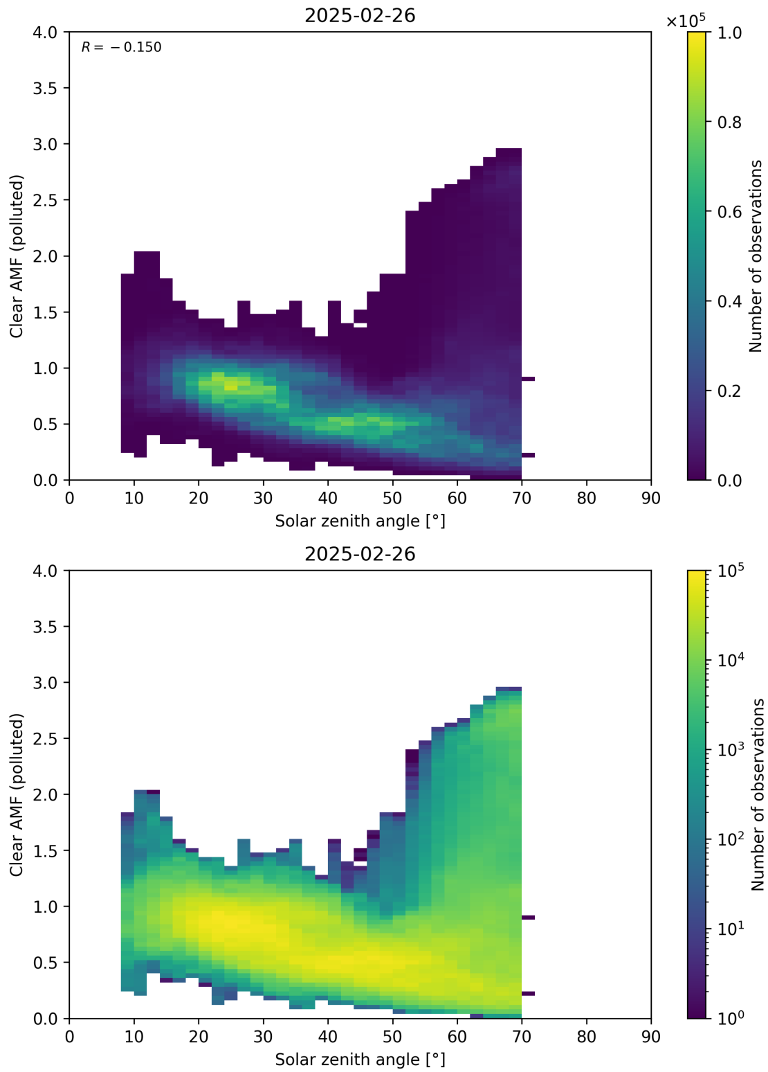
Figure 178: Scatter density plot of “Solar zenith angle” against “Clear AMF (polluted)” for 2025-02-25 to 2025-02-27.
