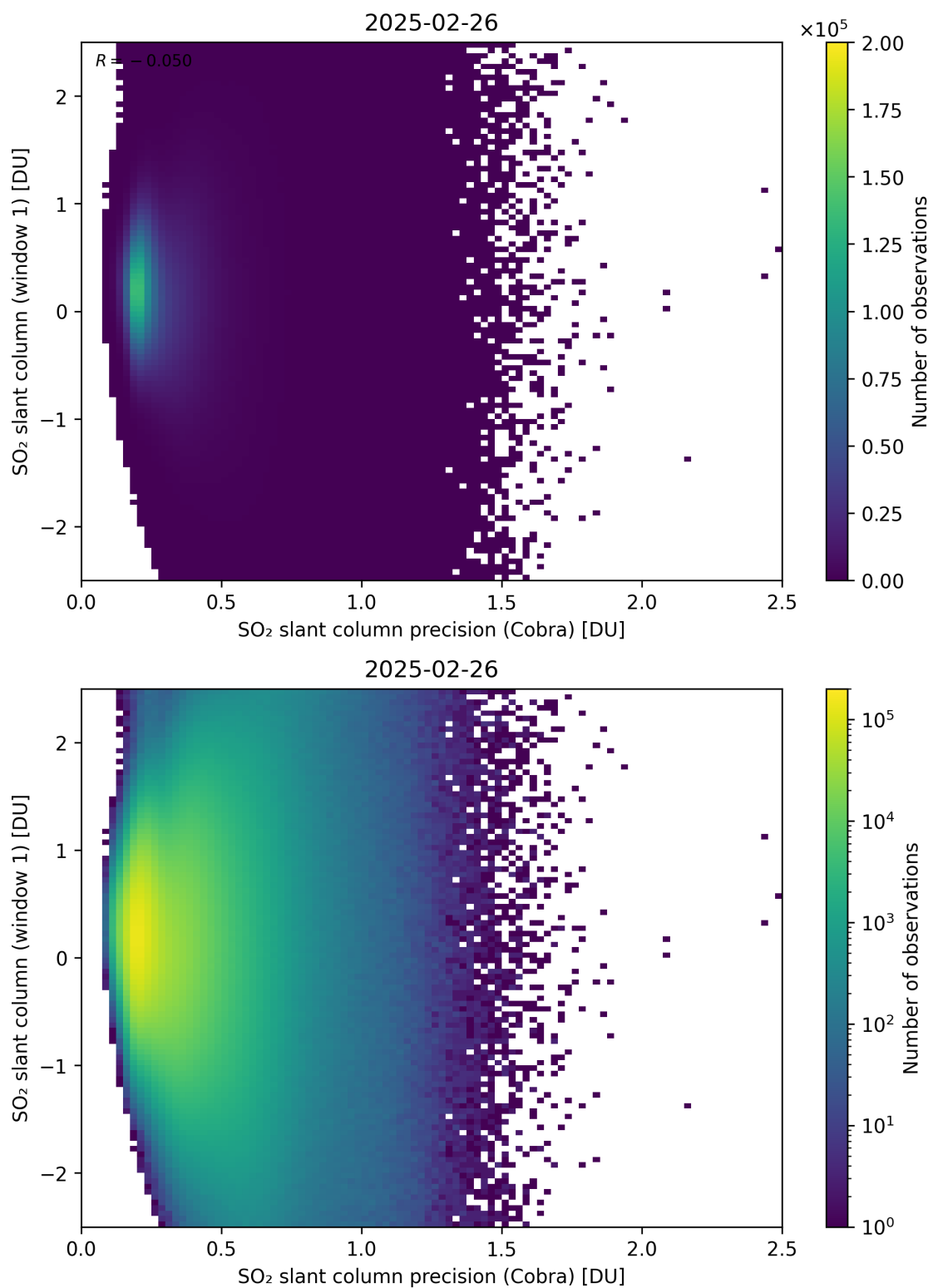
Figure 208: Scatter density plot of “SO 2 slant column precision (Cobra)” against “SO 2 slant column (window 1)” for 2025-02-25 to 2025-02-27.
