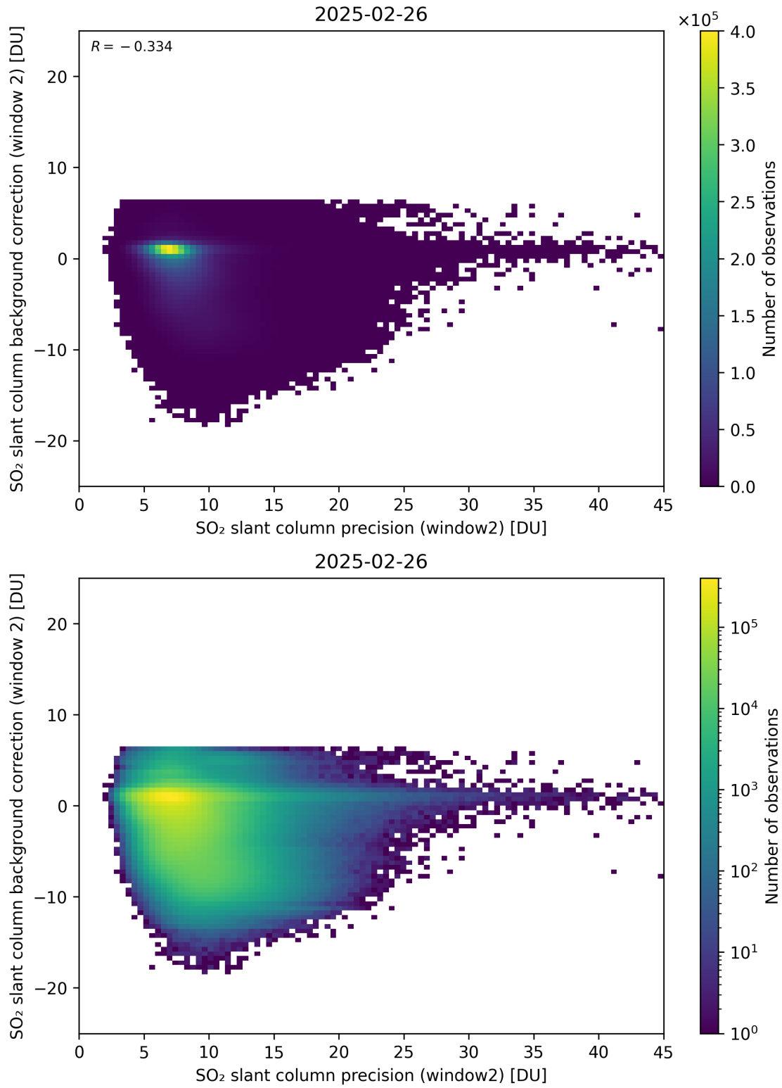
Figure 291: Scatter density plot of “SO 2 slant column precision (window2)” against “SO 2 slant column background correction (window 2)” for 2025-02-25 to 2025-02-27.
