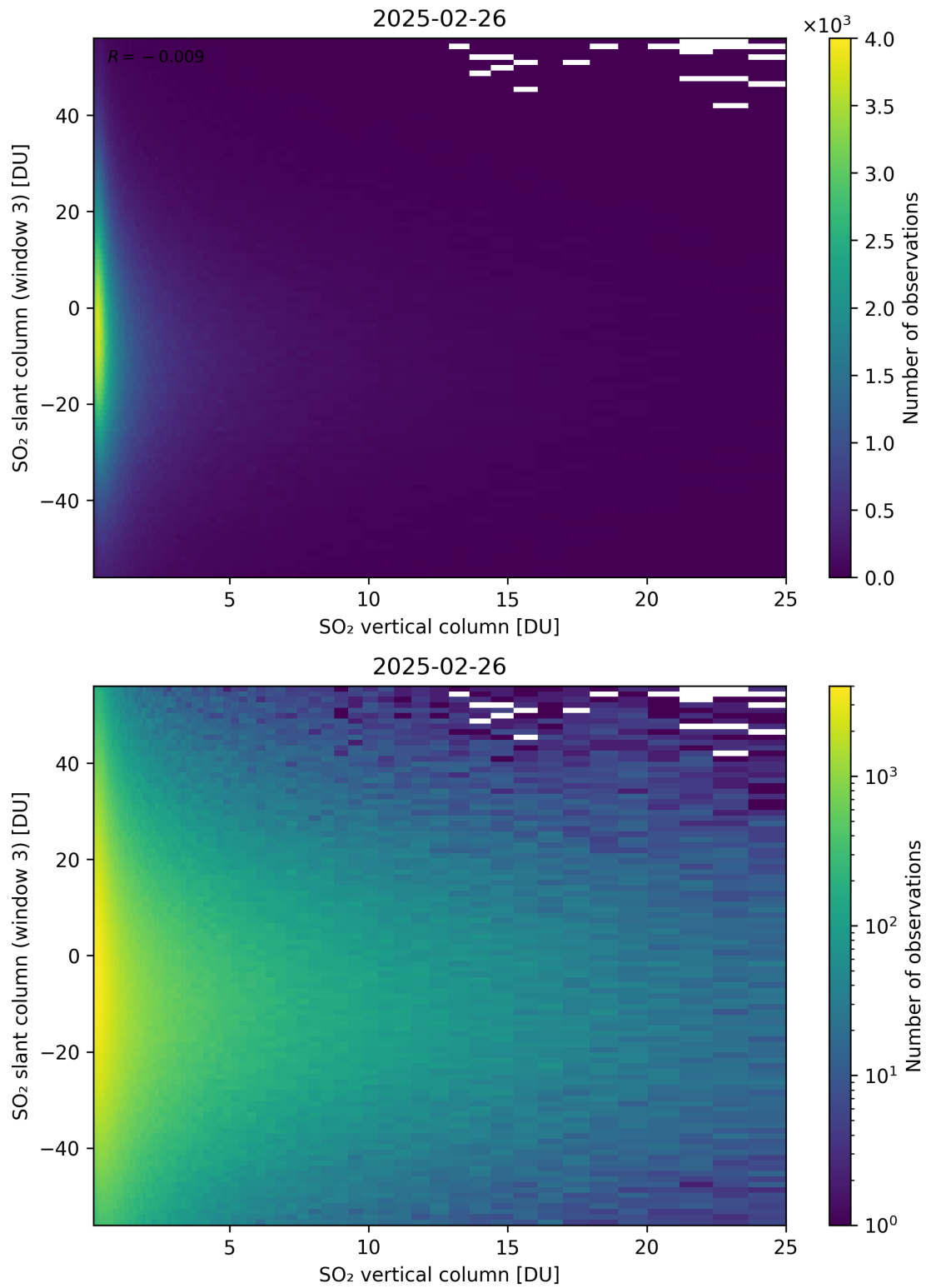
Figure 357: Scatter density plot of “SO 2 vertical column” against “SO 2 slant column (window 3)” for 2025-02-25 to 2025-02-27.
