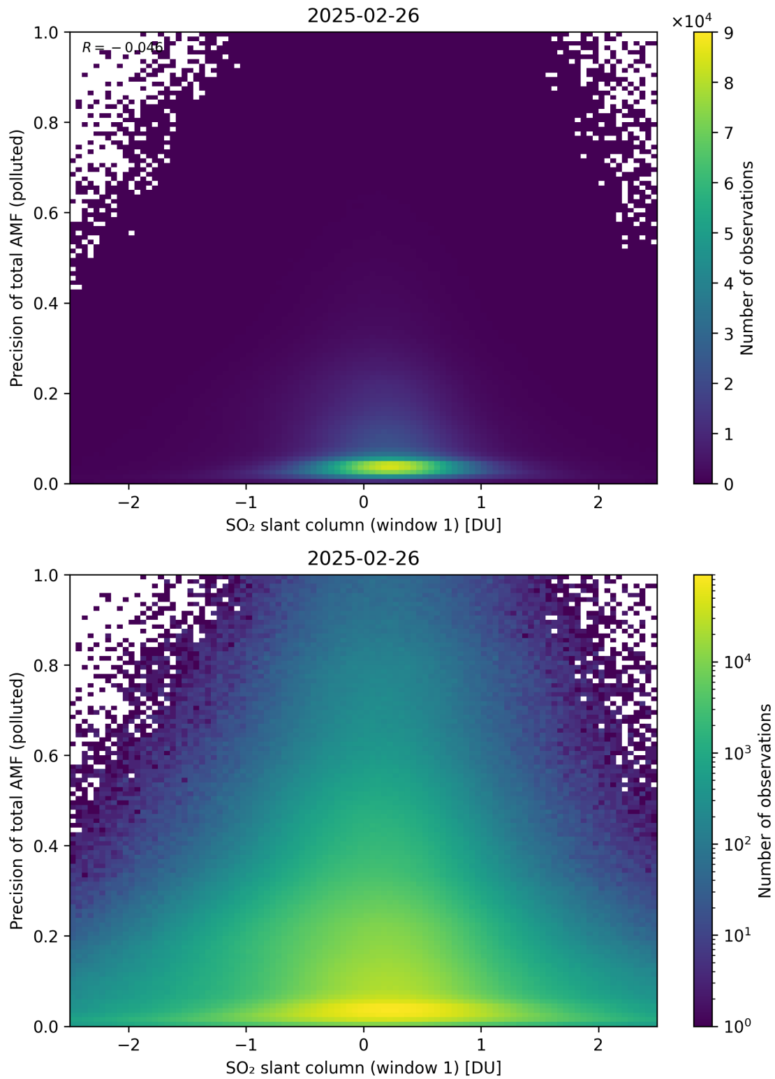
Figure 290: Scatter density plot of “SO 2 slant column (window 1)” against “Precision of total AMF (polluted)” for 2025-02-25 to 2025-02-27.
