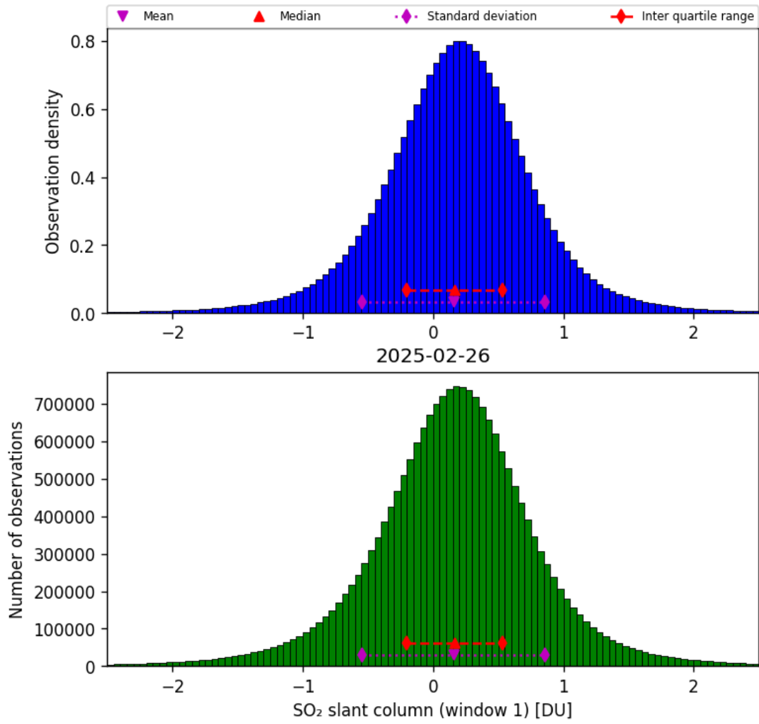
Figure 63: Histogram of “SO 2 slant column (window 1)” for 2025-02-25 to 2025-02-27
