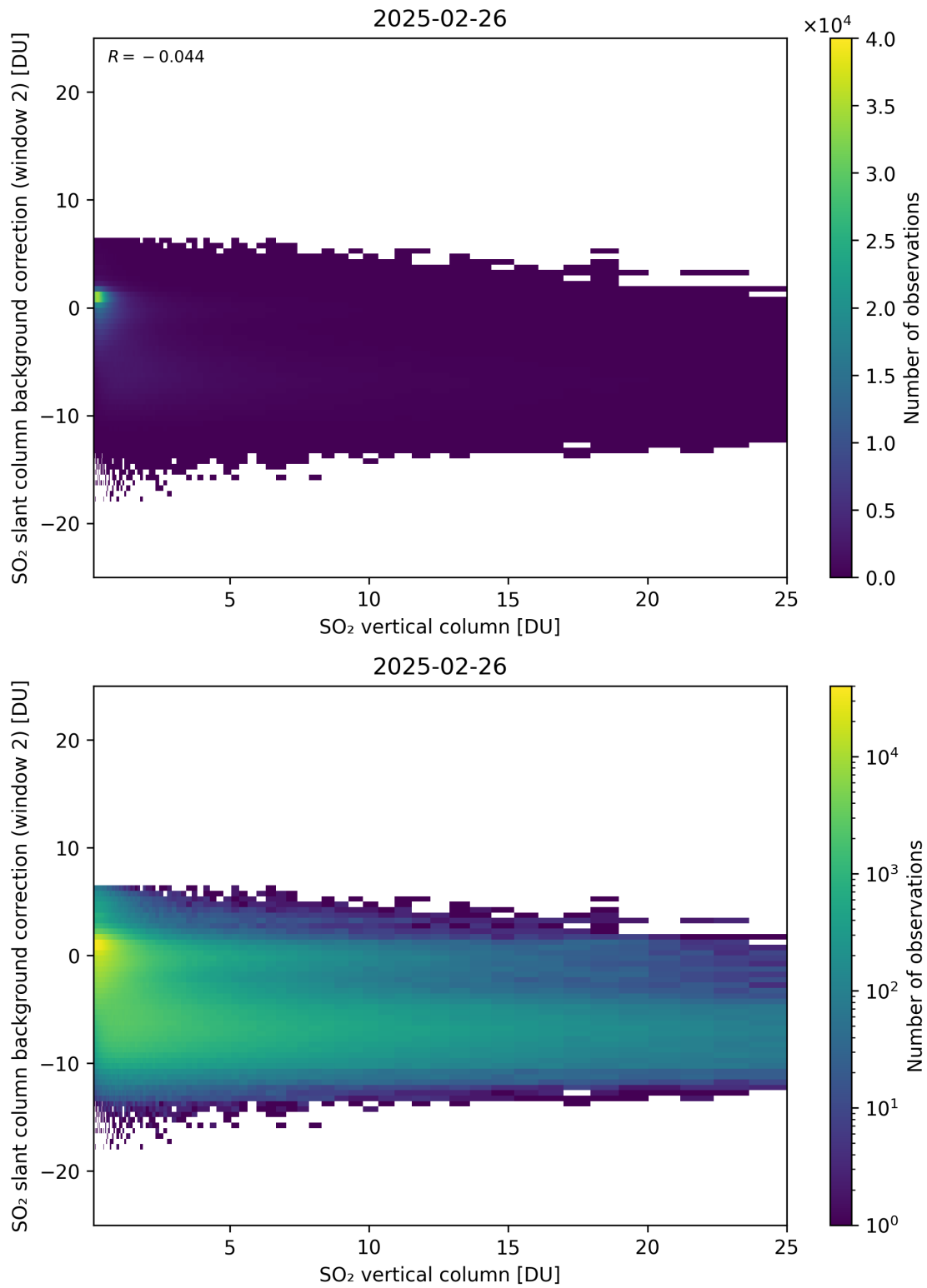
Figure 324: Scatter density plot of “SO 2 vertical column” against “SO 2 slant column background correction (window 2)” for 2025-02-25 to 2025-02-27.
