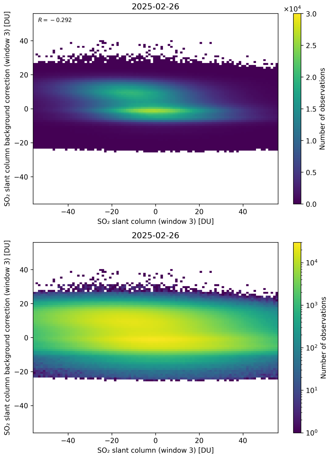
Figure 303: Scatter density plot of “SO 2 slant column (window 3)” against “SO 2 slant column background correction (window 3)” for 2025-02-25 to 2025-02-27.
