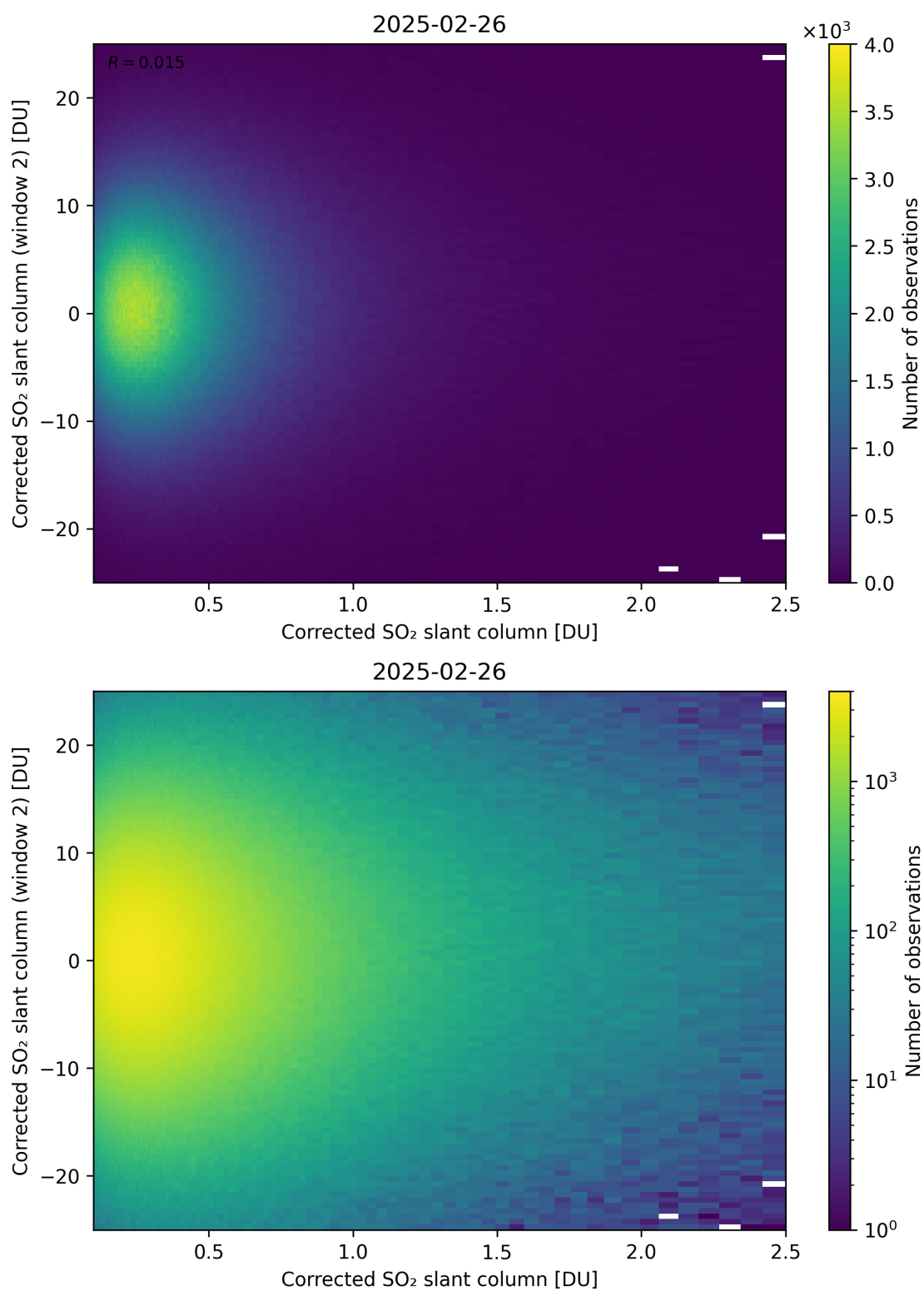
Figure 235: Scatter density plot of “Corrected SO 2 slant column” against “Corrected SO 2 slant column (window 2)” for 2025-02-25 to 2025-02-27.
