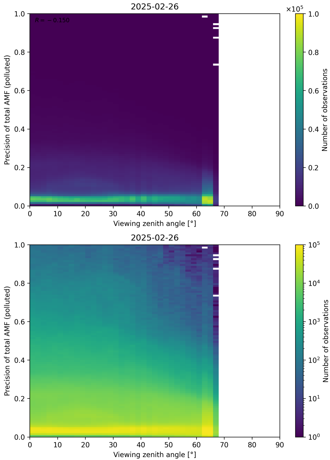
Figure 382: Scatter density plot of “Viewing zenith angle” against “Precision of total AMF (polluted)” for 2025-02-25 to 2025-02-27.
