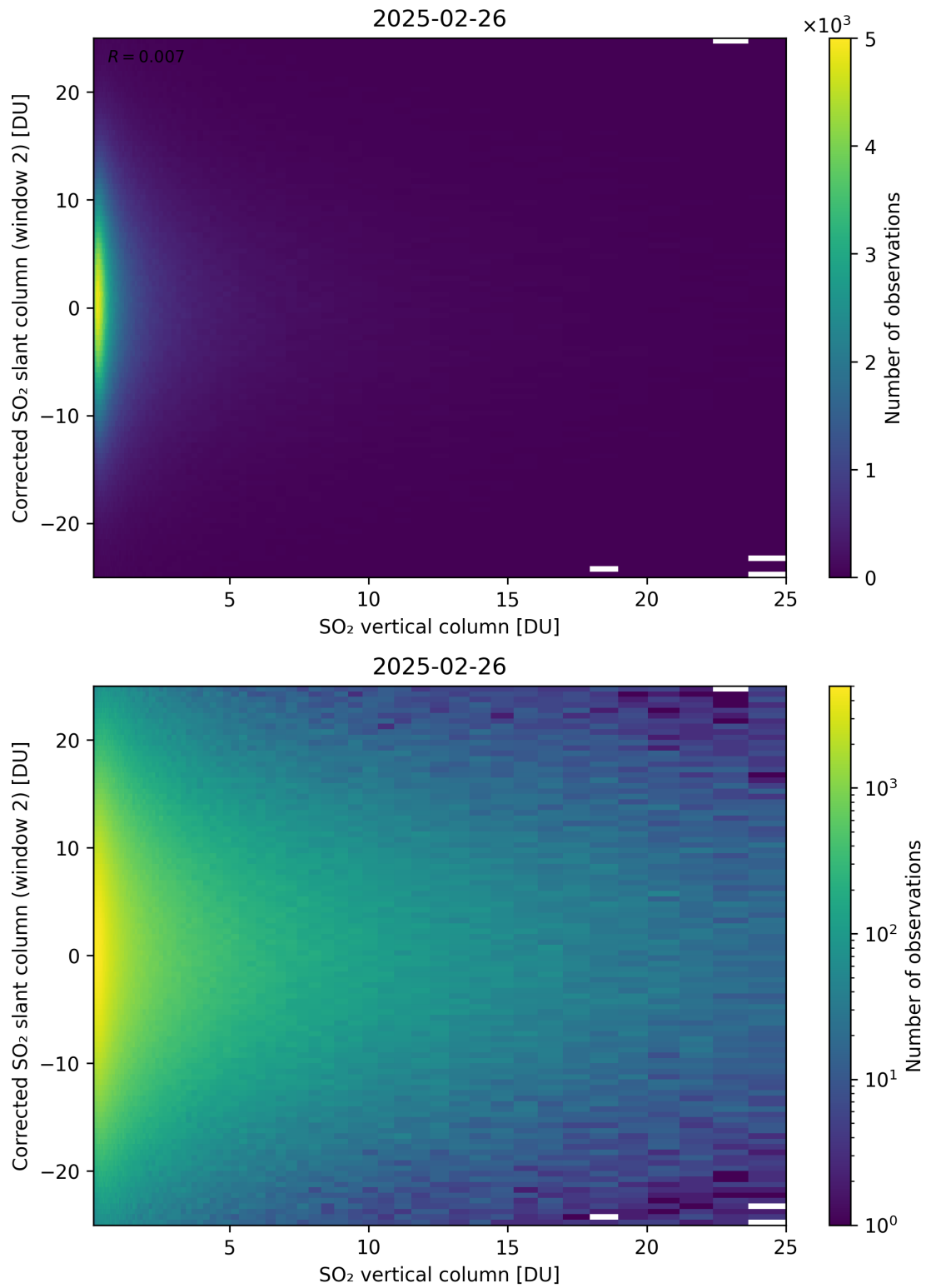
Figure 352: Scatter density plot of “SO 2 vertical column” against “Corrected SO 2 slant column (window 2)” for 2025-02-25 to 2025-02-27.
