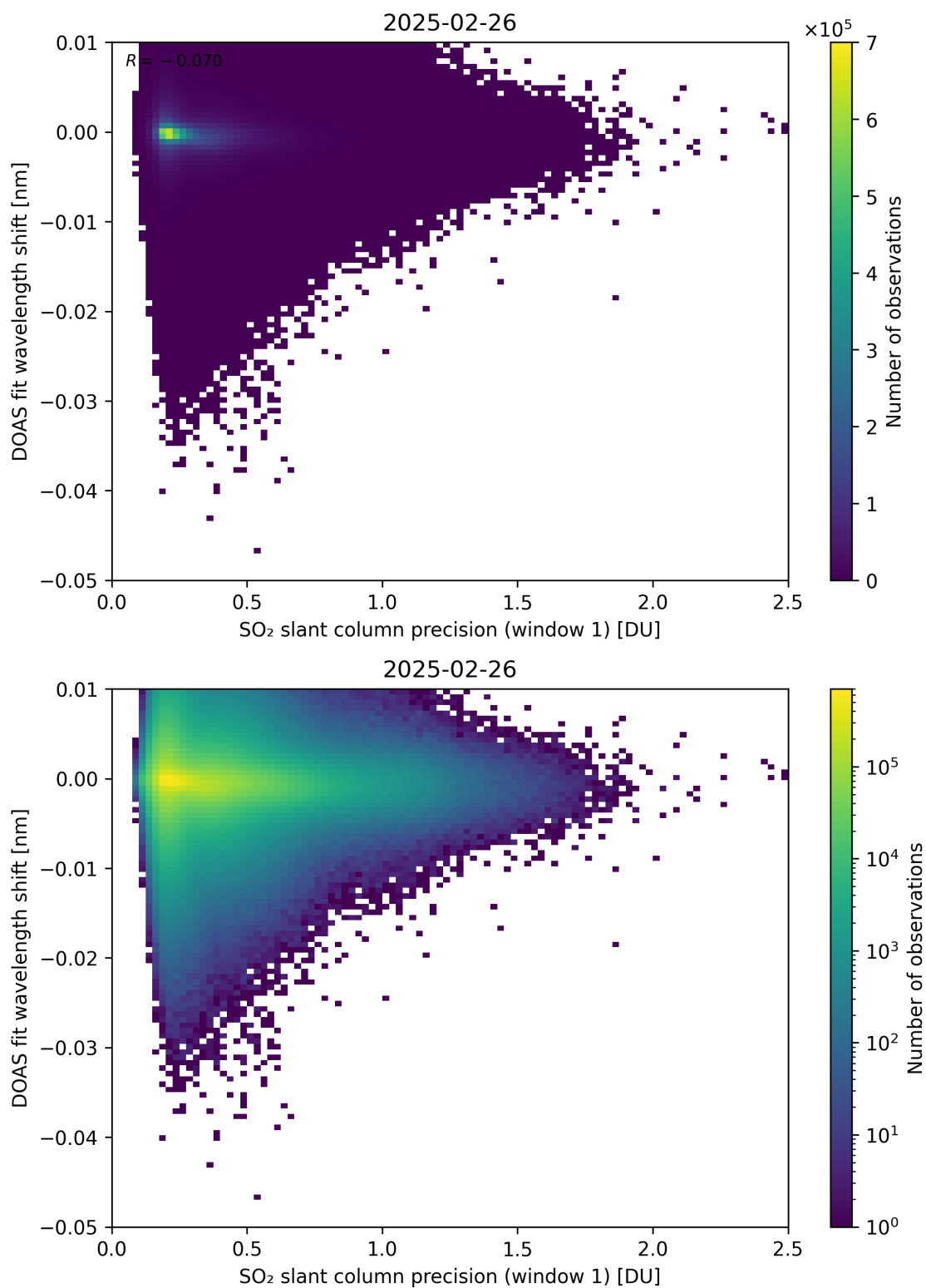
Figure 271: Scatter density plot of “SO 2 slant column precision (window 1)” against “DOAS fit wavelength shift” for 2025-02-25 to 2025-02-27.
