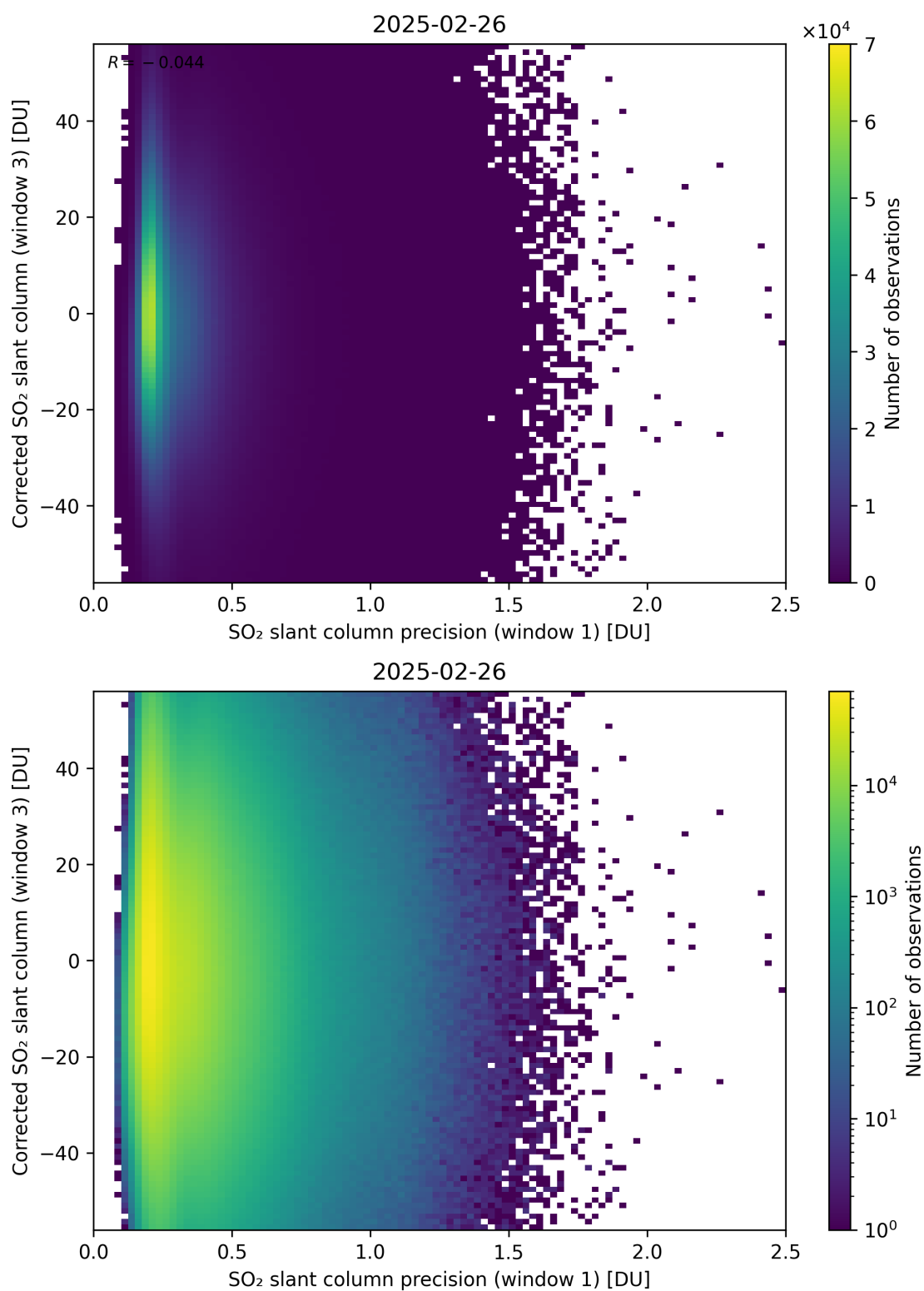
Figure 276: Scatter density plot of “SO 2 slant column precision (window 1)” against “Corrected SO 2 slant column (window 3)” for 2025-02-25 to 2025-02-27.
