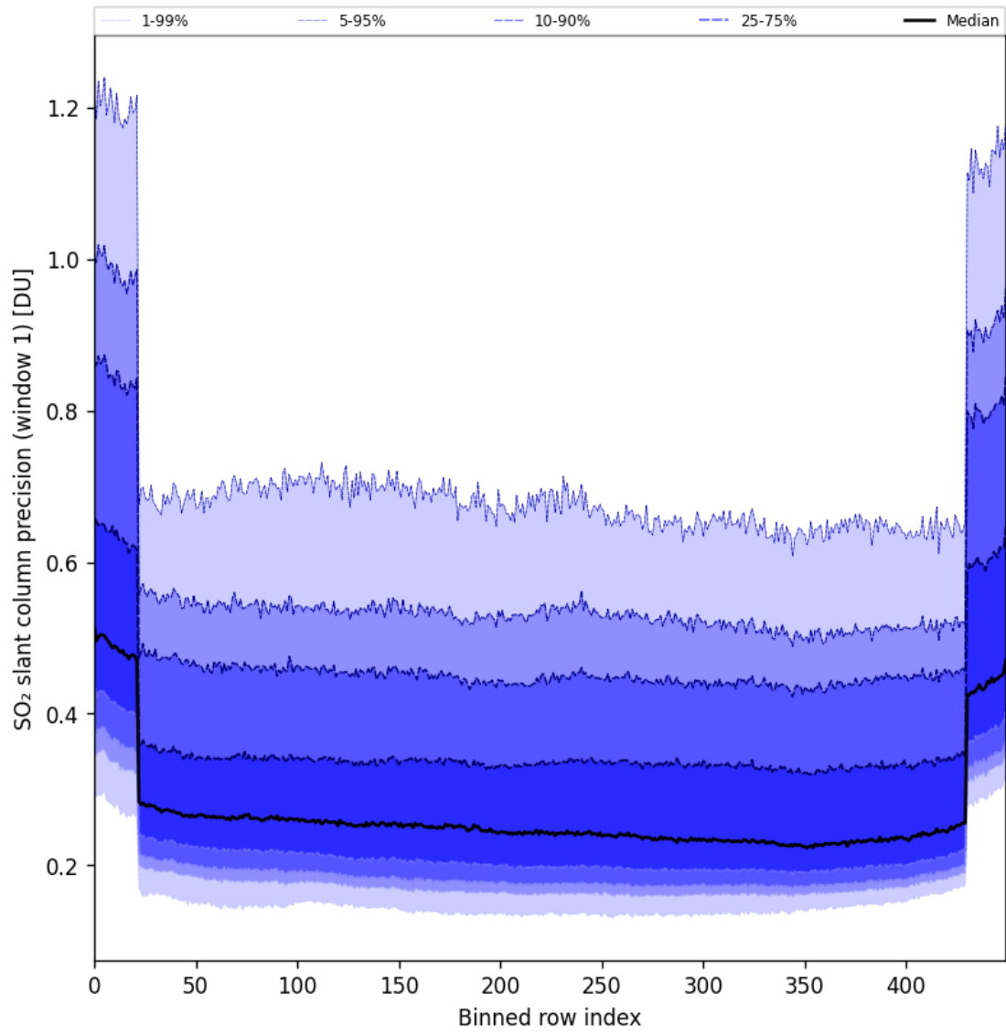
Figure 90: Along track statistics of “SO 2 slant column precision (window 1)” for 2025-02-25 to 2025-02-27
