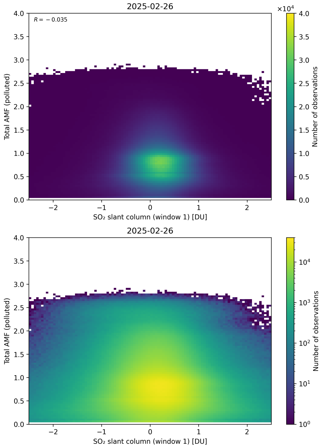
Figure 289: Scatter density plot of “SO 2 slant column (window 1)” against “Total AMF (polluted)” for 2025-02-25 to 2025-02-27.
