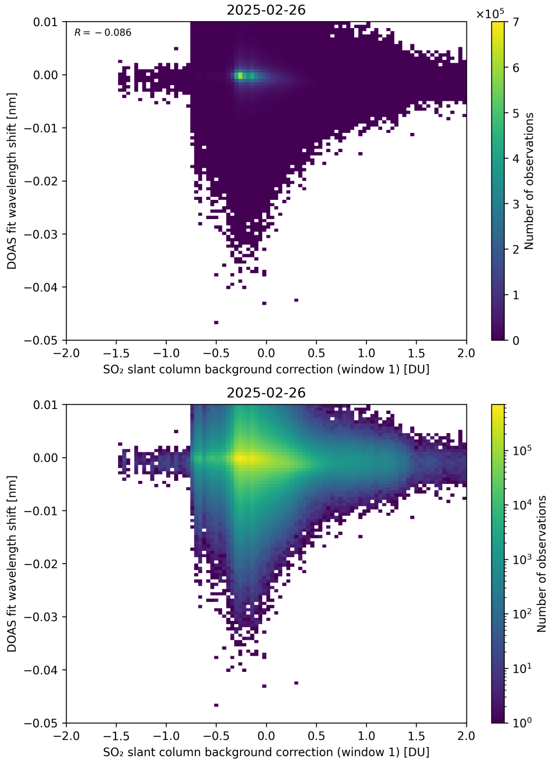
Figure 111: Scatter density plot of “SO 2 slant column background correction (window 1)” against “DOAS fit wavelength shift” for 2025-02-25 to 2025-02-27.
