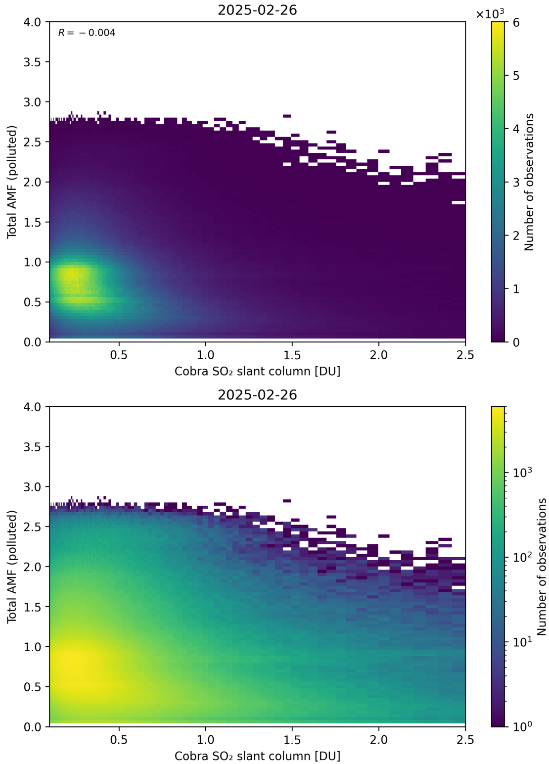
Figure 224: Scatter density plot of “Cobra SO 2 slant column” against “Total AMF (polluted)” for 2025-02-25 to 2025-02-27.
