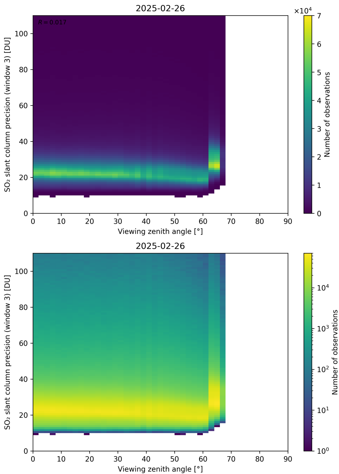
Figure 380: Scatter density plot of “Viewing zenith angle” against “SO 2 slant column precision (window 3)” for 2025-02-25 to 2025-02-27.
