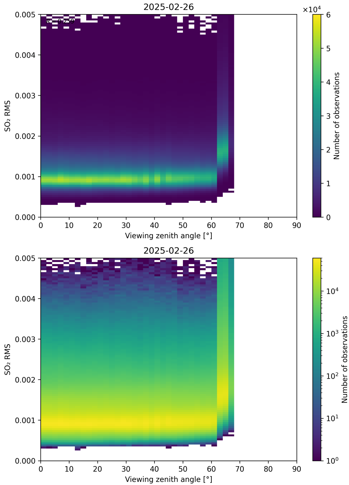
Figure 367: Scatter density plot of “Viewing zenith angle” against “SO 2 RMS” for 2025-02-25 to 2025-02-27.
