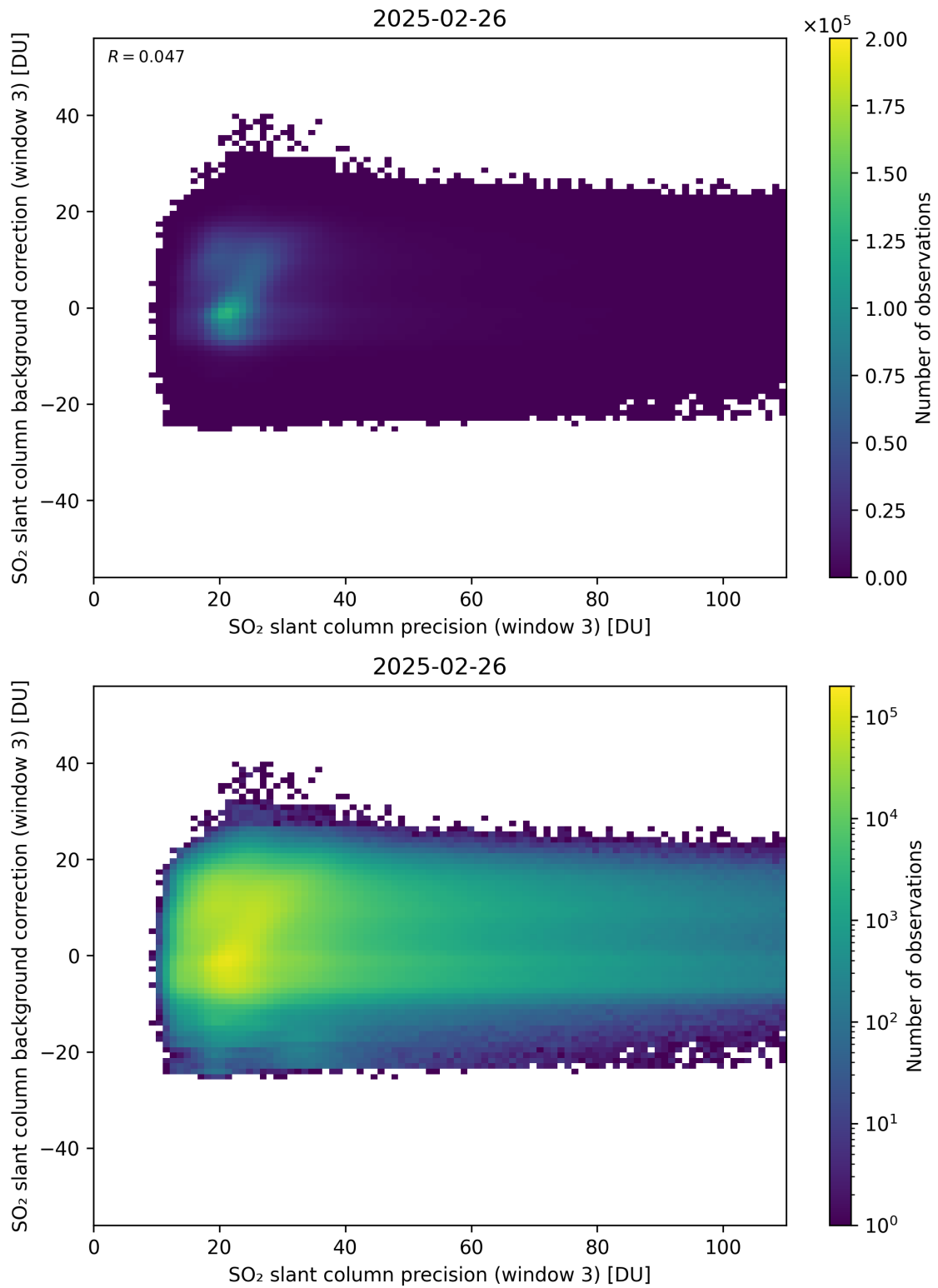
Figure 307: Scatter density plot of “SO 2 slant column precision (window 3)” against “SO 2 slant column background correction (window 3)” for 2025-02-25 to 2025-02-27.
