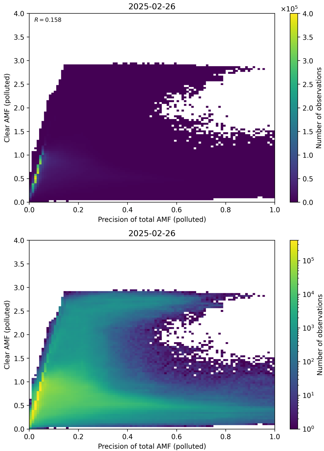
Figure 320: Scatter density plot of “Precision of total AMF (polluted)” against “Clear AMF (polluted)” for 2025-02-25 to 2025-02-27.
