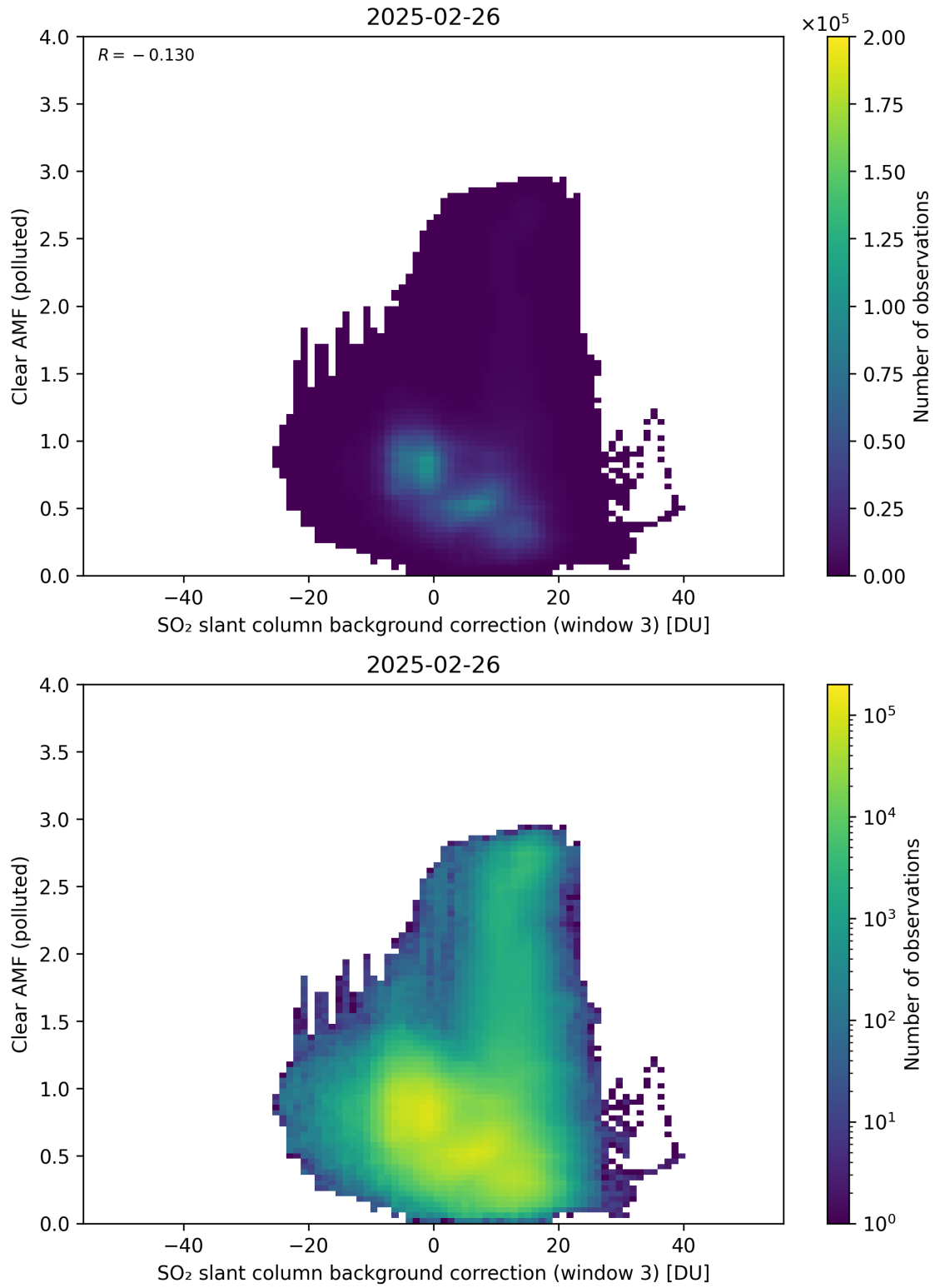
Figure 135: Scatter density plot of “SO 2 slant column background correction (window 3)” against “Clear AMF (polluted)” for 2025-02-25 to 2025-02-27.
