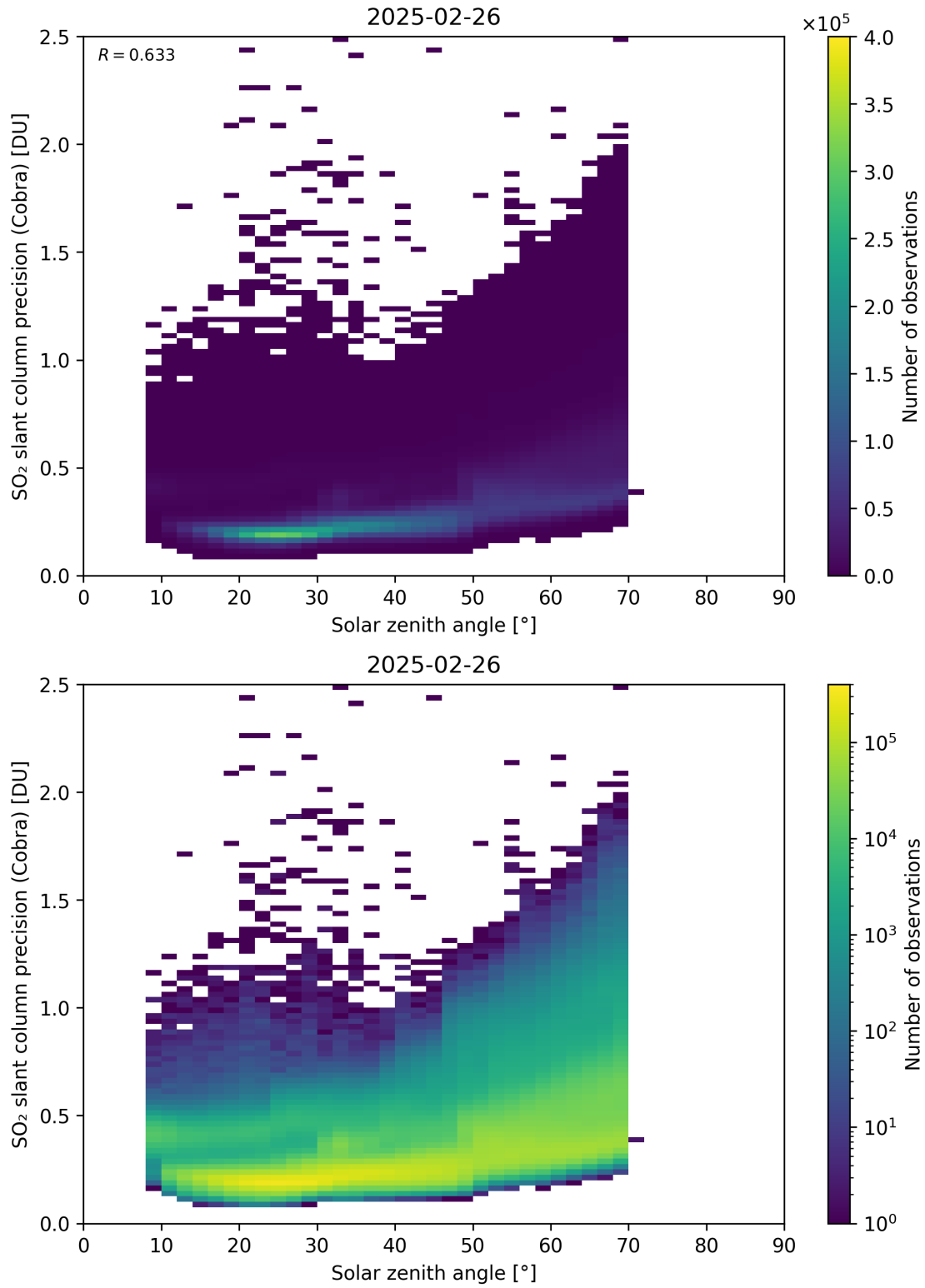
Figure 180: Scatter density plot of “Solar zenith angle” against “SO 2 slant column precision (Cobra)” for 2025-02-25 to 2025-02-27.
