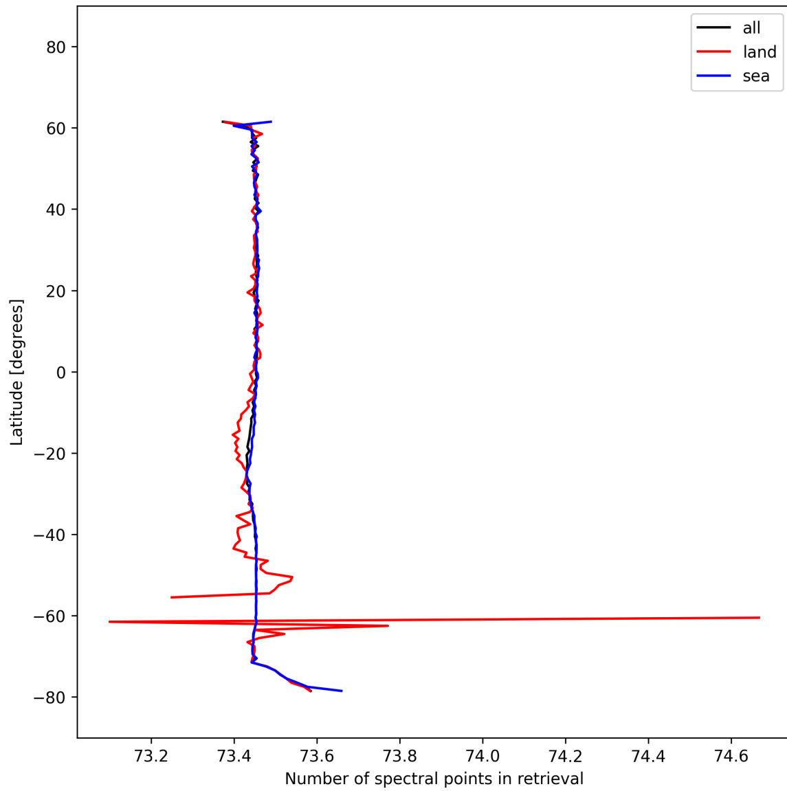
Figure 56: Zonal average of “Number of spectral points in retrieval” for 2025-02-25 to 2025-02-27.
