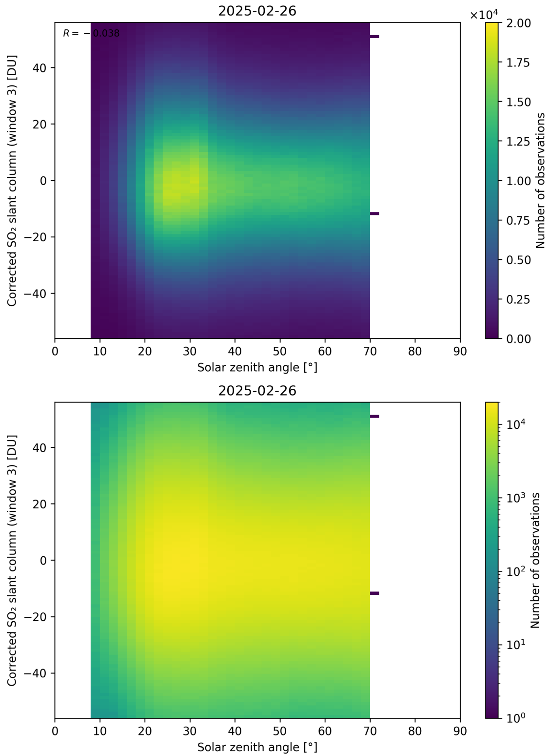
Figure 183: Scatter density plot of “Solar zenith angle” against “Corrected SO 2 slant column (window 3)” for 2025-02-25 to 2025-02-27.
