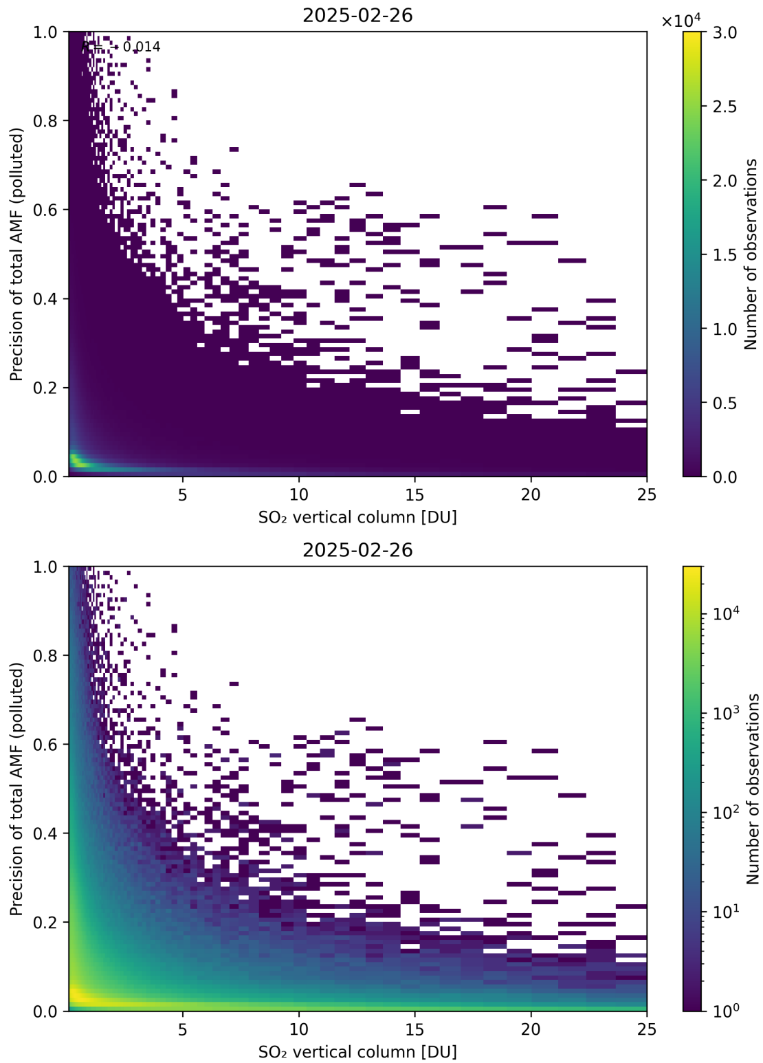
Figure 360: Scatter density plot of “SO 2 vertical column” against “Precision of total AMF (polluted)” for 2025-02-25 to 2025-02-27.
