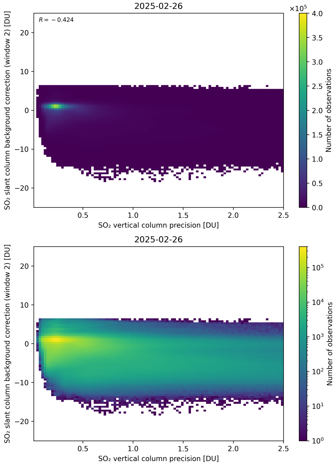
Figure 330: Scatter density plot of “SO 2 vertical column precision” against “SO 2 slant column background correction (window 2)” for 2025-02-25 to 2025-02-27.
