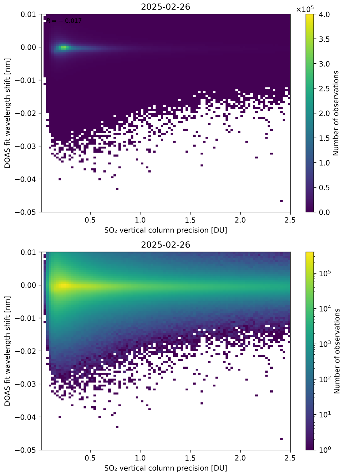
Figure 332: Scatter density plot of “SO 2 vertical column precision” against “DOAS fit wavelength shift” for 2025-02-25 to 2025-02-27.
