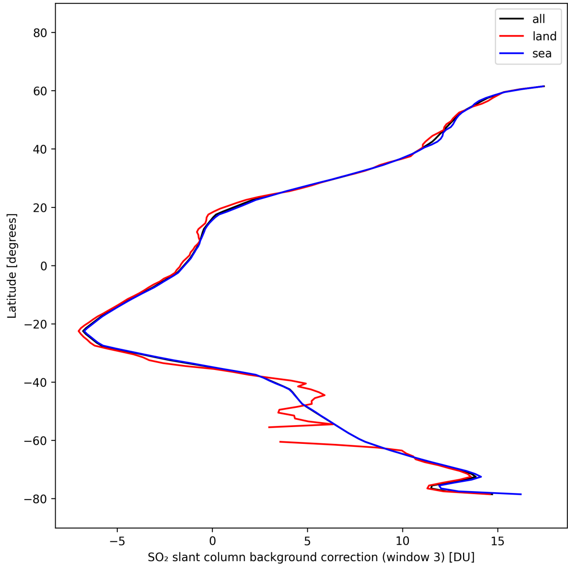
Figure 48: Zonal average of “SO 2 slant column background correction (window 3)” for 2025-02-25 to 2025-02-27.
