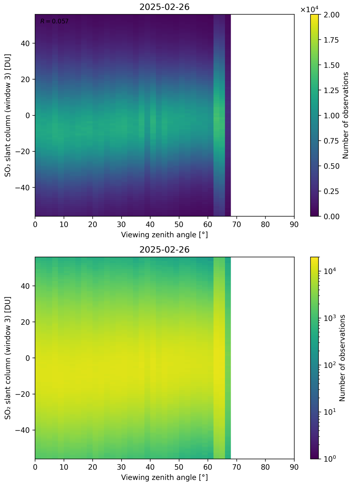
Figure 379: Scatter density plot of “Viewing zenith angle” against “SO 2 slant column (window 3)” for 2025-02-25 to 2025-02-27.
