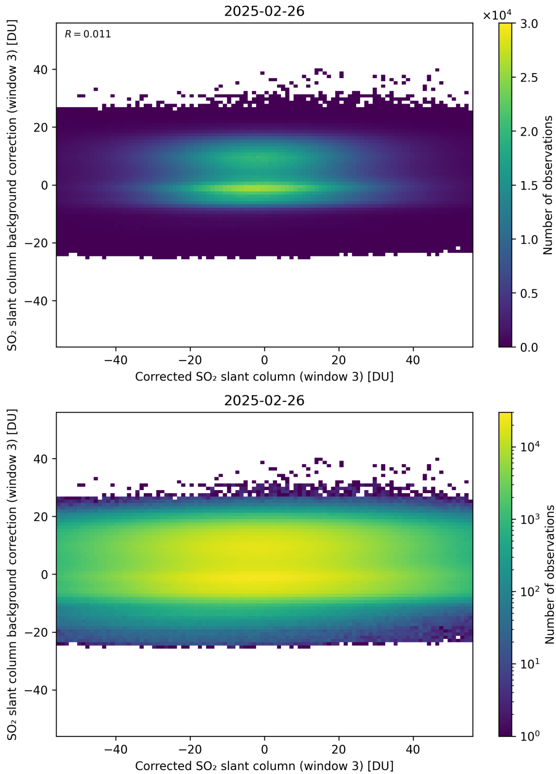
Figure 255: Scatter density plot of “Corrected SO 2 slant column (window 3)” against “SO 2 slant column background correction (window 3)” for 2025-02-25 to 2025-02-27.
