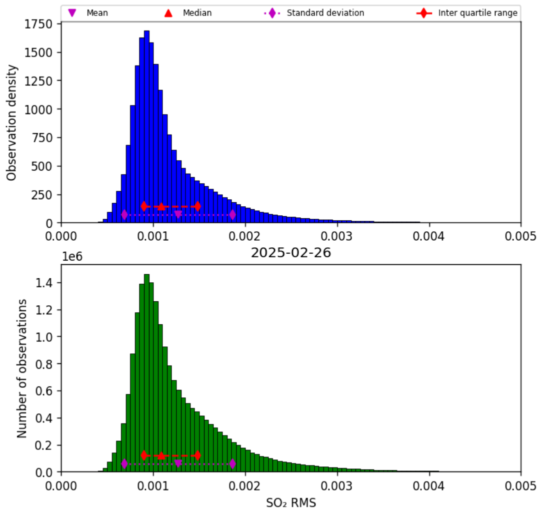
Figure 78: Histogram of “SO 2 RMS” for 2025-02-25 to 2025-02-27
