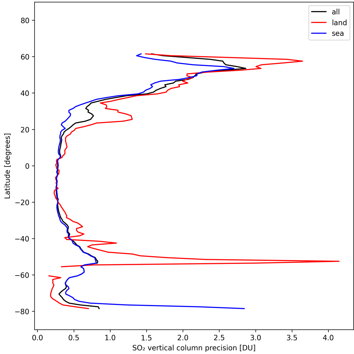
Figure 33: Zonal average of “SO 2 vertical column precision” for 2025-02-25 to 2025-02-27.
