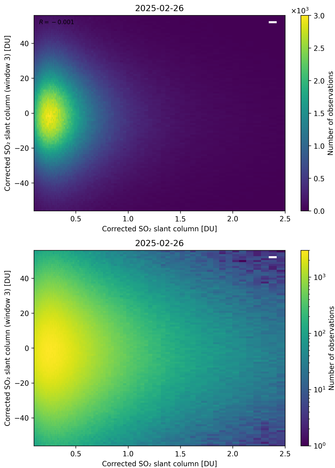
Figure 236: Scatter density plot of “Corrected SO 2 slant column” against “Corrected SO 2 slant column (window 3)” for 2025-02-25 to 2025-02-27.
