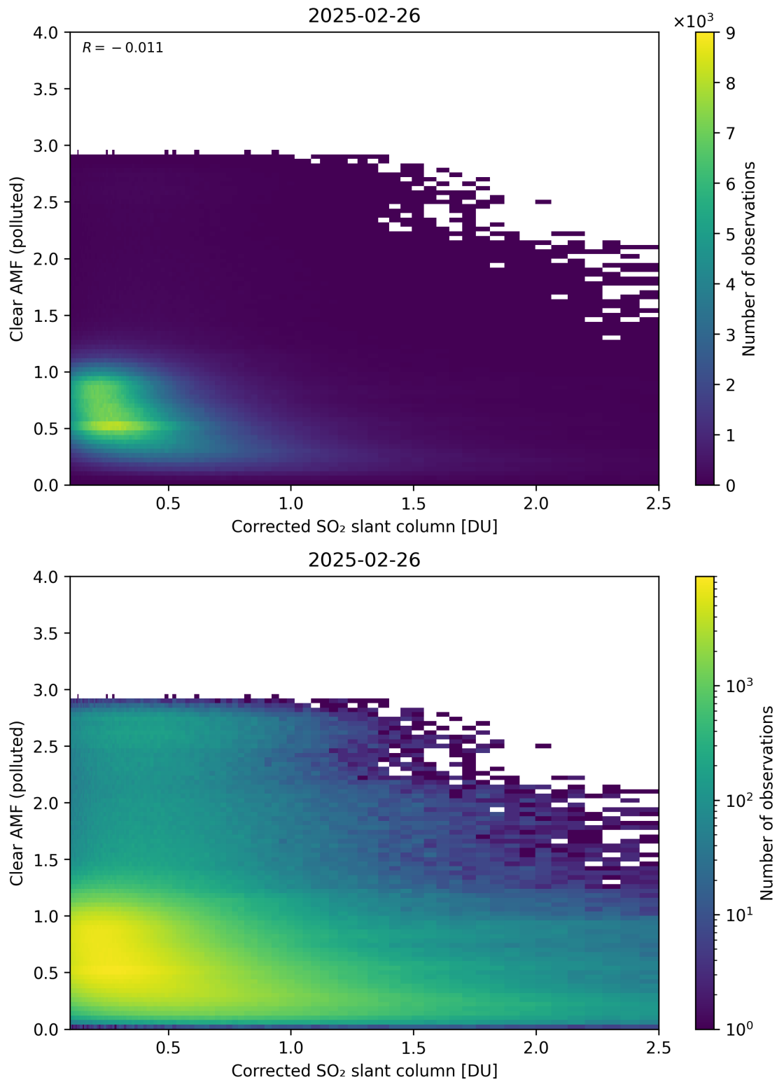
Figure 232: Scatter density plot of “Corrected SO 2 slant column” against “Clear AMF (polluted)” for 2025-02-25 to 2025-02-27.
