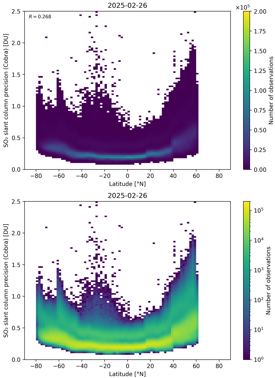
Figure 158: Scatter density plot of “Latitude” against “SO 2 slant column precision (Cobra)” for 2025-02-25 to 2025-02-27.
