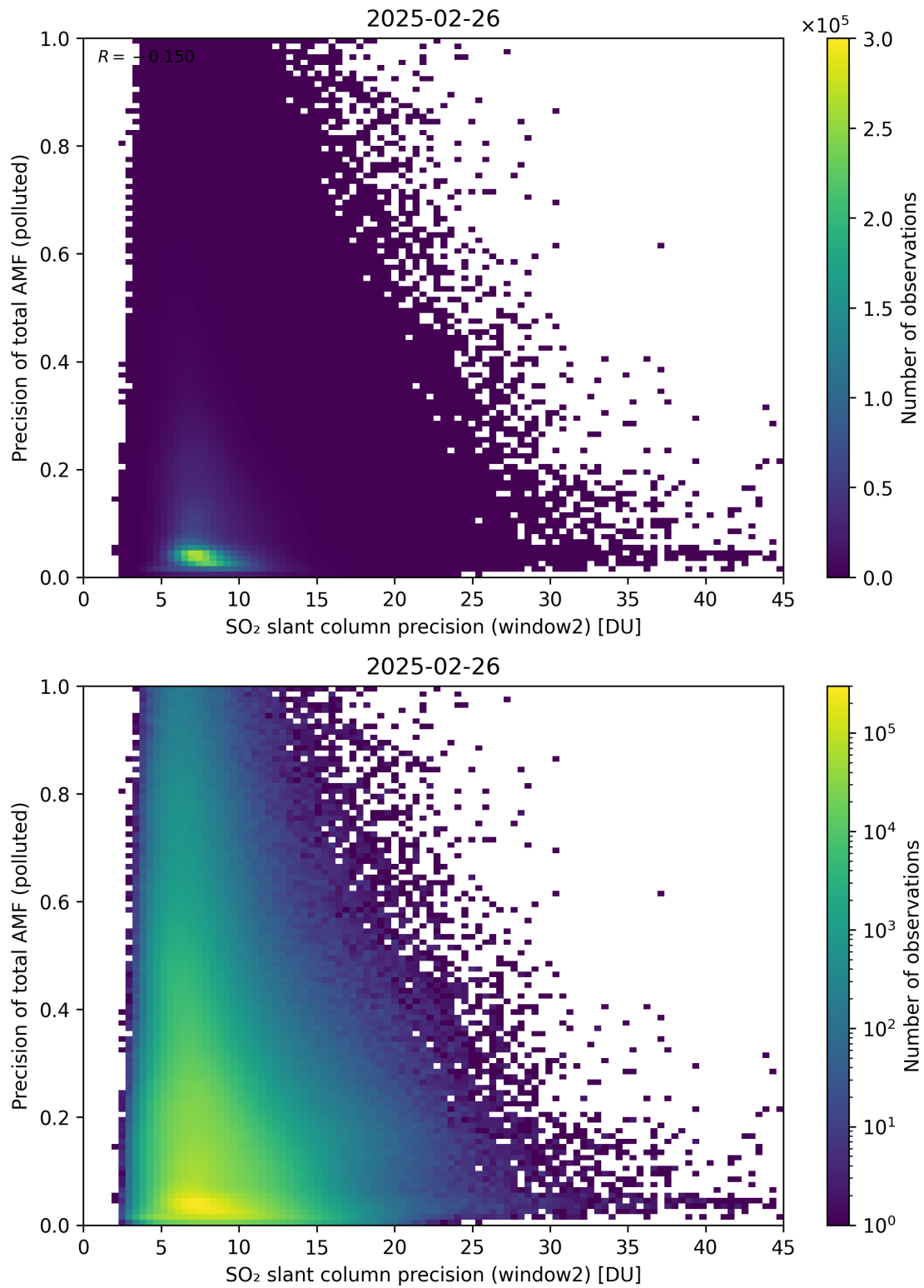
Figure 302: Scatter density plot of “SO 2 slant column precision (window2)” against “Precision of total AMF (polluted)” for 2025-02-25 to 2025-02-27.
