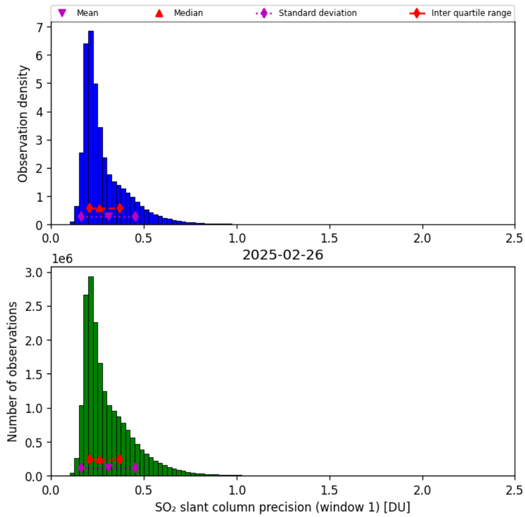
Figure 64: Histogram of “SO 2 slant column precision (window 1)” for 2025-02-25 to 2025-02-27
