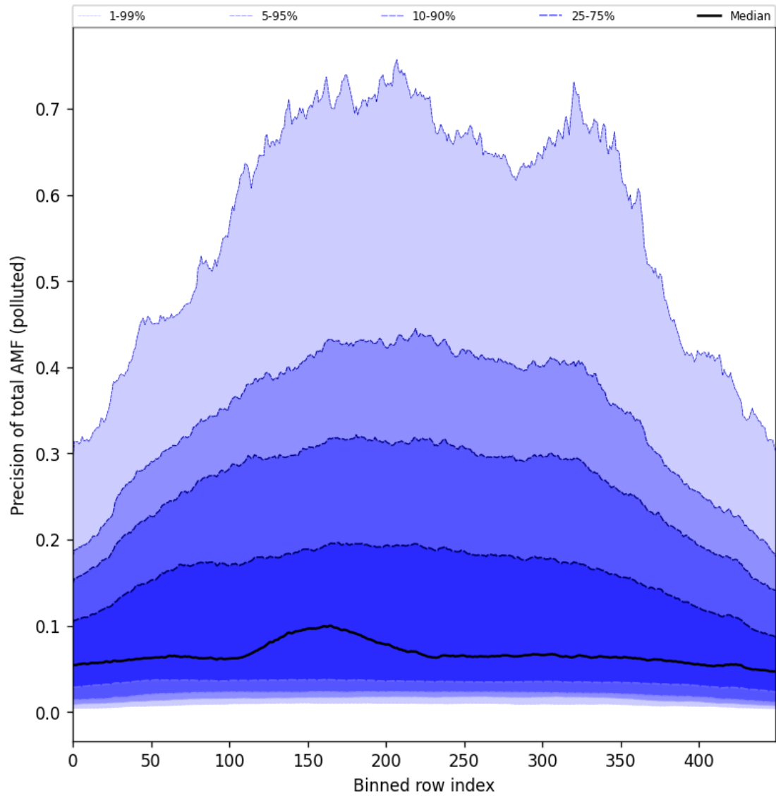
Figure 106: Along track statistics of “Precision of total AMF (polluted)” for 2025-02-25 to 2025-02-27
