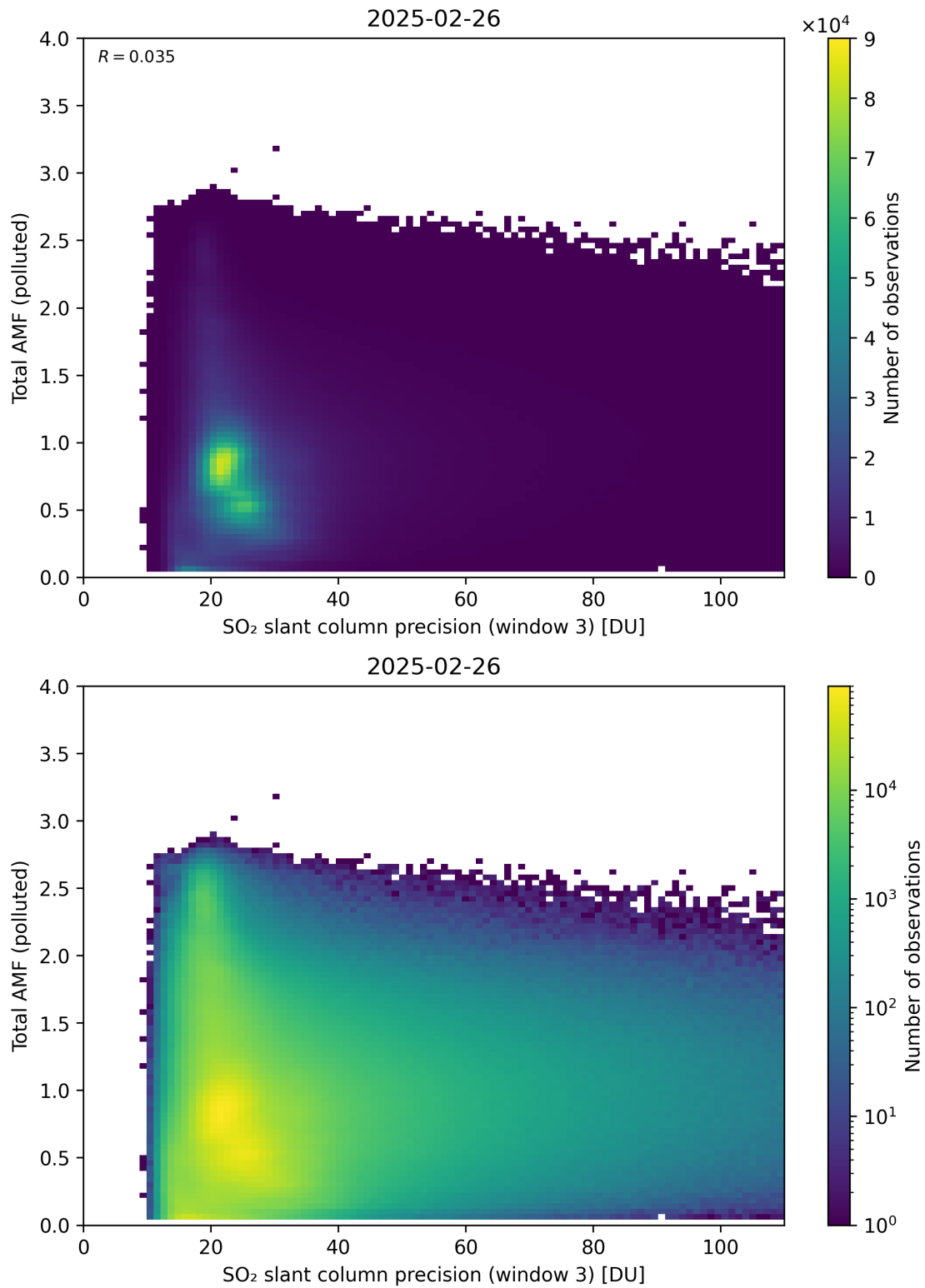
Figure 313: Scatter density plot of “SO 2 slant column precision (window 3)” against “Total AMF (polluted)” for 2025-02-25 to 2025-02-27.
