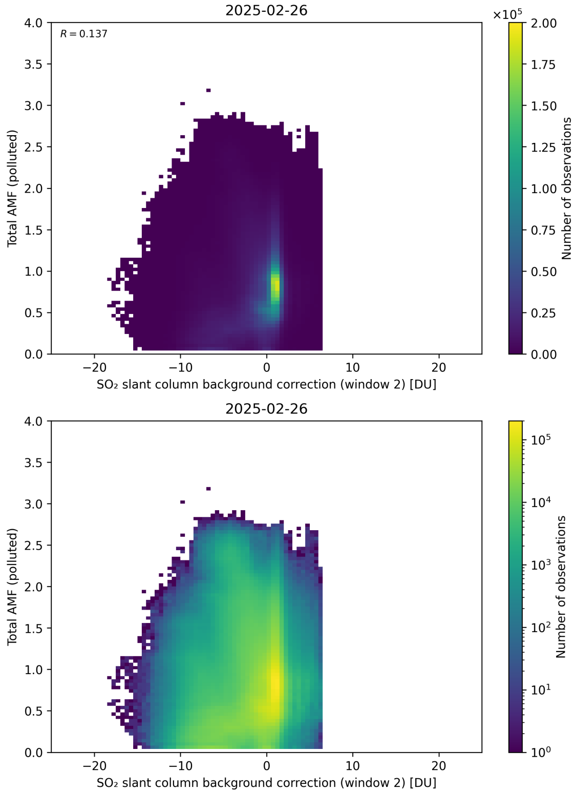
Figure 130: Scatter density plot of “SO 2 slant column background correction (window 2)” against “Total AMF (polluted)” for 2025-02-25 to 2025-02-27.
