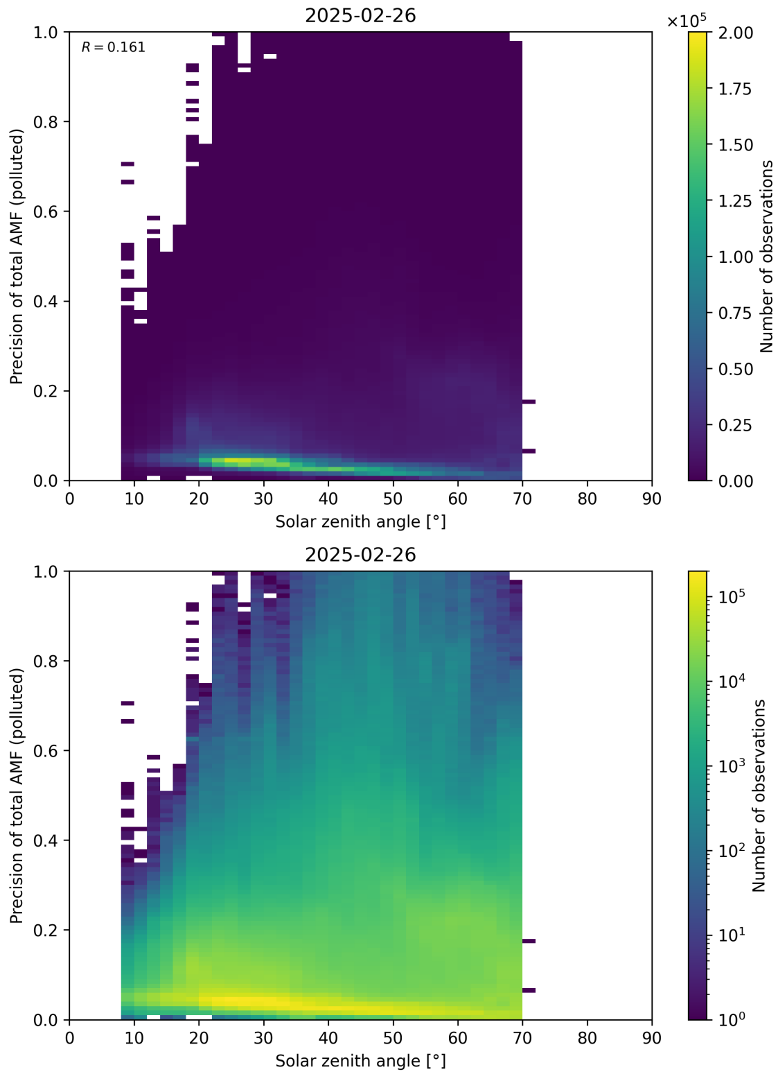
Figure 190: Scatter density plot of “Solar zenith angle” against “Precision of total AMF (polluted)” for 2025-02-25 to 2025-02-27.
