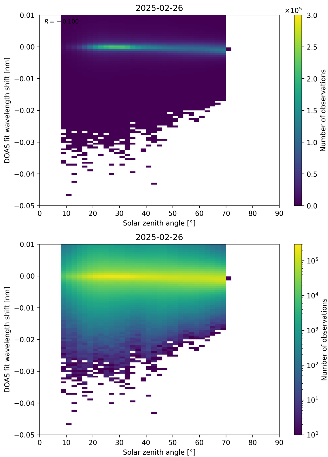
Figure 174: Scatter density plot of “Solar zenith angle” against “DOAS fit wavelength shift” for 2025-02-25 to 2025-02-27.
