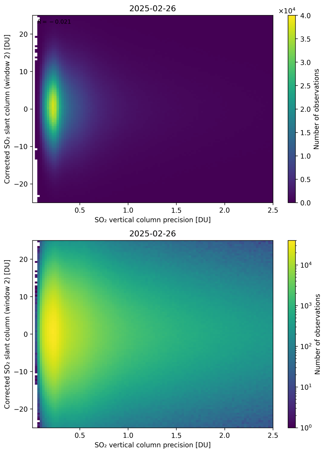
Figure 339: Scatter density plot of “SO 2 vertical column precision” against “Corrected SO 2 slant column (window 2)” for 2025-02-25 to 2025-02-27.
