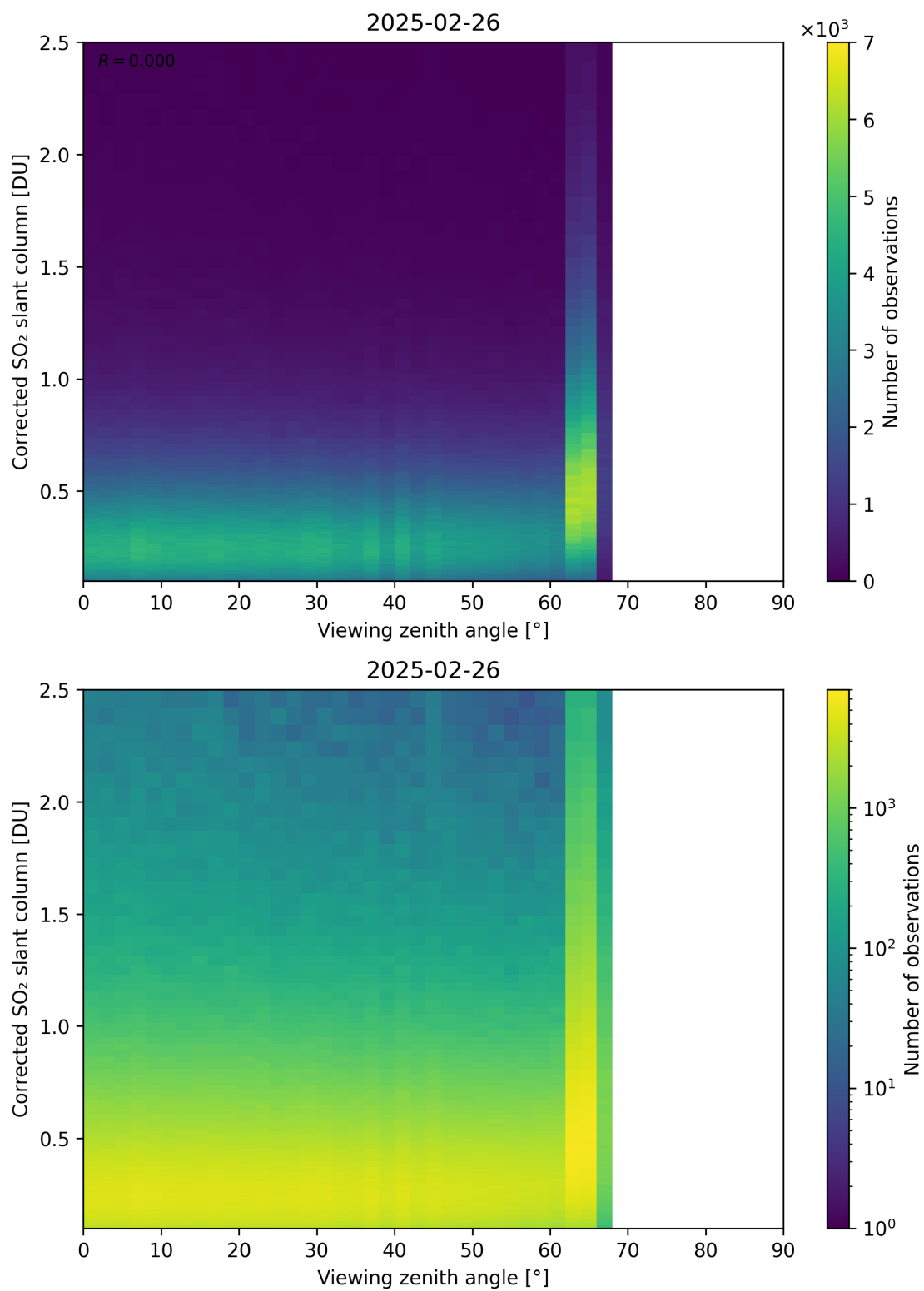
Figure 373: Scatter density plot of “Viewing zenith angle” against “Corrected SO 2 slant column” for 2025-02-25 to 2025-02-27.
