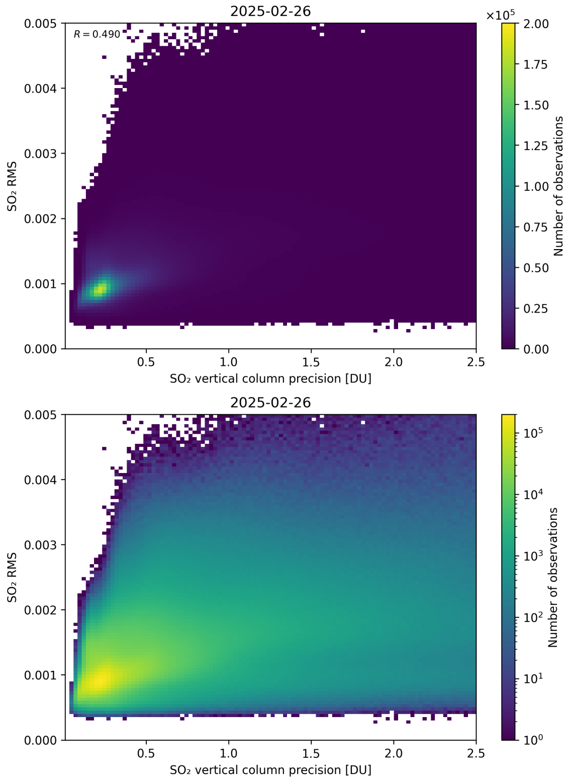
Figure 334: Scatter density plot of “SO 2 vertical column precision” against “SO 2 RMS” for 2025-02-25 to 2025-02-27.
