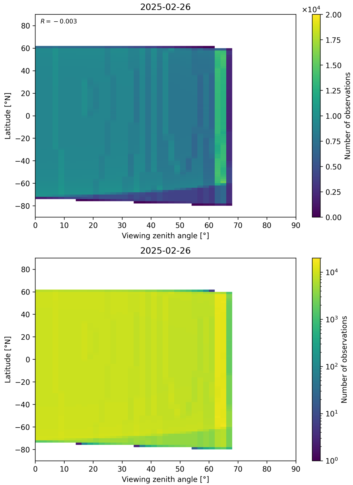
Figure 368: Scatter density plot of “Viewing zenith angle” against “Latitude” for 2025-02-25 to 2025-02-27.
