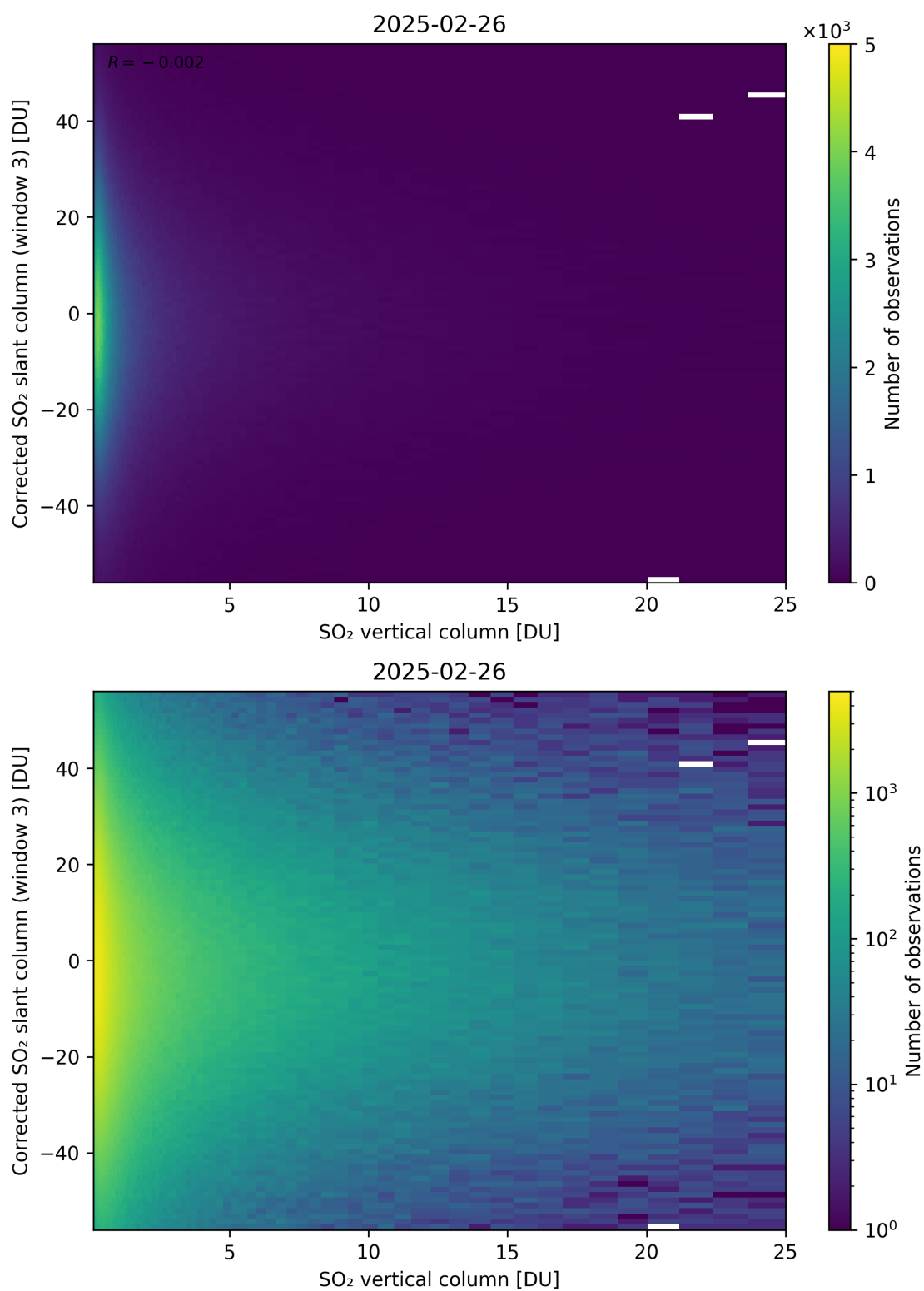
Figure 353: Scatter density plot of “SO 2 vertical column” against “Corrected SO 2 slant column (window 3)” for 2025-02-25 to 2025-02-27.
