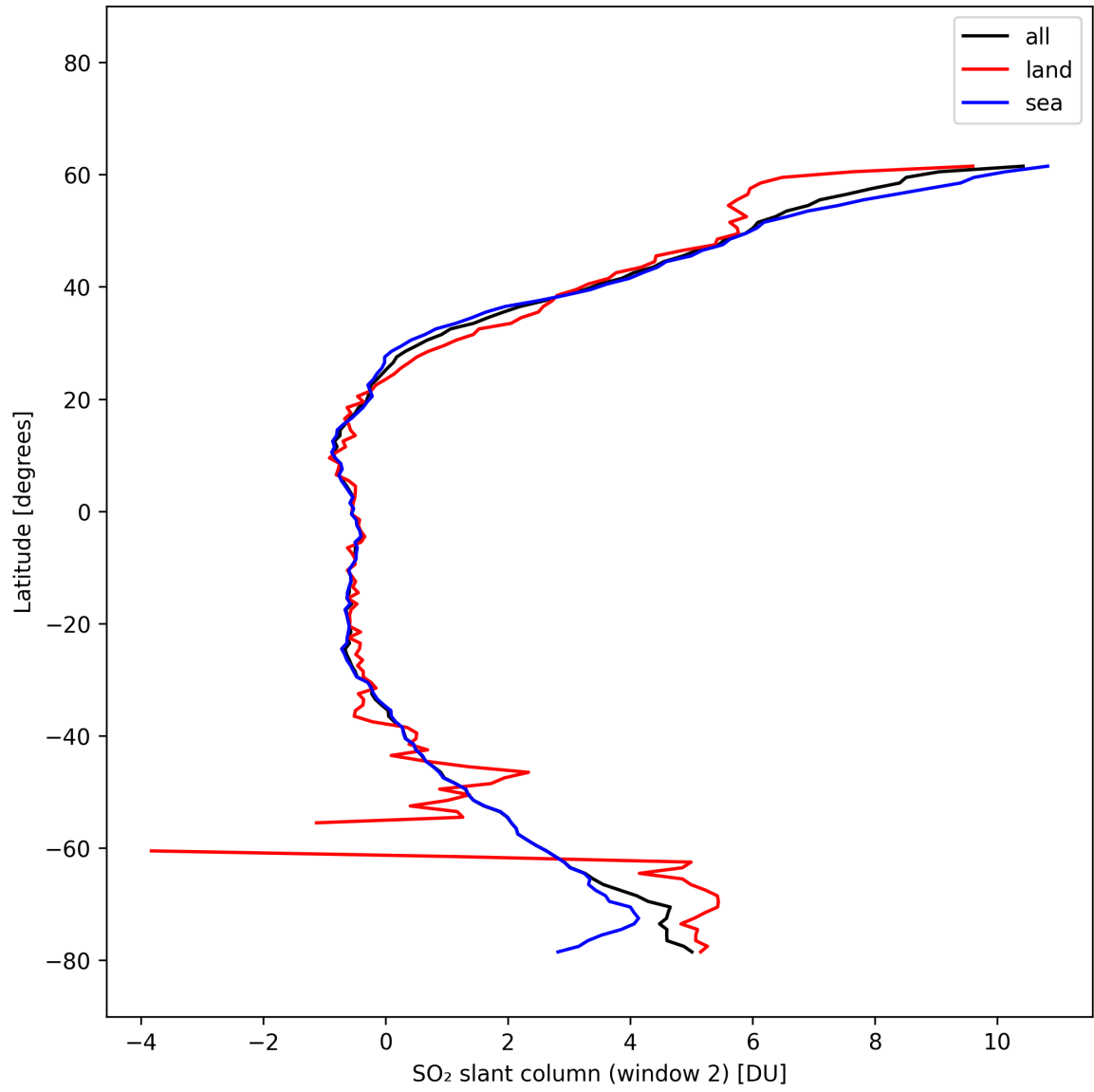
Figure 41: Zonal average of “SO 2 slant column (window 2)” for 2025-02-25 to 2025-02-27.
