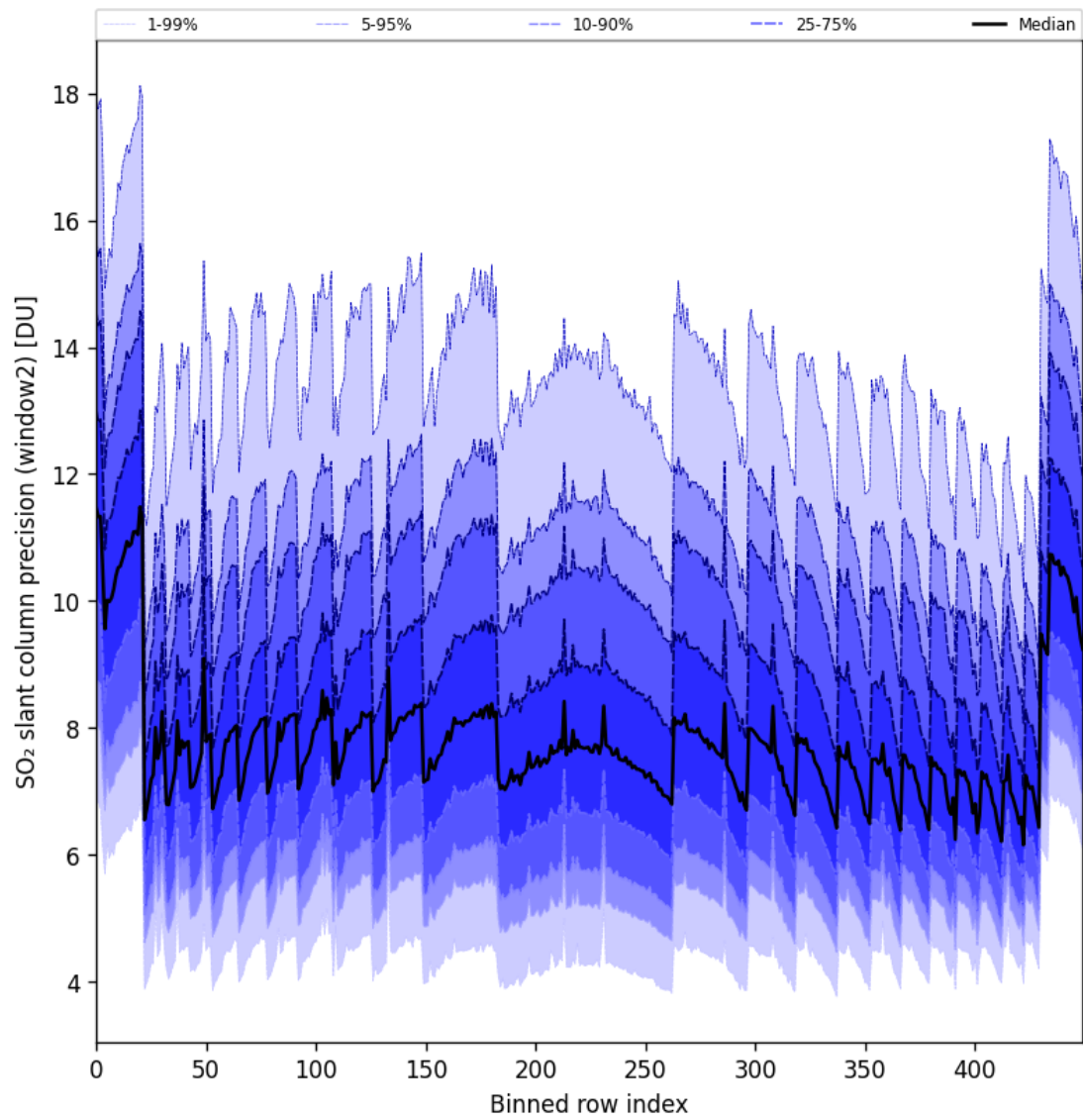
Figure 94: Along track statistics of “SO 2 slant column precision (window2)” for 2025-02-25 to 2025-02-27
