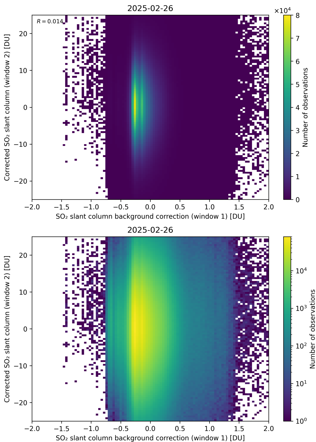
Figure 115: Scatter density plot of “SO 2 slant column background correction (window 1)” against “Corrected SO 2 slant column (window 2)” for 2025-02-25 to 2025-02-27.
