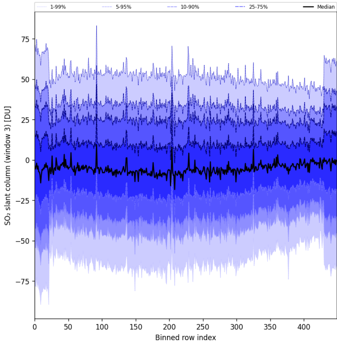
Figure 97: Along track statistics of “SO 2 slant column (window 3)” for 2025-02-25 to 2025-02-27
