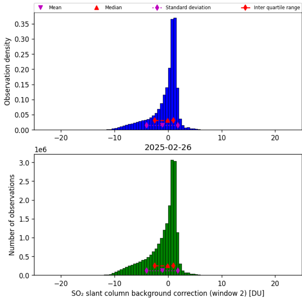
Figure 70: Histogram of “SO 2 slant column background correction (window 2)” for 2025-02-25 to 2025-02-27
