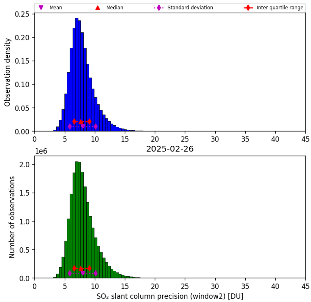
Figure 68: Histogram of “SO 2 slant column precision (window2)” for 2025-02-25 to 2025-02-27
