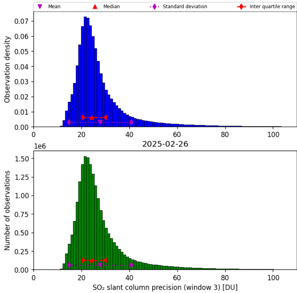
Figure 72: Histogram of “SO 2 slant column precision (window 3)” for 2025-02-25 to 2025-02-27
