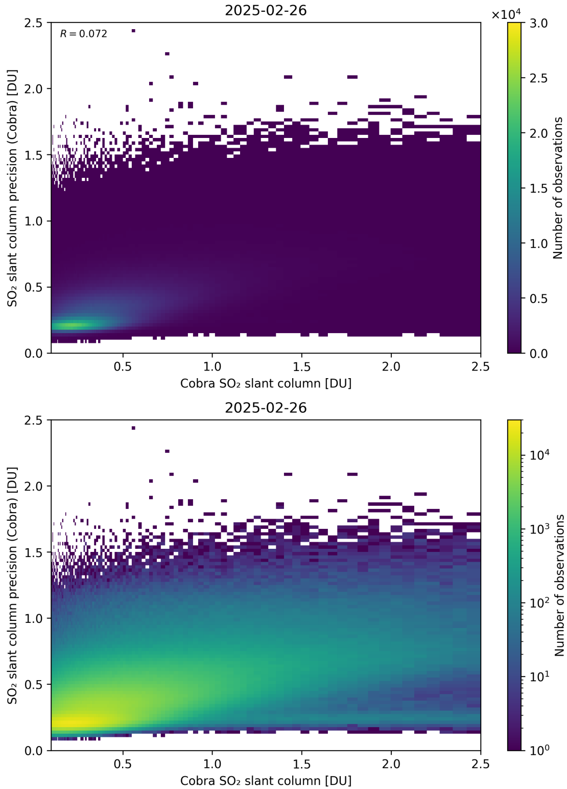
Figure 216: Scatter density plot of “Cobra SO 2 slant column” against “SO 2 slant column precision (Cobra)” for 2025-02-25 to 2025-02-27.
