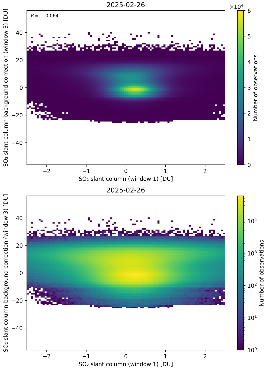
Figure 264: Scatter density plot of “SO 2 slant column (window 1)” against “SO 2 slant column background correction (window 3)” for 2025-02-25 to 2025-02-27.
