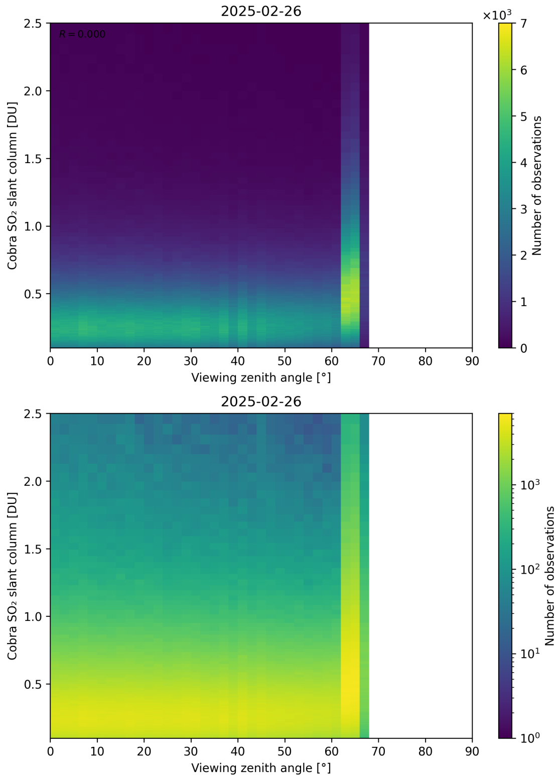
Figure 371: Scatter density plot of “Viewing zenith angle” against “Cobra SO 2 slant column” for 2025-02-25 to 2025-02-27.
