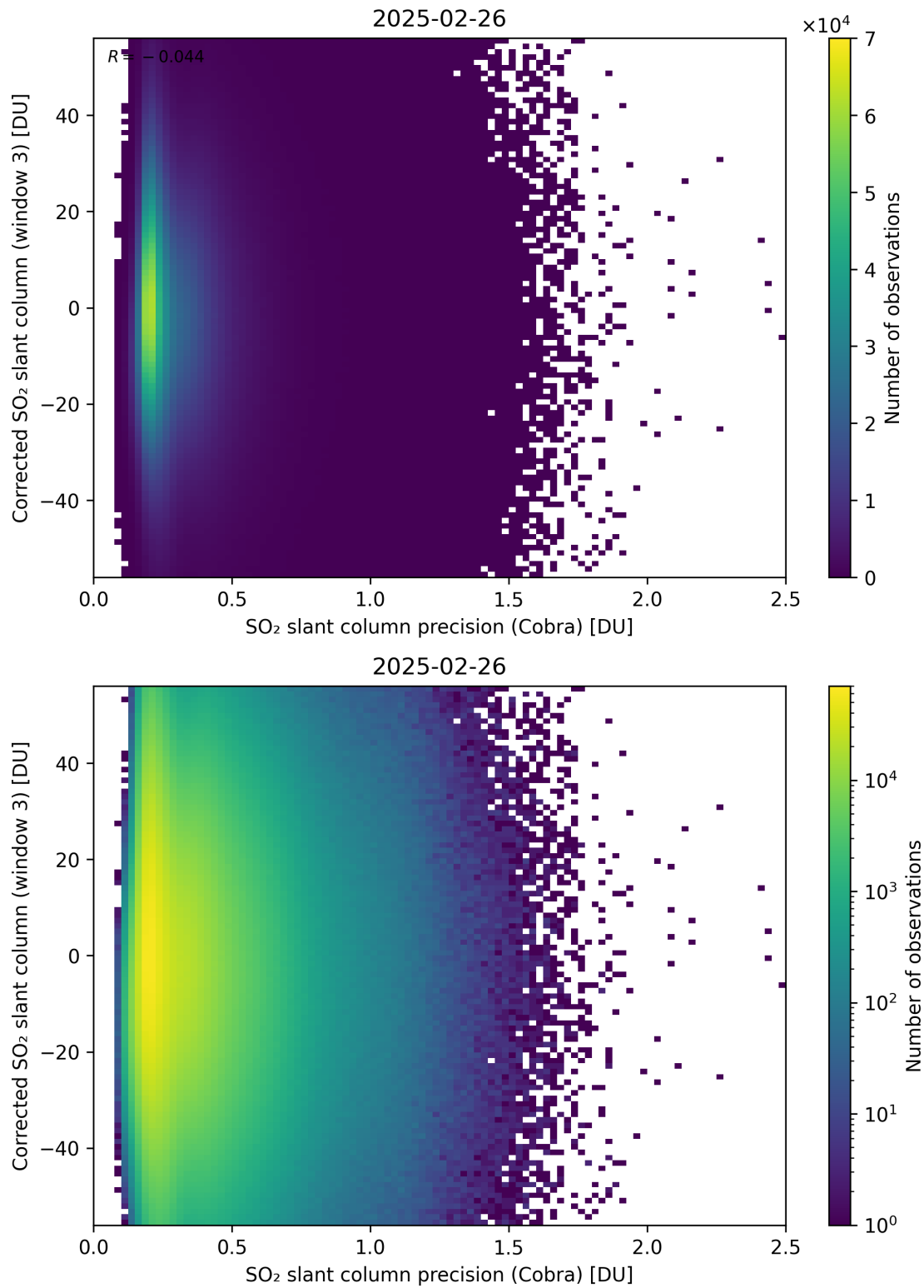
Figure 207: Scatter density plot of “SO 2 slant column precision (Cobra)” against “Corrected SO 2 slant column (window 3)” for 2025-02-25 to 2025-02-27.
