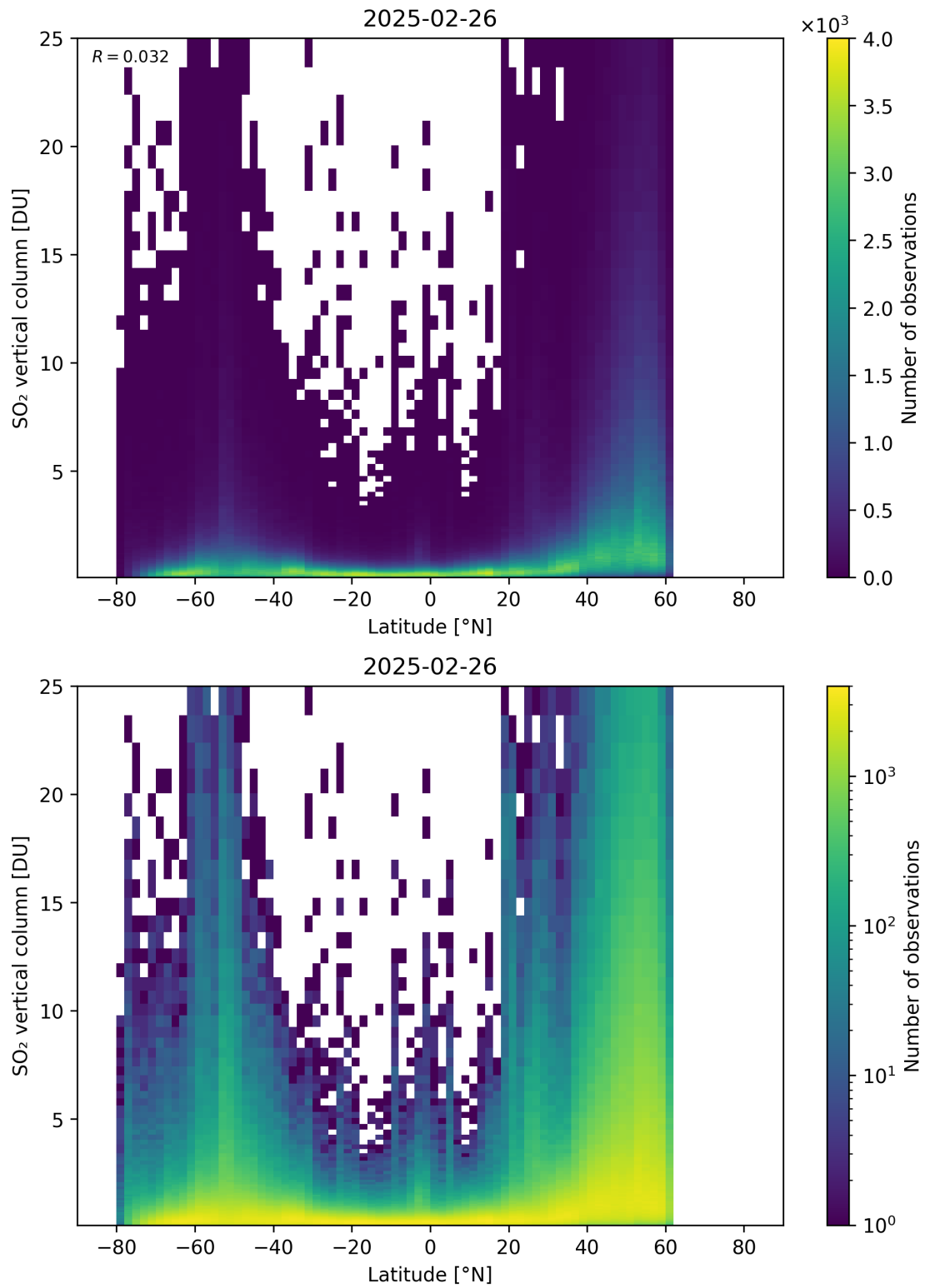
Figure 169: Scatter density plot of “Latitude” against “SO 2 vertical column” for 2025-02-25 to 2025-02-27.
