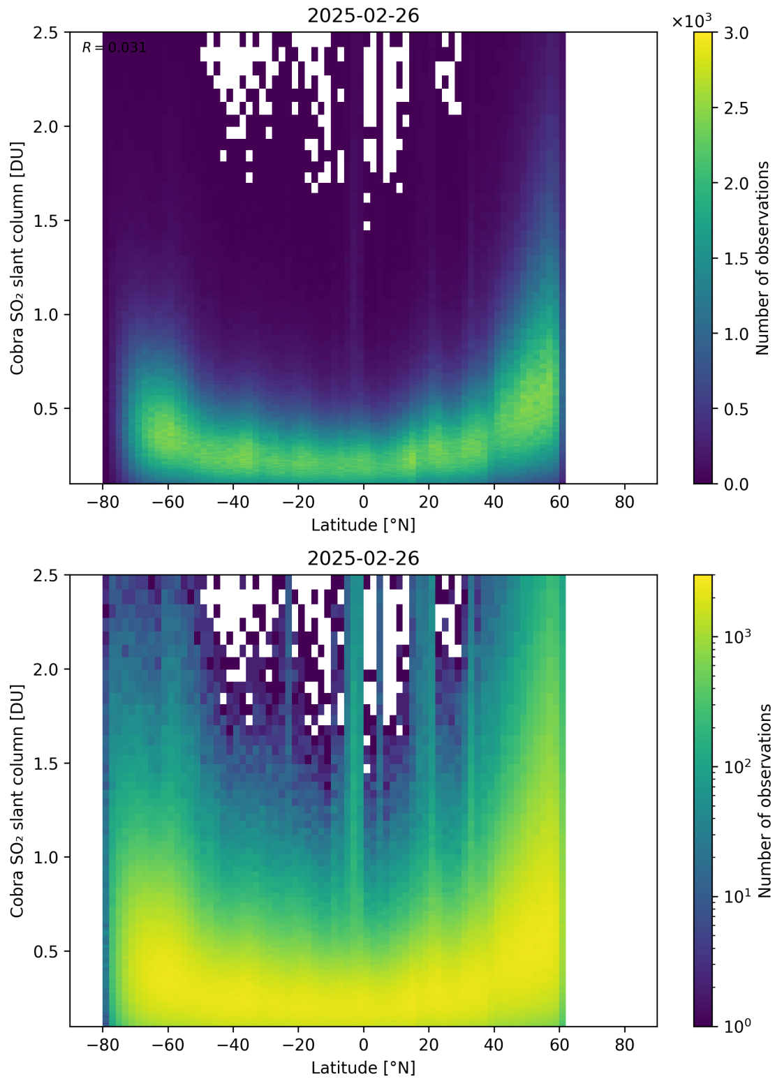
Figure 157: Scatter density plot of “Latitude” against “Cobra SO 2 slant column” for 2025-02-25 to 2025-02-27.
