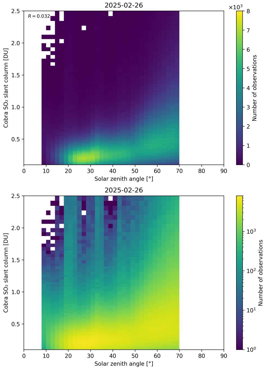
Figure 179: Scatter density plot of “Solar zenith angle” against “Cobra SO 2 slant column” for 2025-02-25 to 2025-02-27.
