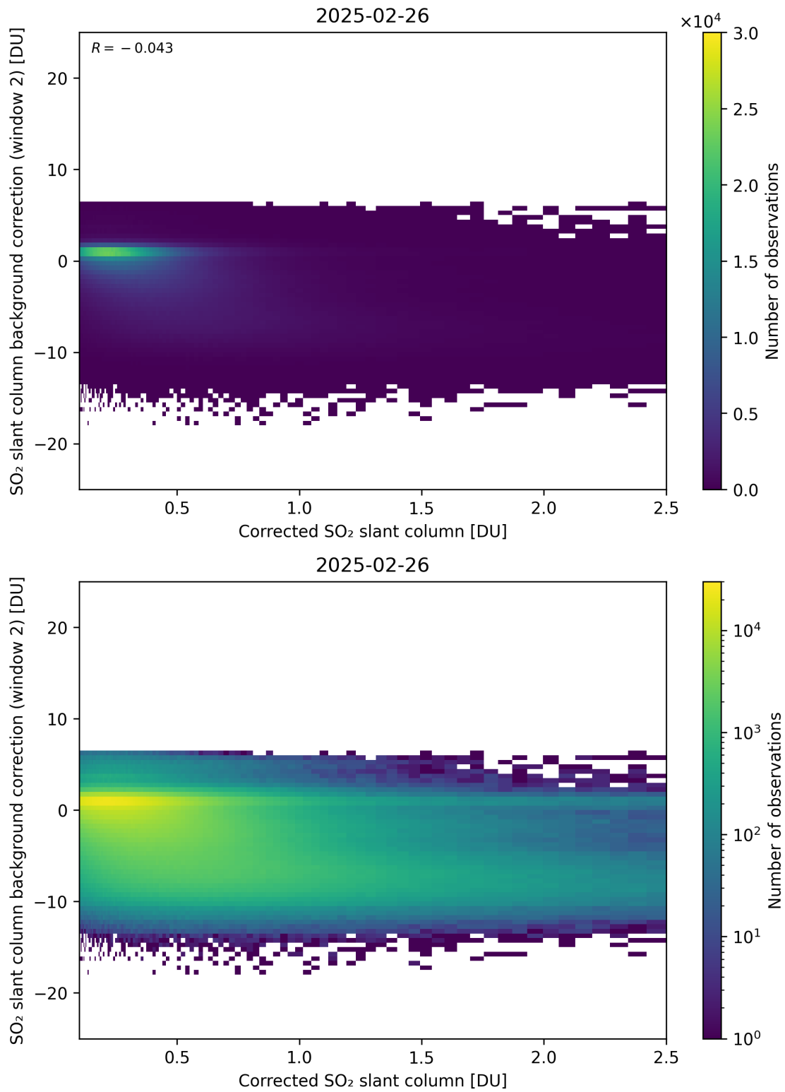
Figure 227: Scatter density plot of “Corrected SO 2 slant column” against “SO 2 slant column background correction (window 2)” for 2025-02-25 to 2025-02-27.
