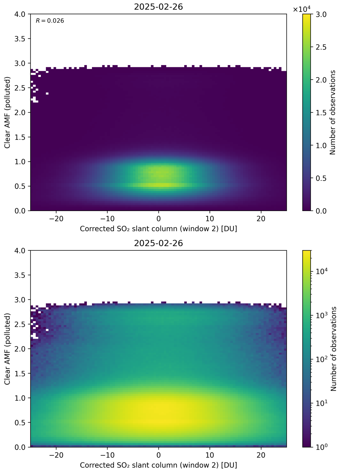
Figure 249: Scatter density plot of “Corrected SO 2 slant column (window 2)” against “Clear AMF (polluted)” for 2025-02-25 to 2025-02-27.
