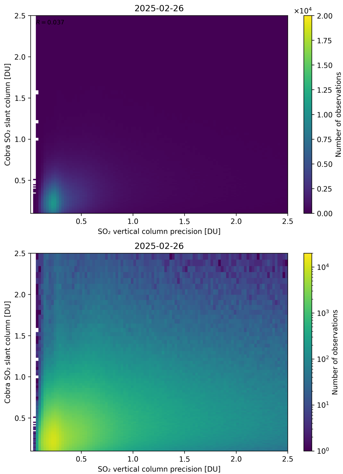
Figure 336: Scatter density plot of “SO 2 vertical column precision” against “Cobra SO 2 slant column” for 2025-02-25 to 2025-02-27.
