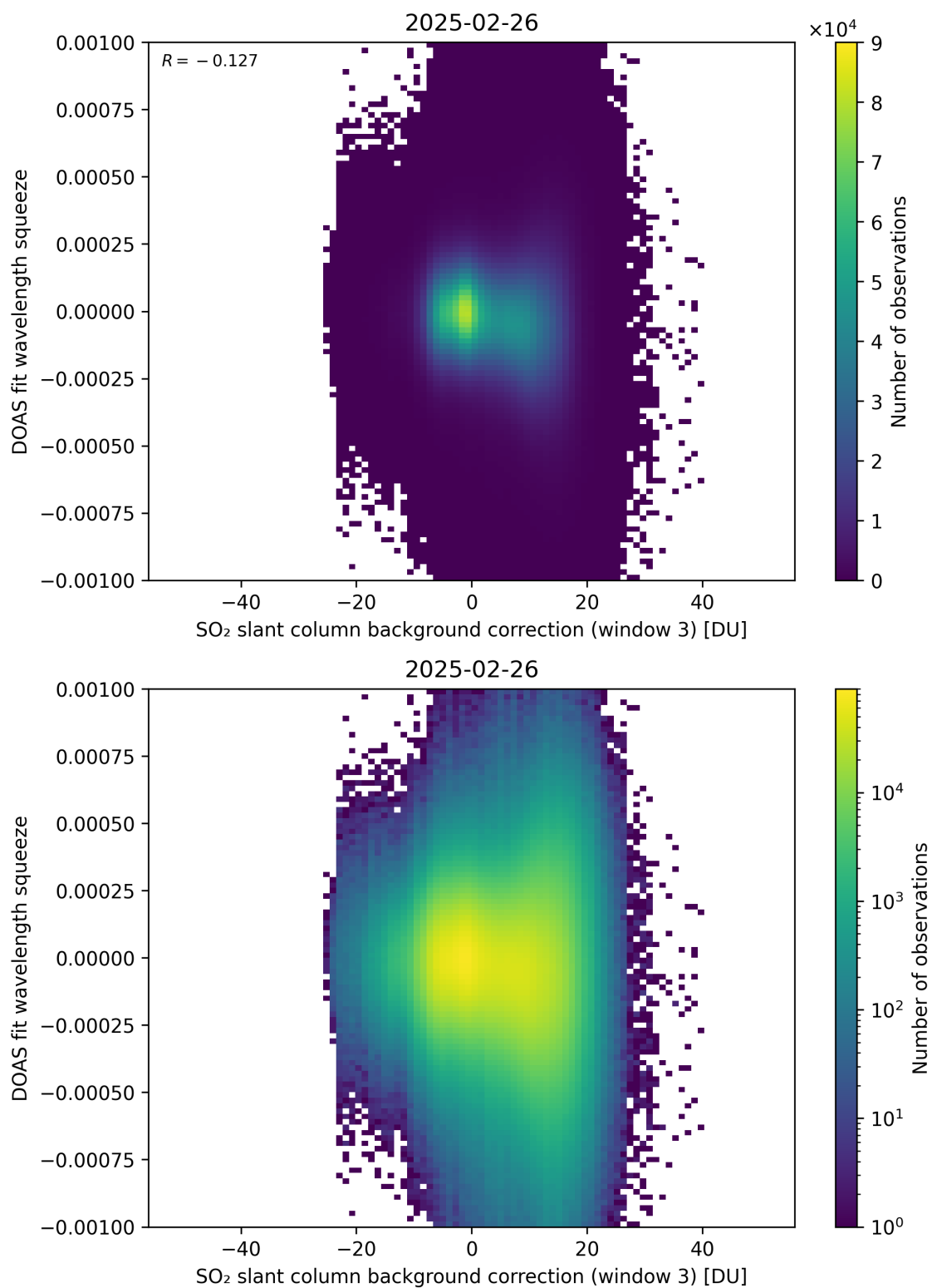
Figure 133: Scatter density plot of “SO 2 slant column background correction (window 3)” against “DOAS fit wavelength squeeze” for 2025-02-25 to 2025-02-27.
