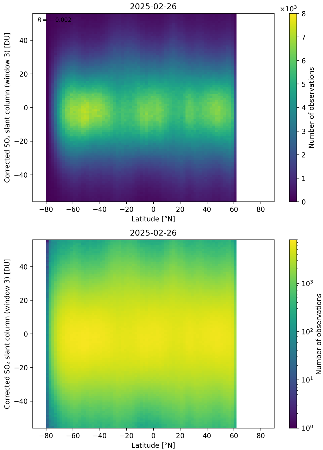
Figure 161: Scatter density plot of “Latitude” against “Corrected SO 2 slant column (window 3)” for 2025-02-25 to 2025-02-27.
