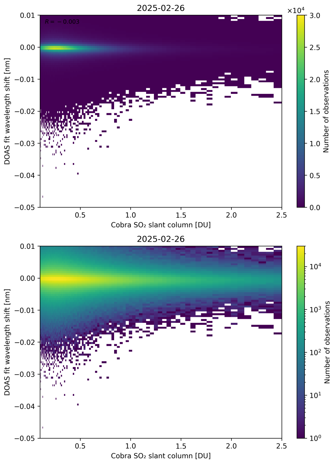
Figure 196: Scatter density plot of “Cobra SO 2 slant column” against “DOAS fit wavelength shift” for 2025-02-25 to 2025-02-27.
