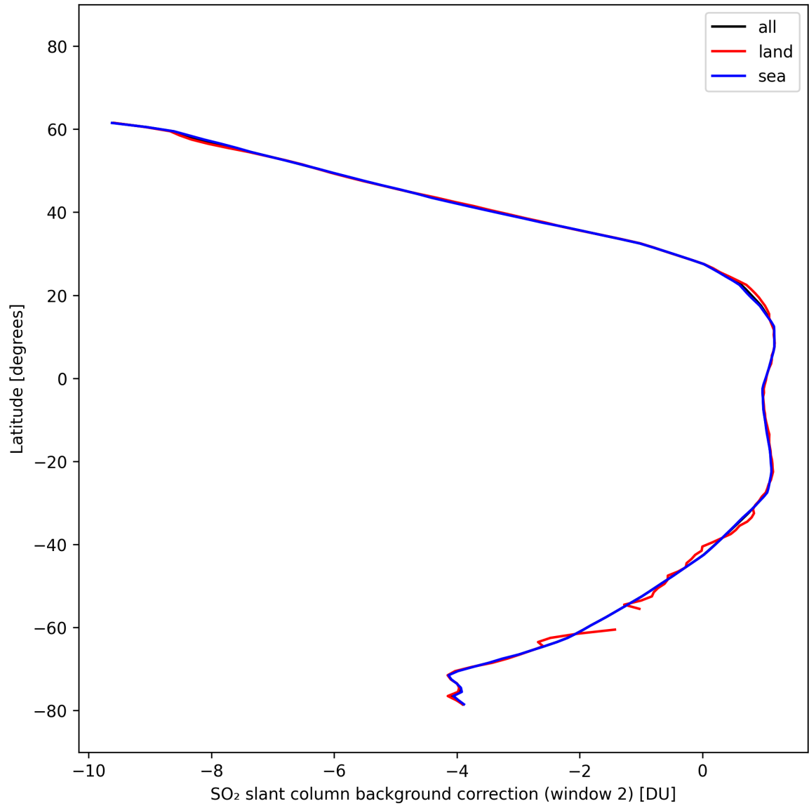
Figure 44: Zonal average of “SO 2 slant column background correction (window 2)” for 2025-02-25 to 2025-02-27.
