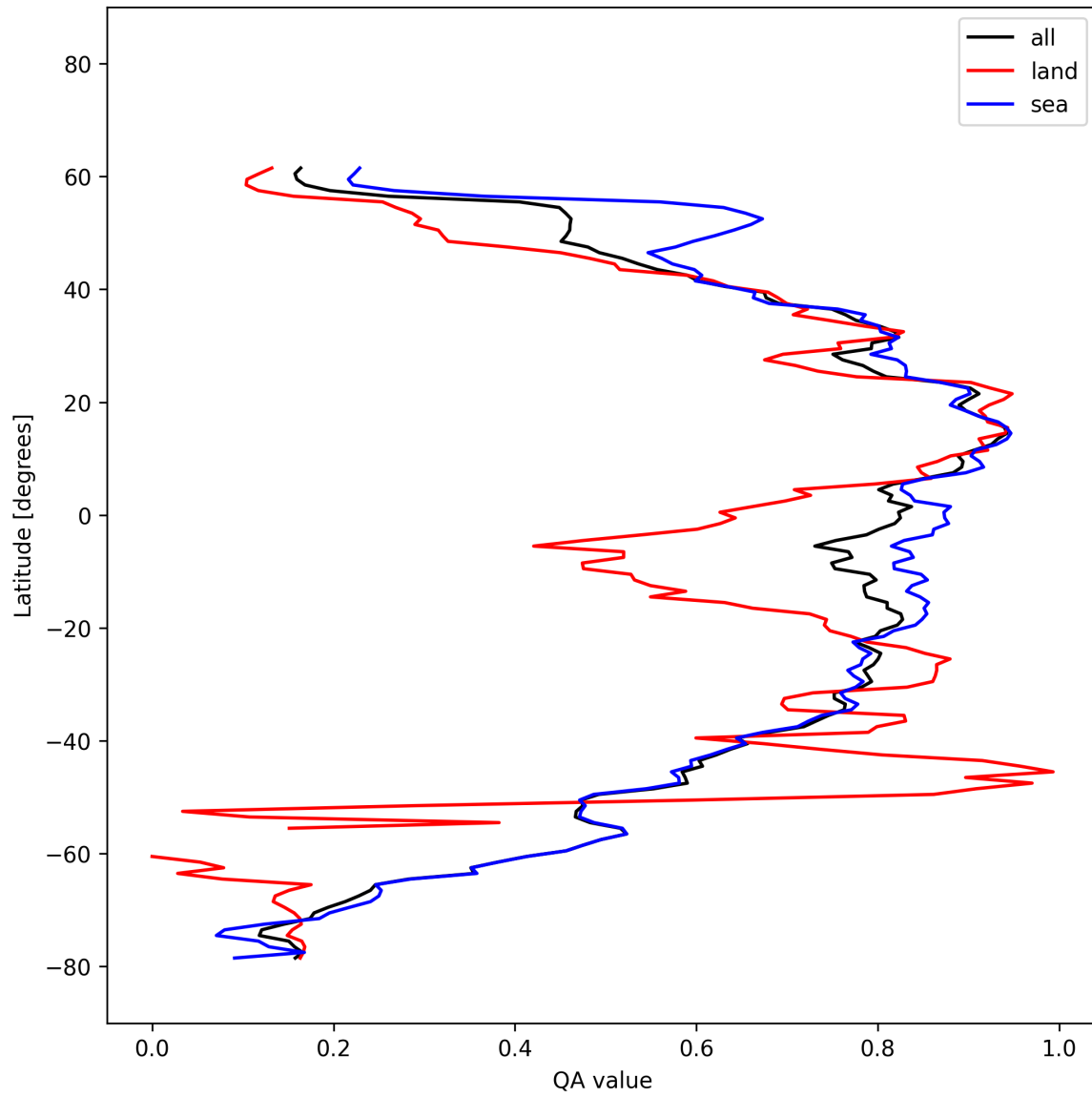
Figure 31: Zonal average of “QA value” for 2025-02-25 to 2025-02-27.
