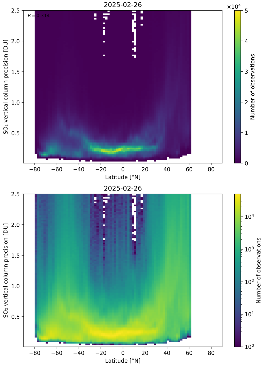
Figure 170: Scatter density plot of “Latitude” against “SO 2 vertical column precision” for 2025-02-25 to 2025-02-27.
