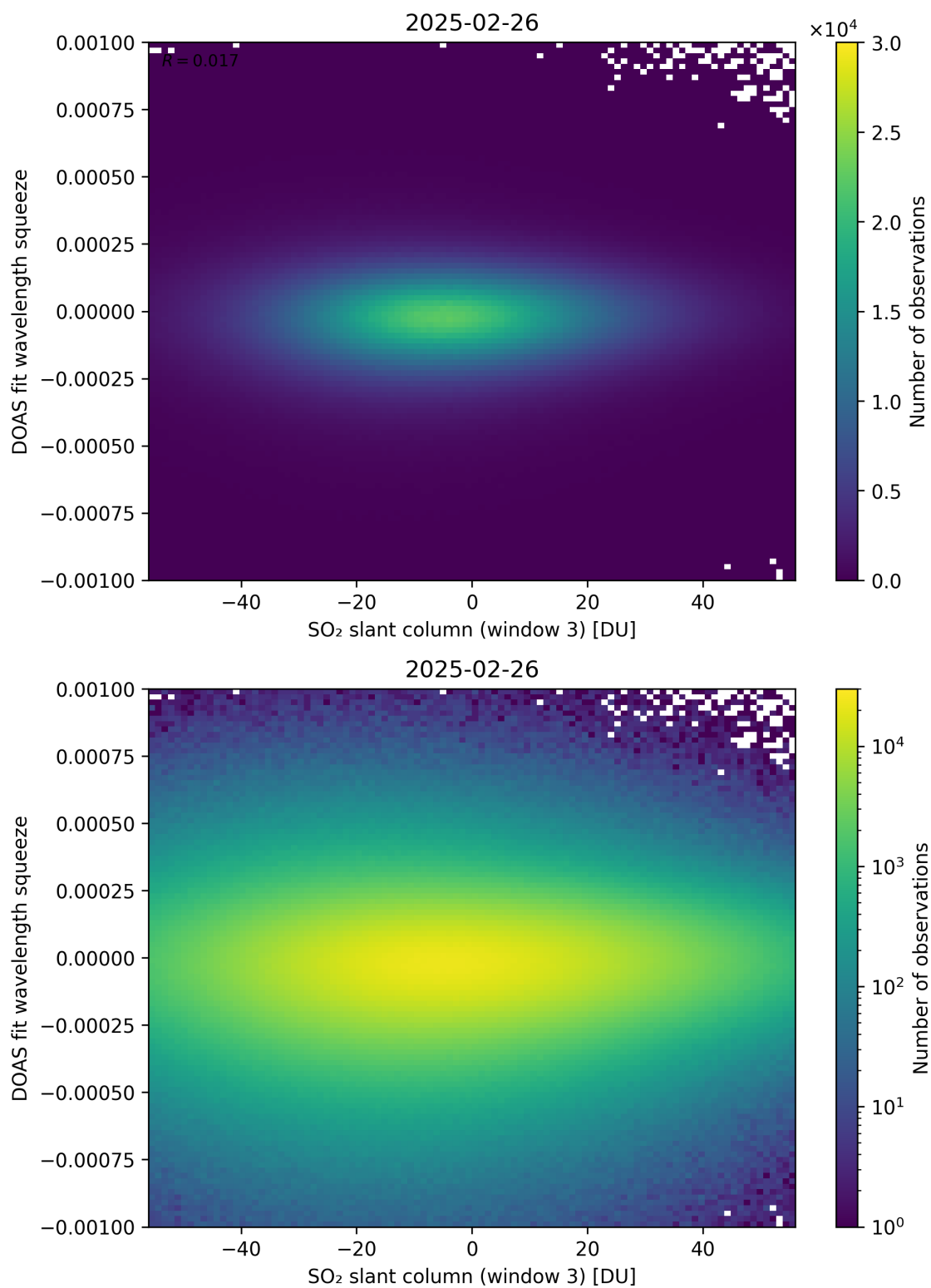
Figure 305: Scatter density plot of “SO 2 slant column (window 3)” against “DOAS fit wavelength squeeze” for 2025-02-25 to 2025-02-27.
