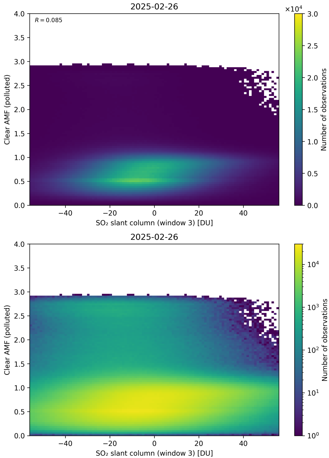
Figure 315: Scatter density plot of “SO 2 slant column (window 3)” against “Clear AMF (polluted)” for 2025-02-25 to 2025-02-27.
