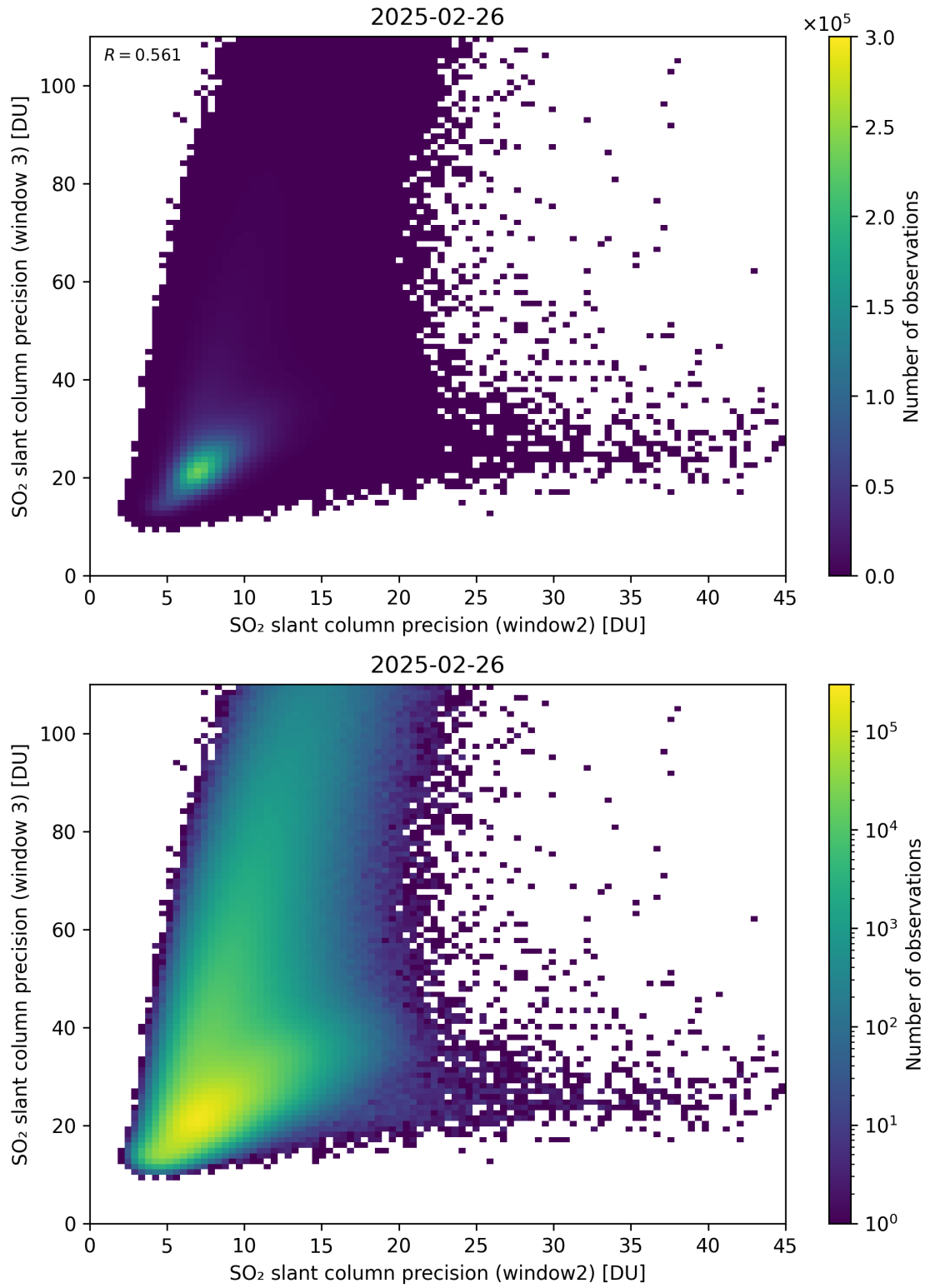
Figure 300: Scatter density plot of “SO 2 slant column precision (window2)” against “SO 2 slant column precision (window 3)” for 2025-02-25 to 2025-02-27.
