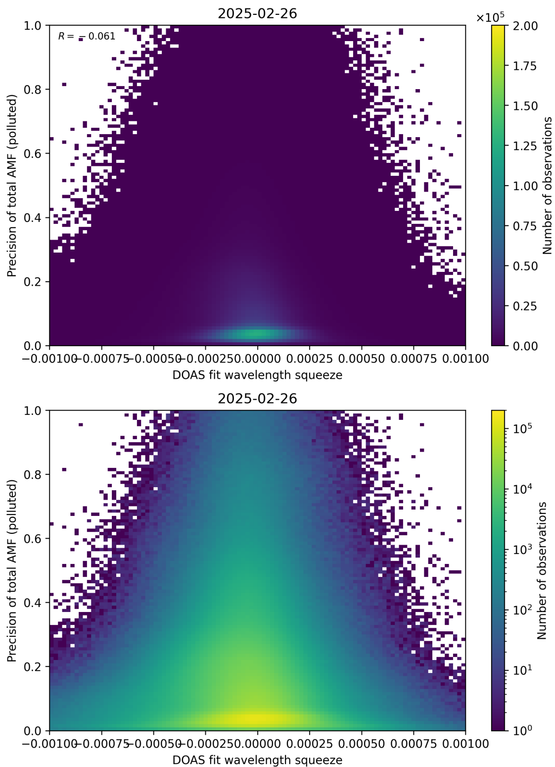
Figure 146: Scatter density plot of “DOAS fit wavelength squeeze” against “Precision of total AMF (polluted)” for 2025-02-25 to 2025-02-27.
