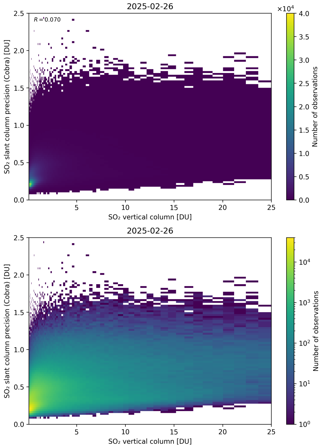
Figure 350: Scatter density plot of “SO 2 vertical column” against “SO 2 slant column precision (Cobra)” for 2025-02-25 to 2025-02-27.
