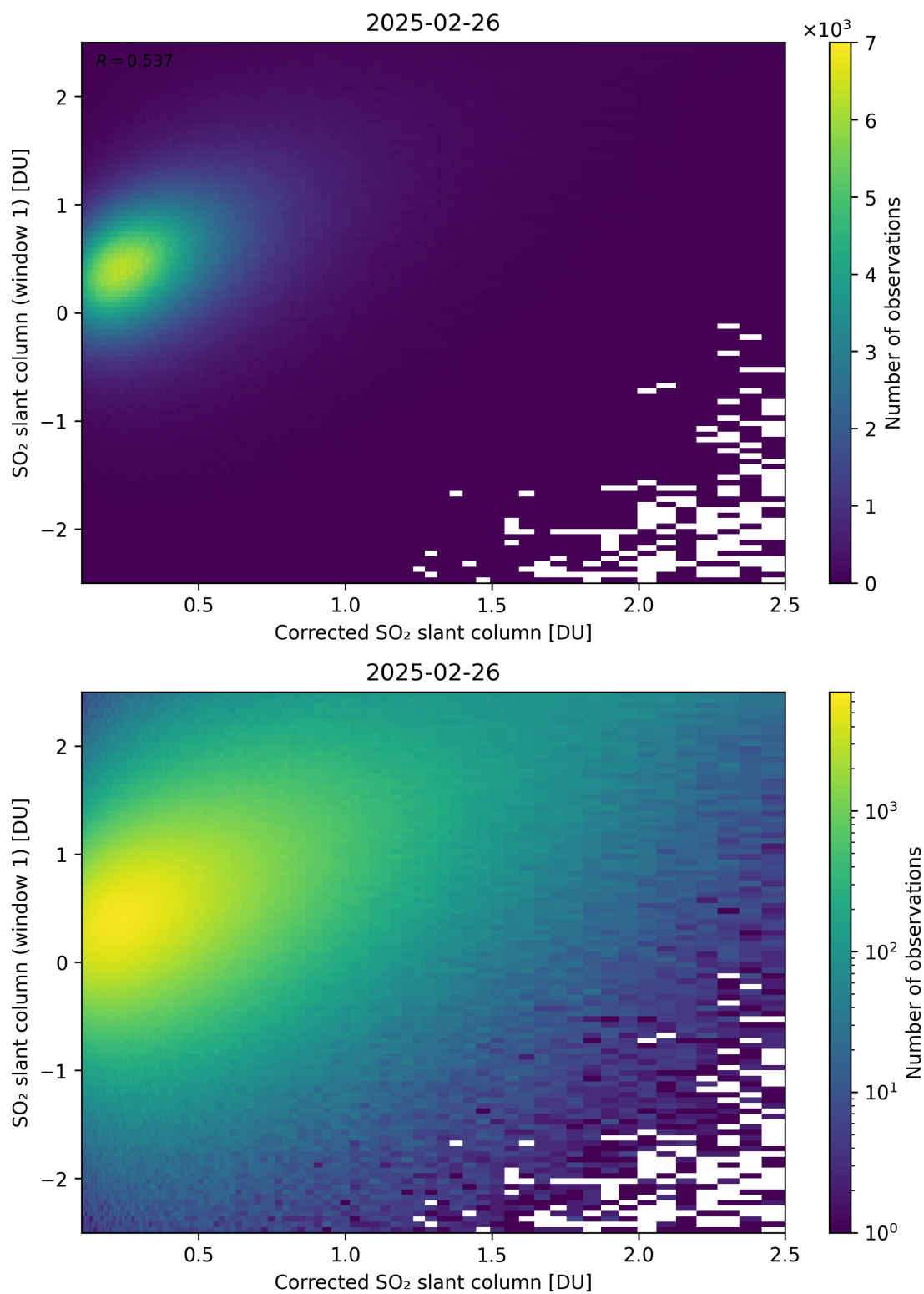
Figure 237: Scatter density plot of “Corrected SO 2 slant column” against “SO 2 slant column (window 1)” for 2025-02-25 to 2025-02-27.
