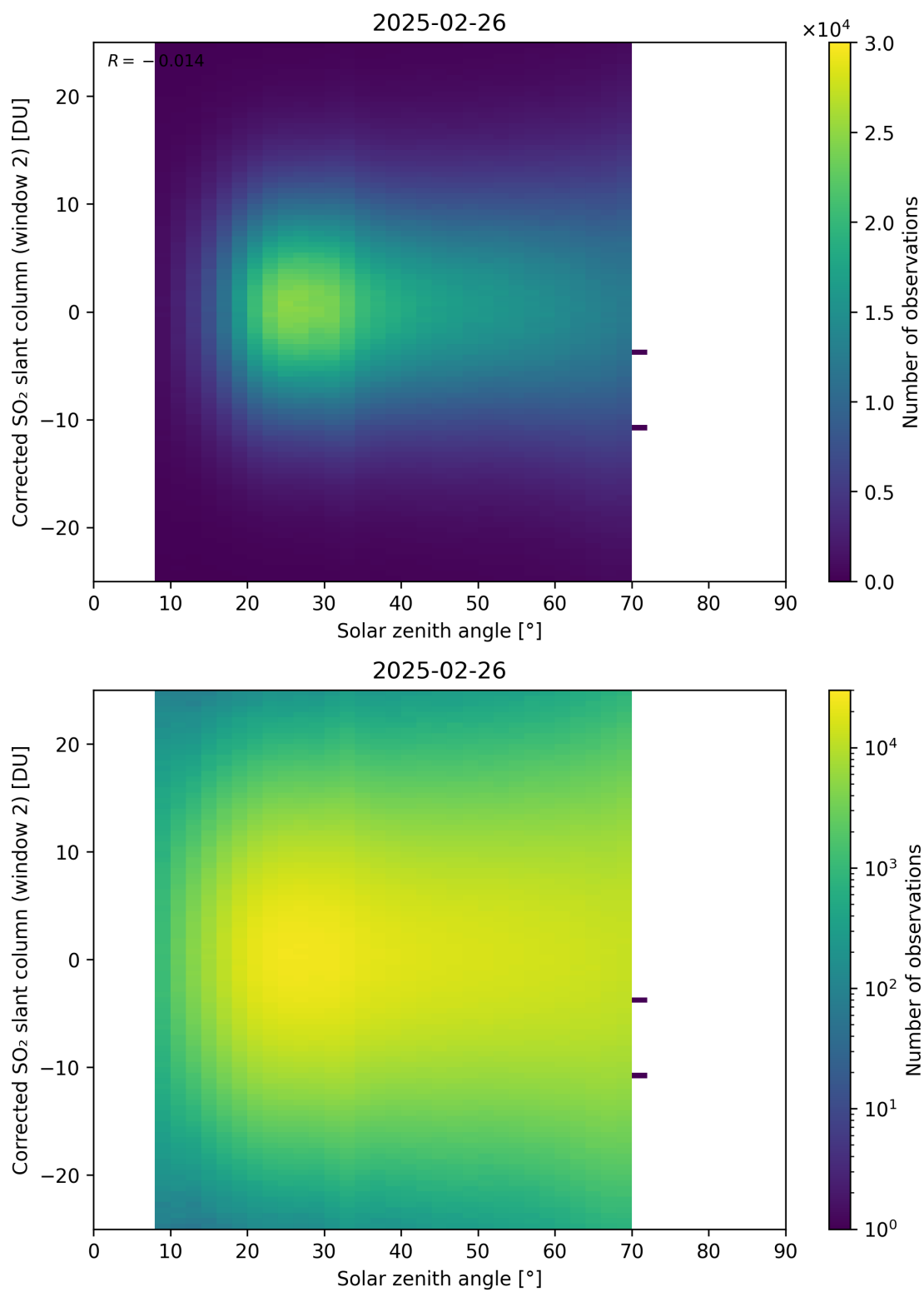
Figure 182: Scatter density plot of “Solar zenith angle” against “Corrected SO 2 slant column (window 2)” for 2025-02-25 to 2025-02-27.
