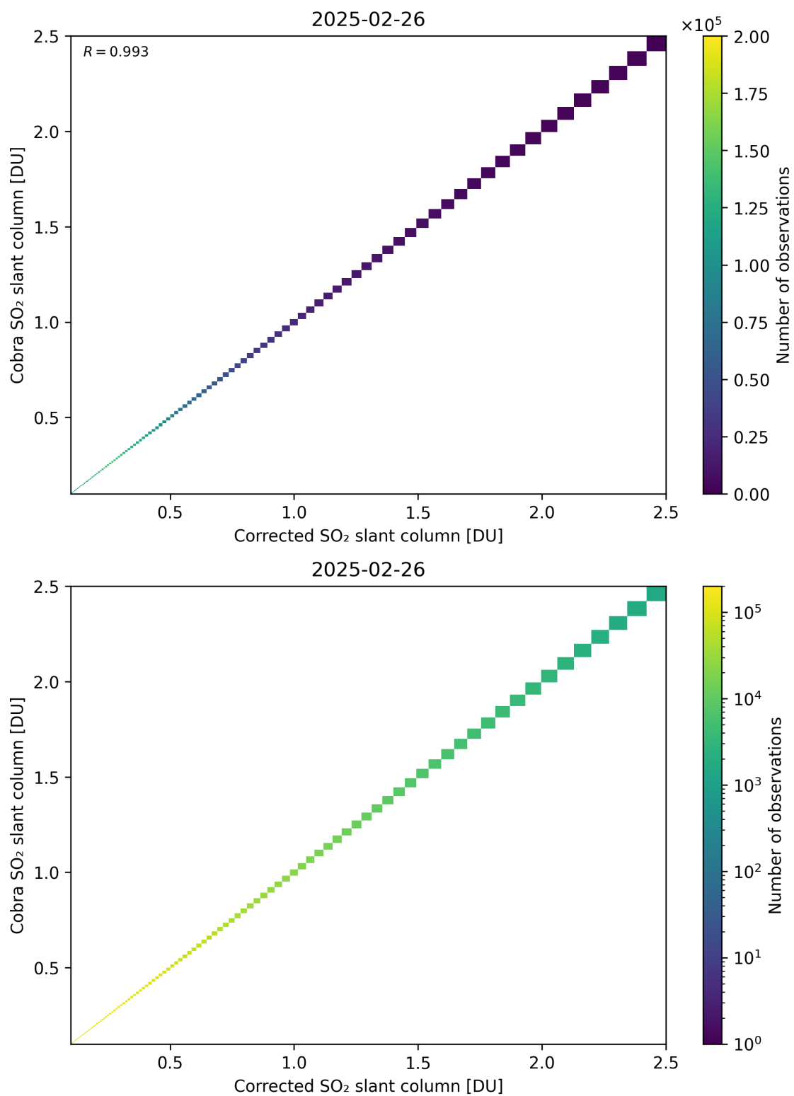
Figure 233: Scatter density plot of “Corrected SO 2 slant column” against “Cobra SO 2 slant column” for 2025-02-25 to 2025-02-27.
