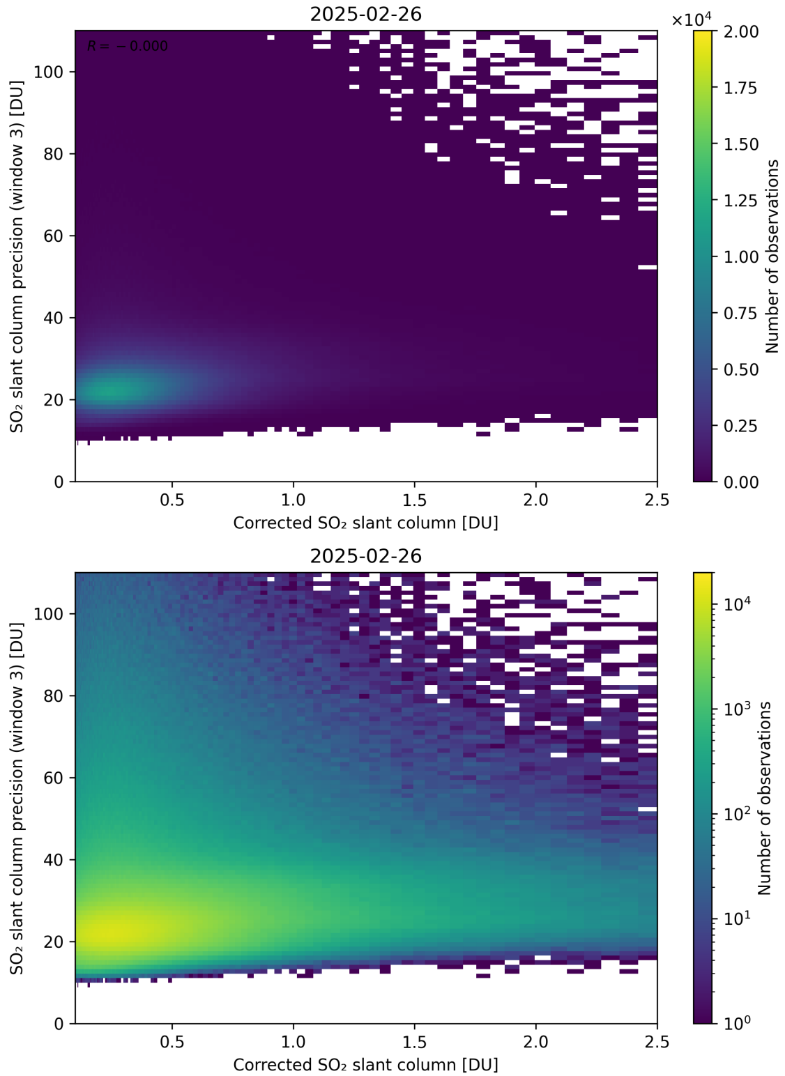
Figure 241: Scatter density plot of “Corrected SO 2 slant column” against “SO 2 slant column precision (window 3)” for 2025-02-25 to 2025-02-27.
