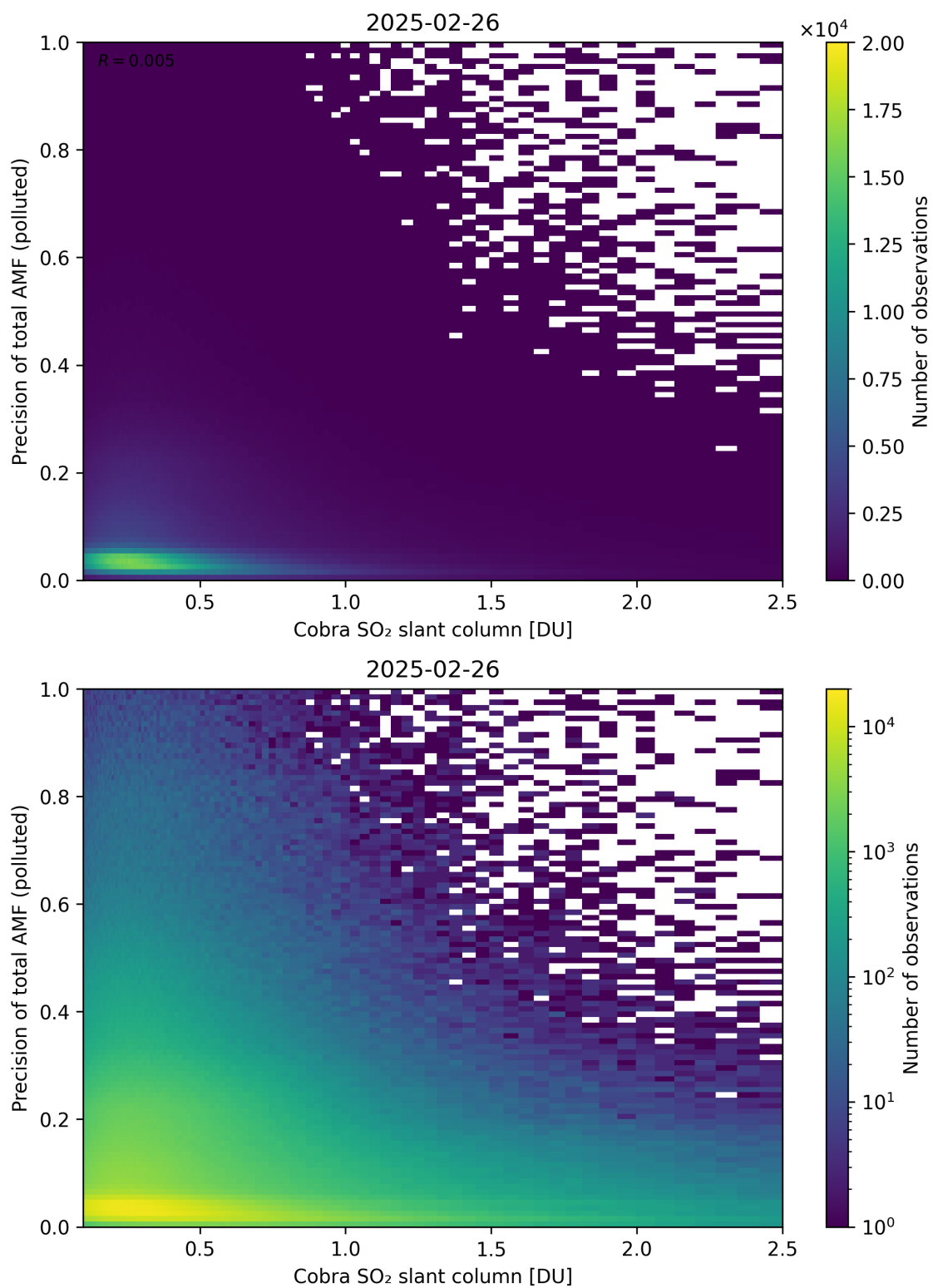
Figure 225: Scatter density plot of “Cobra SO 2 slant column” against “Precision of total AMF (polluted)” for 2025-02-25 to 2025-02-27.
