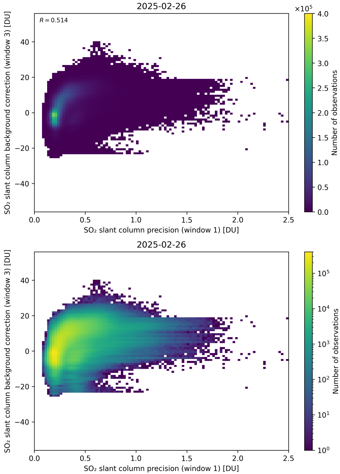
Figure 270: Scatter density plot of “SO 2 slant column precision (window 1)” against “SO 2 slant column background correction (window 3)” for 2025-02-25 to 2025-02-27.
