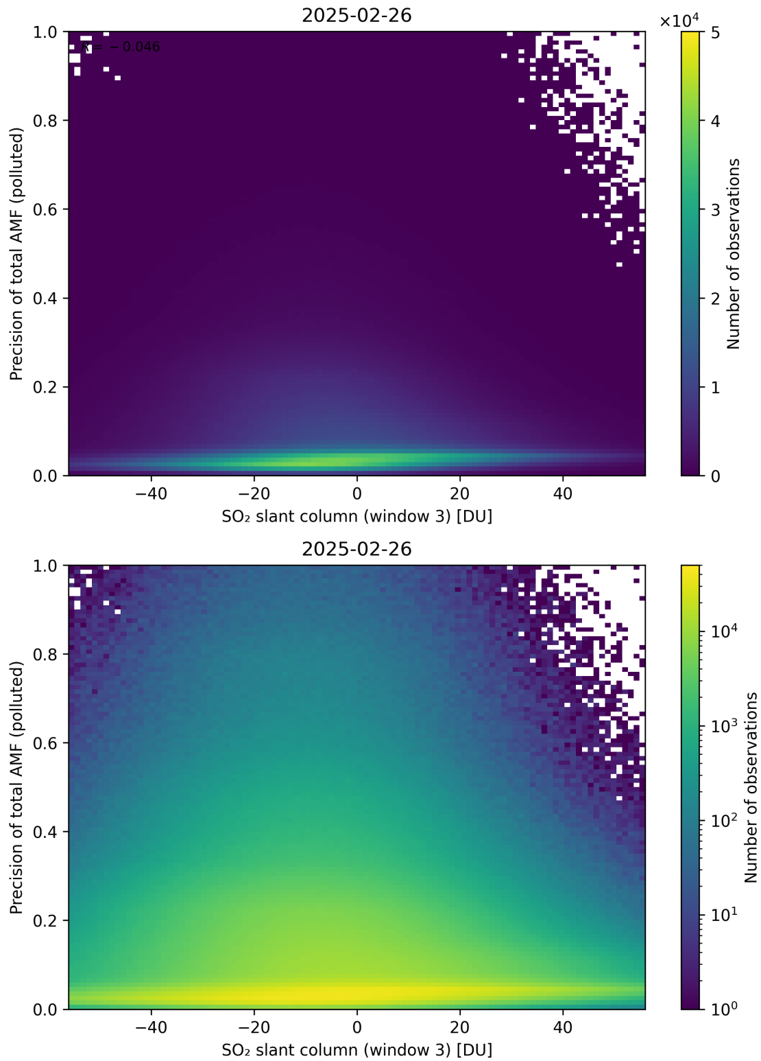
Figure 319: Scatter density plot of “SO 2 slant column (window 3)” against “Precision of total AMF (polluted)” for 2025-02-25 to 2025-02-27.
