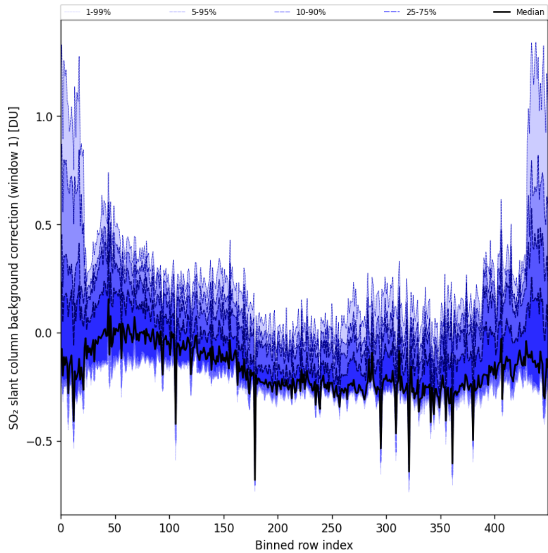
Figure 92: Along track statistics of “SO 2 slant column background correction (window 1)” for 2025-02-25 to 2025-02-27
