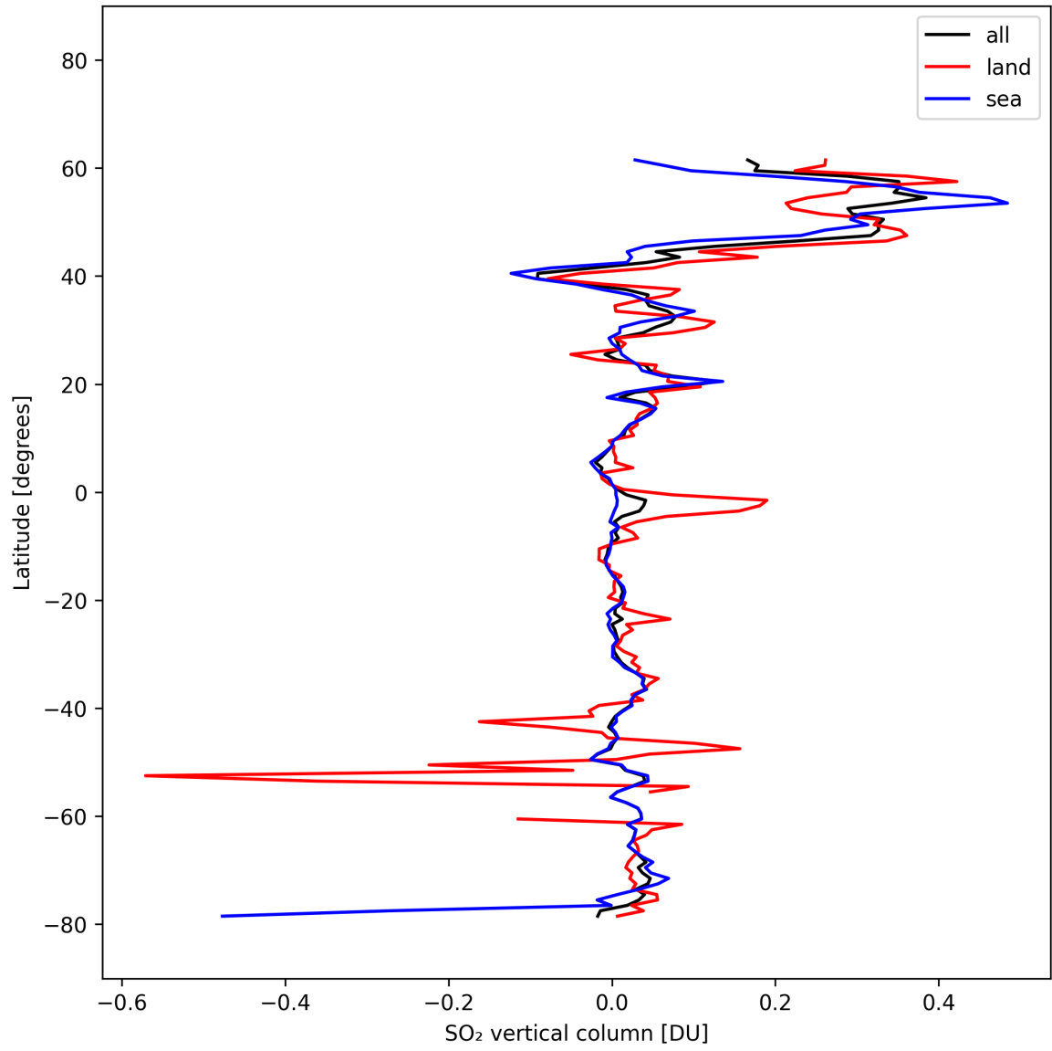
Figure 32: Zonal average of “SO 2 vertical column” for 2025-02-25 to 2025-02-27.
