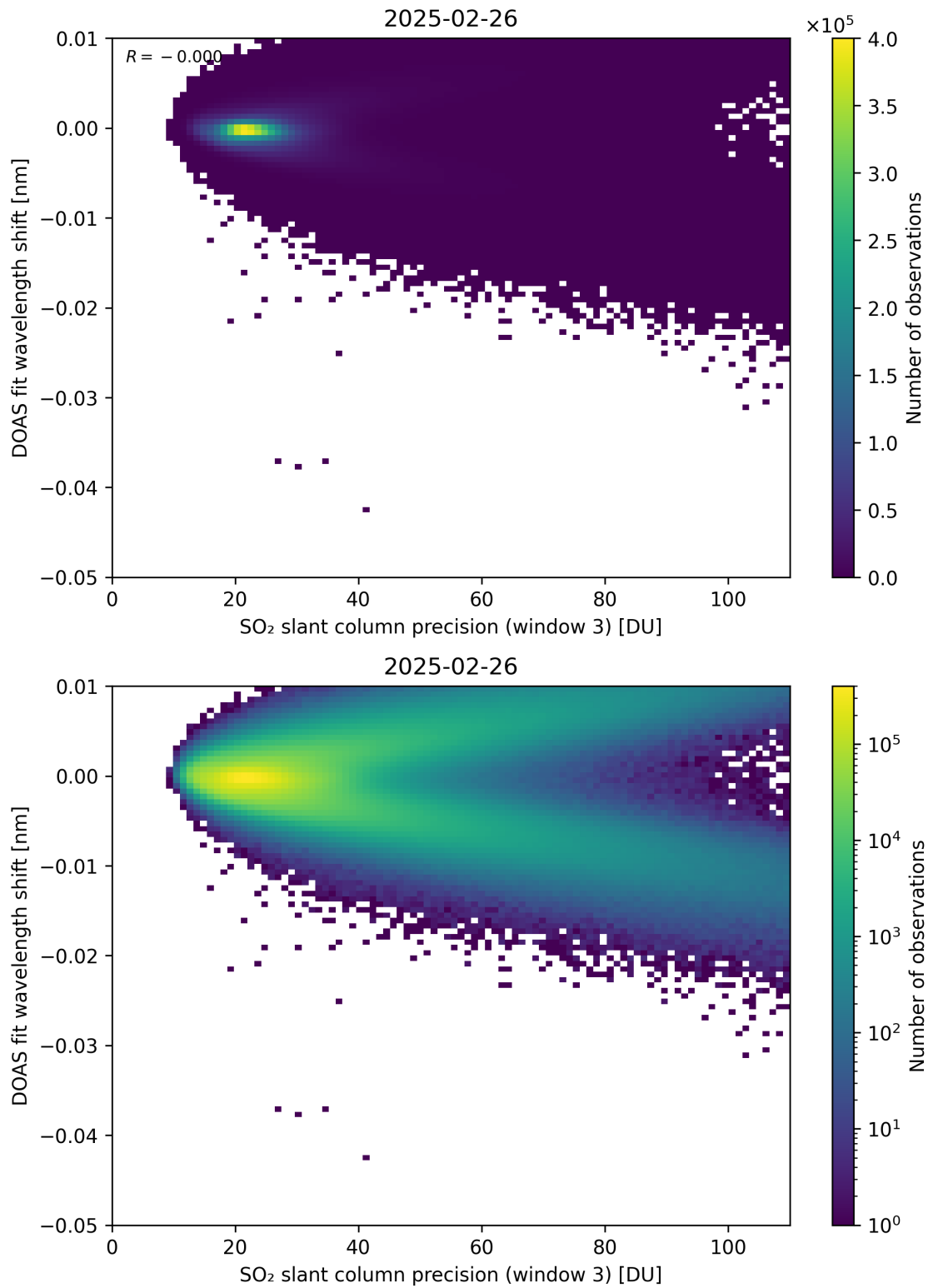
Figure 308: Scatter density plot of “SO 2 slant column precision (window 3)” against “DOAS fit wavelength shift” for 2025-02-25 to 2025-02-27.
