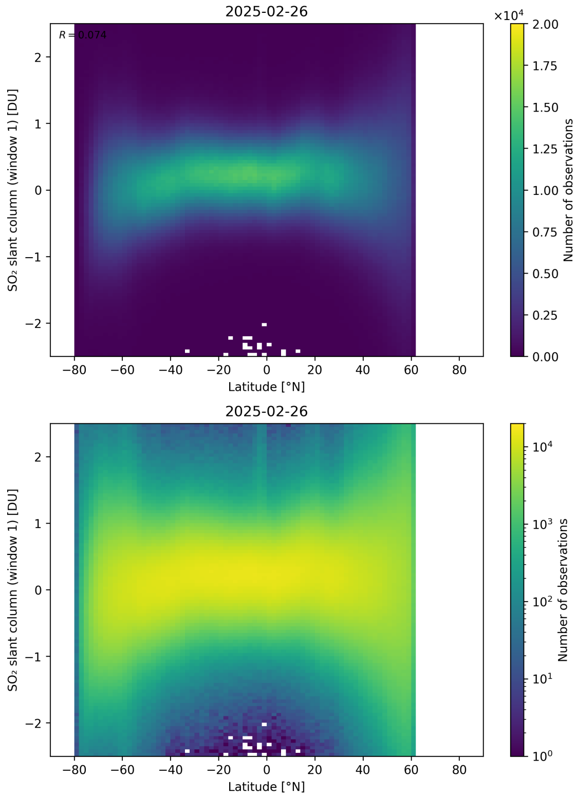
Figure 162: Scatter density plot of “Latitude” against “SO 2 slant column (window 1)” for 2025-02-25 to 2025-02-27.
