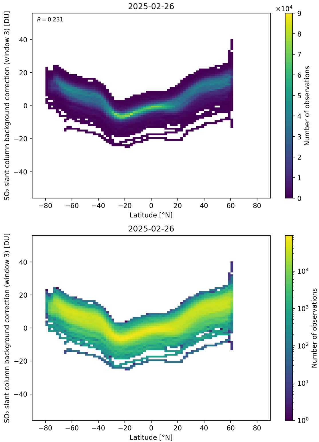
Figure 152: Scatter density plot of “Latitude” against “SO 2 slant column background correction (window 3)” for 2025-02-25 to 2025-02-27.
