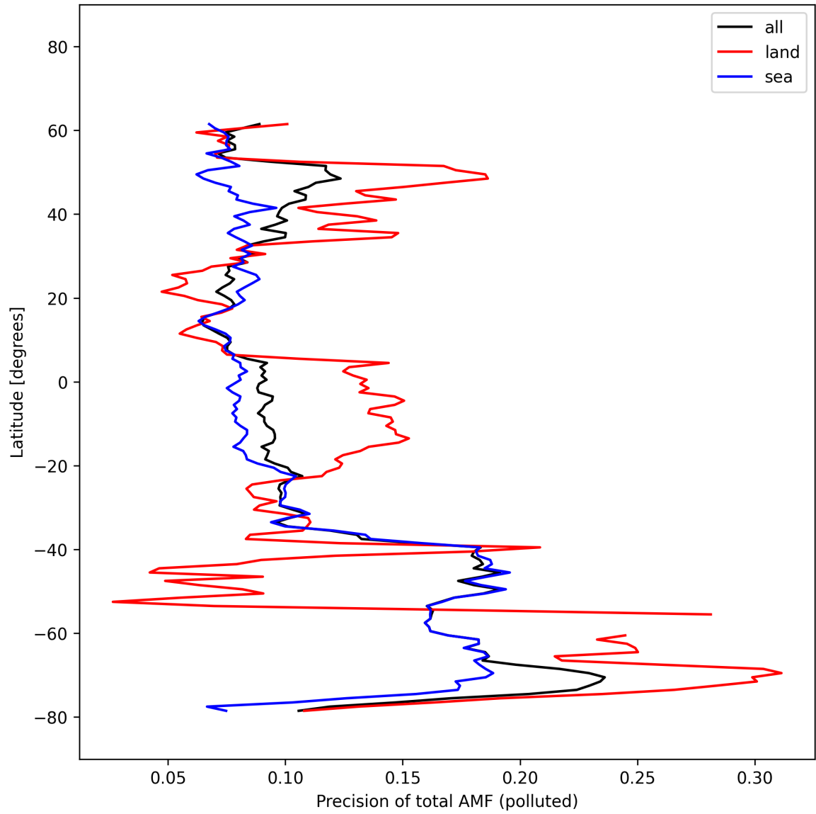
Figure 54: Zonal average of “Precision of total AMF (polluted)” for 2025-02-25 to 2025-02-27.
