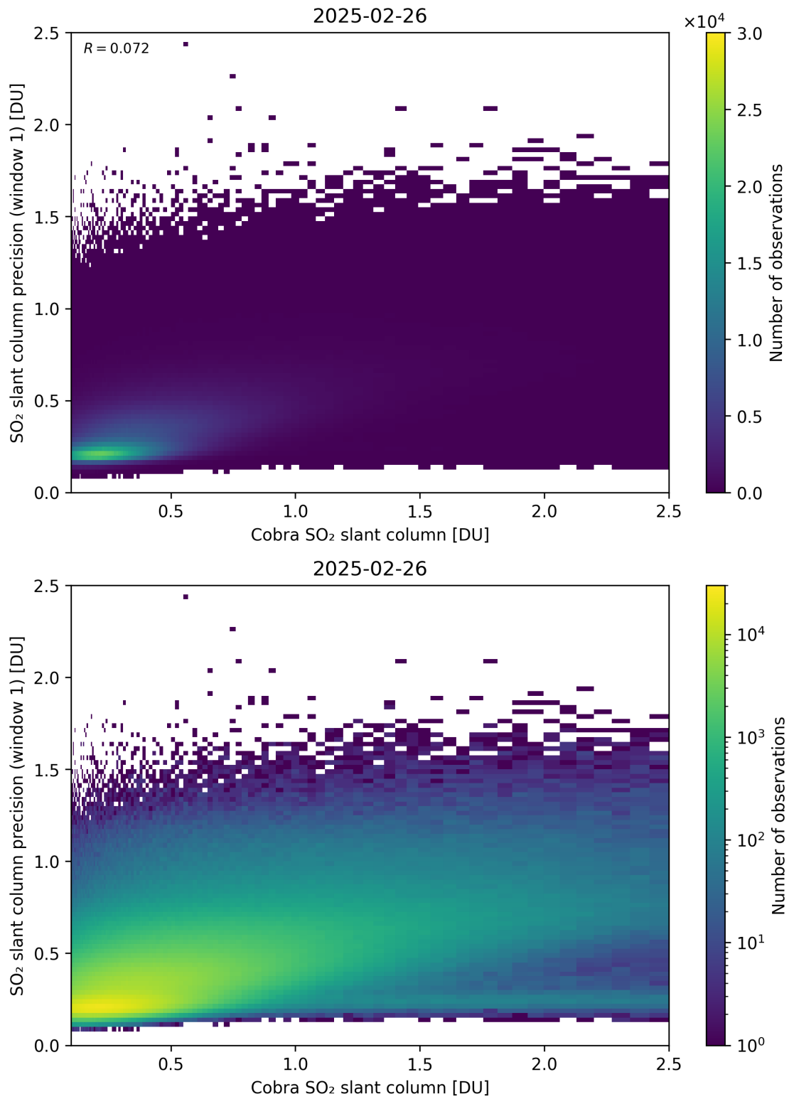
Figure 220: Scatter density plot of “Cobra SO 2 slant column” against “SO 2 slant column precision (window 1)” for 2025-02-25 to 2025-02-27.
