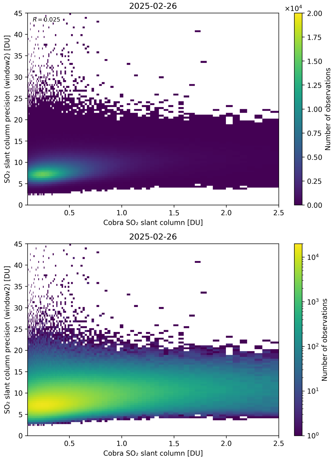
Figure 221: Scatter density plot of “Cobra SO 2 slant column” against “SO 2 slant column precision (window2)” for 2025-02-25 to 2025-02-27.
