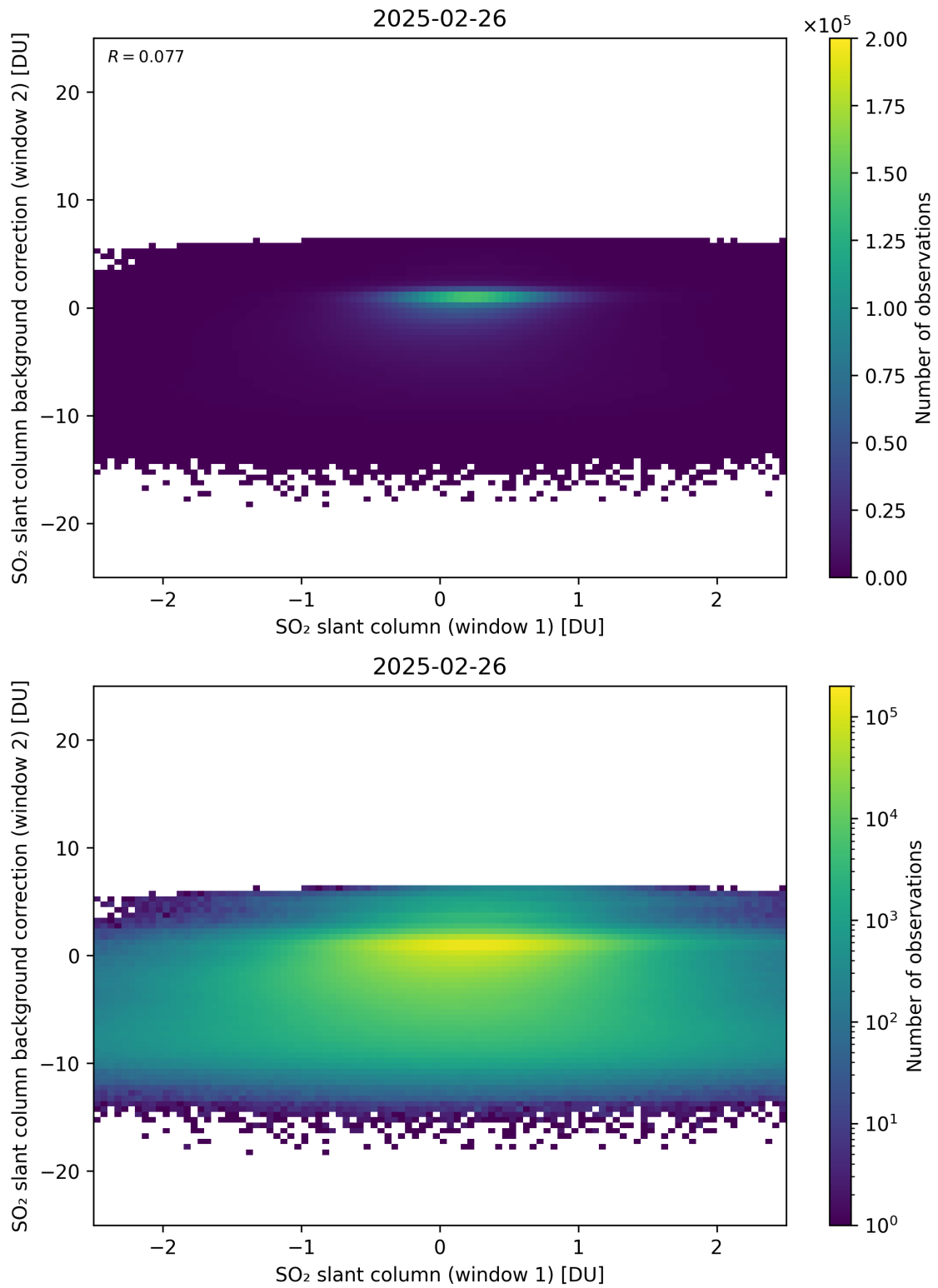
Figure 263: Scatter density plot of “SO 2 slant column (window 1)” against “SO 2 slant column background correction (window 2)” for 2025-02-25 to 2025-02-27.
