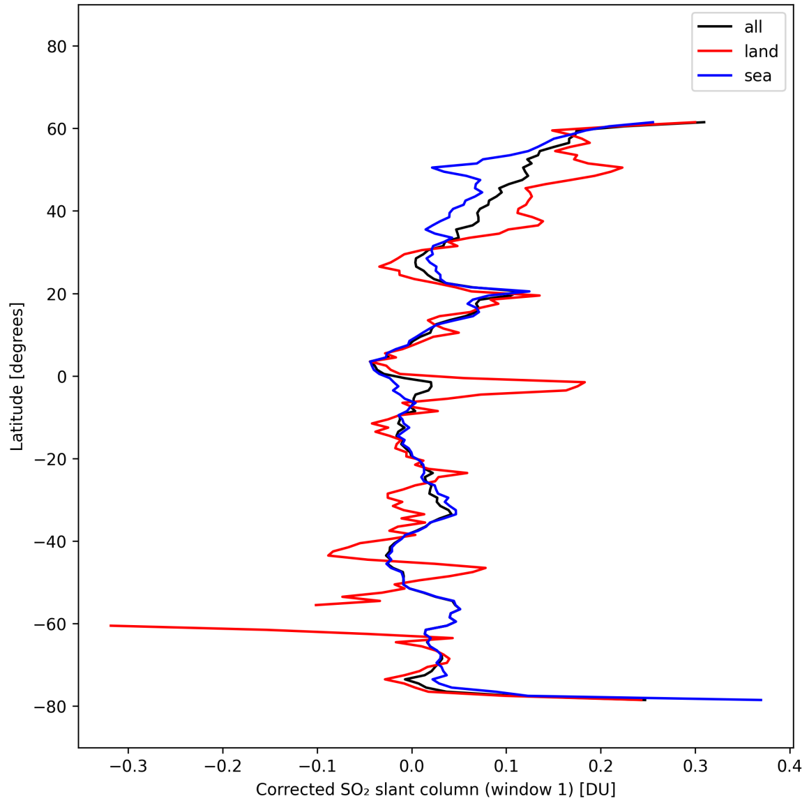
Figure 39: Zonal average of “Corrected SO 2 slant column (window 1)” for 2025-02-25 to 2025-02-27.
