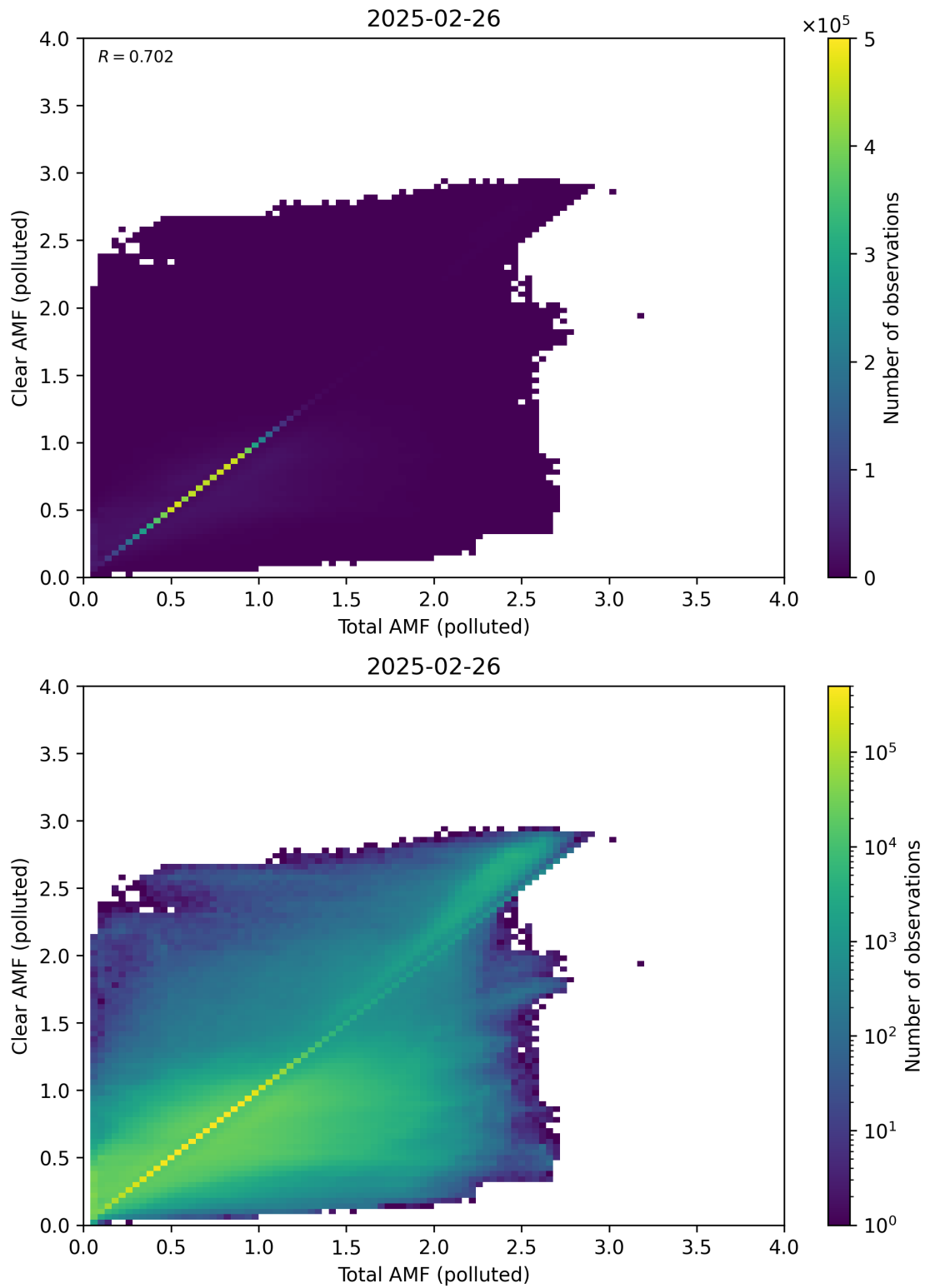
Figure 321: Scatter density plot of “Total AMF (polluted)” against “Clear AMF (polluted)” for 2025-02-25 to 2025-02-27.
