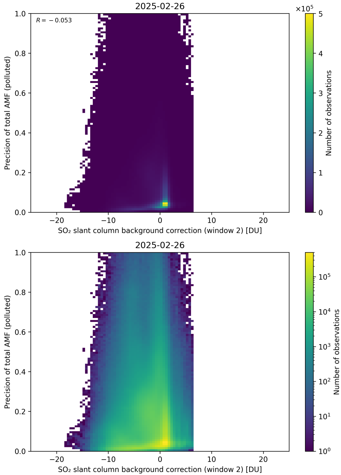
Figure 131: Scatter density plot of “SO 2 slant column background correction (window 2)” against “Precision of total AMF (polluted)” for 2025-02-25 to 2025-02-27.
