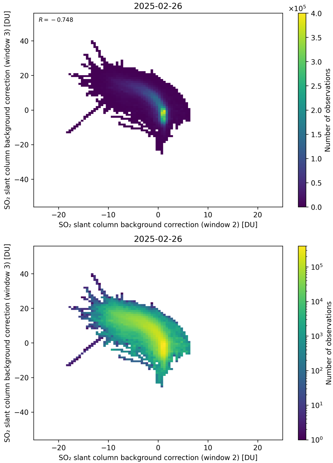
Figure 122: Scatter density plot of “SO 2 slant column background correction (window 2)” against “SO 2 slant column background correction (window 3)” for 2025-02-25 to 2025-02-27.
