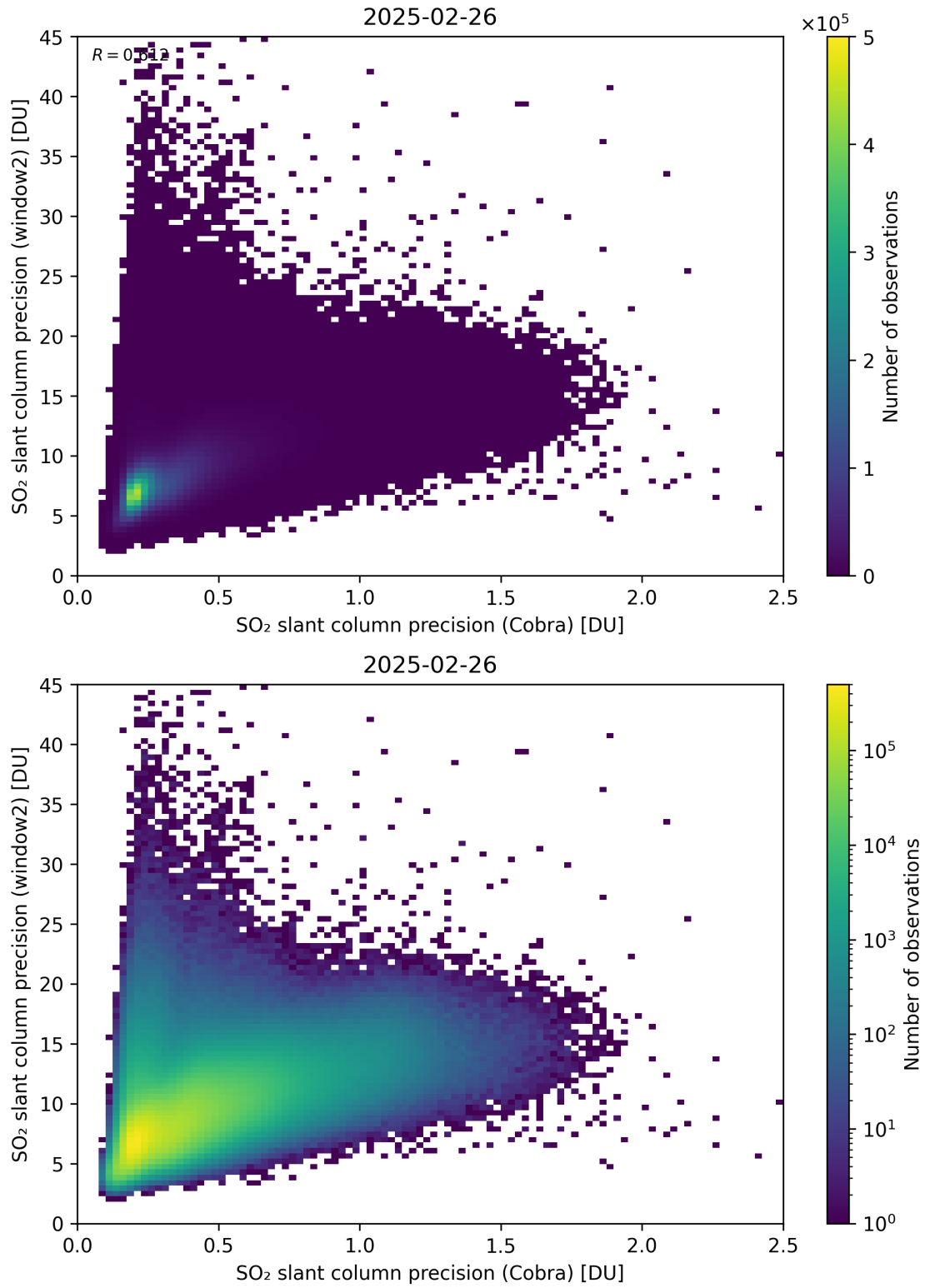
Figure 210: Scatter density plot of “SO 2 slant column precision (Cobra)” against “SO 2 slant column precision (window2)” for 2025-02-25 to 2025-02-27.
