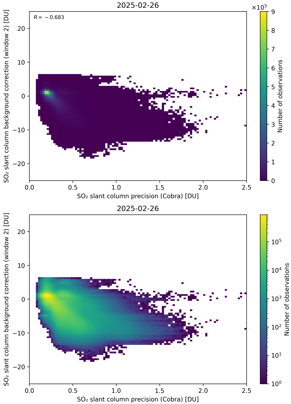
Figure 200: Scatter density plot of “SO 2 slant column precision (Cobra)” against “SO 2 slant column background correction (window 2)” for 2025-02-25 to 2025-02-27.
