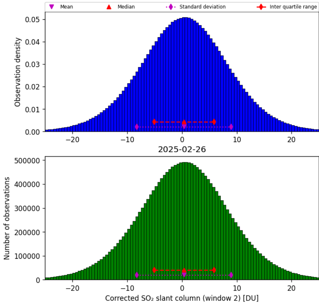
Figure 69: Histogram of "Corrected SO 2 slant column (window 2)" for 2025-02-25 to 2025-02-27
