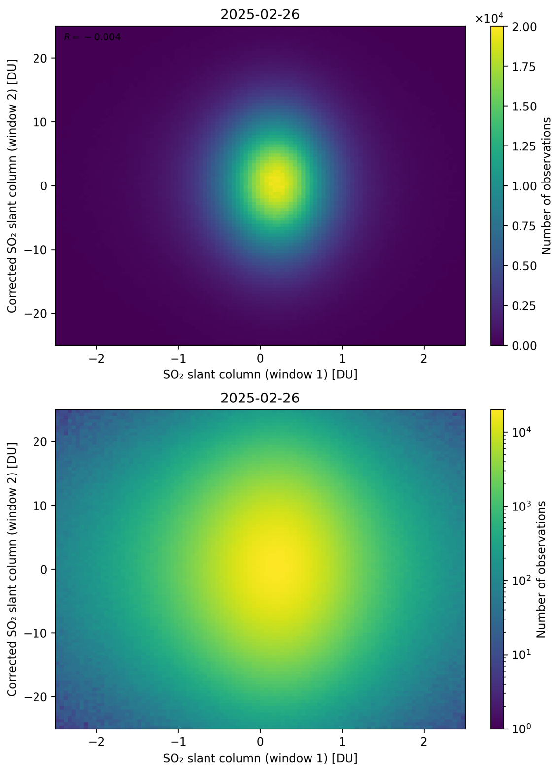
Figure 283: Scatter density plot of “SO 2 slant column (window 1)” against “Corrected SO 2 slant column (window 2)” for 2025-02-25 to 2025-02-27.
