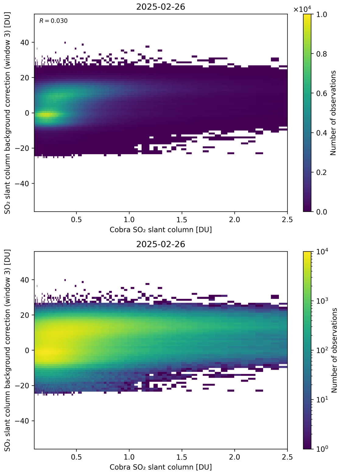
Figure 195: Scatter density plot of “Cobra SO 2 slant column” against “SO 2 slant column background correction (window 3)” for 2025-02-25 to 2025-02-27.
