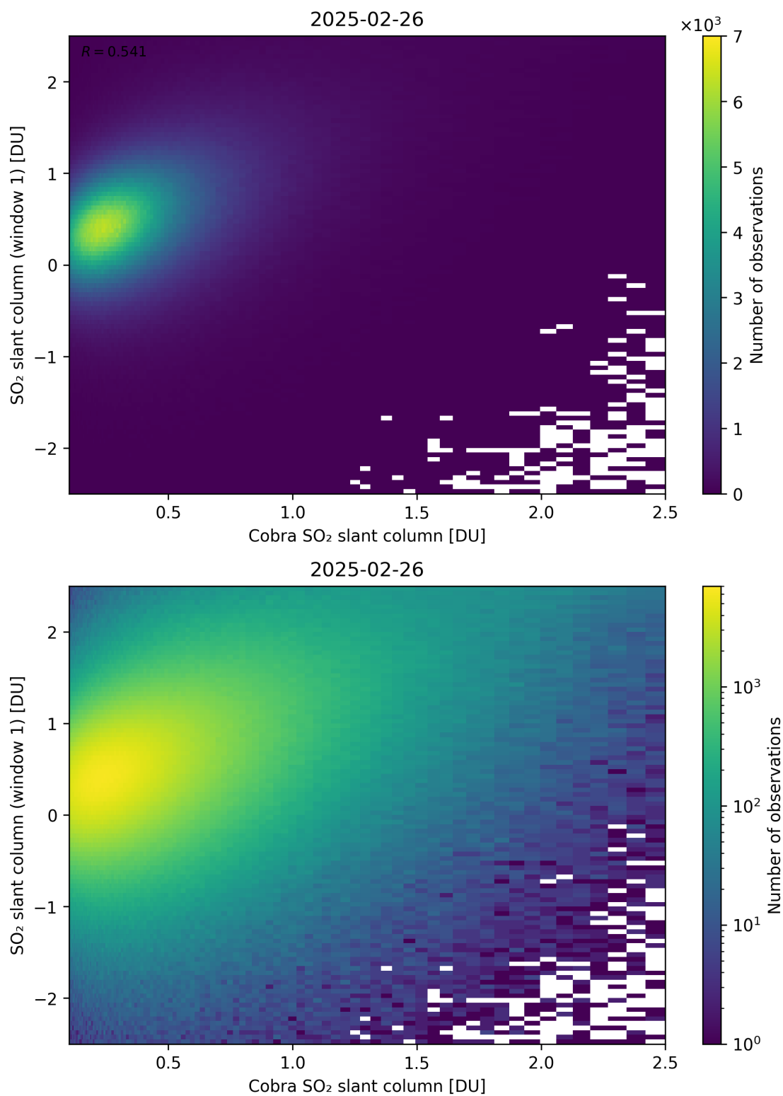
Figure 219: Scatter density plot of “Cobra SO 2 slant column” against “SO 2 slant column (window 1)” for 2025-02-25 to 2025-02-27.
