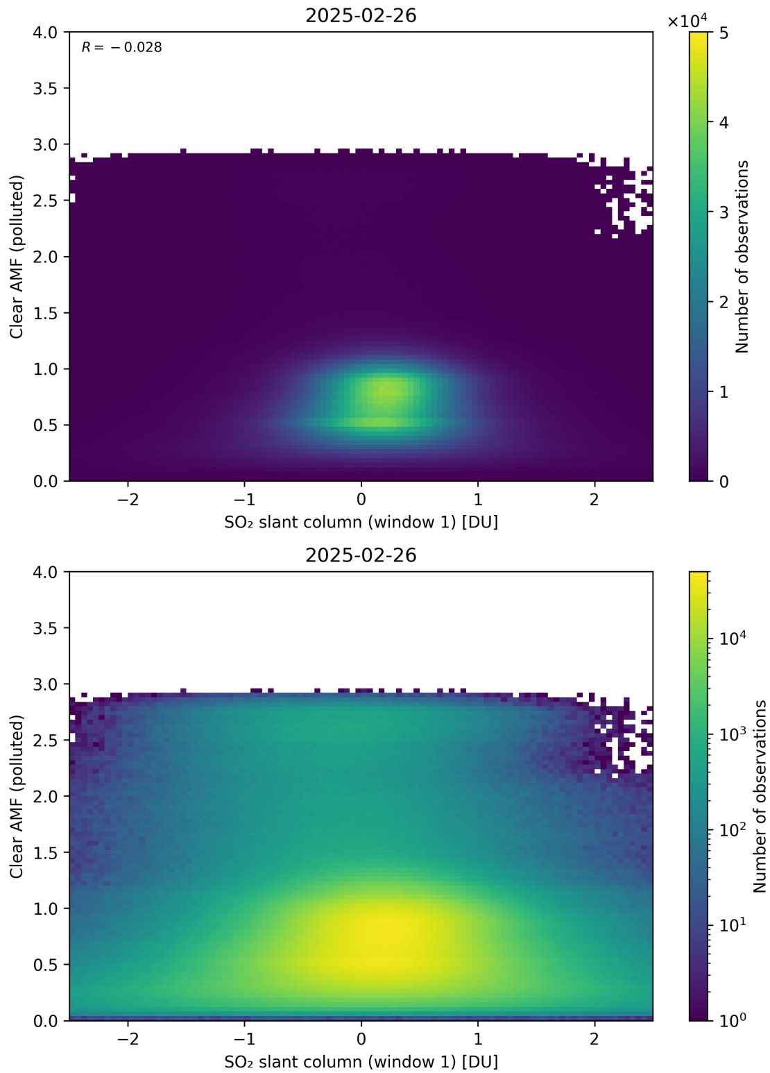
Figure 282: Scatter density plot of “SO 2 slant column (window 1)” against “Clear AMF (polluted)” for 2025-02-25 to 2025-02-27.
