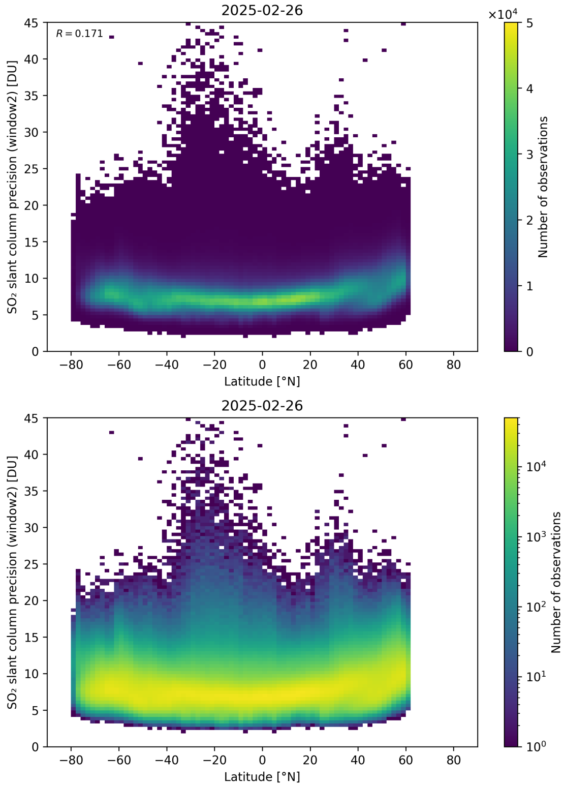
Figure 164: Scatter density plot of “Latitude” against “SO 2 slant column precision (window2)” for 2025-02-25 to 2025-02-27.
