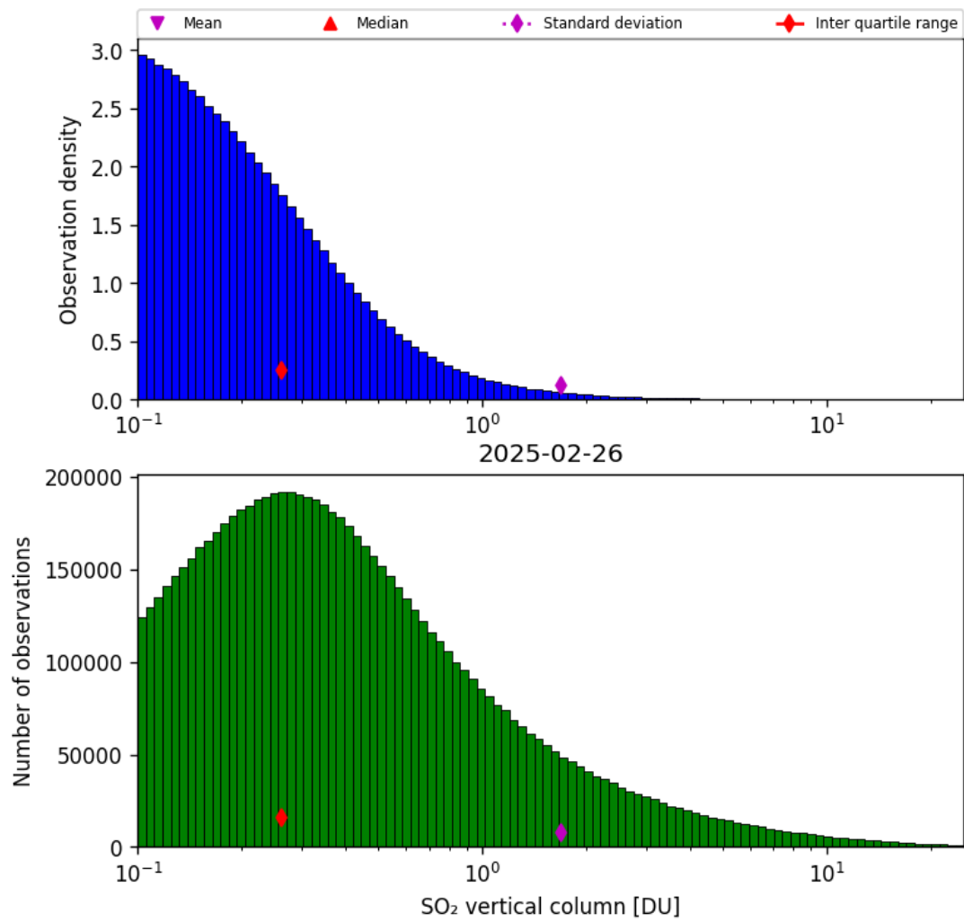
Figure 58: Histogram of “SO 2 vertical column” for 2025-02-25 to 2025-02-27
