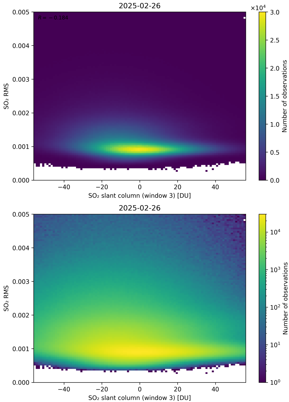
Figure 306: Scatter density plot of “SO 2 slant column (window 3)” against “SO 2 RMS” for 2025-02-25 to 2025-02-27.
