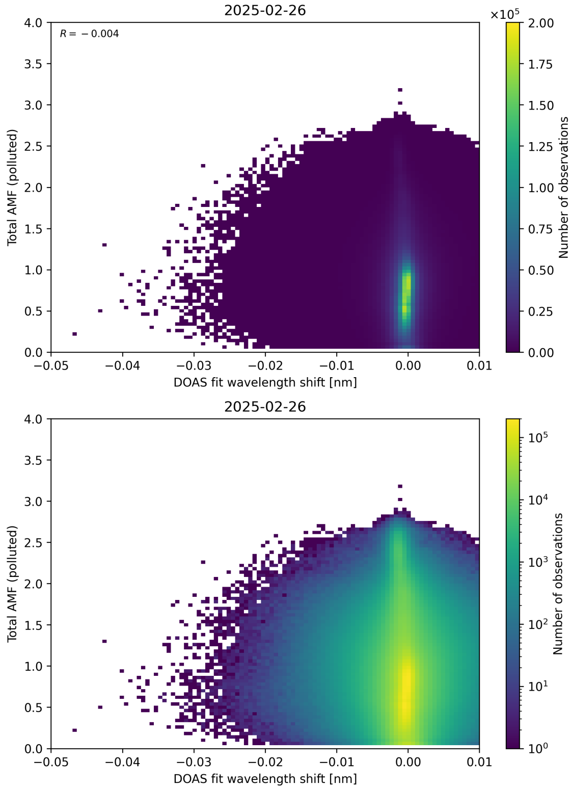
Figure 141: Scatter density plot of “DOAS fit wavelength shift” against “Total AMF (polluted)” for 2025-02-25 to 2025-02-27.
