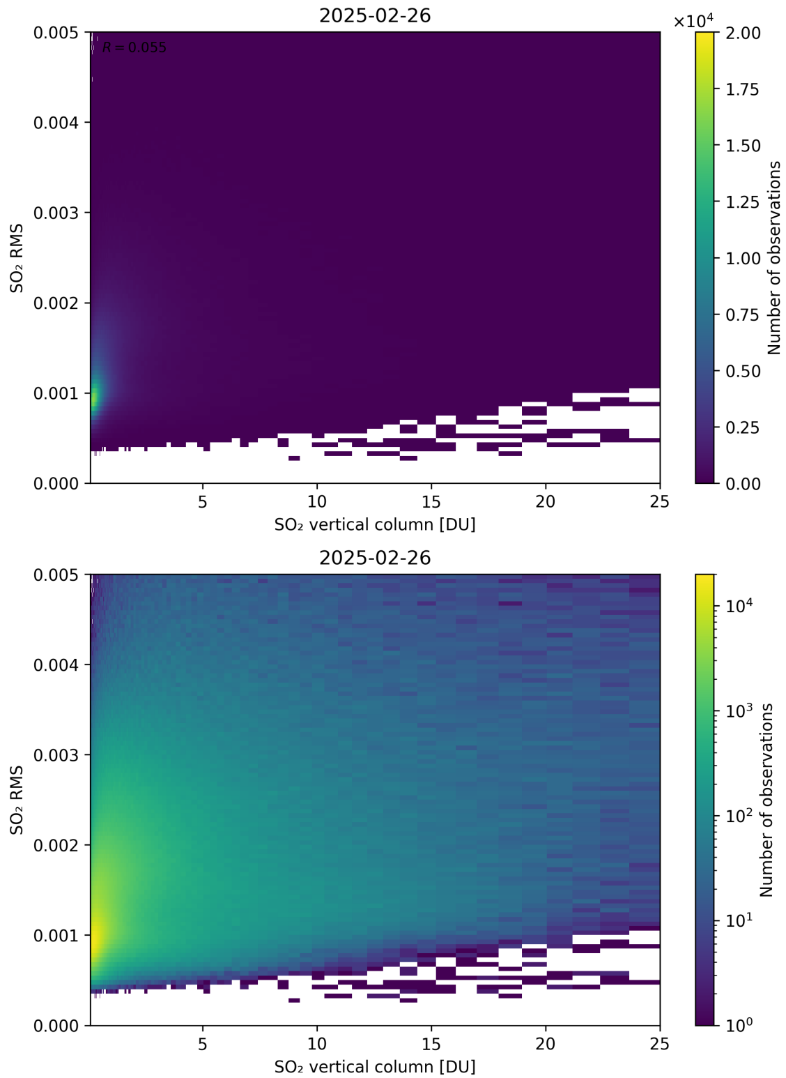
Figure 328: Scatter density plot of “SO 2 vertical column” against “SO 2 RMS” for 2025-02-25 to 2025-02-27.
