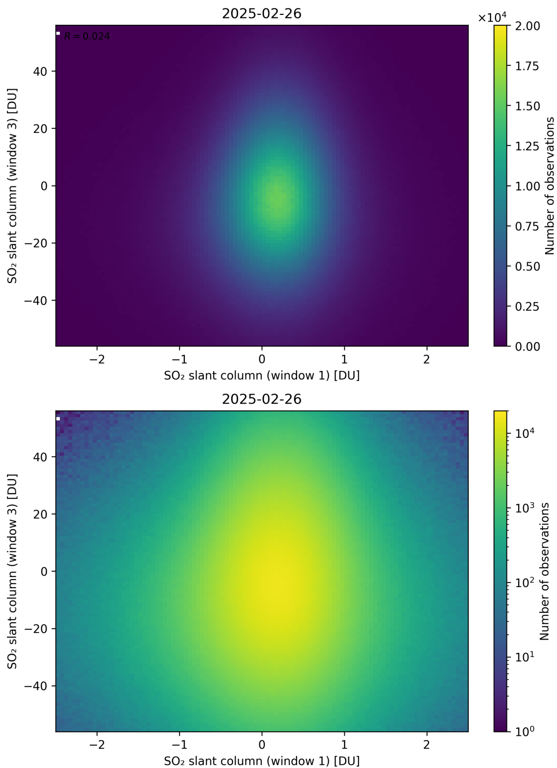
Figure 287: Scatter density plot of “SO 2 slant column (window 1)” against “SO 2 slant column (window 3)” for 2025-02-25 to 2025-02-27.
