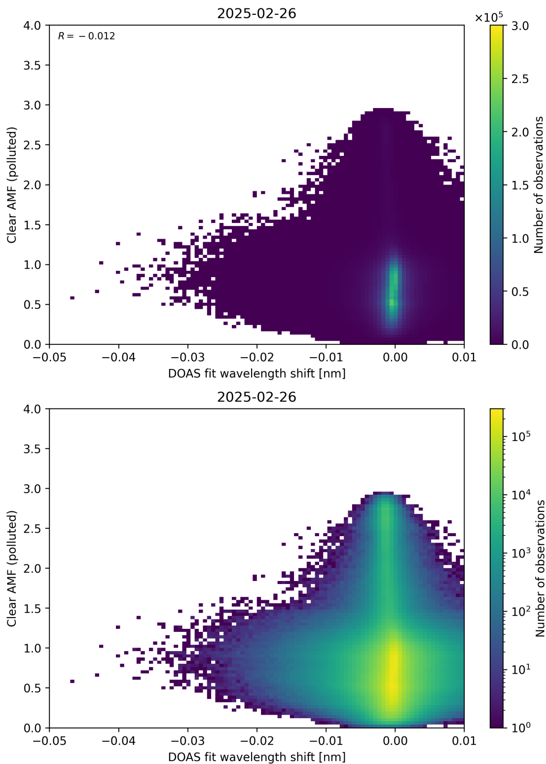
Figure 140: Scatter density plot of “DOAS fit wavelength shift” against “Clear AMF (polluted)” for 2025-02-25 to 2025-02-27.
