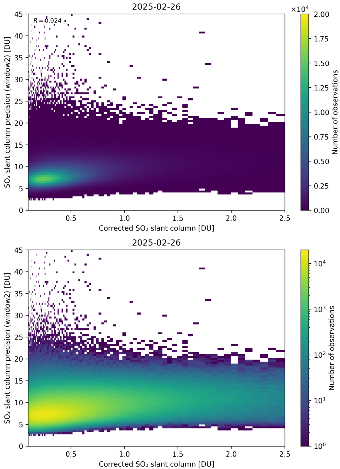
Figure 239: Scatter density plot of “Corrected SO 2 slant column” against “SO 2 slant column precision (window2)” for 2025-02-25 to 2025-02-27.
