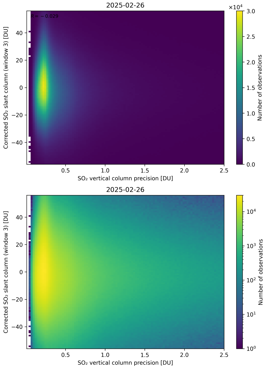
Figure 340: Scatter density plot of “SO 2 vertical column precision” against “Corrected SO 2 slant column (window 3)” for 2025-02-25 to 2025-02-27.
