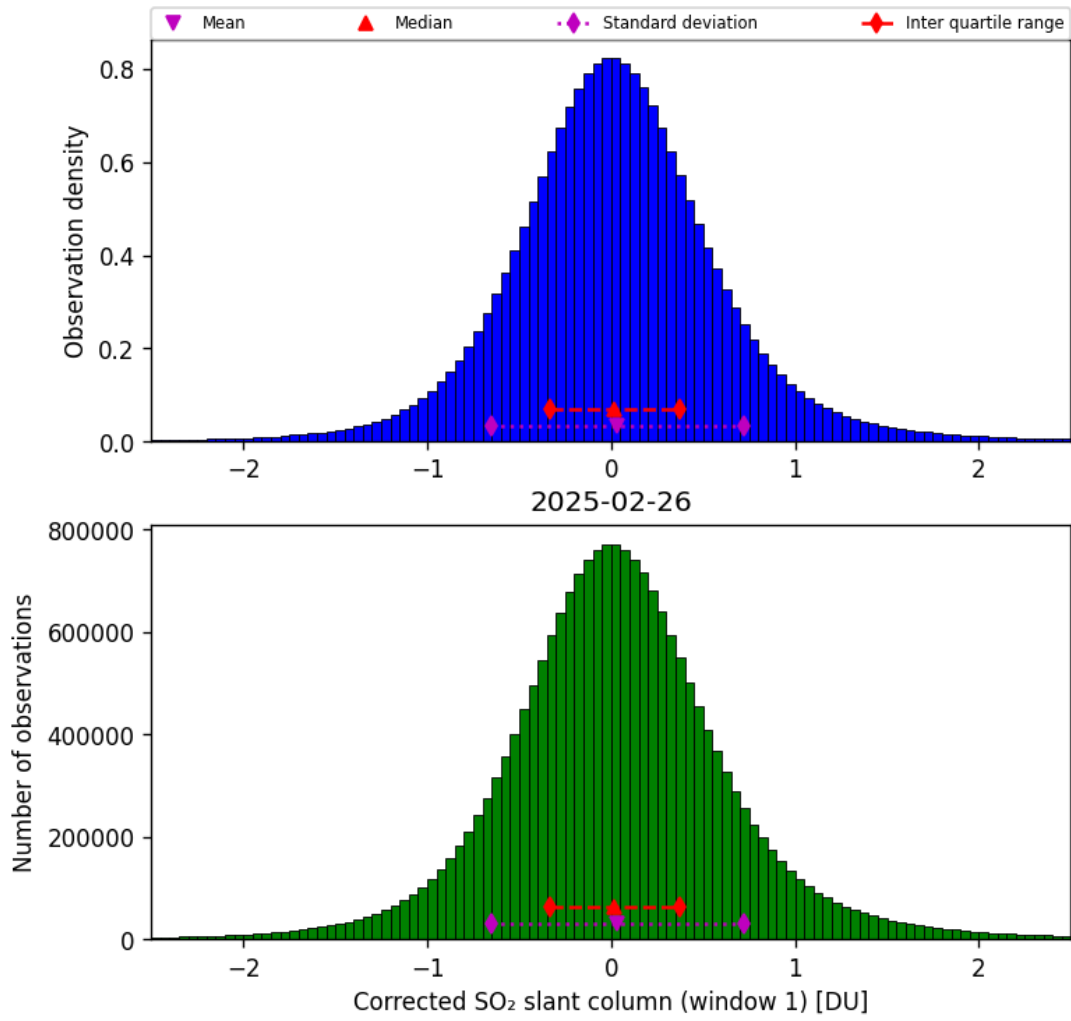
Figure 65: Histogram of “Corrected SO 2 slant column (window 1)” for 2025-02-25 to 2025-02-27
