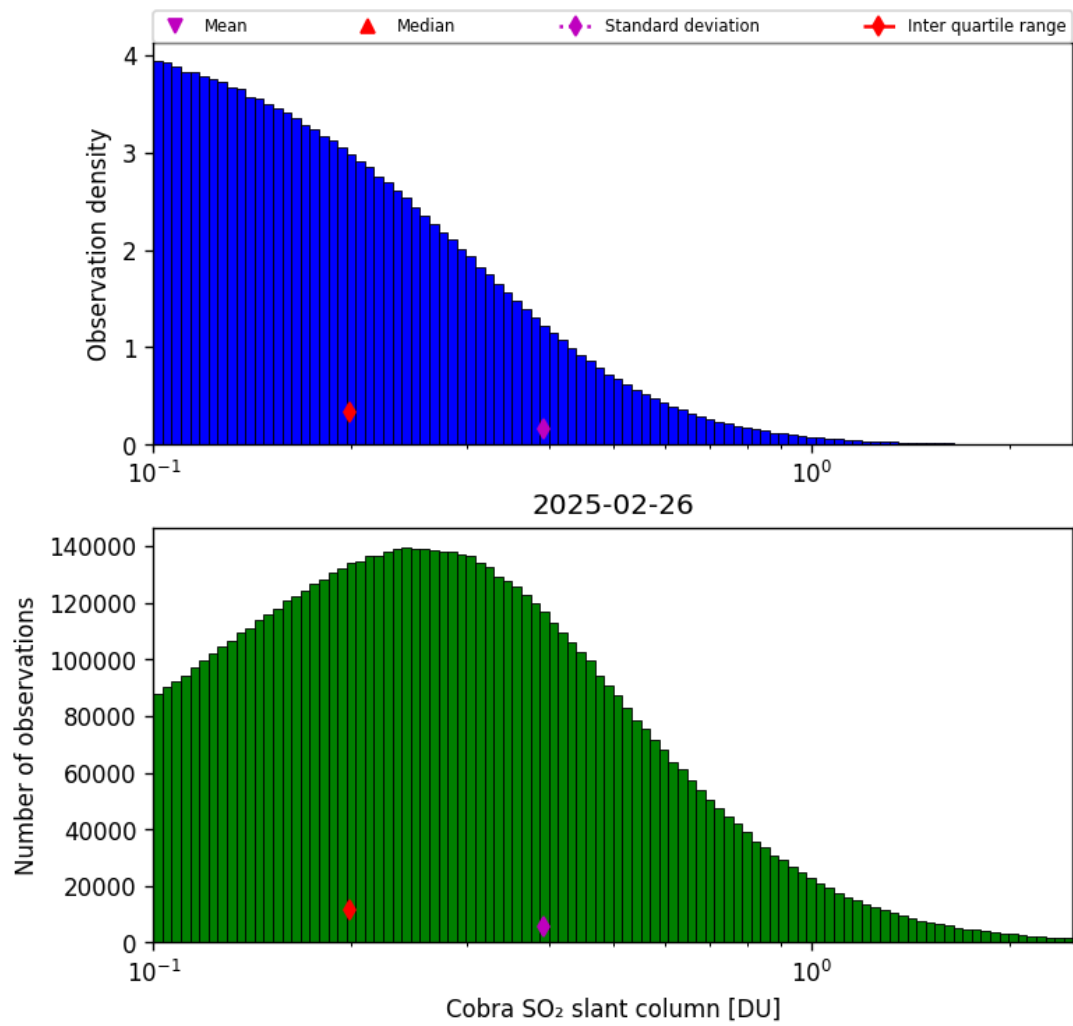
Figure 61: Histogram of “Cobra SO 2 slant column” for 2025-02-25 to 2025-02-27
