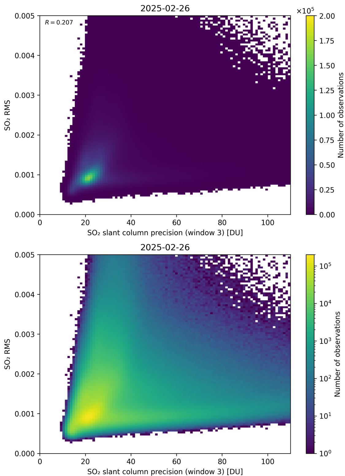
Figure 310: Scatter density plot of “SO 2 slant column precision (window 3)” against “SO 2 RMS” for 2025-02-25 to 2025-02-27.
