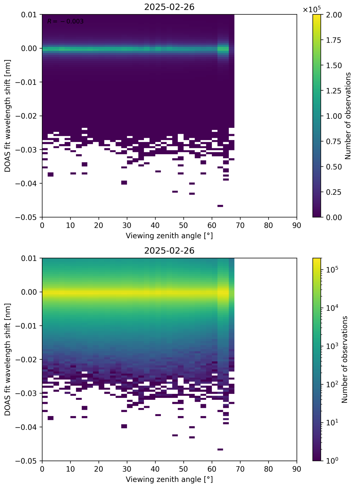
Figure 365: Scatter density plot of “Viewing zenith angle” against “DOAS fit wavelength shift” for 2025-02-25 to 2025-02-27.
