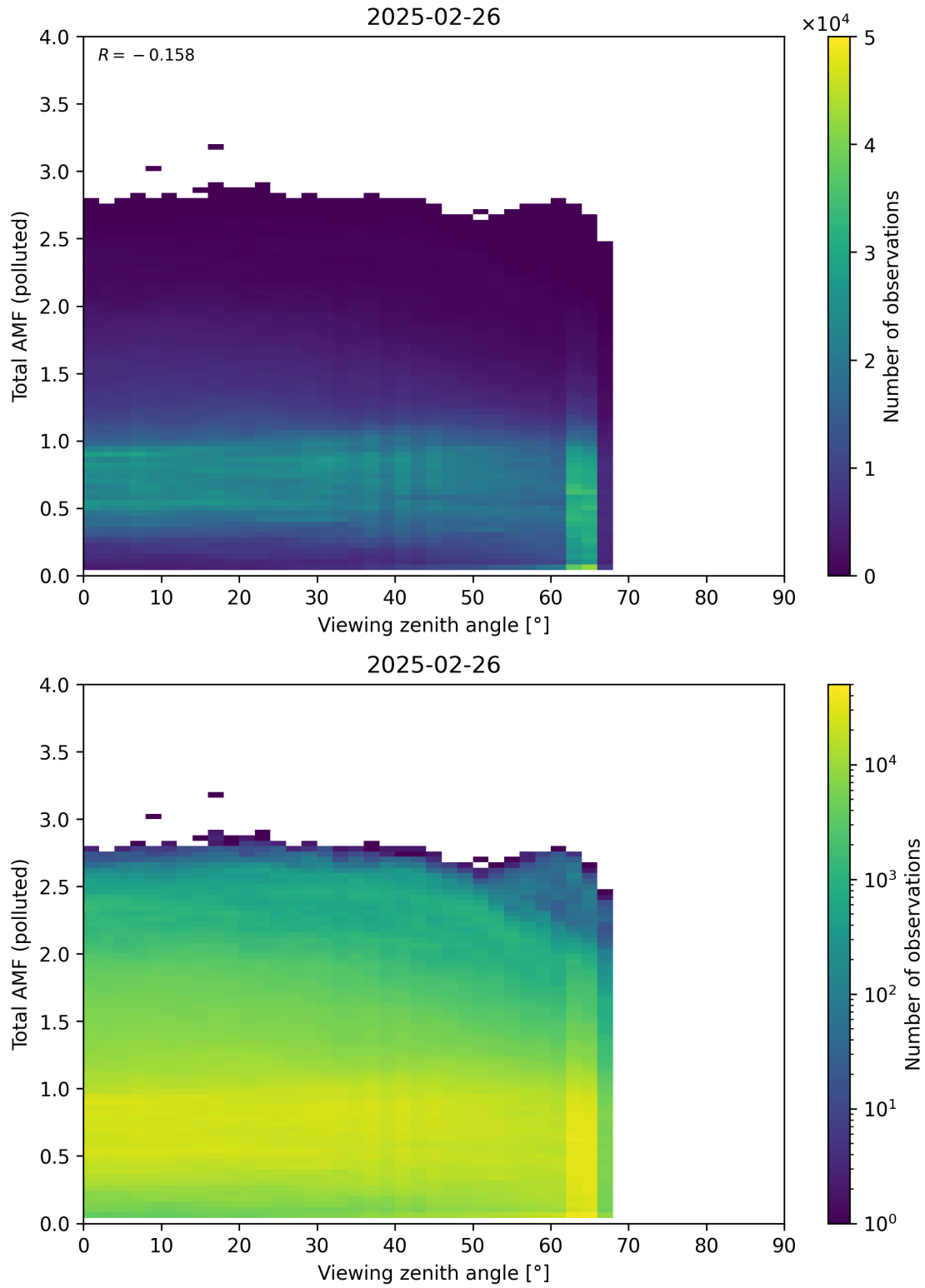
Figure 381: Scatter density plot of “Viewing zenith angle” against “Total AMF (polluted)” for 2025-02-25 to 2025-02-27.
