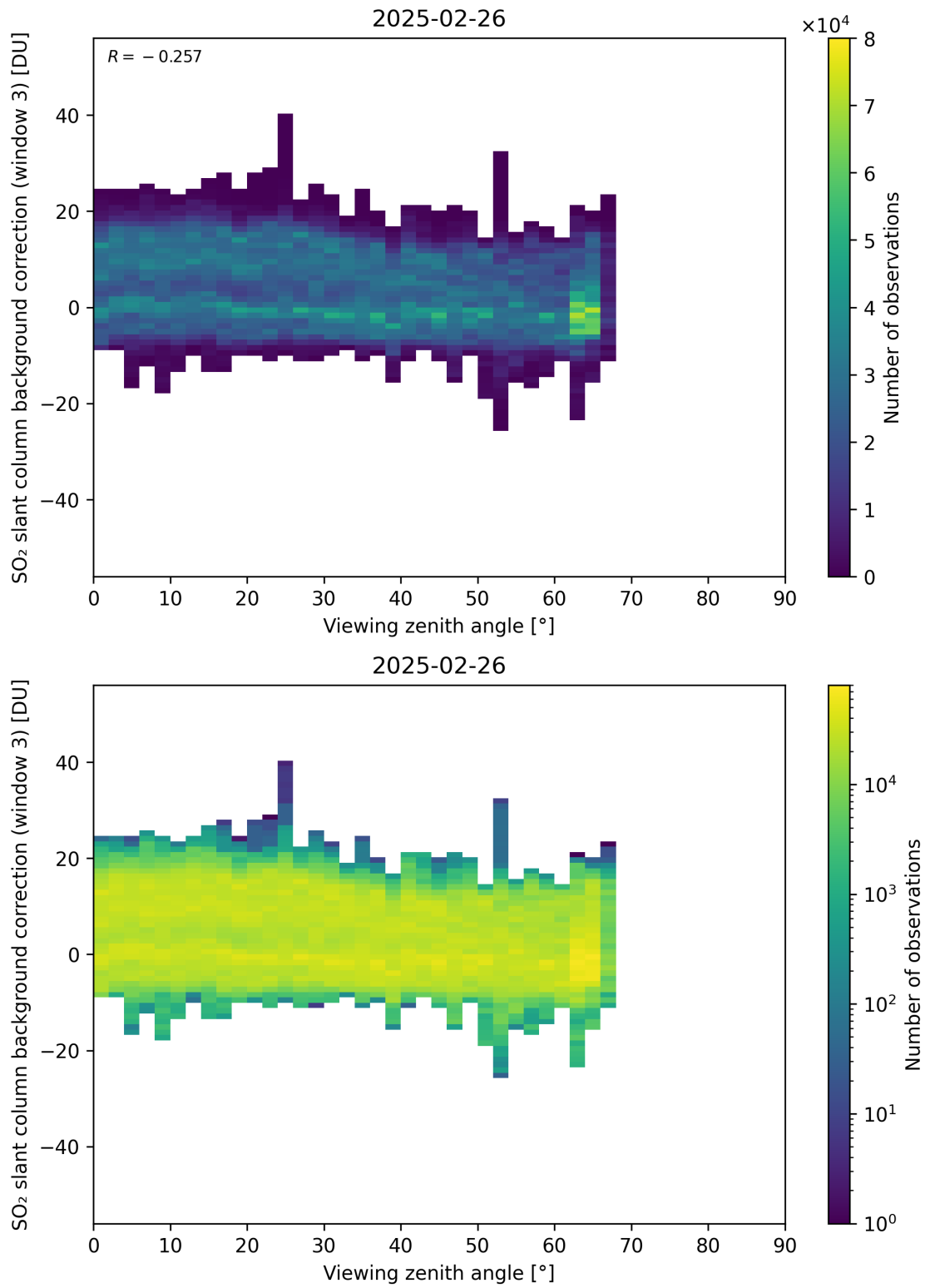
Figure 364: Scatter density plot of “Viewing zenith angle” against “SO 2 slant column background correction (window 3)” for 2025-02-25 to 2025-02-27.
