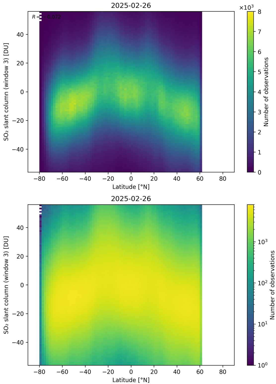
Figure 165: Scatter density plot of “Latitude” against “SO 2 slant column (window 3)” for 2025-02-25 to 2025-02-27.
