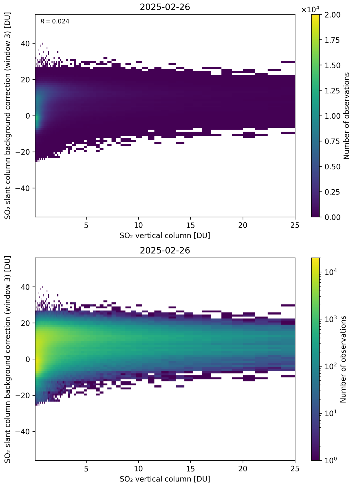
Figure 325: Scatter density plot of “SO 2 vertical column” against “SO 2 slant column background correction (window 3)” for 2025-02-25 to 2025-02-27.
