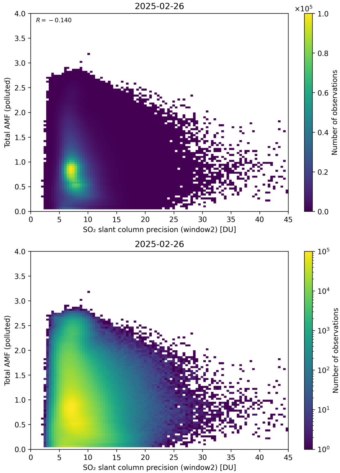
Figure 301: Scatter density plot of “SO 2 slant column precision (window2)” against “Total AMF (polluted)” for 2025-02-25 to 2025-02-27.
