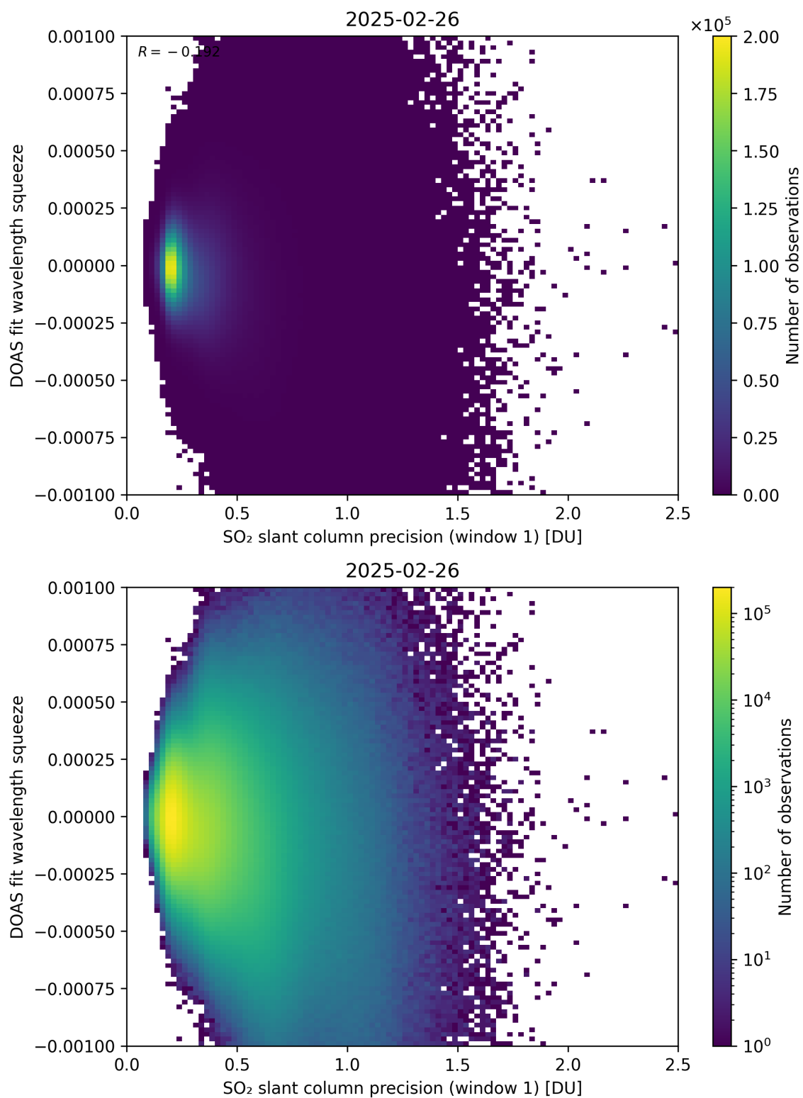
Figure 272: Scatter density plot of “SO 2 slant column precision (window 1)” against “DOAS fit wavelength squeeze” for 2025-02-25 to 2025-02-27.
