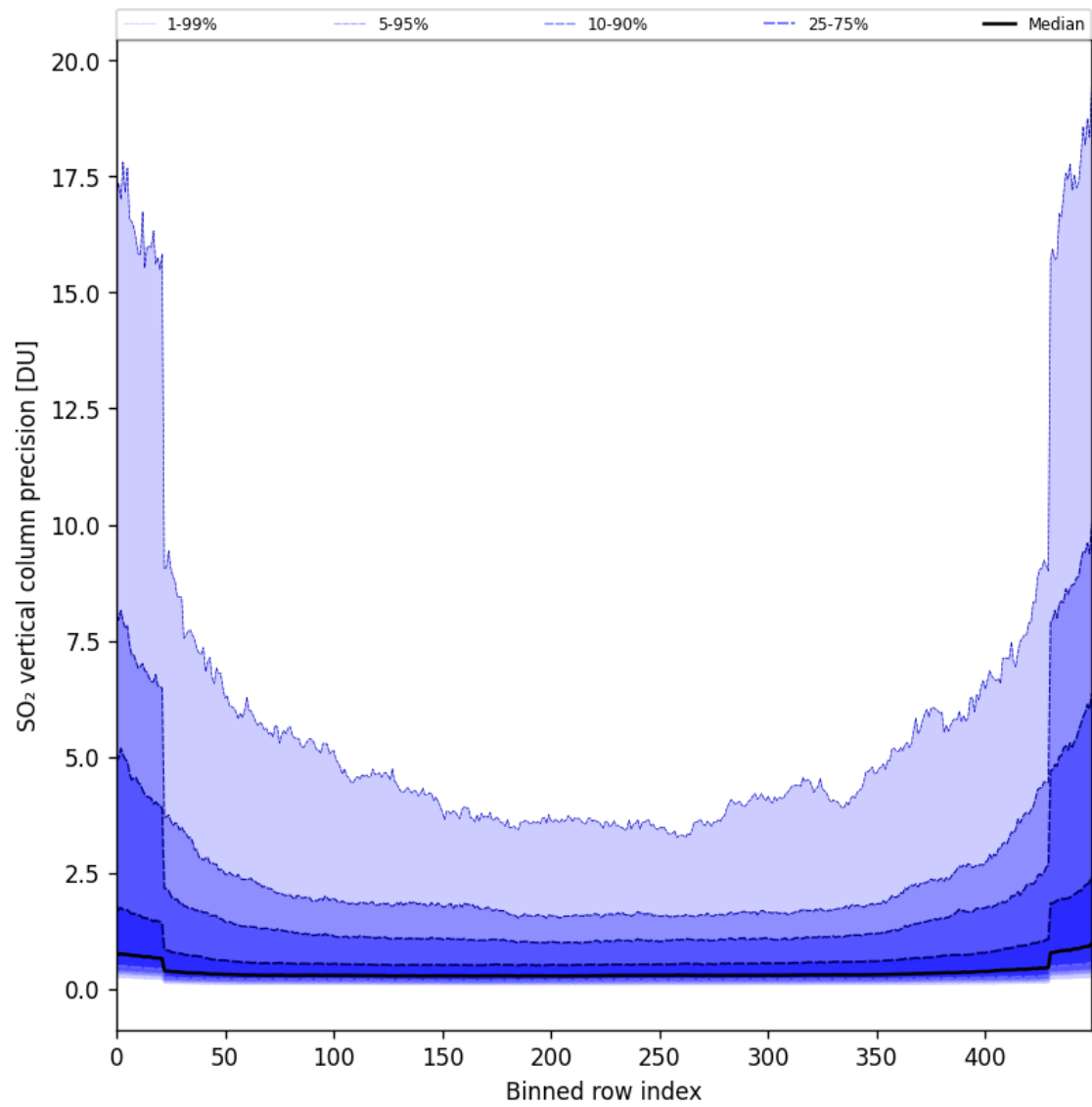
Figure 85: Along track statistics of "SO 2 vertical column precision" for 2025-02-25 to 2025-02-27
