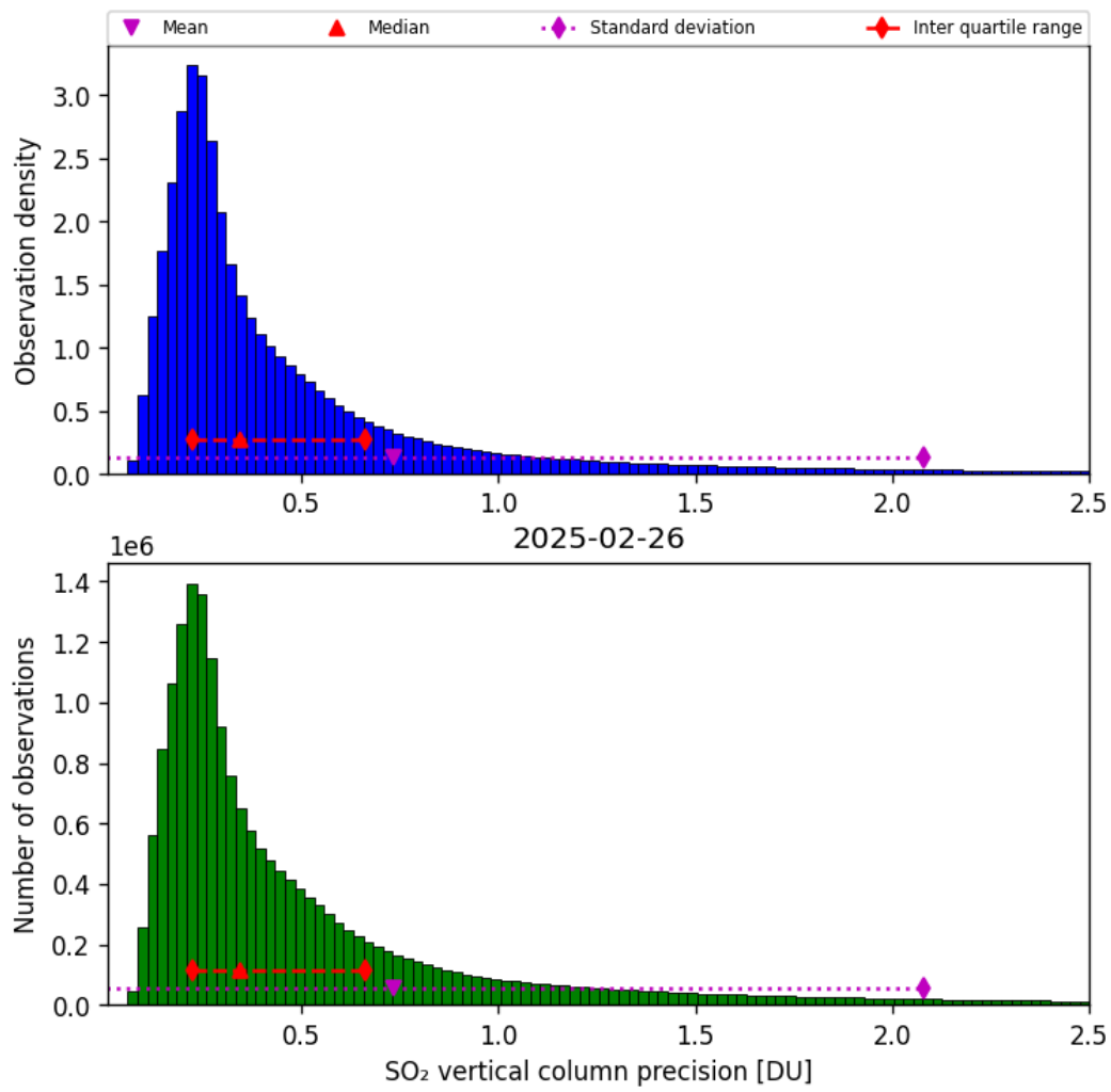
Figure 59: Histogram of “SO 2 vertical column precision” for 2025-02-25 to 2025-02-27
