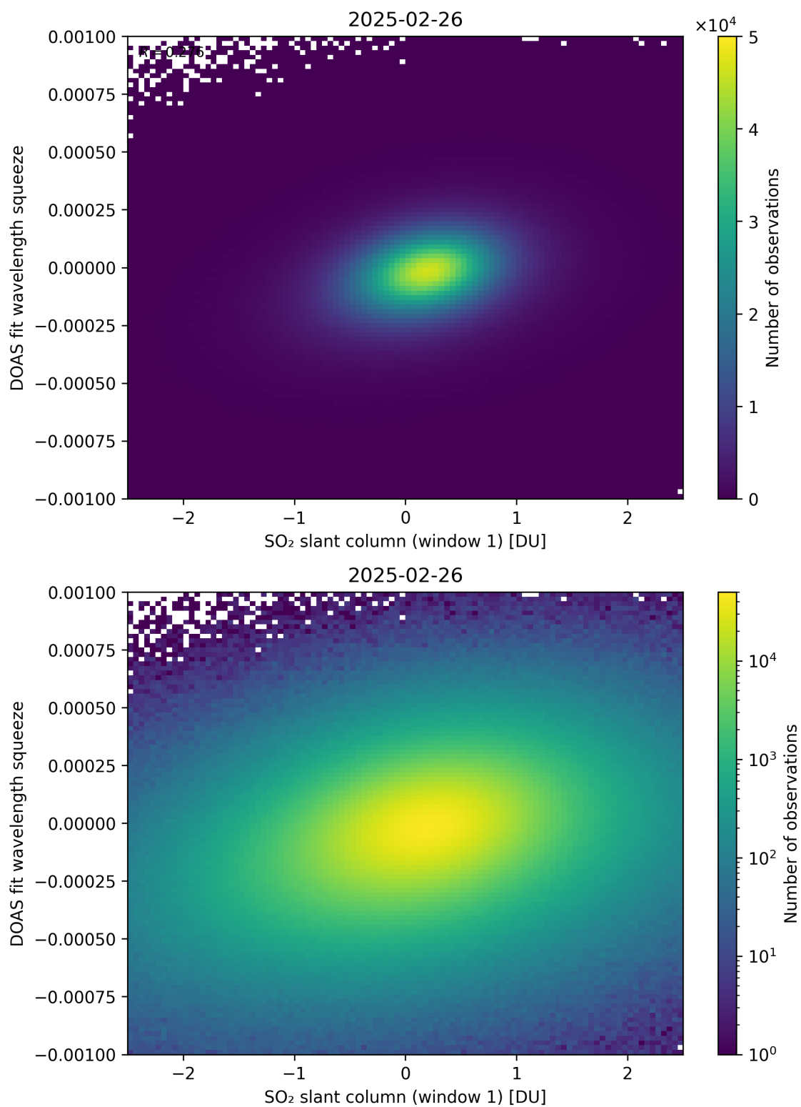
Figure 266: Scatter density plot of “SO 2 slant column (window 1)” against “DOAS fit wavelength squeeze” for 2025-02-25 to 2025-02-27.
