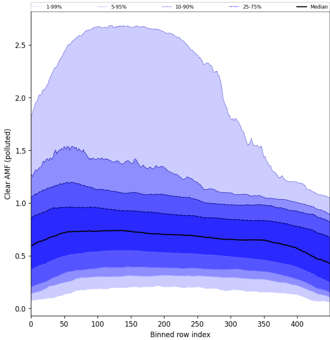
Figure 107: Along track statistics of “Clear AMF (polluted)” for 2025-02-25 to 2025-02-27
