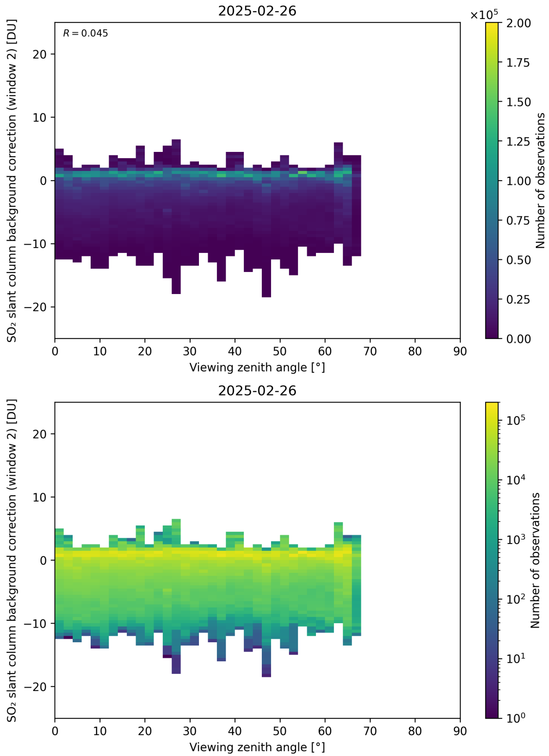
Figure 363: Scatter density plot of “Viewing zenith angle” against “SO 2 slant column background correction (window 2)” for 2025-02-25 to 2025-02-27.
