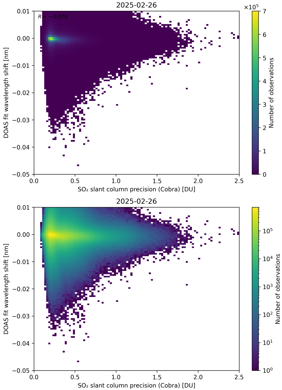
Figure 202: Scatter density plot of “SO 2 slant column precision (Cobra)” against “DOAS fit wavelength shift” for 2025-02-25 to 2025-02-27.
