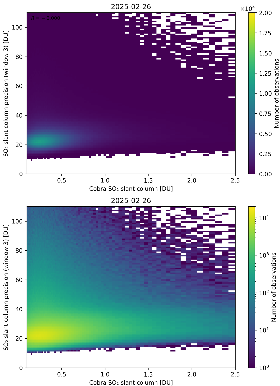
Figure 223: Scatter density plot of “Cobra SO 2 slant column” against “SO 2 slant column precision (window 3)” for 2025-02-25 to 2025-02-27.
