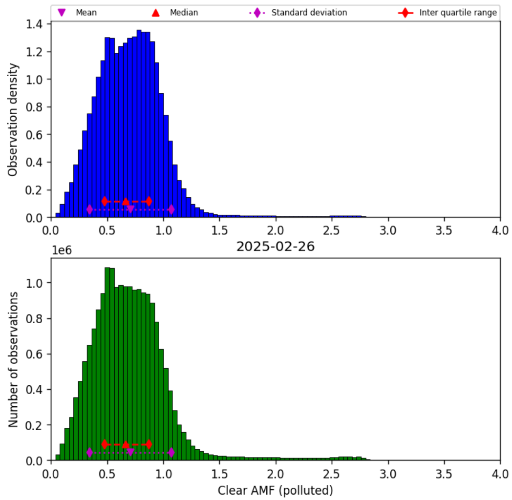
Figure 81: Histogram of “Clear AMF (polluted)” for 2025-02-25 to 2025-02-27
