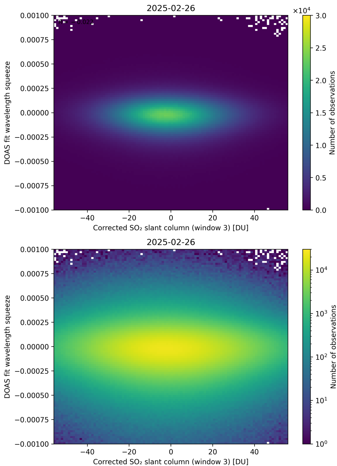
Figure 257: Scatter density plot of “Corrected SO 2 slant column (window 3)” against “DOAS fit wavelength squeeze” for 2025-02-25 to 2025-02-27.
