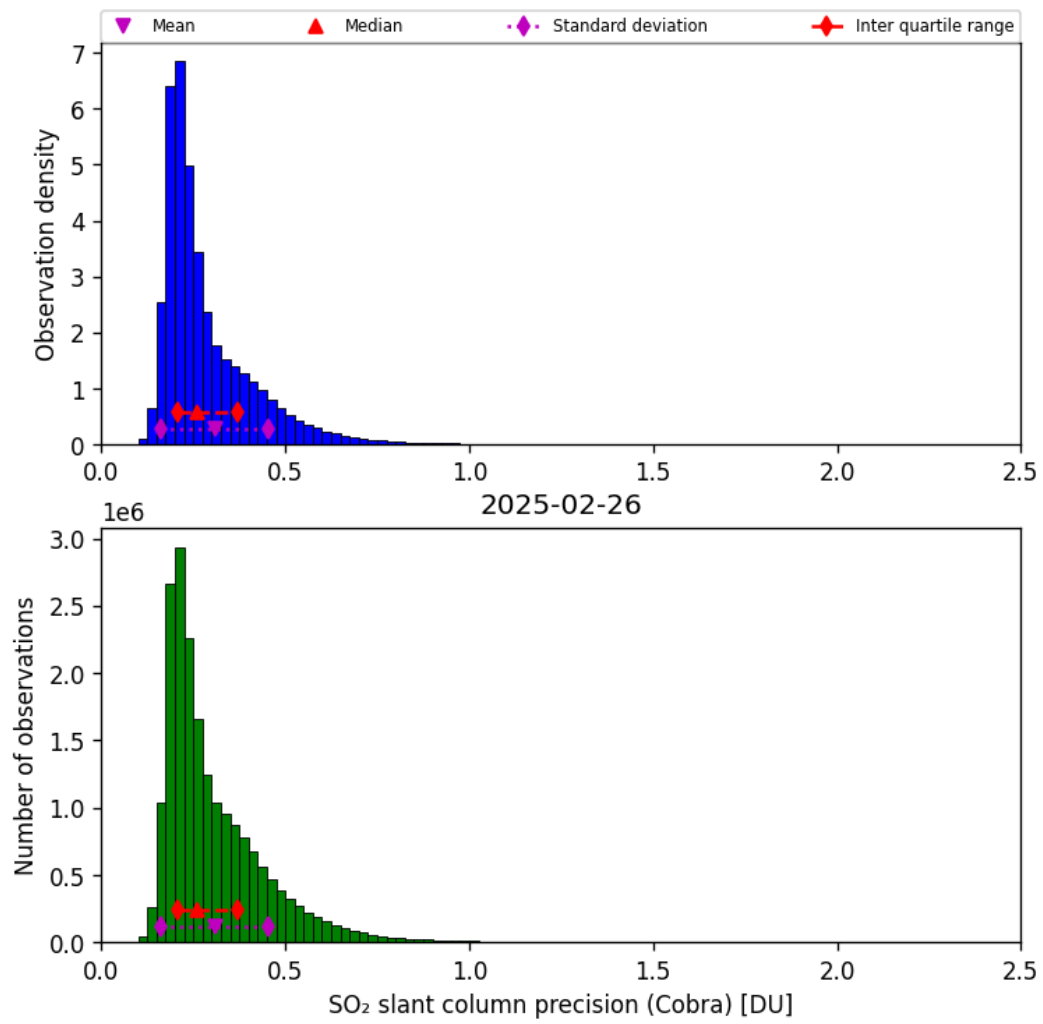
Figure 62: Histogram of “SO 2 slant column precision (Cobra)” for 2025-02-25 to 2025-02-27
