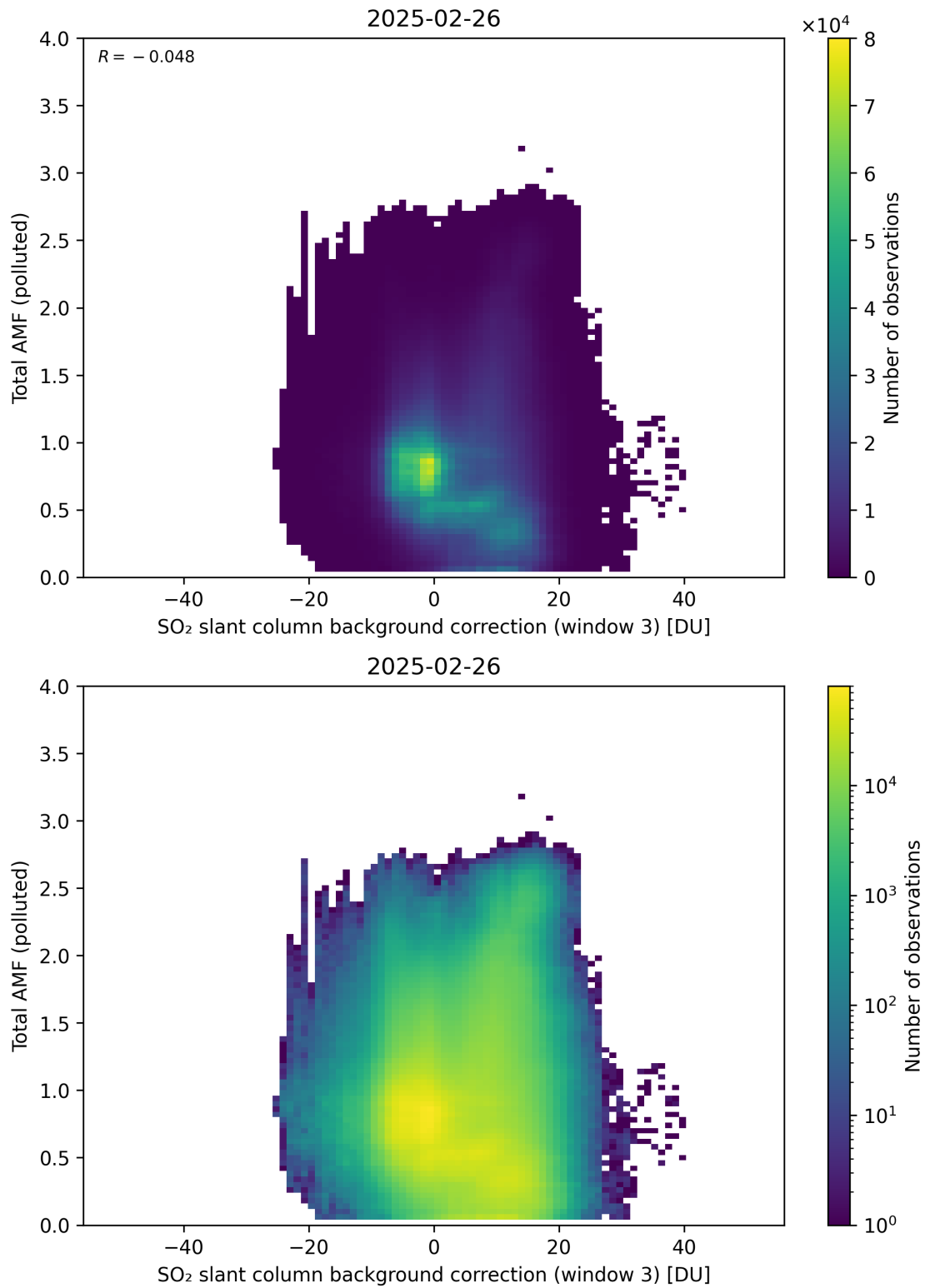
Figure 136: Scatter density plot of “SO 2 slant column background correction (window 3)” against “Total AMF (polluted)” for 2025-02-25 to 2025-02-27.
