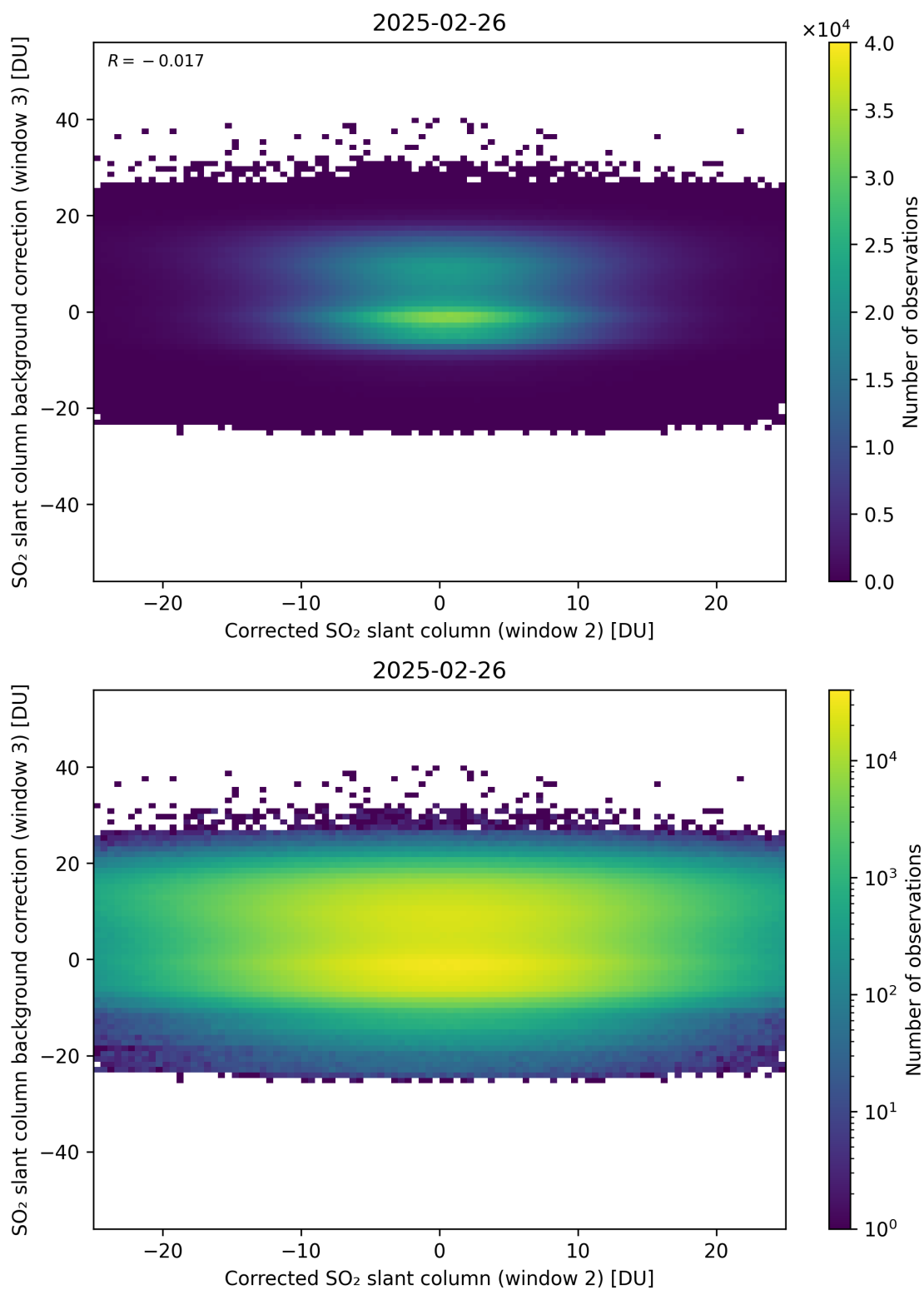
Figure 245: Scatter density plot of “Corrected SO 2 slant column (window 2)” against “SO 2 slant column background correction (window 3)” for 2025-02-25 to 2025-02-27.
