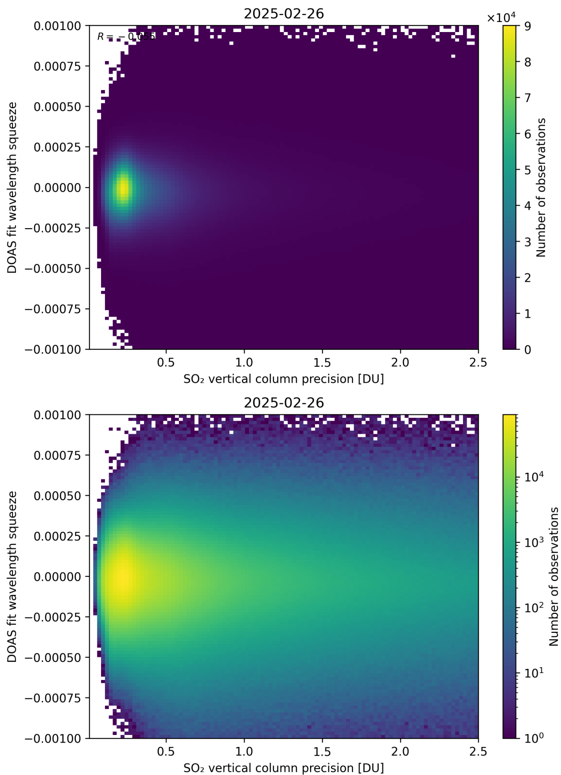
Figure 333: Scatter density plot of “SO 2 vertical column precision” against “DOAS fit wavelength squeeze” for 2025-02-25 to 2025-02-27.
