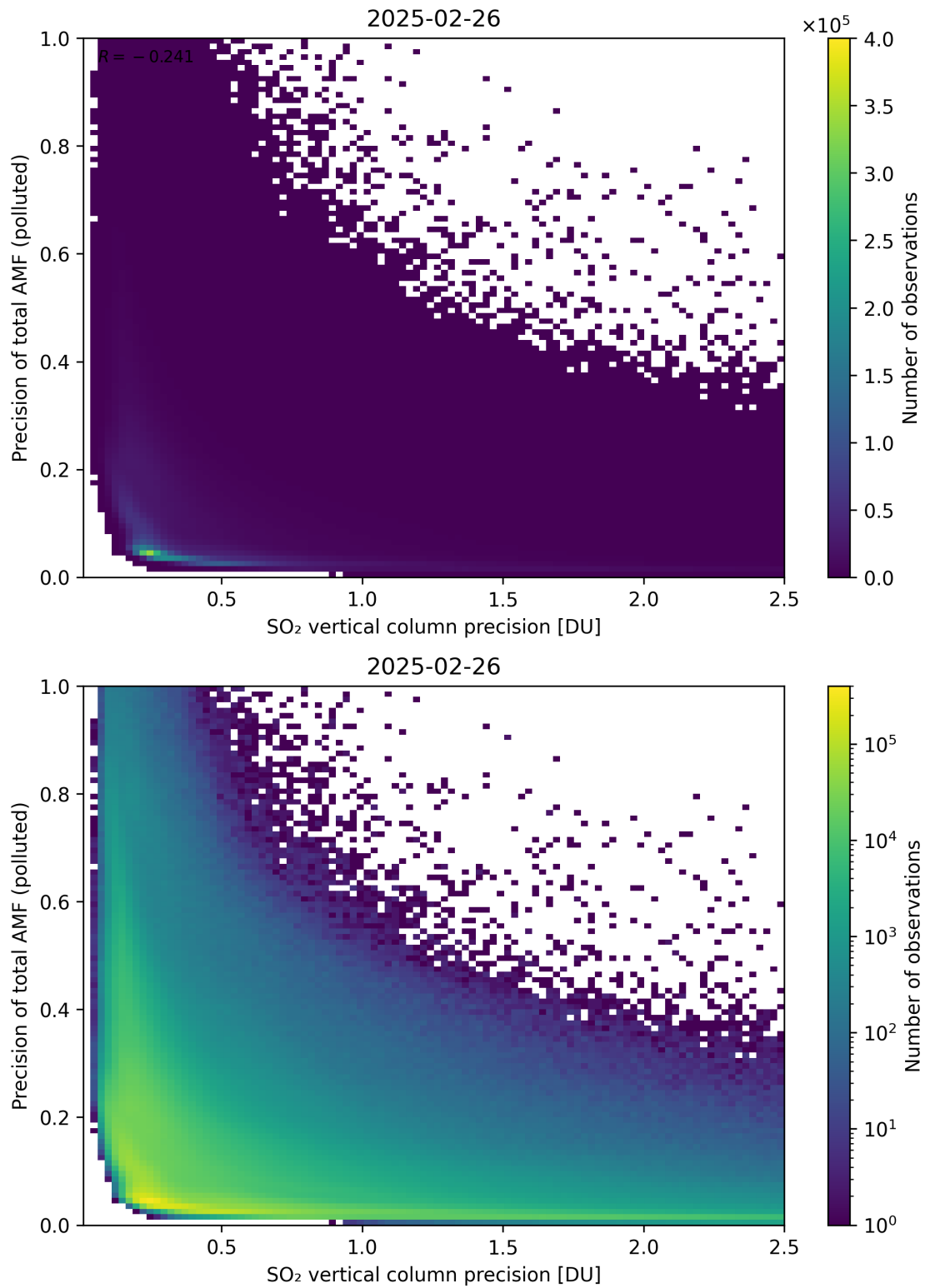
Figure 347: Scatter density plot of “SO 2 vertical column precision” against “Precision of total AMF (polluted)” for 2025-02-25 to 2025-02-27.
