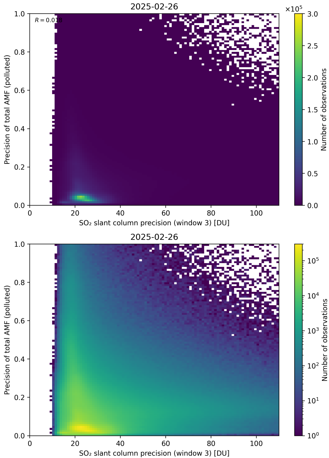
Figure 314: Scatter density plot of “SO 2 slant column precision (window 3)” against “Precision of total AMF (polluted)” for 2025-02-25 to 2025-02-27.
