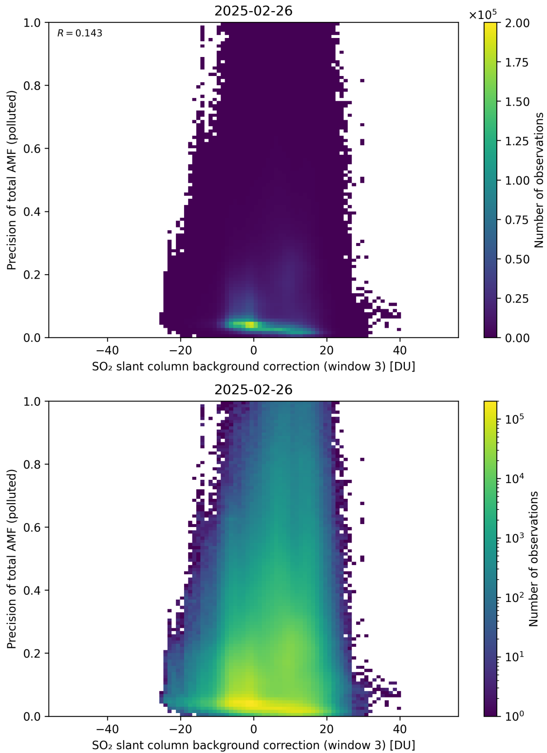
Figure 137: Scatter density plot of “SO 2 slant column background correction (window 3)” against “Precision of total AMF (polluted)” for 2025-02-25 to 2025-02-27.
