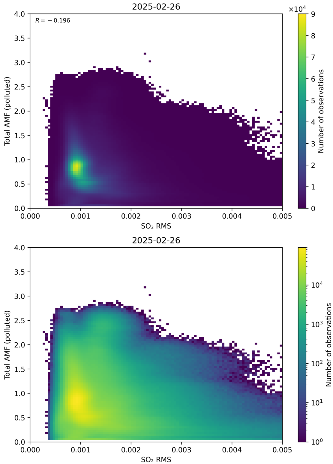
Figure 148: Scatter density plot of “SO 2 RMS” against “Total AMF (polluted)” for 2025-02-25 to 2025-02-27.
