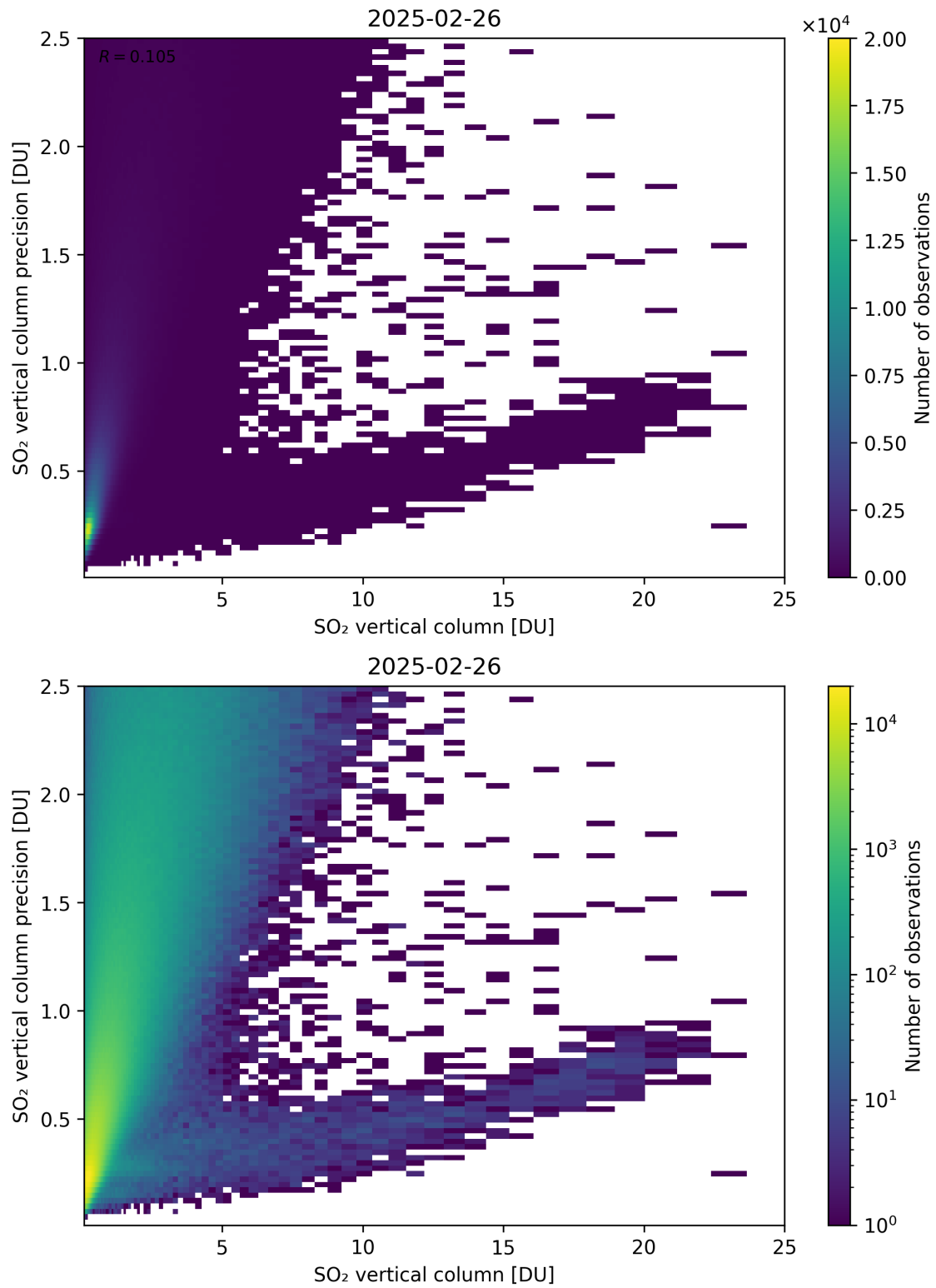
Figure 361: Scatter density plot of “SO 2 vertical column” against “SO 2 vertical column precision” for 2025-02-25 to 2025-02-27.
