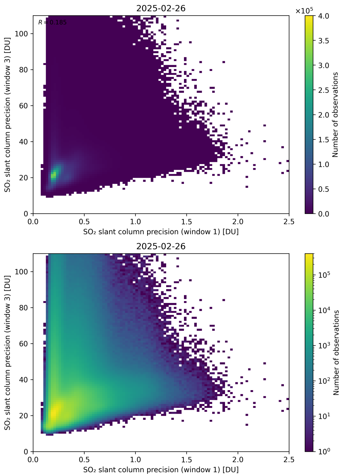
Figure 279: Scatter density plot of “SO 2 slant column precision (window 1)” against “SO 2 slant column precision (window 3)” for 2025-02-25 to 2025-02-27.
