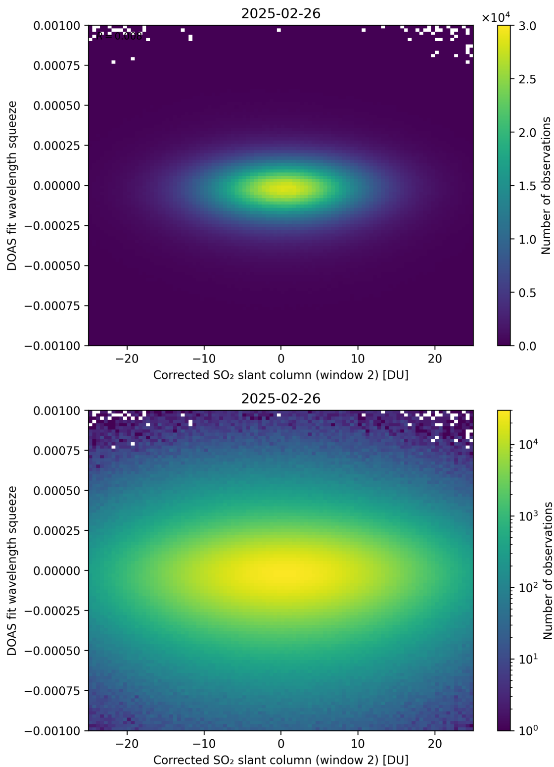
Figure 247: Scatter density plot of “Corrected SO 2 slant column (window 2)” against “DOAS fit wavelength squeeze” for 2025-02-25 to 2025-02-27.
