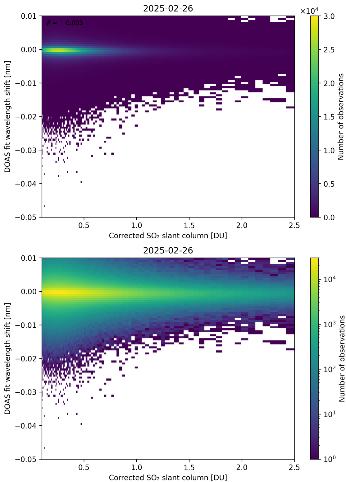
Figure 229: Scatter density plot of “Corrected SO 2 slant column” against “DOAS fit wavelength shift” for 2025-02-25 to 2025-02-27.
