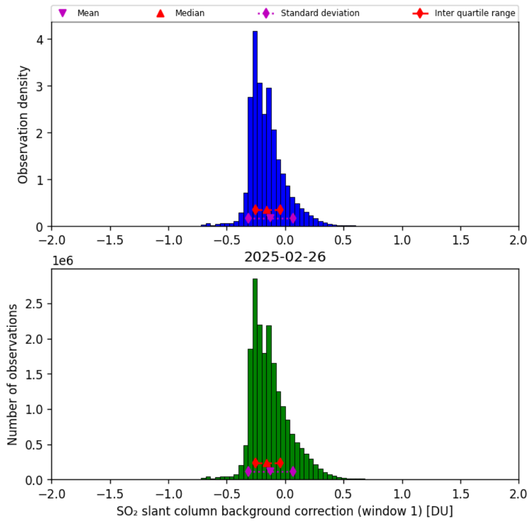
Figure 66: Histogram of “SO 2 slant column background correction (window 1)” for 2025-02-25 to 2025-02-27
