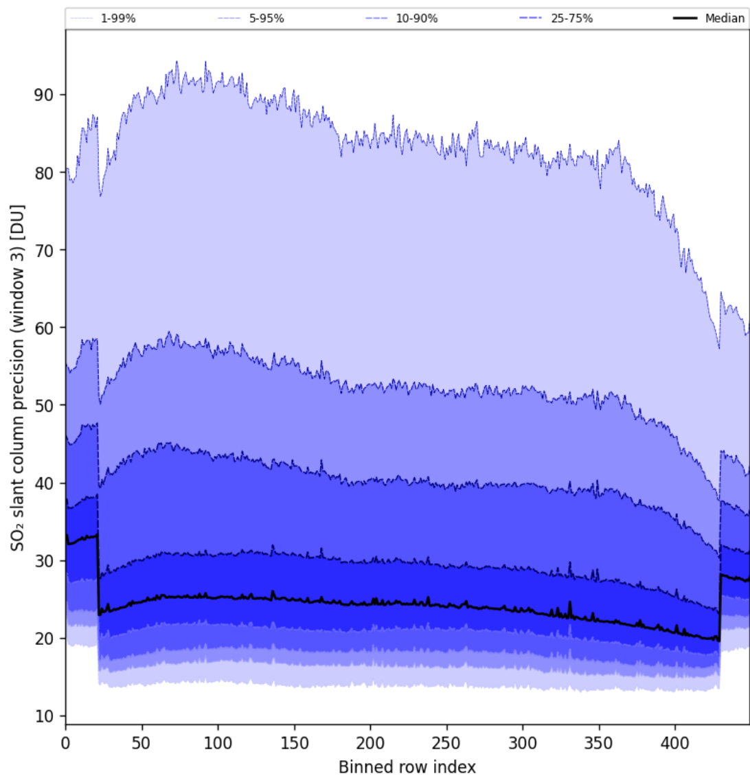
Figure 98: Along track statistics of “SO 2 slant column precision (window 3)” for 2025-02-25 to 2025-02-27
