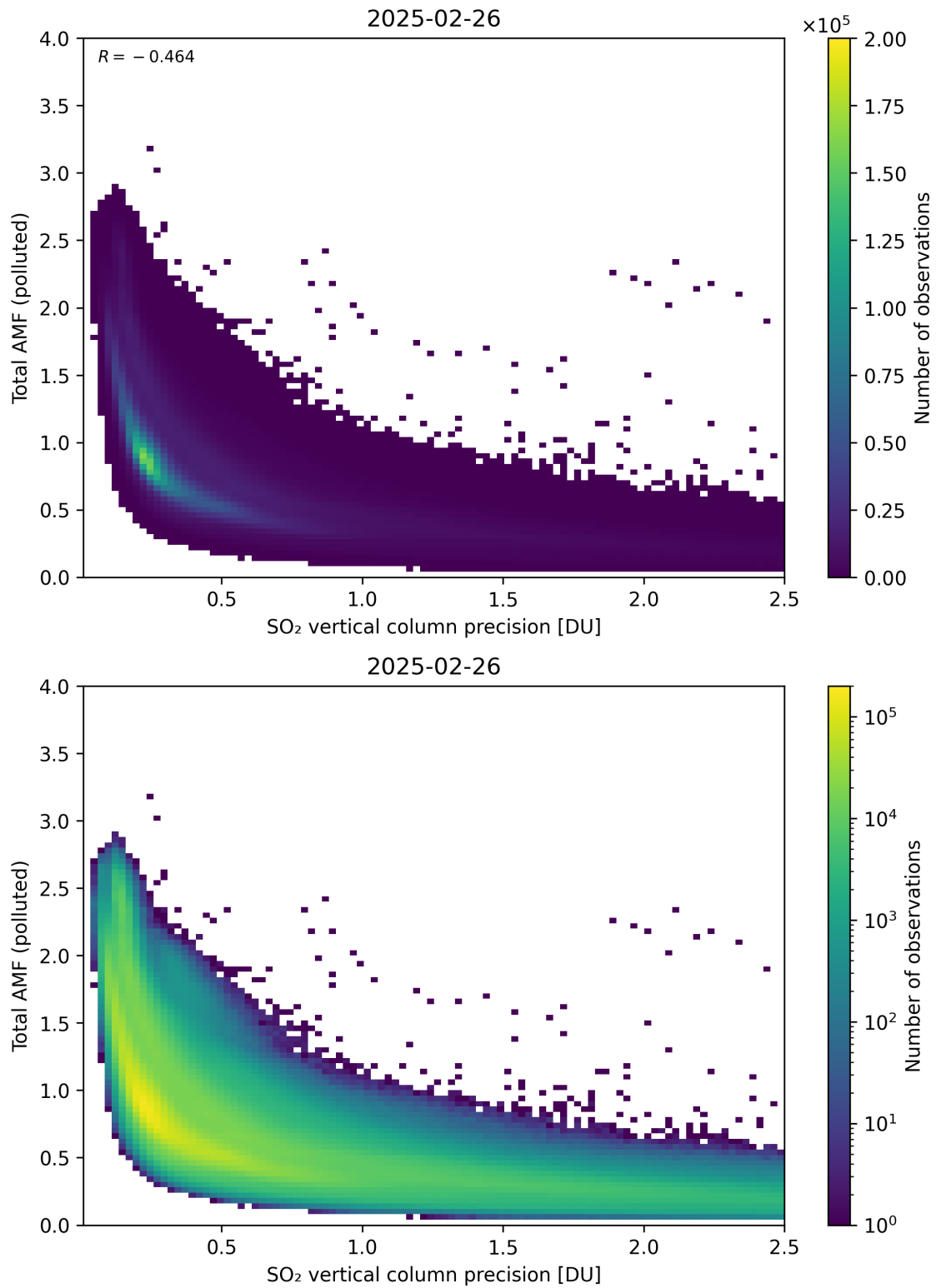
Figure 346: Scatter density plot of “SO 2 vertical column precision” against “Total AMF (polluted)” for 2025-02-25 to 2025-02-27.
