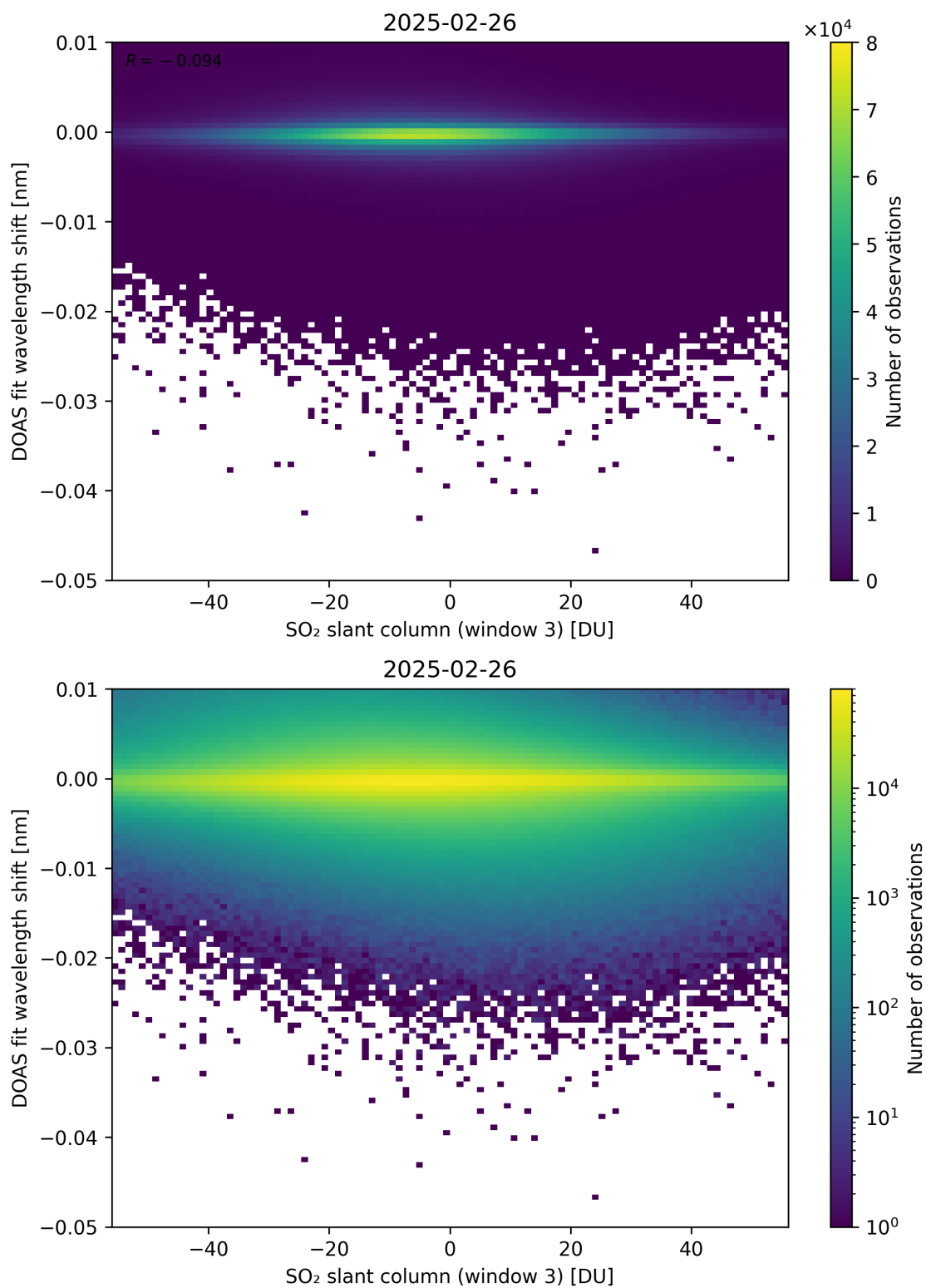
Figure 304: Scatter density plot of “SO 2 slant column (window 3)” against “DOAS fit wavelength shift” for 2025-02-25 to 2025-02-27.
