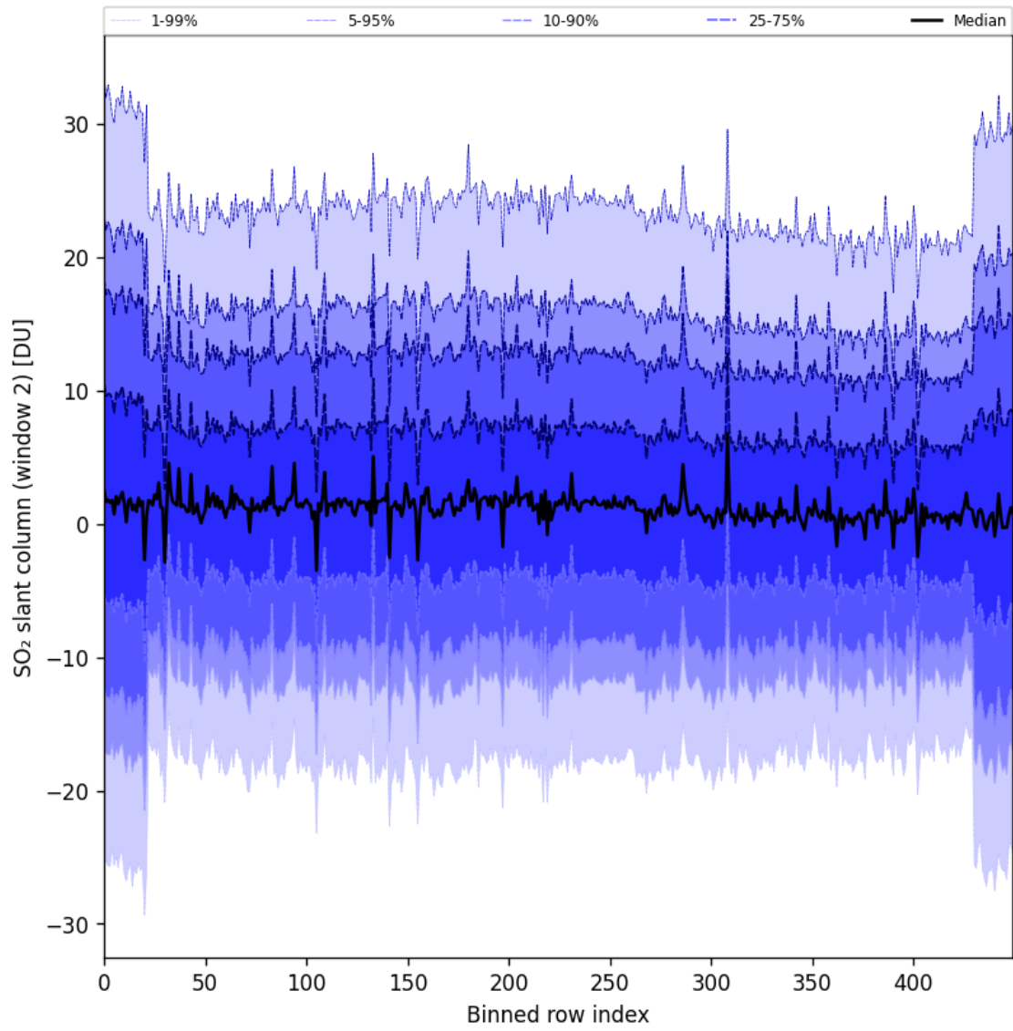
Figure 93: Along track statistics of “SO 2 slant column (window 2)” for 2025-02-25 to 2025-02-27
