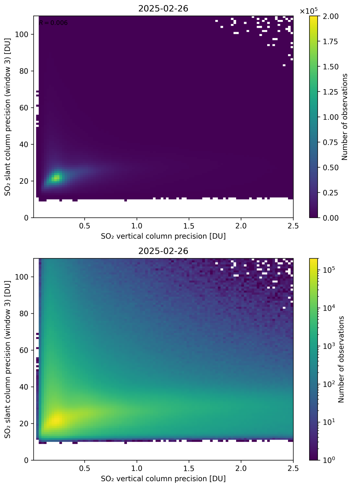
Figure 345: Scatter density plot of “SO 2 vertical column precision” against “SO 2 slant column precision (window 3)” for 2025-02-25 to 2025-02-27.
