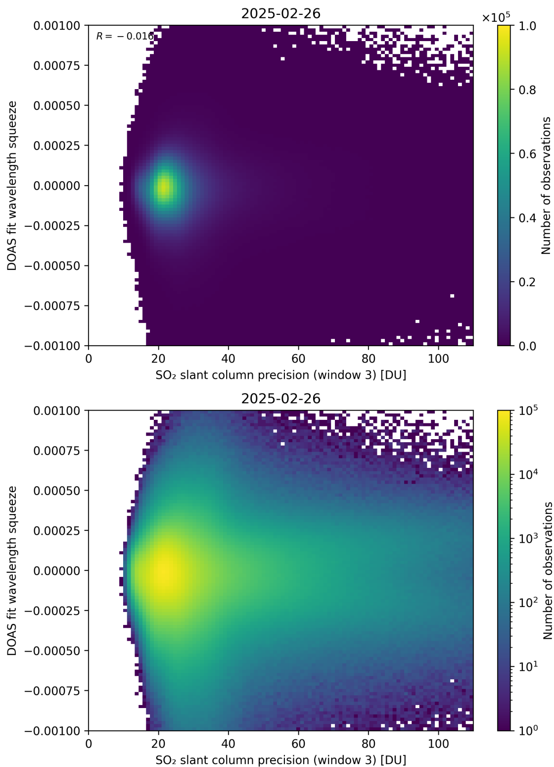
Figure 309: Scatter density plot of “SO 2 slant column precision (window 3)” against “DOAS fit wavelength squeeze” for 2025-02-25 to 2025-02-27.
