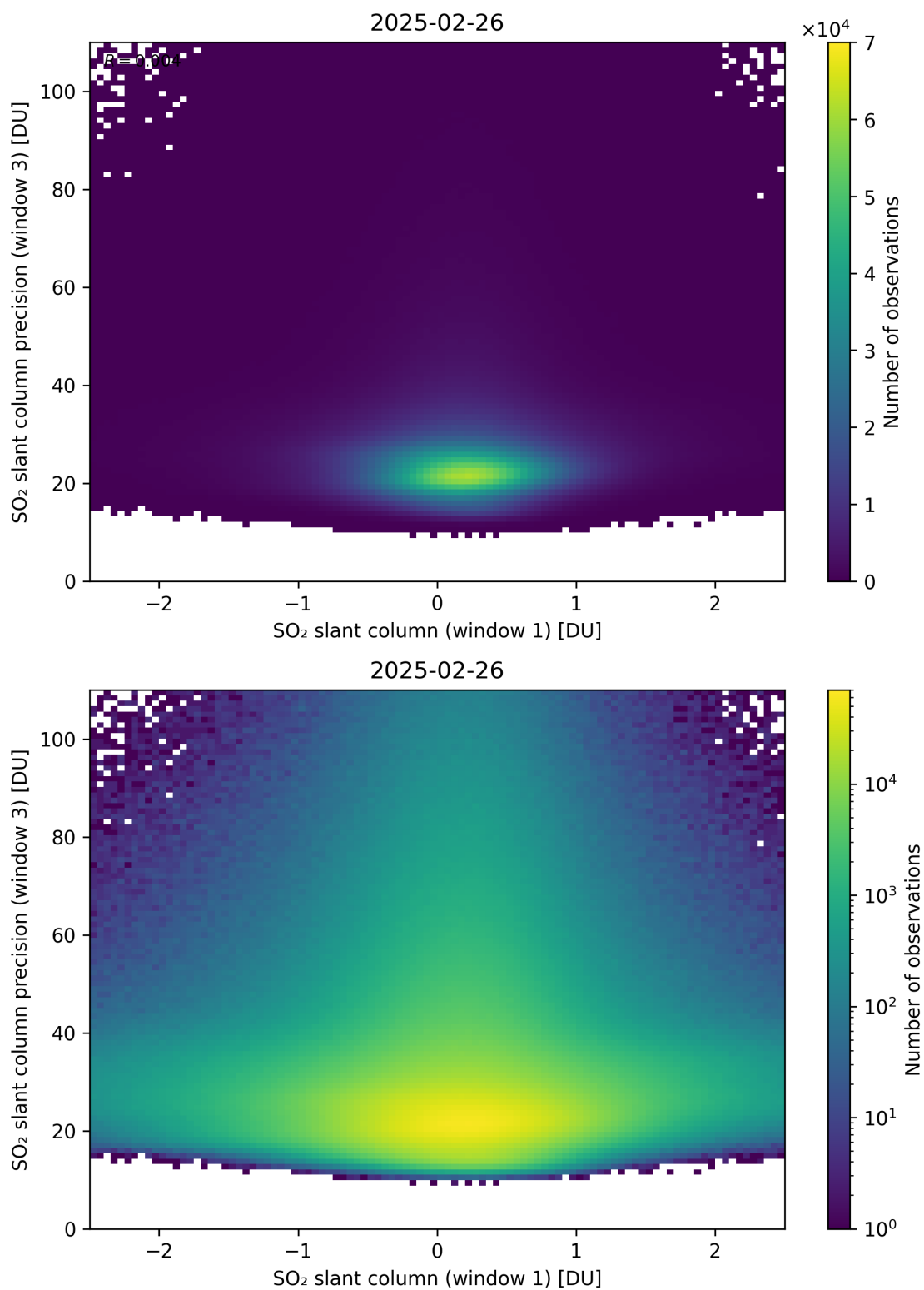
Figure 288: Scatter density plot of “SO 2 slant column (window 1)” against “SO 2 slant column precision (window 3)” for 2025-02-25 to 2025-02-27.
