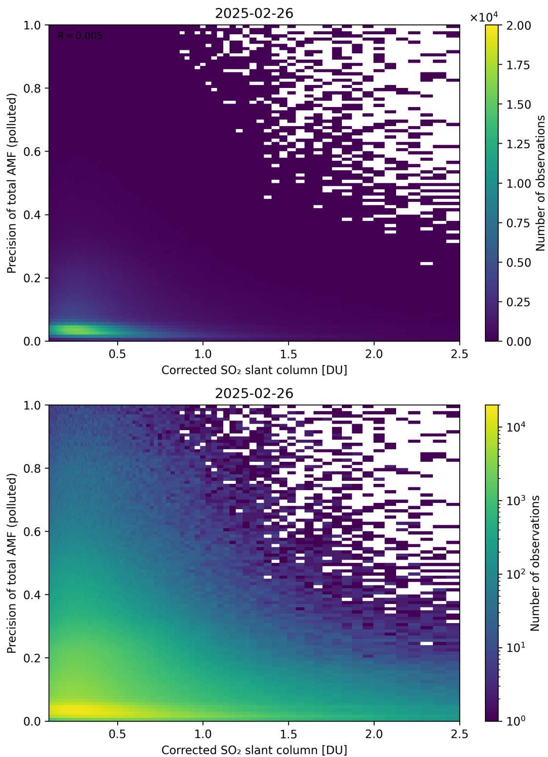
Figure 243: Scatter density plot of “Corrected SO 2 slant column” against “Precision of total AMF (polluted)” for 2025-02-25 to 2025-02-27.
