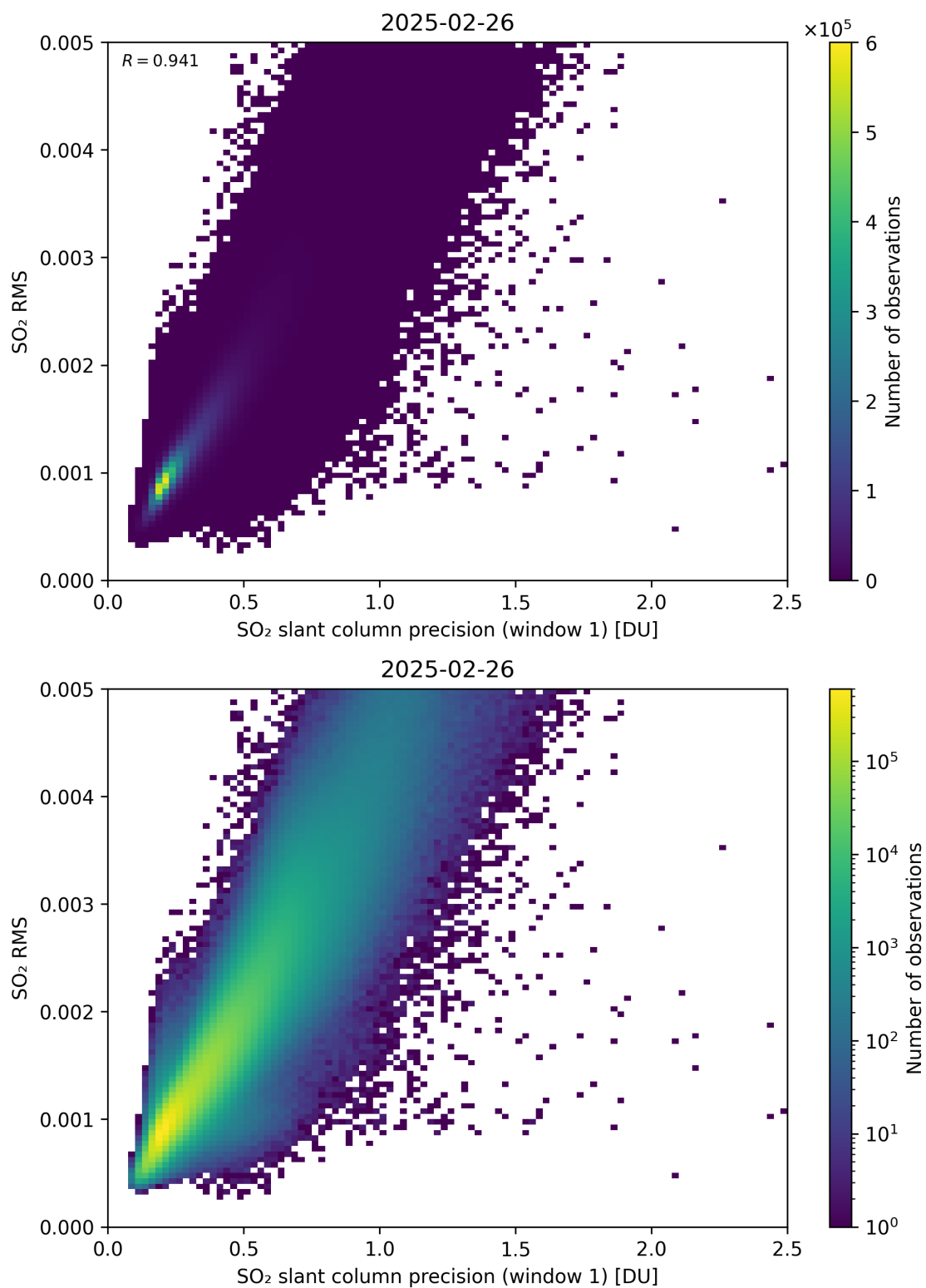
Figure 273: Scatter density plot of “SO 2 slant column precision (window 1)” against “SO 2 RMS” for 2025-02-25 to 2025-02-27.
