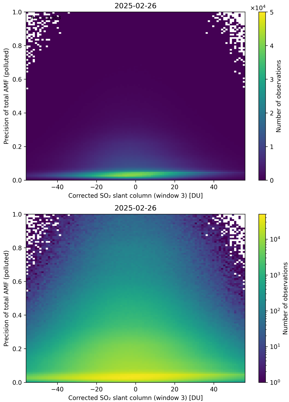
Figure 261: Scatter density plot of “Corrected SO 2 slant column (window 3)” against “Precision of total AMF (polluted)” for 2025-02-25 to 2025-02-27.
