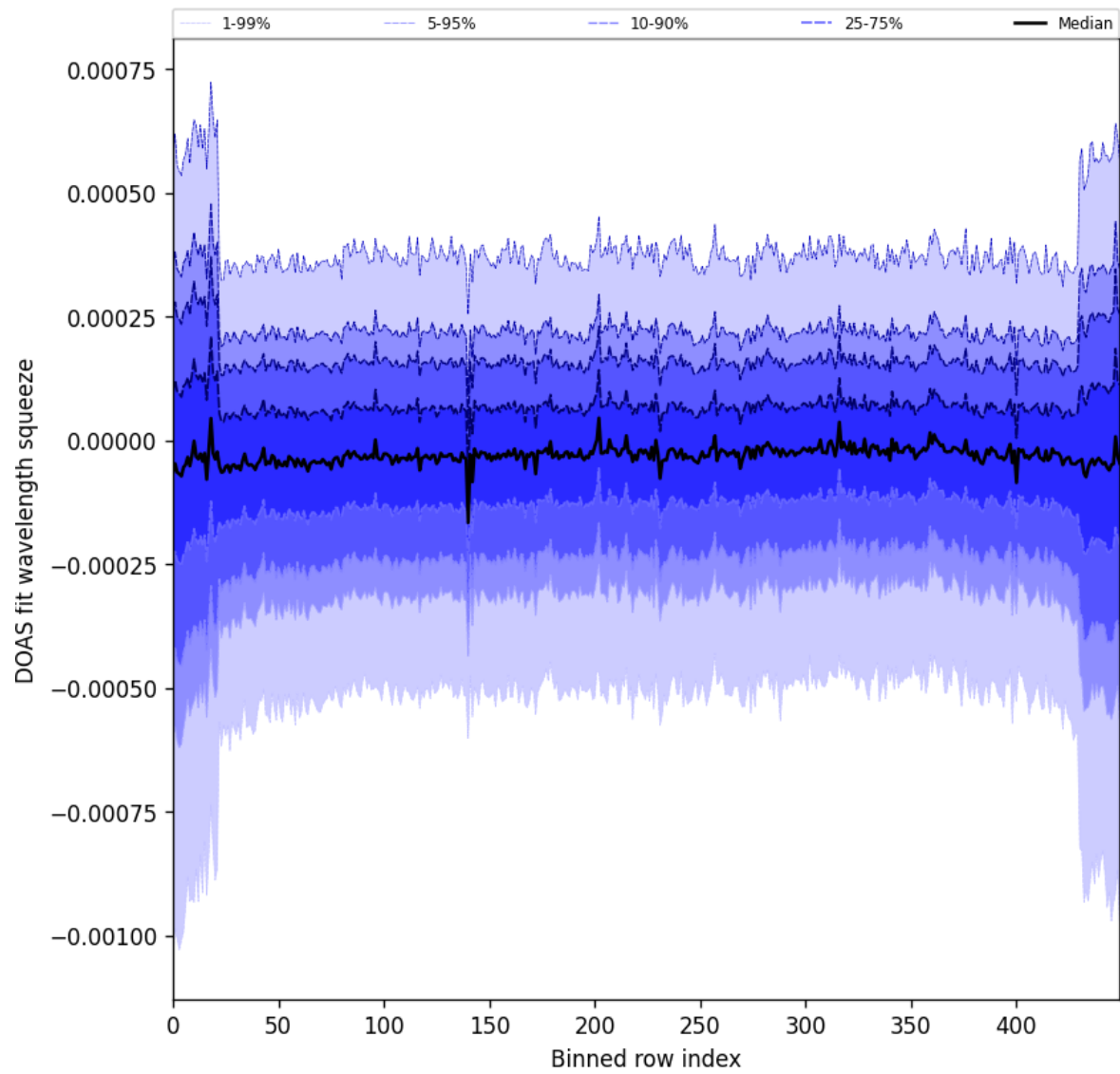
Figure 103: Along track statistics of “DOAS fit wavelength squeeze” for 2025-02-25 to 2025-02-27
