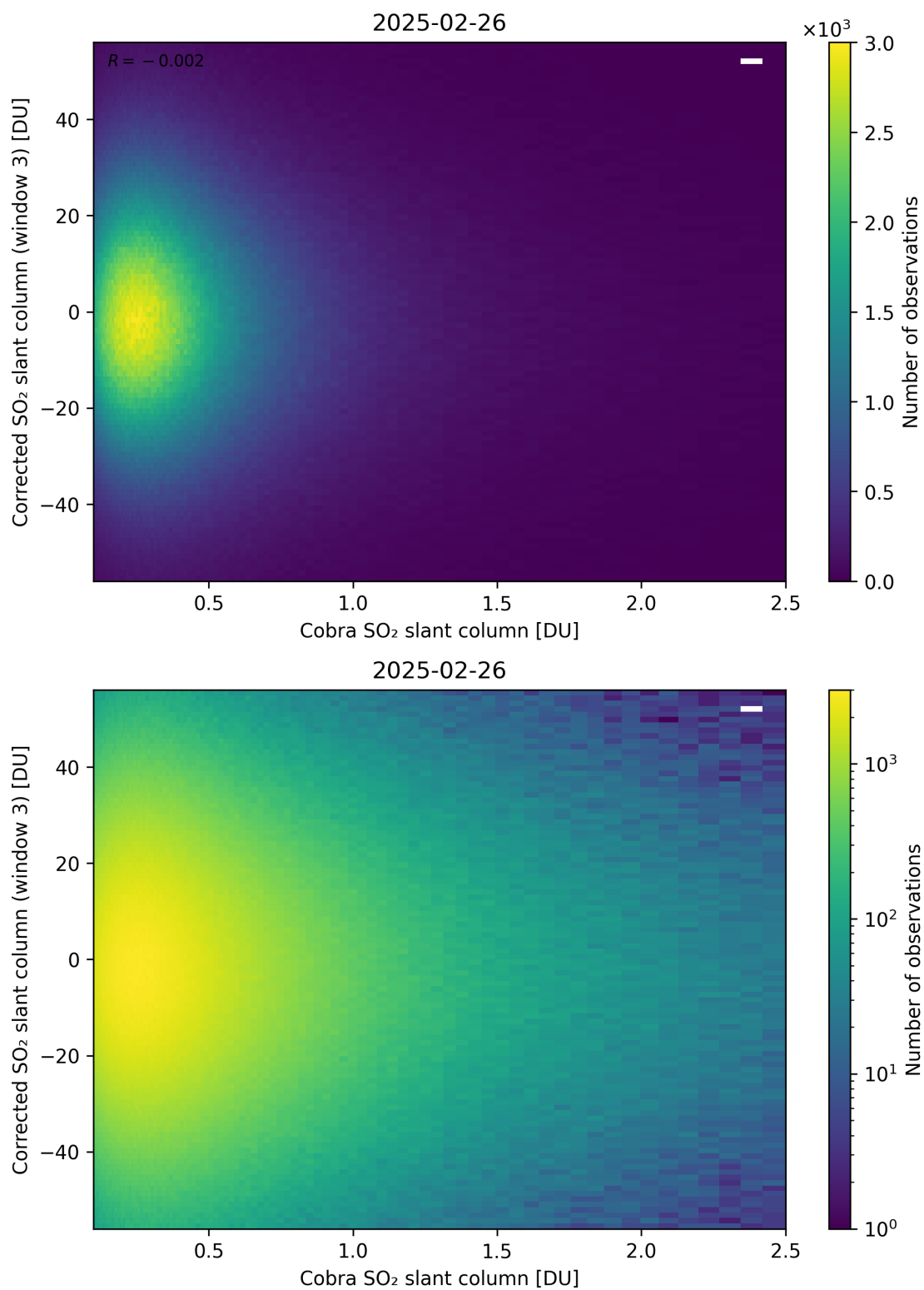
Figure 218: Scatter density plot of “Cobra SO 2 slant column” against “Corrected SO 2 slant column (window 3)” for 2025-02-25 to 2025-02-27.
