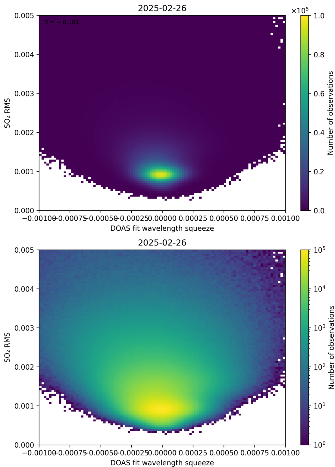
Figure 143: Scatter density plot of “DOAS fit wavelength squeeze” against “SO 2 RMS” for 2025-02-25 to 2025-02-27.
