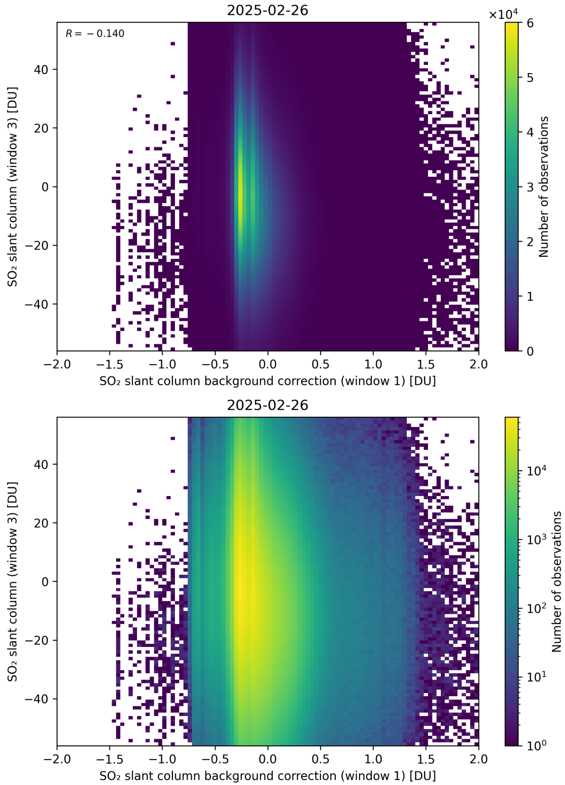
Figure 118: Scatter density plot of “SO 2 slant column background correction (window 1)” against “SO 2 slant column (window 3)” for 2025-02-25 to 2025-02-27.
