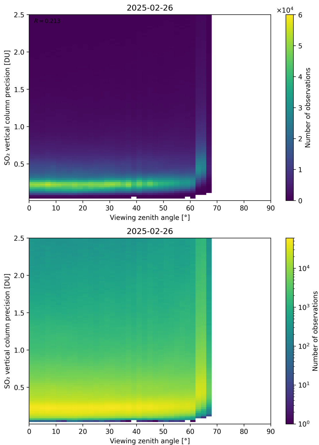
Figure 384: Scatter density plot of “Viewing zenith angle” against “SO 2 vertical column precision” for 2025-02-25 to 2025-02-27.
