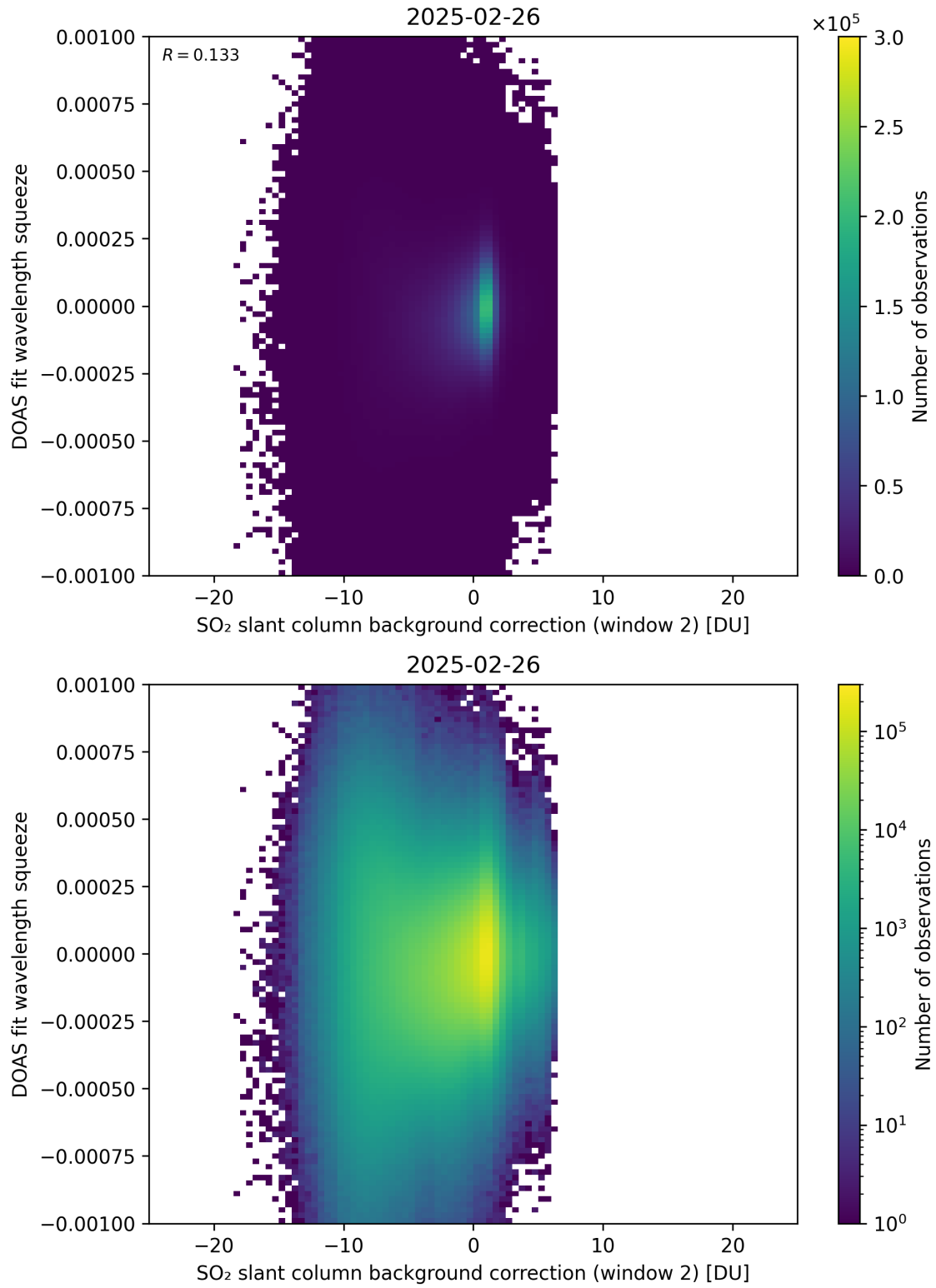
Figure 124: Scatter density plot of “SO 2 slant column background correction (window 2)” against “DOAS fit wavelength squeeze” for 2025-02-25 to 2025-02-27.
