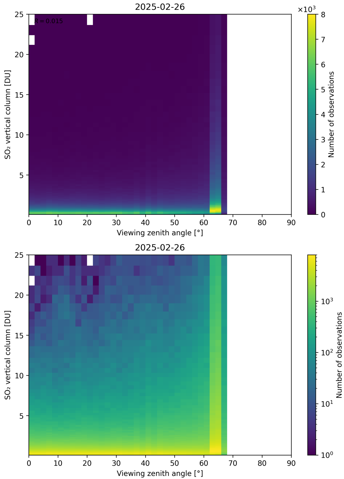
Figure 383: Scatter density plot of “Viewing zenith angle” against “SO 2 vertical column” for 2025-02-25 to 2025-02-27.
