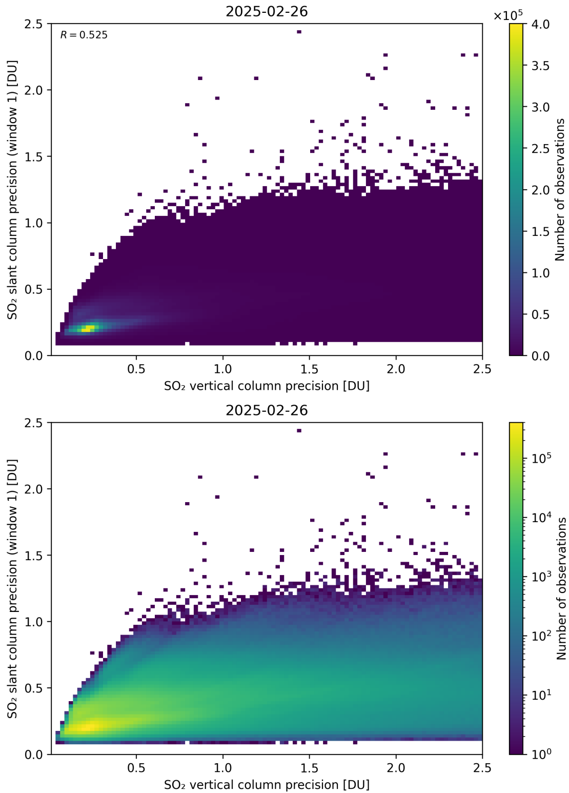
Figure 342: Scatter density plot of “SO 2 vertical column precision” against “SO 2 slant column precision (window 1)” for 2025-02-25 to 2025-02-27.
