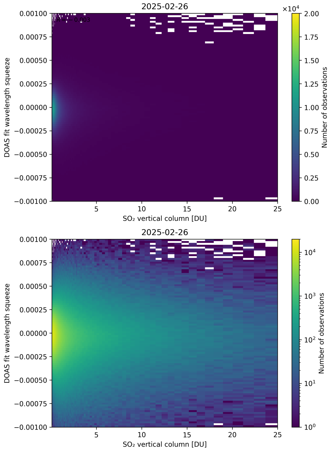
Figure 327: Scatter density plot of “SO 2 vertical column” against “DOAS fit wavelength squeeze” for 2025-02-25 to 2025-02-27.
