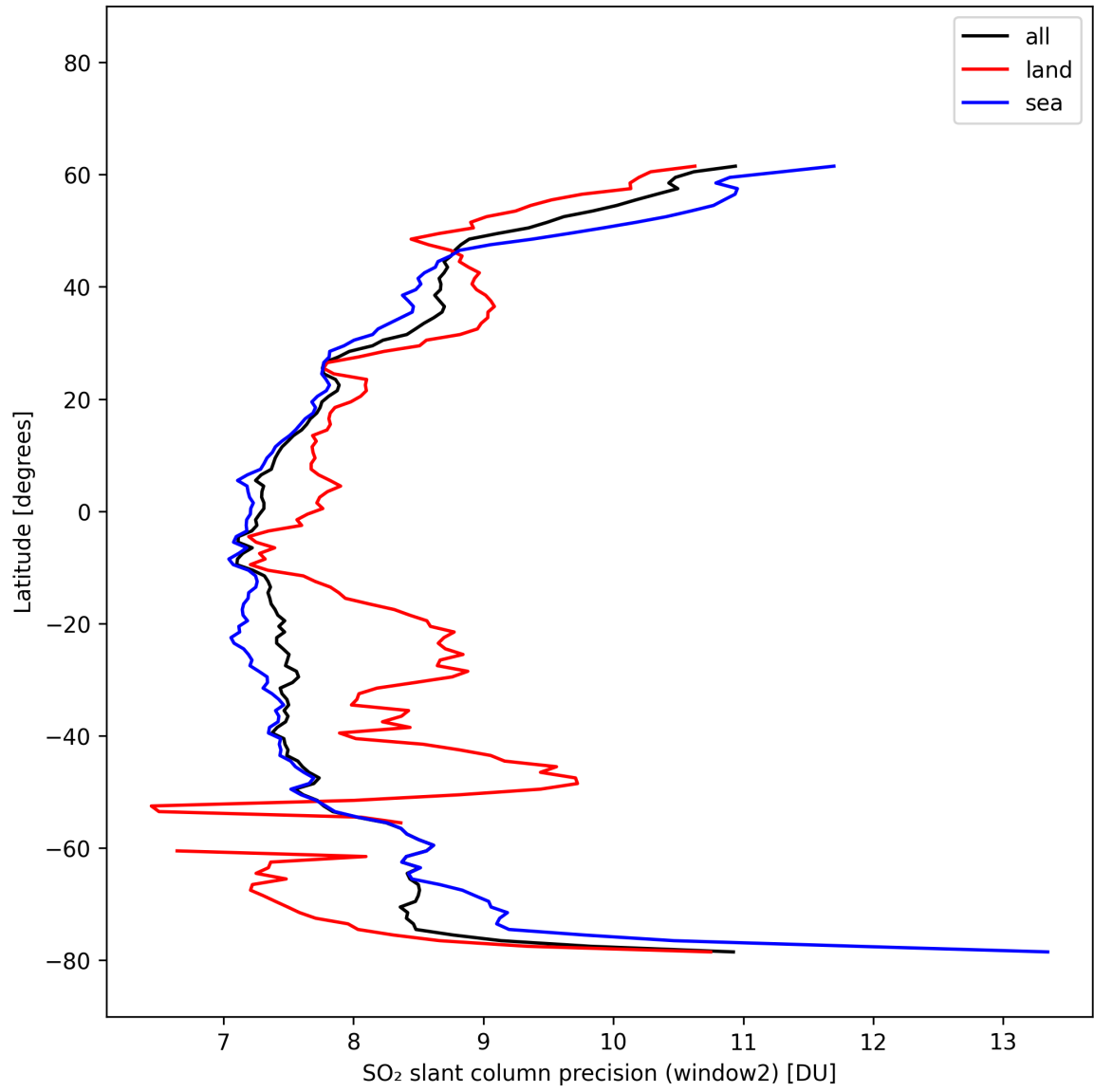
Figure 42: Zonal average of “SO 2 slant column precision (window2)” for 2025-02-25 to 2025-02-27.
