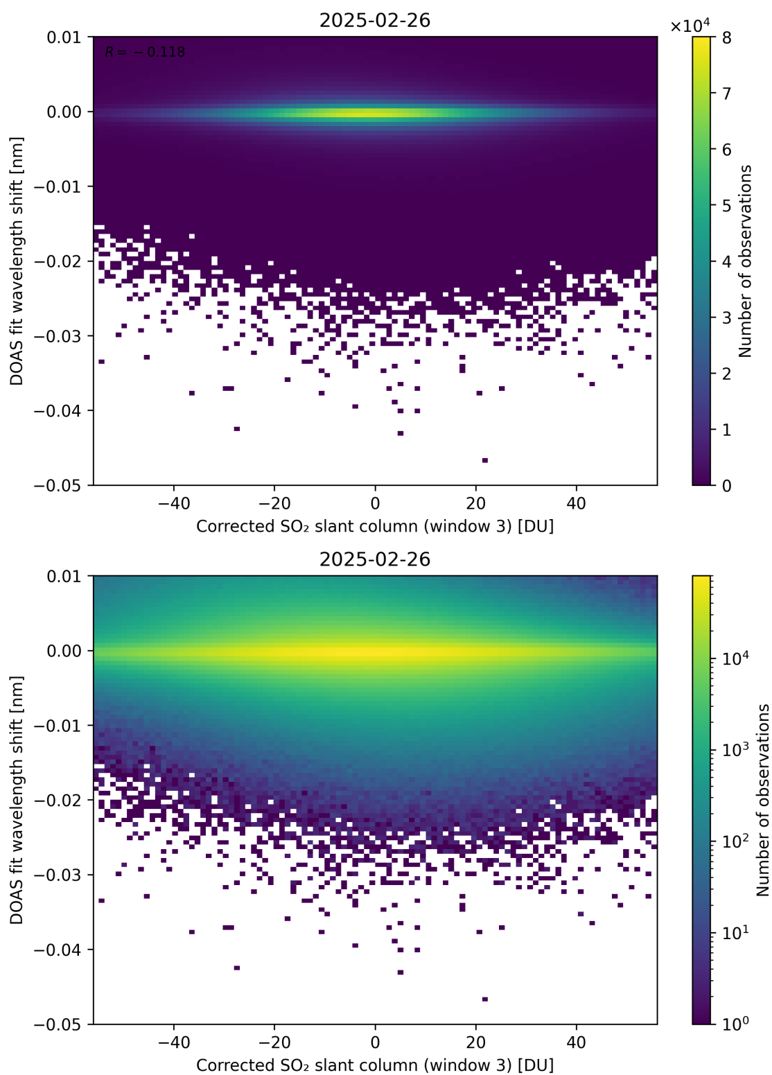
Figure 256: Scatter density plot of “Corrected SO 2 slant column (window 3)” against “DOAS fit wavelength shift” for 2025-02-25 to 2025-02-27.
