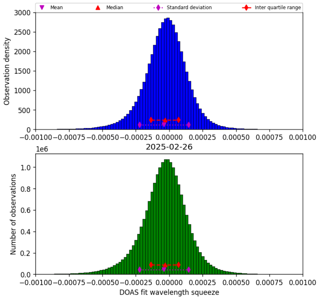
Figure 77: Histogram of “DOAS fit wavelength squeeze” for 2025-02-25 to 2025-02-27
