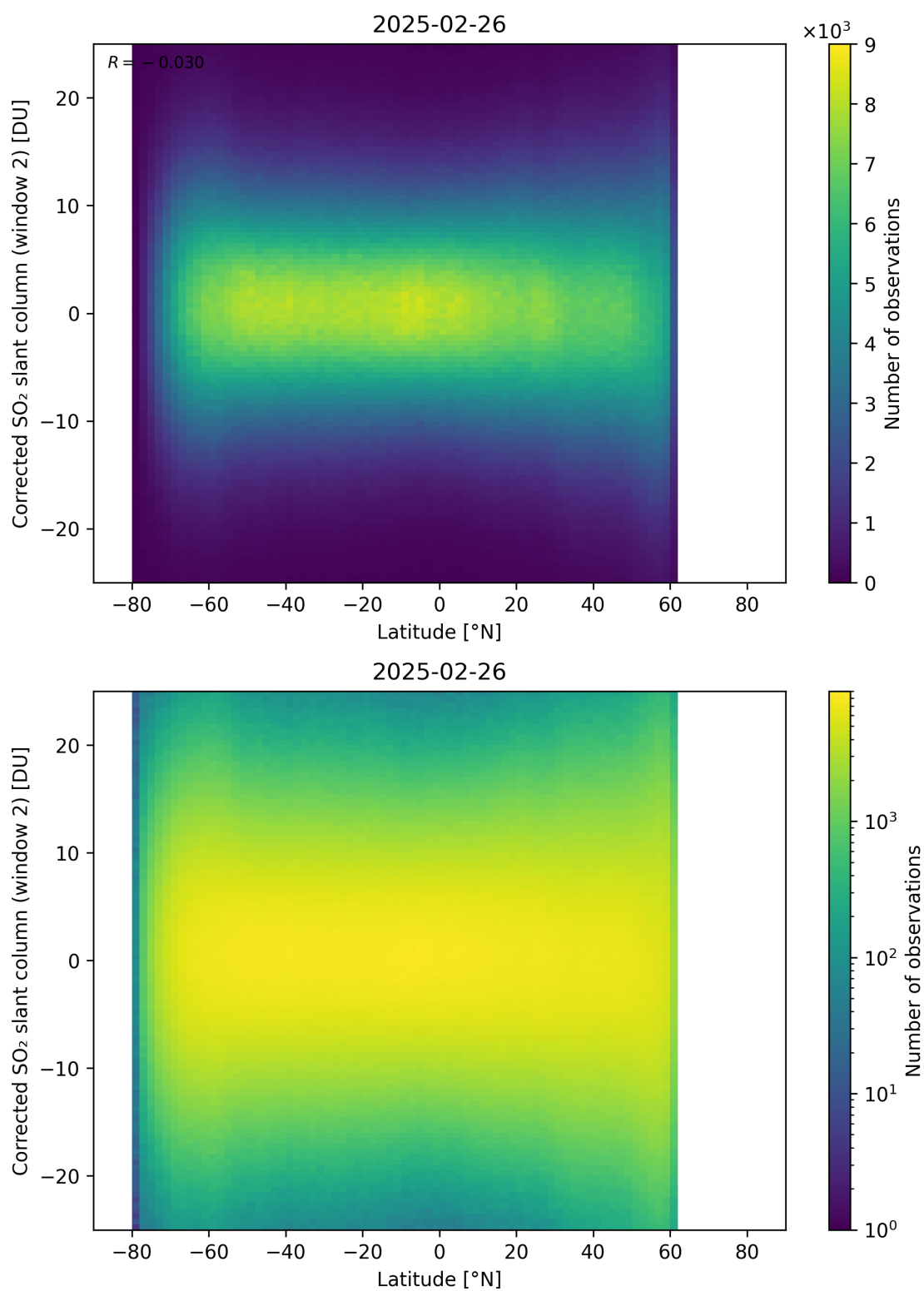
Figure 160: Scatter density plot of “Latitude” against “Corrected SO 2 slant column (window 2)” for 2025-02-25 to 2025-02-27.
