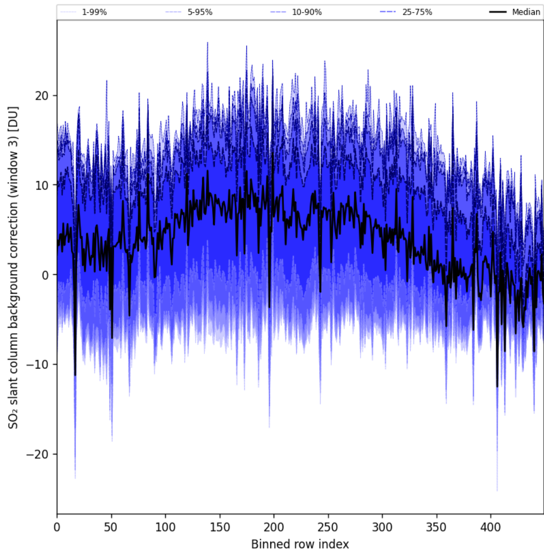
Figure 100: Along track statistics of “SO 2 slant column background correction (window 3)” for 2025-02-25 to 2025-02-27
