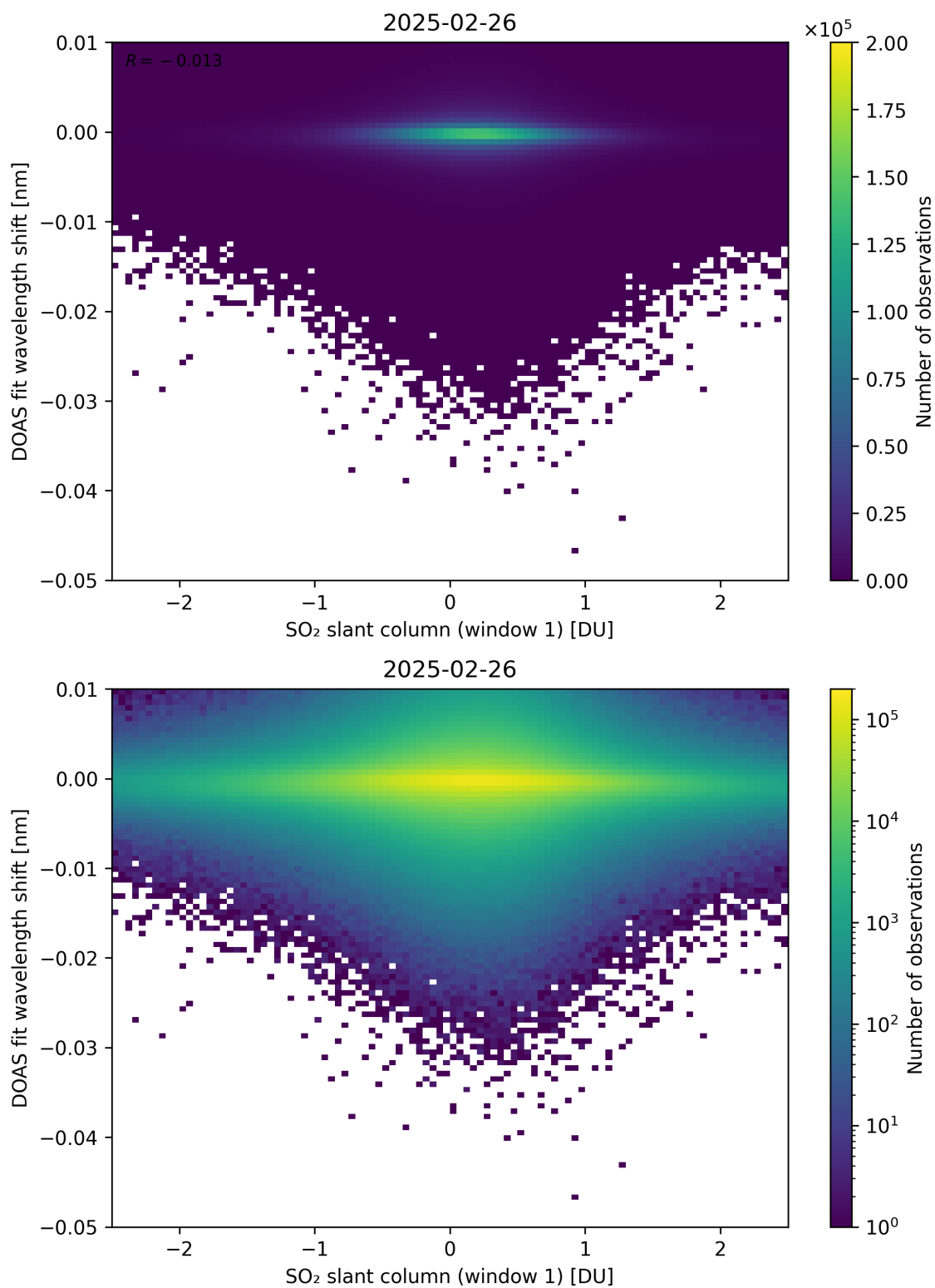
Figure 265: Scatter density plot of “SO 2 slant column (window 1)” against “DOAS fit wavelength shift” for 2025-02-25 to 2025-02-27.
