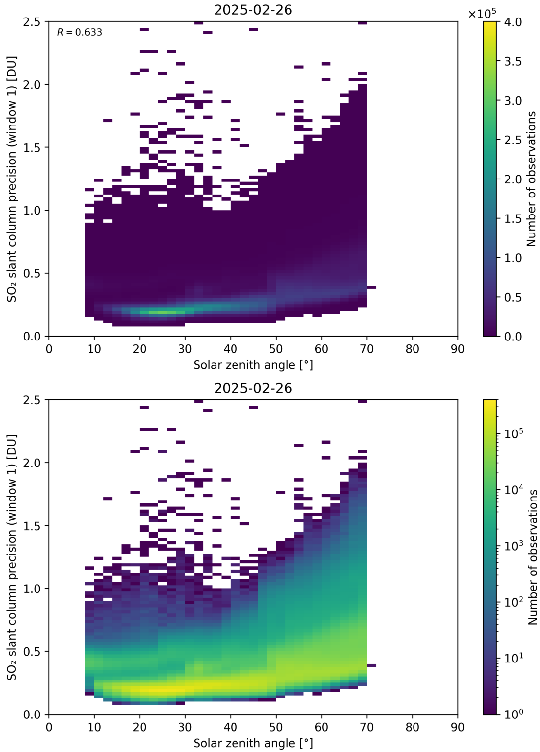
Figure 185: Scatter density plot of “Solar zenith angle” against “SO 2 slant column precision (window 1)” for 2025-02-25 to 2025-02-27.
