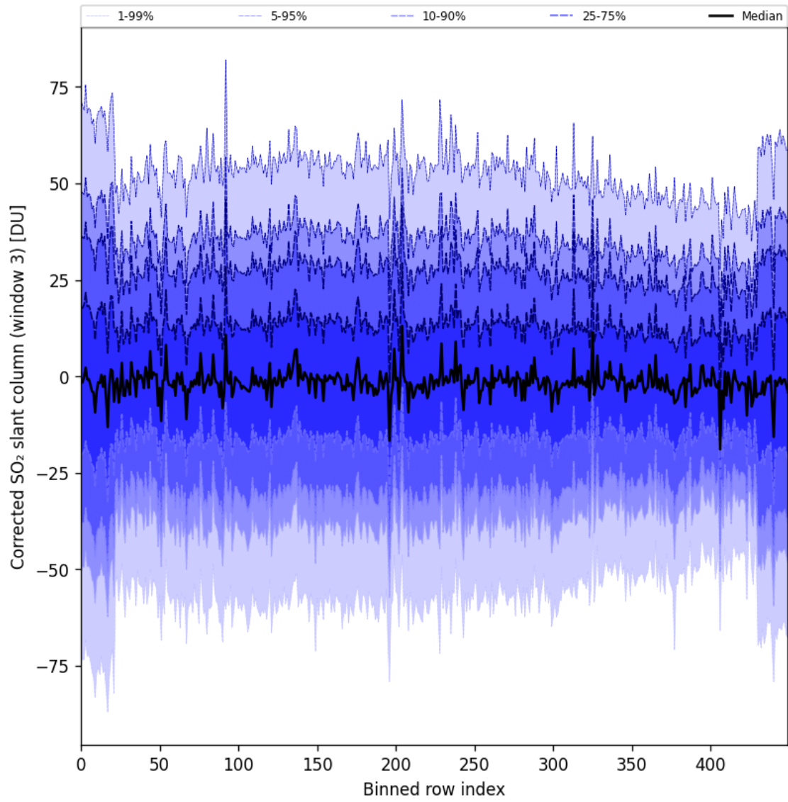
Figure 99: Along track statistics of “Corrected SO 2 slant column (window 3)” for 2025-02-25 to 2025-02-27
