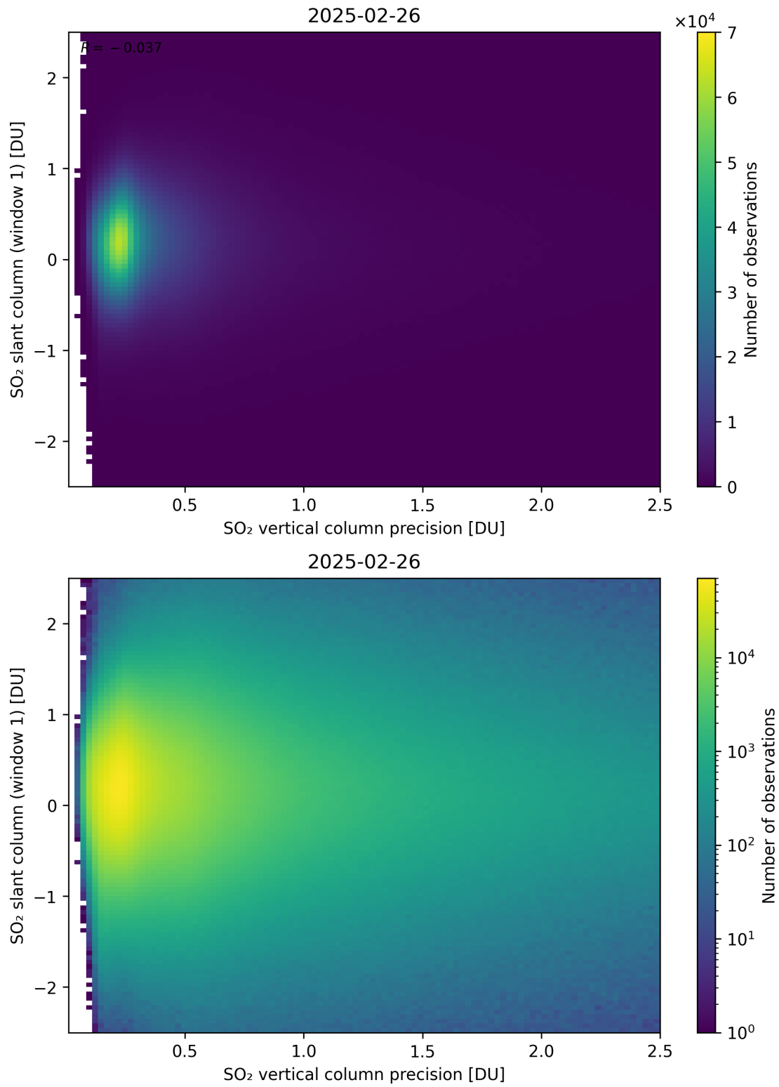
Figure 341: Scatter density plot of “SO 2 vertical column precision” against “SO 2 slant column (window 1)” for 2025-02-25 to 2025-02-27.
