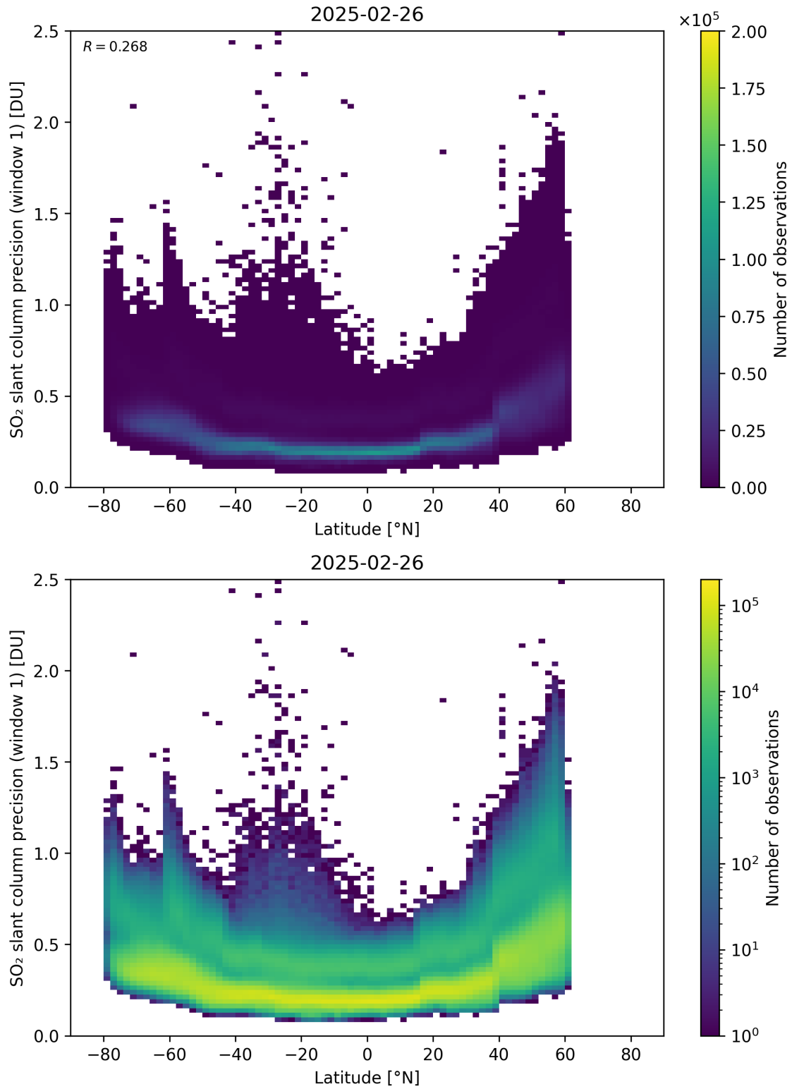
Figure 163: Scatter density plot of “Latitude” against “SO 2 slant column precision (window 1)” for 2025-02-25 to 2025-02-27.
