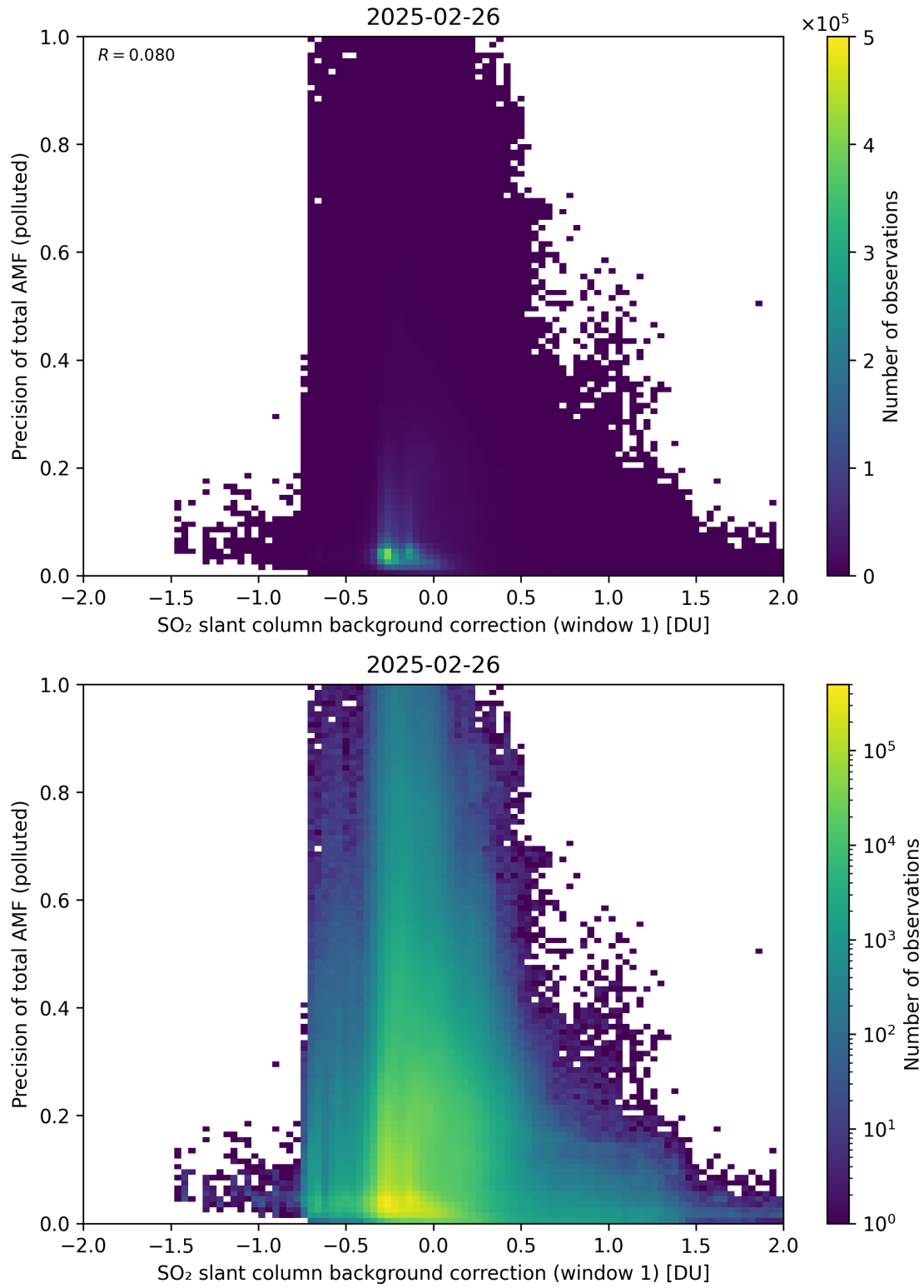
Figure 121: Scatter density plot of “SO 2 slant column background correction (window 1)” against “Precision of total AMF (polluted)” for 2025-02-25 to 2025-02-27.
