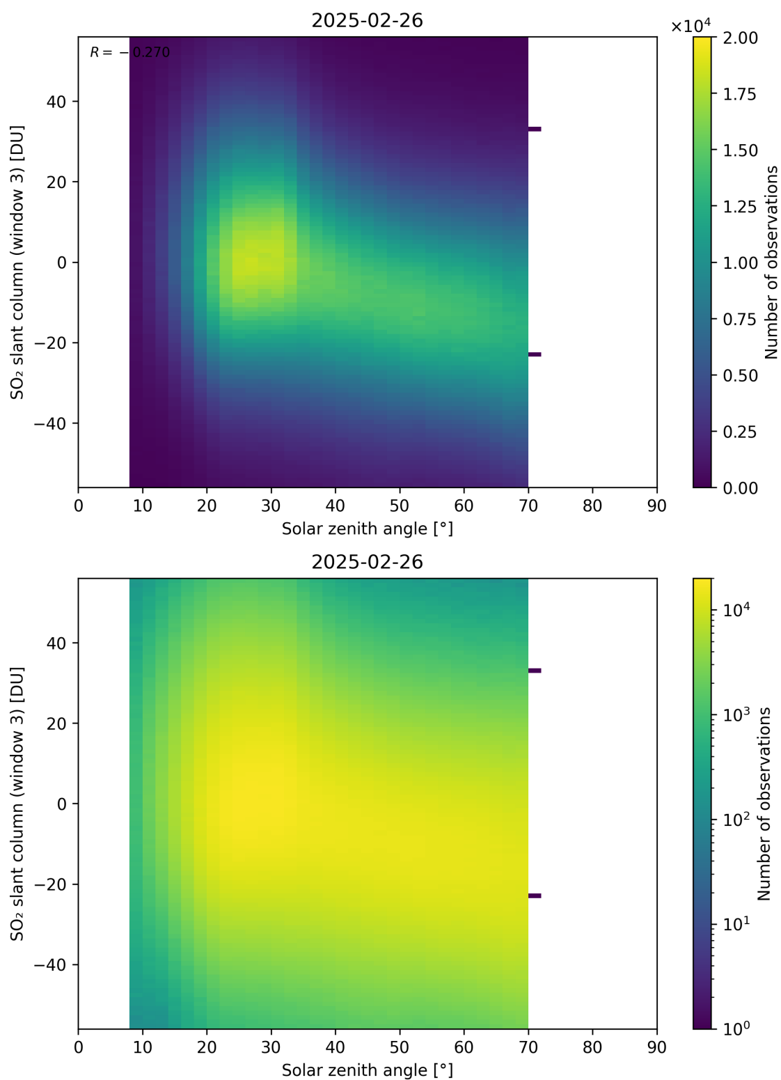
Figure 187: Scatter density plot of “Solar zenith angle” against “SO 2 slant column (window 3)” for 2025-02-25 to 2025-02-27.
