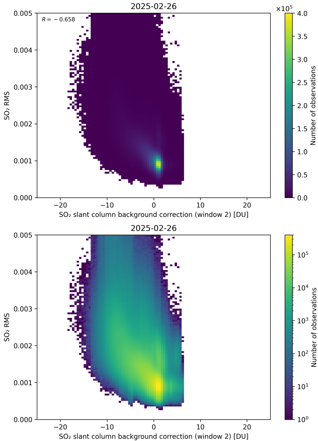
Figure 125: Scatter density plot of “SO 2 slant column background correction (window 2)” against “SO 2 RMS” for 2025-02-25 to 2025-02-27.
