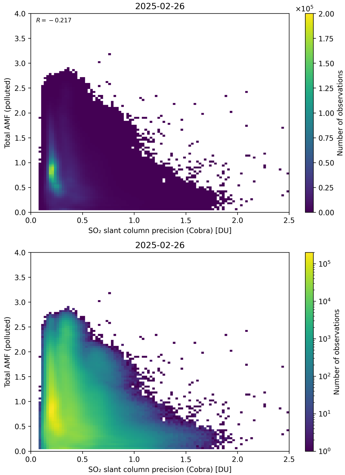
Figure 213: Scatter density plot of “SO 2 slant column precision (Cobra)” against “Total AMF (polluted)” for 2025-02-25 to 2025-02-27.
