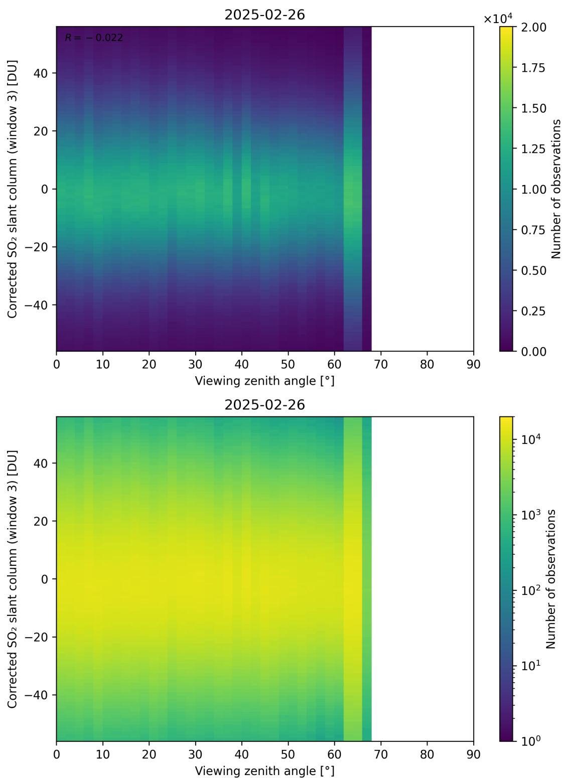
Figure 375: Scatter density plot of “Viewing zenith angle” against “Corrected SO 2 slant column (window 3)” for 2025-02-25 to 2025-02-27.
