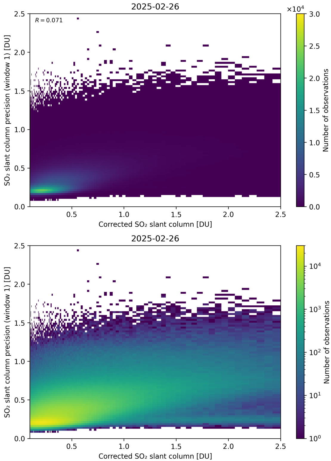
Figure 238: Scatter density plot of “Corrected SO 2 slant column” against “SO 2 slant column precision (window 1)” for 2025-02-25 to 2025-02-27.
