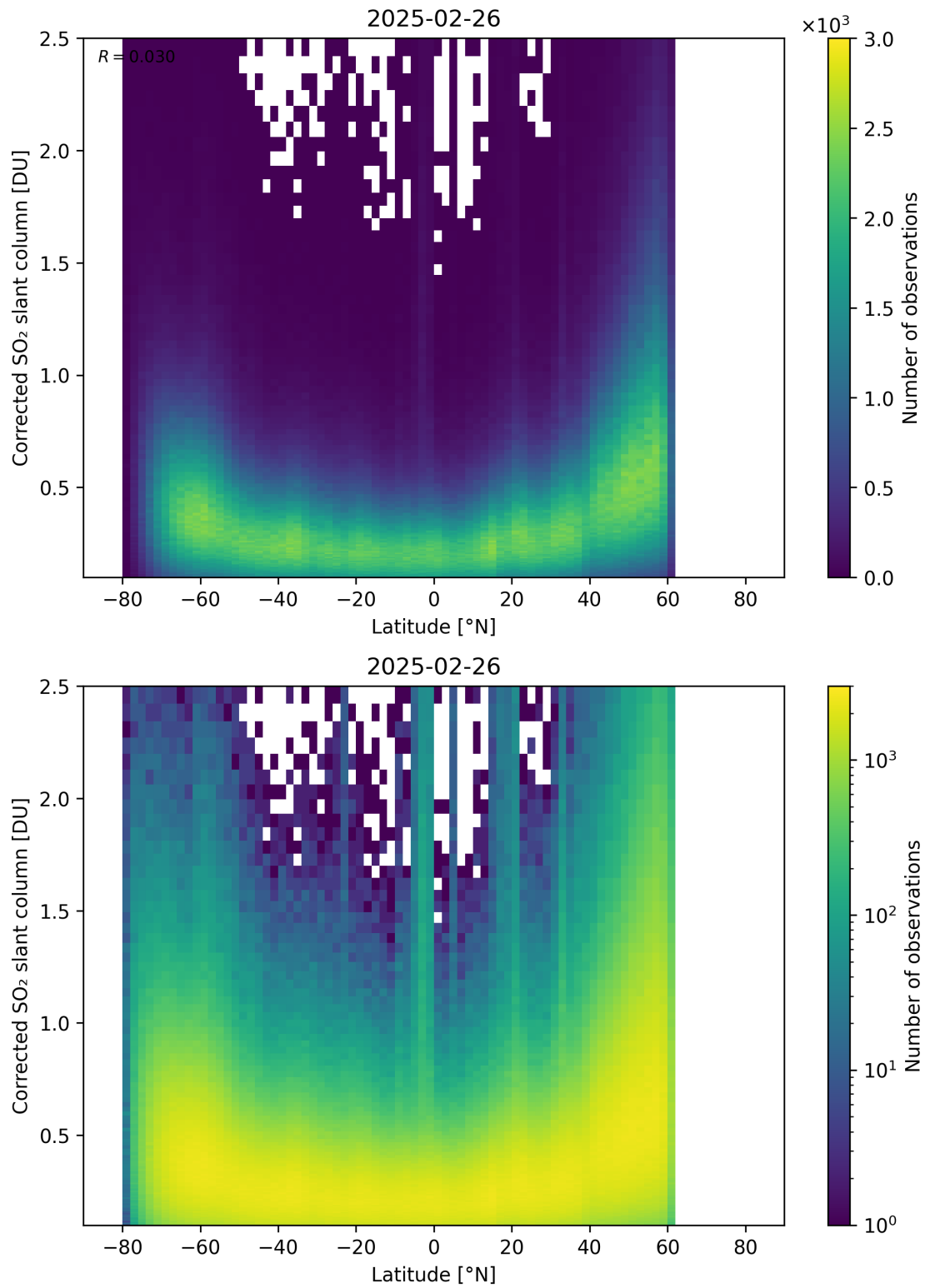
Figure 159: Scatter density plot of “Latitude” against “Corrected SO 2 slant column” for 2025-02-25 to 2025-02-27.
