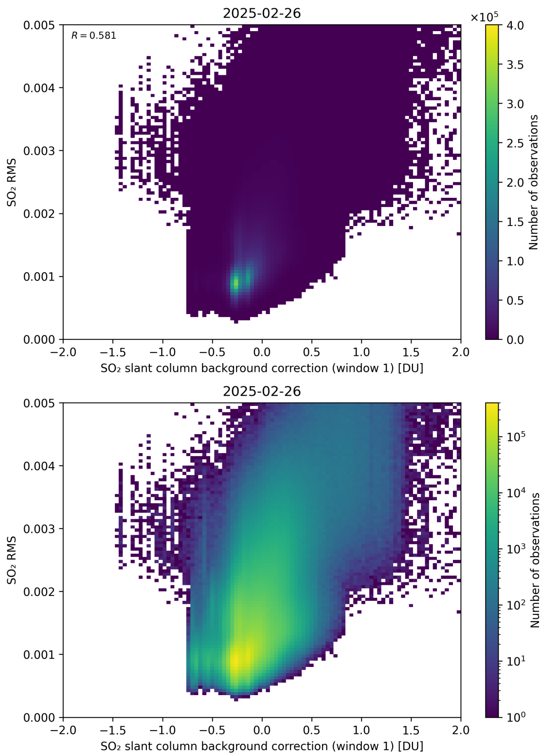
Figure 113: Scatter density plot of “SO 2 slant column background correction (window 1)” against “SO 2 RMS” for 2025-02-25 to 2025-02-27.
