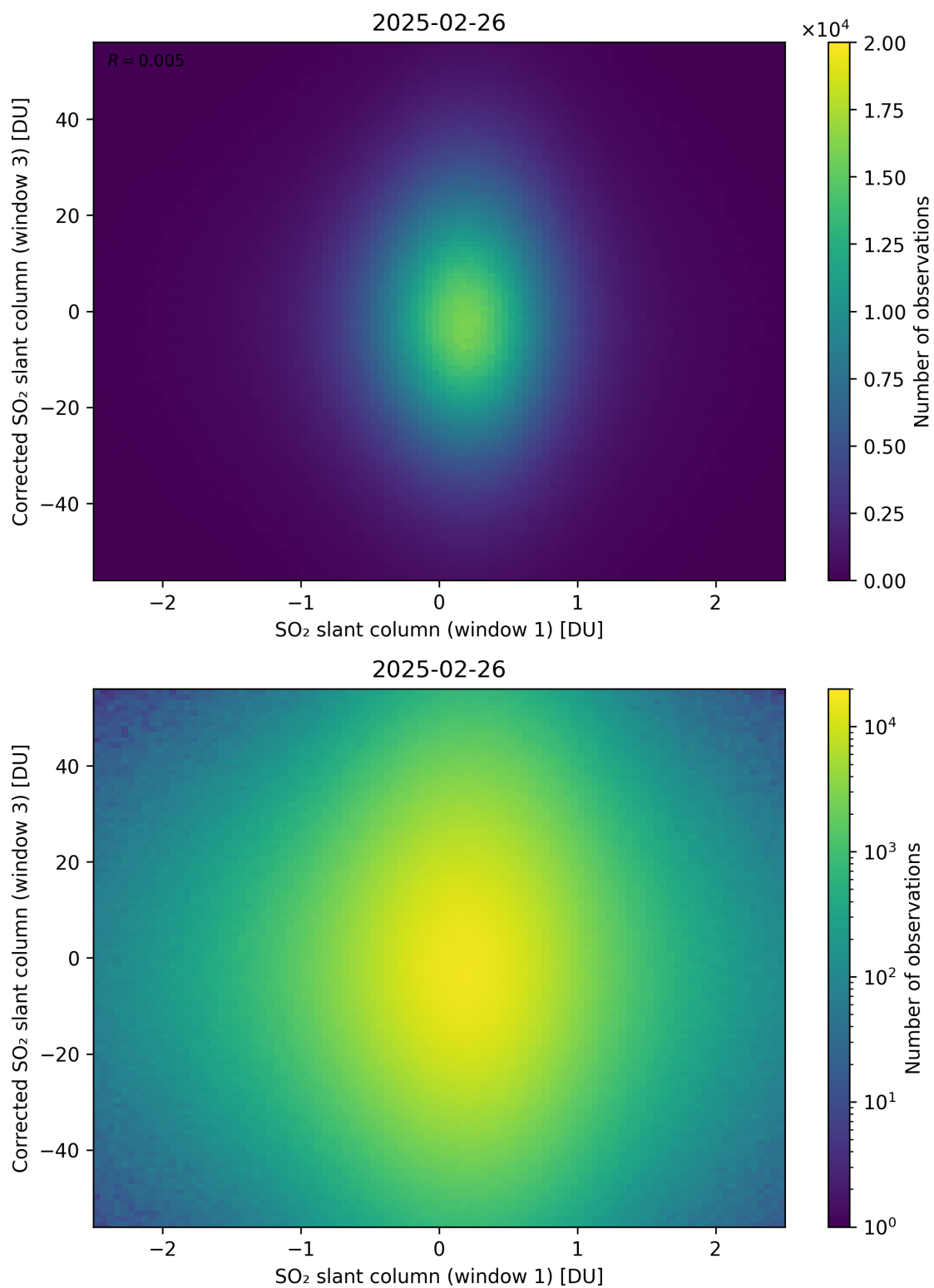
Figure 284: Scatter density plot of “SO 2 slant column (window 1)” against “Corrected SO 2 slant column (window 3)” for 2025-02-25 to 2025-02-27.
