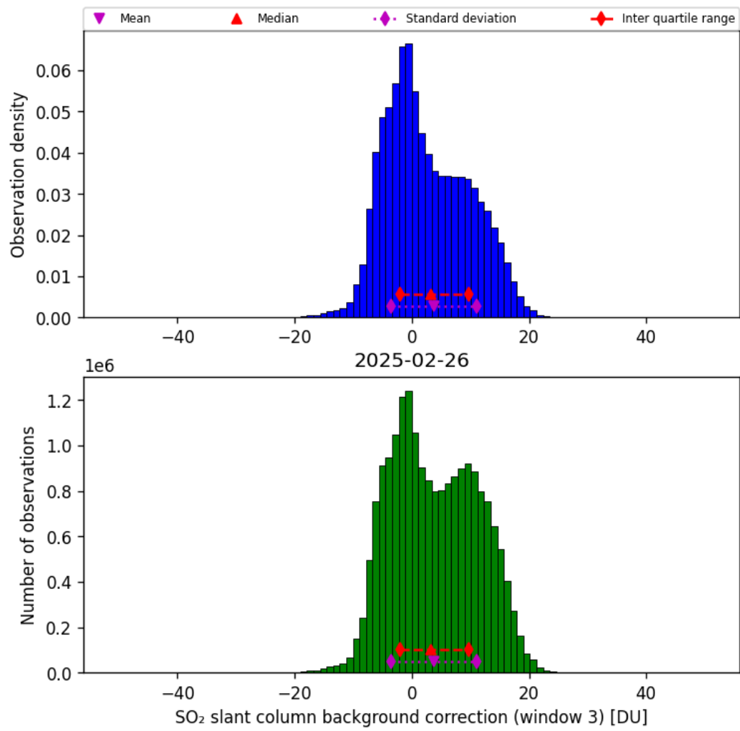
Figure 74: Histogram of “SO 2 slant column background correction (window 3)” for 2025-02-25 to 2025-02-27
