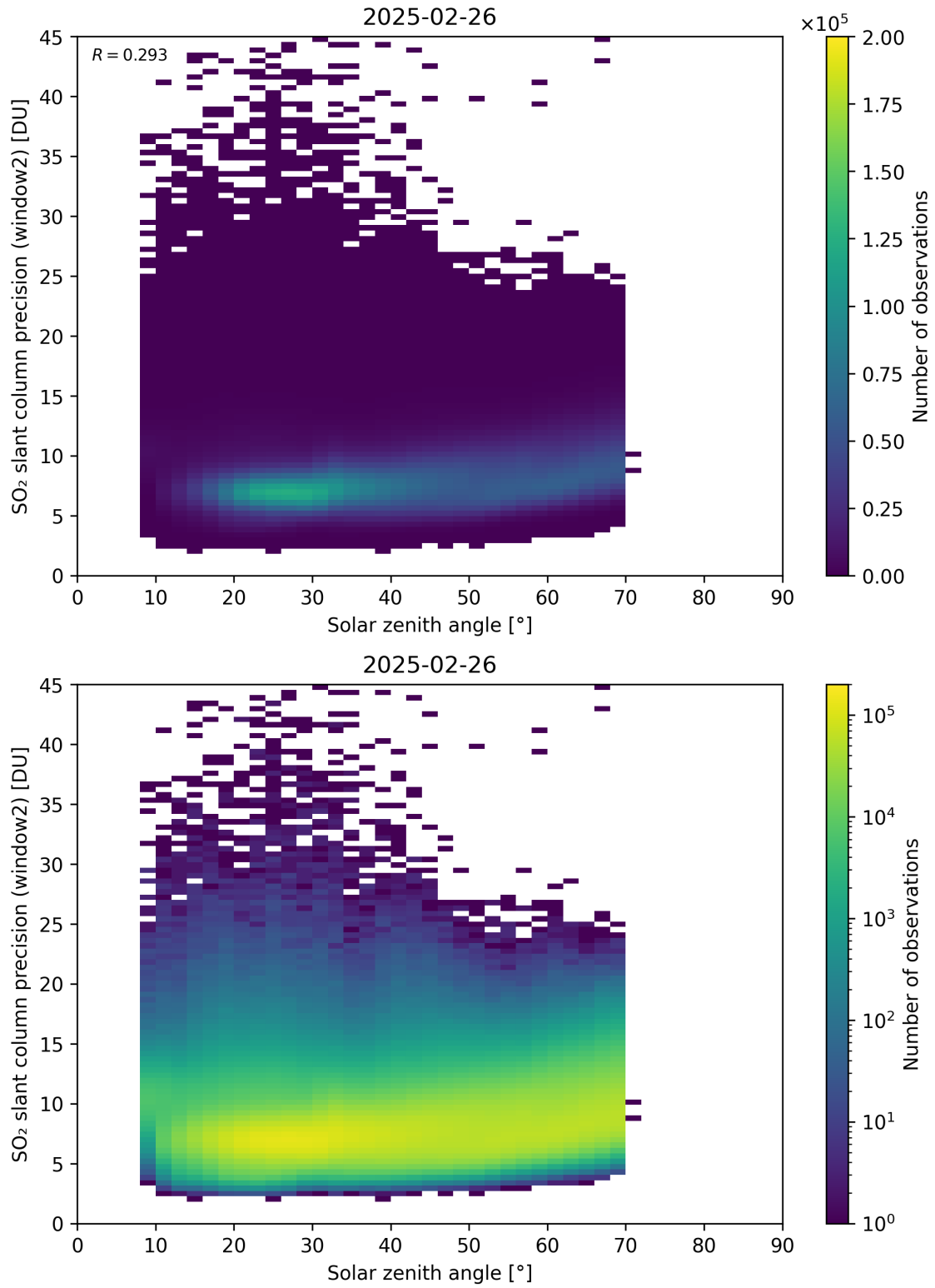
Figure 186: Scatter density plot of “Solar zenith angle” against “SO 2 slant column precision (window2)” for 2025-02-25 to 2025-02-27.
