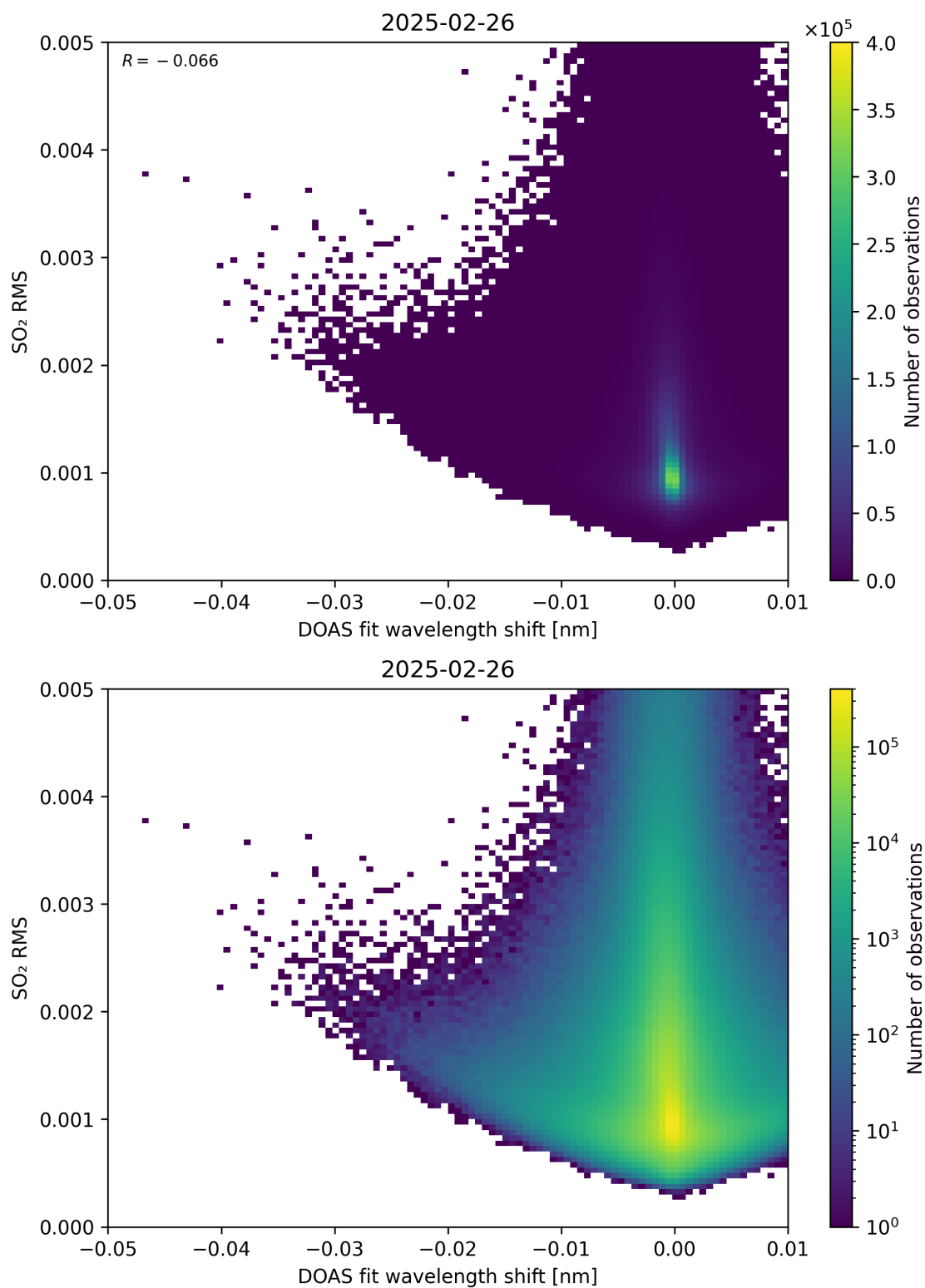
Figure 139: Scatter density plot of “DOAS fit wavelength shift” against “SO 2 RMS” for 2025-02-25 to 2025-02-27.
