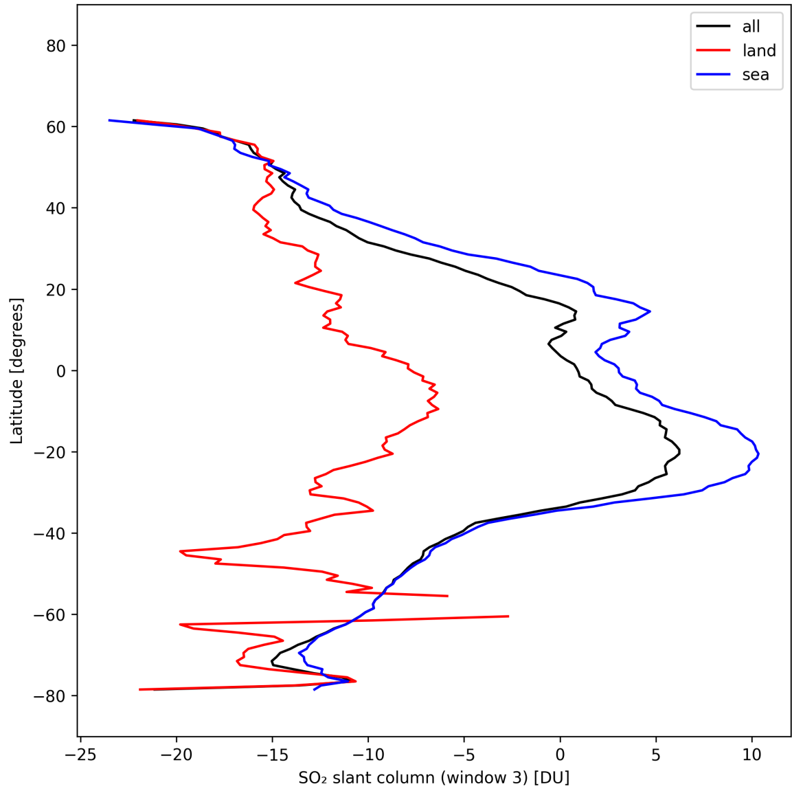
Figure 45: Zonal average of “SO 2 slant column (window 3)” for 2025-02-25 to 2025-02-27.
