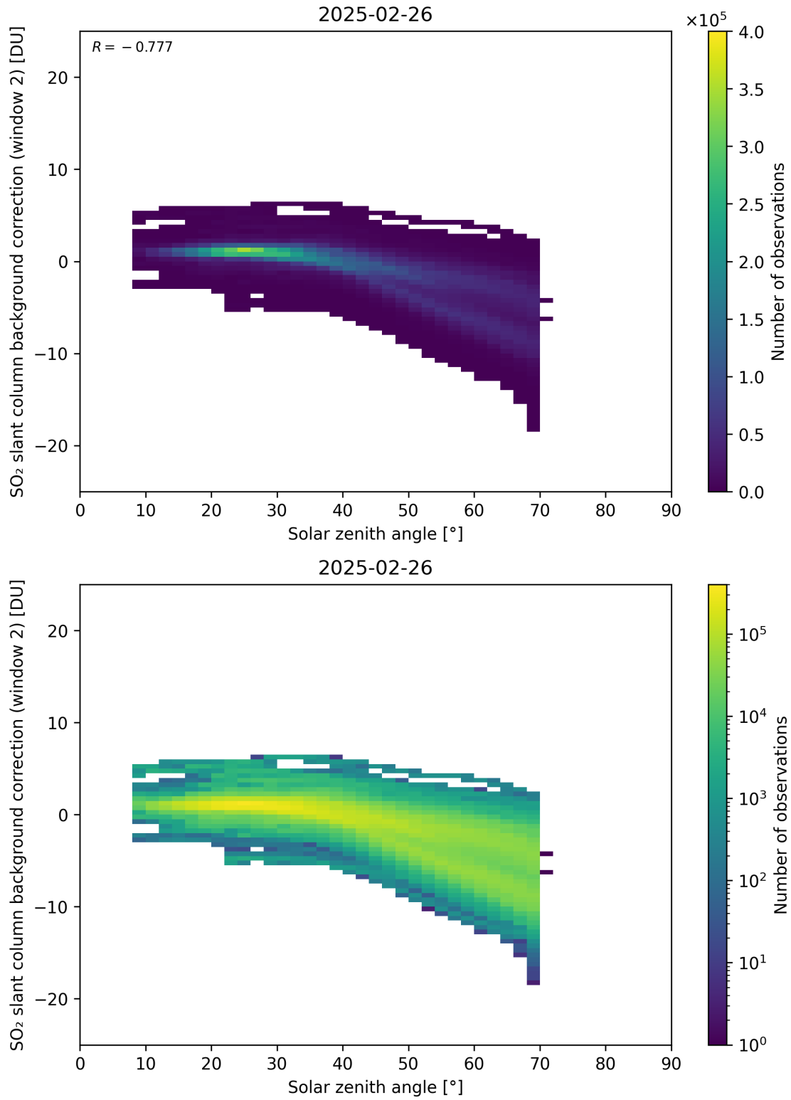
Figure 172: Scatter density plot of “Solar zenith angle” against “SO 2 slant column background correction (window 2)” for 2025-02-25 to 2025-02-27.
