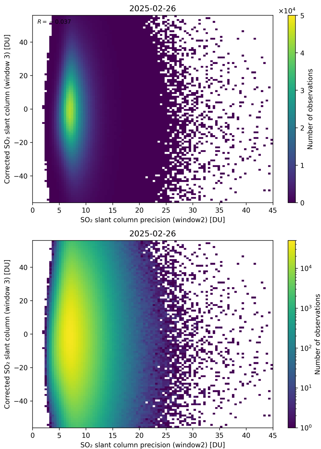
Figure 298: Scatter density plot of “SO 2 slant column precision (window2)” against “Corrected SO 2 slant column (window 3)” for 2025-02-25 to 2025-02-27.
