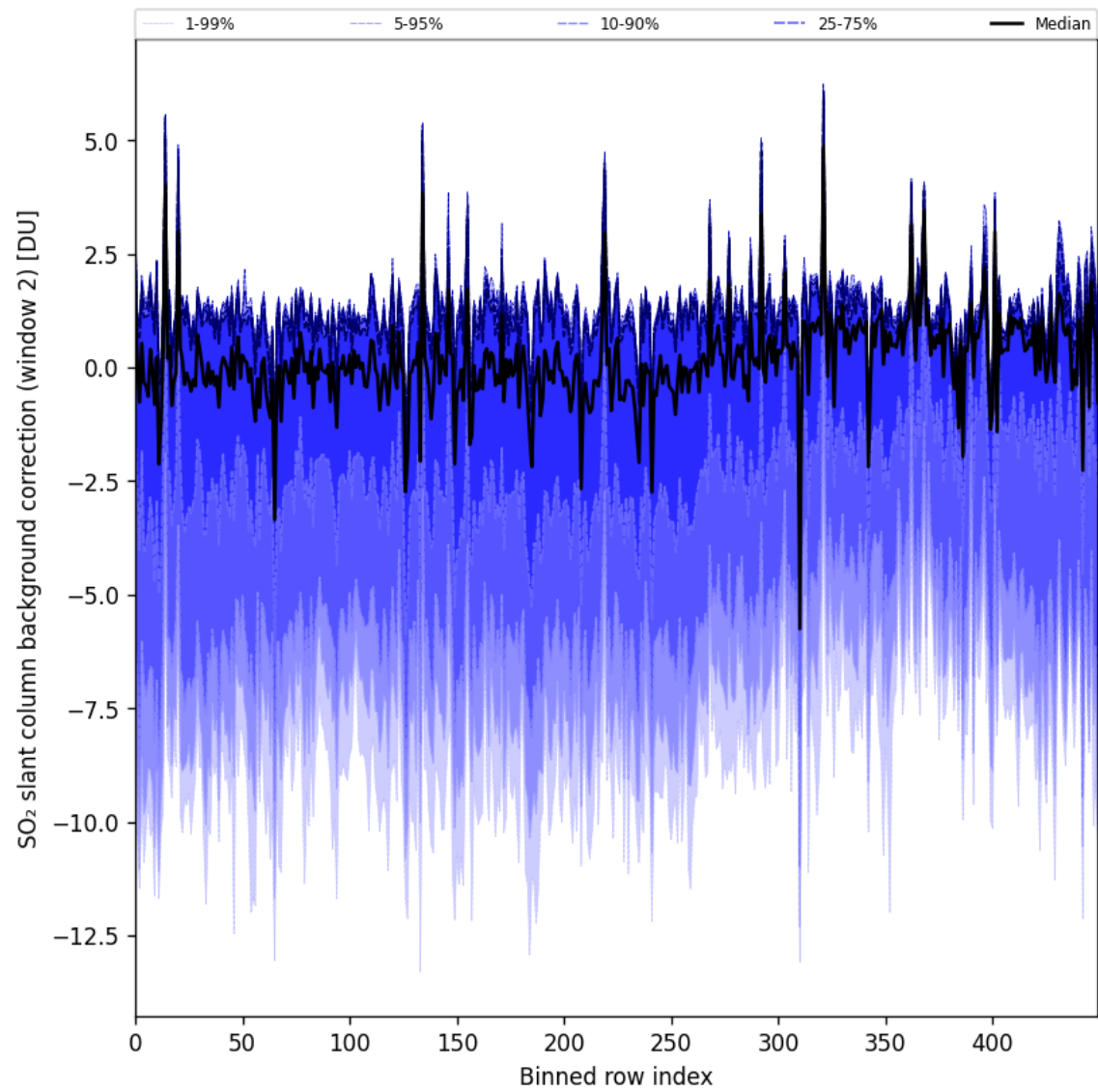
Figure 96: Along track statistics of “SO 2 slant column background correction (window 2)” for 2025-02-25 to 2025-02-27
