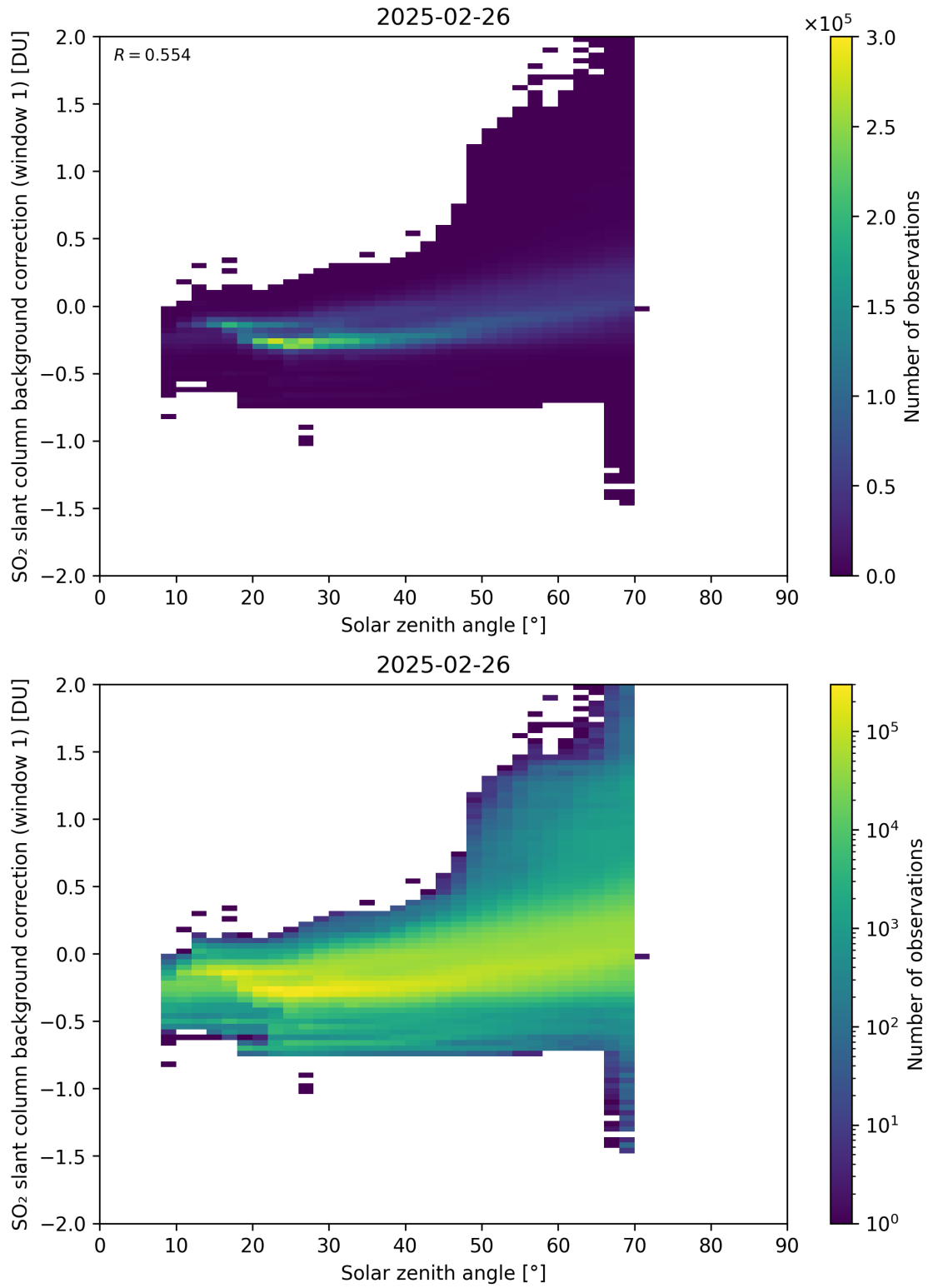
Figure 171: Scatter density plot of “Solar zenith angle” against “SO 2 slant column background correction (window 1)” for 2025-02-25 to 2025-02-27.
