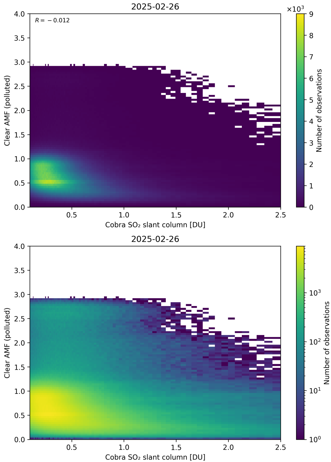
Figure 215: Scatter density plot of “Cobra SO 2 slant column” against “Clear AMF (polluted)” for 2025-02-25 to 2025-02-27.
