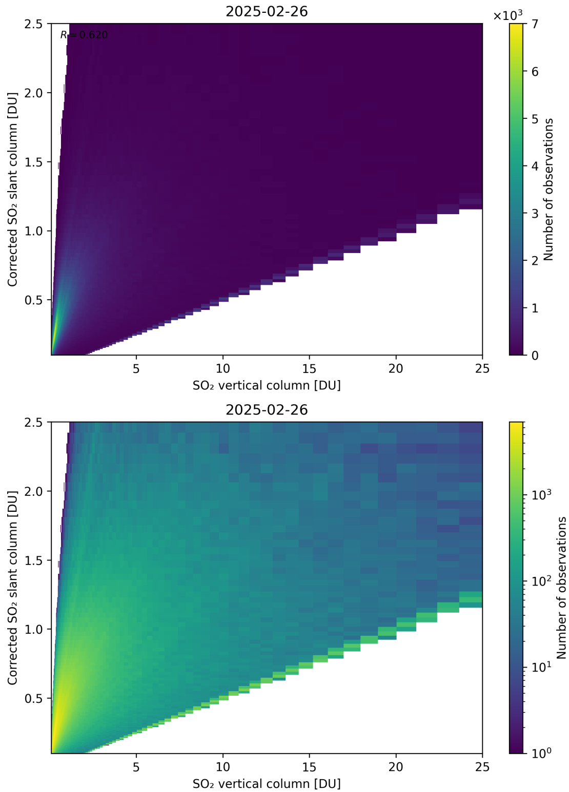
Figure 351: Scatter density plot of “SO 2 vertical column” against “Corrected SO 2 slant column” for 2025-02-25 to 2025-02-27.
