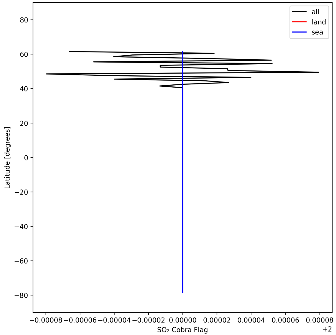
Figure 49: Zonal average of “SO 2 Cobra Flag” for 2025-02-25 to 2025-02-27.
