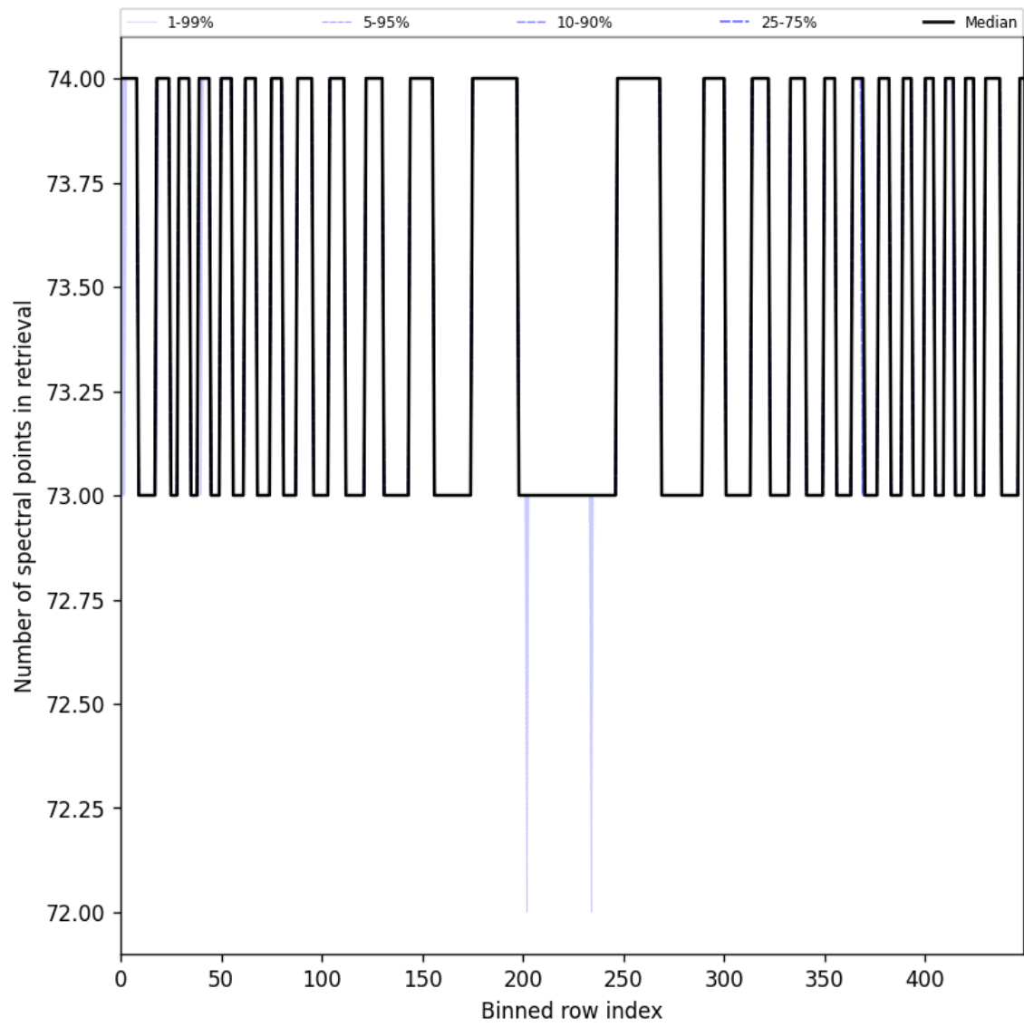
Figure 108: Along track statistics of “Number of spectral points in retrieval” for 2025-02-25 to 2025-02-27
