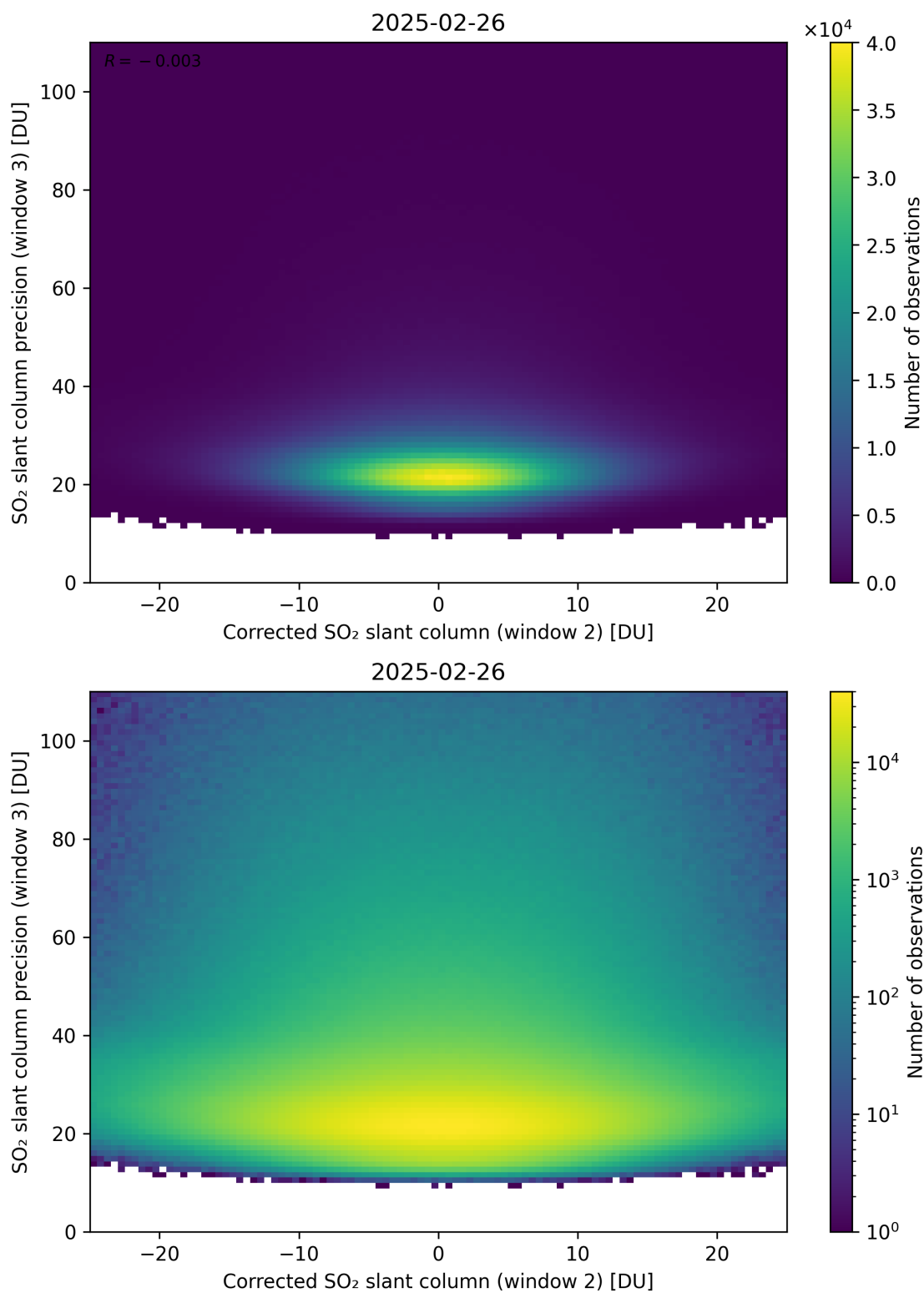
Figure 252: Scatter density plot of “Corrected SO 2 slant column (window 2)” against “SO 2 slant column precision (window 3)” for 2025-02-25 to 2025-02-27.
