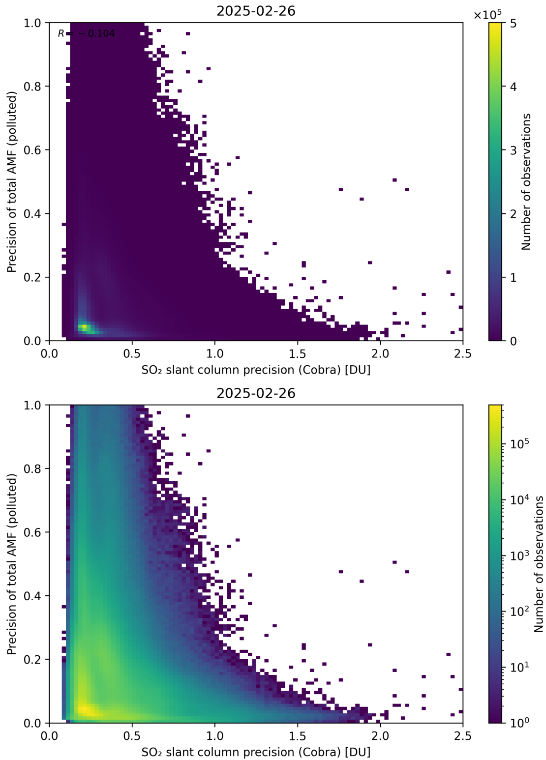
Figure 214: Scatter density plot of “SO 2 slant column precision (Cobra)” against “Precision of total AMF (polluted)” for 2025-02-25 to 2025-02-27.
