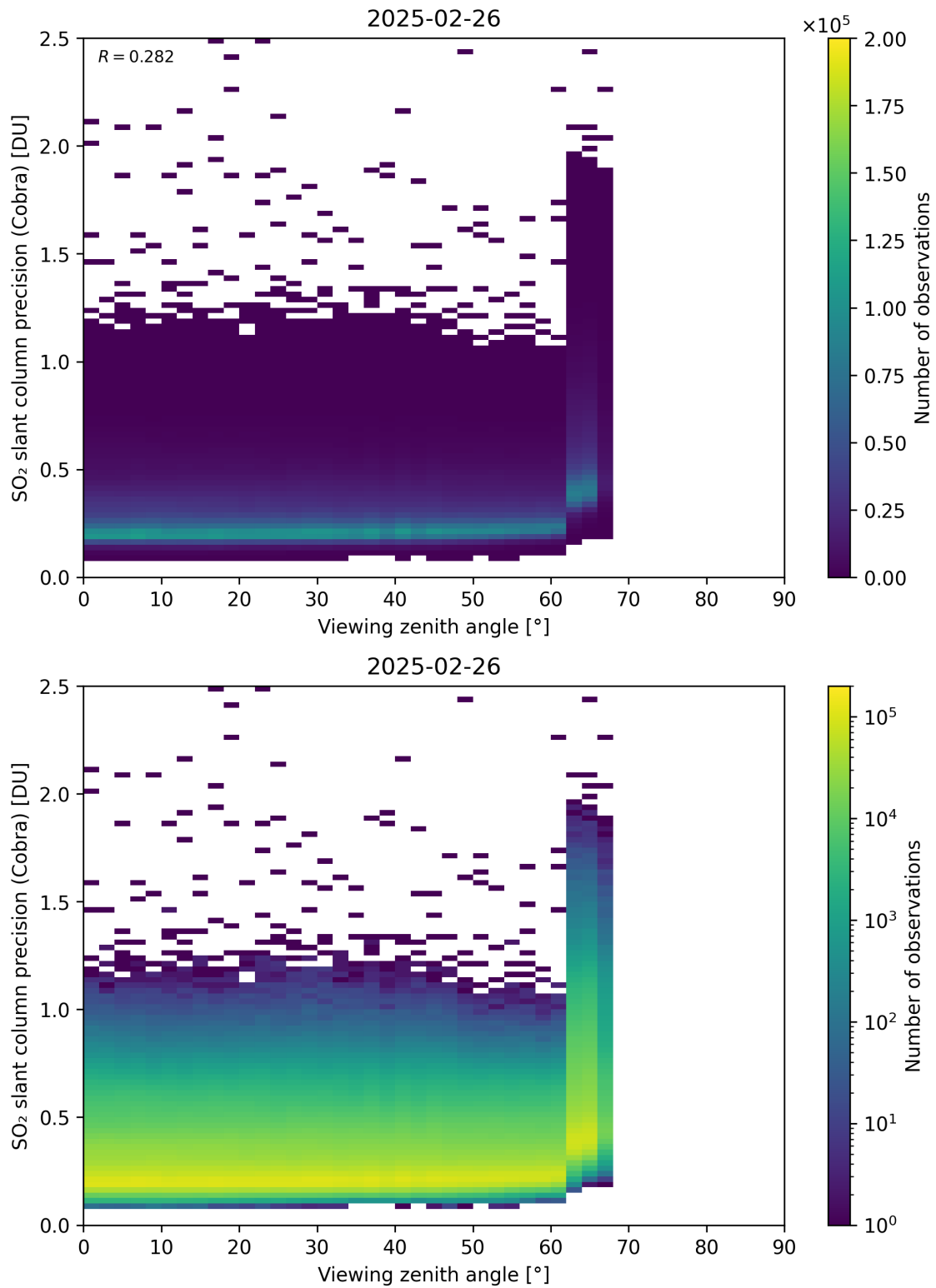
Figure 372: Scatter density plot of “Viewing zenith angle” against “SO 2 slant column precision (Cobra)” for 2025-02-25 to 2025-02-27.
