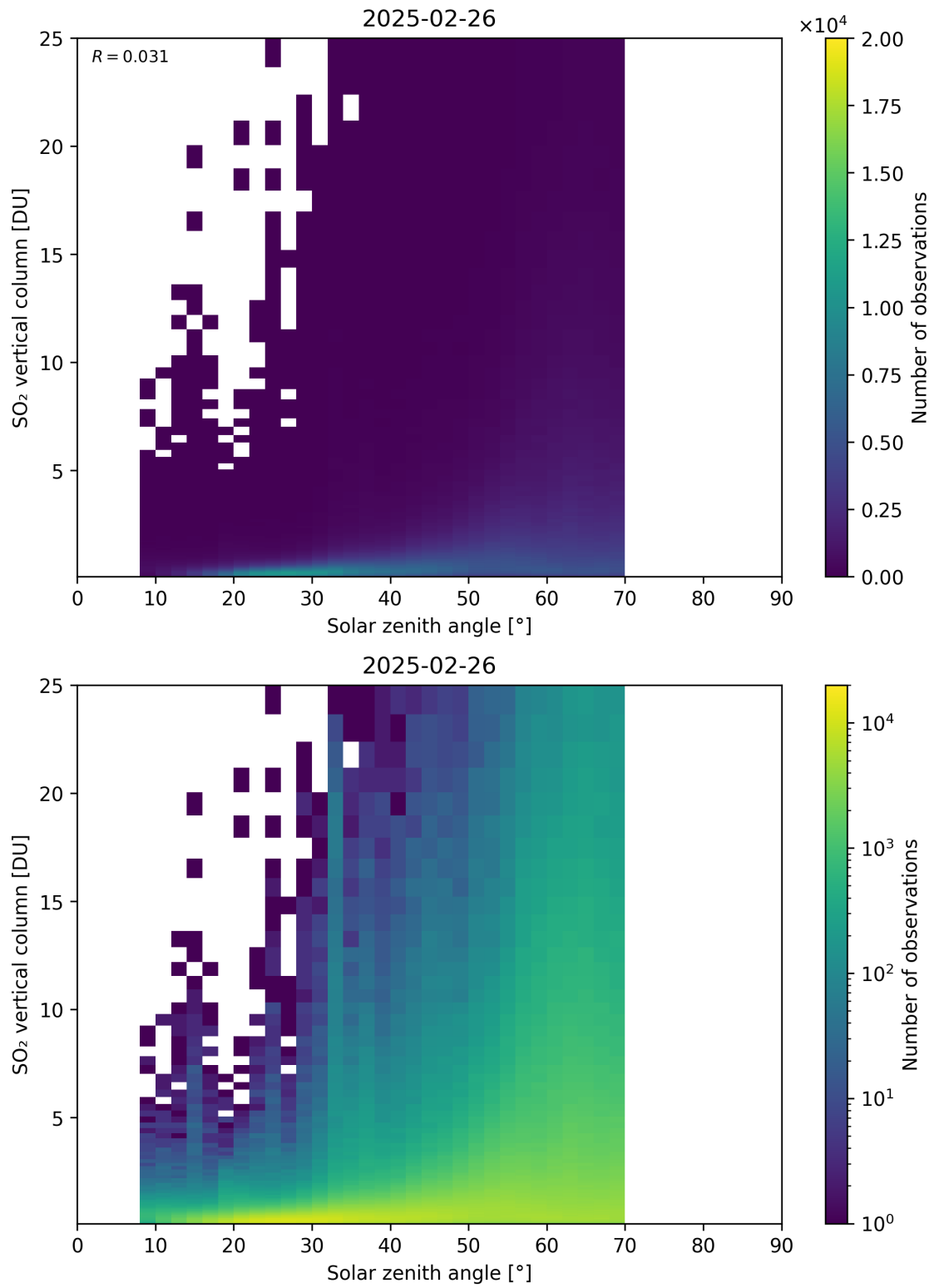
Figure 191: Scatter density plot of “Solar zenith angle” against “SO 2 vertical column” for 2025-02-25 to 2025-02-27.
