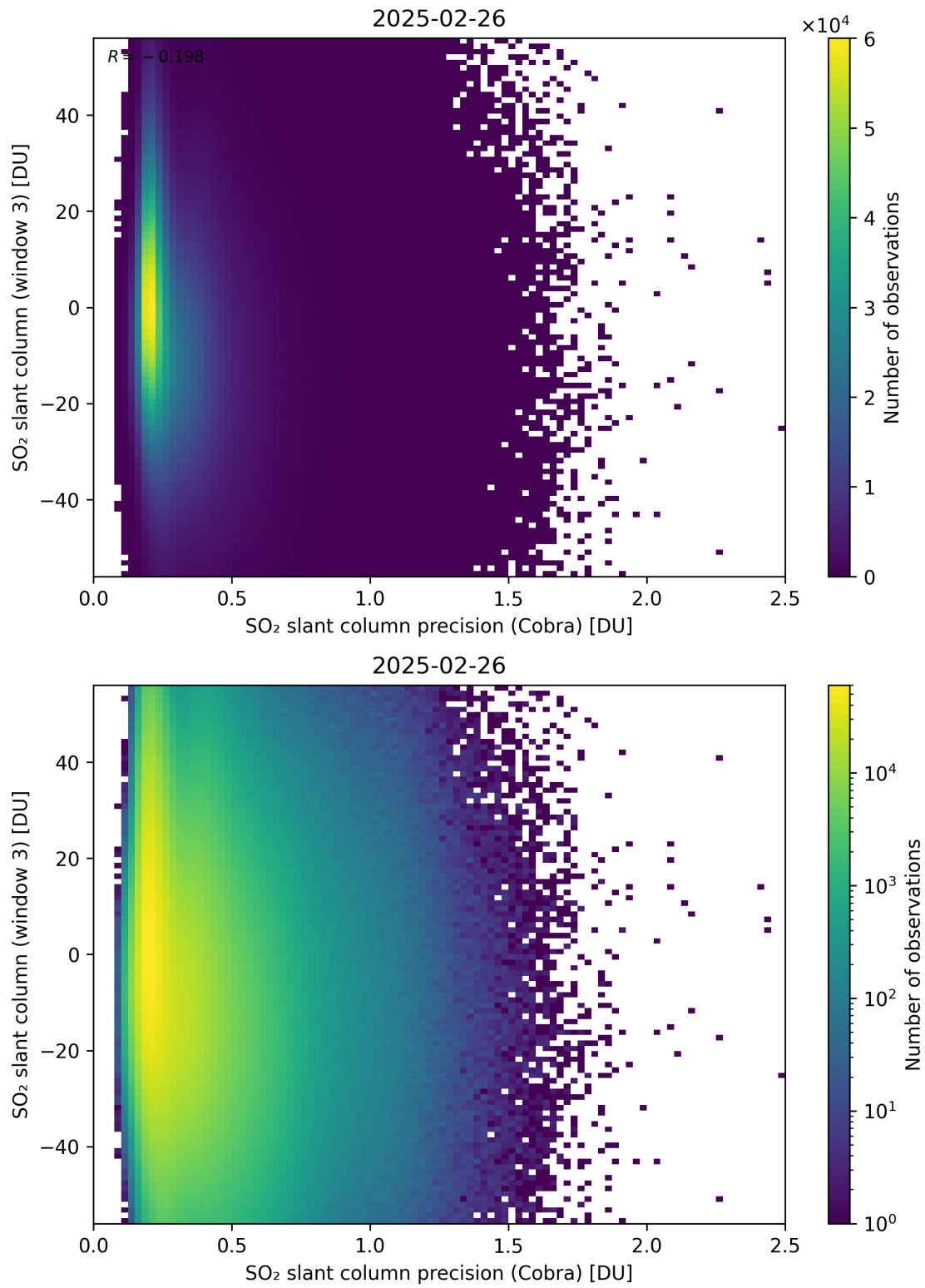
Figure 211: Scatter density plot of “SO 2 slant column precision (Cobra)” against “SO 2 slant column (window 3)” for 2025-02-25 to 2025-02-27.
