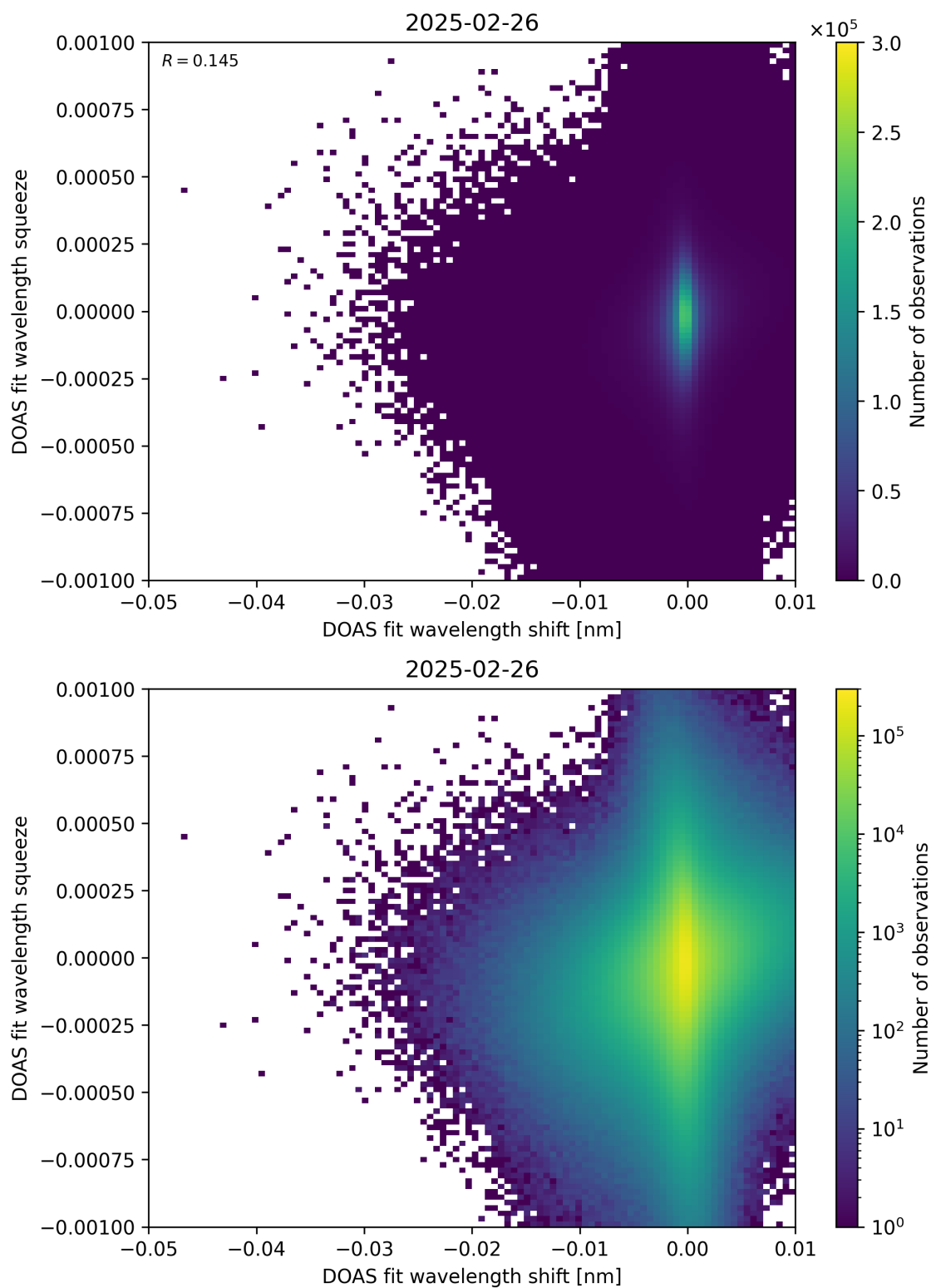
Figure 138: Scatter density plot of “DOAS fit wavelength shift” against “DOAS fit wavelength squeeze” for 2025-02-25 to 2025-02-27.
