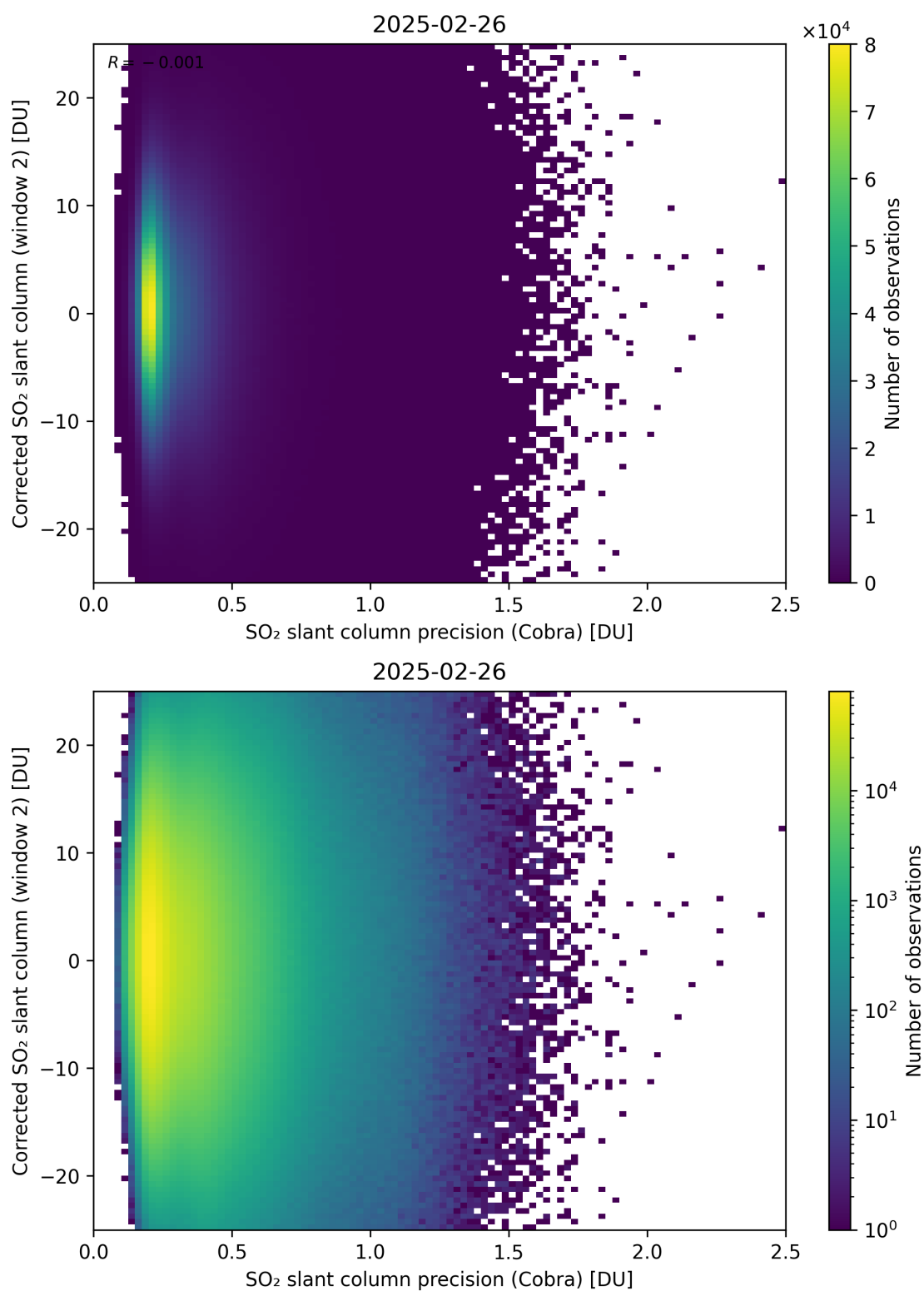
Figure 206: Scatter density plot of “SO 2 slant column precision (Cobra)” against “Corrected SO 2 slant column (window 2)” for 2025-02-25 to 2025-02-27.
