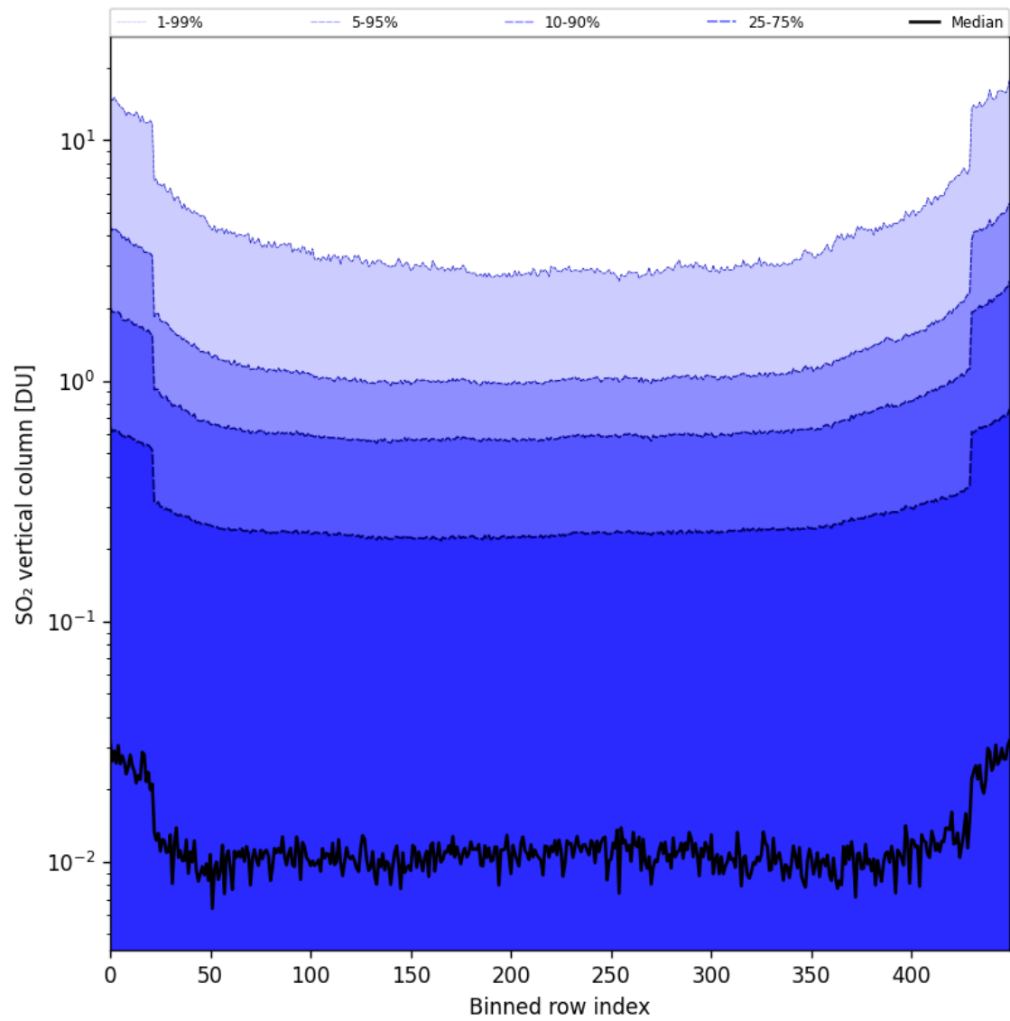
Figure 84: Along track statistics of “SO 2 vertical column” for 2025-02-25 to 2025-02-27
