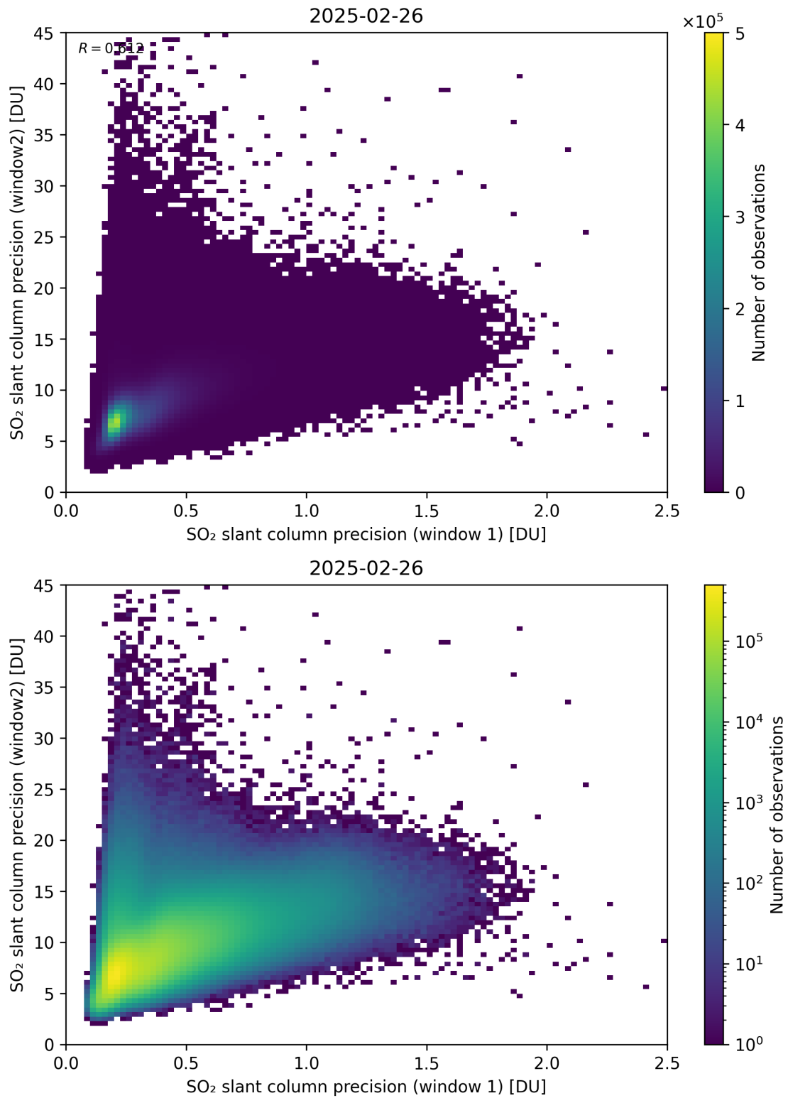
Figure 277: Scatter density plot of “SO 2 slant column precision (window 1)” against “SO 2 slant column precision (window2)” for 2025-02-25 to 2025-02-27.
