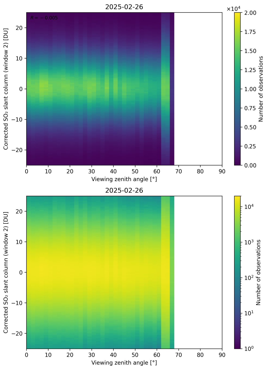
Figure 374: Scatter density plot of “Viewing zenith angle” against “Corrected SO 2 slant column (window 2)” for 2025-02-25 to 2025-02-27.
