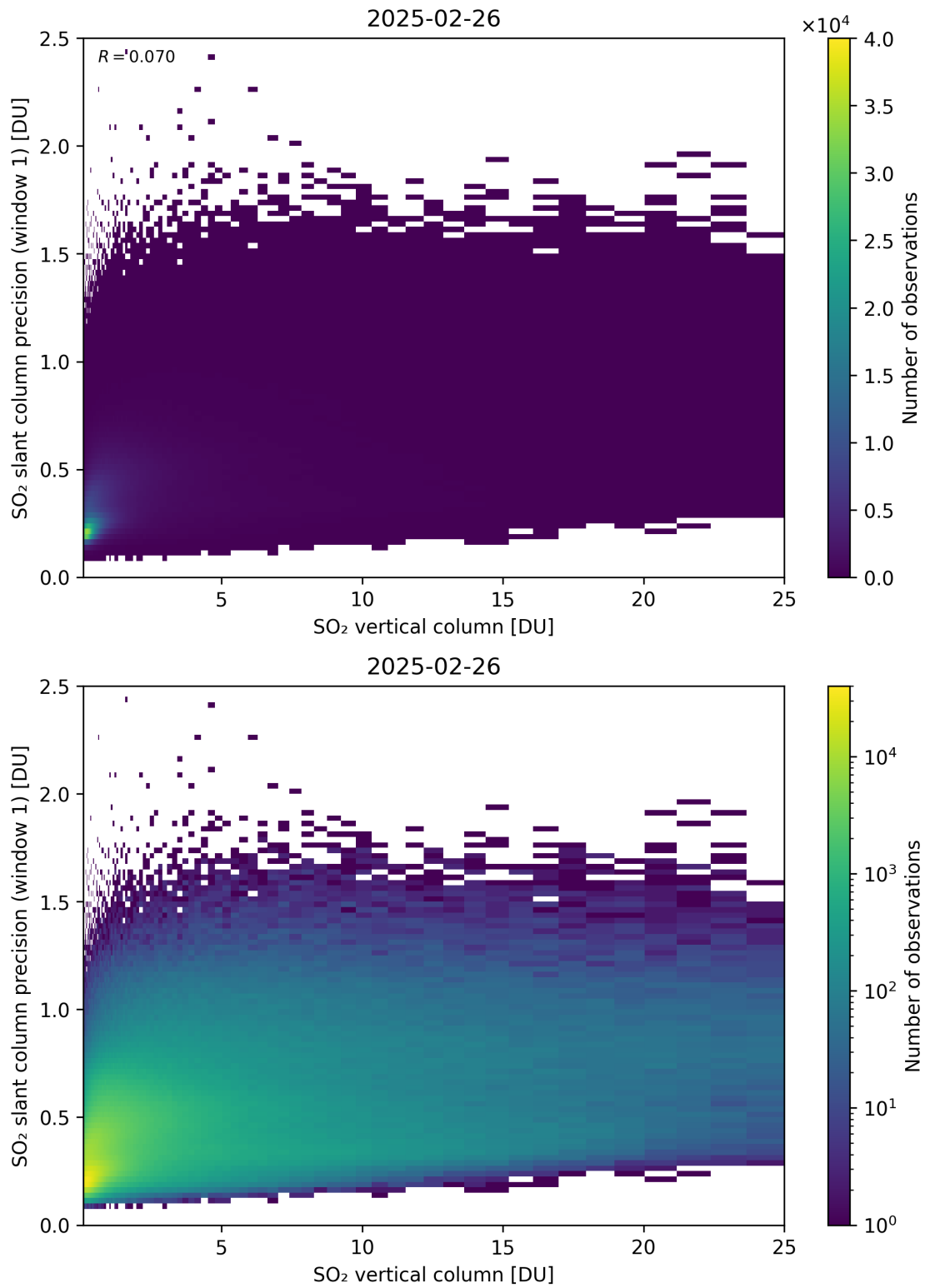
Figure 355: Scatter density plot of “SO 2 vertical column” against “SO 2 slant column precision (window 1)” for 2025-02-25 to 2025-02-27.
