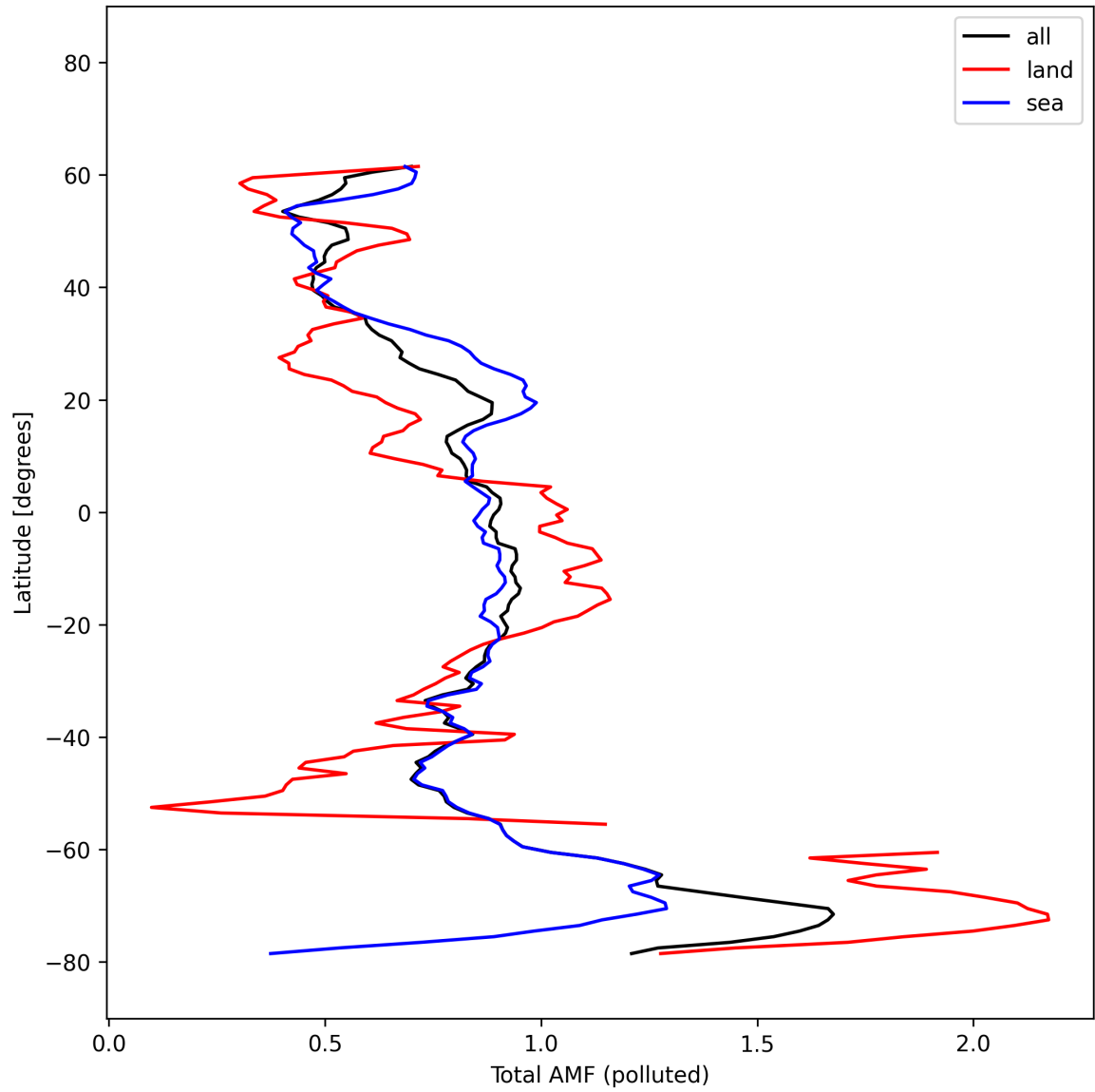
Figure 53: Zonal average of “Total AMF (polluted)” for 2025-02-25 to 2025-02-27.
