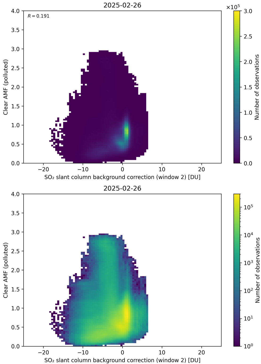
Figure 126: Scatter density plot of “SO 2 slant column background correction (window 2)” against “Clear AMF (polluted)” for 2025-02-25 to 2025-02-27.
