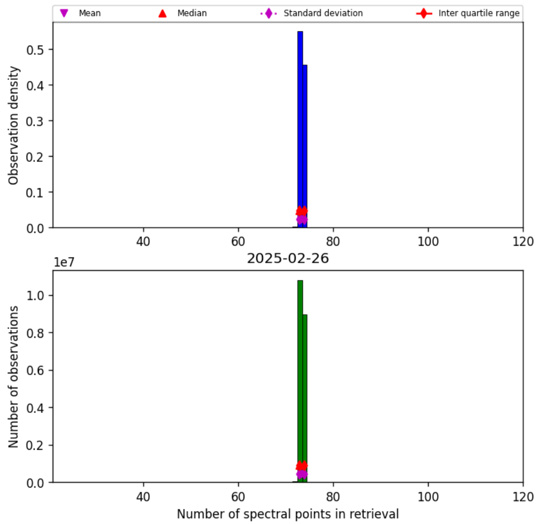
Figure 82: Histogram of “Number of spectral points in retrieval” for 2025-02-25 to 2025-02-27
