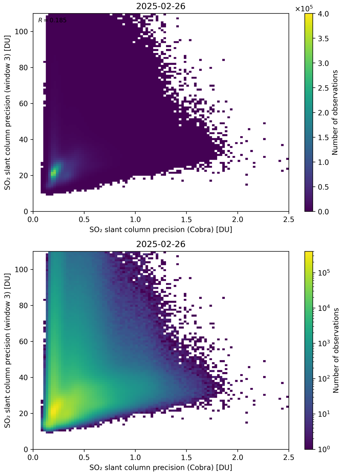
Figure 212: Scatter density plot of “SO 2 slant column precision (Cobra)” against “SO 2 slant column precision (window 3)” for 2025-02-25 to 2025-02-27.
