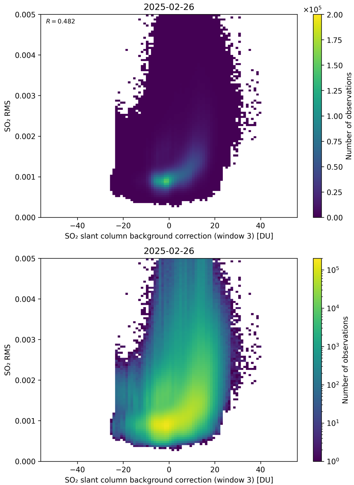
Figure 134: Scatter density plot of “SO 2 slant column background correction (window 3)” against “SO 2 RMS” for 2025-02-25 to 2025-02-27.
