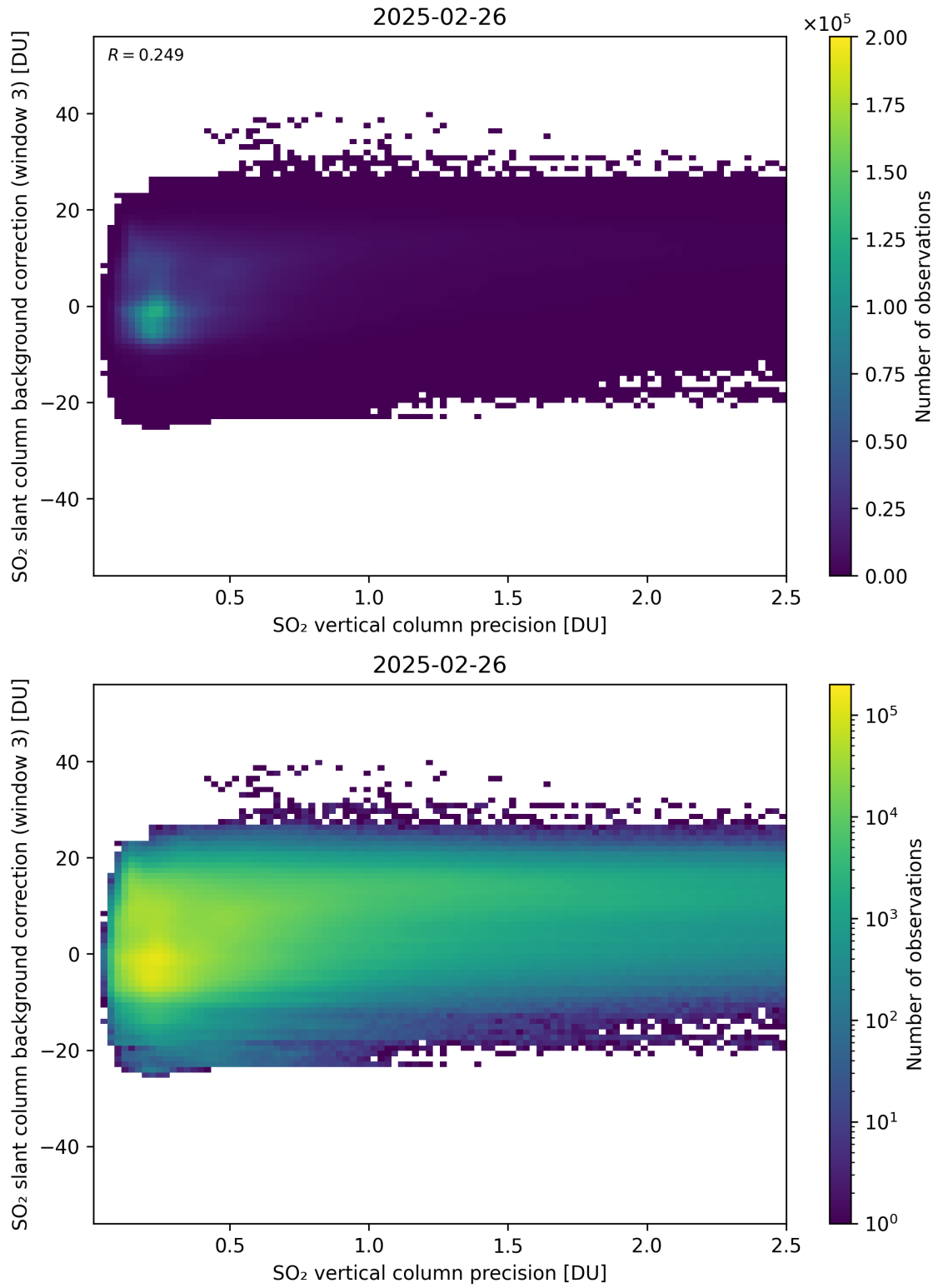
Figure 331: Scatter density plot of “SO 2 vertical column precision” against “SO 2 slant column background correction (window 3)” for 2025-02-25 to 2025-02-27.
