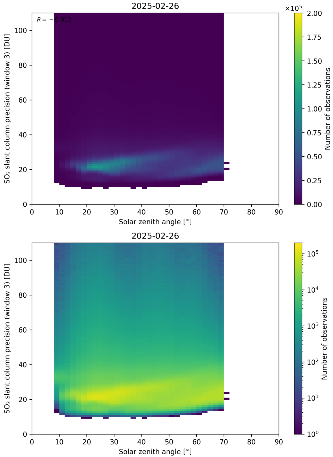
Figure 188: Scatter density plot of “Solar zenith angle” against “SO 2 slant column precision (window 3)” for 2025-02-25 to 2025-02-27.
