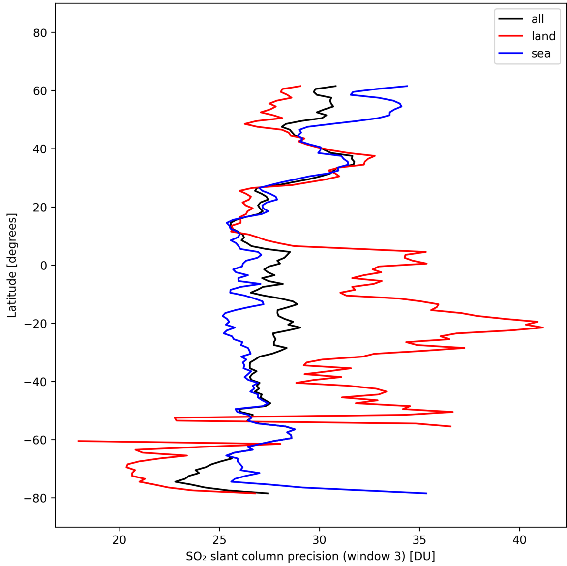
Figure 46: Zonal average of “SO 2 slant column precision (window 3)” for 2025-02-25 to 2025-02-27.
