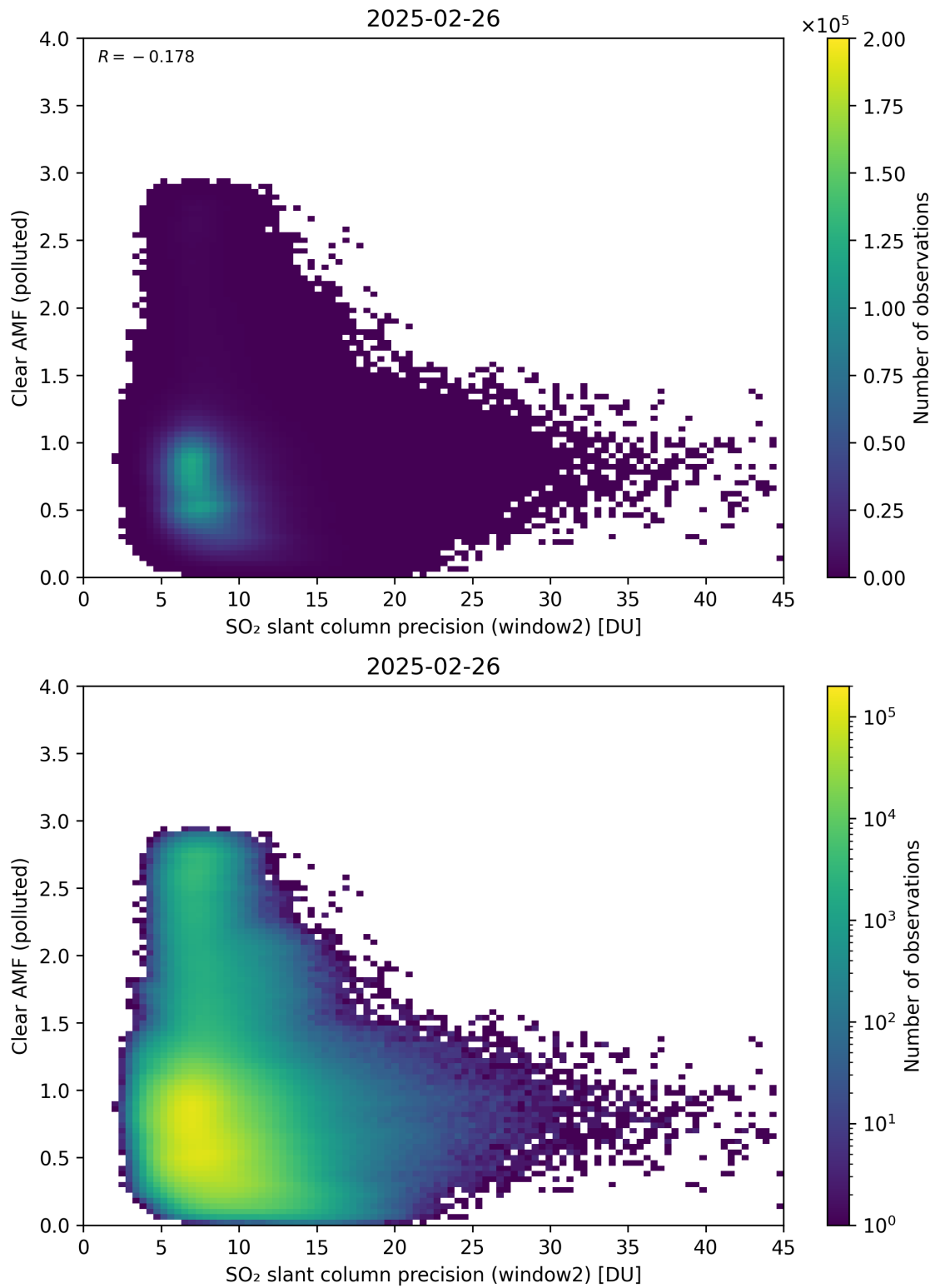
Figure 296: Scatter density plot of “SO 2 slant column precision (window2)” against “Clear AMF (polluted)” for 2025-02-25 to 2025-02-27.
