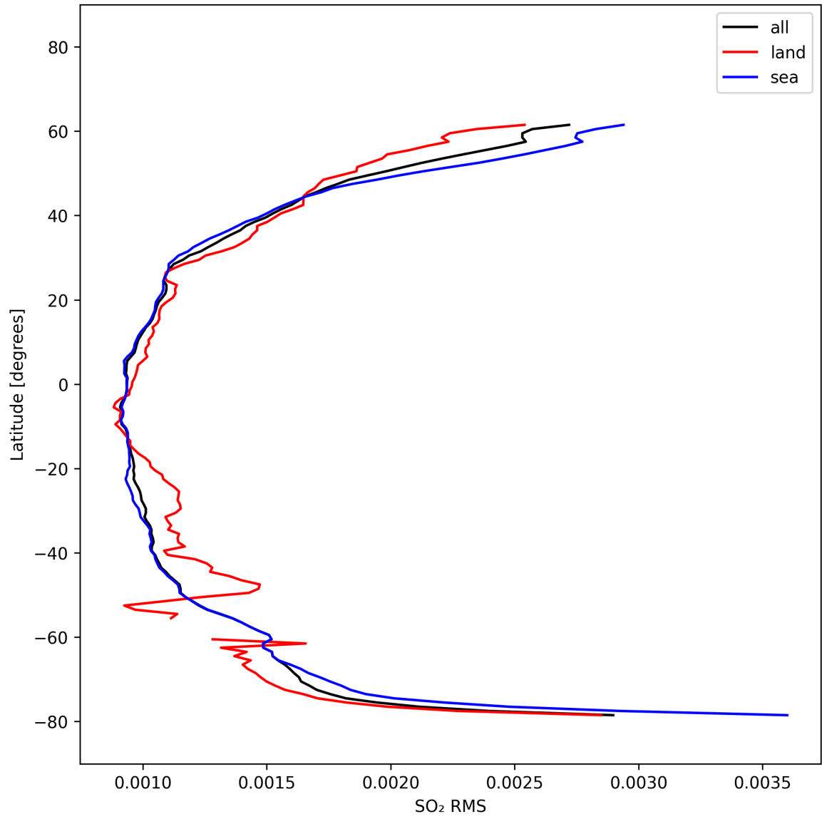
Figure 52: Zonal average of “SO 2 RMS” for 2025-02-25 to 2025-02-27.
