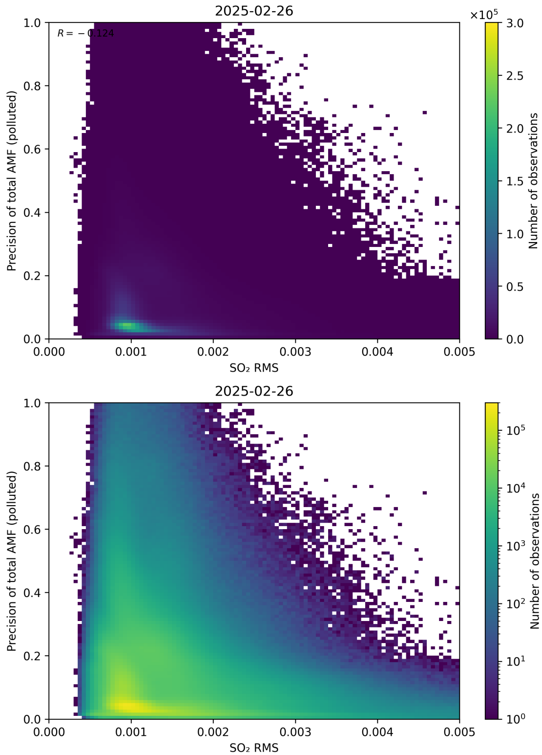
Figure 149: Scatter density plot of “SO 2 RMS” against “Precision of total AMF (polluted)” for 2025-02-25 to 2025-02-27.
