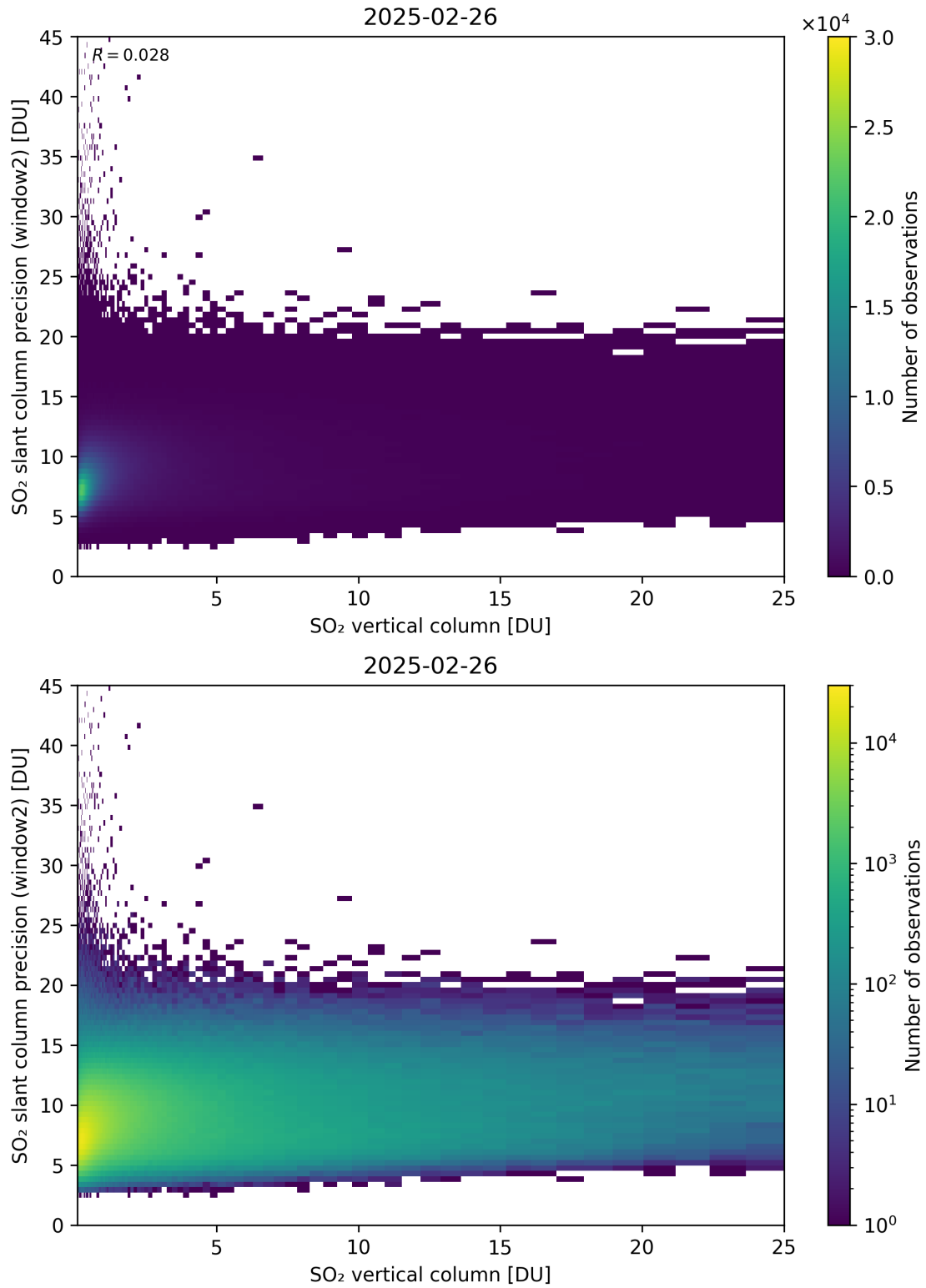
Figure 356: Scatter density plot of “SO 2 vertical column” against “SO 2 slant column precision (window2)” for 2025-02-25 to 2025-02-27.
