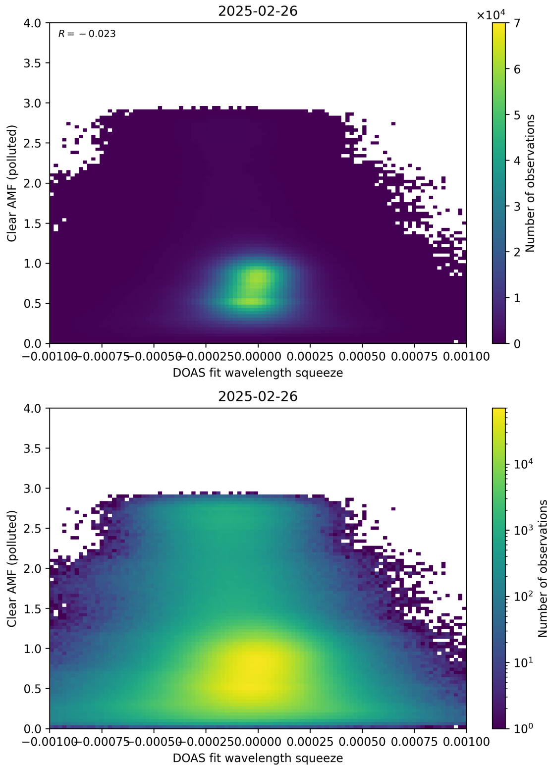
Figure 144: Scatter density plot of “DOAS fit wavelength squeeze” against “Clear AMF (polluted)” for 2025-02-25 to 2025-02-27.
