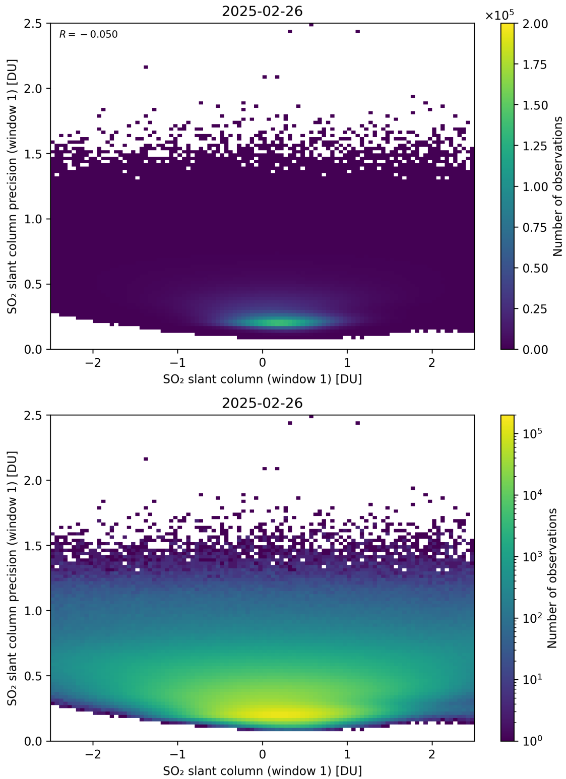
Figure 285: Scatter density plot of “SO 2 slant column (window 1)” against “SO 2 slant column precision (window 1)” for 2025-02-25 to 2025-02-27.
