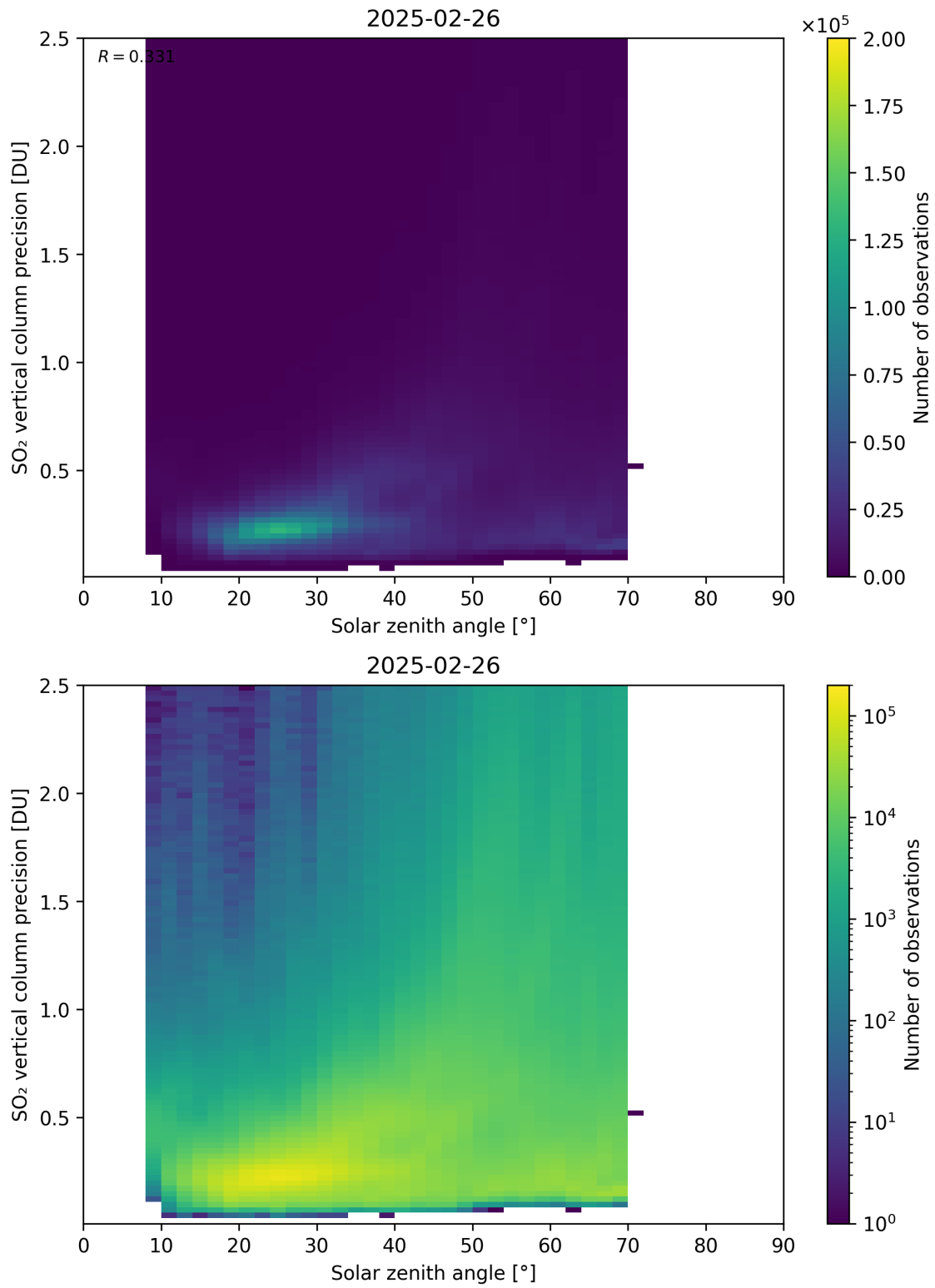
Figure 192: Scatter density plot of “Solar zenith angle” against “SO 2 vertical column precision” for 2025-02-25 to 2025-02-27.
