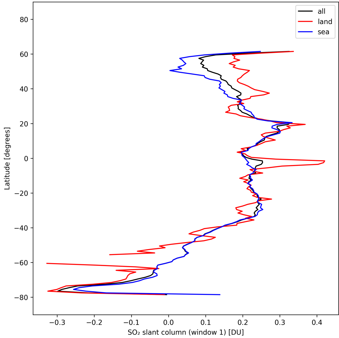
Figure 37: Zonal average of “SO 2 slant column (window 1)” for 2025-02-25 to 2025-02-27.
