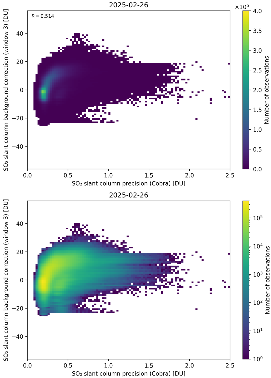
Figure 201: Scatter density plot of “SO 2 slant column precision (Cobra)” against “SO 2 slant column background correction (window 3)” for 2025-02-25 to 2025-02-27.
