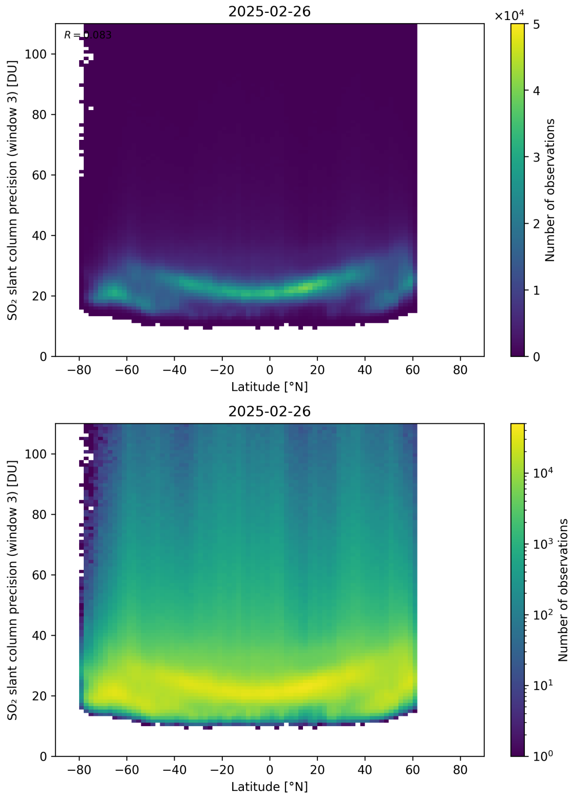
Figure 166: Scatter density plot of “Latitude” against “SO 2 slant column precision (window 3)” for 2025-02-25 to 2025-02-27.
