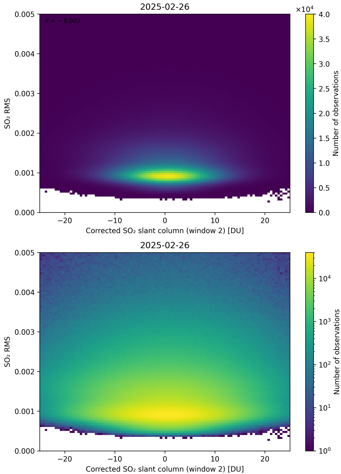
Figure 248: Scatter density plot of “Corrected SO 2 slant column (window 2)” against “SO 2 RMS” for 2025-02-25 to 2025-02-27.
