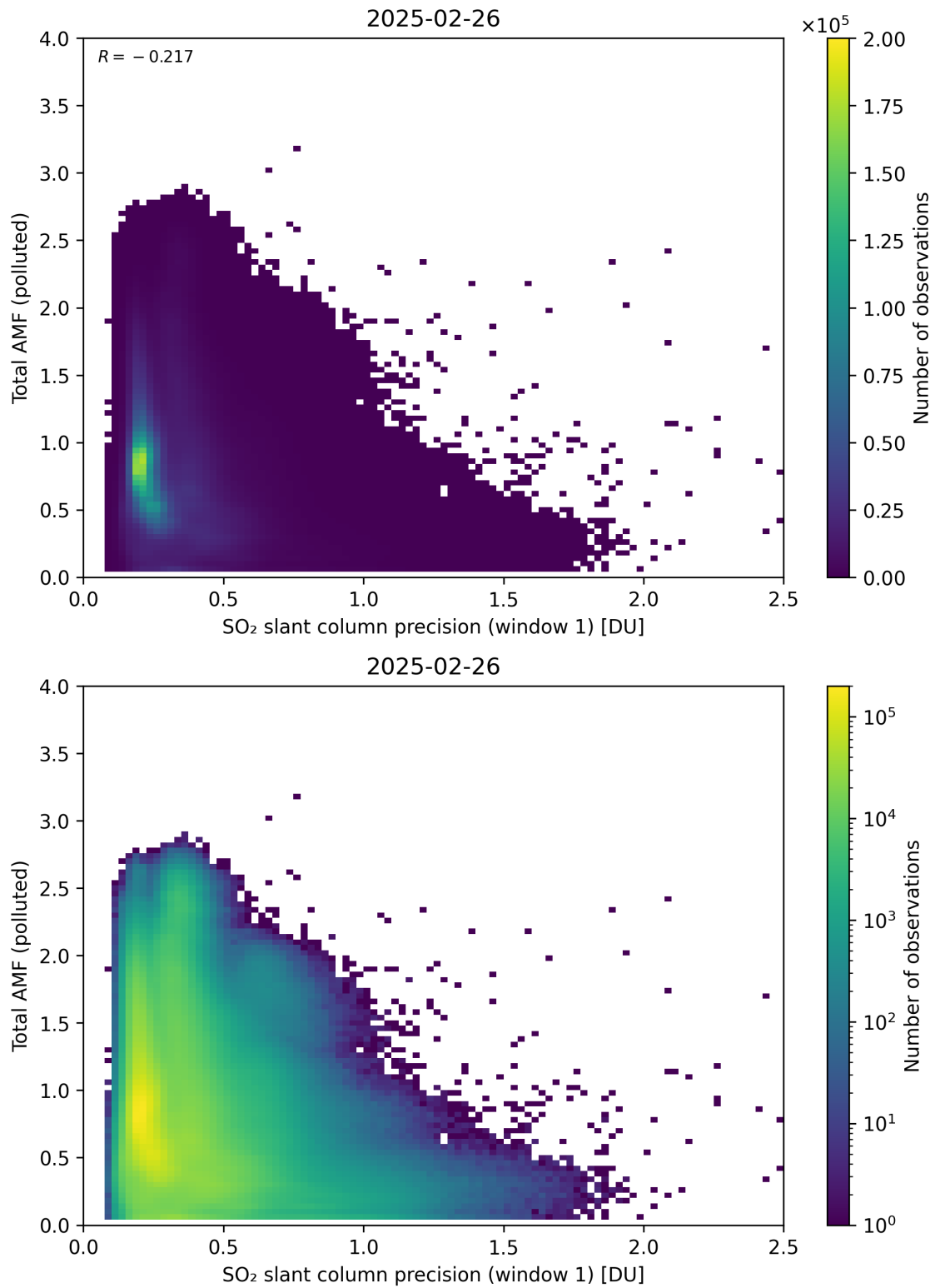
Figure 280: Scatter density plot of “SO 2 slant column precision (window 1)” against “Total AMF (polluted)” for 2025-02-25 to 2025-02-27.
