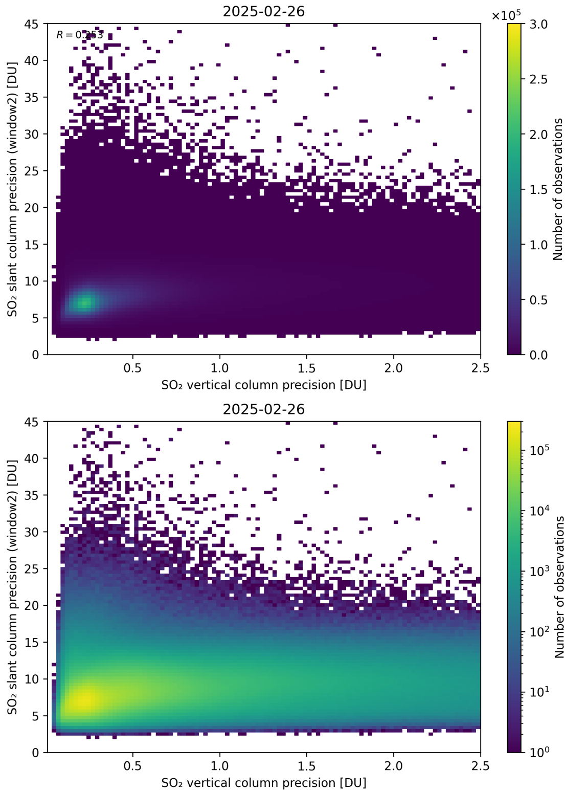
Figure 343: Scatter density plot of “SO 2 vertical column precision” against “SO 2 slant column precision (window2)” for 2025-02-25 to 2025-02-27.
