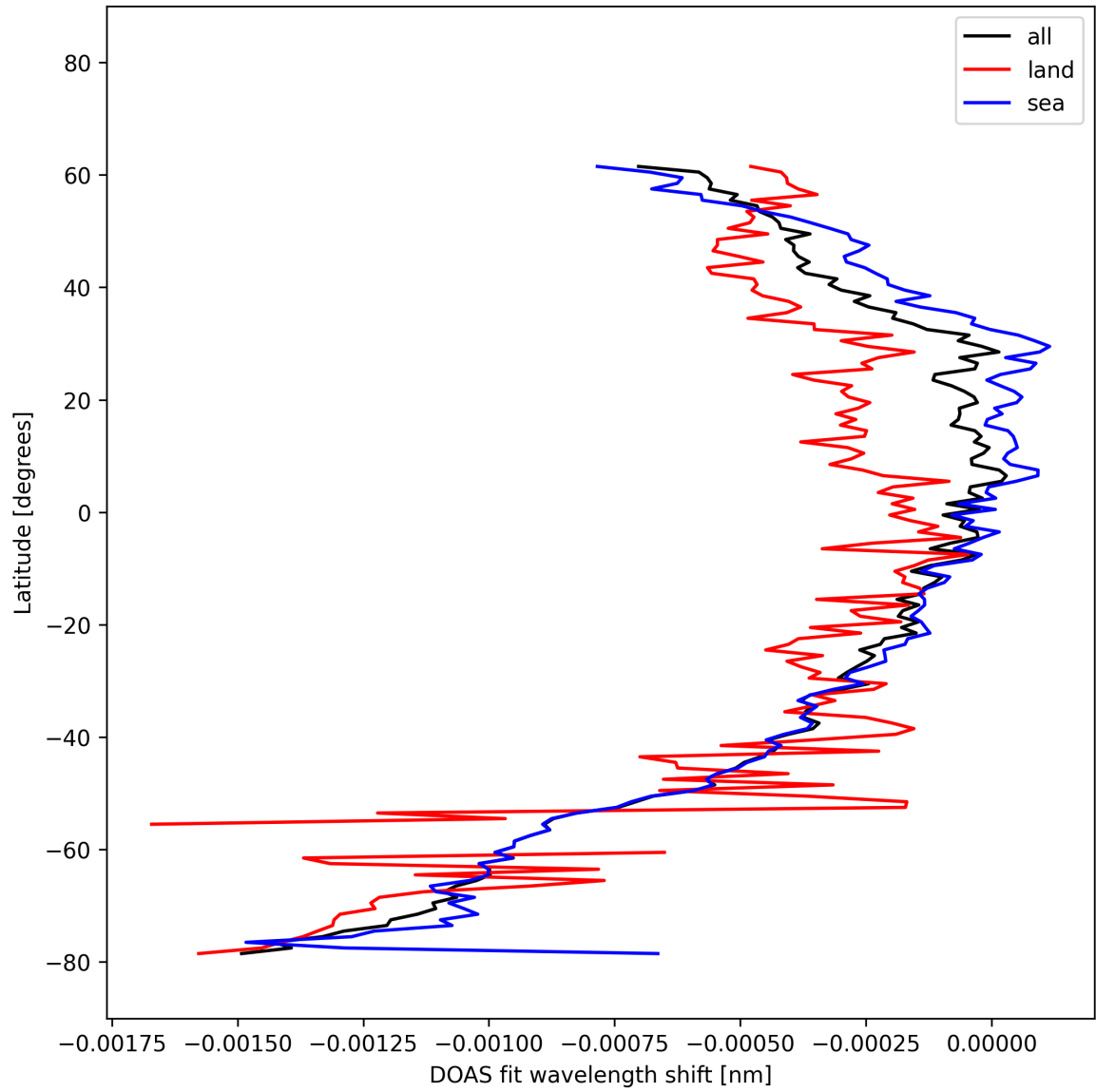
Figure 50: Zonal average of “DOAS fit wavelength shift” for 2025-02-25 to 2025-02-27.
