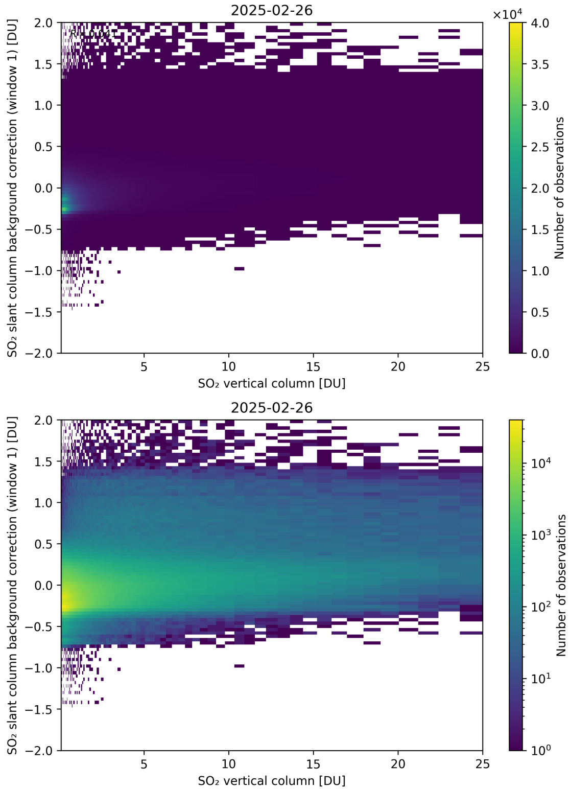
Figure 323: Scatter density plot of “SO 2 vertical column” against “SO 2 slant column background correction (window 1)” for 2025-02-25 to 2025-02-27.
