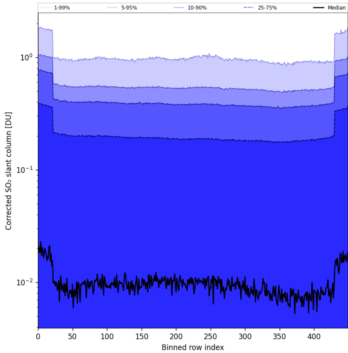
Figure 86: Along track statistics of “Corrected SO 2 slant column” for 2025-02-25 to 2025-02-27
