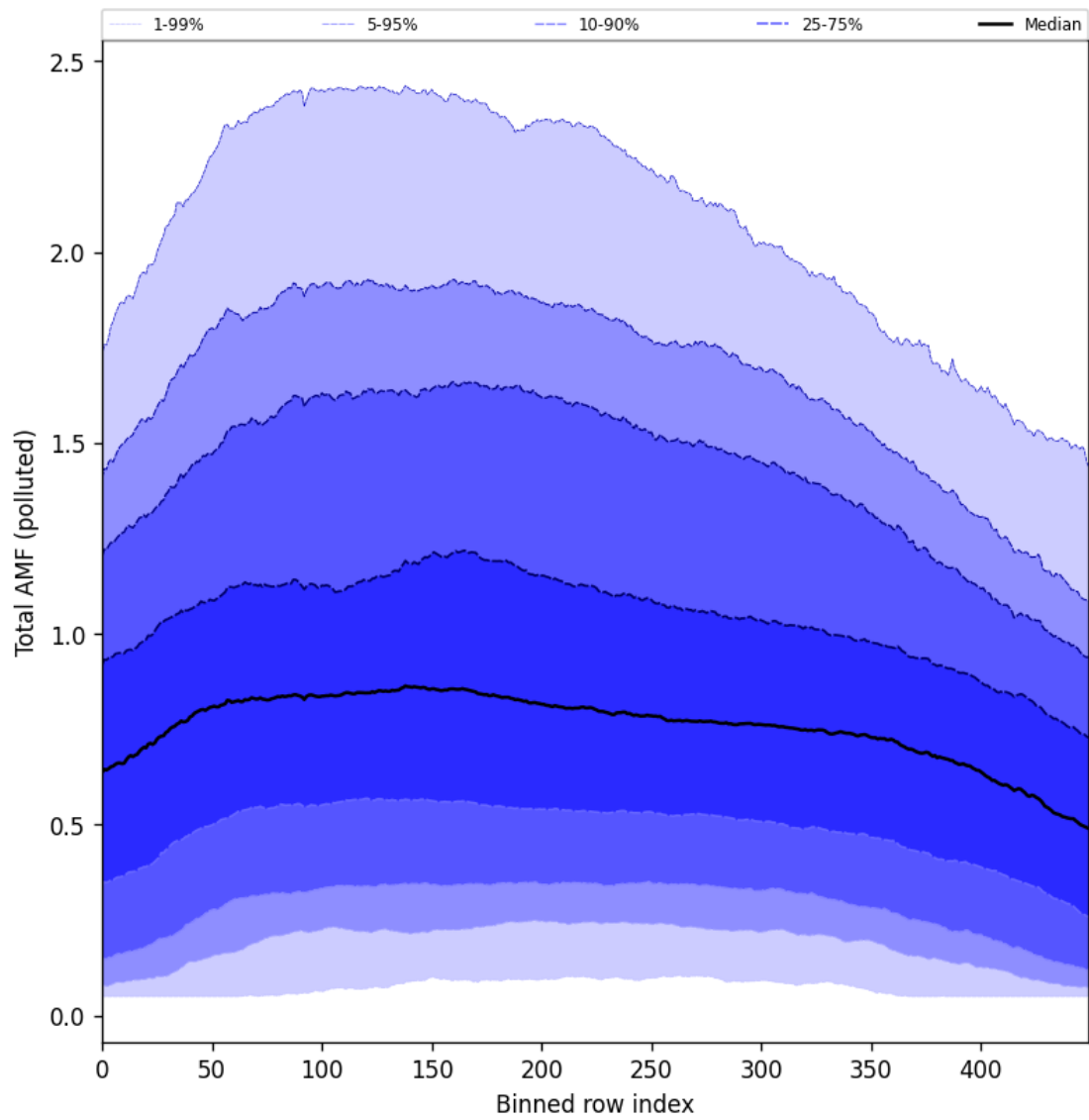
Figure 105: Along track statistics of “Total AMF (polluted)” for 2025-02-25 to 2025-02-27
