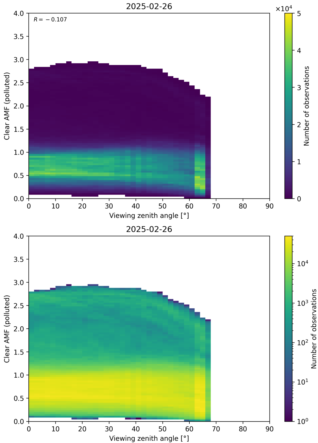
Figure 370: Scatter density plot of “Viewing zenith angle” against “Clear AMF (polluted)” for 2025-02-25 to 2025-02-27.
