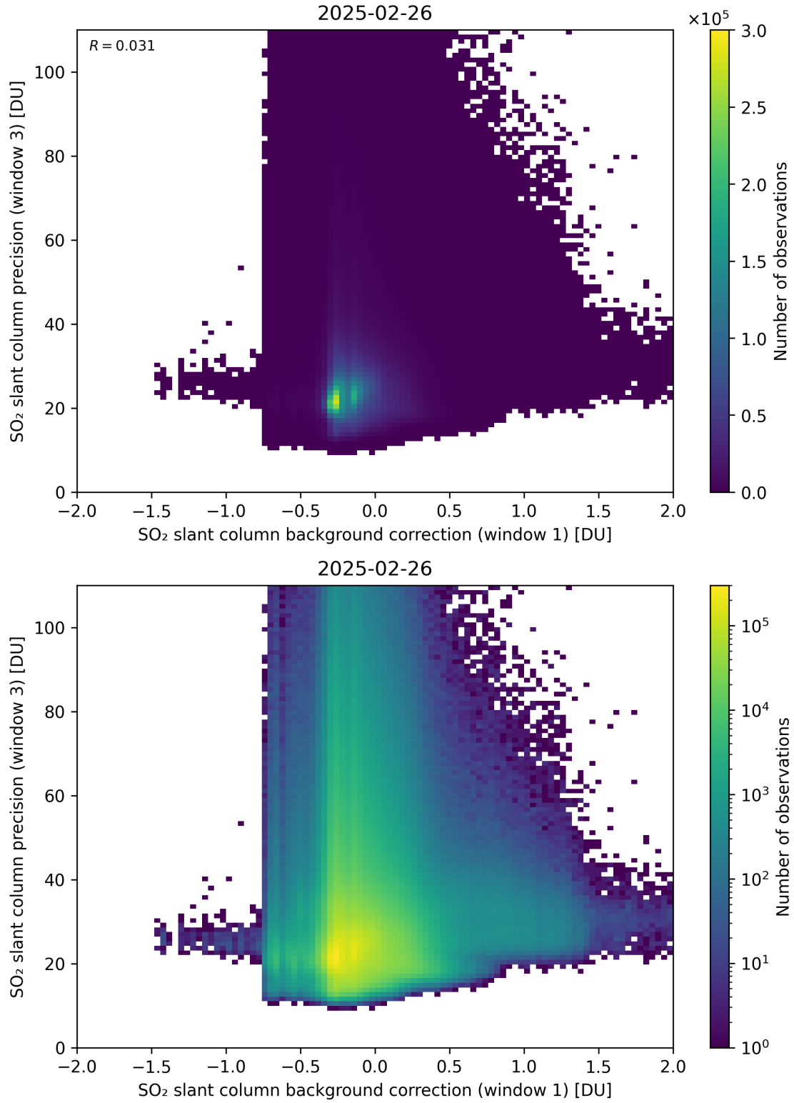
Figure 119: Scatter density plot of “SO 2 slant column background correction (window 1)” against “SO 2 slant column precision (window 3)” for 2025-02-25 to 2025-02-27.
