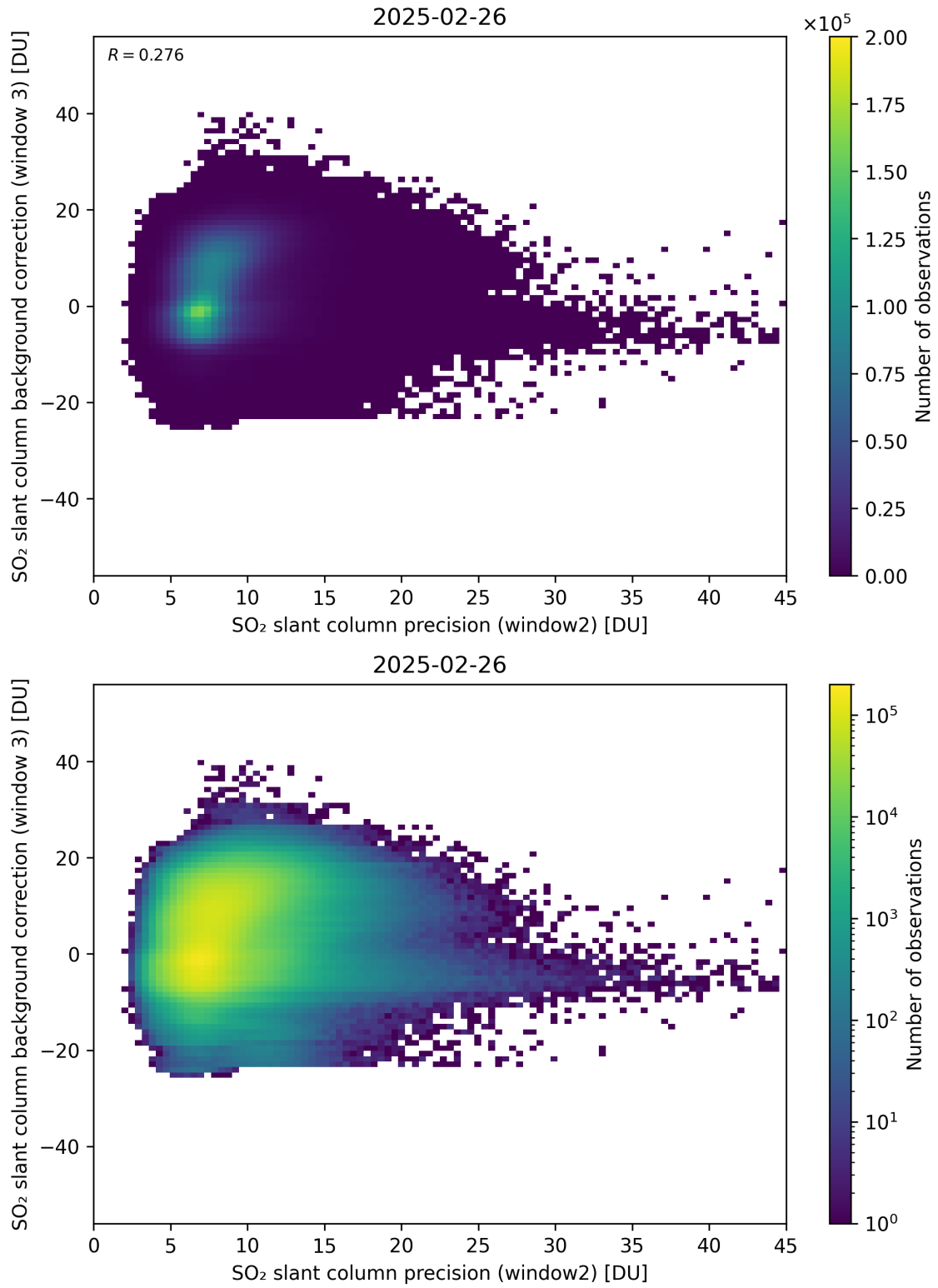
Figure 292: Scatter density plot of “SO 2 slant column precision (window2)” against “SO 2 slant column background correction (window 3)” for 2025-02-25 to 2025-02-27.
