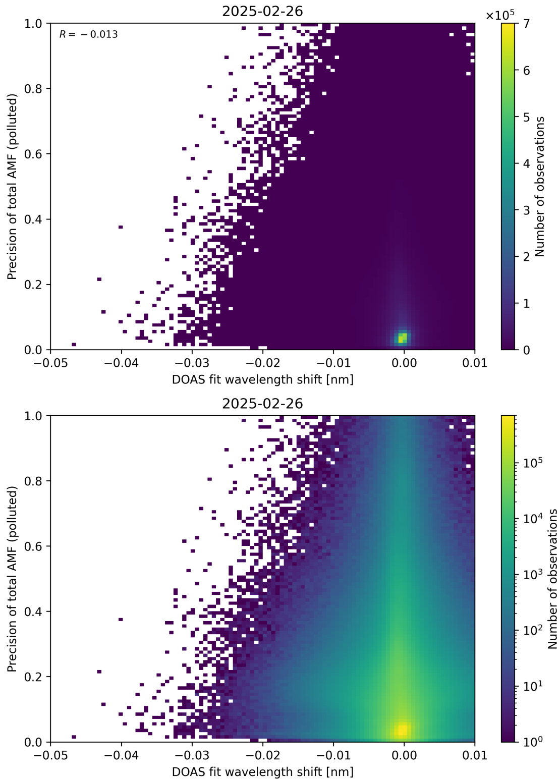
Figure 142: Scatter density plot of “DOAS fit wavelength shift” against “Precision of total AMF (polluted)” for 2025-02-25 to 2025-02-27.
