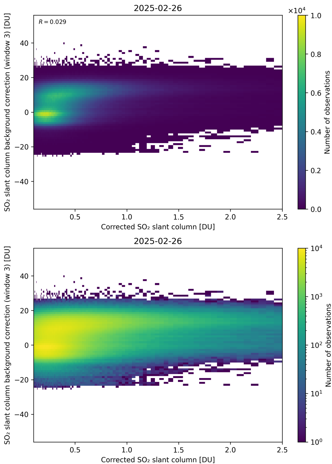
Figure 228: Scatter density plot of “Corrected SO 2 slant column” against “SO 2 slant column background correction (window 3)” for 2025-02-25 to 2025-02-27.
