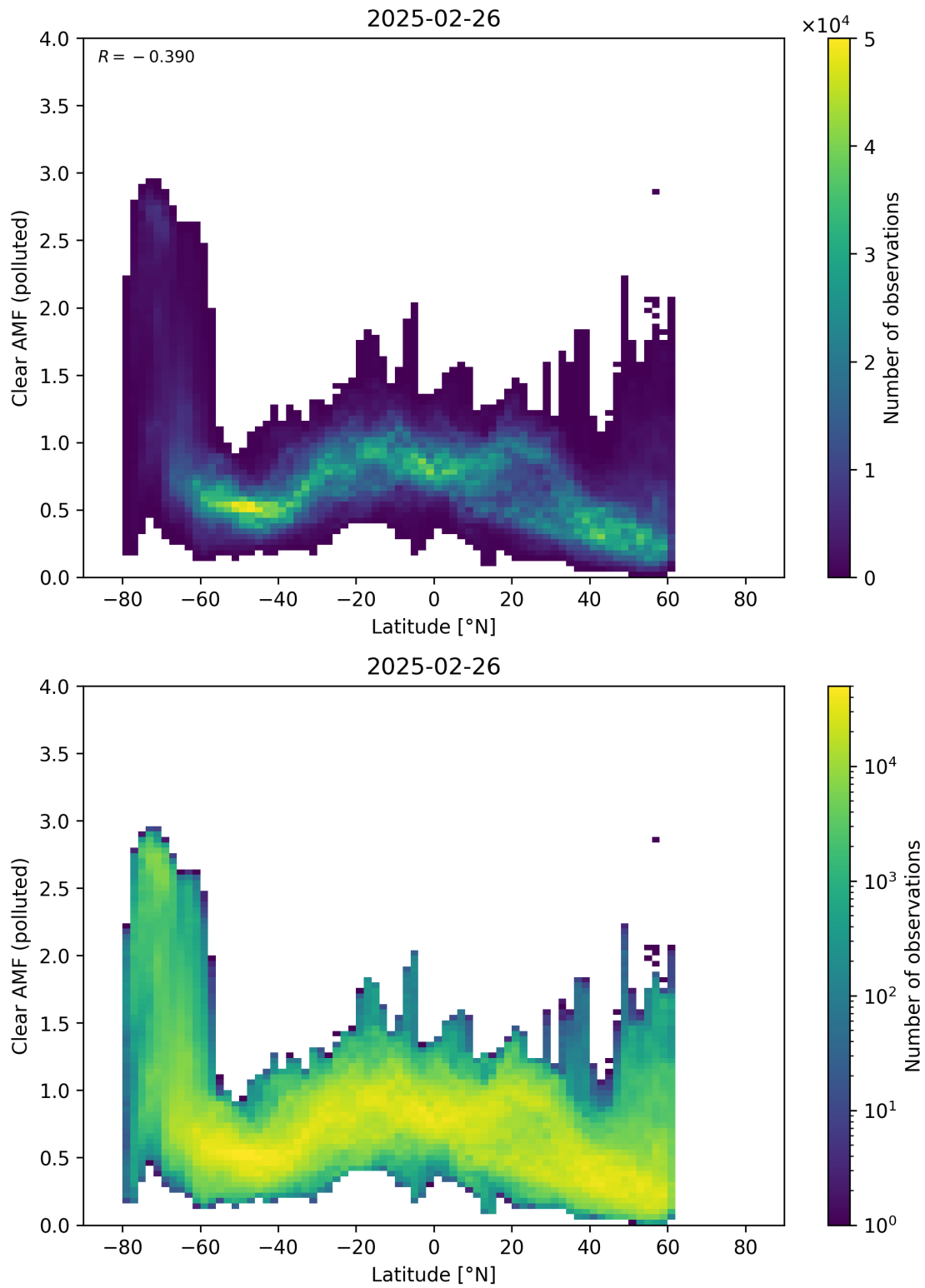
Figure 156: Scatter density plot of “Latitude” against “Clear AMF (polluted)” for 2025-02-25 to 2025-02-27.
