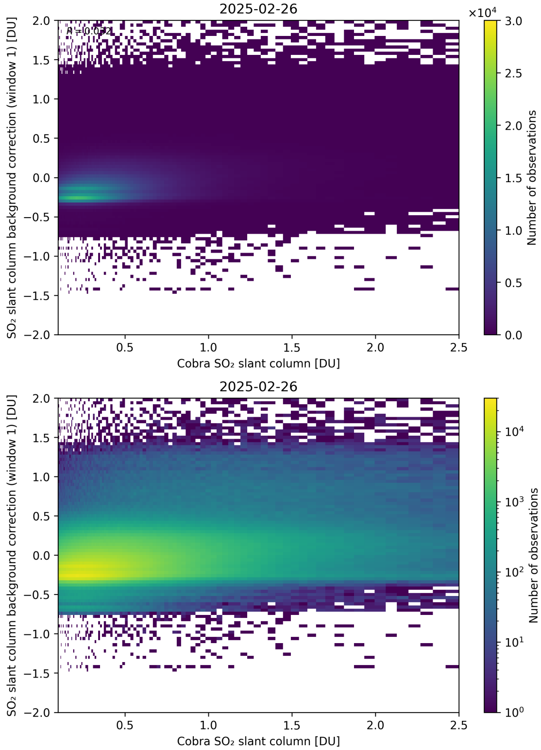
Figure 193: Scatter density plot of “Cobra SO 2 slant column” against “SO 2 slant column background correction (window 1)” for 2025-02-25 to 2025-02-27.
