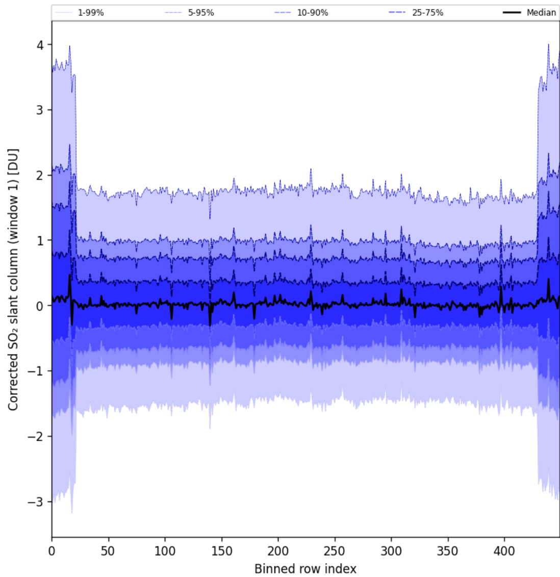
Figure 91: Along track statistics of “Corrected SO 2 slant column (window 1)” for 2025-02-25 to 2025-02-27
