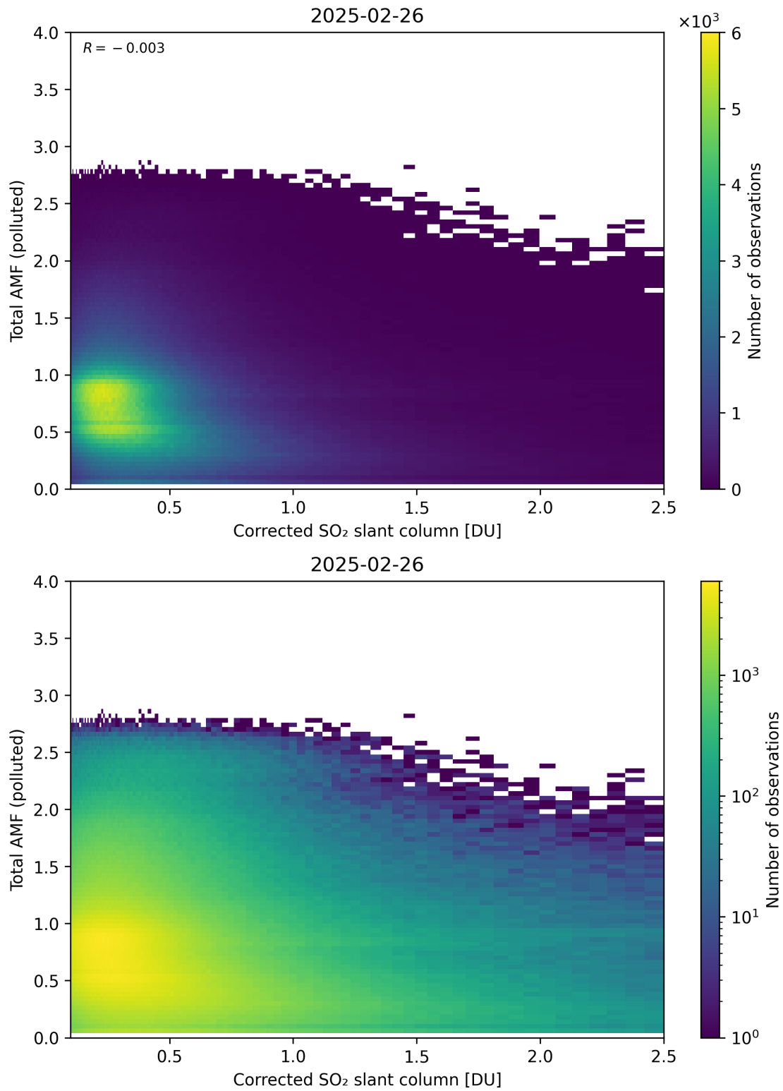
Figure 242: Scatter density plot of “Corrected SO 2 slant column” against “Total AMF (polluted)” for 2025-02-25 to 2025-02-27.
