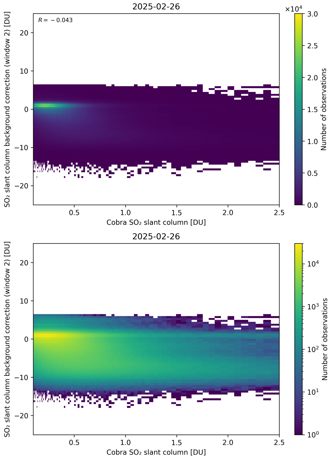
Figure 194: Scatter density plot of “Cobra SO 2 slant column” against “SO 2 slant column background correction (window 2)” for 2025-02-25 to 2025-02-27.
