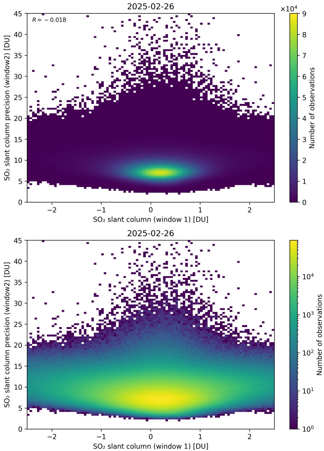
Figure 286: Scatter density plot of “SO 2 slant column (window 1)” against “SO 2 slant column precision (window2)” for 2025-02-25 to 2025-02-27.
