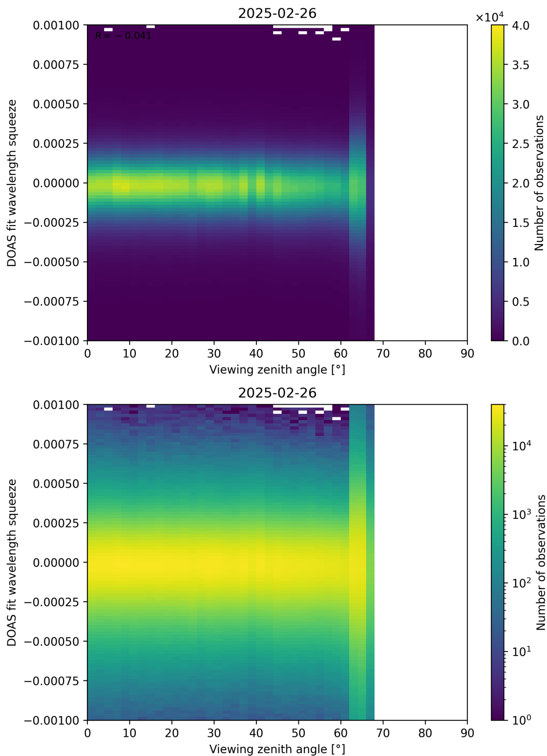
Figure 366: Scatter density plot of “Viewing zenith angle” against “DOAS fit wavelength squeeze” for 2025-02-25 to 2025-02-27.
