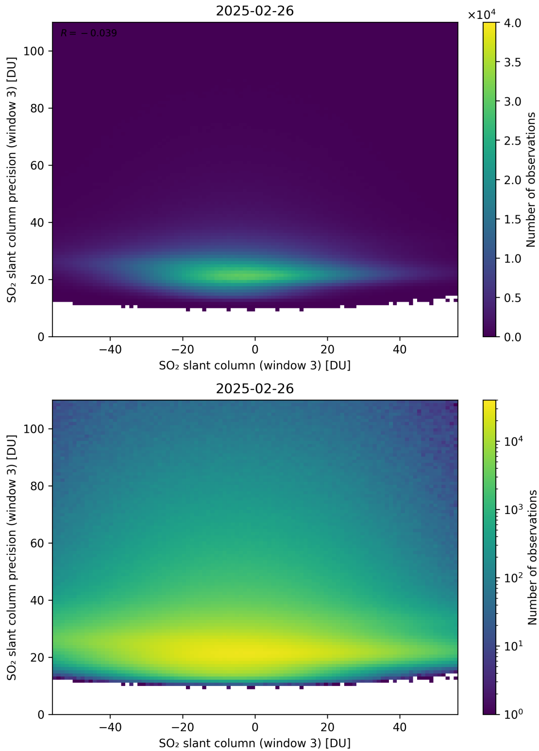
Figure 317: Scatter density plot of “SO 2 slant column (window 3)” against “SO 2 slant column precision (window 3)” for 2025-02-25 to 2025-02-27.
