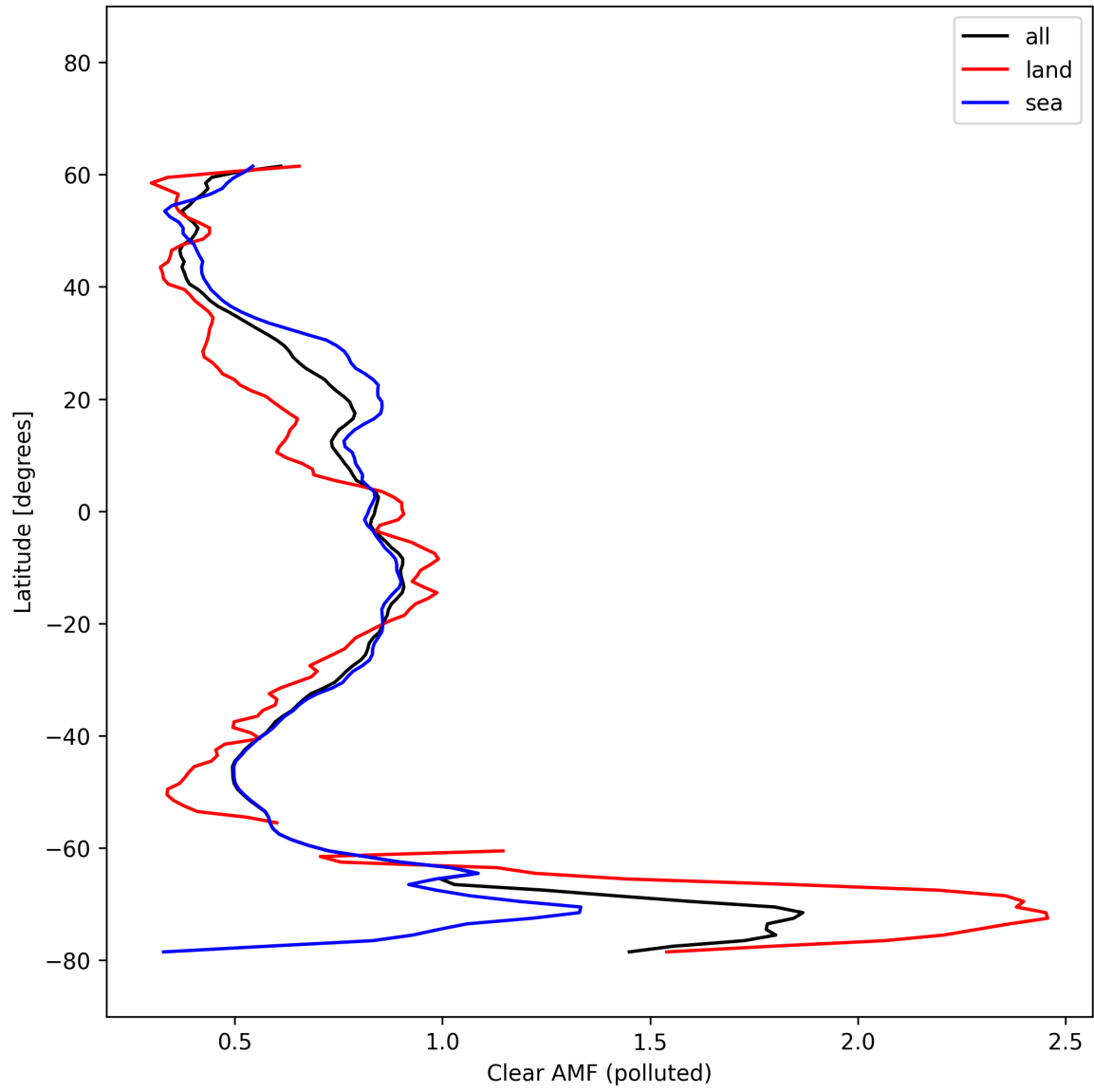
Figure 55: Zonal average of “Clear AMF (polluted)” for 2025-02-25 to 2025-02-27.
