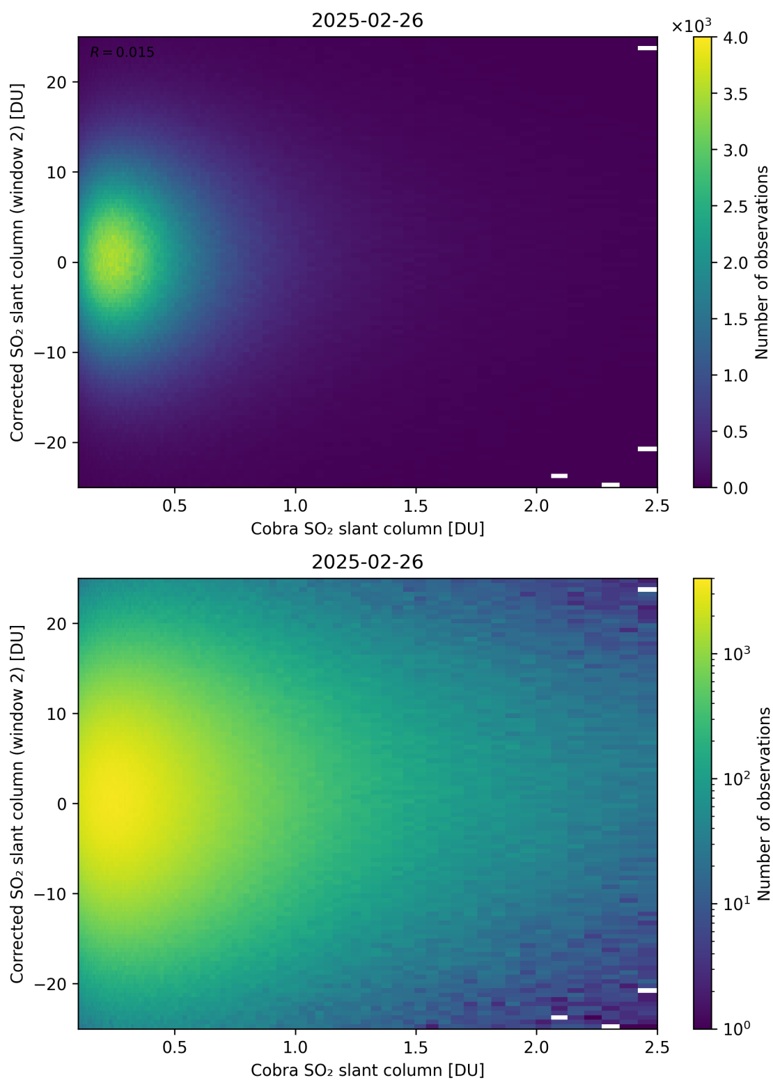
Figure 217: Scatter density plot of “Cobra SO 2 slant column” against “Corrected SO 2 slant column (window 2)” for 2025-02-25 to 2025-02-27.
