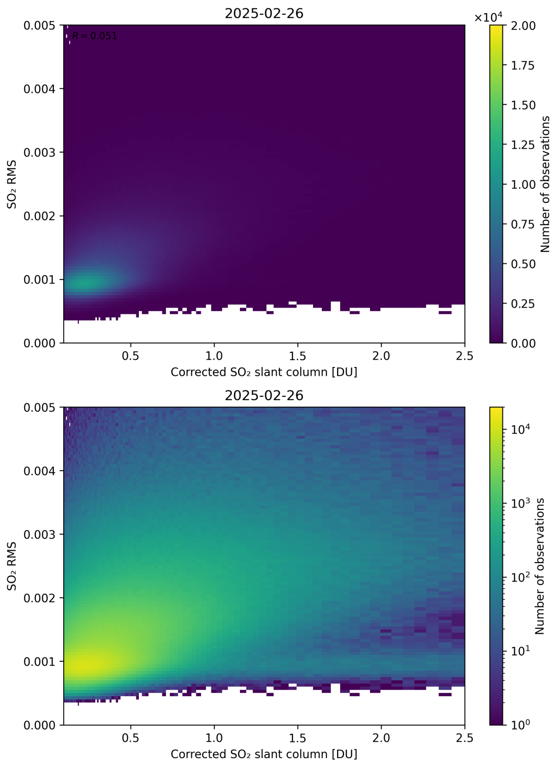
Figure 231: Scatter density plot of “Corrected SO 2 slant column” against “SO 2 RMS” for 2025-02-25 to 2025-02-27.
