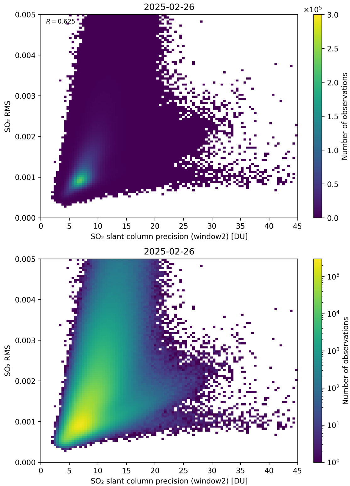
Figure 295: Scatter density plot of “SO 2 slant column precision (window2)” against “SO 2 RMS” for 2025-02-25 to 2025-02-27.
