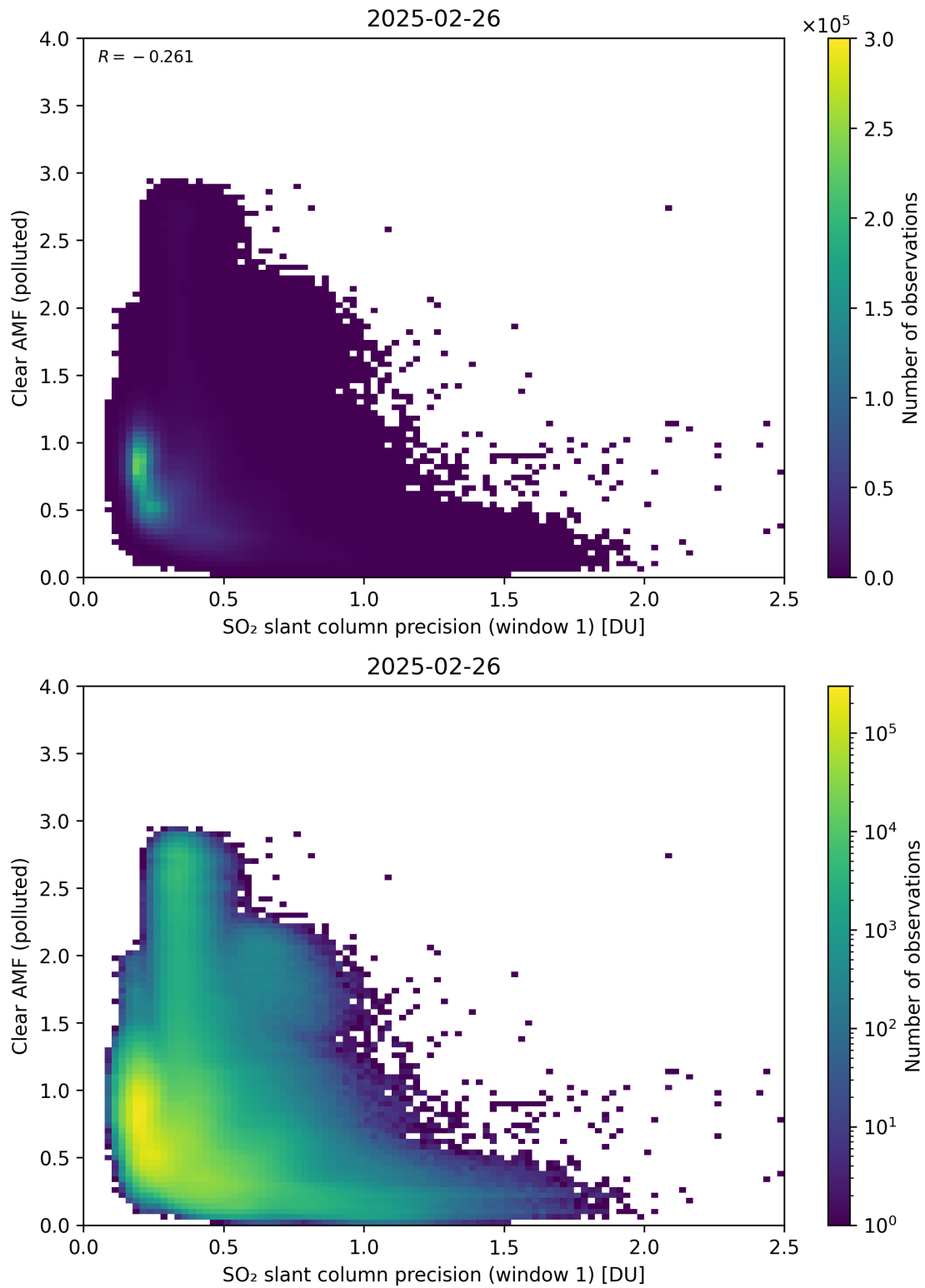
Figure 274: Scatter density plot of “SO 2 slant column precision (window 1)” against “Clear AMF (polluted)” for 2025-02-25 to 2025-02-27.
