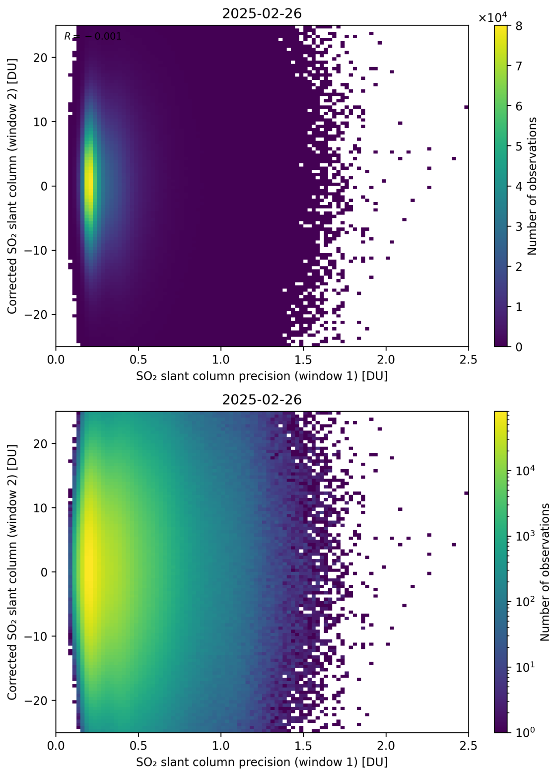
Figure 275: Scatter density plot of “SO 2 slant column precision (window 1)” against “Corrected SO 2 slant column (window 2)” for 2025-02-25 to 2025-02-27.
