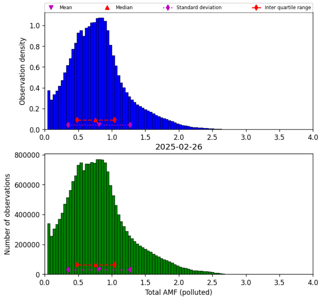
Figure 79: Histogram of “Total AMF (polluted)” for 2025-02-25 to 2025-02-27
