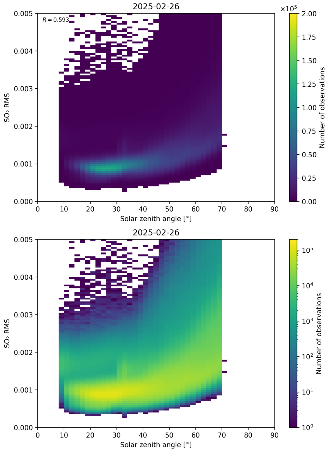
Figure 176: Scatter density plot of “Solar zenith angle” against “SO 2 RMS” for 2025-02-25 to 2025-02-27.
