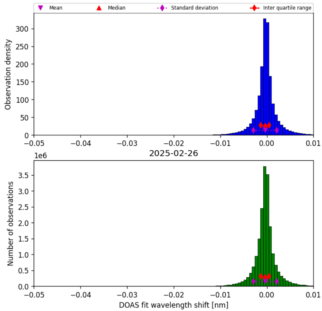
Figure 76: Histogram of “DOAS fit wavelength shift” for 2025-02-25 to 2025-02-27
