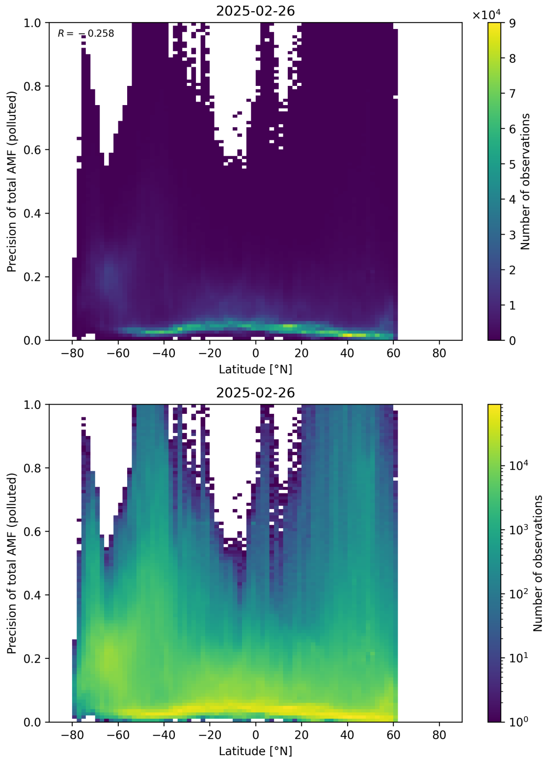
Figure 168: Scatter density plot of “Latitude” against “Precision of total AMF (polluted)” for 2025-02-25 to 2025-02-27.
