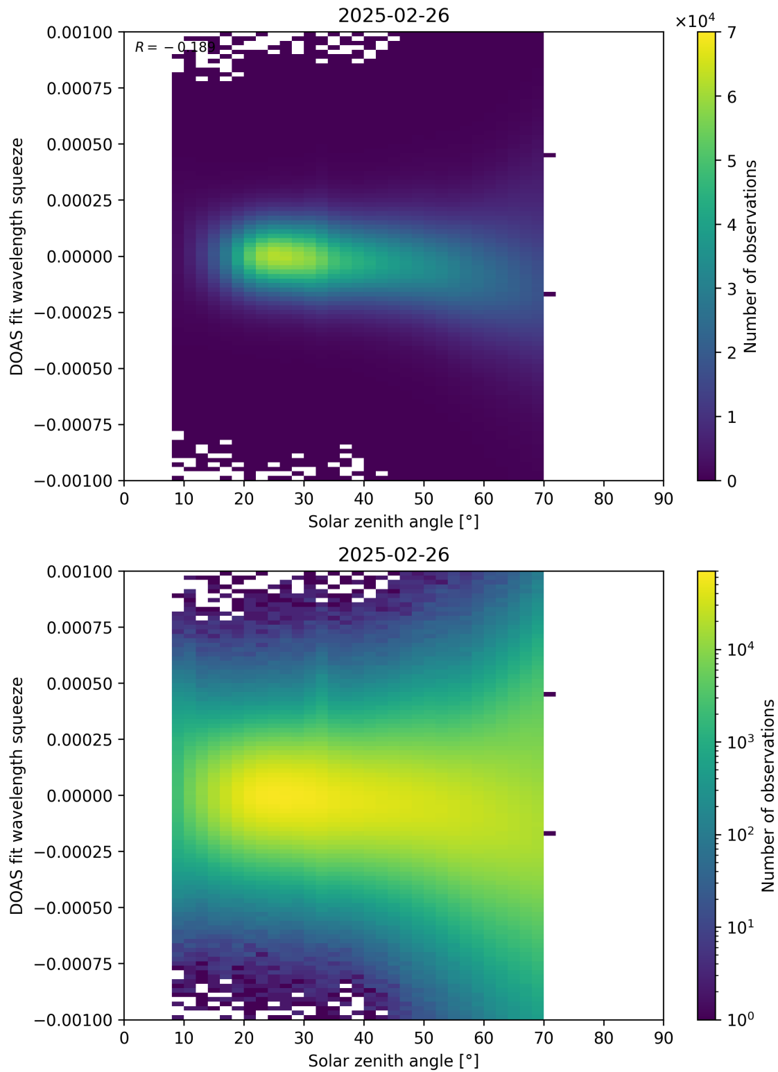
Figure 175: Scatter density plot of “Solar zenith angle” against “DOAS fit wavelength squeeze” for 2025-02-25 to 2025-02-27.
