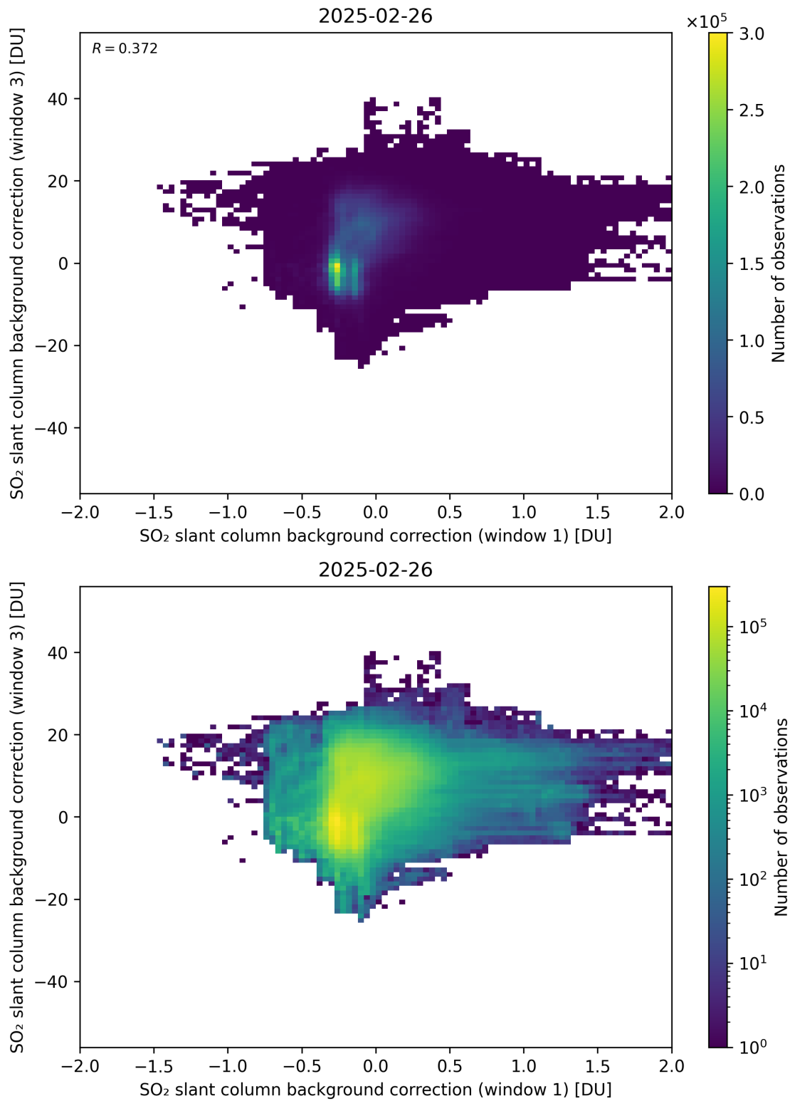
Figure 110: Scatter density plot of “SO 2 slant column background correction (window 1)” against “SO 2 slant column background correction (window 3)” for 2025-02-25 to 2025-02-27.
