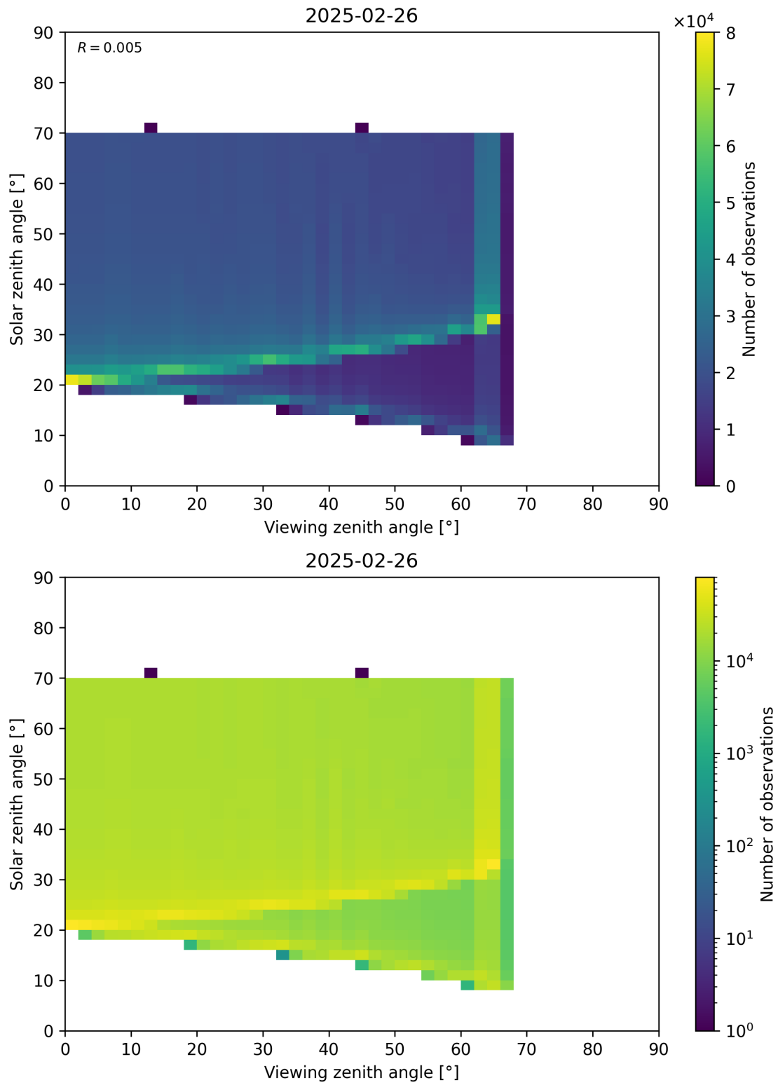
Figure 369: Scatter density plot of “Viewing zenith angle” against “Solar zenith angle” for 2025-02-25 to 2025-02-27.
