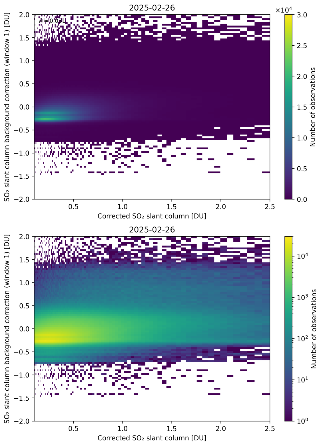
Figure 226: Scatter density plot of “Corrected SO 2 slant column” against “SO 2 slant column background correction (window 1)” for 2025-02-25 to 2025-02-27.
