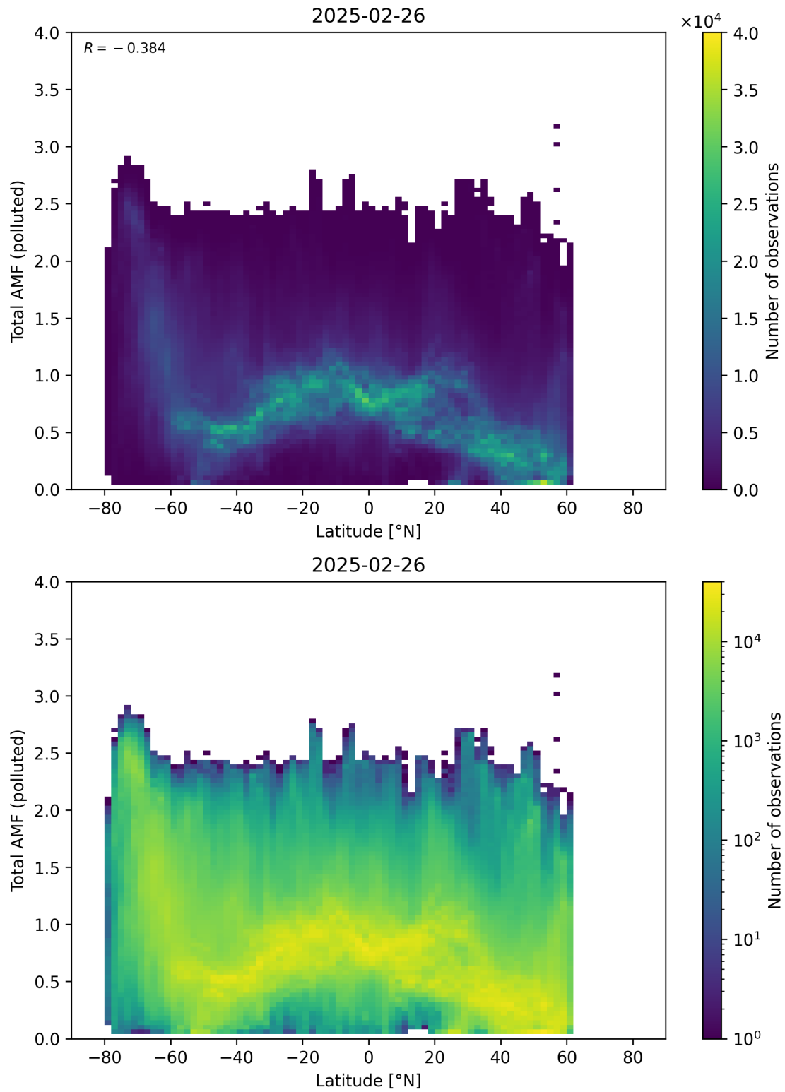
Figure 167: Scatter density plot of “Latitude” against “Total AMF (polluted)” for 2025-02-25 to 2025-02-27.
