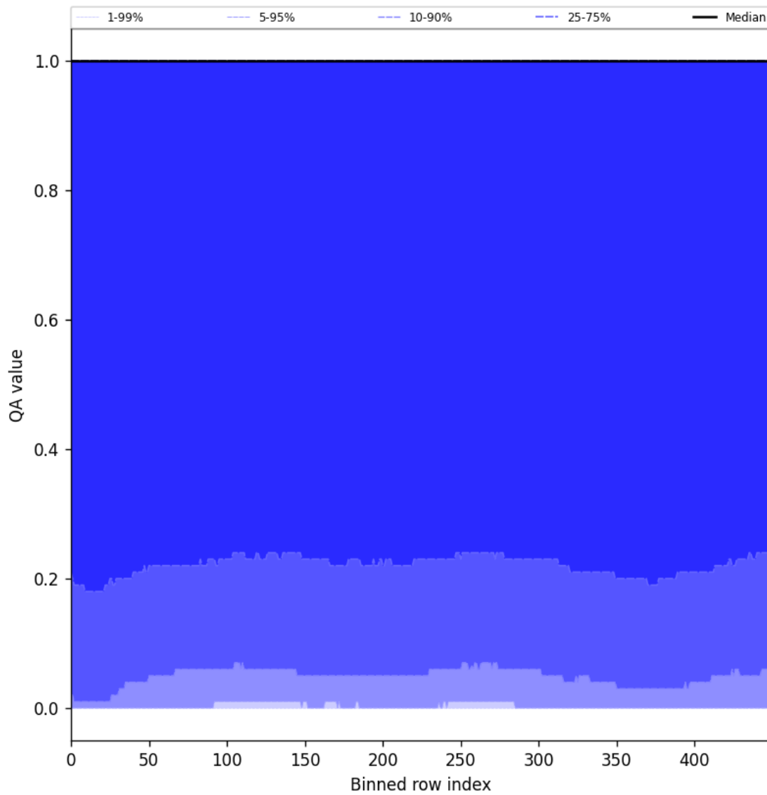
Figure 83: Along track statistics of “QA value” for 2025-02-25 to 2025-02-27
