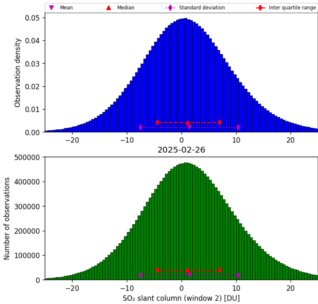
Figure 67: Histogram of “SO 2 slant column (window 2)” for 2025-02-25 to 2025-02-27
