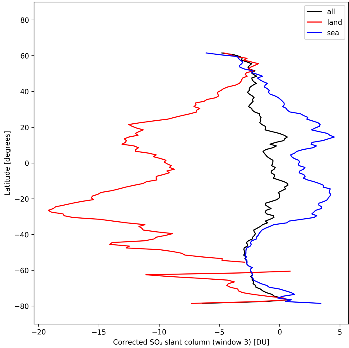
Figure 47: Zonal average of “Corrected SO 2 slant column (window 3)” for 2025-02-25 to 2025-02-27.
