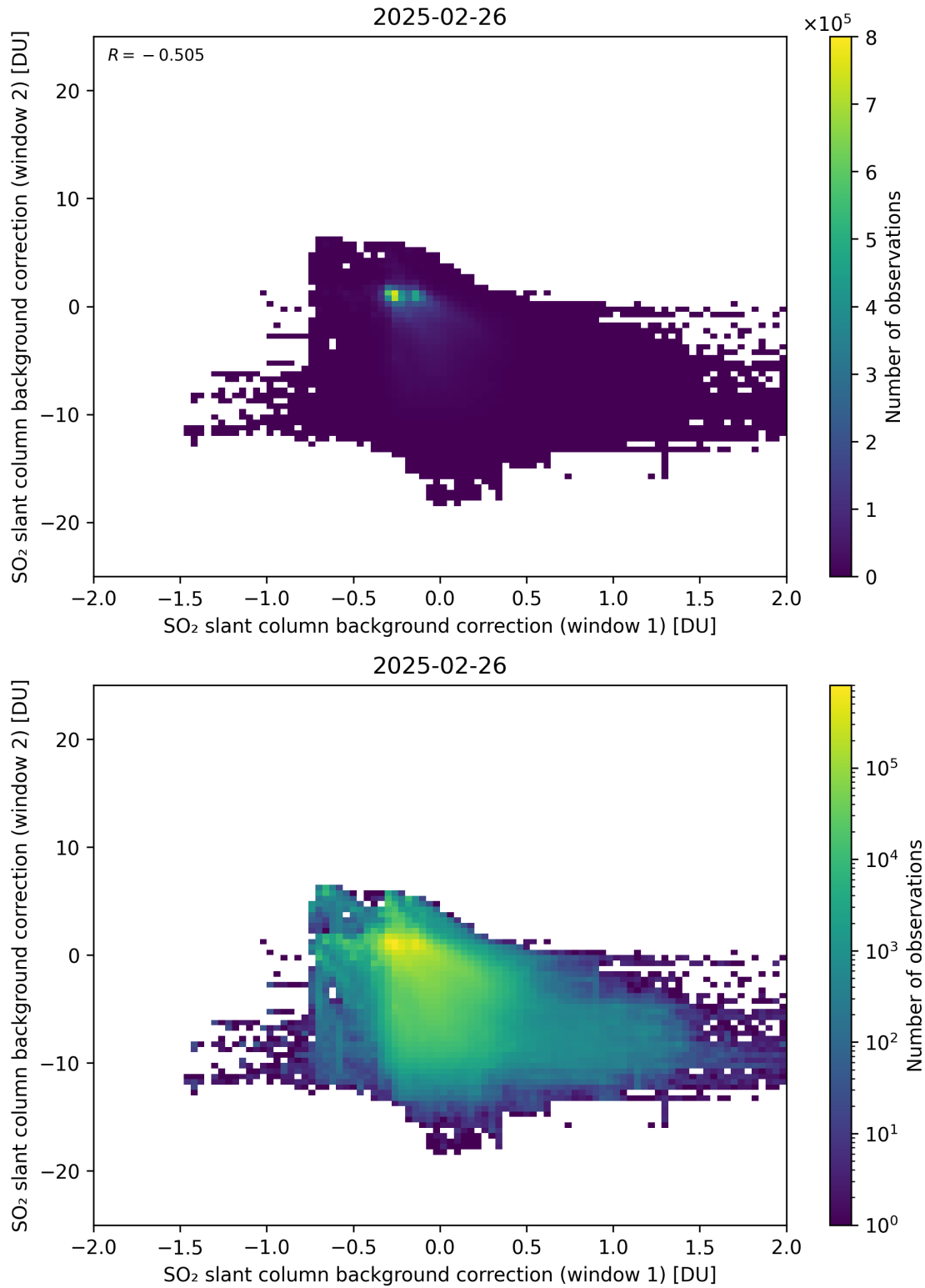
Figure 109: Scatter density plot of “SO 2 slant column background correction (window 1)” against “SO 2 slant column background correction (window 2)” for 2025-02-25 to 2025-02-27.
