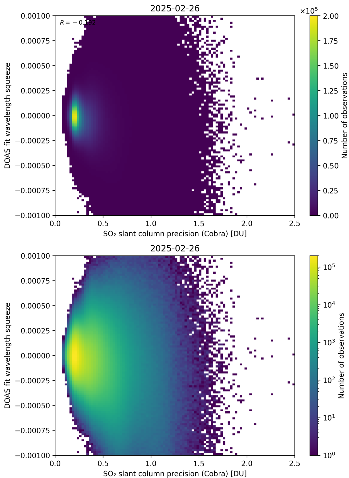
Figure 203: Scatter density plot of “SO 2 slant column precision (Cobra)” against “DOAS fit wavelength squeeze” for 2025-02-25 to 2025-02-27.
