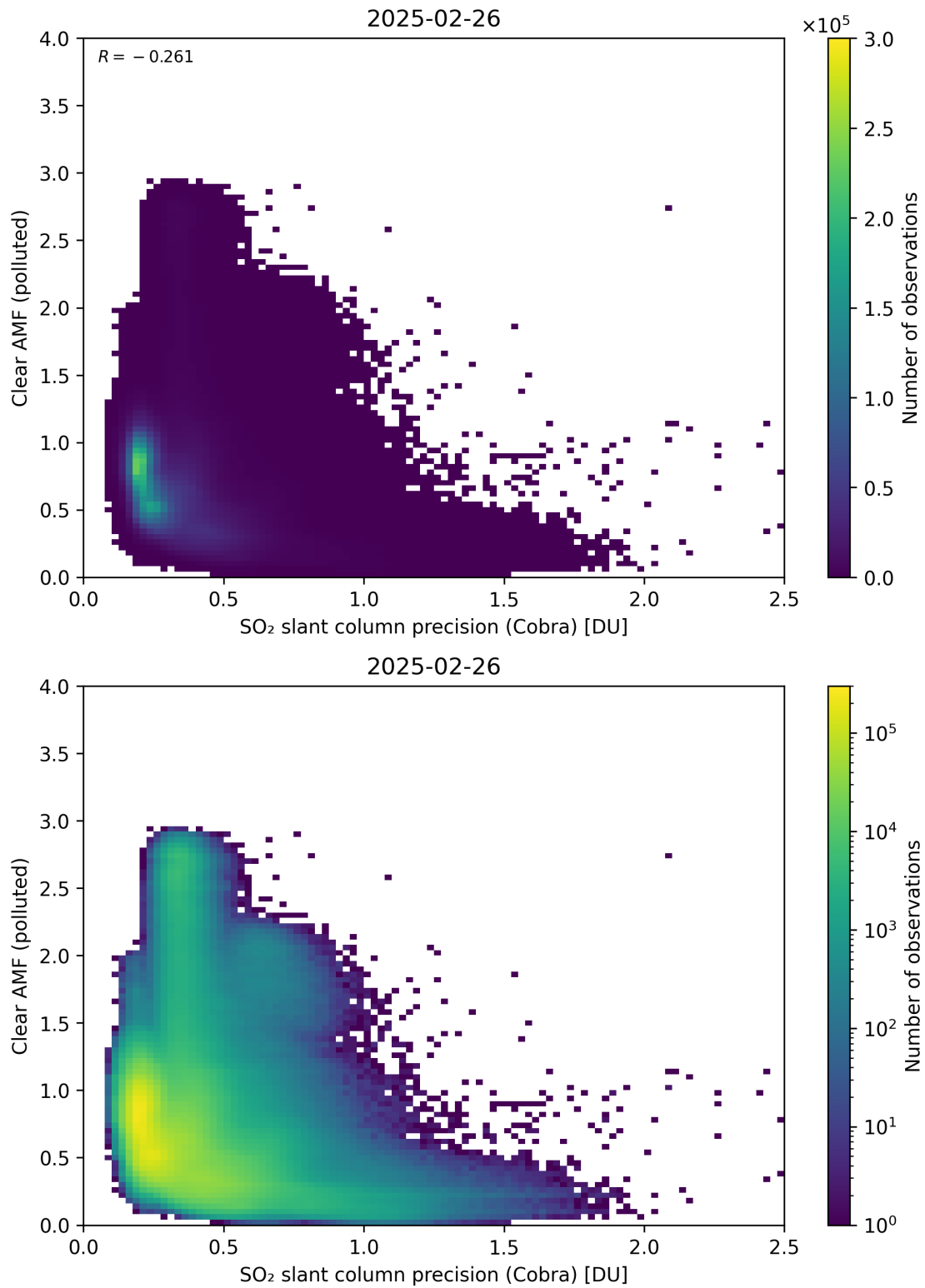
Figure 205: Scatter density plot of “SO 2 slant column precision (Cobra)” against “Clear AMF (polluted)” for 2025-02-25 to 2025-02-27.
