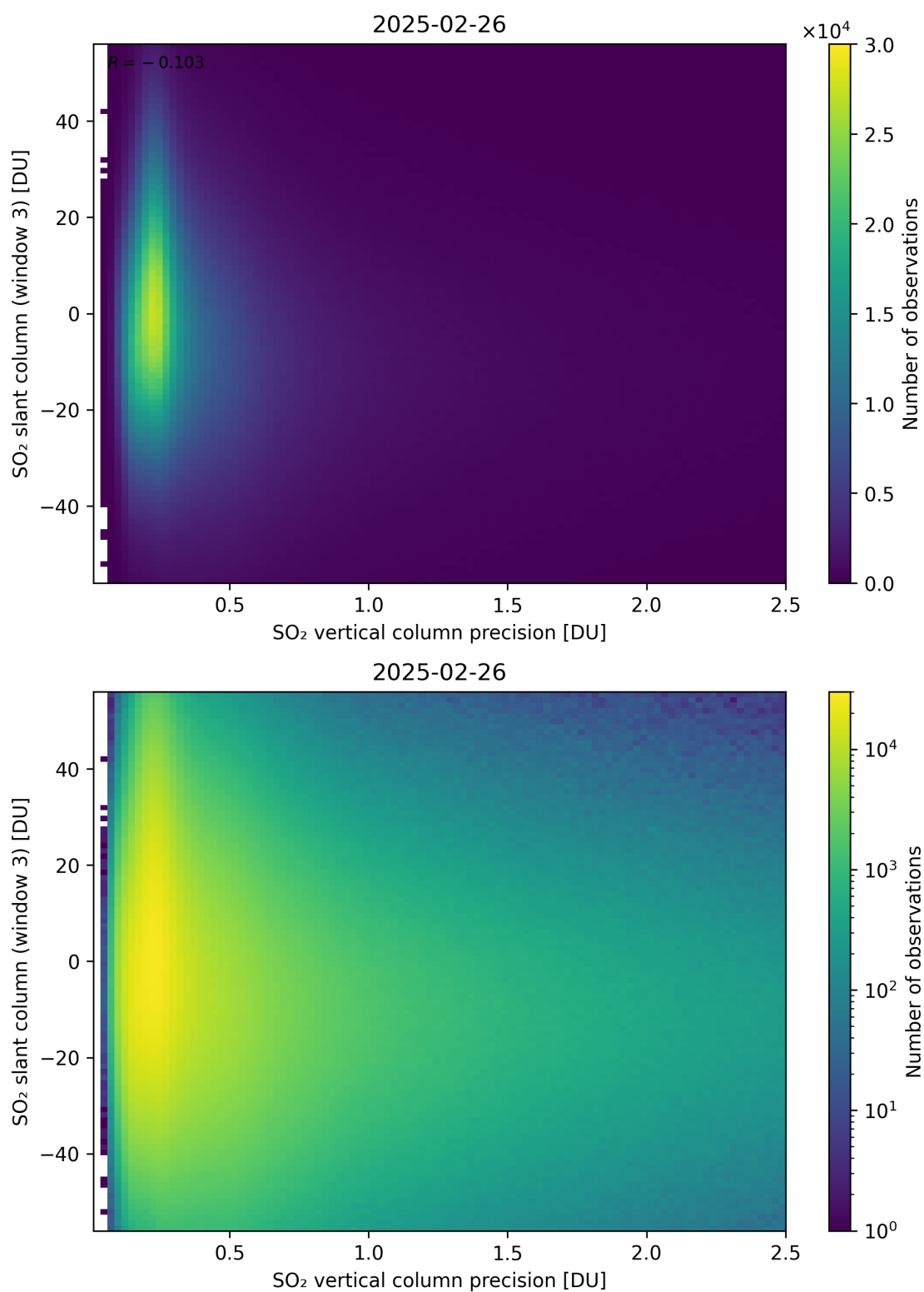
Figure 344: Scatter density plot of “SO 2 vertical column precision” against “SO 2 slant column (window 3)” for 2025-02-25 to 2025-02-27.
