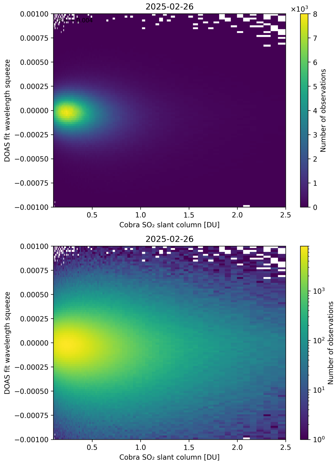
Figure 197: Scatter density plot of “Cobra SO 2 slant column” against “DOAS fit wavelength squeeze” for 2025-02-25 to 2025-02-27.
