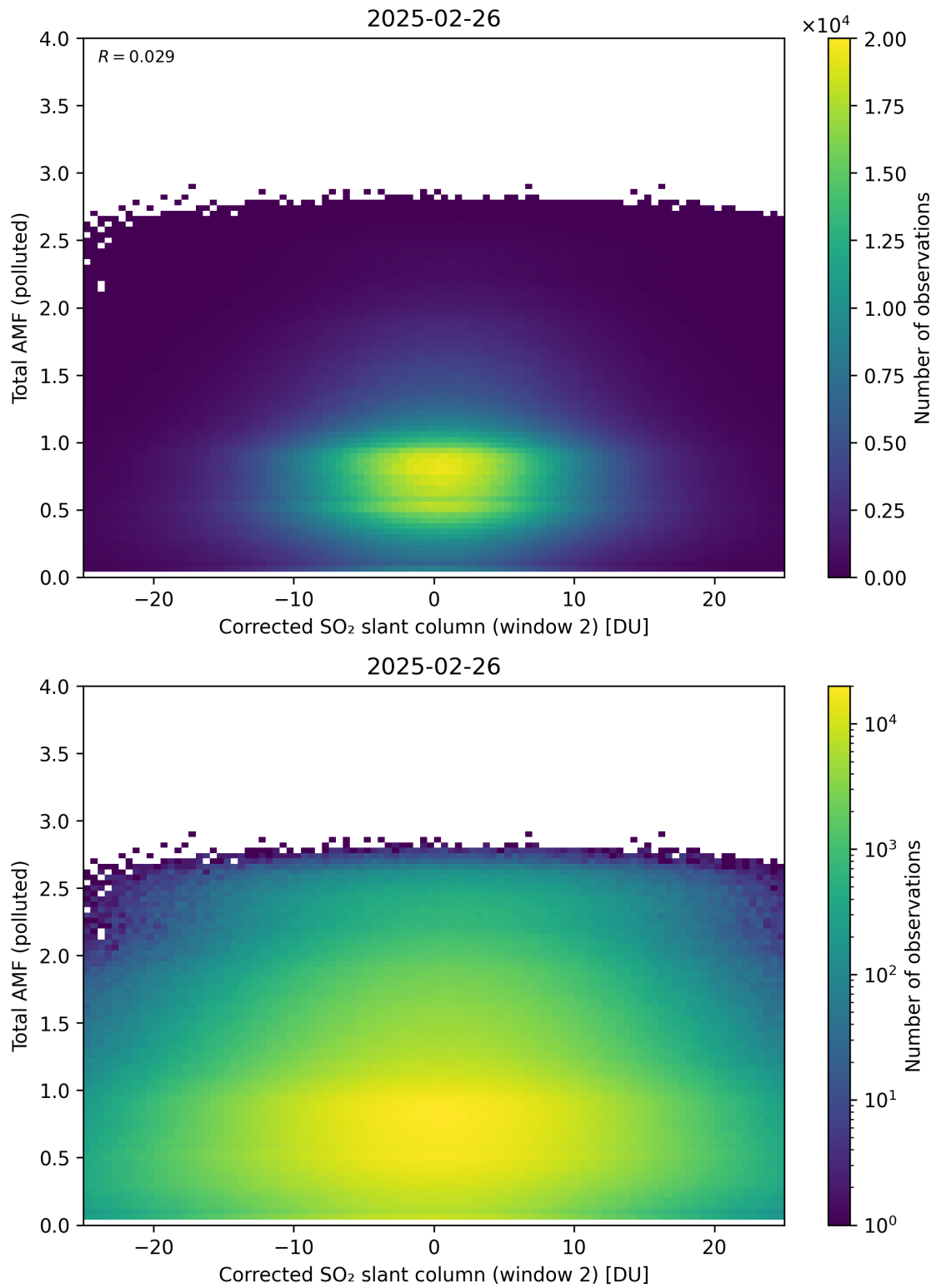
Figure 253: Scatter density plot of “Corrected SO 2 slant column (window 2)” against “Total AMF (polluted)” for 2025-02-25 to 2025-02-27.
