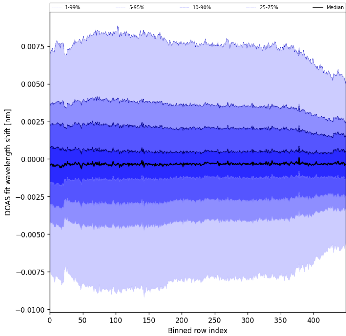
Figure 102: Along track statistics of “DOAS fit wavelength shift” for 2025-02-25 to 2025-02-27
