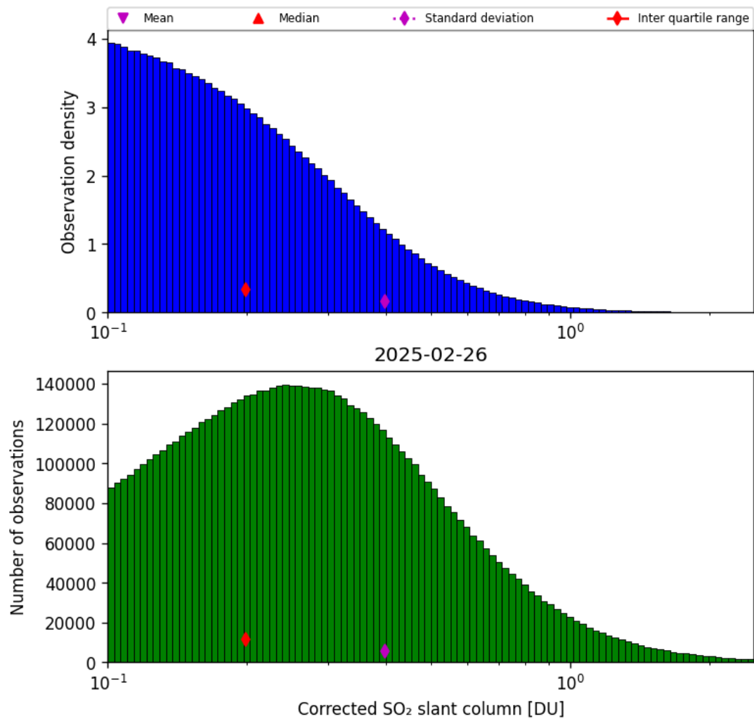
Figure 60: Histogram of “Corrected SO 2 slant column” for 2025-02-25 to 2025-02-27
