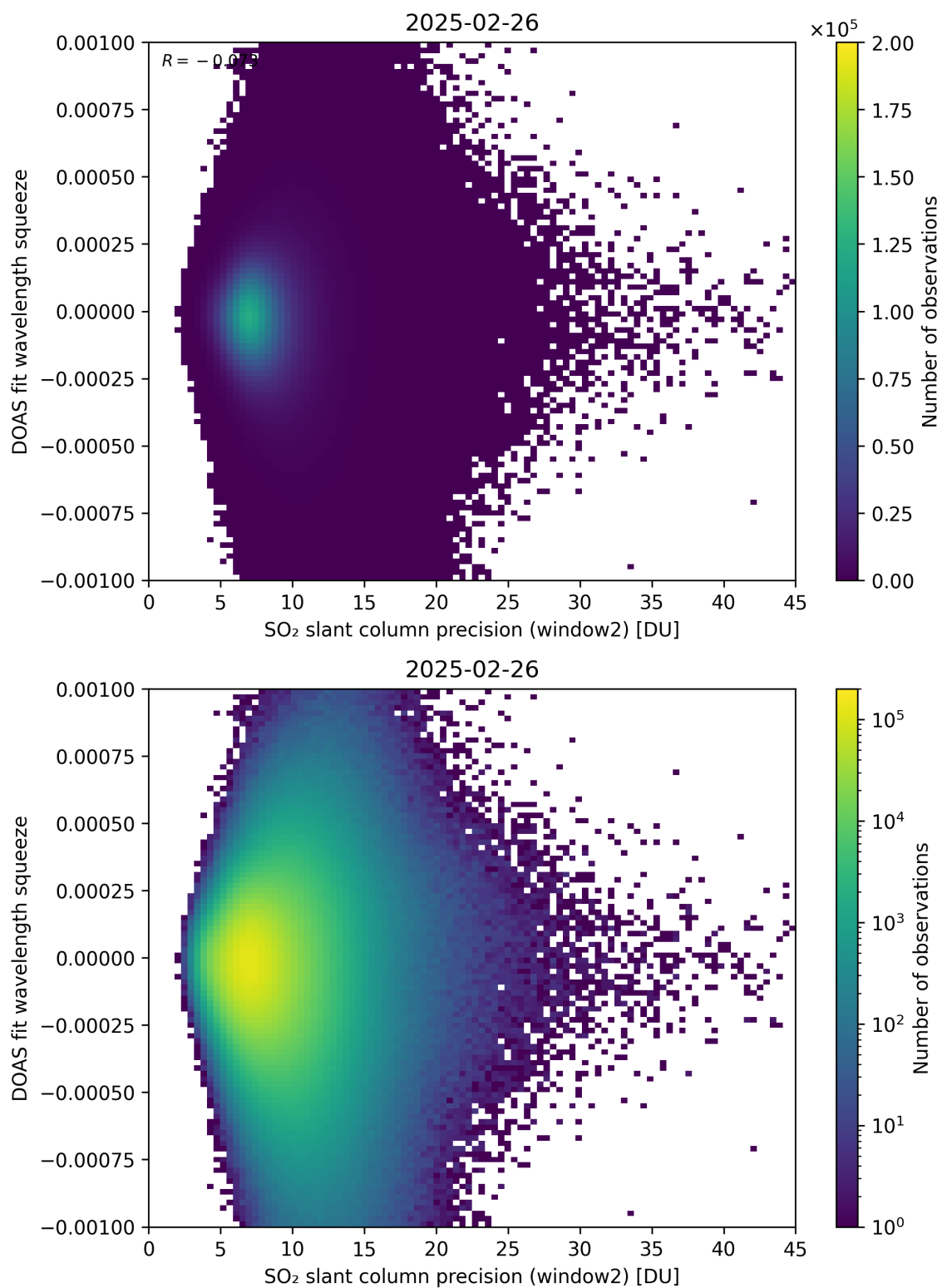
Figure 294: Scatter density plot of “SO 2 slant column precision (window2)” against “DOAS fit wavelength squeeze” for 2025-02-25 to 2025-02-27.
