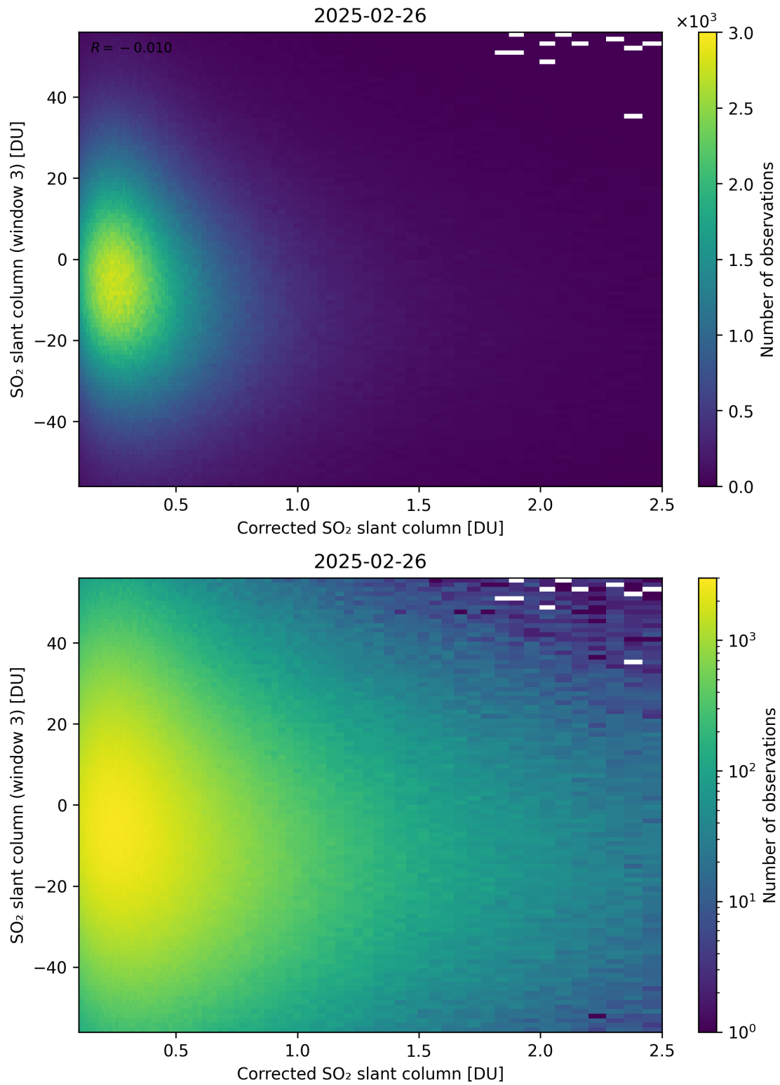
Figure 240: Scatter density plot of “Corrected SO 2 slant column” against “SO 2 slant column (window 3)” for 2025-02-25 to 2025-02-27.
