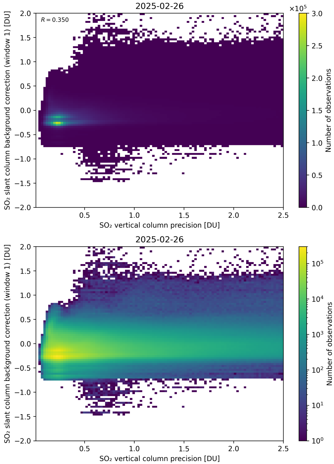
Figure 329: Scatter density plot of “SO 2 vertical column precision” against “SO 2 slant column background correction (window 1)” for 2025-02-25 to 2025-02-27.
