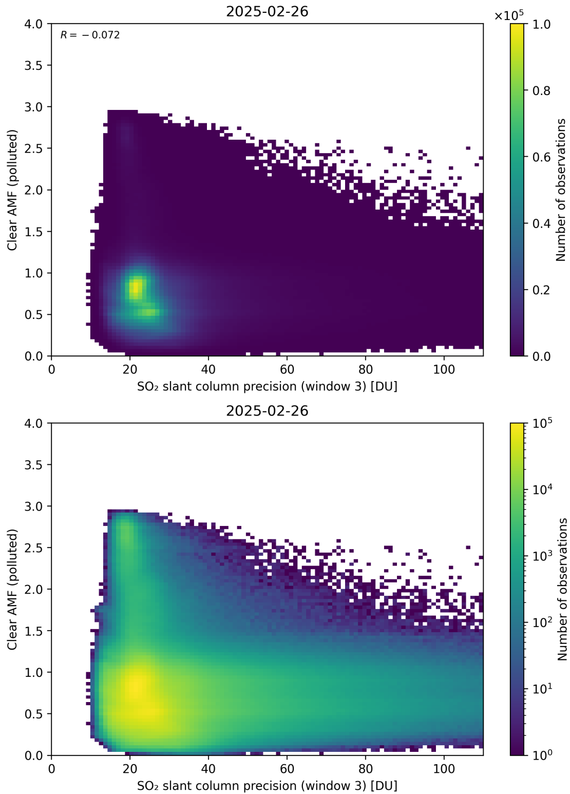
Figure 311: Scatter density plot of “SO 2 slant column precision (window 3)” against “Clear AMF (polluted)” for 2025-02-25 to 2025-02-27.
