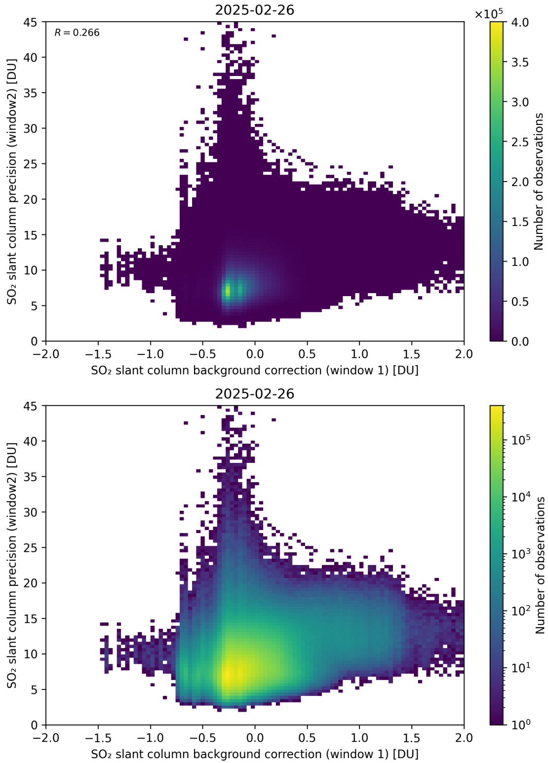
Figure 117: Scatter density plot of “SO 2 slant column background correction (window 1)” against “SO 2 slant column precision (window2)” for 2025-02-25 to 2025-02-27.
