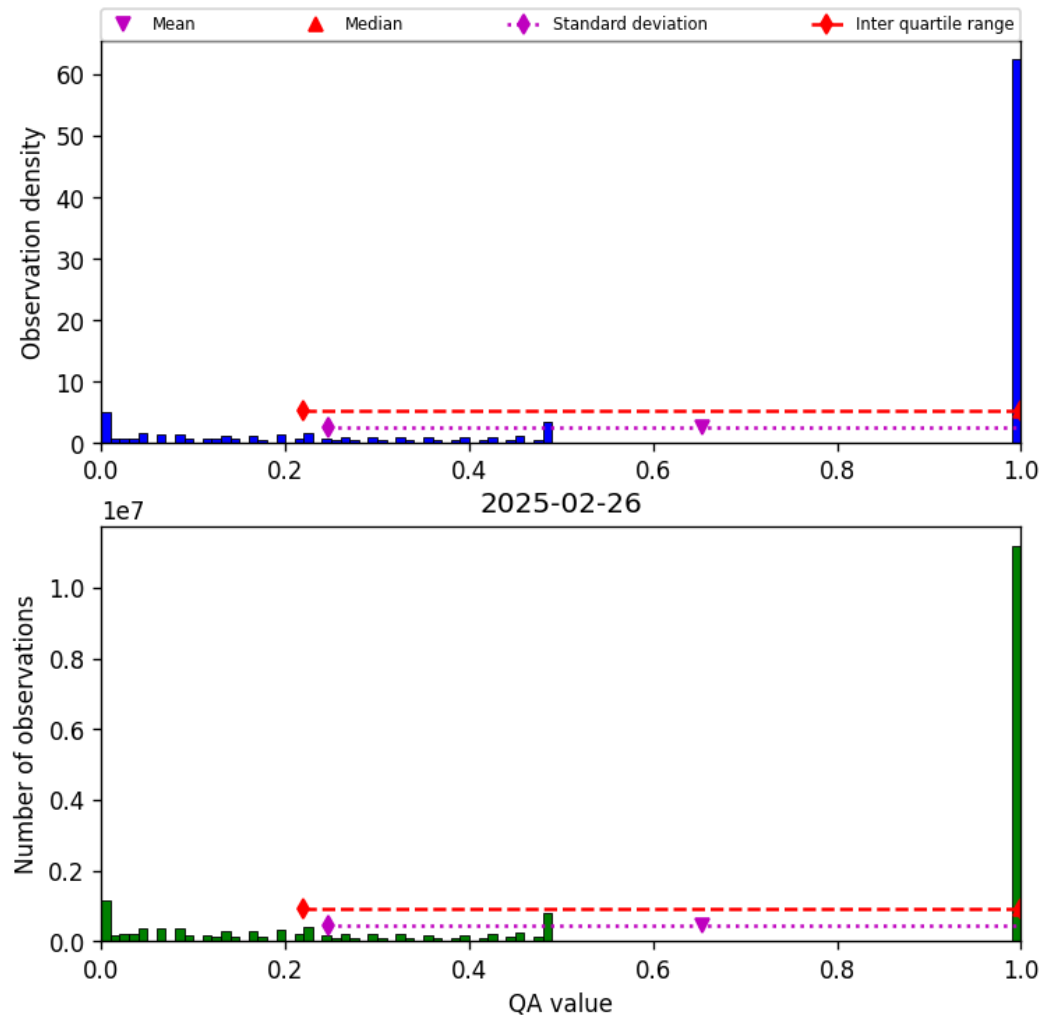
Figure 57: Histogram of “QA value” for 2025-02-25 to 2025-02-27
