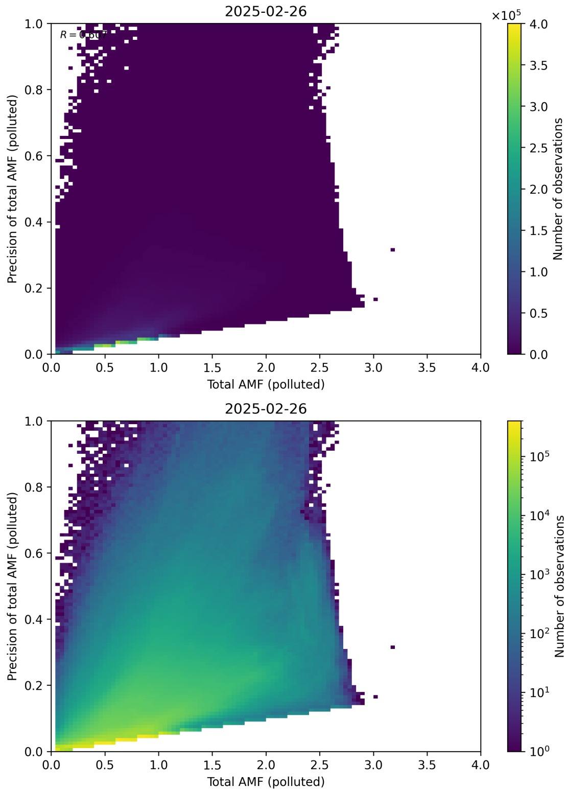
Figure 322: Scatter density plot of “Total AMF (polluted)” against “Precision of total AMF (polluted)” for 2025-02-25 to 2025-02-27.
