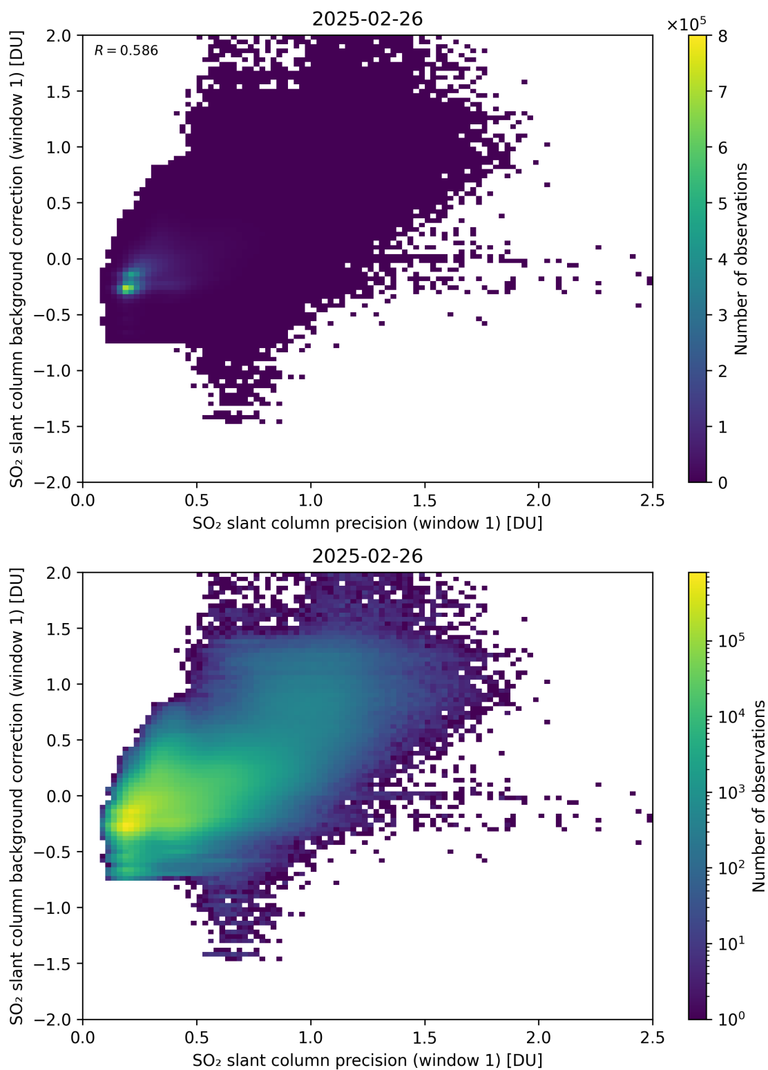
Figure 268: Scatter density plot of “SO 2 slant column precision (window 1)” against “SO 2 slant column background correction (window 1)” for 2025-02-25 to 2025-02-27.
