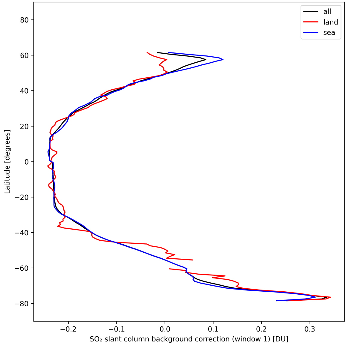
Figure 40: Zonal average of “SO 2 slant column background correction (window 1)” for 2025-02-25 to 2025-02-27.
