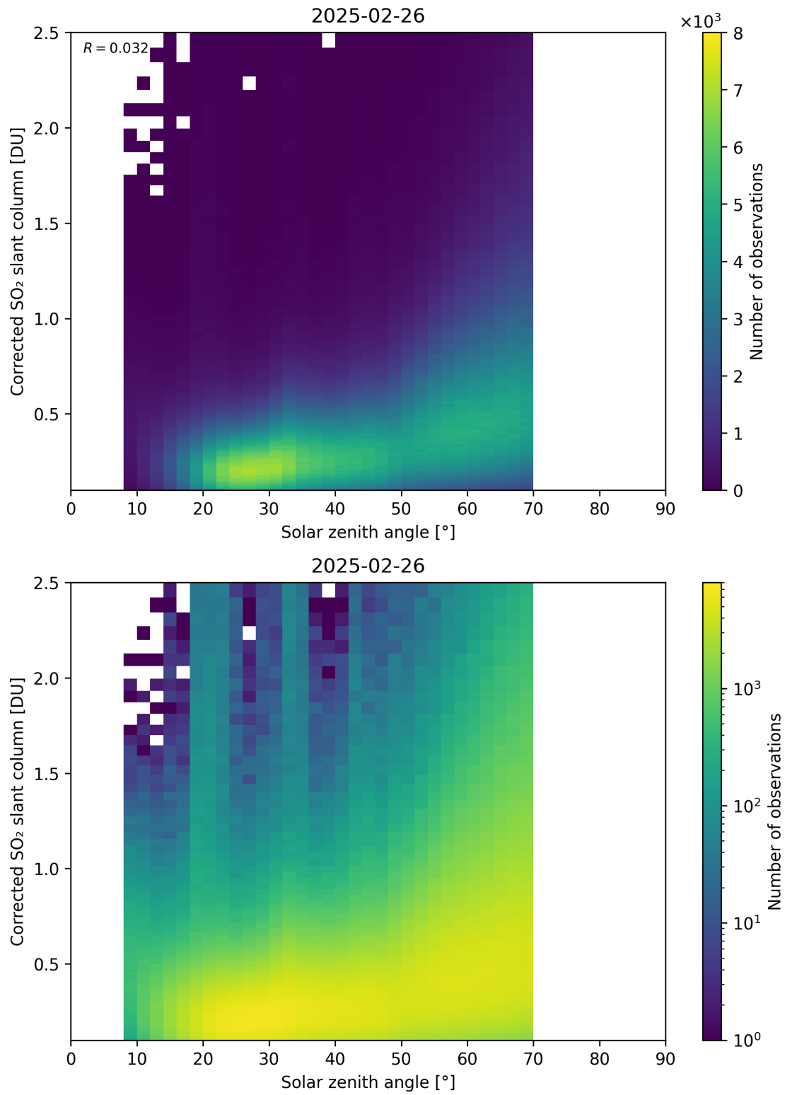
Figure 181: Scatter density plot of “Solar zenith angle” against “Corrected SO 2 slant column” for 2025-02-25 to 2025-02-27.
