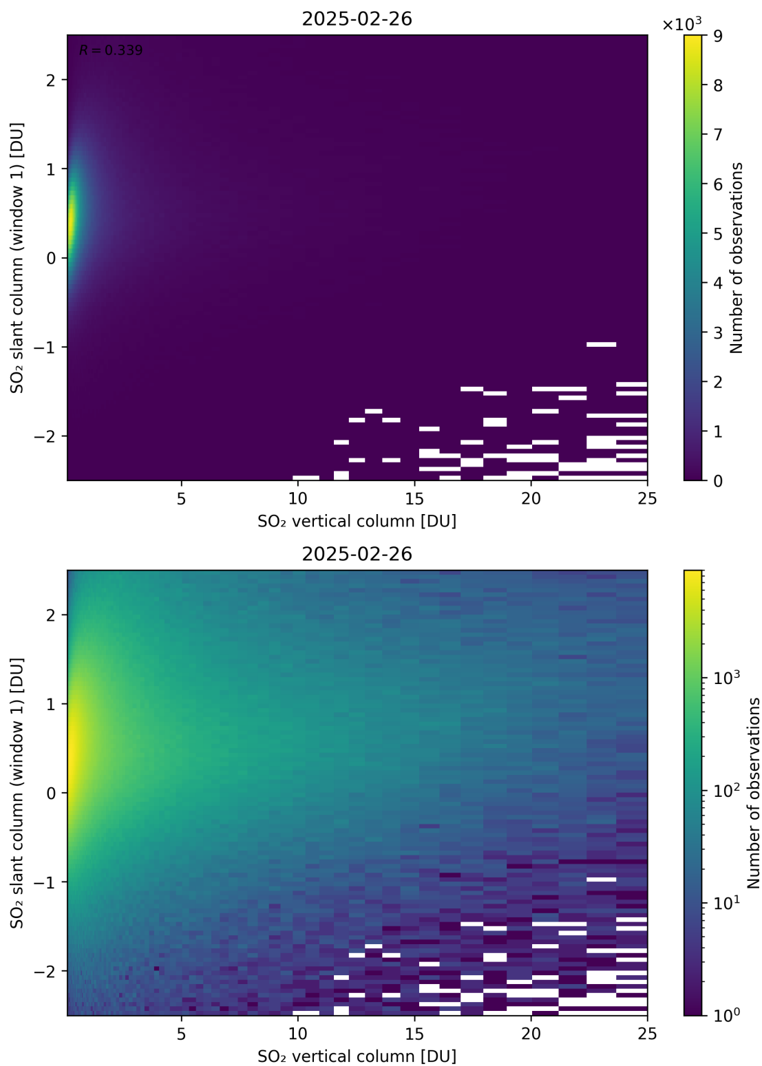
Figure 354: Scatter density plot of “SO 2 vertical column” against “SO 2 slant column (window 1)” for 2025-02-25 to 2025-02-27.
