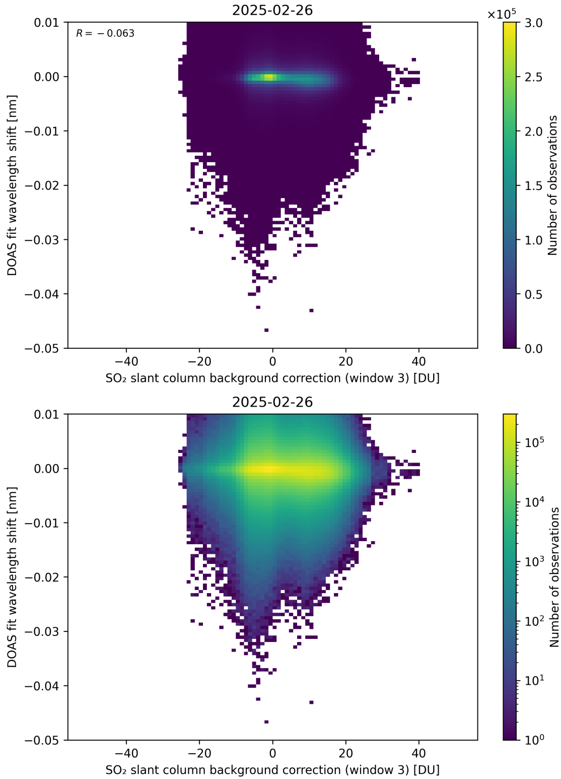
Figure 132: Scatter density plot of “SO 2 slant column background correction (window 3)” against “DOAS fit wavelength shift” for 2025-02-25 to 2025-02-27.
