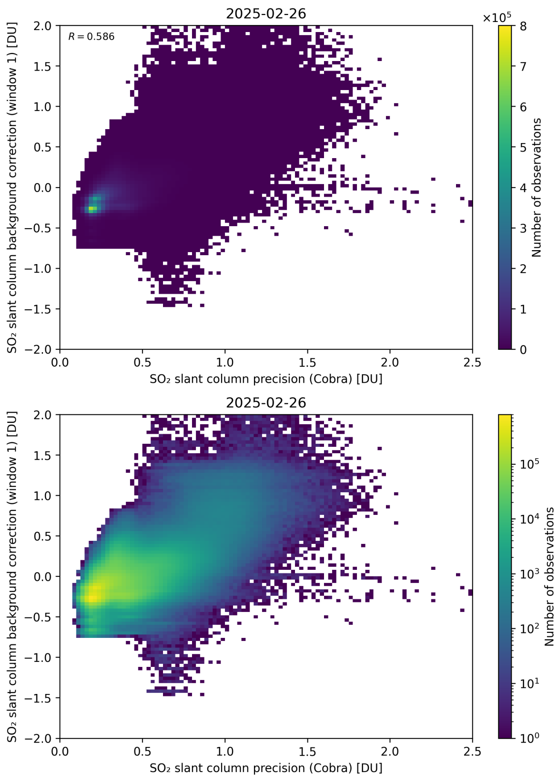
Figure 199: Scatter density plot of “SO 2 slant column precision (Cobra)” against “SO 2 slant column background correction (window 1)” for 2025-02-25 to 2025-02-27.
