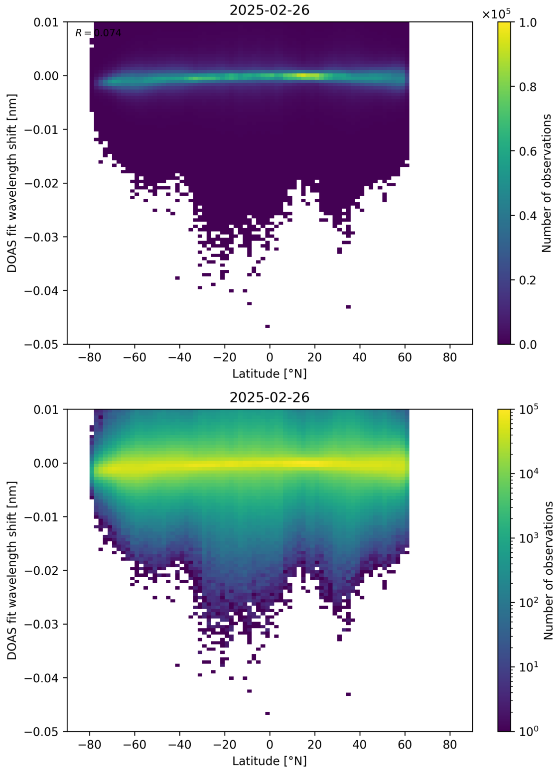
Figure 153: Scatter density plot of “Latitude” against “DOAS fit wavelength shift” for 2025-02-25 to 2025-02-27.
