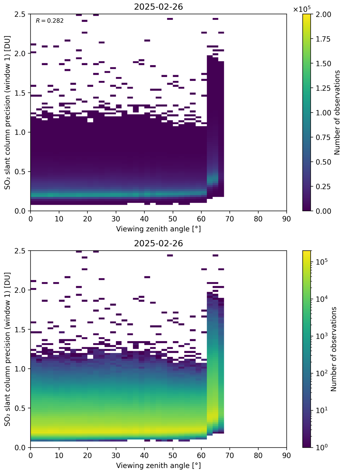
Figure 377: Scatter density plot of “Viewing zenith angle” against “SO 2 slant column precision (window 1)” for 2025-02-25 to 2025-02-27.
