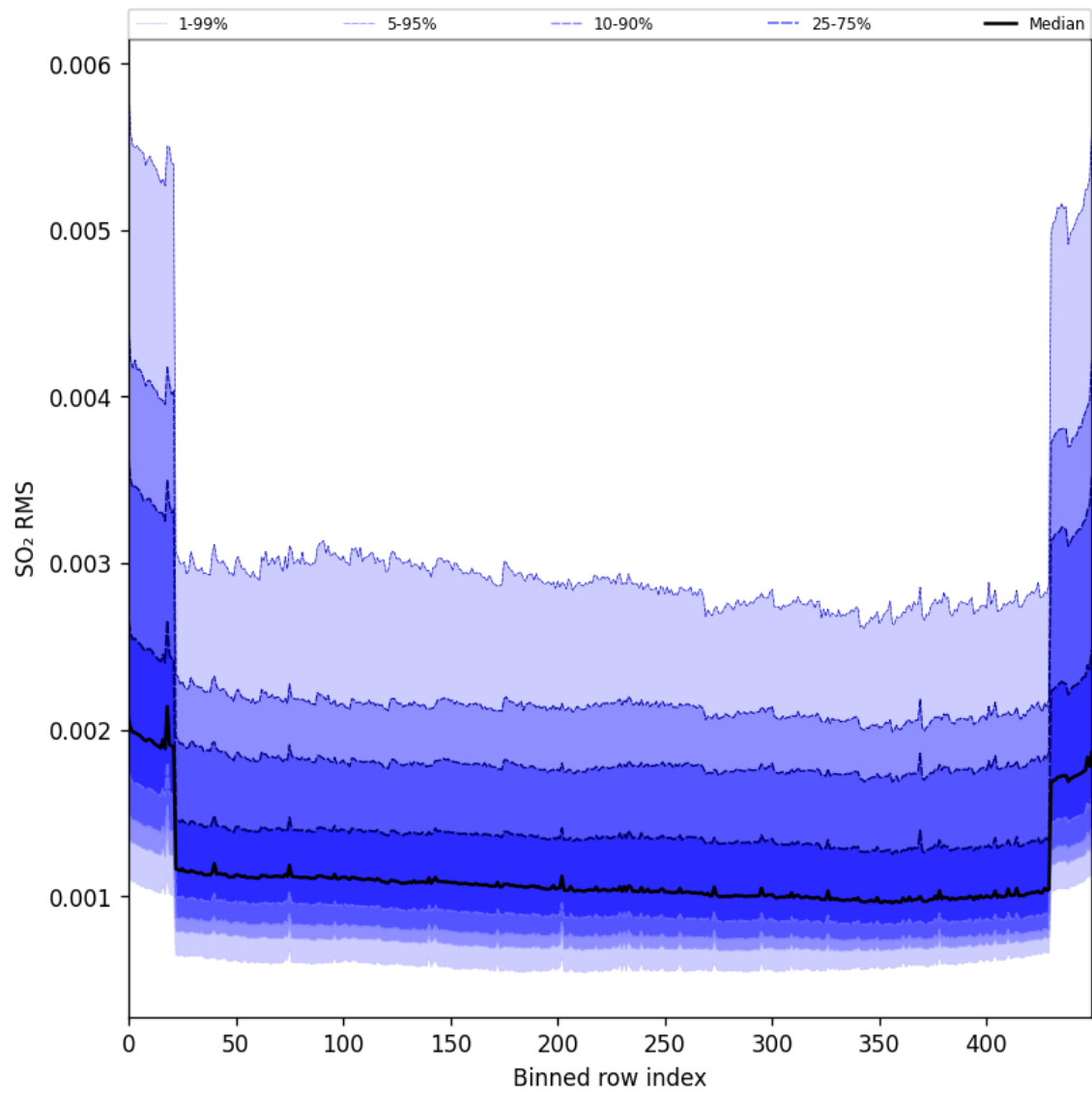
Figure 104: Along track statistics of “SO 2 RMS” for 2025-02-25 to 2025-02-27
