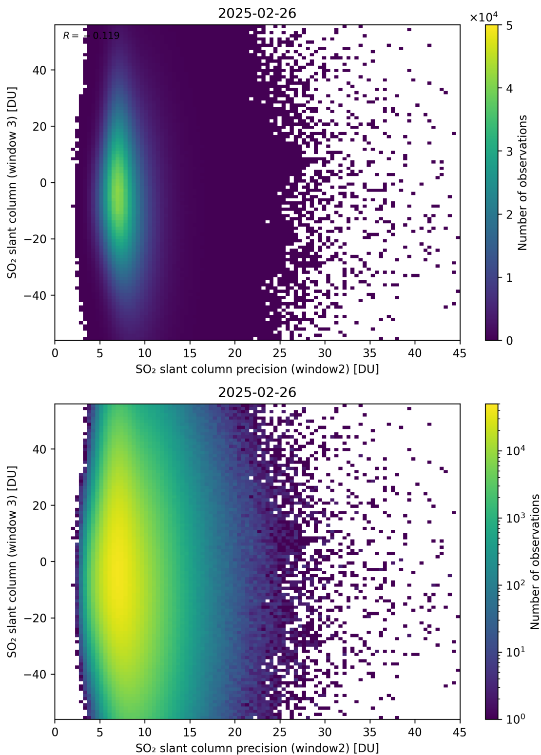
Figure 299: Scatter density plot of “SO 2 slant column precision (window2)” against “SO 2 slant column (window 3)” for 2025-02-25 to 2025-02-27.
