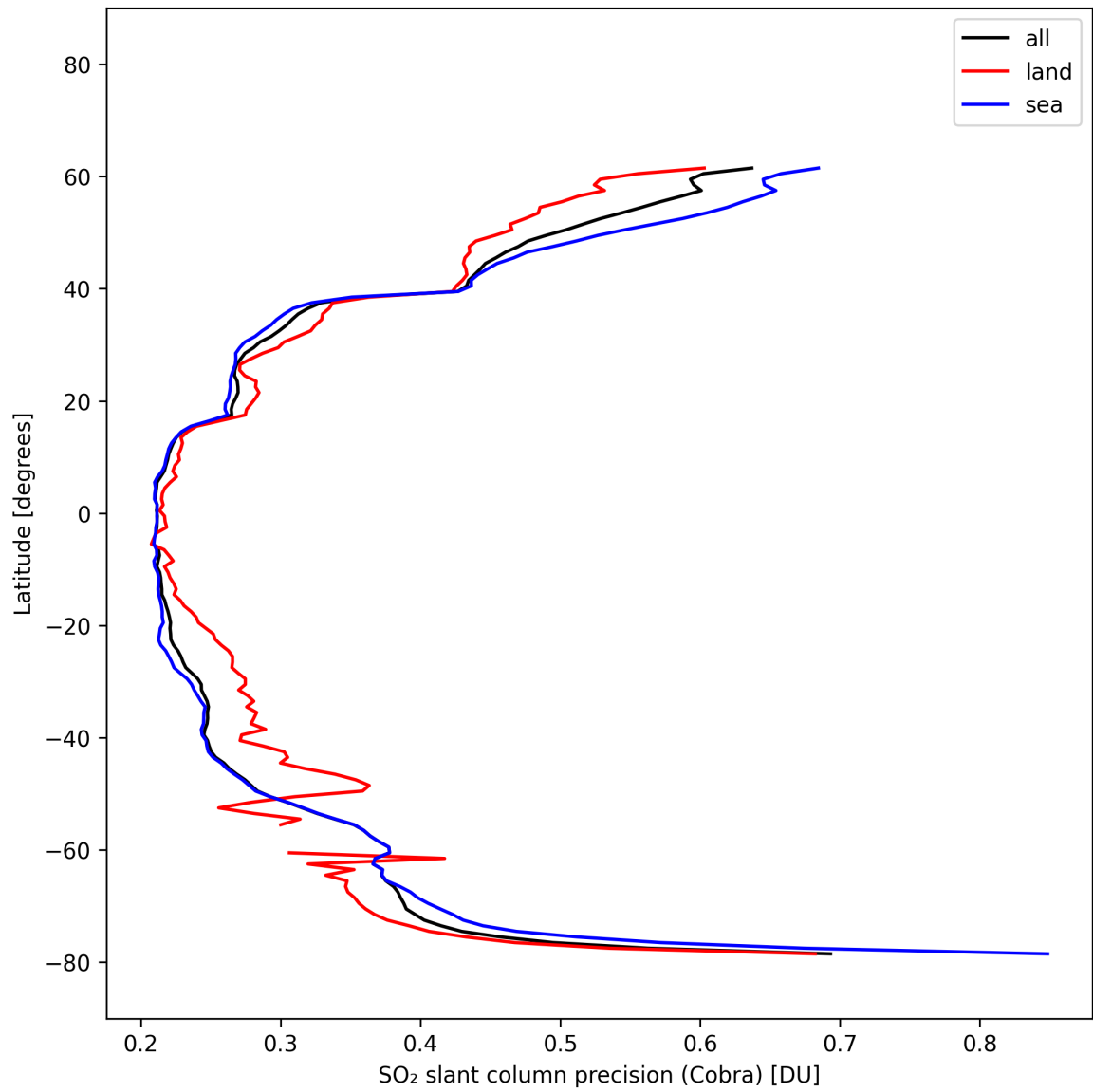
Figure 36: Zonal average of “SO 2 slant column precision (Cobra)” for 2025-02-25 to 2025-02-27.
