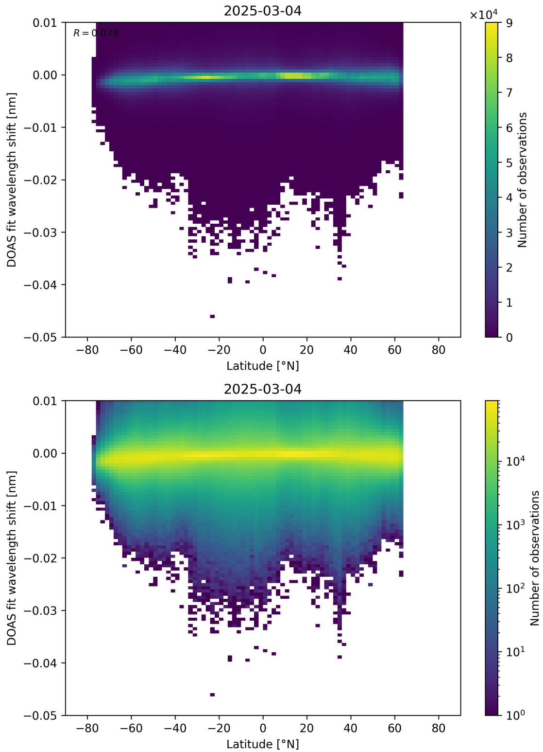
Figure 153: Scatter density plot of “Latitude” against “DOAS fit wavelength shift” for 2025-03-03 to 2025-03-05.
