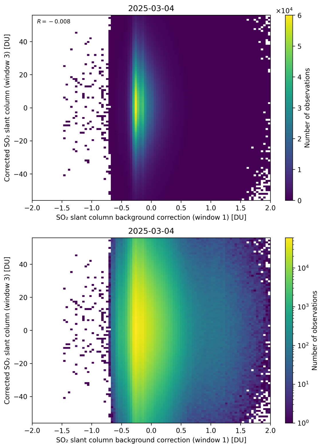
Figure 116: Scatter density plot of “SO 2 slant column background correction (window 1)” against “Corrected SO 2 slant column (window 3)” for 2025-03-03 to 2025-03-05.
