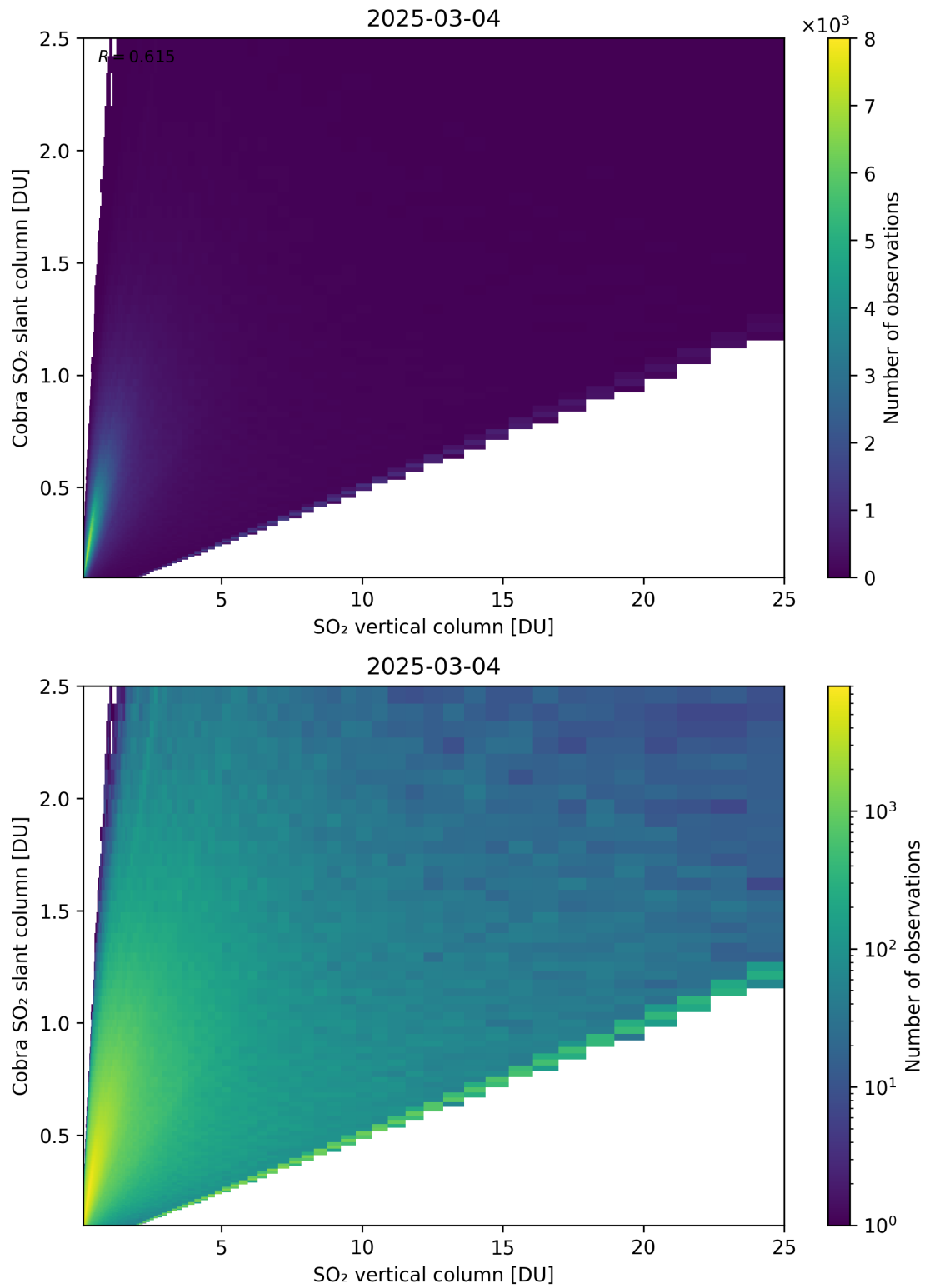
Figure 349: Scatter density plot of “SO 2 vertical column” against “Cobra SO 2 slant column” for 2025-03-03 to 2025-03-05.
