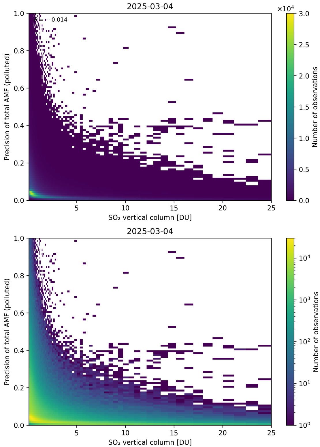
Figure 360: Scatter density plot of “SO 2 vertical column” against “Precision of total AMF (polluted)” for 2025-03-03 to 2025-03-05.
