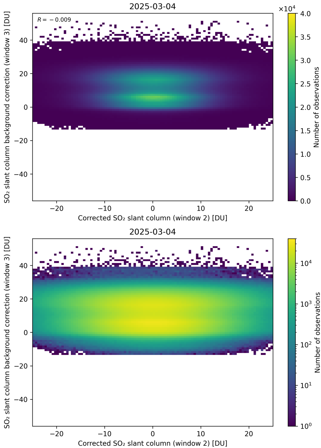
Figure 245: Scatter density plot of “Corrected SO 2 slant column (window 2)” against “SO 2 slant column background correction (window 3)” for 2025-03-03 to 2025-03-05.
