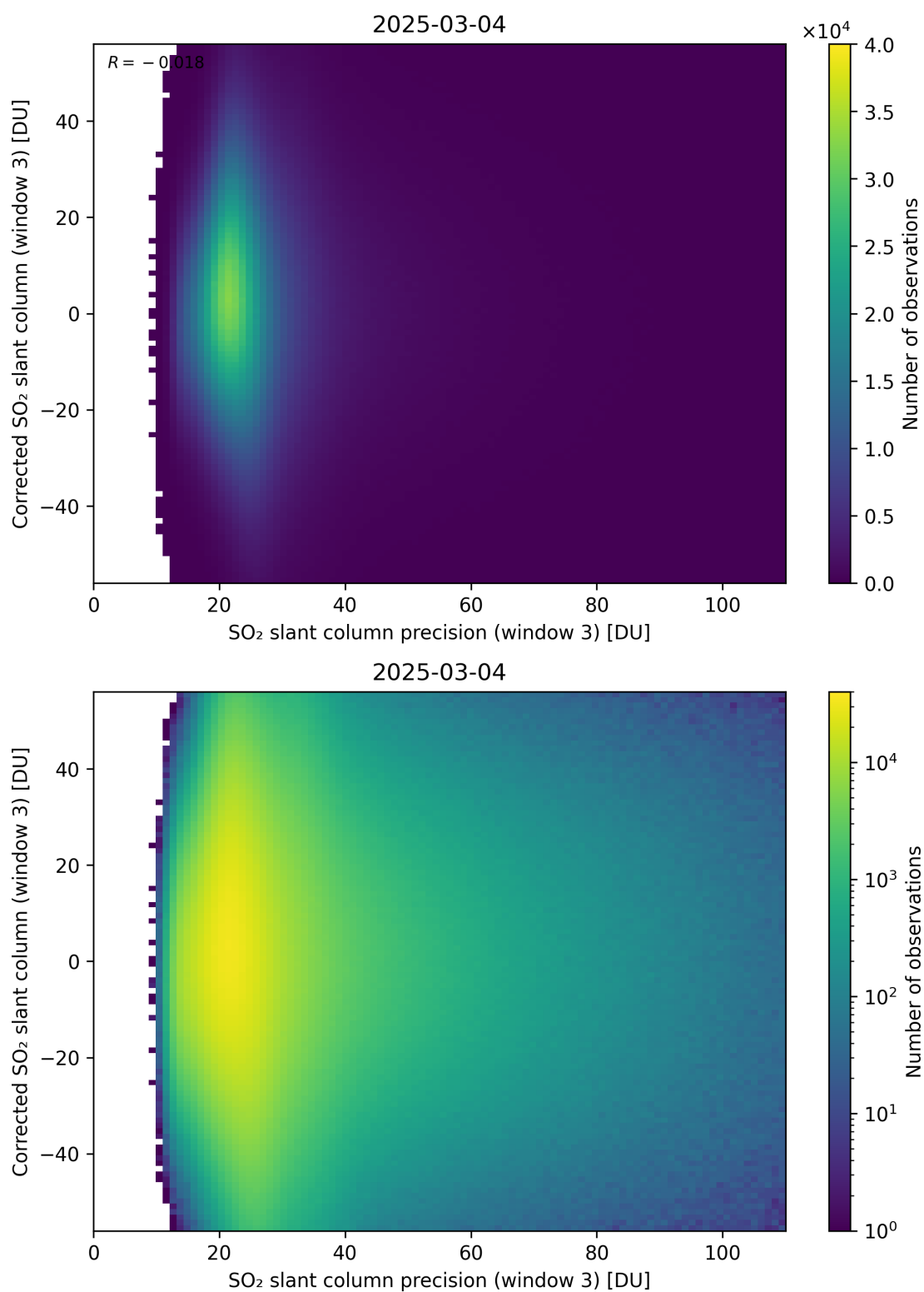
Figure 312: Scatter density plot of “SO 2 slant column precision (window 3)” against “Corrected SO 2 slant column (window 3)” for 2025-03-03 to 2025-03-05.
