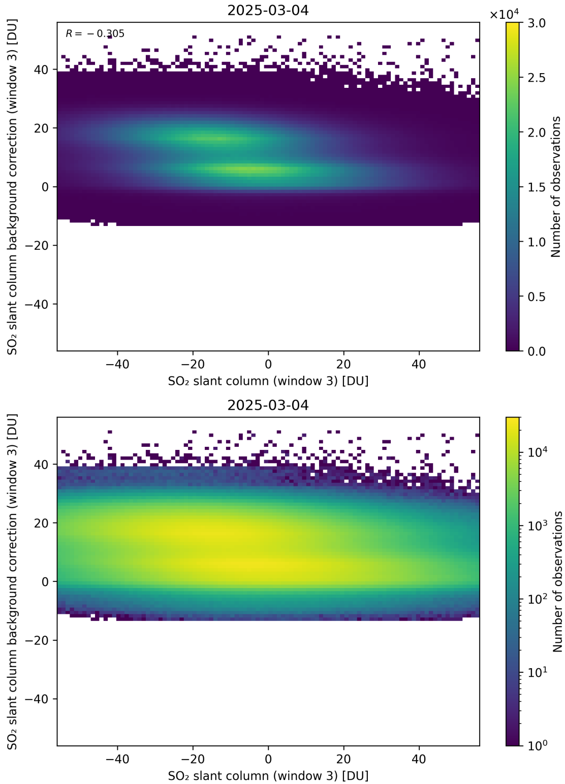
Figure 303: Scatter density plot of “SO 2 slant column (window 3)” against “SO 2 slant column background correction (window 3)” for 2025-03-03 to 2025-03-05.
