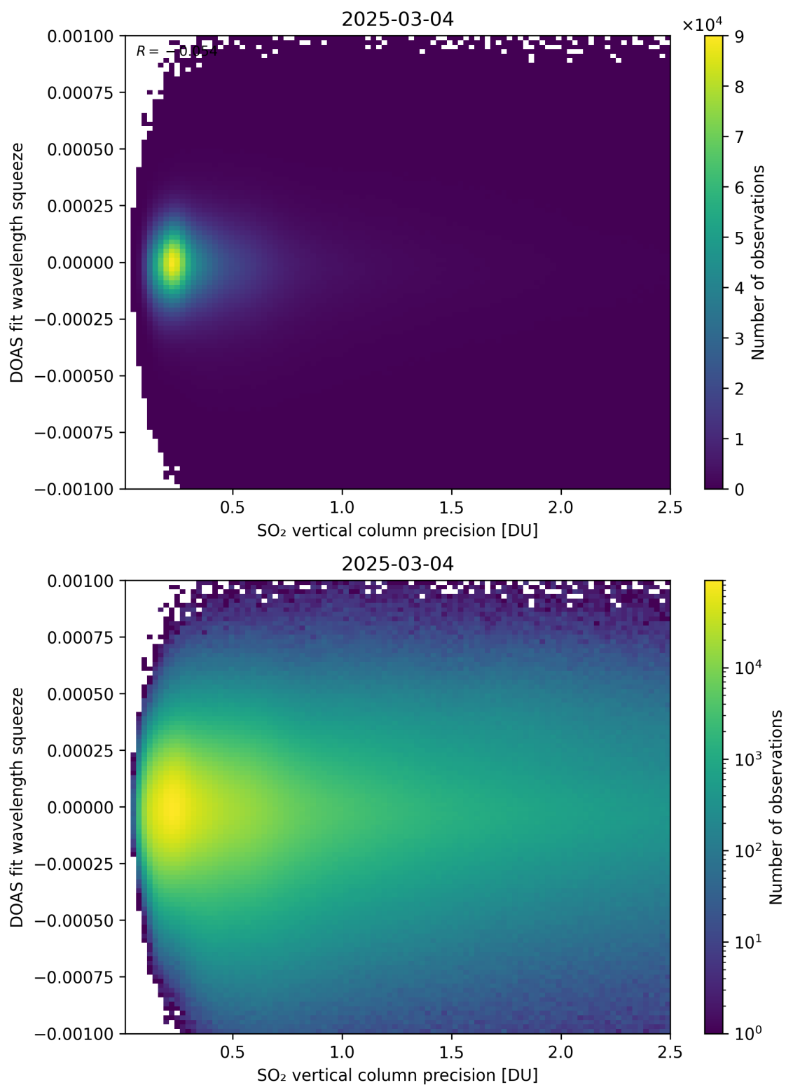
Figure 333: Scatter density plot of “SO 2 vertical column precision” against “DOAS fit wavelength squeeze” for 2025-03-03 to 2025-03-05.
