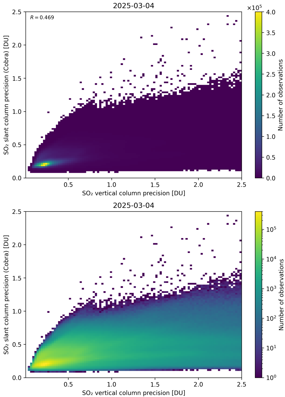
Figure 337: Scatter density plot of “SO 2 vertical column precision” against “SO 2 slant column precision (Cobra)” for 2025-03-03 to 2025-03-05.
