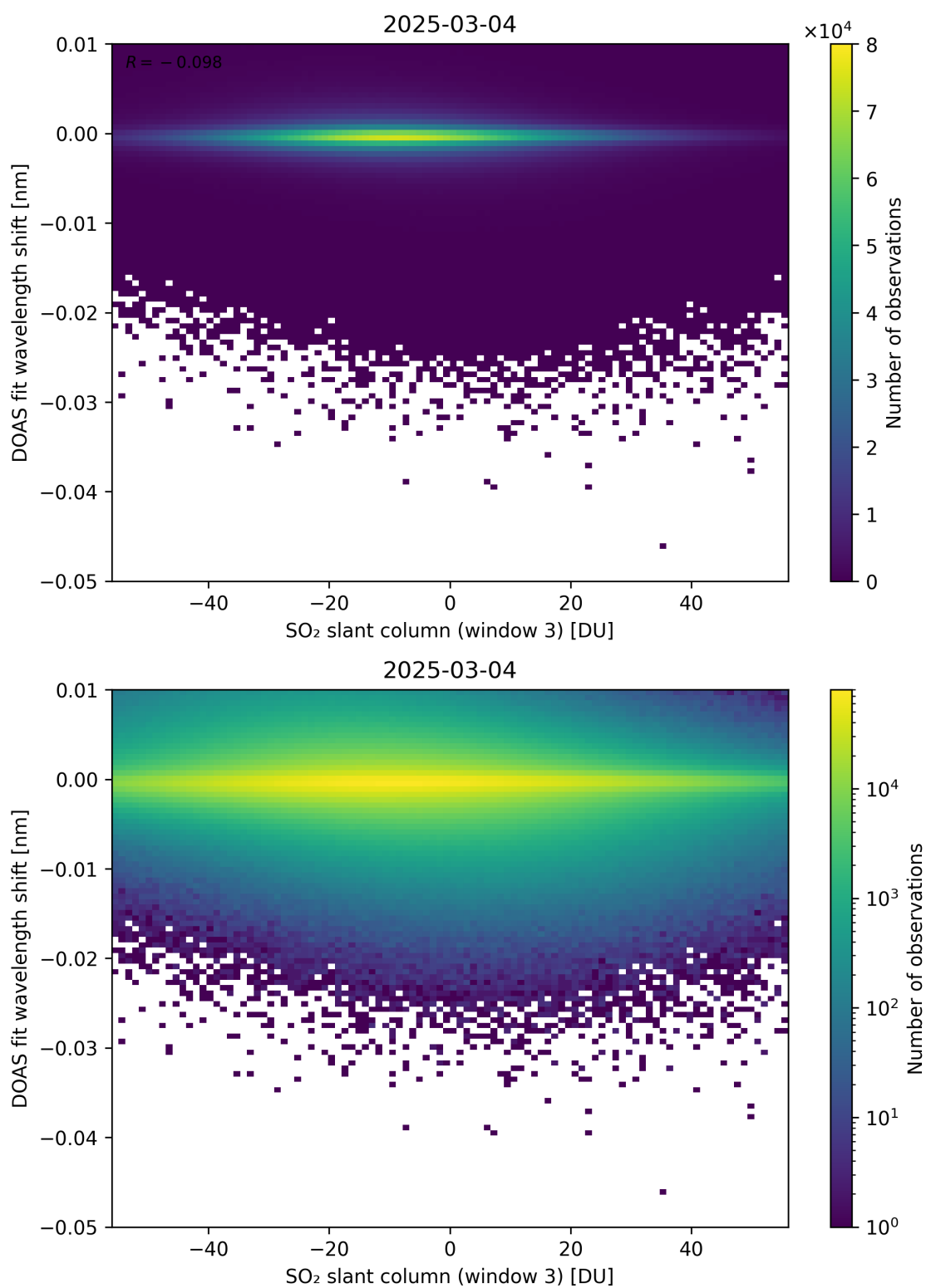
Figure 304: Scatter density plot of “SO 2 slant column (window 3)” against “DOAS fit wavelength shift” for 2025-03-03 to 2025-03-05.
