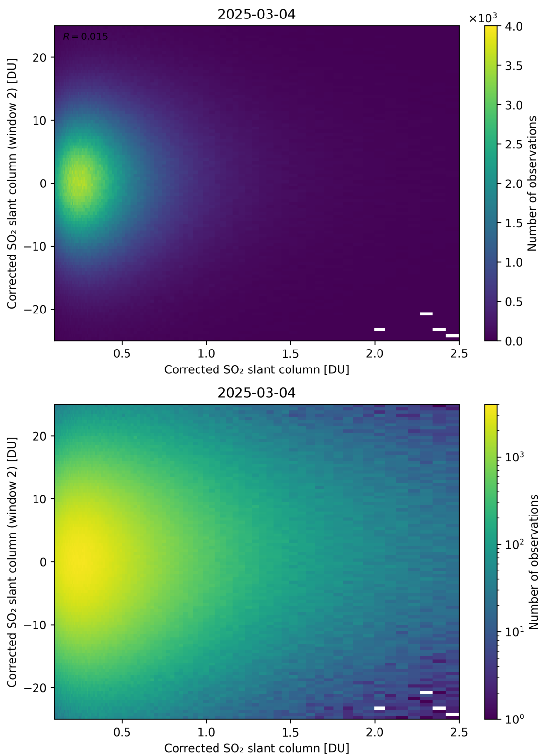
Figure 235: Scatter density plot of “Corrected SO 2 slant column” against “Corrected SO 2 slant column (window 2)” for 2025-03-03 to 2025-03-05.
