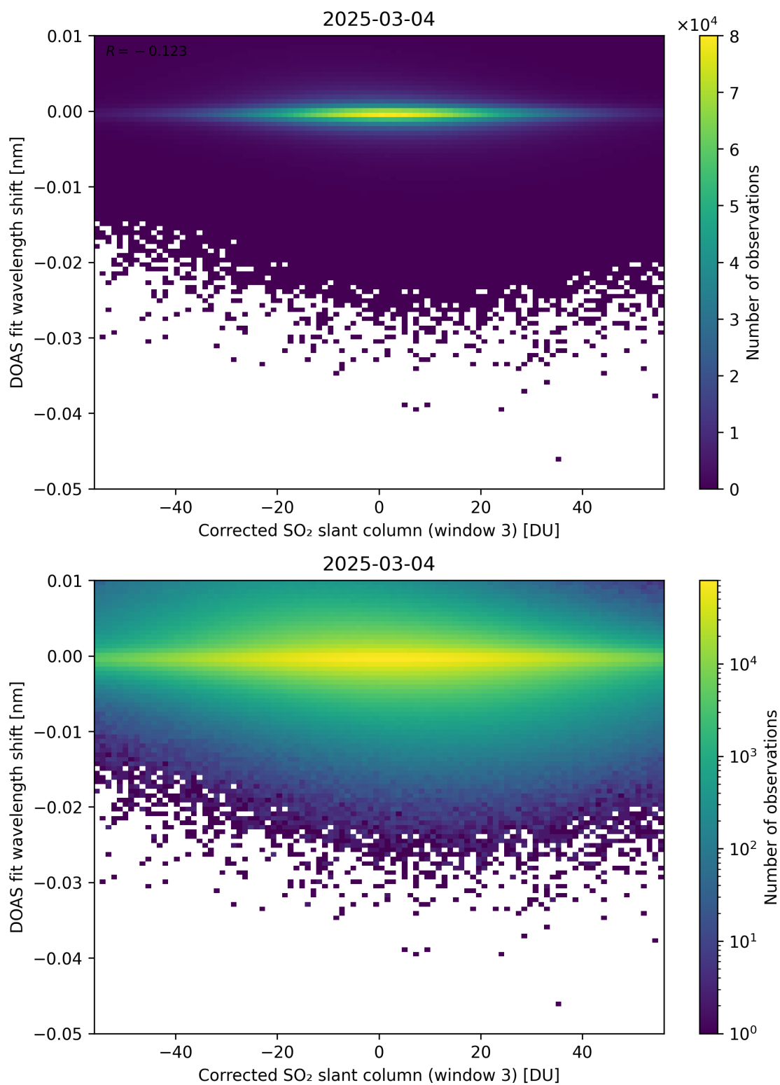
Figure 256: Scatter density plot of “Corrected SO 2 slant column (window 3)” against “DOAS fit wavelength shift” for 2025-03-03 to 2025-03-05.
