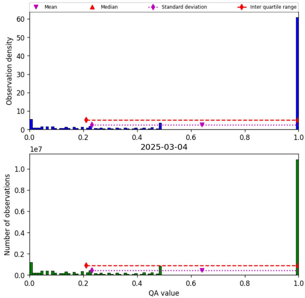
Figure 57: Histogram of “QA value” for 2025-03-03 to 2025-03-05
