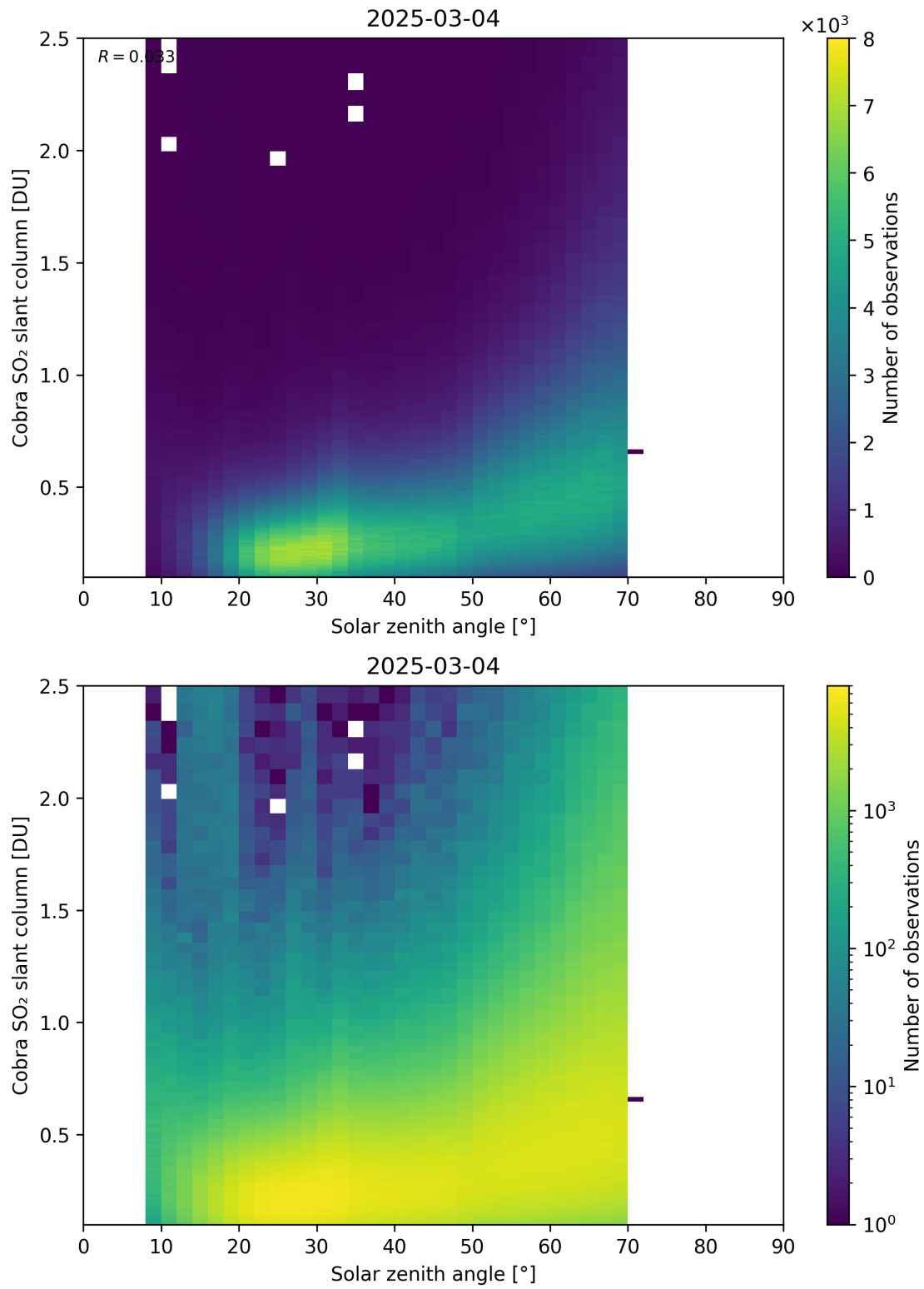
Figure 179: Scatter density plot of “Solar zenith angle” against “Cobra SO 2 slant column” for 2025-03-03 to 2025-03-05.
