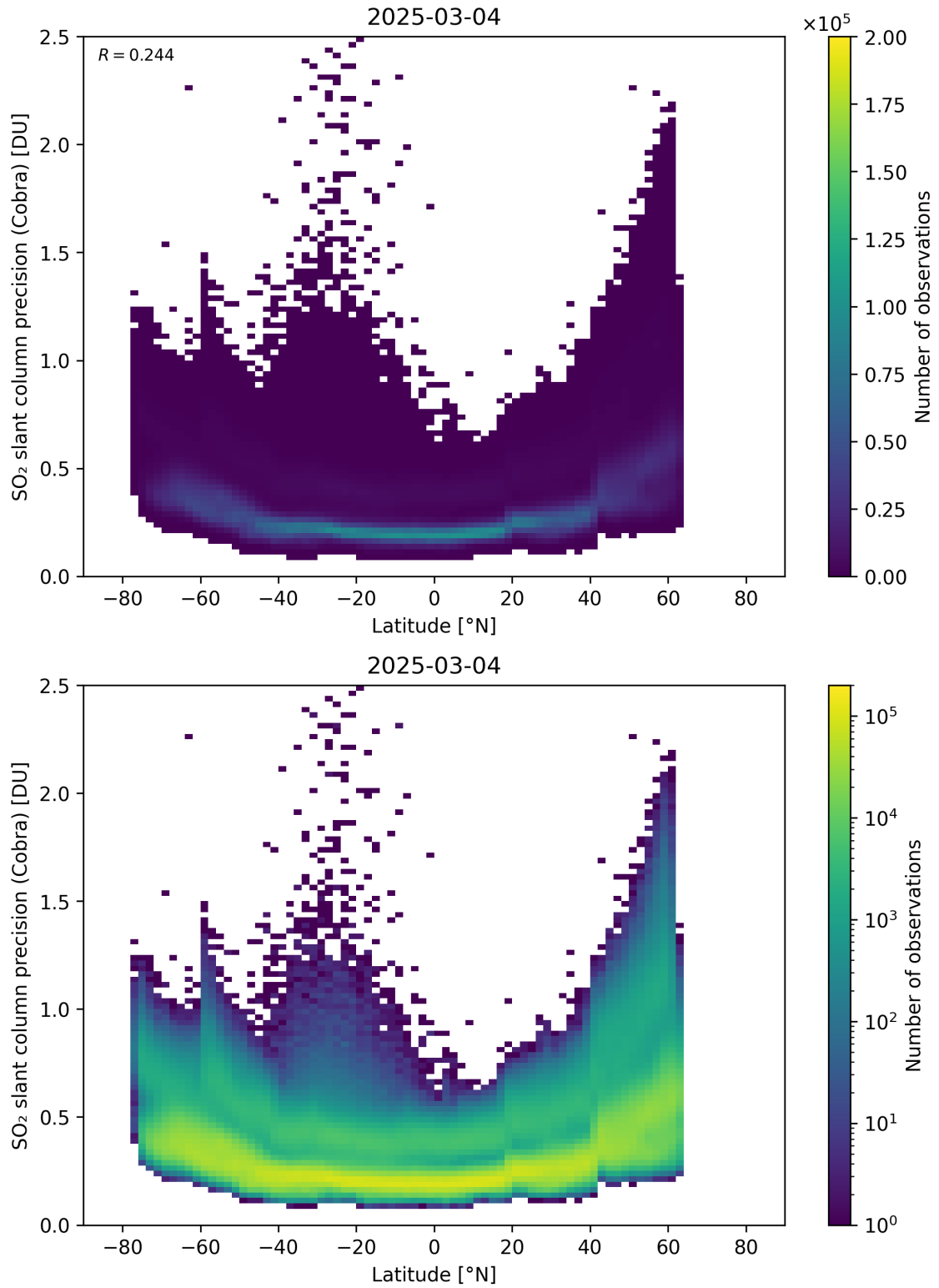
Figure 158: Scatter density plot of “Latitude” against “SO 2 slant column precision (Cobra)” for 2025-03-03 to 2025-03-05.
