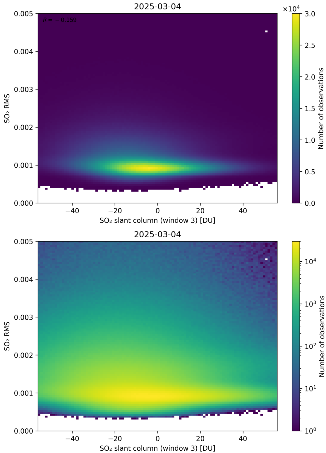
Figure 306: Scatter density plot of “SO 2 slant column (window 3)” against “SO 2 RMS” for 2025-03-03 to 2025-03-05.
