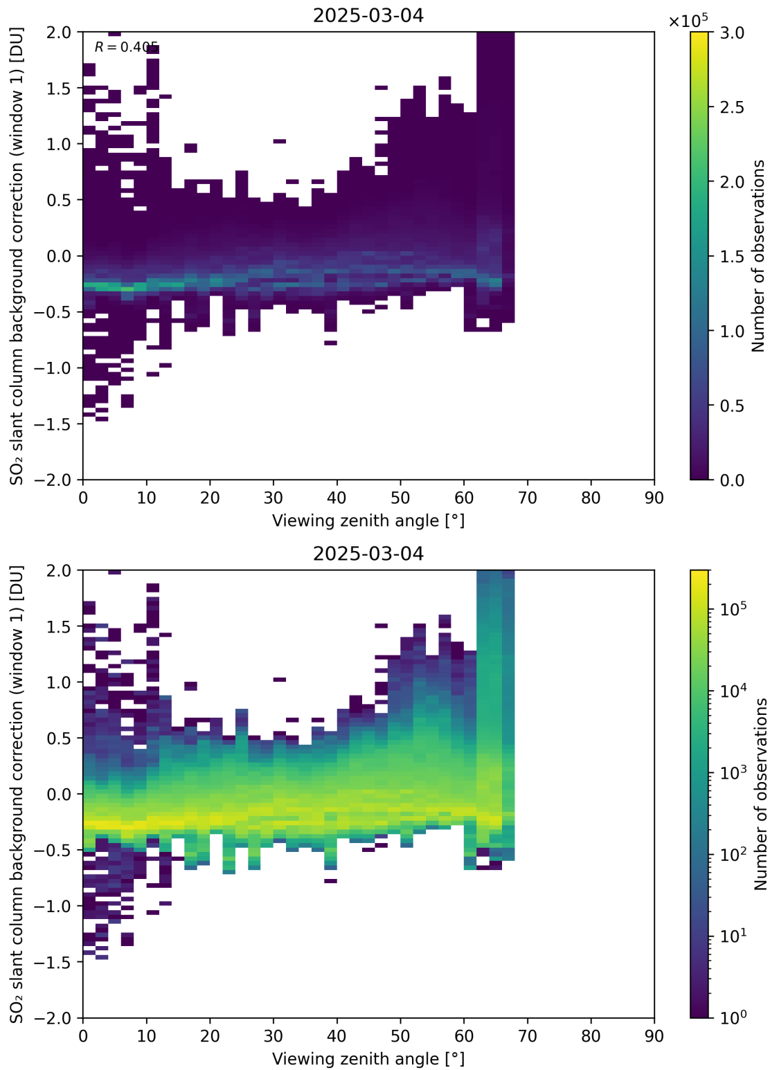
Figure 362: Scatter density plot of “Viewing zenith angle” against “SO 2 slant column background correction (window 1)” for 2025-03-03 to 2025-03-05.
