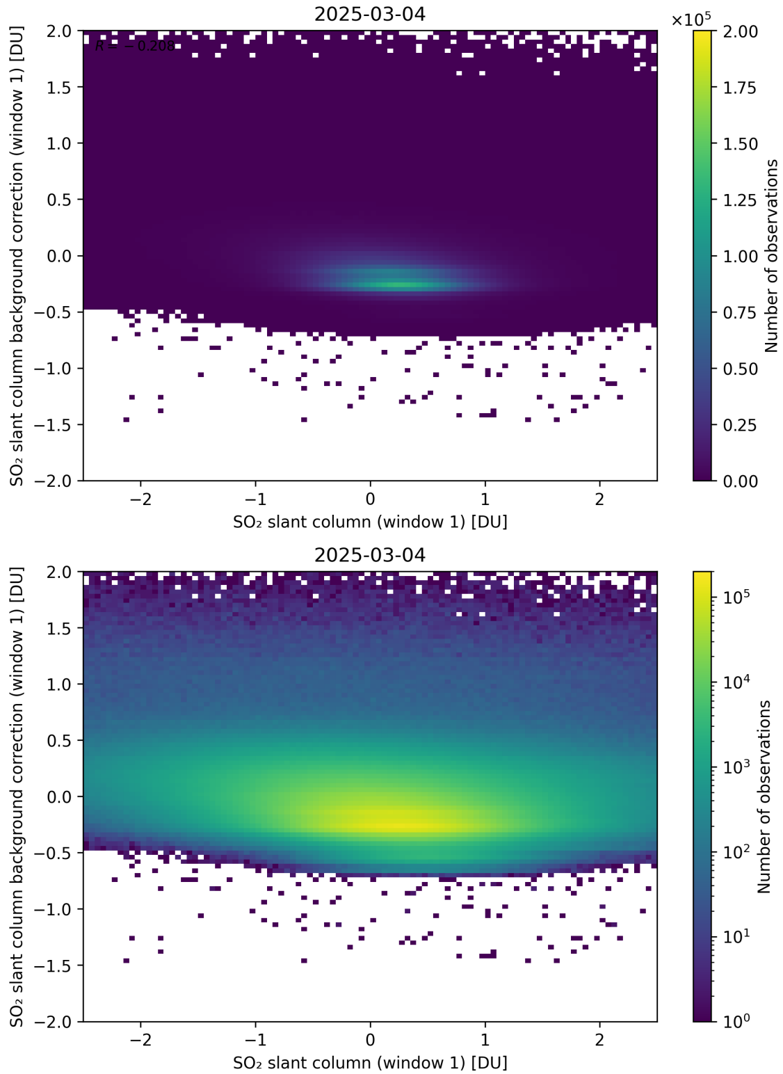
Figure 262: Scatter density plot of “SO 2 slant column (window 1)” against “SO 2 slant column background correction (window 1)” for 2025-03-03 to 2025-03-05.
