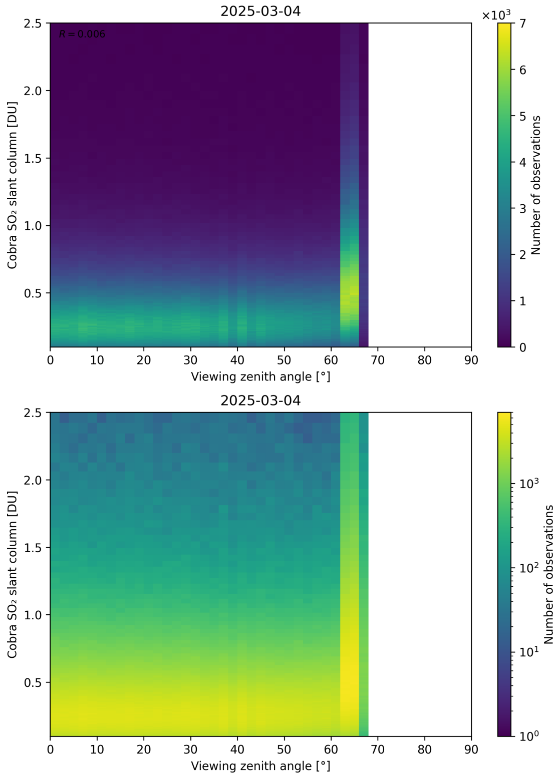
Figure 371: Scatter density plot of “Viewing zenith angle” against “Cobra SO 2 slant column” for 2025-03-03 to 2025-03-05.
