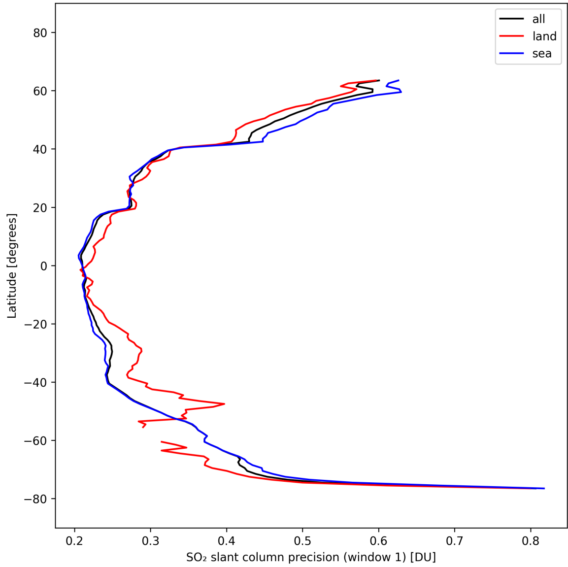
Figure 38: Zonal average of “SO 2 slant column precision (window 1)” for 2025-03-03 to 2025-03-05.
