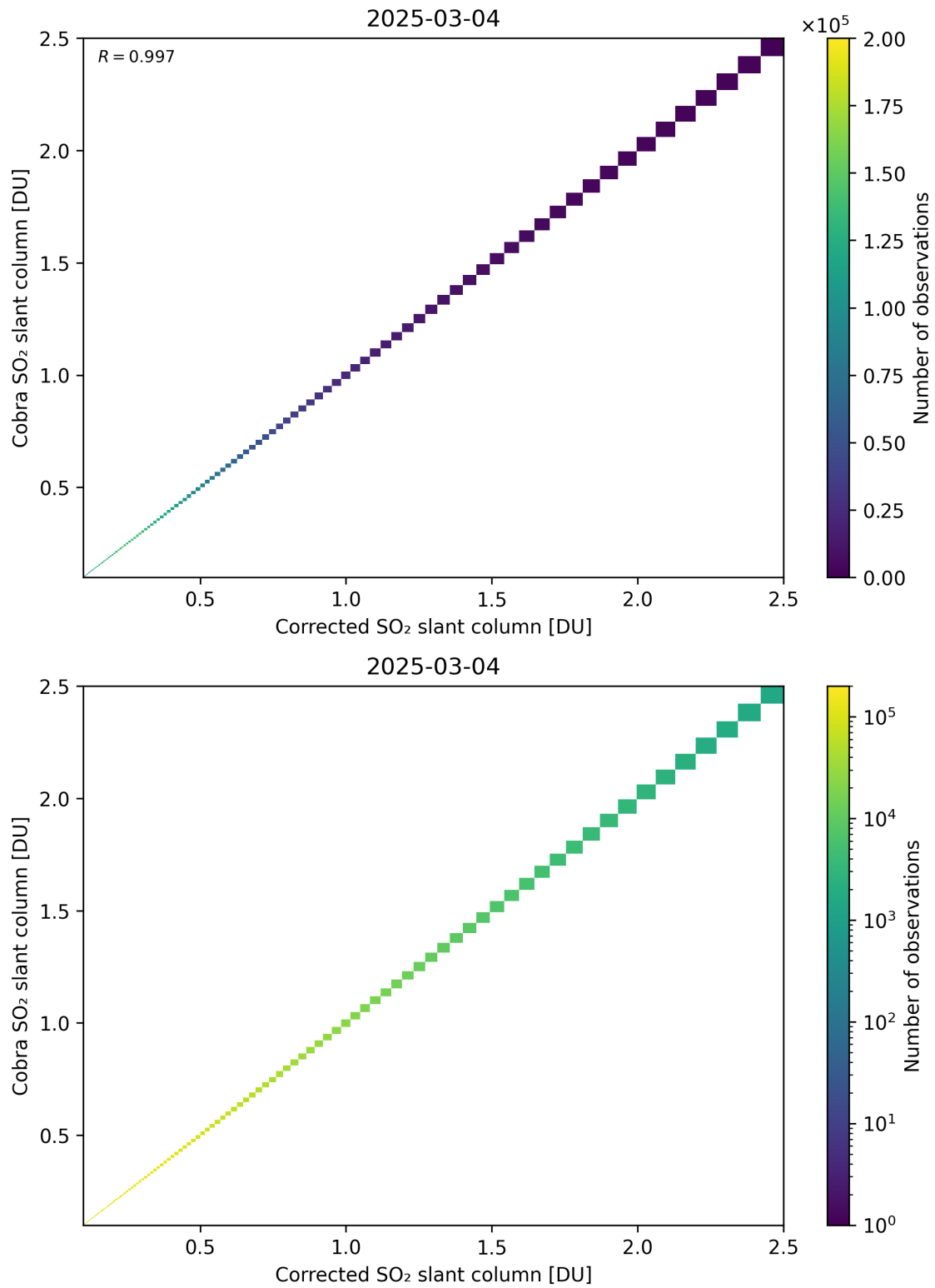
Figure 233: Scatter density plot of “Corrected SO 2 slant column” against “Cobra SO 2 slant column” for 2025-03-03 to 2025-03-05.
