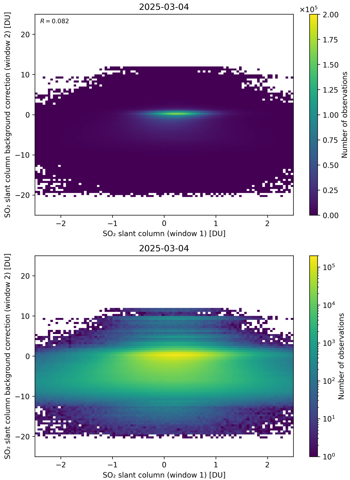
Figure 263: Scatter density plot of “SO 2 slant column (window 1)” against “SO 2 slant column background correction (window 2)” for 2025-03-03 to 2025-03-05.
