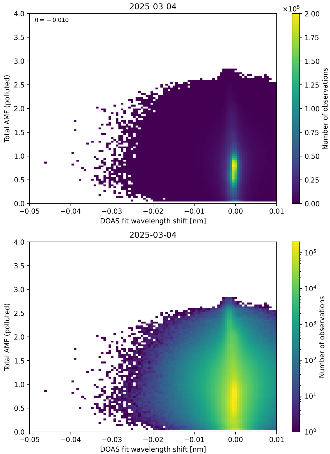
Figure 141: Scatter density plot of “DOAS fit wavelength shift” against “Total AMF (polluted)” for 2025-03-03 to 2025-03-05.
