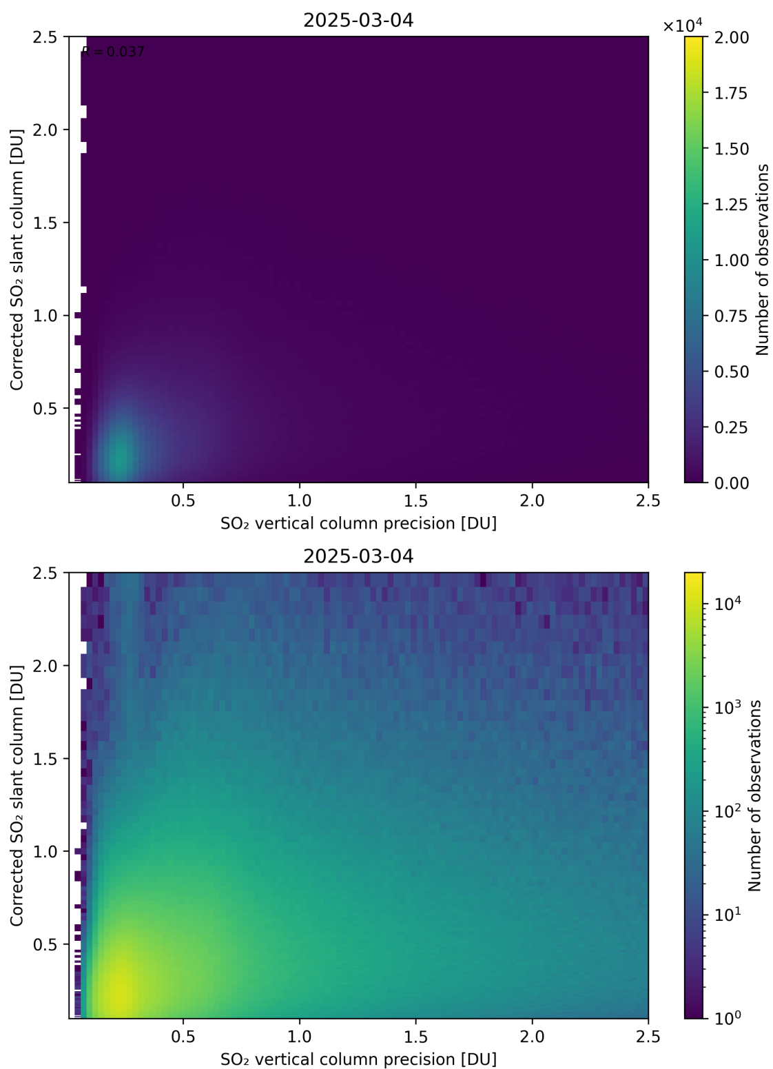
Figure 338: Scatter density plot of “SO 2 vertical column precision” against “Corrected SO 2 slant column” for 2025-03-03 to 2025-03-05.
