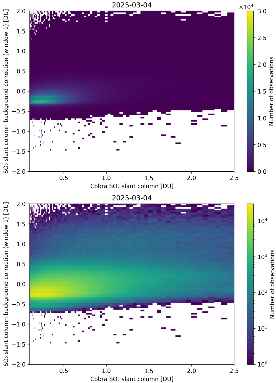
Figure 193: Scatter density plot of “Cobra SO 2 slant column” against “SO 2 slant column background correction (window 1)” for 2025-03-03 to 2025-03-05.
