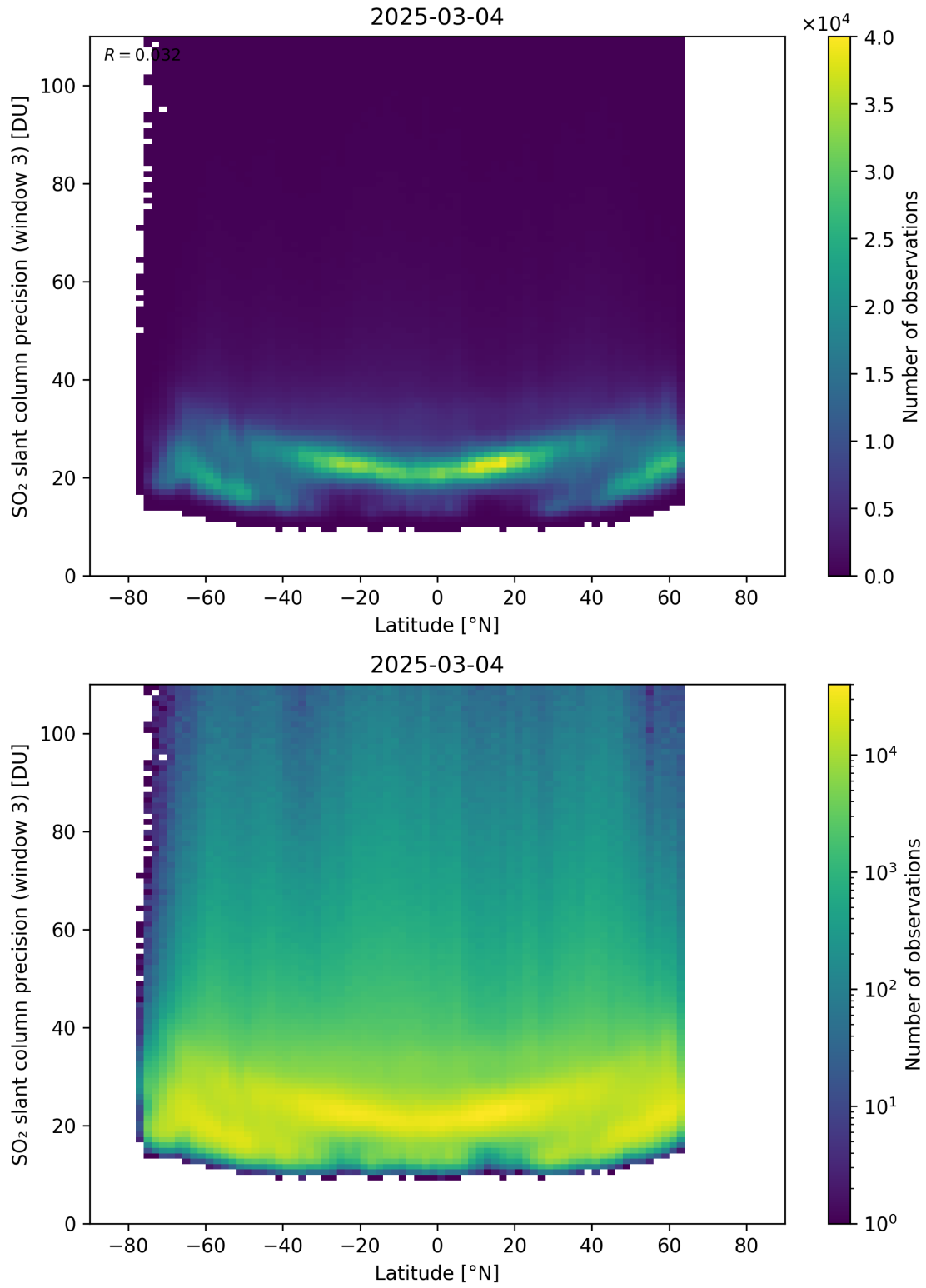
Figure 166: Scatter density plot of “Latitude” against “SO 2 slant column precision (window 3)” for 2025-03-03 to 2025-03-05.
