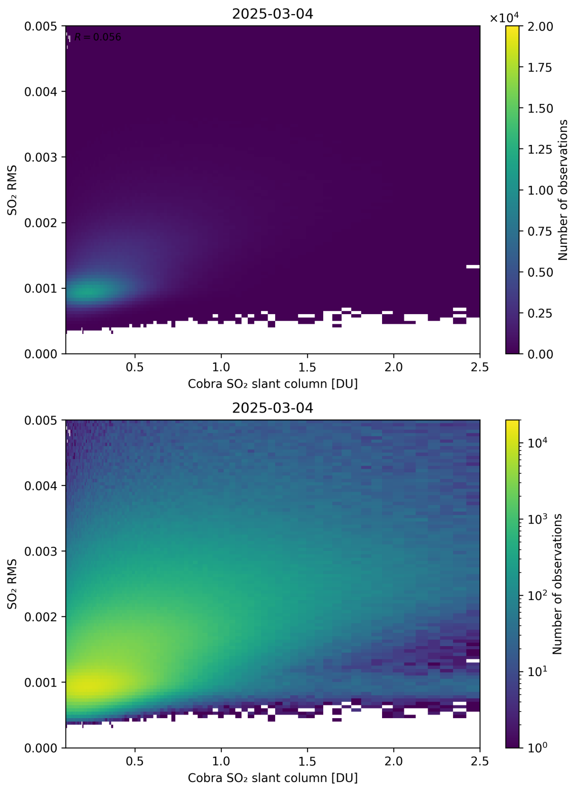
Figure 198: Scatter density plot of “Cobra SO 2 slant column” against “SO 2 RMS” for 2025-03-03 to 2025-03-05.
