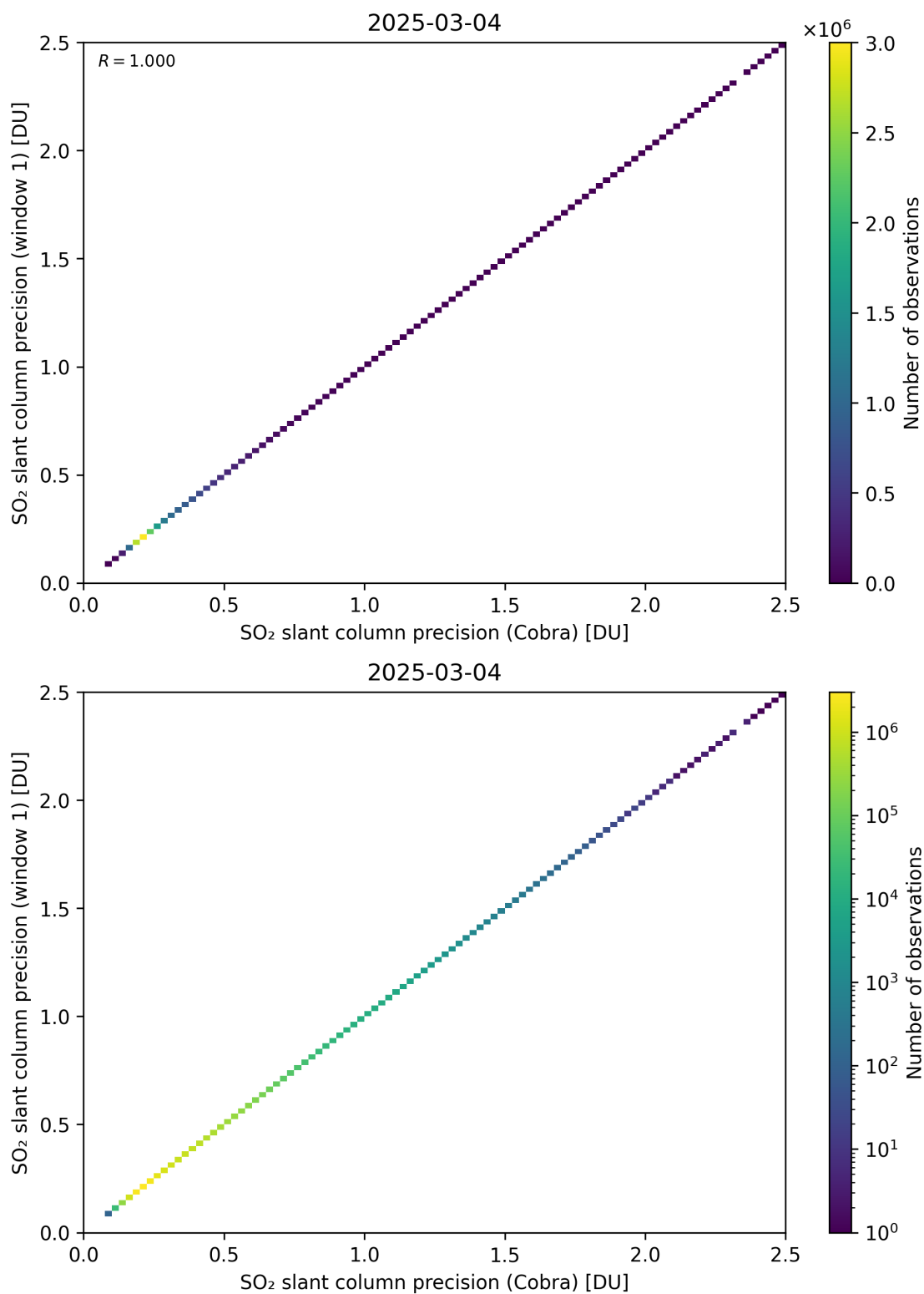
Figure 209: Scatter density plot of “SO 2 slant column precision (Cobra)” against “SO 2 slant column precision (window 1)” for 2025-03-03 to 2025-03-05.
