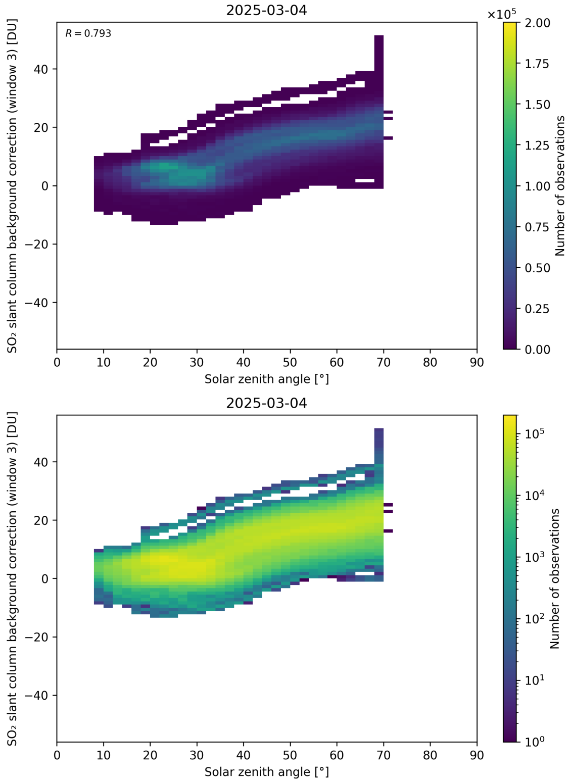
Figure 173: Scatter density plot of “Solar zenith angle” against “SO 2 slant column background correction (window 3)” for 2025-03-03 to 2025-03-05.
