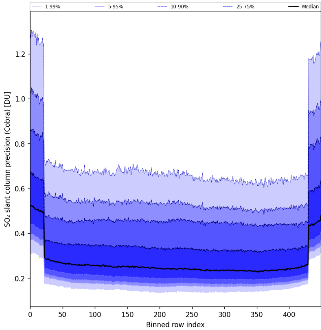
Figure 88: Along track statistics of “SO 2 slant column precision (Cobra)” for 2025-03-03 to 2025-03-05
