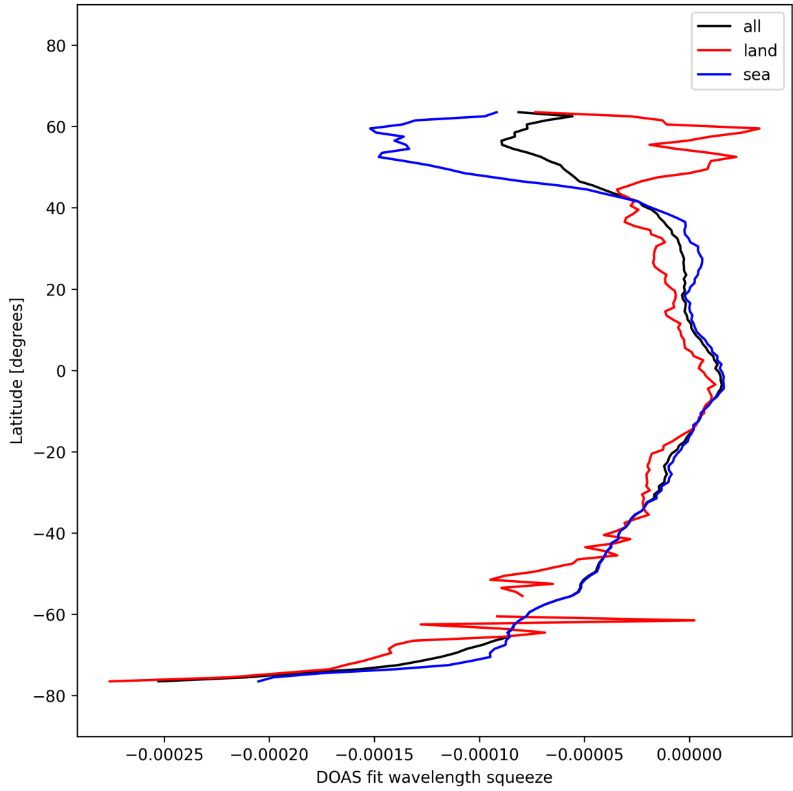
Figure 51: Zonal average of “DOAS fit wavelength squeeze” for 2025-03-03 to 2025-03-05.
