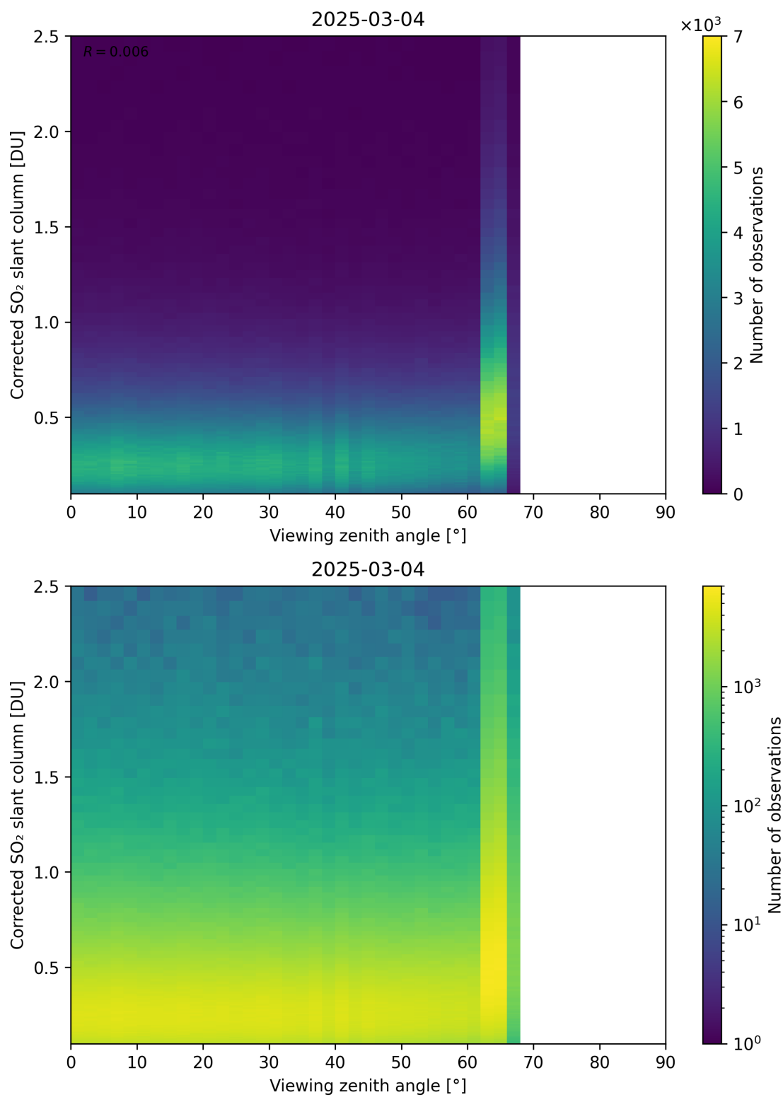
Figure 373: Scatter density plot of “Viewing zenith angle” against “Corrected SO 2 slant column” for 2025-03-03 to 2025-03-05.
