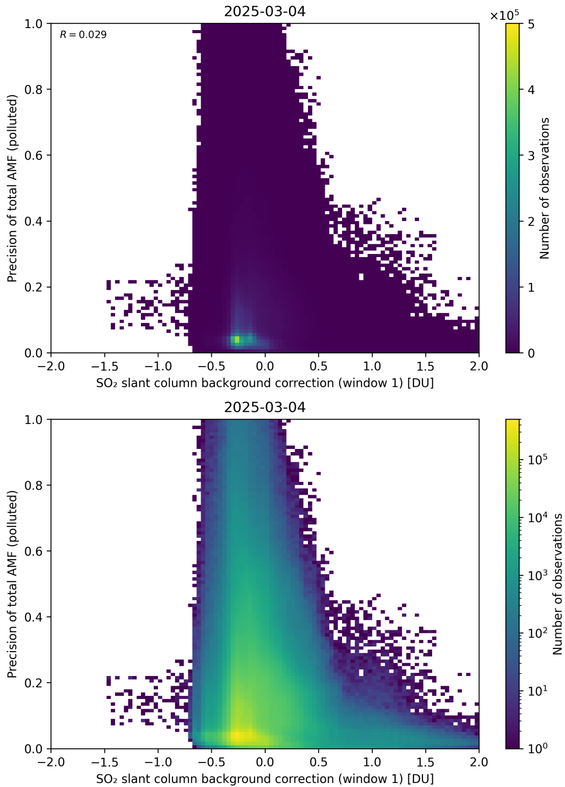
Figure 121: Scatter density plot of “SO 2 slant column background correction (window 1)” against “Precision of total AMF (polluted)” for 2025-03-03 to 2025-03-05.
