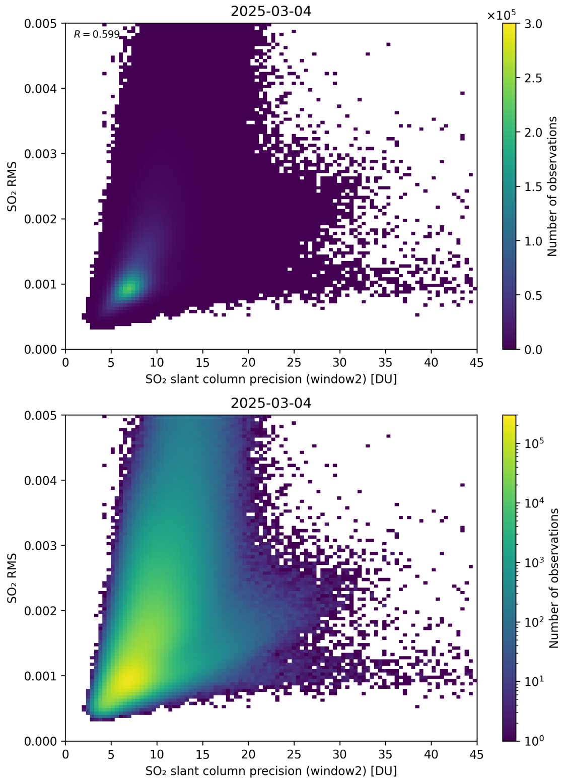
Figure 295: Scatter density plot of “SO 2 slant column precision (window2)” against “SO 2 RMS” for 2025-03-03 to 2025-03-05.
