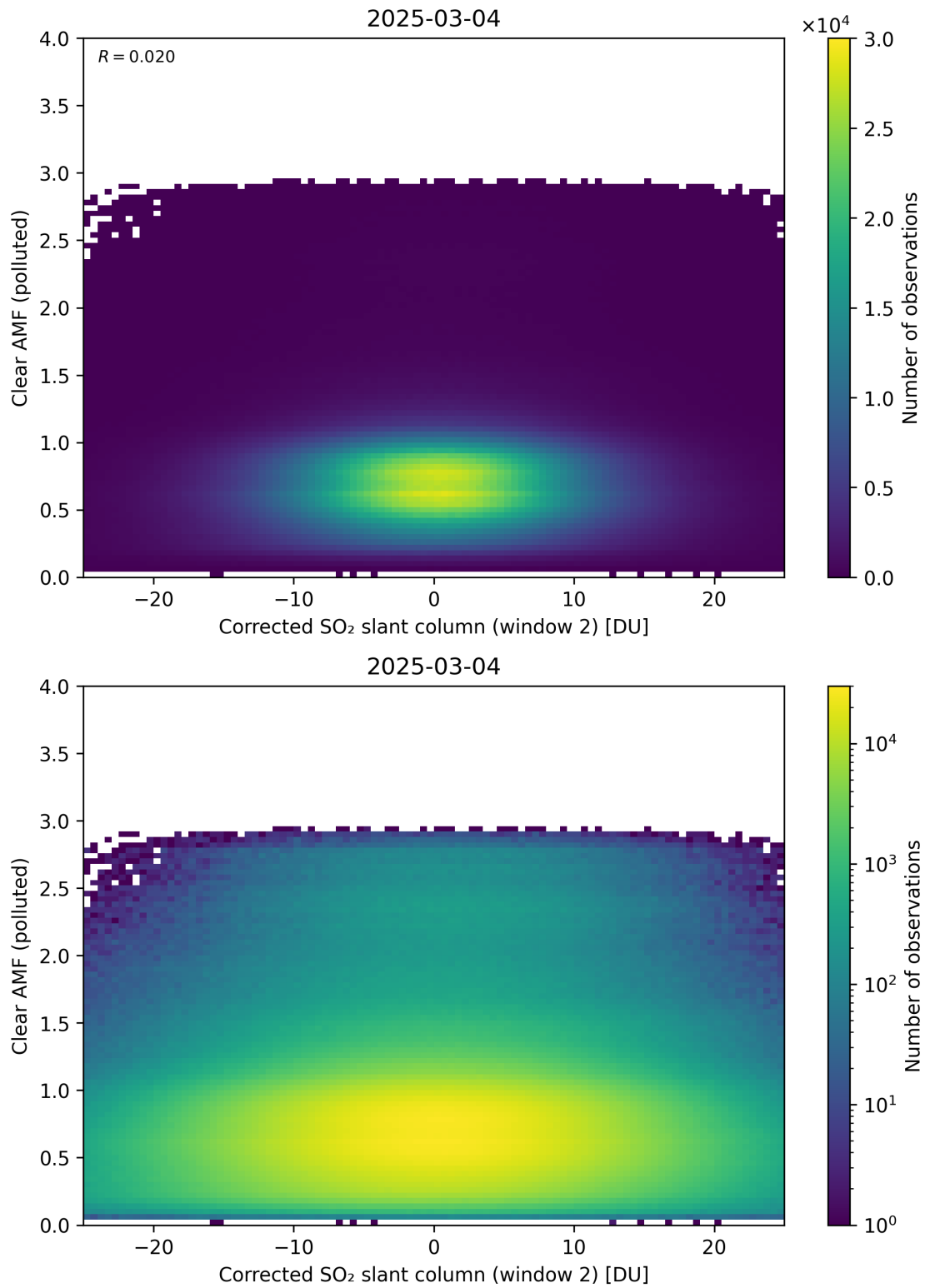
Figure 249: Scatter density plot of “Corrected SO 2 slant column (window 2)” against “Clear AMF (polluted)” for 2025-03-03 to 2025-03-05.
