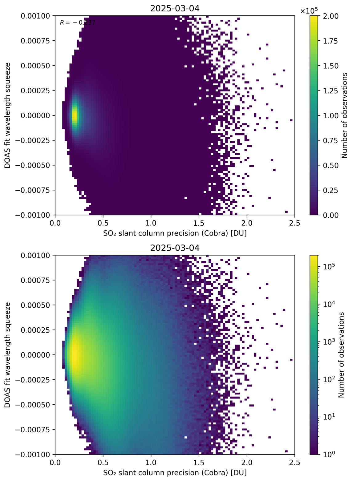
Figure 203: Scatter density plot of “SO 2 slant column precision (Cobra)” against “DOAS fit wavelength squeeze” for 2025-03-03 to 2025-03-05.
