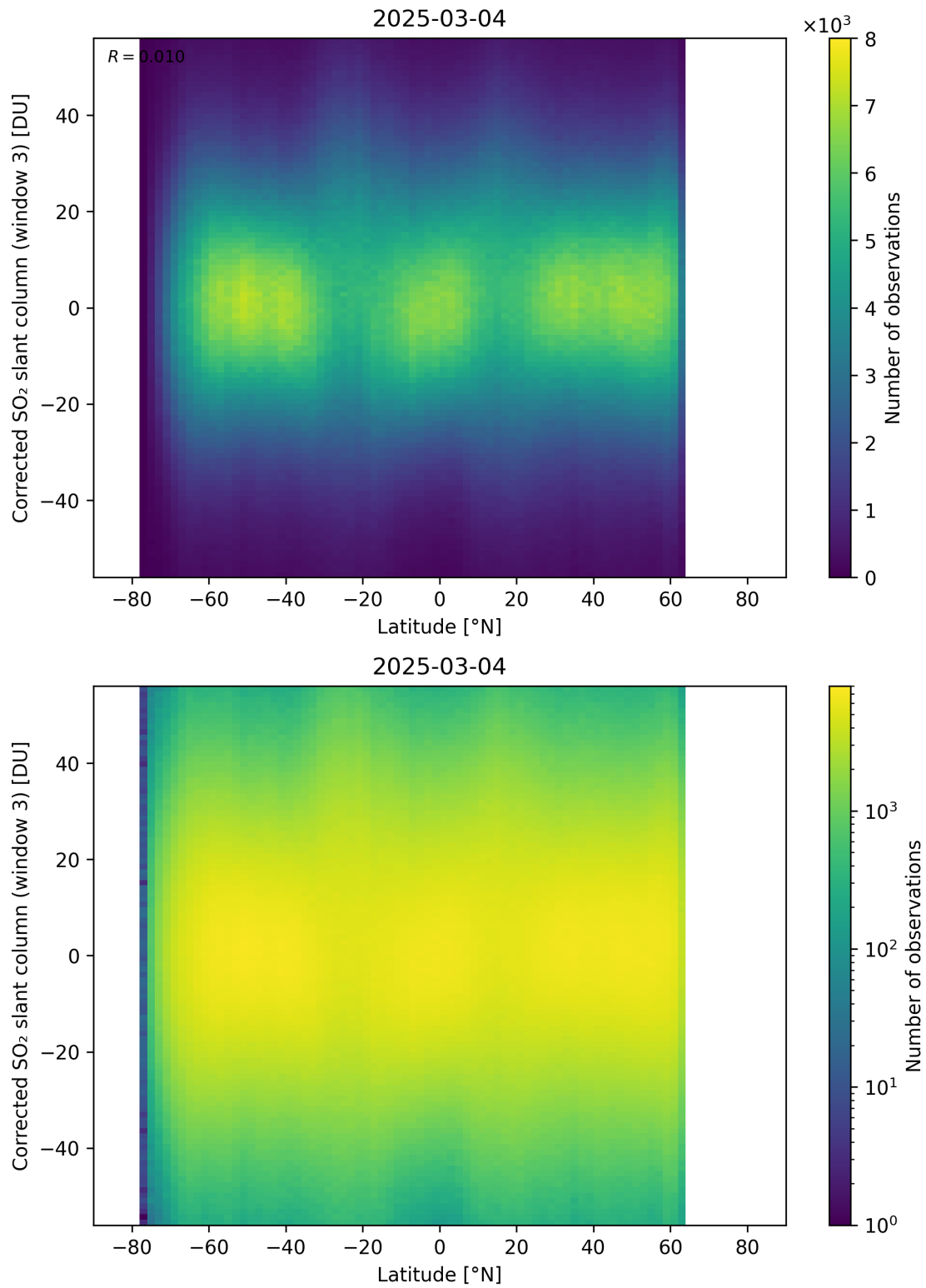
Figure 161: Scatter density plot of “Latitude” against “Corrected SO 2 slant column (window 3)” for 2025-03-03 to 2025-03-05.
