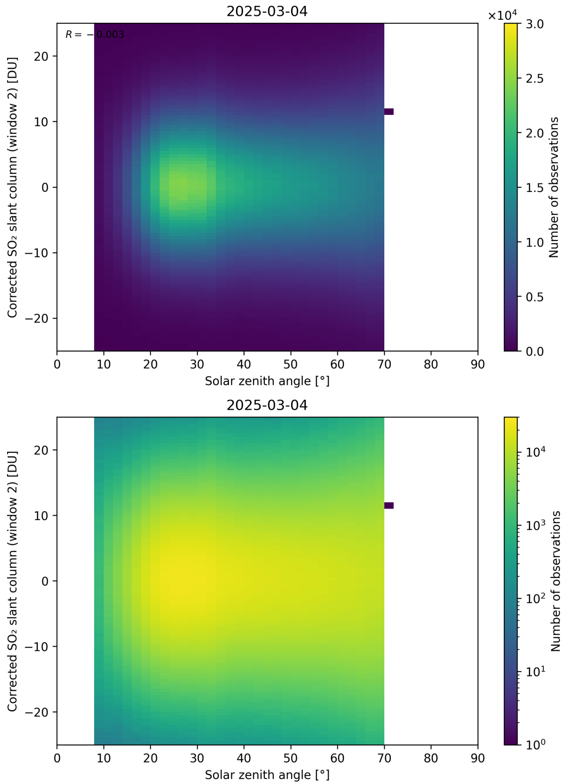
Figure 182: Scatter density plot of “Solar zenith angle” against “Corrected SO 2 slant column (window 2)” for 2025-03-03 to 2025-03-05.
