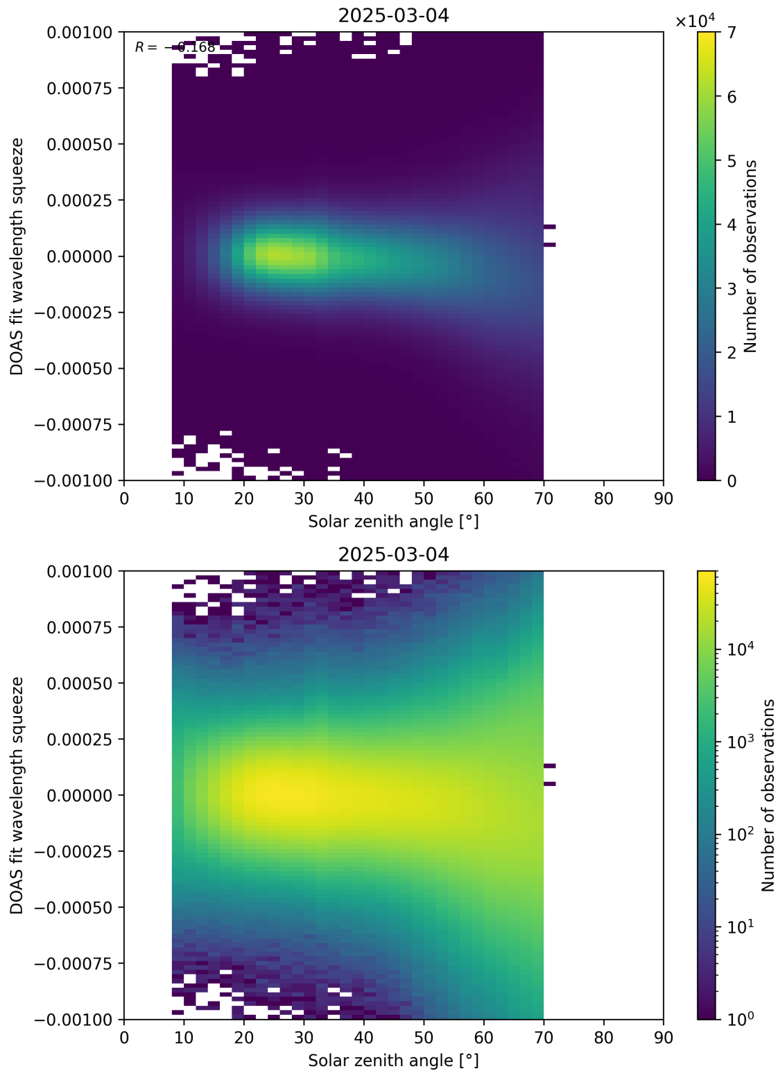
Figure 175: Scatter density plot of “Solar zenith angle” against “DOAS fit wavelength squeeze” for 2025-03-03 to 2025-03-05.
