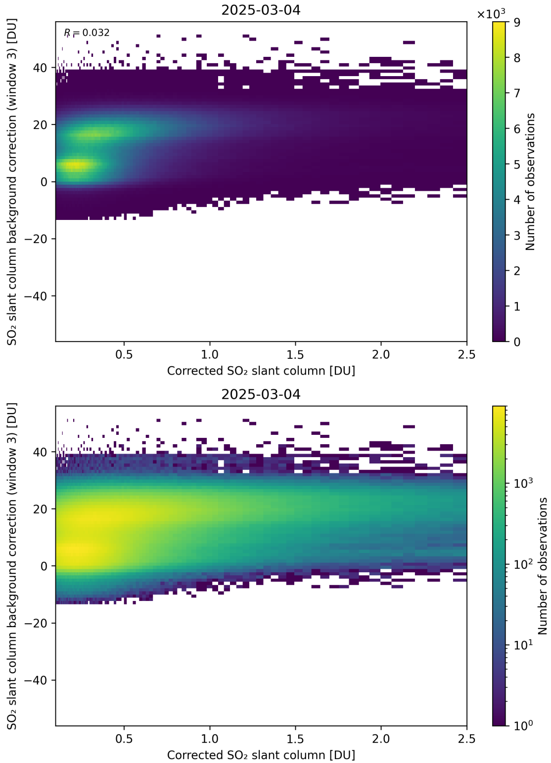
Figure 228: Scatter density plot of “Corrected SO 2 slant column” against “SO 2 slant column background correction (window 3)” for 2025-03-03 to 2025-03-05.
