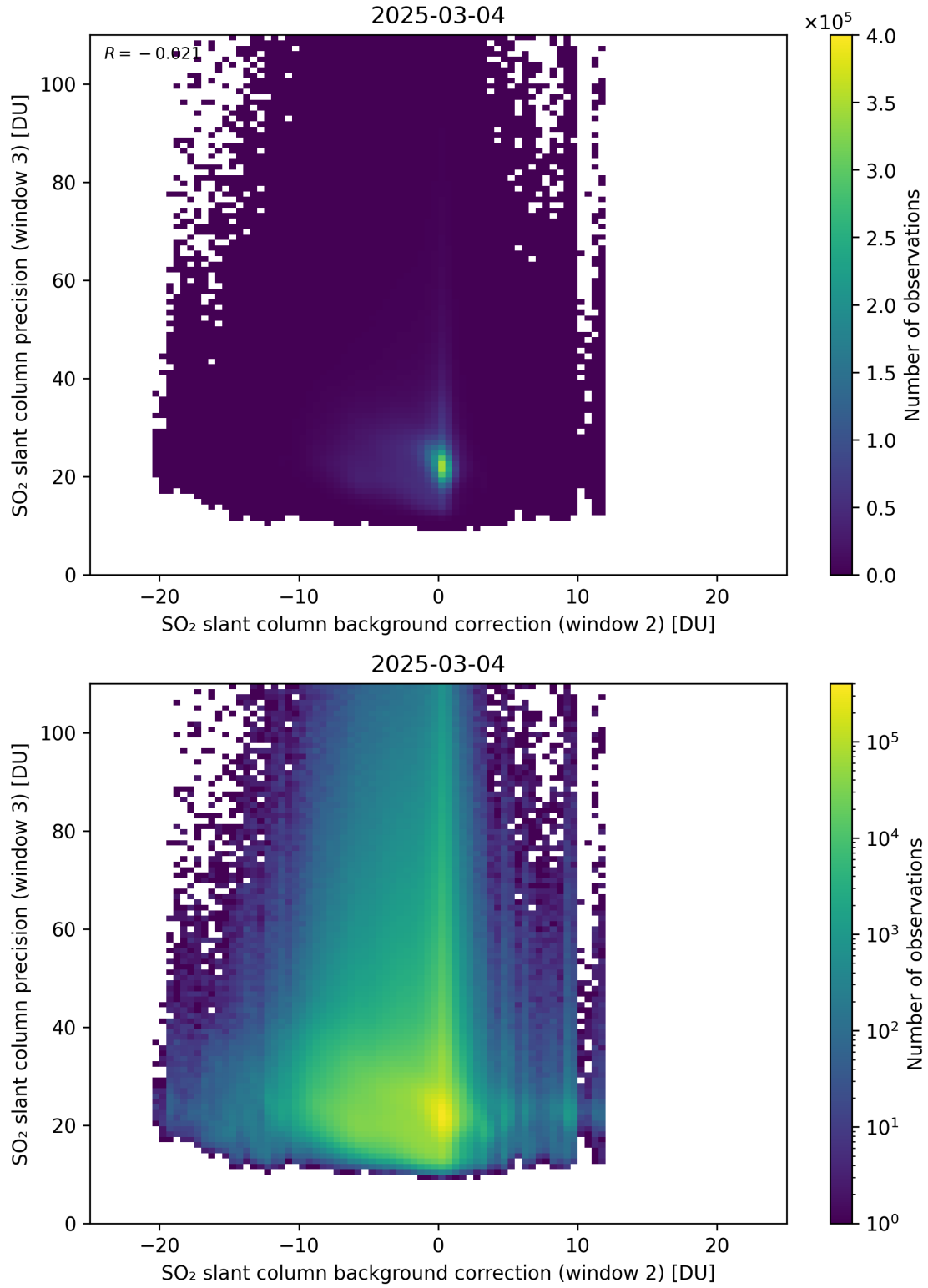
Figure 129: Scatter density plot of “SO 2 slant column background correction (window 2)” against “SO 2 slant column precision (window 3)” for 2025-03-03 to 2025-03-05.
