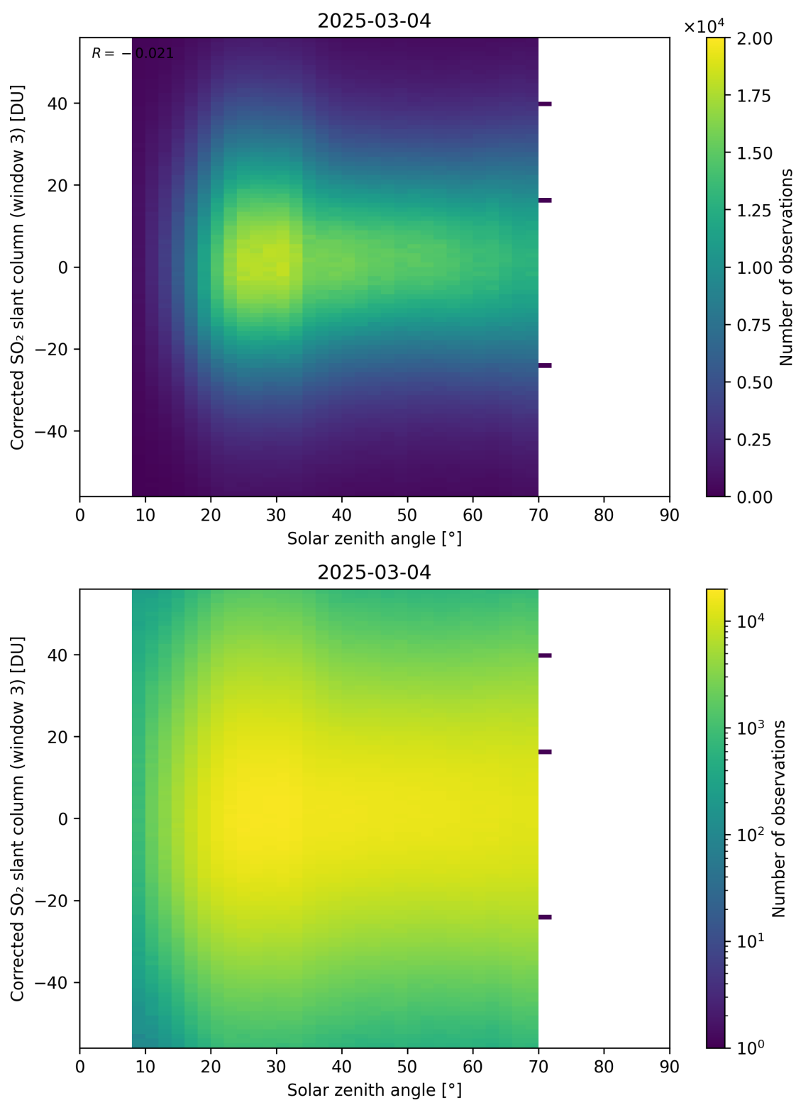
Figure 183: Scatter density plot of “Solar zenith angle” against “Corrected SO 2 slant column (window 3)” for 2025-03-03 to 2025-03-05.
