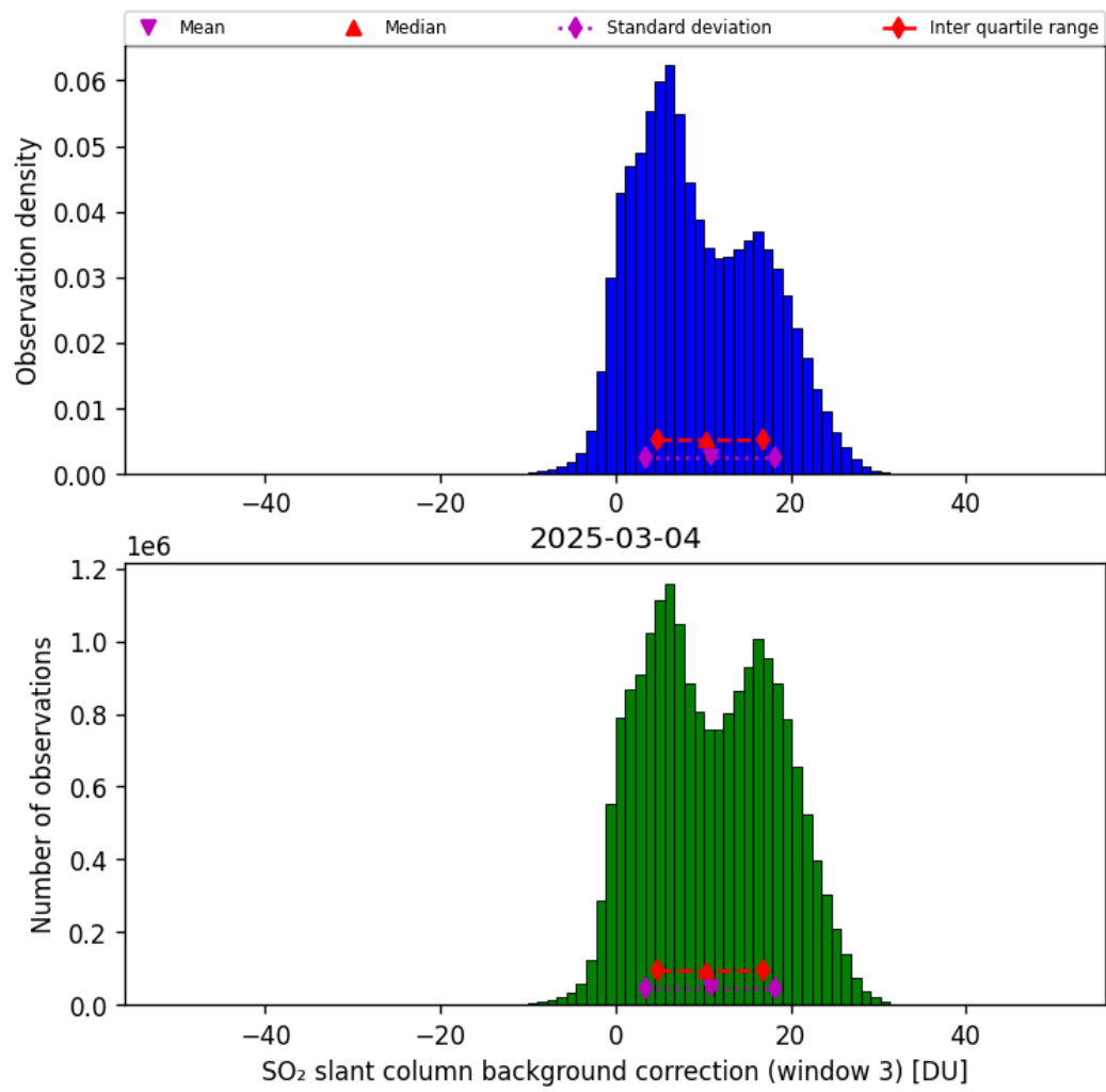
Figure 74: Histogram of “SO 2 slant column background correction (window 3)” for 2025-03-03 to 2025-03-05
