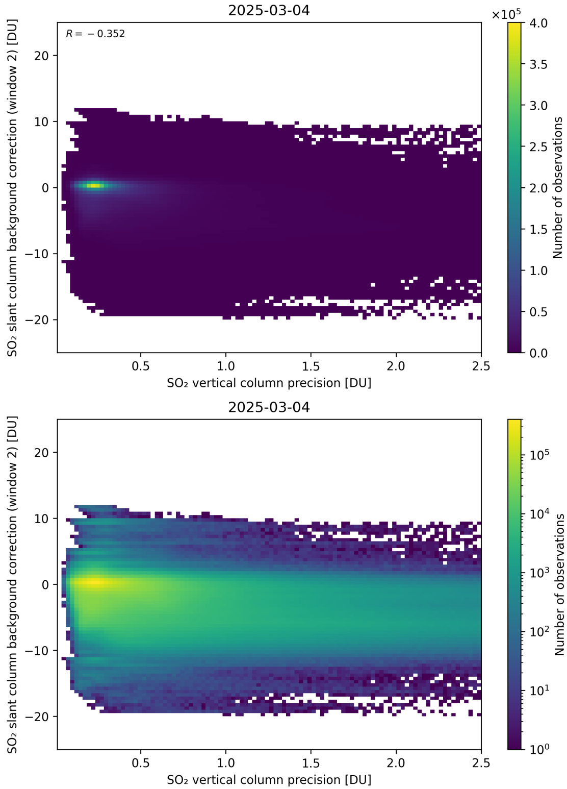
Figure 330: Scatter density plot of “SO 2 vertical column precision” against “SO 2 slant column background correction (window 2)” for 2025-03-03 to 2025-03-05.
