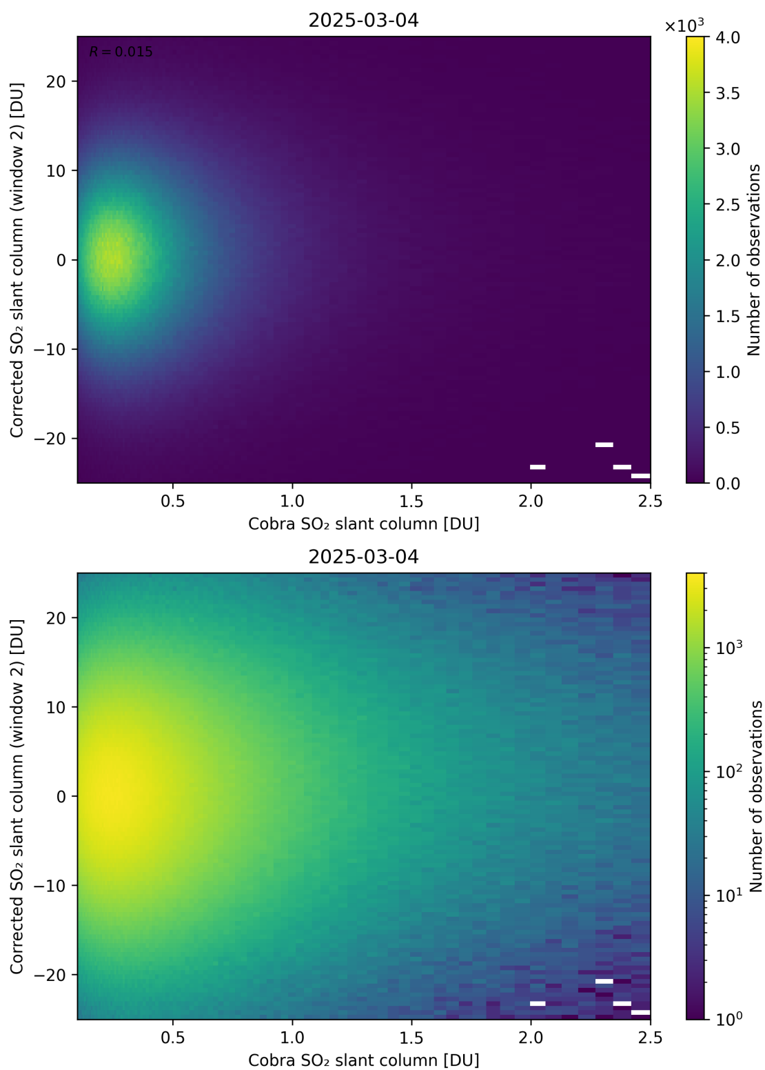
Figure 217: Scatter density plot of “Cobra SO 2 slant column” against “Corrected SO 2 slant column (window 2)” for 2025-03-03 to 2025-03-05.
