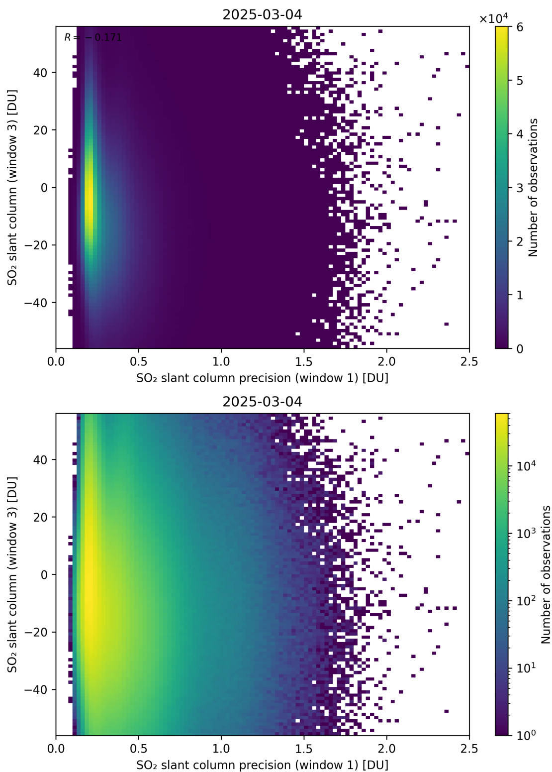
Figure 278: Scatter density plot of “SO 2 slant column precision (window 1)” against “SO 2 slant column (window 3)” for 2025-03-03 to 2025-03-05.
