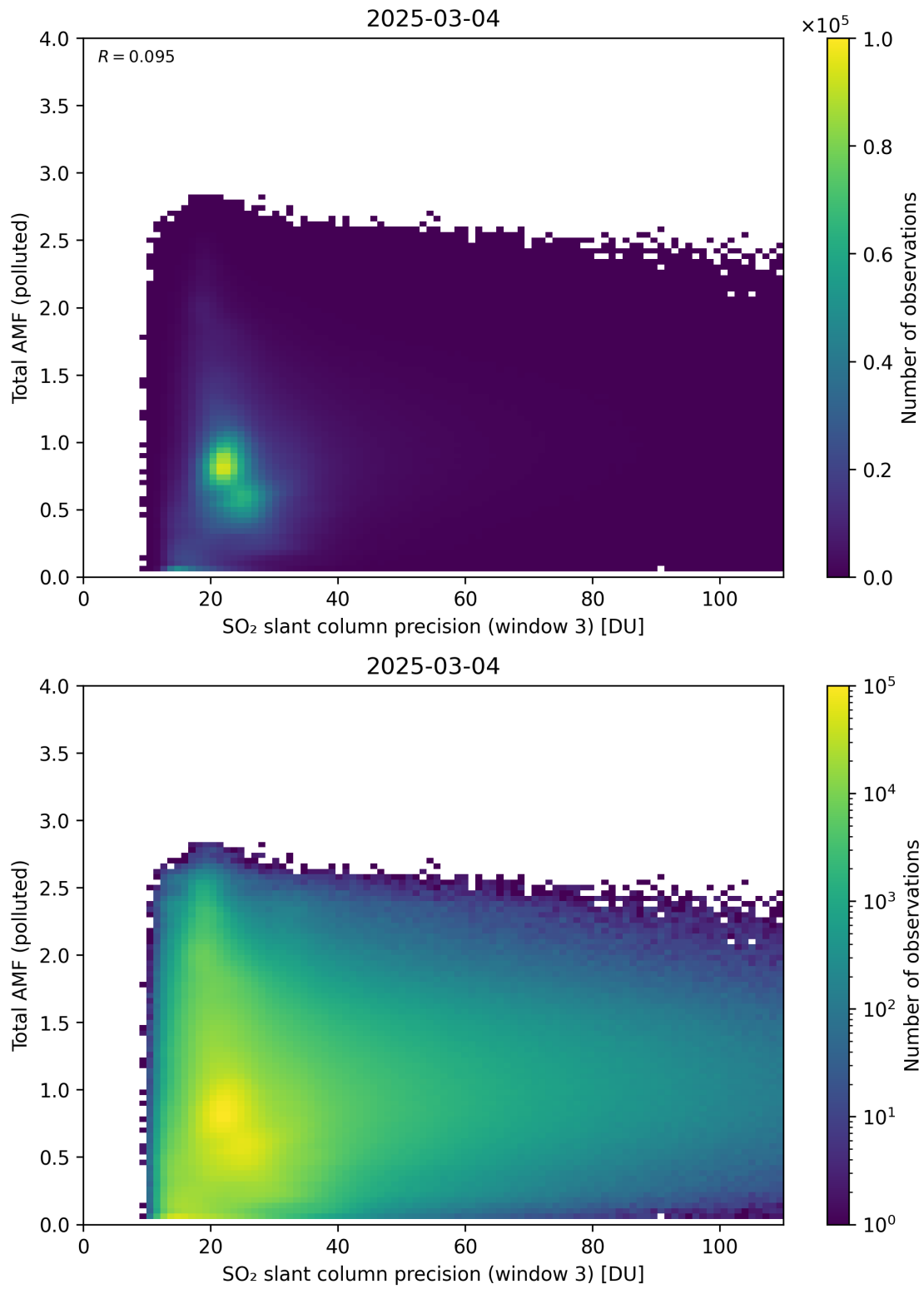
Figure 313: Scatter density plot of “SO 2 slant column precision (window 3)” against “Total AMF (polluted)” for 2025-03-03 to 2025-03-05.
