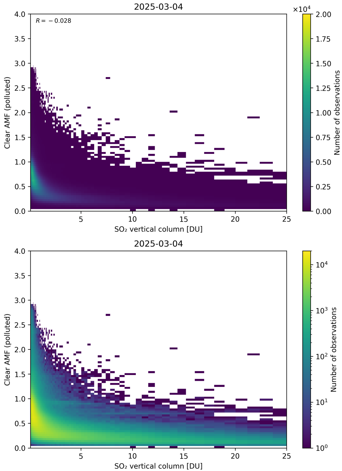
Figure 348: Scatter density plot of “SO 2 vertical column” against “Clear AMF (polluted)” for 2025-03-03 to 2025-03-05.
