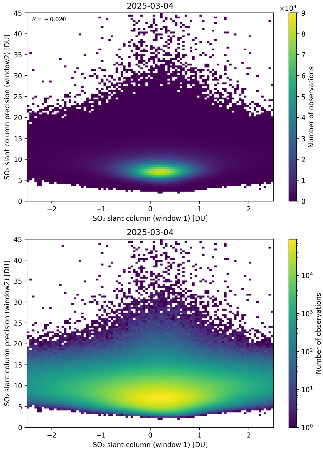
Figure 286: Scatter density plot of “SO 2 slant column (window 1)” against “SO 2 slant column precision (window2)” for 2025-03-03 to 2025-03-05.
