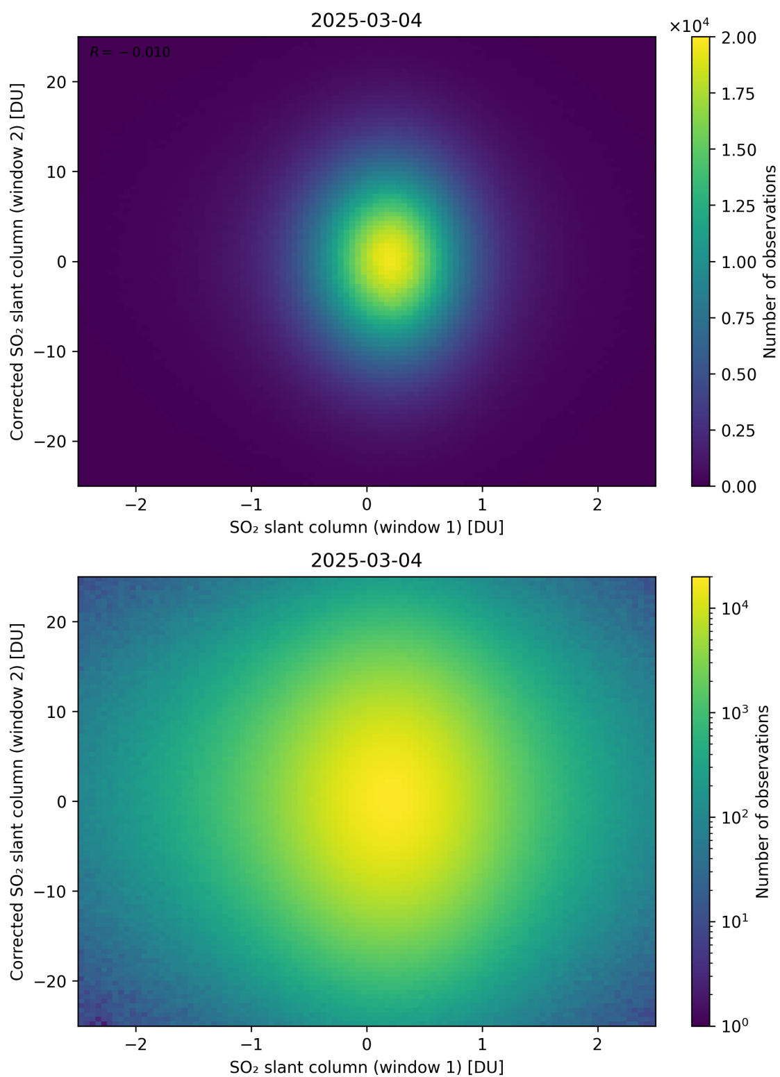
Figure 283: Scatter density plot of “SO 2 slant column (window 1)” against “Corrected SO 2 slant column (window 2)” for 2025-03-03 to 2025-03-05.
