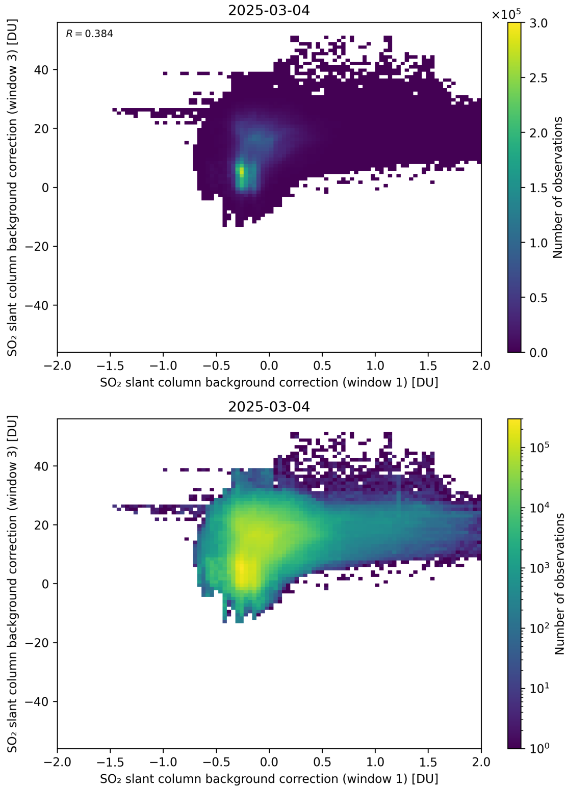
Figure 110: Scatter density plot of “SO 2 slant column background correction (window 1)” against “SO 2 slant column background correction (window 3)” for 2025-03-03 to 2025-03-05.
