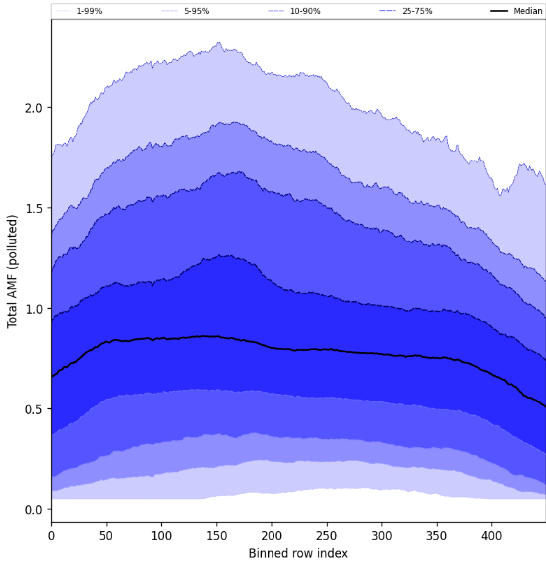
Figure 105: Along track statistics of “Total AMF (polluted)” for 2025-03-03 to 2025-03-05
