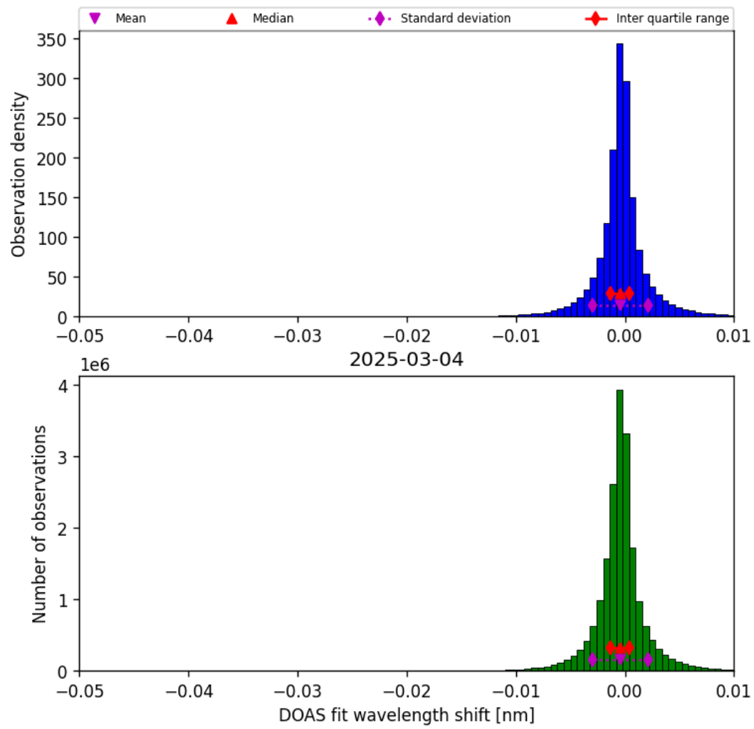
Figure 76: Histogram of “DOAS fit wavelength shift” for 2025-03-03 to 2025-03-05
