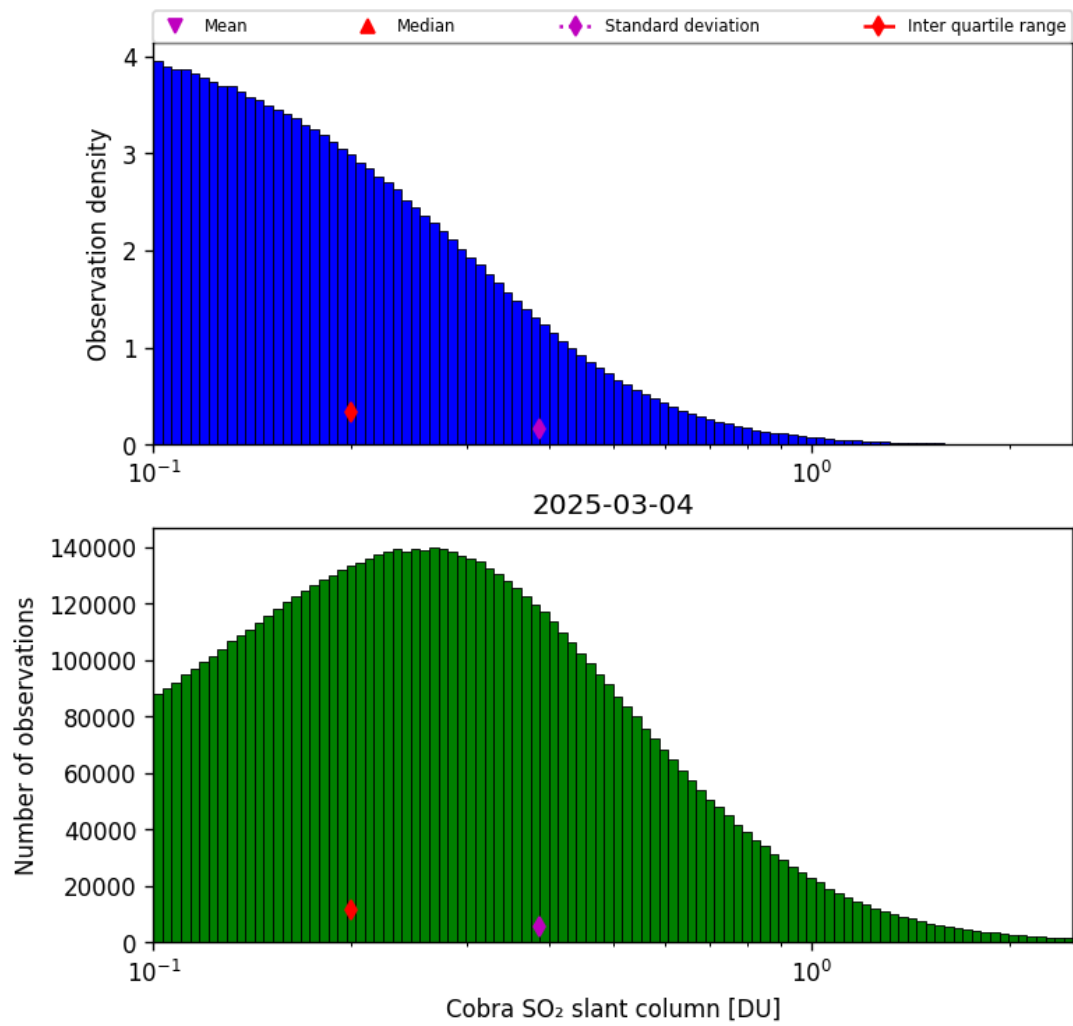
Figure 61: Histogram of “Cobra SO 2 slant column” for 2025-03-03 to 2025-03-05
