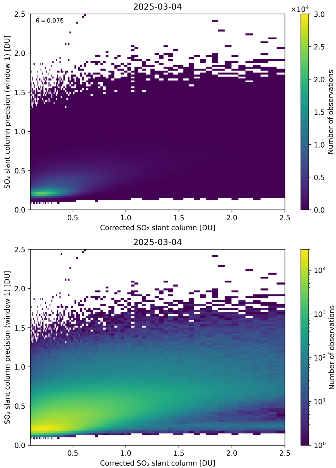
Figure 238: Scatter density plot of “Corrected SO 2 slant column” against “SO 2 slant column precision (window 1)” for 2025-03-03 to 2025-03-05.
