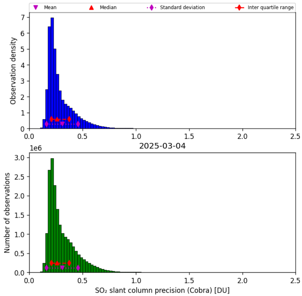
Figure 62: Histogram of “SO 2 slant column precision (Cobra)” for 2025-03-03 to 2025-03-05
