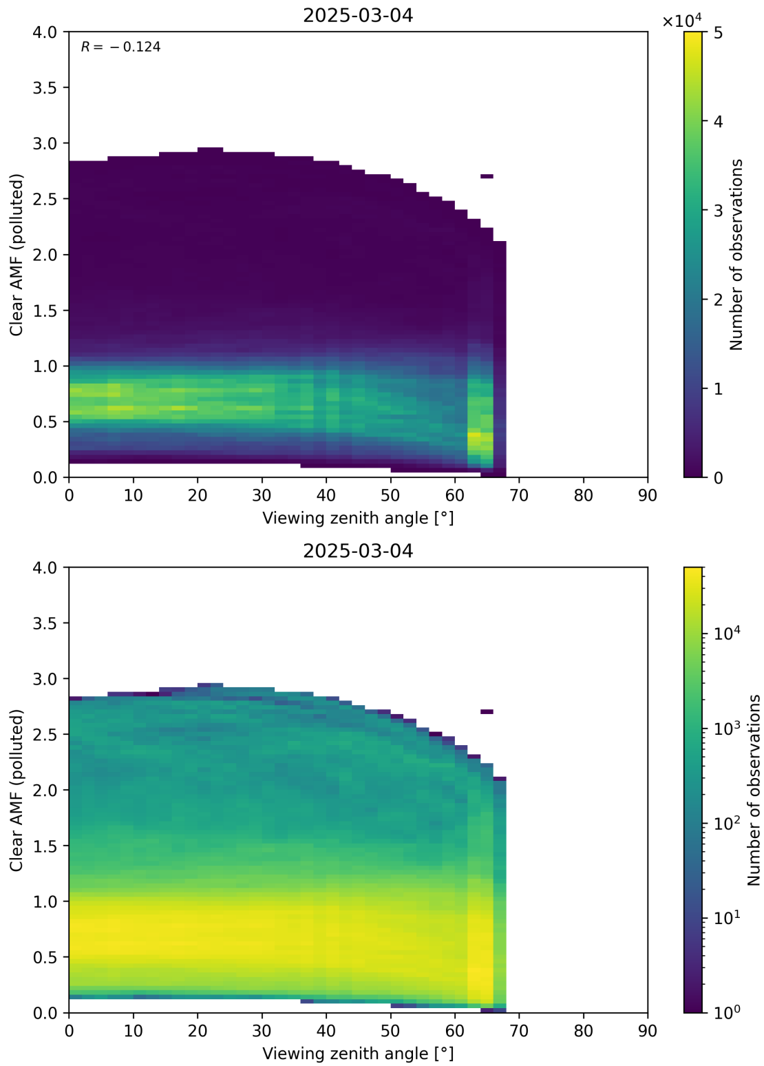
Figure 370: Scatter density plot of “Viewing zenith angle” against “Clear AMF (polluted)” for 2025-03-03 to 2025-03-05.
