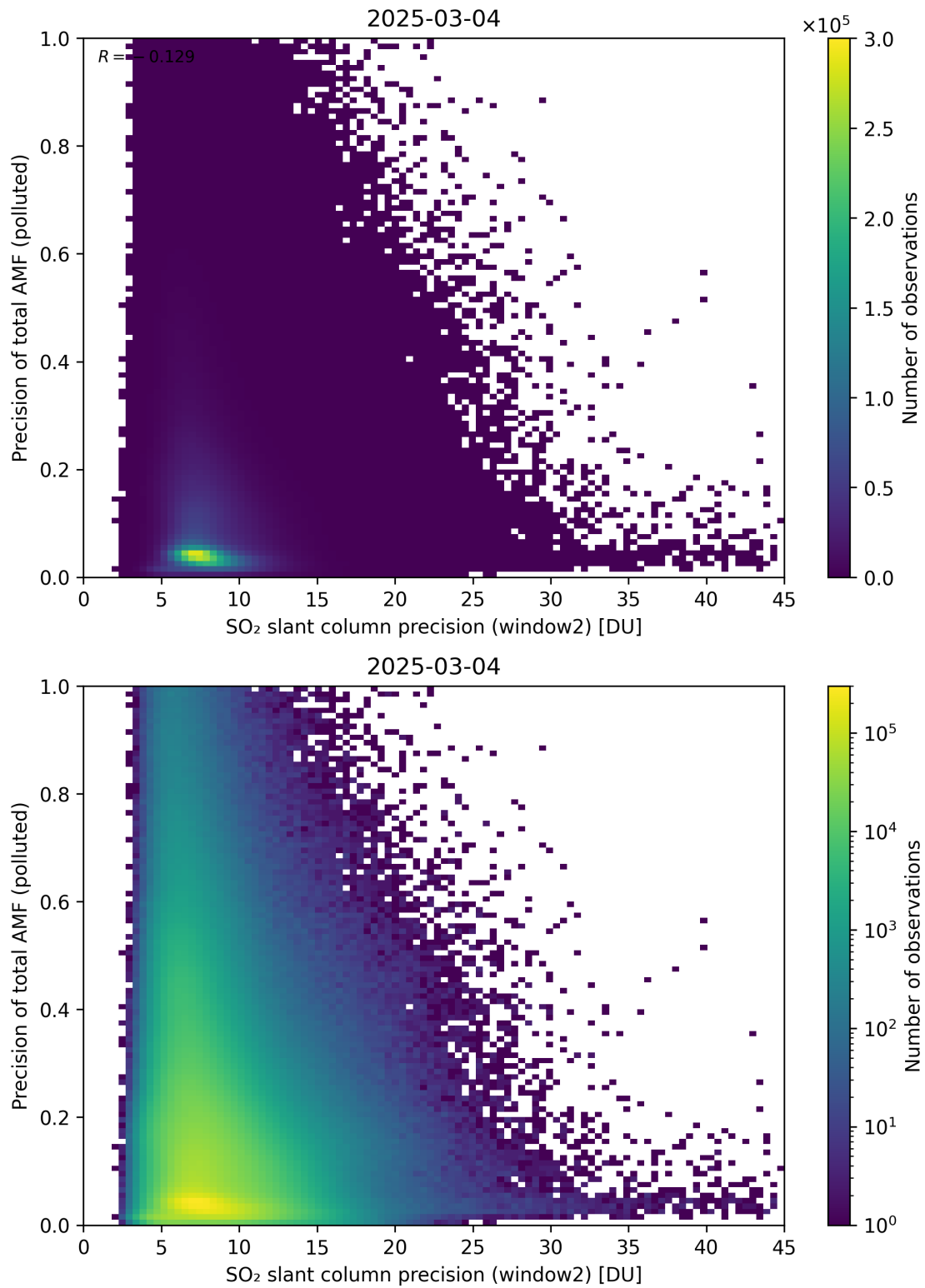
Figure 302: Scatter density plot of “SO 2 slant column precision (window2)” against “Precision of total AMF (polluted)” for 2025-03-03 to 2025-03-05.
