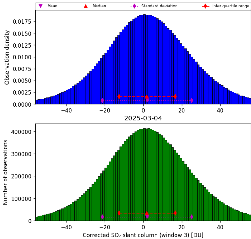
Figure 73: Histogram of “Corrected SO 2 slant column (window 3)” for 2025-03-03 to 2025-03-05
