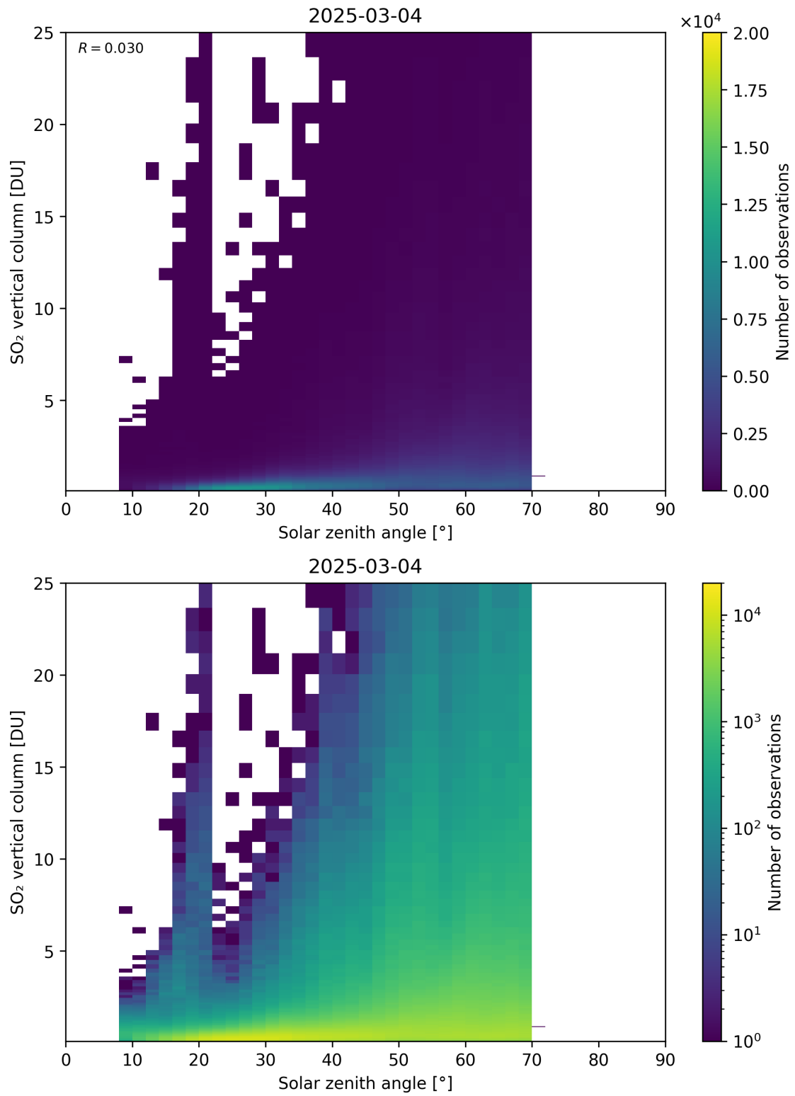
Figure 191: Scatter density plot of “Solar zenith angle” against “SO 2 vertical column” for 2025-03-03 to 2025-03-05.
