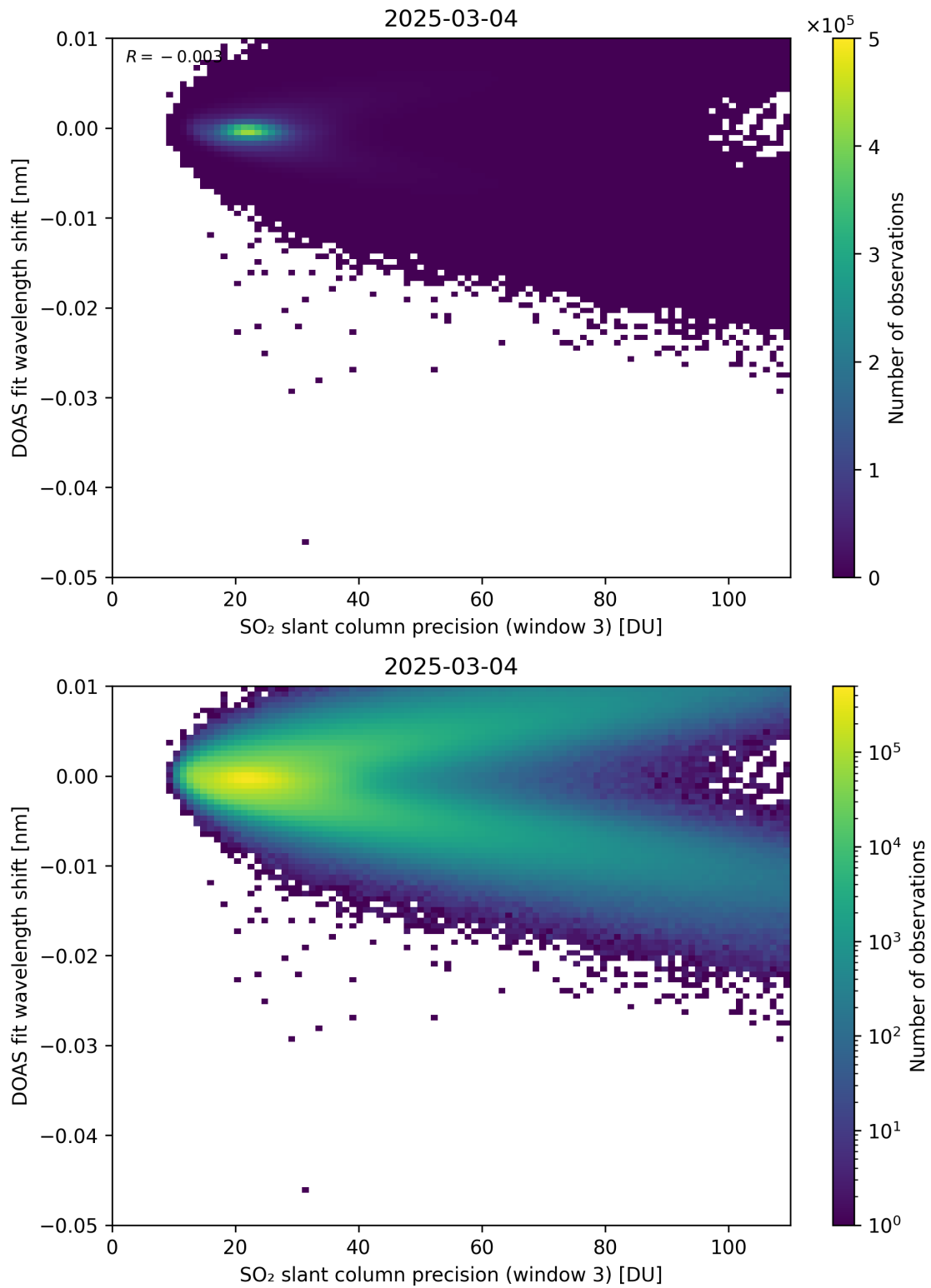
Figure 308: Scatter density plot of “SO 2 slant column precision (window 3)” against “DOAS fit wavelength shift” for 2025-03-03 to 2025-03-05.
