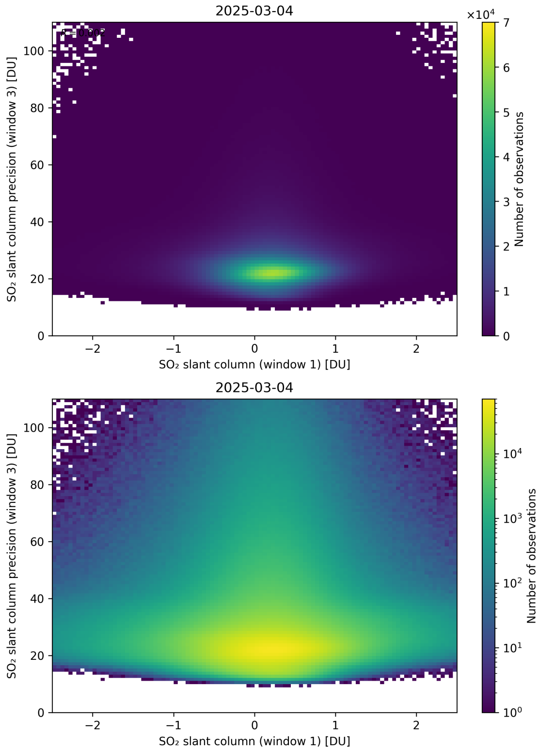
Figure 288: Scatter density plot of “SO 2 slant column (window 1)” against “SO 2 slant column precision (window 3)” for 2025-03-03 to 2025-03-05.
