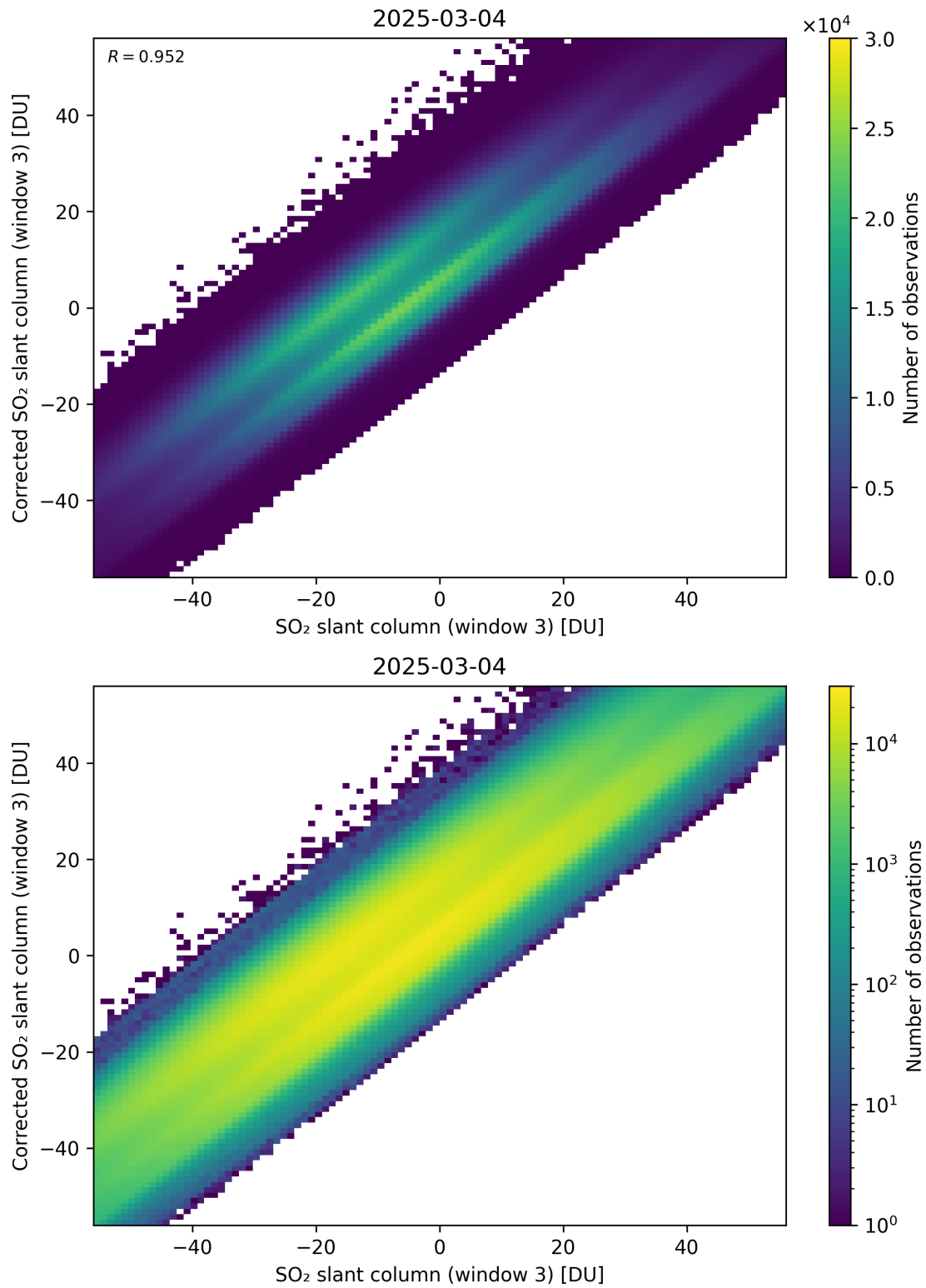
Figure 316: Scatter density plot of “SO 2 slant column (window 3)” against “Corrected SO 2 slant column (window 3)” for 2025-03-03 to 2025-03-05.
