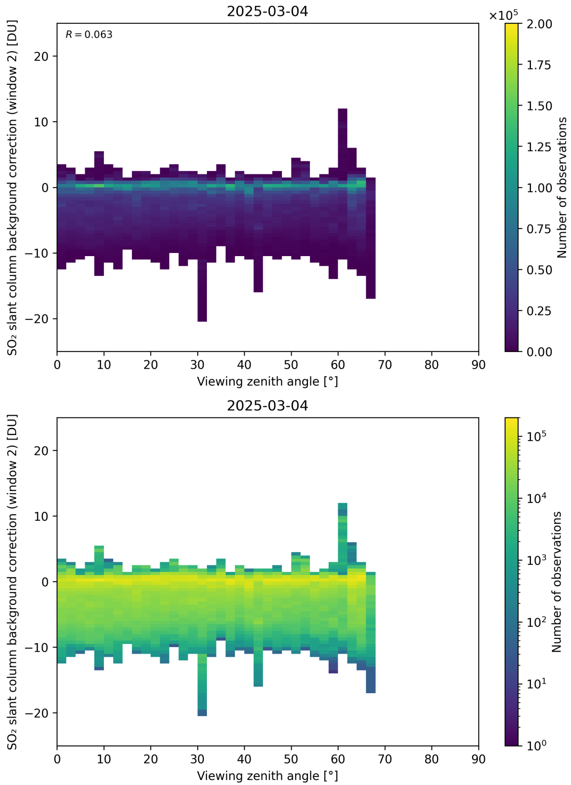
Figure 363: Scatter density plot of “Viewing zenith angle” against “SO 2 slant column background correction (window 2)” for 2025-03-03 to 2025-03-05.
