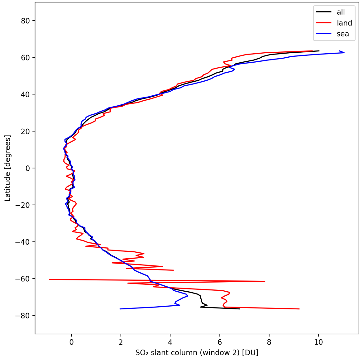
Figure 41: Zonal average of “SO 2 slant column (window 2)” for 2025-03-03 to 2025-03-05.
