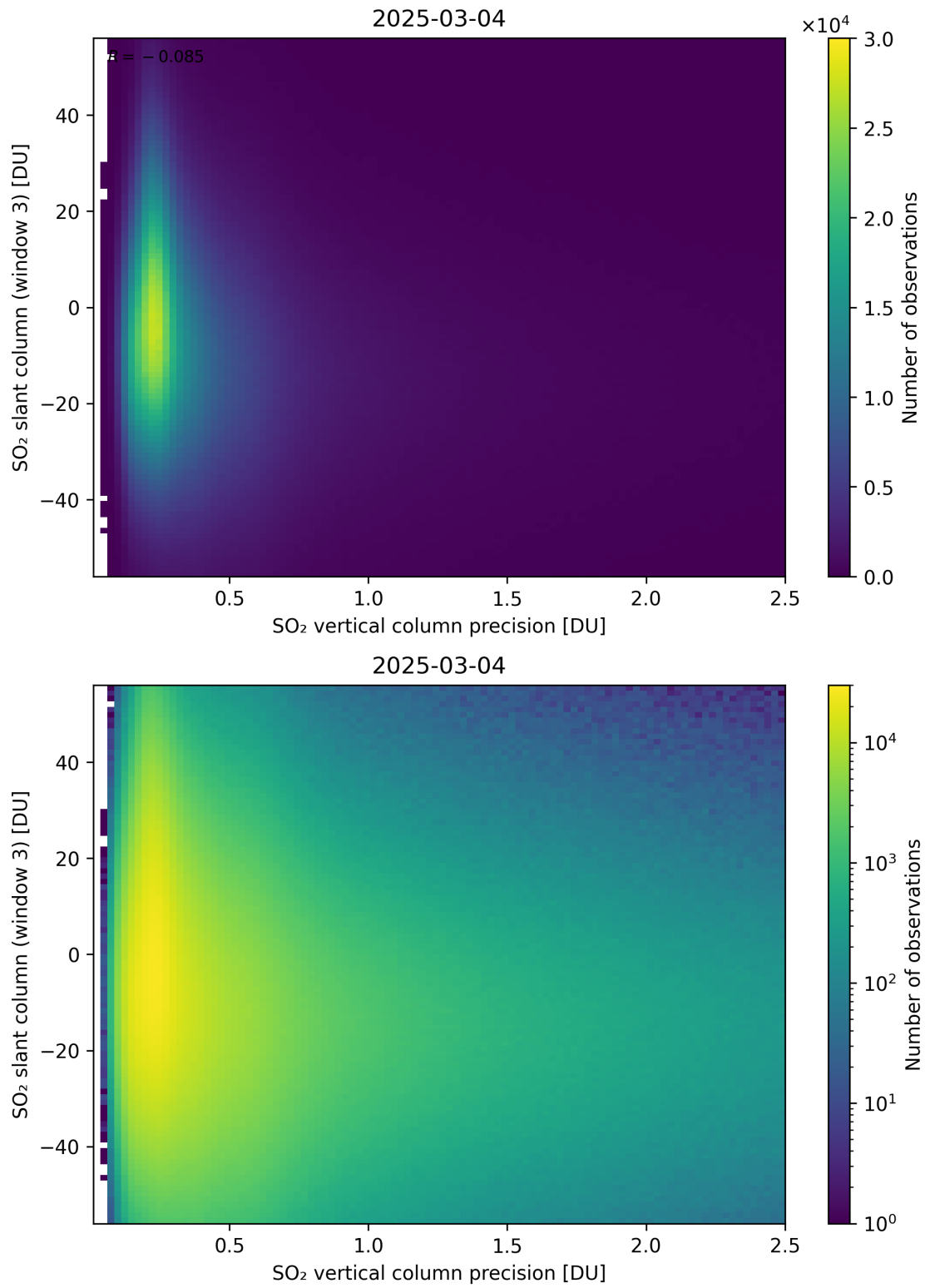
Figure 344: Scatter density plot of “SO 2 vertical column precision” against “SO 2 slant column (window 3)” for 2025-03-03 to 2025-03-05.
