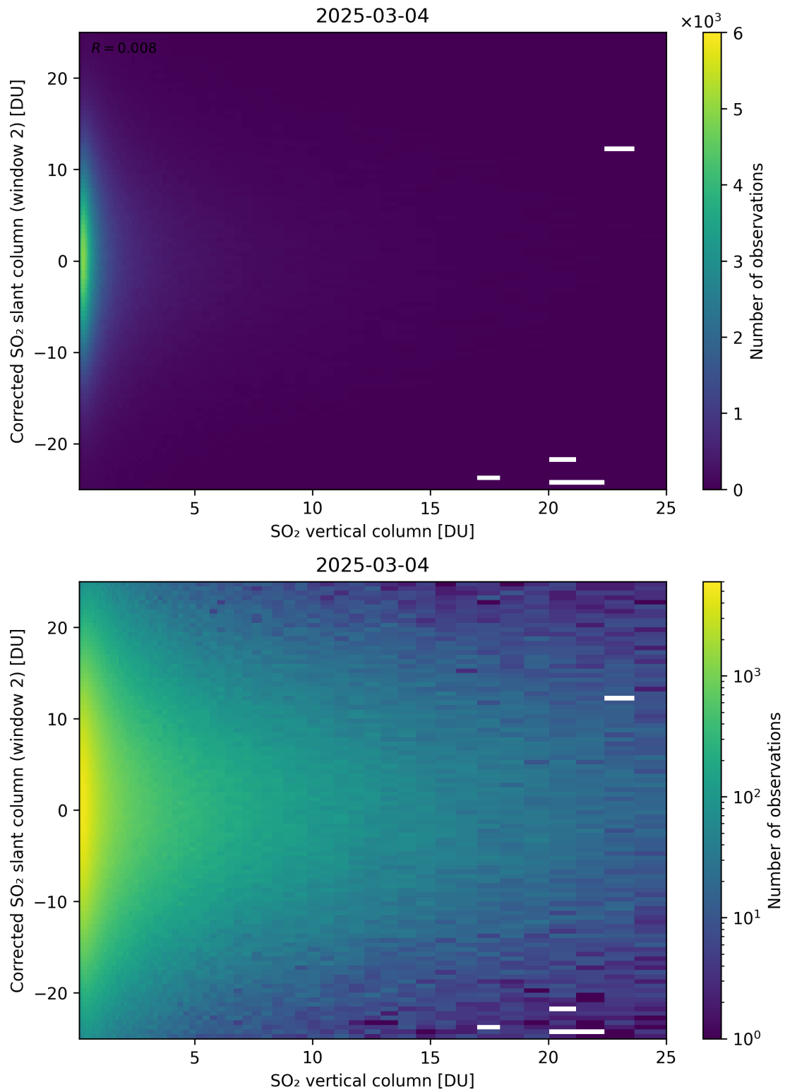
Figure 352: Scatter density plot of “SO 2 vertical column” against “Corrected SO 2 slant column (window 2)” for 2025-03-03 to 2025-03-05.
