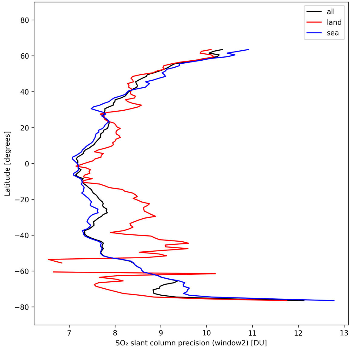
Figure 42: Zonal average of “SO 2 slant column precision (window2)” for 2025-03-03 to 2025-03-05.
