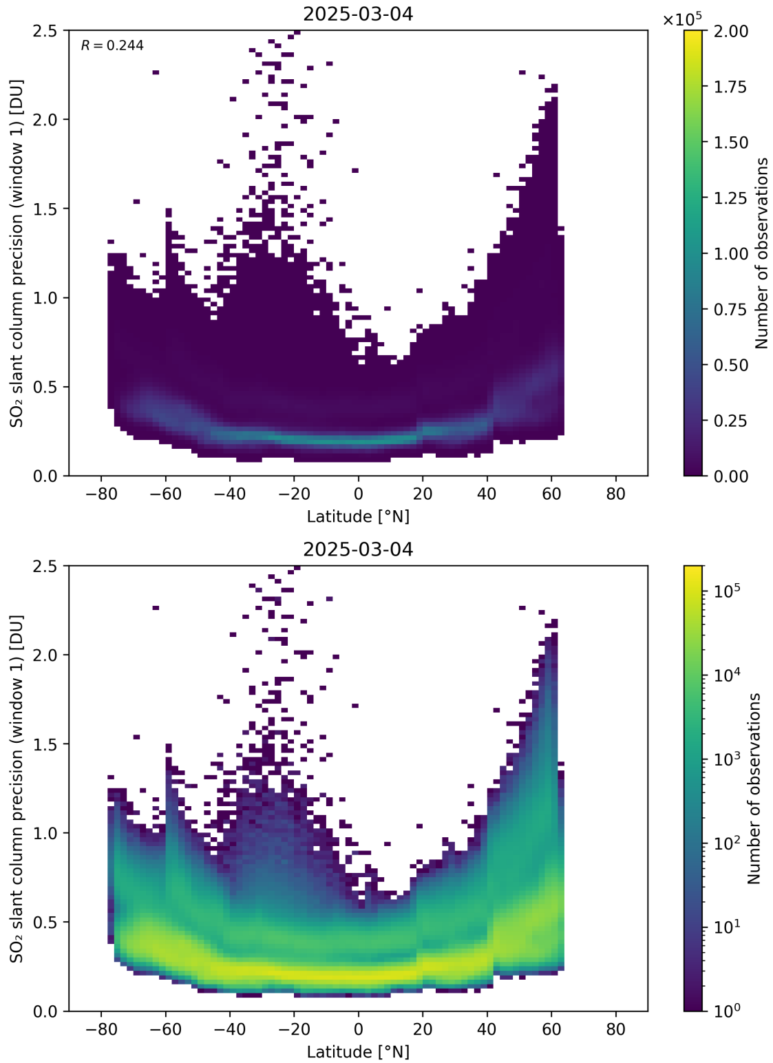
Figure 163: Scatter density plot of “Latitude” against “SO 2 slant column precision (window 1)” for 2025-03-03 to 2025-03-05.
