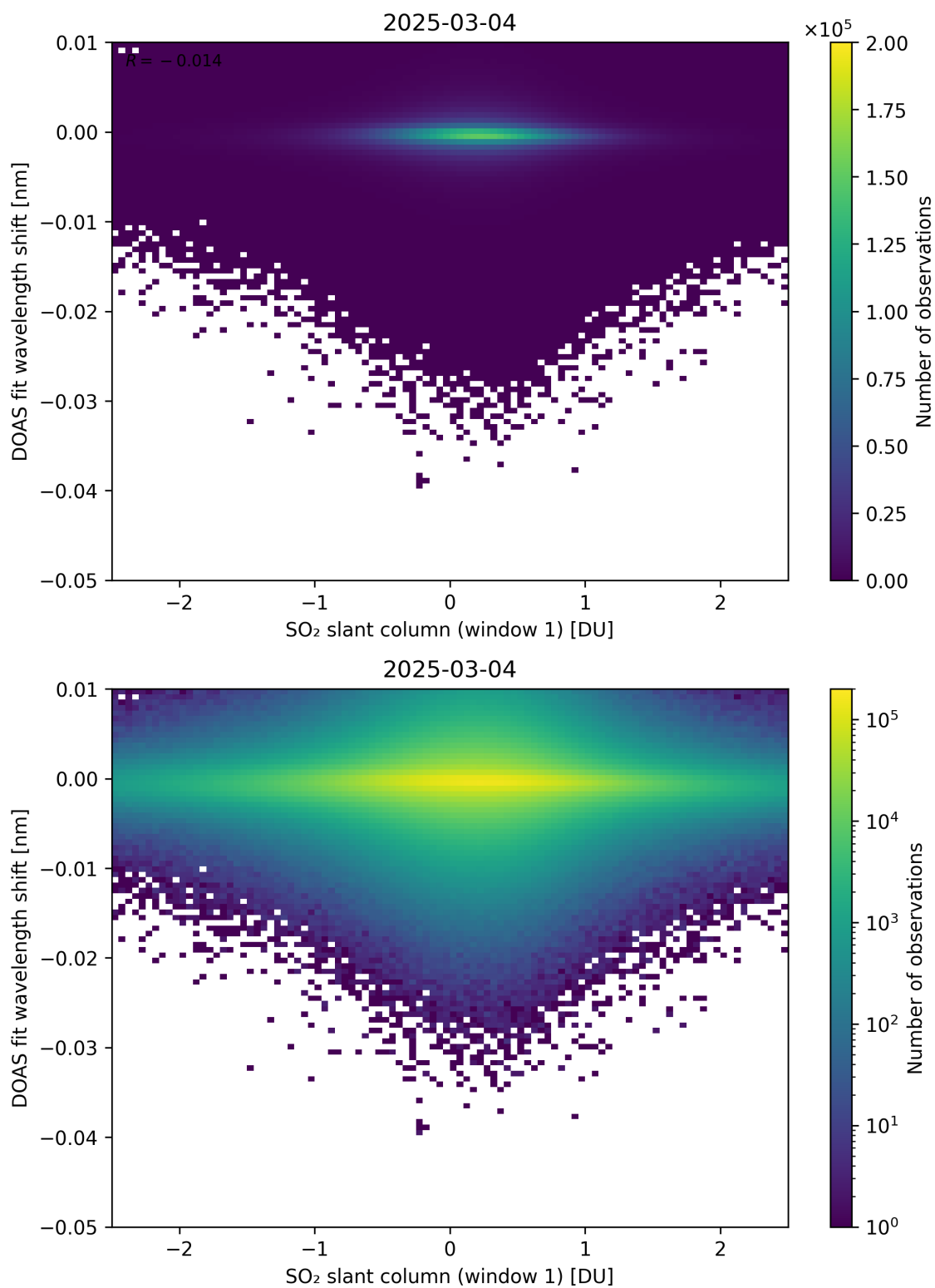
Figure 265: Scatter density plot of “SO 2 slant column (window 1)” against “DOAS fit wavelength shift” for 2025-03-03 to 2025-03-05.
