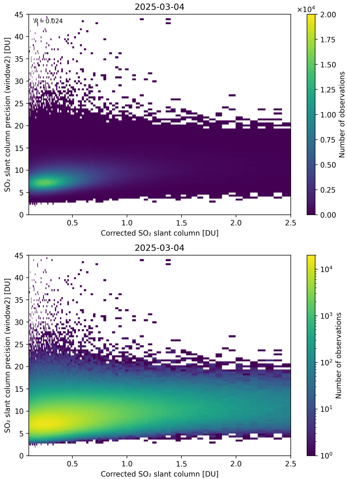
Figure 239: Scatter density plot of “Corrected SO 2 slant column” against “SO 2 slant column precision (window2)” for 2025-03-03 to 2025-03-05.
