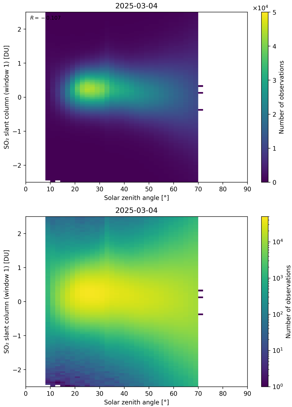
Figure 184: Scatter density plot of “Solar zenith angle” against “SO 2 slant column (window 1)” for 2025-03-03 to 2025-03-05.
