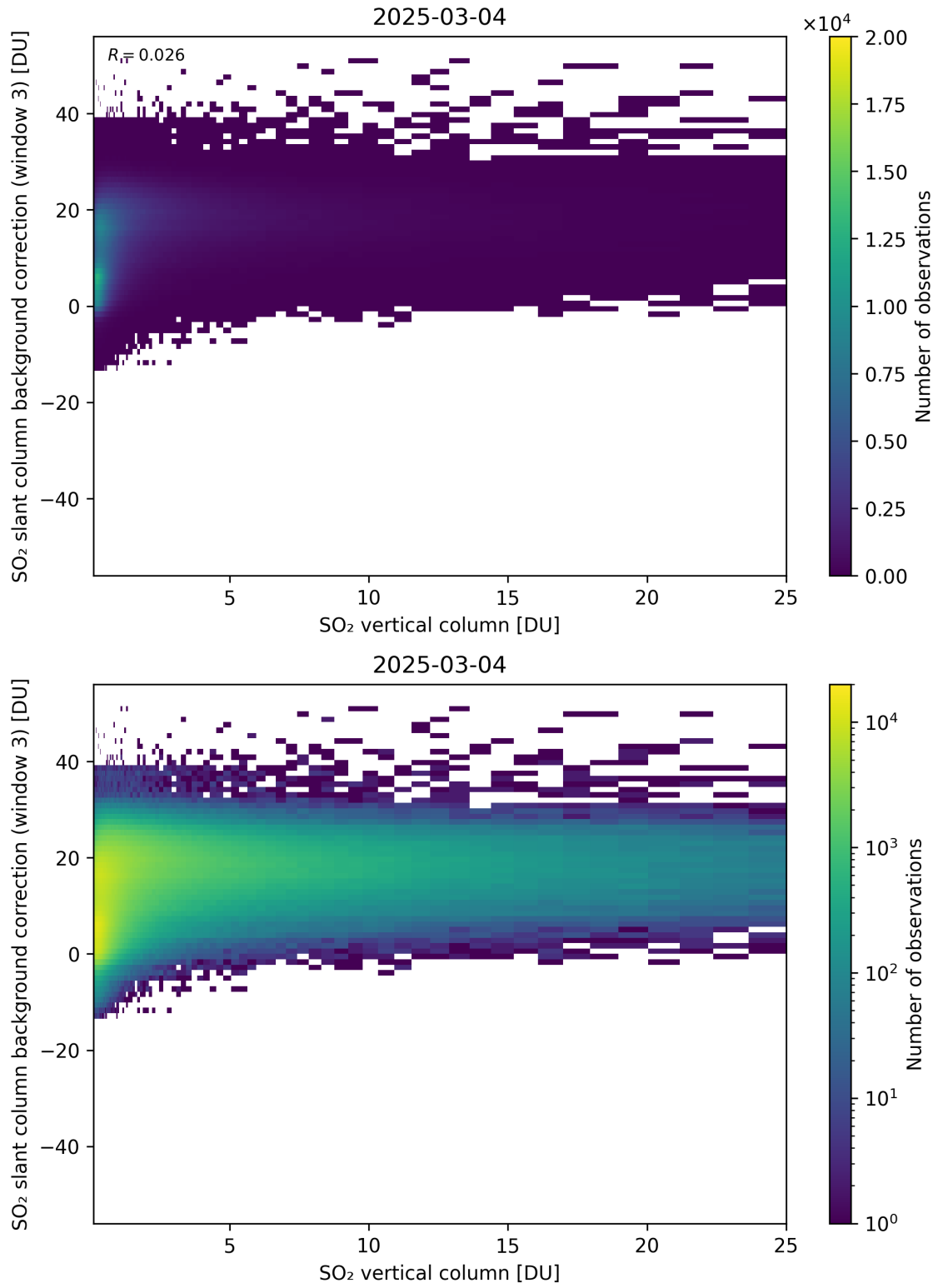
Figure 325: Scatter density plot of “SO 2 vertical column” against “SO 2 slant column background correction (window 3)” for 2025-03-03 to 2025-03-05.
