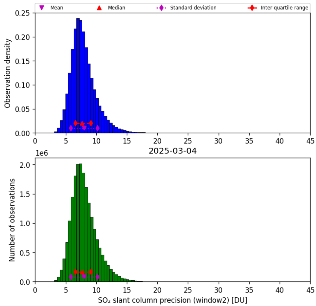
Figure 68: Histogram of “SO 2 slant column precision (window2)” for 2025-03-03 to 2025-03-05
