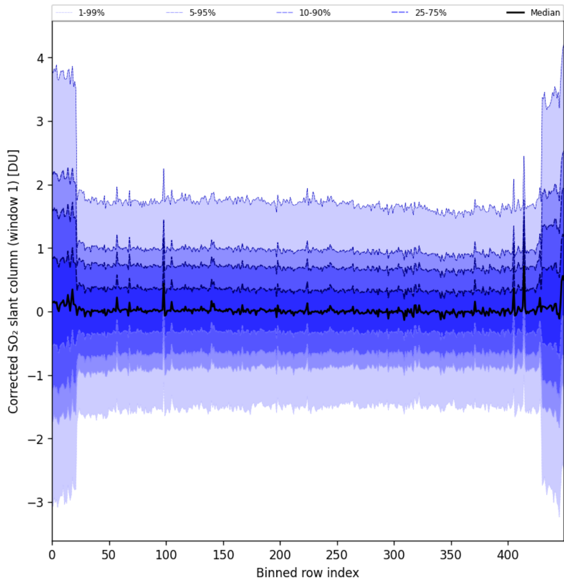
Figure 91: Along track statistics of “Corrected SO 2 slant column (window 1)” for 2025-03-03 to 2025-03-05
