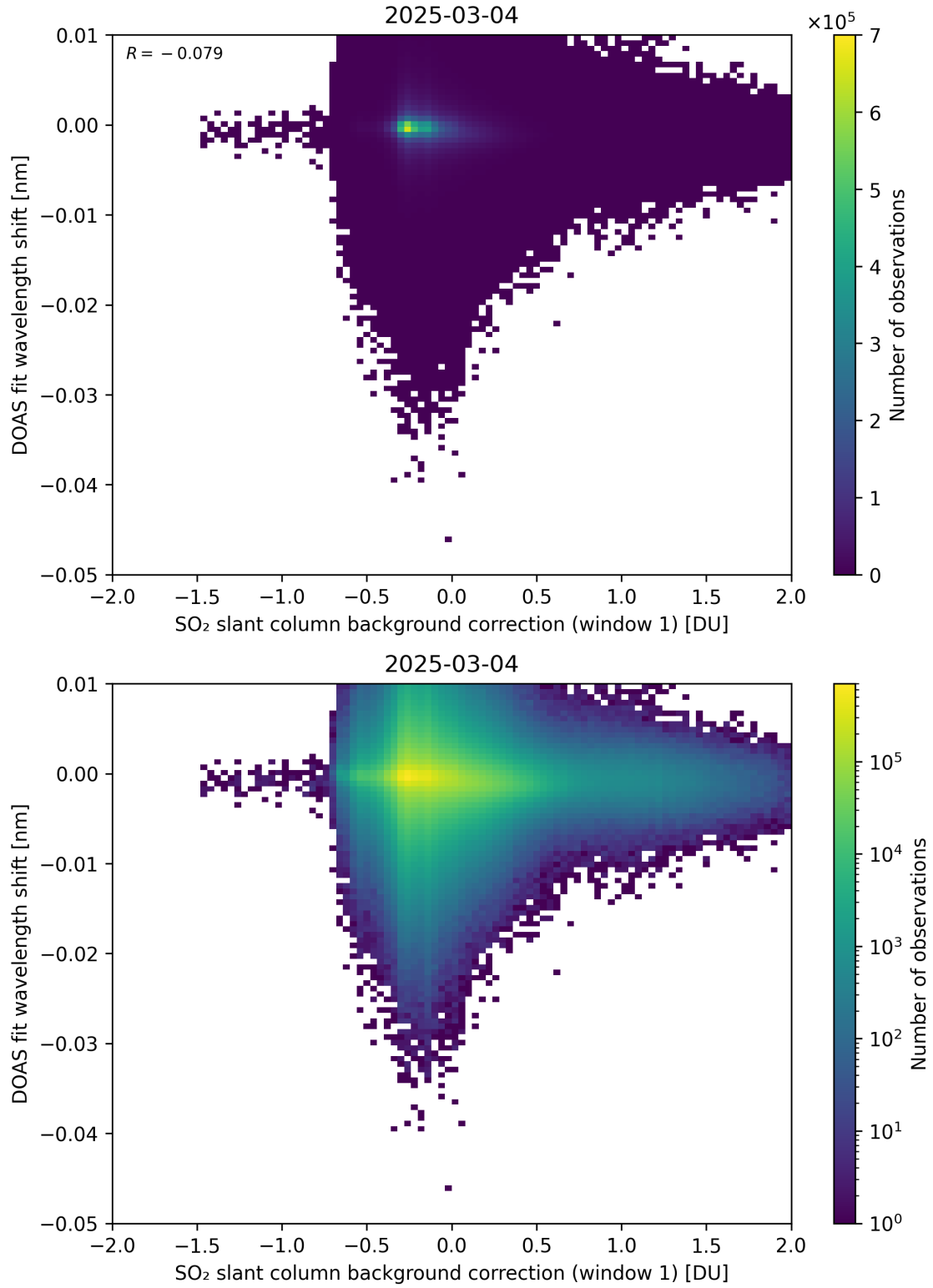
Figure 111: Scatter density plot of “SO 2 slant column background correction (window 1)” against “DOAS fit wavelength shift” for 2025-03-03 to 2025-03-05.
