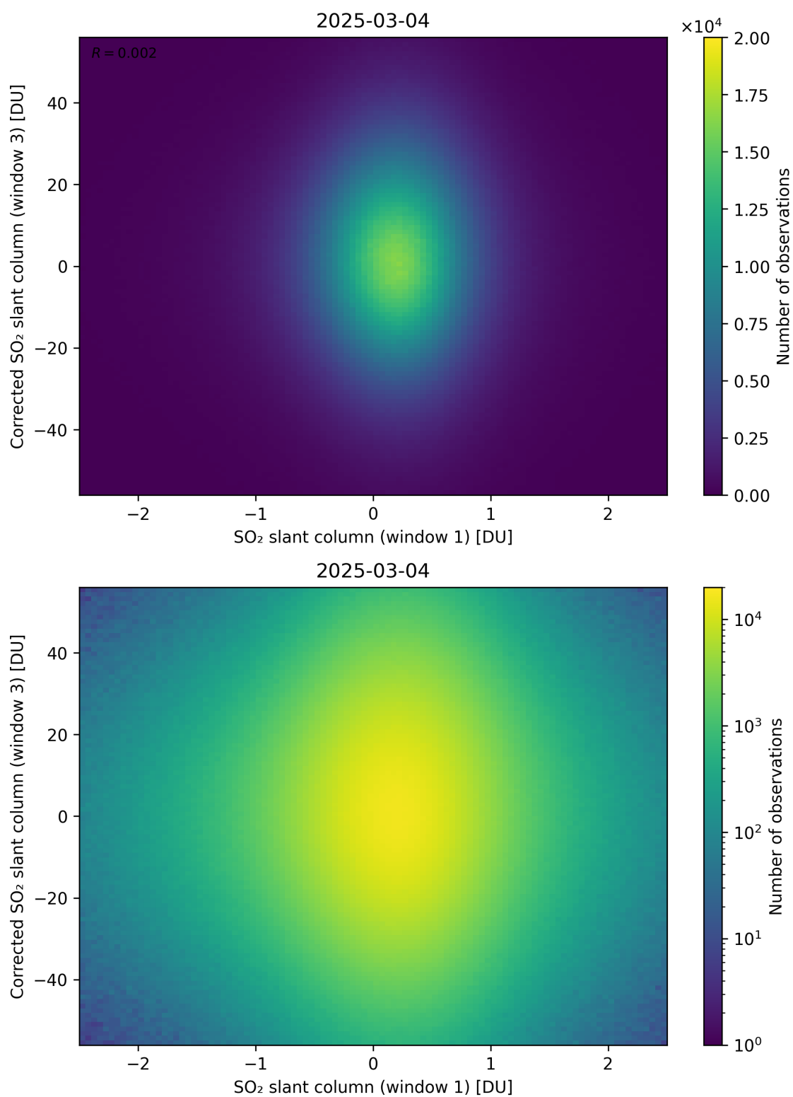
Figure 284: Scatter density plot of “SO 2 slant column (window 1)” against “Corrected SO 2 slant column (window 3)” for 2025-03-03 to 2025-03-05.
