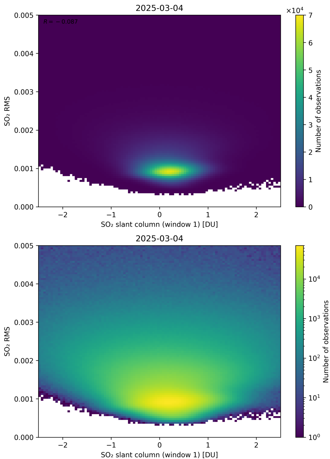
Figure 267: Scatter density plot of “SO 2 slant column (window 1)” against “SO 2 RMS” for 2025-03-03 to 2025-03-05.
