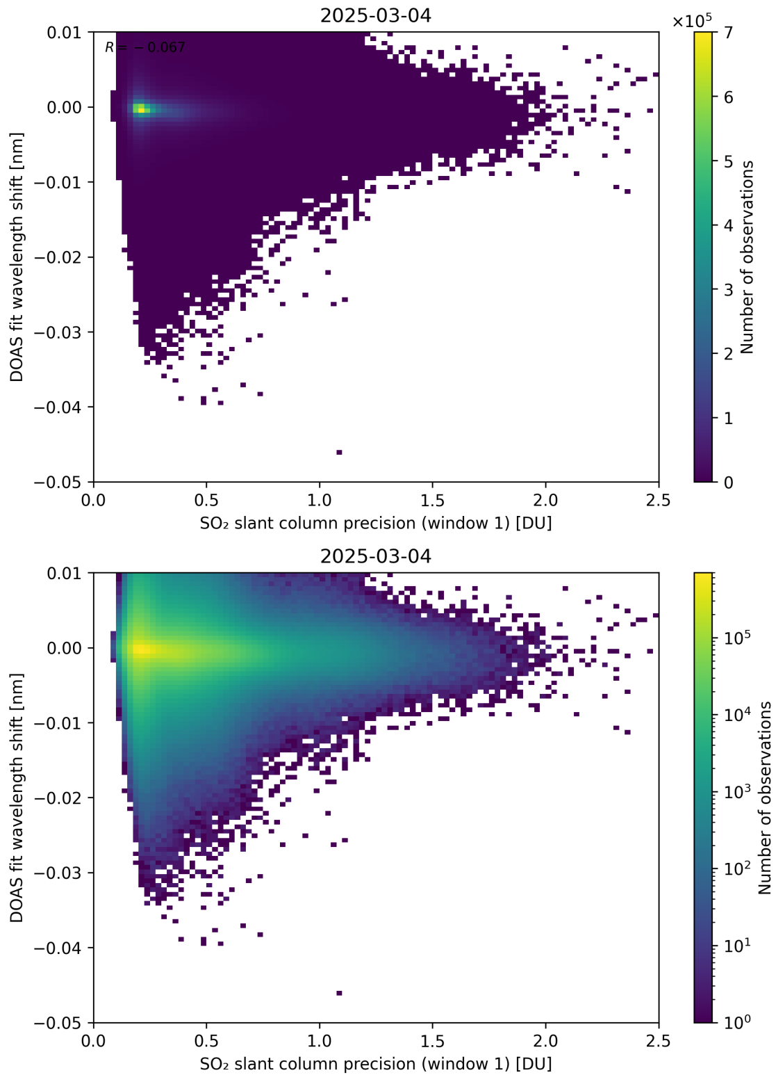
Figure 271: Scatter density plot of “SO 2 slant column precision (window 1)” against “DOAS fit wavelength shift” for 2025-03-03 to 2025-03-05.
