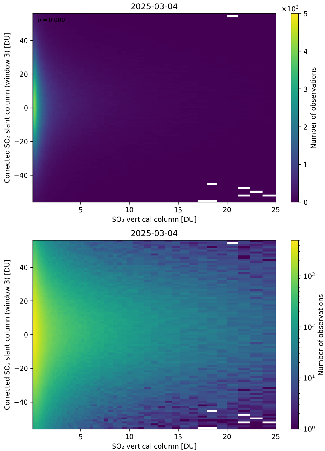
Figure 353: Scatter density plot of “SO 2 vertical column” against “Corrected SO 2 slant column (window 3)” for 2025-03-03 to 2025-03-05.
