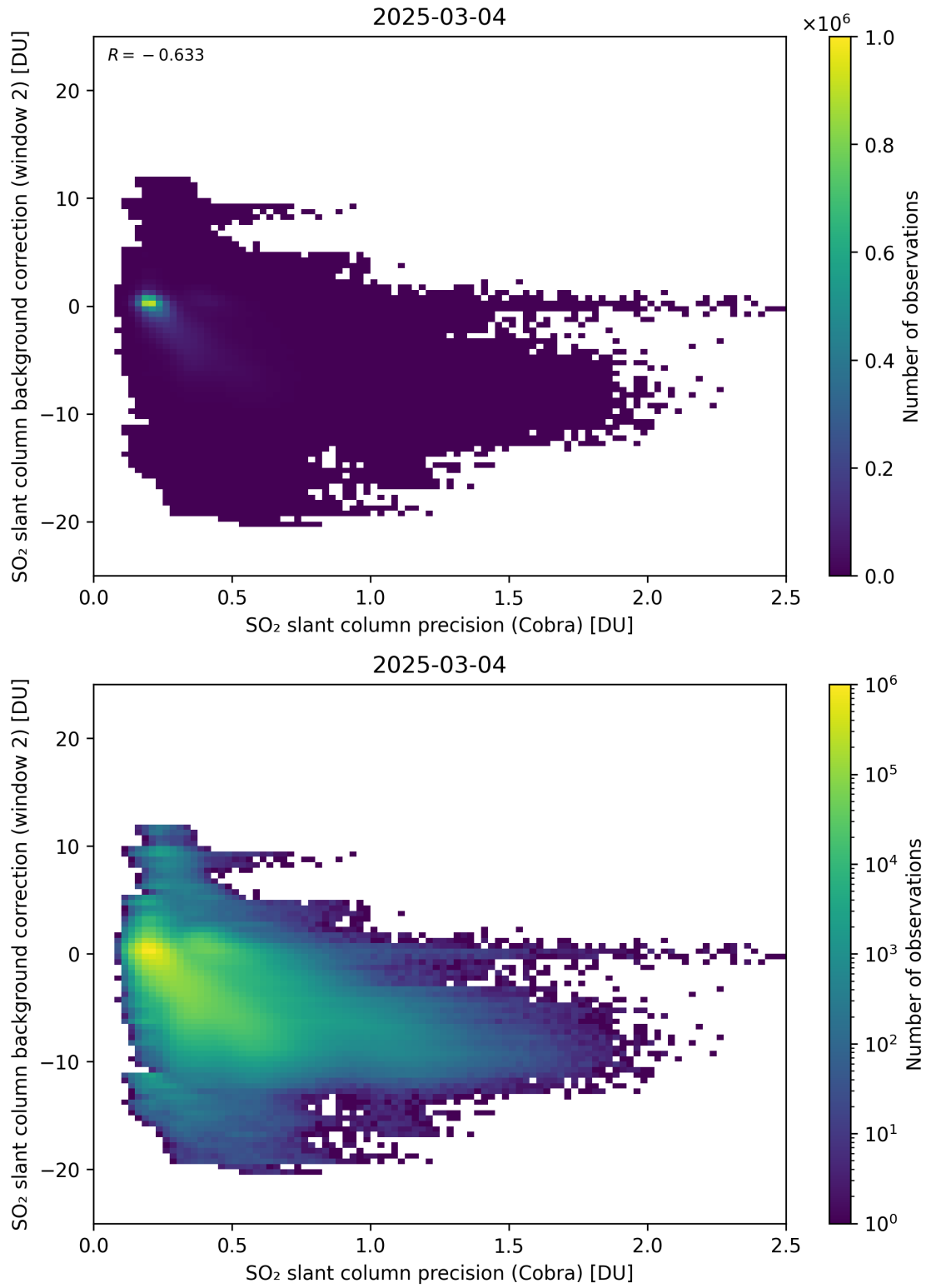
Figure 200: Scatter density plot of “SO 2 slant column precision (Cobra)” against “SO 2 slant column background correction (window 2)” for 2025-03-03 to 2025-03-05.
