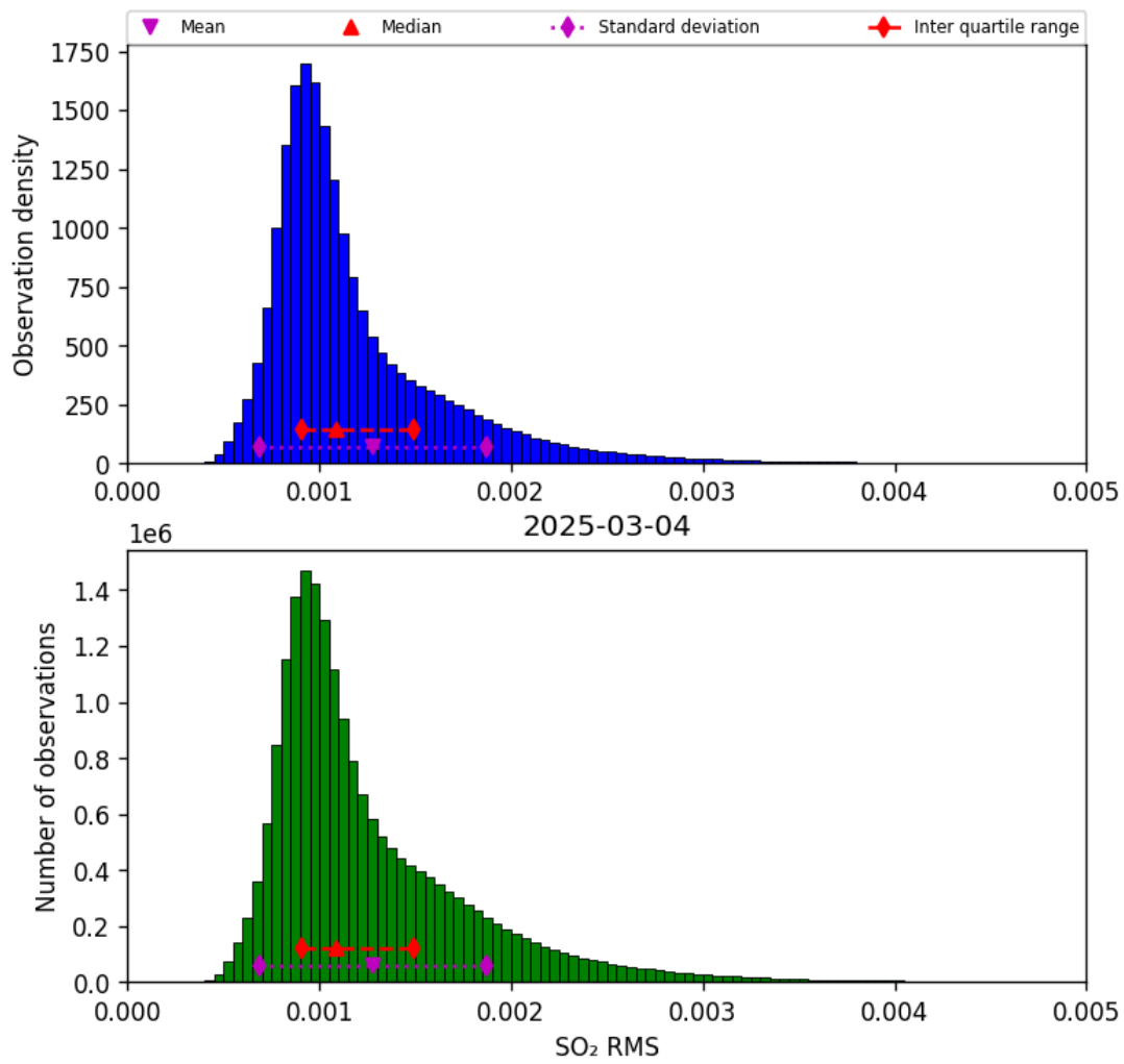
Figure 78: Histogram of “SO 2 RMS” for 2025-03-03 to 2025-03-05
