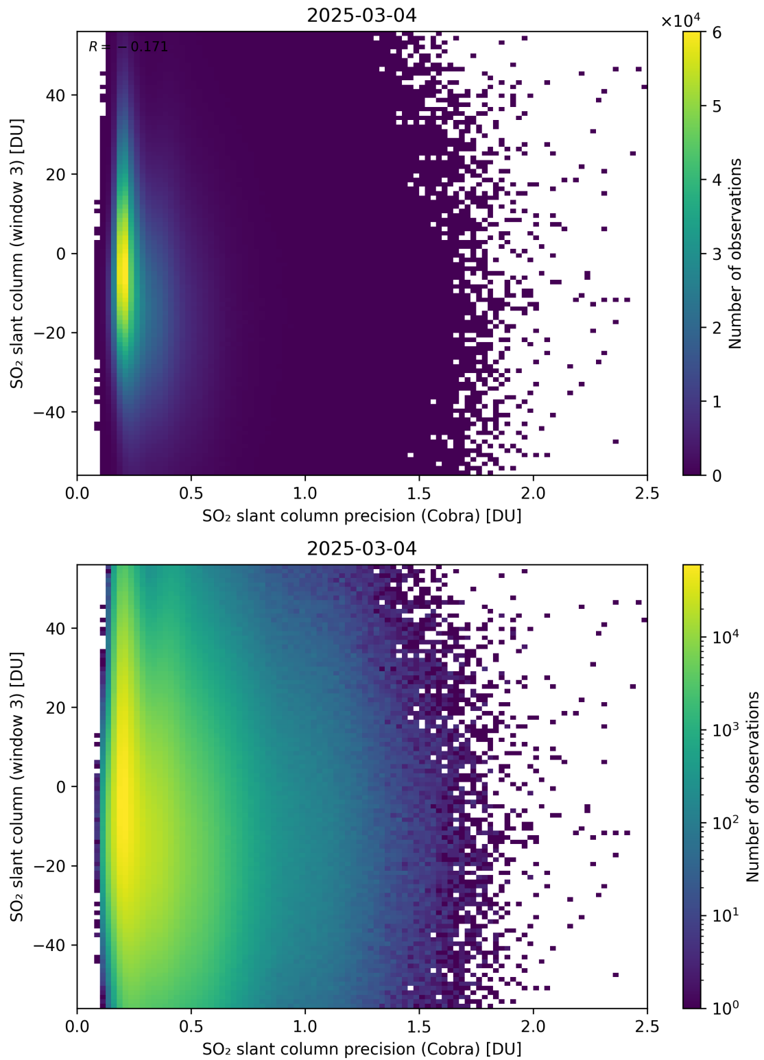
Figure 211: Scatter density plot of “SO 2 slant column precision (Cobra)” against “SO 2 slant column (window 3)” for 2025-03-03 to 2025-03-05.
