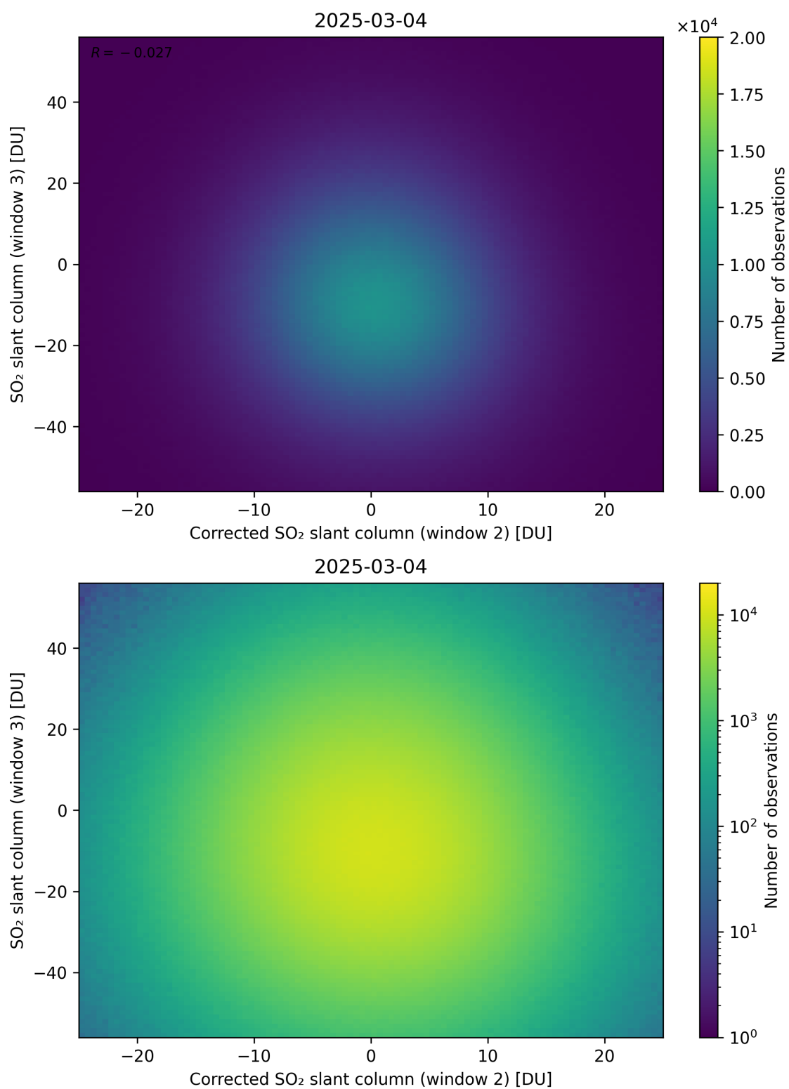
Figure 251: Scatter density plot of “Corrected SO 2 slant column (window 2)” against “SO 2 slant column (window 3)” for 2025-03-03 to 2025-03-05.
