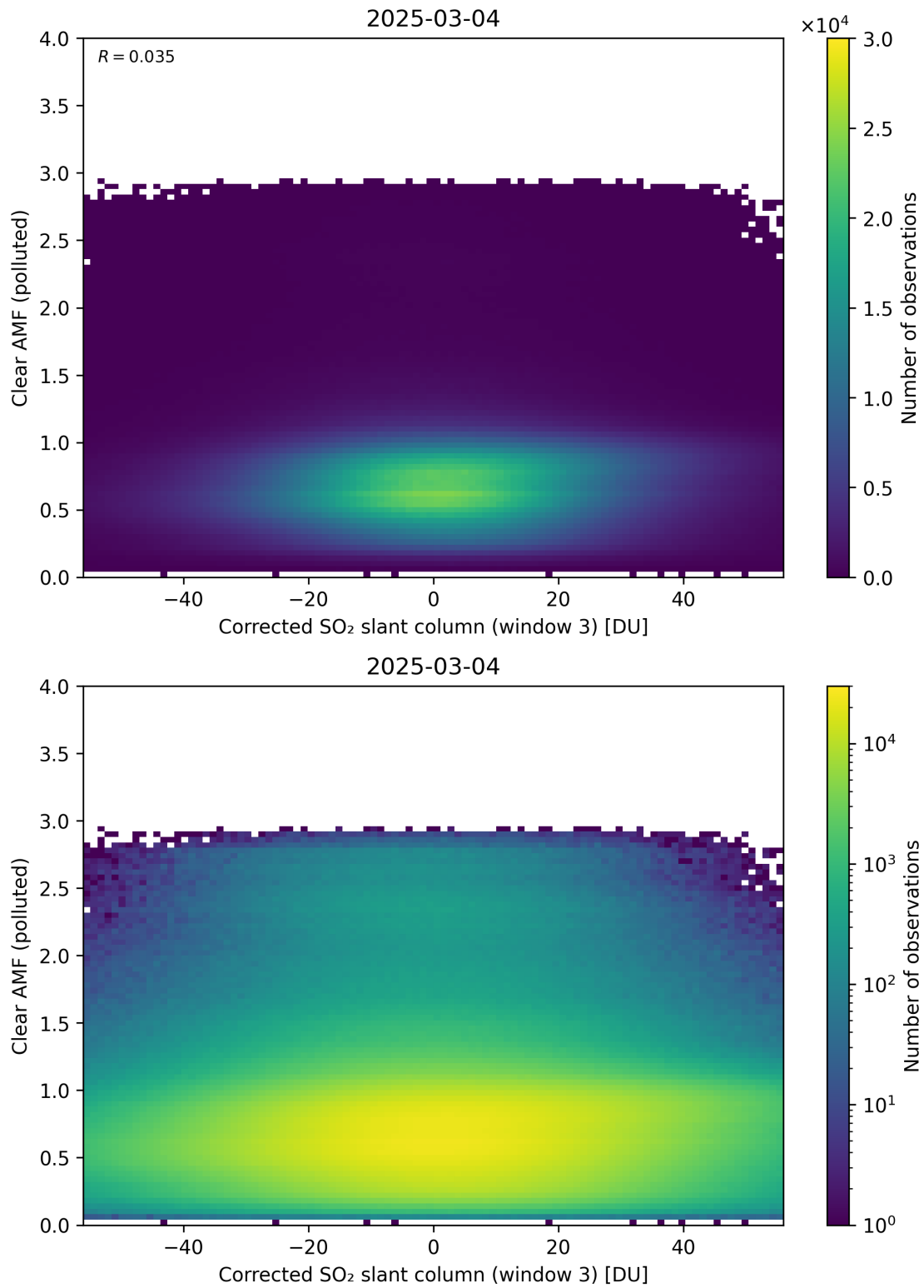
Figure 259: Scatter density plot of “Corrected SO 2 slant column (window 3)” against “Clear AMF (polluted)” for 2025-03-03 to 2025-03-05.
