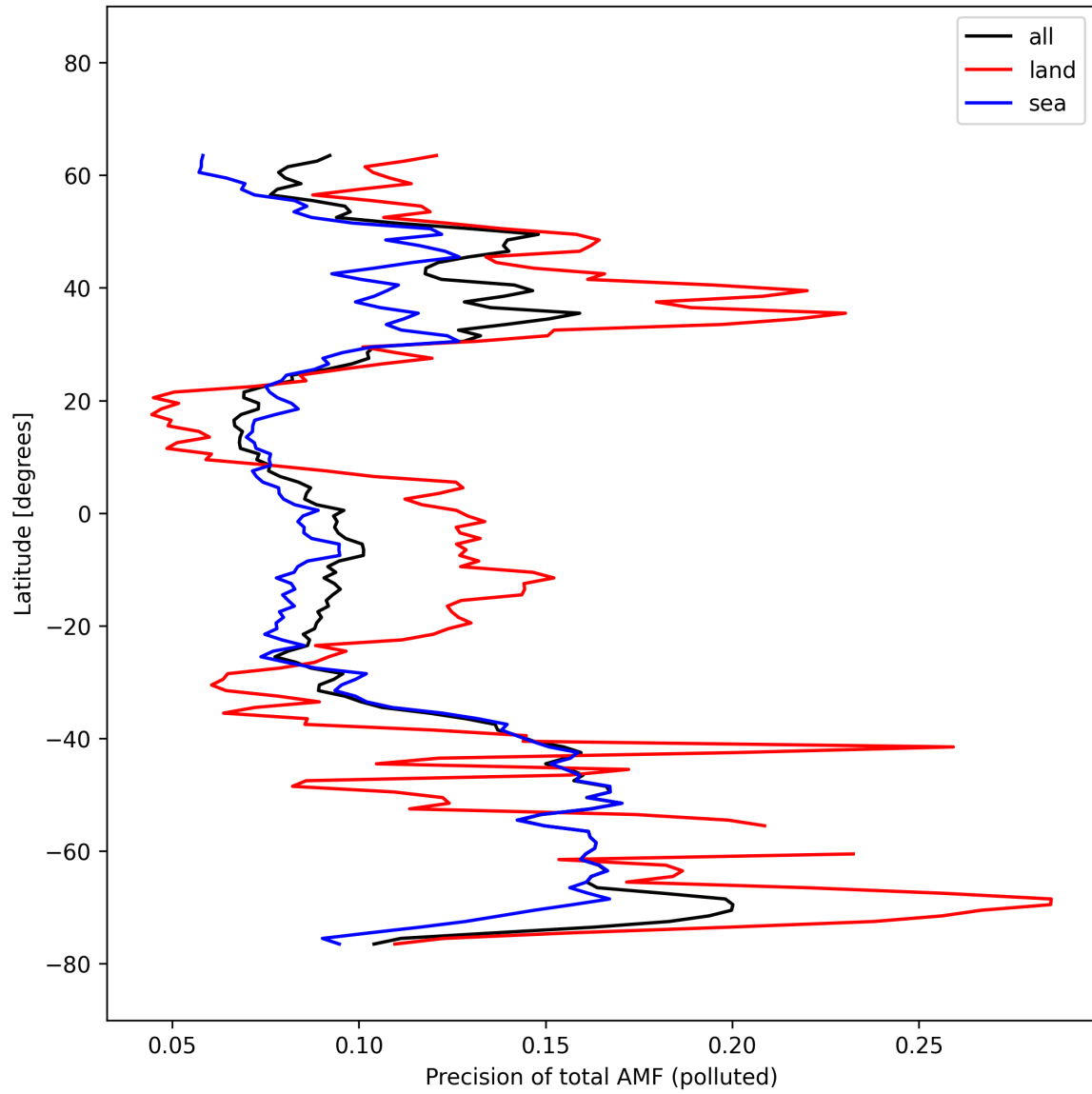
Figure 54: Zonal average of “Precision of total AMF (polluted)” for 2025-03-03 to 2025-03-05.
