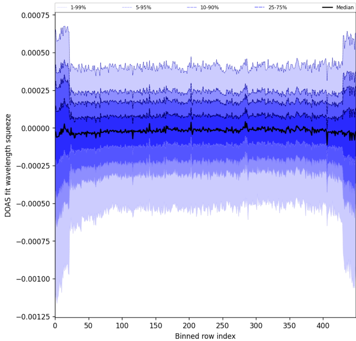
Figure 103: Along track statistics of “DOAS fit wavelength squeeze” for 2025-03-03 to 2025-03-05
