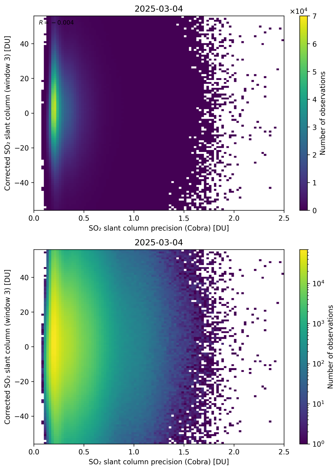
Figure 207: Scatter density plot of “SO 2 slant column precision (Cobra)” against “Corrected SO 2 slant column (window 3)” for 2025-03-03 to 2025-03-05.
