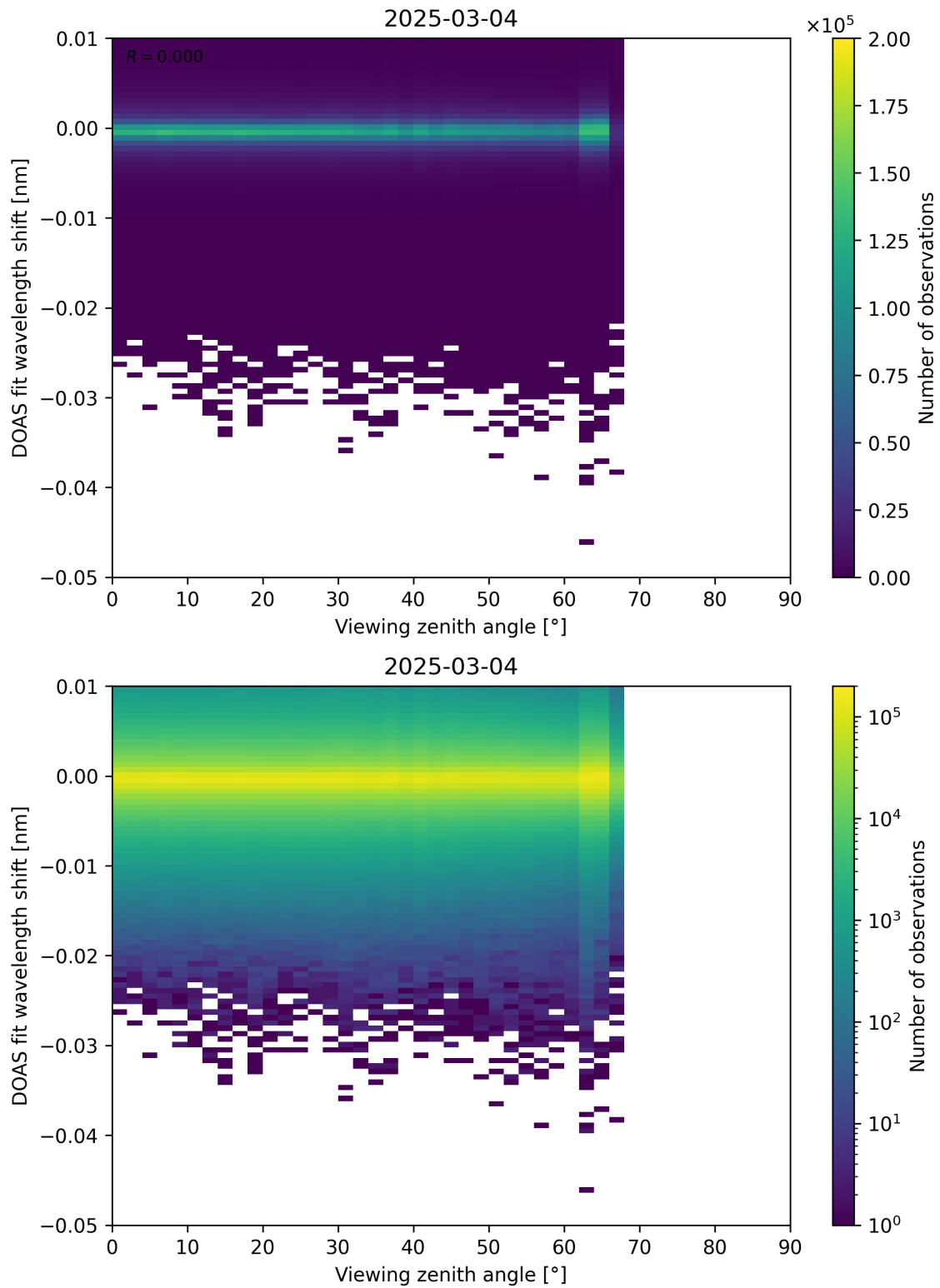
Figure 365: Scatter density plot of “Viewing zenith angle” against “DOAS fit wavelength shift” for 2025-03-03 to 2025-03-05.
