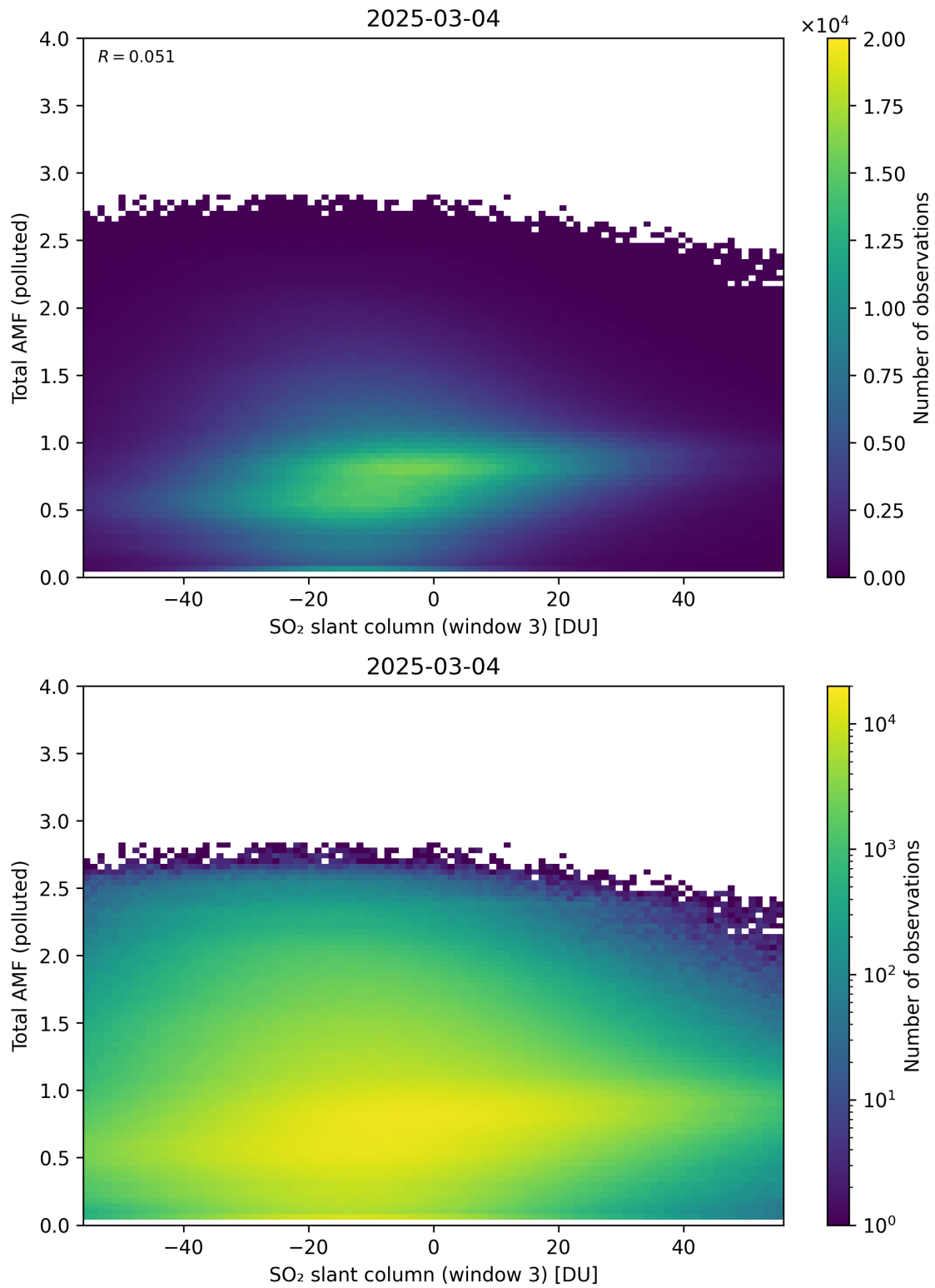
Figure 318: Scatter density plot of “SO 2 slant column (window 3)” against “Total AMF (polluted)” for 2025-03-03 to 2025-03-05.
