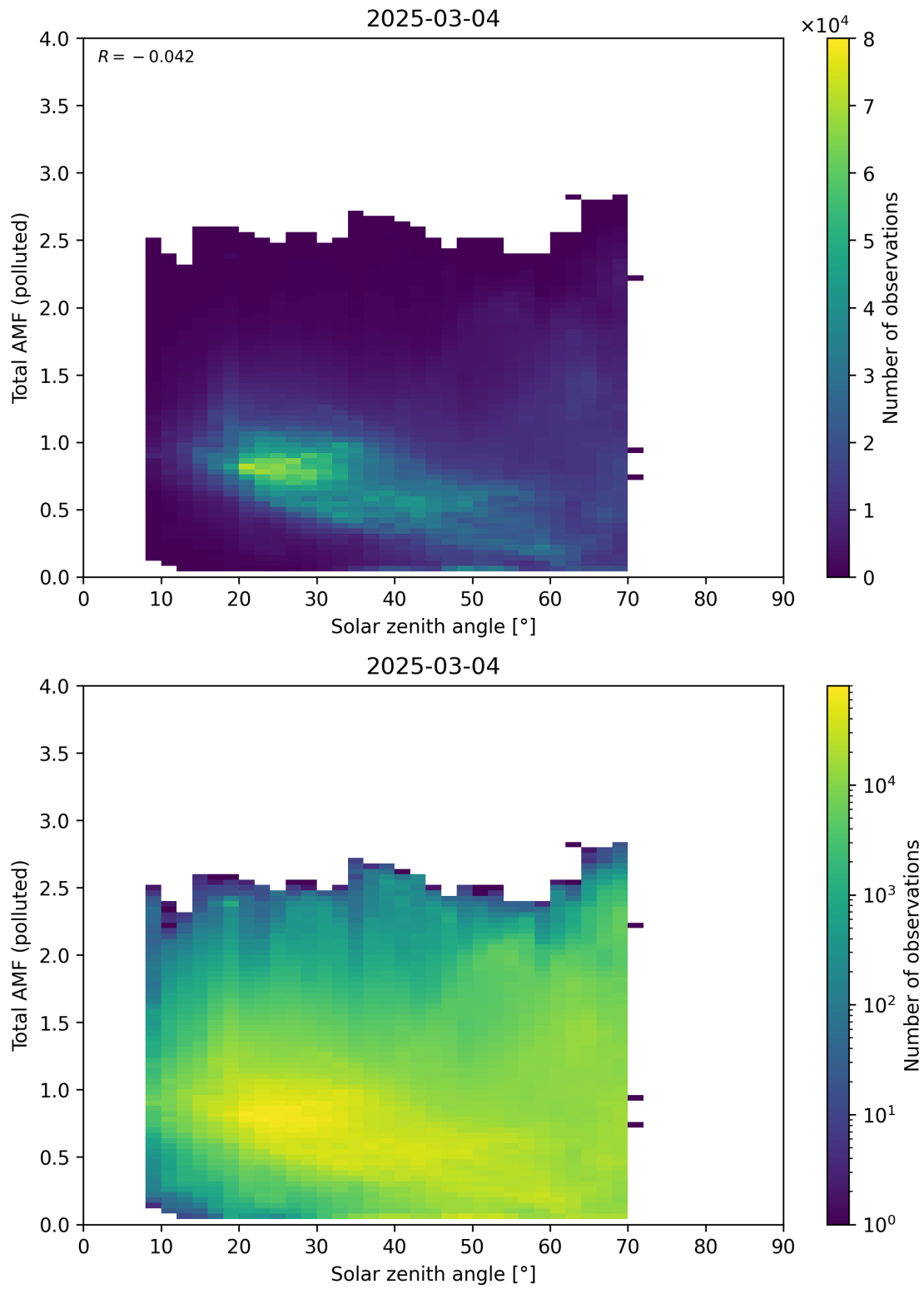
Figure 189: Scatter density plot of “Solar zenith angle” against “Total AMF (polluted)” for 2025-03-03 to 2025-03-05.
