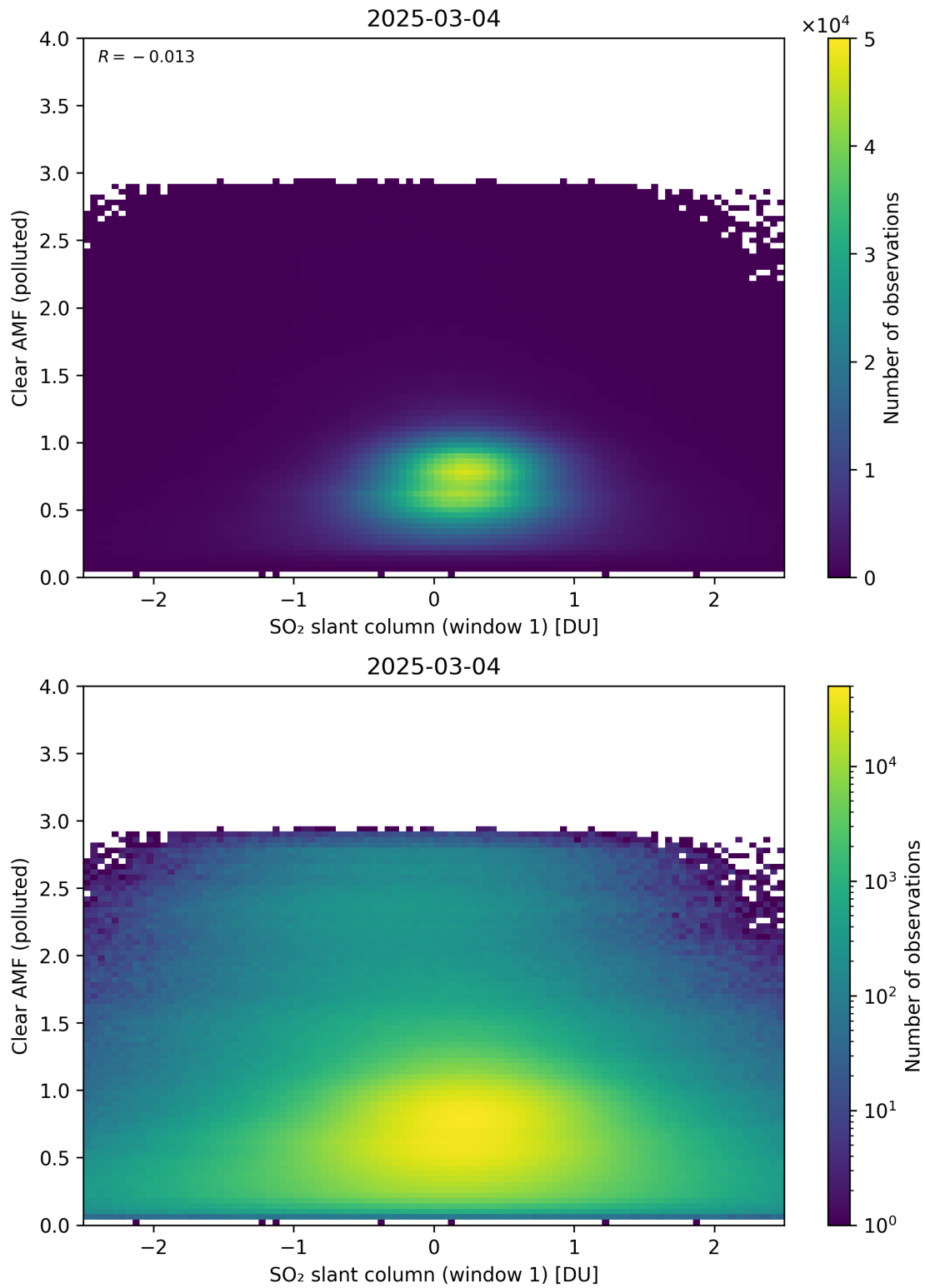
Figure 282: Scatter density plot of “SO 2 slant column (window 1)” against “Clear AMF (polluted)” for 2025-03-03 to 2025-03-05.
