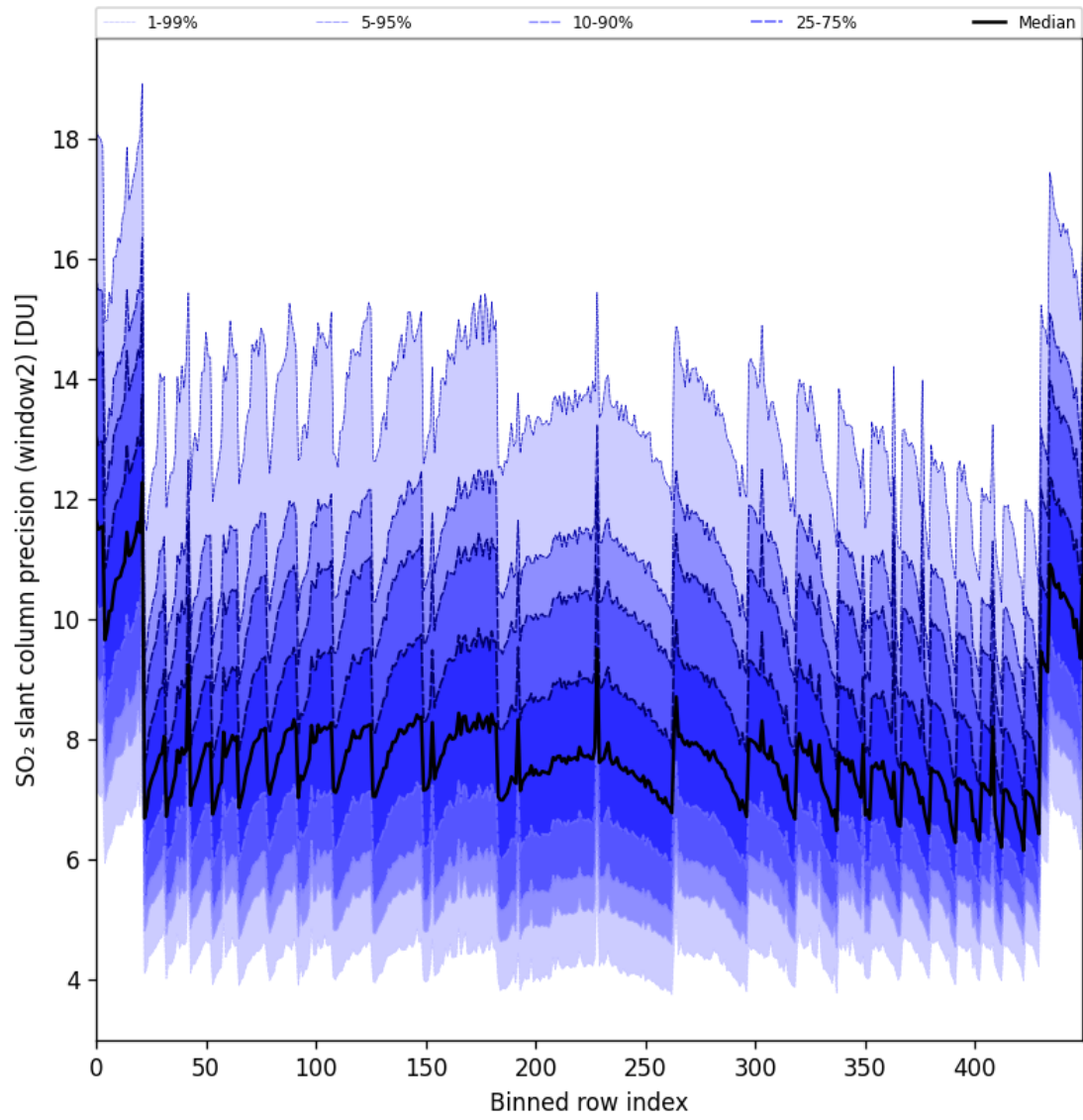
Figure 94: Along track statistics of “SO 2 slant column precision (window2)” for 2025-03-03 to 2025-03-05
