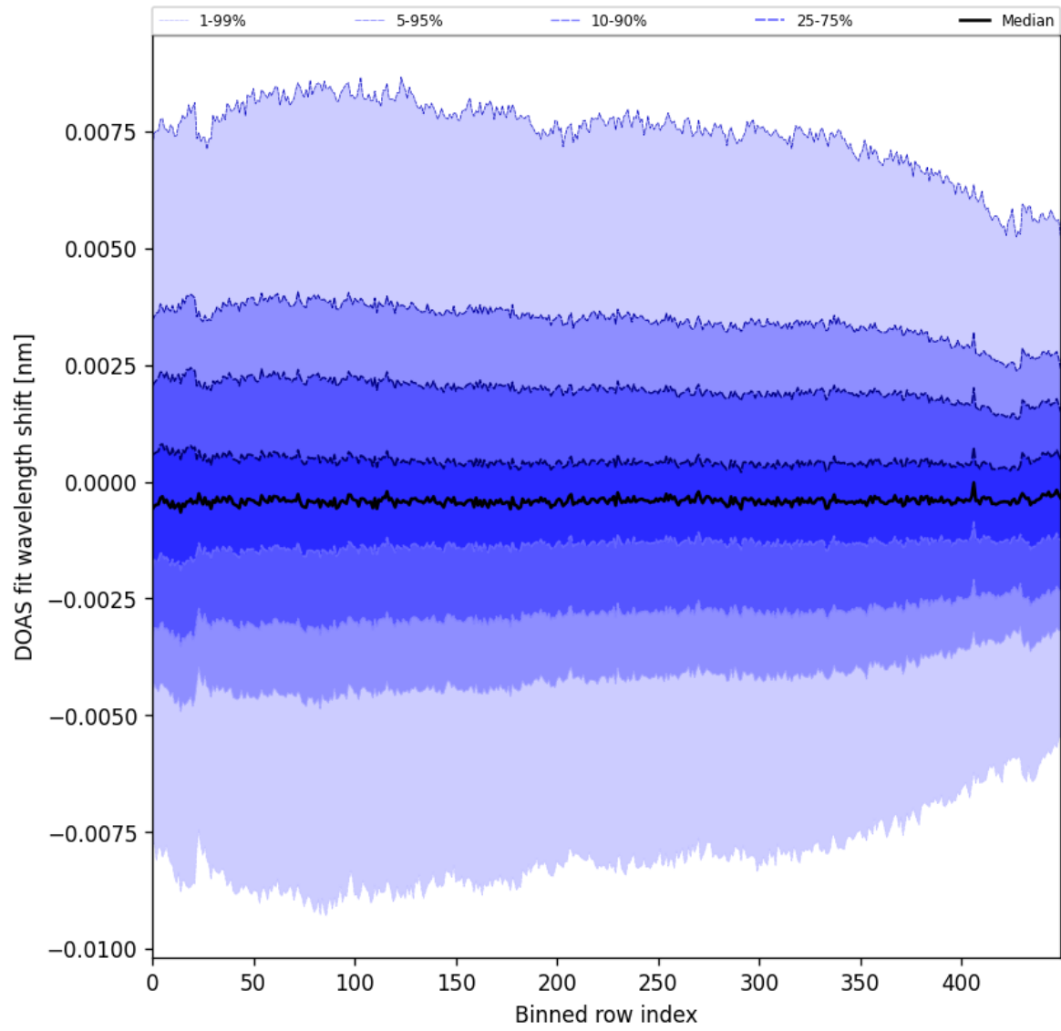
Figure 102: Along track statistics of “DOAS fit wavelength shift” for 2025-03-03 to 2025-03-05
