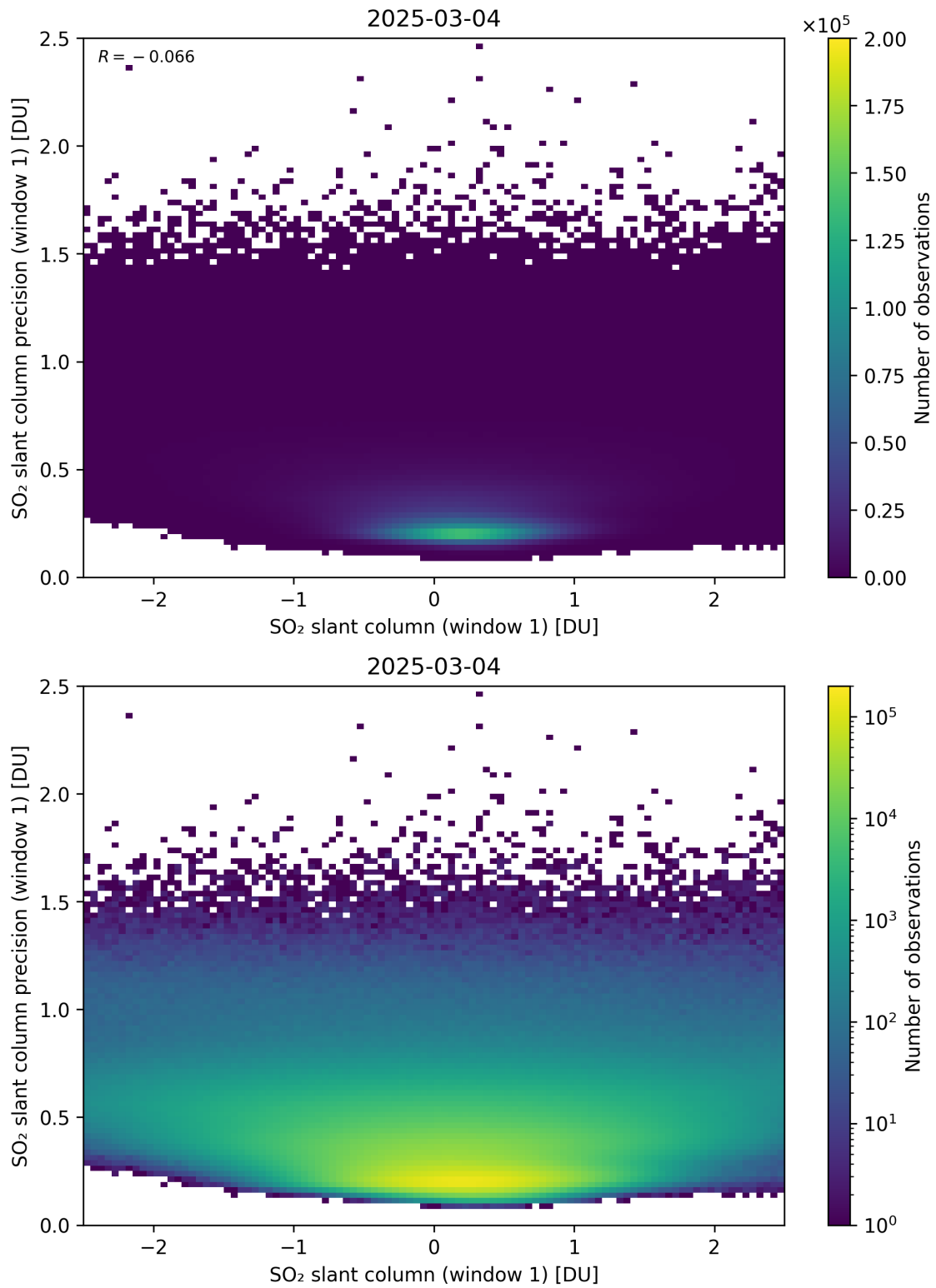
Figure 285: Scatter density plot of “SO 2 slant column (window 1)” against “SO 2 slant column precision (window 1)” for 2025-03-03 to 2025-03-05.
