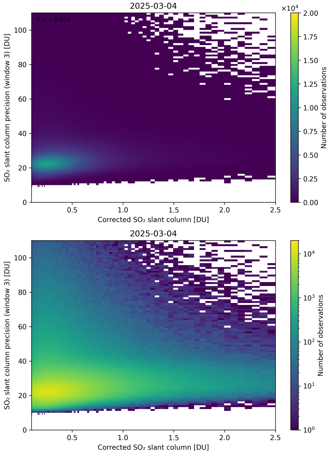
Figure 241: Scatter density plot of “Corrected SO 2 slant column” against “SO 2 slant column precision (window 3)” for 2025-03-03 to 2025-03-05.
