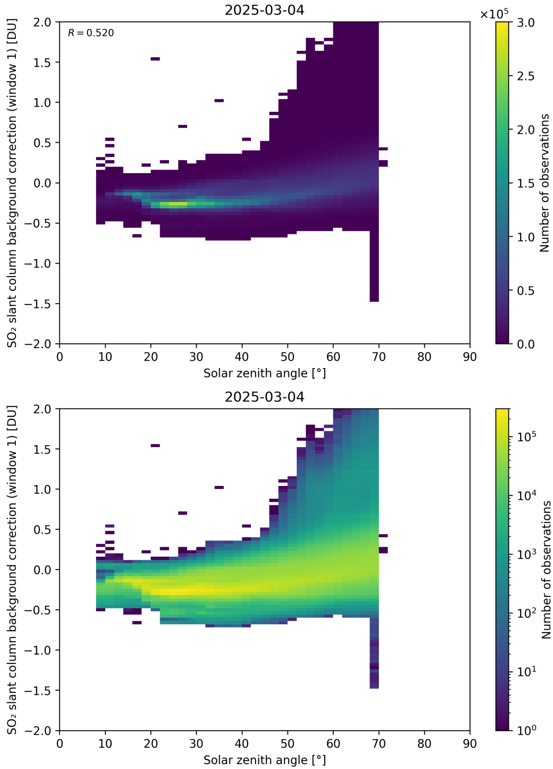
Figure 171: Scatter density plot of “Solar zenith angle” against “SO 2 slant column background correction (window 1)” for 2025-03-03 to 2025-03-05.
