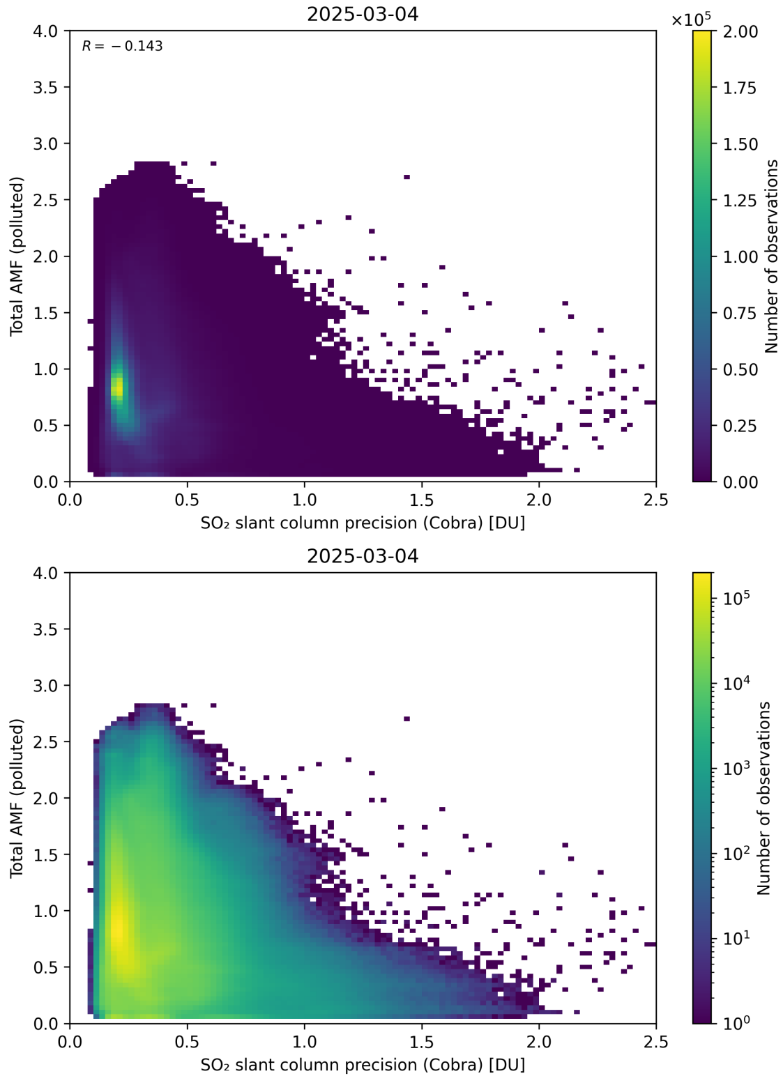
Figure 213: Scatter density plot of “SO 2 slant column precision (Cobra)” against “Total AMF (polluted)” for 2025-03-03 to 2025-03-05.
