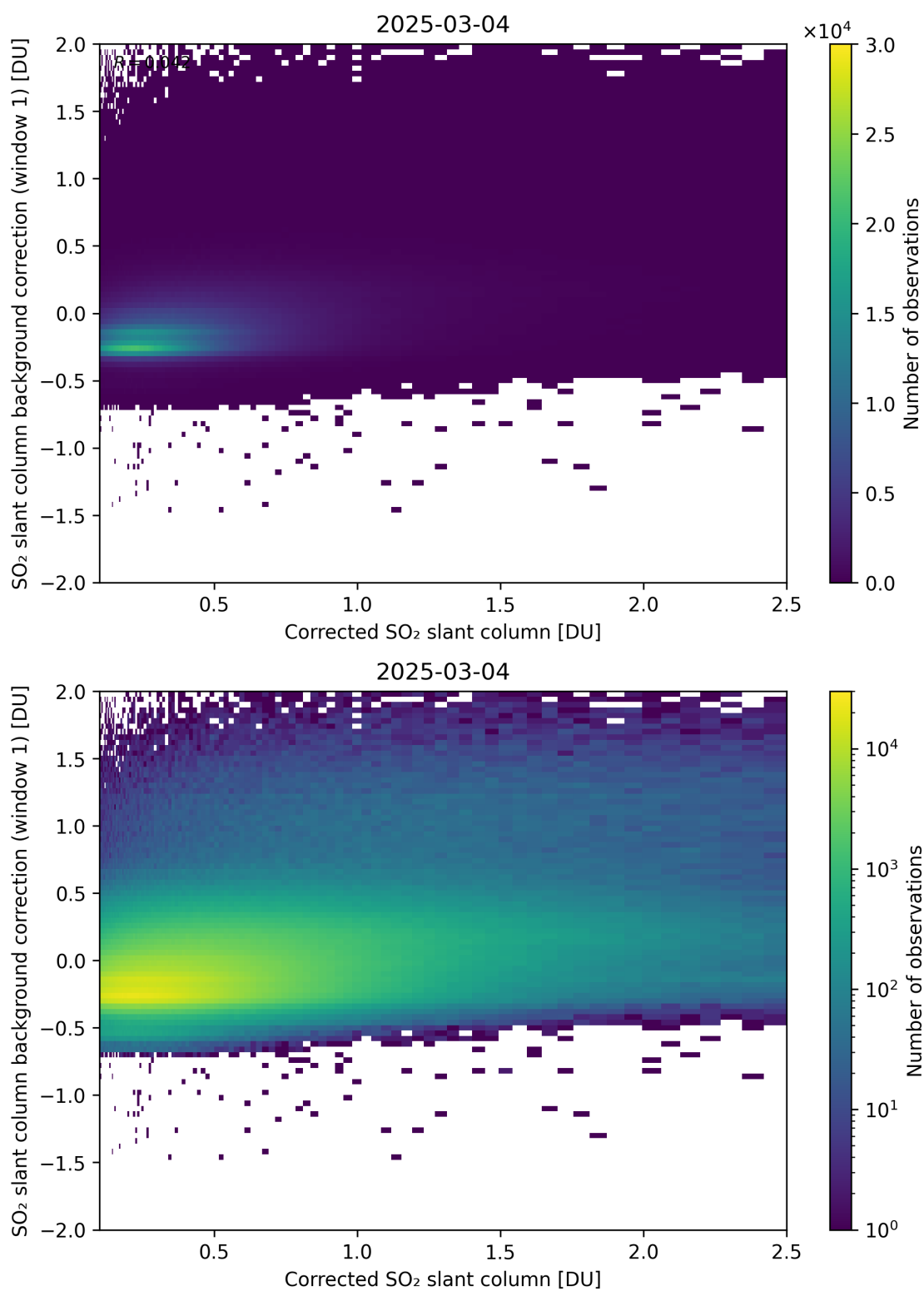
Figure 226: Scatter density plot of “Corrected SO 2 slant column” against “SO 2 slant column background correction (window 1)” for 2025-03-03 to 2025-03-05.
