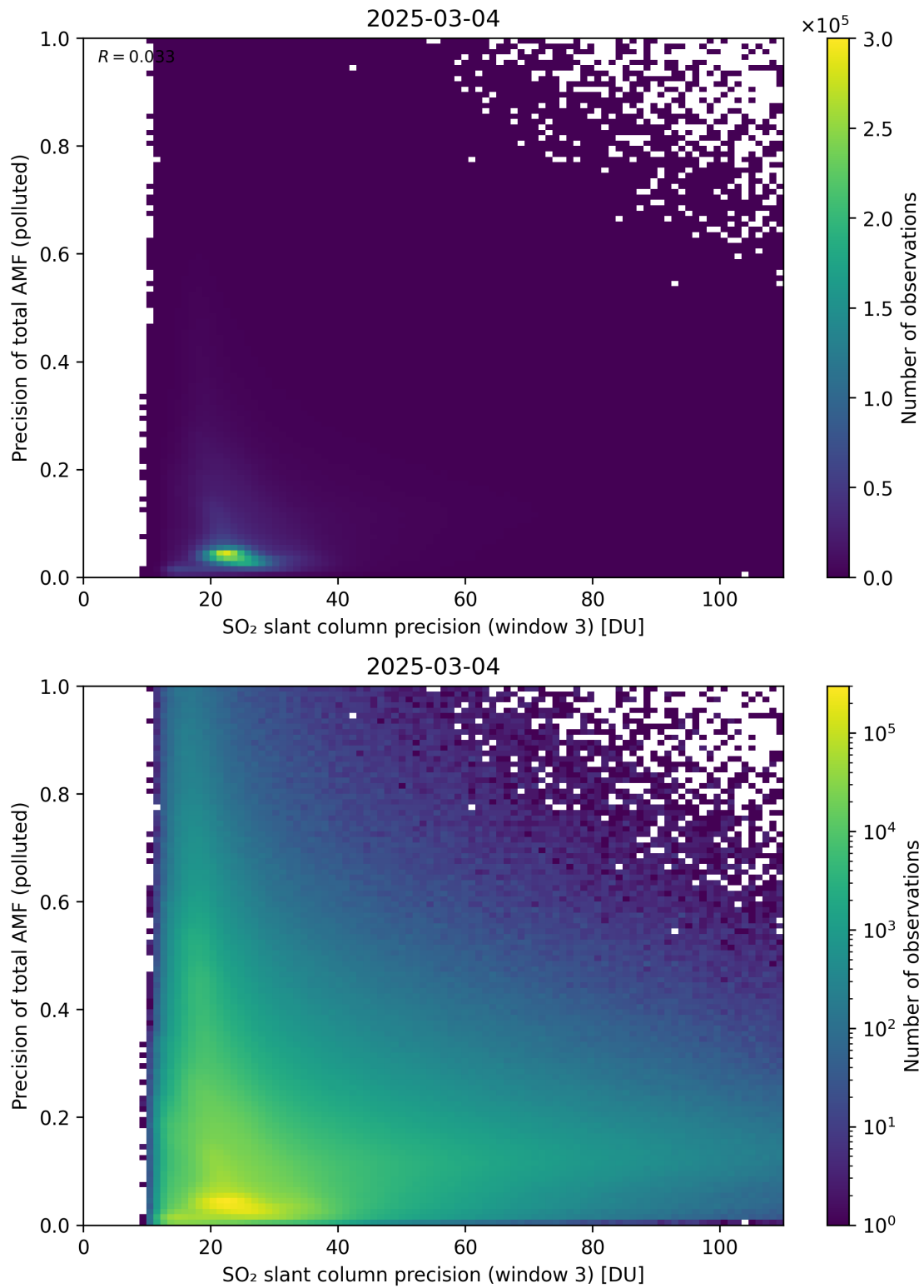
Figure 314: Scatter density plot of “SO 2 slant column precision (window 3)” against “Precision of total AMF (polluted)” for 2025-03-03 to 2025-03-05.
