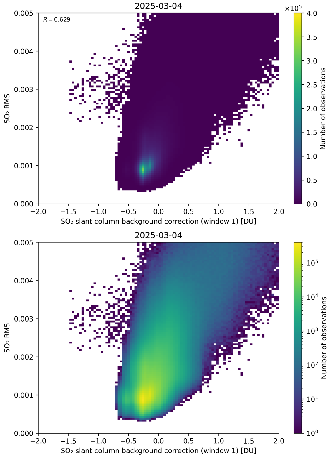
Figure 113: Scatter density plot of “SO 2 slant column background correction (window 1)” against “SO 2 RMS” for 2025-03-03 to 2025-03-05.
