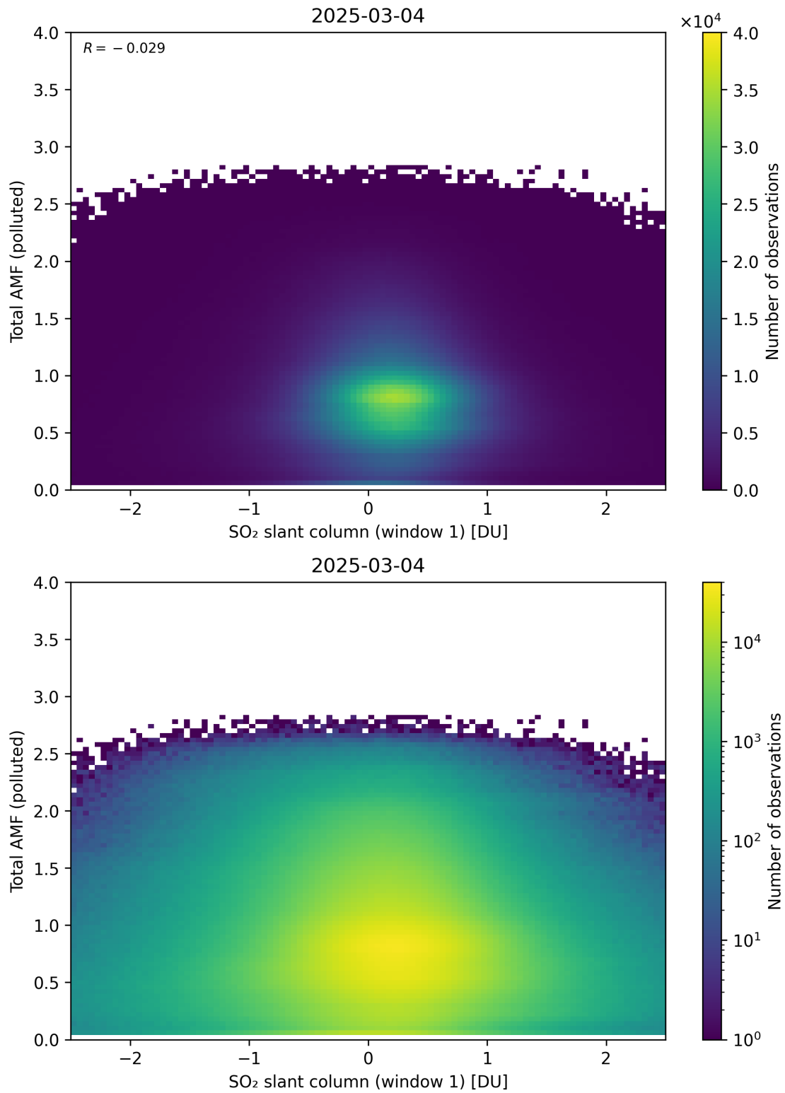
Figure 289: Scatter density plot of “SO 2 slant column (window 1)” against “Total AMF (polluted)” for 2025-03-03 to 2025-03-05.
