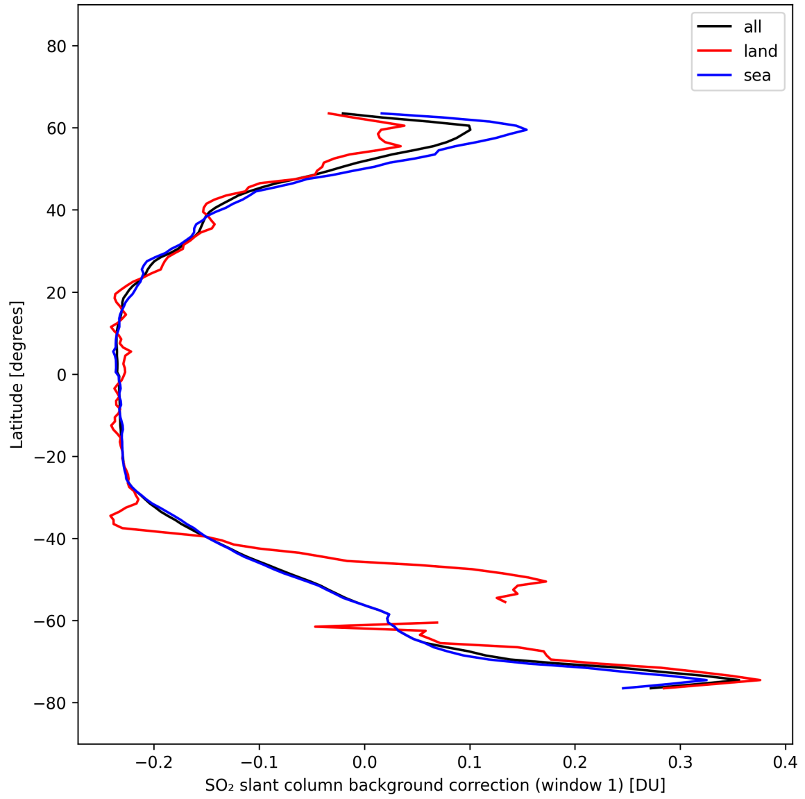
Figure 40: Zonal average of "SO 2 slant column background correction (window 1)" for 2025-03-03 to 2025-03-05.
