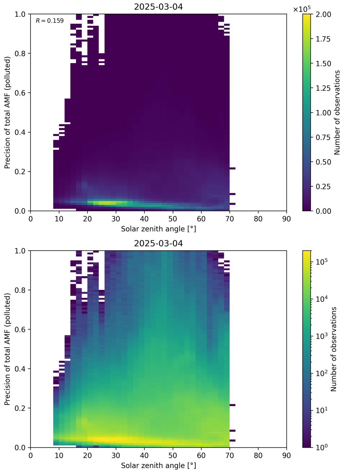
Figure 190: Scatter density plot of “Solar zenith angle” against “Precision of total AMF (polluted)” for 2025-03-03 to 2025-03-05.
