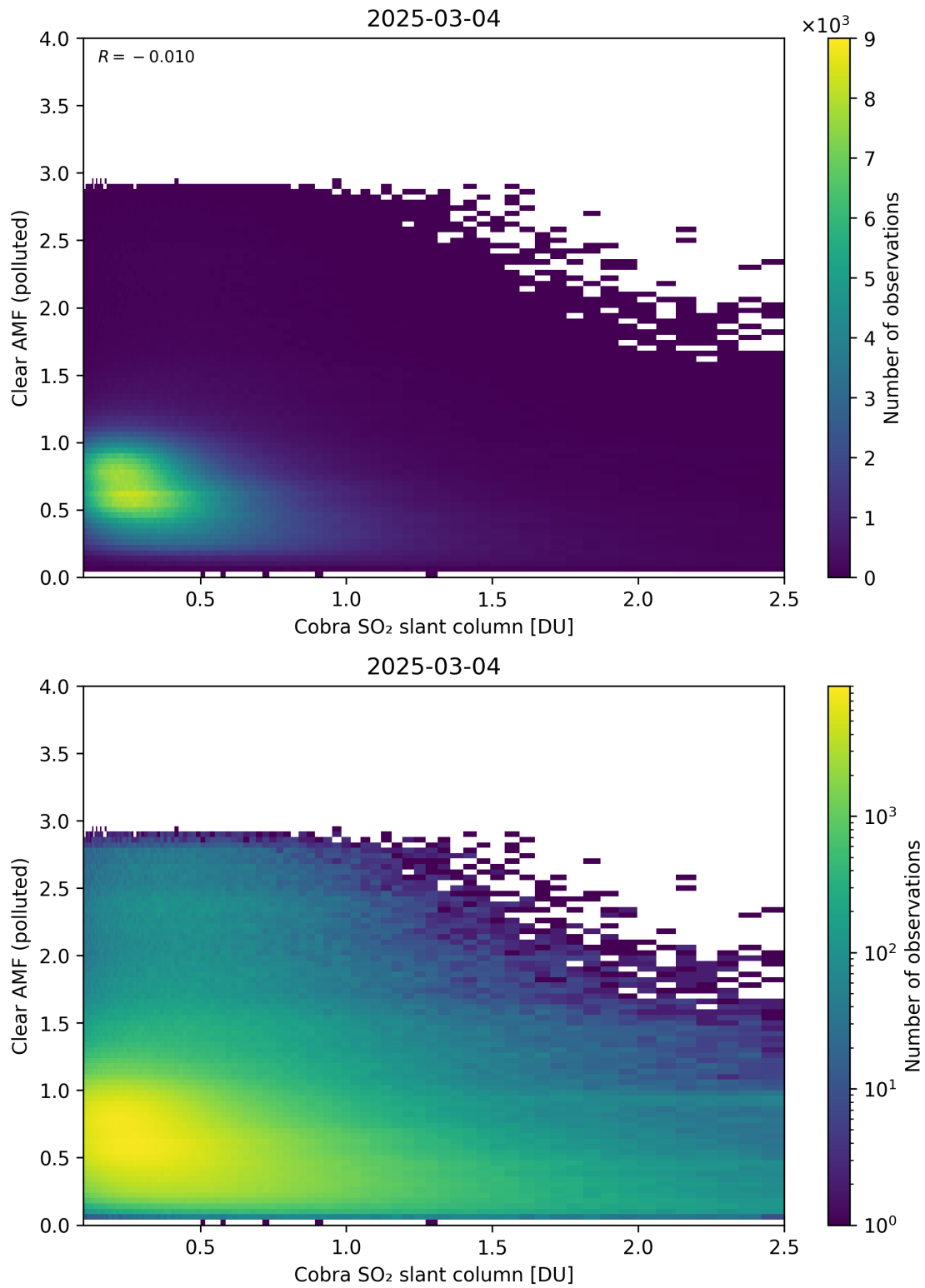
Figure 215: Scatter density plot of “Cobra SO 2 slant column” against “Clear AMF (polluted)” for 2025-03-03 to 2025-03-05.
