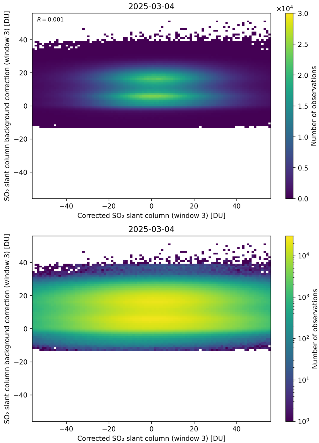
Figure 255: Scatter density plot of “Corrected SO 2 slant column (window 3)” against “SO 2 slant column background correction (window 3)” for 2025-03-03 to 2025-03-05.
