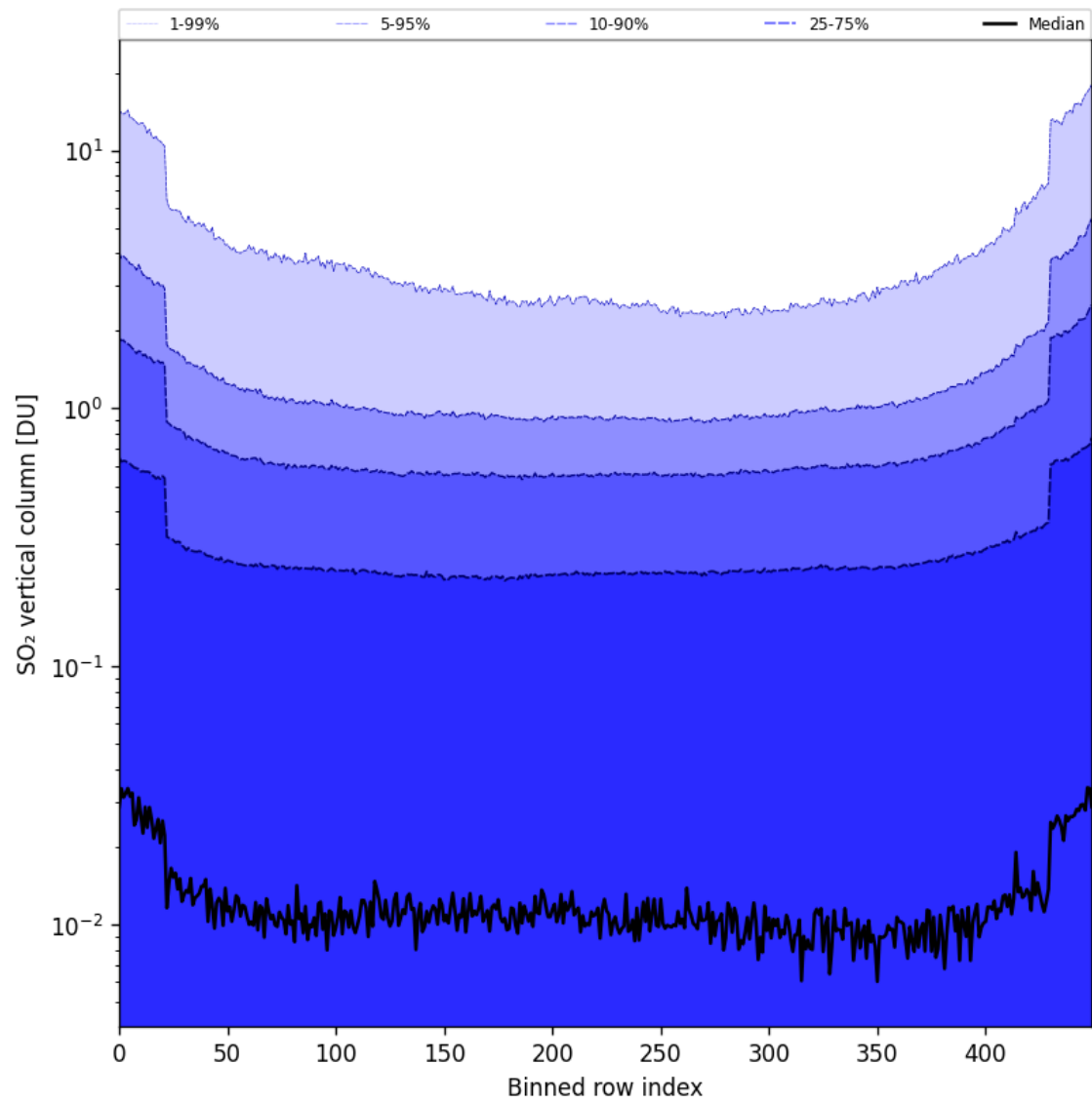
Figure 84: Along track statistics of “SO 2 vertical column” for 2025-03-03 to 2025-03-05
