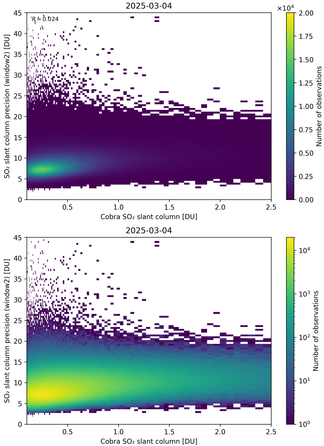
Figure 221: Scatter density plot of “Cobra SO 2 slant column” against “SO 2 slant column precision (window2)” for 2025-03-03 to 2025-03-05.
