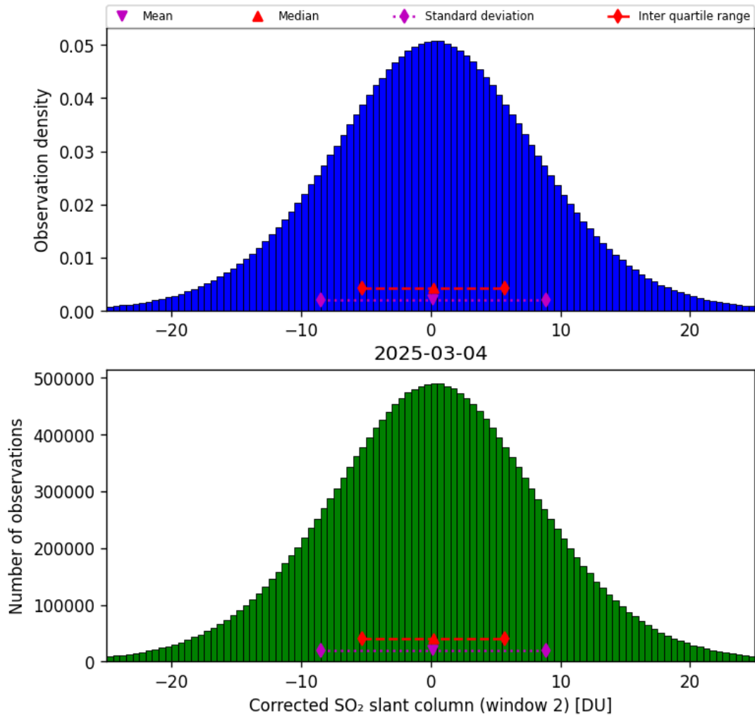
Figure 69: Histogram of “Corrected SO 2 slant column (window 2)” for 2025-03-03 to 2025-03-05
