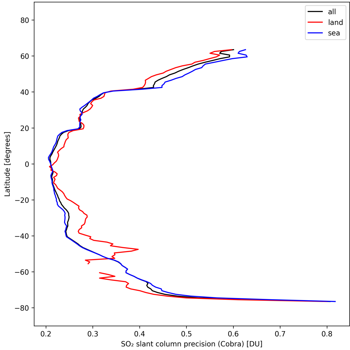
Figure 36: Zonal average of “SO 2 slant column precision (Cobra)” for 2025-03-03 to 2025-03-05.
