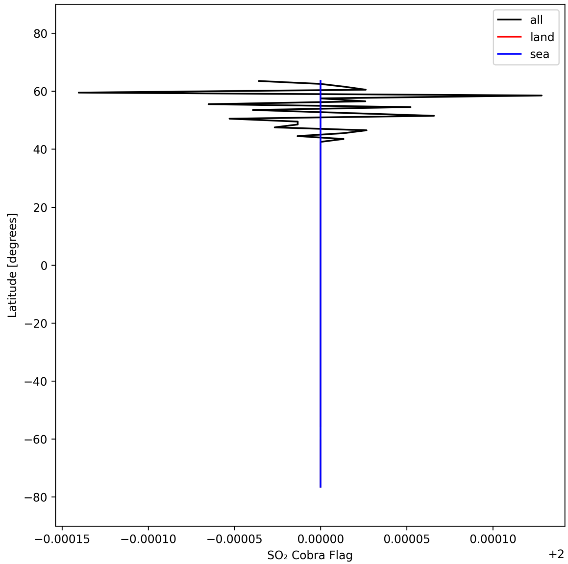
Figure 49: Zonal average of “SO 2 Cobra Flag” for 2025-03-03 to 2025-03-05.
