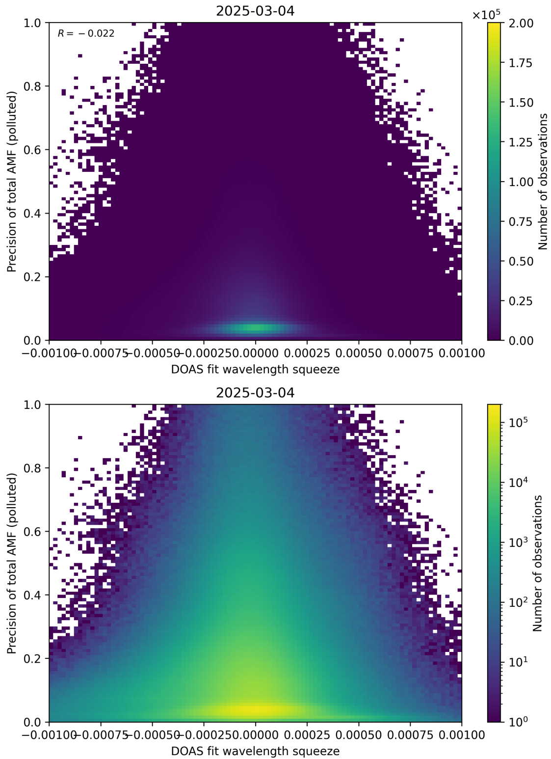
Figure 146: Scatter density plot of “DOAS fit wavelength squeeze” against “Precision of total AMF (polluted)” for 2025-03-03 to 2025-03-05.
