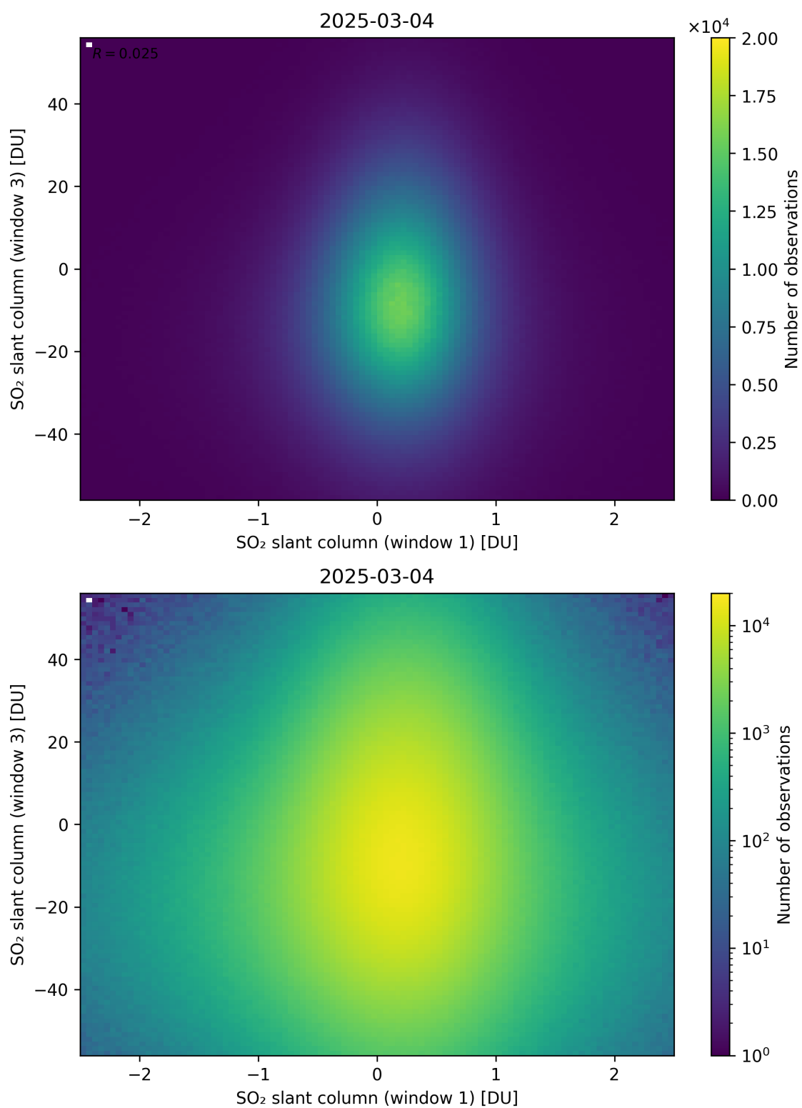
Figure 287: Scatter density plot of “SO 2 slant column (window 1)” against “SO 2 slant column (window 3)” for 2025-03-03 to 2025-03-05.
