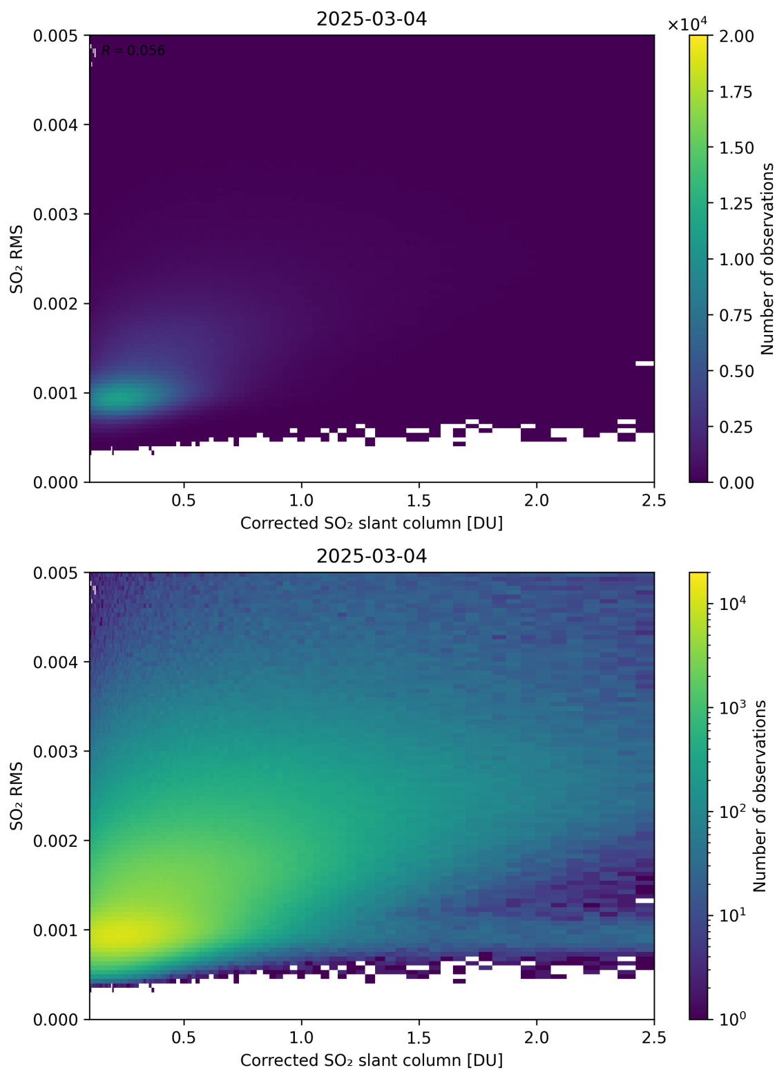
Figure 231: Scatter density plot of “Corrected SO 2 slant column” against “SO 2 RMS” for 2025-03-03 to 2025-03-05.
