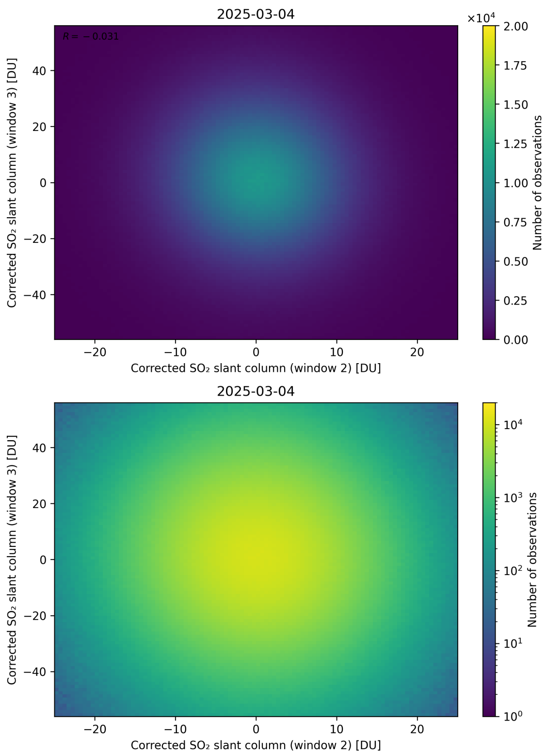
Figure 250: Scatter density plot of “Corrected SO 2 slant column (window 2)” against “Corrected SO 2 slant column (window 3)” for 2025-03-03 to 2025-03-05.
