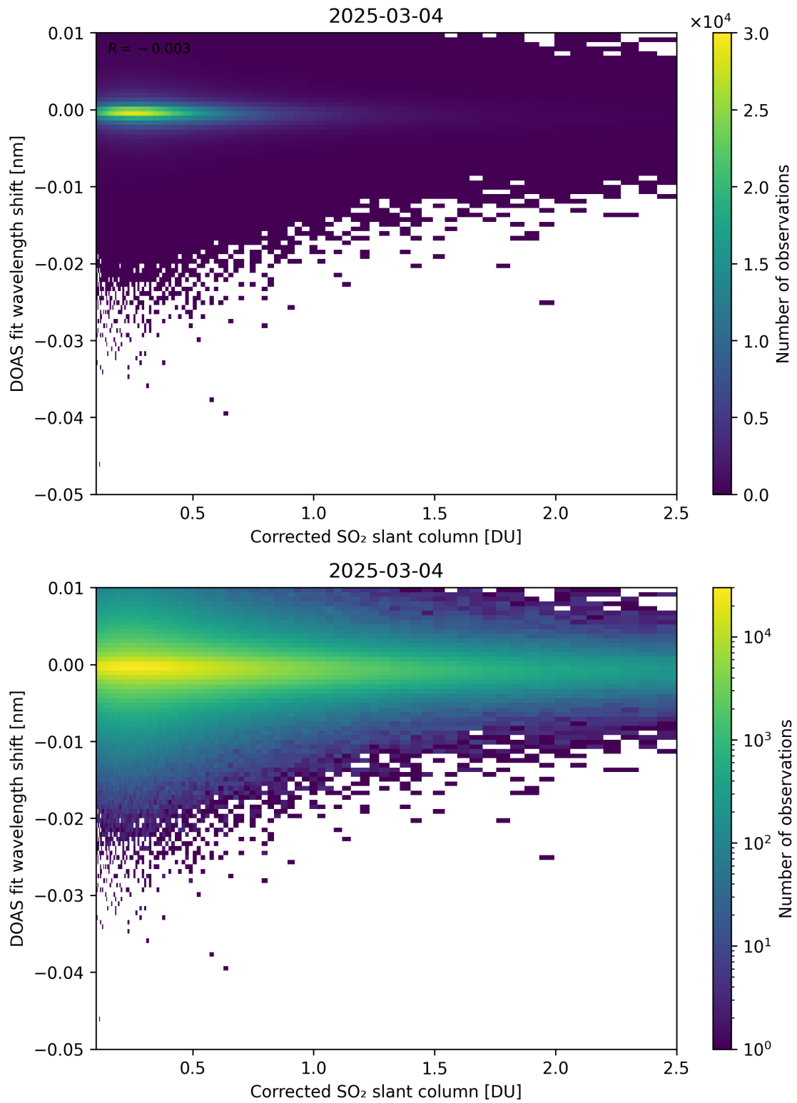
Figure 229: Scatter density plot of “Corrected SO 2 slant column” against “DOAS fit wavelength shift” for 2025-03-03 to 2025-03-05.
