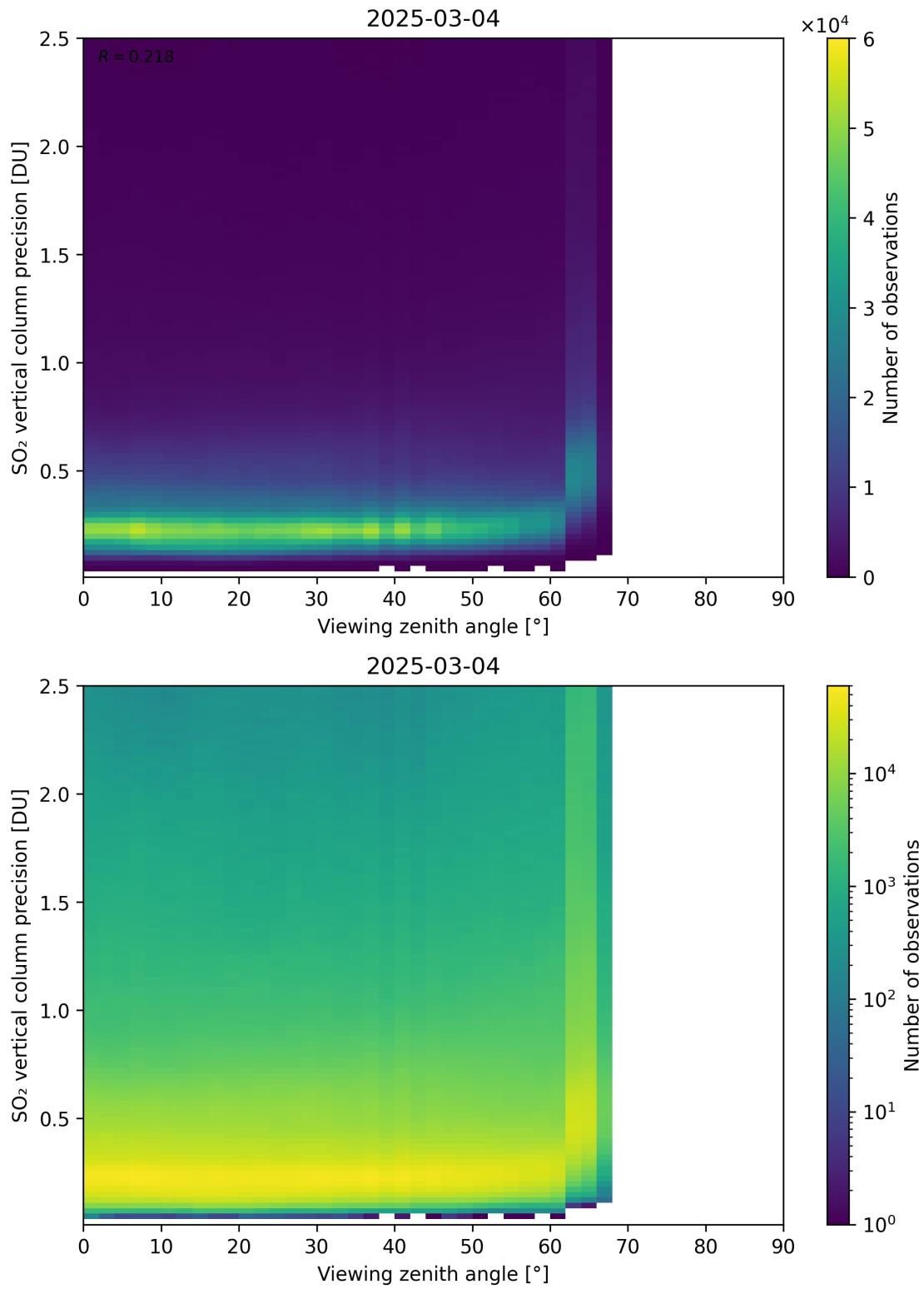
Figure 384: Scatter density plot of “Viewing zenith angle” against “SO 2 vertical column precision” for 2025-03-03 to 2025-03-05.
