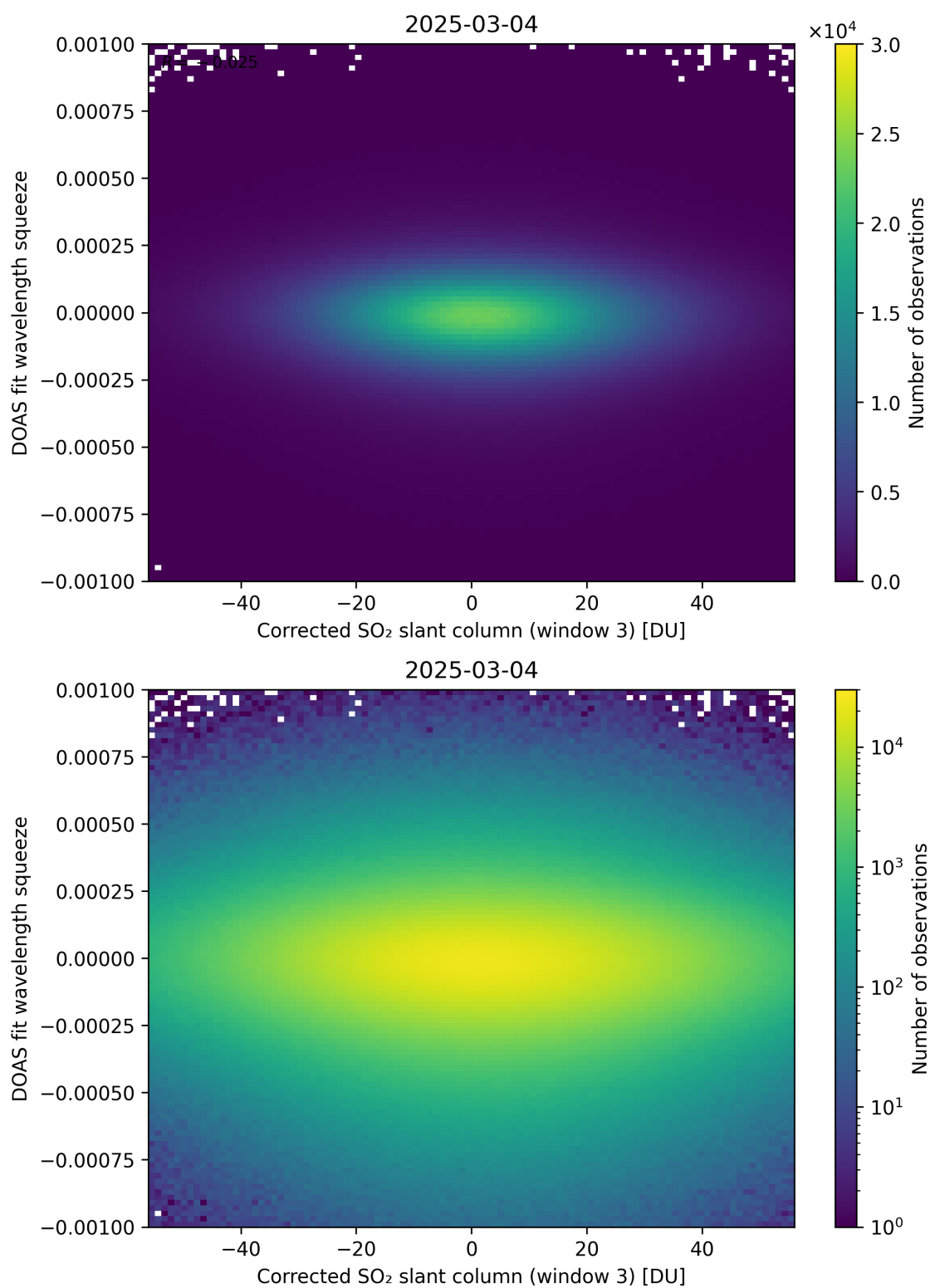
Figure 257: Scatter density plot of “Corrected SO 2 slant column (window 3)” against “DOAS fit wavelength squeeze” for 2025-03-03 to 2025-03-05.
