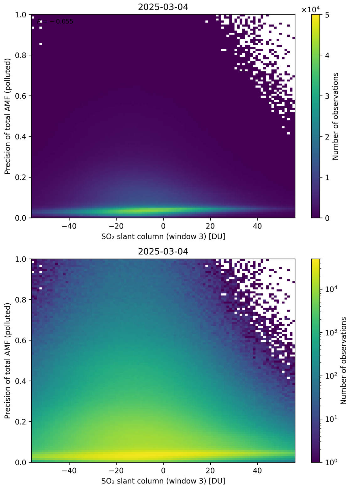
Figure 319: Scatter density plot of “SO 2 slant column (window 3)” against “Precision of total AMF (polluted)” for 2025-03-03 to 2025-03-05.
