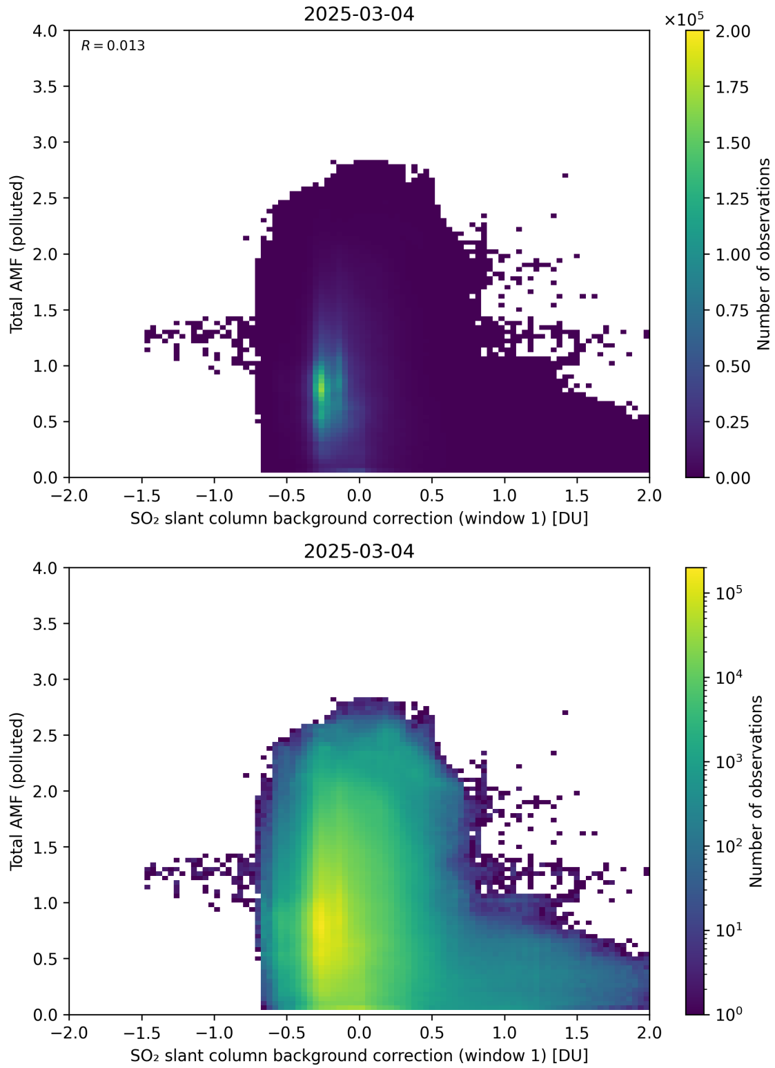
Figure 120: Scatter density plot of “SO 2 slant column background correction (window 1)” against “Total AMF (polluted)” for 2025-03-03 to 2025-03-05.
