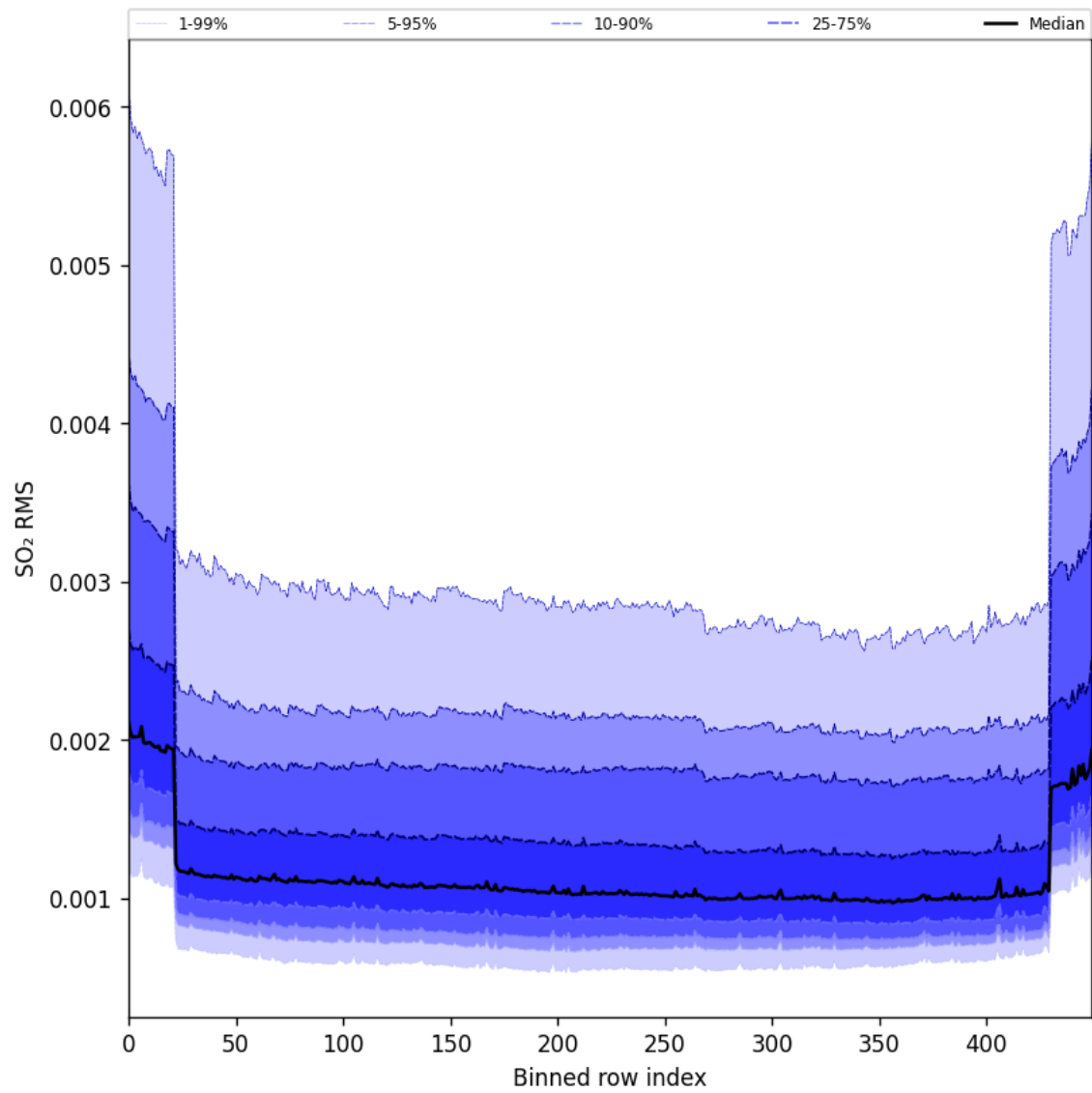
Figure 104: Along track statistics of “SO 2 RMS” for 2025-03-03 to 2025-03-05
