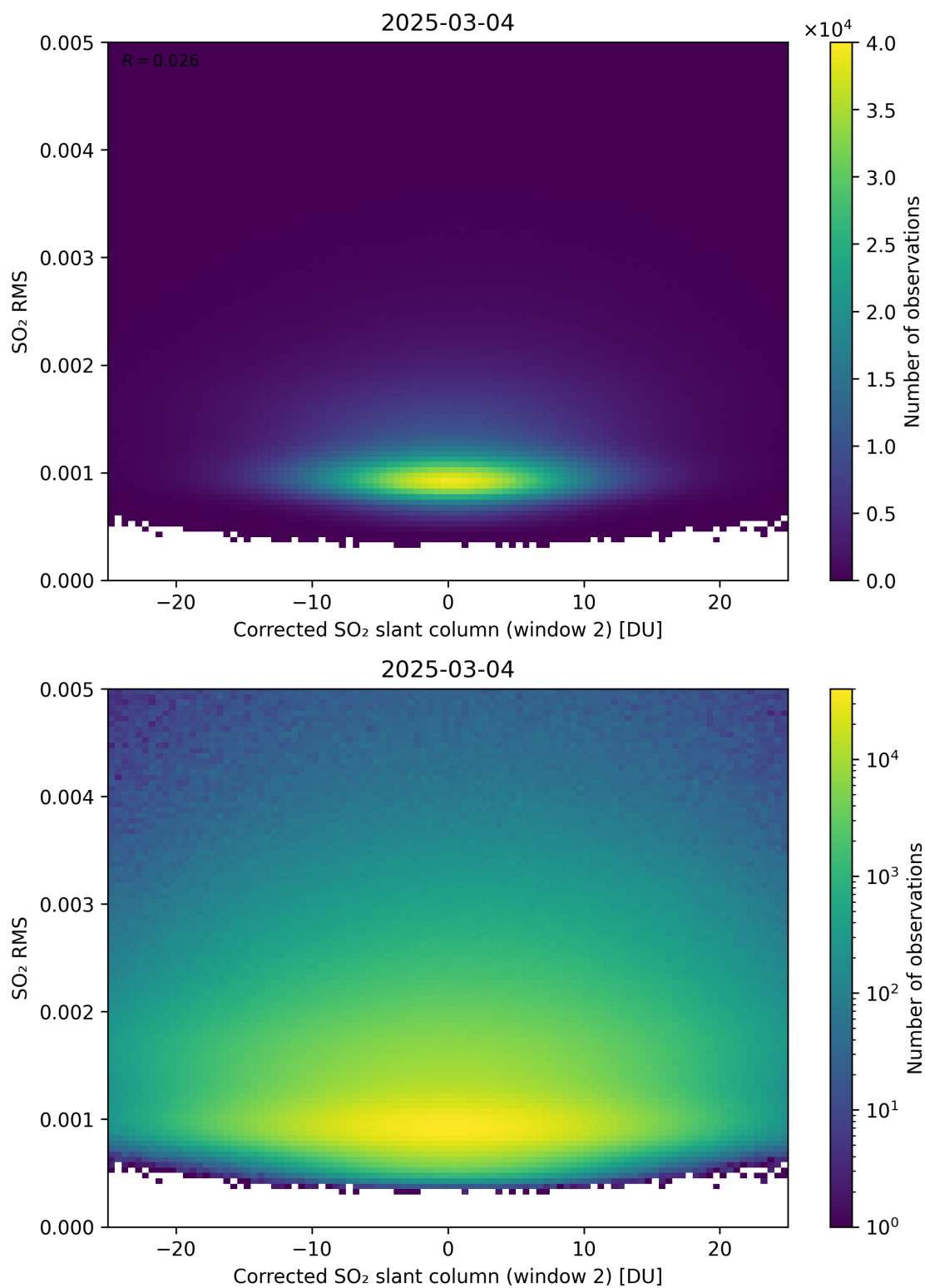
Figure 248: Scatter density plot of “Corrected SO 2 slant column (window 2)” against “SO 2 RMS” for 2025-03-03 to 2025-03-05.
