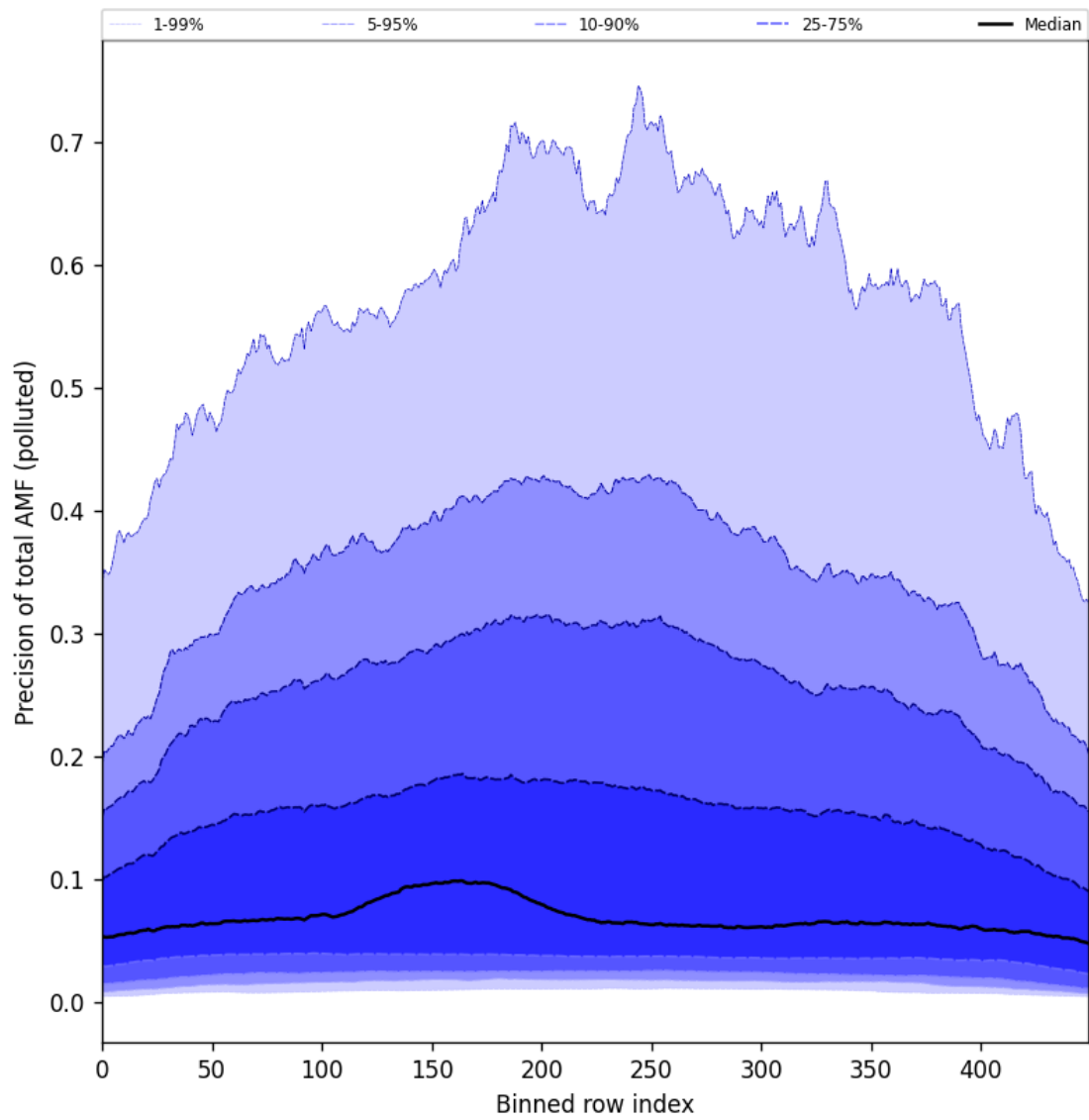
Figure 106: Along track statistics of “Precision of total AMF (polluted)” for 2025-03-03 to 2025-03-05
