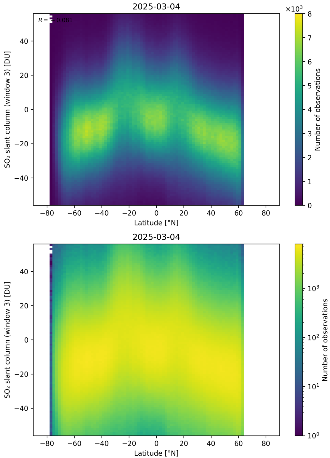
Figure 165: Scatter density plot of “Latitude” against “SO 2 slant column (window 3)” for 2025-03-03 to 2025-03-05.
