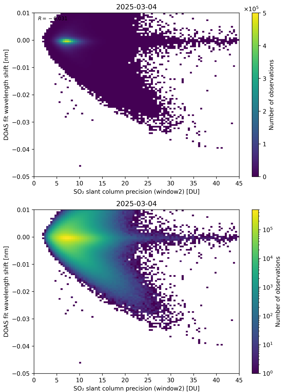
Figure 293: Scatter density plot of “SO 2 slant column precision (window2)” against “DOAS fit wavelength shift” for 2025-03-03 to 2025-03-05.
