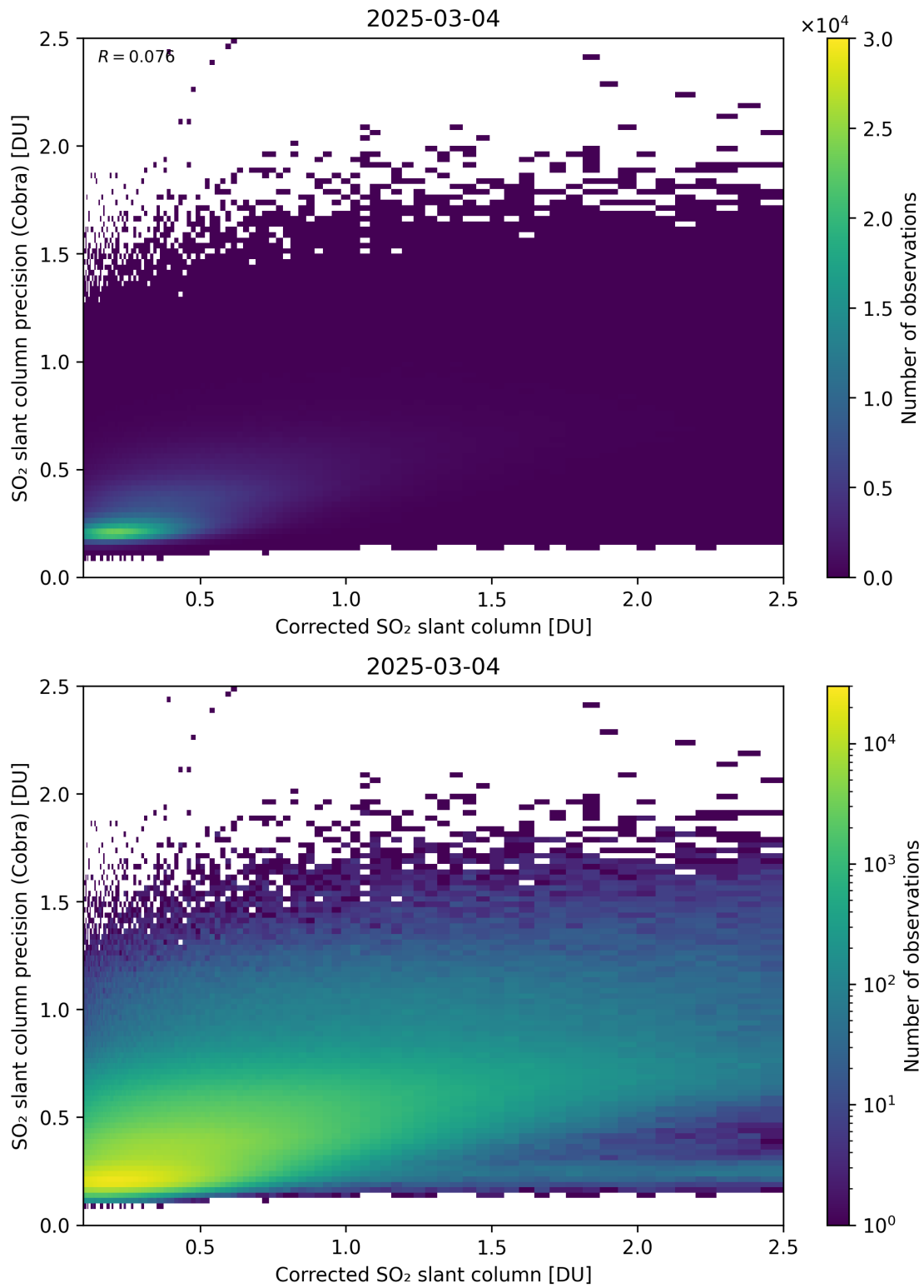
Figure 234: Scatter density plot of “Corrected SO 2 slant column” against “SO 2 slant column precision (Cobra)” for 2025-03-03 to 2025-03-05.
