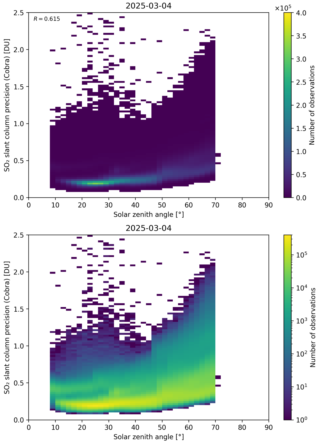
Figure 180: Scatter density plot of “Solar zenith angle” against “SO 2 slant column precision (Cobra)” for 2025-03-03 to 2025-03-05.
