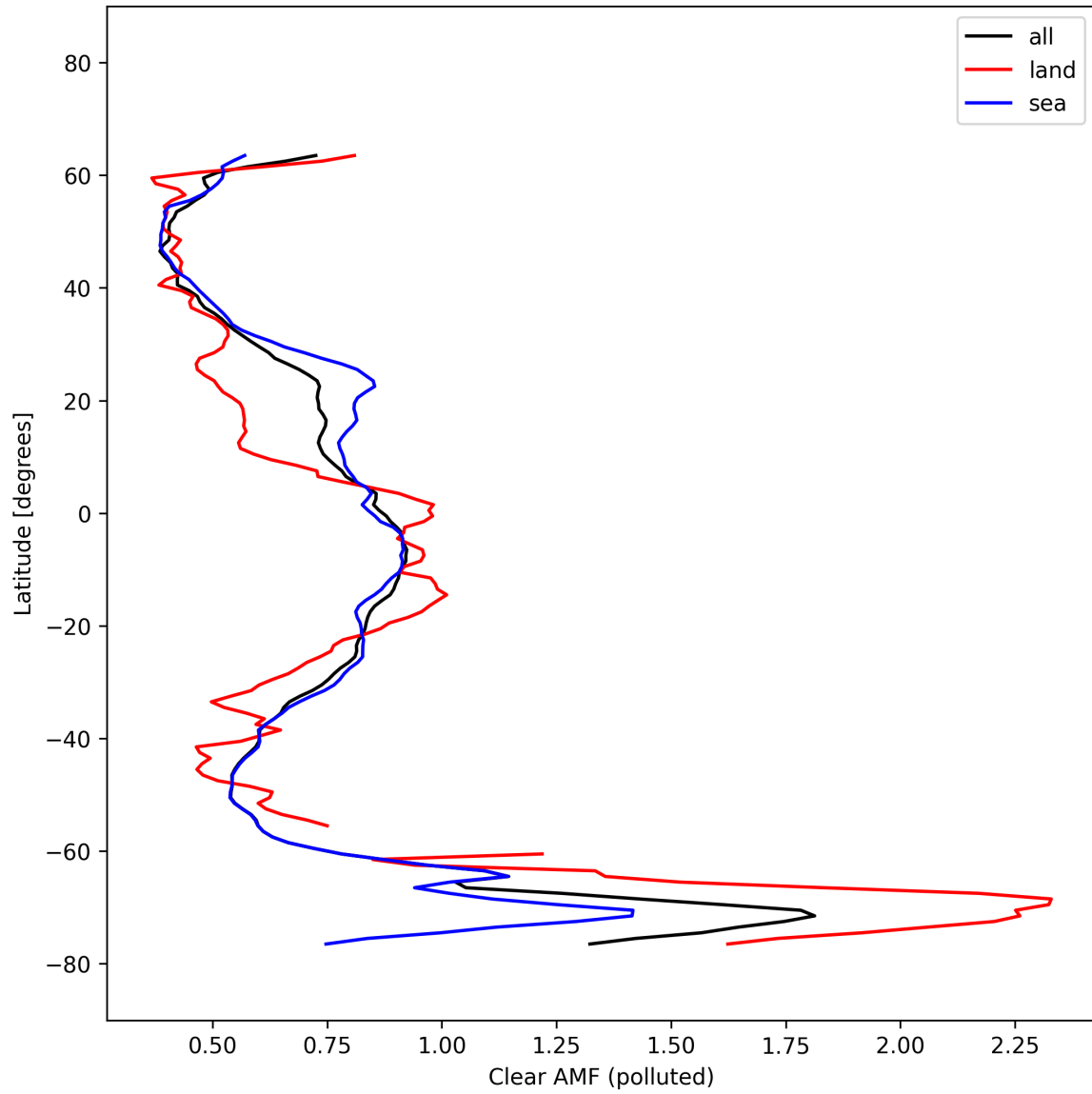
Figure 55: Zonal average of “Clear AMF (polluted)” for 2025-03-03 to 2025-03-05.
