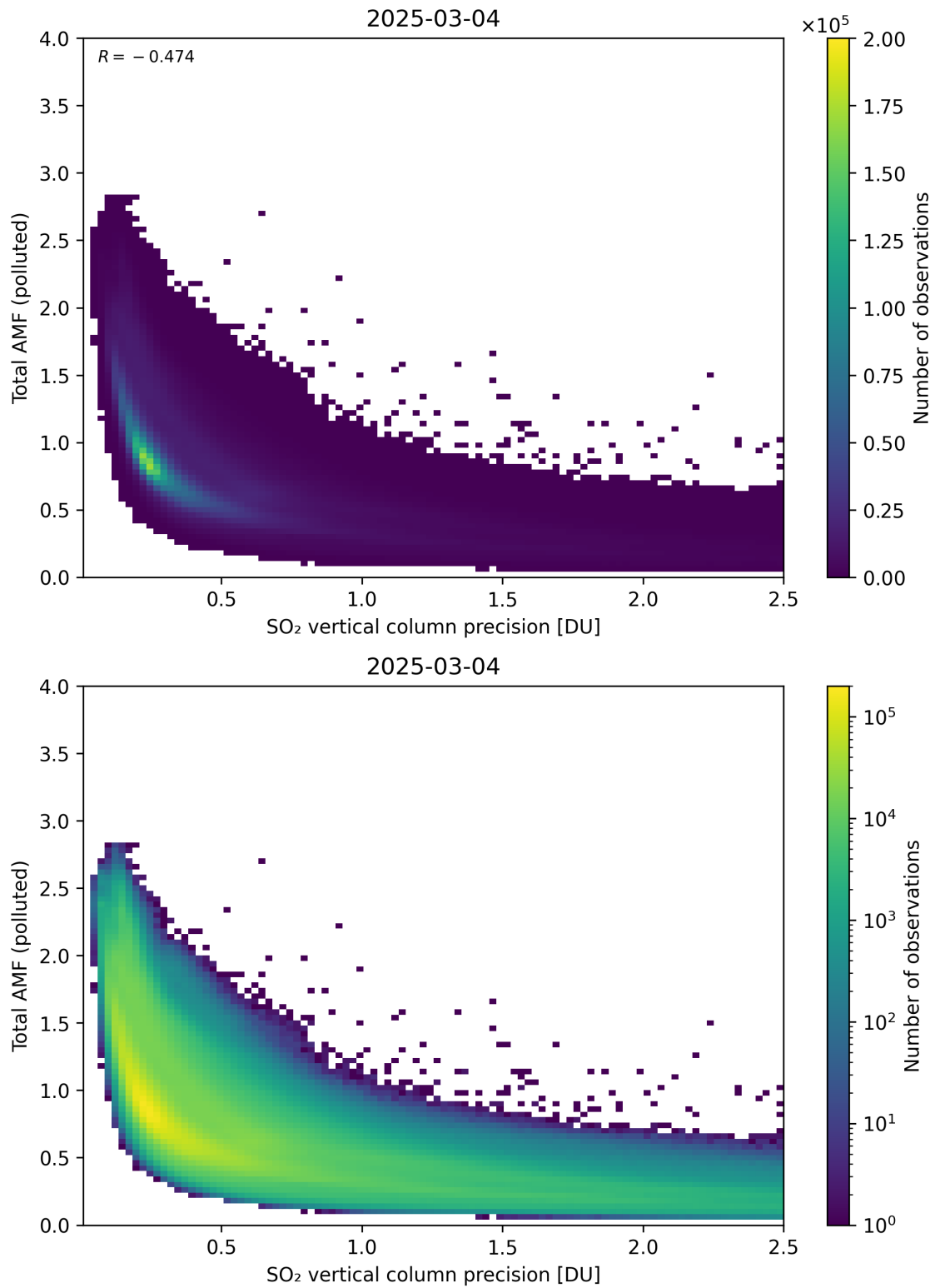
Figure 346: Scatter density plot of “SO 2 vertical column precision” against “Total AMF (polluted)” for 2025-03-03 to 2025-03-05.
