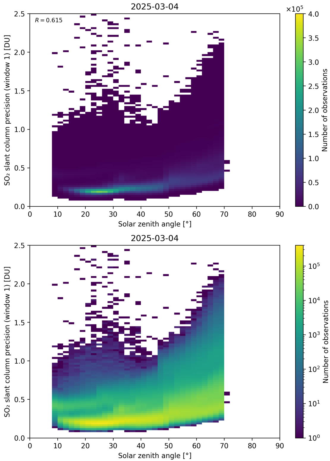
Figure 185: Scatter density plot of “Solar zenith angle” against “SO 2 slant column precision (window 1)” for 2025-03-03 to 2025-03-05.
