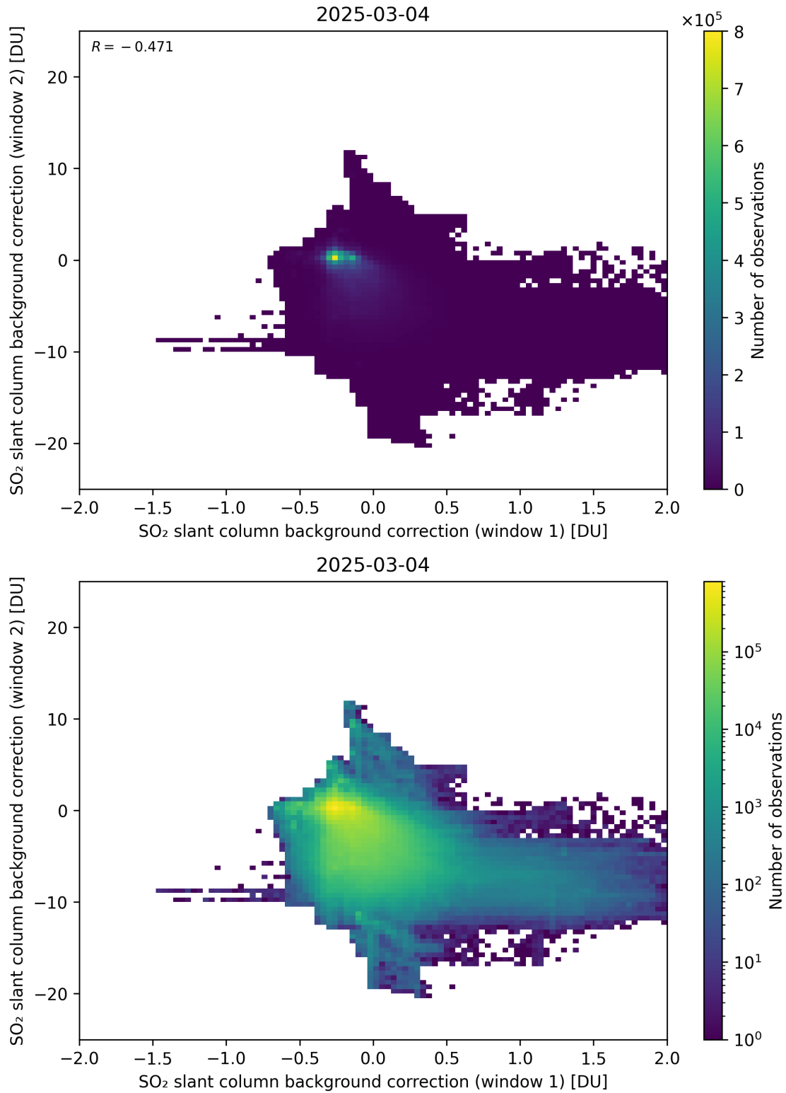
Figure 109: Scatter density plot of “SO 2 slant column background correction (window 1)” against “SO 2 slant column background correction (window 2)” for 2025-03-03 to 2025-03-05.
