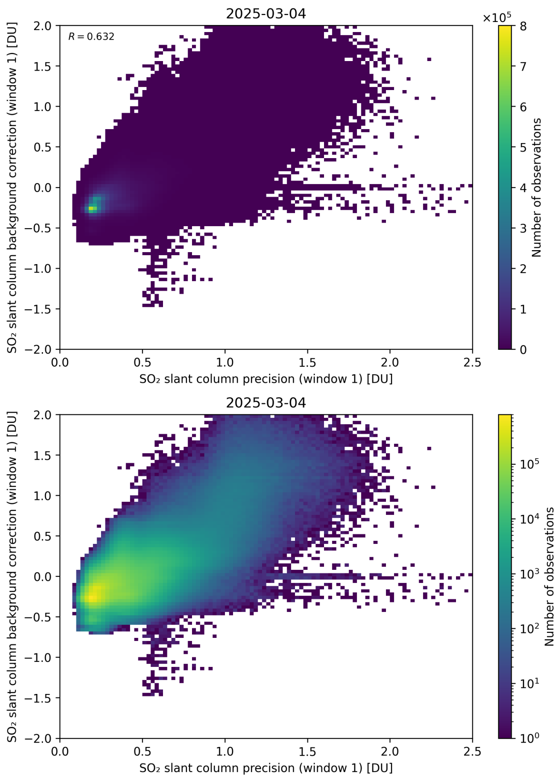
Figure 268: Scatter density plot of “SO 2 slant column precision (window 1)” against “SO 2 slant column background correction (window 1)” for 2025-03-03 to 2025-03-05.
