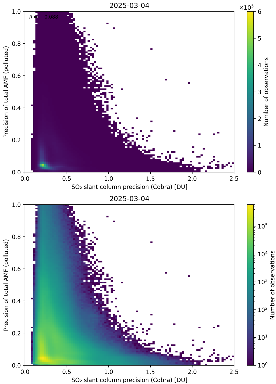
Figure 214: Scatter density plot of “SO 2 slant column precision (Cobra)” against “Precision of total AMF (polluted)” for 2025-03-03 to 2025-03-05.
