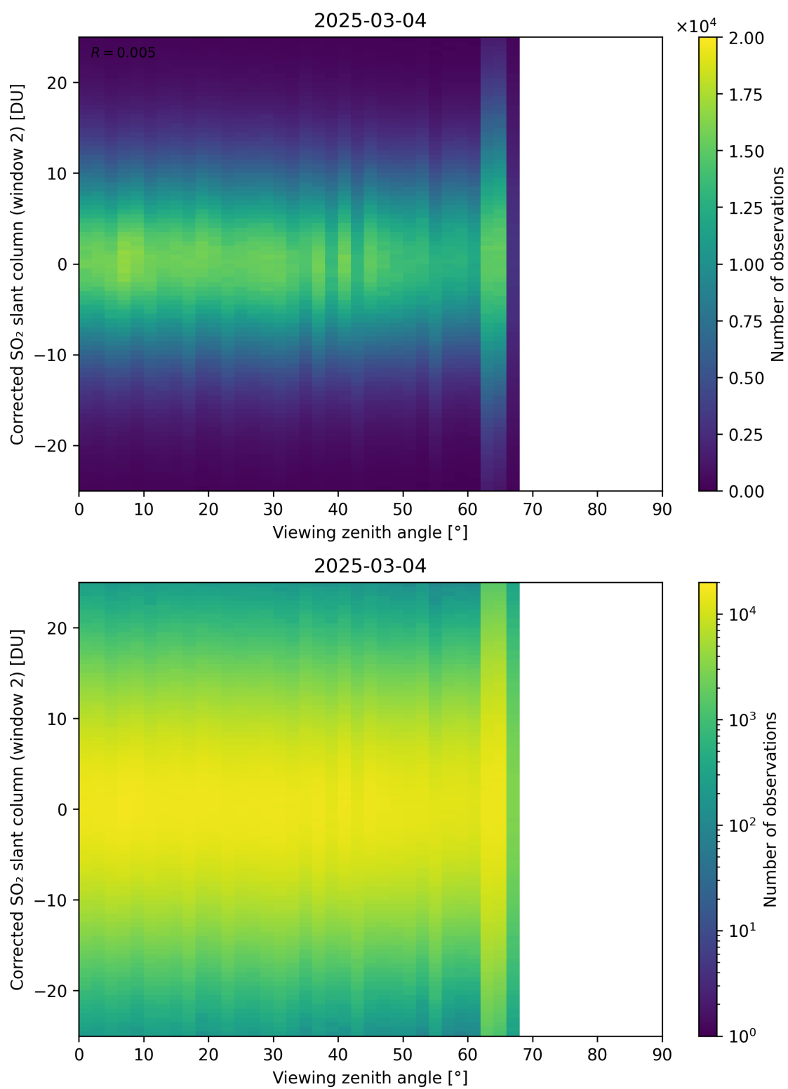
Figure 374: Scatter density plot of “Viewing zenith angle” against “Corrected SO 2 slant column (window 2)” for 2025-03-03 to 2025-03-05.
