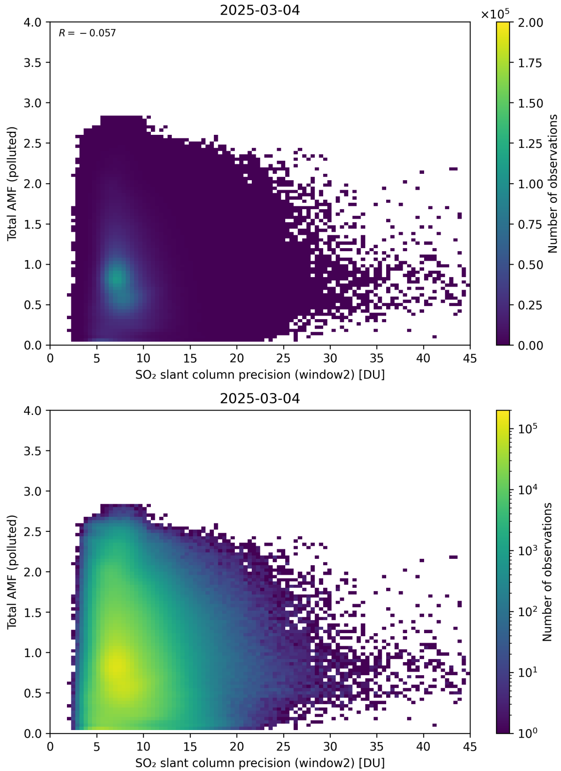
Figure 301: Scatter density plot of “SO 2 slant column precision (window2)” against “Total AMF (polluted)” for 2025-03-03 to 2025-03-05.
