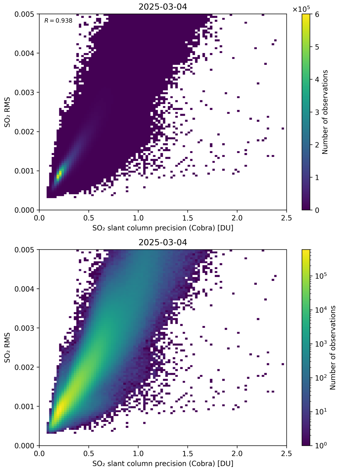
Figure 204: Scatter density plot of “SO 2 slant column precision (Cobra)” against “SO 2 RMS” for 2025-03-03 to 2025-03-05.
