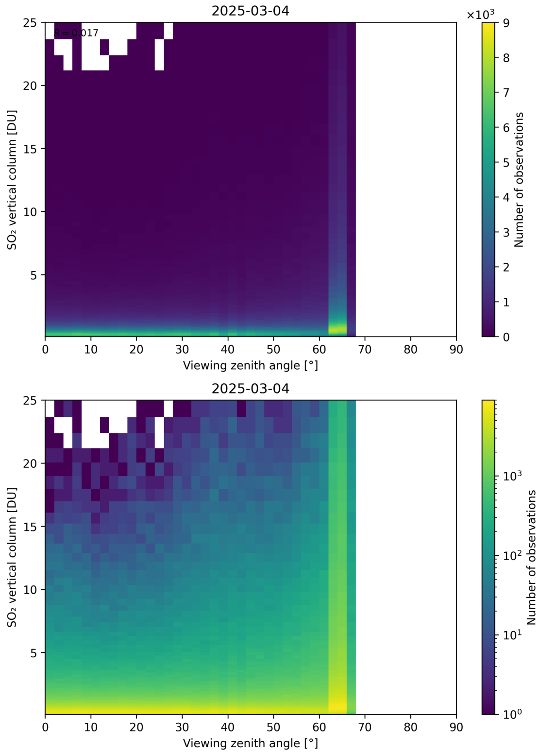
Figure 383: Scatter density plot of “Viewing zenith angle” against “SO 2 vertical column” for 2025-03-03 to 2025-03-05.
