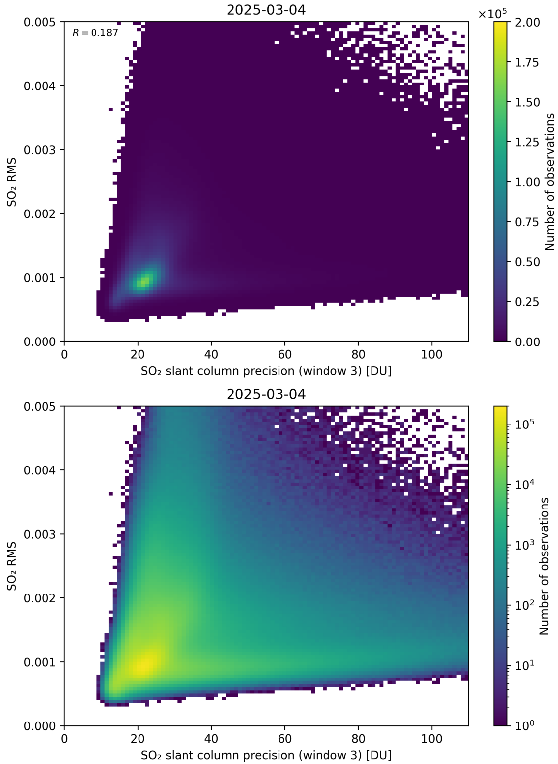
Figure 310: Scatter density plot of “SO 2 slant column precision (window 3)” against “SO 2 RMS” for 2025-03-03 to 2025-03-05.
