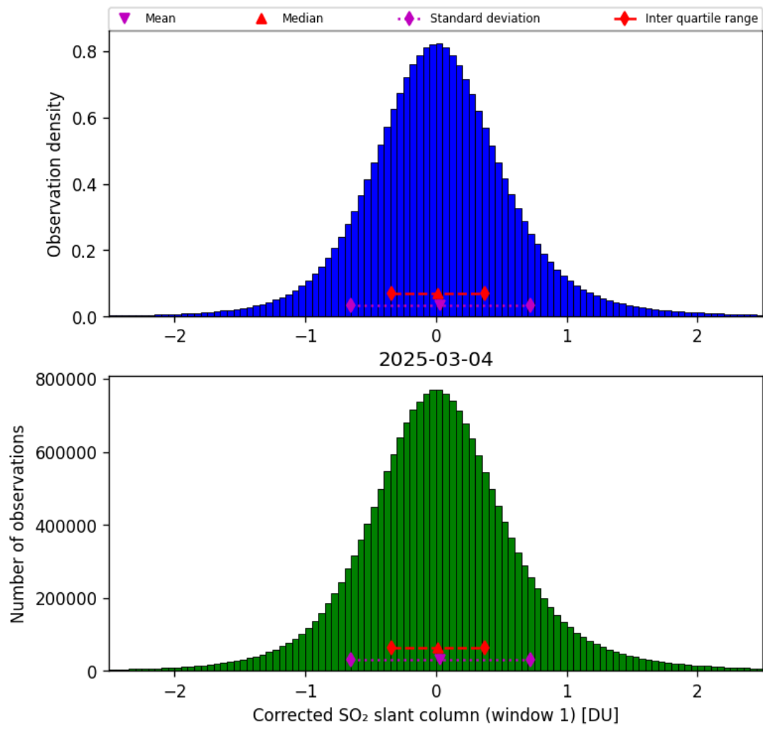
Figure 65: Histogram of “Corrected SO 2 slant column (window 1)” for 2025-03-03 to 2025-03-05
