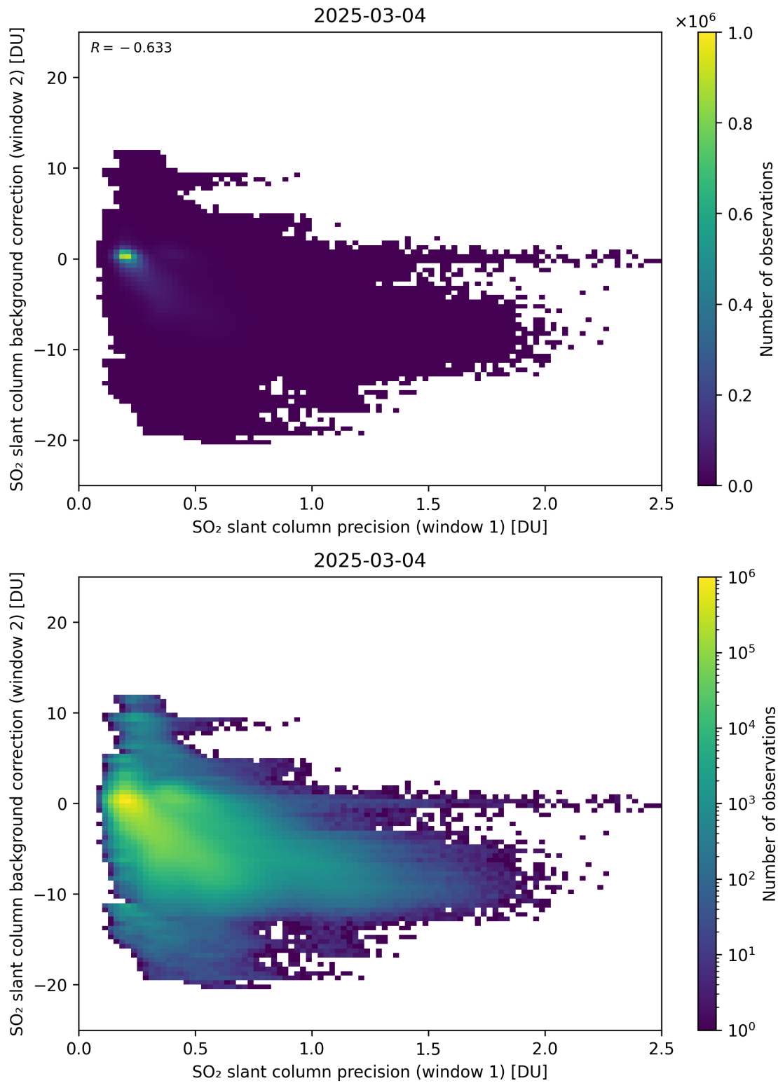
Figure 269: Scatter density plot of “SO 2 slant column precision (window 1)” against “SO 2 slant column background correction (window 2)” for 2025-03-03 to 2025-03-05.
