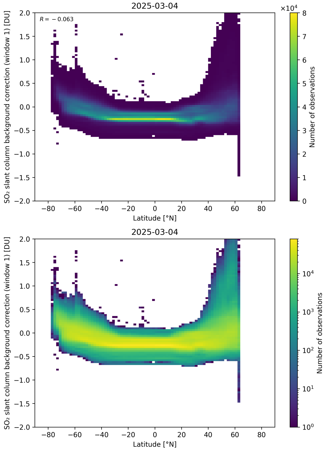
Figure 150: Scatter density plot of “Latitude” against “SO 2 slant column background correction (window 1)” for 2025-03-03 to 2025-03-05.
