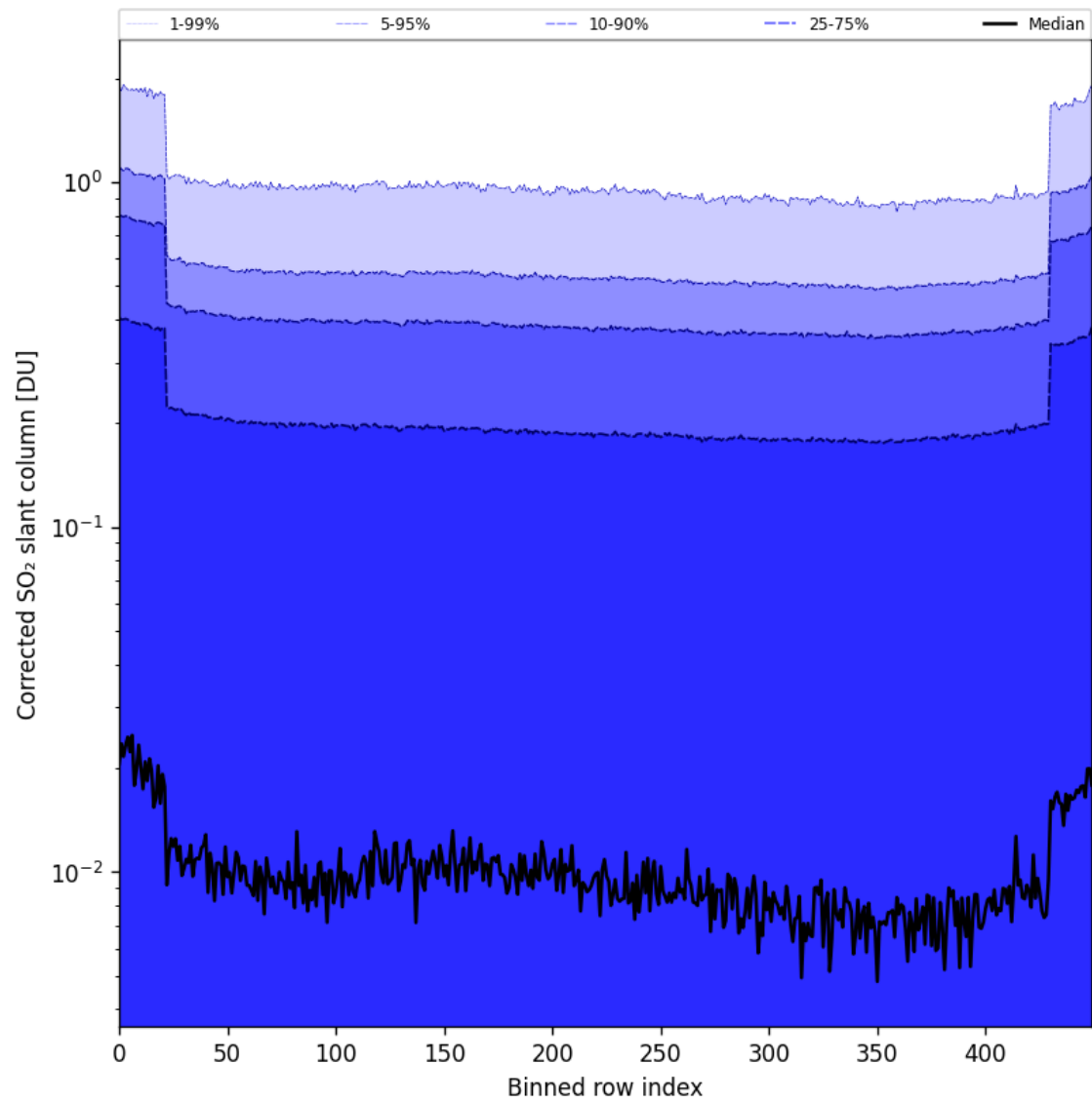
Figure 86: Along track statistics of “Corrected SO 2 slant column” for 2025-03-03 to 2025-03-05
