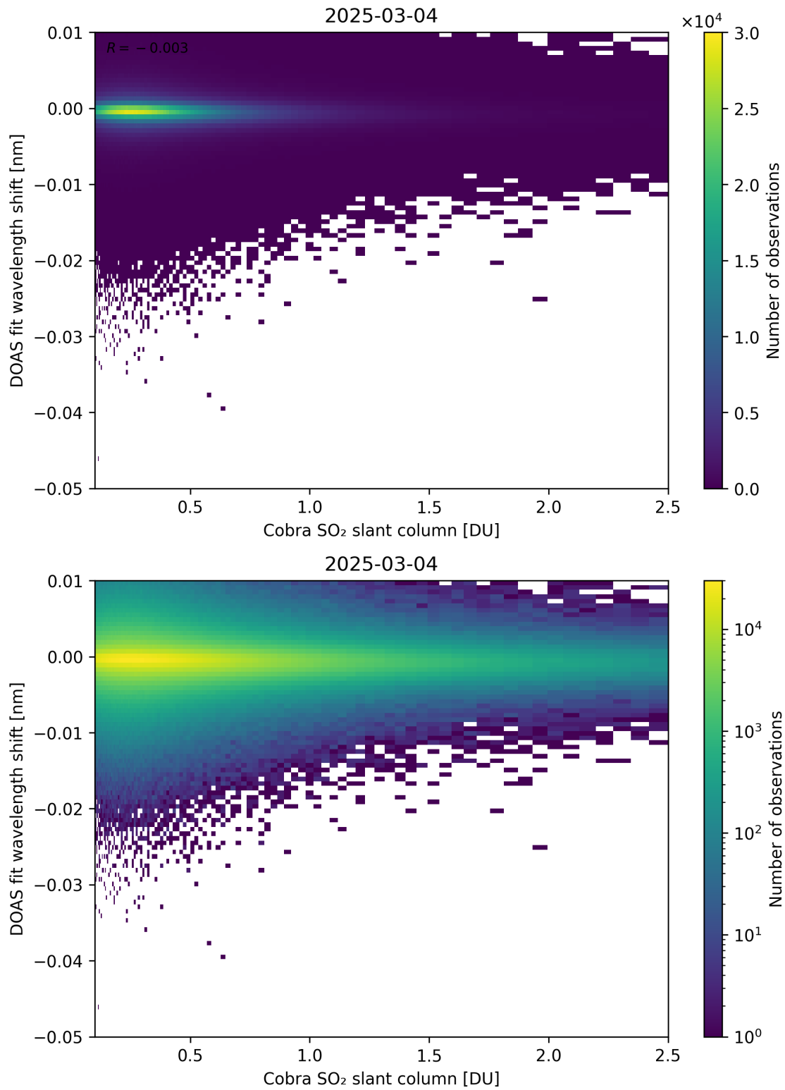
Figure 196: Scatter density plot of “Cobra SO 2 slant column” against “DOAS fit wavelength shift” for 2025-03-03 to 2025-03-05.
