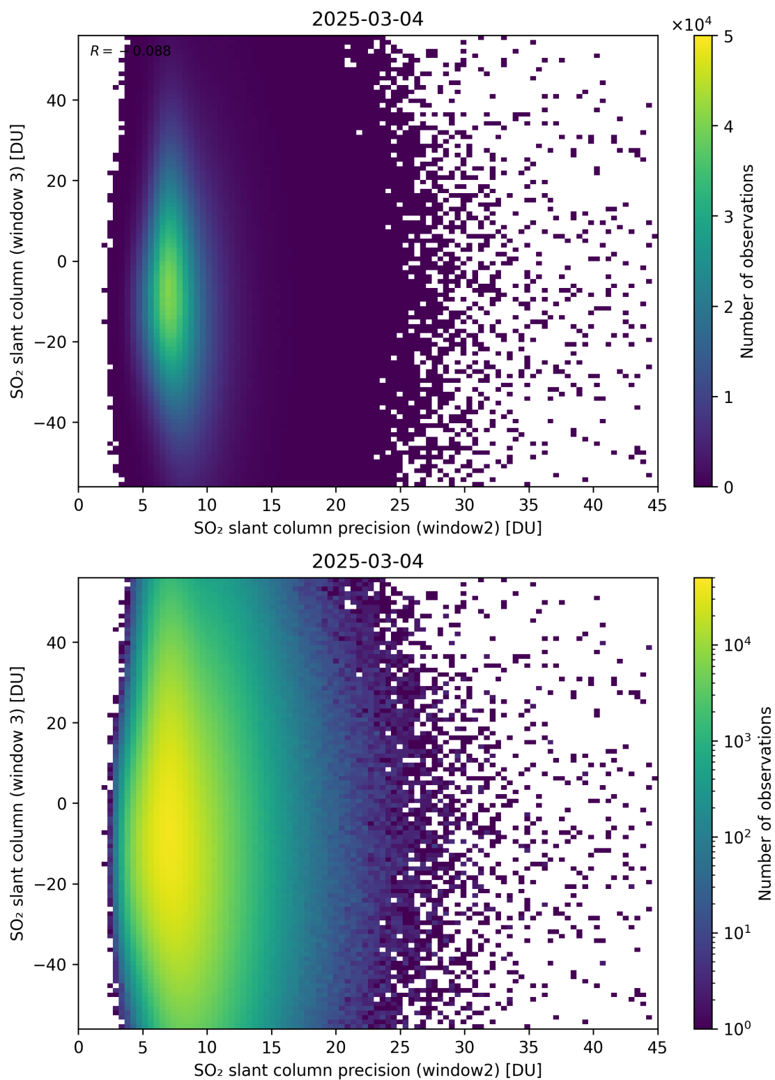
Figure 299: Scatter density plot of “SO 2 slant column precision (window2)” against “SO 2 slant column (window 3)” for 2025-03-03 to 2025-03-05.
