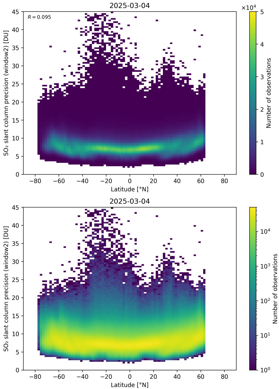
Figure 164: Scatter density plot of “Latitude” against “SO 2 slant column precision (window2)” for 2025-03-03 to 2025-03-05.
