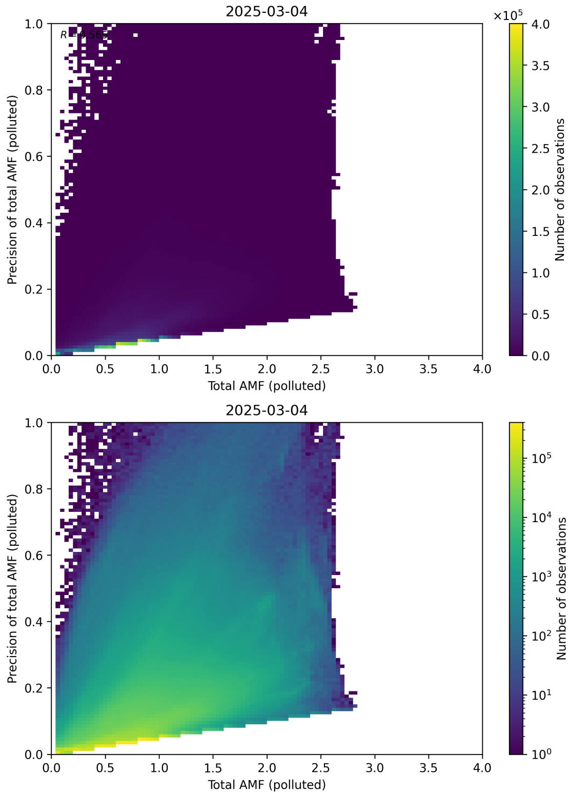
Figure 322: Scatter density plot of “Total AMF (polluted)” against “Precision of total AMF (polluted)” for 2025-03-03 to 2025-03-05.
