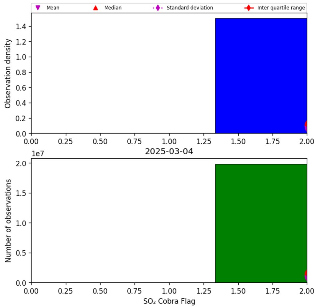
Figure 75: Histogram of “SO 2 Cobra Flag” for 2025-03-03 to 2025-03-05
