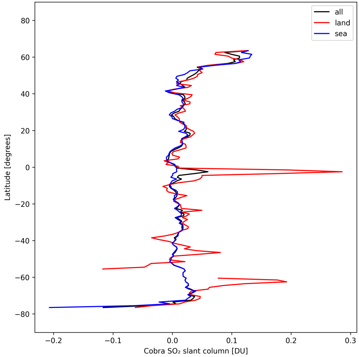
Figure 35: Zonal average of “Cobra SO 2 slant column” for 2025-03-03 to 2025-03-05.
