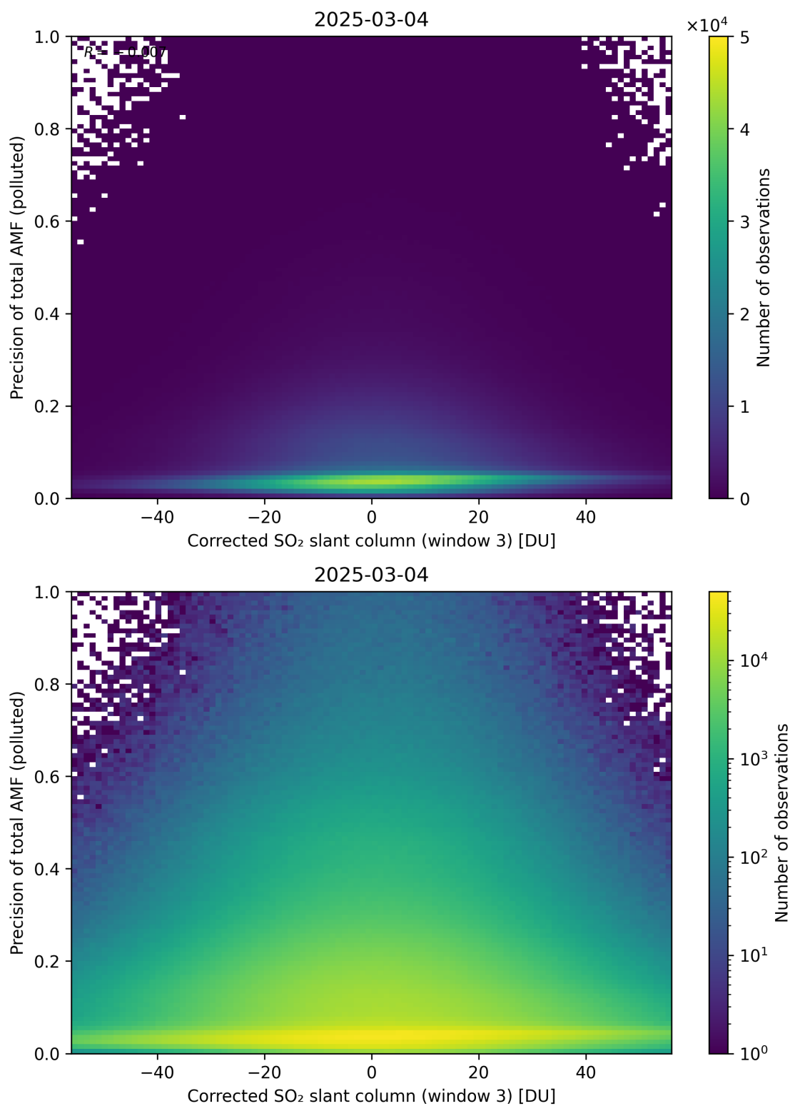
Figure 261: Scatter density plot of “Corrected SO 2 slant column (window 3)” against “Precision of total AMF (polluted)” for 2025-03-03 to 2025-03-05.
