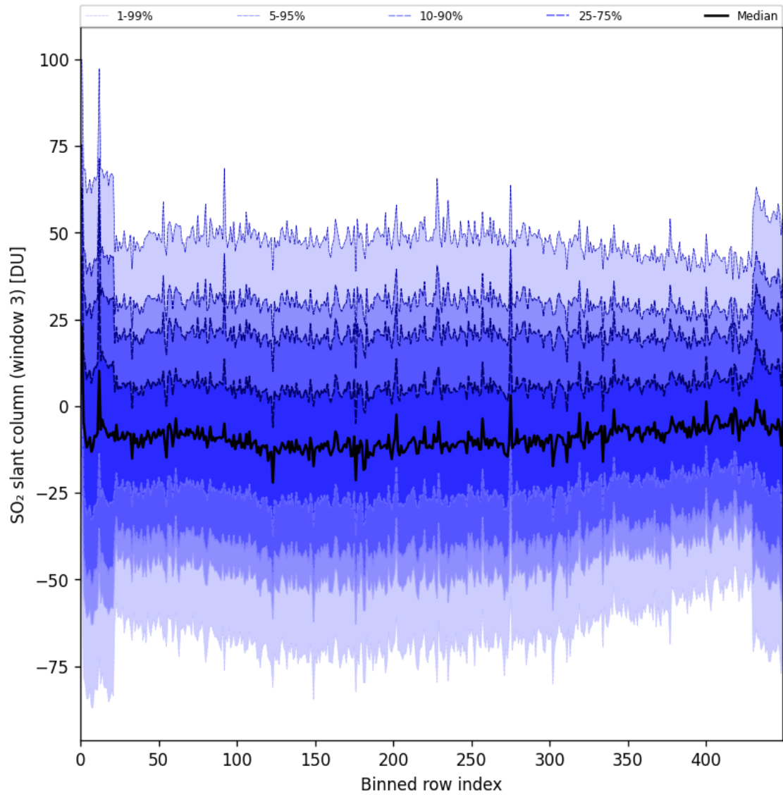
Figure 97: Along track statistics of “SO 2 slant column (window 3)” for 2025-03-03 to 2025-03-05
