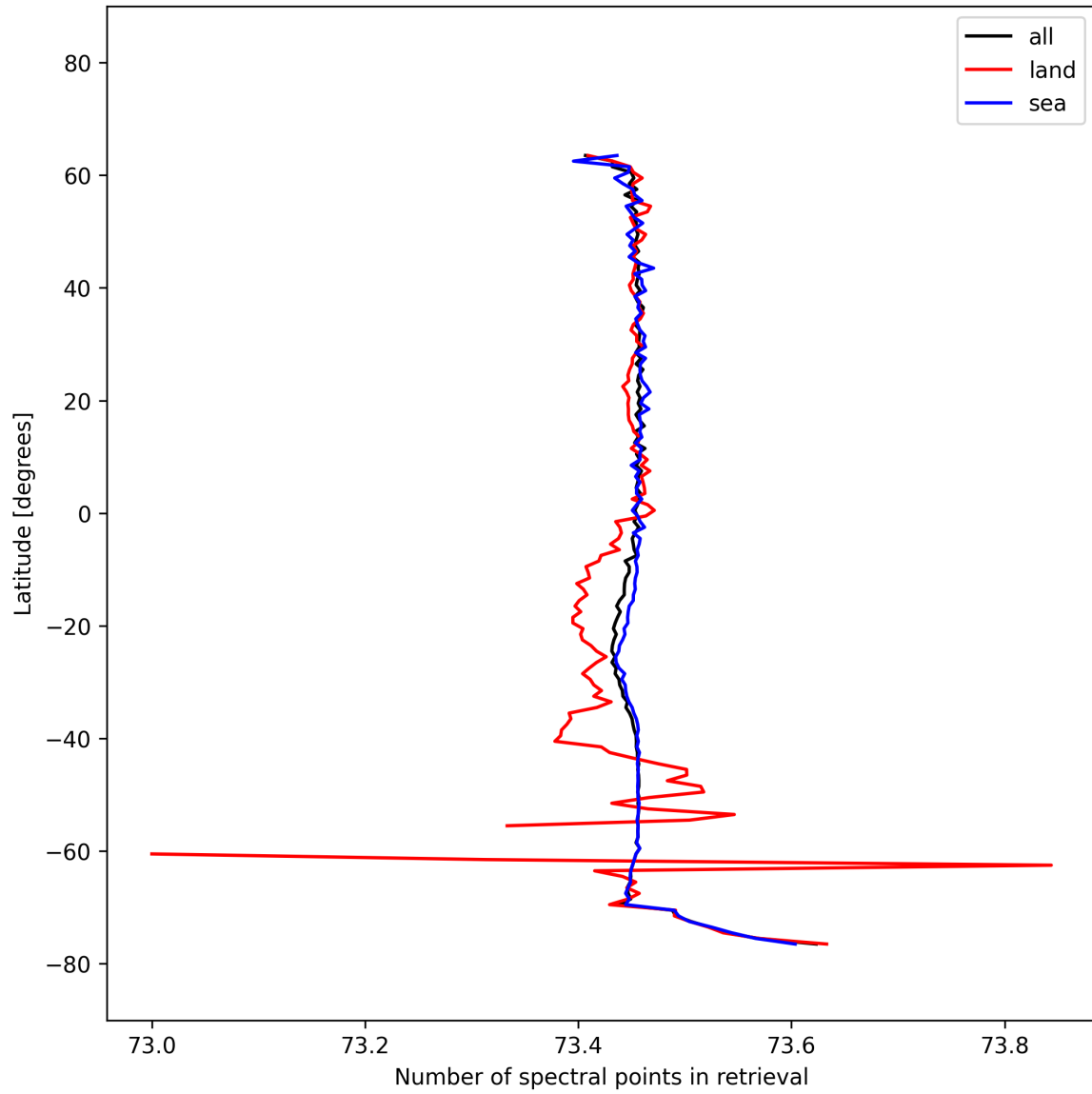
Figure 56: Zonal average of “Number of spectral points in retrieval” for 2025-03-03 to 2025-03-05.
