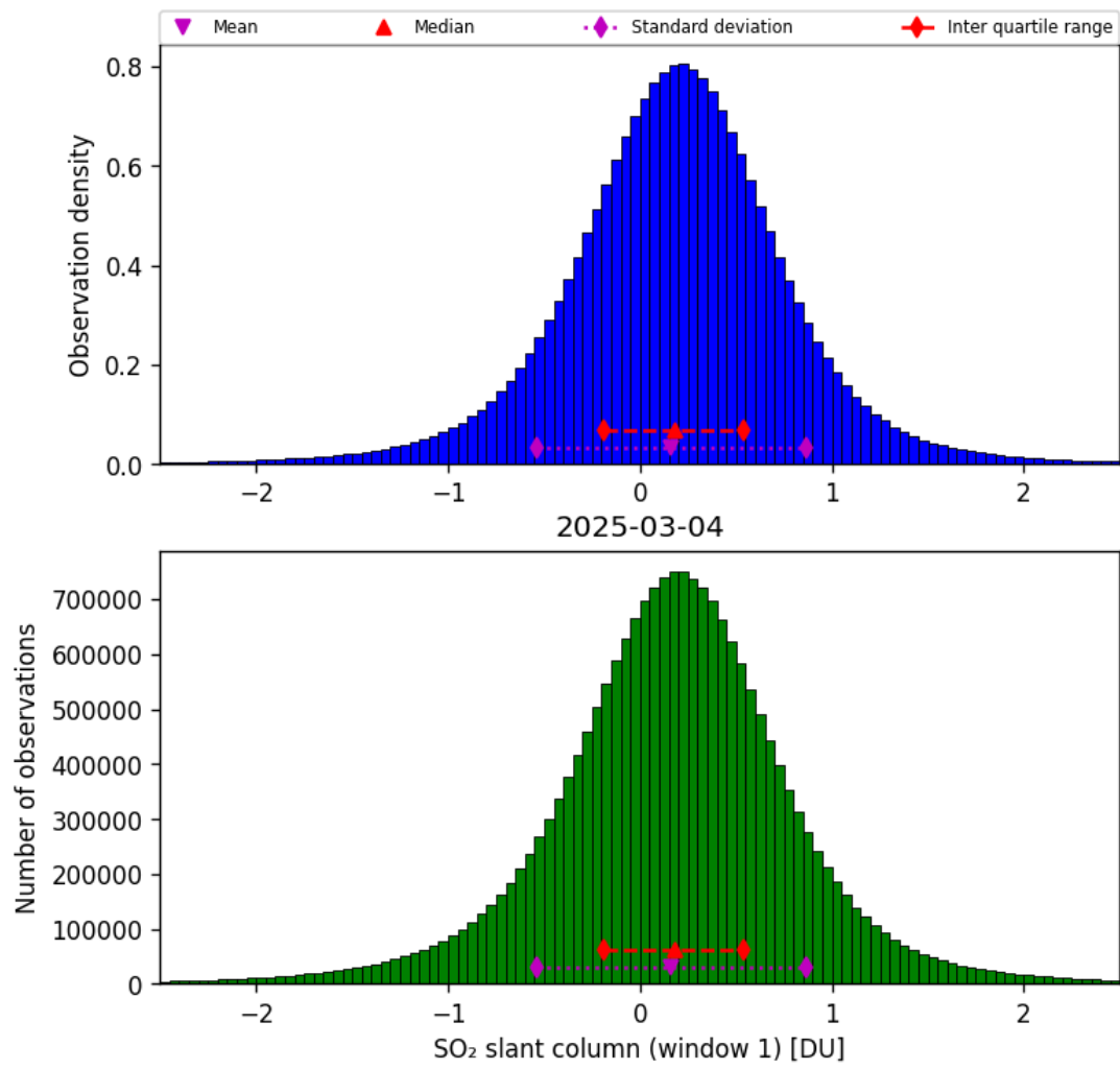
Figure 63: Histogram of “SO 2 slant column (window 1)” for 2025-03-03 to 2025-03-05
