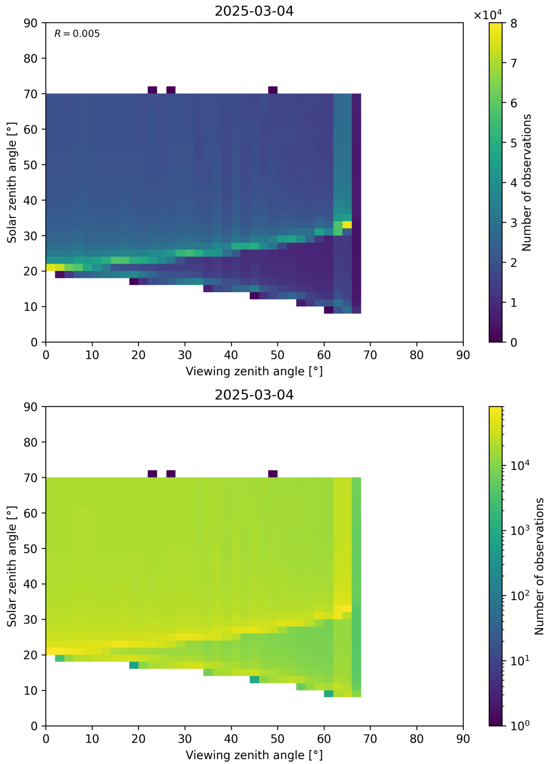
Figure 369: Scatter density plot of “Viewing zenith angle” against “Solar zenith angle” for 2025-03-03 to 2025-03-05.
