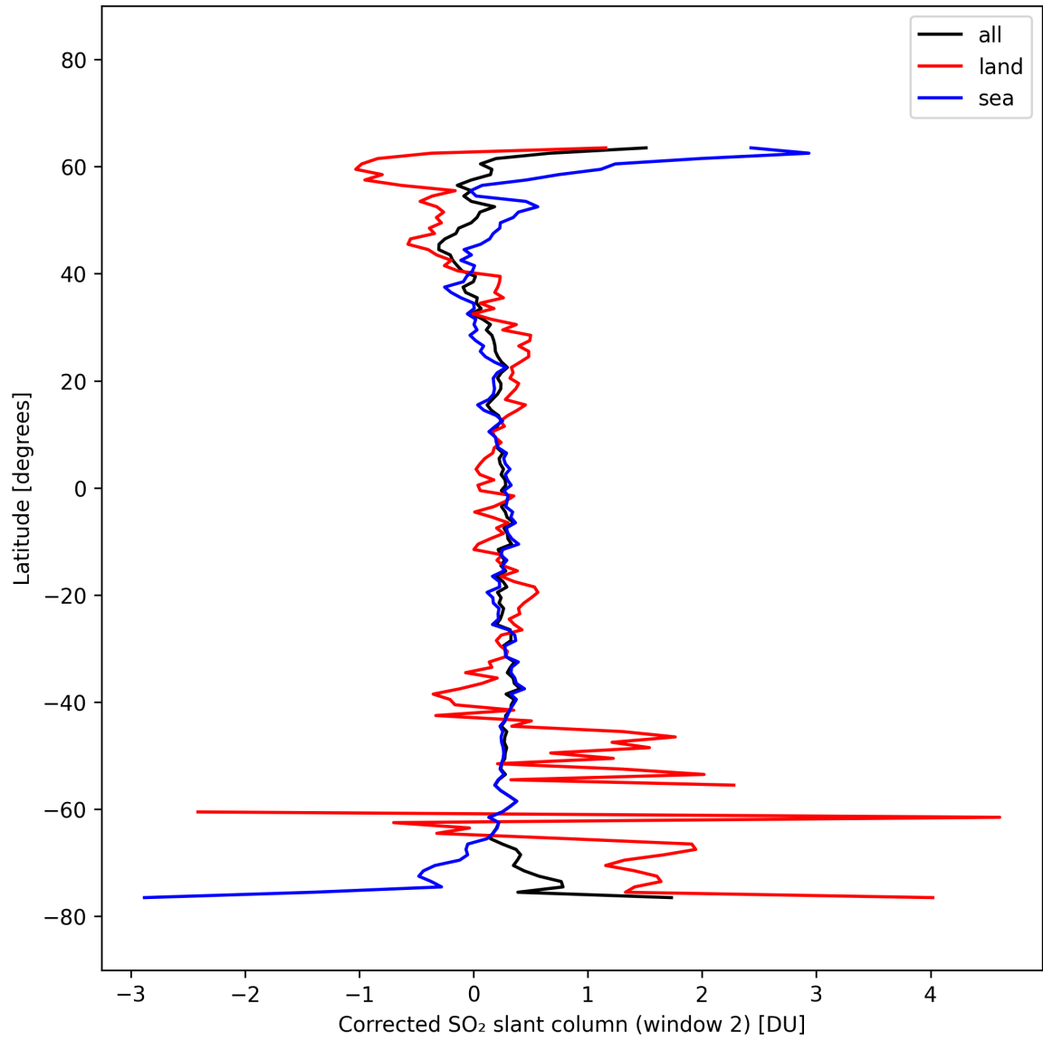
Figure 43: Zonal average of “Corrected SO 2 slant column (window 2)” for 2025-03-03 to 2025-03-05.
