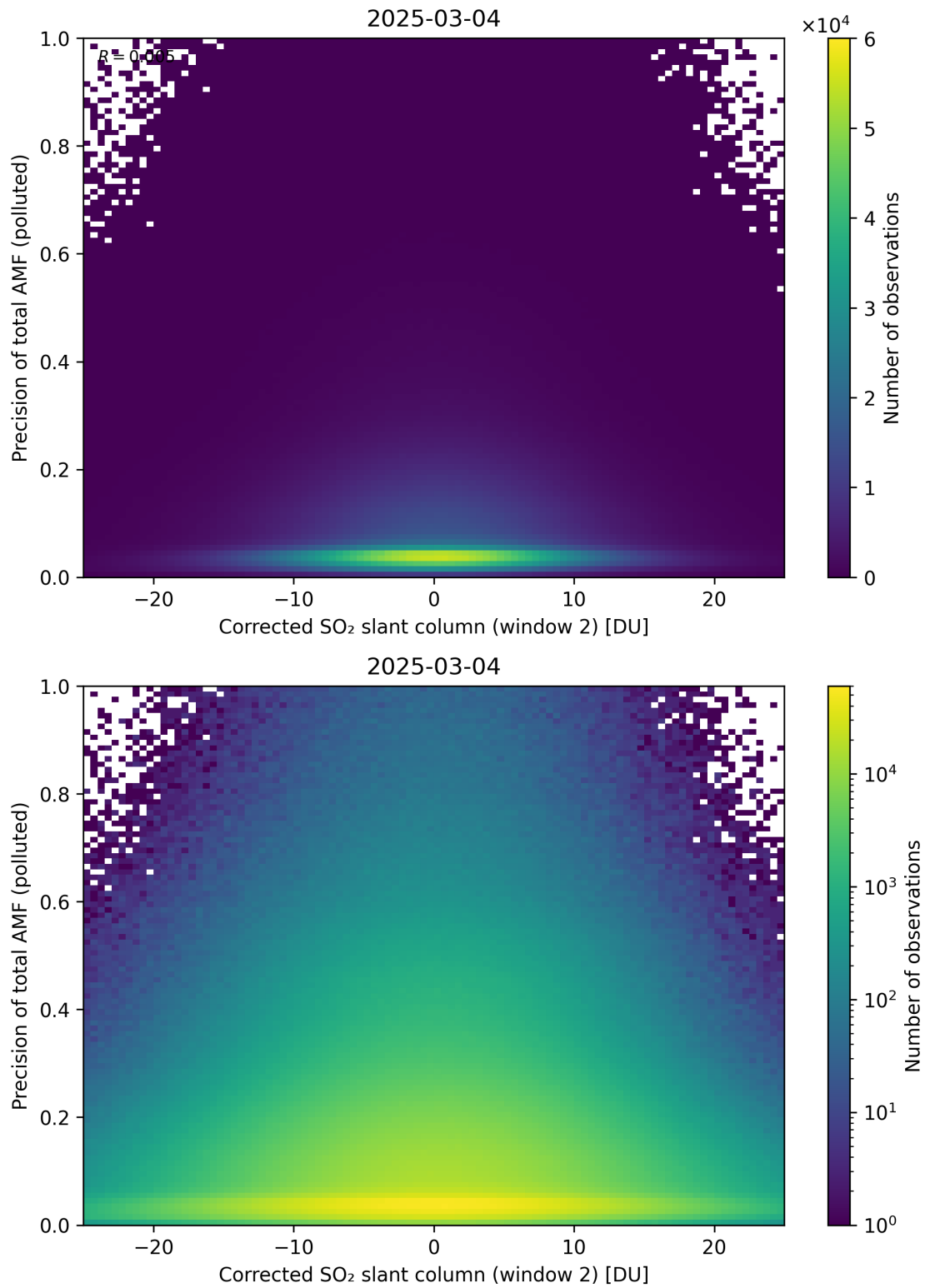
Figure 254: Scatter density plot of “Corrected SO 2 slant column (window 2)” against “Precision of total AMF (polluted)” for 2025-03-03 to 2025-03-05.
