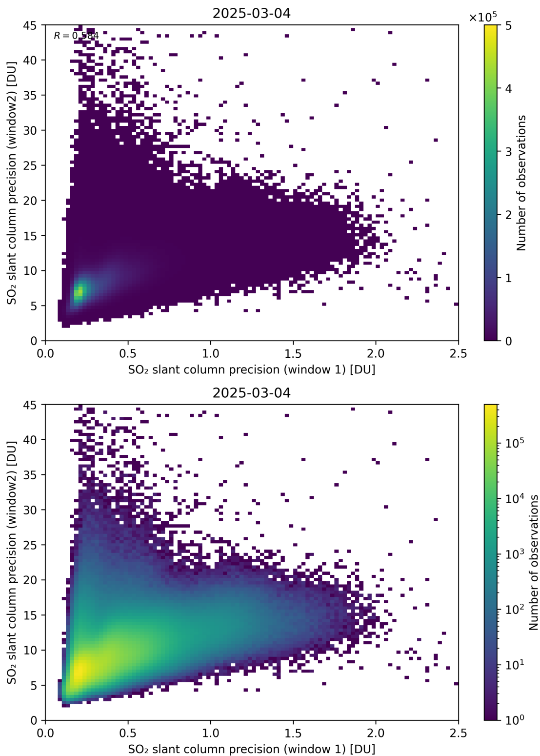
Figure 277: Scatter density plot of “SO 2 slant column precision (window 1)” against “SO 2 slant column precision (window2)” for 2025-03-03 to 2025-03-05.
