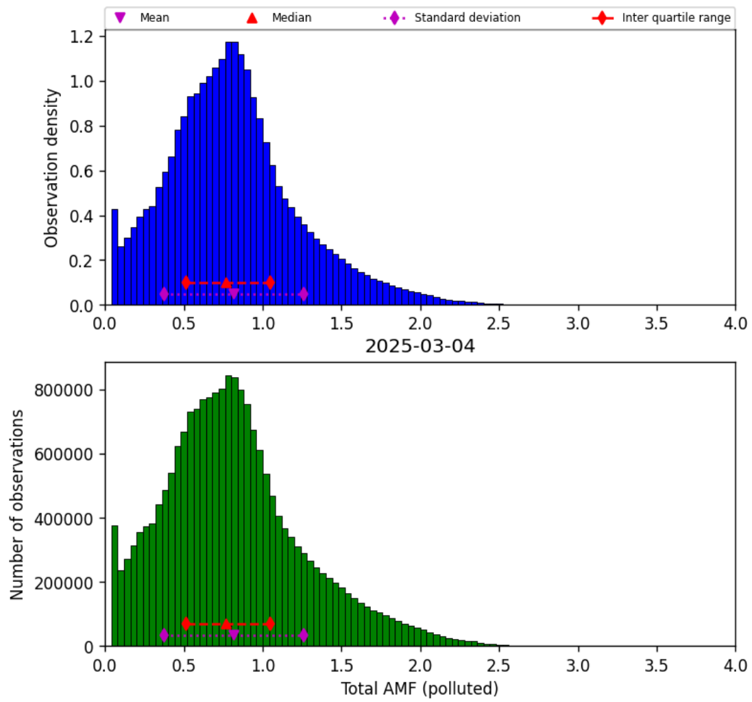
Figure 79: Histogram of “Total AMF (polluted)” for 2025-03-03 to 2025-03-05
