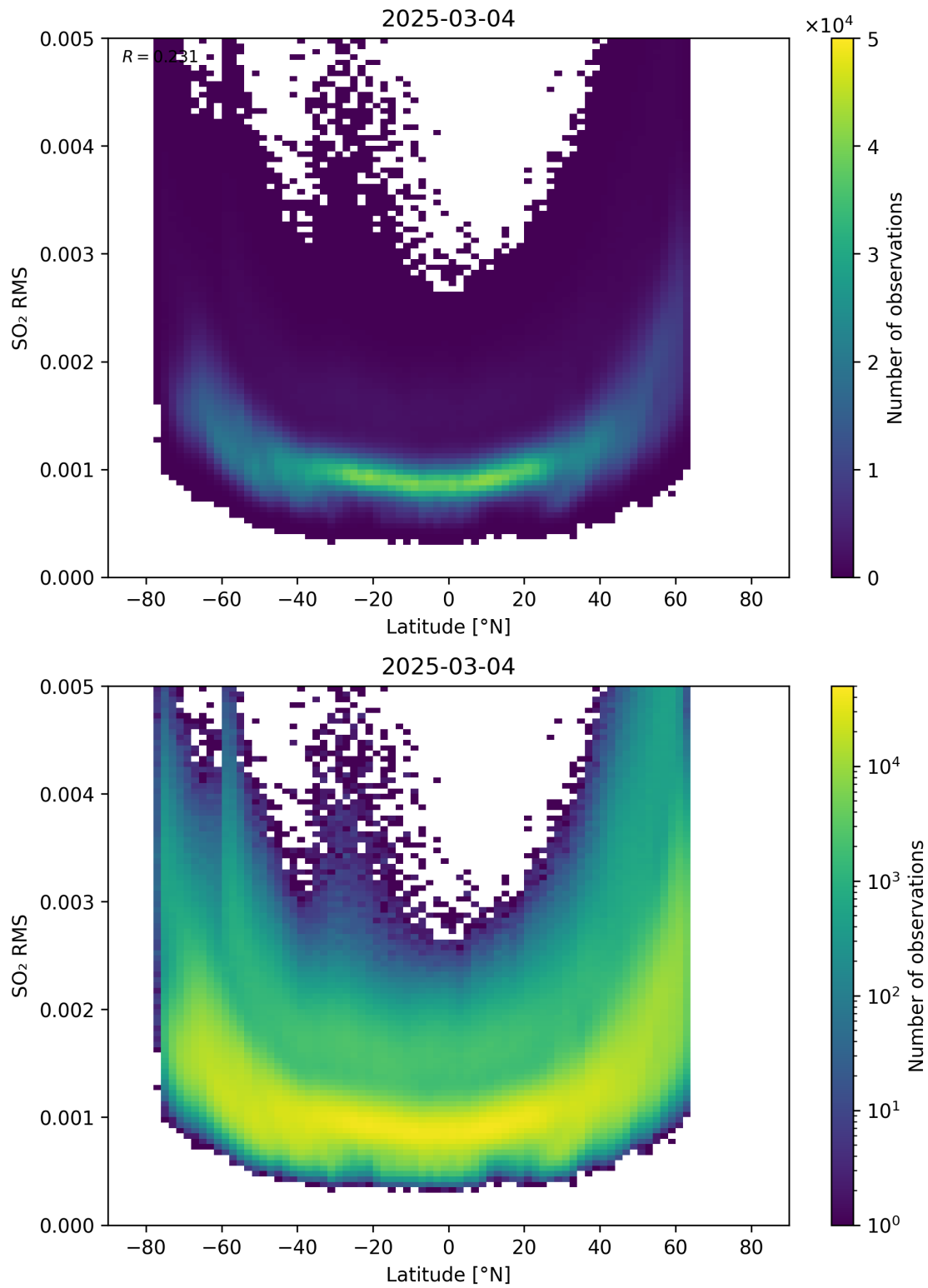
Figure 155: Scatter density plot of “Latitude” against “SO 2 RMS” for 2025-03-03 to 2025-03-05.
