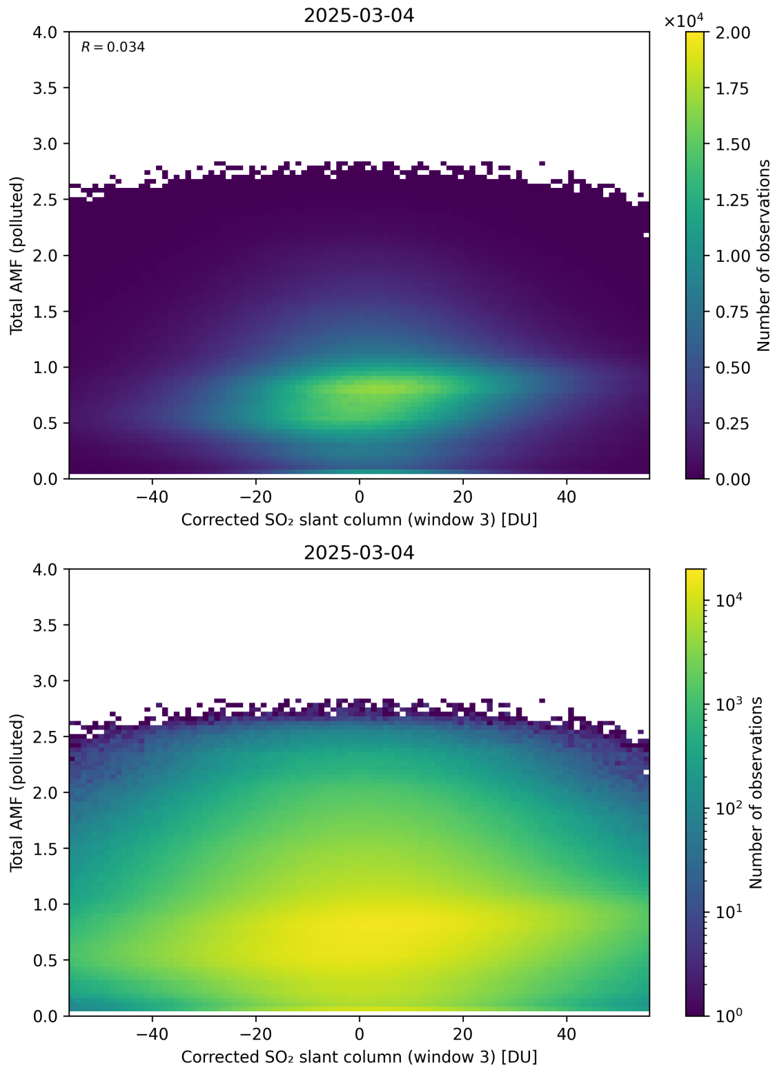
Figure 260: Scatter density plot of “Corrected SO 2 slant column (window 3)” against “Total AMF (polluted)” for 2025-03-03 to 2025-03-05.
