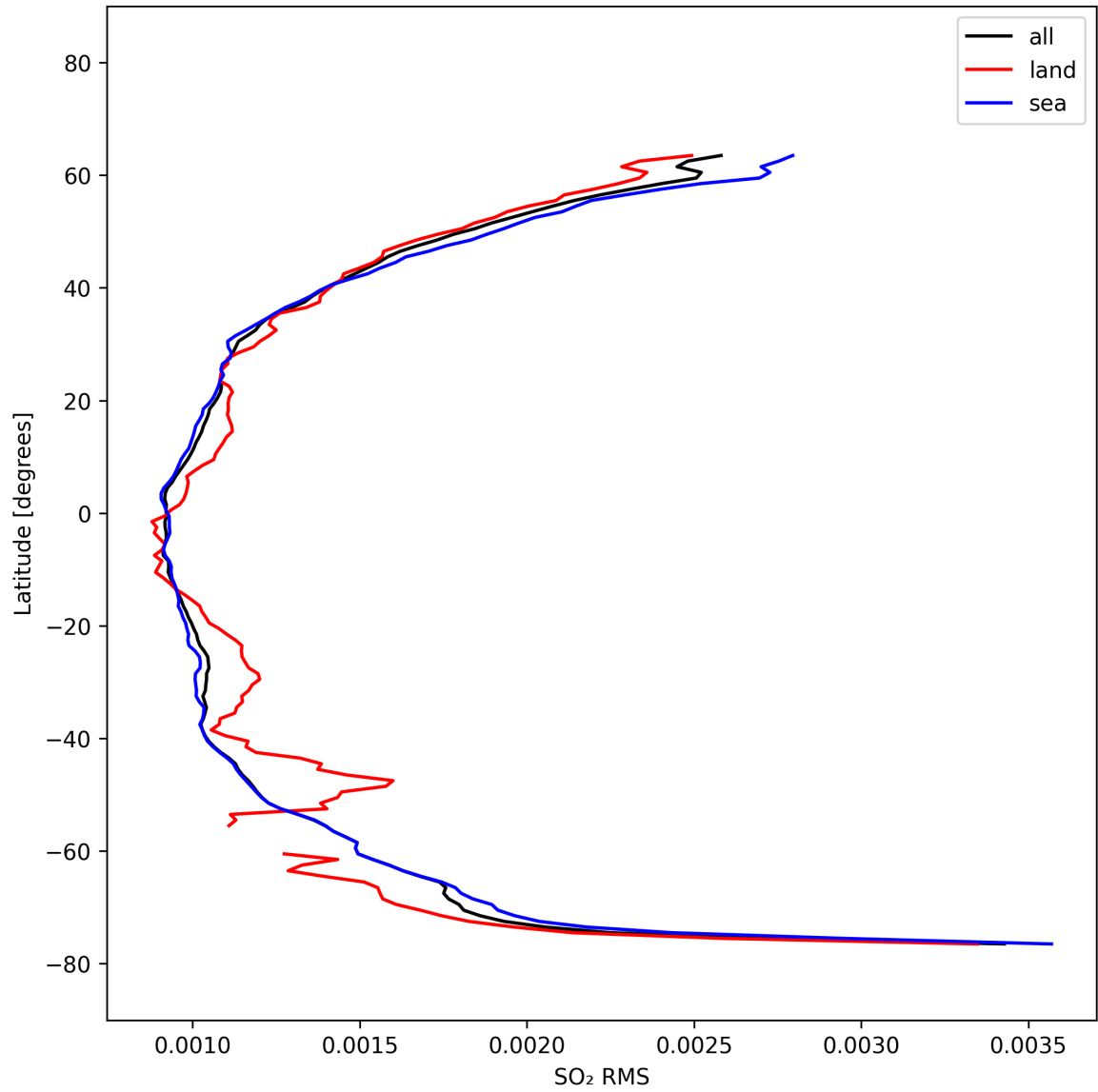
Figure 52: Zonal average of “SO 2 RMS” for 2025-03-03 to 2025-03-05.
