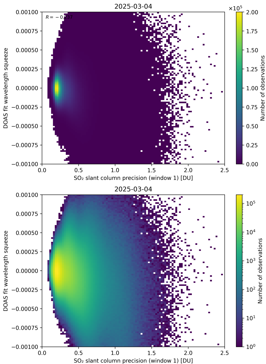
Figure 272: Scatter density plot of “SO 2 slant column precision (window 1)” against “DOAS fit wavelength squeeze” for 2025-03-03 to 2025-03-05.
