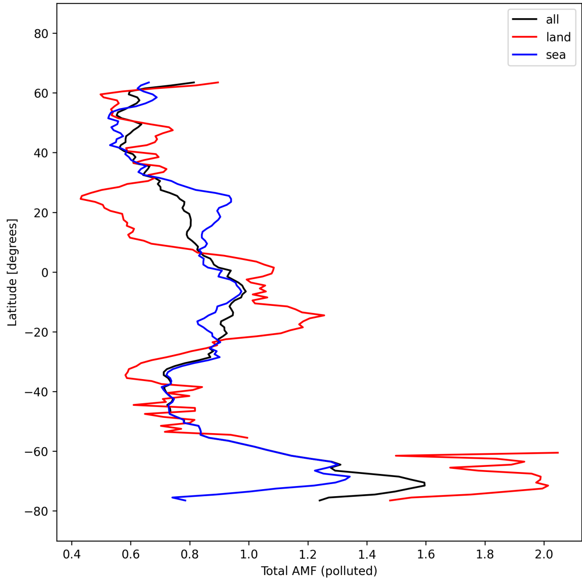
Figure 53: Zonal average of “Total AMF (polluted)” for 2025-03-03 to 2025-03-05.
