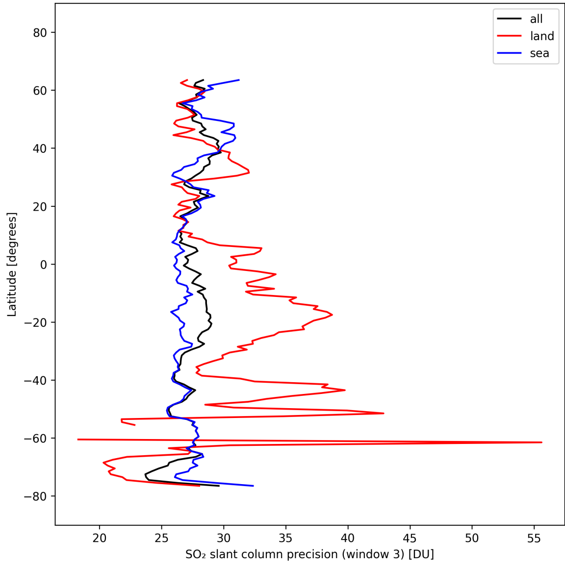
Figure 46: Zonal average of “SO 2 slant column precision (window 3)” for 2025-03-03 to 2025-03-05.
