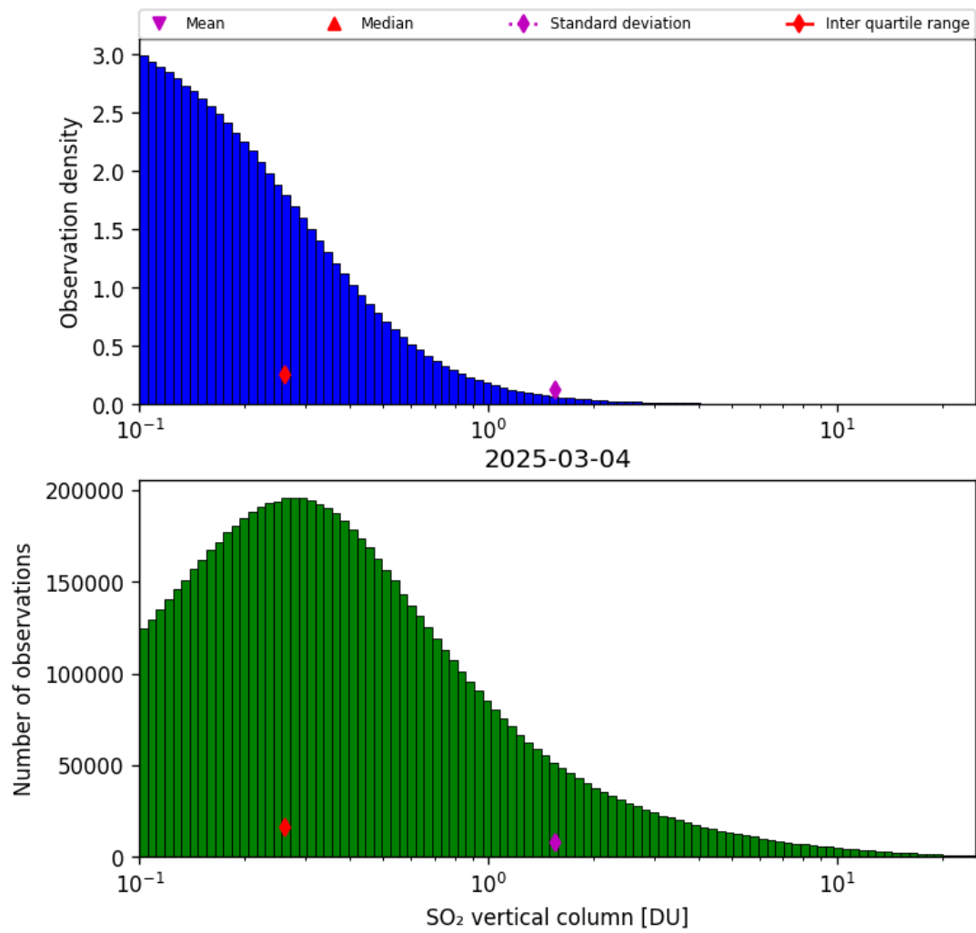
Figure 58: Histogram of “SO 2 vertical column” for 2025-03-03 to 2025-03-05
