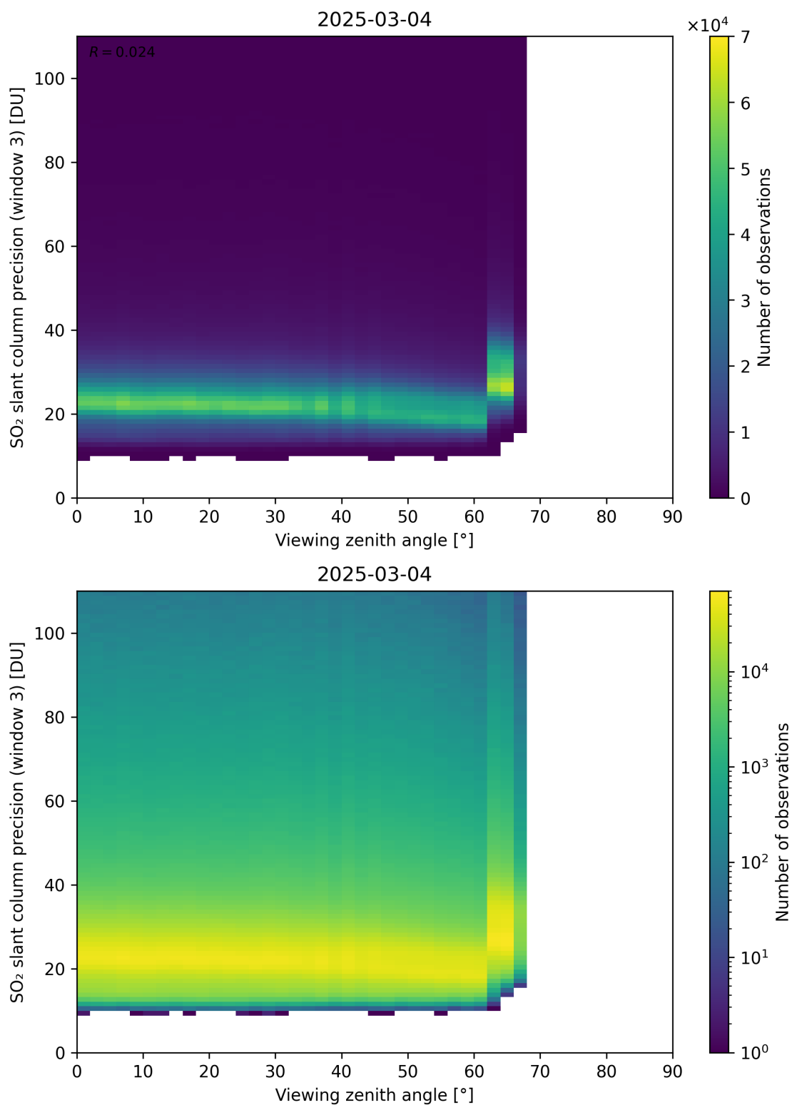
Figure 380: Scatter density plot of “Viewing zenith angle” against “SO 2 slant column precision (window 3)” for 2025-03-03 to 2025-03-05.
