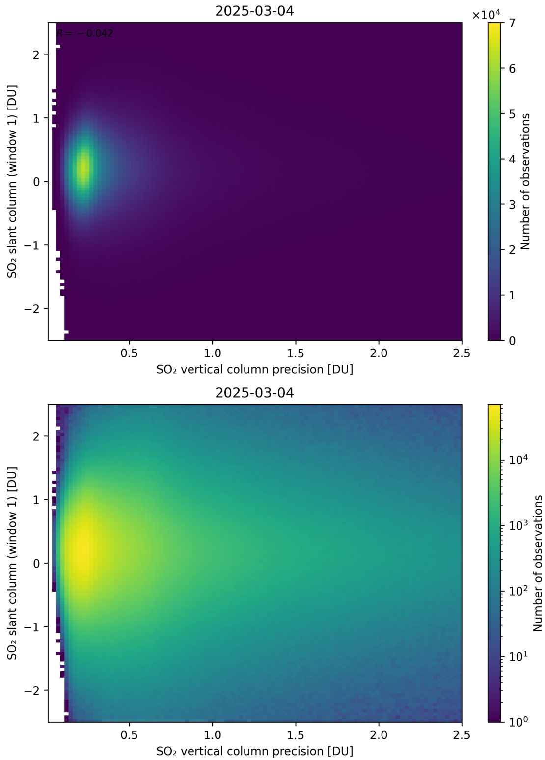
Figure 341: Scatter density plot of “SO 2 vertical column precision” against “SO 2 slant column (window 1)” for 2025-03-03 to 2025-03-05.
