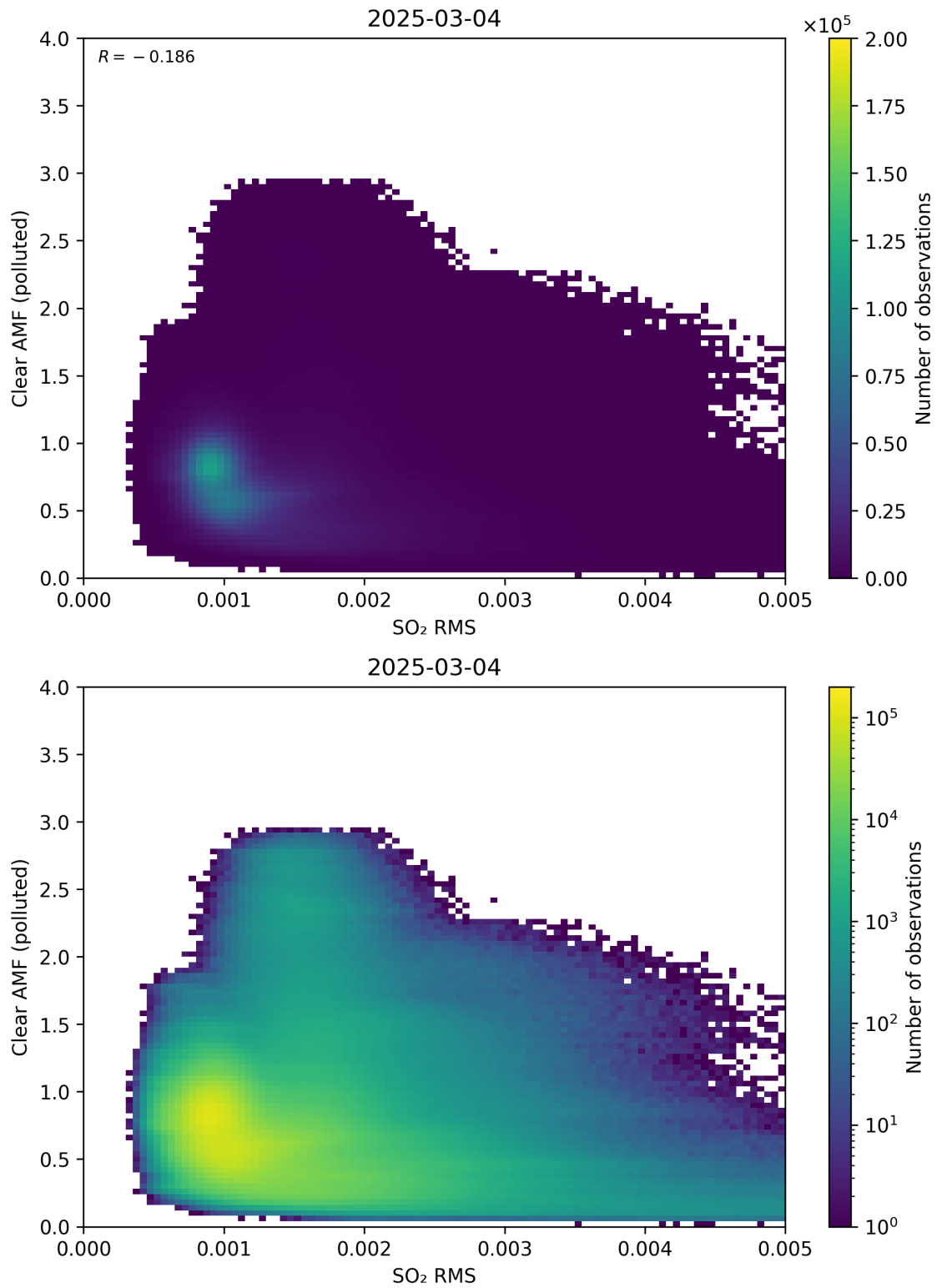
Figure 147: Scatter density plot of “SO 2 RMS” against “Clear AMF (polluted)” for 2025-03-03 to 2025-03-05.
