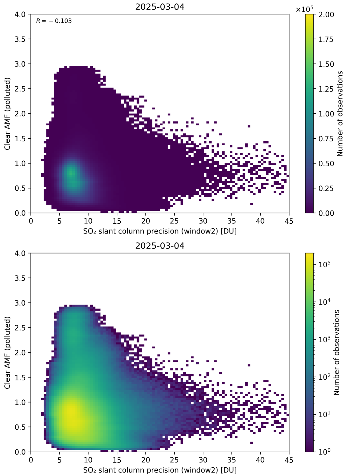
Figure 296: Scatter density plot of “SO 2 slant column precision (window2)” against “Clear AMF (polluted)” for 2025-03-03 to 2025-03-05.
