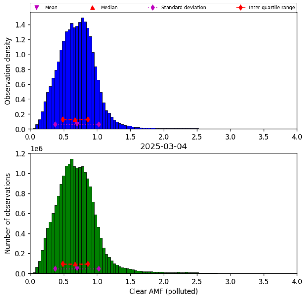
Figure 81: Histogram of “Clear AMF (polluted)” for 2025-03-03 to 2025-03-05
