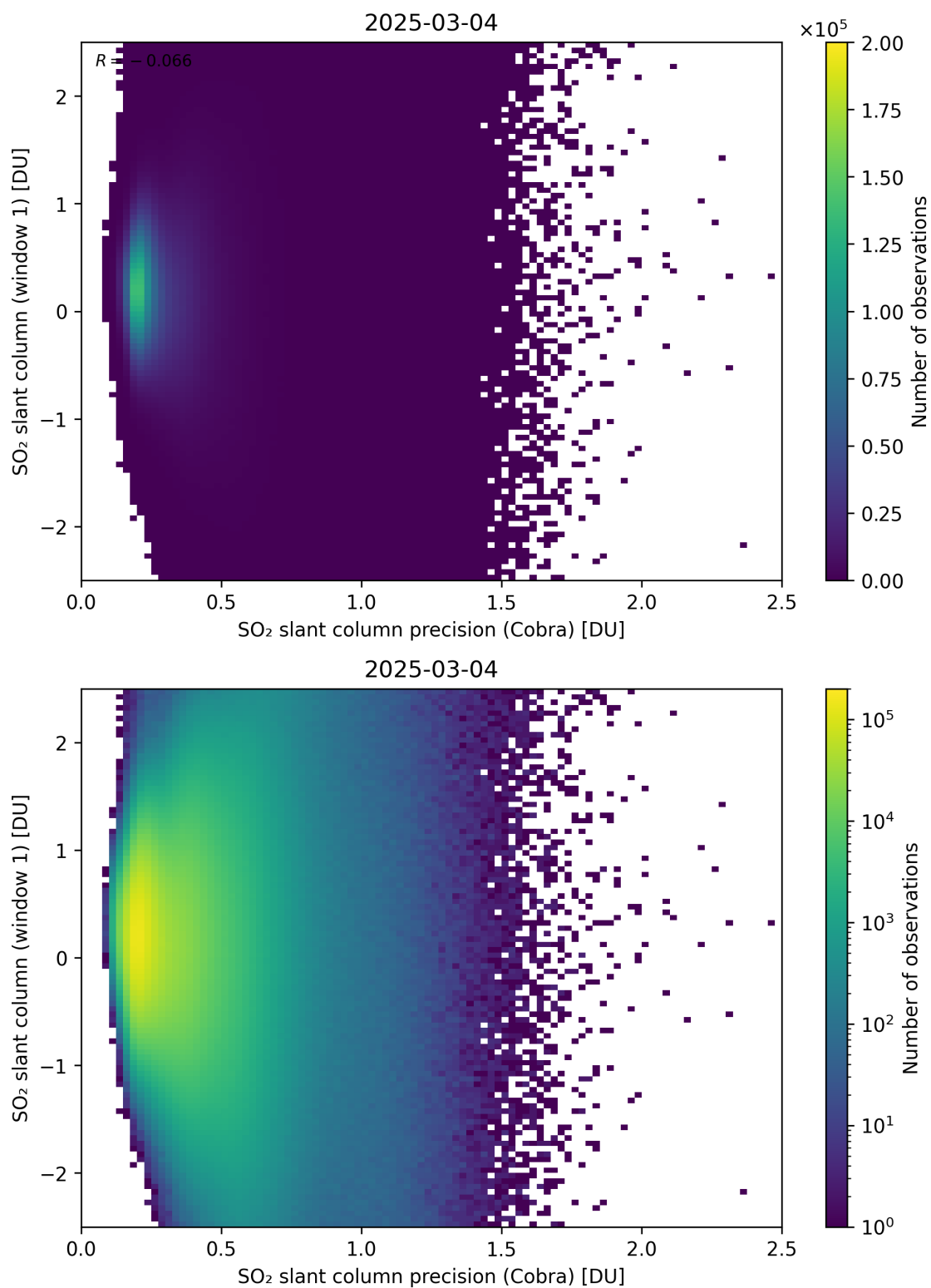
Figure 208: Scatter density plot of “SO 2 slant column precision (Cobra)” against “SO 2 slant column (window 1)” for 2025-03-03 to 2025-03-05.
