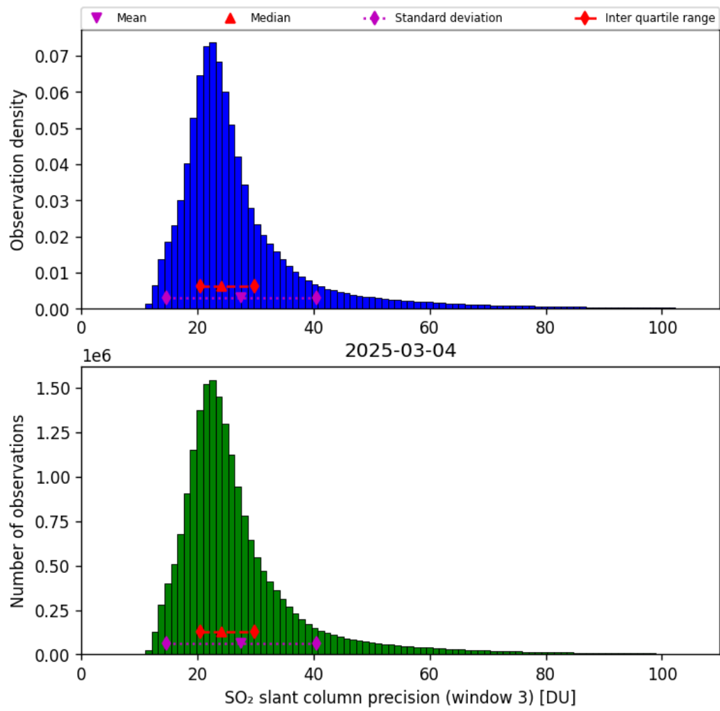
Figure 72: Histogram of “SO 2 slant column precision (window 3)” for 2025-03-03 to 2025-03-05
