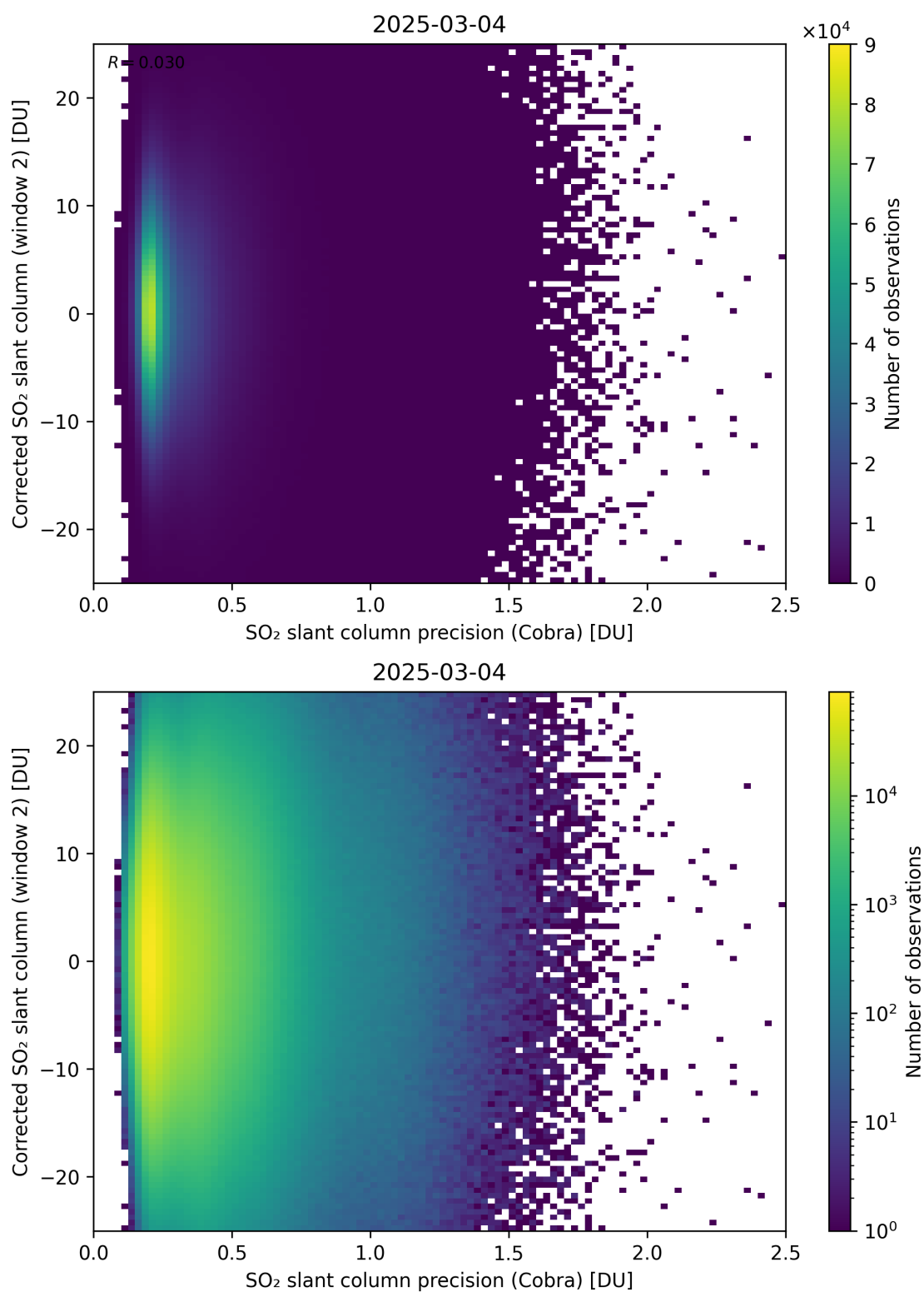
Figure 206: Scatter density plot of “SO 2 slant column precision (Cobra)” against “Corrected SO 2 slant column (window 2)” for 2025-03-03 to 2025-03-05.
