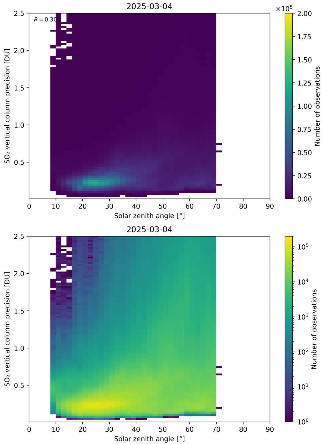
Figure 192: Scatter density plot of “Solar zenith angle” against “SO 2 vertical column precision” for 2025-03-03 to 2025-03-05.
