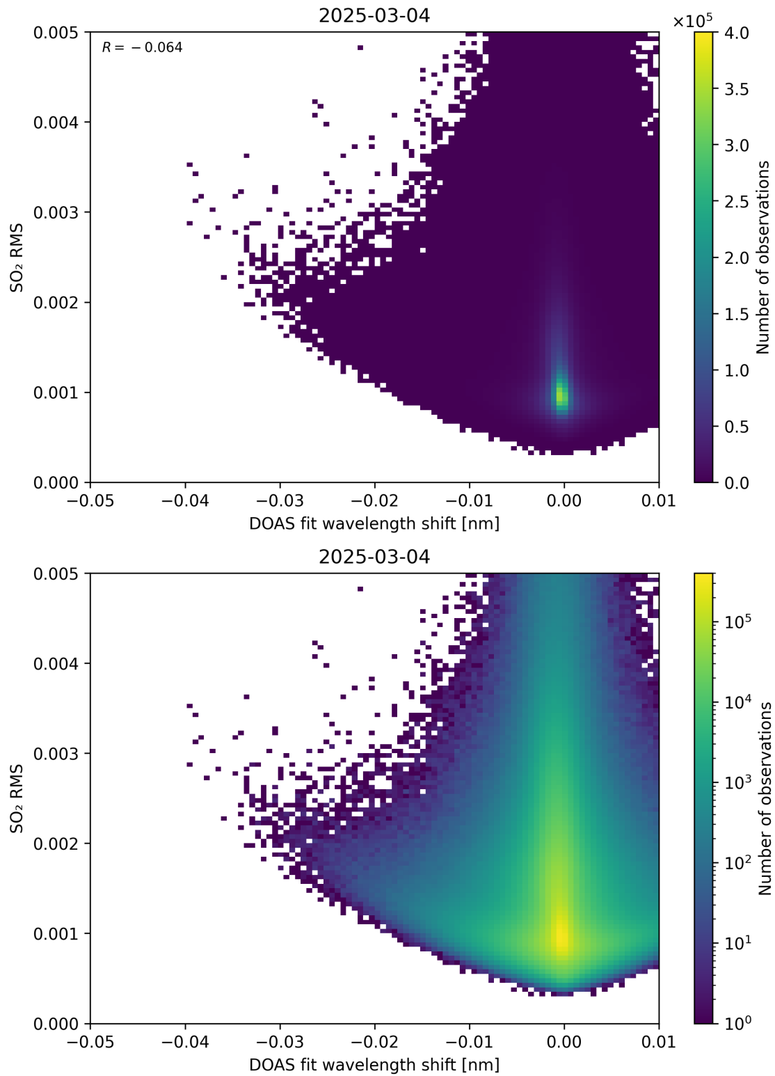
Figure 139: Scatter density plot of “DOAS fit wavelength shift” against “SO 2 RMS” for 2025-03-03 to 2025-03-05.
