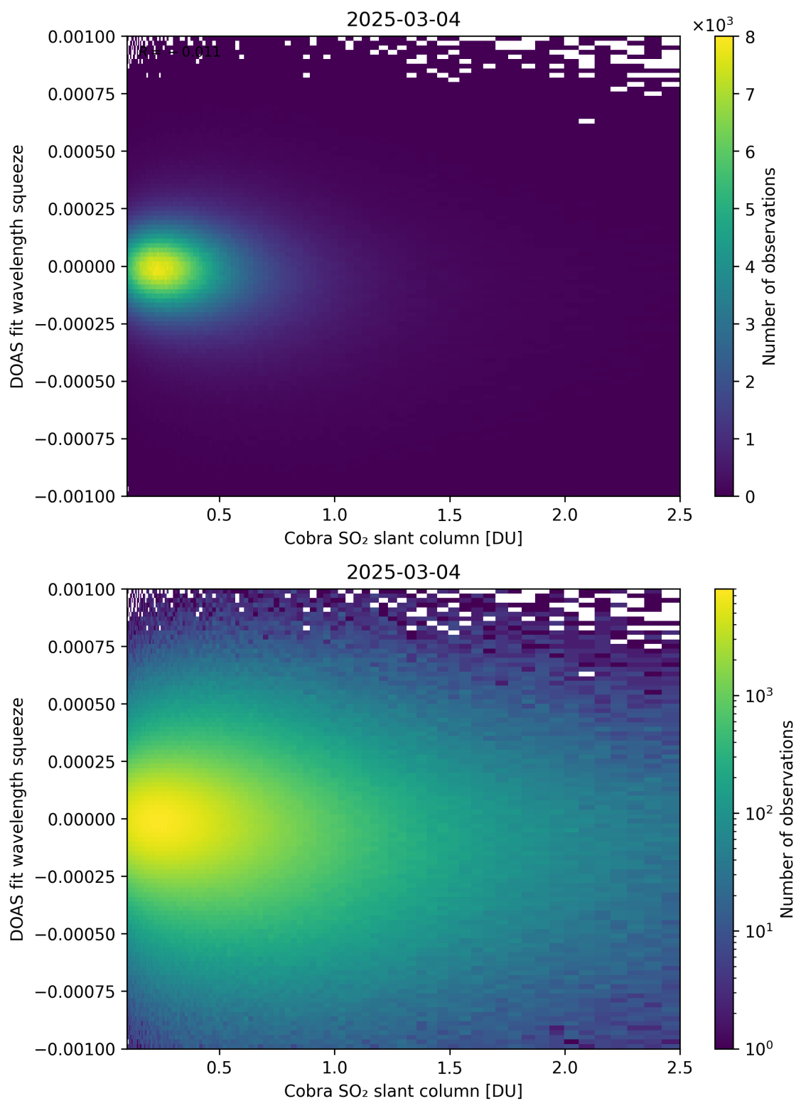
Figure 197: Scatter density plot of “Cobra SO 2 slant column” against “DOAS fit wavelength squeeze” for 2025-03-03 to 2025-03-05.
