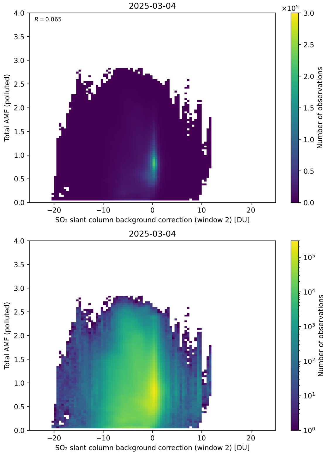
Figure 130: Scatter density plot of “SO 2 slant column background correction (window 2)” against “Total AMF (polluted)” for 2025-03-03 to 2025-03-05.
