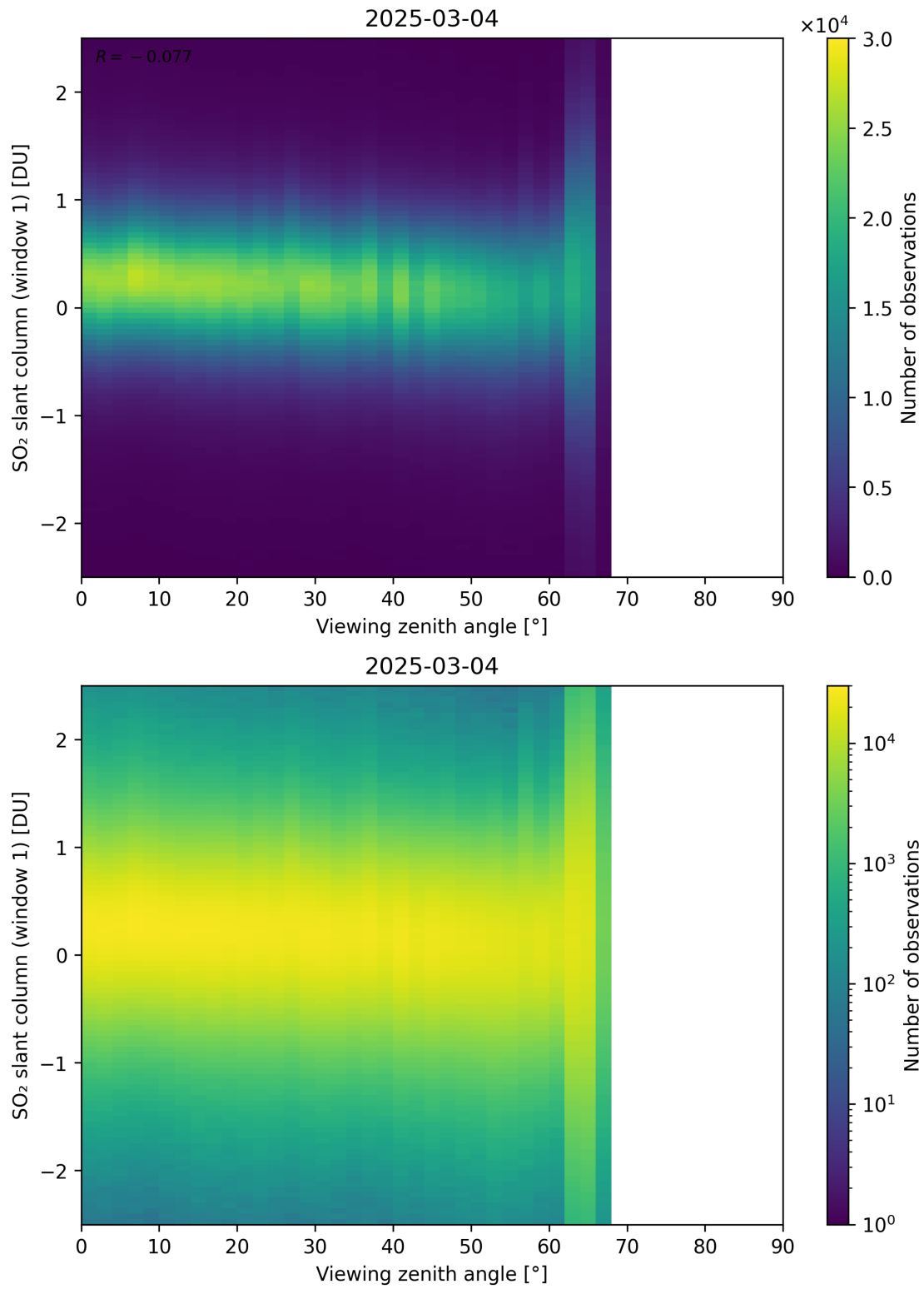
Figure 376: Scatter density plot of “Viewing zenith angle” against “SO 2 slant column (window 1)” for 2025-03-03 to 2025-03-05.
