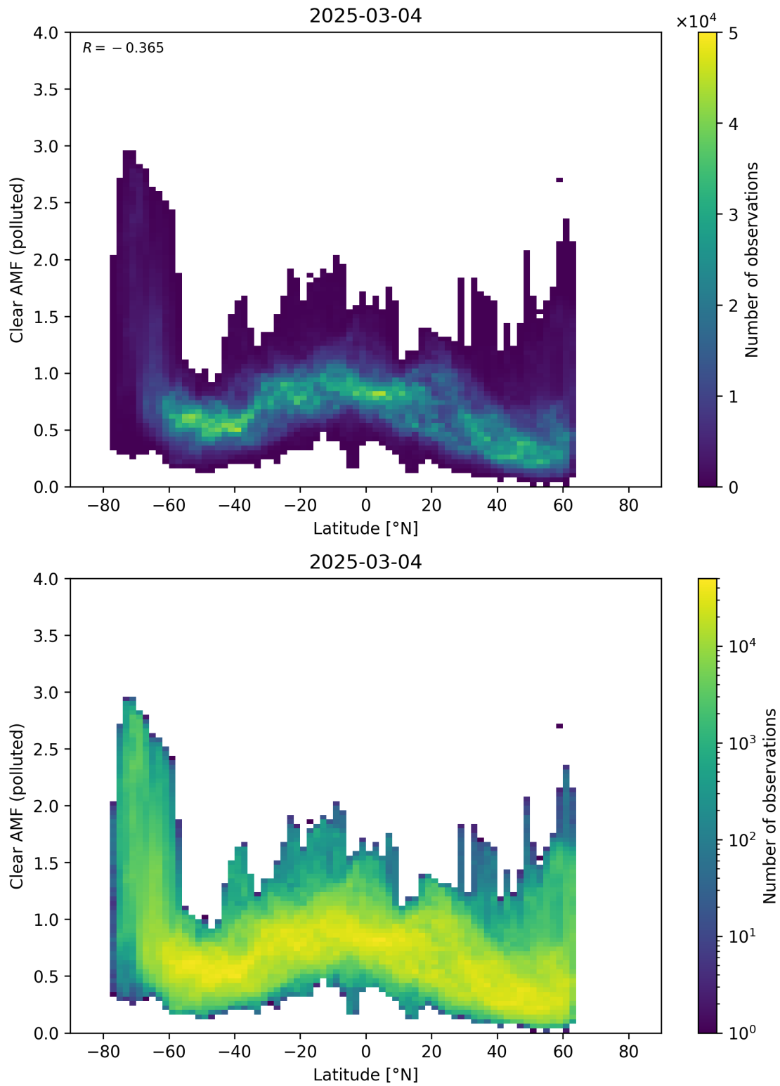
Figure 156: Scatter density plot of “Latitude” against “Clear AMF (polluted)” for 2025-03-03 to 2025-03-05.
