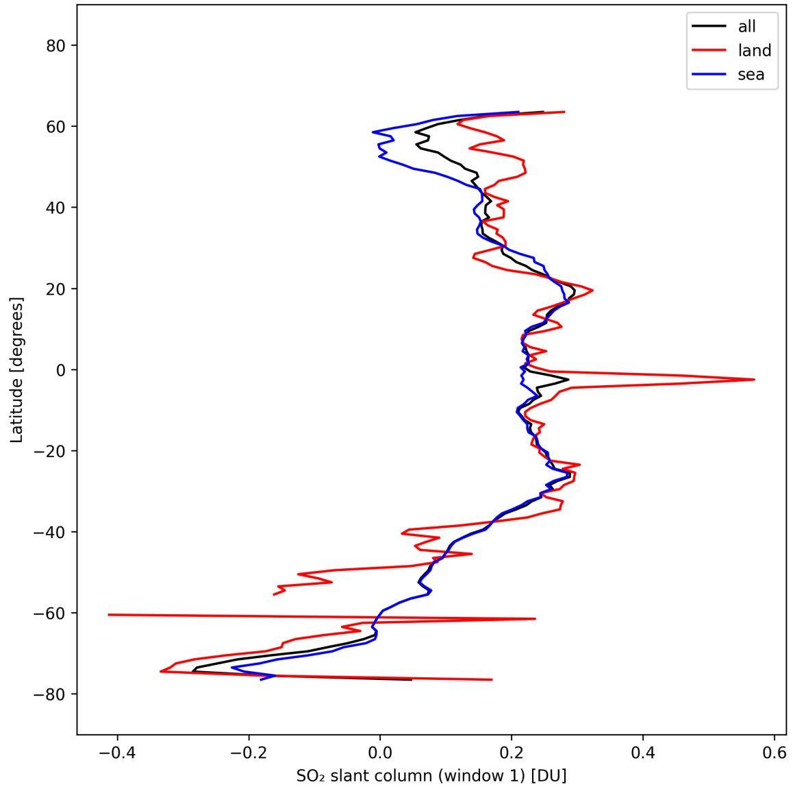
Figure 37: Zonal average of “SO 2 slant column (window 1)” for 2025-03-03 to 2025-03-05.
