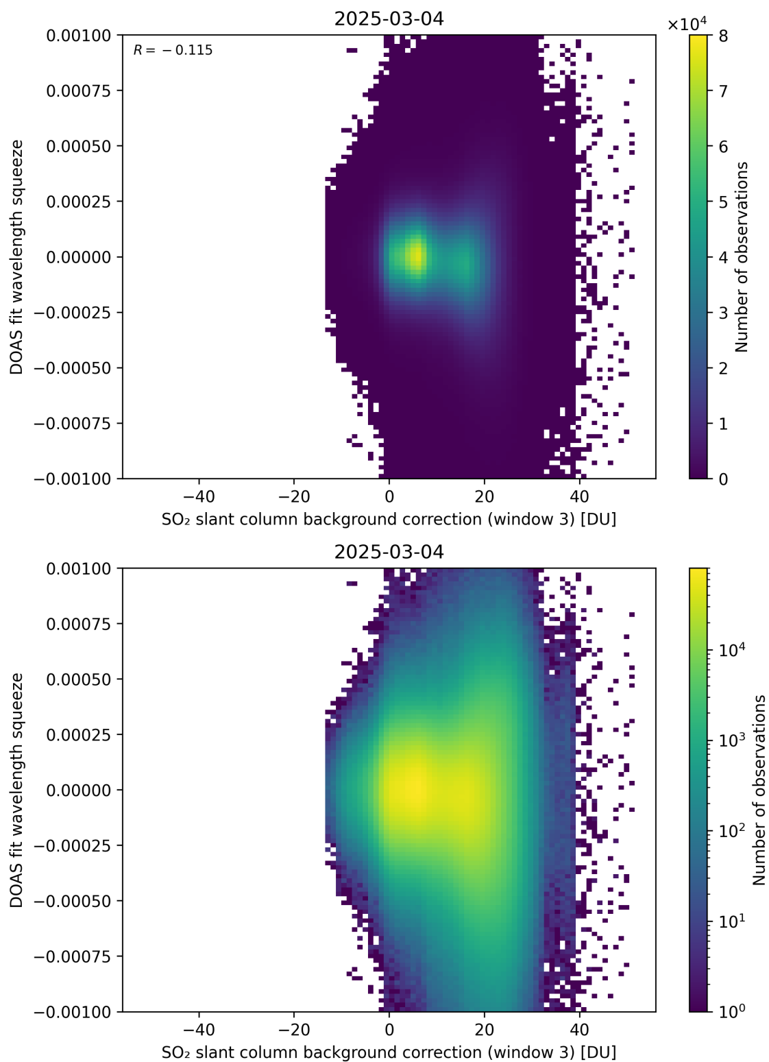
Figure 133: Scatter density plot of “SO 2 slant column background correction (window 3)” against “DOAS fit wavelength squeeze” for 2025-03-03 to 2025-03-05.
