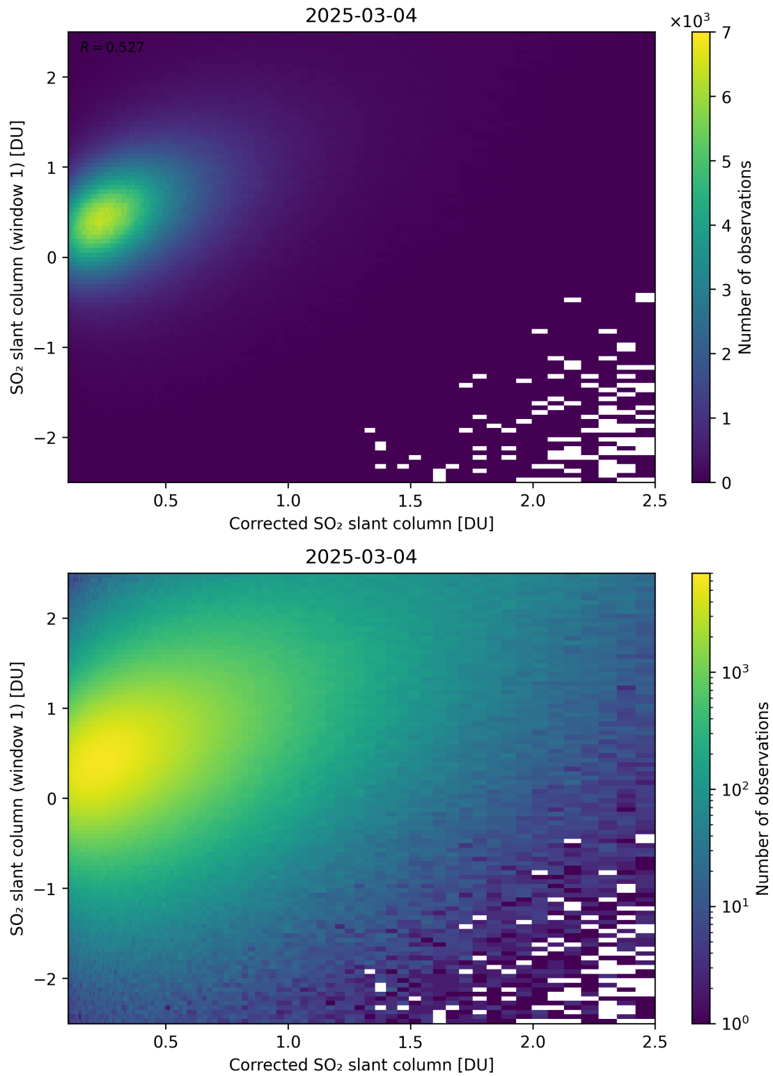
Figure 237: Scatter density plot of “Corrected SO 2 slant column” against “SO 2 slant column (window 1)” for 2025-03-03 to 2025-03-05.
