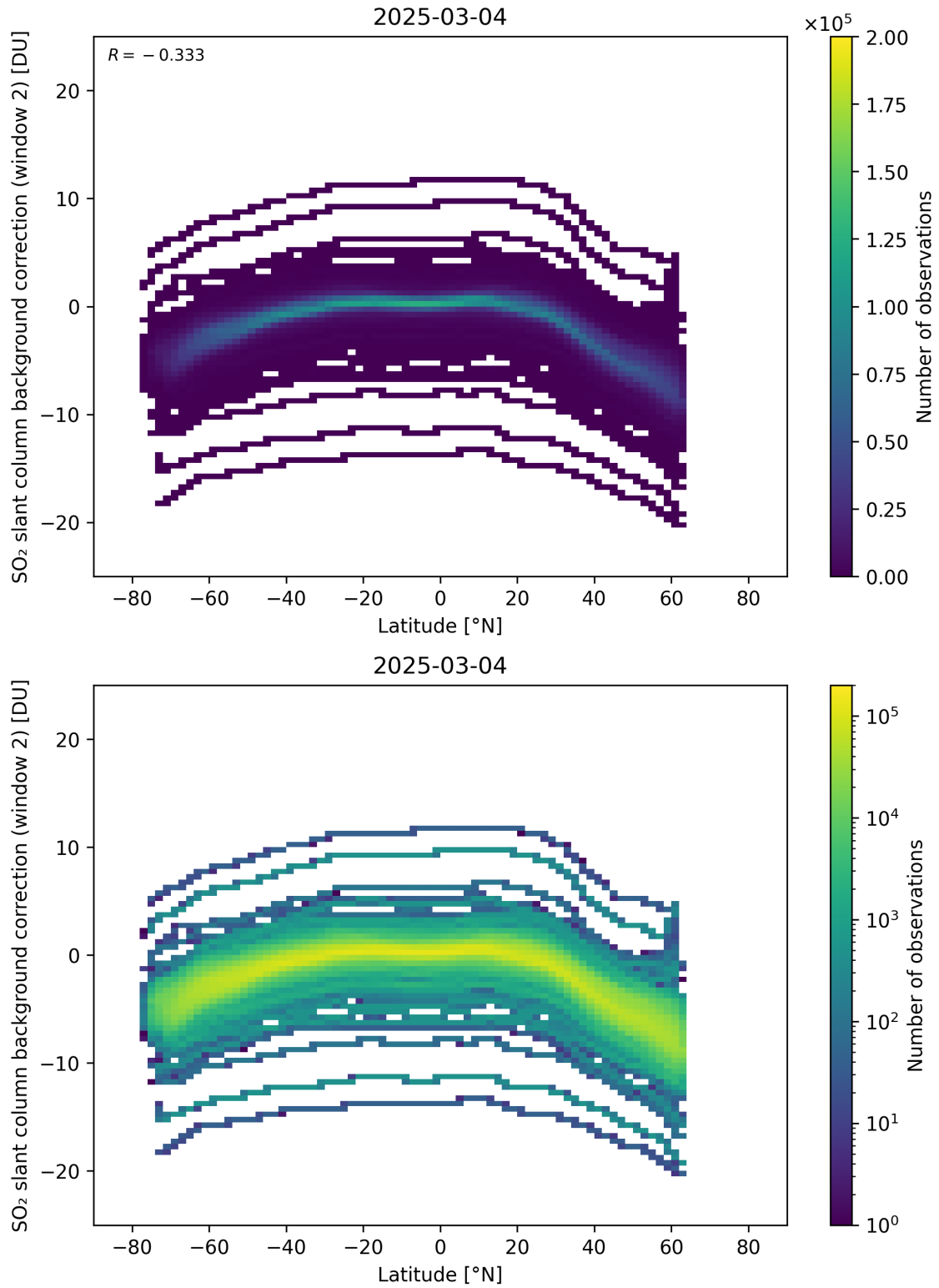
Figure 151: Scatter density plot of “Latitude” against “SO 2 slant column background correction (window 2)” for 2025-03-03 to 2025-03-05.
