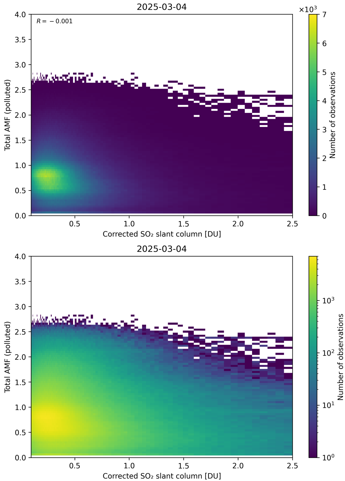
Figure 242: Scatter density plot of “Corrected SO 2 slant column” against “Total AMF (polluted)” for 2025-03-03 to 2025-03-05.
