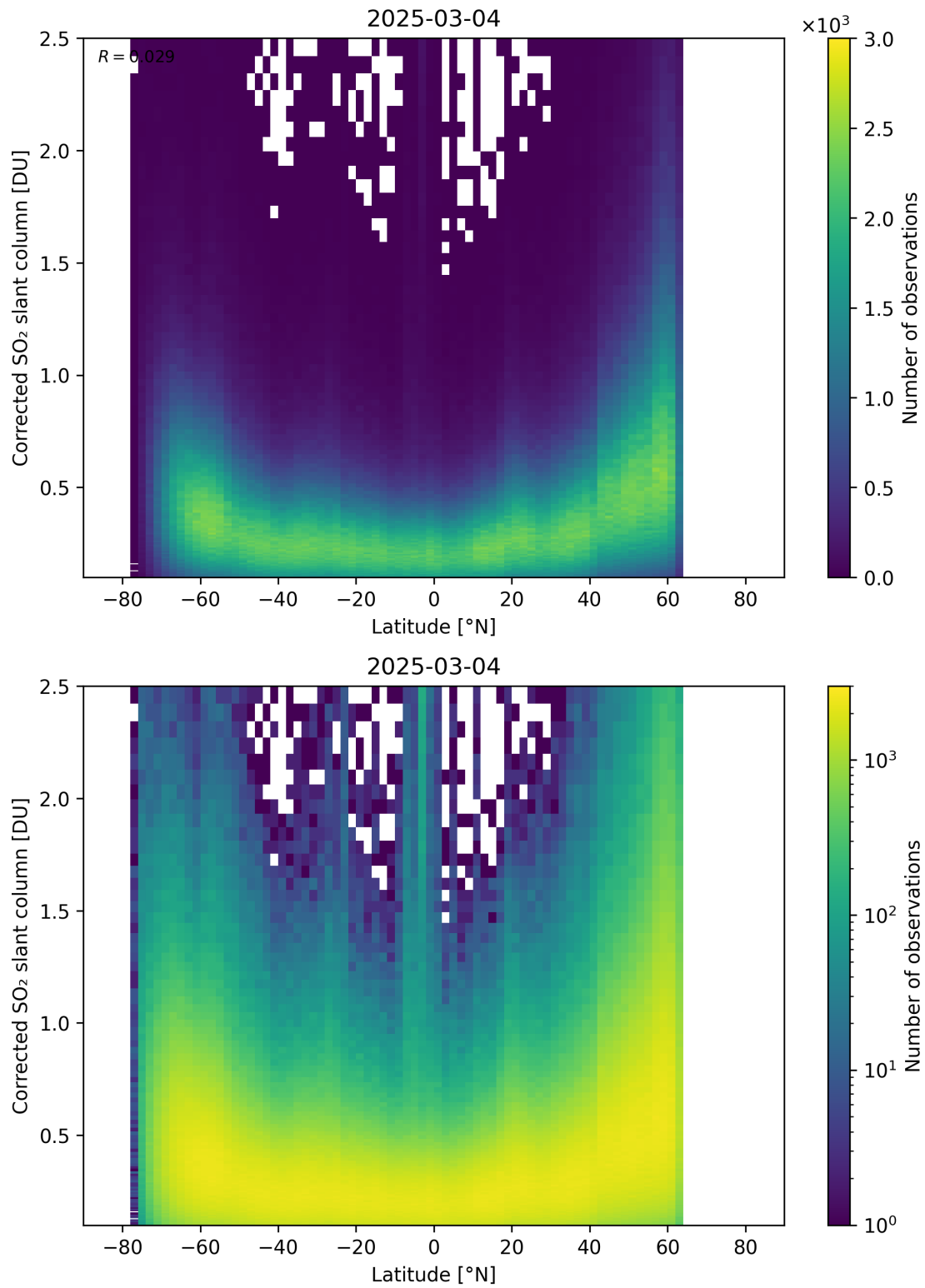
Figure 159: Scatter density plot of “Latitude” against “Corrected SO 2 slant column” for 2025-03-03 to 2025-03-05.
