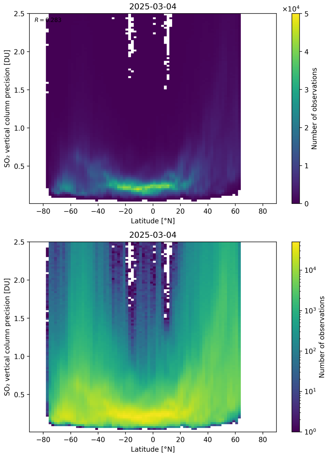
Figure 170: Scatter density plot of “Latitude” against “SO 2 vertical column precision” for 2025-03-03 to 2025-03-05.
