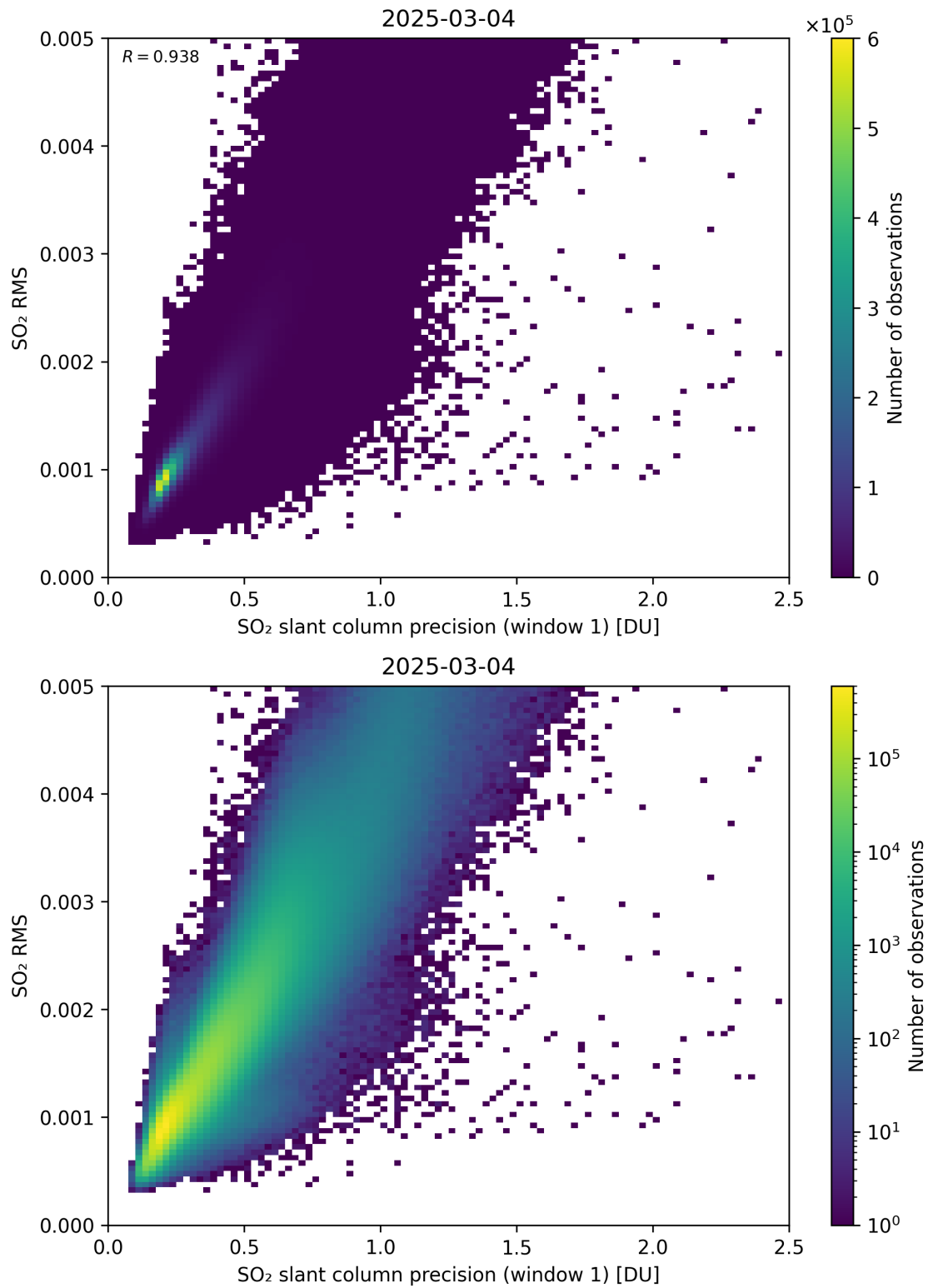
Figure 273: Scatter density plot of “SO 2 slant column precision (window 1)” against “SO 2 RMS” for 2025-03-03 to 2025-03-05.
