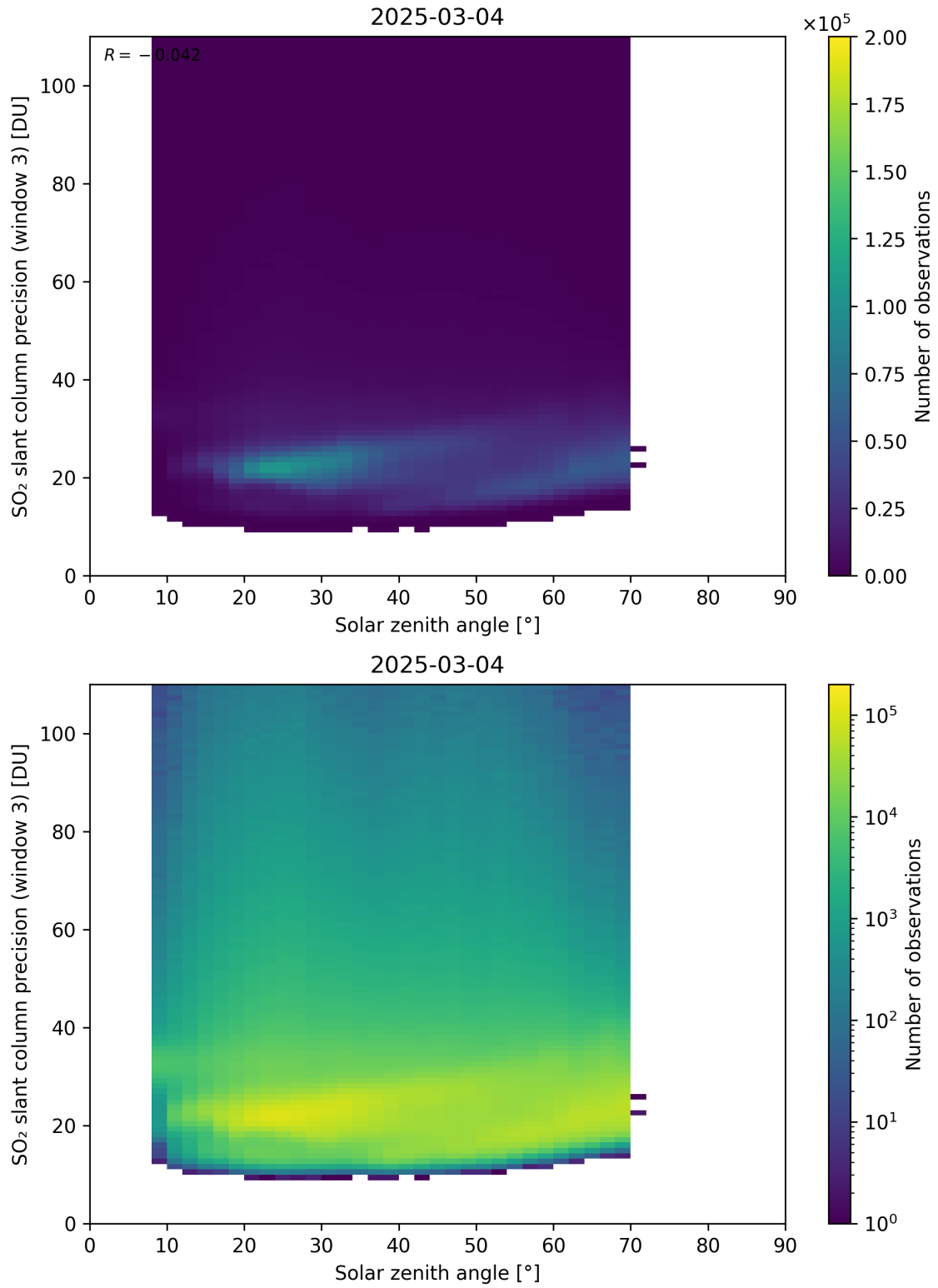
Figure 188: Scatter density plot of “Solar zenith angle” against “SO 2 slant column precision (window 3)” for 2025-03-03 to 2025-03-05.
