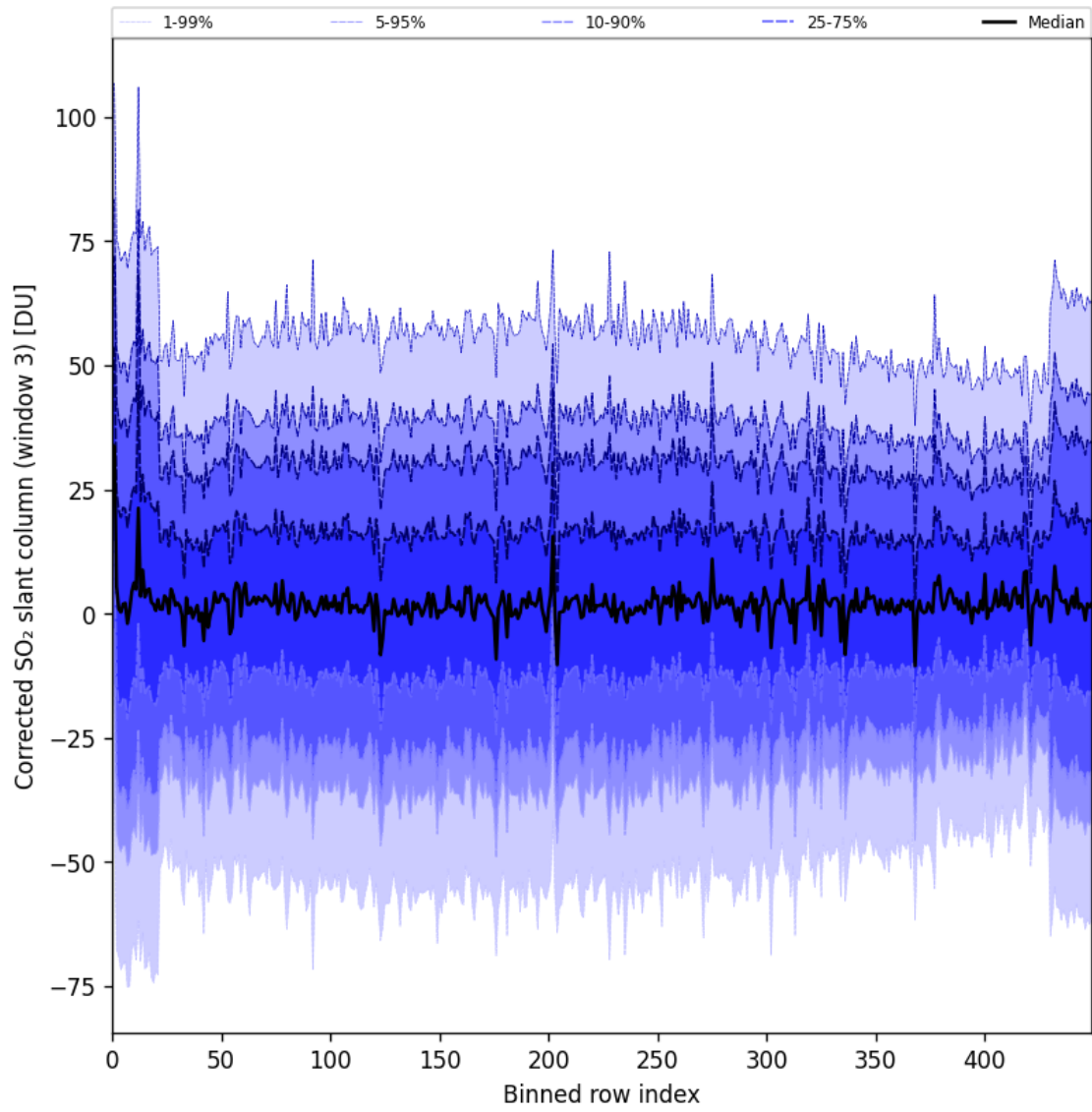
Figure 99: Along track statistics of "Corrected SO 2 slant column (window 3)" for 2025-03-03 to 2025-03-05
