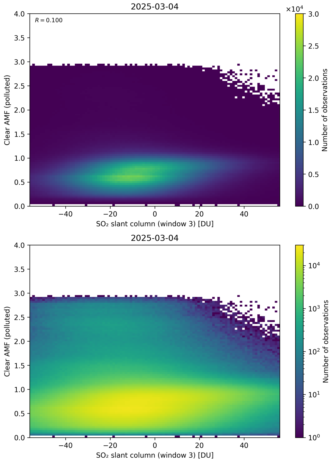
Figure 315: Scatter density plot of “SO 2 slant column (window 3)” against “Clear AMF (polluted)” for 2025-03-03 to 2025-03-05.
