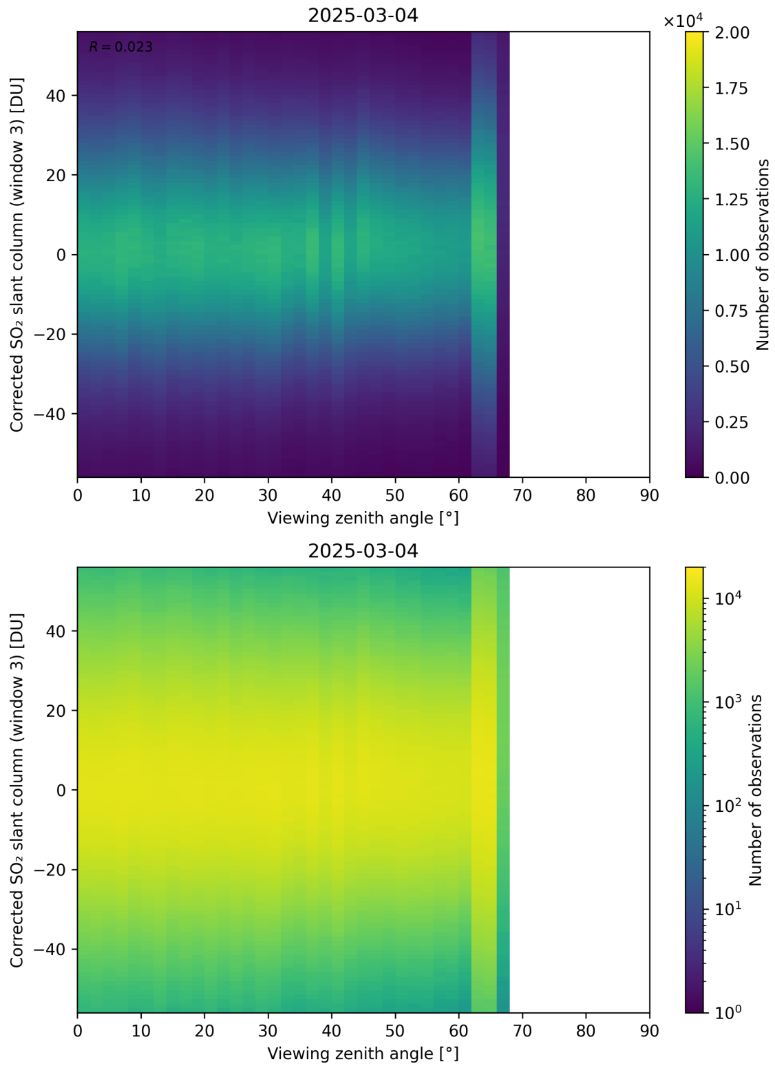
Figure 375: Scatter density plot of “Viewing zenith angle” against “Corrected SO 2 slant column (window 3)” for 2025-03-03 to 2025-03-05.
