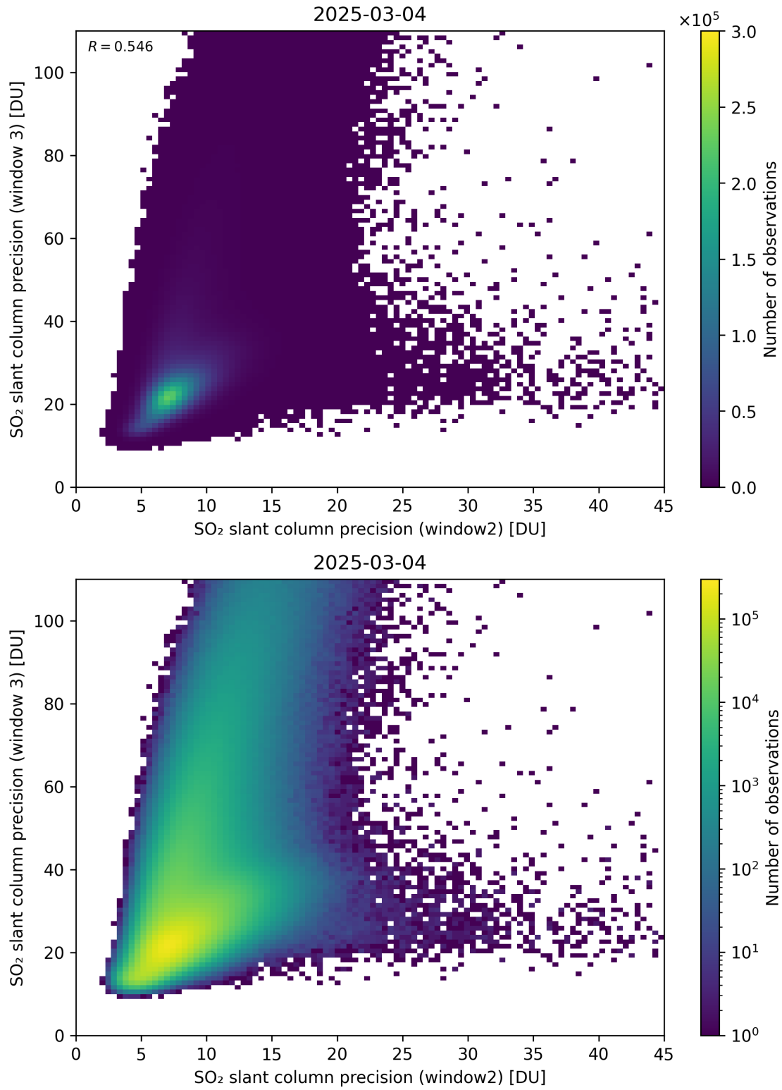
Figure 300: Scatter density plot of “SO 2 slant column precision (window2)” against “SO 2 slant column precision (window 3)” for 2025-03-03 to 2025-03-05.
