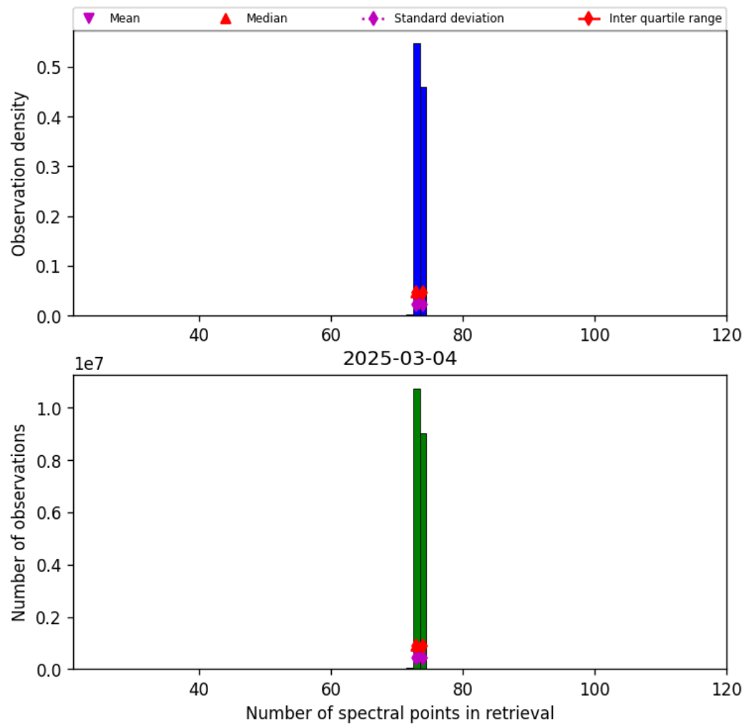
Figure 82: Histogram of “Number of spectral points in retrieval” for 2025-03-03 to 2025-03-05
