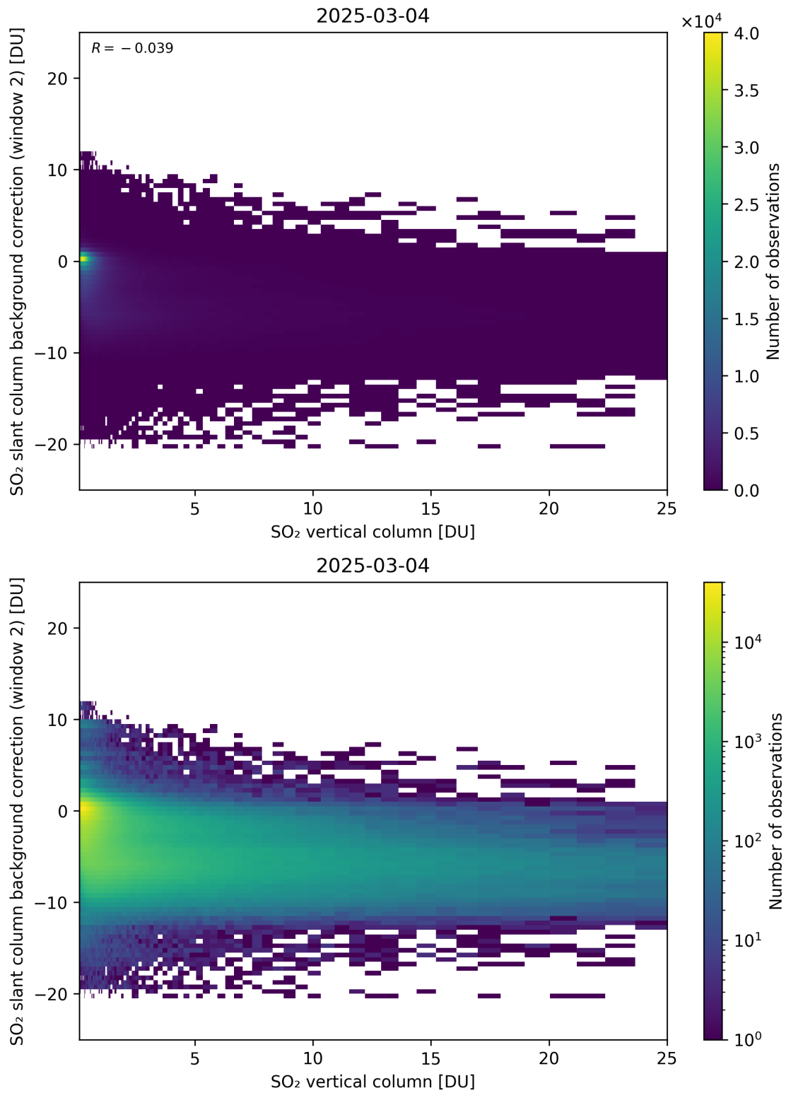
Figure 324: Scatter density plot of “SO 2 vertical column” against “SO 2 slant column background correction (window 2)” for 2025-03-03 to 2025-03-05.
