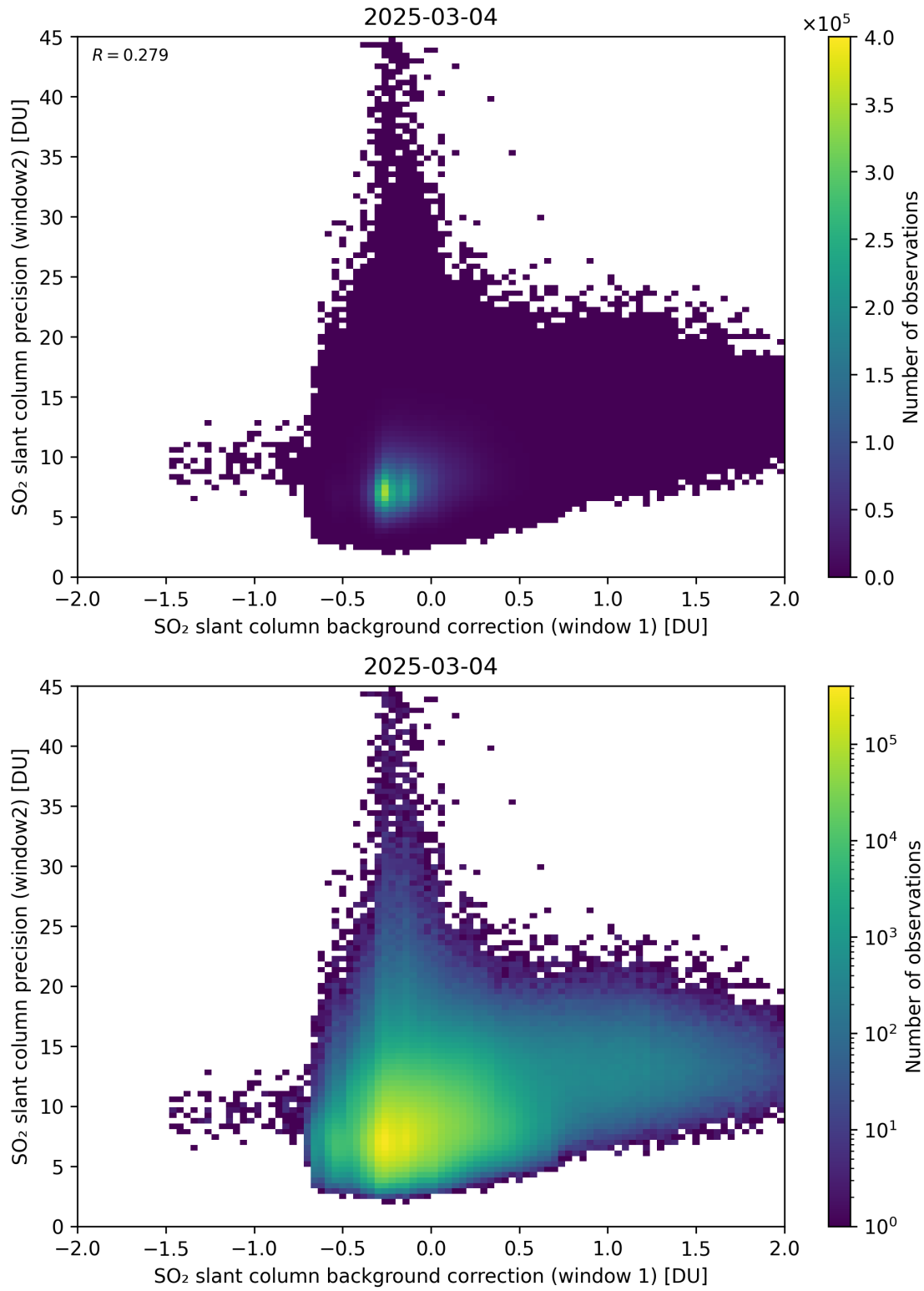
Figure 117: Scatter density plot of “SO 2 slant column background correction (window 1)” against “SO 2 slant column precision (window2)” for 2025-03-03 to 2025-03-05.
