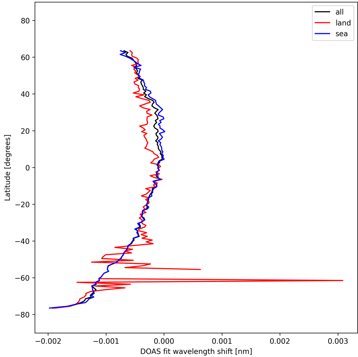
Figure 50: Zonal average of "DOAS fit wavelength shift" for 2025-03-03 to 2025-03-05.
