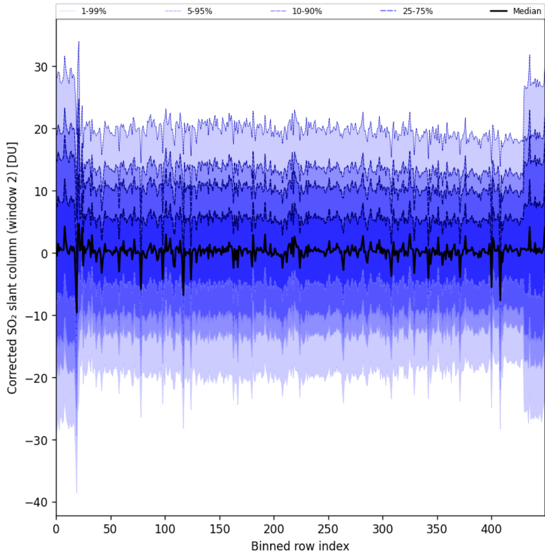
Figure 95: Along track statistics of “Corrected SO 2 slant column (window 2)” for 2025-03-03 to 2025-03-05
