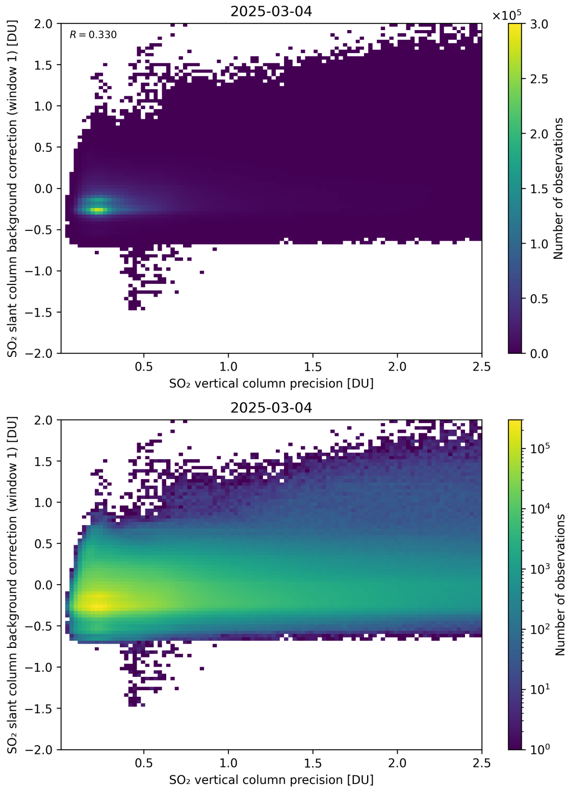
Figure 329: Scatter density plot of “SO 2 vertical column precision” against “SO 2 slant column background correction (window 1)” for 2025-03-03 to 2025-03-05.
