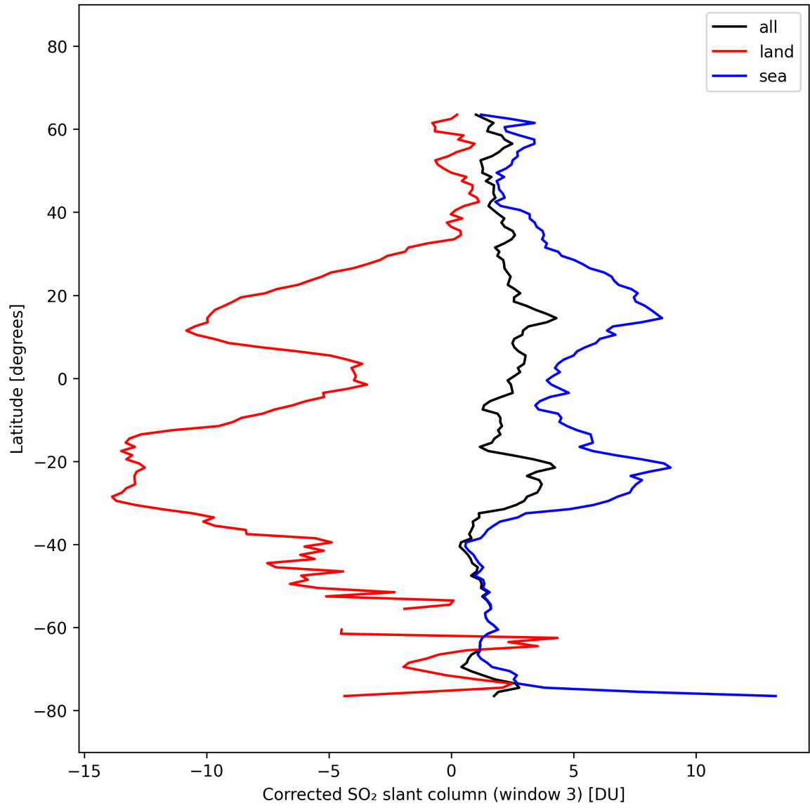
Figure 47: Zonal average of “Corrected SO 2 slant column (window 3)” for 2025-03-03 to 2025-03-05.
