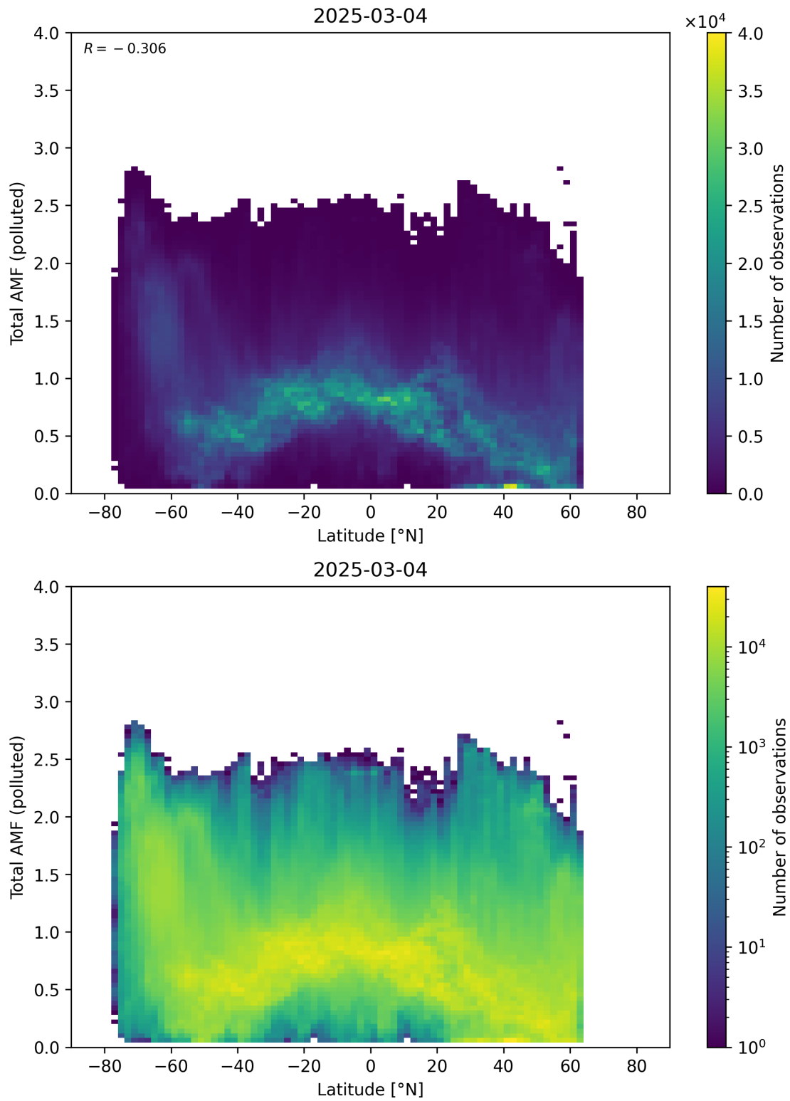
Figure 167: Scatter density plot of “Latitude” against “Total AMF (polluted)” for 2025-03-03 to 2025-03-05.
