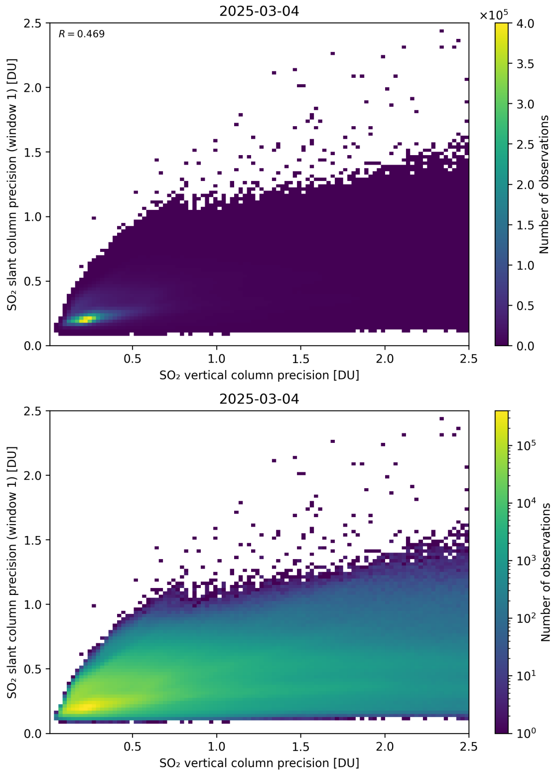
Figure 342: Scatter density plot of “SO 2 vertical column precision” against “SO 2 slant column precision (window 1)” for 2025-03-03 to 2025-03-05.
