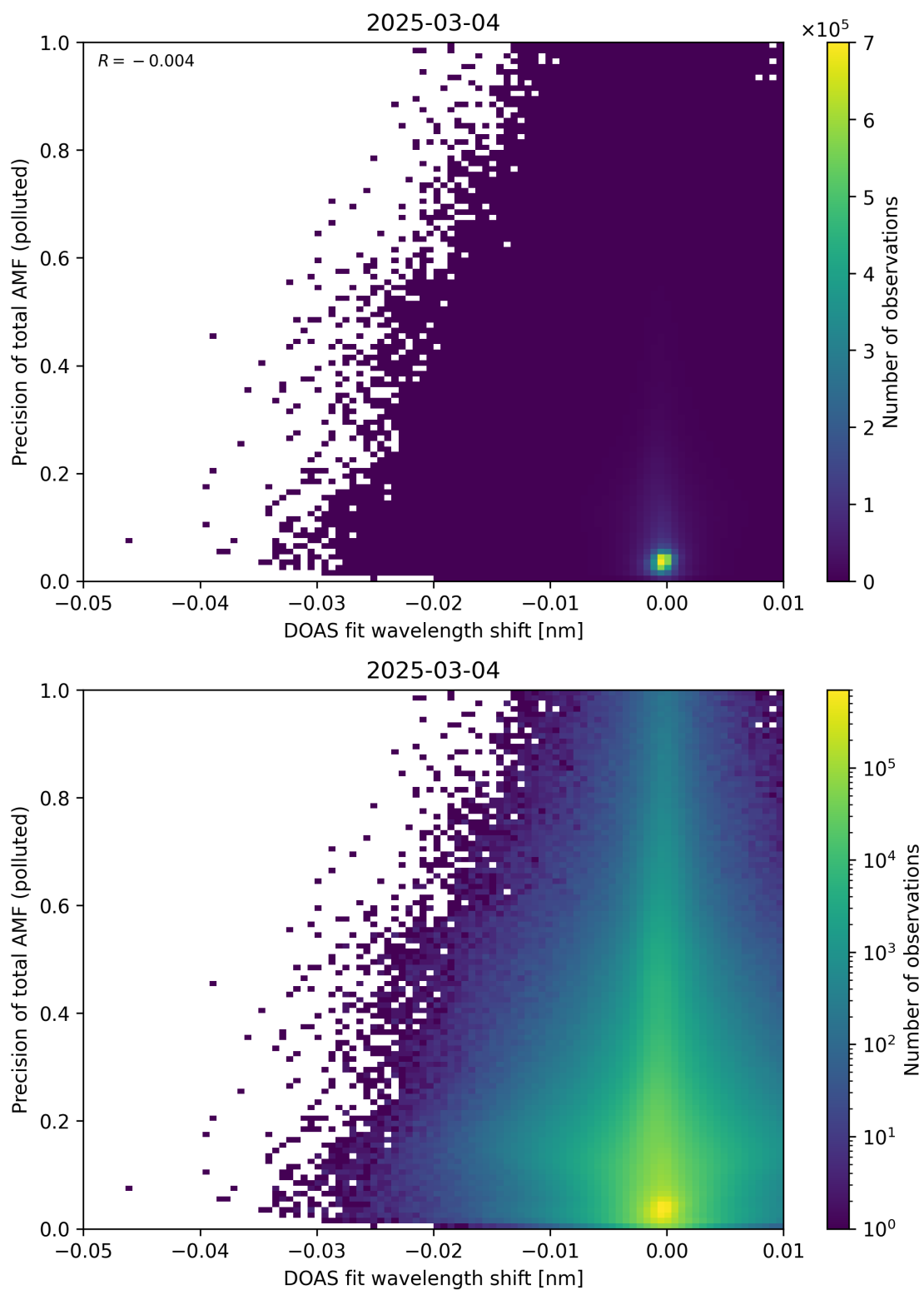
Figure 142: Scatter density plot of “DOAS fit wavelength shift” against “Precision of total AMF (polluted)” for 2025-03-03 to 2025-03-05.
