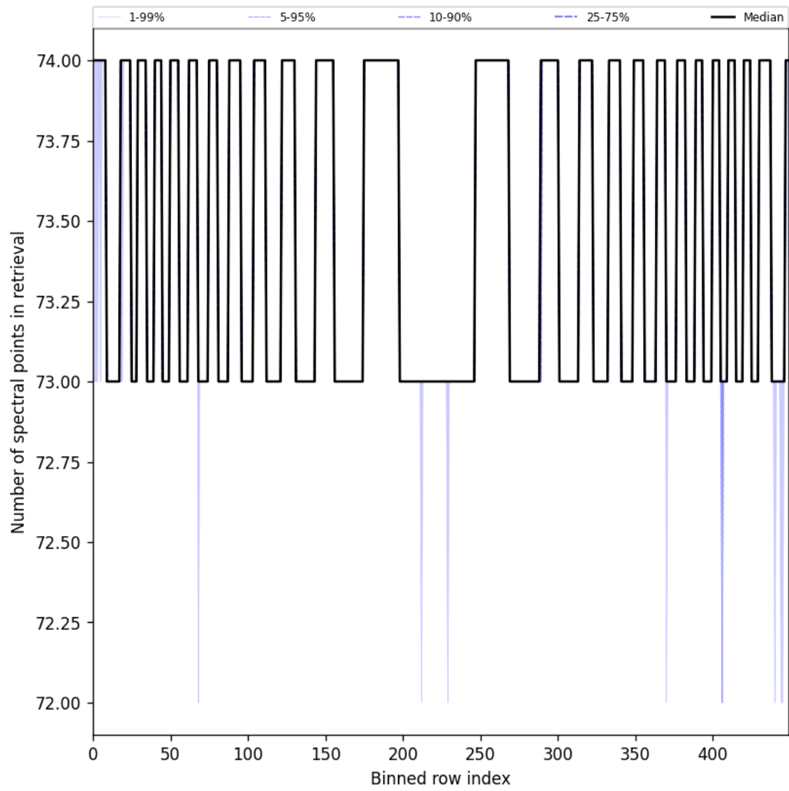
Figure 108: Along track statistics of “Number of spectral points in retrieval” for 2025-03-03 to 2025-03-05
