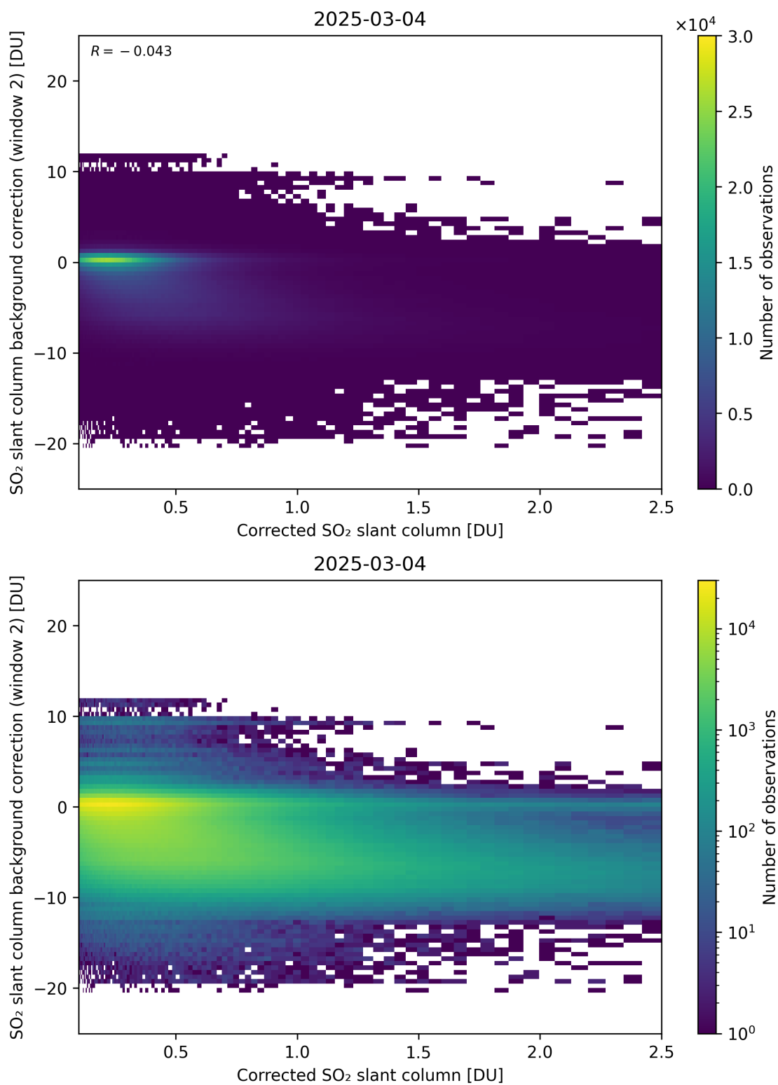
Figure 227: Scatter density plot of “Corrected SO 2 slant column” against “SO 2 slant column background correction (window 2)” for 2025-03-03 to 2025-03-05.
