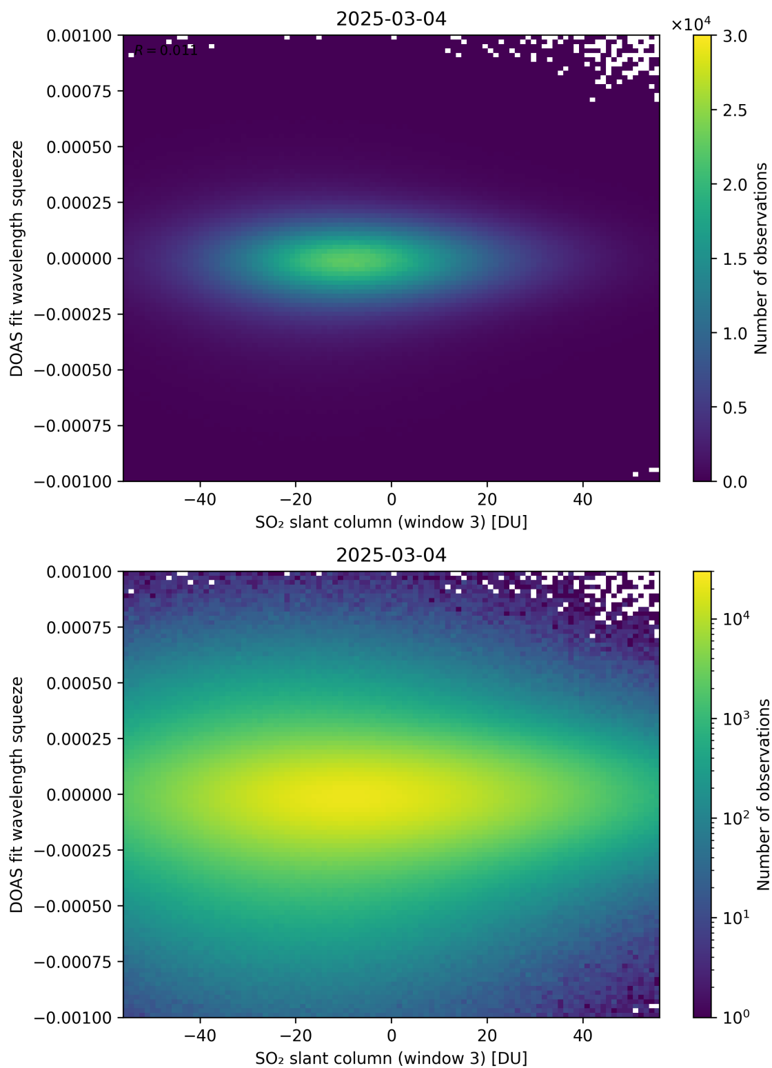
Figure 305: Scatter density plot of “SO 2 slant column (window 3)” against “DOAS fit wavelength squeeze” for 2025-03-03 to 2025-03-05.
