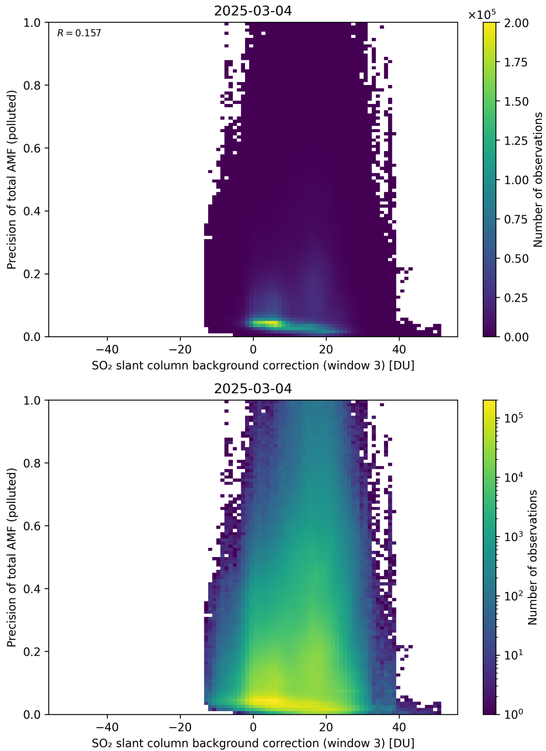
Figure 137: Scatter density plot of “SO 2 slant column background correction (window 3)” against “Precision of total AMF (polluted)” for 2025-03-03 to 2025-03-05.
