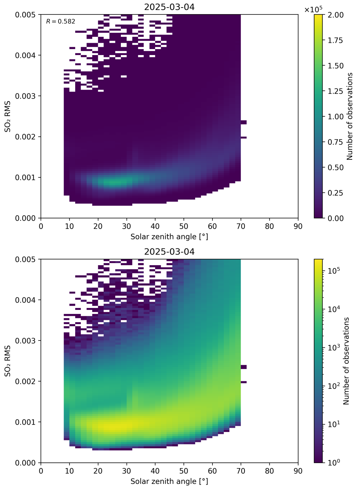
Figure 176: Scatter density plot of “Solar zenith angle” against “SO 2 RMS” for 2025-03-03 to 2025-03-05.
