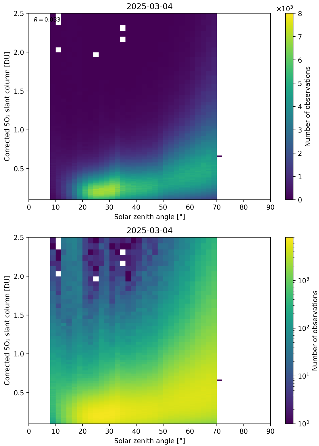
Figure 181: Scatter density plot of “Solar zenith angle” against “Corrected SO 2 slant column” for 2025-03-03 to 2025-03-05.
