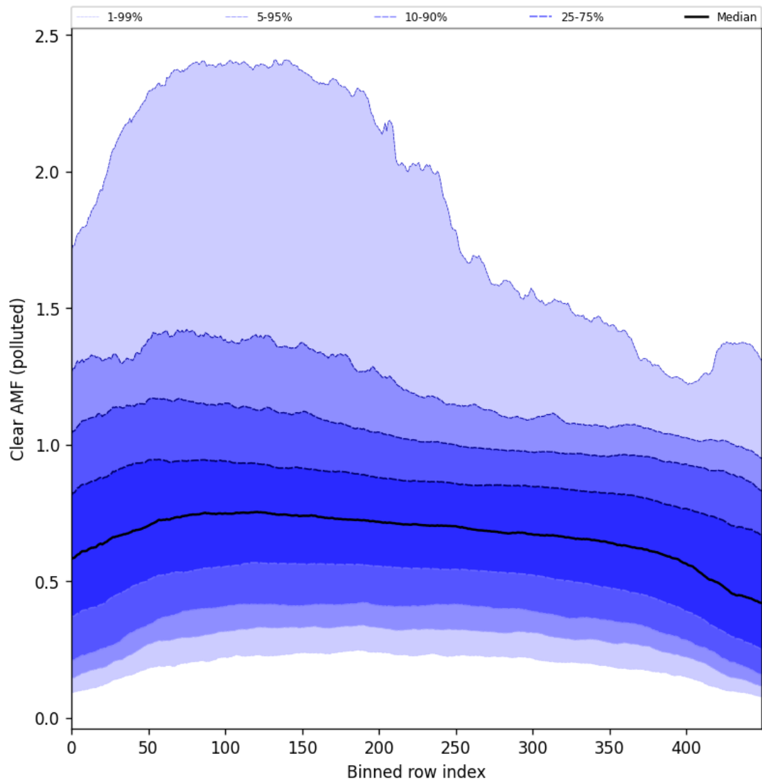
Figure 107: Along track statistics of “Clear AMF (polluted)” for 2025-03-03 to 2025-03-05
