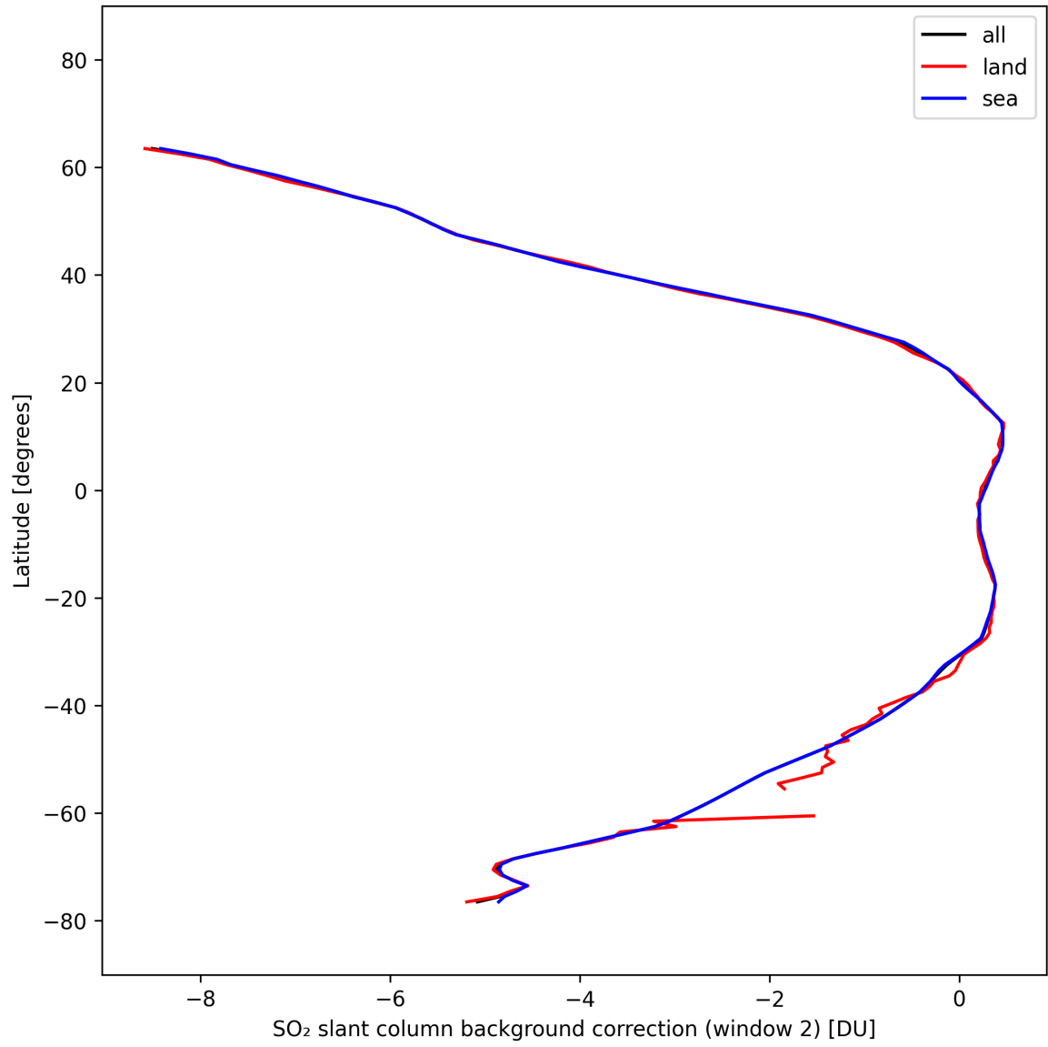
Figure 44: Zonal average of “SO 2 slant column background correction (window 2)” for 2025-03-03 to 2025-03-05.
