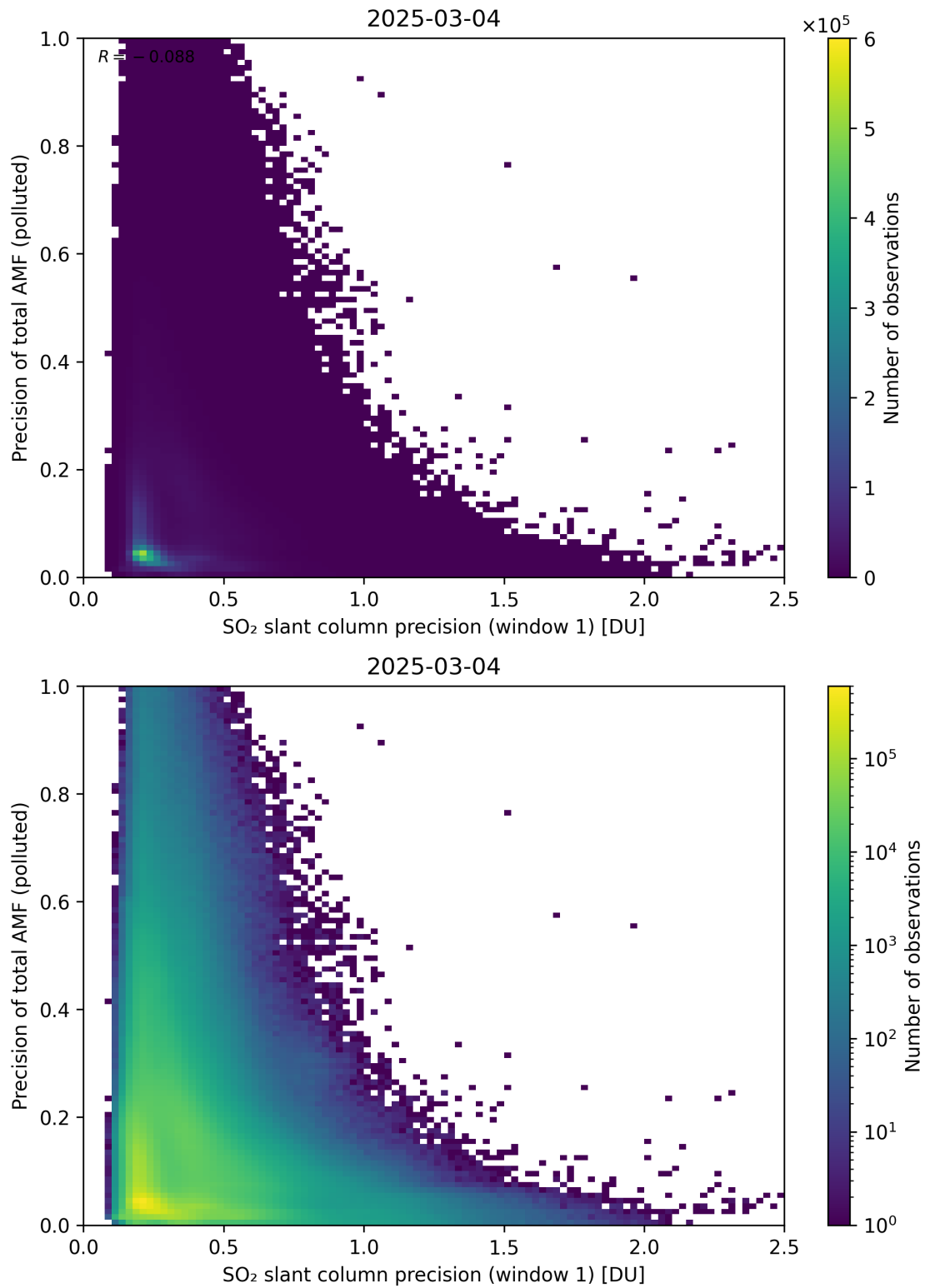
Figure 281: Scatter density plot of “SO 2 slant column precision (window 1)” against “Precision of total AMF (polluted)” for 2025-03-03 to 2025-03-05.
