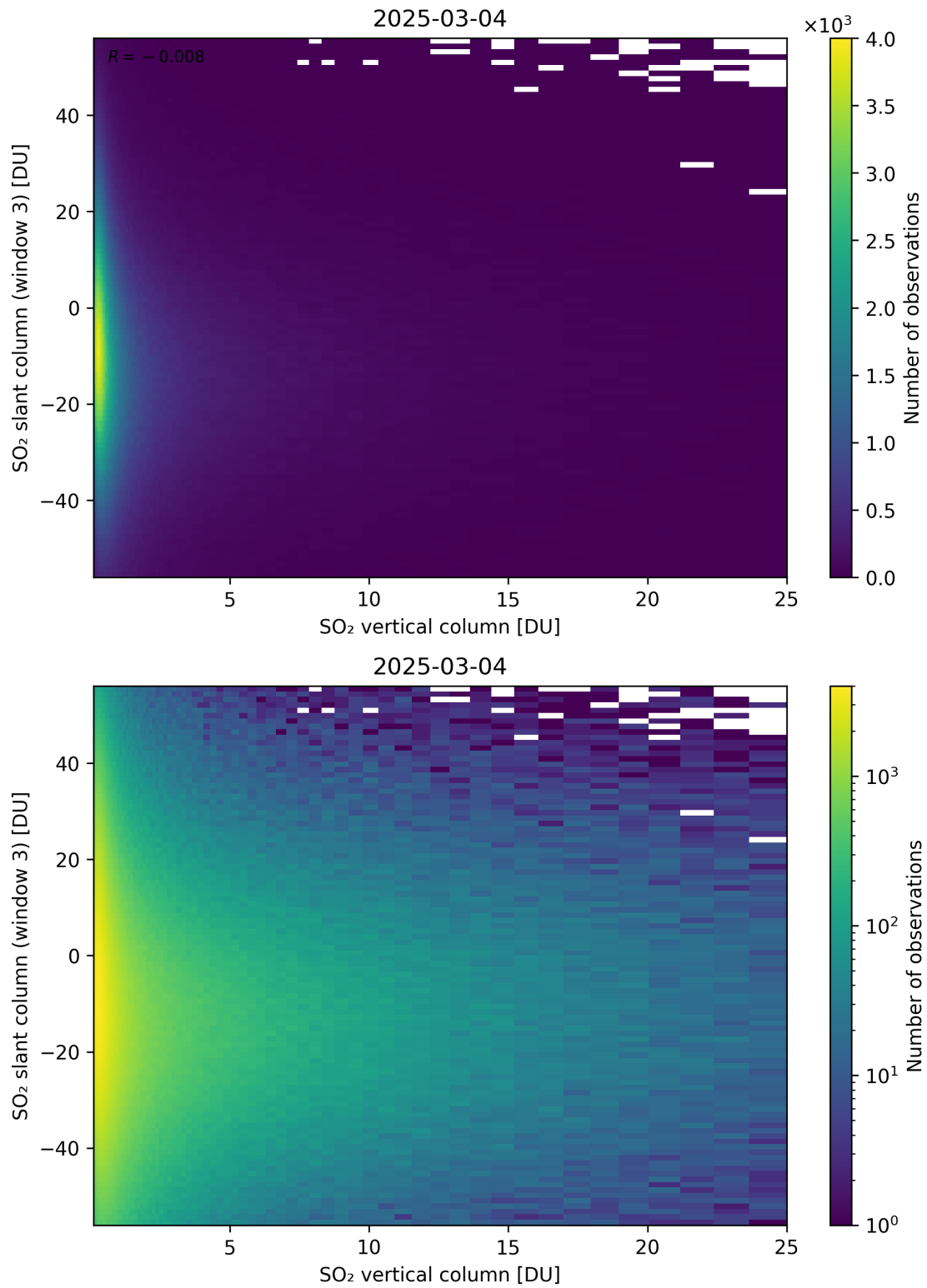
Figure 357: Scatter density plot of “SO 2 vertical column” against “SO 2 slant column (window 3)” for 2025-03-03 to 2025-03-05.
