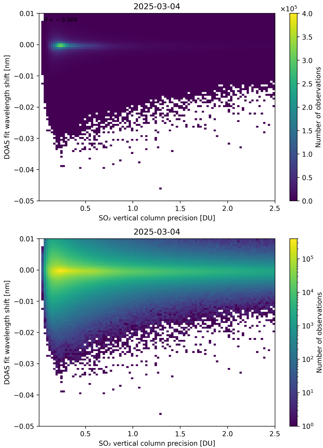
Figure 332: Scatter density plot of “SO 2 vertical column precision” against “DOAS fit wavelength shift” for 2025-03-03 to 2025-03-05.
