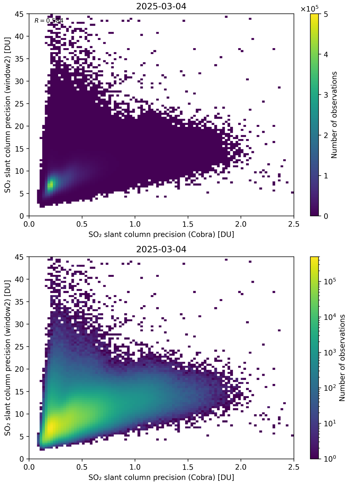
Figure 210: Scatter density plot of “SO 2 slant column precision (Cobra)” against “SO 2 slant column precision (window2)” for 2025-03-03 to 2025-03-05.
