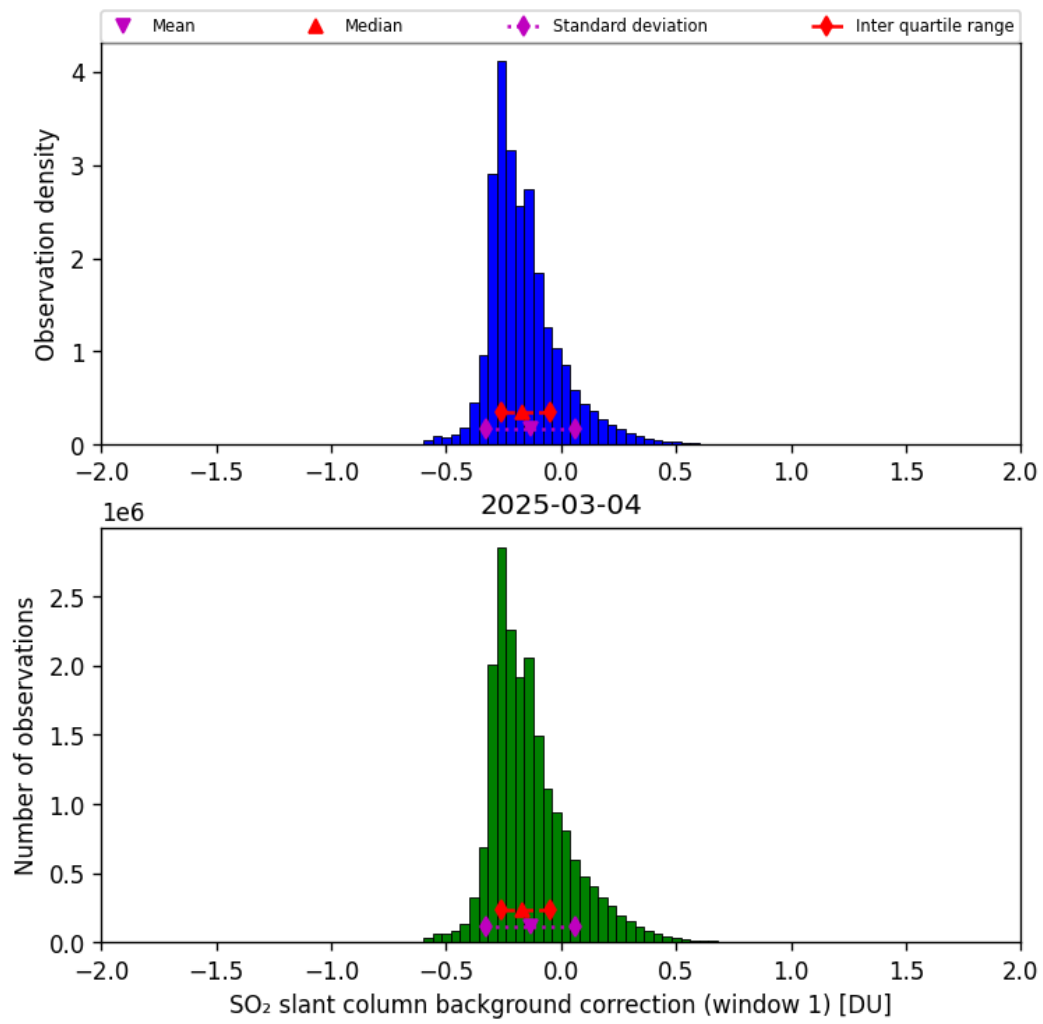
Figure 66: Histogram of “SO 2 slant column background correction (window 1)” for 2025-03-03 to 2025-03-05
