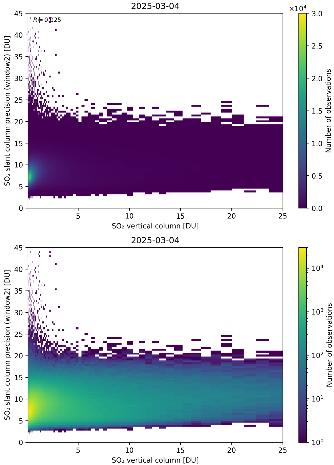
Figure 356: Scatter density plot of “SO 2 vertical column” against “SO 2 slant column precision (window2)” for 2025-03-03 to 2025-03-05.
