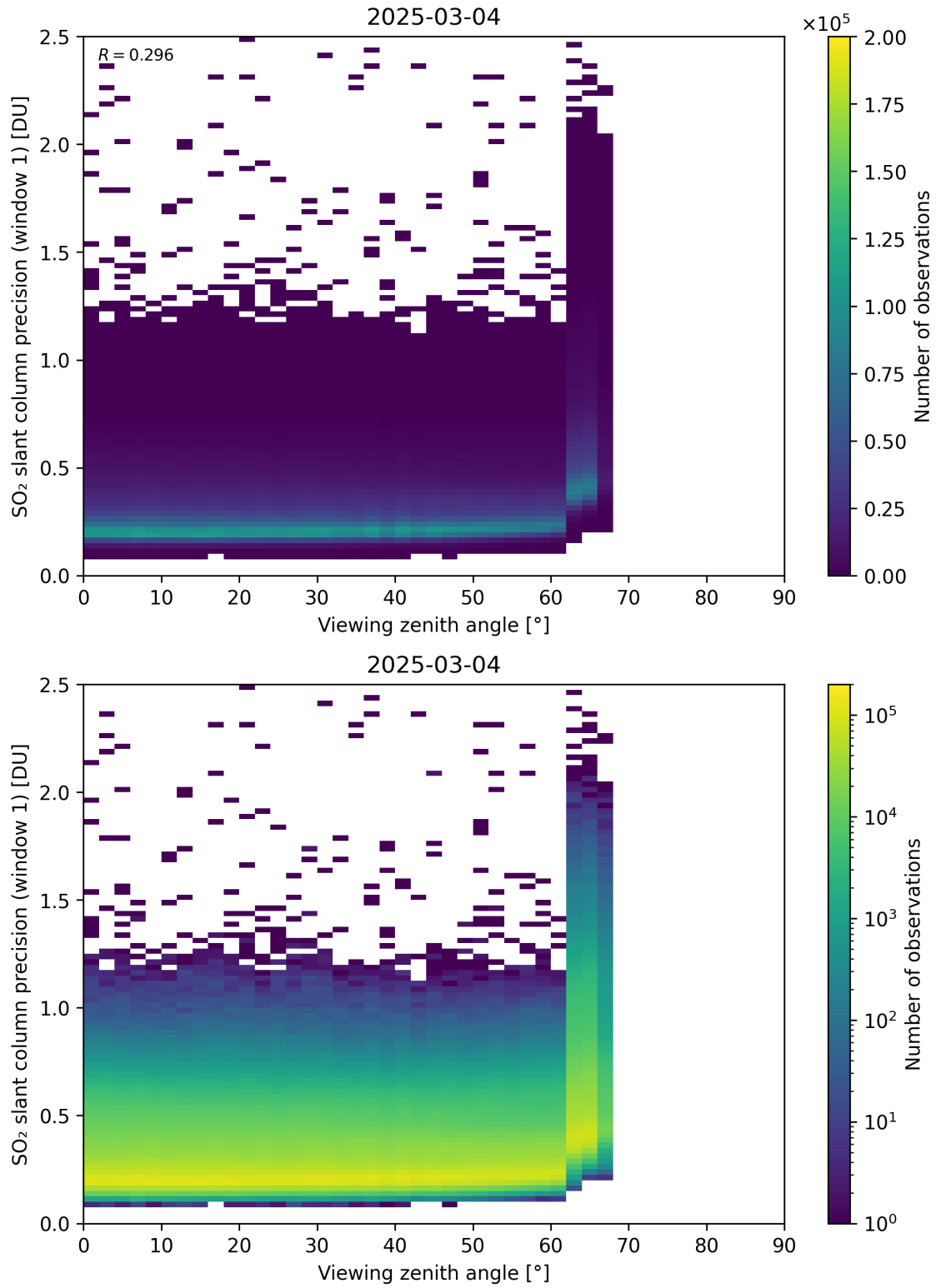
Figure 377: Scatter density plot of “Viewing zenith angle” against “SO 2 slant column precision (window 1)” for 2025-03-03 to 2025-03-05.
