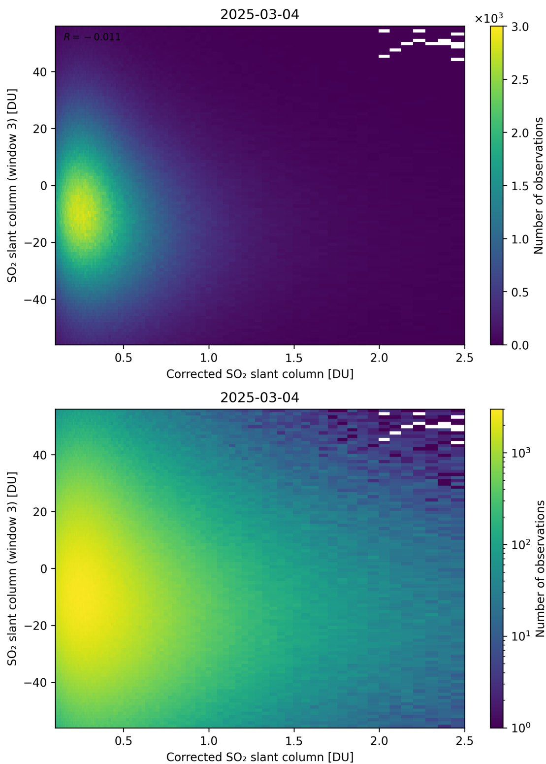
Figure 240: Scatter density plot of “Corrected SO 2 slant column” against “SO 2 slant column (window 3)” for 2025-03-03 to 2025-03-05.
