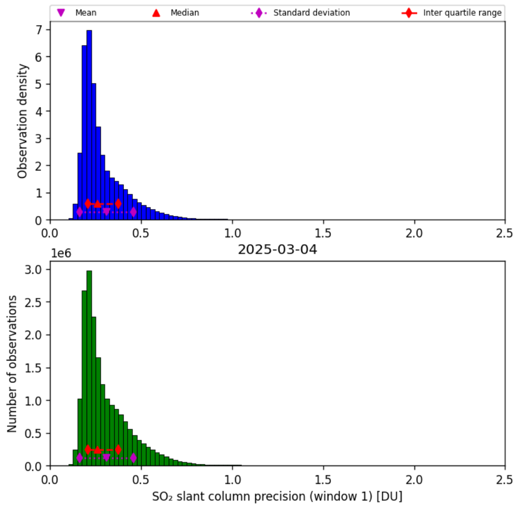
Figure 64: Histogram of “SO 2 slant column precision (window 1)” for 2025-03-03 to 2025-03-05
