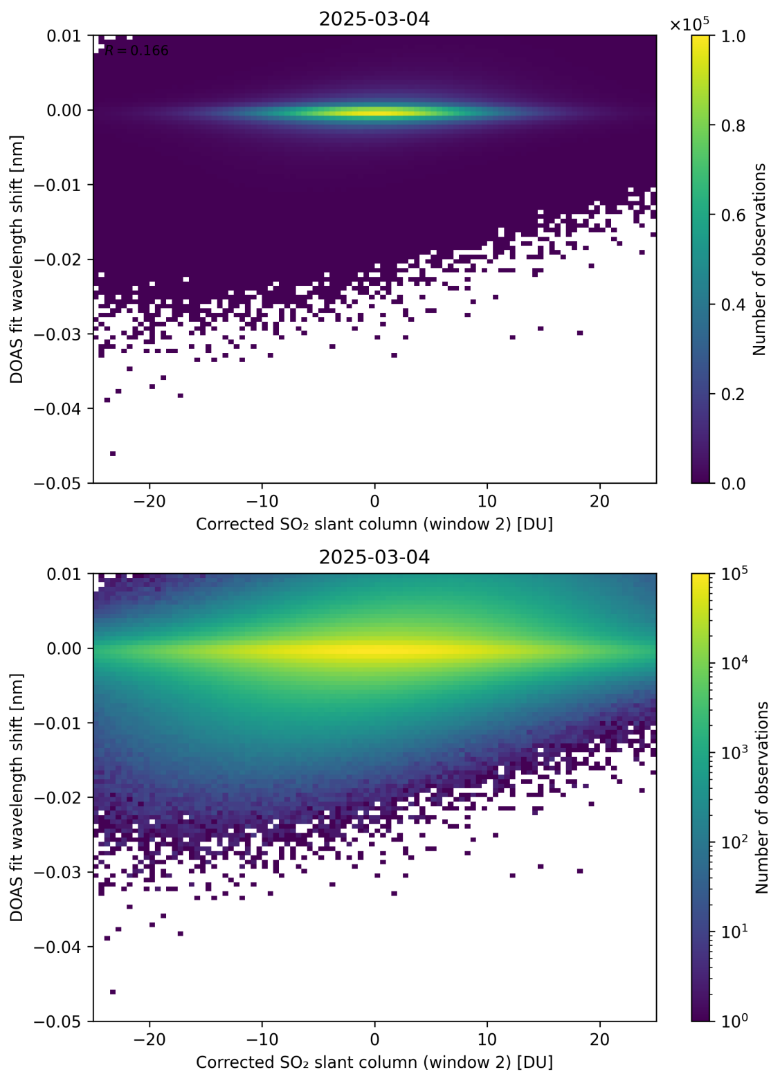
Figure 246: Scatter density plot of “Corrected SO 2 slant column (window 2)” against “DOAS fit wavelength shift” for 2025-03-03 to 2025-03-05.
