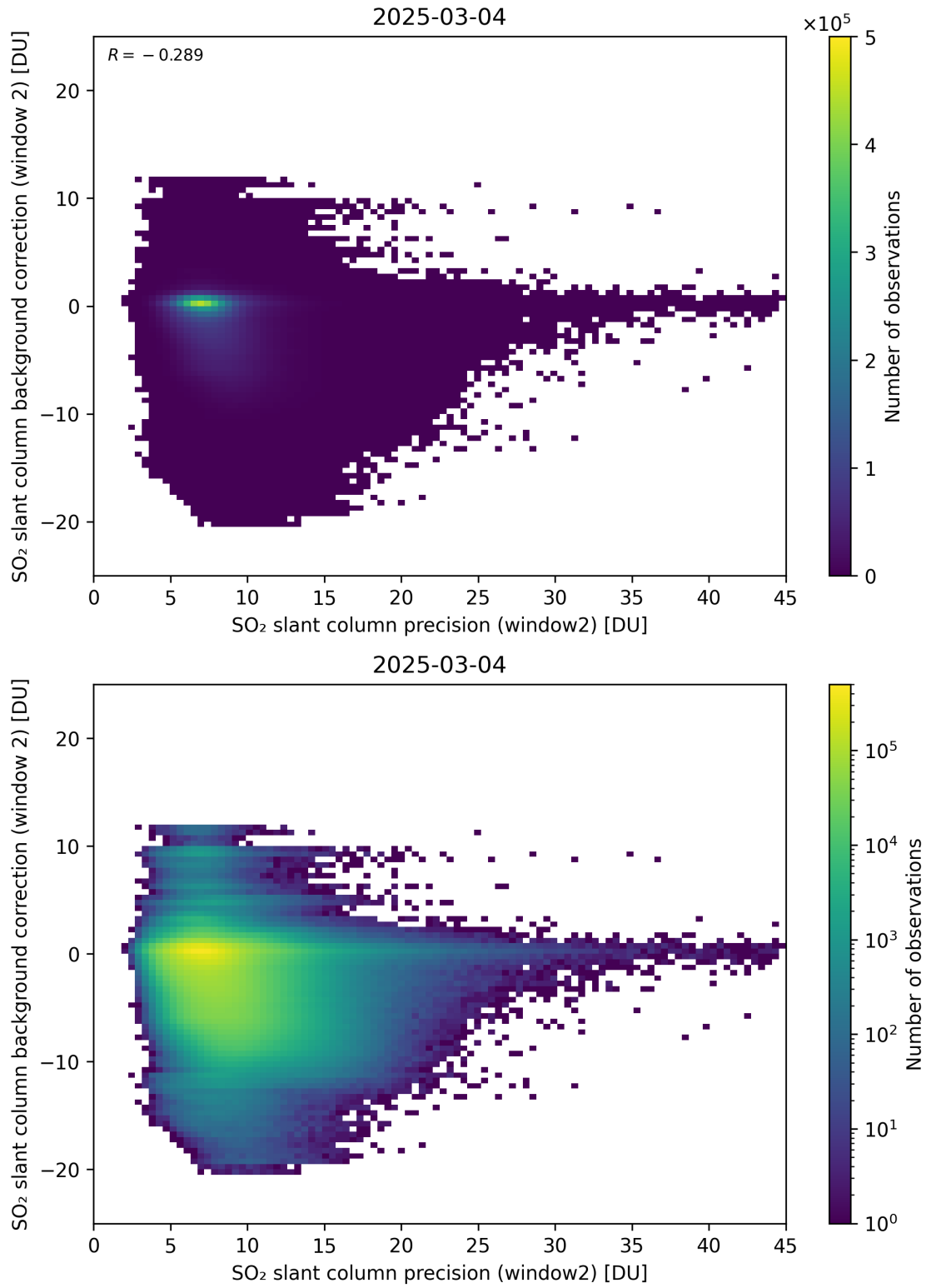
Figure 291: Scatter density plot of “SO 2 slant column precision (window2)” against “SO 2 slant column background correction (window 2)” for 2025-03-03 to 2025-03-05.
