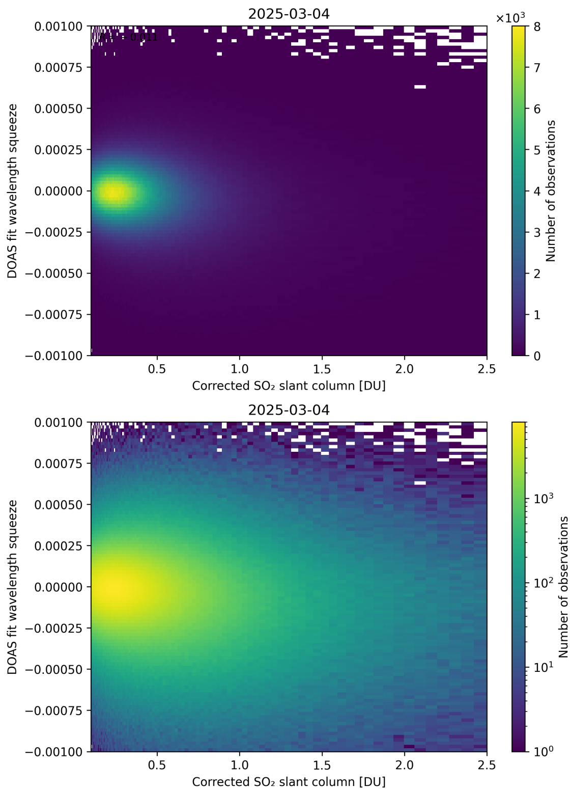
Figure 230: Scatter density plot of “Corrected SO 2 slant column” against “DOAS fit wavelength squeeze” for 2025-03-03 to 2025-03-05.
