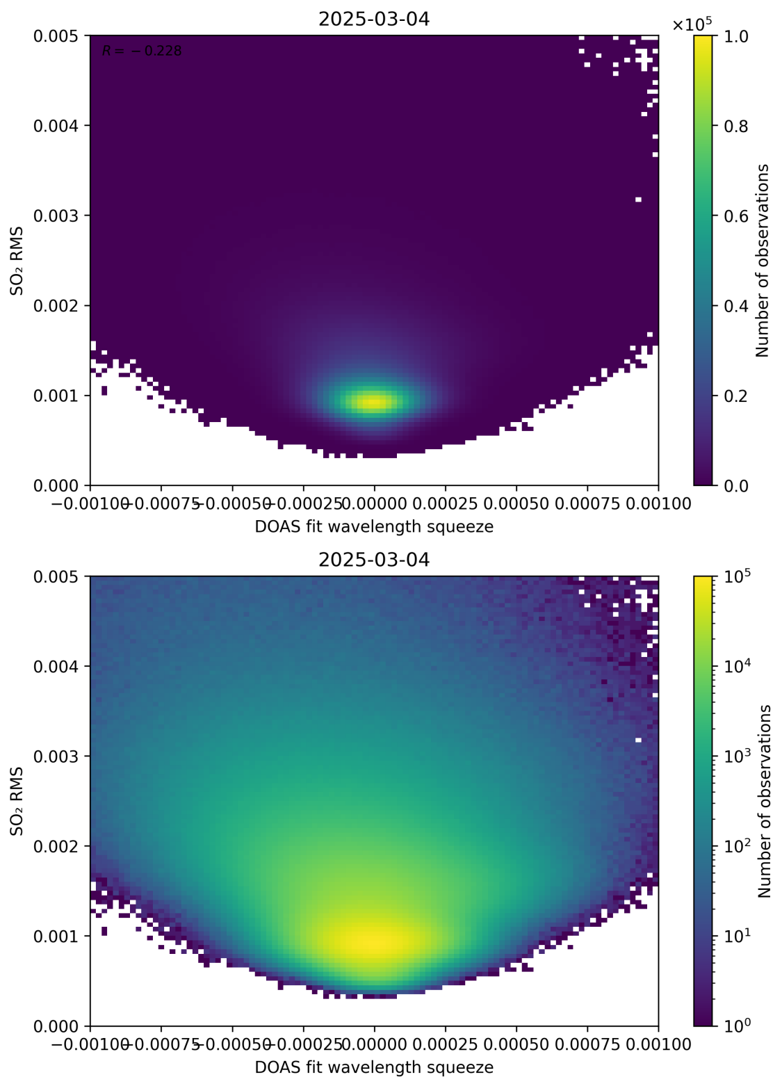
Figure 143: Scatter density plot of “DOAS fit wavelength squeeze” against “SO 2 RMS” for 2025-03-03 to 2025-03-05.
