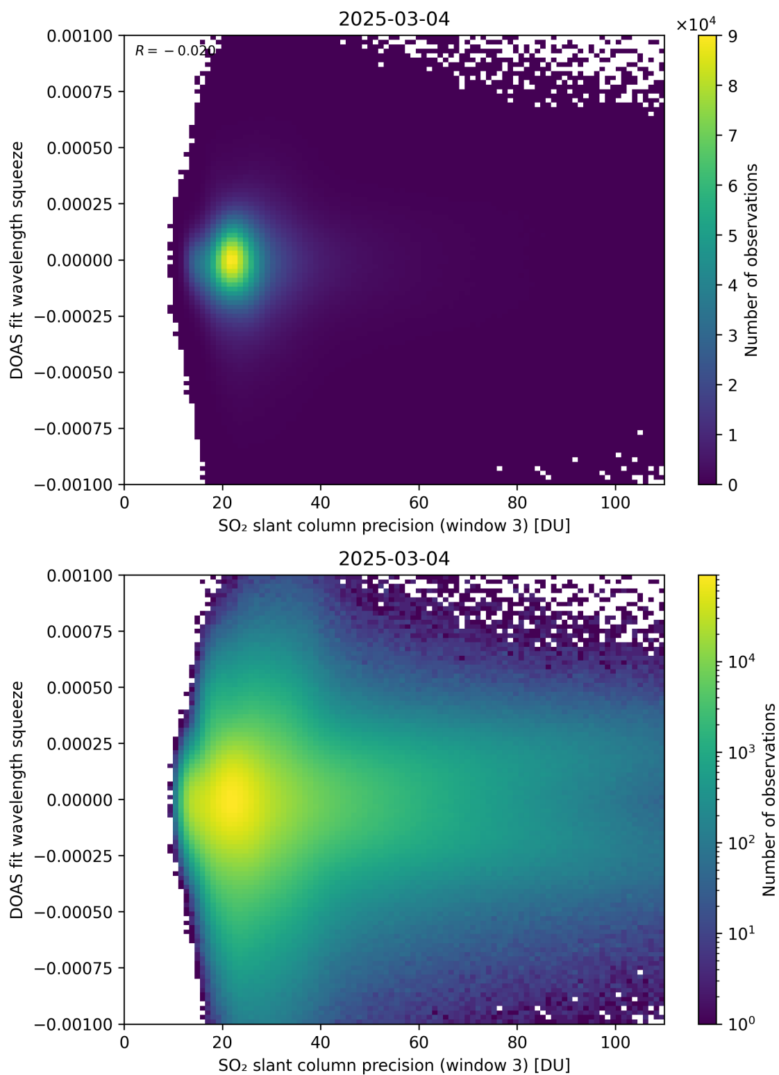
Figure 309: Scatter density plot of “SO 2 slant column precision (window 3)” against “DOAS fit wavelength squeeze” for 2025-03-03 to 2025-03-05.
