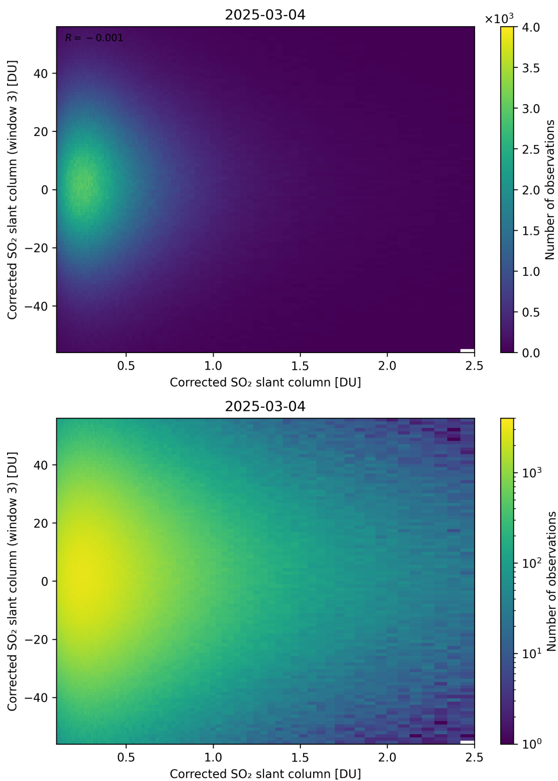
Figure 236: Scatter density plot of “Corrected SO 2 slant column” against “Corrected SO 2 slant column (window 3)” for 2025-03-03 to 2025-03-05.
