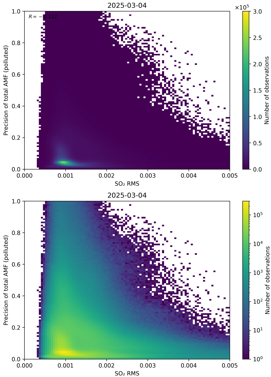
Figure 149: Scatter density plot of “SO 2 RMS” against “Precision of total AMF (polluted)” for 2025-03-03 to 2025-03-05.
