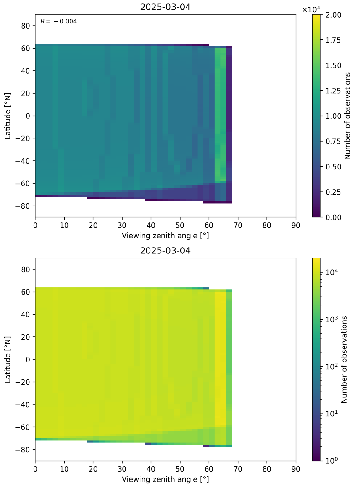
Figure 368: Scatter density plot of “Viewing zenith angle” against “Latitude” for 2025-03-03 to 2025-03-05.
