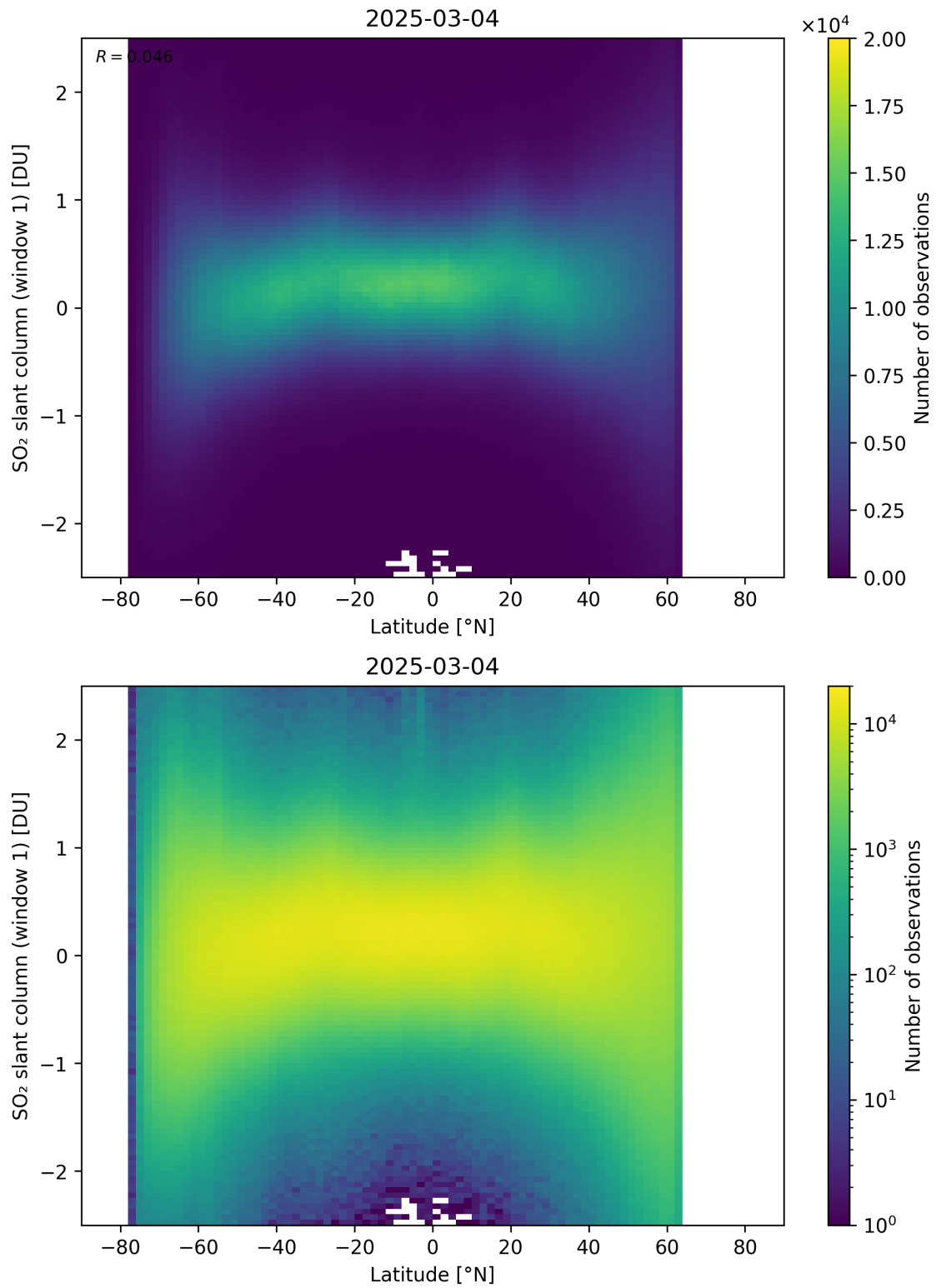
Figure 162: Scatter density plot of “Latitude” against “SO 2 slant column (window 1)” for 2025-03-03 to 2025-03-05.
