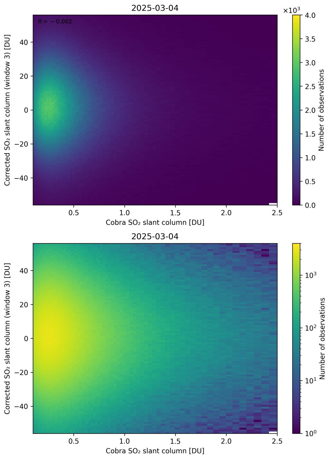
Figure 218: Scatter density plot of “Cobra SO 2 slant column” against “Corrected SO 2 slant column (window 3)” for 2025-03-03 to 2025-03-05.
