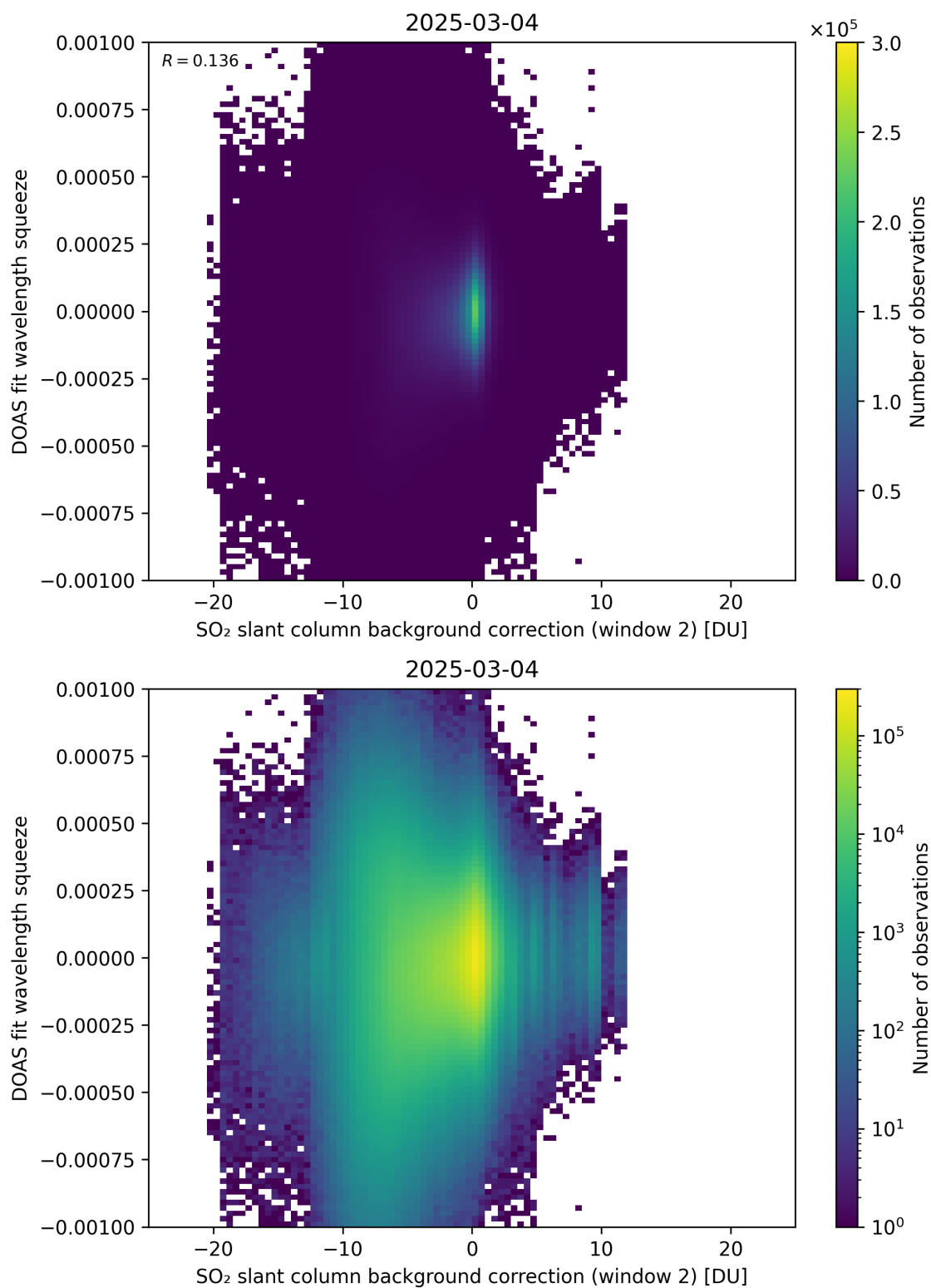
Figure 124: Scatter density plot of “SO 2 slant column background correction (window 2)” against “DOAS fit wavelength squeeze” for 2025-03-03 to 2025-03-05.
