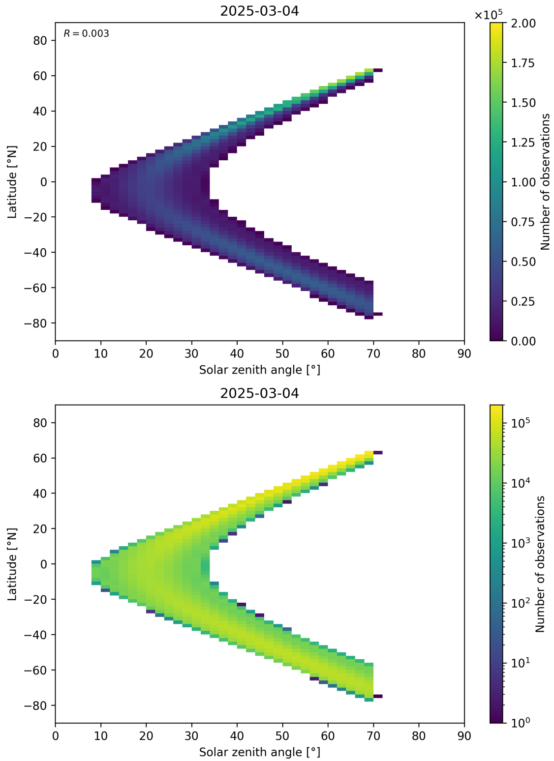
Figure 177: Scatter density plot of “Solar zenith angle” against “Latitude” for 2025-03-03 to 2025-03-05.
