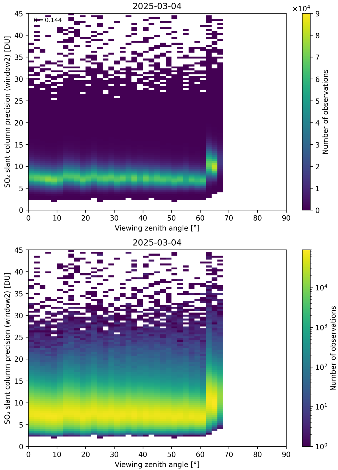
Figure 378: Scatter density plot of “Viewing zenith angle” against “SO 2 slant column precision (window2)” for 2025-03-03 to 2025-03-05.
