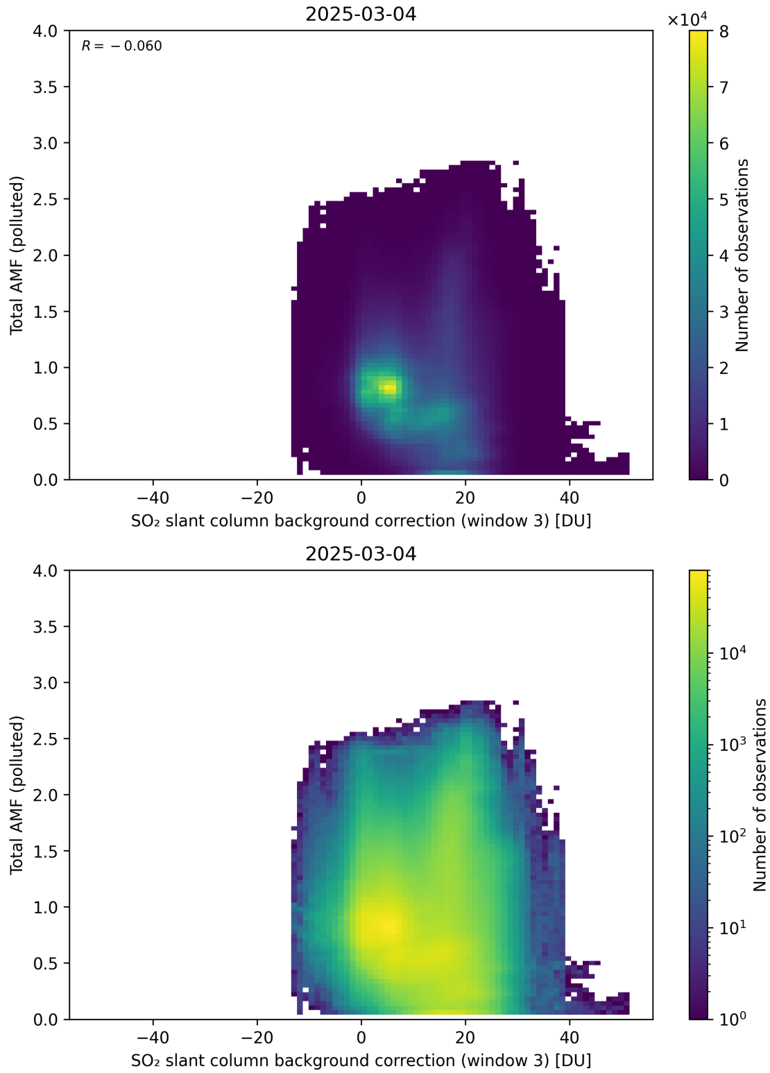
Figure 136: Scatter density plot of “SO 2 slant column background correction (window 3)” against “Total AMF (polluted)” for 2025-03-03 to 2025-03-05.
