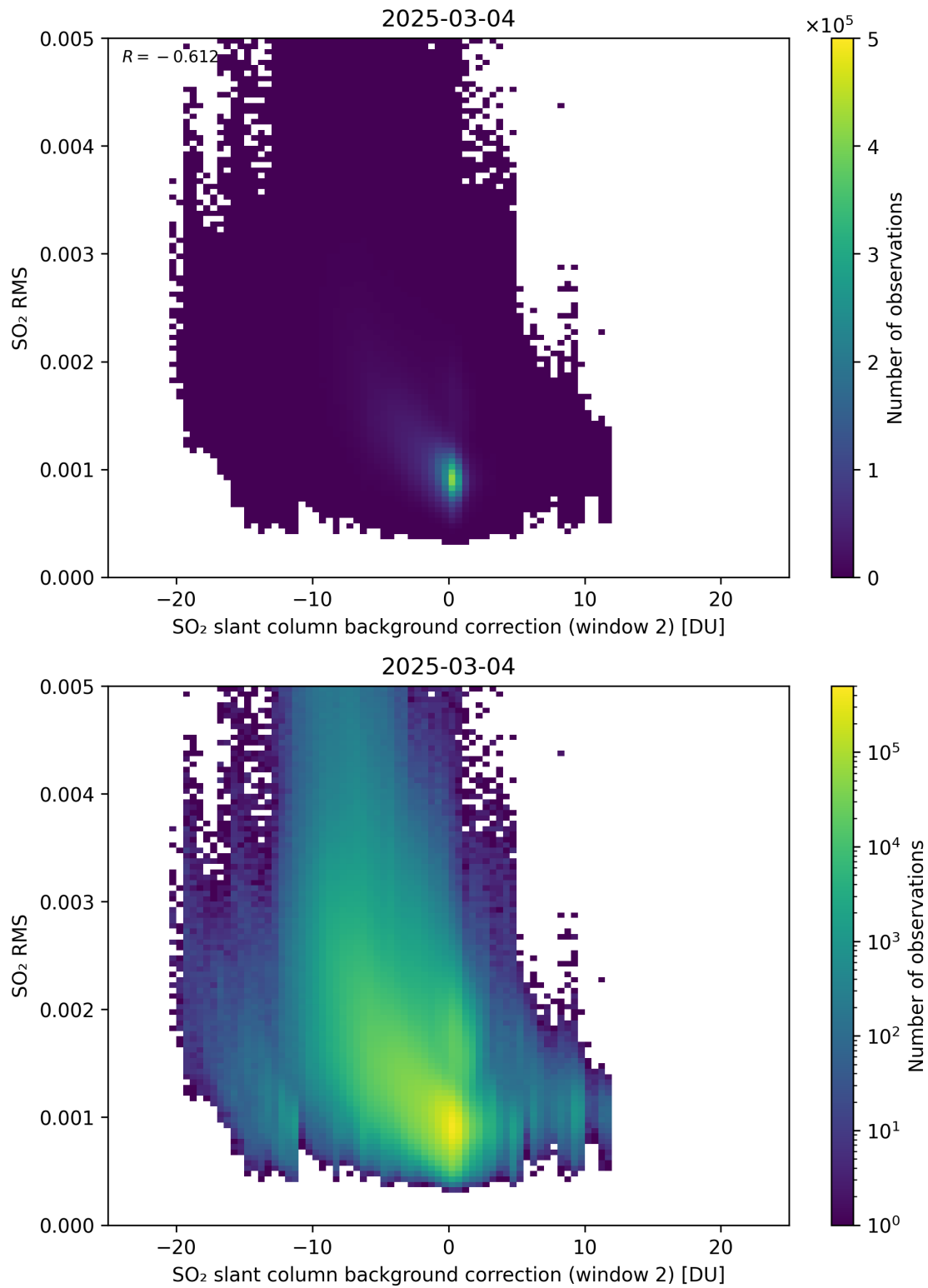
Figure 125: Scatter density plot of “SO 2 slant column background correction (window 2)” against “SO 2 RMS” for 2025-03-03 to 2025-03-05.
