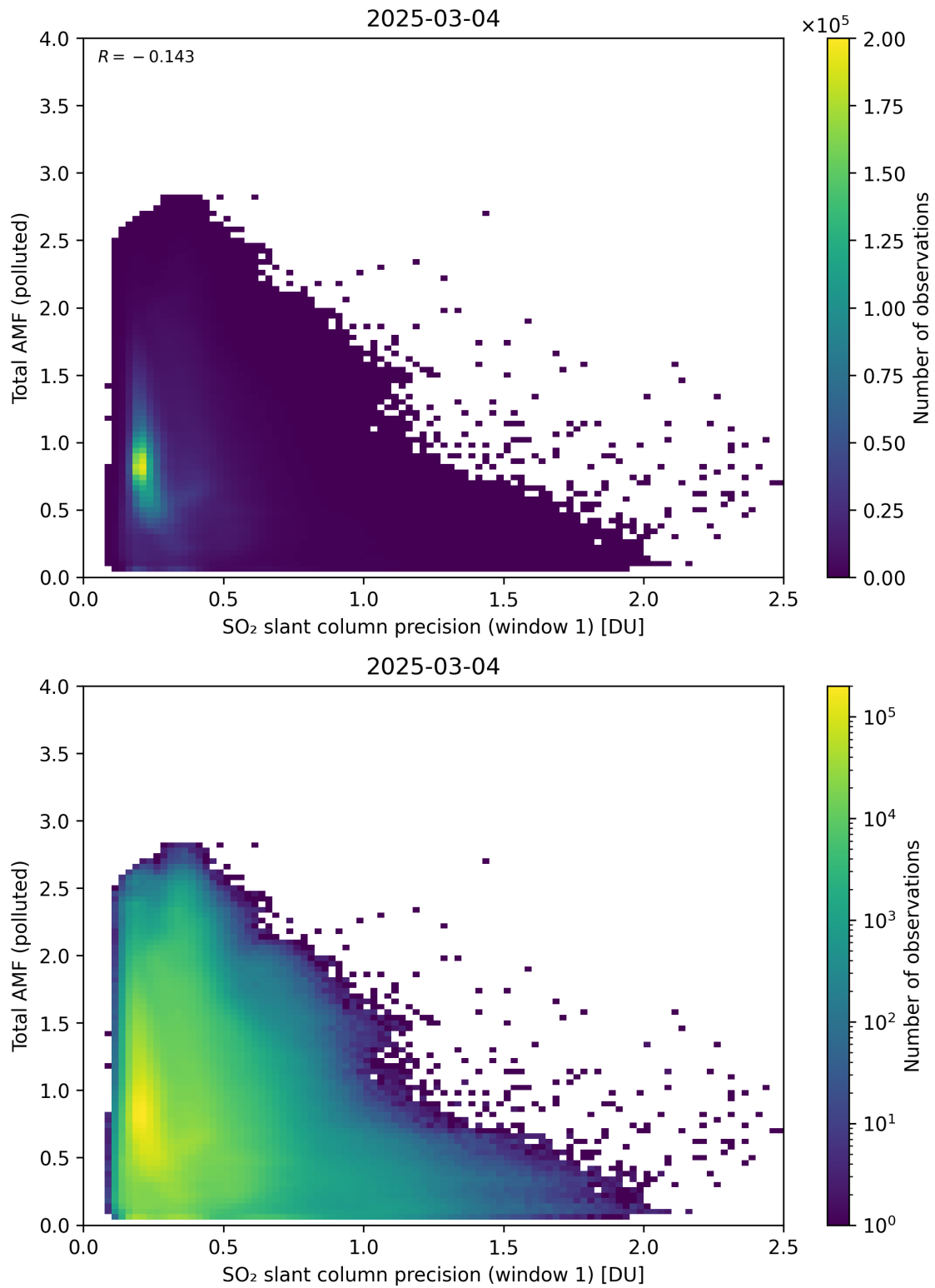
Figure 280: Scatter density plot of “SO 2 slant column precision (window 1)” against “Total AMF (polluted)” for 2025-03-03 to 2025-03-05.
