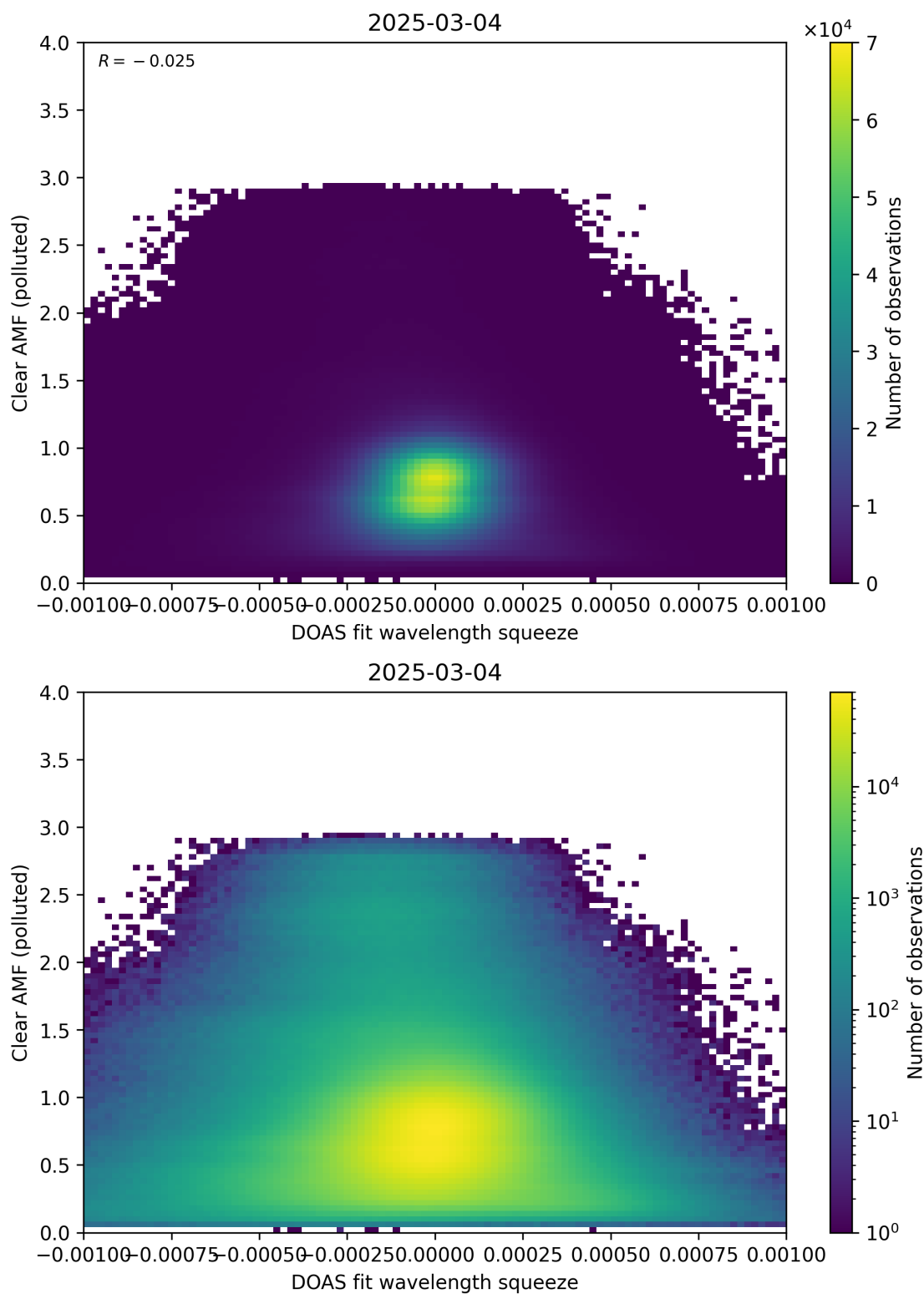
Figure 144: Scatter density plot of “DOAS fit wavelength squeeze” against “Clear AMF (polluted)” for 2025-03-03 to 2025-03-05.
