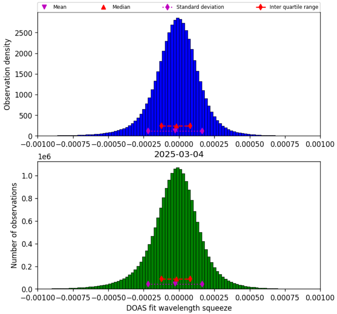
Figure 77: Histogram of “DOAS fit wavelength squeeze” for 2025-03-03 to 2025-03-05
