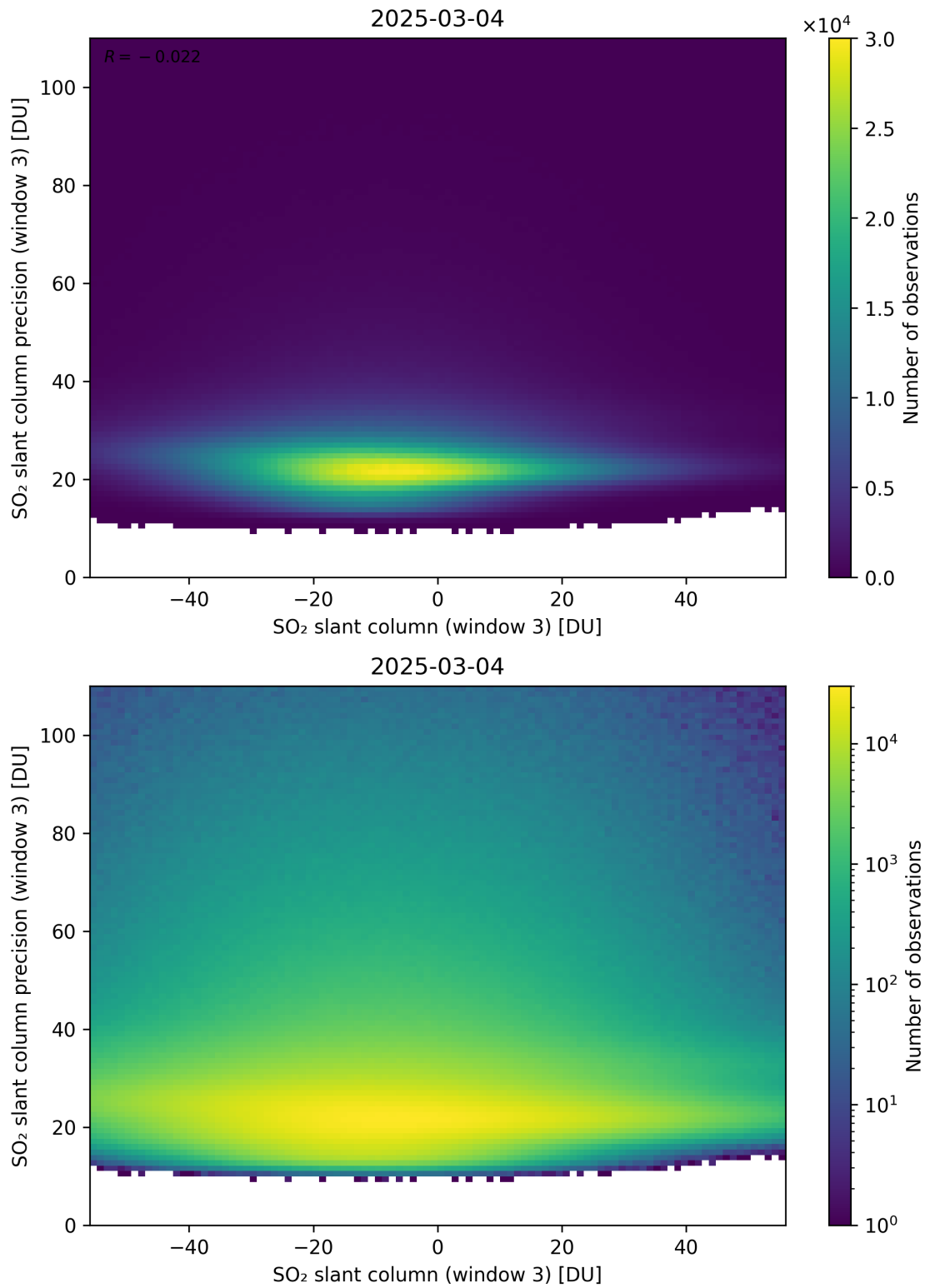
Figure 317: Scatter density plot of “SO 2 slant column (window 3)” against “SO 2 slant column precision (window 3)” for 2025-03-03 to 2025-03-05.
