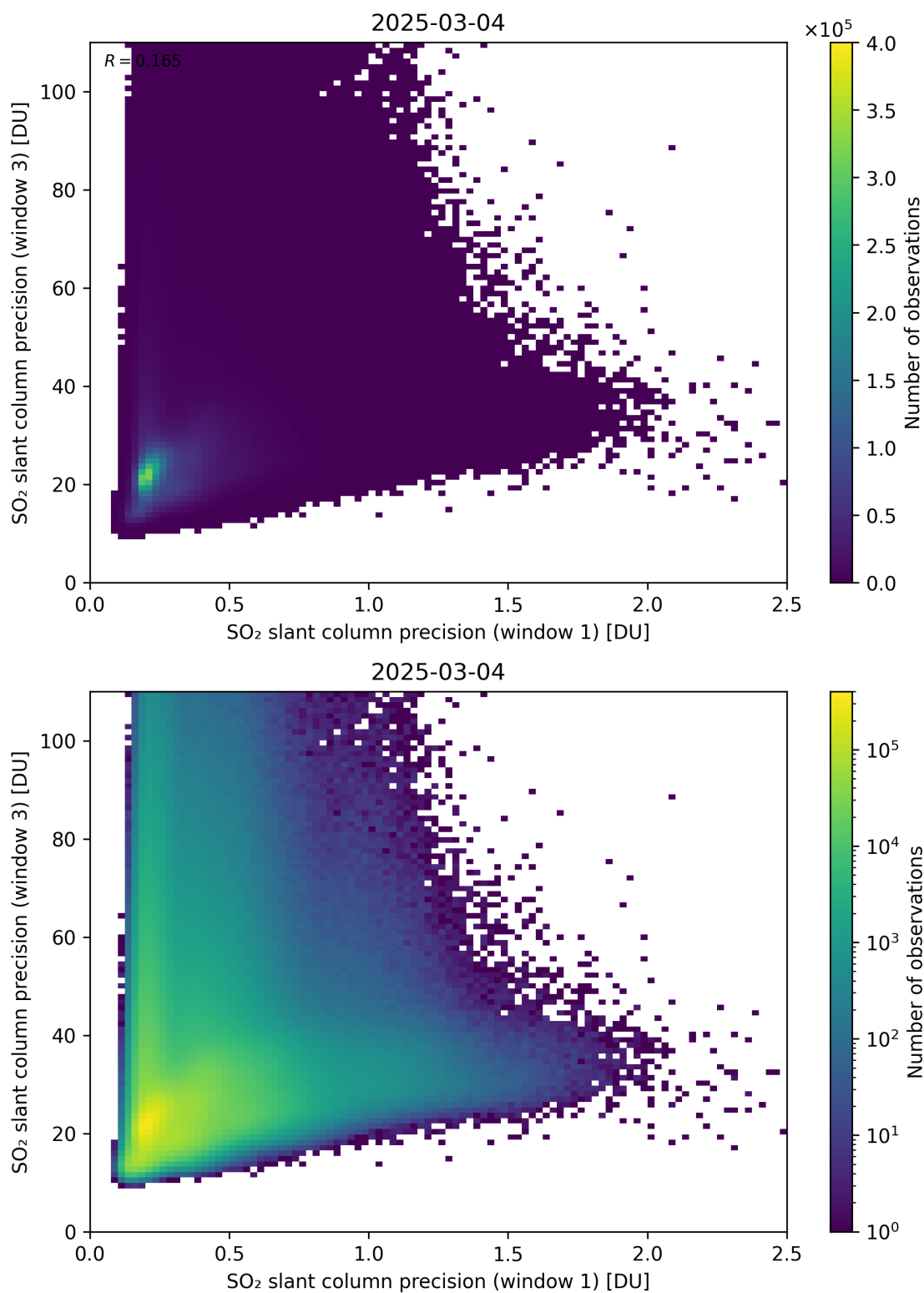
Figure 279: Scatter density plot of “SO 2 slant column precision (window 1)” against “SO 2 slant column precision (window 3)” for 2025-03-03 to 2025-03-05.
