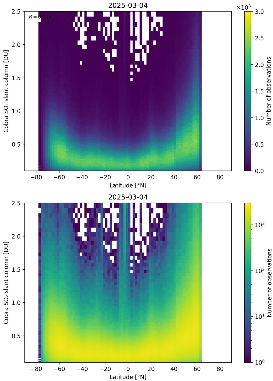
Figure 157: Scatter density plot of “Latitude” against “Cobra SO 2 slant column” for 2025-03-03 to 2025-03-05.
