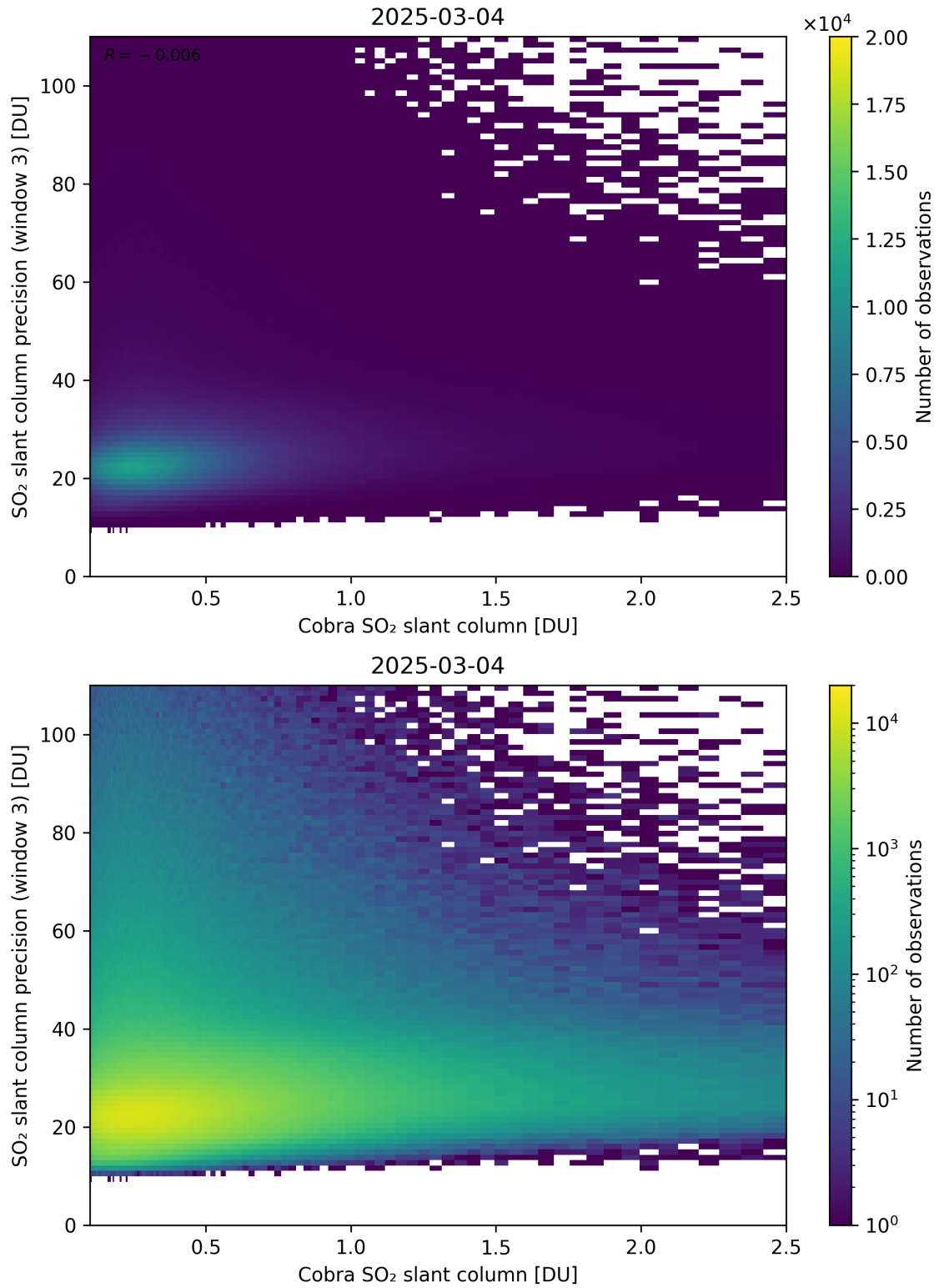
Figure 223: Scatter density plot of “Cobra SO 2 slant column” against “SO 2 slant column precision (window 3)” for 2025-03-03 to 2025-03-05.
