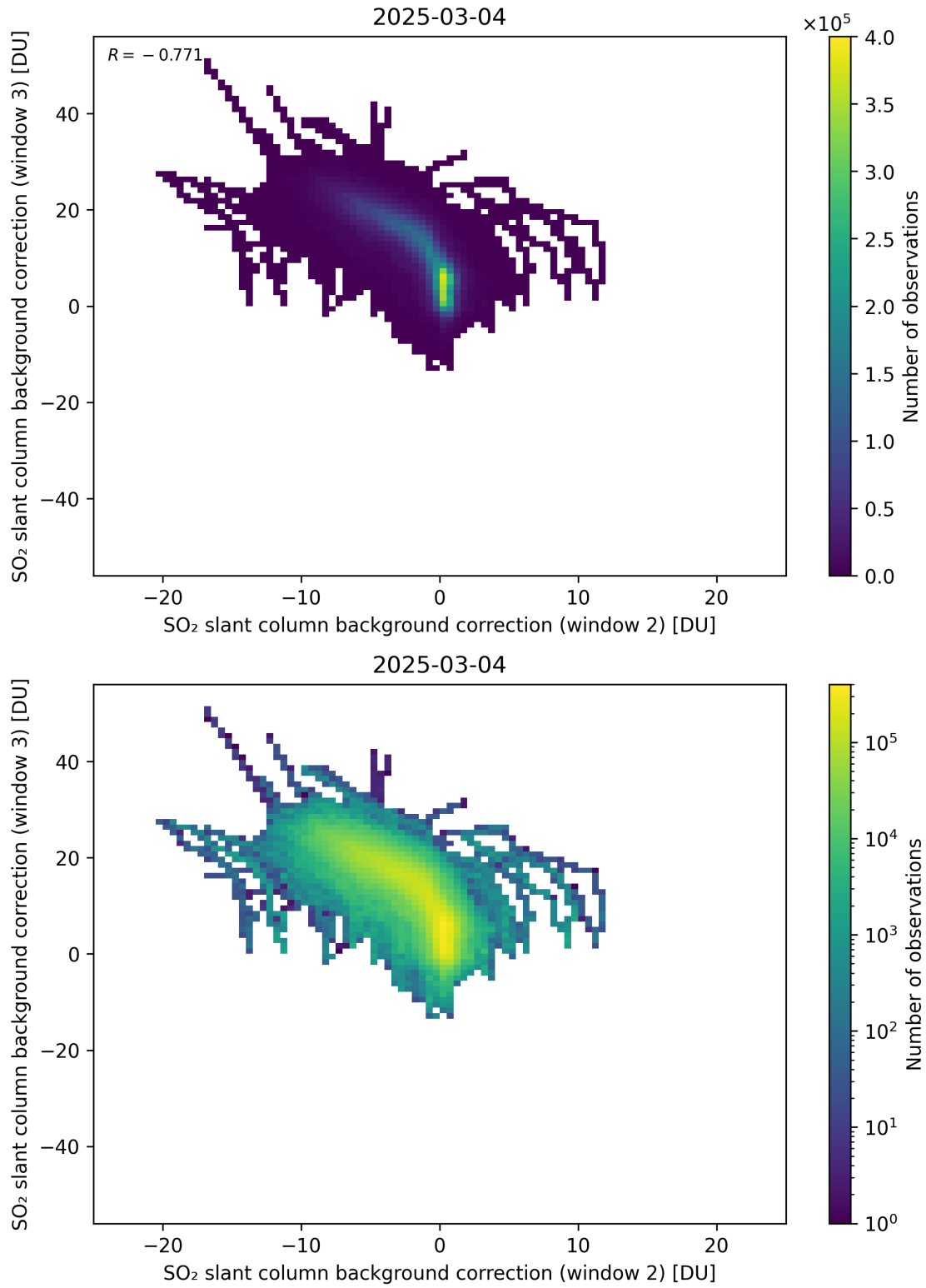
Figure 122: Scatter density plot of “SO 2 slant column background correction (window 2)” against “SO 2 slant column background correction (window 3)” for 2025-03-03 to 2025-03-05.
