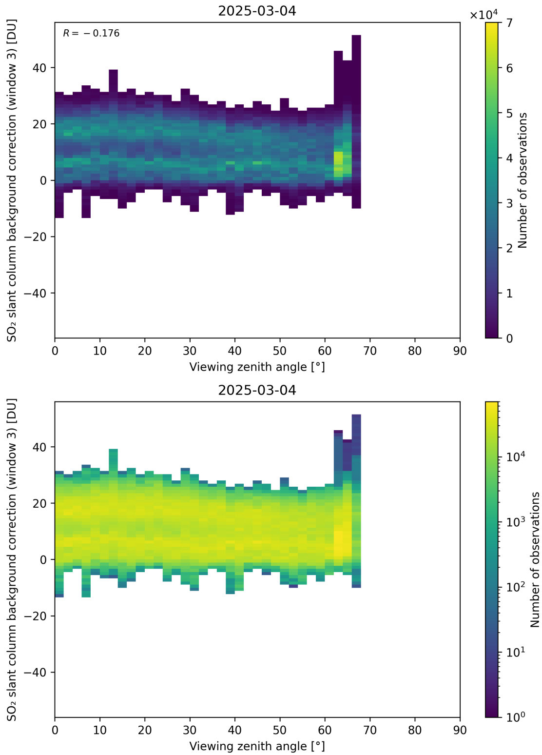
Figure 364: Scatter density plot of “Viewing zenith angle” against “SO 2 slant column background correction (window 3)” for 2025-03-03 to 2025-03-05.
