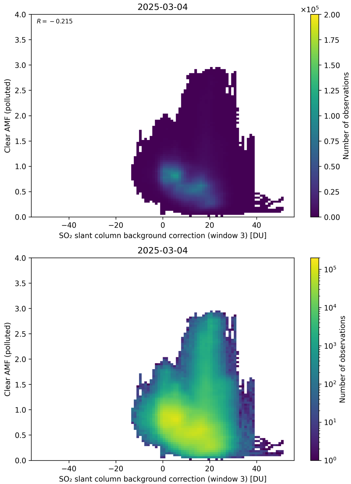
Figure 135: Scatter density plot of “SO 2 slant column background correction (window 3)” against “Clear AMF (polluted)” for 2025-03-03 to 2025-03-05.
