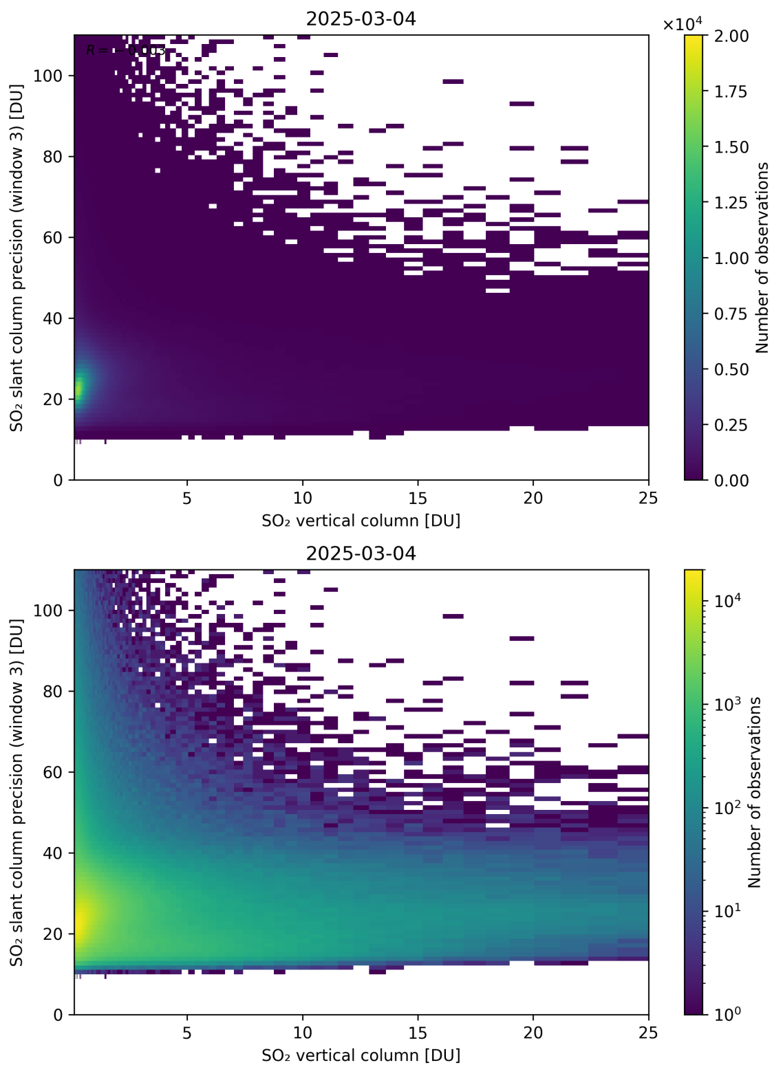
Figure 358: Scatter density plot of “SO 2 vertical column” against “SO 2 slant column precision (window 3)” for 2025-03-03 to 2025-03-05.
