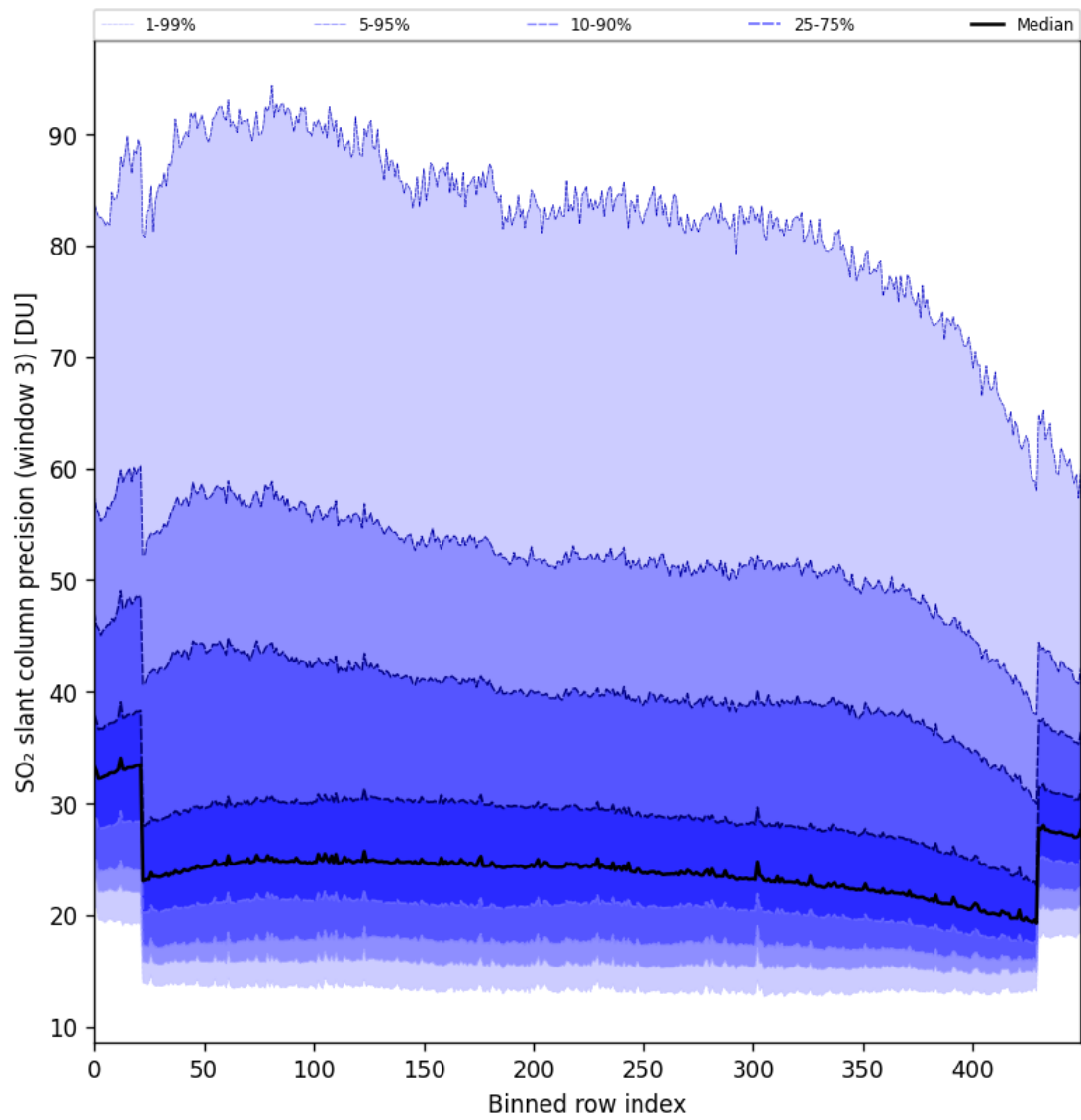
Figure 98: Along track statistics of “SO 2 slant column precision (window 3)” for 2025-03-03 to 2025-03-05
