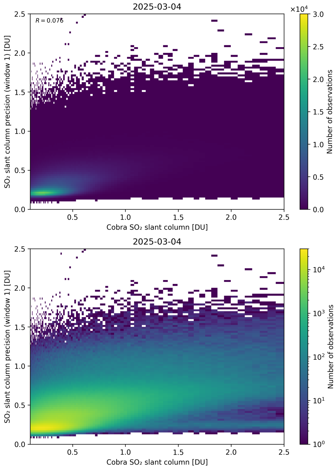
Figure 220: Scatter density plot of “Cobra SO 2 slant column” against “SO 2 slant column precision (window 1)” for 2025-03-03 to 2025-03-05.
