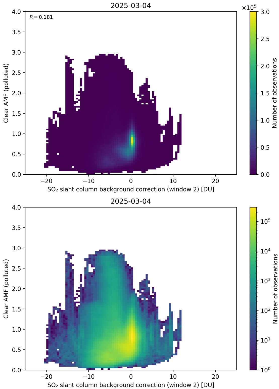
Figure 126: Scatter density plot of “SO 2 slant column background correction (window 2)” against “Clear AMF (polluted)” for 2025-03-03 to 2025-03-05.
