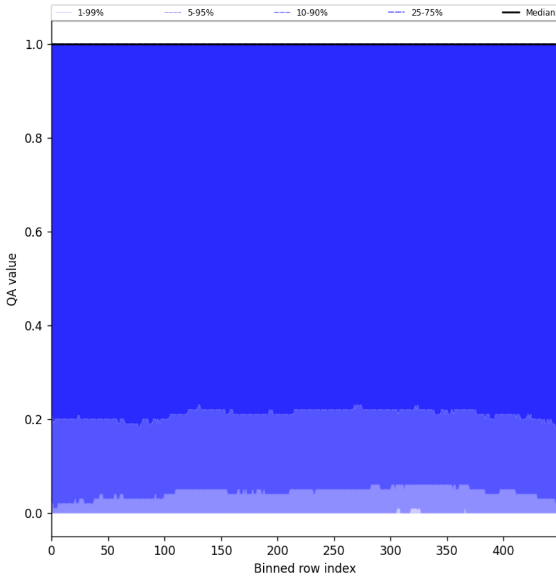
Figure 83: Along track statistics of “QA value” for 2025-03-03 to 2025-03-05
