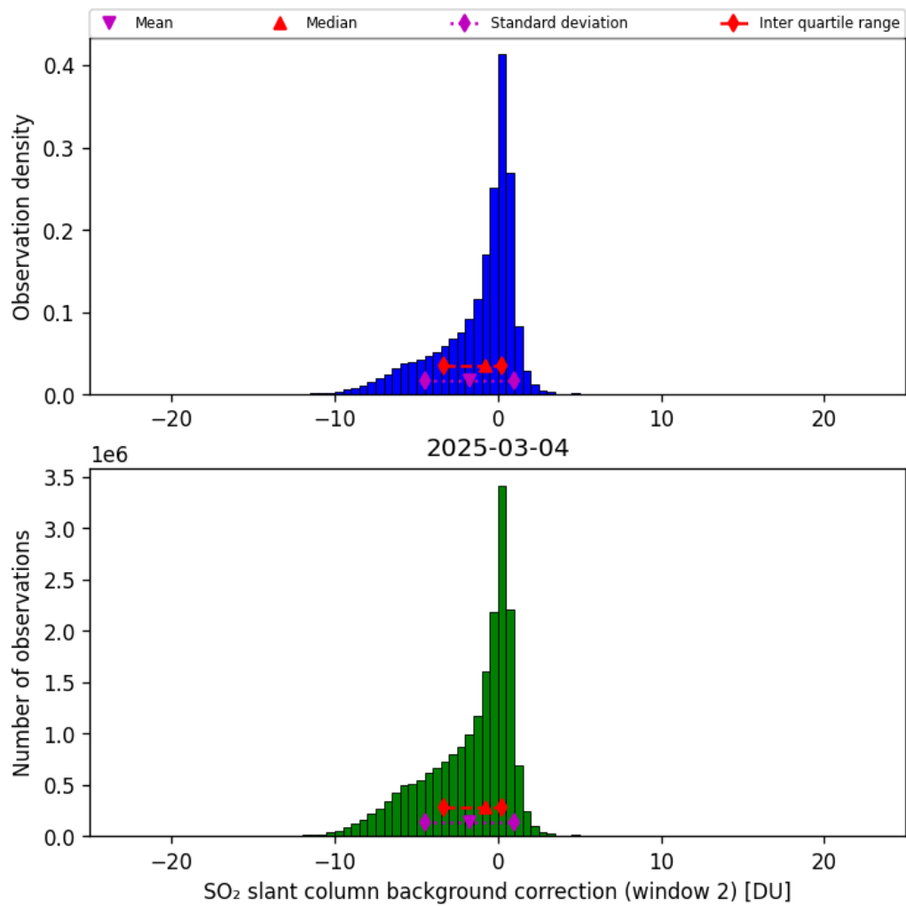
Figure 70: Histogram of “SO 2 slant column background correction (window 2)” for 2025-03-03 to 2025-03-05
