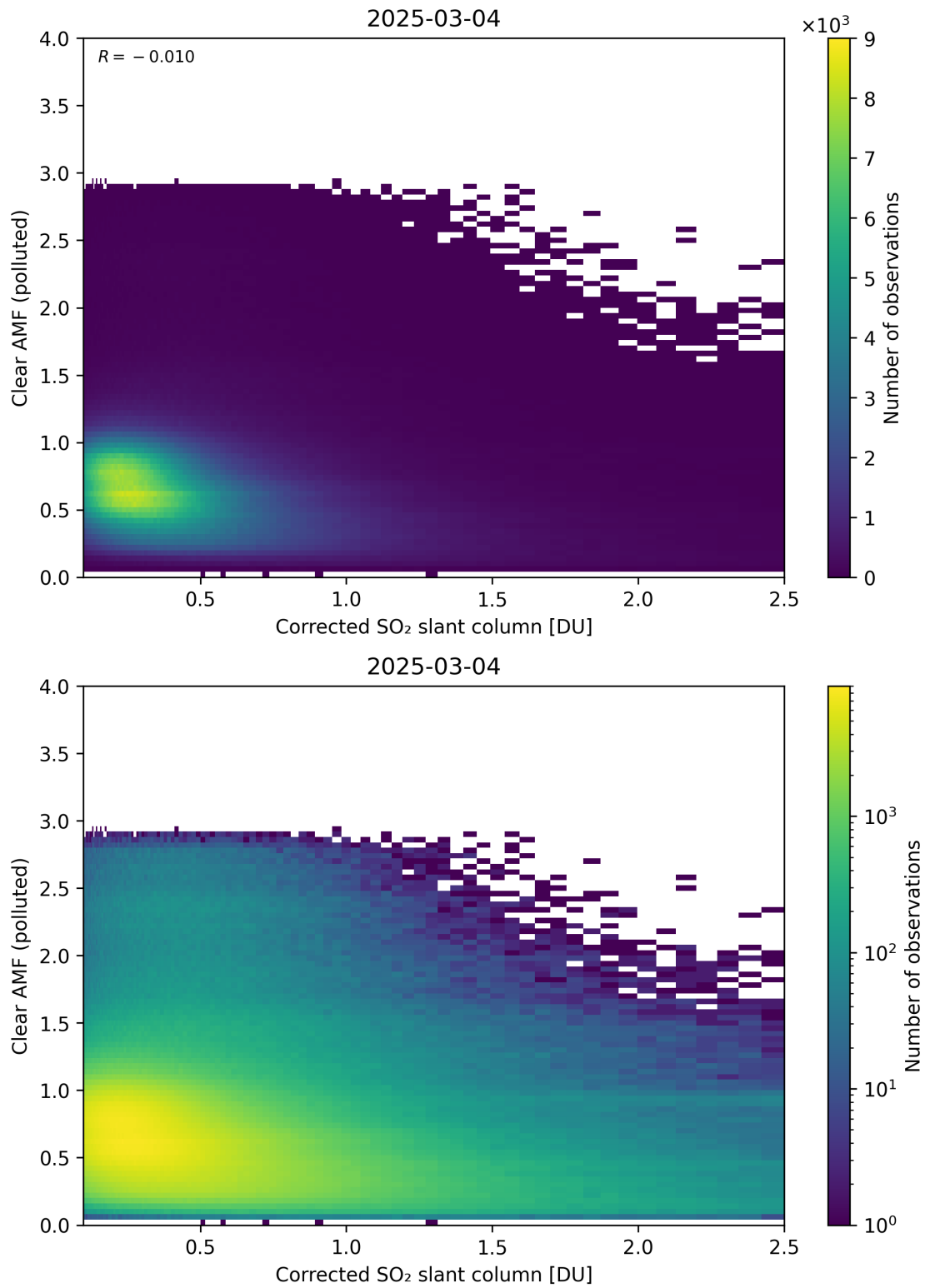
Figure 232: Scatter density plot of “Corrected SO 2 slant column” against “Clear AMF (polluted)” for 2025-03-03 to 2025-03-05.
