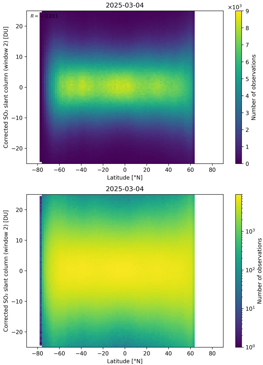
Figure 160: Scatter density plot of “Latitude” against “Corrected SO 2 slant column (window 2)” for 2025-03-03 to 2025-03-05.
