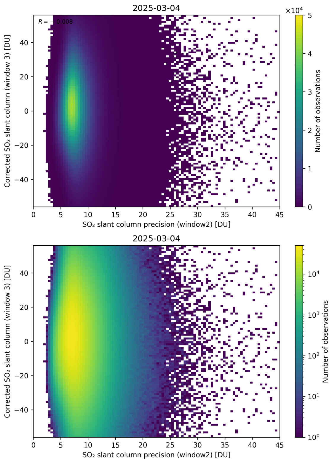
Figure 298: Scatter density plot of “SO 2 slant column precision (window2)” against “Corrected SO 2 slant column (window 3)” for 2025-03-03 to 2025-03-05.
