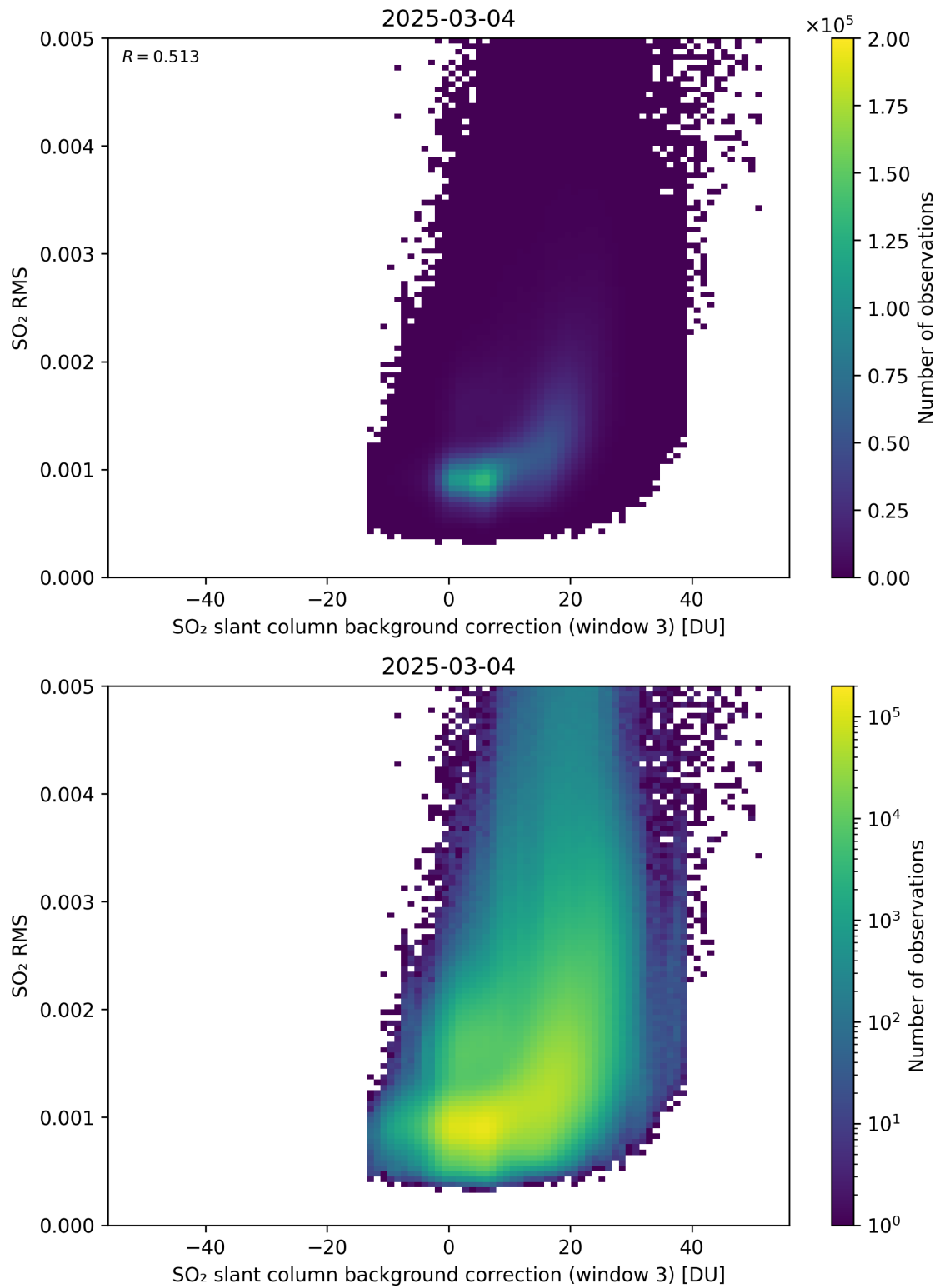
Figure 134: Scatter density plot of “SO 2 slant column background correction (window 3)” against “SO 2 RMS” for 2025-03-03 to 2025-03-05.
