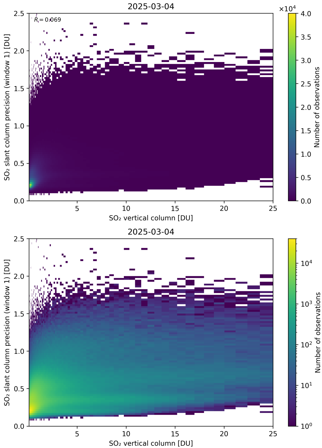
Figure 355: Scatter density plot of “SO 2 vertical column” against “SO 2 slant column precision (window 1)” for 2025-03-03 to 2025-03-05.
