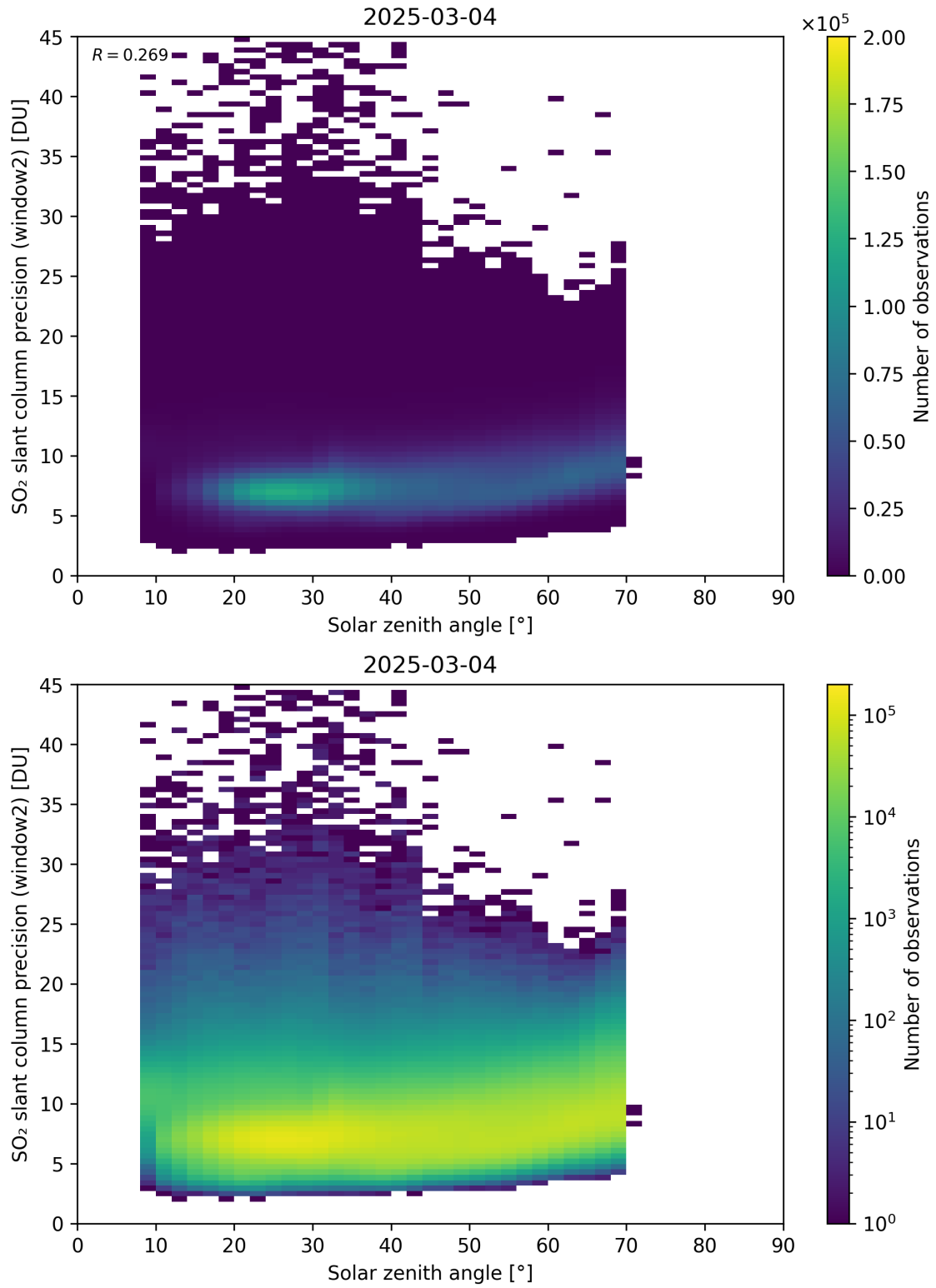
Figure 186: Scatter density plot of “Solar zenith angle” against “SO 2 slant column precision (window2)” for 2025-03-03 to 2025-03-05.
