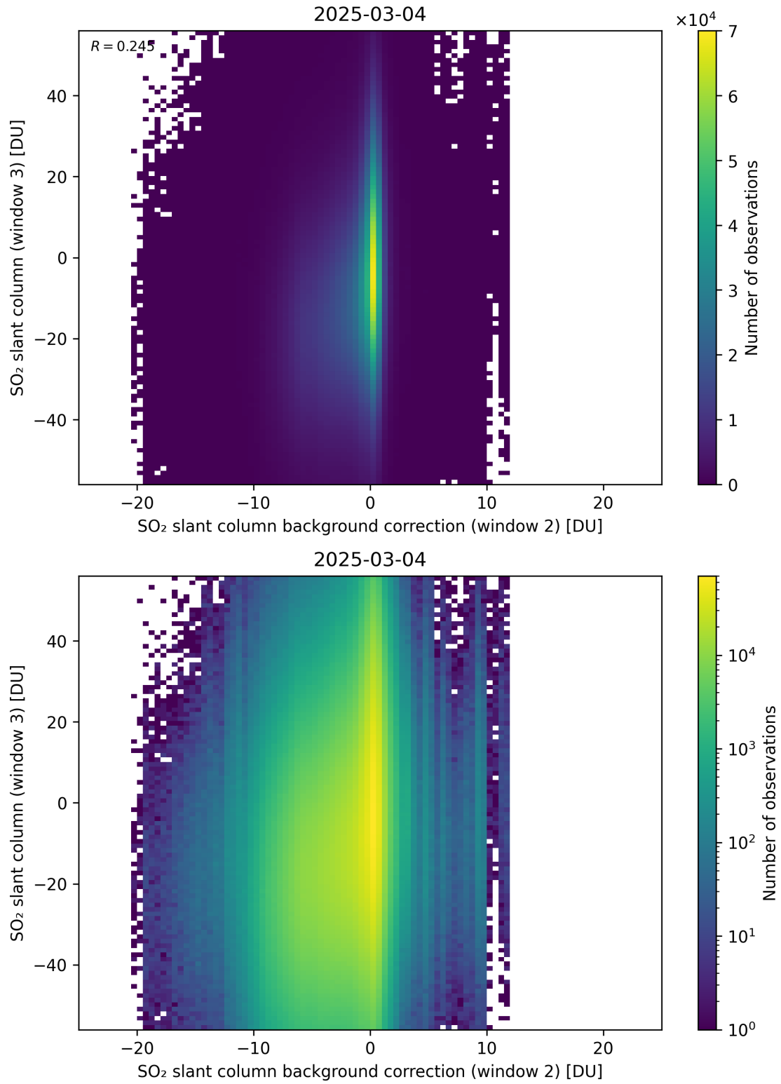
Figure 128: Scatter density plot of “SO 2 slant column background correction (window 2)” against “SO 2 slant column (window 3)” for 2025-03-03 to 2025-03-05.
