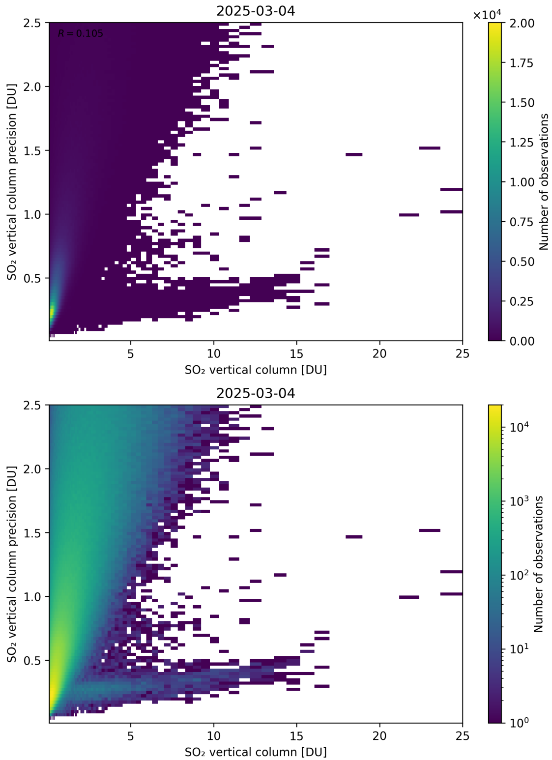
Figure 361: Scatter density plot of “SO 2 vertical column” against “SO 2 vertical column precision” for 2025-03-03 to 2025-03-05.
