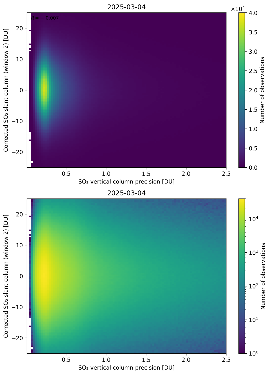
Figure 339: Scatter density plot of “SO 2 vertical column precision” against “Corrected SO 2 slant column (window 2)” for 2025-03-03 to 2025-03-05.
