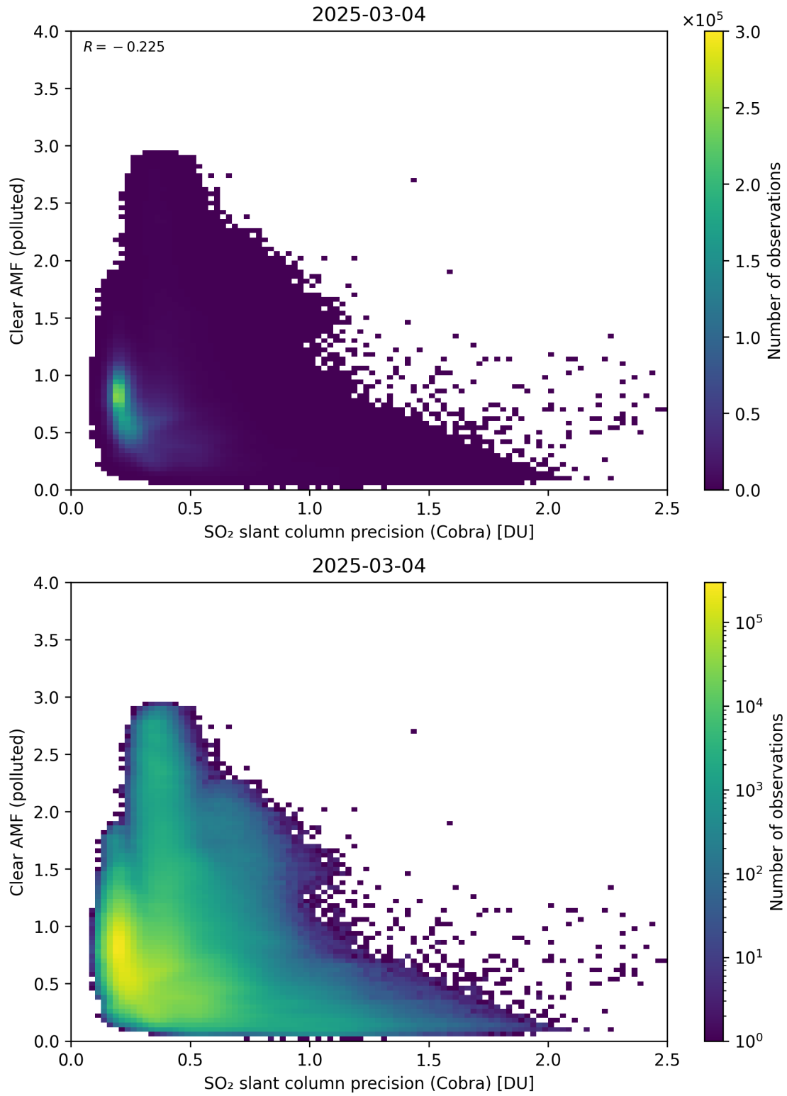
Figure 205: Scatter density plot of “SO 2 slant column precision (Cobra)” against “Clear AMF (polluted)” for 2025-03-03 to 2025-03-05.
