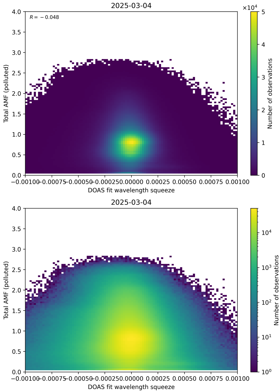
Figure 145: Scatter density plot of “DOAS fit wavelength squeeze” against “Total AMF (polluted)” for 2025-03-03 to 2025-03-05.
