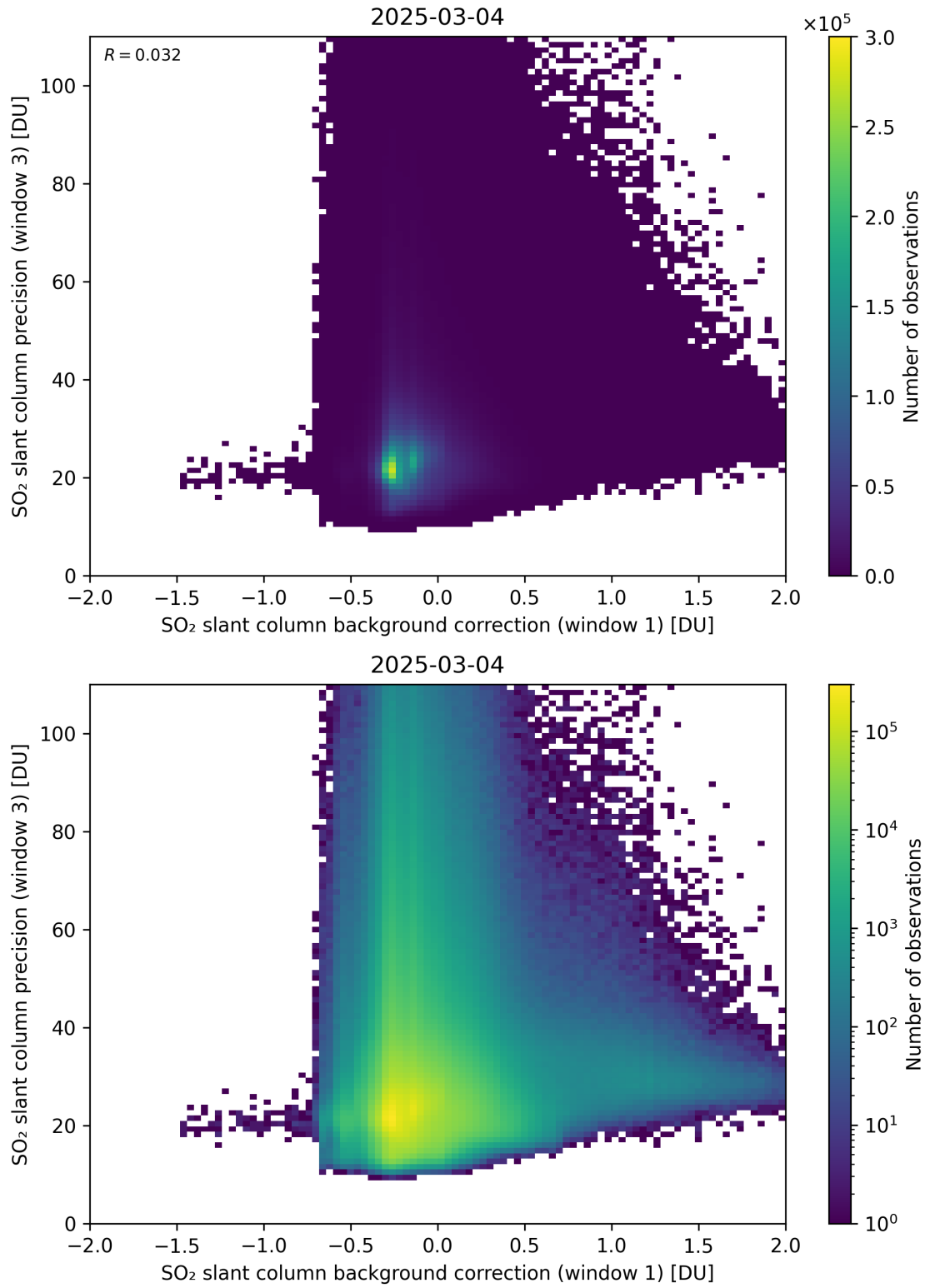
Figure 119: Scatter density plot of “SO 2 slant column background correction (window 1)” against “SO 2 slant column precision (window 3)” for 2025-03-03 to 2025-03-05.
