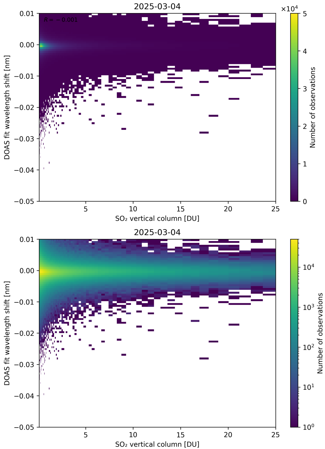
Figure 326: Scatter density plot of “SO 2 vertical column” against “DOAS fit wavelength shift” for 2025-03-03 to 2025-03-05.
