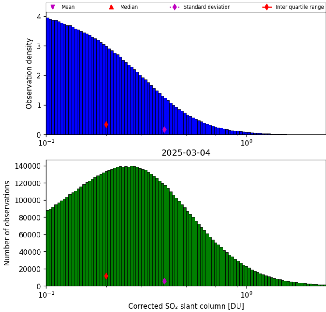
Figure 60: Histogram of “Corrected SO 2 slant column” for 2025-03-03 to 2025-03-05
