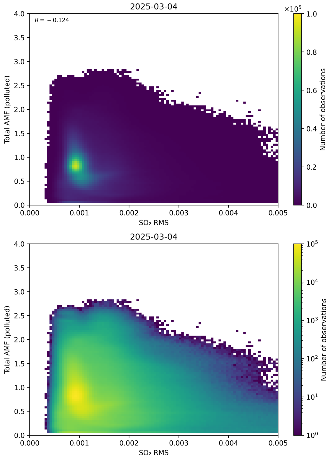
Figure 148: Scatter density plot of “SO 2 RMS” against “Total AMF (polluted)” for 2025-03-03 to 2025-03-05.
