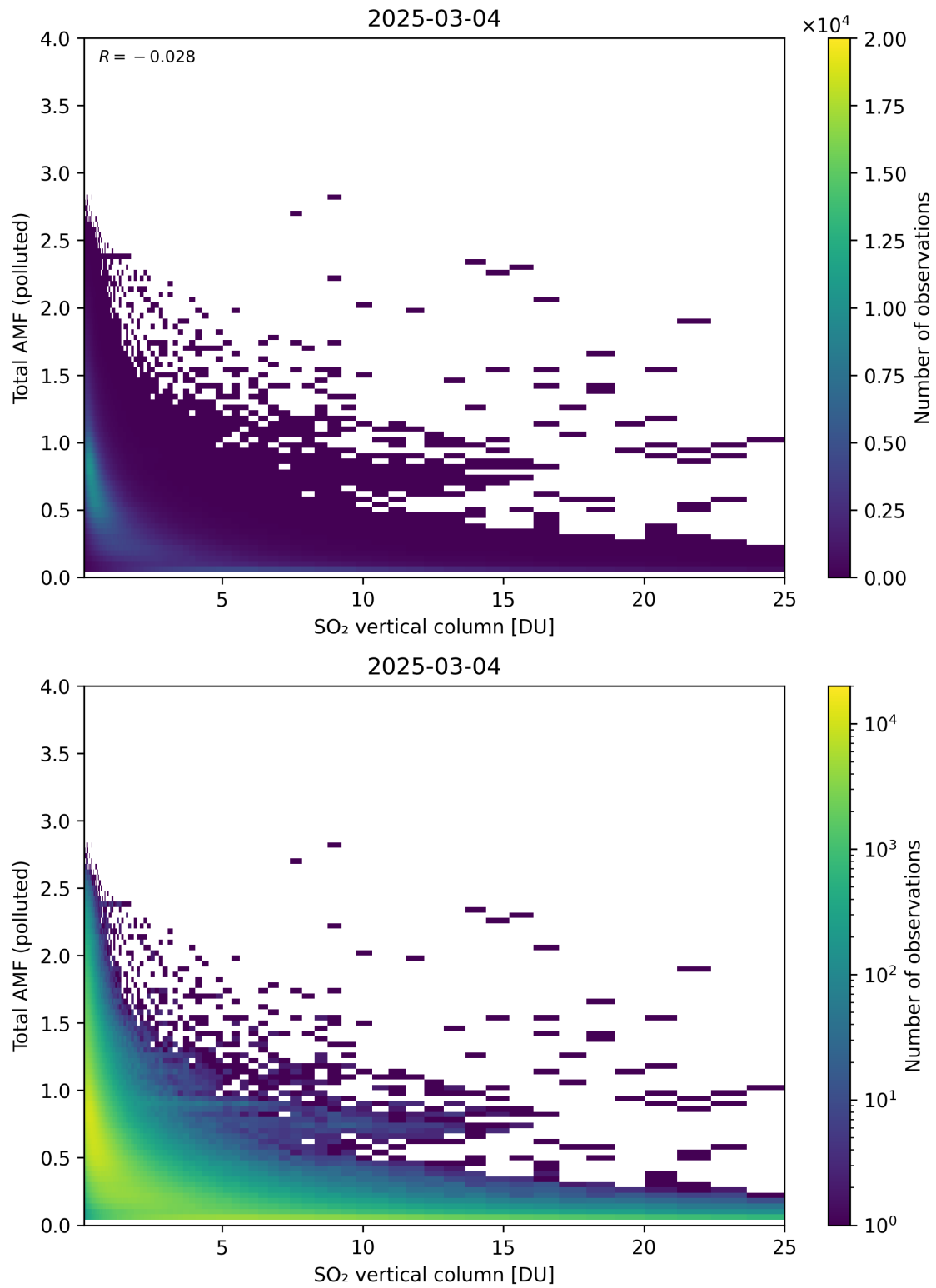
Figure 359: Scatter density plot of “SO 2 vertical column” against “Total AMF (polluted)” for 2025-03-03 to 2025-03-05.
