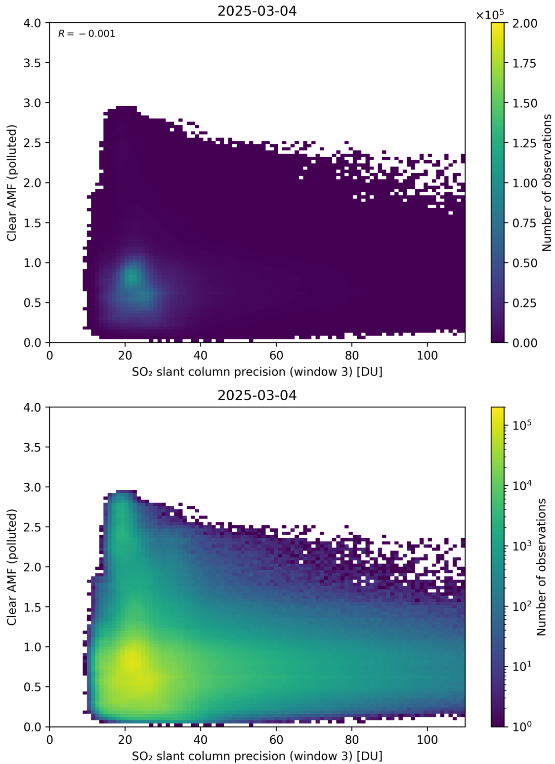
Figure 311: Scatter density plot of “SO 2 slant column precision (window 3)” against “Clear AMF (polluted)” for 2025-03-03 to 2025-03-05.
