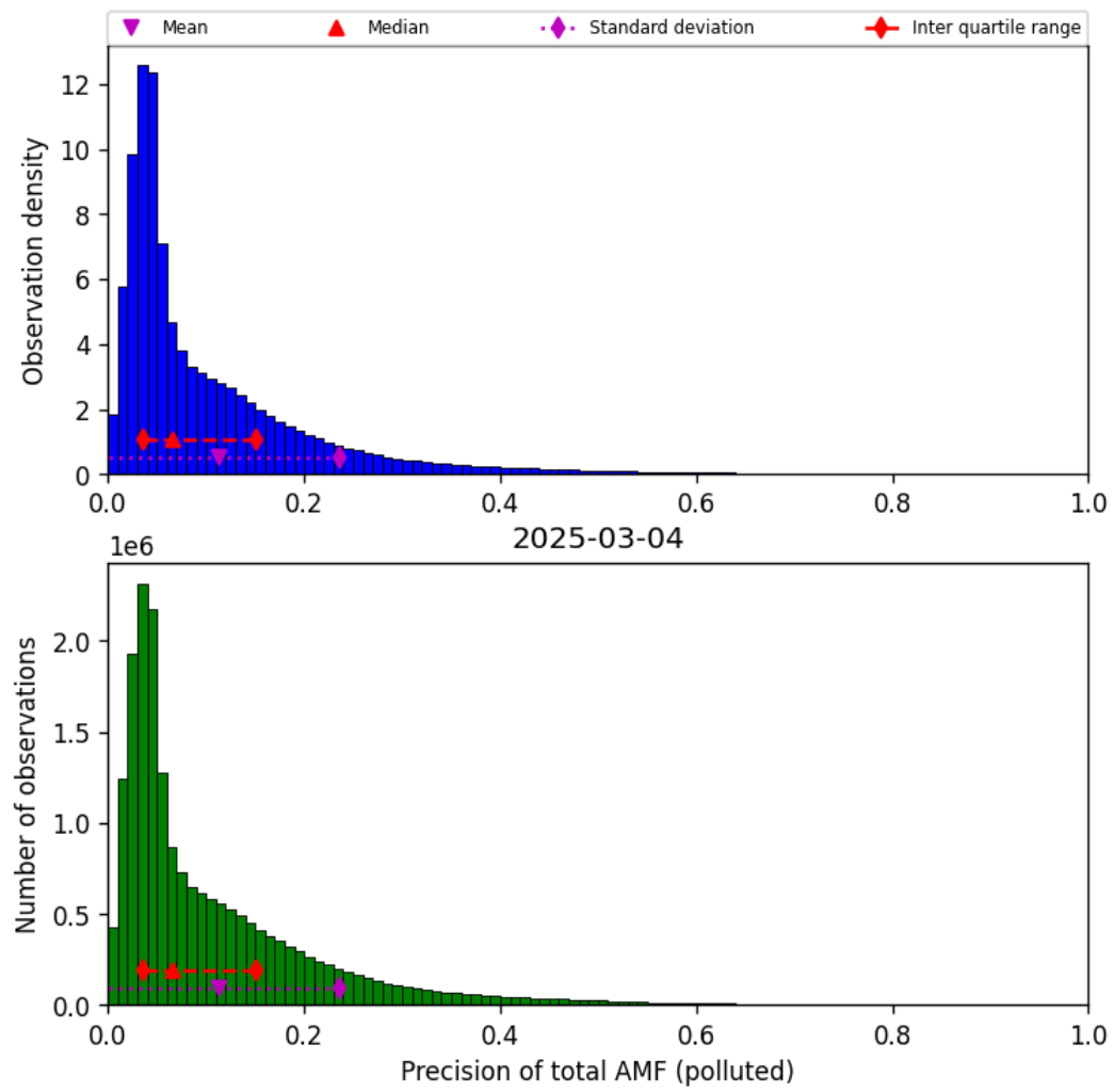
Figure 80: Histogram of “Precision of total AMF (polluted)” for 2025-03-03 to 2025-03-05
