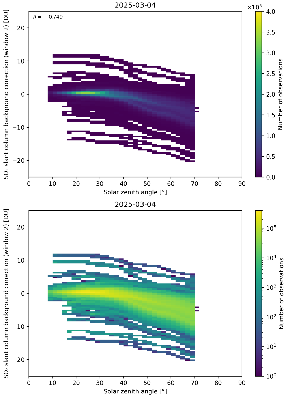
Figure 172: Scatter density plot of “Solar zenith angle” against “SO 2 slant column background correction (window 2)” for 2025-03-03 to 2025-03-05.
