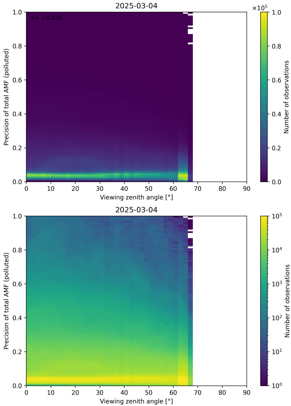
Figure 382: Scatter density plot of “Viewing zenith angle” against “Precision of total AMF (polluted)” for 2025-03-03 to 2025-03-05.
