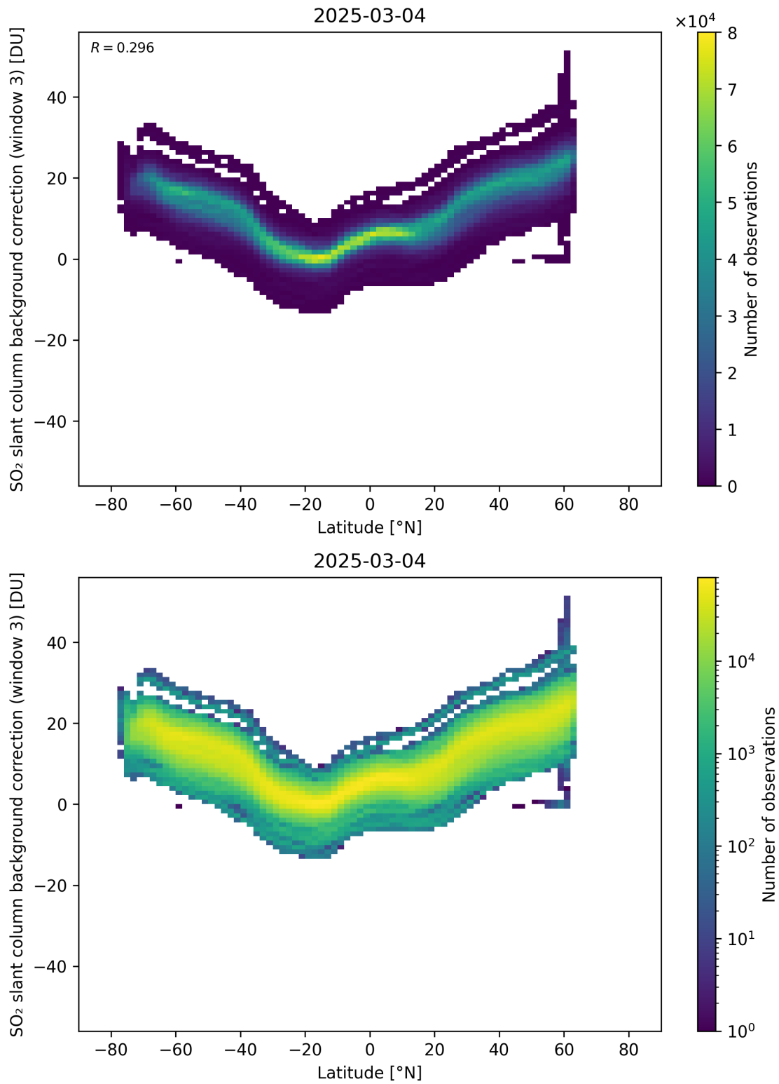
Figure 152: Scatter density plot of “Latitude” against “SO 2 slant column background correction (window 3)” for 2025-03-03 to 2025-03-05.
