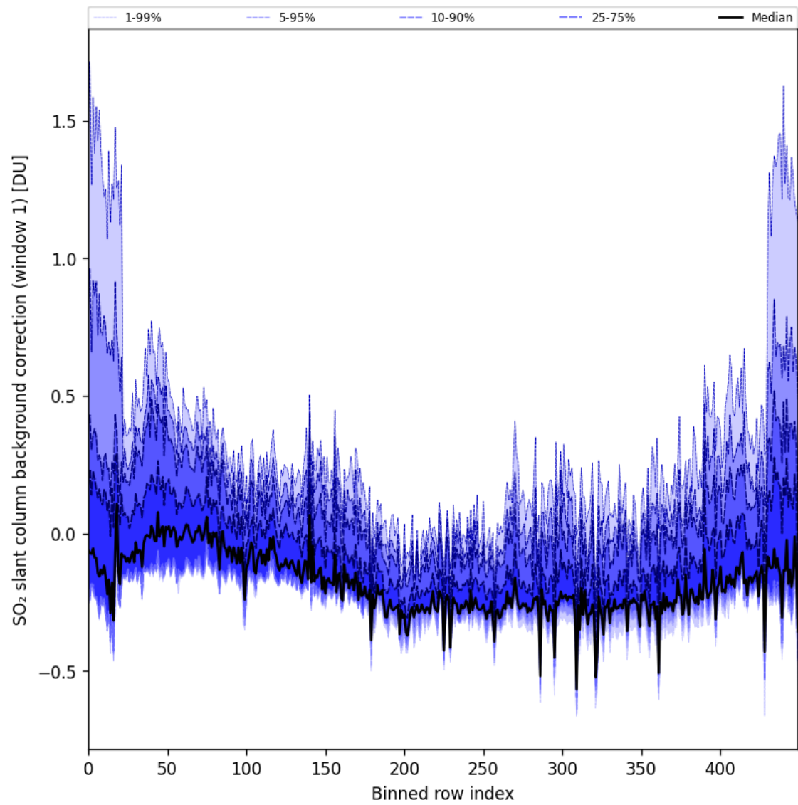
Figure 92: Along track statistics of “SO 2 slant column background correction (window 1)” for 2025-03-03 to 2025-03-05
