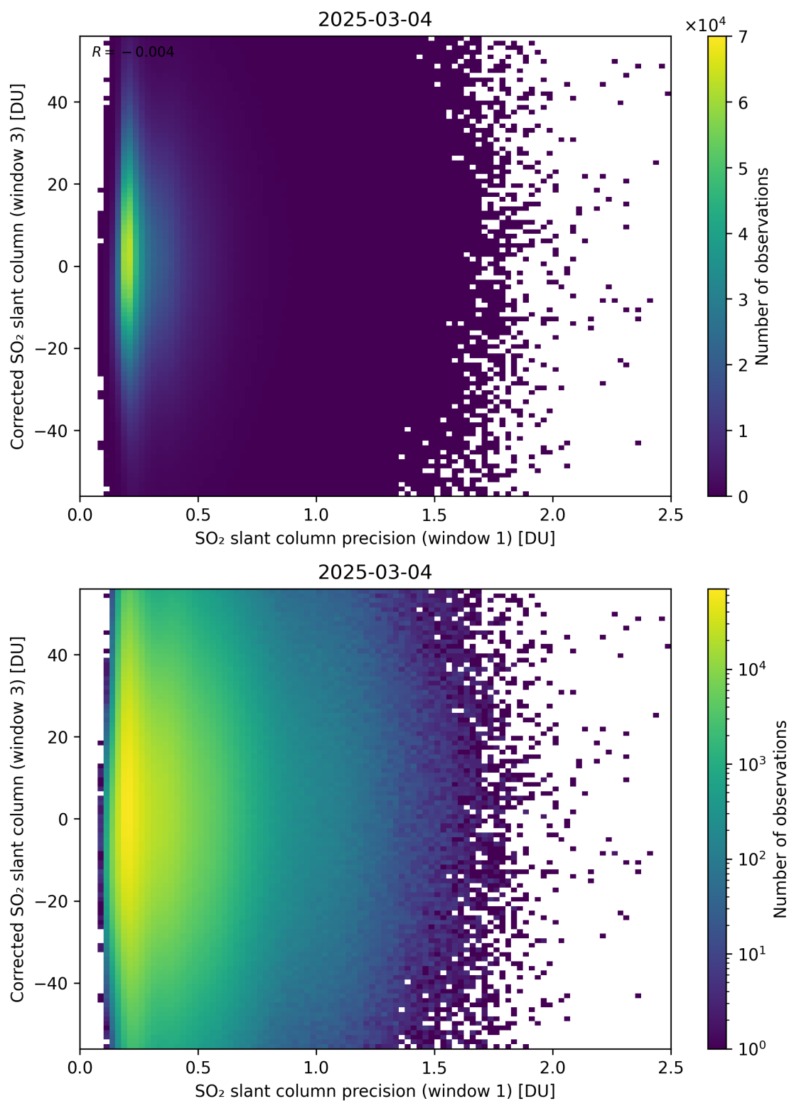
Figure 276: Scatter density plot of “SO 2 slant column precision (window 1)” against “Corrected SO 2 slant column (window 3)” for 2025-03-03 to 2025-03-05.
