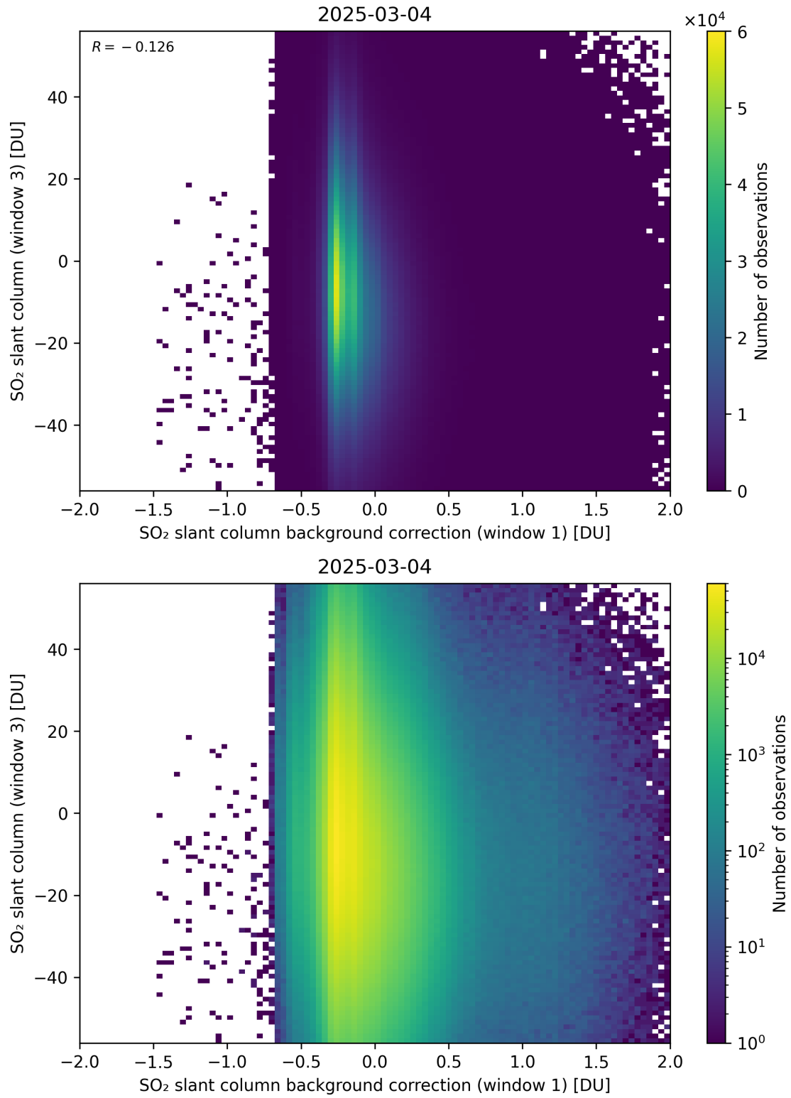
Figure 118: Scatter density plot of “SO 2 slant column background correction (window 1)” against “SO 2 slant column (window 3)” for 2025-03-03 to 2025-03-05.
