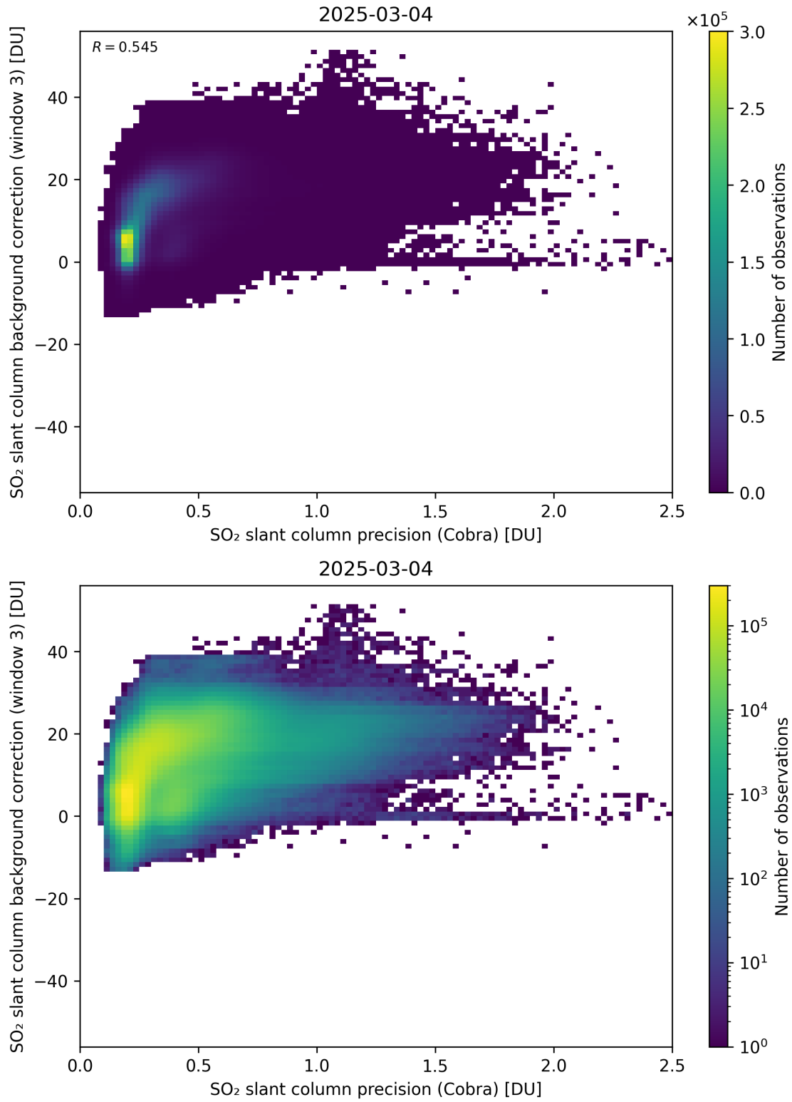
Figure 201: Scatter density plot of “SO 2 slant column precision (Cobra)” against “SO 2 slant column background correction (window 3)” for 2025-03-03 to 2025-03-05.
