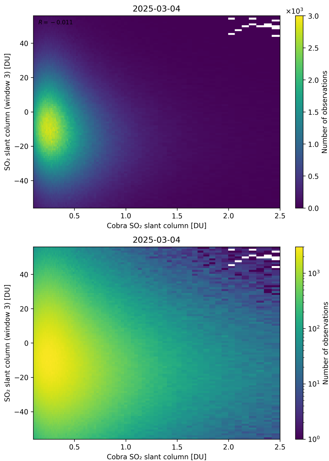
Figure 222: Scatter density plot of “Cobra SO 2 slant column” against “SO 2 slant column (window 3)” for 2025-03-03 to 2025-03-05.
