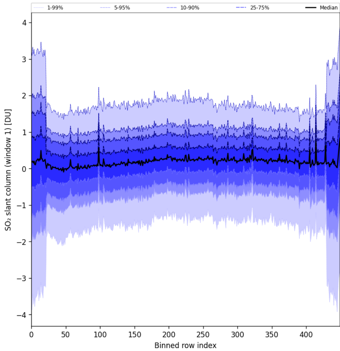
Figure 89: Along track statistics of “SO 2 slant column (window 1)” for 2025-03-03 to 2025-03-05
