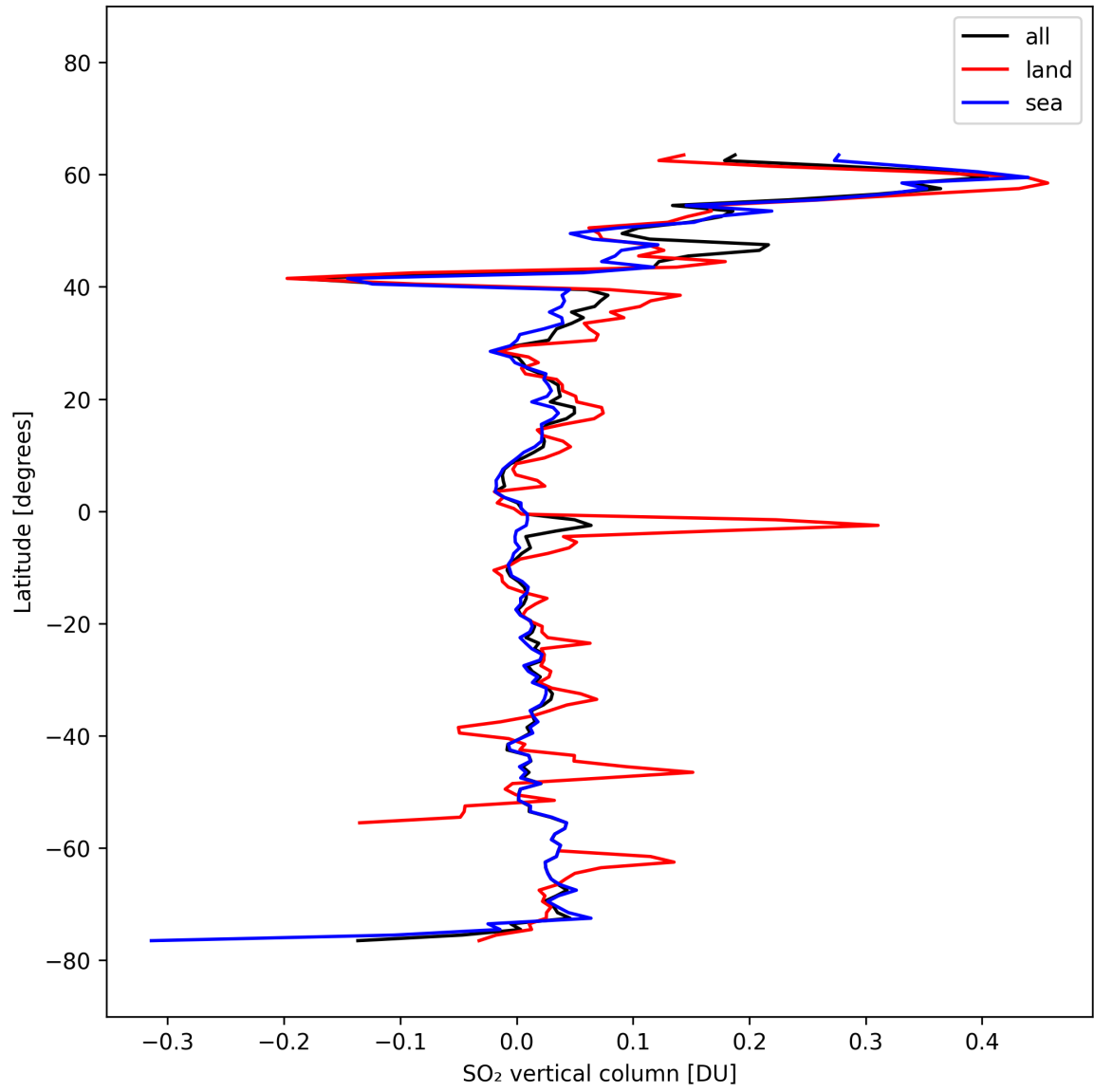
Figure 32: Zonal average of “SO 2 vertical column” for 2025-03-03 to 2025-03-05.
