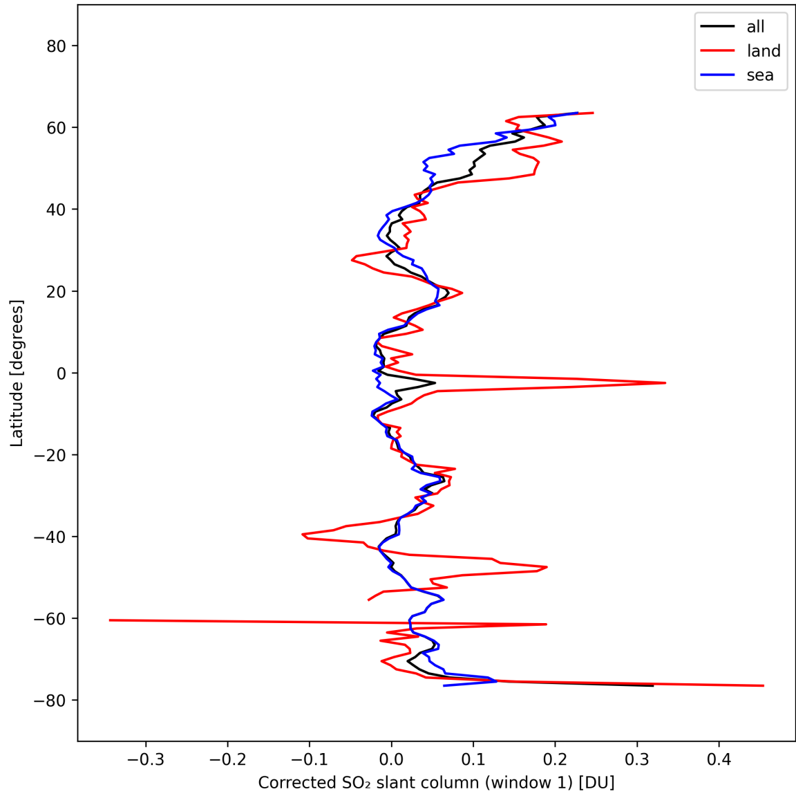
Figure 39: Zonal average of “Corrected SO 2 slant column (window 1)” for 2025-03-03 to 2025-03-05.
