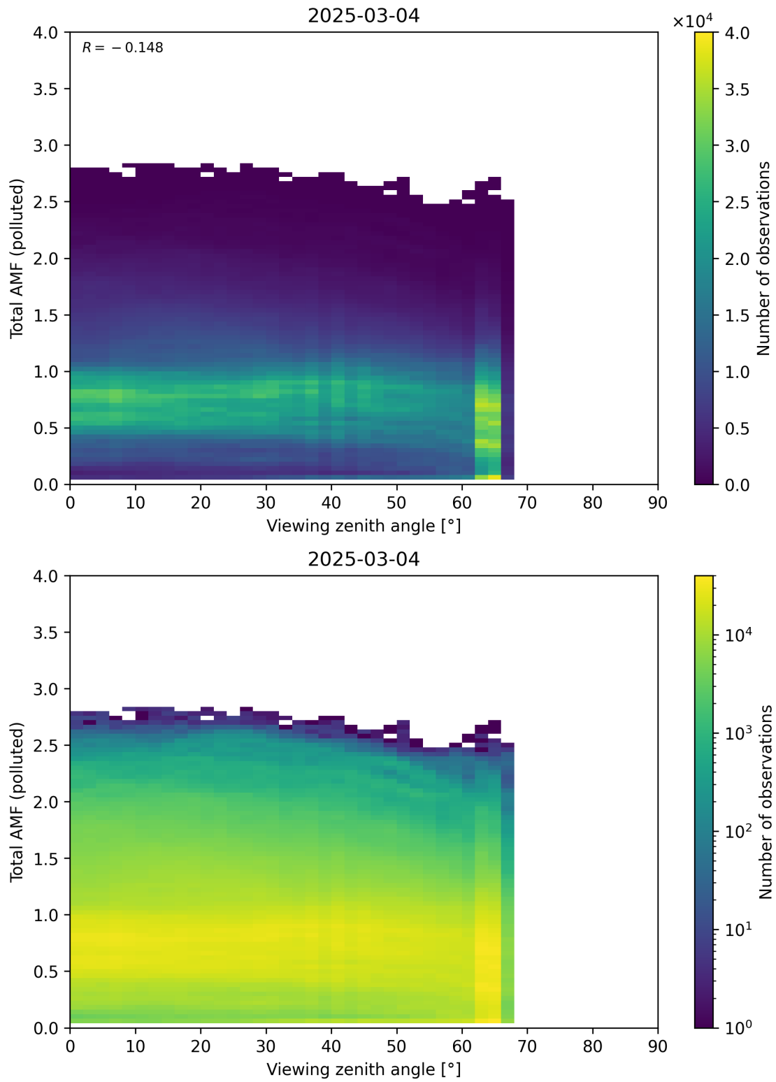
Figure 381: Scatter density plot of “Viewing zenith angle” against “Total AMF (polluted)” for 2025-03-03 to 2025-03-05.
