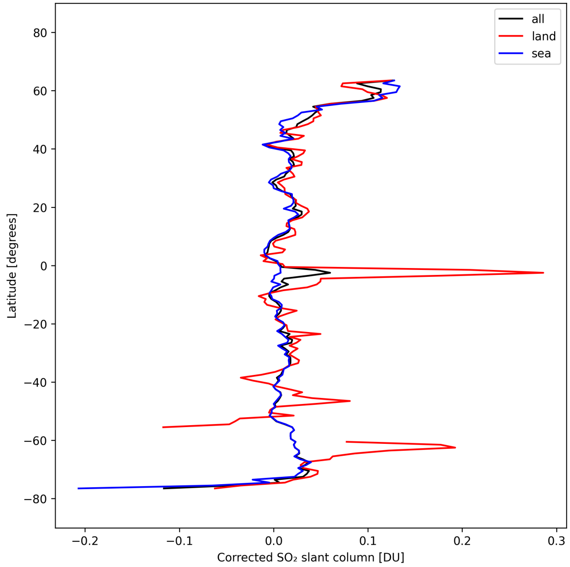
Figure 34: Zonal average of “Corrected SO 2 slant column” for 2025-03-03 to 2025-03-05.
