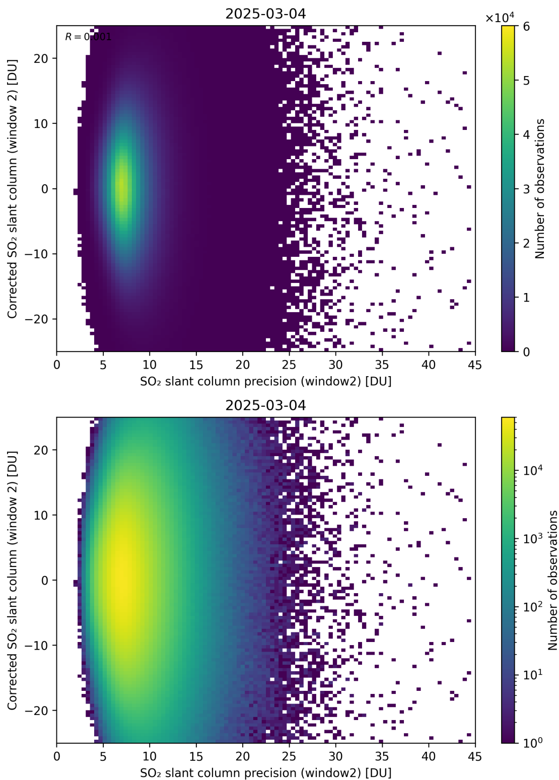
Figure 297: Scatter density plot of “SO 2 slant column precision (window2)” against “Corrected SO 2 slant column (window 2)” for 2025-03-03 to 2025-03-05.
