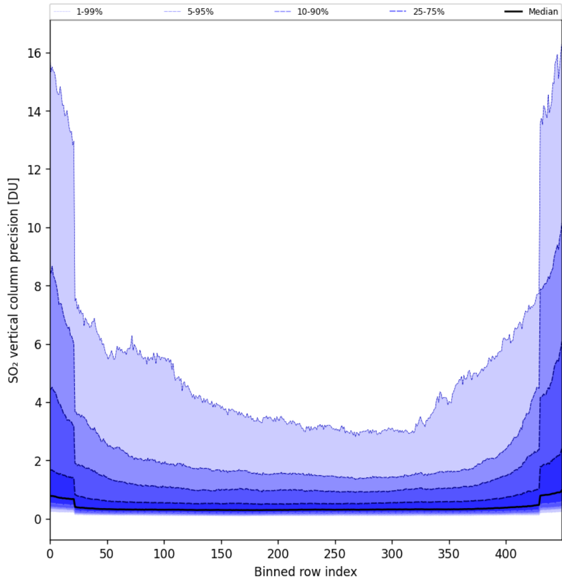
Figure 85: Along track statistics of “SO 2 vertical column precision” for 2025-03-03 to 2025-03-05
