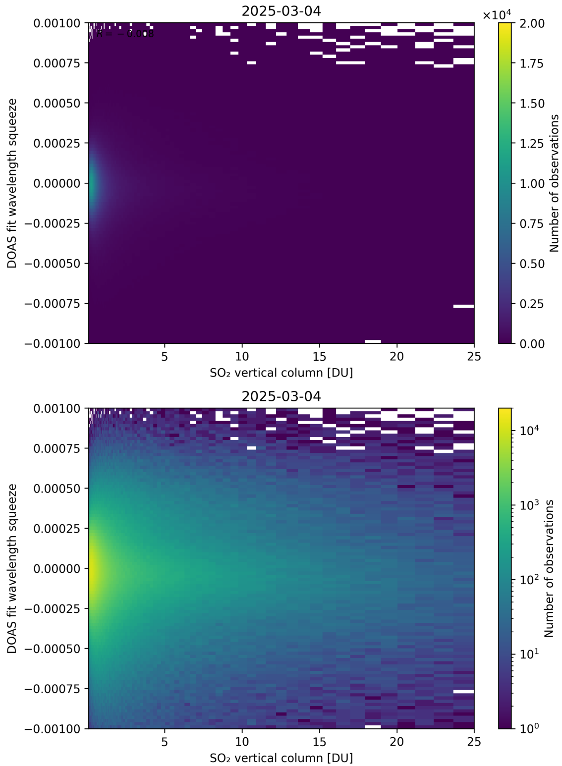
Figure 327: Scatter density plot of “SO 2 vertical column” against “DOAS fit wavelength squeeze” for 2025-03-03 to 2025-03-05.
