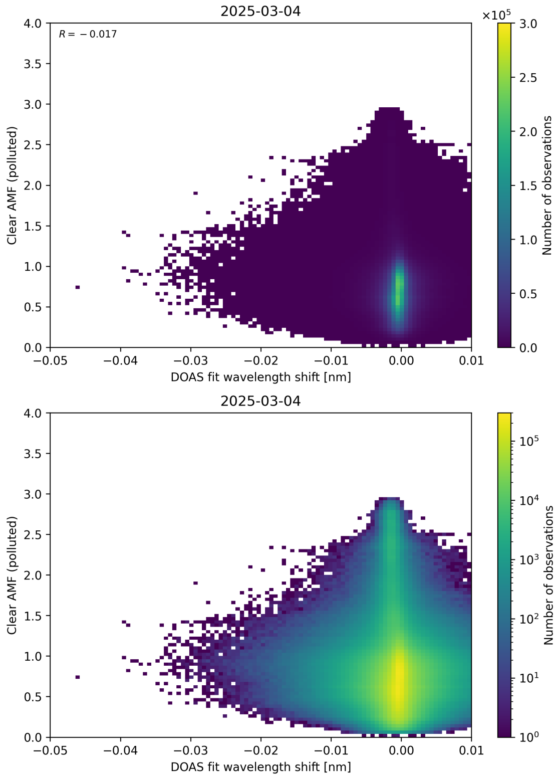
Figure 140: Scatter density plot of “DOAS fit wavelength shift” against “Clear AMF (polluted)” for 2025-03-03 to 2025-03-05.
