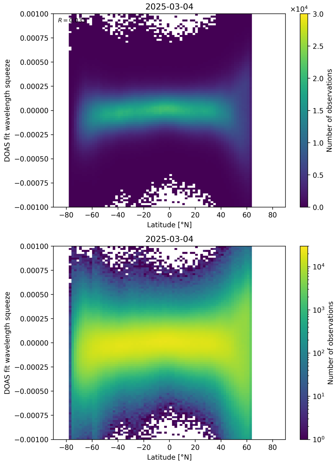
Figure 154: Scatter density plot of “Latitude” against “DOAS fit wavelength squeeze” for 2025-03-03 to 2025-03-05.
