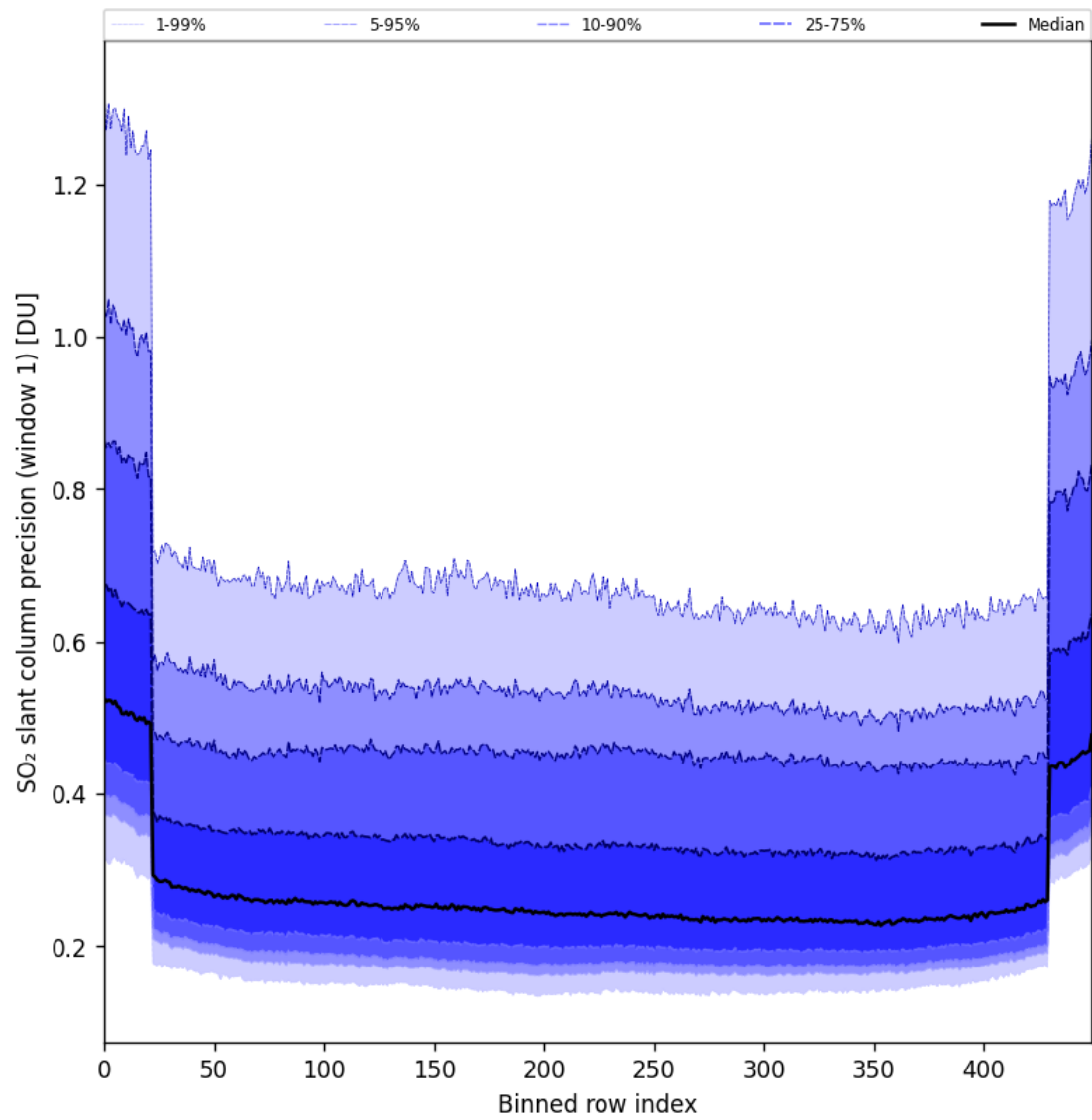
Figure 90: Along track statistics of “SO 2 slant column precision (window 1)” for 2025-03-03 to 2025-03-05
