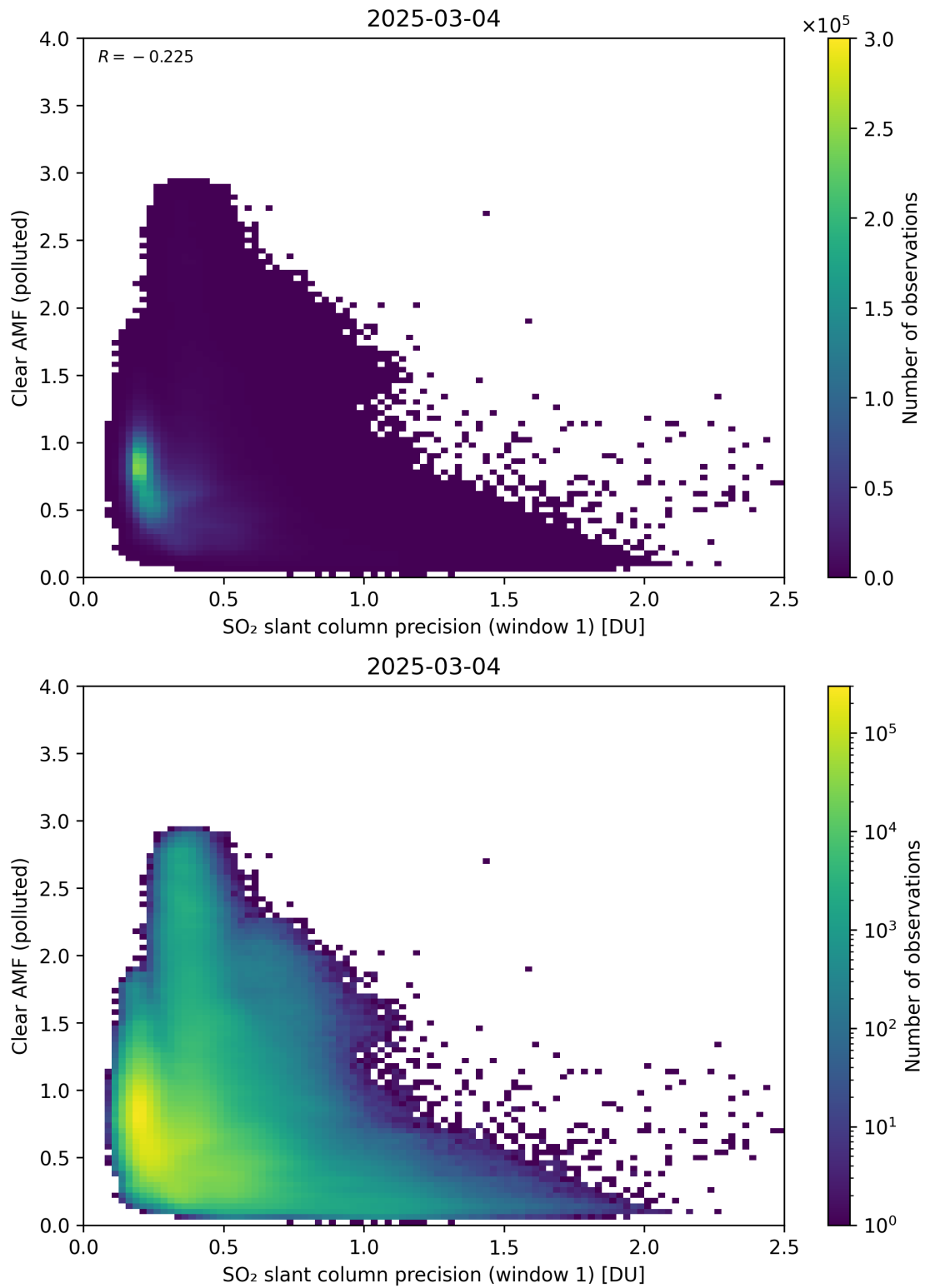
Figure 274: Scatter density plot of “SO 2 slant column precision (window 1)” against “Clear AMF (polluted)” for 2025-03-03 to 2025-03-05.
