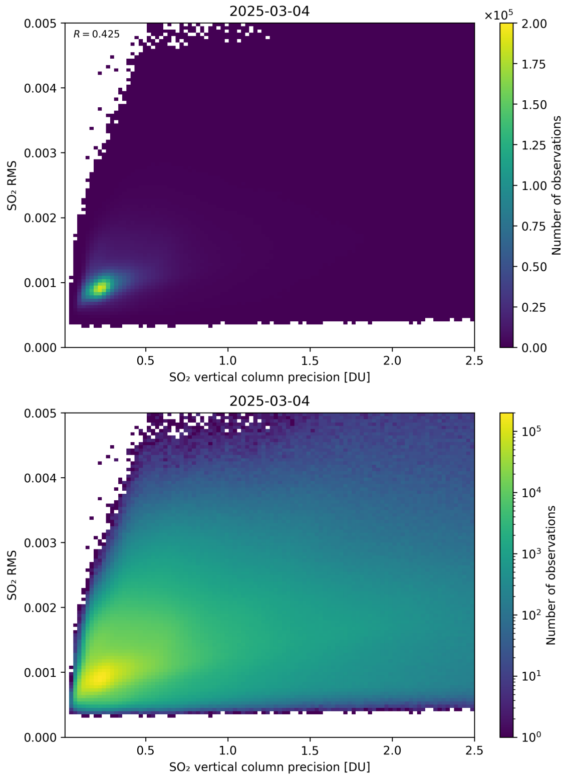
Figure 334: Scatter density plot of “SO 2 vertical column precision” against “SO 2 RMS” for 2025-03-03 to 2025-03-05.
