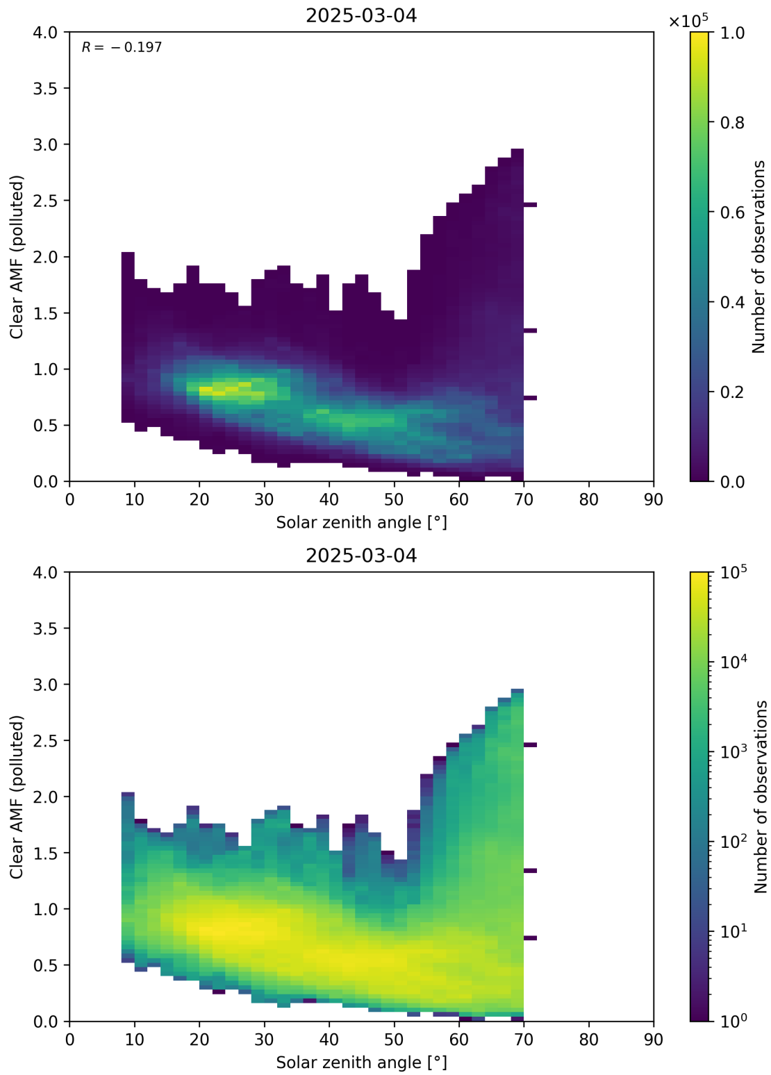
Figure 178: Scatter density plot of “Solar zenith angle” against “Clear AMF (polluted)” for 2025-03-03 to 2025-03-05.
