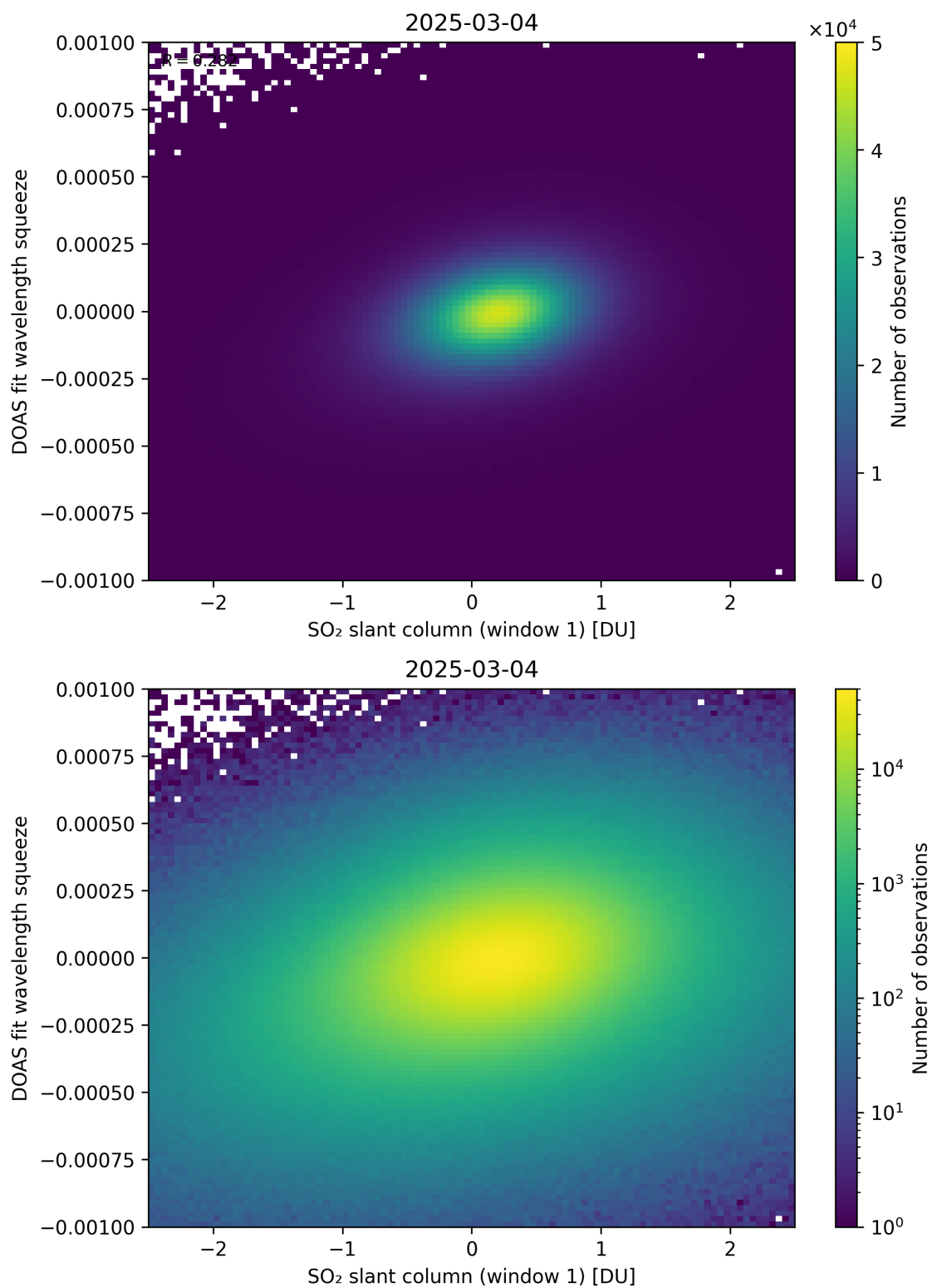
Figure 266: Scatter density plot of “SO 2 slant column (window 1)” against “DOAS fit wavelength squeeze” for 2025-03-03 to 2025-03-05.
