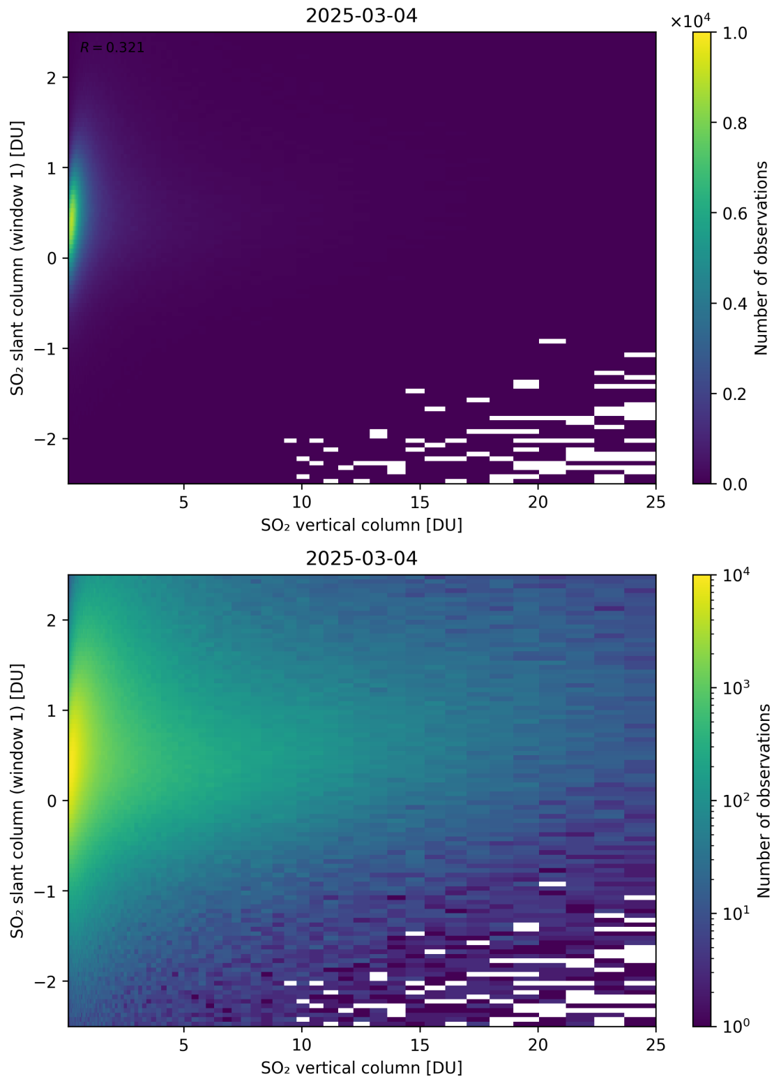
Figure 354: Scatter density plot of “SO 2 vertical column” against “SO 2 slant column (window 1)” for 2025-03-03 to 2025-03-05.
