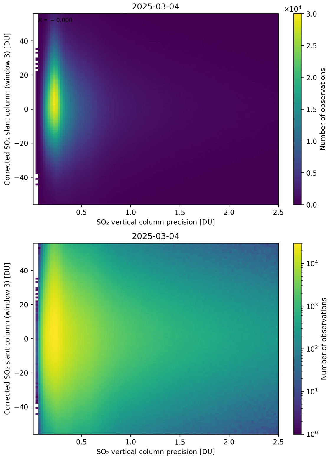
Figure 340: Scatter density plot of “SO 2 vertical column precision” against “Corrected SO 2 slant column (window 3)” for 2025-03-03 to 2025-03-05.
