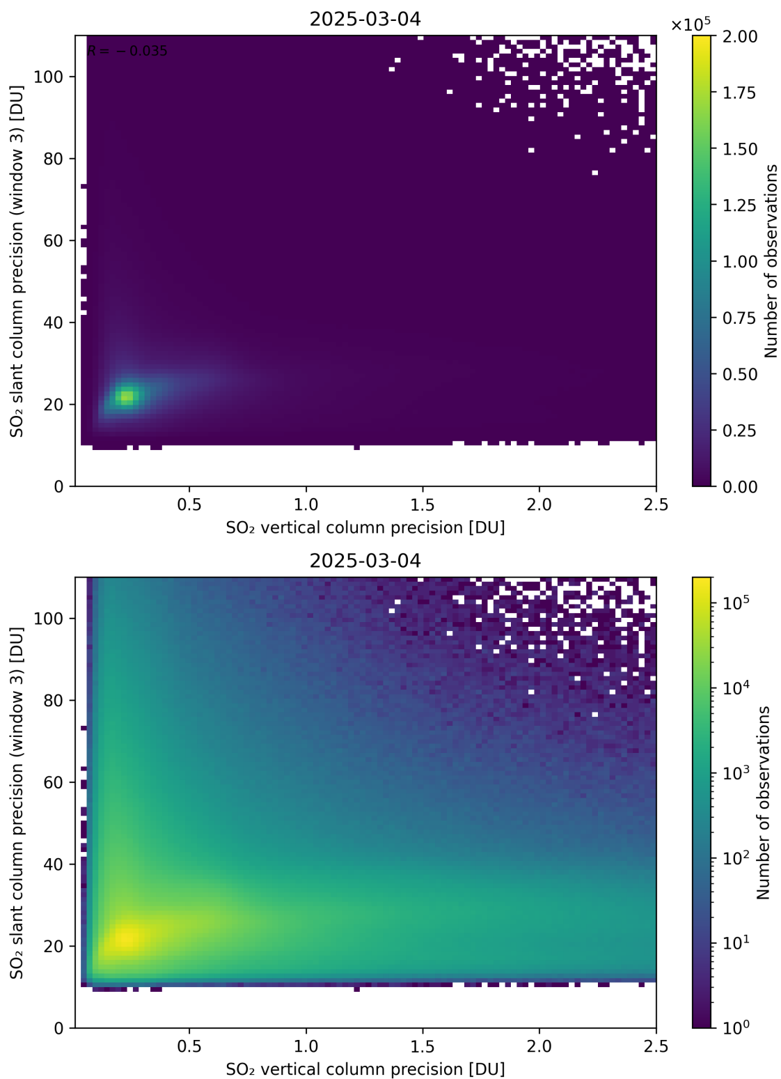
Figure 345: Scatter density plot of “SO 2 vertical column precision” against “SO 2 slant column precision (window 3)” for 2025-03-03 to 2025-03-05.
