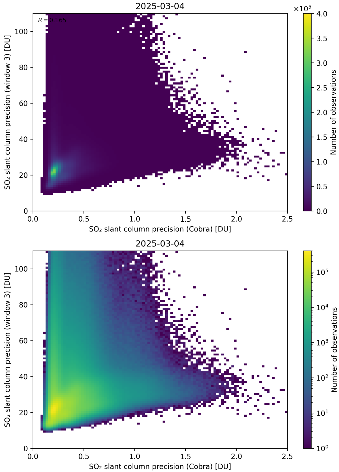
Figure 212: Scatter density plot of “SO 2 slant column precision (Cobra)” against “SO 2 slant column precision (window 3)” for 2025-03-03 to 2025-03-05.
