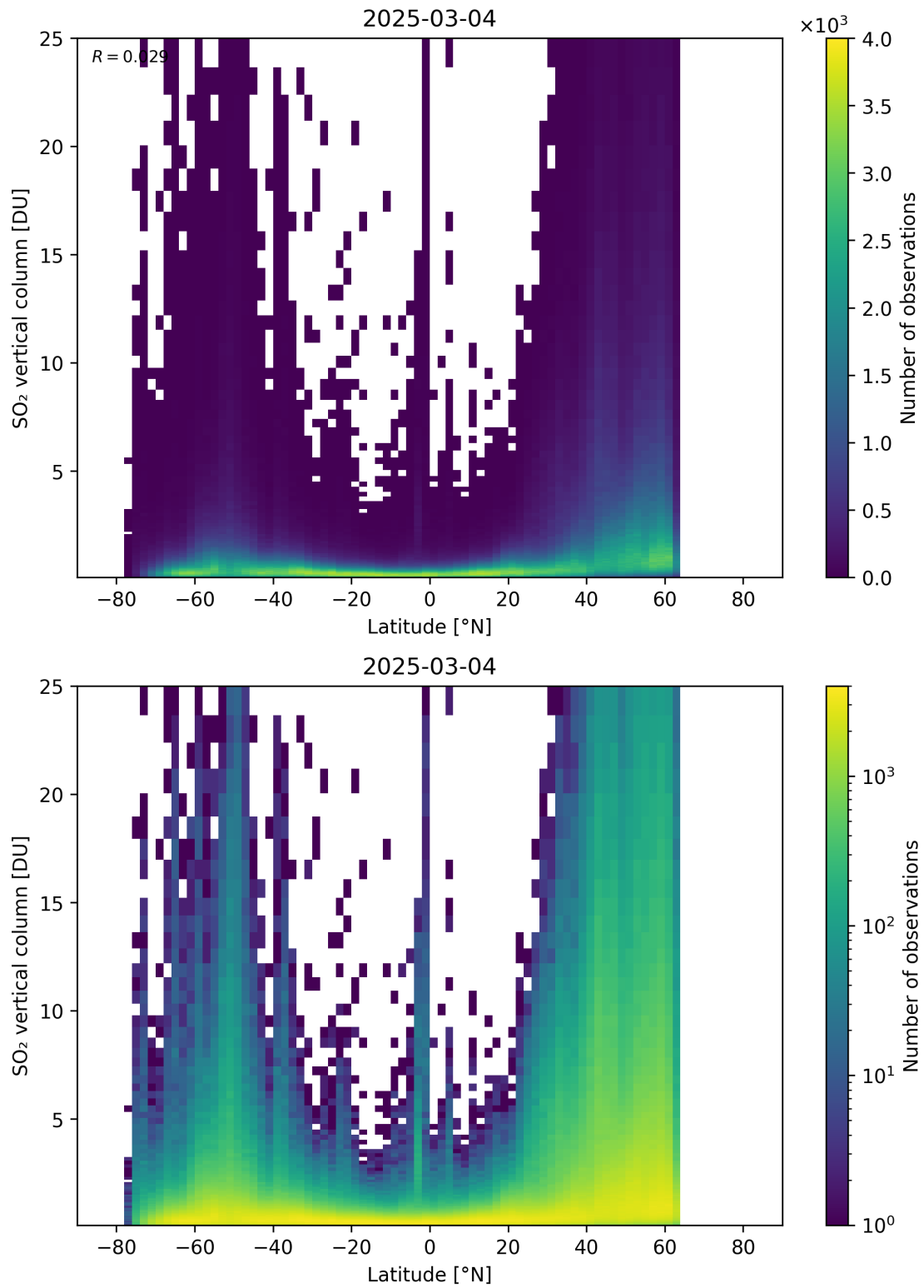
Figure 169: Scatter density plot of “Latitude” against “SO 2 vertical column” for 2025-03-03 to 2025-03-05.
