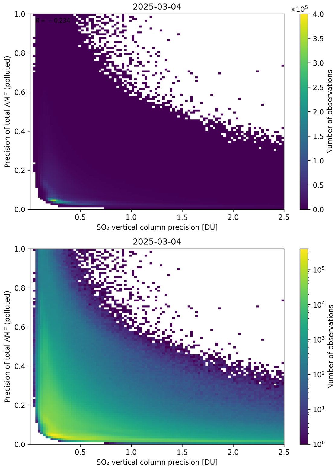
Figure 347: Scatter density plot of “SO 2 vertical column precision” against “Precision of total AMF (polluted)” for 2025-03-03 to 2025-03-05.
