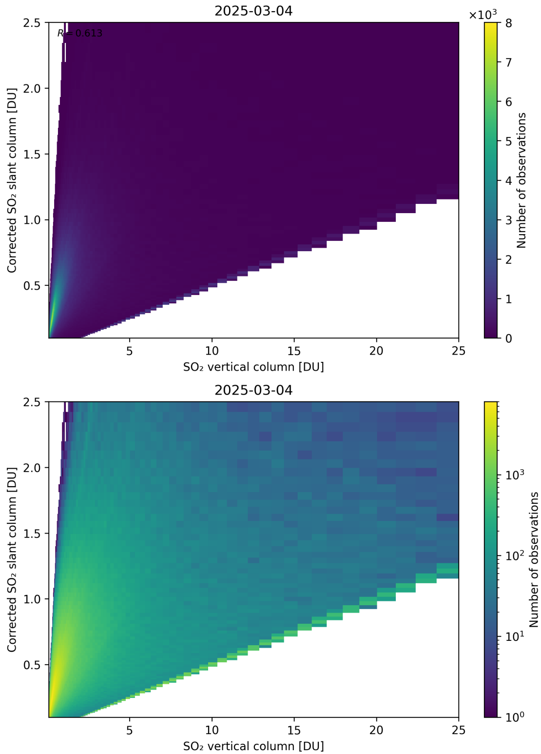
Figure 351: Scatter density plot of “SO 2 vertical column” against “Corrected SO 2 slant column” for 2025-03-03 to 2025-03-05.
