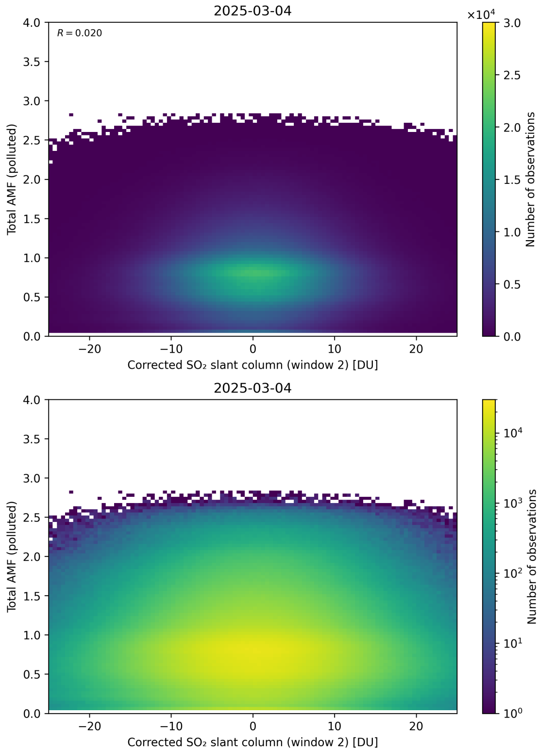
Figure 253: Scatter density plot of “Corrected SO 2 slant column (window 2)” against “Total AMF (polluted)” for 2025-03-03 to 2025-03-05.
