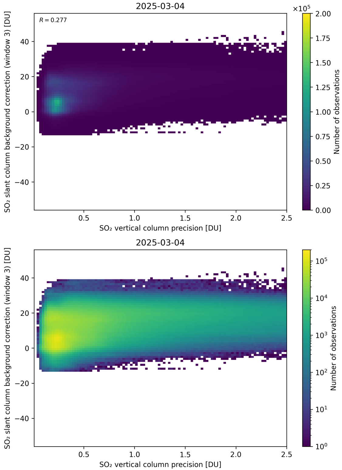
Figure 331: Scatter density plot of “SO 2 vertical column precision” against “SO 2 slant column background correction (window 3)” for 2025-03-03 to 2025-03-05.
