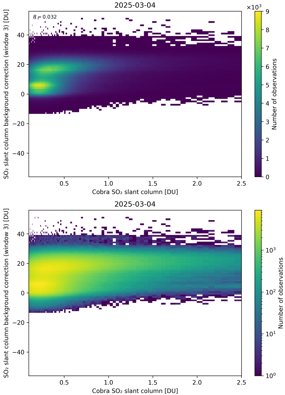
Figure 195: Scatter density plot of “Cobra SO 2 slant column” against “SO 2 slant column background correction (window 3)” for 2025-03-03 to 2025-03-05.
