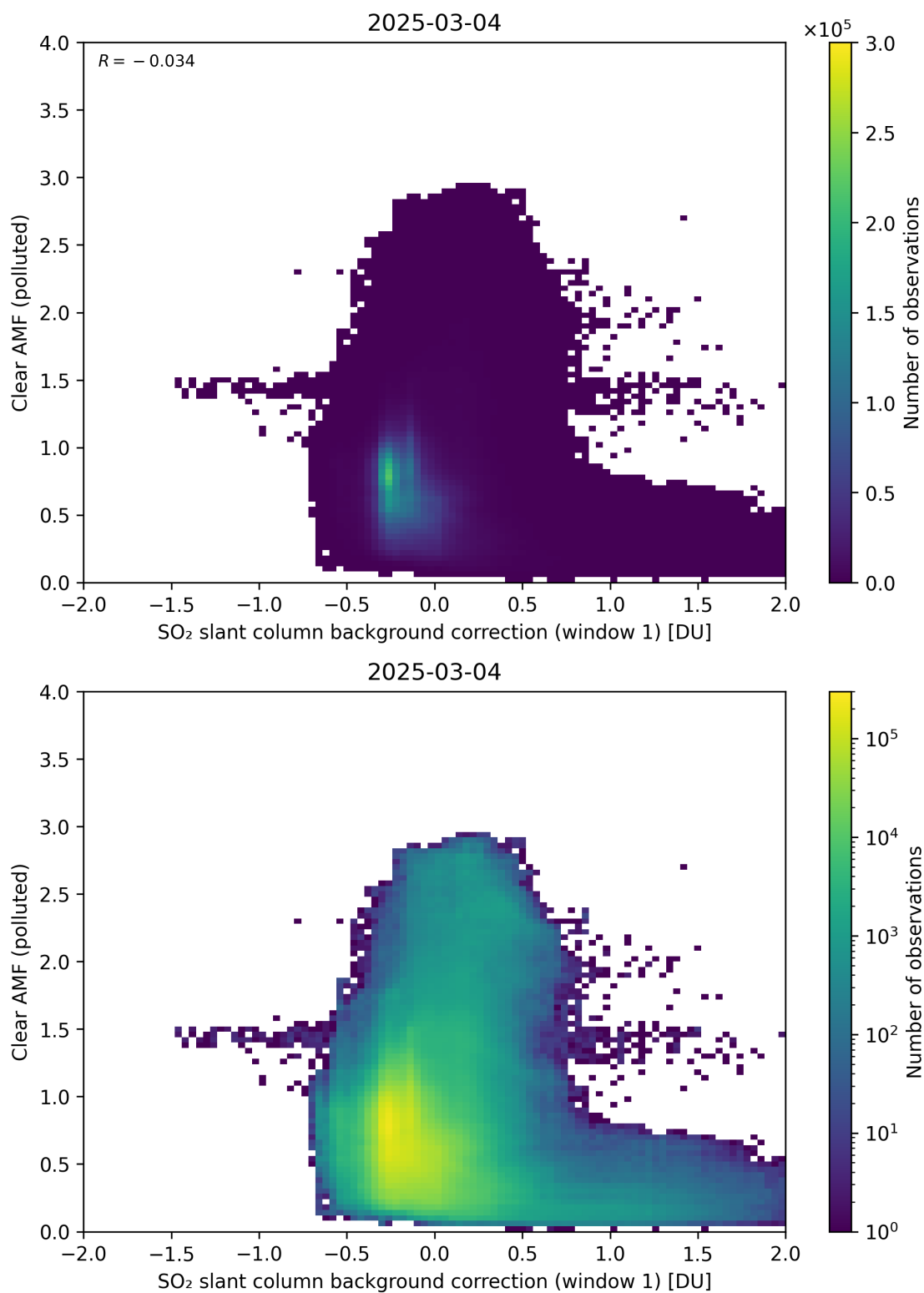
Figure 114: Scatter density plot of “SO 2 slant column background correction (window 1)” against “Clear AMF (polluted)” for 2025-03-03 to 2025-03-05.
