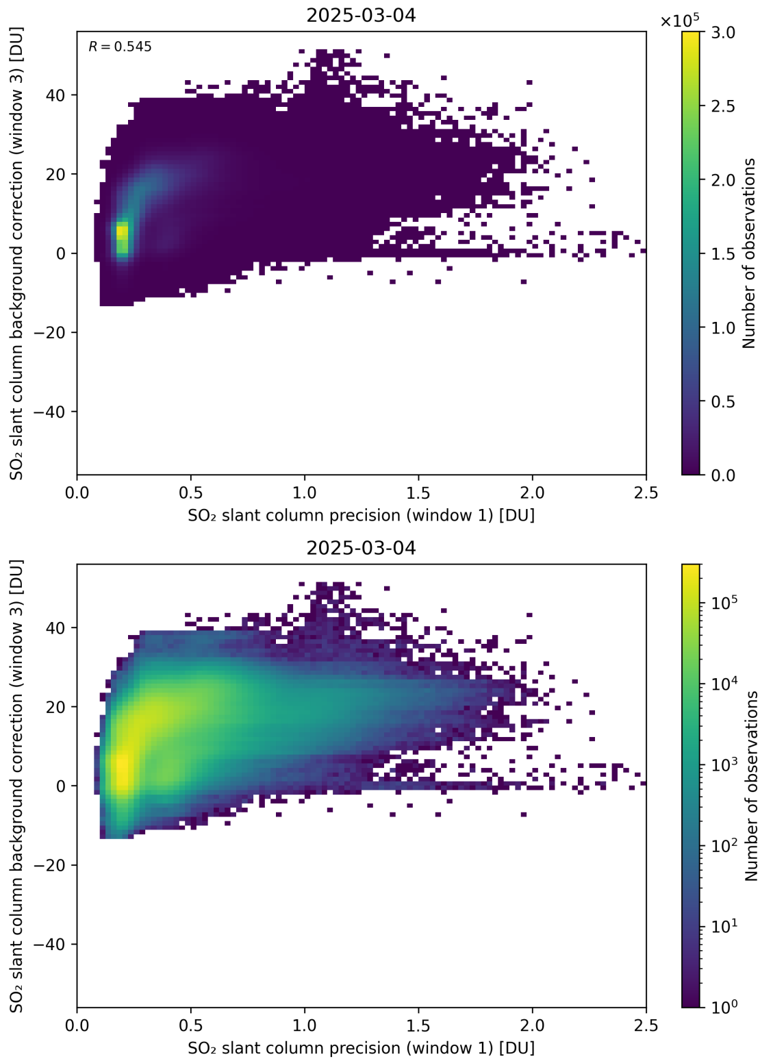
Figure 270: Scatter density plot of “SO 2 slant column precision (window 1)” against “SO 2 slant column background correction (window 3)” for 2025-03-03 to 2025-03-05.
