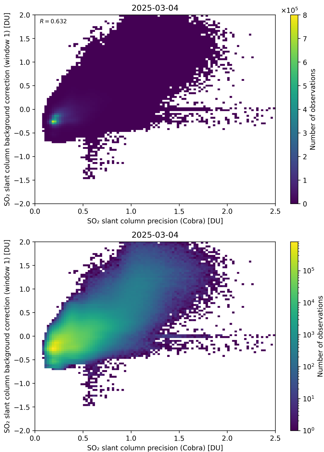
Figure 199: Scatter density plot of “SO 2 slant column precision (Cobra)” against “SO 2 slant column background correction (window 1)” for 2025-03-03 to 2025-03-05.
