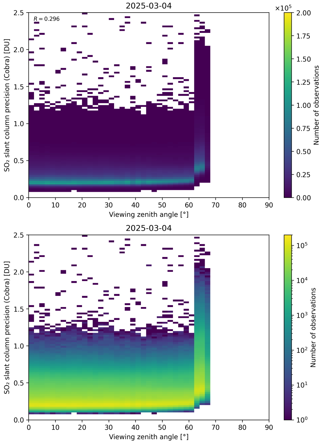
Figure 372: Scatter density plot of “Viewing zenith angle” against “SO 2 slant column precision (Cobra)” for 2025-03-03 to 2025-03-05.
