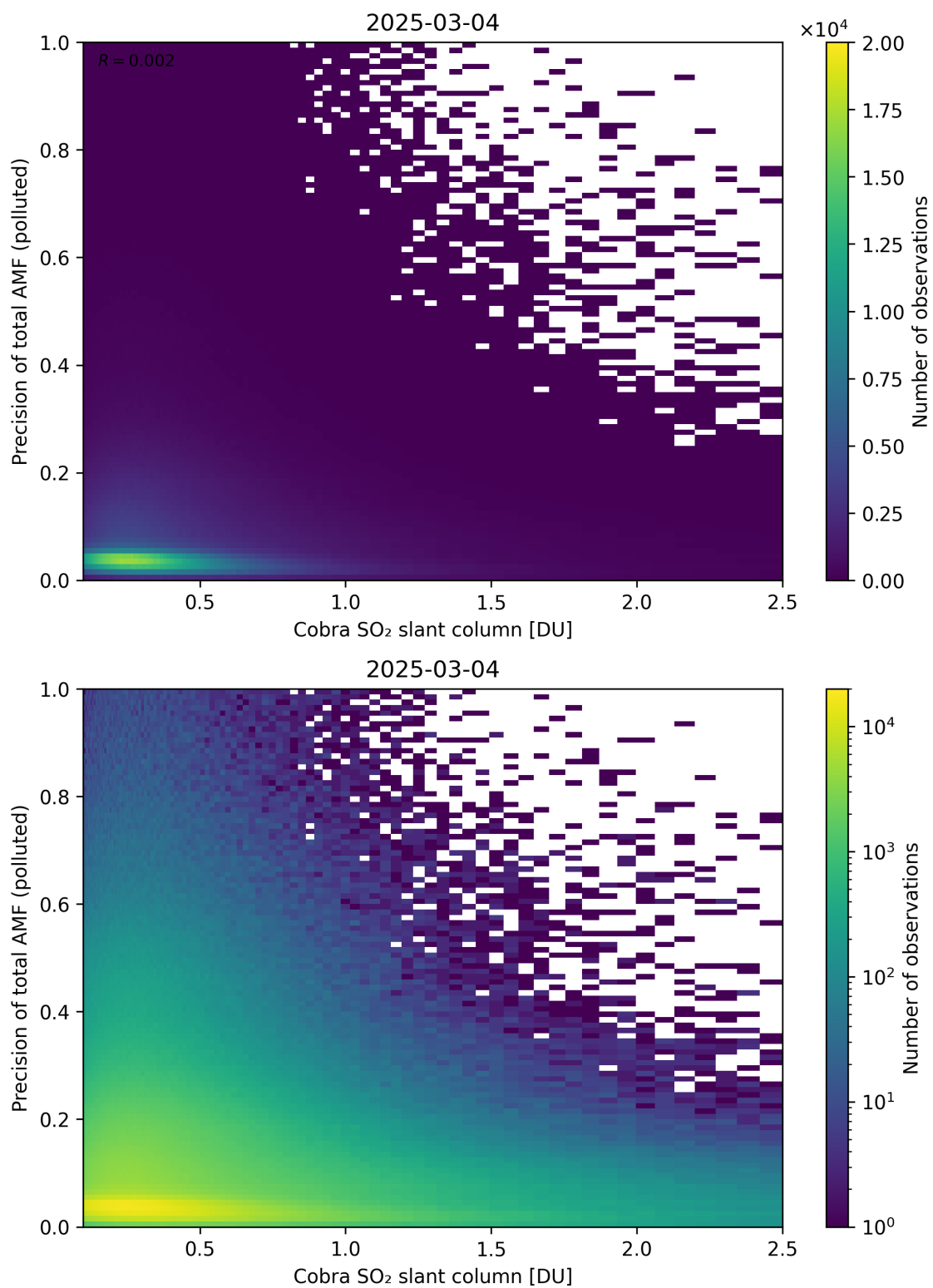
Figure 225: Scatter density plot of “Cobra SO 2 slant column” against “Precision of total AMF (polluted)” for 2025-03-03 to 2025-03-05.
