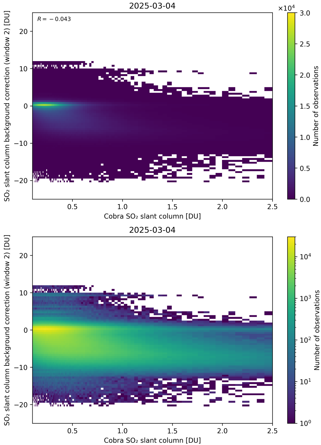
Figure 194: Scatter density plot of “Cobra SO 2 slant column” against “SO 2 slant column background correction (window 2)” for 2025-03-03 to 2025-03-05.
