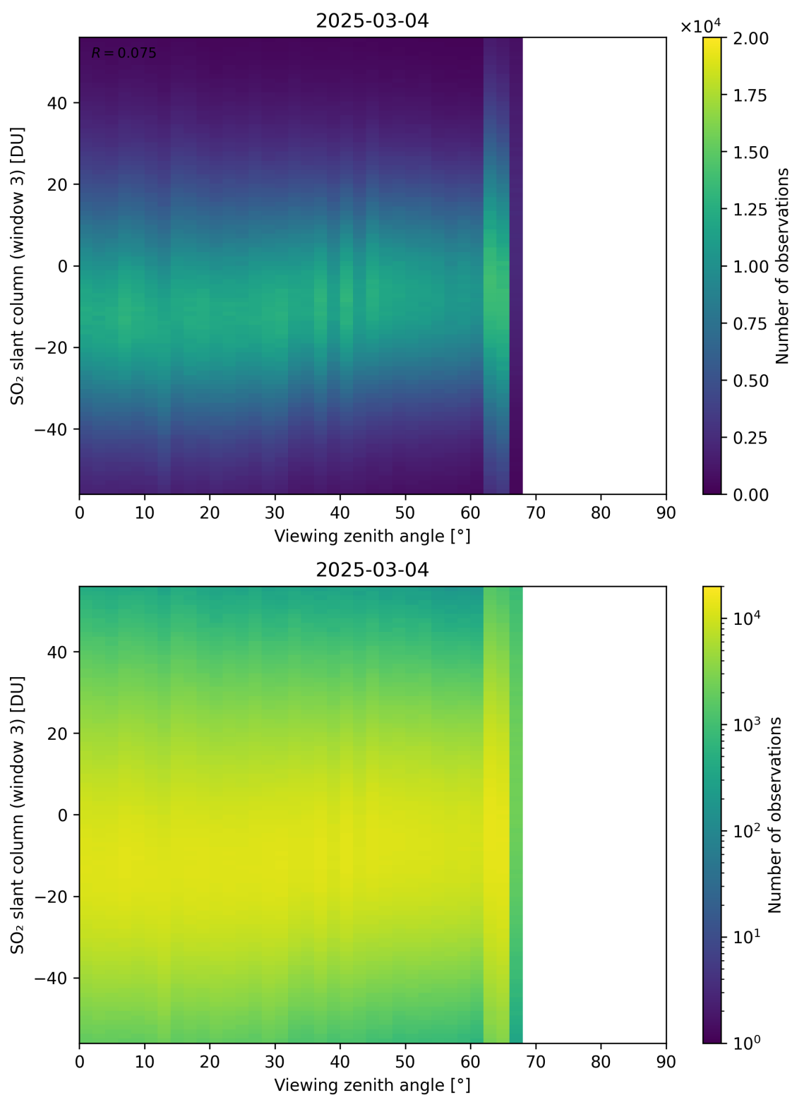
Figure 379: Scatter density plot of “Viewing zenith angle” against “SO 2 slant column (window 3)” for 2025-03-03 to 2025-03-05.
