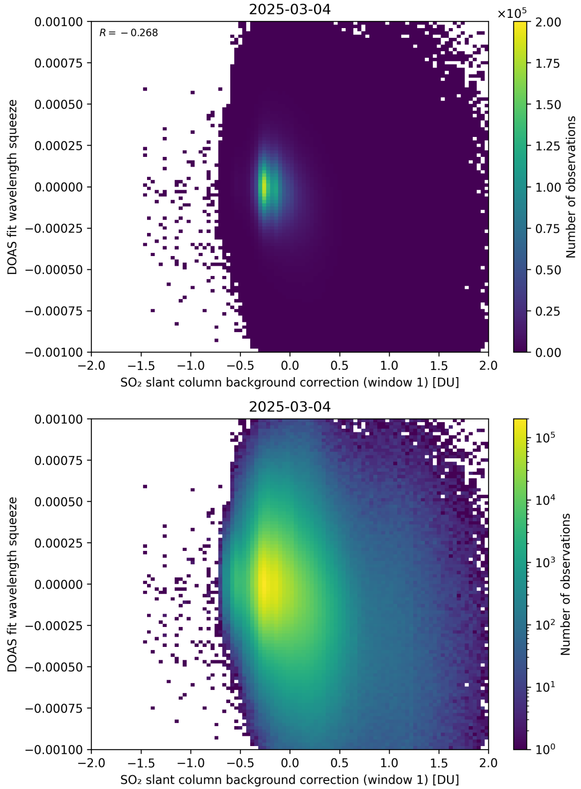
Figure 112: Scatter density plot of “SO 2 slant column background correction (window 1)” against “DOAS fit wavelength squeeze” for 2025-03-03 to 2025-03-05.
