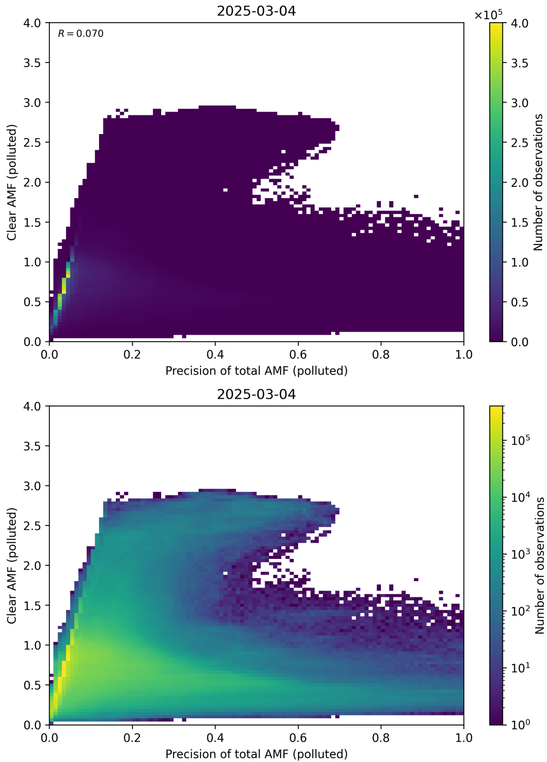
Figure 320: Scatter density plot of “Precision of total AMF (polluted)” against “Clear AMF (polluted)” for 2025-03-03 to 2025-03-05.
