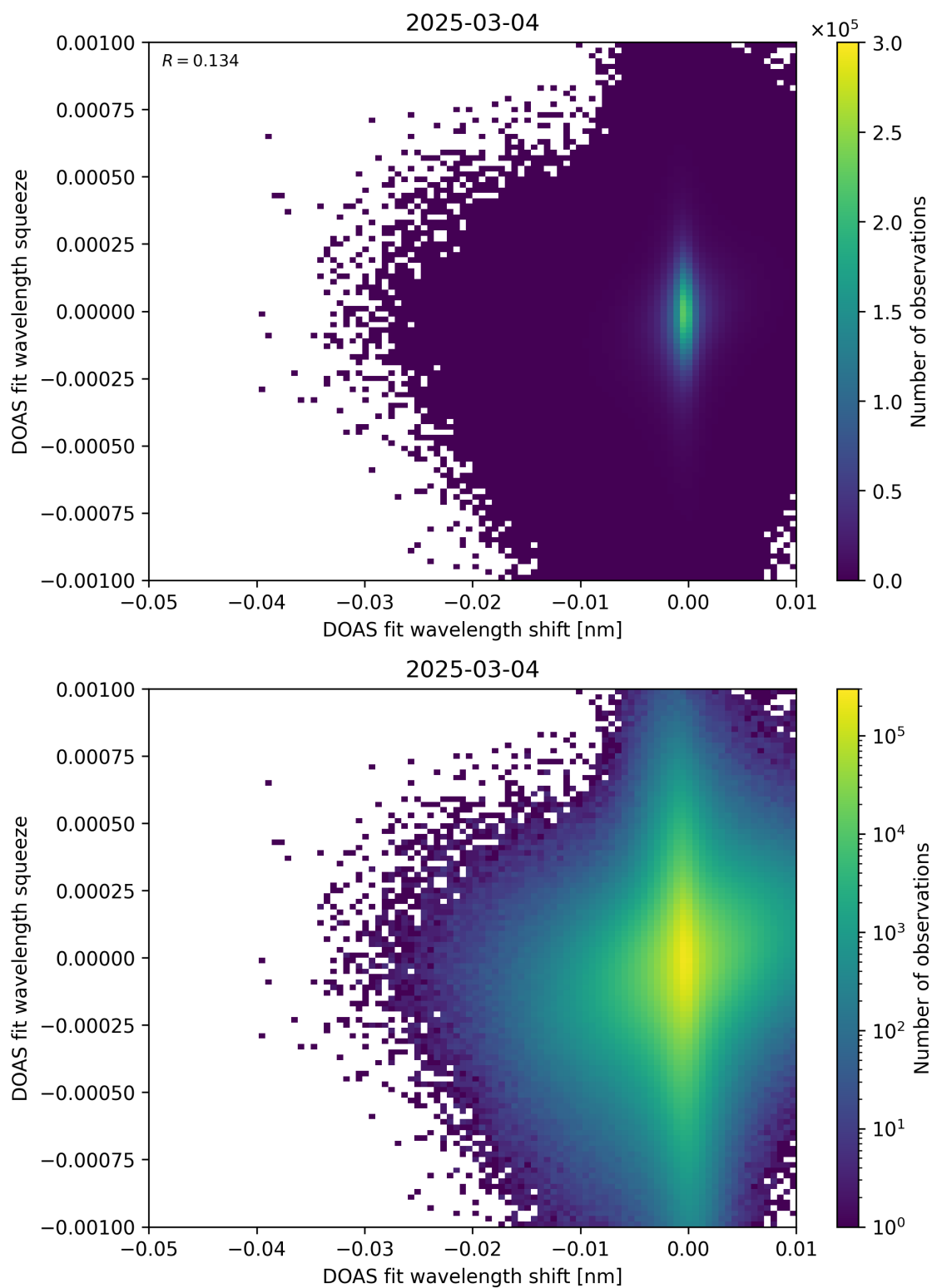
Figure 138: Scatter density plot of “DOAS fit wavelength shift” against “DOAS fit wavelength squeeze” for 2025-03-03 to 2025-03-05.
