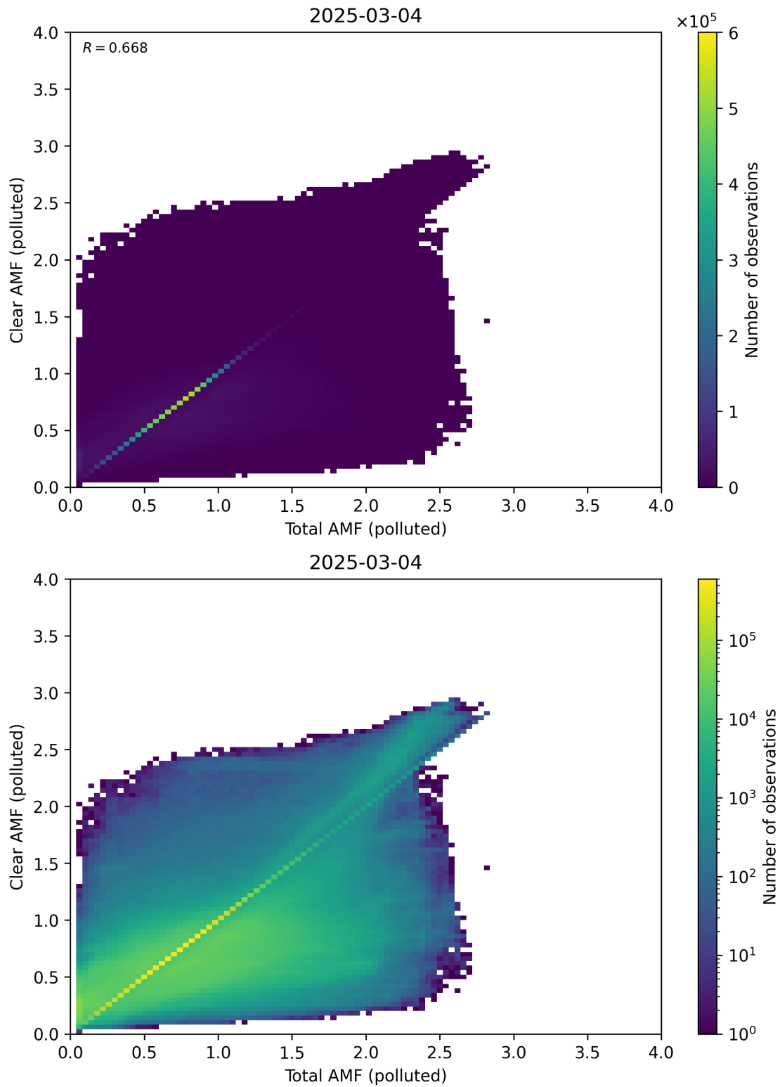
Figure 321: Scatter density plot of “Total AMF (polluted)” against “Clear AMF (polluted)” for 2025-03-03 to 2025-03-05.
