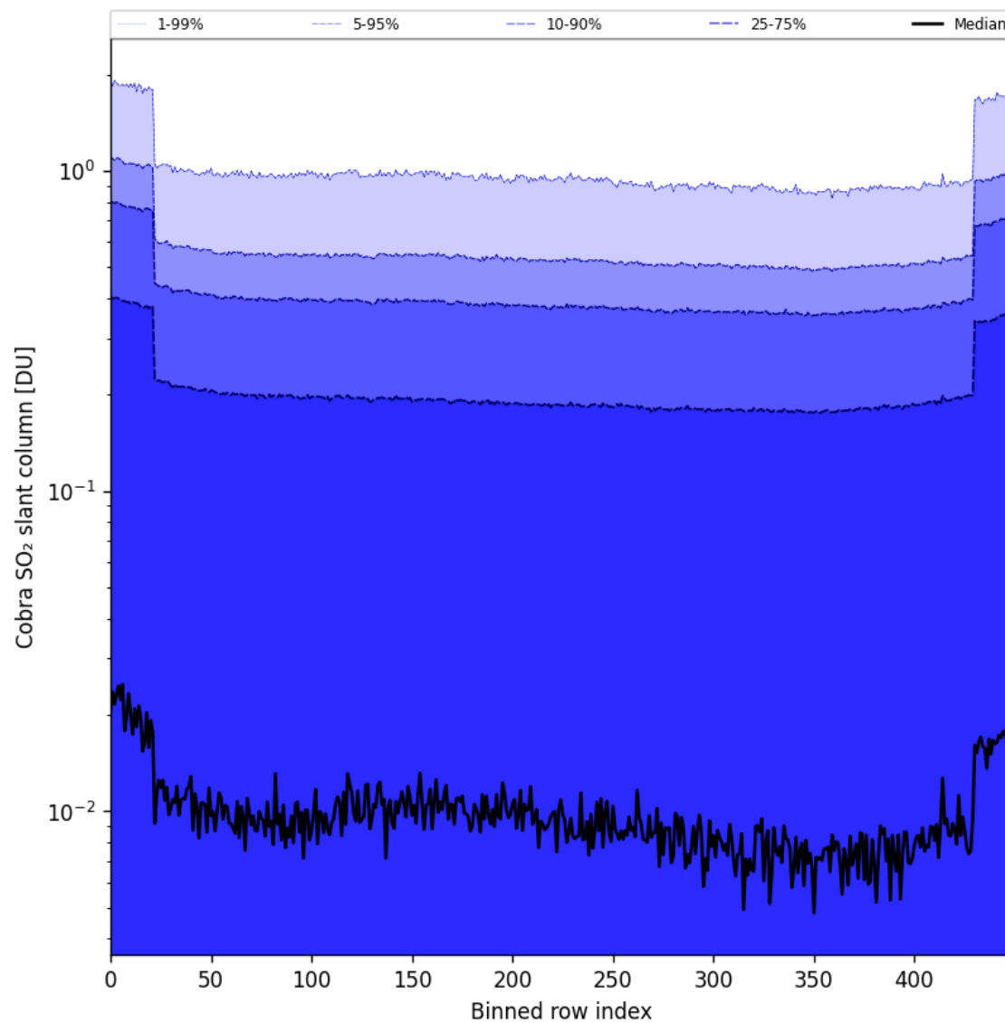
Figure 87: Along track statistics of “Cobra SO 2 slant column” for 2025-03-03 to 2025-03-05
