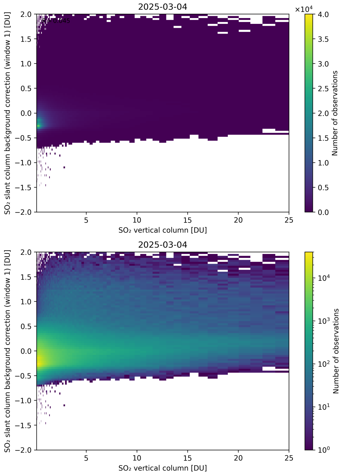
Figure 323: Scatter density plot of “SO 2 vertical column” against “SO 2 slant column background correction (window 1)” for 2025-03-03 to 2025-03-05.
