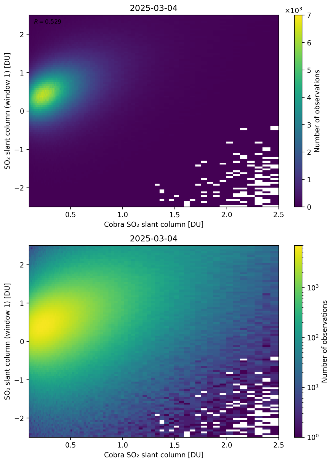
Figure 219: Scatter density plot of “Cobra SO 2 slant column” against “SO 2 slant column (window 1)” for 2025-03-03 to 2025-03-05.
