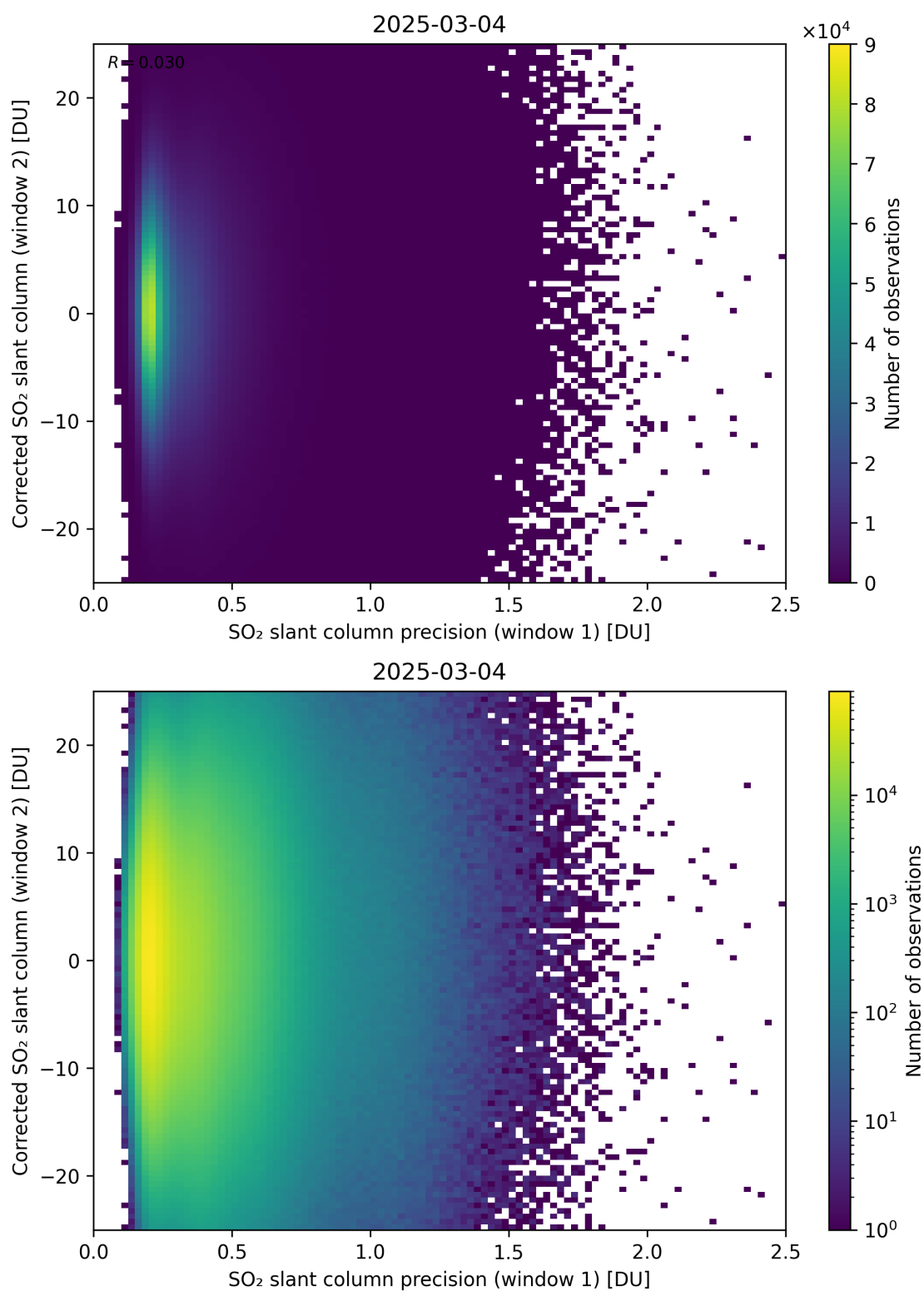
Figure 275: Scatter density plot of “SO 2 slant column precision (window 1)” against “Corrected SO 2 slant column (window 2)” for 2025-03-03 to 2025-03-05.
