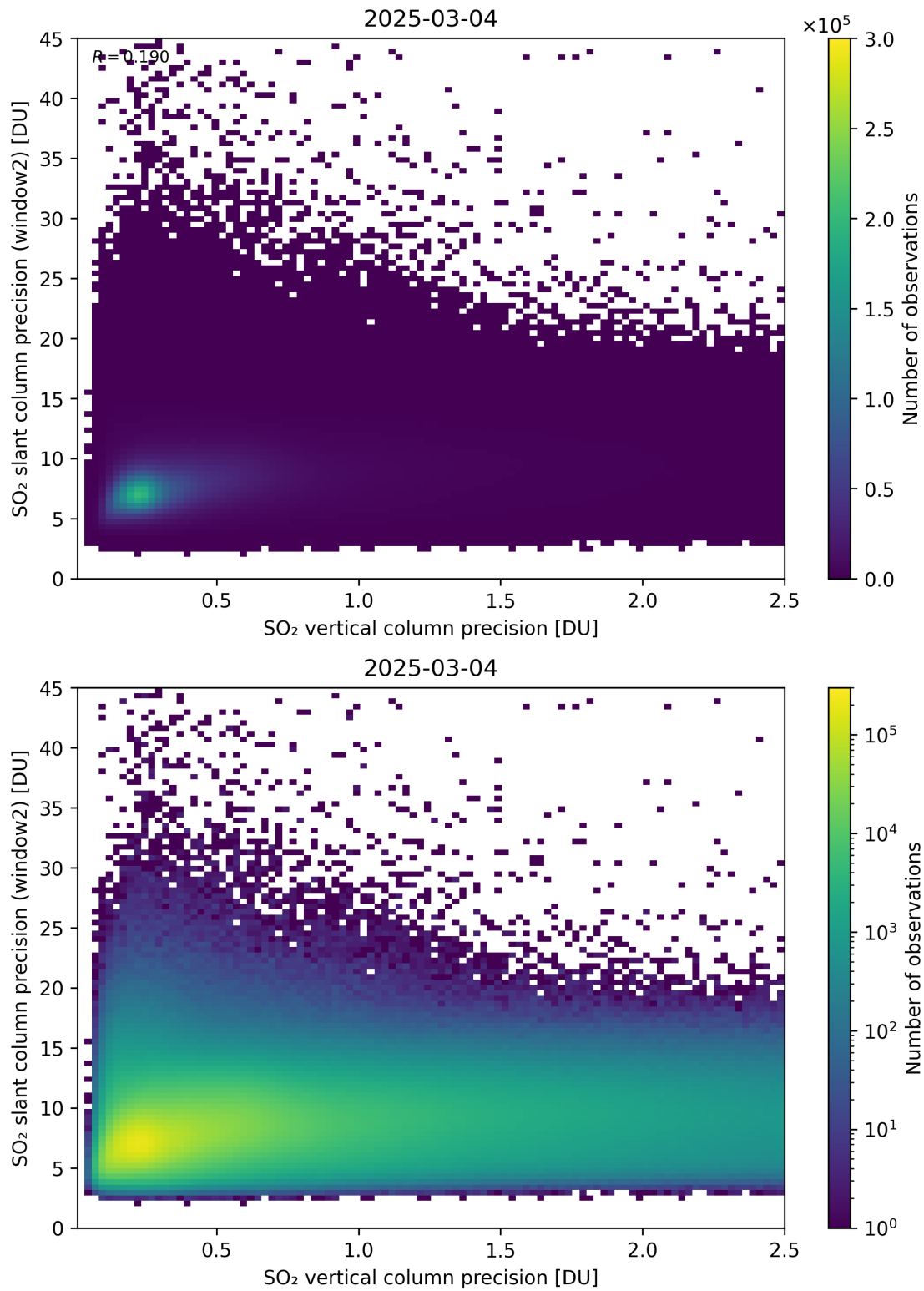
Figure 343: Scatter density plot of “SO 2 vertical column precision” against “SO 2 slant column precision (window2)” for 2025-03-03 to 2025-03-05.
