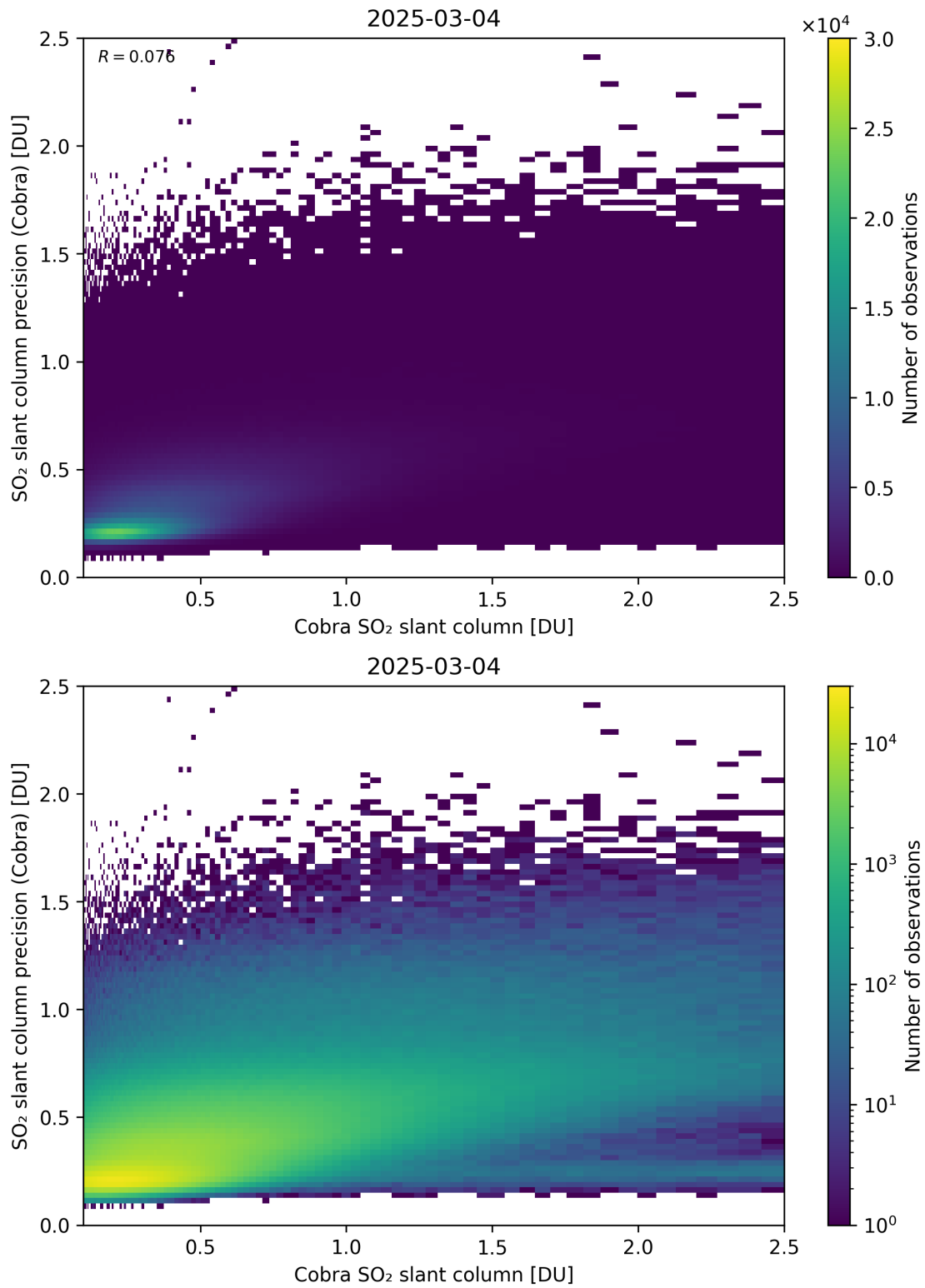
Figure 216: Scatter density plot of “Cobra SO 2 slant column” against “SO 2 slant column precision (Cobra)” for 2025-03-03 to 2025-03-05.
