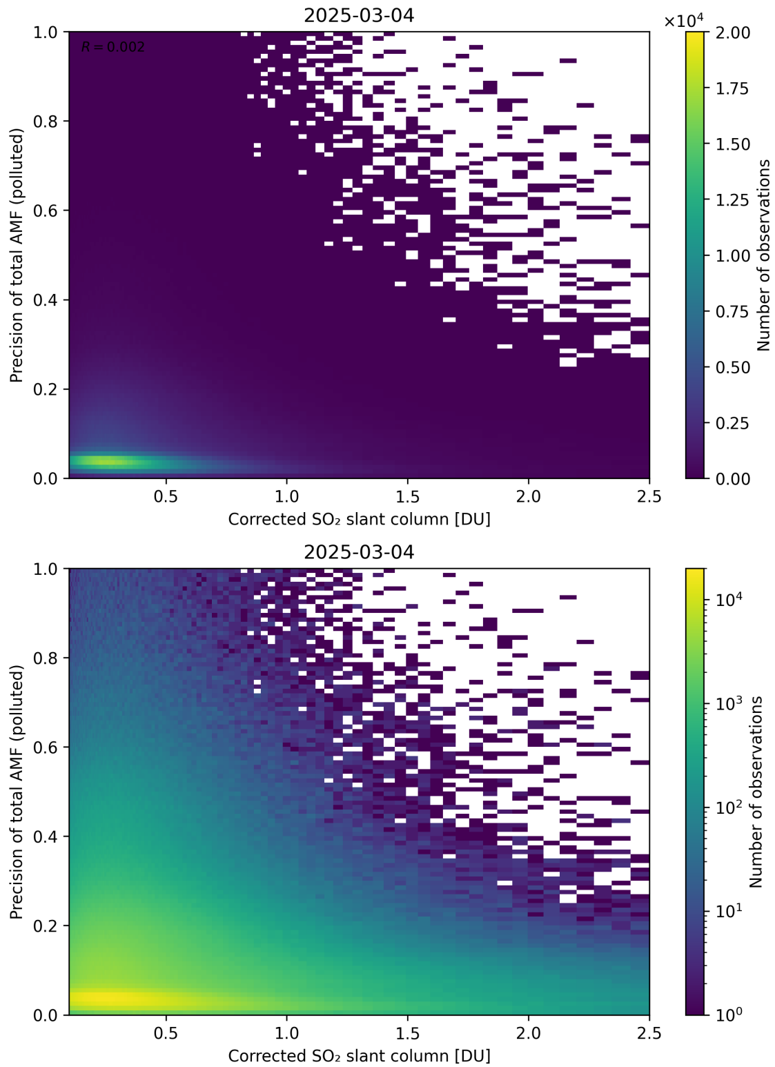
Figure 243: Scatter density plot of “Corrected SO 2 slant column” against “Precision of total AMF (polluted)” for 2025-03-03 to 2025-03-05.
