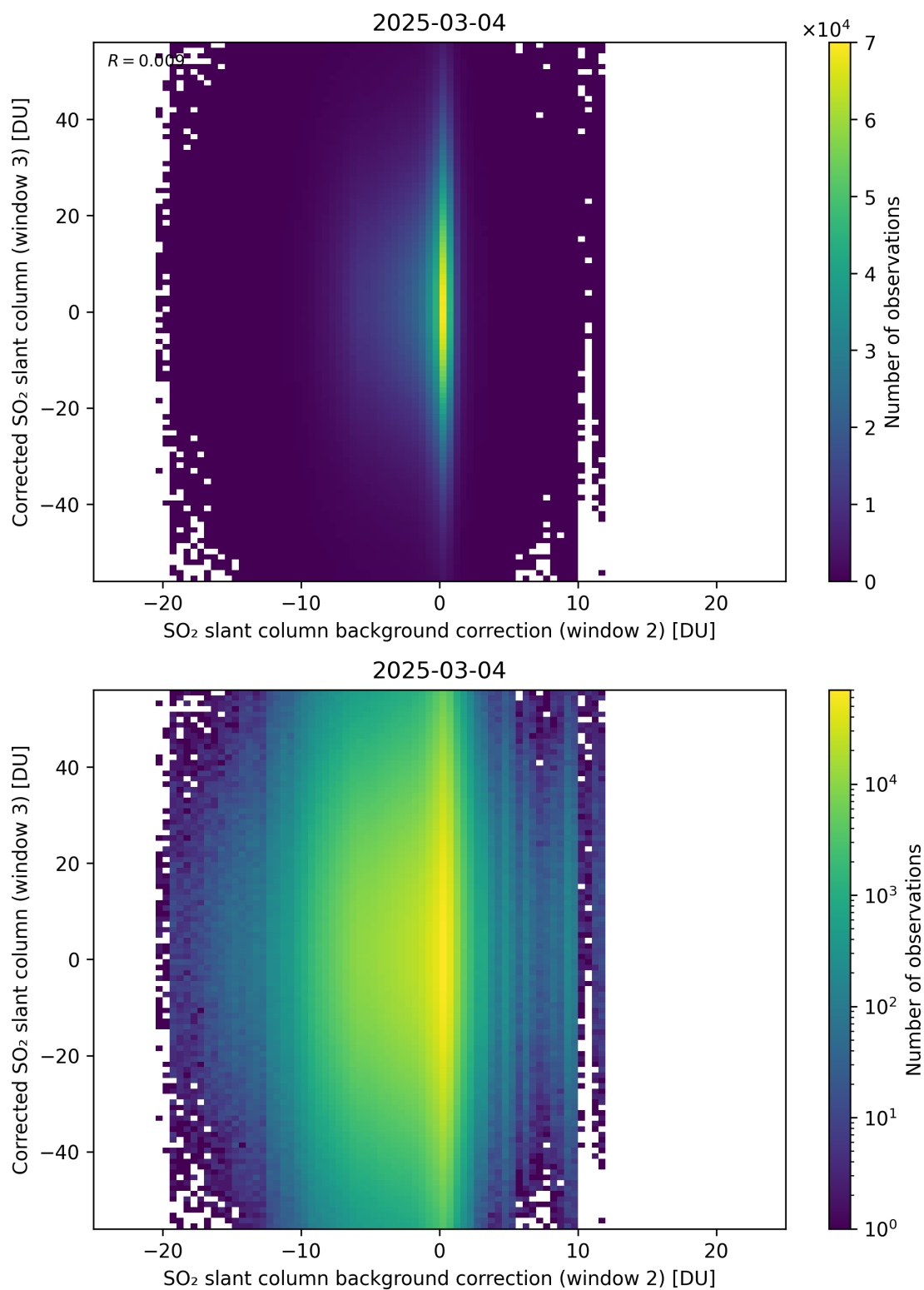
Figure 127: Scatter density plot of “SO 2 slant column background correction (window 2)” against “Corrected SO 2 slant column (window 3)” for 2025-03-03 to 2025-03-05.
