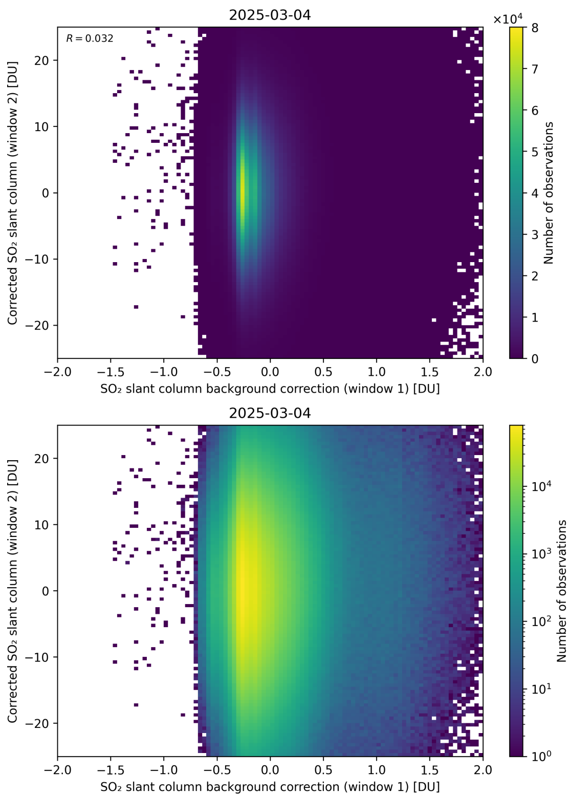
Figure 115: Scatter density plot of “SO 2 slant column background correction (window 1)” against “Corrected SO 2 slant column (window 2)” for 2025-03-03 to 2025-03-05.
