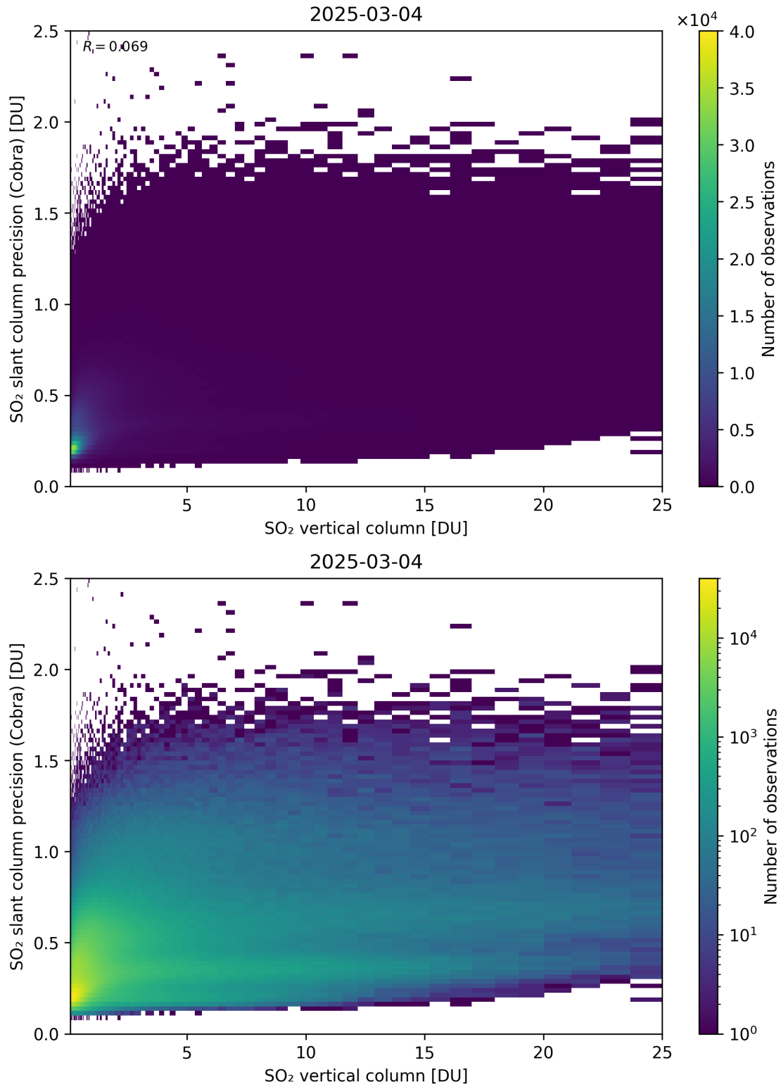
Figure 350: Scatter density plot of “SO 2 vertical column” against “SO 2 slant column precision (Cobra)” for 2025-03-03 to 2025-03-05.
