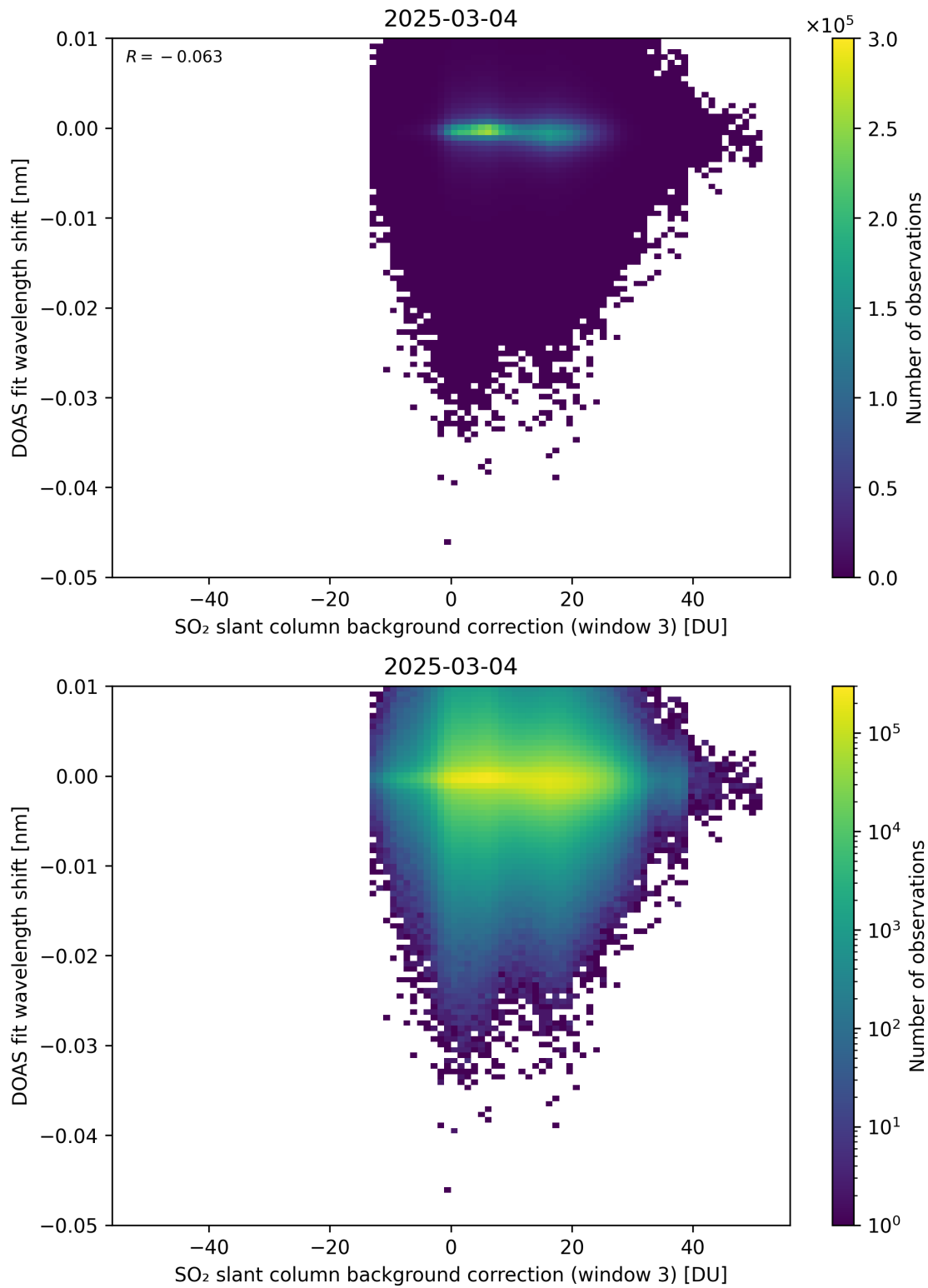
Figure 132: Scatter density plot of “SO 2 slant column background correction (window 3)” against “DOAS fit wavelength shift” for 2025-03-03 to 2025-03-05.
