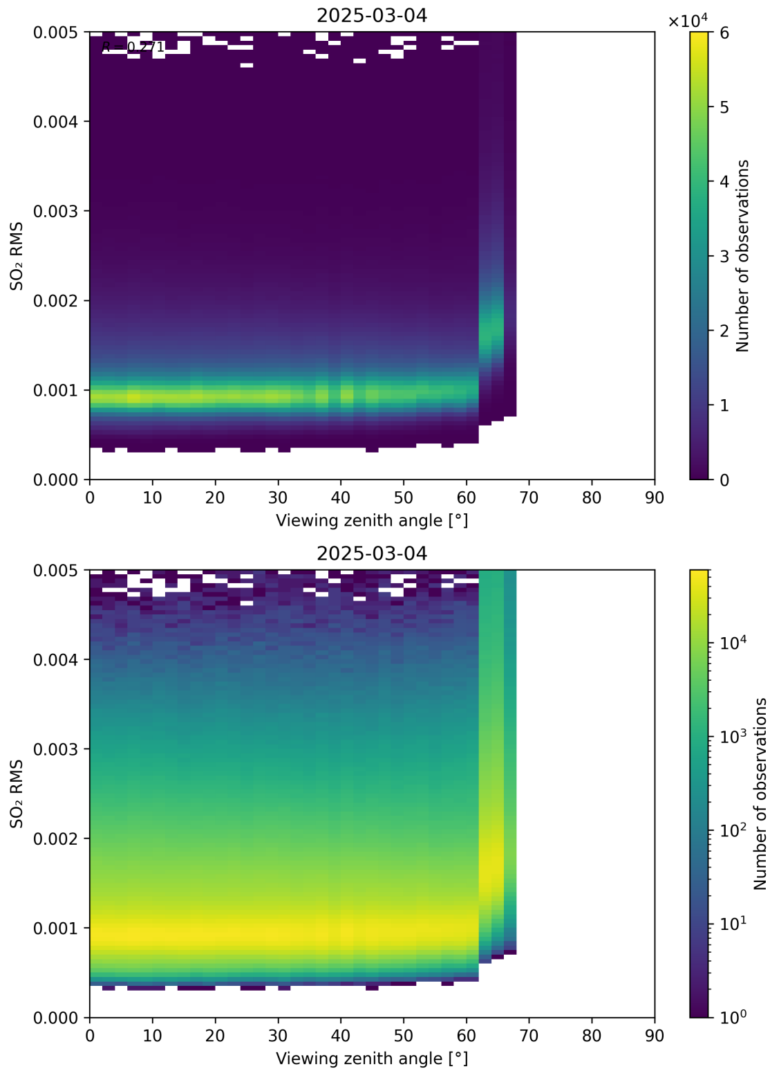
Figure 367: Scatter density plot of “Viewing zenith angle” against “SO 2 RMS” for 2025-03-03 to 2025-03-05.
