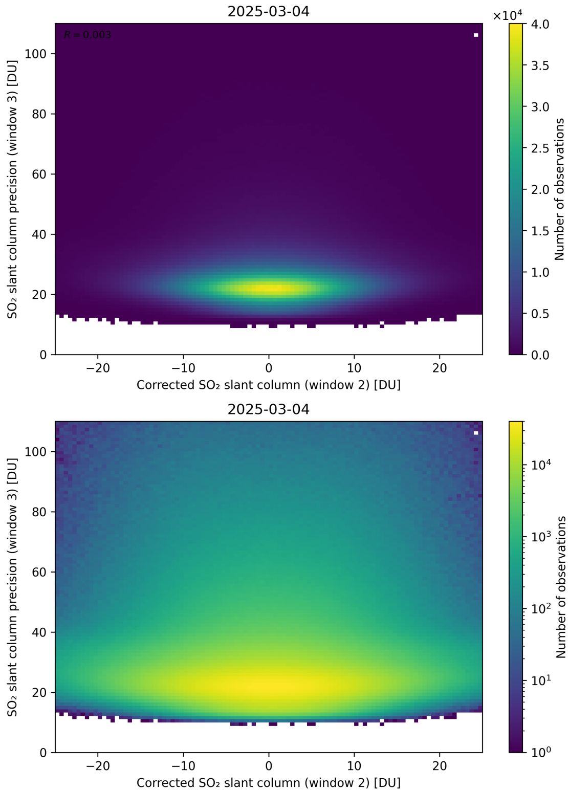
Figure 252: Scatter density plot of “Corrected SO 2 slant column (window 2)” against “SO 2 slant column precision (window 3)” for 2025-03-03 to 2025-03-05.
