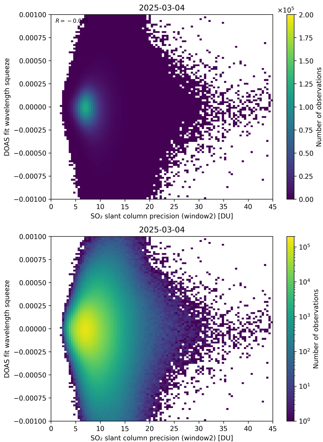
Figure 294: Scatter density plot of “SO 2 slant column precision (window2)” against “DOAS fit wavelength squeeze” for 2025-03-03 to 2025-03-05.
