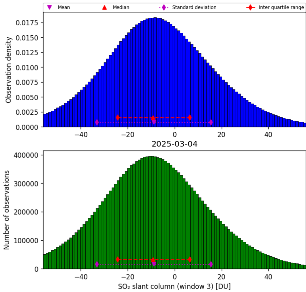
Figure 71: Histogram of “SO 2 slant column (window 3)” for 2025-03-03 to 2025-03-05
