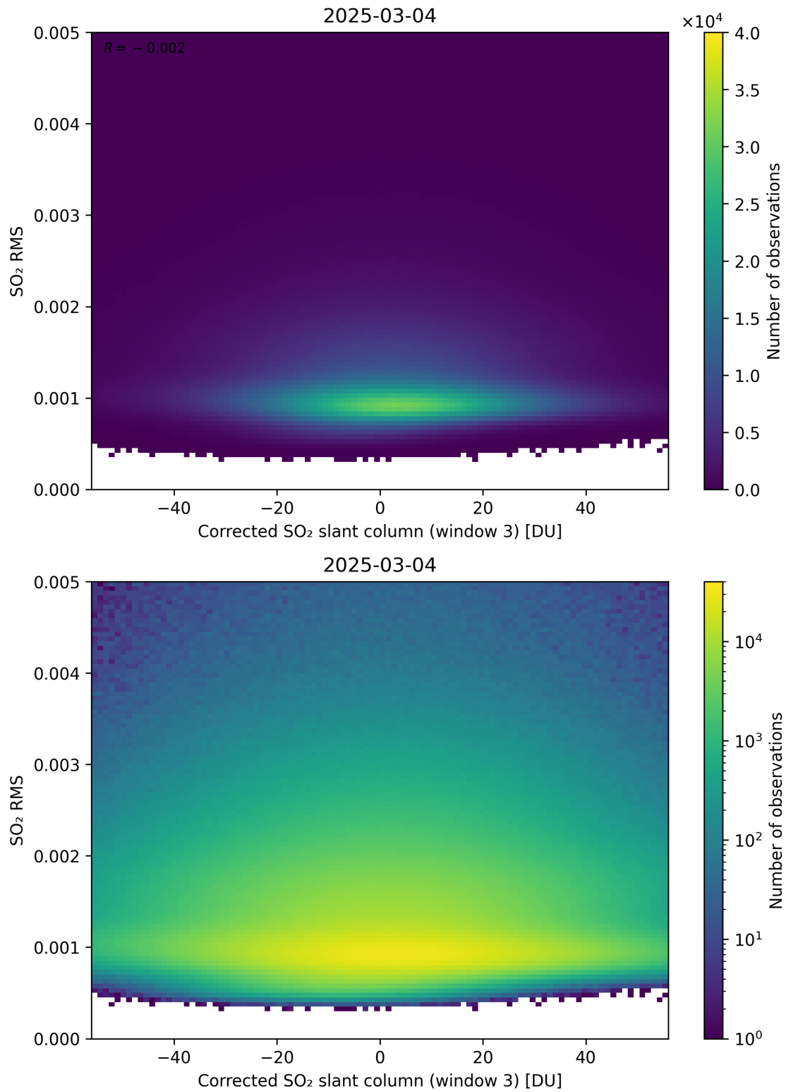
Figure 258: Scatter density plot of “Corrected SO 2 slant column (window 3)” against “SO 2 RMS” for 2025-03-03 to 2025-03-05.
