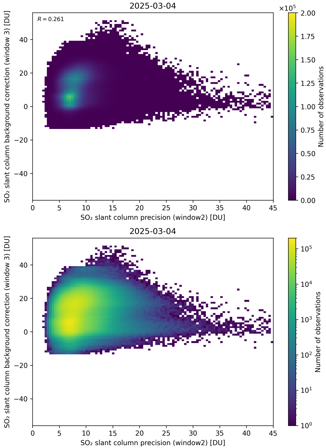
Figure 292: Scatter density plot of “SO 2 slant column precision (window2)” against “SO 2 slant column background correction (window 3)” for 2025-03-03 to 2025-03-05.
