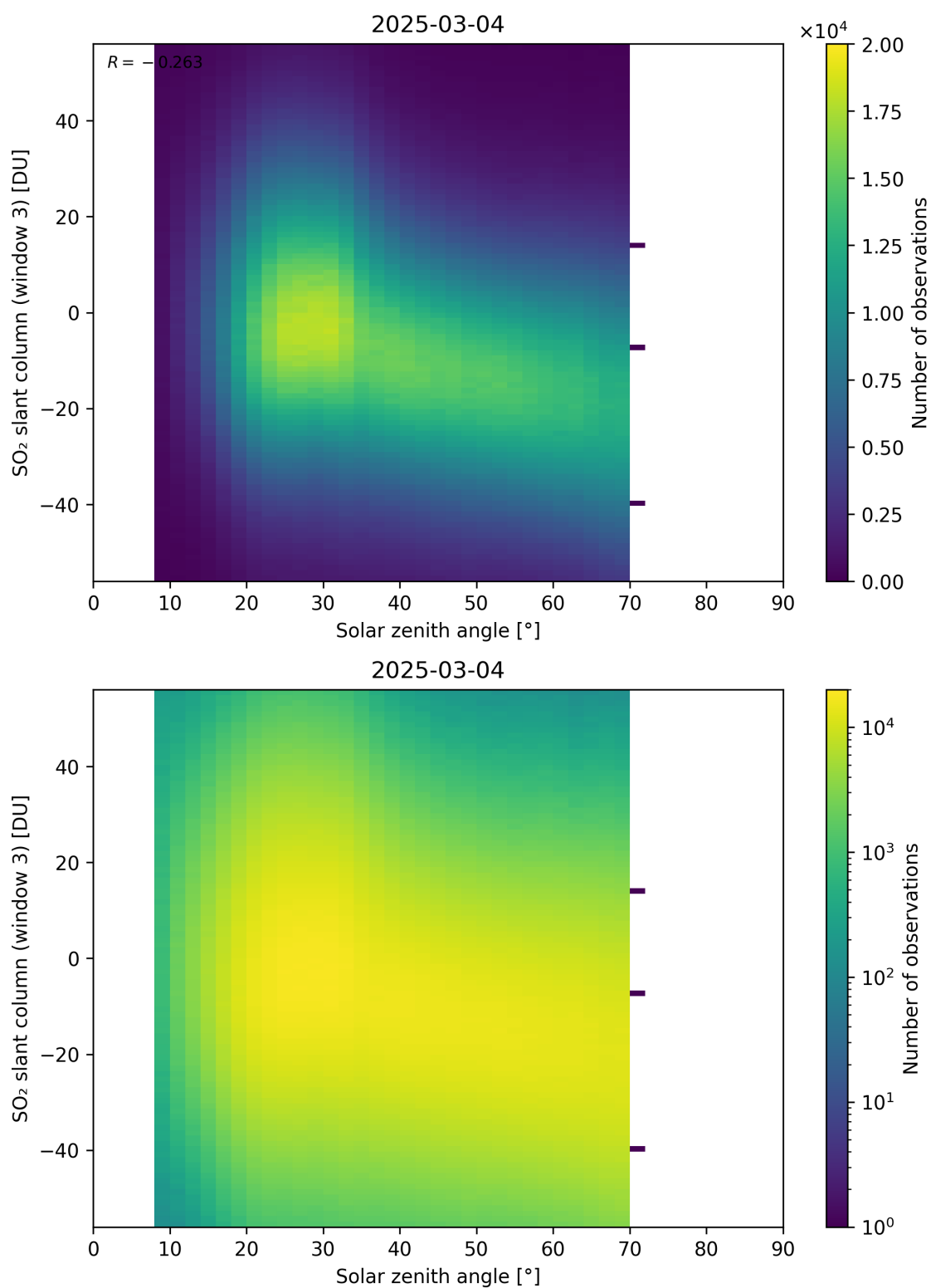
Figure 187: Scatter density plot of “Solar zenith angle” against “SO 2 slant column (window 3)” for 2025-03-03 to 2025-03-05.
