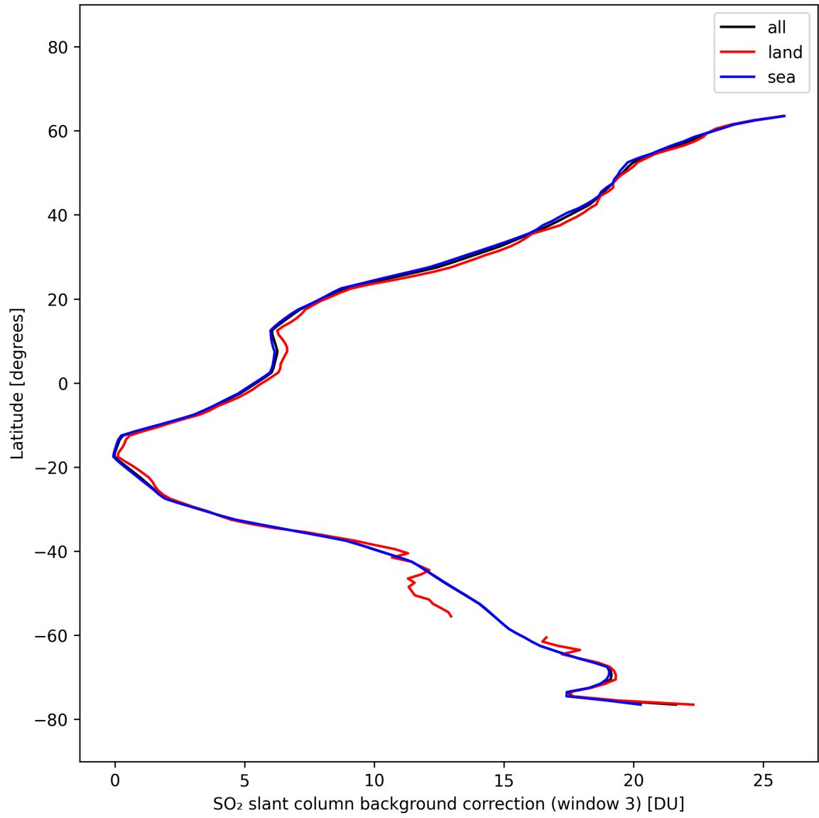
Figure 48: Zonal average of “SO 2 slant column background correction (window 3)” for 2025-03-03 to 2025-03-05.
