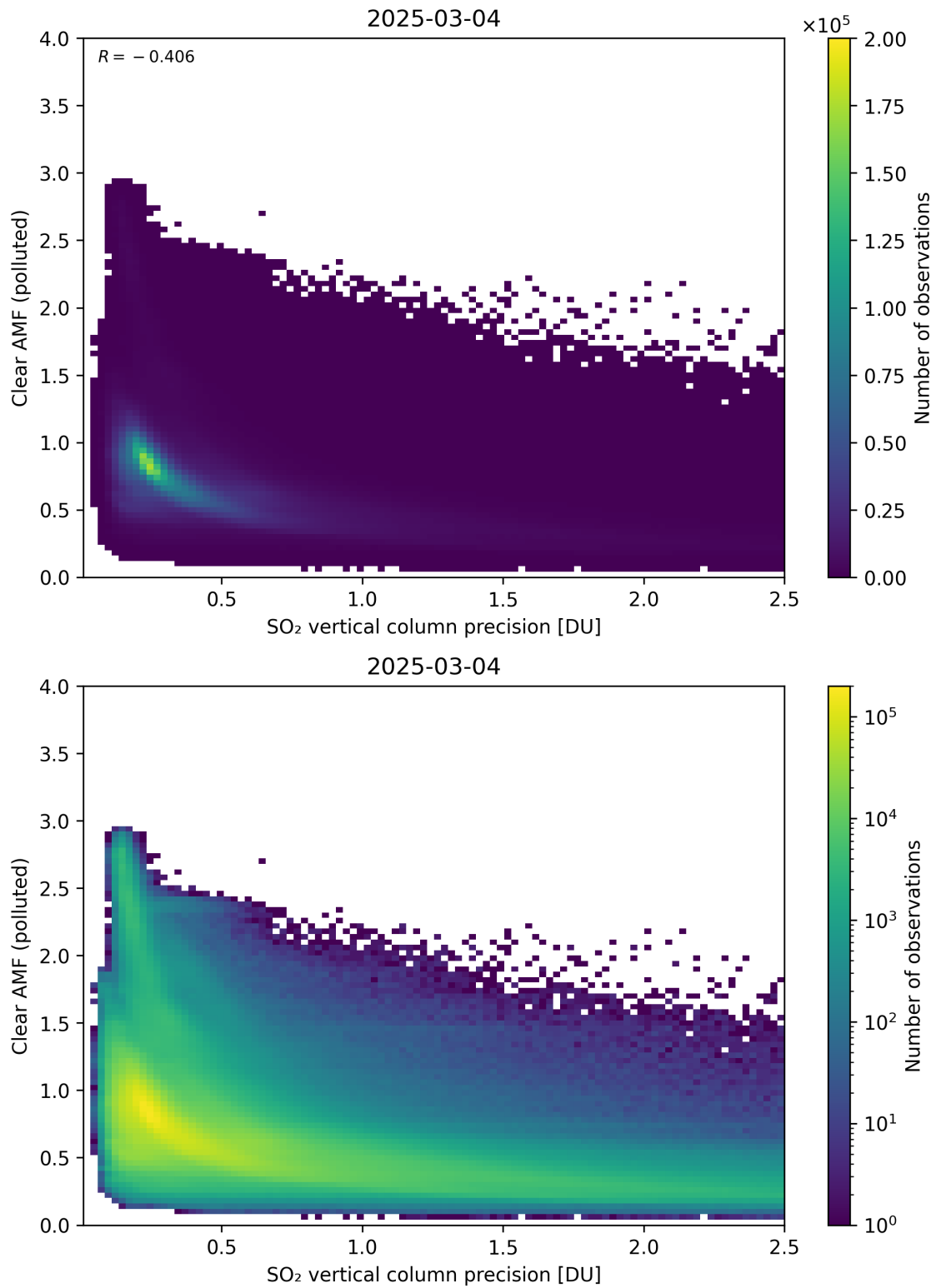
Figure 335: Scatter density plot of “SO 2 vertical column precision” against “Clear AMF (polluted)” for 2025-03-03 to 2025-03-05.
