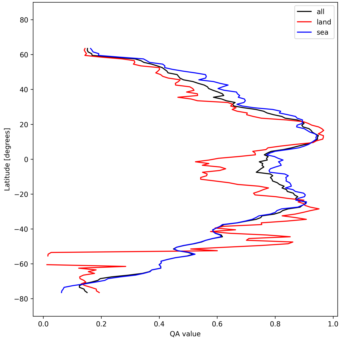
Figure 31: Zonal average of “QA value” for 2025-03-03 to 2025-03-05.
