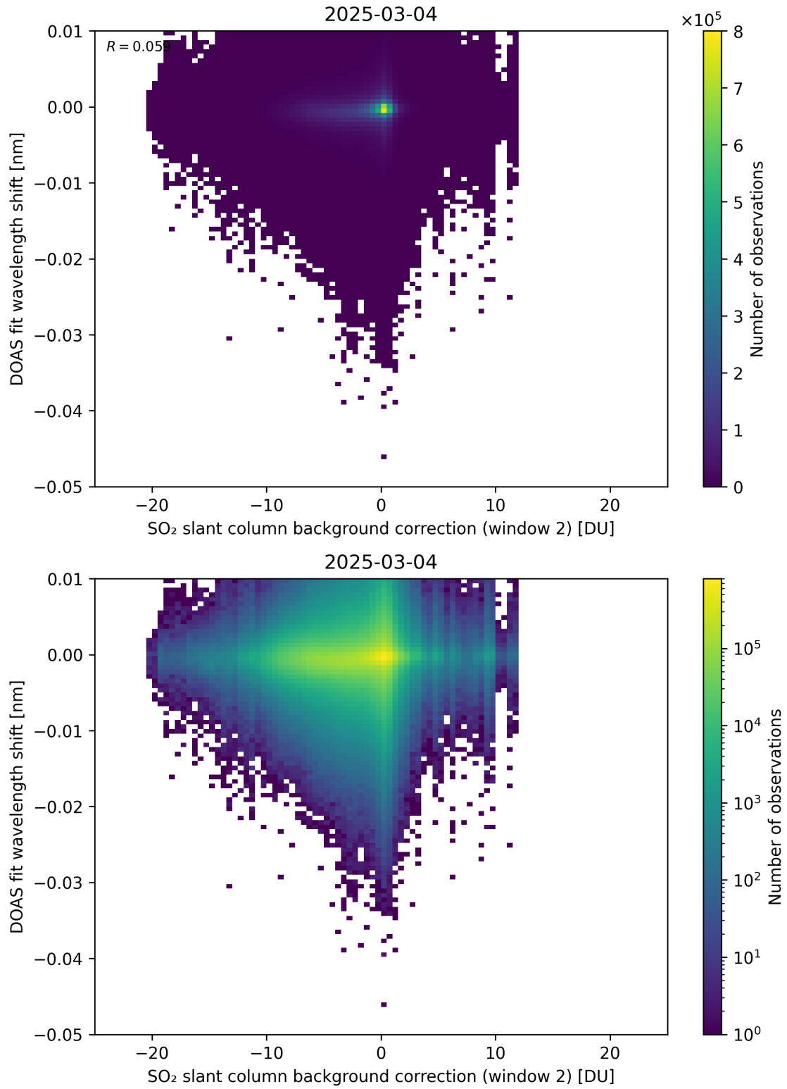
Figure 123: Scatter density plot of “SO 2 slant column background correction (window 2)” against “DOAS fit wavelength shift” for 2025-03-03 to 2025-03-05.
