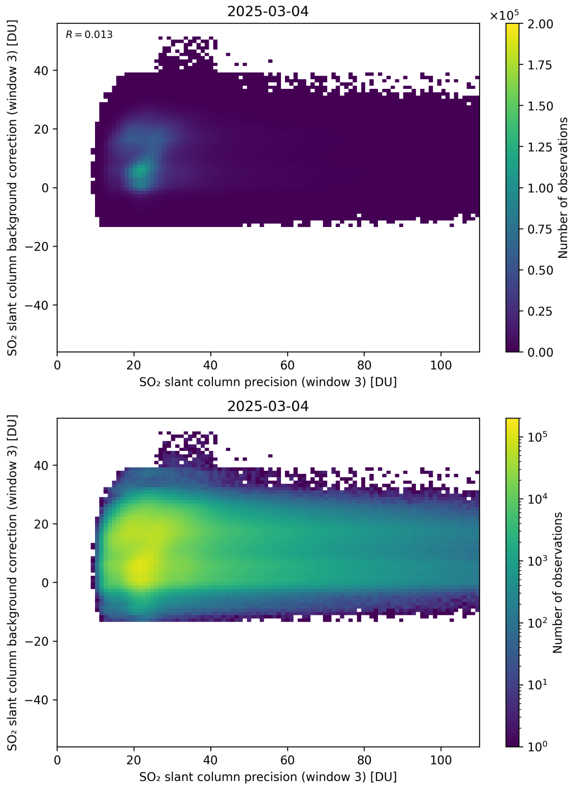
Figure 307: Scatter density plot of “SO 2 slant column precision (window 3)” against “SO 2 slant column background correction (window 3)” for 2025-03-03 to 2025-03-05.
