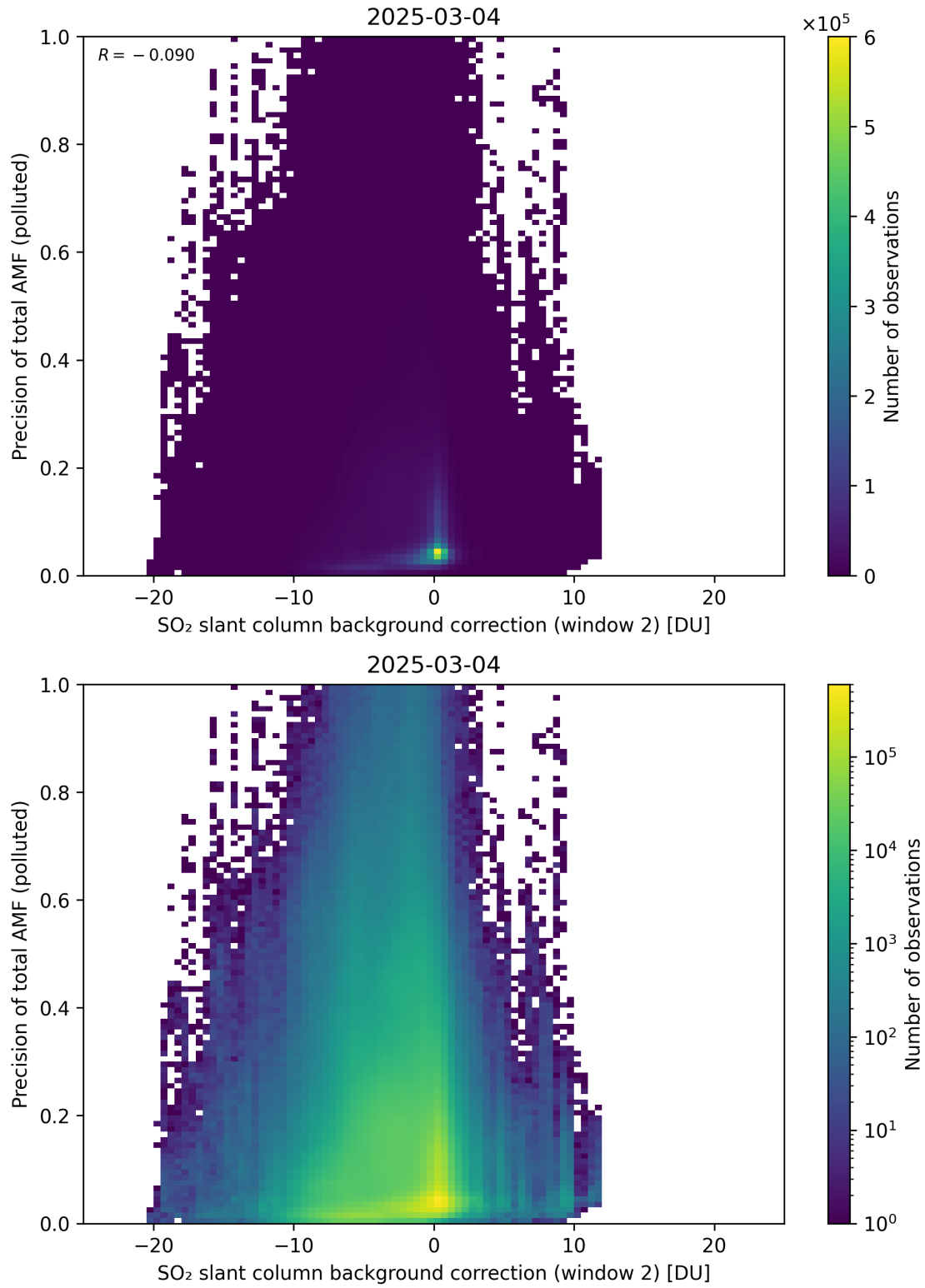
Figure 131: Scatter density plot of “SO 2 slant column background correction (window 2)” against “Precision of total AMF (polluted)” for 2025-03-03 to 2025-03-05.
