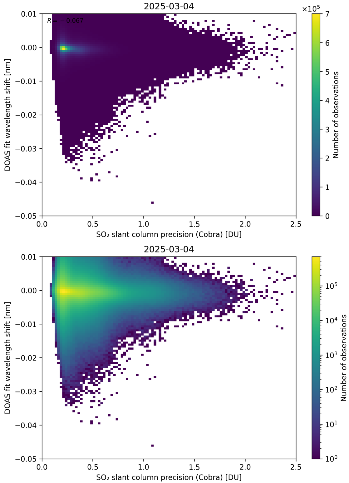
Figure 202: Scatter density plot of “SO 2 slant column precision (Cobra)” against “DOAS fit wavelength shift” for 2025-03-03 to 2025-03-05.
