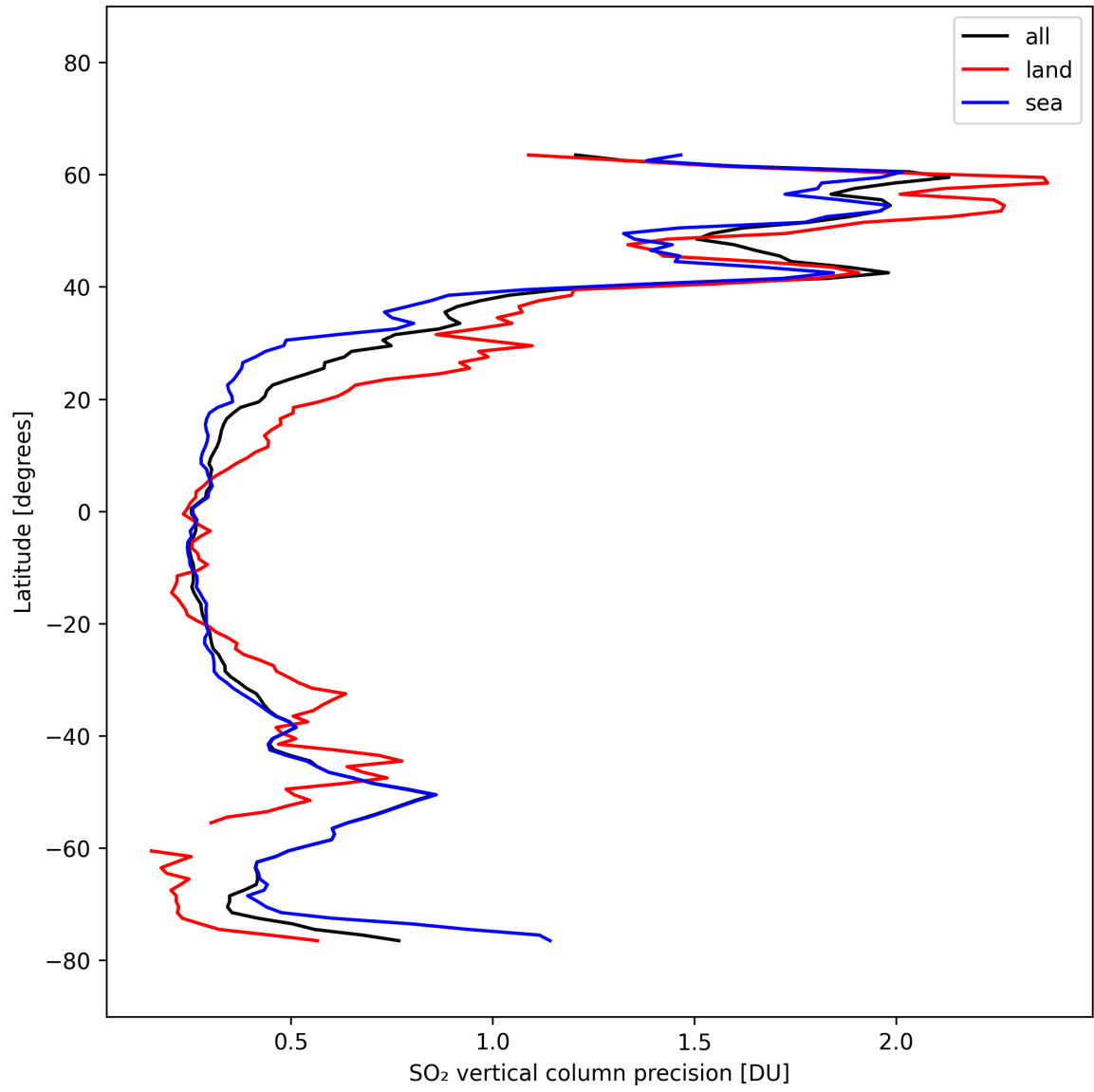
Figure 33: Zonal average of “SO 2 vertical column precision” for 2025-03-03 to 2025-03-05.
