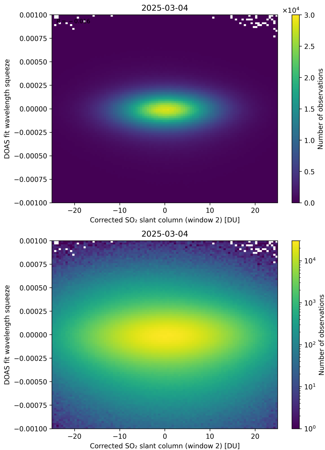
Figure 247: Scatter density plot of “Corrected SO 2 slant column (window 2)” against “DOAS fit wavelength squeeze” for 2025-03-03 to 2025-03-05.
