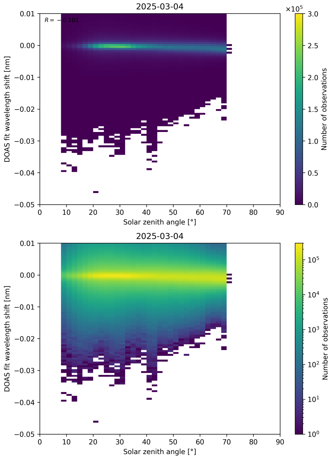
Figure 174: Scatter density plot of “Solar zenith angle” against “DOAS fit wavelength shift” for 2025-03-03 to 2025-03-05.
