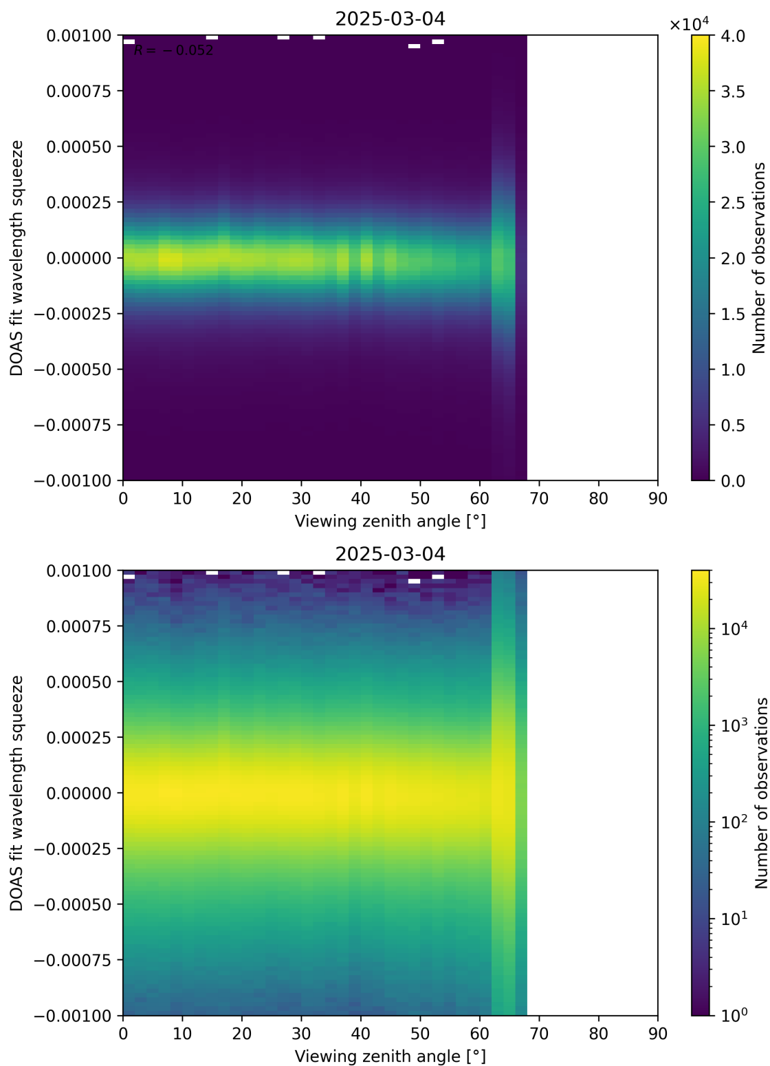
Figure 366: Scatter density plot of “Viewing zenith angle” against “DOAS fit wavelength squeeze” for 2025-03-03 to 2025-03-05.
