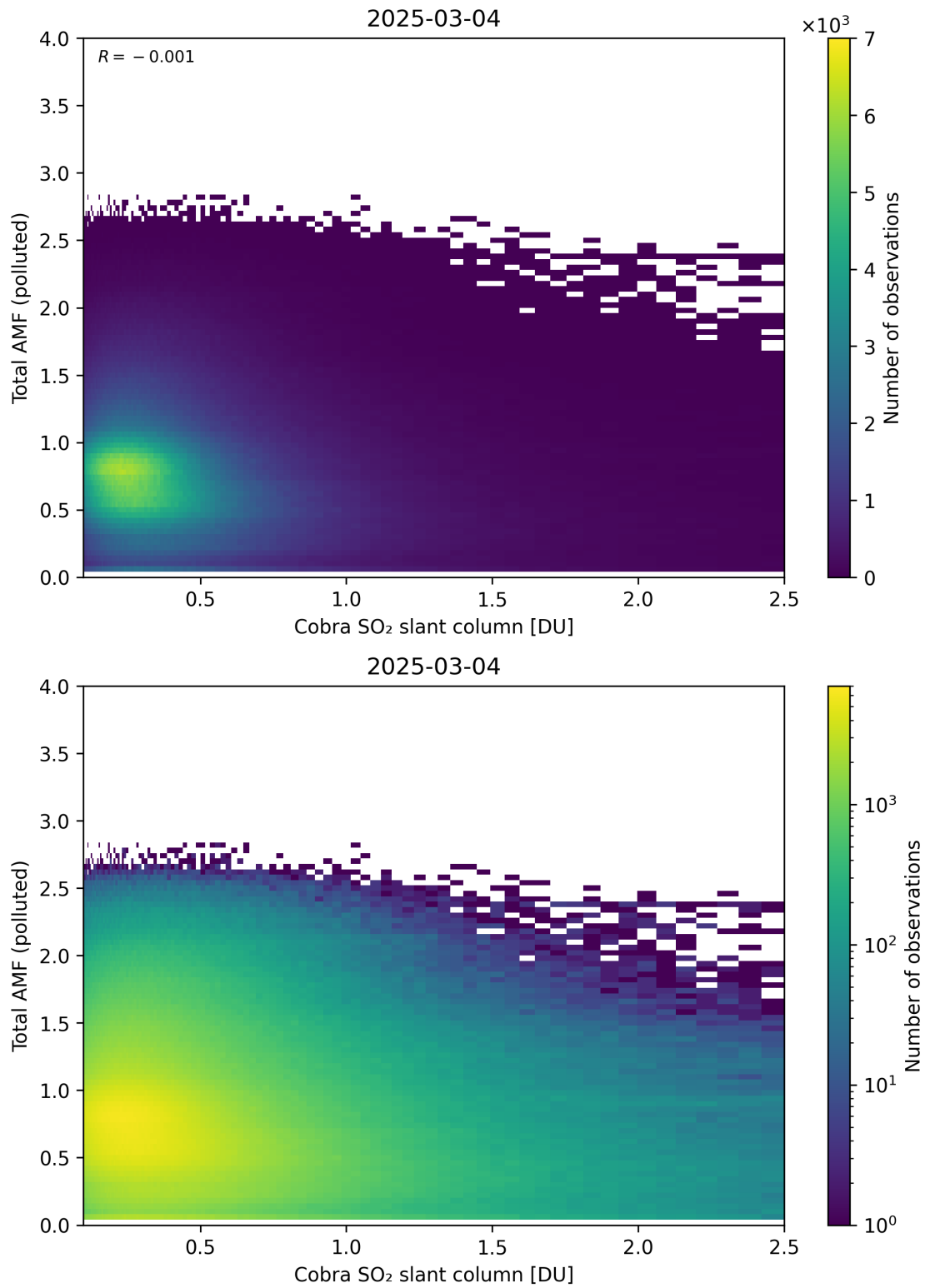
Figure 224: Scatter density plot of “Cobra SO 2 slant column” against “Total AMF (polluted)” for 2025-03-03 to 2025-03-05.
