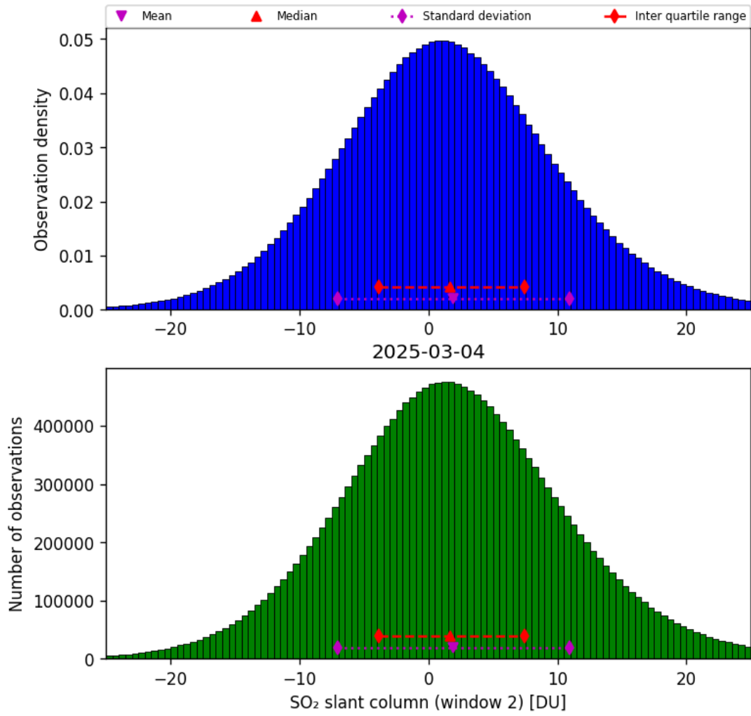
Figure 67: Histogram of “SO 2 slant column (window 2)” for 2025-03-03 to 2025-03-05
