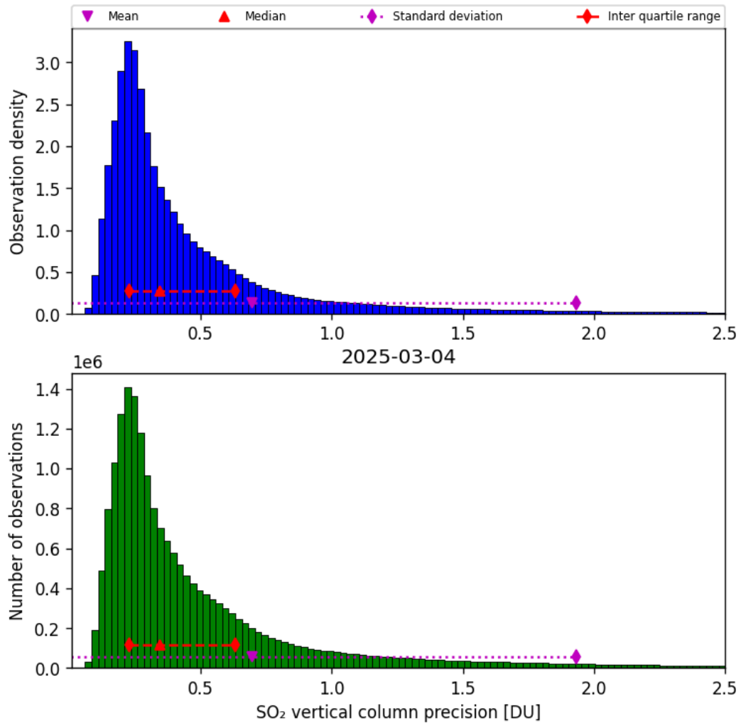
Figure 59: Histogram of “SO 2 vertical column precision” for 2025-03-03 to 2025-03-05
