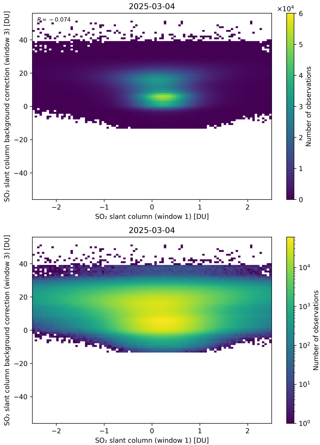
Figure 264: Scatter density plot of “SO 2 slant column (window 1)” against “SO 2 slant column background correction (window 3)” for 2025-03-03 to 2025-03-05.
