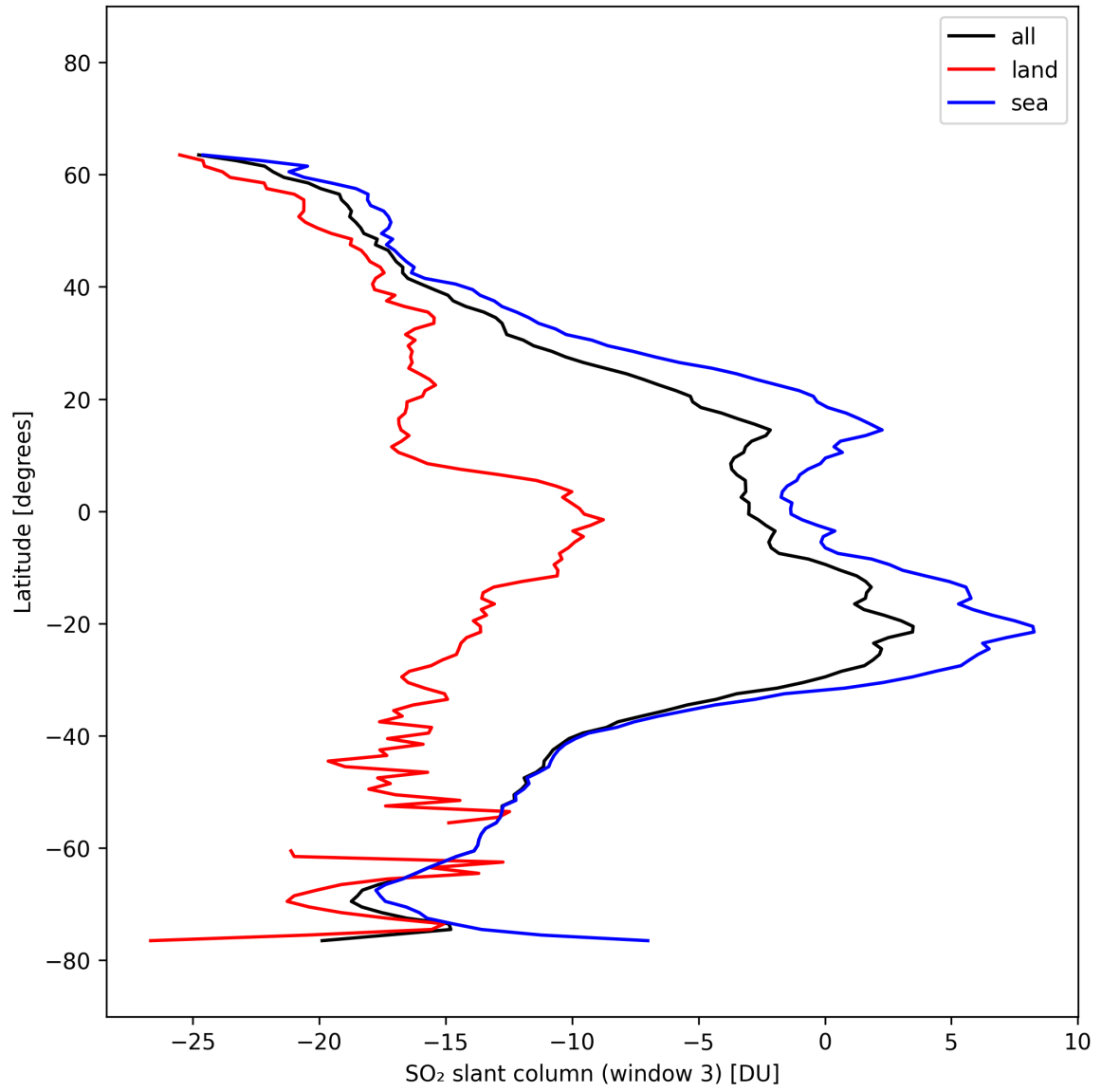
Figure 45: Zonal average of “SO 2 slant column (window 3)” for 2025-03-03 to 2025-03-05.
