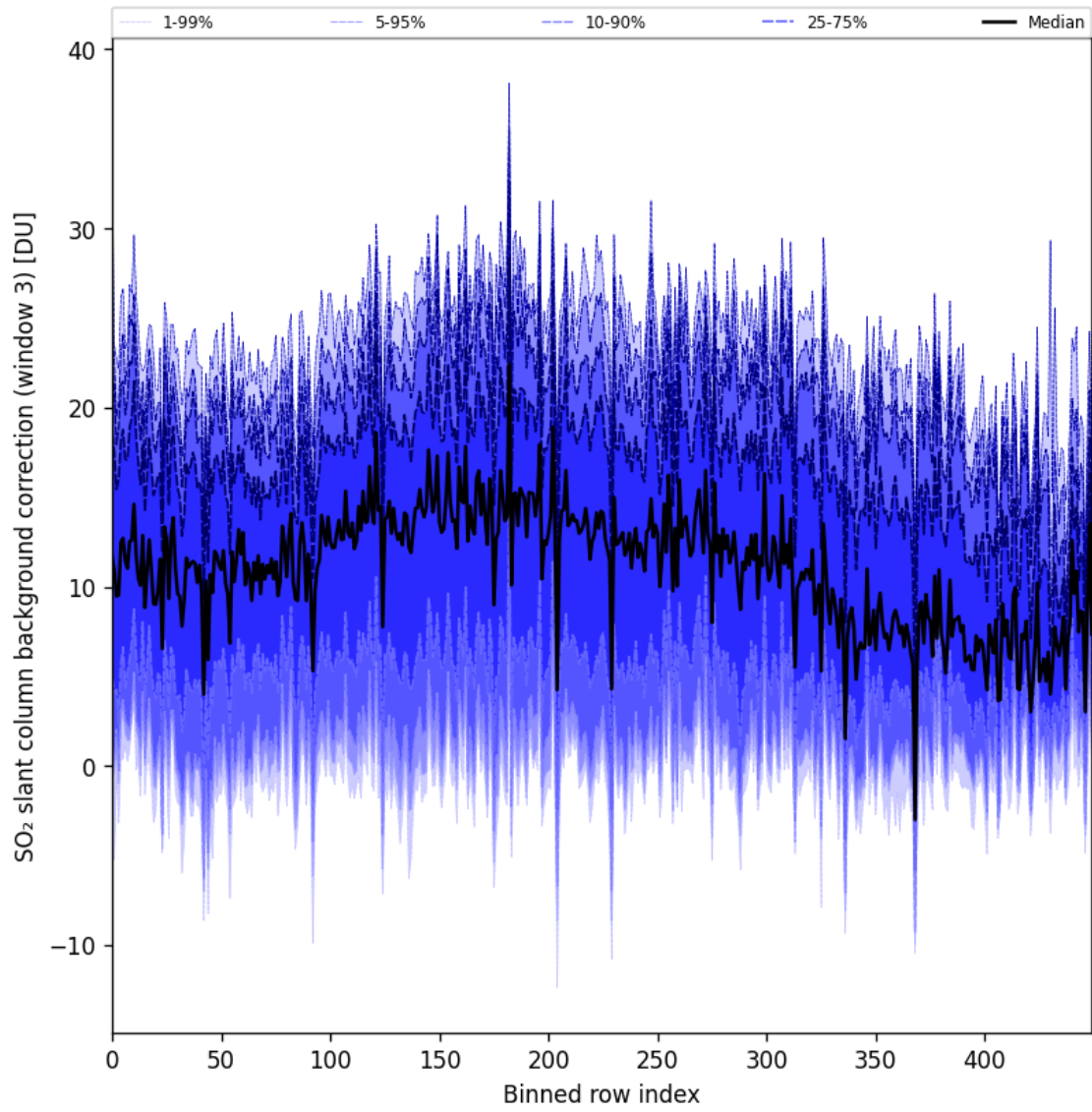
Figure 100: Along track statistics of “SO 2 slant column background correction (window 3)” for 2025-03-03 to 2025-03-05
