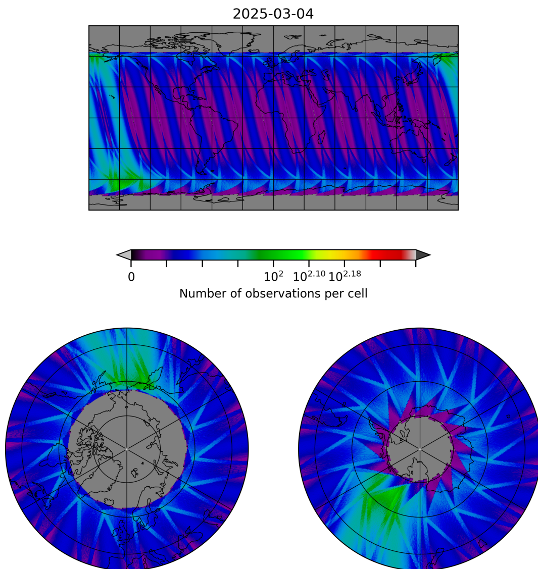
Figure 30: Map of the number of observations for 2025-03-03 to 2025-03-05
