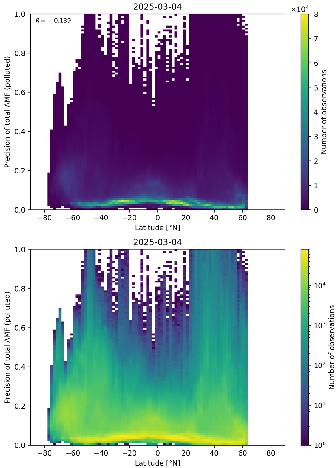
Figure 168: Scatter density plot of “Latitude” against “Precision of total AMF (polluted)” for 2025-03-03 to 2025-03-05.
