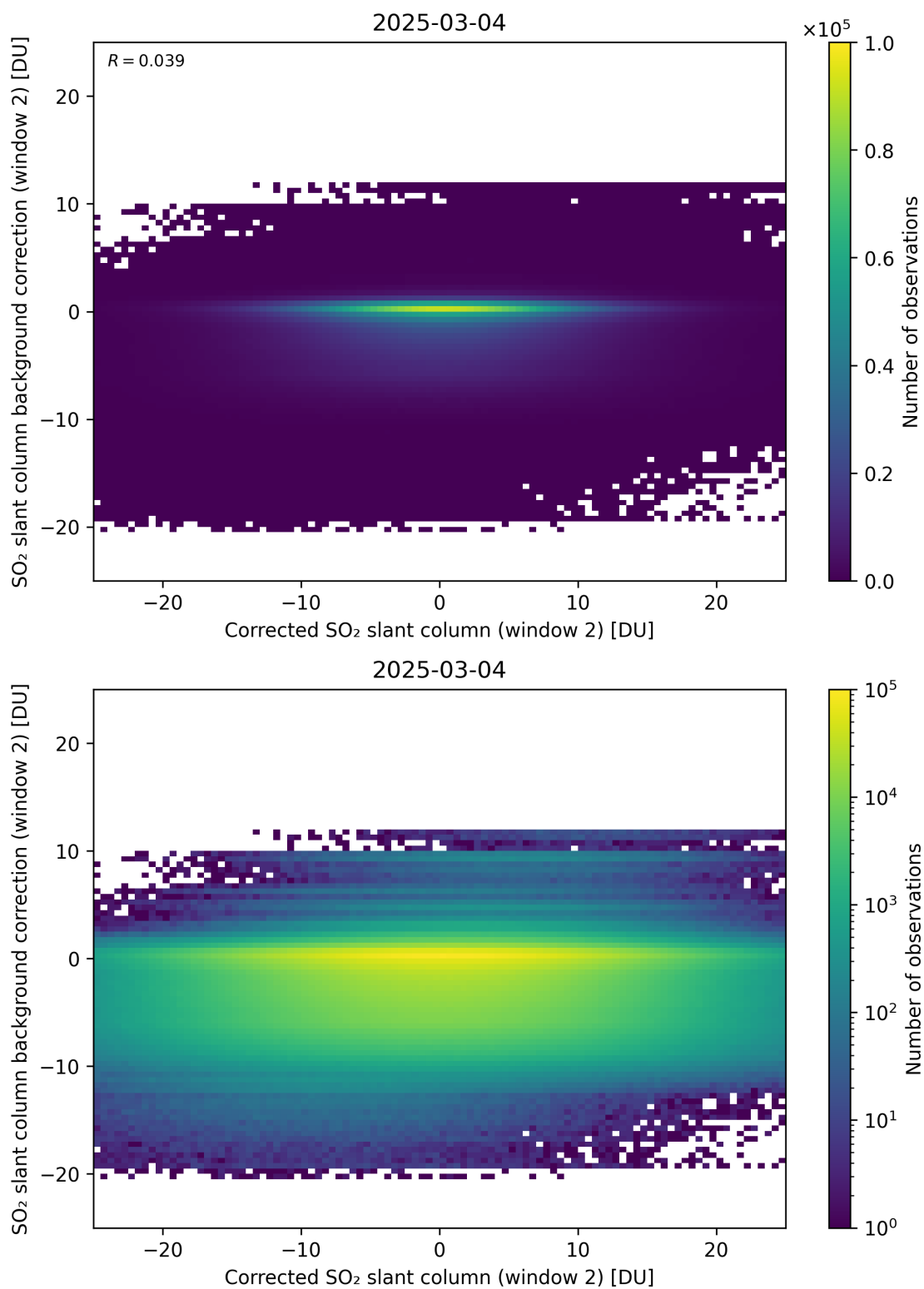
Figure 244: Scatter density plot of “Corrected SO 2 slant column (window 2)” against “SO 2 slant column background correction (window 2)” for 2025-03-03 to 2025-03-05.
