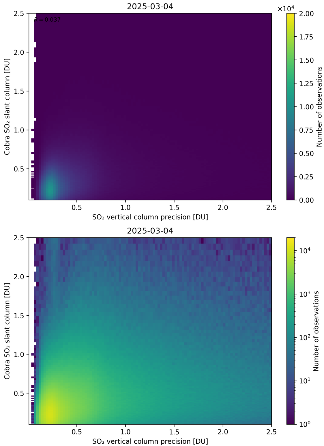
Figure 336: Scatter density plot of “SO 2 vertical column precision” against “Cobra SO 2 slant column” for 2025-03-03 to 2025-03-05.
