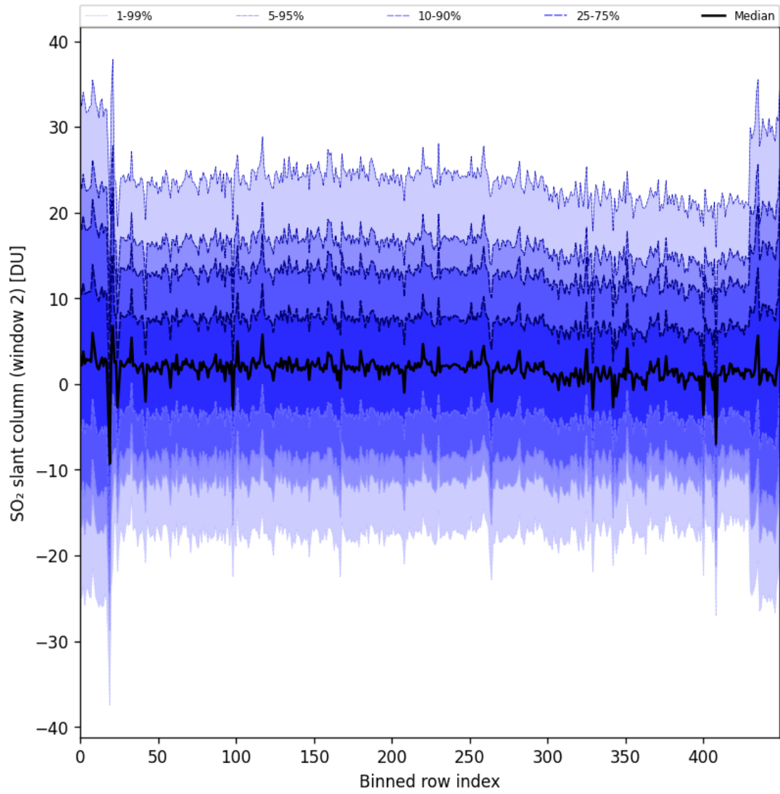
Figure 93: Along track statistics of “SO 2 slant column (window 2)” for 2025-03-03 to 2025-03-05
