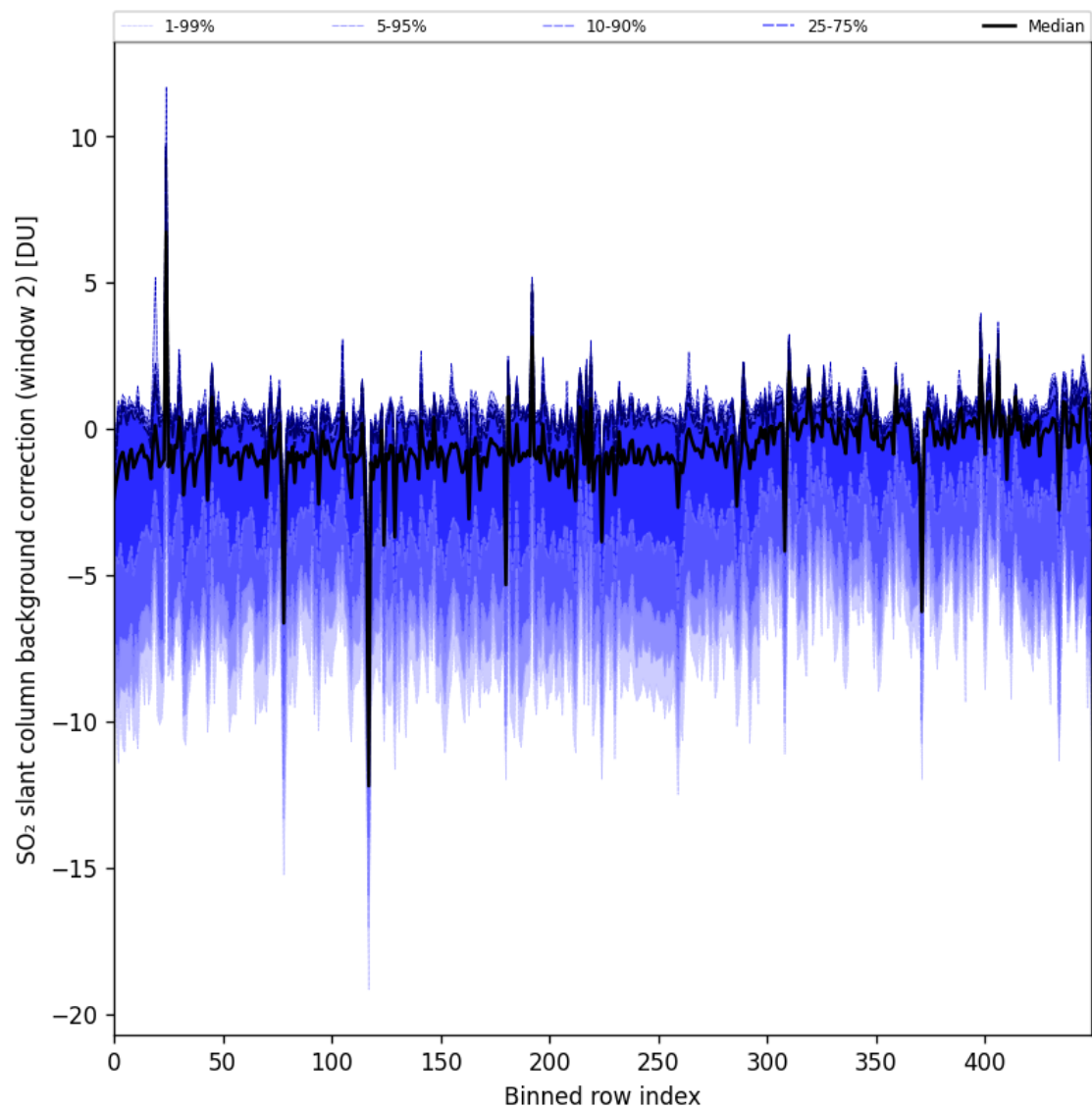
Figure 96: Along track statistics of “SO 2 slant column background correction (window 2)” for 2025-03-03 to 2025-03-05
