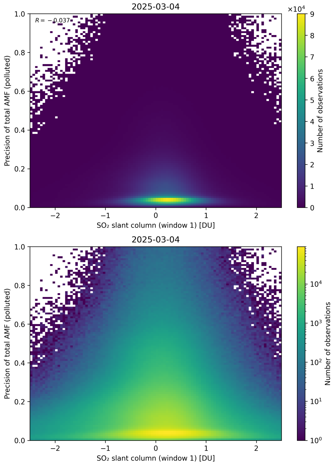
Figure 290: Scatter density plot of “SO 2 slant column (window 1)” against “Precision of total AMF (polluted)” for 2025-03-03 to 2025-03-05.
