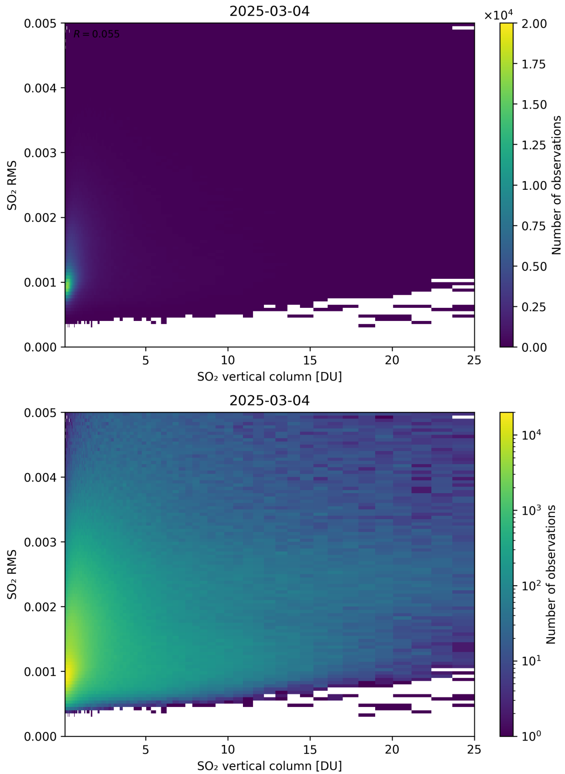
Figure 328: Scatter density plot of “SO 2 vertical column” against “SO 2 RMS” for 2025-03-03 to 2025-03-05.
