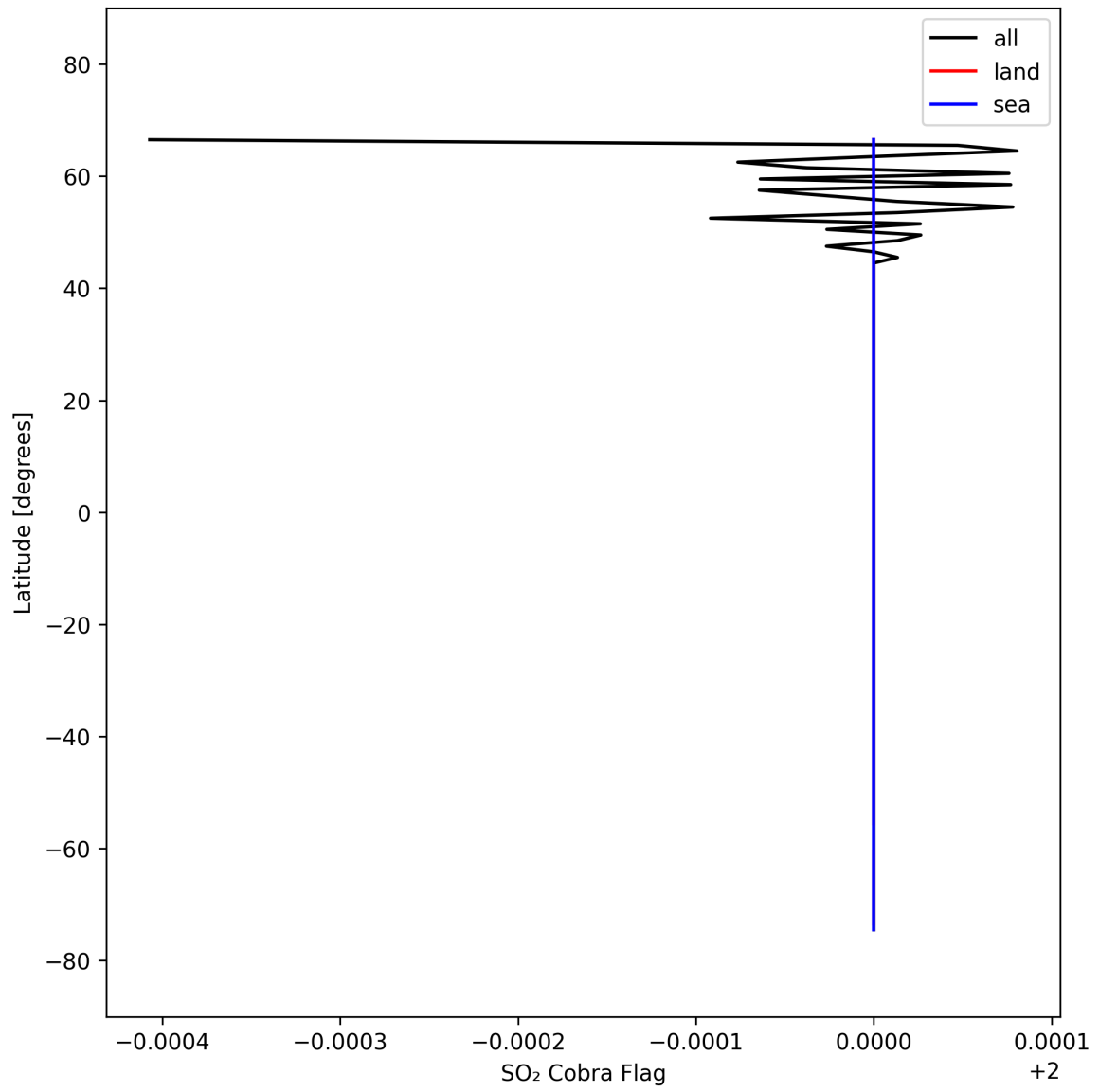
Figure 49: Zonal average of “SO 2 Cobra Flag” for 2025-03-09 to 2025-03-11.
