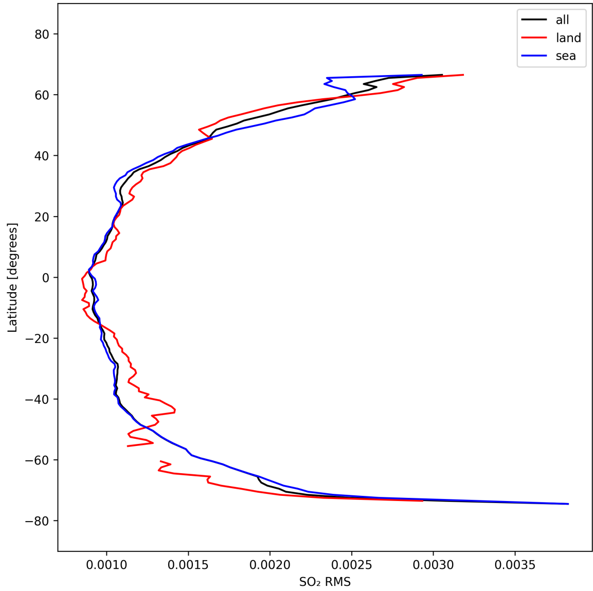
Figure 52: Zonal average of “SO 2 RMS” for 2025-03-09 to 2025-03-11.
