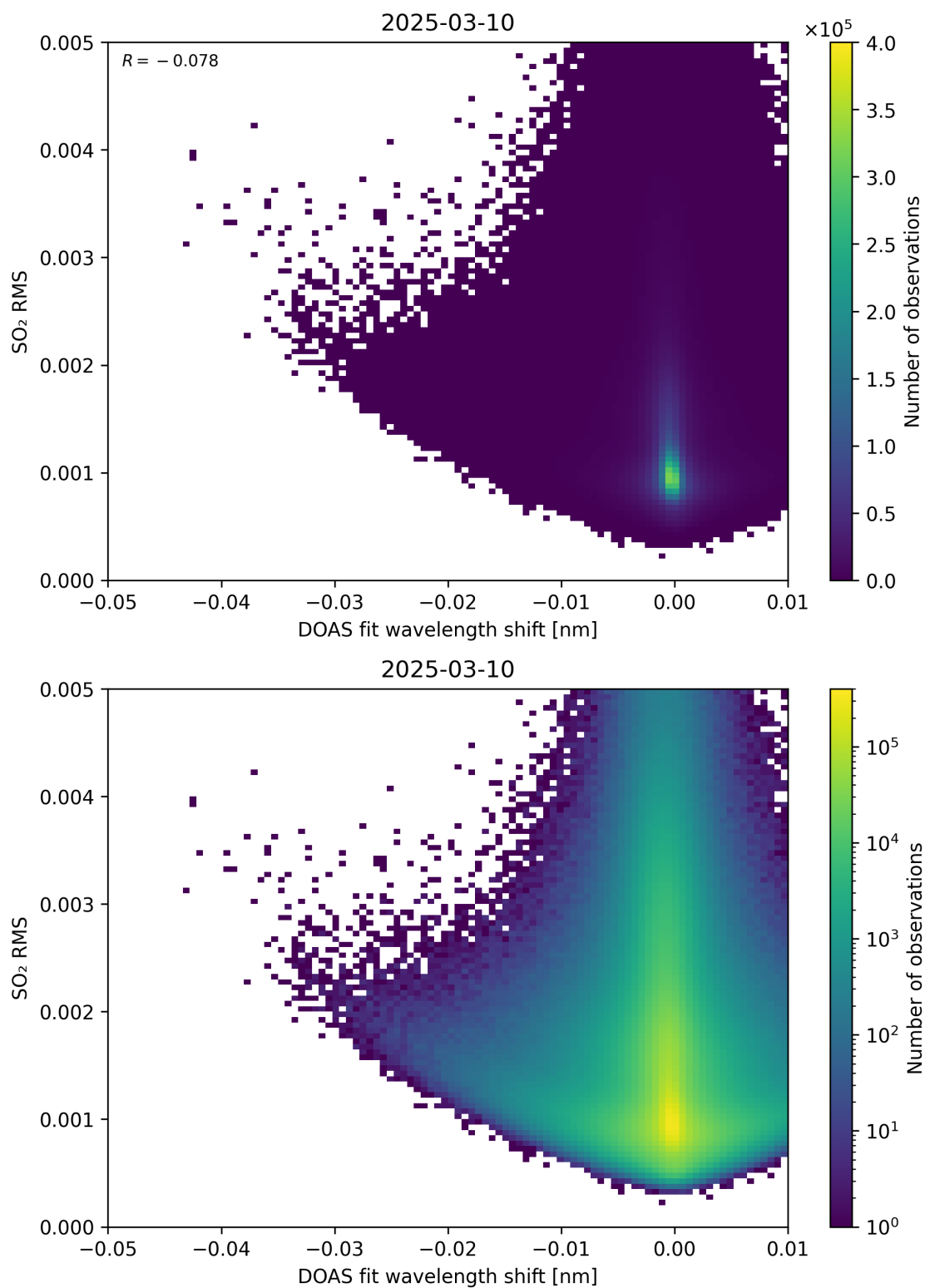
Figure 139: Scatter density plot of “DOAS fit wavelength shift” against “SO 2 RMS” for 2025-03-09 to 2025-03-11.
