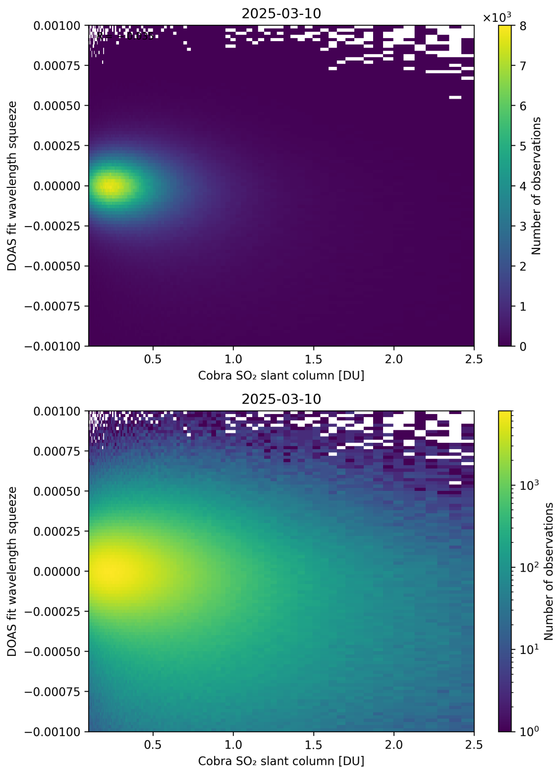
Figure 197: Scatter density plot of “Cobra SO 2 slant column” against “DOAS fit wavelength squeeze” for 2025-03-09 to 2025-03-11.
