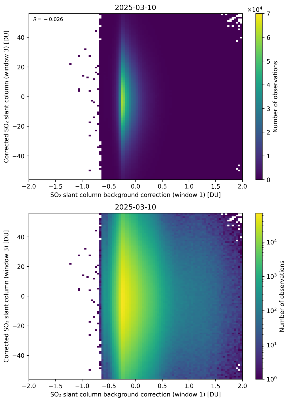
Figure 116: Scatter density plot of “SO 2 slant column background correction (window 1)” against “Corrected SO 2 slant column (window 3)” for 2025-03-09 to 2025-03-11.
