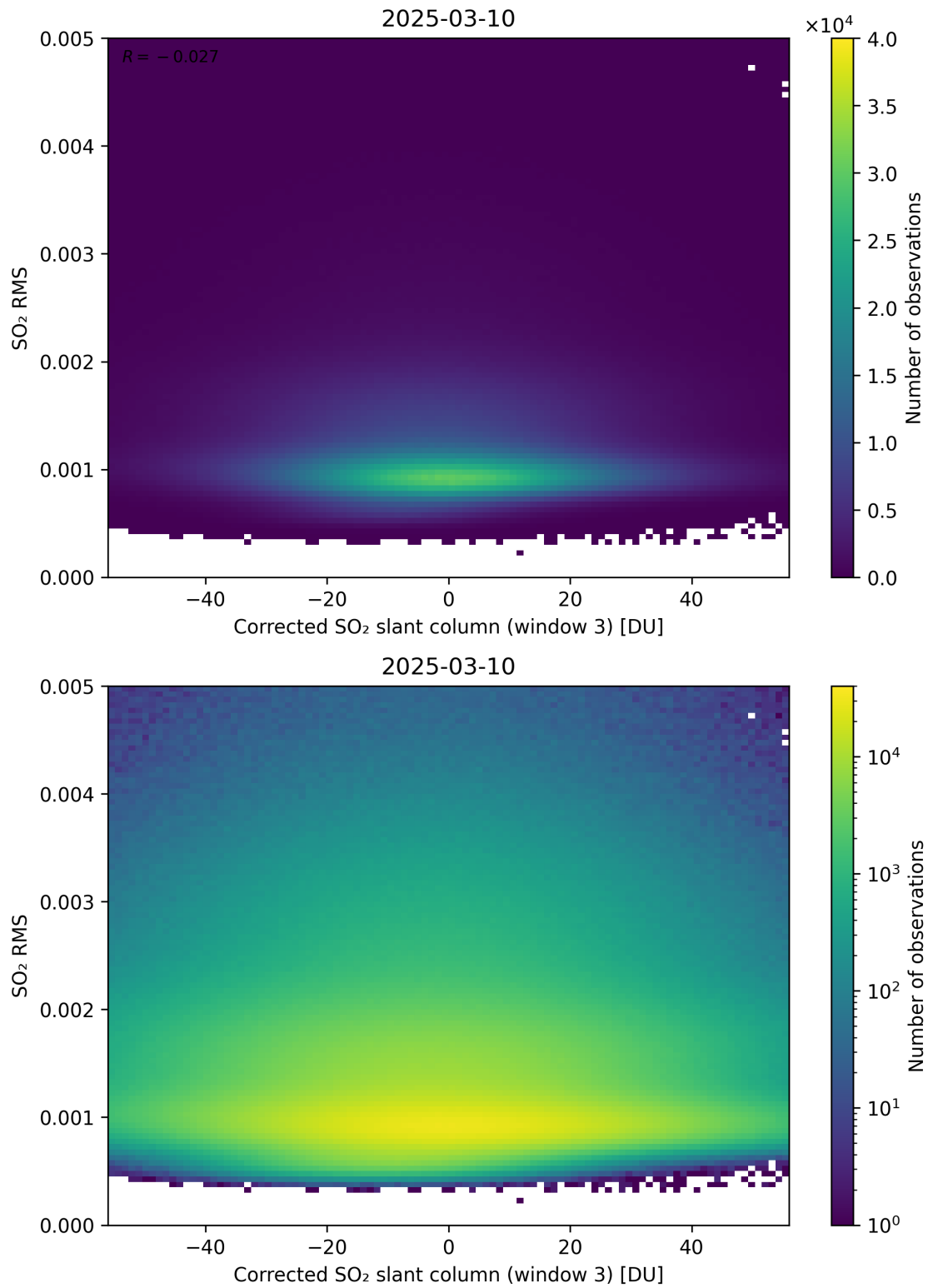
Figure 258: Scatter density plot of “Corrected SO 2 slant column (window 3)” against “SO 2 RMS” for 2025-03-09 to 2025-03-11.
