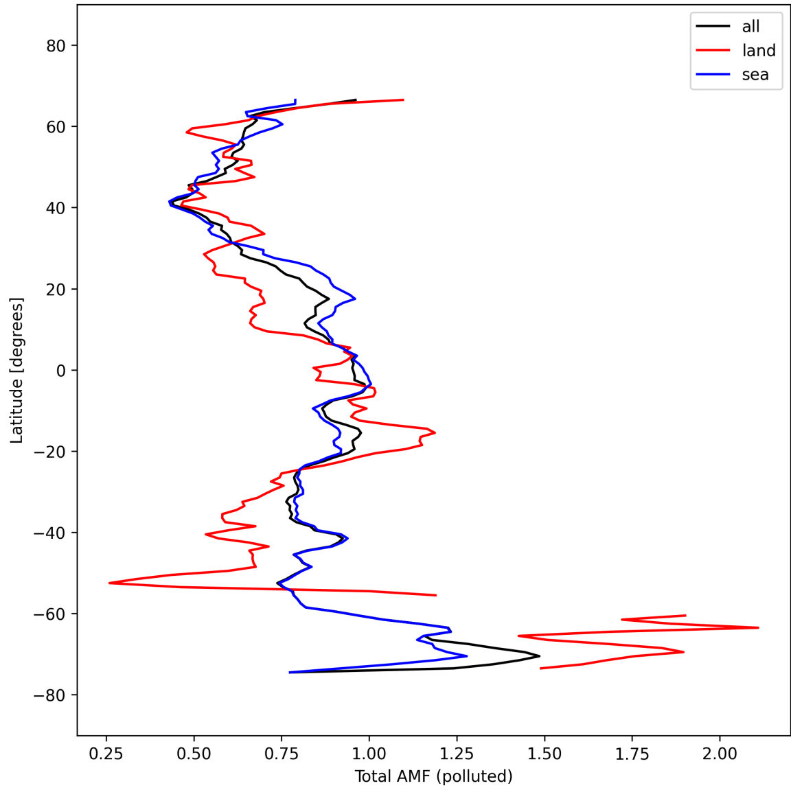
Figure 53: Zonal average of “Total AMF (polluted)” for 2025-03-09 to 2025-03-11.
