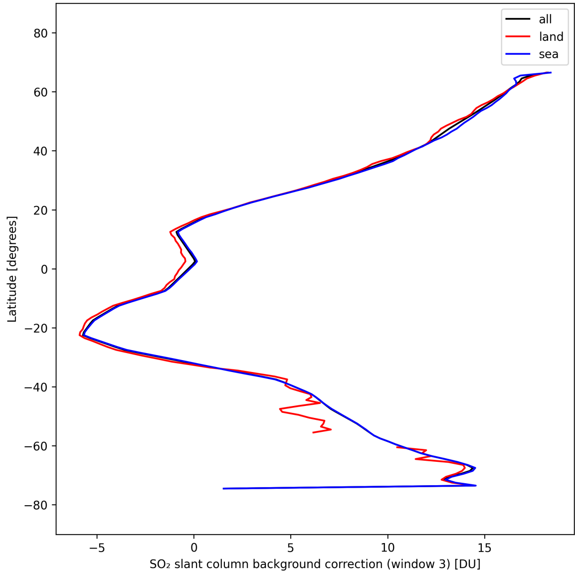
Figure 48: Zonal average of “SO 2 slant column background correction (window 3)” for 2025-03-09 to 2025-03-11.
