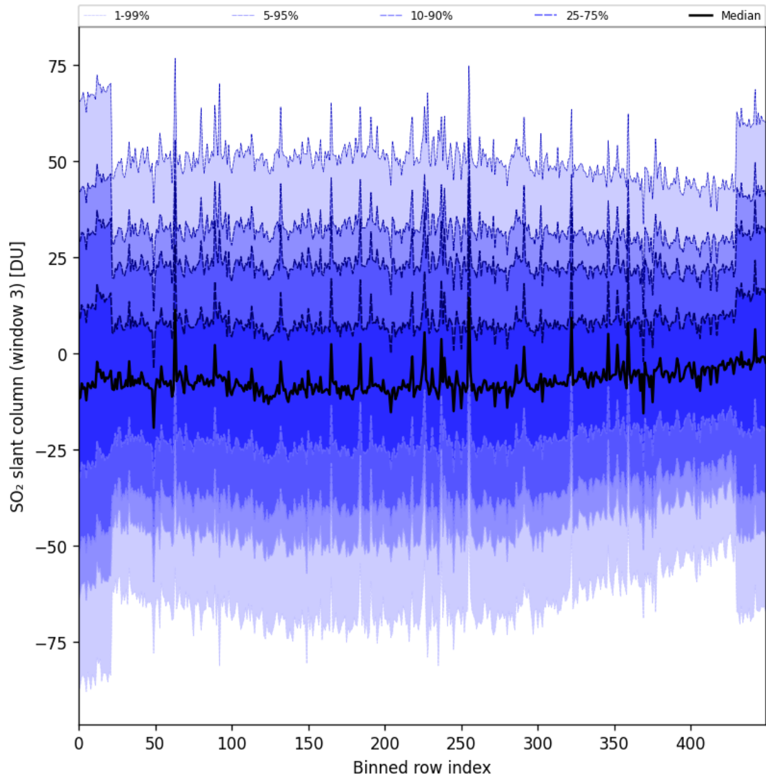
Figure 97: Along track statistics of “SO 2 slant column (window 3)” for 2025-03-09 to 2025-03-11
