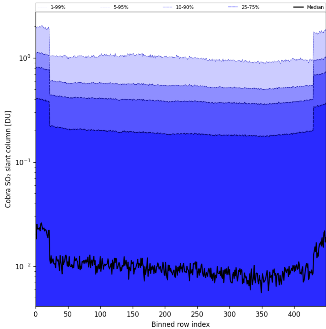
Figure 87: Along track statistics of “Cobra SO 2 slant column” for 2025-03-09 to 2025-03-11
