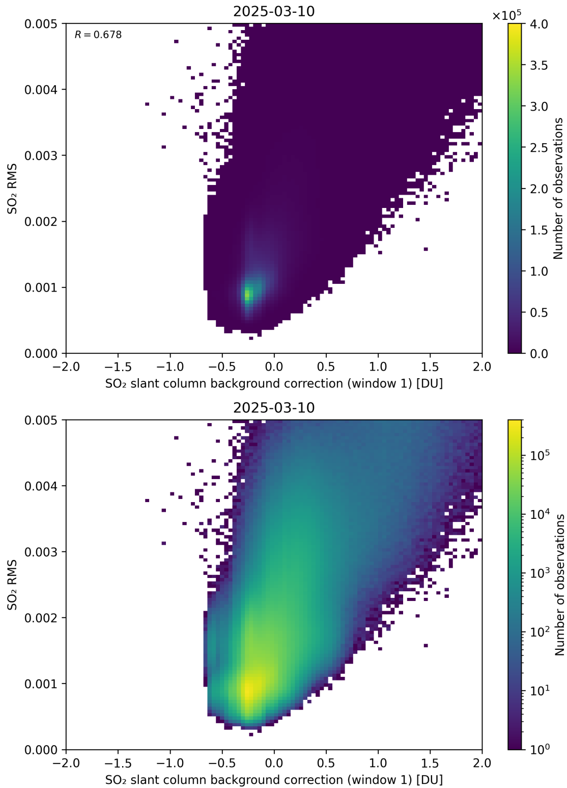
Figure 113: Scatter density plot of “SO 2 slant column background correction (window 1)” against “SO 2 RMS” for 2025-03-09 to 2025-03-11.
