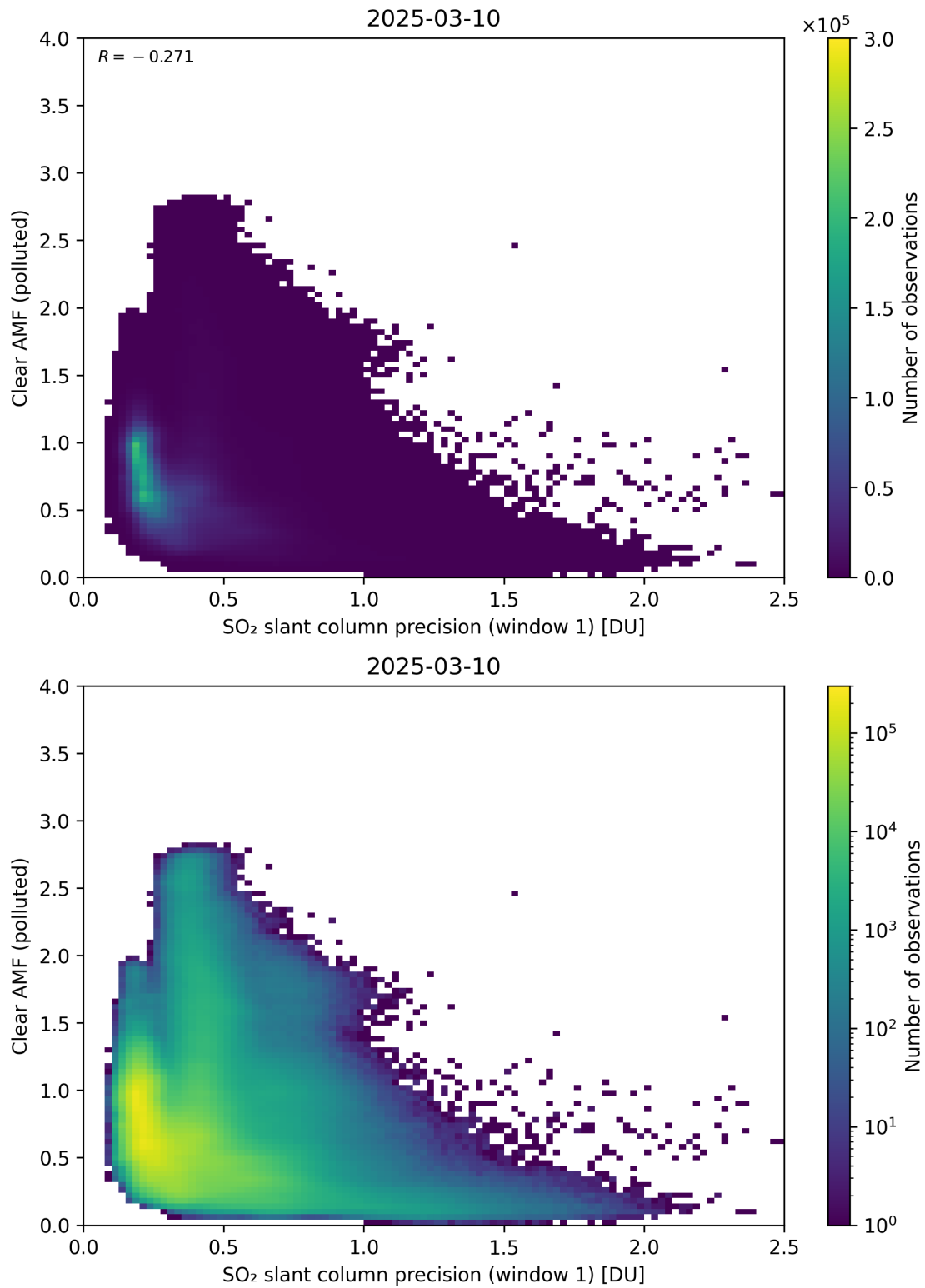
Figure 274: Scatter density plot of “SO 2 slant column precision (window 1)” against “Clear AMF (polluted)” for 2025-03-09 to 2025-03-11.
