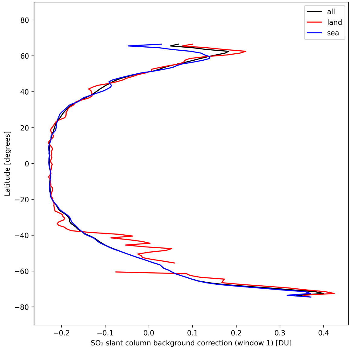
Figure 40: Zonal average of “SO 2 slant column background correction (window 1)” for 2025-03-09 to 2025-03-11.
