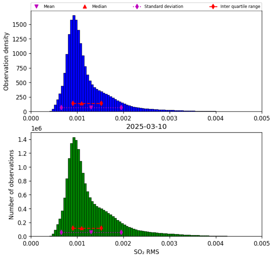
Figure 78: Histogram of “SO 2 RMS” for 2025-03-09 to 2025-03-11
