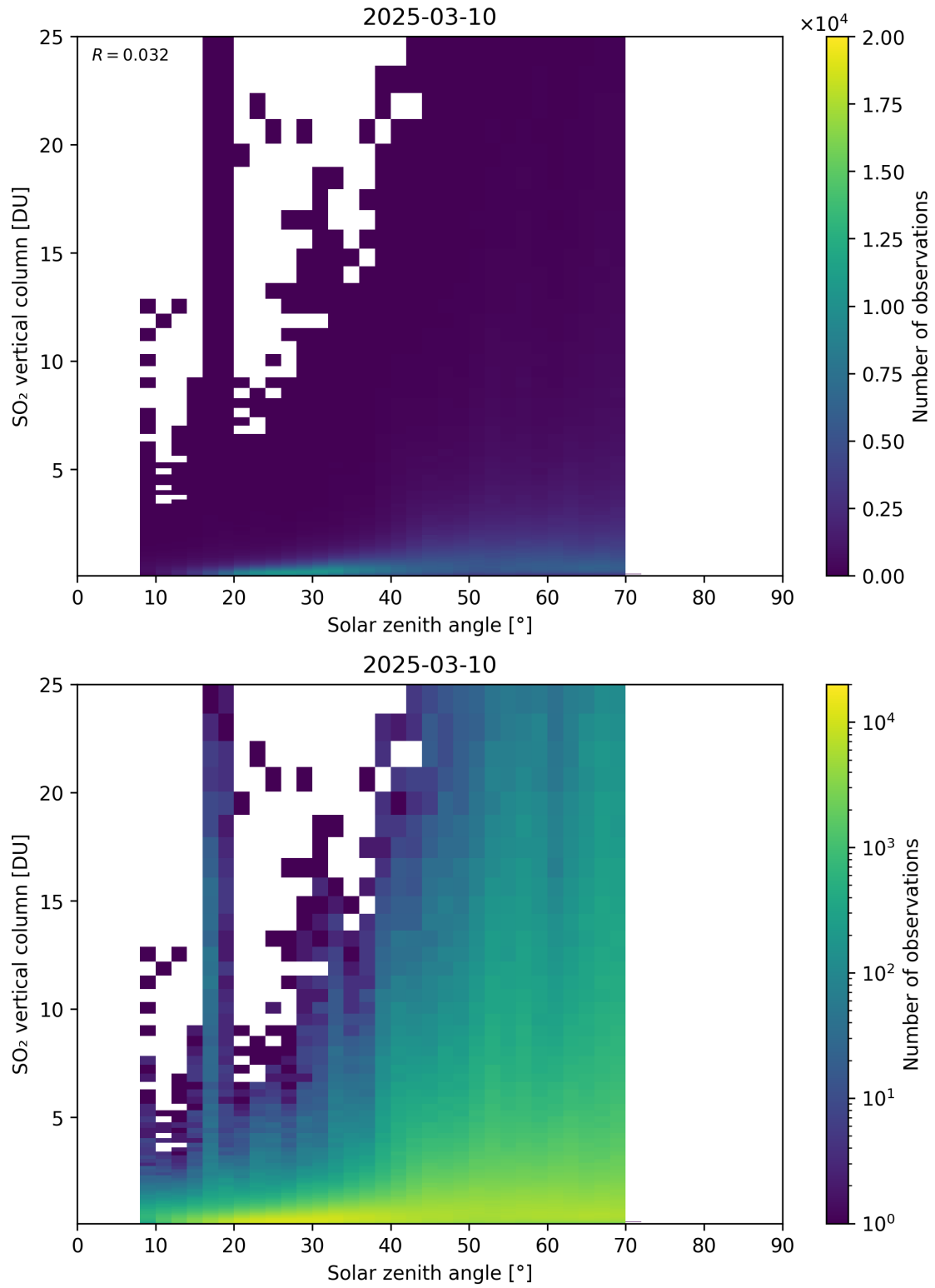
Figure 191: Scatter density plot of “Solar zenith angle” against “SO 2 vertical column” for 2025-03-09 to 2025-03-11.
