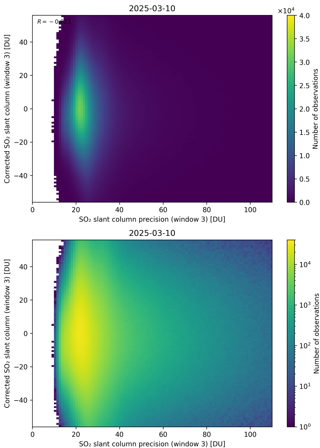
Figure 312: Scatter density plot of “SO 2 slant column precision (window 3)” against “Corrected SO 2 slant column (window 3)” for 2025-03-09 to 2025-03-11.
