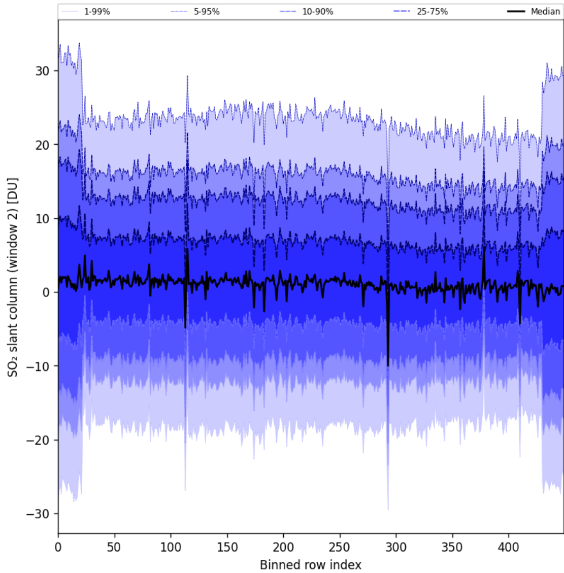
Figure 93: Along track statistics of “SO 2 slant column (window 2)” for 2025-03-09 to 2025-03-11
