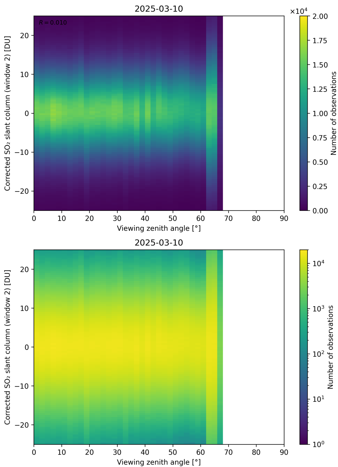
Figure 374: Scatter density plot of “Viewing zenith angle” against “Corrected SO 2 slant column (window 2)” for 2025-03-09 to 2025-03-11.
