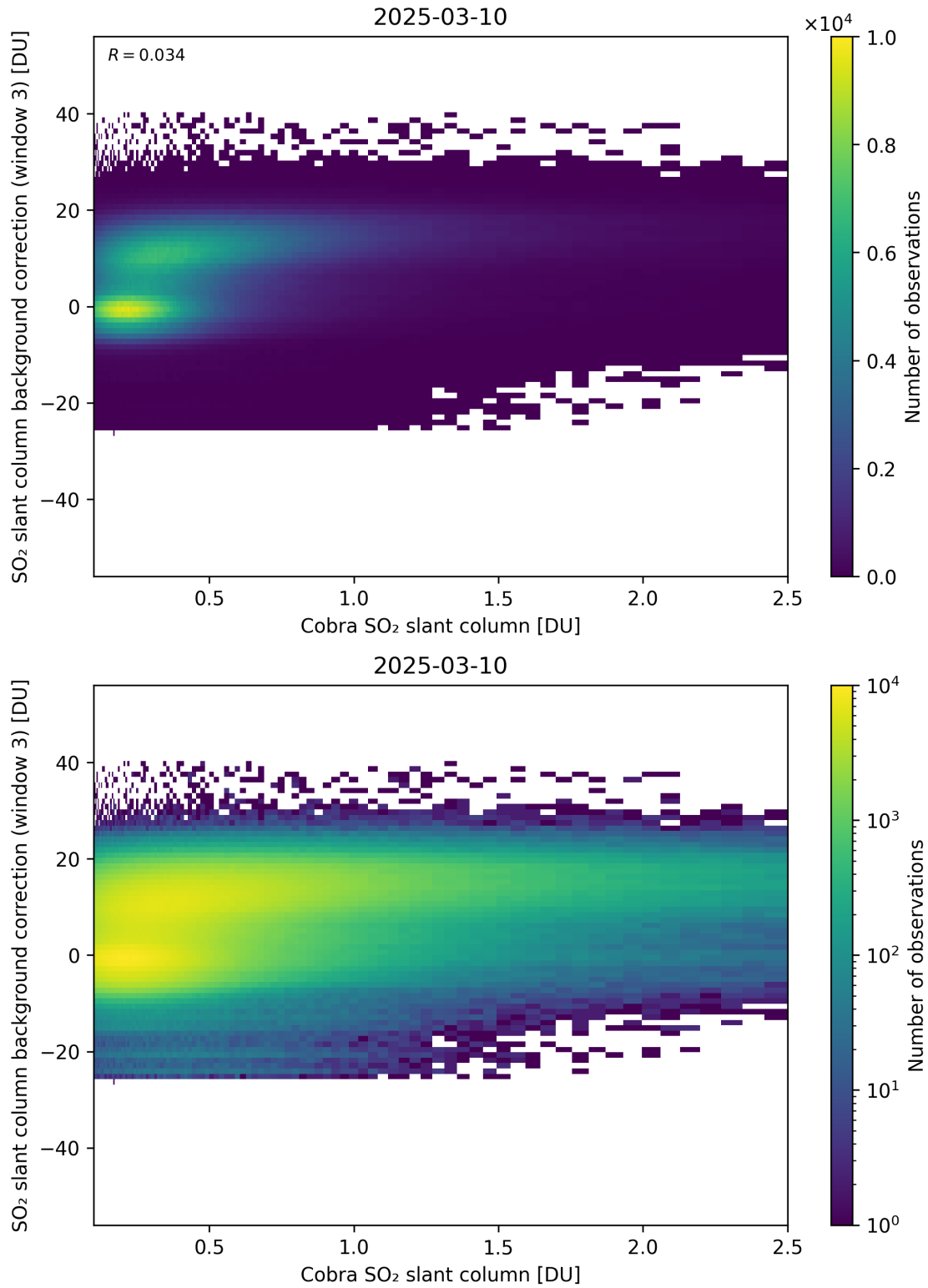
Figure 195: Scatter density plot of “Cobra SO 2 slant column” against “SO 2 slant column background correction (window 3)” for 2025-03-09 to 2025-03-11.
