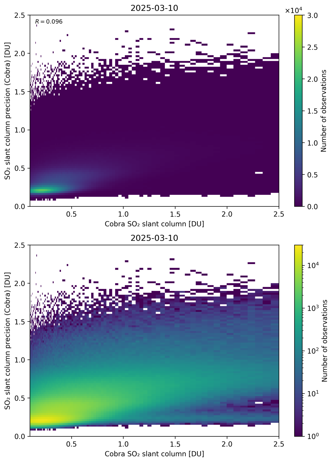
Figure 216: Scatter density plot of “Cobra SO 2 slant column” against “SO 2 slant column precision (Cobra)” for 2025-03-09 to 2025-03-11.
