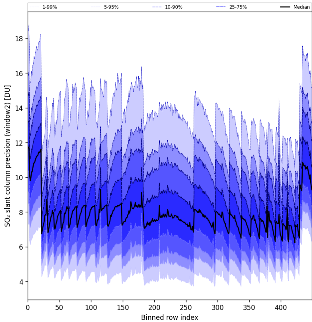
Figure 94: Along track statistics of “SO 2 slant column precision (window2)” for 2025-03-09 to 2025-03-11
