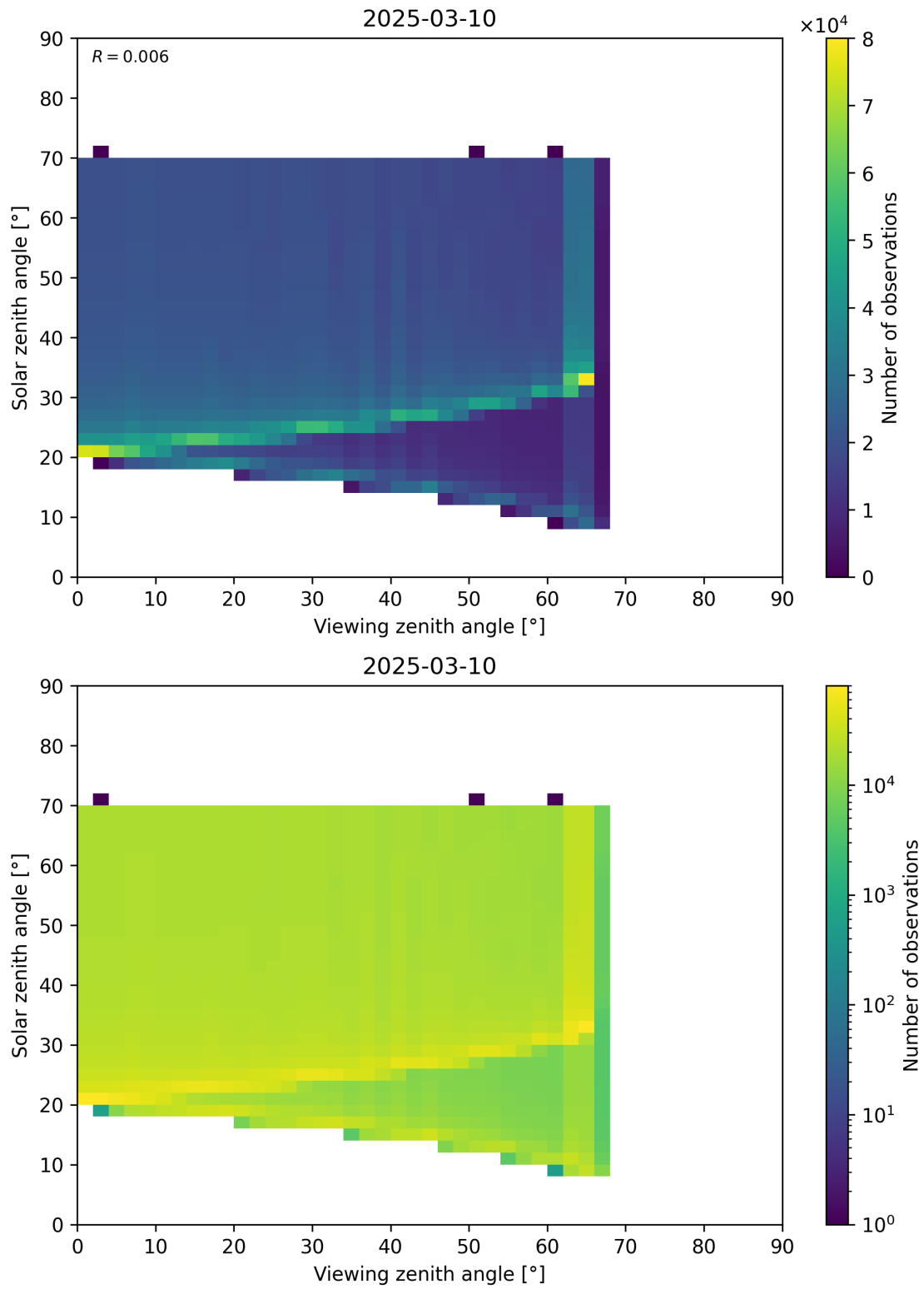
Figure 369: Scatter density plot of “Viewing zenith angle” against “Solar zenith angle” for 2025-03-09 to 2025-03-11.
