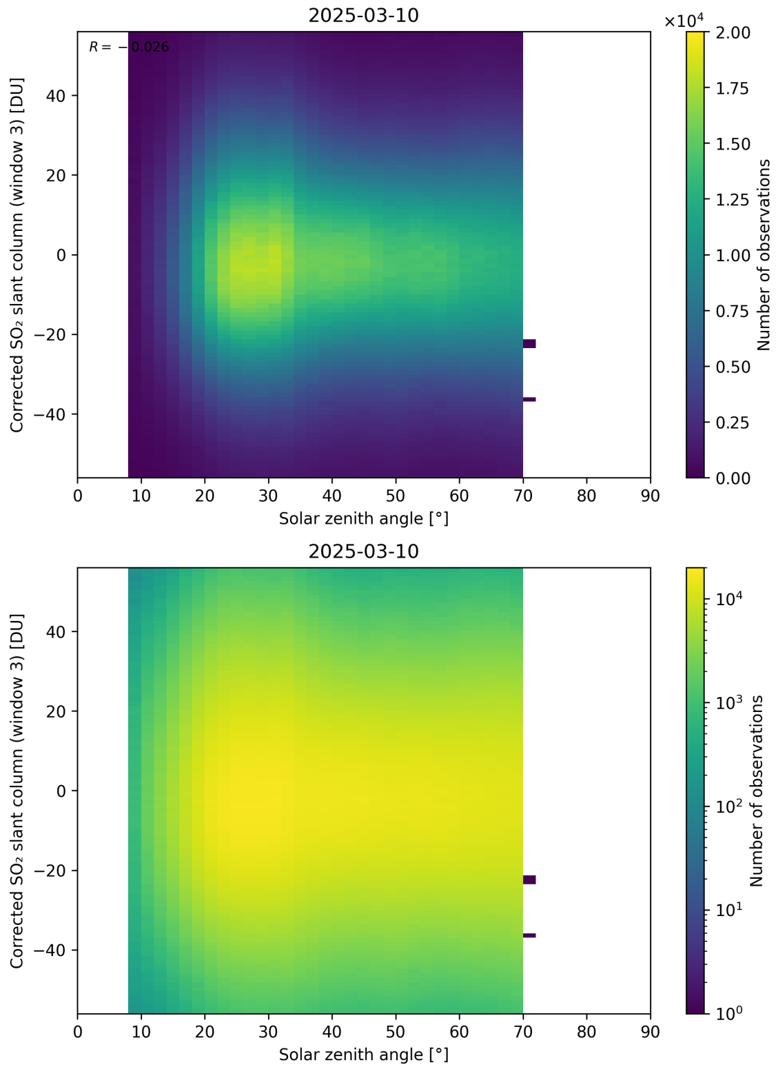
Figure 183: Scatter density plot of “Solar zenith angle” against “Corrected SO 2 slant column (window 3)” for 2025-03-09 to 2025-03-11.
