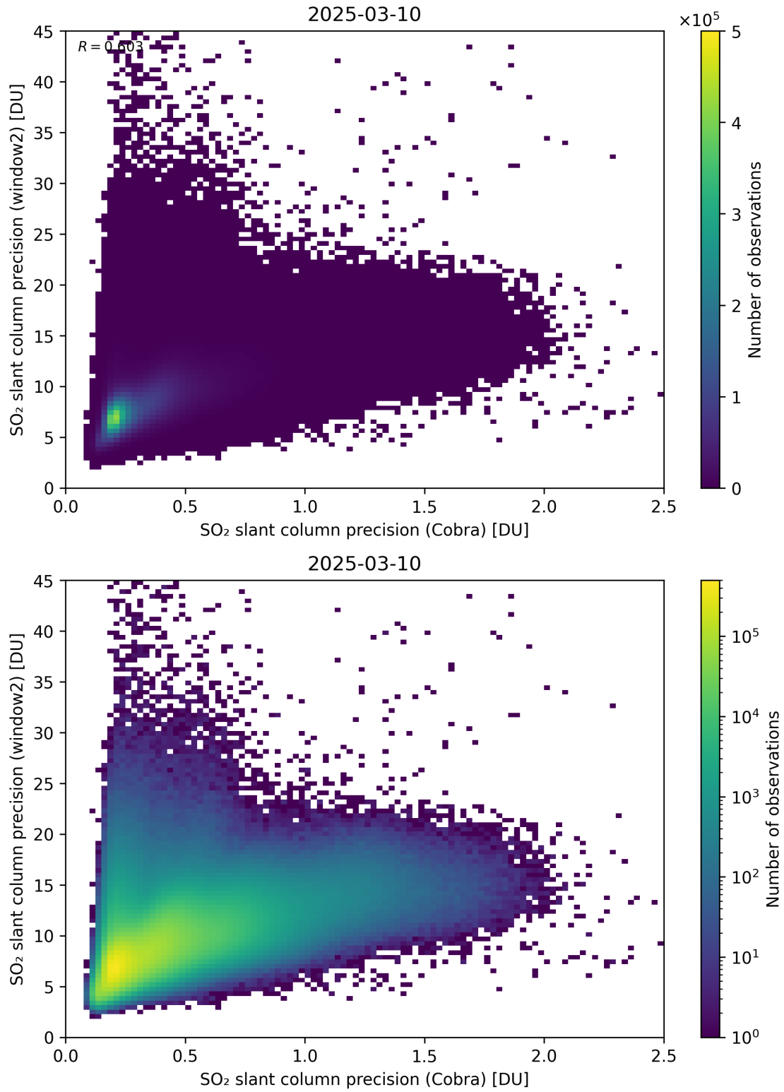
Figure 210: Scatter density plot of “SO 2 slant column precision (Cobra)” against “SO 2 slant column precision (window2)” for 2025-03-09 to 2025-03-11.
