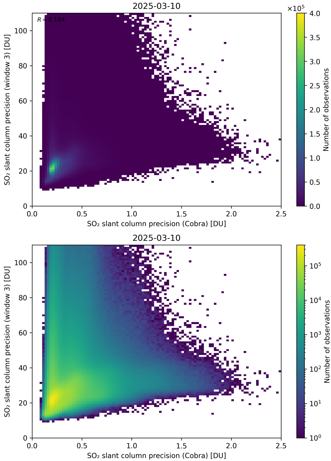
Figure 212: Scatter density plot of “SO 2 slant column precision (Cobra)” against “SO 2 slant column precision (window 3)” for 2025-03-09 to 2025-03-11.
