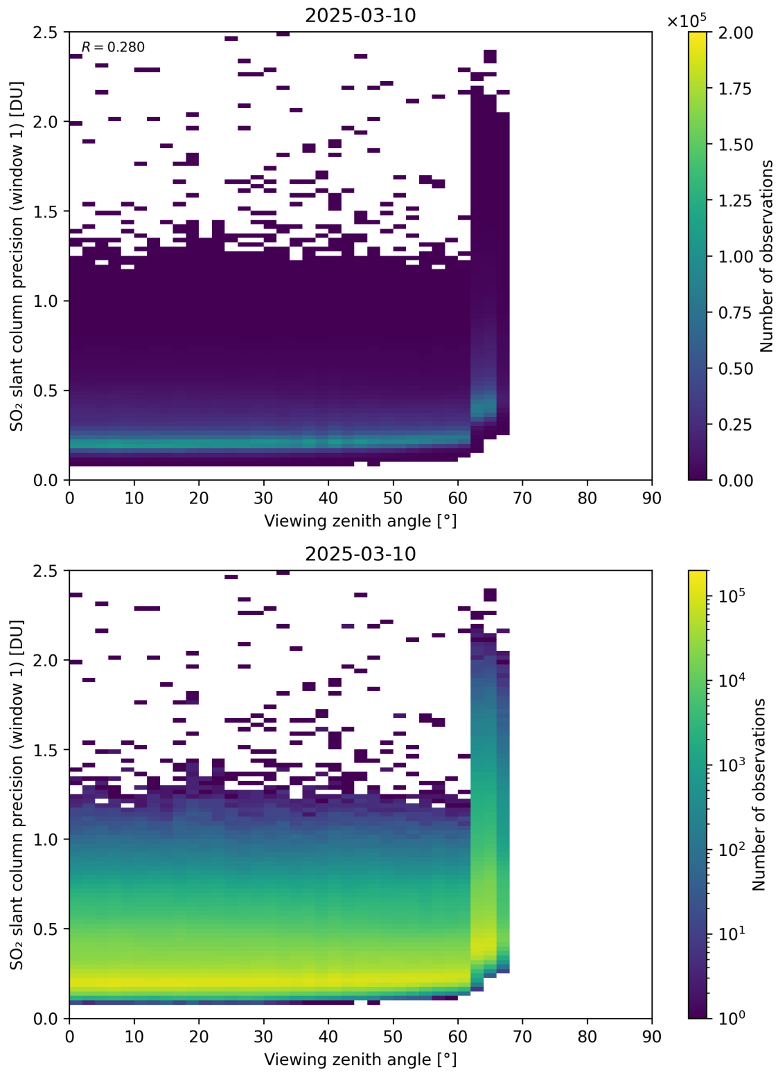
Figure 377: Scatter density plot of “Viewing zenith angle” against “SO 2 slant column precision (window 1)” for 2025-03-09 to 2025-03-11.
