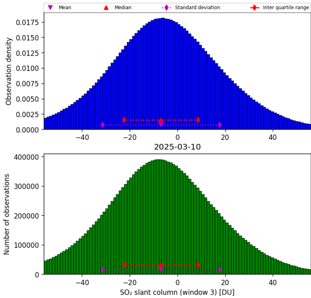
Figure 71: Histogram of “SO 2 slant column (window 3)” for 2025-03-09 to 2025-03-11
