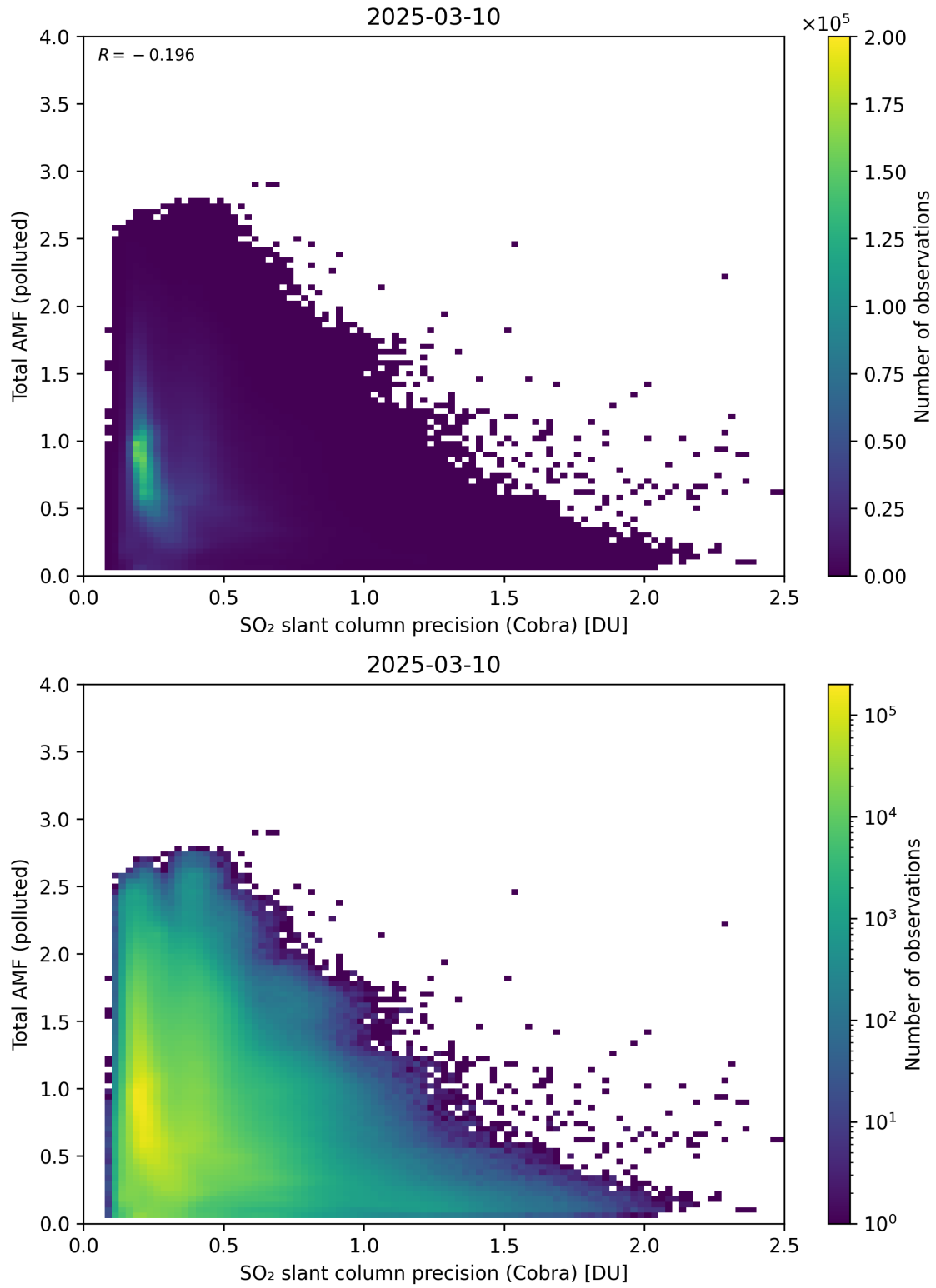
Figure 213: Scatter density plot of “SO 2 slant column precision (Cobra)” against “Total AMF (polluted)” for 2025-03-09 to 2025-03-11.
