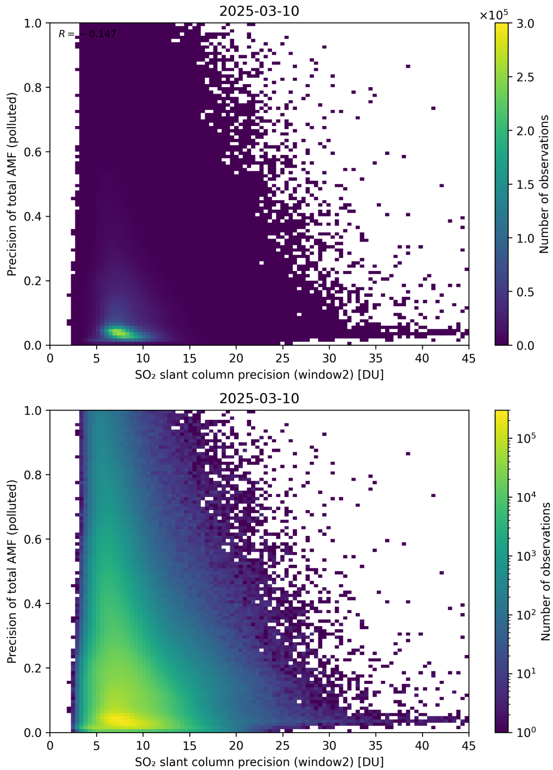
Figure 302: Scatter density plot of “SO 2 slant column precision (window2)” against “Precision of total AMF (polluted)” for 2025-03-09 to 2025-03-11.
