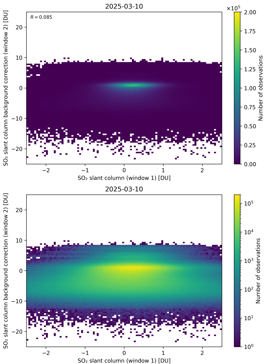
Figure 263: Scatter density plot of “SO 2 slant column (window 1)” against “SO 2 slant column background correction (window 2)” for 2025-03-09 to 2025-03-11.
