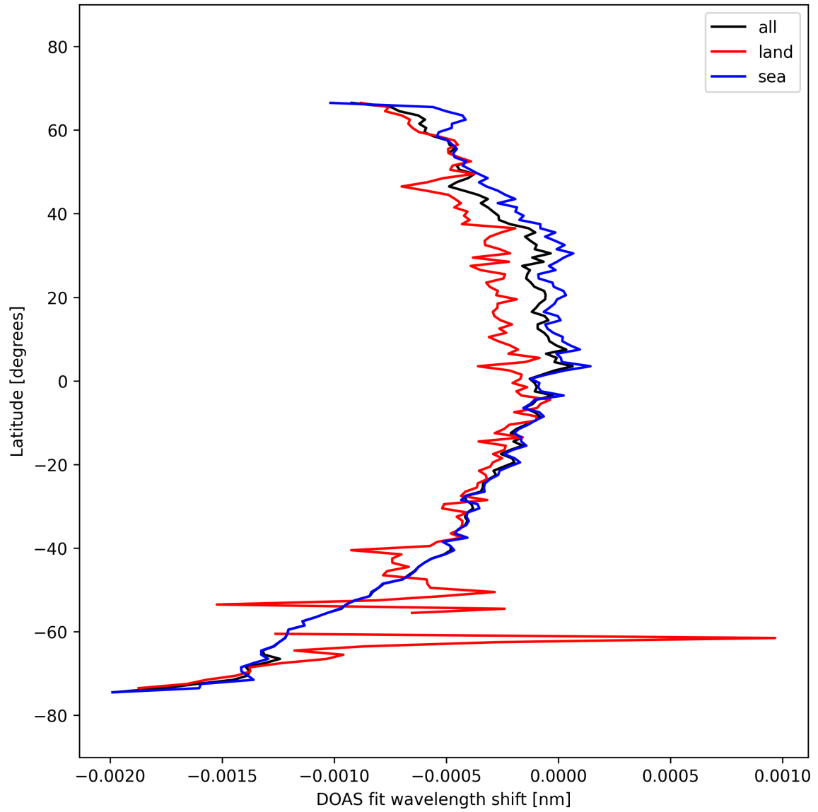
Figure 50: Zonal average of "DOAS fit wavelength shift" for 2025-03-09 to 2025-03-11.
