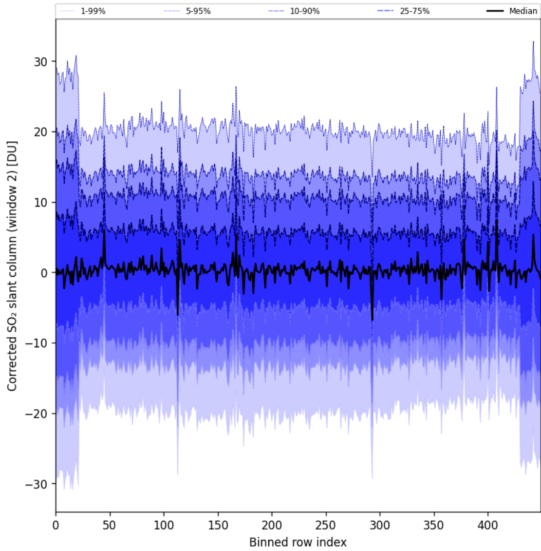
Figure 95: Along track statistics of “Corrected SO 2 slant column (window 2)” for 2025-03-09 to 2025-03-11
