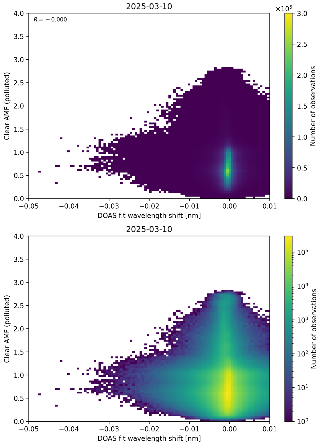
Figure 140: Scatter density plot of “DOAS fit wavelength shift” against “Clear AMF (polluted)” for 2025-03-09 to 2025-03-11.
