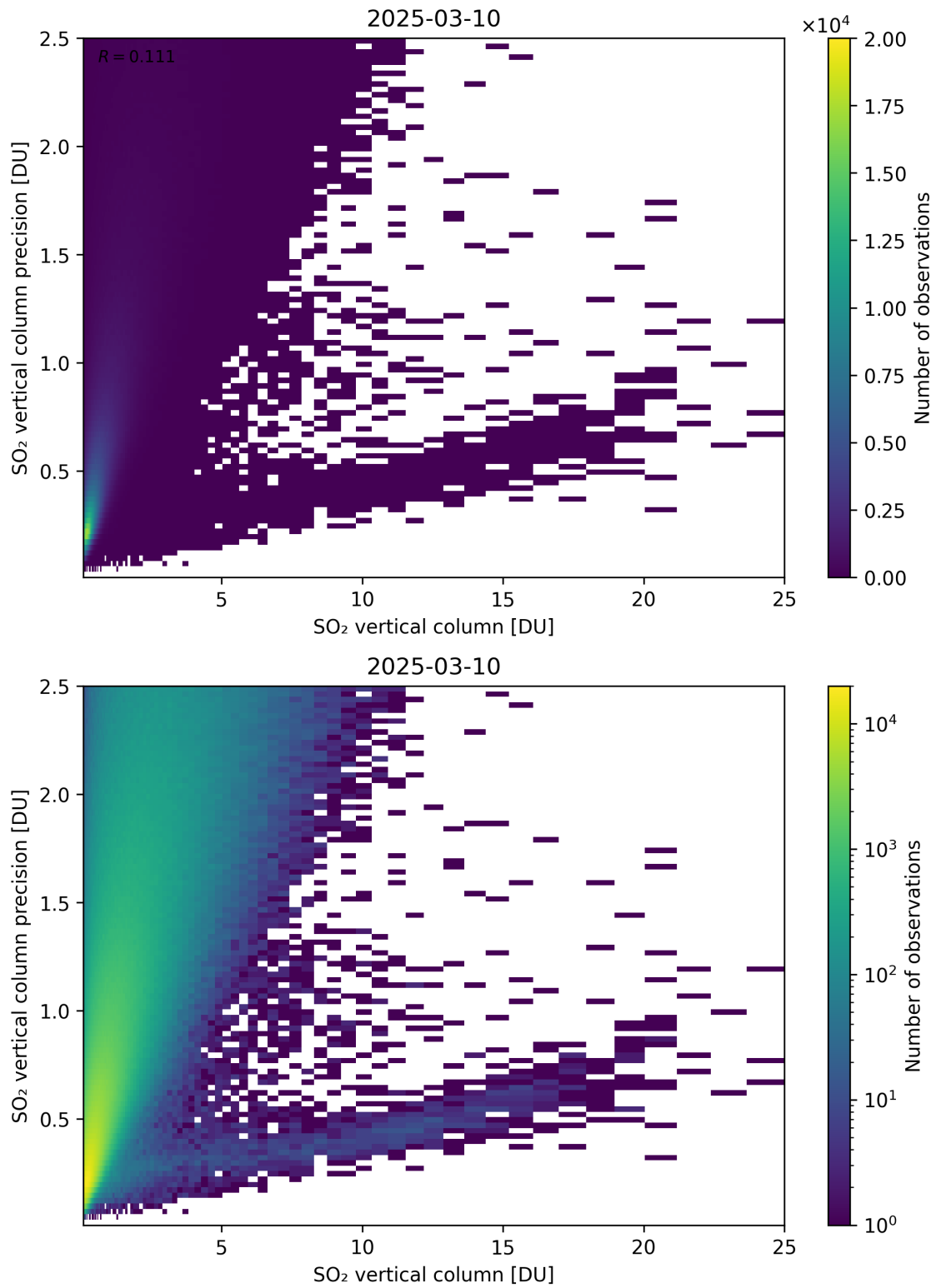
Figure 361: Scatter density plot of “SO 2 vertical column” against “SO 2 vertical column precision” for 2025-03-09 to 2025-03-11.
