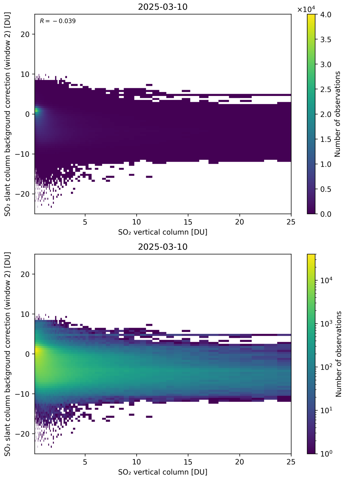
Figure 324: Scatter density plot of “SO 2 vertical column” against “SO 2 slant column background correction (window 2)” for 2025-03-09 to 2025-03-11.
