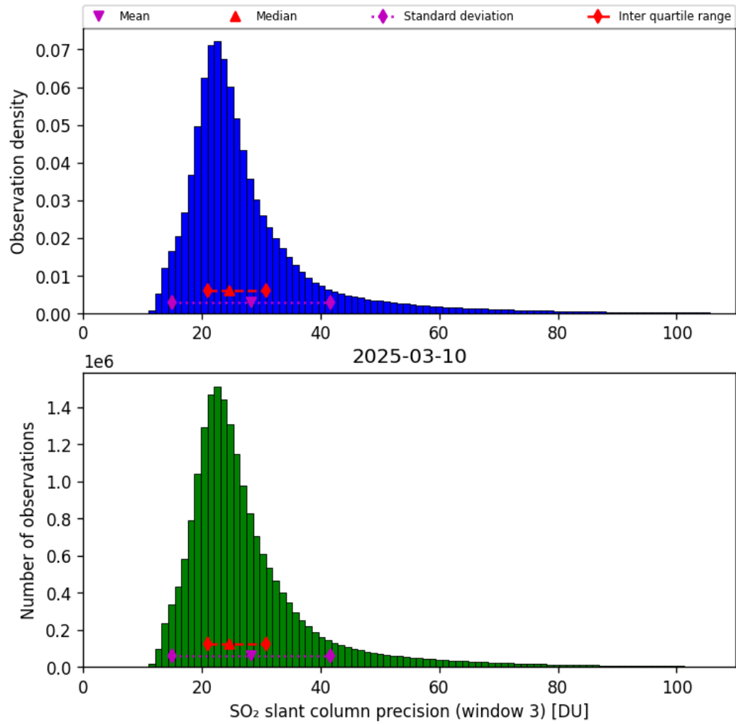
Figure 72: Histogram of “SO 2 slant column precision (window 3)” for 2025-03-09 to 2025-03-11
