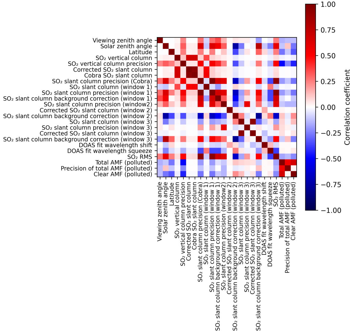
Figure 2: Map of correlation matrix for 2025-03-09 to 2025-03-11.
