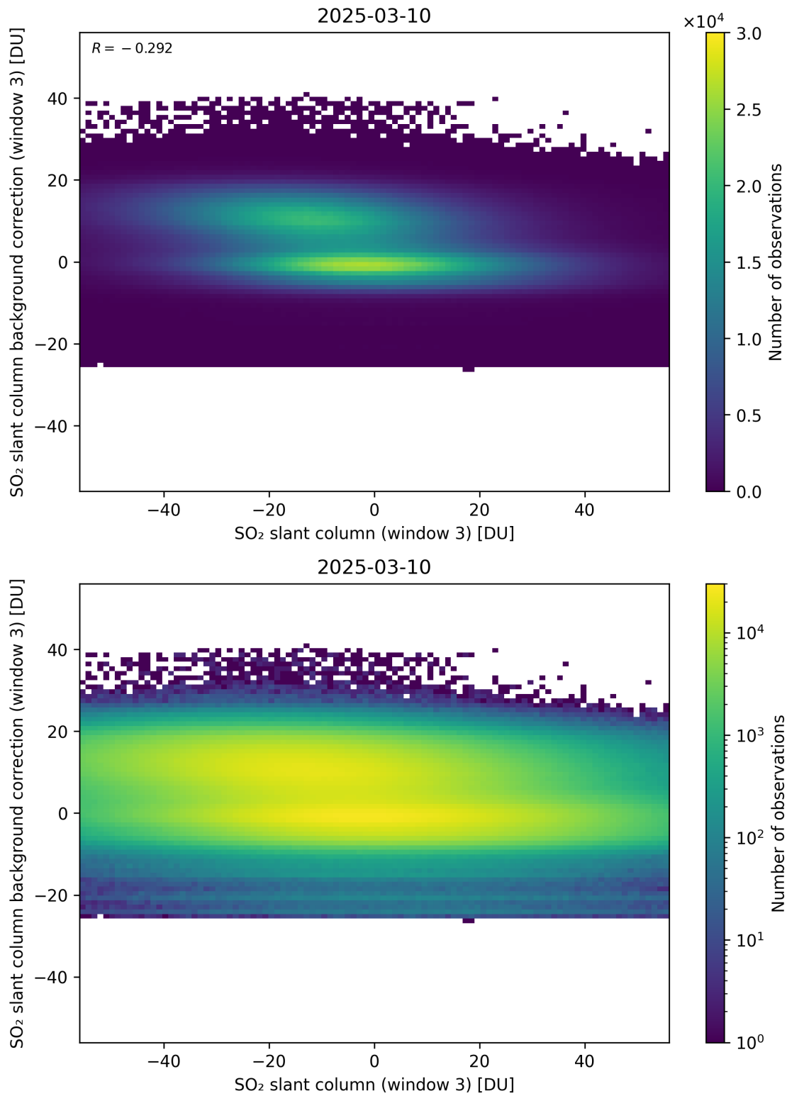
Figure 303: Scatter density plot of “SO 2 slant column (window 3)” against “SO 2 slant column background correction (window 3)” for 2025-03-09 to 2025-03-11.
