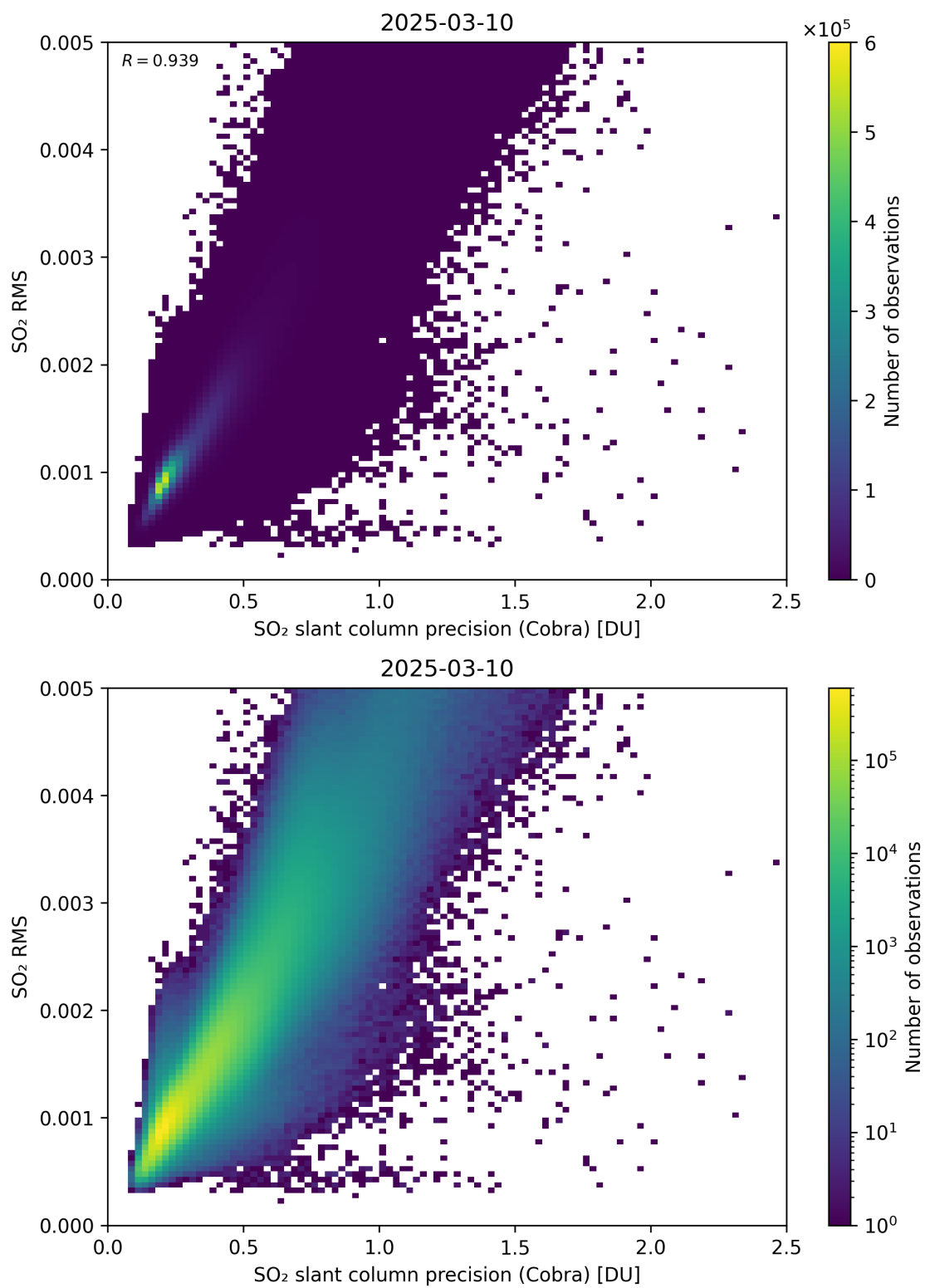
Figure 204: Scatter density plot of “SO 2 slant column precision (Cobra)” against “SO 2 RMS” for 2025-03-09 to 2025-03-11.
