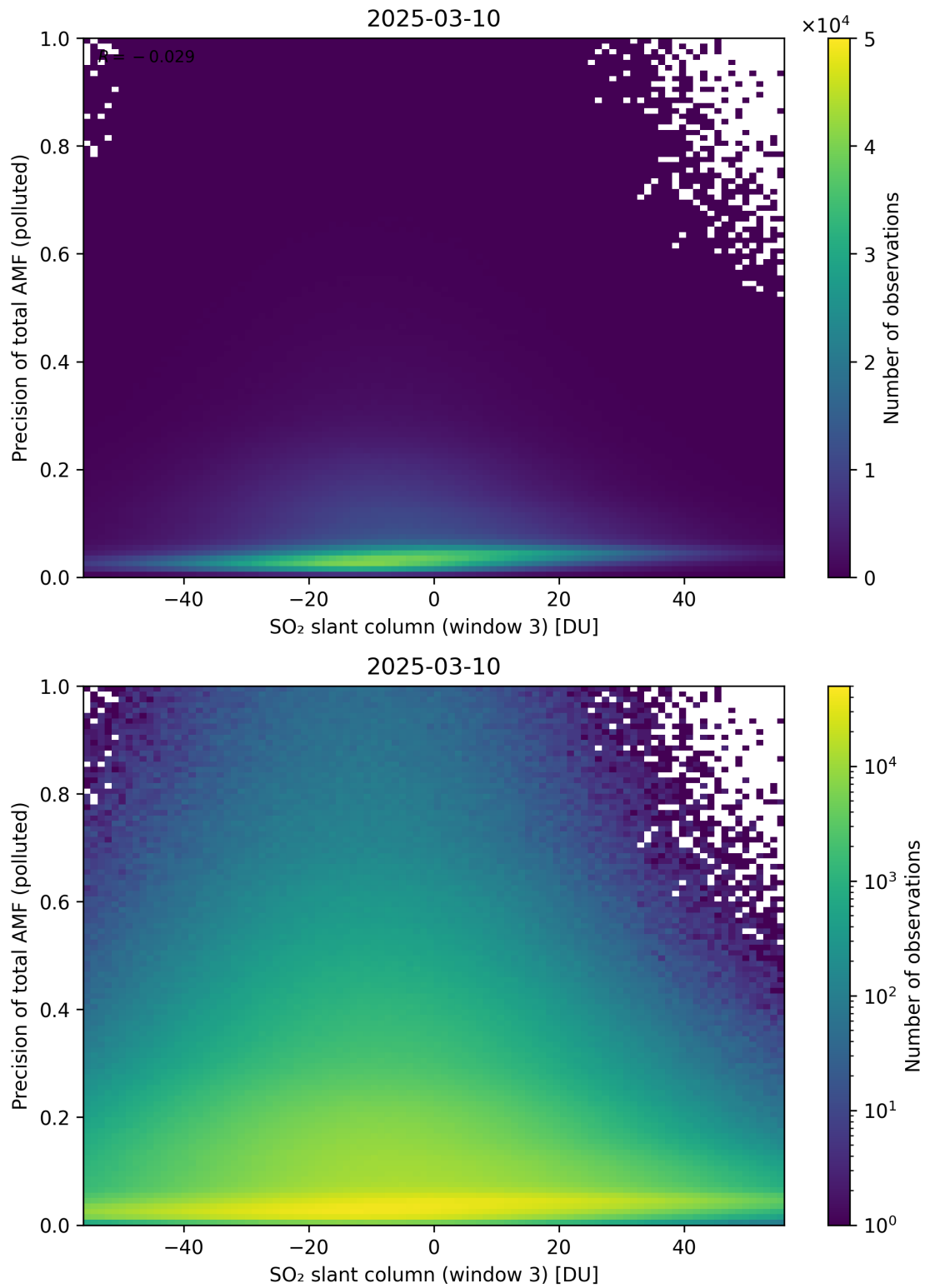
Figure 319: Scatter density plot of “SO 2 slant column (window 3)” against “Precision of total AMF (polluted)” for 2025-03-09 to 2025-03-11.
