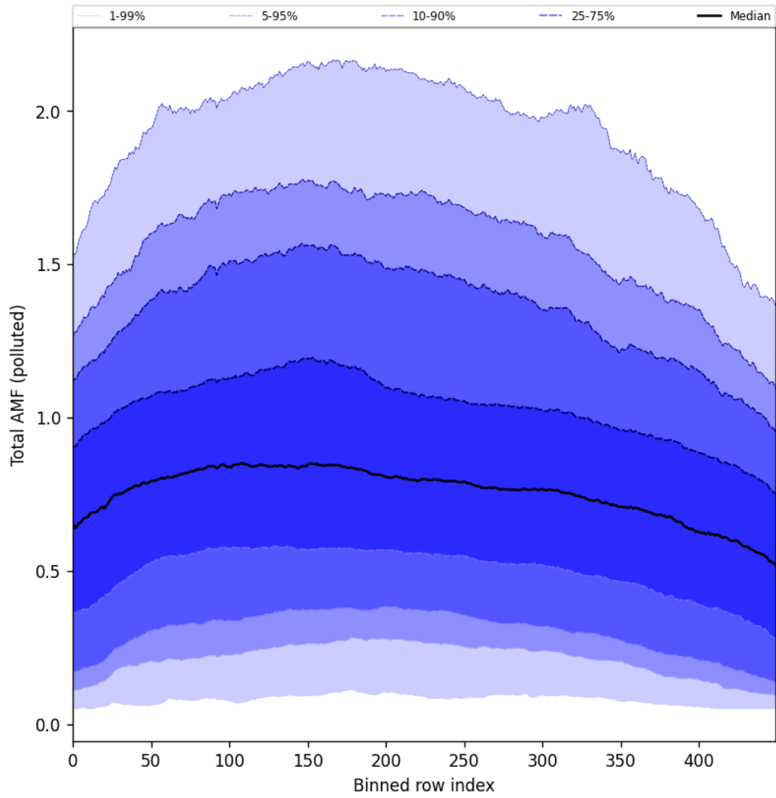
Figure 105: Along track statistics of “Total AMF (polluted)” for 2025-03-09 to 2025-03-11
