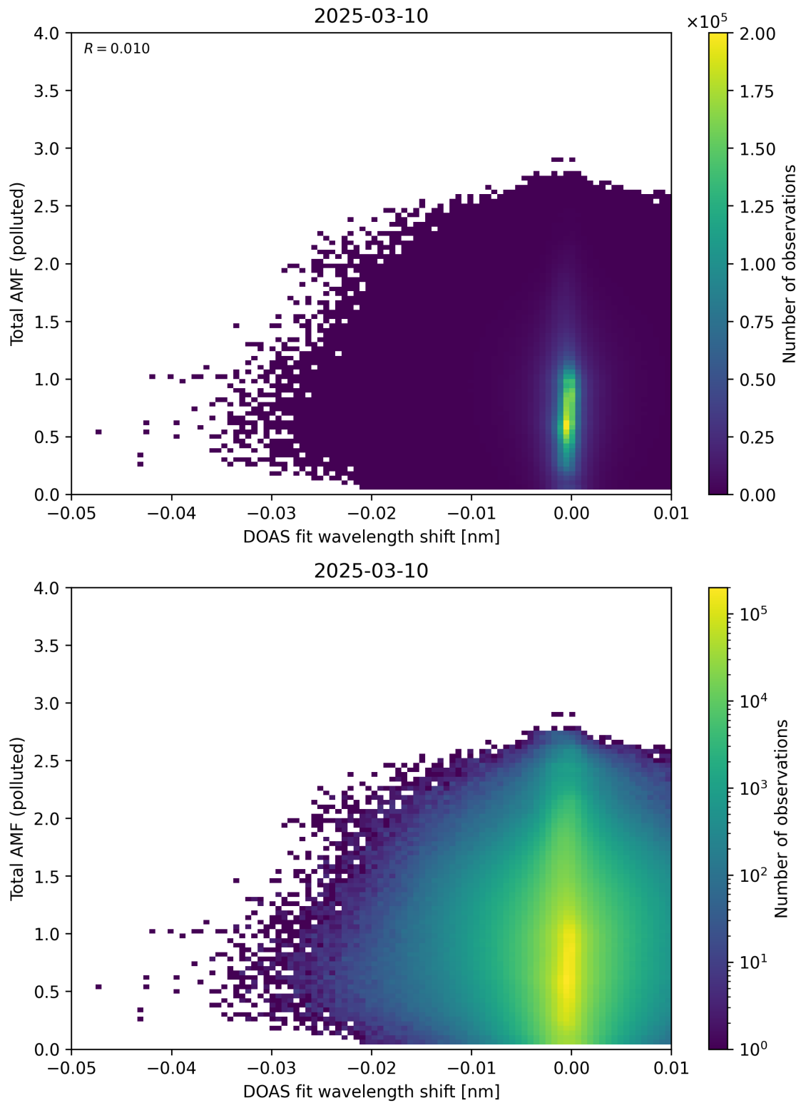
Figure 141: Scatter density plot of “DOAS fit wavelength shift” against “Total AMF (polluted)” for 2025-03-09 to 2025-03-11.
