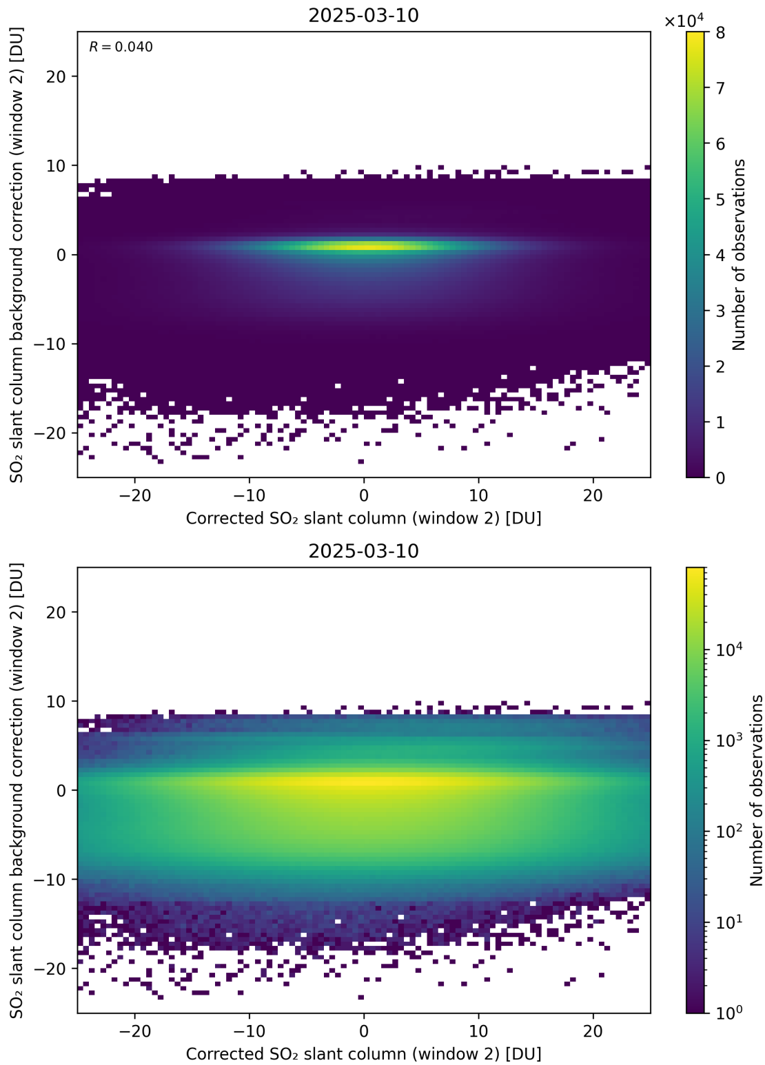
Figure 244: Scatter density plot of “Corrected SO 2 slant column (window 2)” against “SO 2 slant column background correction (window 2)” for 2025-03-09 to 2025-03-11.
