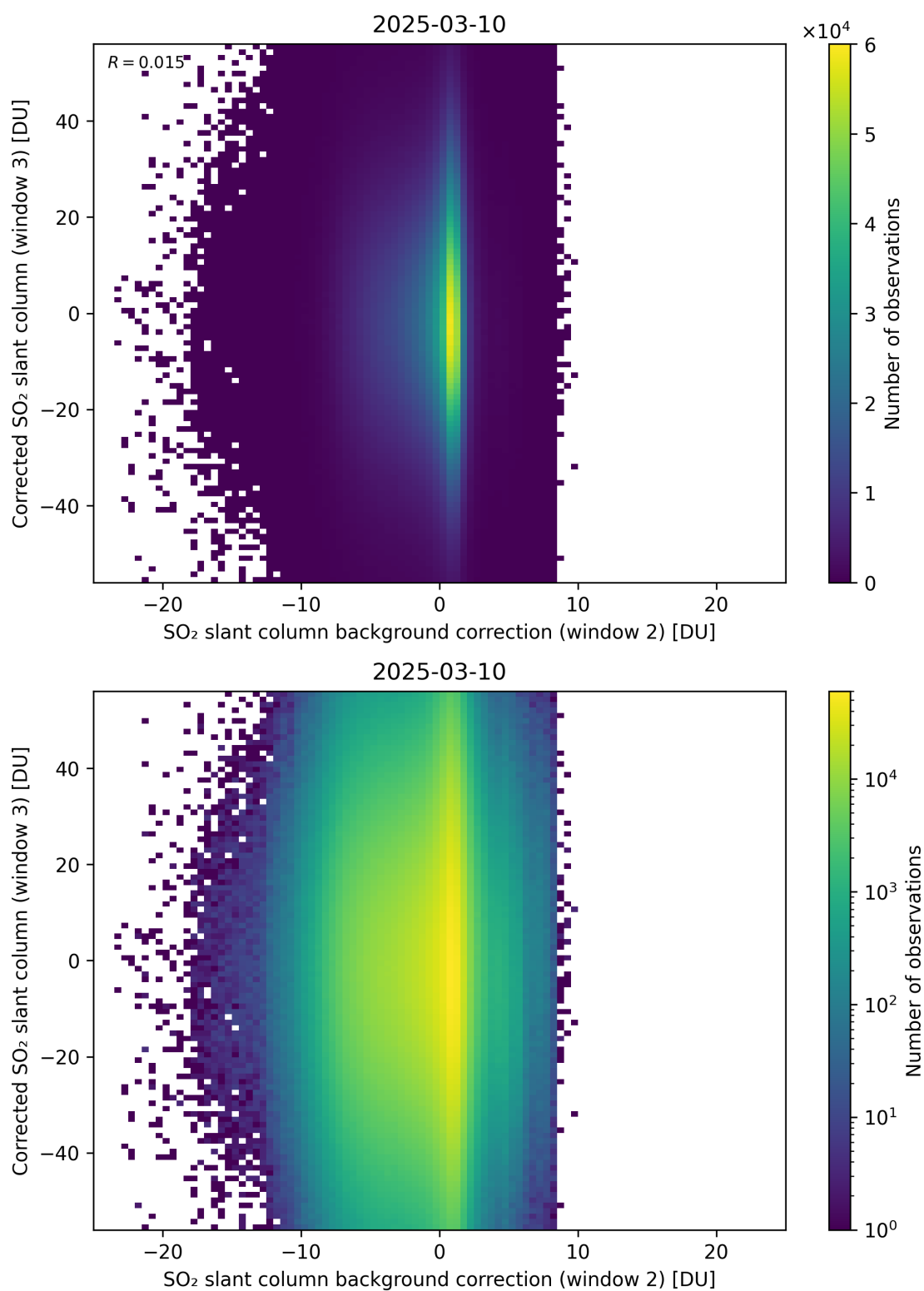
Figure 127: Scatter density plot of “SO 2 slant column background correction (window 2)” against “Corrected SO 2 slant column (window 3)” for 2025-03-09 to 2025-03-11.
