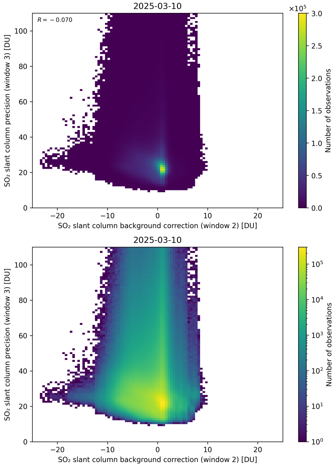
Figure 129: Scatter density plot of “SO 2 slant column background correction (window 2)” against “SO 2 slant column precision (window 3)” for 2025-03-09 to 2025-03-11.
