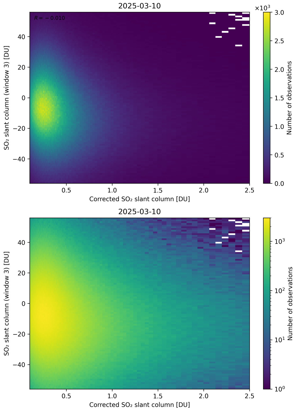
Figure 240: Scatter density plot of “Corrected SO 2 slant column” against “SO 2 slant column (window 3)” for 2025-03-09 to 2025-03-11.
