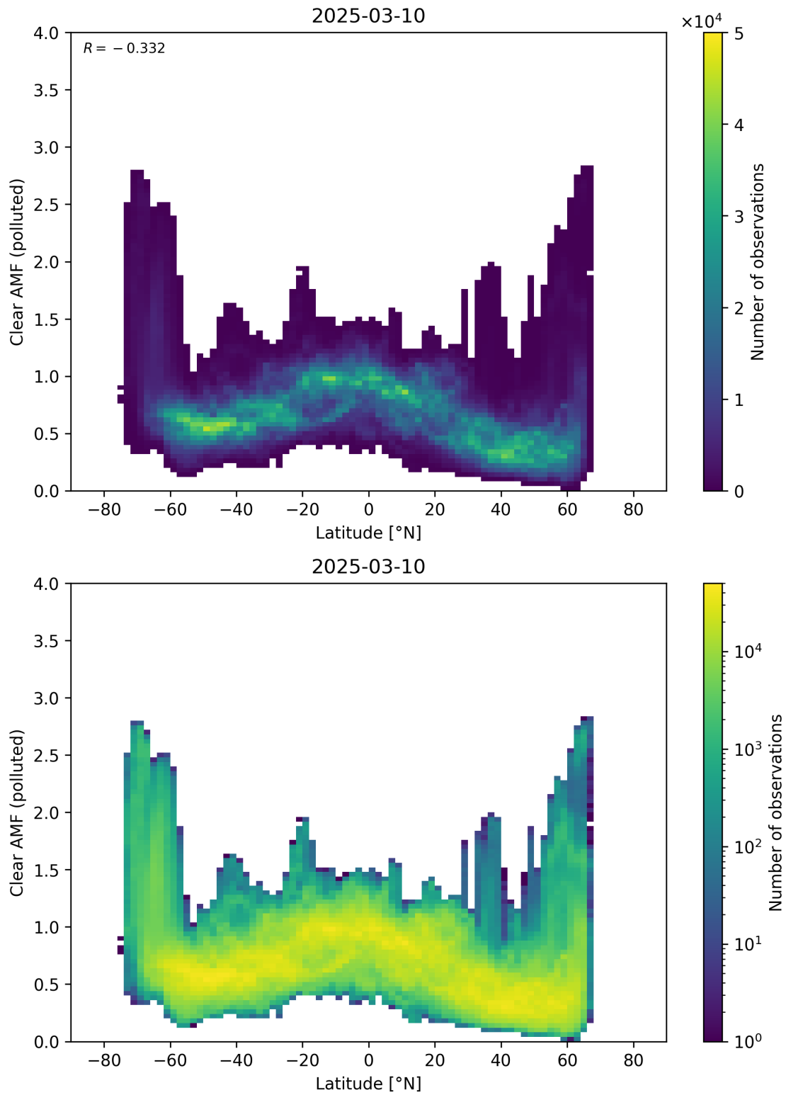
Figure 156: Scatter density plot of “Latitude” against “Clear AMF (polluted)” for 2025-03-09 to 2025-03-11.
