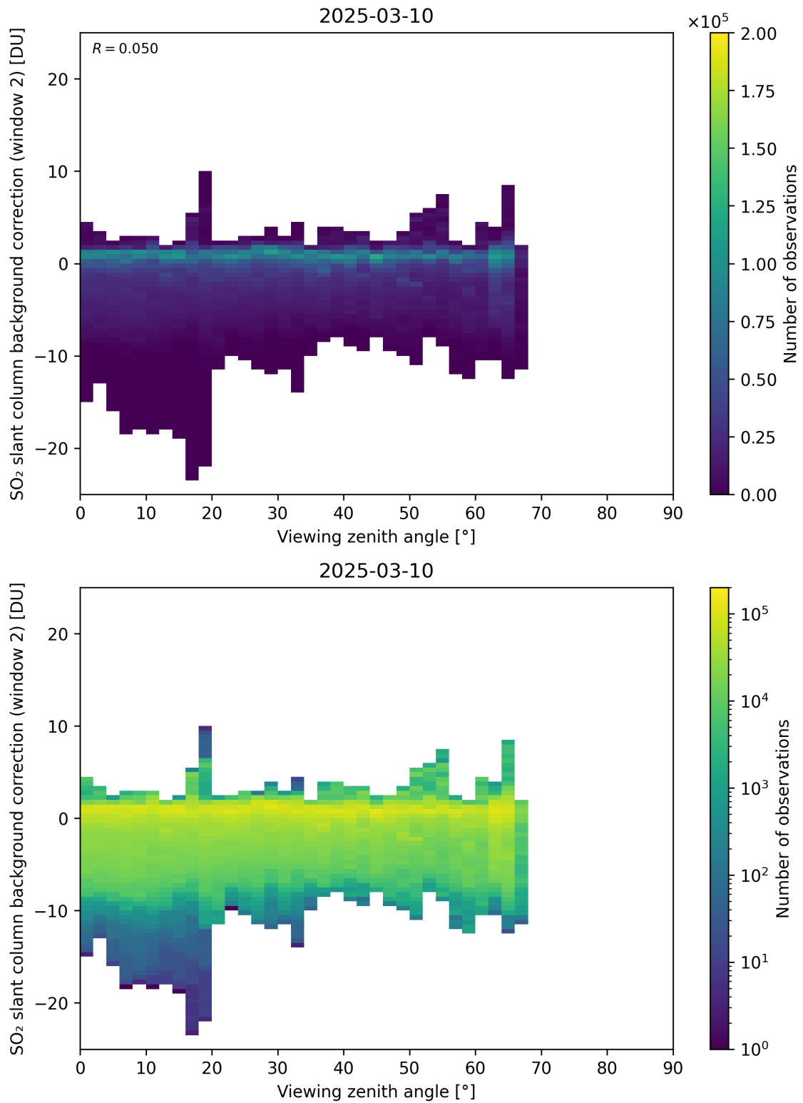
Figure 363: Scatter density plot of “Viewing zenith angle” against “SO 2 slant column background correction (window 2)” for 2025-03-09 to 2025-03-11.
