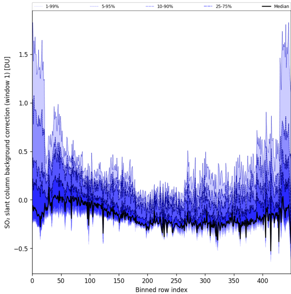
Figure 92: Along track statistics of “SO 2 slant column background correction (window 1)” for 2025-03-09 to 2025-03-11
