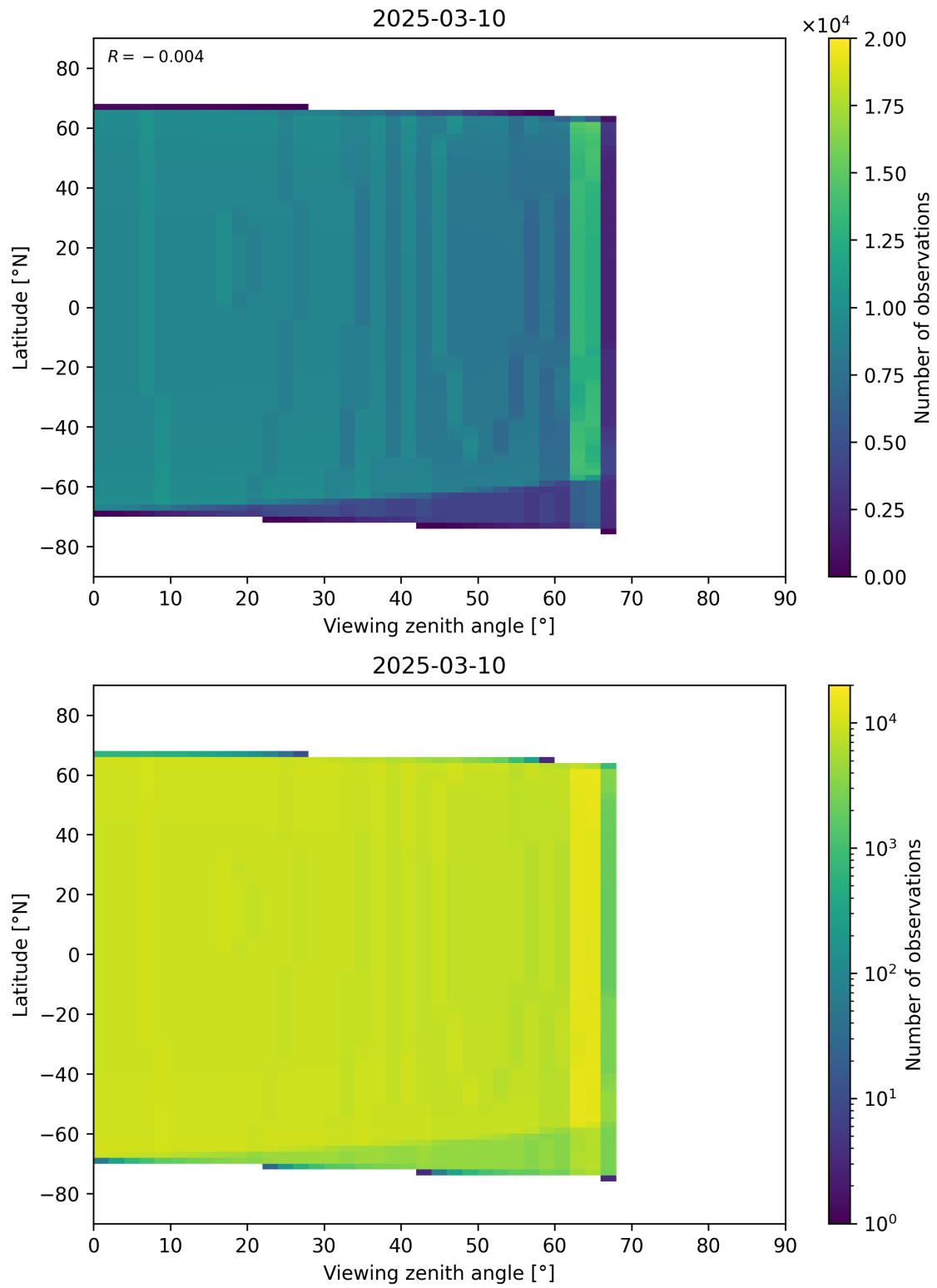
Figure 368: Scatter density plot of “Viewing zenith angle” against “Latitude” for 2025-03-09 to 2025-03-11.
