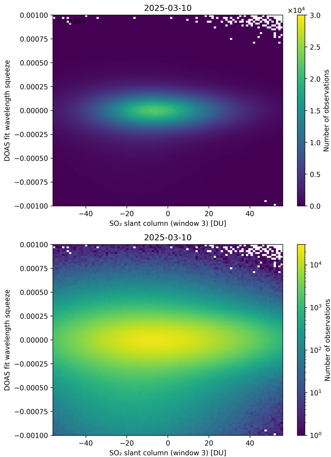
Figure 305: Scatter density plot of “SO 2 slant column (window 3)” against “DOAS fit wavelength squeeze” for 2025-03-09 to 2025-03-11.
