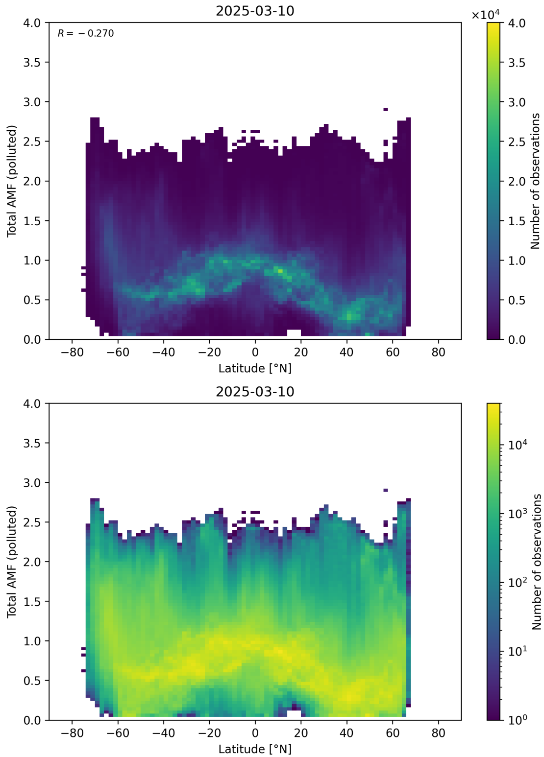
Figure 167: Scatter density plot of “Latitude” against “Total AMF (polluted)” for 2025-03-09 to 2025-03-11.
