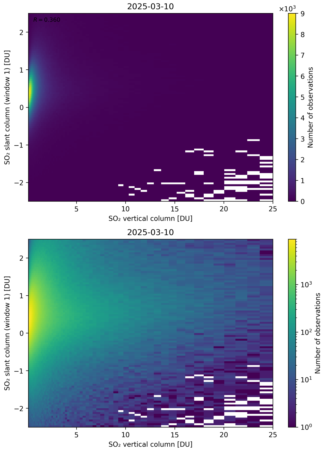
Figure 354: Scatter density plot of “SO 2 vertical column” against “SO 2 slant column (window 1)” for 2025-03-09 to 2025-03-11.
