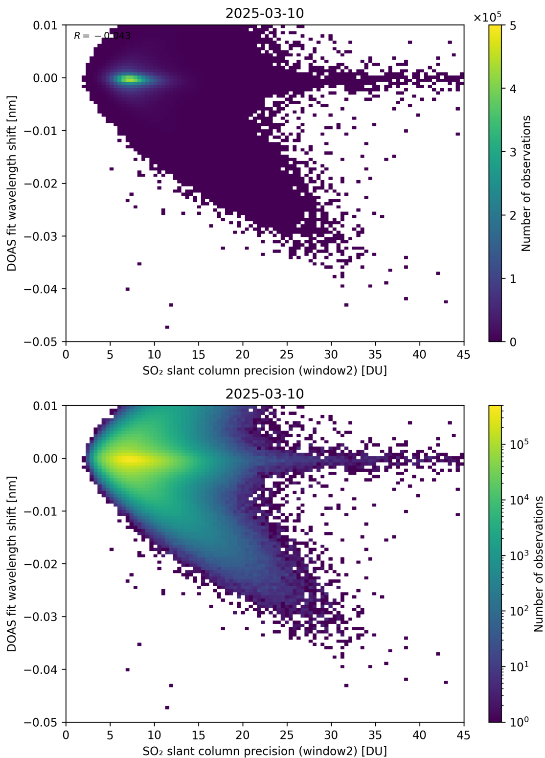
Figure 293: Scatter density plot of “SO 2 slant column precision (window2)” against “DOAS fit wavelength shift” for 2025-03-09 to 2025-03-11.
