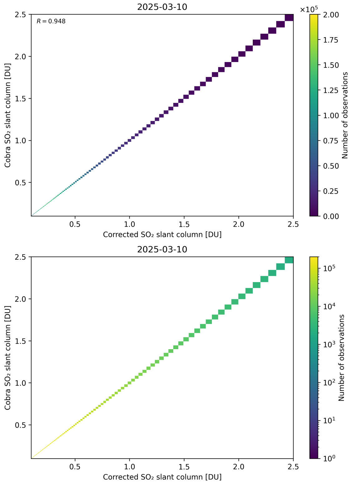
Figure 233: Scatter density plot of “Corrected SO 2 slant column” against “Cobra SO 2 slant column” for 2025-03-09 to 2025-03-11.
