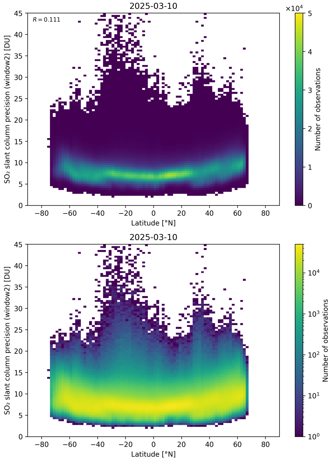
Figure 164: Scatter density plot of “Latitude” against “SO 2 slant column precision (window2)” for 2025-03-09 to 2025-03-11.
