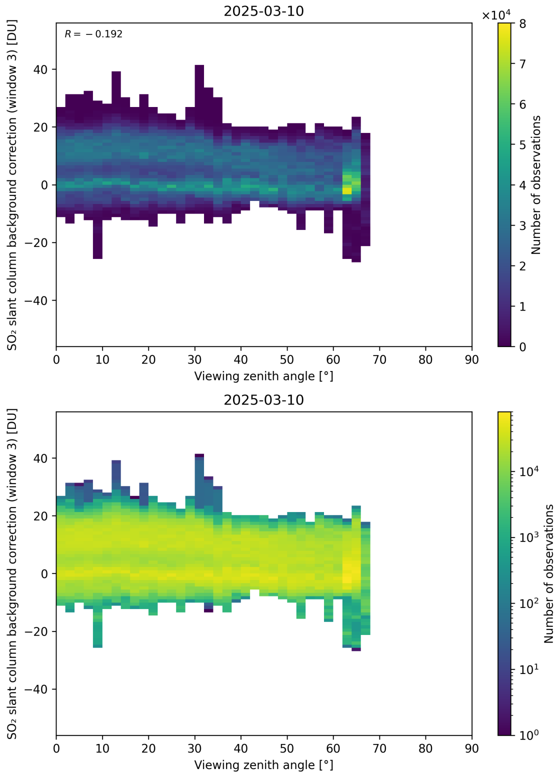
Figure 364: Scatter density plot of “Viewing zenith angle” against “SO 2 slant column background correction (window 3)” for 2025-03-09 to 2025-03-11.
