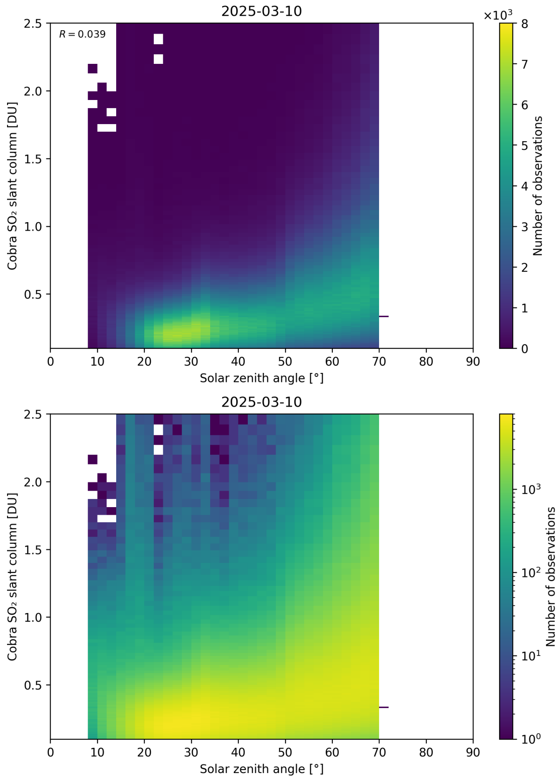
Figure 179: Scatter density plot of “Solar zenith angle” against “Cobra SO 2 slant column” for 2025-03-09 to 2025-03-11.
