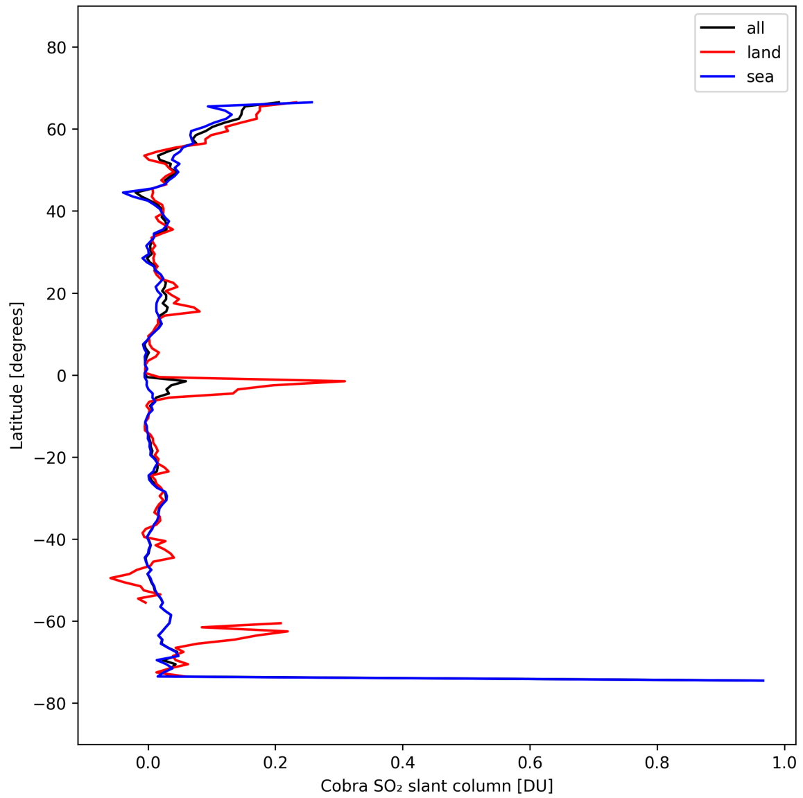
Figure 35: Zonal average of “Cobra SO 2 slant column” for 2025-03-09 to 2025-03-11.
