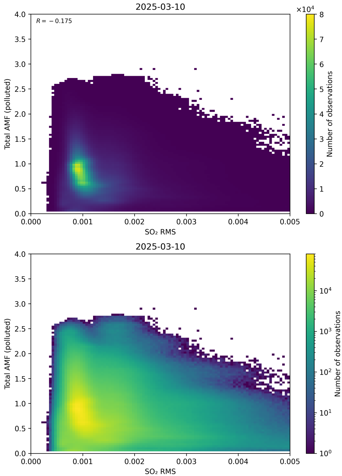
Figure 148: Scatter density plot of “SO 2 RMS” against “Total AMF (polluted)” for 2025-03-09 to 2025-03-11.
