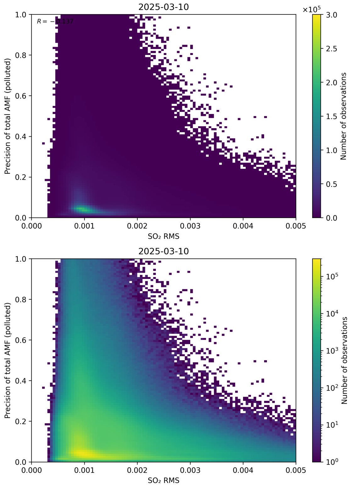
Figure 149: Scatter density plot of “SO 2 RMS” against “Precision of total AMF (polluted)” for 2025-03-09 to 2025-03-11.
