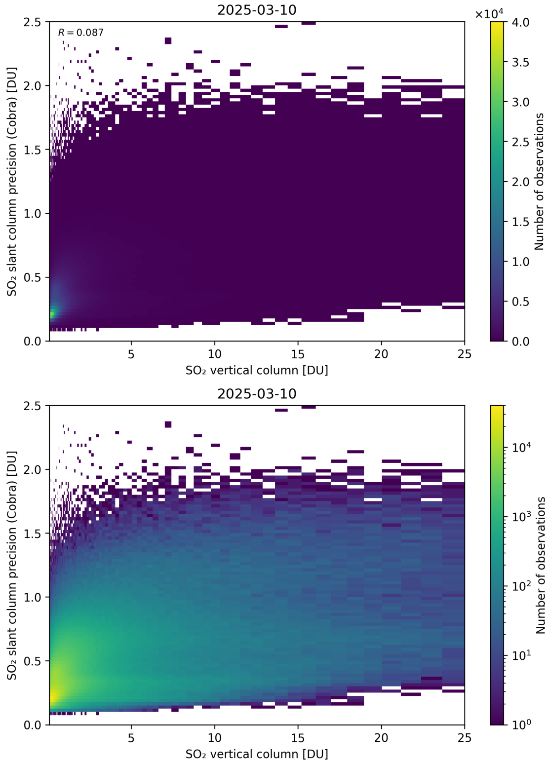
Figure 350: Scatter density plot of “SO 2 vertical column” against “SO 2 slant column precision (Cobra)” for 2025-03-09 to 2025-03-11.
