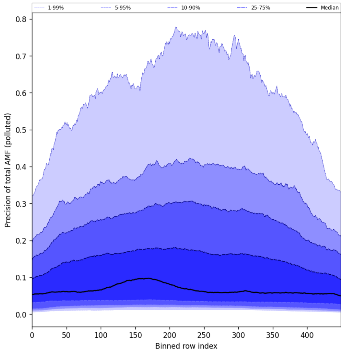
Figure 106: Along track statistics of “Precision of total AMF (polluted)” for 2025-03-09 to 2025-03-11
