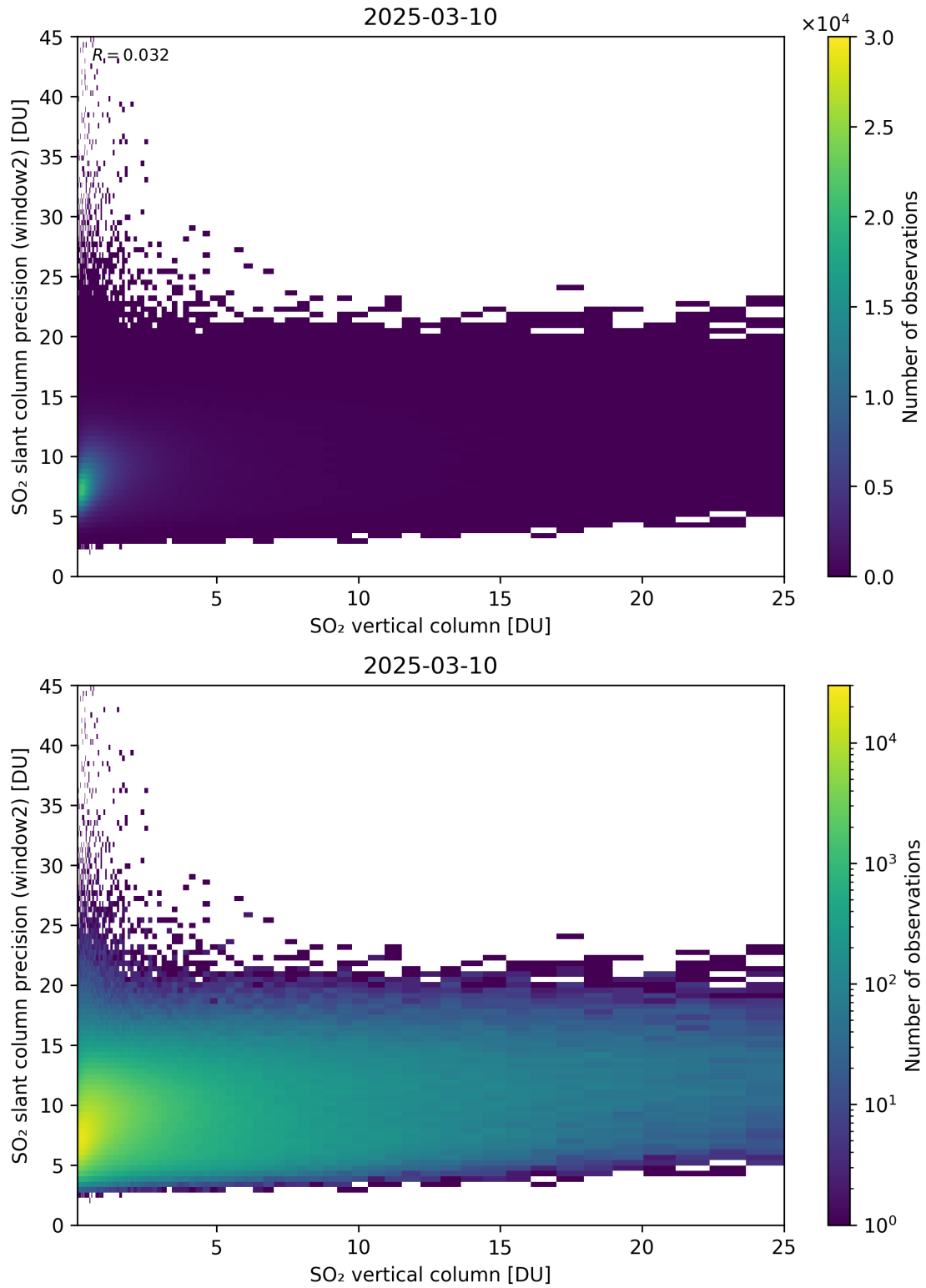
Figure 356: Scatter density plot of “SO 2 vertical column” against “SO 2 slant column precision (window2)” for 2025-03-09 to 2025-03-11.
