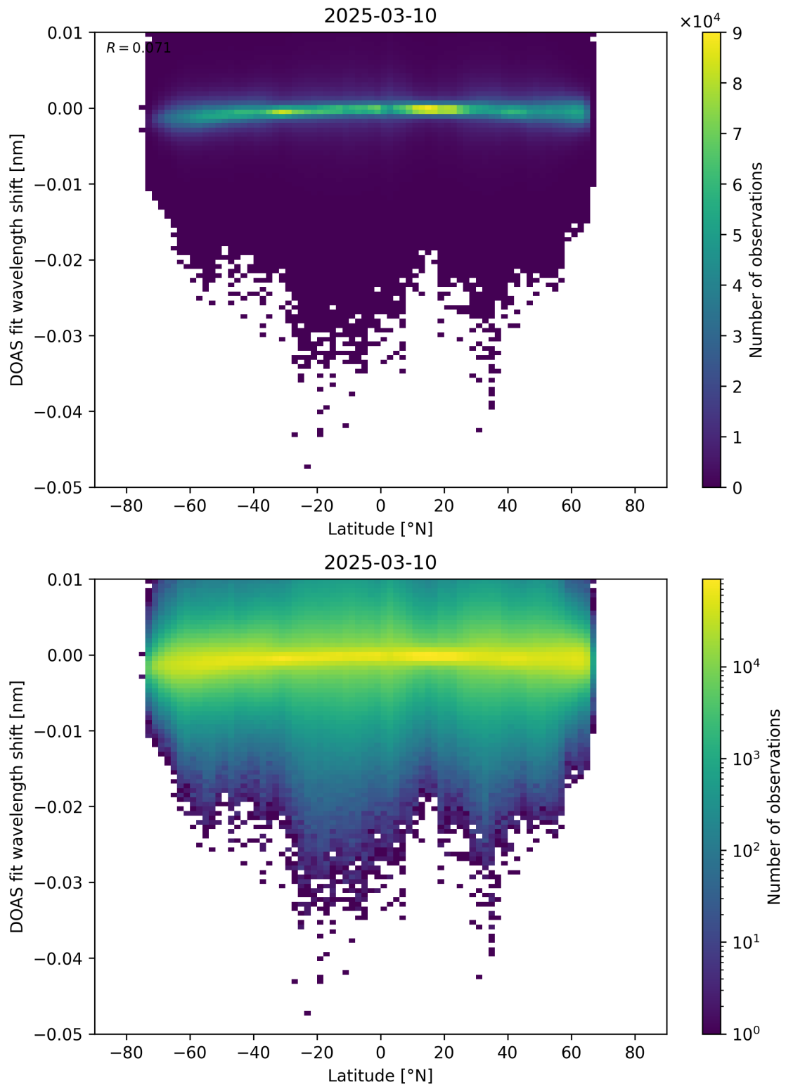
Figure 153: Scatter density plot of “Latitude” against “DOAS fit wavelength shift” for 2025-03-09 to 2025-03-11.
