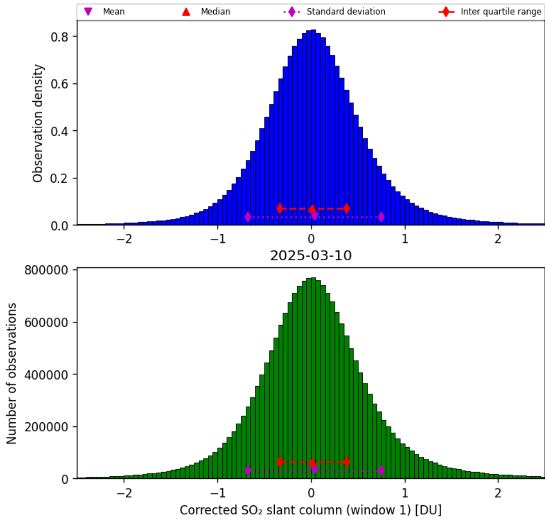
Figure 65: Histogram of “Corrected SO 2 slant column (window 1)” for 2025-03-09 to 2025-03-11
