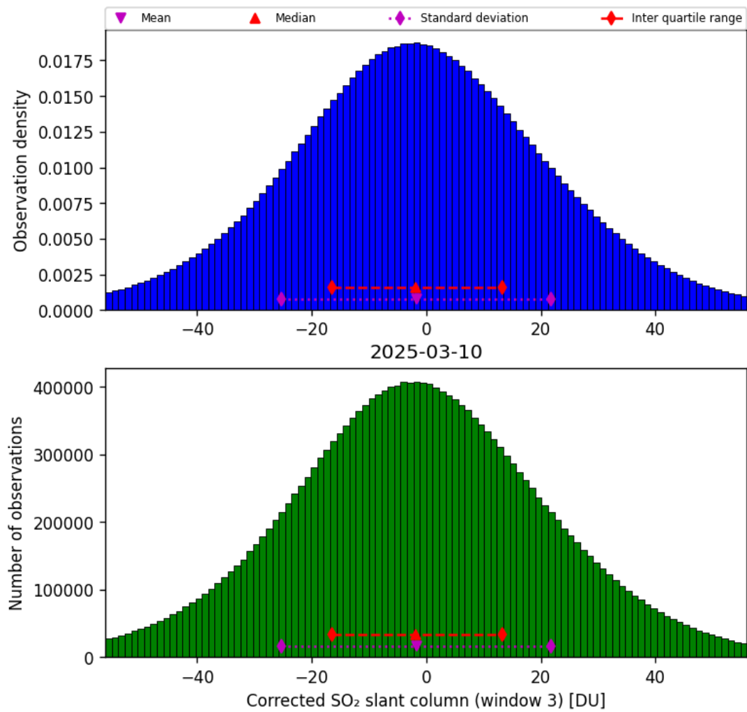
Figure 73: Histogram of “Corrected SO 2 slant column (window 3)” for 2025-03-09 to 2025-03-11
