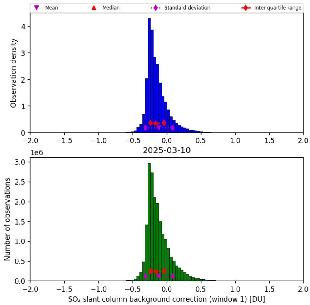
Figure 66: Histogram of “SO 2 slant column background correction (window 1)” for 2025-03-09 to 2025-03-11
