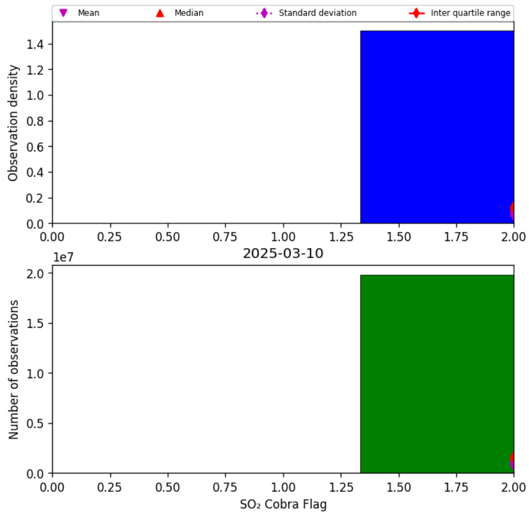
Figure 75: Histogram of “SO 2 Cobra Flag” for 2025-03-09 to 2025-03-11
