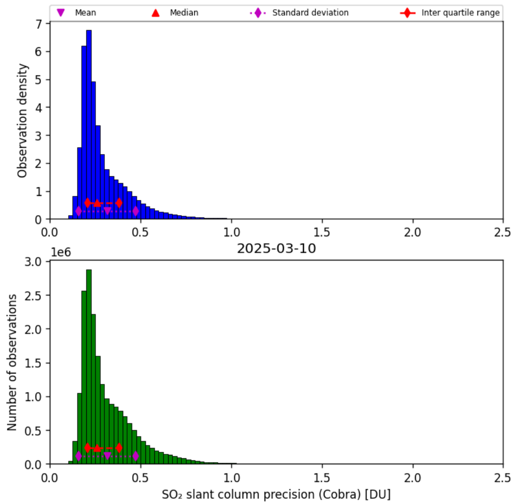
Figure 62: Histogram of “SO 2 slant column precision (Cobra)” for 2025-03-09 to 2025-03-11
