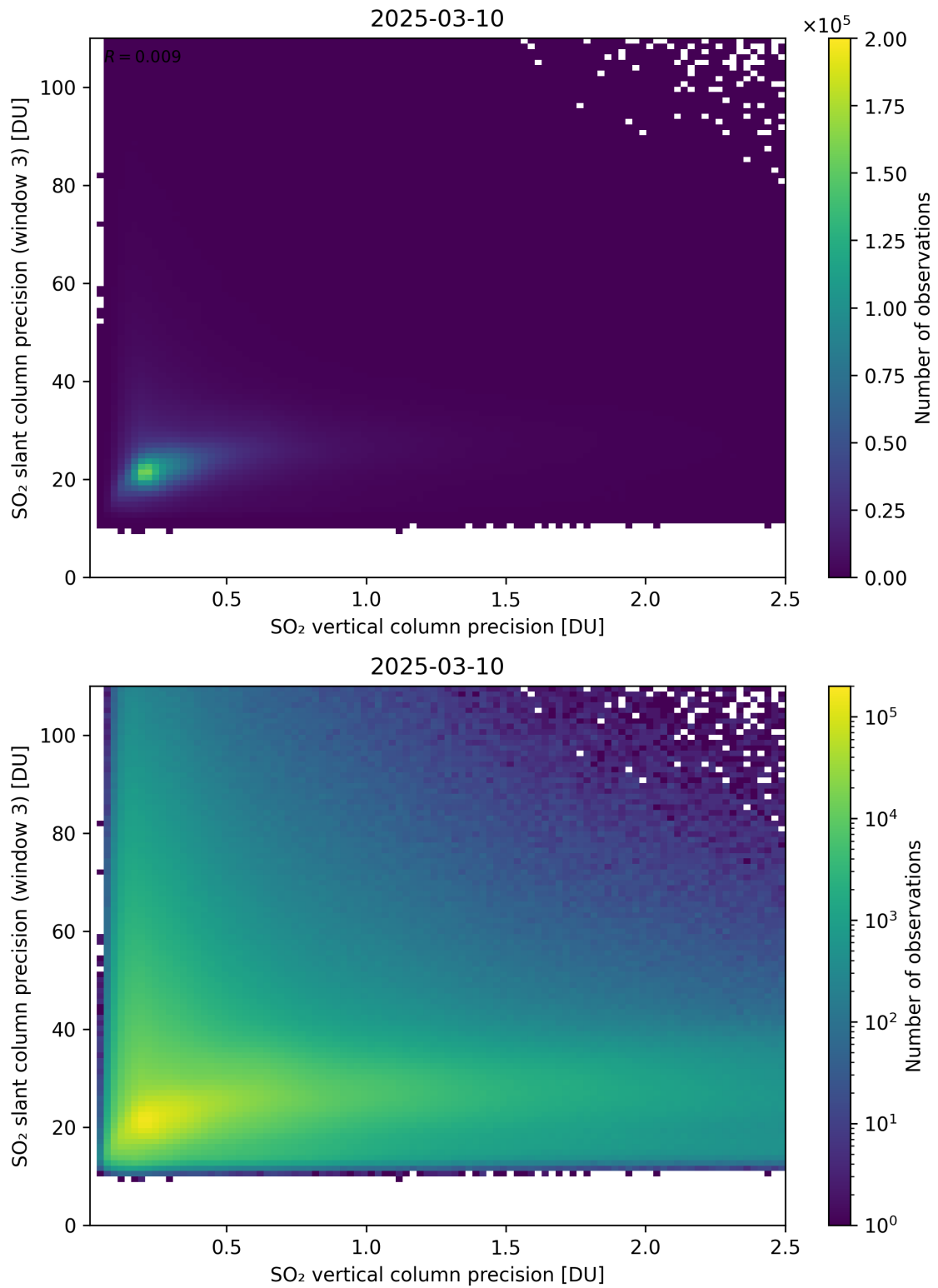
Figure 345: Scatter density plot of “SO 2 vertical column precision” against “SO 2 slant column precision (window 3)” for 2025-03-09 to 2025-03-11.
