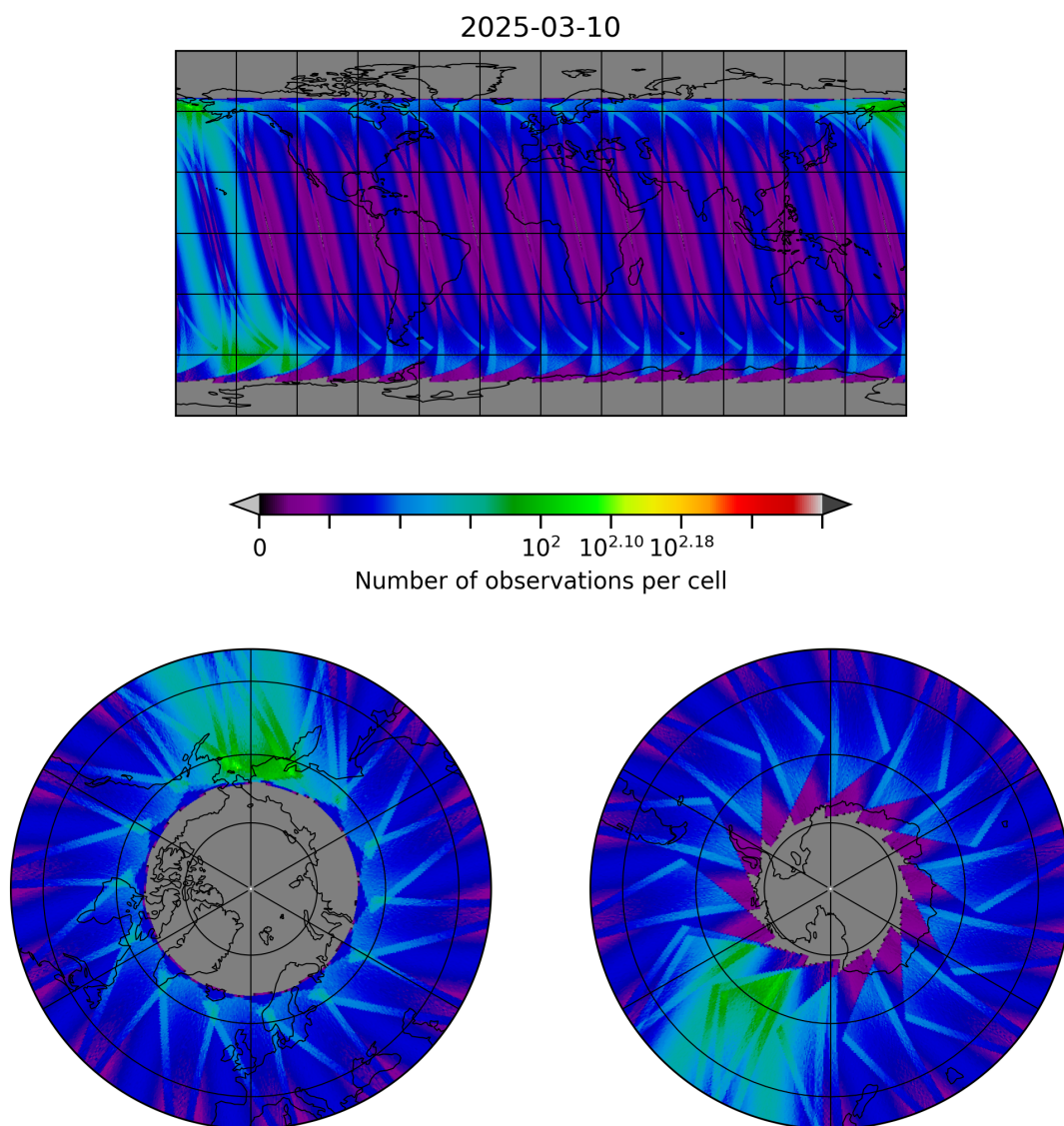
Figure 30: Map of the number of observations for 2025-03-09 to 2025-03-11
