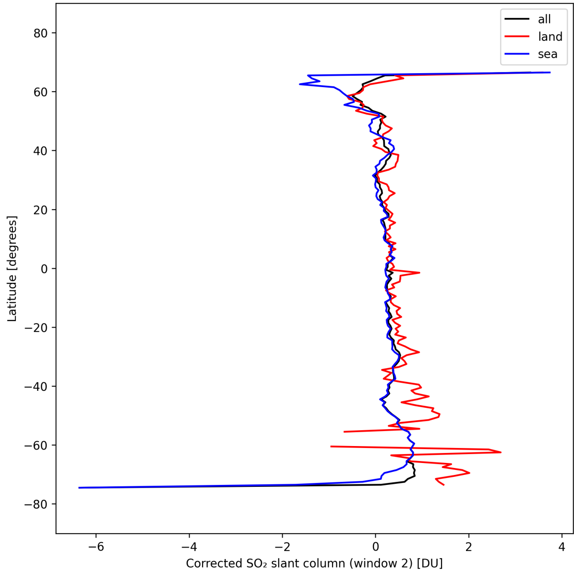
Figure 43: Zonal average of “Corrected SO 2 slant column (window 2)” for 2025-03-09 to 2025-03-11.
