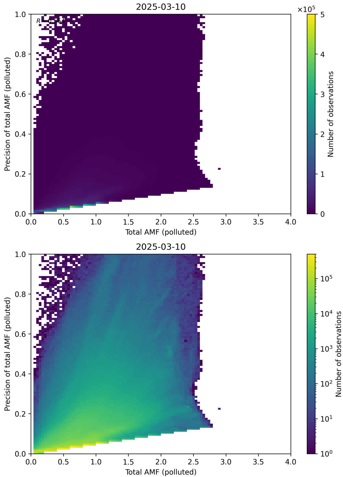
Figure 322: Scatter density plot of “Total AMF (polluted)” against “Precision of total AMF (polluted)” for 2025-03-09 to 2025-03-11.
