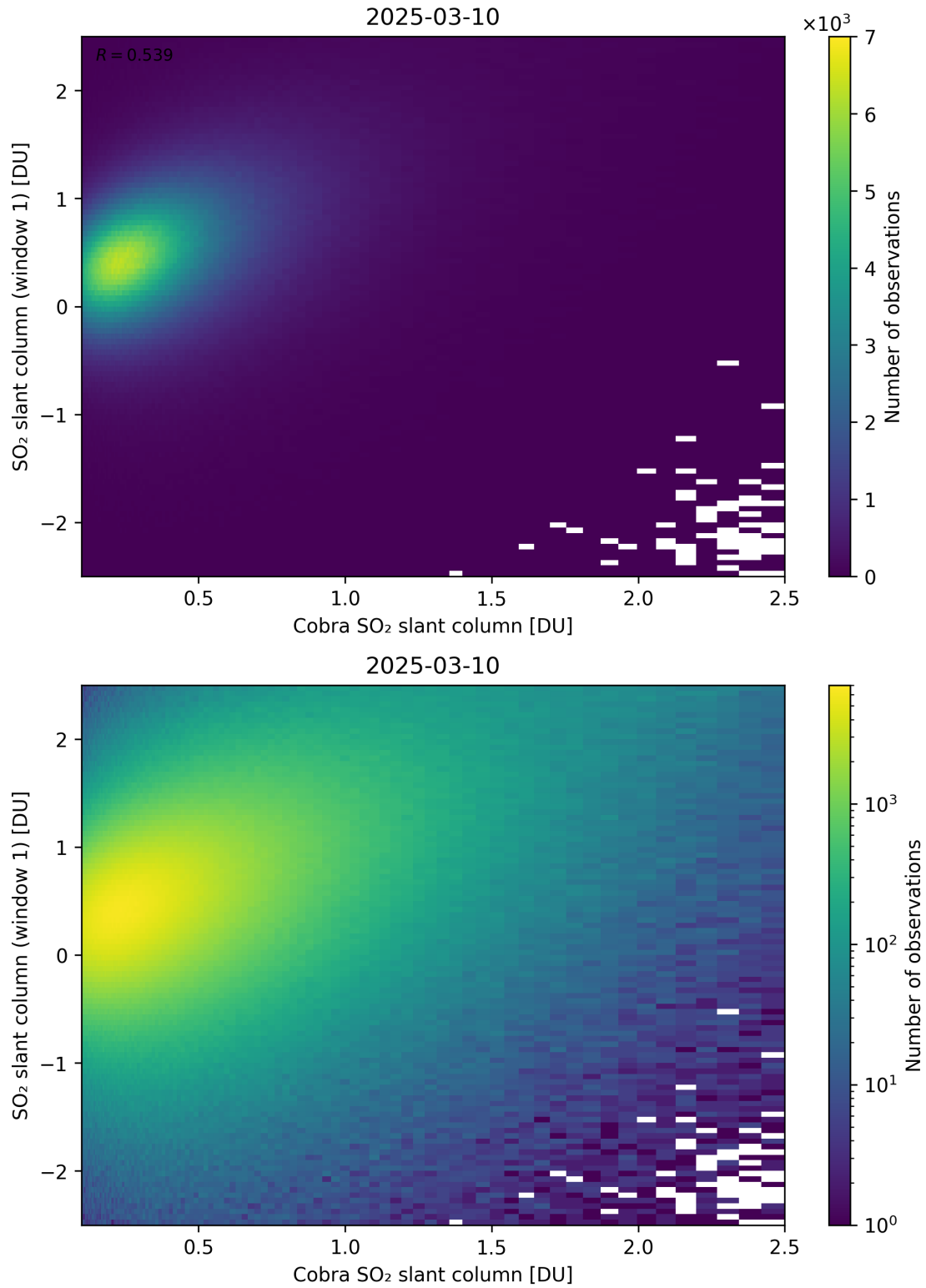
Figure 219: Scatter density plot of “Cobra SO 2 slant column” against “SO 2 slant column (window 1)” for 2025-03-09 to 2025-03-11.
