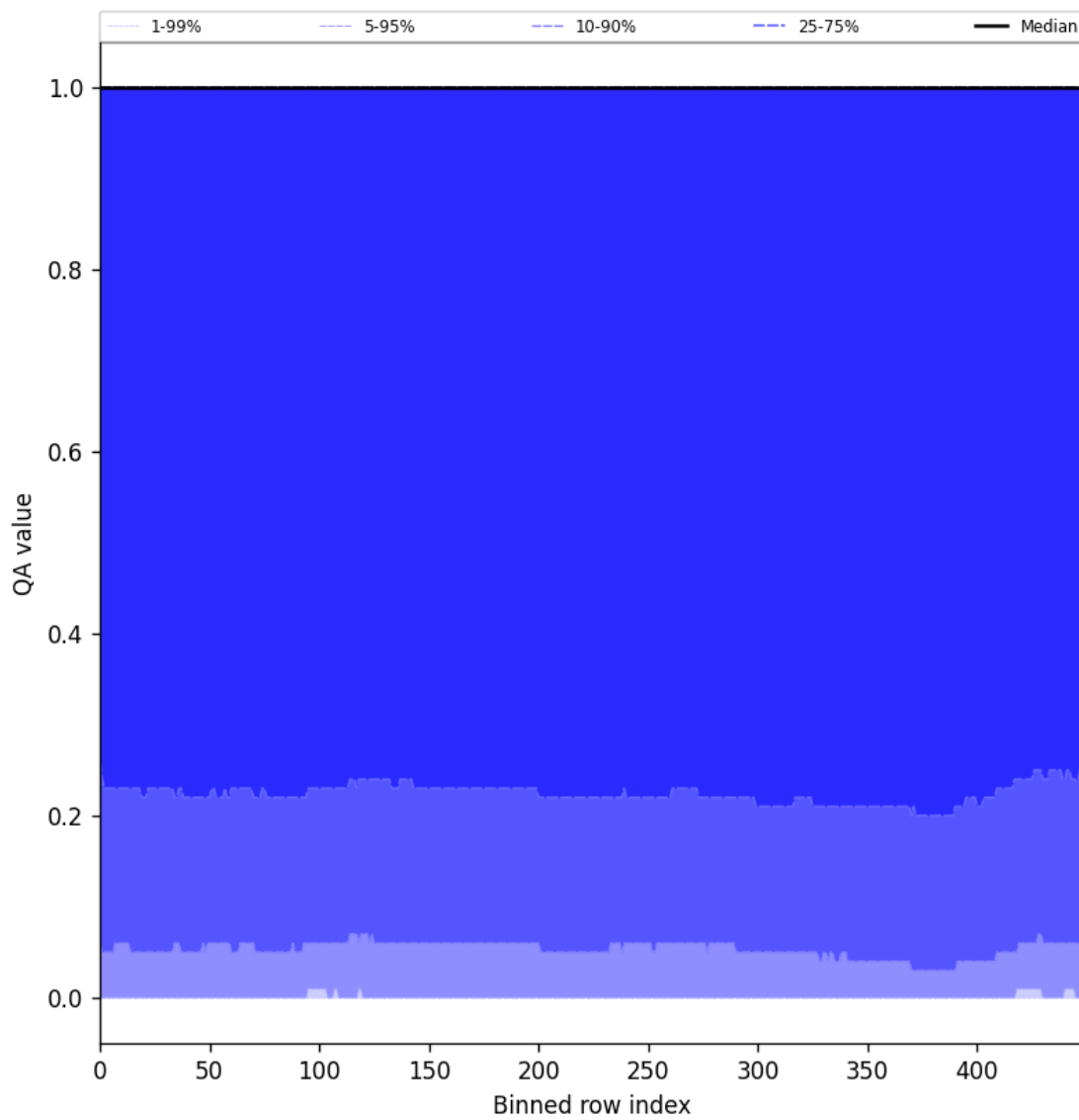
Figure 83: Along track statistics of “QA value” for 2025-03-09 to 2025-03-11
