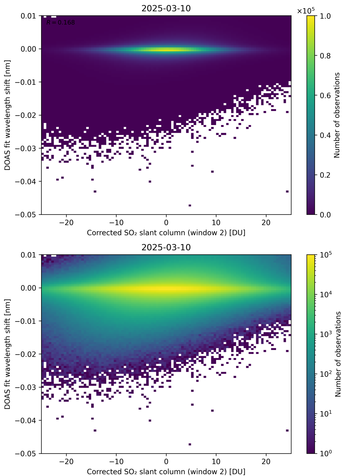
Figure 246: Scatter density plot of “Corrected SO 2 slant column (window 2)” against “DOAS fit wavelength shift” for 2025-03-09 to 2025-03-11.
