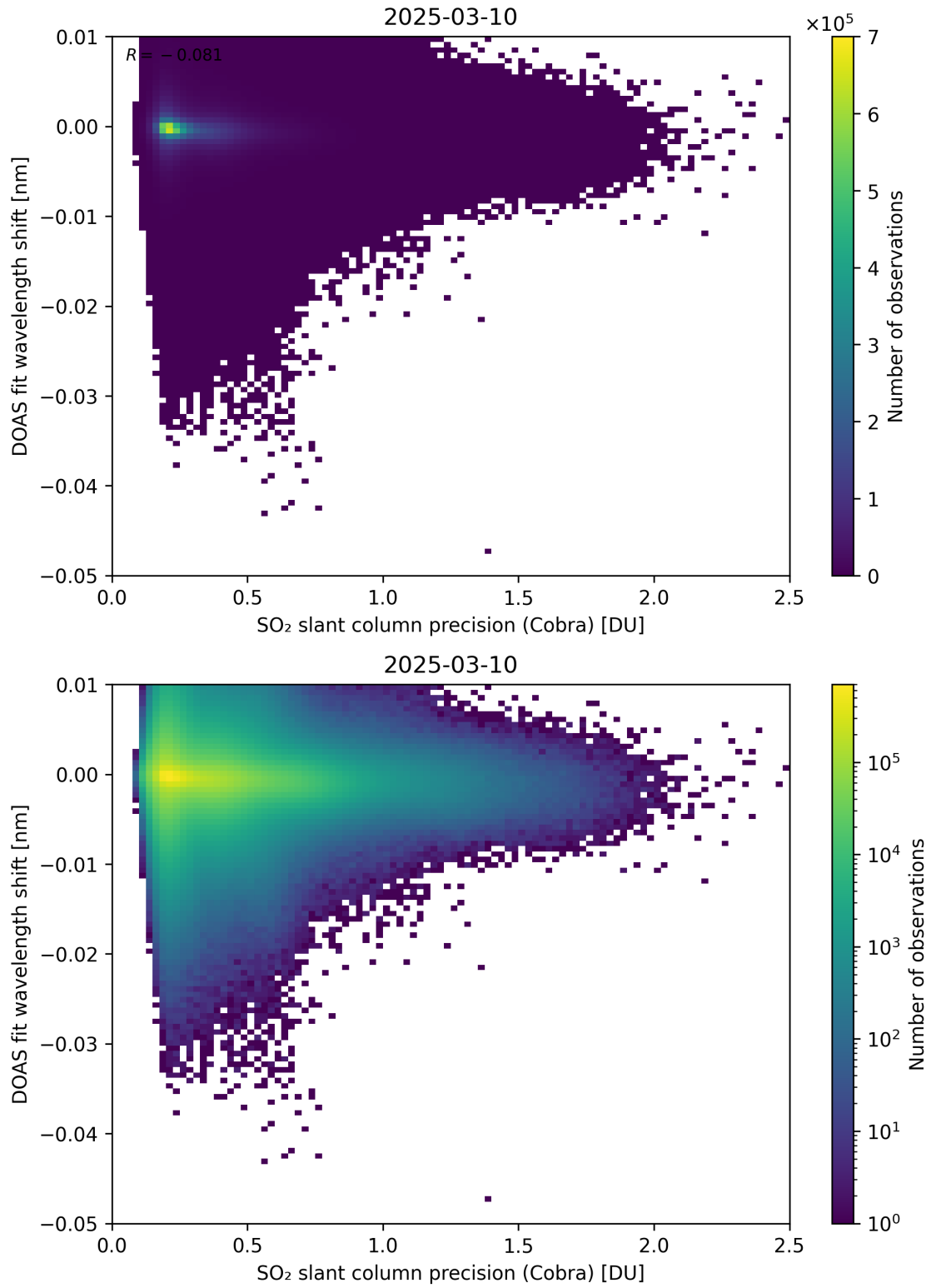
Figure 202: Scatter density plot of “SO 2 slant column precision (Cobra)” against “DOAS fit wavelength shift” for 2025-03-09 to 2025-03-11.
