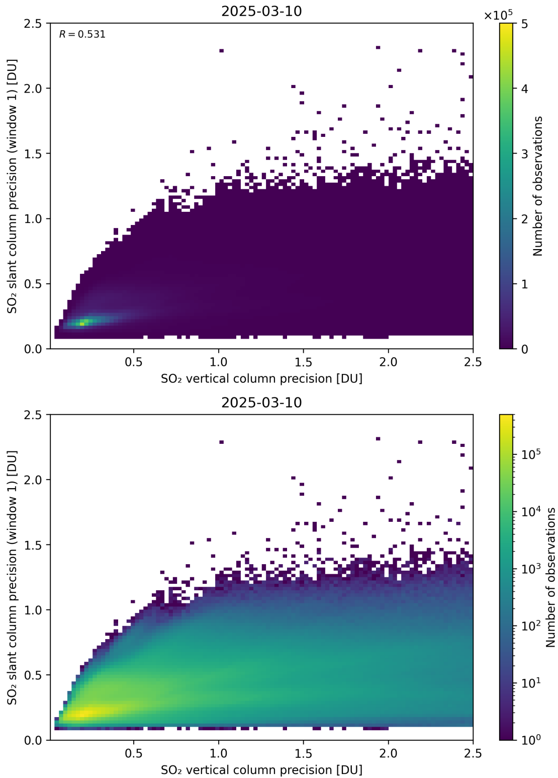
Figure 342: Scatter density plot of “SO 2 vertical column precision” against “SO 2 slant column precision (window 1)” for 2025-03-09 to 2025-03-11.
