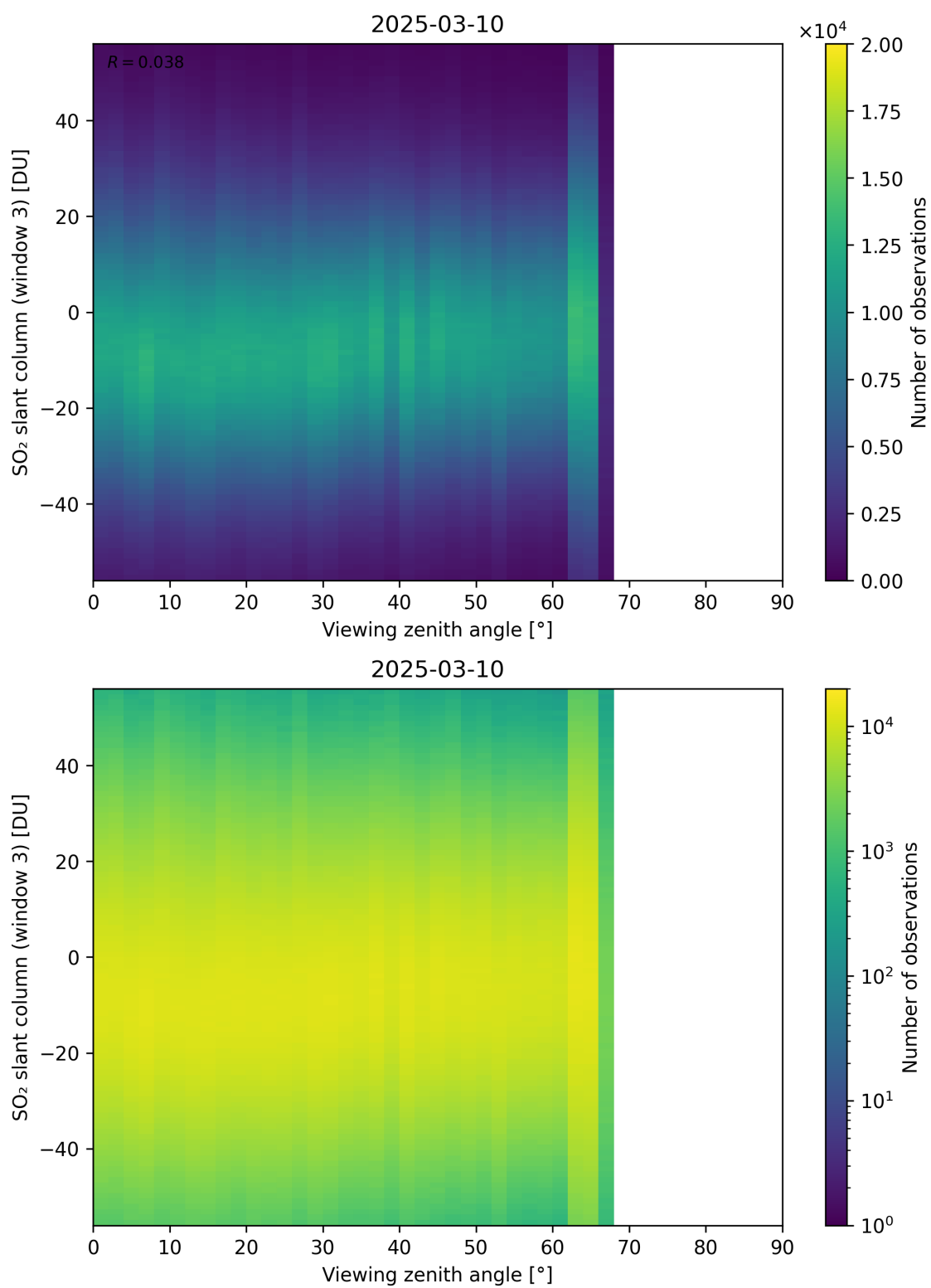
Figure 379: Scatter density plot of “Viewing zenith angle” against “SO 2 slant column (window 3)” for 2025-03-09 to 2025-03-11.
