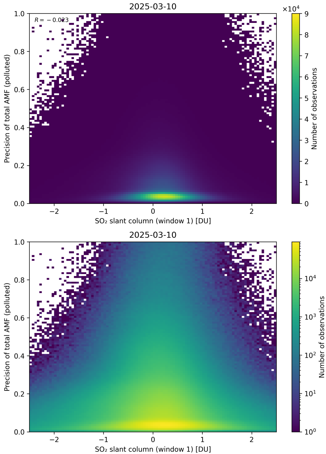
Figure 290: Scatter density plot of “SO 2 slant column (window 1)” against “Precision of total AMF (polluted)” for 2025-03-09 to 2025-03-11.
