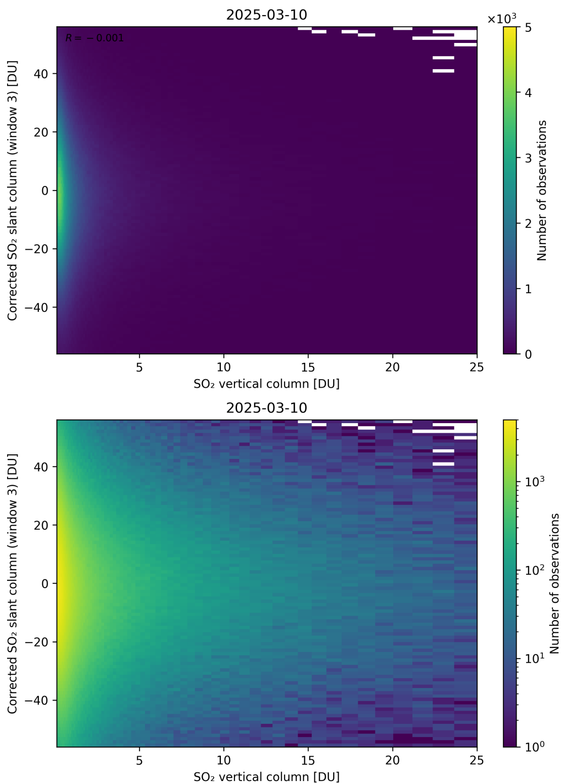
Figure 353: Scatter density plot of “SO 2 vertical column” against “Corrected SO 2 slant column (window 3)” for 2025-03-09 to 2025-03-11.
