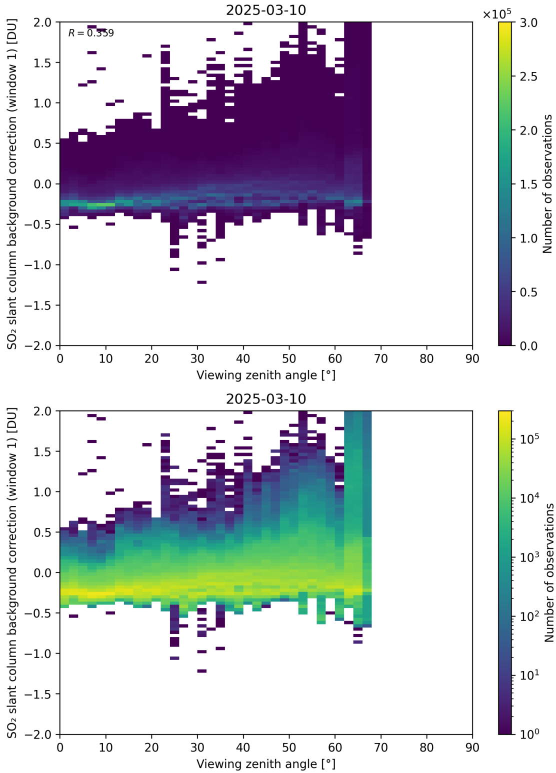
Figure 362: Scatter density plot of “Viewing zenith angle” against “SO 2 slant column background correction (window 1)” for 2025-03-09 to 2025-03-11.
