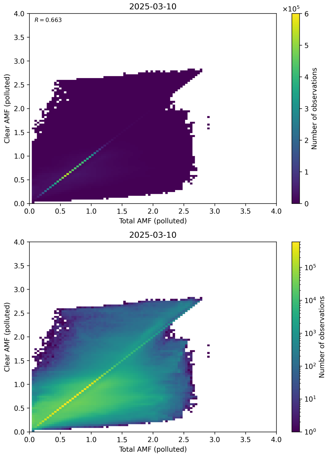
Figure 321: Scatter density plot of “Total AMF (polluted)” against “Clear AMF (polluted)” for 2025-03-09 to 2025-03-11.
