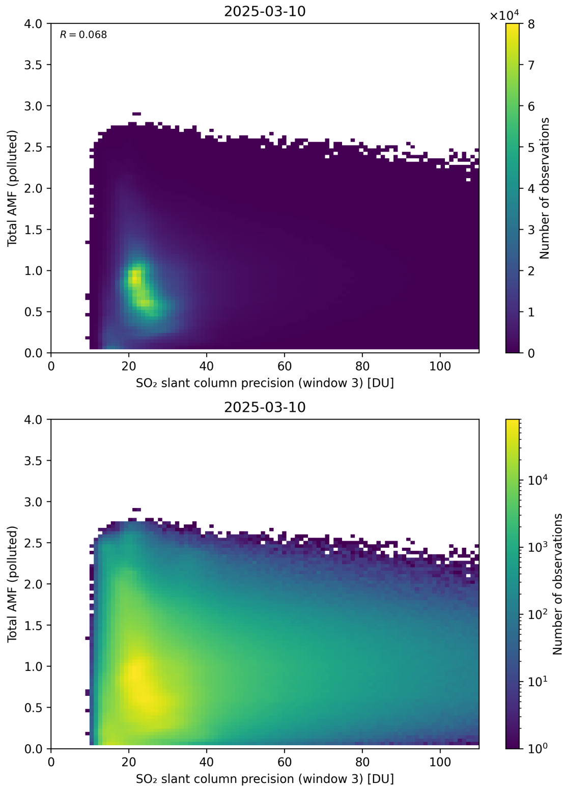
Figure 313: Scatter density plot of “SO 2 slant column precision (window 3)” against “Total AMF (polluted)” for 2025-03-09 to 2025-03-11.
