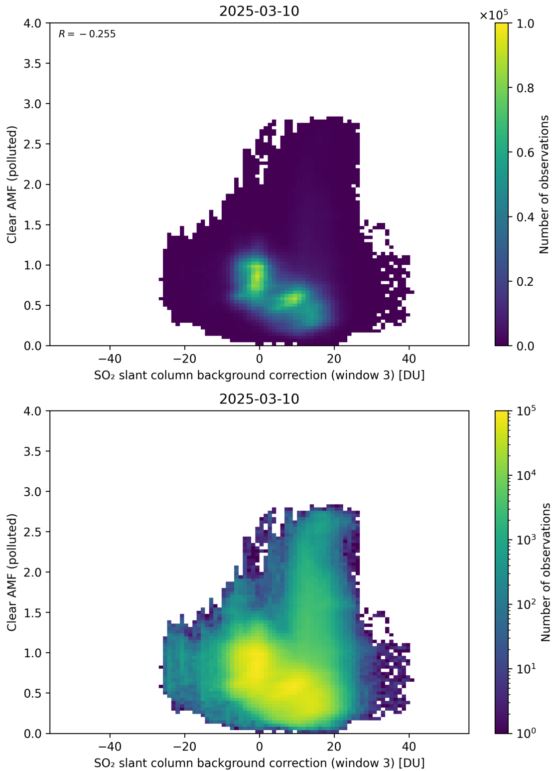
Figure 135: Scatter density plot of “SO 2 slant column background correction (window 3)” against “Clear AMF (polluted)” for 2025-03-09 to 2025-03-11.
