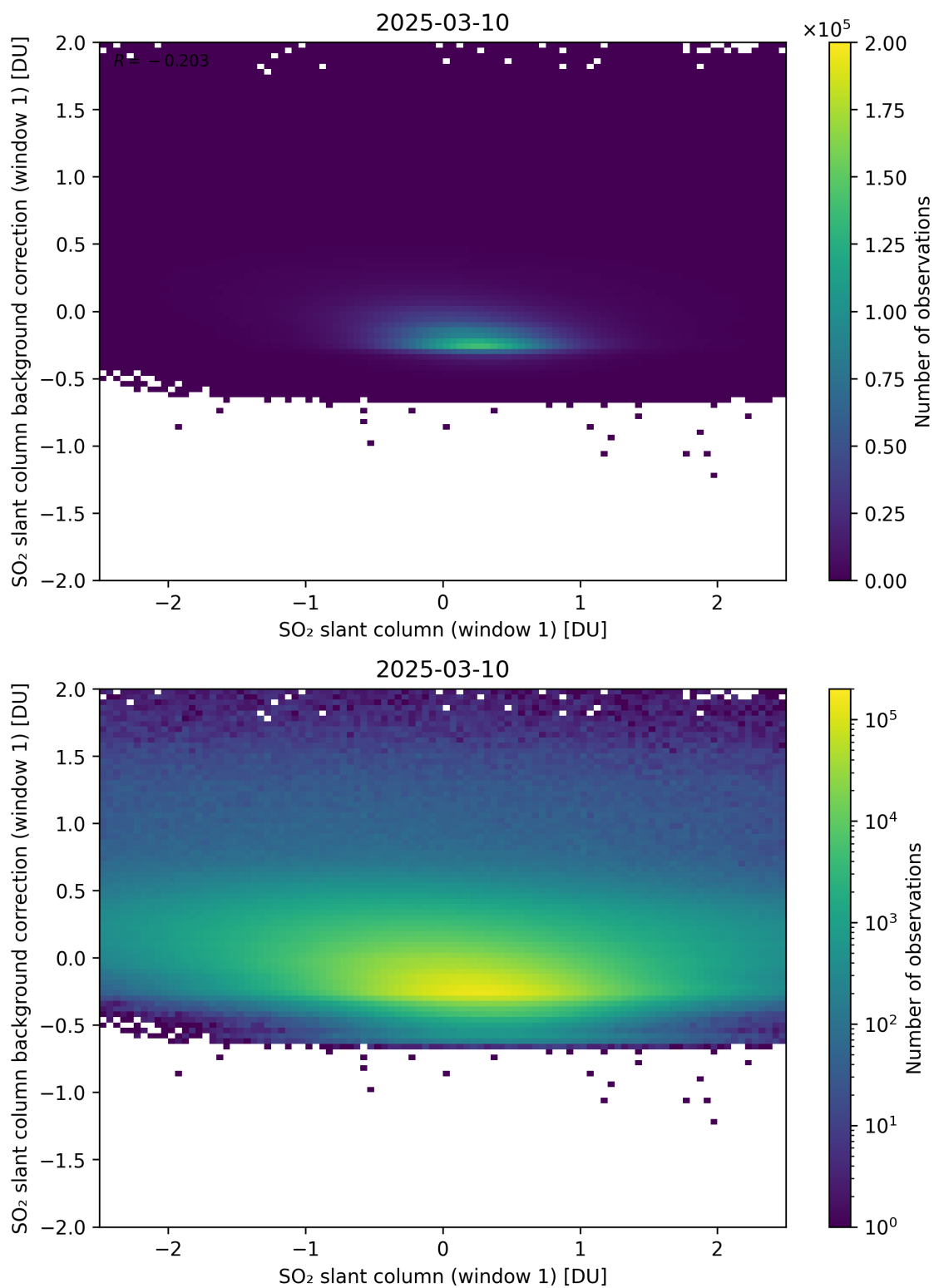
Figure 262: Scatter density plot of “SO 2 slant column (window 1)” against “SO 2 slant column background correction (window 1)” for 2025-03-09 to 2025-03-11.
