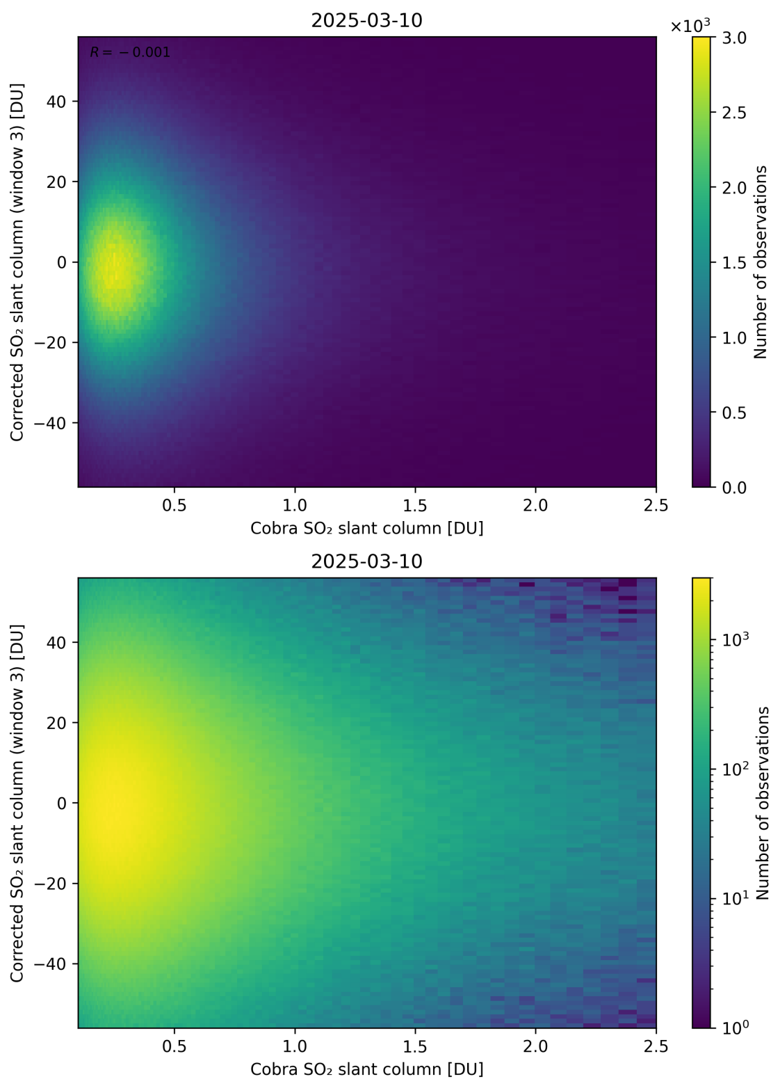
Figure 218: Scatter density plot of “Cobra SO 2 slant column” against “Corrected SO 2 slant column (window 3)” for 2025-03-09 to 2025-03-11.
