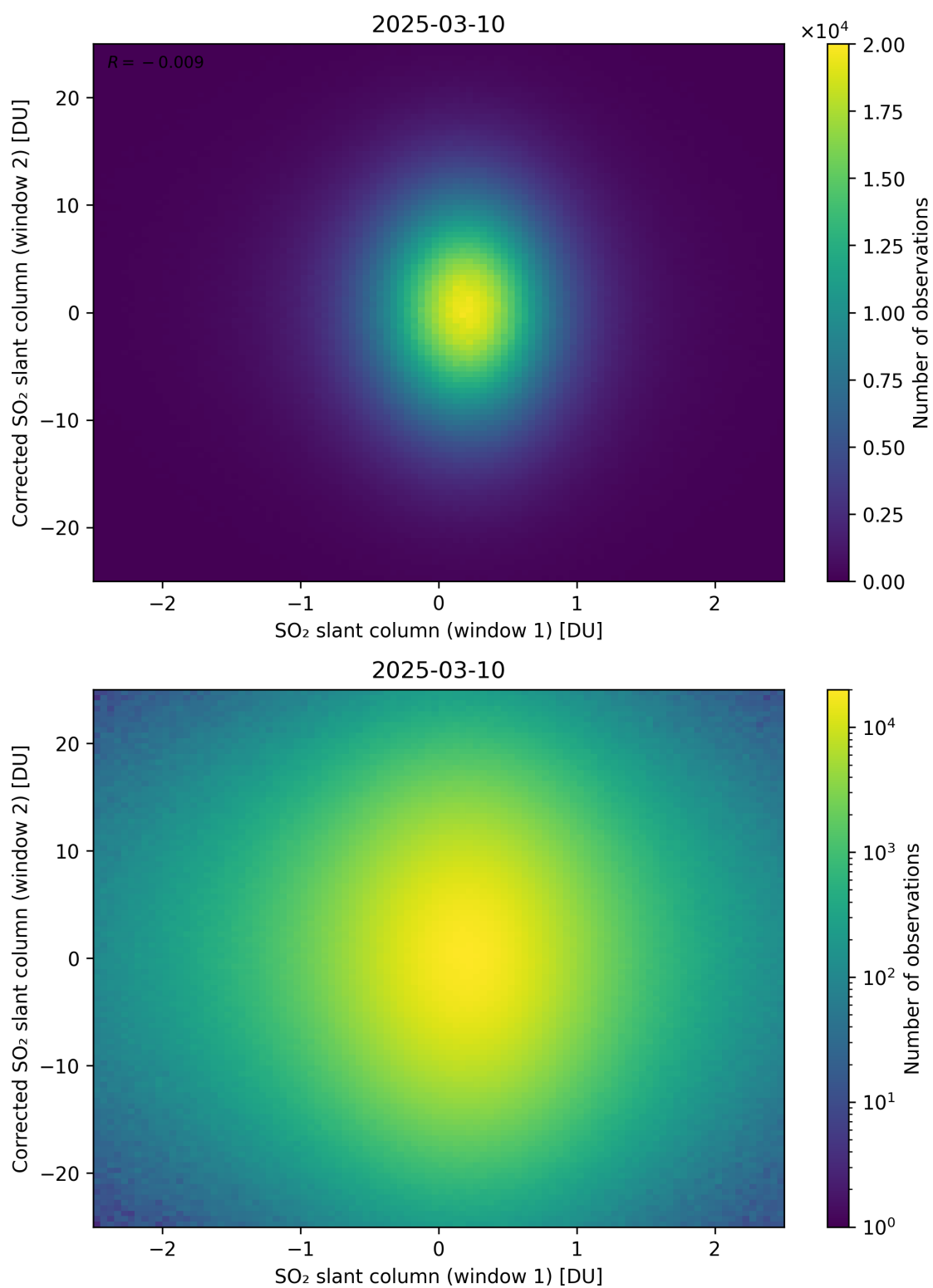
Figure 283: Scatter density plot of “SO 2 slant column (window 1)” against “Corrected SO 2 slant column (window 2)” for 2025-03-09 to 2025-03-11.
