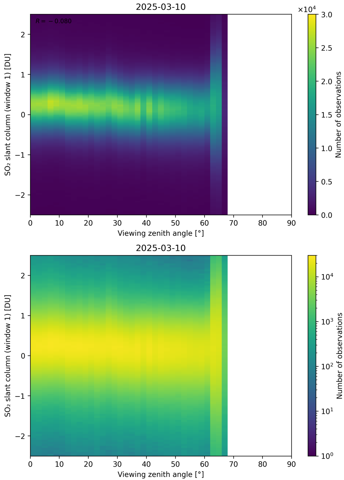
Figure 376: Scatter density plot of “Viewing zenith angle” against “SO 2 slant column (window 1)” for 2025-03-09 to 2025-03-11.
