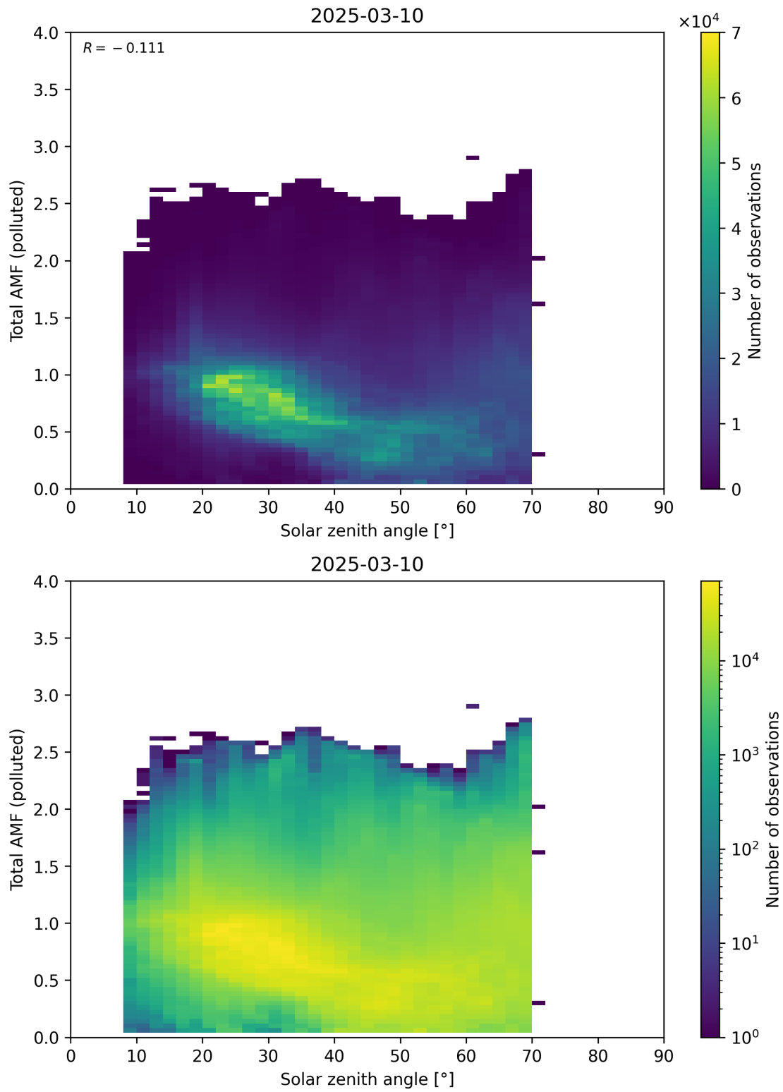
Figure 189: Scatter density plot of “Solar zenith angle” against “Total AMF (polluted)” for 2025-03-09 to 2025-03-11.
