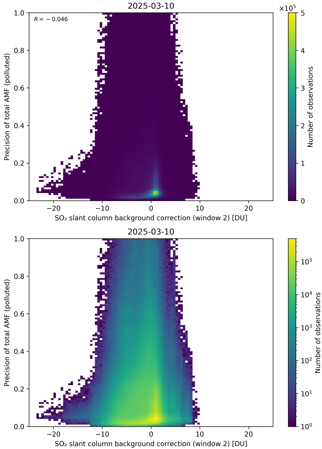
Figure 131: Scatter density plot of “SO 2 slant column background correction (window 2)” against “Precision of total AMF (polluted)” for 2025-03-09 to 2025-03-11.
