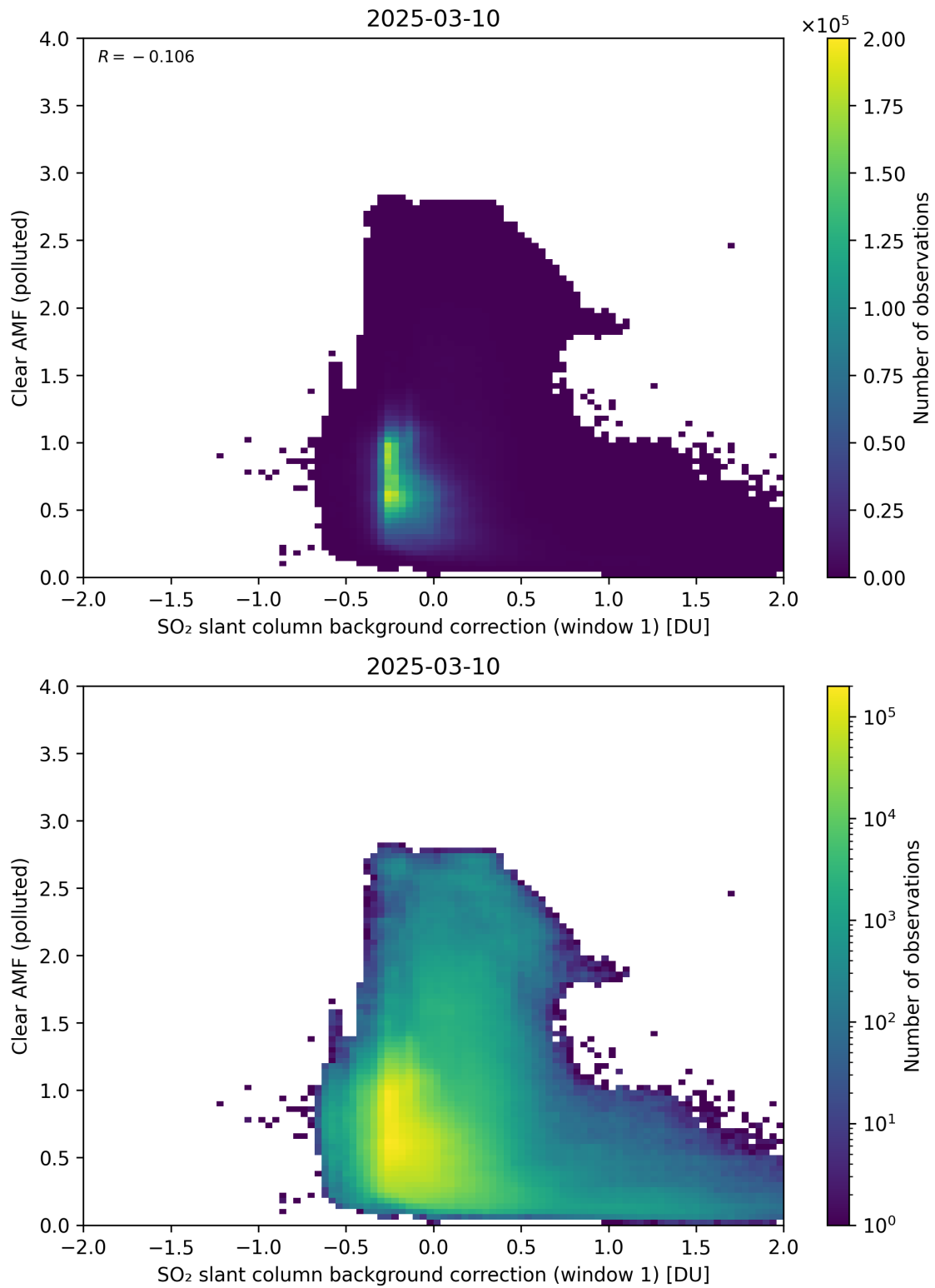
Figure 114: Scatter density plot of “SO 2 slant column background correction (window 1)” against “Clear AMF (polluted)” for 2025-03-09 to 2025-03-11.
