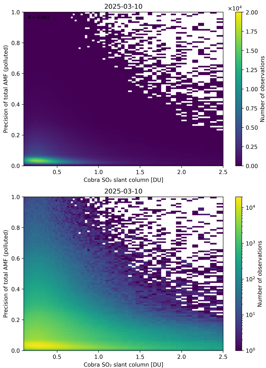
Figure 225: Scatter density plot of “Cobra SO 2 slant column” against “Precision of total AMF (polluted)” for 2025-03-09 to 2025-03-11.
