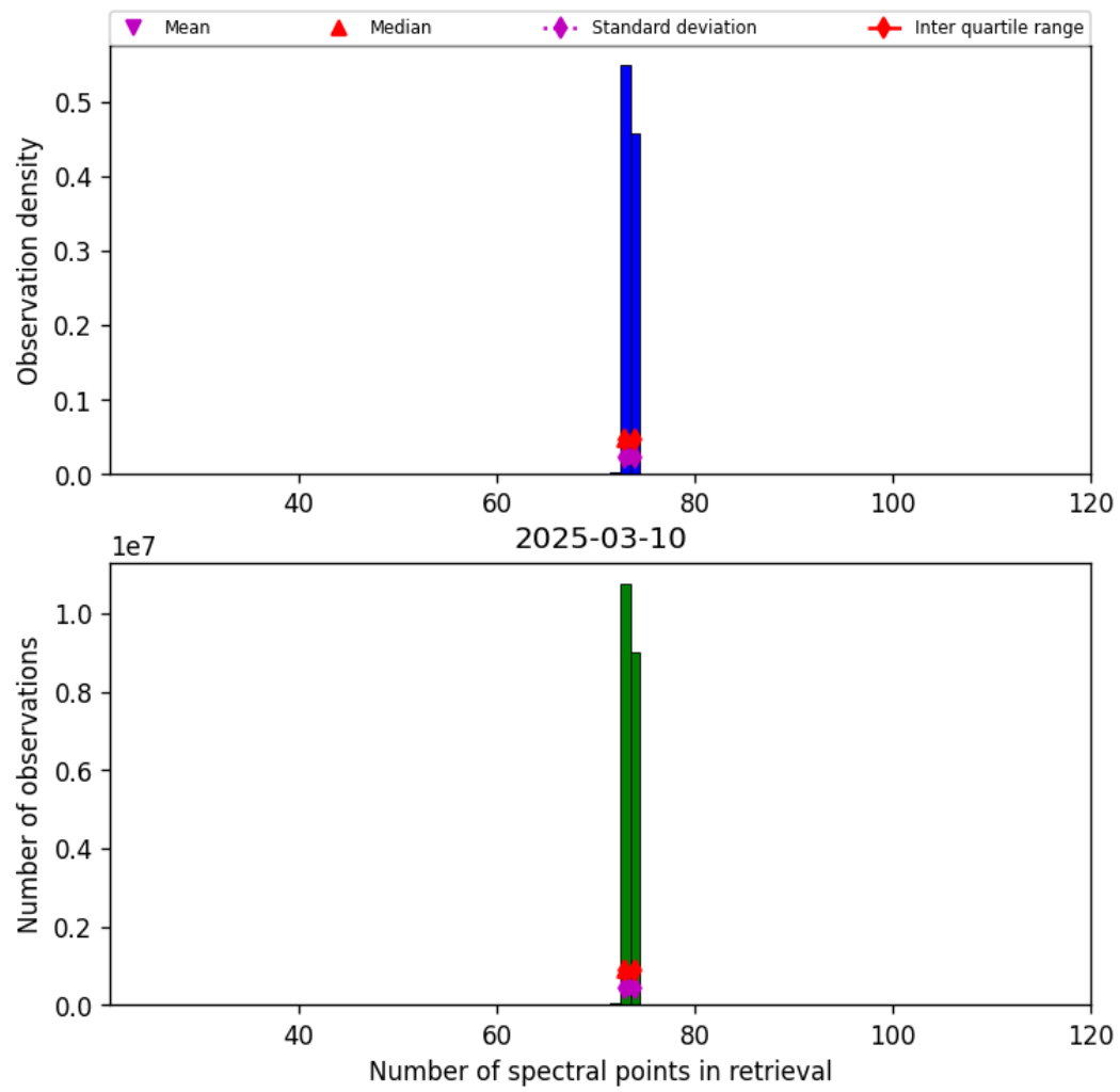
Figure 82: Histogram of “Number of spectral points in retrieval” for 2025-03-09 to 2025-03-11
