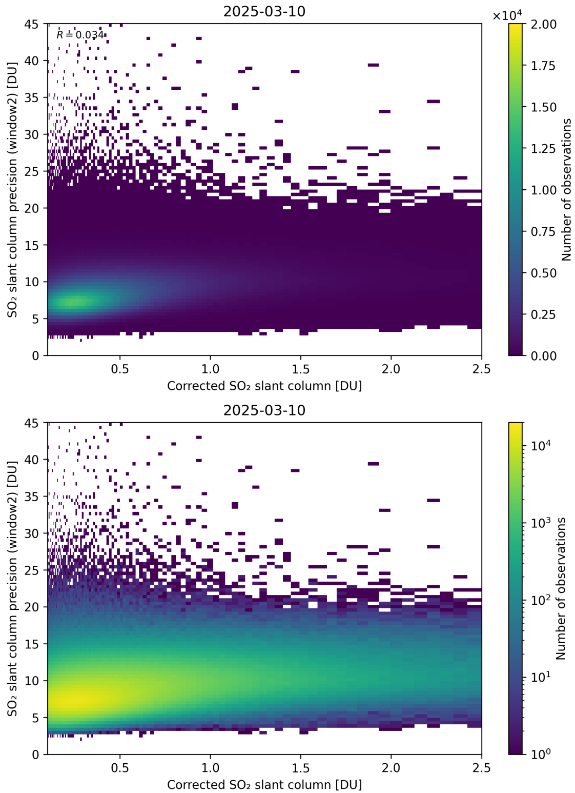
Figure 239: Scatter density plot of “Corrected SO 2 slant column” against “SO 2 slant column precision (window2)” for 2025-03-09 to 2025-03-11.
