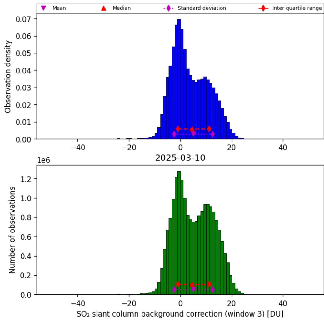
Figure 74: Histogram of “SO 2 slant column background correction (window 3)” for 2025-03-09 to 2025-03-11
