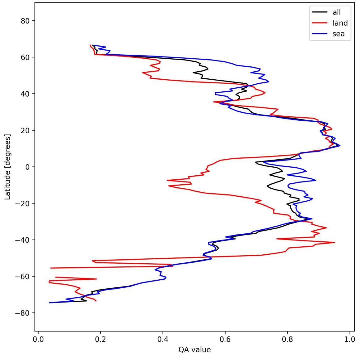
Figure 31: Zonal average of “QA value” for 2025-03-09 to 2025-03-11.
