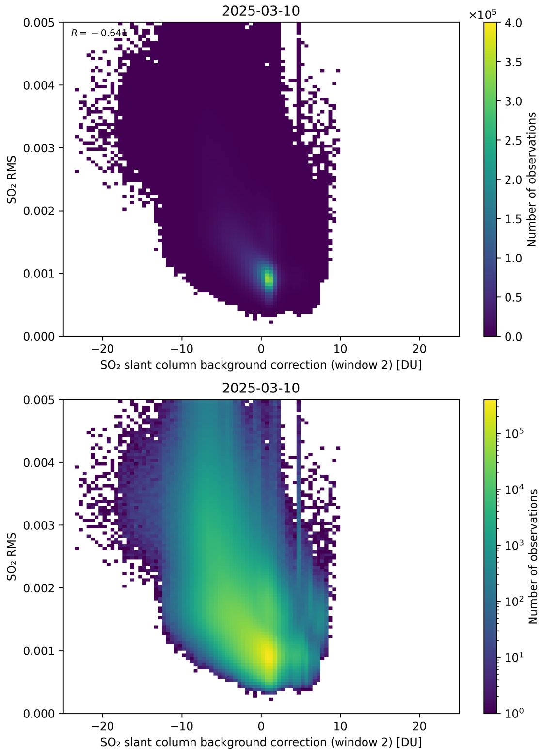
Figure 125: Scatter density plot of “SO 2 slant column background correction (window 2)” against “SO 2 RMS” for 2025-03-09 to 2025-03-11.
