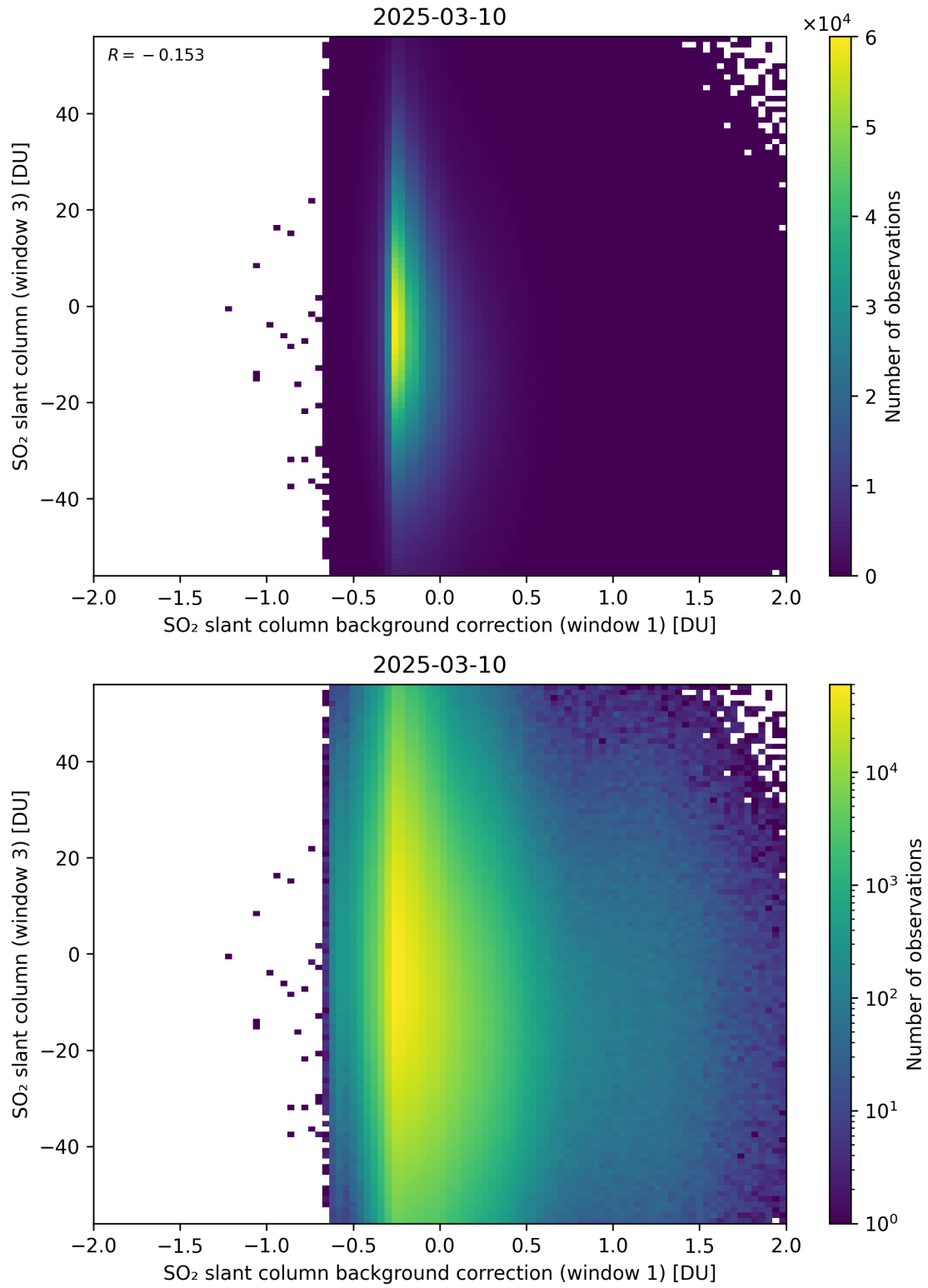
Figure 118: Scatter density plot of “SO 2 slant column background correction (window 1)” against “SO 2 slant column (window 3)” for 2025-03-09 to 2025-03-11.
