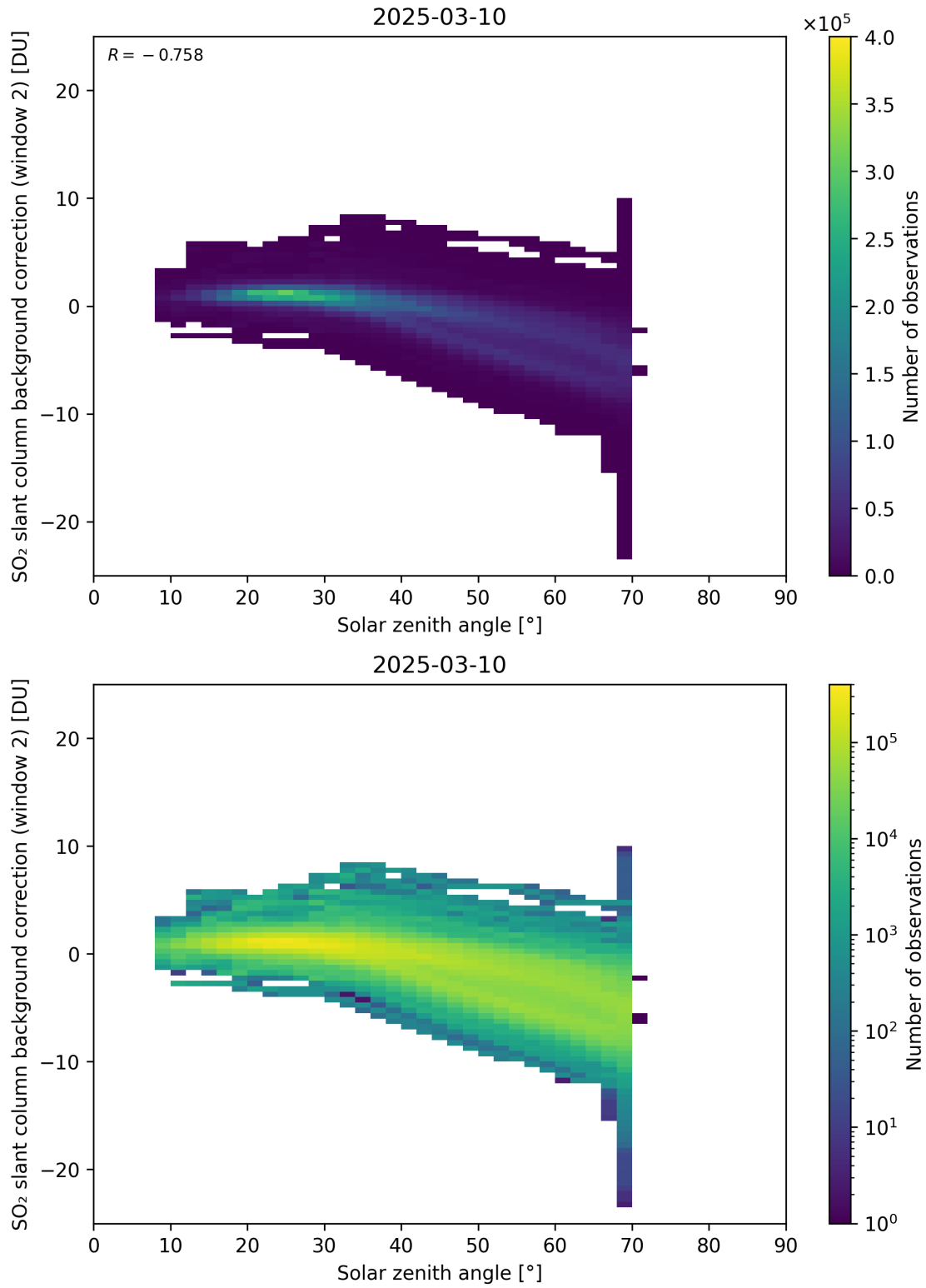
Figure 172: Scatter density plot of “Solar zenith angle” against “SO 2 slant column background correction (window 2)” for 2025-03-09 to 2025-03-11.
