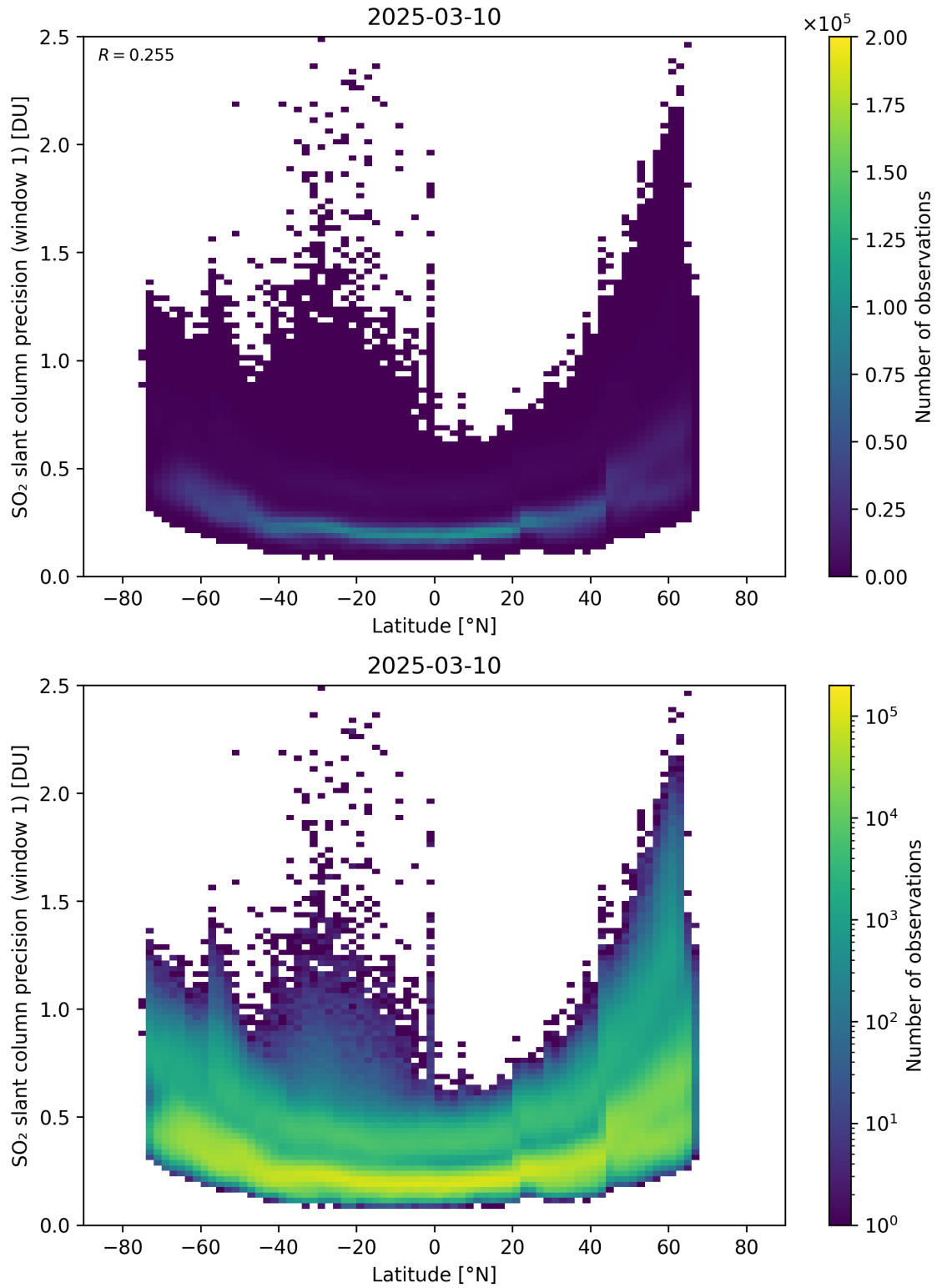
Figure 163: Scatter density plot of “Latitude” against “SO 2 slant column precision (window 1)” for 2025-03-09 to 2025-03-11.
