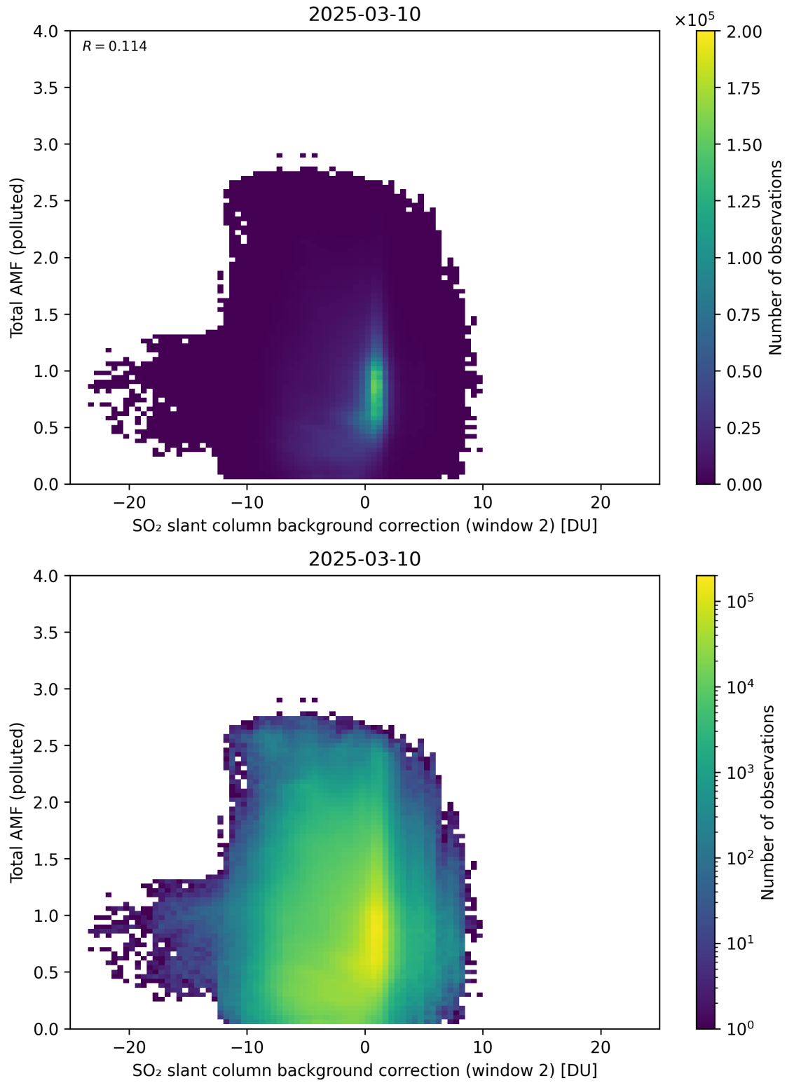
Figure 130: Scatter density plot of “SO 2 slant column background correction (window 2)” against “Total AMF (polluted)” for 2025-03-09 to 2025-03-11.
