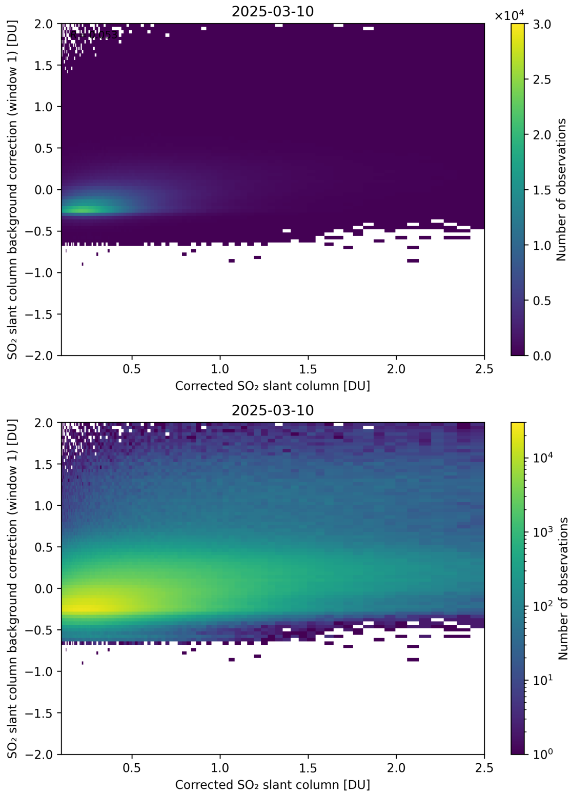
Figure 226: Scatter density plot of “Corrected SO 2 slant column” against “SO 2 slant column background correction (window 1)” for 2025-03-09 to 2025-03-11.
