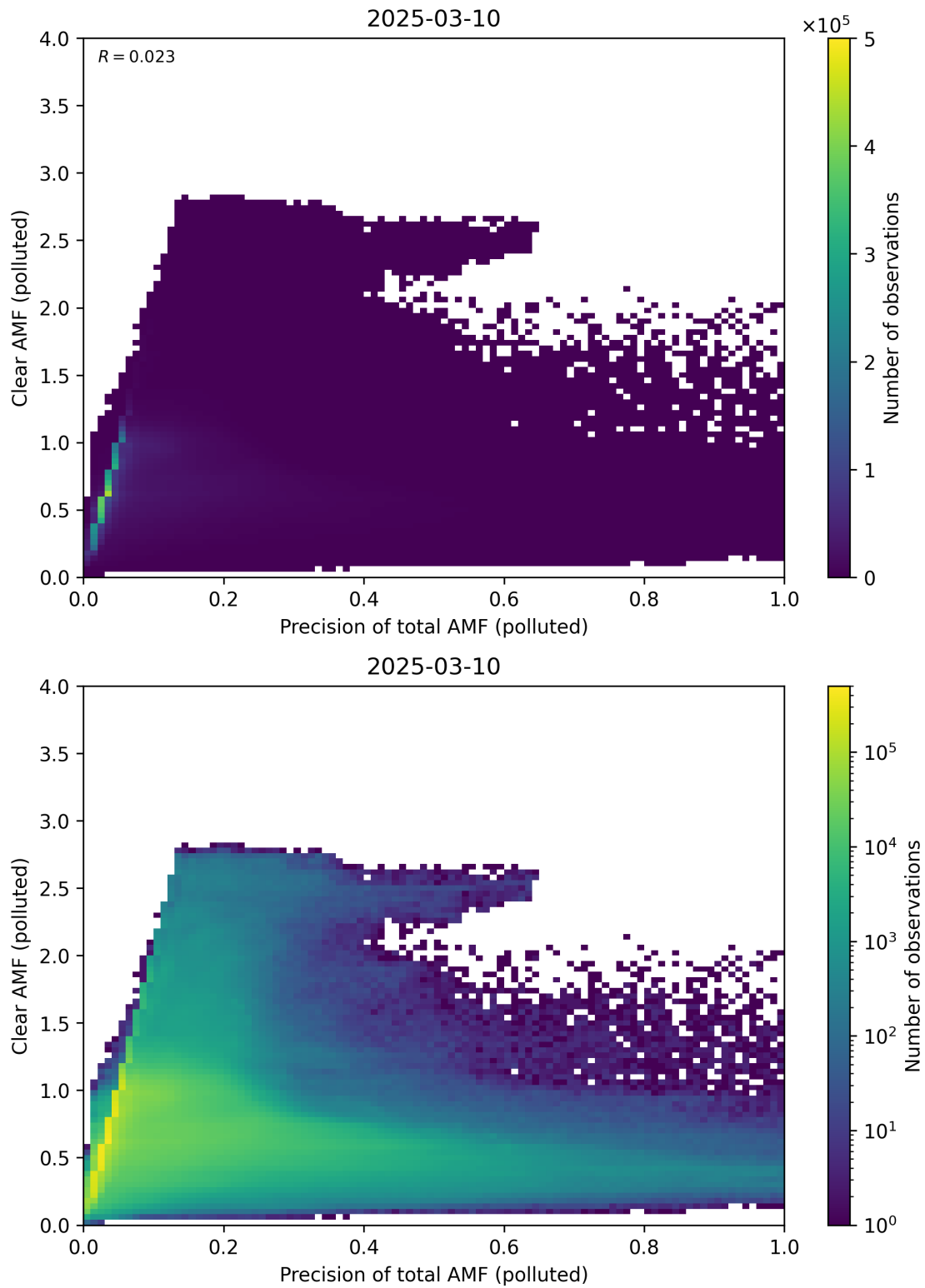
Figure 320: Scatter density plot of “Precision of total AMF (polluted)” against “Clear AMF (polluted)” for 2025-03-09 to 2025-03-11.
