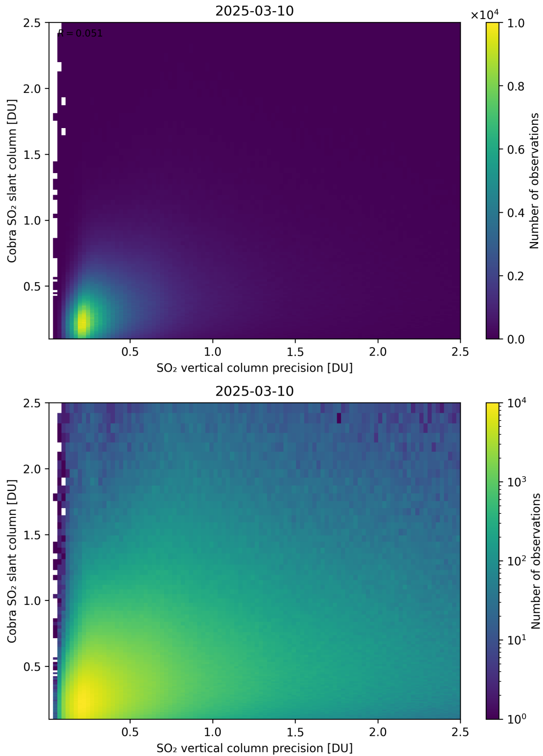
Figure 336: Scatter density plot of “SO 2 vertical column precision” against “Cobra SO 2 slant column” for 2025-03-09 to 2025-03-11.
