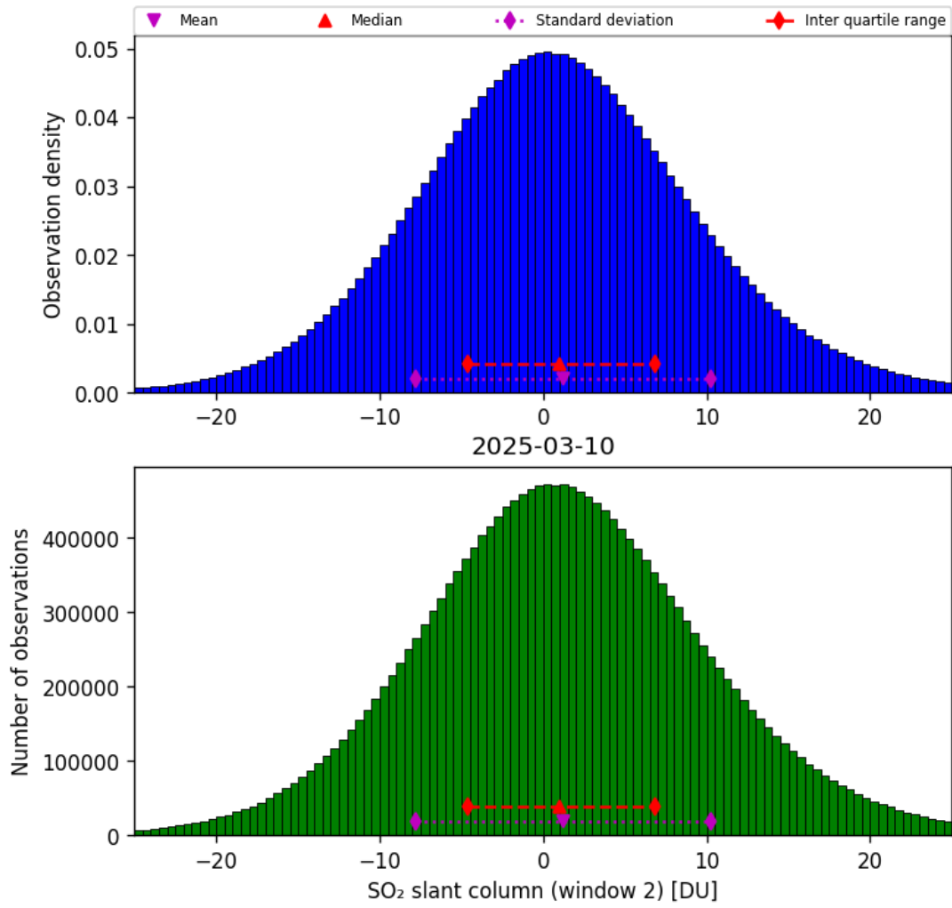
Figure 67: Histogram of “SO 2 slant column (window 2)” for 2025-03-09 to 2025-03-11
