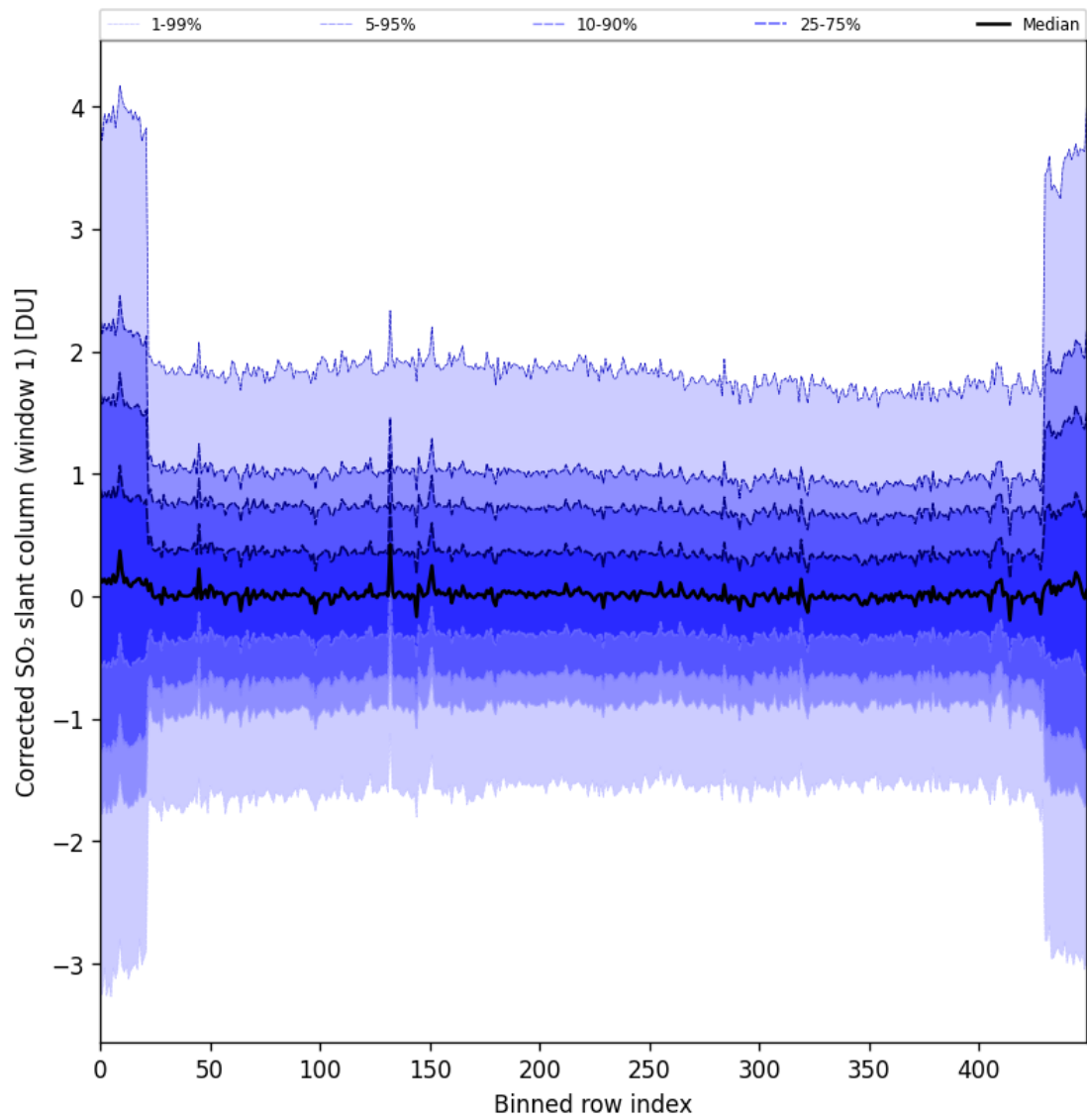
Figure 91: Along track statistics of “Corrected SO 2 slant column (window 1)” for 2025-03-09 to 2025-03-11
