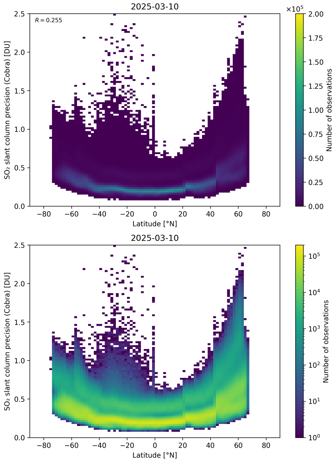
Figure 158: Scatter density plot of “Latitude” against “SO 2 slant column precision (Cobra)” for 2025-03-09 to 2025-03-11.
