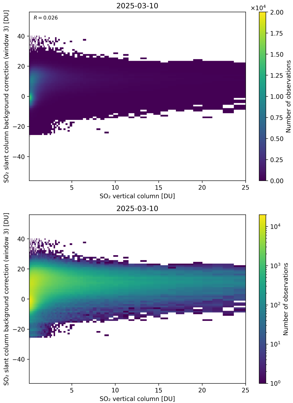
Figure 325: Scatter density plot of “SO 2 vertical column” against “SO 2 slant column background correction (window 3)” for 2025-03-09 to 2025-03-11.
