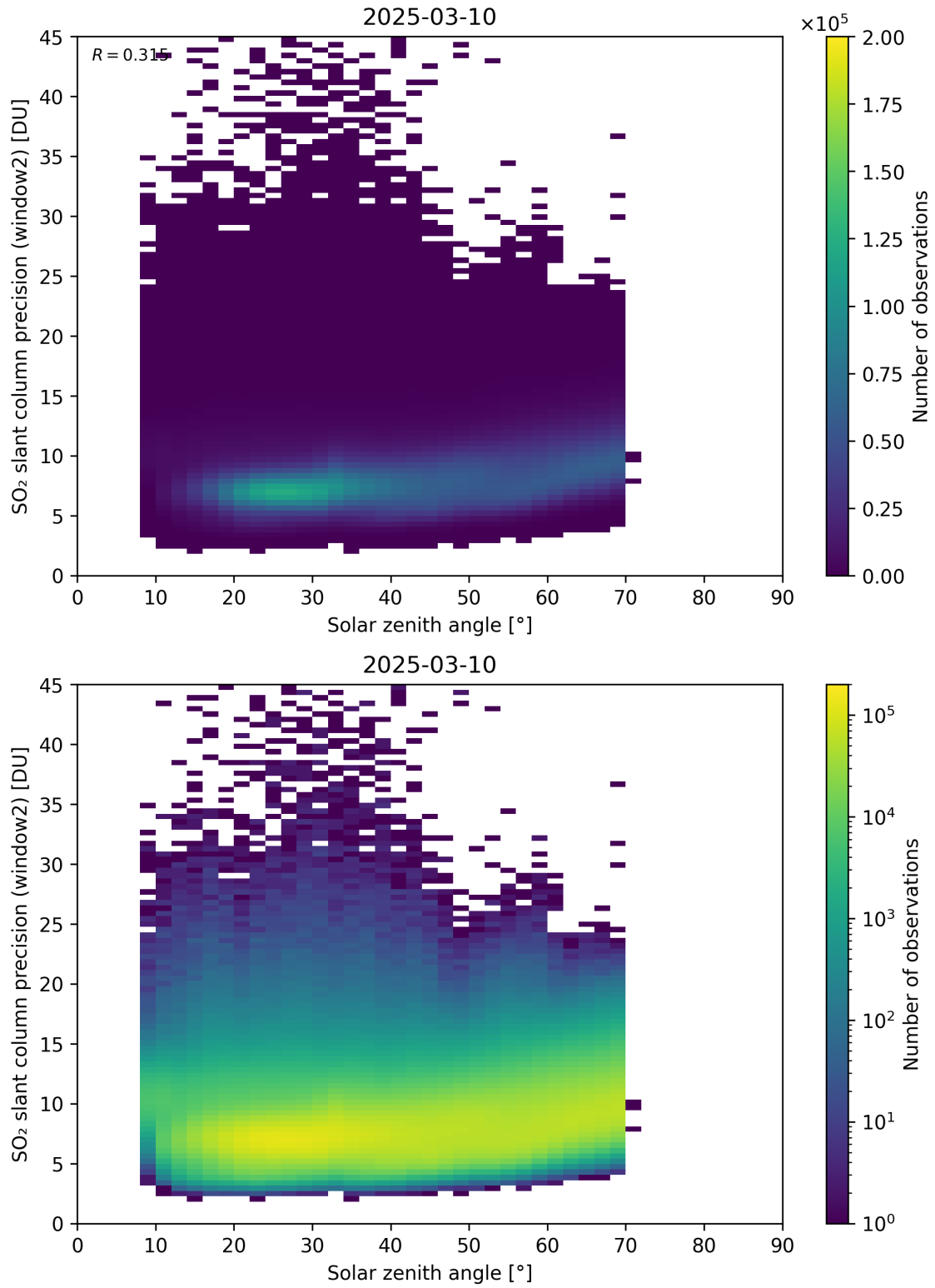
Figure 186: Scatter density plot of “Solar zenith angle” against “SO 2 slant column precision (window2)” for 2025-03-09 to 2025-03-11.
