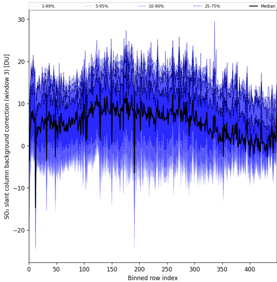
Figure 100: Along track statistics of “SO 2 slant column background correction (window 3)” for 2025-03-09 to 2025-03-11
