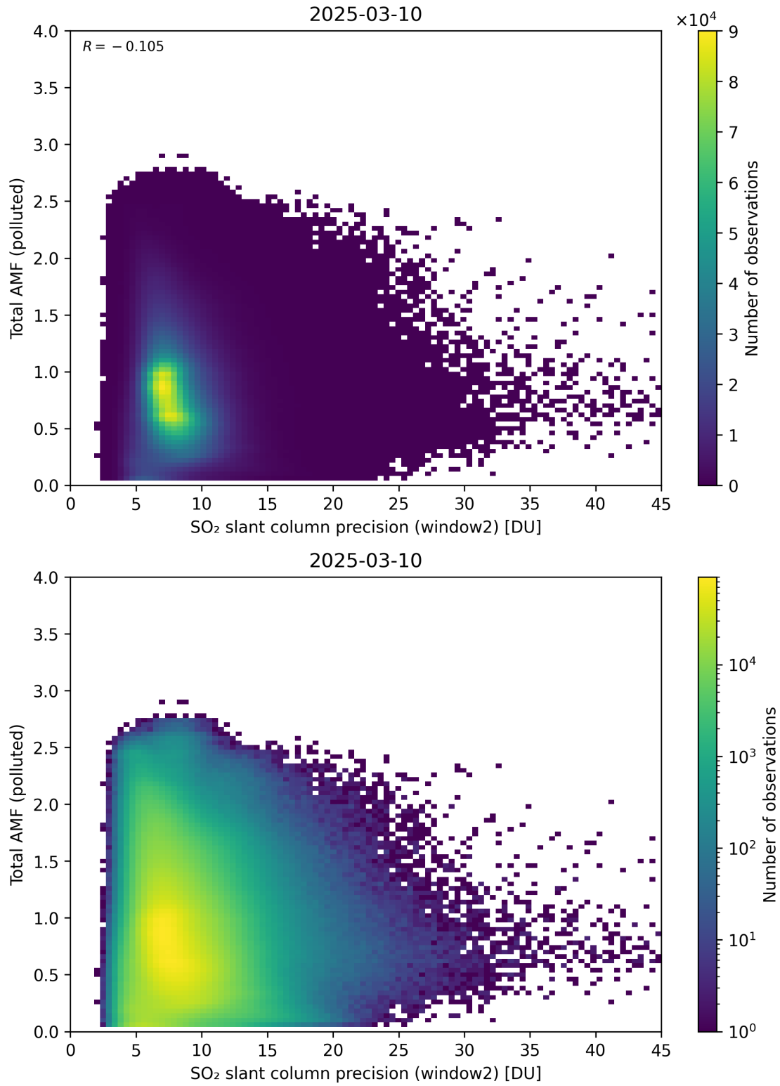
Figure 301: Scatter density plot of “SO 2 slant column precision (window2)” against “Total AMF (polluted)” for 2025-03-09 to 2025-03-11.
