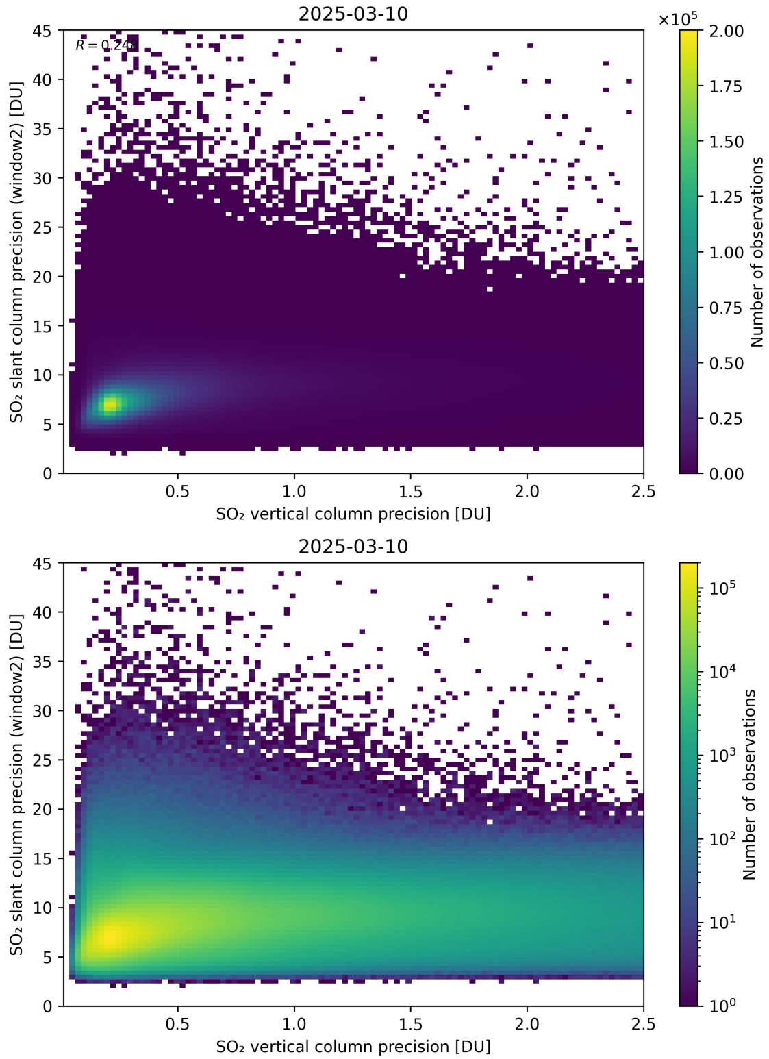
Figure 343: Scatter density plot of “SO 2 vertical column precision” against “SO 2 slant column precision (window2)” for 2025-03-09 to 2025-03-11.
