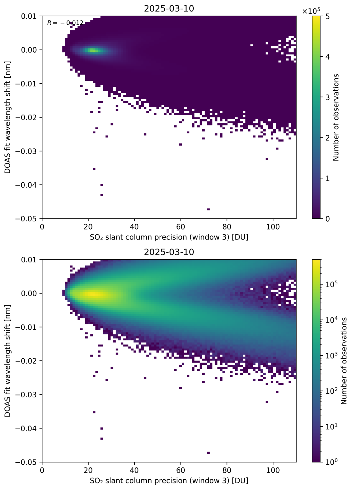
Figure 308: Scatter density plot of “SO 2 slant column precision (window 3)” against “DOAS fit wavelength shift” for 2025-03-09 to 2025-03-11.
