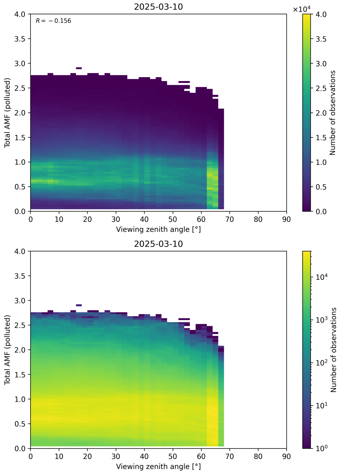
Figure 381: Scatter density plot of “Viewing zenith angle” against “Total AMF (polluted)” for 2025-03-09 to 2025-03-11.
