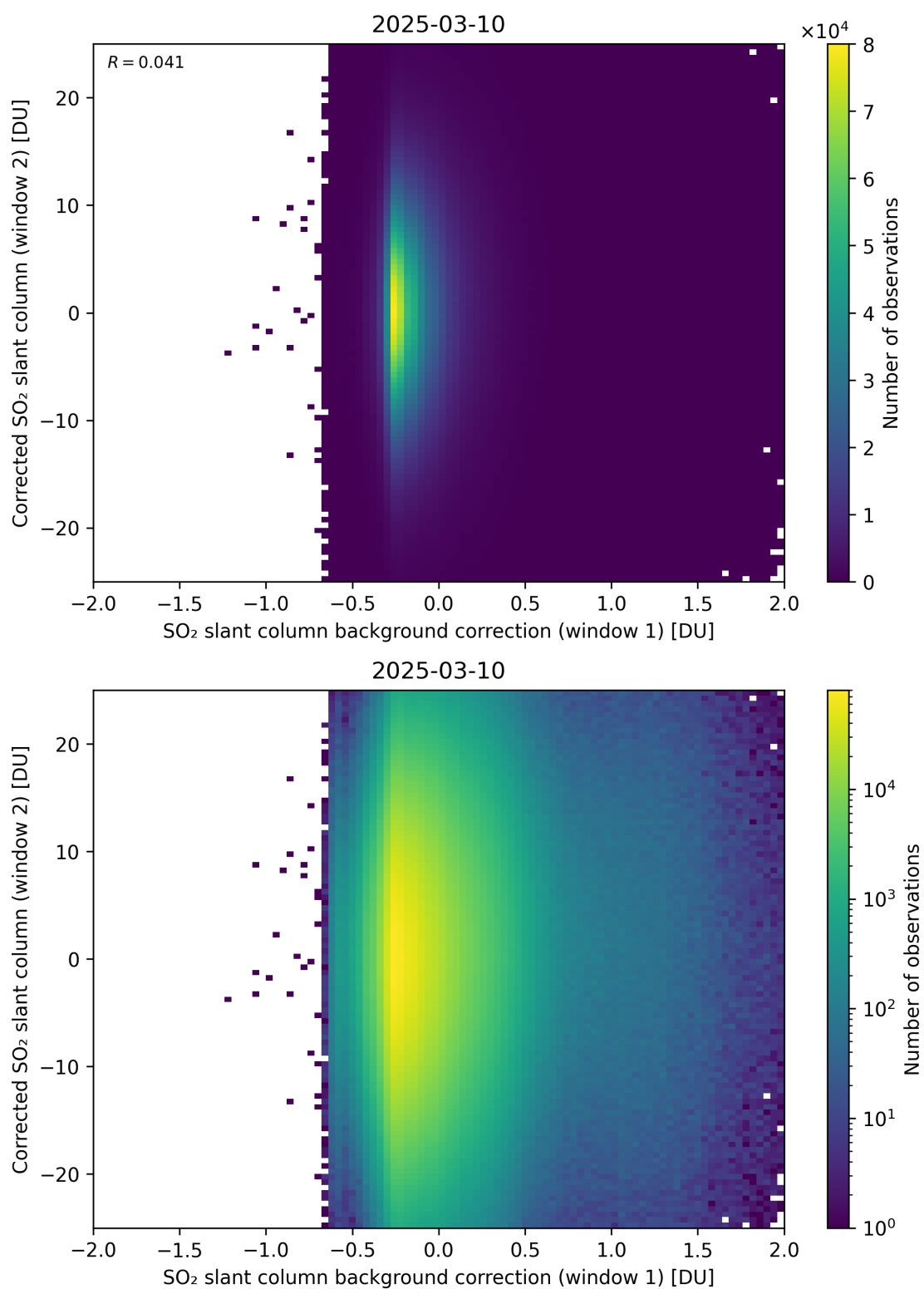
Figure 115: Scatter density plot of “SO 2 slant column background correction (window 1)” against “Corrected SO 2 slant column (window 2)” for 2025-03-09 to 2025-03-11.
