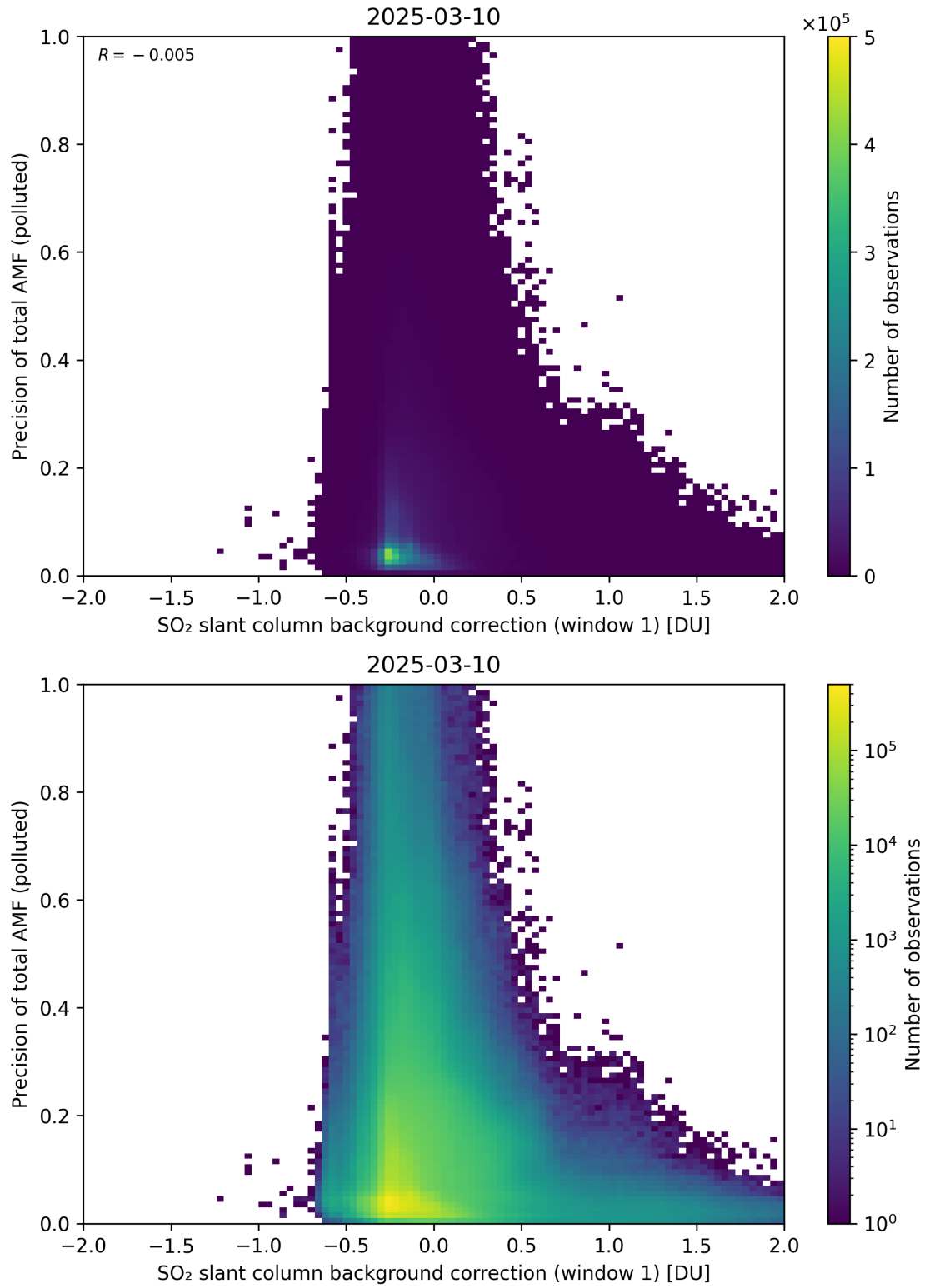
Figure 121: Scatter density plot of “SO 2 slant column background correction (window 1)” against “Precision of total AMF (polluted)” for 2025-03-09 to 2025-03-11.
