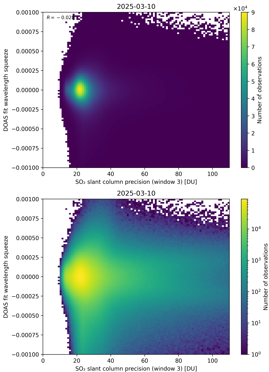
Figure 309: Scatter density plot of “SO 2 slant column precision (window 3)” against “DOAS fit wavelength squeeze” for 2025-03-09 to 2025-03-11.
