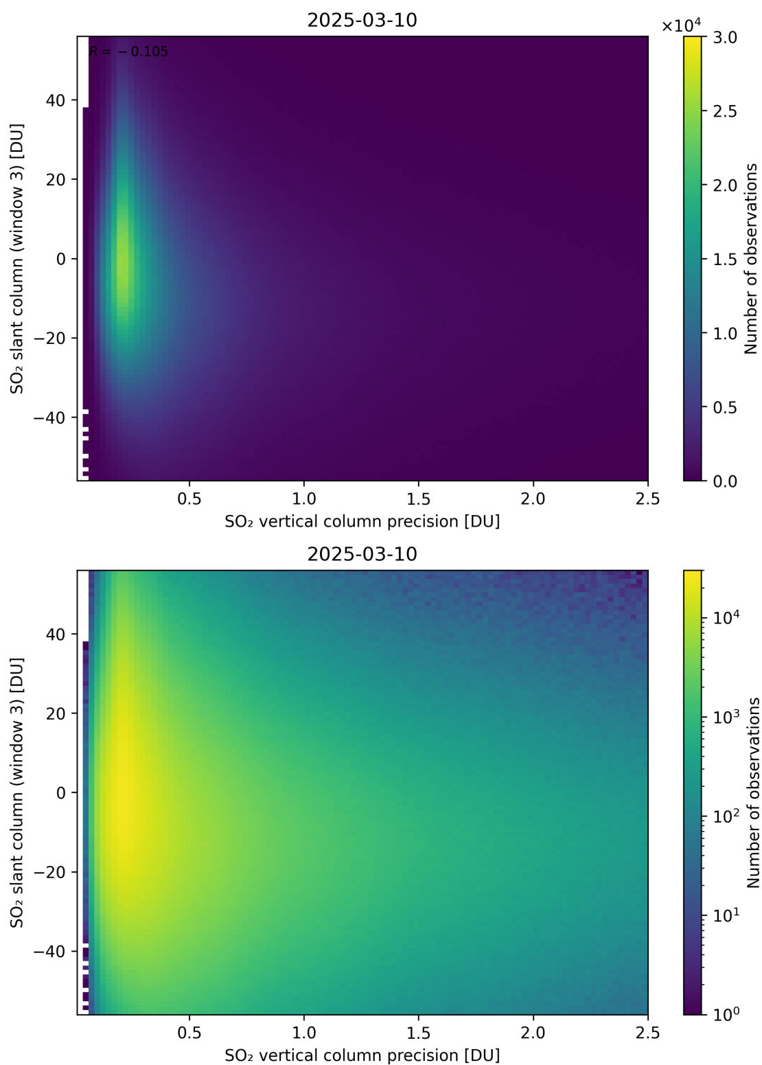
Figure 344: Scatter density plot of “SO 2 vertical column precision” against “SO 2 slant column (window 3)” for 2025-03-09 to 2025-03-11.
