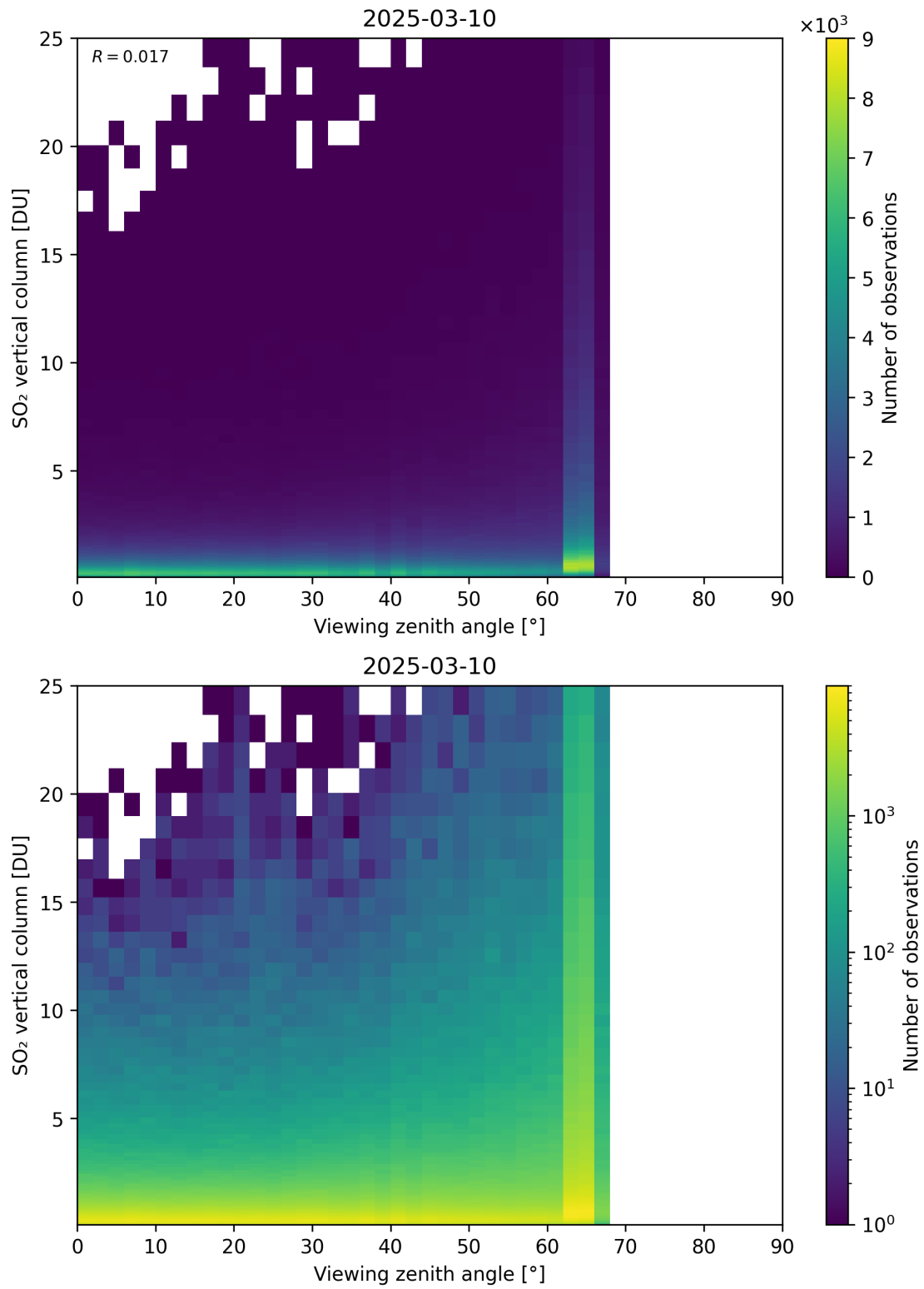
Figure 383: Scatter density plot of “Viewing zenith angle” against “SO 2 vertical column” for 2025-03-09 to 2025-03-11.
