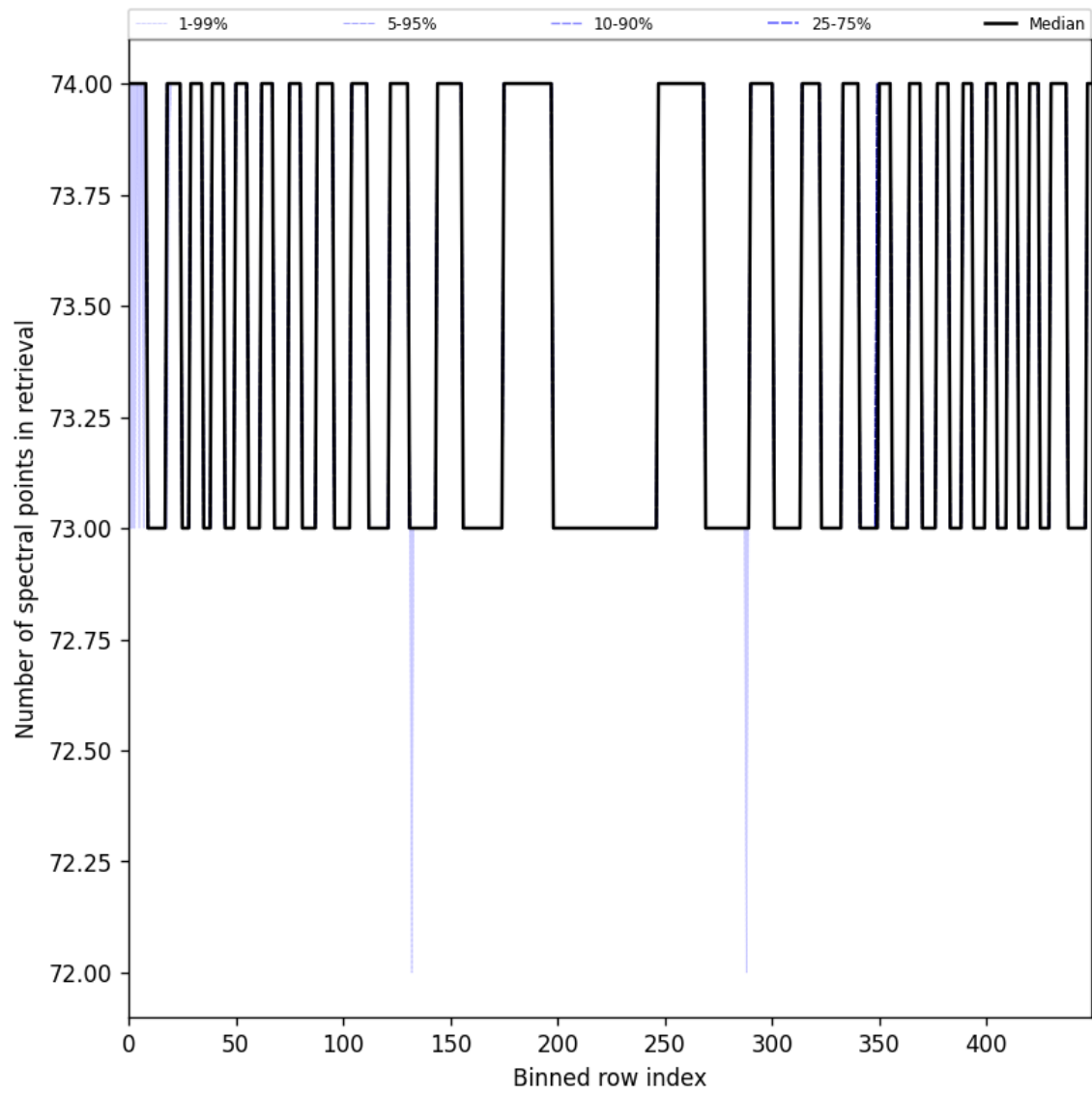
Figure 108: Along track statistics of “Number of spectral points in retrieval” for 2025-03-09 to 2025-03-11
