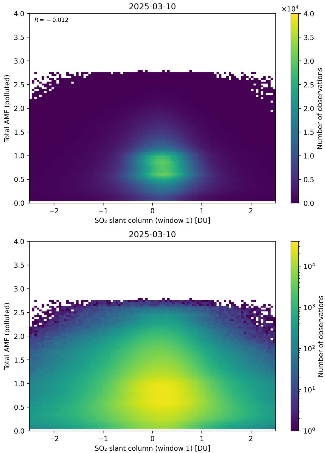
Figure 289: Scatter density plot of “SO 2 slant column (window 1)” against “Total AMF (polluted)” for 2025-03-09 to 2025-03-11.
