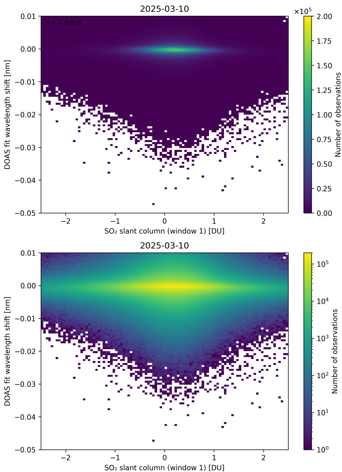
Figure 265: Scatter density plot of “SO 2 slant column (window 1)” against “DOAS fit wavelength shift” for 2025-03-09 to 2025-03-11.
