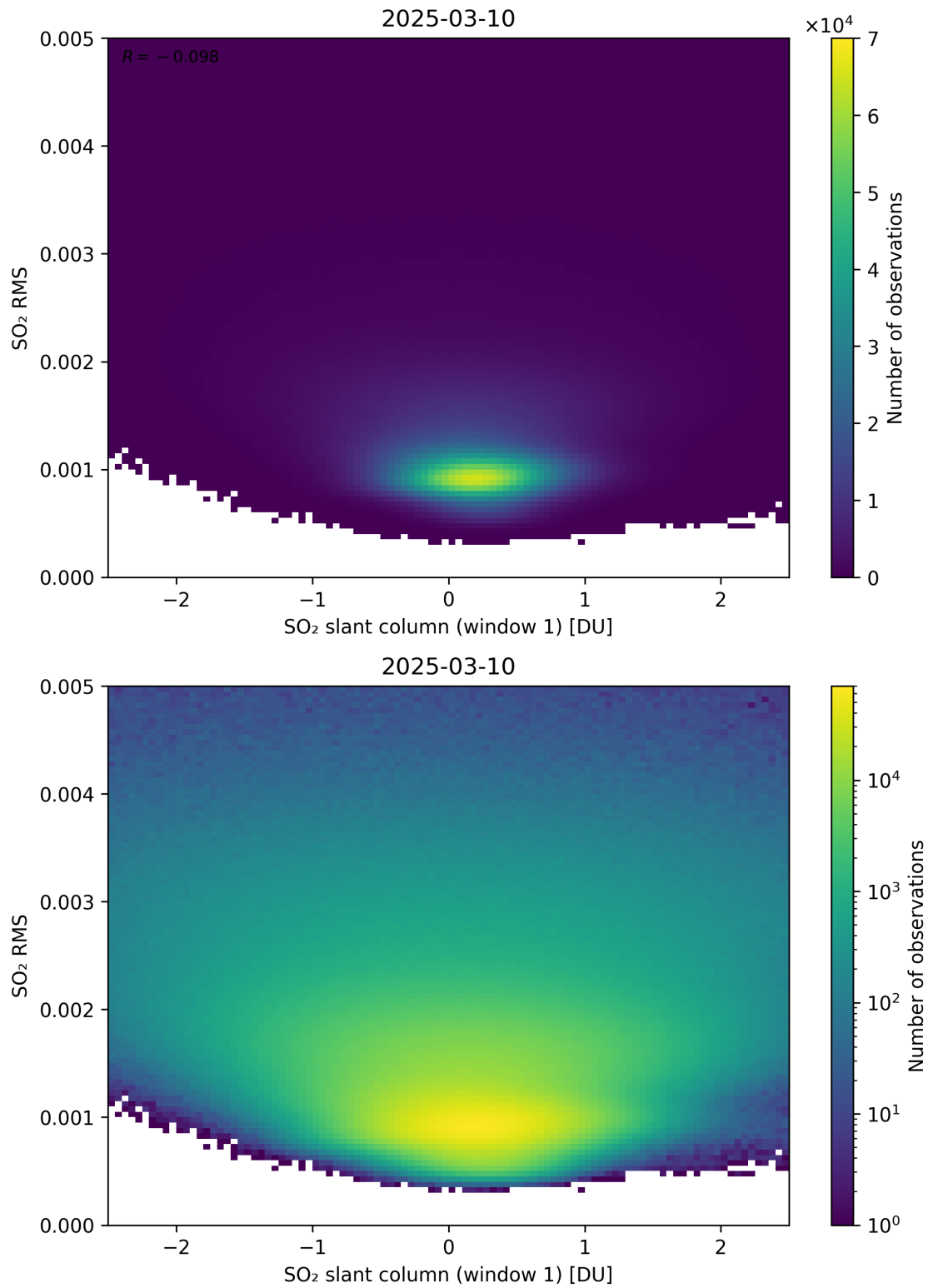
Figure 267: Scatter density plot of “SO 2 slant column (window 1)” against “SO 2 RMS” for 2025-03-09 to 2025-03-11.
