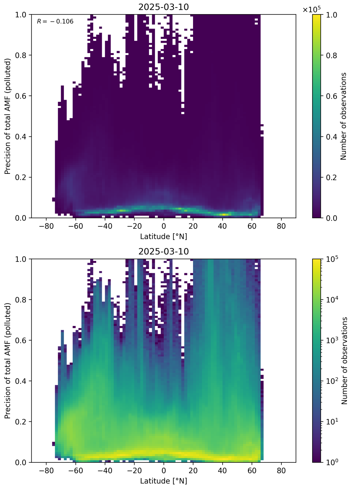
Figure 168: Scatter density plot of “Latitude” against “Precision of total AMF (polluted)” for 2025-03-09 to 2025-03-11.
