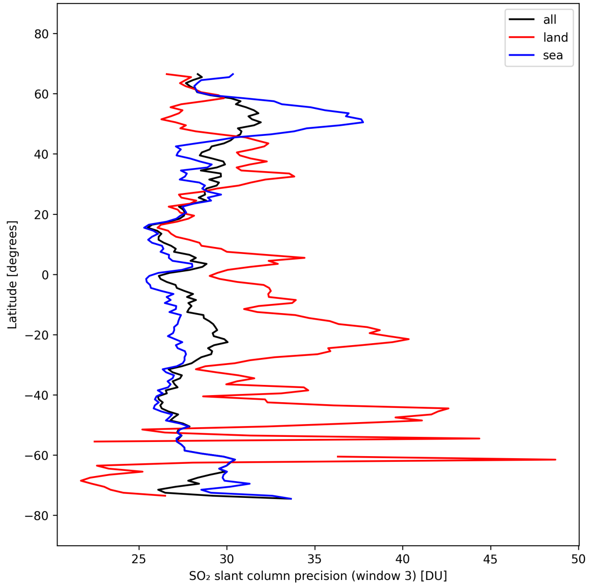
Figure 46: Zonal average of “SO 2 slant column precision (window 3)” for 2025-03-09 to 2025-03-11.
