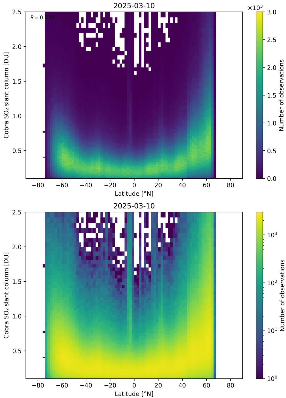
Figure 157: Scatter density plot of “Latitude” against “Cobra SO 2 slant column” for 2025-03-09 to 2025-03-11.
