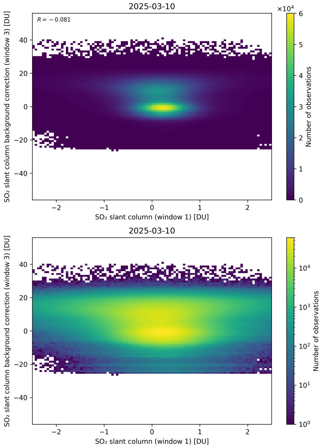
Figure 264: Scatter density plot of “SO 2 slant column (window 1)” against “SO 2 slant column background correction (window 3)” for 2025-03-09 to 2025-03-11.
