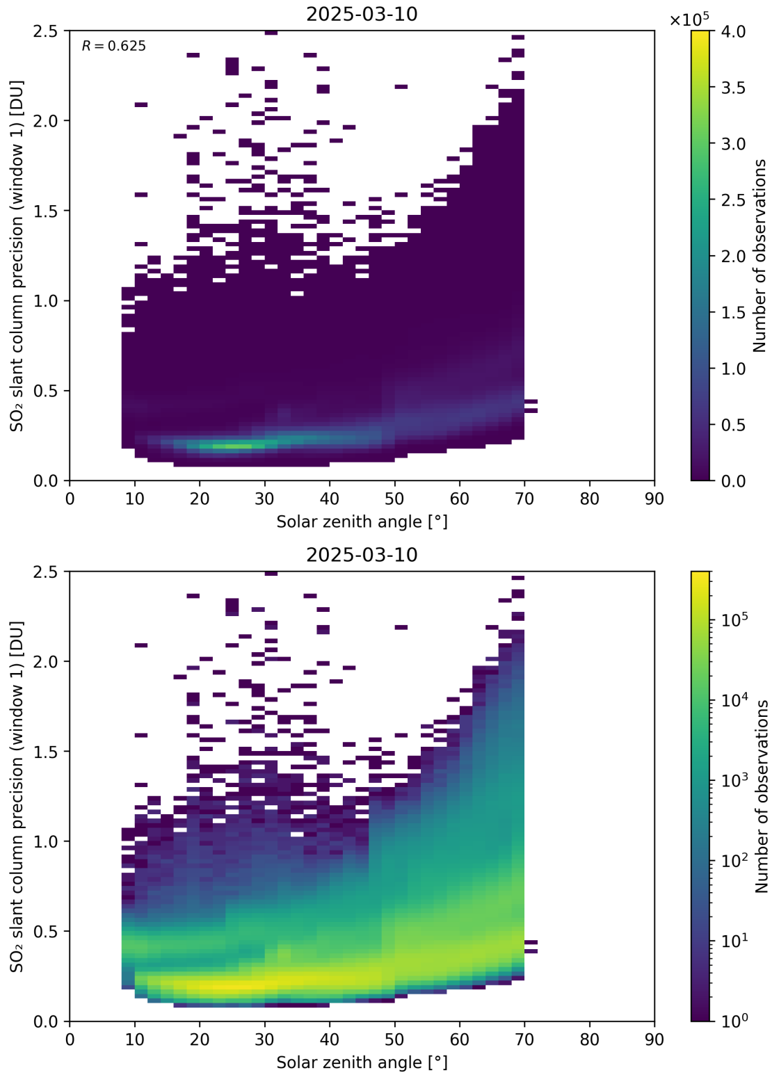
Figure 185: Scatter density plot of “Solar zenith angle” against “SO 2 slant column precision (window 1)” for 2025-03-09 to 2025-03-11.
