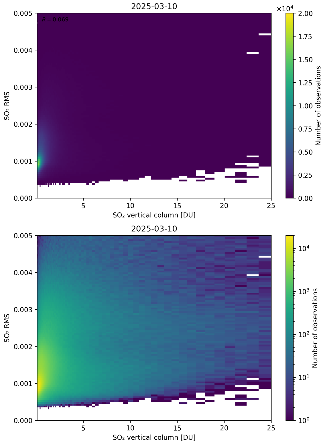
Figure 328: Scatter density plot of “SO 2 vertical column” against “SO 2 RMS” for 2025-03-09 to 2025-03-11.
