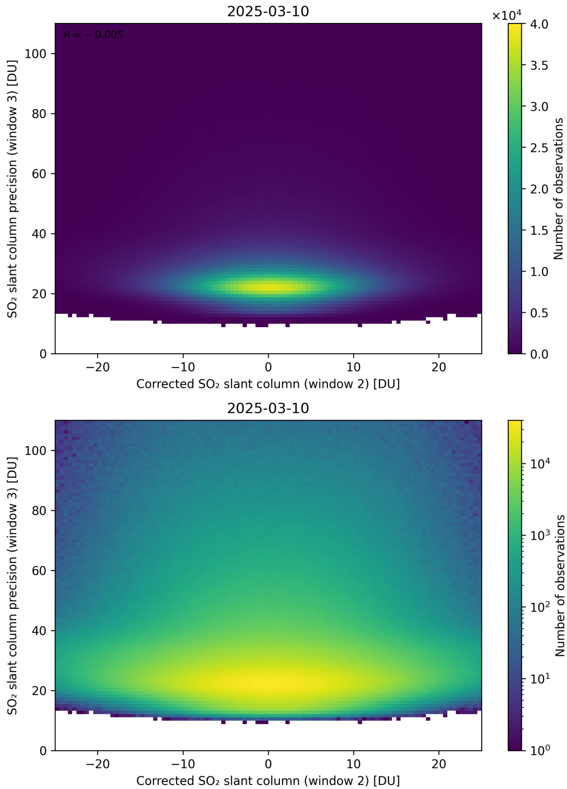
Figure 252: Scatter density plot of “Corrected SO 2 slant column (window 2)” against “SO 2 slant column precision (window 3)” for 2025-03-09 to 2025-03-11.
