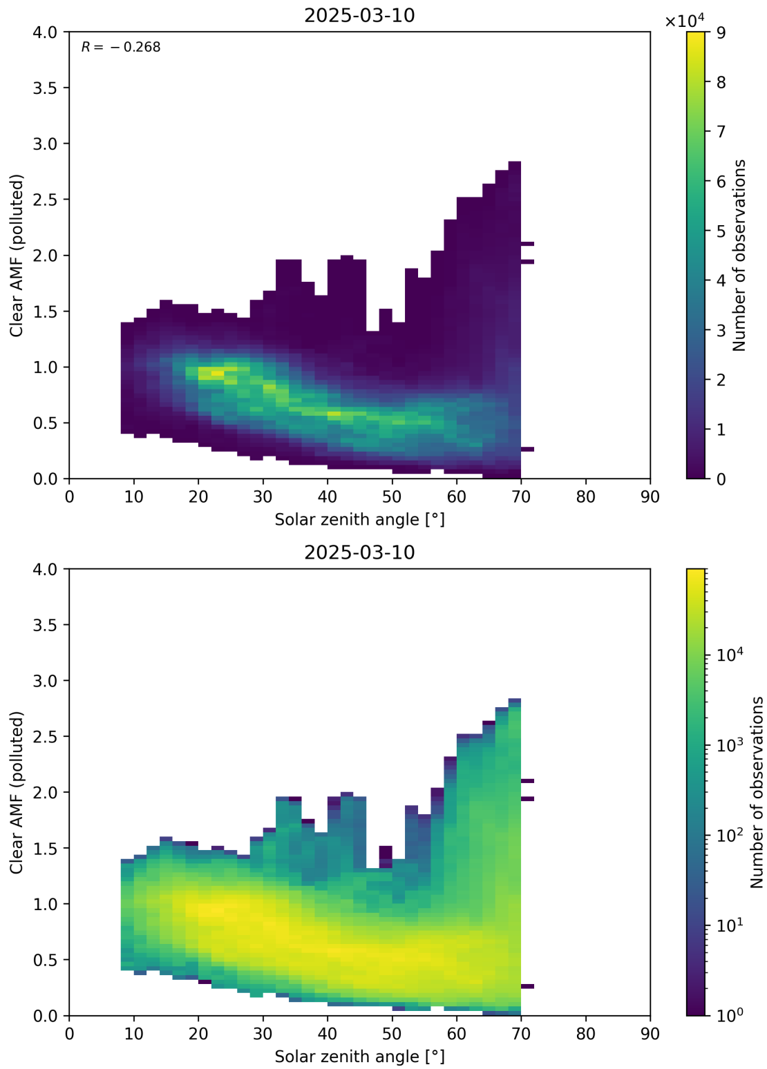
Figure 178: Scatter density plot of “Solar zenith angle” against “Clear AMF (polluted)” for 2025-03-09 to 2025-03-11.
