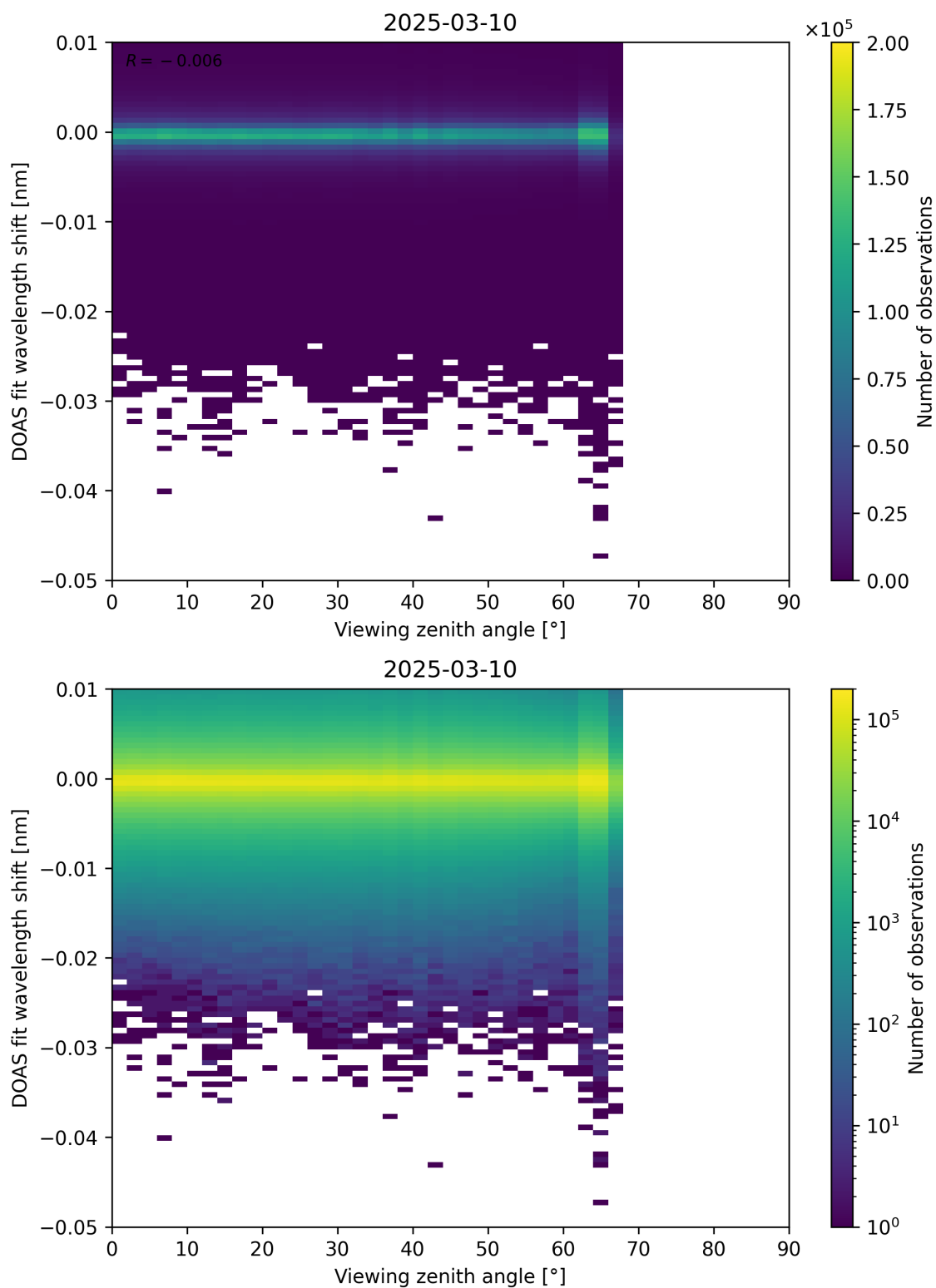
Figure 365: Scatter density plot of “Viewing zenith angle” against “DOAS fit wavelength shift” for 2025-03-09 to 2025-03-11.
