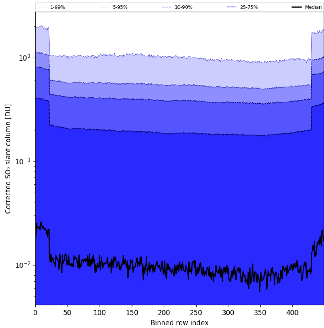
Figure 86: Along track statistics of “Corrected SO 2 slant column” for 2025-03-09 to 2025-03-11
