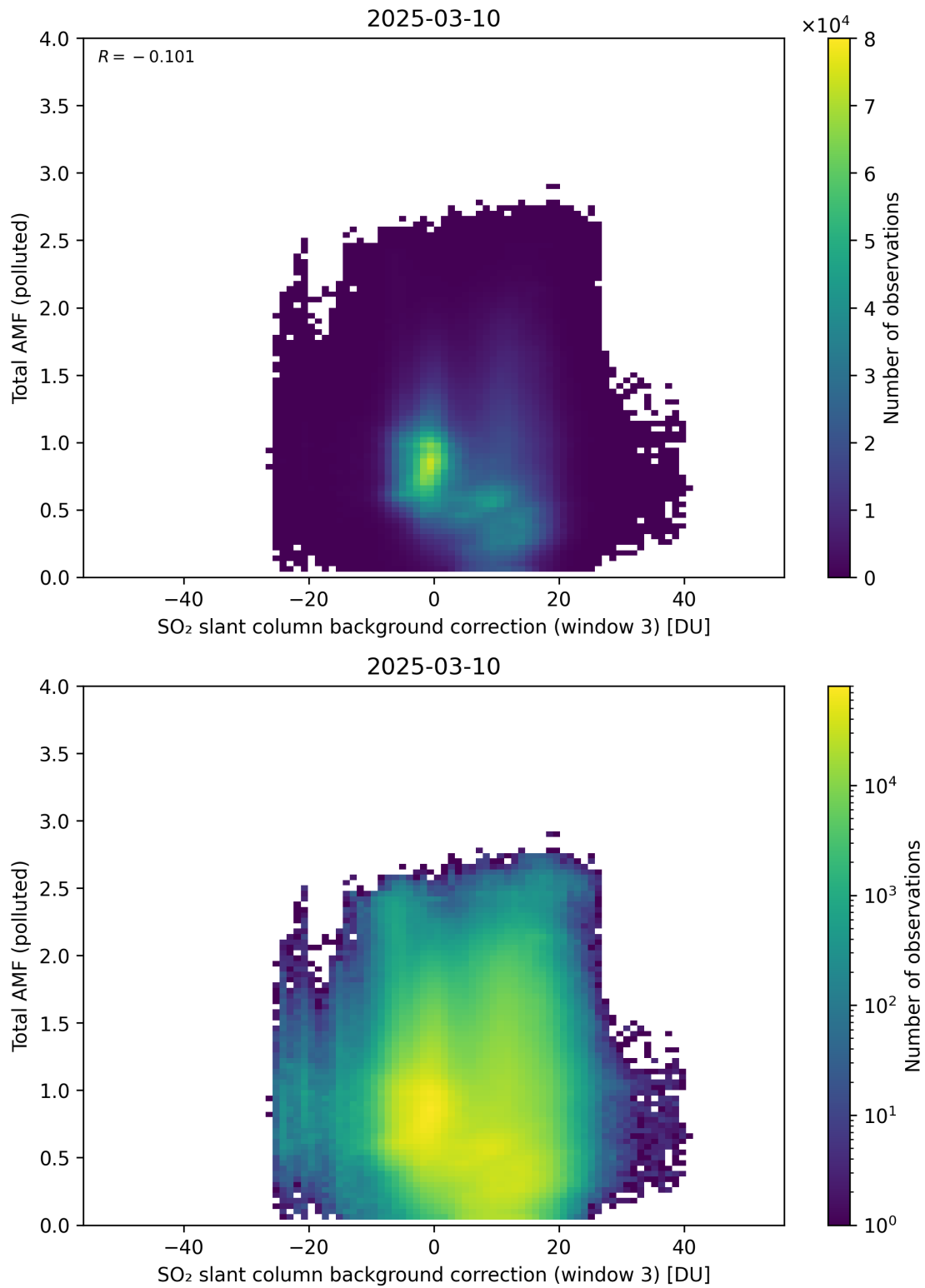
Figure 136: Scatter density plot of “SO 2 slant column background correction (window 3)” against “Total AMF (polluted)” for 2025-03-09 to 2025-03-11.
