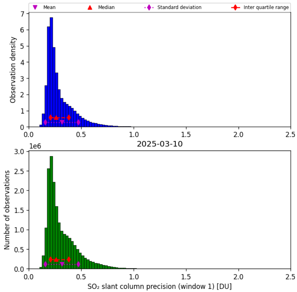
Figure 64: Histogram of “SO 2 slant column precision (window 1)” for 2025-03-09 to 2025-03-11
