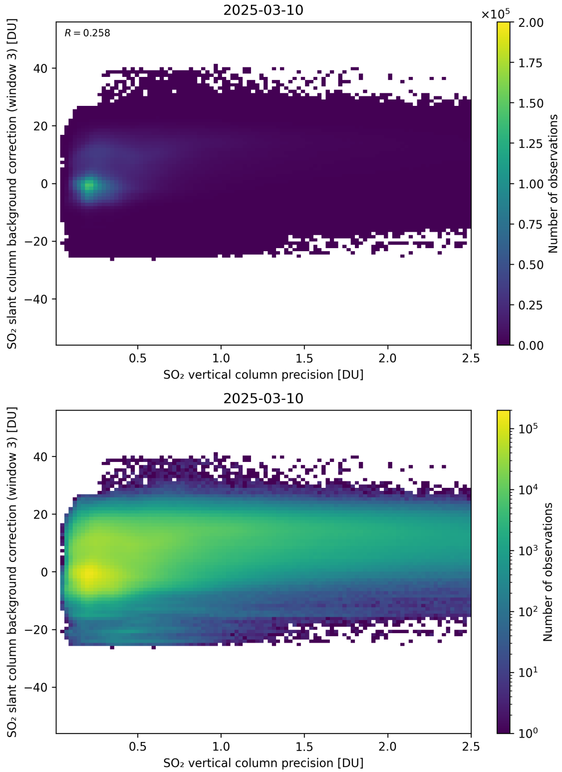
Figure 331: Scatter density plot of “SO 2 vertical column precision” against “SO 2 slant column background correction (window 3)” for 2025-03-09 to 2025-03-11.
