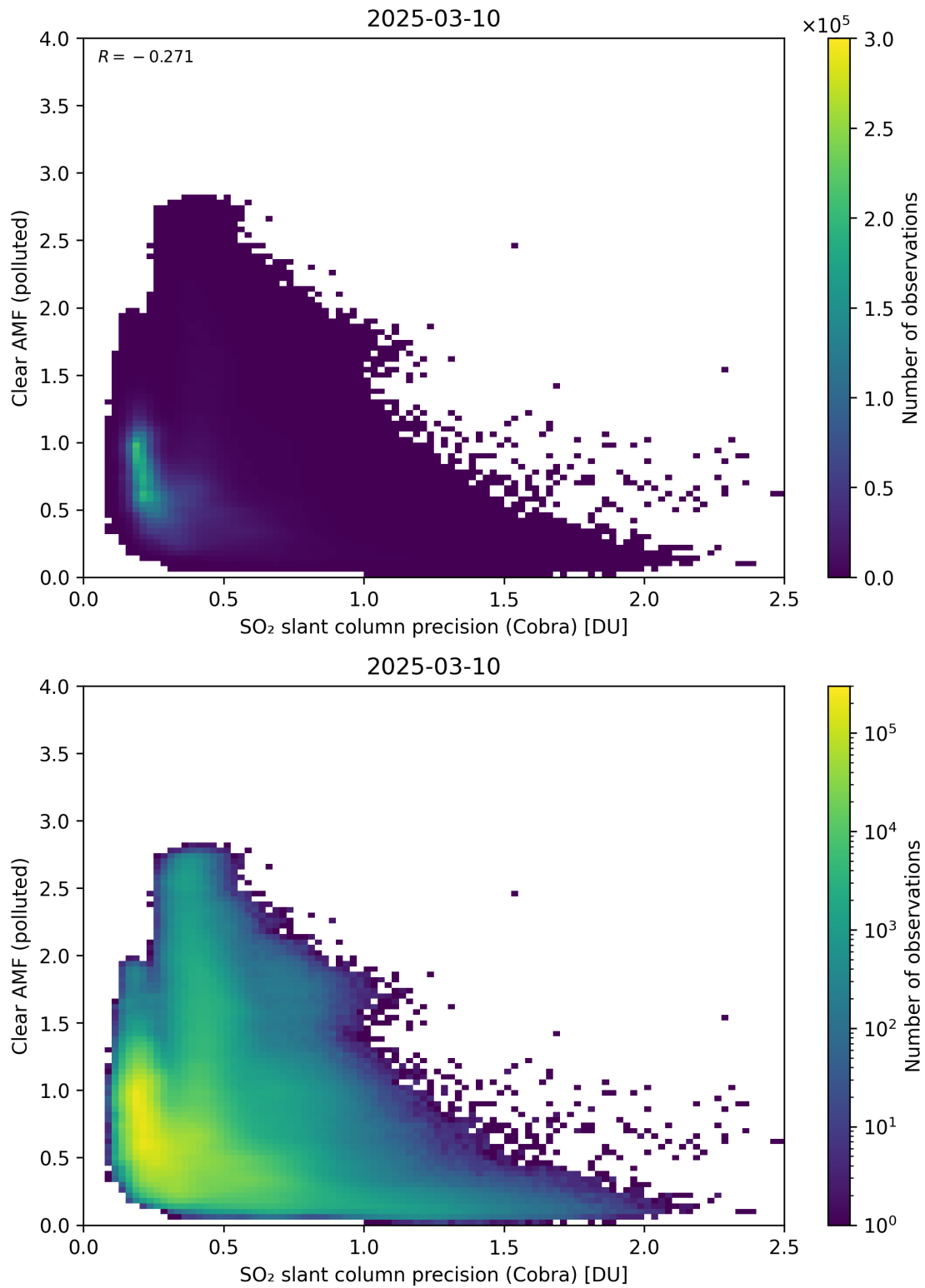
Figure 205: Scatter density plot of “SO 2 slant column precision (Cobra)” against “Clear AMF (polluted)” for 2025-03-09 to 2025-03-11.
