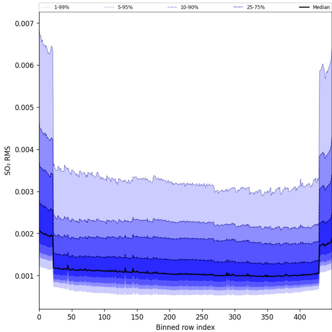
Figure 104: Along track statistics of “SO 2 RMS” for 2025-03-09 to 2025-03-11
