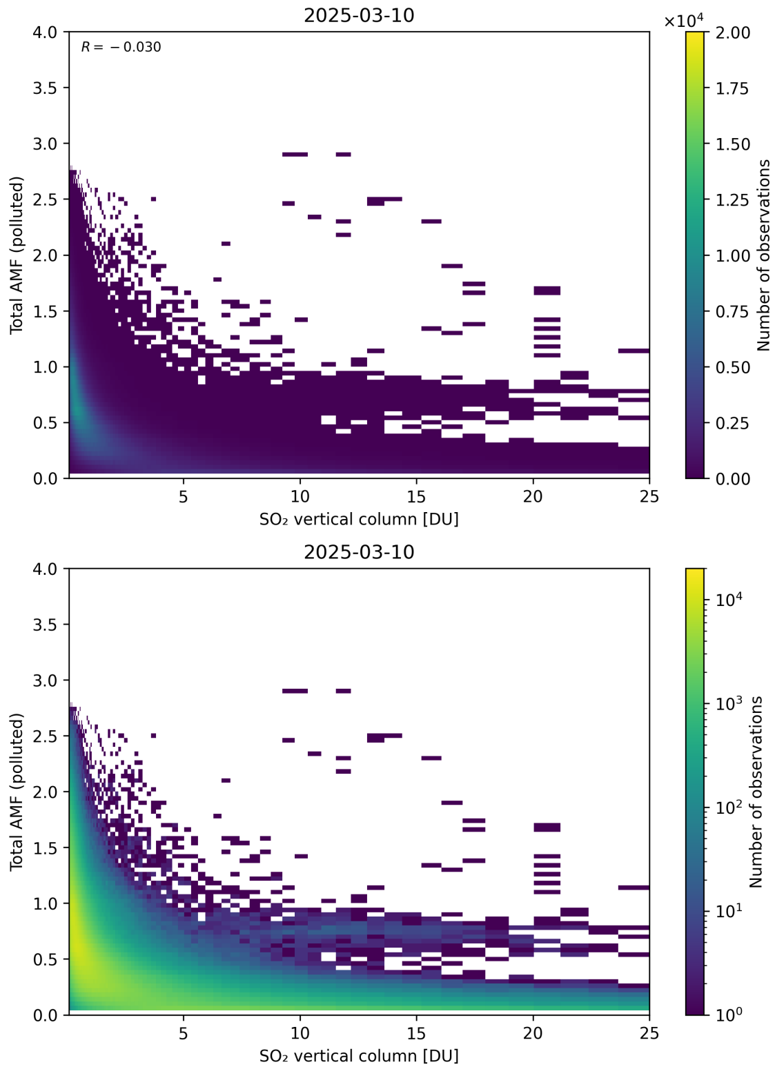
Figure 359: Scatter density plot of “SO 2 vertical column” against “Total AMF (polluted)” for 2025-03-09 to 2025-03-11.
