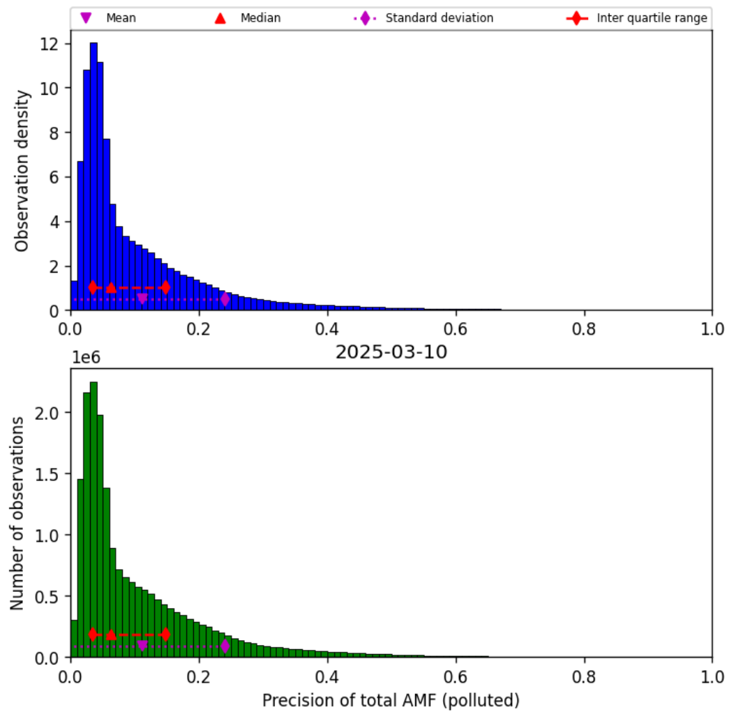
Figure 80: Histogram of “Precision of total AMF (polluted)” for 2025-03-09 to 2025-03-11
