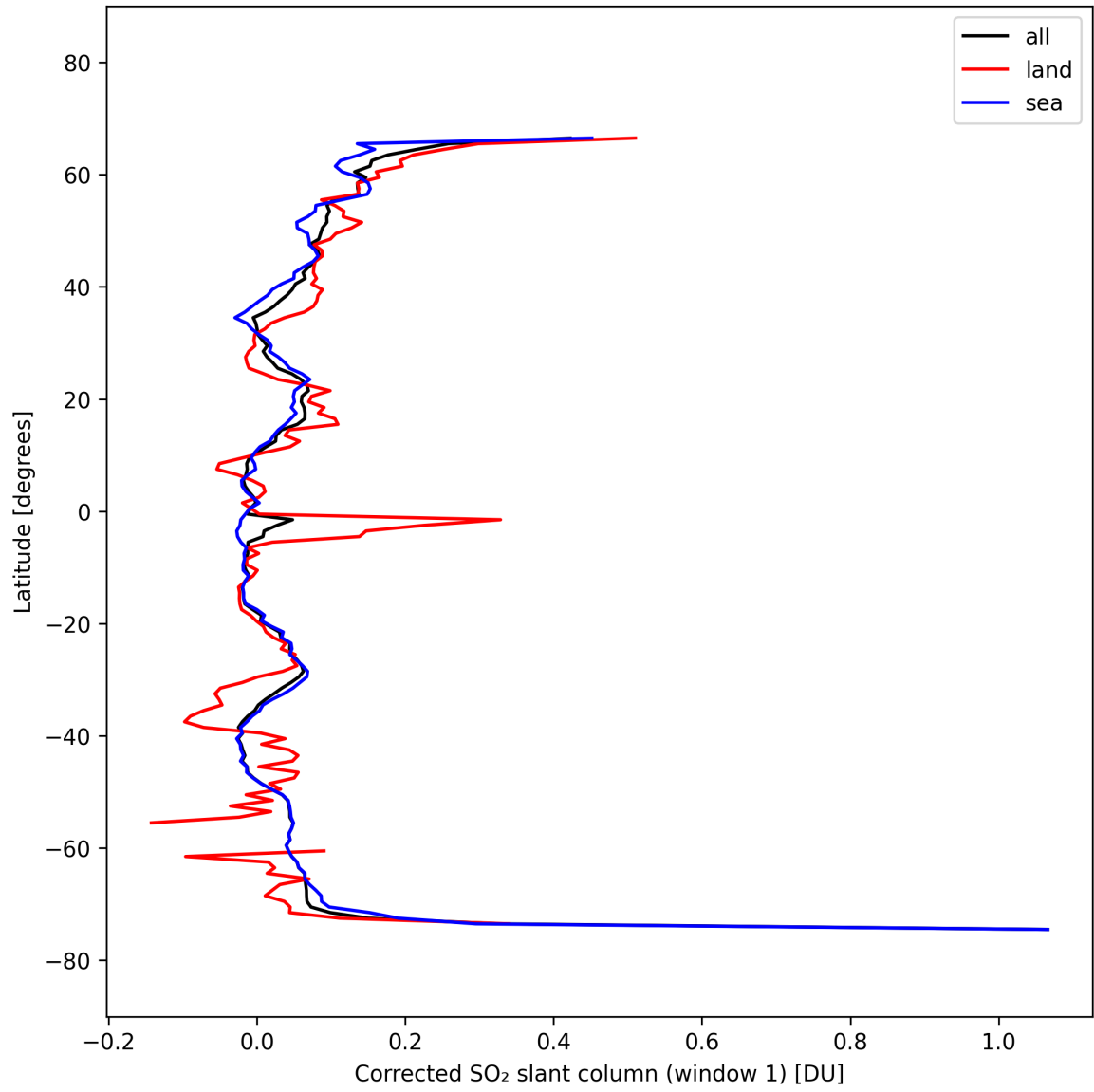
Figure 39: Zonal average of “Corrected SO 2 slant column (window 1)” for 2025-03-09 to 2025-03-11.
