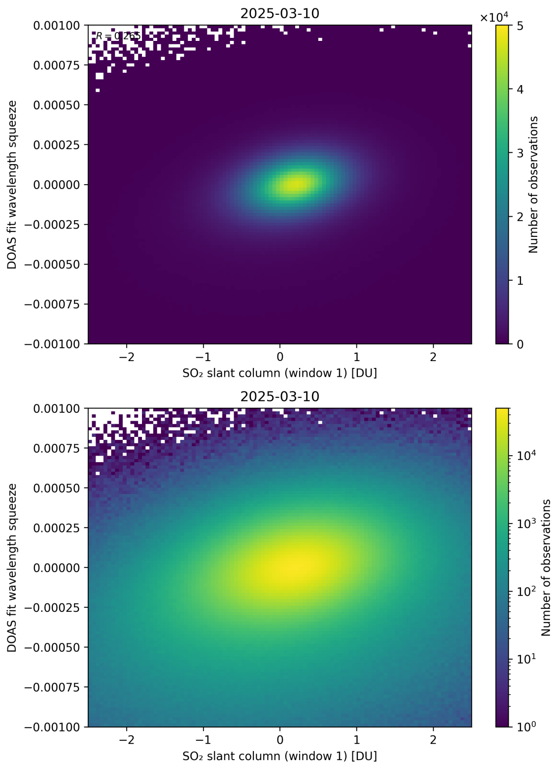
Figure 266: Scatter density plot of “SO 2 slant column (window 1)” against “DOAS fit wavelength squeeze” for 2025-03-09 to 2025-03-11.
