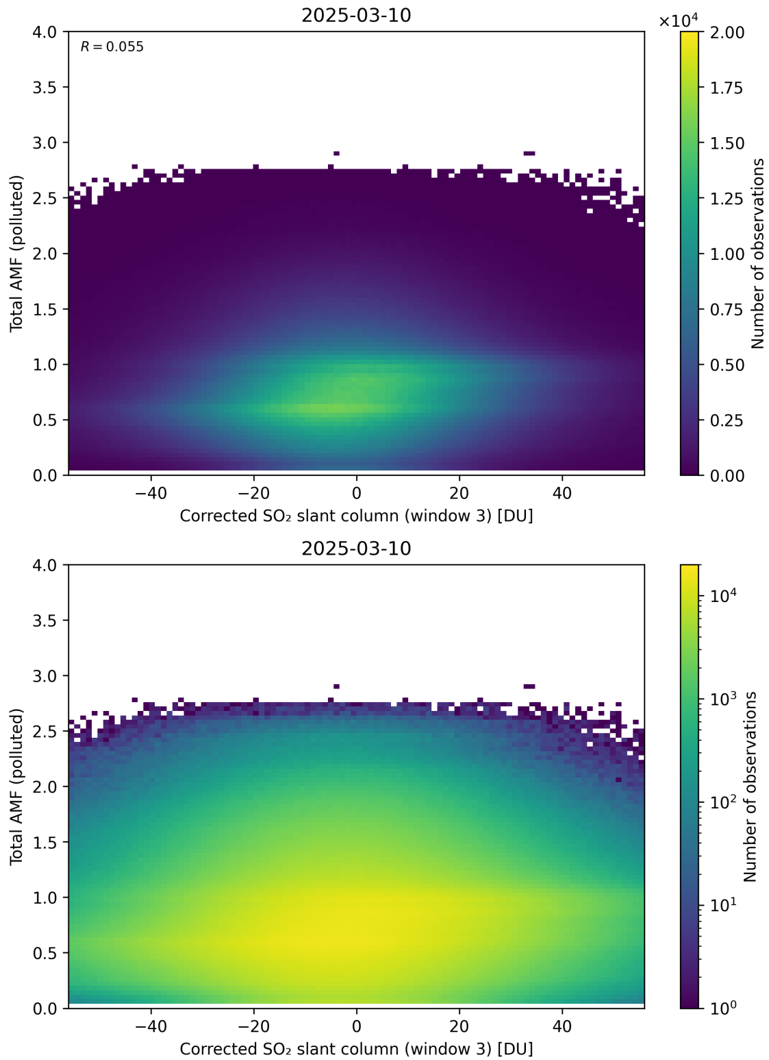
Figure 260: Scatter density plot of “Corrected SO 2 slant column (window 3)” against “Total AMF (polluted)” for 2025-03-09 to 2025-03-11.
