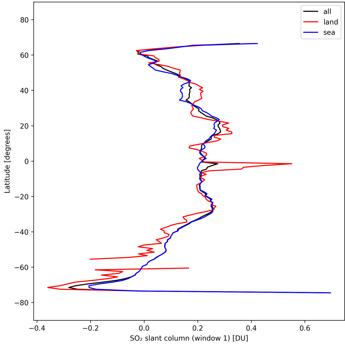
Figure 37: Zonal average of “SO 2 slant column (window 1)” for 2025-03-09 to 2025-03-11.
