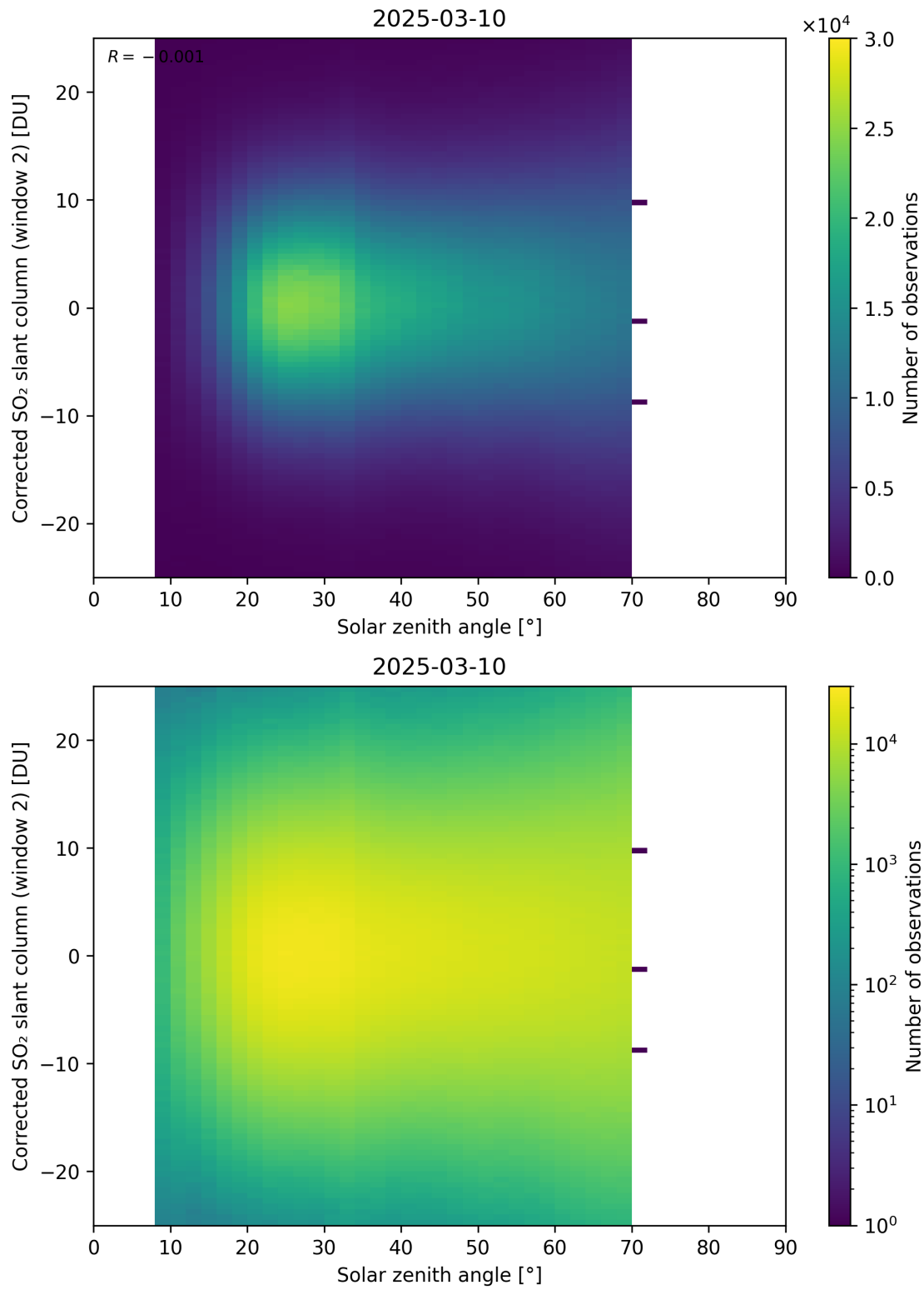
Figure 182: Scatter density plot of “Solar zenith angle” against “Corrected SO 2 slant column (window 2)” for 2025-03-09 to 2025-03-11.
