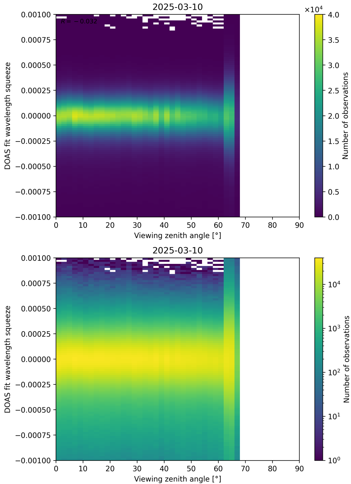
Figure 366: Scatter density plot of “Viewing zenith angle” against “DOAS fit wavelength squeeze” for 2025-03-09 to 2025-03-11.
