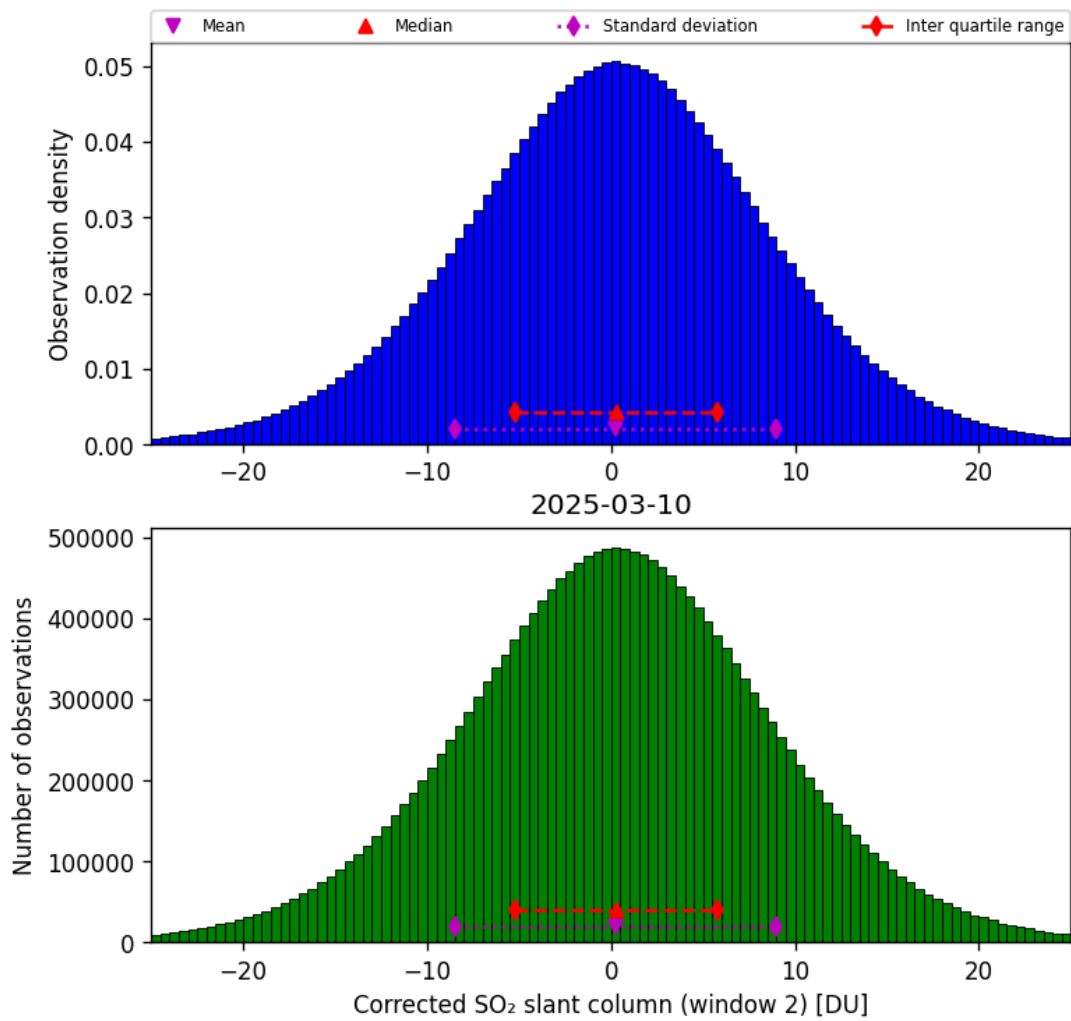
Figure 69: Histogram of “Corrected SO 2 slant column (window 2)” for 2025-03-09 to 2025-03-11
