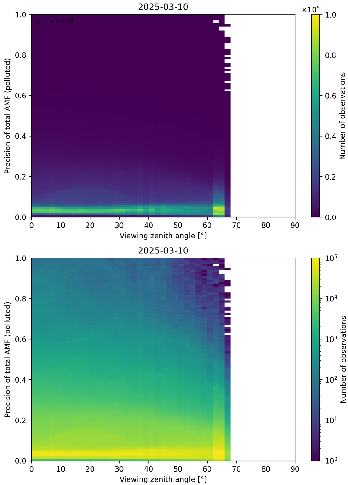
Figure 382: Scatter density plot of “Viewing zenith angle” against “Precision of total AMF (polluted)” for 2025-03-09 to 2025-03-11.
