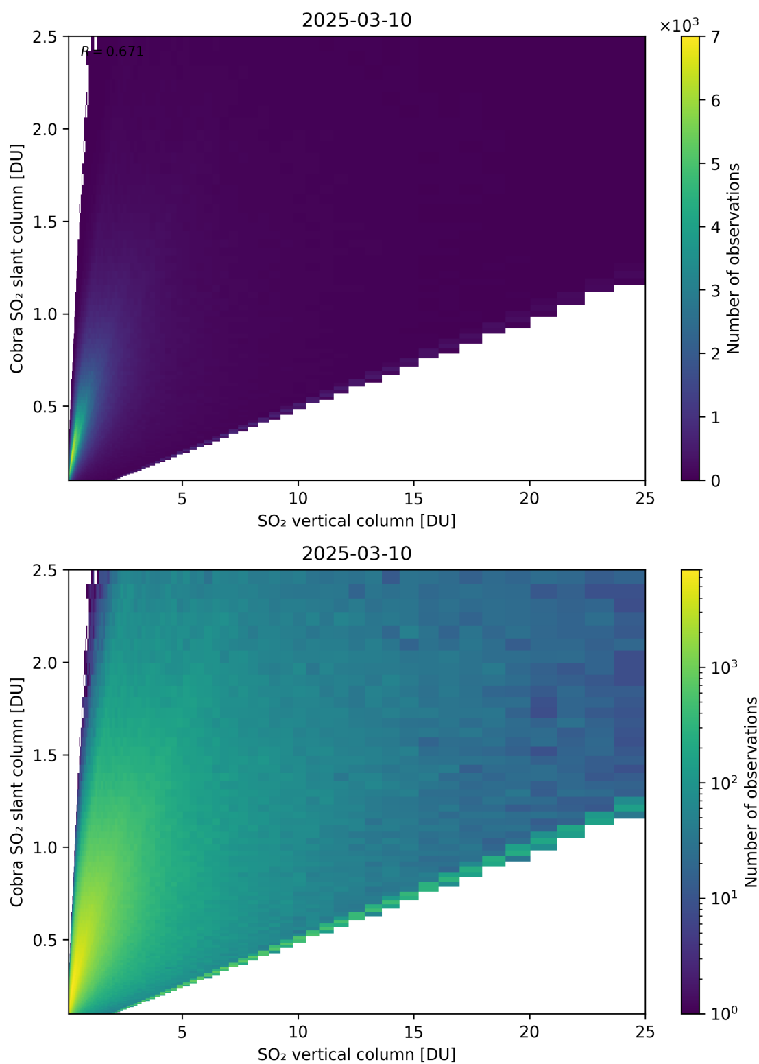
Figure 349: Scatter density plot of “SO 2 vertical column” against “Cobra SO 2 slant column” for 2025-03-09 to 2025-03-11.
