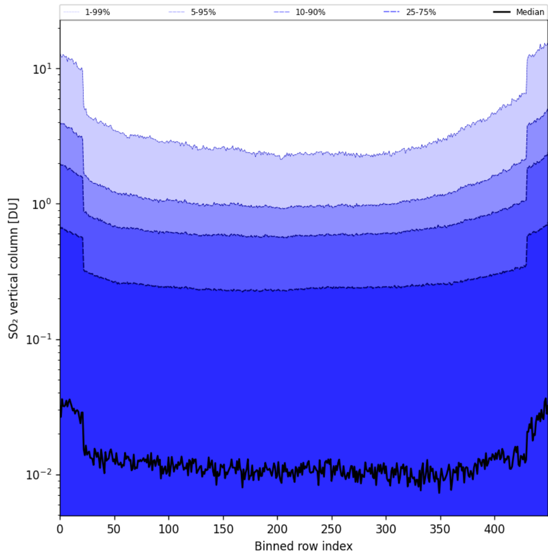
Figure 84: Along track statistics of “SO 2 vertical column” for 2025-03-09 to 2025-03-11
