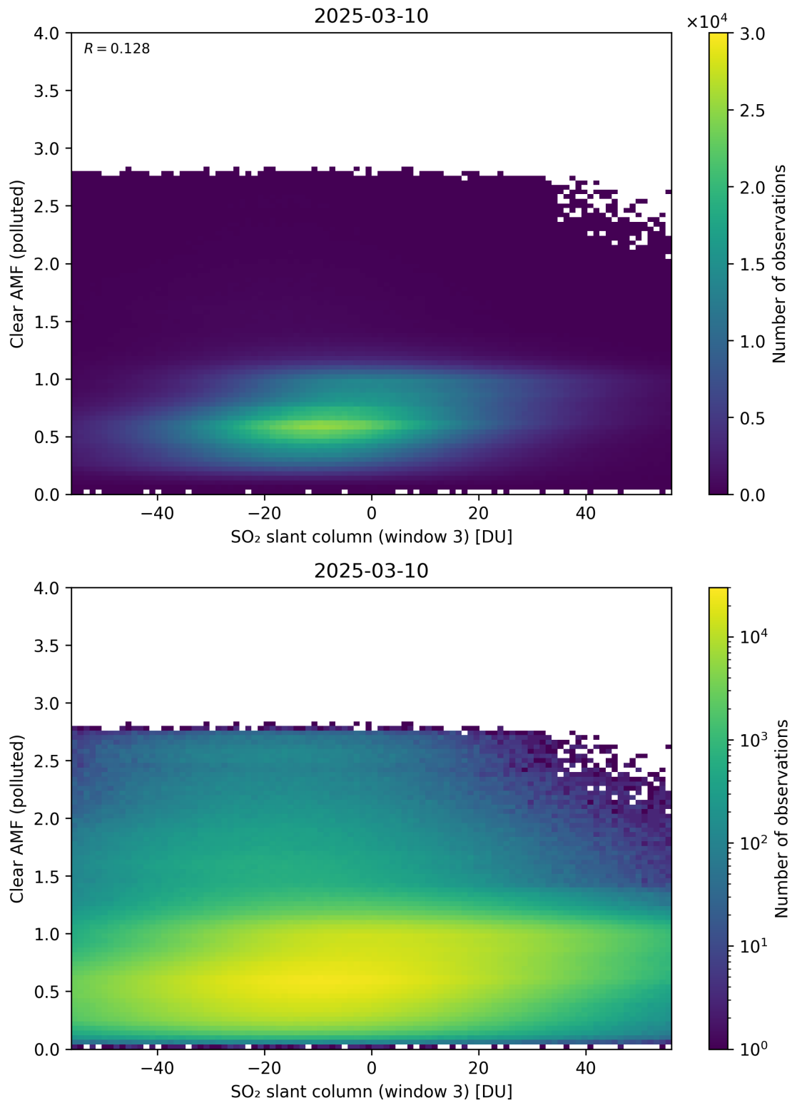
Figure 315: Scatter density plot of “SO 2 slant column (window 3)” against “Clear AMF (polluted)” for 2025-03-09 to 2025-03-11.
