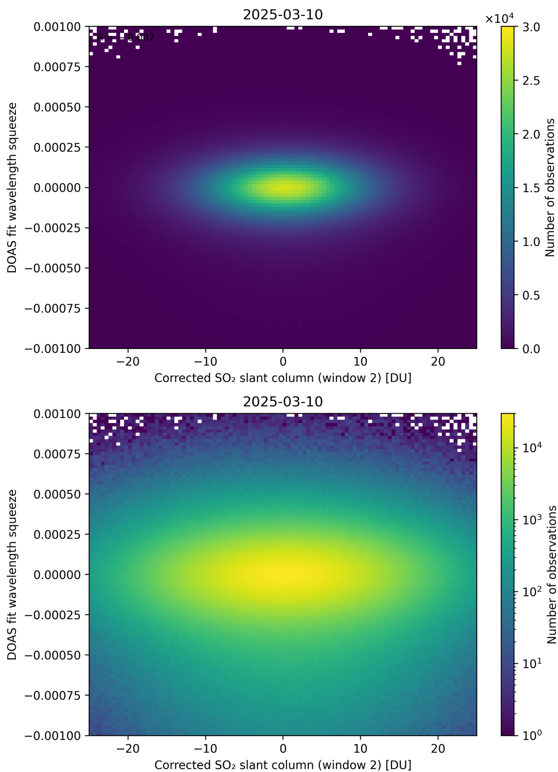
Figure 247: Scatter density plot of “Corrected SO 2 slant column (window 2)” against “DOAS fit wavelength squeeze” for 2025-03-09 to 2025-03-11.
