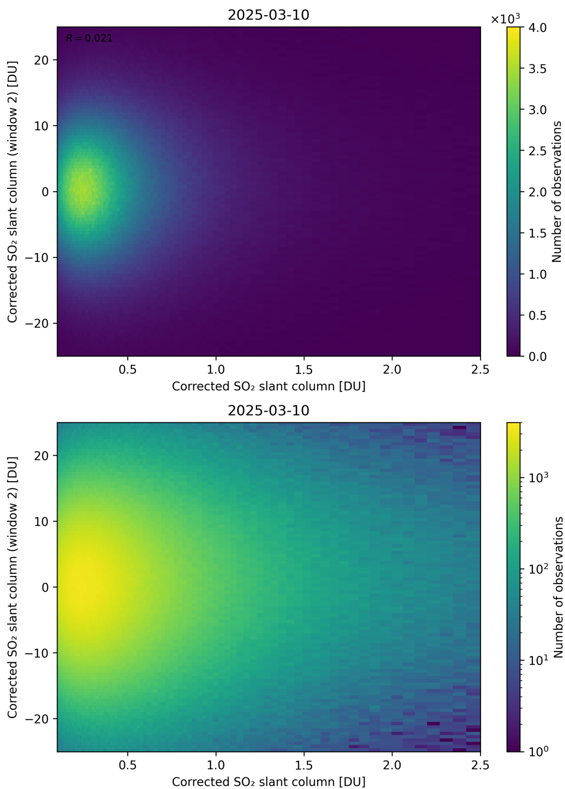
Figure 235: Scatter density plot of “Corrected SO 2 slant column” against “Corrected SO 2 slant column (window 2)” for 2025-03-09 to 2025-03-11.
