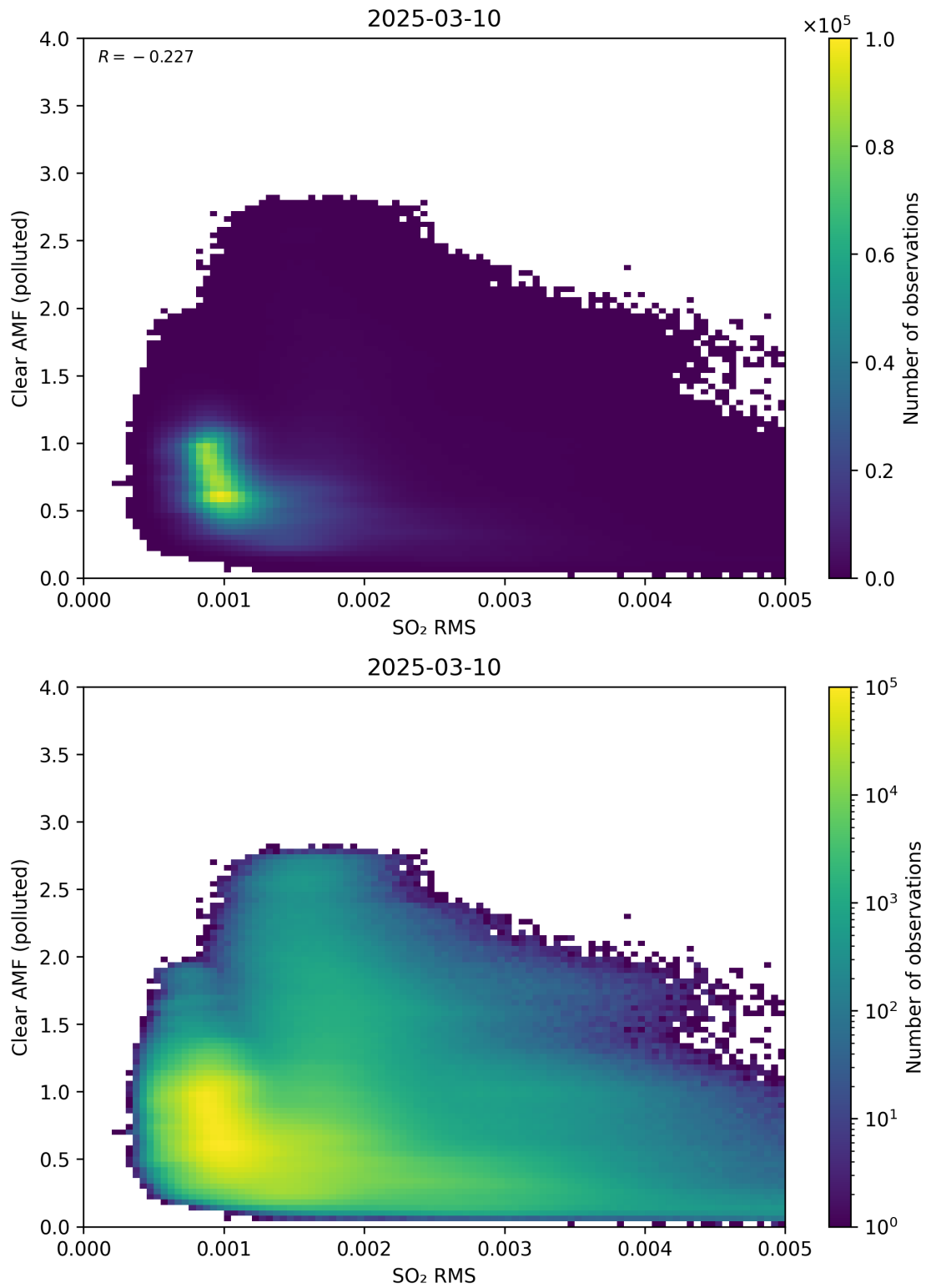
Figure 147: Scatter density plot of “SO 2 RMS” against “Clear AMF (polluted)” for 2025-03-09 to 2025-03-11.
