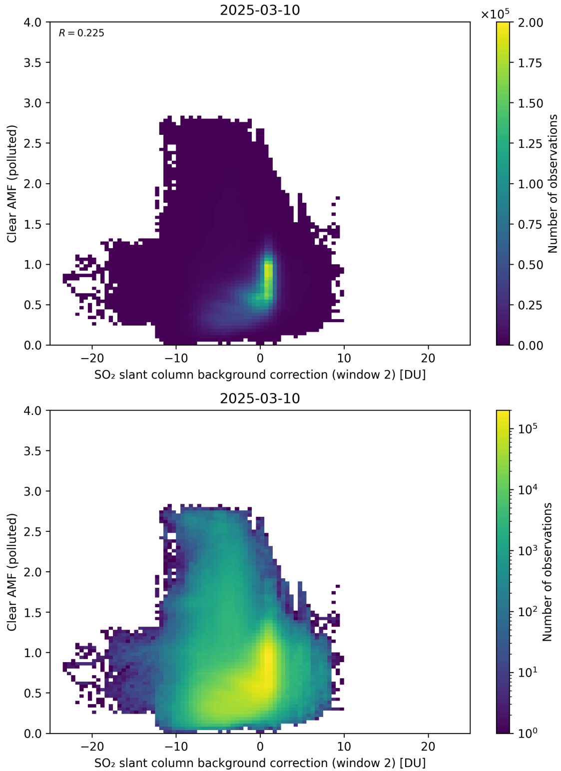
Figure 126: Scatter density plot of “SO 2 slant column background correction (window 2)” against “Clear AMF (polluted)” for 2025-03-09 to 2025-03-11.
