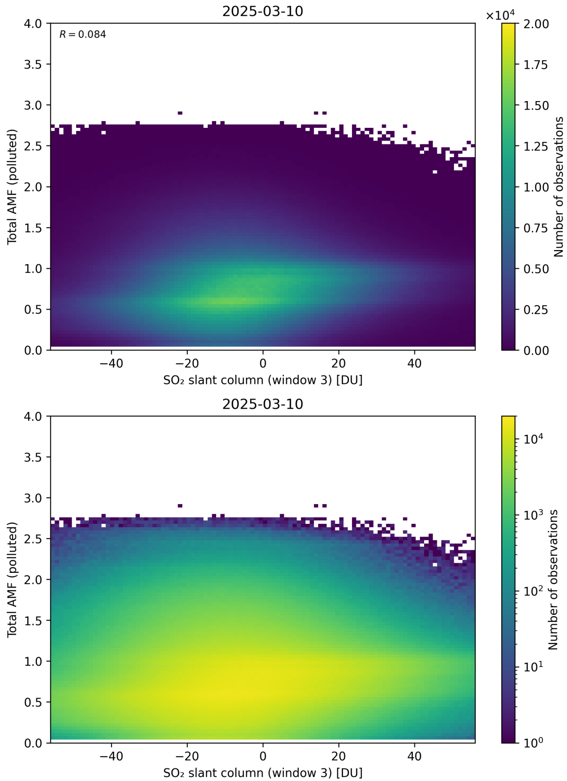
Figure 318: Scatter density plot of “SO 2 slant column (window 3)” against “Total AMF (polluted)” for 2025-03-09 to 2025-03-11.
