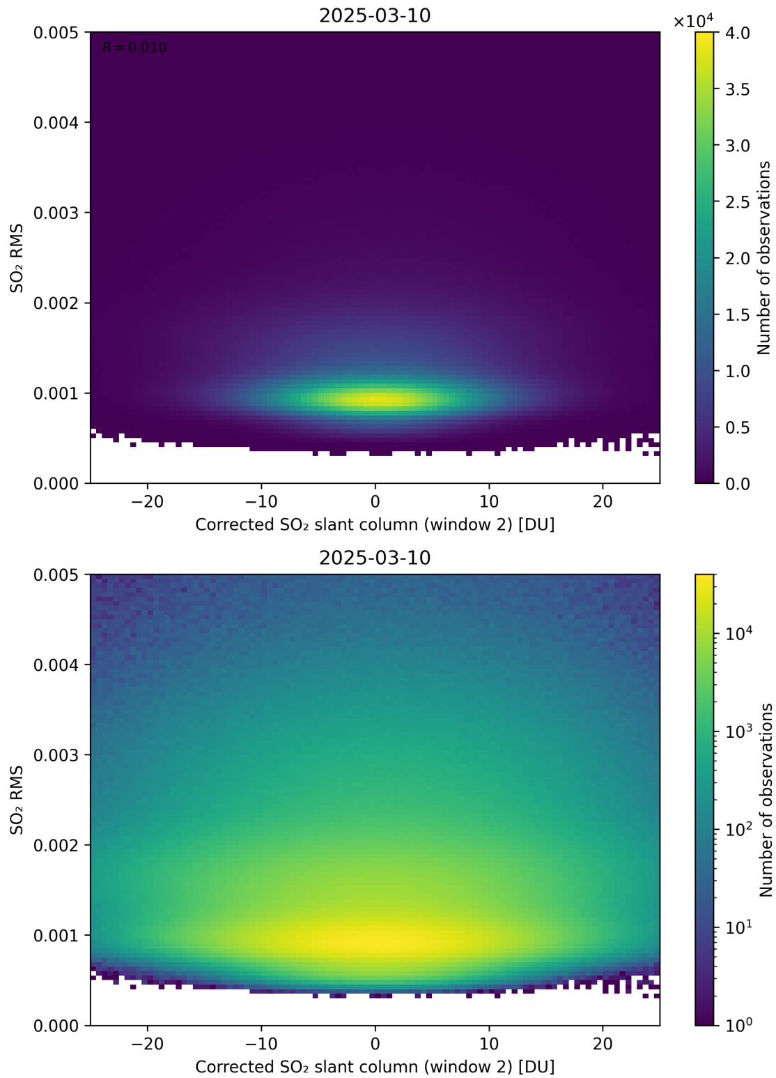
Figure 248: Scatter density plot of “Corrected SO 2 slant column (window 2)” against “SO 2 RMS” for 2025-03-09 to 2025-03-11.
