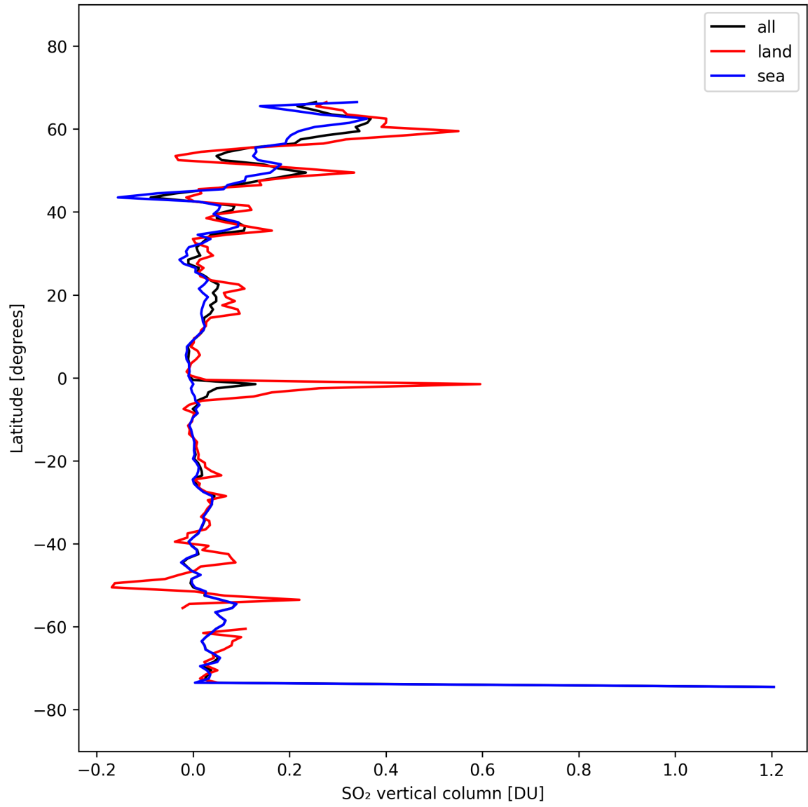
Figure 32: Zonal average of “SO 2 vertical column” for 2025-03-09 to 2025-03-11.
