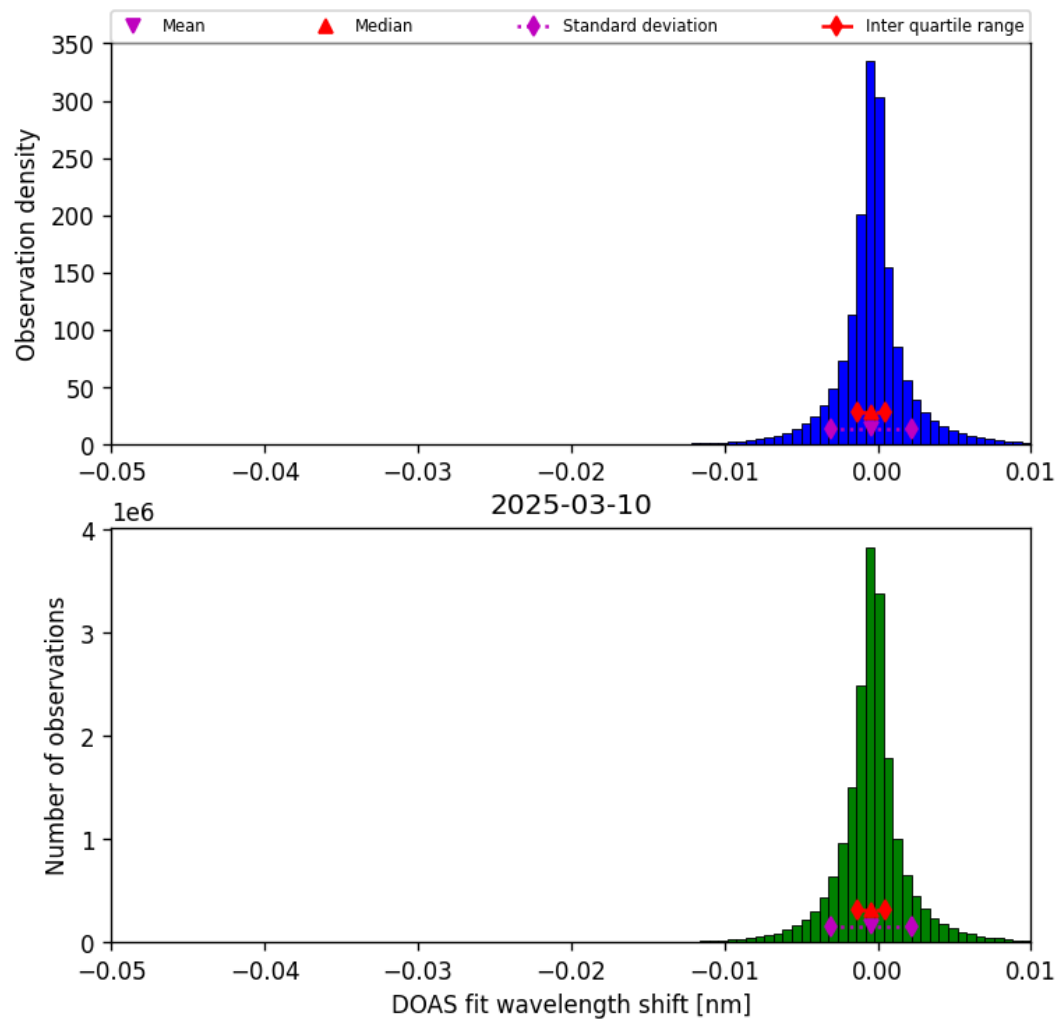
Figure 76: Histogram of “DOAS fit wavelength shift” for 2025-03-09 to 2025-03-11
