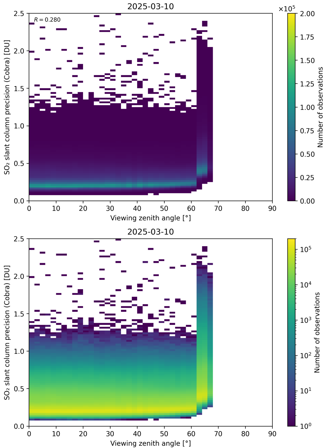
Figure 372: Scatter density plot of “Viewing zenith angle” against “SO 2 slant column precision (Cobra)” for 2025-03-09 to 2025-03-11.
