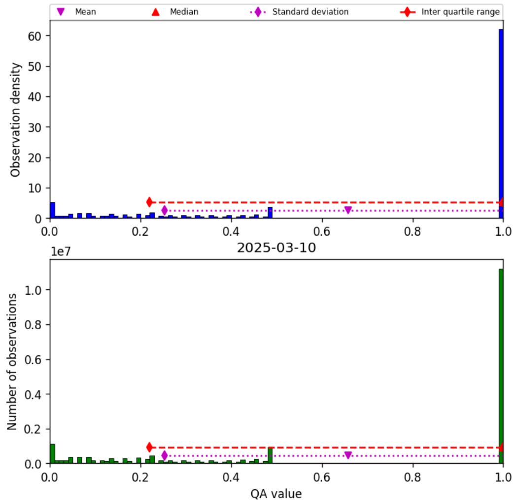
Figure 57: Histogram of “QA value” for 2025-03-09 to 2025-03-11
