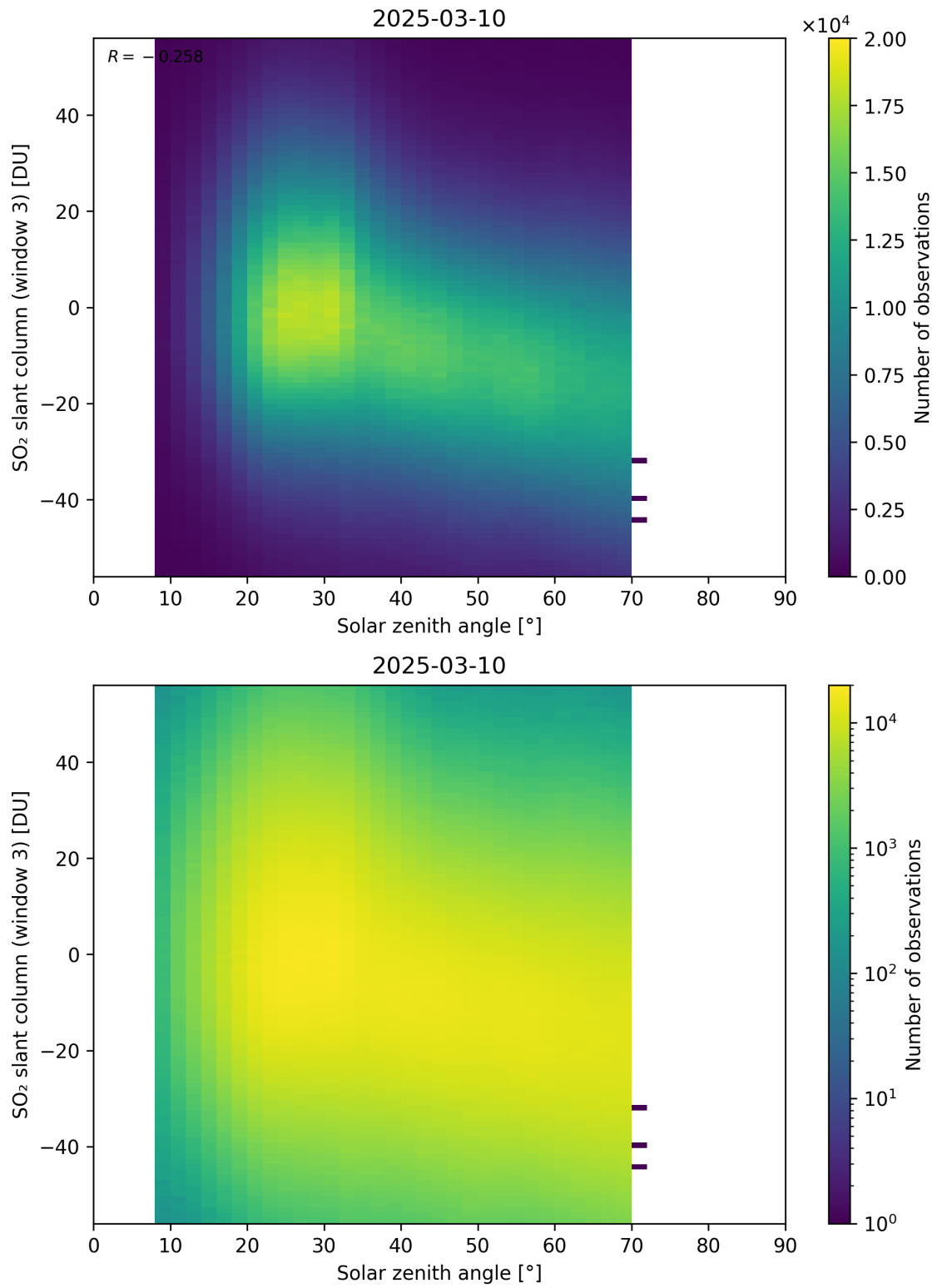
Figure 187: Scatter density plot of “Solar zenith angle” against “SO 2 slant column (window 3)” for 2025-03-09 to 2025-03-11.
