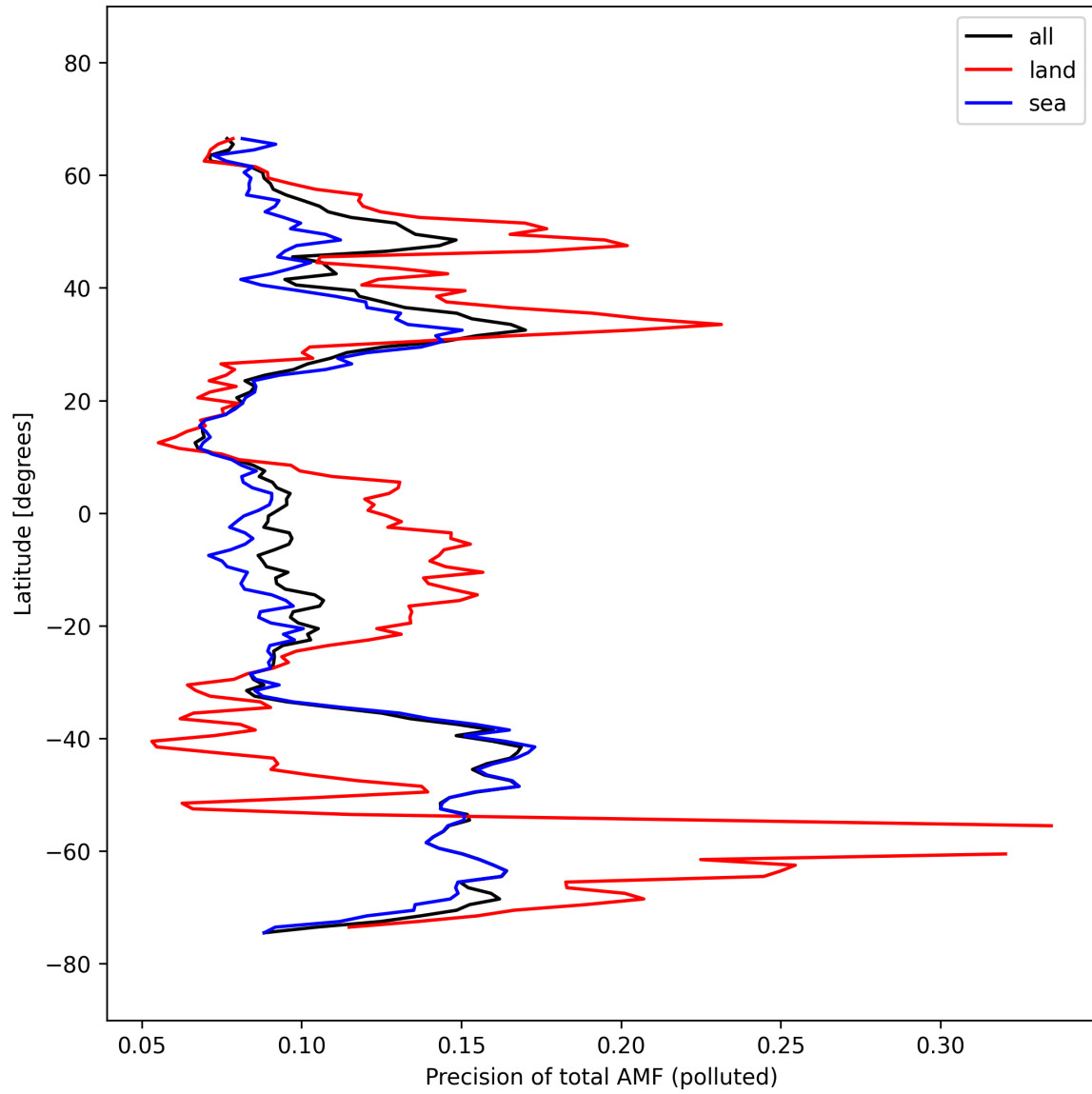
Figure 54: Zonal average of “Precision of total AMF (polluted)” for 2025-03-09 to 2025-03-11.
