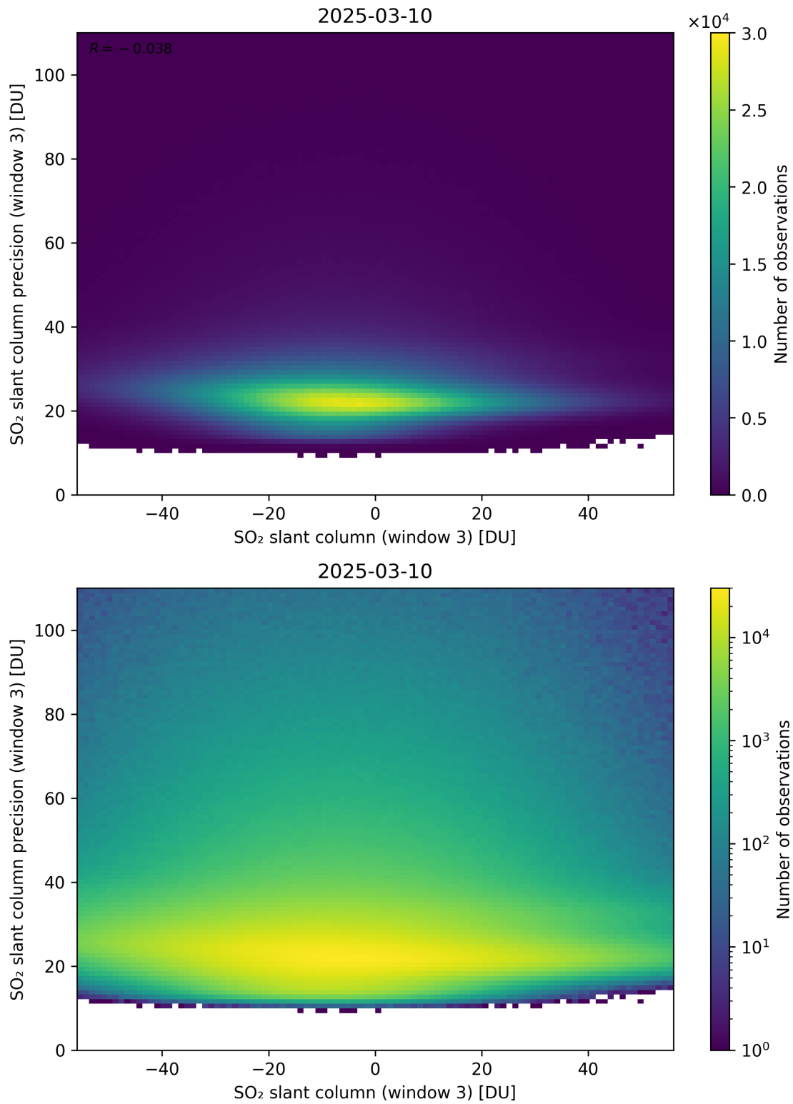
Figure 317: Scatter density plot of “SO 2 slant column (window 3)” against “SO 2 slant column precision (window 3)” for 2025-03-09 to 2025-03-11.
