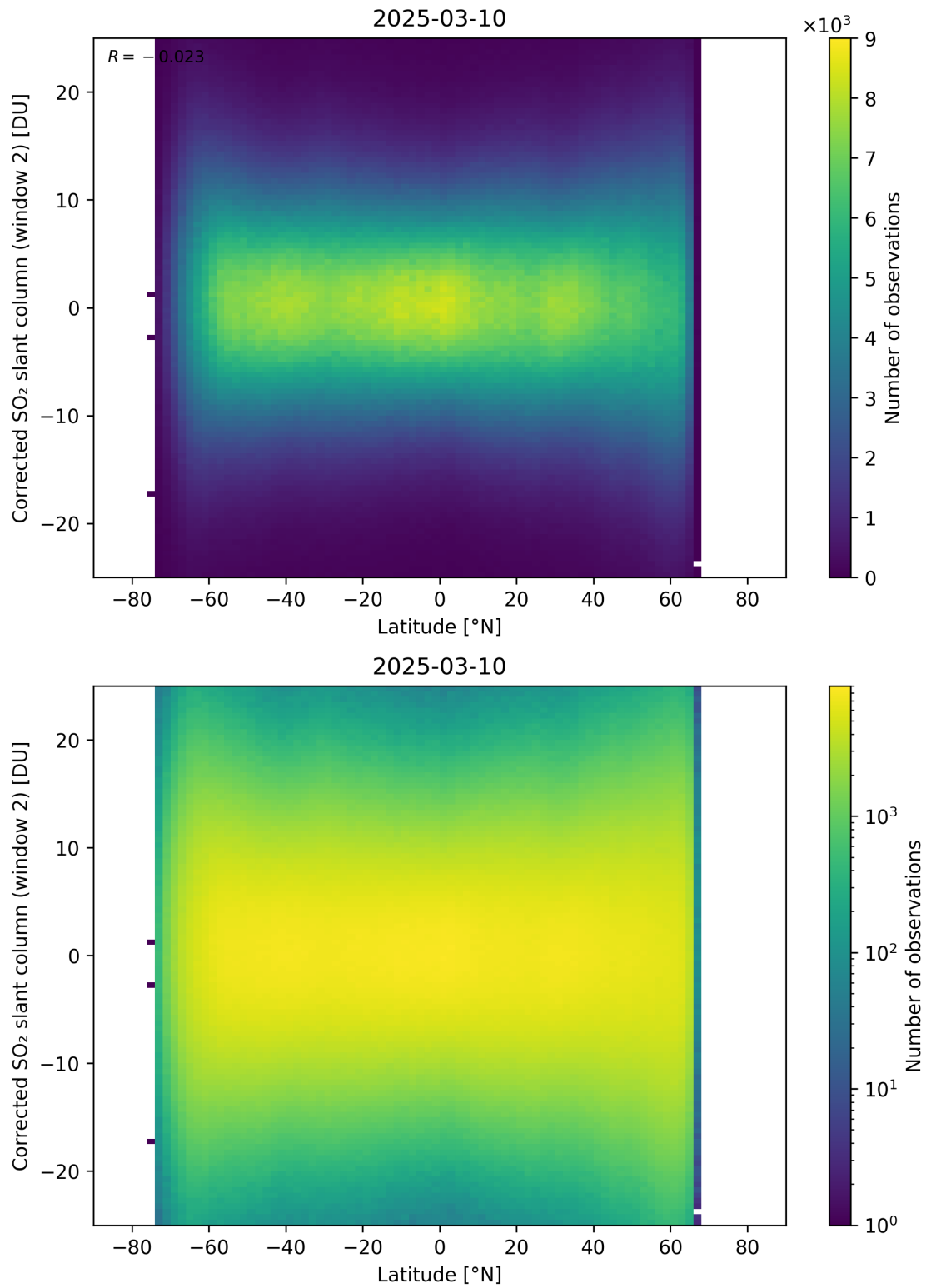
Figure 160: Scatter density plot of “Latitude” against “Corrected SO 2 slant column (window 2)” for 2025-03-09 to 2025-03-11.
