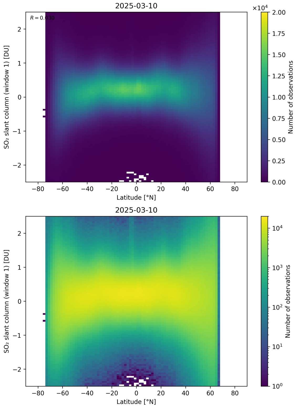
Figure 162: Scatter density plot of “Latitude” against “SO 2 slant column (window 1)” for 2025-03-09 to 2025-03-11.
