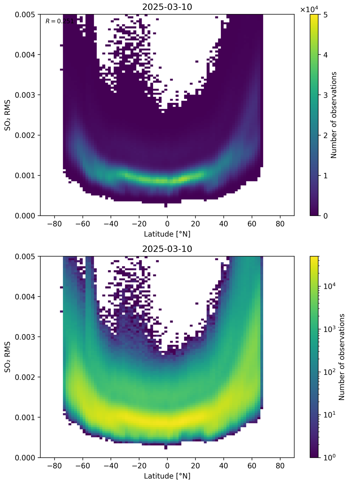
Figure 155: Scatter density plot of “Latitude” against “SO 2 RMS” for 2025-03-09 to 2025-03-11.
