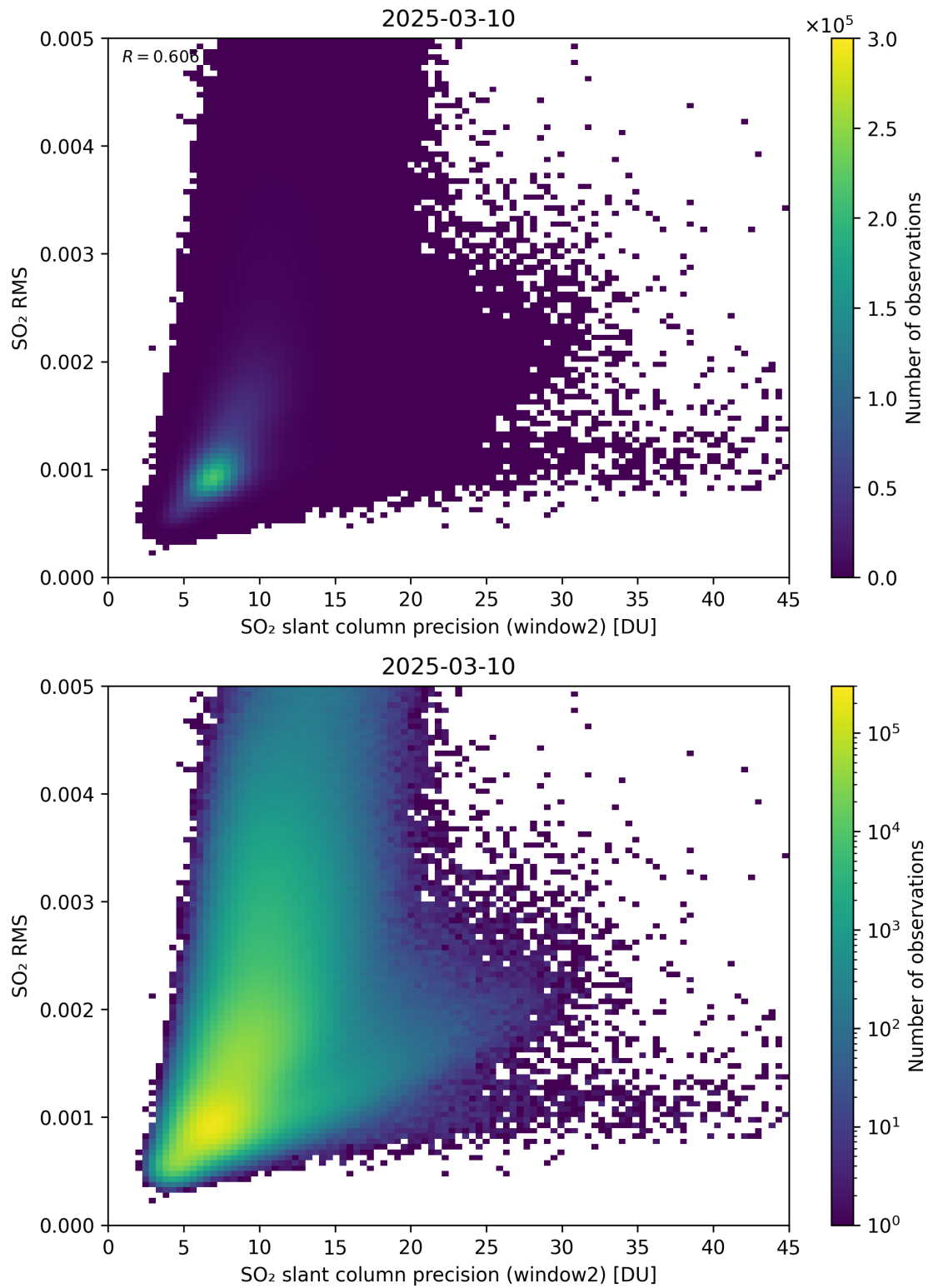
Figure 295: Scatter density plot of “SO 2 slant column precision (window2)” against “SO 2 RMS” for 2025-03-09 to 2025-03-11.
