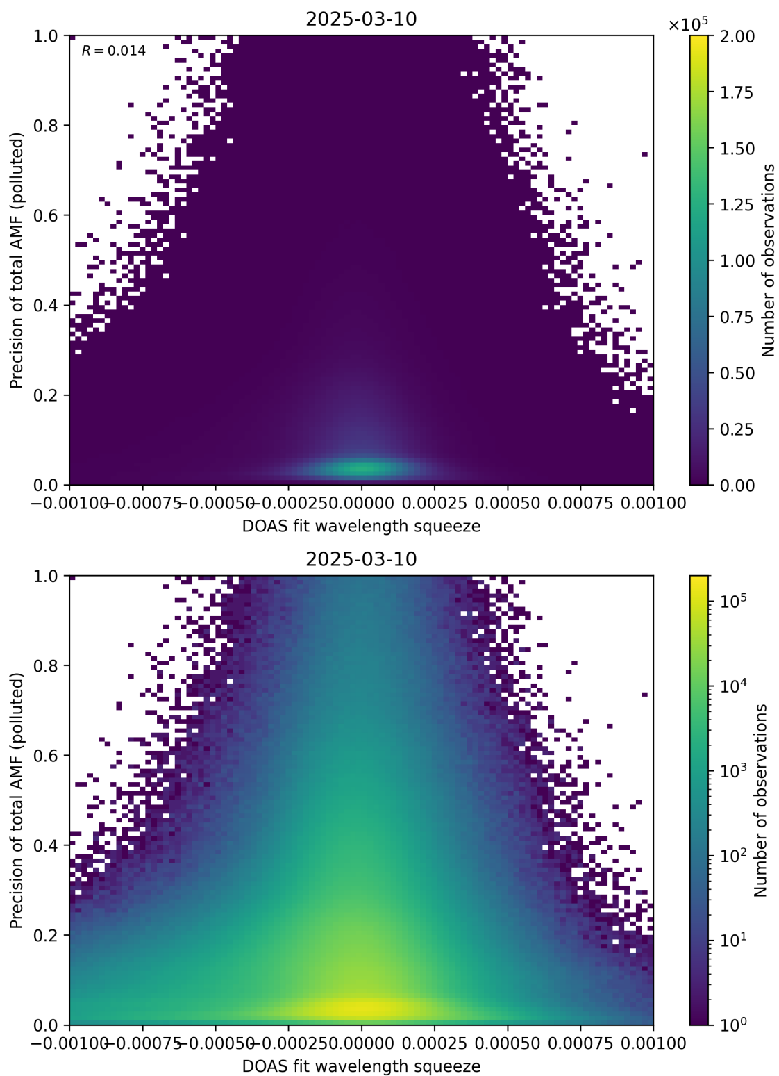
Figure 146: Scatter density plot of “DOAS fit wavelength squeeze” against “Precision of total AMF (polluted)” for 2025-03-09 to 2025-03-11.
