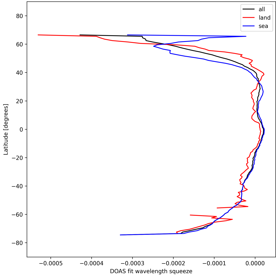
Figure 51: Zonal average of “DOAS fit wavelength squeeze” for 2025-03-09 to 2025-03-11.
