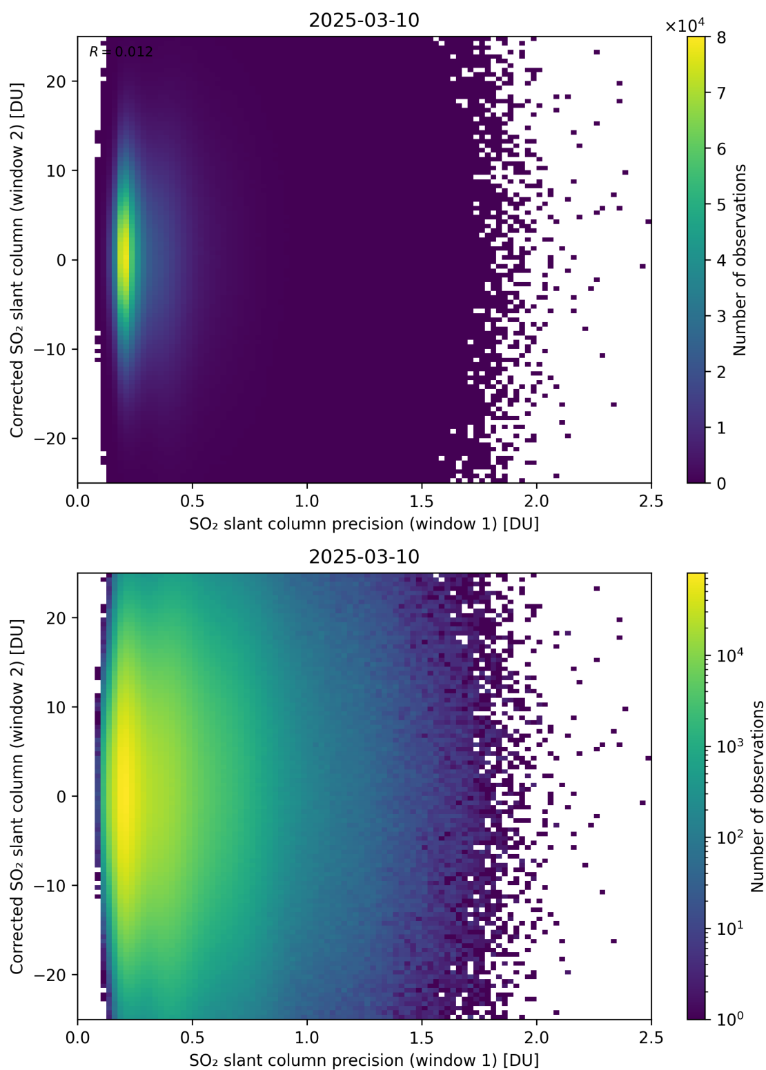
Figure 275: Scatter density plot of “SO 2 slant column precision (window 1)” against “Corrected SO 2 slant column (window 2)” for 2025-03-09 to 2025-03-11.
