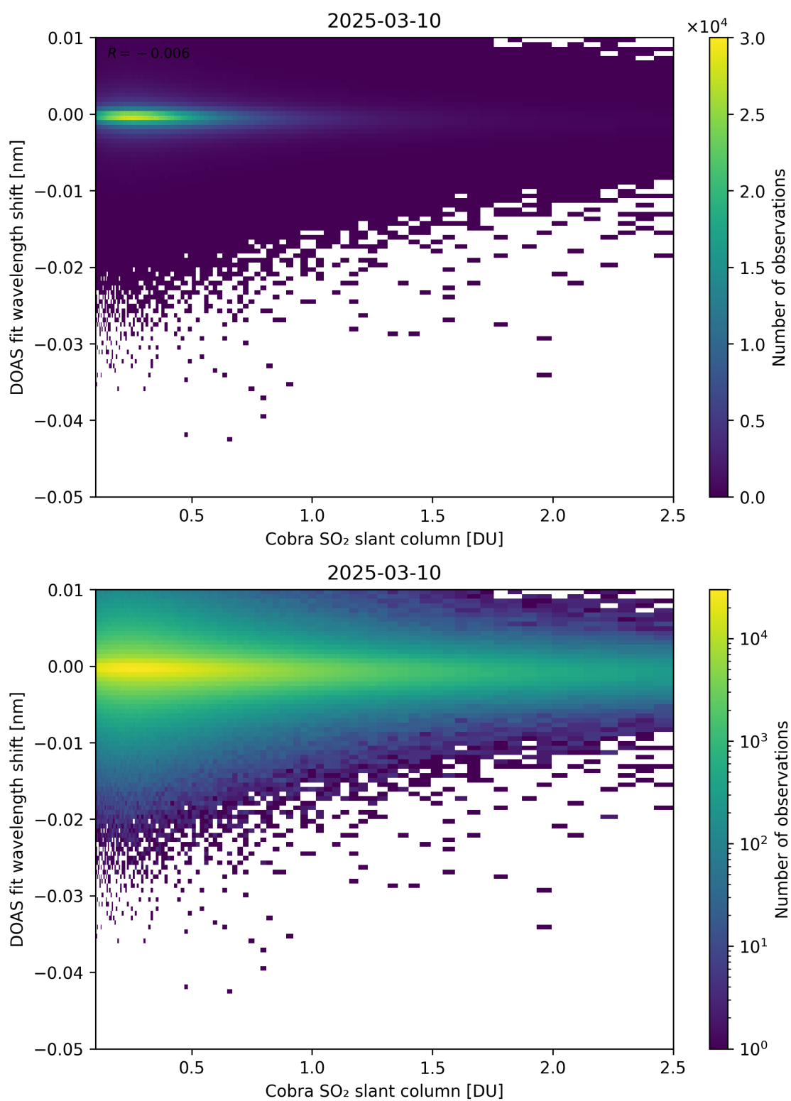
Figure 196: Scatter density plot of “Cobra SO 2 slant column” against “DOAS fit wavelength shift” for 2025-03-09 to 2025-03-11.
