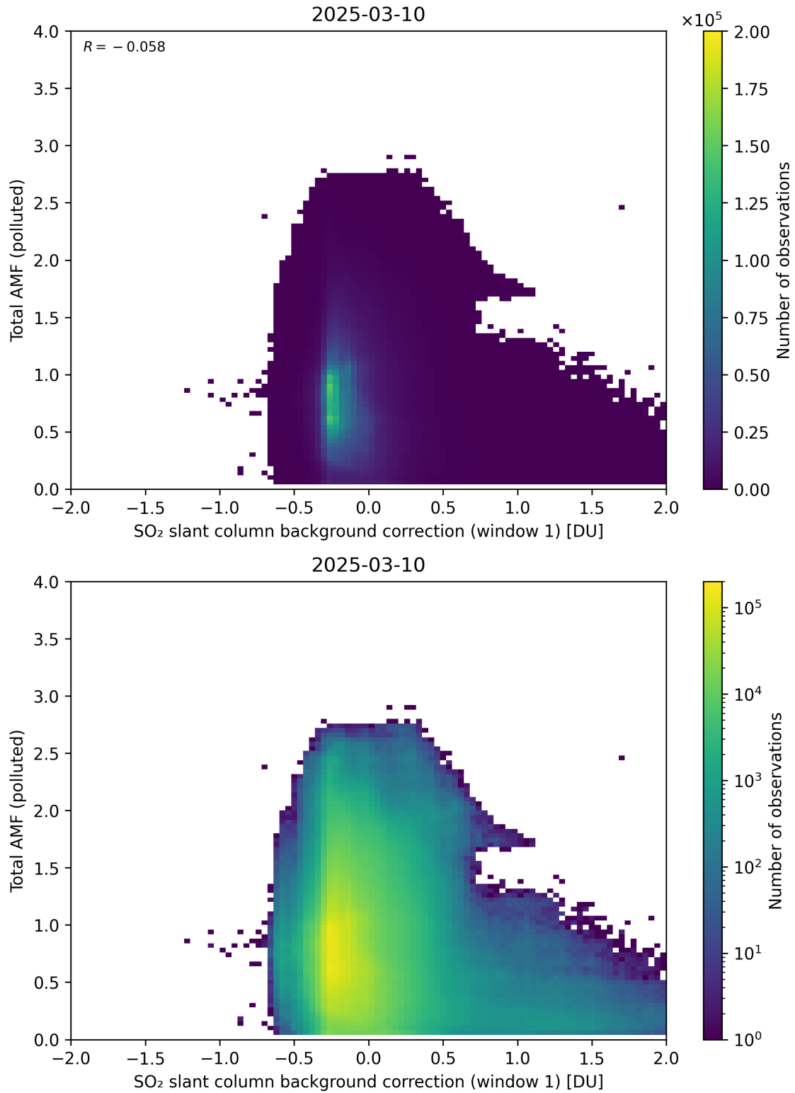
Figure 120: Scatter density plot of “SO 2 slant column background correction (window 1)” against “Total AMF (polluted)” for 2025-03-09 to 2025-03-11.
