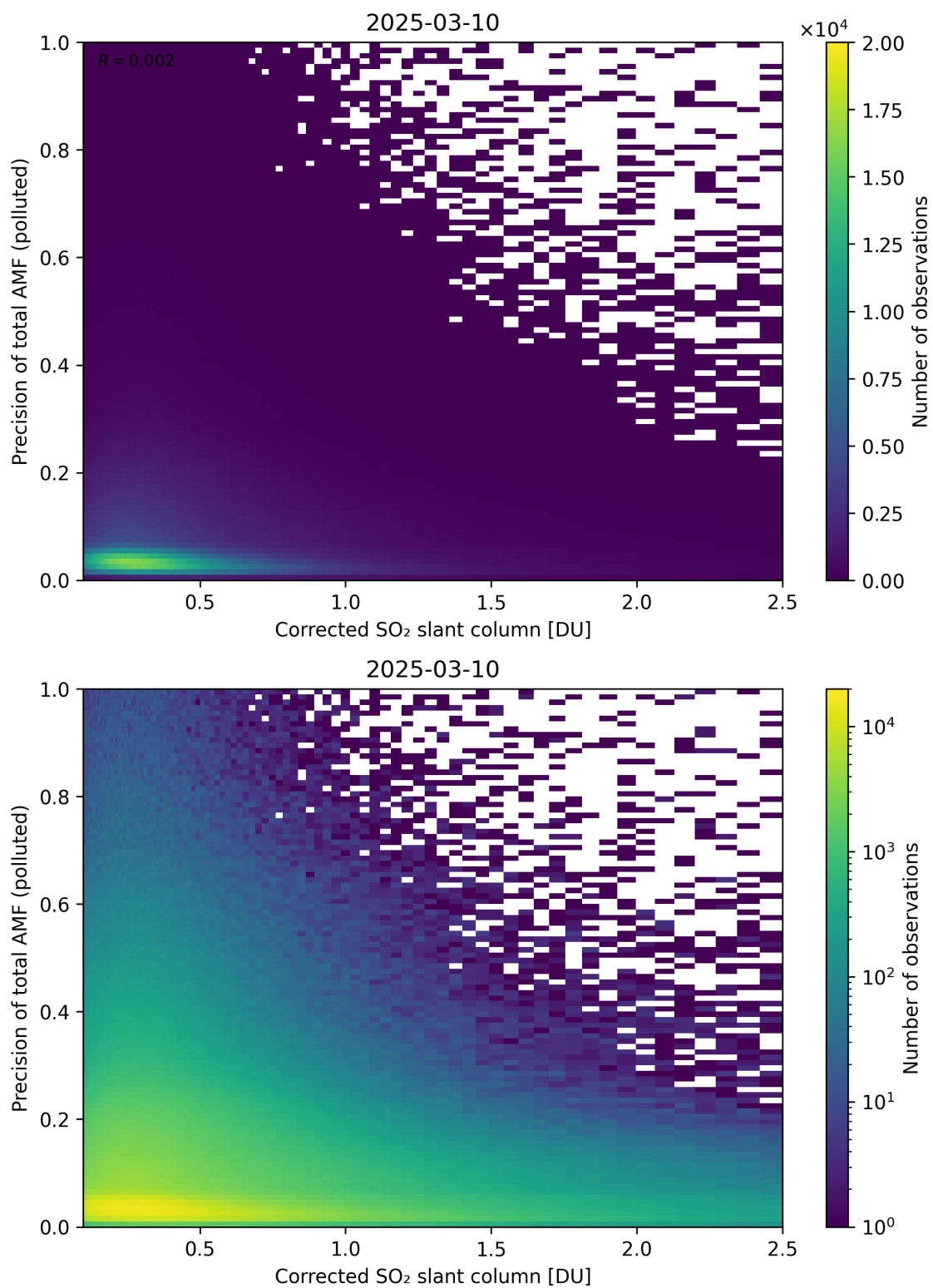
Figure 243: Scatter density plot of “Corrected SO 2 slant column” against “Precision of total AMF (polluted)” for 2025-03-09 to 2025-03-11.
