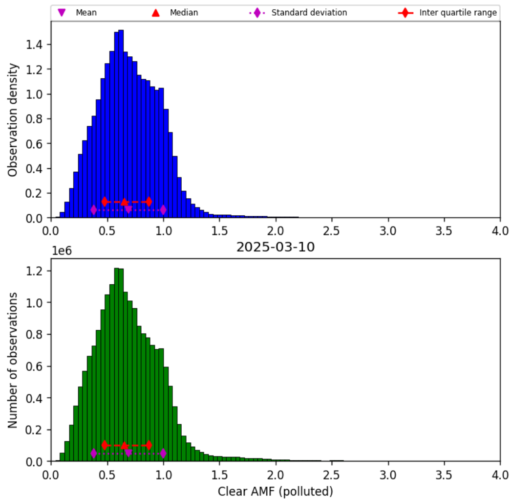
Figure 81: Histogram of “Clear AMF (polluted)” for 2025-03-09 to 2025-03-11
