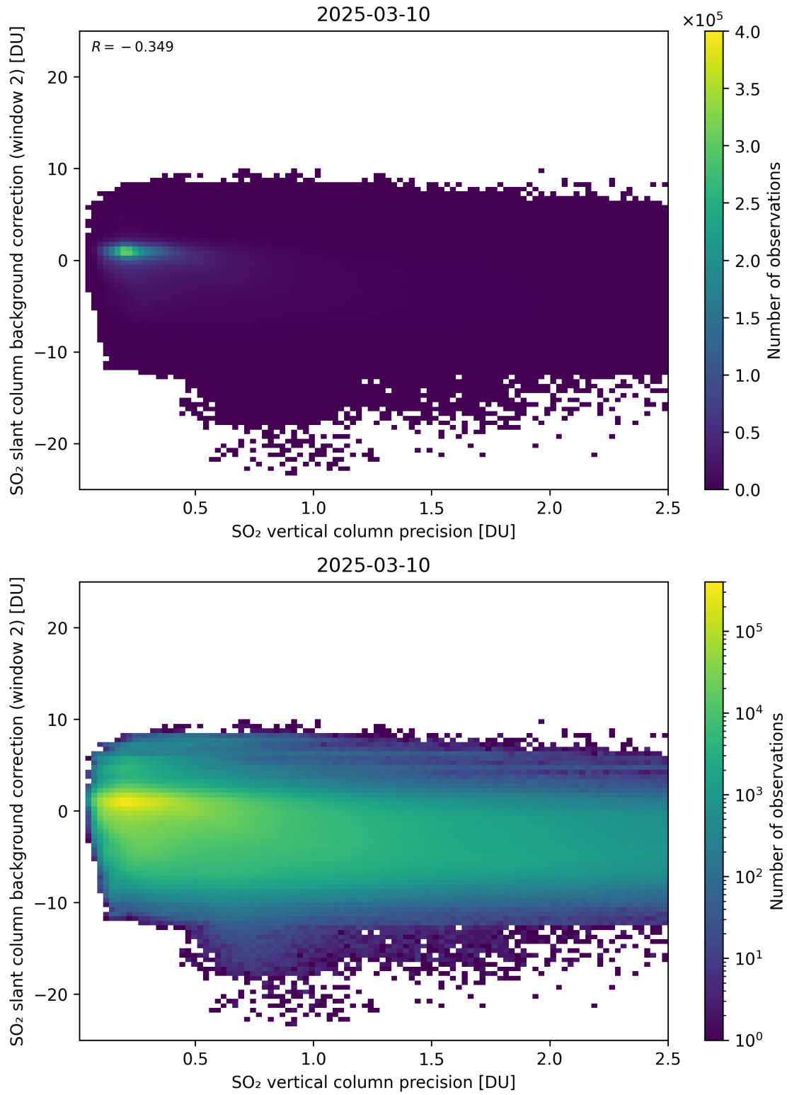
Figure 330: Scatter density plot of “SO 2 vertical column precision” against “SO 2 slant column background correction (window 2)” for 2025-03-09 to 2025-03-11.
