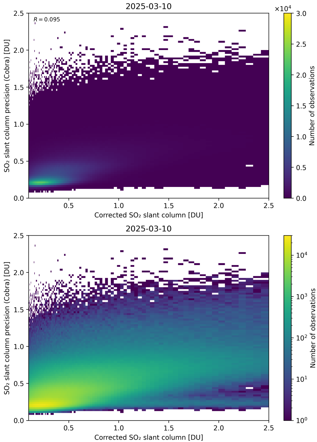
Figure 234: Scatter density plot of “Corrected SO 2 slant column” against “SO 2 slant column precision (Cobra)” for 2025-03-09 to 2025-03-11.
