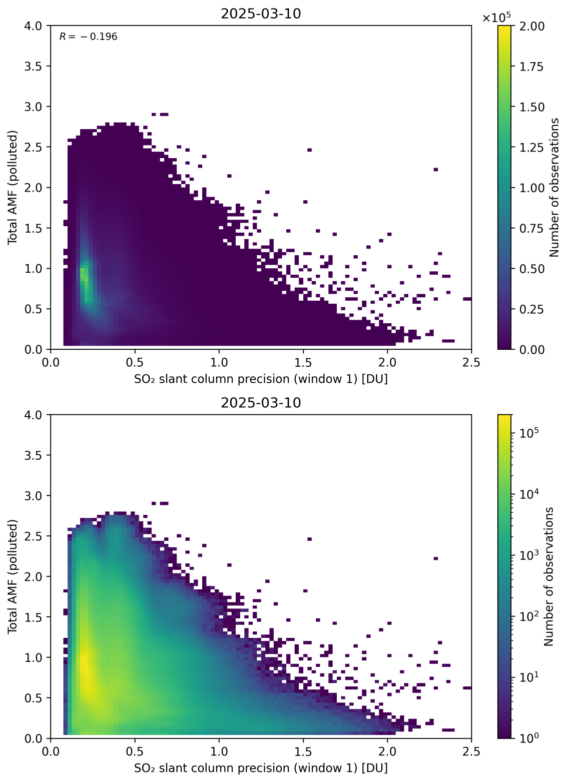
Figure 280: Scatter density plot of “SO 2 slant column precision (window 1)” against “Total AMF (polluted)” for 2025-03-09 to 2025-03-11.
