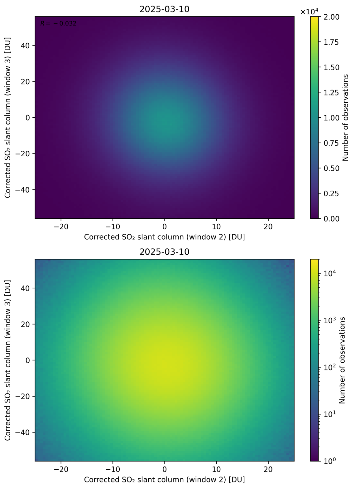
Figure 250: Scatter density plot of “Corrected SO 2 slant column (window 2)” against “Corrected SO 2 slant column (window 3)” for 2025-03-09 to 2025-03-11.
