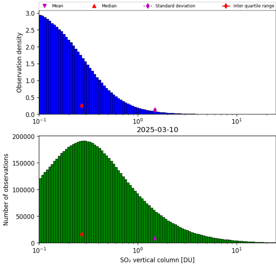
Figure 58: Histogram of “SO 2 vertical column” for 2025-03-09 to 2025-03-11
