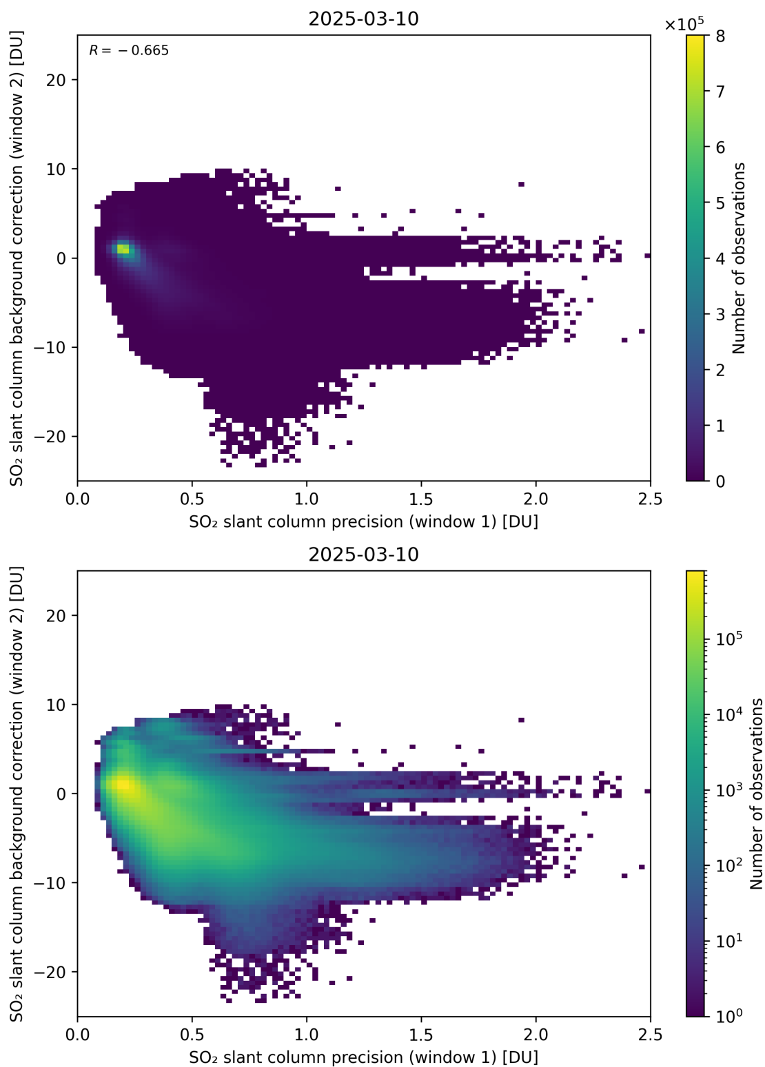
Figure 269: Scatter density plot of “SO 2 slant column precision (window 1)” against “SO 2 slant column background correction (window 2)” for 2025-03-09 to 2025-03-11.
