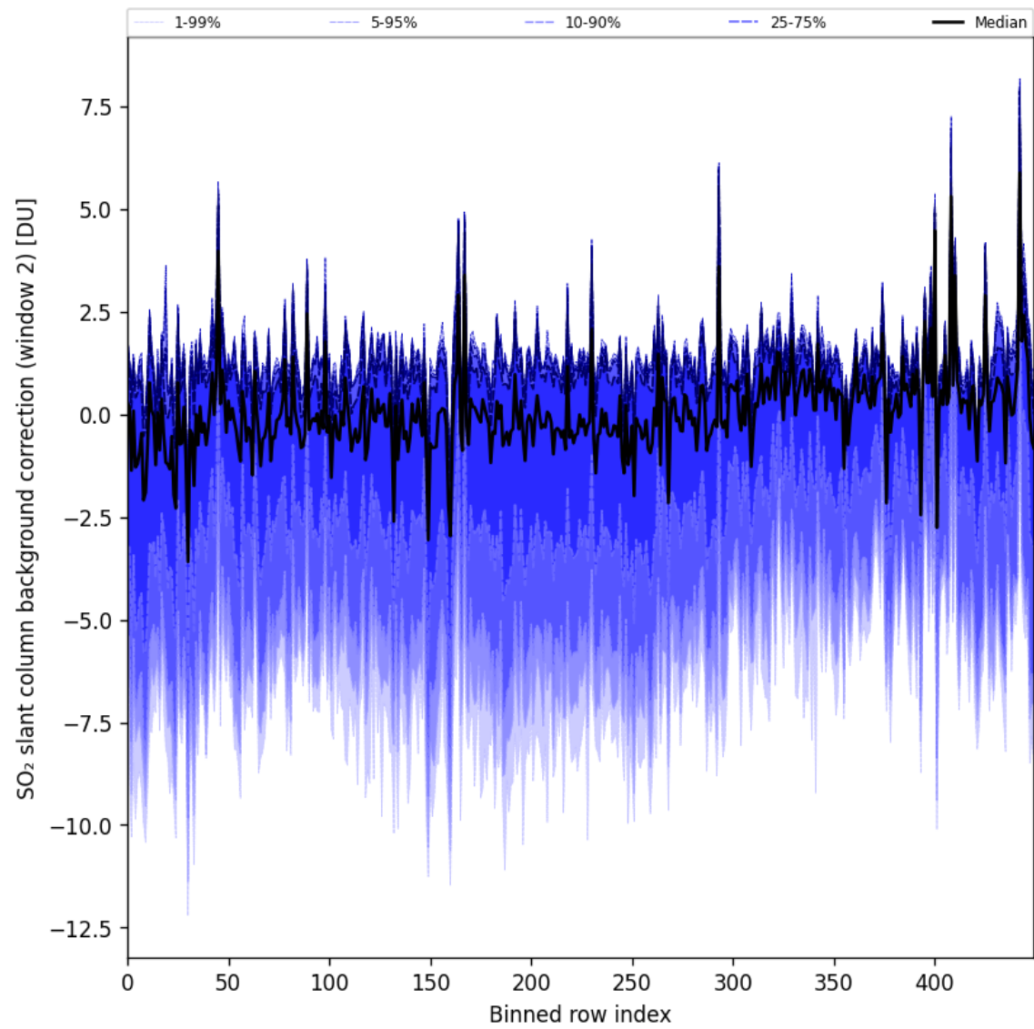
Figure 96: Along track statistics of “SO 2 slant column background correction (window 2)” for 2025-03-09 to 2025-03-11
