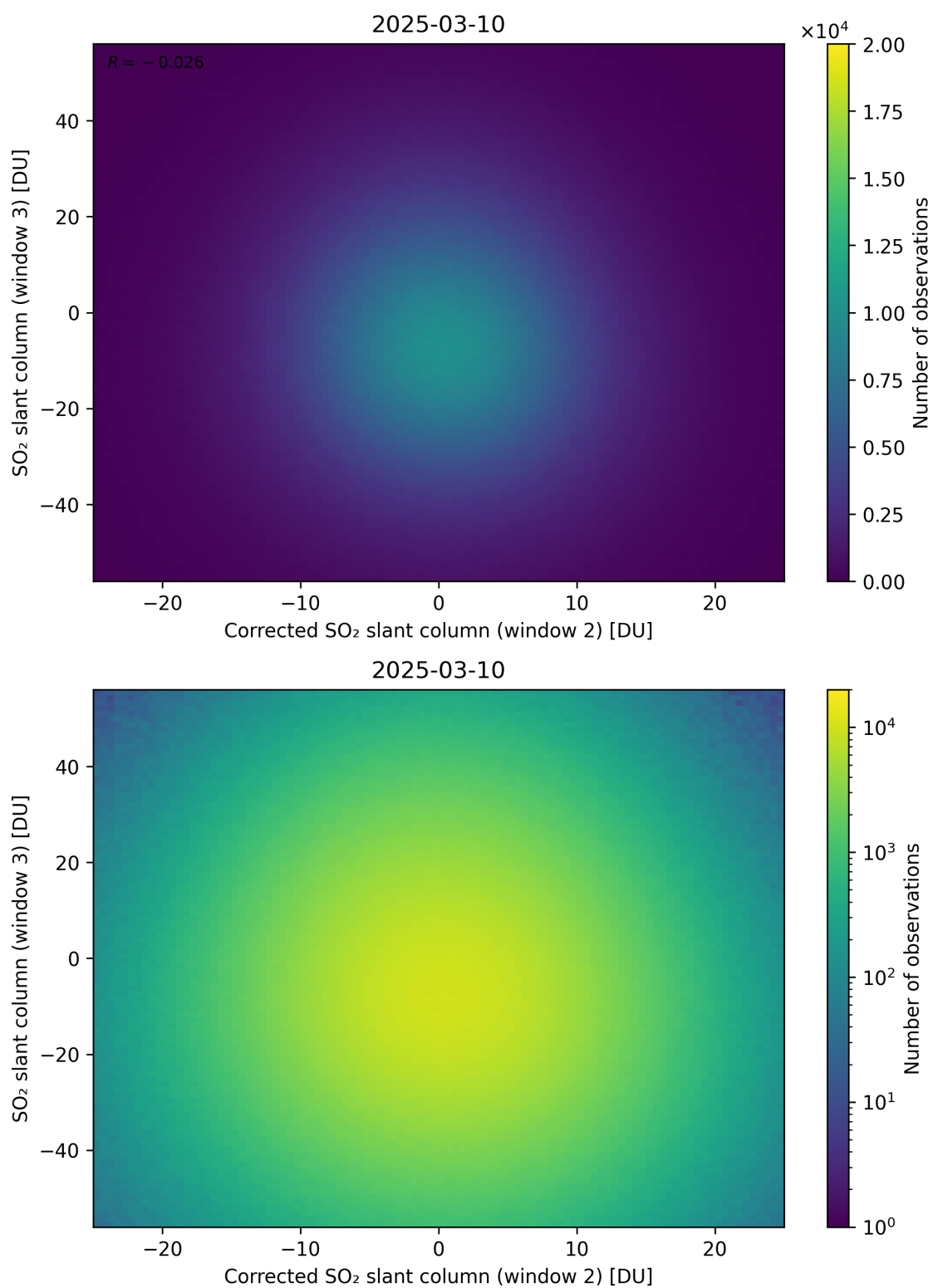
Figure 251: Scatter density plot of “Corrected SO 2 slant column (window 2)” against “SO 2 slant column (window 3)” for 2025-03-09 to 2025-03-11.
