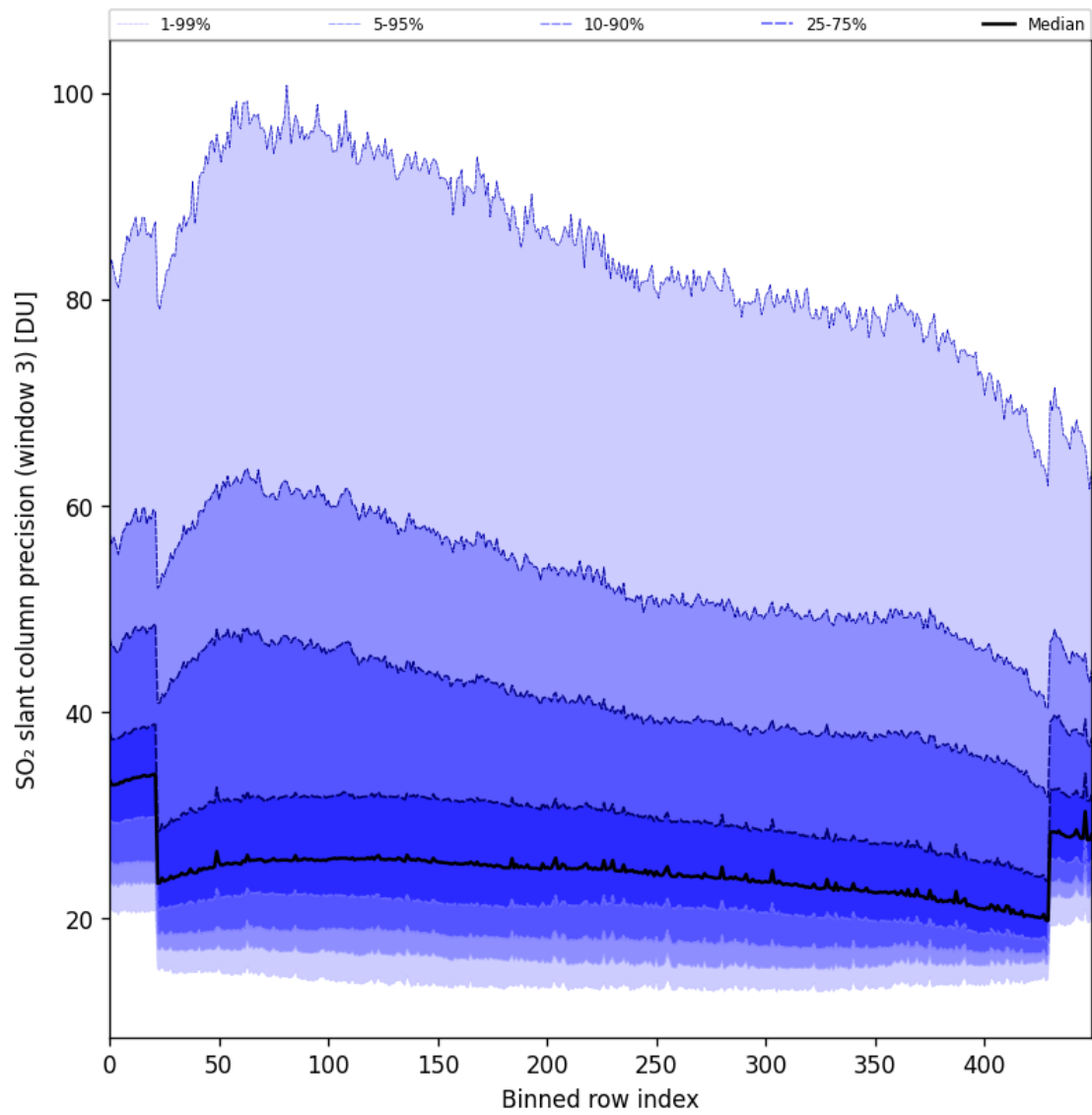
Figure 98: Along track statistics of “SO 2 slant column precision (window 3)” for 2025-03-09 to 2025-03-11
