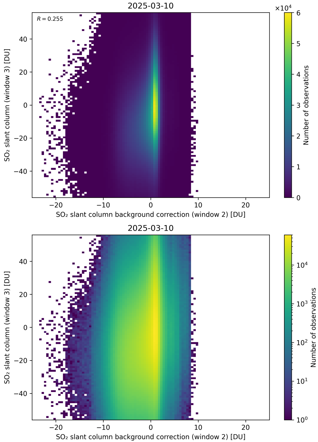
Figure 128: Scatter density plot of “SO 2 slant column background correction (window 2)” against “SO 2 slant column (window 3)” for 2025-03-09 to 2025-03-11.
