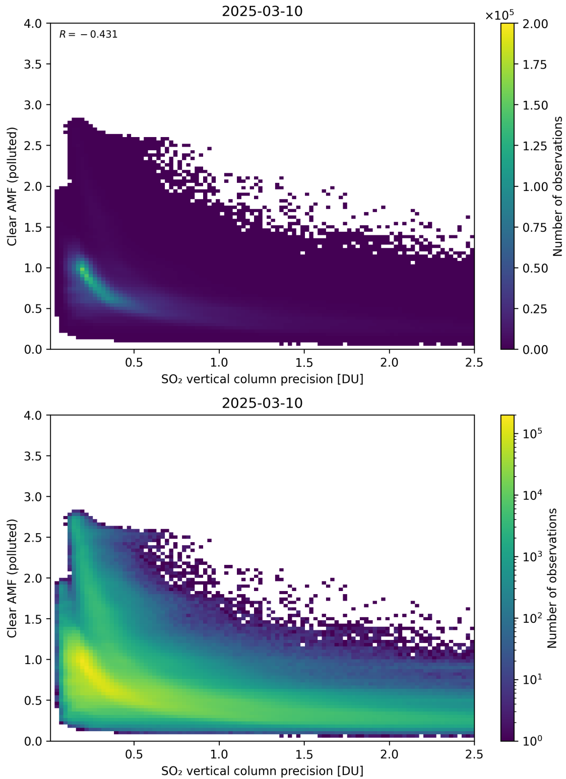
Figure 335: Scatter density plot of “SO 2 vertical column precision” against “Clear AMF (polluted)” for 2025-03-09 to 2025-03-11.
