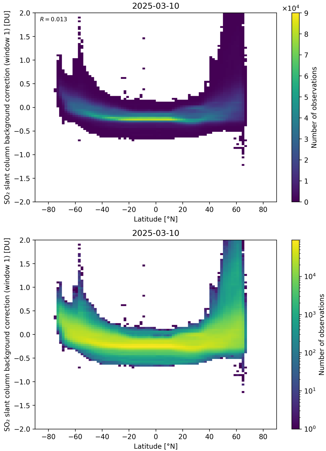
Figure 150: Scatter density plot of “Latitude” against “SO 2 slant column background correction (window 1)” for 2025-03-09 to 2025-03-11.
