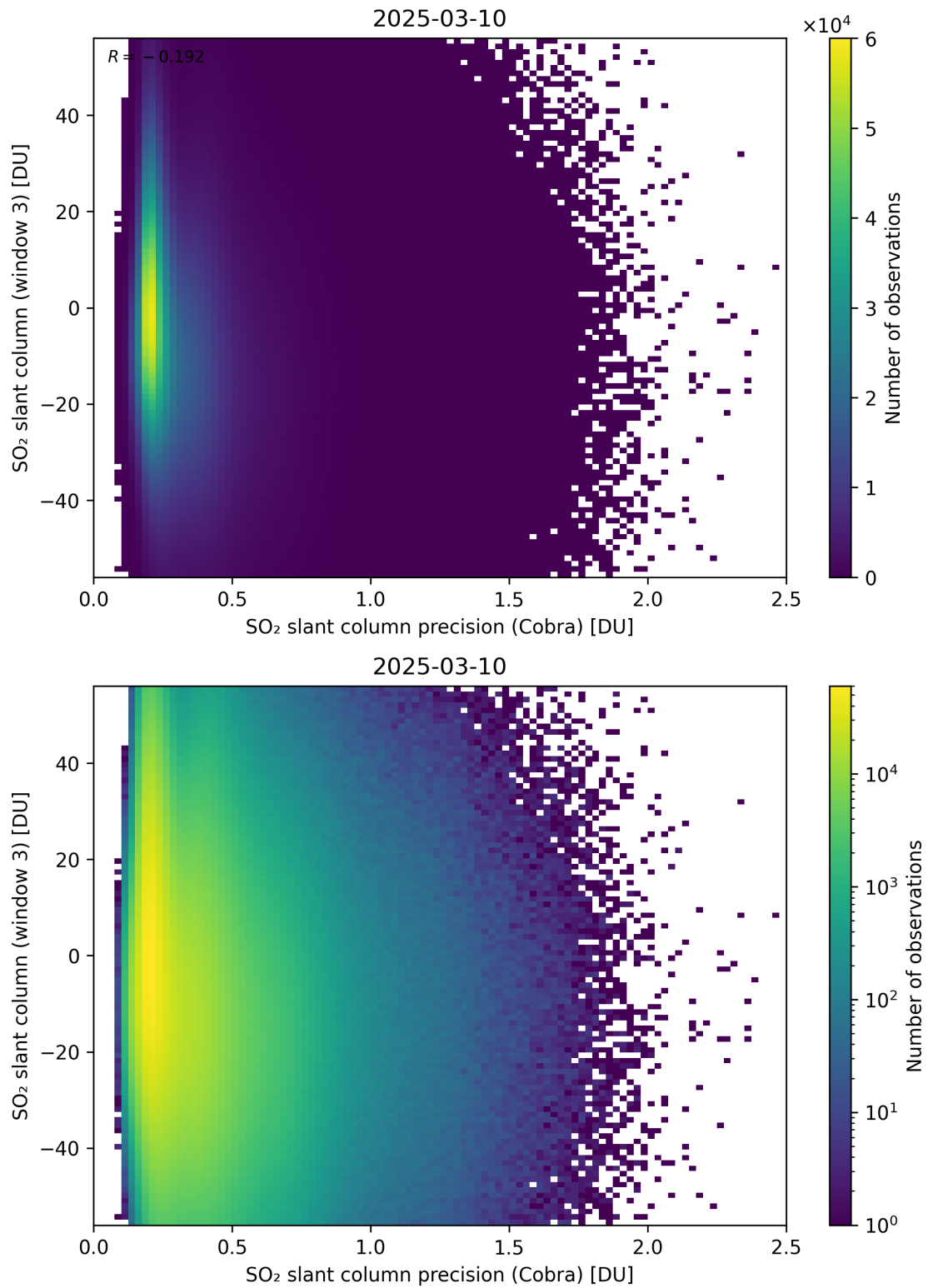
Figure 211: Scatter density plot of “SO 2 slant column precision (Cobra)” against “SO 2 slant column (window 3)” for 2025-03-09 to 2025-03-11.
