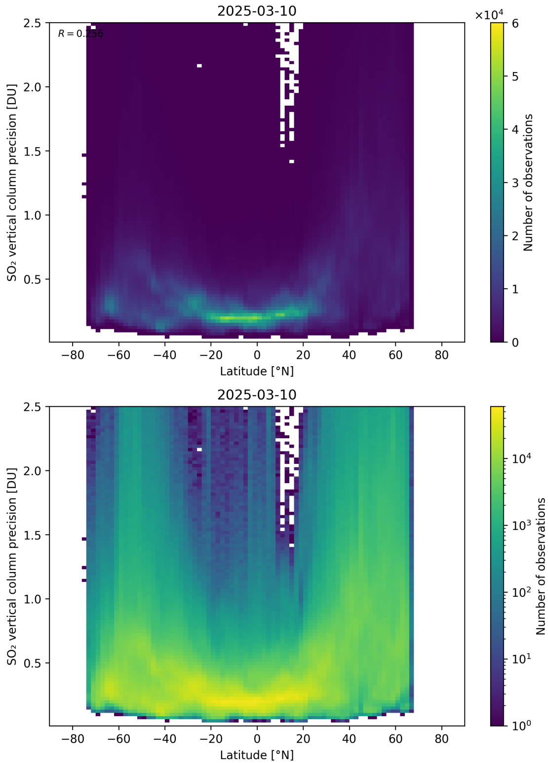
Figure 170: Scatter density plot of “Latitude” against “SO 2 vertical column precision” for 2025-03-09 to 2025-03-11.
