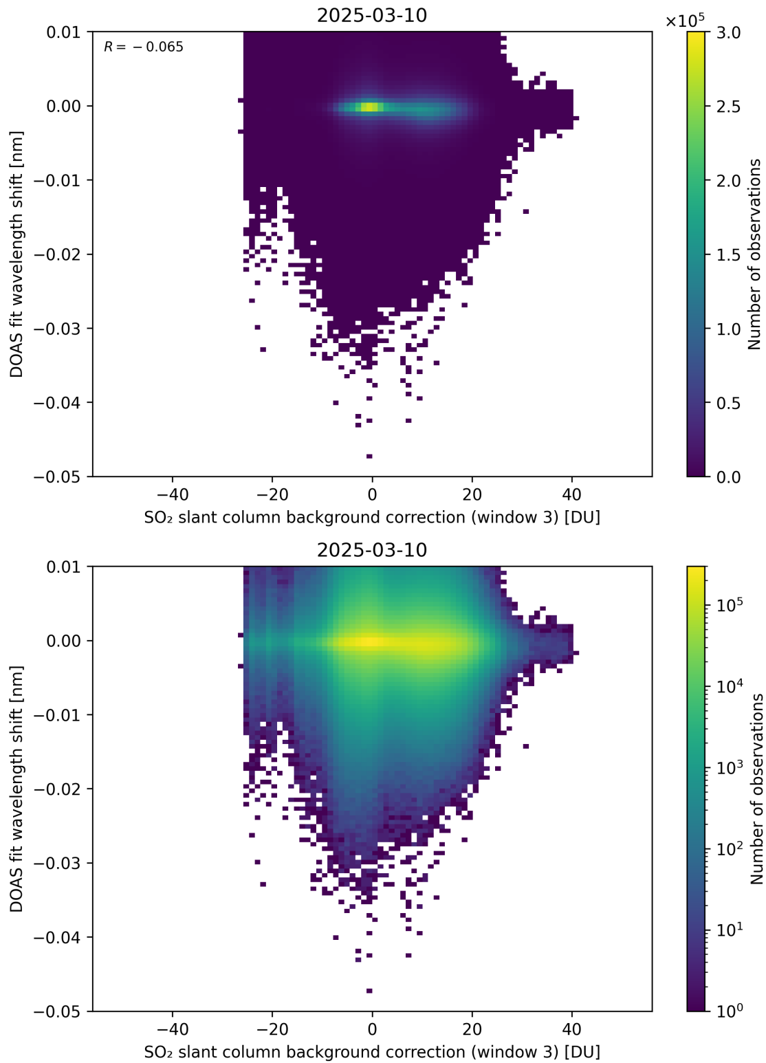
Figure 132: Scatter density plot of “SO 2 slant column background correction (window 3)” against “DOAS fit wavelength shift” for 2025-03-09 to 2025-03-11.
