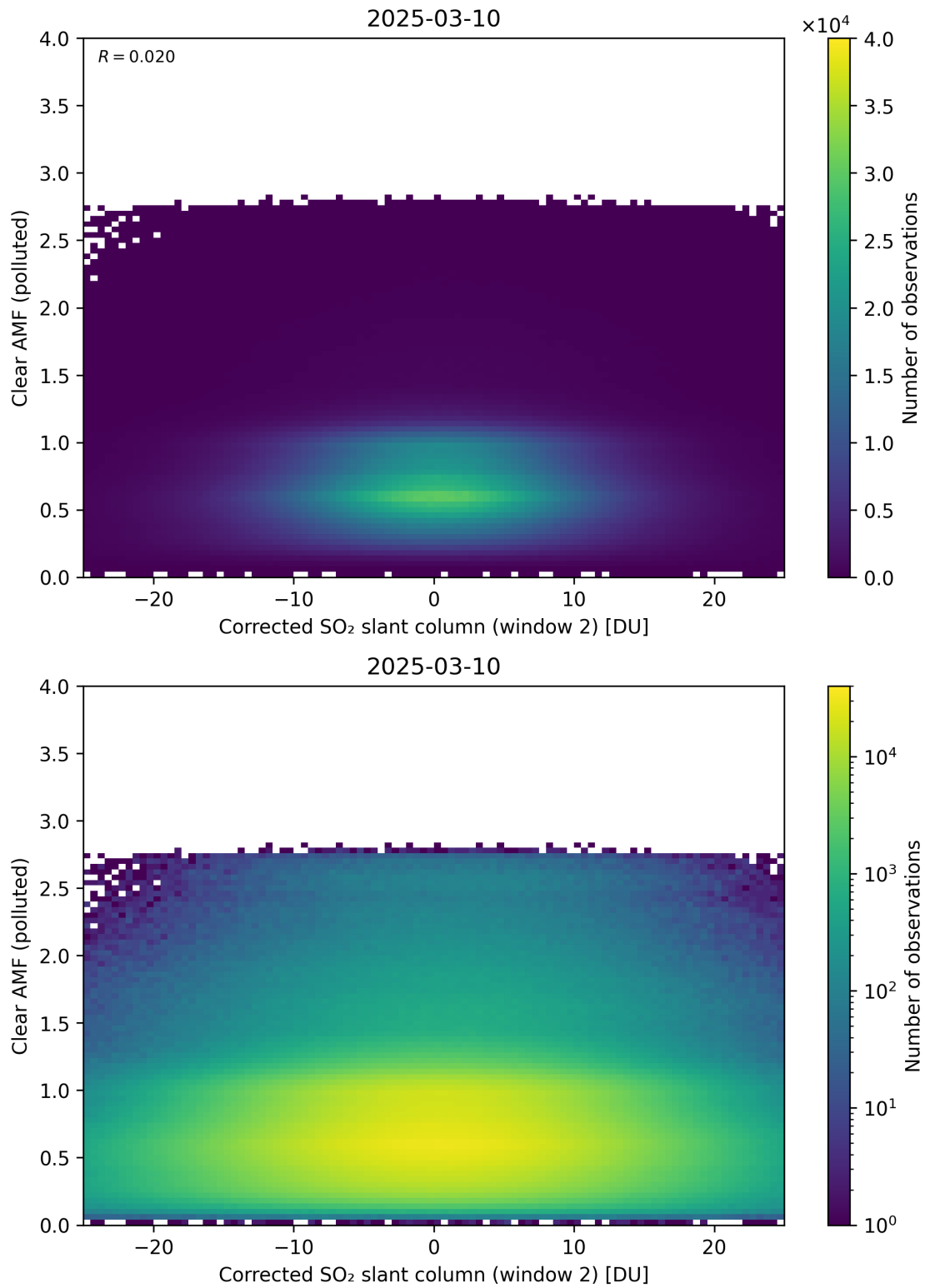
Figure 249: Scatter density plot of “Corrected SO 2 slant column (window 2)” against “Clear AMF (polluted)” for 2025-03-09 to 2025-03-11.
