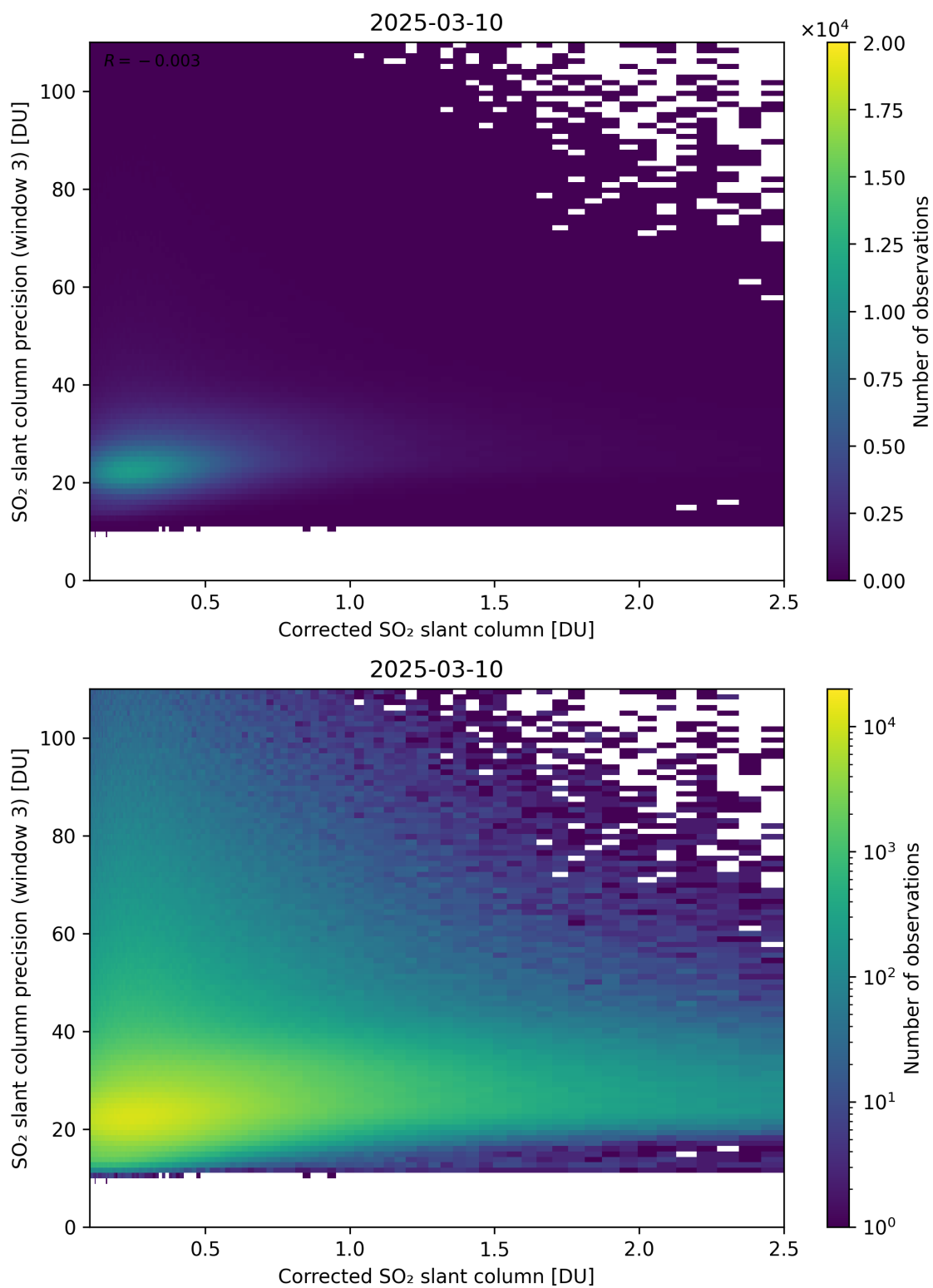
Figure 241: Scatter density plot of “Corrected SO 2 slant column” against “SO 2 slant column precision (window 3)” for 2025-03-09 to 2025-03-11.
