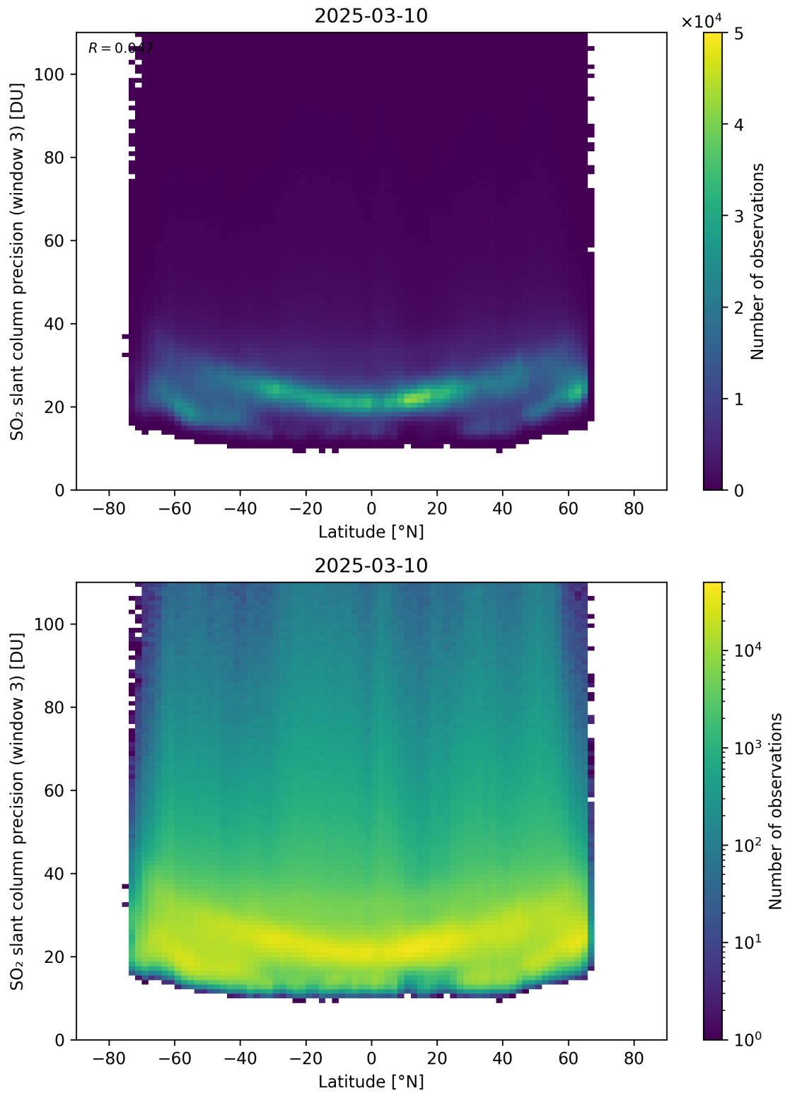
Figure 166: Scatter density plot of “Latitude” against “SO 2 slant column precision (window 3)” for 2025-03-09 to 2025-03-11.
