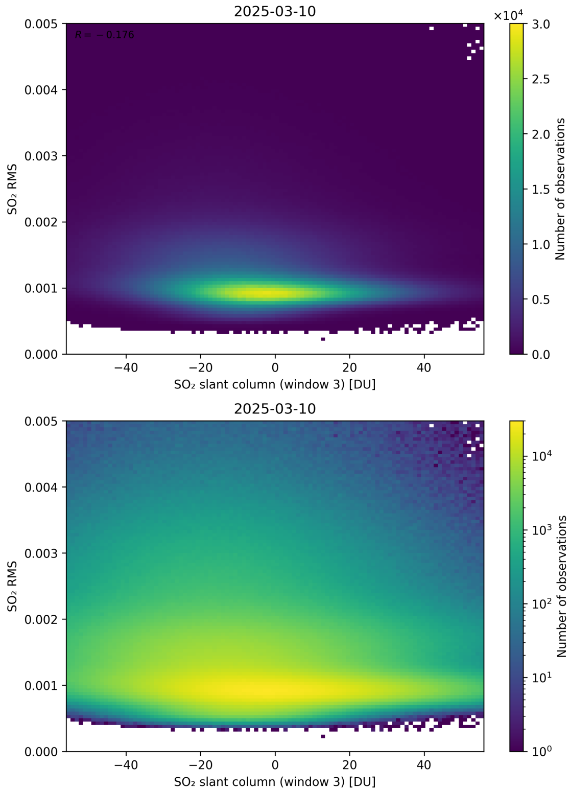
Figure 306: Scatter density plot of “SO 2 slant column (window 3)” against “SO 2 RMS” for 2025-03-09 to 2025-03-11.
