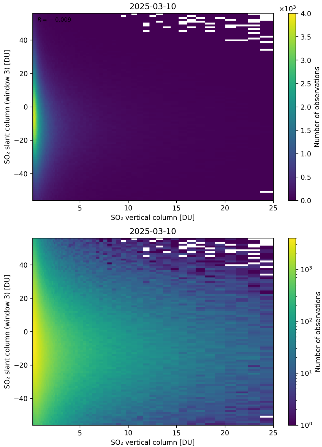
Figure 357: Scatter density plot of “SO 2 vertical column” against “SO 2 slant column (window 3)” for 2025-03-09 to 2025-03-11.
