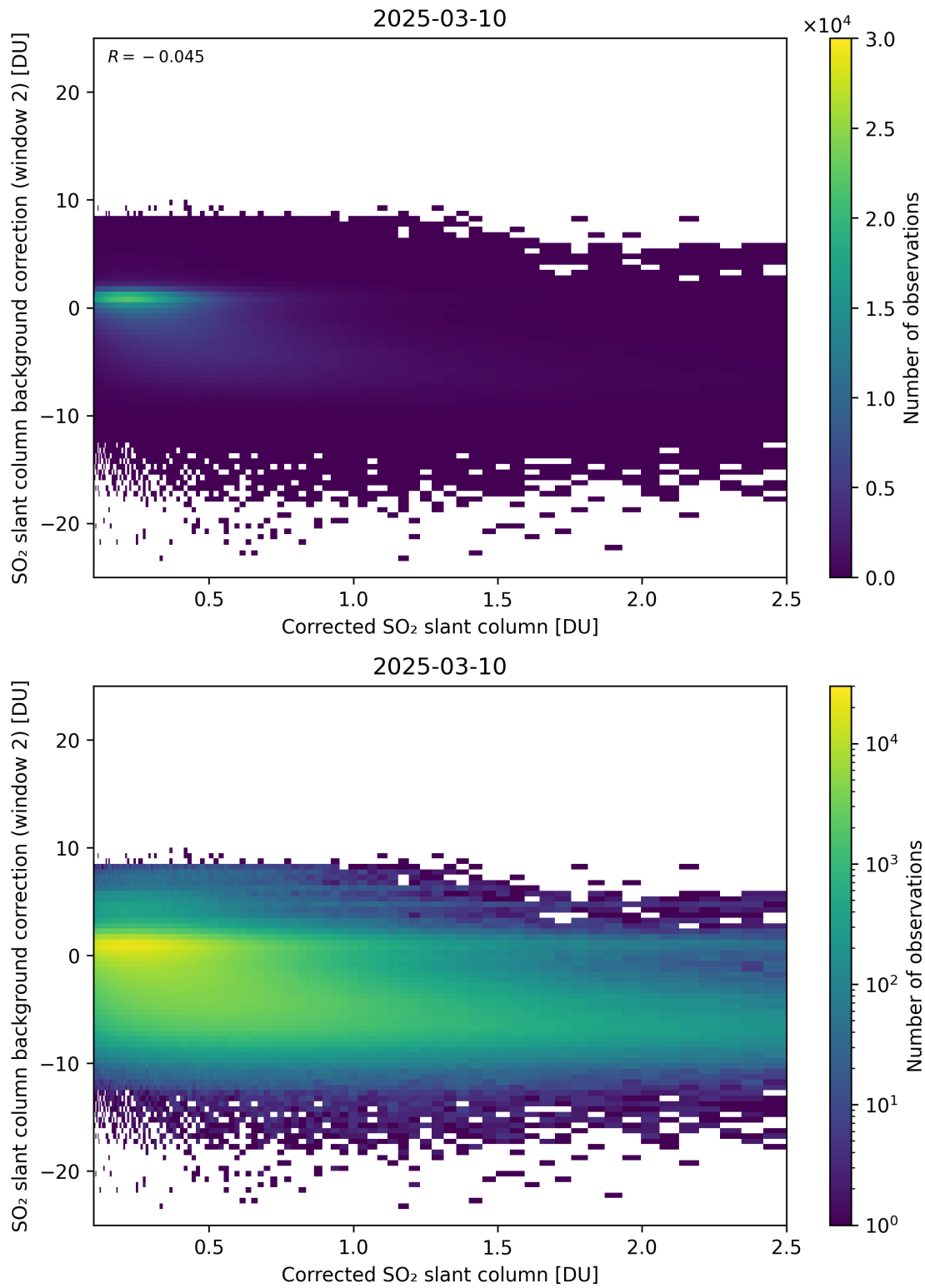
Figure 227: Scatter density plot of “Corrected SO 2 slant column” against “SO 2 slant column background correction (window 2)” for 2025-03-09 to 2025-03-11.
