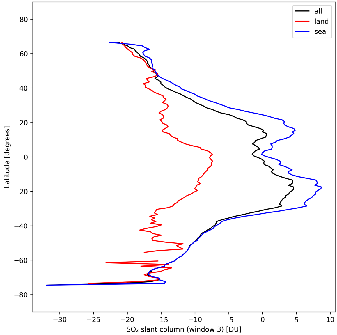
Figure 45: Zonal average of “SO 2 slant column (window 3)” for 2025-03-09 to 2025-03-11.
