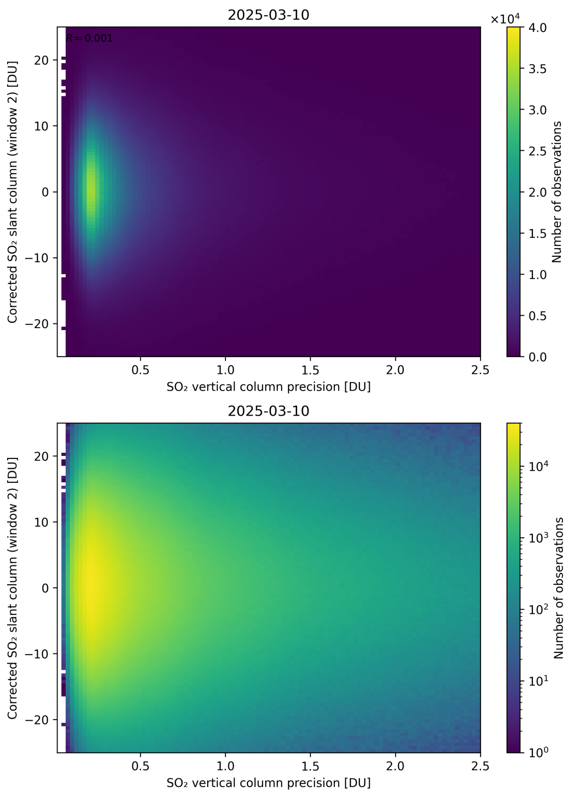
Figure 339: Scatter density plot of “SO 2 vertical column precision” against “Corrected SO 2 slant column (window 2)” for 2025-03-09 to 2025-03-11.
