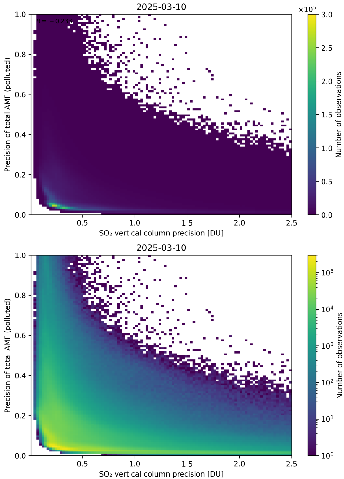
Figure 347: Scatter density plot of “SO 2 vertical column precision” against “Precision of total AMF (polluted)” for 2025-03-09 to 2025-03-11.
