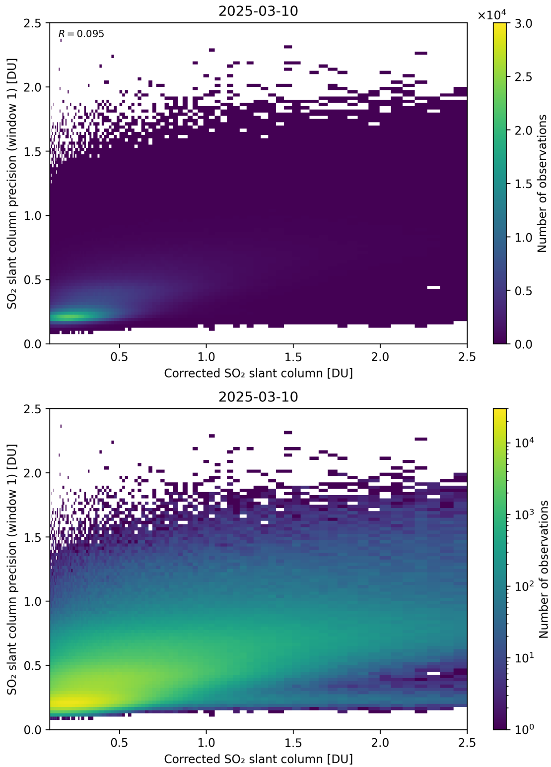
Figure 238: Scatter density plot of “Corrected SO 2 slant column” against “SO 2 slant column precision (window 1)” for 2025-03-09 to 2025-03-11.
