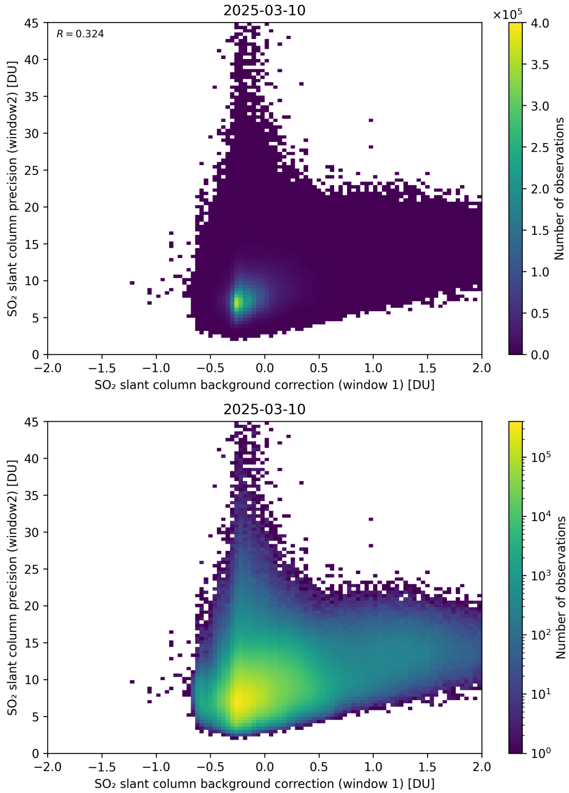
Figure 117: Scatter density plot of “SO 2 slant column background correction (window 1)” against “SO 2 slant column precision (window2)” for 2025-03-09 to 2025-03-11.
