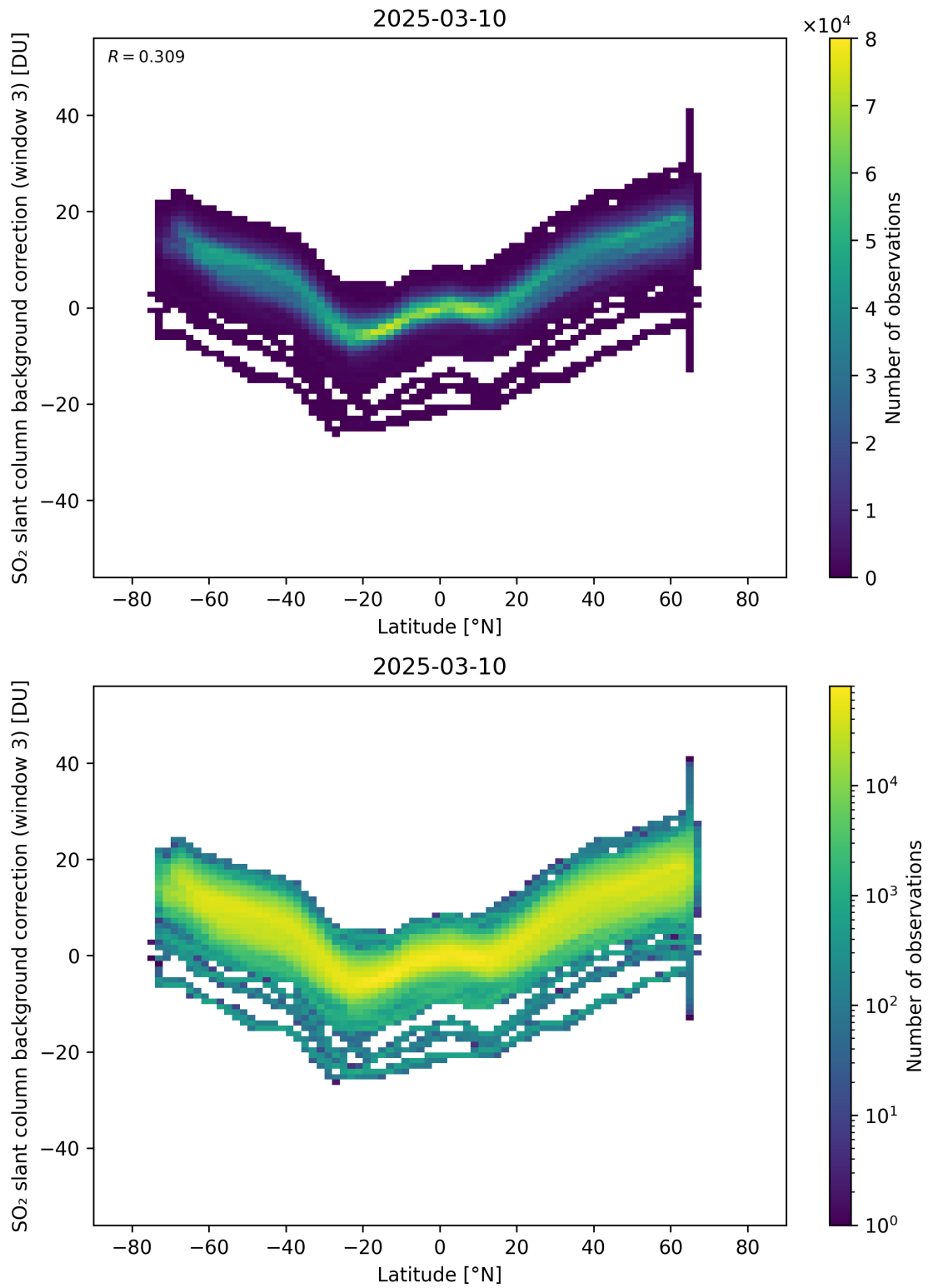
Figure 152: Scatter density plot of “Latitude” against “SO 2 slant column background correction (window 3)” for 2025-03-09 to 2025-03-11.
