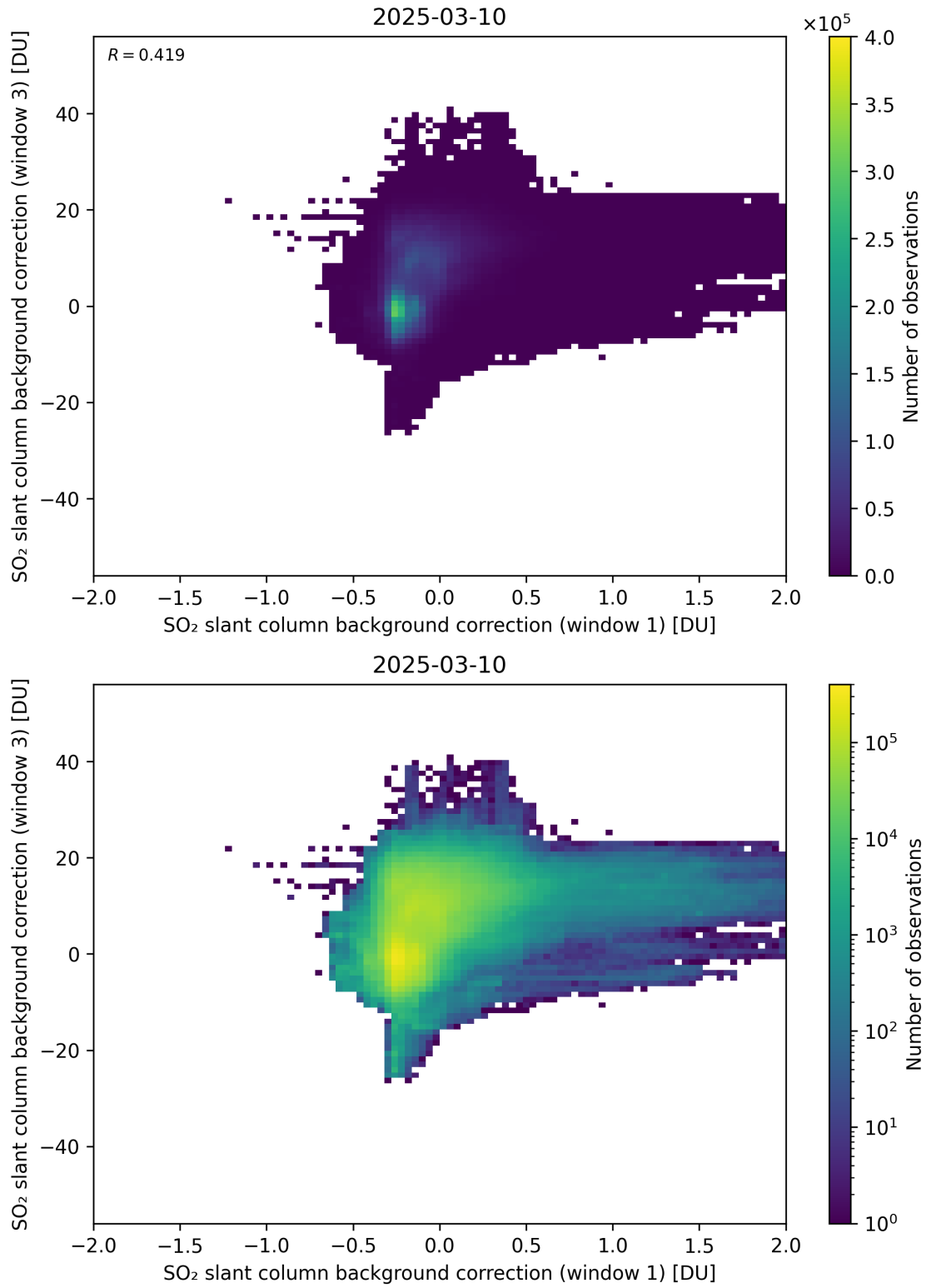
Figure 110: Scatter density plot of “SO 2 slant column background correction (window 1)” against “SO 2 slant column background correction (window 3)” for 2025-03-09 to 2025-03-11.
