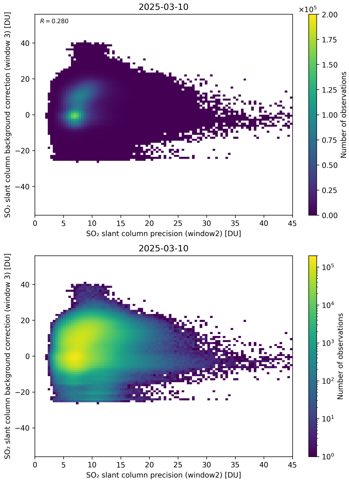
Figure 292: Scatter density plot of “SO 2 slant column precision (window2)” against “SO 2 slant column background correction (window 3)” for 2025-03-09 to 2025-03-11.
