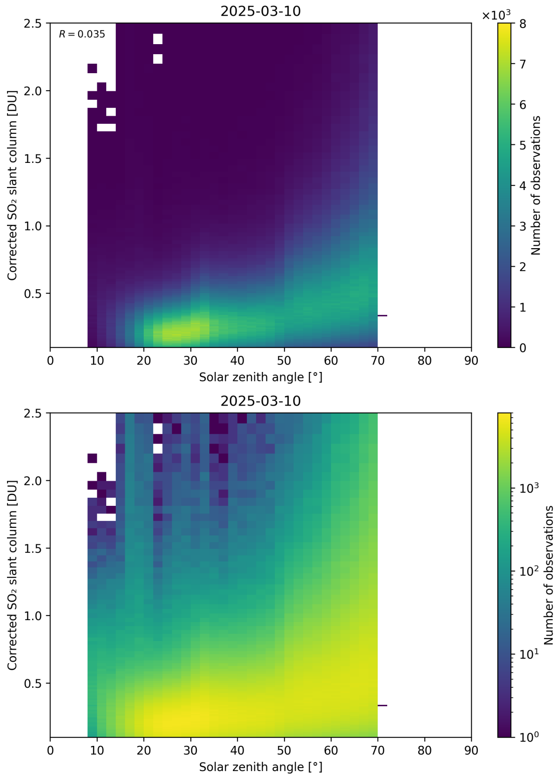
Figure 181: Scatter density plot of “Solar zenith angle” against “Corrected SO 2 slant column” for 2025-03-09 to 2025-03-11.
