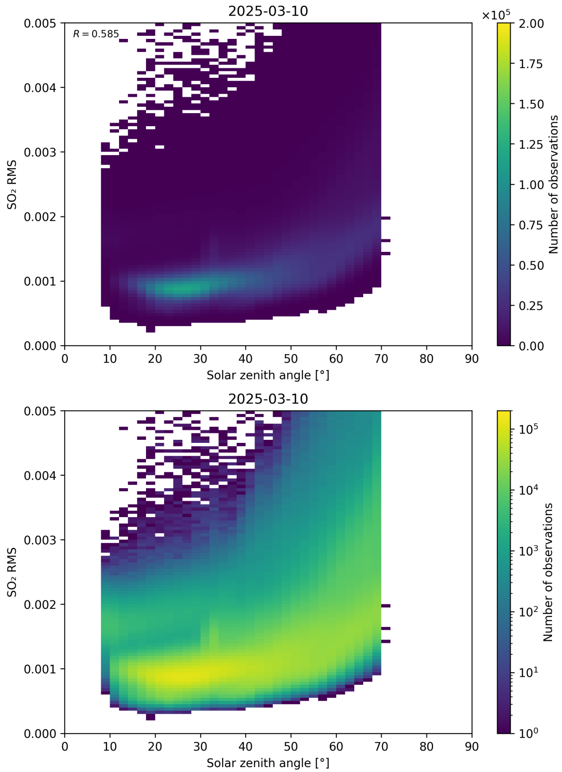
Figure 176: Scatter density plot of “Solar zenith angle” against “SO 2 RMS” for 2025-03-09 to 2025-03-11.
