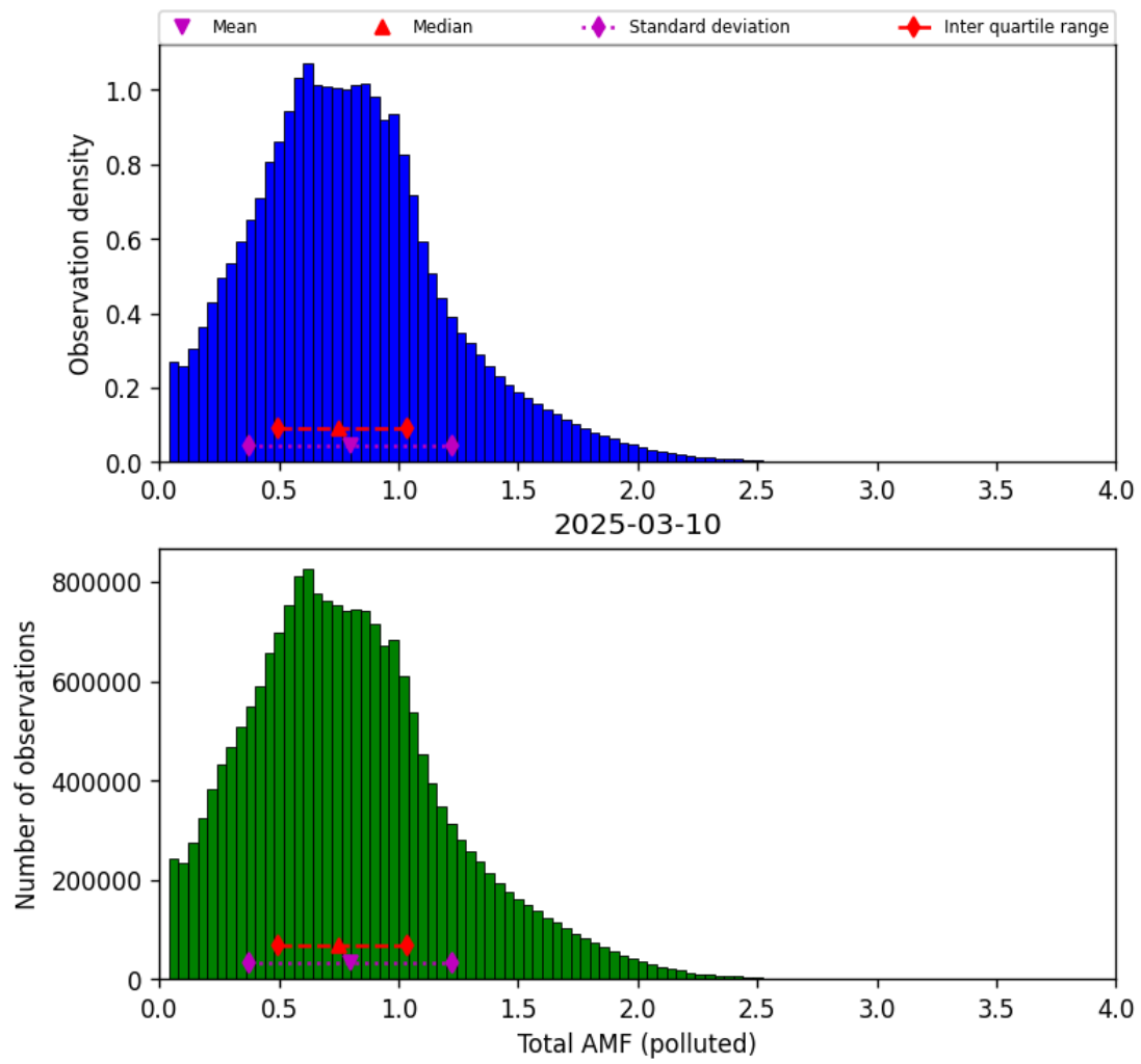
Figure 79: Histogram of “Total AMF (polluted)” for 2025-03-09 to 2025-03-11
