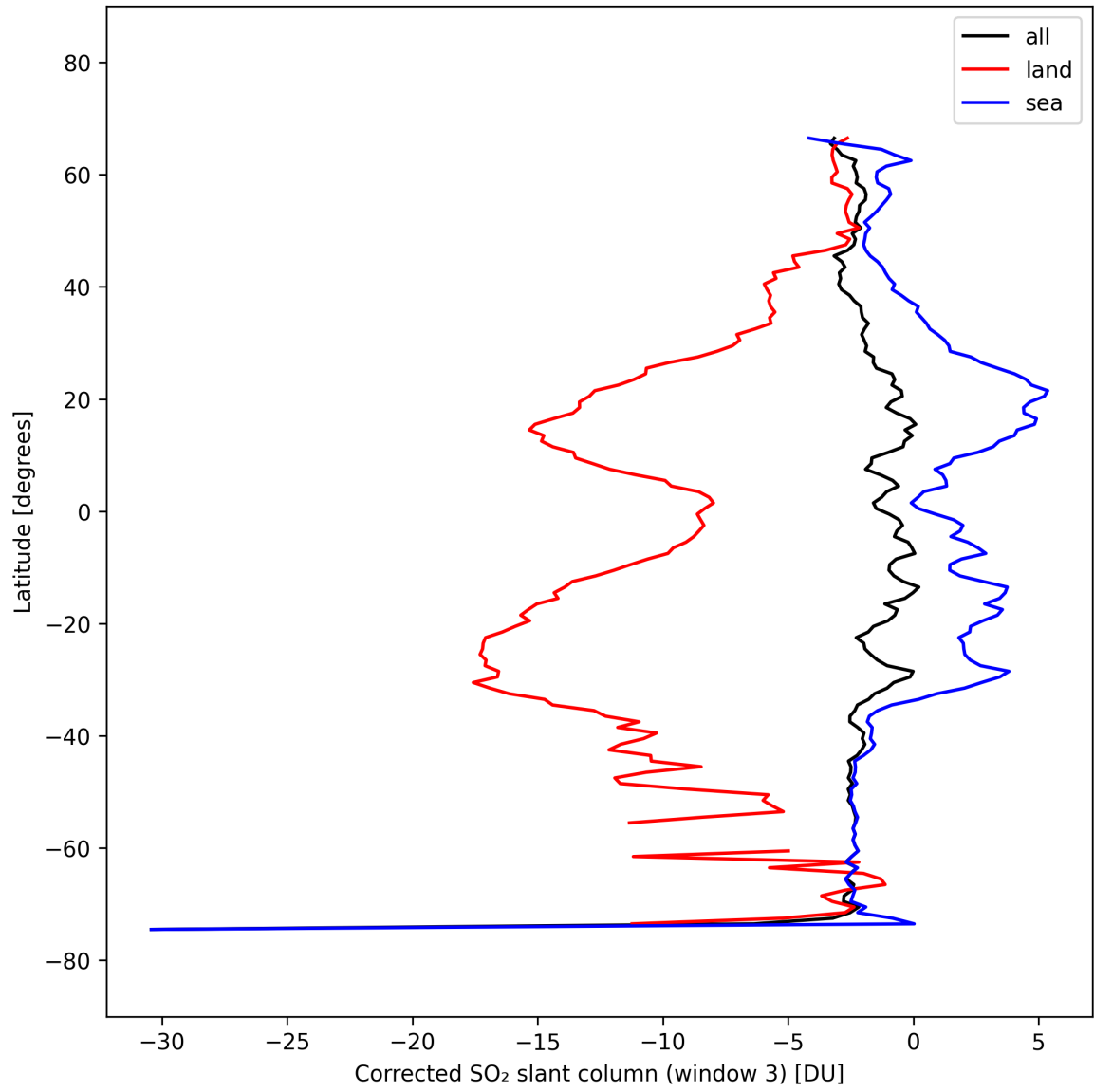
Figure 47: Zonal average of “Corrected SO 2 slant column (window 3)” for 2025-03-09 to 2025-03-11.
