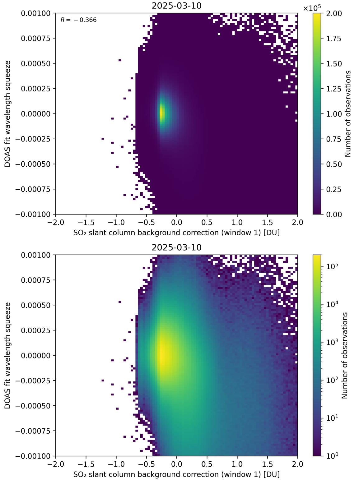
Figure 112: Scatter density plot of “SO 2 slant column background correction (window 1)” against “DOAS fit wavelength squeeze” for 2025-03-09 to 2025-03-11.
