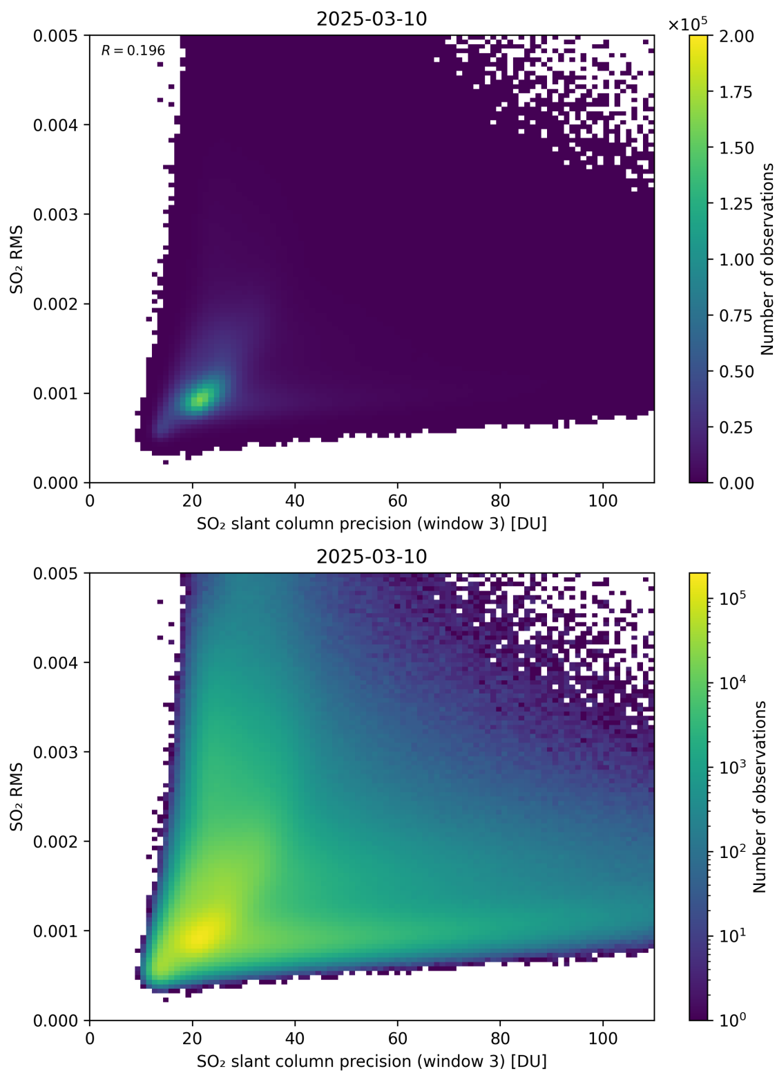
Figure 310: Scatter density plot of “SO 2 slant column precision (window 3)” against “SO 2 RMS” for 2025-03-09 to 2025-03-11.
