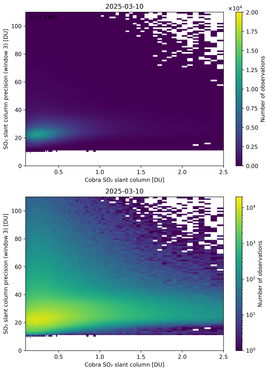
Figure 223: Scatter density plot of “Cobra SO 2 slant column” against “SO 2 slant column precision (window 3)” for 2025-03-09 to 2025-03-11.
