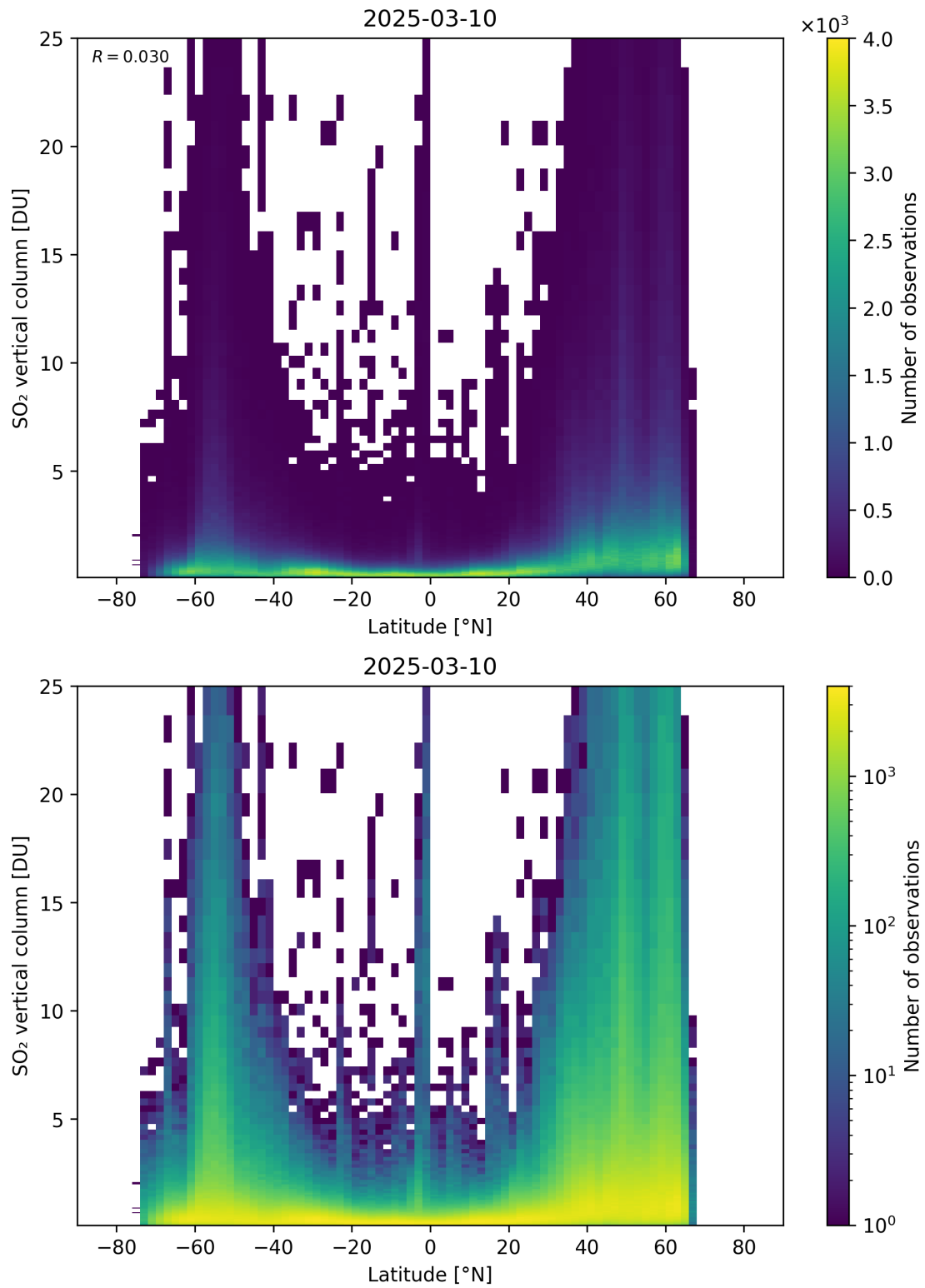
Figure 169: Scatter density plot of “Latitude” against “SO 2 vertical column” for 2025-03-09 to 2025-03-11.
