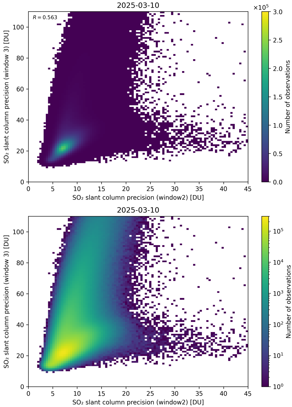
Figure 300: Scatter density plot of “SO 2 slant column precision (window2)” against “SO 2 slant column precision (window 3)” for 2025-03-09 to 2025-03-11.
