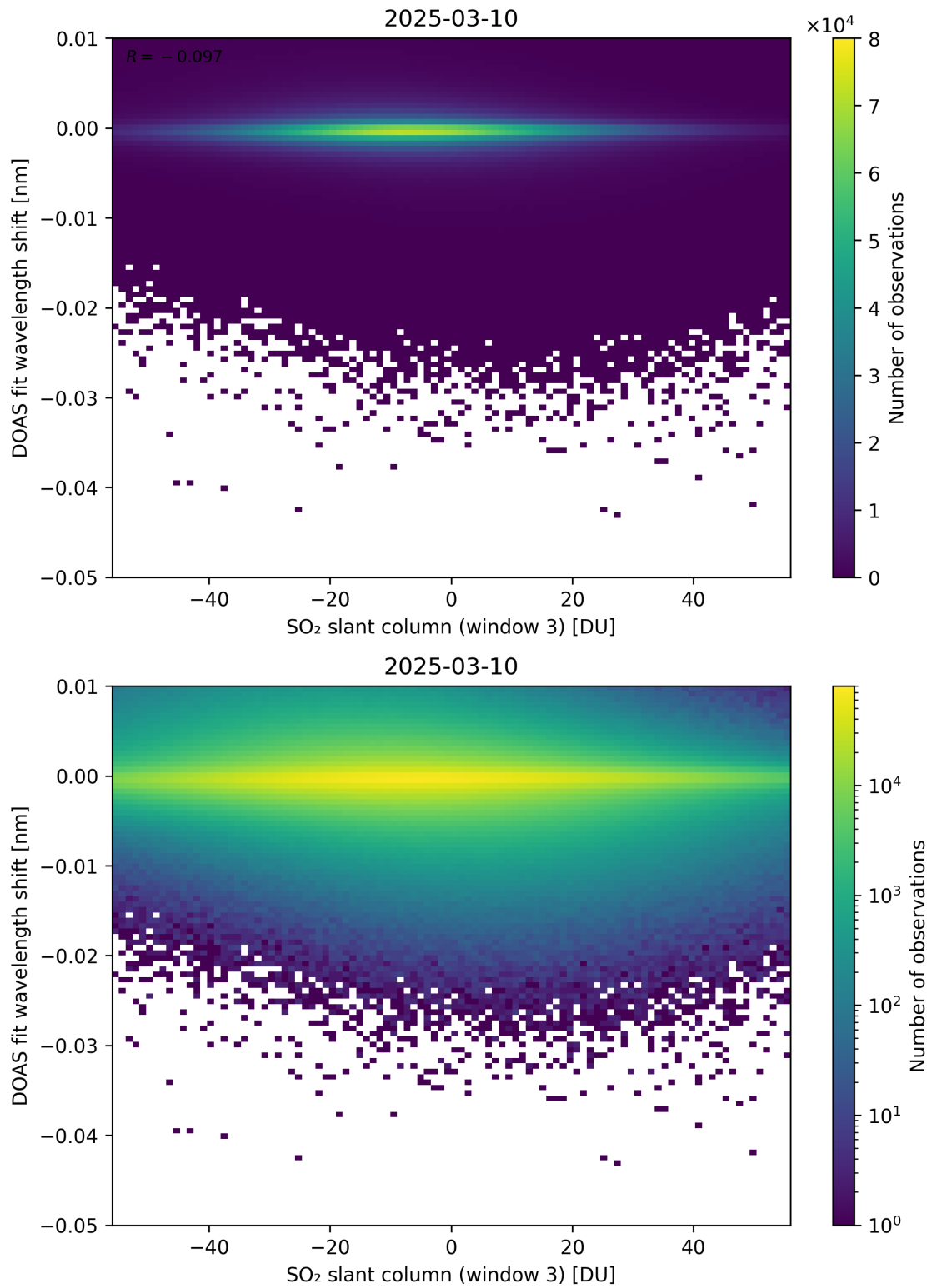
Figure 304: Scatter density plot of “SO 2 slant column (window 3)” against “DOAS fit wavelength shift” for 2025-03-09 to 2025-03-11.
