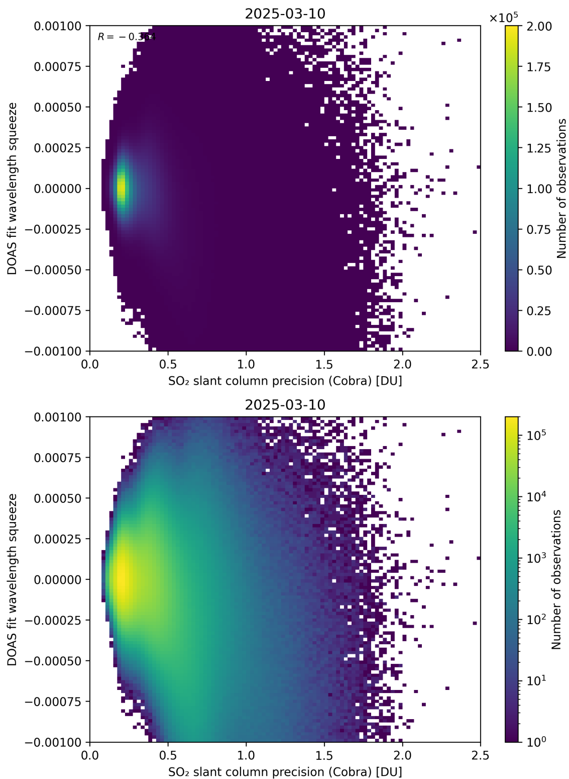
Figure 203: Scatter density plot of “SO 2 slant column precision (Cobra)” against “DOAS fit wavelength squeeze” for 2025-03-09 to 2025-03-11.
