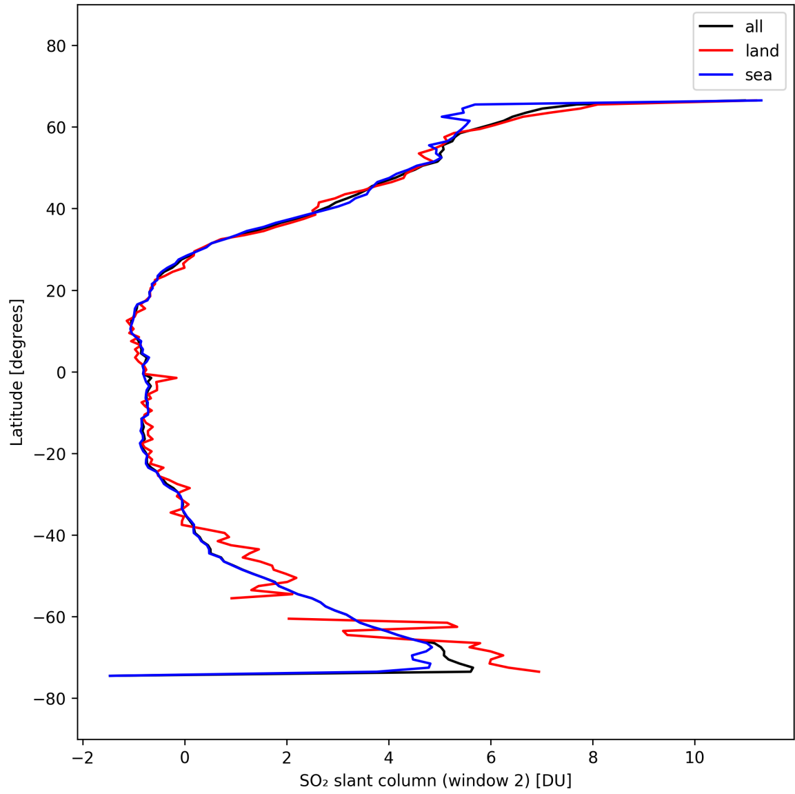
Figure 41: Zonal average of “SO 2 slant column (window 2)” for 2025-03-09 to 2025-03-11.
