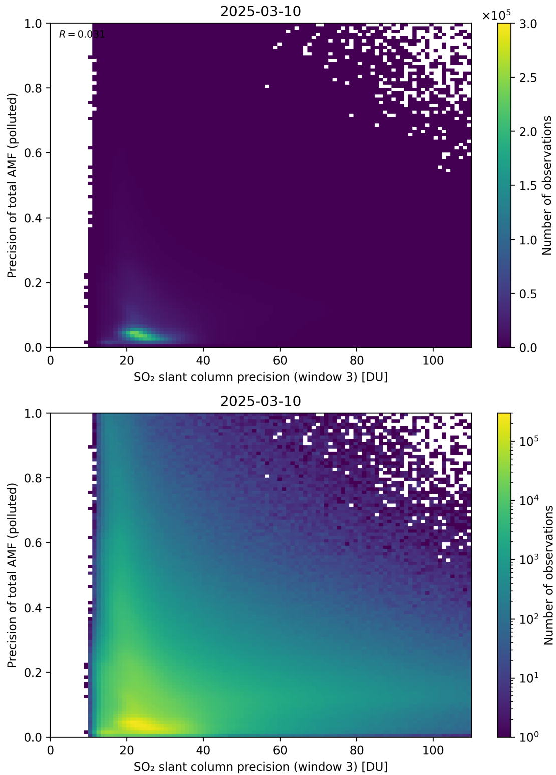
Figure 314: Scatter density plot of “SO 2 slant column precision (window 3)” against “Precision of total AMF (polluted)” for 2025-03-09 to 2025-03-11.
