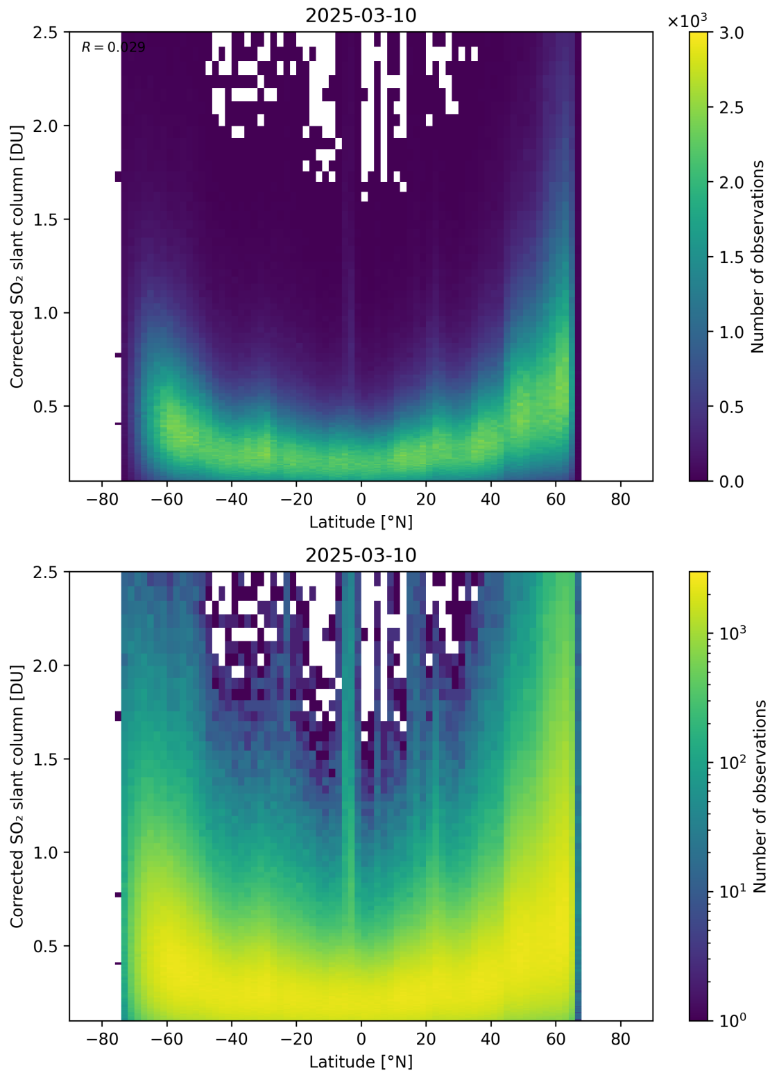
Figure 159: Scatter density plot of “Latitude” against “Corrected SO 2 slant column” for 2025-03-09 to 2025-03-11.
