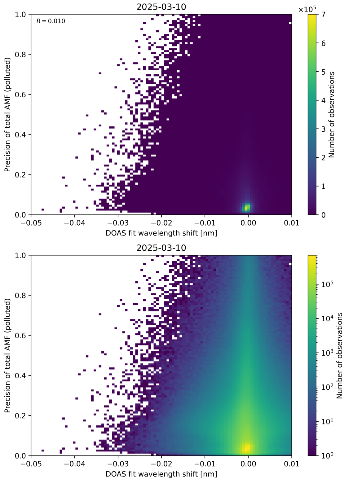
Figure 142: Scatter density plot of “DOAS fit wavelength shift” against “Precision of total AMF (polluted)” for 2025-03-09 to 2025-03-11.
