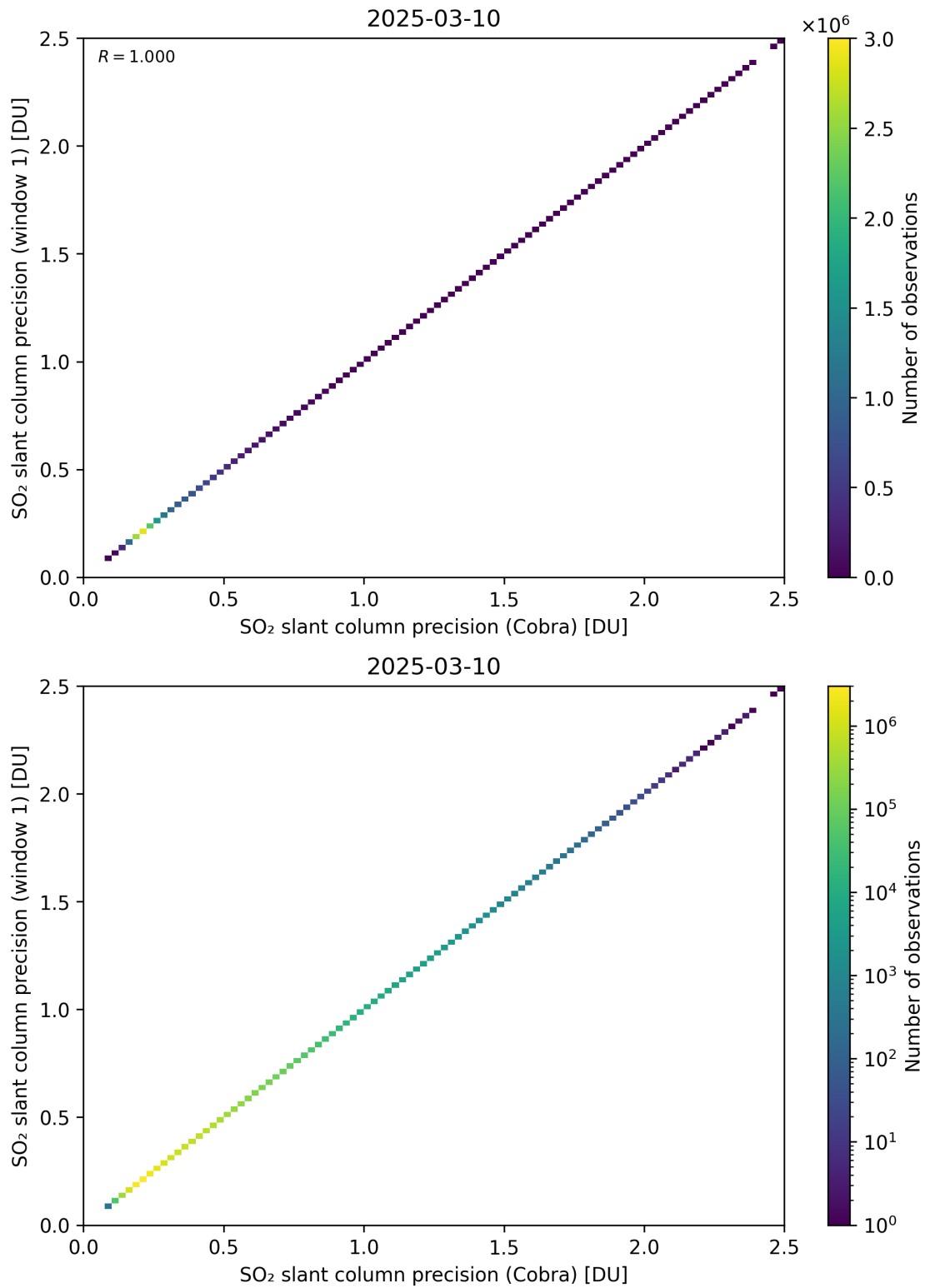
Figure 209: Scatter density plot of “SO 2 slant column precision (Cobra)” against “SO 2 slant column precision (window 1)” for 2025-03-09 to 2025-03-11.
