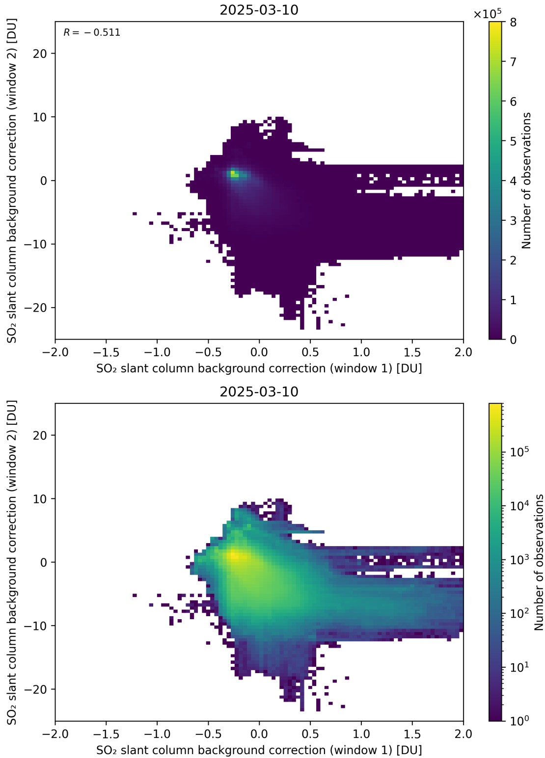
Figure 109: Scatter density plot of “SO 2 slant column background correction (window 1)” against “SO 2 slant column background correction (window 2)” for 2025-03-09 to 2025-03-11.
