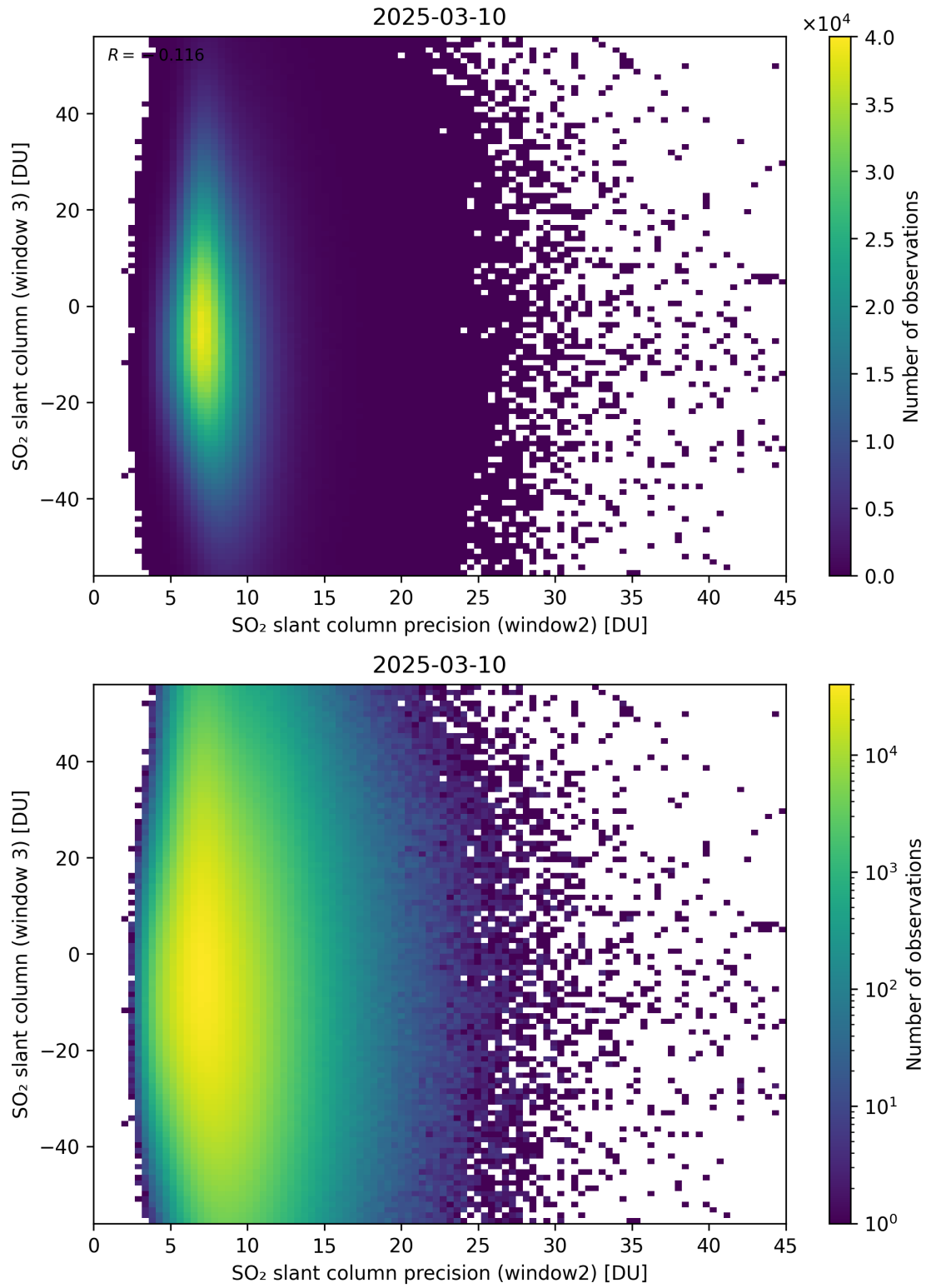
Figure 299: Scatter density plot of “SO 2 slant column precision (window2)” against “SO 2 slant column (window 3)” for 2025-03-09 to 2025-03-11.
