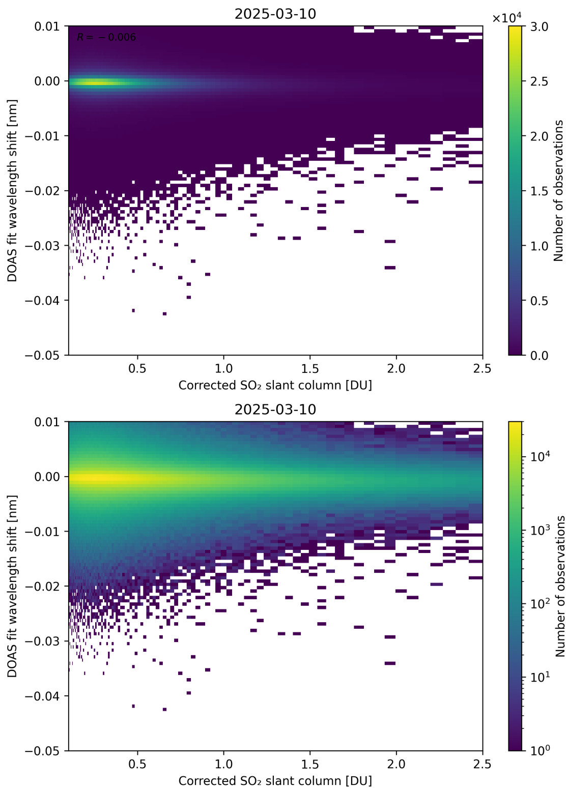
Figure 229: Scatter density plot of “Corrected SO 2 slant column” against “DOAS fit wavelength shift” for 2025-03-09 to 2025-03-11.
