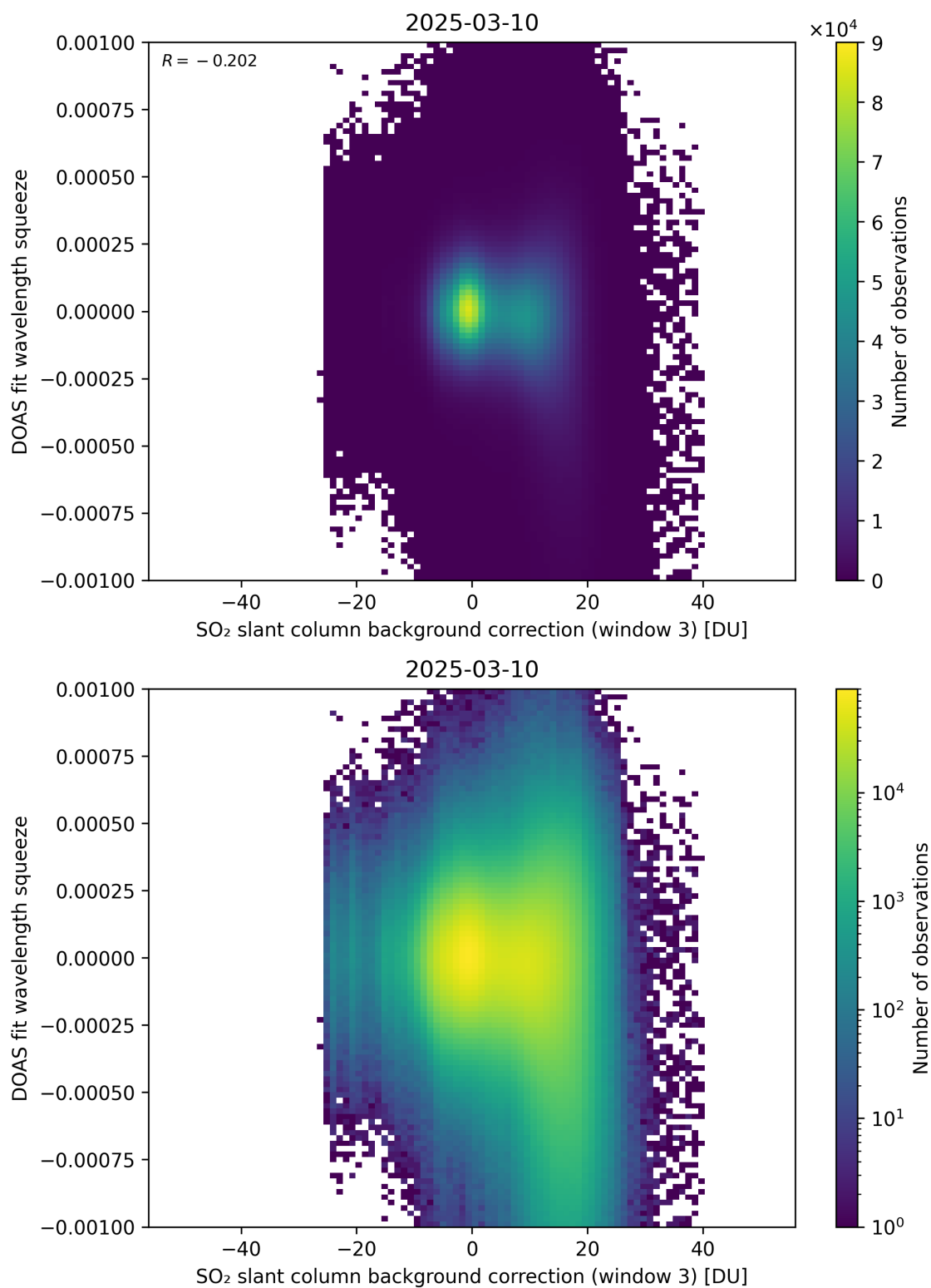
Figure 133: Scatter density plot of “SO 2 slant column background correction (window 3)” against “DOAS fit wavelength squeeze” for 2025-03-09 to 2025-03-11.
