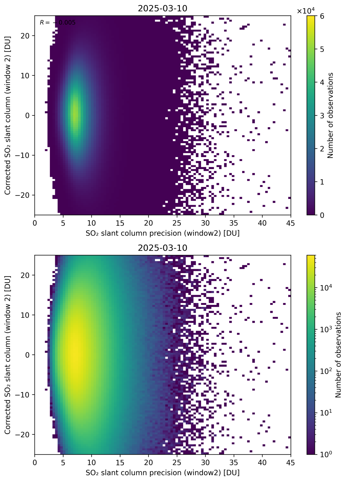
Figure 297: Scatter density plot of “SO 2 slant column precision (window2)” against “Corrected SO 2 slant column (window 2)” for 2025-03-09 to 2025-03-11.
