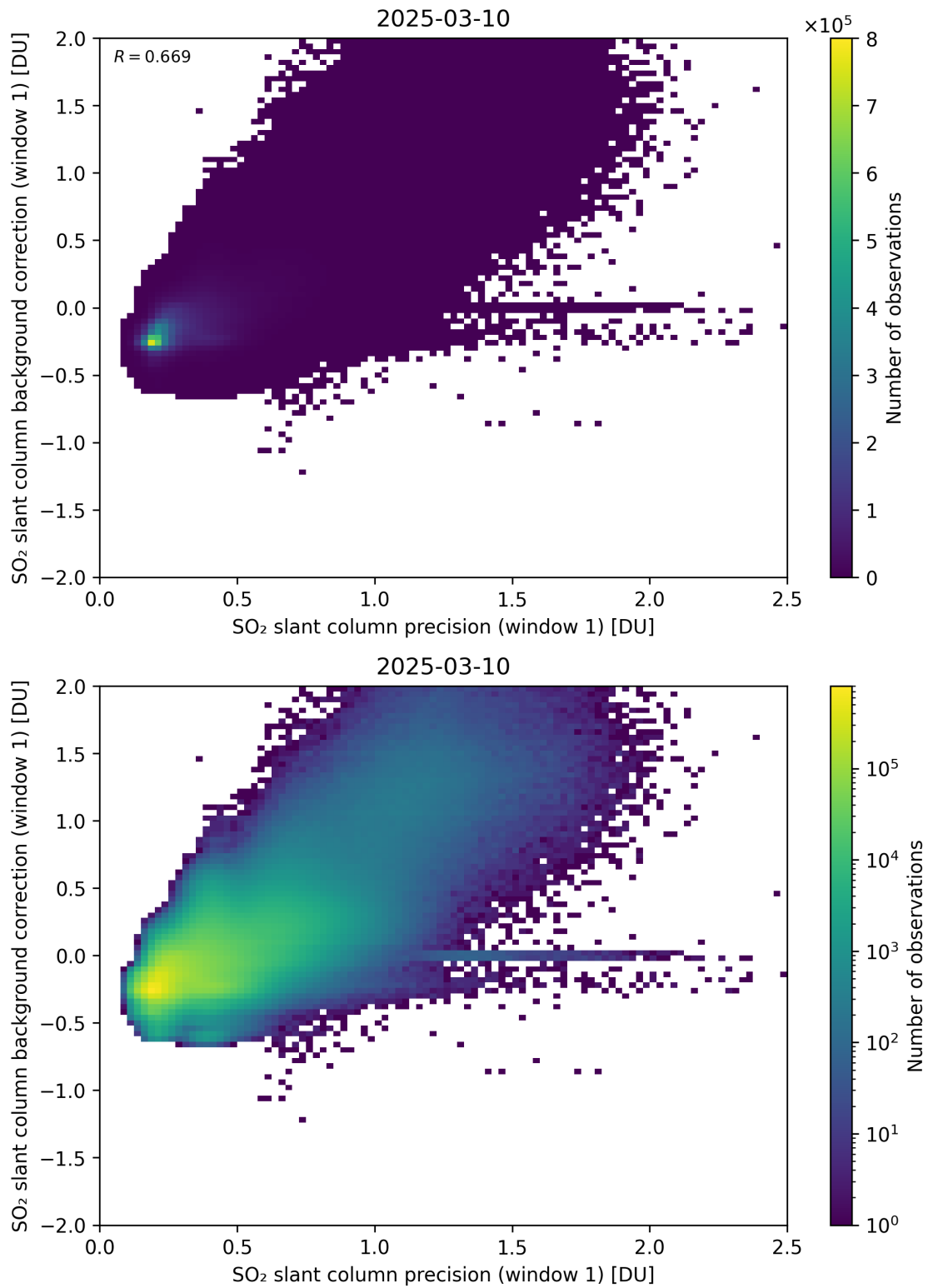
Figure 268: Scatter density plot of “SO 2 slant column precision (window 1)” against “SO 2 slant column background correction (window 1)” for 2025-03-09 to 2025-03-11.
