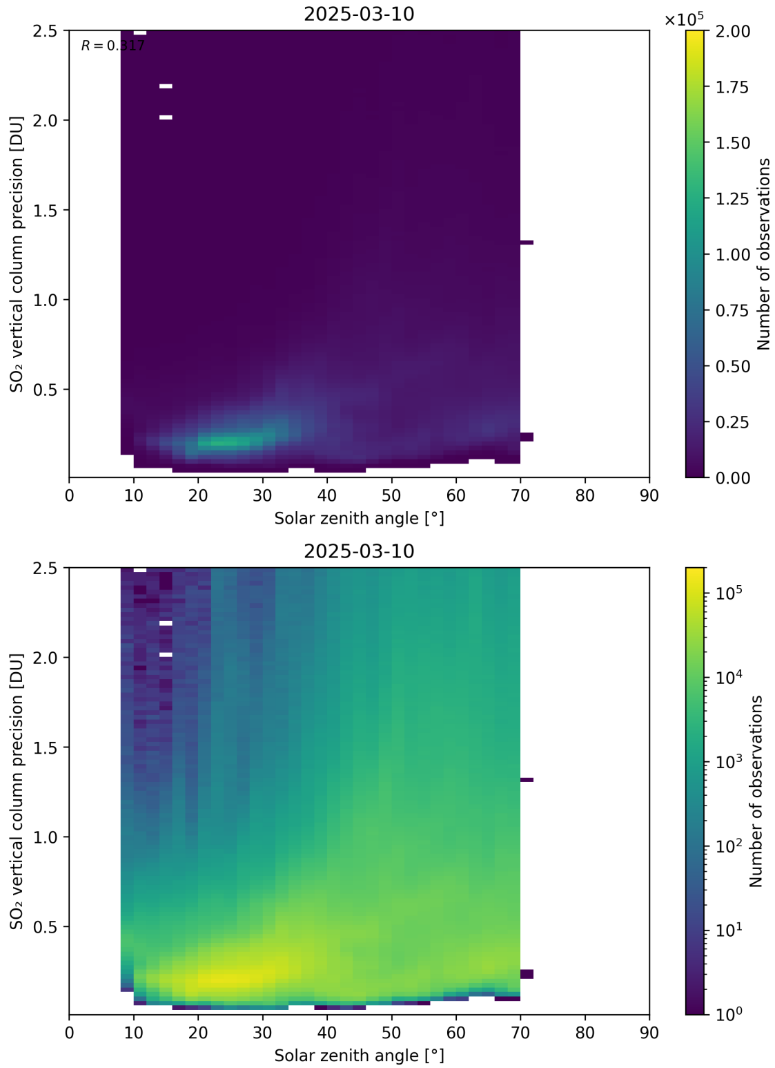
Figure 192: Scatter density plot of “Solar zenith angle” against “SO 2 vertical column precision” for 2025-03-09 to 2025-03-11.
