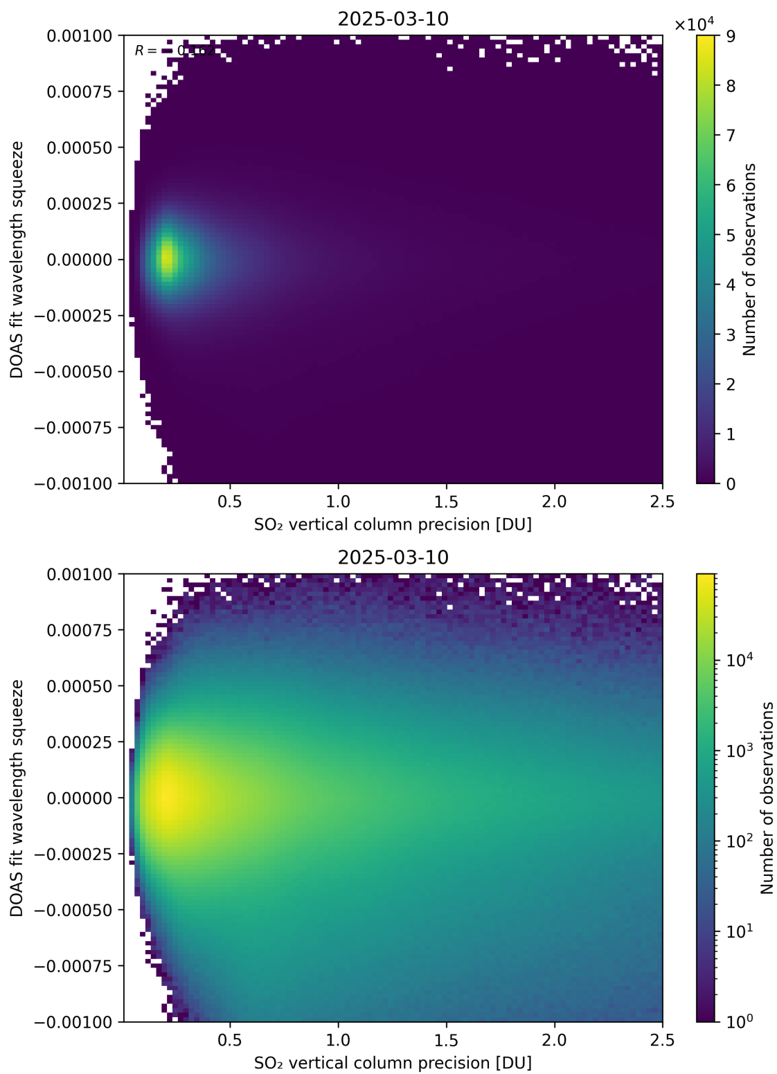
Figure 333: Scatter density plot of “SO 2 vertical column precision” against “DOAS fit wavelength squeeze” for 2025-03-09 to 2025-03-11.
