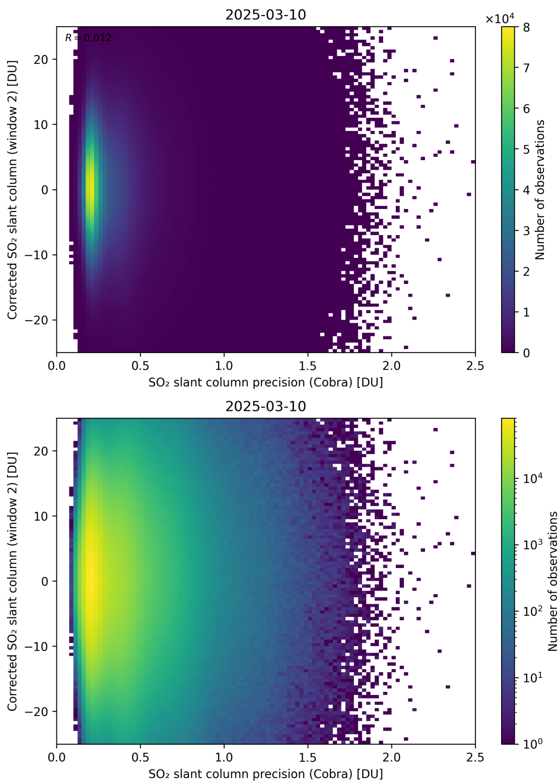
Figure 206: Scatter density plot of “SO 2 slant column precision (Cobra)” against “Corrected SO 2 slant column (window 2)” for 2025-03-09 to 2025-03-11.
