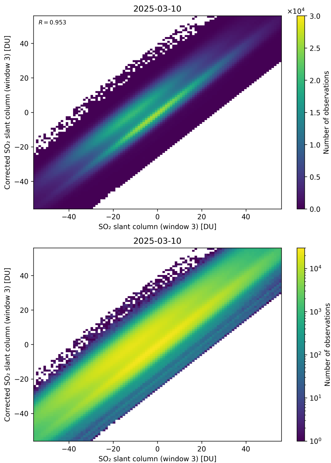
Figure 316: Scatter density plot of “SO 2 slant column (window 3)” against “Corrected SO 2 slant column (window 3)” for 2025-03-09 to 2025-03-11.
