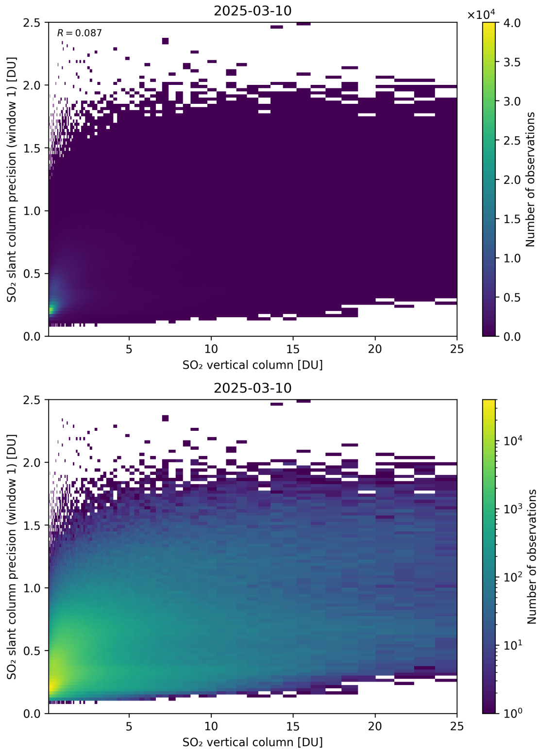
Figure 355: Scatter density plot of “SO 2 vertical column” against “SO 2 slant column precision (window 1)” for 2025-03-09 to 2025-03-11.
