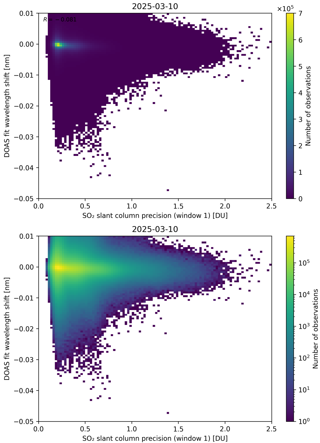
Figure 271: Scatter density plot of “SO 2 slant column precision (window 1)” against “DOAS fit wavelength shift” for 2025-03-09 to 2025-03-11.
