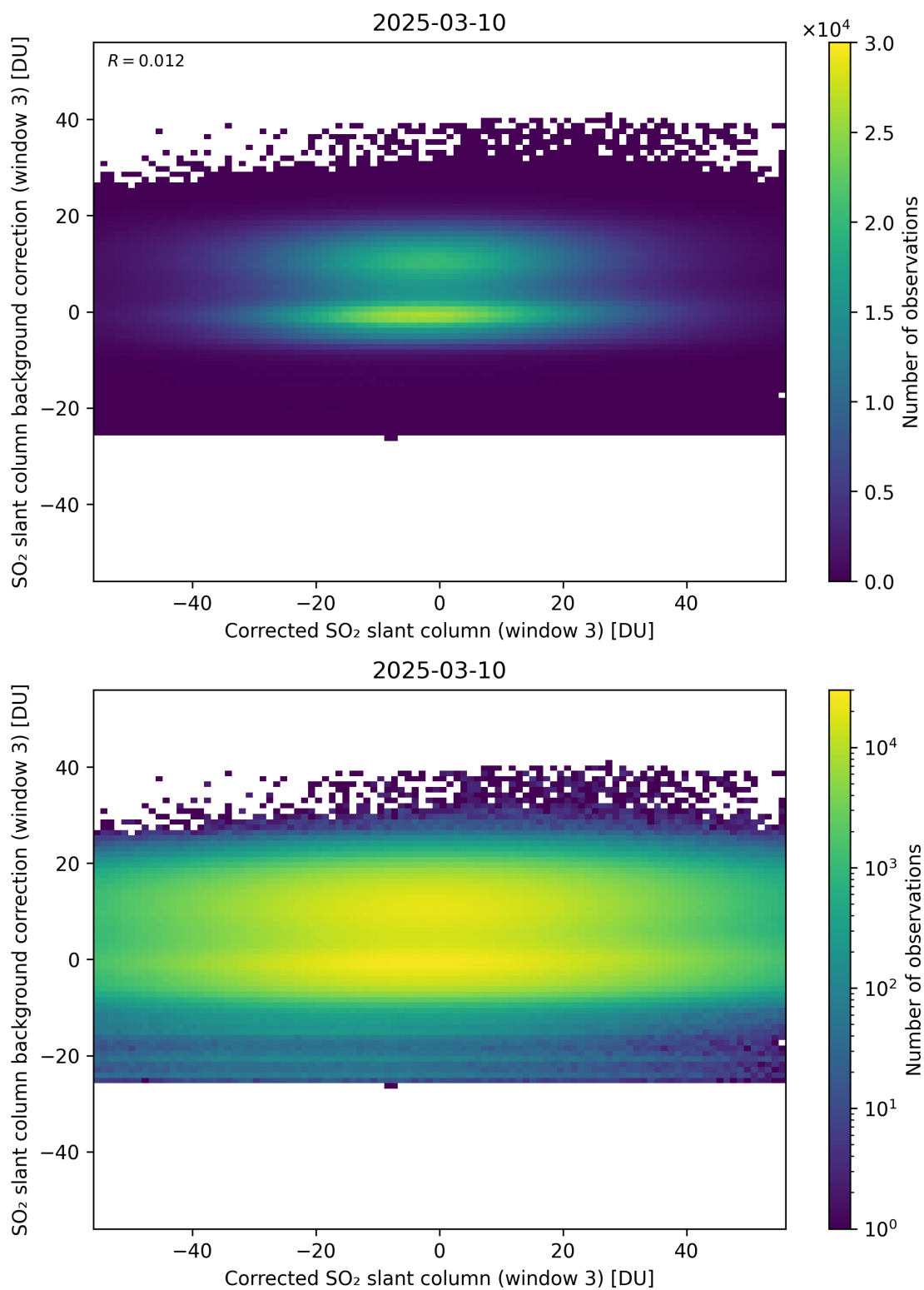
Figure 255: Scatter density plot of “Corrected SO 2 slant column (window 3)” against “SO 2 slant column background correction (window 3)” for 2025-03-09 to 2025-03-11.
