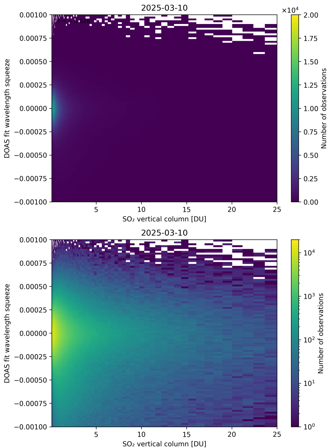
Figure 327: Scatter density plot of “SO 2 vertical column” against “DOAS fit wavelength squeeze” for 2025-03-09 to 2025-03-11.
