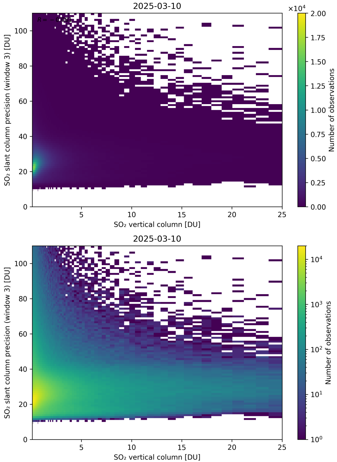
Figure 358: Scatter density plot of “SO 2 vertical column” against “SO 2 slant column precision (window 3)” for 2025-03-09 to 2025-03-11.
