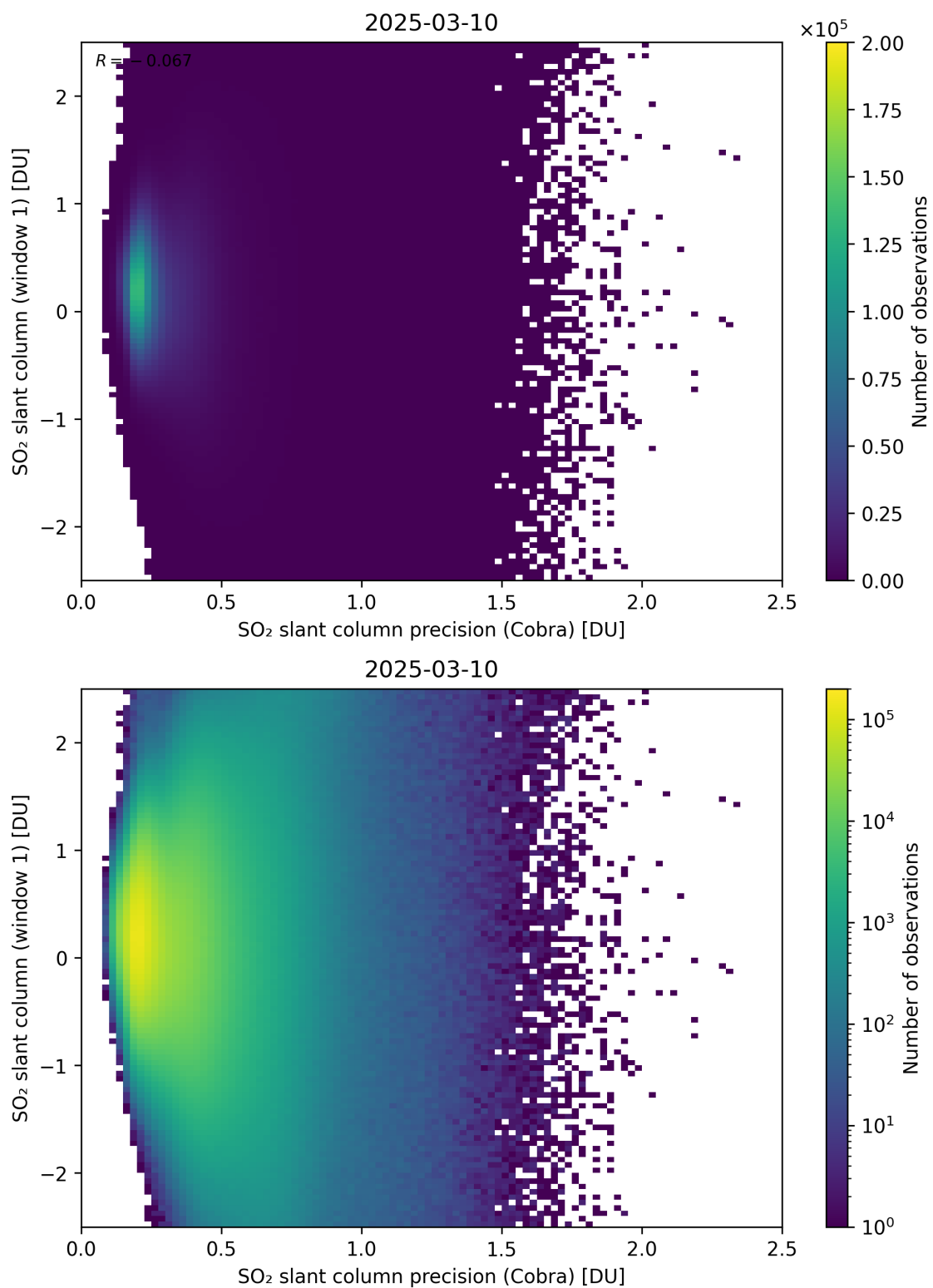
Figure 208: Scatter density plot of “SO 2 slant column precision (Cobra)” against “SO 2 slant column (window 1)” for 2025-03-09 to 2025-03-11.
