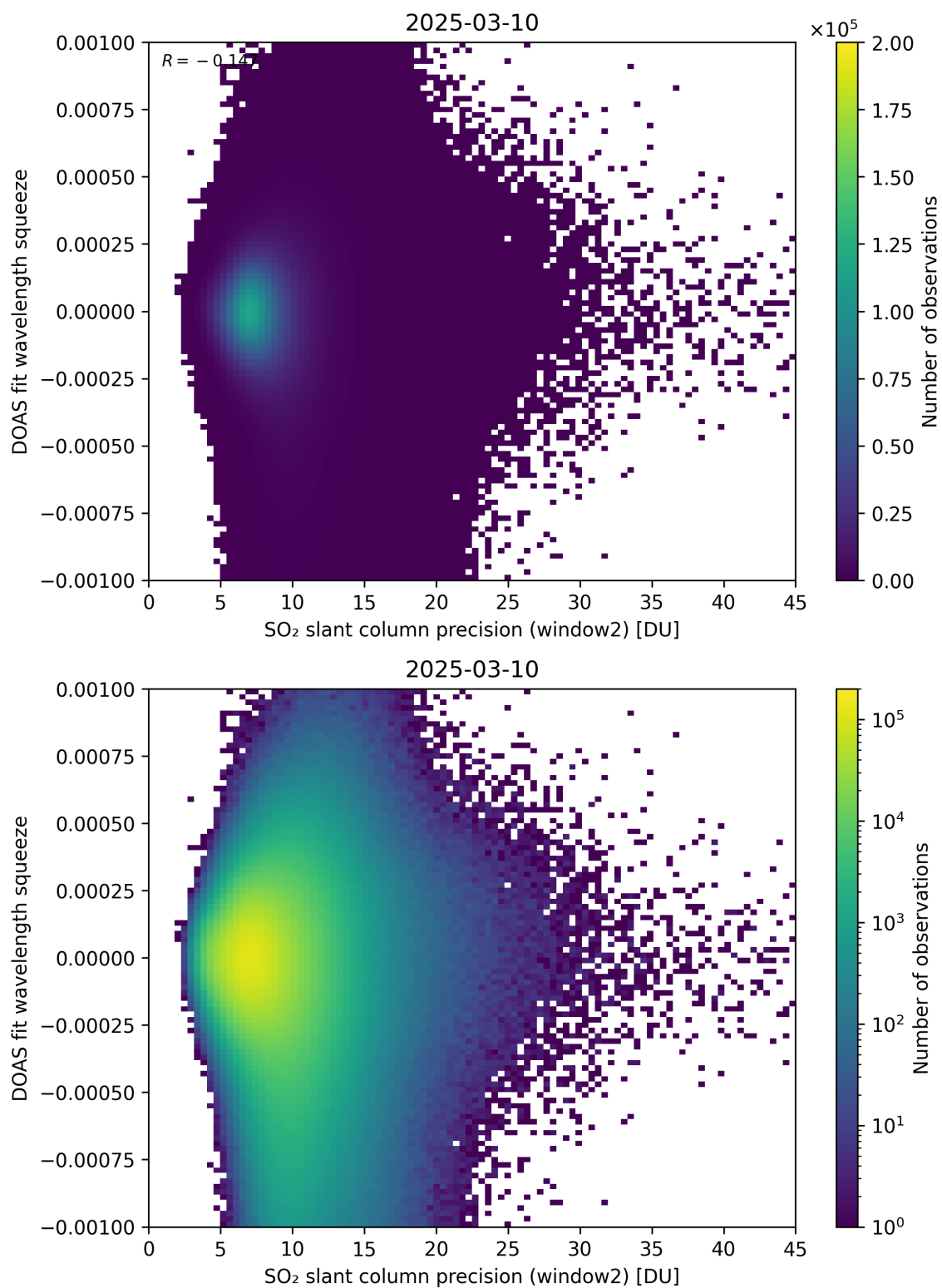
Figure 294: Scatter density plot of “SO 2 slant column precision (window2)” against “DOAS fit wavelength squeeze” for 2025-03-09 to 2025-03-11.
