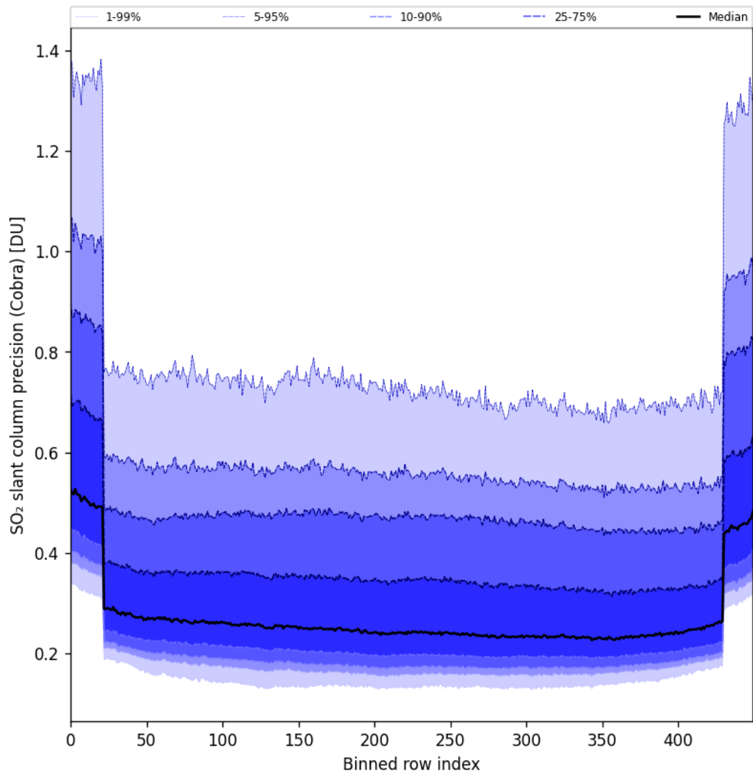
Figure 88: Along track statistics of “SO 2 slant column precision (Cobra)” for 2025-03-09 to 2025-03-11
