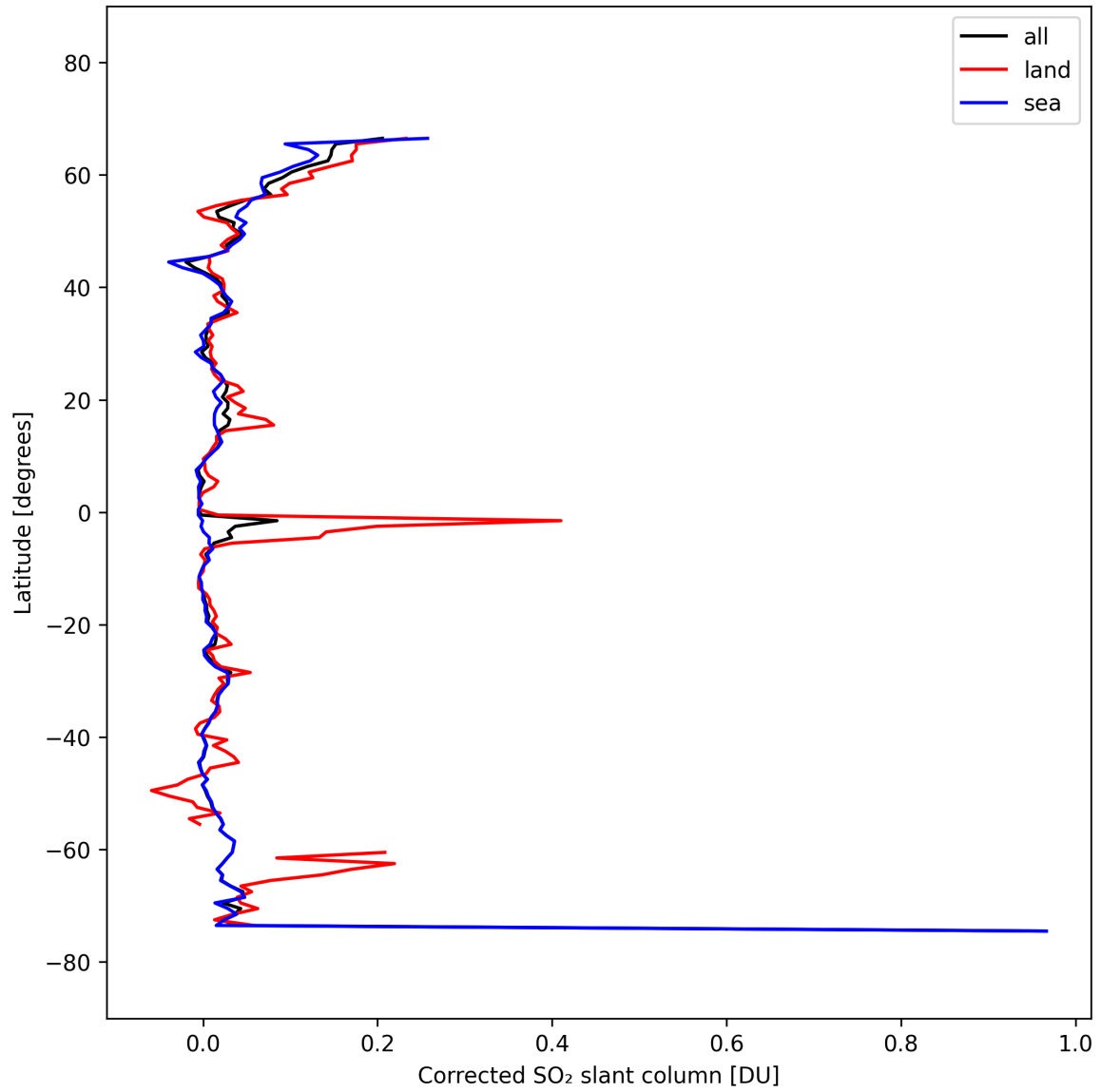
Figure 34: Zonal average of “Corrected SO 2 slant column” for 2025-03-09 to 2025-03-11.
