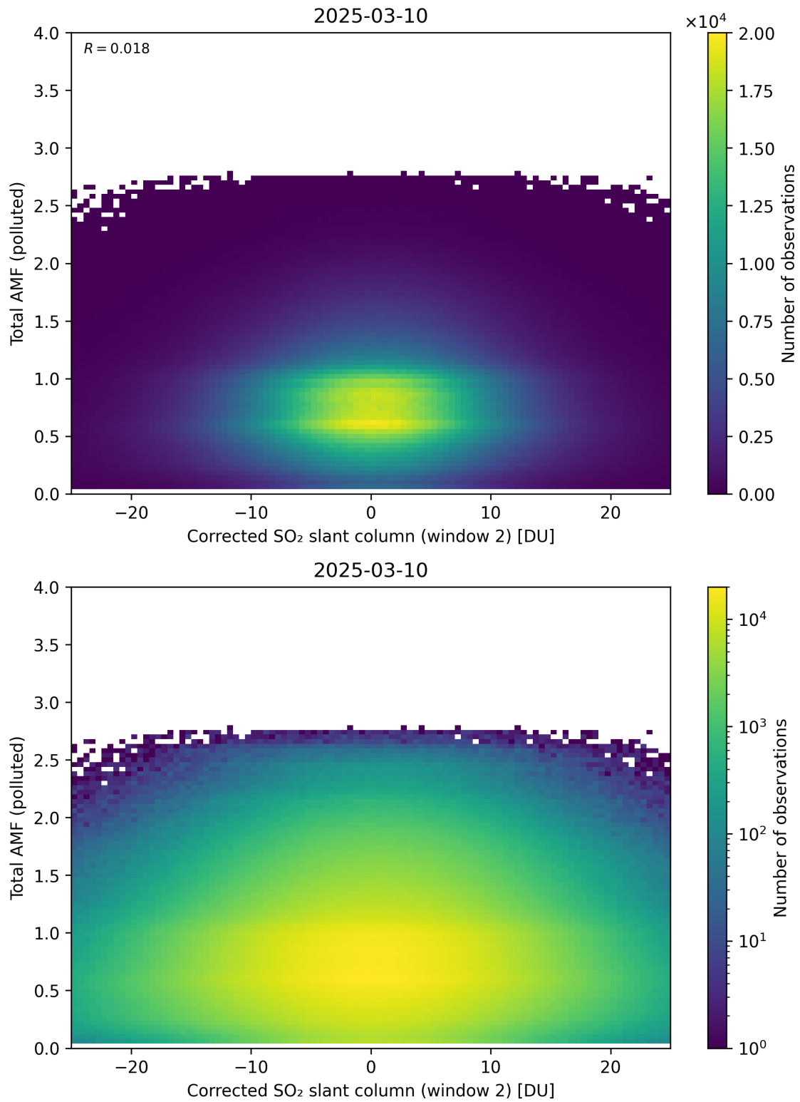
Figure 253: Scatter density plot of “Corrected SO 2 slant column (window 2)” against “Total AMF (polluted)” for 2025-03-09 to 2025-03-11.
