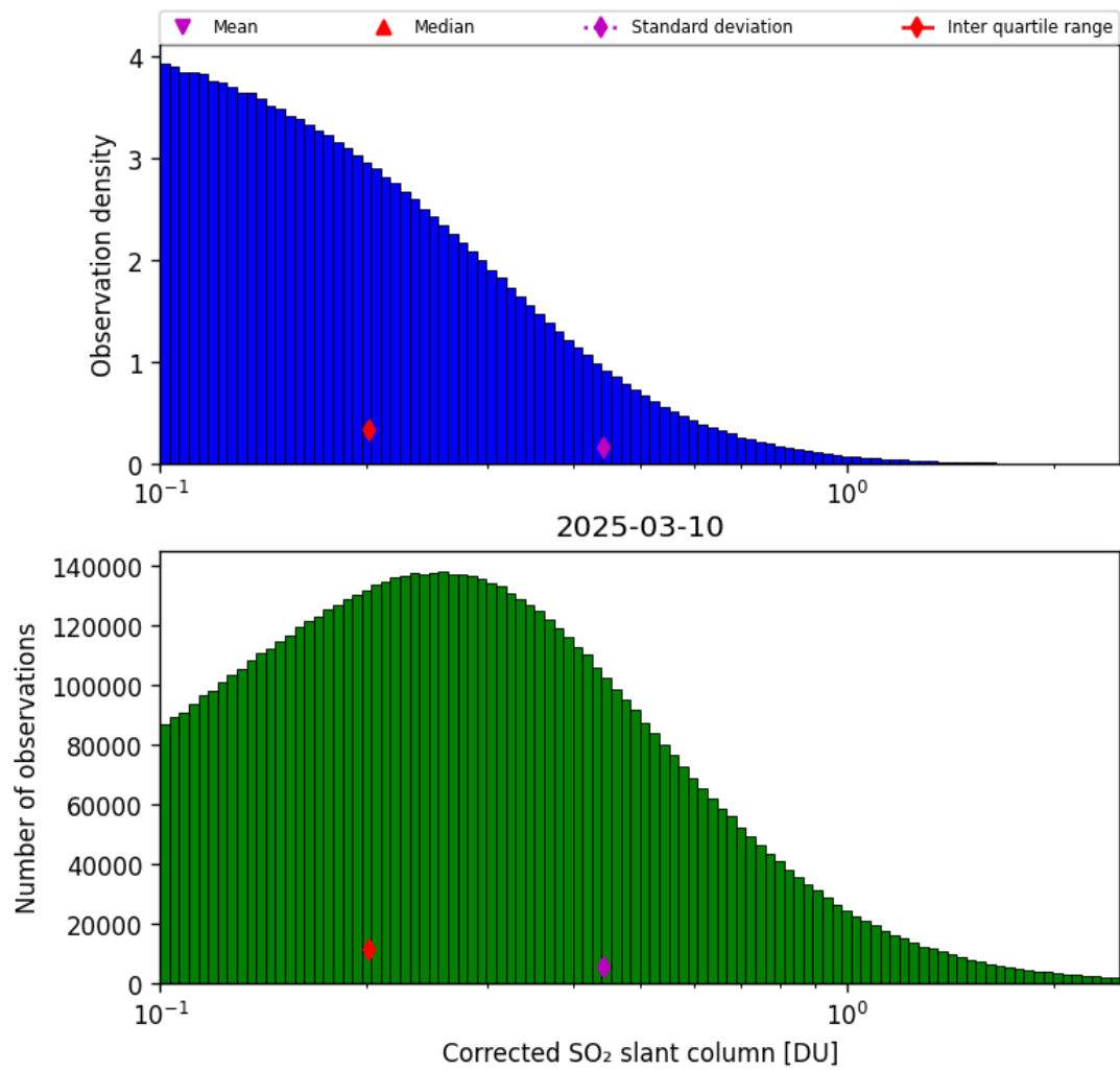
Figure 60: Histogram of “Corrected SO 2 slant column” for 2025-03-09 to 2025-03-11
