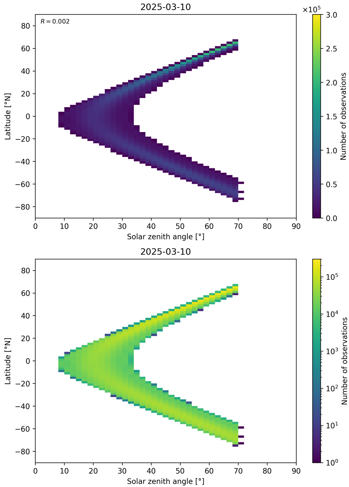
Figure 177: Scatter density plot of “Solar zenith angle” against “Latitude” for 2025-03-09 to 2025-03-11.
