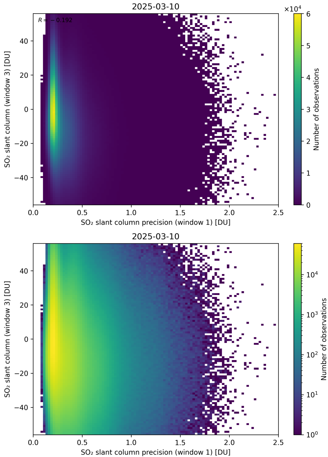
Figure 278: Scatter density plot of “SO 2 slant column precision (window 1)” against “SO 2 slant column (window 3)” for 2025-03-09 to 2025-03-11.
