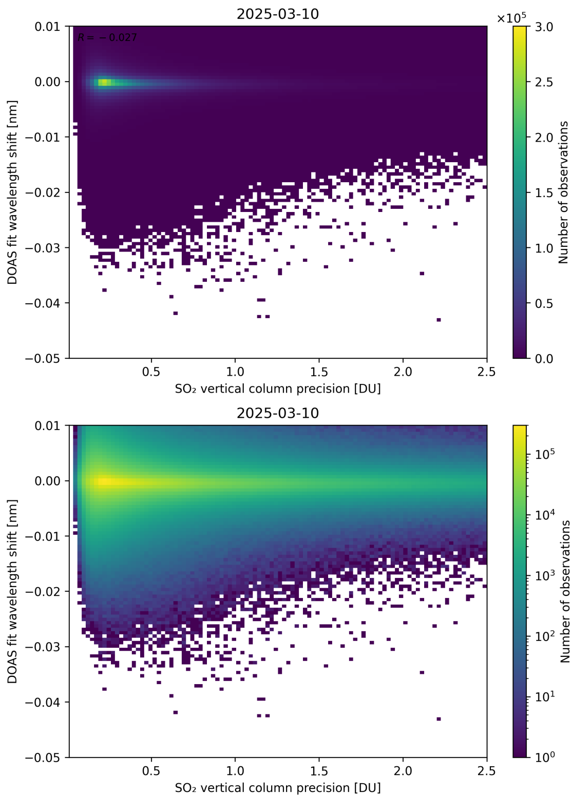
Figure 332: Scatter density plot of “SO 2 vertical column precision” against “DOAS fit wavelength shift” for 2025-03-09 to 2025-03-11.
