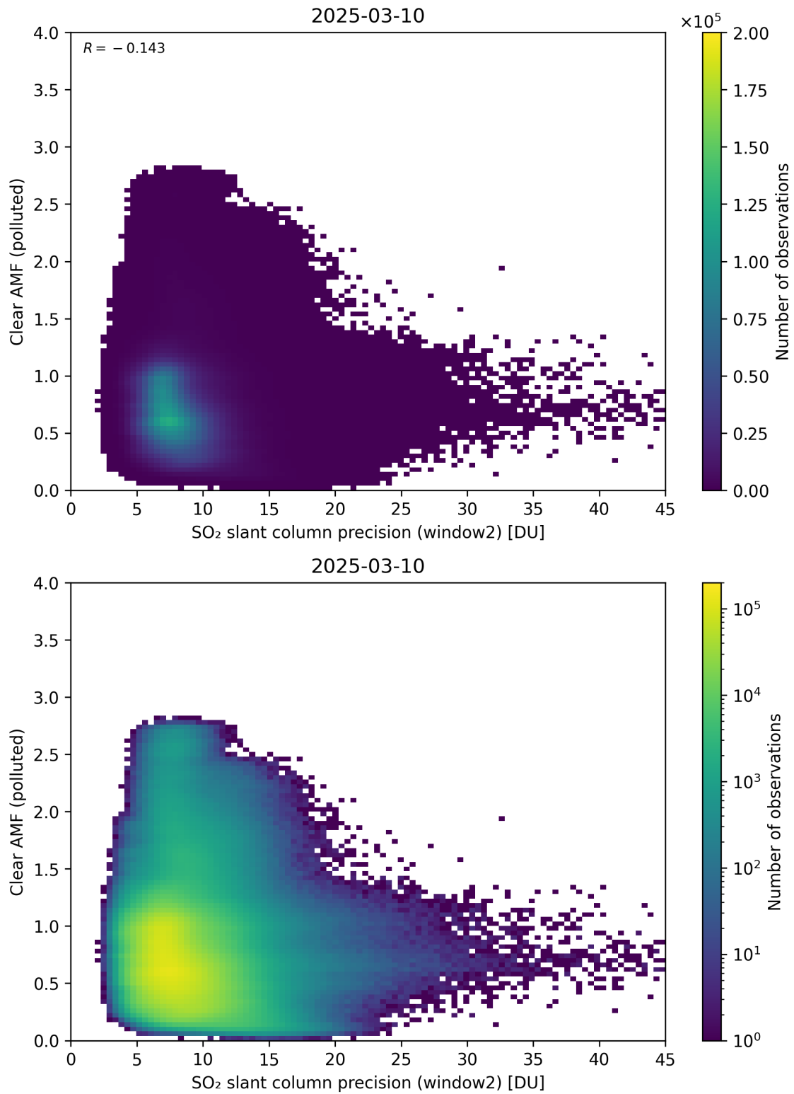
Figure 296: Scatter density plot of “SO 2 slant column precision (window2)” against “Clear AMF (polluted)” for 2025-03-09 to 2025-03-11.
