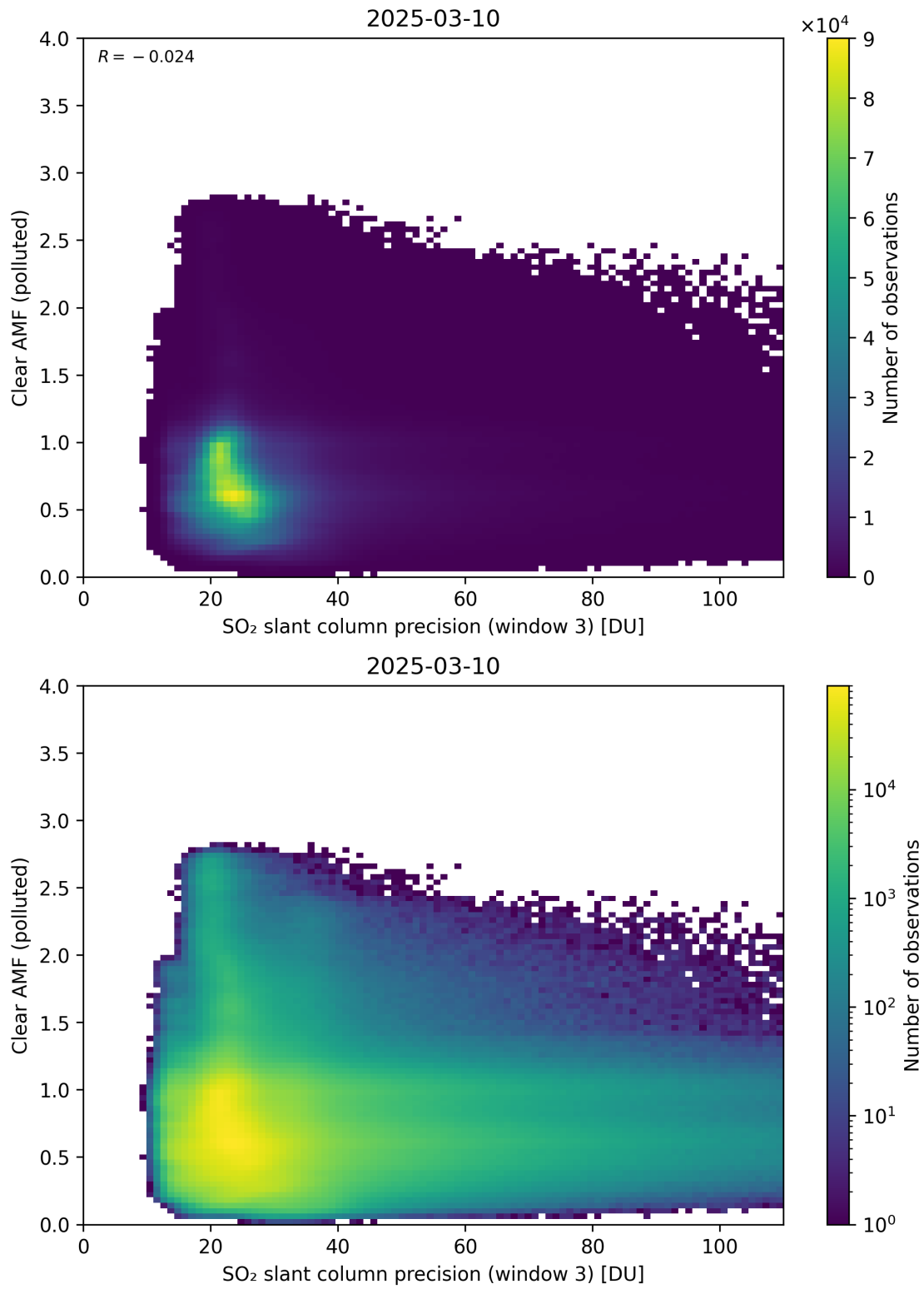
Figure 311: Scatter density plot of “SO 2 slant column precision (window 3)” against “Clear AMF (polluted)” for 2025-03-09 to 2025-03-11.
