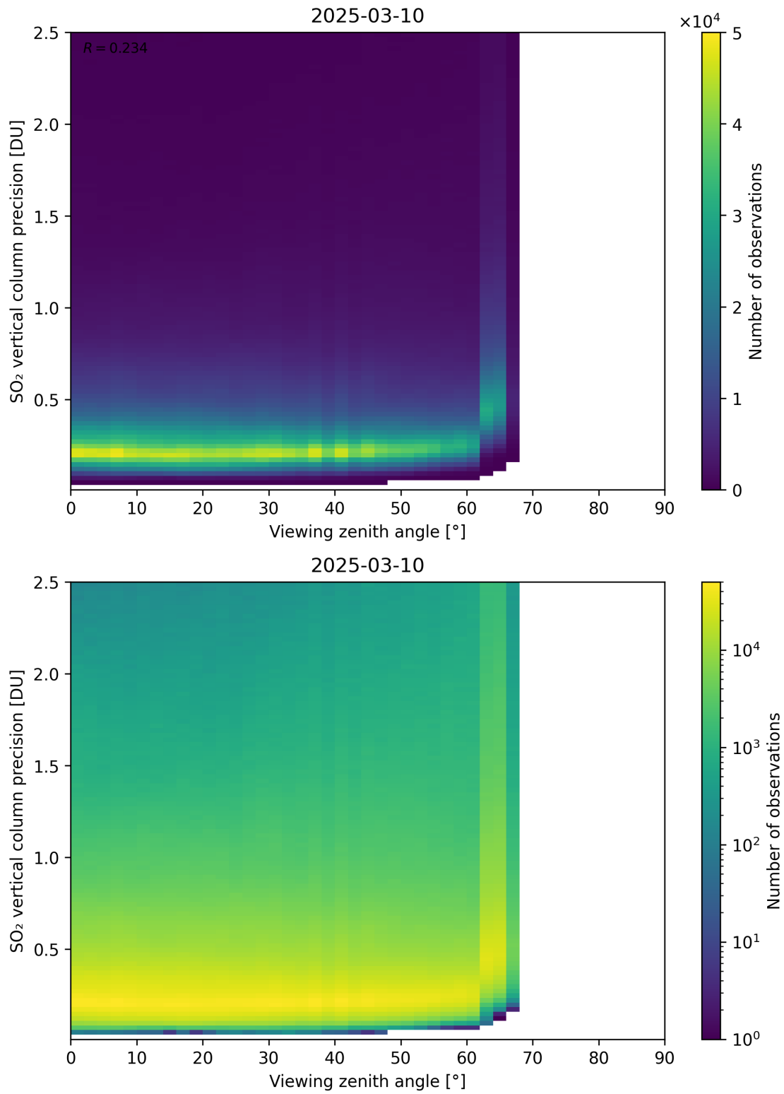
Figure 384: Scatter density plot of “Viewing zenith angle” against “SO 2 vertical column precision” for 2025-03-09 to 2025-03-11.
