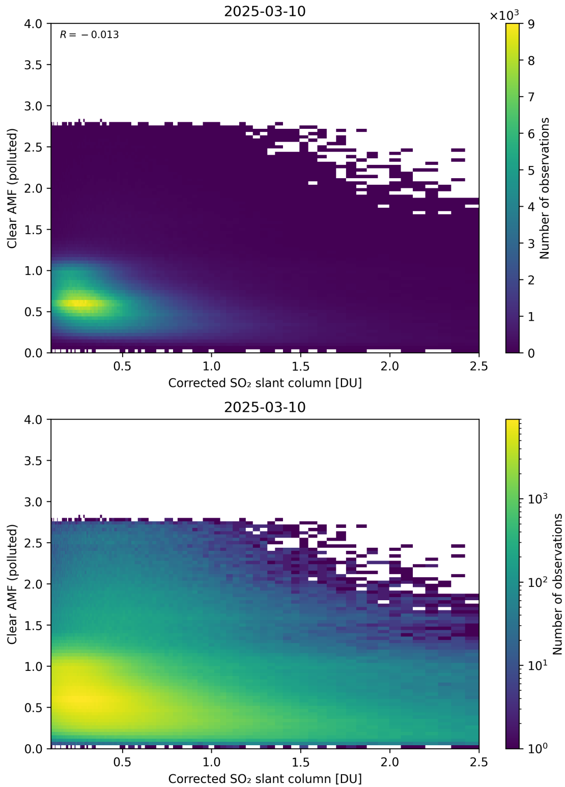
Figure 232: Scatter density plot of “Corrected SO 2 slant column” against “Clear AMF (polluted)” for 2025-03-09 to 2025-03-11.
