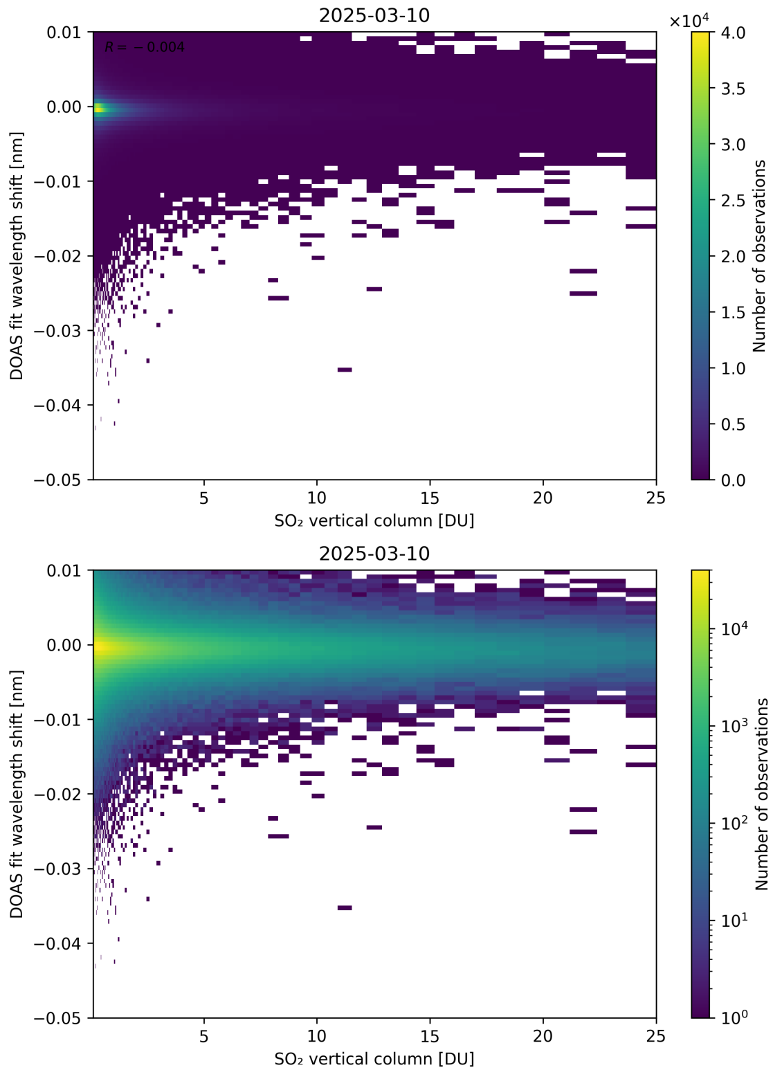
Figure 326: Scatter density plot of “SO 2 vertical column” against “DOAS fit wavelength shift” for 2025-03-09 to 2025-03-11.
