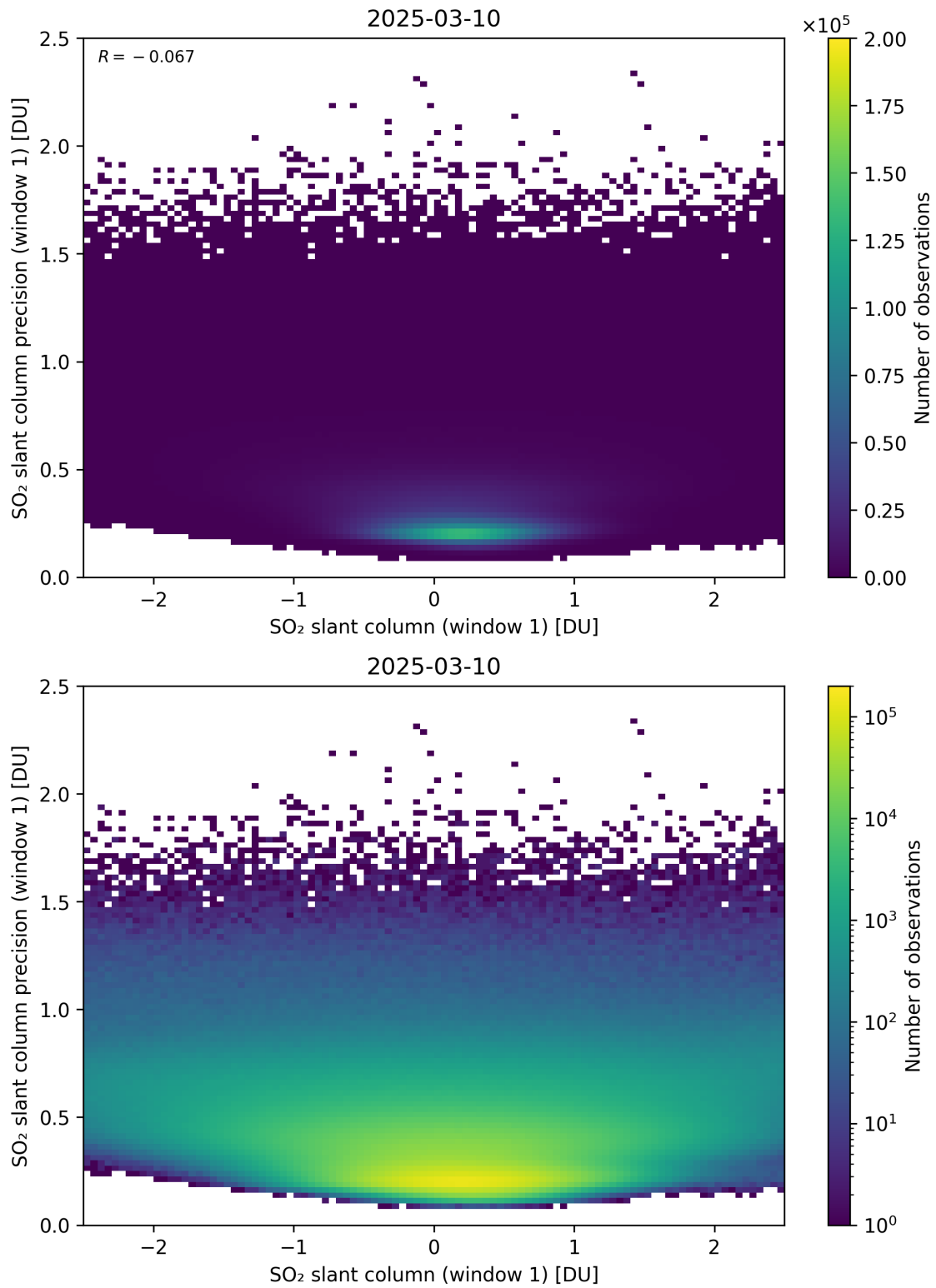
Figure 285: Scatter density plot of “SO 2 slant column (window 1)” against “SO 2 slant column precision (window 1)” for 2025-03-09 to 2025-03-11.
