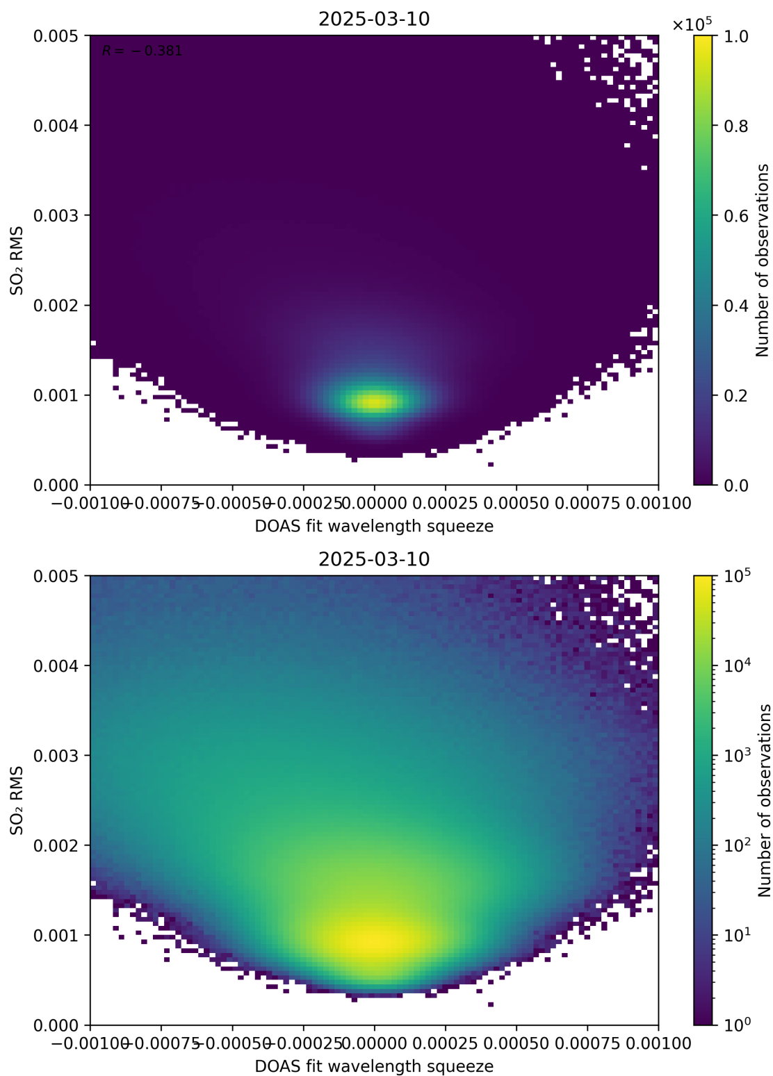
Figure 143: Scatter density plot of “DOAS fit wavelength squeeze” against “SO 2 RMS” for 2025-03-09 to 2025-03-11.
