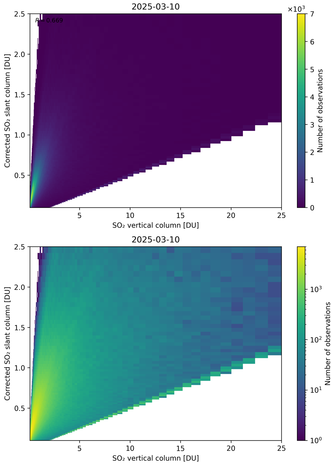
Figure 351: Scatter density plot of “SO 2 vertical column” against “Corrected SO 2 slant column” for 2025-03-09 to 2025-03-11.
