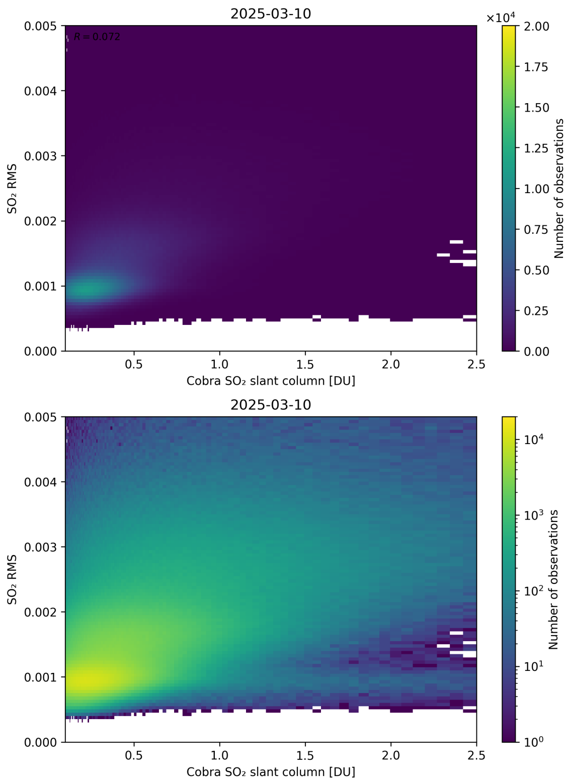
Figure 198: Scatter density plot of “Cobra SO 2 slant column” against “SO 2 RMS” for 2025-03-09 to 2025-03-11.
