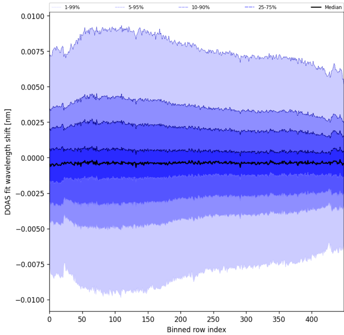
Figure 102: Along track statistics of “DOAS fit wavelength shift” for 2025-03-09 to 2025-03-11
