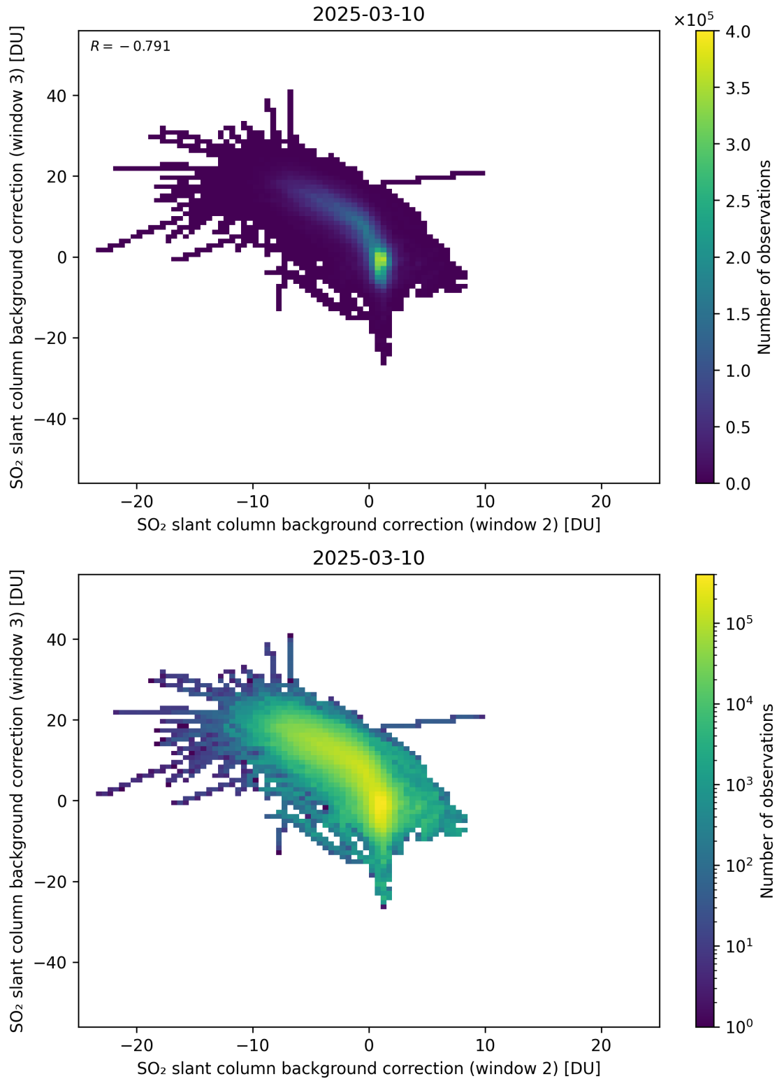
Figure 122: Scatter density plot of “SO 2 slant column background correction (window 2)” against “SO 2 slant column background correction (window 3)” for 2025-03-09 to 2025-03-11.
