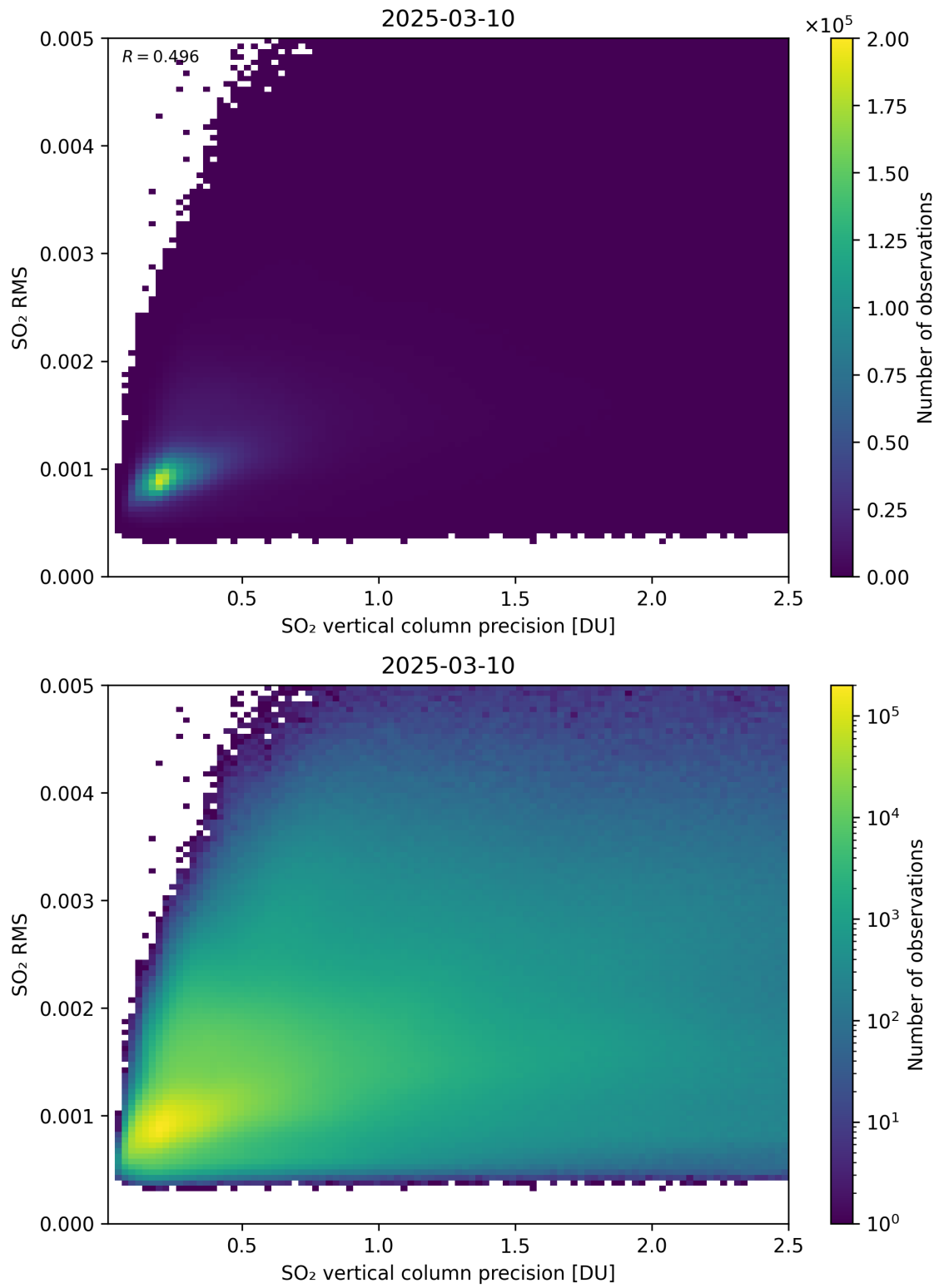
Figure 334: Scatter density plot of “SO 2 vertical column precision” against “SO 2 RMS” for 2025-03-09 to 2025-03-11.
