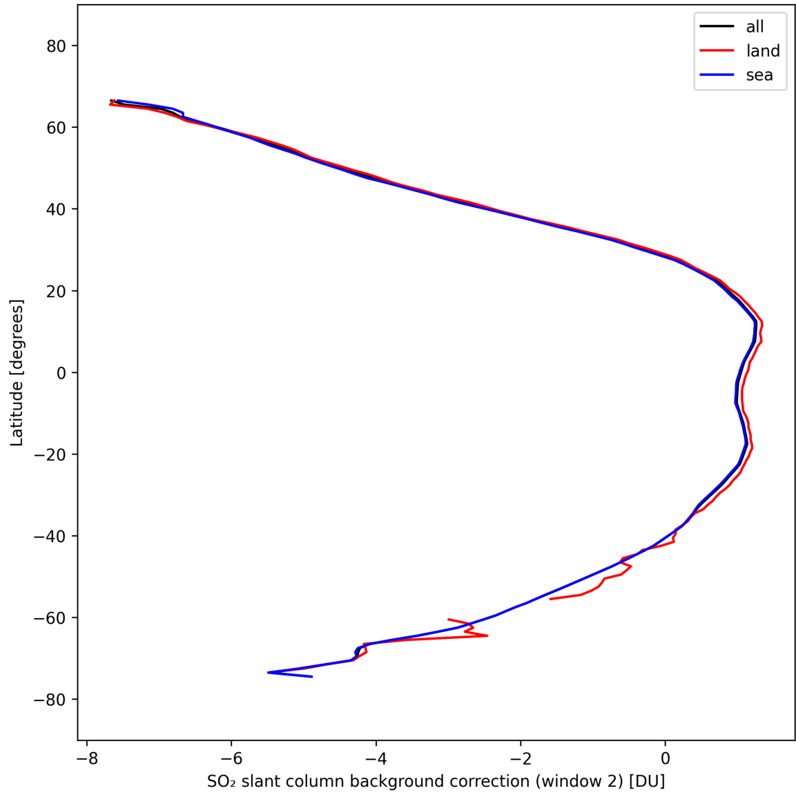
Figure 44: Zonal average of “SO 2 slant column background correction (window 2)” for 2025-03-09 to 2025-03-11.
