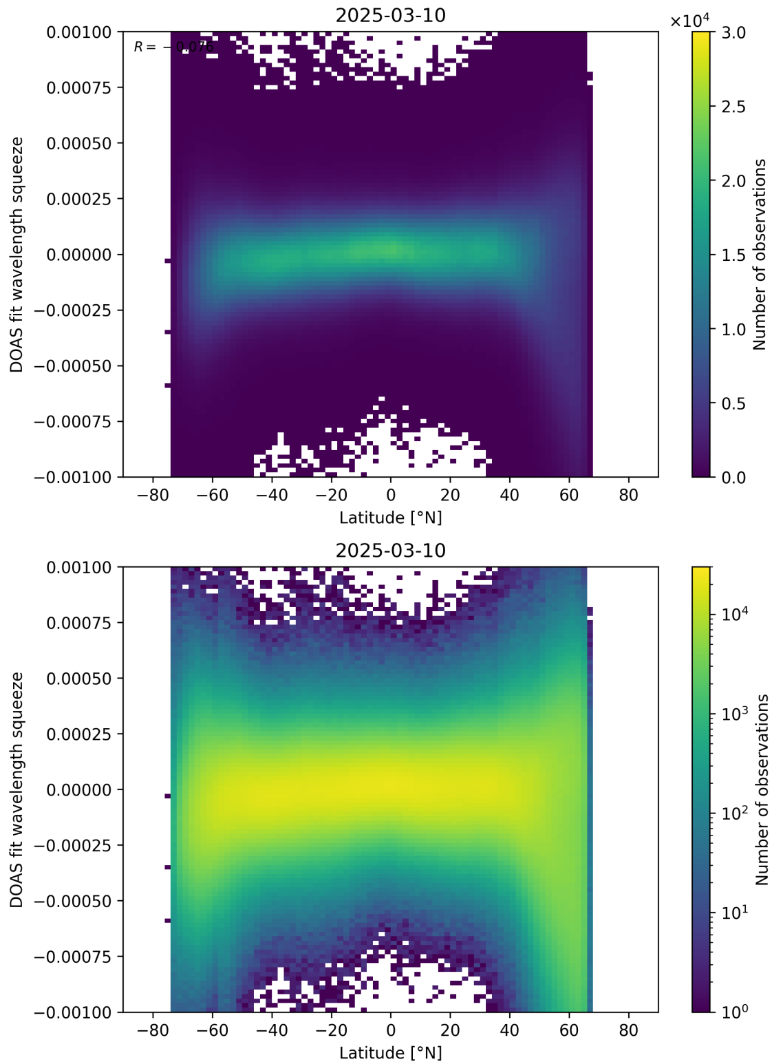
Figure 154: Scatter density plot of “Latitude” against “DOAS fit wavelength squeeze” for 2025-03-09 to 2025-03-11.
