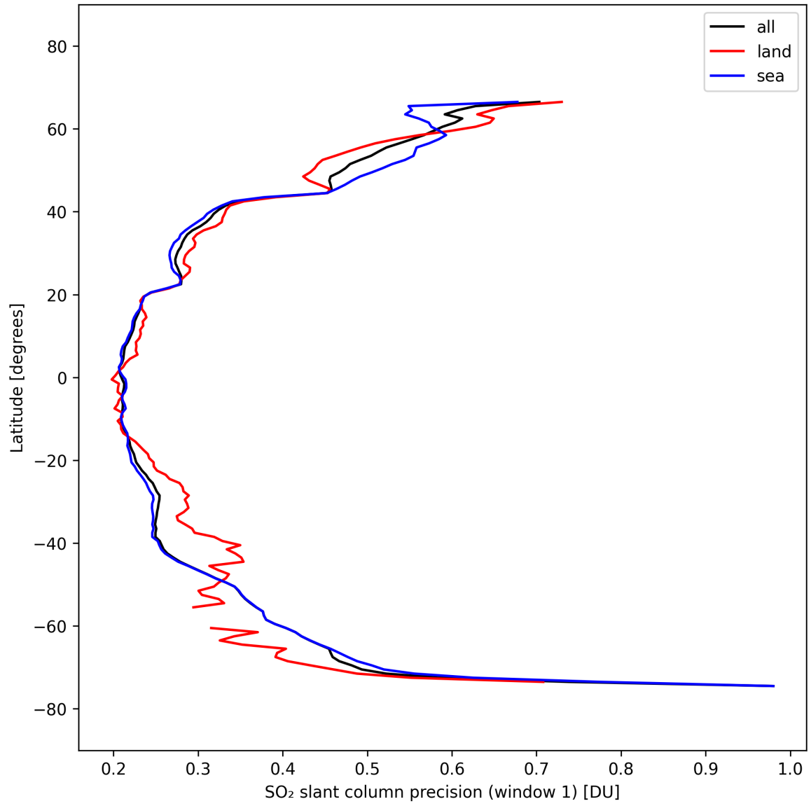
Figure 38: Zonal average of “SO 2 slant column precision (window 1)” for 2025-03-09 to 2025-03-11.
