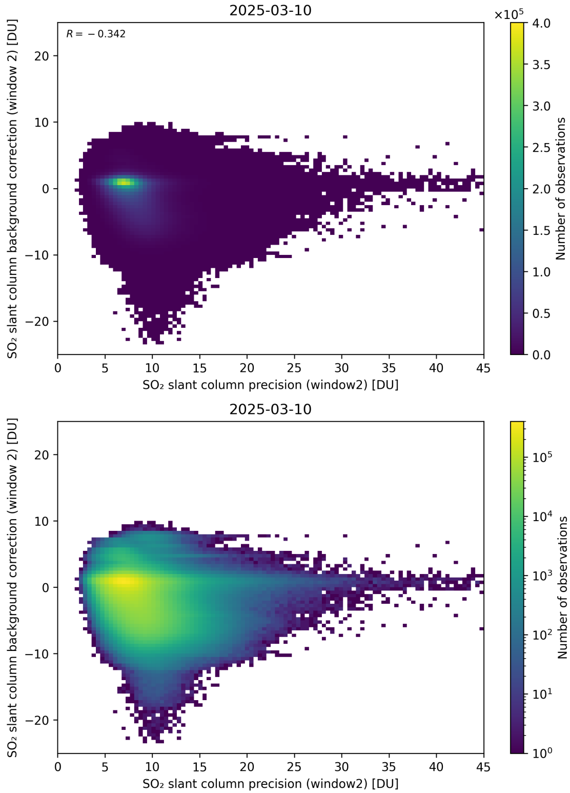
Figure 291: Scatter density plot of “SO 2 slant column precision (window2)” against “SO 2 slant column background correction (window 2)” for 2025-03-09 to 2025-03-11.
