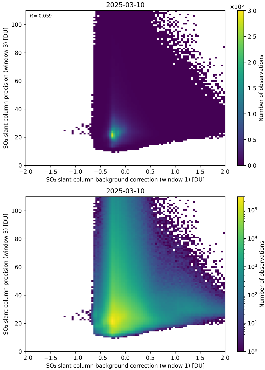
Figure 119: Scatter density plot of “SO 2 slant column background correction (window 1)” against “SO 2 slant column precision (window 3)” for 2025-03-09 to 2025-03-11.
