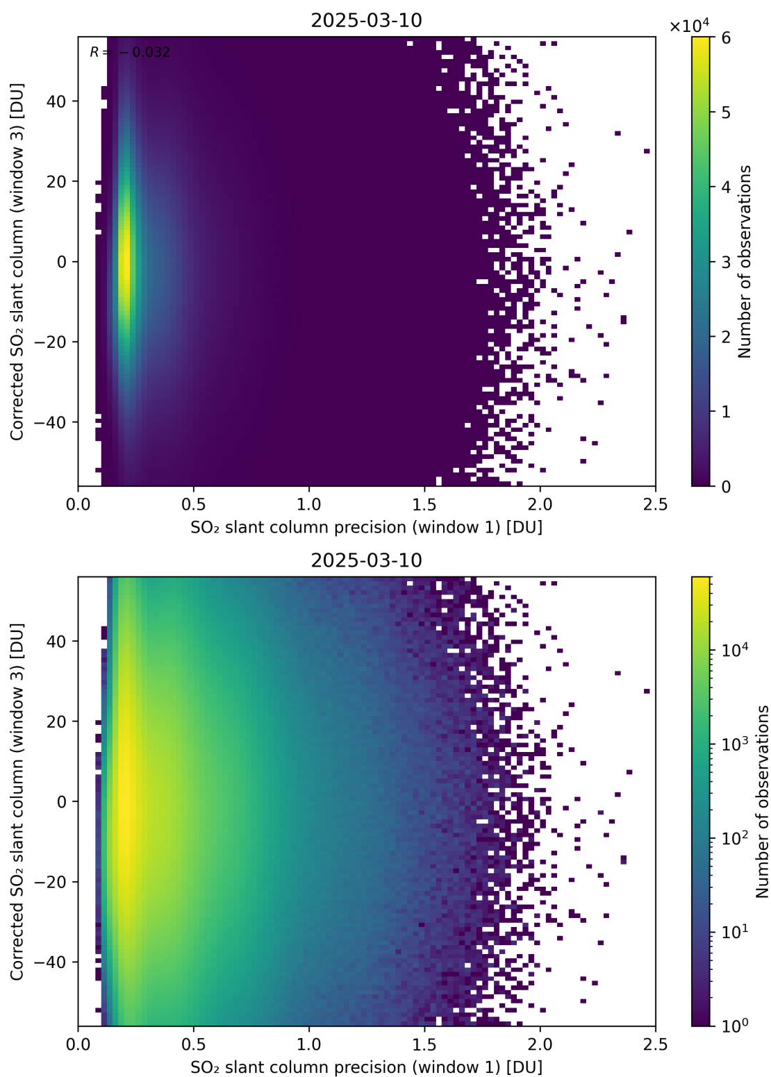
Figure 276: Scatter density plot of “SO 2 slant column precision (window 1)” against “Corrected SO 2 slant column (window 3)” for 2025-03-09 to 2025-03-11.
