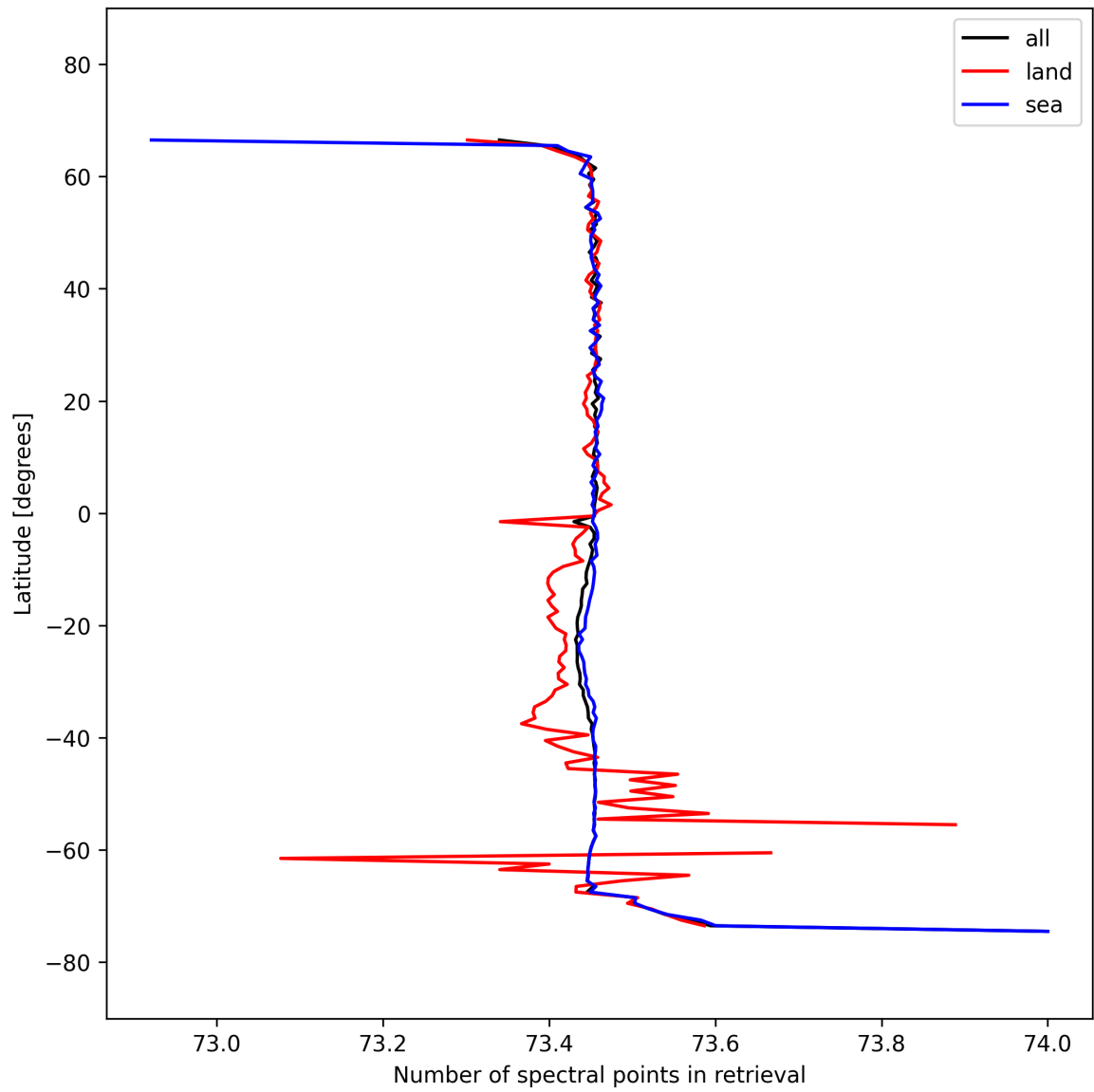
Figure 56: Zonal average of “Number of spectral points in retrieval” for 2025-03-09 to 2025-03-11.
