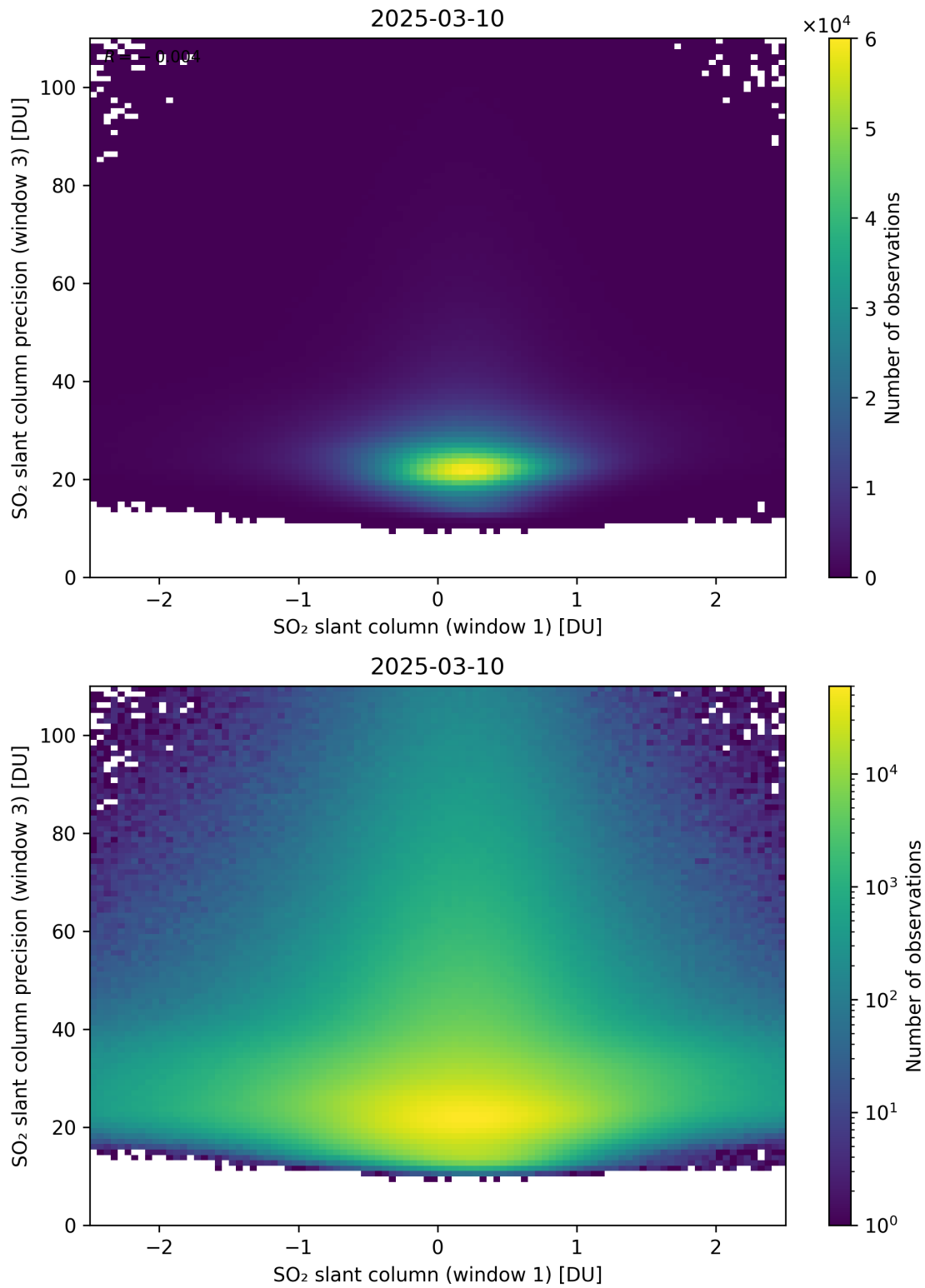
Figure 288: Scatter density plot of “SO 2 slant column (window 1)” against “SO 2 slant column precision (window 3)” for 2025-03-09 to 2025-03-11.
