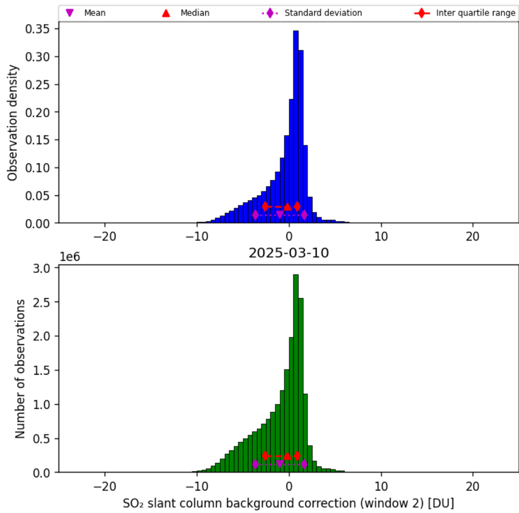
Figure 70: Histogram of “SO 2 slant column background correction (window 2)” for 2025-03-09 to 2025-03-11
