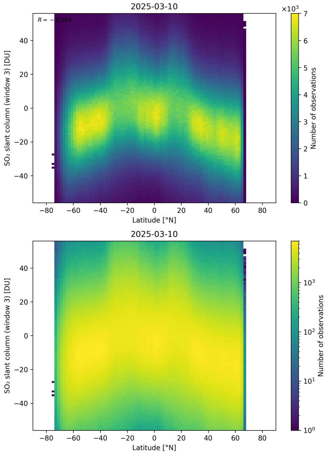
Figure 165: Scatter density plot of “Latitude” against “SO 2 slant column (window 3)” for 2025-03-09 to 2025-03-11.
