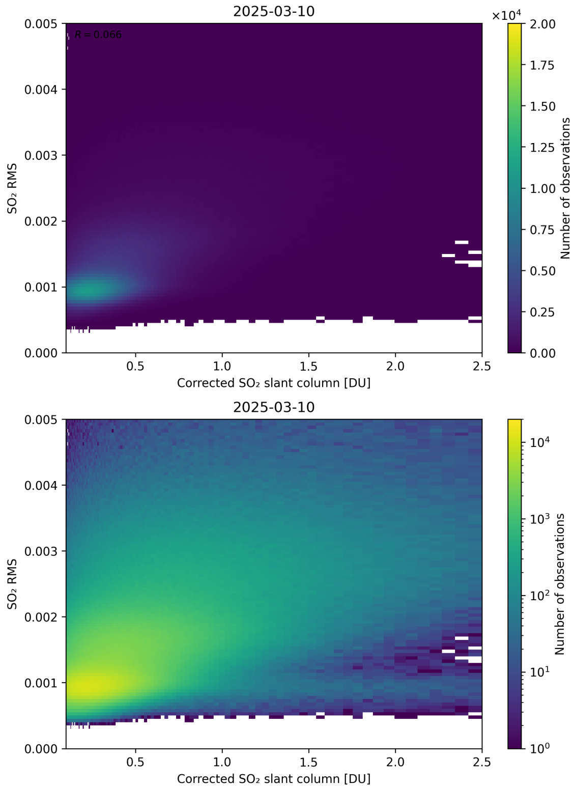
Figure 231: Scatter density plot of “Corrected SO 2 slant column” against “SO 2 RMS” for 2025-03-09 to 2025-03-11.
