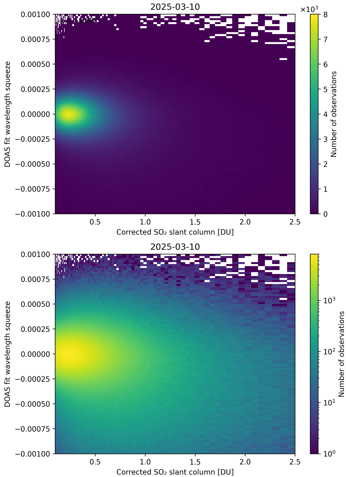
Figure 230: Scatter density plot of "Corrected SO 2 slant column" against "DOAS fit wavelength squeeze" for 2025-03-09 to 2025-03-11.
