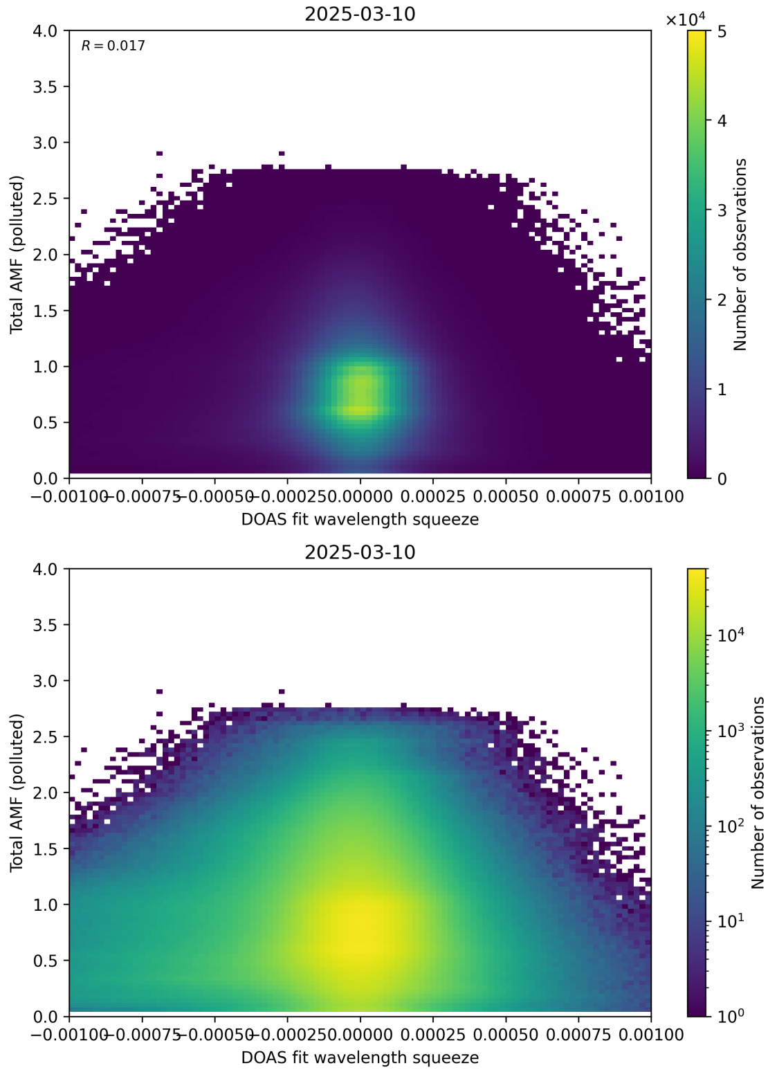
Figure 145: Scatter density plot of “DOAS fit wavelength squeeze” against “Total AMF (polluted)” for 2025-03-09 to 2025-03-11.
