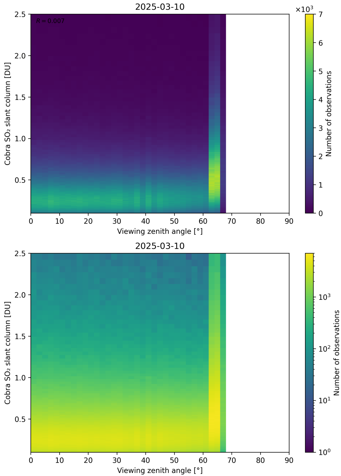
Figure 371: Scatter density plot of “Viewing zenith angle” against “Cobra SO 2 slant column” for 2025-03-09 to 2025-03-11.
