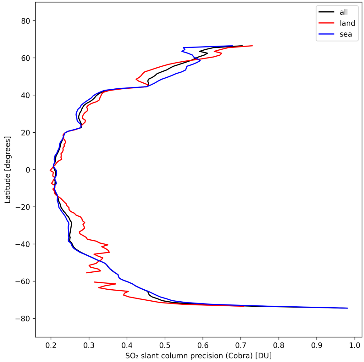
Figure 36: Zonal average of “SO 2 slant column precision (Cobra)” for 2025-03-09 to 2025-03-11.
