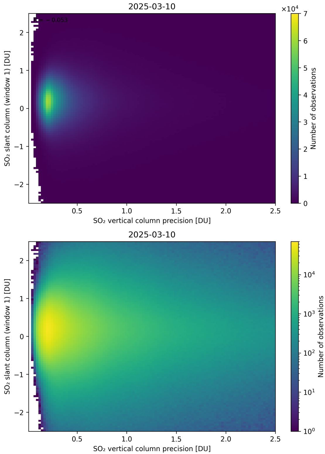
Figure 341: Scatter density plot of “SO 2 vertical column precision” against “SO 2 slant column (window 1)” for 2025-03-09 to 2025-03-11.
