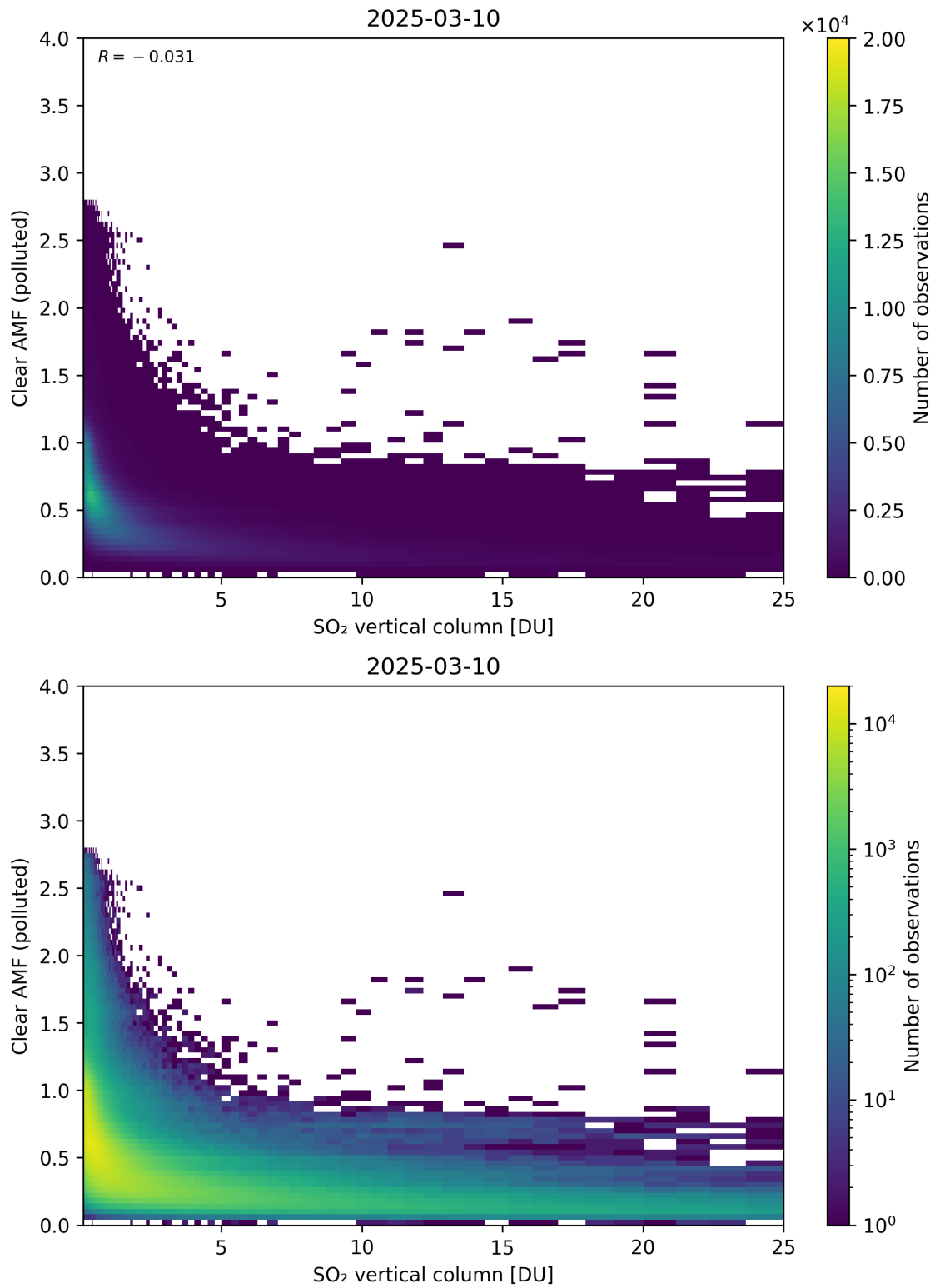
Figure 348: Scatter density plot of “SO 2 vertical column” against “Clear AMF (polluted)” for 2025-03-09 to 2025-03-11.
