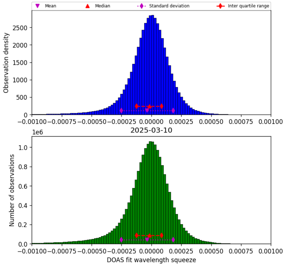
Figure 77: Histogram of “DOAS fit wavelength squeeze” for 2025-03-09 to 2025-03-11
