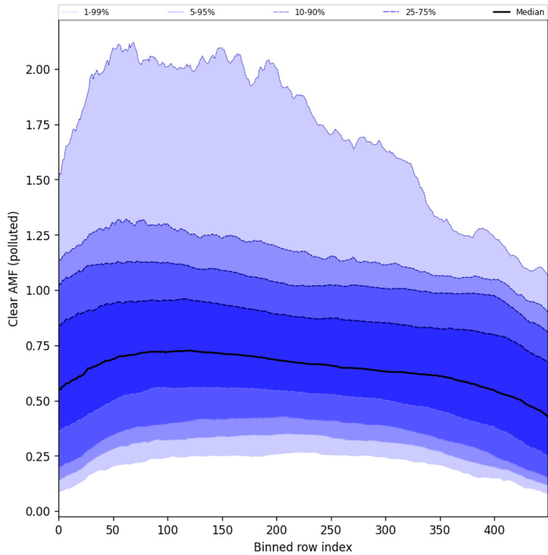
Figure 107: Along track statistics of “Clear AMF (polluted)” for 2025-03-09 to 2025-03-11
