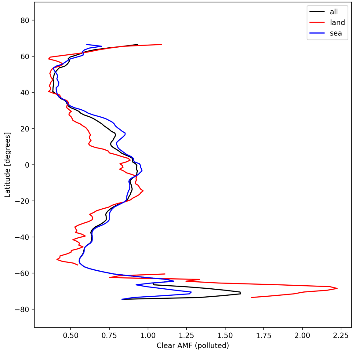
Figure 55: Zonal average of “Clear AMF (polluted)” for 2025-03-09 to 2025-03-11.
