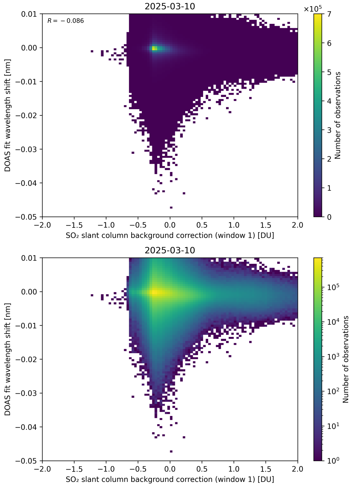
Figure 111: Scatter density plot of “SO 2 slant column background correction (window 1)” against “DOAS fit wavelength shift” for 2025-03-09 to 2025-03-11.
