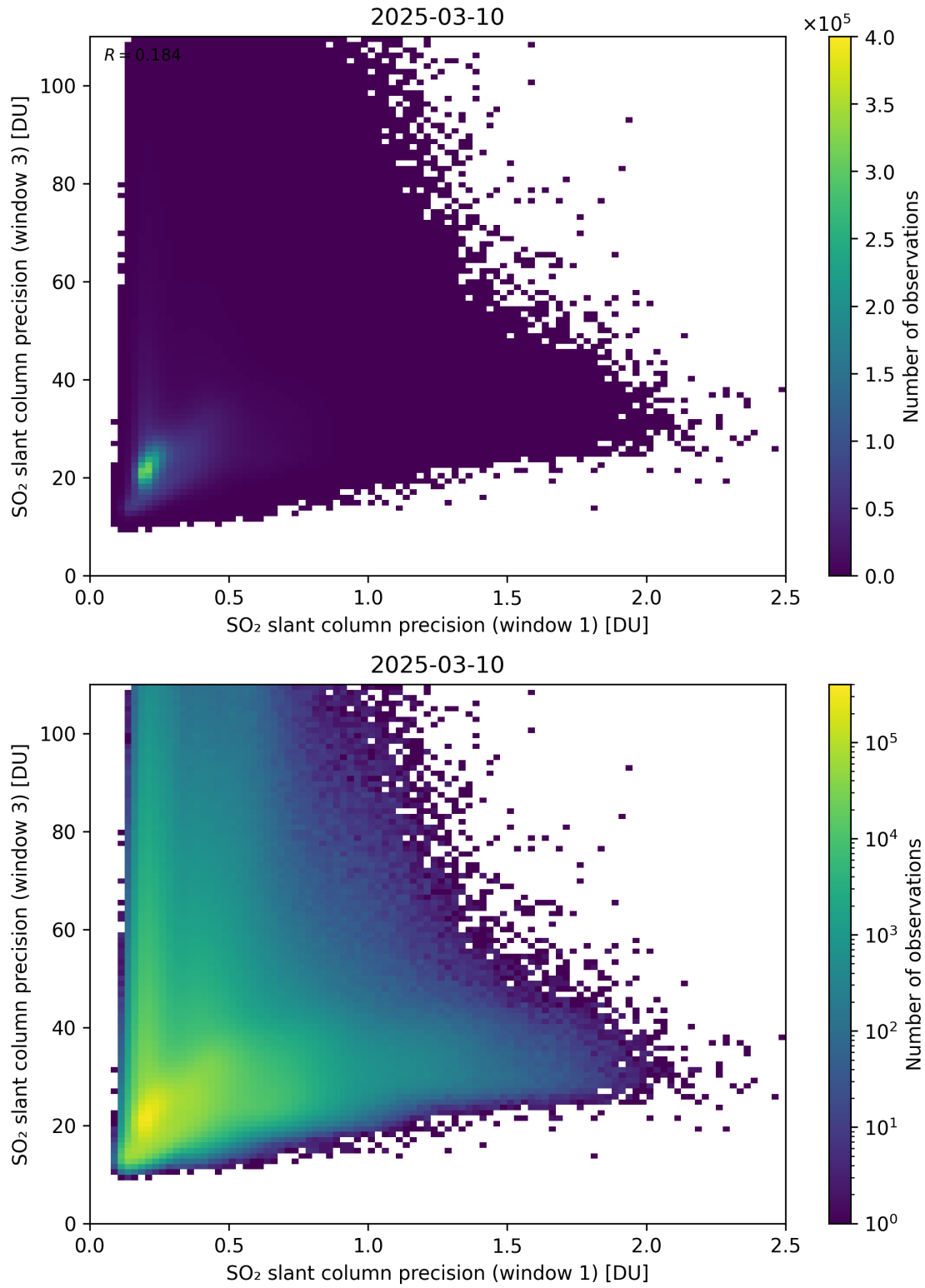
Figure 279: Scatter density plot of “SO 2 slant column precision (window 1)” against “SO 2 slant column precision (window 3)” for 2025-03-09 to 2025-03-11.
