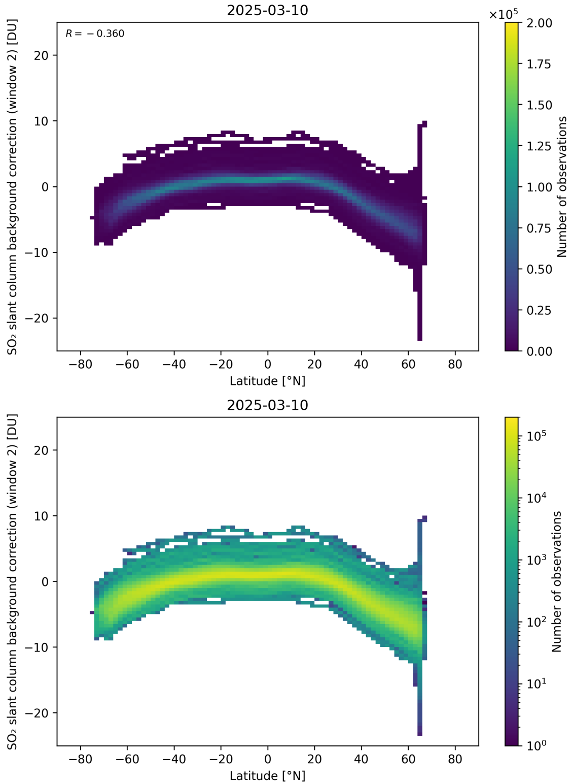
Figure 151: Scatter density plot of “Latitude” against “SO 2 slant column background correction (window 2)” for 2025-03-09 to 2025-03-11.
