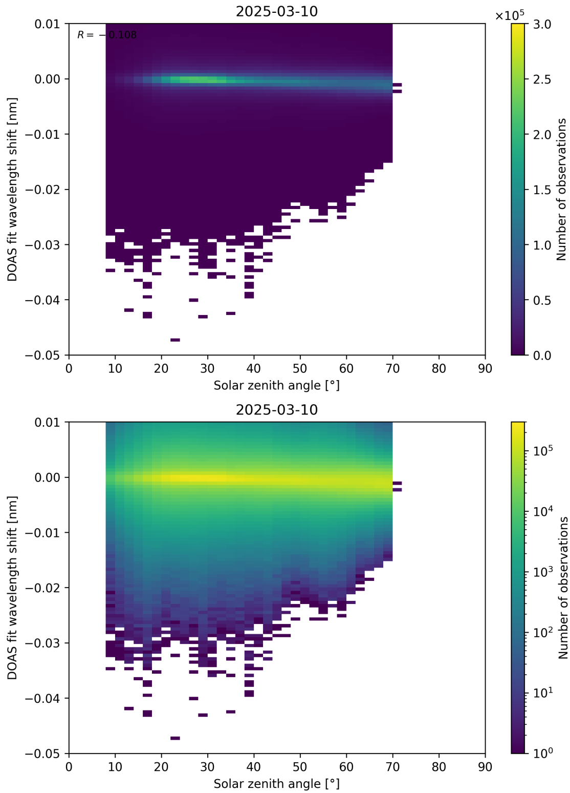
Figure 174: Scatter density plot of “Solar zenith angle” against “DOAS fit wavelength shift” for 2025-03-09 to 2025-03-11.
