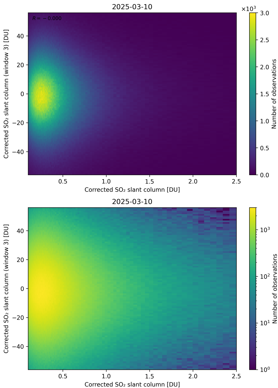
Figure 236: Scatter density plot of “Corrected SO 2 slant column” against “Corrected SO 2 slant column (window 3)” for 2025-03-09 to 2025-03-11.
