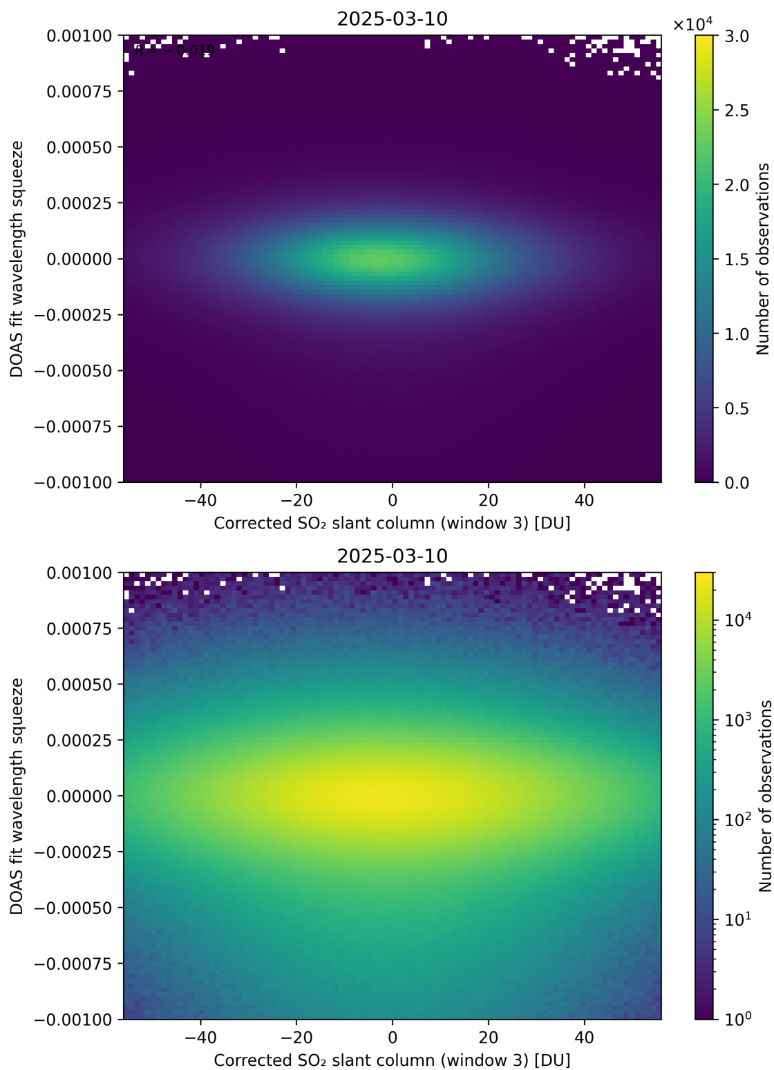
Figure 257: Scatter density plot of “Corrected SO 2 slant column (window 3)” against “DOAS fit wavelength squeeze” for 2025-03-09 to 2025-03-11.
