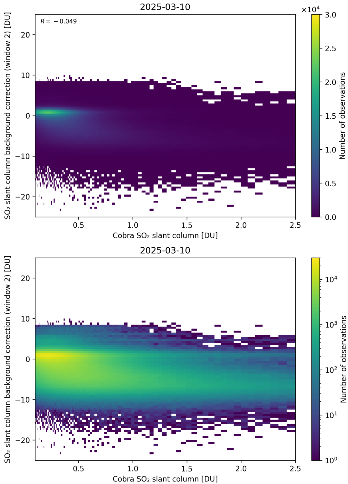
Figure 194: Scatter density plot of “Cobra SO 2 slant column” against “SO 2 slant column background correction (window 2)” for 2025-03-09 to 2025-03-11.
