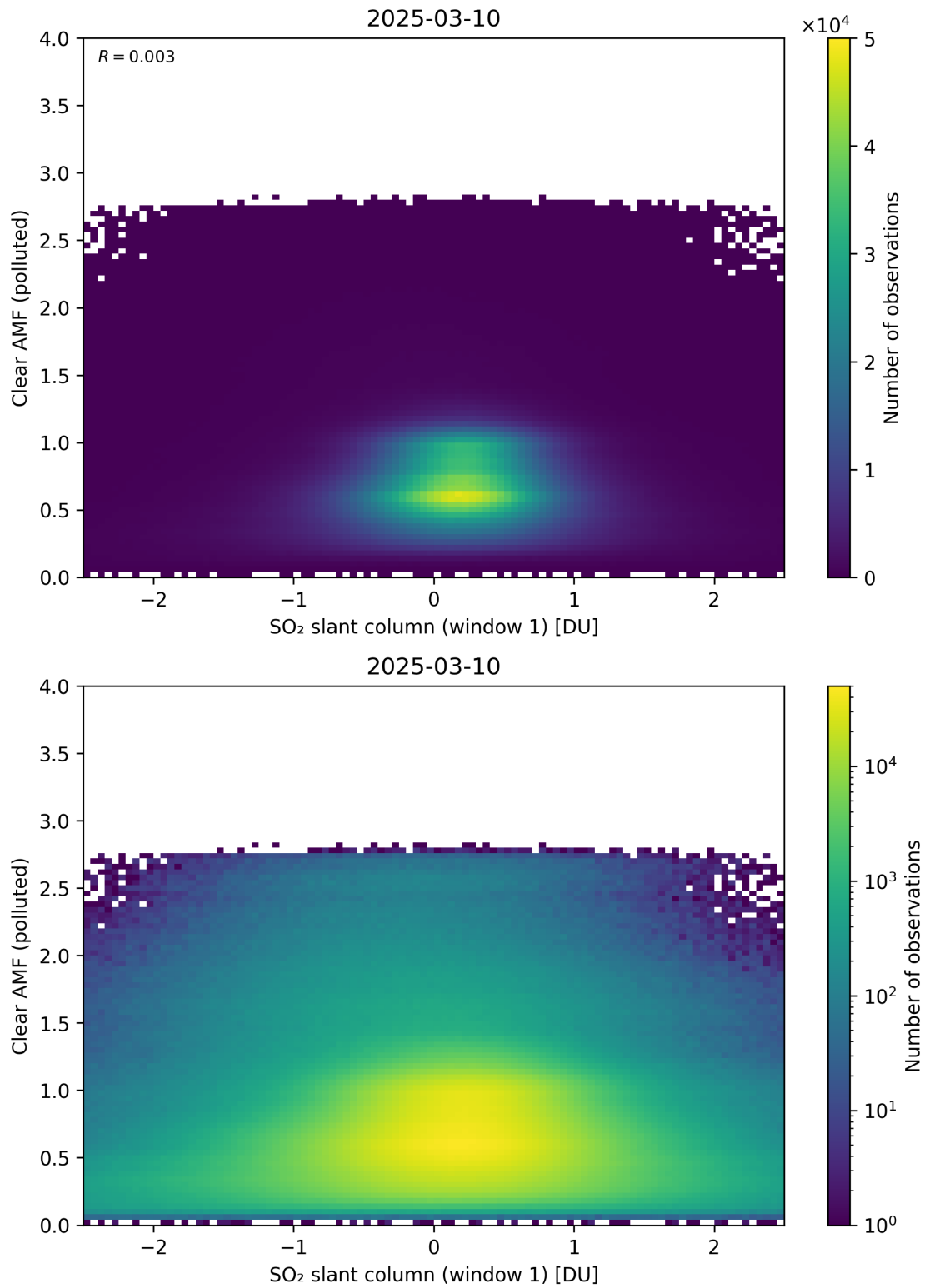
Figure 282: Scatter density plot of “SO 2 slant column (window 1)” against “Clear AMF (polluted)” for 2025-03-09 to 2025-03-11.
