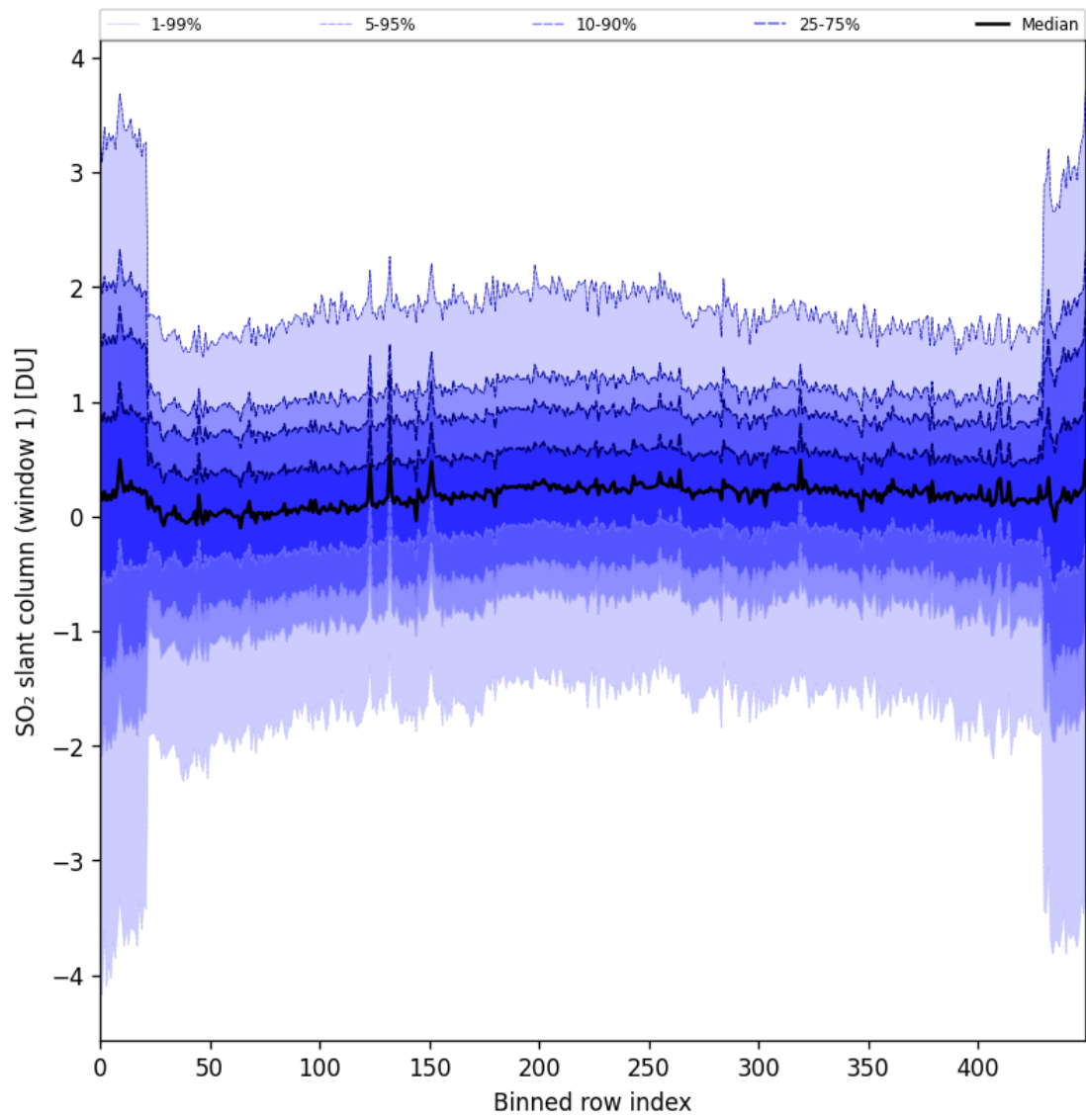
Figure 89: Along track statistics of “SO 2 slant column (window 1)” for 2025-03-09 to 2025-03-11
