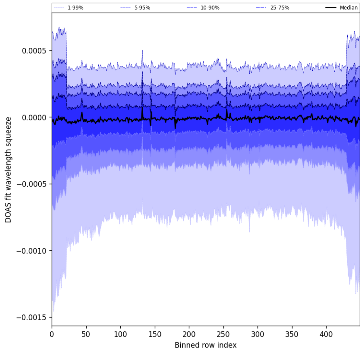
Figure 103: Along track statistics of “DOAS fit wavelength squeeze” for 2025-03-09 to 2025-03-11
