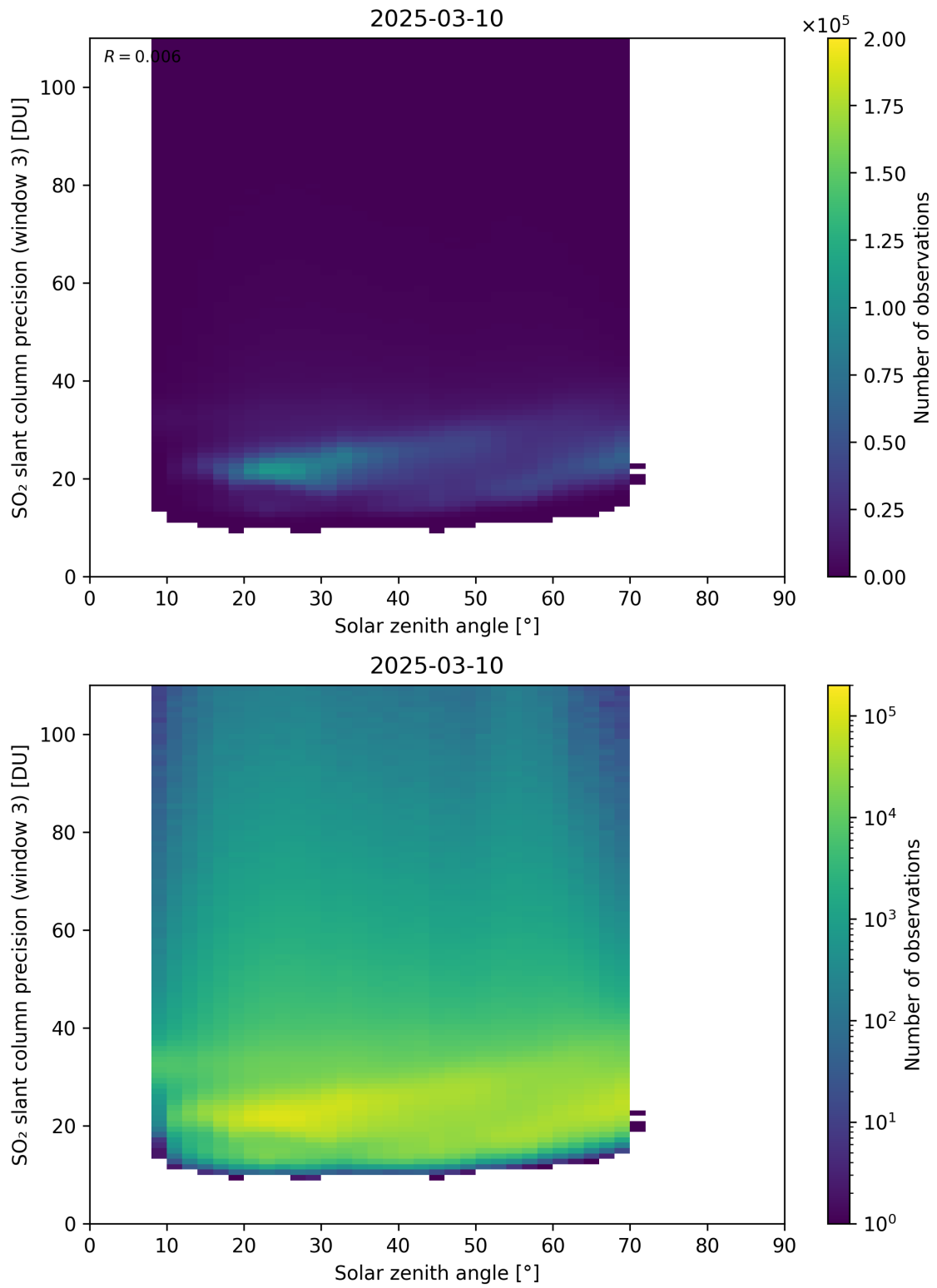
Figure 188: Scatter density plot of “Solar zenith angle” against “SO 2 slant column precision (window 3)” for 2025-03-09 to 2025-03-11.
