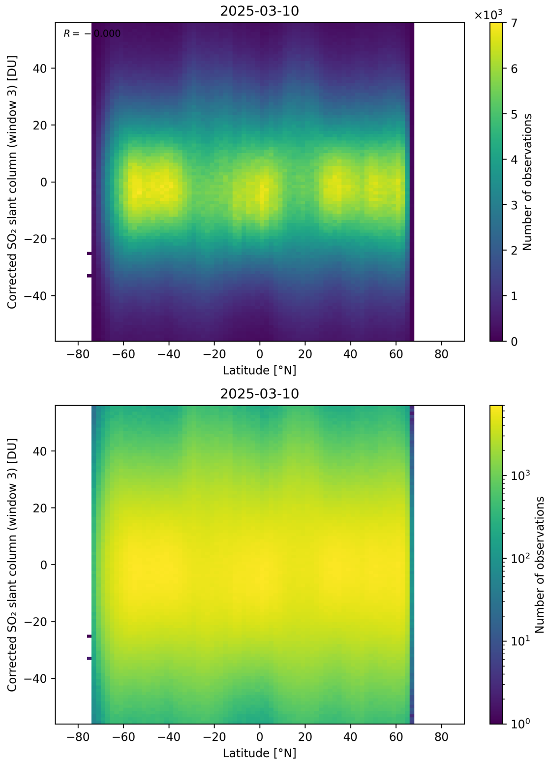
Figure 161: Scatter density plot of “Latitude” against “Corrected SO 2 slant column (window 3)” for 2025-03-09 to 2025-03-11.
