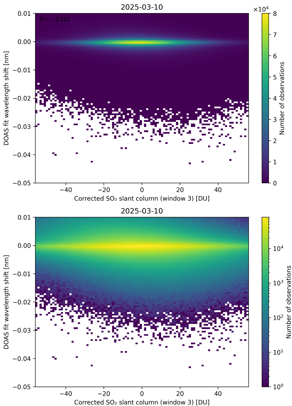
Figure 256: Scatter density plot of “Corrected SO 2 slant column (window 3)” against “DOAS fit wavelength shift” for 2025-03-09 to 2025-03-11.
