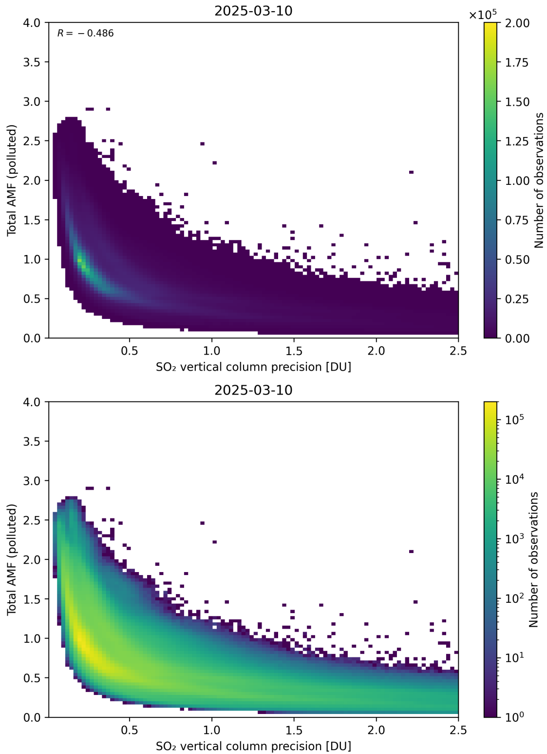
Figure 346: Scatter density plot of “SO 2 vertical column precision” against “Total AMF (polluted)” for 2025-03-09 to 2025-03-11.
