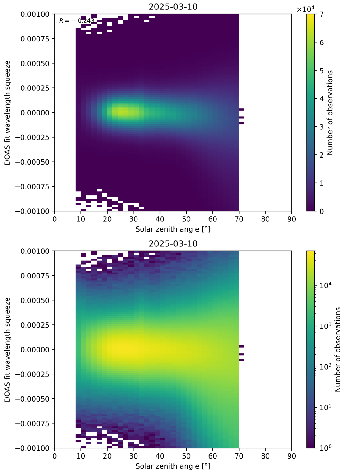
Figure 175: Scatter density plot of “Solar zenith angle” against “DOAS fit wavelength squeeze” for 2025-03-09 to 2025-03-11.
