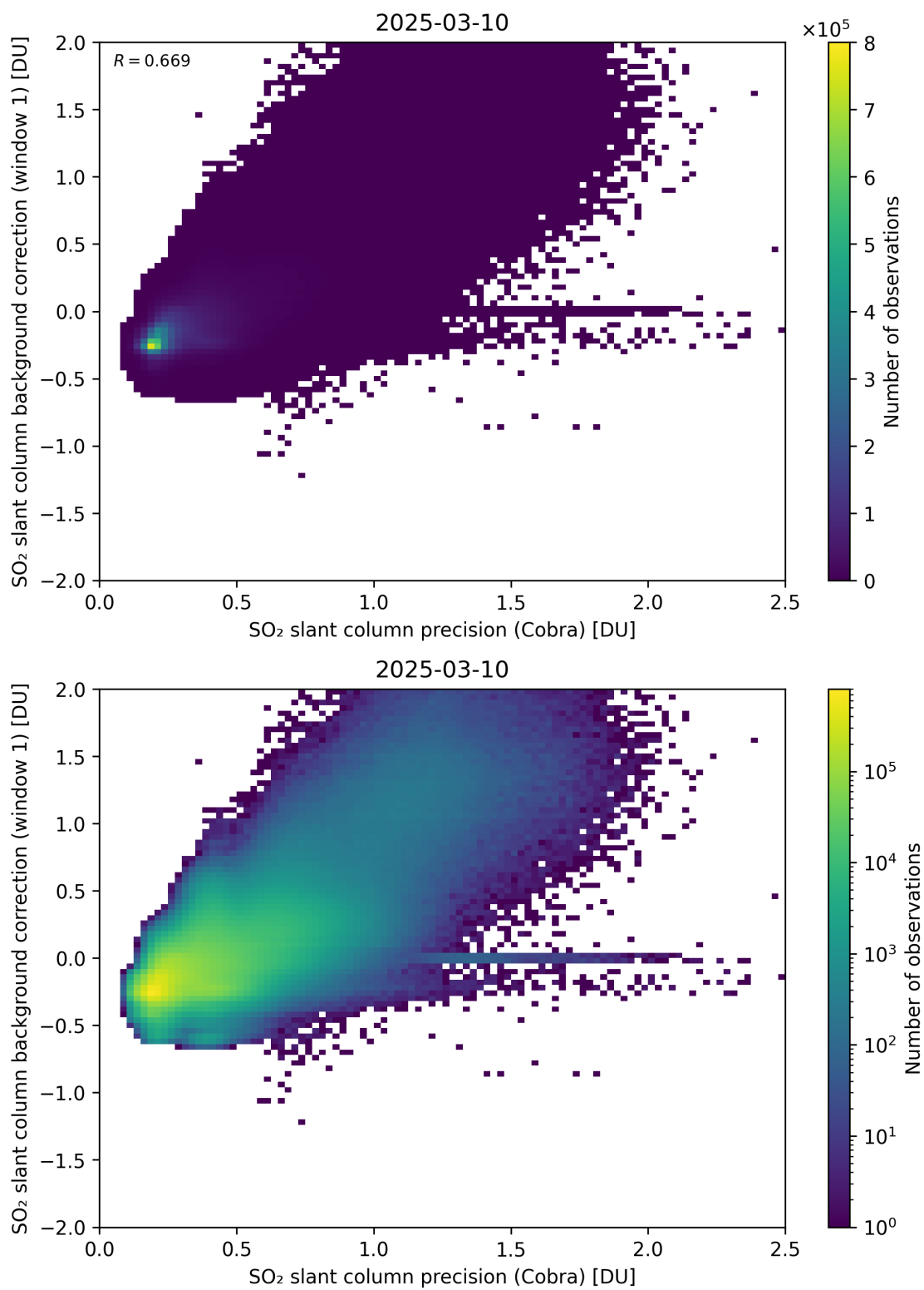
Figure 199: Scatter density plot of “SO 2 slant column precision (Cobra)” against “SO 2 slant column background correction (window 1)” for 2025-03-09 to 2025-03-11.
