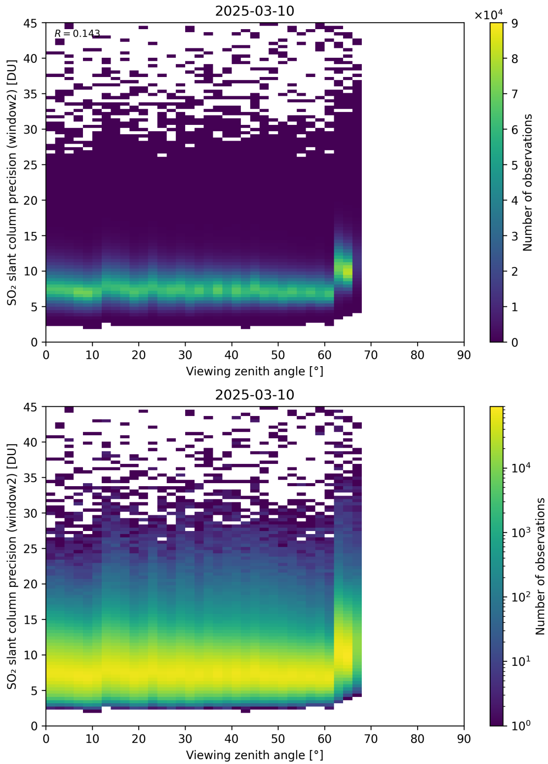
Figure 378: Scatter density plot of “Viewing zenith angle” against “SO 2 slant column precision (window2)” for 2025-03-09 to 2025-03-11.
