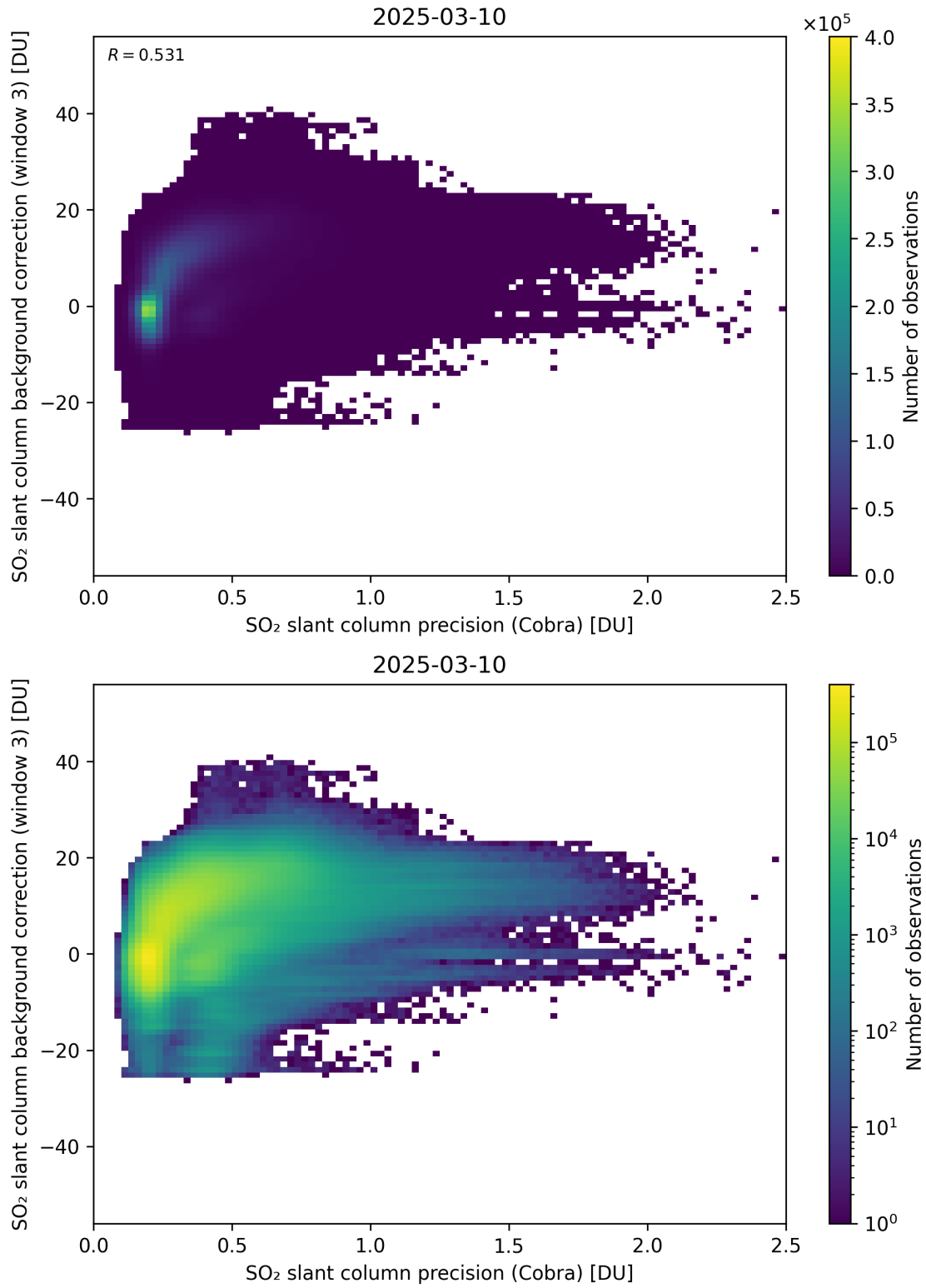
Figure 201: Scatter density plot of “SO 2 slant column precision (Cobra)” against “SO 2 slant column background correction (window 3)” for 2025-03-09 to 2025-03-11.
