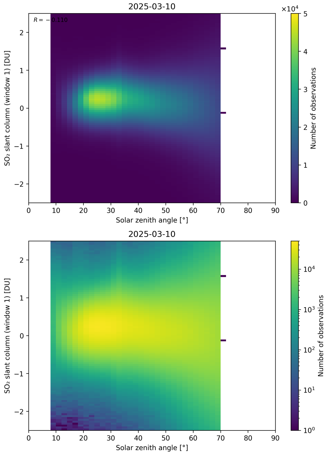
Figure 184: Scatter density plot of “Solar zenith angle” against “SO 2 slant column (window 1)” for 2025-03-09 to 2025-03-11.
