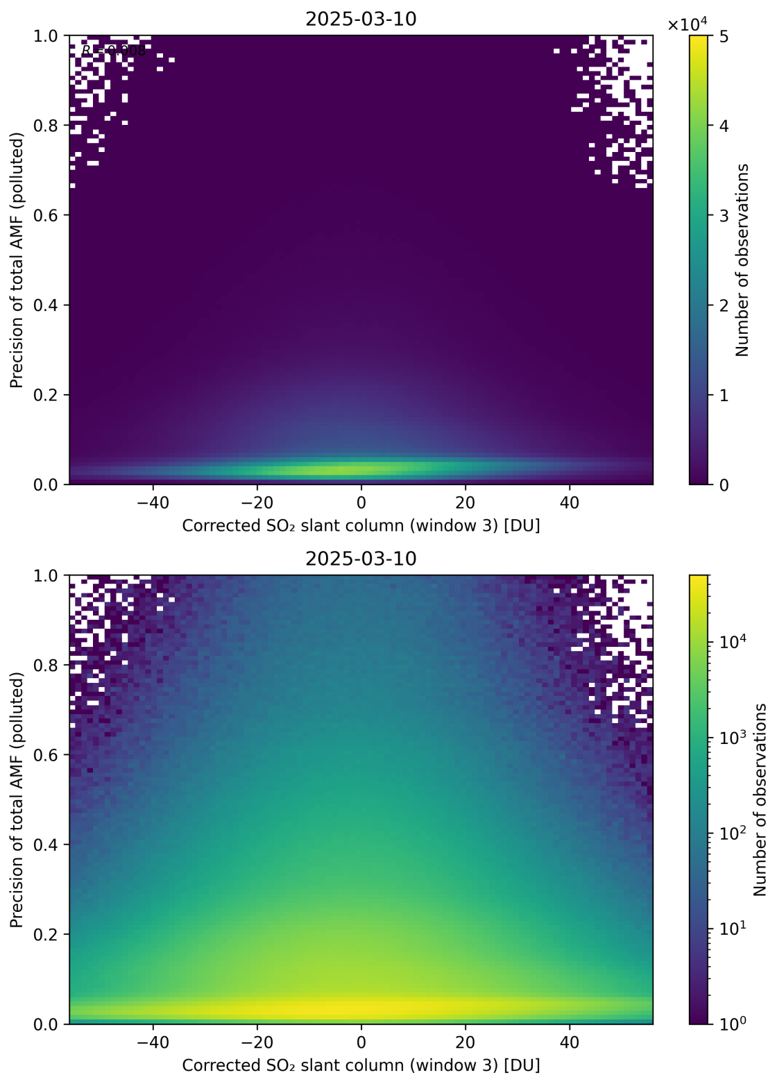
Figure 261: Scatter density plot of “Corrected SO 2 slant column (window 3)” against “Precision of total AMF (polluted)” for 2025-03-09 to 2025-03-11.
