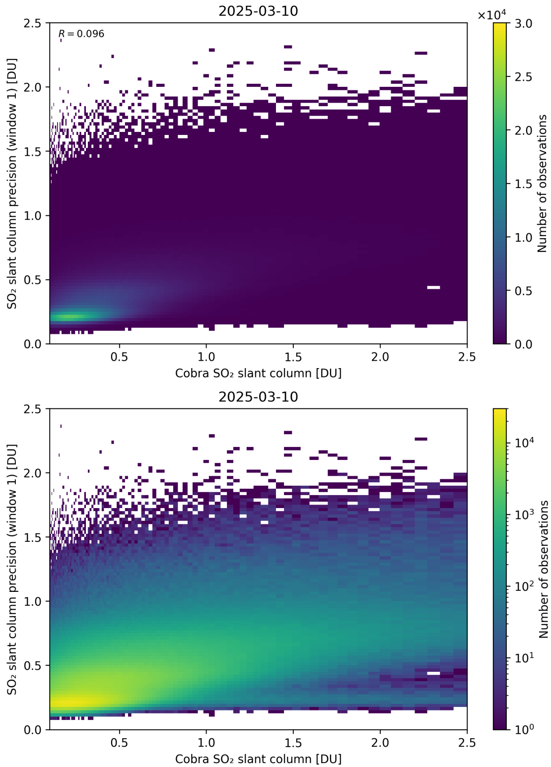
Figure 220: Scatter density plot of “Cobra SO 2 slant column” against “SO 2 slant column precision (window 1)” for 2025-03-09 to 2025-03-11.
