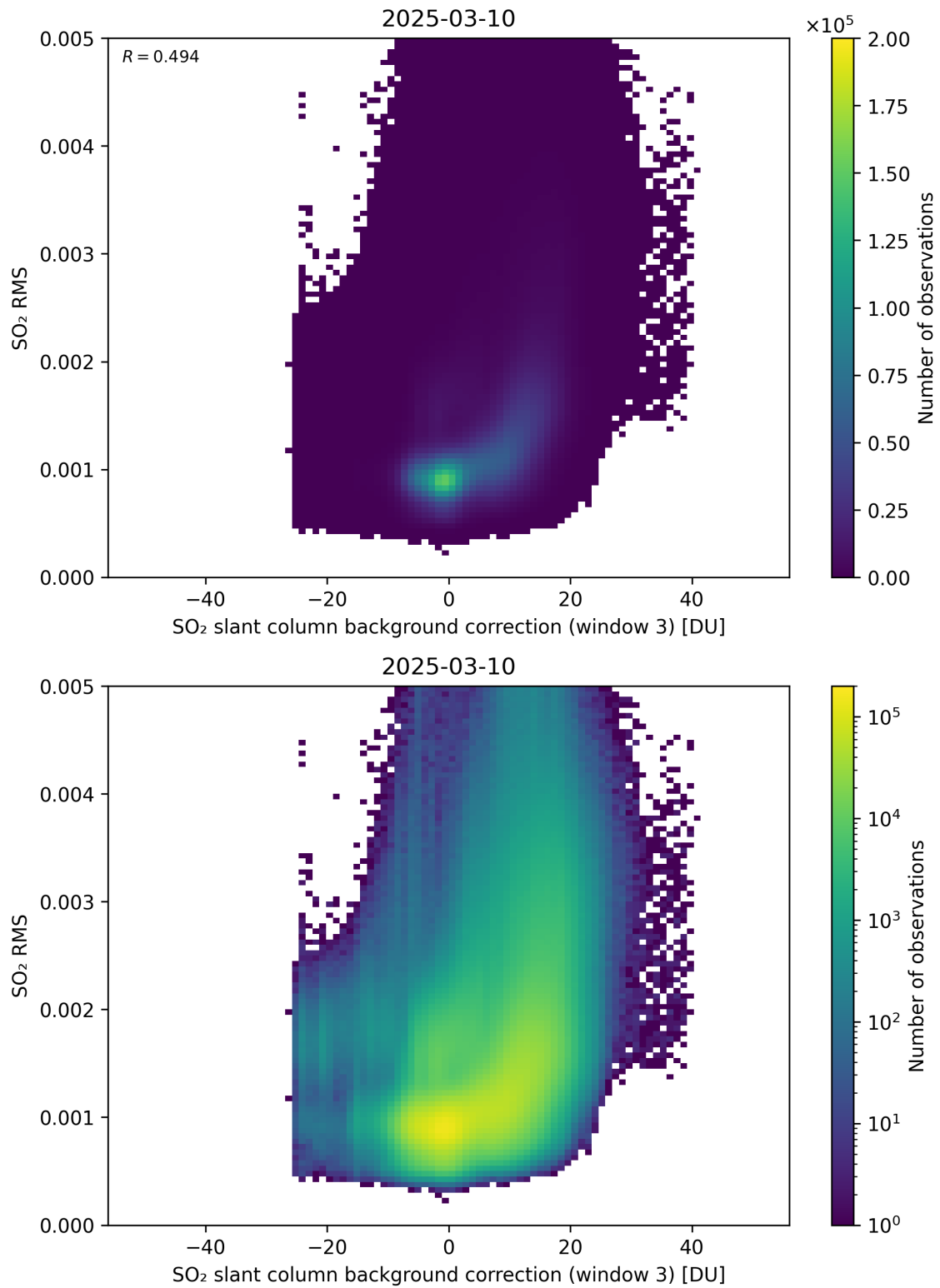
Figure 134: Scatter density plot of “SO 2 slant column background correction (window 3)” against “SO 2 RMS” for 2025-03-09 to 2025-03-11.
