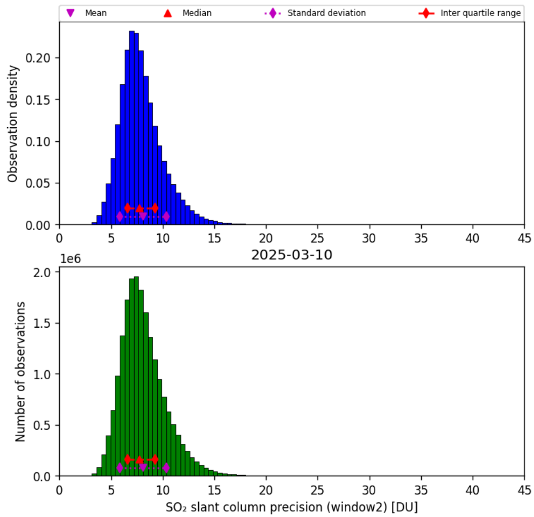
Figure 68: Histogram of “SO 2 slant column precision (window2)” for 2025-03-09 to 2025-03-11
