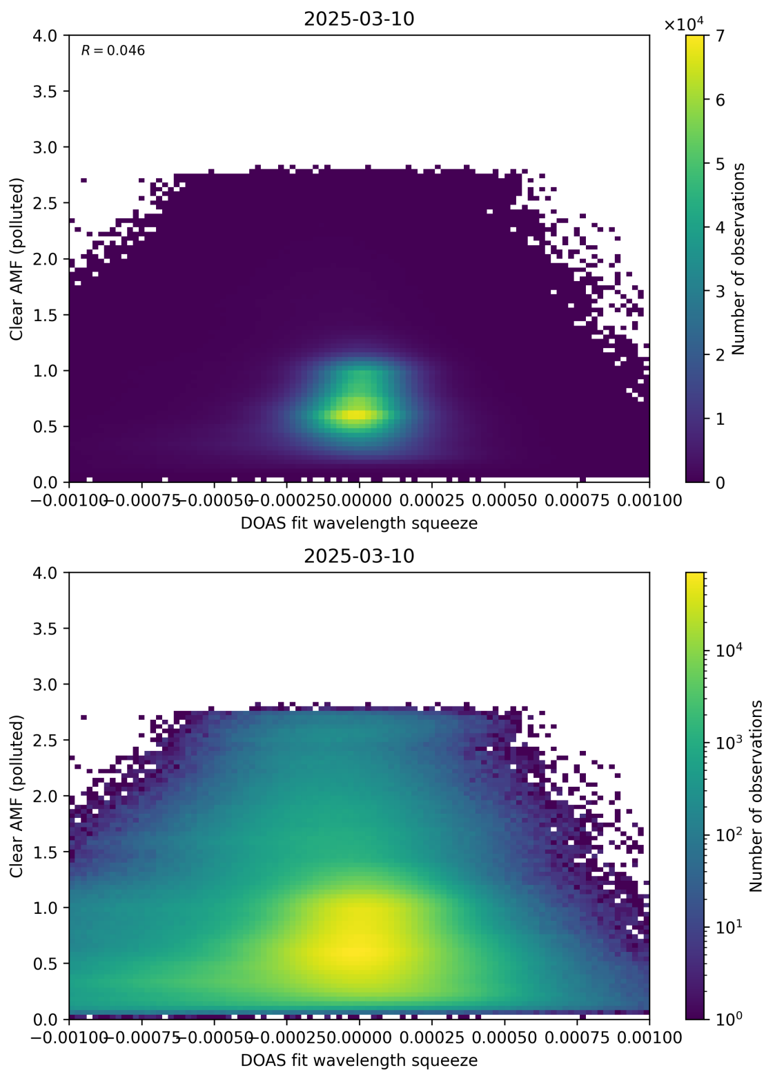
Figure 144: Scatter density plot of “DOAS fit wavelength squeeze” against “Clear AMF (polluted)” for 2025-03-09 to 2025-03-11.
