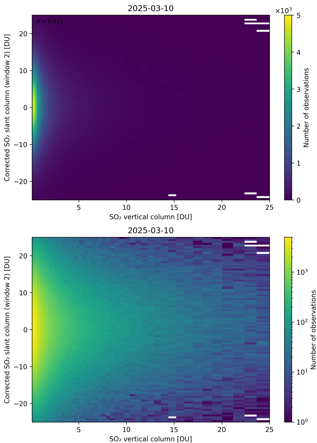
Figure 352: Scatter density plot of “SO 2 vertical column” against “Corrected SO 2 slant column (window 2)” for 2025-03-09 to 2025-03-11.
