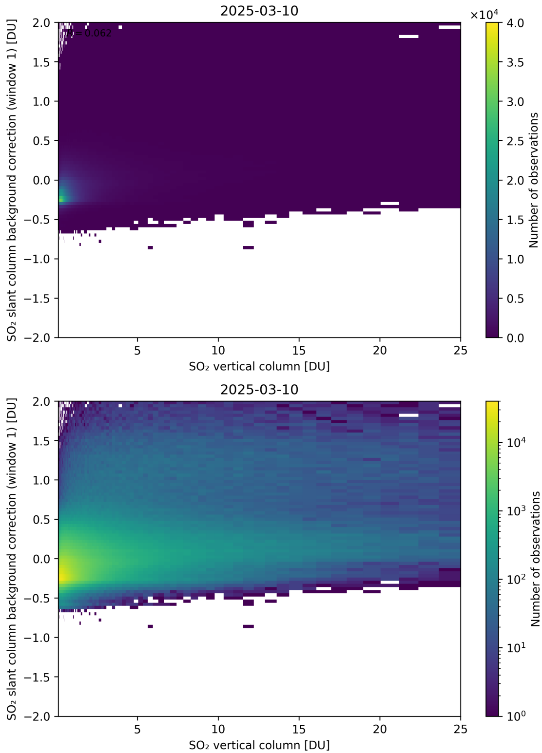
Figure 323: Scatter density plot of “SO 2 vertical column” against “SO 2 slant column background correction (window 1)” for 2025-03-09 to 2025-03-11.
