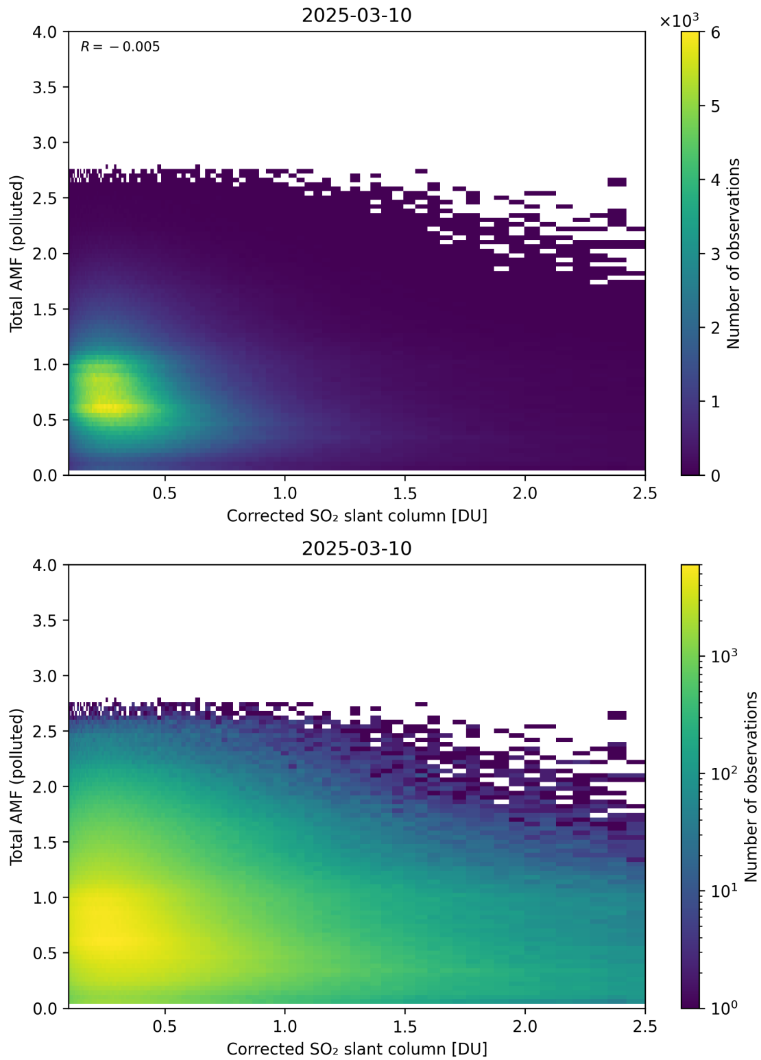
Figure 242: Scatter density plot of “Corrected SO 2 slant column” against “Total AMF (polluted)” for 2025-03-09 to 2025-03-11.
