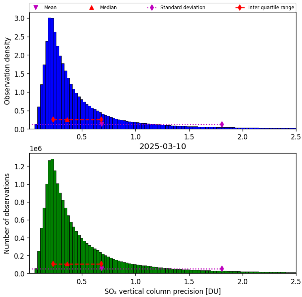
Figure 59: Histogram of “SO 2 vertical column precision” for 2025-03-09 to 2025-03-11
