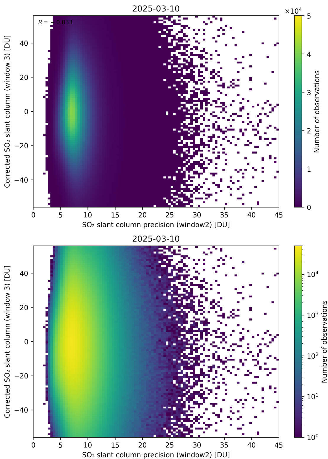
Figure 298: Scatter density plot of “SO 2 slant column precision (window2)” against “Corrected SO 2 slant column (window 3)” for 2025-03-09 to 2025-03-11.
