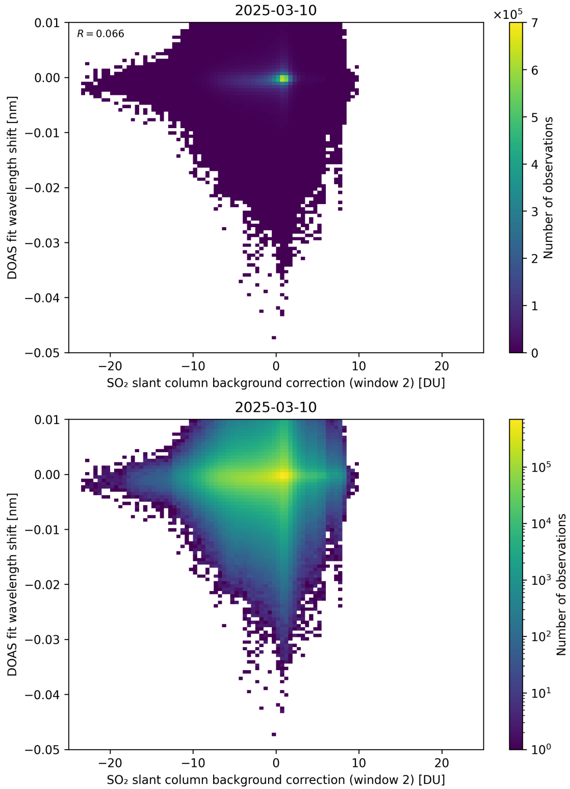
Figure 123: Scatter density plot of “SO 2 slant column background correction (window 2)” against “DOAS fit wavelength shift” for 2025-03-09 to 2025-03-11.
