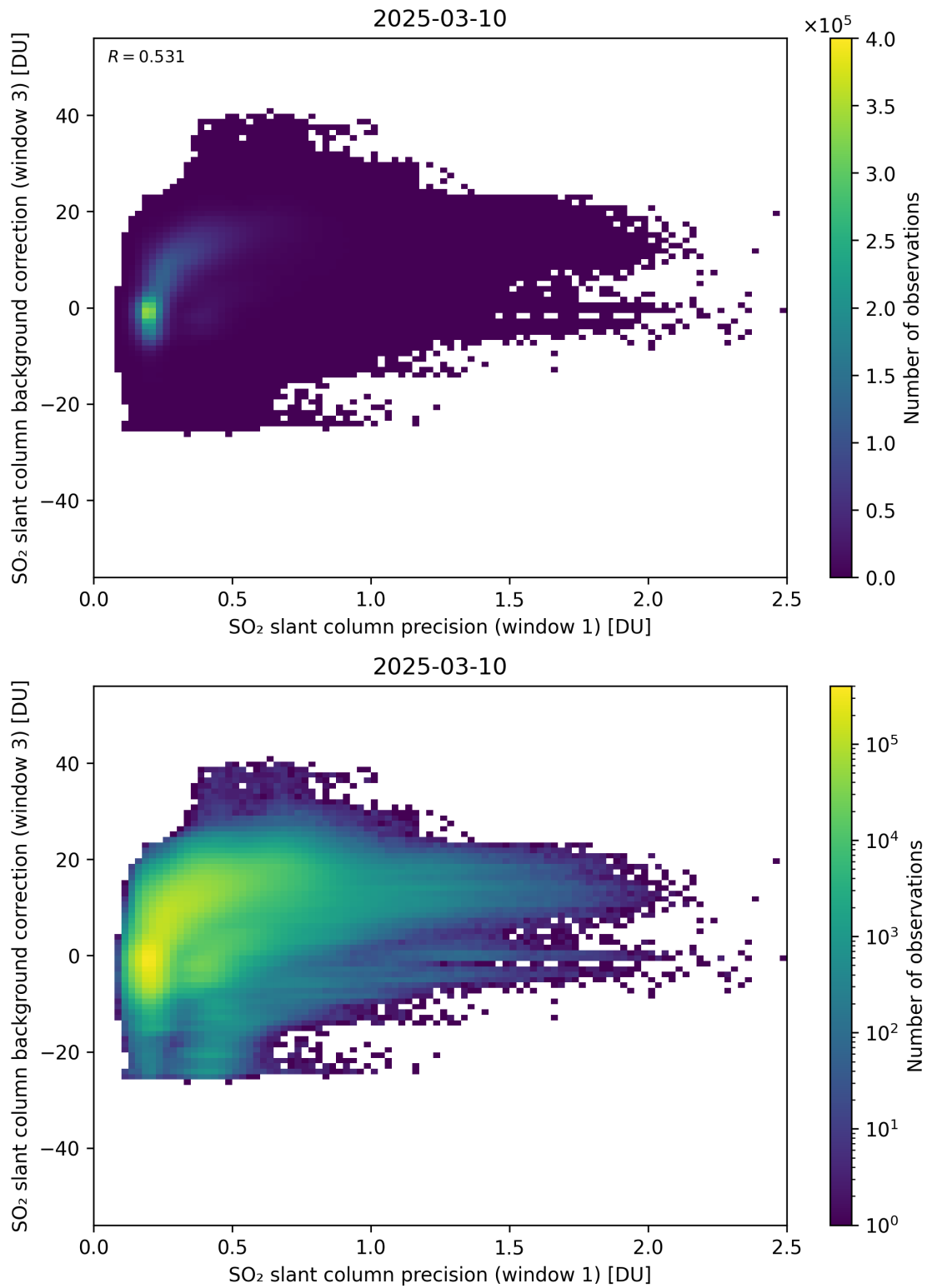
Figure 270: Scatter density plot of “SO 2 slant column precision (window 1)” against “SO 2 slant column background correction (window 3)” for 2025-03-09 to 2025-03-11.
