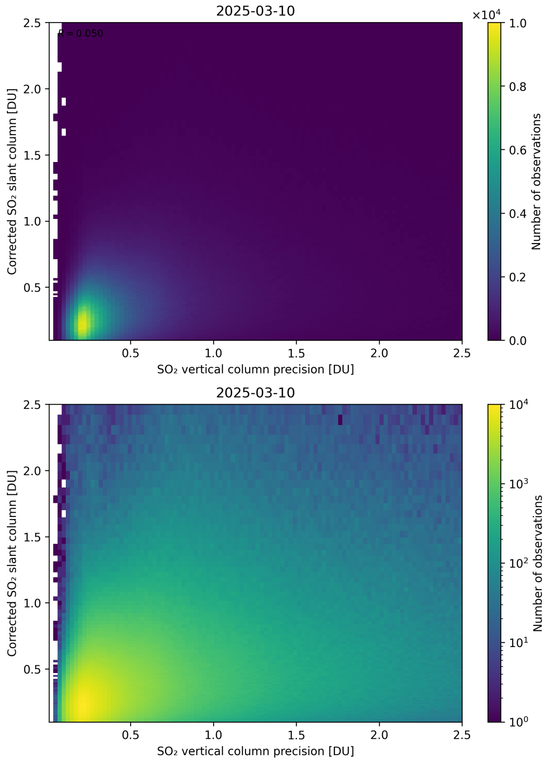
Figure 338: Scatter density plot of “SO 2 vertical column precision” against “Corrected SO 2 slant column” for 2025-03-09 to 2025-03-11.
