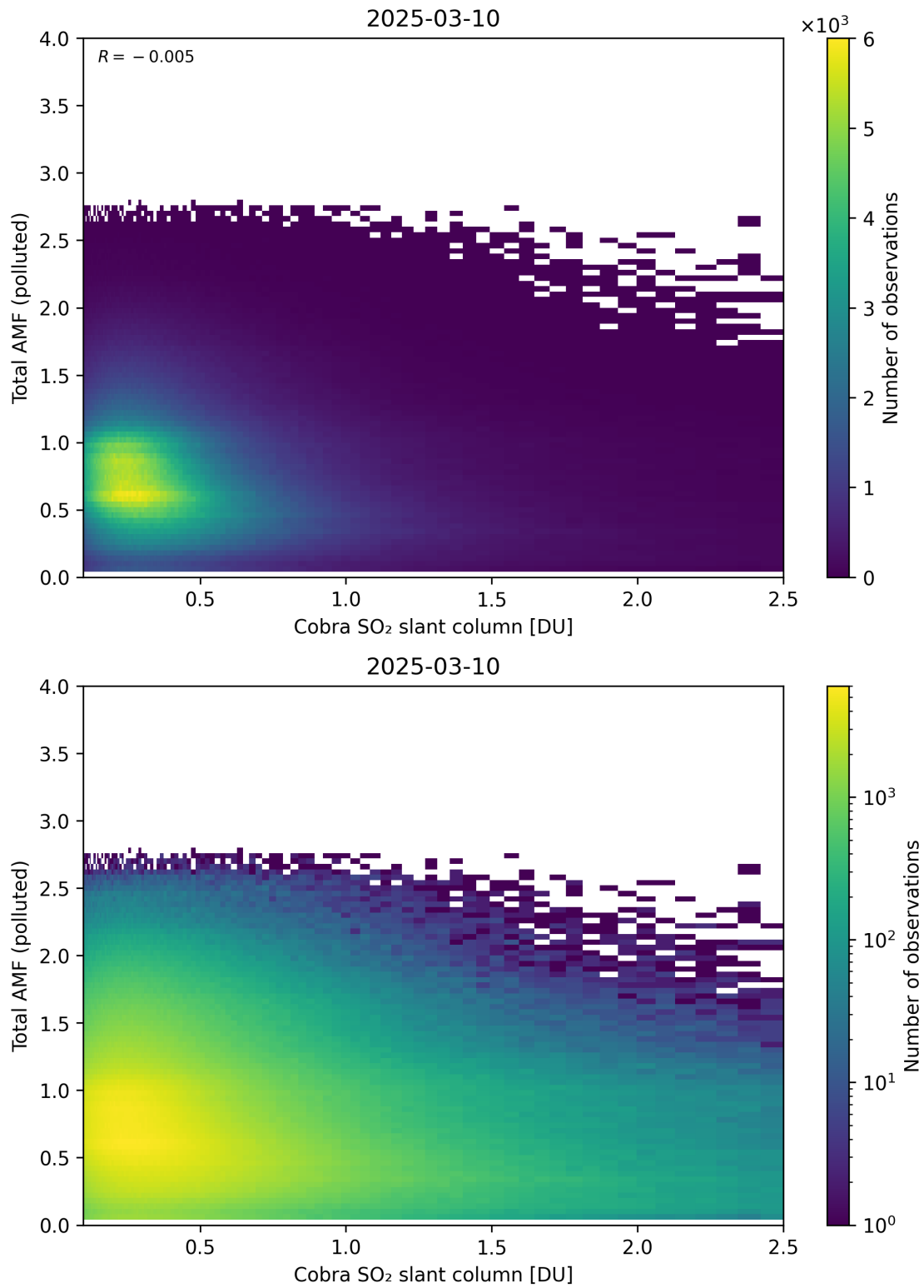
Figure 224: Scatter density plot of “Cobra SO 2 slant column” against “Total AMF (polluted)” for 2025-03-09 to 2025-03-11.
