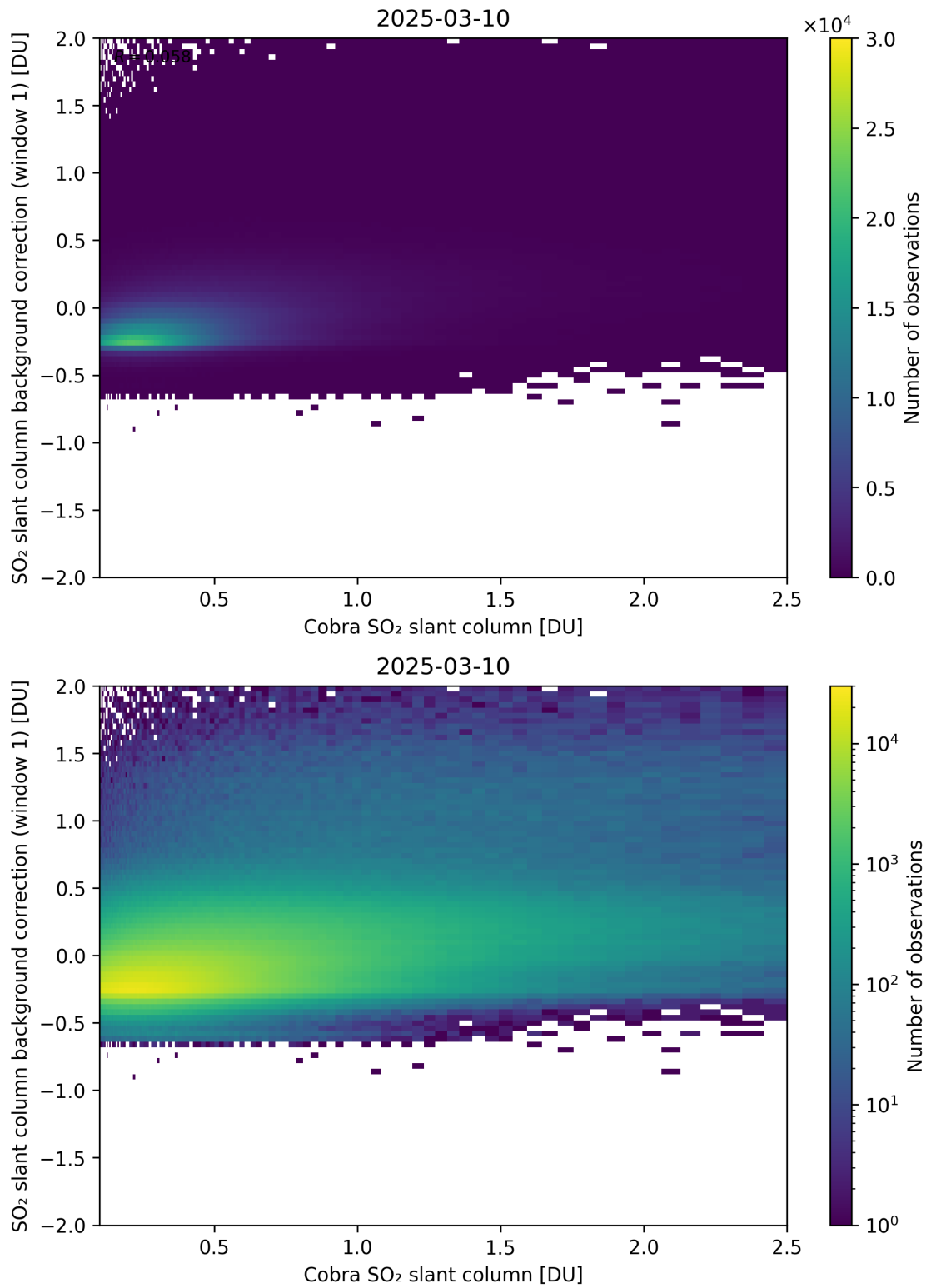
Figure 193: Scatter density plot of “Cobra SO 2 slant column” against “SO 2 slant column background correction (window 1)” for 2025-03-09 to 2025-03-11.
