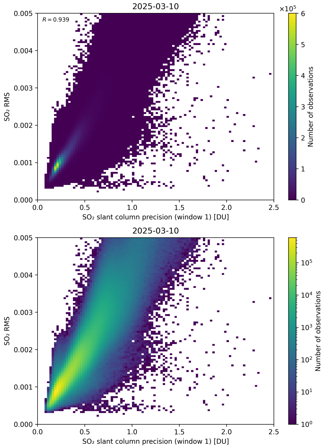
Figure 273: Scatter density plot of “SO 2 slant column precision (window 1)” against “SO 2 RMS” for 2025-03-09 to 2025-03-11.
