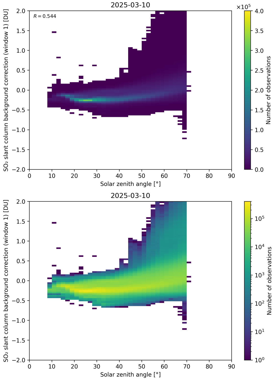
Figure 171: Scatter density plot of “Solar zenith angle” against “SO 2 slant column background correction (window 1)” for 2025-03-09 to 2025-03-11.
