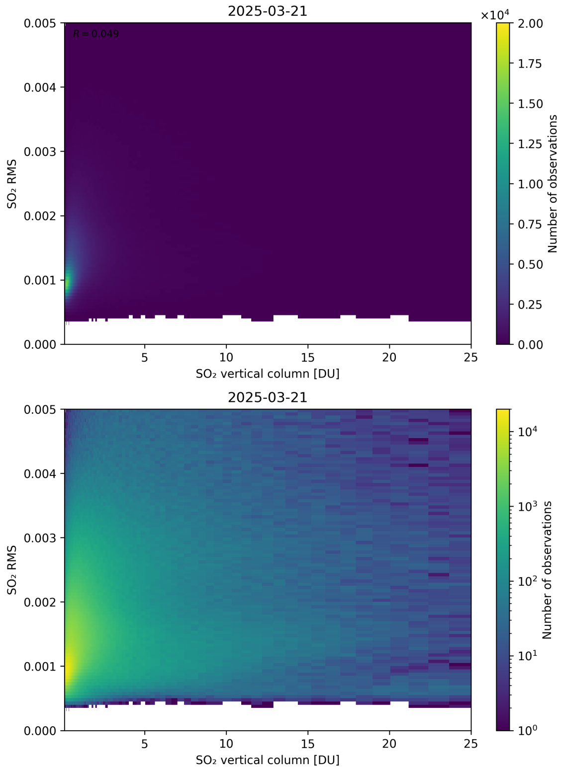
Figure 328: Scatter density plot of “SO 2 vertical column” against “SO 2 RMS” for 2025-03-20 to 2025-03-22.
