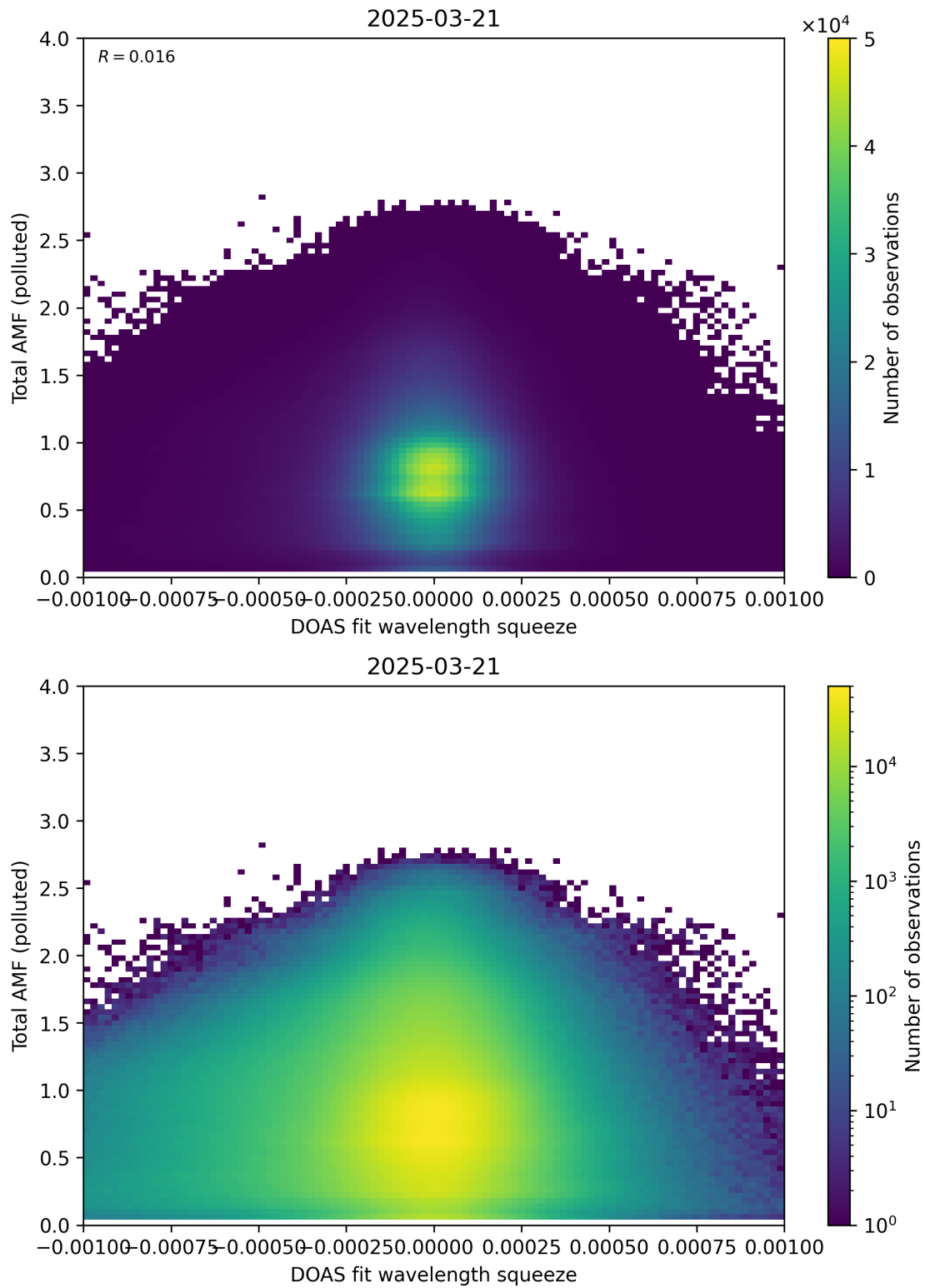
Figure 145: Scatter density plot of “DOAS fit wavelength squeeze” against “Total AMF (polluted)” for 2025-03-20 to 2025-03-22.
