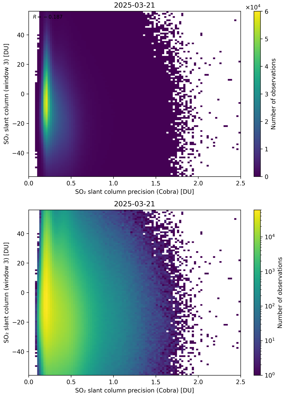
Figure 211: Scatter density plot of “SO 2 slant column precision (Cobra)” against “SO 2 slant column (window 3)” for 2025-03-20 to 2025-03-22.
