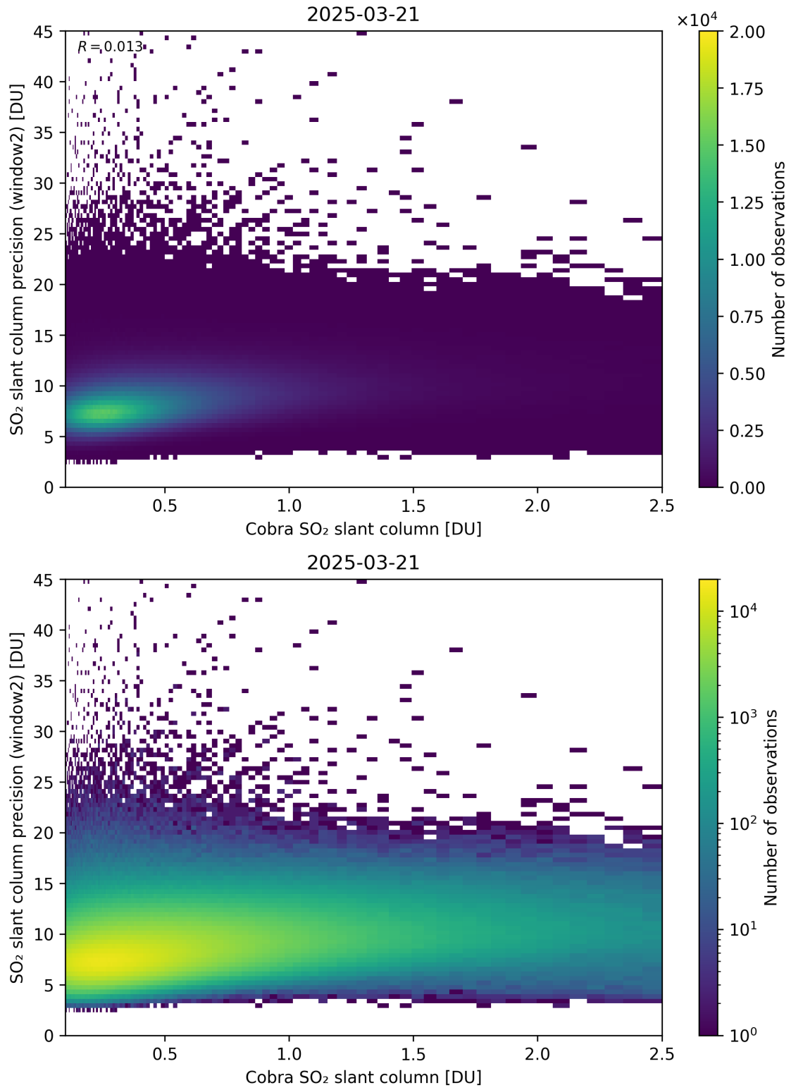
Figure 221: Scatter density plot of “Cobra SO 2 slant column” against “SO 2 slant column precision (window2)” for 2025-03-20 to 2025-03-22.
