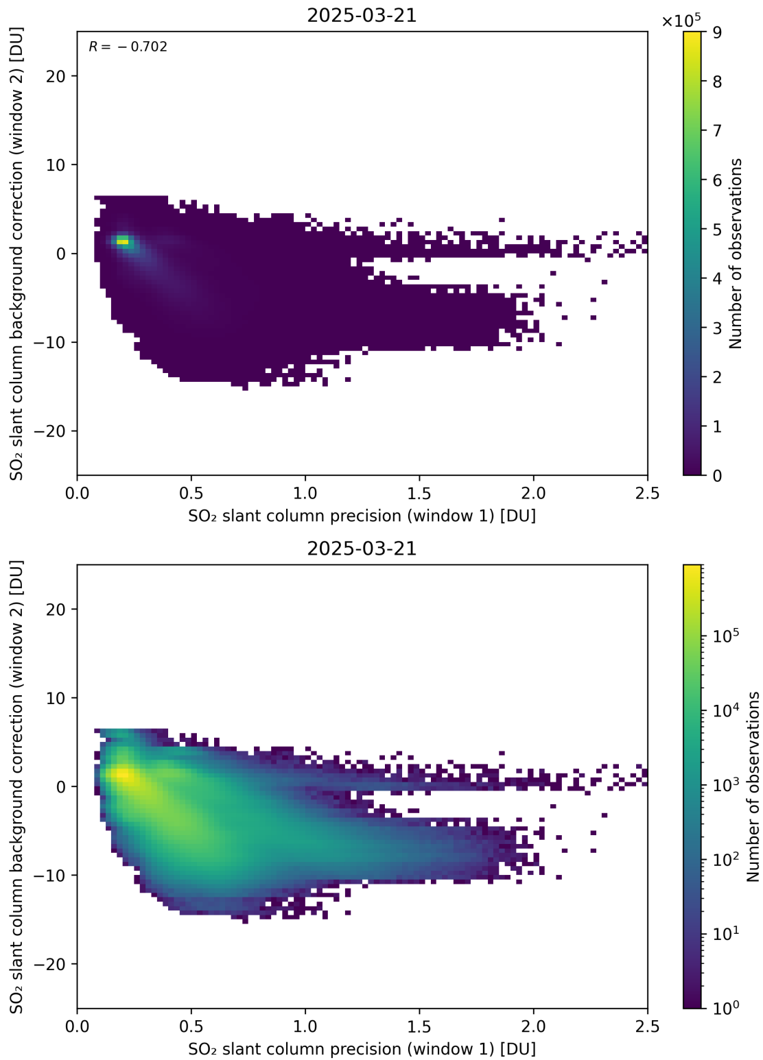
Figure 269: Scatter density plot of “SO 2 slant column precision (window 1)” against “SO 2 slant column background correction (window 2)” for 2025-03-20 to 2025-03-22.
