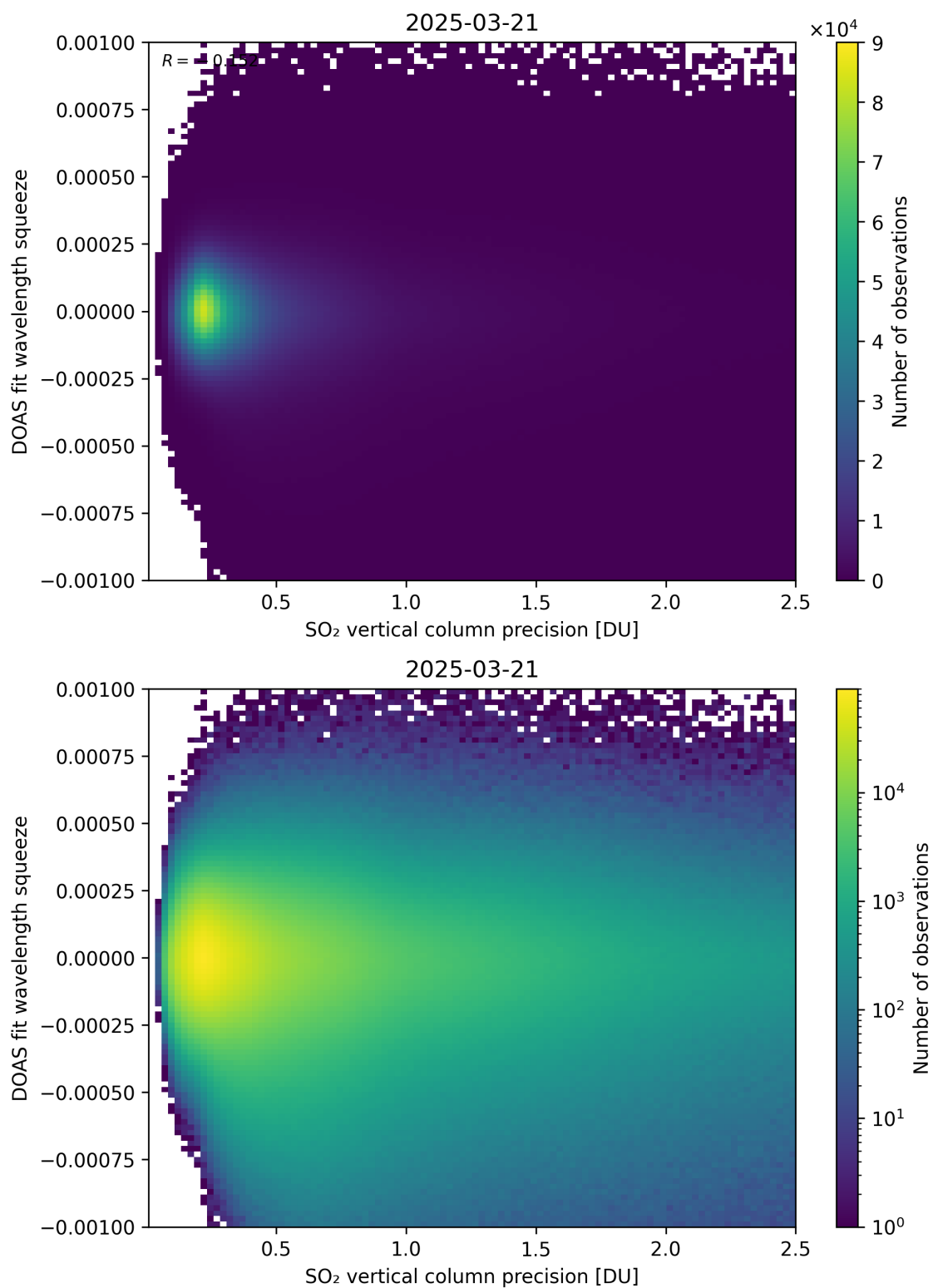
Figure 333: Scatter density plot of “SO 2 vertical column precision” against “DOAS fit wavelength squeeze” for 2025-03-20 to 2025-03-22.
