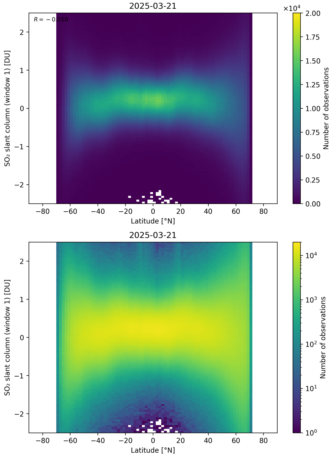
Figure 162: Scatter density plot of “Latitude” against “SO 2 slant column (window 1)” for 2025-03-20 to 2025-03-22.
