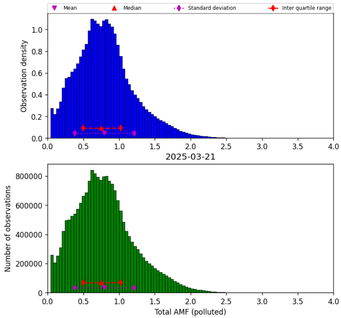
Figure 79: Histogram of “Total AMF (polluted)” for 2025-03-20 to 2025-03-22
