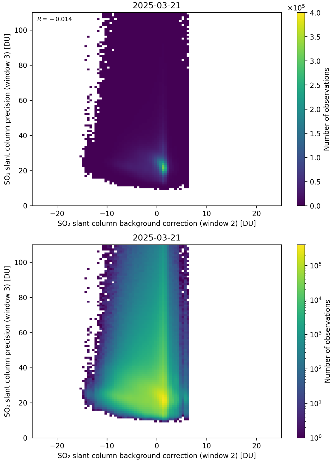
Figure 129: Scatter density plot of “SO 2 slant column background correction (window 2)” against “SO 2 slant column precision (window 3)” for 2025-03-20 to 2025-03-22.
