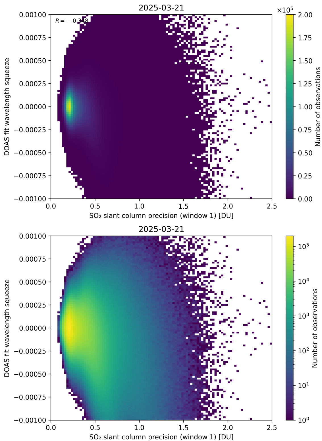
Figure 272: Scatter density plot of “SO 2 slant column precision (window 1)” against “DOAS fit wavelength squeeze” for 2025-03-20 to 2025-03-22.
