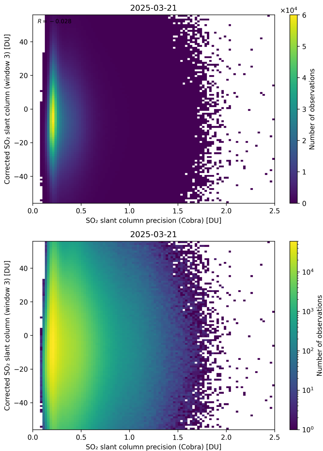
Figure 207: Scatter density plot of “SO 2 slant column precision (Cobra)” against “Corrected SO 2 slant column (window 3)” for 2025-03-20 to 2025-03-22.
