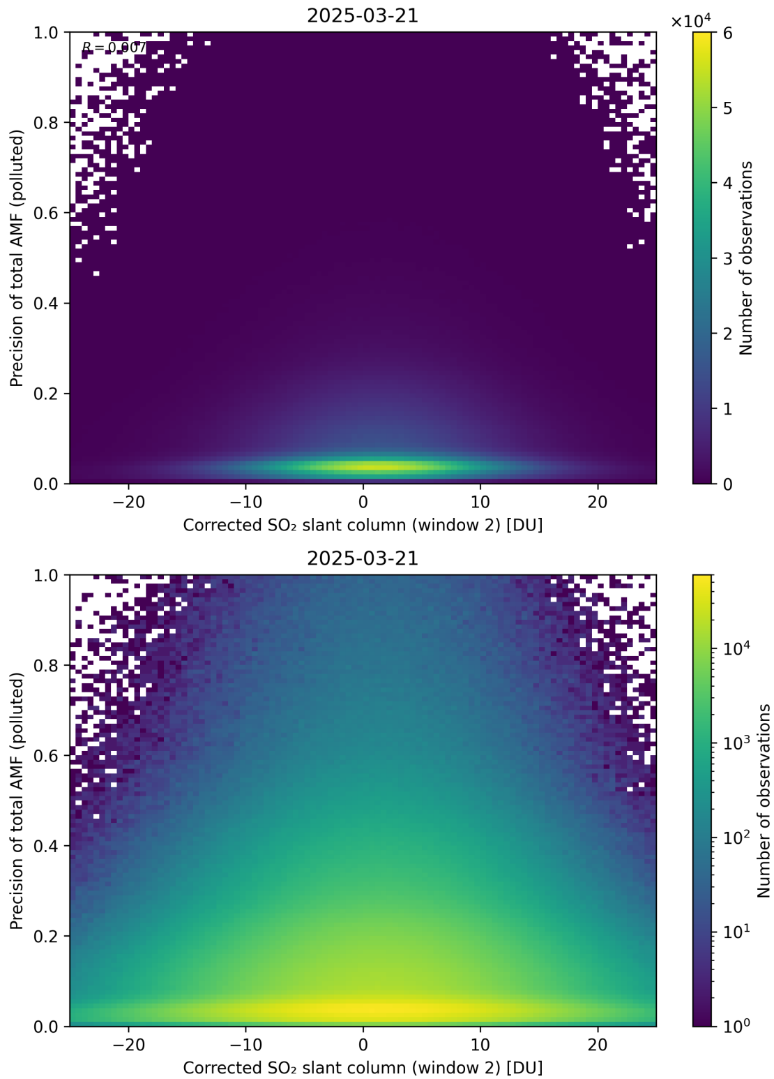
Figure 254: Scatter density plot of “Corrected SO 2 slant column (window 2)” against “Precision of total AMF (polluted)” for 2025-03-20 to 2025-03-22.
