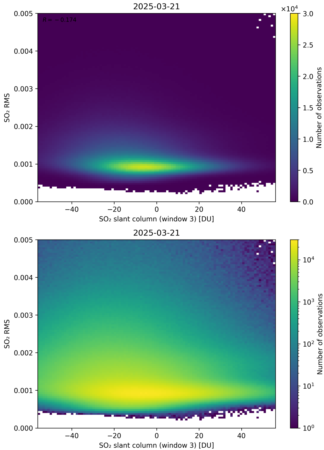
Figure 306: Scatter density plot of “SO 2 slant column (window 3)” against “SO 2 RMS” for 2025-03-20 to 2025-03-22.
