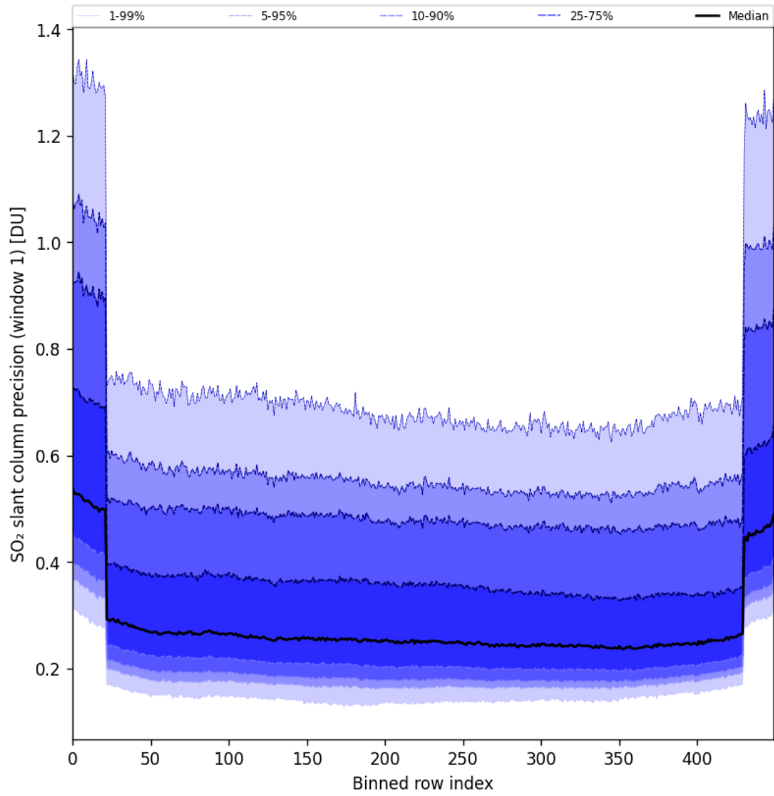
Figure 90: Along track statistics of “SO 2 slant column precision (window 1)” for 2025-03-20 to 2025-03-22
