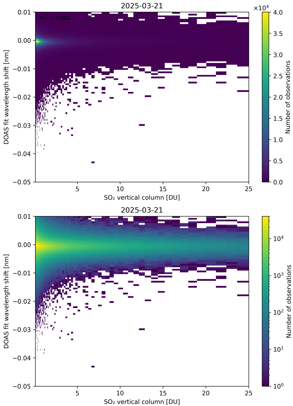
Figure 326: Scatter density plot of “SO 2 vertical column” against “DOAS fit wavelength shift” for 2025-03-20 to 2025-03-22.
