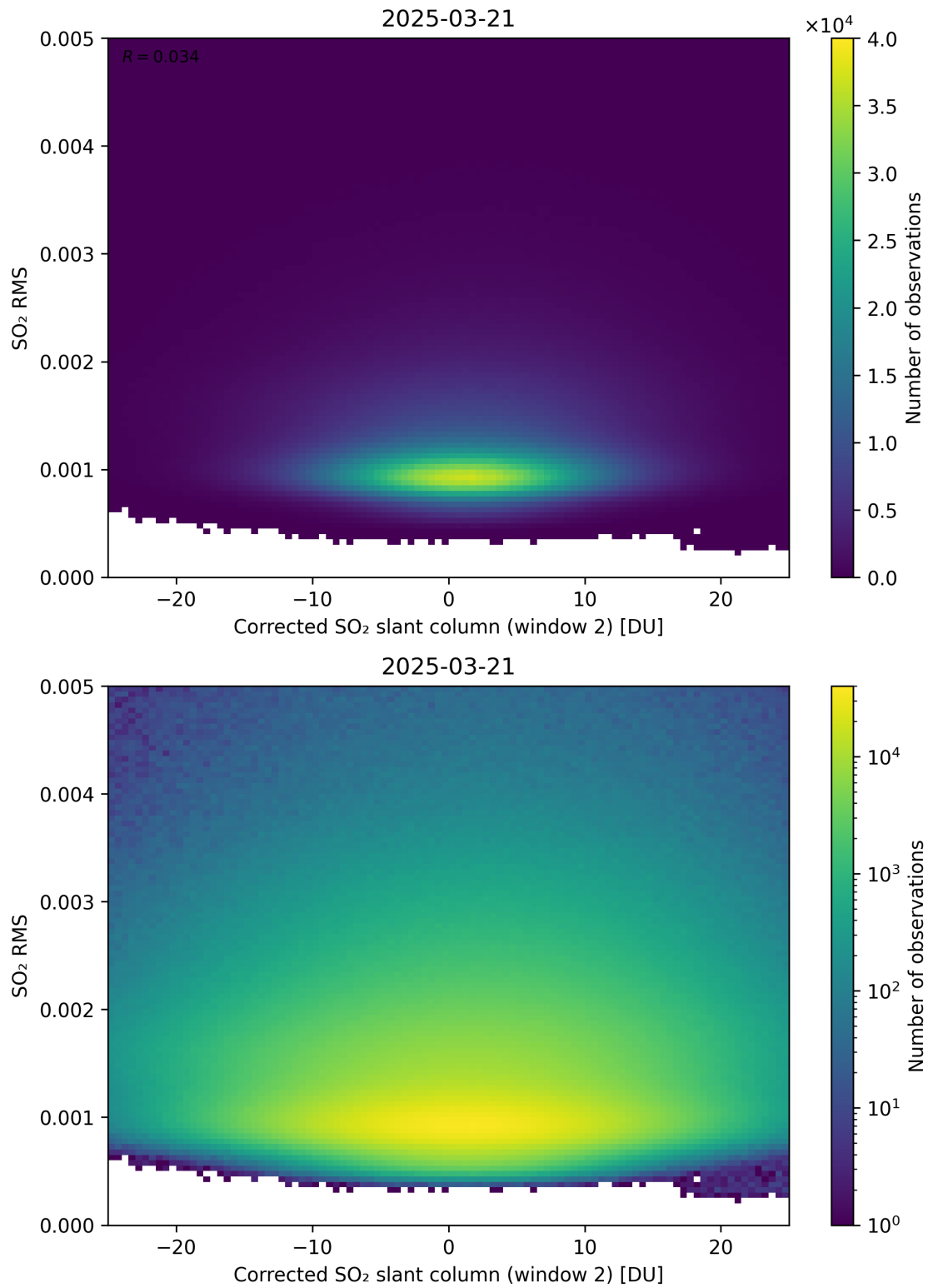
Figure 248: Scatter density plot of “Corrected SO 2 slant column (window 2)” against “SO 2 RMS” for 2025-03-20 to 2025-03-22.
