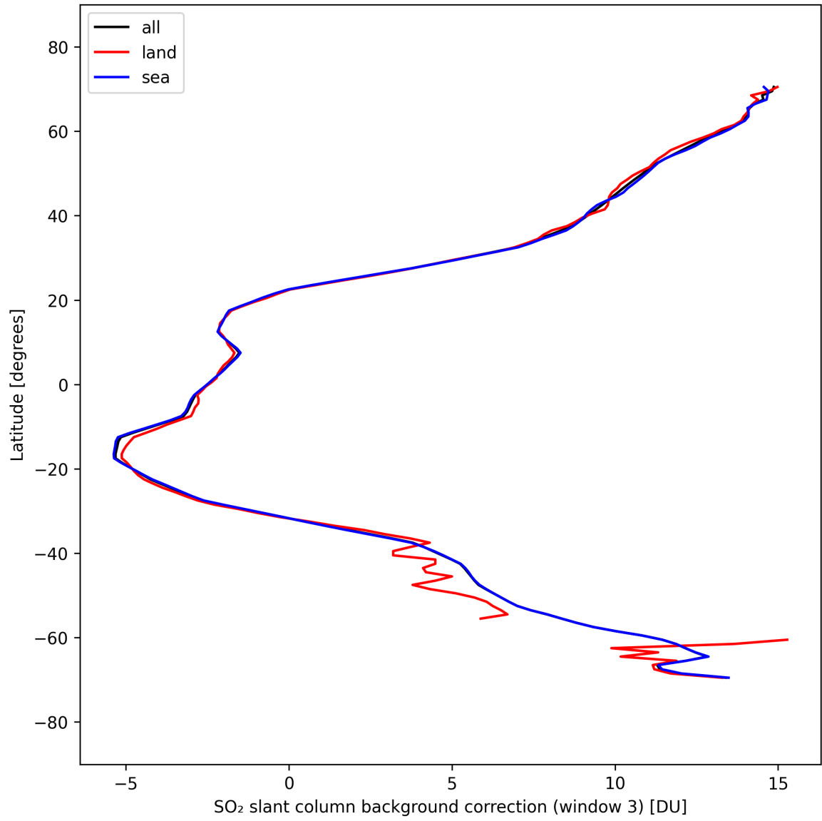
Figure 48: Zonal average of “SO 2 slant column background correction (window 3)” for 2025-03-20 to 2025-03-22.
