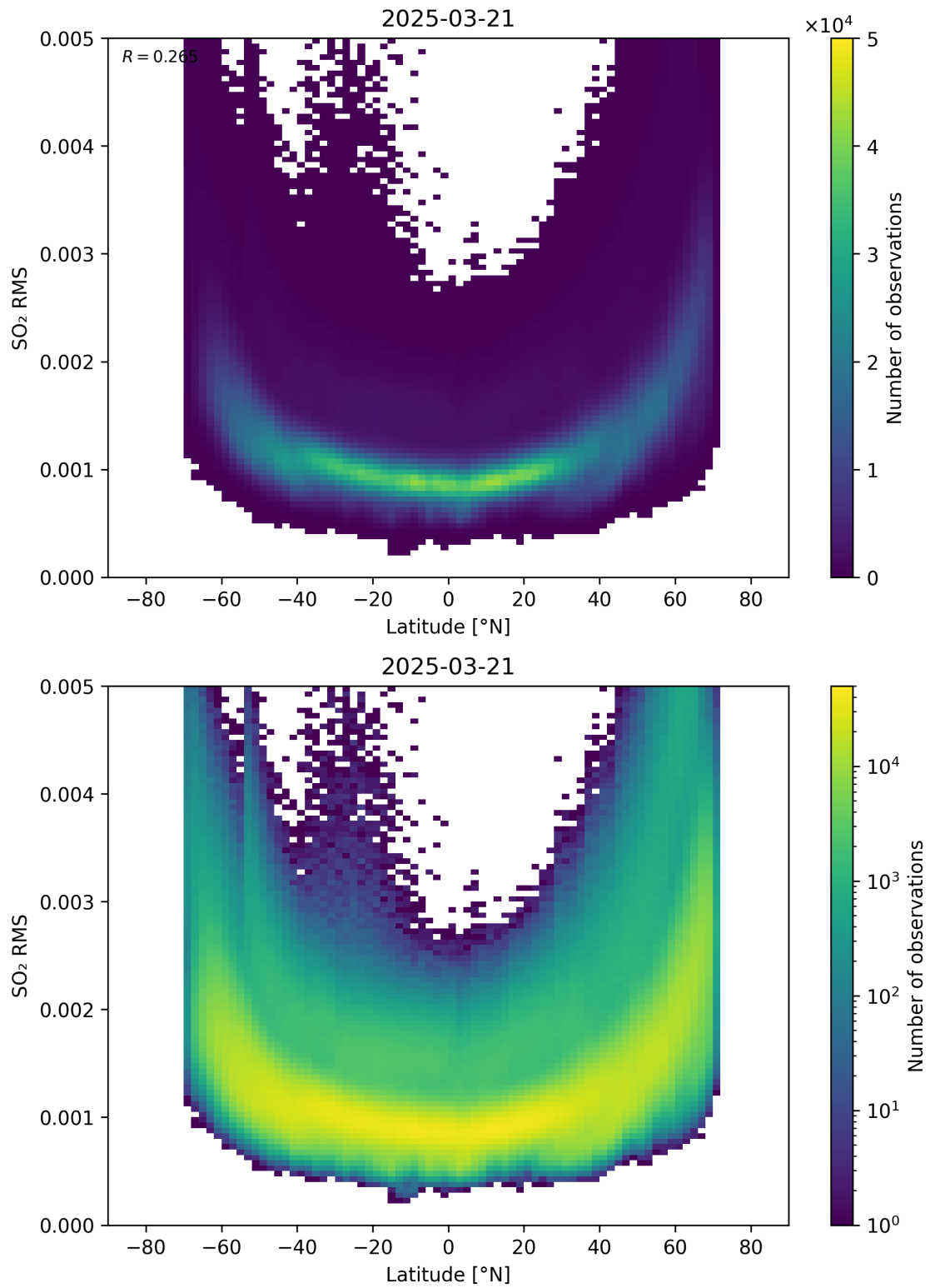
Figure 155: Scatter density plot of “Latitude” against “SO 2 RMS” for 2025-03-20 to 2025-03-22.
