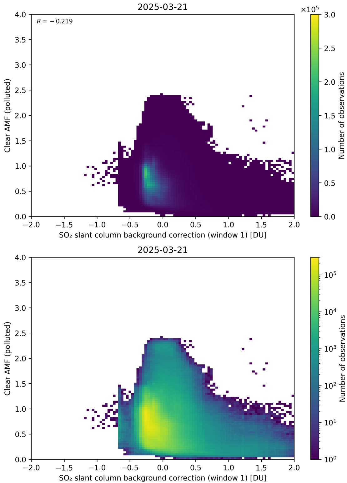
Figure 114: Scatter density plot of “SO 2 slant column background correction (window 1)” against “Clear AMF (polluted)” for 2025-03-20 to 2025-03-22.
