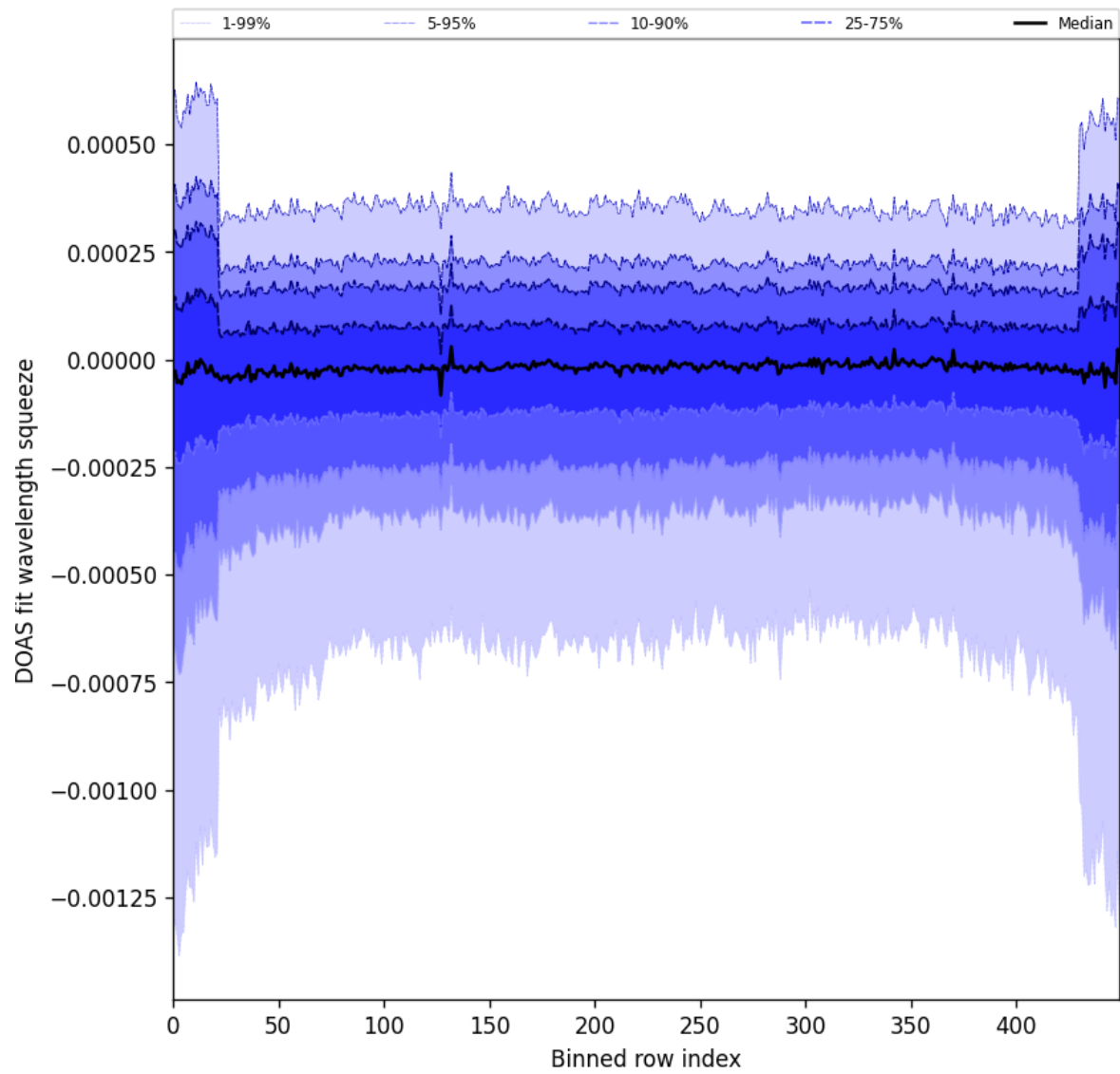
Figure 103: Along track statistics of “DOAS fit wavelength squeeze” for 2025-03-20 to 2025-03-22
