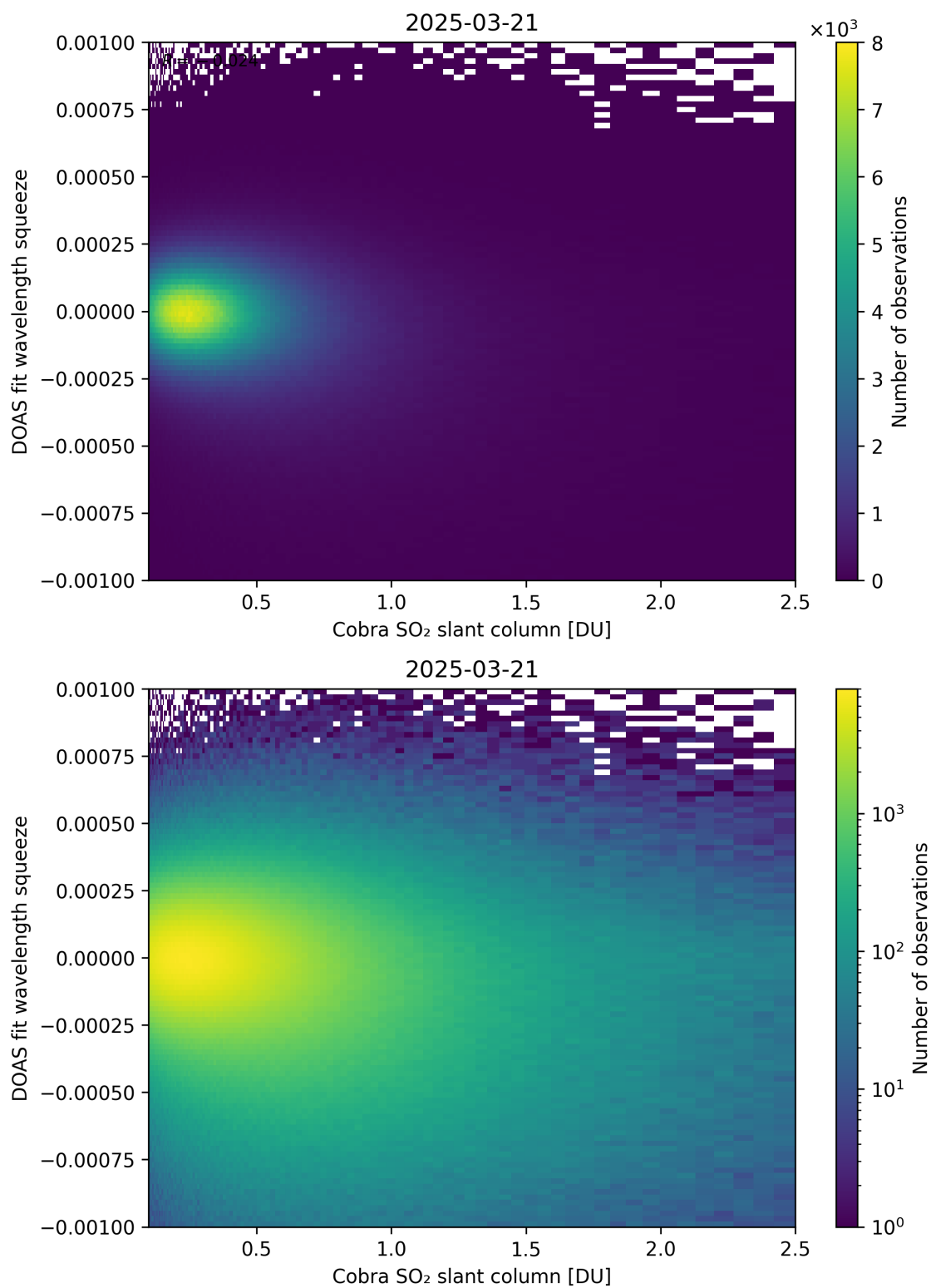
Figure 197: Scatter density plot of “Cobra SO 2 slant column” against “DOAS fit wavelength squeeze” for 2025-03-20 to 2025-03-22.
