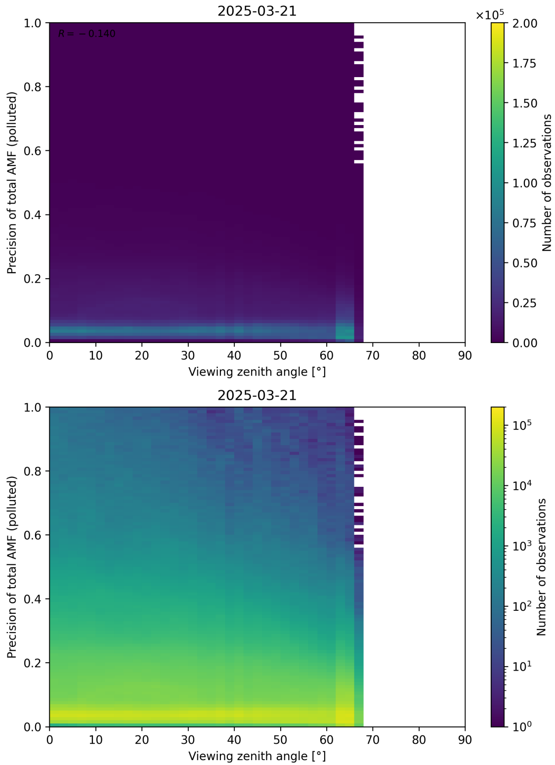
Figure 382: Scatter density plot of “Viewing zenith angle” against “Precision of total AMF (polluted)” for 2025-03-20 to 2025-03-22.
