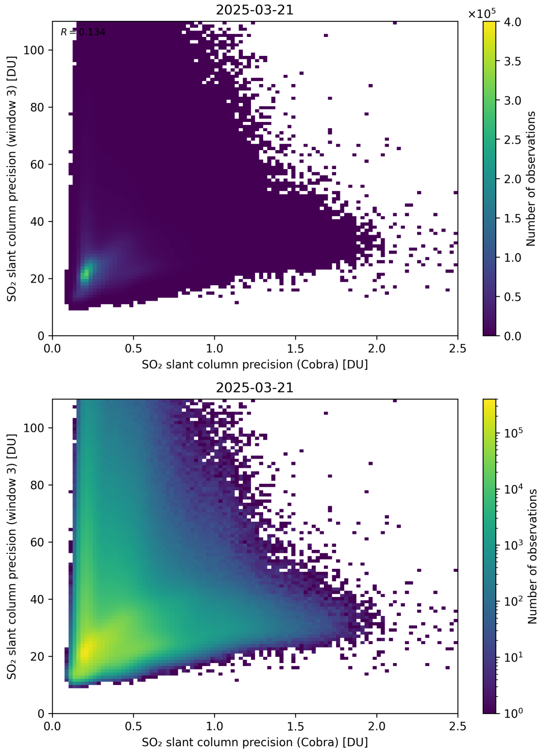
Figure 212: Scatter density plot of “SO 2 slant column precision (Cobra)” against “SO 2 slant column precision (window 3)” for 2025-03-20 to 2025-03-22.
