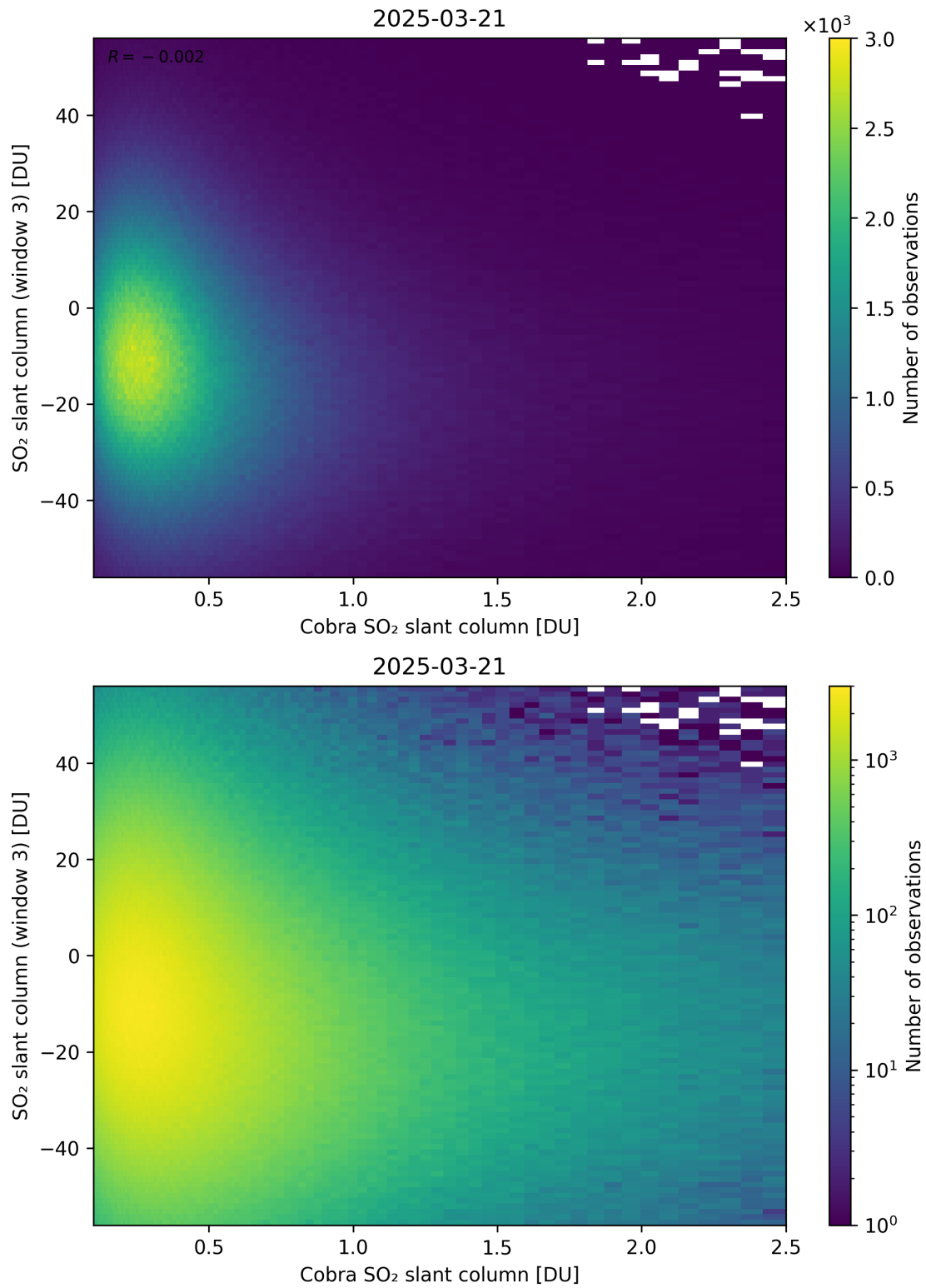
Figure 222: Scatter density plot of “Cobra SO 2 slant column” against “SO 2 slant column (window 3)” for 2025-03-20 to 2025-03-22.
