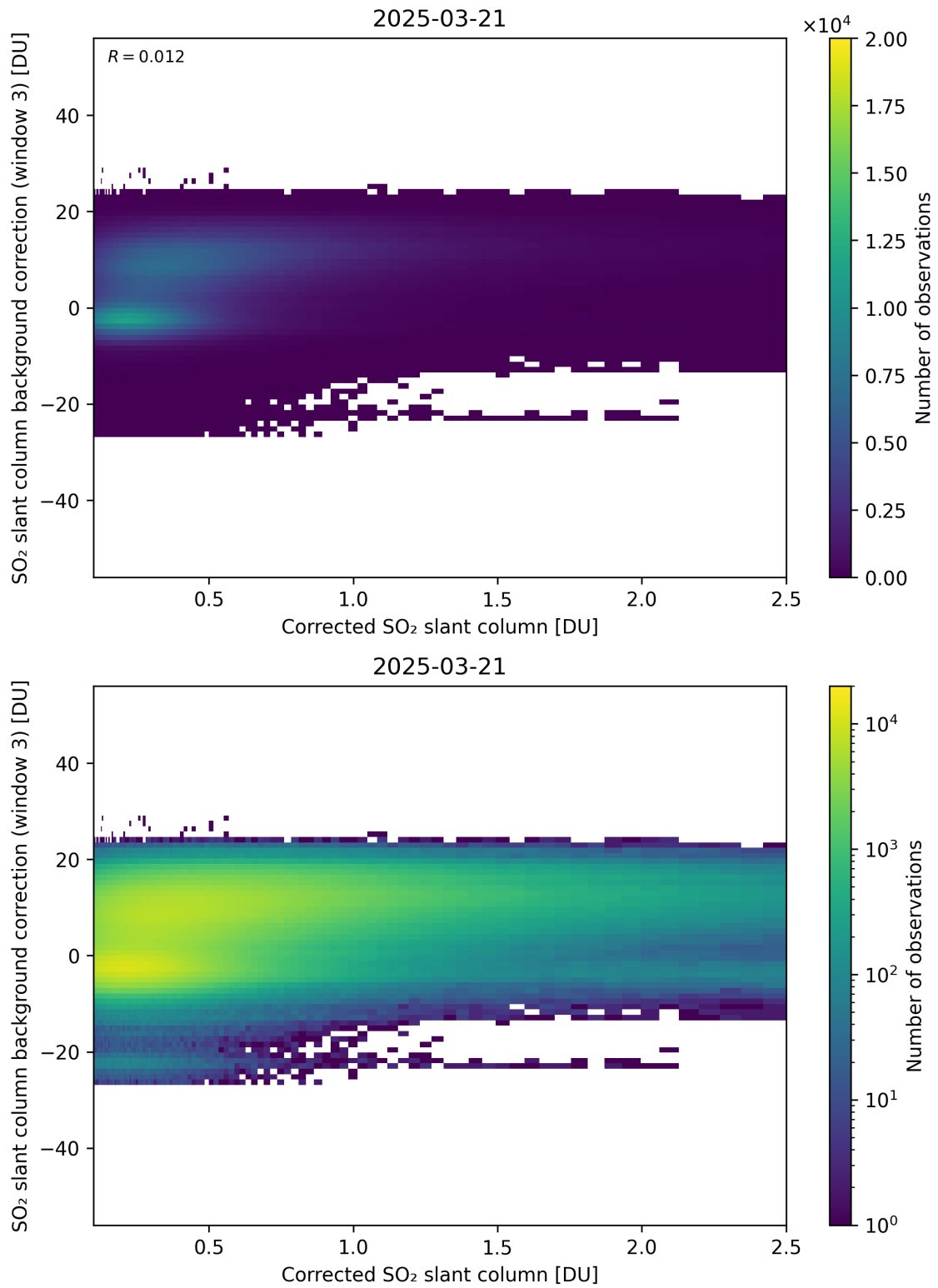
Figure 228: Scatter density plot of “Corrected SO 2 slant column” against “SO 2 slant column background correction (window 3)” for 2025-03-20 to 2025-03-22.
