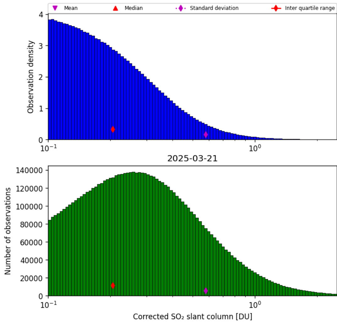
Figure 60: Histogram of "Corrected SO 2 slant column" for 2025-03-20 to 2025-03-22
