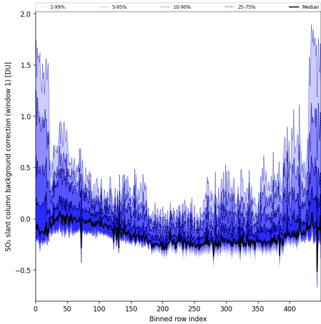
Figure 92: Along track statistics of “SO 2 slant column background correction (window 1)” for 2025-03-20 to 2025-03-22
