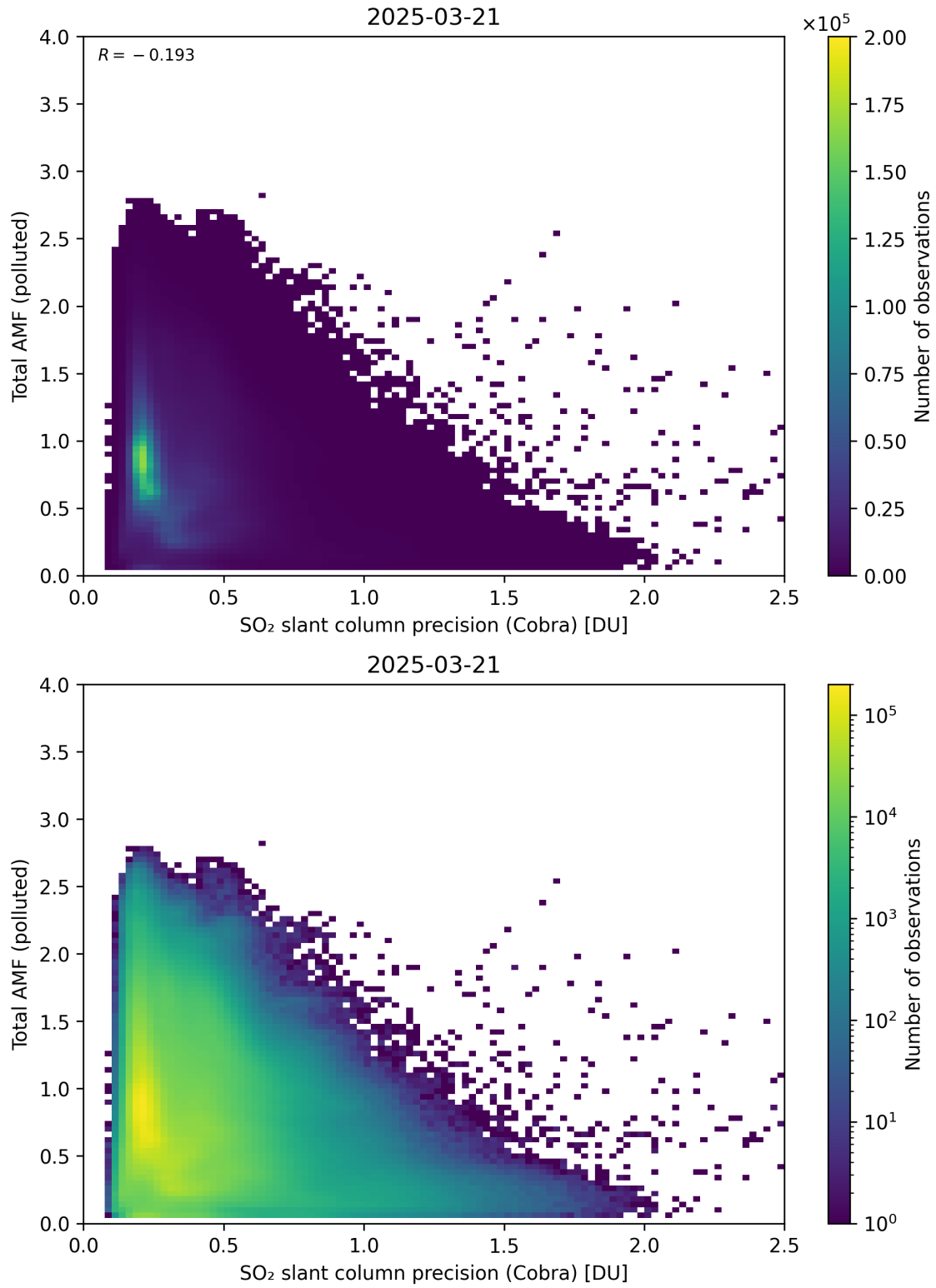
Figure 213: Scatter density plot of “SO 2 slant column precision (Cobra)” against “Total AMF (polluted)” for 2025-03-20 to 2025-03-22.
