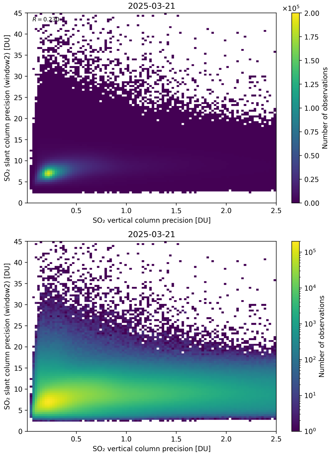
Figure 343: Scatter density plot of “SO 2 vertical column precision” against “SO 2 slant column precision (window2)” for 2025-03-20 to 2025-03-22.
