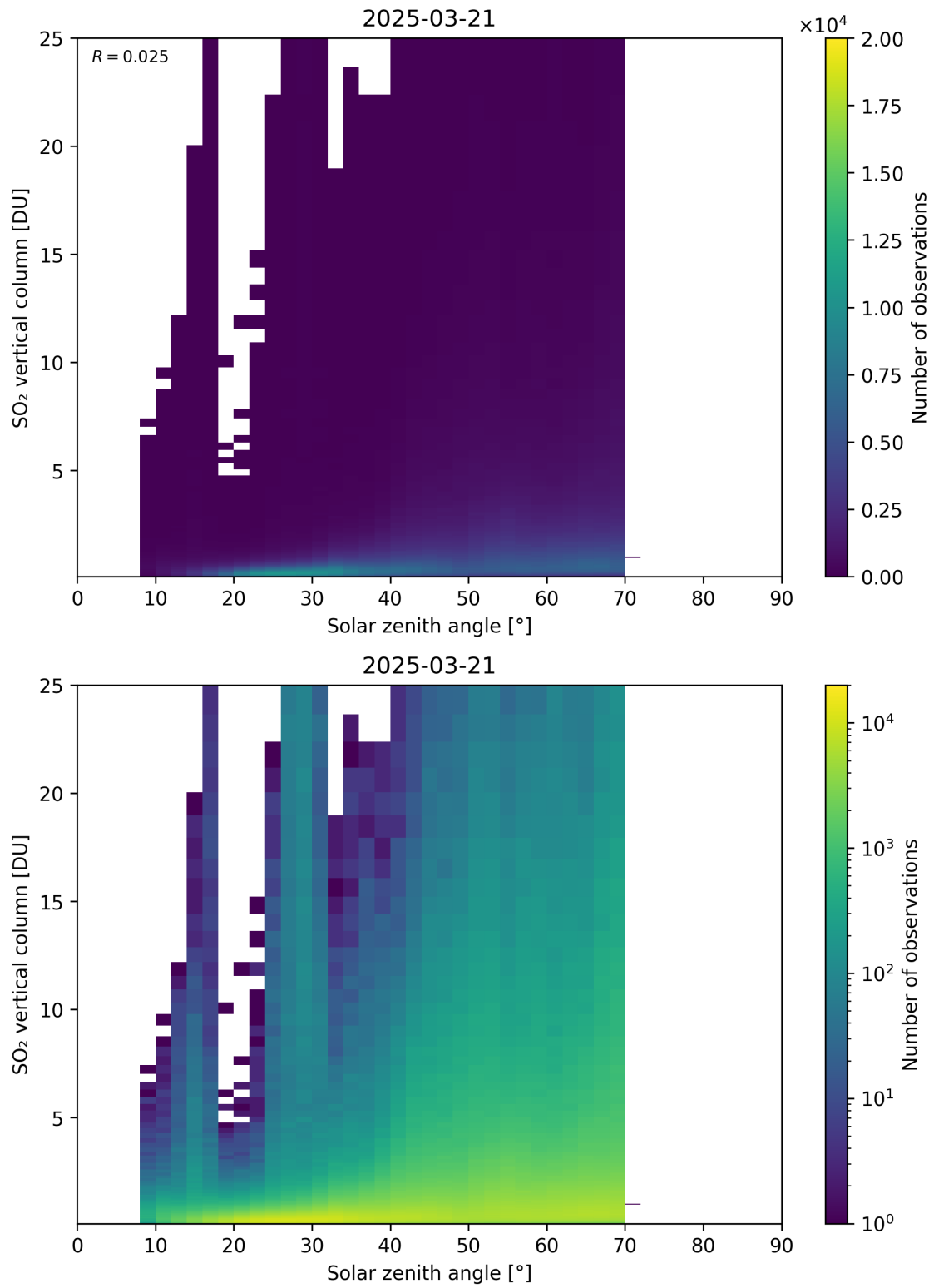
Figure 191: Scatter density plot of “Solar zenith angle” against “SO 2 vertical column” for 2025-03-20 to 2025-03-22.
