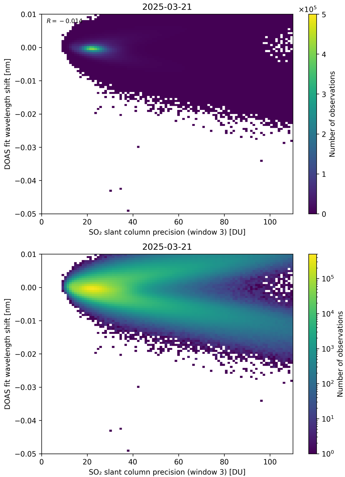
Figure 308: Scatter density plot of “SO 2 slant column precision (window 3)” against “DOAS fit wavelength shift” for 2025-03-20 to 2025-03-22.
