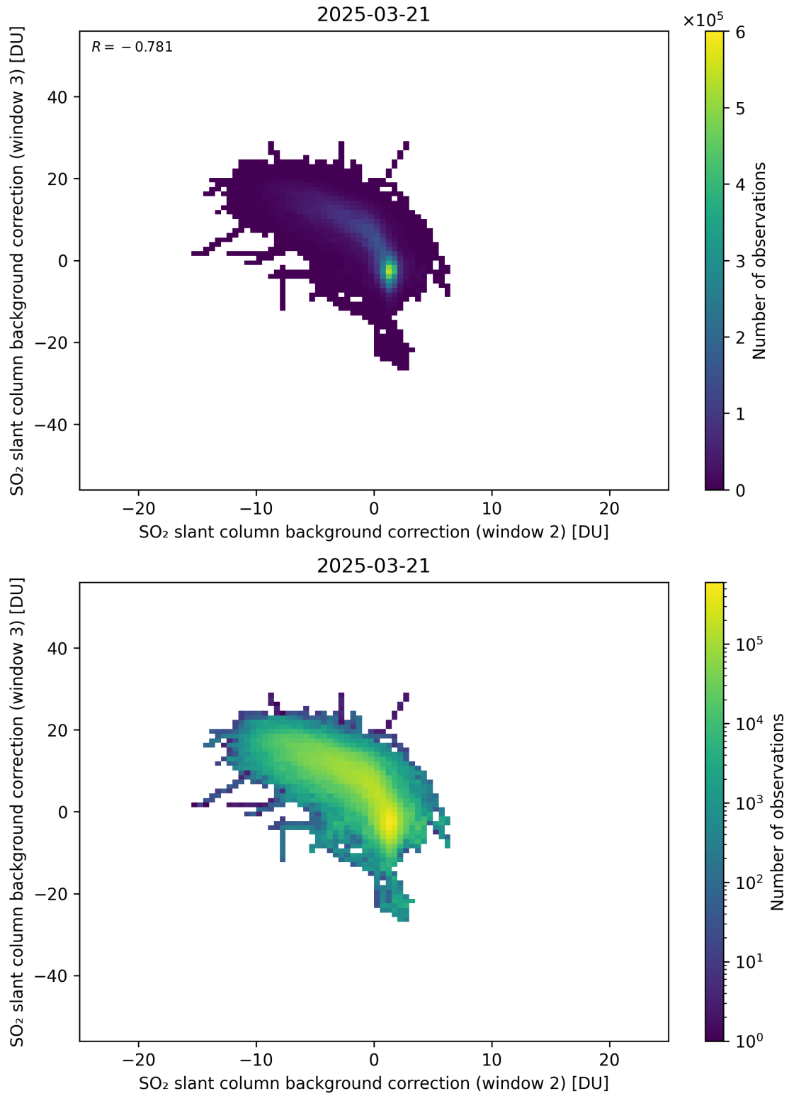
Figure 122: Scatter density plot of “SO 2 slant column background correction (window 2)” against “SO 2 slant column background correction (window 3)” for 2025-03-20 to 2025-03-22.
