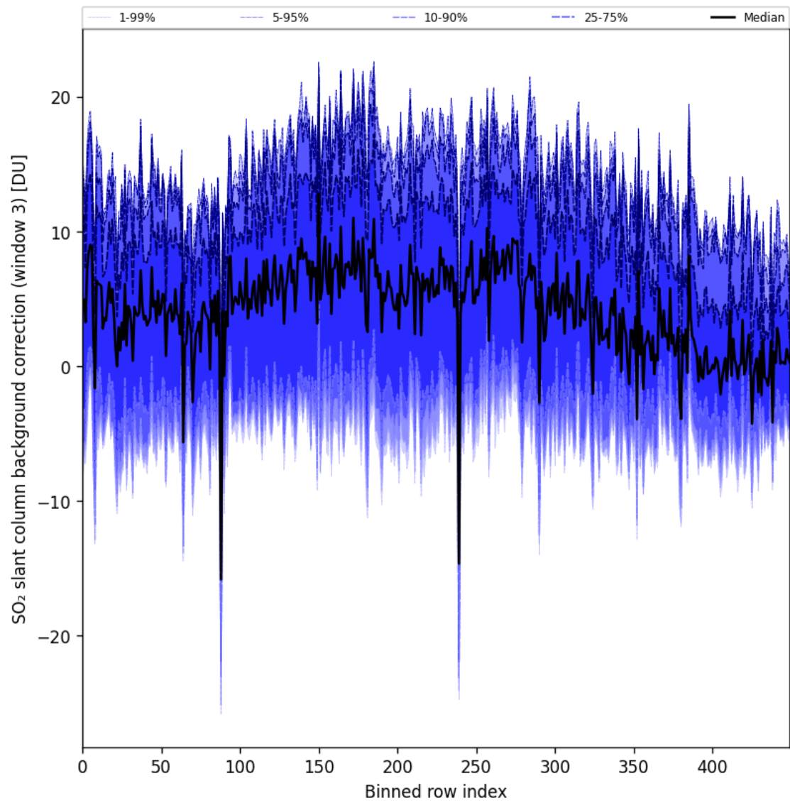
Figure 100: Along track statistics of “SO 2 slant column background correction (window 3)” for 2025-03-20 to 2025-03-22
