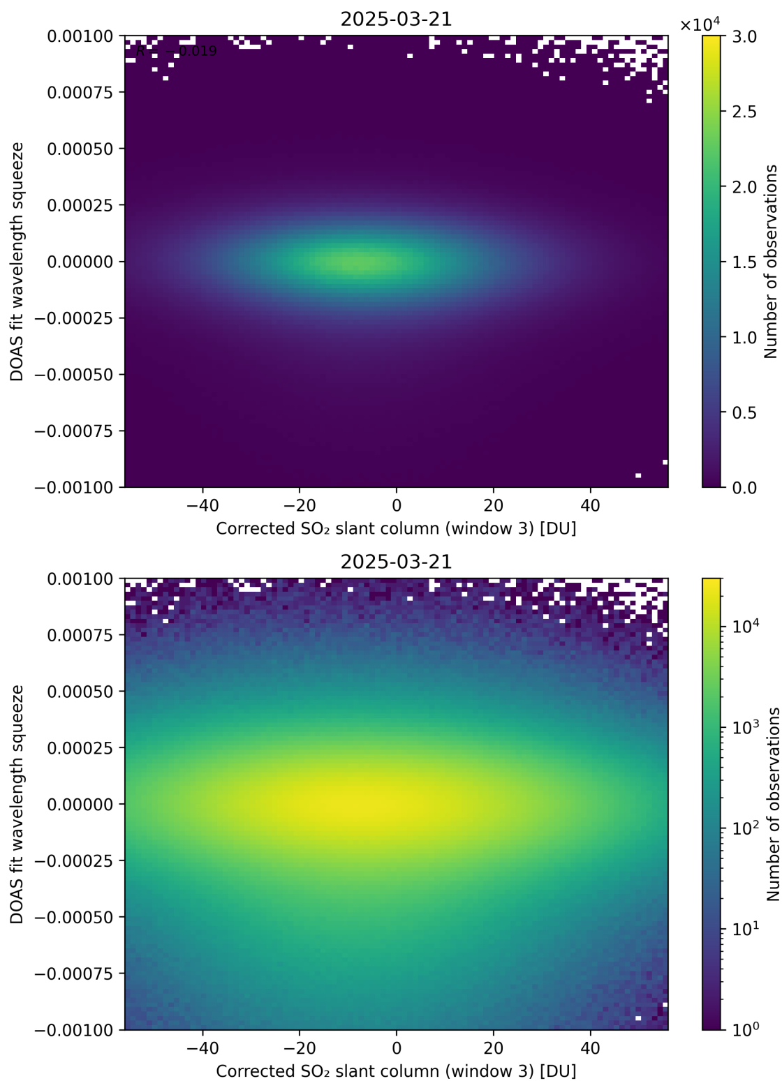
Figure 257: Scatter density plot of “Corrected SO 2 slant column (window 3)” against “DOAS fit wavelength squeeze” for 2025-03-20 to 2025-03-22.
