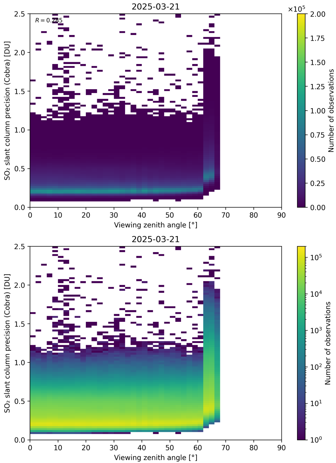
Figure 372: Scatter density plot of “Viewing zenith angle” against “SO 2 slant column precision (Cobra)” for 2025-03-20 to 2025-03-22.
