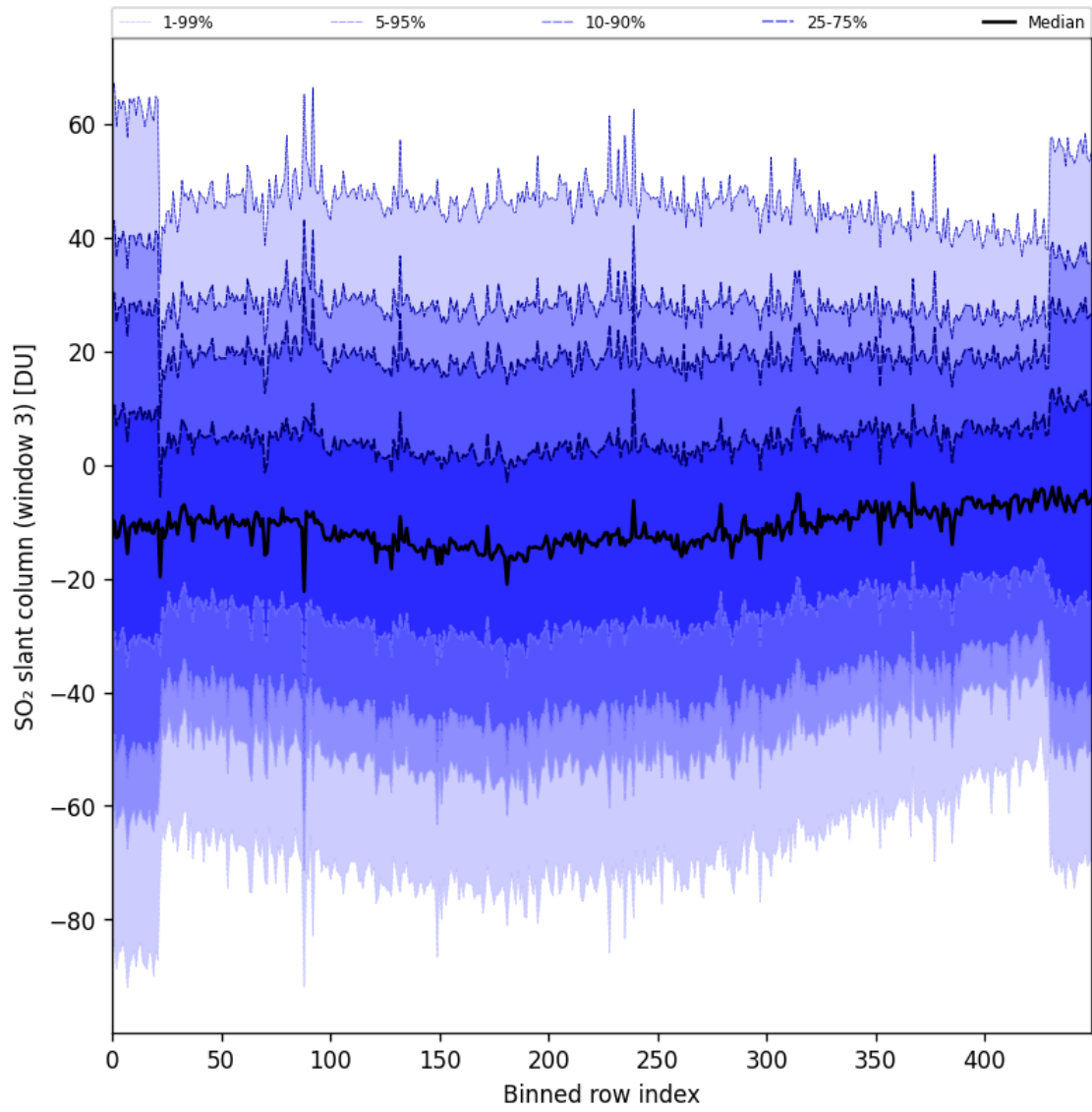
Figure 97: Along track statistics of “SO 2 slant column (window 3)” for 2025-03-20 to 2025-03-22
