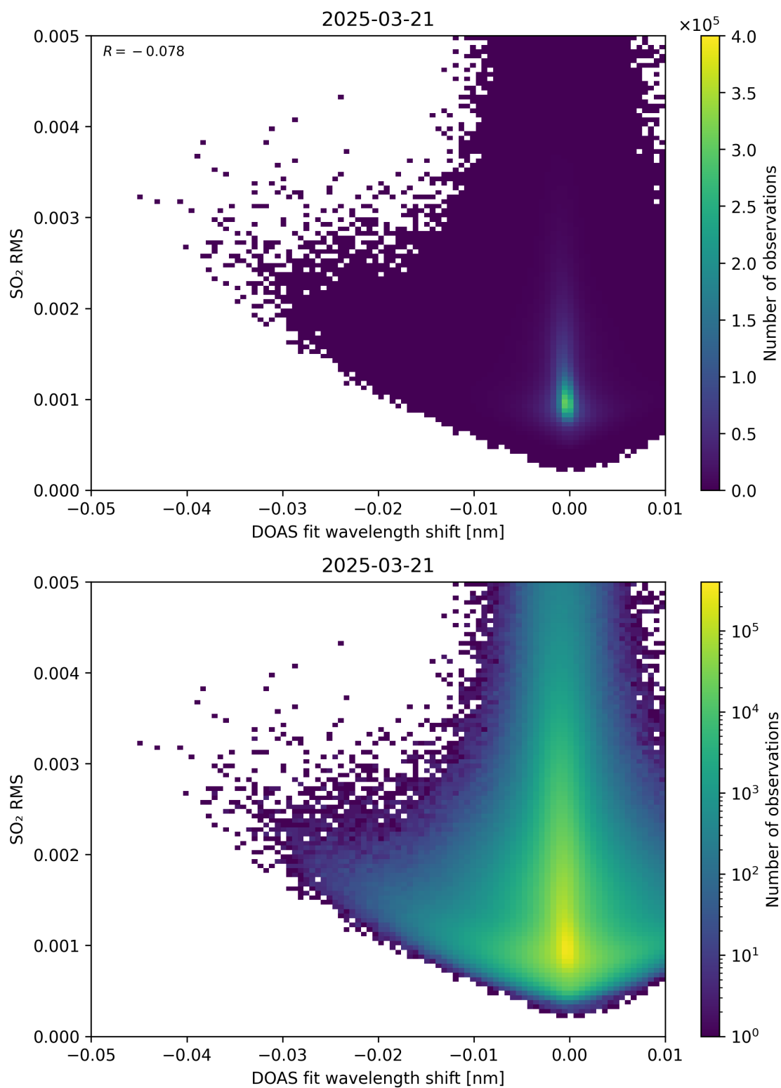
Figure 139: Scatter density plot of “DOAS fit wavelength shift” against “SO 2 RMS” for 2025-03-20 to 2025-03-22.
