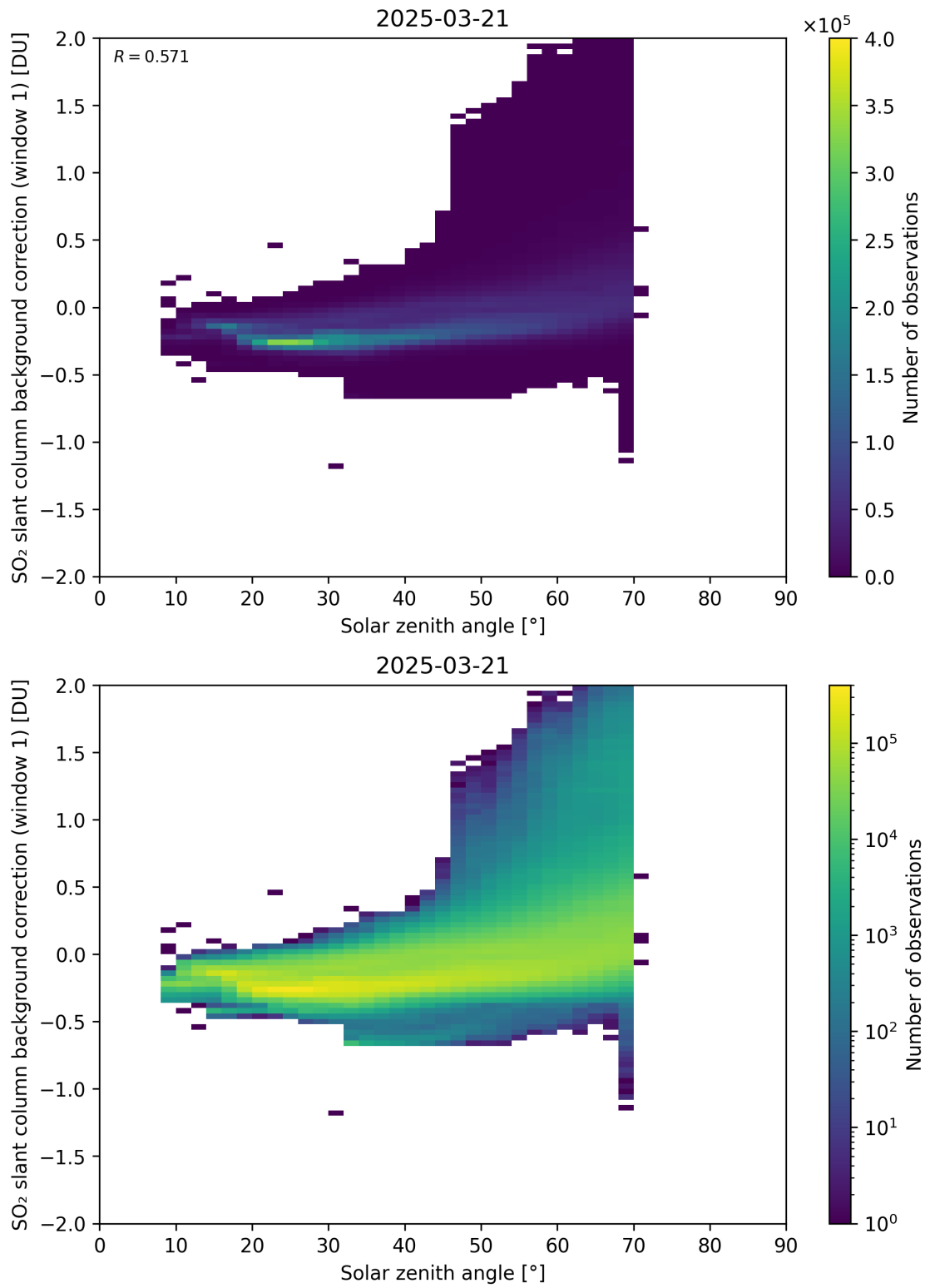
Figure 171: Scatter density plot of “Solar zenith angle” against “SO 2 slant column background correction (window 1)” for 2025-03-20 to 2025-03-22.
