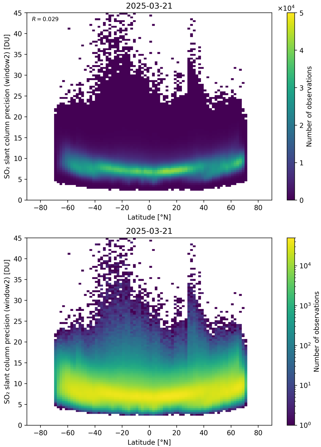
Figure 164: Scatter density plot of “Latitude” against “SO 2 slant column precision (window2)” for 2025-03-20 to 2025-03-22.
