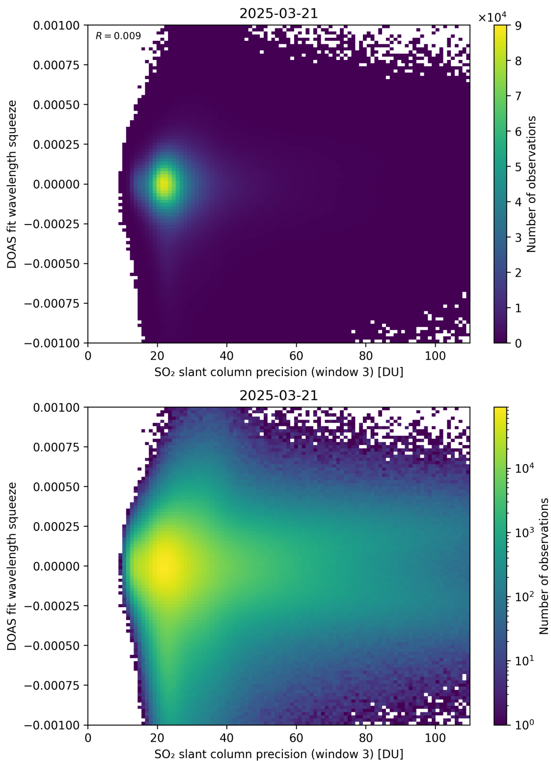
Figure 309: Scatter density plot of “SO 2 slant column precision (window 3)” against “DOAS fit wavelength squeeze” for 2025-03-20 to 2025-03-22.
