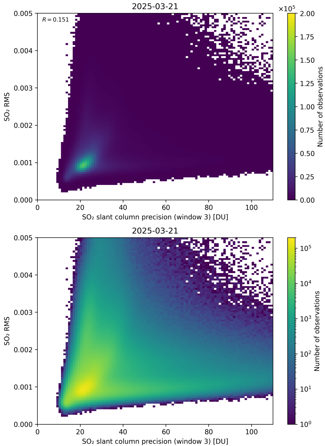
Figure 310: Scatter density plot of “SO 2 slant column precision (window 3)” against “SO 2 RMS” for 2025-03-20 to 2025-03-22.
