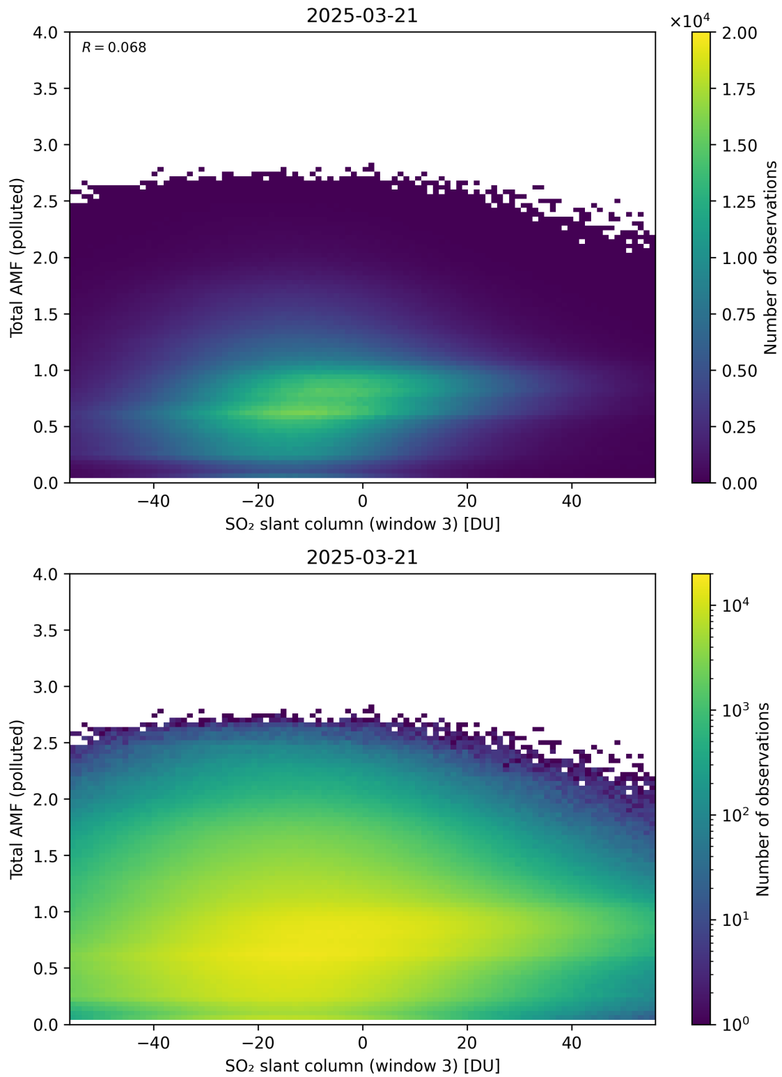
Figure 318: Scatter density plot of “SO 2 slant column (window 3)” against “Total AMF (polluted)” for 2025-03-20 to 2025-03-22.
