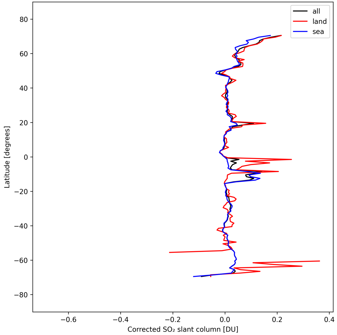
Figure 34: Zonal average of “Corrected SO 2 slant column” for 2025-03-20 to 2025-03-22.
