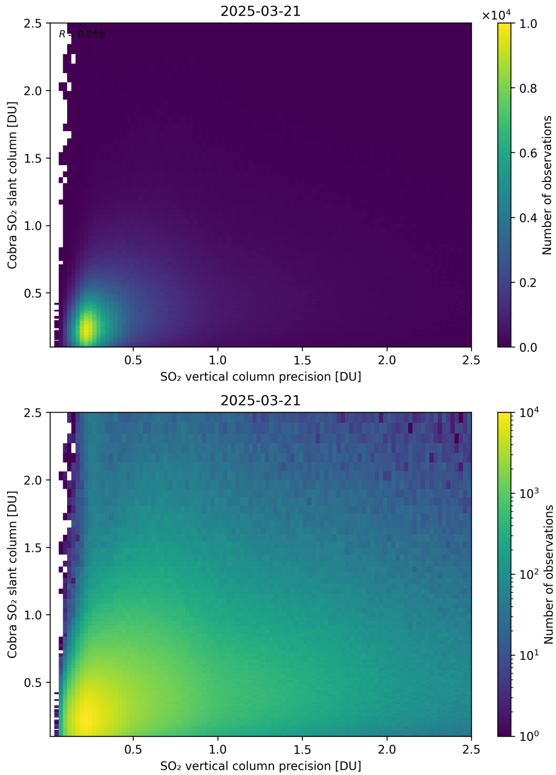
Figure 336: Scatter density plot of “SO 2 vertical column precision” against “Cobra SO 2 slant column” for 2025-03-20 to 2025-03-22.
