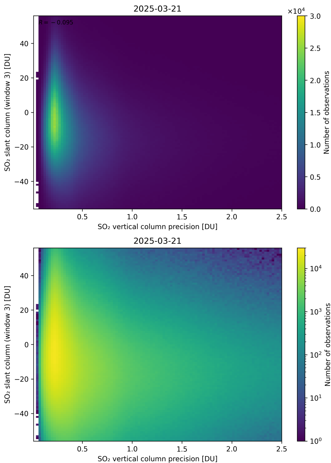
Figure 344: Scatter density plot of “SO 2 vertical column precision” against “SO 2 slant column (window 3)” for 2025-03-20 to 2025-03-22.
