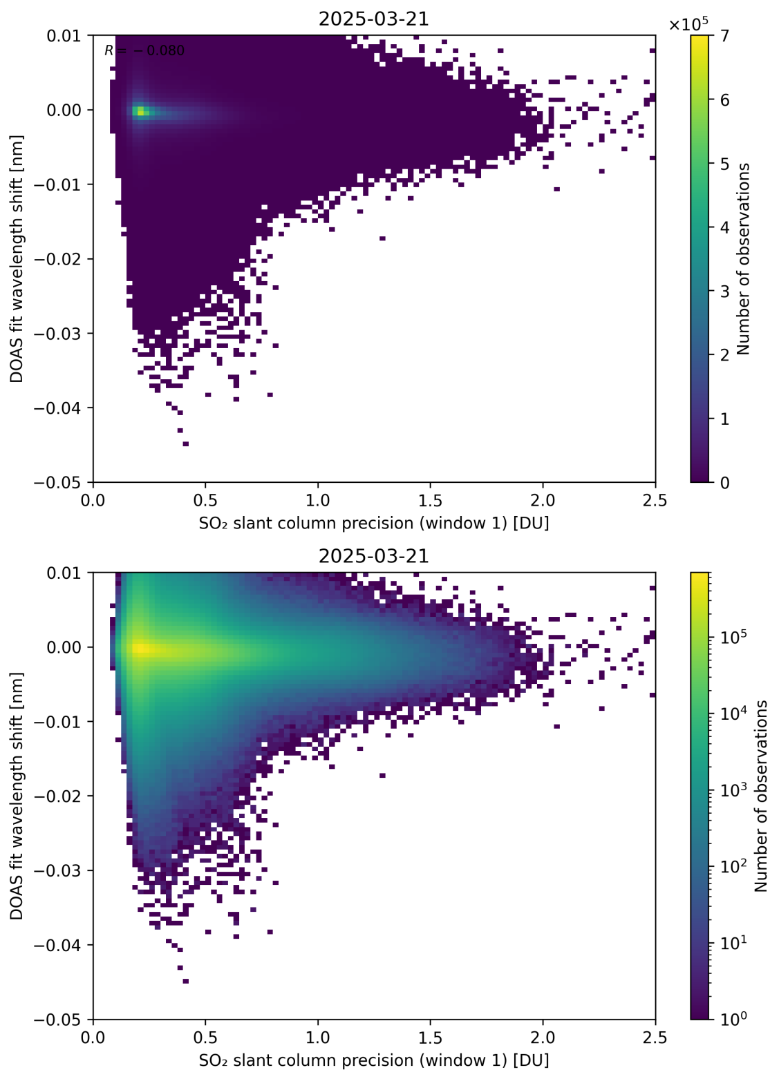
Figure 271: Scatter density plot of “SO 2 slant column precision (window 1)” against “DOAS fit wavelength shift” for 2025-03-20 to 2025-03-22.
