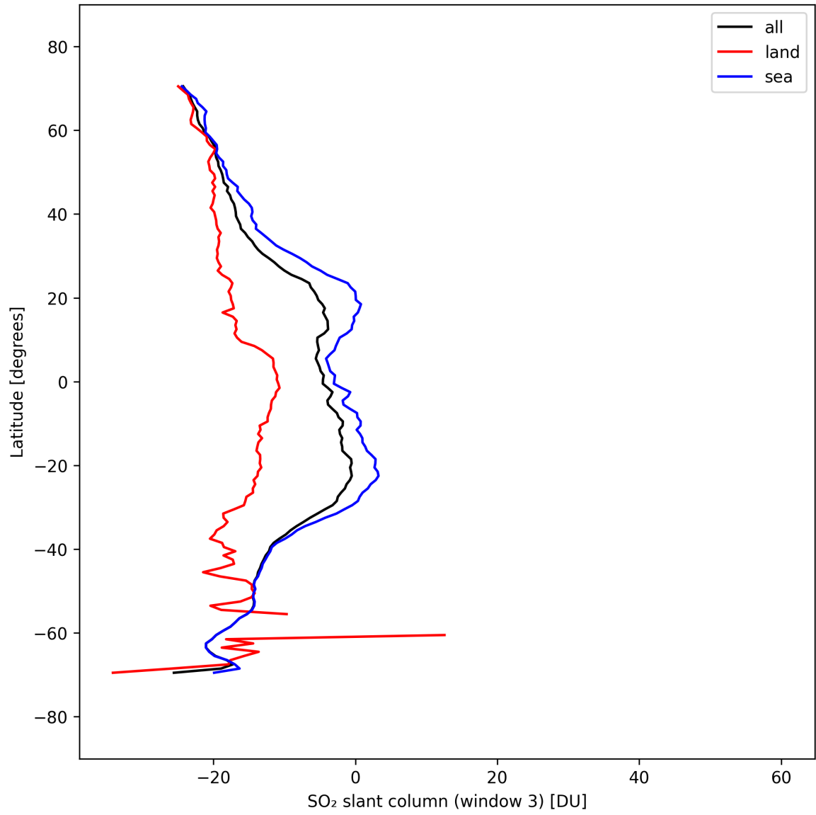
Figure 45: Zonal average of “SO 2 slant column (window 3)” for 2025-03-20 to 2025-03-22.
