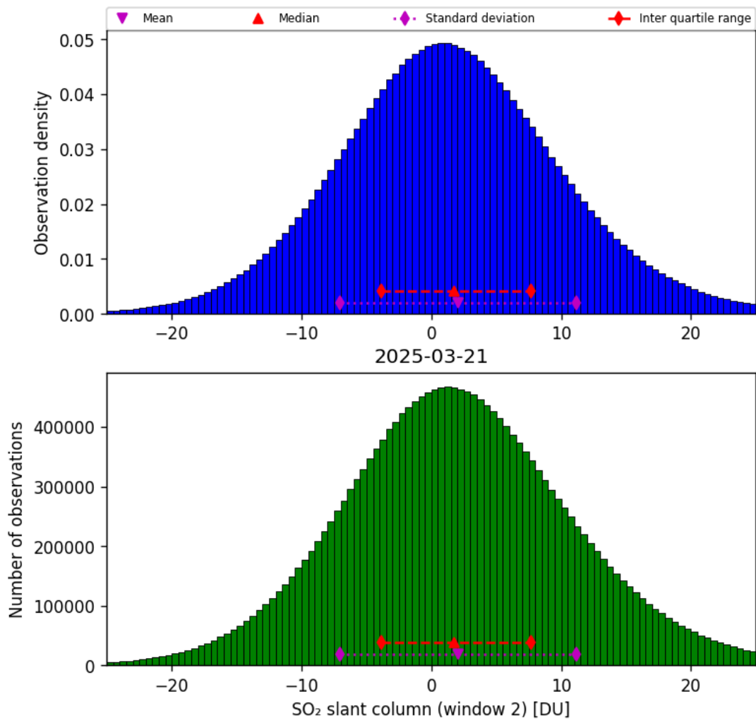
Figure 67: Histogram of “SO 2 slant column (window 2)” for 2025-03-20 to 2025-03-22
