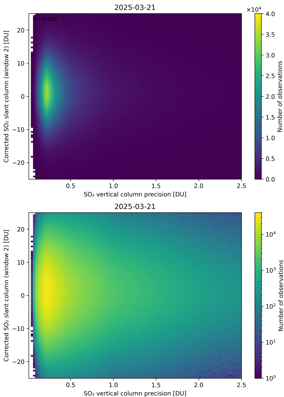
Figure 339: Scatter density plot of “SO 2 vertical column precision” against “Corrected SO 2 slant column (window 2)” for 2025-03-20 to 2025-03-22.
