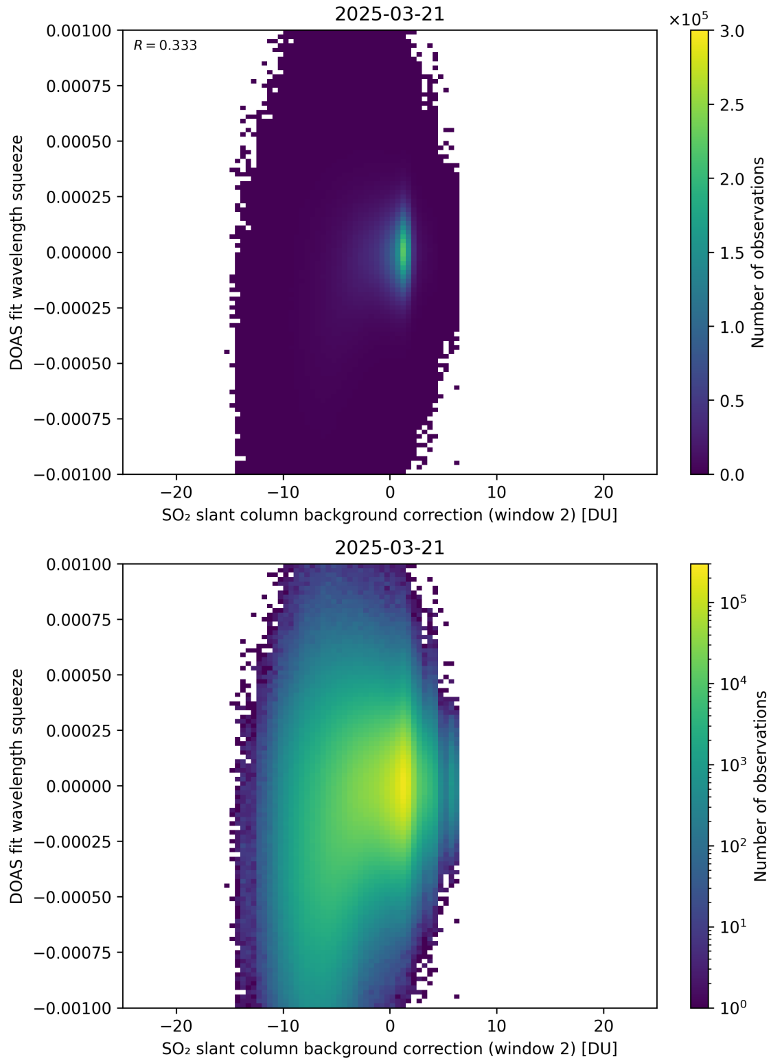
Figure 124: Scatter density plot of “SO 2 slant column background correction (window 2)” against “DOAS fit wavelength squeeze” for 2025-03-20 to 2025-03-22.
