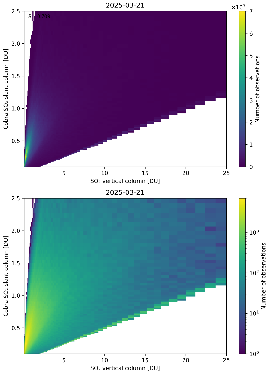
Figure 349: Scatter density plot of “SO 2 vertical column” against “Cobra SO 2 slant column” for 2025-03-20 to 2025-03-22.
