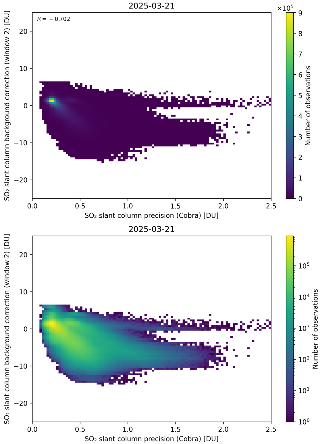
Figure 200: Scatter density plot of “SO 2 slant column precision (Cobra)” against “SO 2 slant column background correction (window 2)” for 2025-03-20 to 2025-03-22.
