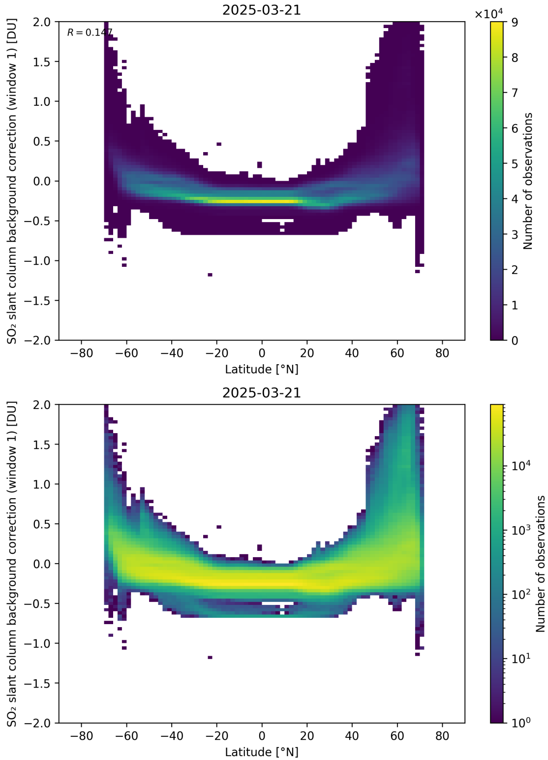
Figure 150: Scatter density plot of “Latitude” against “SO 2 slant column background correction (window 1)” for 2025-03-20 to 2025-03-22.
