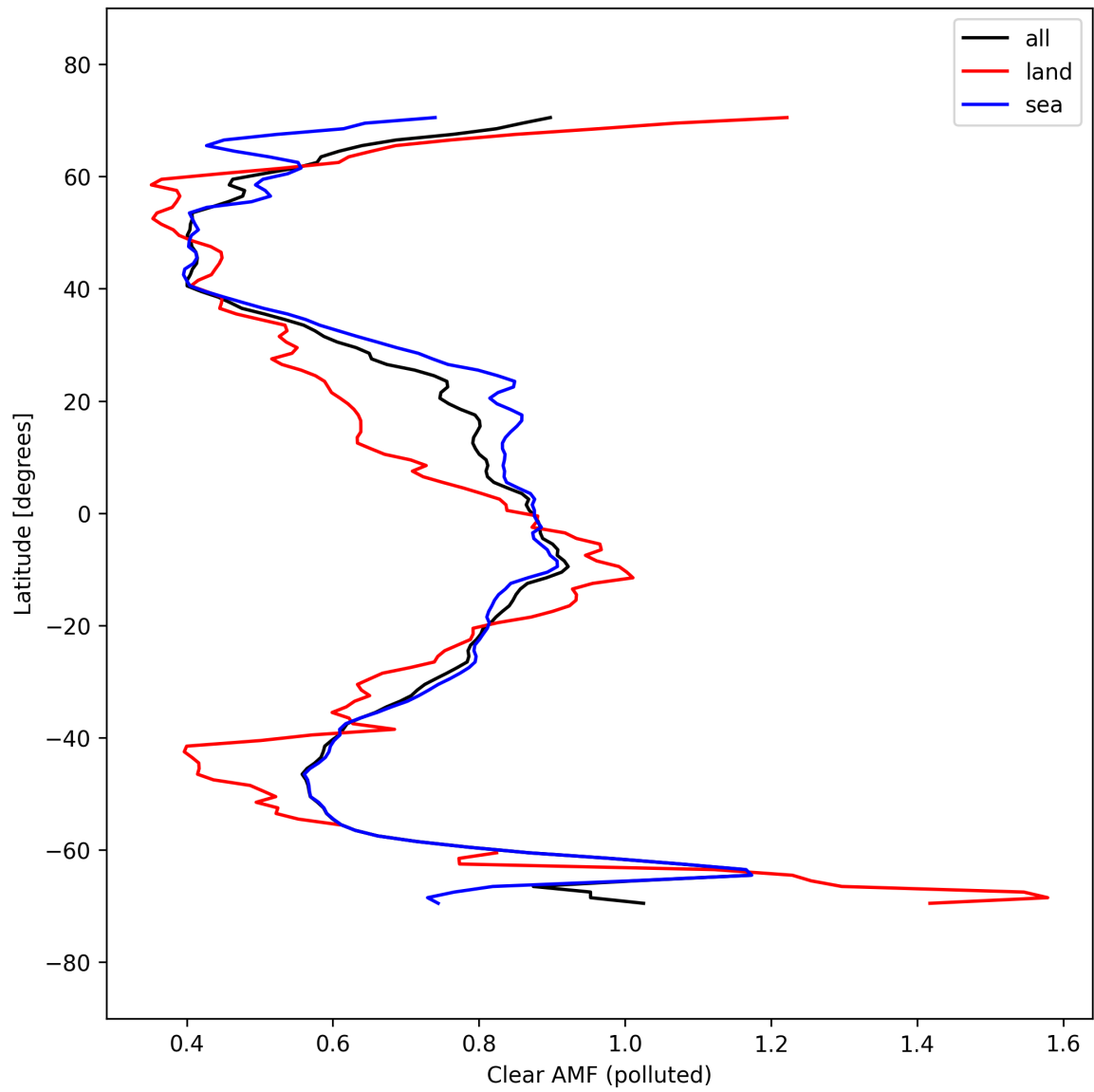
Figure 55: Zonal average of “Clear AMF (polluted)” for 2025-03-20 to 2025-03-22.
