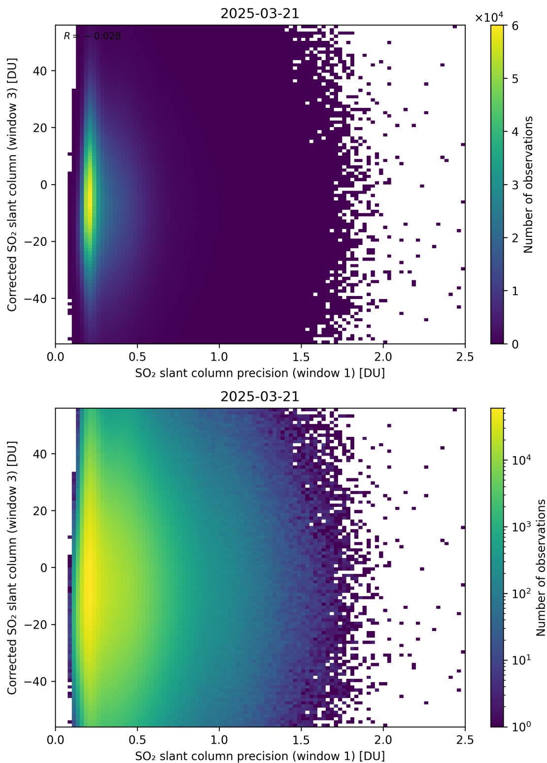
Figure 276: Scatter density plot of “SO 2 slant column precision (window 1)” against “Corrected SO 2 slant column (window 3)” for 2025-03-20 to 2025-03-22.
