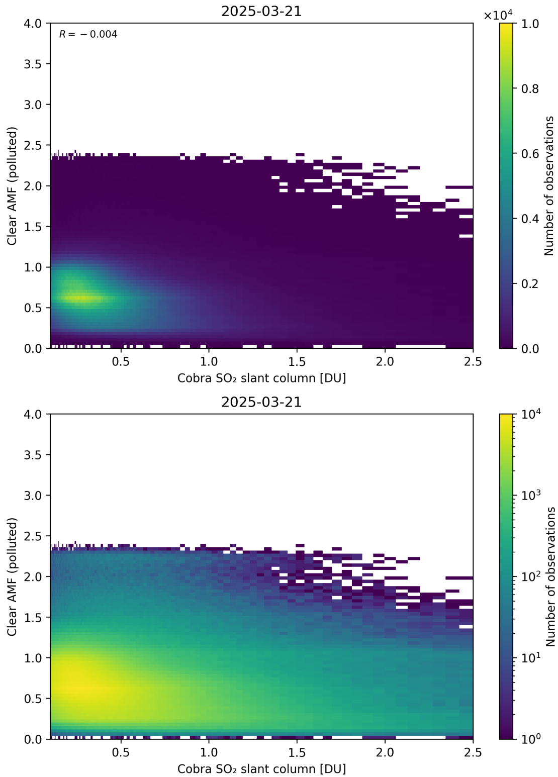
Figure 215: Scatter density plot of “Cobra SO 2 slant column” against “Clear AMF (polluted)” for 2025-03-20 to 2025-03-22.
