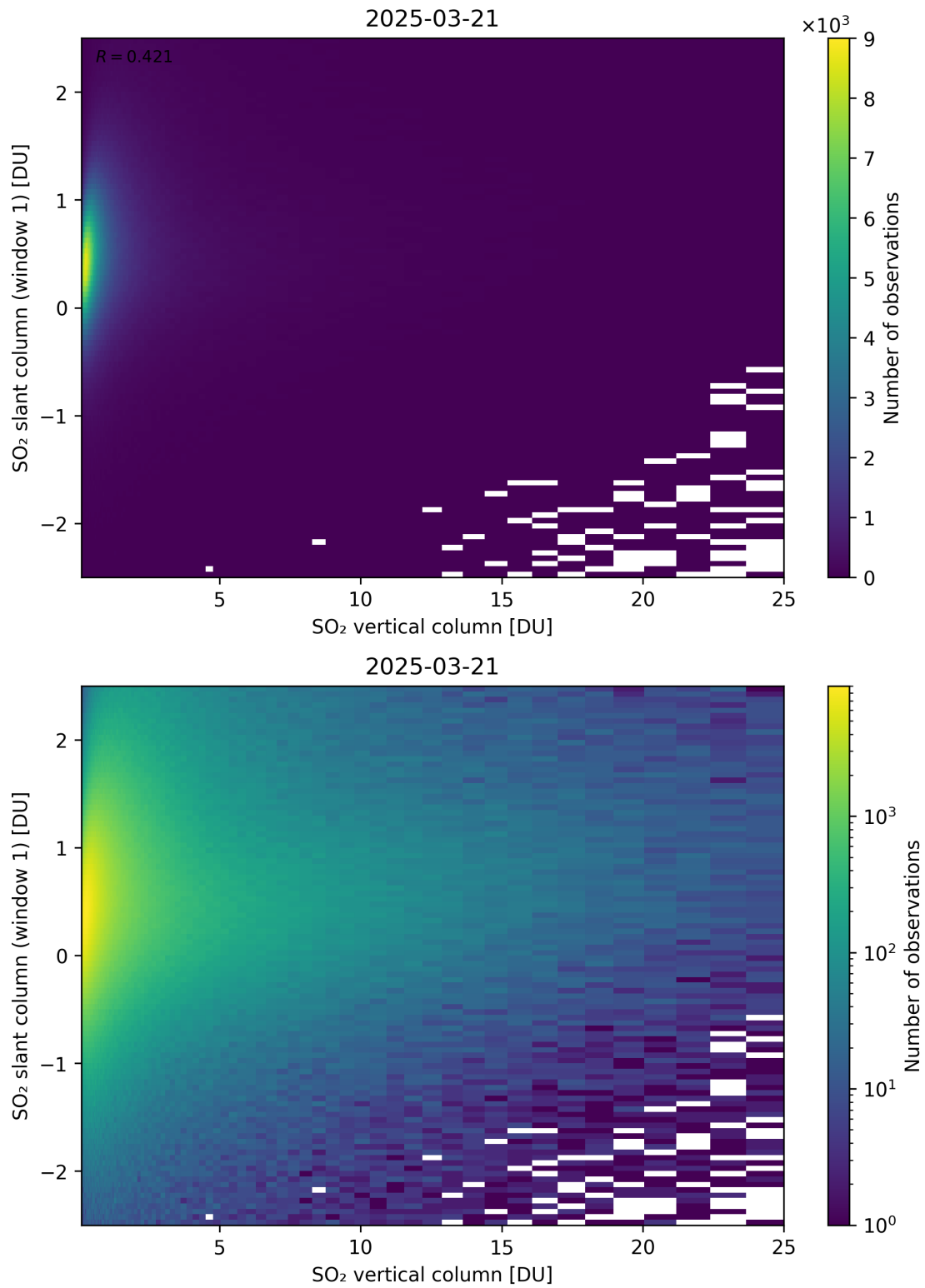
Figure 354: Scatter density plot of “SO 2 vertical column” against “SO 2 slant column (window 1)” for 2025-03-20 to 2025-03-22.
