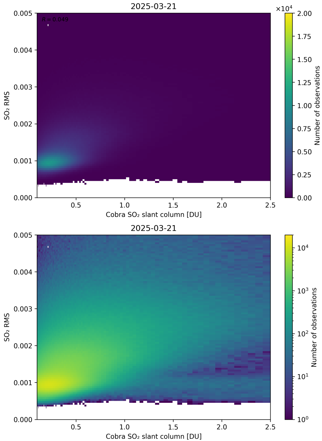
Figure 198: Scatter density plot of “Cobra SO 2 slant column” against “SO 2 RMS” for 2025-03-20 to 2025-03-22.
