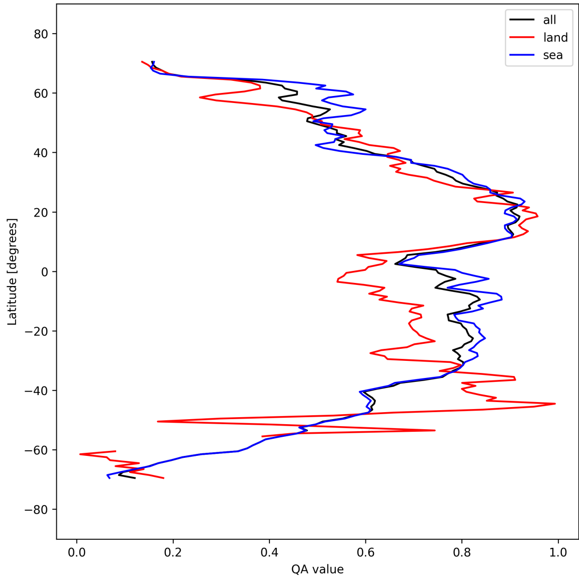
Figure 31: Zonal average of “QA value” for 2025-03-20 to 2025-03-22.
