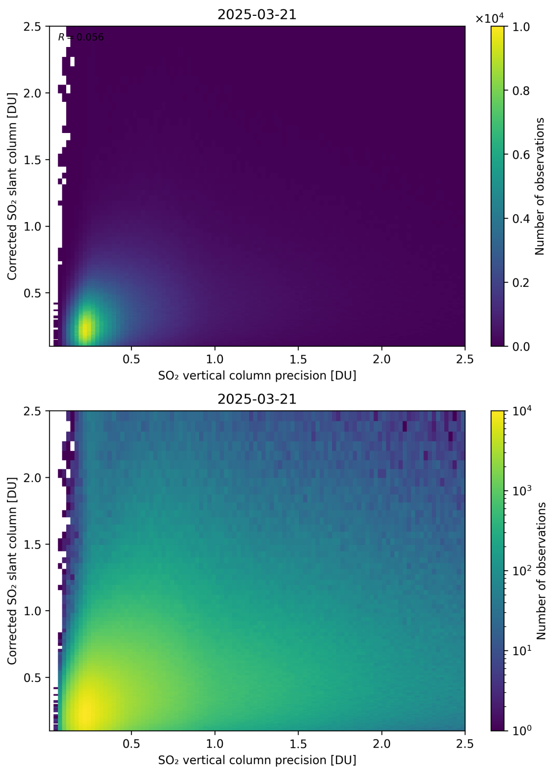
Figure 338: Scatter density plot of “SO 2 vertical column precision” against “Corrected SO 2 slant column” for 2025-03-20 to 2025-03-22.
