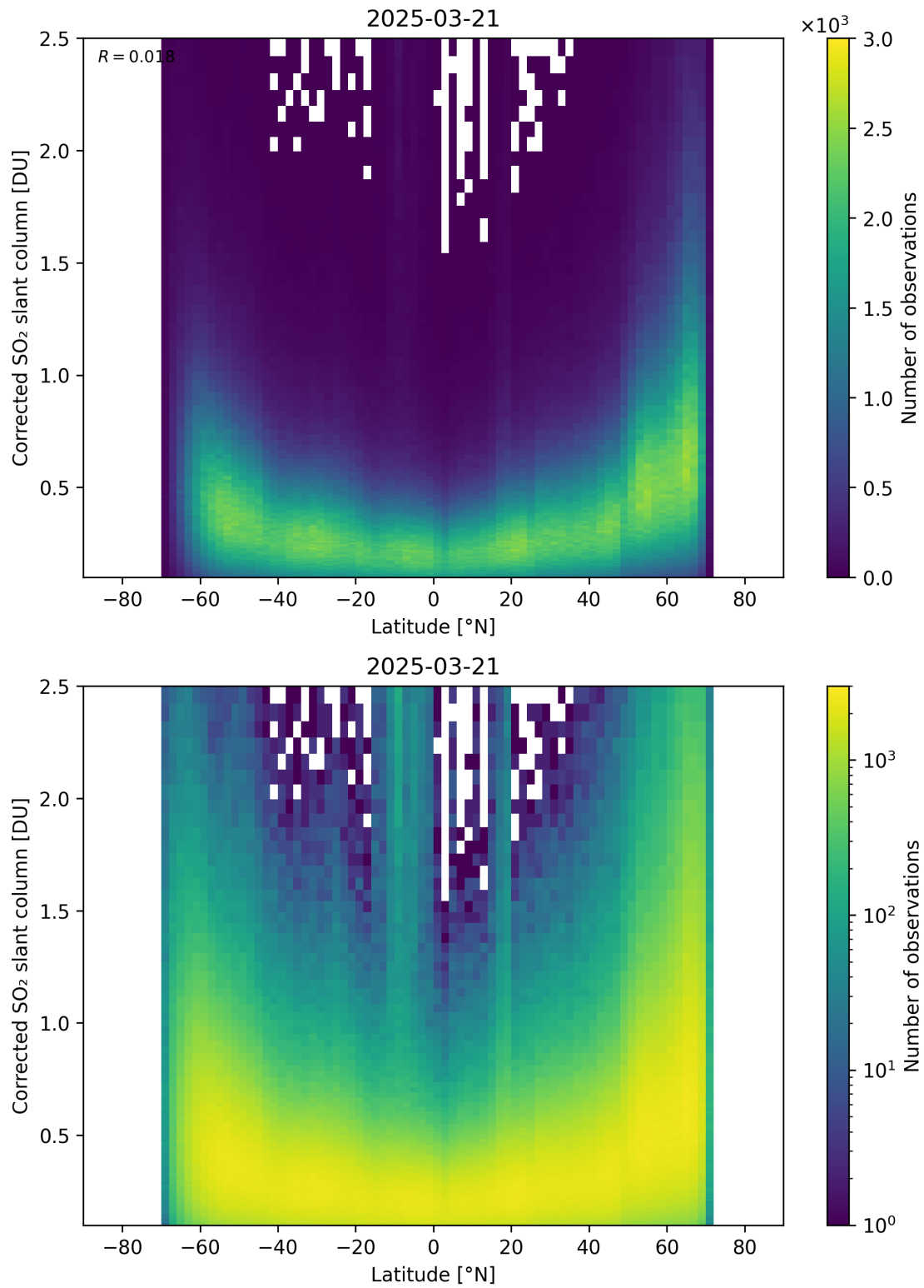
Figure 159: Scatter density plot of “Latitude” against “Corrected SO 2 slant column” for 2025-03-20 to 2025-03-22.
