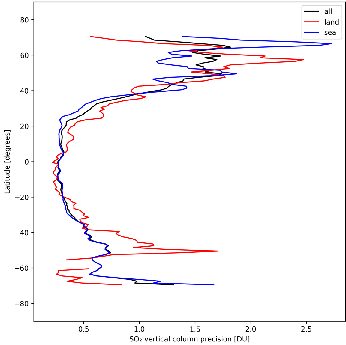
Figure 33: Zonal average of “SO 2 vertical column precision” for 2025-03-20 to 2025-03-22.
