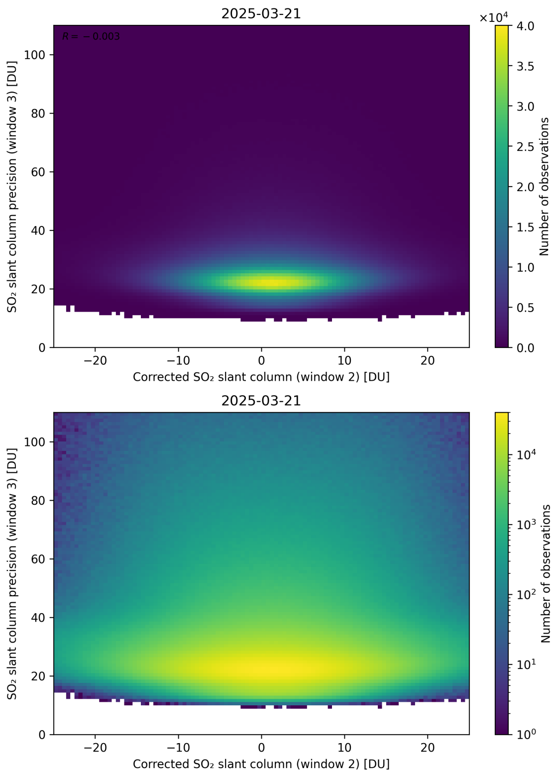
Figure 252: Scatter density plot of “Corrected SO 2 slant column (window 2)” against “SO 2 slant column precision (window 3)” for 2025-03-20 to 2025-03-22.
