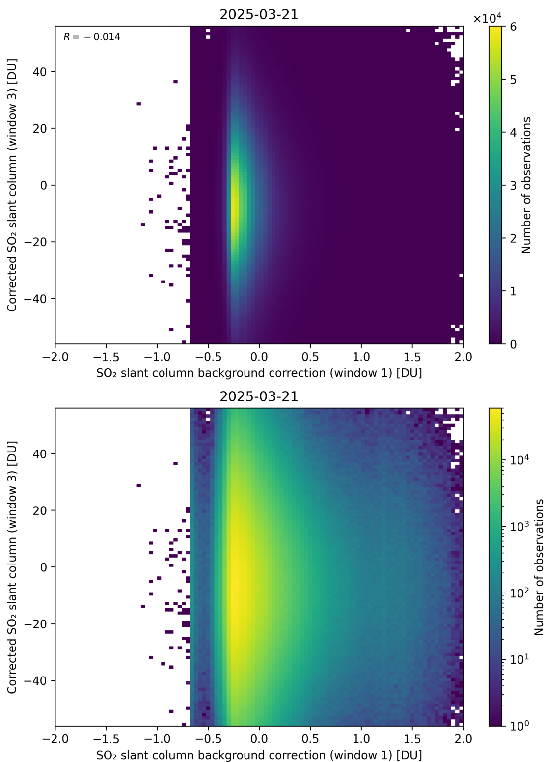
Figure 116: Scatter density plot of “SO 2 slant column background correction (window 1)” against “Corrected SO 2 slant column (window 3)” for 2025-03-20 to 2025-03-22.
