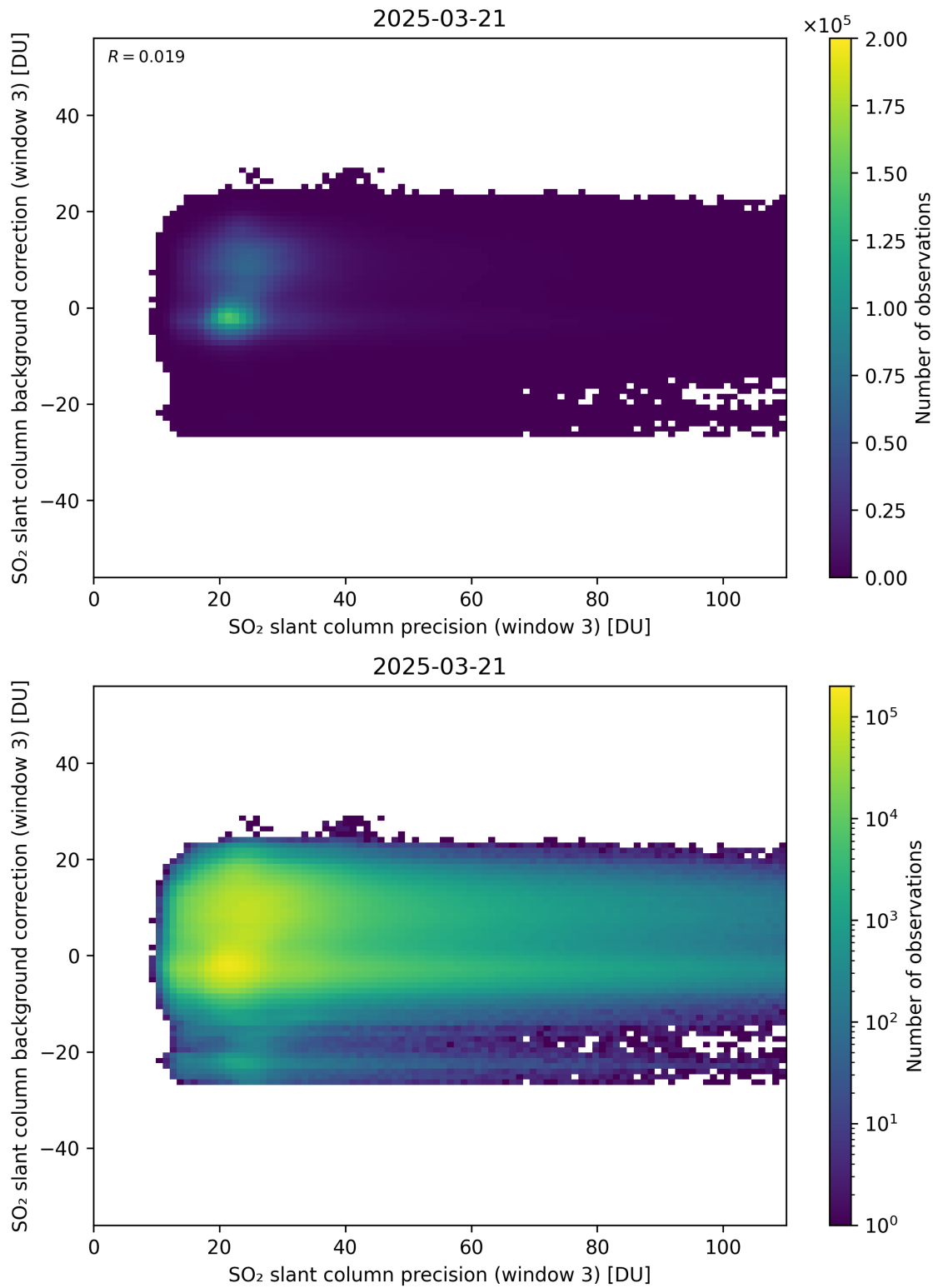
Figure 307: Scatter density plot of “SO 2 slant column precision (window 3)” against “SO 2 slant column background correction (window 3)” for 2025-03-20 to 2025-03-22.
