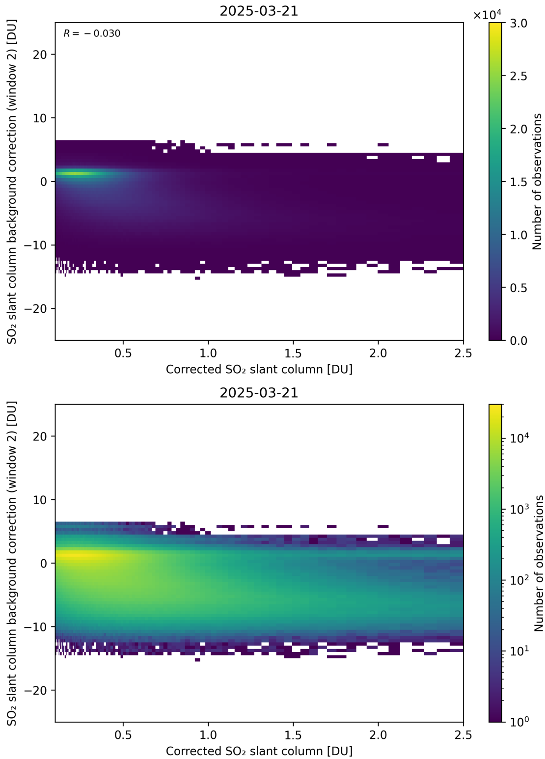
Figure 227: Scatter density plot of “Corrected SO 2 slant column” against “SO 2 slant column background correction (window 2)” for 2025-03-20 to 2025-03-22.
