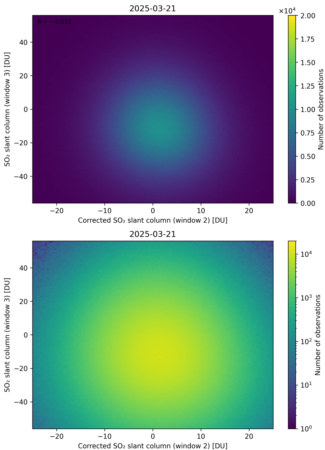
Figure 251: Scatter density plot of “Corrected SO 2 slant column (window 2)” against “SO 2 slant column (window 3)” for 2025-03-20 to 2025-03-22.
