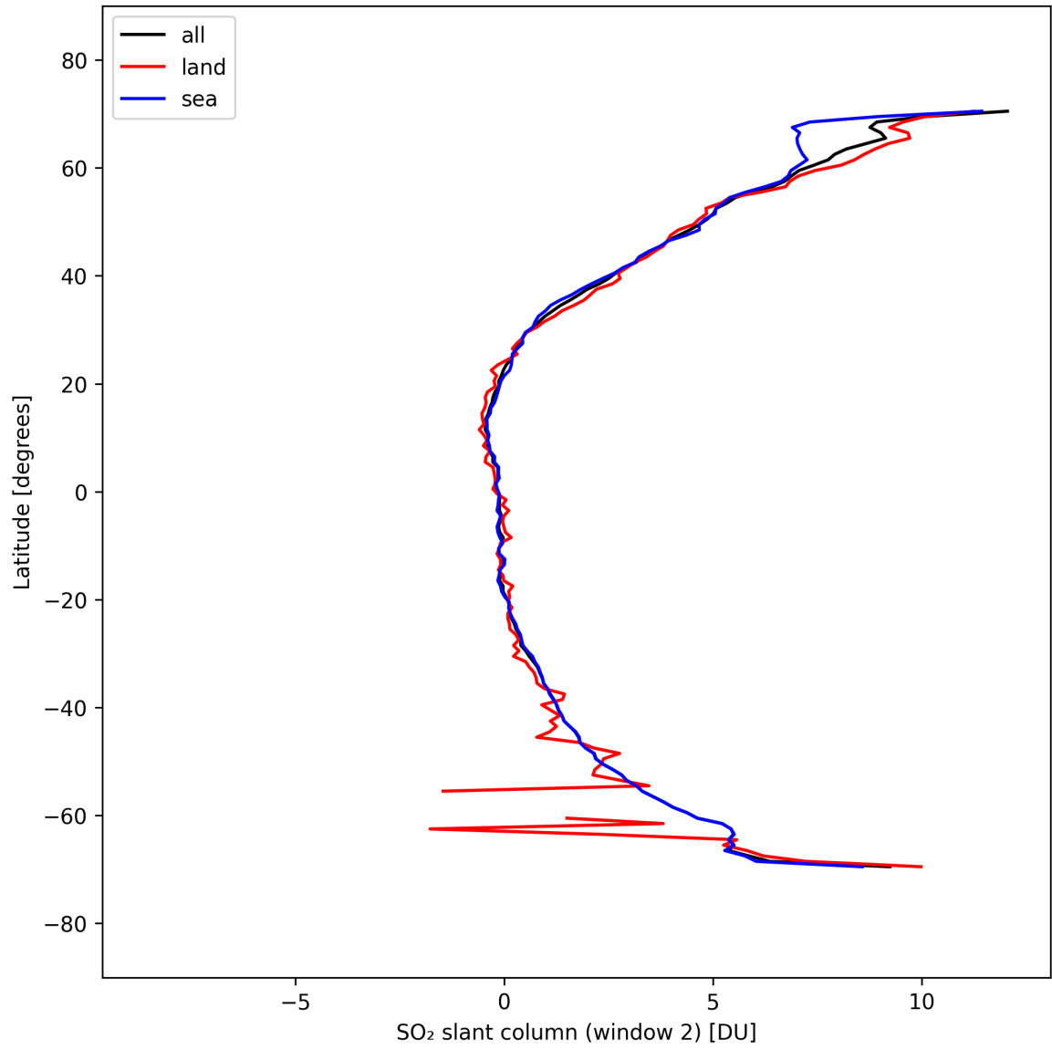
Figure 41: Zonal average of “SO 2 slant column (window 2)” for 2025-03-20 to 2025-03-22.
