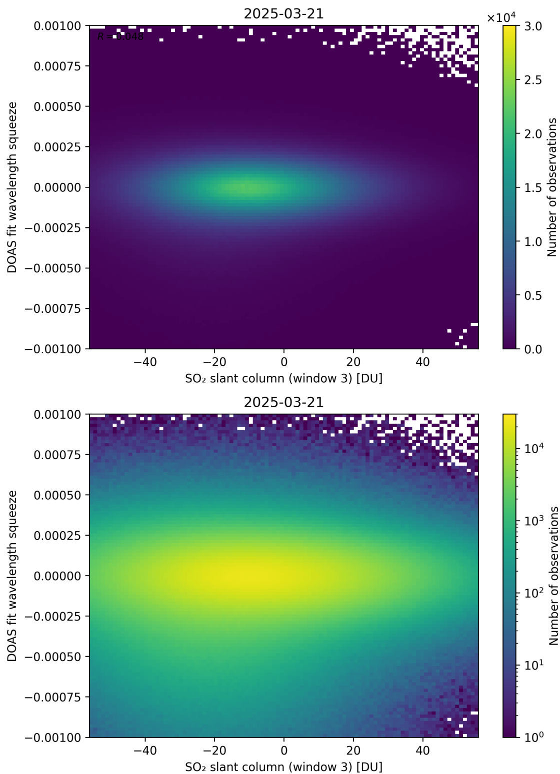
Figure 305: Scatter density plot of “SO 2 slant column (window 3)” against “DOAS fit wavelength squeeze” for 2025-03-20 to 2025-03-22.
