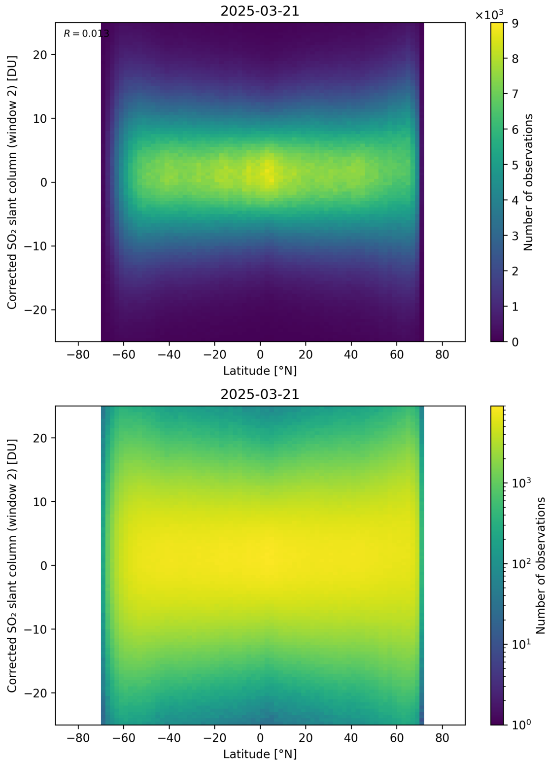
Figure 160: Scatter density plot of “Latitude” against “Corrected SO 2 slant column (window 2)” for 2025-03-20 to 2025-03-22.
