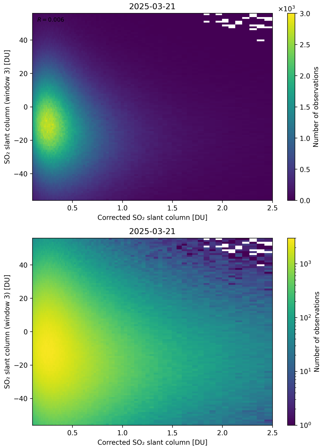
Figure 240: Scatter density plot of “Corrected SO 2 slant column” against “SO 2 slant column (window 3)” for 2025-03-20 to 2025-03-22.
