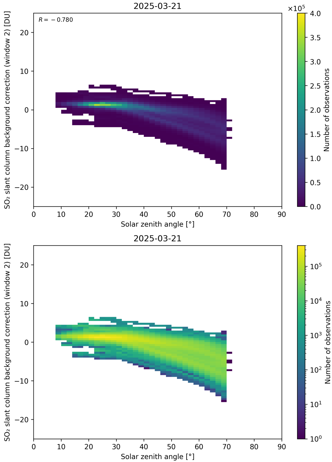
Figure 172: Scatter density plot of “Solar zenith angle” against “SO 2 slant column background correction (window 2)” for 2025-03-20 to 2025-03-22.
