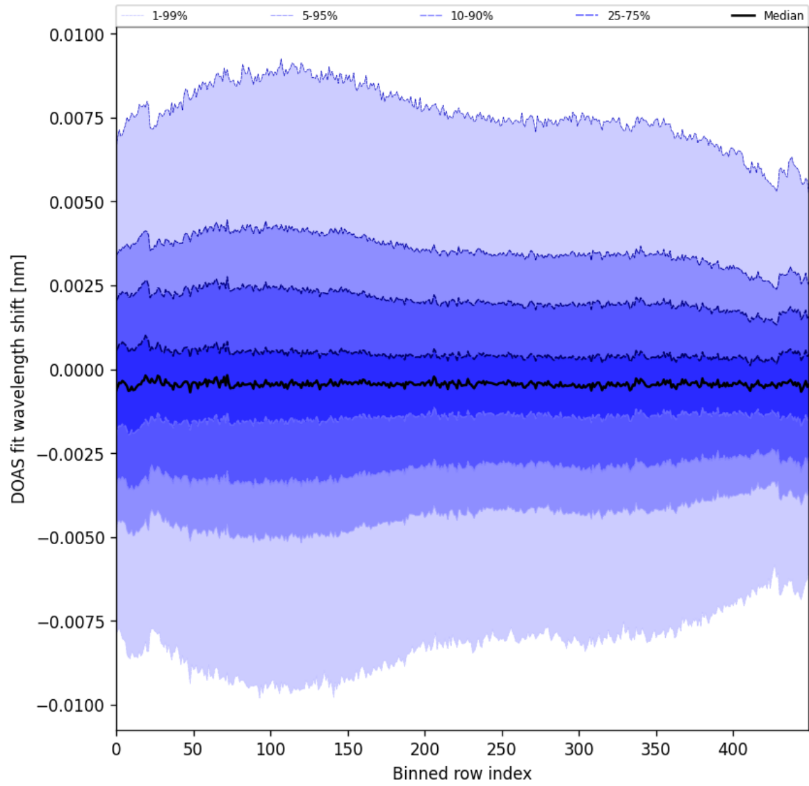
Figure 102: Along track statistics of “DOAS fit wavelength shift” for 2025-03-20 to 2025-03-22
