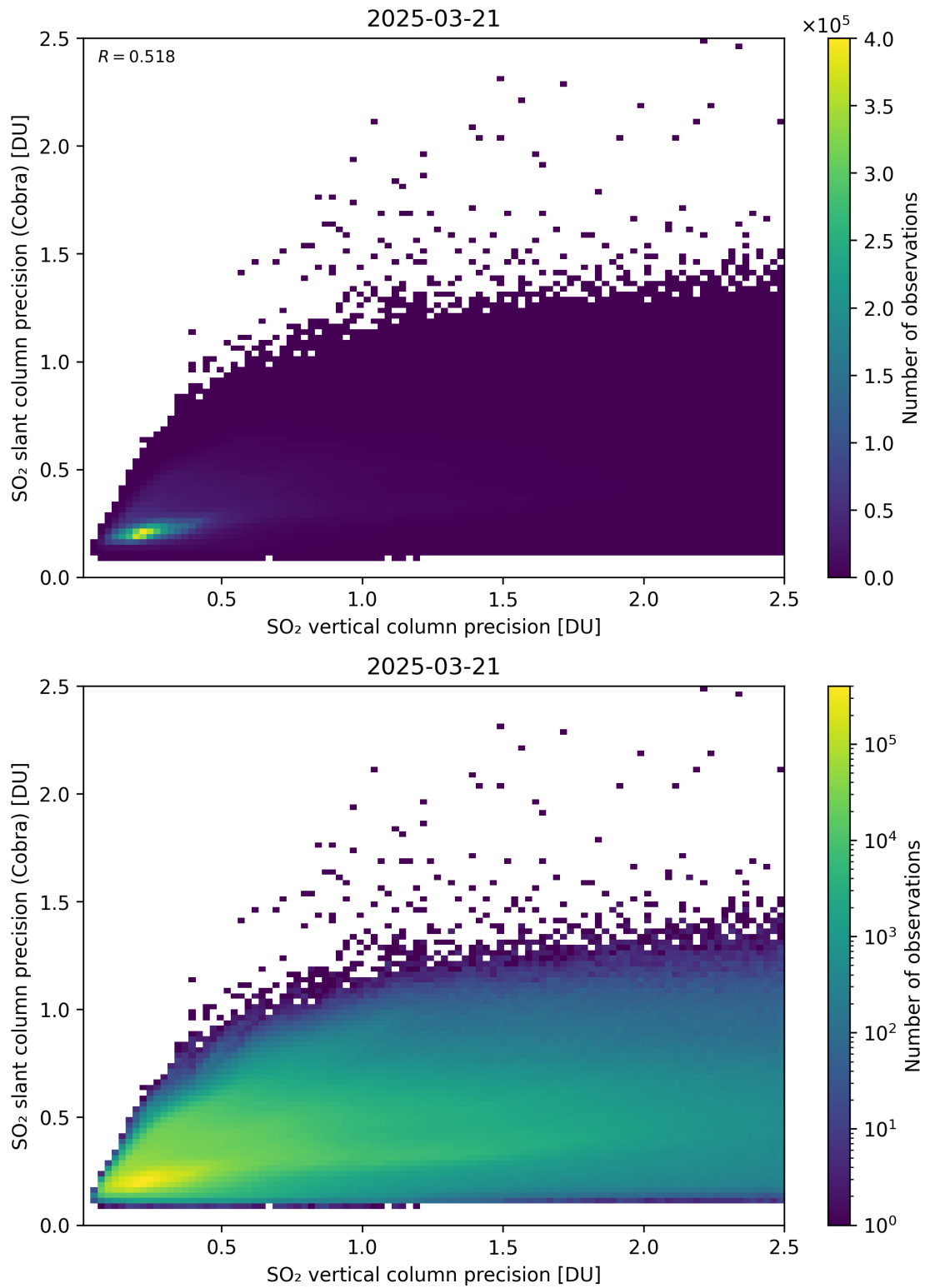
Figure 337: Scatter density plot of “SO 2 vertical column precision” against “SO 2 slant column precision (Cobra)” for 2025-03-20 to 2025-03-22.
