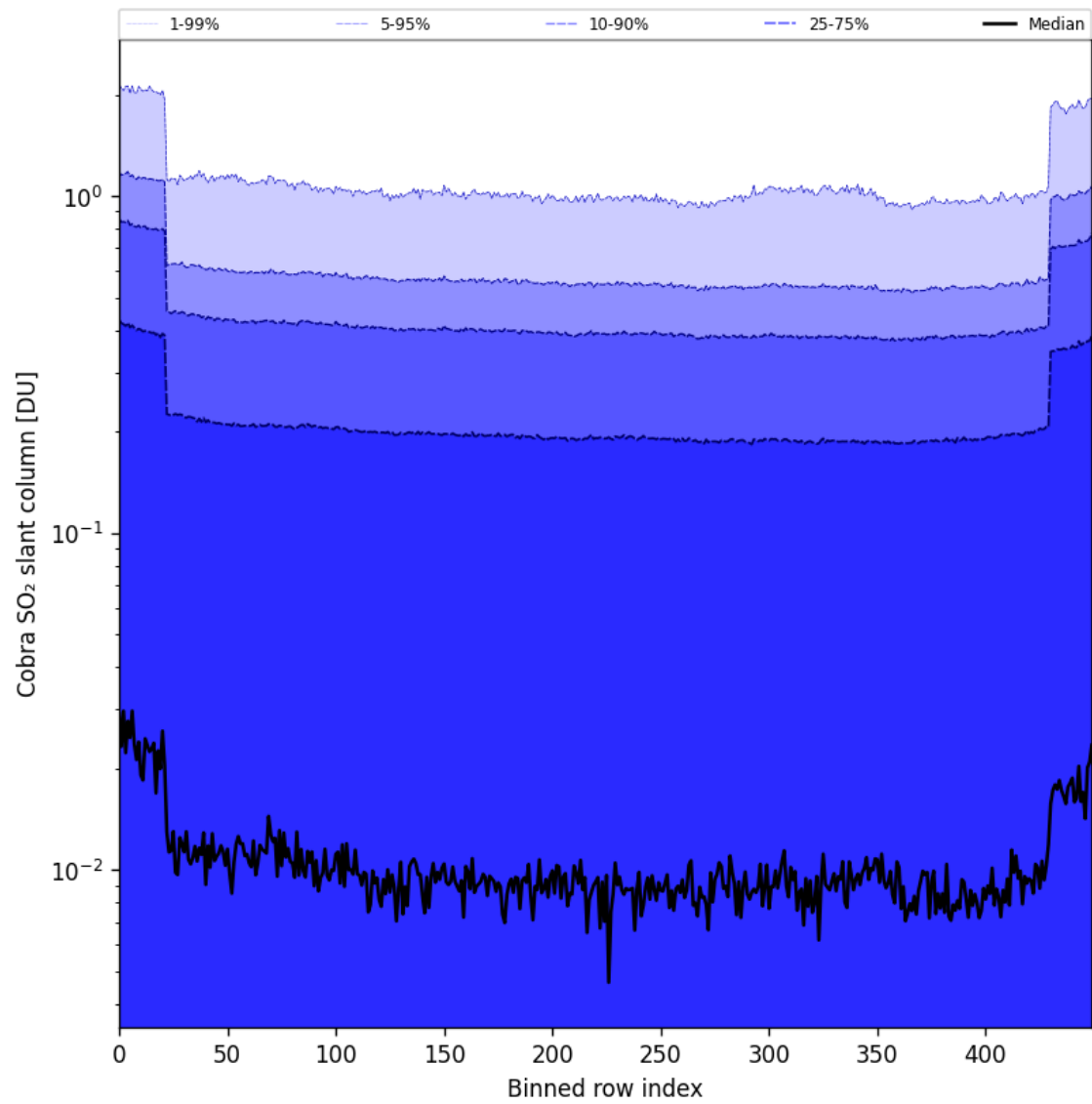
Figure 87: Along track statistics of "Cobra SO 2 slant column" for 2025-03-20 to 2025-03-22
