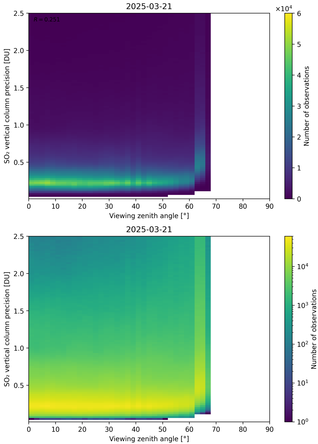
Figure 384: Scatter density plot of “Viewing zenith angle” against “SO 2 vertical column precision” for 2025-03-20 to 2025-03-22.
