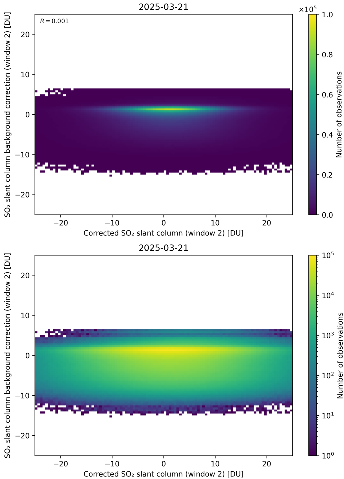
Figure 244: Scatter density plot of “Corrected SO 2 slant column (window 2)” against “SO 2 slant column background correction (window 2)” for 2025-03-20 to 2025-03-22.
