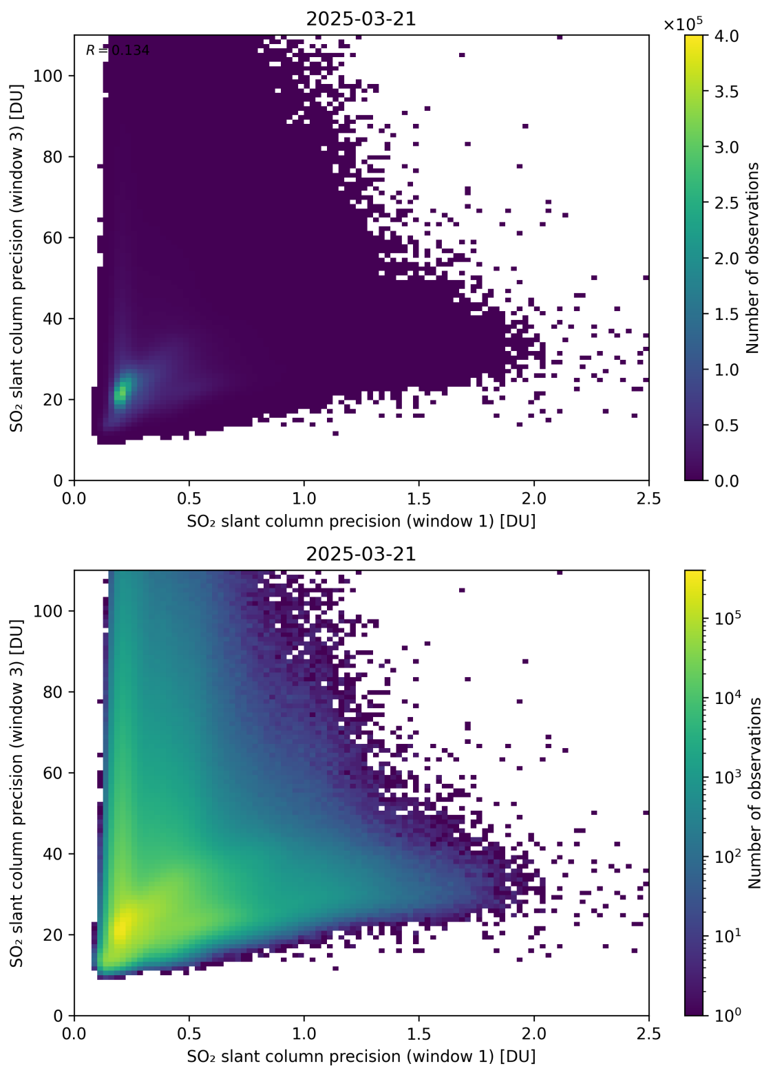
Figure 279: Scatter density plot of “SO 2 slant column precision (window 1)” against “SO 2 slant column precision (window 3)” for 2025-03-20 to 2025-03-22.
