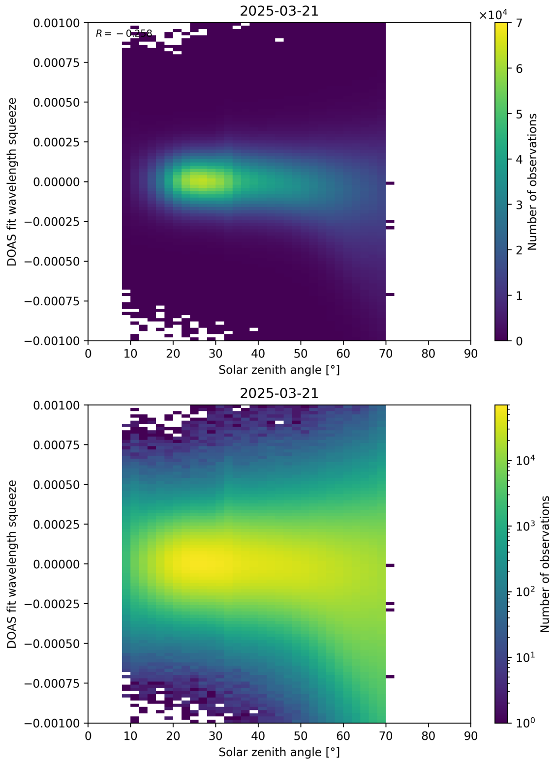
Figure 175: Scatter density plot of “Solar zenith angle” against “DOAS fit wavelength squeeze” for 2025-03-20 to 2025-03-22.
