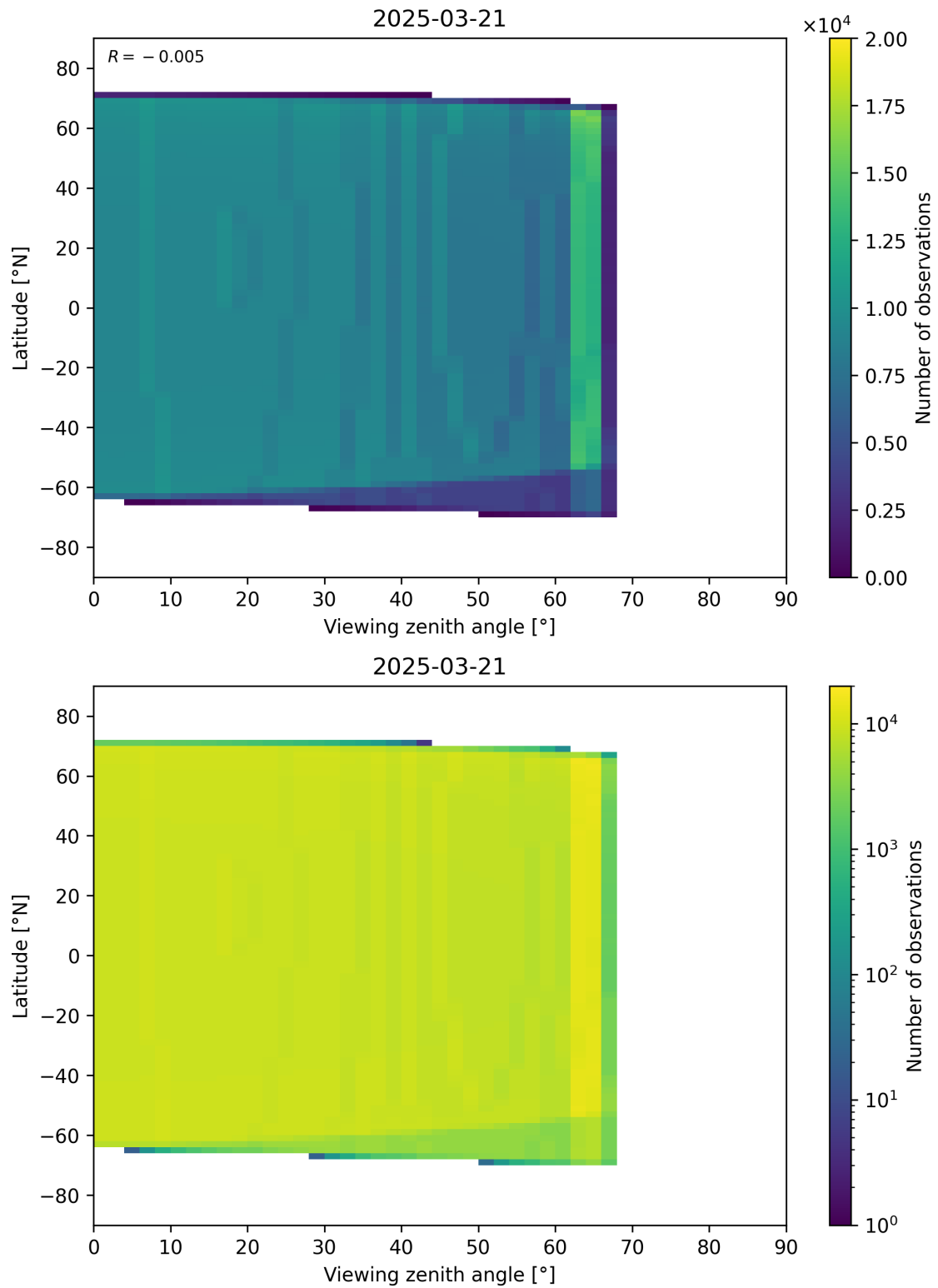
Figure 368: Scatter density plot of “Viewing zenith angle” against “Latitude” for 2025-03-20 to 2025-03-22.
