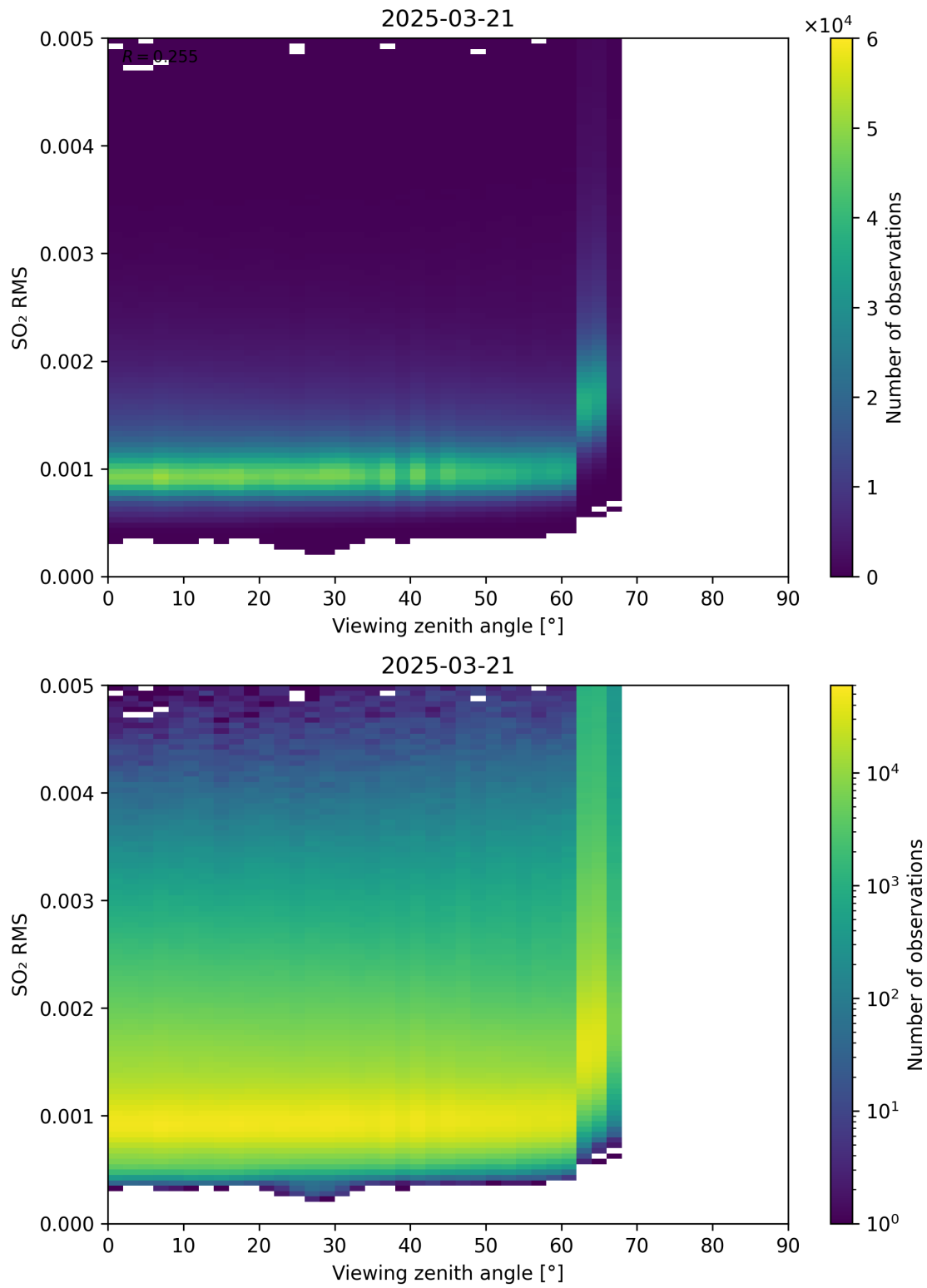
Figure 367: Scatter density plot of “Viewing zenith angle” against “SO 2 RMS” for 2025-03-20 to 2025-03-22.
