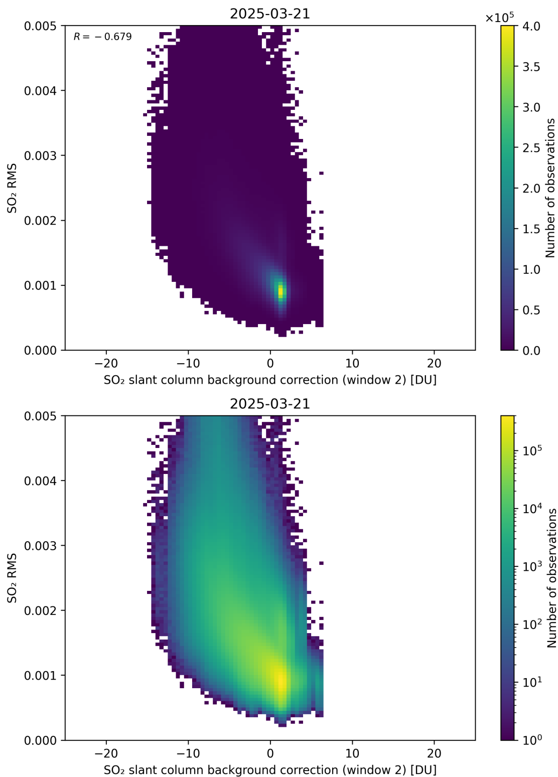
Figure 125: Scatter density plot of “SO 2 slant column background correction (window 2)” against “SO 2 RMS” for 2025-03-20 to 2025-03-22.
