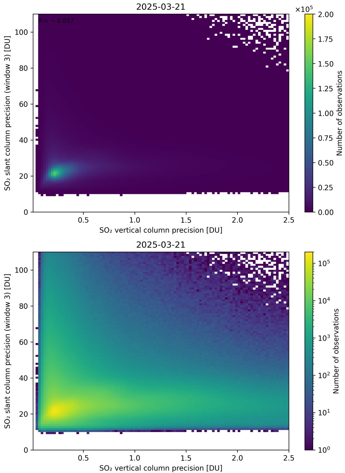
Figure 345: Scatter density plot of “SO 2 vertical column precision” against “SO 2 slant column precision (window 3)” for 2025-03-20 to 2025-03-22.
