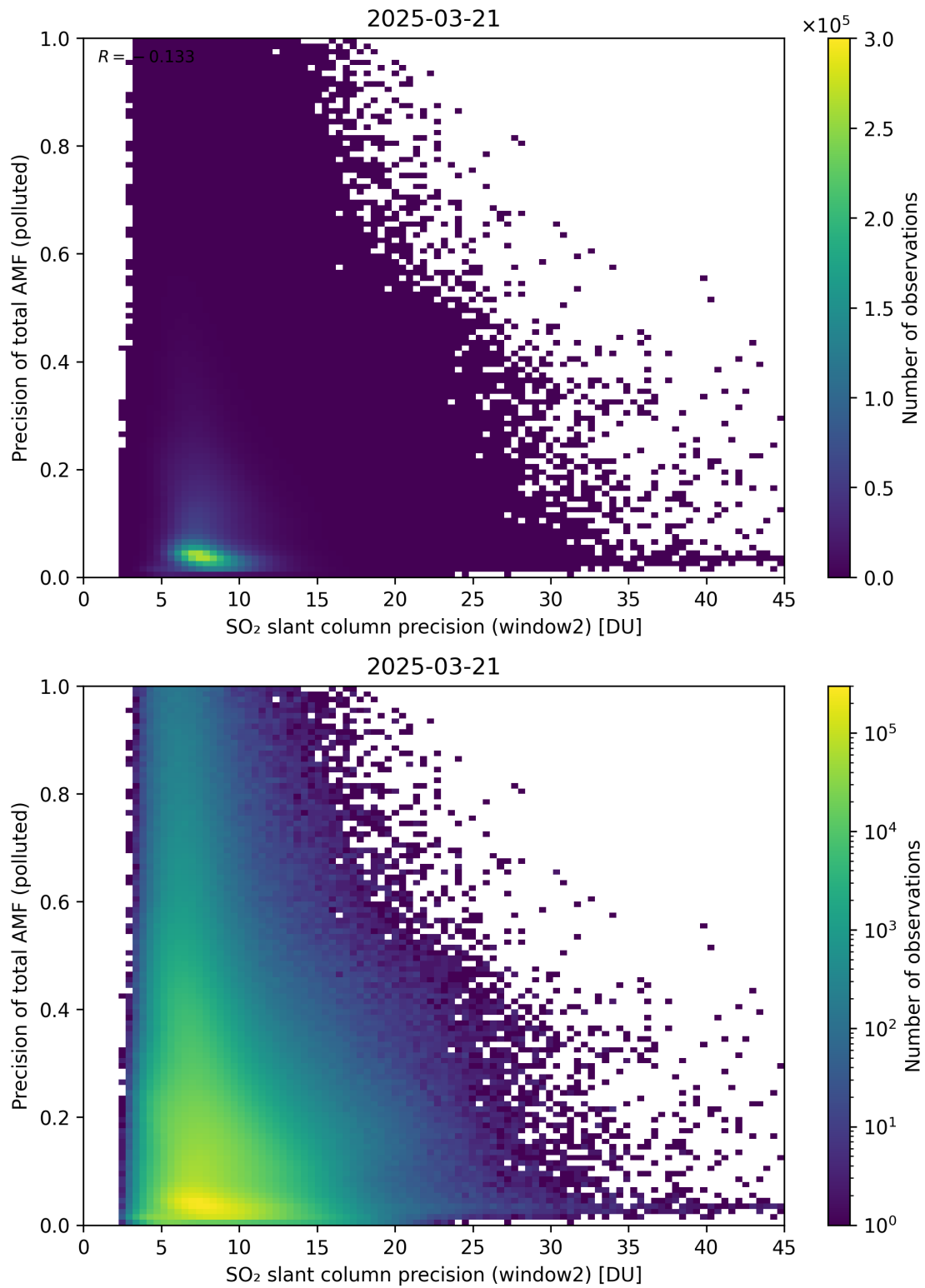
Figure 302: Scatter density plot of “SO 2 slant column precision (window2)” against “Precision of total AMF (polluted)” for 2025-03-20 to 2025-03-22.
