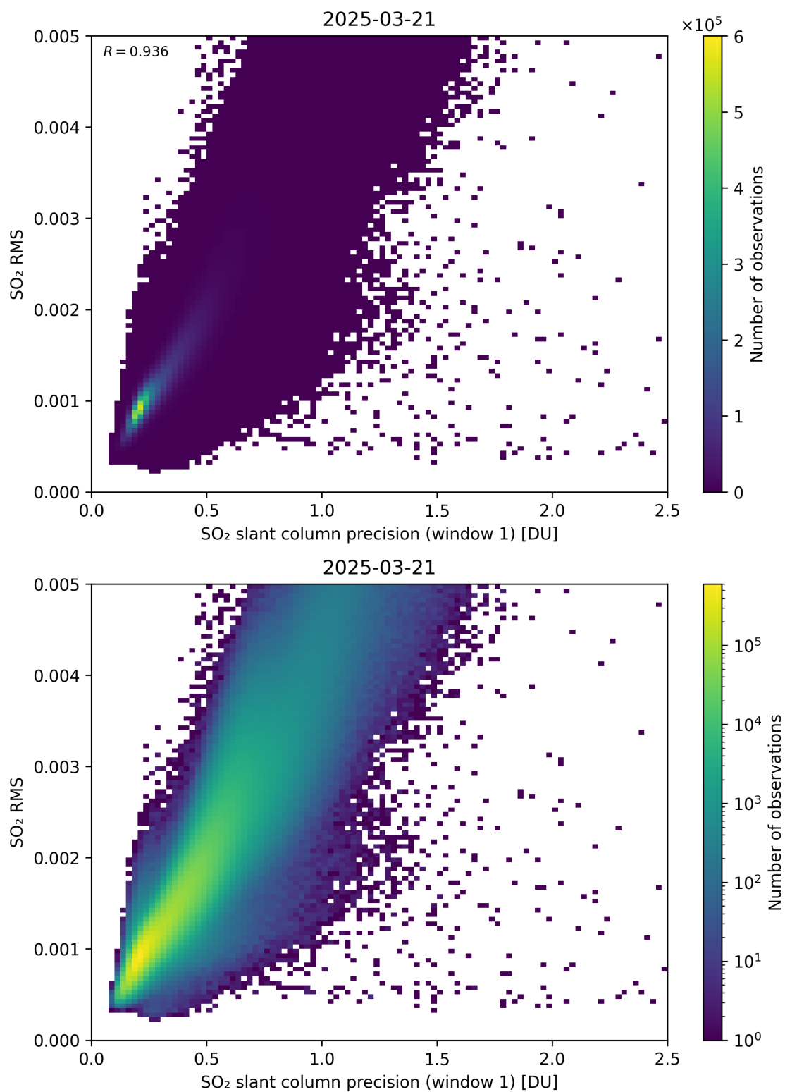
Figure 273: Scatter density plot of “SO 2 slant column precision (window 1)” against “SO 2 RMS” for 2025-03-20 to 2025-03-22.
