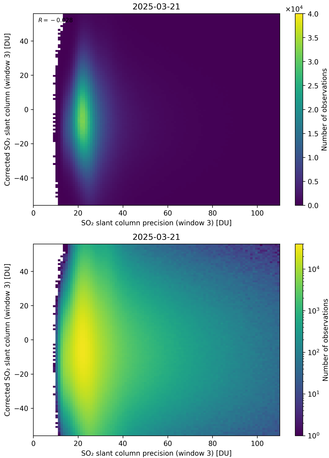
Figure 312: Scatter density plot of “SO 2 slant column precision (window 3)” against “Corrected SO 2 slant column (window 3)” for 2025-03-20 to 2025-03-22.
