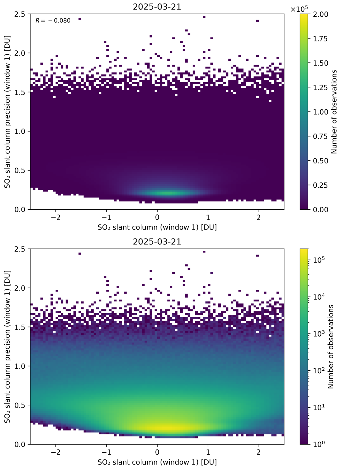
Figure 285: Scatter density plot of “SO 2 slant column (window 1)” against “SO 2 slant column precision (window 1)” for 2025-03-20 to 2025-03-22.
