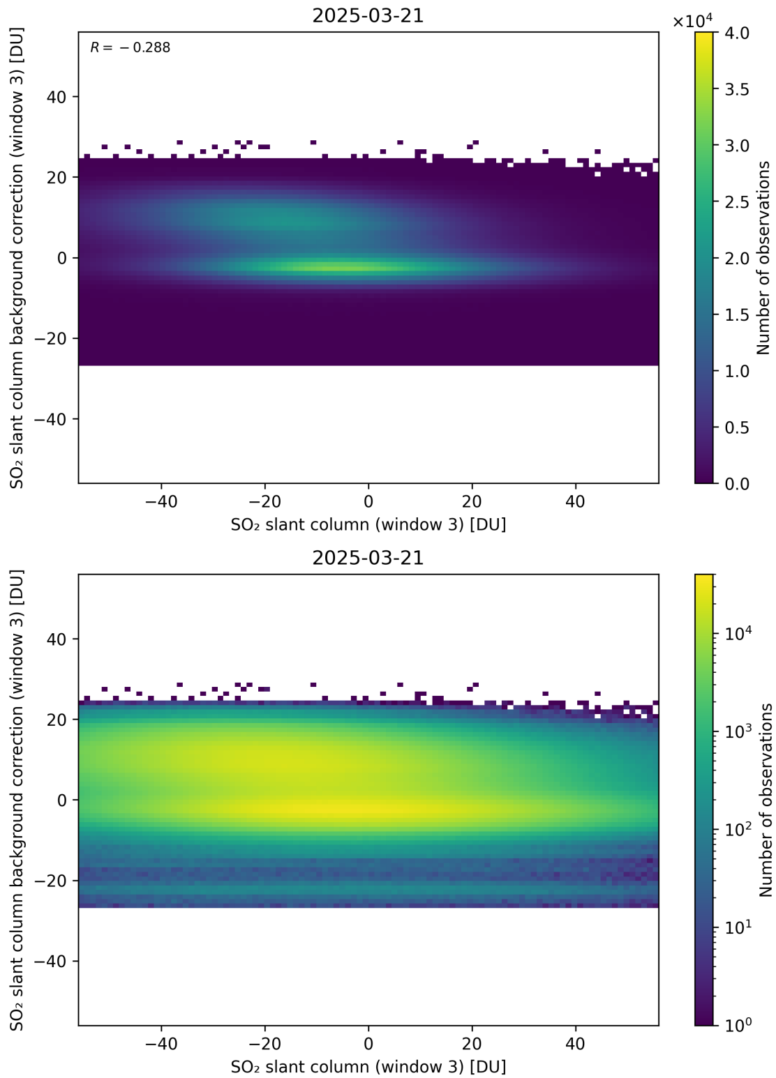
Figure 303: Scatter density plot of “SO 2 slant column (window 3)” against “SO 2 slant column background correction (window 3)” for 2025-03-20 to 2025-03-22.
