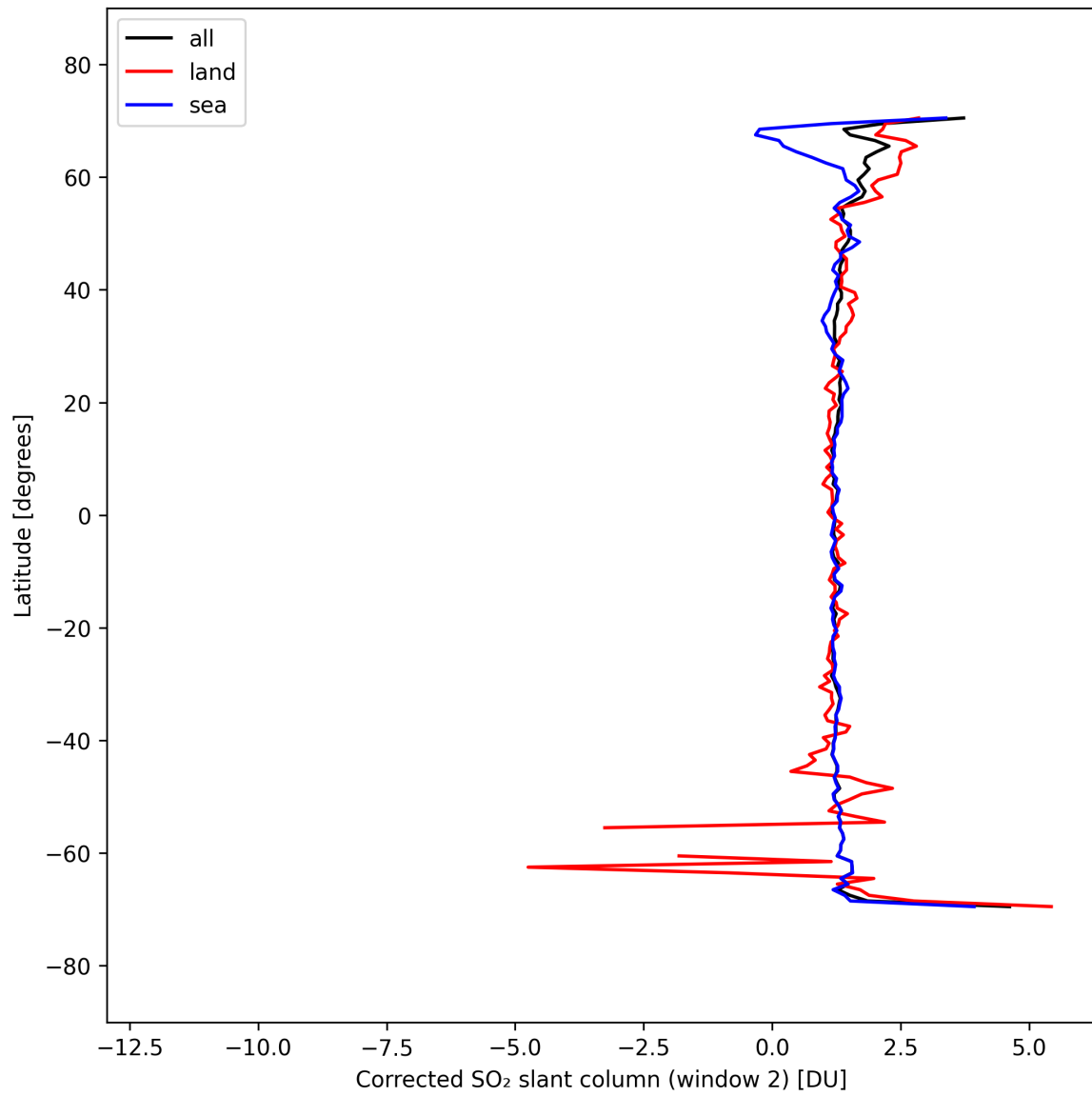
Figure 43: Zonal average of “Corrected SO 2 slant column (window 2)” for 2025-03-20 to 2025-03-22.
