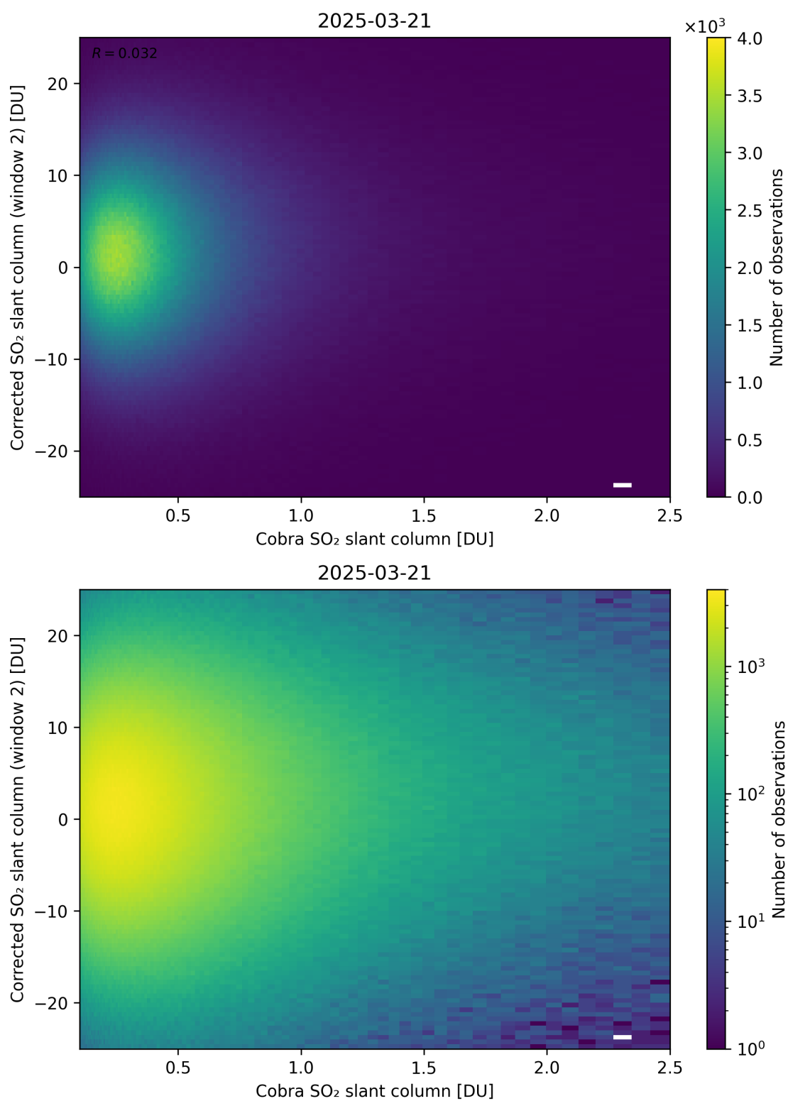
Figure 217: Scatter density plot of “Cobra SO 2 slant column” against “Corrected SO 2 slant column (window 2)” for 2025-03-20 to 2025-03-22.
