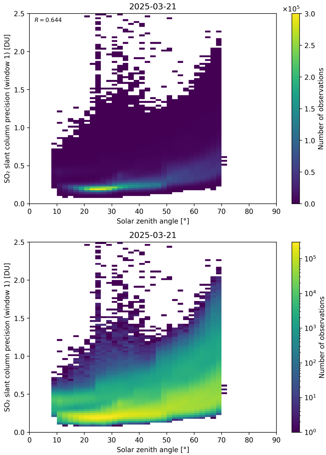
Figure 185: Scatter density plot of “Solar zenith angle” against “SO 2 slant column precision (window 1)” for 2025-03-20 to 2025-03-22.
