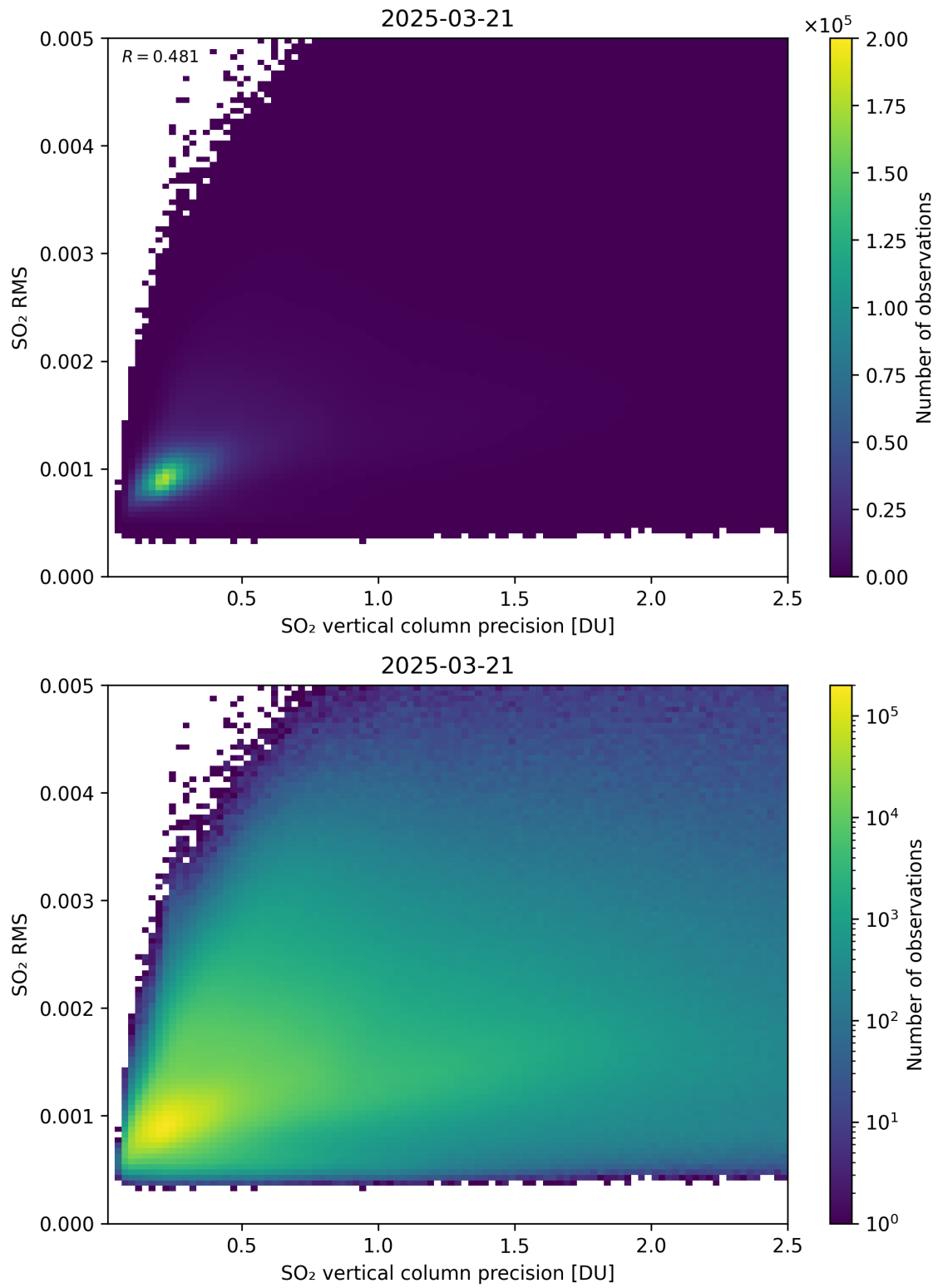
Figure 334: Scatter density plot of “SO 2 vertical column precision” against “SO 2 RMS” for 2025-03-20 to 2025-03-22.
