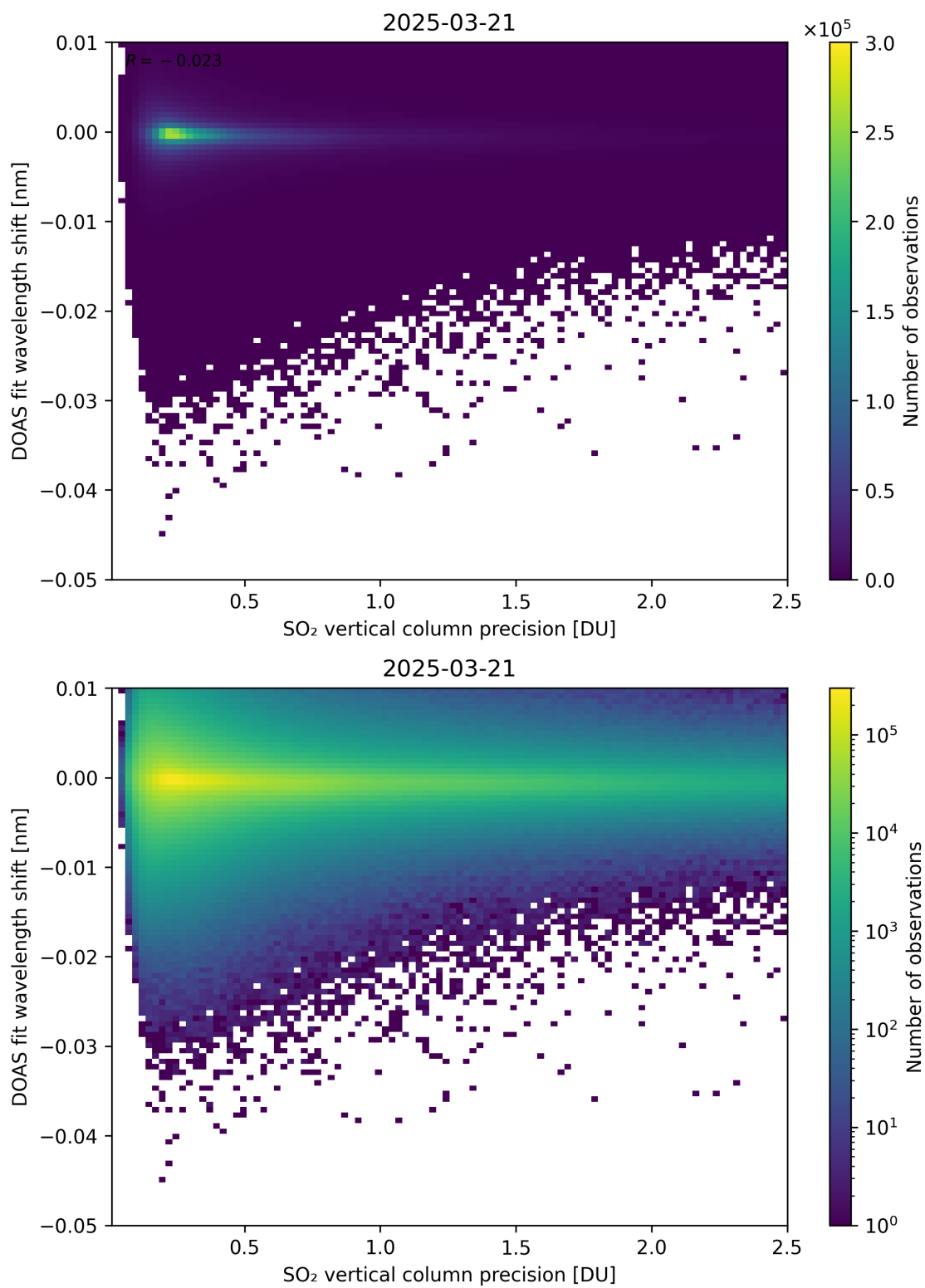
Figure 332: Scatter density plot of “SO 2 vertical column precision” against “DOAS fit wavelength shift” for 2025-03-20 to 2025-03-22.
