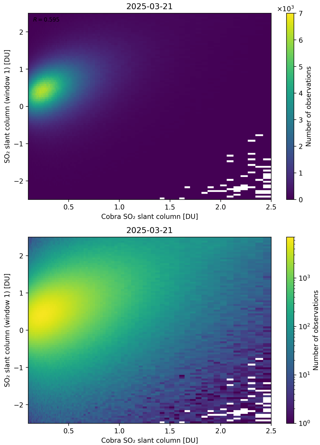
Figure 219: Scatter density plot of “Cobra SO 2 slant column” against “SO 2 slant column (window 1)” for 2025-03-20 to 2025-03-22.
