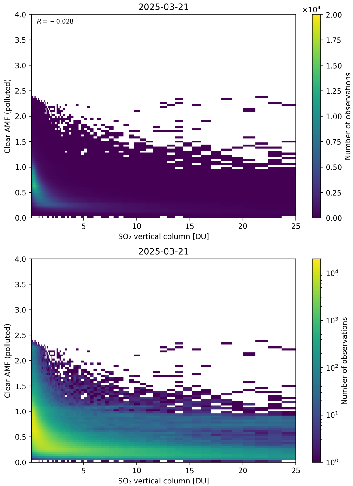
Figure 348: Scatter density plot of “SO 2 vertical column” against “Clear AMF (polluted)” for 2025-03-20 to 2025-03-22.
