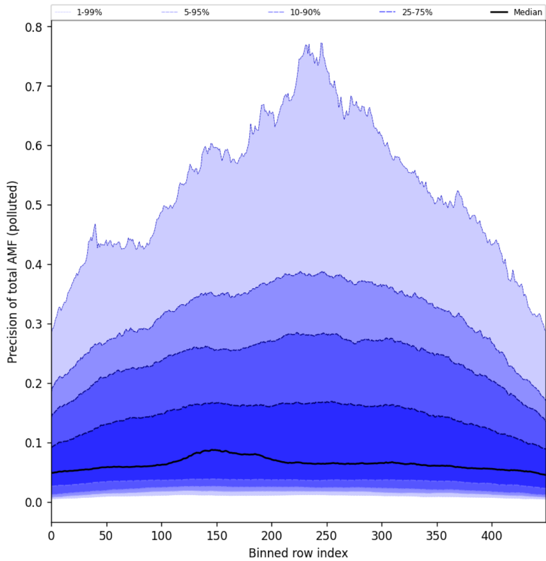
Figure 106: Along track statistics of “Precision of total AMF (polluted)” for 2025-03-20 to 2025-03-22
