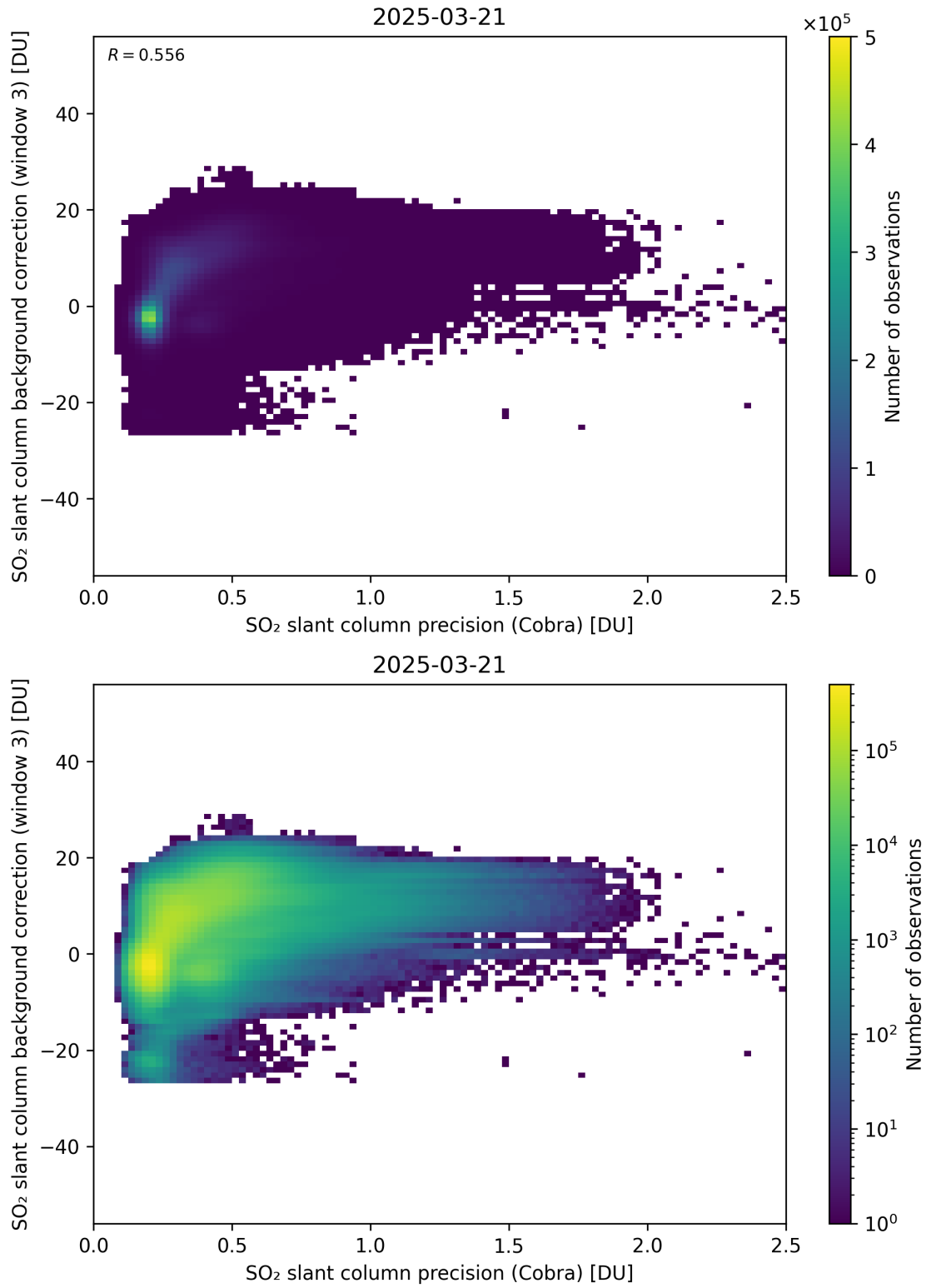
Figure 201: Scatter density plot of “SO 2 slant column precision (Cobra)” against “SO 2 slant column background correction (window 3)” for 2025-03-20 to 2025-03-22.
