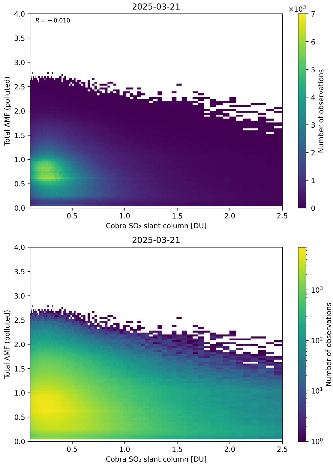
Figure 224: Scatter density plot of “Cobra SO 2 slant column” against “Total AMF (polluted)” for 2025-03-20 to 2025-03-22.
