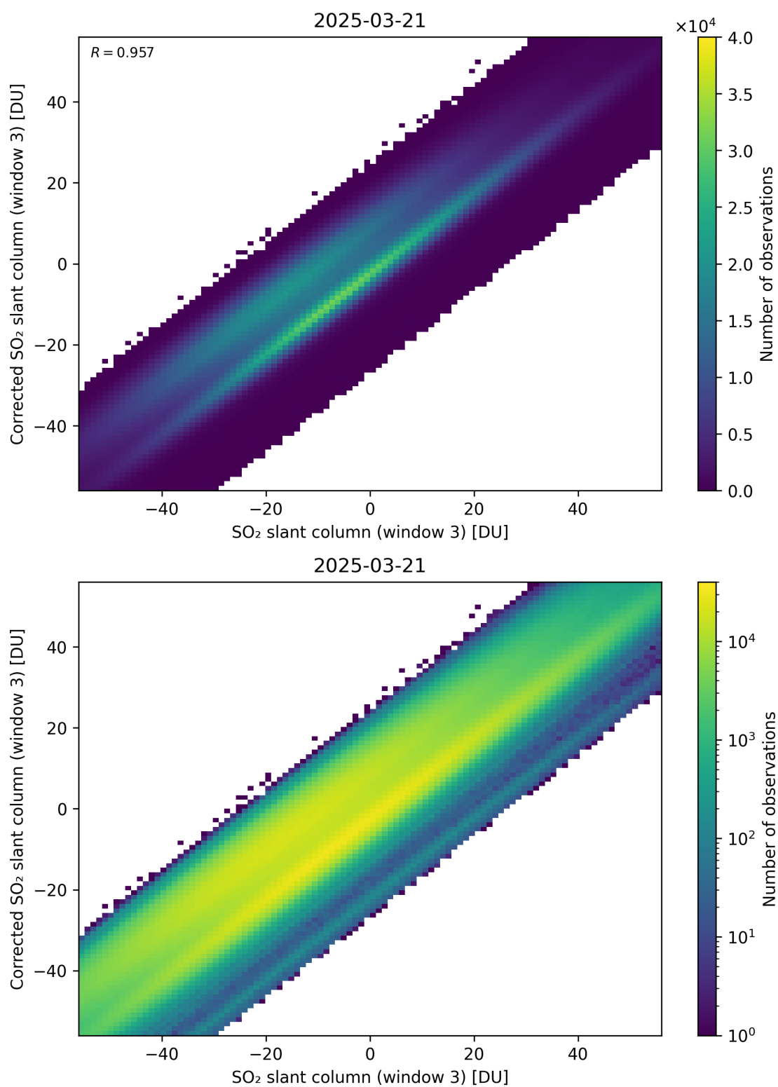
Figure 316: Scatter density plot of “SO 2 slant column (window 3)” against “Corrected SO 2 slant column (window 3)” for 2025-03-20 to 2025-03-22.
