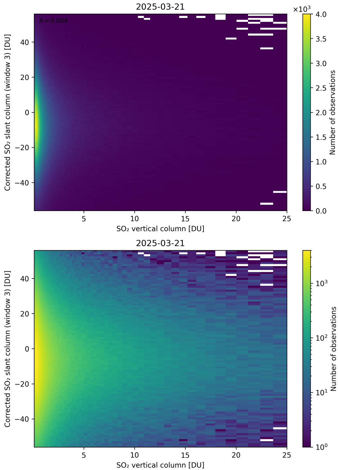
Figure 353: Scatter density plot of “SO 2 vertical column” against “Corrected SO 2 slant column (window 3)” for 2025-03-20 to 2025-03-22.
