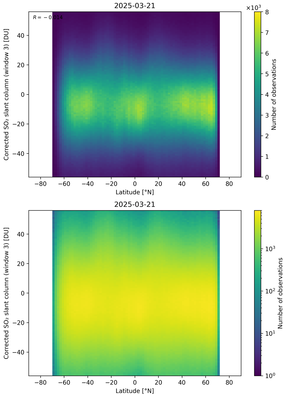
Figure 161: Scatter density plot of “Latitude” against “Corrected SO 2 slant column (window 3)” for 2025-03-20 to 2025-03-22.
