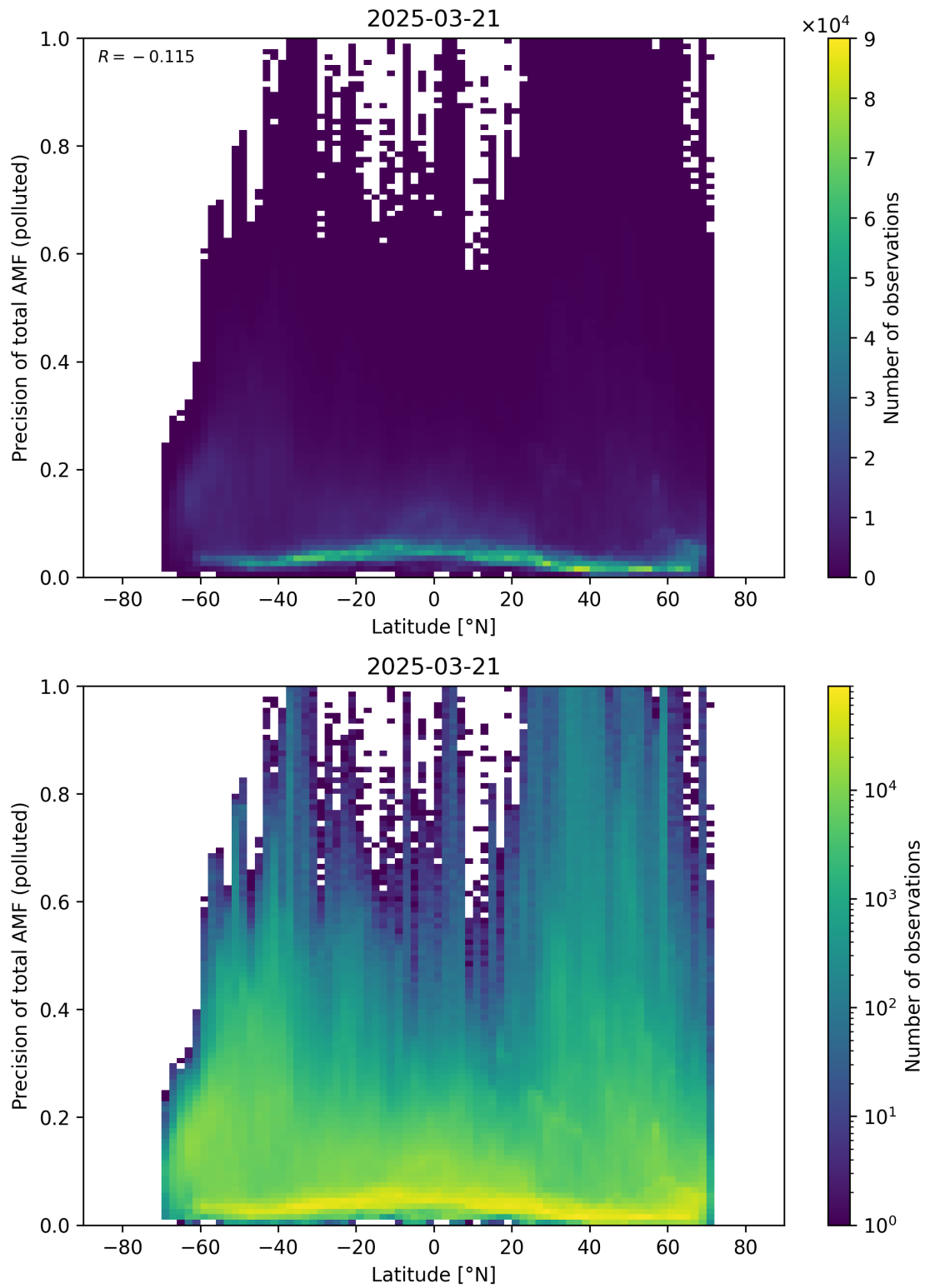
Figure 168: Scatter density plot of “Latitude” against “Precision of total AMF (polluted)” for 2025-03-20 to 2025-03-22.
