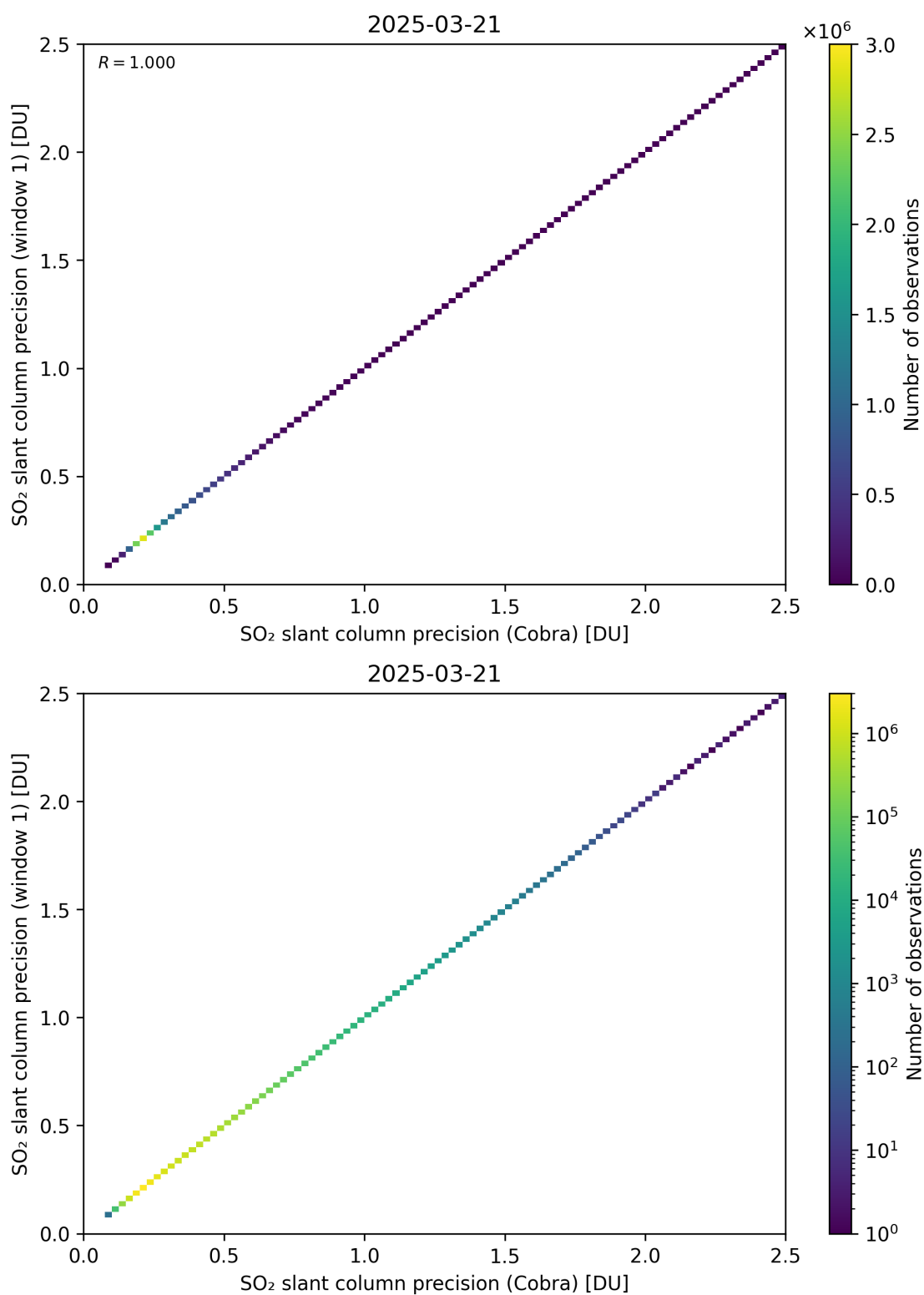
Figure 209: Scatter density plot of “SO 2 slant column precision (Cobra)” against “SO 2 slant column precision (window 1)” for 2025-03-20 to 2025-03-22.
