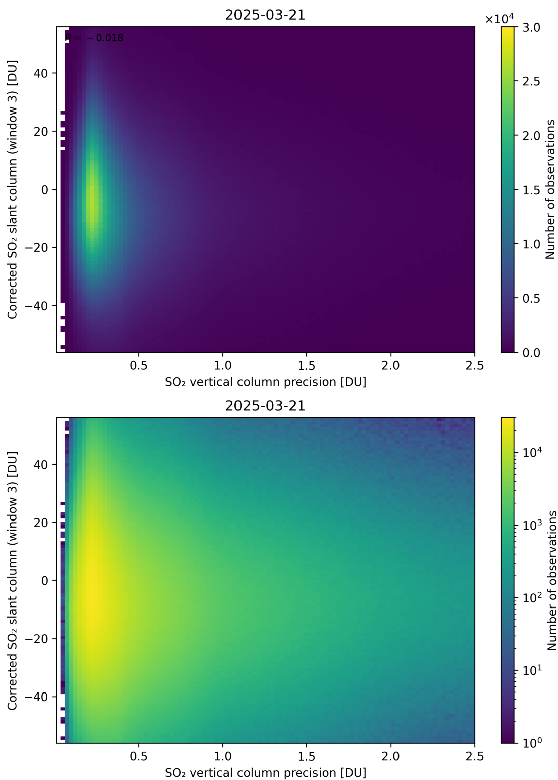
Figure 340: Scatter density plot of “SO 2 vertical column precision” against “Corrected SO 2 slant column (window 3)” for 2025-03-20 to 2025-03-22.
