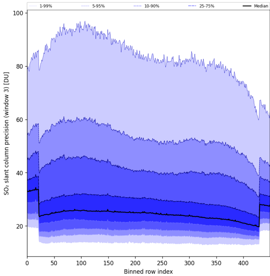
Figure 98: Along track statistics of “SO 2 slant column precision (window 3)” for 2025-03-20 to 2025-03-22
