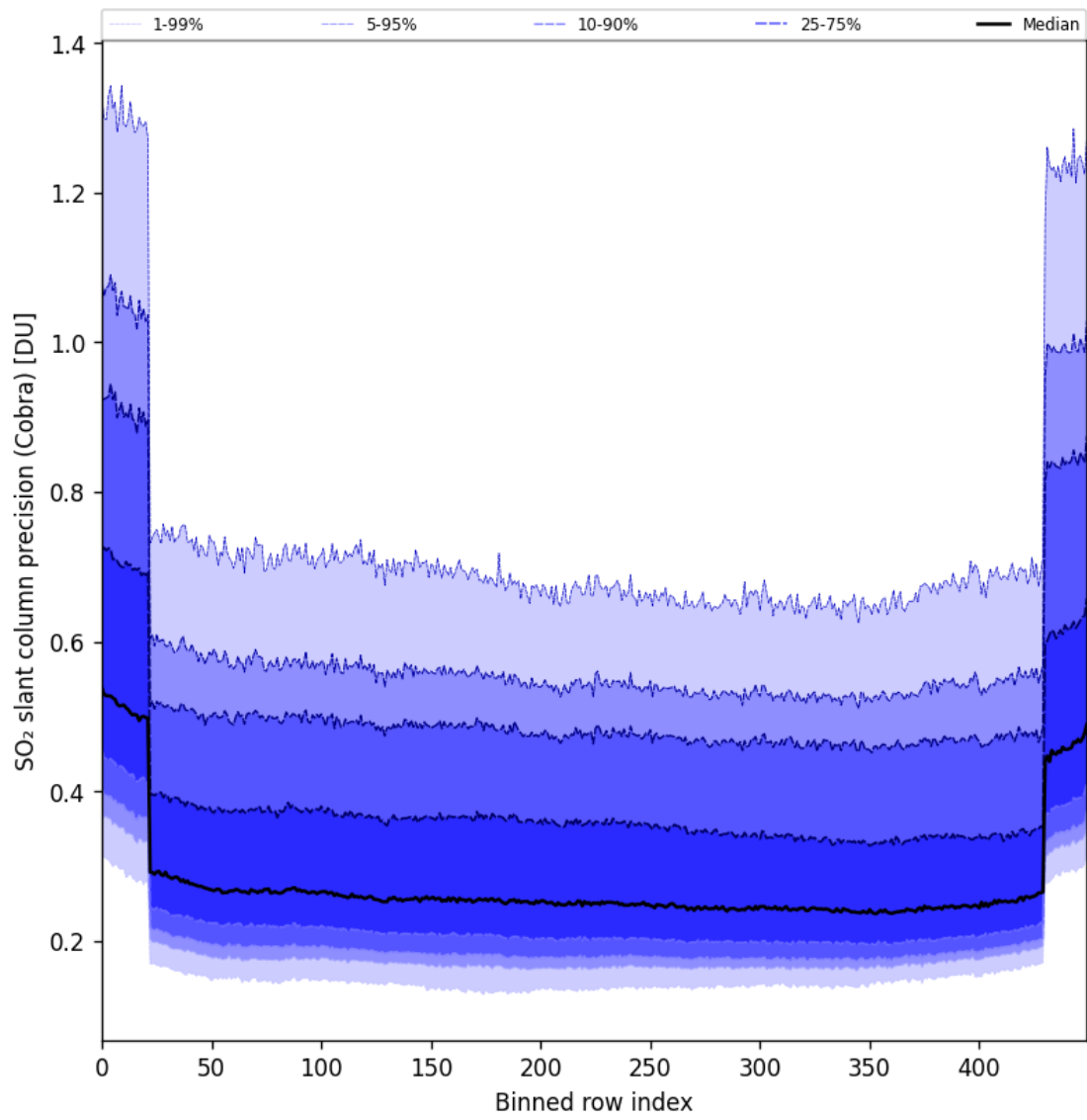
Figure 88: Along track statistics of “SO 2 slant column precision (Cobra)” for 2025-03-20 to 2025-03-22
