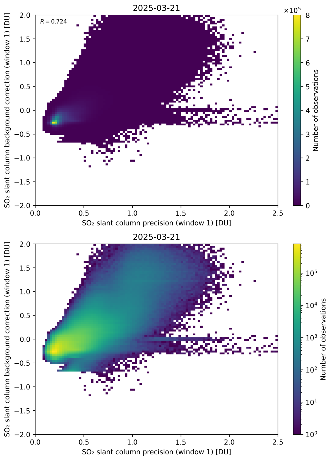
Figure 268: Scatter density plot of “SO 2 slant column precision (window 1)” against “SO 2 slant column background correction (window 1)” for 2025-03-20 to 2025-03-22.
