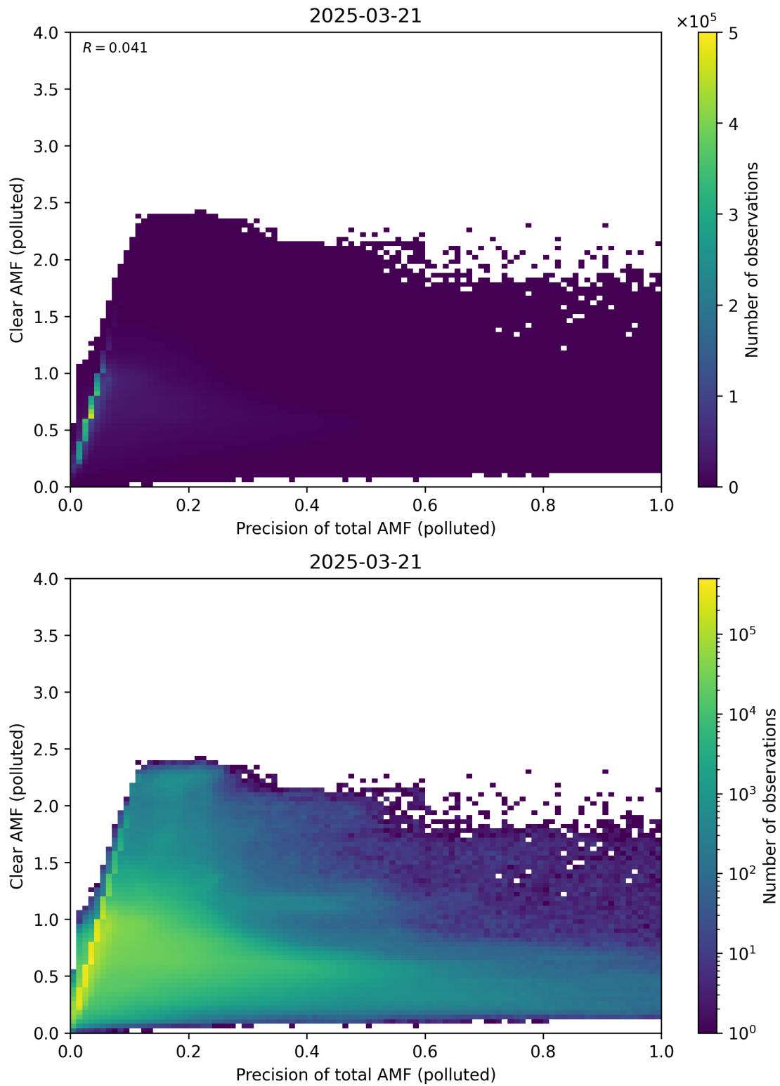
Figure 320: Scatter density plot of “Precision of total AMF (polluted)” against “Clear AMF (polluted)” for 2025-03-20 to 2025-03-22.
