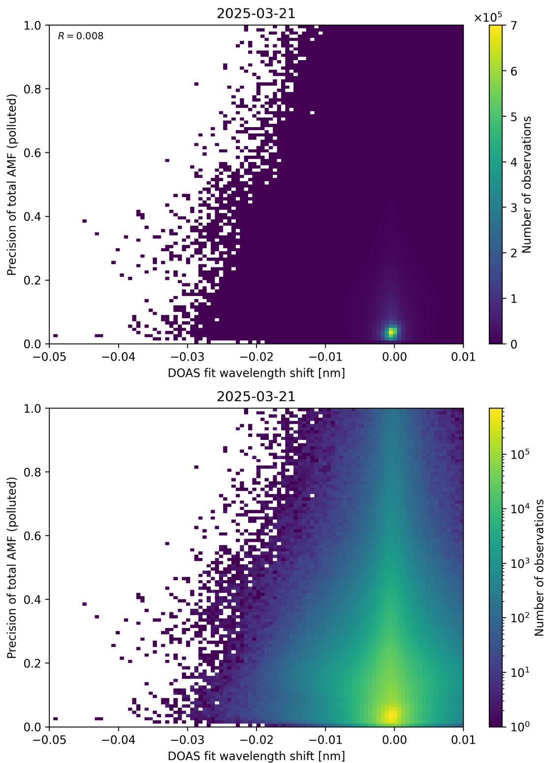
Figure 142: Scatter density plot of “DOAS fit wavelength shift” against “Precision of total AMF (polluted)” for 2025-03-20 to 2025-03-22.
