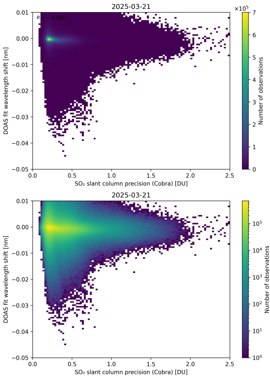
Figure 202: Scatter density plot of “SO 2 slant column precision (Cobra)” against “DOAS fit wavelength shift” for 2025-03-20 to 2025-03-22.
