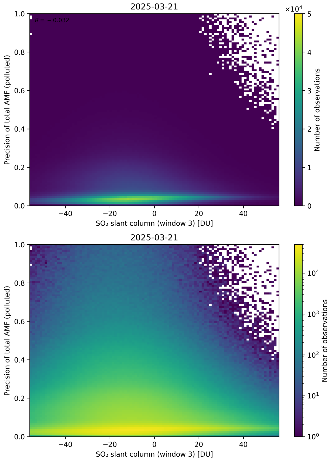
Figure 319: Scatter density plot of “SO 2 slant column (window 3)” against “Precision of total AMF (polluted)” for 2025-03-20 to 2025-03-22.
