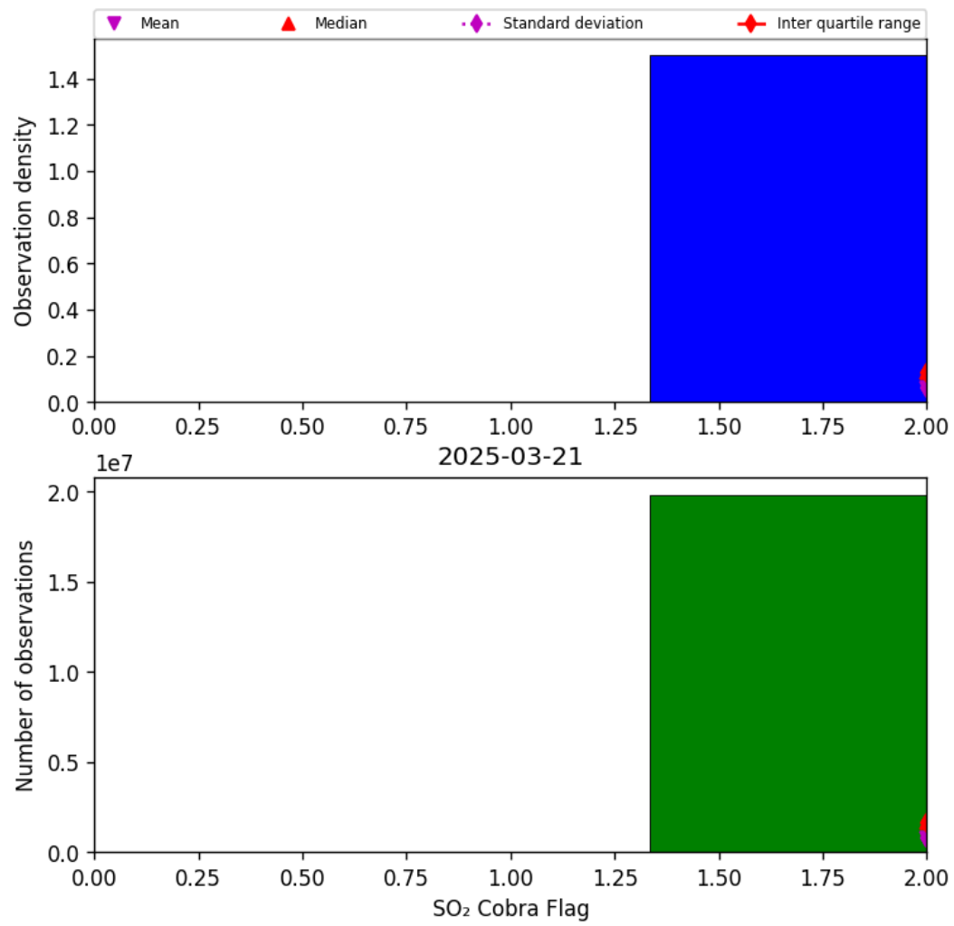
Figure 75: Histogram of “SO 2 Cobra Flag” for 2025-03-20 to 2025-03-22
