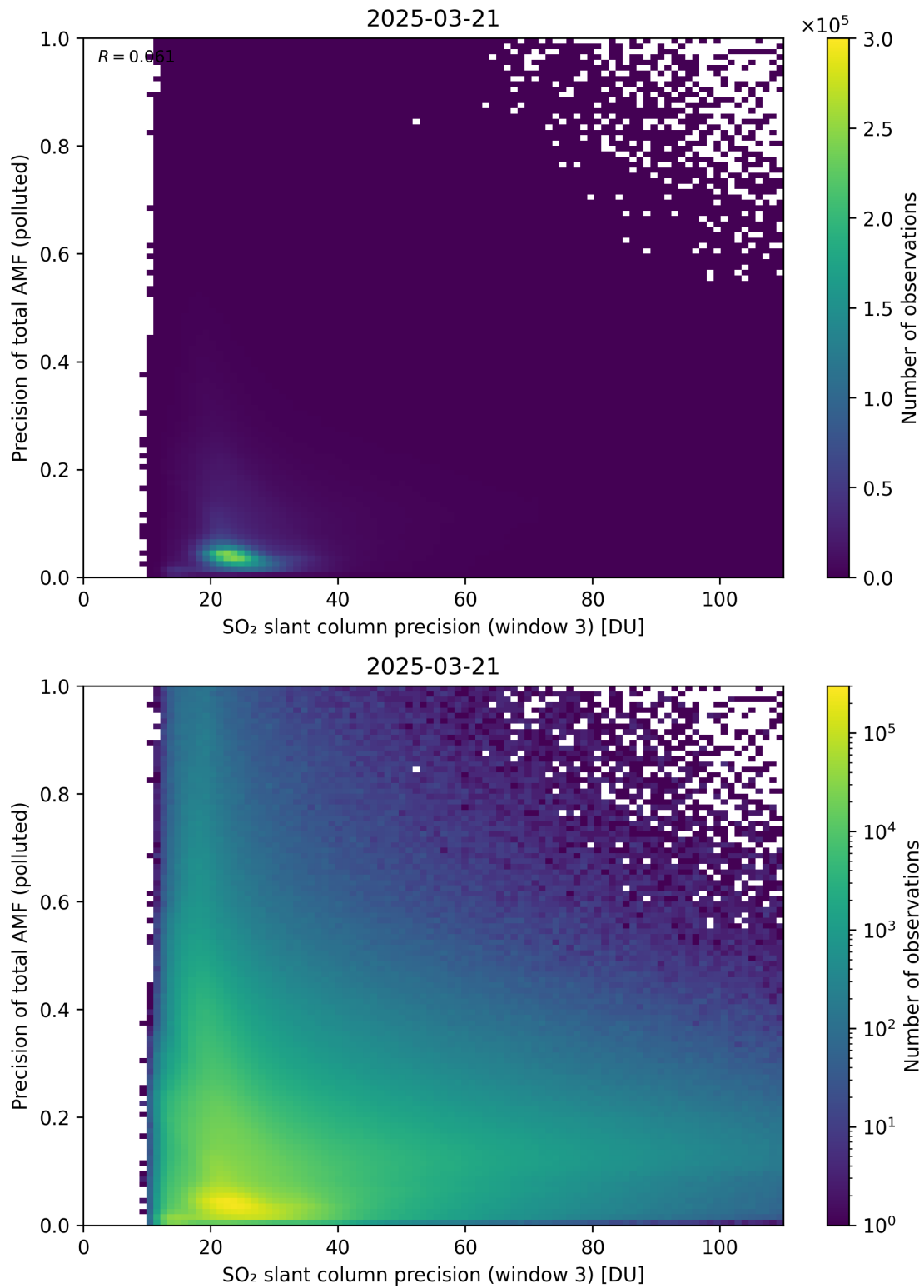
Figure 314: Scatter density plot of “SO 2 slant column precision (window 3)” against “Precision of total AMF (polluted)” for 2025-03-20 to 2025-03-22.
