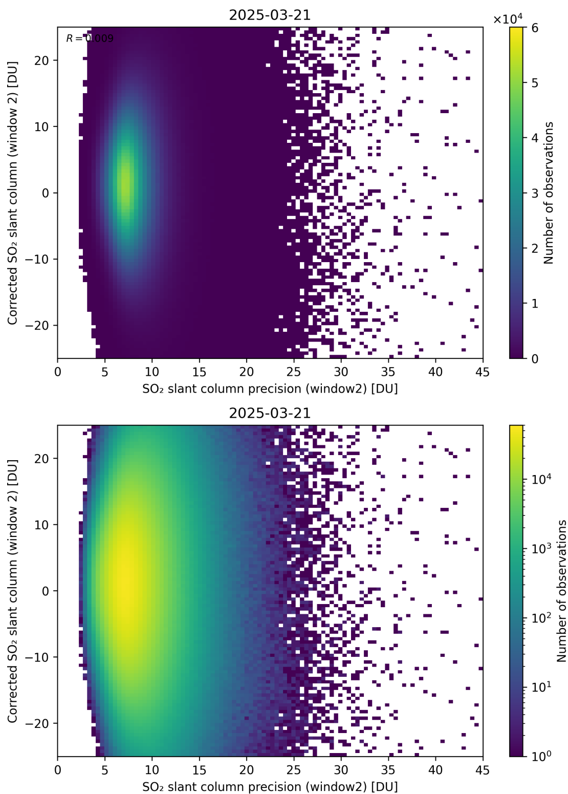
Figure 297: Scatter density plot of “SO 2 slant column precision (window2)” against “Corrected SO 2 slant column (window 2)” for 2025-03-20 to 2025-03-22.
