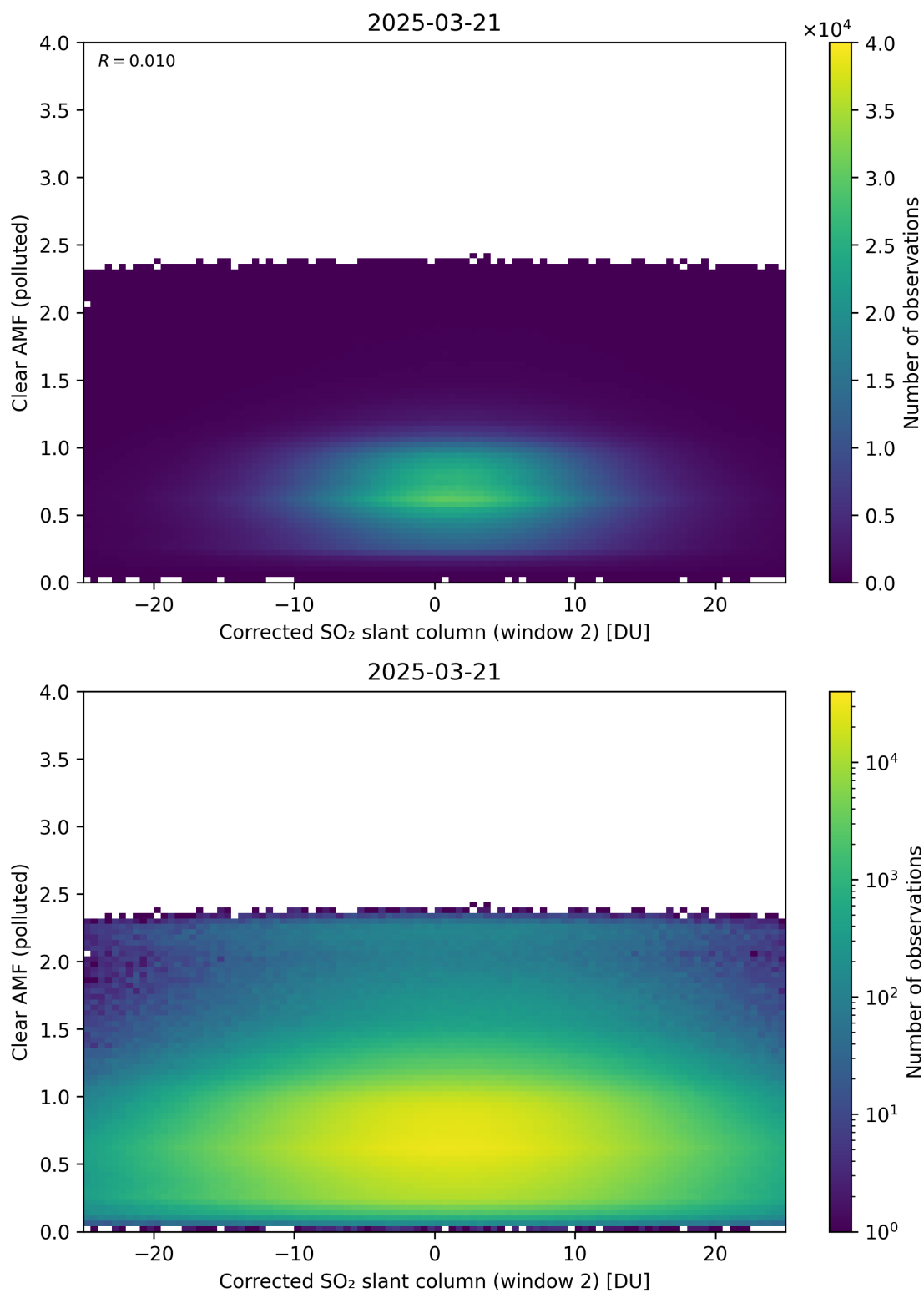
Figure 249: Scatter density plot of “Corrected SO 2 slant column (window 2)” against “Clear AMF (polluted)” for 2025-03-20 to 2025-03-22.
