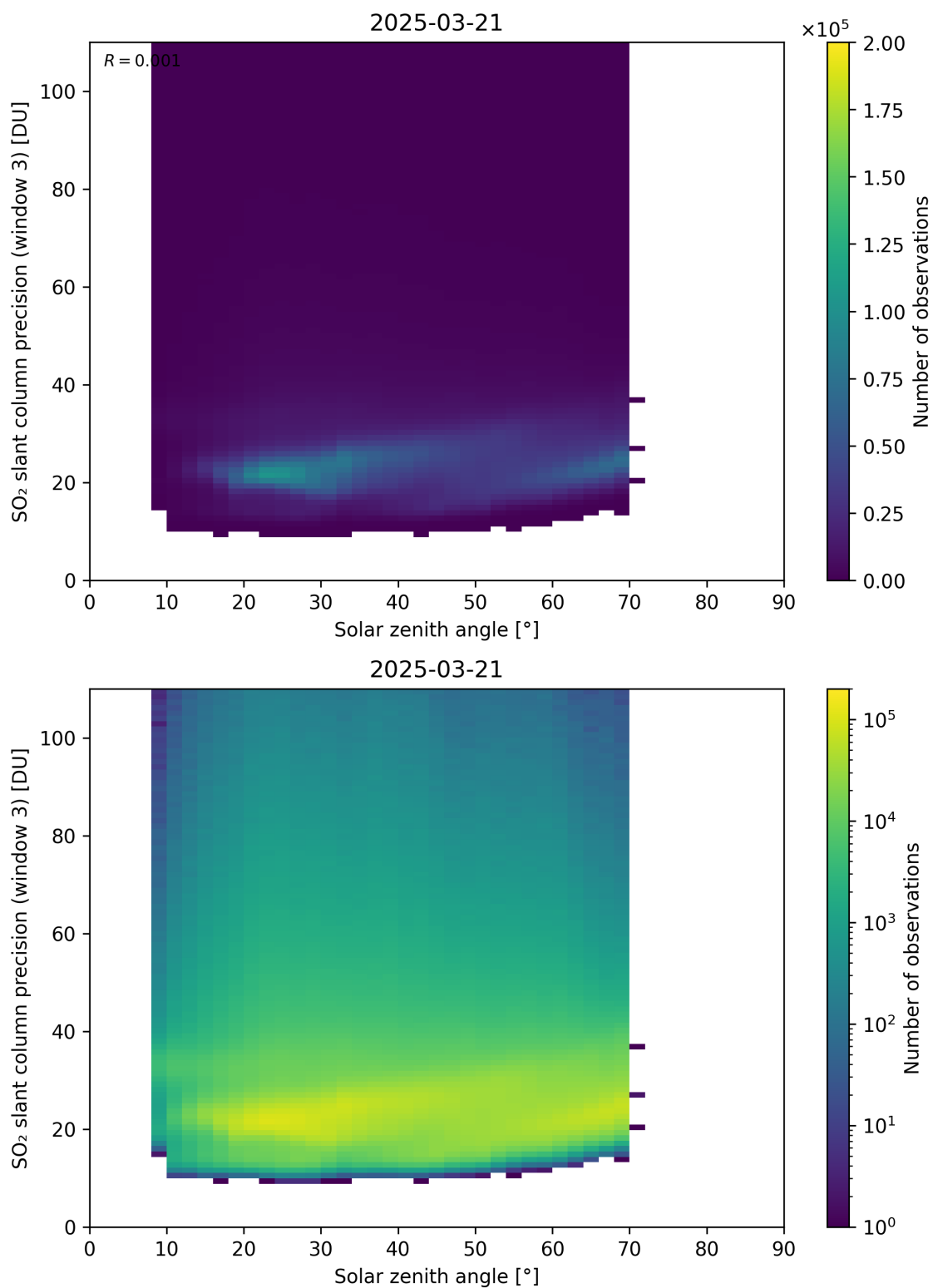
Figure 188: Scatter density plot of “Solar zenith angle” against “SO 2 slant column precision (window 3)” for 2025-03-20 to 2025-03-22.
