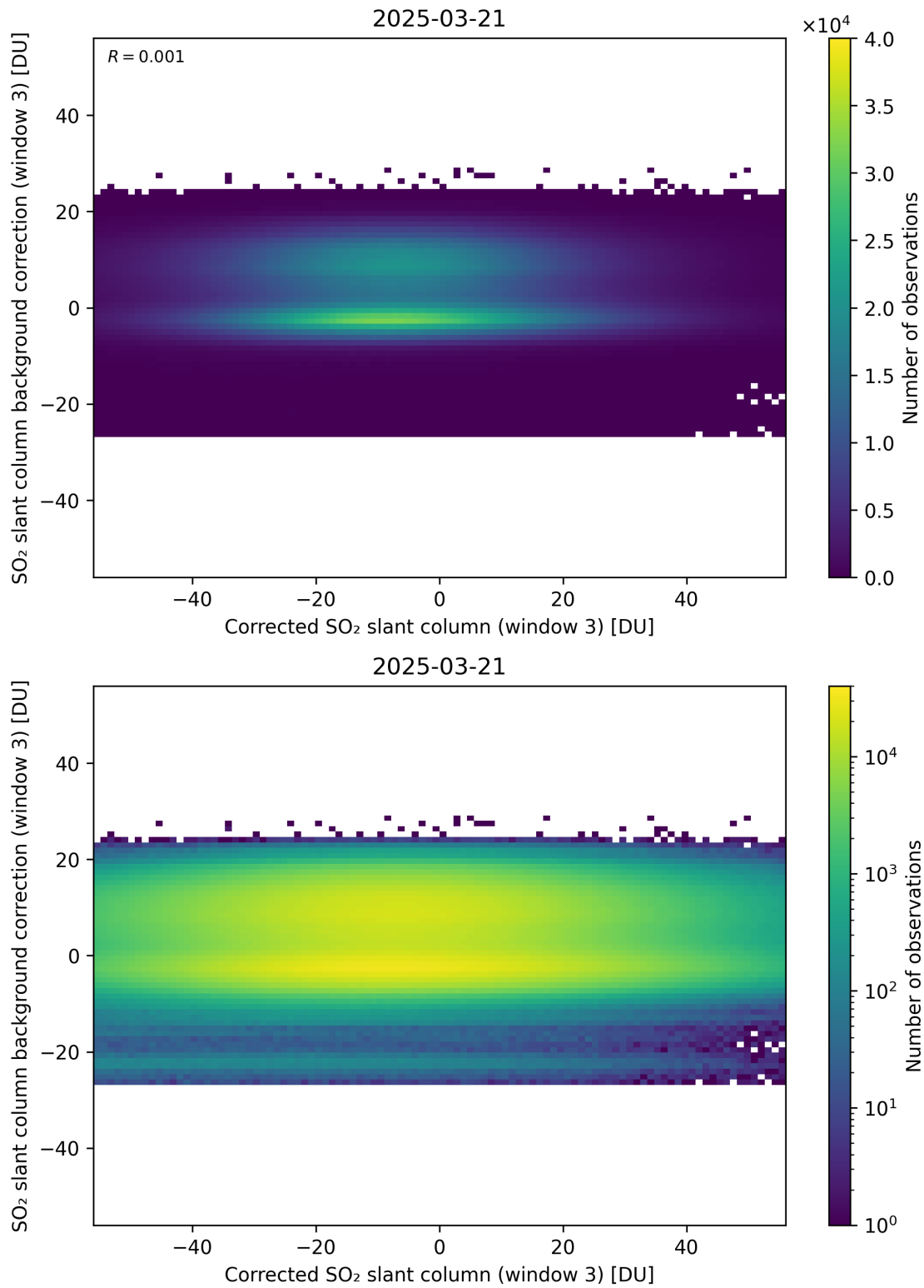
Figure 255: Scatter density plot of “Corrected SO 2 slant column (window 3)” against “SO 2 slant column background correction (window 3)” for 2025-03-20 to 2025-03-22.
