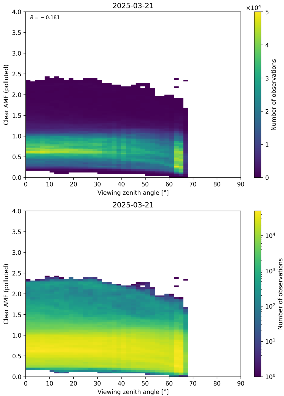
Figure 370: Scatter density plot of “Viewing zenith angle” against “Clear AMF (polluted)” for 2025-03-20 to 2025-03-22.
