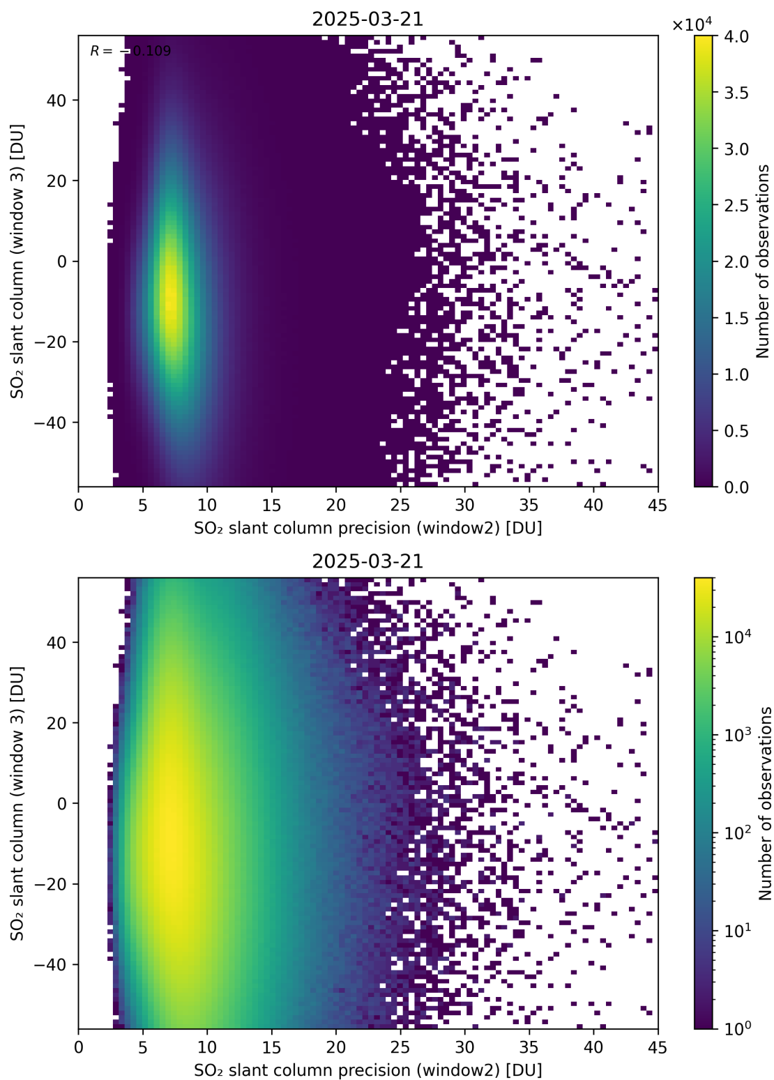
Figure 299: Scatter density plot of “SO 2 slant column precision (window2)” against “SO 2 slant column (window 3)” for 2025-03-20 to 2025-03-22.
