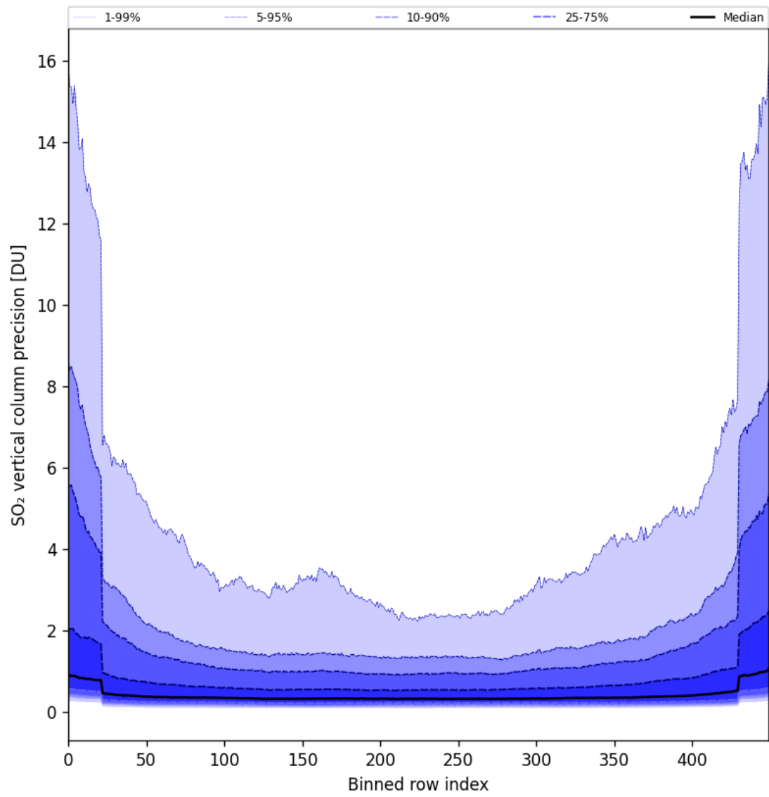
Figure 85: Along track statistics of “SO 2 vertical column precision” for 2025-03-20 to 2025-03-22
