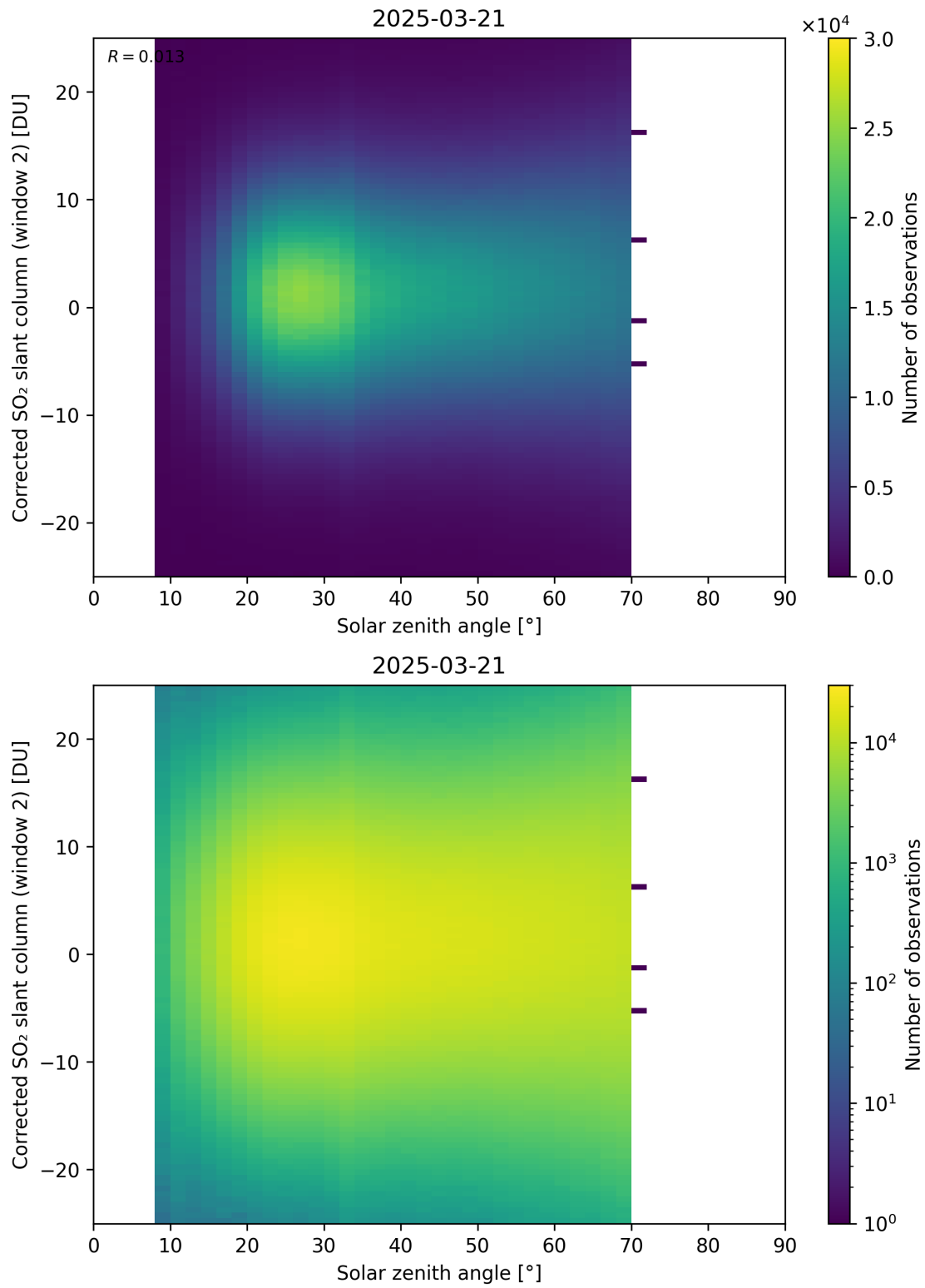
Figure 182: Scatter density plot of “Solar zenith angle” against “Corrected SO 2 slant column (window 2)” for 2025-03-20 to 2025-03-22.
