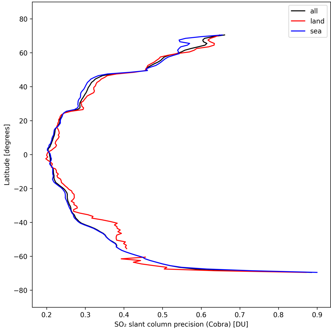
Figure 36: Zonal average of "SO 2 slant column precision (Cobra)" for 2025-03-20 to 2025-03-22.
