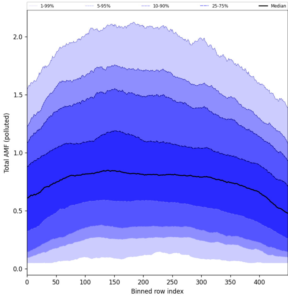
Figure 105: Along track statistics of “Total AMF (polluted)” for 2025-03-20 to 2025-03-22
