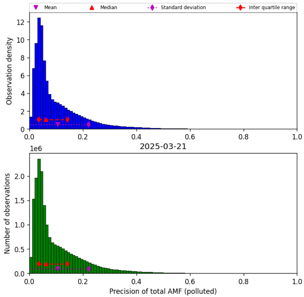
Figure 80: Histogram of “Precision of total AMF (polluted)” for 2025-03-20 to 2025-03-22
