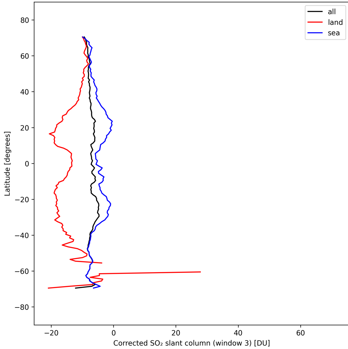
Figure 47: Zonal average of “Corrected SO 2 slant column (window 3)” for 2025-03-20 to 2025-03-22.
