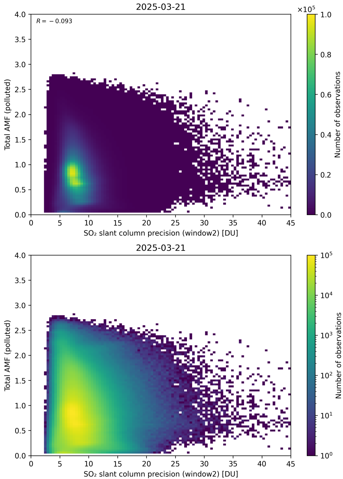
Figure 301: Scatter density plot of “SO 2 slant column precision (window2)” against “Total AMF (polluted)” for 2025-03-20 to 2025-03-22.
