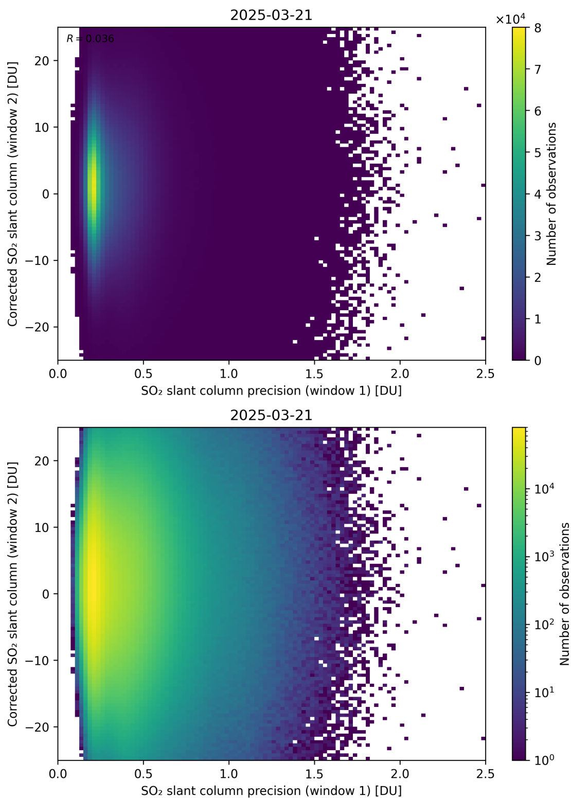
Figure 275: Scatter density plot of “SO 2 slant column precision (window 1)” against “Corrected SO 2 slant column (window 2)” for 2025-03-20 to 2025-03-22.
