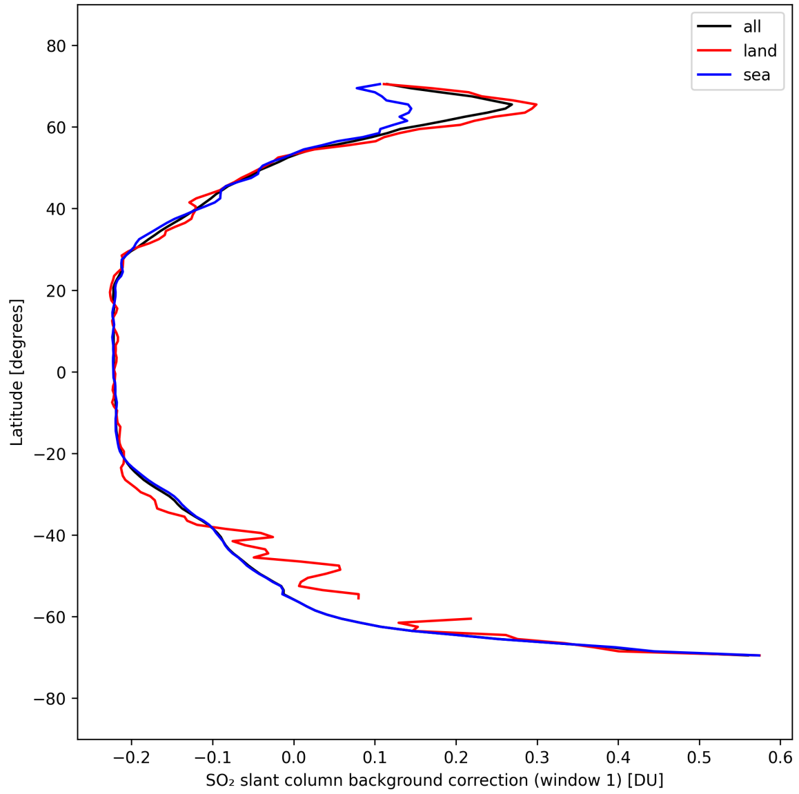
Figure 40: Zonal average of “SO 2 slant column background correction (window 1)” for 2025-03-20 to 2025-03-22.
