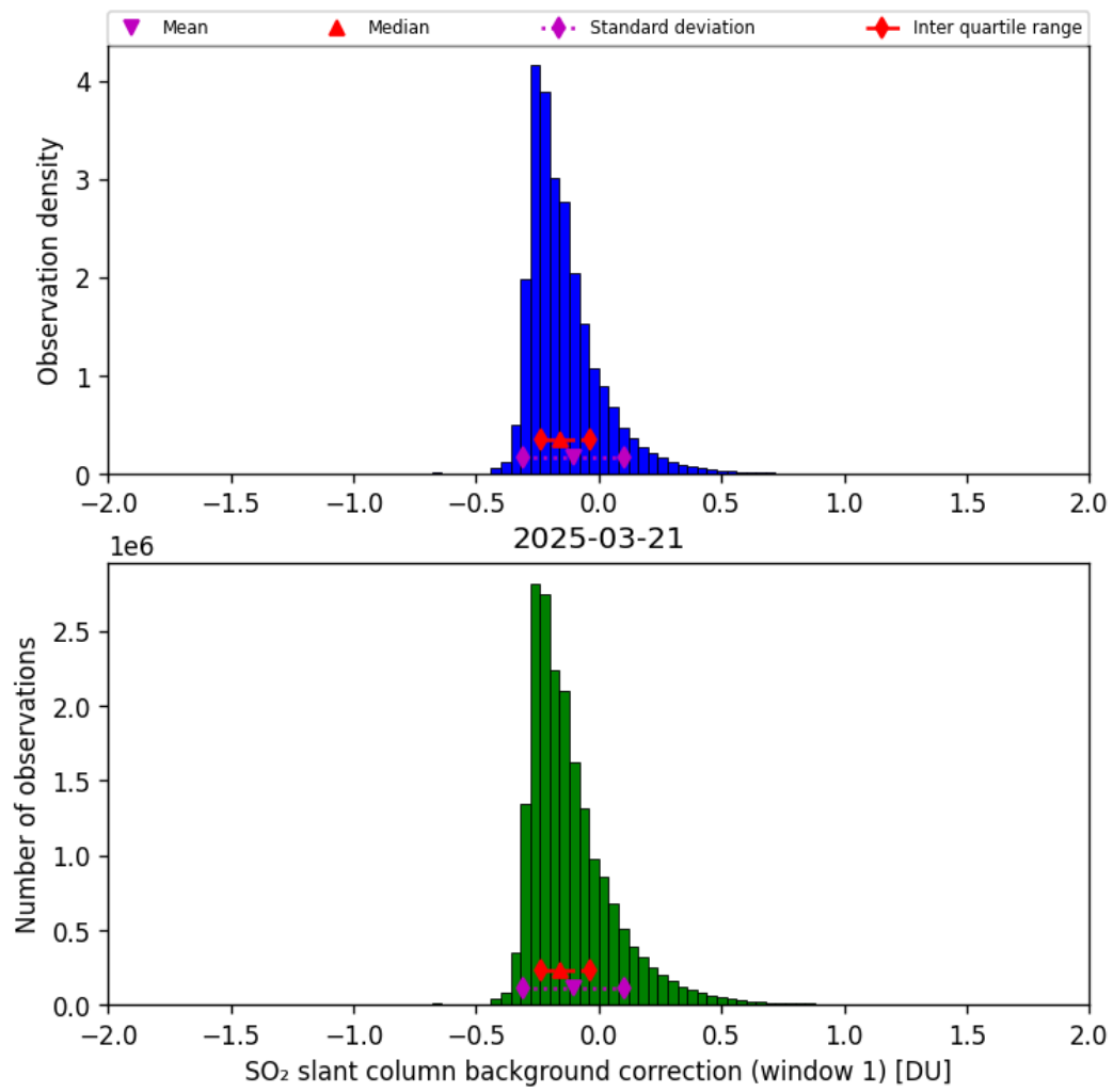
Figure 66: Histogram of “SO 2 slant column background correction (window 1)” for 2025-03-20 to 2025-03-22
