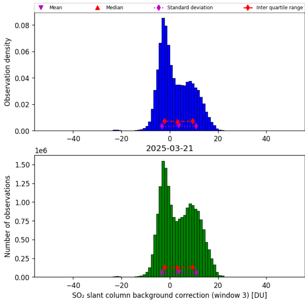
Figure 74: Histogram of “SO 2 slant column background correction (window 3)” for 2025-03-20 to 2025-03-22
