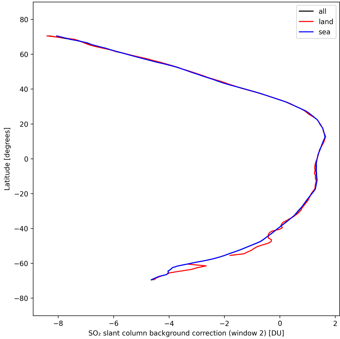
Figure 44: Zonal average of “SO 2 slant column background correction (window 2)” for 2025-03-20 to 2025-03-22.
