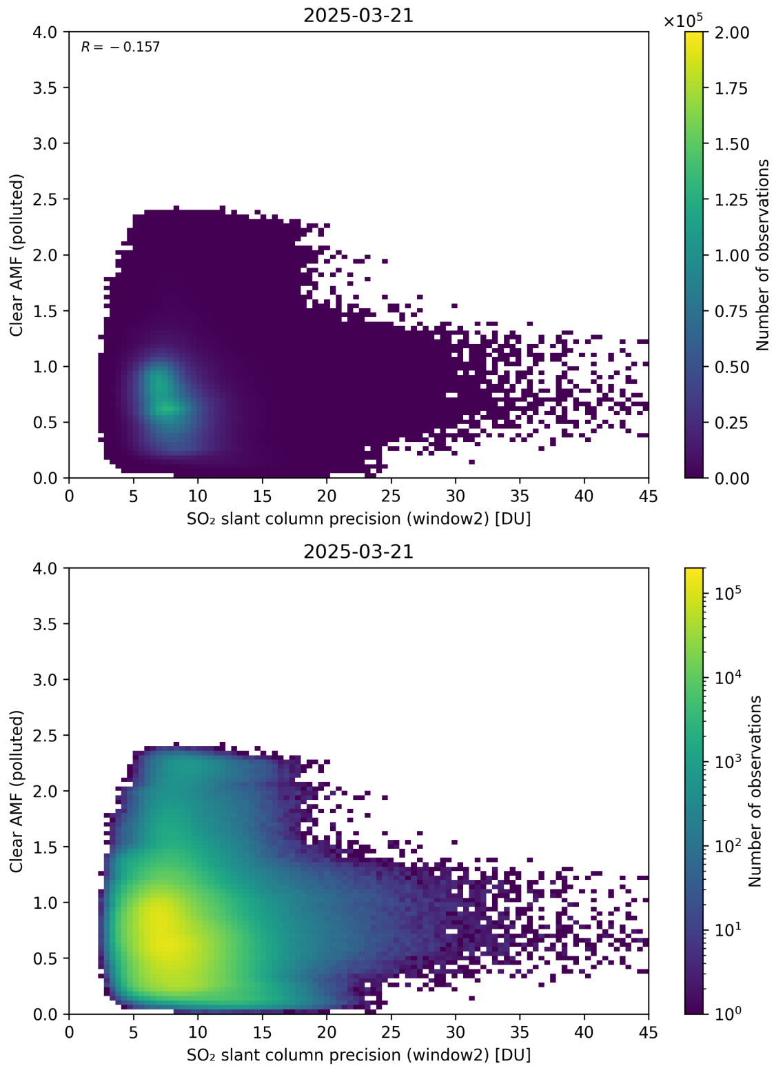
Figure 296: Scatter density plot of “SO 2 slant column precision (window2)” against “Clear AMF (polluted)” for 2025-03-20 to 2025-03-22.
