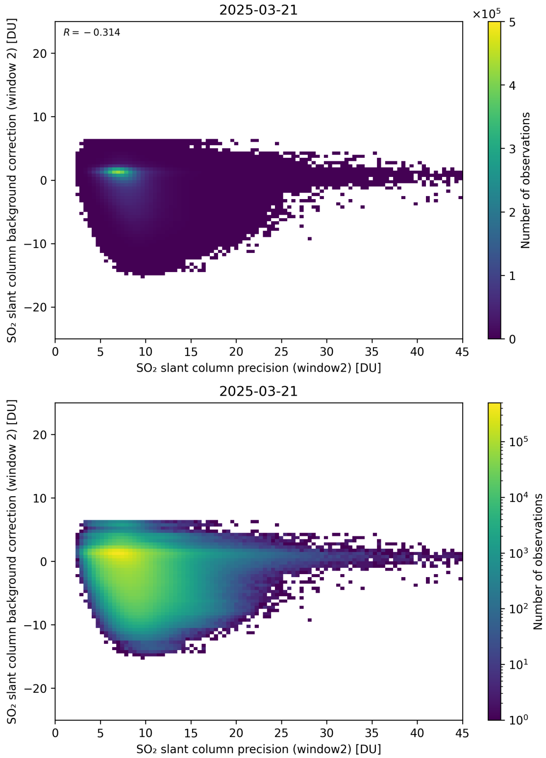
Figure 291: Scatter density plot of “SO 2 slant column precision (window2)” against “SO 2 slant column background correction (window 2)” for 2025-03-20 to 2025-03-22.
