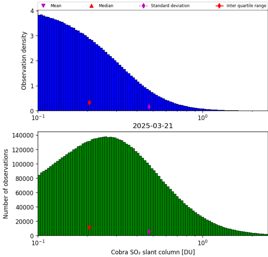
Figure 61: Histogram of “Cobra SO 2 slant column” for 2025-03-20 to 2025-03-22
