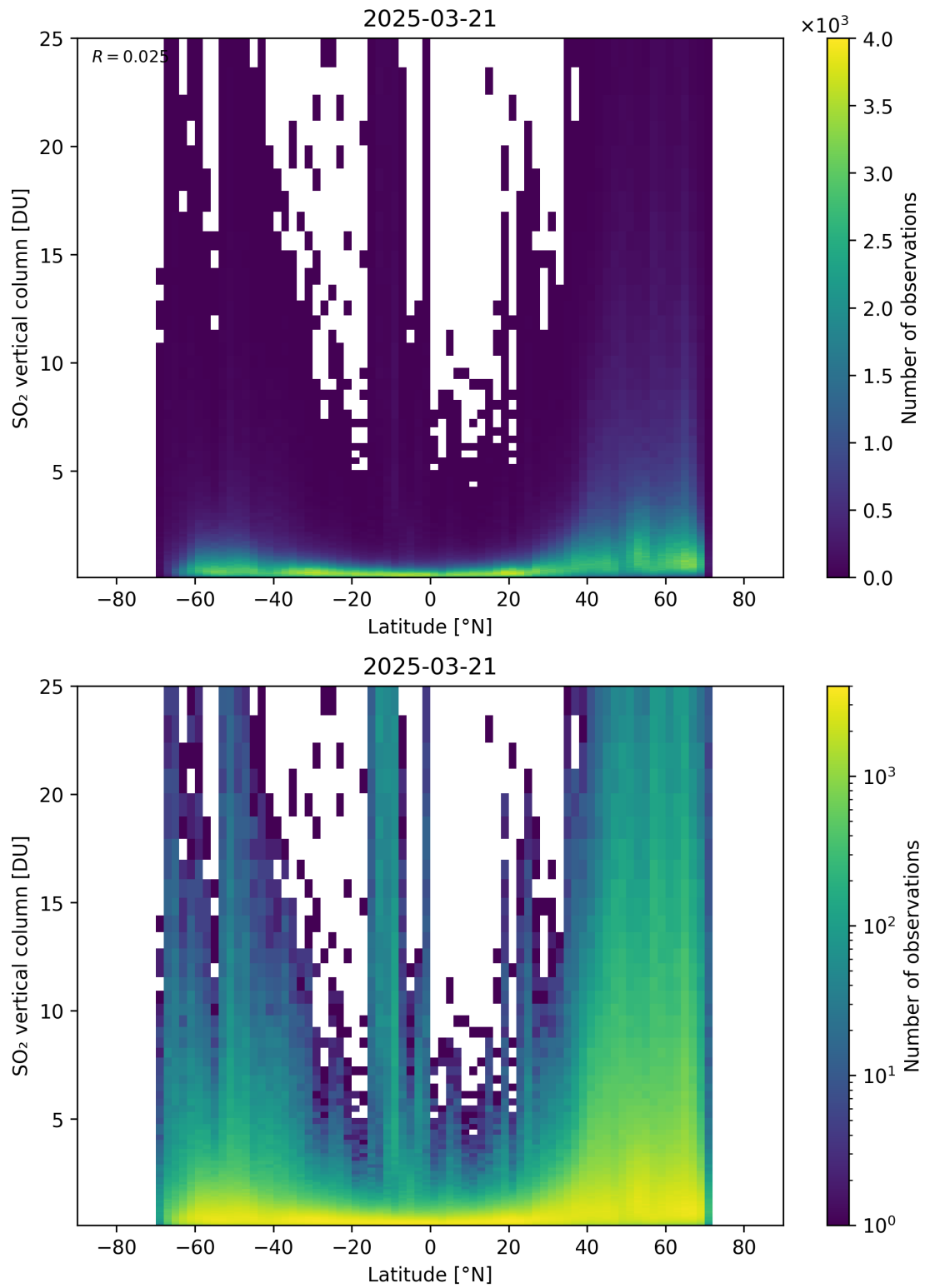
Figure 169: Scatter density plot of “Latitude” against “SO 2 vertical column” for 2025-03-20 to 2025-03-22.
