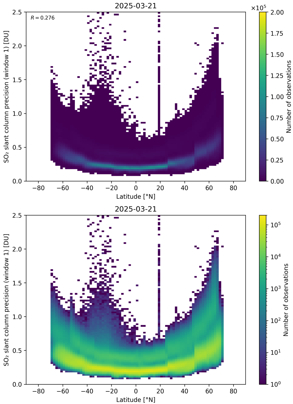
Figure 163: Scatter density plot of “Latitude” against “SO 2 slant column precision (window 1)” for 2025-03-20 to 2025-03-22.
