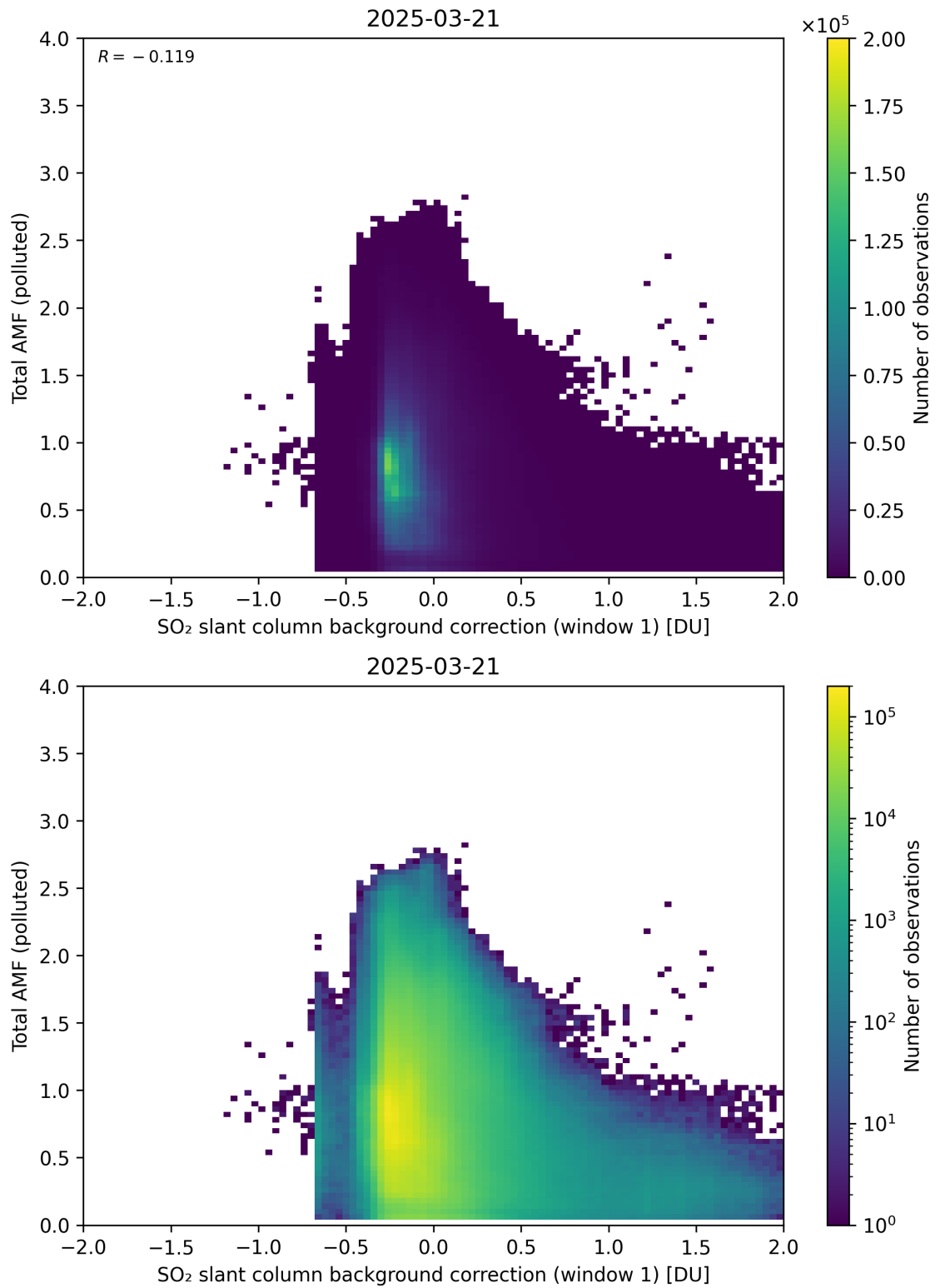
Figure 120: Scatter density plot of “SO 2 slant column background correction (window 1)” against “Total AMF (polluted)” for 2025-03-20 to 2025-03-22.
