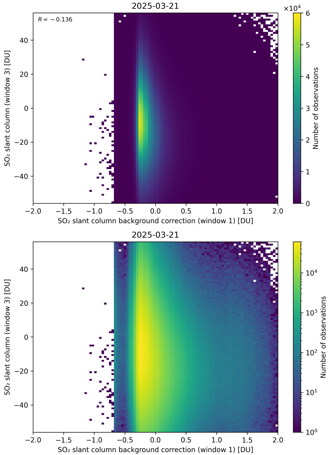
Figure 118: Scatter density plot of “SO 2 slant column background correction (window 1)” against “SO 2 slant column (window 3)” for 2025-03-20 to 2025-03-22.
