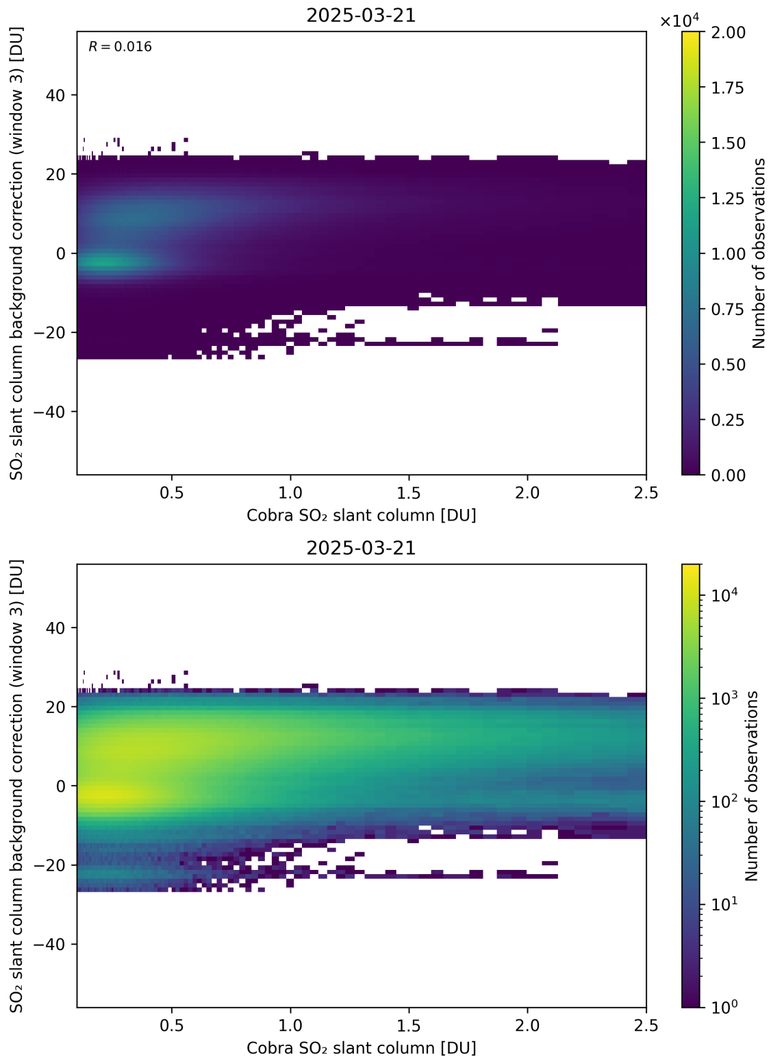
Figure 195: Scatter density plot of “Cobra SO 2 slant column” against “SO 2 slant column background correction (window 3)” for 2025-03-20 to 2025-03-22.
