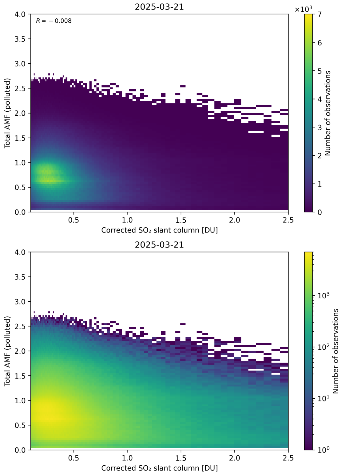
Figure 242: Scatter density plot of “Corrected SO 2 slant column” against “Total AMF (polluted)” for 2025-03-20 to 2025-03-22.
