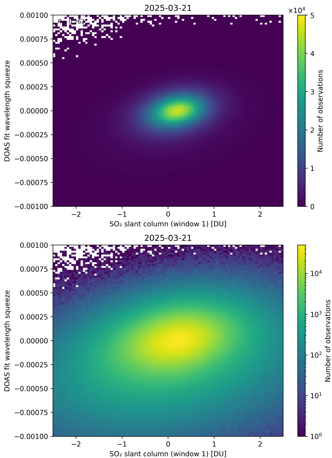
Figure 266: Scatter density plot of “SO 2 slant column (window 1)” against “DOAS fit wavelength squeeze” for 2025-03-20 to 2025-03-22.
