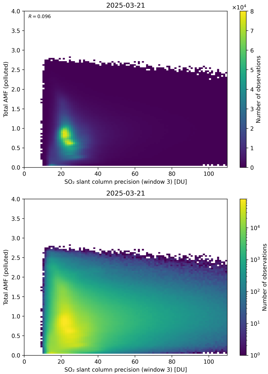
Figure 313: Scatter density plot of “SO 2 slant column precision (window 3)” against “Total AMF (polluted)” for 2025-03-20 to 2025-03-22.
