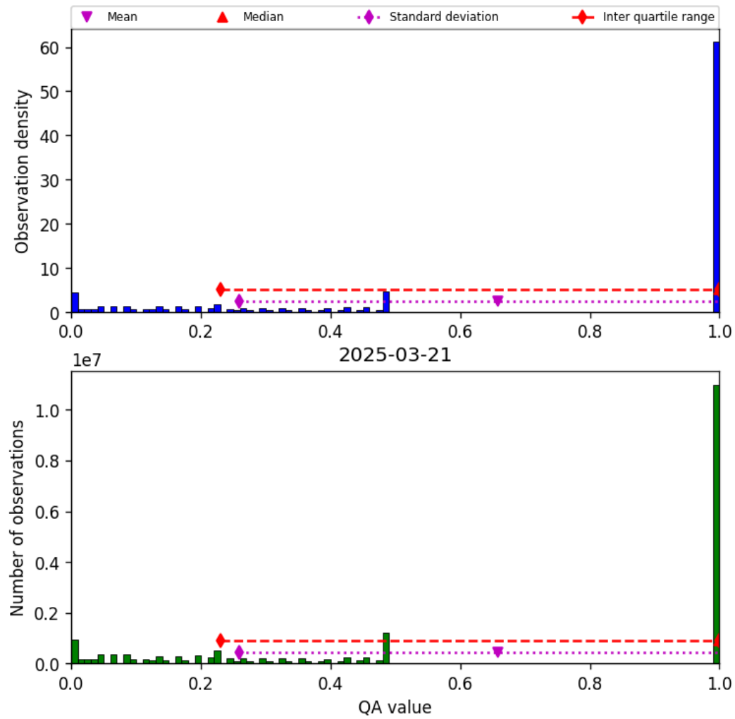
Figure 57: Histogram of “QA value” for 2025-03-20 to 2025-03-22
