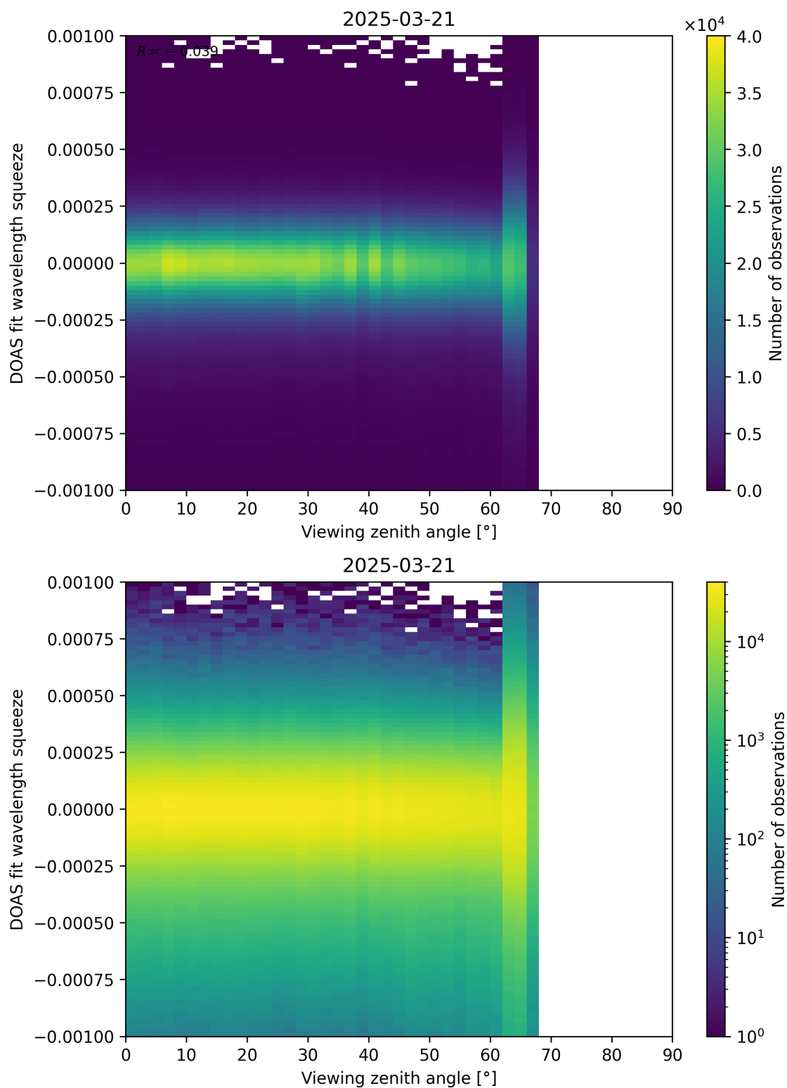
Figure 366: Scatter density plot of “Viewing zenith angle” against “DOAS fit wavelength squeeze” for 2025-03-20 to 2025-03-22.
