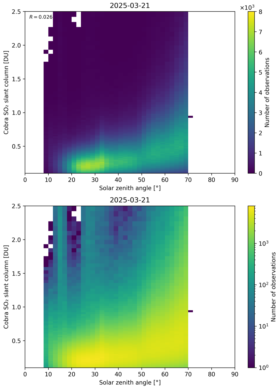
Figure 179: Scatter density plot of “Solar zenith angle” against “Cobra SO 2 slant column” for 2025-03-20 to 2025-03-22.
