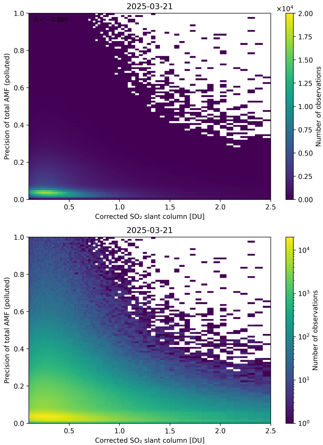
Figure 243: Scatter density plot of “Corrected SO 2 slant column” against “Precision of total AMF (polluted)” for 2025-03-20 to 2025-03-22.
