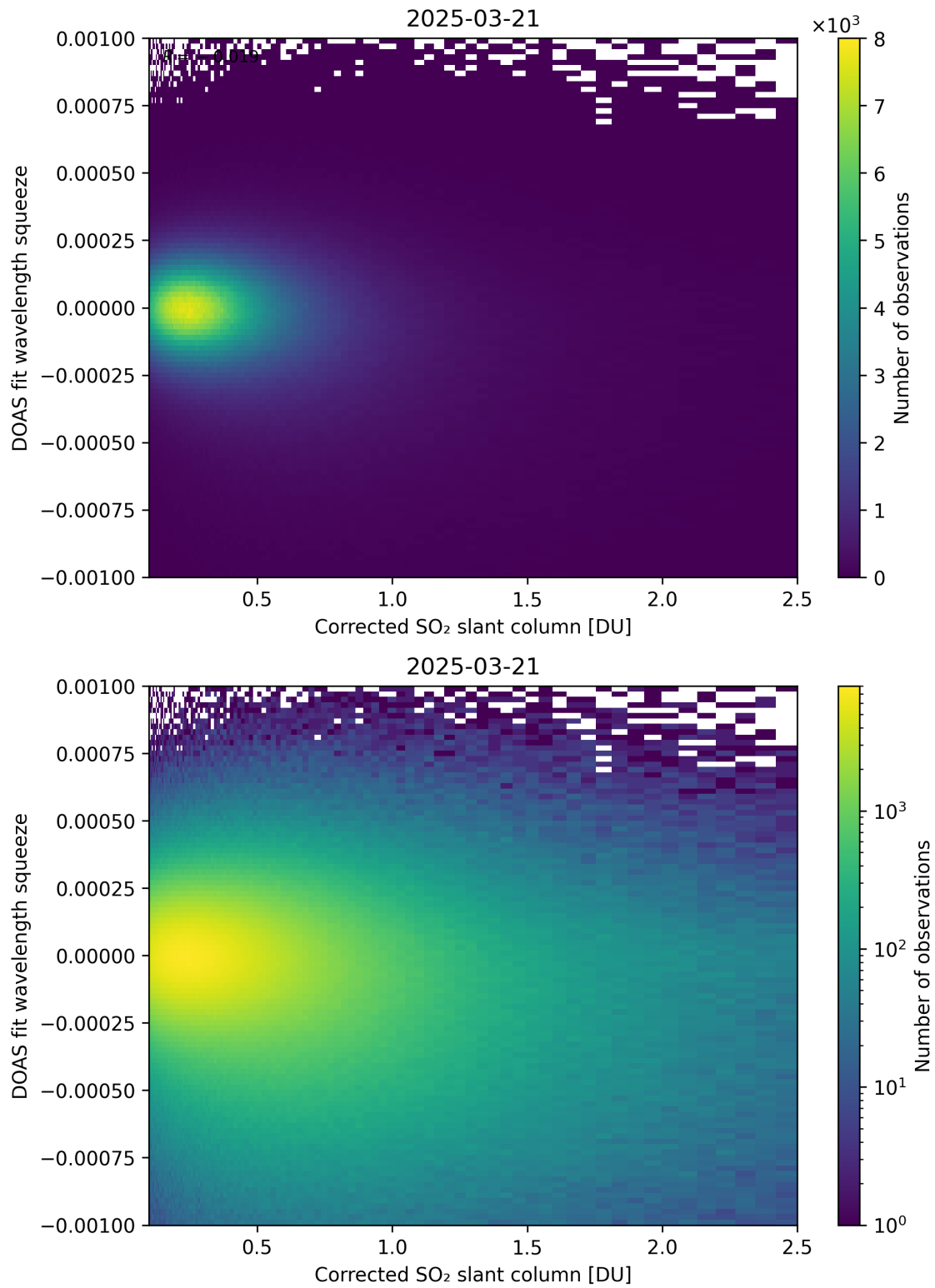
Figure 230: Scatter density plot of “Corrected SO 2 slant column” against “DOAS fit wavelength squeeze” for 2025-03-20 to 2025-03-22.
