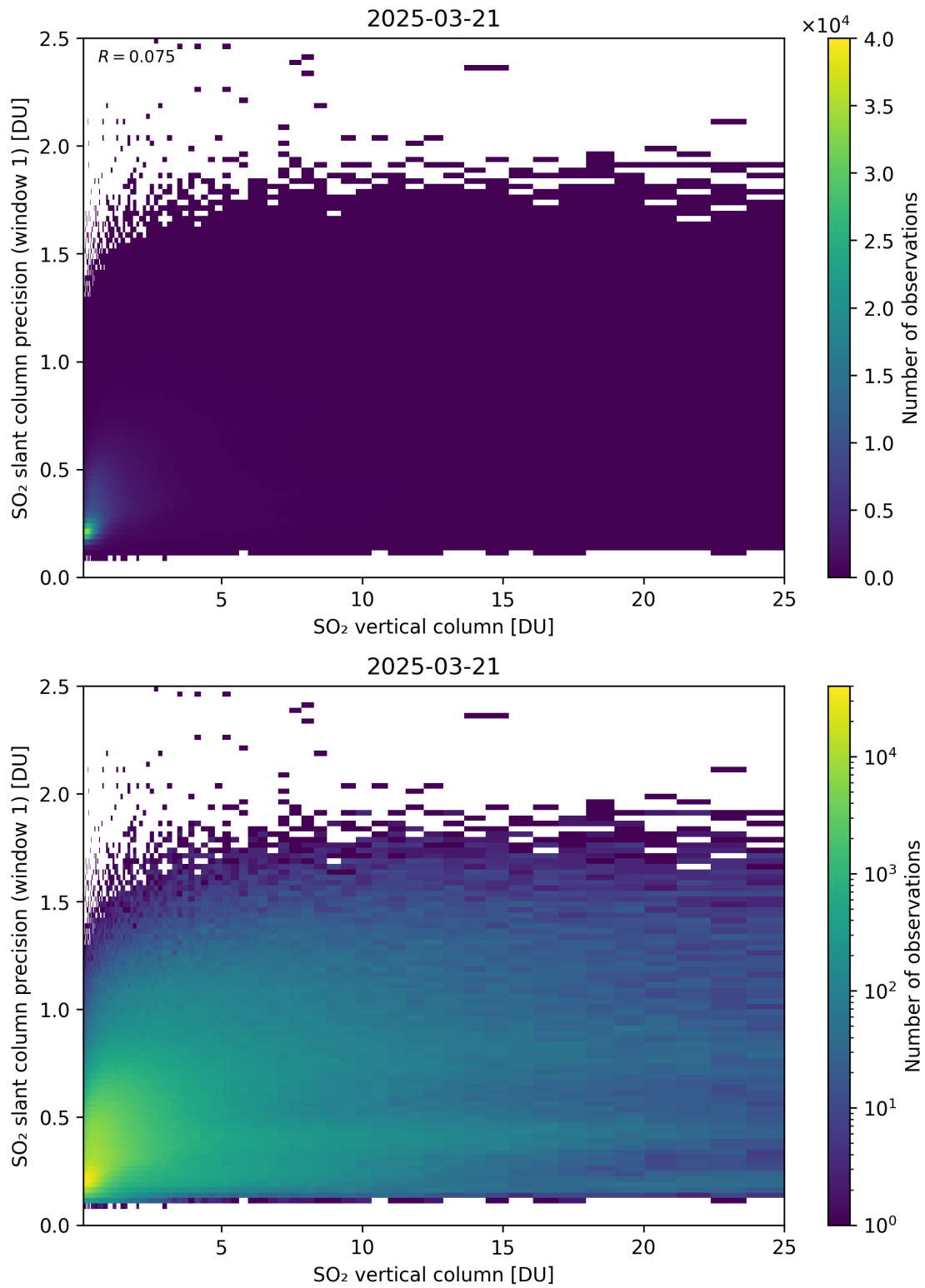
Figure 355: Scatter density plot of “SO 2 vertical column” against “SO 2 slant column precision (window 1)” for 2025-03-20 to 2025-03-22.
