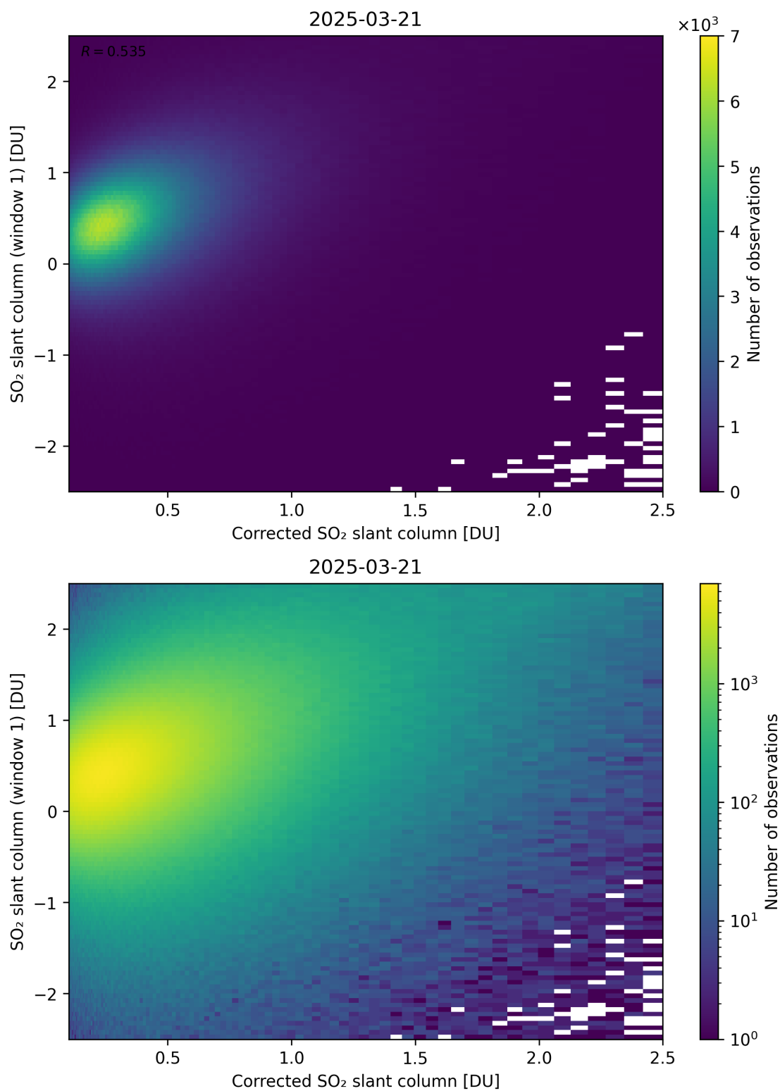
Figure 237: Scatter density plot of “Corrected SO 2 slant column” against “SO 2 slant column (window 1)” for 2025-03-20 to 2025-03-22.
