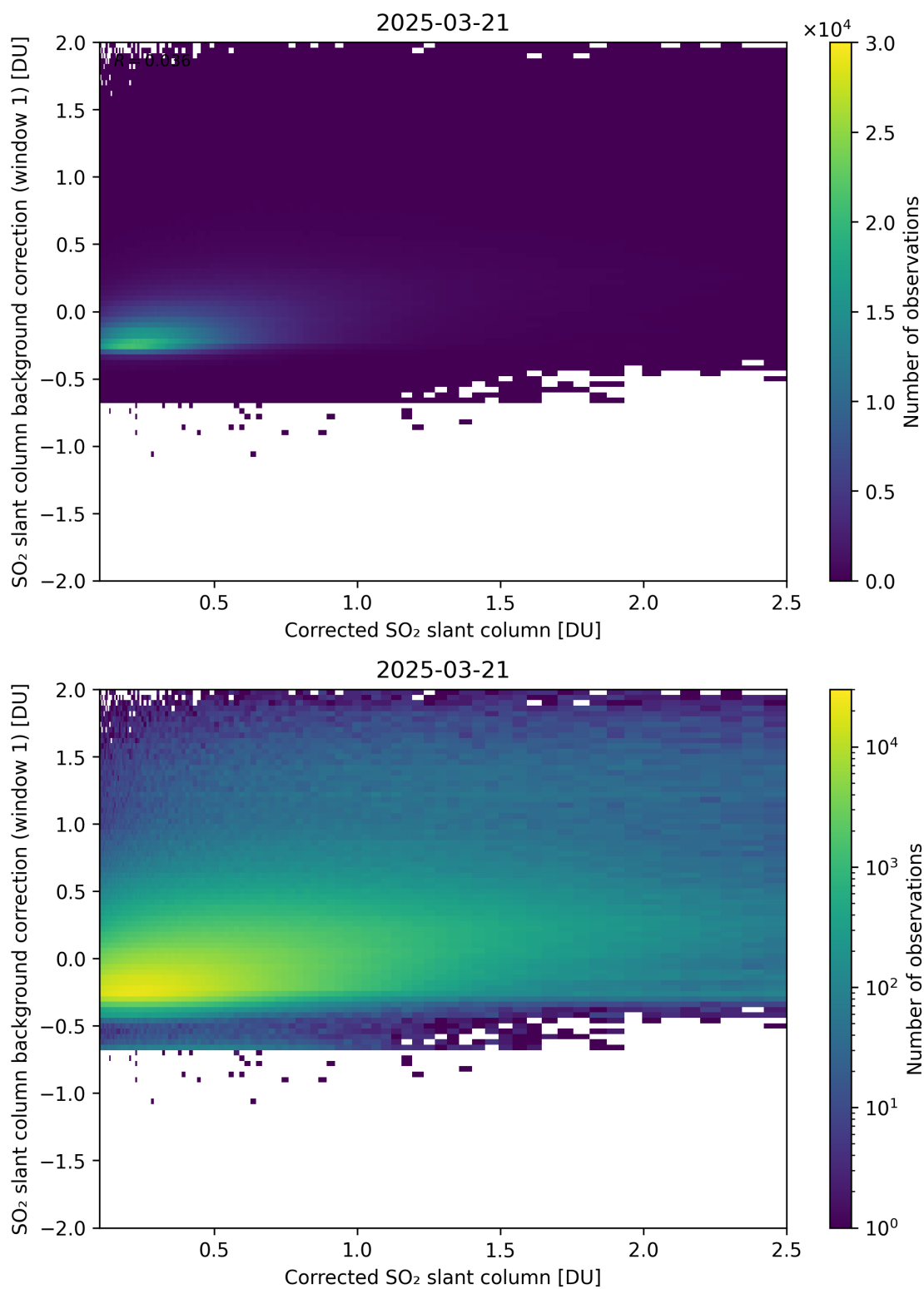
Figure 226: Scatter density plot of “Corrected SO 2 slant column” against “SO 2 slant column background correction (window 1)” for 2025-03-20 to 2025-03-22.
