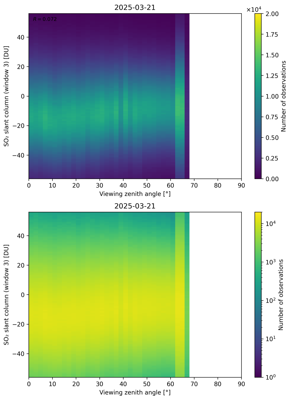
Figure 379: Scatter density plot of “Viewing zenith angle” against “SO 2 slant column (window 3)” for 2025-03-20 to 2025-03-22.
