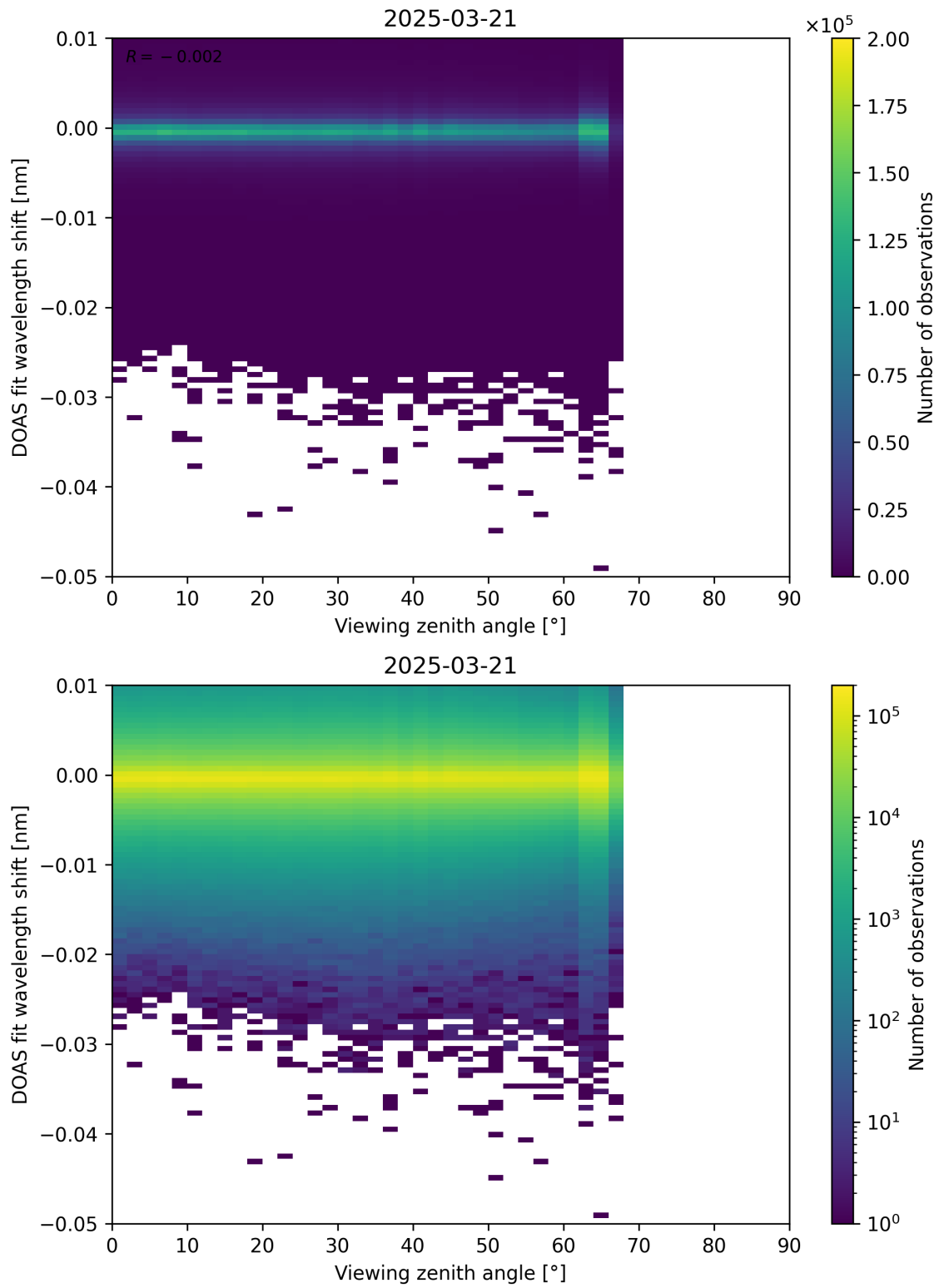
Figure 365: Scatter density plot of “Viewing zenith angle” against “DOAS fit wavelength shift” for 2025-03-20 to 2025-03-22.
