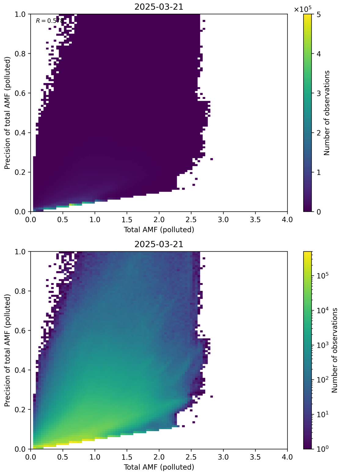
Figure 322: Scatter density plot of “Total AMF (polluted)” against “Precision of total AMF (polluted)” for 2025-03-20 to 2025-03-22.
