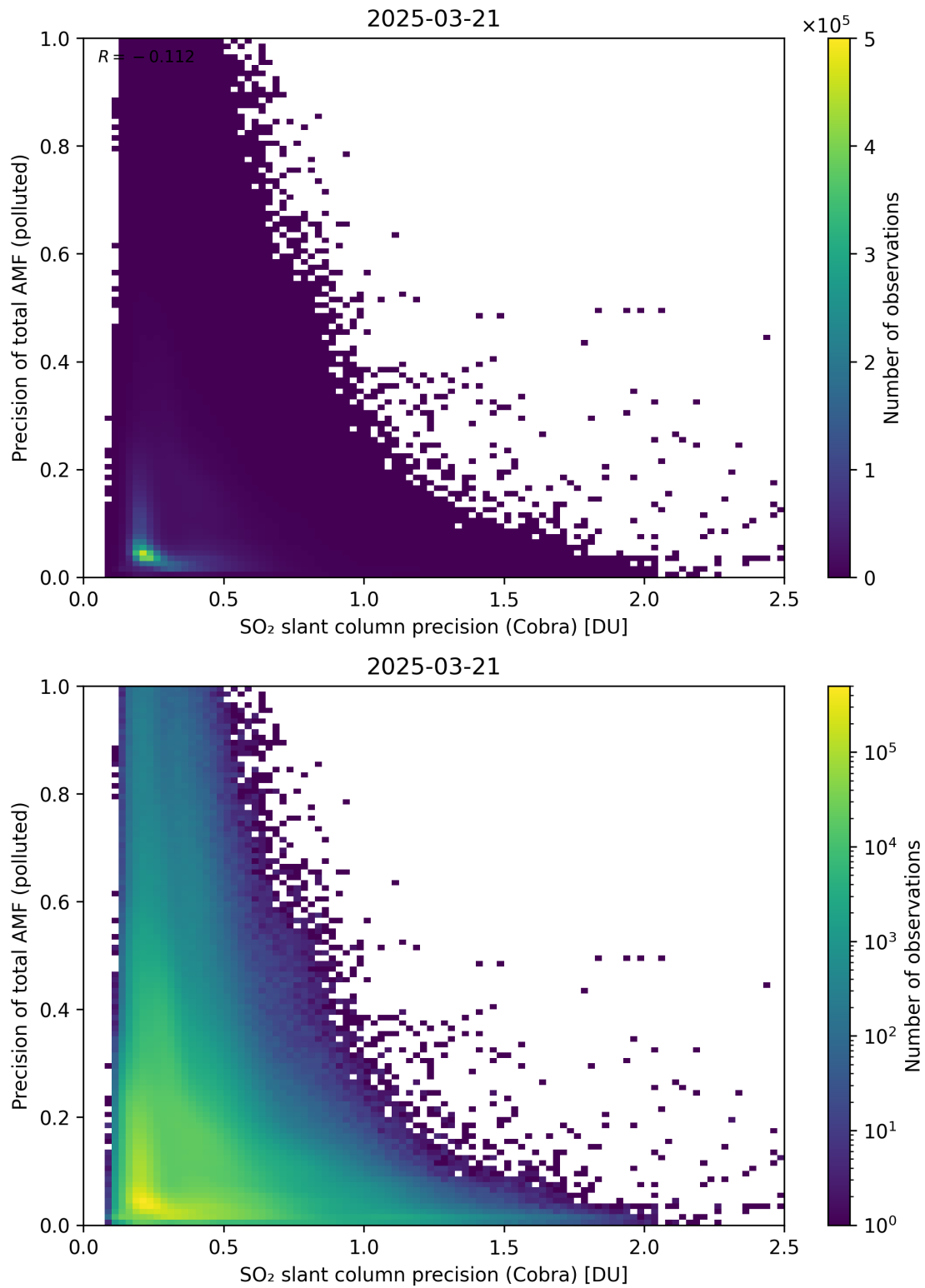
Figure 214: Scatter density plot of “SO 2 slant column precision (Cobra)” against “Precision of total AMF (polluted)” for 2025-03-20 to 2025-03-22.
