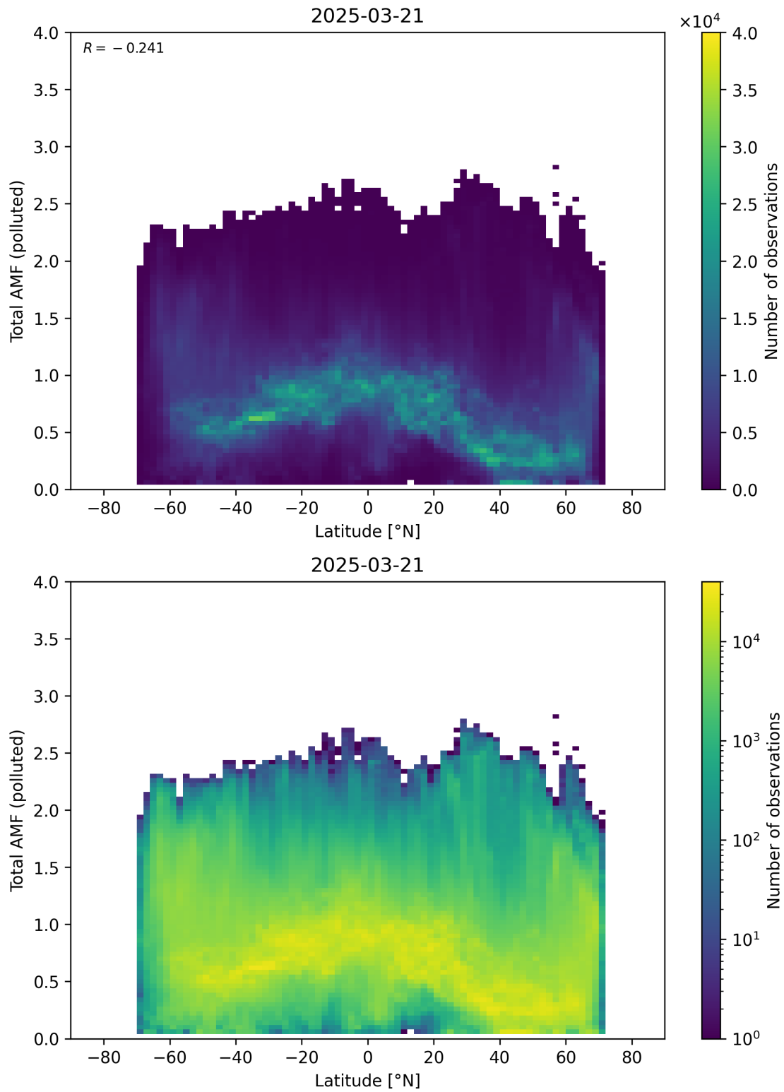
Figure 167: Scatter density plot of “Latitude” against “Total AMF (polluted)” for 2025-03-20 to 2025-03-22.
