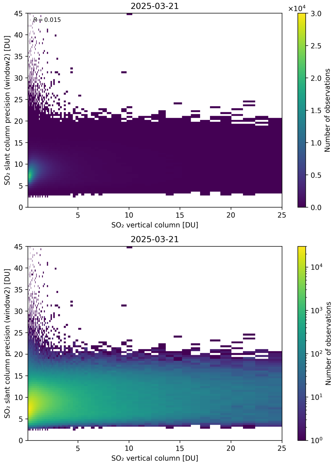
Figure 356: Scatter density plot of “SO 2 vertical column” against “SO 2 slant column precision (window2)” for 2025-03-20 to 2025-03-22.
