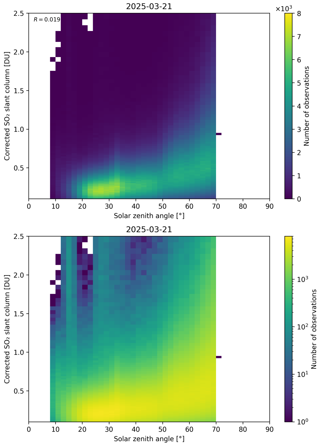
Figure 181: Scatter density plot of “Solar zenith angle” against “Corrected SO 2 slant column” for 2025-03-20 to 2025-03-22.
