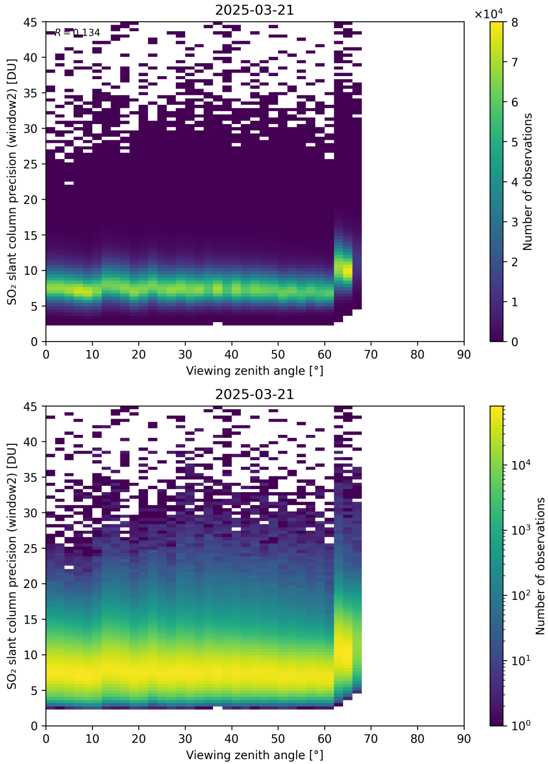
Figure 378: Scatter density plot of “Viewing zenith angle” against “SO 2 slant column precision (window2)” for 2025-03-20 to 2025-03-22.
