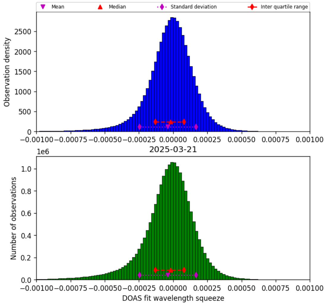
Figure 77: Histogram of “DOAS fit wavelength squeeze” for 2025-03-20 to 2025-03-22
