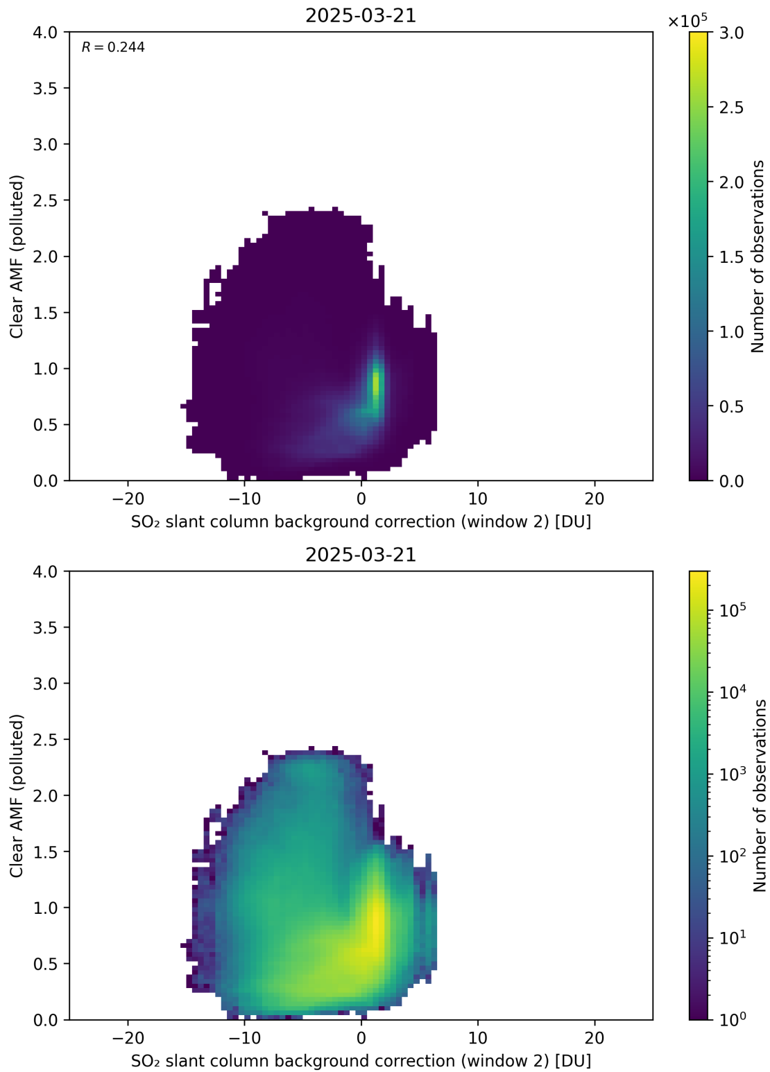
Figure 126: Scatter density plot of “SO 2 slant column background correction (window 2)” against “Clear AMF (polluted)” for 2025-03-20 to 2025-03-22.
