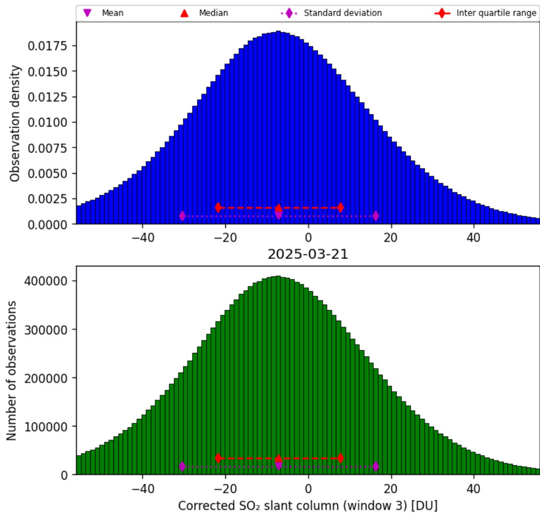
Figure 73: Histogram of “Corrected SO 2 slant column (window 3)” for 2025-03-20 to 2025-03-22
