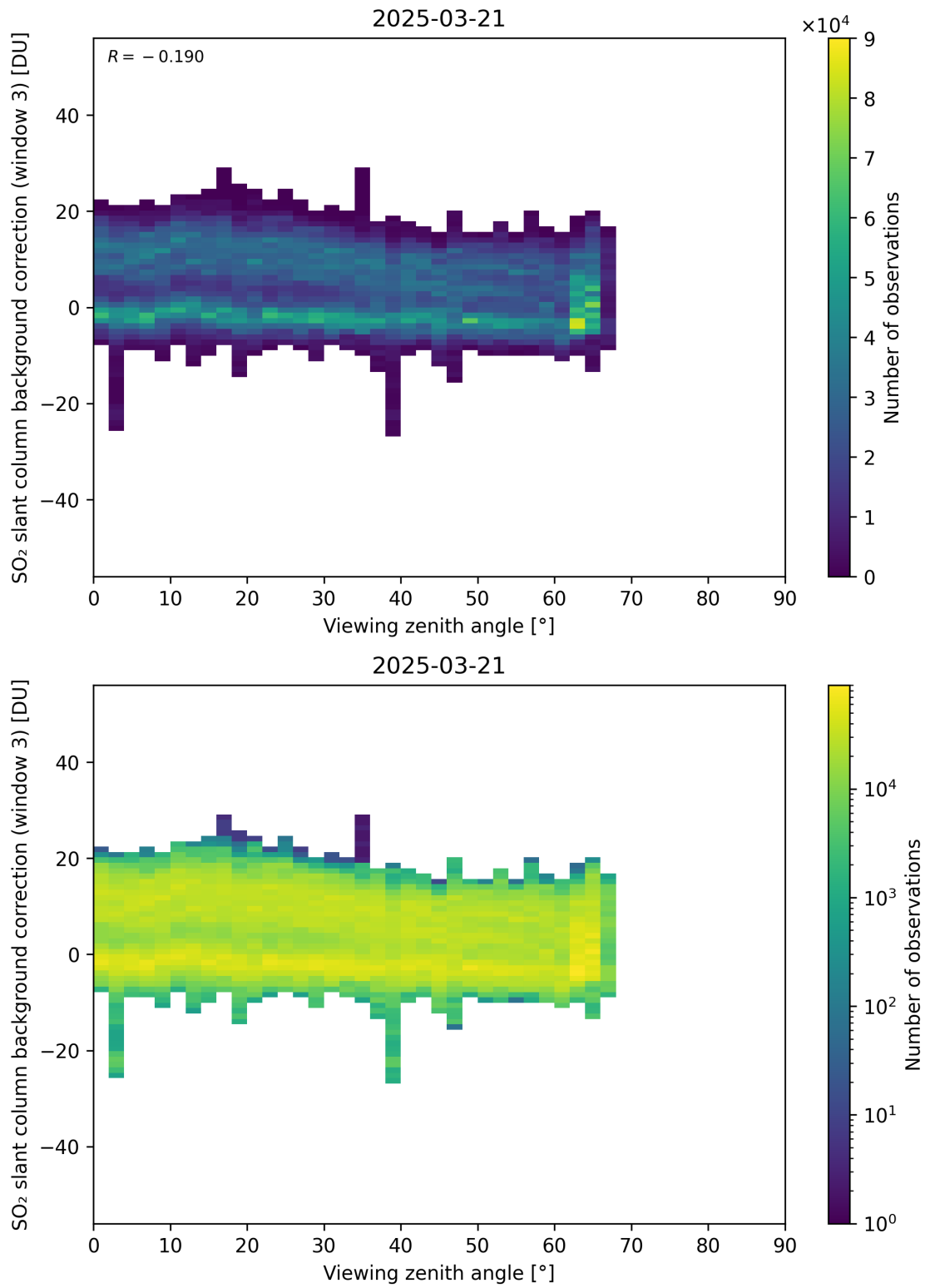
Figure 364: Scatter density plot of “Viewing zenith angle” against “SO 2 slant column background correction (window 3)” for 2025-03-20 to 2025-03-22.
