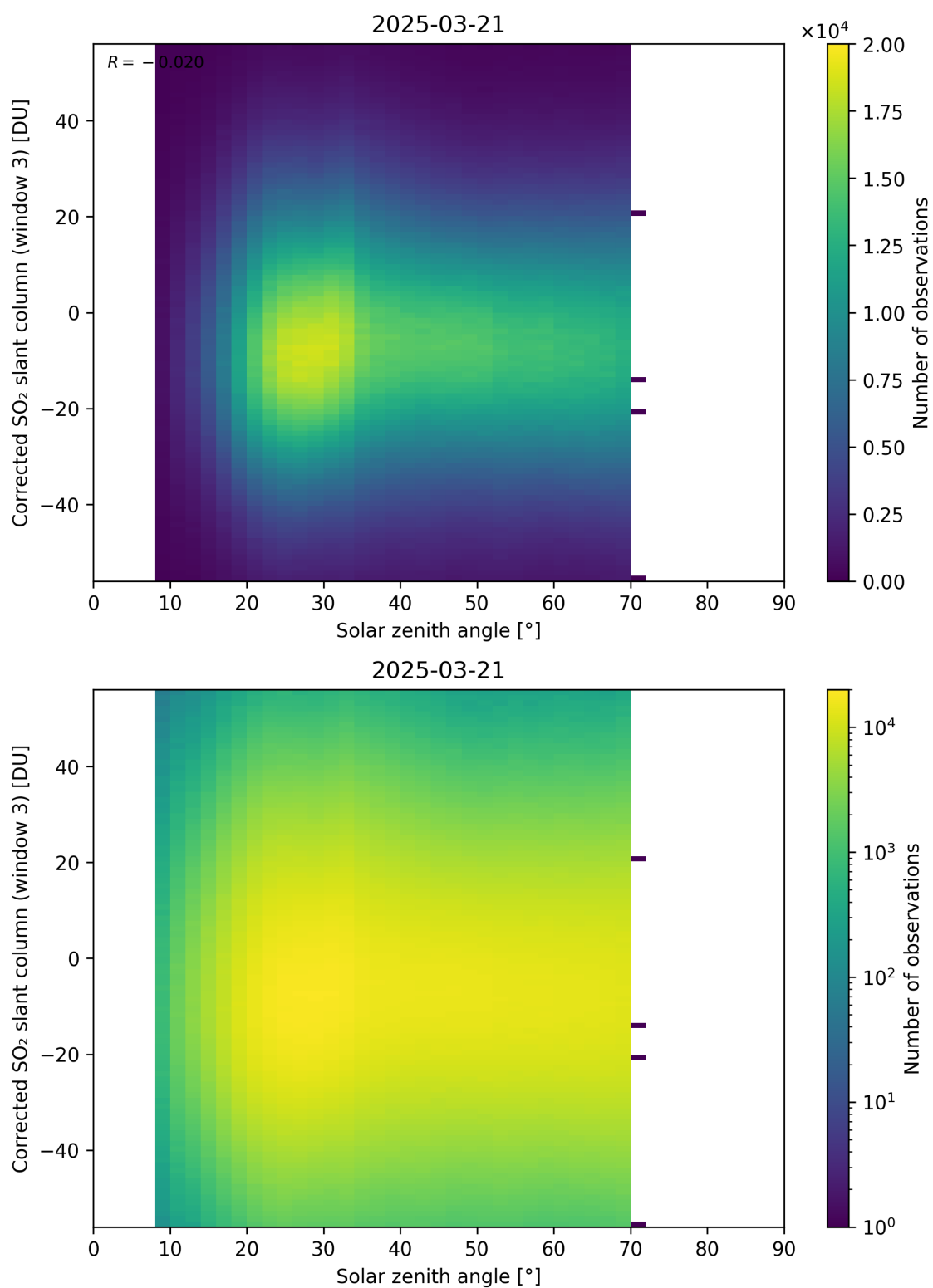
Figure 183: Scatter density plot of “Solar zenith angle” against “Corrected SO 2 slant column (window 3)” for 2025-03-20 to 2025-03-22.
