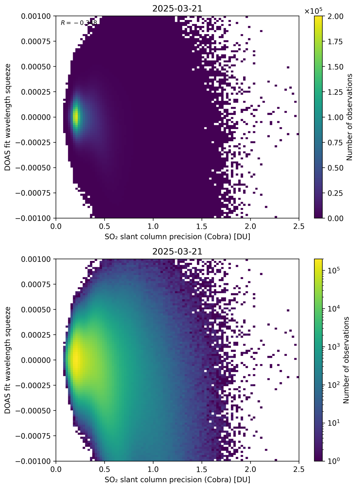
Figure 203: Scatter density plot of “SO 2 slant column precision (Cobra)” against “DOAS fit wavelength squeeze” for 2025-03-20 to 2025-03-22.
