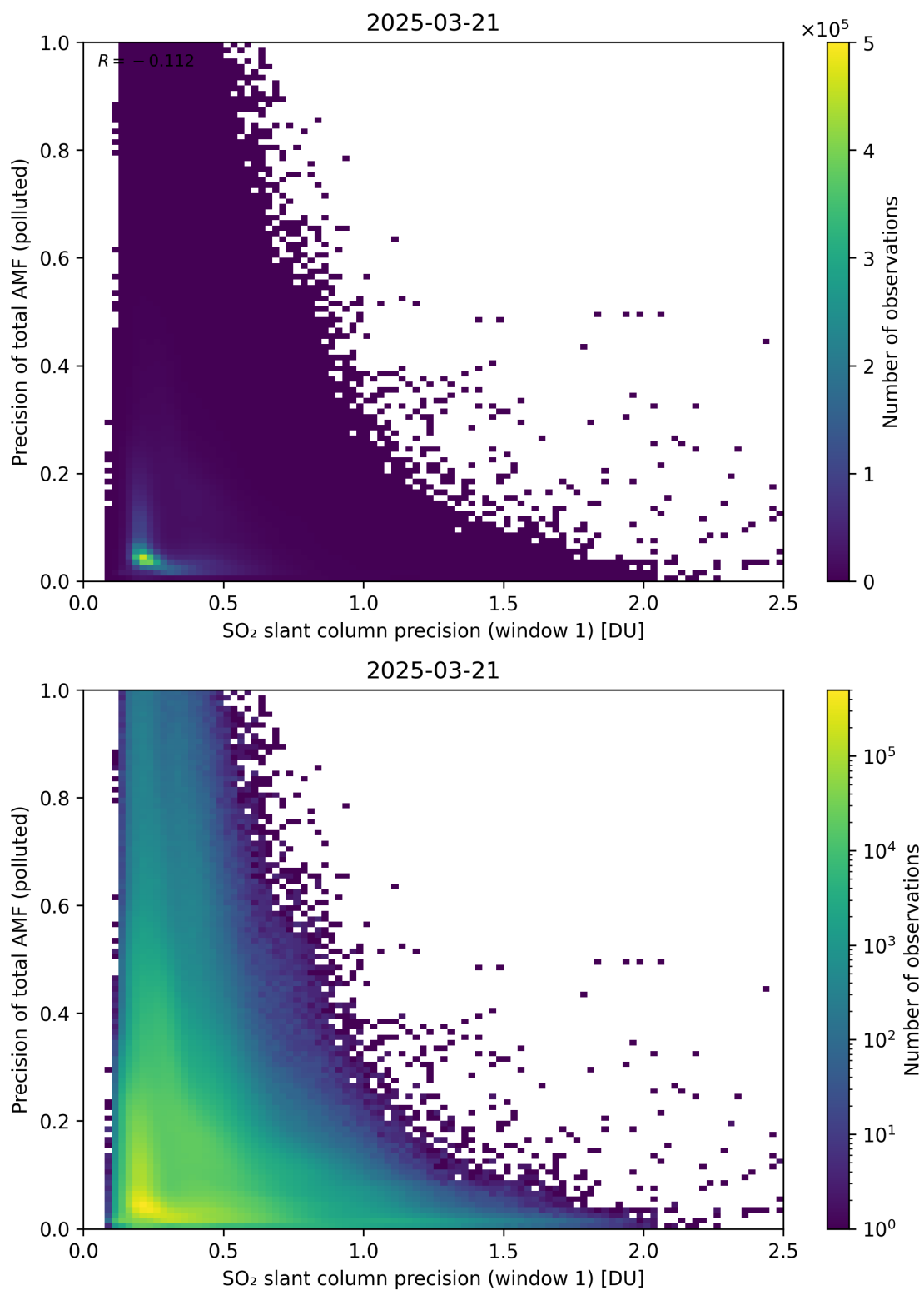
Figure 281: Scatter density plot of “SO 2 slant column precision (window 1)” against “Precision of total AMF (polluted)” for 2025-03-20 to 2025-03-22.
