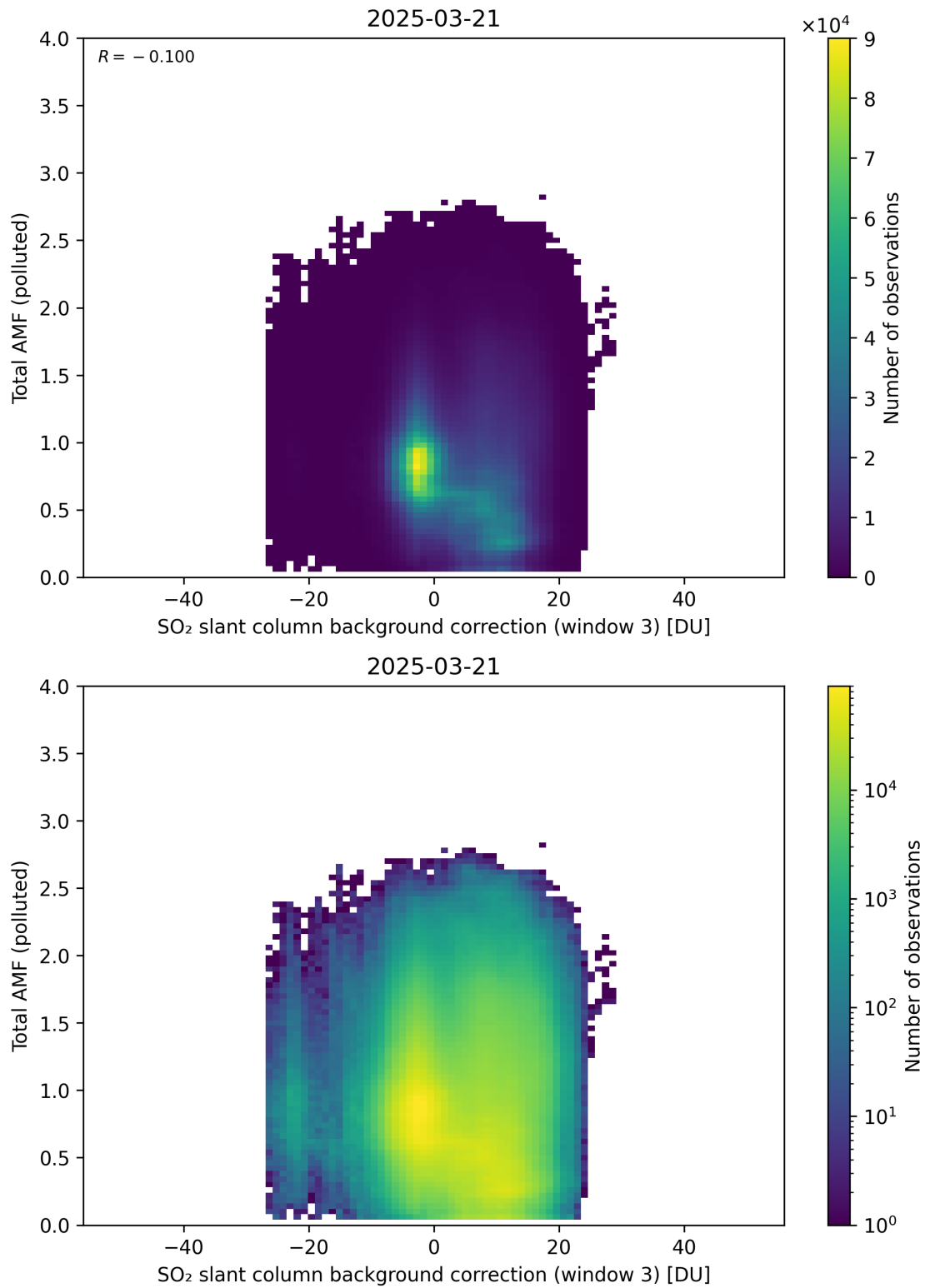
Figure 136: Scatter density plot of “SO 2 slant column background correction (window 3)” against “Total AMF (polluted)” for 2025-03-20 to 2025-03-22.
