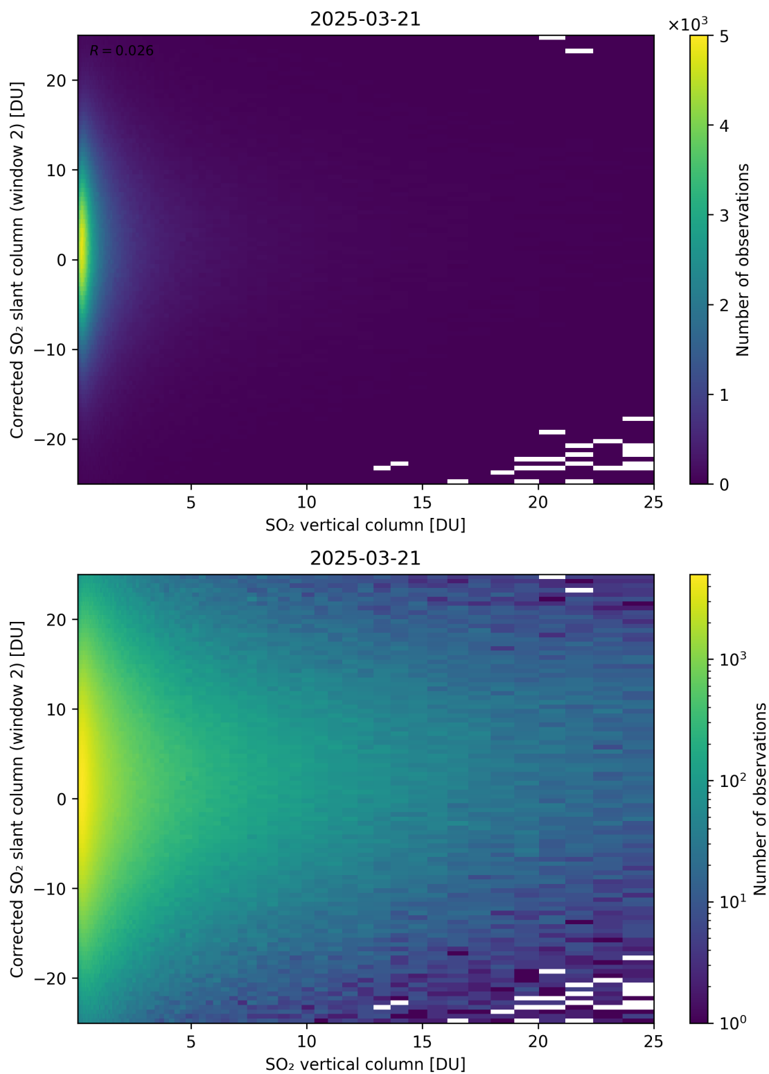
Figure 352: Scatter density plot of “SO 2 vertical column” against “Corrected SO 2 slant column (window 2)” for 2025-03-20 to 2025-03-22.
