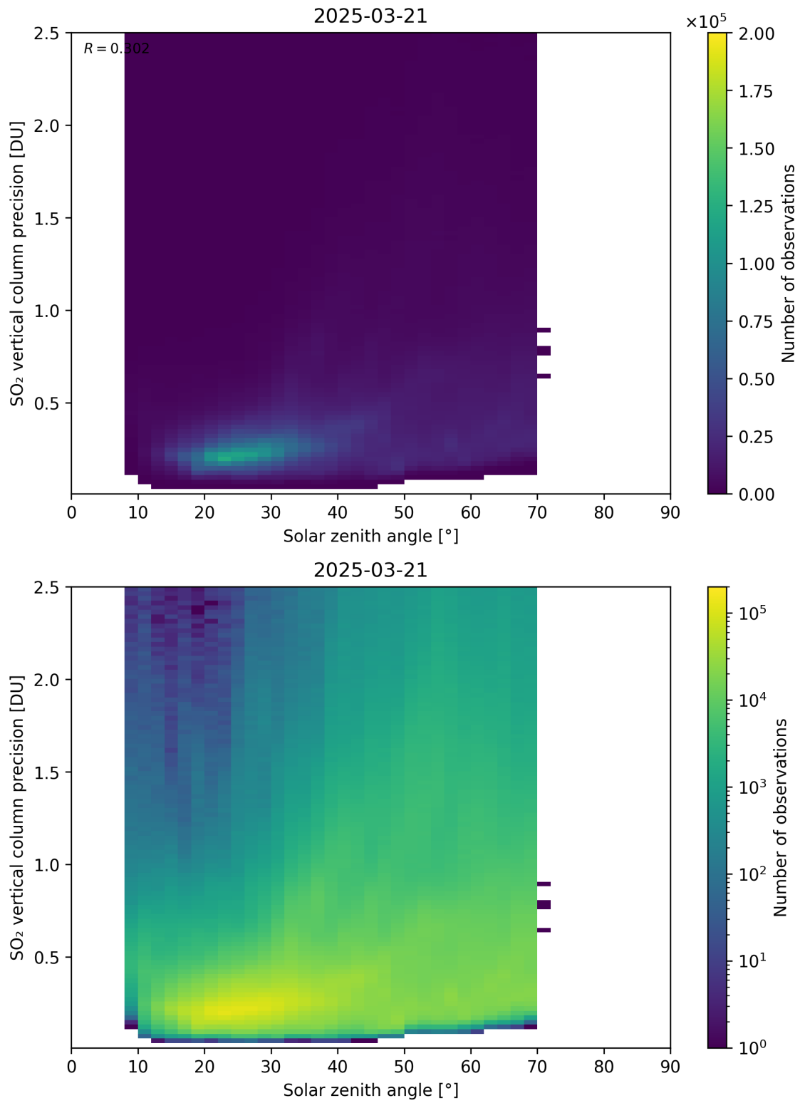
Figure 192: Scatter density plot of “Solar zenith angle” against “SO 2 vertical column precision” for 2025-03-20 to 2025-03-22.
