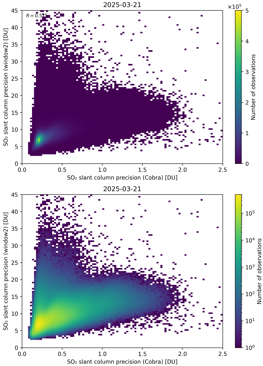
Figure 210: Scatter density plot of “SO 2 slant column precision (Cobra)” against “SO 2 slant column precision (window2)” for 2025-03-20 to 2025-03-22.
