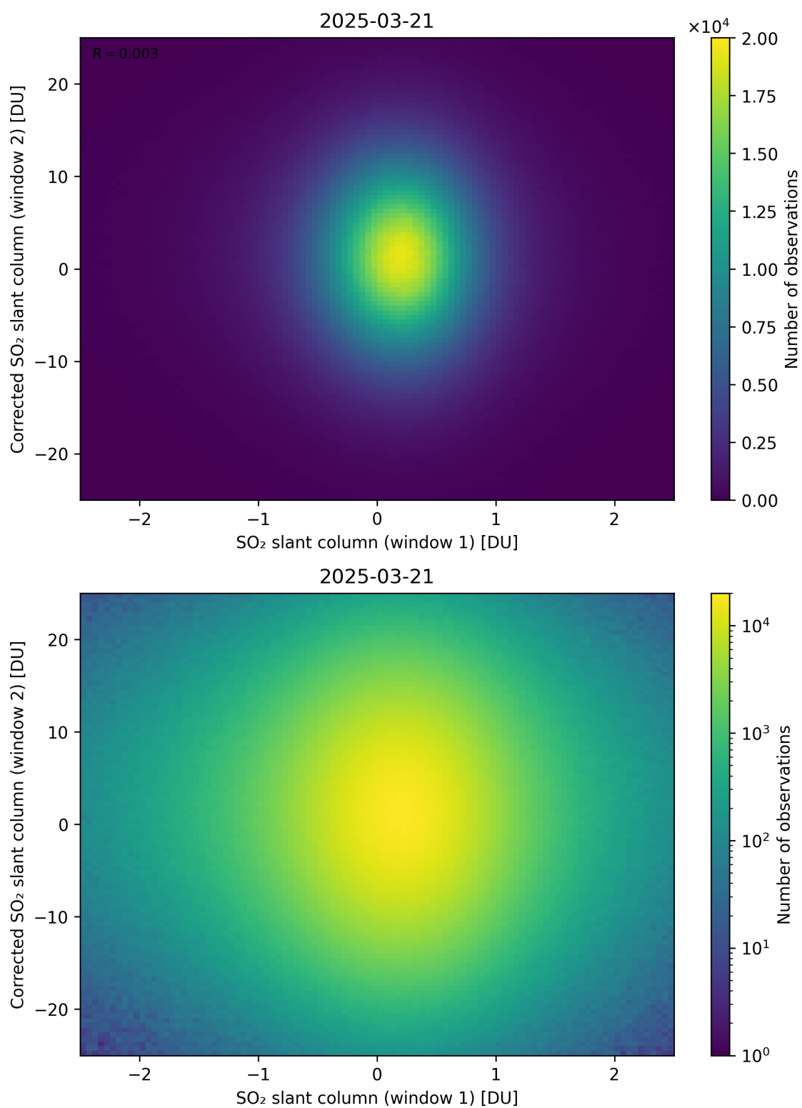
Figure 283: Scatter density plot of “SO 2 slant column (window 1)” against “Corrected SO 2 slant column (window 2)” for 2025-03-20 to 2025-03-22.
