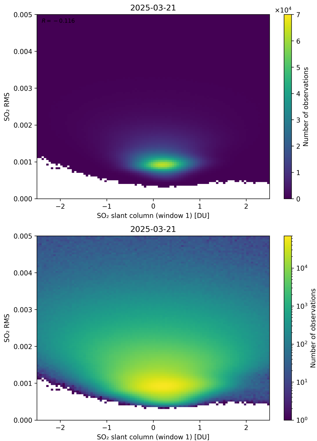
Figure 267: Scatter density plot of “SO 2 slant column (window 1)” against “SO 2 RMS” for 2025-03-20 to 2025-03-22.
