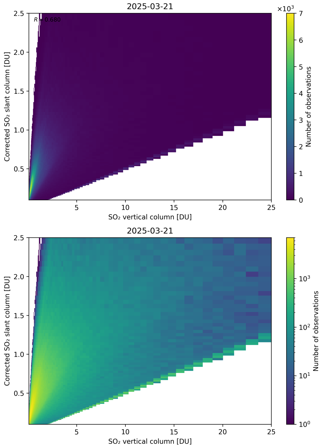
Figure 351: Scatter density plot of “SO 2 vertical column” against “Corrected SO 2 slant column” for 2025-03-20 to 2025-03-22.
