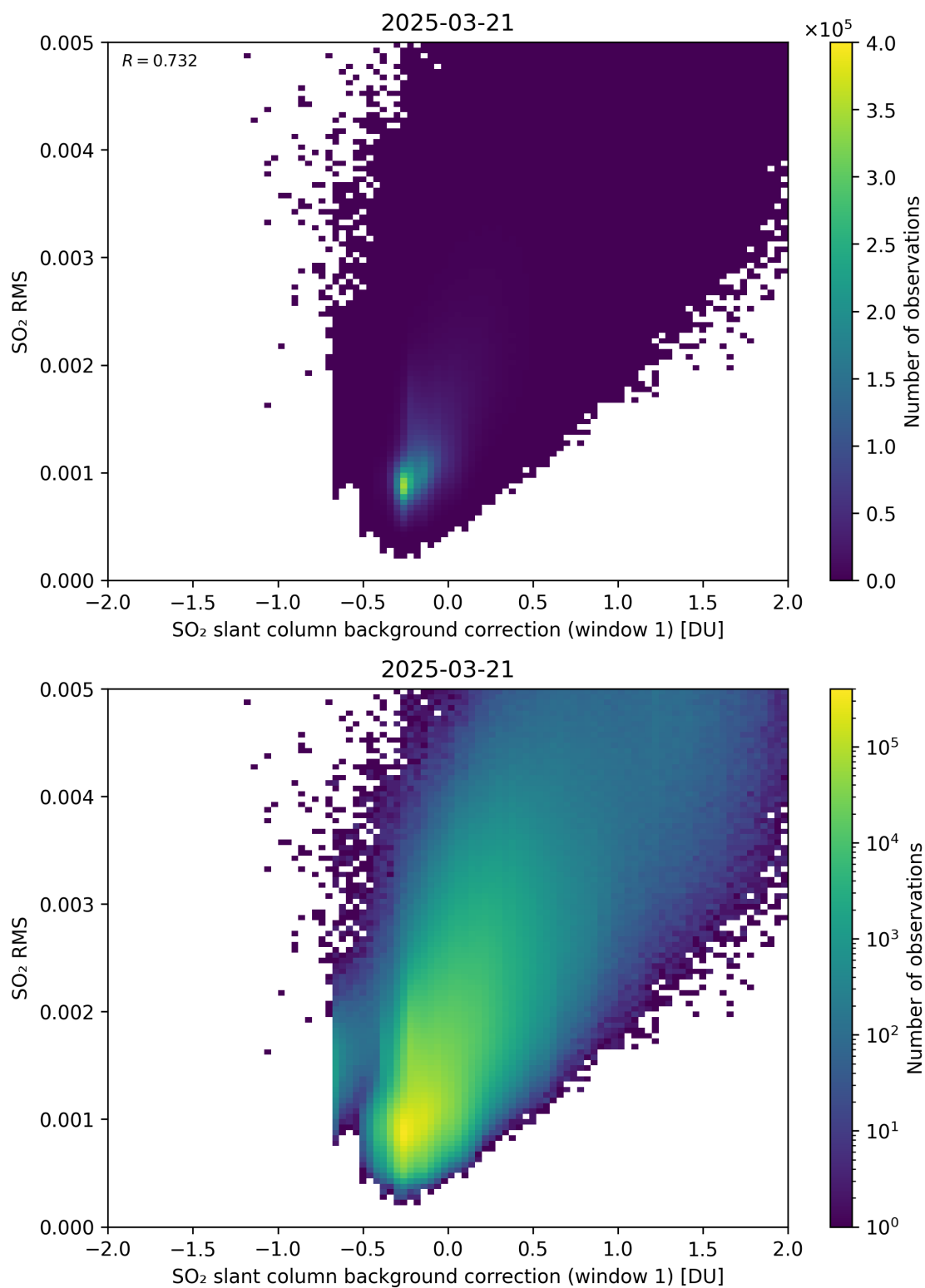
Figure 113: Scatter density plot of “SO 2 slant column background correction (window 1)” against “SO 2 RMS” for 2025-03-20 to 2025-03-22.
