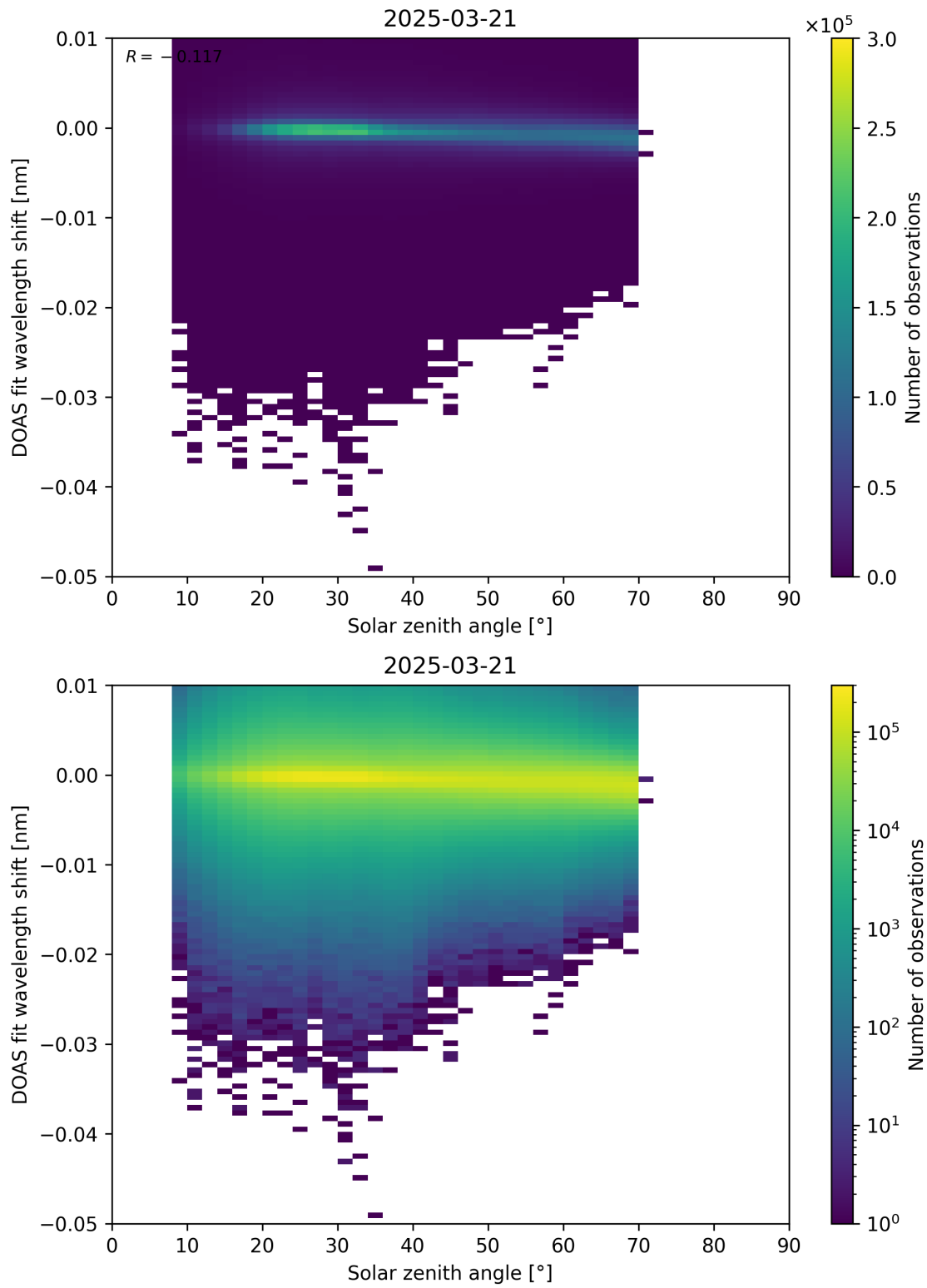
Figure 174: Scatter density plot of “Solar zenith angle” against “DOAS fit wavelength shift” for 2025-03-20 to 2025-03-22.
