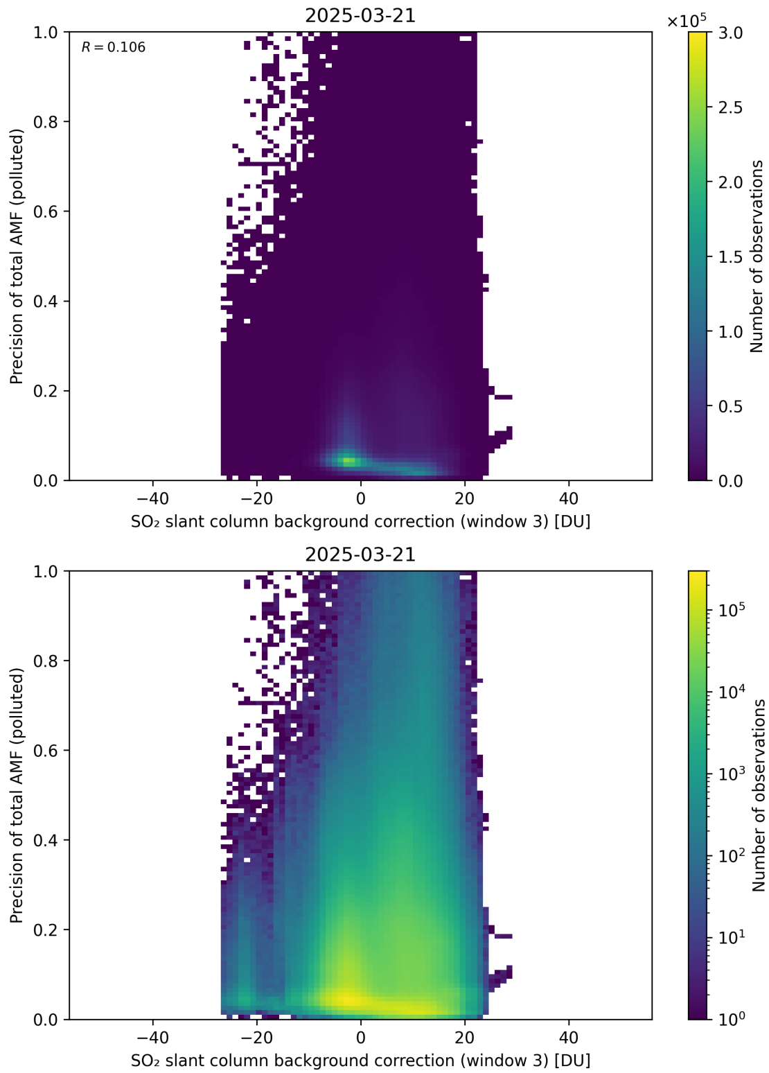
Figure 137: Scatter density plot of “SO 2 slant column background correction (window 3)” against “Precision of total AMF (polluted)” for 2025-03-20 to 2025-03-22.
