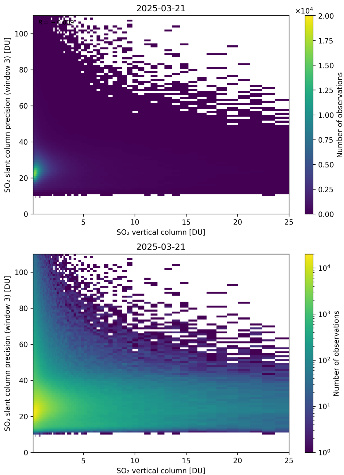
Figure 358: Scatter density plot of “SO 2 vertical column” against “SO 2 slant column precision (window 3)” for 2025-03-20 to 2025-03-22.
