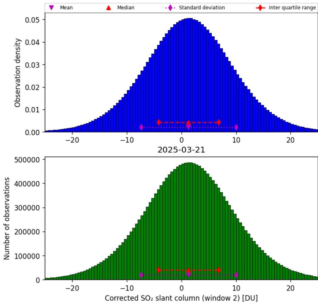
Figure 69: Histogram of “Corrected SO 2 slant column (window 2)” for 2025-03-20 to 2025-03-22
