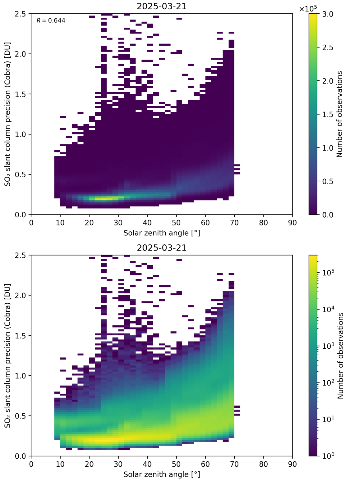
Figure 180: Scatter density plot of “Solar zenith angle” against “SO 2 slant column precision (Cobra)” for 2025-03-20 to 2025-03-22.
