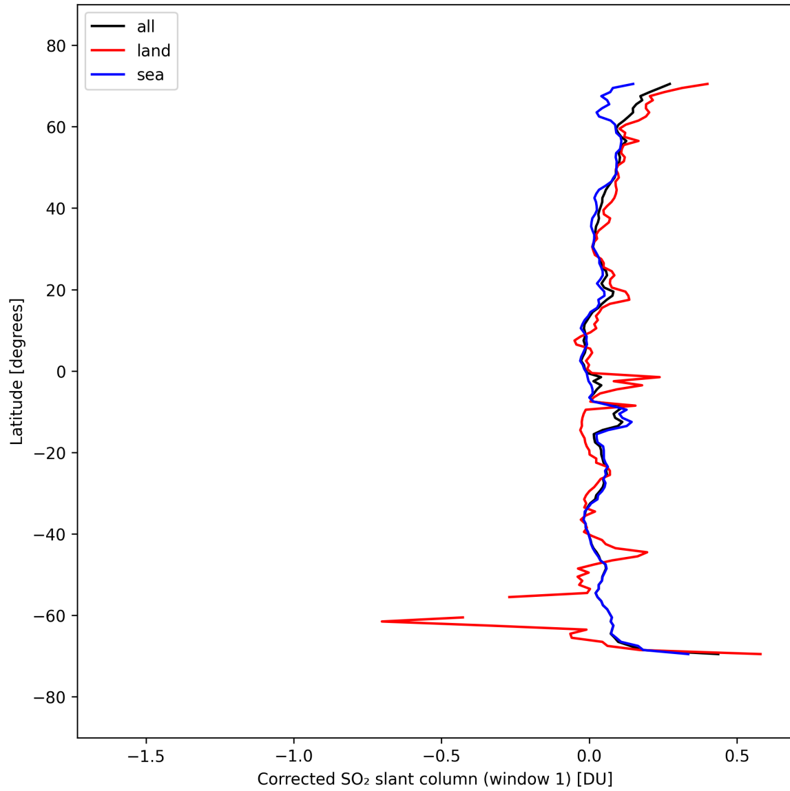
Figure 39: Zonal average of “Corrected SO 2 slant column (window 1)” for 2025-03-20 to 2025-03-22.
