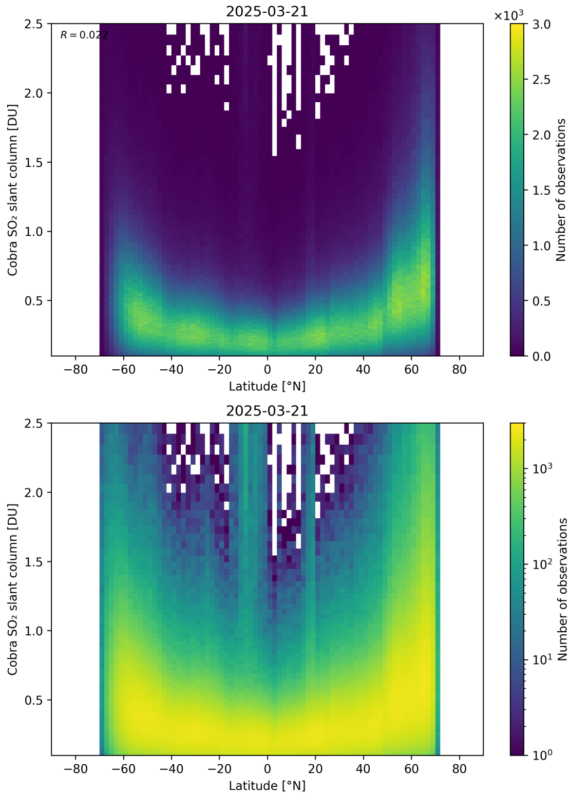
Figure 157: Scatter density plot of “Latitude” against “Cobra SO 2 slant column” for 2025-03-20 to 2025-03-22.
