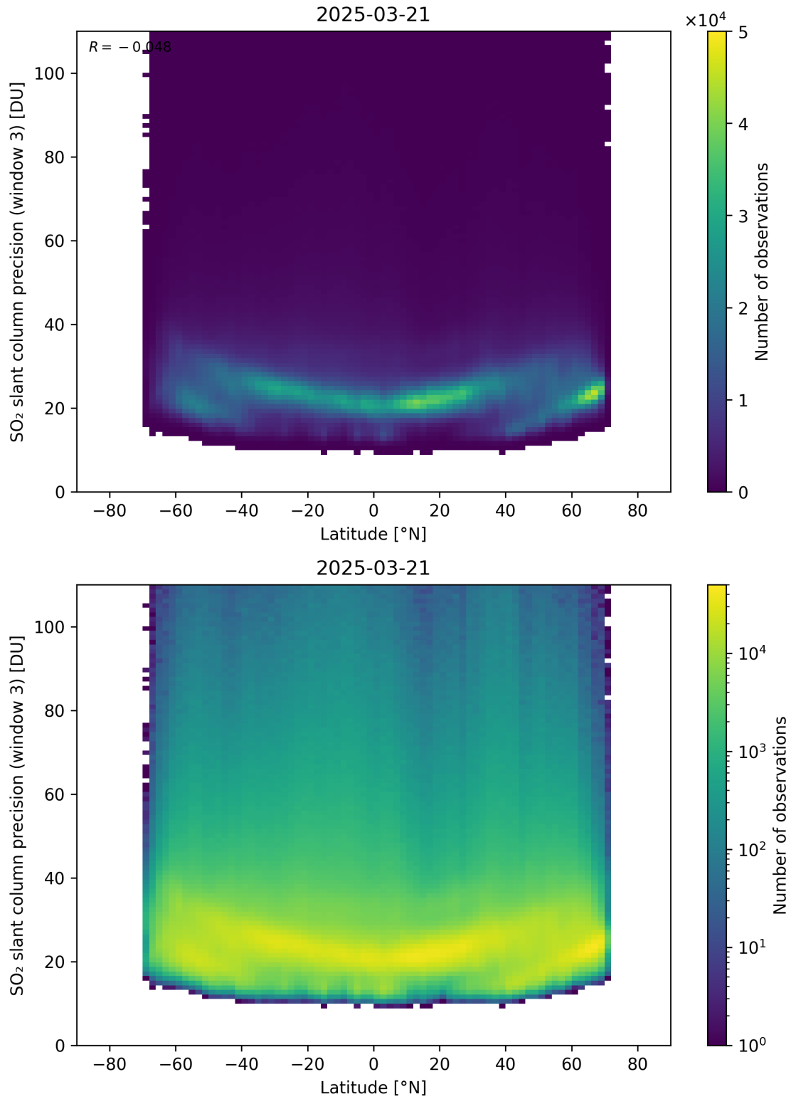
Figure 166: Scatter density plot of “Latitude” against “SO 2 slant column precision (window 3)” for 2025-03-20 to 2025-03-22.
