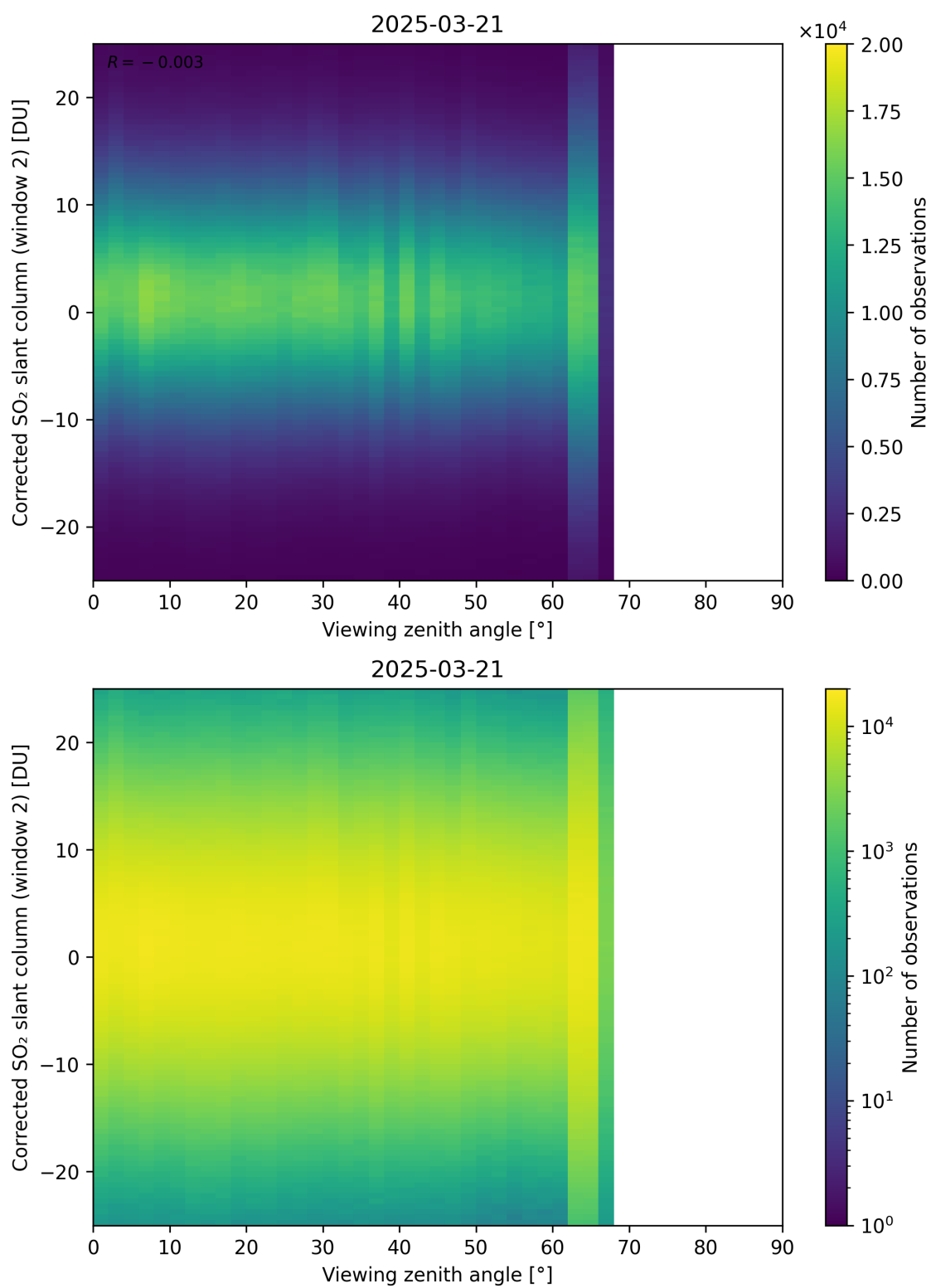
Figure 374: Scatter density plot of “Viewing zenith angle” against “Corrected SO 2 slant column (window 2)” for 2025-03-20 to 2025-03-22.
