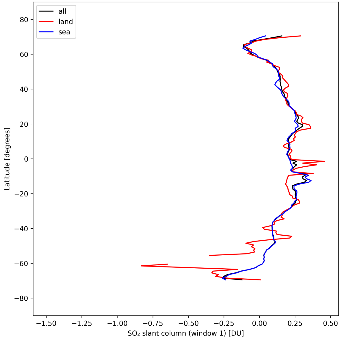
Figure 37: Zonal average of “SO 2 slant column (window 1)” for 2025-03-20 to 2025-03-22.
