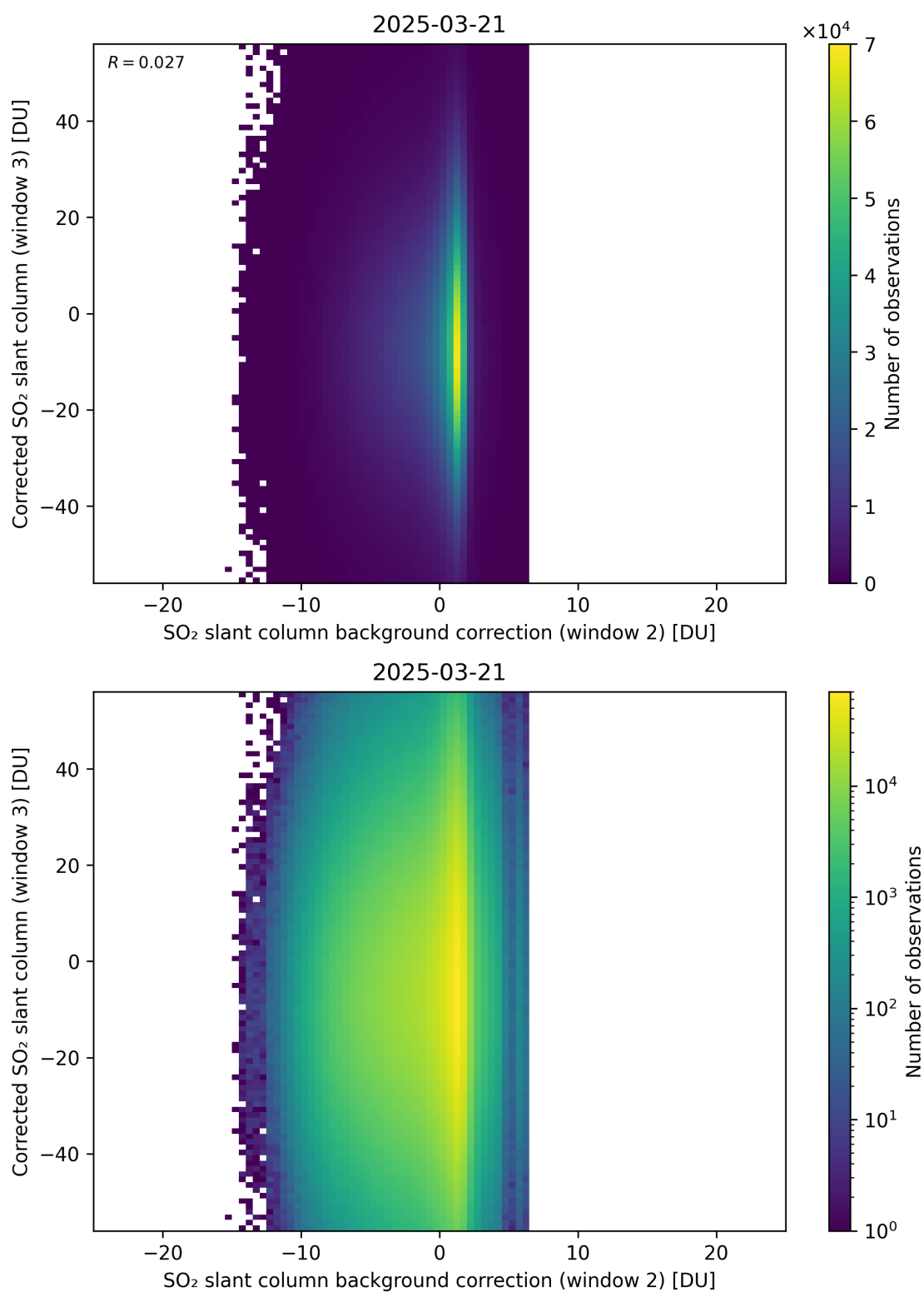
Figure 127: Scatter density plot of “SO 2 slant column background correction (window 2)” against “Corrected SO 2 slant column (window 3)” for 2025-03-20 to 2025-03-22.
