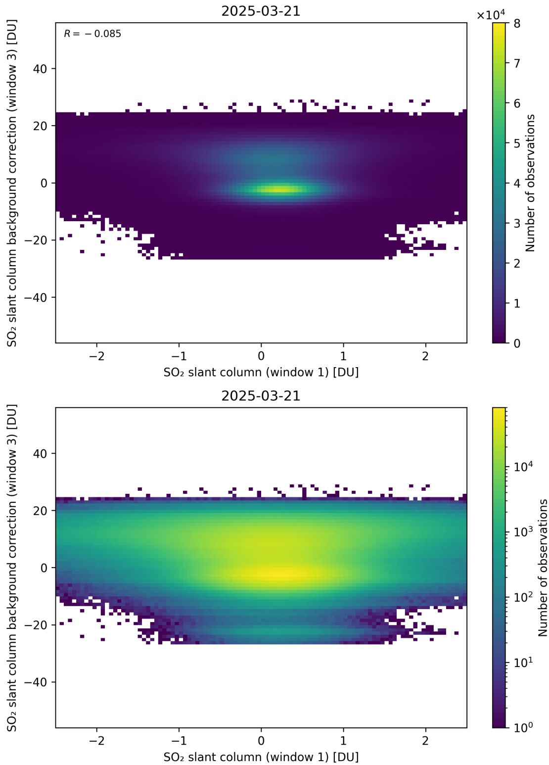
Figure 264: Scatter density plot of “SO 2 slant column (window 1)” against “SO 2 slant column background correction (window 3)” for 2025-03-20 to 2025-03-22.
