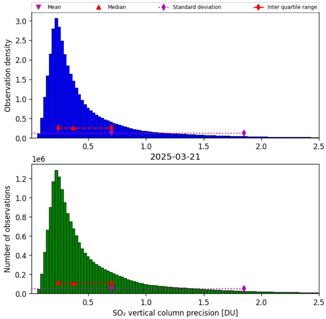
Figure 59: Histogram of "SO 2 vertical column precision" for 2025-03-20 to 2025-03-22
