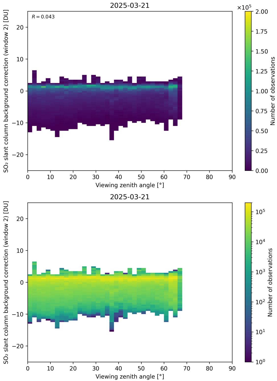
Figure 363: Scatter density plot of “Viewing zenith angle” against “SO 2 slant column background correction (window 2)” for 2025-03-20 to 2025-03-22.
