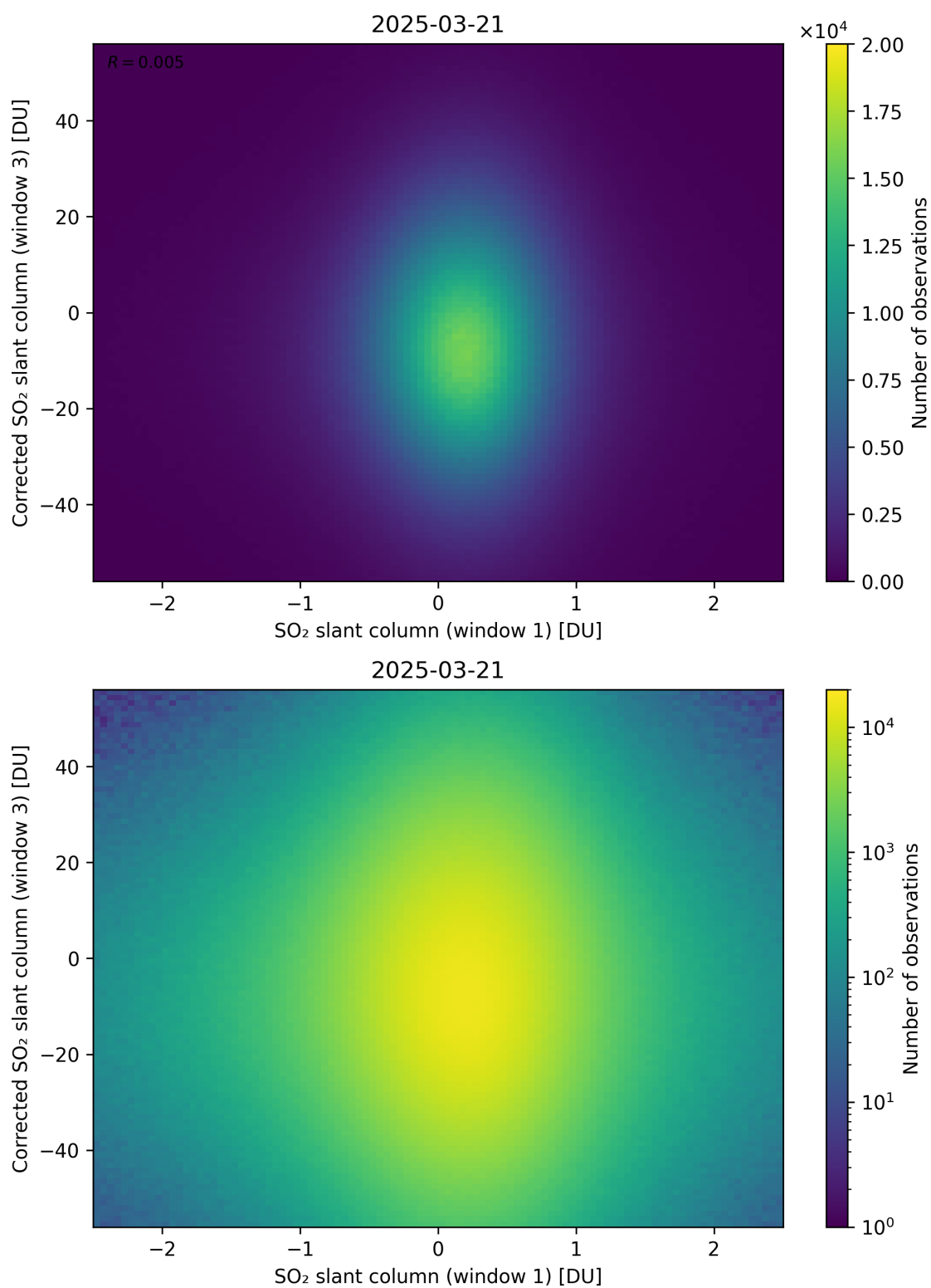
Figure 284: Scatter density plot of “SO 2 slant column (window 1)” against “Corrected SO 2 slant column (window 3)” for 2025-03-20 to 2025-03-22.
