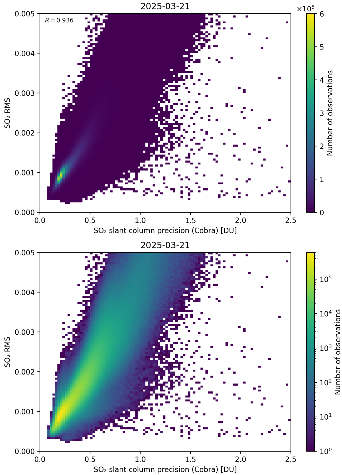
Figure 204: Scatter density plot of “SO 2 slant column precision (Cobra)” against “SO 2 RMS” for 2025-03-20 to 2025-03-22.
