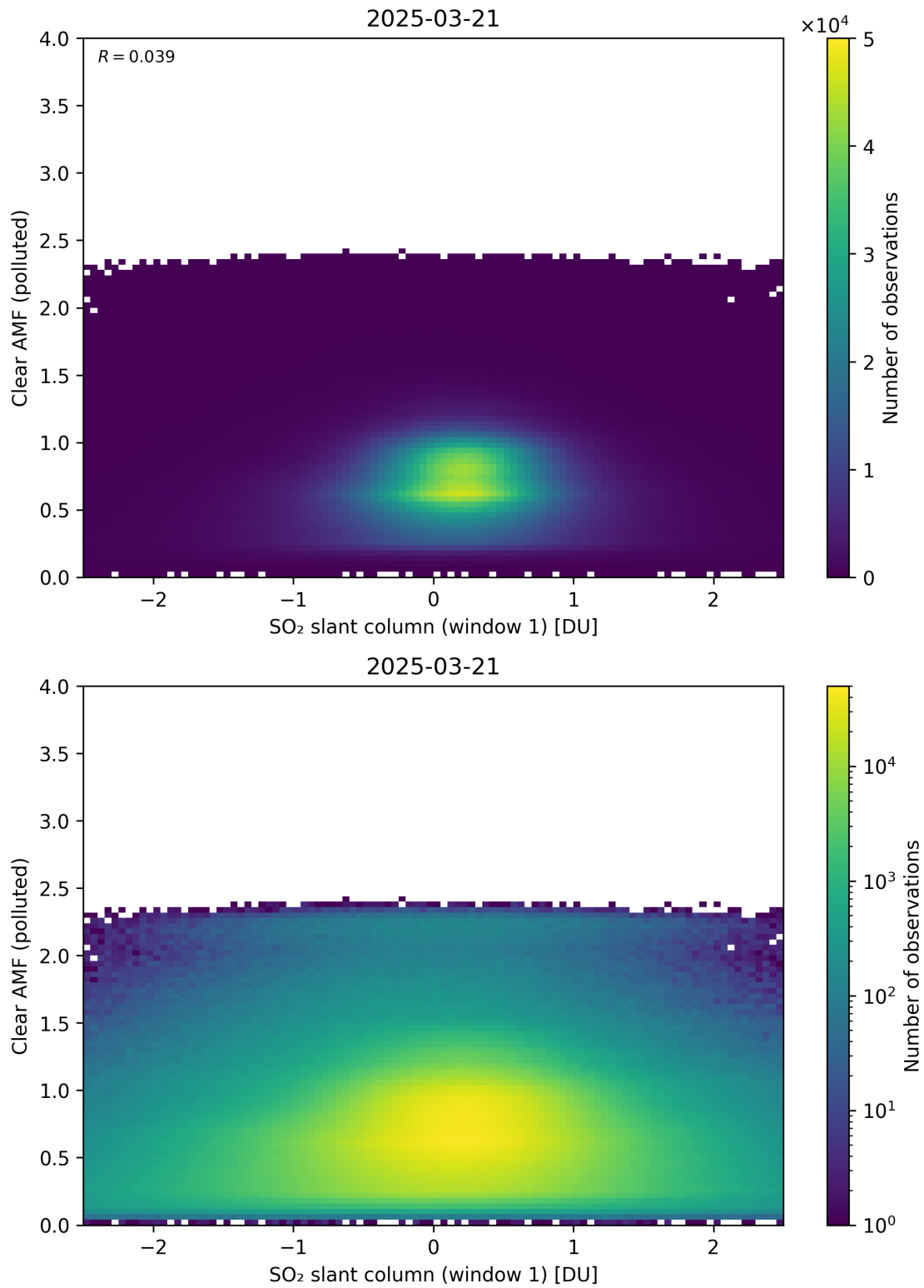
Figure 282: Scatter density plot of “SO 2 slant column (window 1)” against “Clear AMF (polluted)” for 2025-03-20 to 2025-03-22.
