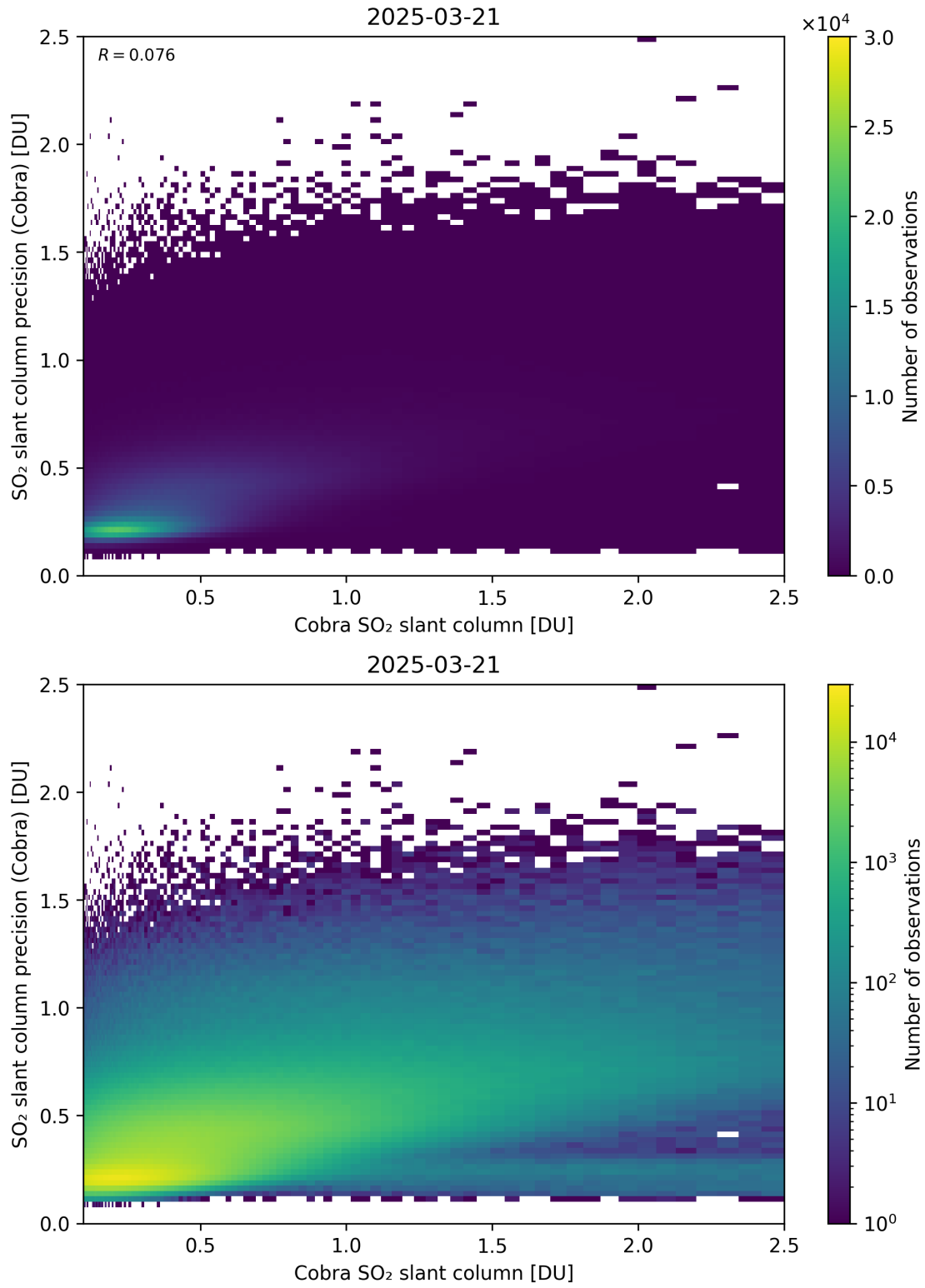
Figure 216: Scatter density plot of “Cobra SO 2 slant column” against “SO 2 slant column precision (Cobra)” for 2025-03-20 to 2025-03-22.
