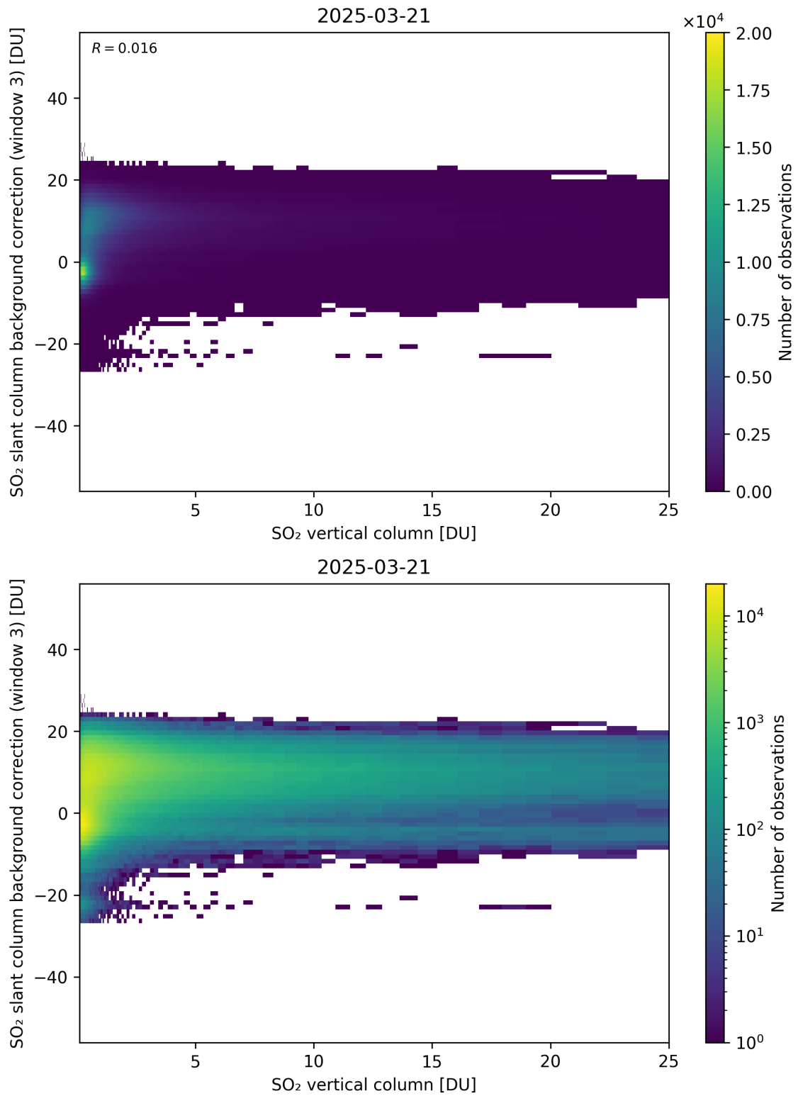
Figure 325: Scatter density plot of “SO 2 vertical column” against “SO 2 slant column background correction (window 3)” for 2025-03-20 to 2025-03-22.
