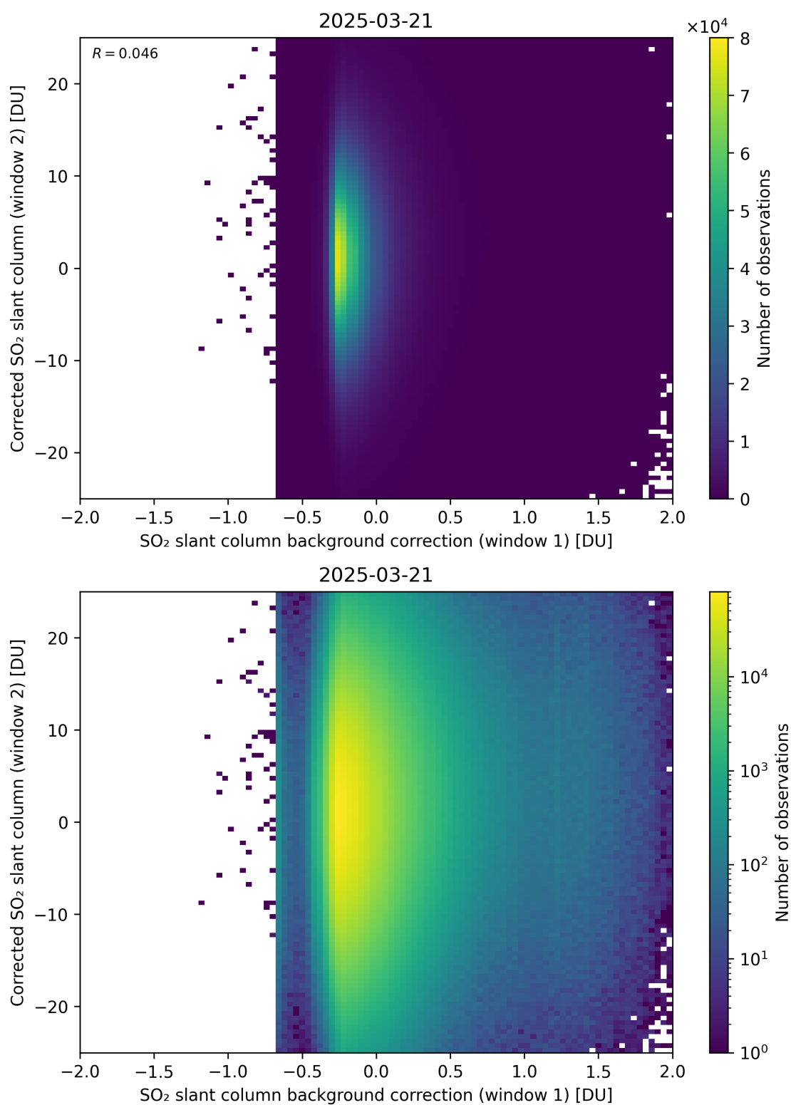
Figure 115: Scatter density plot of “SO 2 slant column background correction (window 1)” against “Corrected SO 2 slant column (window 2)” for 2025-03-20 to 2025-03-22.
