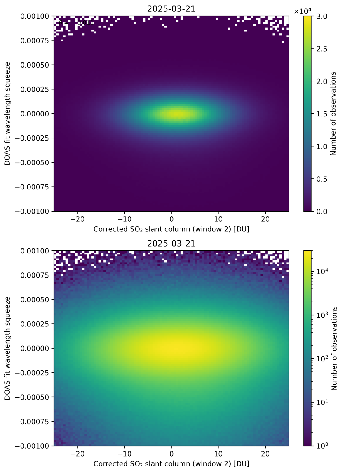
Figure 247: Scatter density plot of “Corrected SO 2 slant column (window 2)” against “DOAS fit wavelength squeeze” for 2025-03-20 to 2025-03-22.
