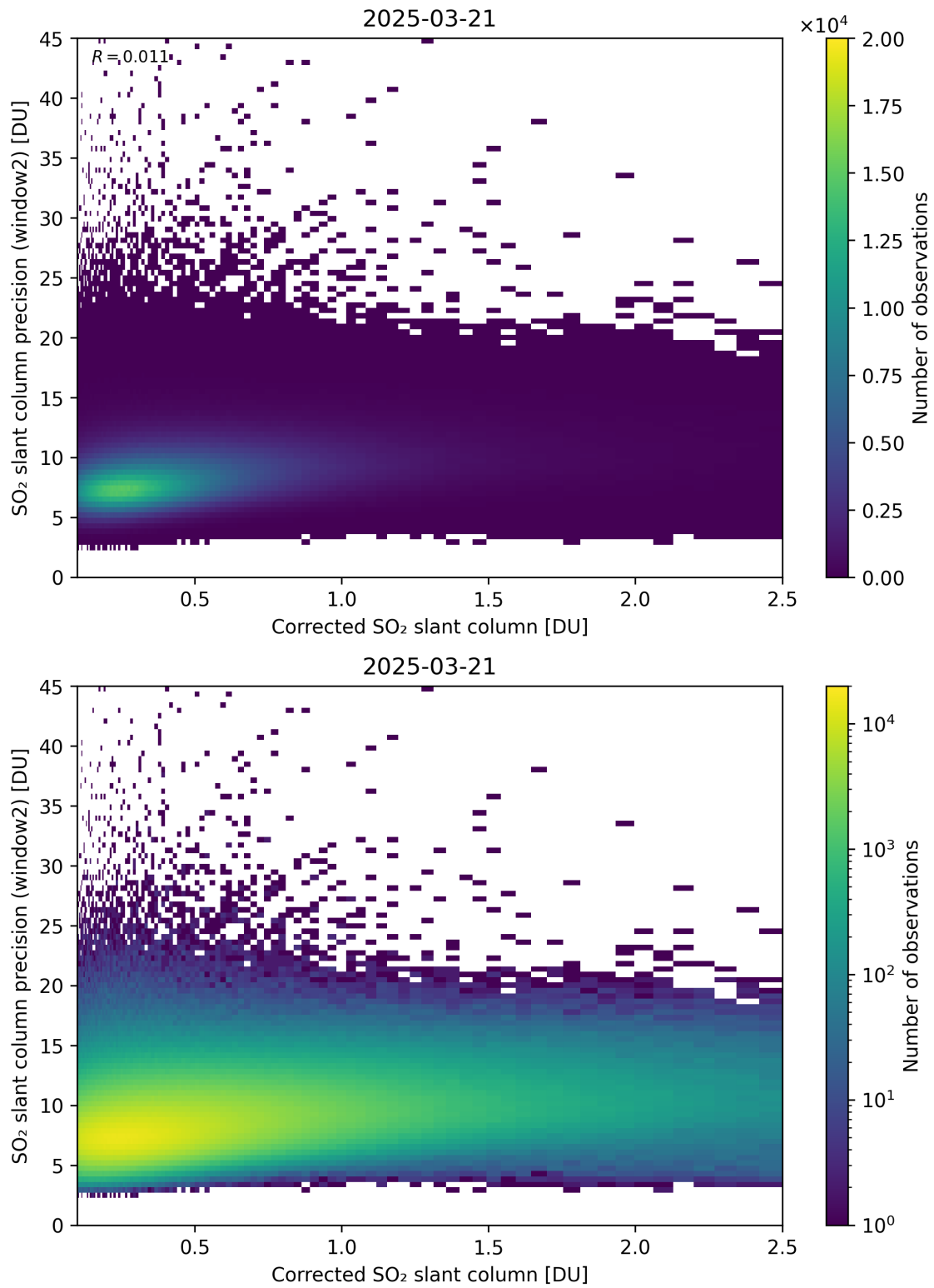
Figure 239: Scatter density plot of “Corrected SO 2 slant column” against “SO 2 slant column precision (window2)” for 2025-03-20 to 2025-03-22.
