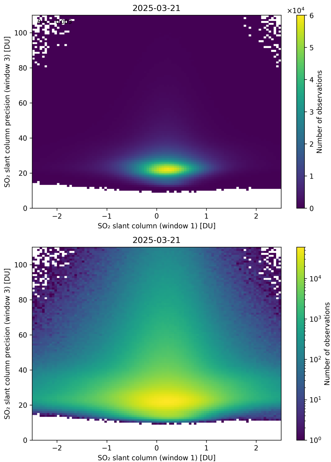
Figure 288: Scatter density plot of “SO 2 slant column (window 1)” against “SO 2 slant column precision (window 3)” for 2025-03-20 to 2025-03-22.
