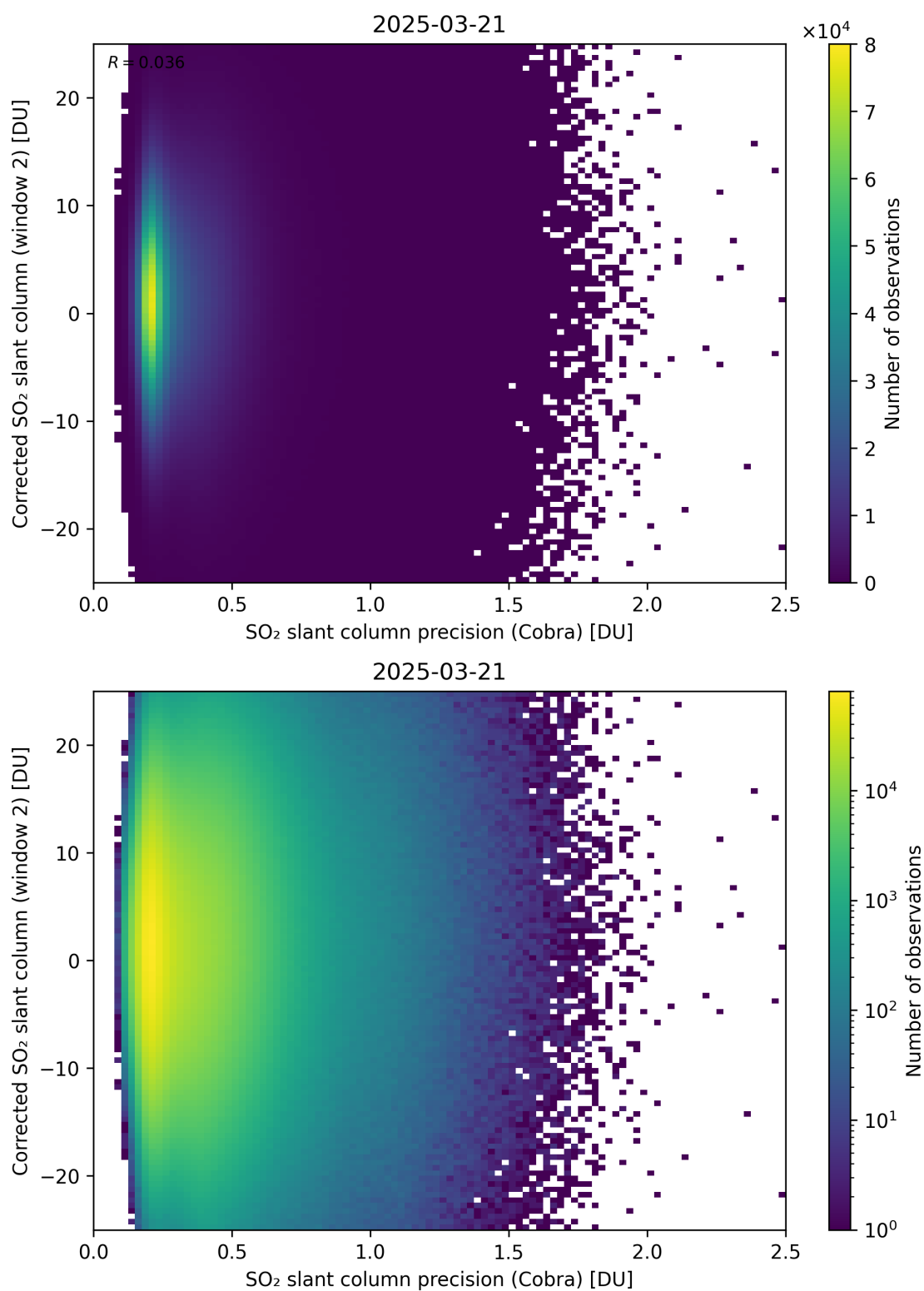
Figure 206: Scatter density plot of “SO 2 slant column precision (Cobra)” against “Corrected SO 2 slant column (window 2)” for 2025-03-20 to 2025-03-22.
