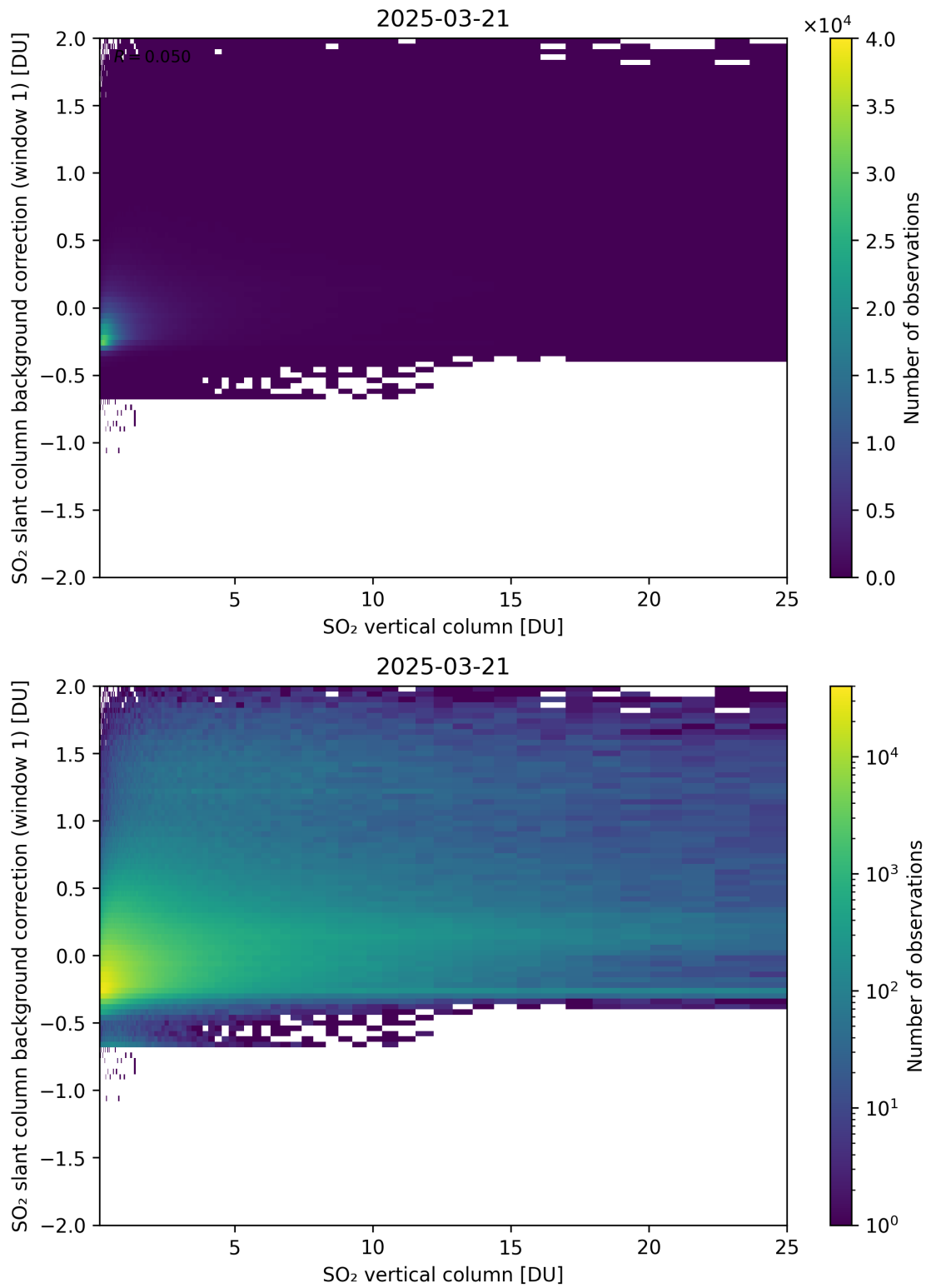
Figure 323: Scatter density plot of “SO 2 vertical column” against “SO 2 slant column background correction (window 1)” for 2025-03-20 to 2025-03-22.
