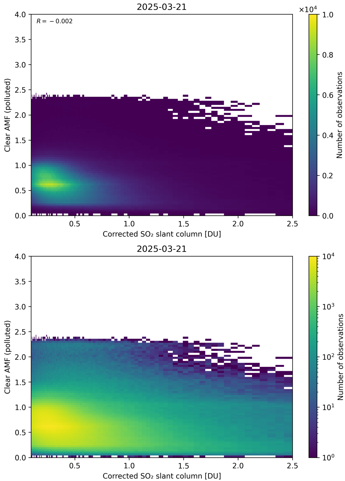
Figure 232: Scatter density plot of “Corrected SO 2 slant column” against “Clear AMF (polluted)” for 2025-03-20 to 2025-03-22.
