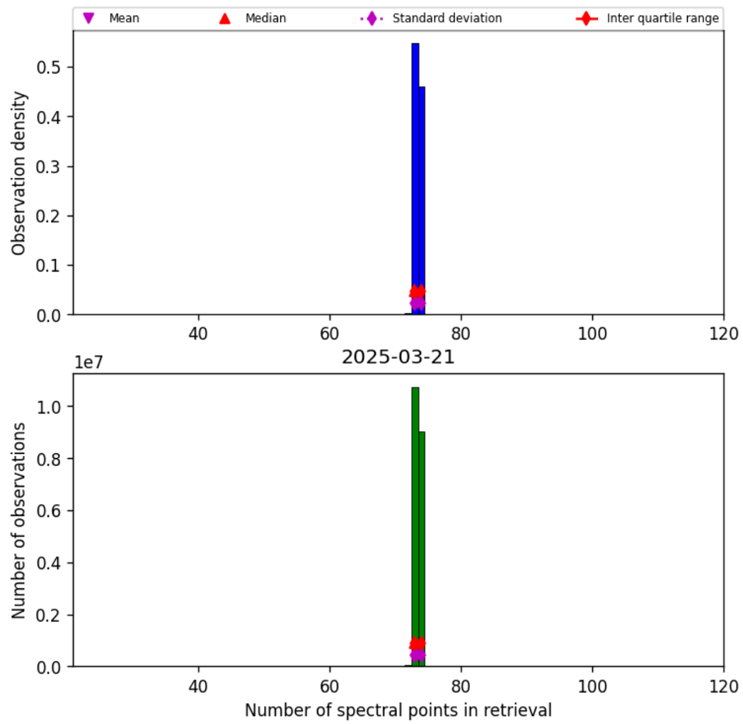
Figure 82: Histogram of “Number of spectral points in retrieval” for 2025-03-20 to 2025-03-22
