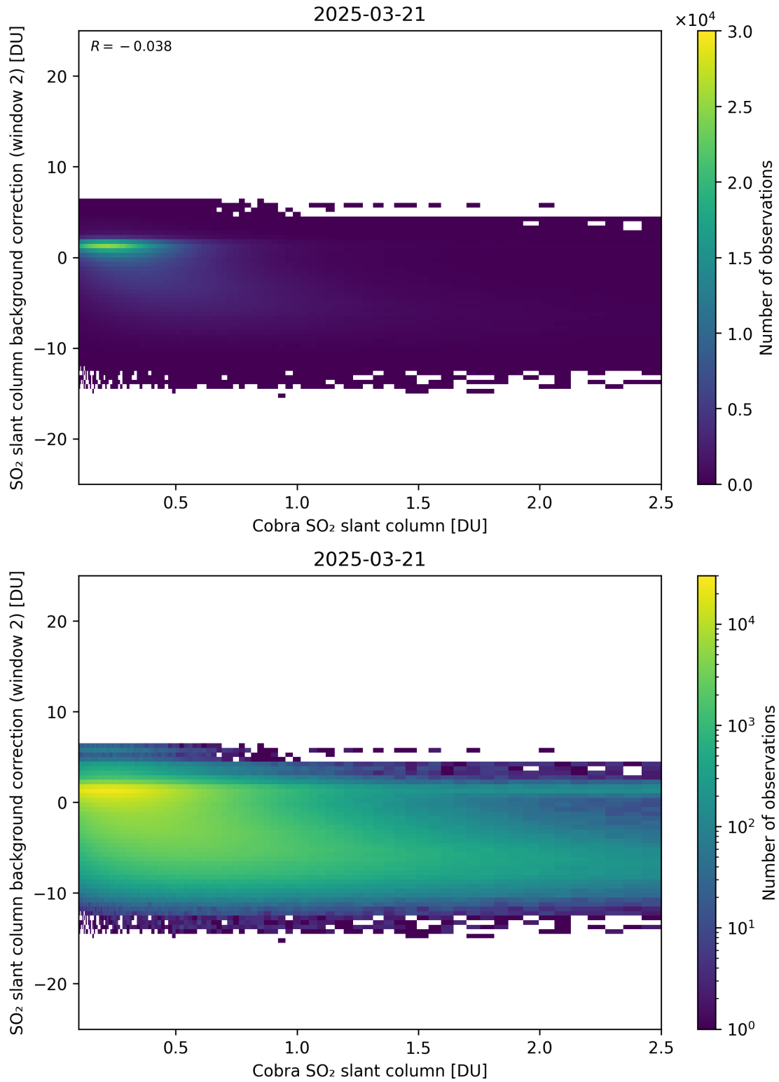
Figure 194: Scatter density plot of “Cobra SO 2 slant column” against “SO 2 slant column background correction (window 2)” for 2025-03-20 to 2025-03-22.
