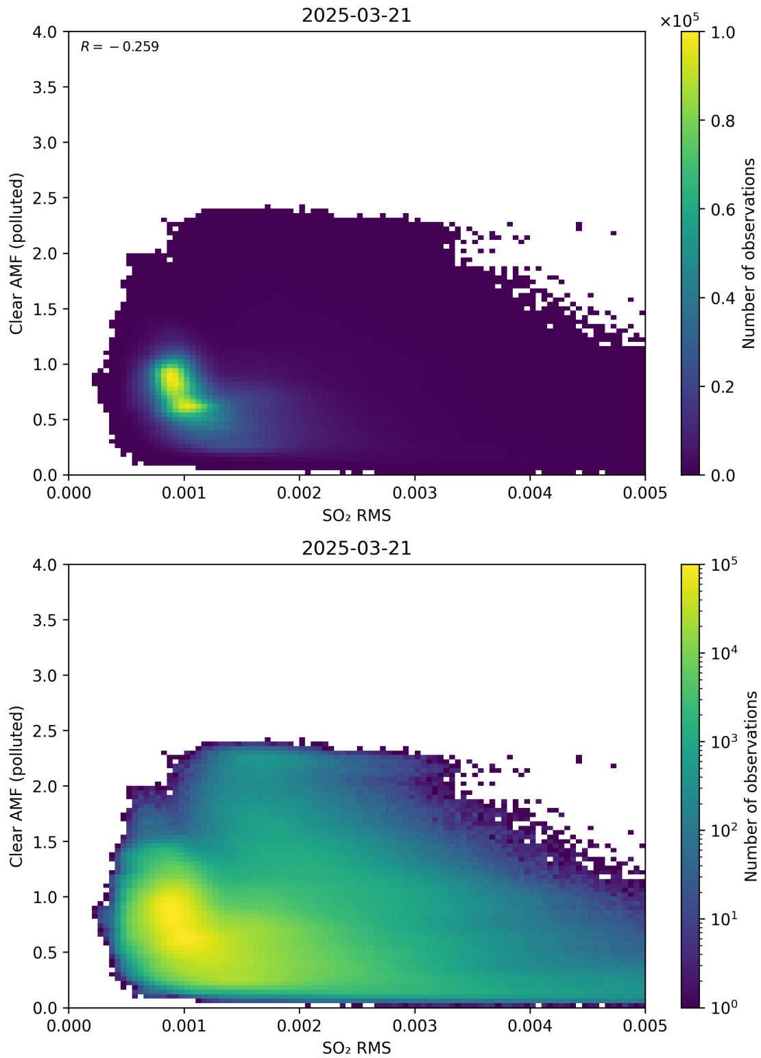
Figure 147: Scatter density plot of “SO 2 RMS” against “Clear AMF (polluted)” for 2025-03-20 to 2025-03-22.
