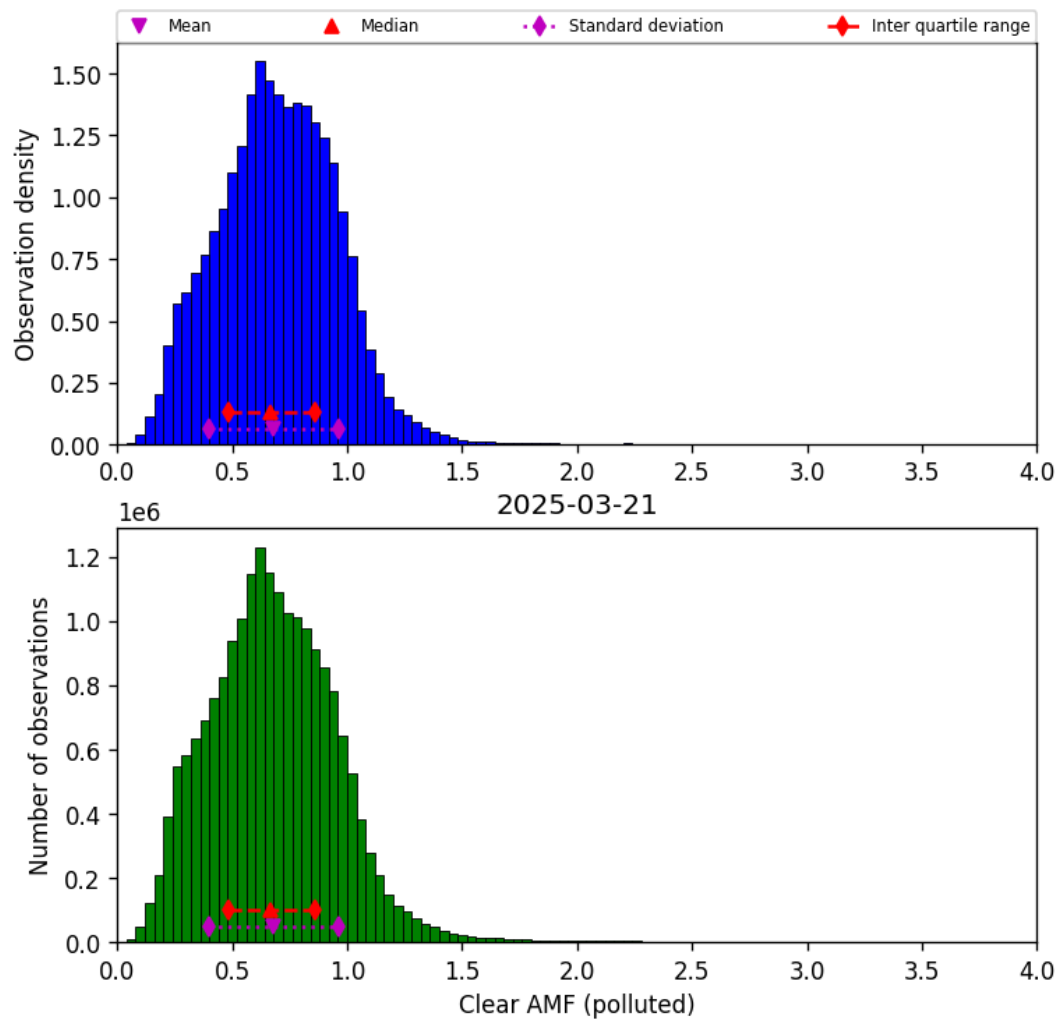
Figure 81: Histogram of “Clear AMF (polluted)” for 2025-03-20 to 2025-03-22
