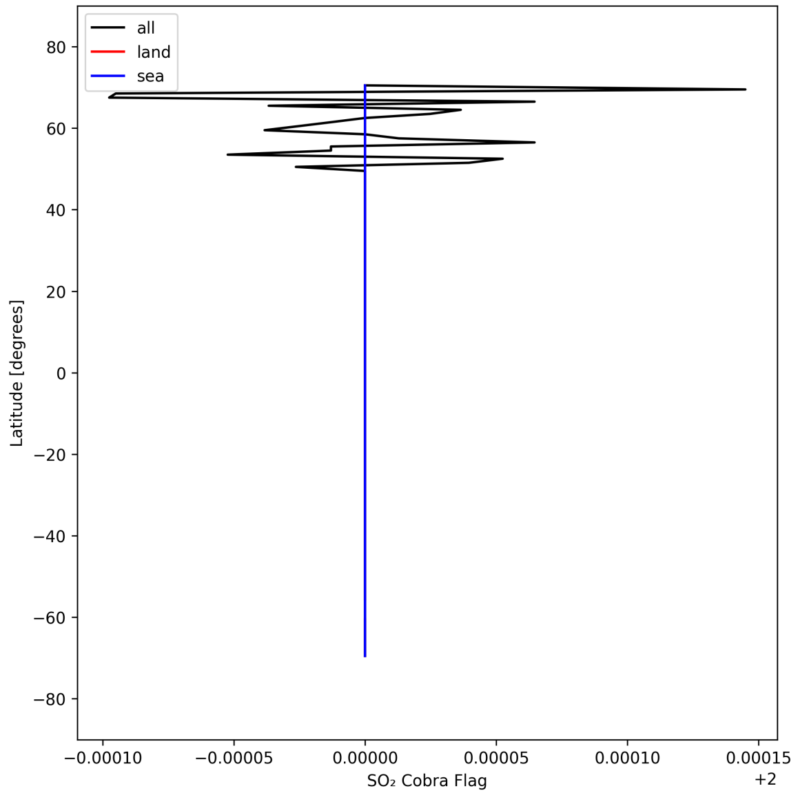
Figure 49: Zonal average of "SO 2 Cobra Flag" for 2025-03-20 to 2025-03-22.
