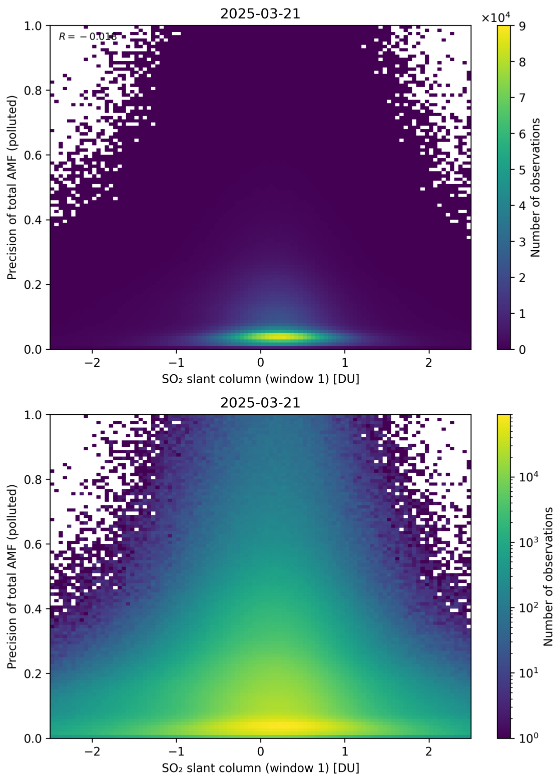
Figure 290: Scatter density plot of “SO 2 slant column (window 1)” against “Precision of total AMF (polluted)” for 2025-03-20 to 2025-03-22.
