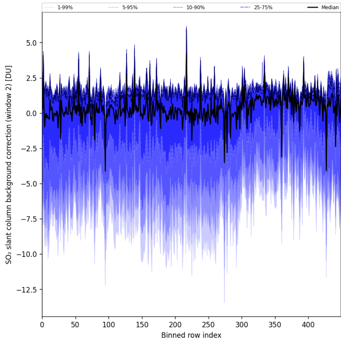
Figure 96: Along track statistics of “SO 2 slant column background correction (window 2)” for 2025-03-20 to 2025-03-22
