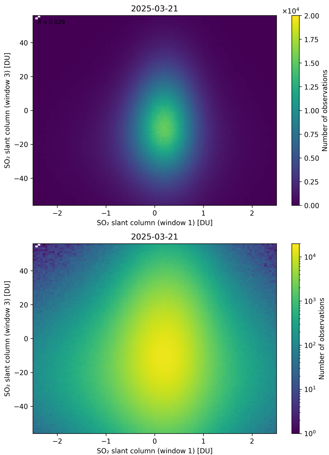
Figure 287: Scatter density plot of “SO 2 slant column (window 1)” against “SO 2 slant column (window 3)” for 2025-03-20 to 2025-03-22.
