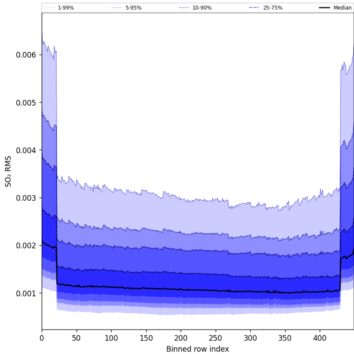
Figure 104: Along track statistics of “SO 2 RMS” for 2025-03-20 to 2025-03-22
