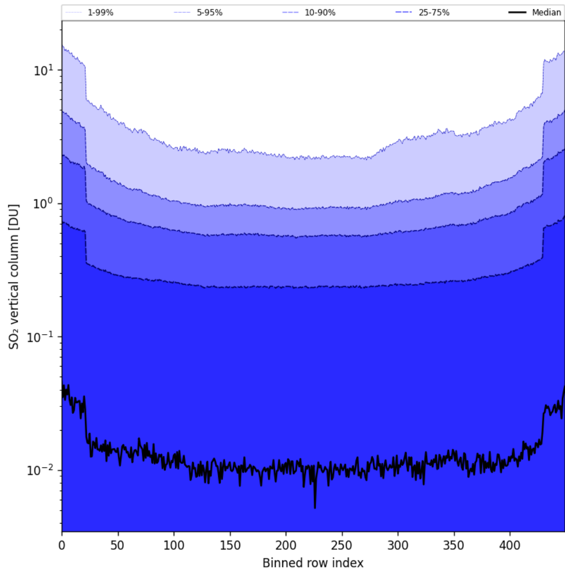
Figure 84: Along track statistics of “SO 2 vertical column” for 2025-03-20 to 2025-03-22
