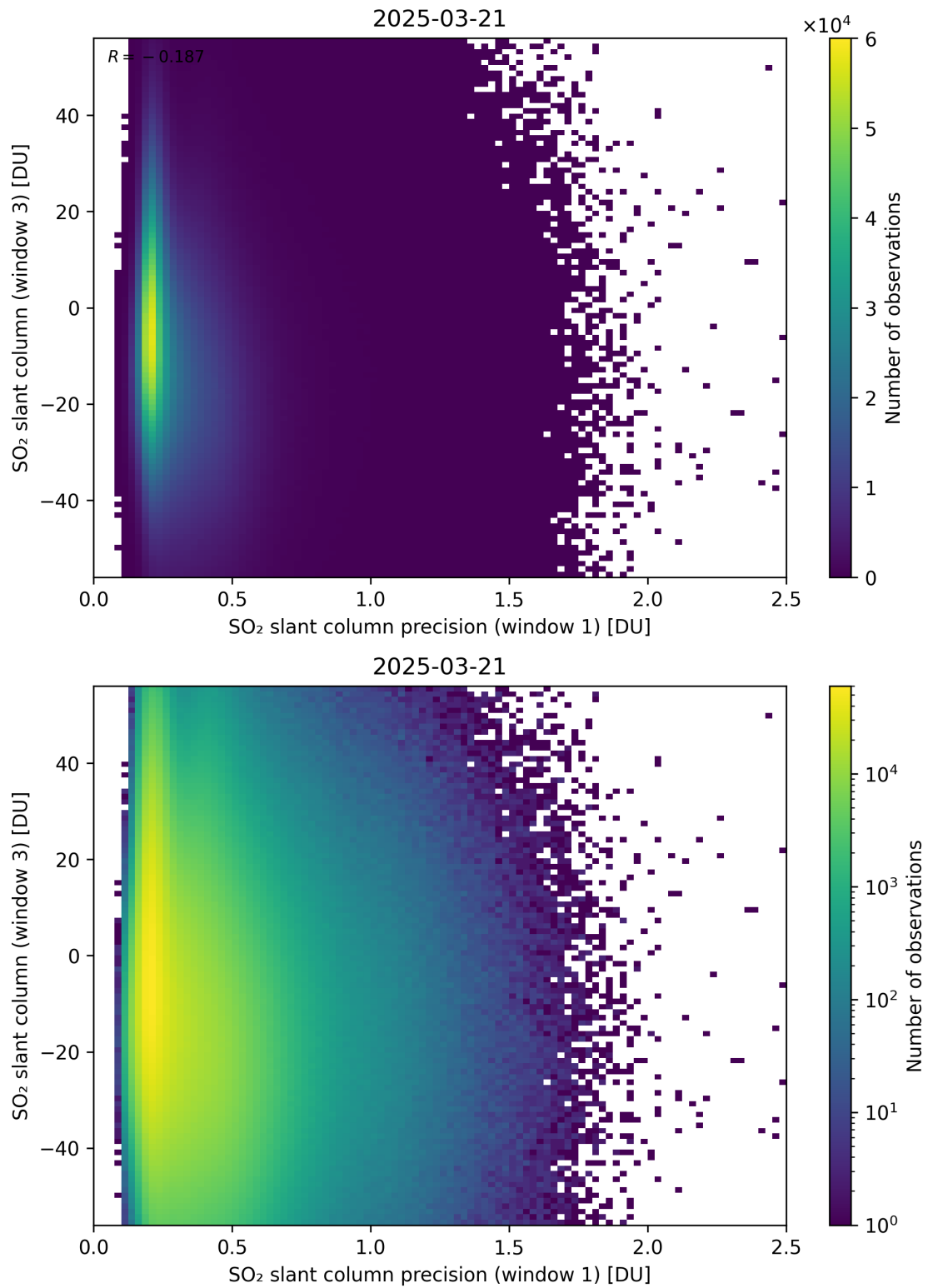
Figure 278: Scatter density plot of “SO 2 slant column precision (window 1)” against “SO 2 slant column (window 3)” for 2025-03-20 to 2025-03-22.
