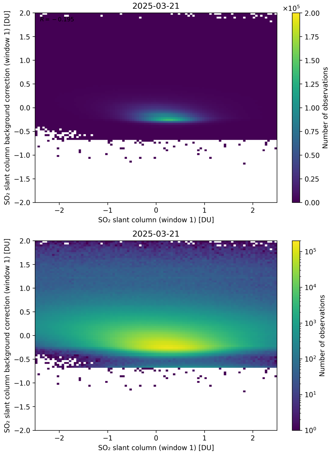
Figure 262: Scatter density plot of “SO 2 slant column (window 1)” against “SO 2 slant column background correction (window 1)” for 2025-03-20 to 2025-03-22.
