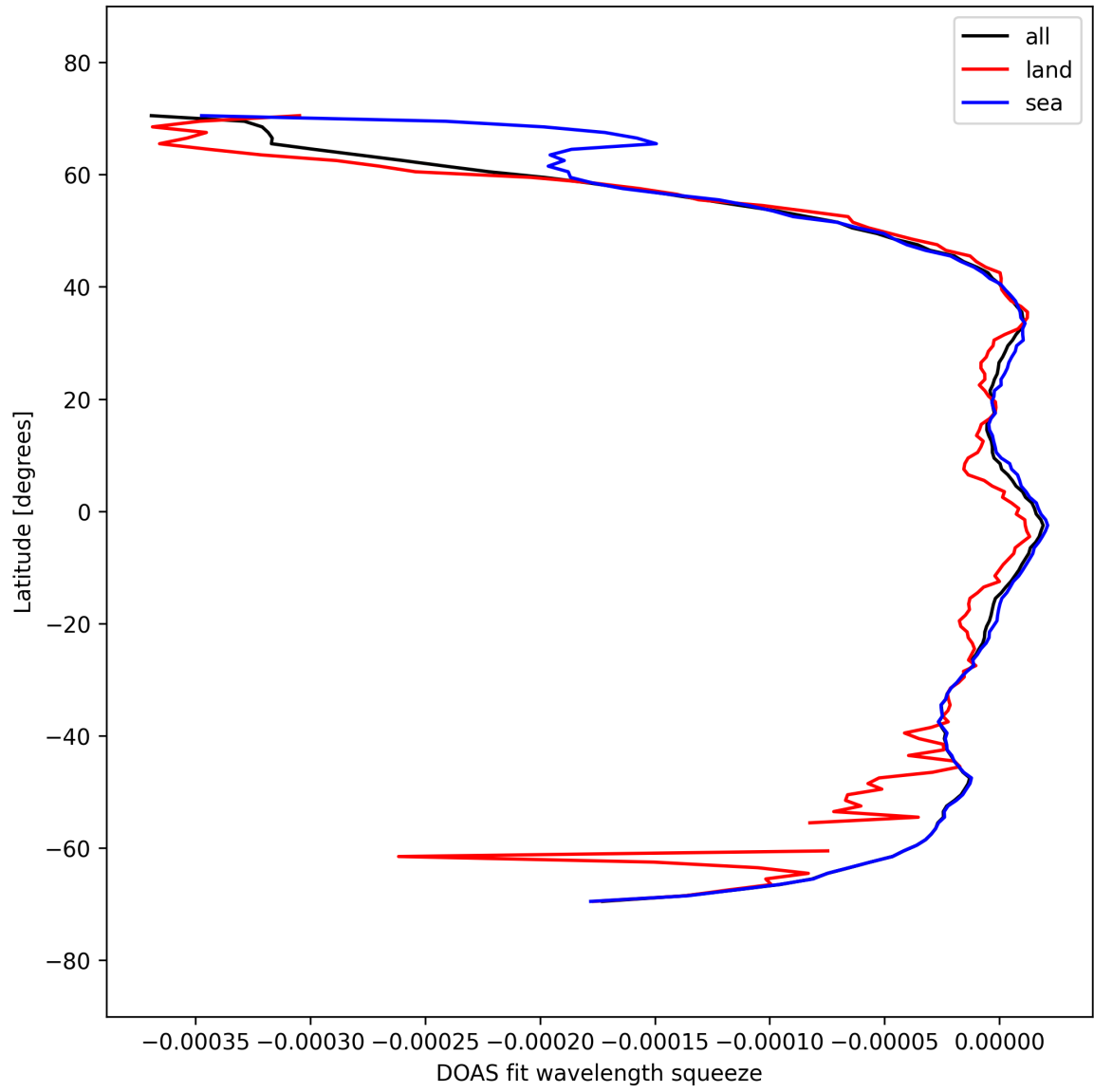
Figure 51: Zonal average of “DOAS fit wavelength squeeze” for 2025-03-20 to 2025-03-22.
