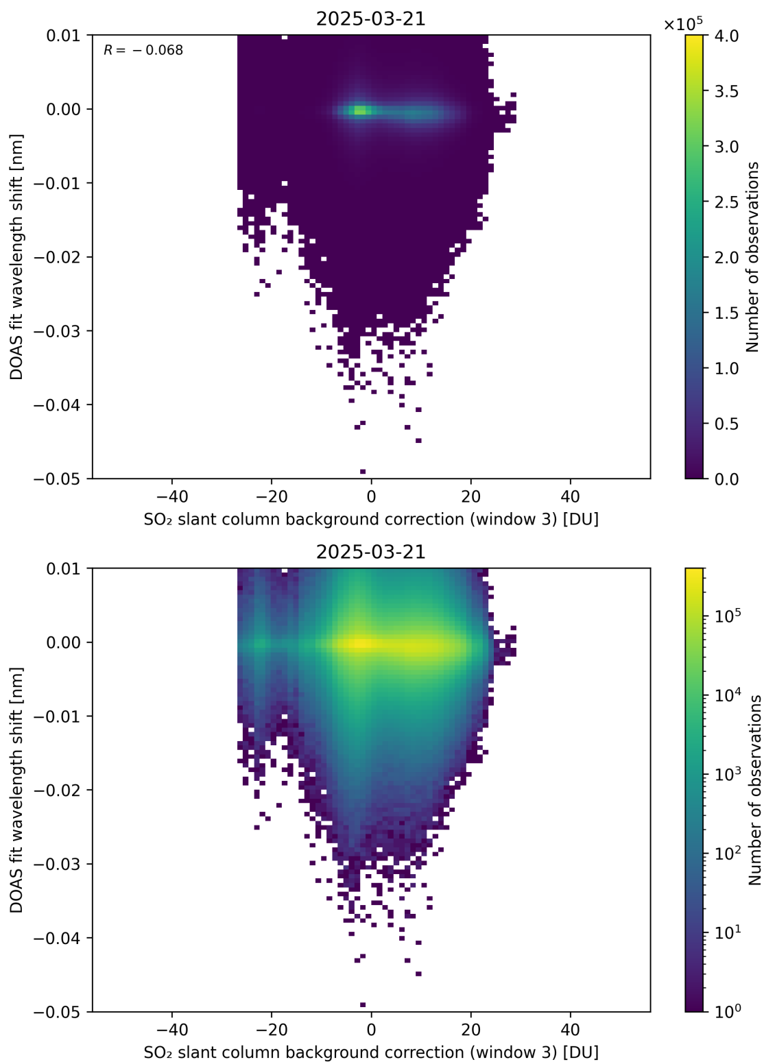
Figure 132: Scatter density plot of “SO 2 slant column background correction (window 3)” against “DOAS fit wavelength shift” for 2025-03-20 to 2025-03-22.
