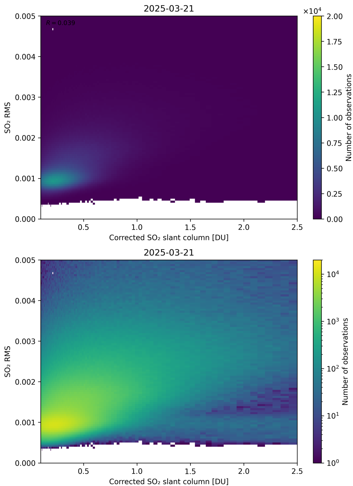
Figure 231: Scatter density plot of “Corrected SO 2 slant column” against “SO 2 RMS” for 2025-03-20 to 2025-03-22.
