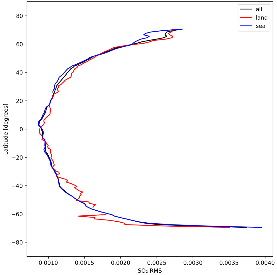
Figure 52: Zonal average of “SO 2 RMS” for 2025-03-20 to 2025-03-22.
