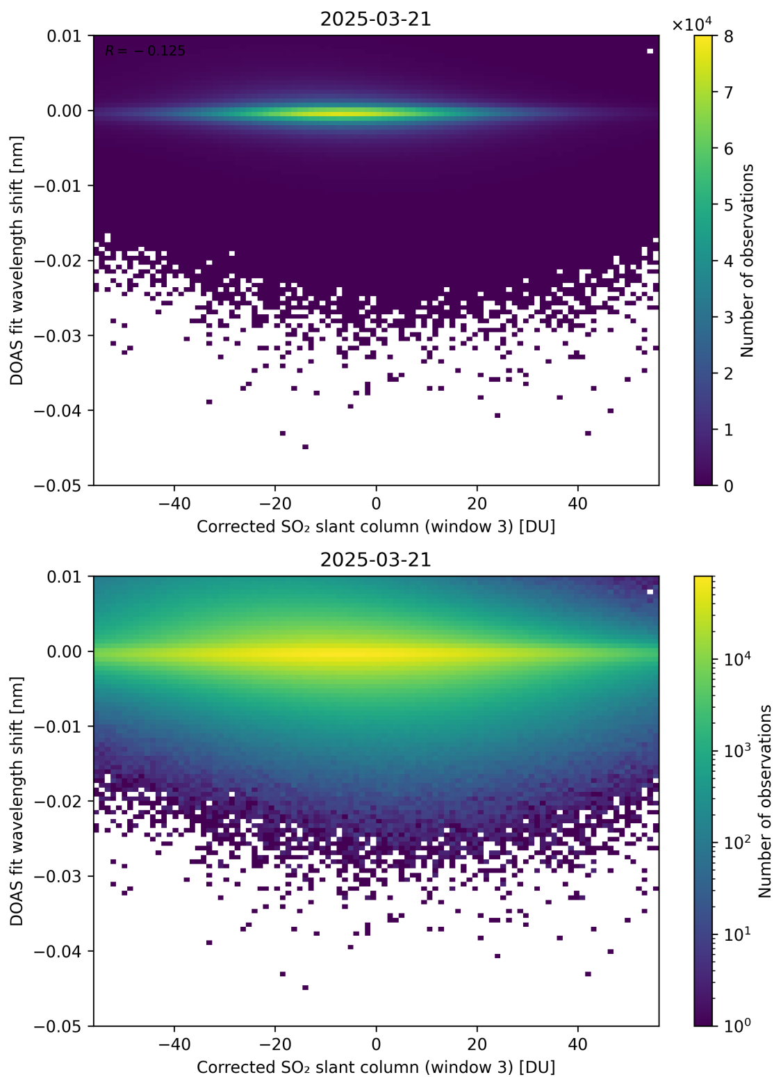
Figure 256: Scatter density plot of “Corrected SO 2 slant column (window 3)” against “DOAS fit wavelength shift” for 2025-03-20 to 2025-03-22.
