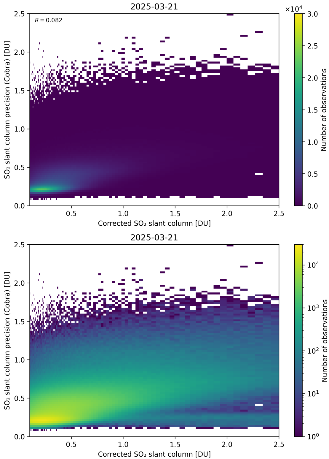
Figure 234: Scatter density plot of “Corrected SO 2 slant column” against “SO 2 slant column precision (Cobra)” for 2025-03-20 to 2025-03-22.
