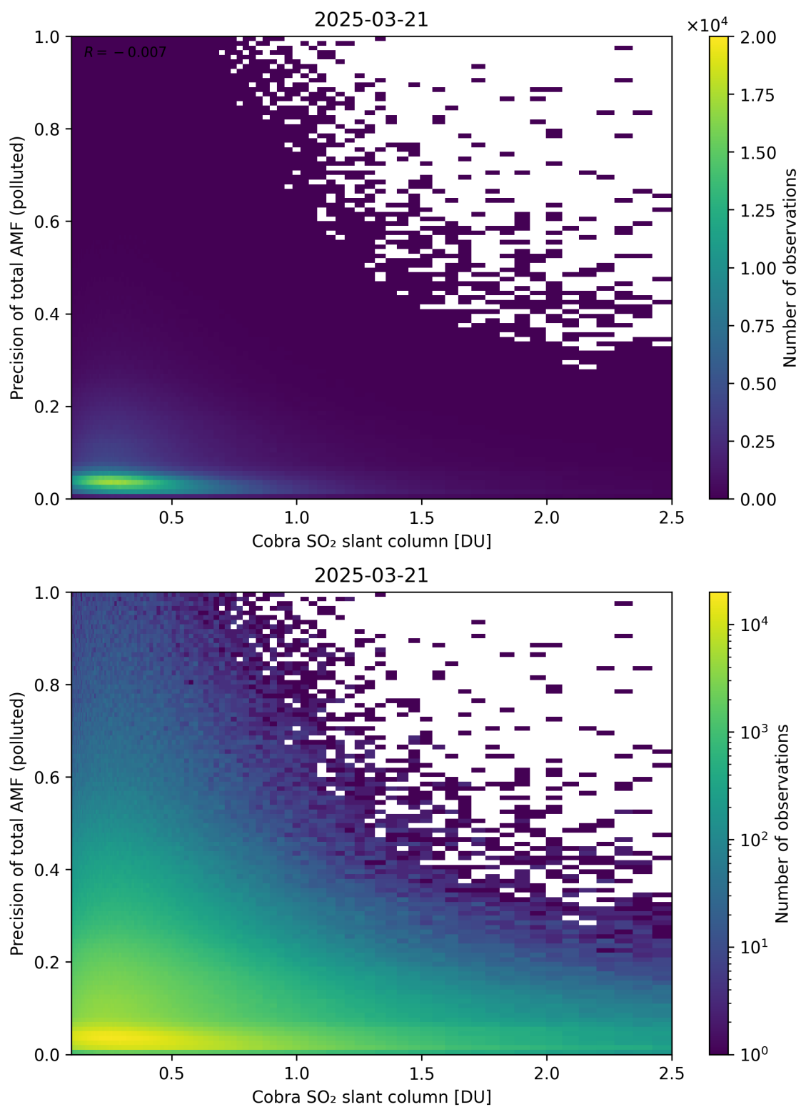
Figure 225: Scatter density plot of “Cobra SO 2 slant column” against “Precision of total AMF (polluted)” for 2025-03-20 to 2025-03-22.
