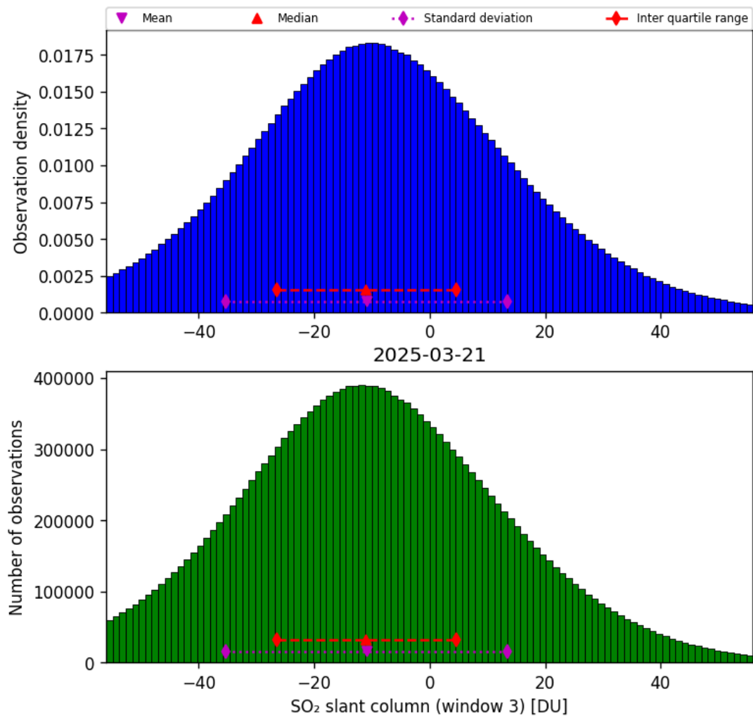
Figure 71: Histogram of “SO 2 slant column (window 3)” for 2025-03-20 to 2025-03-22
