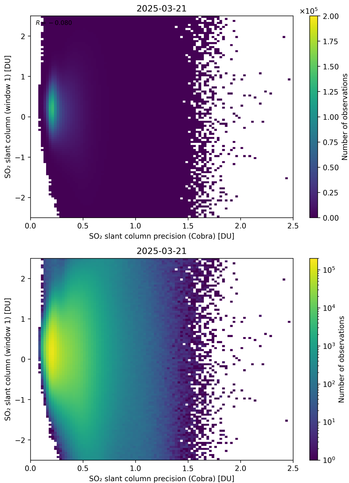
Figure 208: Scatter density plot of “SO 2 slant column precision (Cobra)” against “SO 2 slant column (window 1)” for 2025-03-20 to 2025-03-22.
