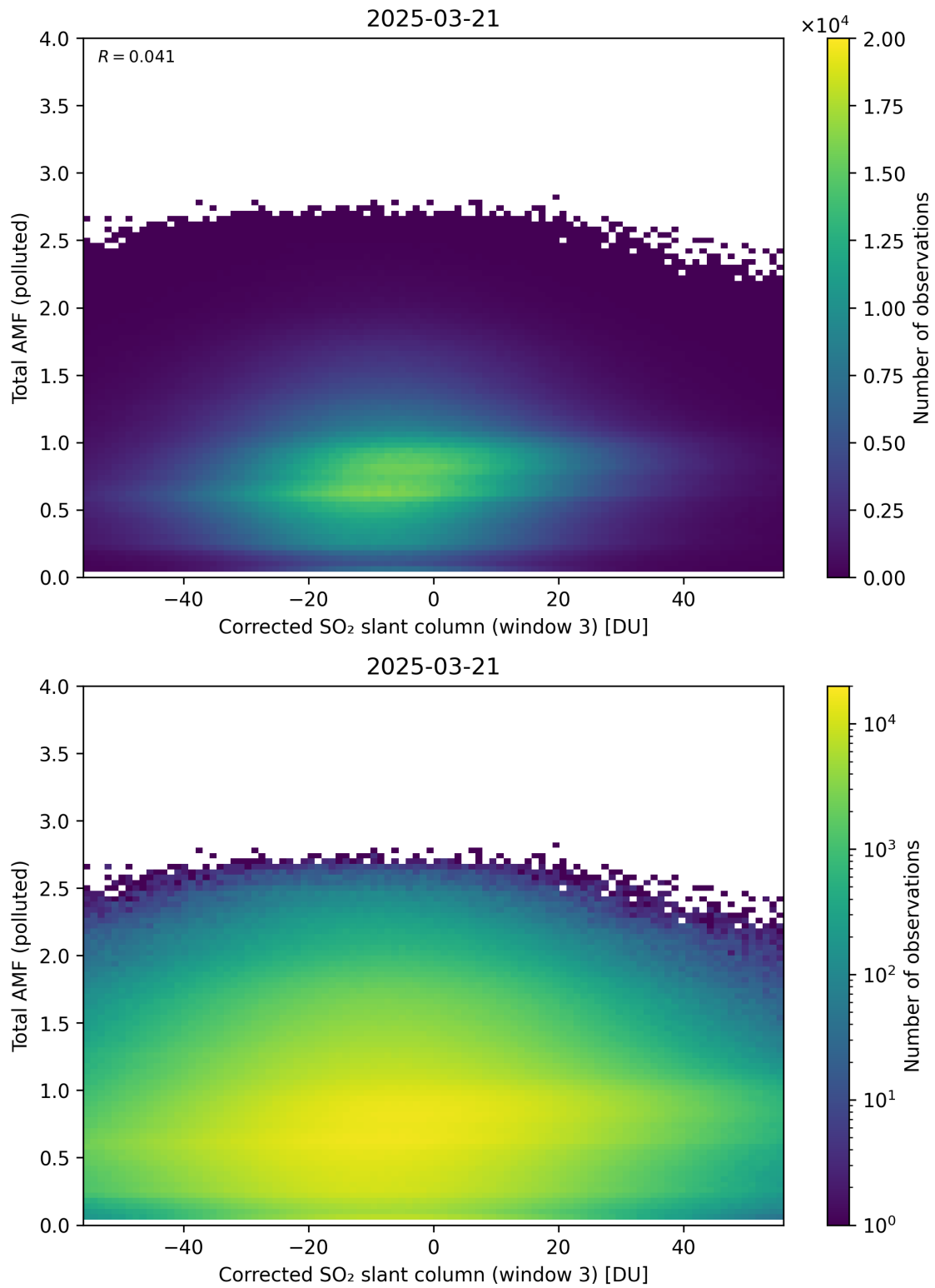
Figure 260: Scatter density plot of “Corrected SO 2 slant column (window 3)” against “Total AMF (polluted)” for 2025-03-20 to 2025-03-22.
