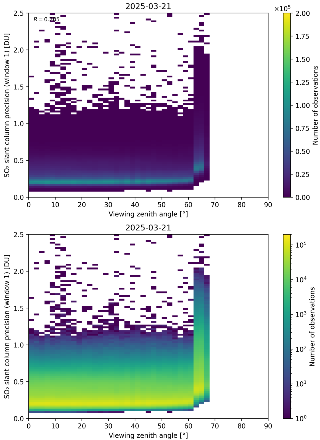
Figure 377: Scatter density plot of “Viewing zenith angle” against “SO 2 slant column precision (window 1)” for 2025-03-20 to 2025-03-22.
