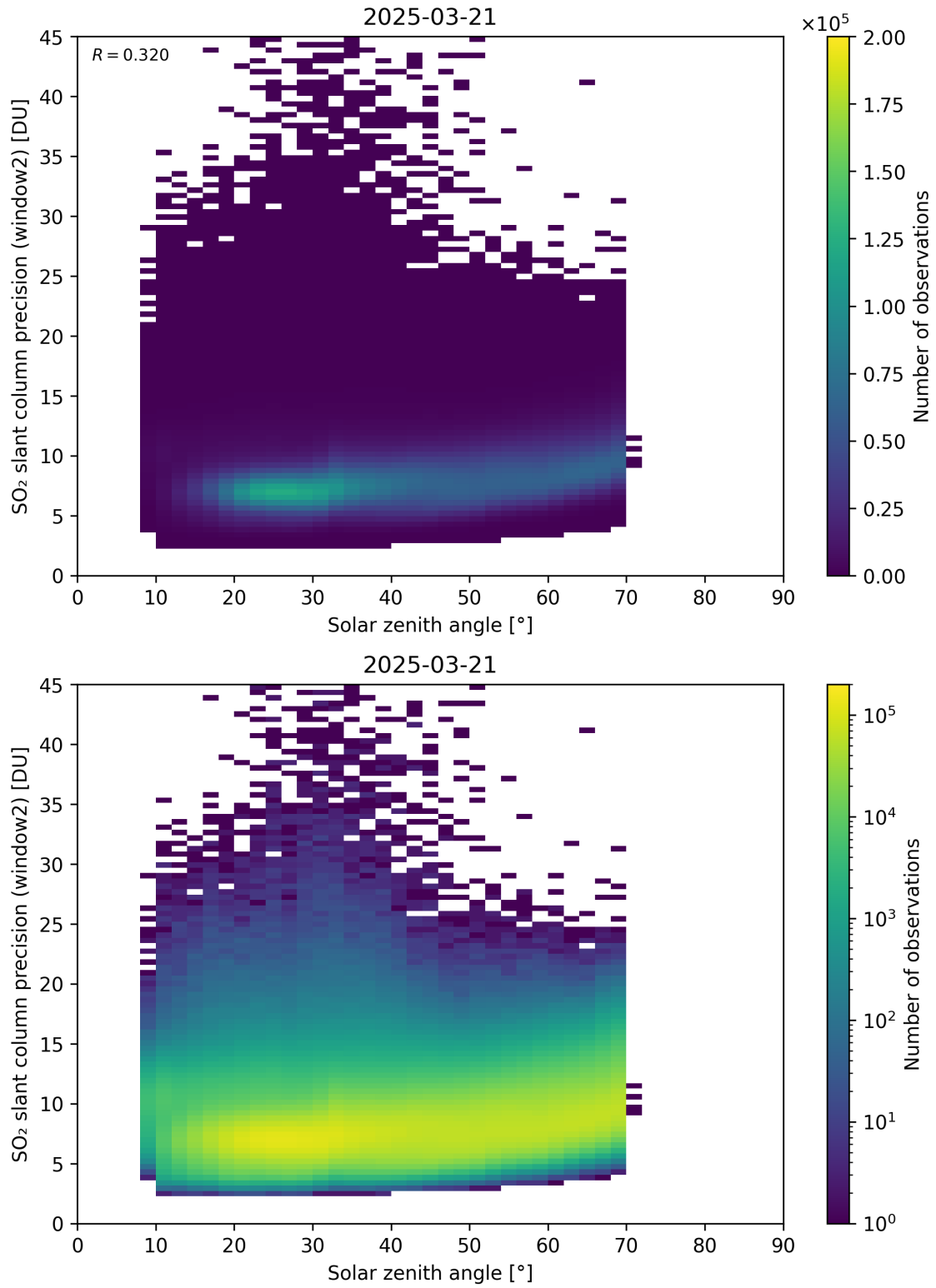
Figure 186: Scatter density plot of “Solar zenith angle” against “SO 2 slant column precision (window2)” for 2025-03-20 to 2025-03-22.
