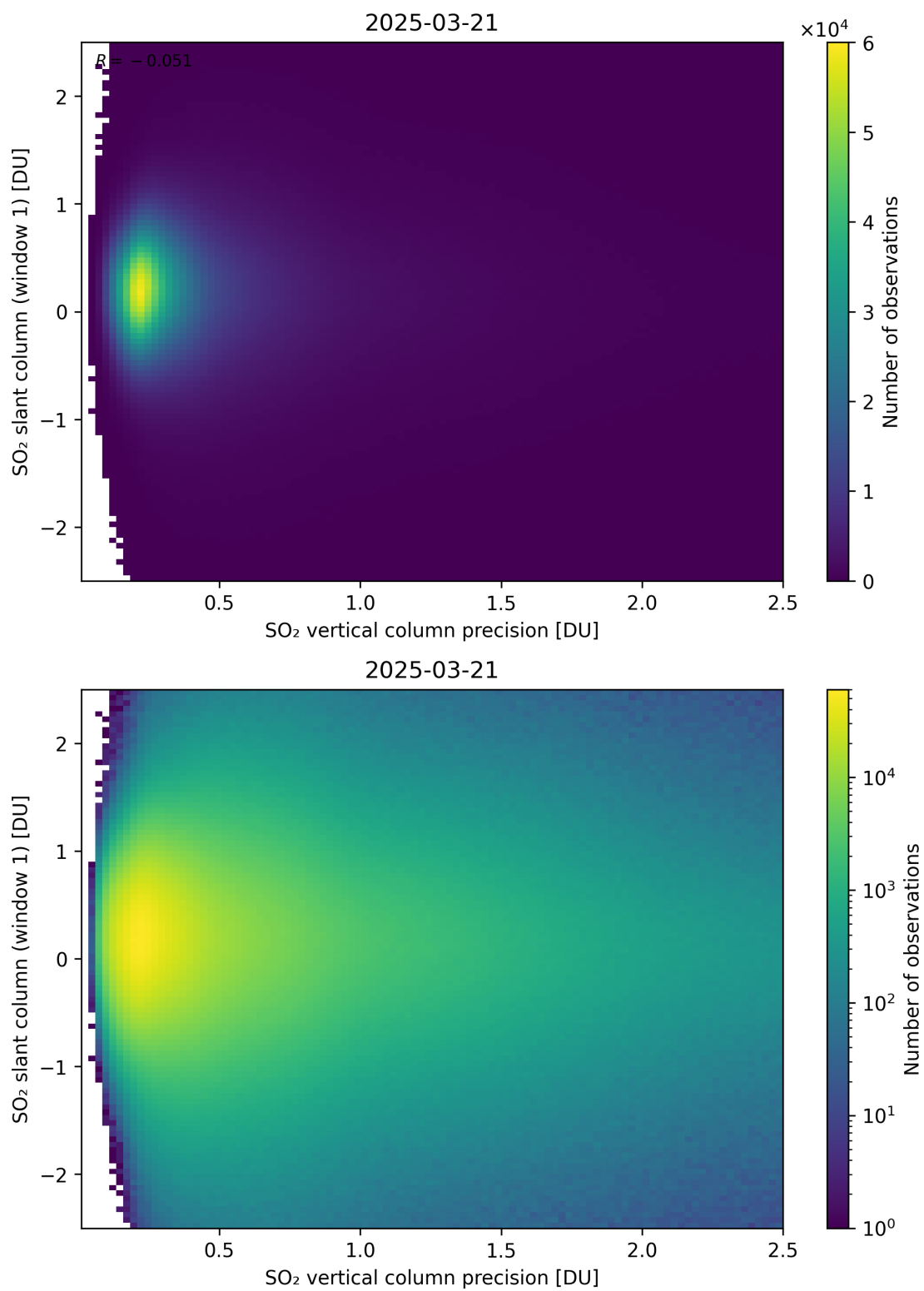
Figure 341: Scatter density plot of “SO 2 vertical column precision” against “SO 2 slant column (window 1)” for 2025-03-20 to 2025-03-22.
