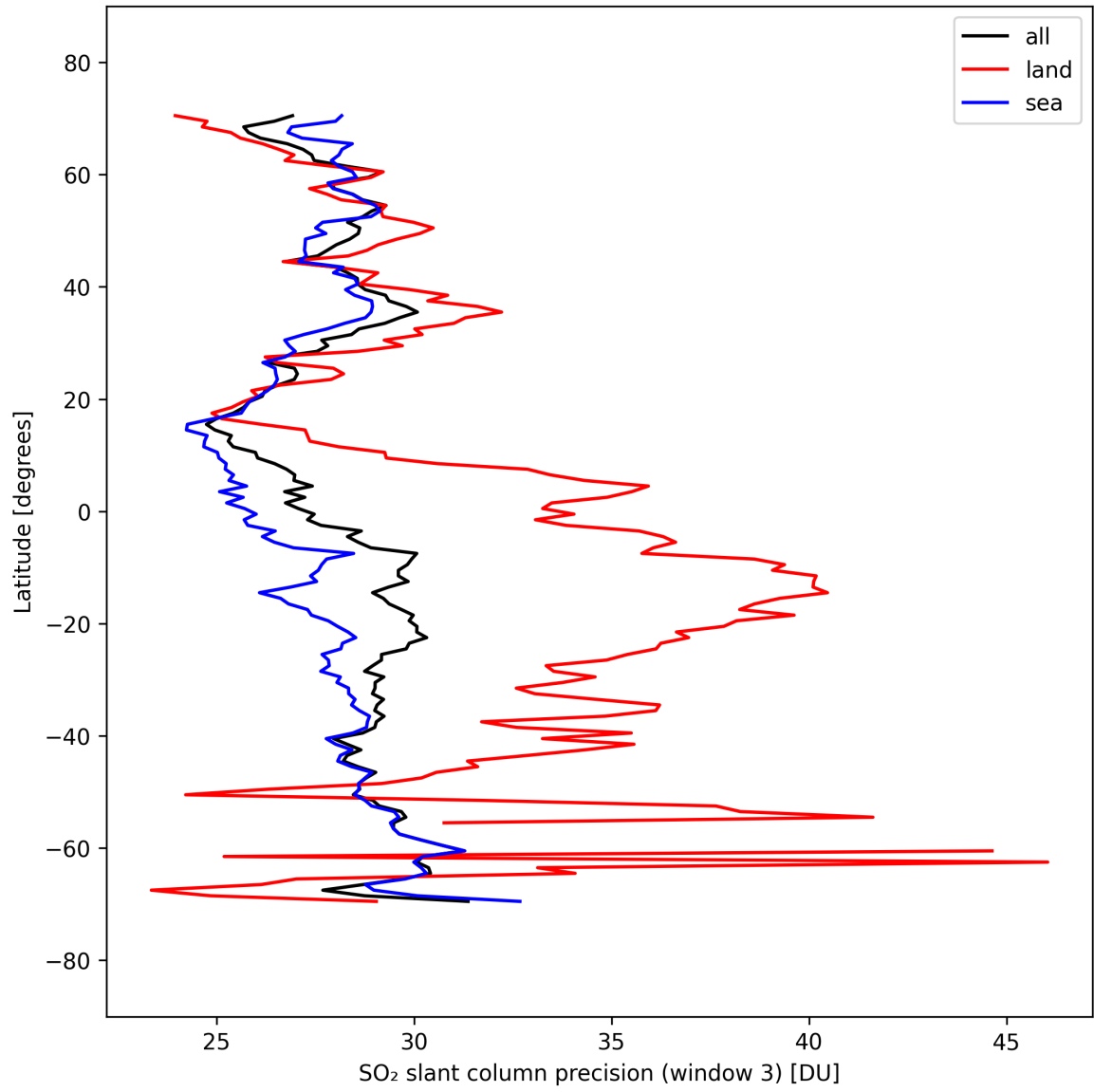
Figure 46: Zonal average of “SO 2 slant column precision (window 3)” for 2025-03-20 to 2025-03-22.
