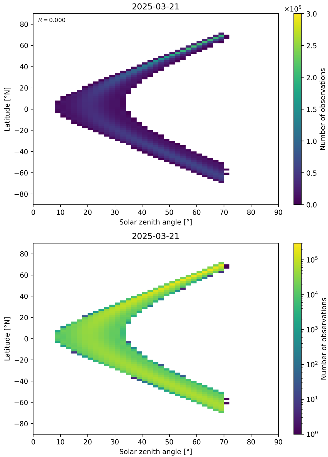
Figure 177: Scatter density plot of “Solar zenith angle” against “Latitude” for 2025-03-20 to 2025-03-22.
