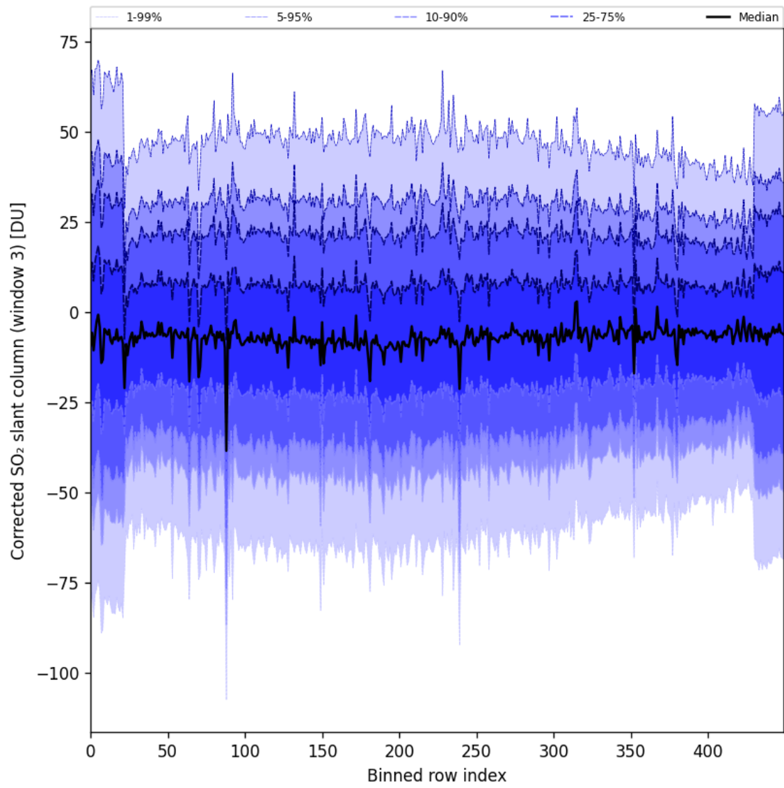
Figure 99: Along track statistics of “Corrected SO 2 slant column (window 3)” for 2025-03-20 to 2025-03-22
