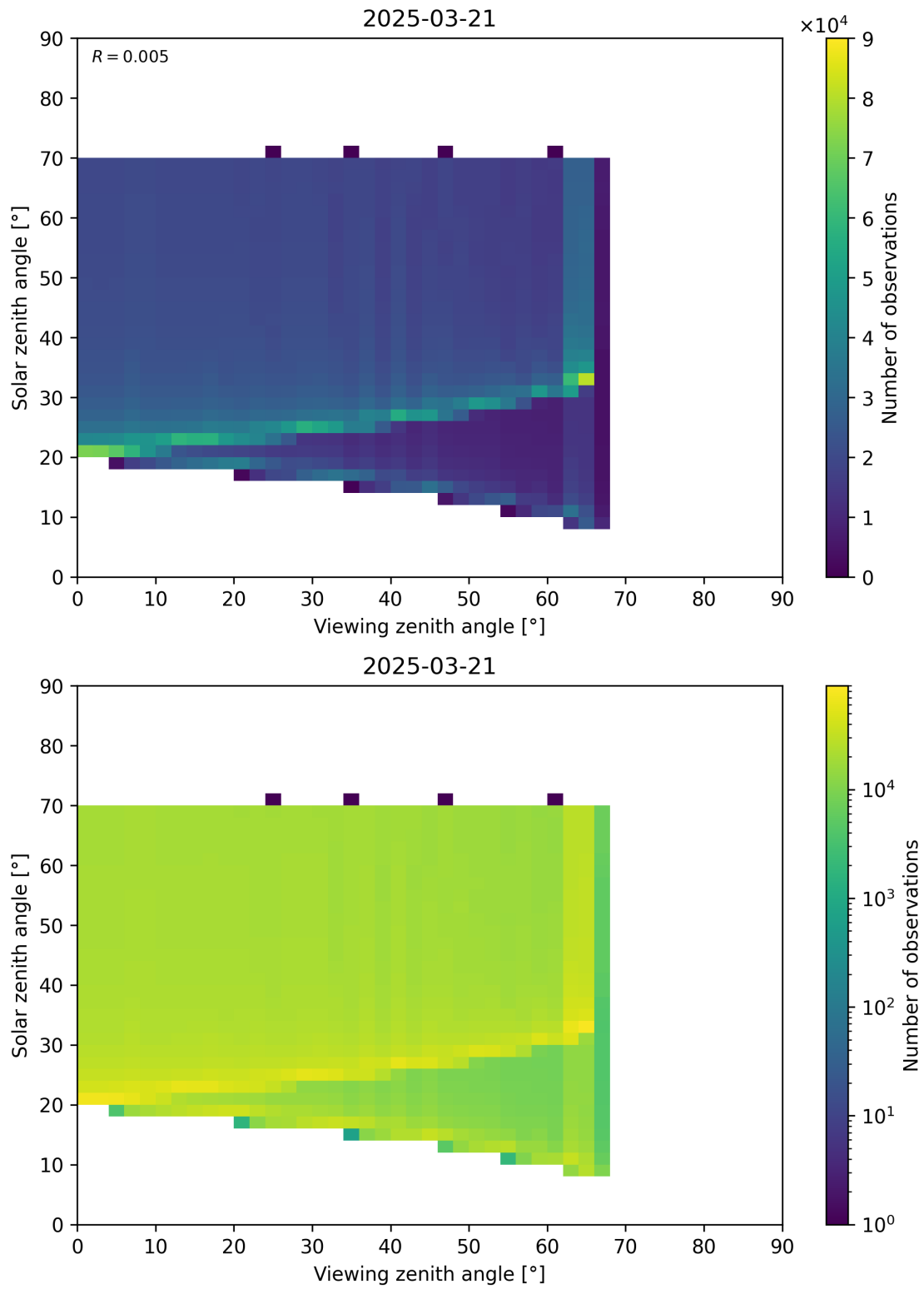
Figure 369: Scatter density plot of “Viewing zenith angle” against “Solar zenith angle” for 2025-03-20 to 2025-03-22.
