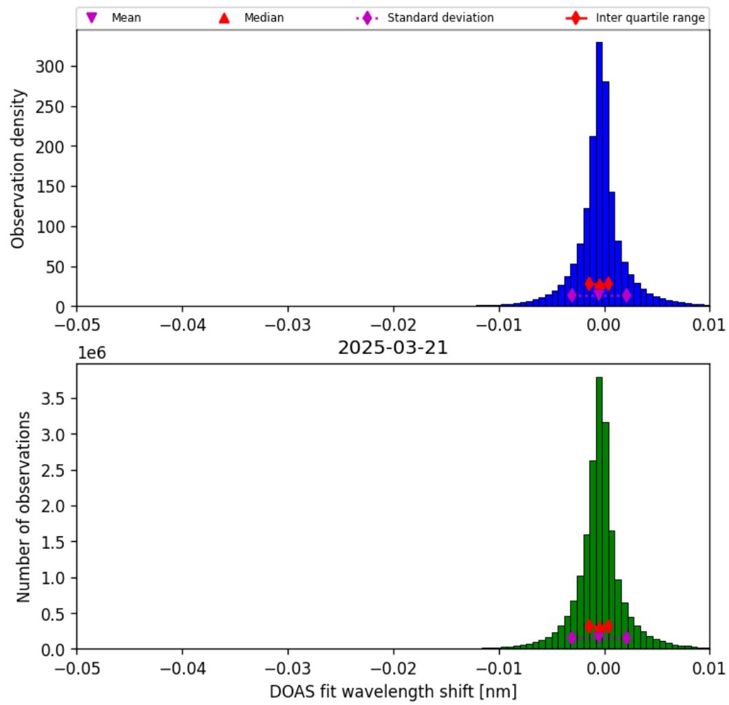
Figure 76: Histogram of “DOAS fit wavelength shift” for 2025-03-20 to 2025-03-22
