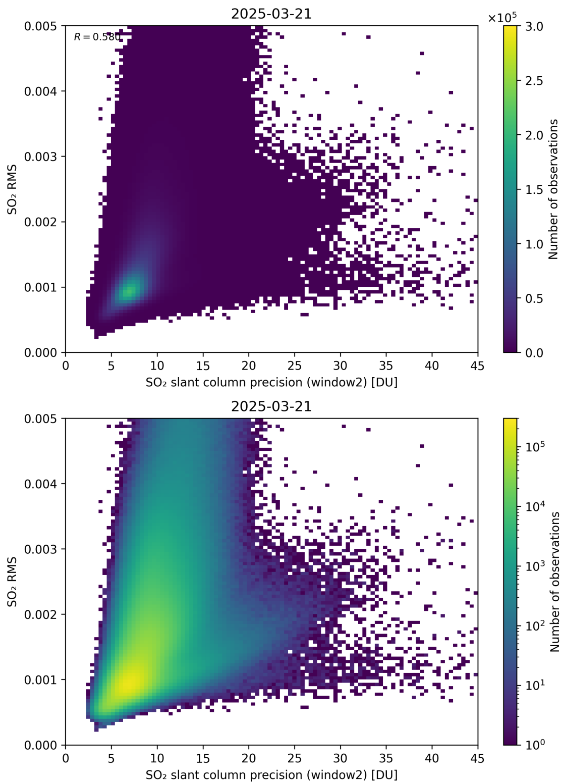
Figure 295: Scatter density plot of “SO 2 slant column precision (window2)” against “SO 2 RMS” for 2025-03-20 to 2025-03-22.
