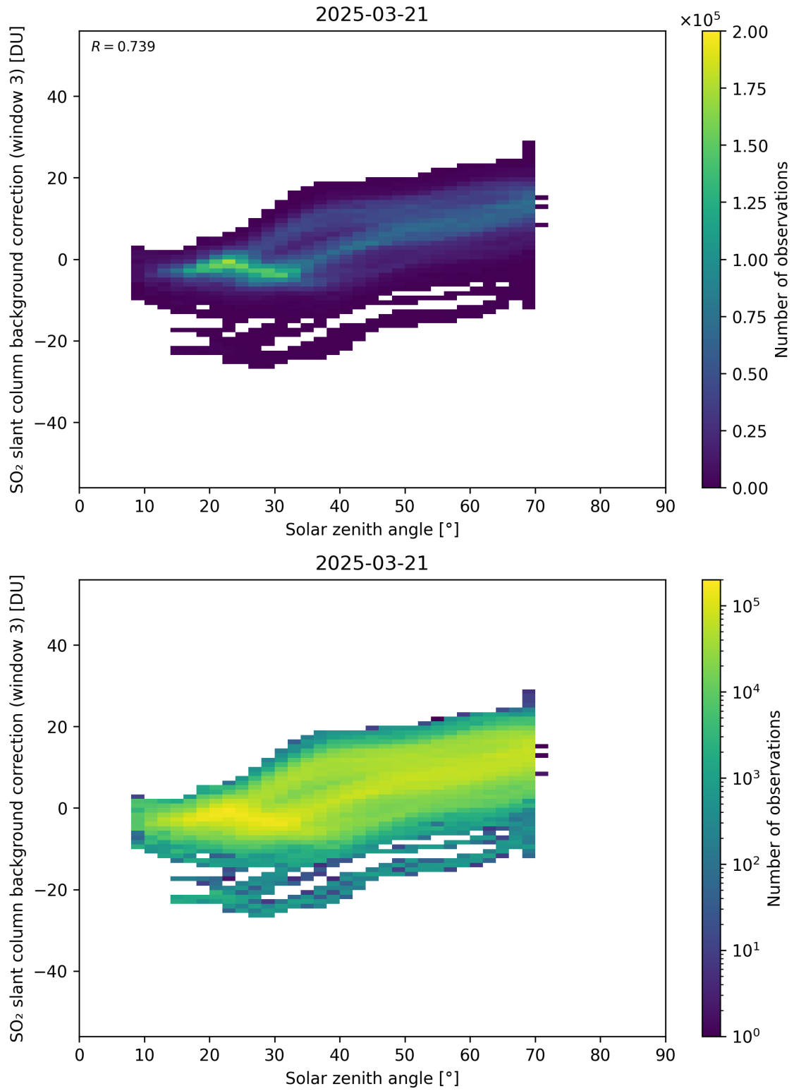
Figure 173: Scatter density plot of “Solar zenith angle” against “SO 2 slant column background correction (window 3)” for 2025-03-20 to 2025-03-22.
