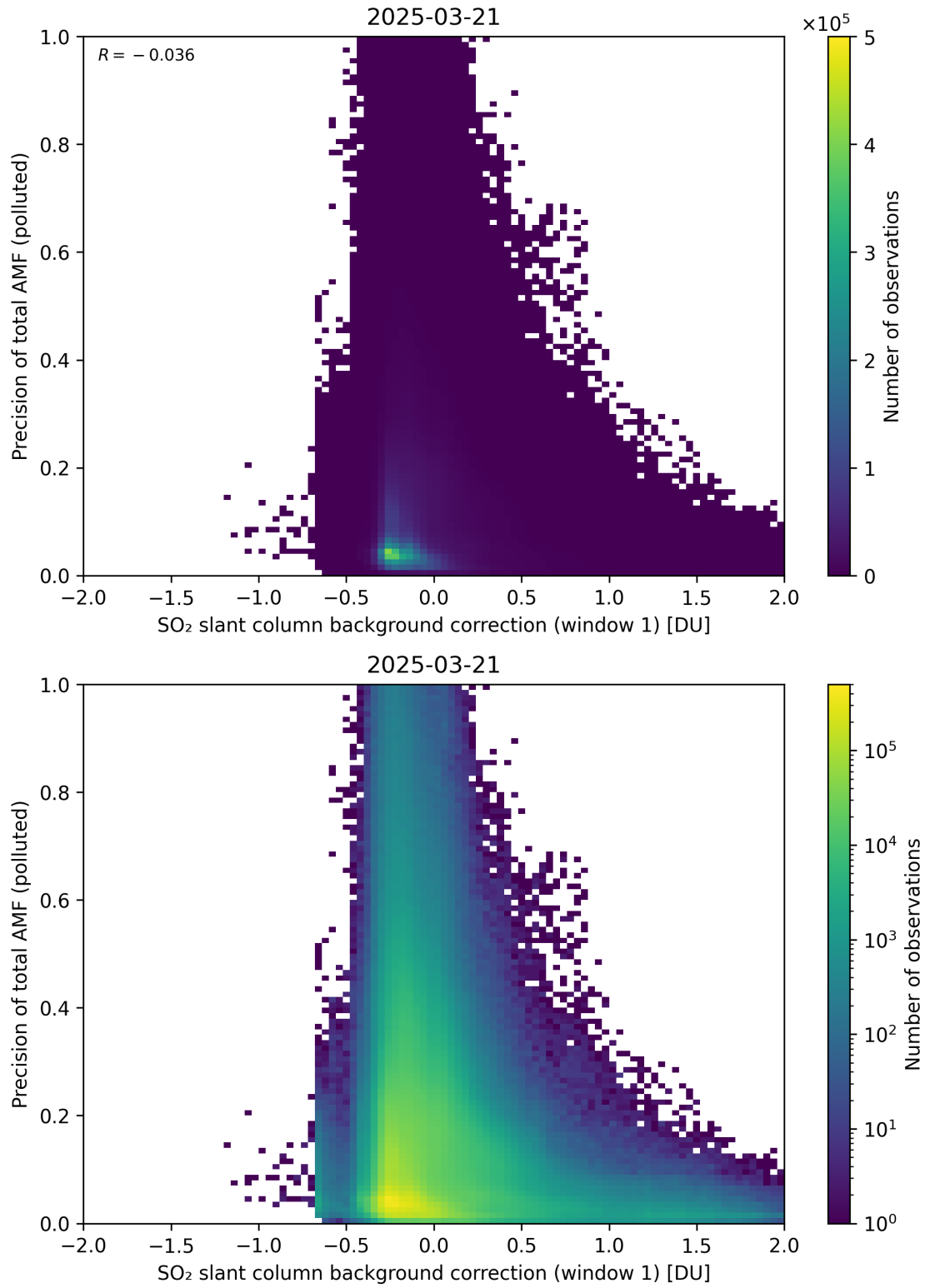
Figure 121: Scatter density plot of “SO 2 slant column background correction (window 1)” against “Precision of total AMF (polluted)” for 2025-03-20 to 2025-03-22.
