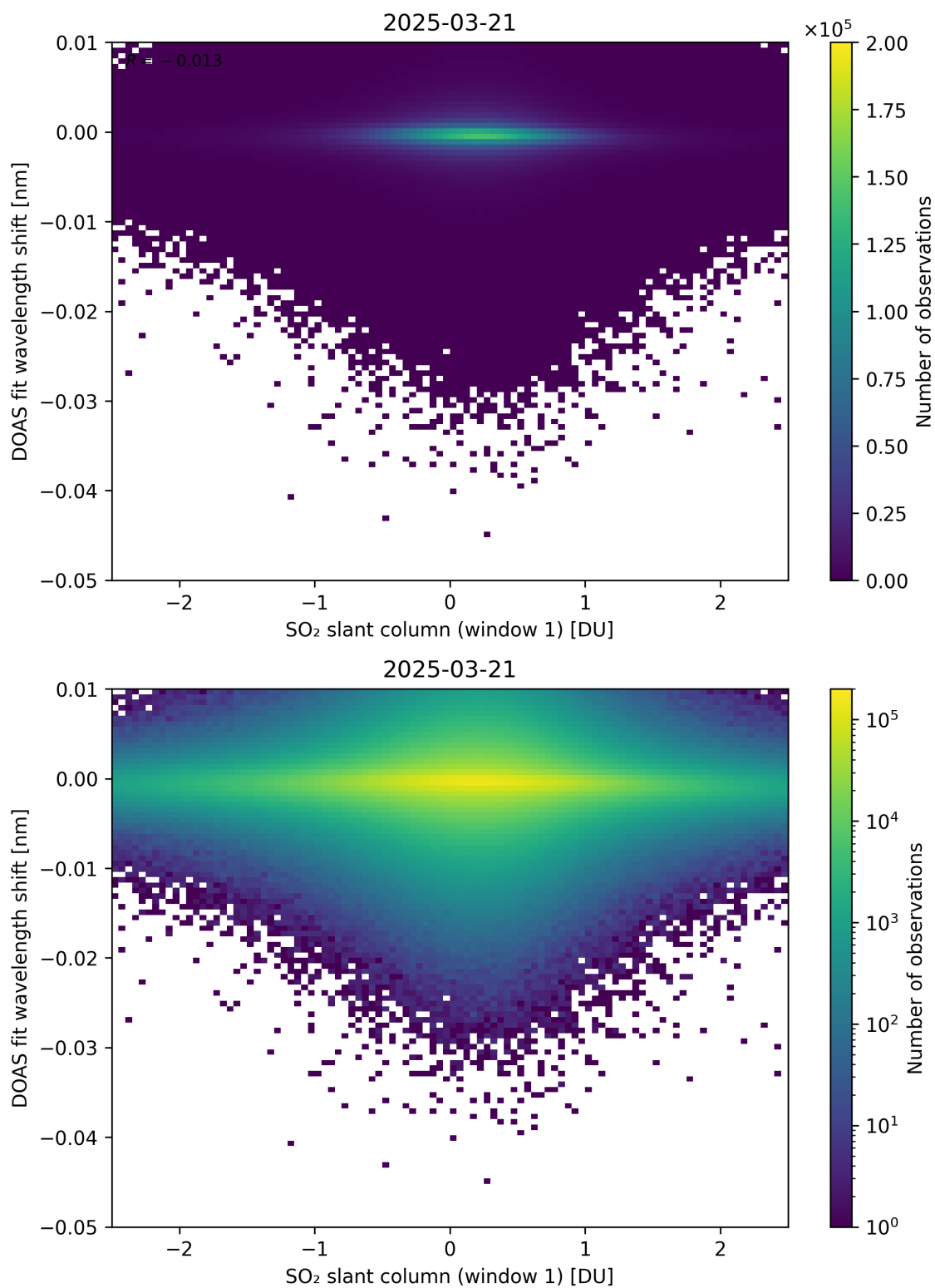
Figure 265: Scatter density plot of “SO 2 slant column (window 1)” against “DOAS fit wavelength shift” for 2025-03-20 to 2025-03-22.
