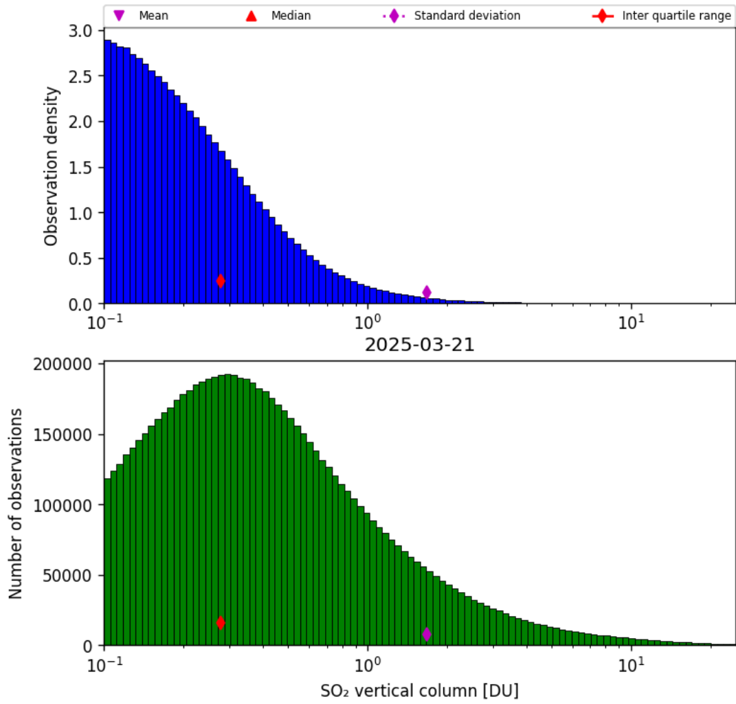
Figure 58: Histogram of “SO 2 vertical column” for 2025-03-20 to 2025-03-22
