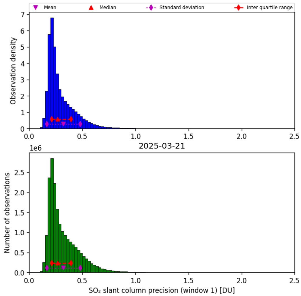
Figure 64: Histogram of “SO 2 slant column precision (window 1)” for 2025-03-20 to 2025-03-22
