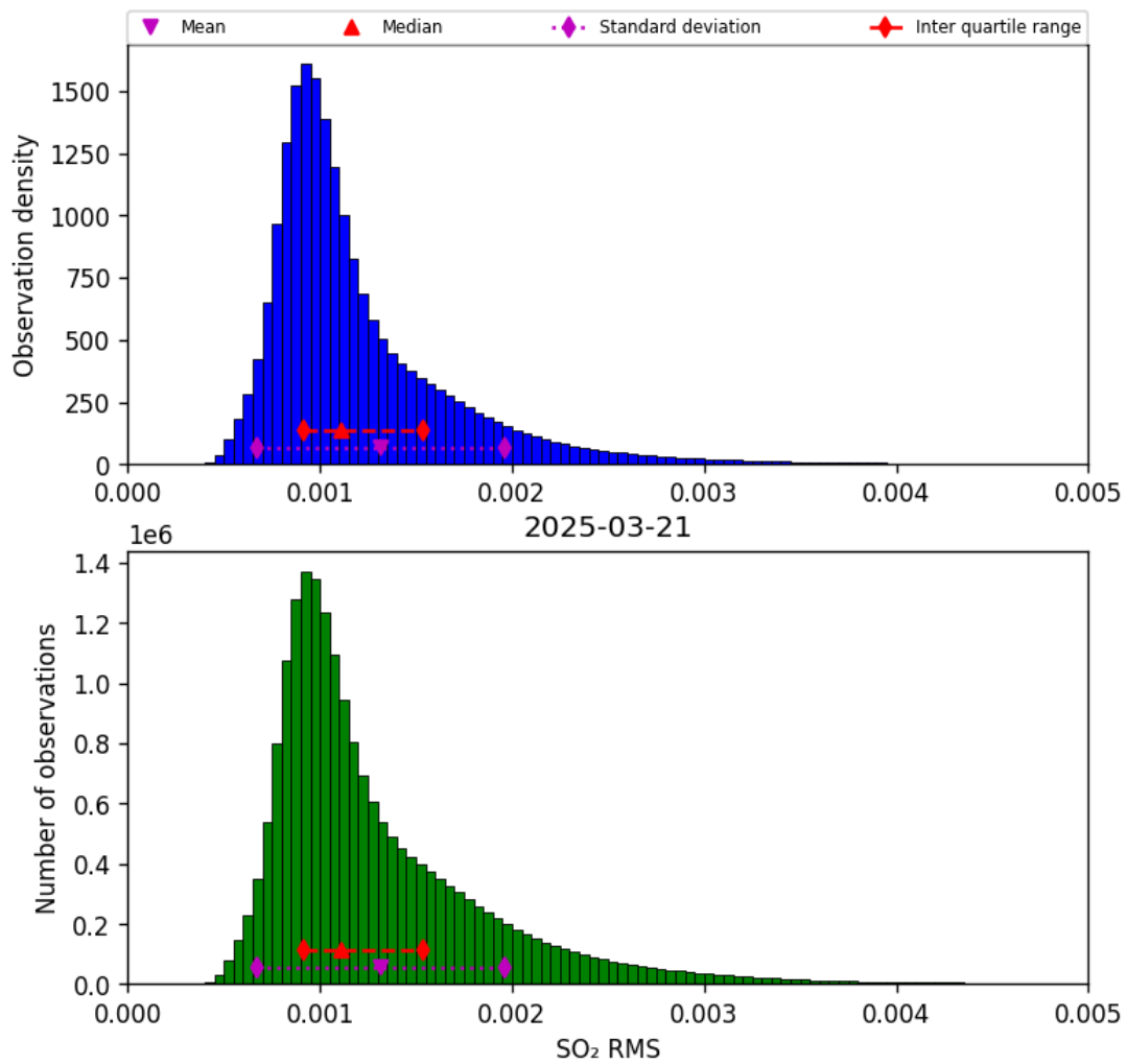
Figure 78: Histogram of “SO 2 RMS” for 2025-03-20 to 2025-03-22
