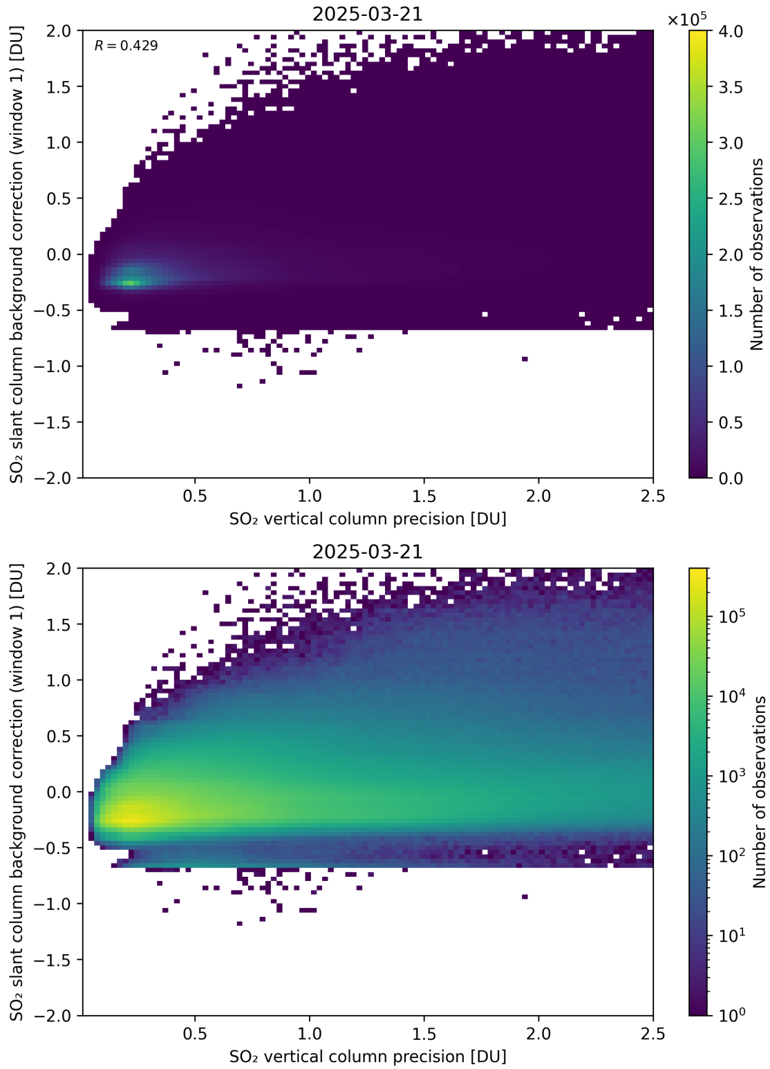
Figure 329: Scatter density plot of “SO 2 vertical column precision” against “SO 2 slant column background correction (window 1)” for 2025-03-20 to 2025-03-22.
