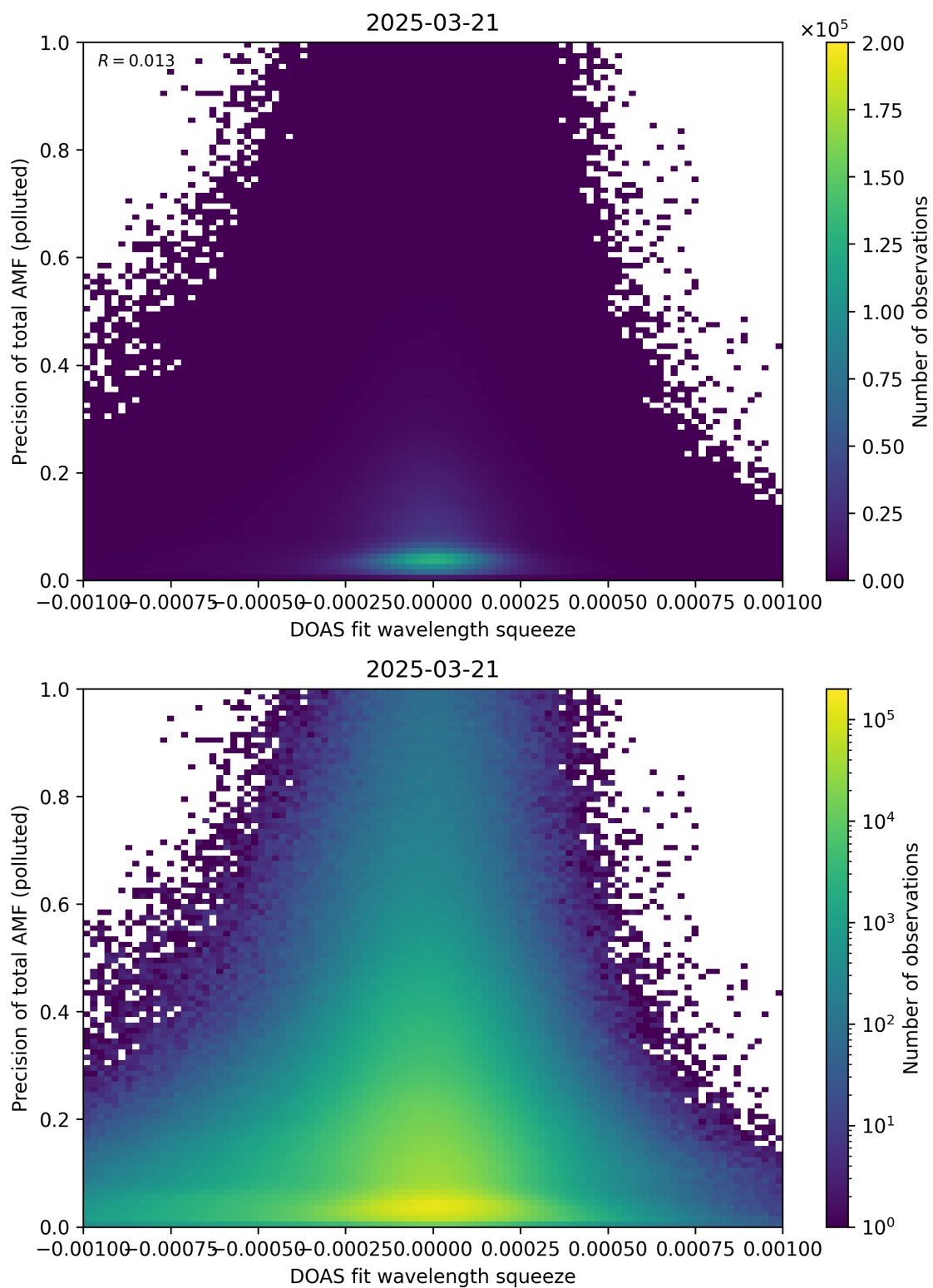
Figure 146: Scatter density plot of “DOAS fit wavelength squeeze” against “Precision of total AMF (polluted)” for 2025-03-20 to 2025-03-22.
