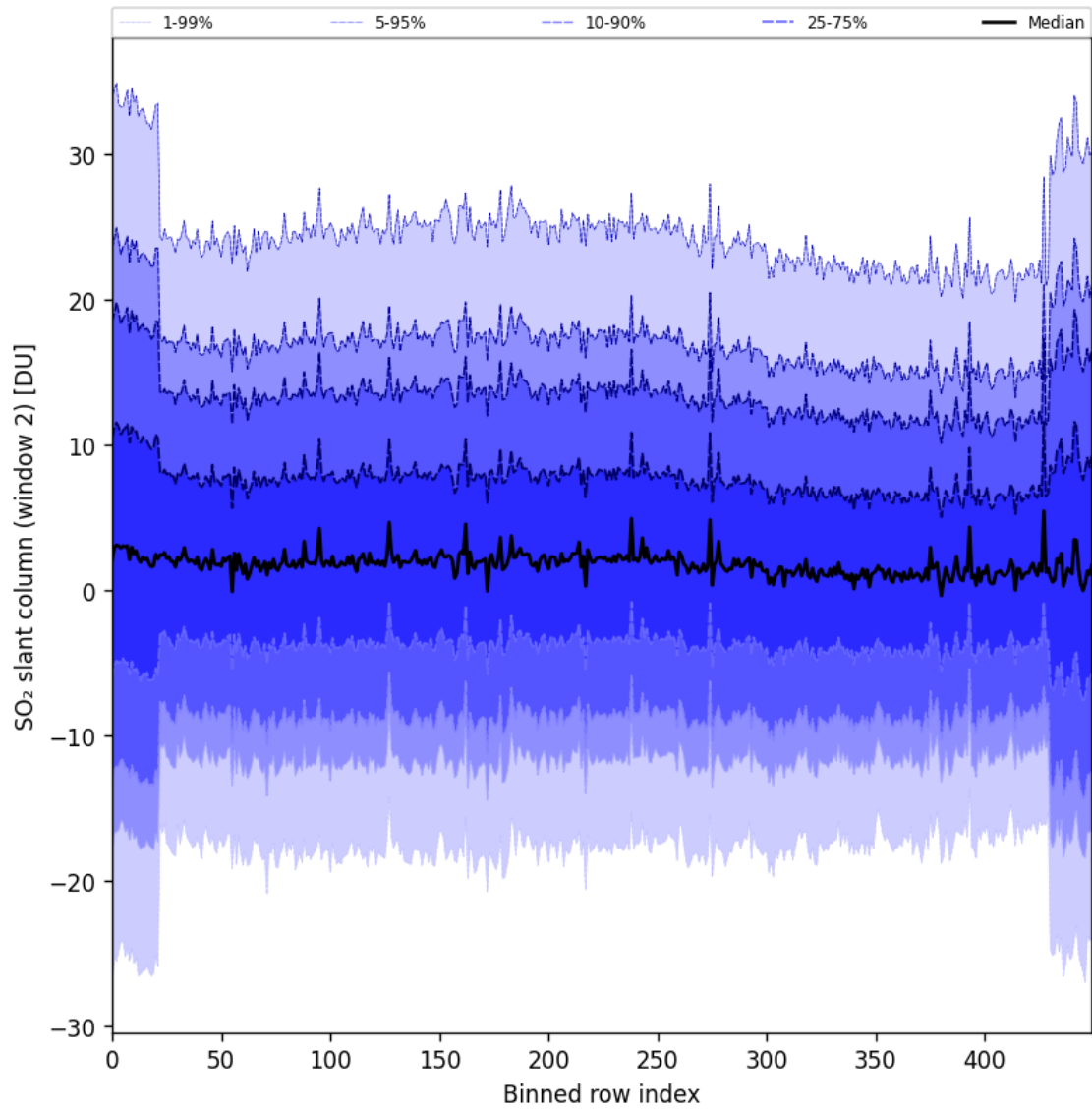
Figure 93: Along track statistics of “SO 2 slant column (window 2)” for 2025-03-20 to 2025-03-22
