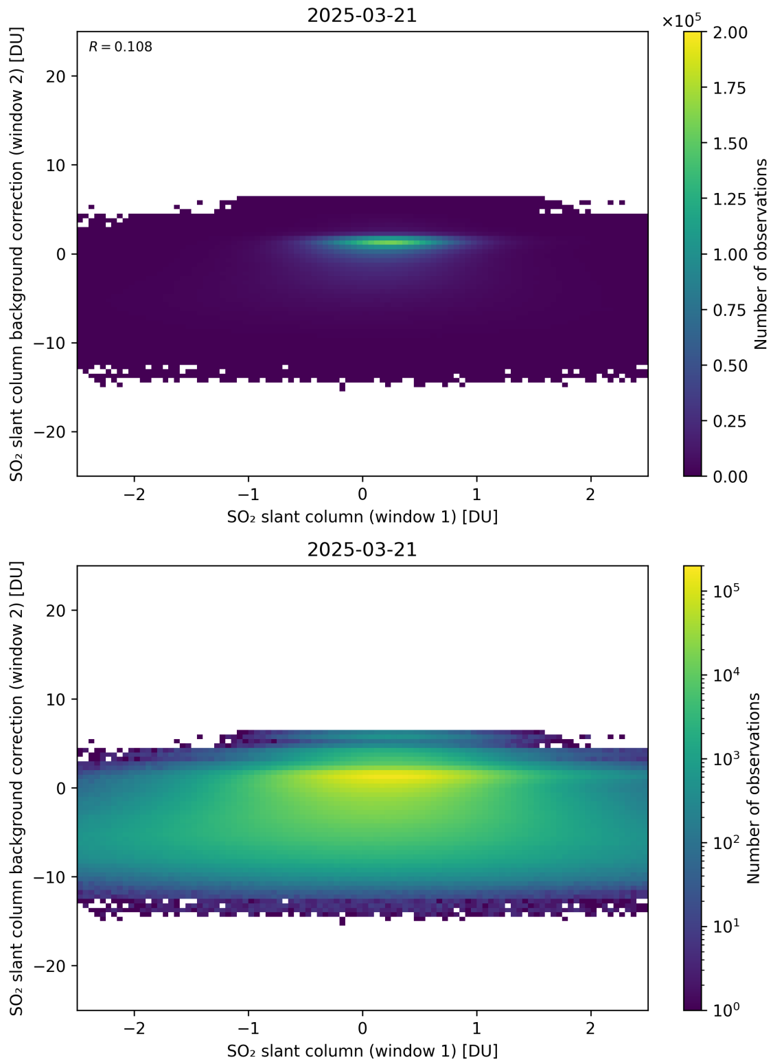
Figure 263: Scatter density plot of “SO 2 slant column (window 1)” against “SO 2 slant column background correction (window 2)” for 2025-03-20 to 2025-03-22.
