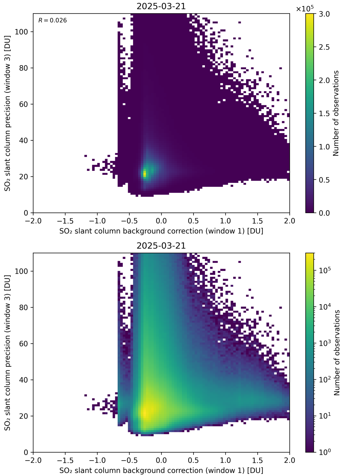
Figure 119: Scatter density plot of “SO 2 slant column background correction (window 1)” against “SO 2 slant column precision (window 3)” for 2025-03-20 to 2025-03-22.
