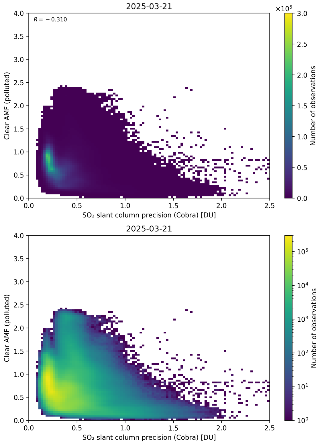
Figure 205: Scatter density plot of “SO 2 slant column precision (Cobra)” against “Clear AMF (polluted)” for 2025-03-20 to 2025-03-22.
