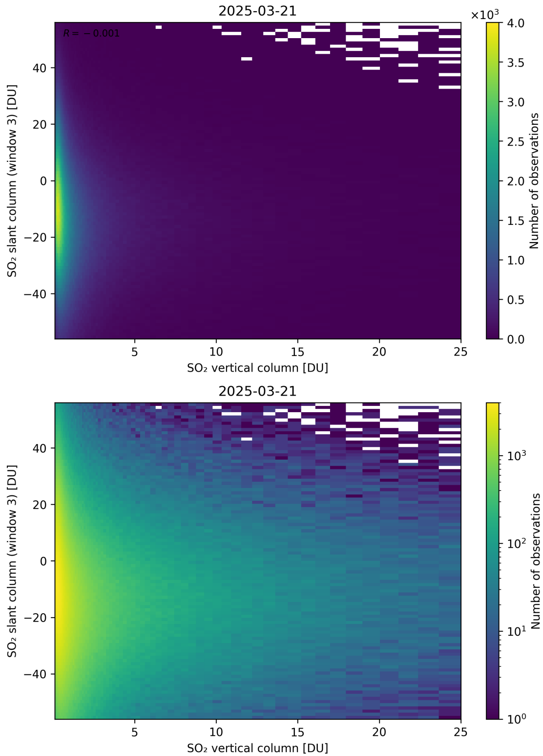
Figure 357: Scatter density plot of “SO 2 vertical column” against “SO 2 slant column (window 3)” for 2025-03-20 to 2025-03-22.
