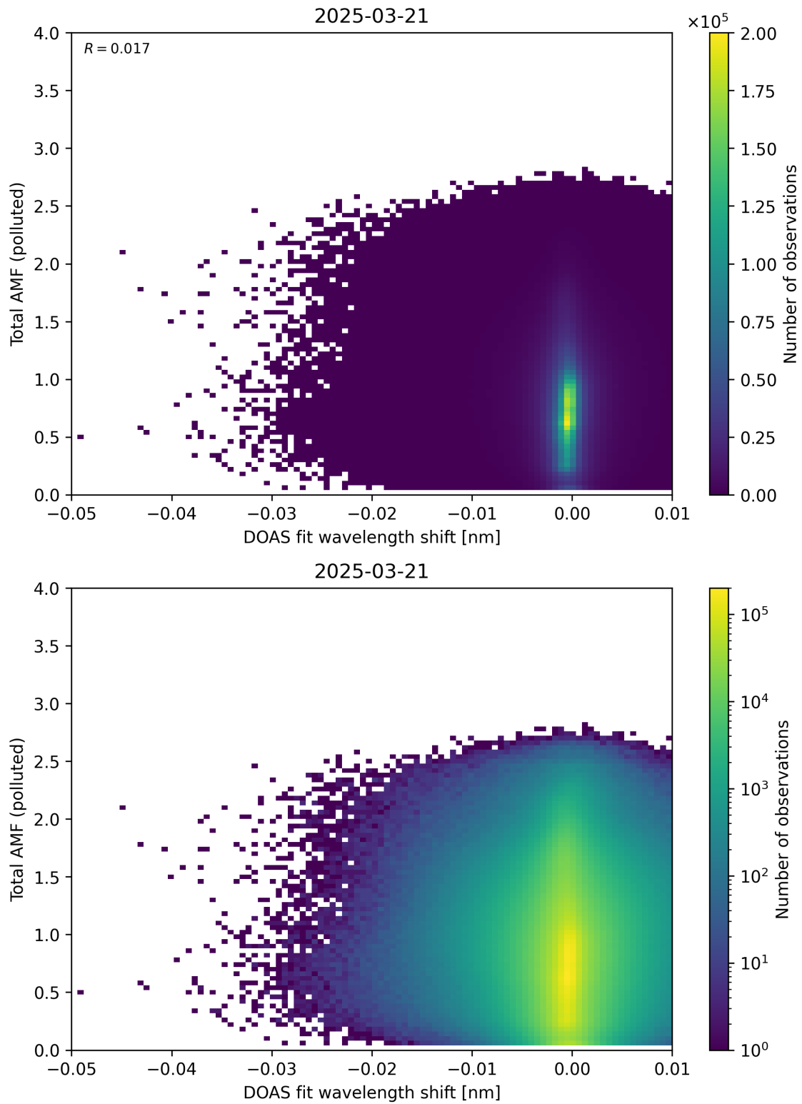
Figure 141: Scatter density plot of “DOAS fit wavelength shift” against “Total AMF (polluted)” for 2025-03-20 to 2025-03-22.
