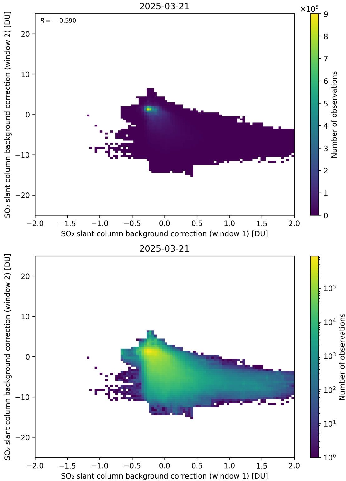
Figure 109: Scatter density plot of “SO 2 slant column background correction (window 1)” against “SO 2 slant column background correction (window 2)” for 2025-03-20 to 2025-03-22.
