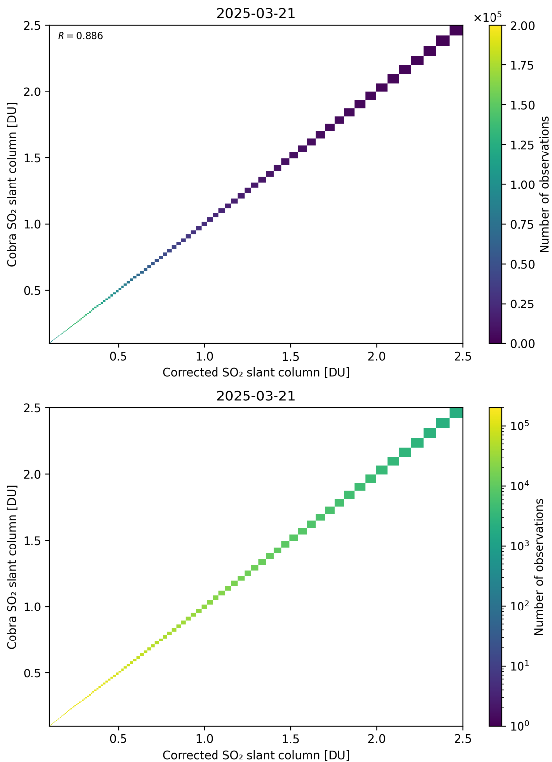
Figure 233: Scatter density plot of “Corrected SO 2 slant column” against “Cobra SO 2 slant column” for 2025-03-20 to 2025-03-22.
