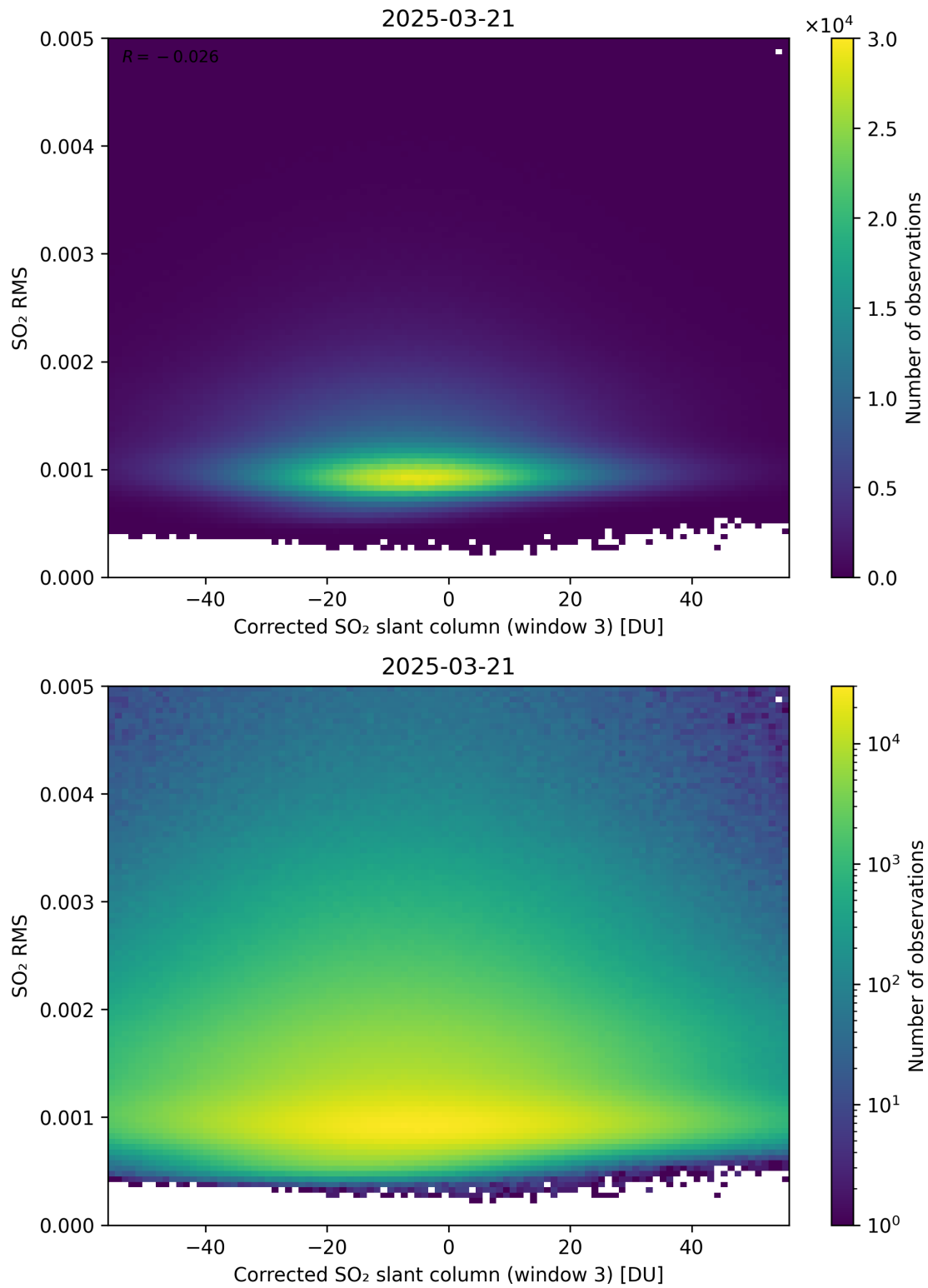
Figure 258: Scatter density plot of “Corrected SO 2 slant column (window 3)” against “SO 2 RMS” for 2025-03-20 to 2025-03-22.
