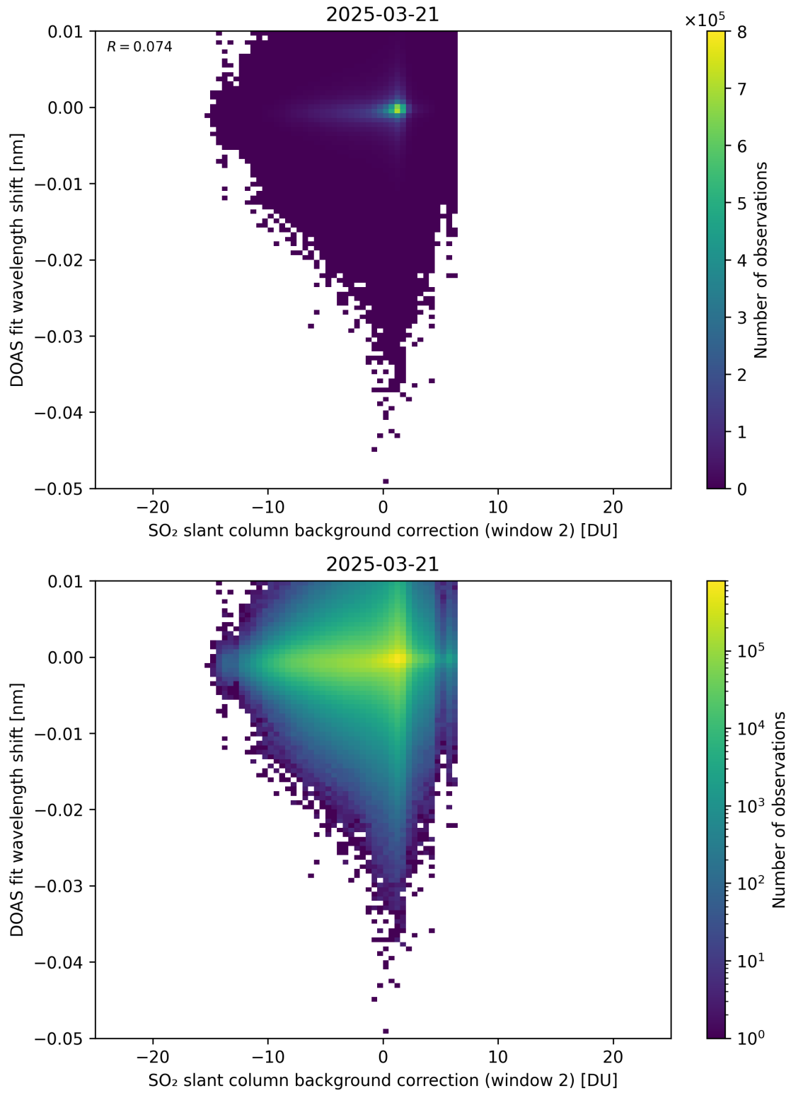
Figure 123: Scatter density plot of “SO 2 slant column background correction (window 2)” against “DOAS fit wavelength shift” for 2025-03-20 to 2025-03-22.
