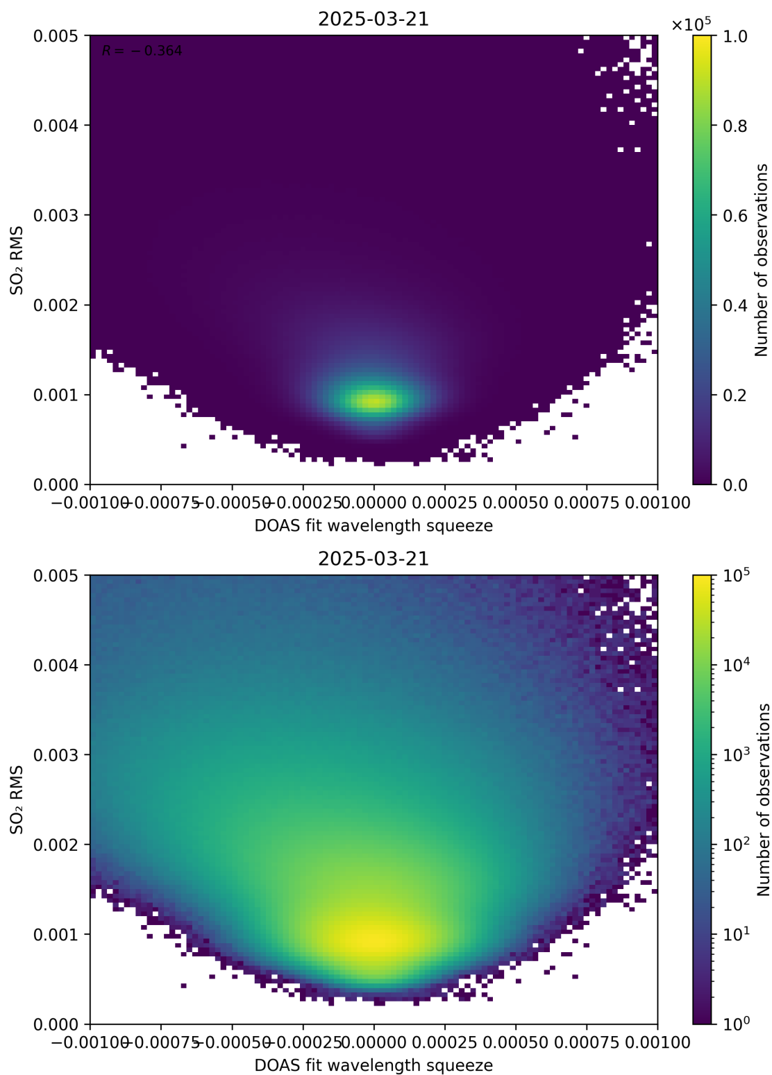
Figure 143: Scatter density plot of “DOAS fit wavelength squeeze” against “SO 2 RMS” for 2025-03-20 to 2025-03-22.
