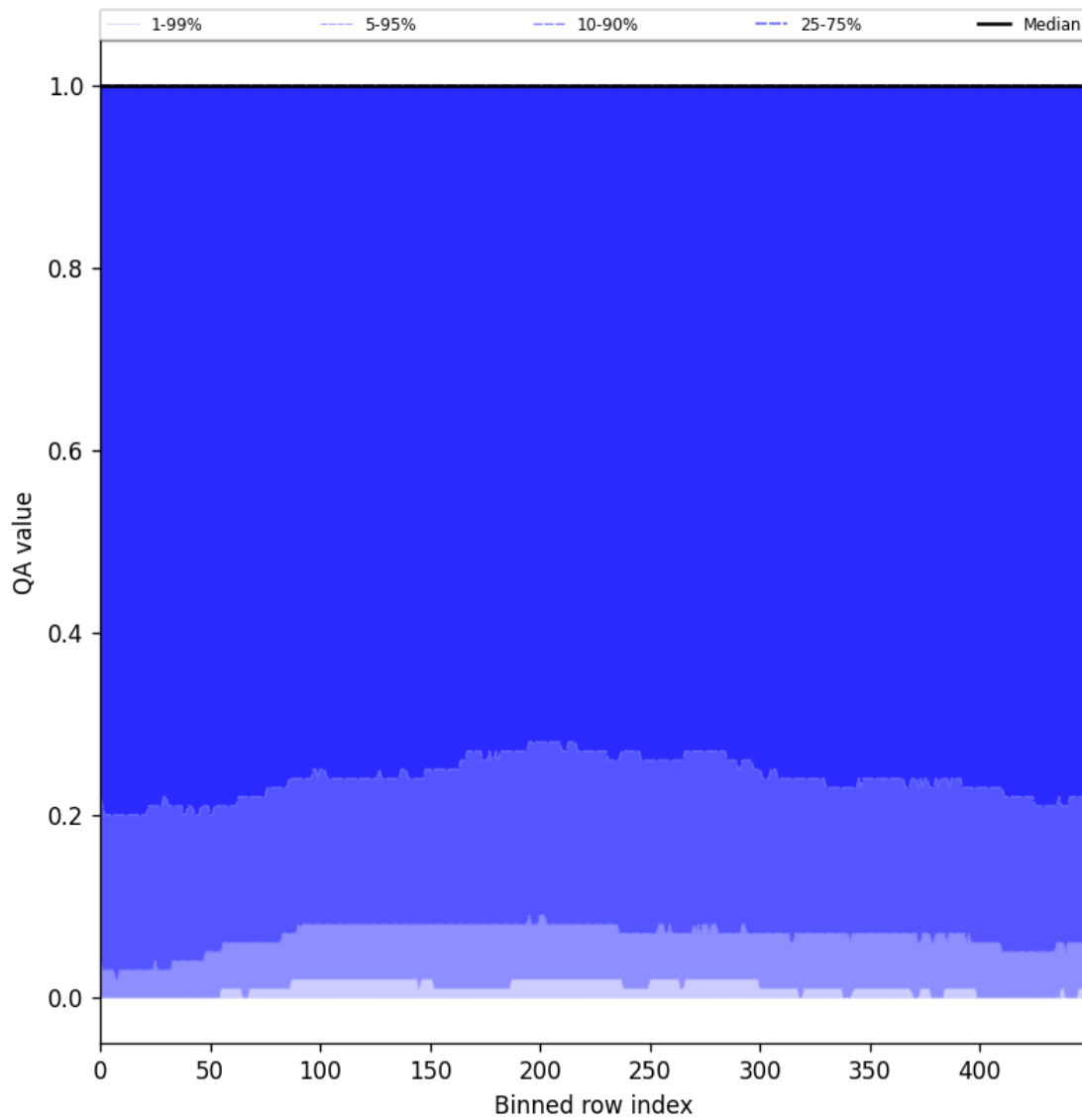
Figure 83: Along track statistics of “QA value” for 2025-03-20 to 2025-03-22
