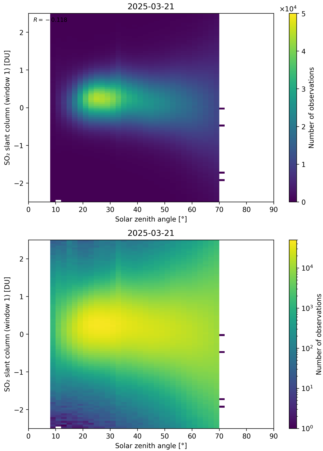
Figure 184: Scatter density plot of “Solar zenith angle” against “SO 2 slant column (window 1)” for 2025-03-20 to 2025-03-22.
