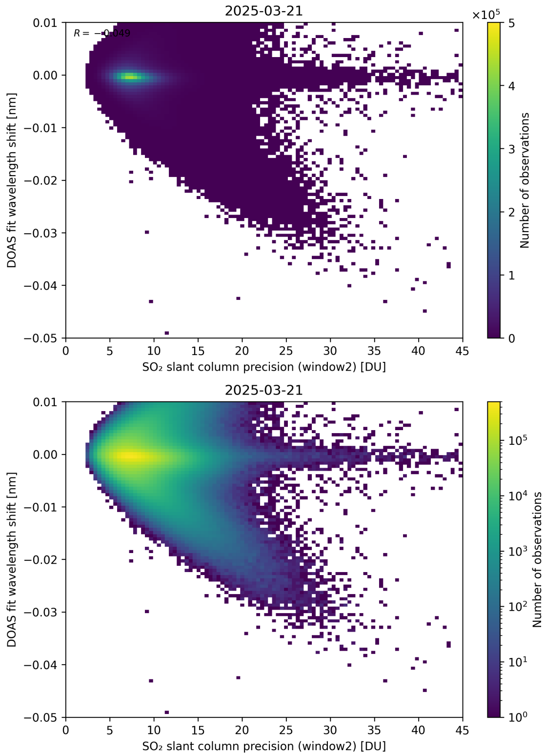
Figure 293: Scatter density plot of “SO 2 slant column precision (window2)” against “DOAS fit wavelength shift” for 2025-03-20 to 2025-03-22.
