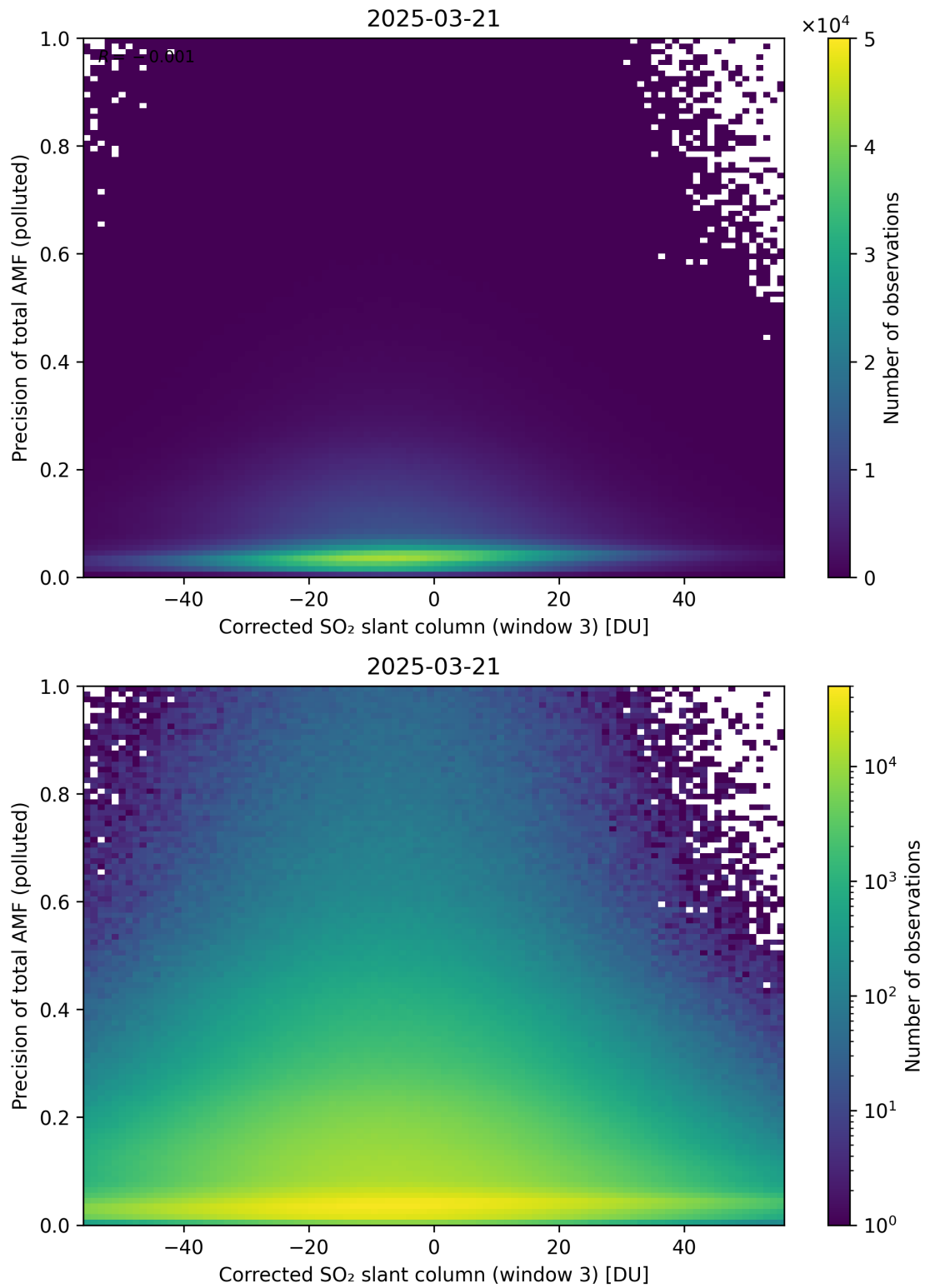
Figure 261: Scatter density plot of “Corrected SO 2 slant column (window 3)” against “Precision of total AMF (polluted)” for 2025-03-20 to 2025-03-22.
