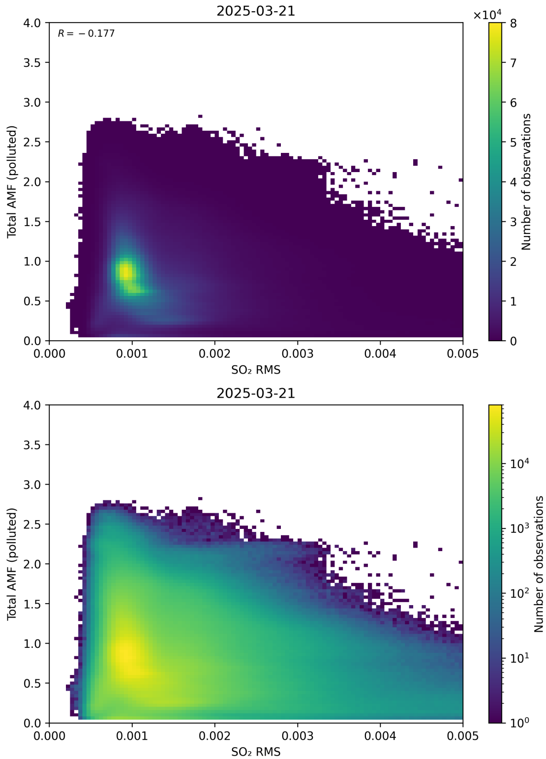
Figure 148: Scatter density plot of “SO 2 RMS” against “Total AMF (polluted)” for 2025-03-20 to 2025-03-22.
