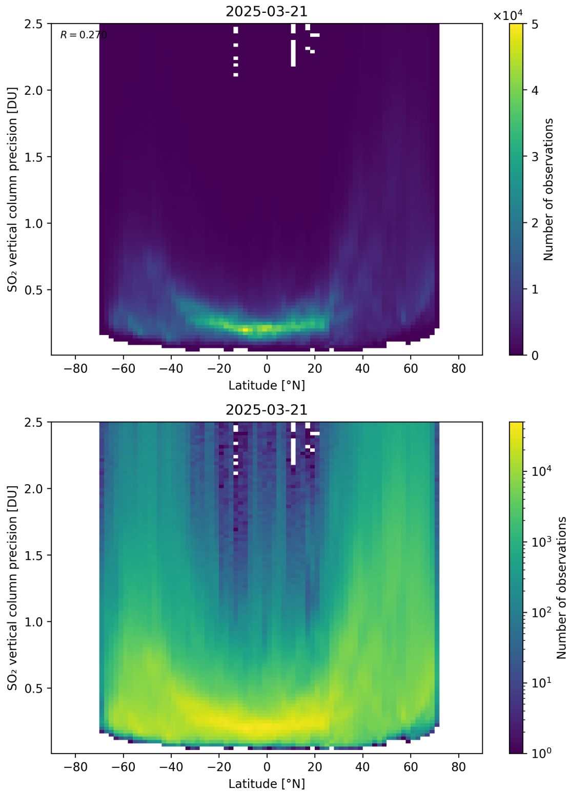
Figure 170: Scatter density plot of “Latitude” against “SO 2 vertical column precision” for 2025-03-20 to 2025-03-22.
