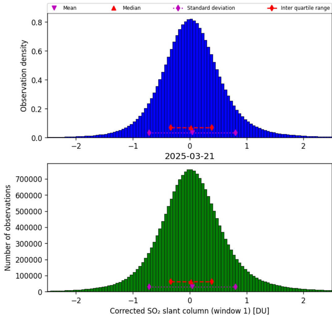
Figure 65: Histogram of “Corrected SO 2 slant column (window 1)” for 2025-03-20 to 2025-03-22
