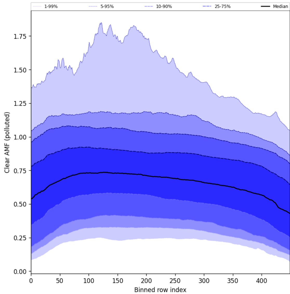
Figure 107: Along track statistics of “Clear AMF (polluted)” for 2025-03-20 to 2025-03-22
