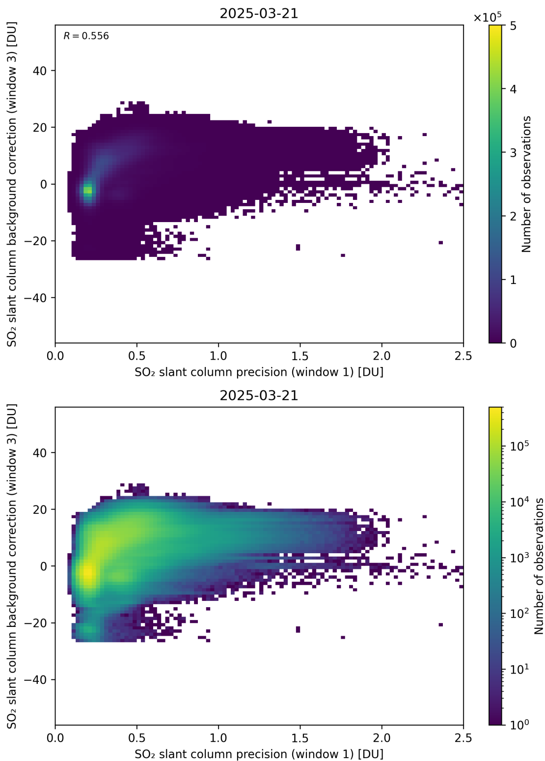
Figure 270: Scatter density plot of “SO 2 slant column precision (window 1)” against “SO 2 slant column background correction (window 3)” for 2025-03-20 to 2025-03-22.
