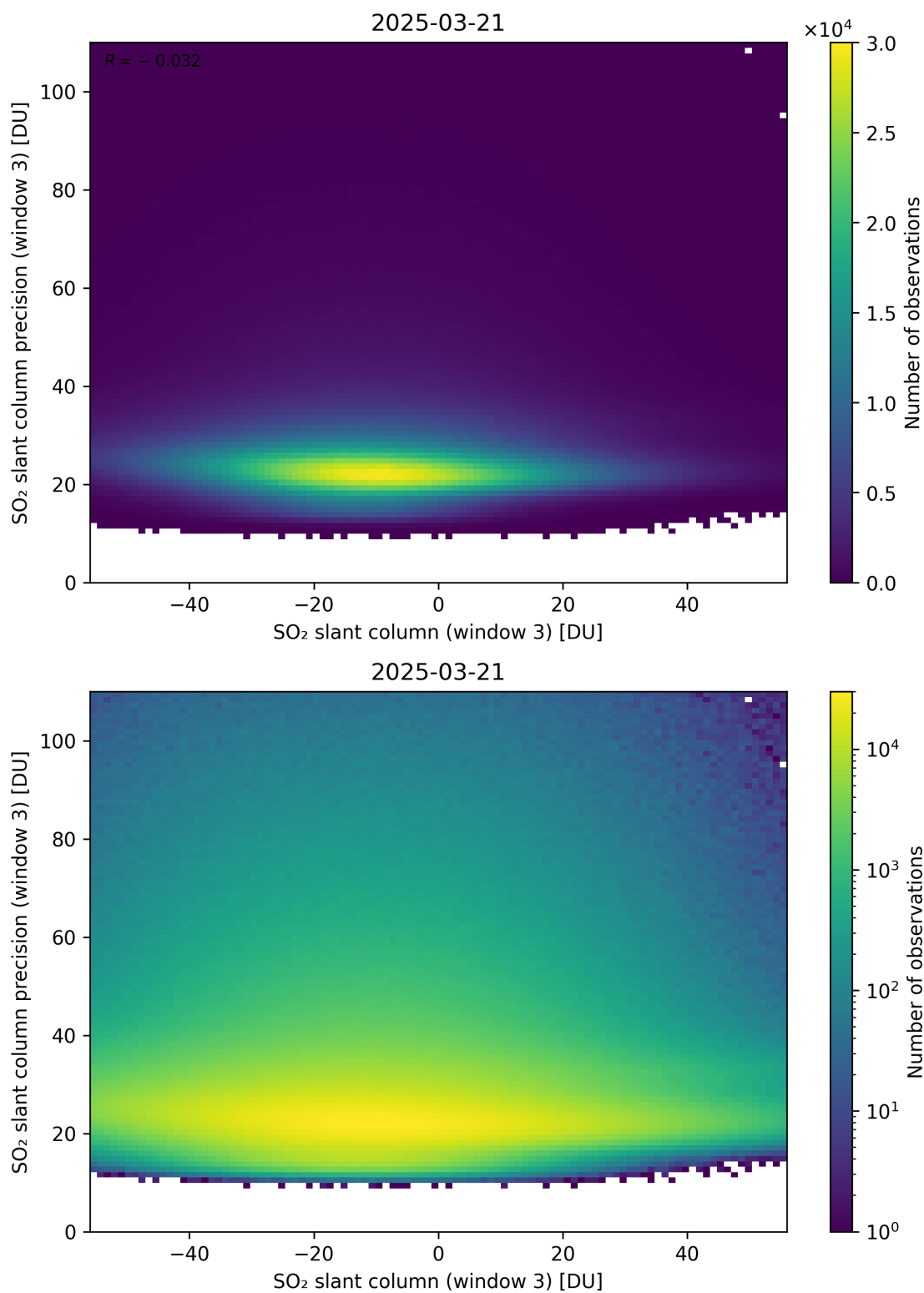
Figure 317: Scatter density plot of “SO 2 slant column (window 3)” against “SO 2 slant column precision (window 3)” for 2025-03-20 to 2025-03-22.
