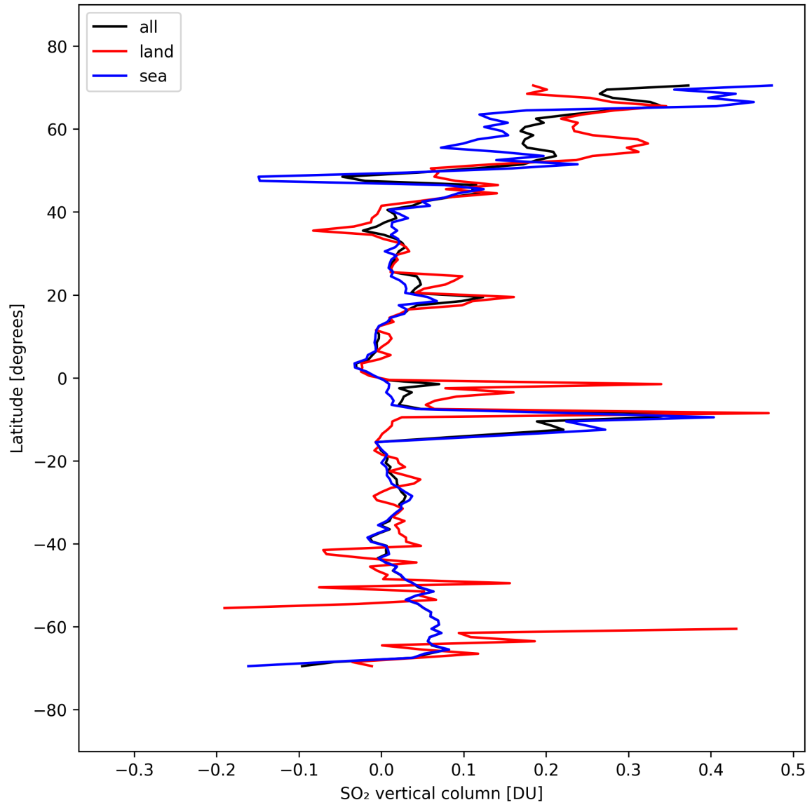
Figure 32: Zonal average of “SO 2 vertical column” for 2025-03-20 to 2025-03-22.
