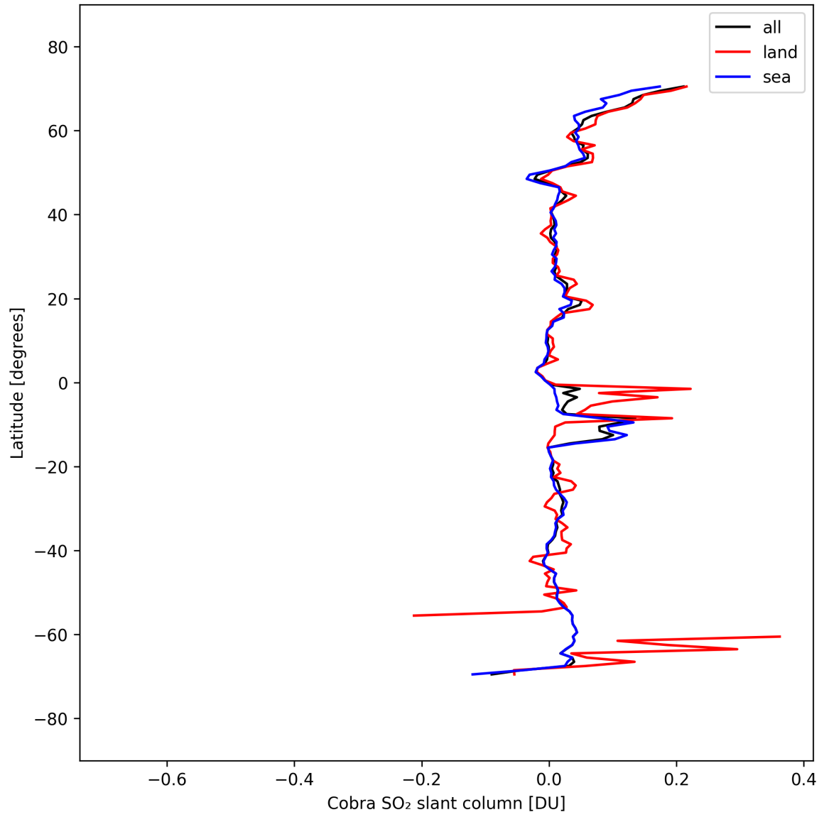
Figure 35: Zonal average of “Cobra SO 2 slant column” for 2025-03-20 to 2025-03-22.
