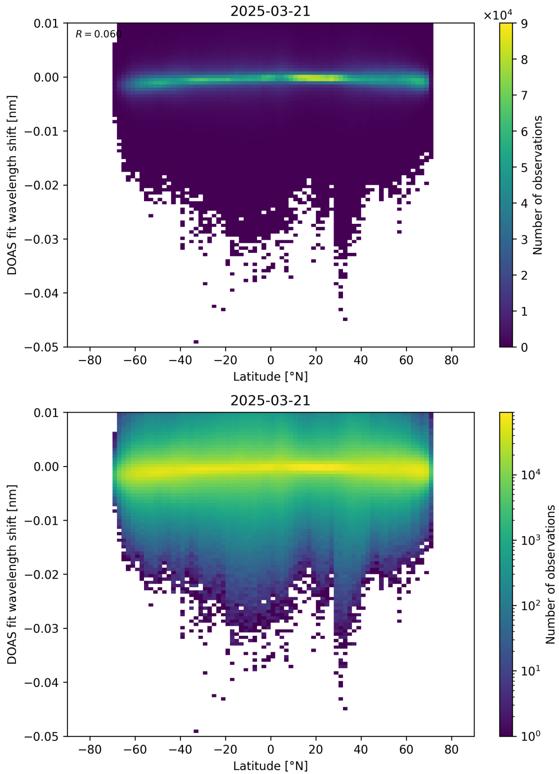
Figure 153: Scatter density plot of “Latitude” against “DOAS fit wavelength shift” for 2025-03-20 to 2025-03-22.
