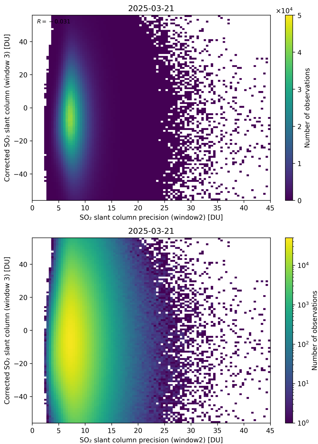
Figure 298: Scatter density plot of “SO 2 slant column precision (window2)” against “Corrected SO 2 slant column (window 3)” for 2025-03-20 to 2025-03-22.
