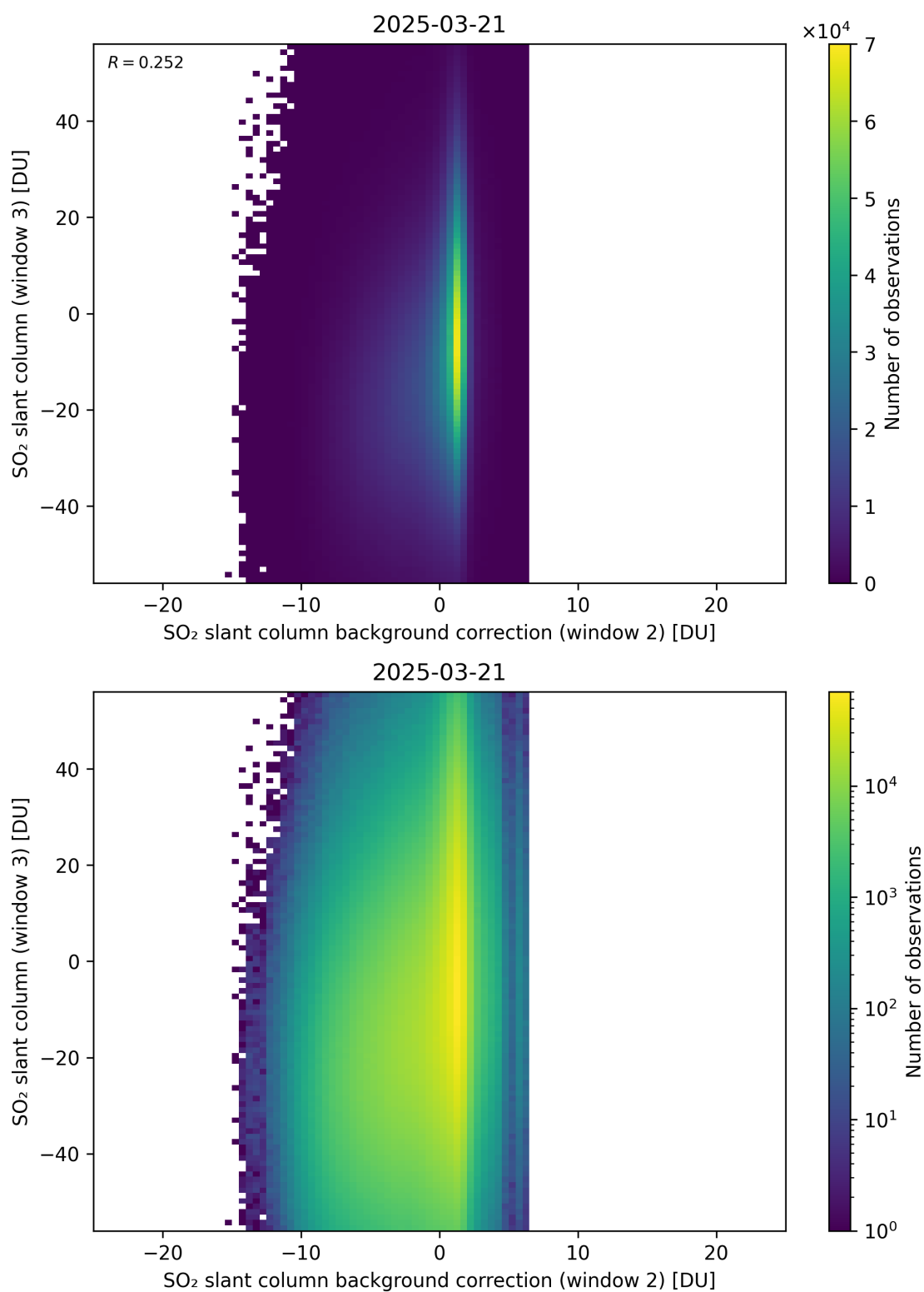
Figure 128: Scatter density plot of “SO 2 slant column background correction (window 2)” against “SO 2 slant column (window 3)” for 2025-03-20 to 2025-03-22.
