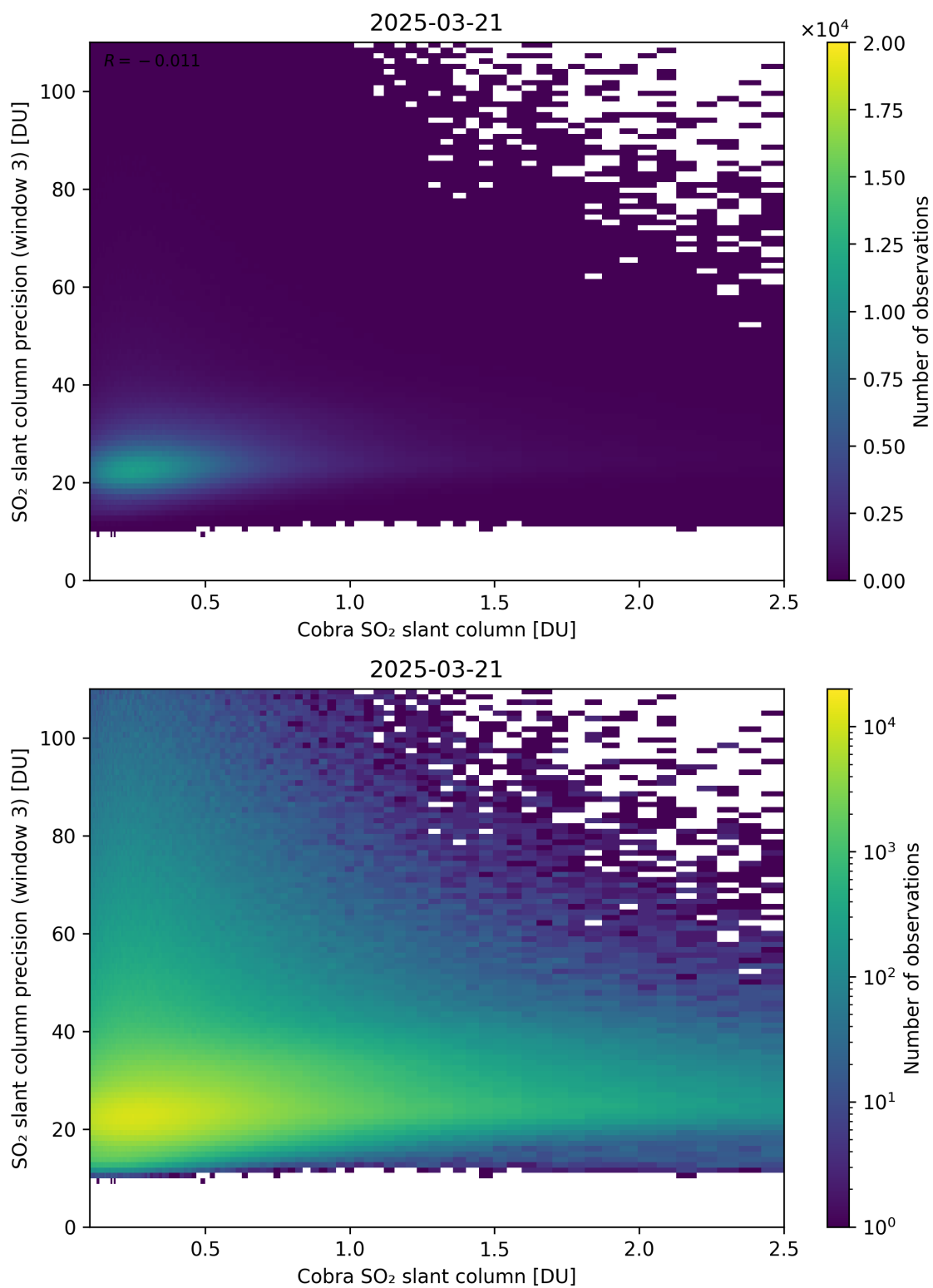
Figure 223: Scatter density plot of “Cobra SO 2 slant column” against “SO 2 slant column precision (window 3)” for 2025-03-20 to 2025-03-22.
