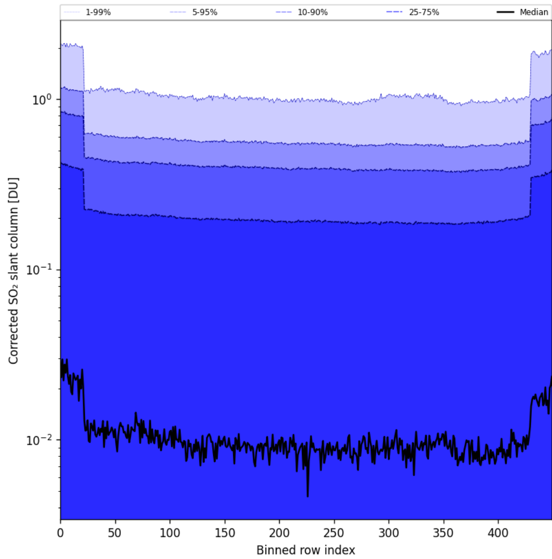
Figure 86: Along track statistics of “Corrected SO 2 slant column” for 2025-03-20 to 2025-03-22
