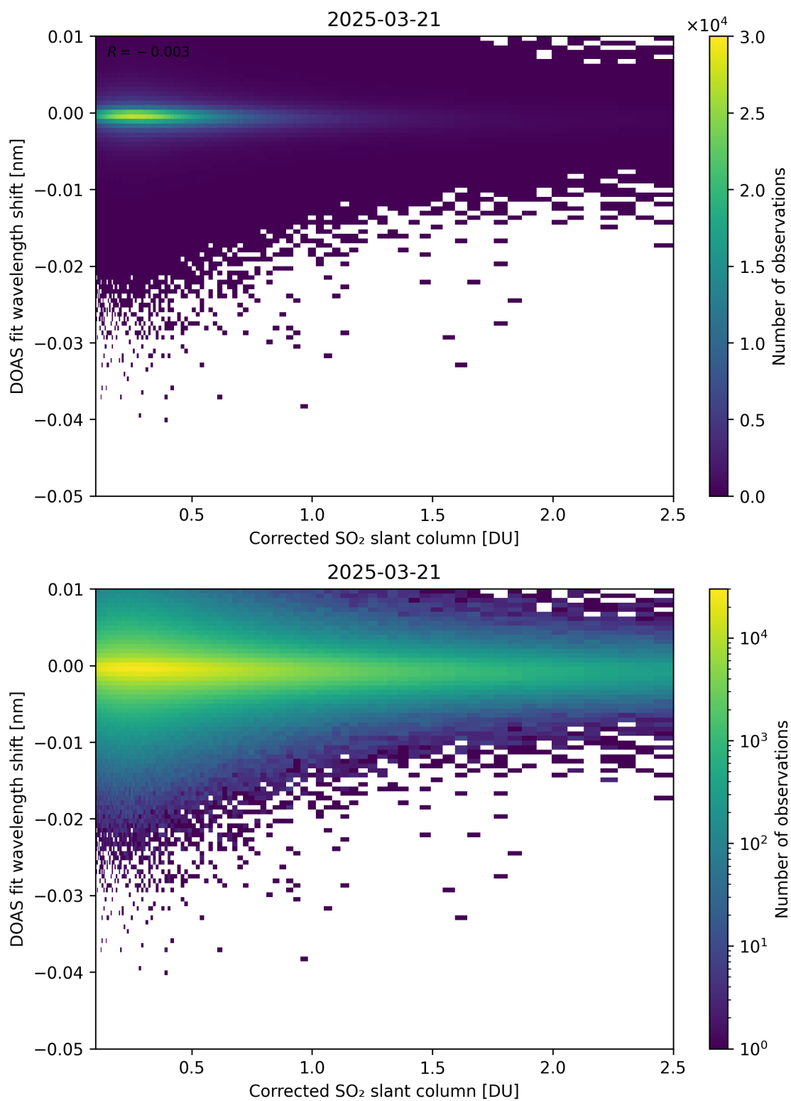
Figure 229: Scatter density plot of “Corrected SO 2 slant column” against “DOAS fit wavelength shift” for 2025-03-20 to 2025-03-22.
