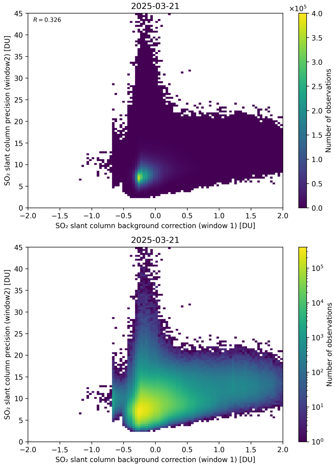
Figure 117: Scatter density plot of “SO 2 slant column background correction (window 1)” against “SO 2 slant column precision (window2)” for 2025-03-20 to 2025-03-22.
