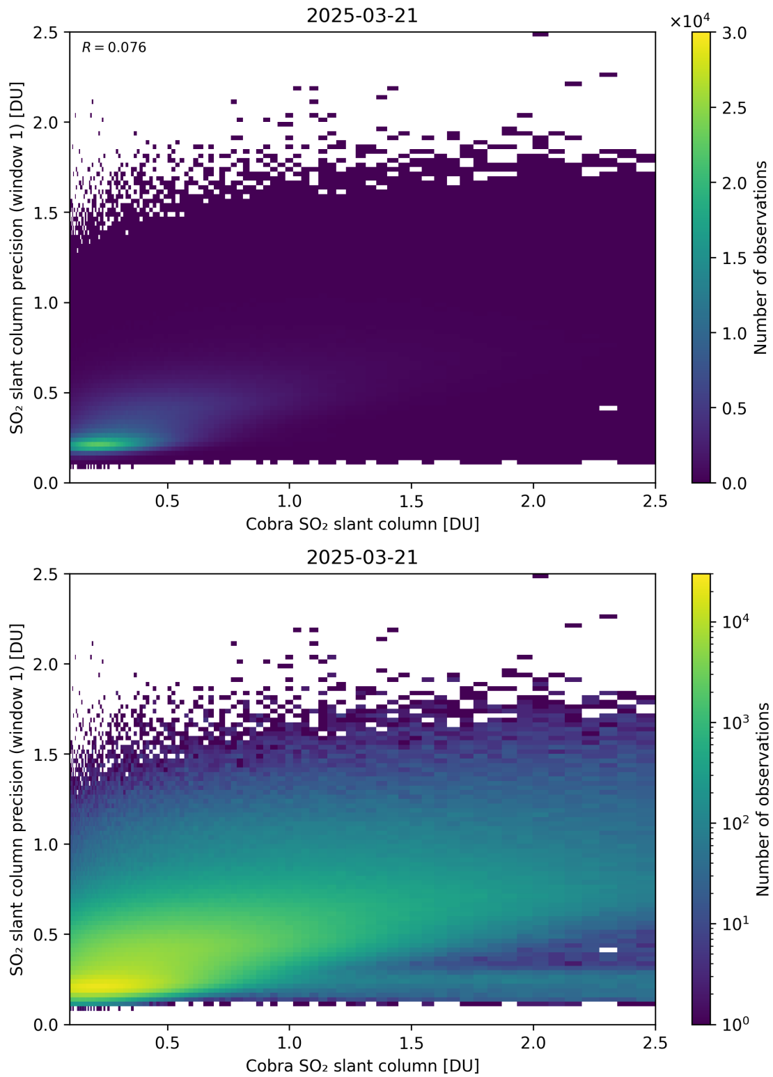
Figure 220: Scatter density plot of “Cobra SO 2 slant column” against “SO 2 slant column precision (window 1)” for 2025-03-20 to 2025-03-22.
