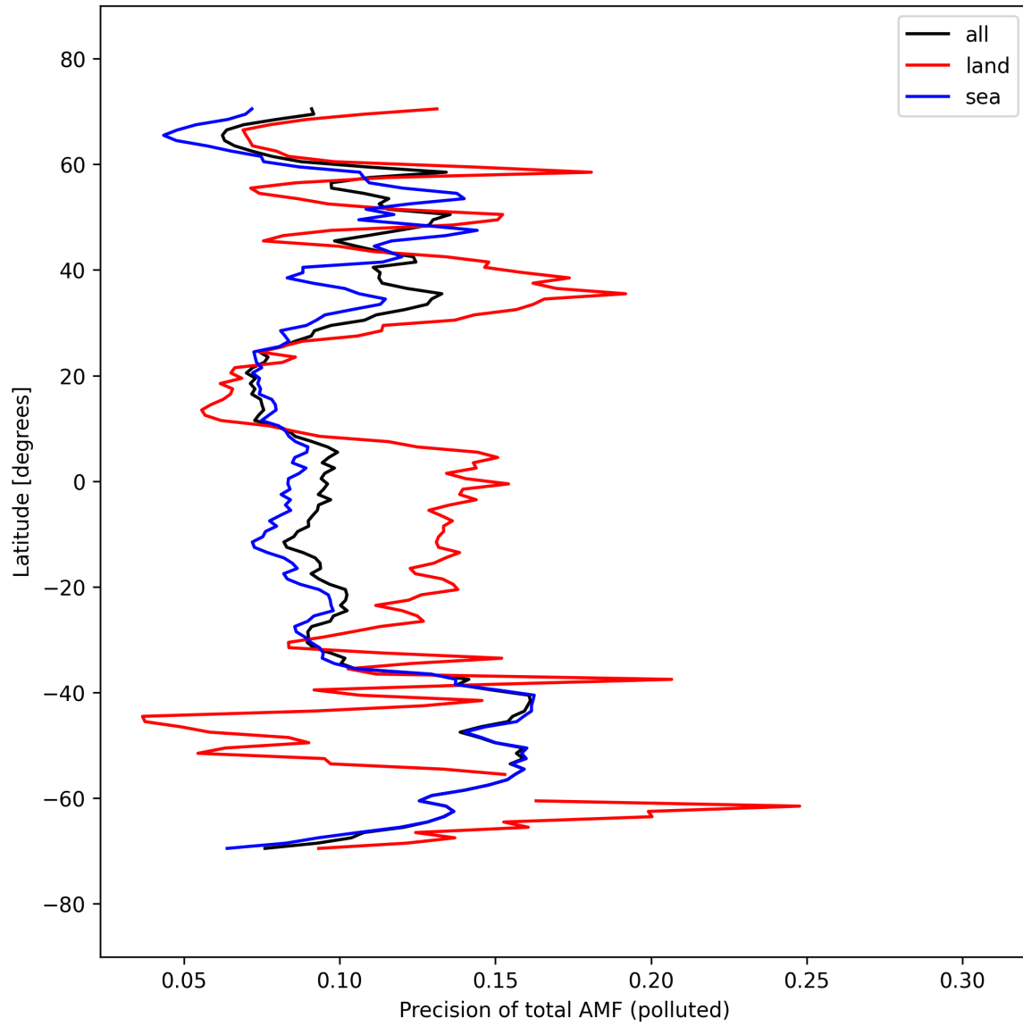
Figure 54: Zonal average of “Precision of total AMF (polluted)” for 2025-03-20 to 2025-03-22.
