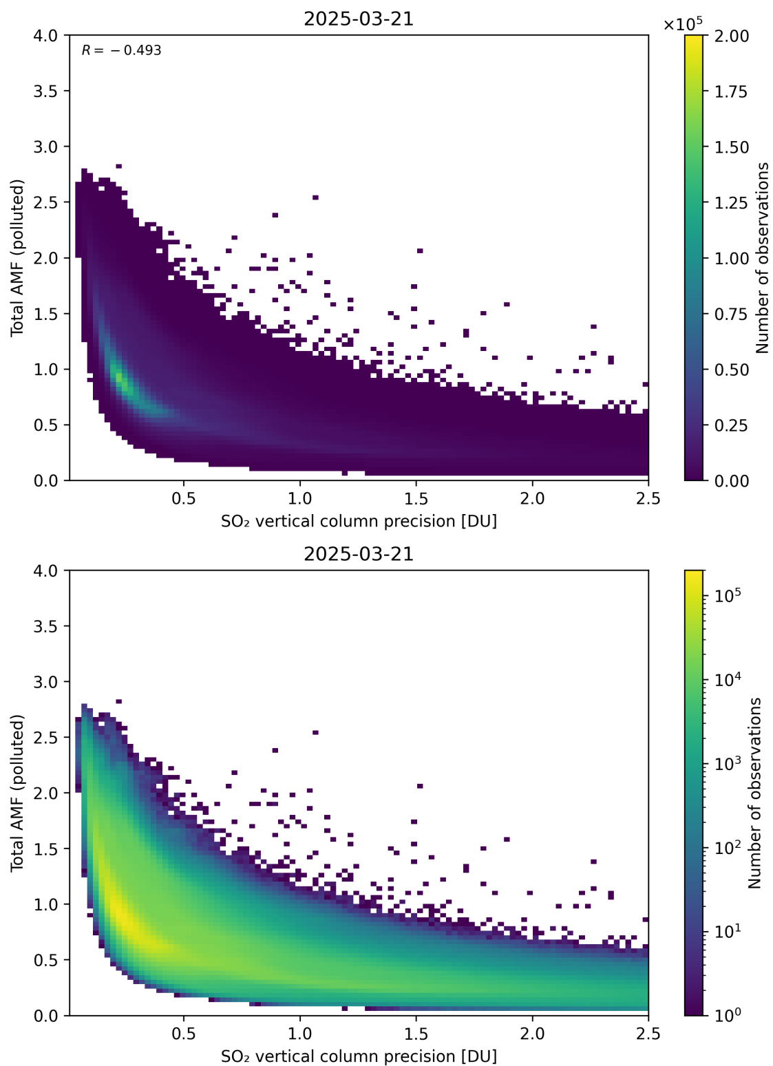
Figure 346: Scatter density plot of “SO 2 vertical column precision” against “Total AMF (polluted)” for 2025-03-20 to 2025-03-22.
