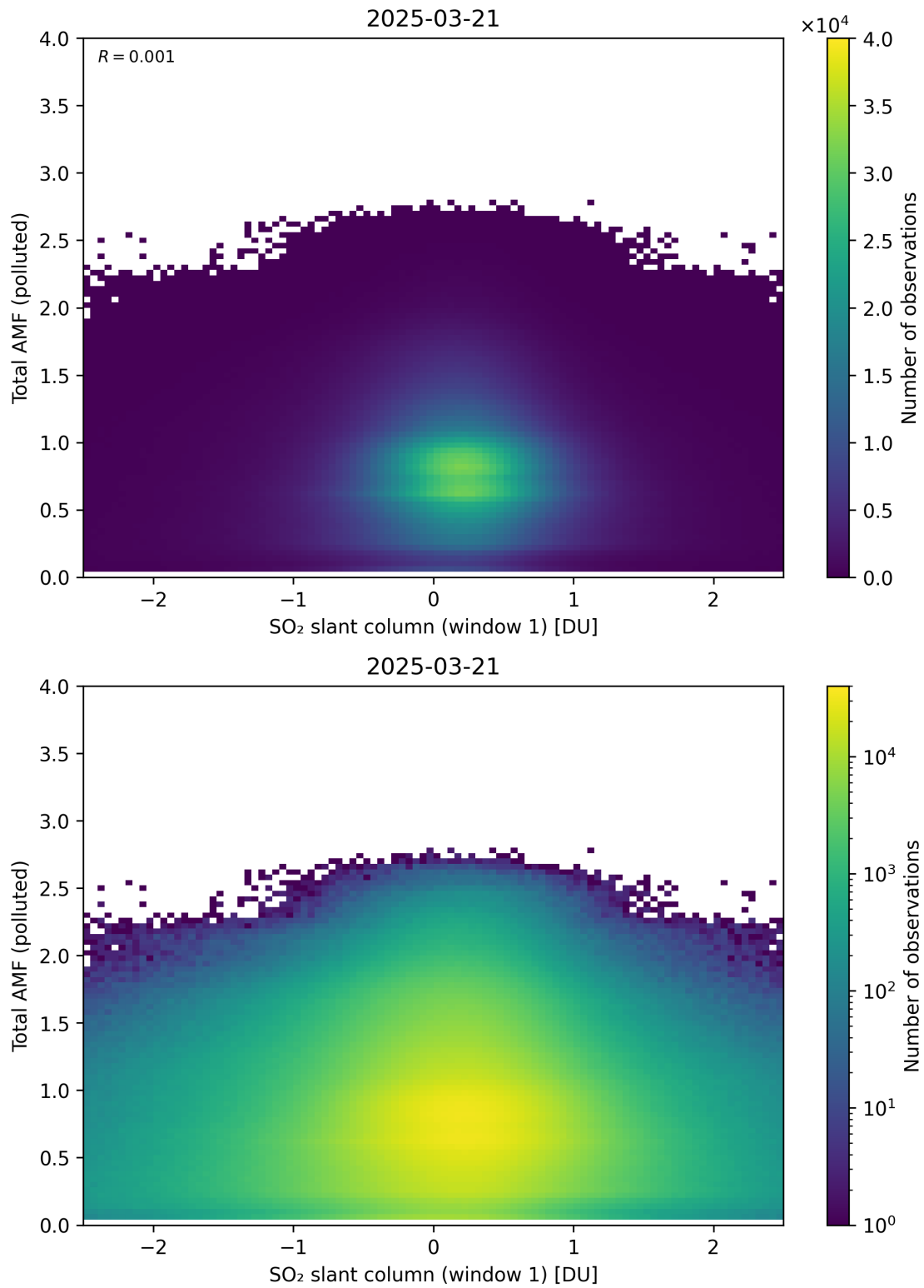
Figure 289: Scatter density plot of “SO 2 slant column (window 1)” against “Total AMF (polluted)” for 2025-03-20 to 2025-03-22.
