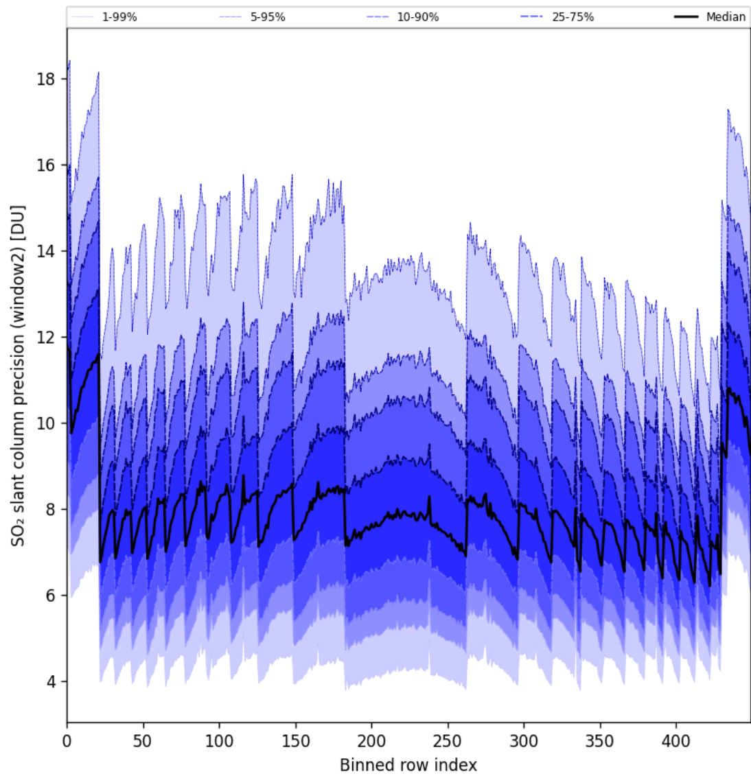
Figure 94: Along track statistics of “SO 2 slant column precision (window2)” for 2025-03-20 to 2025-03-22
