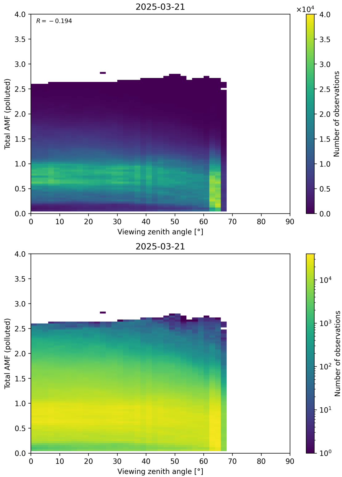
Figure 381: Scatter density plot of “Viewing zenith angle” against “Total AMF (polluted)” for 2025-03-20 to 2025-03-22.
