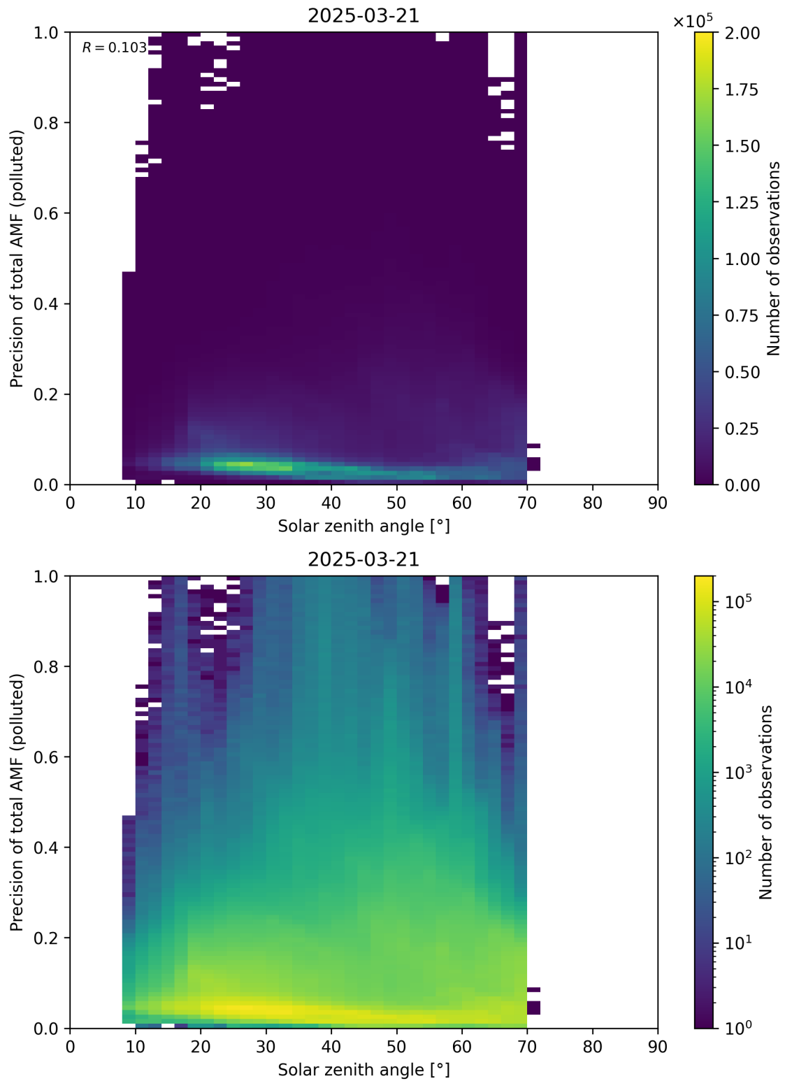
Figure 190: Scatter density plot of “Solar zenith angle” against “Precision of total AMF (polluted)” for 2025-03-20 to 2025-03-22.
