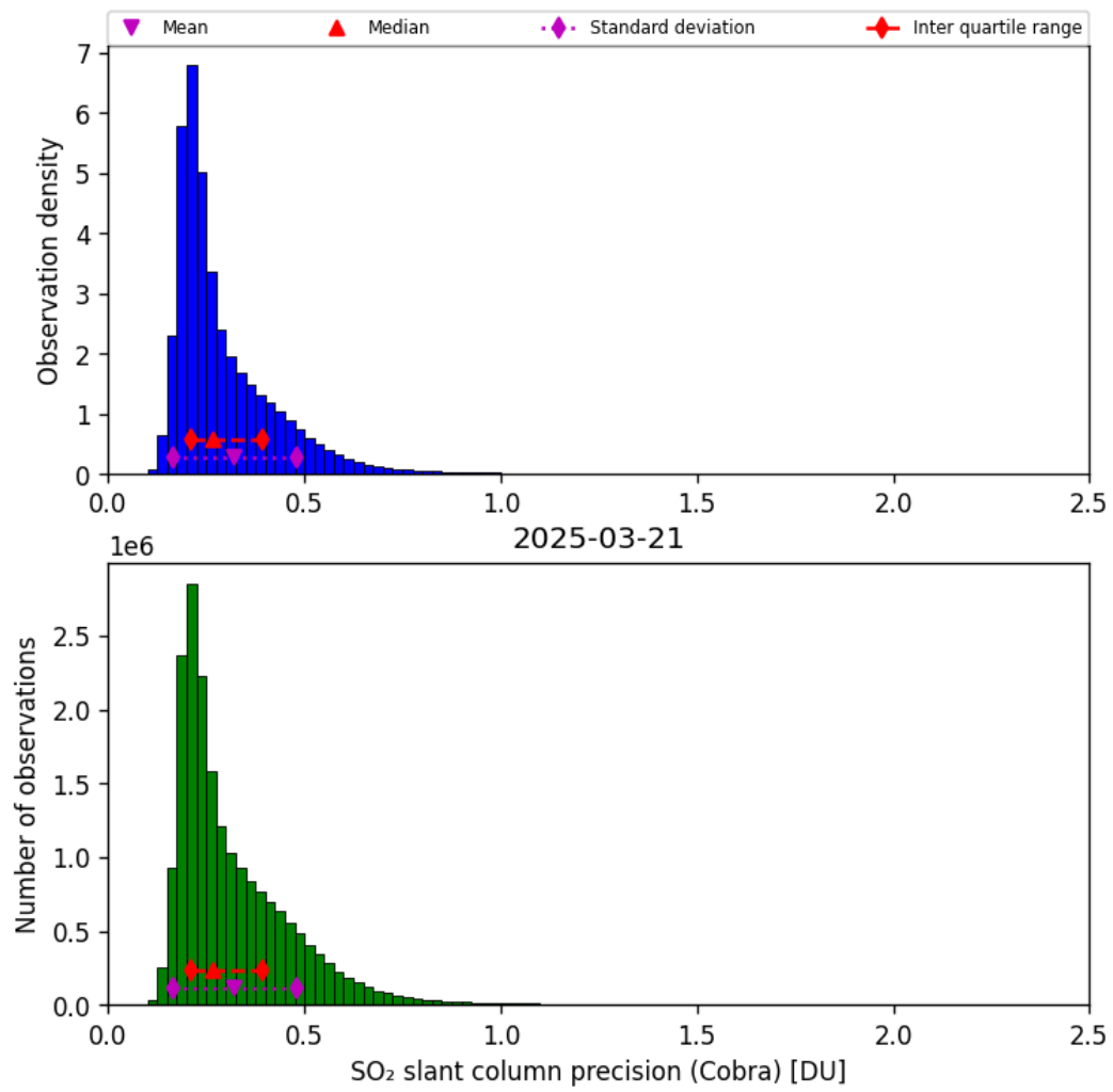
Figure 62: Histogram of “SO 2 slant column precision (Cobra)” for 2025-03-20 to 2025-03-22
