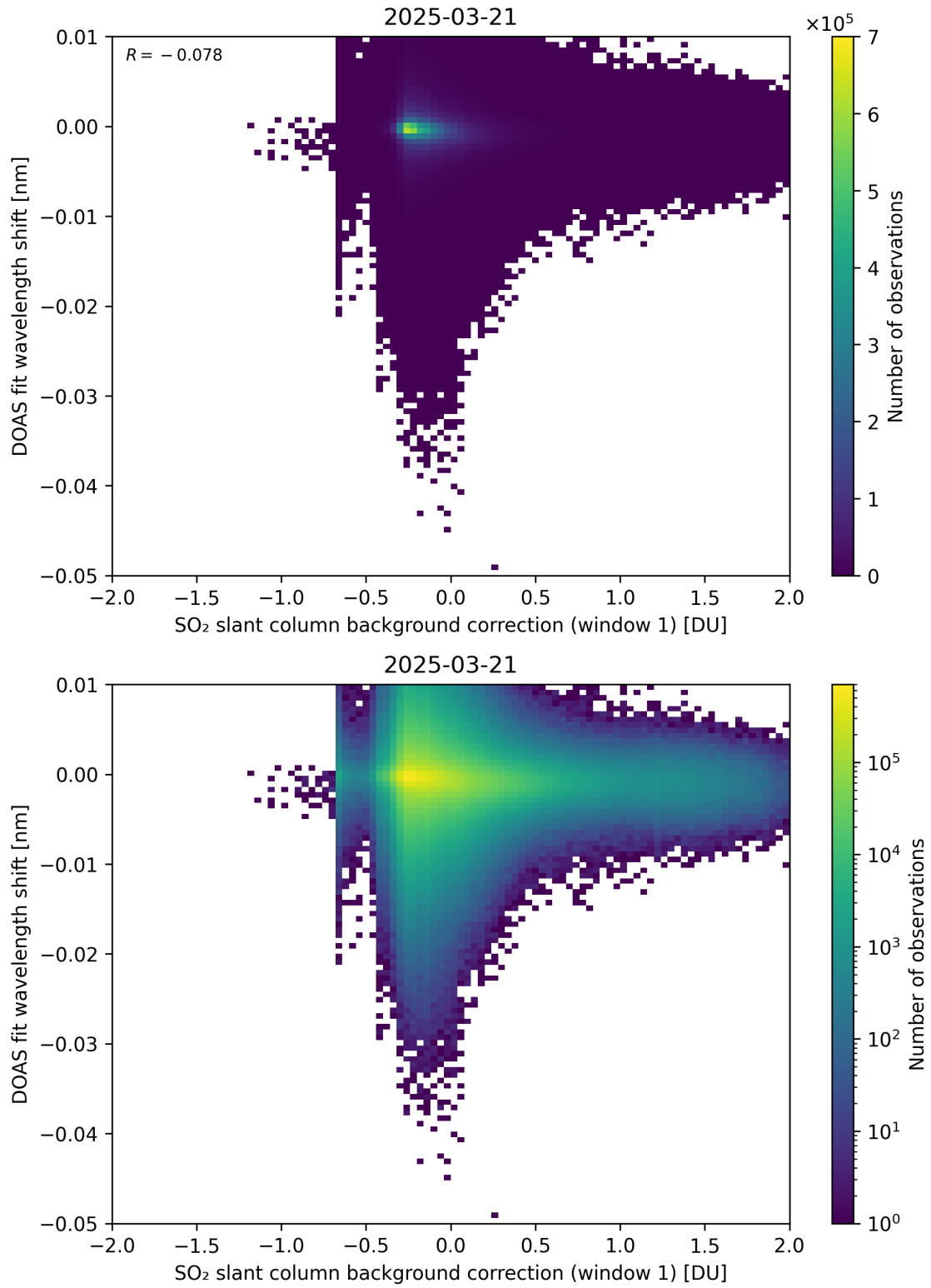
Figure 111: Scatter density plot of “SO 2 slant column background correction (window 1)” against “DOAS fit wavelength shift” for 2025-03-20 to 2025-03-22.
