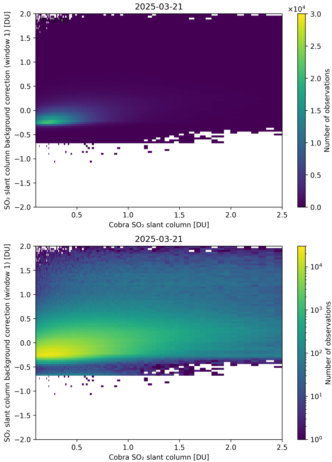
Figure 193: Scatter density plot of “Cobra SO 2 slant column” against “SO 2 slant column background correction (window 1)” for 2025-03-20 to 2025-03-22.
