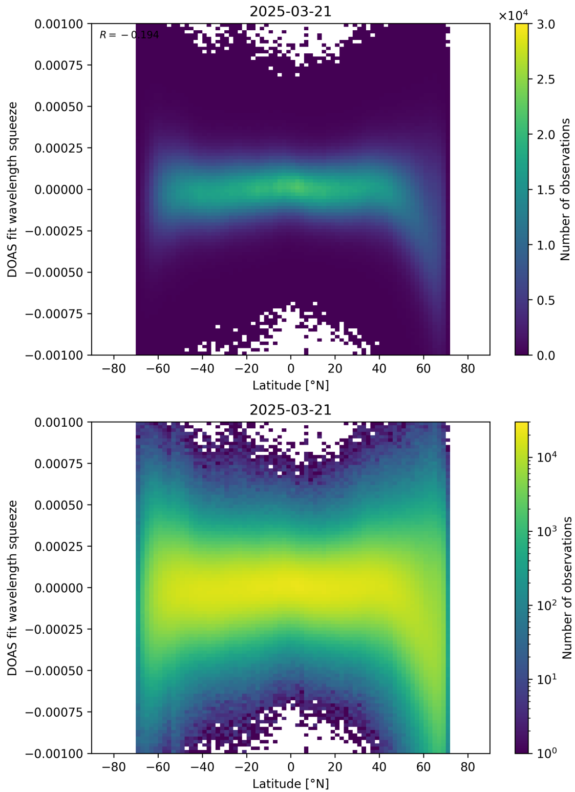
Figure 154: Scatter density plot of “Latitude” against “DOAS fit wavelength squeeze” for 2025-03-20 to 2025-03-22.
