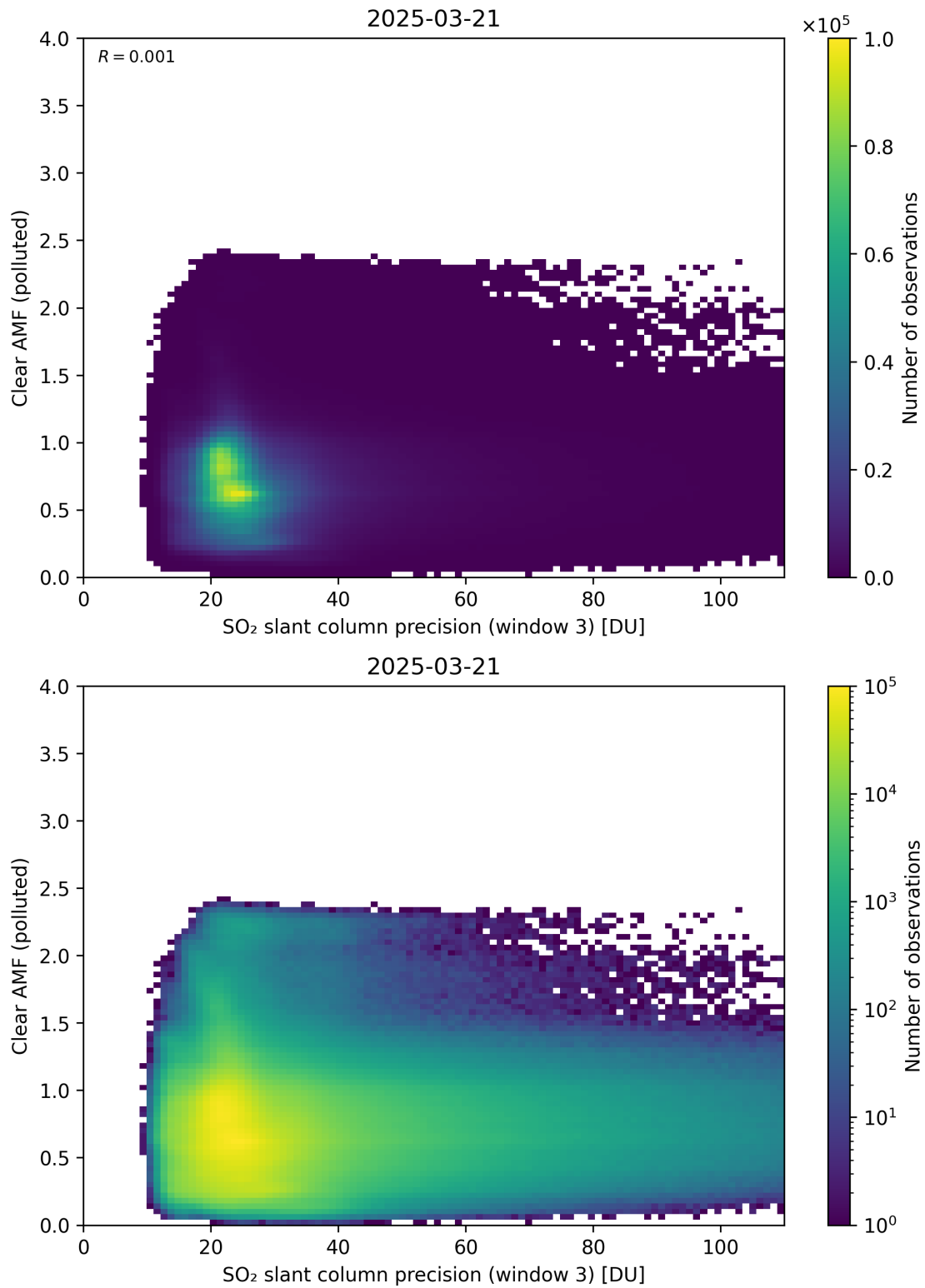
Figure 311: Scatter density plot of “SO 2 slant column precision (window 3)” against “Clear AMF (polluted)” for 2025-03-20 to 2025-03-22.
