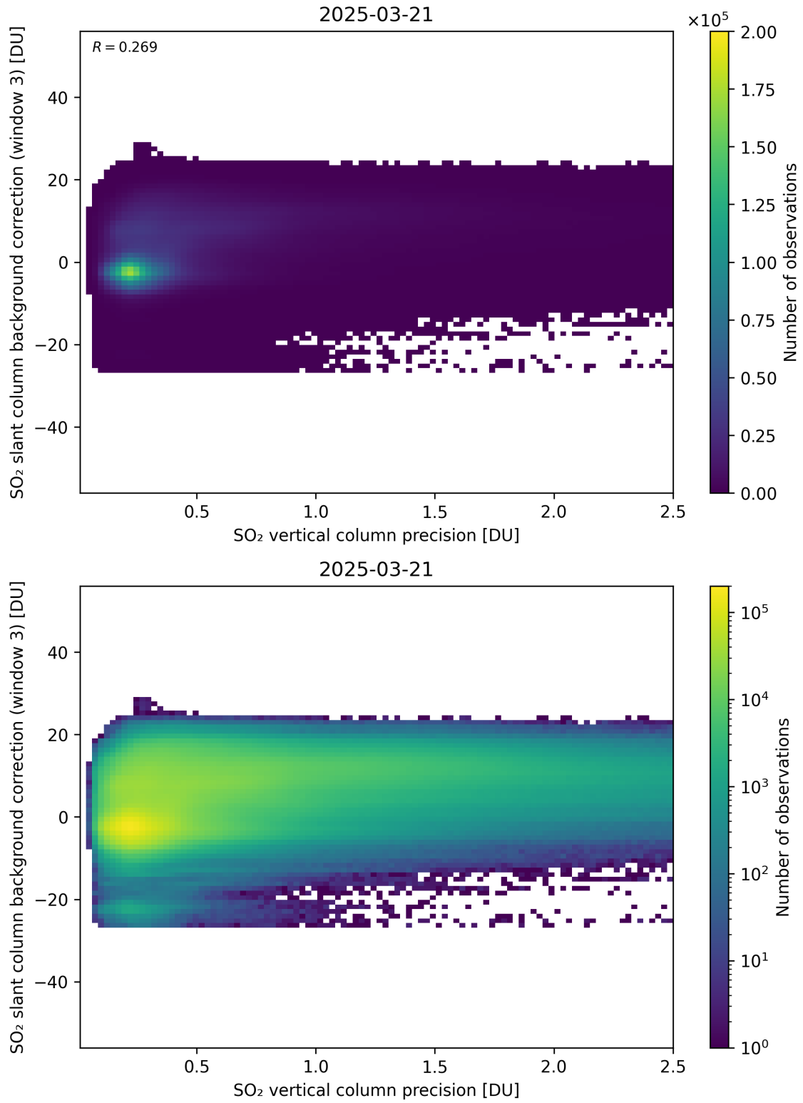
Figure 331: Scatter density plot of “SO 2 vertical column precision” against “SO 2 slant column background correction (window 3)” for 2025-03-20 to 2025-03-22.
