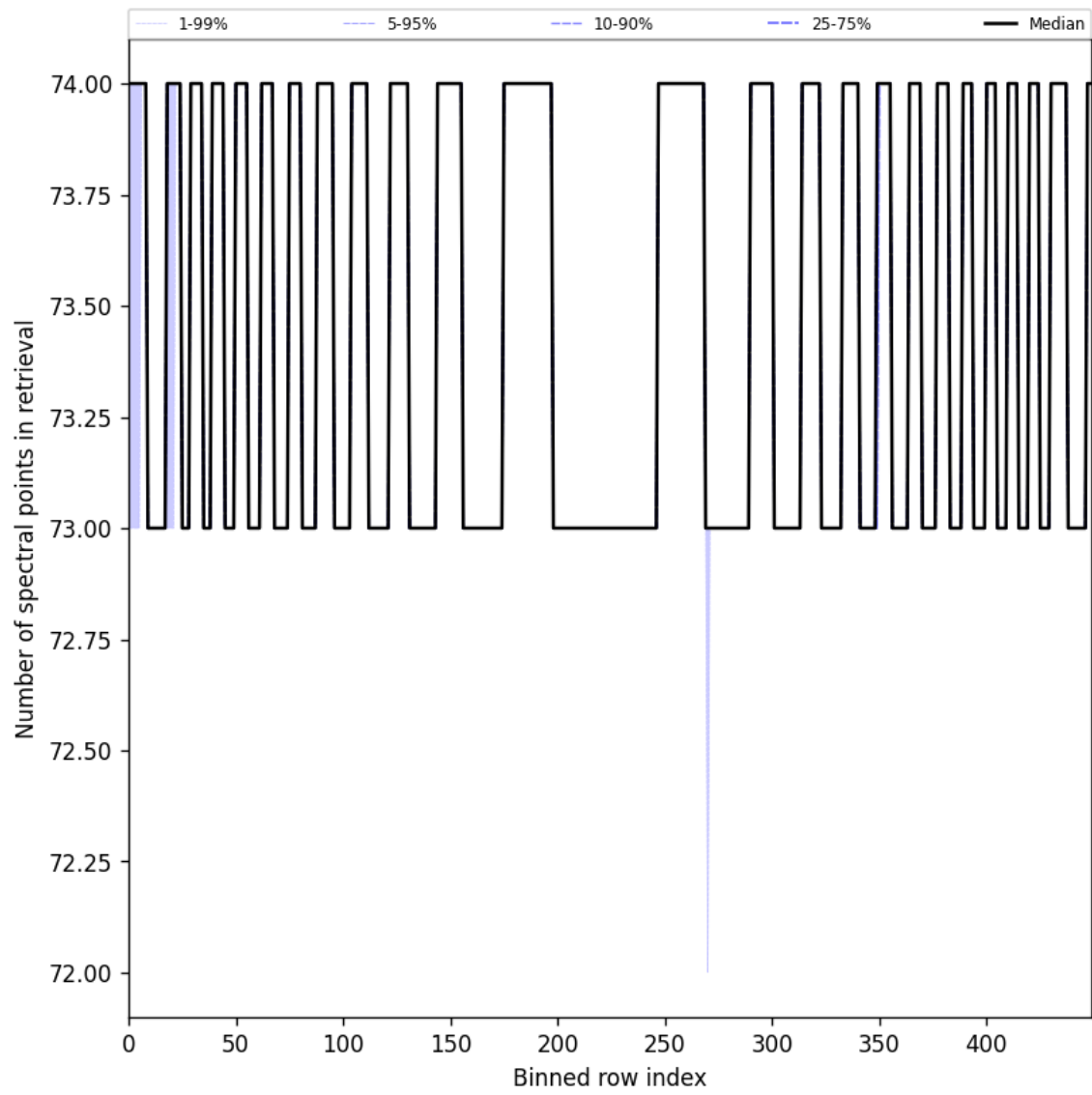
Figure 108: Along track statistics of “Number of spectral points in retrieval” for 2025-03-20 to 2025-03-22
