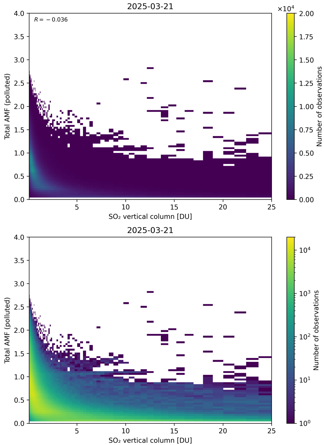
Figure 359: Scatter density plot of “SO 2 vertical column” against “Total AMF (polluted)” for 2025-03-20 to 2025-03-22.
