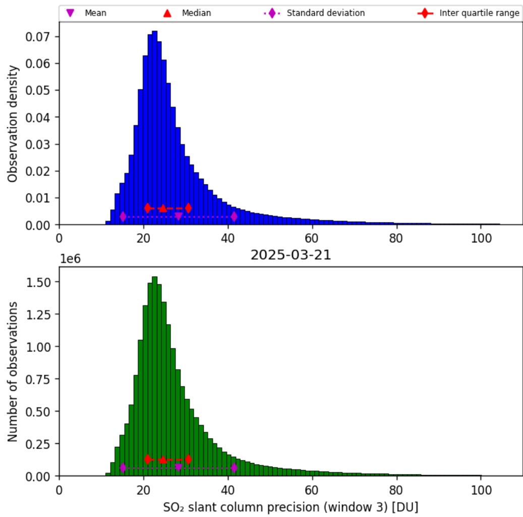
Figure 72: Histogram of “SO 2 slant column precision (window 3)” for 2025-03-20 to 2025-03-22
