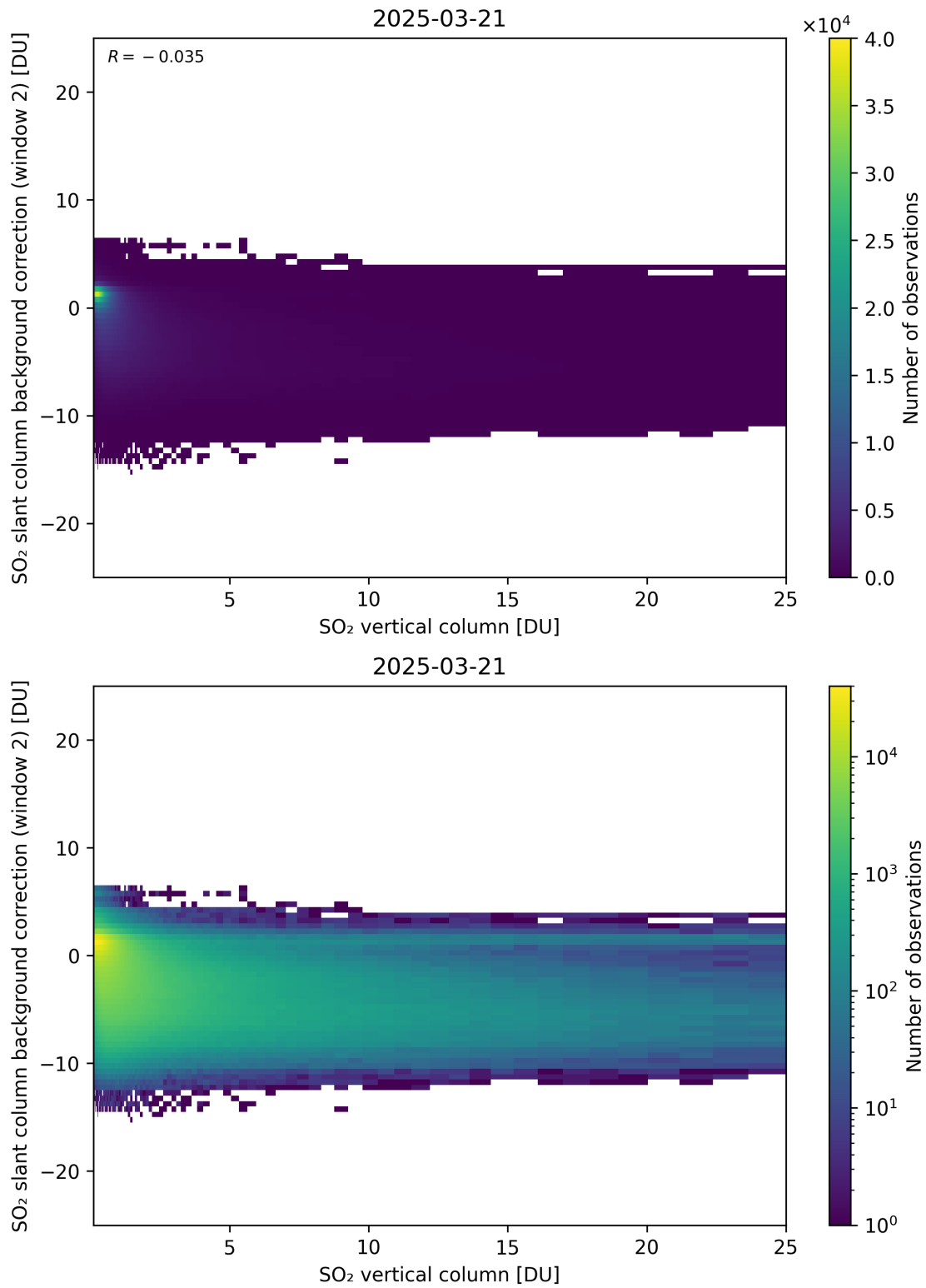
Figure 324: Scatter density plot of “SO 2 vertical column” against “SO 2 slant column background correction (window 2)” for 2025-03-20 to 2025-03-22.
