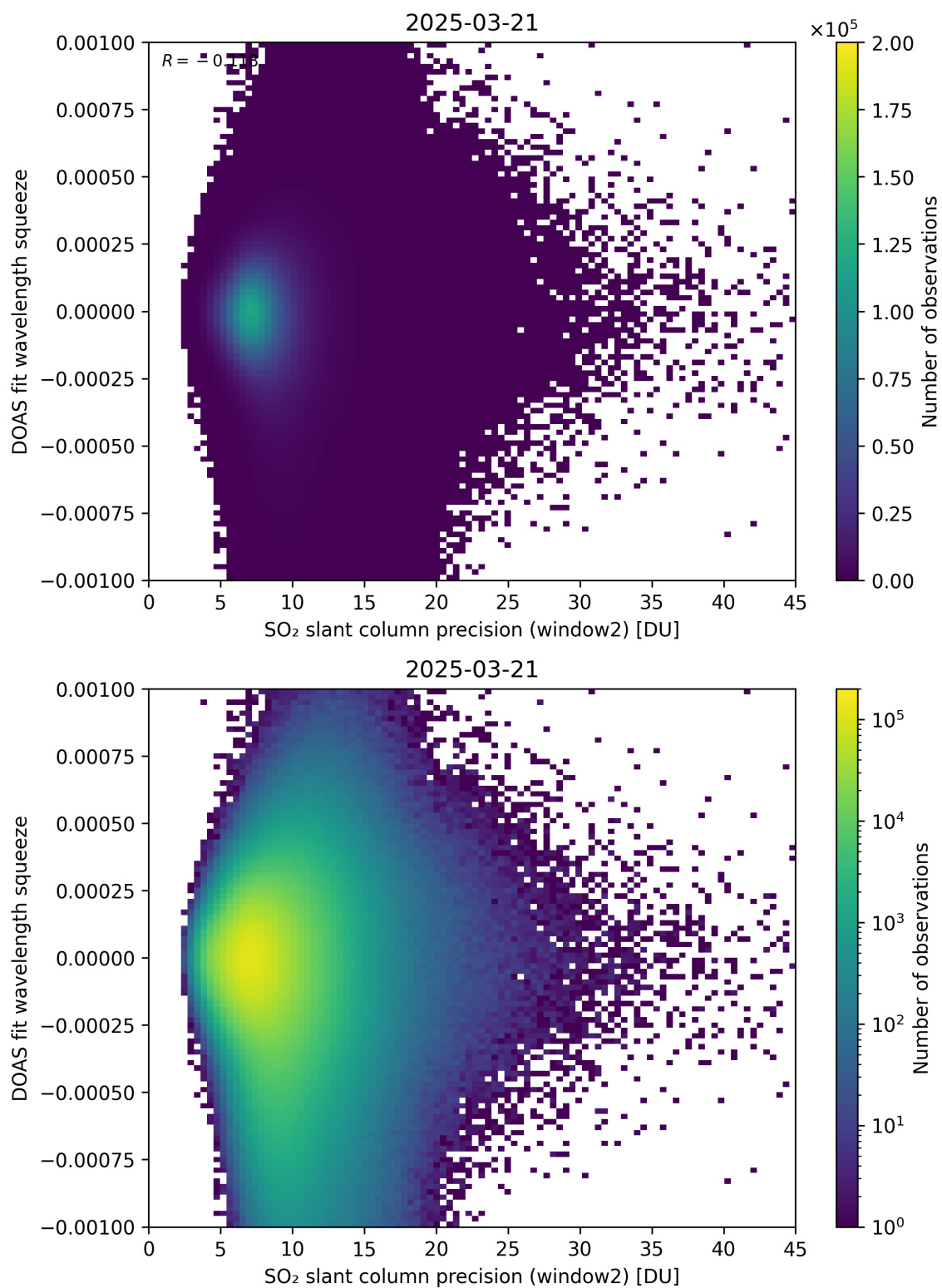
Figure 294: Scatter density plot of “SO 2 slant column precision (window2)” against “DOAS fit wavelength squeeze” for 2025-03-20 to 2025-03-22.
