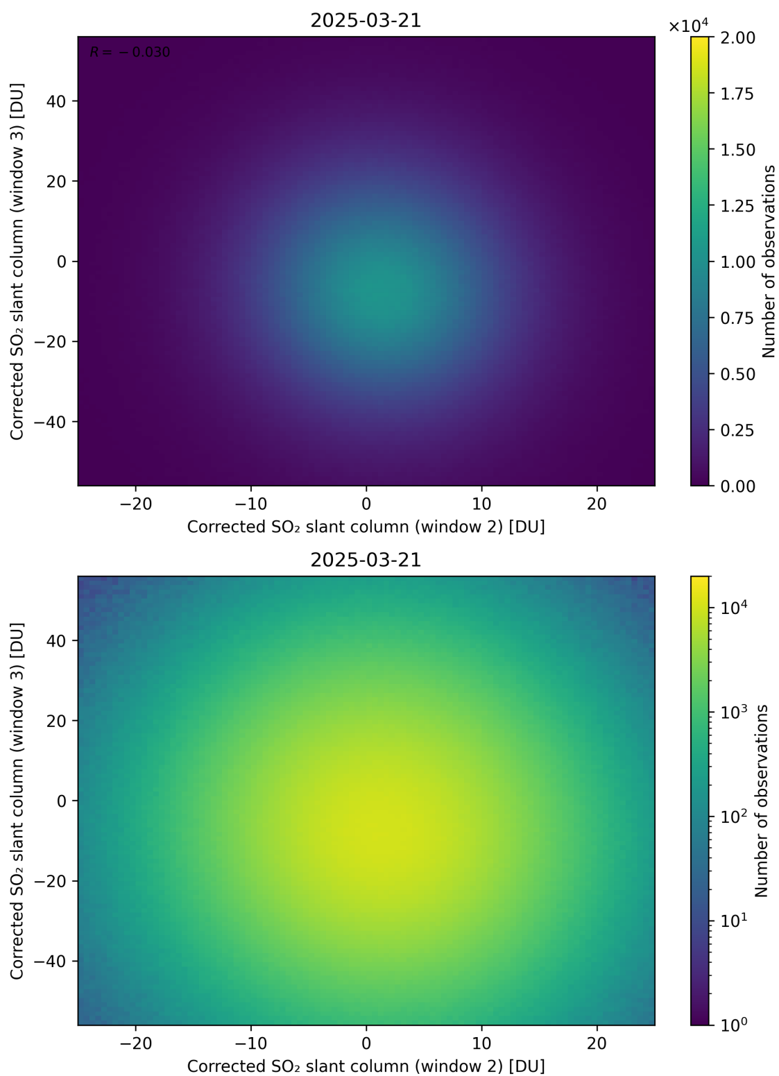
Figure 250: Scatter density plot of “Corrected SO 2 slant column (window 2)” against “Corrected SO 2 slant column (window 3)” for 2025-03-20 to 2025-03-22.
