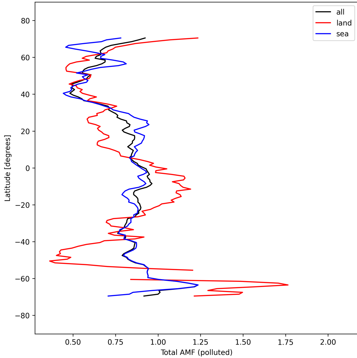
Figure 53: Zonal average of “Total AMF (polluted)” for 2025-03-20 to 2025-03-22.
