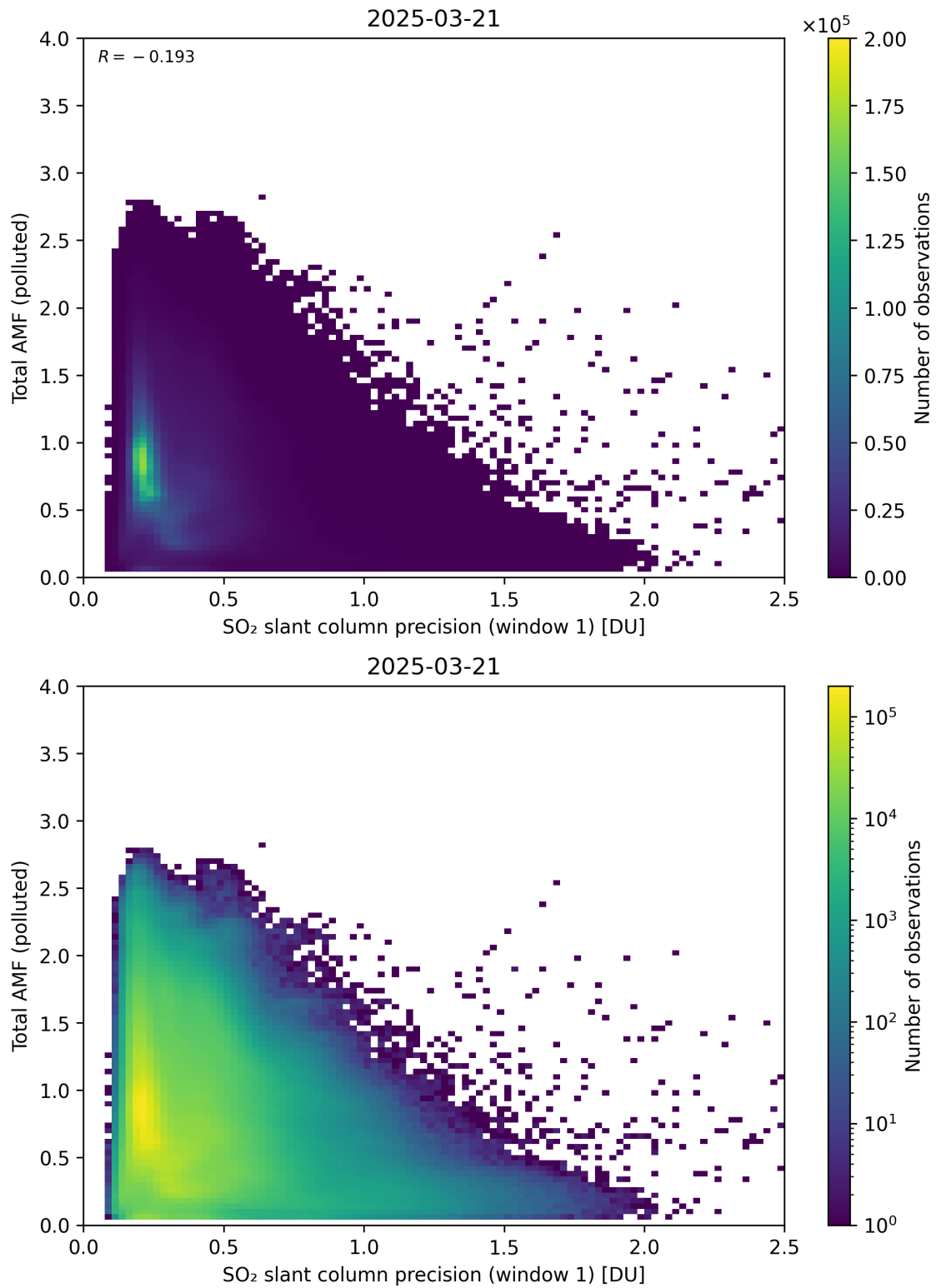
Figure 280: Scatter density plot of “SO 2 slant column precision (window 1)” against “Total AMF (polluted)” for 2025-03-20 to 2025-03-22.
