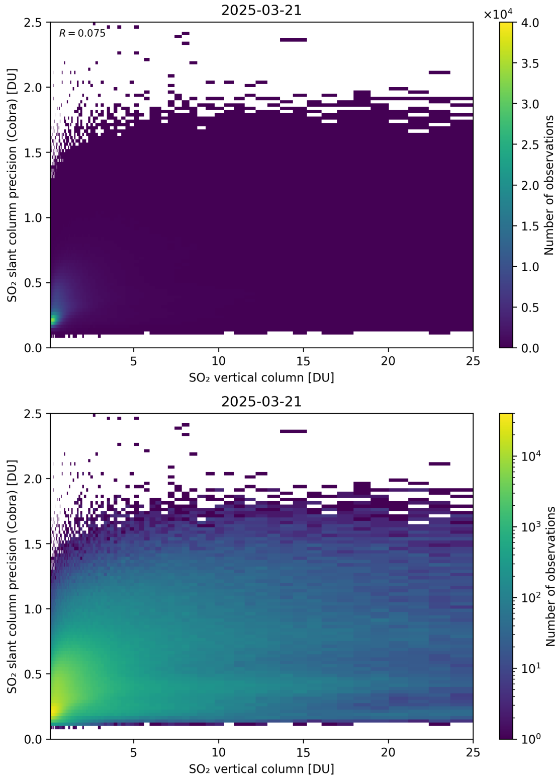
Figure 350: Scatter density plot of “SO 2 vertical column” against “SO 2 slant column precision (Cobra)” for 2025-03-20 to 2025-03-22.
