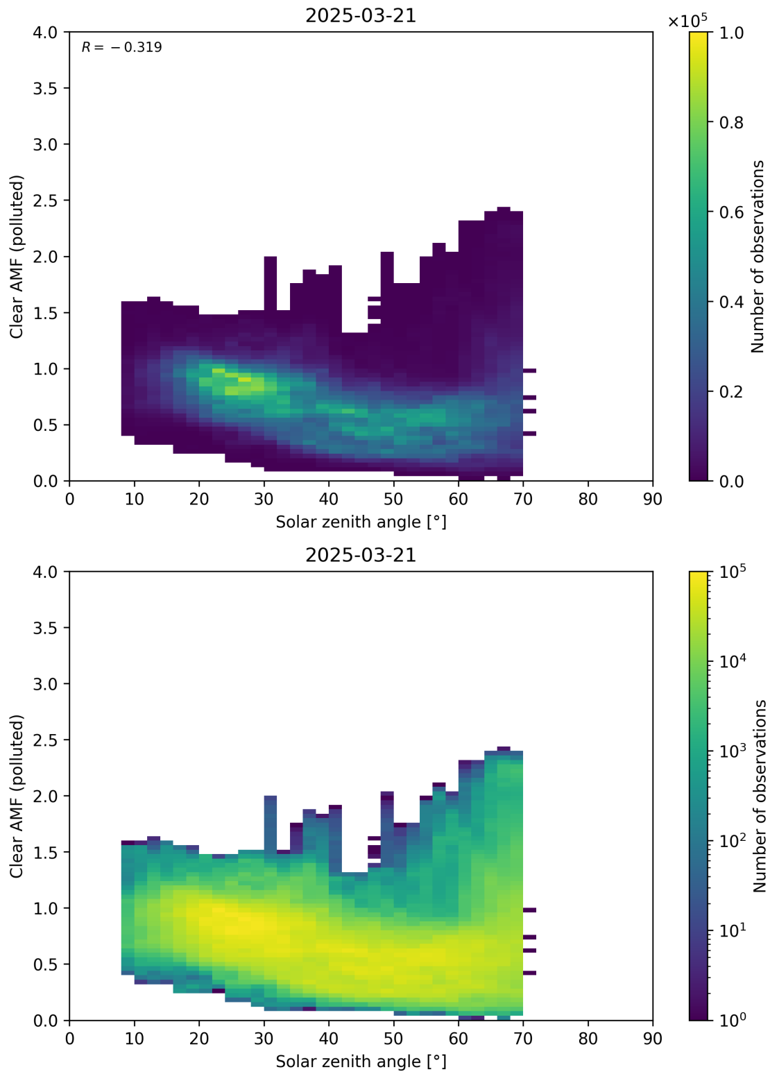
Figure 178: Scatter density plot of “Solar zenith angle” against “Clear AMF (polluted)” for 2025-03-20 to 2025-03-22.
