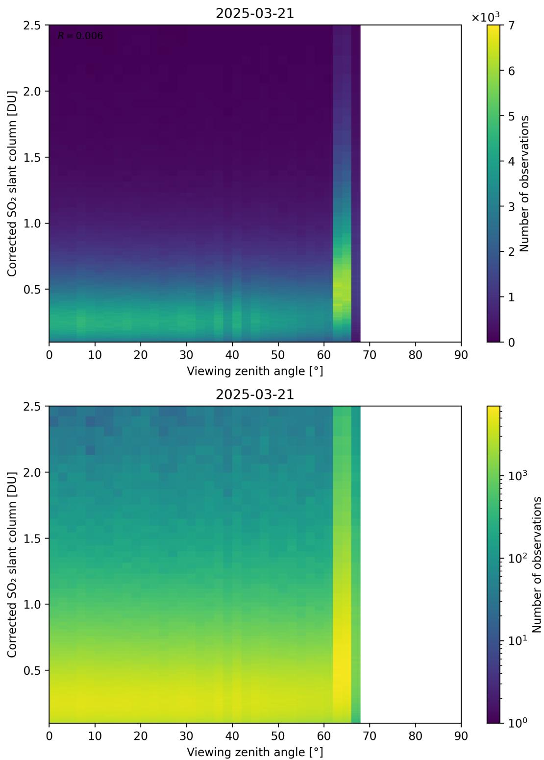
Figure 373: Scatter density plot of “Viewing zenith angle” against “Corrected SO 2 slant column” for 2025-03-20 to 2025-03-22.
