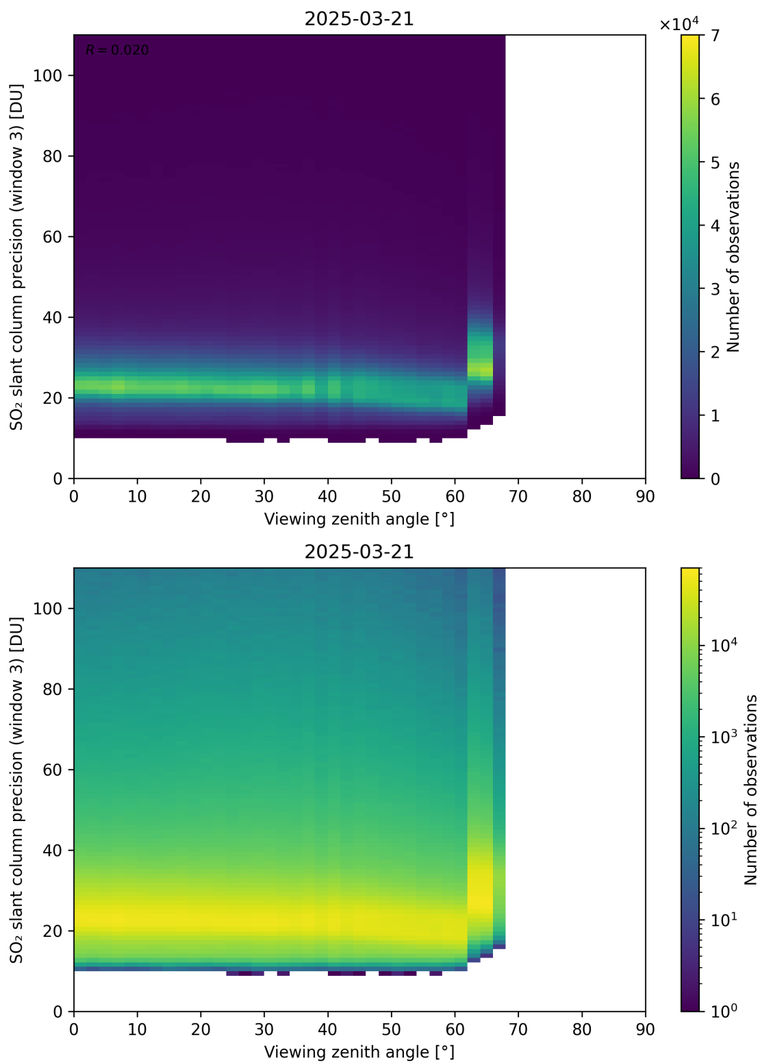
Figure 380: Scatter density plot of “Viewing zenith angle” against “SO 2 slant column precision (window 3)” for 2025-03-20 to 2025-03-22.
