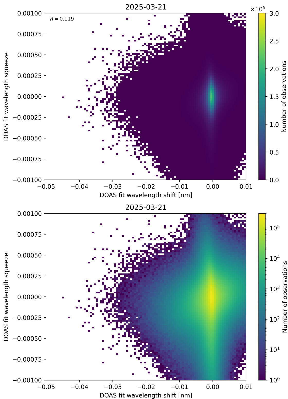
Figure 138: Scatter density plot of “DOAS fit wavelength shift” against “DOAS fit wavelength squeeze” for 2025-03-20 to 2025-03-22.
