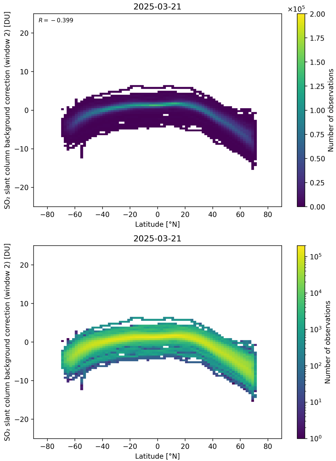
Figure 151: Scatter density plot of “Latitude” against “SO 2 slant column background correction (window 2)” for 2025-03-20 to 2025-03-22.
