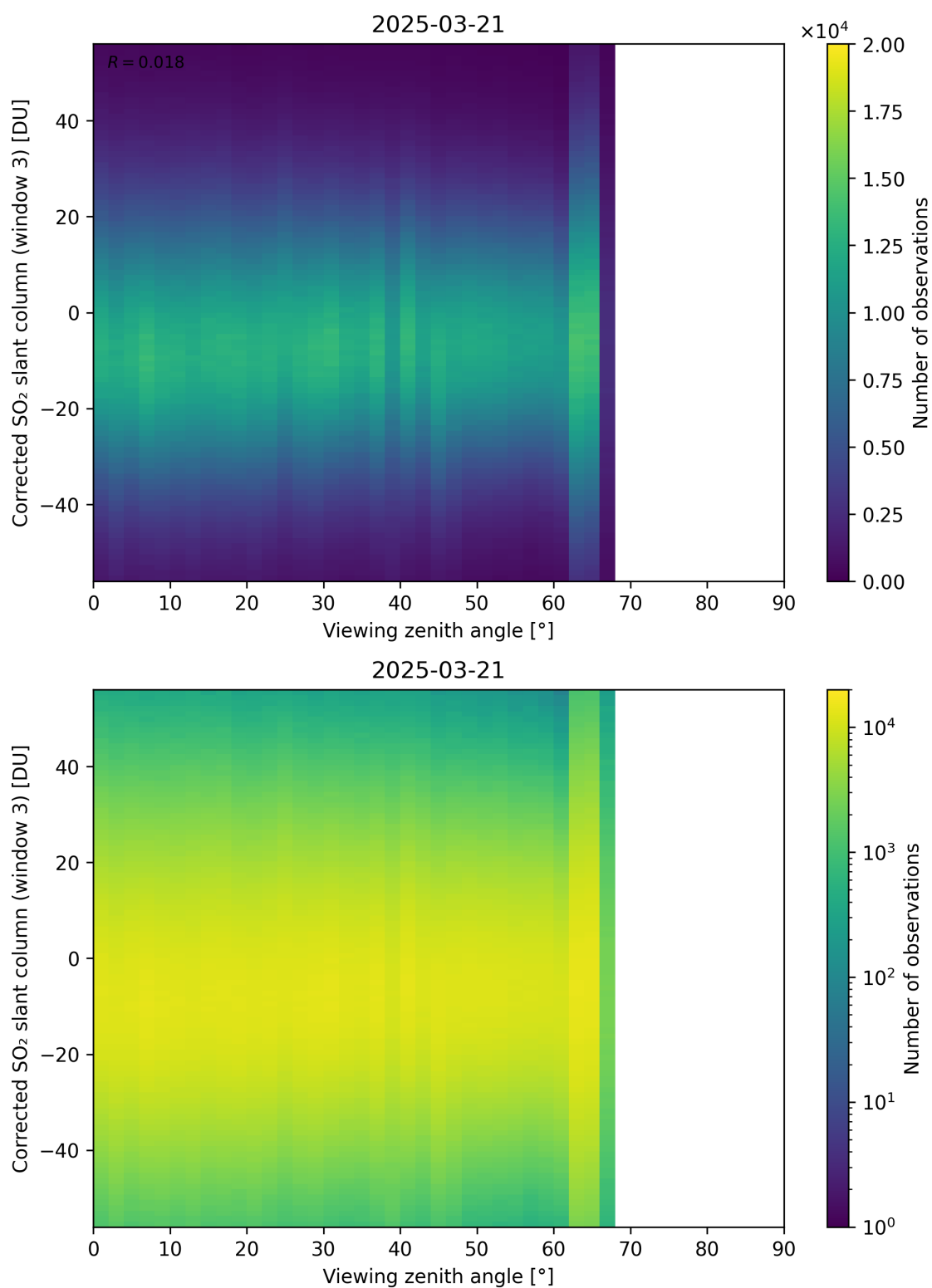
Figure 375: Scatter density plot of “Viewing zenith angle” against “Corrected SO 2 slant column (window 3)” for 2025-03-20 to 2025-03-22.
