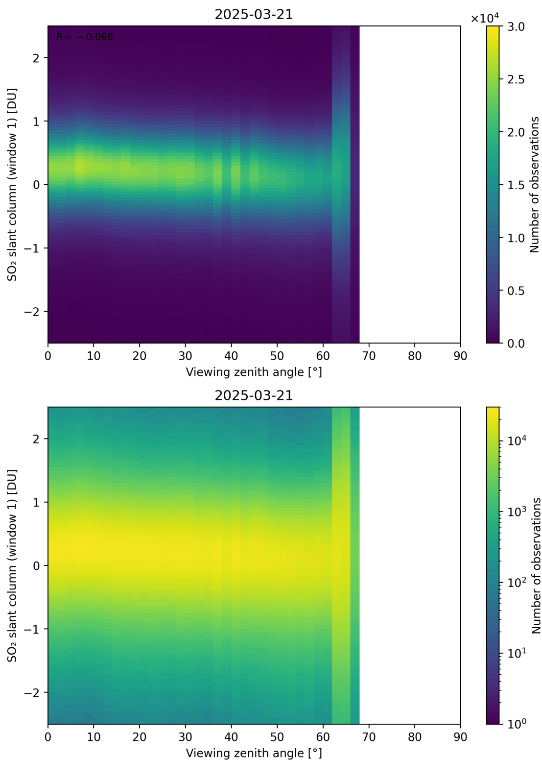
Figure 376: Scatter density plot of “Viewing zenith angle” against “SO 2 slant column (window 1)” for 2025-03-20 to 2025-03-22.
