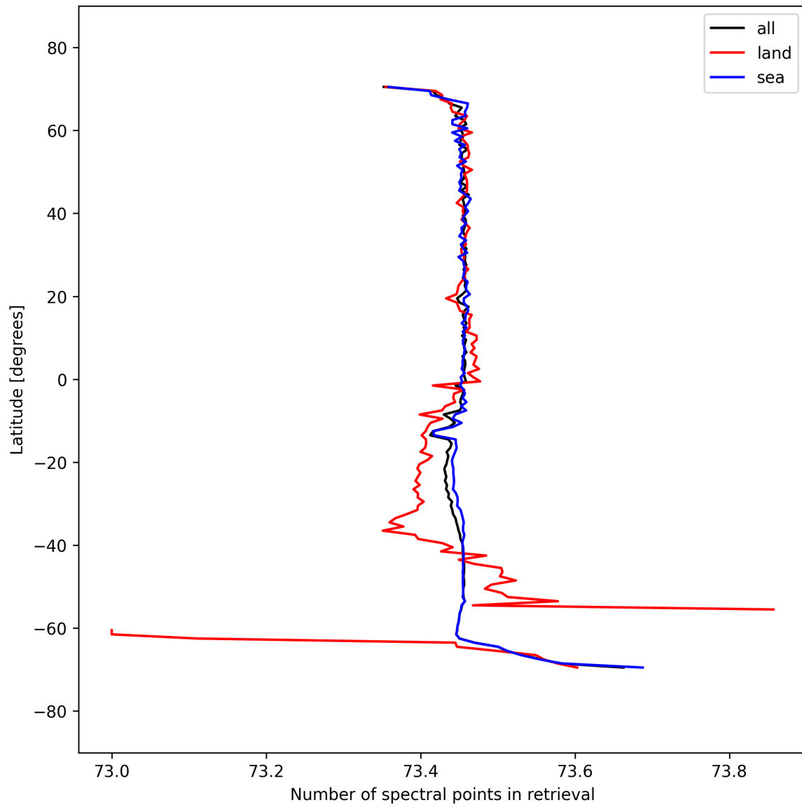
Figure 56: Zonal average of “Number of spectral points in retrieval” for 2025-03-20 to 2025-03-22.
