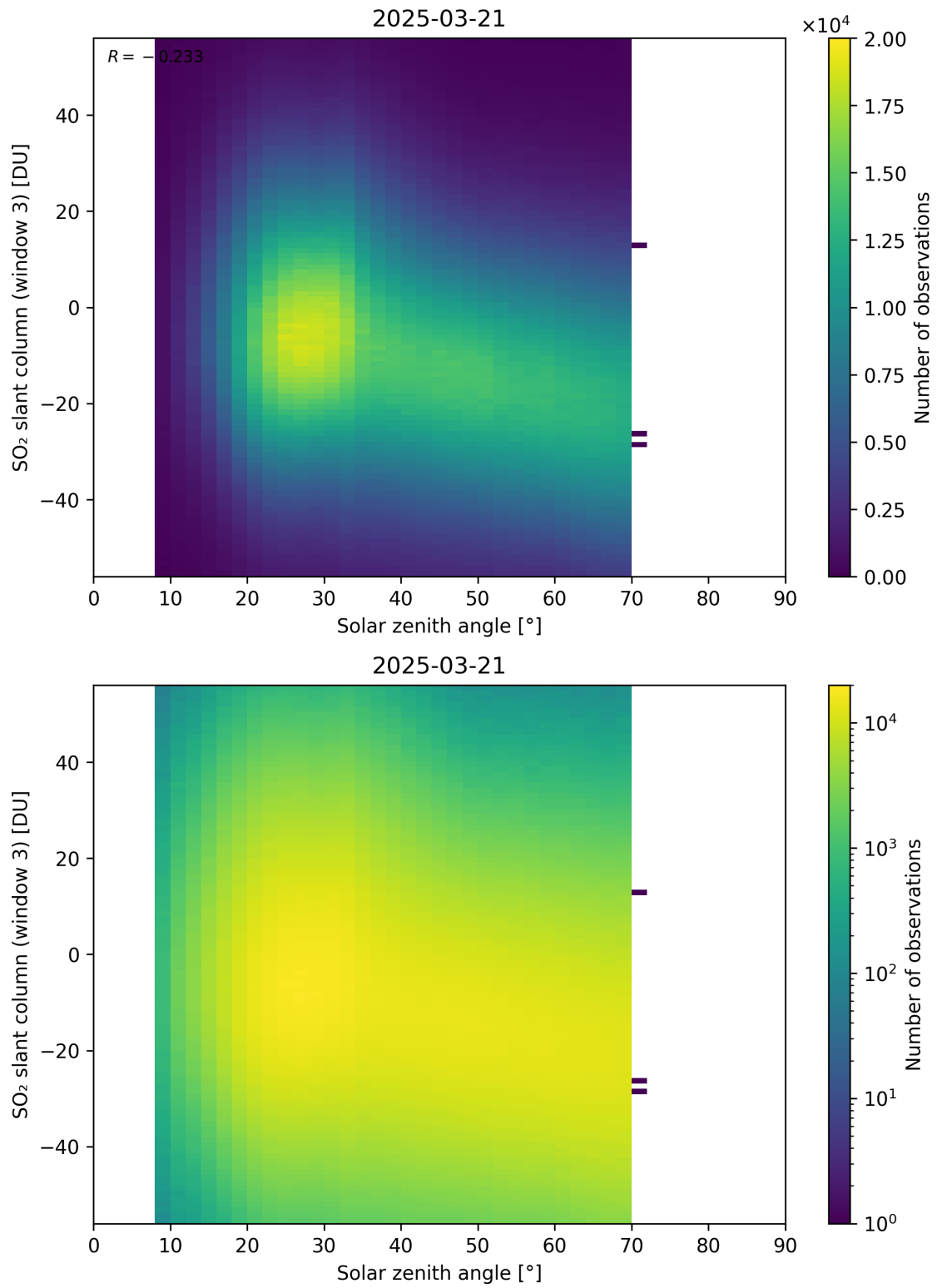
Figure 187: Scatter density plot of “Solar zenith angle” against “SO 2 slant column (window 3)” for 2025-03-20 to 2025-03-22.
