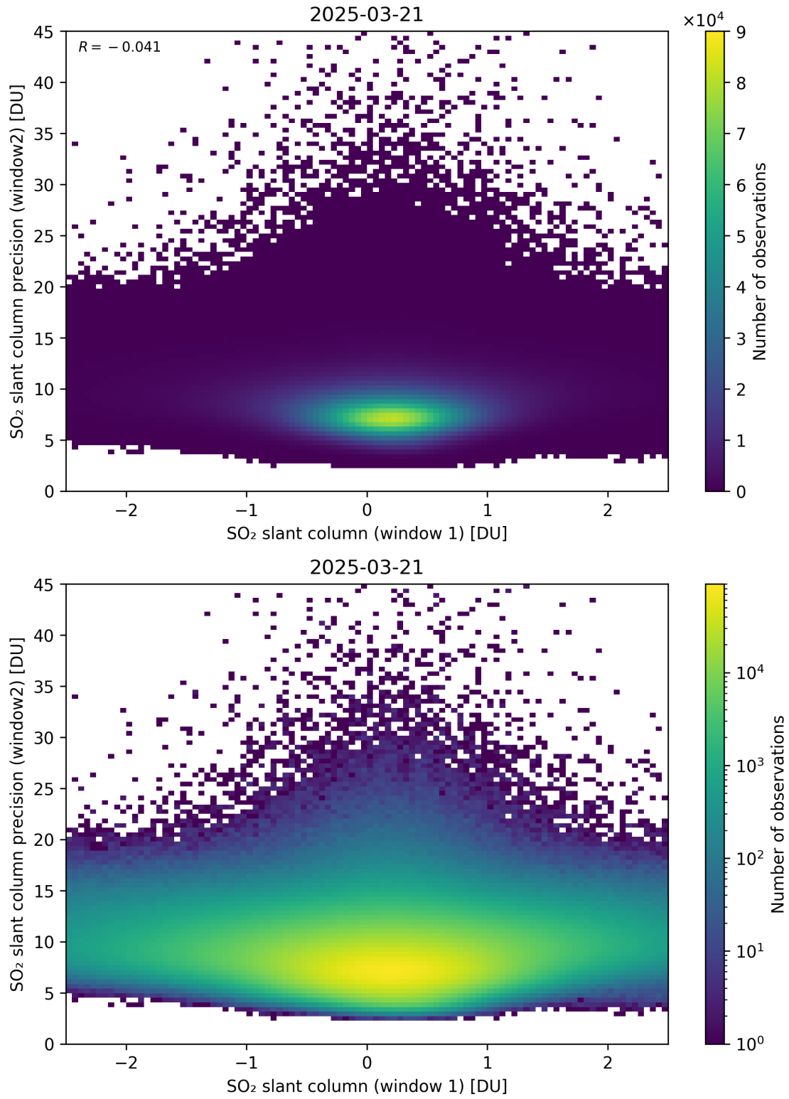
Figure 286: Scatter density plot of “SO 2 slant column (window 1)” against “SO 2 slant column precision (window2)” for 2025-03-20 to 2025-03-22.
