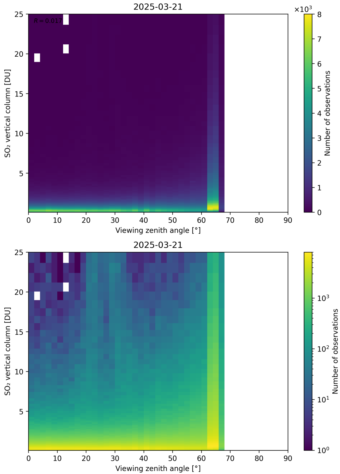
Figure 383: Scatter density plot of “Viewing zenith angle” against “SO 2 vertical column” for 2025-03-20 to 2025-03-22.
