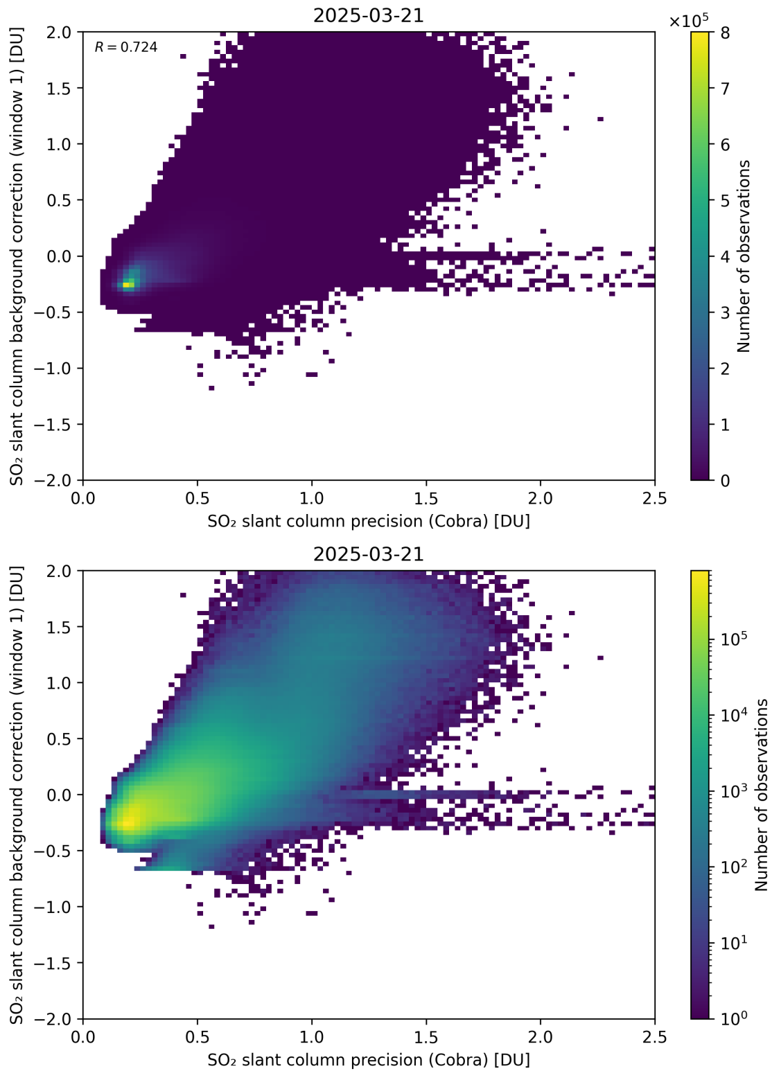
Figure 199: Scatter density plot of “SO 2 slant column precision (Cobra)” against “SO 2 slant column background correction (window 1)” for 2025-03-20 to 2025-03-22.
