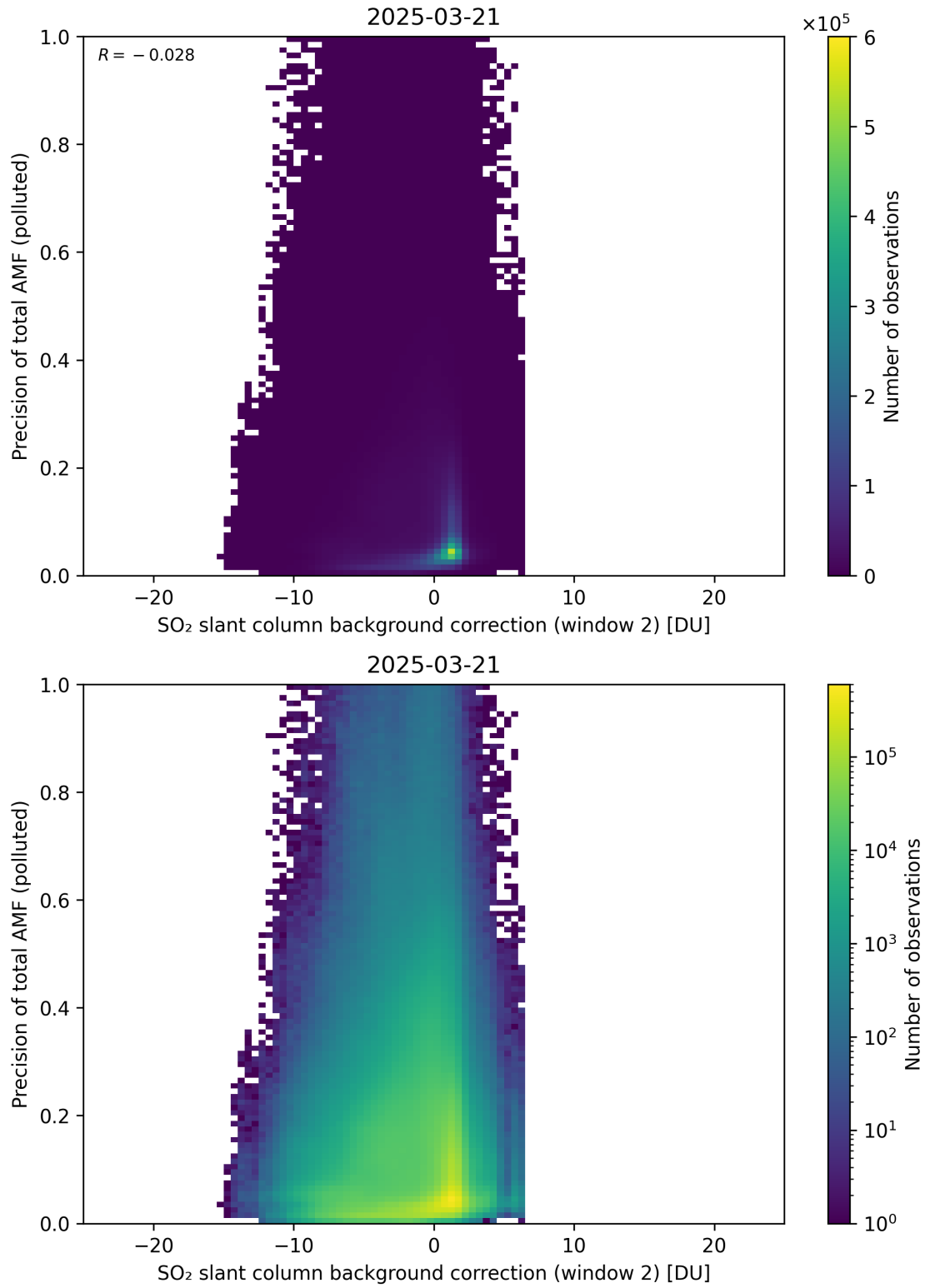
Figure 131: Scatter density plot of “SO 2 slant column background correction (window 2)” against “Precision of total AMF (polluted)” for 2025-03-20 to 2025-03-22.
