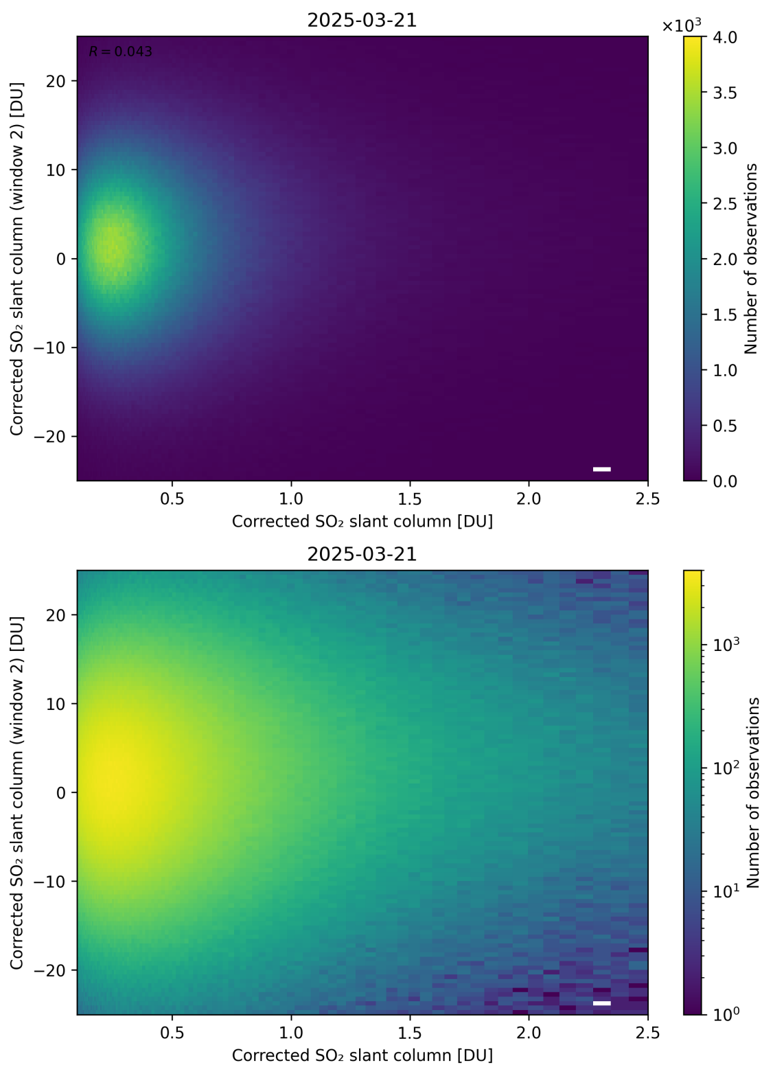
Figure 235: Scatter density plot of “Corrected SO 2 slant column” against “Corrected SO 2 slant column (window 2)” for 2025-03-20 to 2025-03-22.
