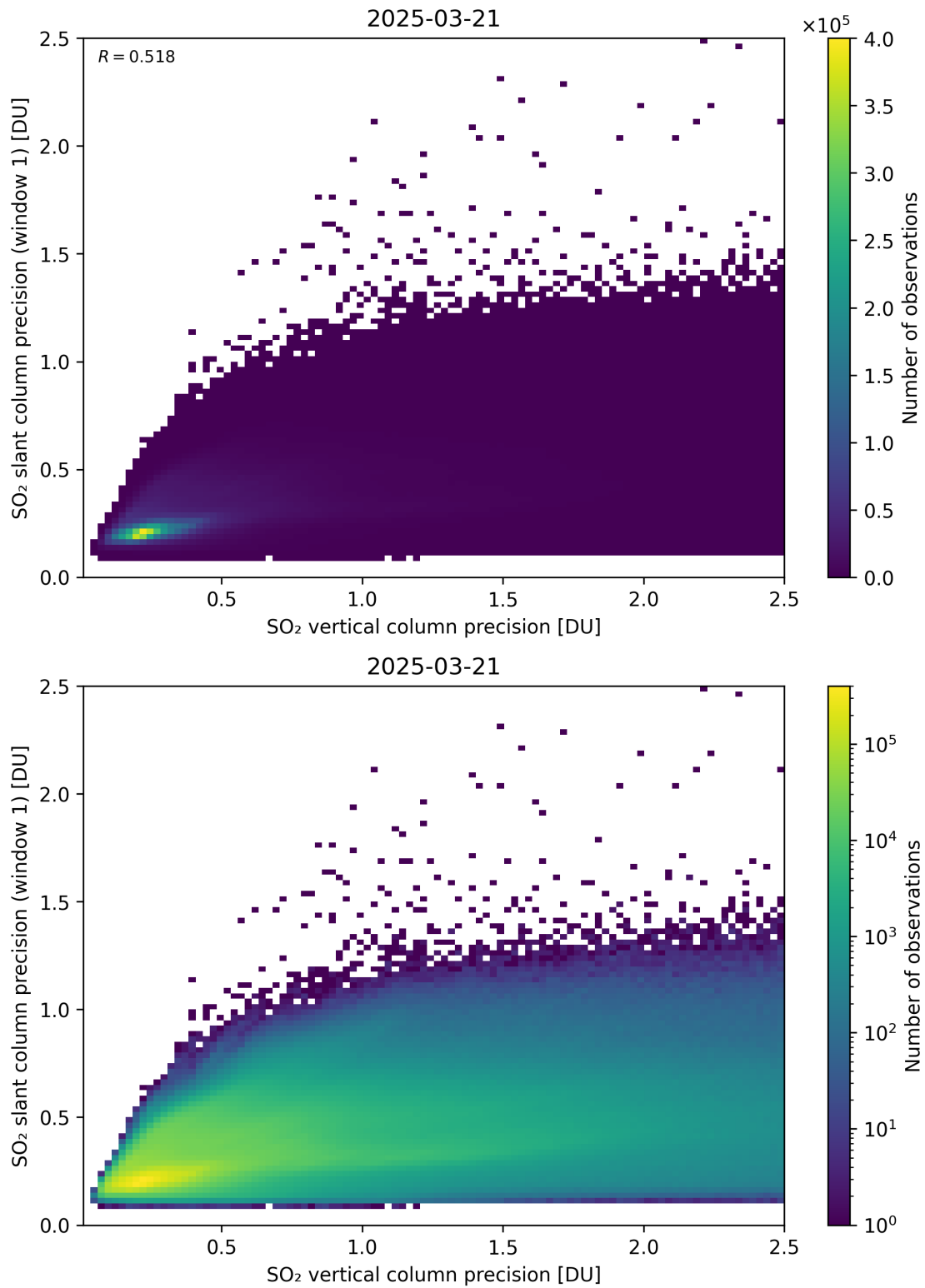
Figure 342: Scatter density plot of “SO 2 vertical column precision” against “SO 2 slant column precision (window 1)” for 2025-03-20 to 2025-03-22.
