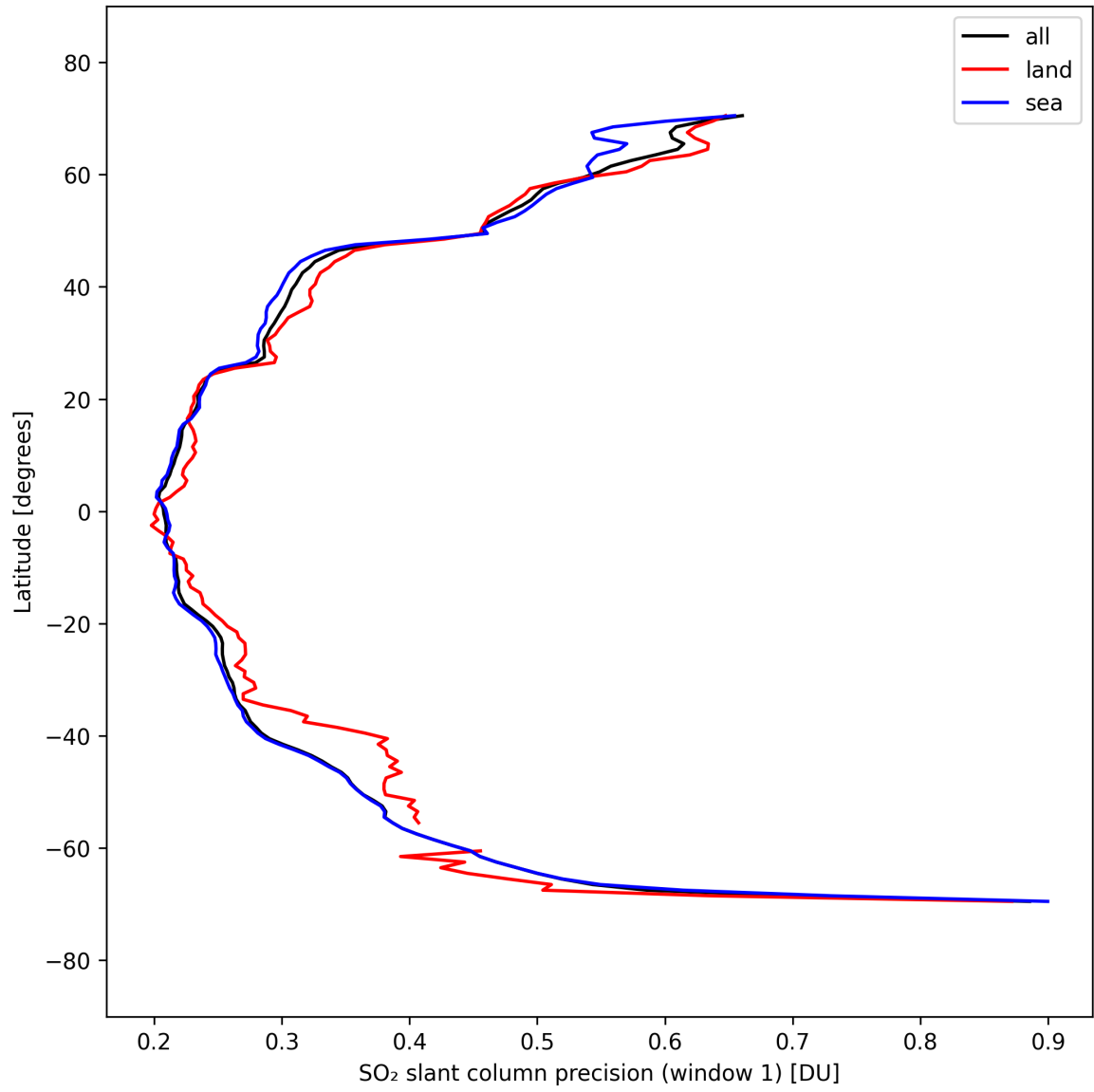
Figure 38: Zonal average of “SO 2 slant column precision (window 1)” for 2025-03-20 to 2025-03-22.
