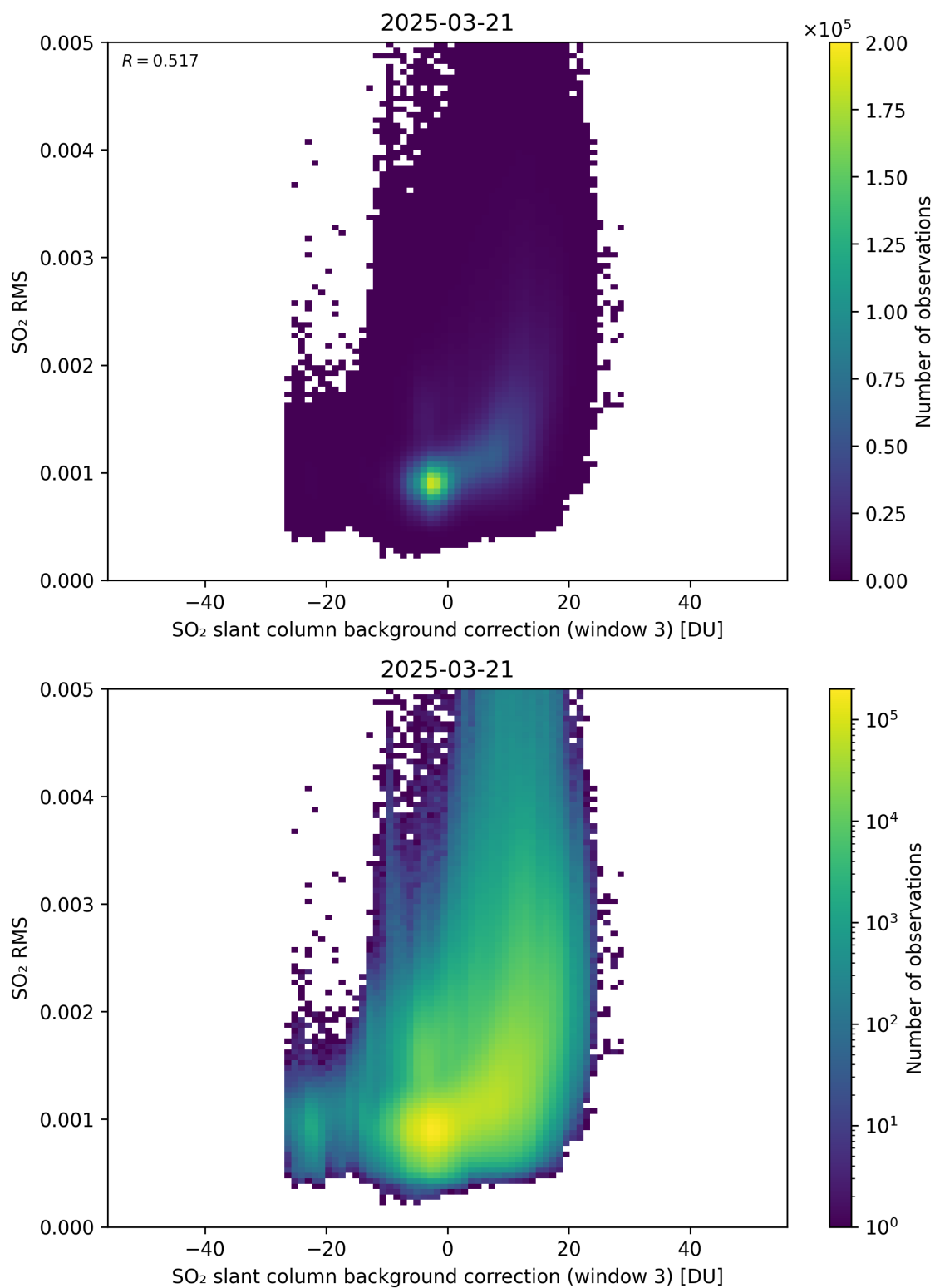
Figure 134: Scatter density plot of “SO 2 slant column background correction (window 3)” against “SO 2 RMS” for 2025-03-20 to 2025-03-22.
