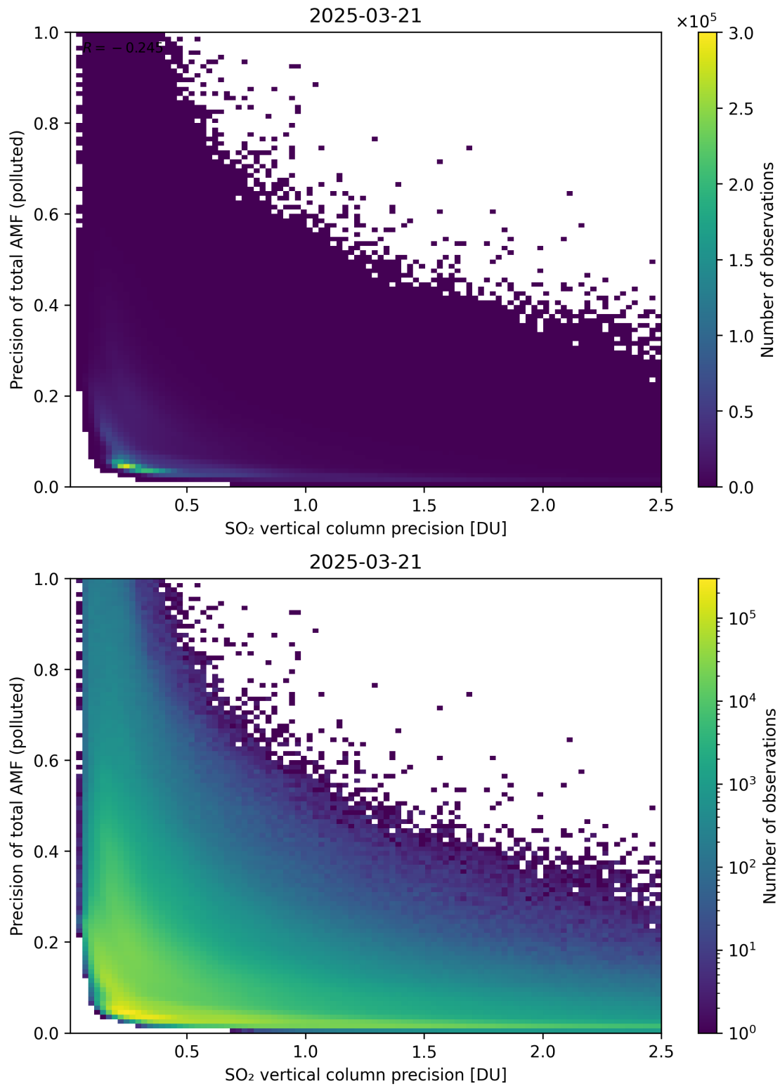
Figure 347: Scatter density plot of “SO 2 vertical column precision” against “Precision of total AMF (polluted)” for 2025-03-20 to 2025-03-22.
