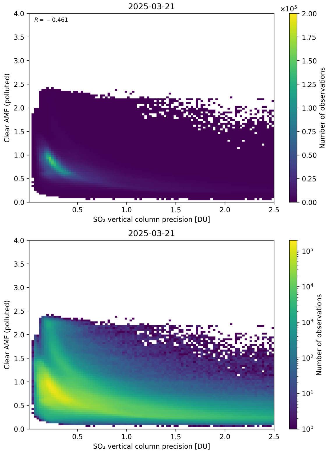
Figure 335: Scatter density plot of “SO 2 vertical column precision” against “Clear AMF (polluted)” for 2025-03-20 to 2025-03-22.
