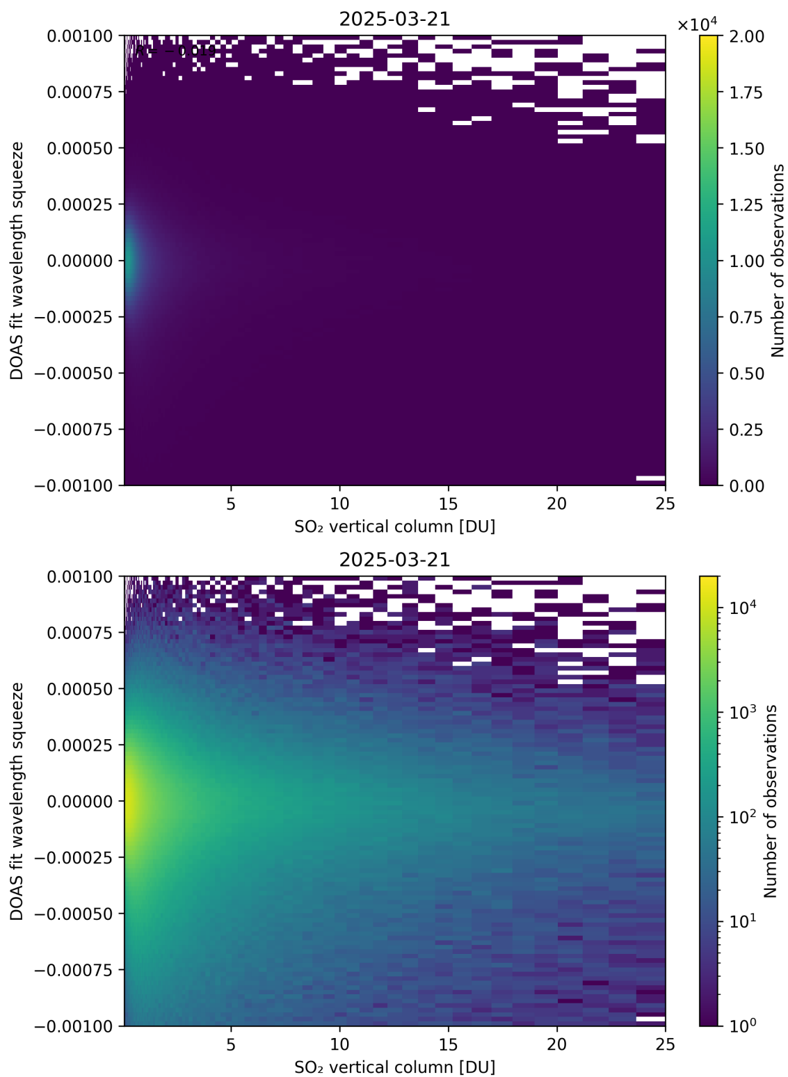
Figure 327: Scatter density plot of “SO 2 vertical column” against “DOAS fit wavelength squeeze” for 2025-03-20 to 2025-03-22.
