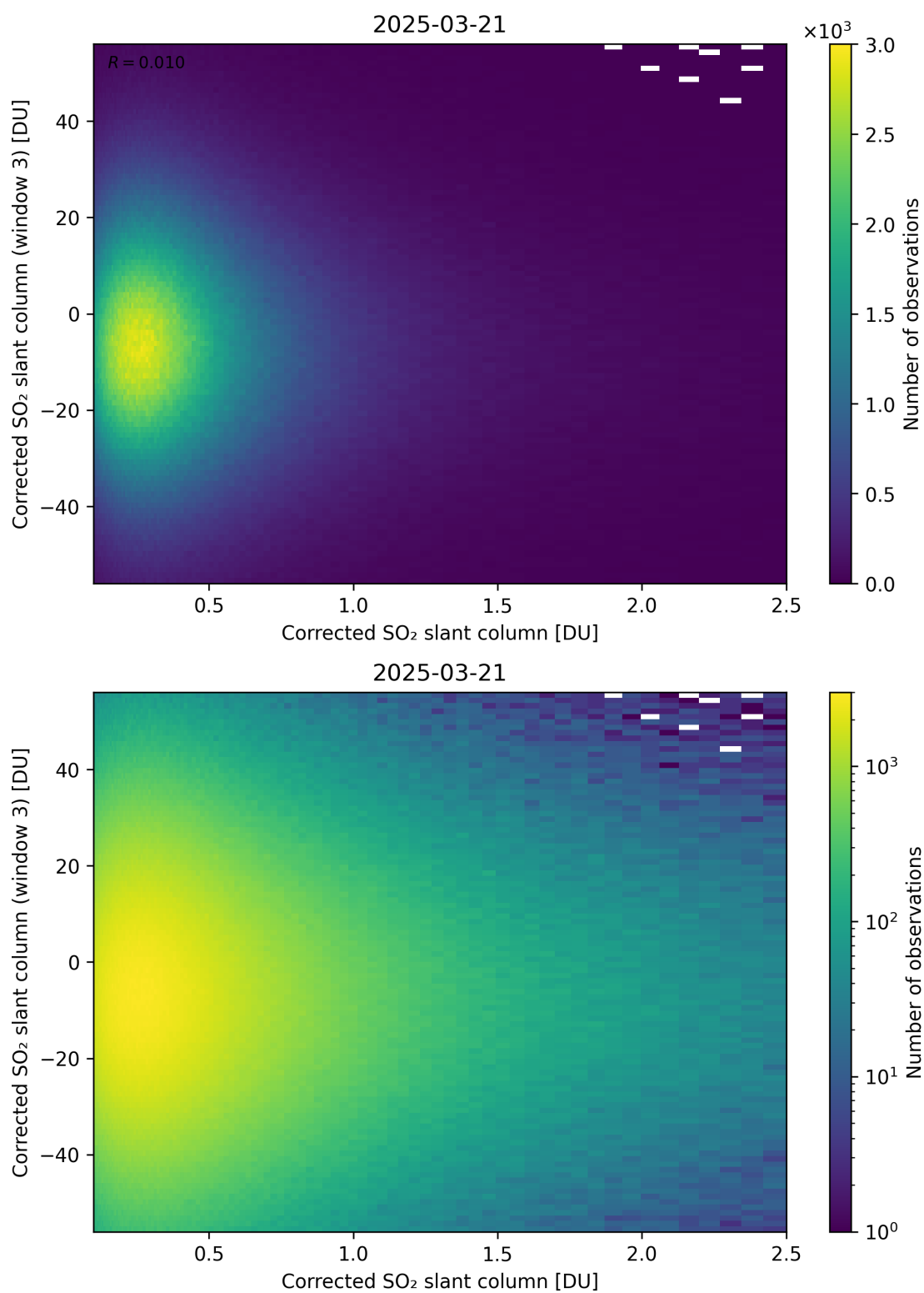
Figure 236: Scatter density plot of “Corrected SO 2 slant column” against “Corrected SO 2 slant column (window 3)” for 2025-03-20 to 2025-03-22.
