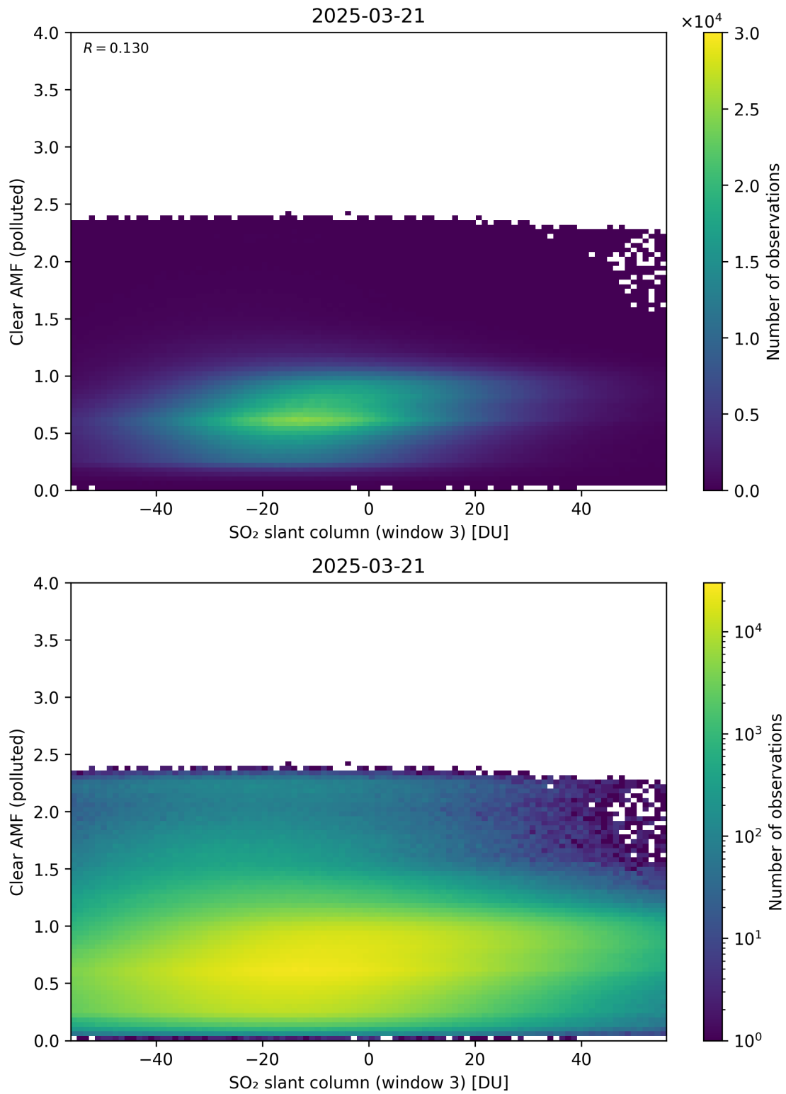
Figure 315: Scatter density plot of “SO 2 slant column (window 3)” against “Clear AMF (polluted)” for 2025-03-20 to 2025-03-22.
