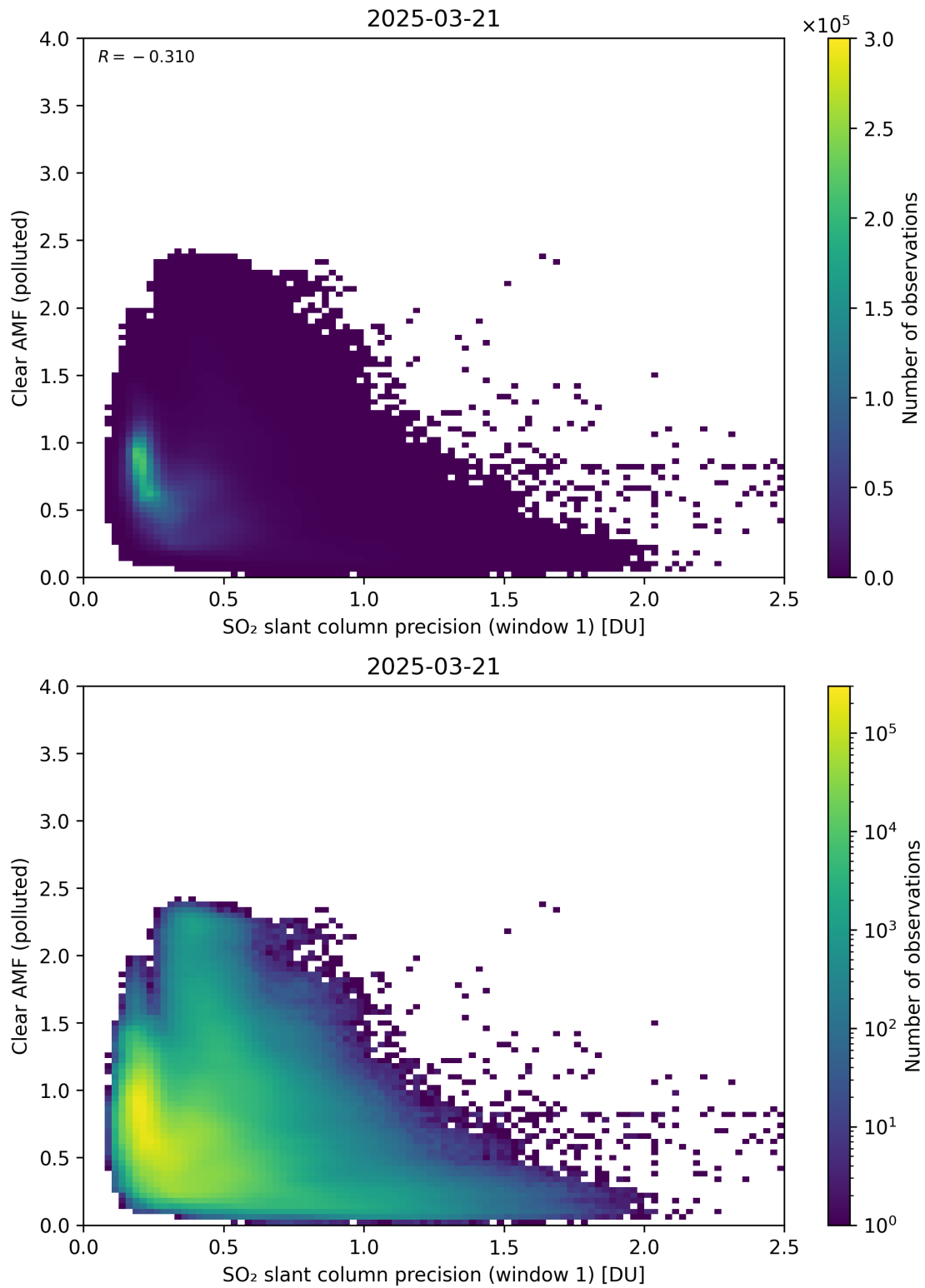
Figure 274: Scatter density plot of “SO 2 slant column precision (window 1)” against “Clear AMF (polluted)” for 2025-03-20 to 2025-03-22.
