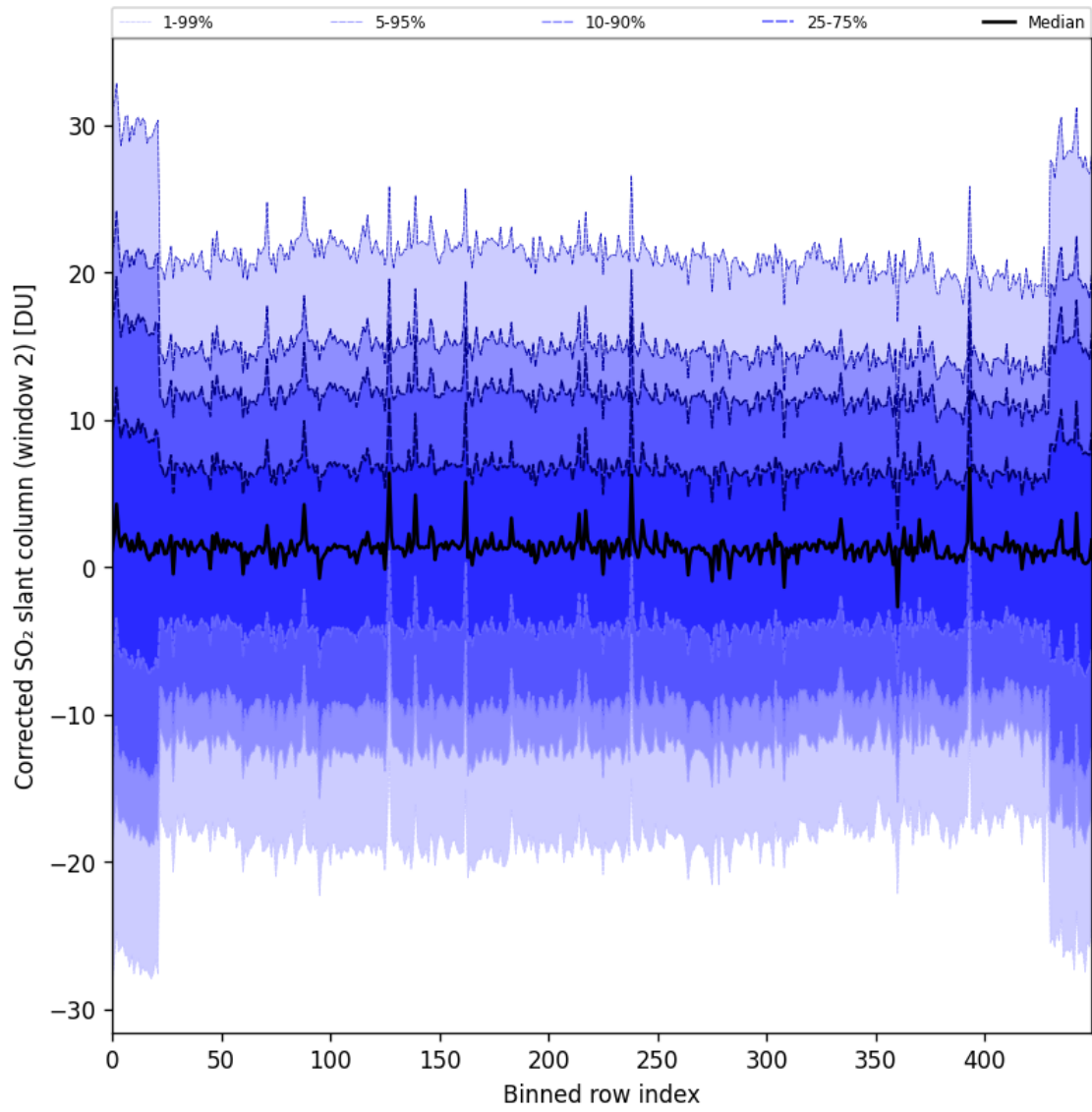
Figure 95: Along track statistics of “Corrected SO 2 slant column (window 2)” for 2025-03-20 to 2025-03-22
