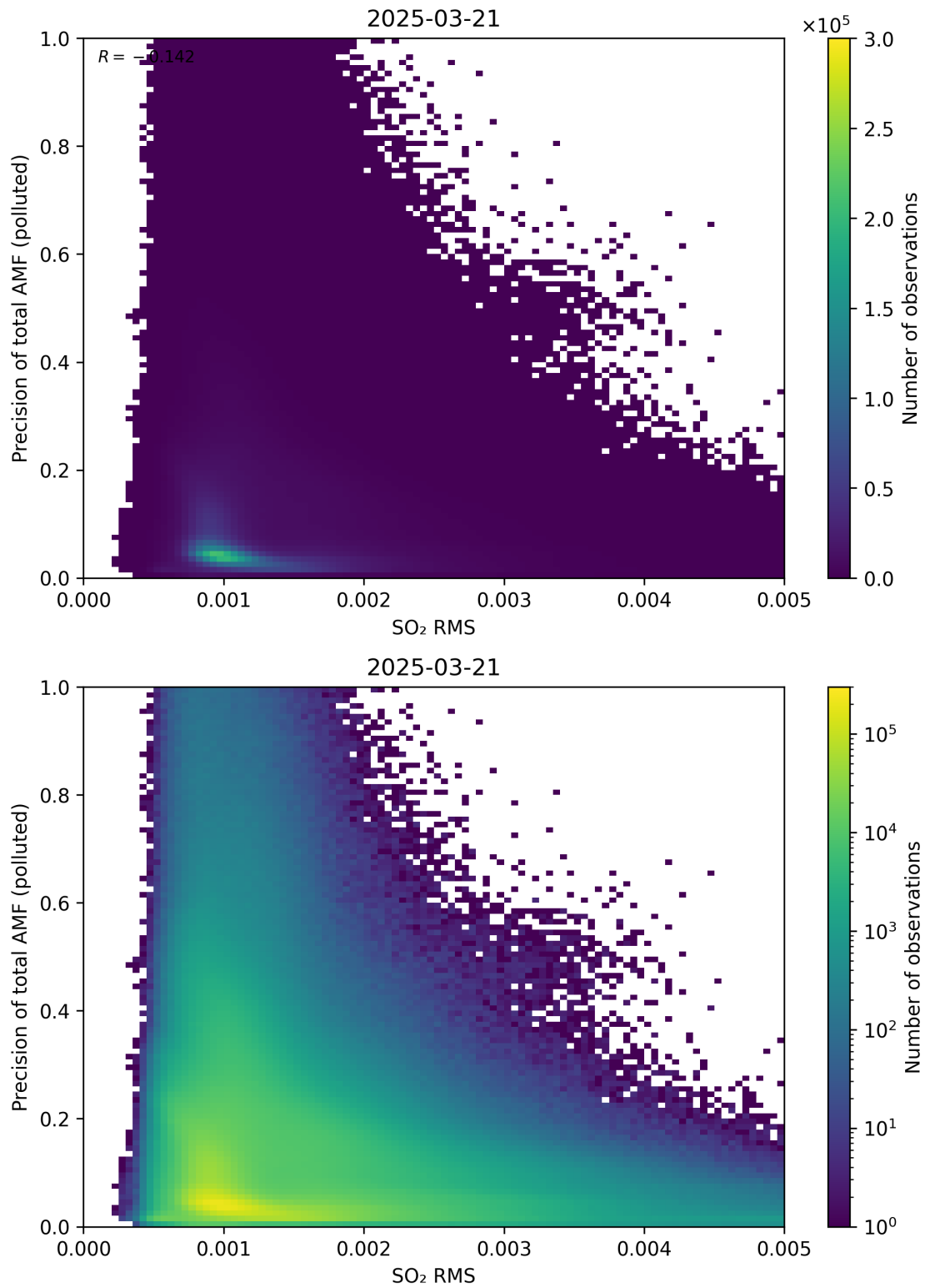
Figure 149: Scatter density plot of “SO 2 RMS” against “Precision of total AMF (polluted)” for 2025-03-20 to 2025-03-22.
