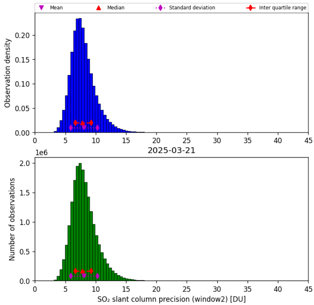
Figure 68: Histogram of “SO 2 slant column precision (window2)” for 2025-03-20 to 2025-03-22
