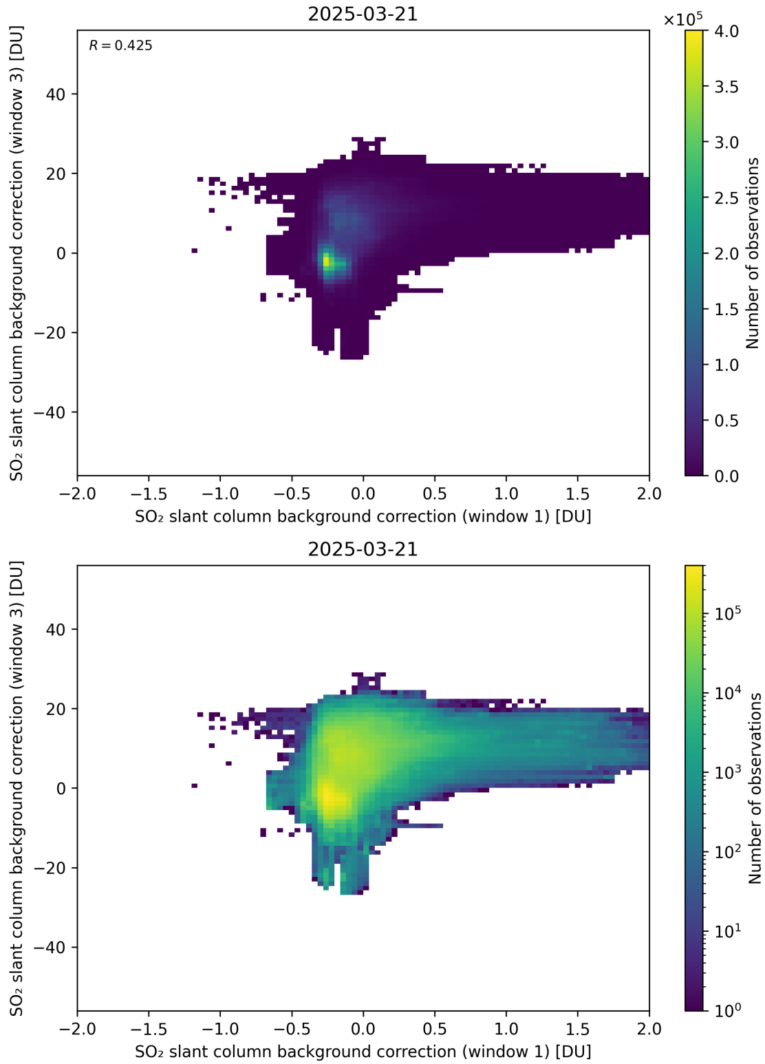
Figure 110: Scatter density plot of “SO 2 slant column background correction (window 1)” against “SO 2 slant column background correction (window 3)” for 2025-03-20 to 2025-03-22.
