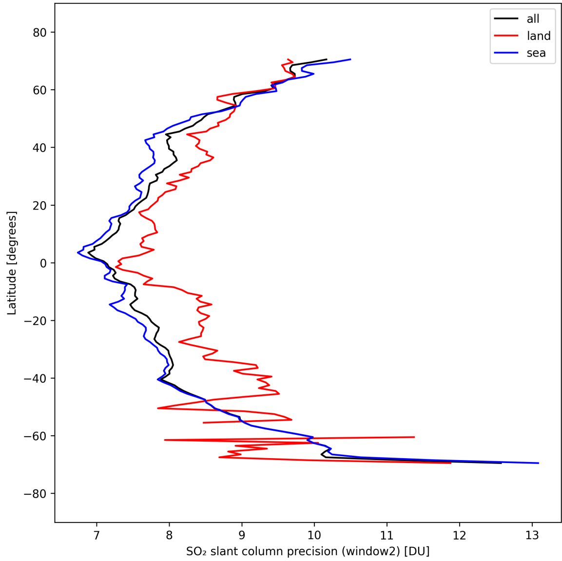
Figure 42: Zonal average of “SO 2 slant column precision (window2)” for 2025-03-20 to 2025-03-22.
