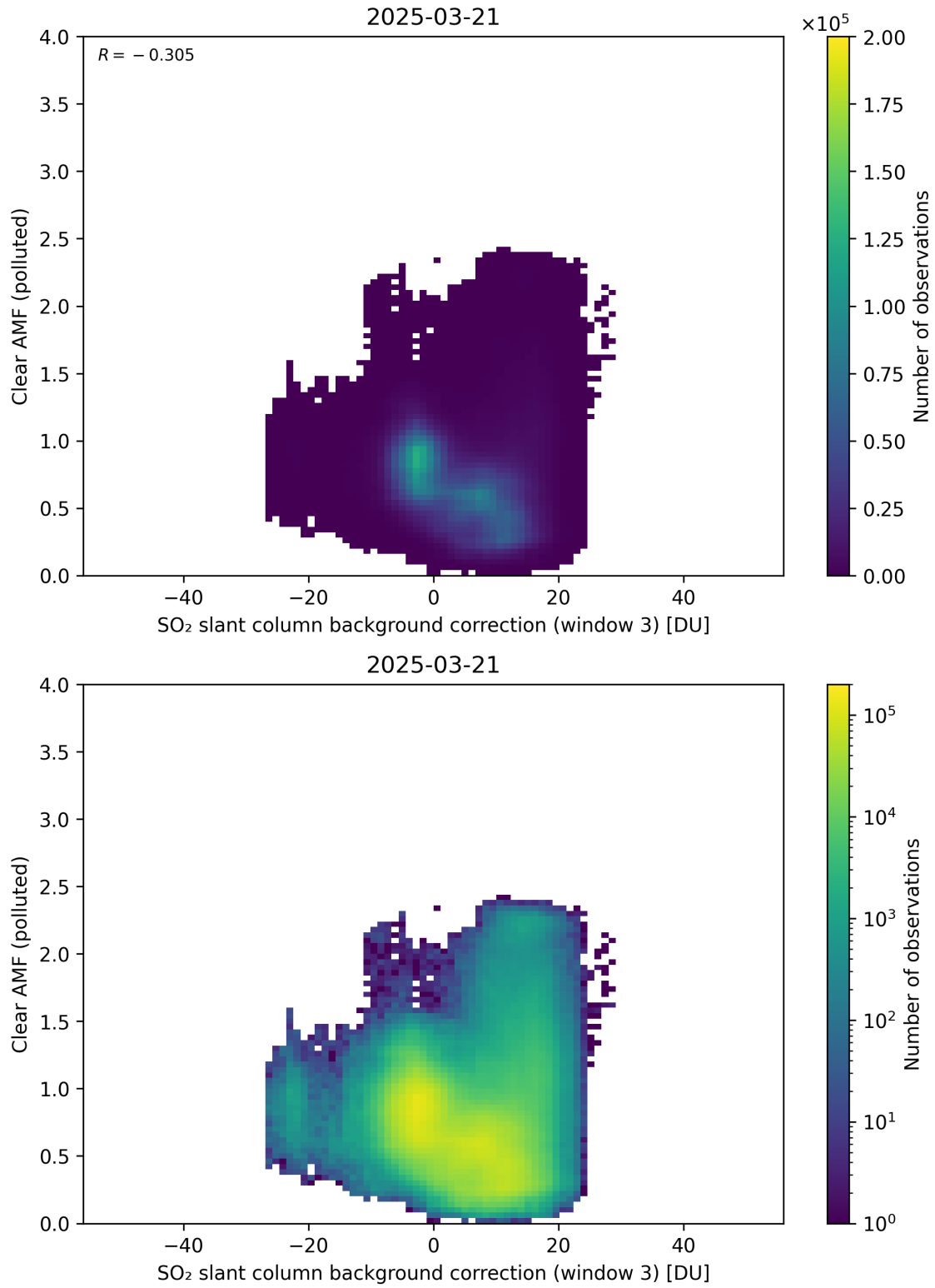
Figure 135: Scatter density plot of “SO 2 slant column background correction (window 3)” against “Clear AMF (polluted)” for 2025-03-20 to 2025-03-22.
