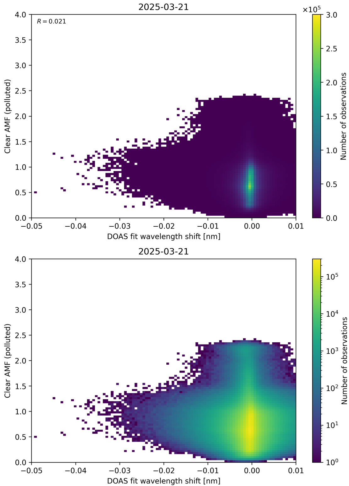
Figure 140: Scatter density plot of “DOAS fit wavelength shift” against “Clear AMF (polluted)” for 2025-03-20 to 2025-03-22.
