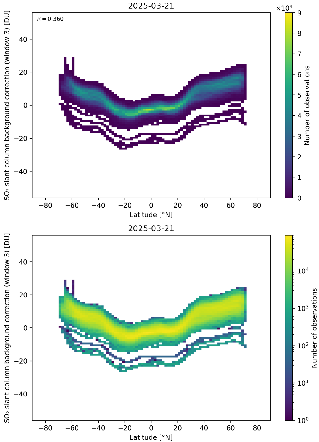
Figure 152: Scatter density plot of “Latitude” against “SO 2 slant column background correction (window 3)” for 2025-03-20 to 2025-03-22.
