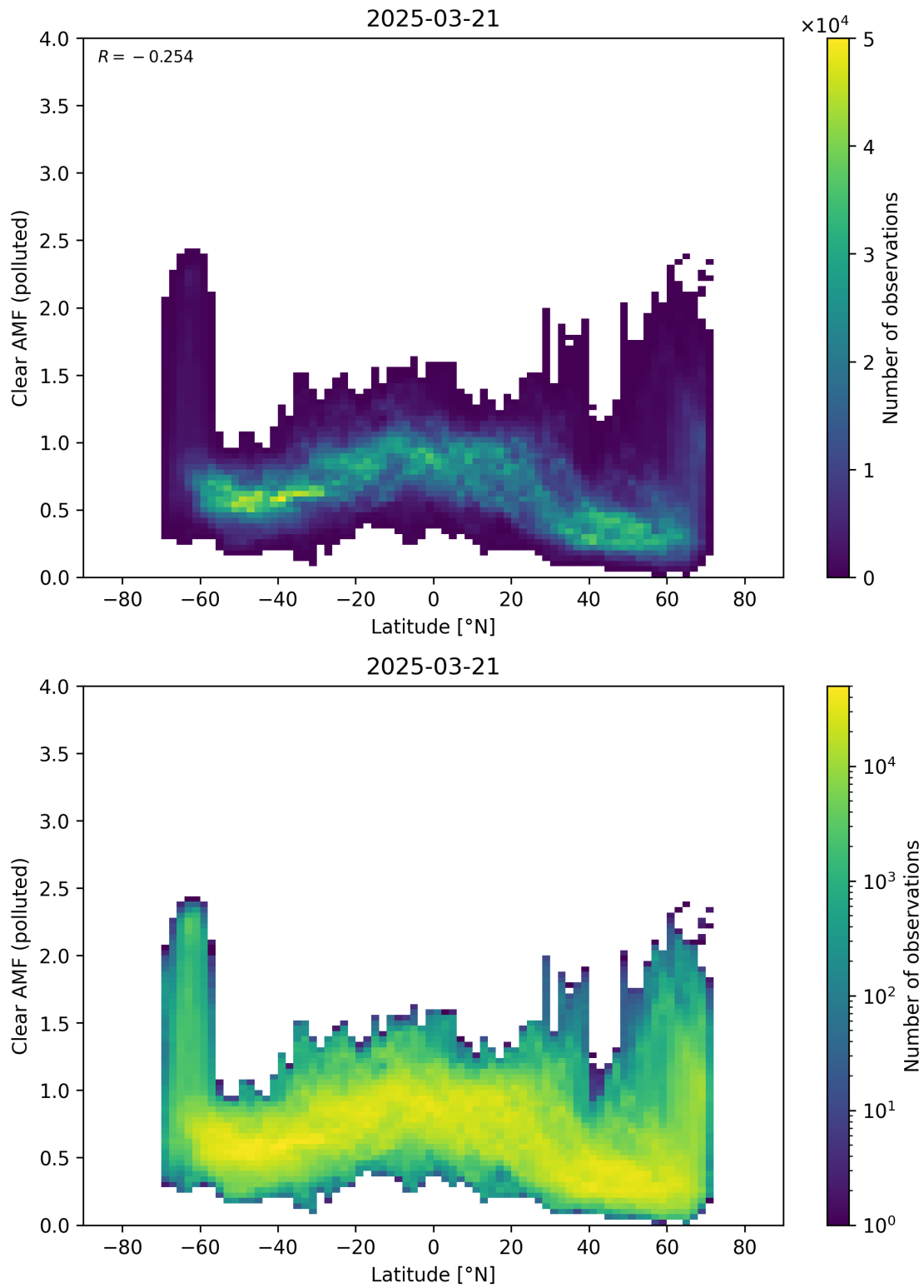
Figure 156: Scatter density plot of “Latitude” against “Clear AMF (polluted)” for 2025-03-20 to 2025-03-22.
