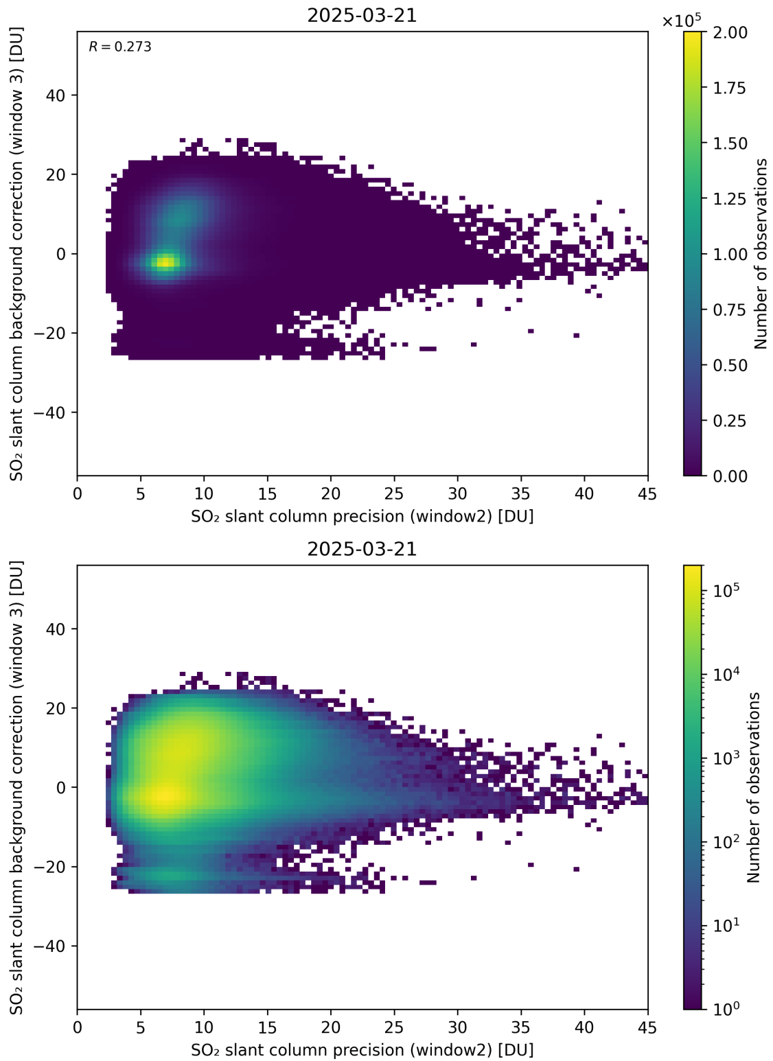
Figure 292: Scatter density plot of “SO 2 slant column precision (window2)” against “SO 2 slant column background correction (window 3)” for 2025-03-20 to 2025-03-22.
