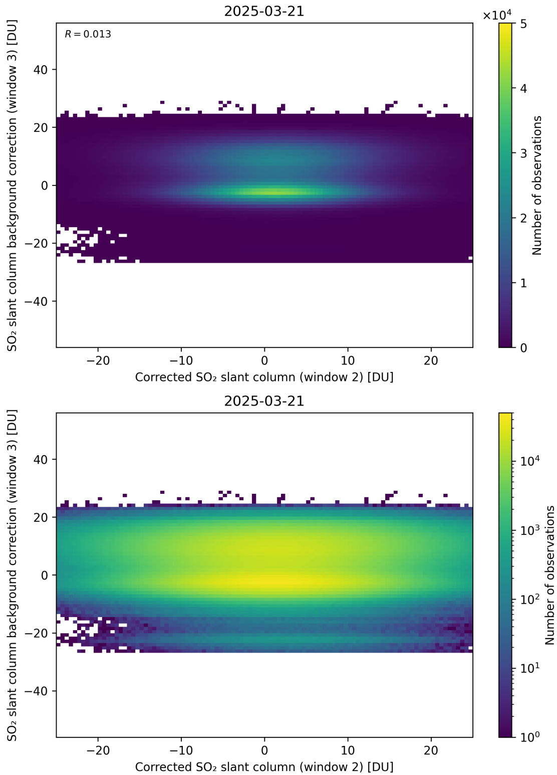
Figure 245: Scatter density plot of “Corrected SO 2 slant column (window 2)” against “SO 2 slant column background correction (window 3)” for 2025-03-20 to 2025-03-22.
