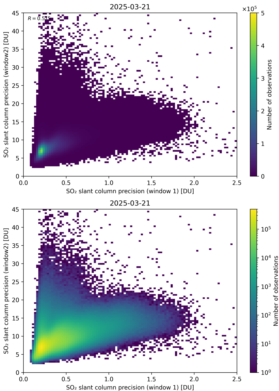
Figure 277: Scatter density plot of “SO 2 slant column precision (window 1)” against “SO 2 slant column precision (window2)” for 2025-03-20 to 2025-03-22.
