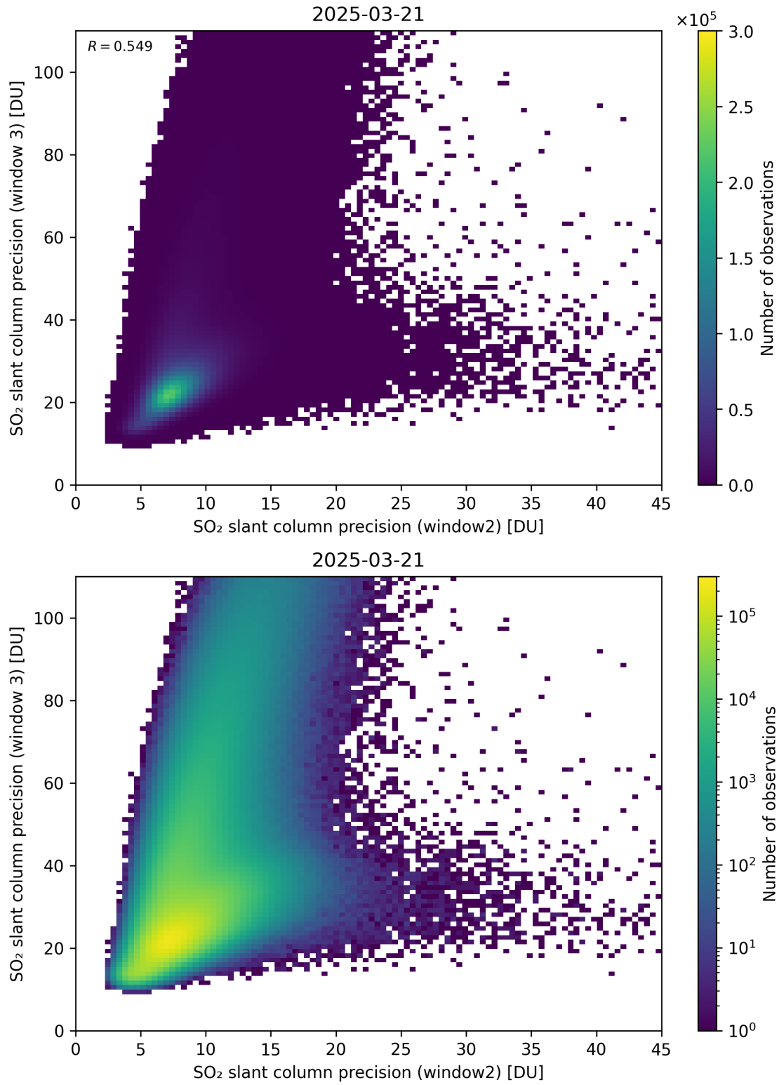
Figure 300: Scatter density plot of “SO 2 slant column precision (window2)” against “SO 2 slant column precision (window 3)” for 2025-03-20 to 2025-03-22.
