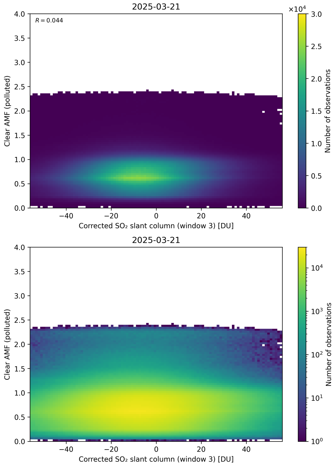
Figure 259: Scatter density plot of “Corrected SO 2 slant column (window 3)” against “Clear AMF (polluted)” for 2025-03-20 to 2025-03-22.
