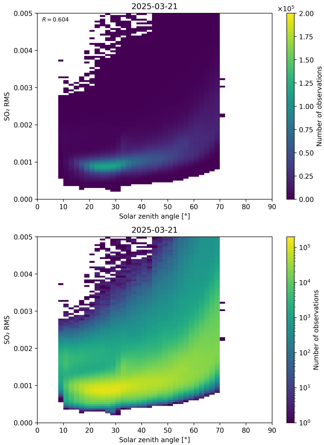
Figure 176: Scatter density plot of “Solar zenith angle” against “SO 2 RMS” for 2025-03-20 to 2025-03-22.
