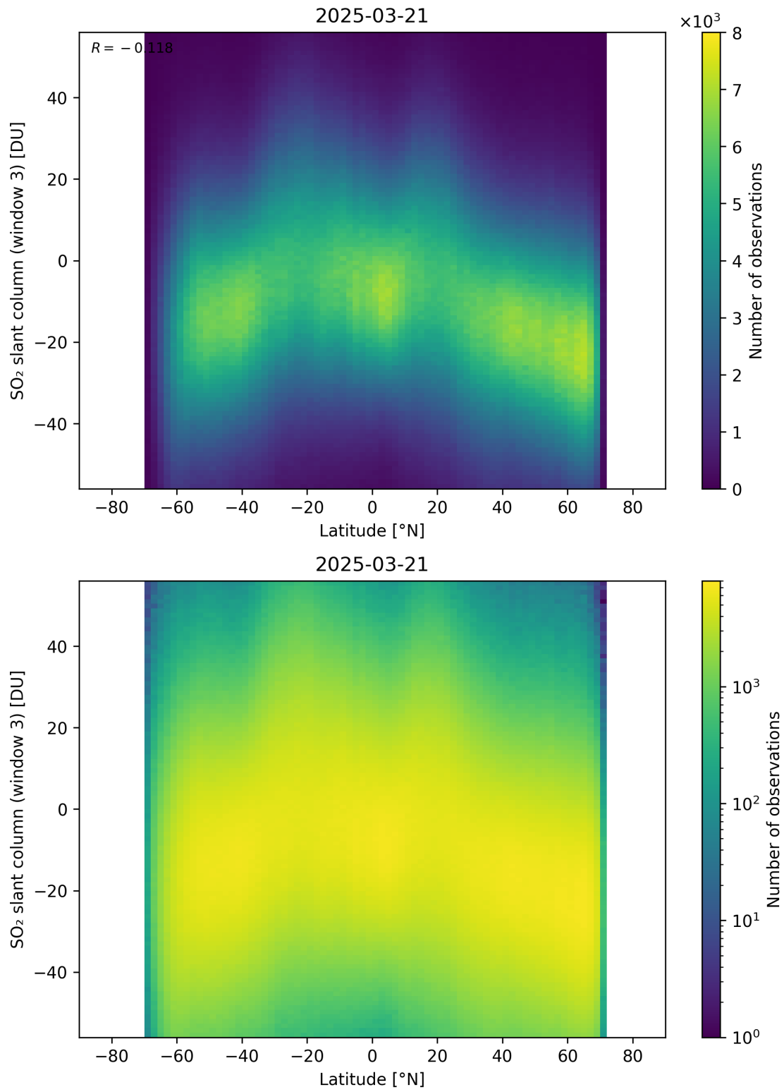
Figure 165: Scatter density plot of “Latitude” against “SO 2 slant column (window 3)” for 2025-03-20 to 2025-03-22.
