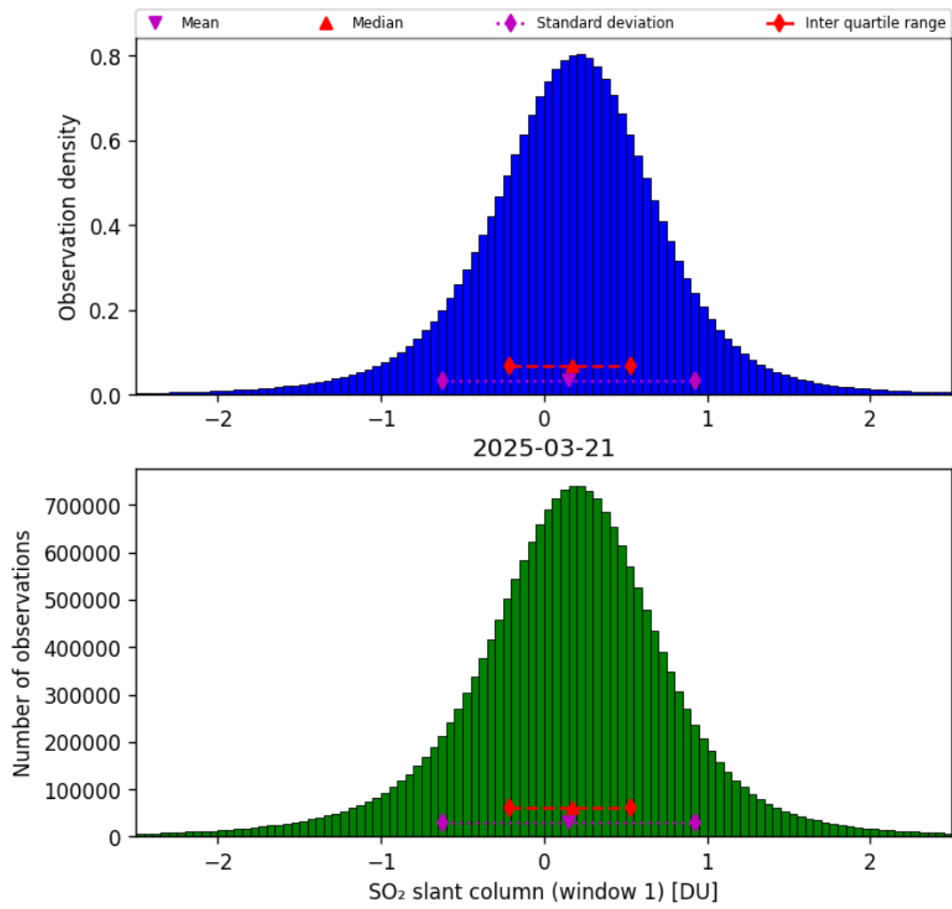
Figure 63: Histogram of “SO 2 slant column (window 1)” for 2025-03-20 to 2025-03-22
