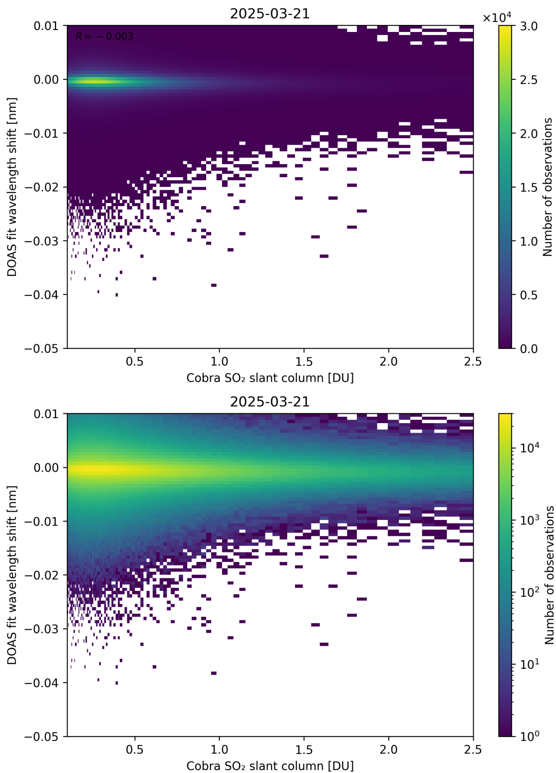
Figure 196: Scatter density plot of “Cobra SO 2 slant column” against “DOAS fit wavelength shift” for 2025-03-20 to 2025-03-22.
