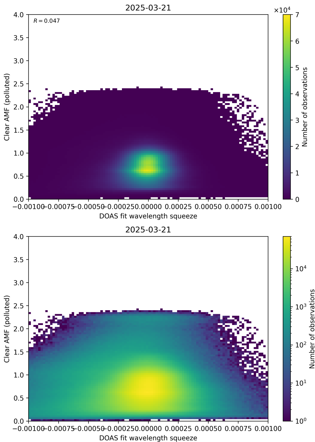
Figure 144: Scatter density plot of “DOAS fit wavelength squeeze” against “Clear AMF (polluted)” for 2025-03-20 to 2025-03-22.
