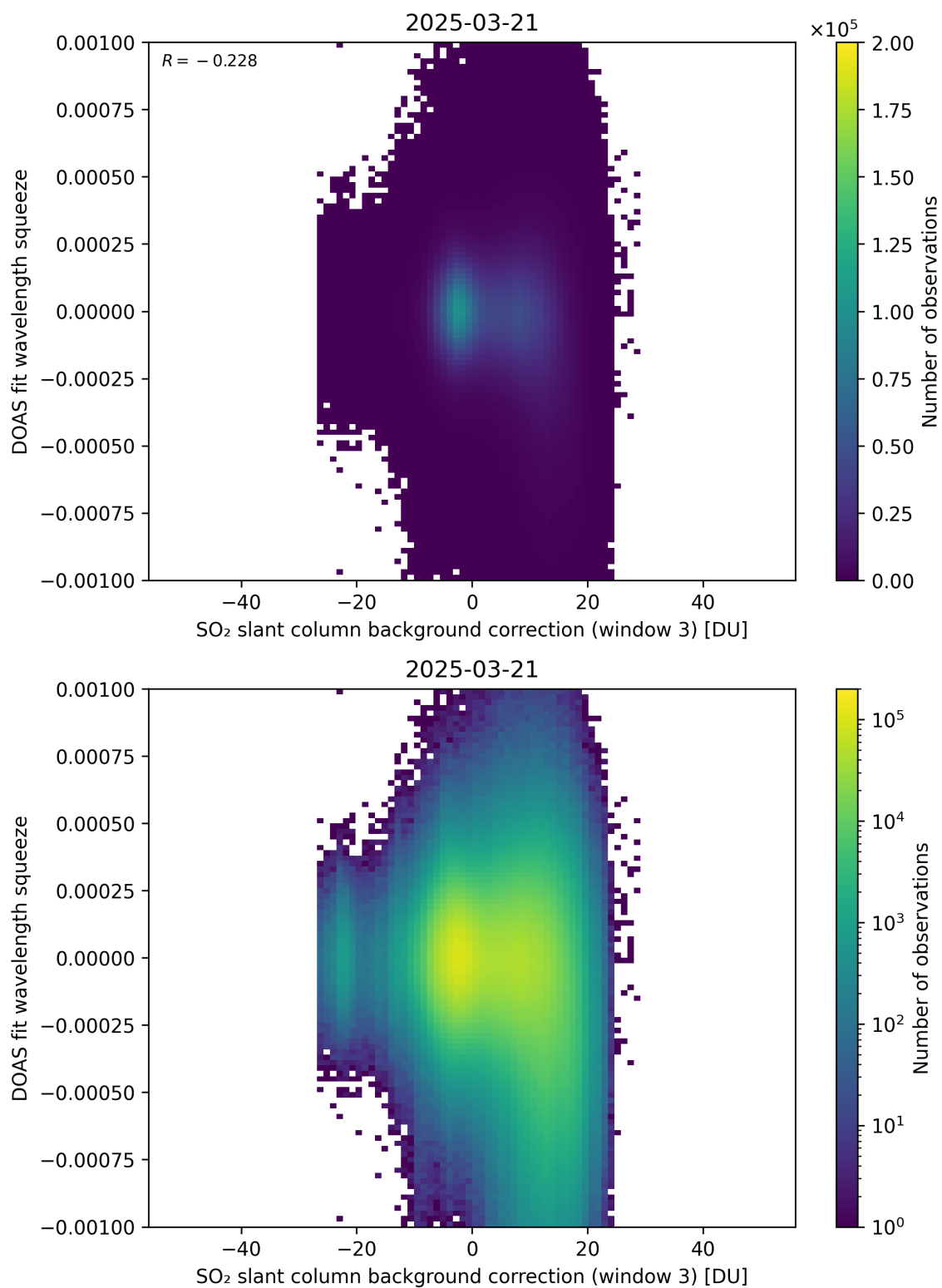
Figure 133: Scatter density plot of “SO 2 slant column background correction (window 3)” against “DOAS fit wavelength squeeze” for 2025-03-20 to 2025-03-22.
