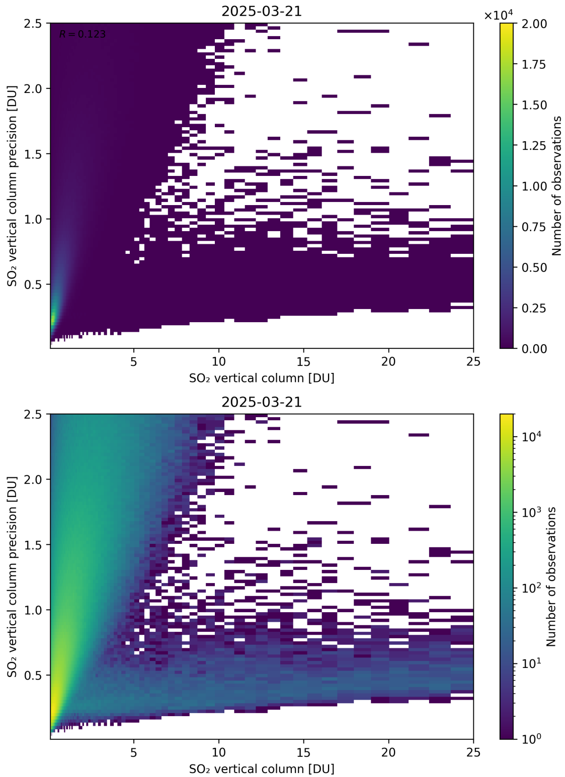
Figure 361: Scatter density plot of “SO 2 vertical column” against “SO 2 vertical column precision” for 2025-03-20 to 2025-03-22.
