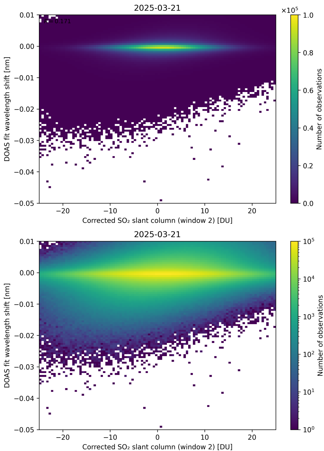
Figure 246: Scatter density plot of “Corrected SO 2 slant column (window 2)” against “DOAS fit wavelength shift” for 2025-03-20 to 2025-03-22.
