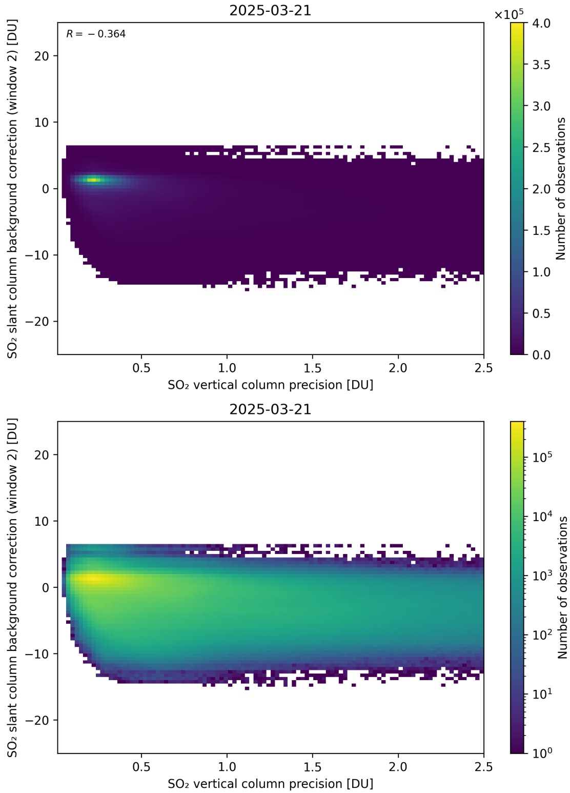
Figure 330: Scatter density plot of “SO 2 vertical column precision” against “SO 2 slant column background correction (window 2)” for 2025-03-20 to 2025-03-22.
