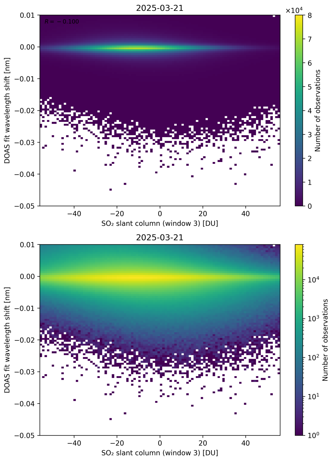
Figure 304: Scatter density plot of “SO 2 slant column (window 3)” against “DOAS fit wavelength shift” for 2025-03-20 to 2025-03-22.
