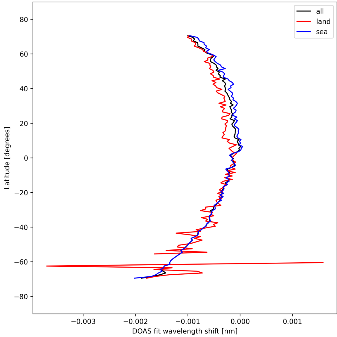
Figure 50: Zonal average of “DOAS fit wavelength shift” for 2025-03-20 to 2025-03-22.
