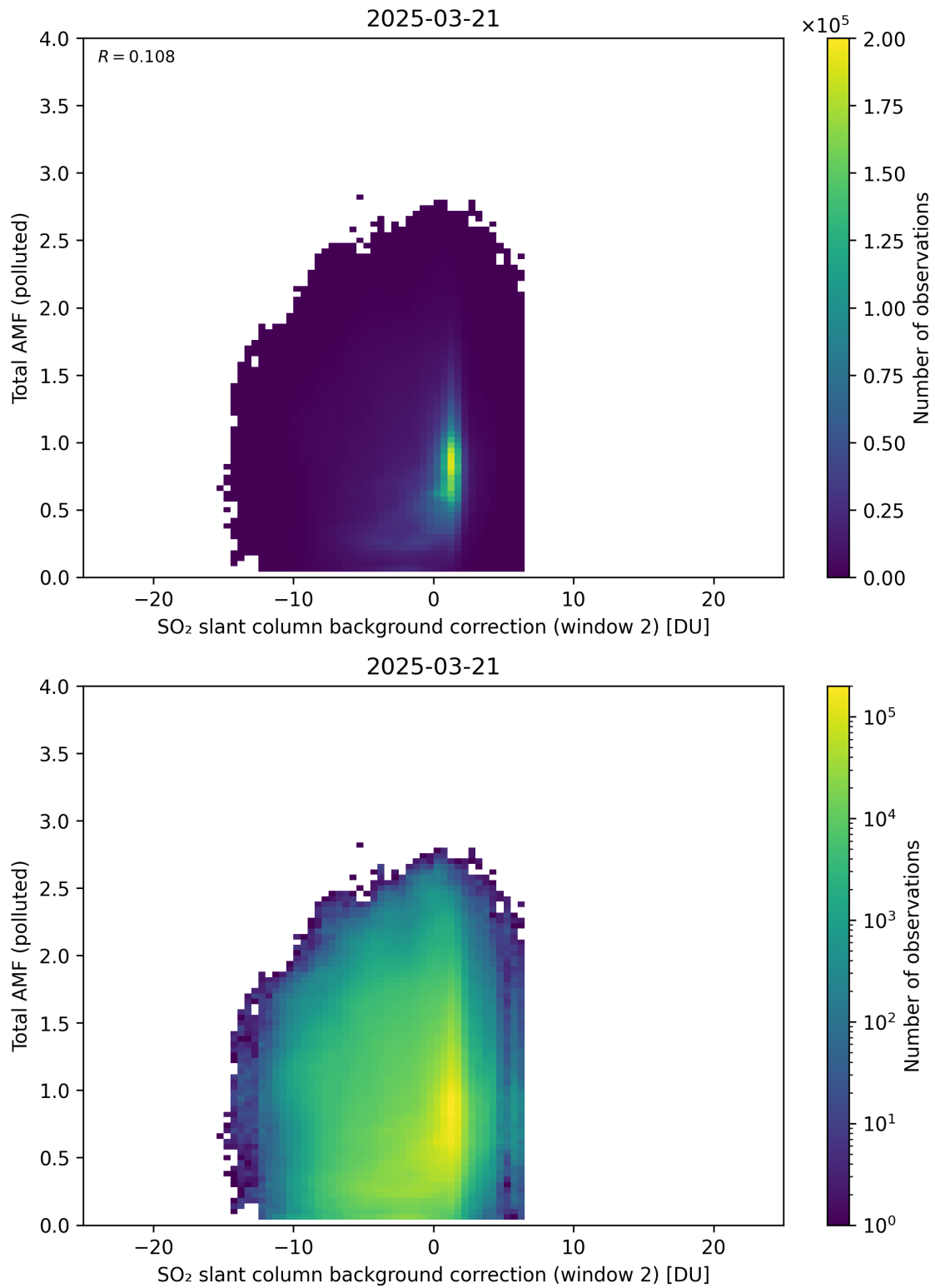
Figure 130: Scatter density plot of “SO 2 slant column background correction (window 2)” against “Total AMF (polluted)” for 2025-03-20 to 2025-03-22.
