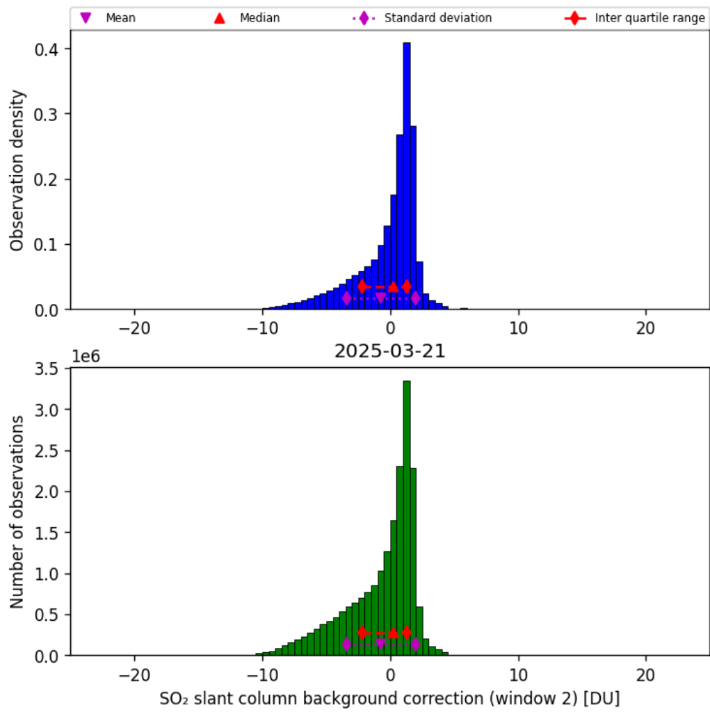
Figure 70: Histogram of “SO 2 slant column background correction (window 2)” for 2025-03-20 to 2025-03-22
