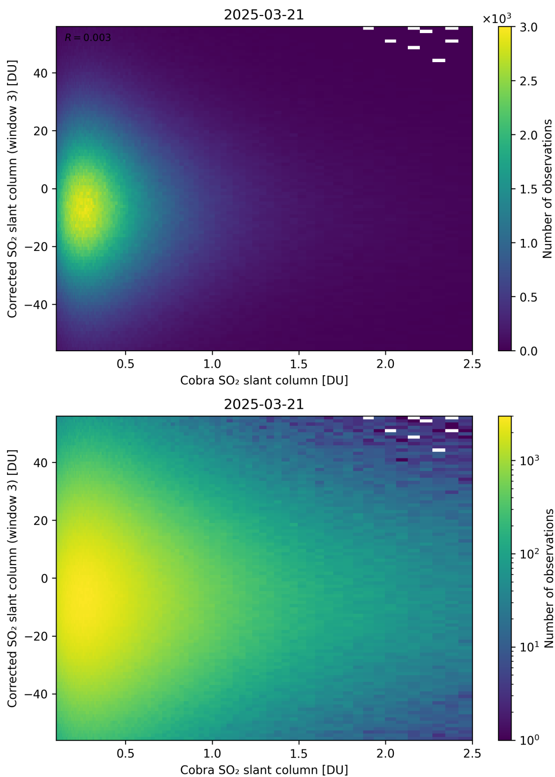
Figure 218: Scatter density plot of “Cobra SO 2 slant column” against “Corrected SO 2 slant column (window 3)” for 2025-03-20 to 2025-03-22.
