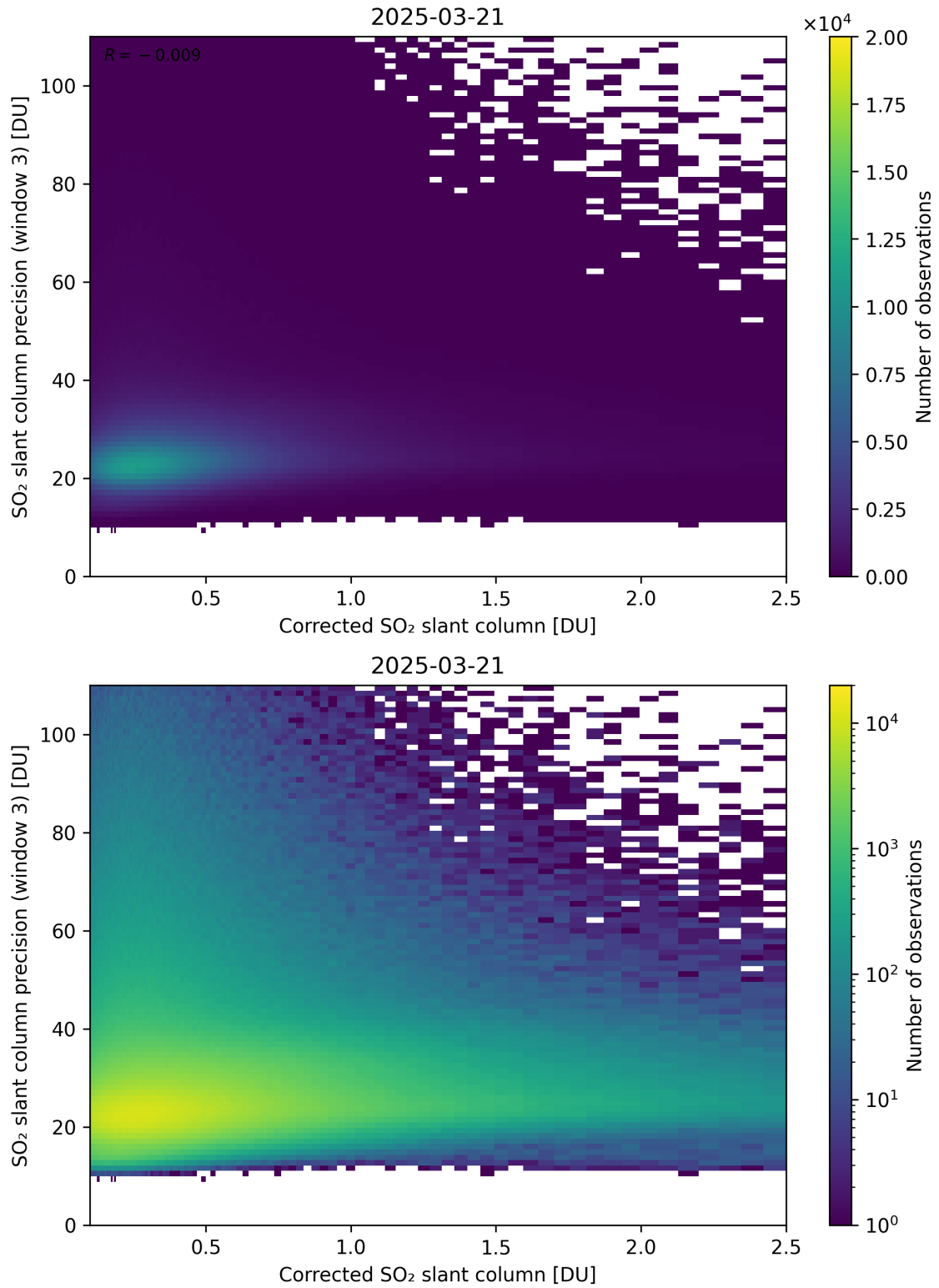
Figure 241: Scatter density plot of “Corrected SO 2 slant column” against “SO 2 slant column precision (window 3)” for 2025-03-20 to 2025-03-22.
