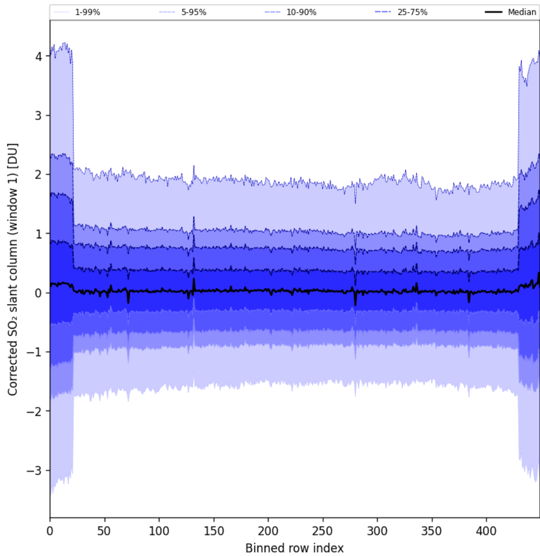
Figure 91: Along track statistics of “Corrected SO 2 slant column (window 1)” for 2025-03-20 to 2025-03-22
