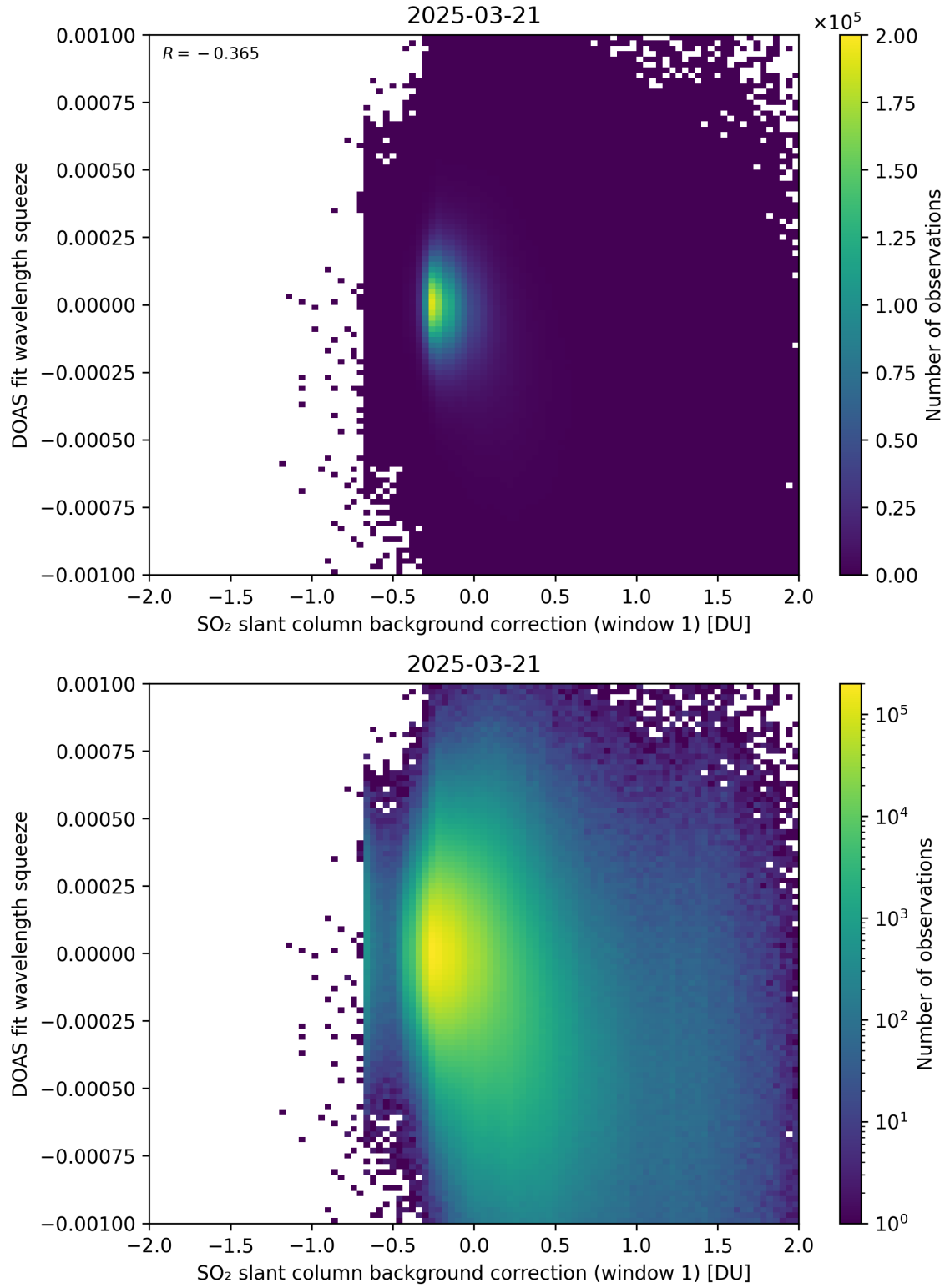
Figure 112: Scatter density plot of “SO 2 slant column background correction (window 1)” against “DOAS fit wavelength squeeze” for 2025-03-20 to 2025-03-22.
