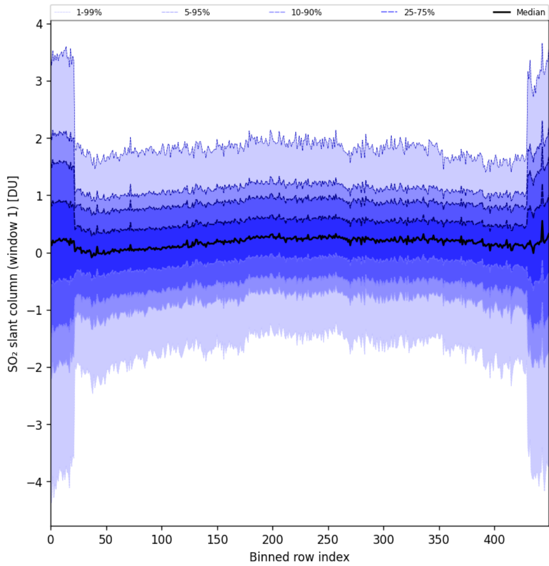
Figure 89: Along track statistics of “SO 2 slant column (window 1)” for 2025-03-20 to 2025-03-22
