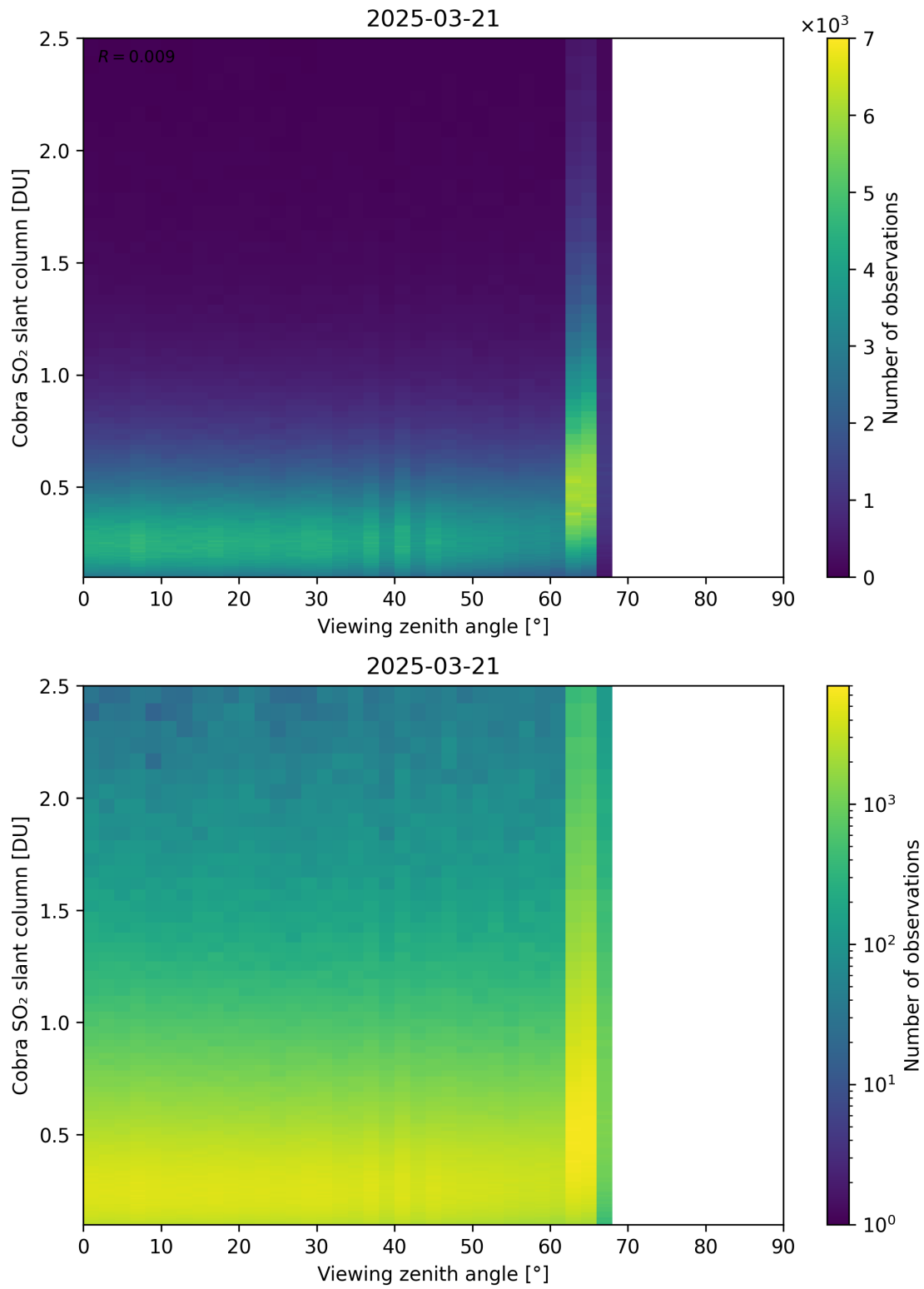
Figure 371: Scatter density plot of “Viewing zenith angle” against “Cobra SO 2 slant column” for 2025-03-20 to 2025-03-22.
