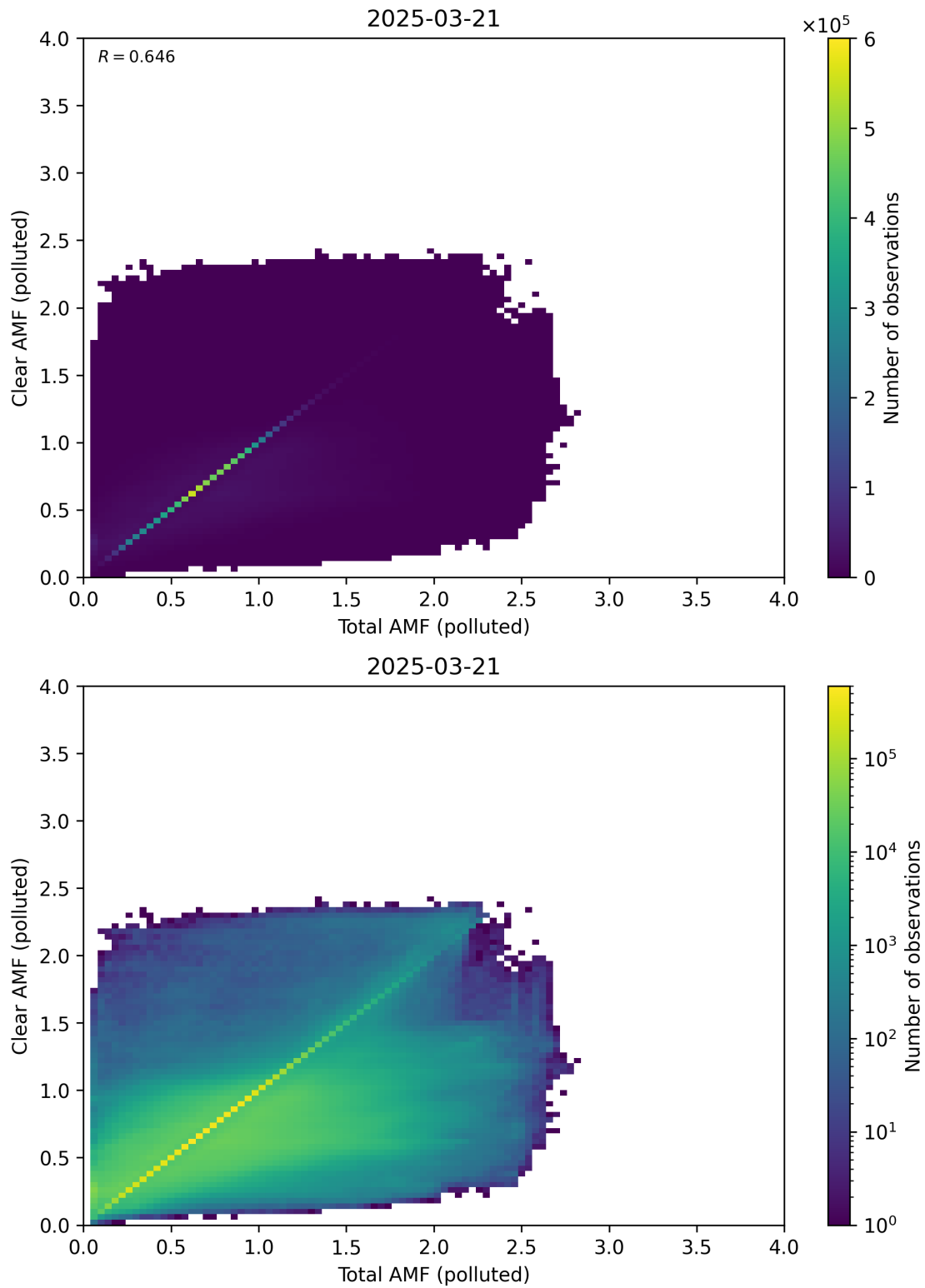
Figure 321: Scatter density plot of “Total AMF (polluted)” against “Clear AMF (polluted)” for 2025-03-20 to 2025-03-22.
