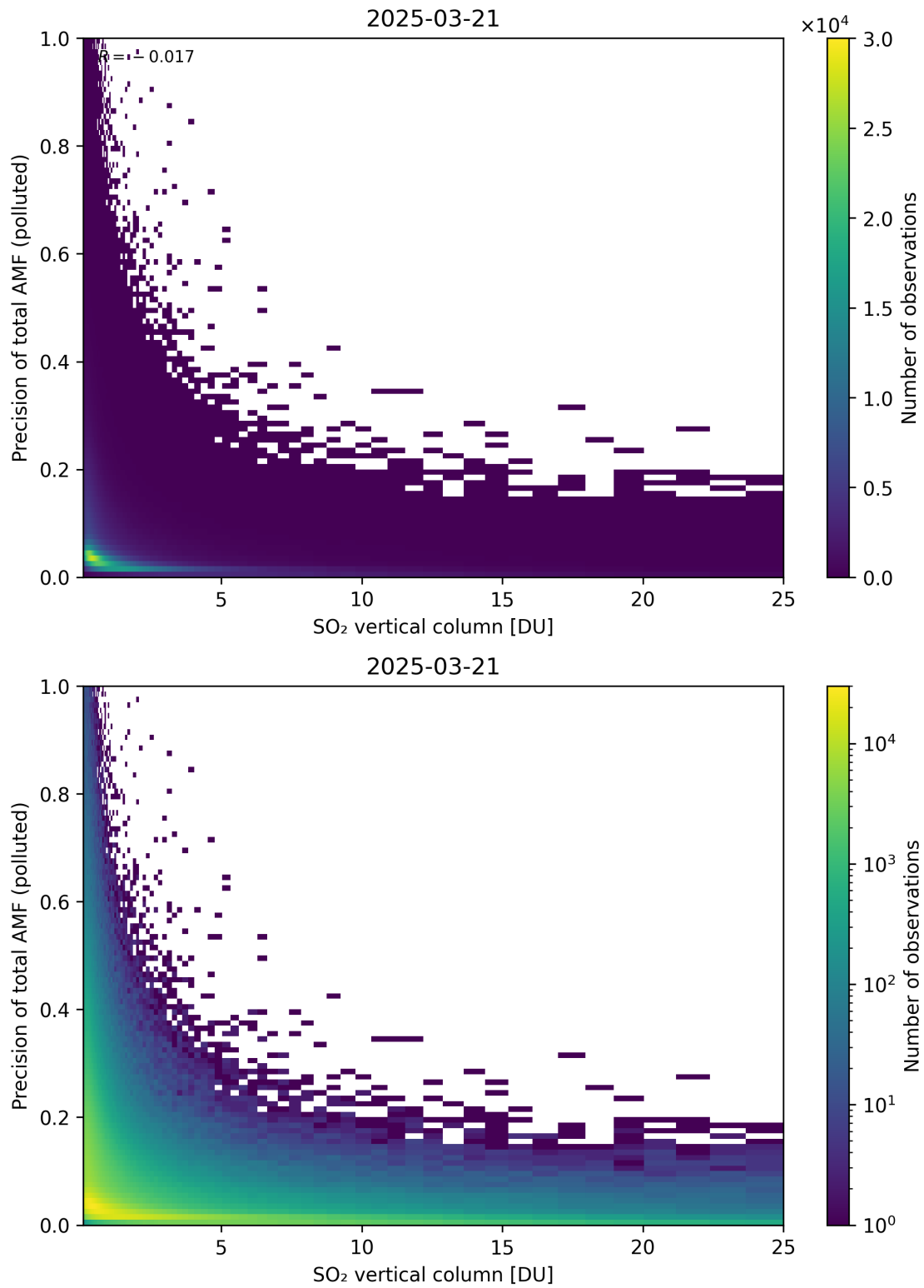
Figure 360: Scatter density plot of “SO 2 vertical column” against “Precision of total AMF (polluted)” for 2025-03-20 to 2025-03-22.
