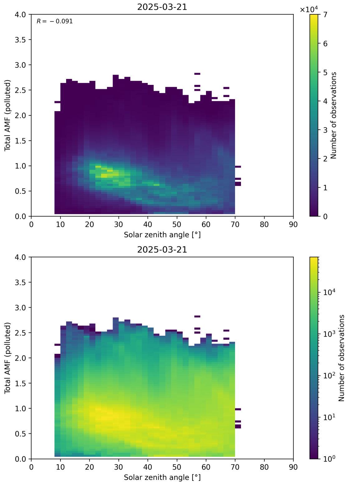
Figure 189: Scatter density plot of “Solar zenith angle” against “Total AMF (polluted)” for 2025-03-20 to 2025-03-22.
