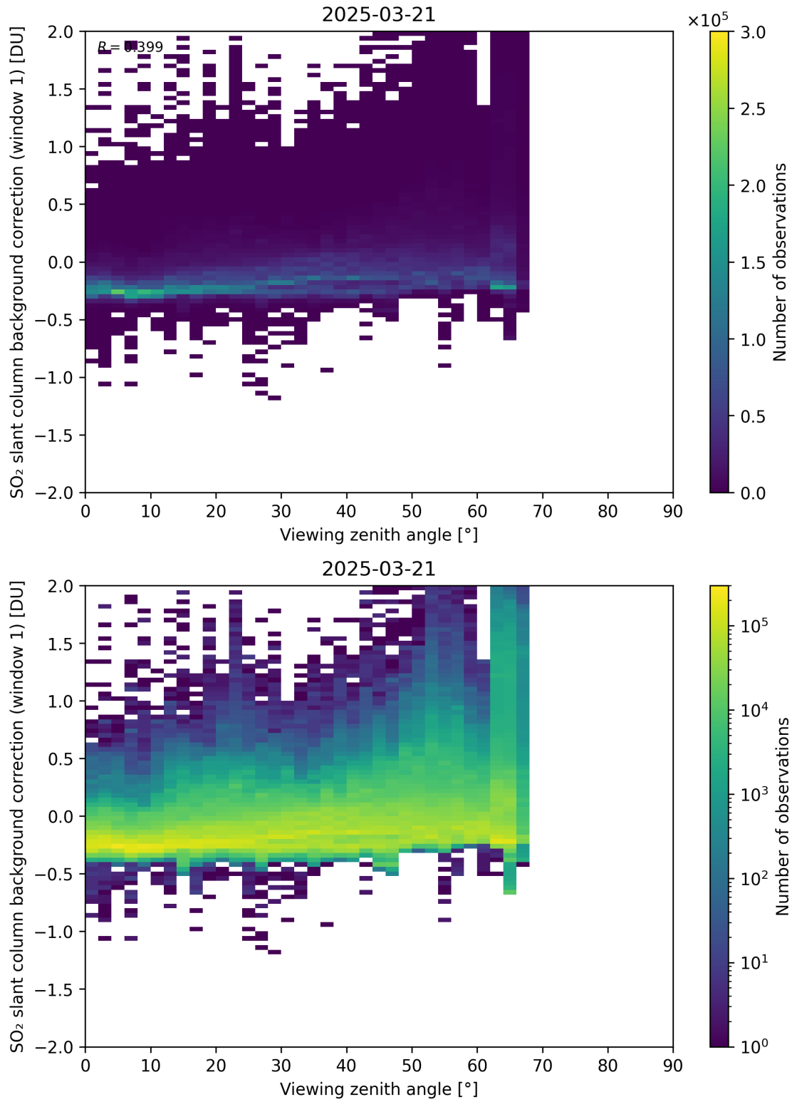
Figure 362: Scatter density plot of “Viewing zenith angle” against “SO 2 slant column background correction (window 1)” for 2025-03-20 to 2025-03-22.
