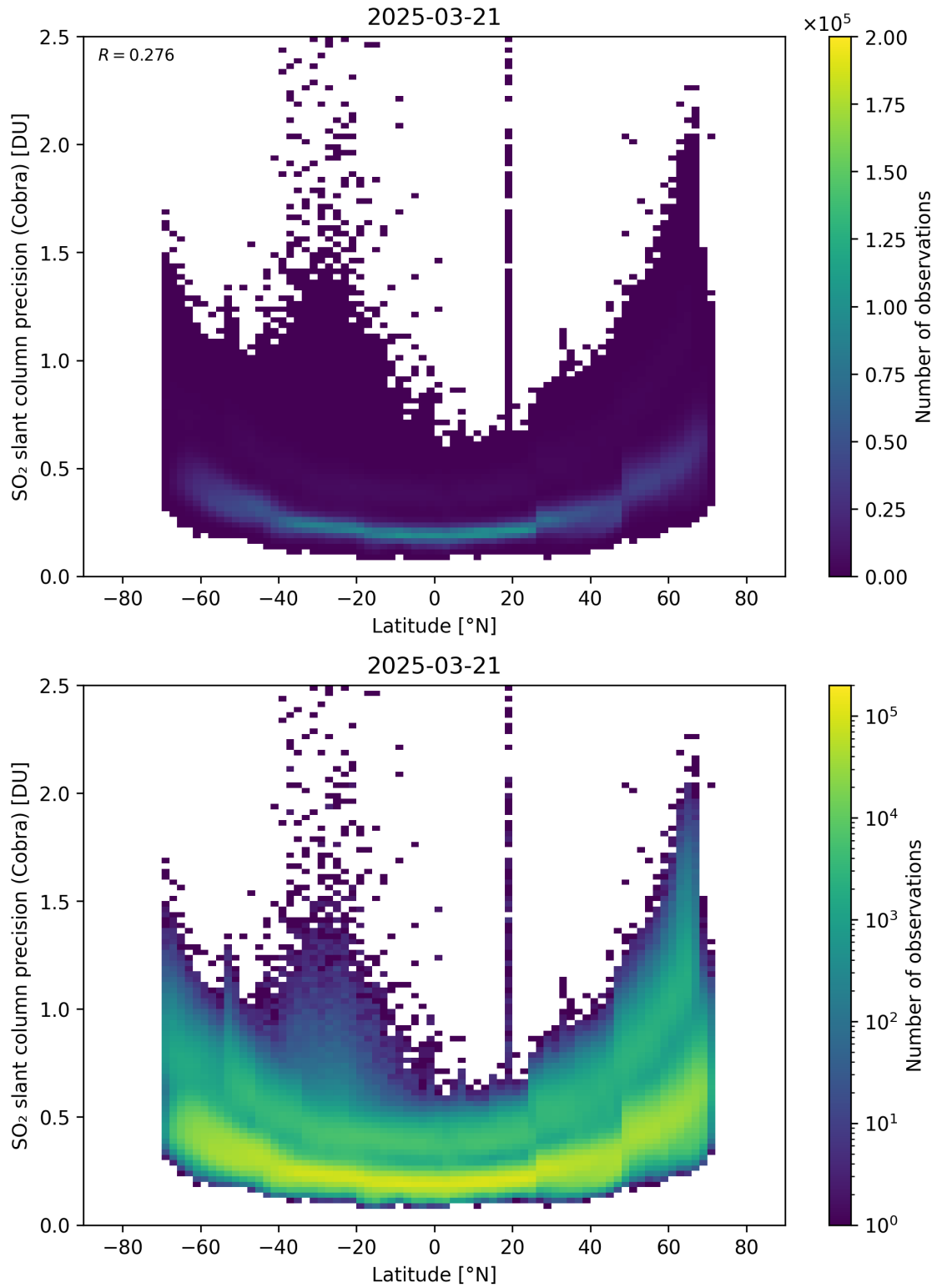
Figure 158: Scatter density plot of “Latitude” against “SO 2 slant column precision (Cobra)” for 2025-03-20 to 2025-03-22.
