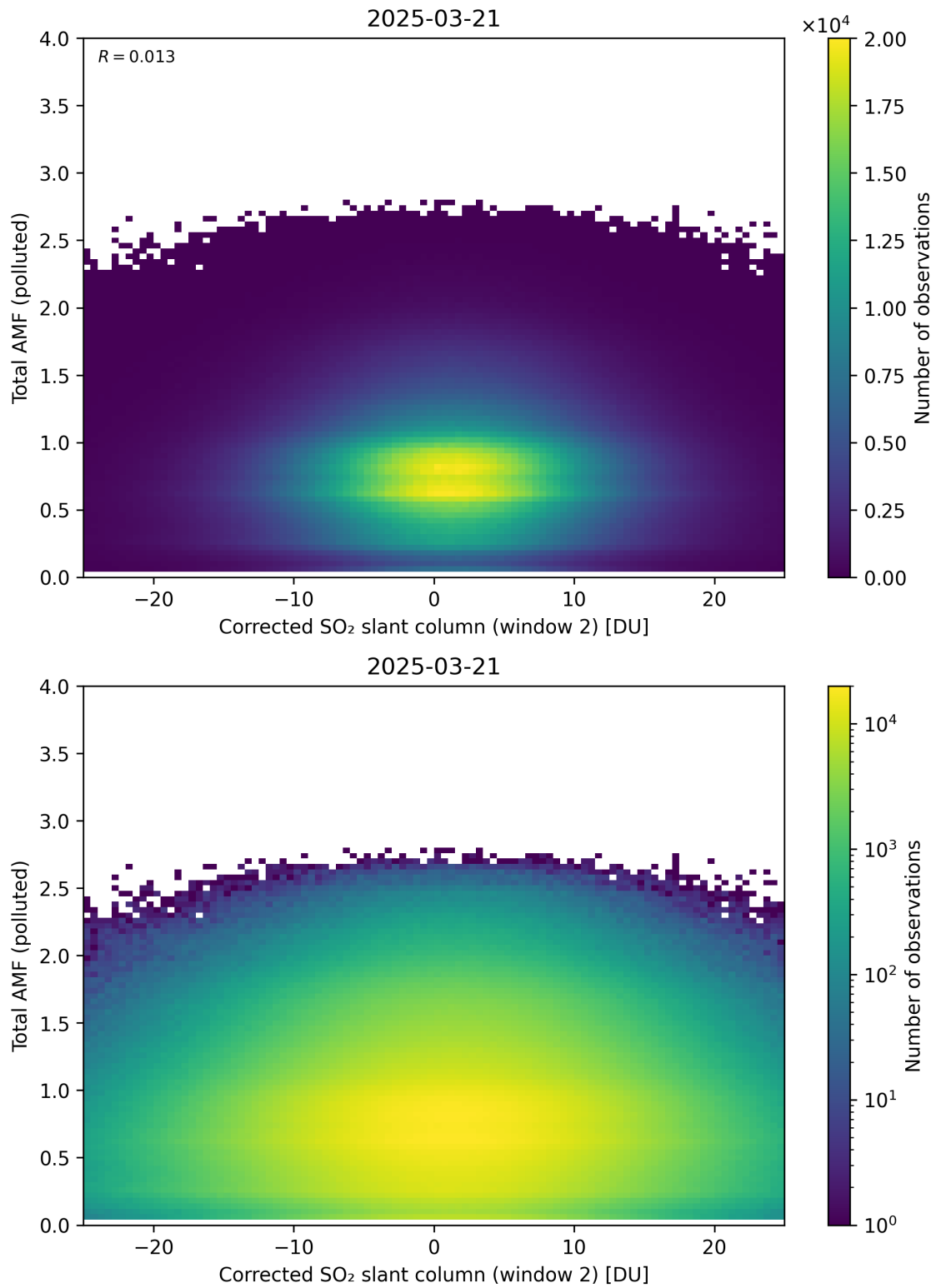
Figure 253: Scatter density plot of “Corrected SO 2 slant column (window 2)” against “Total AMF (polluted)” for 2025-03-20 to 2025-03-22.
