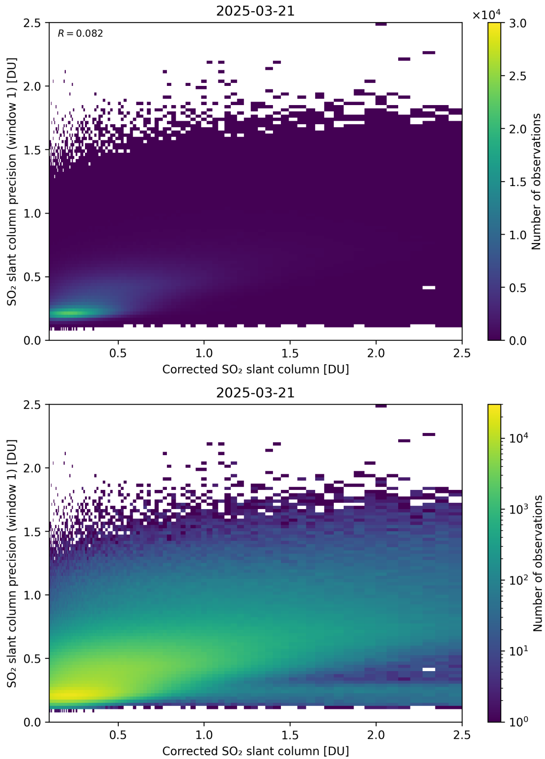
Figure 238: Scatter density plot of “Corrected SO 2 slant column” against “SO 2 slant column precision (window 1)” for 2025-03-20 to 2025-03-22.
