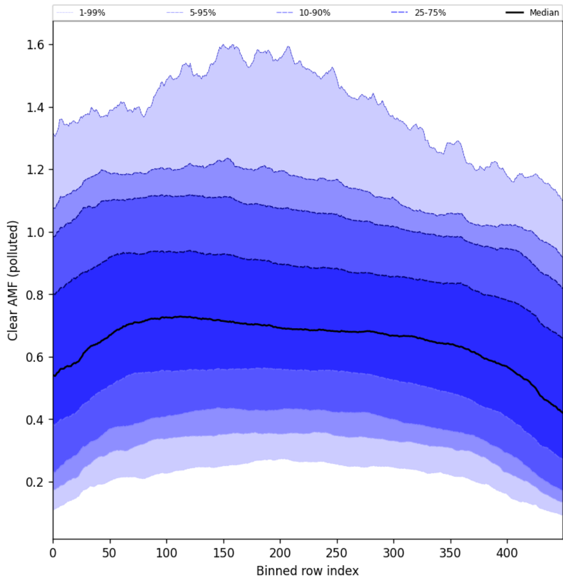
Figure 107: Along track statistics of “Clear AMF (polluted)” for 2025-04-02 to 2025-04-03
