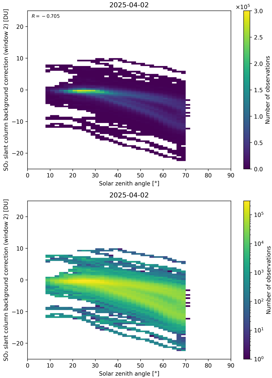
Figure 172: Scatter density plot of “Solar zenith angle” against “SO 2 slant column background correction (window 2)” for 2025-04-02 to 2025-04-03.
