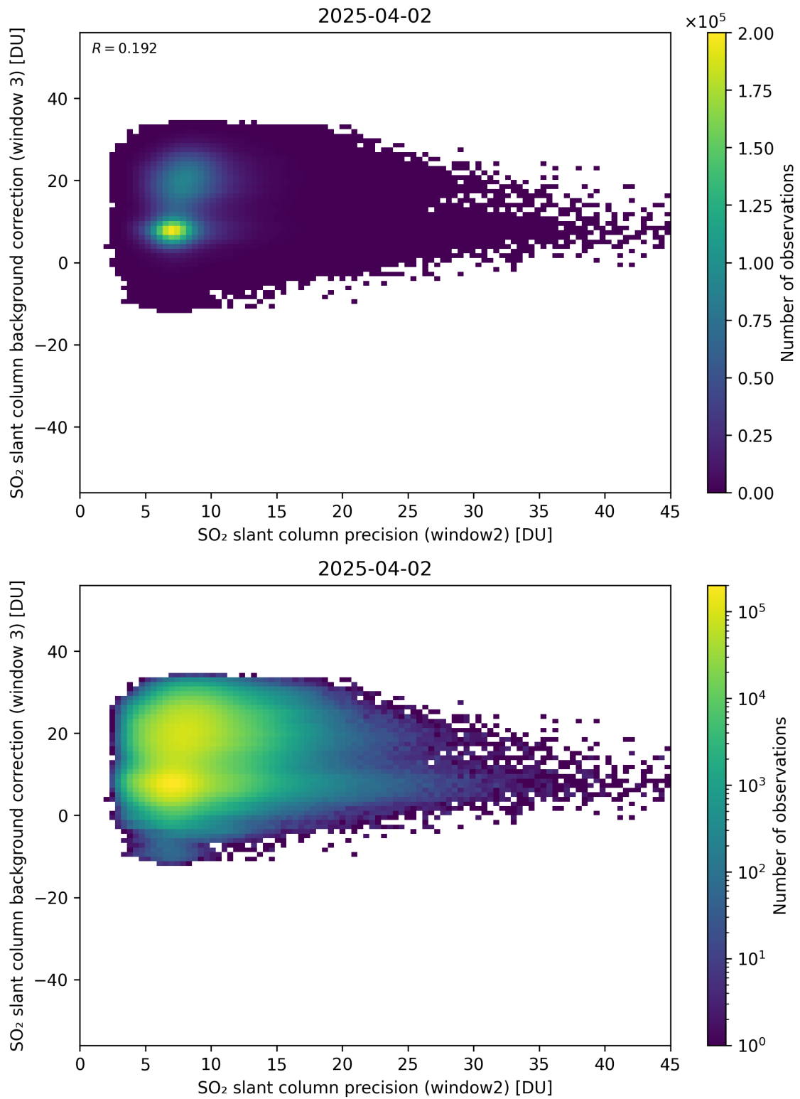
Figure 292: Scatter density plot of “SO 2 slant column precision (window2)” against “SO 2 slant column background correction (window 3)” for 2025-04-02 to 2025-04-03.
