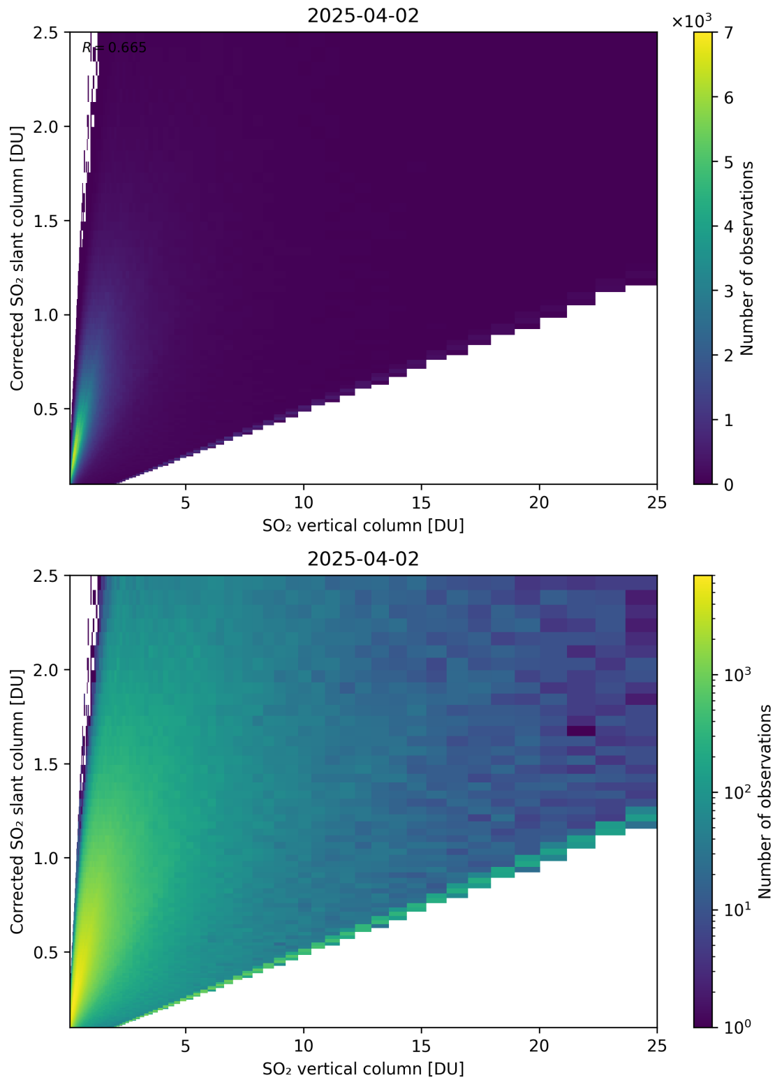
Figure 351: Scatter density plot of “SO 2 vertical column” against “Corrected SO 2 slant column” for 2025-04-02 to 2025-04-03.
