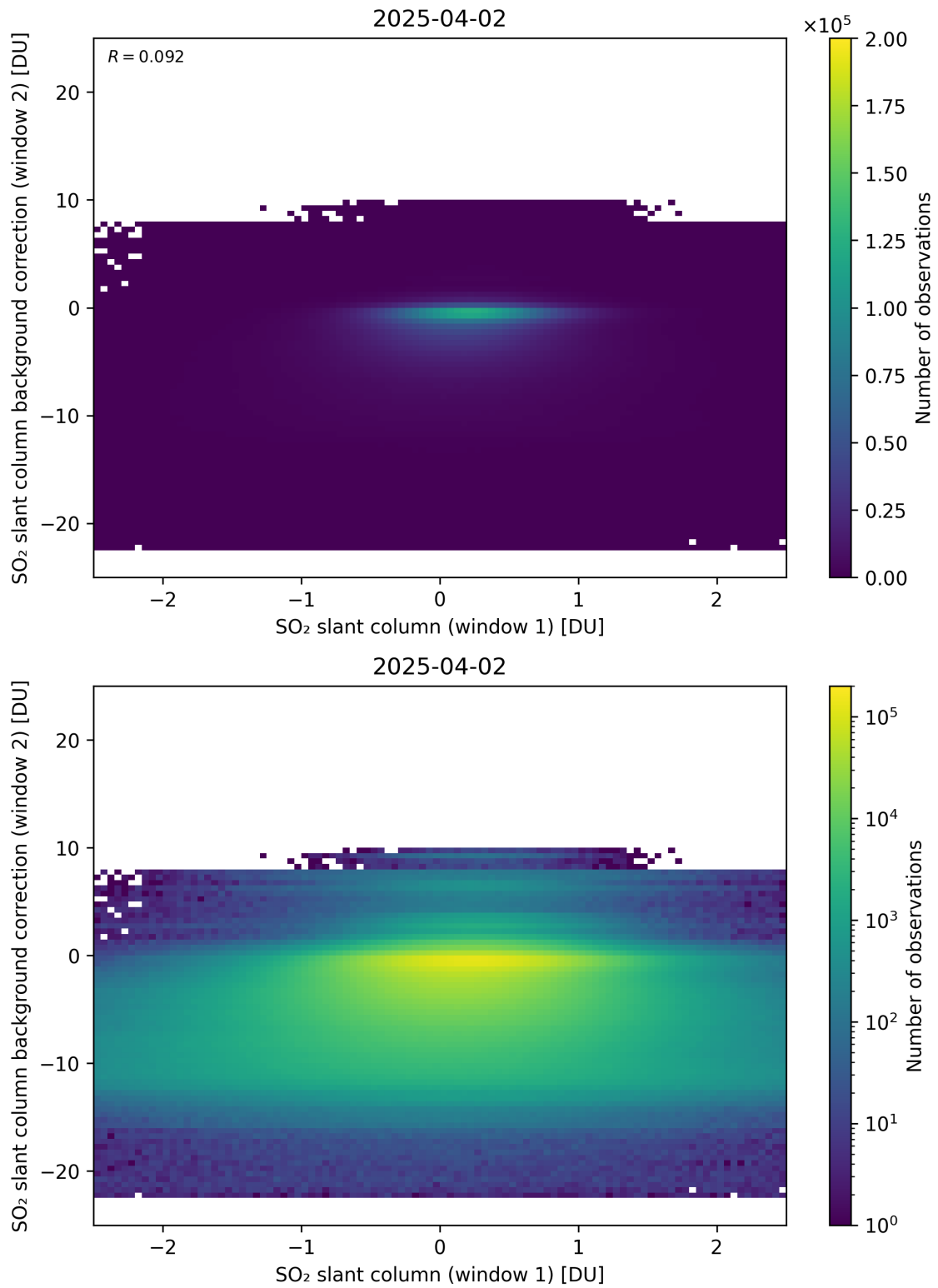
Figure 263: Scatter density plot of “SO 2 slant column (window 1)” against “SO 2 slant column background correction (window 2)” for 2025-04-02 to 2025-04-03.
