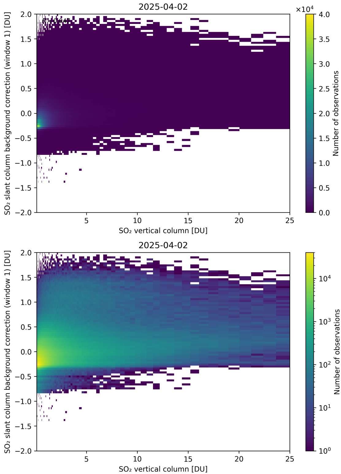
Figure 323: Scatter density plot of “SO 2 vertical column” against “SO 2 slant column background correction (window 1)” for 2025-04-02 to 2025-04-03.
