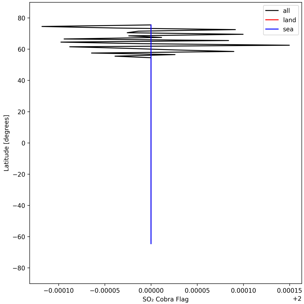
Figure 49: Zonal average of "SO 2 Cobra Flag" for 2025-04-02 to 2025-04-03.
