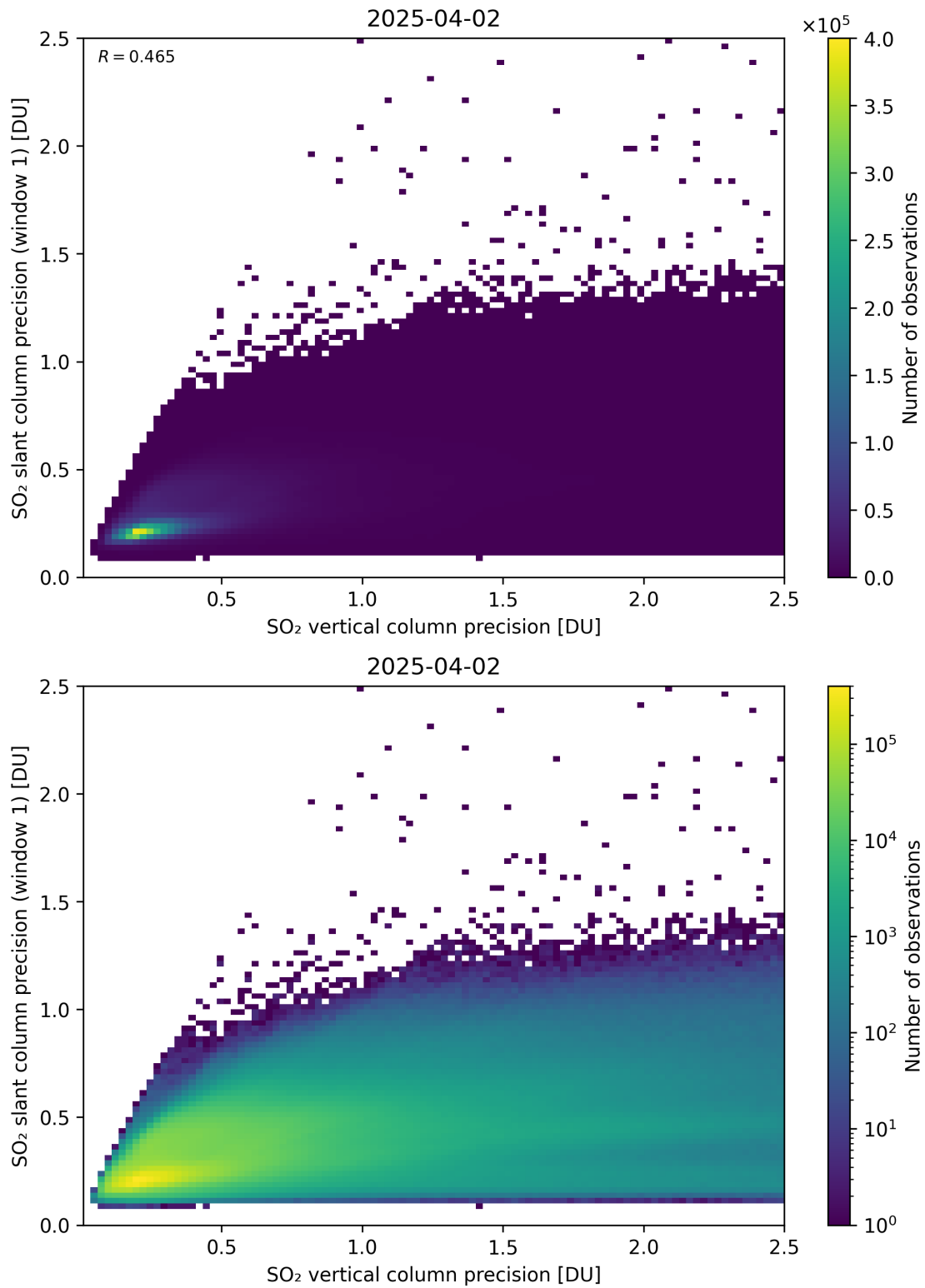
Figure 342: Scatter density plot of “SO 2 vertical column precision” against “SO 2 slant column precision (window 1)” for 2025-04-02 to 2025-04-03.
