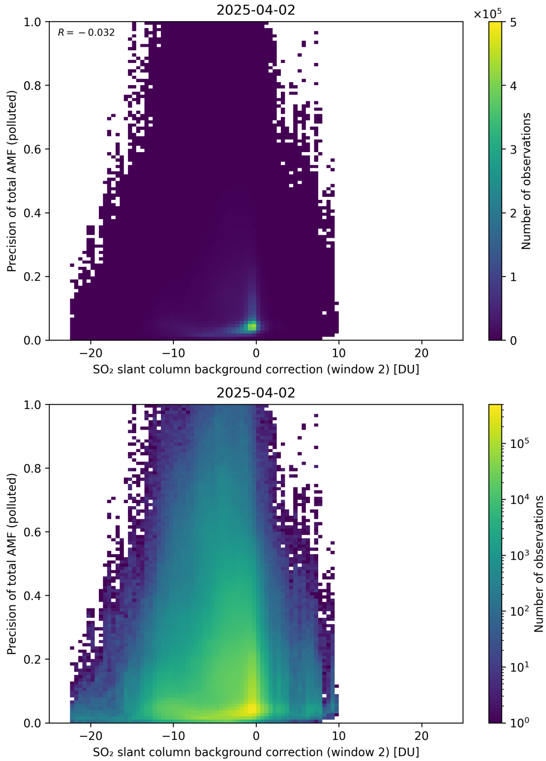
Figure 131: Scatter density plot of “SO 2 slant column background correction (window 2)” against “Precision of total AMF (polluted)” for 2025-04-02 to 2025-04-03.
