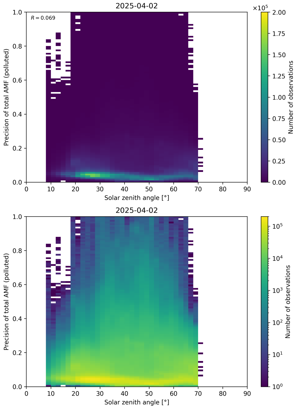
Figure 190: Scatter density plot of “Solar zenith angle” against “Precision of total AMF (polluted)” for 2025-04-02 to 2025-04-03.
