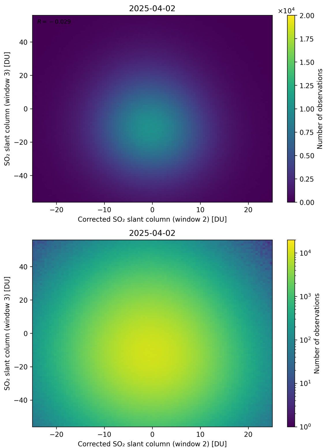
Figure 251: Scatter density plot of “Corrected SO 2 slant column (window 2)” against “SO 2 slant column (window 3)” for 2025-04-02 to 2025-04-03.
