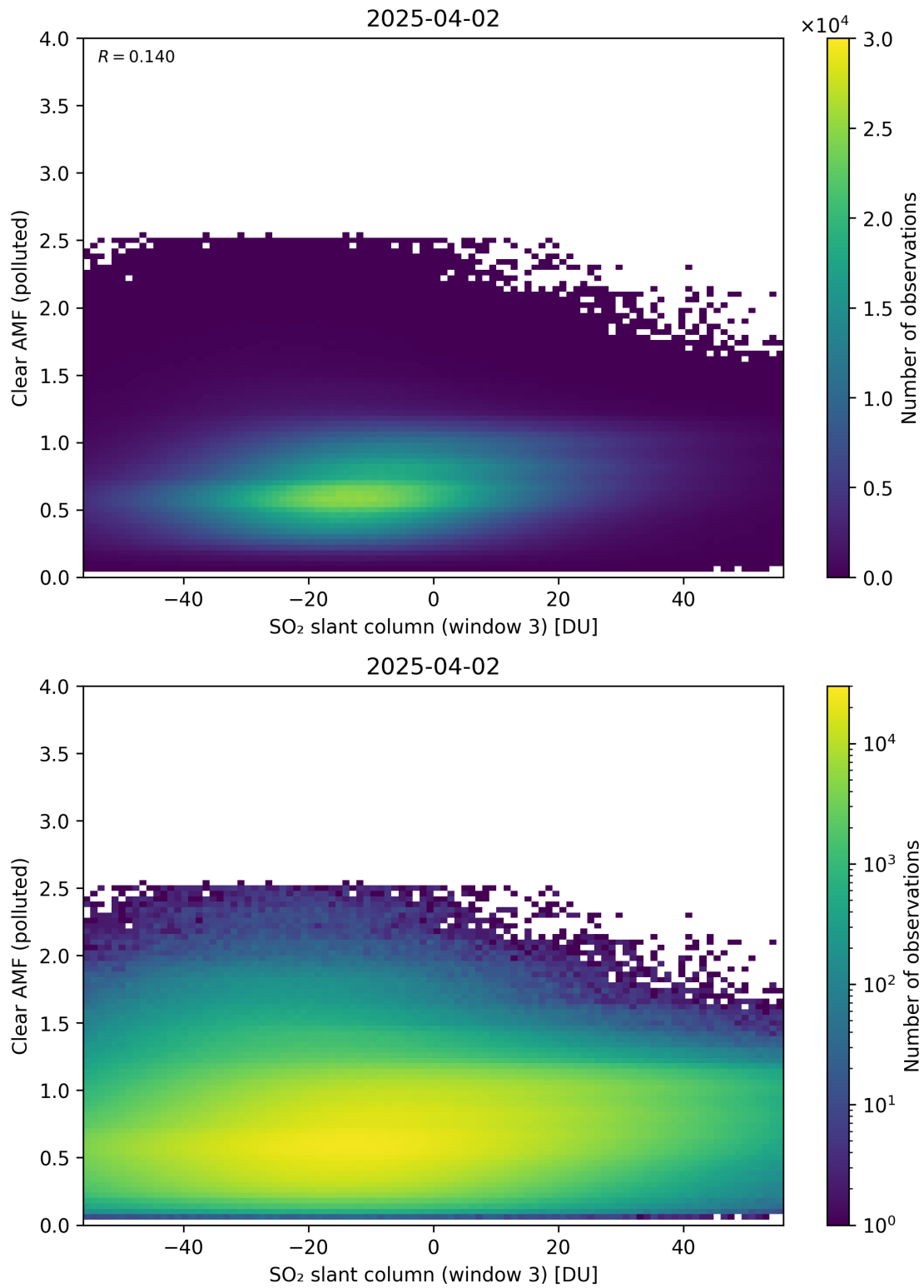
Figure 315: Scatter density plot of “SO 2 slant column (window 3)” against “Clear AMF (polluted)” for 2025-04-02 to 2025-04-03.
