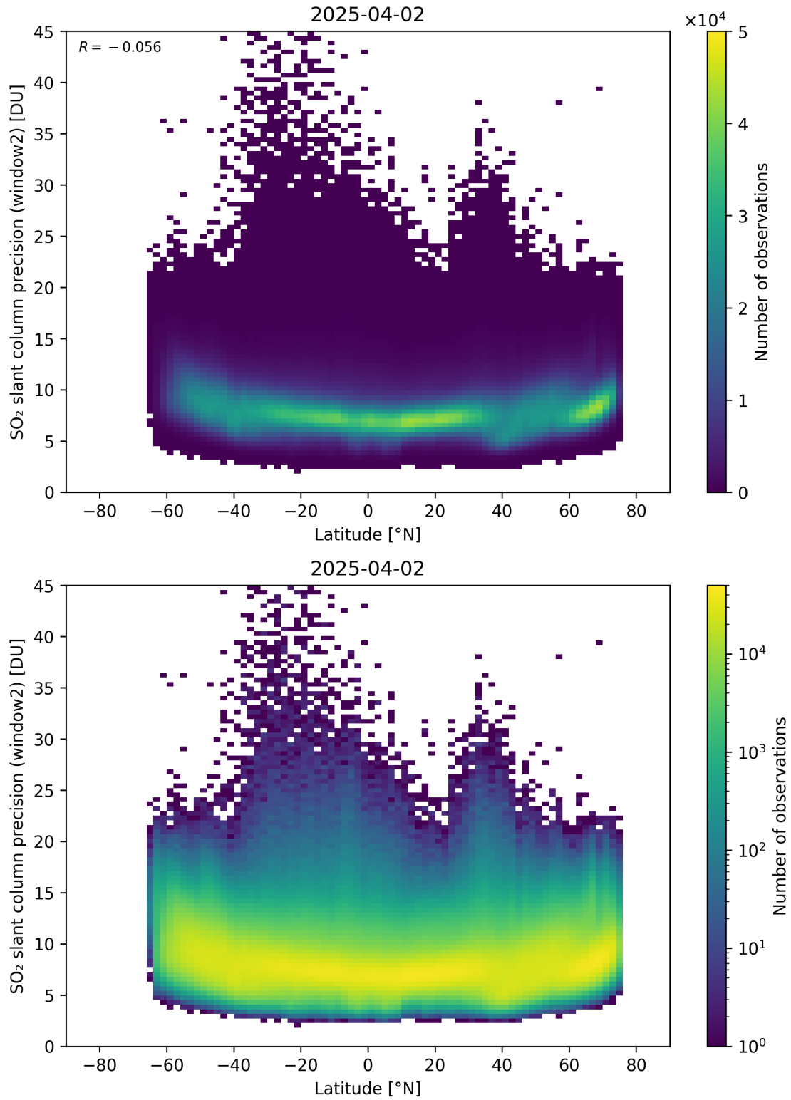
Figure 164: Scatter density plot of “Latitude” against “SO 2 slant column precision (window2)” for 2025-04-02 to 2025-04-03.
