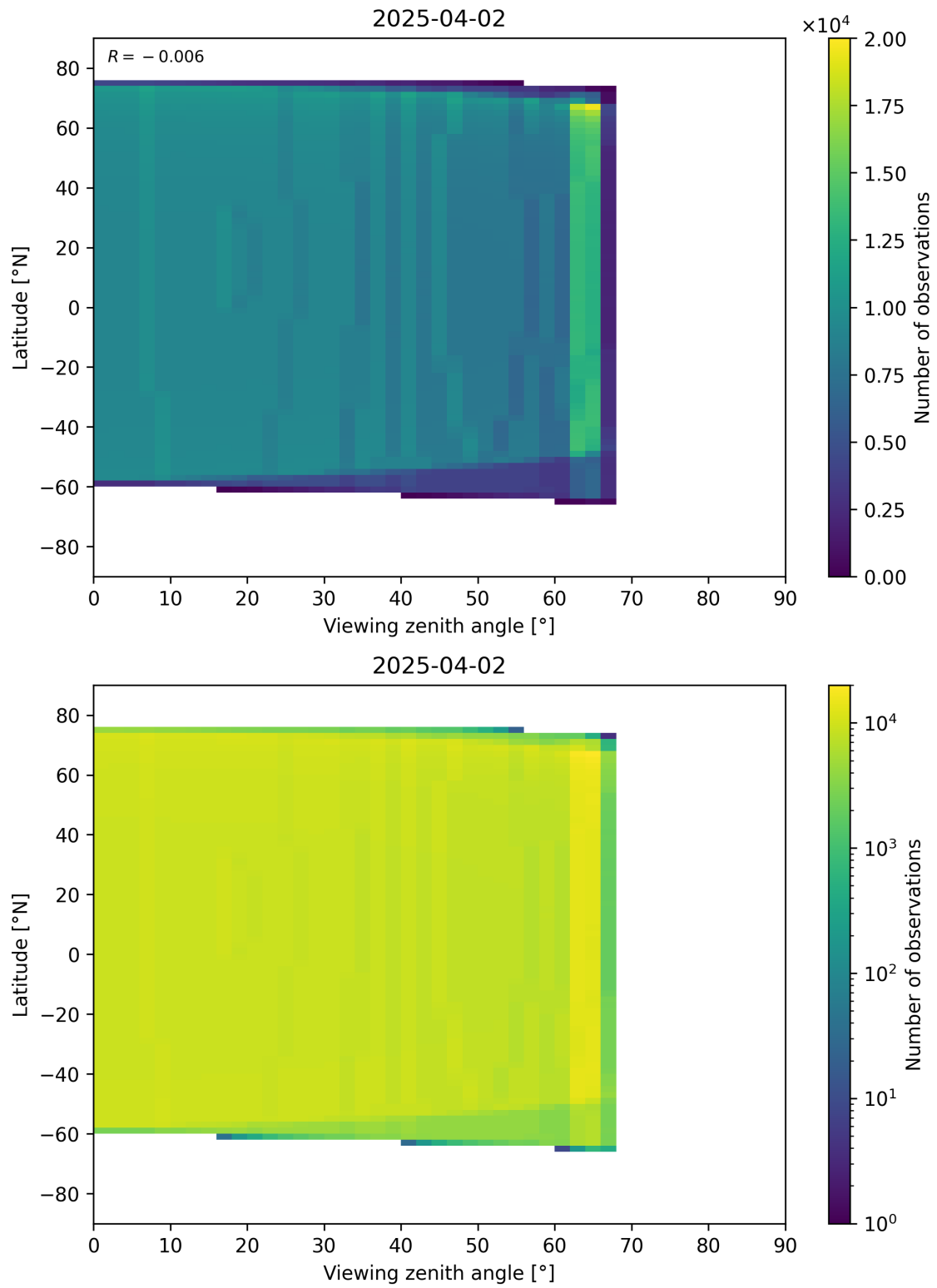
Figure 368: Scatter density plot of “Viewing zenith angle” against “Latitude” for 2025-04-02 to 2025-04-03.
