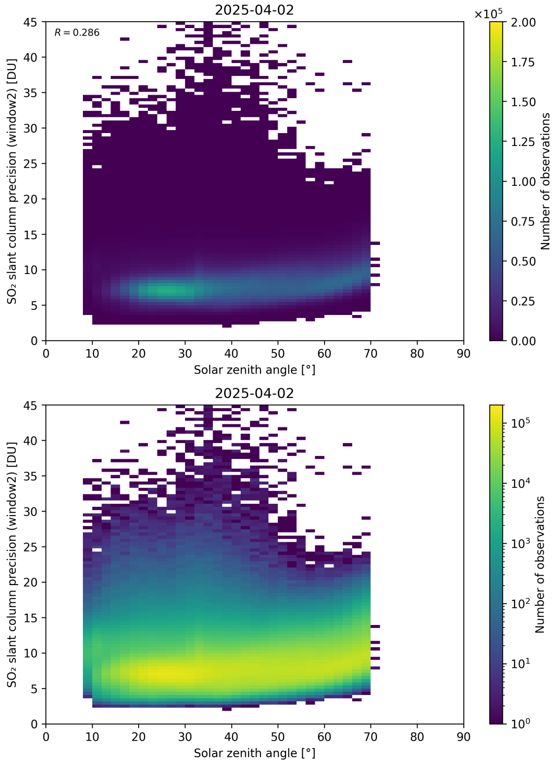
Figure 186: Scatter density plot of “Solar zenith angle” against “SO 2 slant column precision (window2)” for 2025-04-02 to 2025-04-03.
