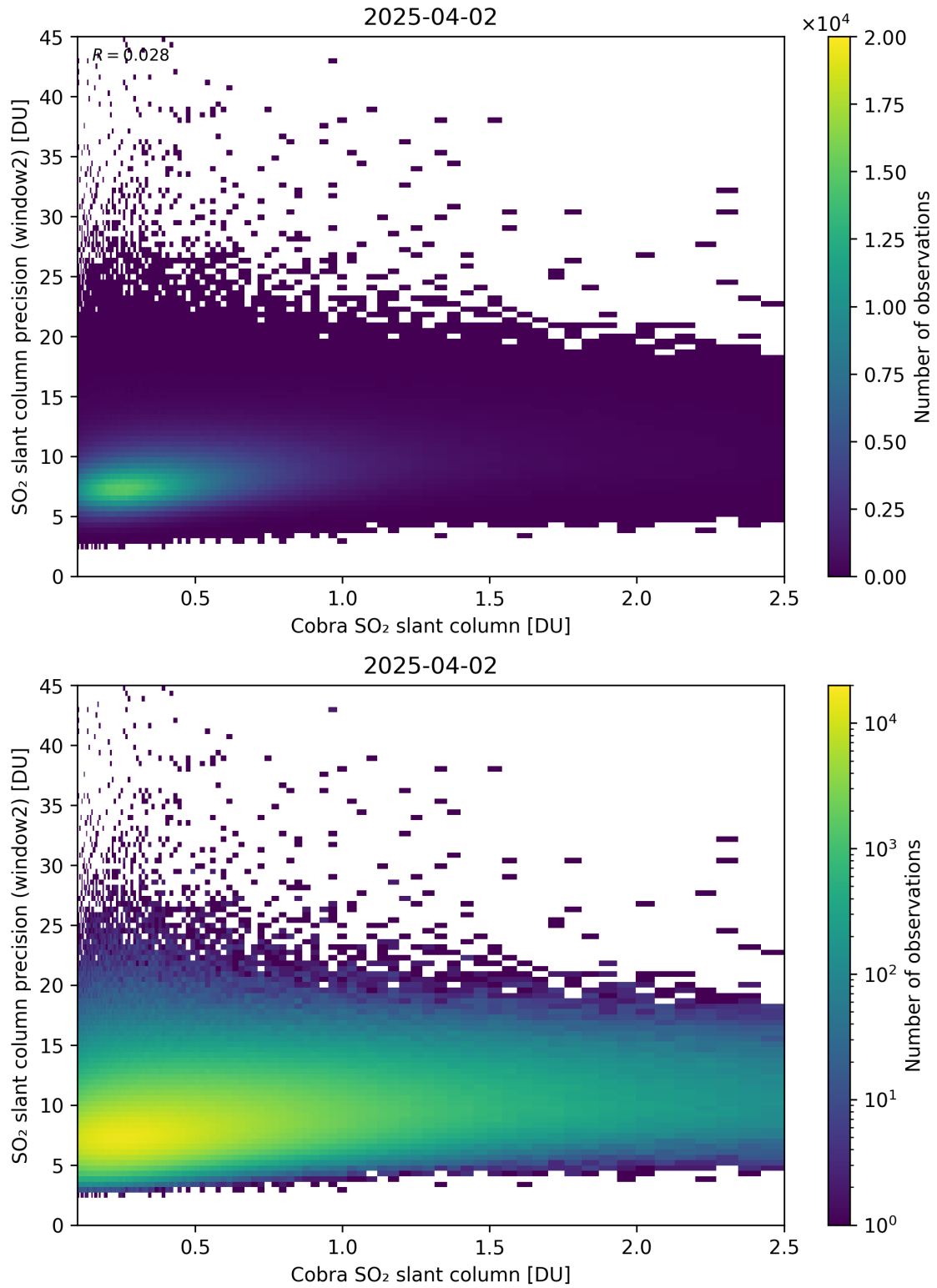
Figure 221: Scatter density plot of “Cobra SO 2 slant column” against “SO 2 slant column precision (window2)” for 2025-04-02 to 2025-04-03.
