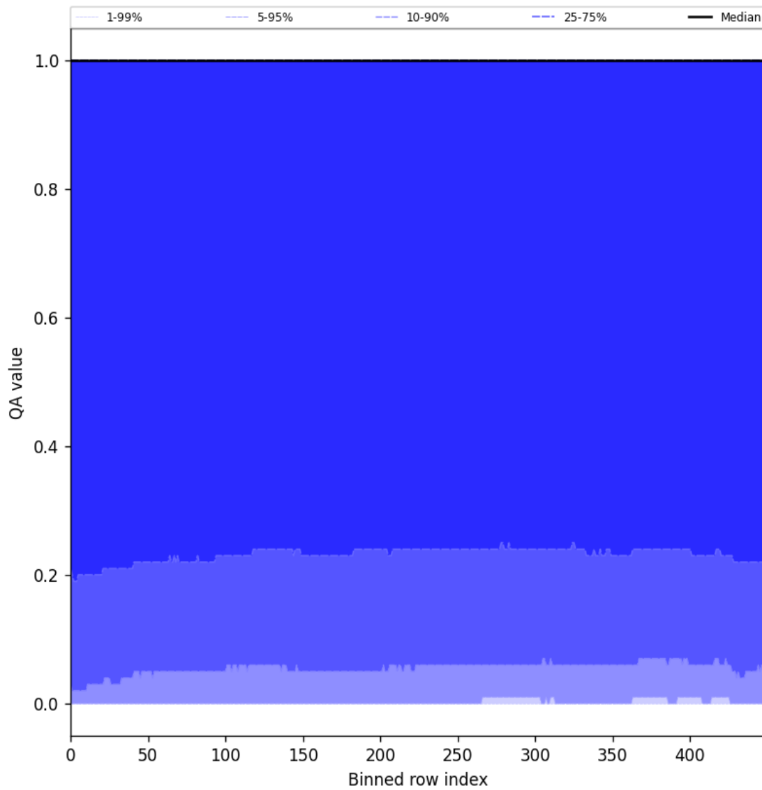
Figure 83: Along track statistics of “QA value” for 2025-04-02 to 2025-04-03
