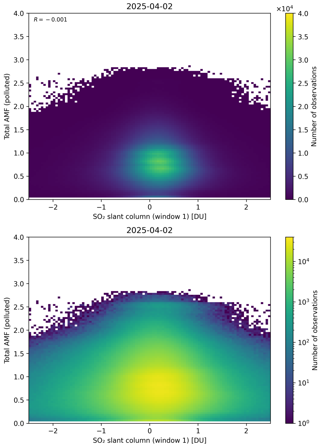
Figure 289: Scatter density plot of “SO 2 slant column (window 1)” against “Total AMF (polluted)” for 2025-04-02 to 2025-04-03.
