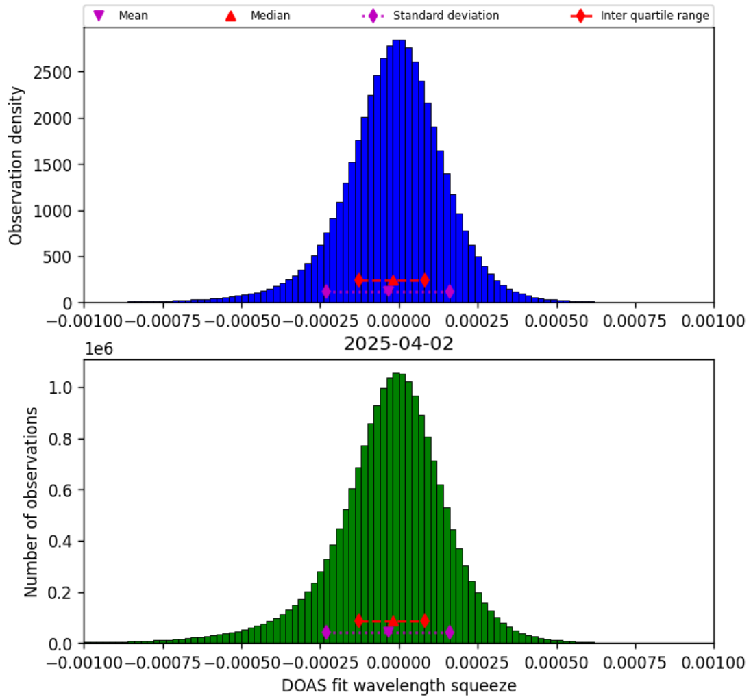
Figure 77: Histogram of “DOAS fit wavelength squeeze” for 2025-04-02 to 2025-04-03
