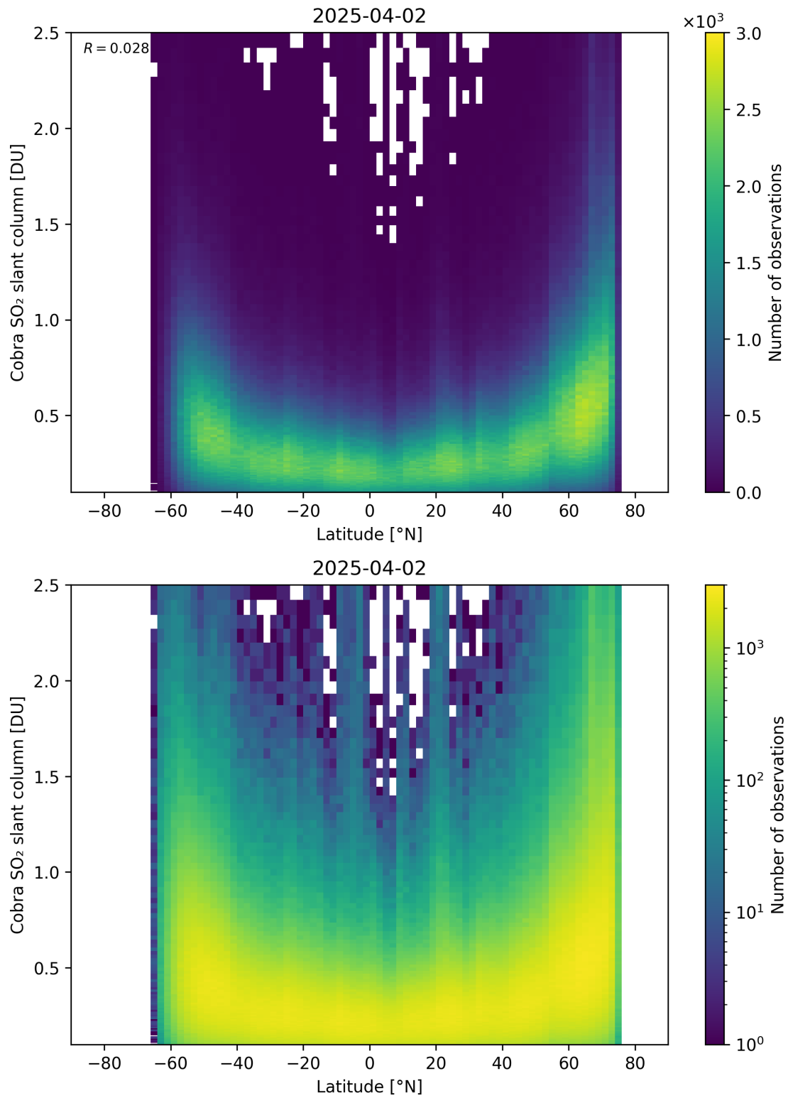
Figure 157: Scatter density plot of “Latitude” against “Cobra SO 2 slant column” for 2025-04-02 to 2025-04-03.
