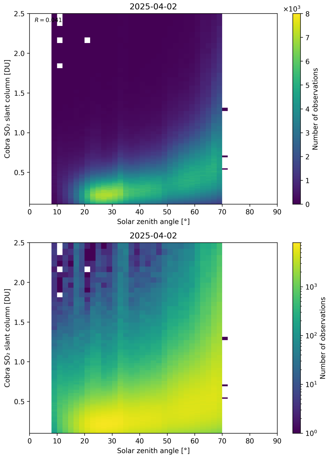
Figure 179: Scatter density plot of “Solar zenith angle” against “Cobra SO 2 slant column” for 2025-04-02 to 2025-04-03.
