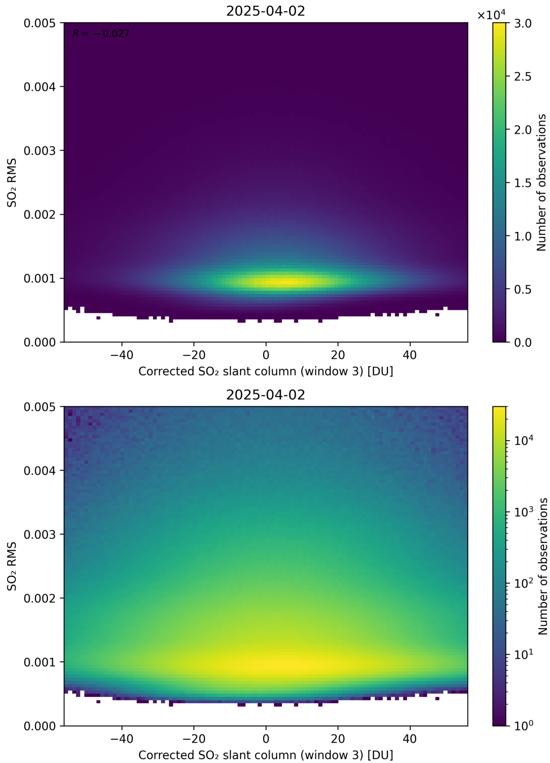
Figure 258: Scatter density plot of “Corrected SO 2 slant column (window 3)” against “SO 2 RMS” for 2025-04-02 to 2025-04-03.
