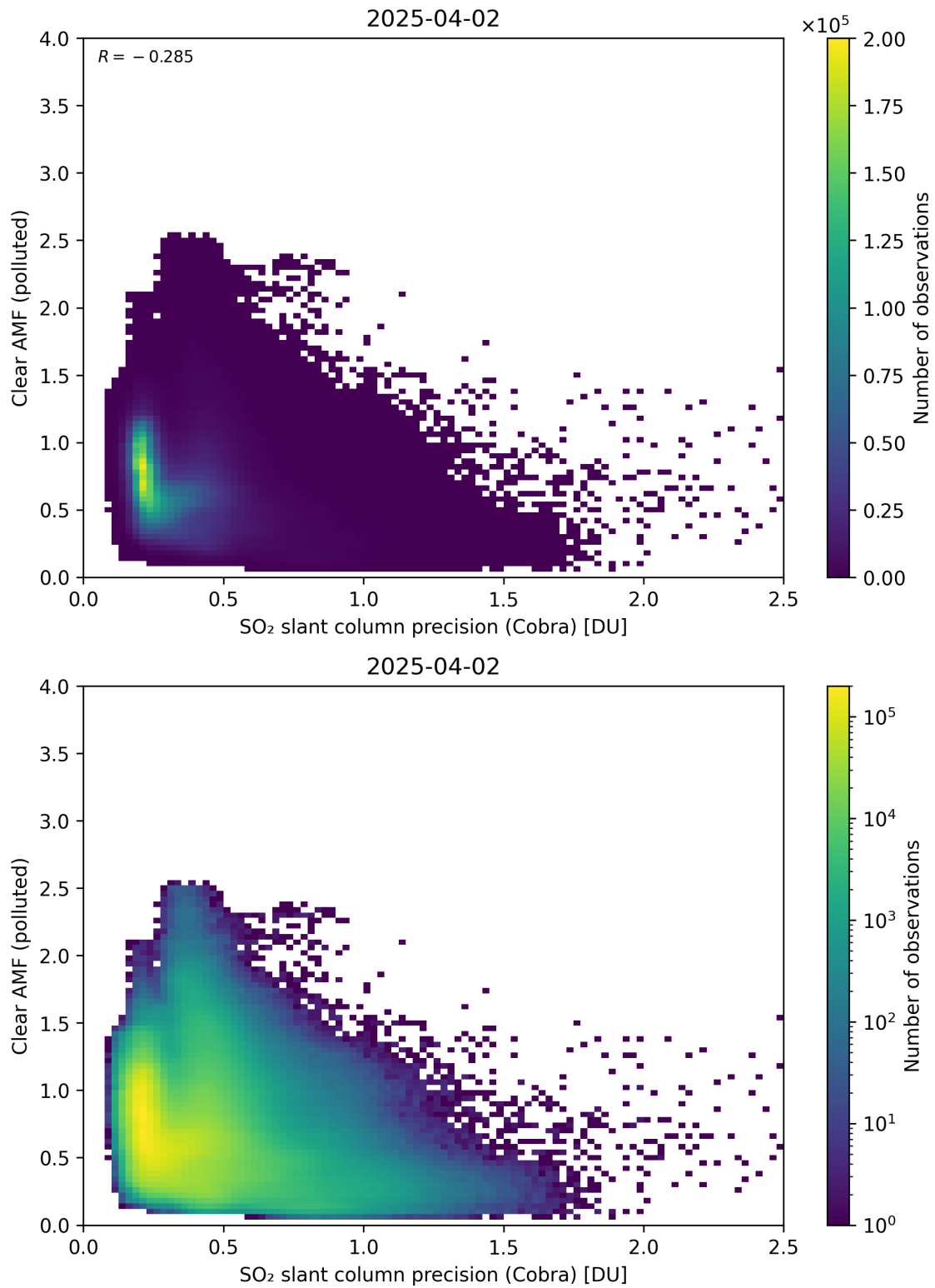
Figure 205: Scatter density plot of “SO 2 slant column precision (Cobra)” against “Clear AMF (polluted)” for 2025-04-02 to 2025-04-03.
