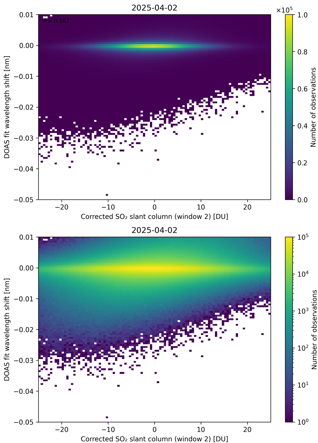
Figure 246: Scatter density plot of “Corrected SO 2 slant column (window 2)” against “DOAS fit wavelength shift” for 2025-04-02 to 2025-04-03.
