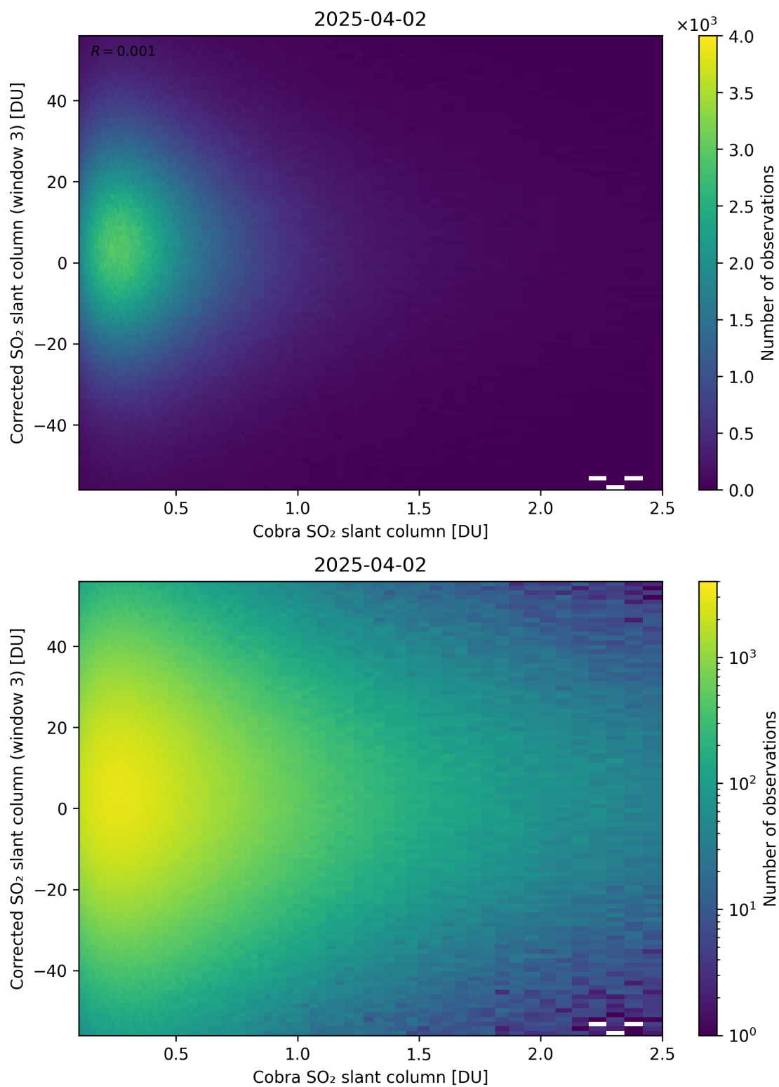
Figure 218: Scatter density plot of “Cobra SO 2 slant column” against “Corrected SO 2 slant column (window 3)” for 2025-04-02 to 2025-04-03.
