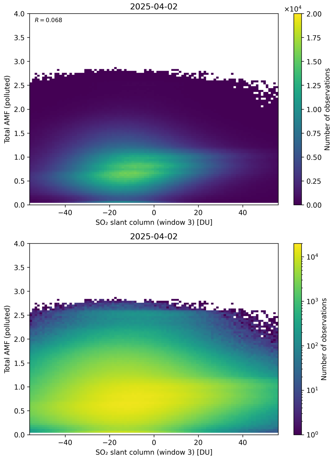
Figure 318: Scatter density plot of “SO 2 slant column (window 3)” against “Total AMF (polluted)” for 2025-04-02 to 2025-04-03.
