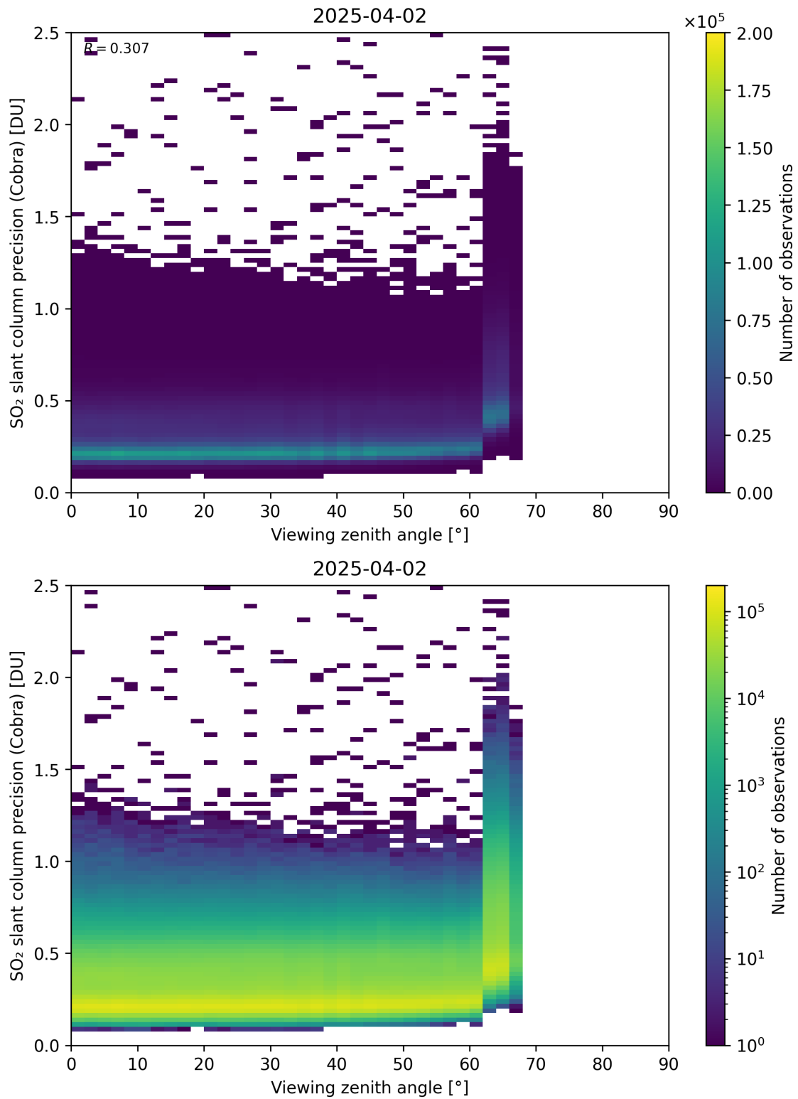
Figure 372: Scatter density plot of “Viewing zenith angle” against “SO 2 slant column precision (Cobra)” for 2025-04-02 to 2025-04-03.
