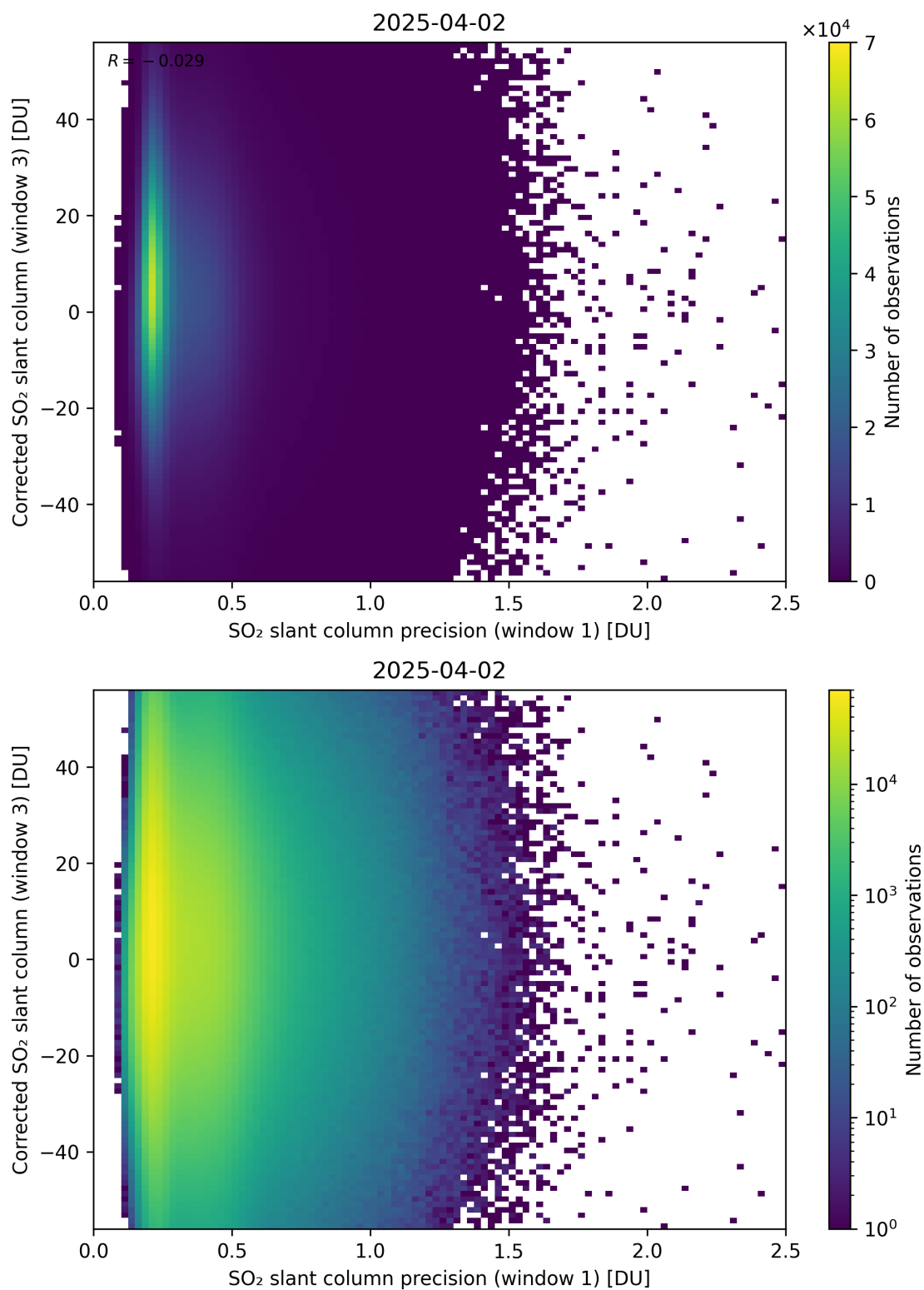
Figure 276: Scatter density plot of “SO 2 slant column precision (window 1)” against “Corrected SO 2 slant column (window 3)” for 2025-04-02 to 2025-04-03.
