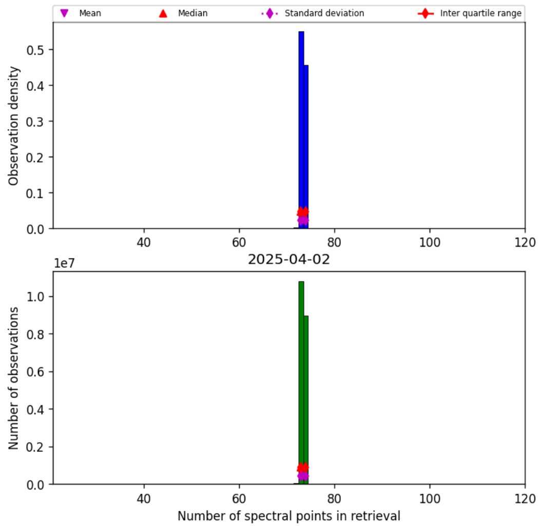
Figure 82: Histogram of “Number of spectral points in retrieval” for 2025-04-02 to 2025-04-03
