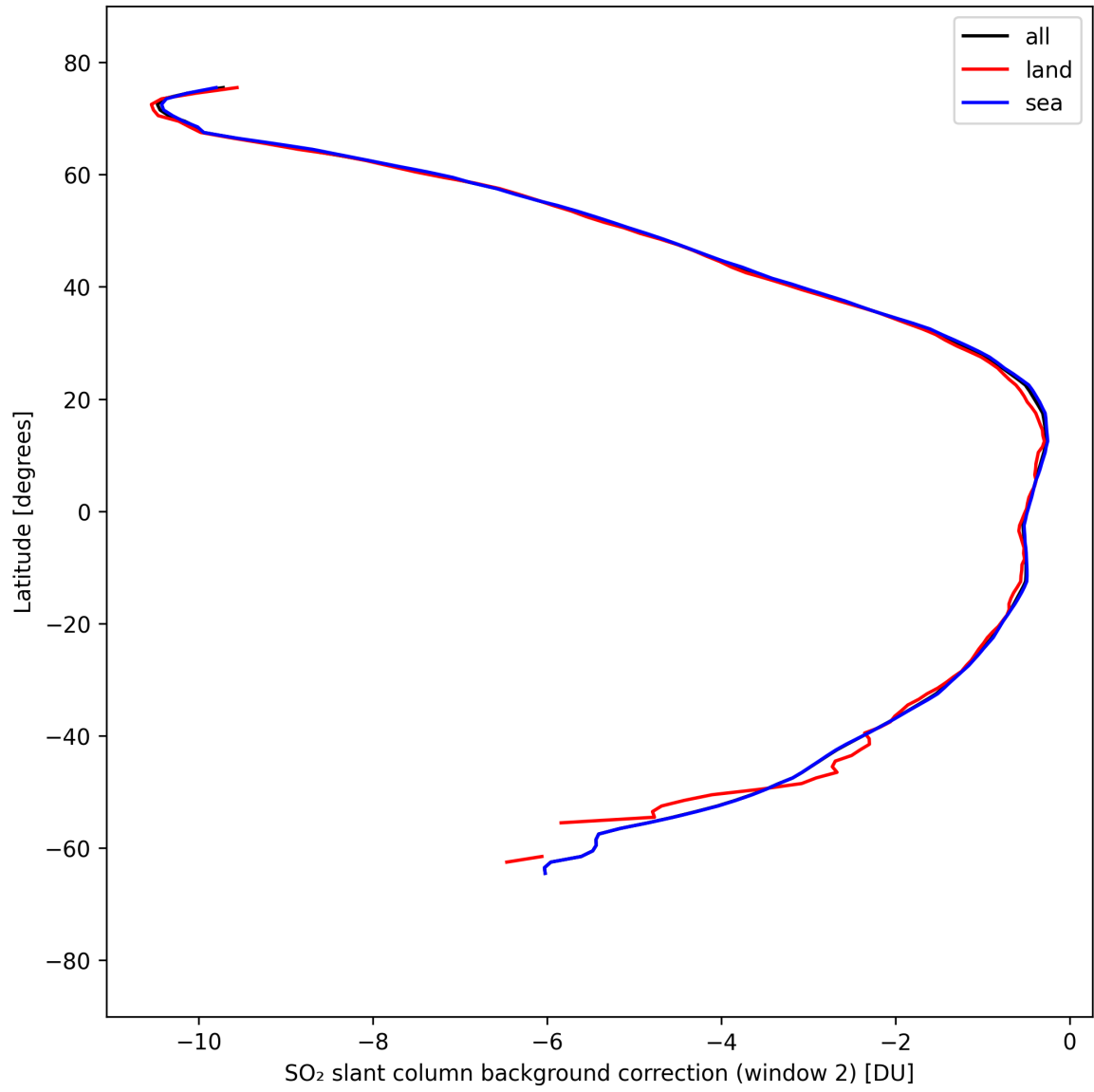
Figure 44: Zonal average of “SO 2 slant column background correction (window 2)” for 2025-04-02 to 2025-04-03.
