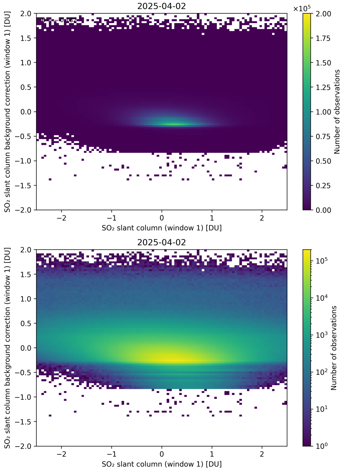
Figure 262: Scatter density plot of “SO 2 slant column (window 1)” against “SO 2 slant column background correction (window 1)” for 2025-04-02 to 2025-04-03.
