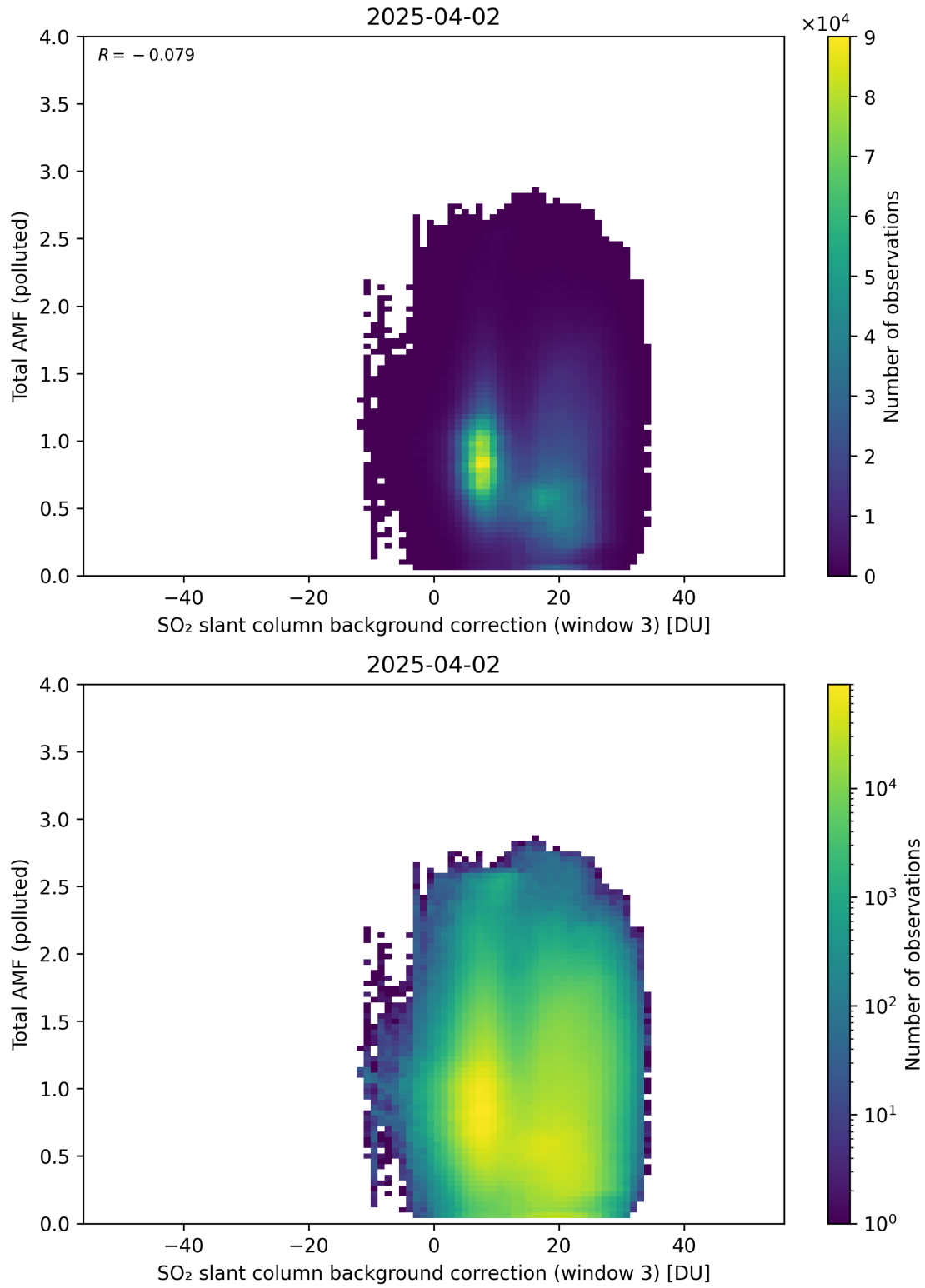
Figure 136: Scatter density plot of “SO 2 slant column background correction (window 3)” against “Total AMF (polluted)” for 2025-04-02 to 2025-04-03.
