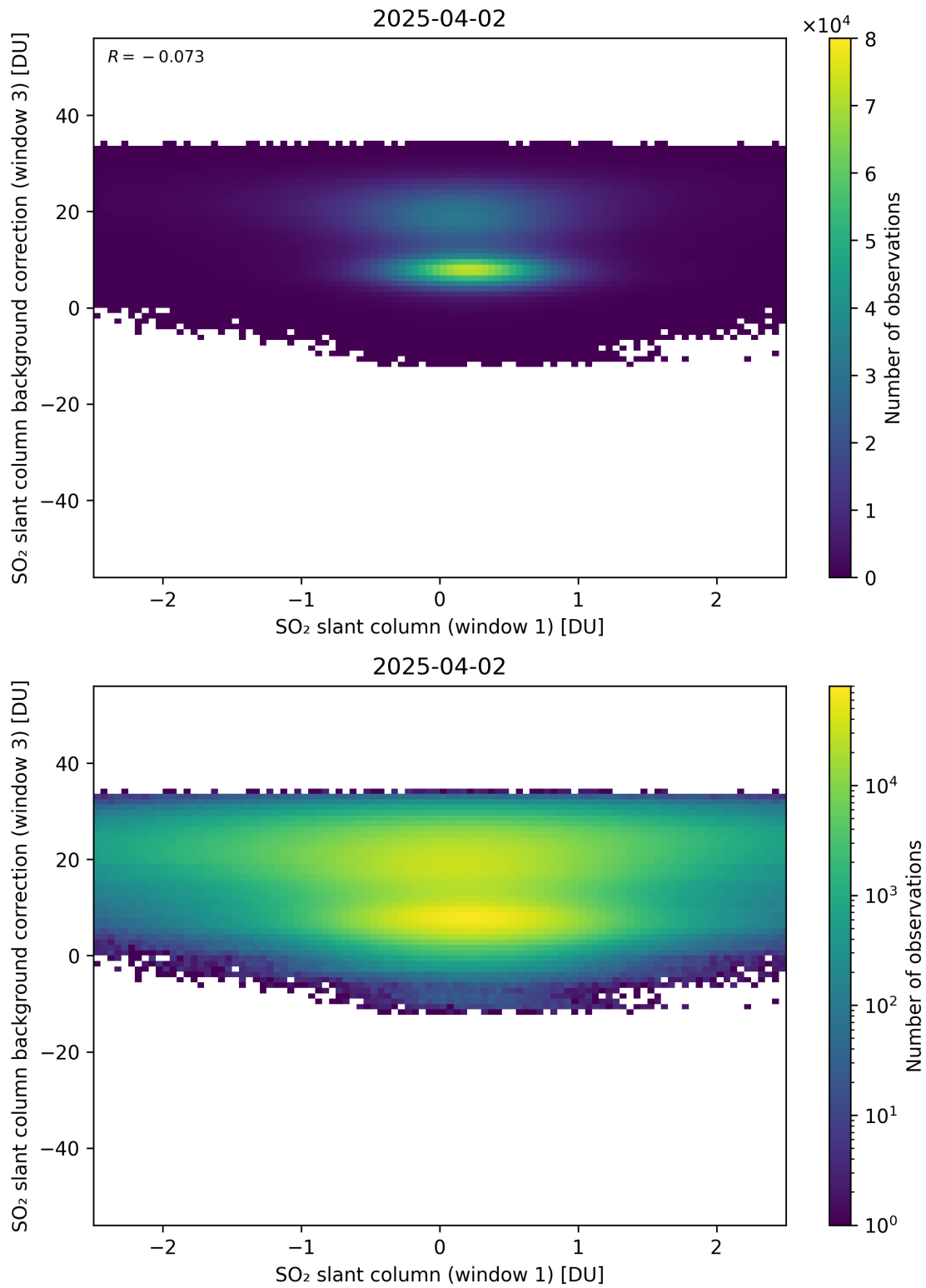
Figure 264: Scatter density plot of “SO 2 slant column (window 1)” against “SO 2 slant column background correction (window 3)” for 2025-04-02 to 2025-04-03.
