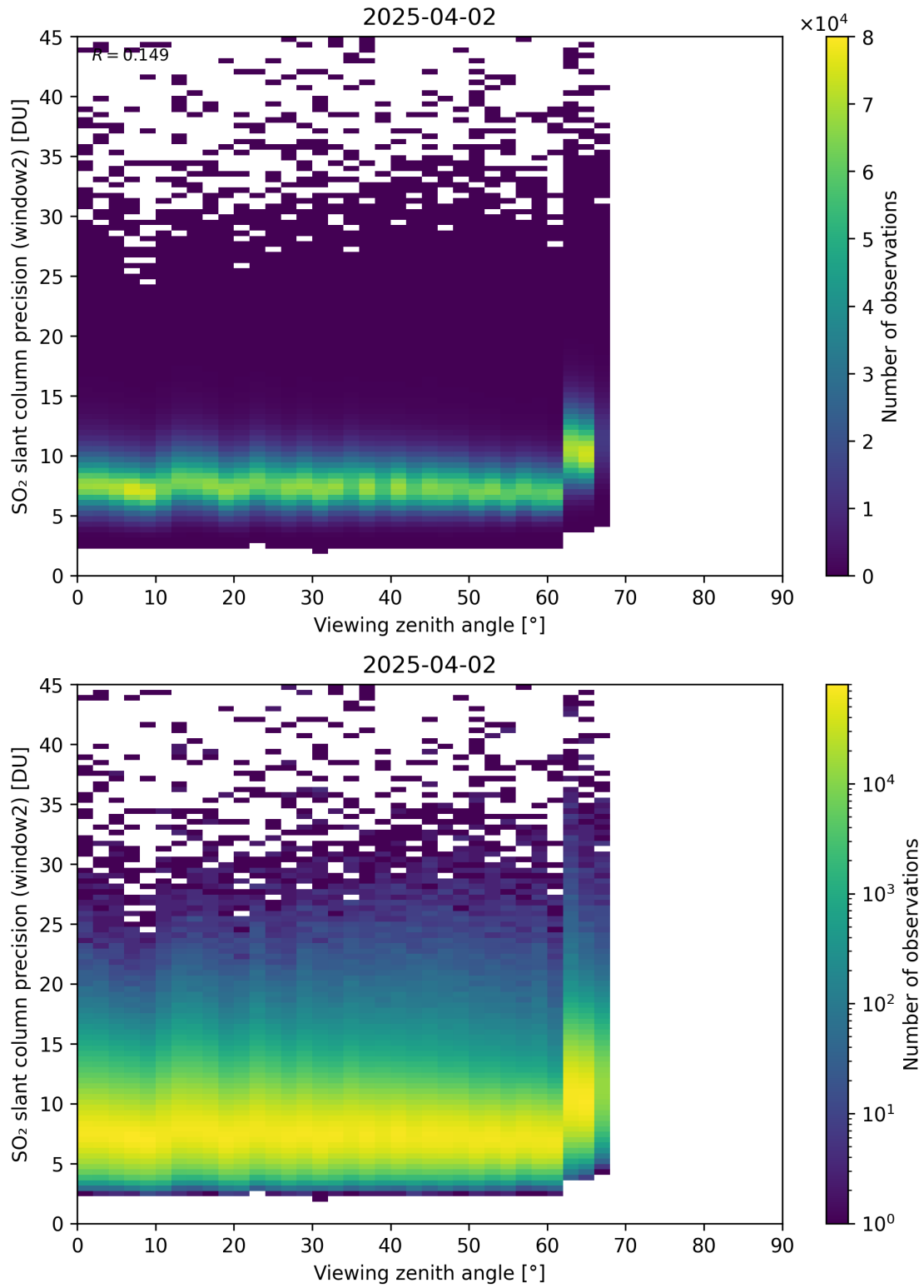
Figure 378: Scatter density plot of “Viewing zenith angle” against “SO 2 slant column precision (window2)” for 2025-04-02 to 2025-04-03.
