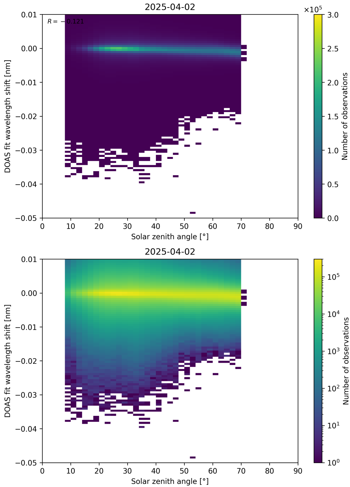
Figure 174: Scatter density plot of “Solar zenith angle” against “DOAS fit wavelength shift” for 2025-04-02 to 2025-04-03.
