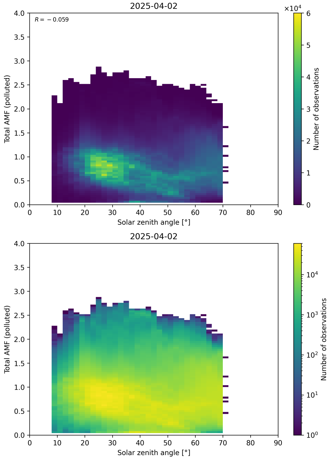
Figure 189: Scatter density plot of “Solar zenith angle” against “Total AMF (polluted)” for 2025-04-02 to 2025-04-03.
