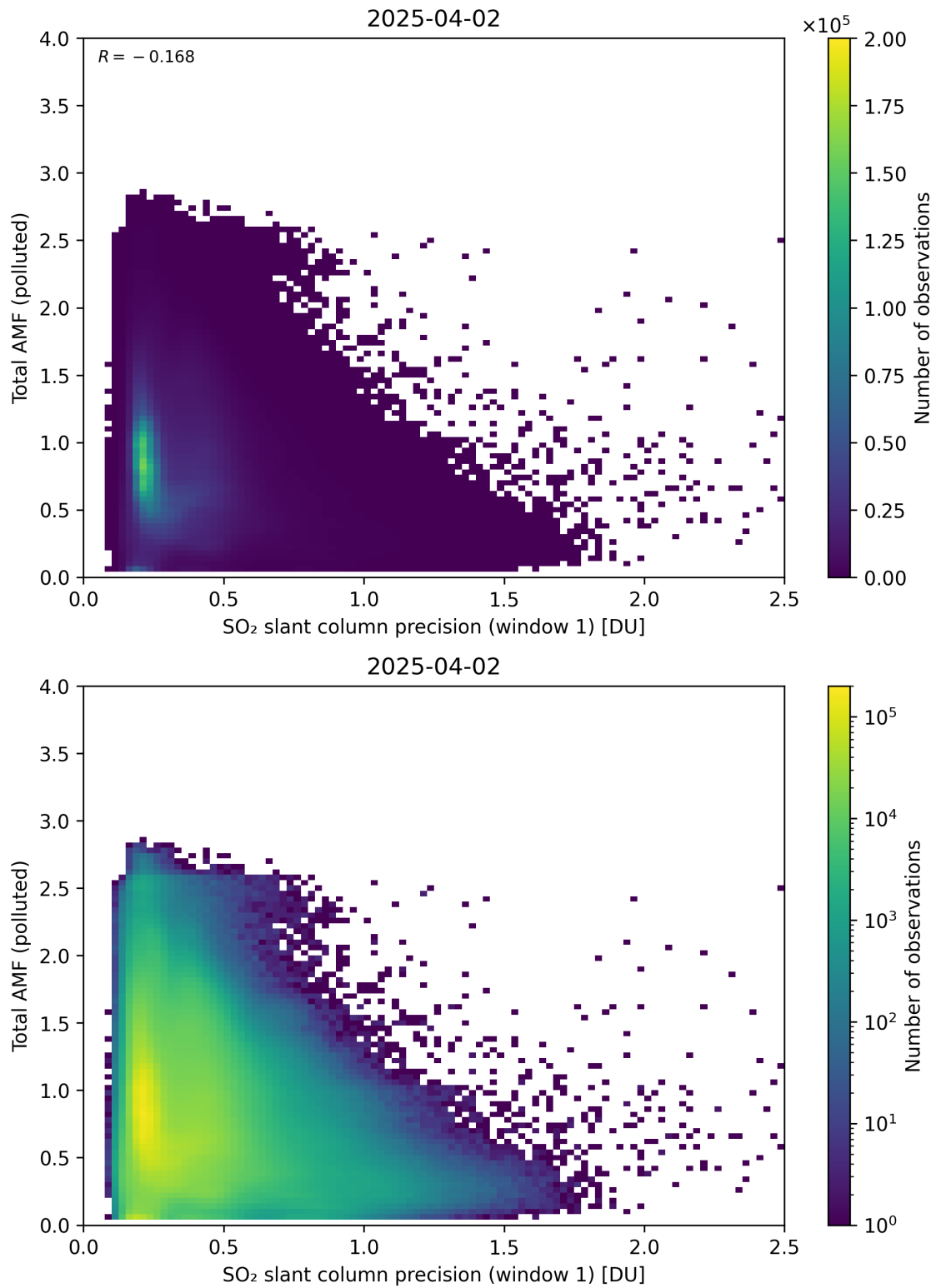
Figure 280: Scatter density plot of “SO 2 slant column precision (window 1)” against “Total AMF (polluted)” for 2025-04-02 to 2025-04-03.
