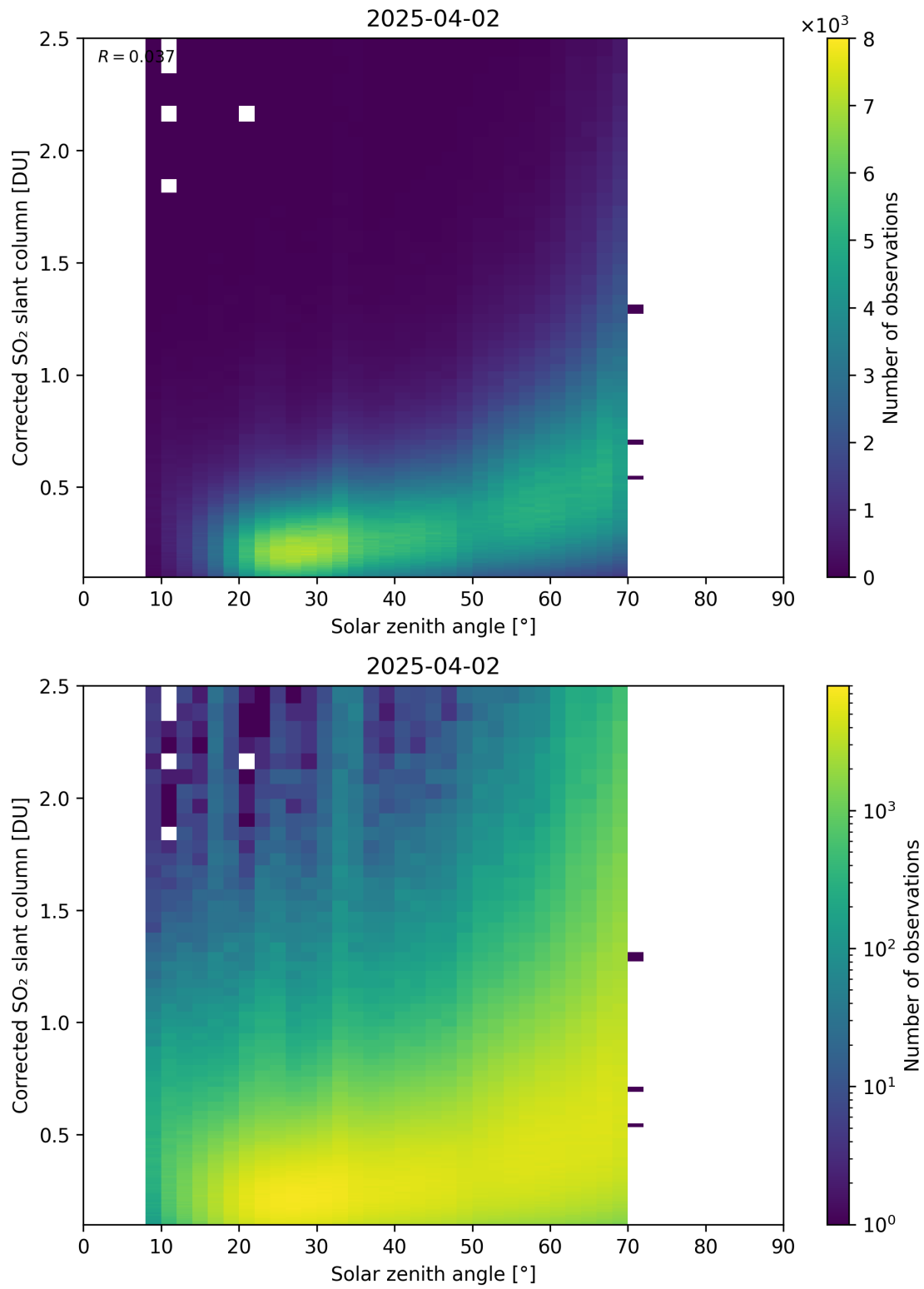
Figure 181: Scatter density plot of “Solar zenith angle” against “Corrected SO 2 slant column” for 2025-04-02 to 2025-04-03.
