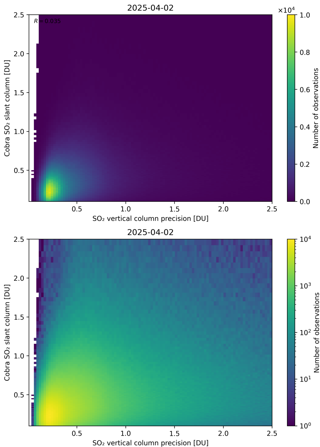
Figure 336: Scatter density plot of “SO 2 vertical column precision” against “Cobra SO 2 slant column” for 2025-04-02 to 2025-04-03.
