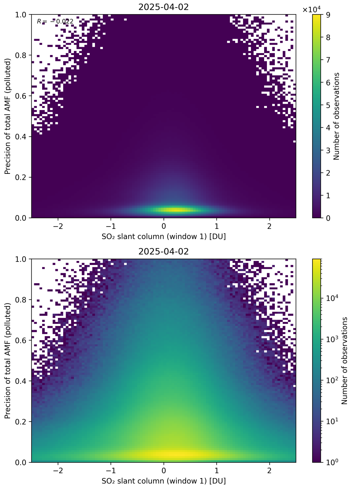
Figure 290: Scatter density plot of “SO 2 slant column (window 1)” against “Precision of total AMF (polluted)” for 2025-04-02 to 2025-04-03.
