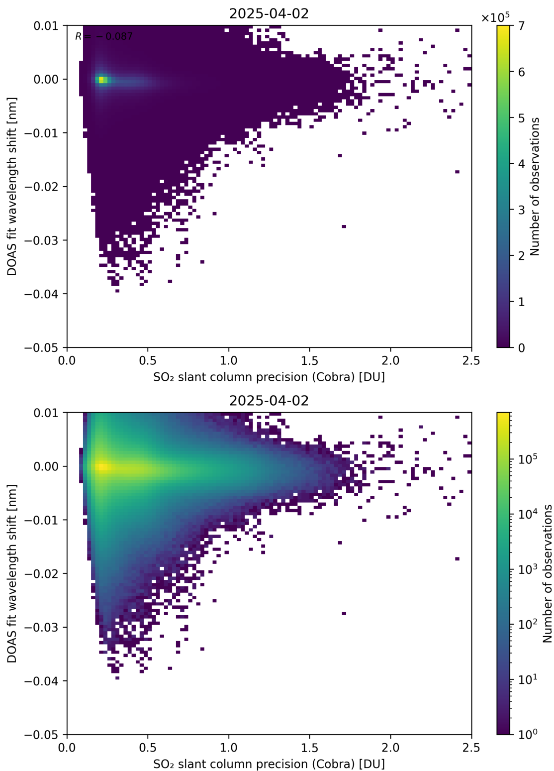
Figure 202: Scatter density plot of “SO 2 slant column precision (Cobra)” against “DOAS fit wavelength shift” for 2025-04-02 to 2025-04-03.
