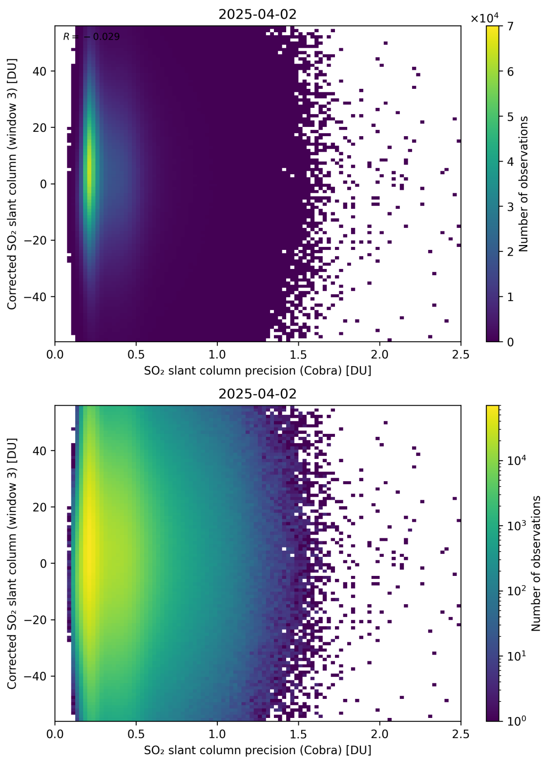
Figure 207: Scatter density plot of “SO 2 slant column precision (Cobra)” against “Corrected SO 2 slant column (window 3)” for 2025-04-02 to 2025-04-03.
