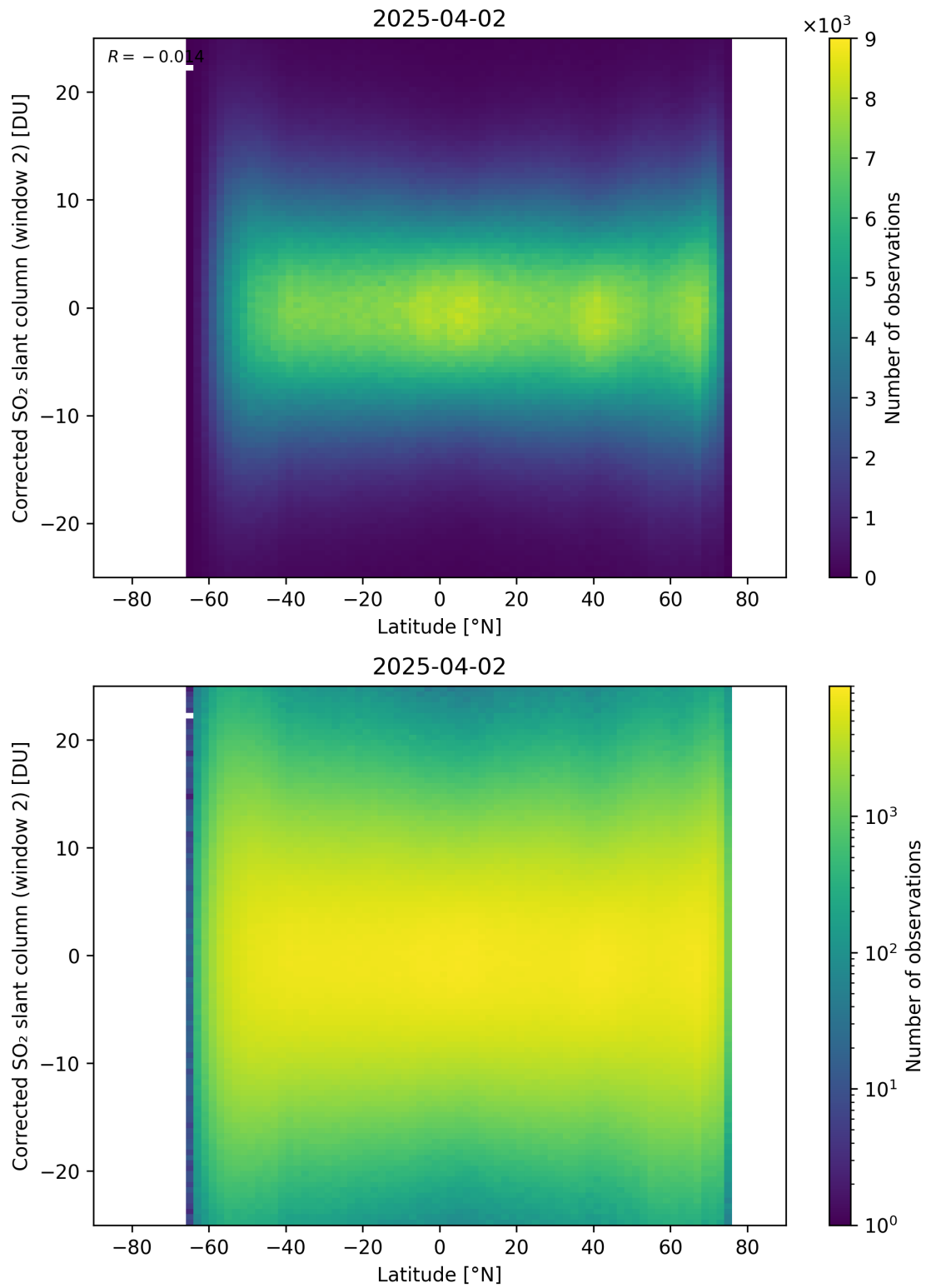
Figure 160: Scatter density plot of “Latitude” against “Corrected SO 2 slant column (window 2)” for 2025-04-02 to 2025-04-03.
