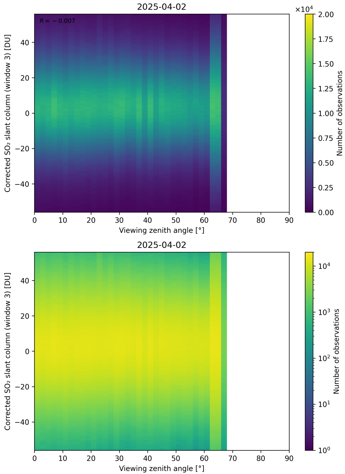
Figure 375: Scatter density plot of “Viewing zenith angle” against “Corrected SO 2 slant column (window 3)” for 2025-04-02 to 2025-04-03.
