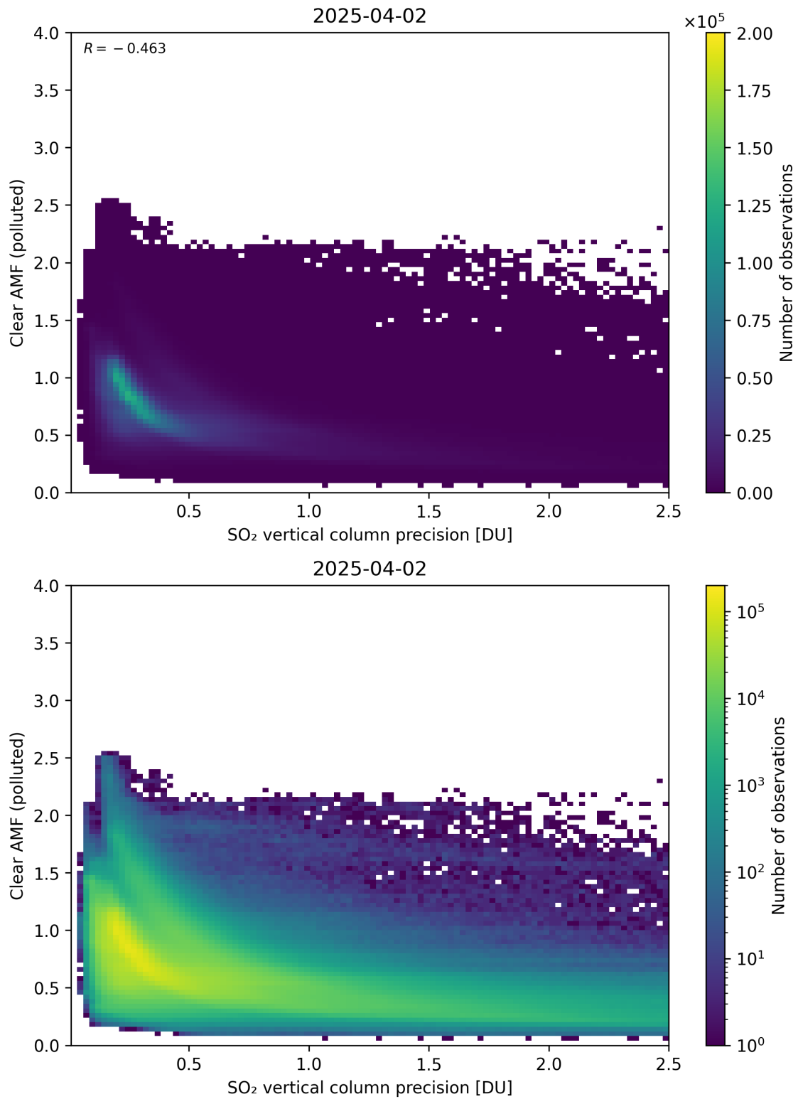
Figure 335: Scatter density plot of “SO 2 vertical column precision” against “Clear AMF (polluted)” for 2025-04-02 to 2025-04-03.
