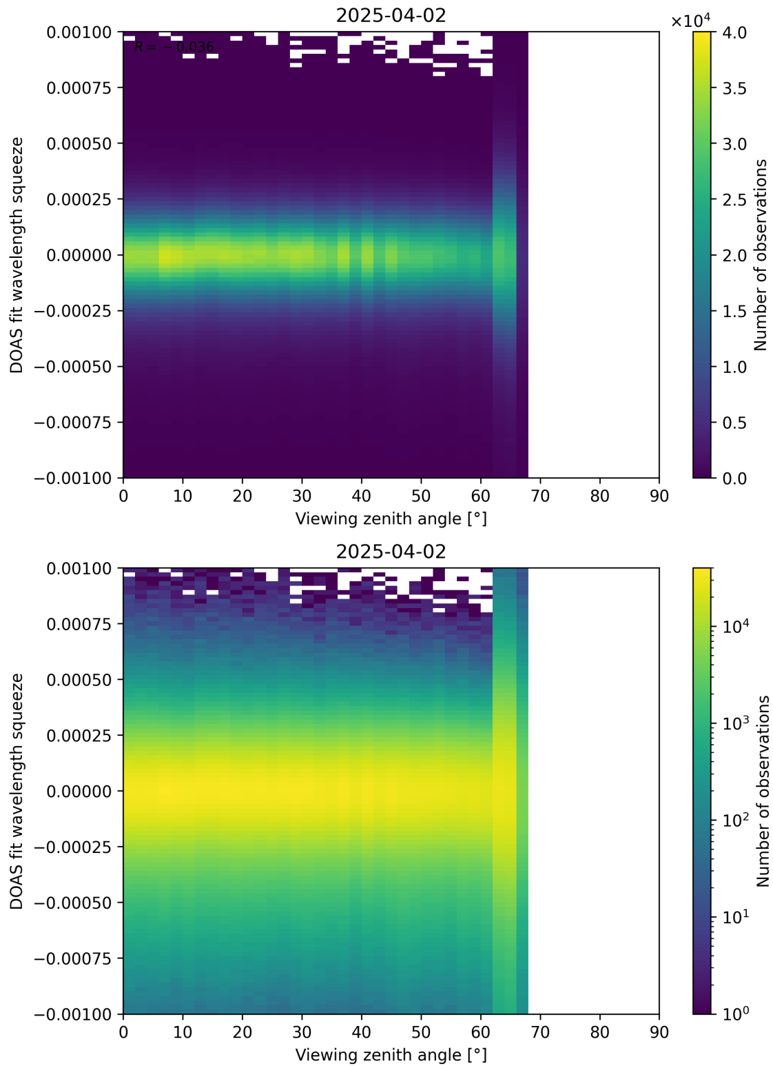
Figure 366: Scatter density plot of “Viewing zenith angle” against “DOAS fit wavelength squeeze” for 2025-04-02 to 2025-04-03.
