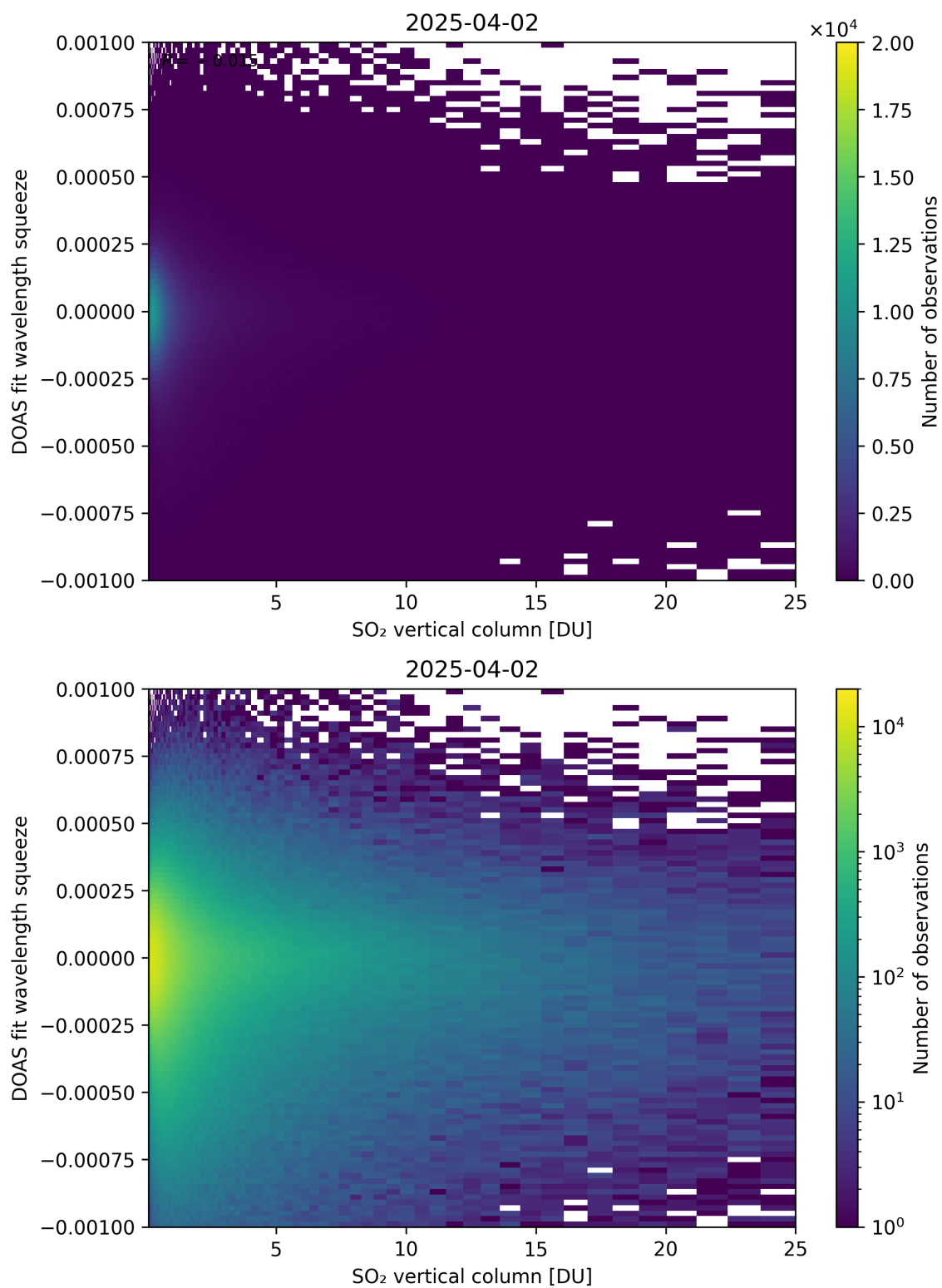
Figure 327: Scatter density plot of “SO 2 vertical column” against “DOAS fit wavelength squeeze” for 2025-04-02 to 2025-04-03.
