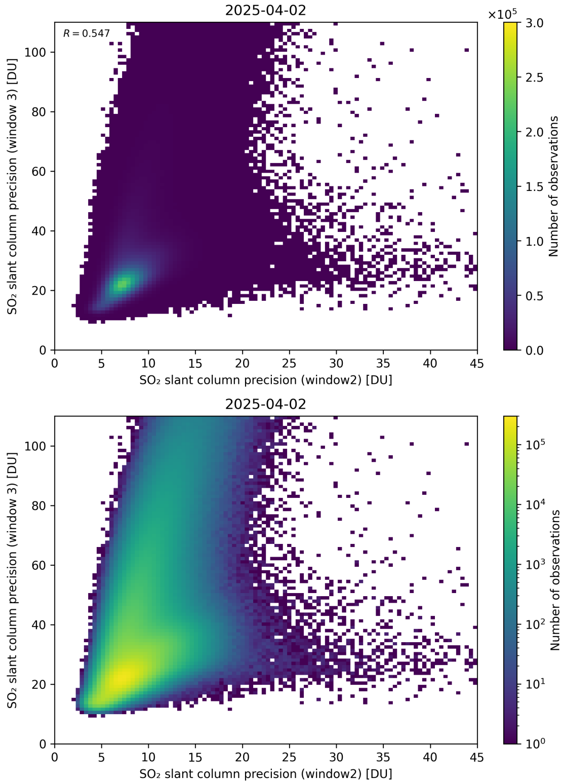
Figure 300: Scatter density plot of “SO 2 slant column precision (window2)” against “SO 2 slant column precision (window 3)” for 2025-04-02 to 2025-04-03.
