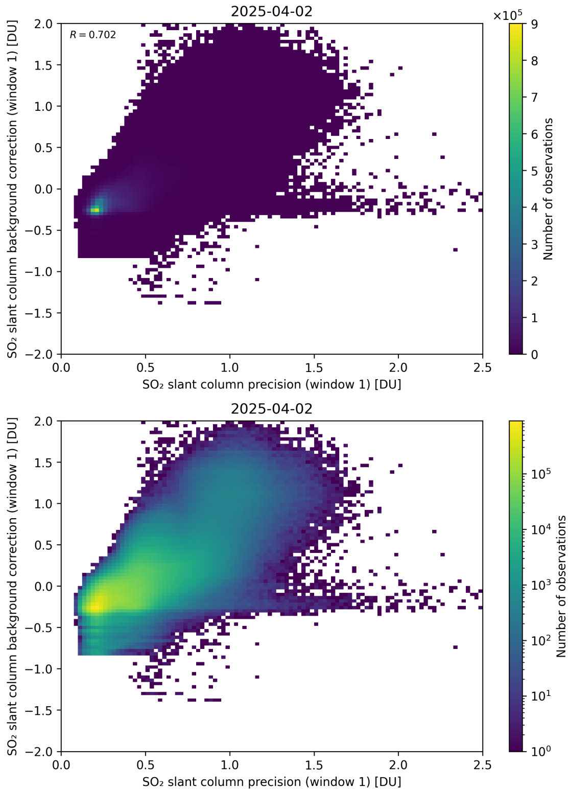
Figure 268: Scatter density plot of “SO 2 slant column precision (window 1)” against “SO 2 slant column background correction (window 1)” for 2025-04-02 to 2025-04-03.
