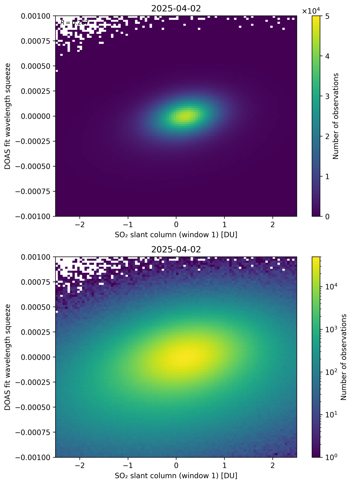
Figure 266: Scatter density plot of “SO 2 slant column (window 1)” against “DOAS fit wavelength squeeze” for 2025-04-02 to 2025-04-03.
