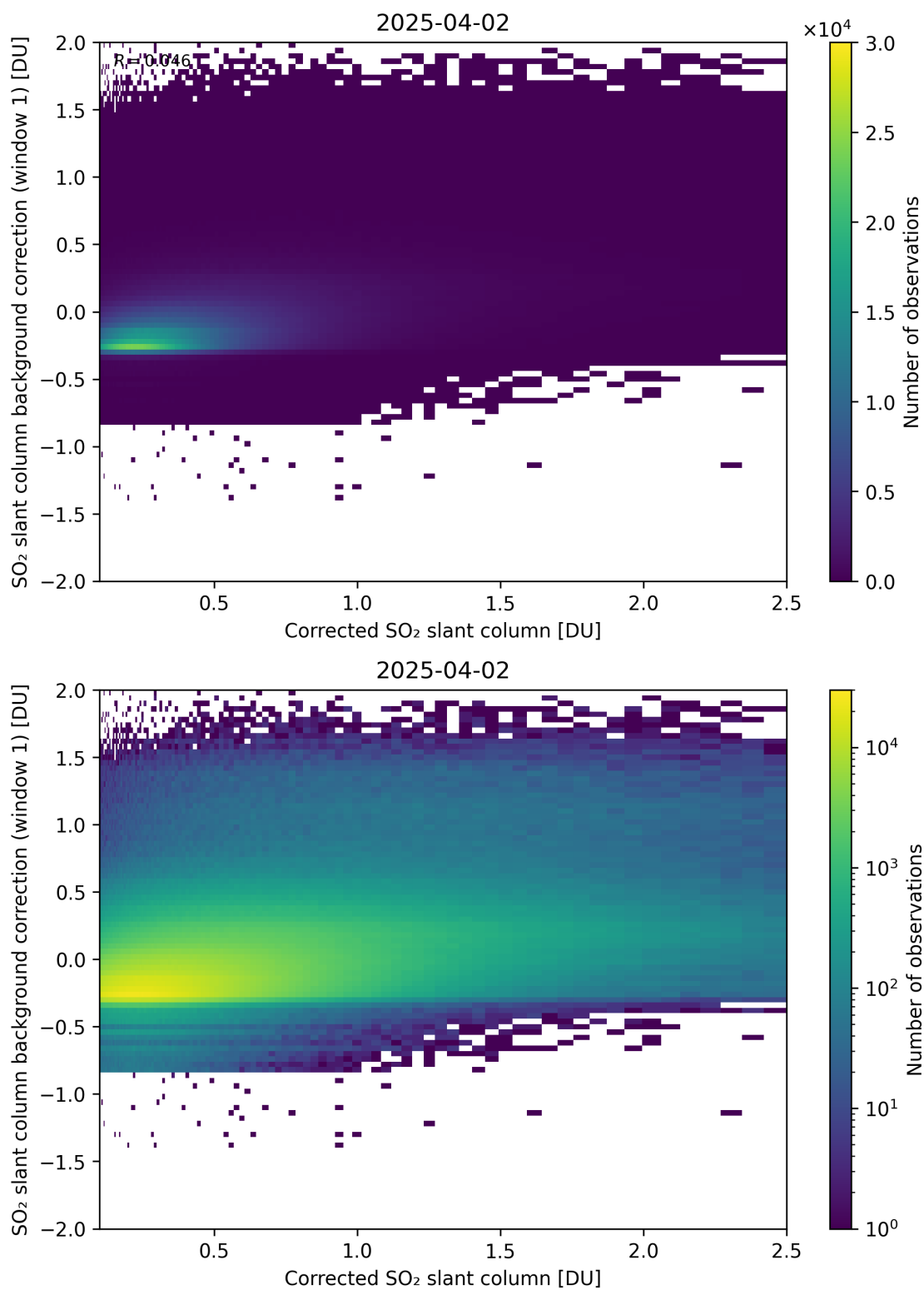
Figure 226: Scatter density plot of “Corrected SO 2 slant column” against “SO 2 slant column background correction (window 1)” for 2025-04-02 to 2025-04-03.
