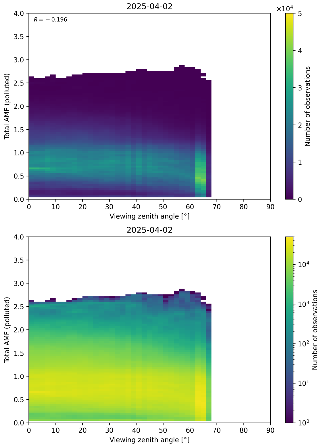
Figure 381: Scatter density plot of “Viewing zenith angle” against “Total AMF (polluted)” for 2025-04-02 to 2025-04-03.
