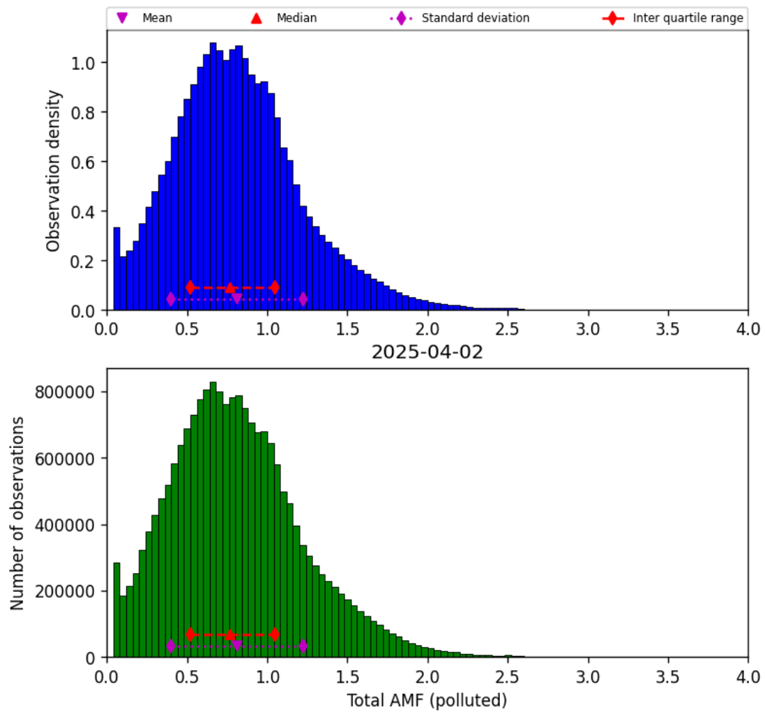
Figure 79: Histogram of “Total AMF (polluted)” for 2025-04-02 to 2025-04-03
