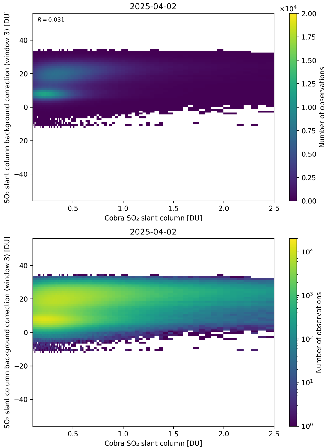
Figure 195: Scatter density plot of “Cobra SO 2 slant column” against “SO 2 slant column background correction (window 3)” for 2025-04-02 to 2025-04-03.
