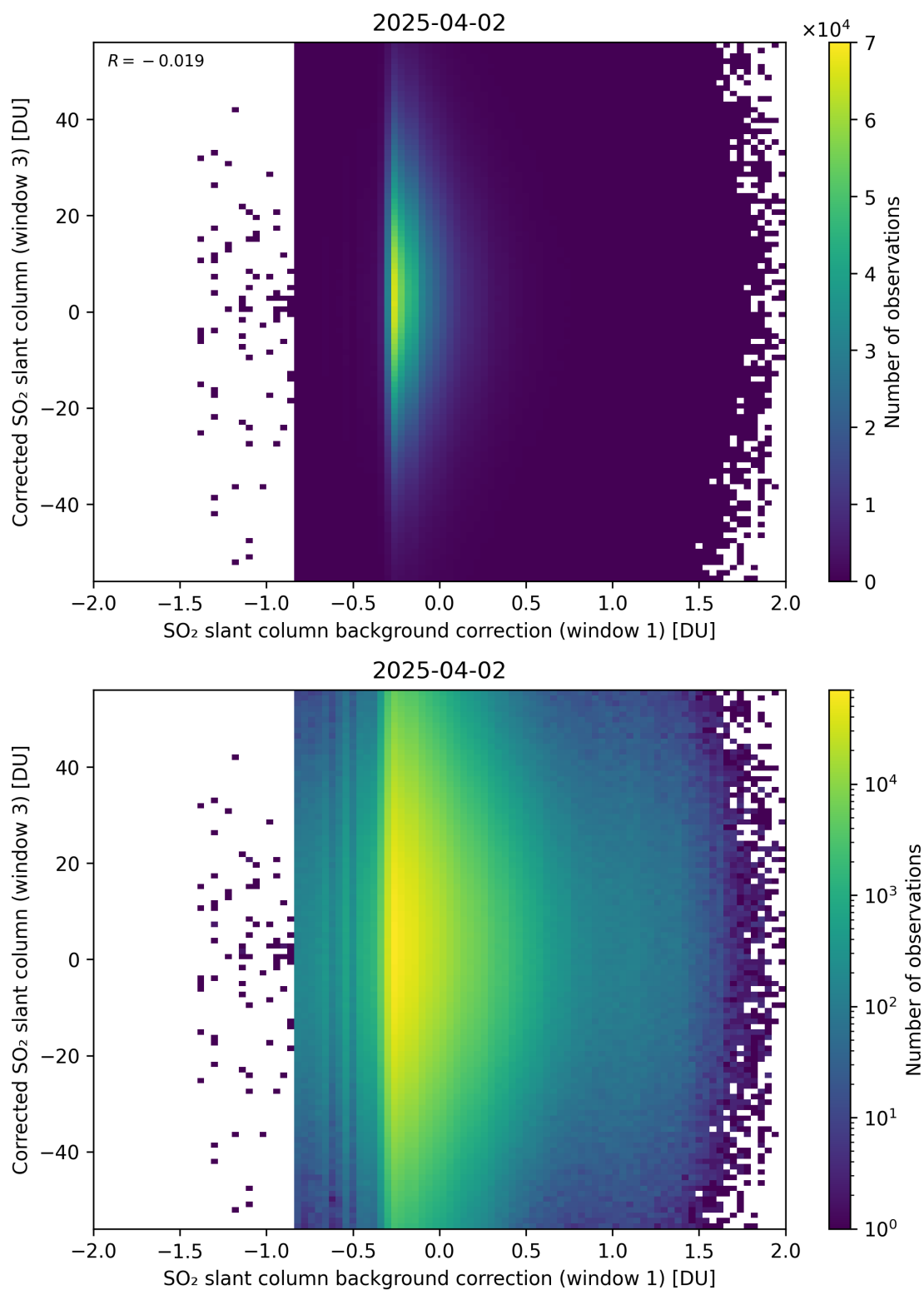
Figure 116: Scatter density plot of “SO 2 slant column background correction (window 1)” against “Corrected SO 2 slant column (window 3)” for 2025-04-02 to 2025-04-03.
