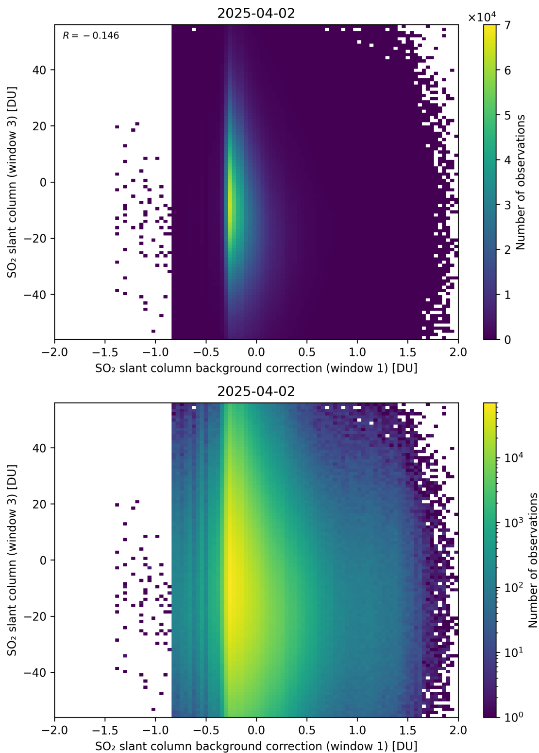
Figure 118: Scatter density plot of “SO 2 slant column background correction (window 1)” against “SO 2 slant column (window 3)” for 2025-04-02 to 2025-04-03.
