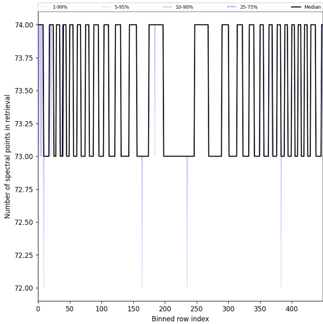
Figure 108: Along track statistics of “Number of spectral points in retrieval” for 2025-04-02 to 2025-04-03
