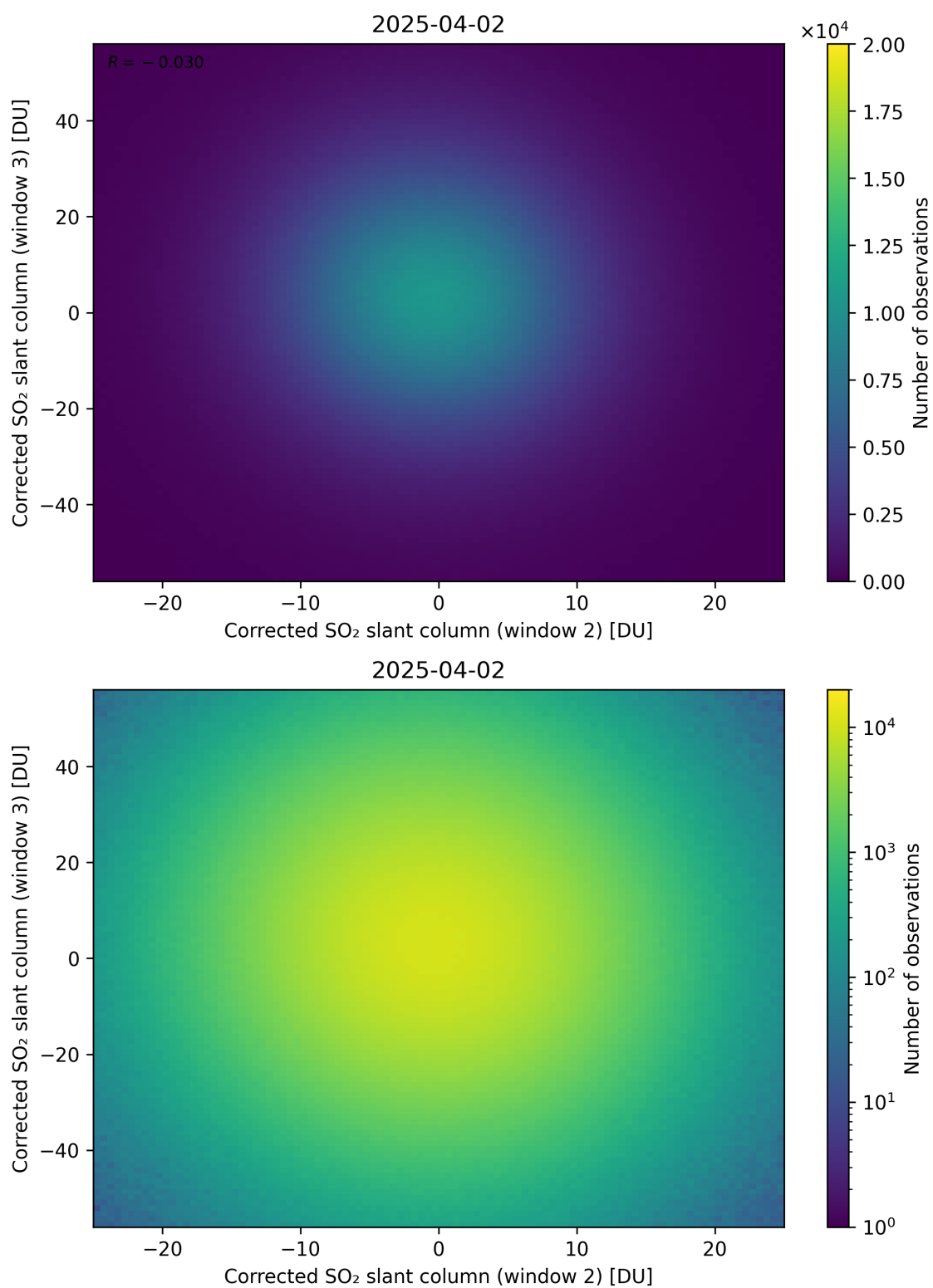
Figure 250: Scatter density plot of “Corrected SO 2 slant column (window 2)” against “Corrected SO 2 slant column (window 3)” for 2025-04-02 to 2025-04-03.
