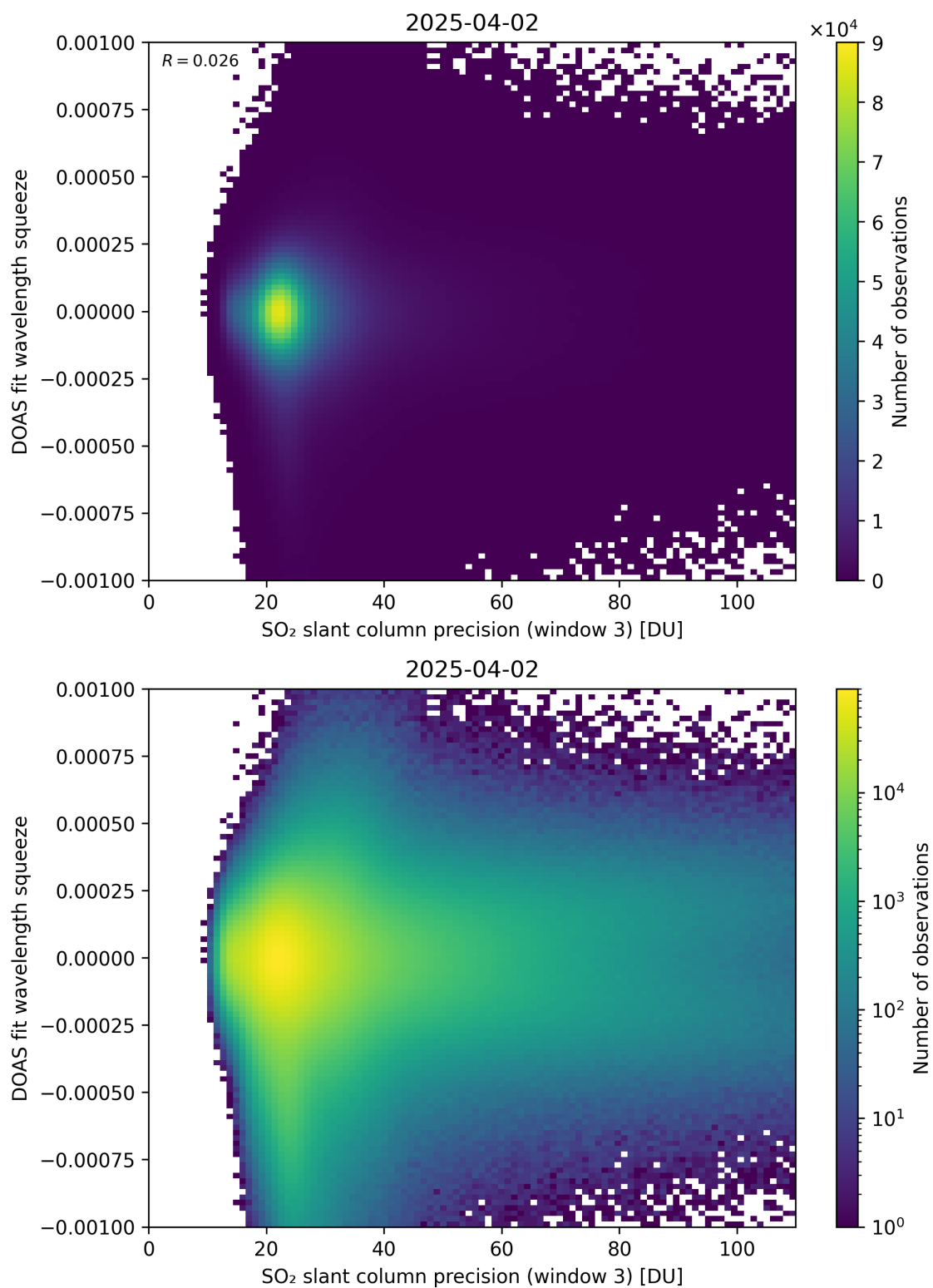
Figure 309: Scatter density plot of “SO 2 slant column precision (window 3)” against “DOAS fit wavelength squeeze” for 2025-04-02 to 2025-04-03.
