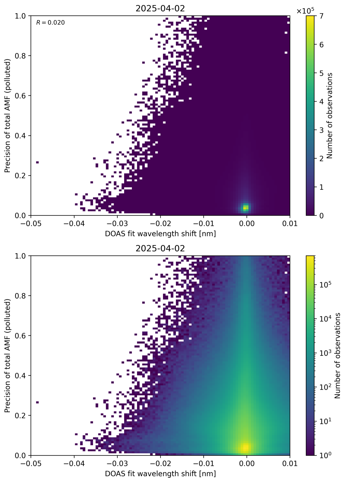
Figure 142: Scatter density plot of “DOAS fit wavelength shift” against “Precision of total AMF (polluted)” for 2025-04-02 to 2025-04-03.
