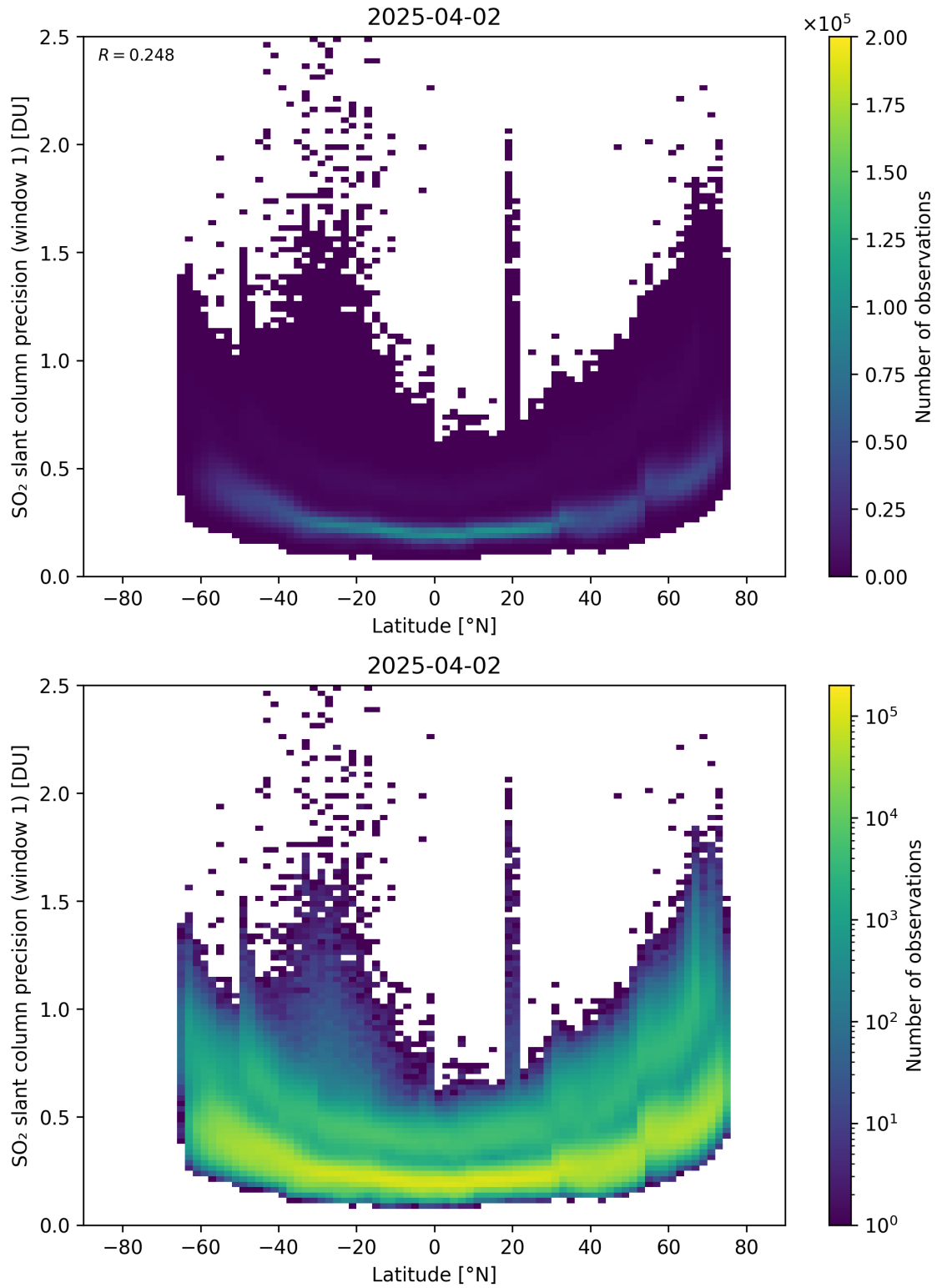
Figure 163: Scatter density plot of “Latitude” against “SO 2 slant column precision (window 1)” for 2025-04-02 to 2025-04-03.
