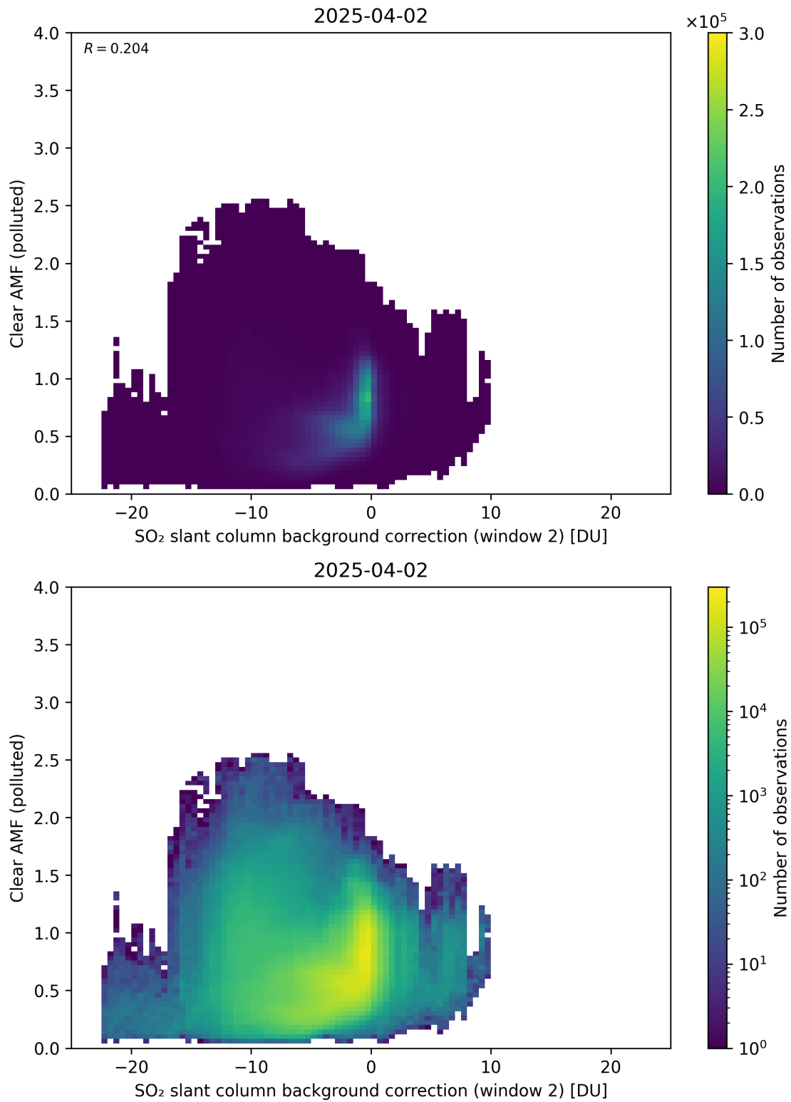
Figure 126: Scatter density plot of “SO 2 slant column background correction (window 2)” against “Clear AMF (polluted)” for 2025-04-02 to 2025-04-03.
