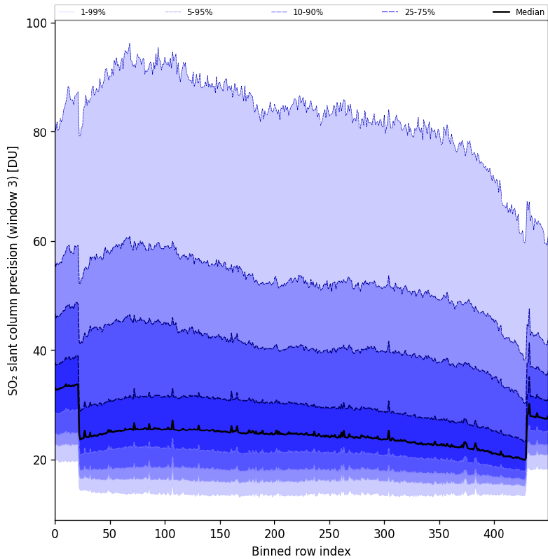
Figure 98: Along track statistics of “SO 2 slant column precision (window 3)” for 2025-04-02 to 2025-04-03
