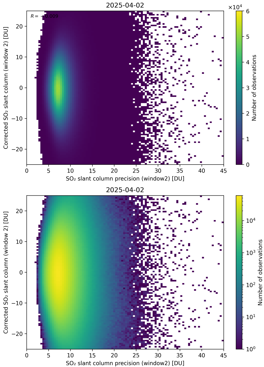
Figure 297: Scatter density plot of “SO 2 slant column precision (window2)” against “Corrected SO 2 slant column (window 2)” for 2025-04-02 to 2025-04-03.
