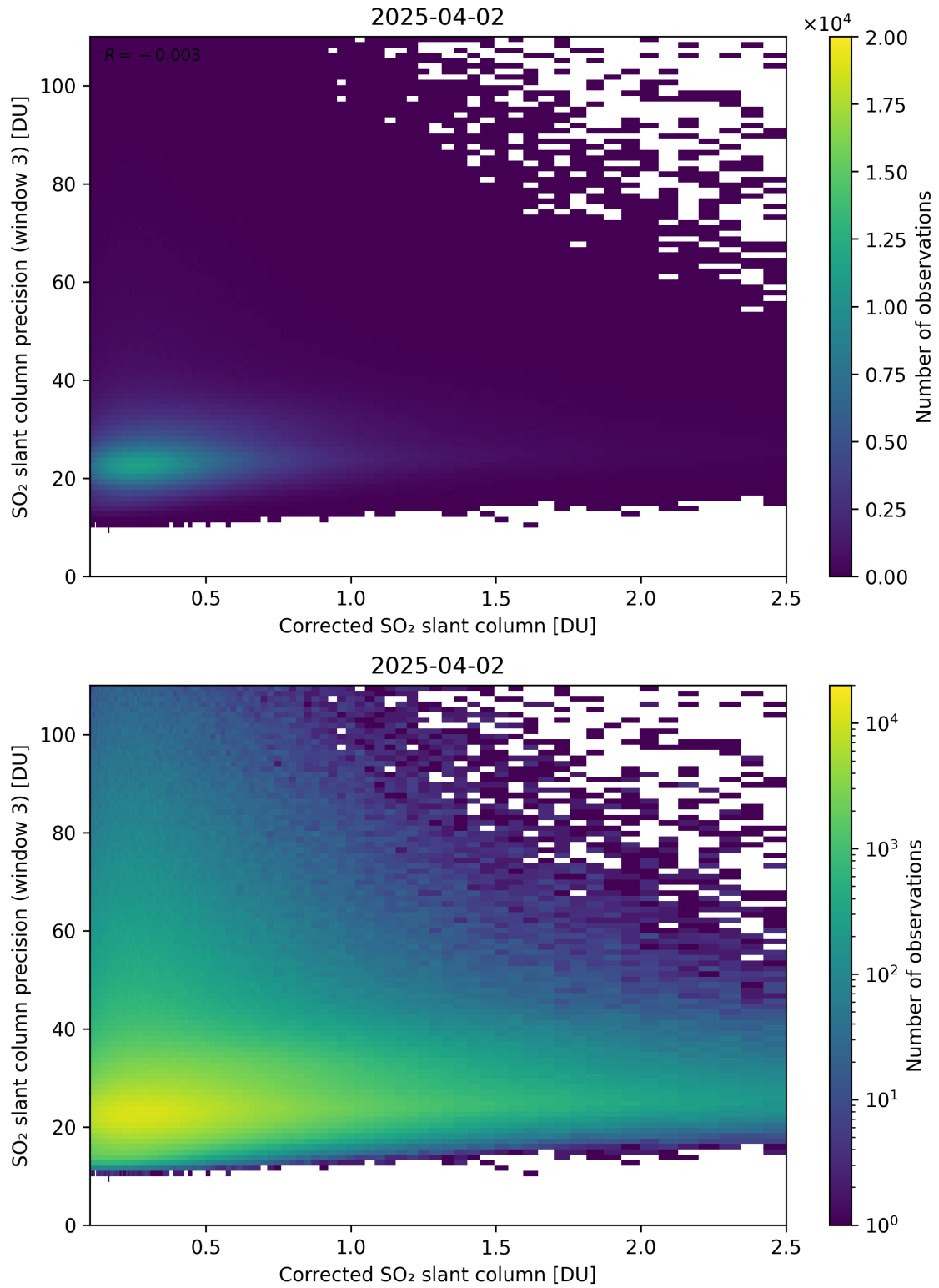
Figure 241: Scatter density plot of “Corrected SO 2 slant column” against “SO 2 slant column precision (window 3)” for 2025-04-02 to 2025-04-03.
