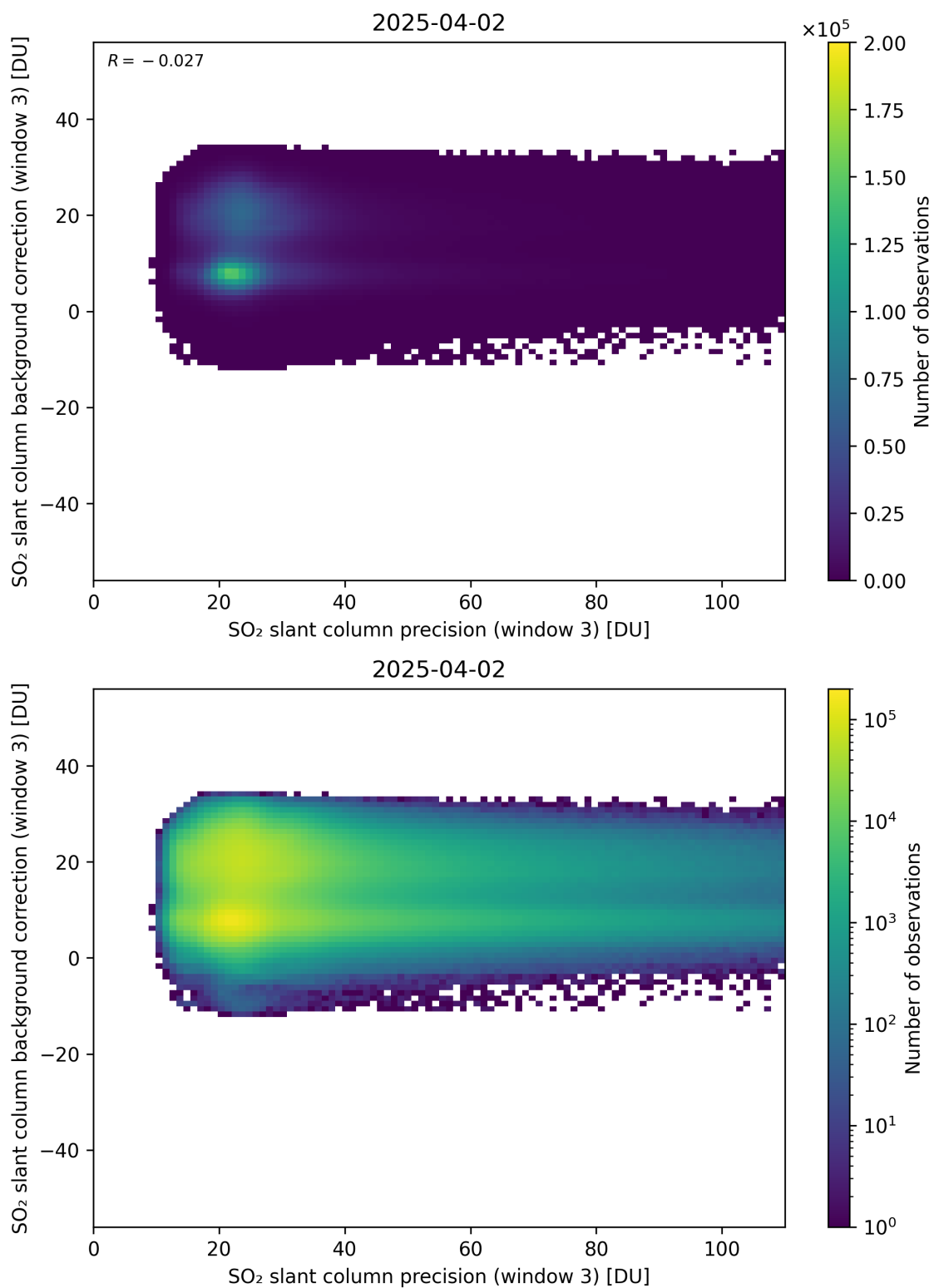
Figure 307: Scatter density plot of “SO 2 slant column precision (window 3)” against “SO 2 slant column background correction (window 3)” for 2025-04-02 to 2025-04-03.
