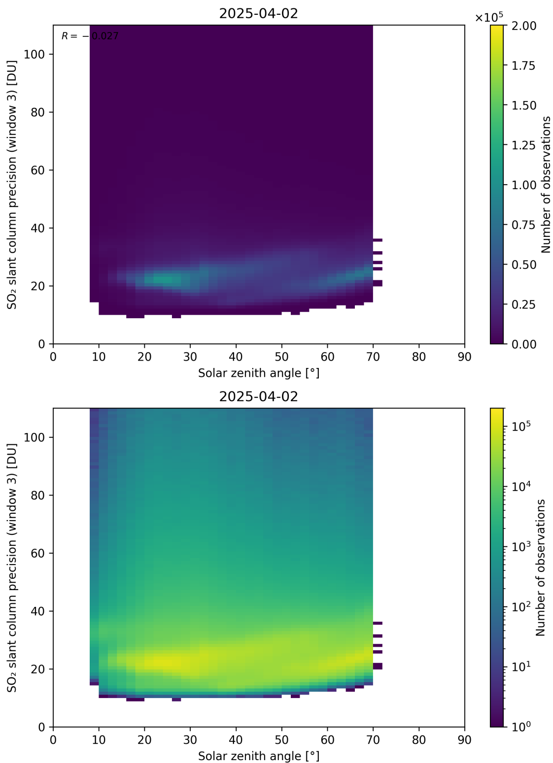
Figure 188: Scatter density plot of “Solar zenith angle” against “SO 2 slant column precision (window 3)” for 2025-04-02 to 2025-04-03.
