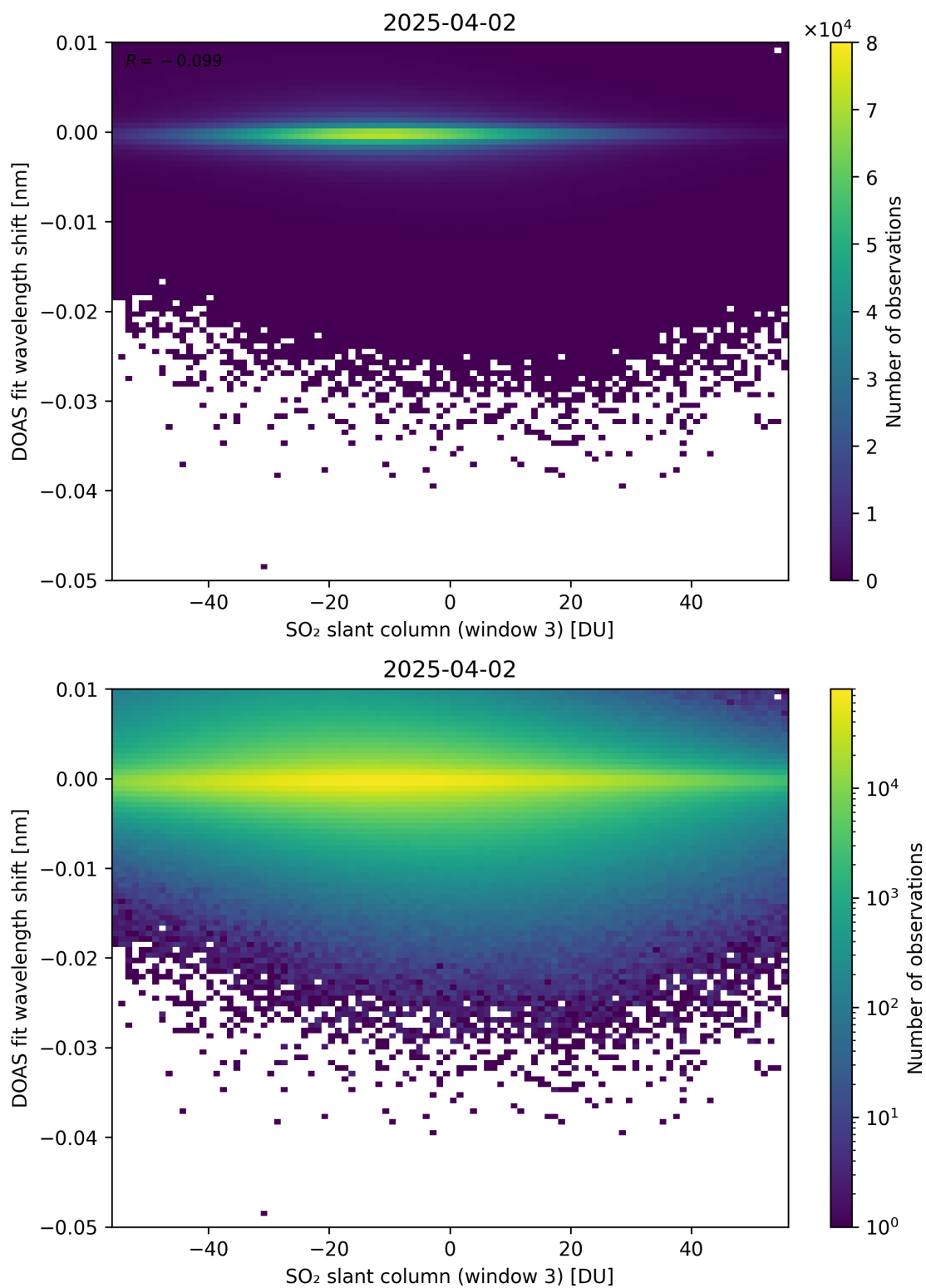
Figure 304: Scatter density plot of “SO 2 slant column (window 3)” against “DOAS fit wavelength shift” for 2025-04-02 to 2025-04-03.
