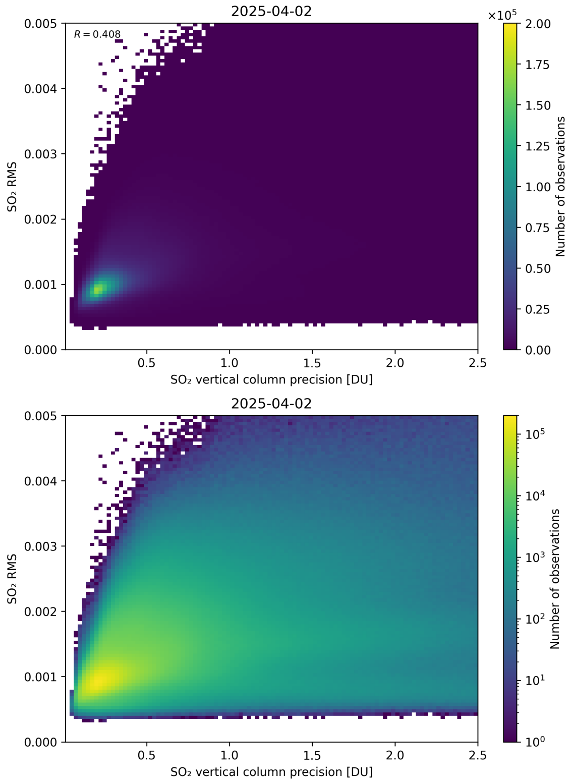
Figure 334: Scatter density plot of “SO 2 vertical column precision” against “SO 2 RMS” for 2025-04-02 to 2025-04-03.
