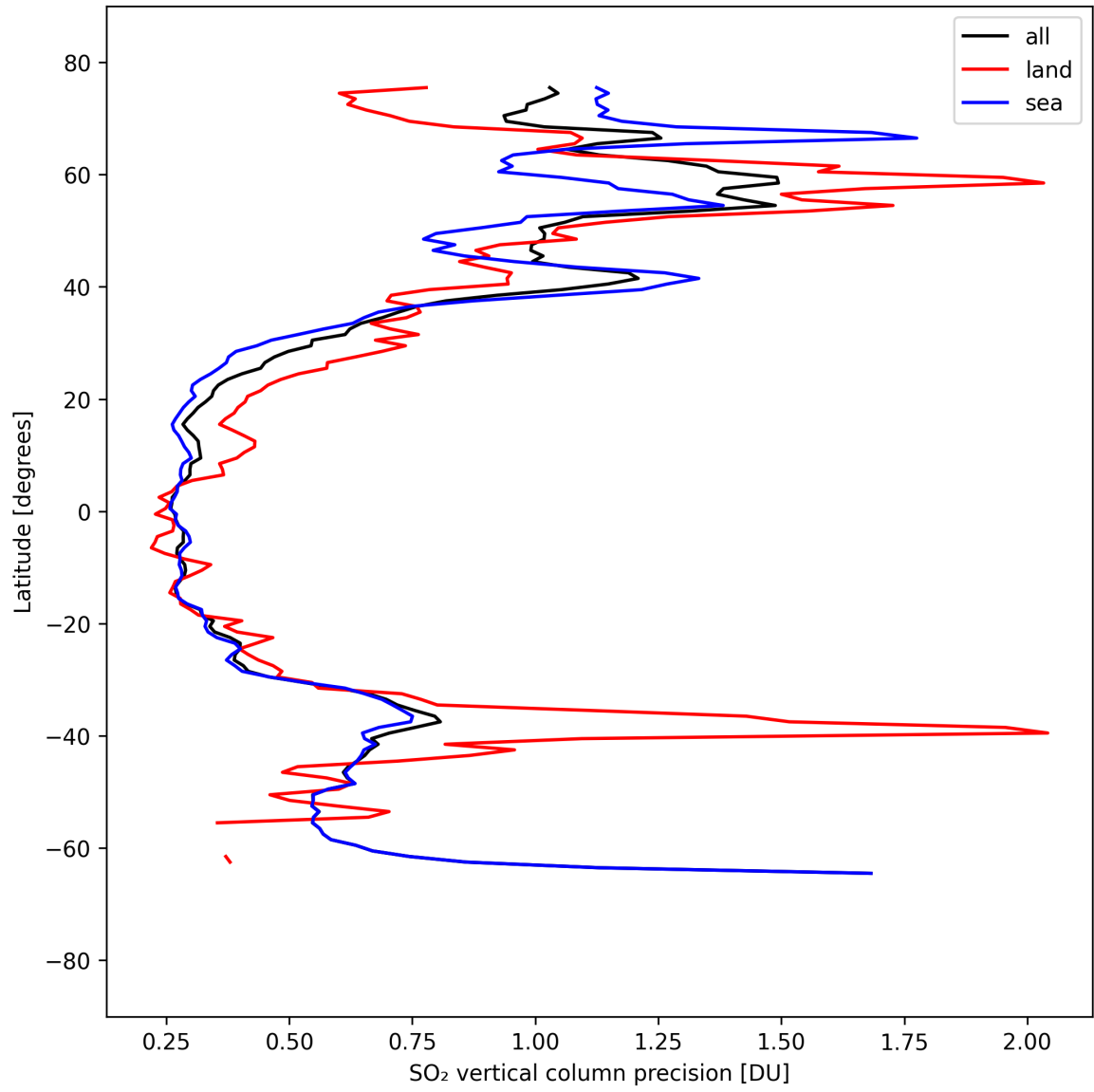
Figure 33: Zonal average of “SO 2 vertical column precision” for 2025-04-02 to 2025-04-03.
