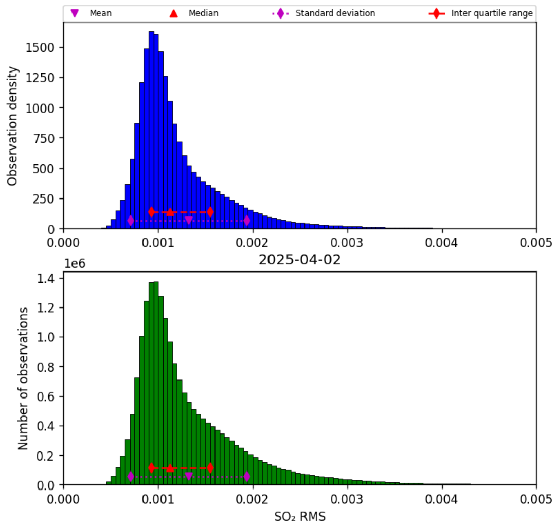
Figure 78: Histogram of "SO 2 RMS" for 2025-04-02 to 2025-04-03
