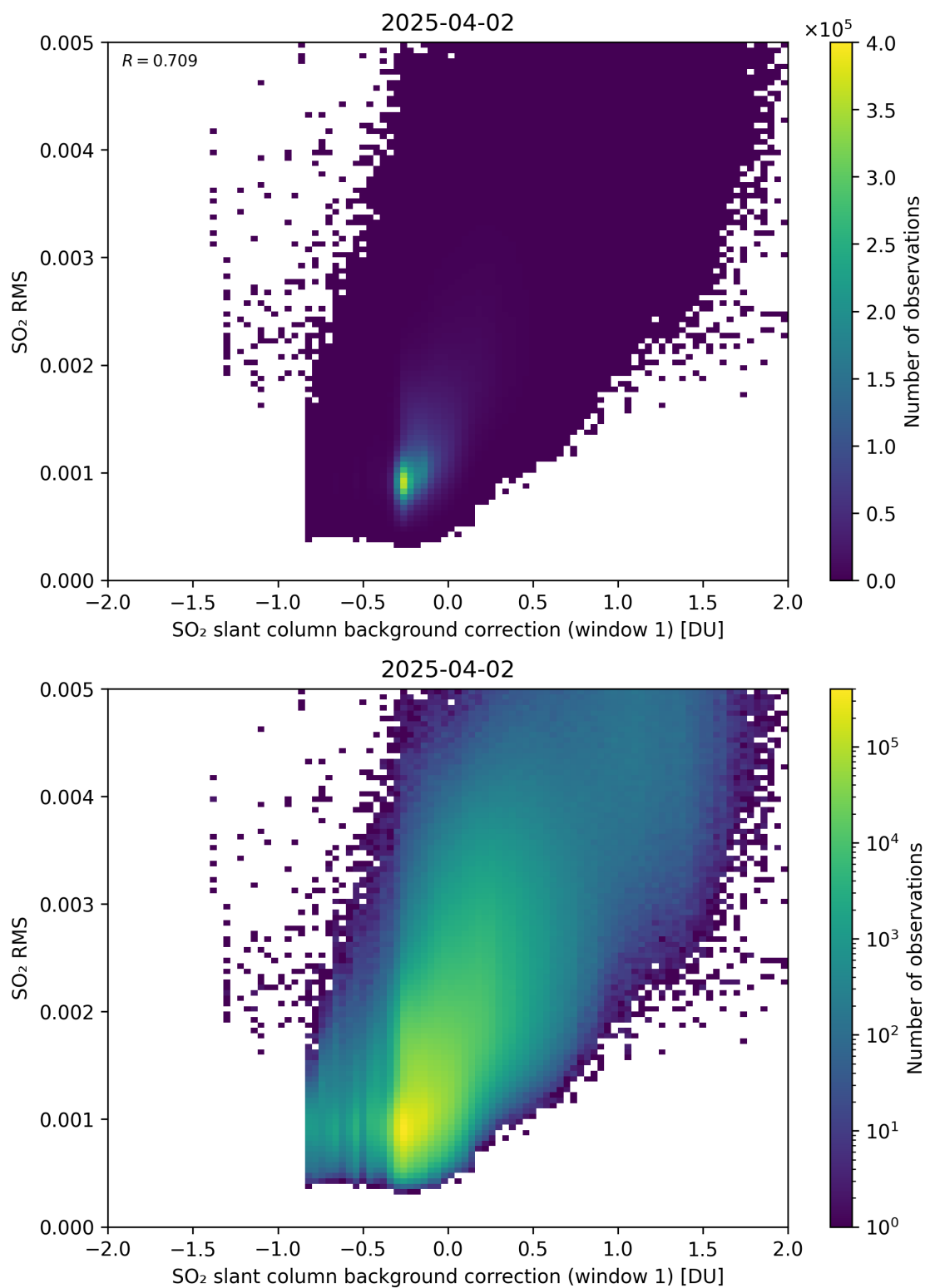
Figure 113: Scatter density plot of “SO 2 slant column background correction (window 1)” against “SO 2 RMS” for 2025-04-02 to 2025-04-03.
