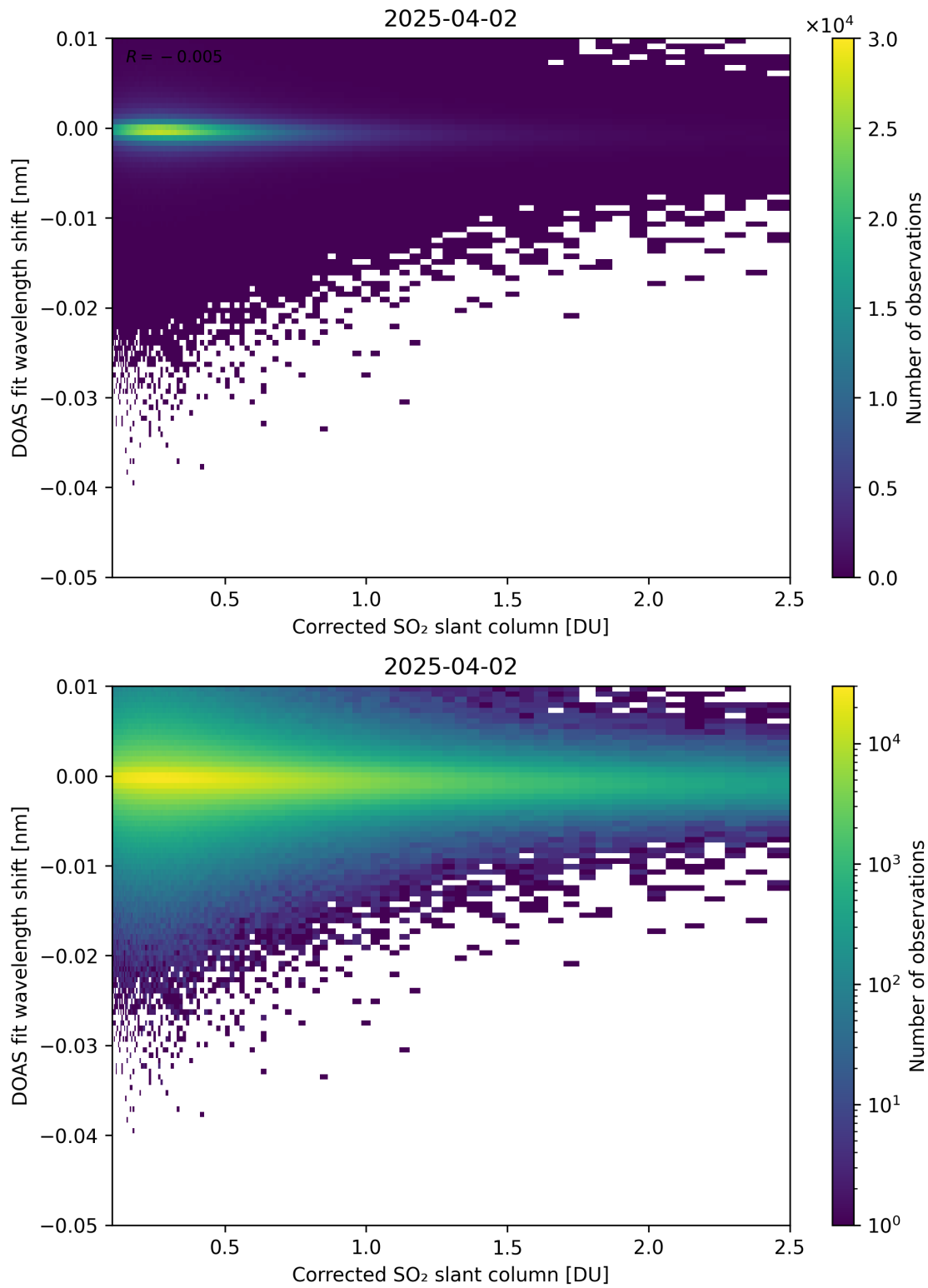
Figure 229: Scatter density plot of “Corrected SO 2 slant column” against “DOAS fit wavelength shift” for 2025-04-02 to 2025-04-03.
