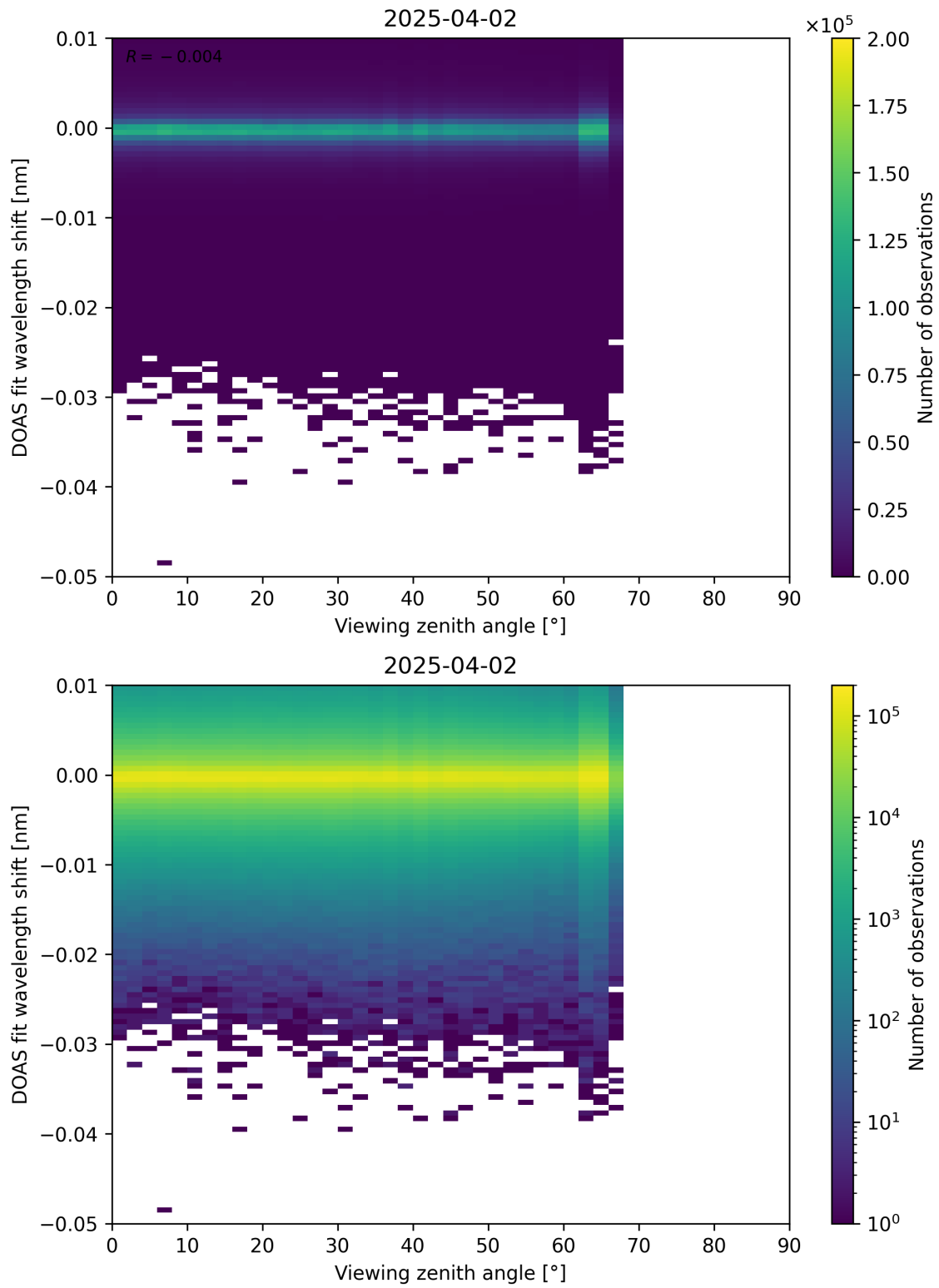
Figure 365: Scatter density plot of “Viewing zenith angle” against “DOAS fit wavelength shift” for 2025-04-02 to 2025-04-03.
