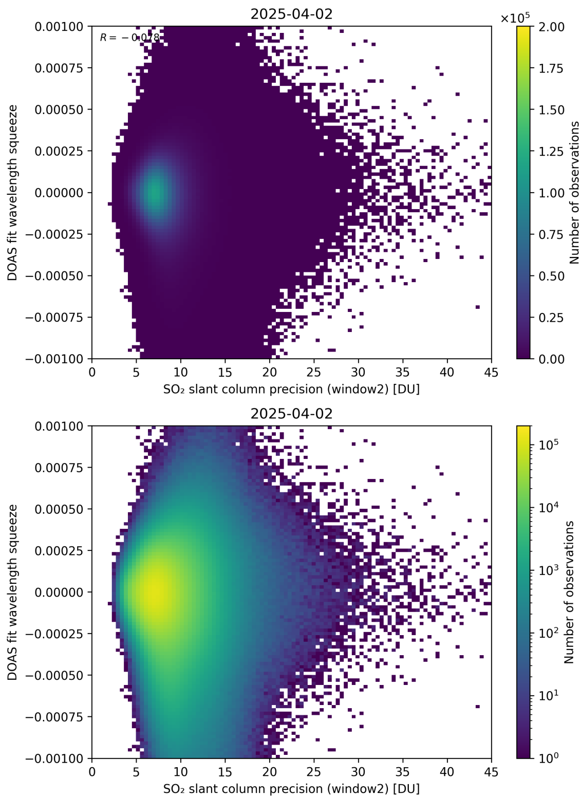
Figure 294: Scatter density plot of “SO 2 slant column precision (window2)” against “DOAS fit wavelength squeeze” for 2025-04-02 to 2025-04-03.
