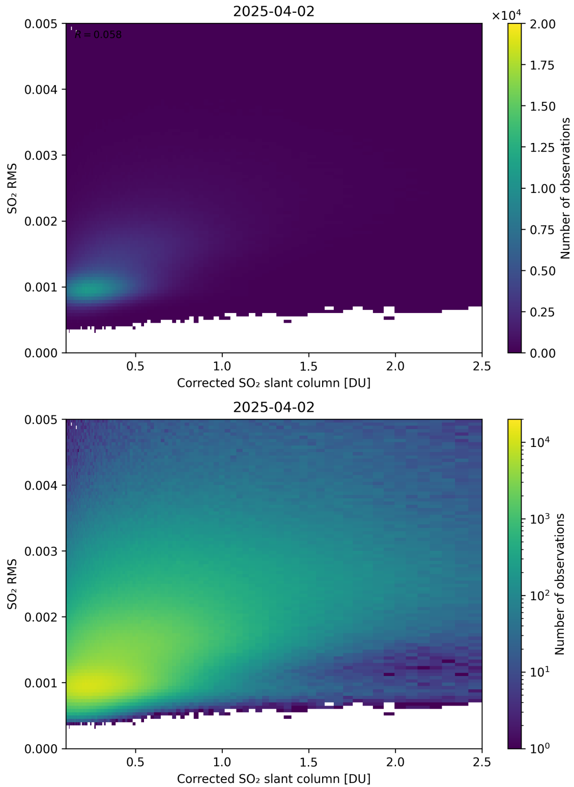
Figure 231: Scatter density plot of “Corrected SO 2 slant column” against “SO 2 RMS” for 2025-04-02 to 2025-04-03.
