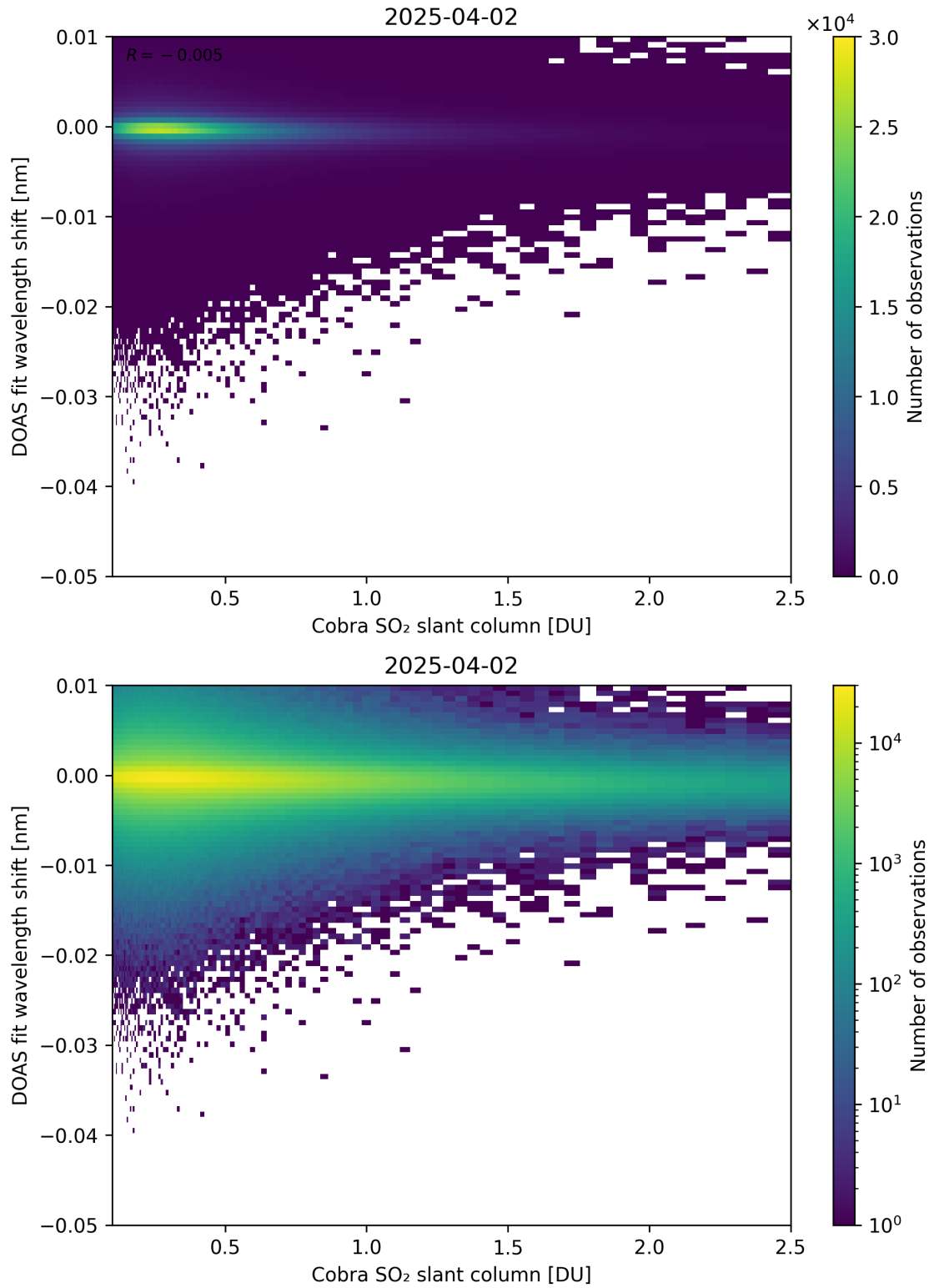
Figure 196: Scatter density plot of “Cobra SO 2 slant column” against “DOAS fit wavelength shift” for 2025-04-02 to 2025-04-03.
