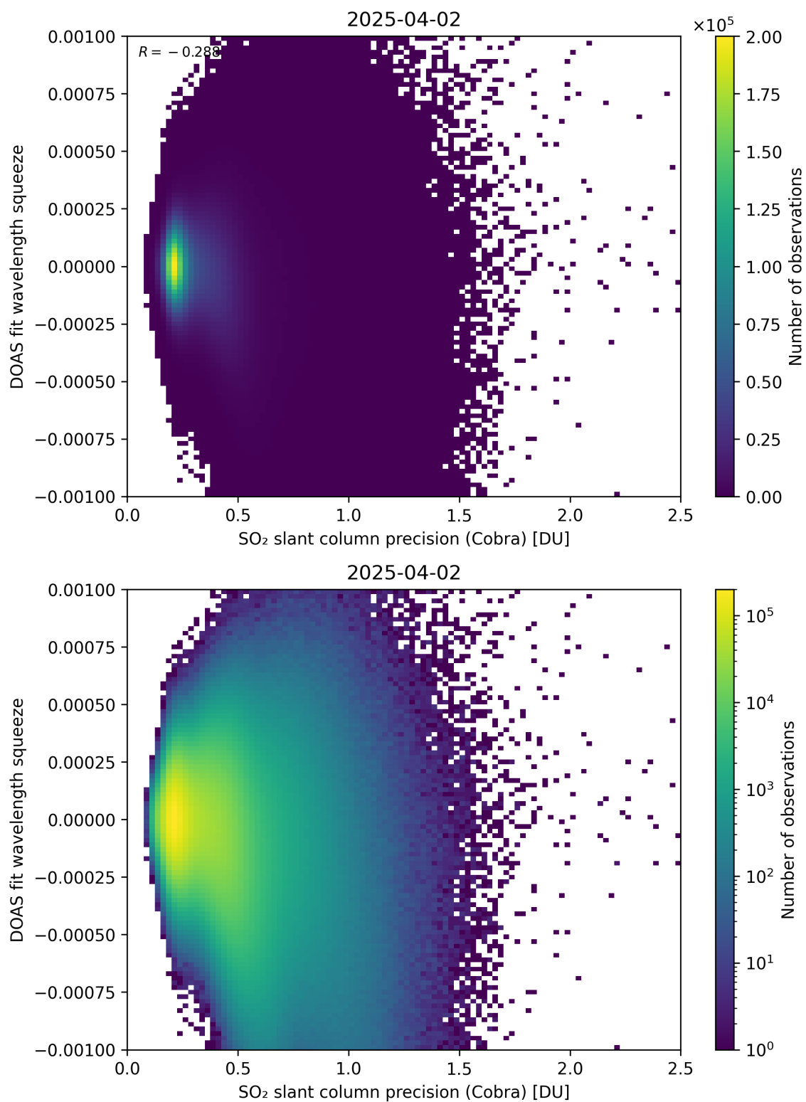
Figure 203: Scatter density plot of “SO 2 slant column precision (Cobra)” against “DOAS fit wavelength squeeze” for 2025-04-02 to 2025-04-03.
