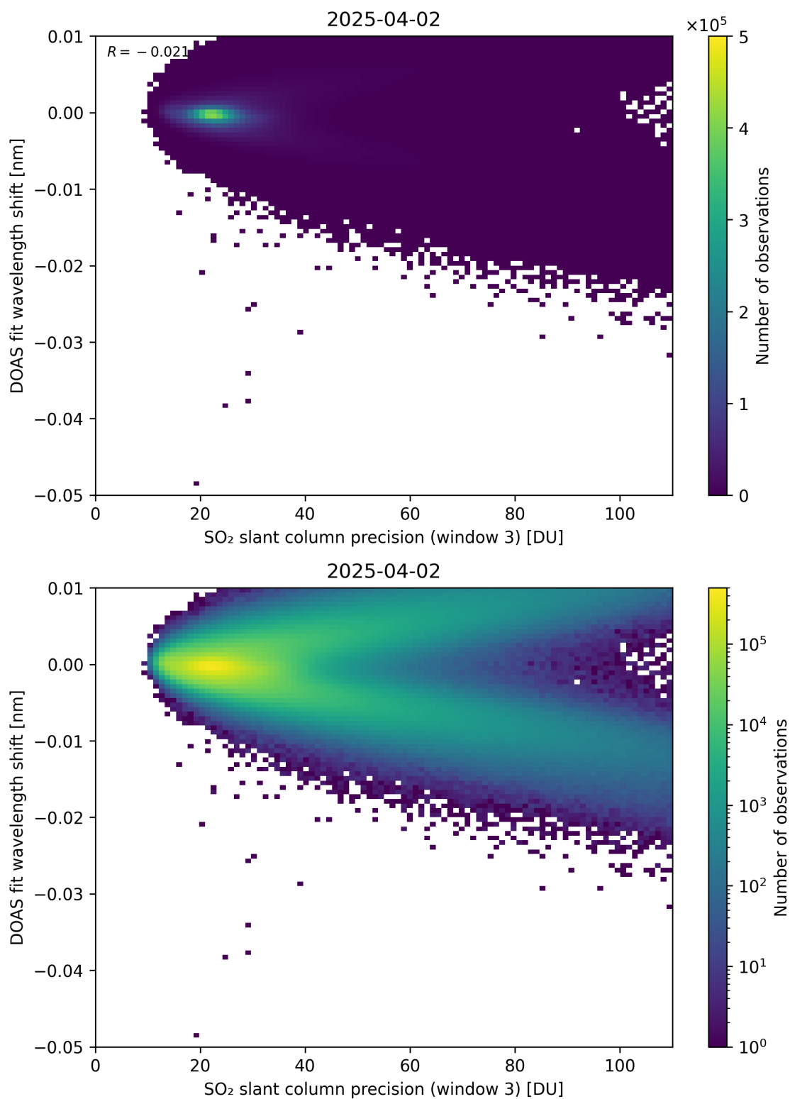
Figure 308: Scatter density plot of “SO 2 slant column precision (window 3)” against “DOAS fit wavelength shift” for 2025-04-02 to 2025-04-03.
