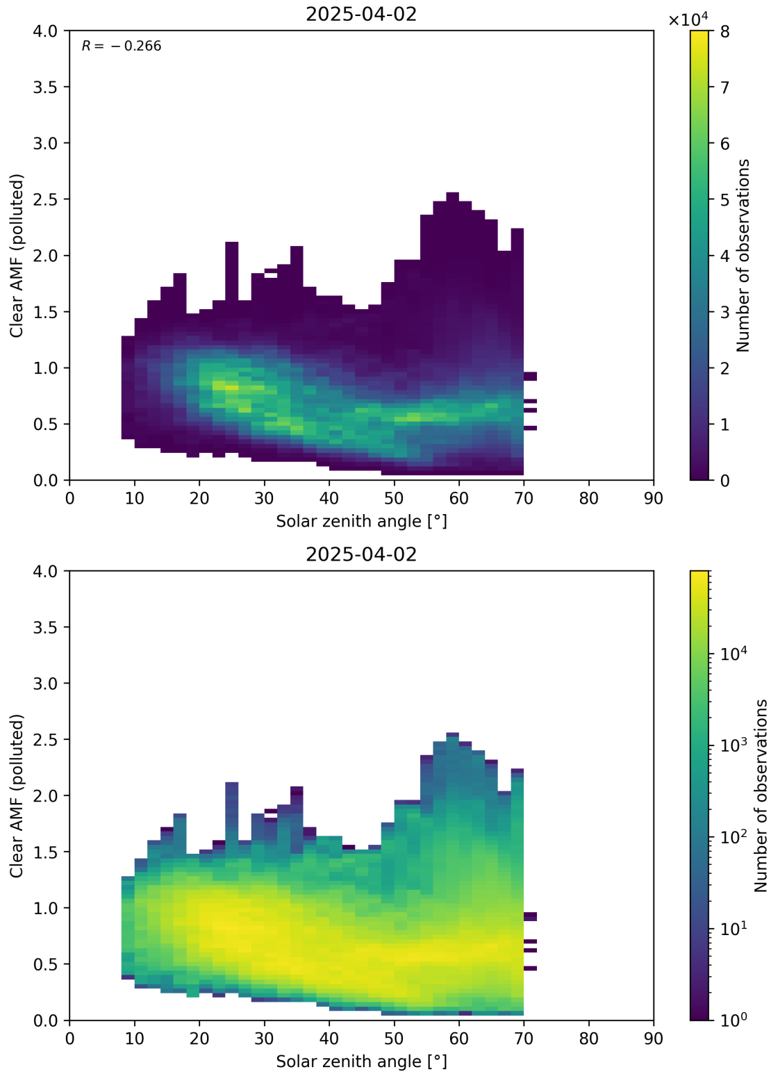
Figure 178: Scatter density plot of “Solar zenith angle” against “Clear AMF (polluted)” for 2025-04-02 to 2025-04-03.
