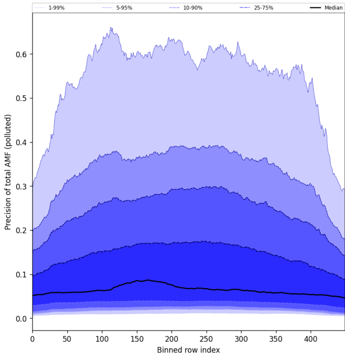
Figure 106: Along track statistics of “Precision of total AMF (polluted)” for 2025-04-02 to 2025-04-03
