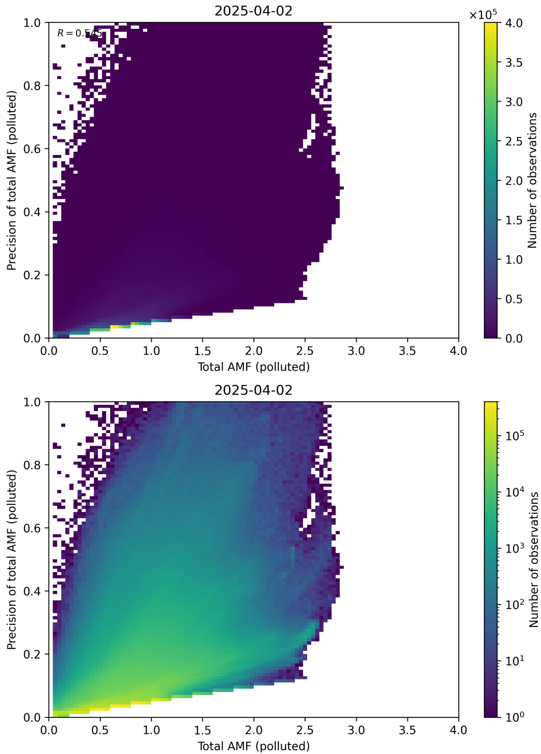
Figure 322: Scatter density plot of “Total AMF (polluted)” against “Precision of total AMF (polluted)” for 2025-04-02 to 2025-04-03.
