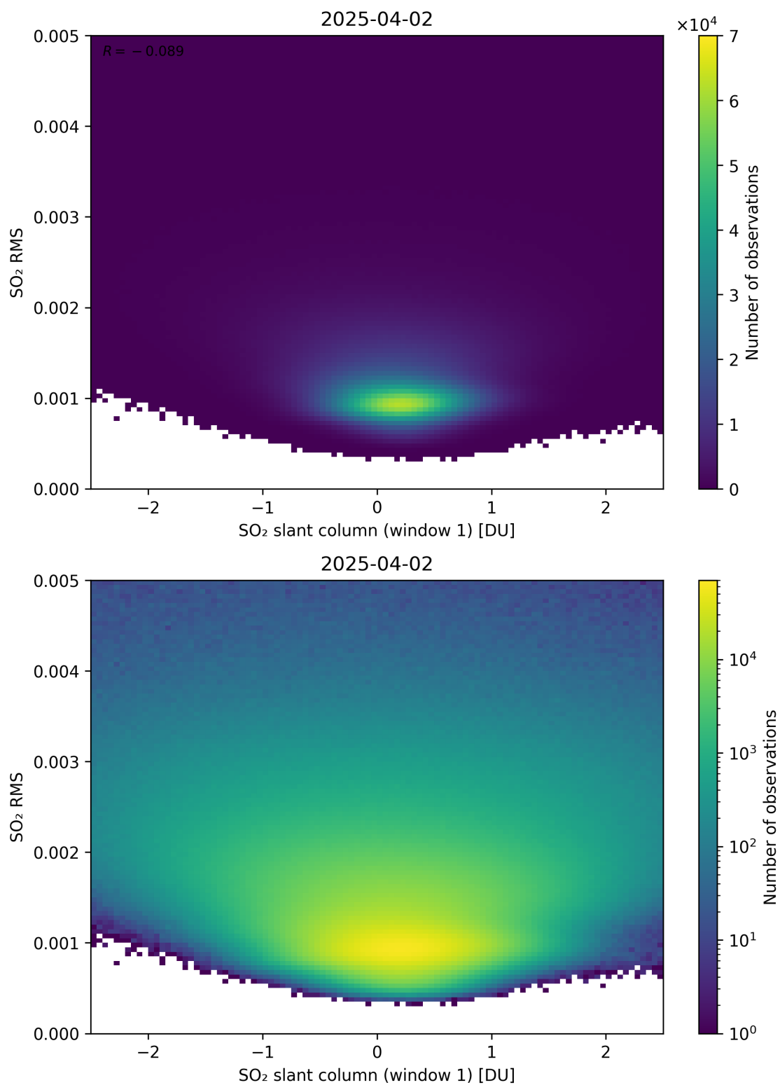
Figure 267: Scatter density plot of “SO 2 slant column (window 1)” against “SO 2 RMS” for 2025-04-02 to 2025-04-03.
