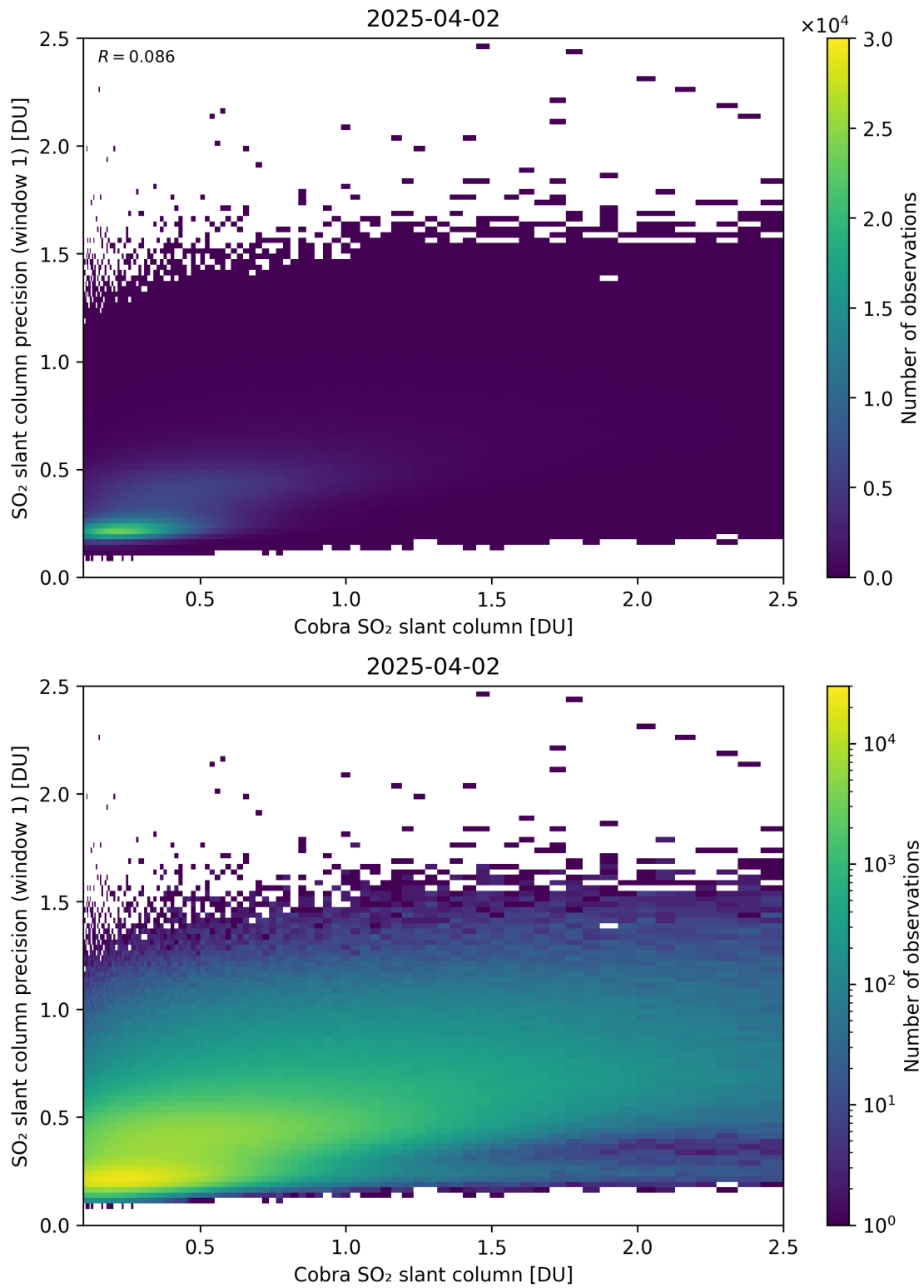
Figure 220: Scatter density plot of “Cobra SO 2 slant column” against “SO 2 slant column precision (window 1)” for 2025-04-02 to 2025-04-03.
