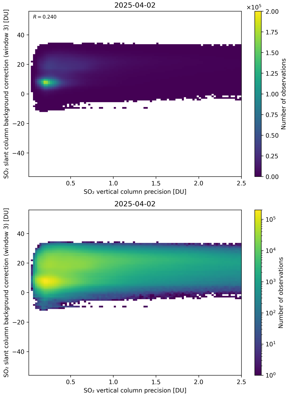
Figure 331: Scatter density plot of “SO 2 vertical column precision” against “SO 2 slant column background correction (window 3)” for 2025-04-02 to 2025-04-03.
