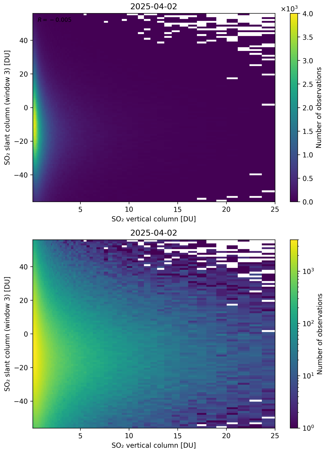
Figure 357: Scatter density plot of “SO 2 vertical column” against “SO 2 slant column (window 3)” for 2025-04-02 to 2025-04-03.
