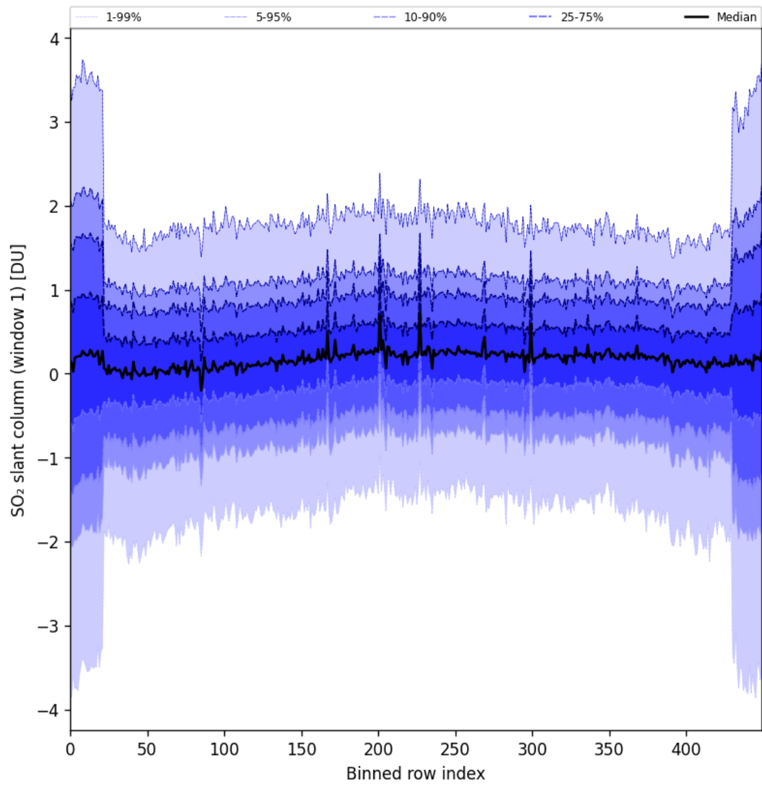
Figure 89: Along track statistics of “SO 2 slant column (window 1)” for 2025-04-02 to 2025-04-03
