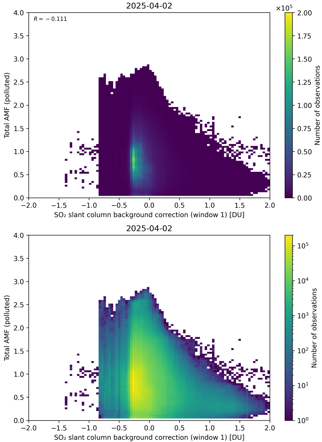
Figure 120: Scatter density plot of “SO 2 slant column background correction (window 1)” against “Total AMF (polluted)” for 2025-04-02 to 2025-04-03.
