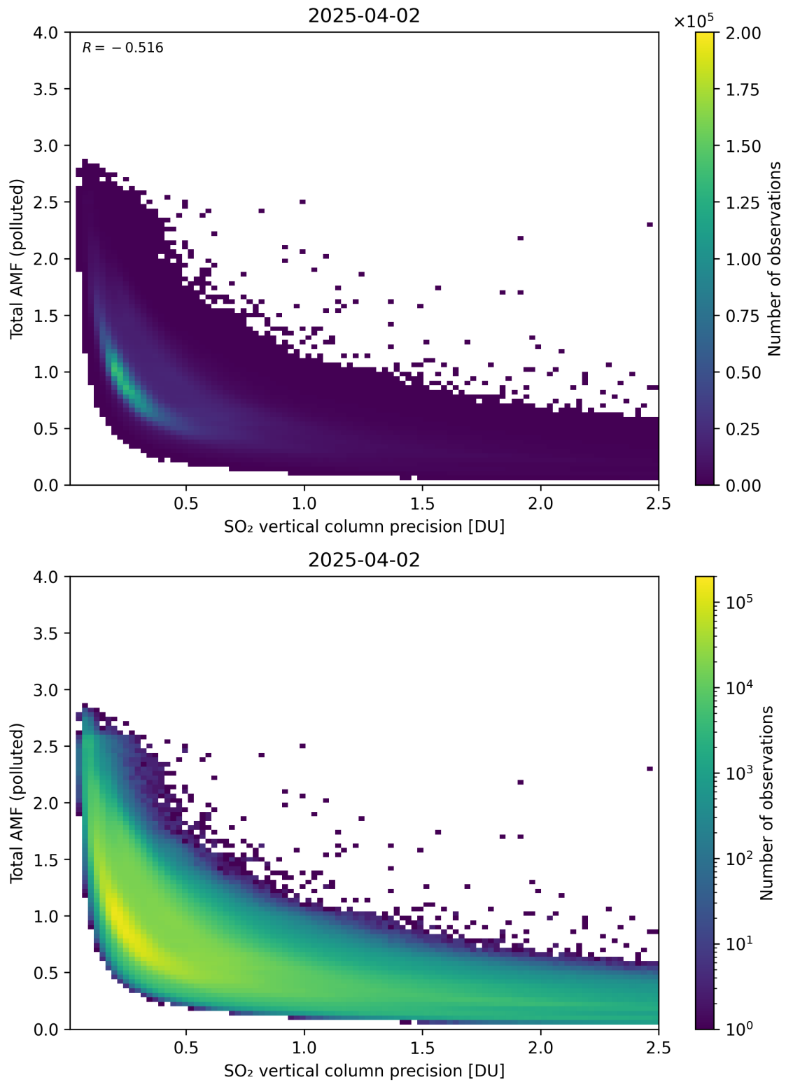
Figure 346: Scatter density plot of “SO 2 vertical column precision” against “Total AMF (polluted)” for 2025-04-02 to 2025-04-03.
