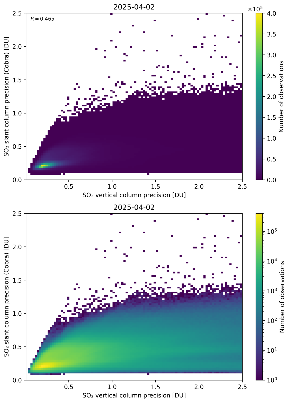
Figure 337: Scatter density plot of “SO 2 vertical column precision” against “SO 2 slant column precision (Cobra)” for 2025-04-02 to 2025-04-03.
