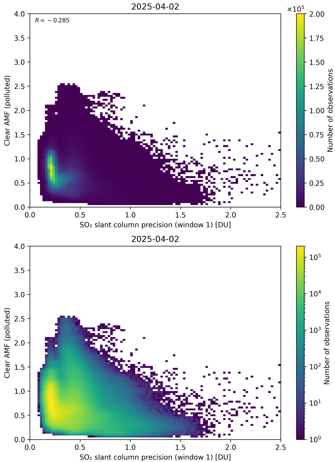
Figure 274: Scatter density plot of “SO 2 slant column precision (window 1)” against “Clear AMF (polluted)” for 2025-04-02 to 2025-04-03.
