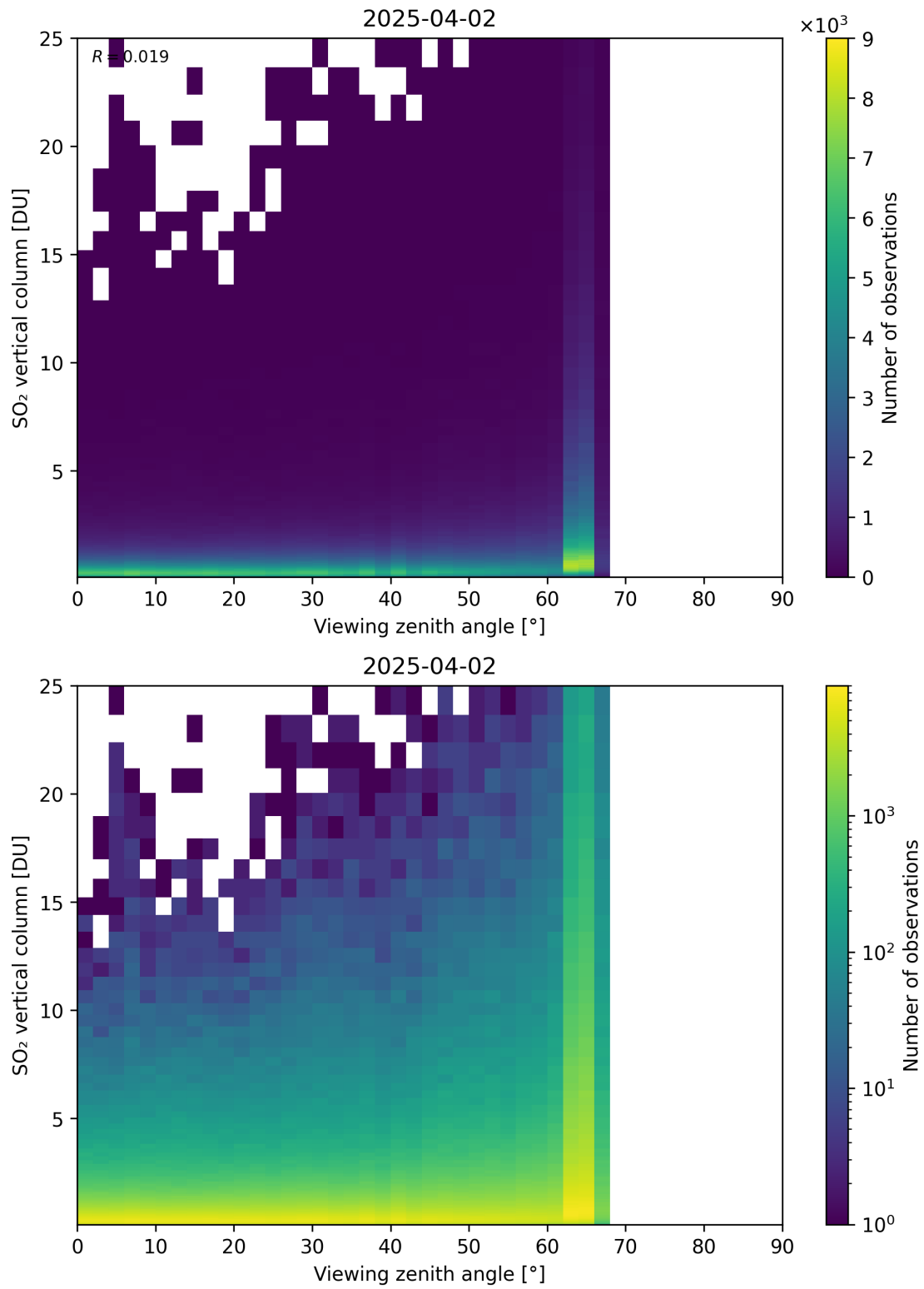
Figure 383: Scatter density plot of “Viewing zenith angle” against “SO 2 vertical column” for 2025-04-02 to 2025-04-03.
