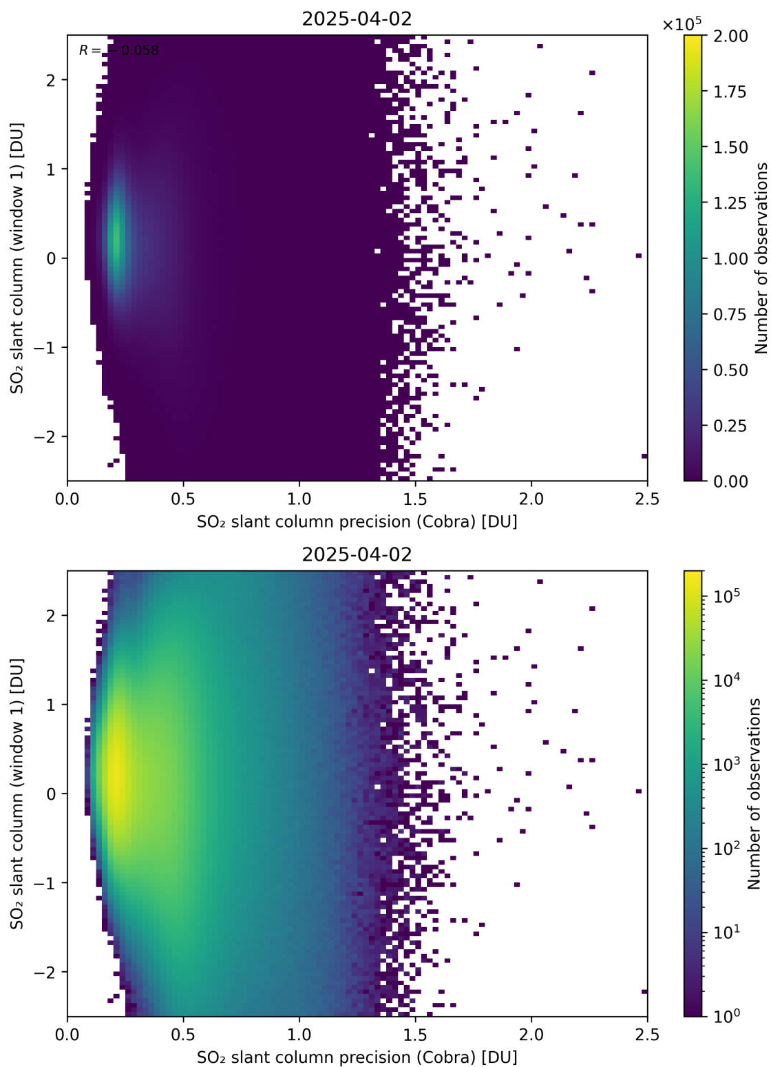
Figure 208: Scatter density plot of “SO 2 slant column precision (Cobra)” against “SO 2 slant column (window 1)” for 2025-04-02 to 2025-04-03.
