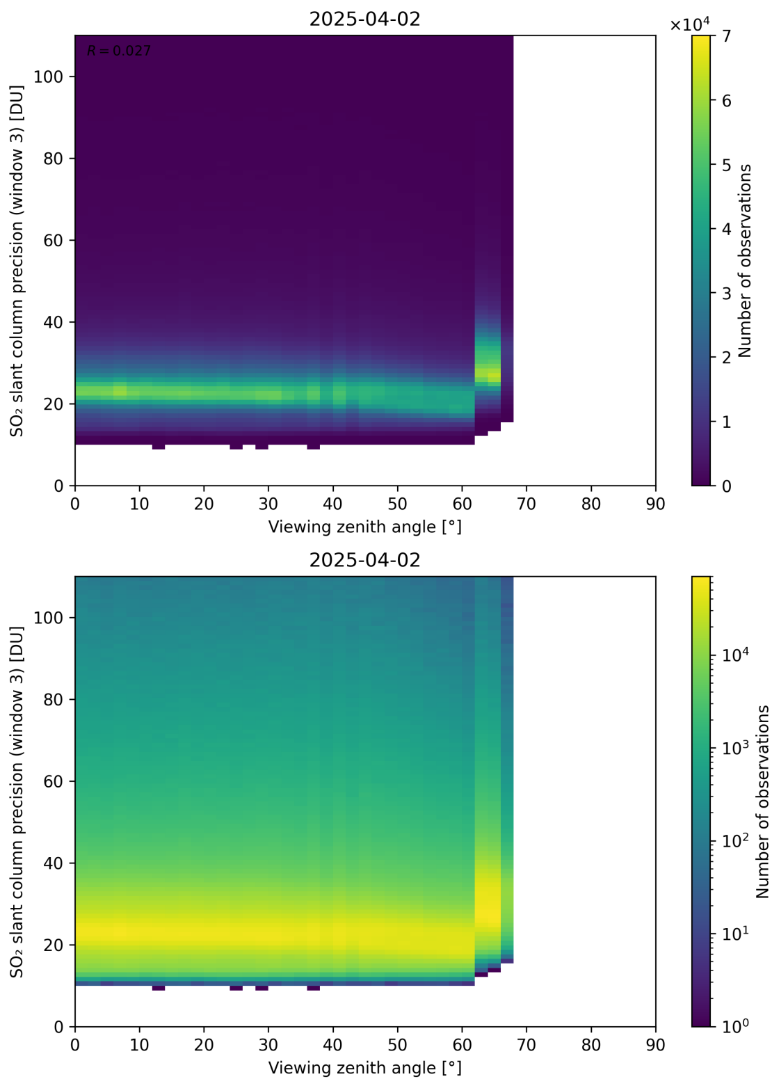
Figure 380: Scatter density plot of “Viewing zenith angle” against “SO 2 slant column precision (window 3)” for 2025-04-02 to 2025-04-03.
