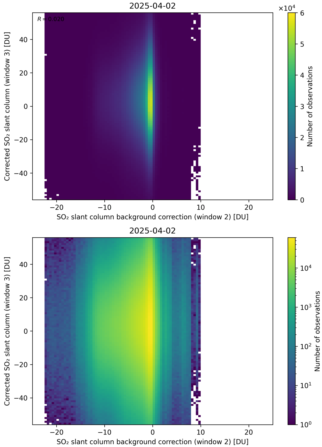
Figure 127: Scatter density plot of “SO 2 slant column background correction (window 2)” against “Corrected SO 2 slant column (window 3)” for 2025-04-02 to 2025-04-03.
