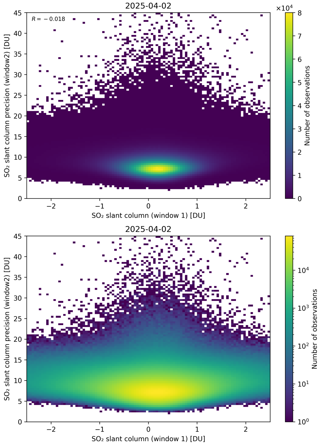
Figure 286: Scatter density plot of “SO 2 slant column (window 1)” against “SO 2 slant column precision (window2)” for 2025-04-02 to 2025-04-03.
