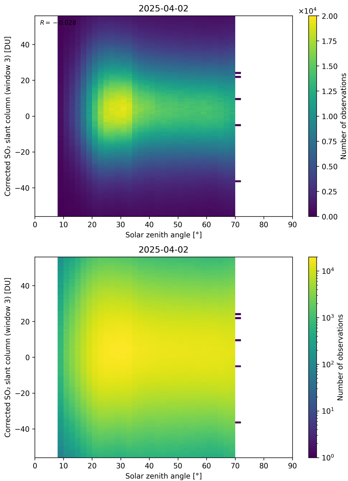
Figure 183: Scatter density plot of “Solar zenith angle” against “Corrected SO 2 slant column (window 3)” for 2025-04-02 to 2025-04-03.
