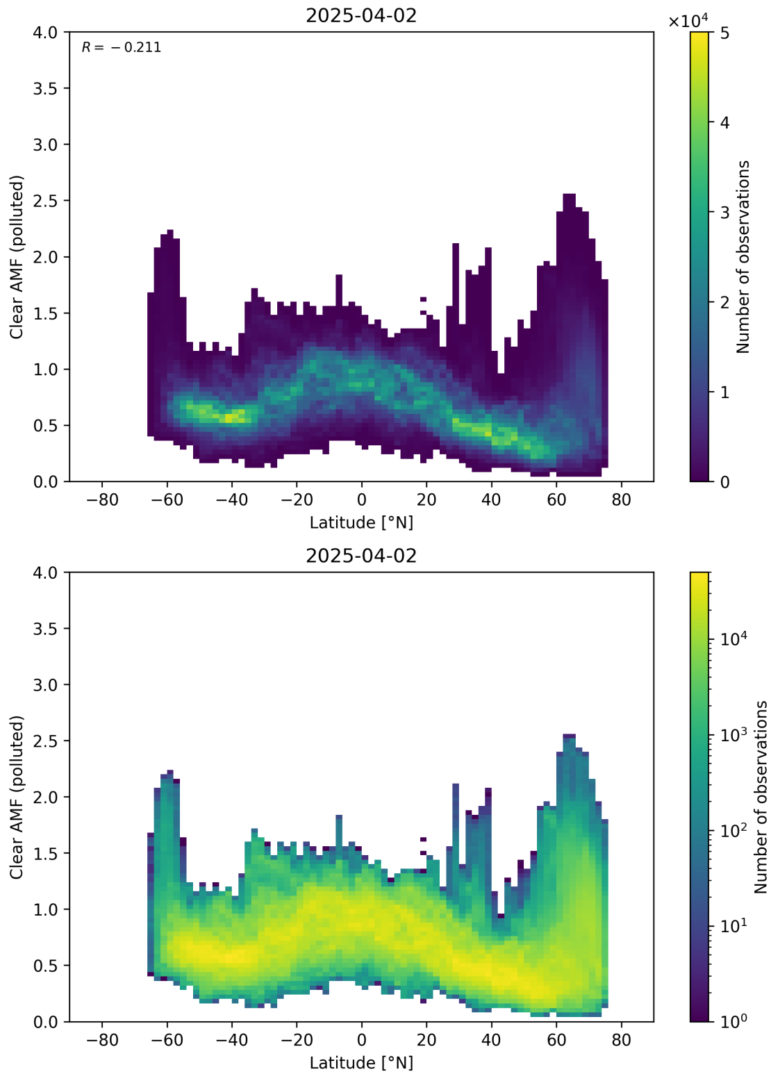
Figure 156: Scatter density plot of “Latitude” against “Clear AMF (polluted)” for 2025-04-02 to 2025-04-03.
