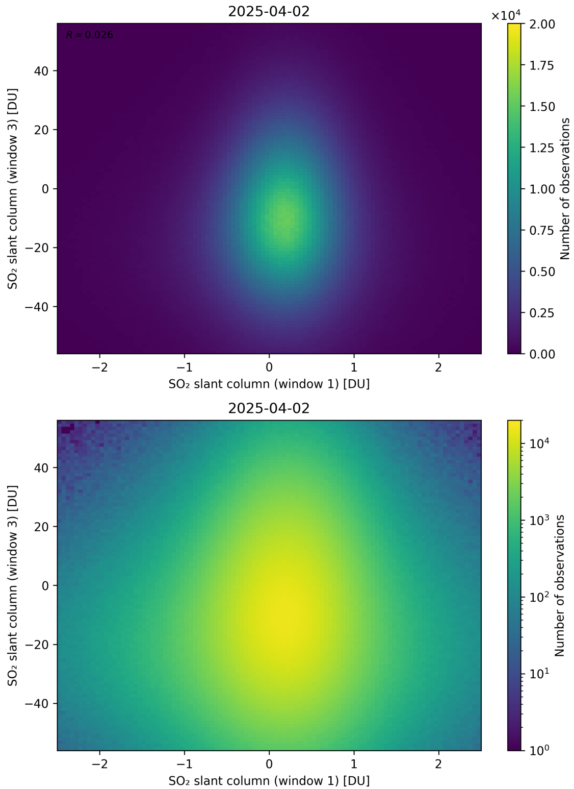
Figure 287: Scatter density plot of “SO 2 slant column (window 1)” against “SO 2 slant column (window 3)” for 2025-04-02 to 2025-04-03.
