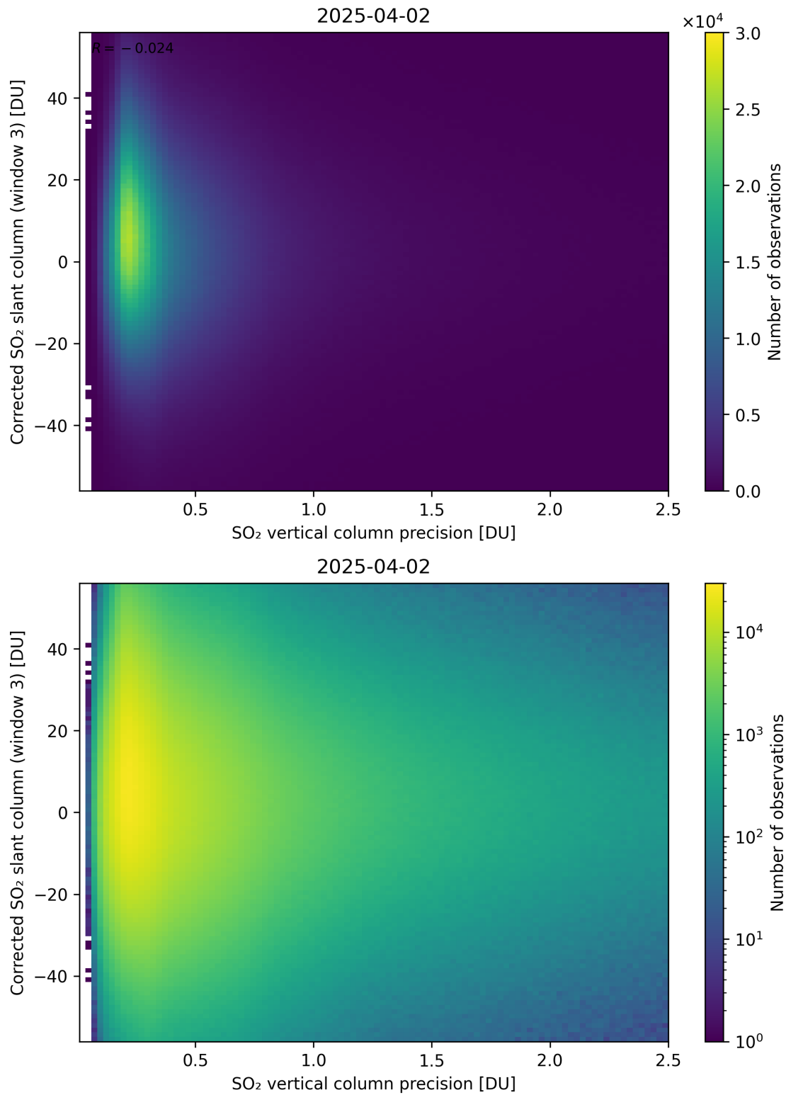
Figure 340: Scatter density plot of “SO 2 vertical column precision” against “Corrected SO 2 slant column (window 3)” for 2025-04-02 to 2025-04-03.
