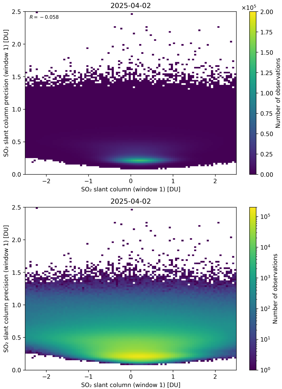
Figure 285: Scatter density plot of “SO 2 slant column (window 1)” against “SO 2 slant column precision (window 1)” for 2025-04-02 to 2025-04-03.
