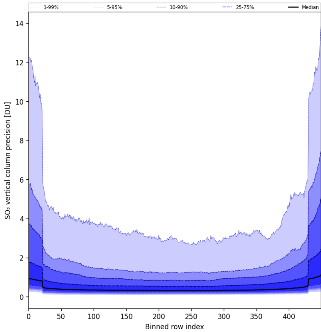
Figure 85: Along track statistics of “SO 2 vertical column precision” for 2025-04-02 to 2025-04-03
