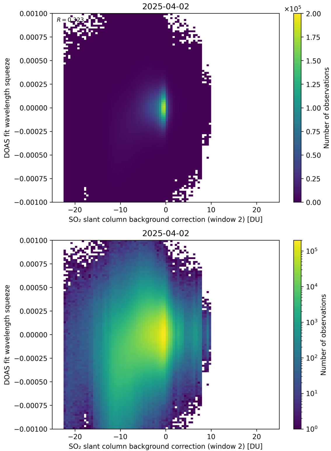
Figure 124: Scatter density plot of “SO 2 slant column background correction (window 2)” against “DOAS fit wavelength squeeze” for 2025-04-02 to 2025-04-03.
