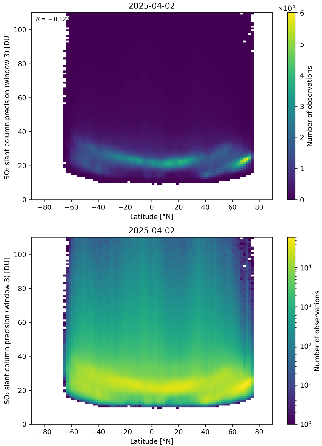
Figure 166: Scatter density plot of “Latitude” against “SO 2 slant column precision (window 3)” for 2025-04-02 to 2025-04-03.
