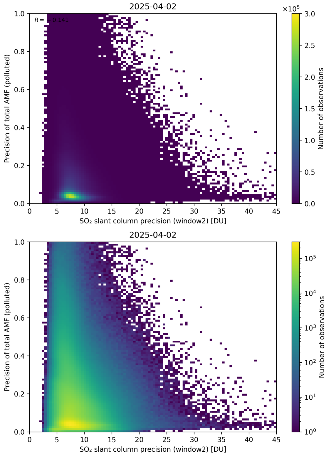
Figure 302: Scatter density plot of “SO 2 slant column precision (window2)” against “Precision of total AMF (polluted)” for 2025-04-02 to 2025-04-03.
