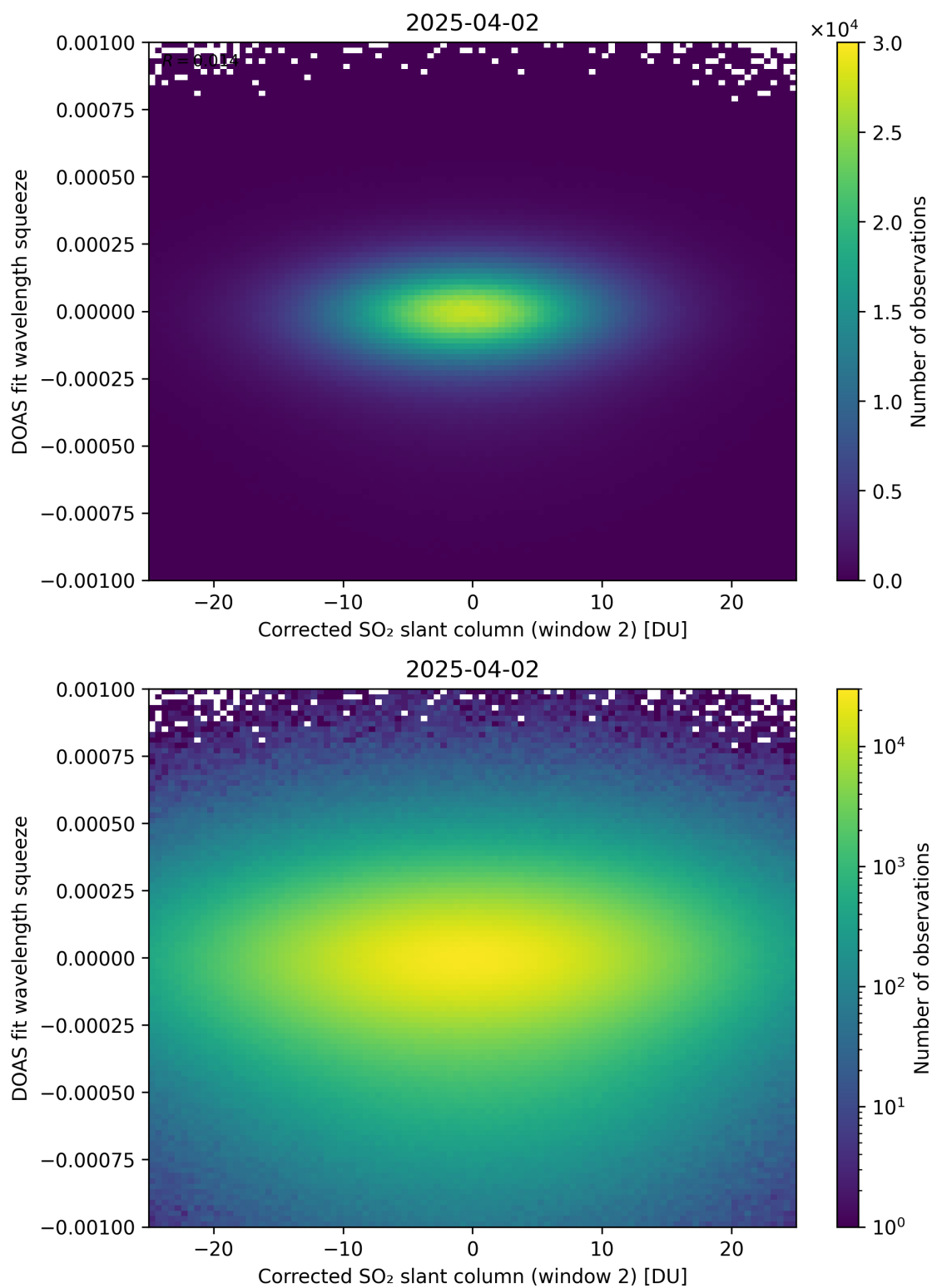
Figure 247: Scatter density plot of “Corrected SO 2 slant column (window 2)” against “DOAS fit wavelength squeeze” for 2025-04-02 to 2025-04-03.
