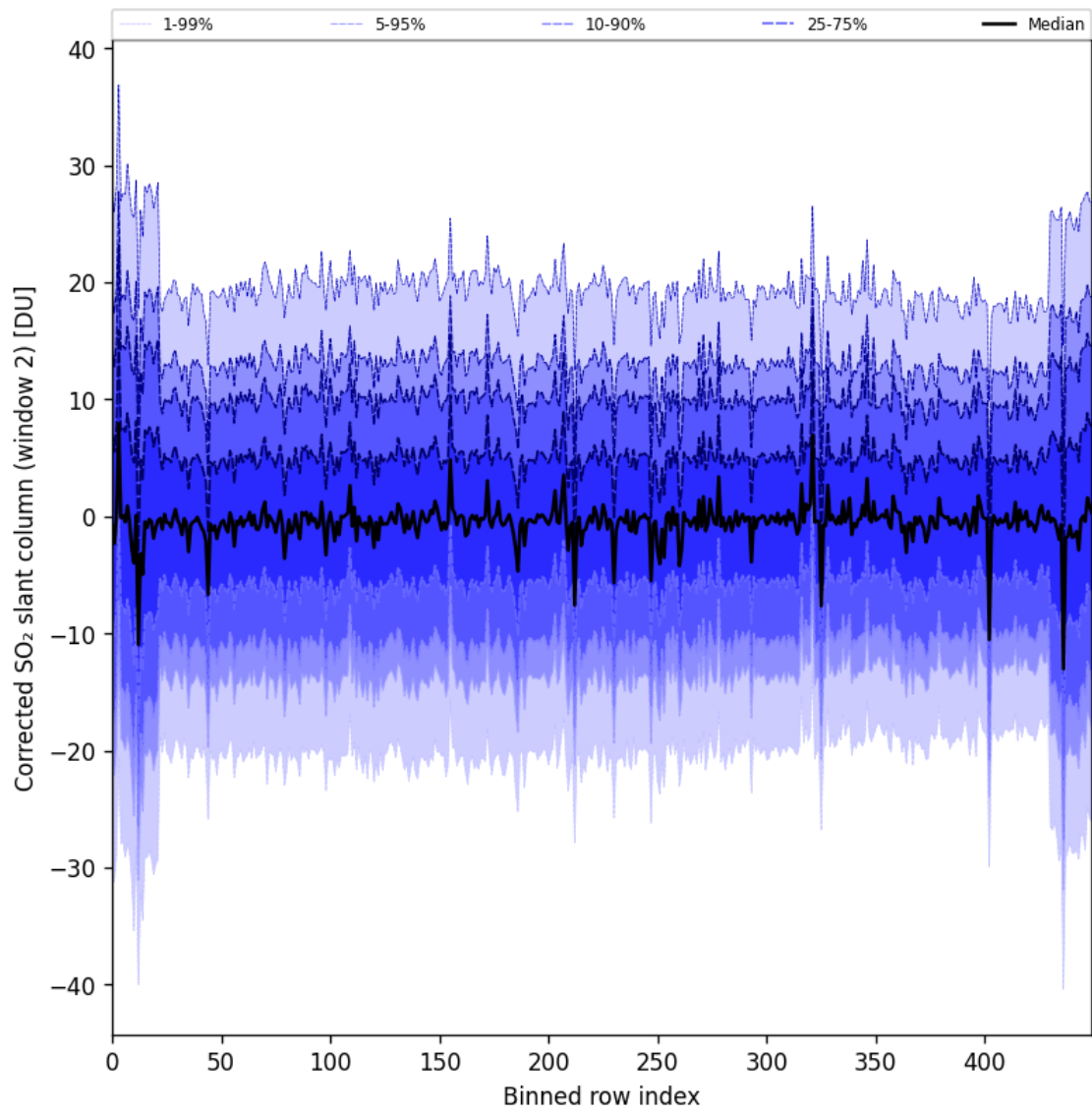
Figure 95: Along track statistics of “Corrected SO 2 slant column (window 2)” for 2025-04-02 to 2025-04-03
