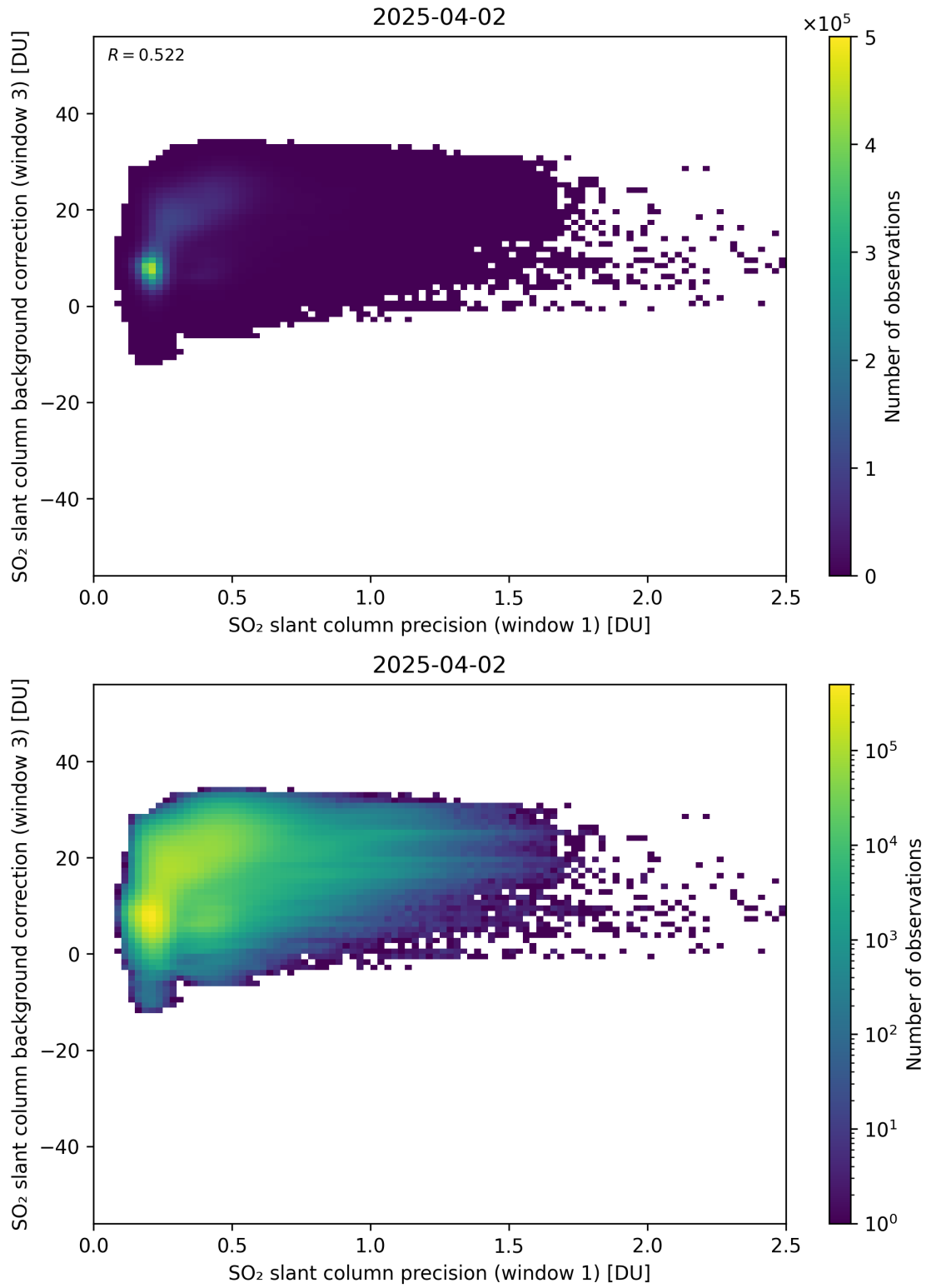
Figure 270: Scatter density plot of “SO 2 slant column precision (window 1)” against “SO 2 slant column background correction (window 3)” for 2025-04-02 to 2025-04-03.
