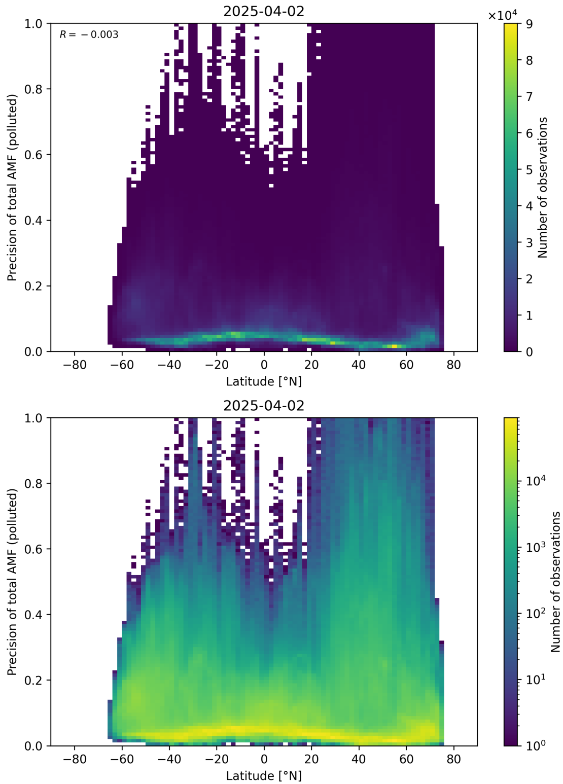
Figure 168: Scatter density plot of “Latitude” against “Precision of total AMF (polluted)” for 2025-04-02 to 2025-04-03.
