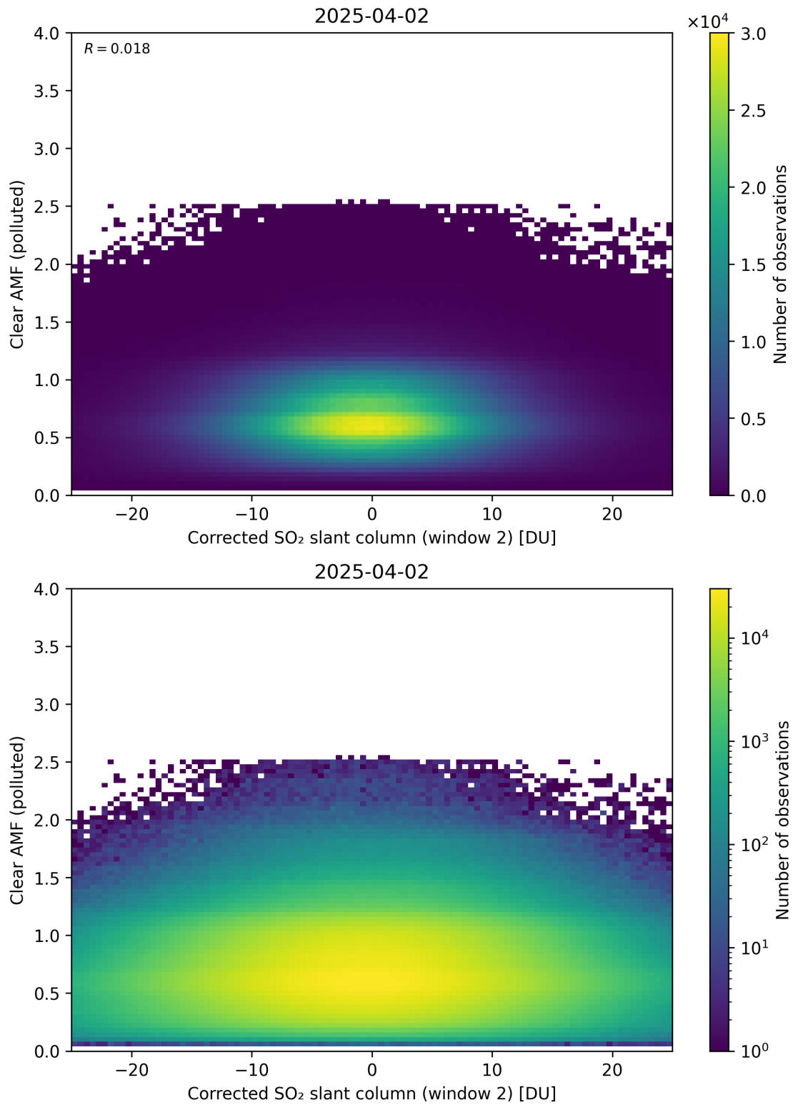
Figure 249: Scatter density plot of “Corrected SO 2 slant column (window 2)” against “Clear AMF (polluted)” for 2025-04-02 to 2025-04-03.
