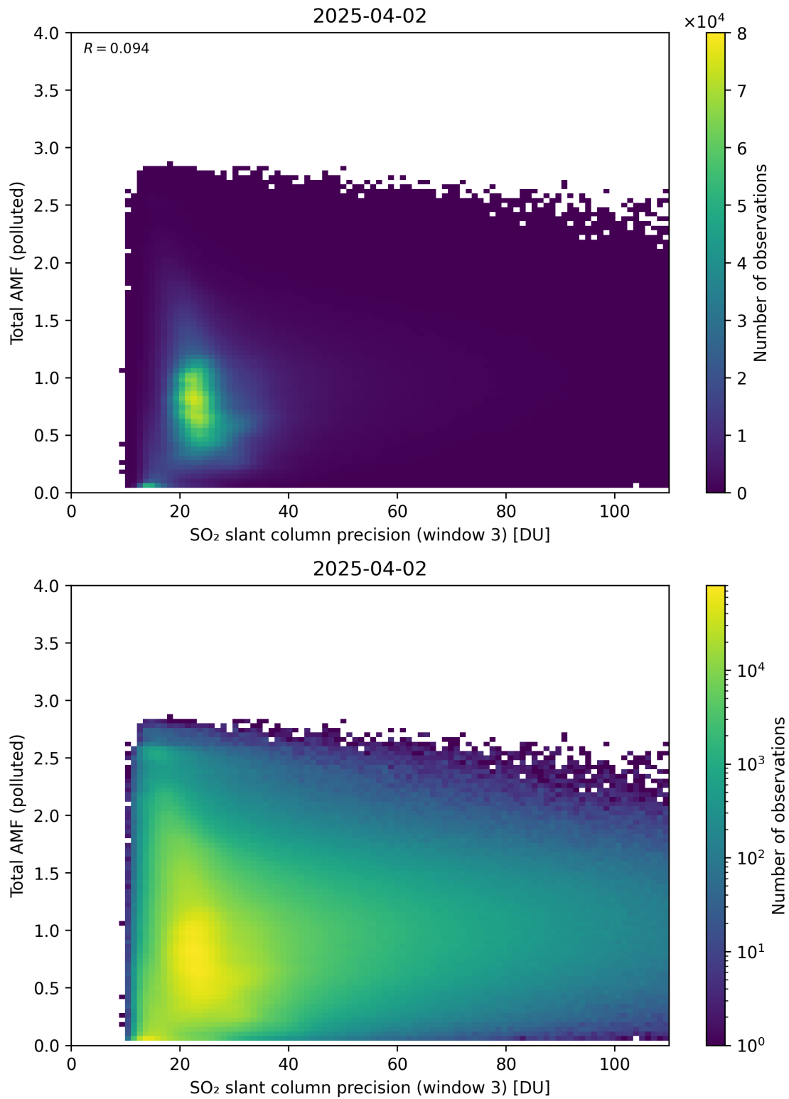
Figure 313: Scatter density plot of “SO 2 slant column precision (window 3)” against “Total AMF (polluted)” for 2025-04-02 to 2025-04-03.
