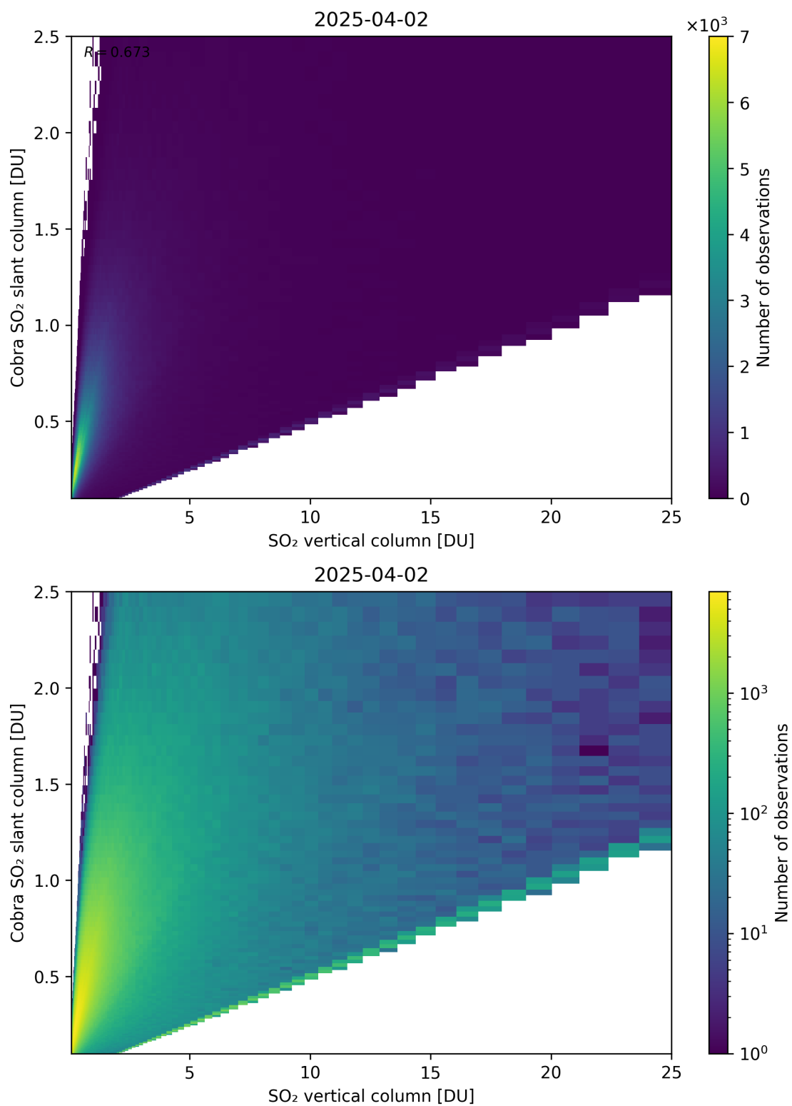
Figure 349: Scatter density plot of “SO 2 vertical column” against “Cobra SO 2 slant column” for 2025-04-02 to 2025-04-03.
