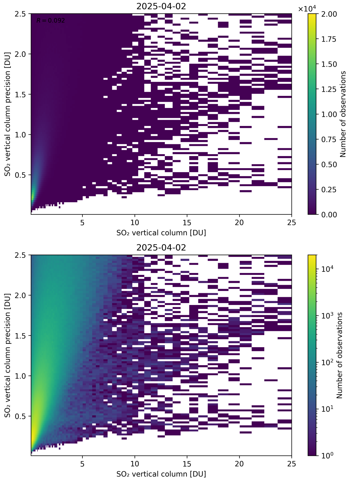
Figure 361: Scatter density plot of “SO 2 vertical column” against “SO 2 vertical column precision” for 2025-04-02 to 2025-04-03.
