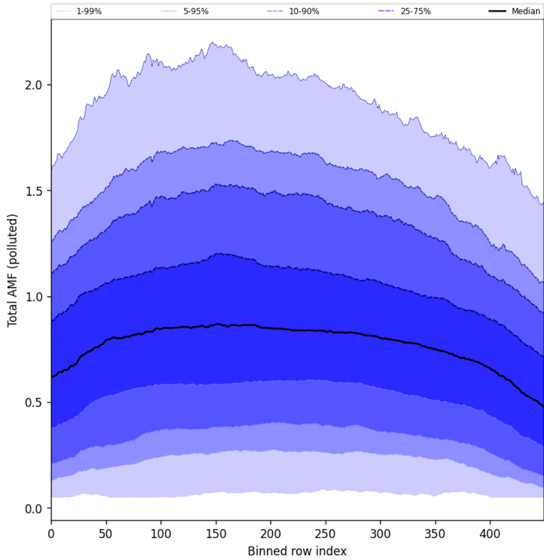
Figure 105: Along track statistics of “Total AMF (polluted)” for 2025-04-02 to 2025-04-03
