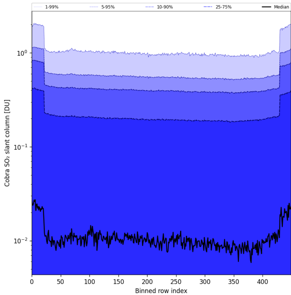
Figure 87: Along track statistics of “Cobra SO 2 slant column” for 2025-04-02 to 2025-04-03
