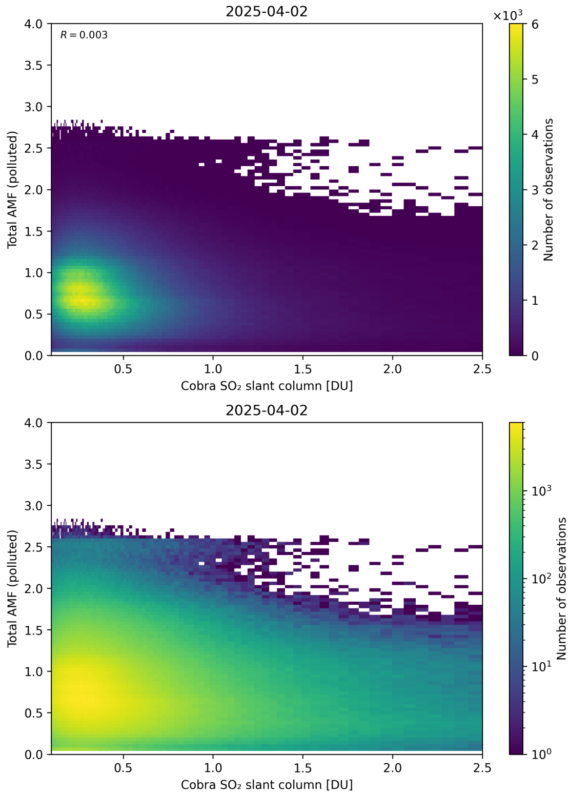
Figure 224: Scatter density plot of “Cobra SO 2 slant column” against “Total AMF (polluted)” for 2025-04-02 to 2025-04-03.
