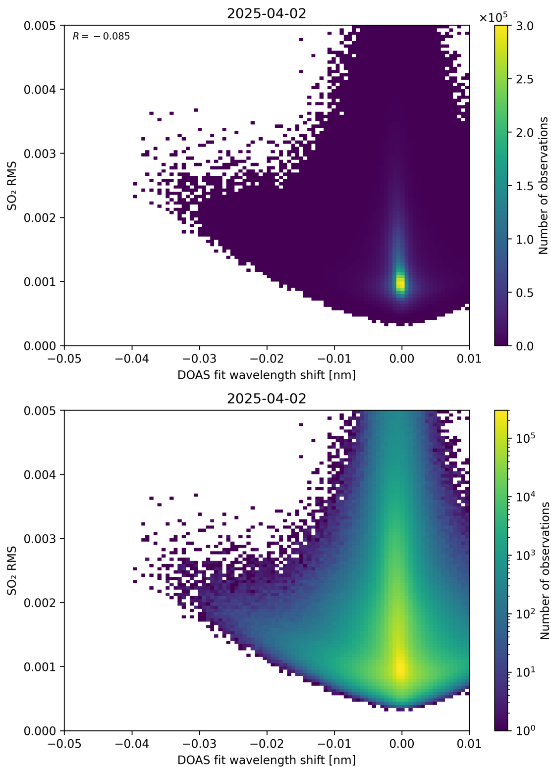
Figure 139: Scatter density plot of “DOAS fit wavelength shift” against “SO 2 RMS” for 2025-04-02 to 2025-04-03.
