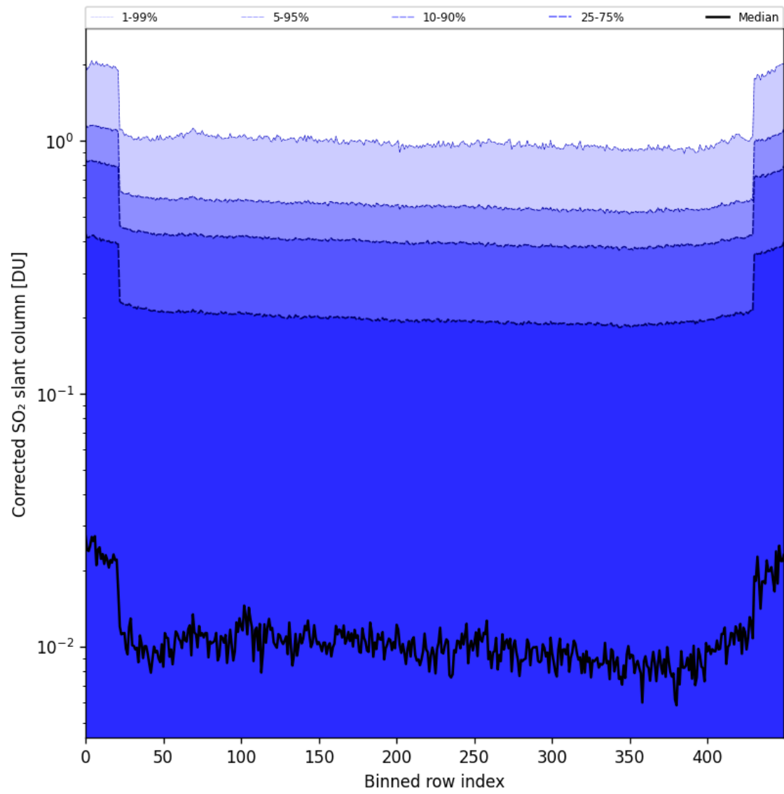
Figure 86: Along track statistics of “Corrected SO 2 slant column” for 2025-04-02 to 2025-04-03
