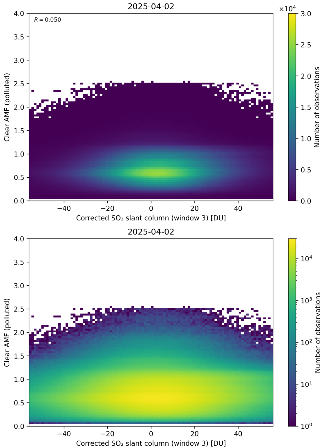
Figure 259: Scatter density plot of “Corrected SO 2 slant column (window 3)” against “Clear AMF (polluted)” for 2025-04-02 to 2025-04-03.
