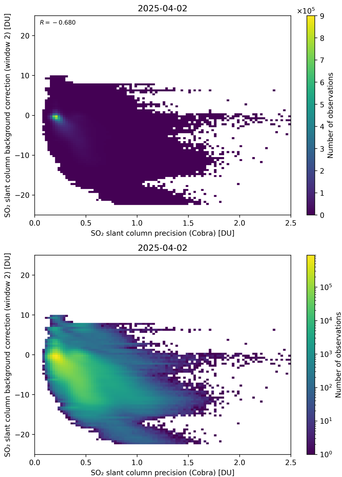
Figure 200: Scatter density plot of “SO 2 slant column precision (Cobra)” against “SO 2 slant column background correction (window 2)” for 2025-04-02 to 2025-04-03.
