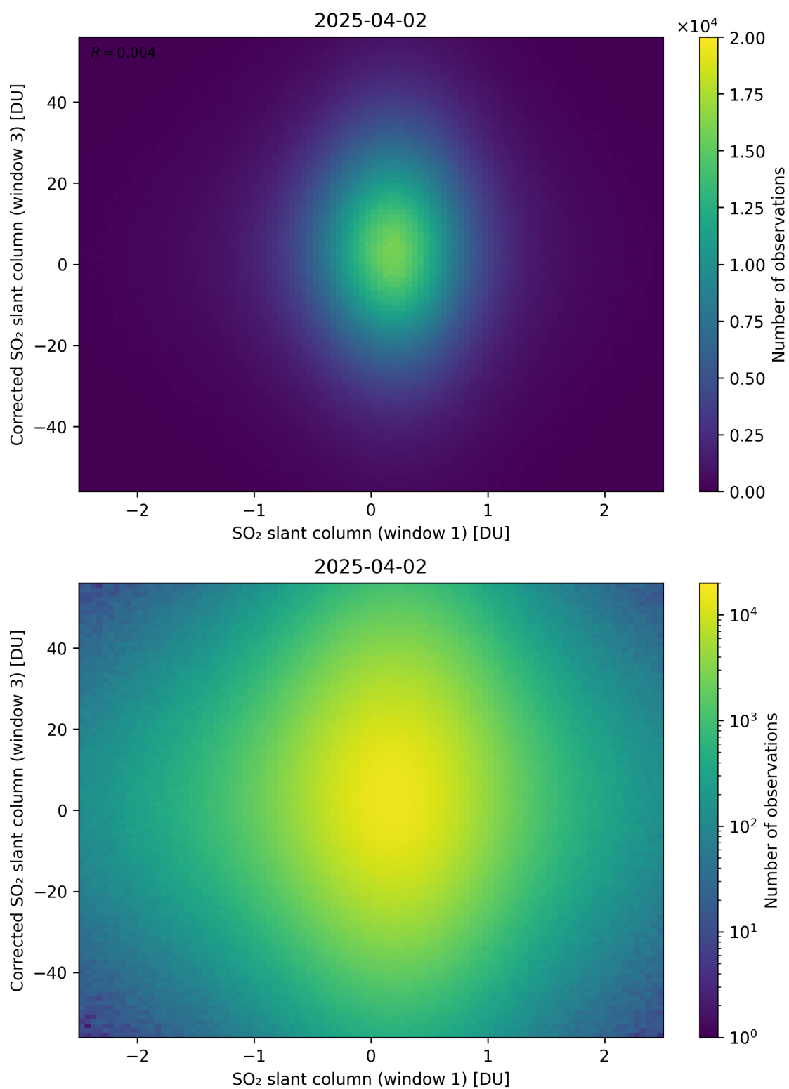
Figure 284: Scatter density plot of “SO 2 slant column (window 1)” against “Corrected SO 2 slant column (window 3)” for 2025-04-02 to 2025-04-03.
