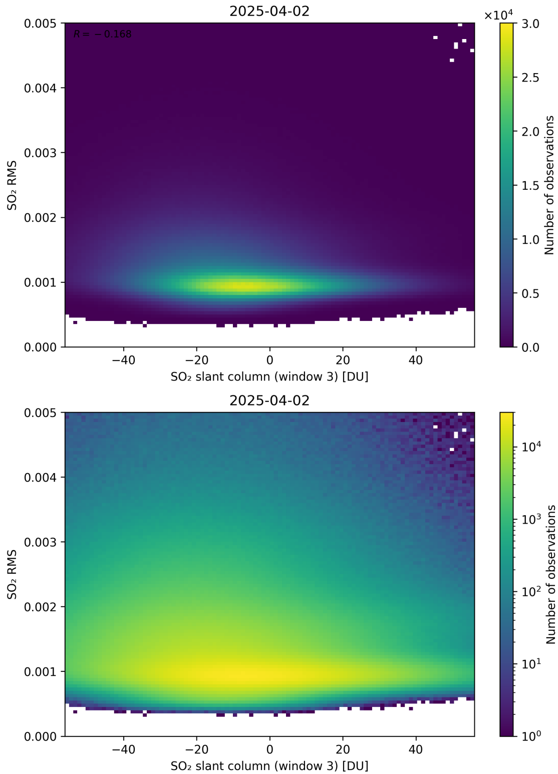
Figure 306: Scatter density plot of “SO 2 slant column (window 3)” against “SO 2 RMS” for 2025-04-02 to 2025-04-03.
