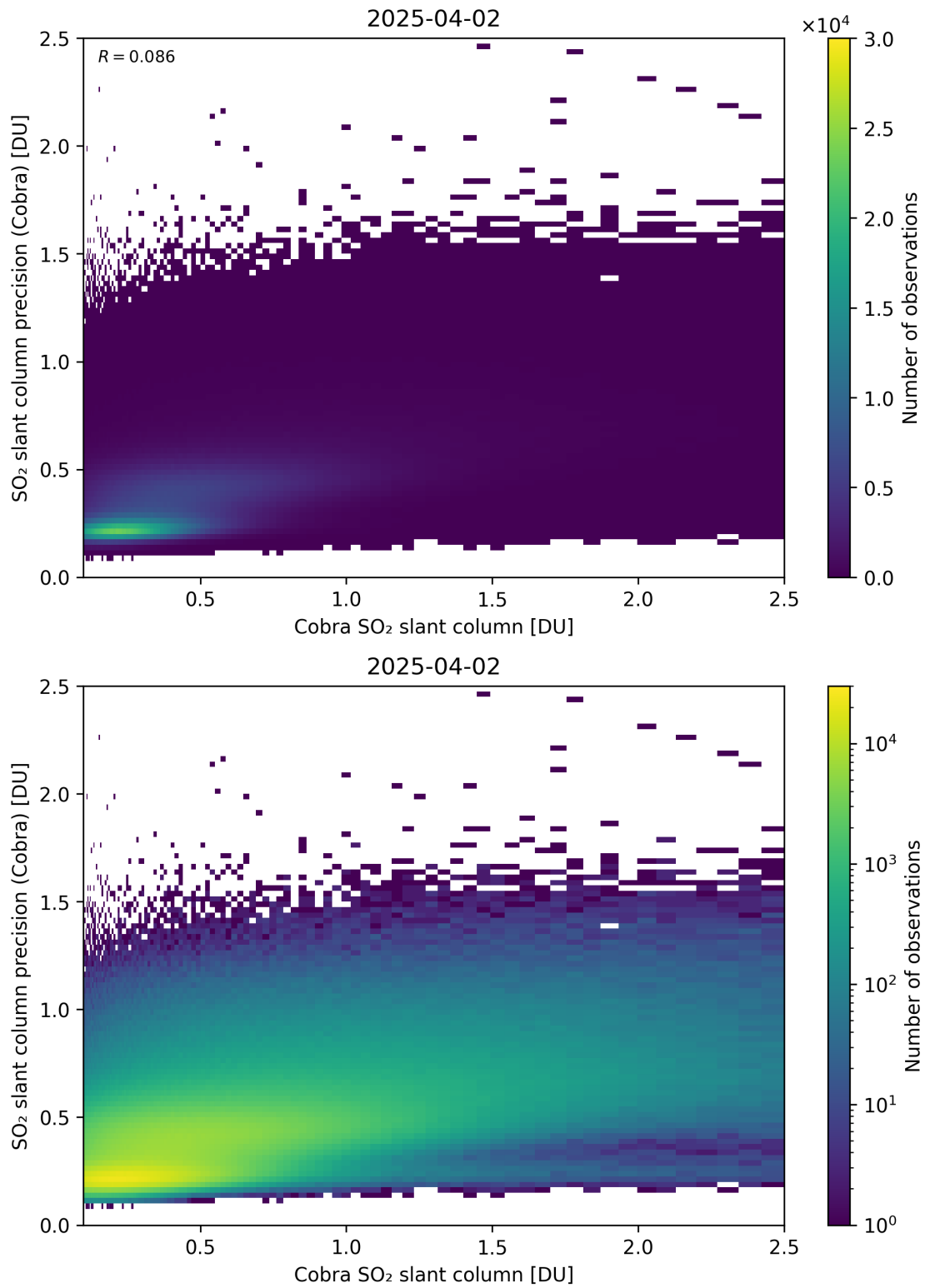
Figure 216: Scatter density plot of “Cobra SO 2 slant column” against “SO 2 slant column precision (Cobra)” for 2025-04-02 to 2025-04-03.
