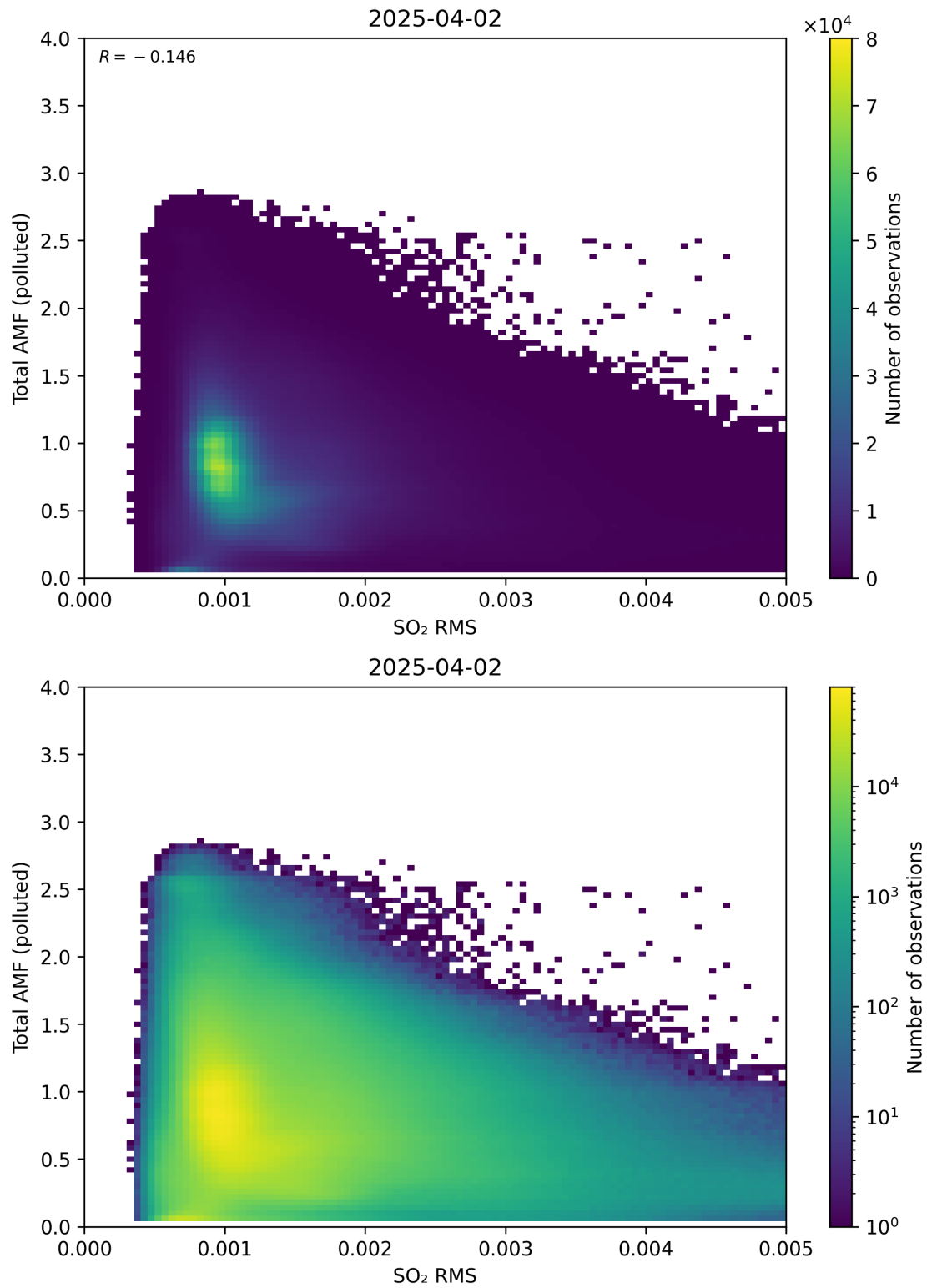
Figure 148: Scatter density plot of “SO 2 RMS” against “Total AMF (polluted)” for 2025-04-02 to 2025-04-03.
