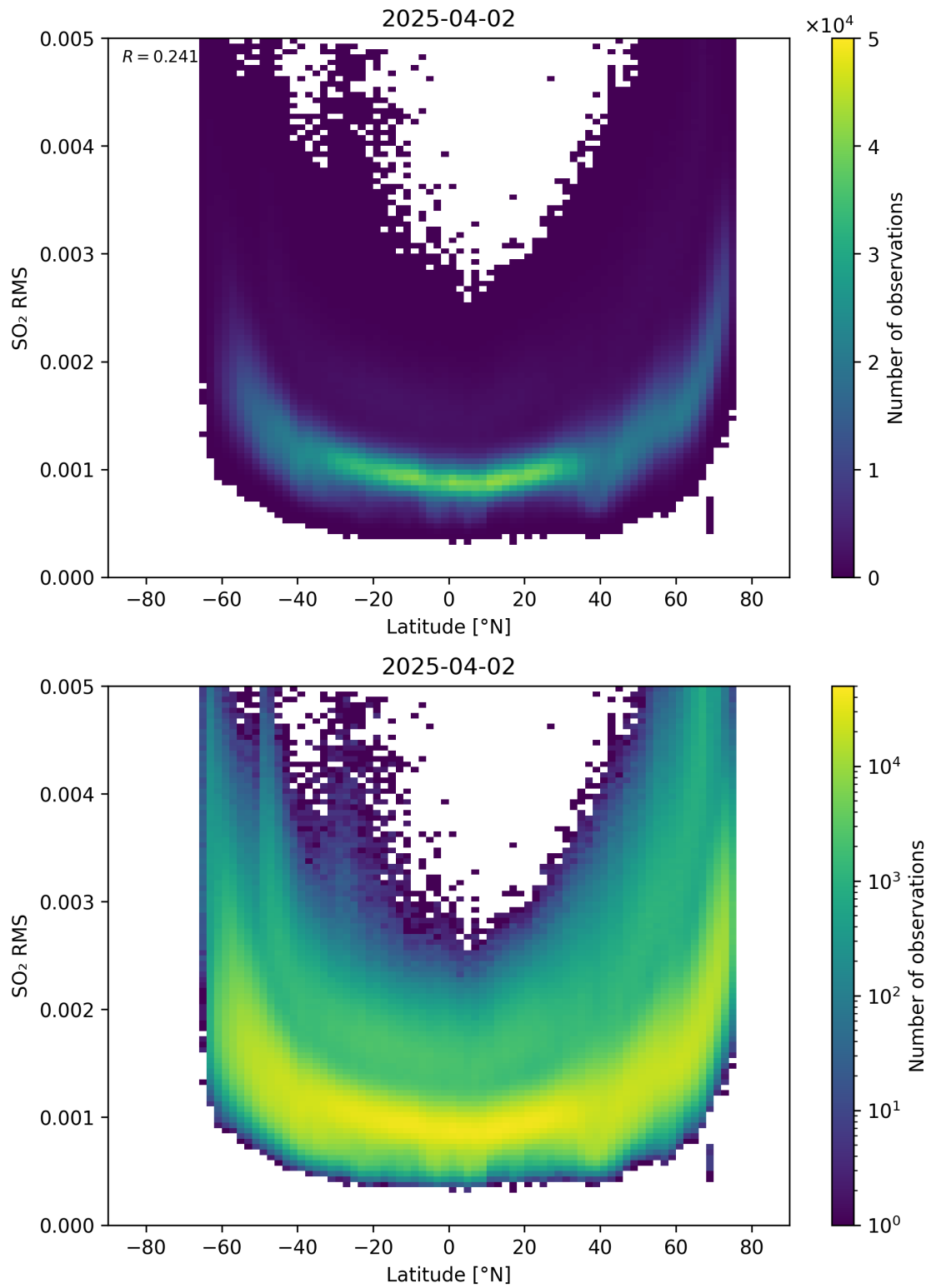
Figure 155: Scatter density plot of “Latitude” against “SO 2 RMS” for 2025-04-02 to 2025-04-03.
