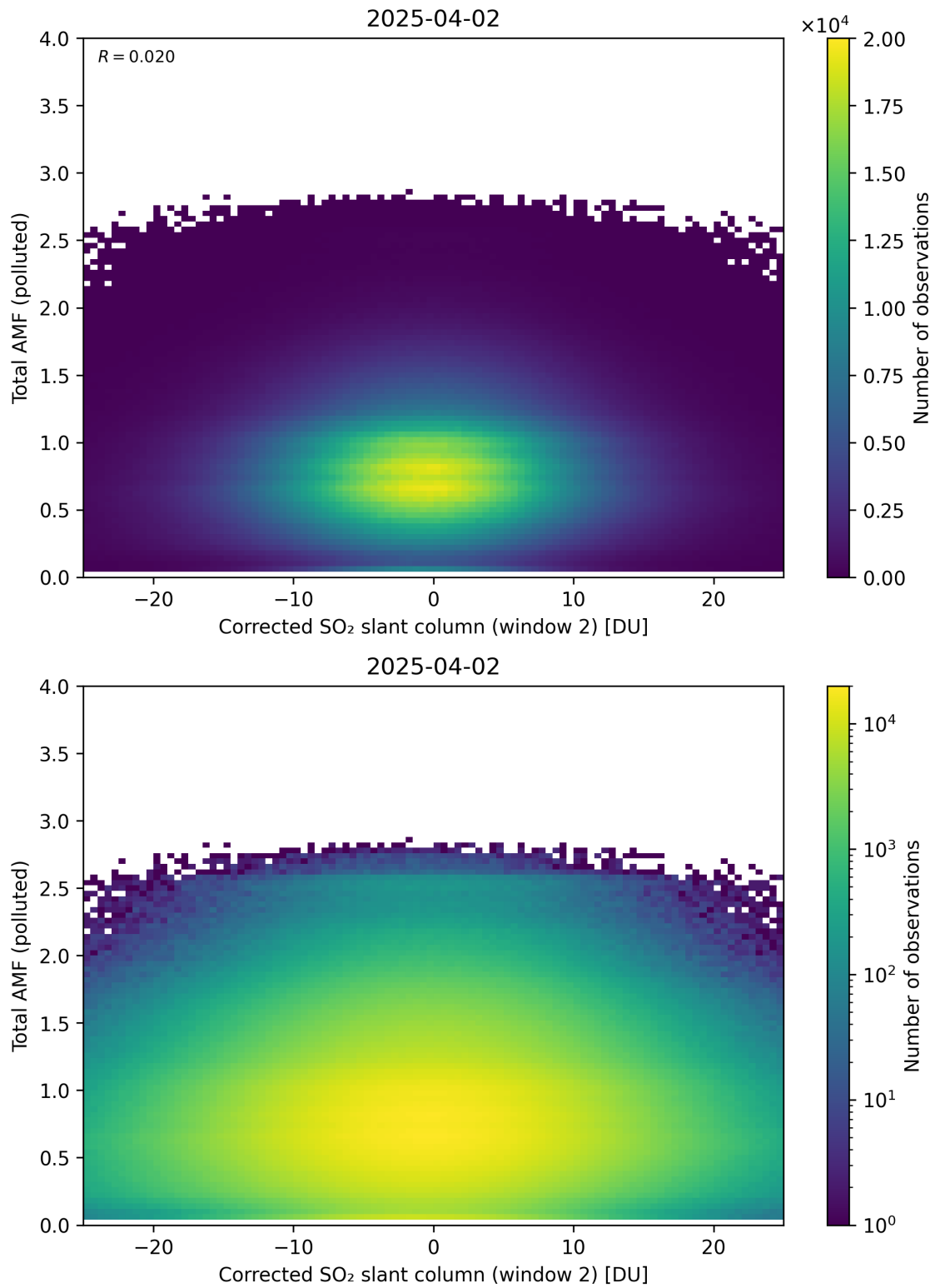
Figure 253: Scatter density plot of “Corrected SO 2 slant column (window 2)” against “Total AMF (polluted)” for 2025-04-02 to 2025-04-03.
