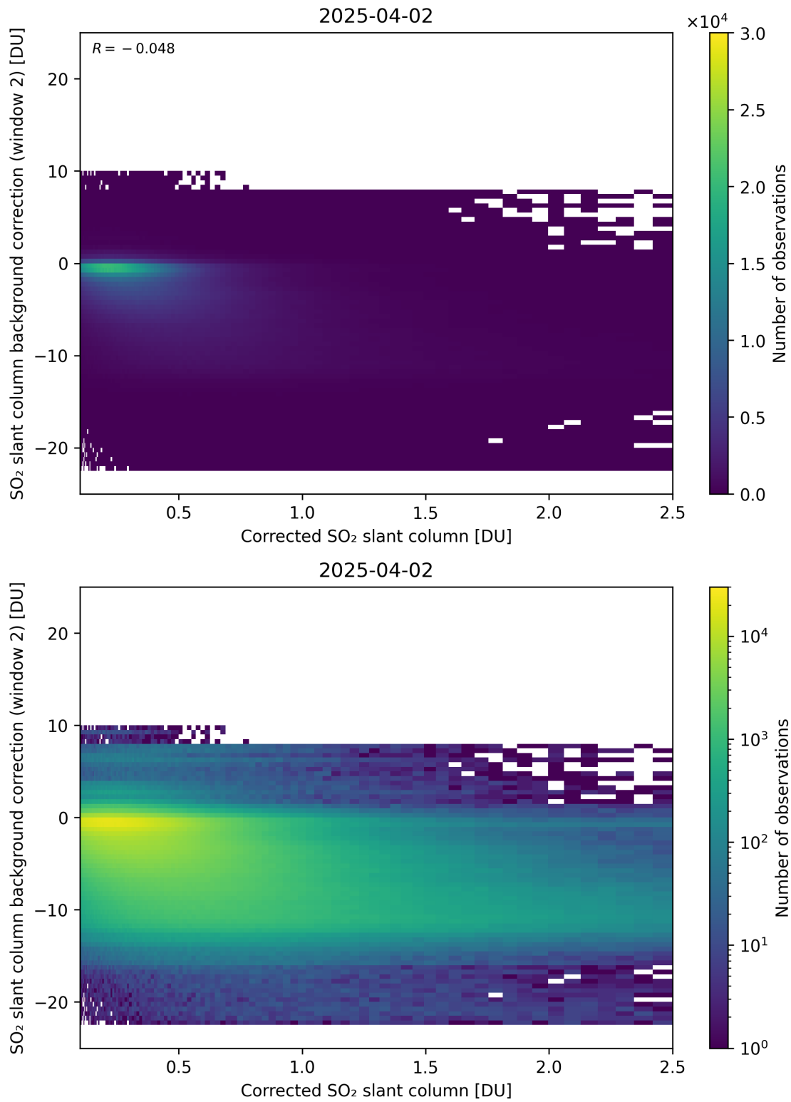
Figure 227: Scatter density plot of “Corrected SO 2 slant column” against “SO 2 slant column background correction (window 2)” for 2025-04-02 to 2025-04-03.
