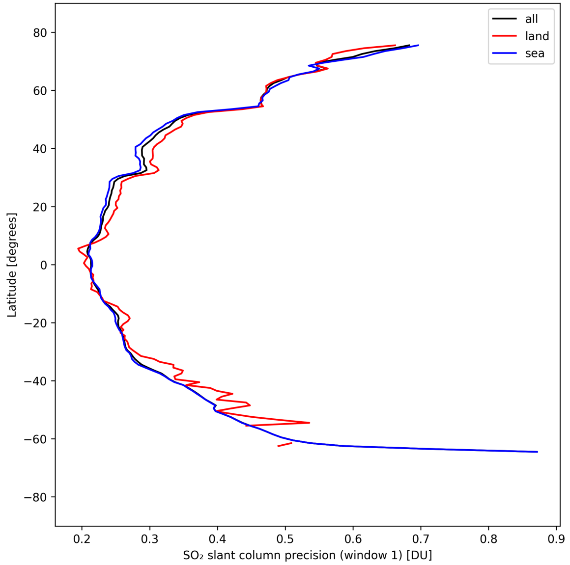
Figure 38: Zonal average of “SO 2 slant column precision (window 1)” for 2025-04-02 to 2025-04-03.
