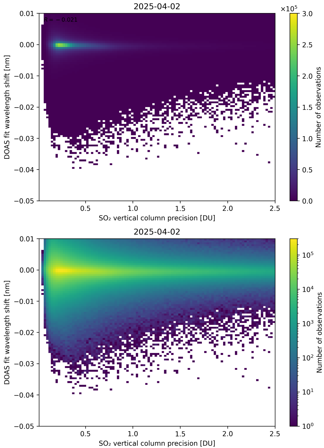
Figure 332: Scatter density plot of “SO 2 vertical column precision” against “DOAS fit wavelength shift” for 2025-04-02 to 2025-04-03.
