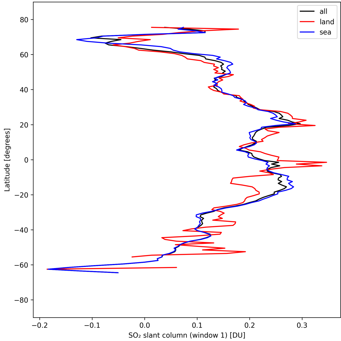
Figure 37: Zonal average of “SO 2 slant column (window 1)” for 2025-04-02 to 2025-04-03.
