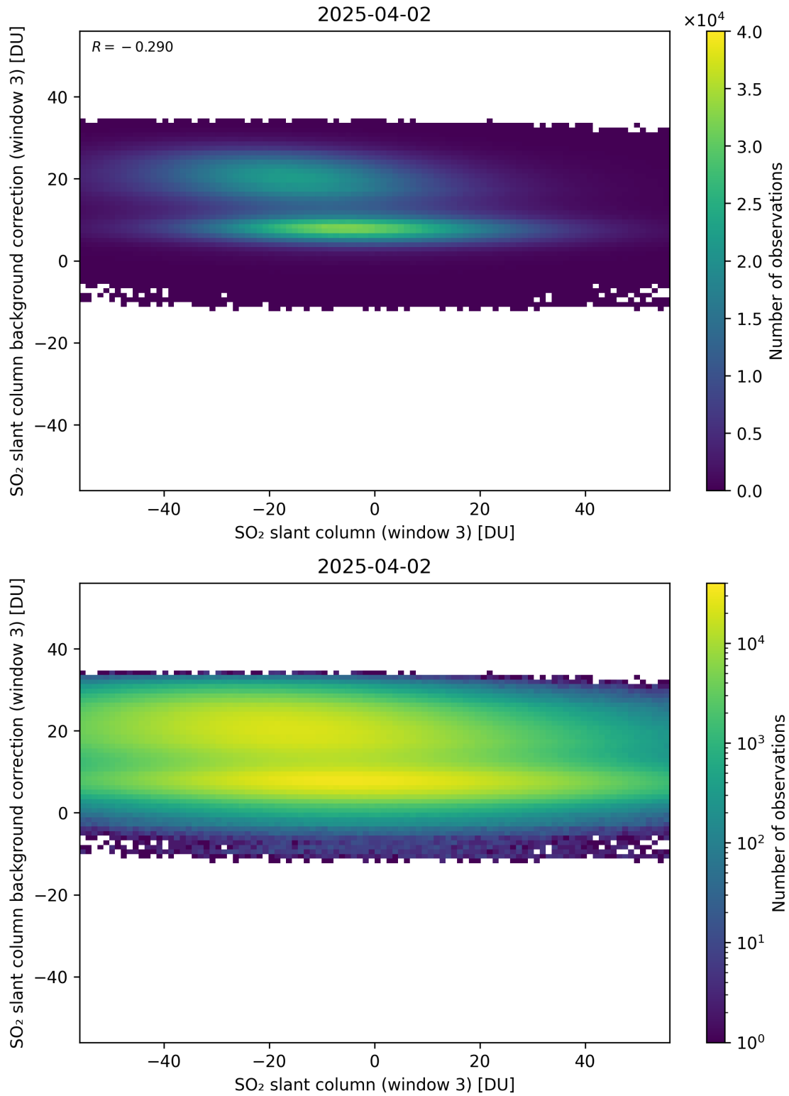
Figure 303: Scatter density plot of “SO 2 slant column (window 3)” against “SO 2 slant column background correction (window 3)” for 2025-04-02 to 2025-04-03.
