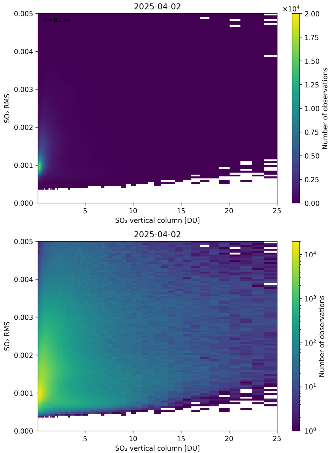
Figure 328: Scatter density plot of “SO 2 vertical column” against “SO 2 RMS” for 2025-04-02 to 2025-04-03.
