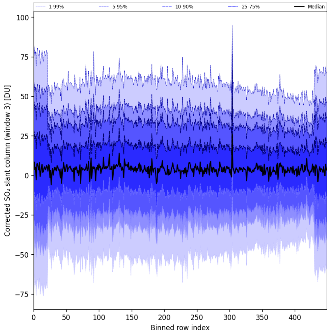
Figure 99: Along track statistics of “Corrected SO 2 slant column (window 3)” for 2025-04-02 to 2025-04-03
