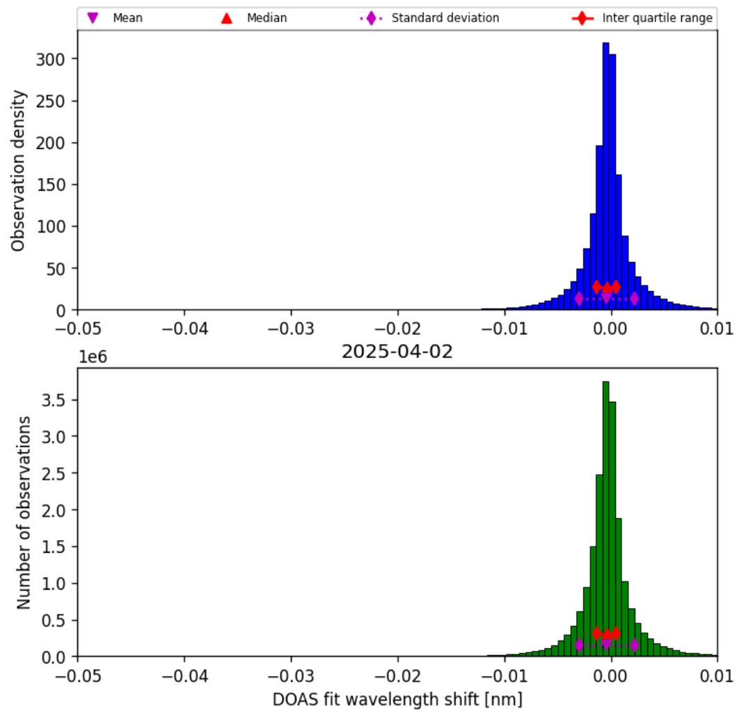
Figure 76: Histogram of “DOAS fit wavelength shift” for 2025-04-02 to 2025-04-03
