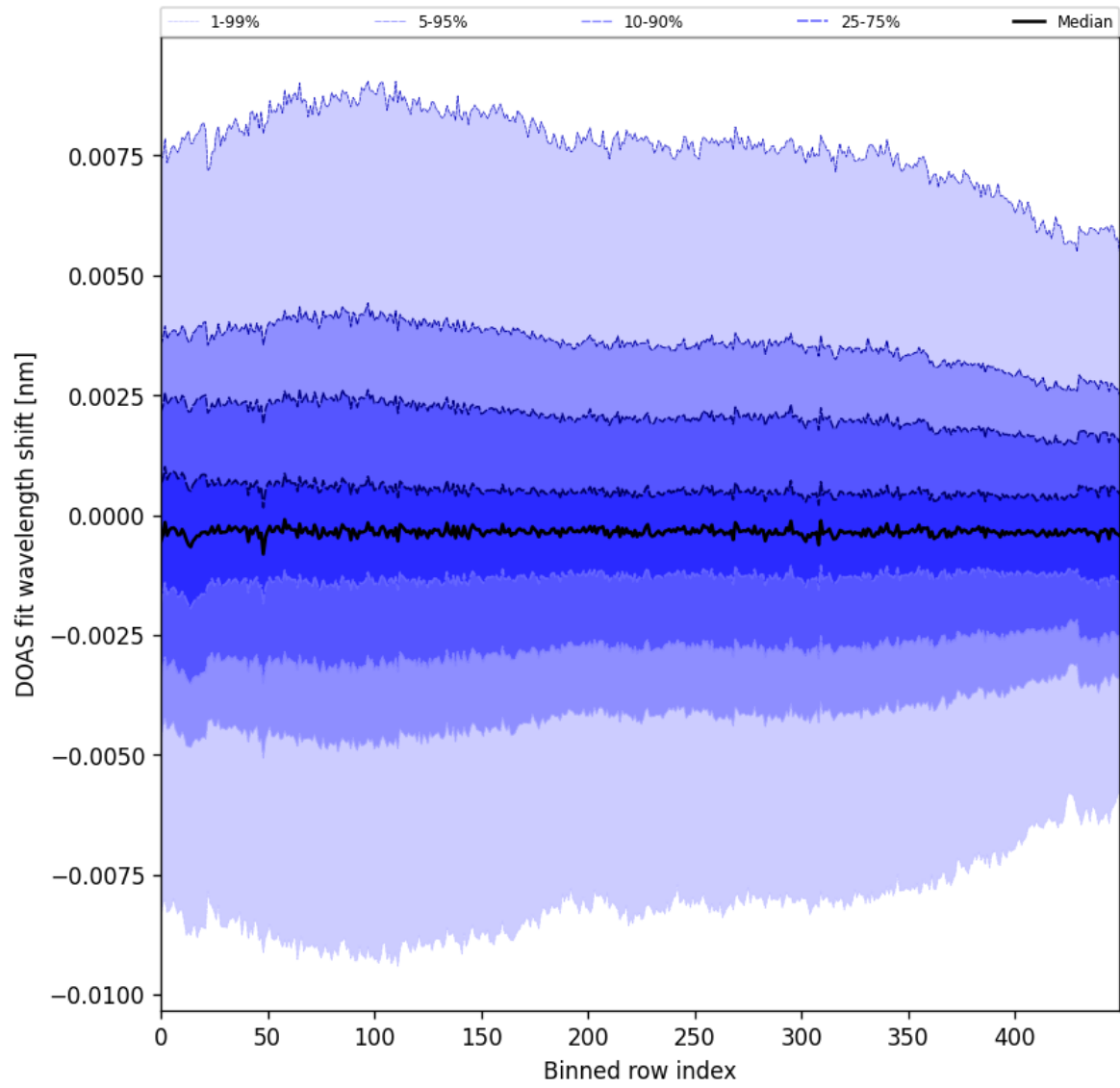
Figure 102: Along track statistics of “DOAS fit wavelength shift” for 2025-04-02 to 2025-04-03
