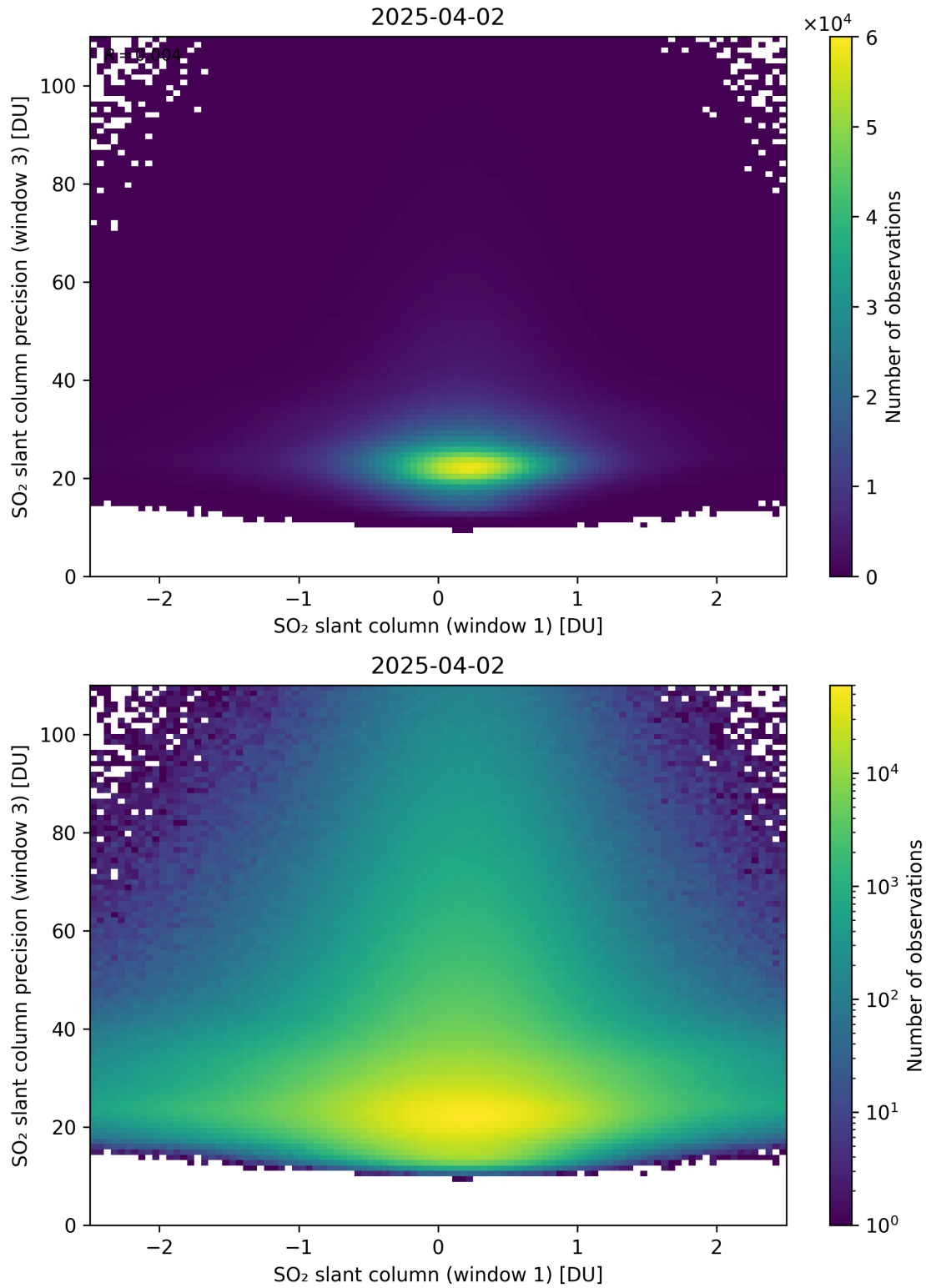
Figure 288: Scatter density plot of “SO 2 slant column (window 1)” against “SO 2 slant column precision (window 3)” for 2025-04-02 to 2025-04-03.
