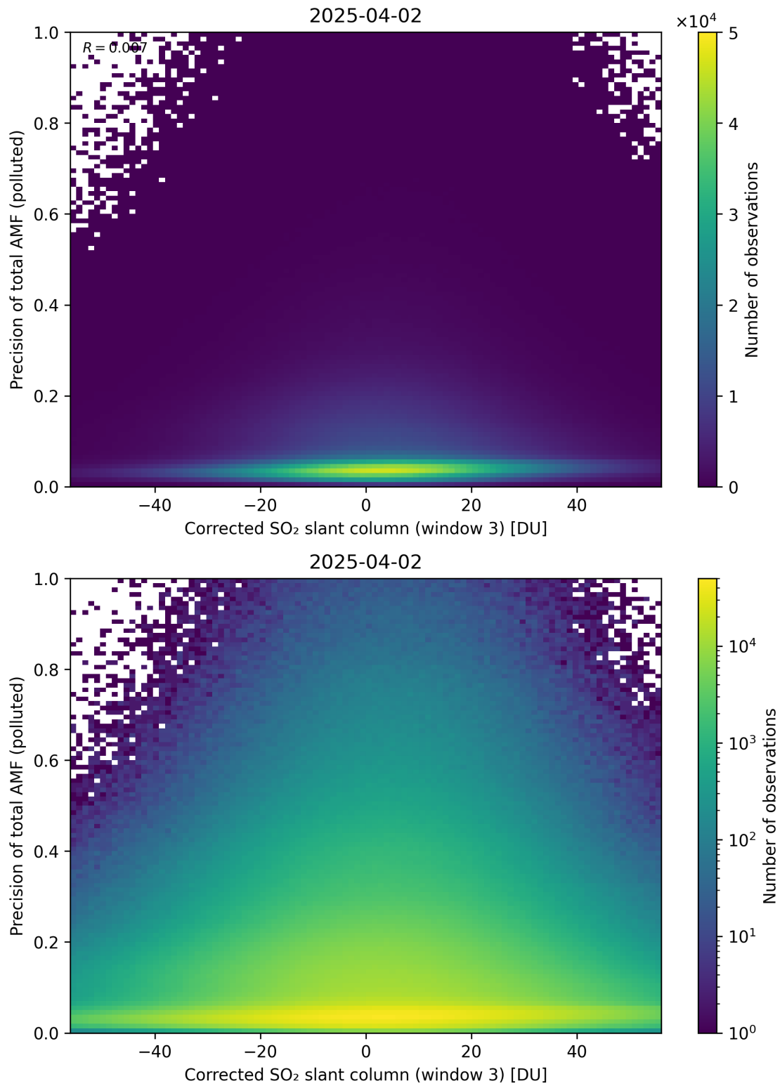
Figure 261: Scatter density plot of “Corrected SO 2 slant column (window 3)” against “Precision of total AMF (polluted)” for 2025-04-02 to 2025-04-03.
