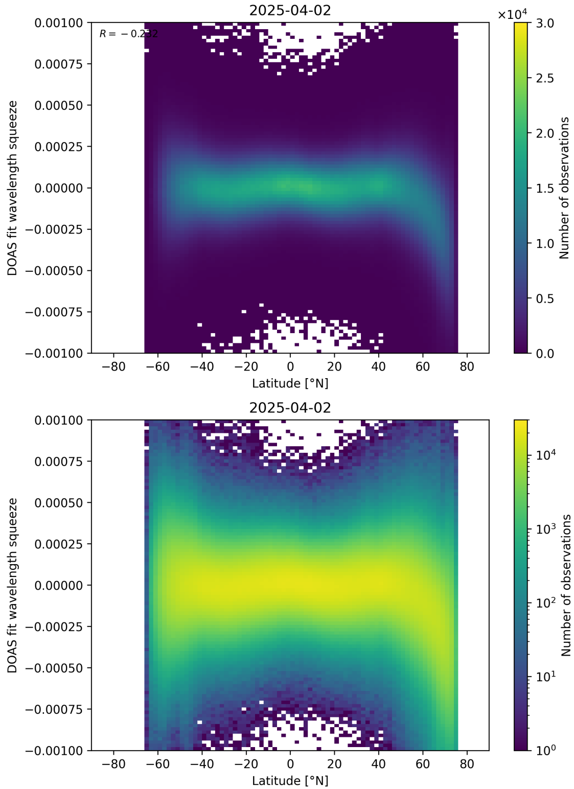
Figure 154: Scatter density plot of “Latitude” against “DOAS fit wavelength squeeze” for 2025-04-02 to 2025-04-03.
