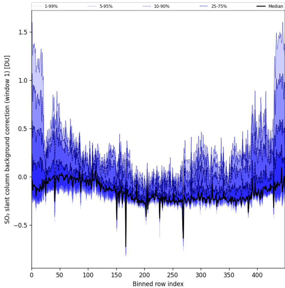
Figure 92: Along track statistics of “SO 2 slant column background correction (window 1)” for 2025-04-02 to 2025-04-03
