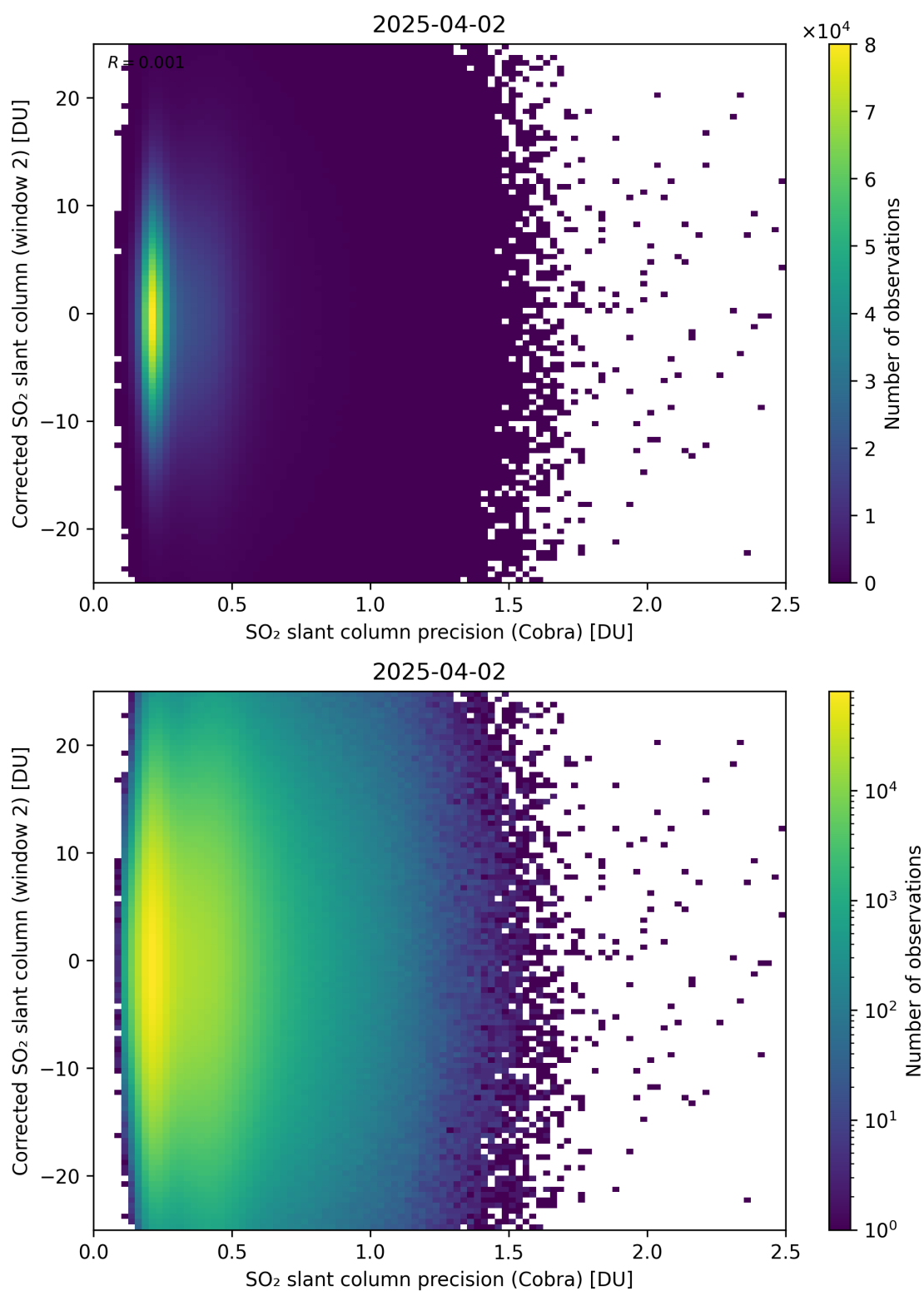
Figure 206: Scatter density plot of “SO 2 slant column precision (Cobra)” against “Corrected SO 2 slant column (window 2)” for 2025-04-02 to 2025-04-03.
