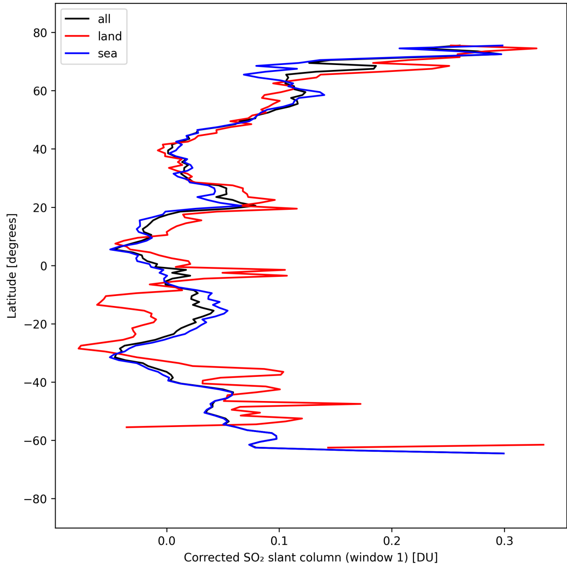
Figure 39: Zonal average of “Corrected SO 2 slant column (window 1)” for 2025-04-02 to 2025-04-03.
