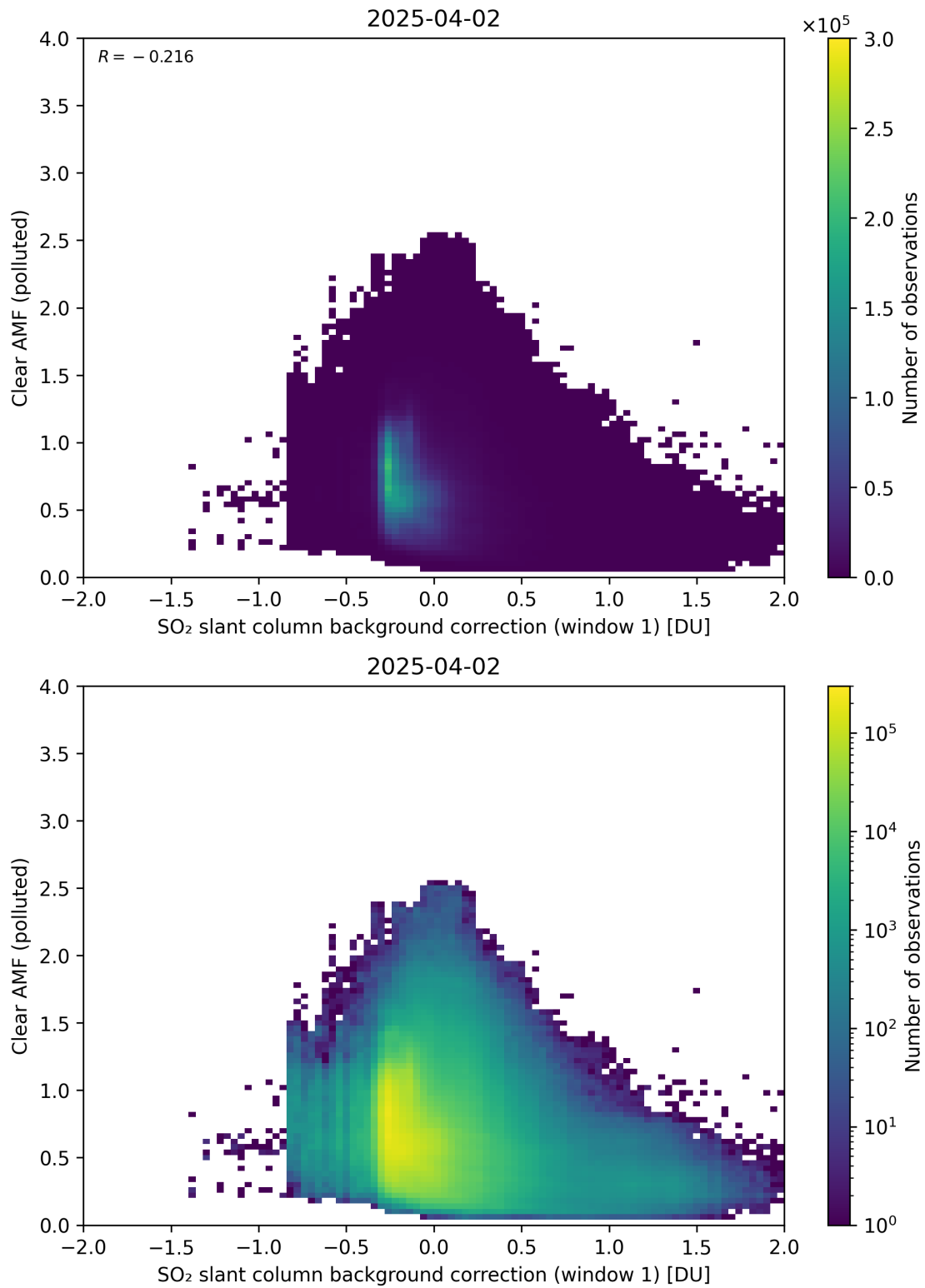
Figure 114: Scatter density plot of “SO 2 slant column background correction (window 1)” against “Clear AMF (polluted)” for 2025-04-02 to 2025-04-03.
