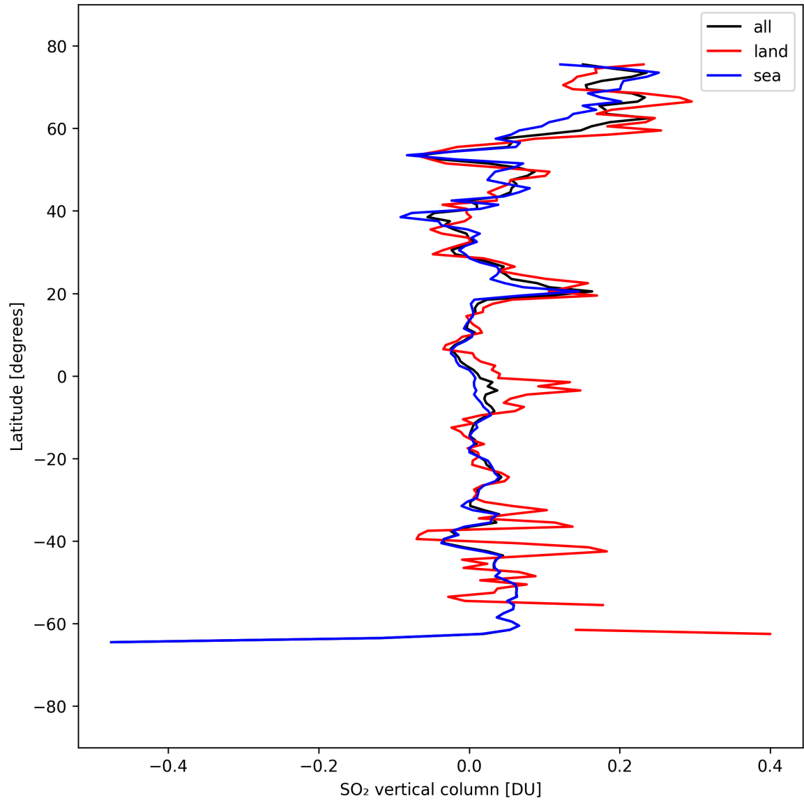
Figure 32: Zonal average of “SO 2 vertical column” for 2025-04-02 to 2025-04-03.
