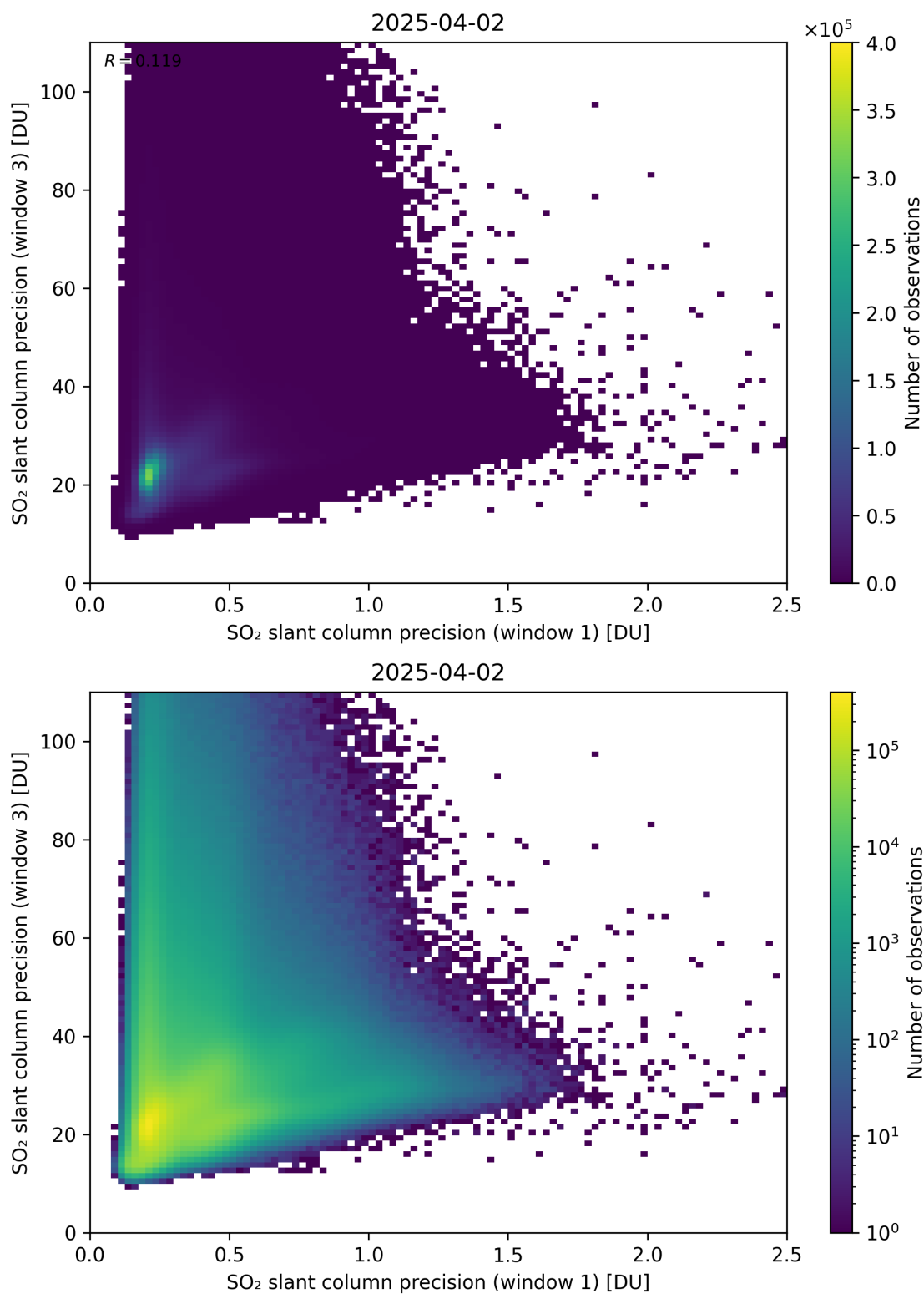
Figure 279: Scatter density plot of “SO 2 slant column precision (window 1)” against “SO 2 slant column precision (window 3)” for 2025-04-02 to 2025-04-03.
