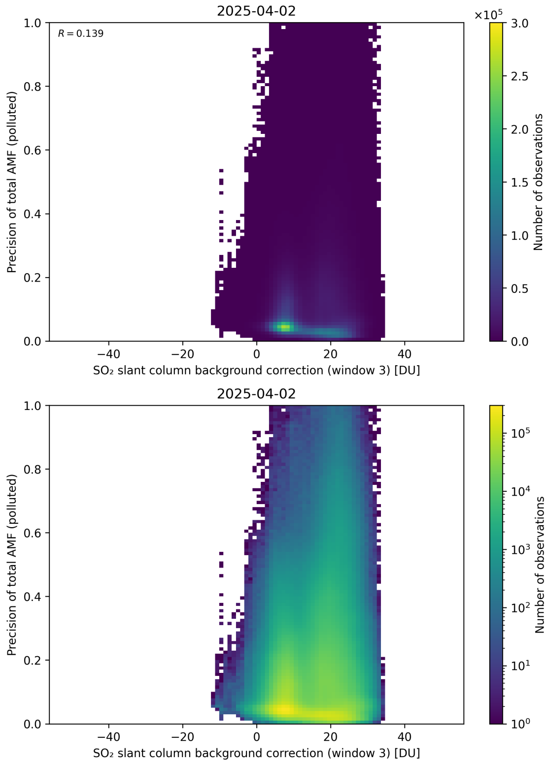
Figure 137: Scatter density plot of “SO 2 slant column background correction (window 3)” against “Precision of total AMF (polluted)” for 2025-04-02 to 2025-04-03.
