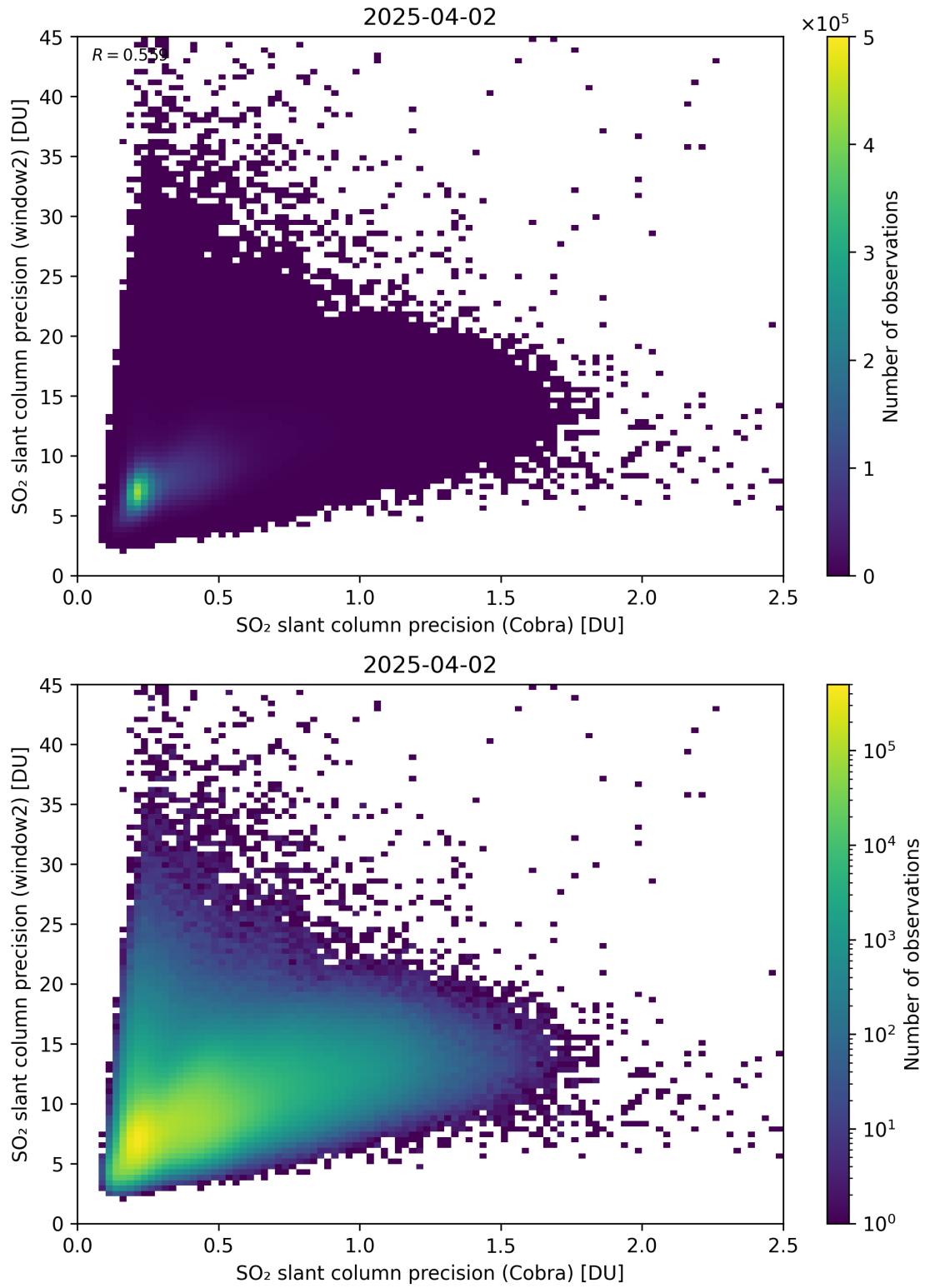
Figure 210: Scatter density plot of “SO 2 slant column precision (Cobra)” against “SO 2 slant column precision (window2)” for 2025-04-02 to 2025-04-03.
