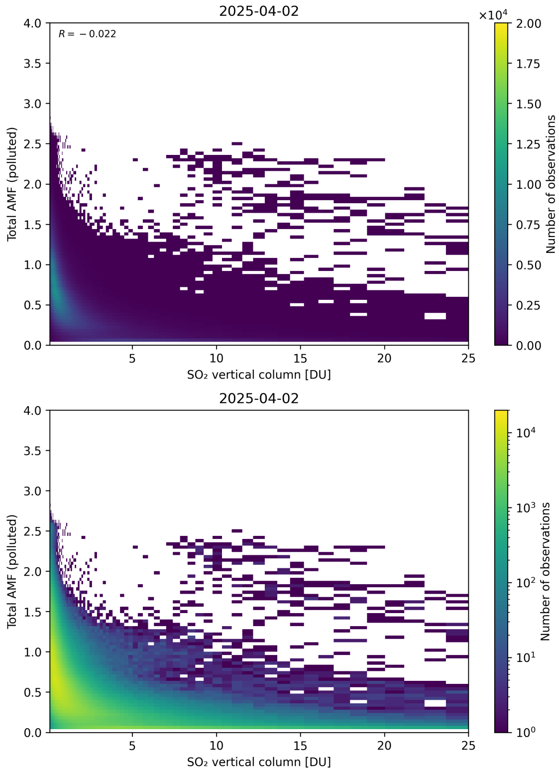
Figure 359: Scatter density plot of “SO 2 vertical column” against “Total AMF (polluted)” for 2025-04-02 to 2025-04-03.
