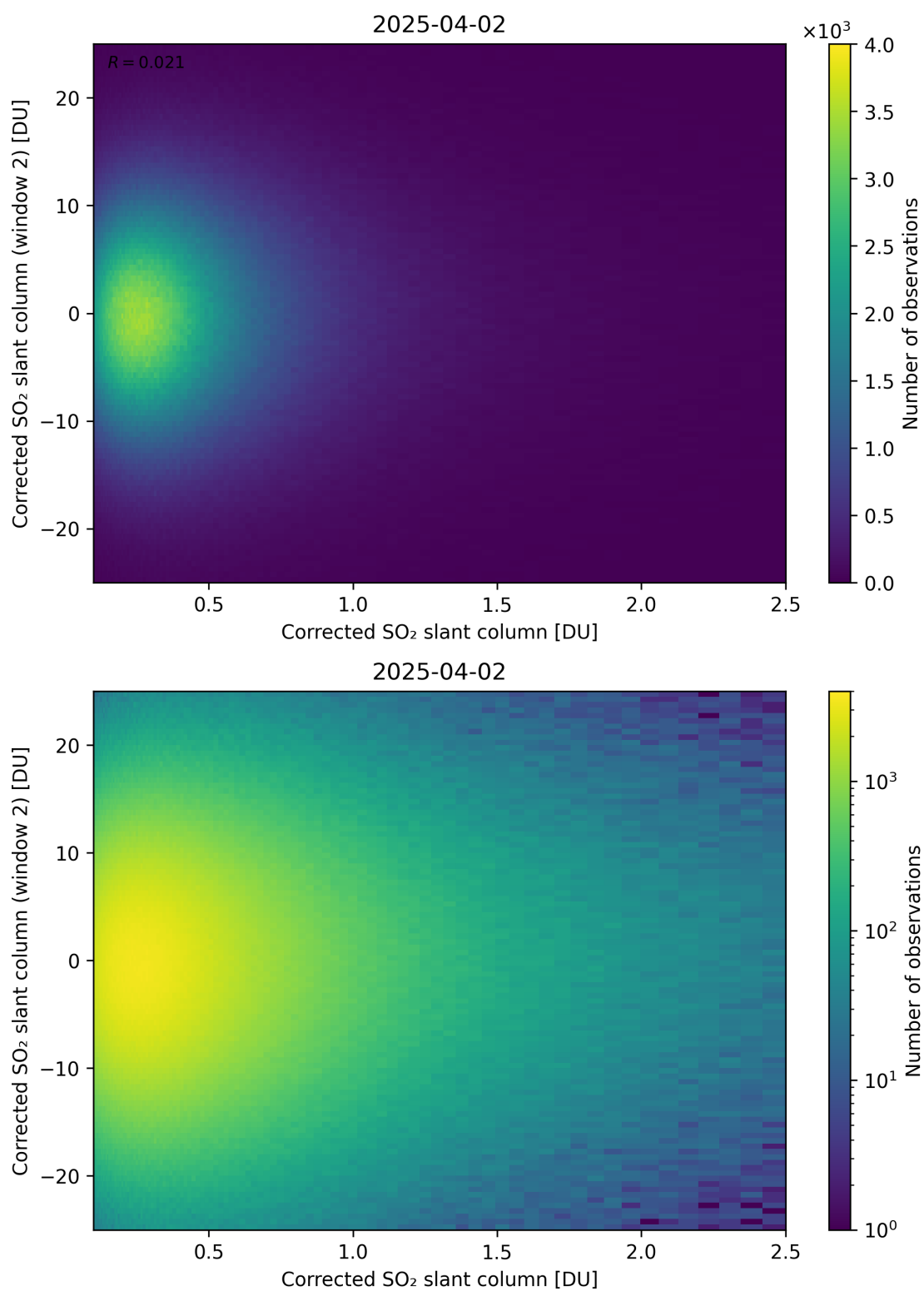
Figure 235: Scatter density plot of “Corrected SO 2 slant column” against “Corrected SO 2 slant column (window 2)” for 2025-04-02 to 2025-04-03.
