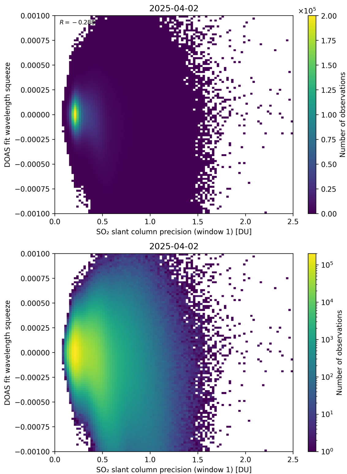
Figure 272: Scatter density plot of “SO 2 slant column precision (window 1)” against “DOAS fit wavelength squeeze” for 2025-04-02 to 2025-04-03.
