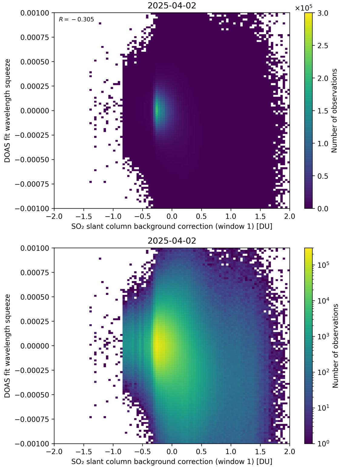
Figure 112: Scatter density plot of “SO 2 slant column background correction (window 1)” against “DOAS fit wavelength squeeze” for 2025-04-02 to 2025-04-03.
