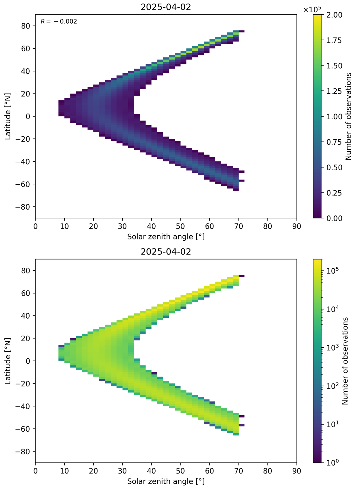
Figure 177: Scatter density plot of “Solar zenith angle” against “Latitude” for 2025-04-02 to 2025-04-03.
