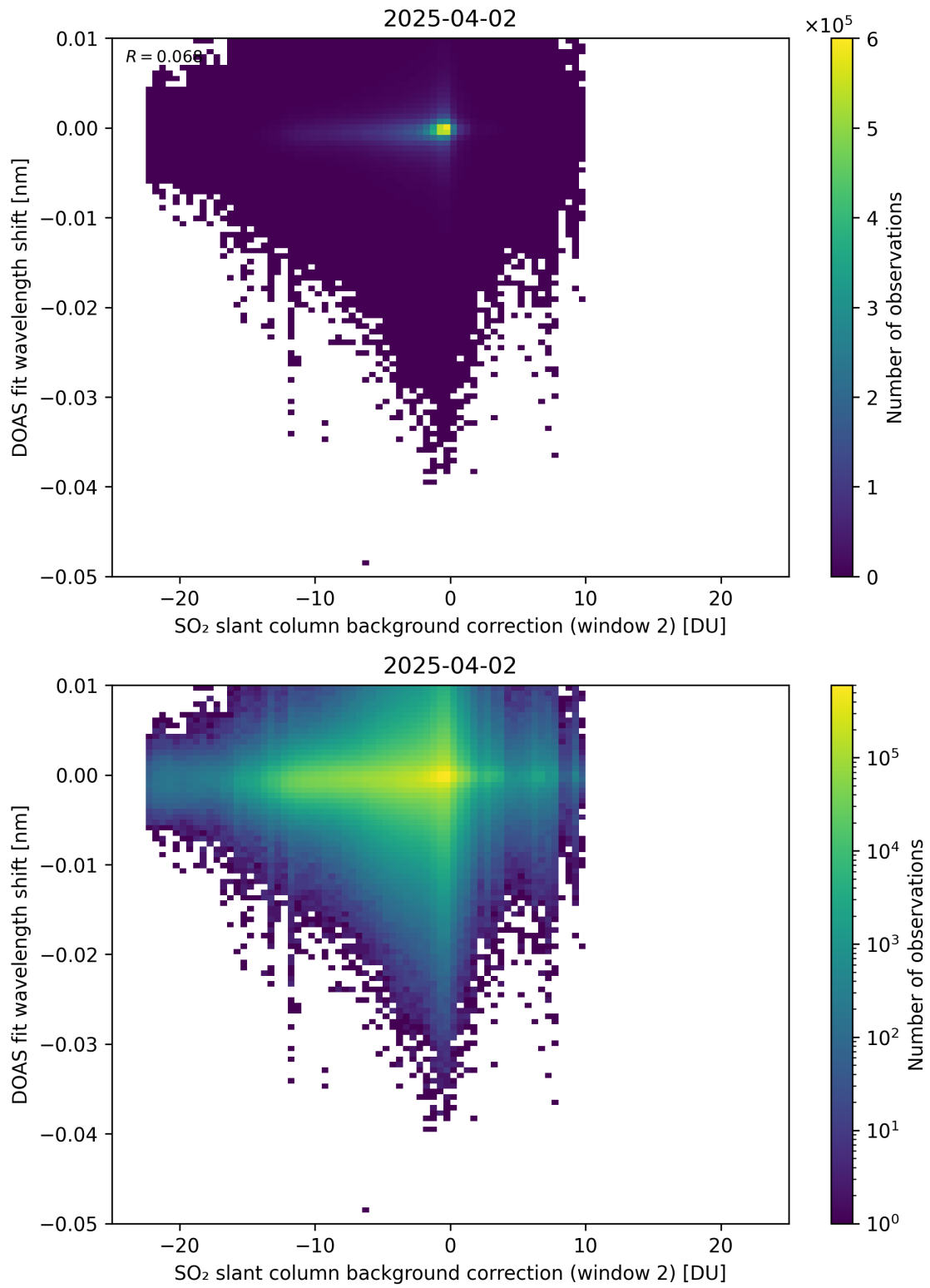
Figure 123: Scatter density plot of “SO 2 slant column background correction (window 2)” against “DOAS fit wavelength shift” for 2025-04-02 to 2025-04-03.
