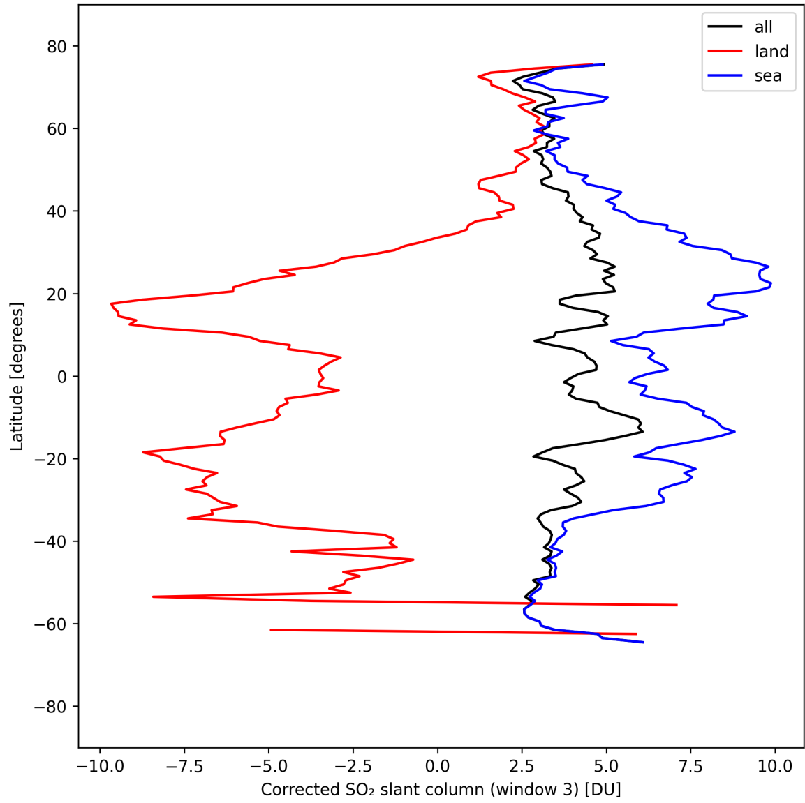
Figure 47: Zonal average of “Corrected SO 2 slant column (window 3)” for 2025-04-02 to 2025-04-03.
