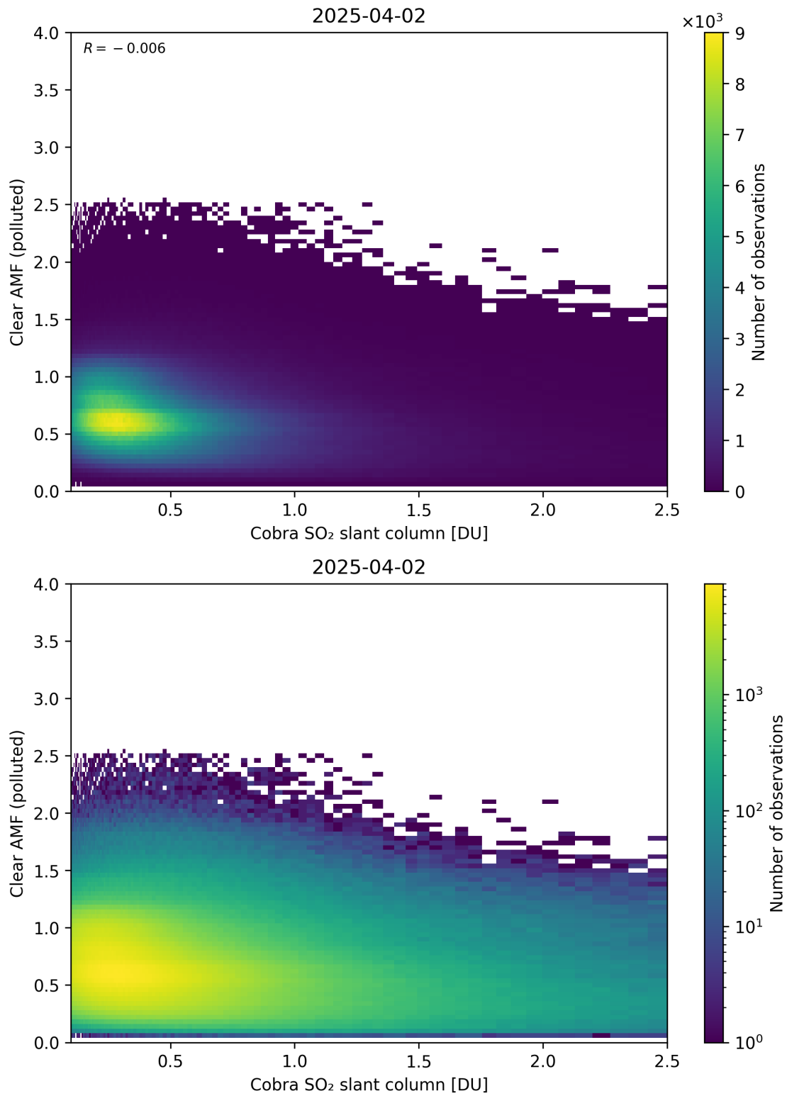
Figure 215: Scatter density plot of “Cobra SO 2 slant column” against “Clear AMF (polluted)” for 2025-04-02 to 2025-04-03.
