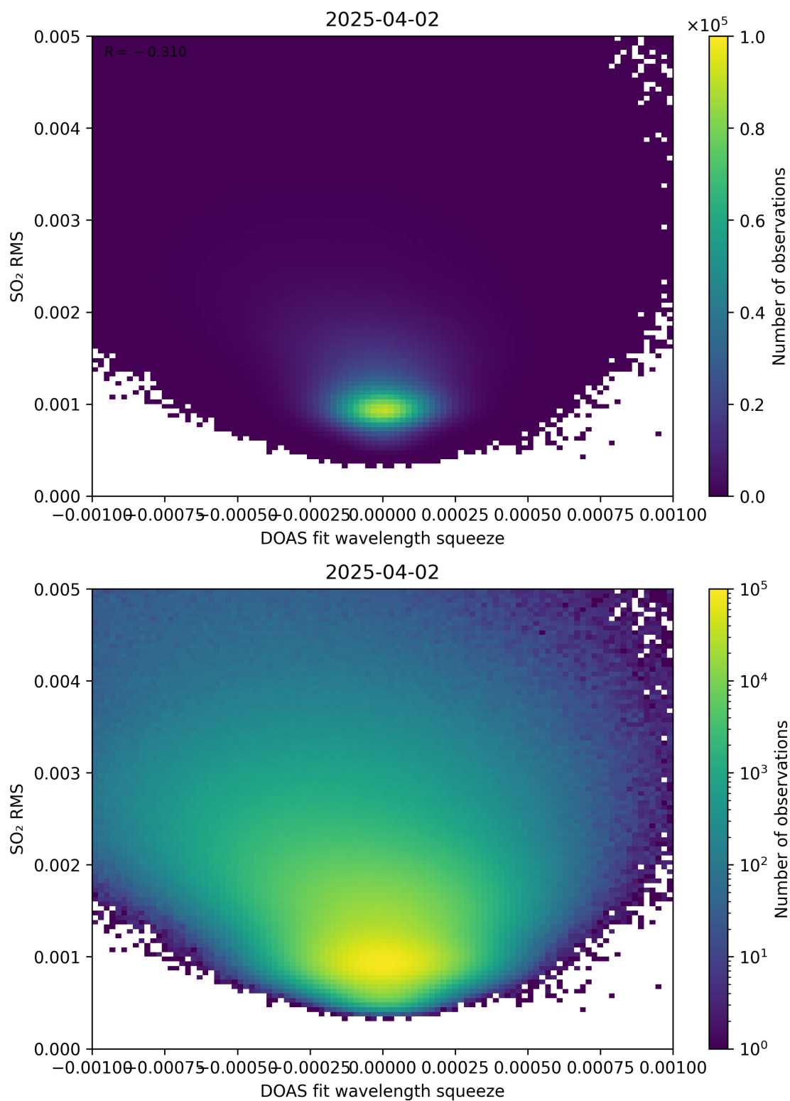
Figure 143: Scatter density plot of “DOAS fit wavelength squeeze” against “SO 2 RMS” for 2025-04-02 to 2025-04-03.
