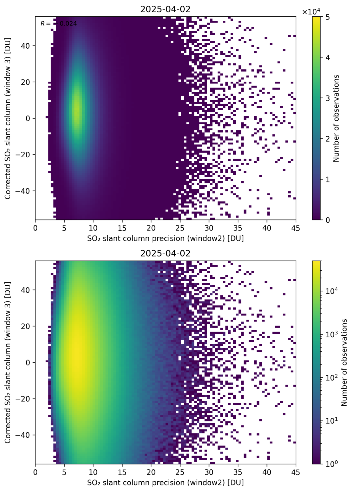
Figure 298: Scatter density plot of “SO 2 slant column precision (window2)” against “Corrected SO 2 slant column (window 3)” for 2025-04-02 to 2025-04-03.
