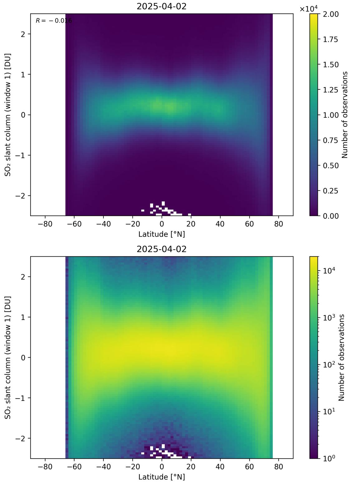
Figure 162: Scatter density plot of “Latitude” against “SO 2 slant column (window 1)” for 2025-04-02 to 2025-04-03.
