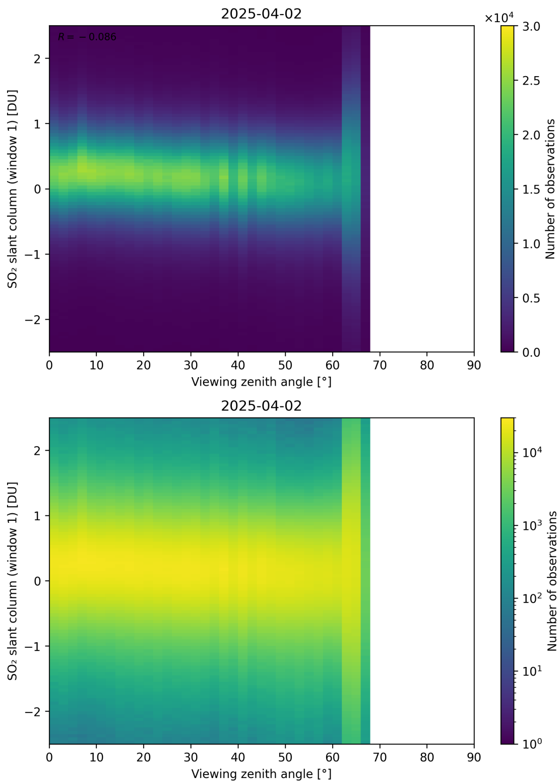
Figure 376: Scatter density plot of “Viewing zenith angle” against “SO 2 slant column (window 1)” for 2025-04-02 to 2025-04-03.
