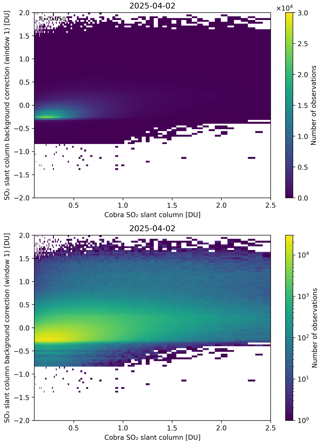
Figure 193: Scatter density plot of “Cobra SO 2 slant column” against “SO 2 slant column background correction (window 1)” for 2025-04-02 to 2025-04-03.
