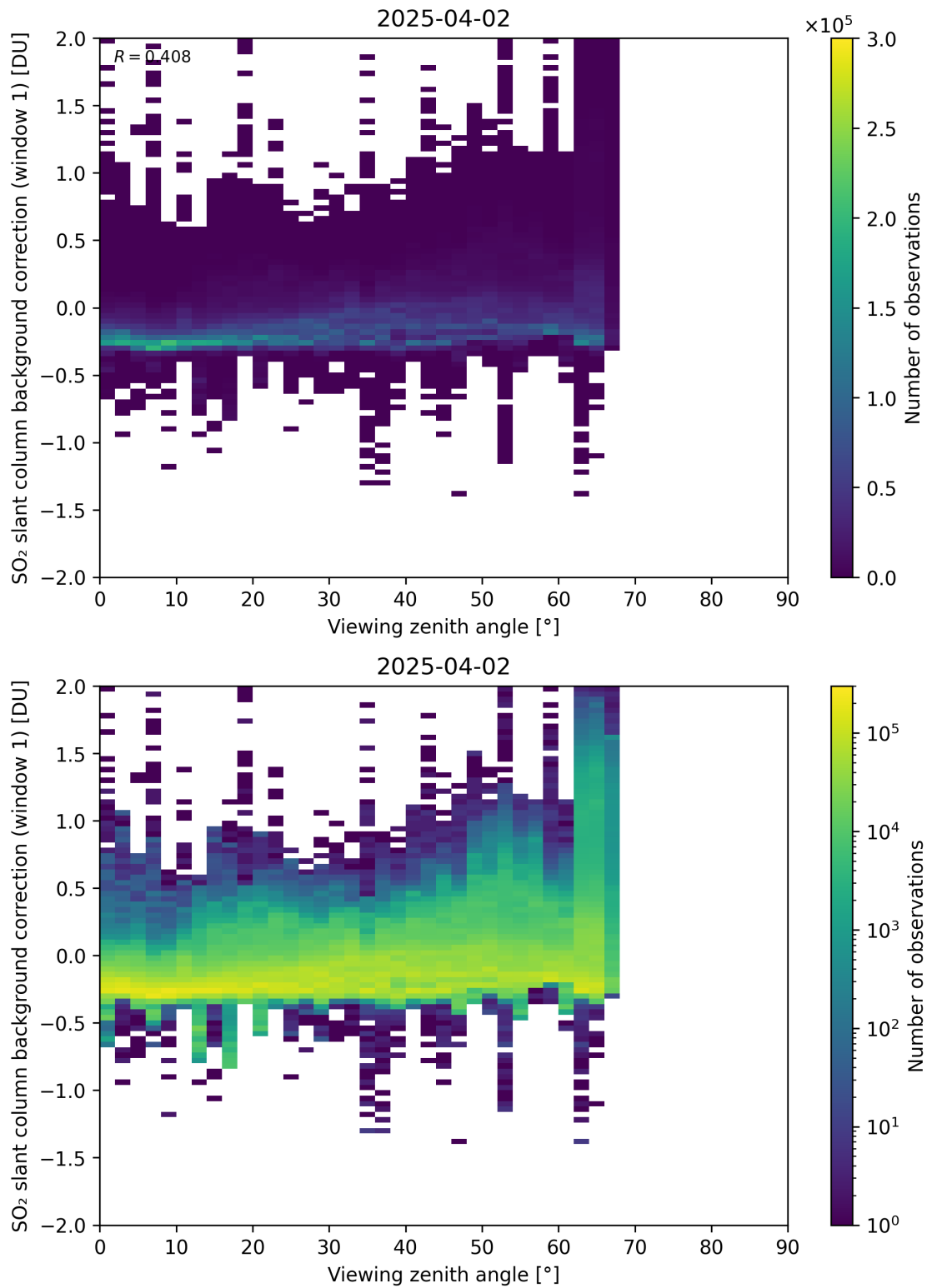
Figure 362: Scatter density plot of “Viewing zenith angle” against “SO 2 slant column background correction (window 1)” for 2025-04-02 to 2025-04-03.
