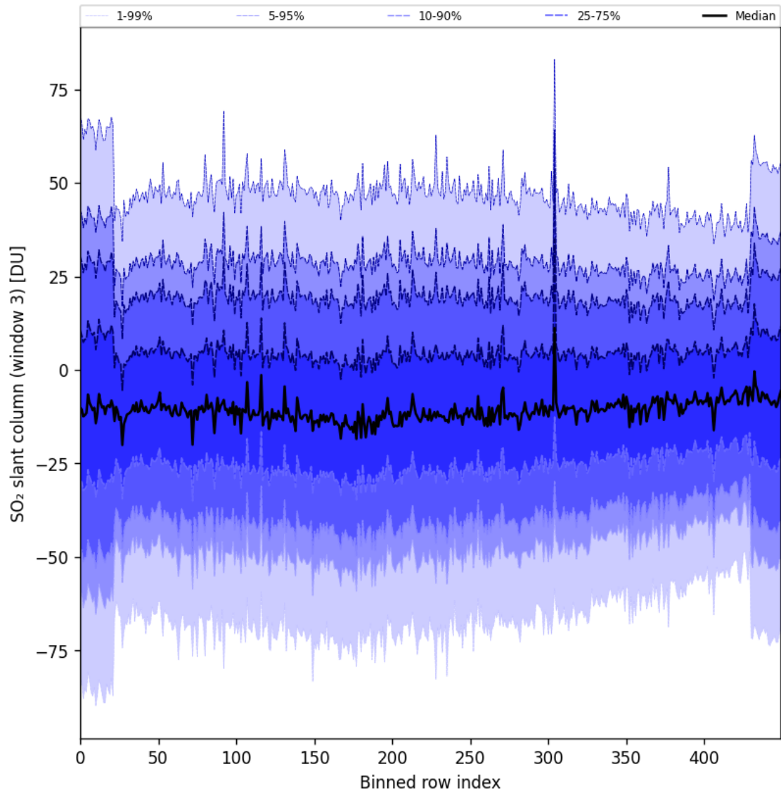
Figure 97: Along track statistics of “SO 2 slant column (window 3)” for 2025-04-02 to 2025-04-03
