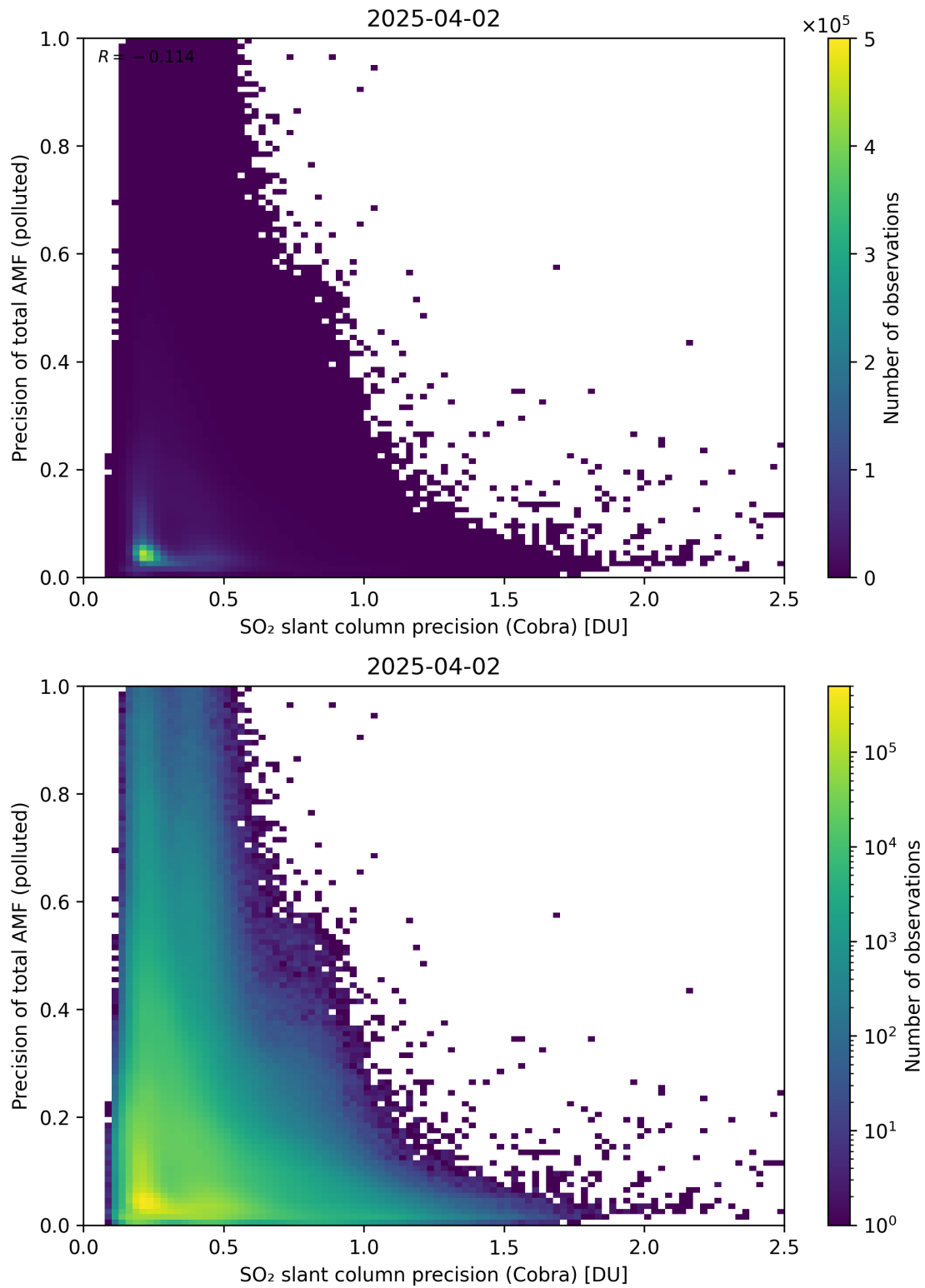
Figure 214: Scatter density plot of “SO 2 slant column precision (Cobra)” against “Precision of total AMF (polluted)” for 2025-04-02 to 2025-04-03.
