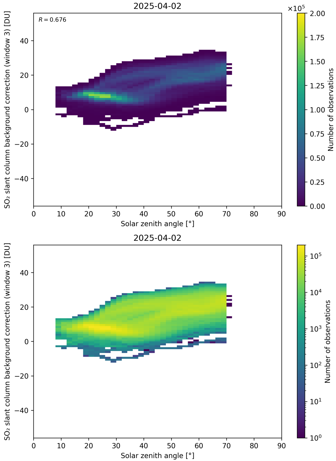
Figure 173: Scatter density plot of “Solar zenith angle” against “SO 2 slant column background correction (window 3)” for 2025-04-02 to 2025-04-03.
