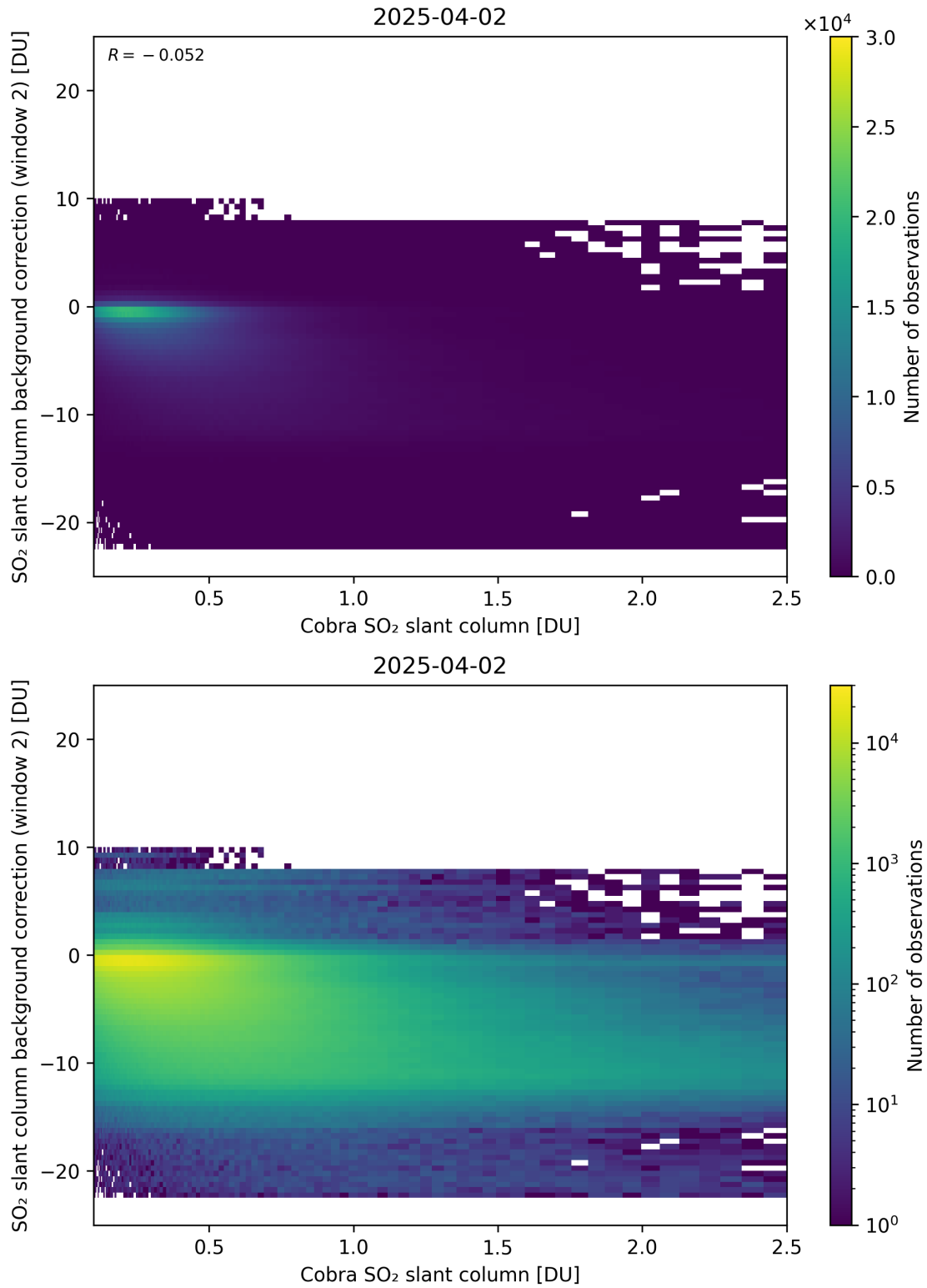
Figure 194: Scatter density plot of “Cobra SO 2 slant column” against “SO 2 slant column background correction (window 2)” for 2025-04-02 to 2025-04-03.
