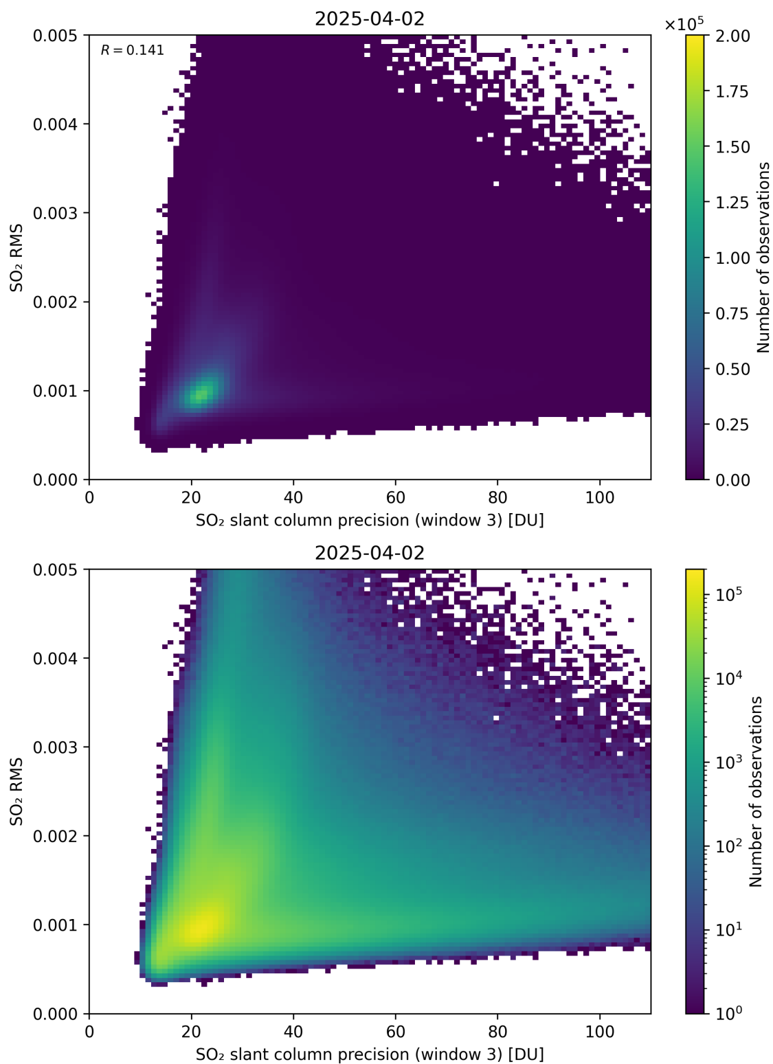
Figure 310: Scatter density plot of “SO 2 slant column precision (window 3)” against “SO 2 RMS” for 2025-04-02 to 2025-04-03.
