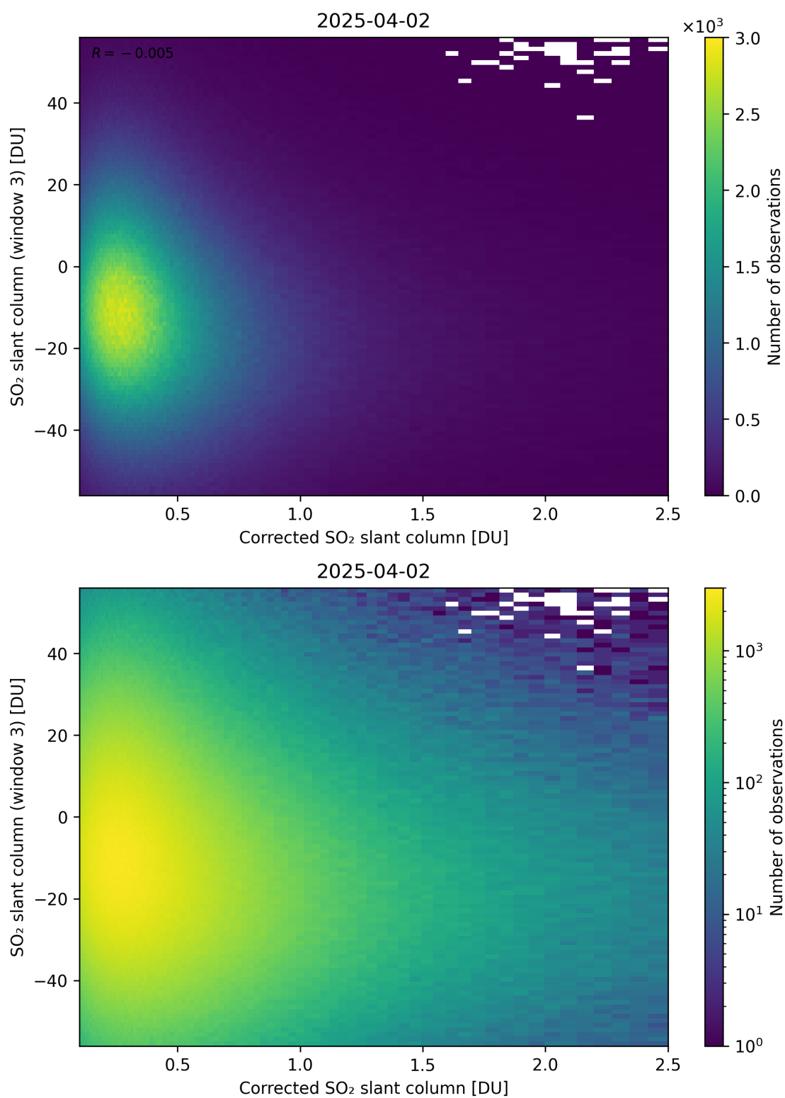
Figure 240: Scatter density plot of “Corrected SO 2 slant column” against “SO 2 slant column (window 3)” for 2025-04-02 to 2025-04-03.
