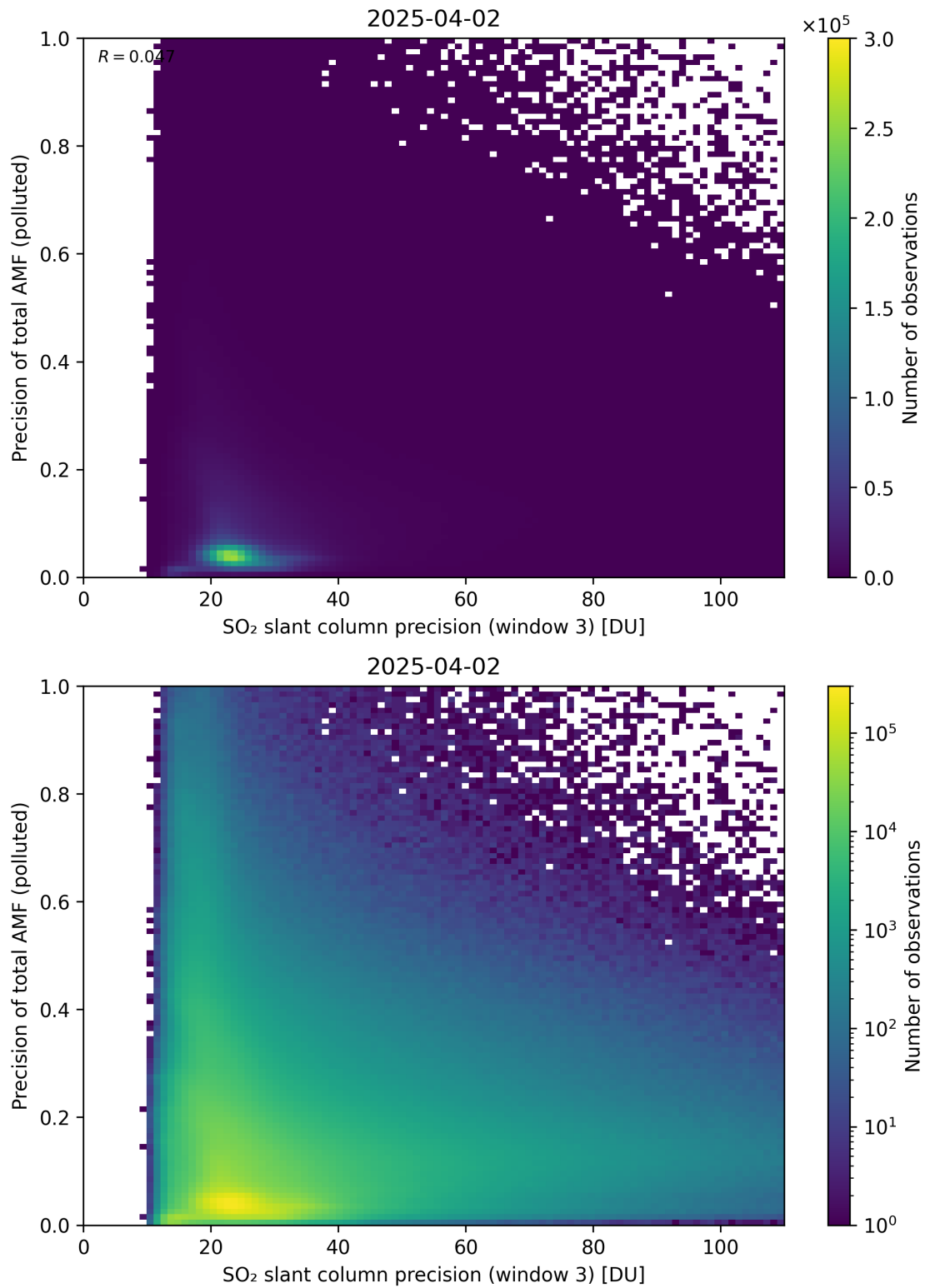
Figure 314: Scatter density plot of “SO 2 slant column precision (window 3)” against “Precision of total AMF (polluted)” for 2025-04-02 to 2025-04-03.
