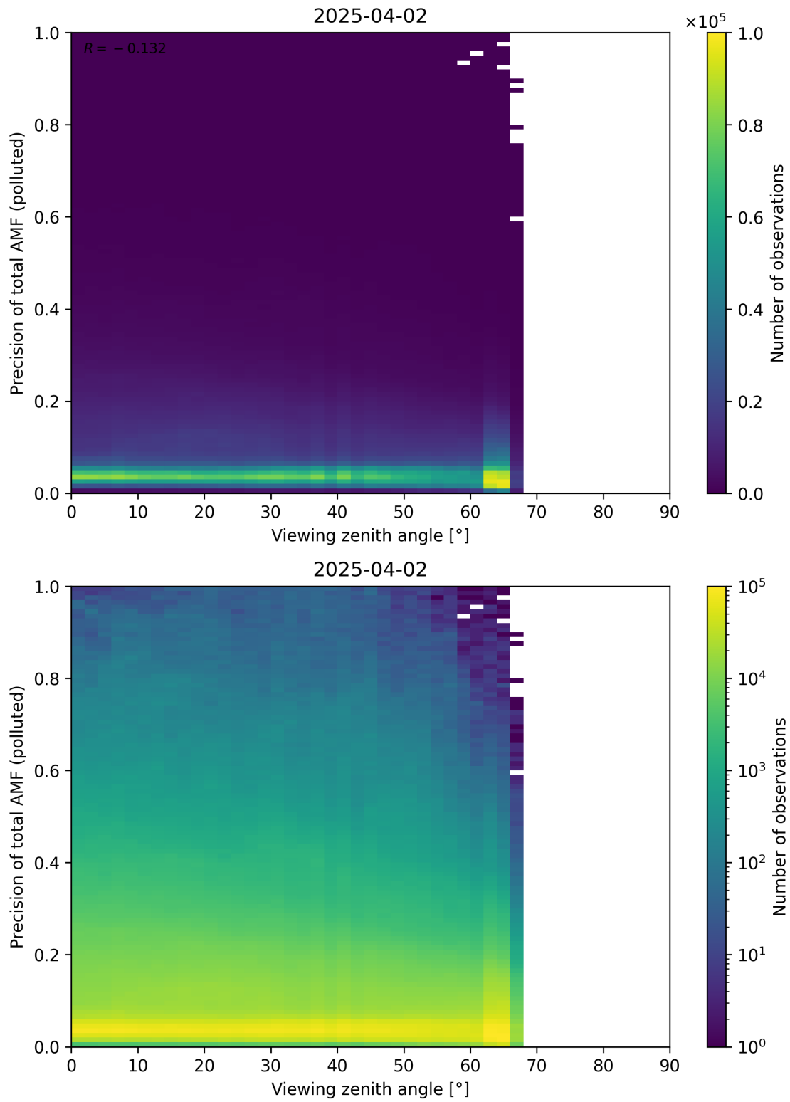
Figure 382: Scatter density plot of “Viewing zenith angle” against “Precision of total AMF (polluted)” for 2025-04-02 to 2025-04-03.
