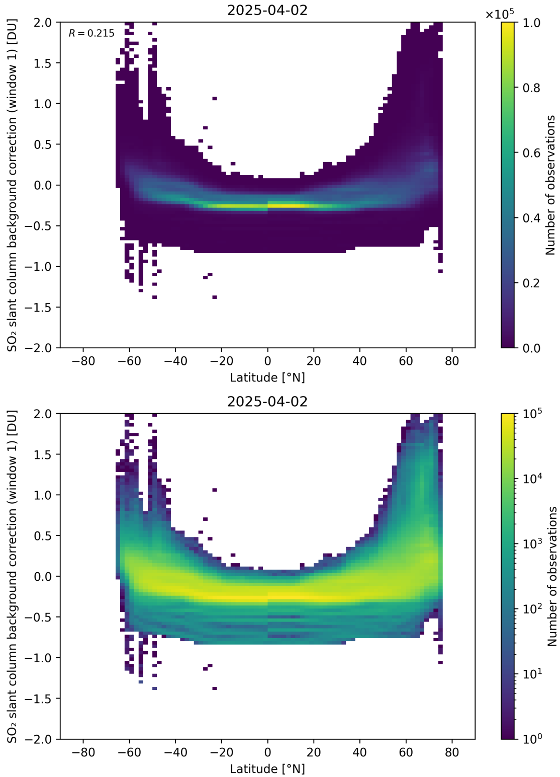
Figure 150: Scatter density plot of “Latitude” against “SO 2 slant column background correction (window 1)” for 2025-04-02 to 2025-04-03.
