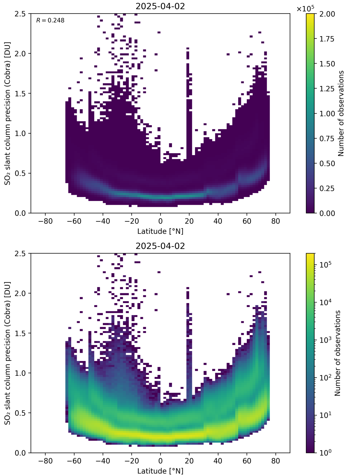
Figure 158: Scatter density plot of “Latitude” against “SO 2 slant column precision (Cobra)” for 2025-04-02 to 2025-04-03.
