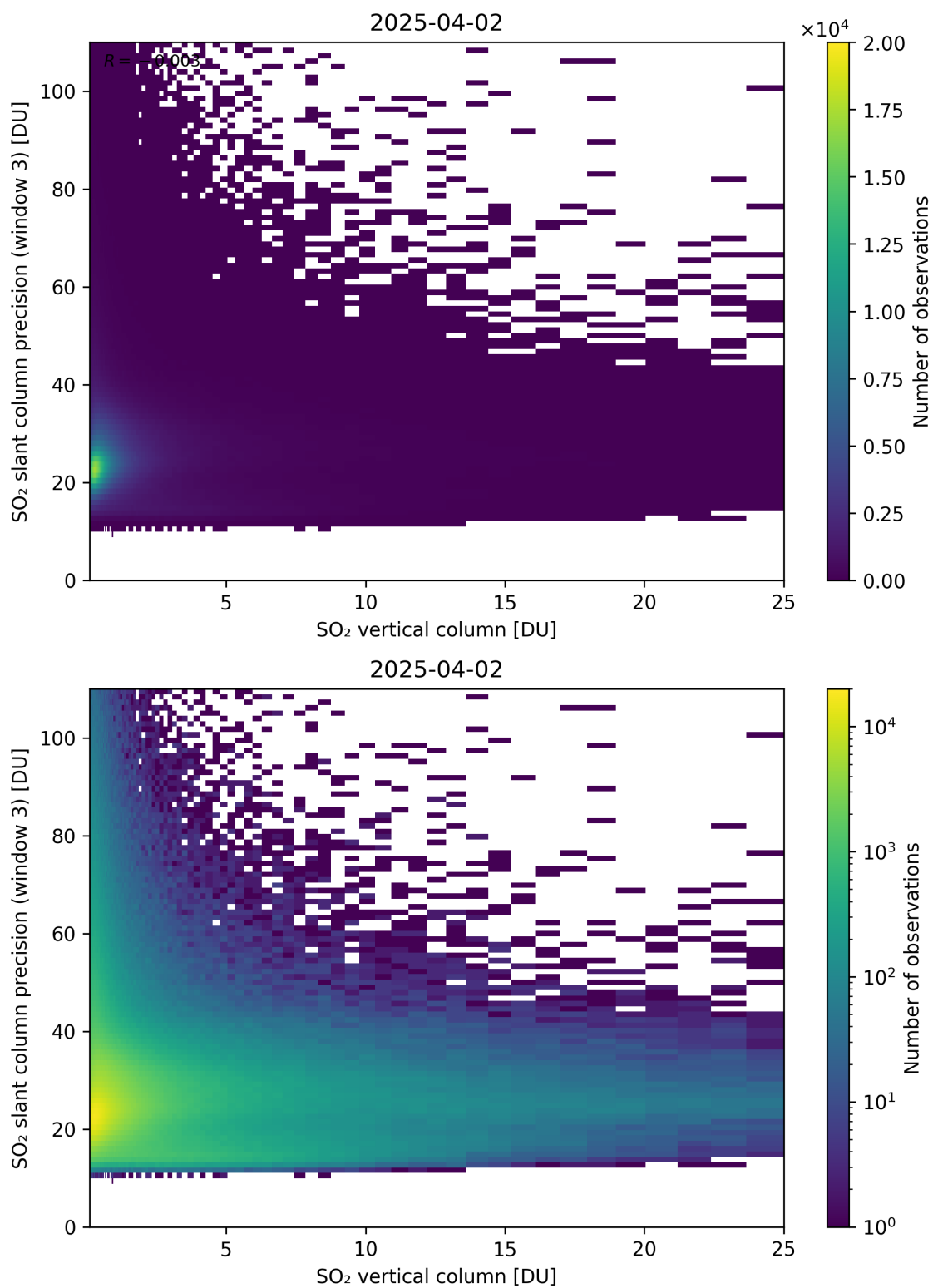
Figure 358: Scatter density plot of “SO 2 vertical column” against “SO 2 slant column precision (window 3)” for 2025-04-02 to 2025-04-03.
