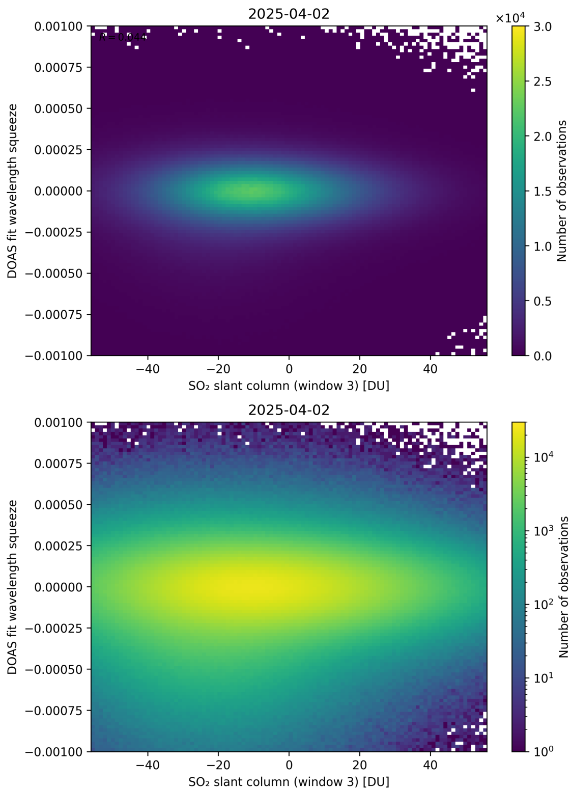
Figure 305: Scatter density plot of “SO 2 slant column (window 3)” against “DOAS fit wavelength squeeze” for 2025-04-02 to 2025-04-03.
