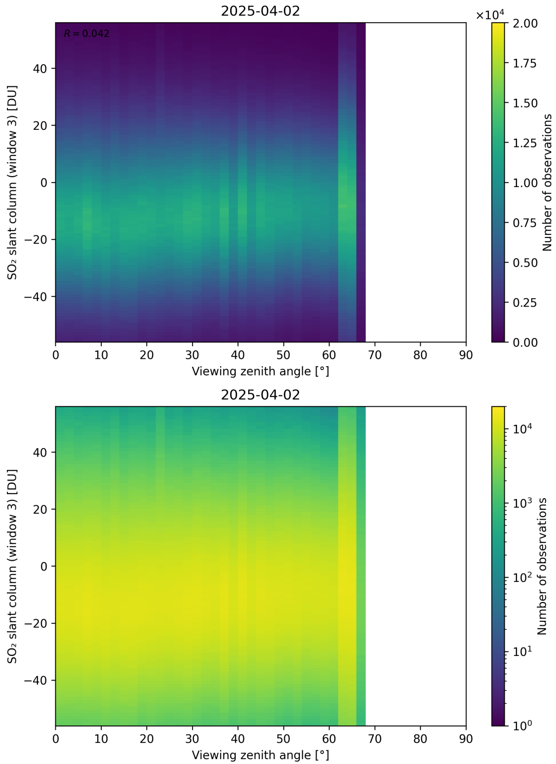
Figure 379: Scatter density plot of “Viewing zenith angle” against “SO 2 slant column (window 3)” for 2025-04-02 to 2025-04-03.
