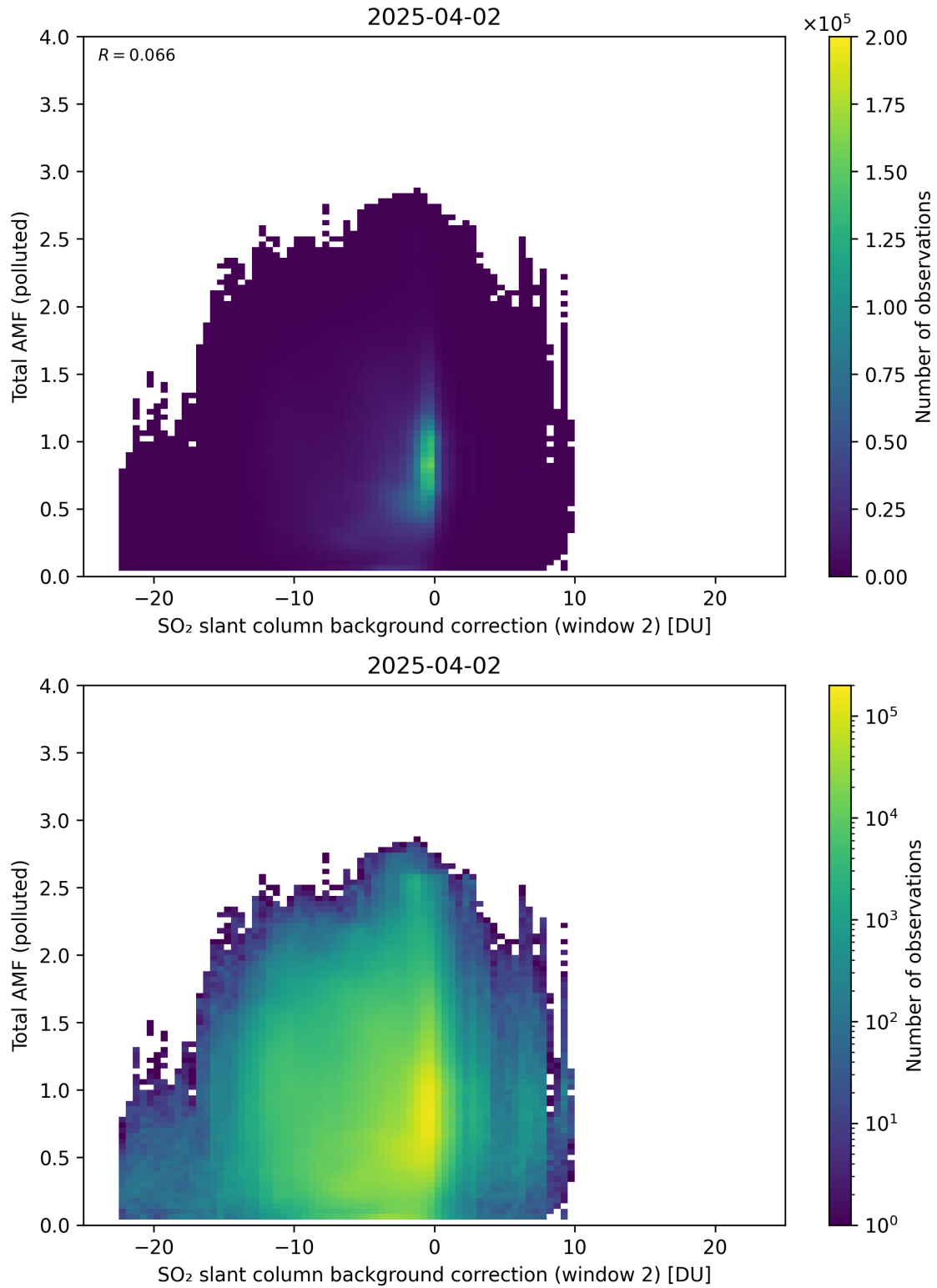
Figure 130: Scatter density plot of “SO 2 slant column background correction (window 2)” against “Total AMF (polluted)” for 2025-04-02 to 2025-04-03.
