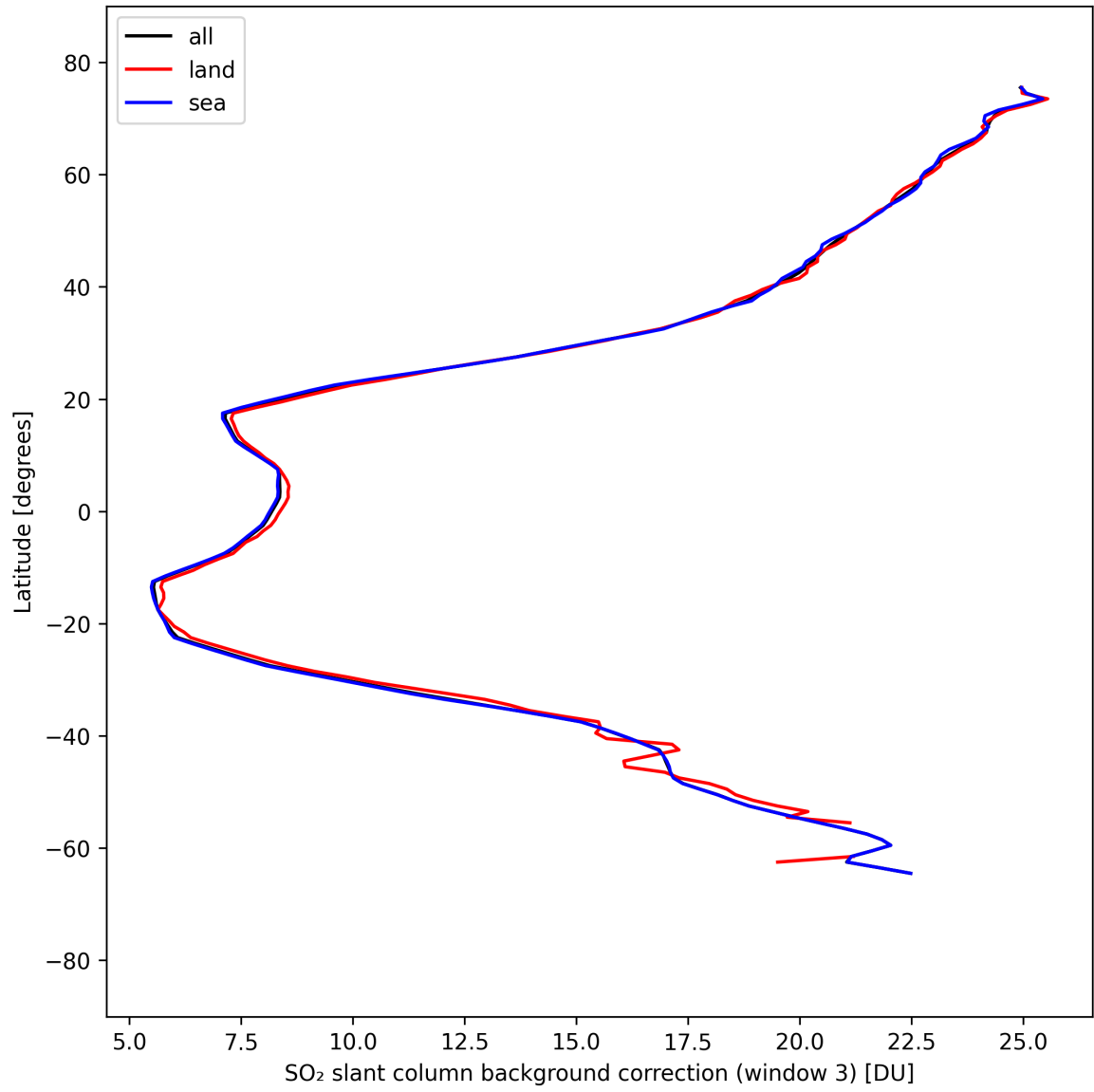
Figure 48: Zonal average of “SO 2 slant column background correction (window 3)” for 2025-04-02 to 2025-04-03.
