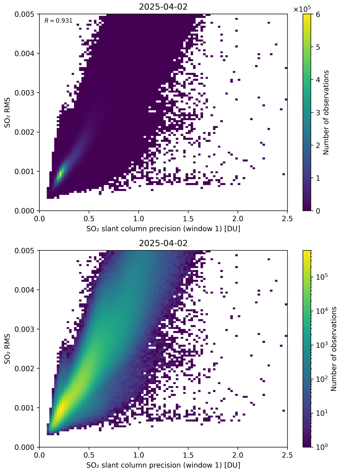
Figure 273: Scatter density plot of “SO 2 slant column precision (window 1)” against “SO 2 RMS” for 2025-04-02 to 2025-04-03.
