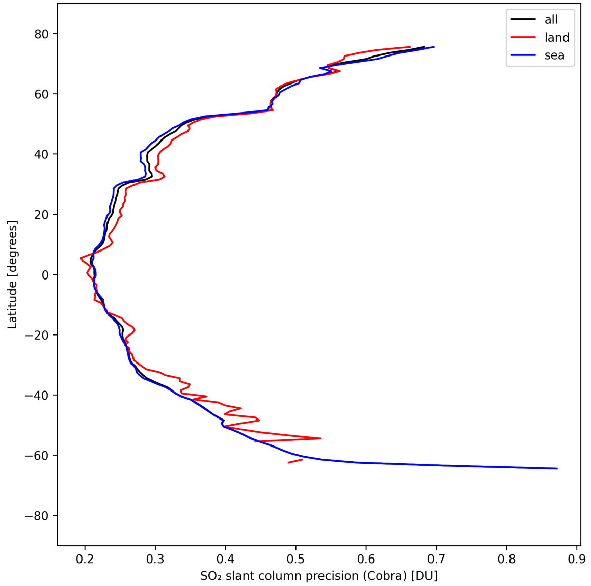
Figure 36: Zonal average of “SO 2 slant column precision (Cobra)” for 2025-04-02 to 2025-04-03.
