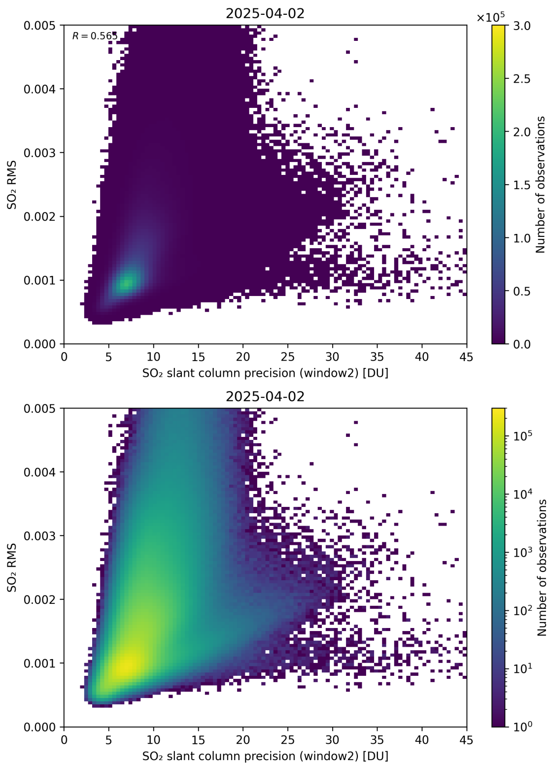
Figure 295: Scatter density plot of “SO 2 slant column precision (window2)” against “SO 2 RMS” for 2025-04-02 to 2025-04-03.
