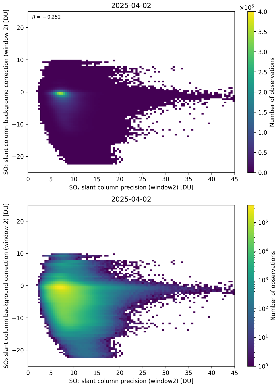
Figure 291: Scatter density plot of “SO 2 slant column precision (window2)” against “SO 2 slant column background correction (window 2)” for 2025-04-02 to 2025-04-03.
