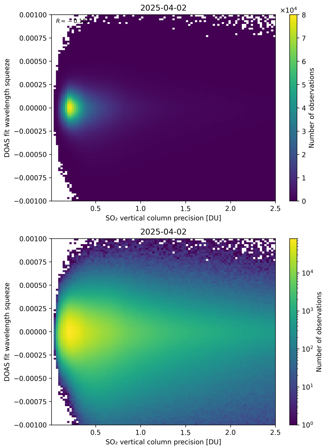
Figure 333: Scatter density plot of “SO 2 vertical column precision” against “DOAS fit wavelength squeeze” for 2025-04-02 to 2025-04-03.
