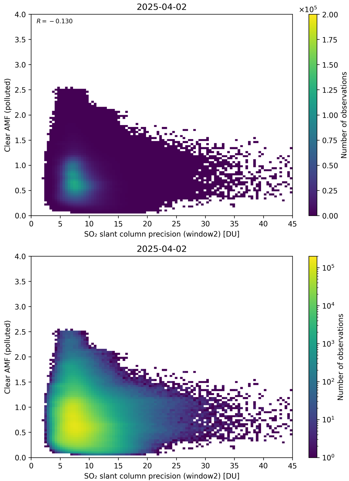
Figure 296: Scatter density plot of “SO 2 slant column precision (window2)” against “Clear AMF (polluted)” for 2025-04-02 to 2025-04-03.
