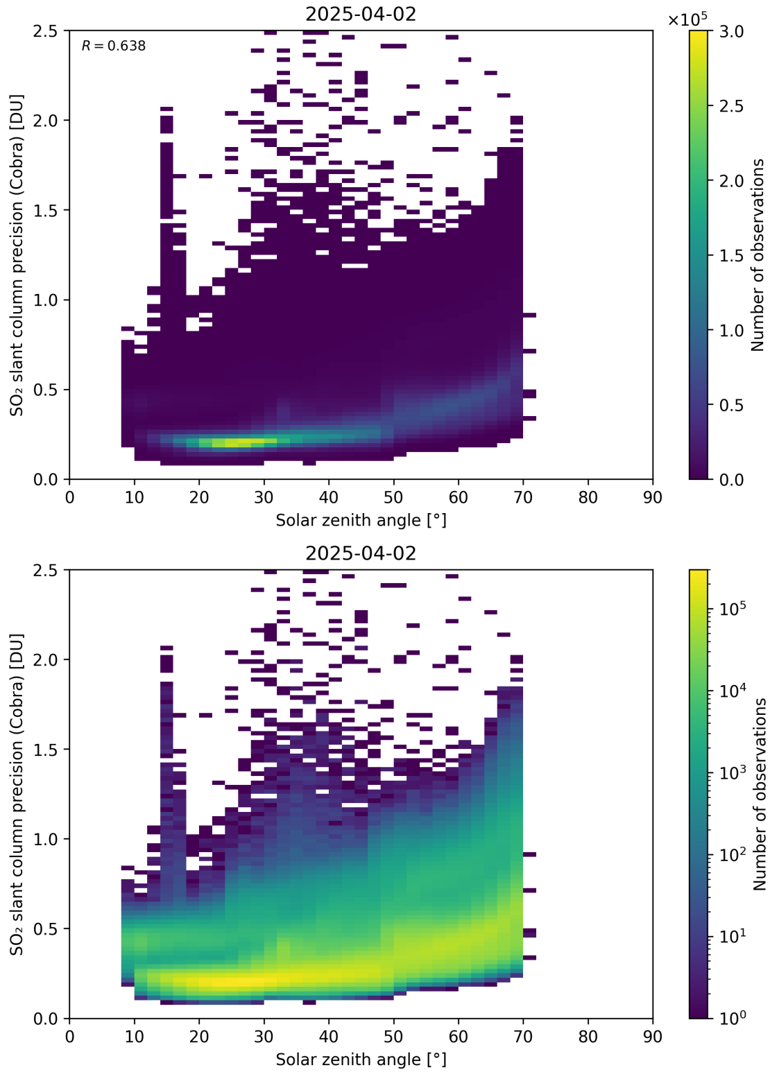
Figure 180: Scatter density plot of “Solar zenith angle” against “SO 2 slant column precision (Cobra)” for 2025-04-02 to 2025-04-03.
