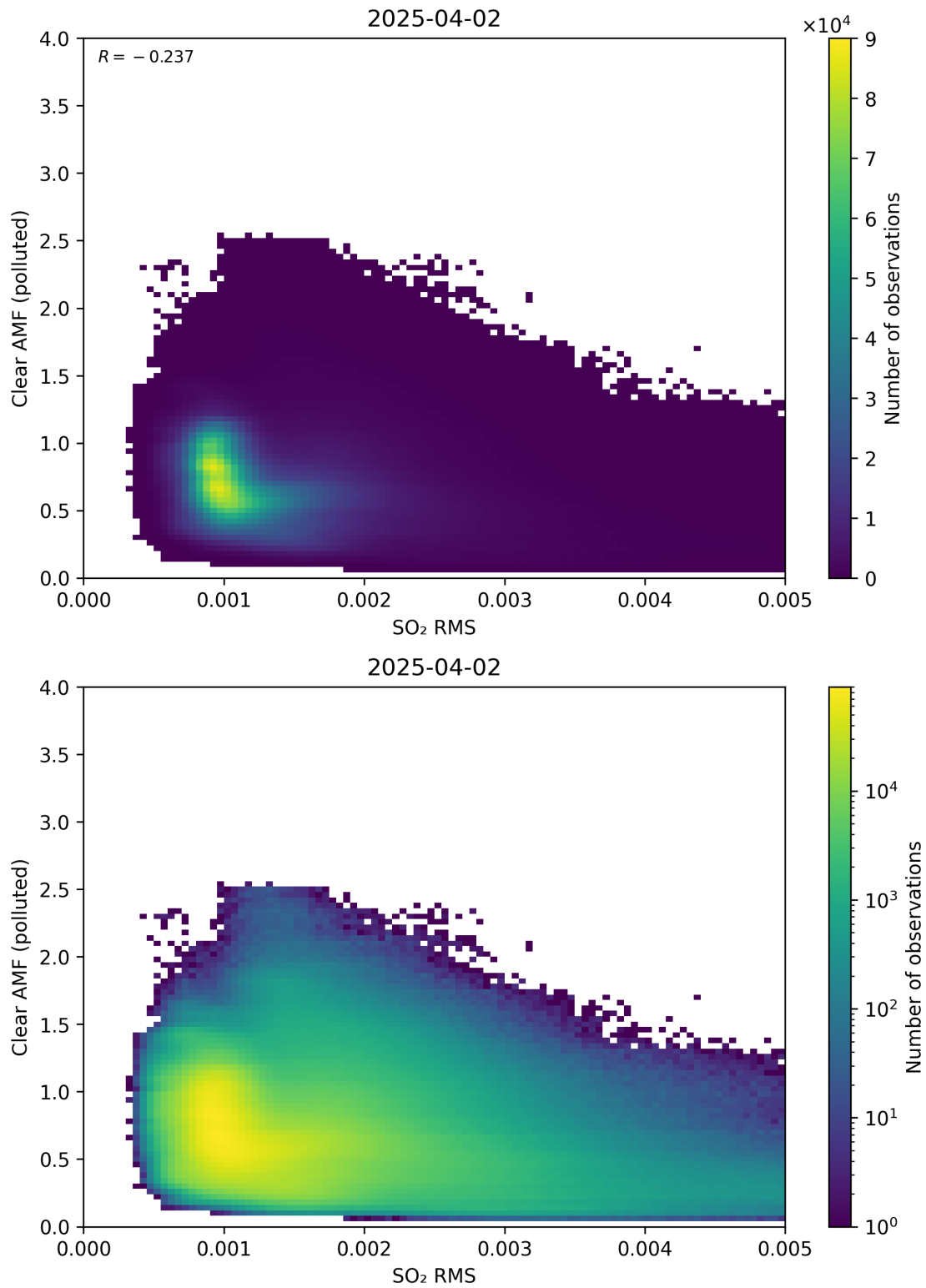
Figure 147: Scatter density plot of “SO 2 RMS” against “Clear AMF (polluted)” for 2025-04-02 to 2025-04-03.
