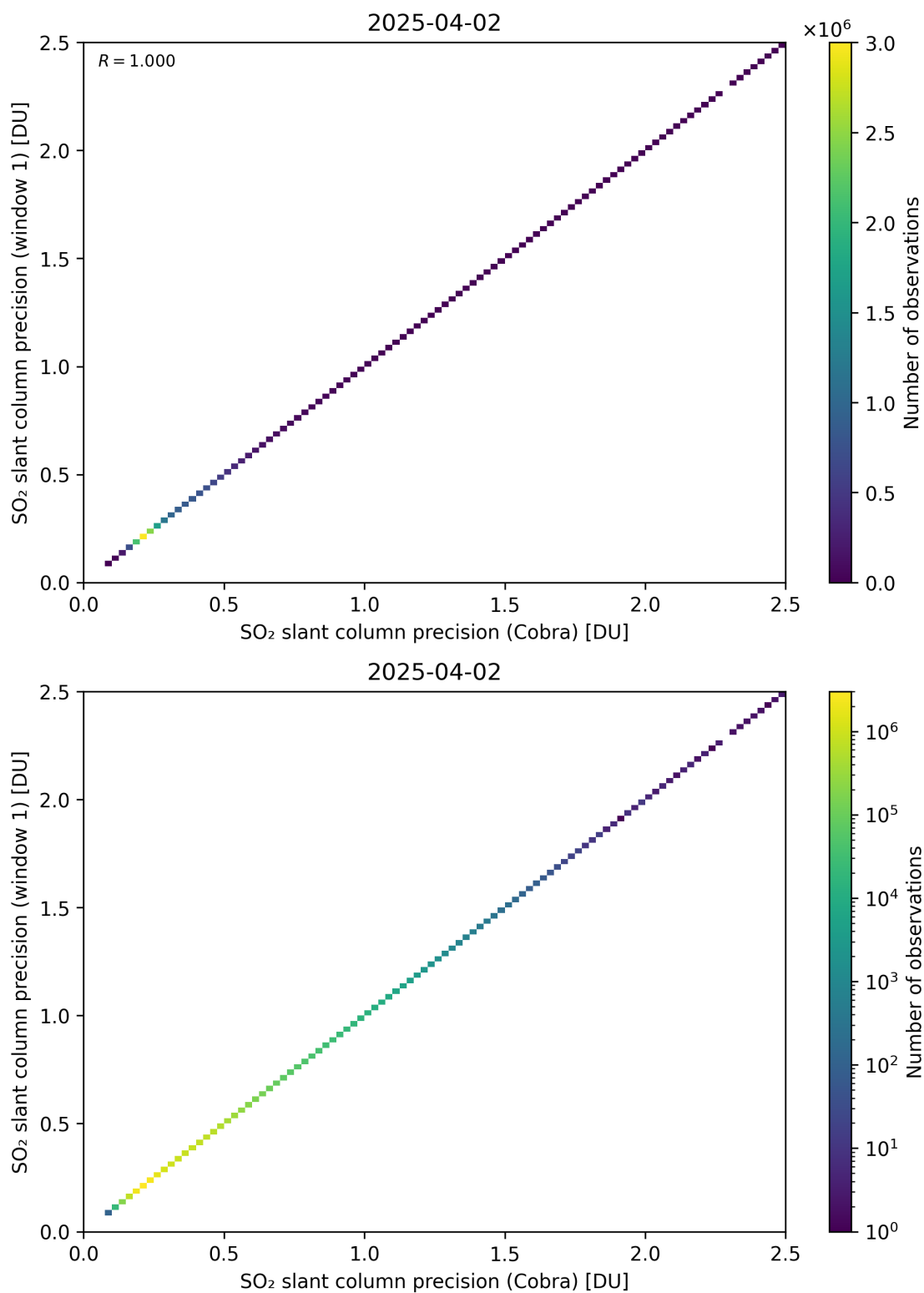
Figure 209: Scatter density plot of “SO 2 slant column precision (Cobra)” against “SO 2 slant column precision (window 1)” for 2025-04-02 to 2025-04-03.
