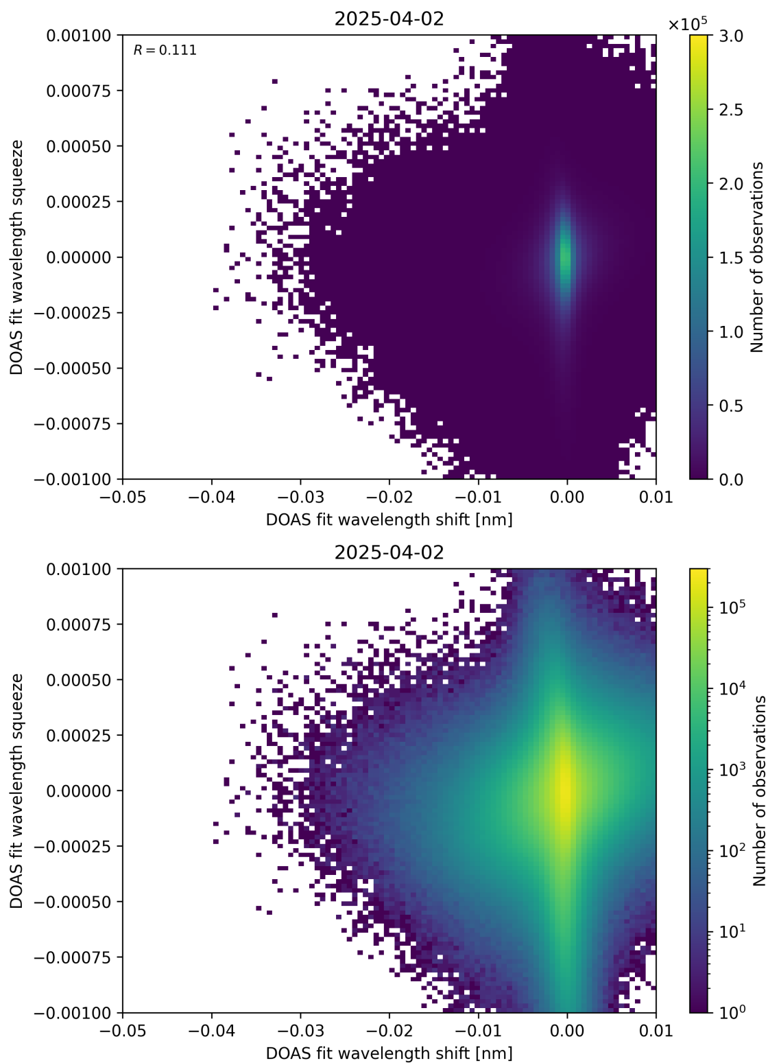
Figure 138: Scatter density plot of “DOAS fit wavelength shift” against “DOAS fit wavelength squeeze” for 2025-04-02 to 2025-04-03.
