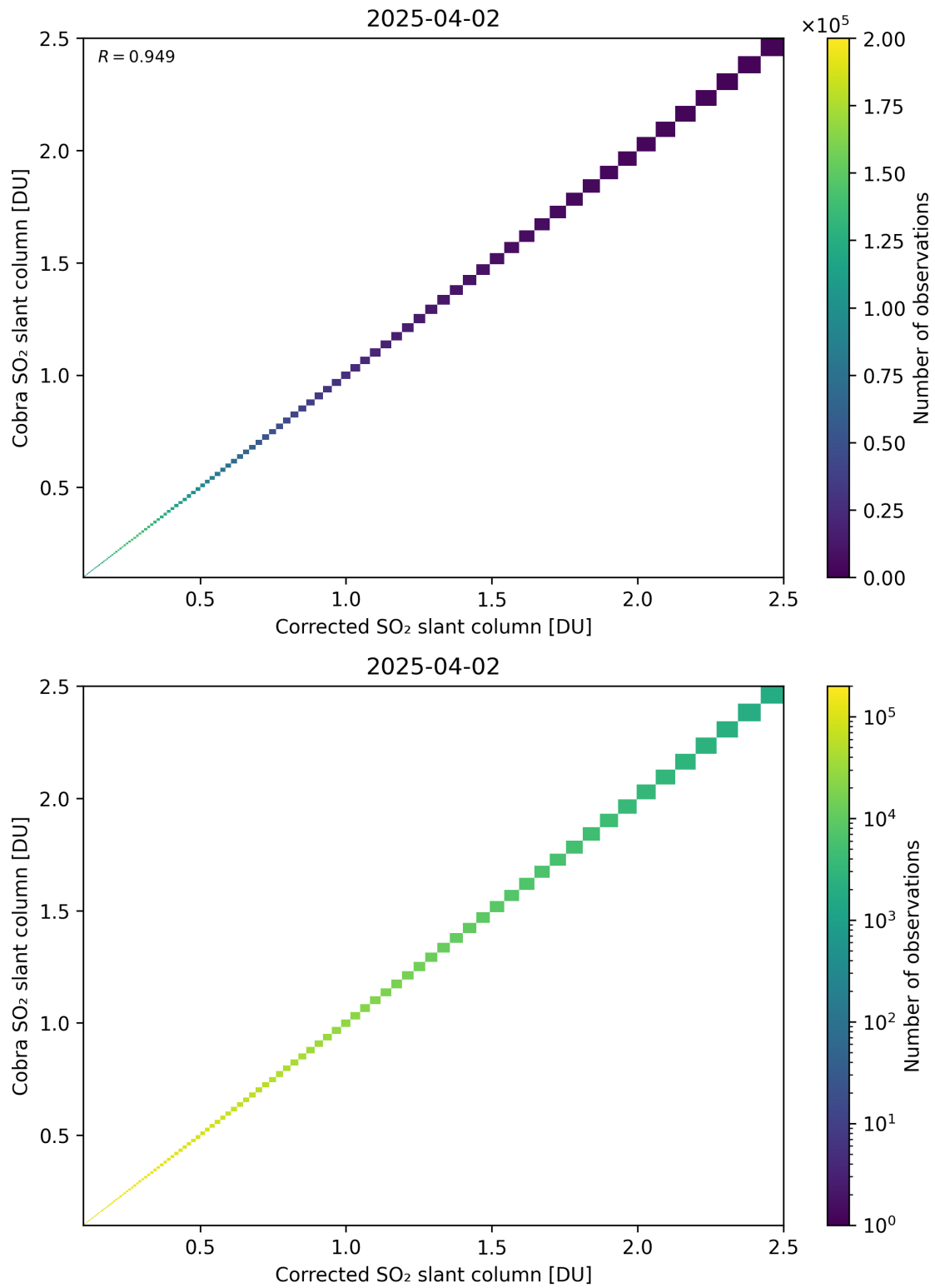
Figure 233: Scatter density plot of “Corrected SO 2 slant column” against “Cobra SO 2 slant column” for 2025-04-02 to 2025-04-03.
