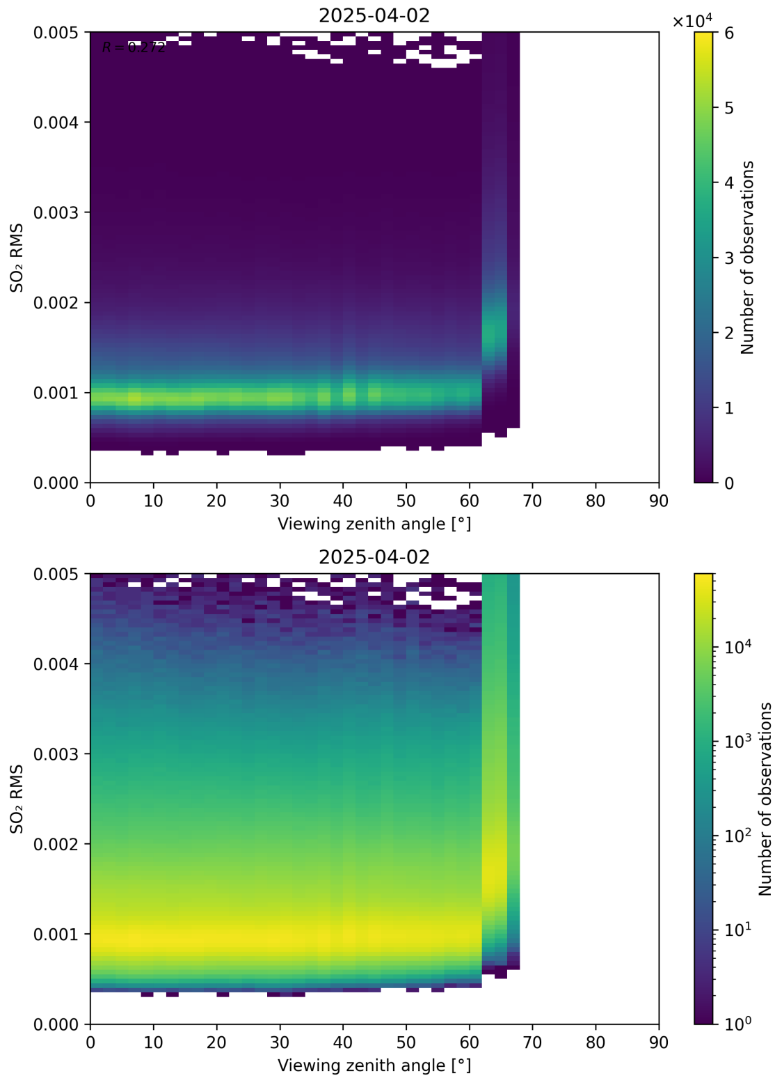
Figure 367: Scatter density plot of “Viewing zenith angle” against “SO 2 RMS” for 2025-04-02 to 2025-04-03.
