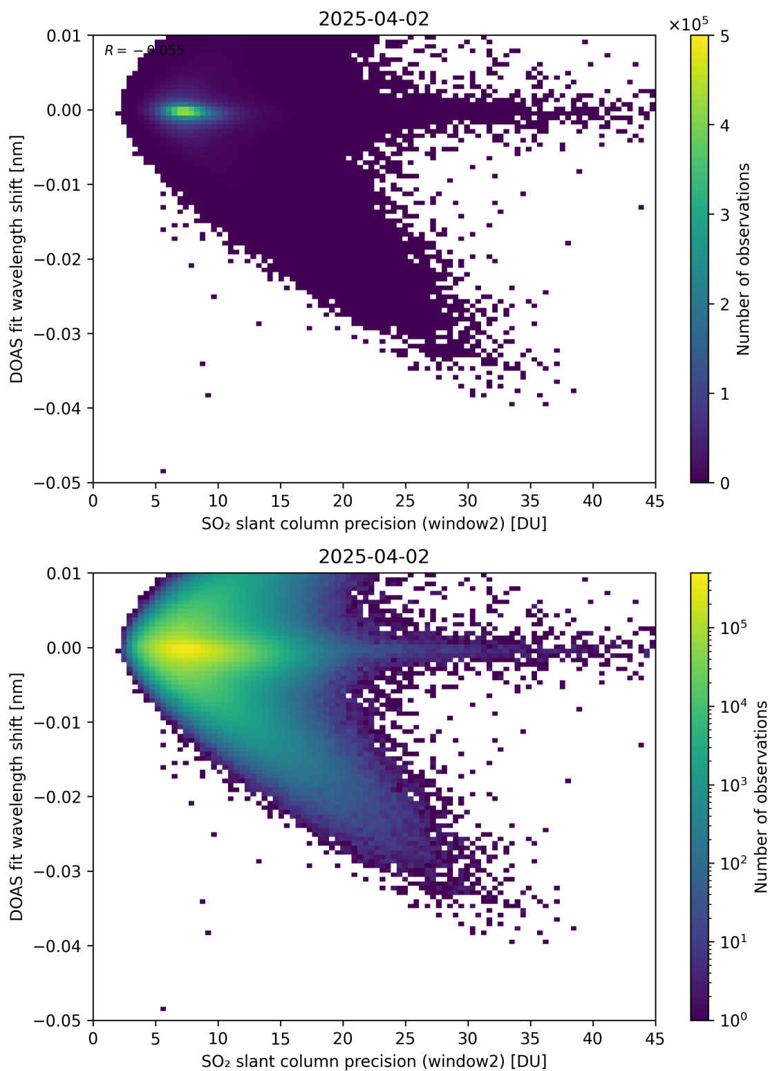
Figure 293: Scatter density plot of “SO 2 slant column precision (window2)” against “DOAS fit wavelength shift” for 2025-04-02 to 2025-04-03.
