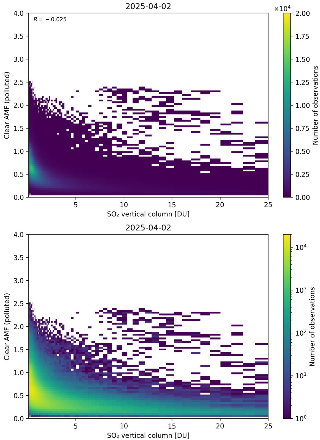
Figure 348: Scatter density plot of “SO 2 vertical column” against “Clear AMF (polluted)” for 2025-04-02 to 2025-04-03.
