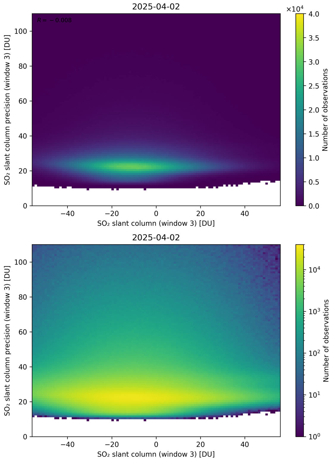
Figure 317: Scatter density plot of “SO 2 slant column (window 3)” against “SO 2 slant column precision (window 3)” for 2025-04-02 to 2025-04-03.
