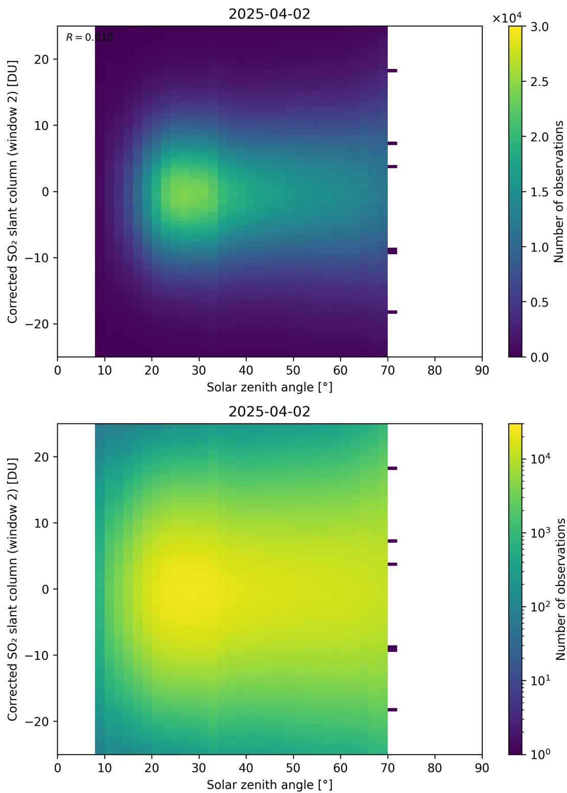
Figure 182: Scatter density plot of “Solar zenith angle” against “Corrected SO 2 slant column (window 2)” for 2025-04-02 to 2025-04-03.
