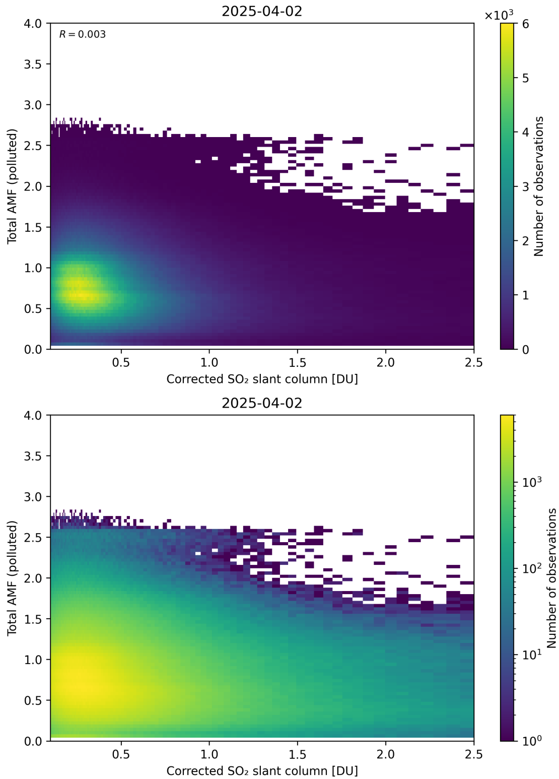
Figure 242: Scatter density plot of “Corrected SO 2 slant column” against “Total AMF (polluted)” for 2025-04-02 to 2025-04-03.
