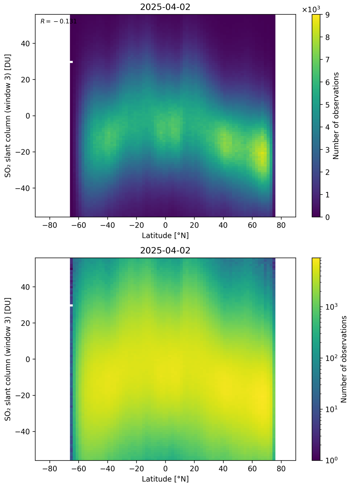
Figure 165: Scatter density plot of “Latitude” against “SO 2 slant column (window 3)” for 2025-04-02 to 2025-04-03.
