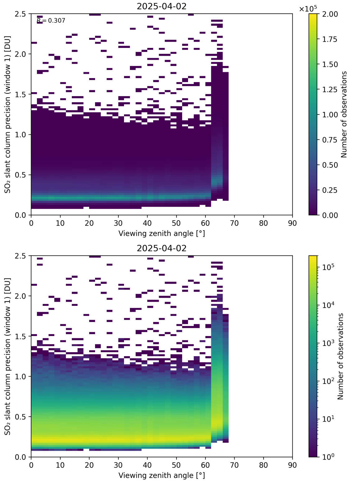
Figure 377: Scatter density plot of “Viewing zenith angle” against “SO 2 slant column precision (window 1)” for 2025-04-02 to 2025-04-03.
