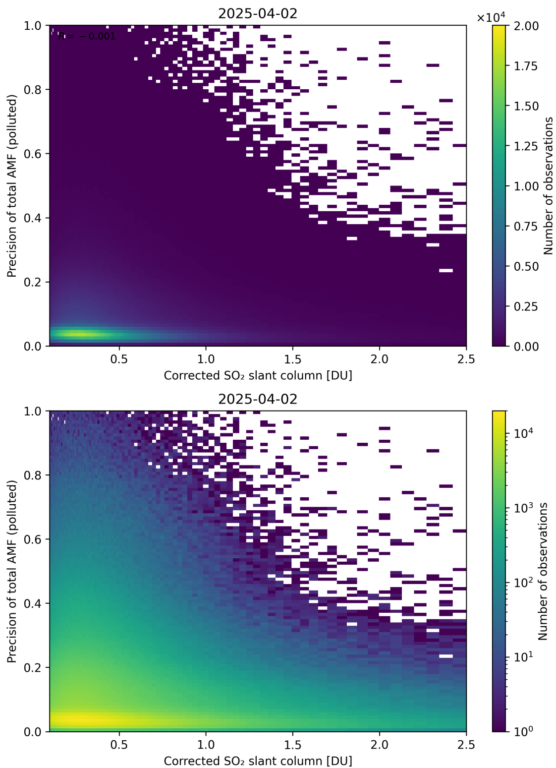
Figure 243: Scatter density plot of “Corrected SO 2 slant column” against “Precision of total AMF (polluted)” for 2025-04-02 to 2025-04-03.
