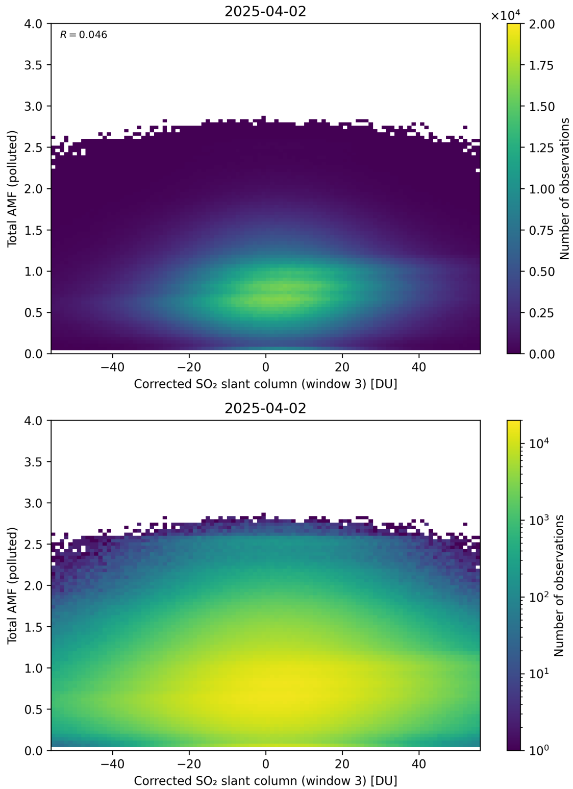
Figure 260: Scatter density plot of “Corrected SO 2 slant column (window 3)” against “Total AMF (polluted)” for 2025-04-02 to 2025-04-03.
