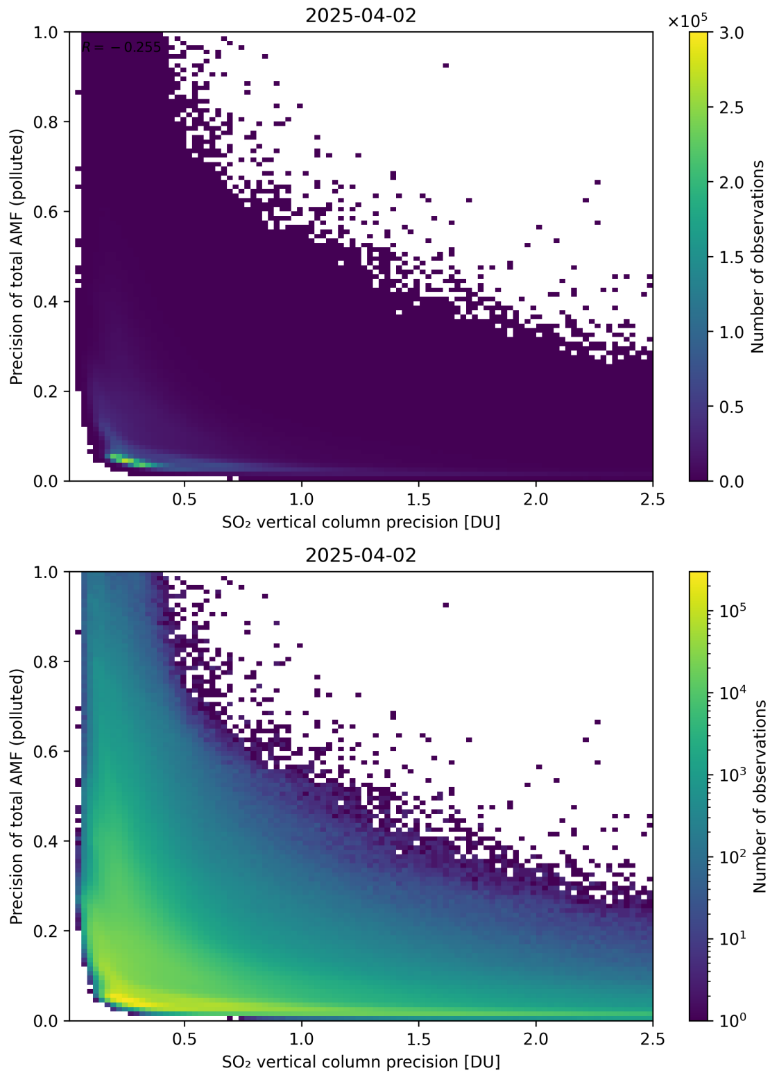
Figure 347: Scatter density plot of “SO 2 vertical column precision” against “Precision of total AMF (polluted)” for 2025-04-02 to 2025-04-03.
