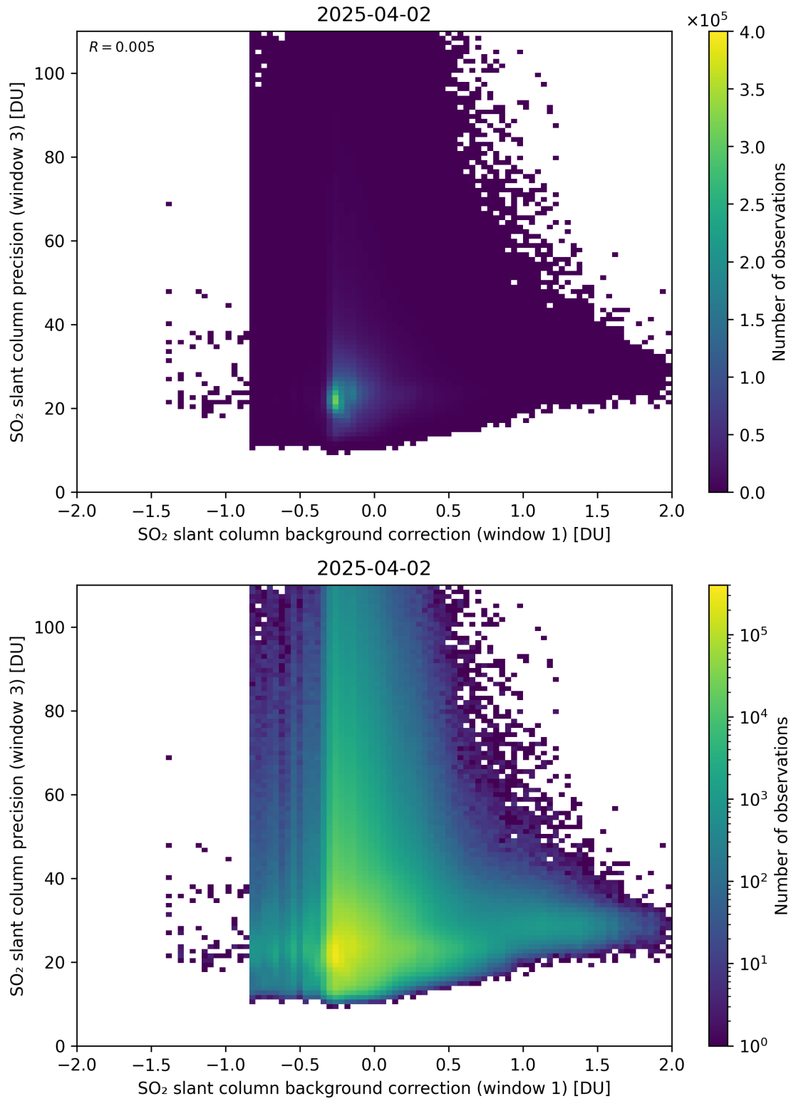
Figure 119: Scatter density plot of “SO 2 slant column background correction (window 1)” against “SO 2 slant column precision (window 3)” for 2025-04-02 to 2025-04-03.
