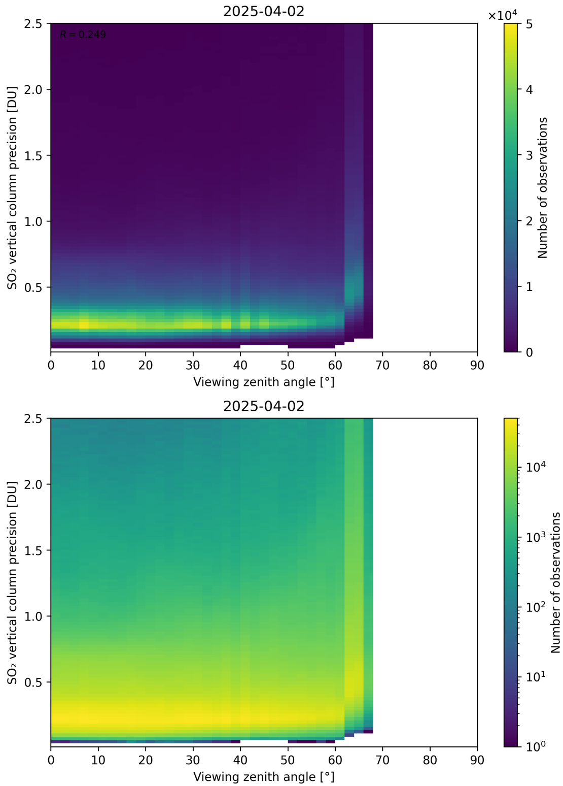
Figure 384: Scatter density plot of “Viewing zenith angle” against “SO 2 vertical column precision” for 2025-04-02 to 2025-04-03.
