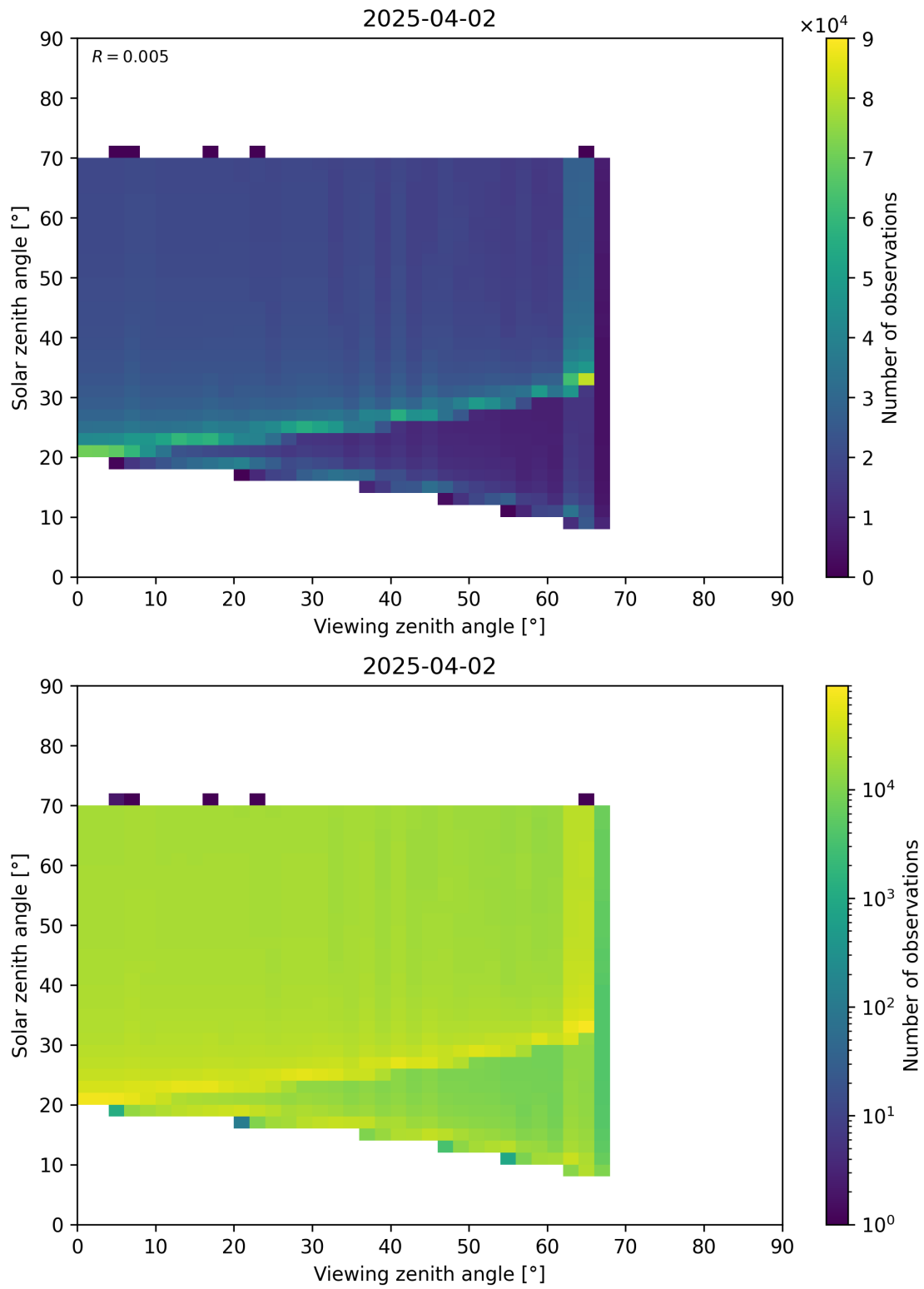
Figure 369: Scatter density plot of “Viewing zenith angle” against “Solar zenith angle” for 2025-04-02 to 2025-04-03.
