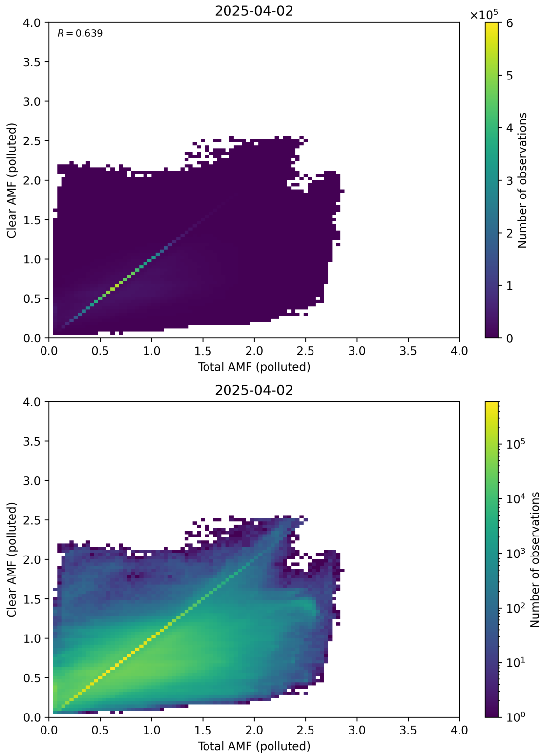
Figure 321: Scatter density plot of “Total AMF (polluted)” against “Clear AMF (polluted)” for 2025-04-02 to 2025-04-03.
