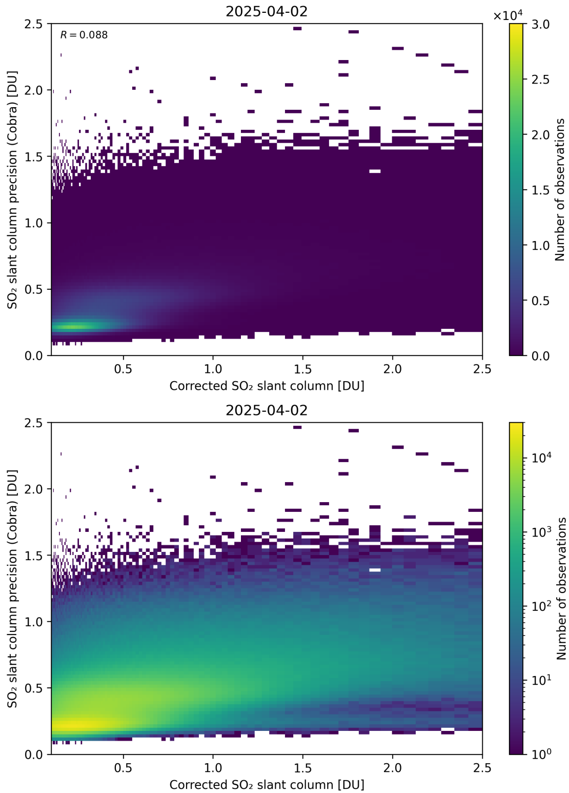
Figure 234: Scatter density plot of “Corrected SO 2 slant column” against “SO 2 slant column precision (Cobra)” for 2025-04-02 to 2025-04-03.
