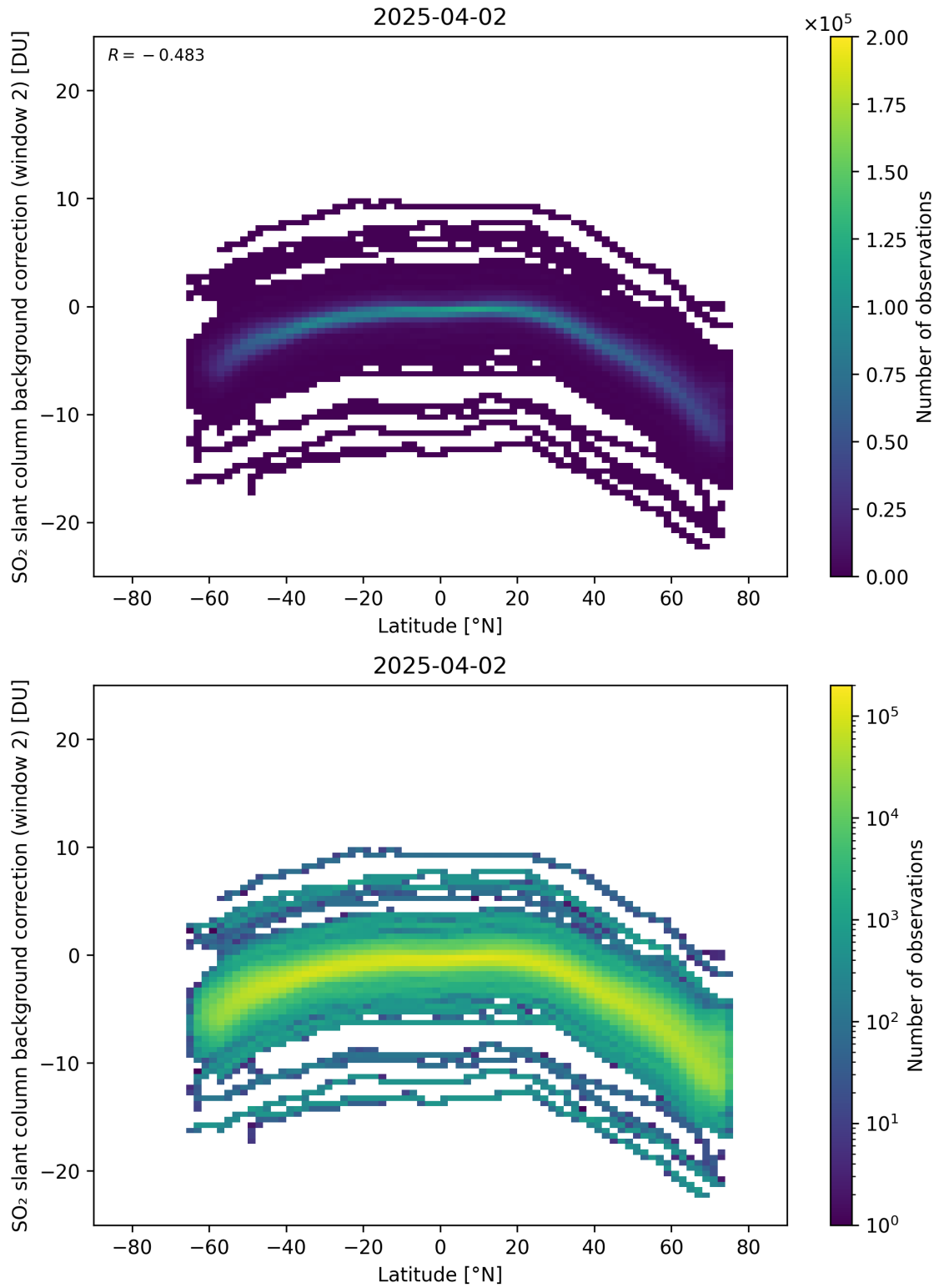
Figure 151: Scatter density plot of “Latitude” against “SO 2 slant column background correction (window 2)” for 2025-04-02 to 2025-04-03.
