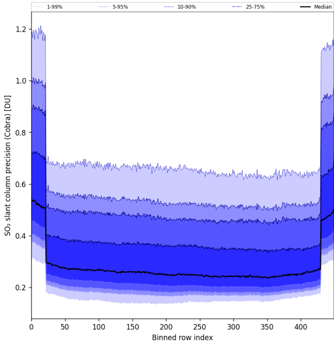
Figure 88: Along track statistics of “SO 2 slant column precision (Cobra)” for 2025-04-02 to 2025-04-03
