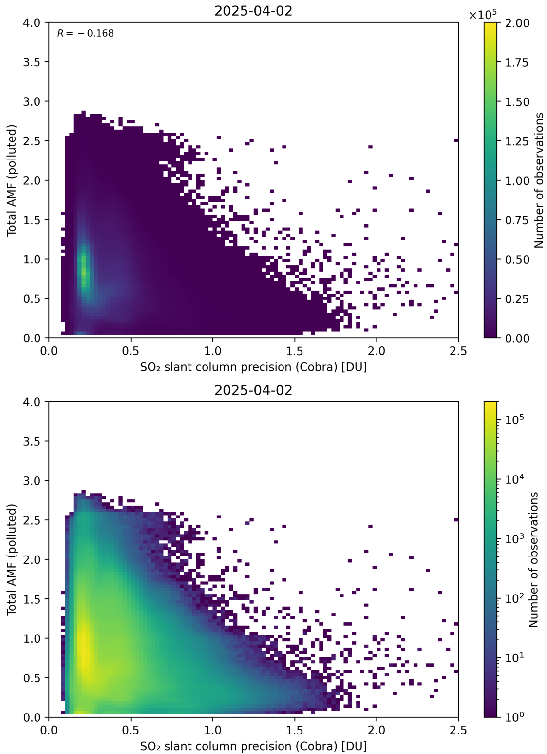
Figure 213: Scatter density plot of “SO 2 slant column precision (Cobra)” against “Total AMF (polluted)” for 2025-04-02 to 2025-04-03.
