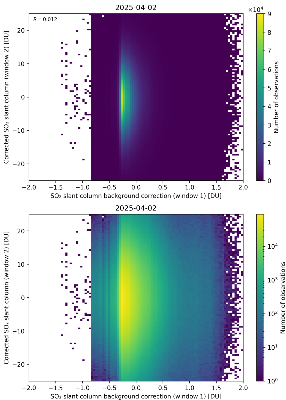
Figure 115: Scatter density plot of “SO 2 slant column background correction (window 1)” against “Corrected SO 2 slant column (window 2)” for 2025-04-02 to 2025-04-03.
