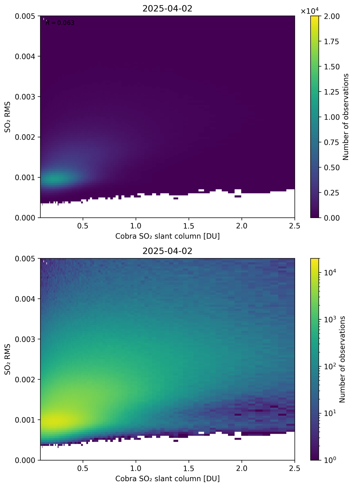
Figure 198: Scatter density plot of “Cobra SO 2 slant column” against “SO 2 RMS” for 2025-04-02 to 2025-04-03.
