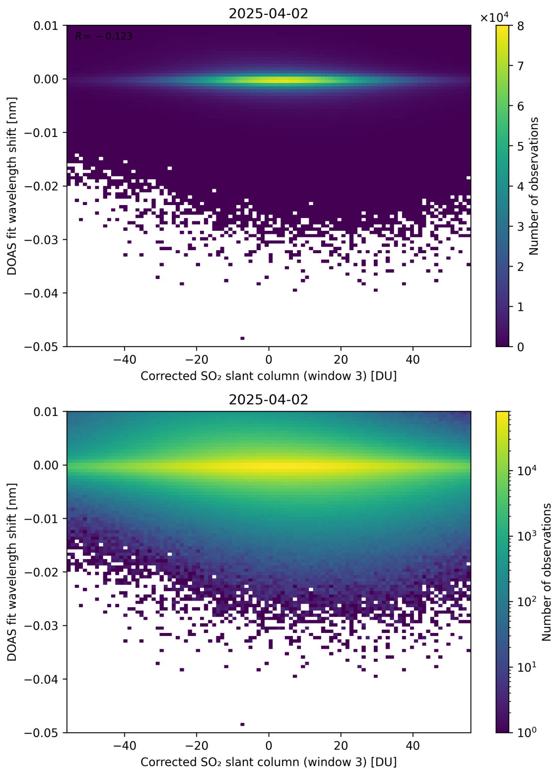
Figure 256: Scatter density plot of “Corrected SO 2 slant column (window 3)” against “DOAS fit wavelength shift” for 2025-04-02 to 2025-04-03.
