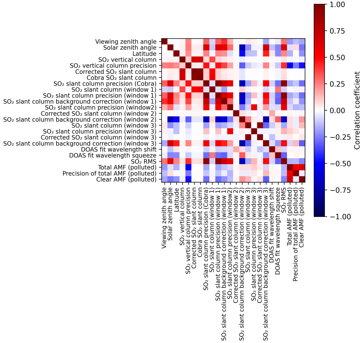
Figure 2: Map of correlation matrix for 2025-04-02 to 2025-04-03.
