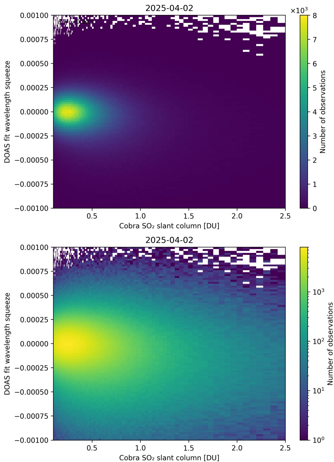
Figure 197: Scatter density plot of “Cobra SO 2 slant column” against “DOAS fit wavelength squeeze” for 2025-04-02 to 2025-04-03.
