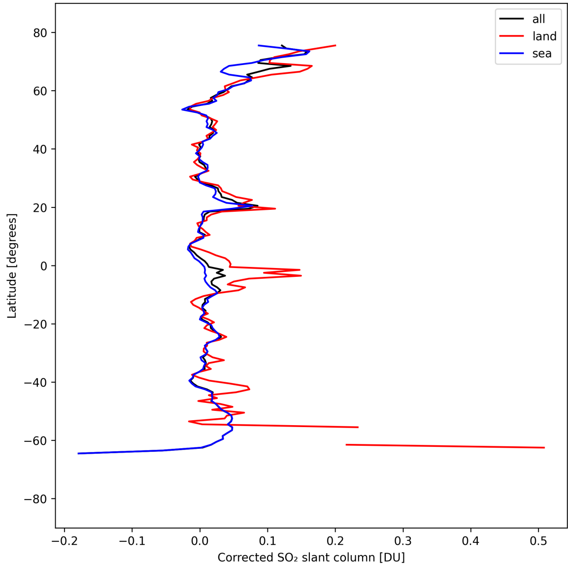
Figure 34: Zonal average of "Corrected SO 2 slant column" for 2025-04-02 to 2025-04-03.
