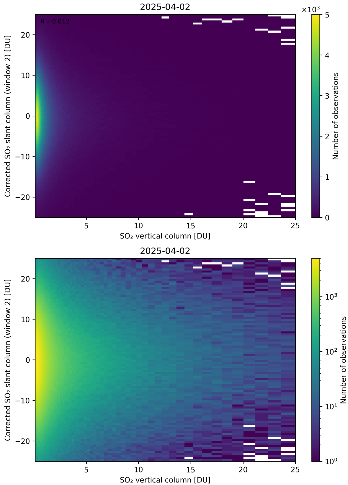
Figure 352: Scatter density plot of “SO 2 vertical column” against “Corrected SO 2 slant column (window 2)” for 2025-04-02 to 2025-04-03.
