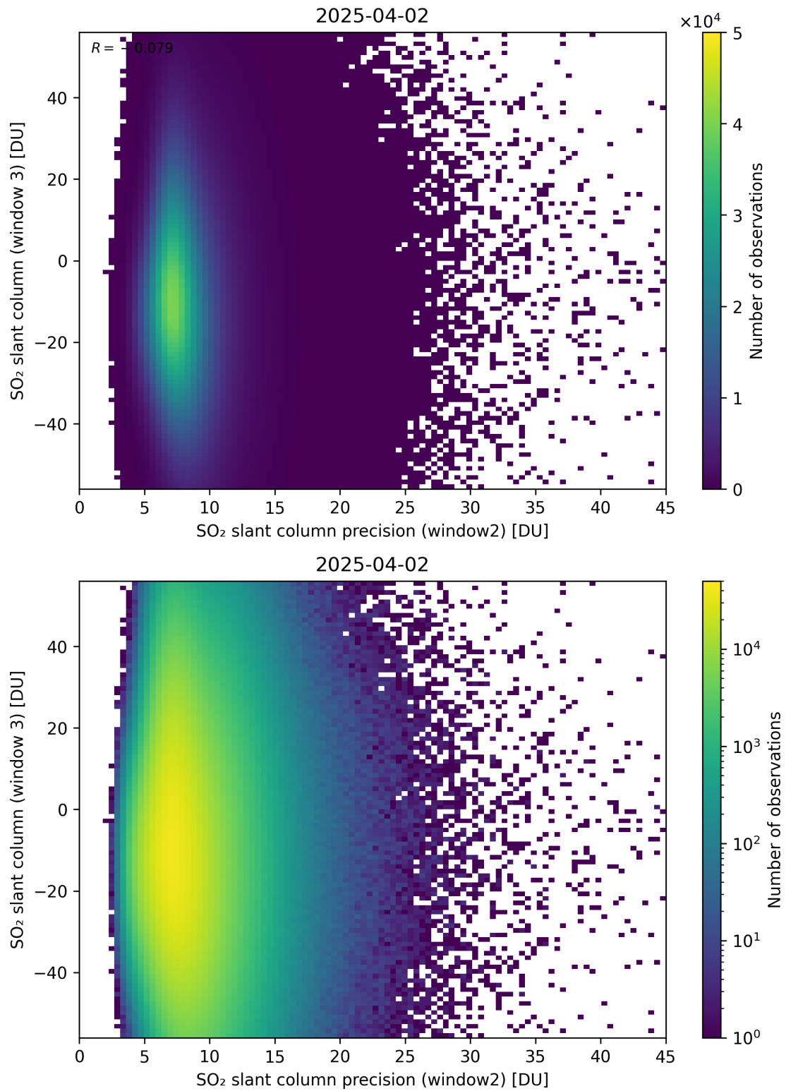
Figure 299: Scatter density plot of “SO 2 slant column precision (window2)” against “SO 2 slant column (window 3)” for 2025-04-02 to 2025-04-03.
