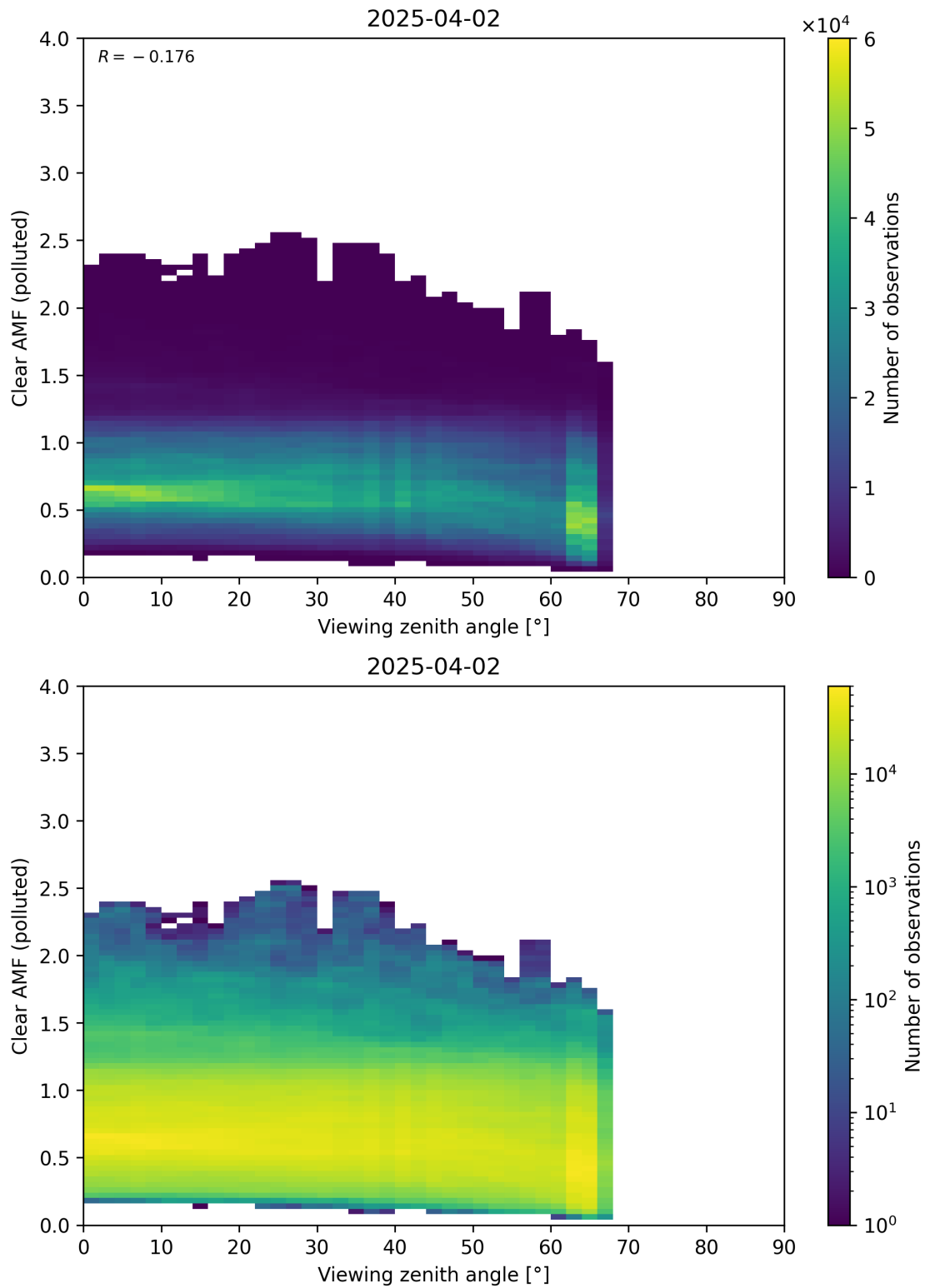
Figure 370: Scatter density plot of “Viewing zenith angle” against “Clear AMF (polluted)” for 2025-04-02 to 2025-04-03.
