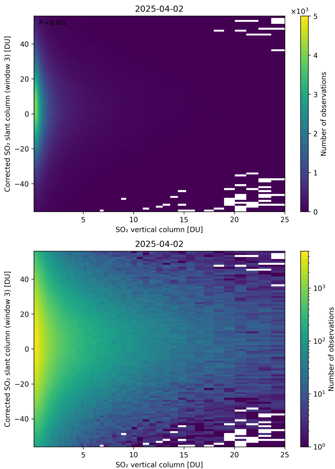
Figure 353: Scatter density plot of “SO 2 vertical column” against “Corrected SO 2 slant column (window 3)” for 2025-04-02 to 2025-04-03.
