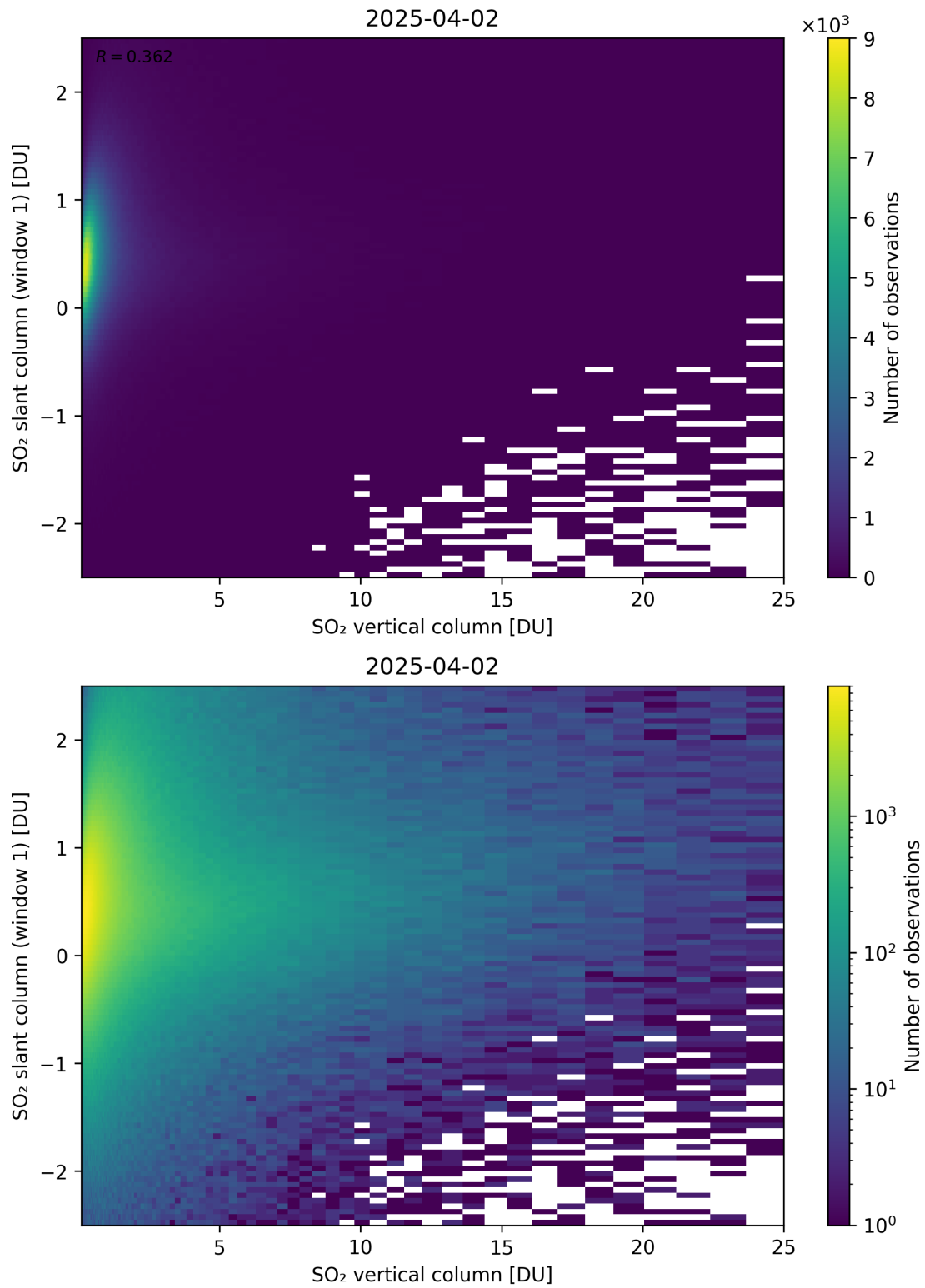
Figure 354: Scatter density plot of “SO 2 vertical column” against “SO 2 slant column (window 1)” for 2025-04-02 to 2025-04-03.
