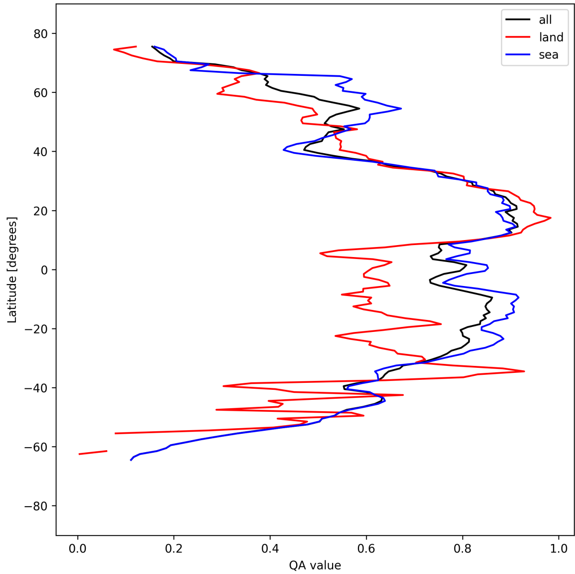
Figure 31: Zonal average of “QA value” for 2025-04-02 to 2025-04-03.
