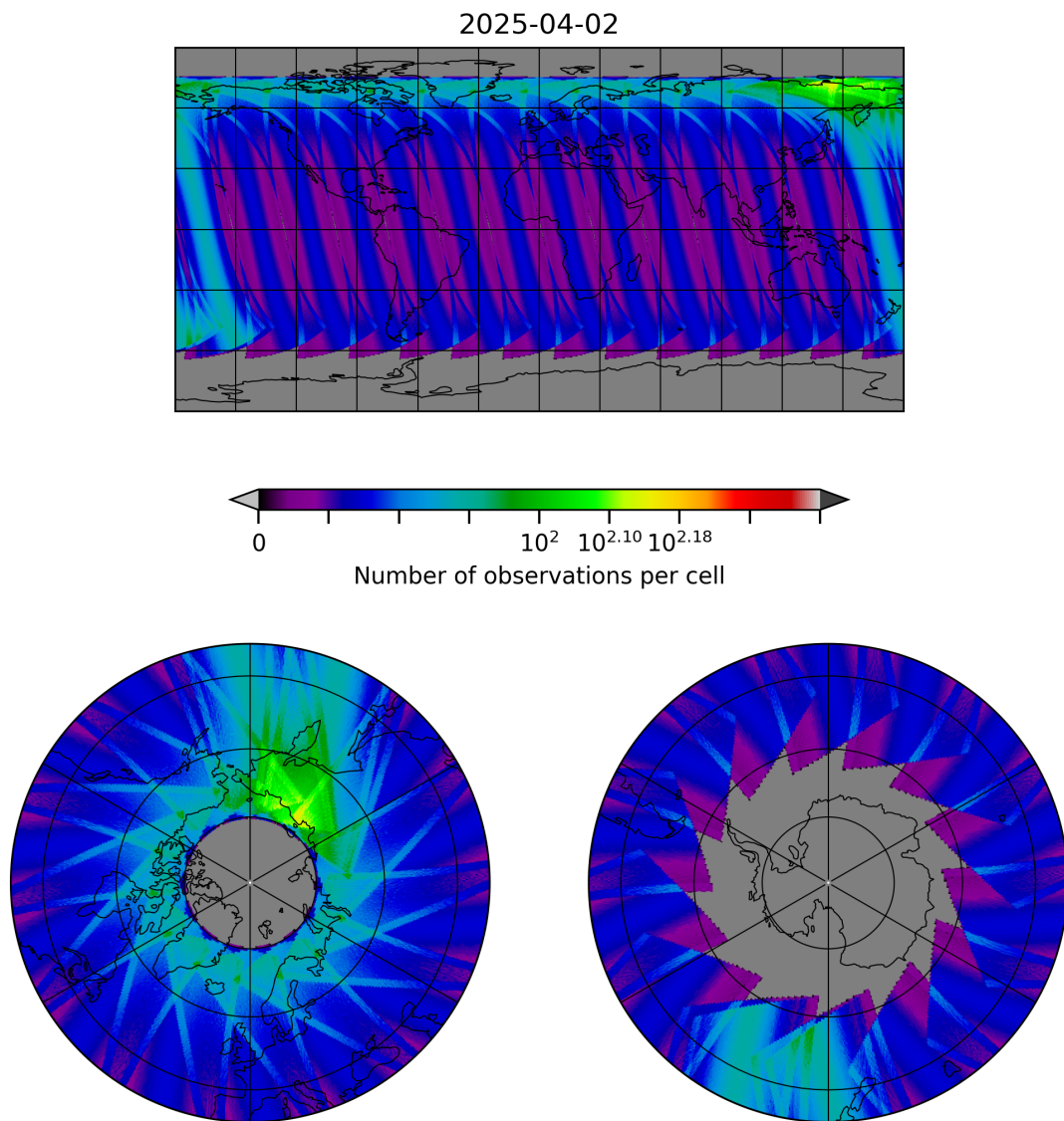
Figure 30: Map of the number of observations for 2025-04-02 to 2025-04-03
