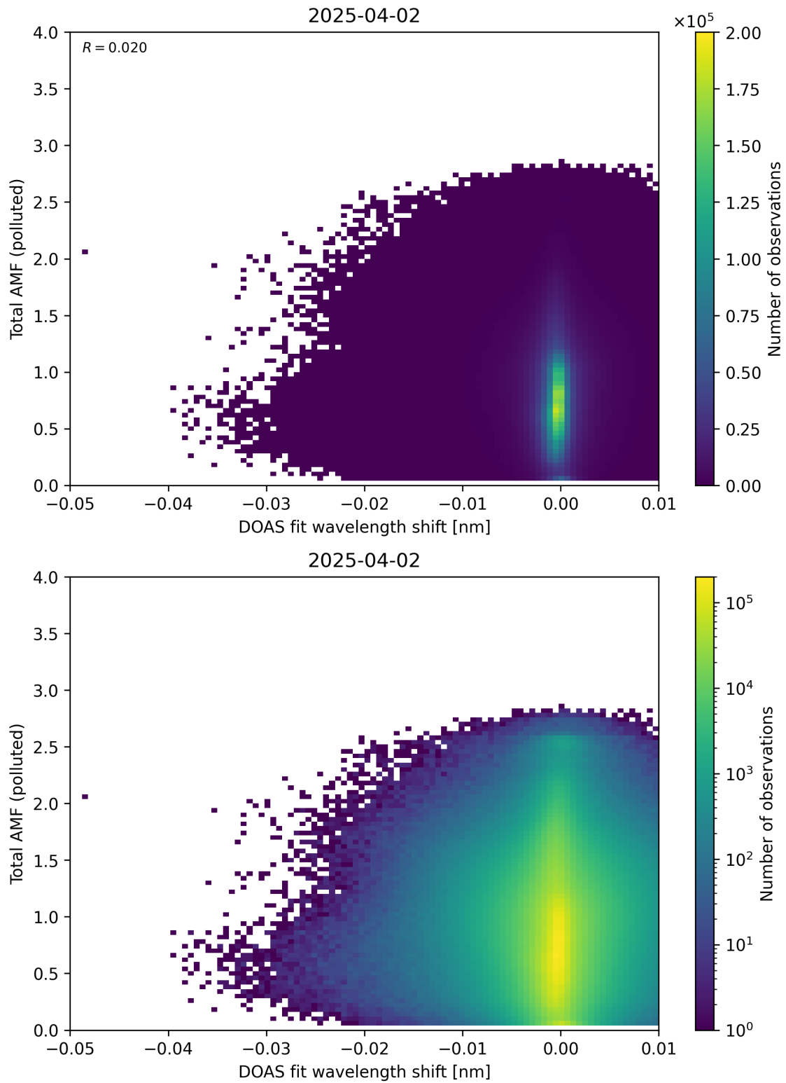
Figure 141: Scatter density plot of “DOAS fit wavelength shift” against “Total AMF (polluted)” for 2025-04-02 to 2025-04-03.
