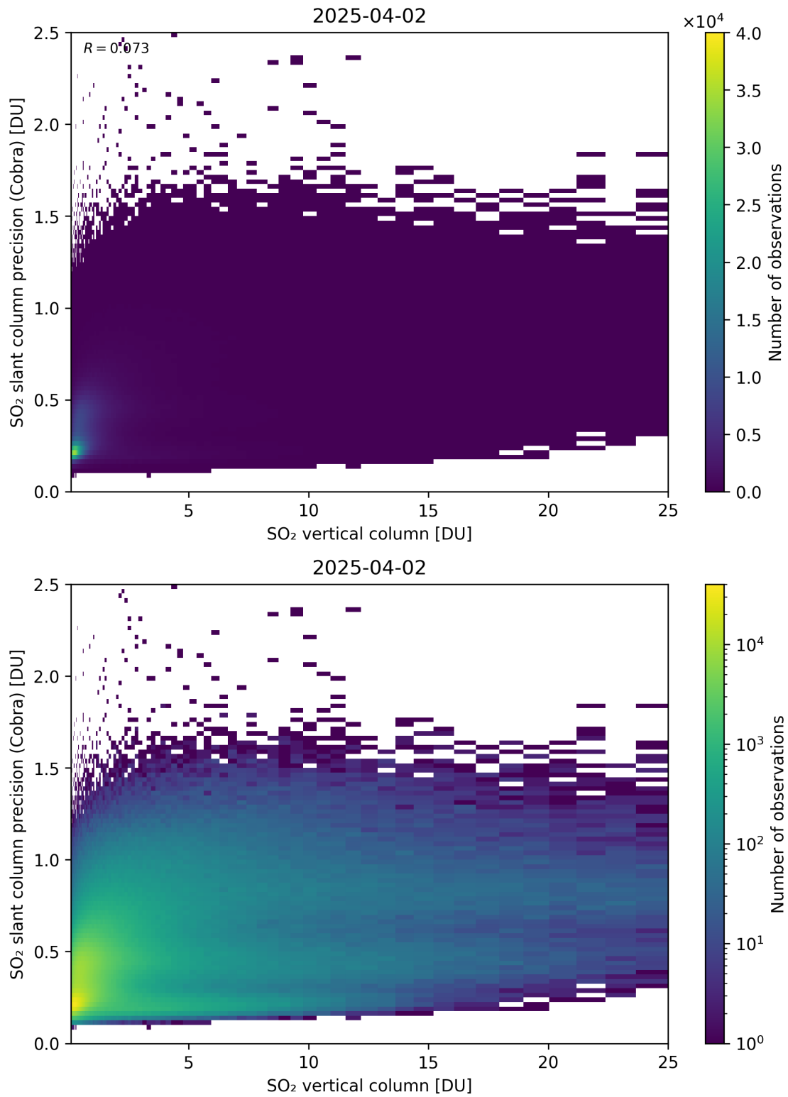
Figure 350: Scatter density plot of “SO 2 vertical column” against “SO 2 slant column precision (Cobra)” for 2025-04-02 to 2025-04-03.
