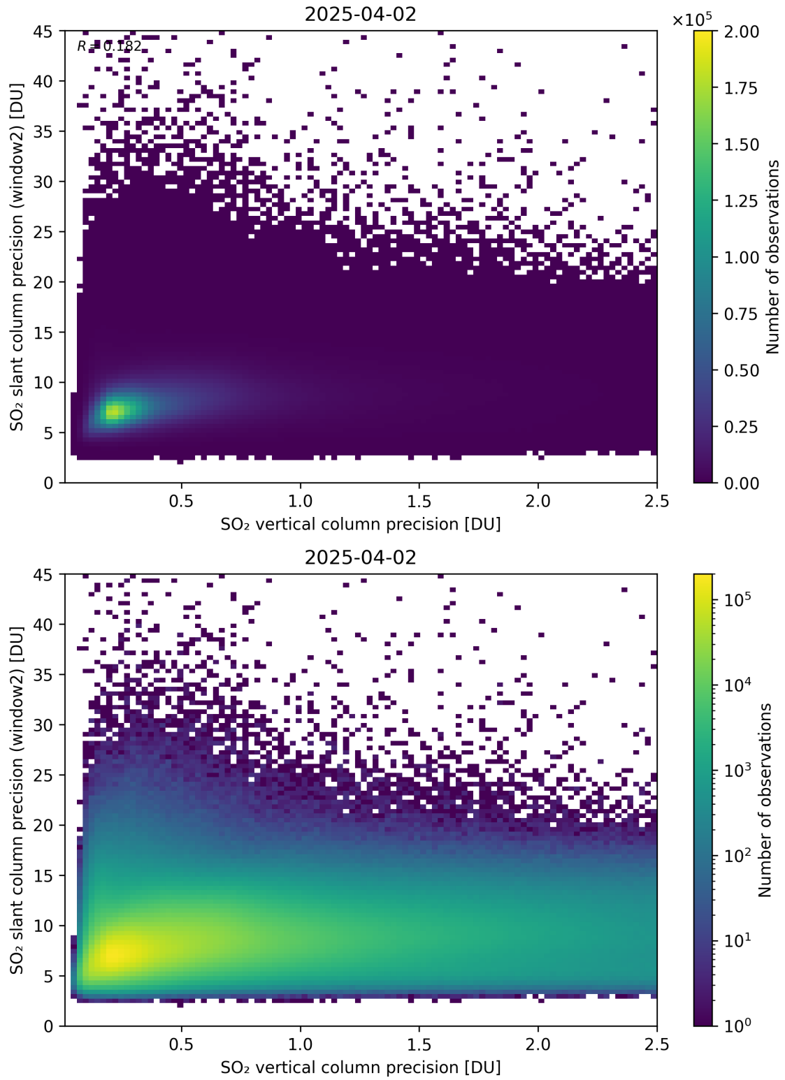
Figure 343: Scatter density plot of “SO 2 vertical column precision” against “SO 2 slant column precision (window2)” for 2025-04-02 to 2025-04-03.
