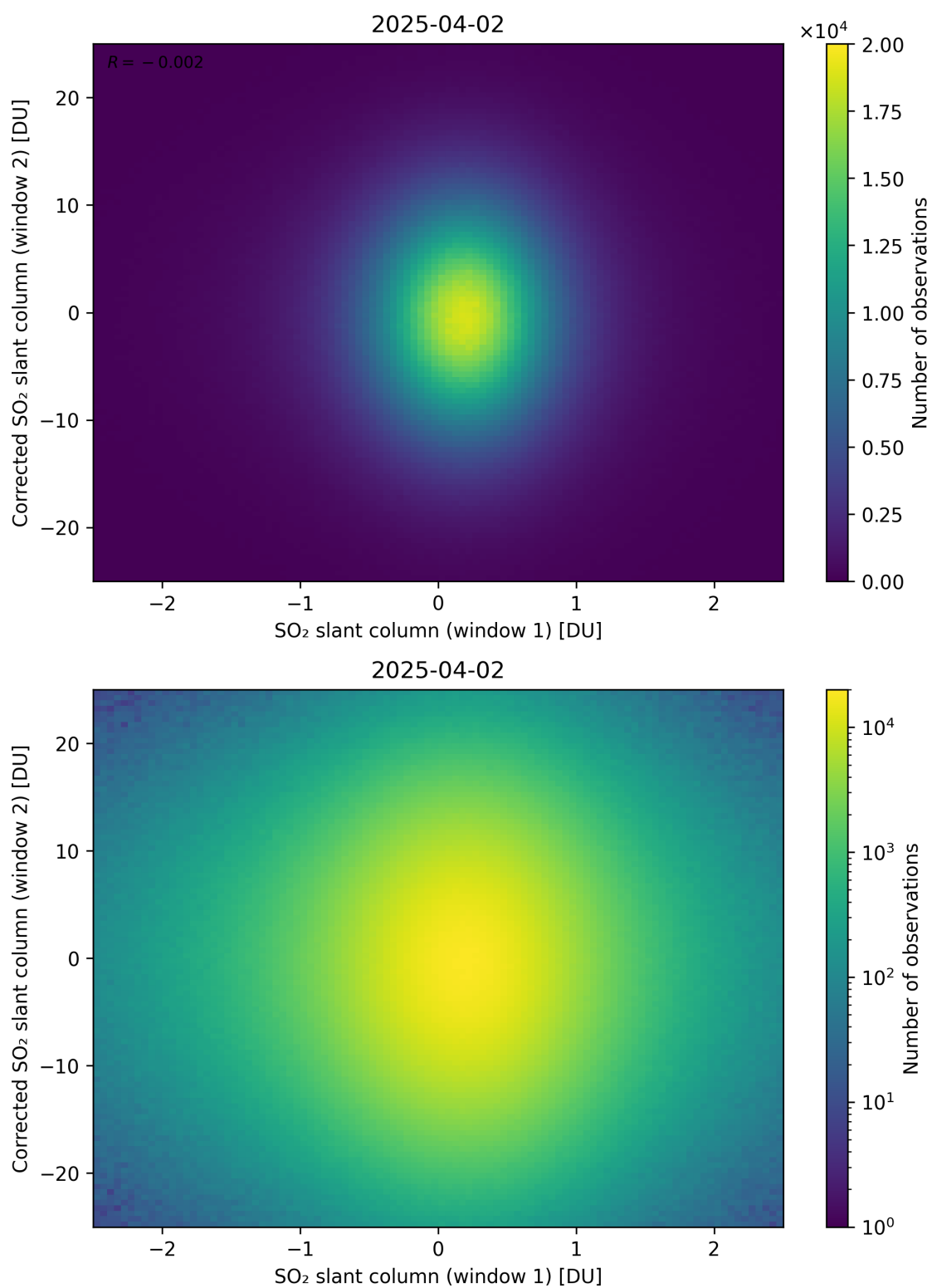
Figure 283: Scatter density plot of “SO 2 slant column (window 1)” against “Corrected SO 2 slant column (window 2)” for 2025-04-02 to 2025-04-03.
