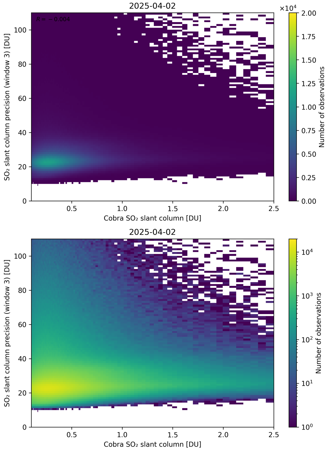
Figure 223: Scatter density plot of “Cobra SO 2 slant column” against “SO 2 slant column precision (window 3)” for 2025-04-02 to 2025-04-03.
