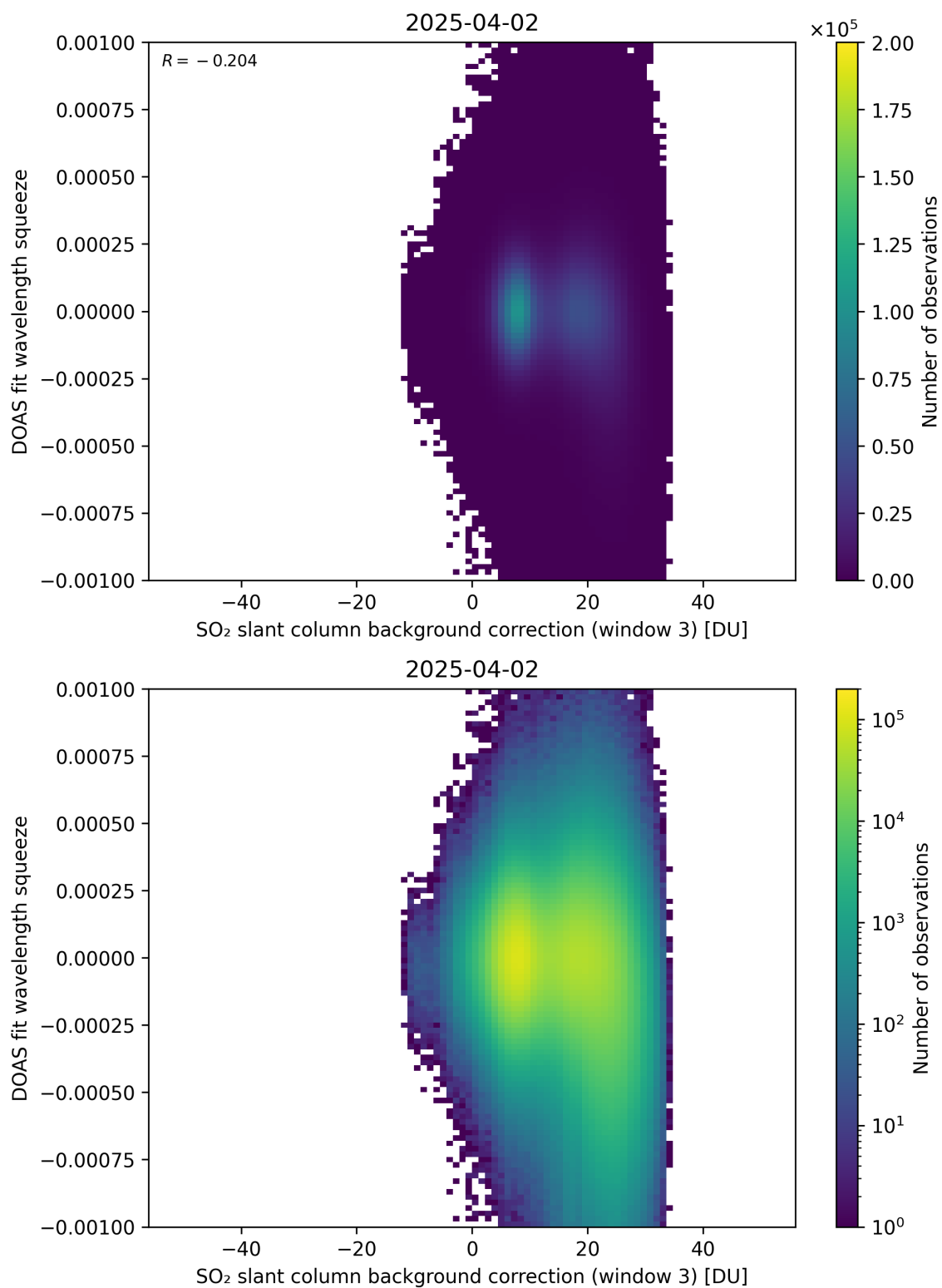
Figure 133: Scatter density plot of “SO 2 slant column background correction (window 3)” against “DOAS fit wavelength squeeze” for 2025-04-02 to 2025-04-03.
