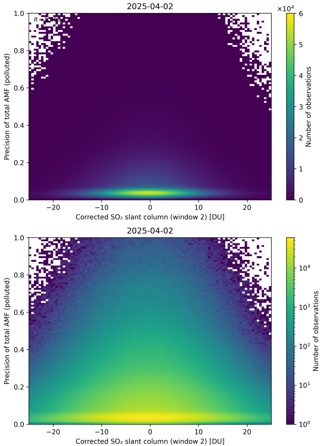
Figure 254: Scatter density plot of “Corrected SO 2 slant column (window 2)” against “Precision of total AMF (polluted)” for 2025-04-02 to 2025-04-03.
