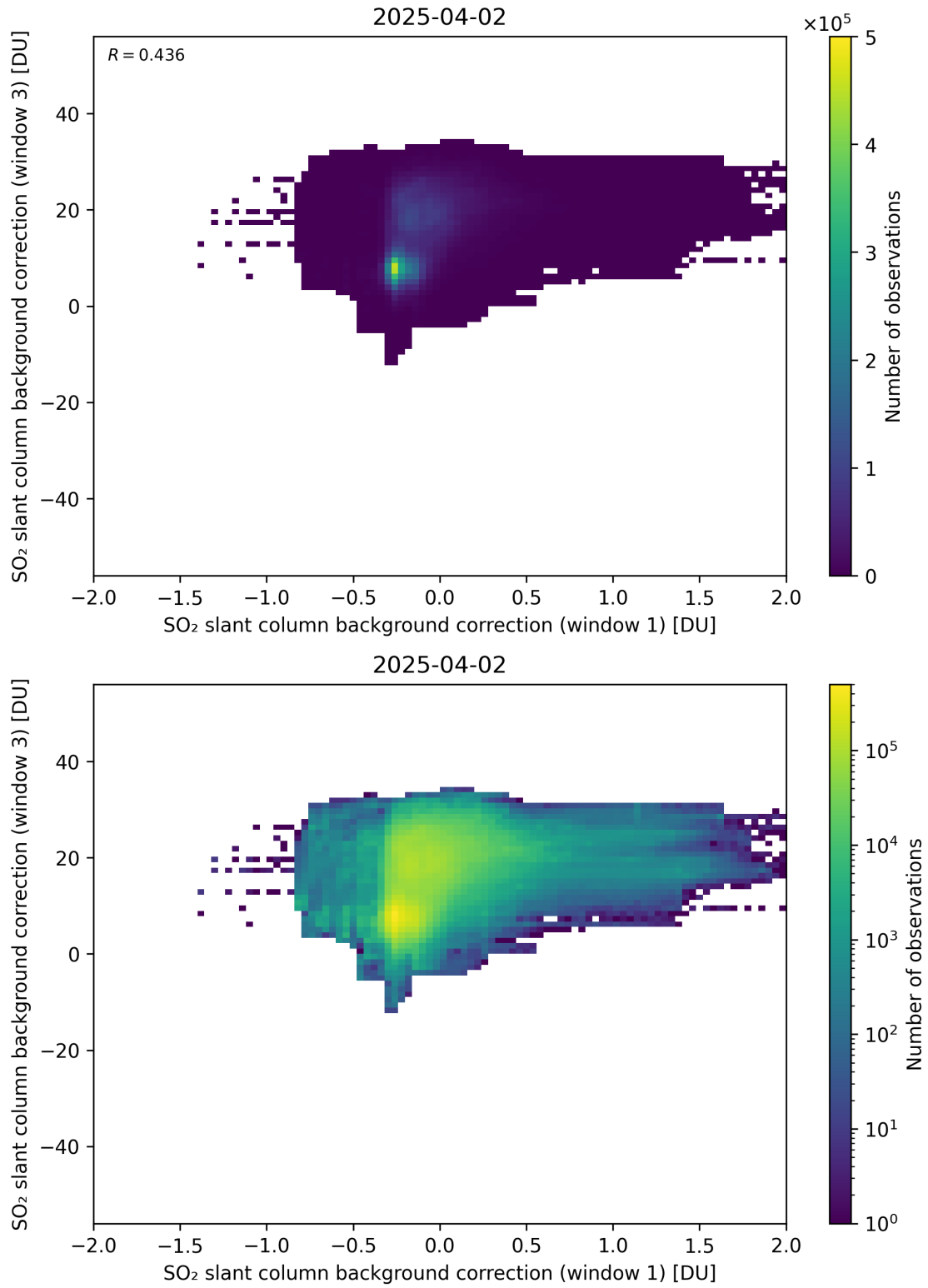
Figure 110: Scatter density plot of “SO 2 slant column background correction (window 1)” against “SO 2 slant column background correction (window 3)” for 2025-04-02 to 2025-04-03.
