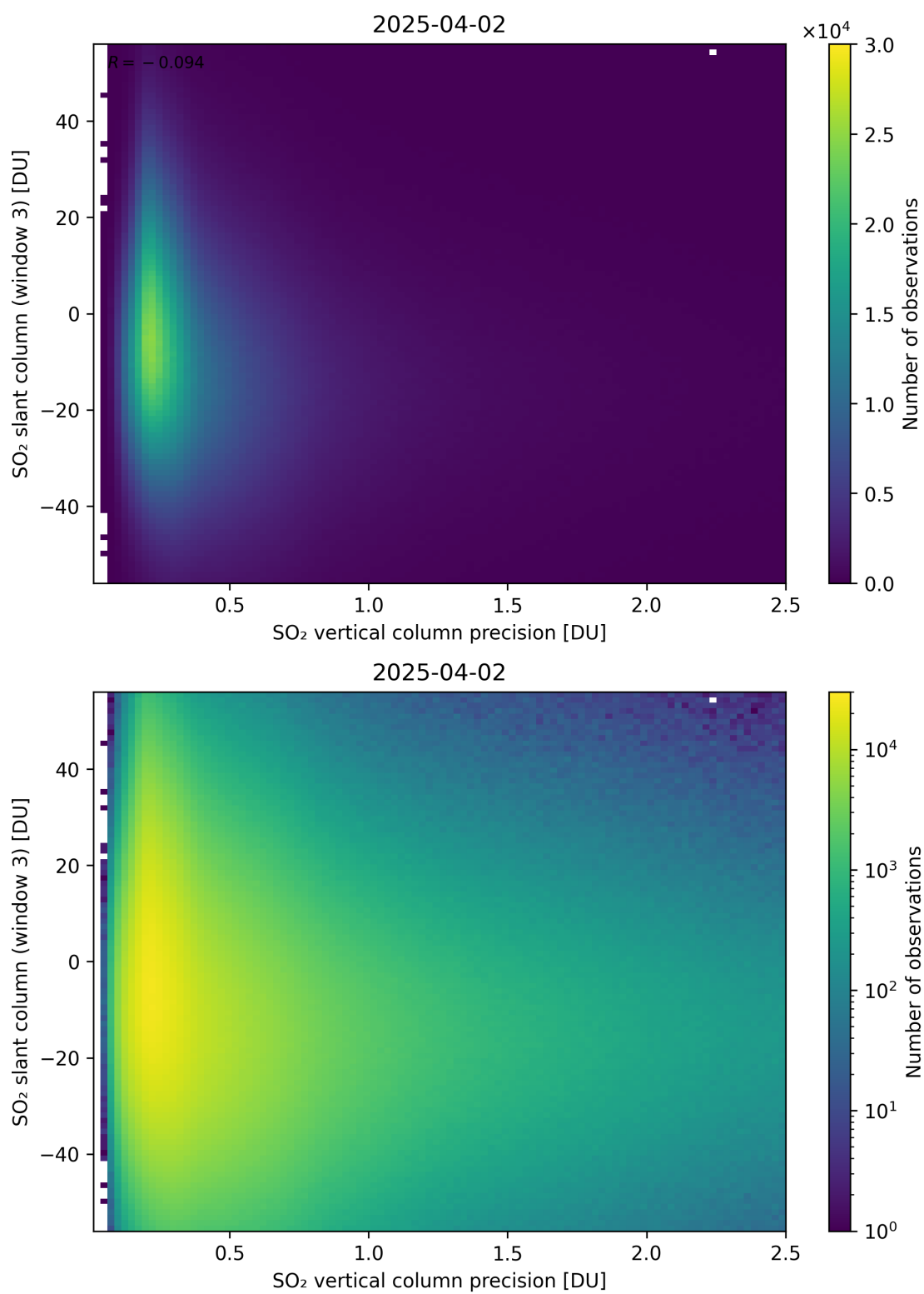
Figure 344: Scatter density plot of “SO 2 vertical column precision” against “SO 2 slant column (window 3)” for 2025-04-02 to 2025-04-03.
