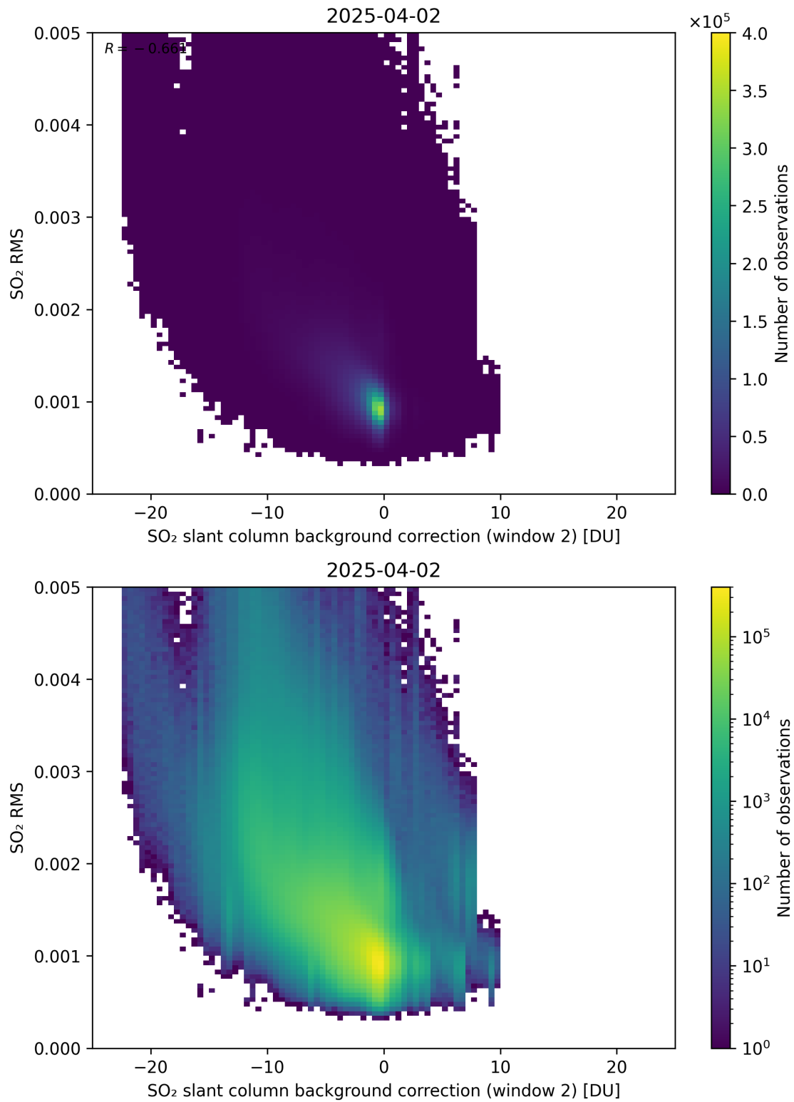
Figure 125: Scatter density plot of “SO 2 slant column background correction (window 2)” against “SO 2 RMS” for 2025-04-02 to 2025-04-03.
