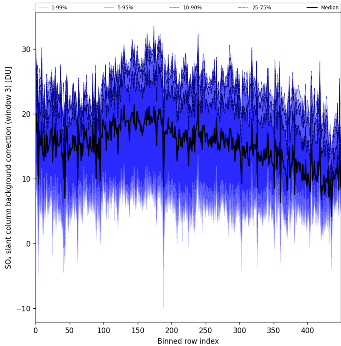
Figure 100: Along track statistics of “SO 2 slant column background correction (window 3)” for 2025-04-02 to 2025-04-03
