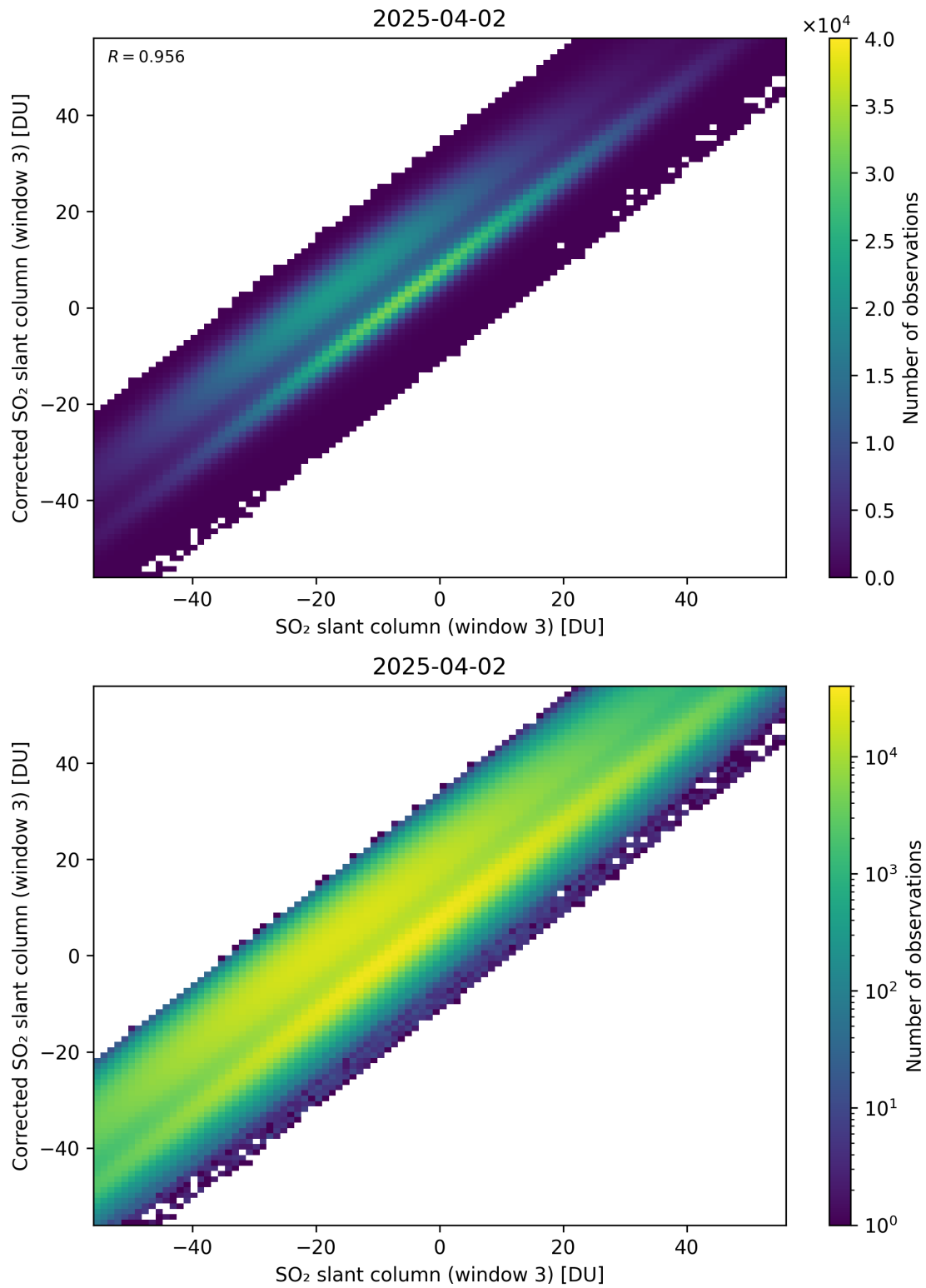
Figure 316: Scatter density plot of “SO 2 slant column (window 3)” against “Corrected SO 2 slant column (window 3)” for 2025-04-02 to 2025-04-03.
