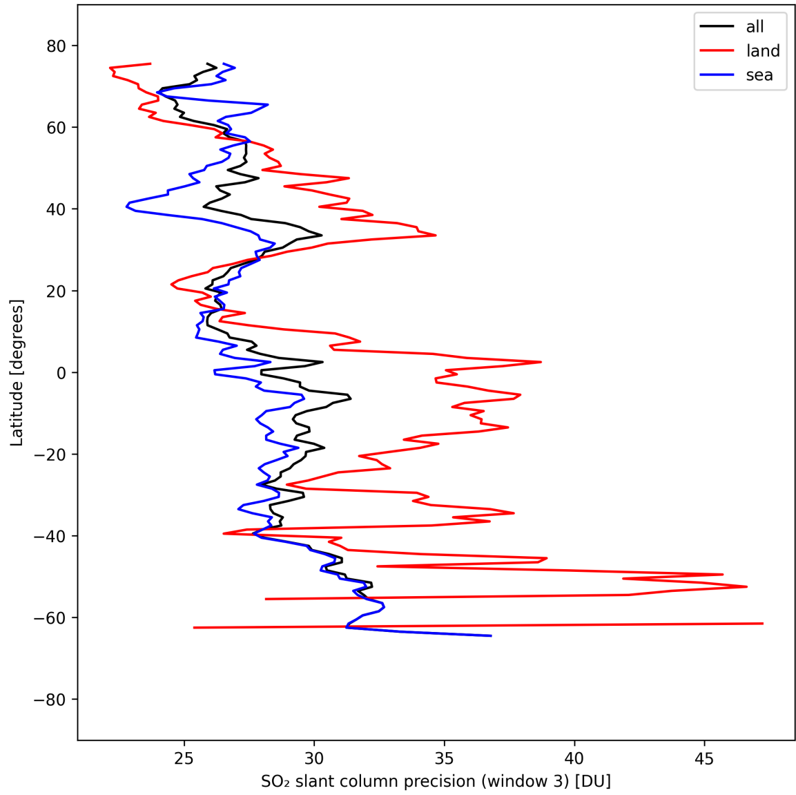
Figure 46: Zonal average of “SO 2 slant column precision (window 3)” for 2025-04-02 to 2025-04-03.
