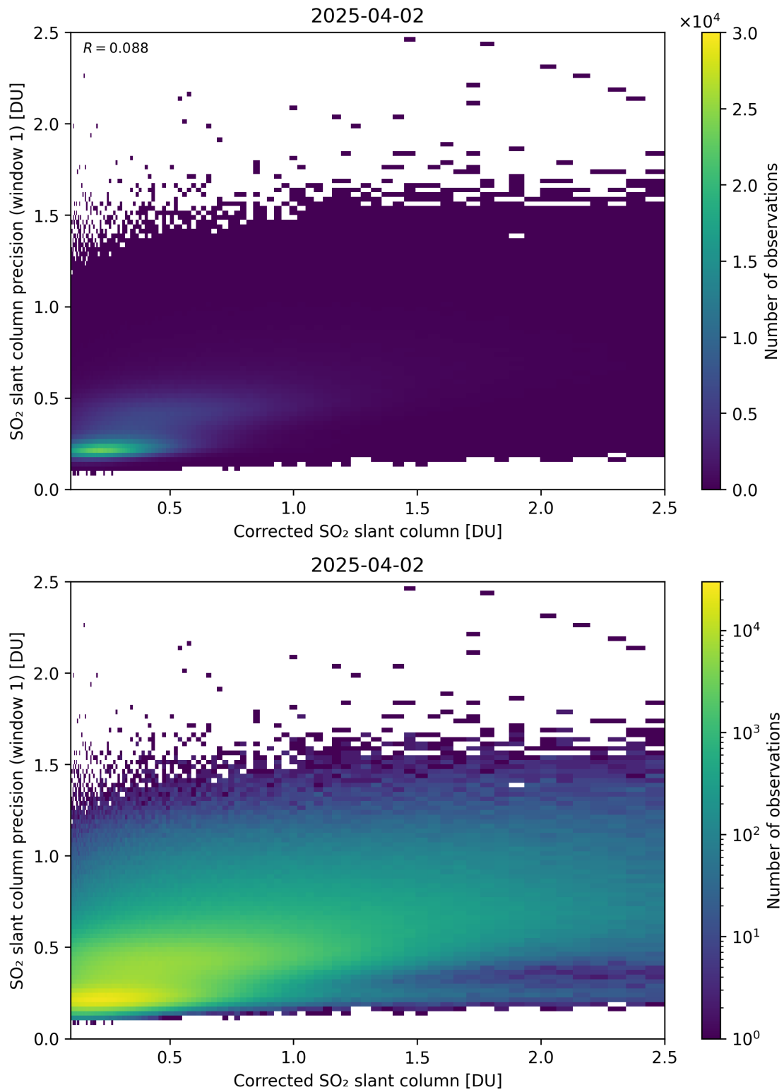
Figure 238: Scatter density plot of “Corrected SO 2 slant column” against “SO 2 slant column precision (window 1)” for 2025-04-02 to 2025-04-03.
