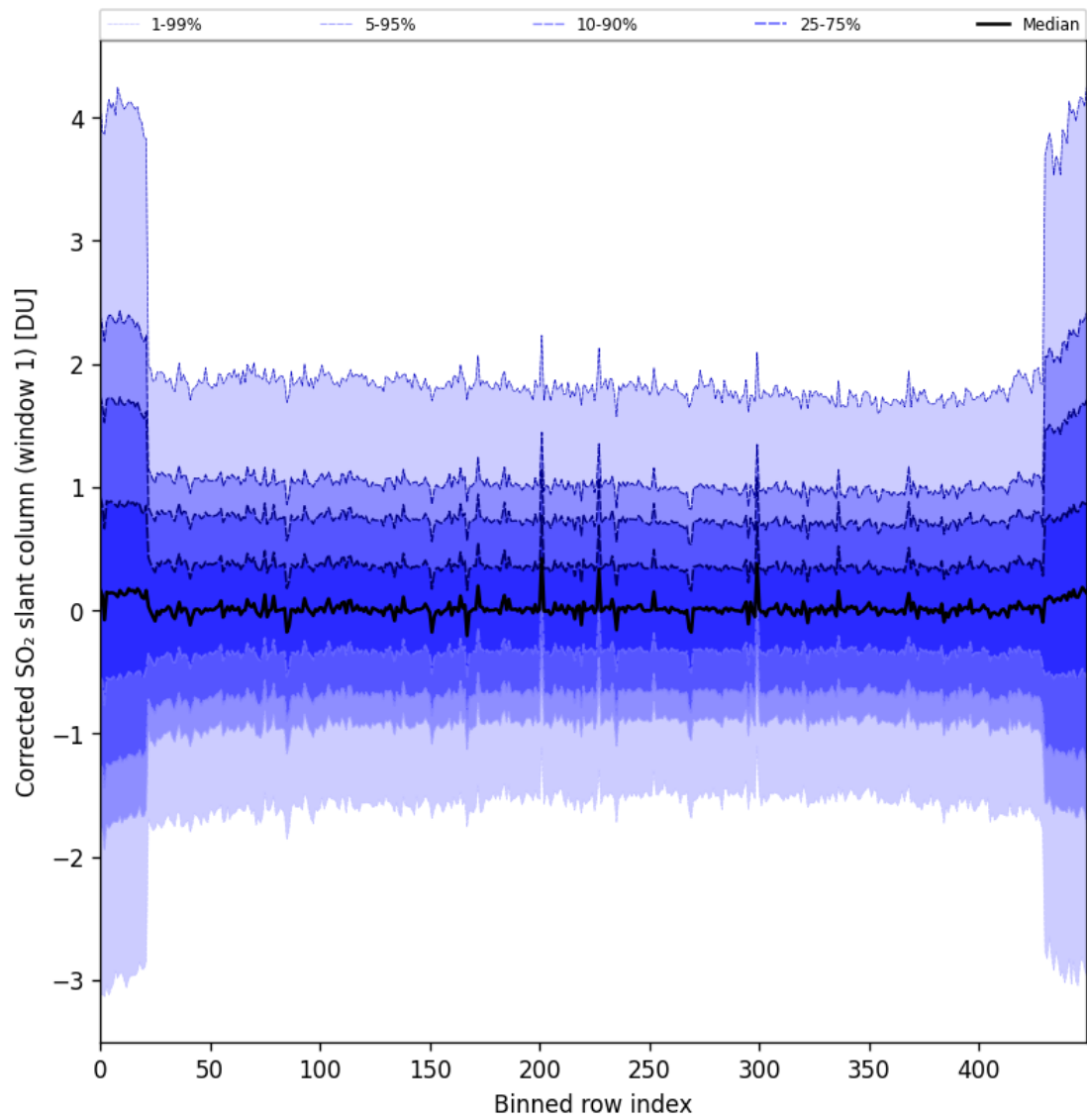
Figure 91: Along track statistics of “Corrected SO 2 slant column (window 1)” for 2025-04-02 to 2025-04-03
