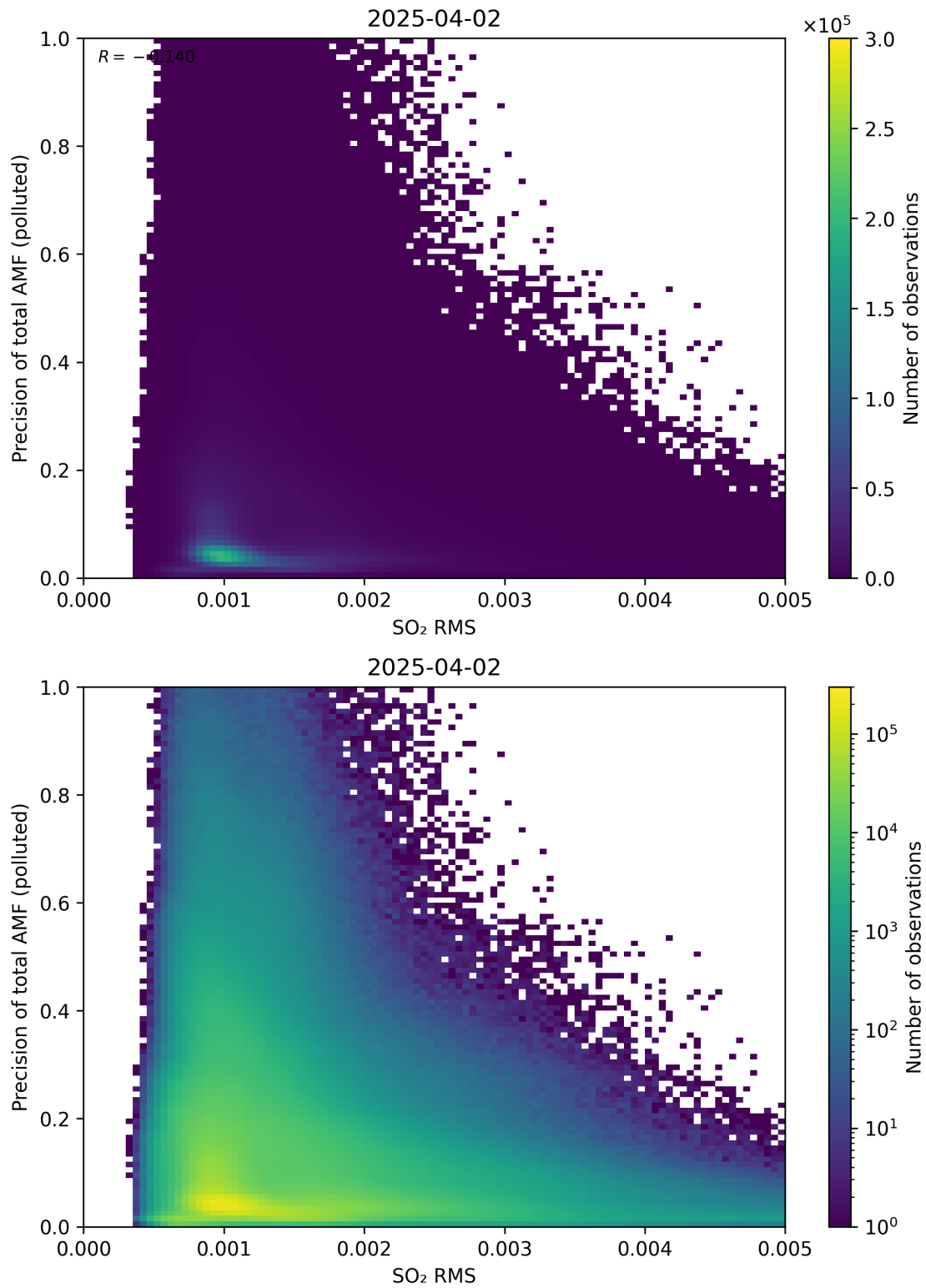
Figure 149: Scatter density plot of “SO 2 RMS” against “Precision of total AMF (polluted)” for 2025-04-02 to 2025-04-03.
