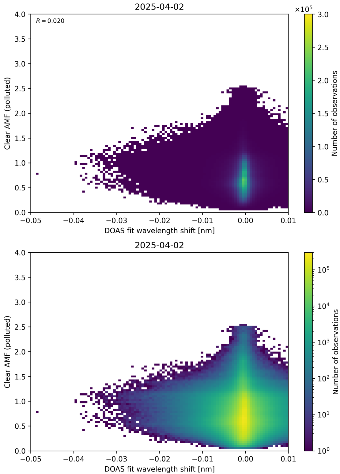
Figure 140: Scatter density plot of “DOAS fit wavelength shift” against “Clear AMF (polluted)” for 2025-04-02 to 2025-04-03.
