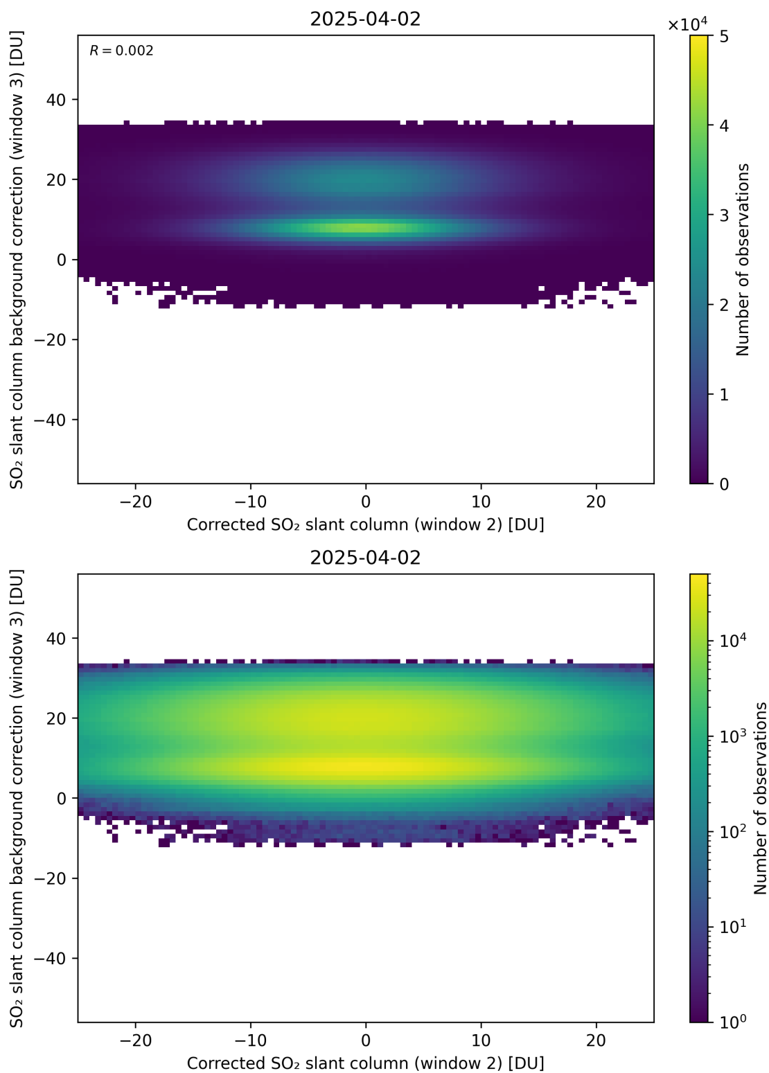
Figure 245: Scatter density plot of “Corrected SO 2 slant column (window 2)” against “SO 2 slant column background correction (window 3)” for 2025-04-02 to 2025-04-03.
