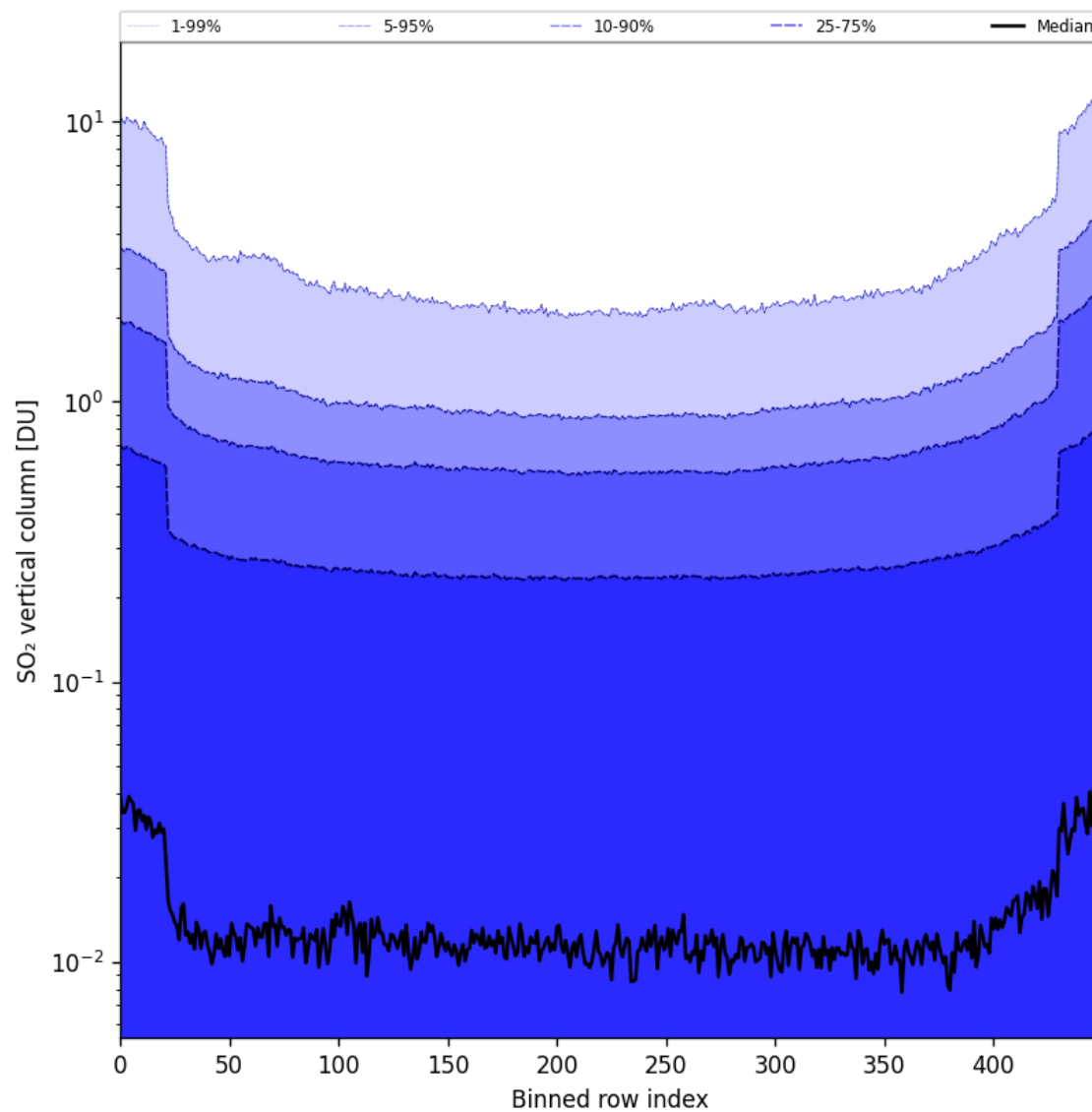
Figure 84: Along track statistics of “SO 2 vertical column” for 2025-04-02 to 2025-04-03
