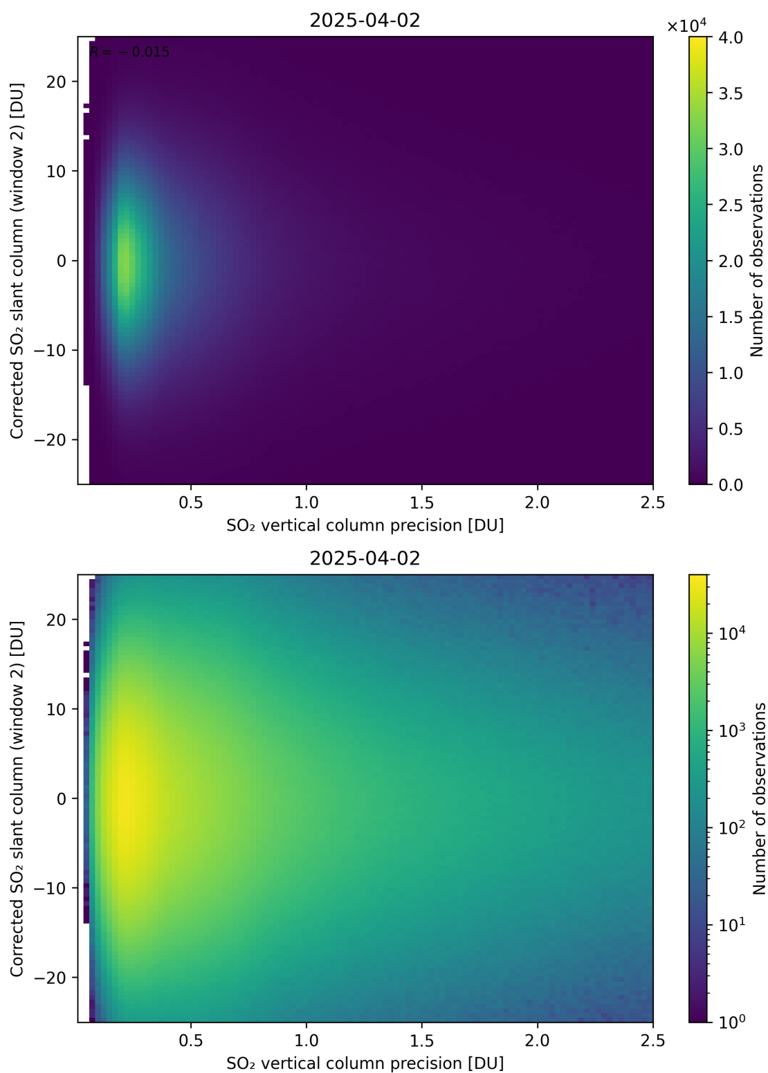
Figure 339: Scatter density plot of “SO 2 vertical column precision” against “Corrected SO 2 slant column (window 2)” for 2025-04-02 to 2025-04-03.
