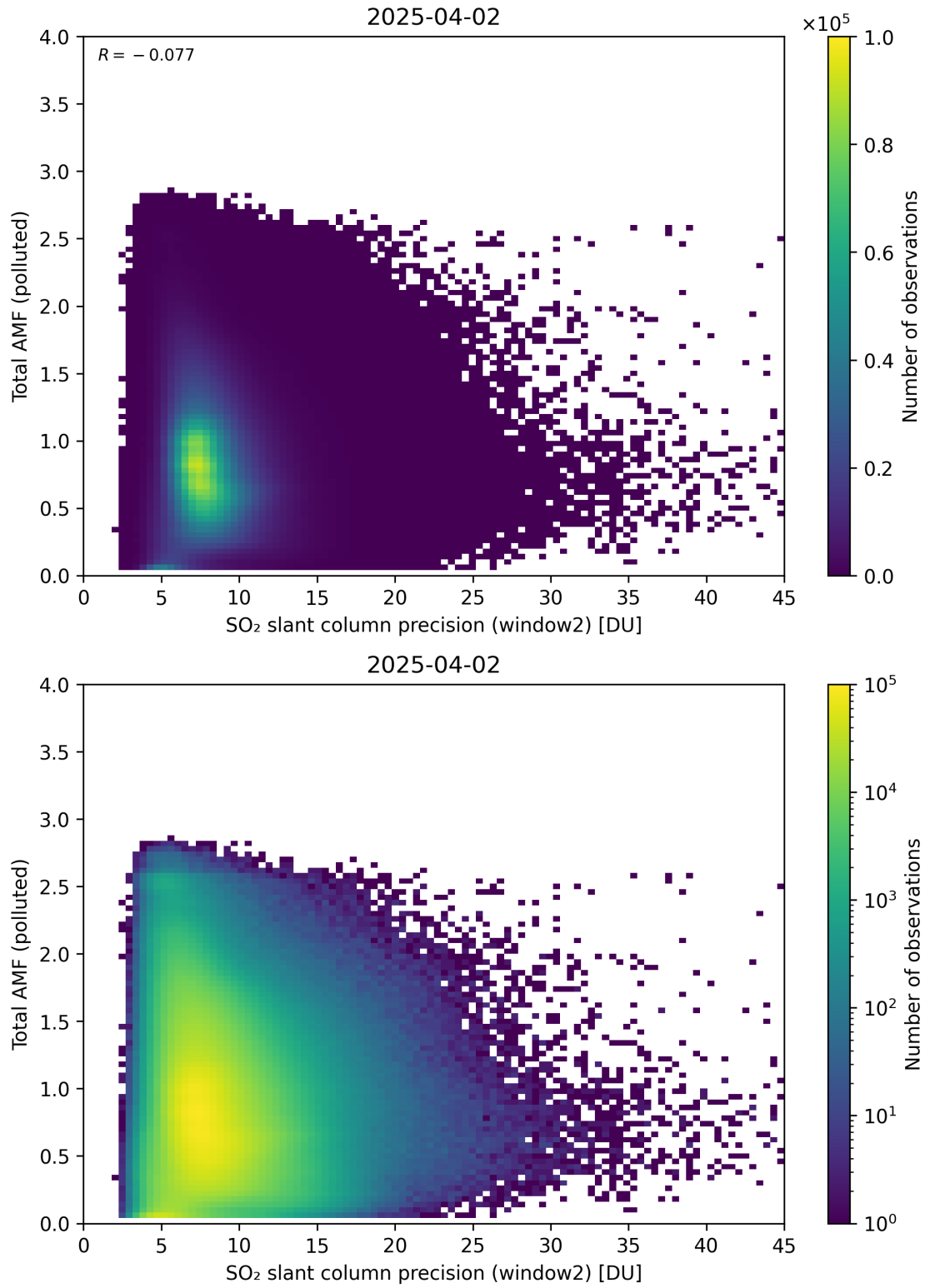
Figure 301: Scatter density plot of “SO 2 slant column precision (window2)” against “Total AMF (polluted)” for 2025-04-02 to 2025-04-03.
