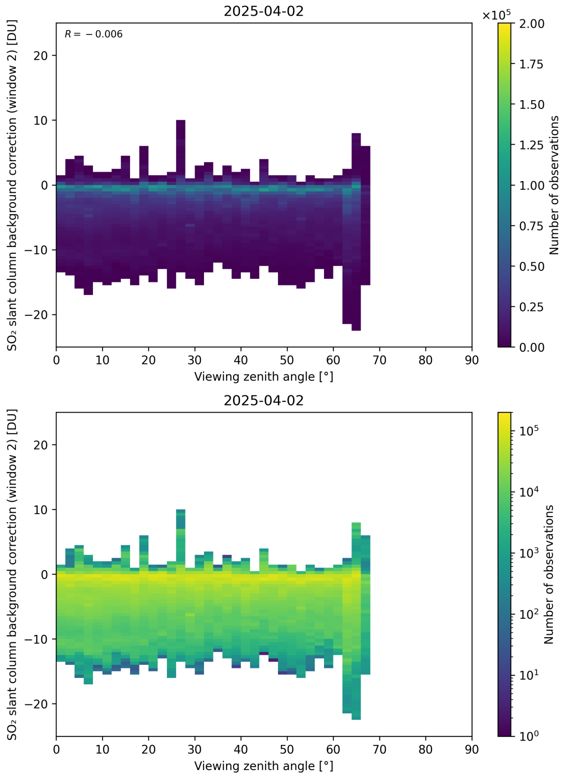
Figure 363: Scatter density plot of “Viewing zenith angle” against “SO 2 slant column background correction (window 2)” for 2025-04-02 to 2025-04-03.
