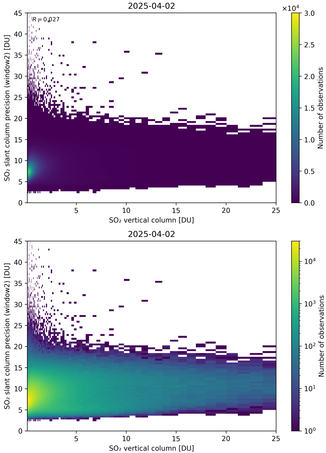
Figure 356: Scatter density plot of “SO 2 vertical column” against “SO 2 slant column precision (window2)” for 2025-04-02 to 2025-04-03.
