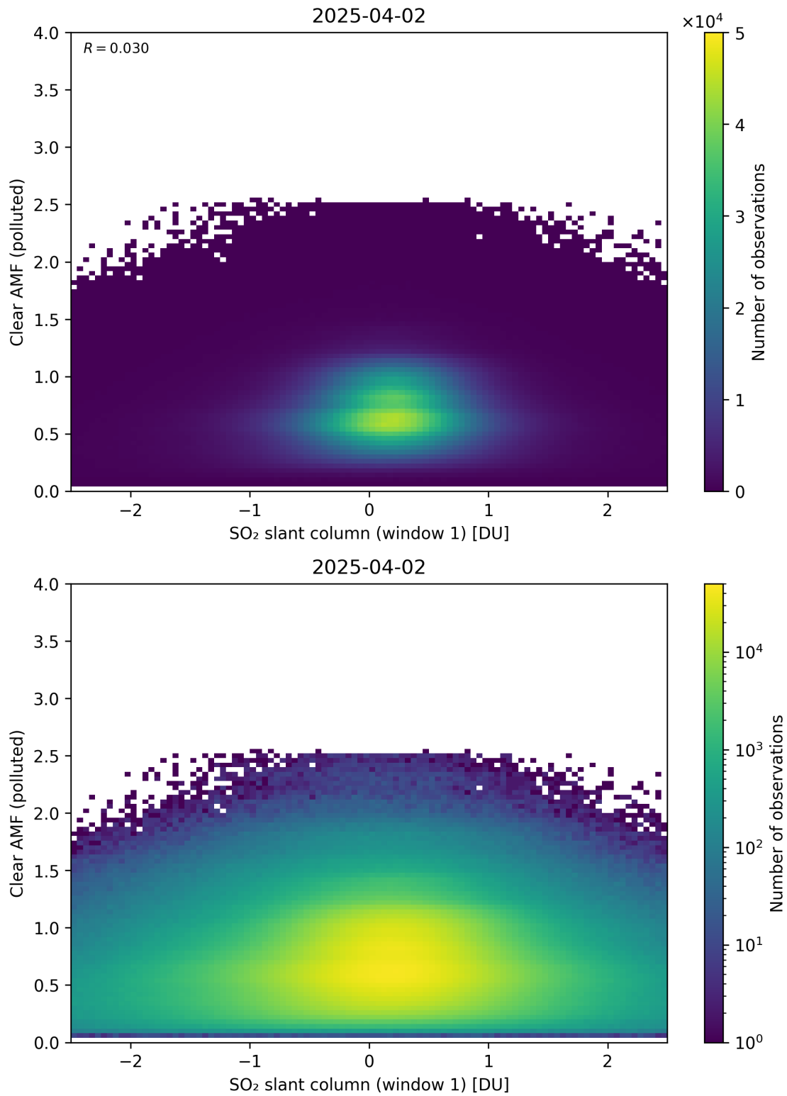
Figure 282: Scatter density plot of “SO 2 slant column (window 1)” against “Clear AMF (polluted)” for 2025-04-02 to 2025-04-03.
