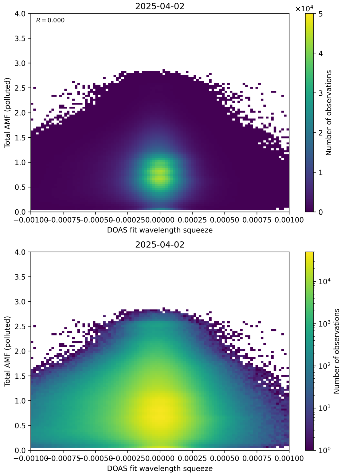
Figure 145: Scatter density plot of “DOAS fit wavelength squeeze” against “Total AMF (polluted)” for 2025-04-02 to 2025-04-03.
