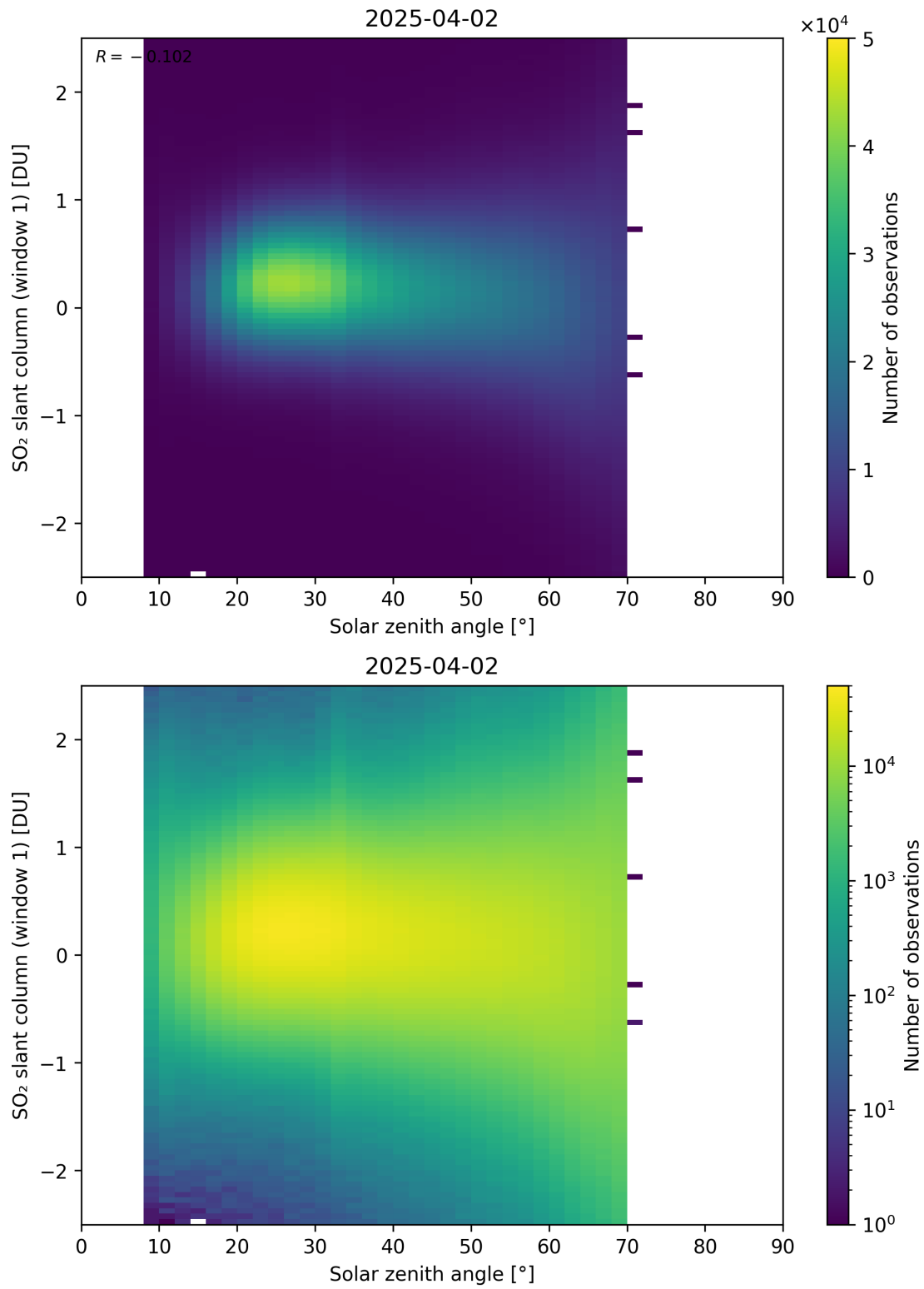
Figure 184: Scatter density plot of “Solar zenith angle” against “SO 2 slant column (window 1)” for 2025-04-02 to 2025-04-03.
