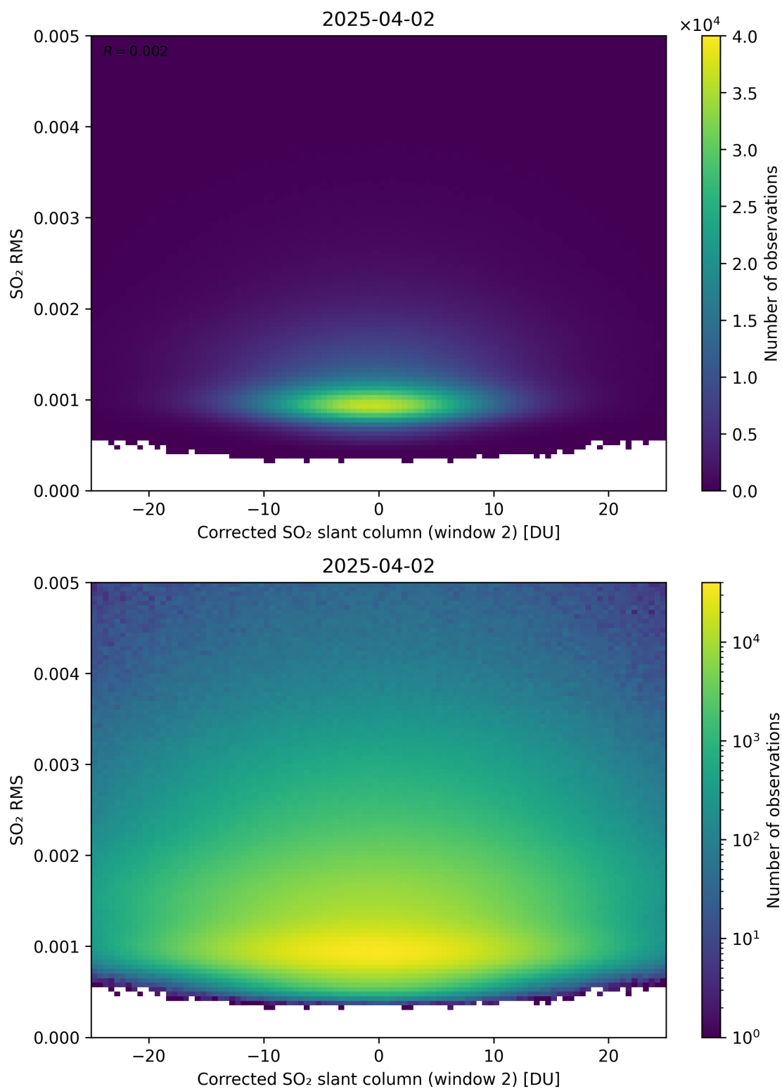
Figure 248: Scatter density plot of “Corrected SO 2 slant column (window 2)” against “SO 2 RMS” for 2025-04-02 to 2025-04-03.
