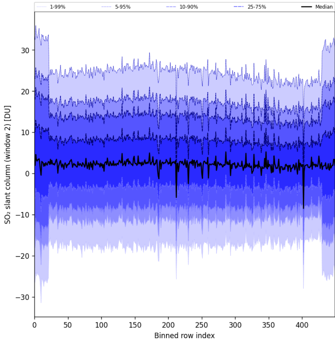
Figure 93: Along track statistics of “SO 2 slant column (window 2)” for 2025-04-02 to 2025-04-03
