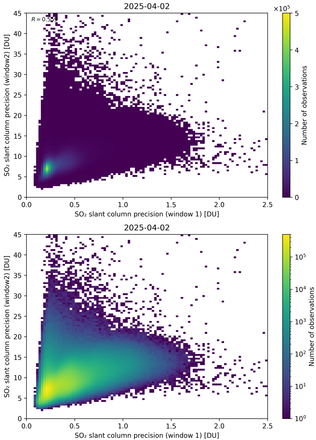
Figure 277: Scatter density plot of “SO 2 slant column precision (window 1)” against “SO 2 slant column precision (window2)” for 2025-04-02 to 2025-04-03.
