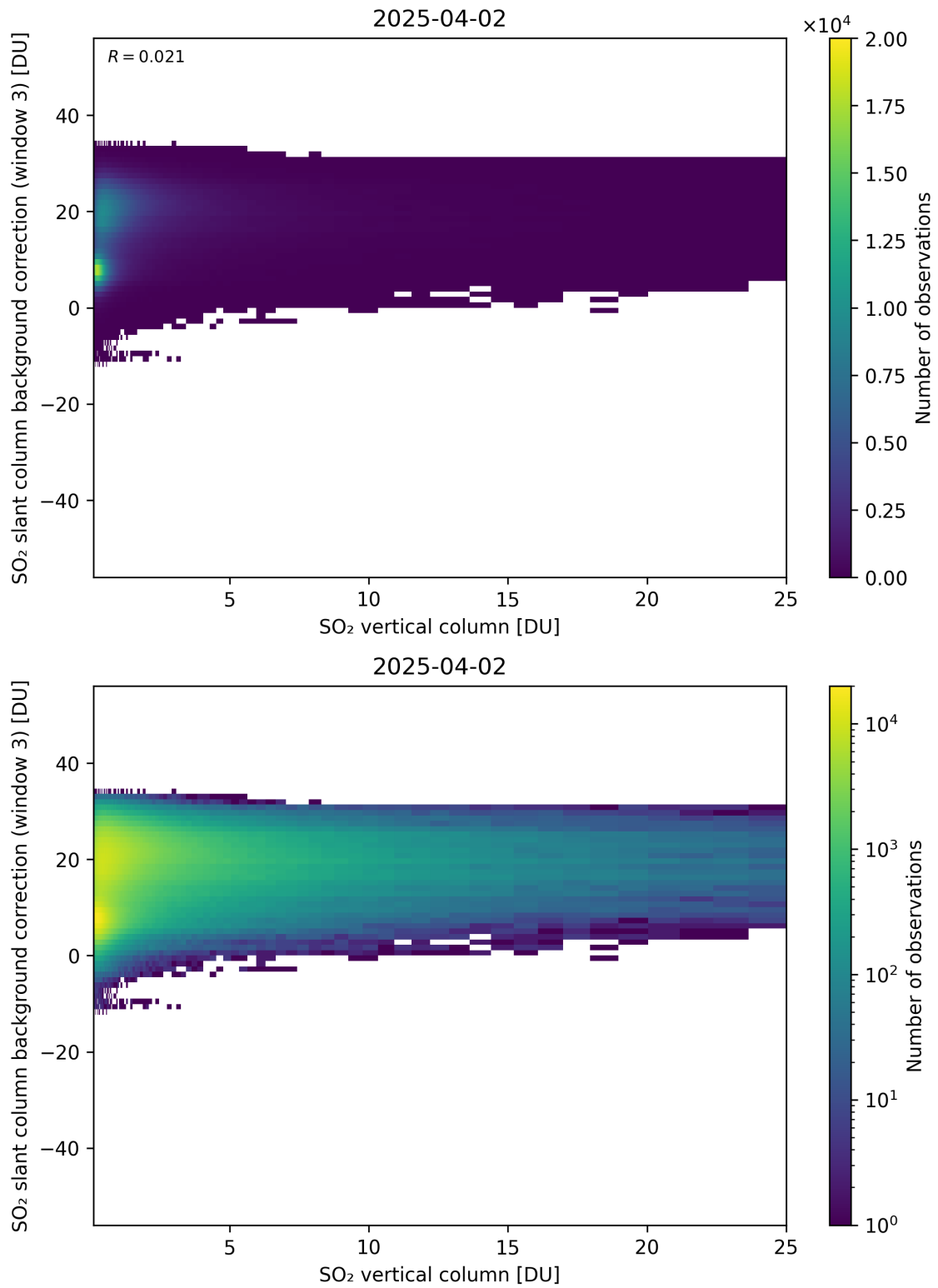
Figure 325: Scatter density plot of “SO 2 vertical column” against “SO 2 slant column background correction (window 3)” for 2025-04-02 to 2025-04-03.
