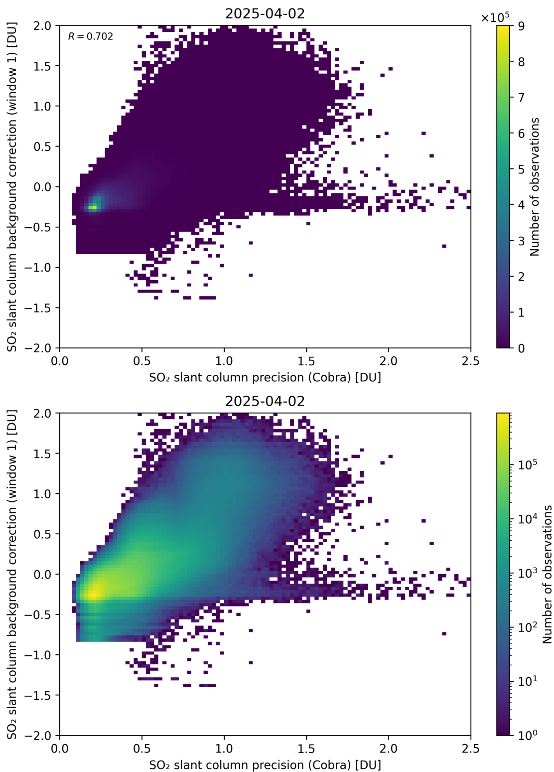
Figure 199: Scatter density plot of “SO 2 slant column precision (Cobra)” against “SO 2 slant column background correction (window 1)” for 2025-04-02 to 2025-04-03.
