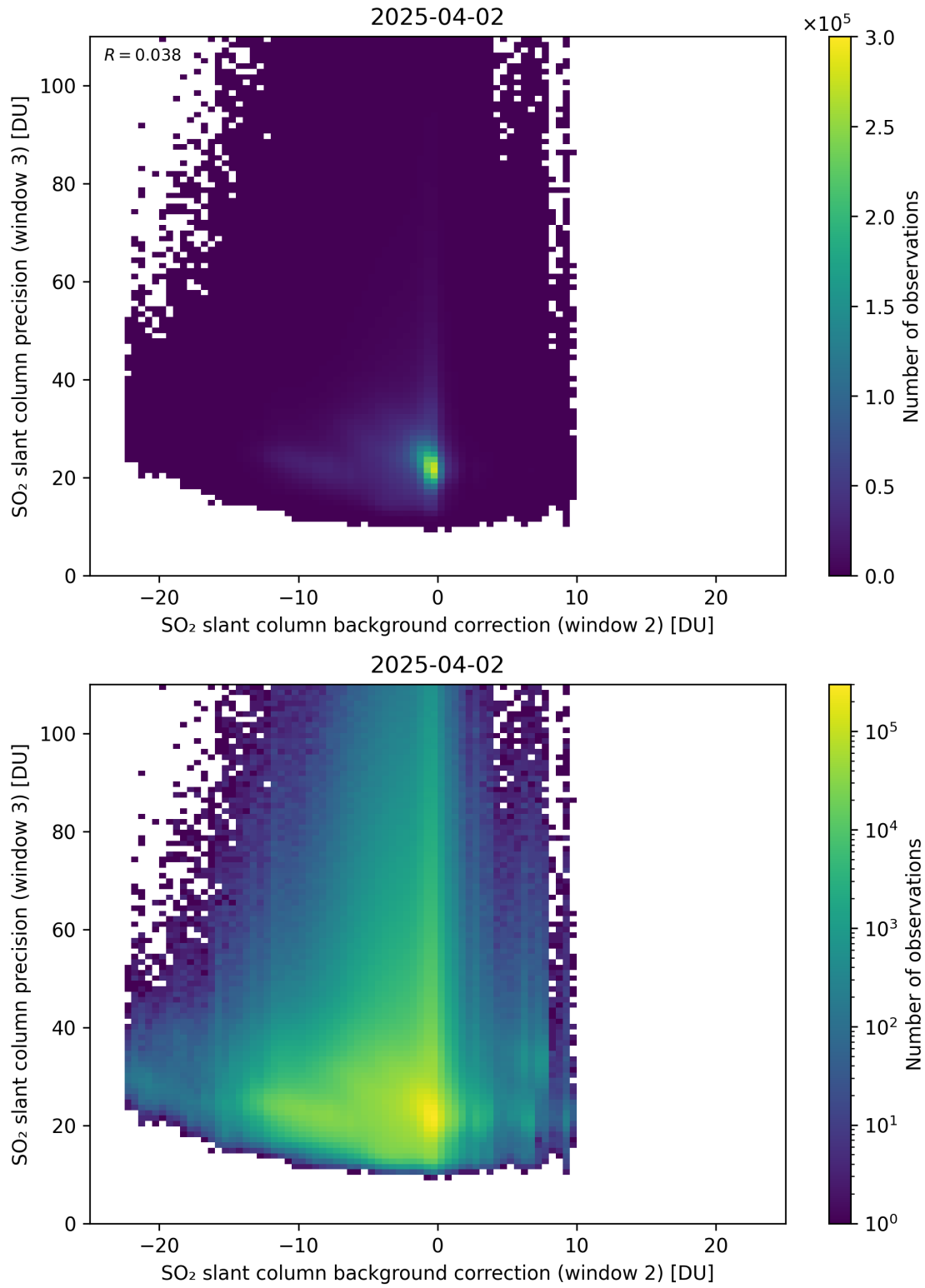
Figure 129: Scatter density plot of “SO 2 slant column background correction (window 2)” against “SO 2 slant column precision (window 3)” for 2025-04-02 to 2025-04-03.
