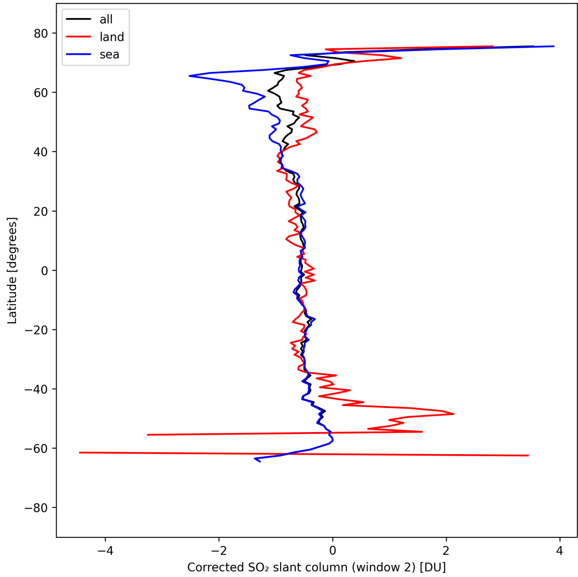
Figure 43: Zonal average of “Corrected SO 2 slant column (window 2)” for 2025-04-02 to 2025-04-03.
