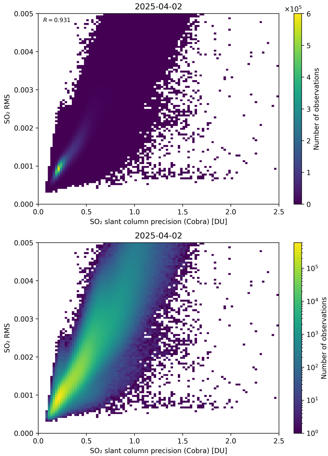
Figure 204: Scatter density plot of “SO 2 slant column precision (Cobra)” against “SO 2 RMS” for 2025-04-02 to 2025-04-03.
