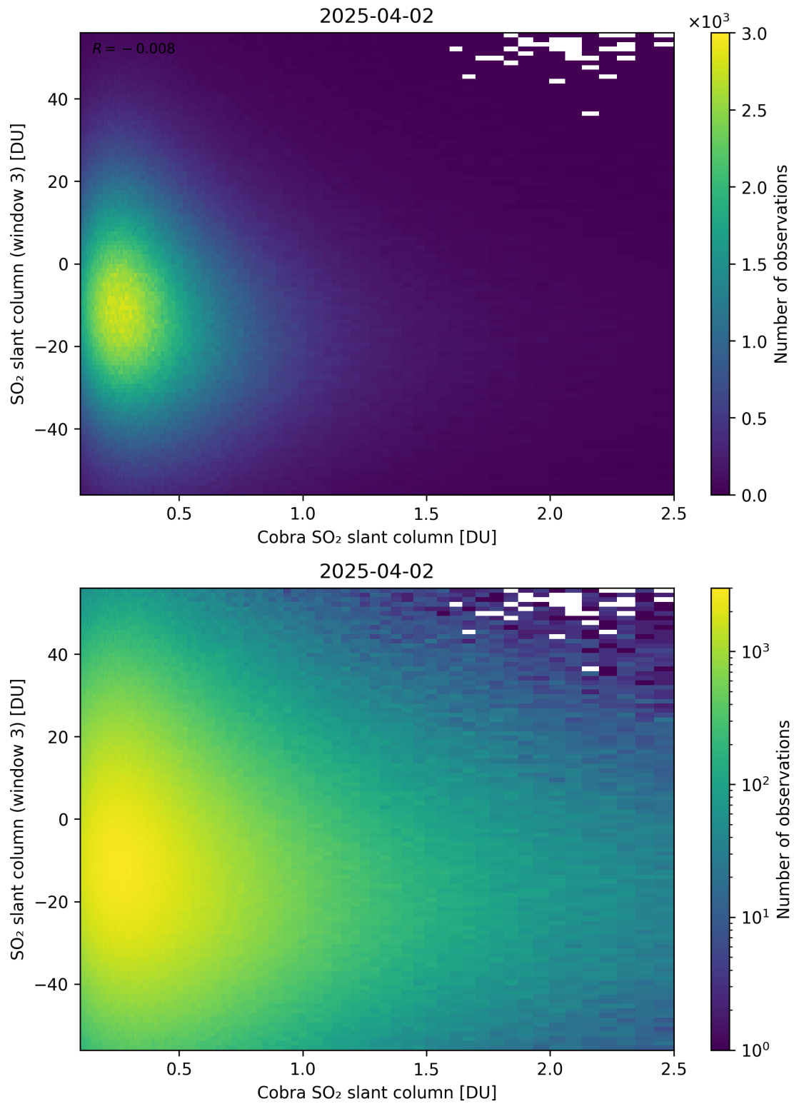
Figure 222: Scatter density plot of “Cobra SO 2 slant column” against “SO 2 slant column (window 3)” for 2025-04-02 to 2025-04-03.
