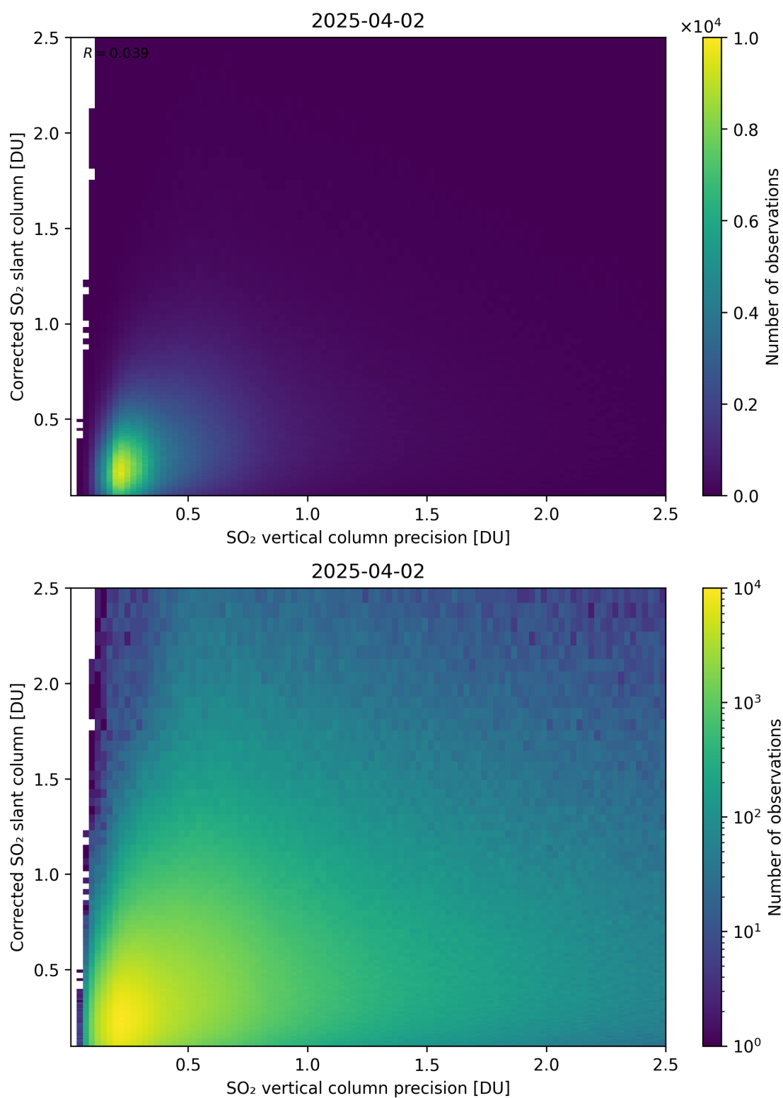
Figure 338: Scatter density plot of “SO 2 vertical column precision” against “Corrected SO 2 slant column” for 2025-04-02 to 2025-04-03.
