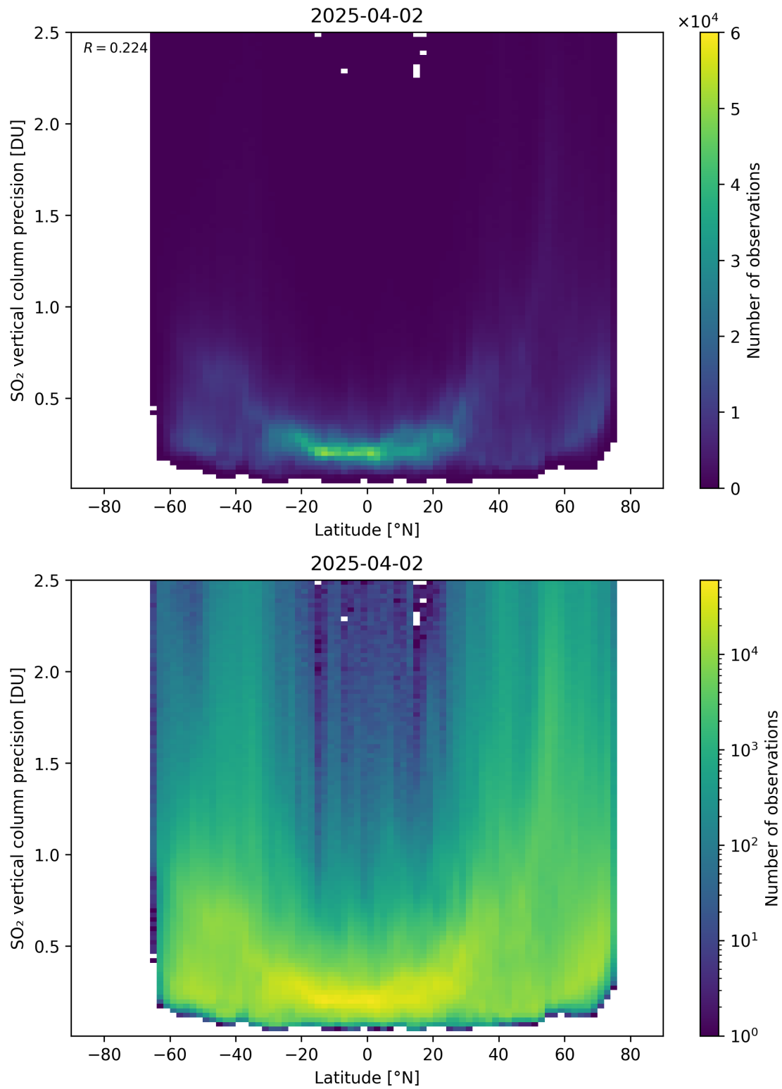
Figure 170: Scatter density plot of “Latitude” against “SO 2 vertical column precision” for 2025-04-02 to 2025-04-03.
