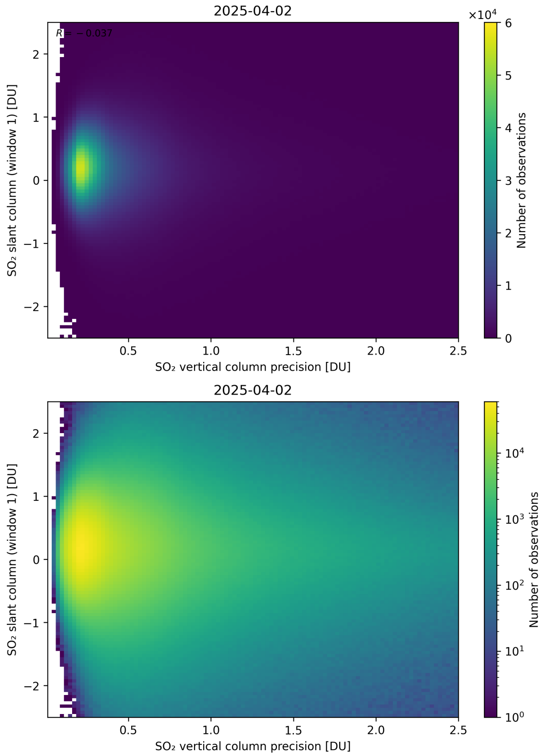
Figure 341: Scatter density plot of “SO 2 vertical column precision” against “SO 2 slant column (window 1)” for 2025-04-02 to 2025-04-03.
