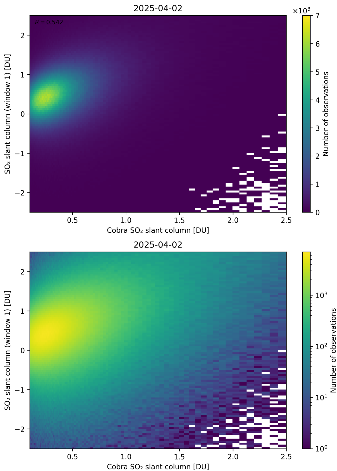
Figure 219: Scatter density plot of “Cobra SO 2 slant column” against “SO 2 slant column (window 1)” for 2025-04-02 to 2025-04-03.
