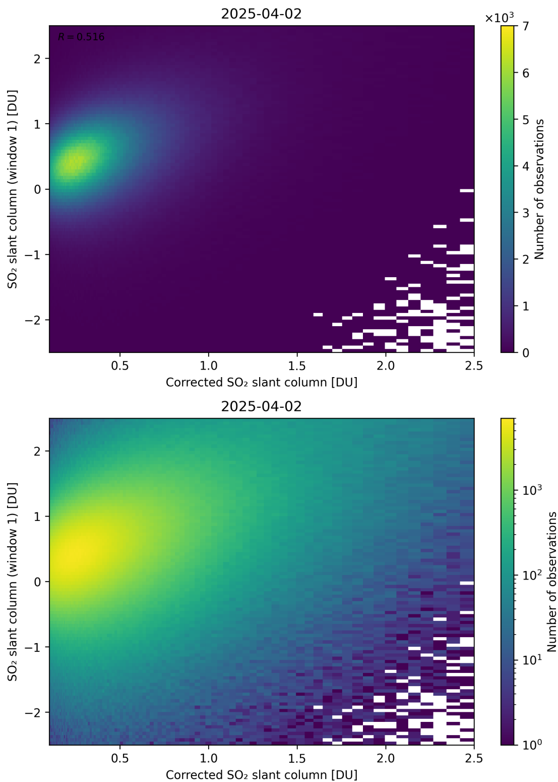
Figure 237: Scatter density plot of “Corrected SO 2 slant column” against “SO 2 slant column (window 1)” for 2025-04-02 to 2025-04-03.
