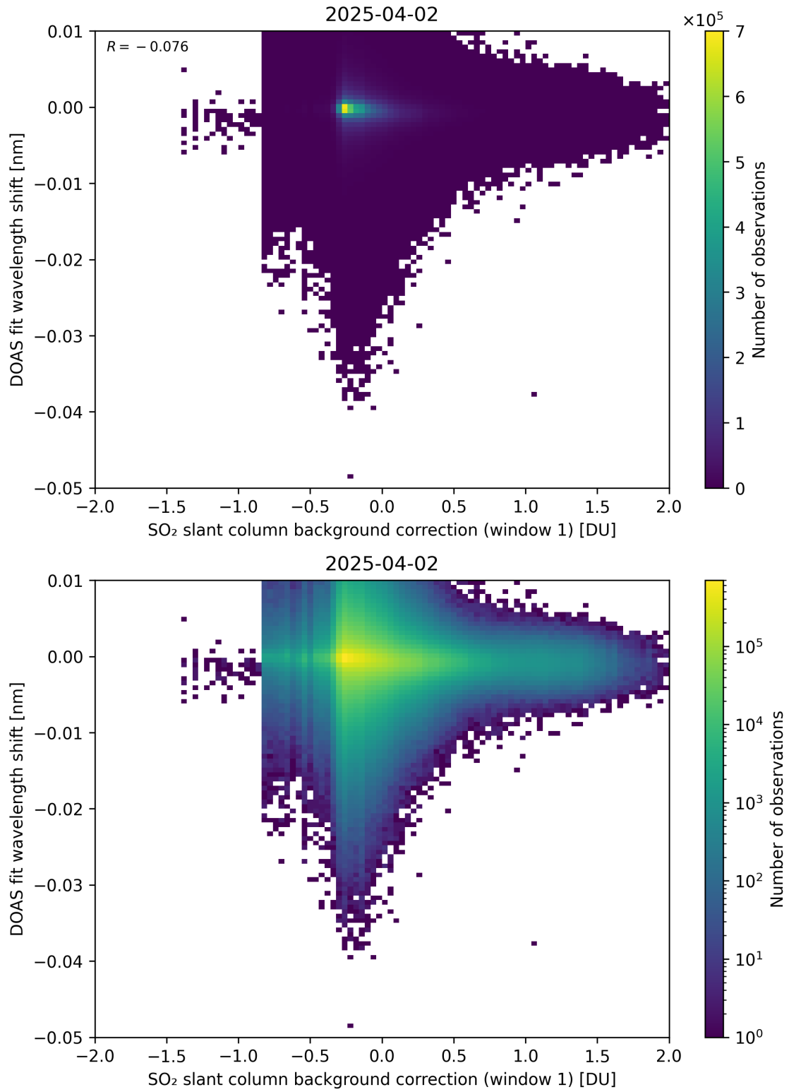
Figure 111: Scatter density plot of “SO 2 slant column background correction (window 1)” against “DOAS fit wavelength shift” for 2025-04-02 to 2025-04-03.
