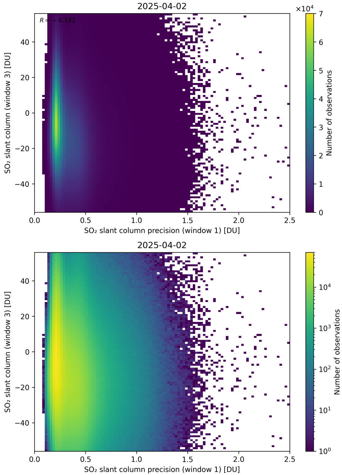
Figure 278: Scatter density plot of “SO 2 slant column precision (window 1)” against “SO 2 slant column (window 3)” for 2025-04-02 to 2025-04-03.
