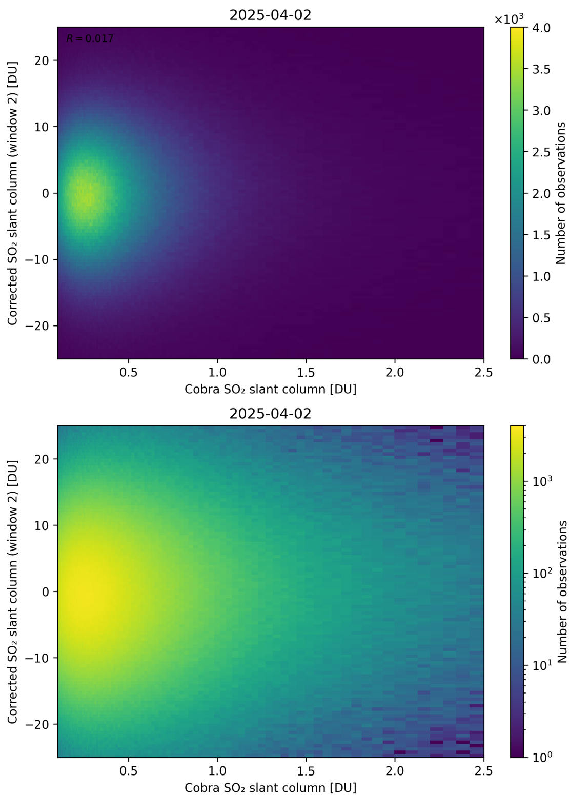
Figure 217: Scatter density plot of “Cobra SO 2 slant column” against “Corrected SO 2 slant column (window 2)” for 2025-04-02 to 2025-04-03.
