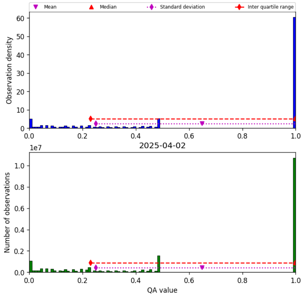
Figure 57: Histogram of “QA value” for 2025-04-02 to 2025-04-03
