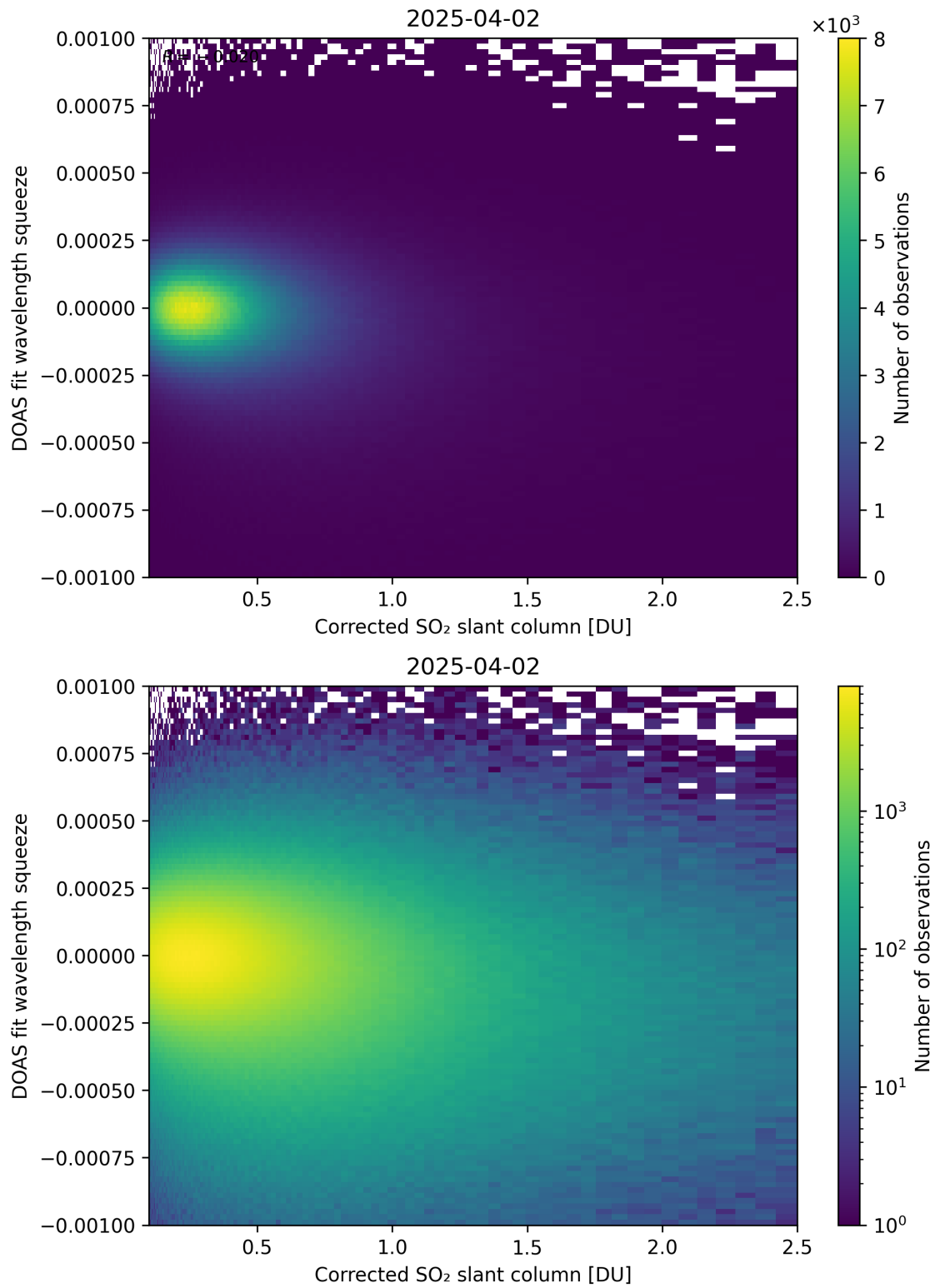
Figure 230: Scatter density plot of “Corrected SO 2 slant column” against “DOAS fit wavelength squeeze” for 2025-04-02 to 2025-04-03.
