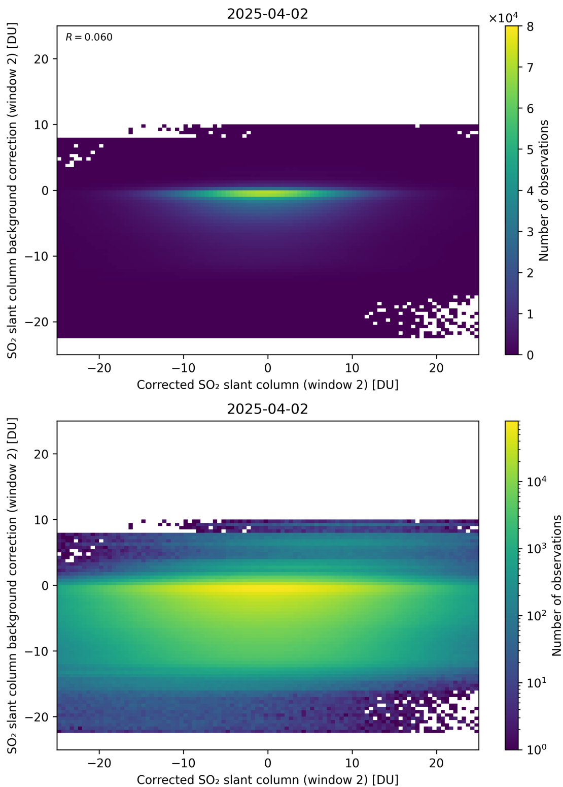
Figure 244: Scatter density plot of “Corrected SO 2 slant column (window 2)” against “SO 2 slant column background correction (window 2)” for 2025-04-02 to 2025-04-03.
