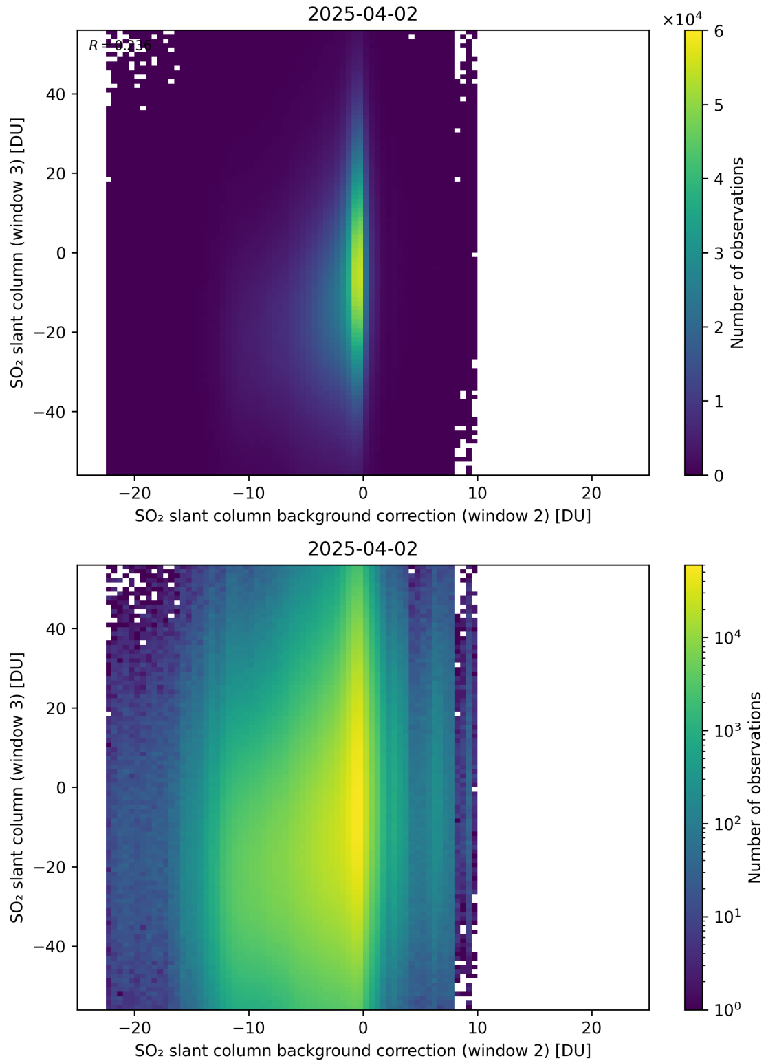
Figure 128: Scatter density plot of “SO 2 slant column background correction (window 2)” against “SO 2 slant column (window 3)” for 2025-04-02 to 2025-04-03.
