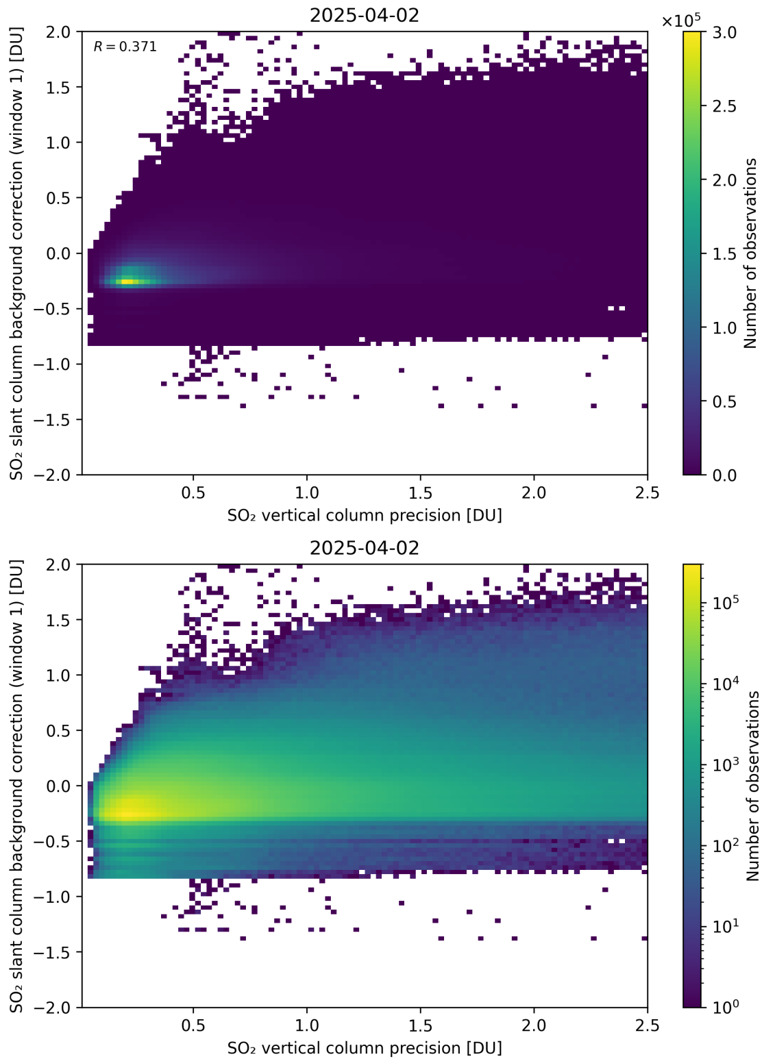
Figure 329: Scatter density plot of “SO 2 vertical column precision” against “SO 2 slant column background correction (window 1)” for 2025-04-02 to 2025-04-03.
