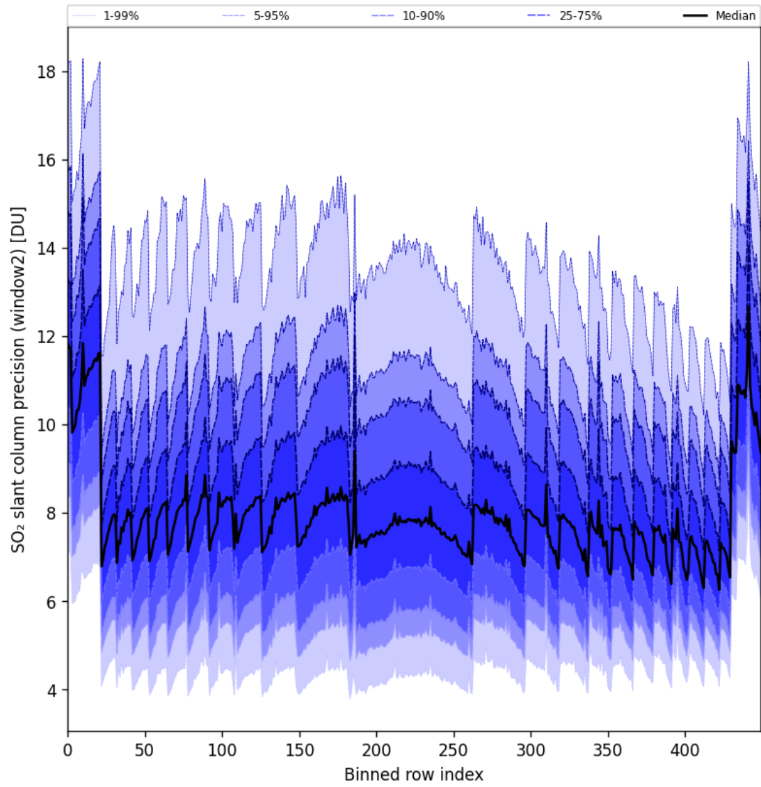
Figure 94: Along track statistics of “SO 2 slant column precision (window2)” for 2025-04-02 to 2025-04-03
