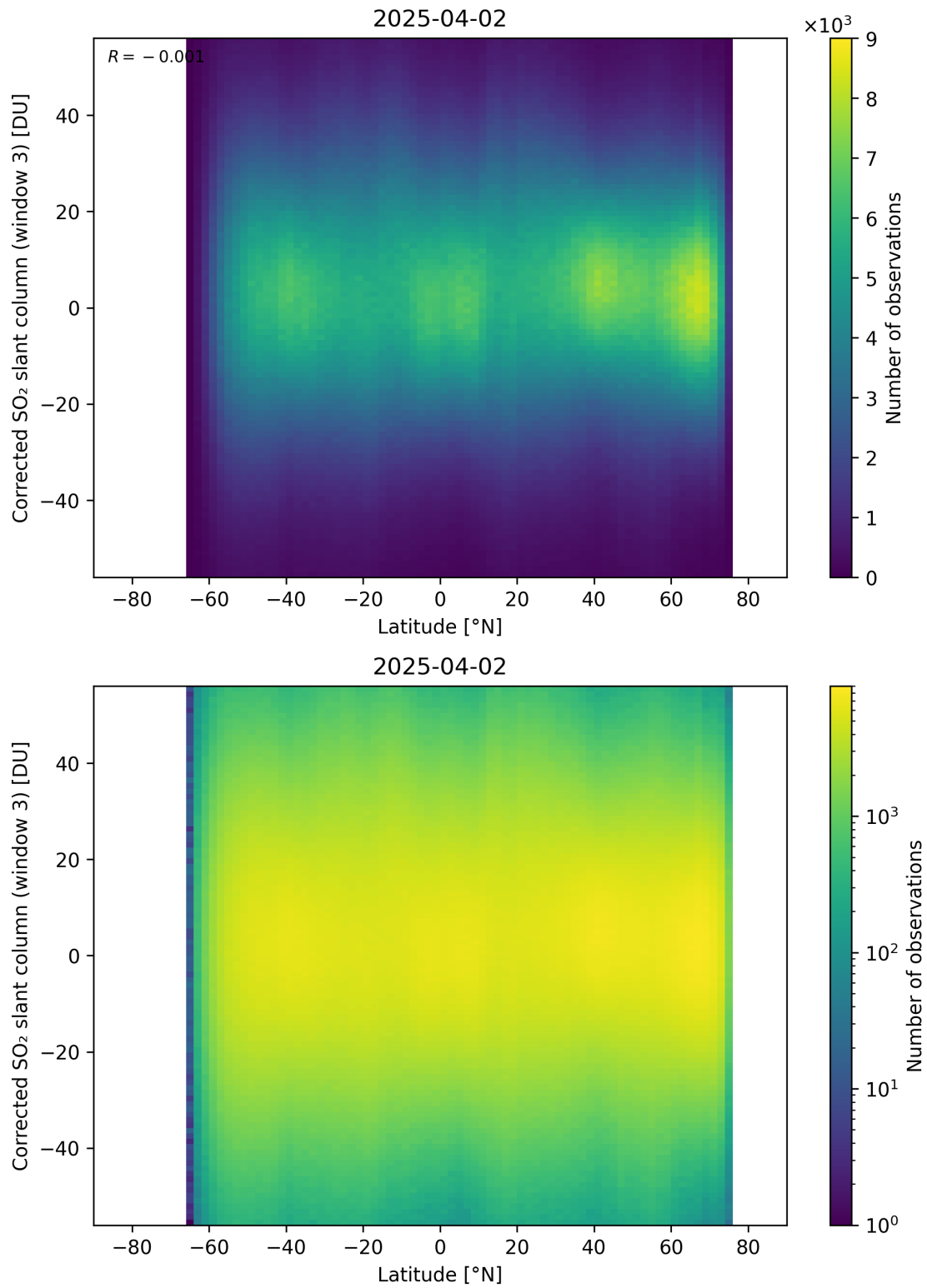
Figure 161: Scatter density plot of “Latitude” against “Corrected SO 2 slant column (window 3)” for 2025-04-02 to 2025-04-03.
