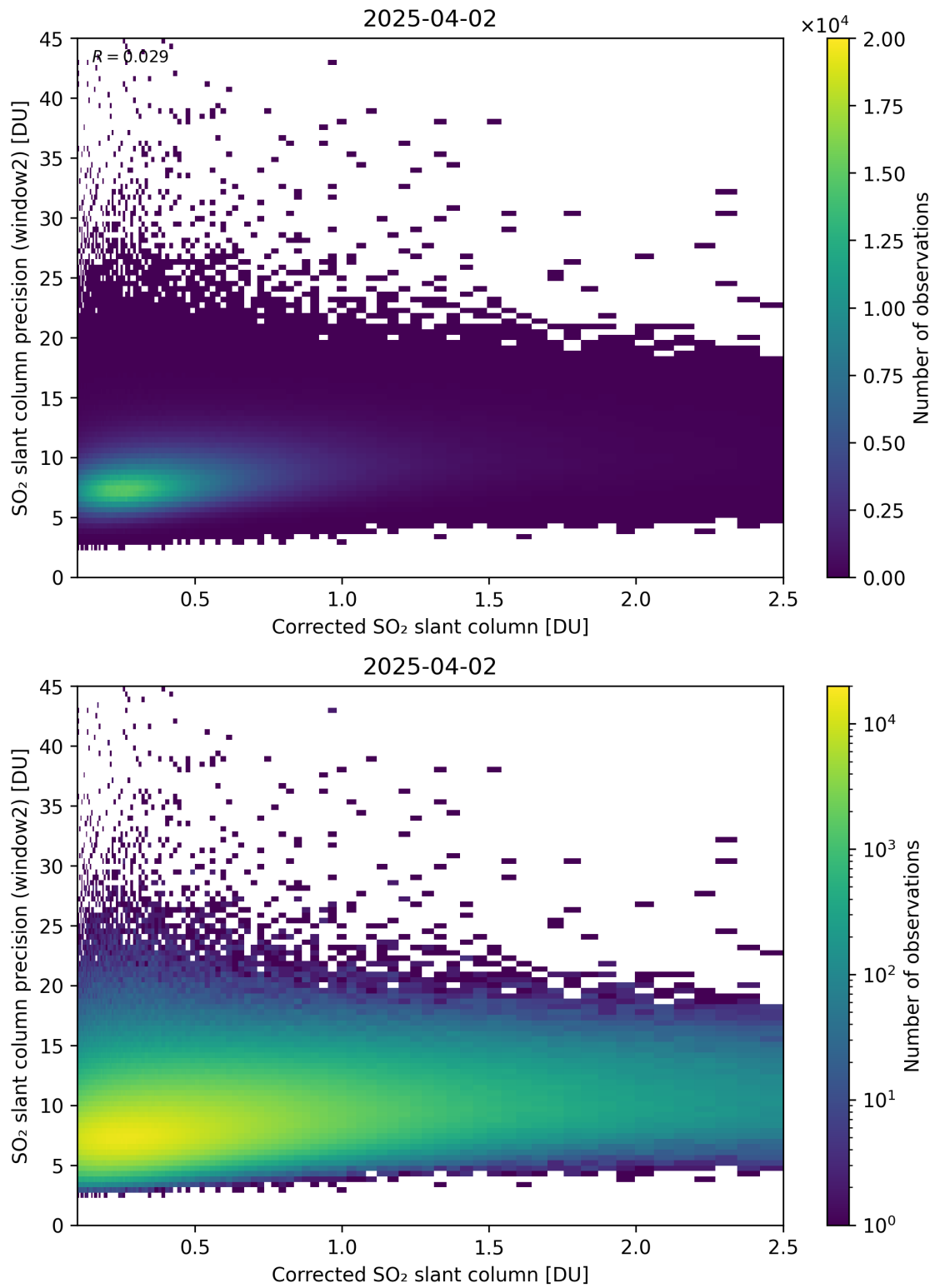
Figure 239: Scatter density plot of “Corrected SO 2 slant column” against “SO 2 slant column precision (window2)” for 2025-04-02 to 2025-04-03.
