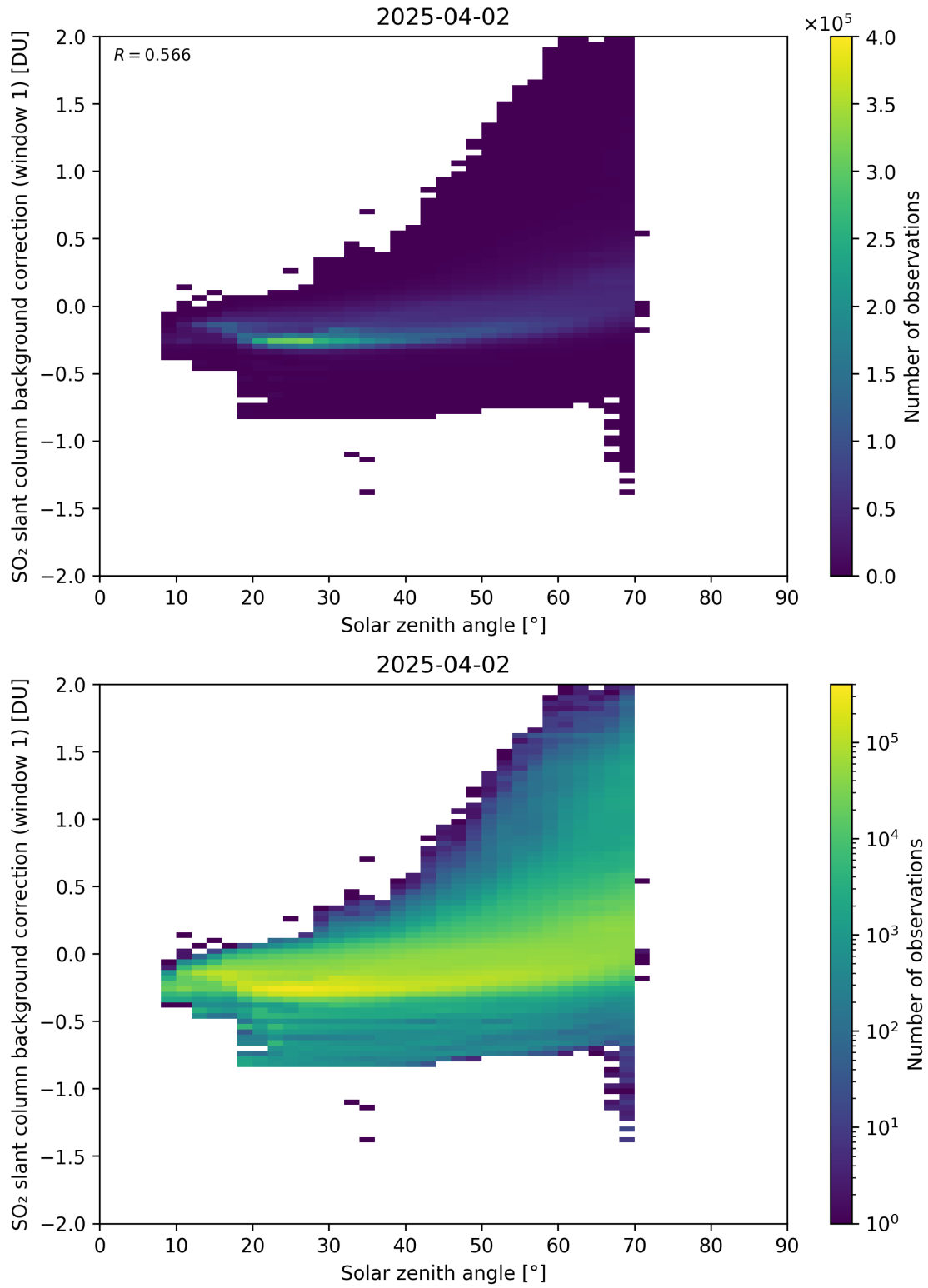
Figure 171: Scatter density plot of “Solar zenith angle” against “SO 2 slant column background correction (window 1)” for 2025-04-02 to 2025-04-03.
