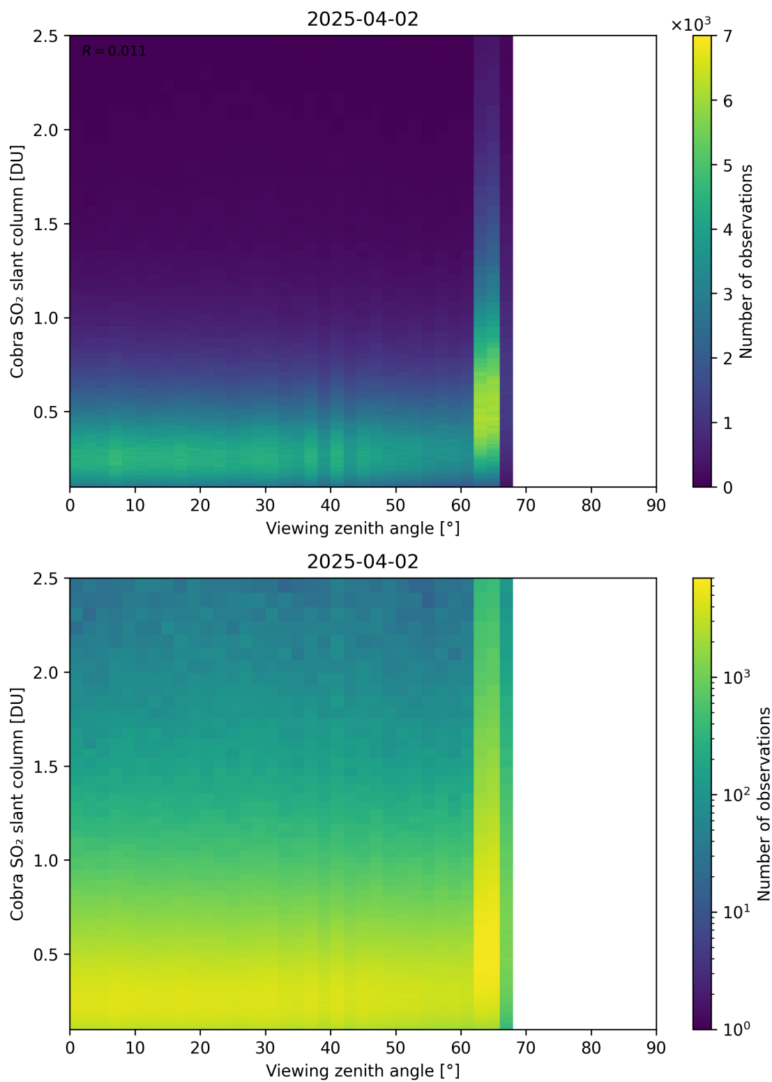
Figure 371: Scatter density plot of “Viewing zenith angle” against “Cobra SO 2 slant column” for 2025-04-02 to 2025-04-03.
