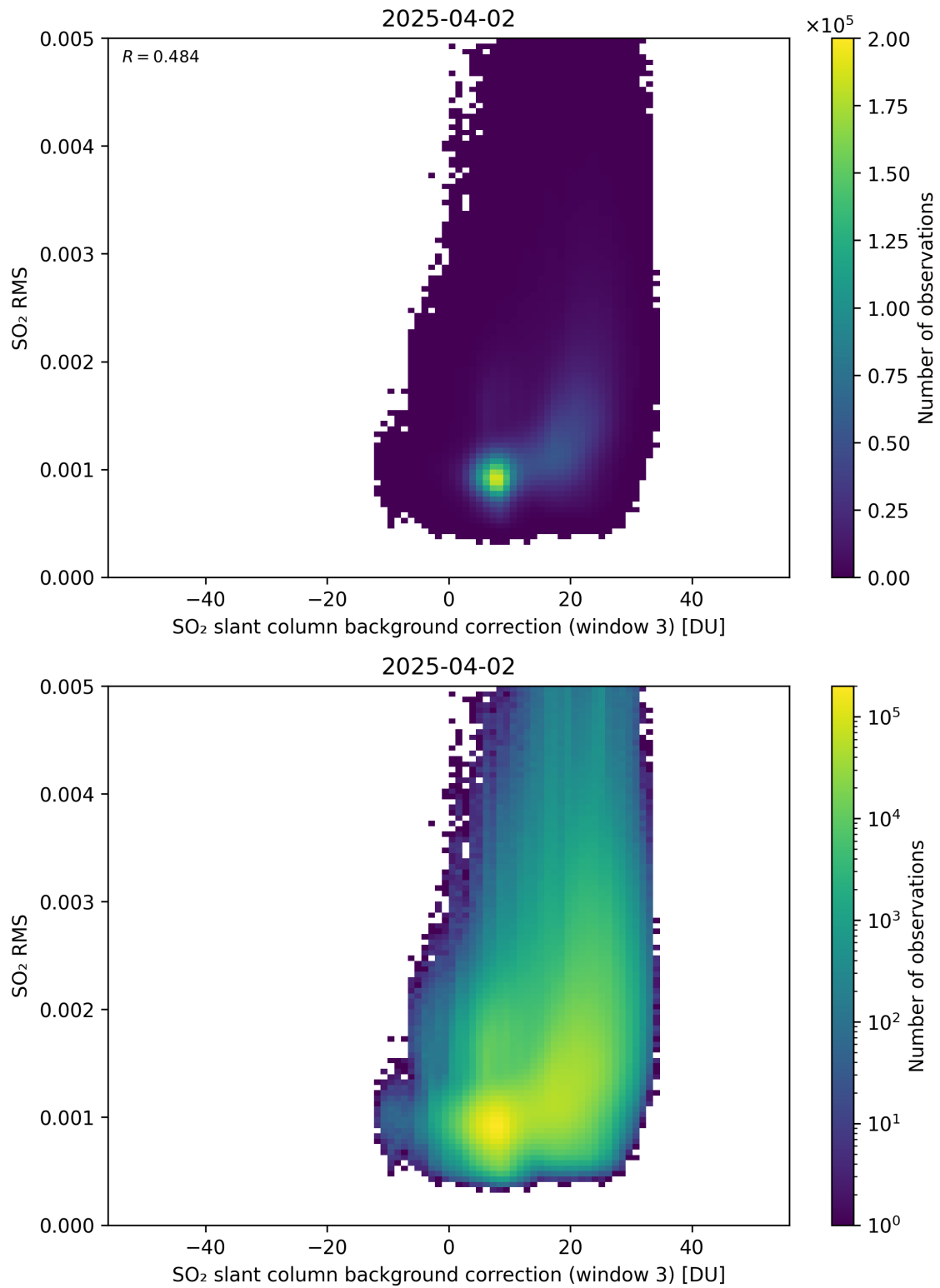
Figure 134: Scatter density plot of “SO 2 slant column background correction (window 3)” against “SO 2 RMS” for 2025-04-02 to 2025-04-03.
