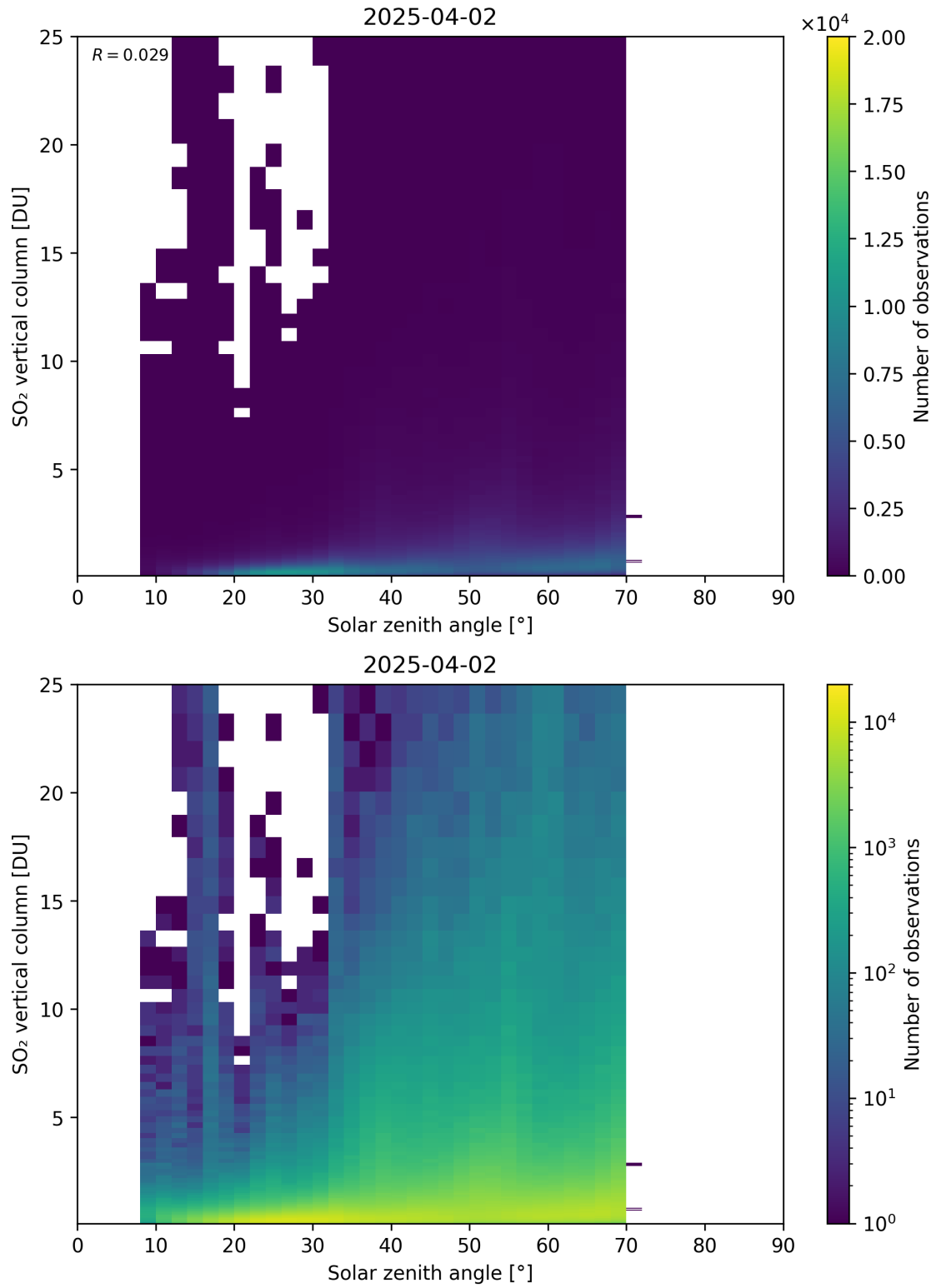
Figure 191: Scatter density plot of “Solar zenith angle” against “SO 2 vertical column” for 2025-04-02 to 2025-04-03.
