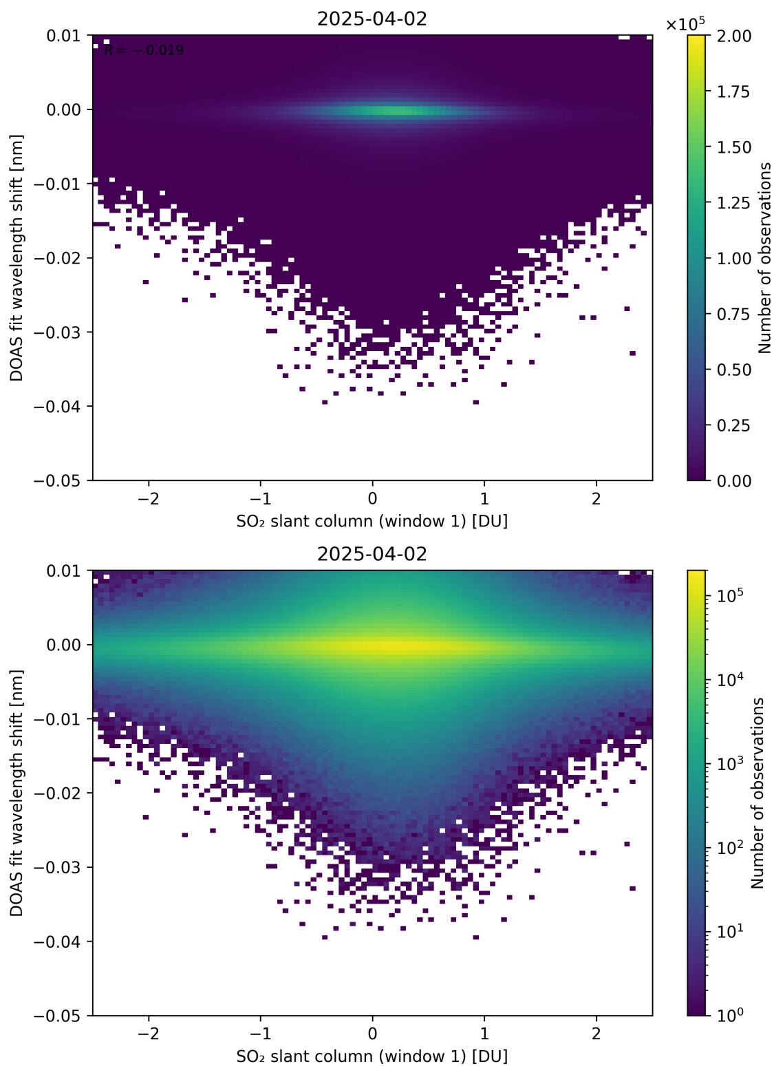
Figure 265: Scatter density plot of “SO 2 slant column (window 1)” against “DOAS fit wavelength shift” for 2025-04-02 to 2025-04-03.
