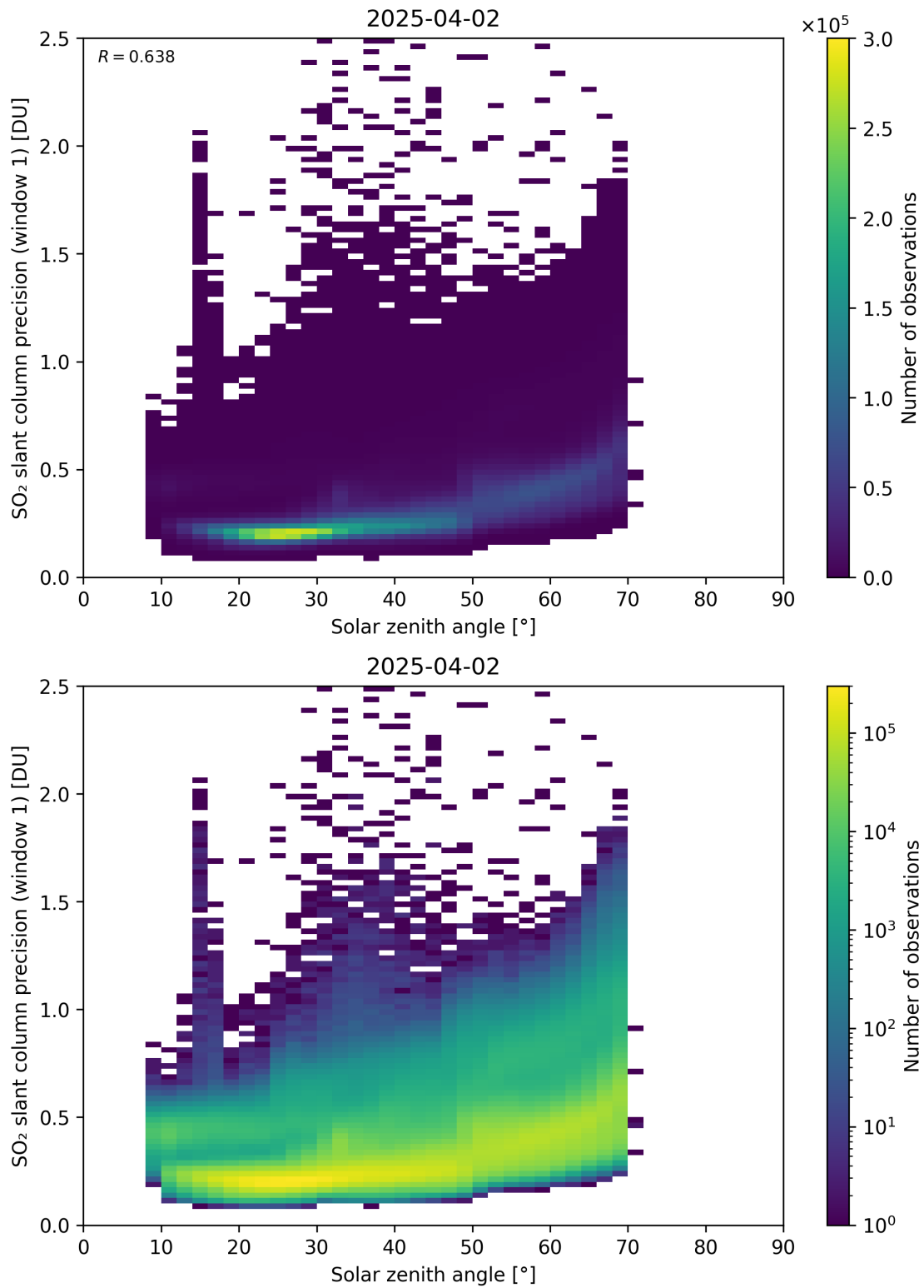
Figure 185: Scatter density plot of “Solar zenith angle” against “SO 2 slant column precision (window 1)” for 2025-04-02 to 2025-04-03.
