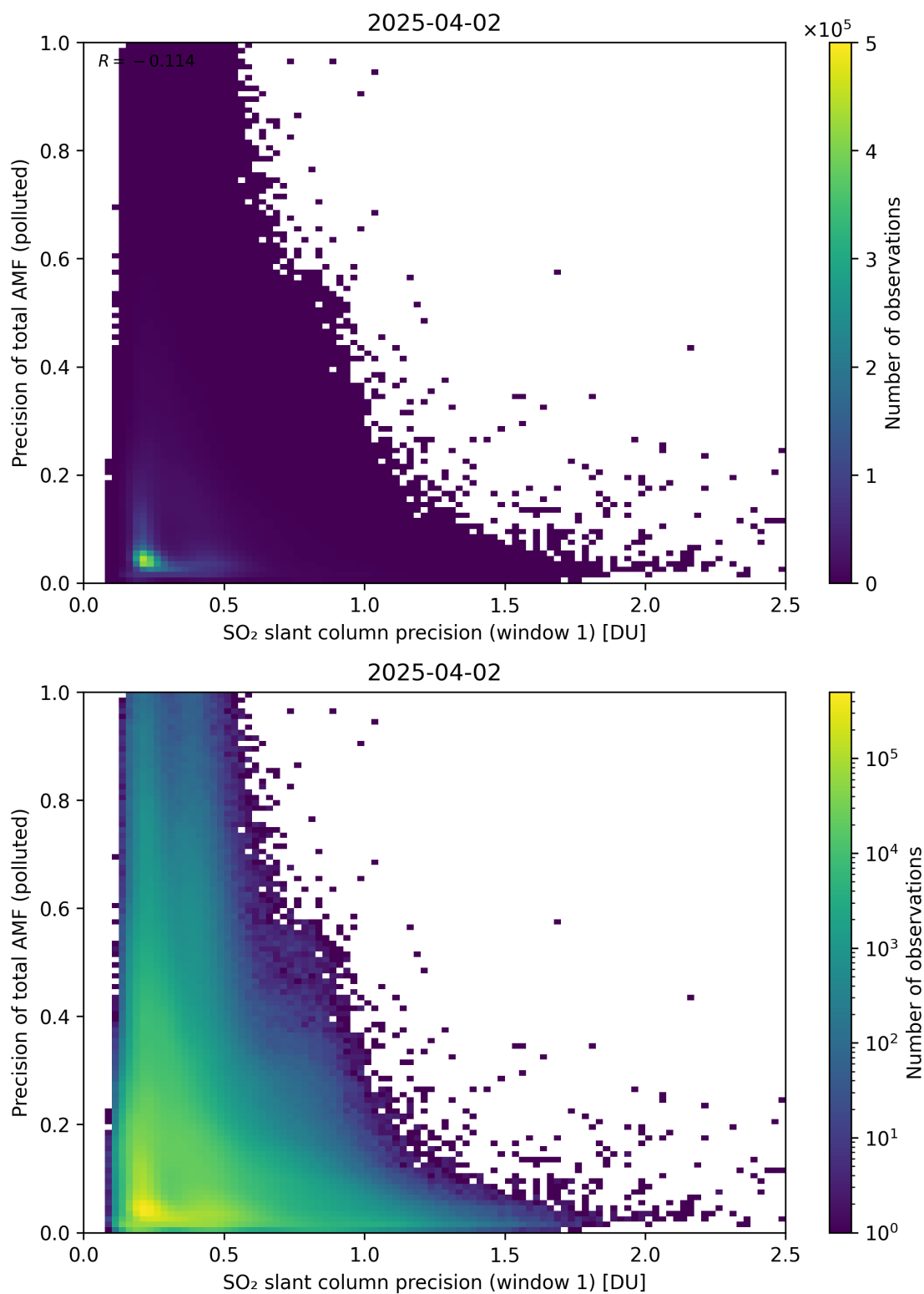
Figure 281: Scatter density plot of “SO 2 slant column precision (window 1)” against “Precision of total AMF (polluted)” for 2025-04-02 to 2025-04-03.
