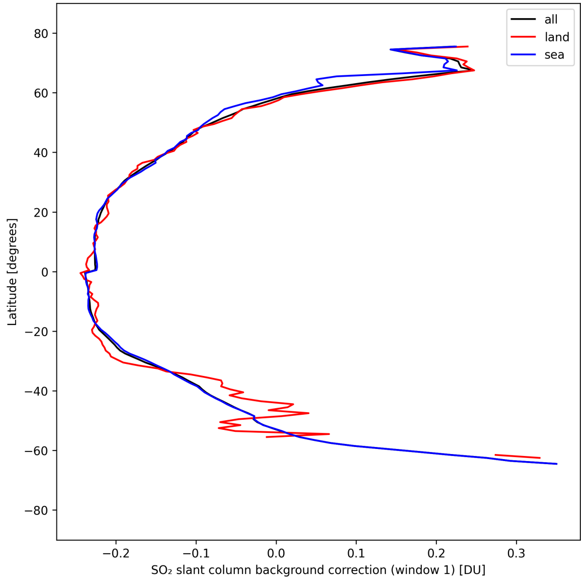
Figure 40: Zonal average of “SO 2 slant column background correction (window 1)” for 2025-04-02 to 2025-04-03.
