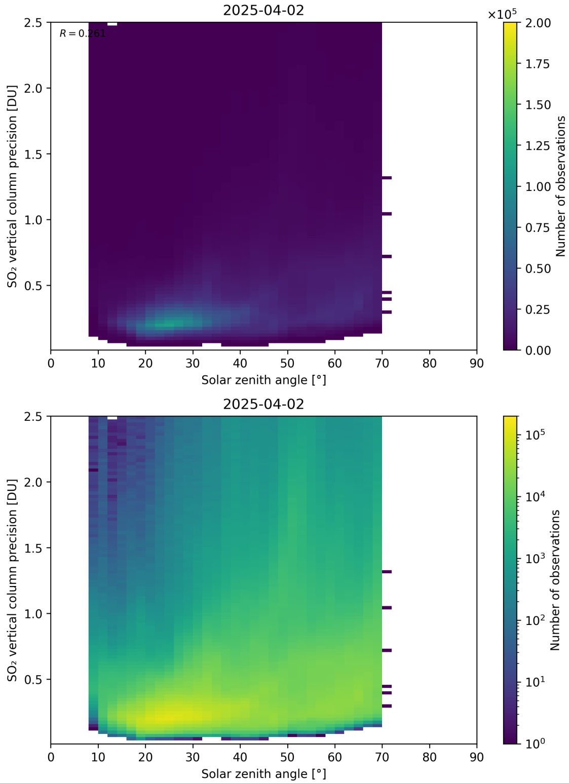
Figure 192: Scatter density plot of “Solar zenith angle” against “SO 2 vertical column precision” for 2025-04-02 to 2025-04-03.
