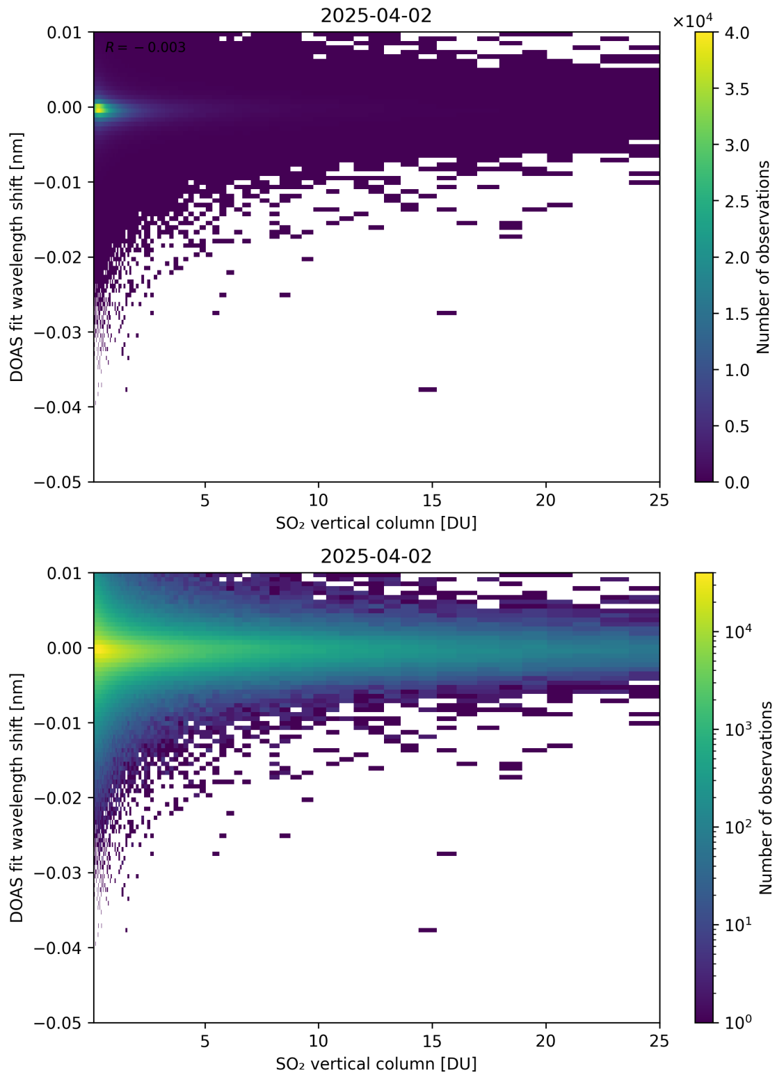
Figure 326: Scatter density plot of “SO 2 vertical column” against “DOAS fit wavelength shift” for 2025-04-02 to 2025-04-03.
