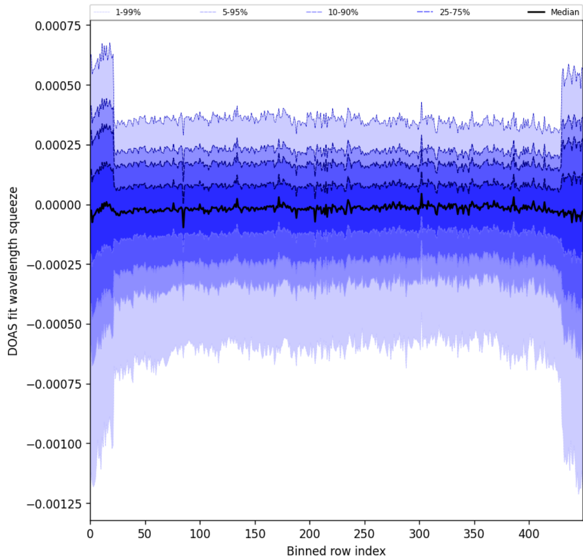
Figure 103: Along track statistics of “DOAS fit wavelength squeeze” for 2025-04-02 to 2025-04-03
