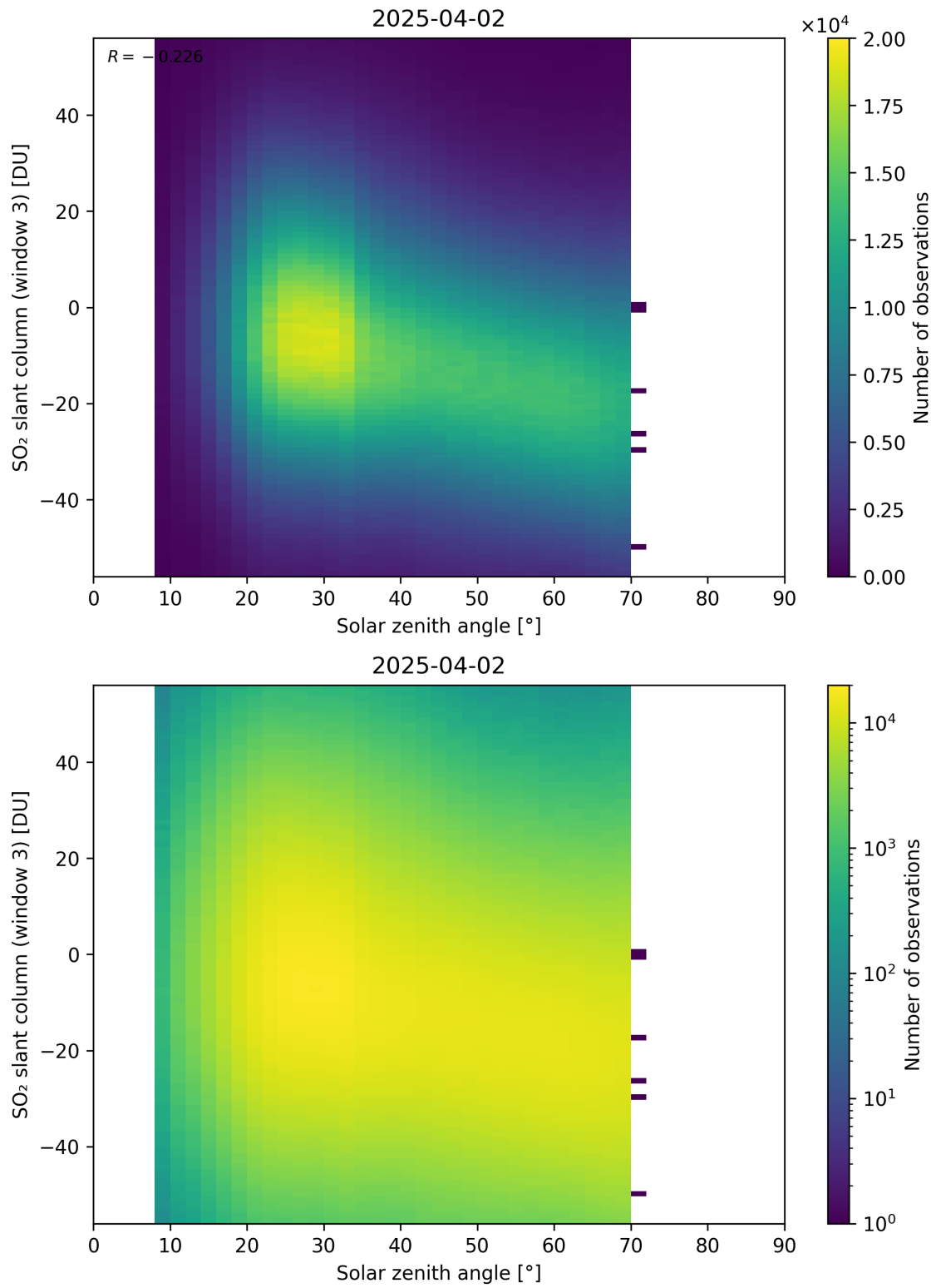
Figure 187: Scatter density plot of “Solar zenith angle” against “SO 2 slant column (window 3)” for 2025-04-02 to 2025-04-03.
