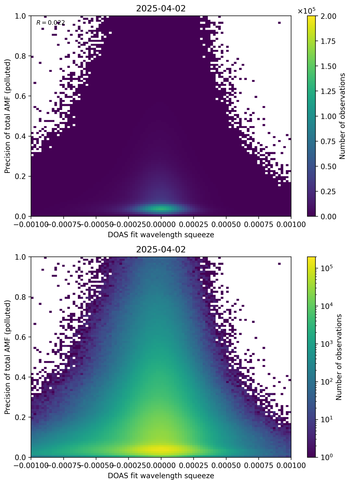
Figure 146: Scatter density plot of “DOAS fit wavelength squeeze” against “Precision of total AMF (polluted)” for 2025-04-02 to 2025-04-03.
