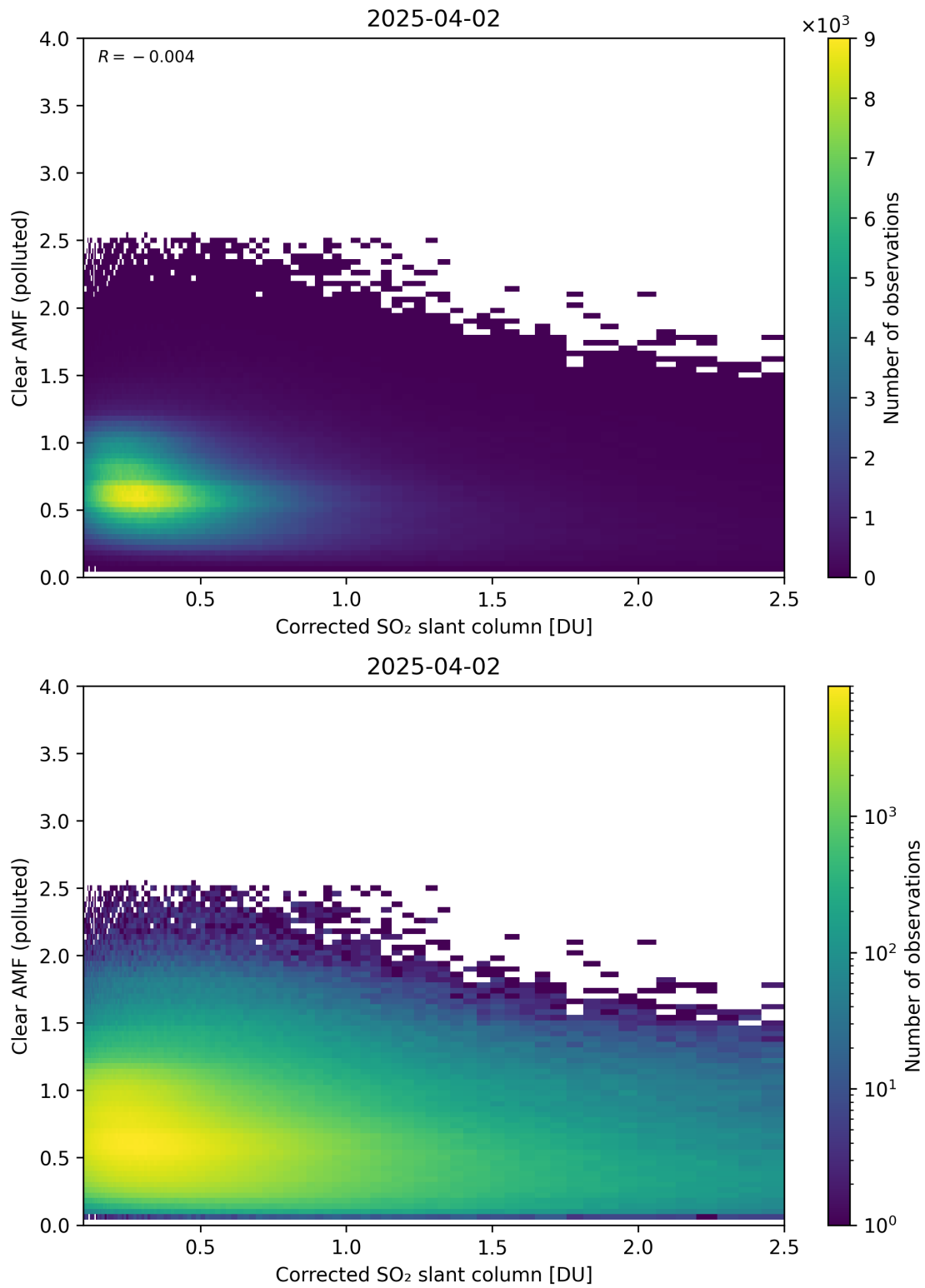
Figure 232: Scatter density plot of “Corrected SO 2 slant column” against “Clear AMF (polluted)” for 2025-04-02 to 2025-04-03.
