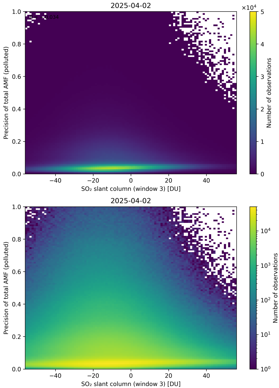
Figure 319: Scatter density plot of “SO 2 slant column (window 3)” against “Precision of total AMF (polluted)” for 2025-04-02 to 2025-04-03.
