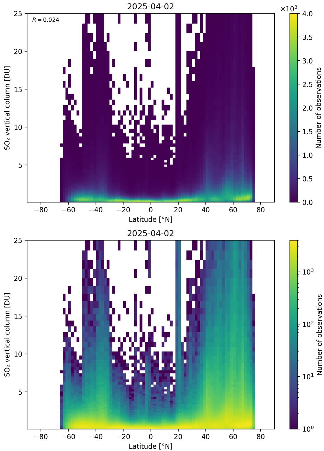
Figure 169: Scatter density plot of “Latitude” against “SO 2 vertical column” for 2025-04-02 to 2025-04-03.
