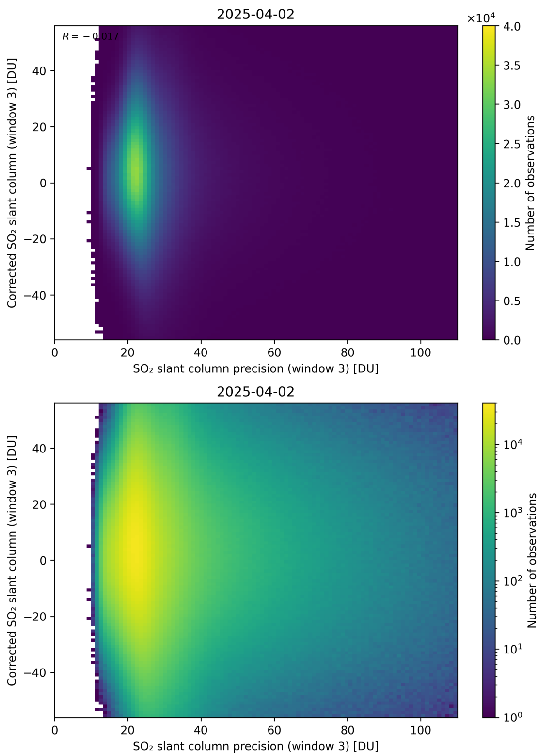
Figure 312: Scatter density plot of “SO 2 slant column precision (window 3)” against “Corrected SO 2 slant column (window 3)” for 2025-04-02 to 2025-04-03.
