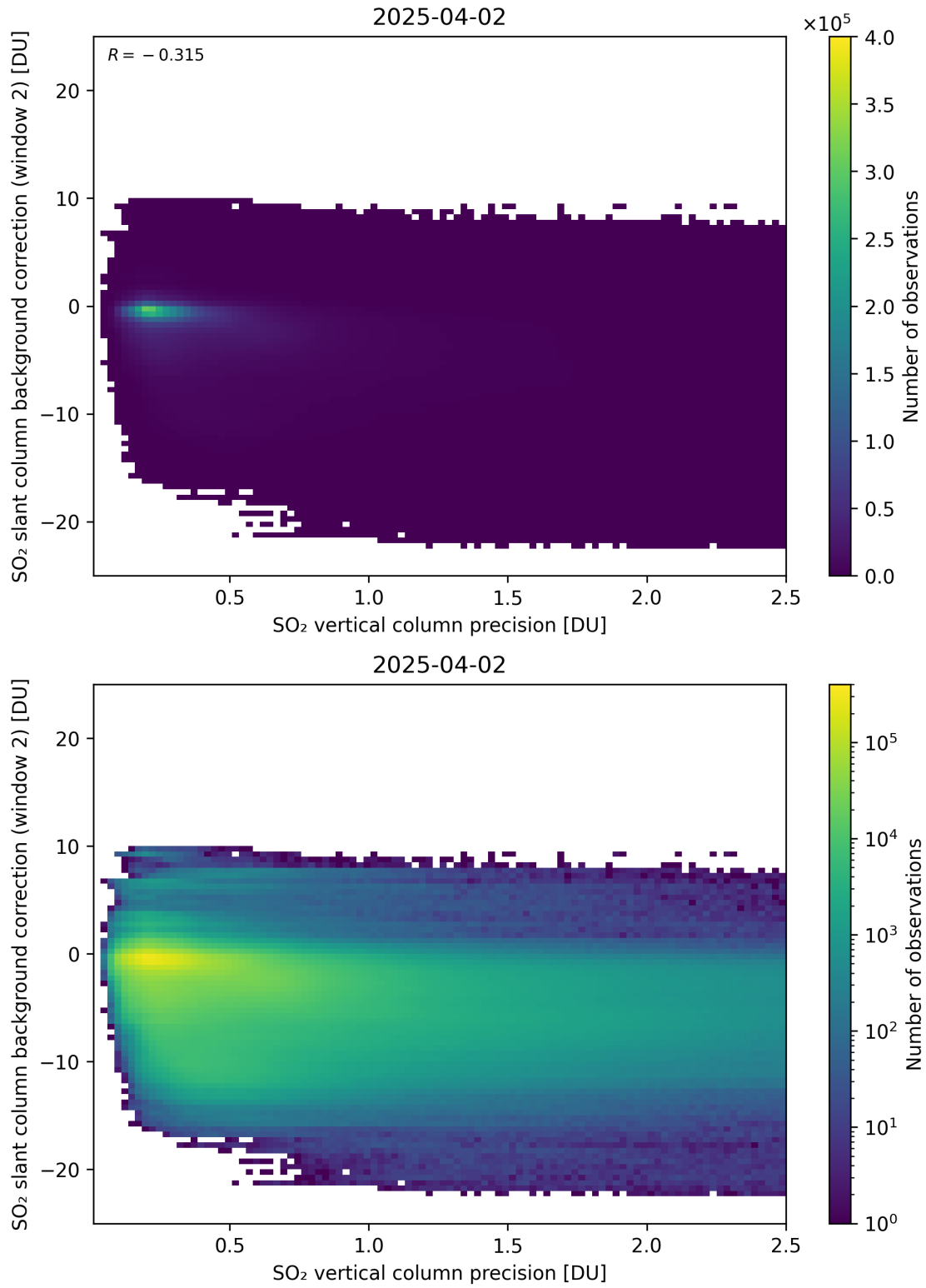
Figure 330: Scatter density plot of “SO 2 vertical column precision” against “SO 2 slant column background correction (window 2)” for 2025-04-02 to 2025-04-03.
