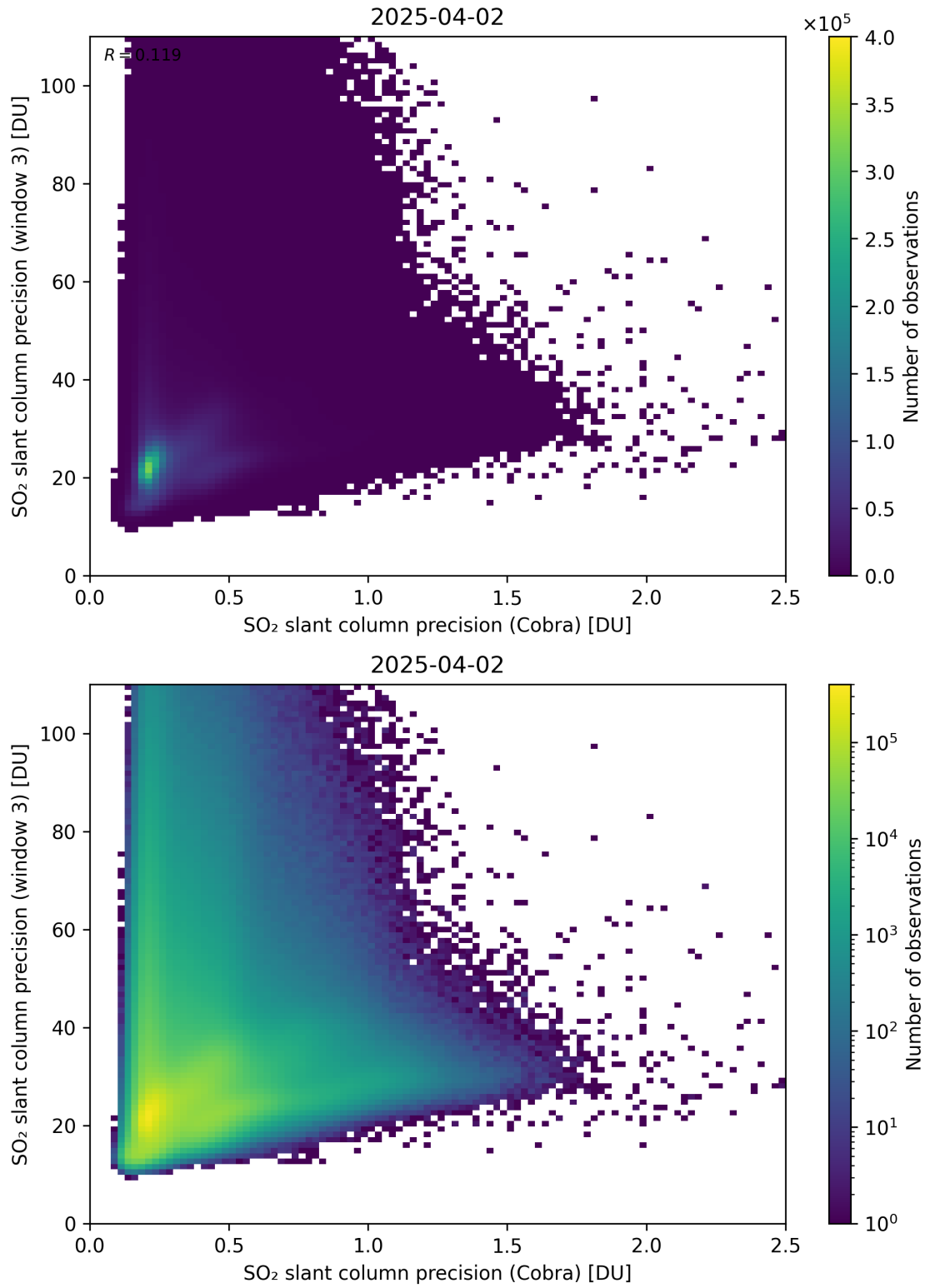
Figure 212: Scatter density plot of “SO 2 slant column precision (Cobra)” against “SO 2 slant column precision (window 3)” for 2025-04-02 to 2025-04-03.
