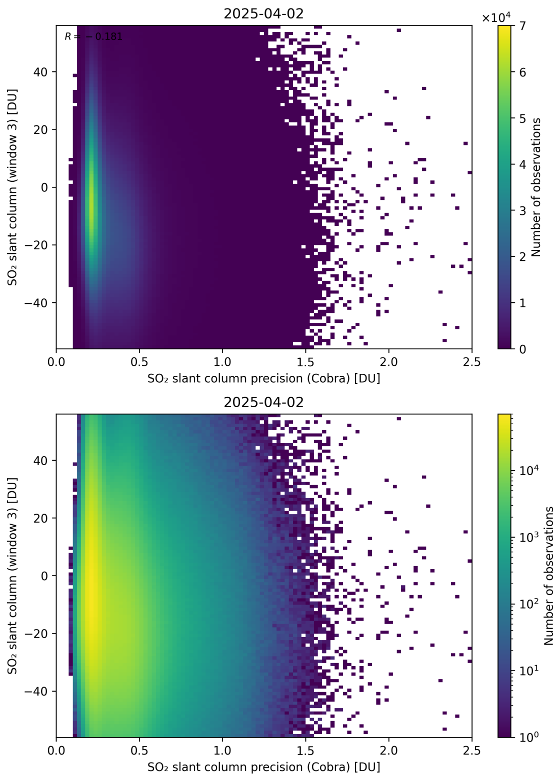
Figure 211: Scatter density plot of “SO 2 slant column precision (Cobra)” against “SO 2 slant column (window 3)” for 2025-04-02 to 2025-04-03.
