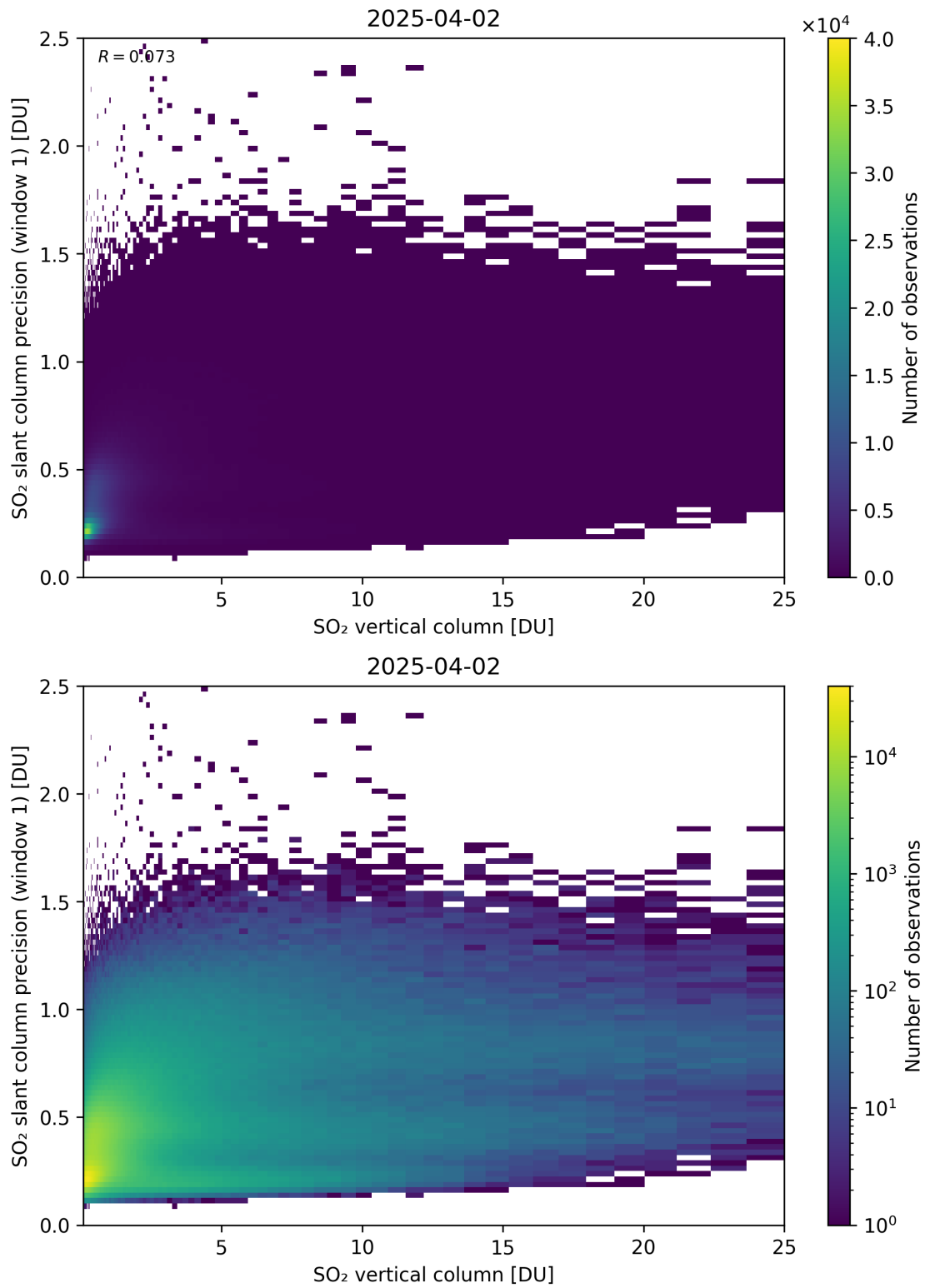
Figure 355: Scatter density plot of “SO 2 vertical column” against “SO 2 slant column precision (window 1)” for 2025-04-02 to 2025-04-03.
