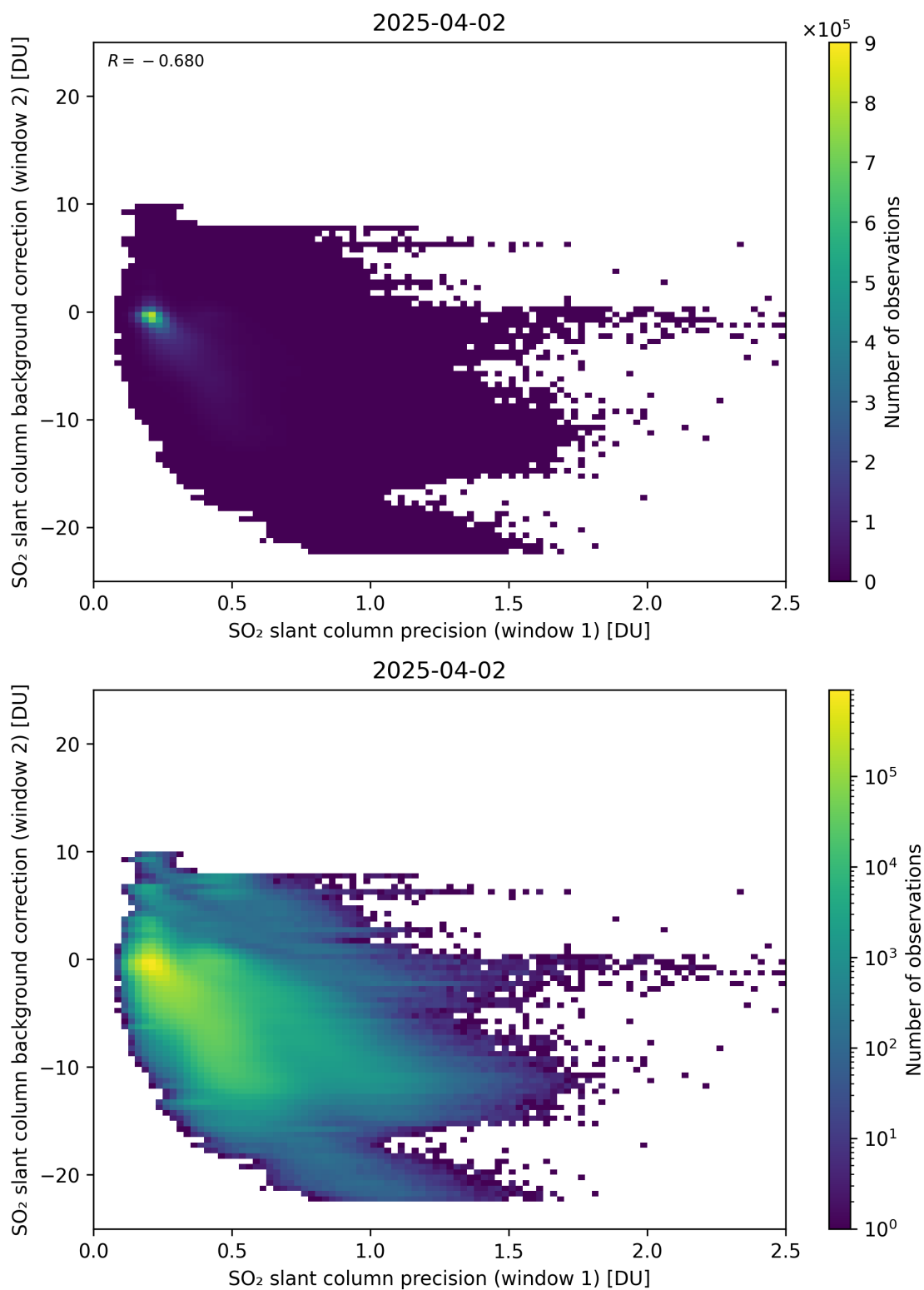
Figure 269: Scatter density plot of “SO 2 slant column precision (window 1)” against “SO 2 slant column background correction (window 2)” for 2025-04-02 to 2025-04-03.
