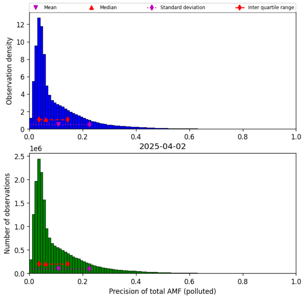
Figure 80: Histogram of “Precision of total AMF (polluted)” for 2025-04-02 to 2025-04-03
