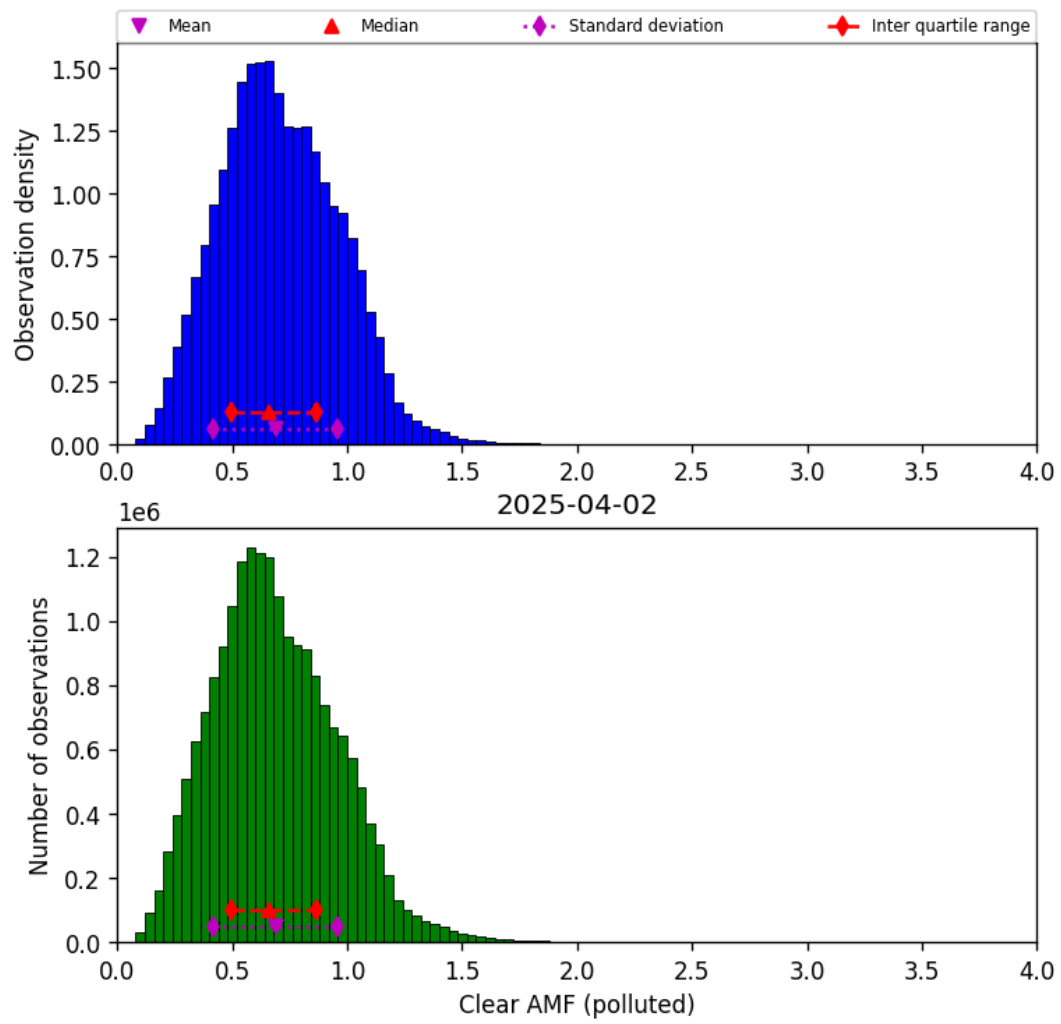
Figure 81: Histogram of “Clear AMF (polluted)” for 2025-04-02 to 2025-04-03
