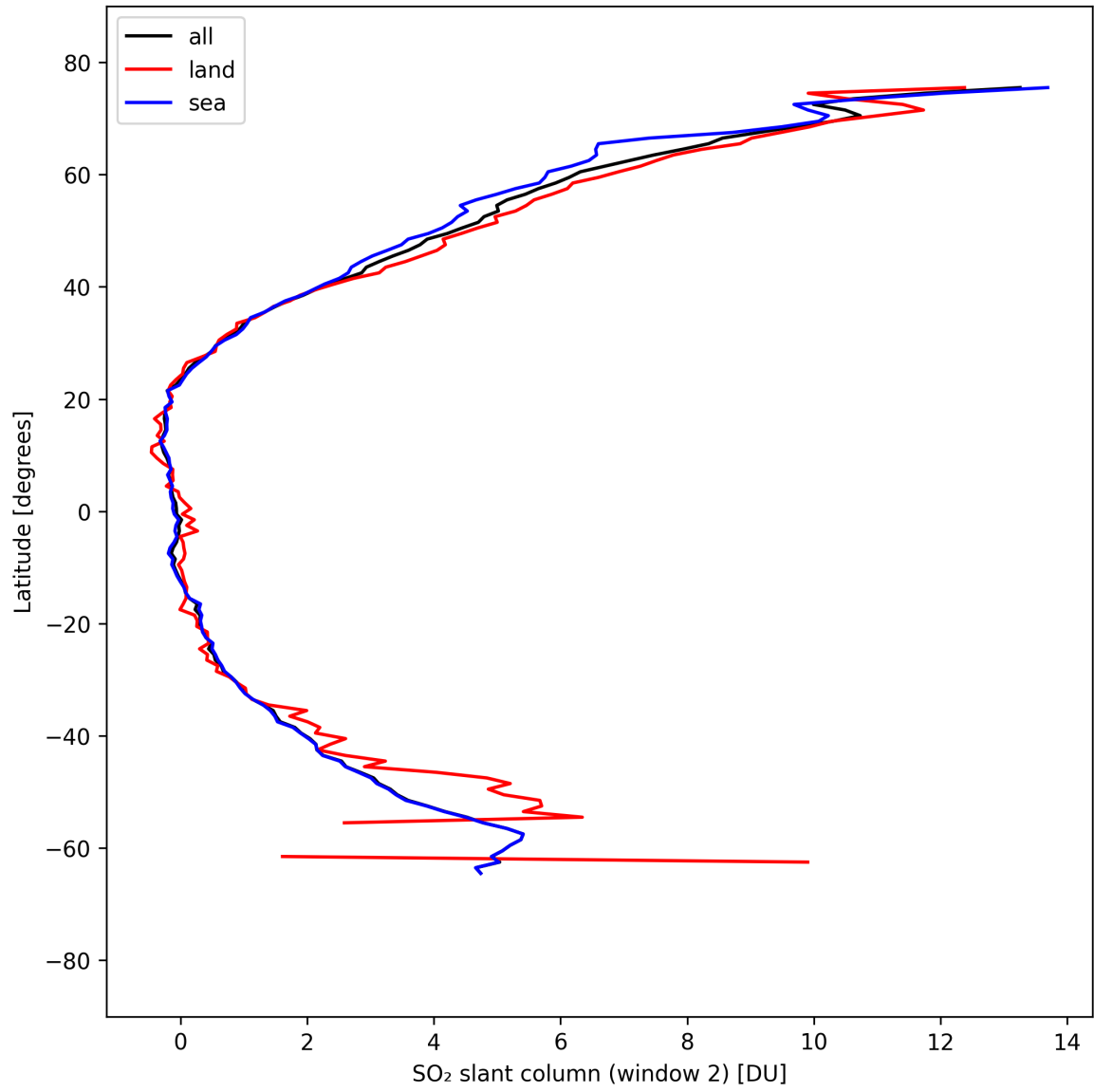
Figure 41: Zonal average of “SO 2 slant column (window 2)” for 2025-04-02 to 2025-04-03.
