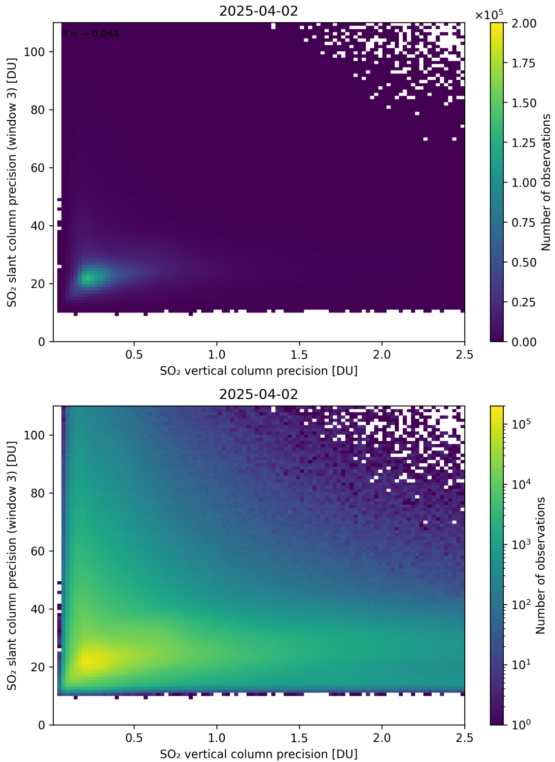
Figure 345: Scatter density plot of “SO 2 vertical column precision” against “SO 2 slant column precision (window 3)” for 2025-04-02 to 2025-04-03.
