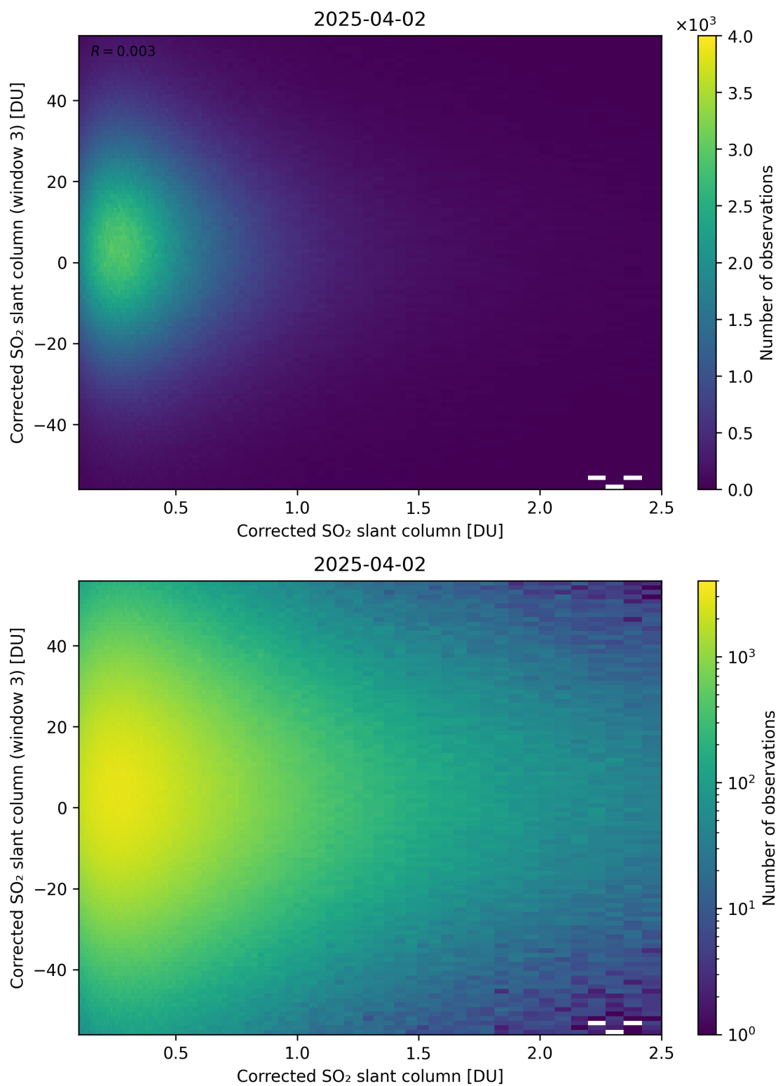
Figure 236: Scatter density plot of “Corrected SO 2 slant column” against “Corrected SO 2 slant column (window 3)” for 2025-04-02 to 2025-04-03.
