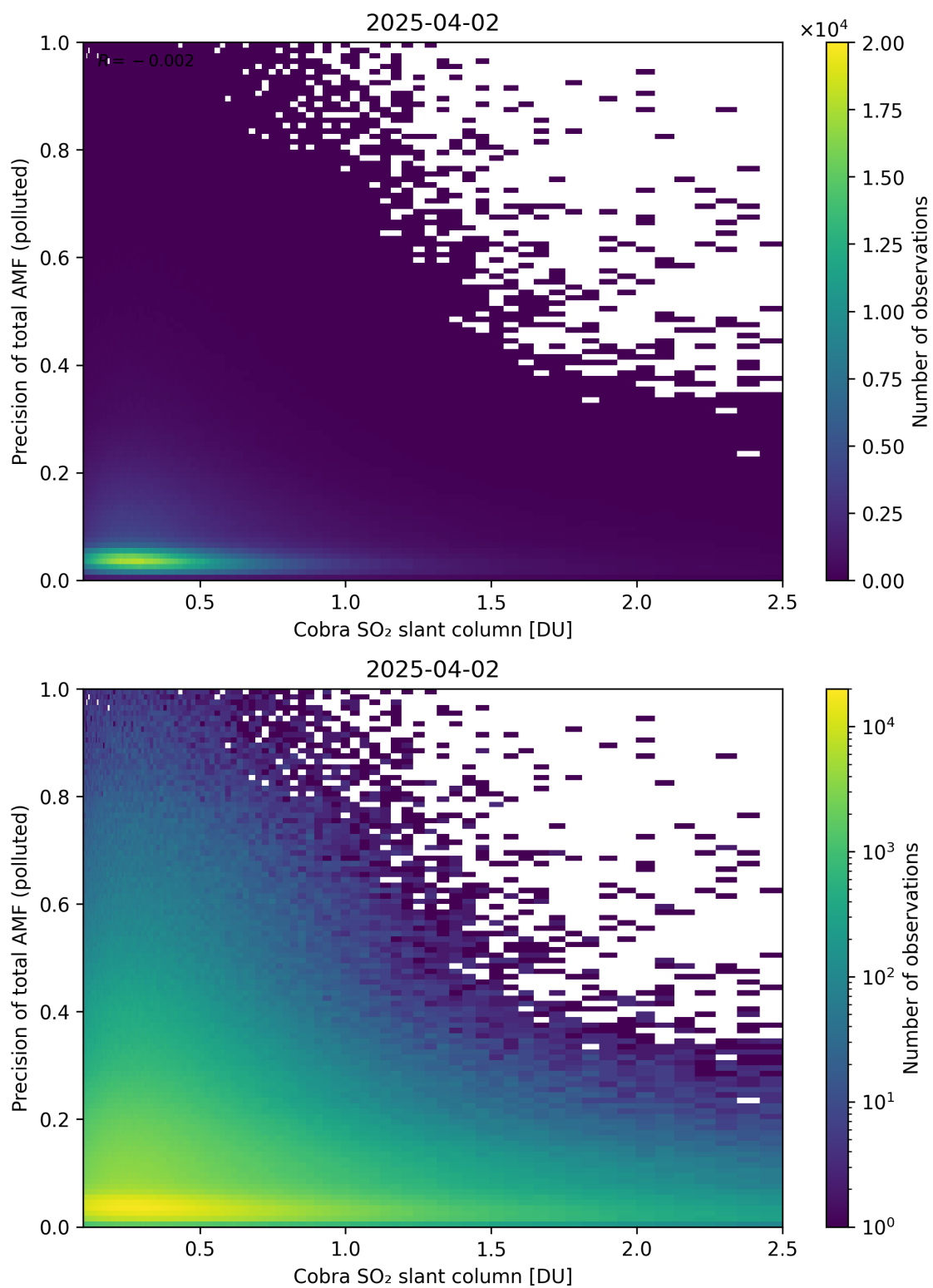
Figure 225: Scatter density plot of “Cobra SO 2 slant column” against “Precision of total AMF (polluted)” for 2025-04-02 to 2025-04-03.
