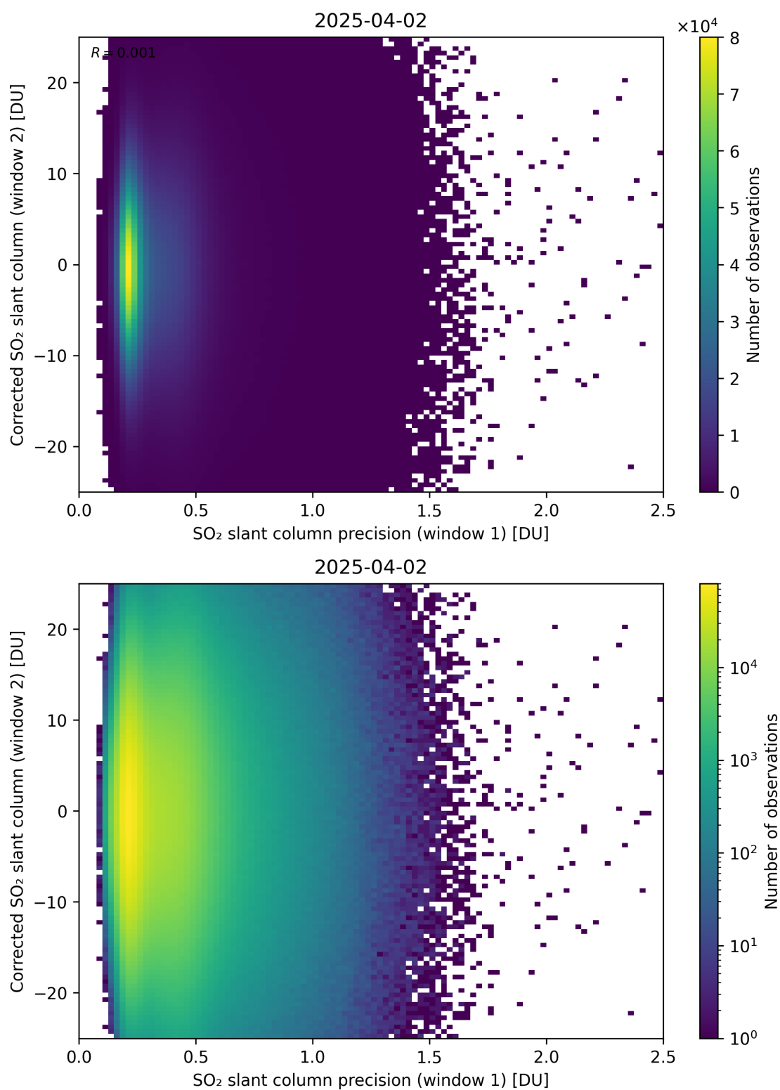
Figure 275: Scatter density plot of “SO 2 slant column precision (window 1)” against “Corrected SO 2 slant column (window 2)” for 2025-04-02 to 2025-04-03.
