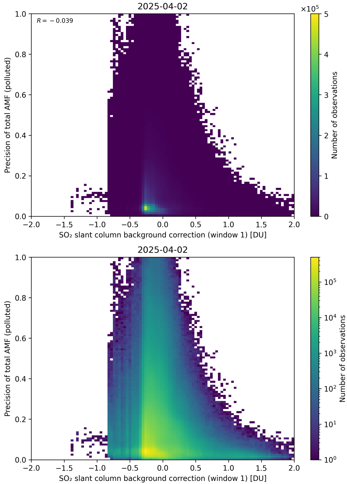
Figure 121: Scatter density plot of “SO 2 slant column background correction (window 1)” against “Precision of total AMF (polluted)” for 2025-04-02 to 2025-04-03.
