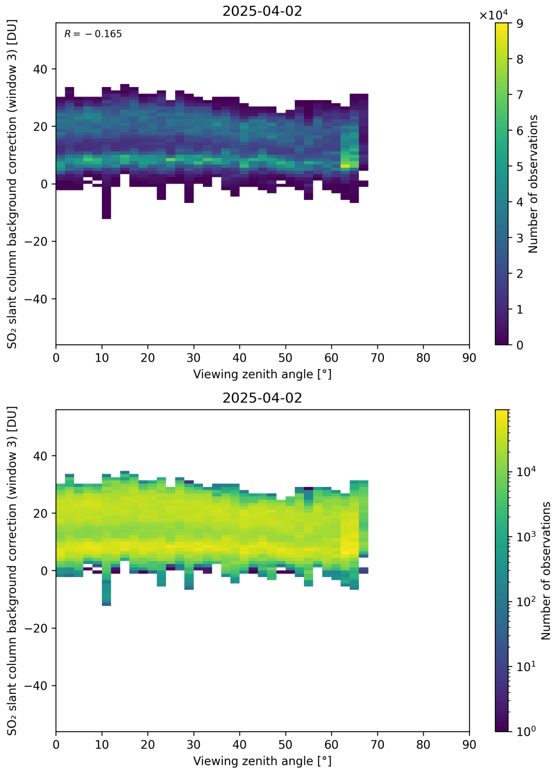
Figure 364: Scatter density plot of “Viewing zenith angle” against “SO 2 slant column background correction (window 3)” for 2025-04-02 to 2025-04-03.
