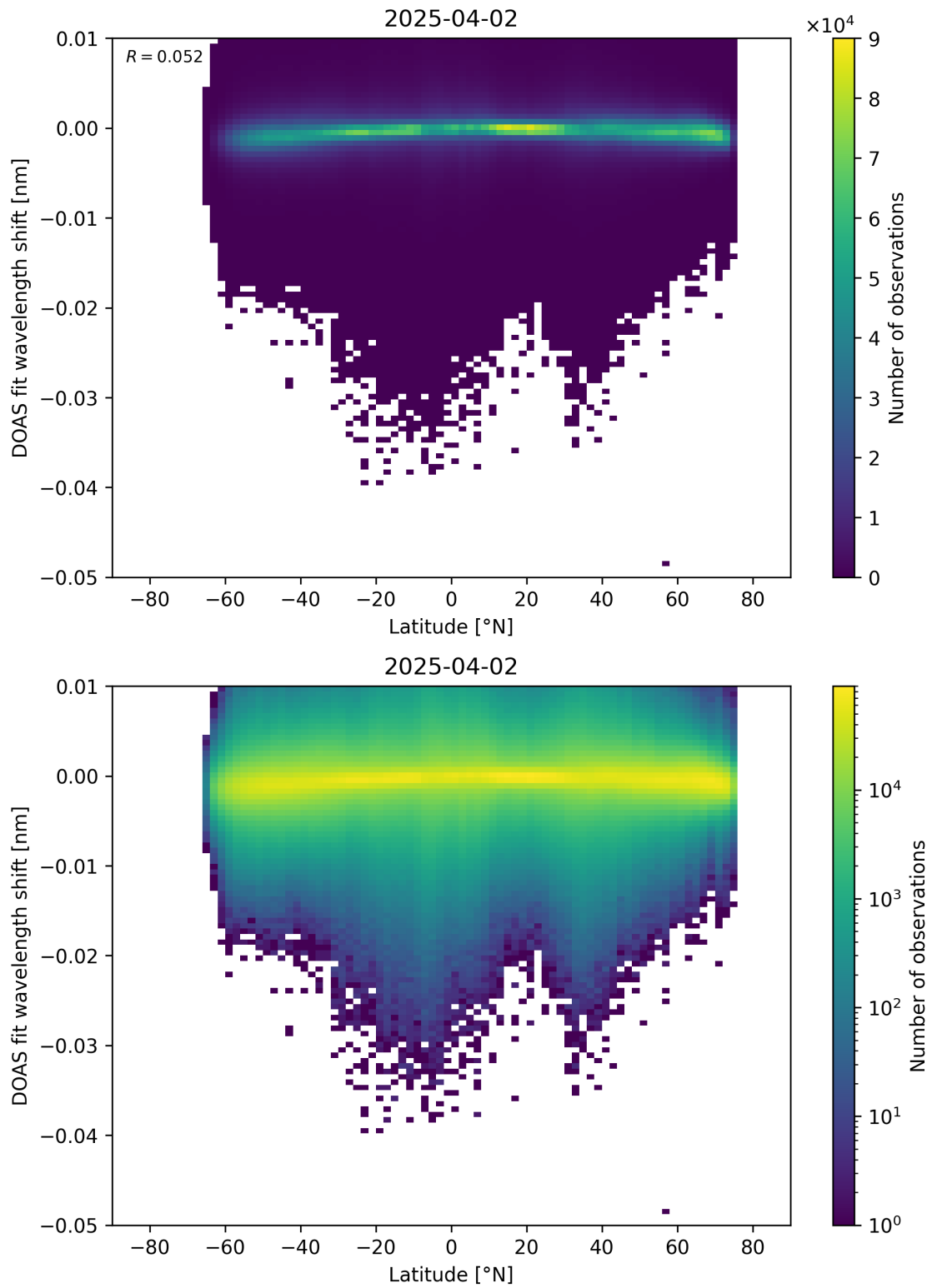
Figure 153: Scatter density plot of “Latitude” against “DOAS fit wavelength shift” for 2025-04-02 to 2025-04-03.
