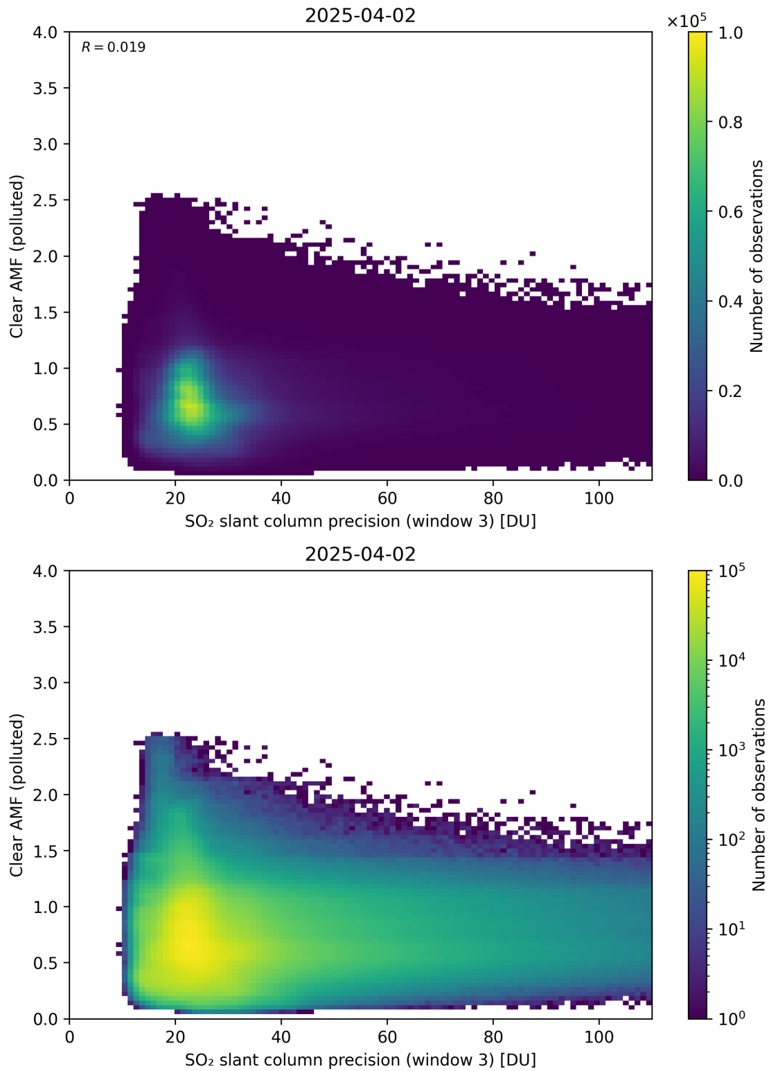
Figure 311: Scatter density plot of “SO 2 slant column precision (window 3)” against “Clear AMF (polluted)” for 2025-04-02 to 2025-04-03.
