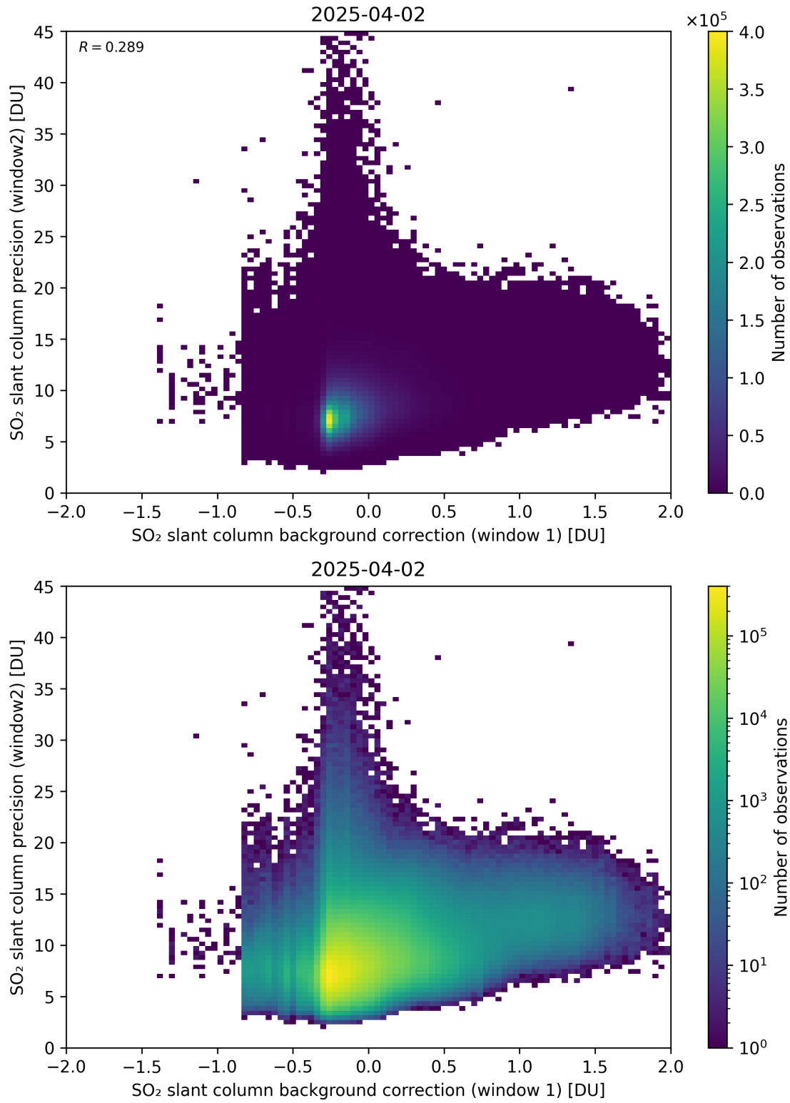
Figure 117: Scatter density plot of “SO 2 slant column background correction (window 1)” against “SO 2 slant column precision (window2)” for 2025-04-02 to 2025-04-03.
