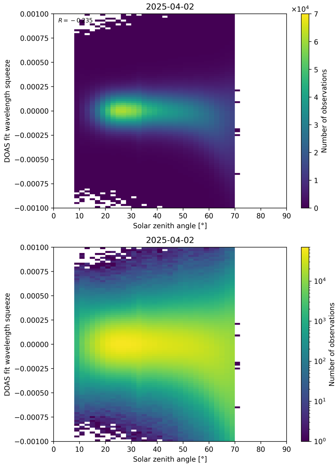
Figure 175: Scatter density plot of “Solar zenith angle” against “DOAS fit wavelength squeeze” for 2025-04-02 to 2025-04-03.
