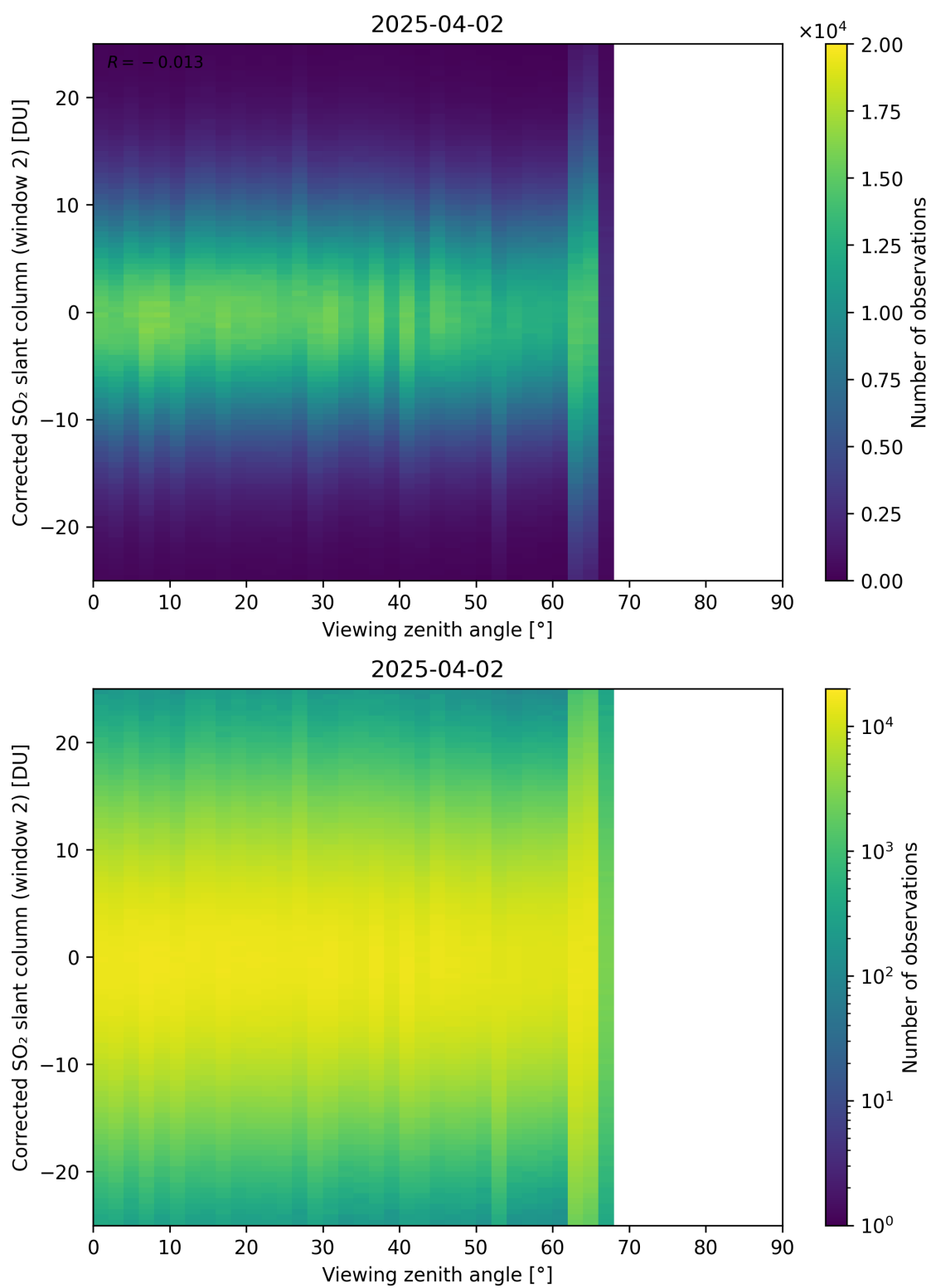
Figure 374: Scatter density plot of “Viewing zenith angle” against “Corrected SO 2 slant column (window 2)” for 2025-04-02 to 2025-04-03.
