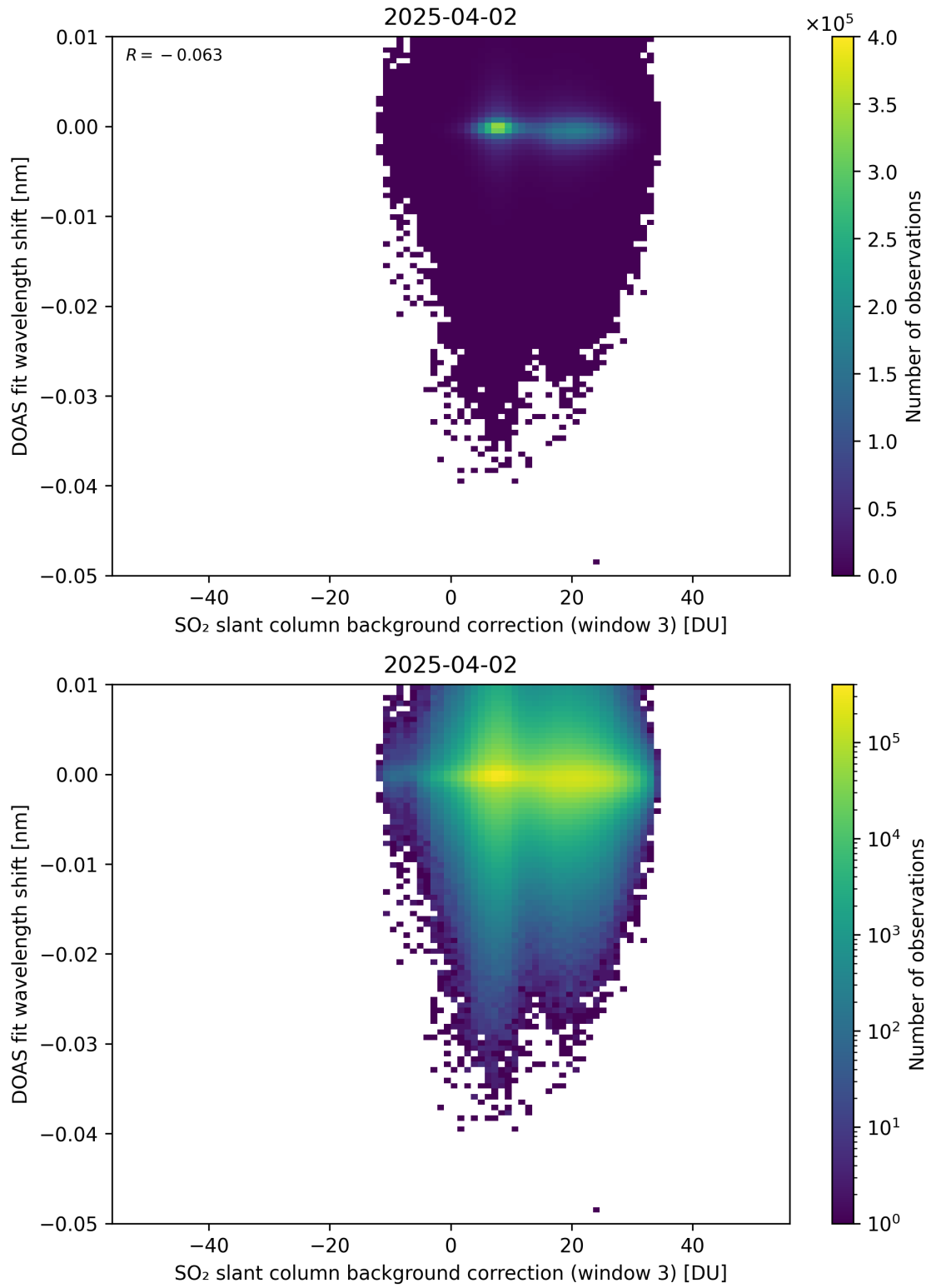
Figure 132: Scatter density plot of “SO 2 slant column background correction (window 3)” against “DOAS fit wavelength shift” for 2025-04-02 to 2025-04-03.
