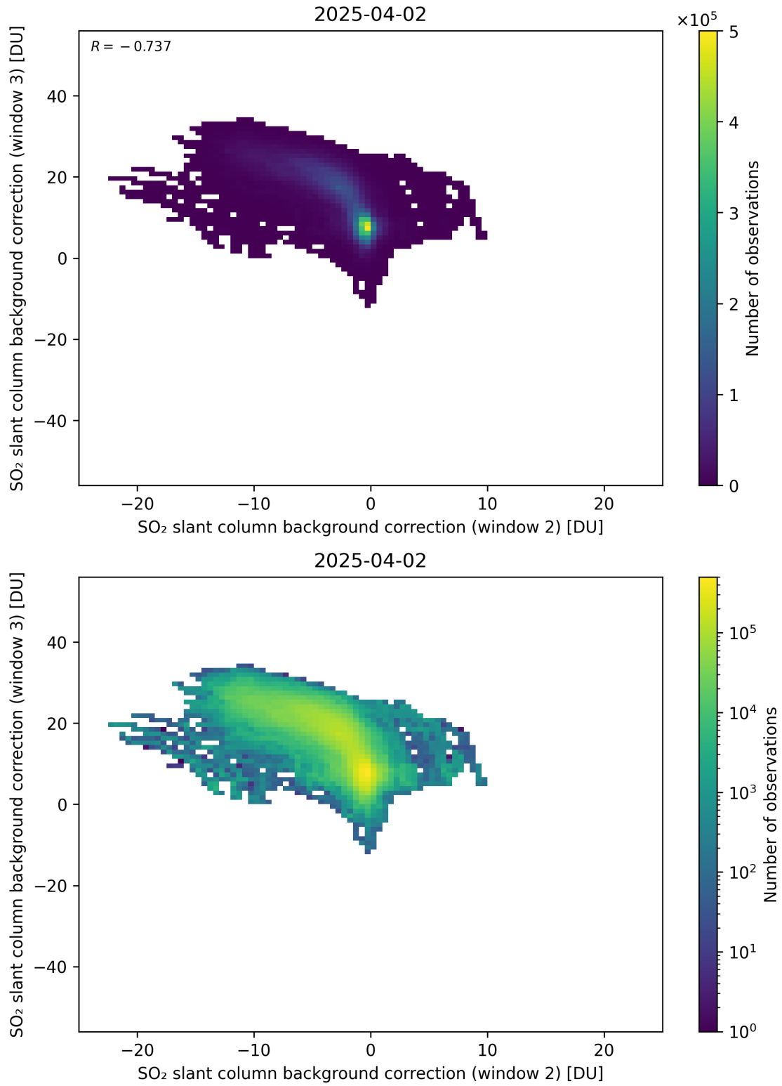
Figure 122: Scatter density plot of “SO 2 slant column background correction (window 2)” against “SO 2 slant column background correction (window 3)” for 2025-04-02 to 2025-04-03.
