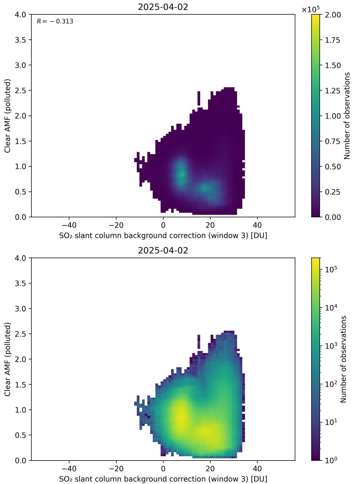
Figure 135: Scatter density plot of “SO 2 slant column background correction (window 3)” against “Clear AMF (polluted)” for 2025-04-02 to 2025-04-03.
