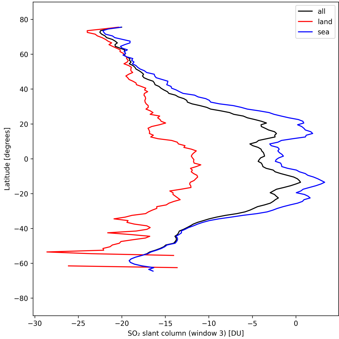
Figure 45: Zonal average of “SO 2 slant column (window 3)” for 2025-04-02 to 2025-04-03.
