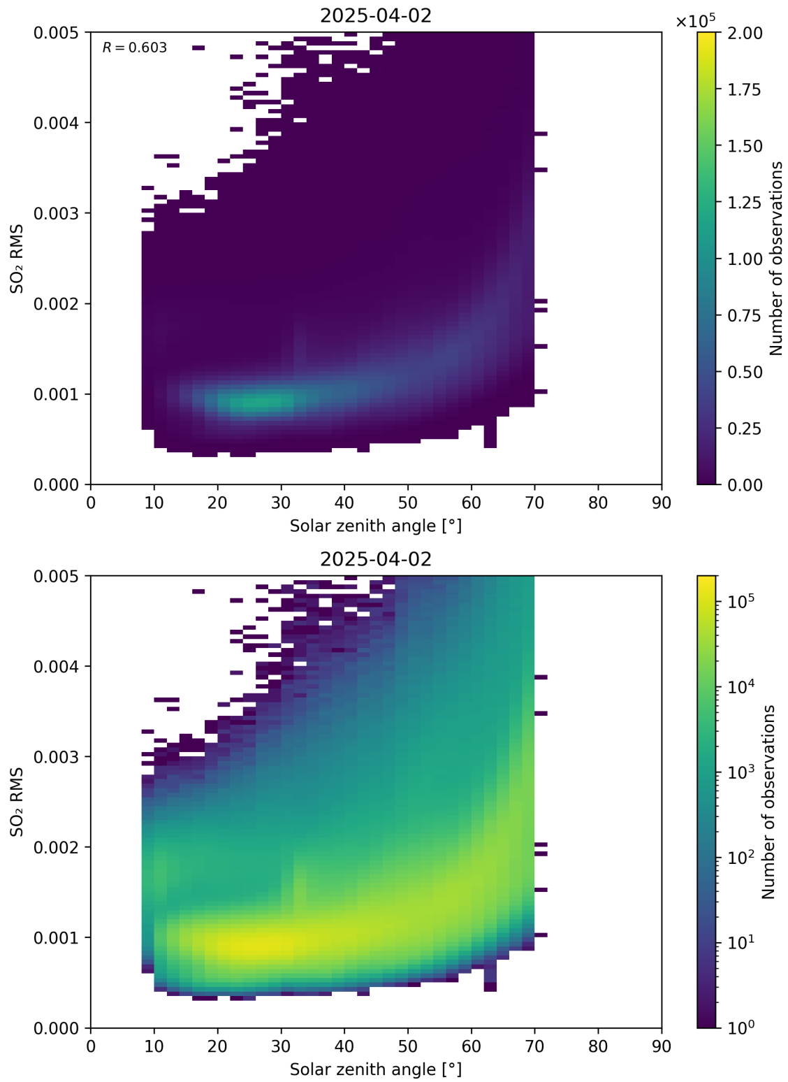
Figure 176: Scatter density plot of “Solar zenith angle” against “SO 2 RMS” for 2025-04-02 to 2025-04-03.
