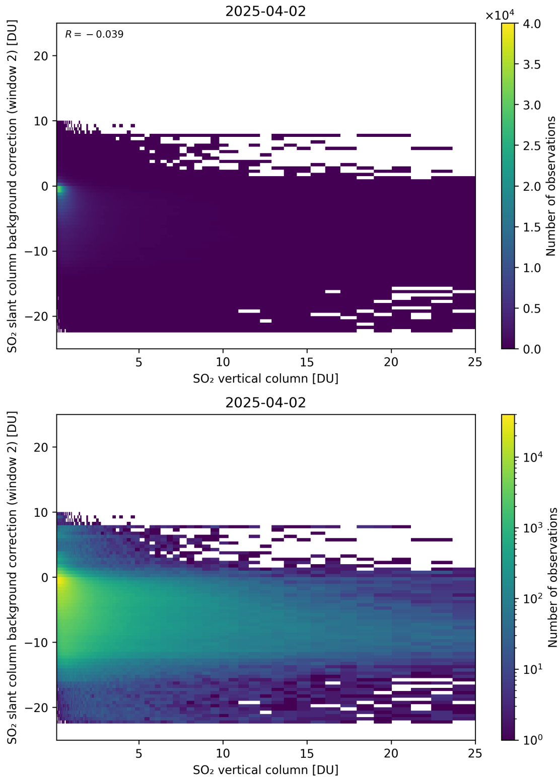
Figure 324: Scatter density plot of “SO 2 vertical column” against “SO 2 slant column background correction (window 2)” for 2025-04-02 to 2025-04-03.
