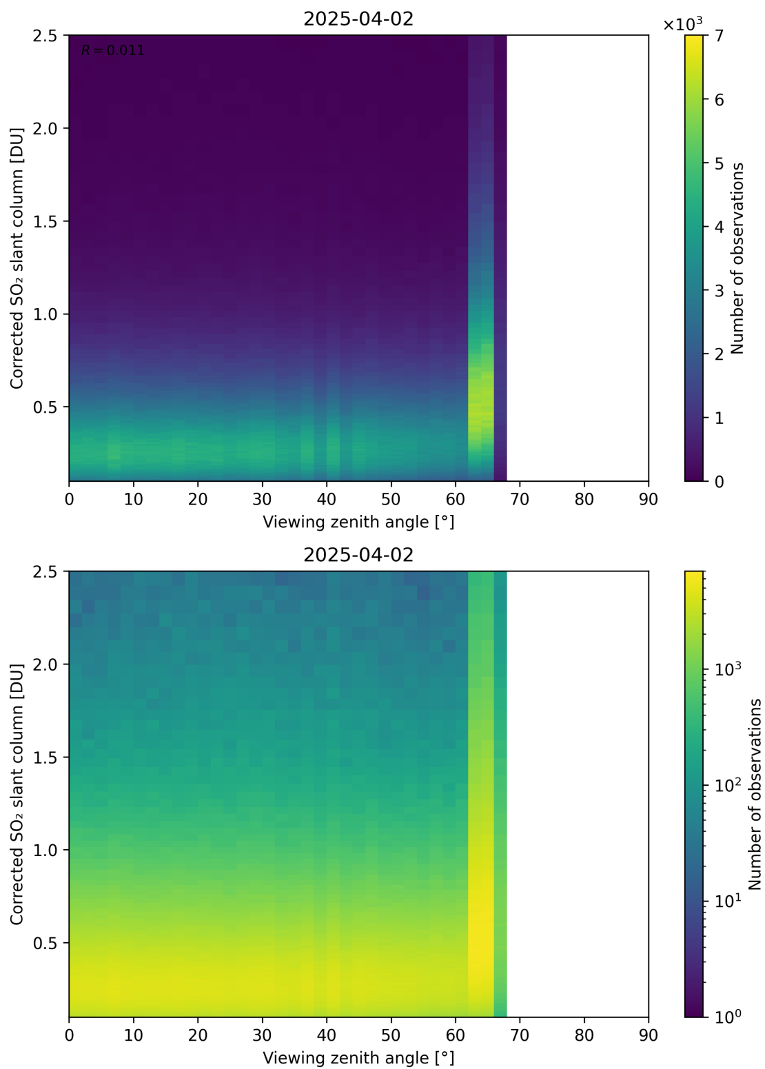
Figure 373: Scatter density plot of “Viewing zenith angle” against “Corrected SO 2 slant column” for 2025-04-02 to 2025-04-03.
