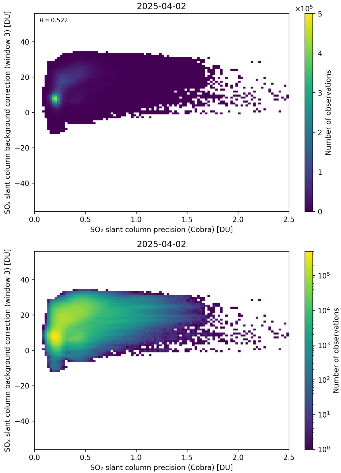
Figure 201: Scatter density plot of “SO 2 slant column precision (Cobra)” against “SO 2 slant column background correction (window 3)” for 2025-04-02 to 2025-04-03.
