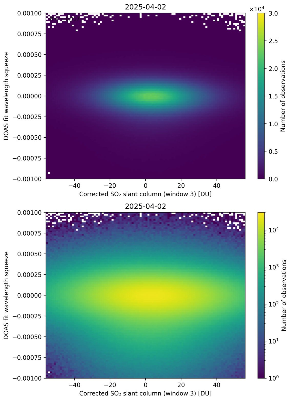
Figure 257: Scatter density plot of “Corrected SO 2 slant column (window 3)” against “DOAS fit wavelength squeeze” for 2025-04-02 to 2025-04-03.
