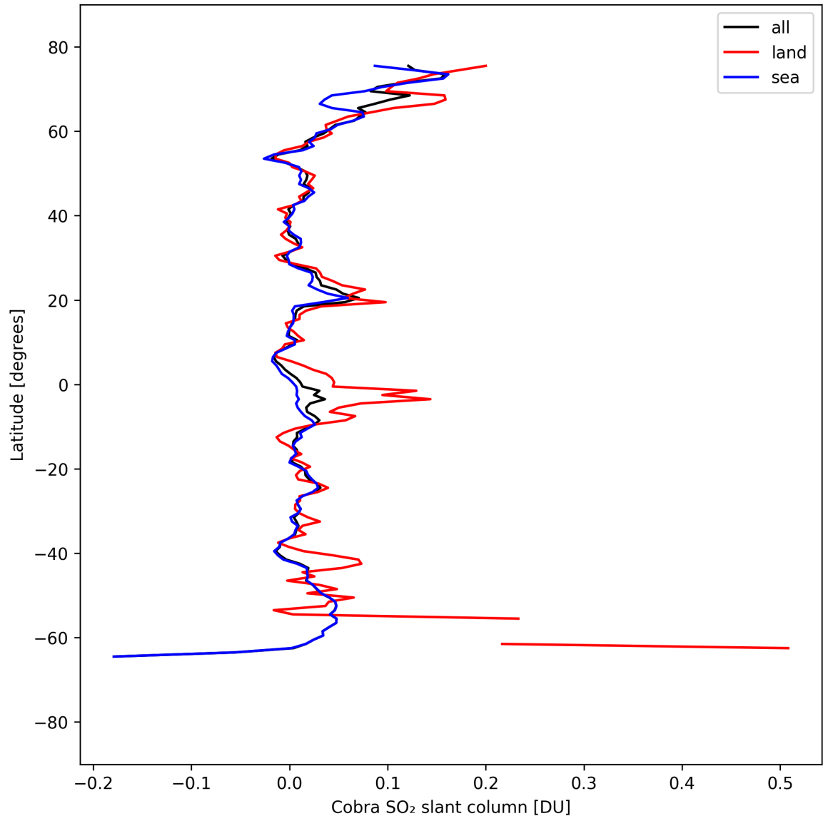
Figure 35: Zonal average of “Cobra SO 2 slant column” for 2025-04-02 to 2025-04-03.
