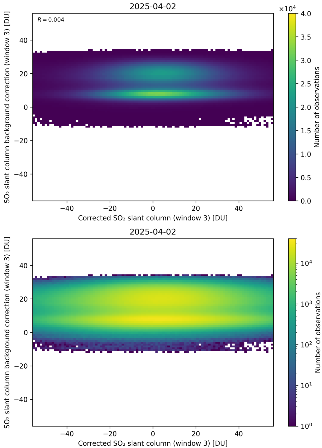
Figure 255: Scatter density plot of “Corrected SO 2 slant column (window 3)” against “SO 2 slant column background correction (window 3)” for 2025-04-02 to 2025-04-03.
