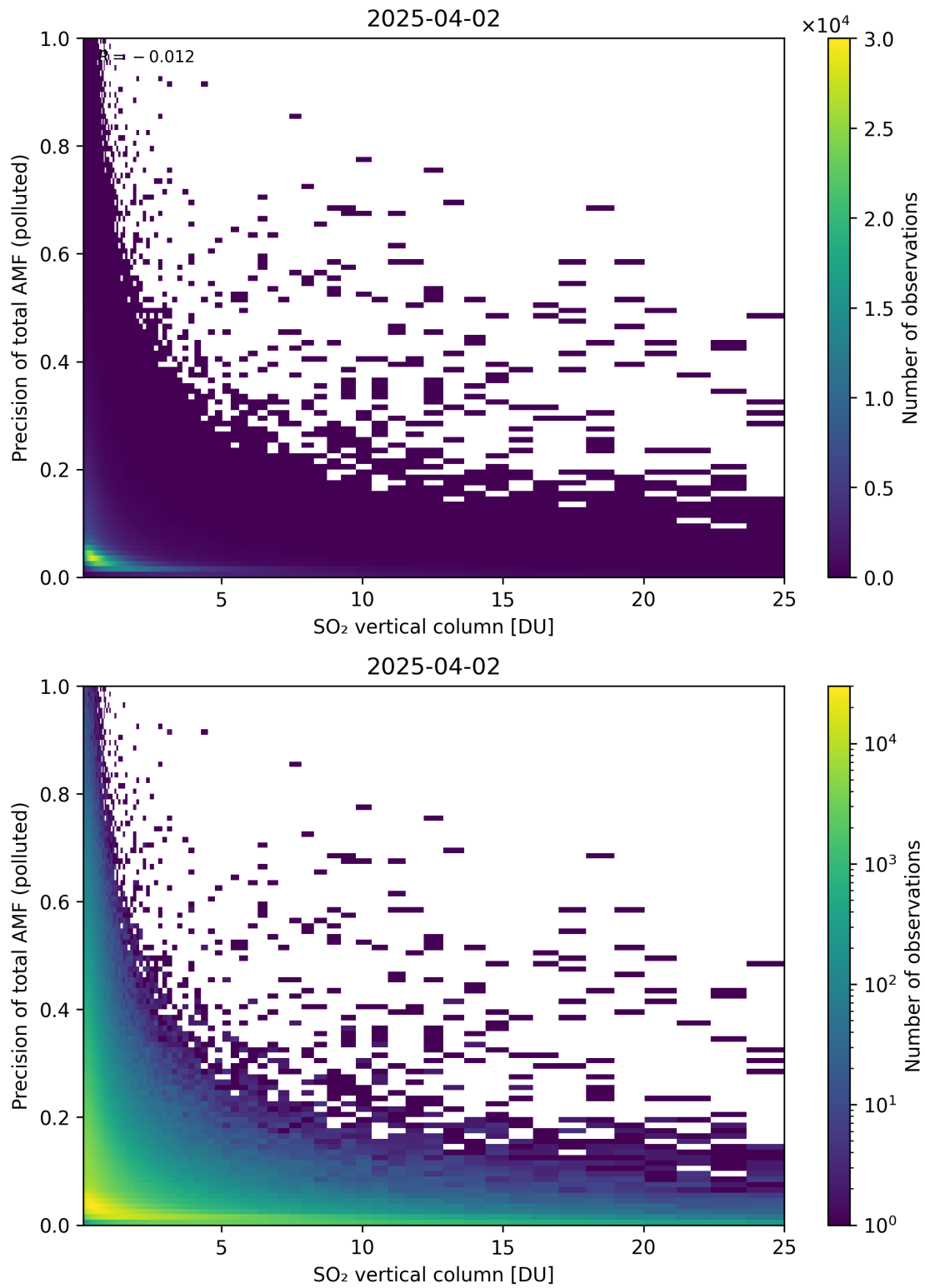
Figure 360: Scatter density plot of “SO 2 vertical column” against “Precision of total AMF (polluted)” for 2025-04-02 to 2025-04-03.
