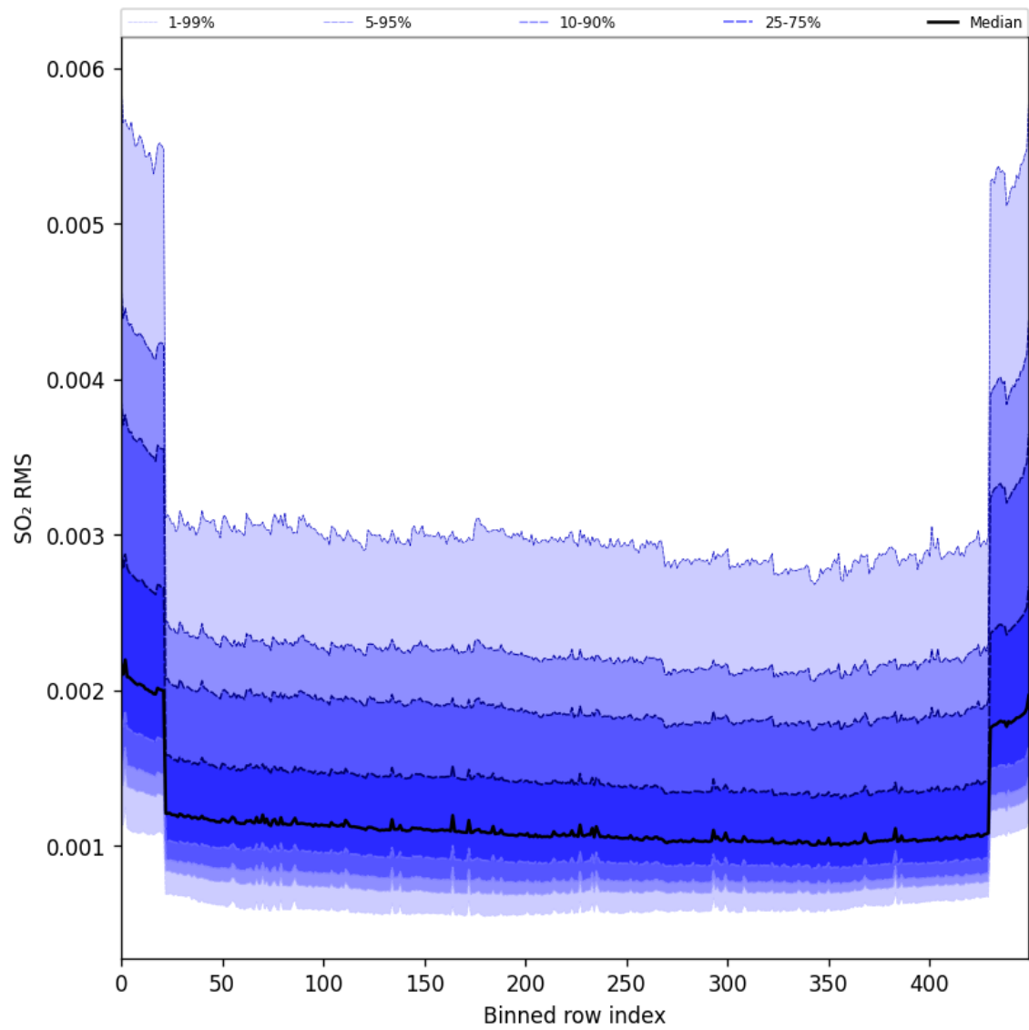
Figure 104: Along track statistics of “SO 2 RMS” for 2025-04-02 to 2025-04-03
