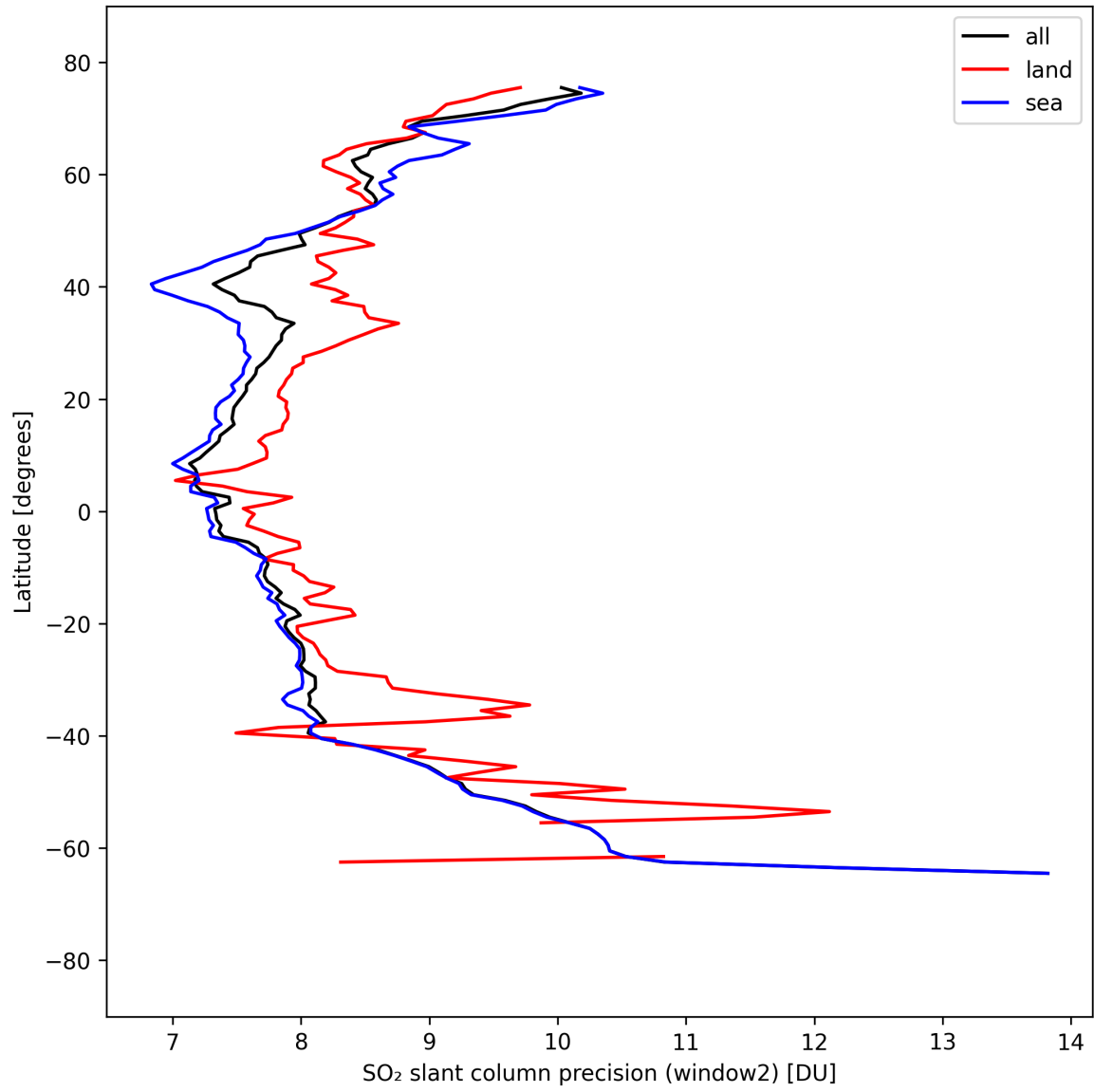
Figure 42: Zonal average of “SO 2 slant column precision (window2)” for 2025-04-02 to 2025-04-03.
