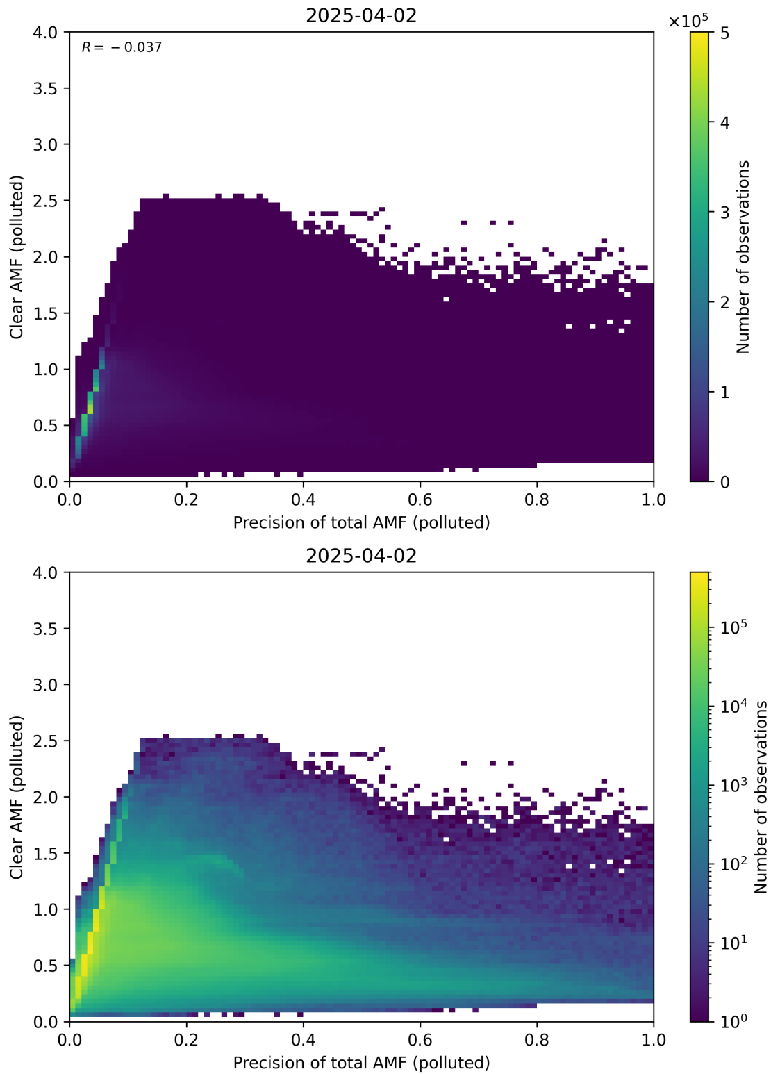
Figure 320: Scatter density plot of “Precision of total AMF (polluted)” against “Clear AMF (polluted)” for 2025-04-02 to 2025-04-03.
