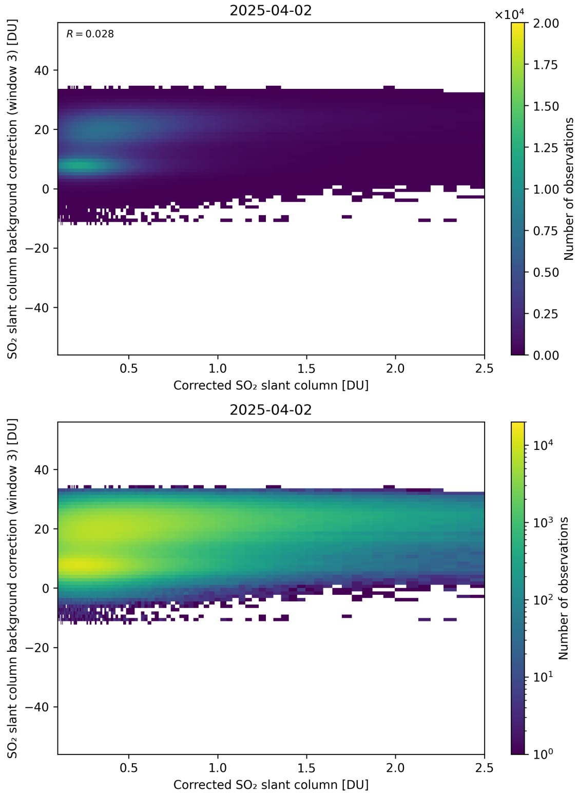
Figure 228: Scatter density plot of “Corrected SO 2 slant column” against “SO 2 slant column background correction (window 3)” for 2025-04-02 to 2025-04-03.
