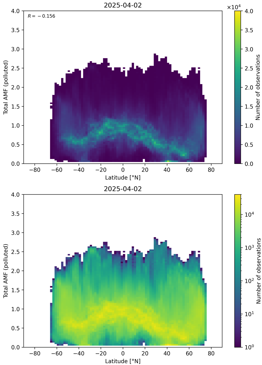
Figure 167: Scatter density plot of “Latitude” against “Total AMF (polluted)” for 2025-04-02 to 2025-04-03.
