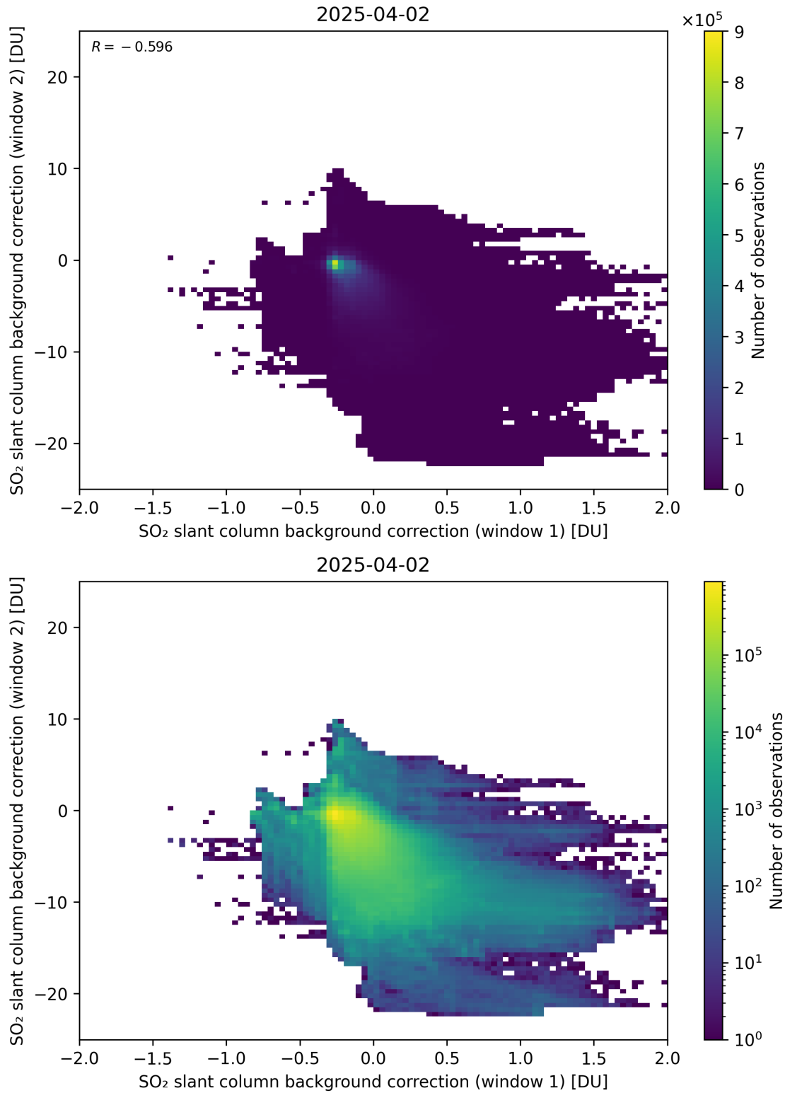
Figure 109: Scatter density plot of “SO 2 slant column background correction (window 1)” against “SO 2 slant column background correction (window 2)” for 2025-04-02 to 2025-04-03.
