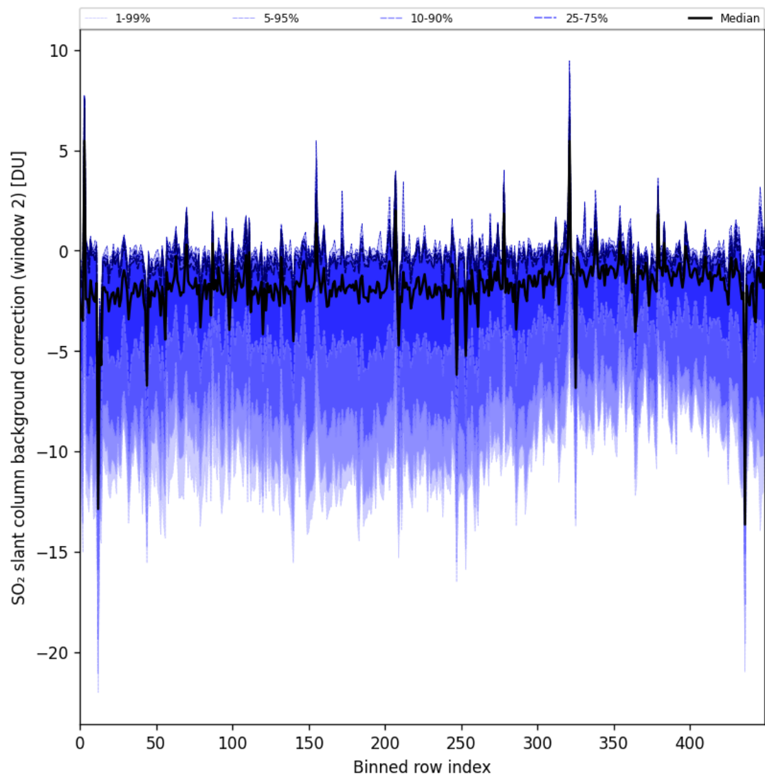
Figure 96: Along track statistics of “SO 2 slant column background correction (window 2)” for 2025-04-02 to 2025-04-03
