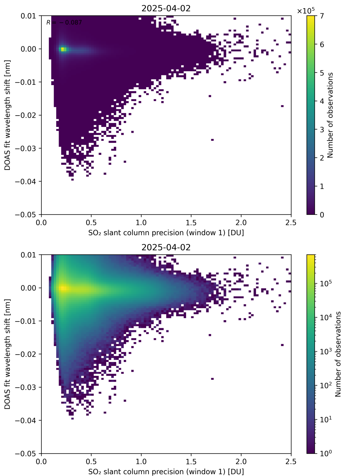
Figure 271: Scatter density plot of “SO 2 slant column precision (window 1)” against “DOAS fit wavelength shift” for 2025-04-02 to 2025-04-03.
