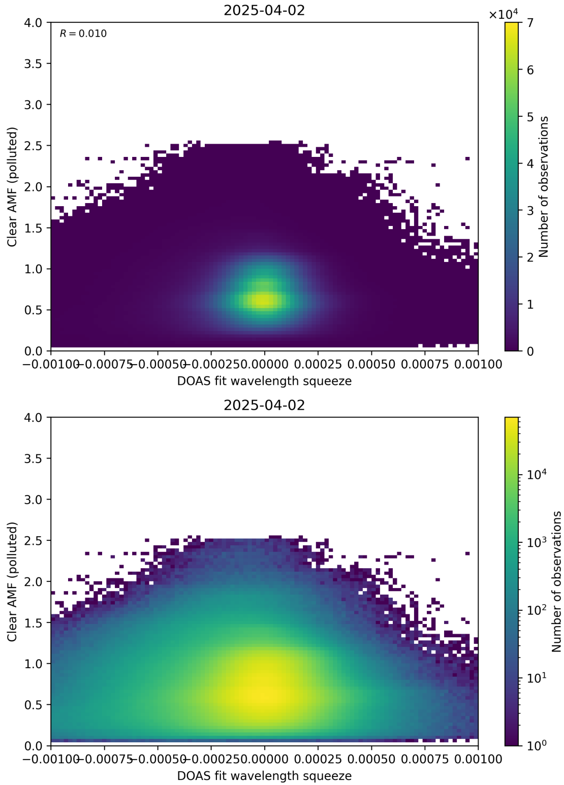
Figure 144: Scatter density plot of “DOAS fit wavelength squeeze” against “Clear AMF (polluted)” for 2025-04-02 to 2025-04-03.
