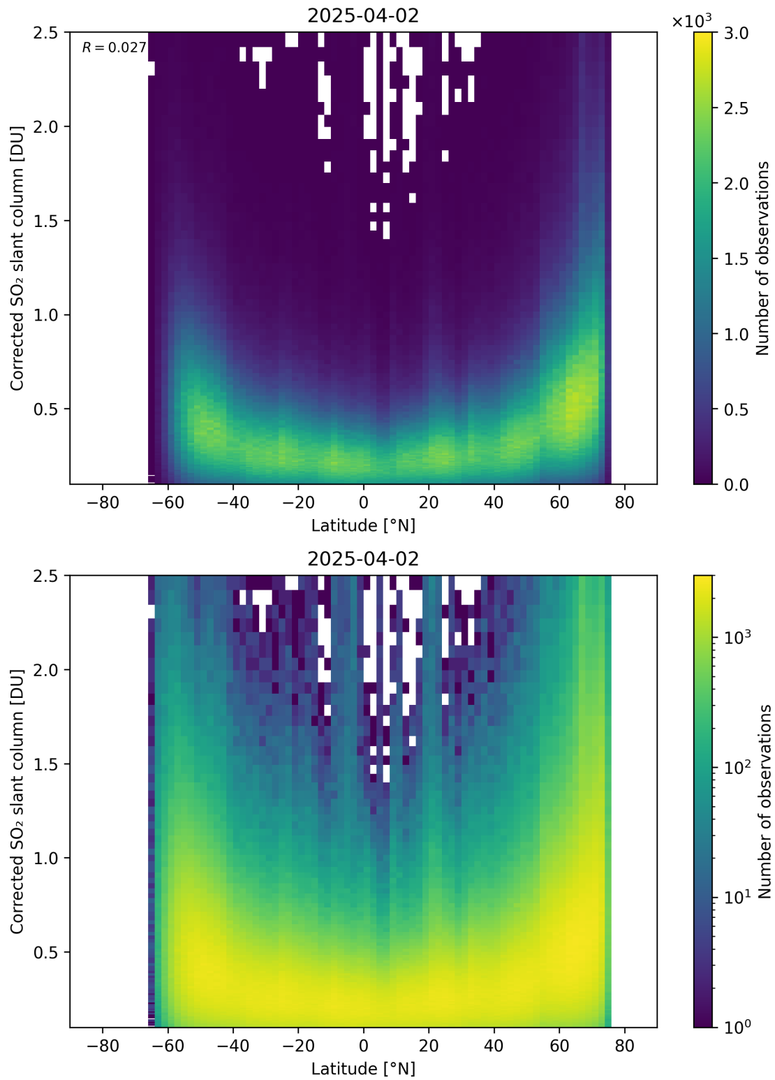
Figure 159: Scatter density plot of “Latitude” against “Corrected SO 2 slant column” for 2025-04-02 to 2025-04-03.
