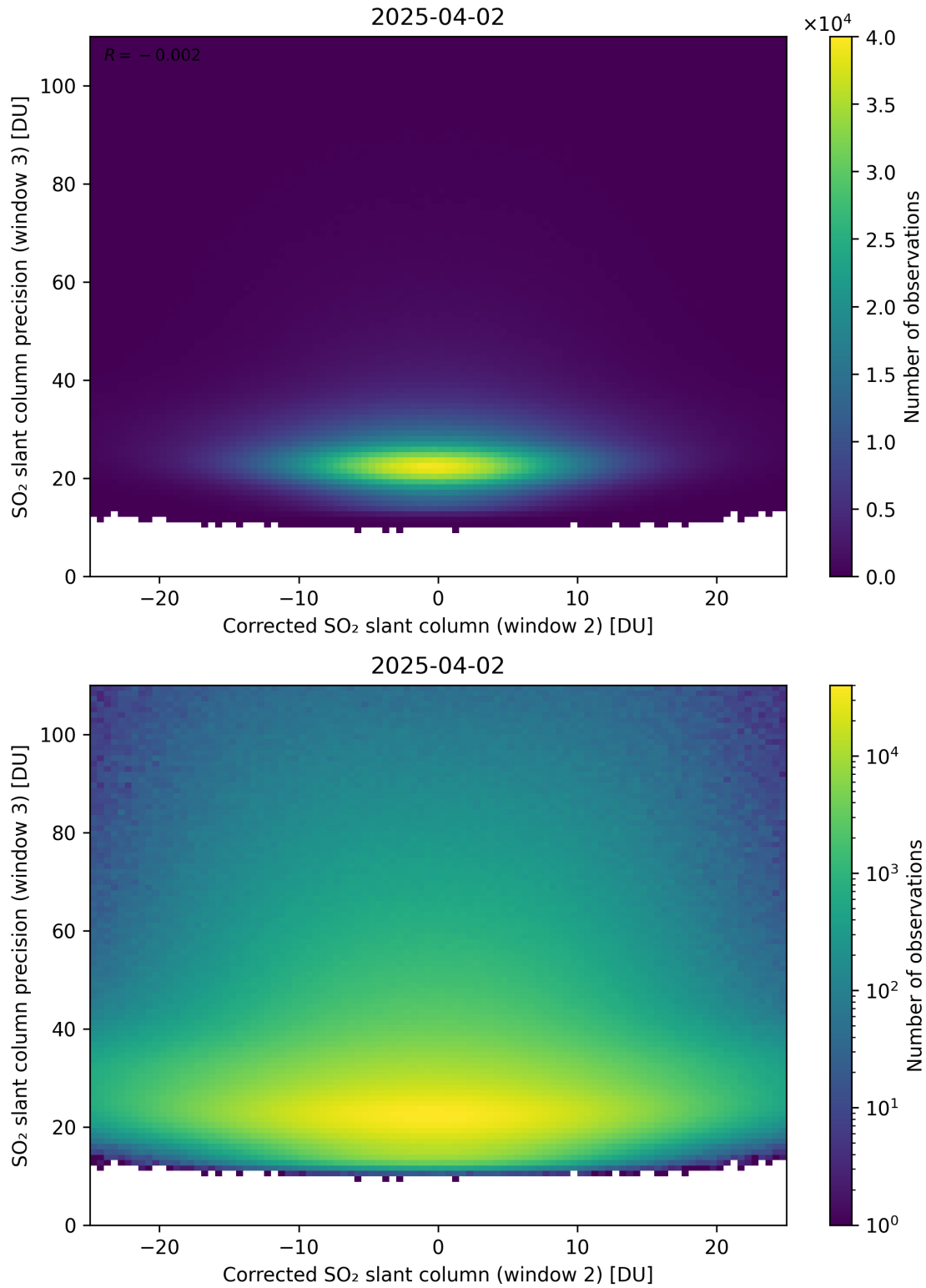
Figure 252: Scatter density plot of “Corrected SO 2 slant column (window 2)” against “SO 2 slant column precision (window 3)” for 2025-04-02 to 2025-04-03.
