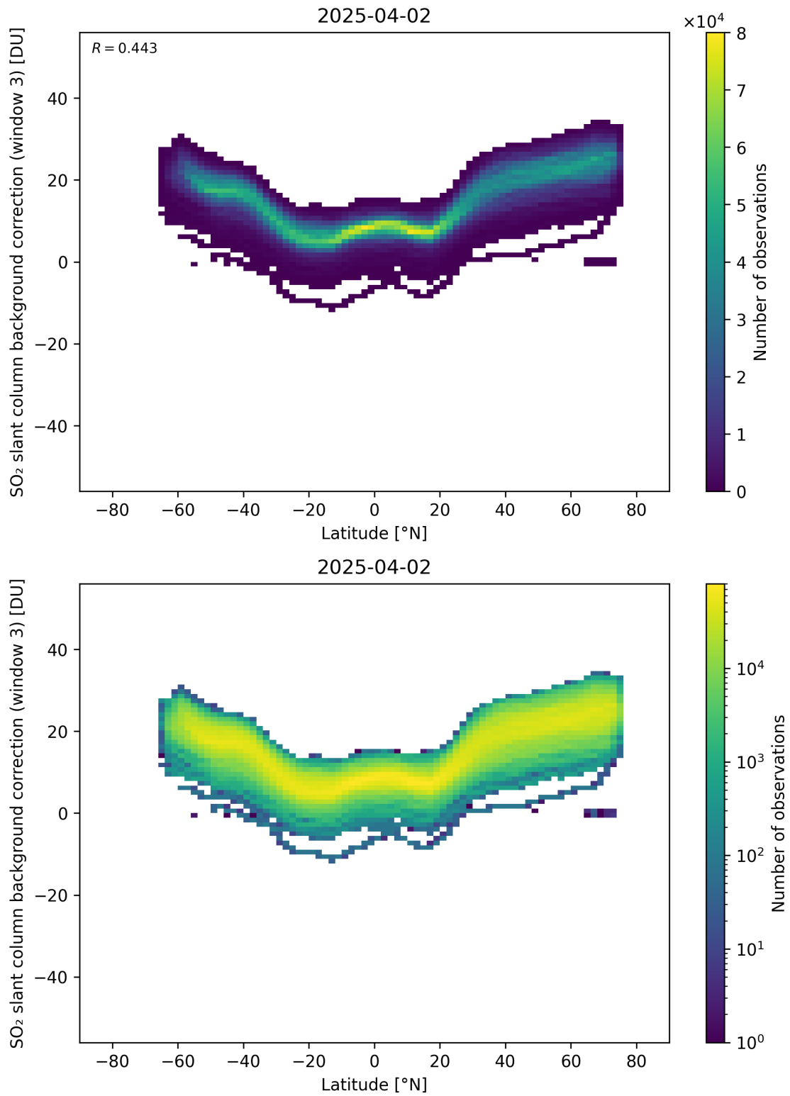
Figure 152: Scatter density plot of “Latitude” against “SO 2 slant column background correction (window 3)” for 2025-04-02 to 2025-04-03.
