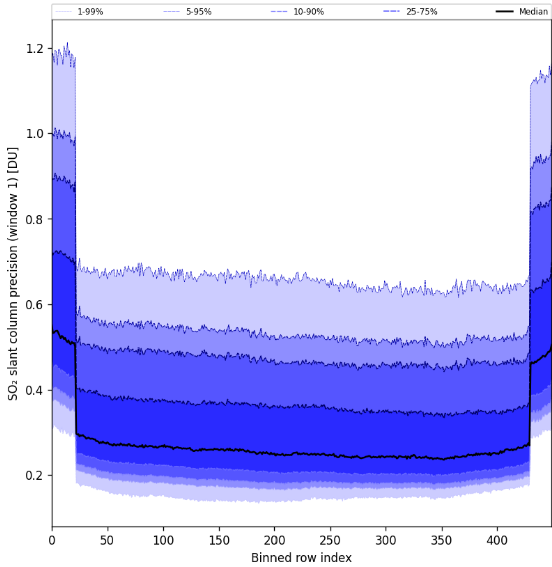
Figure 90: Along track statistics of “SO 2 slant column precision (window 1)” for 2025-04-02 to 2025-04-03
