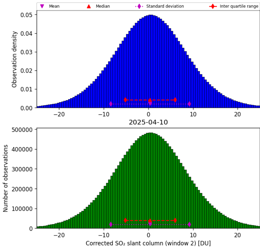
Figure 69: Histogram of “Corrected SO 2 slant column (window 2)” for 2025-04-09 to 2025-04-11
