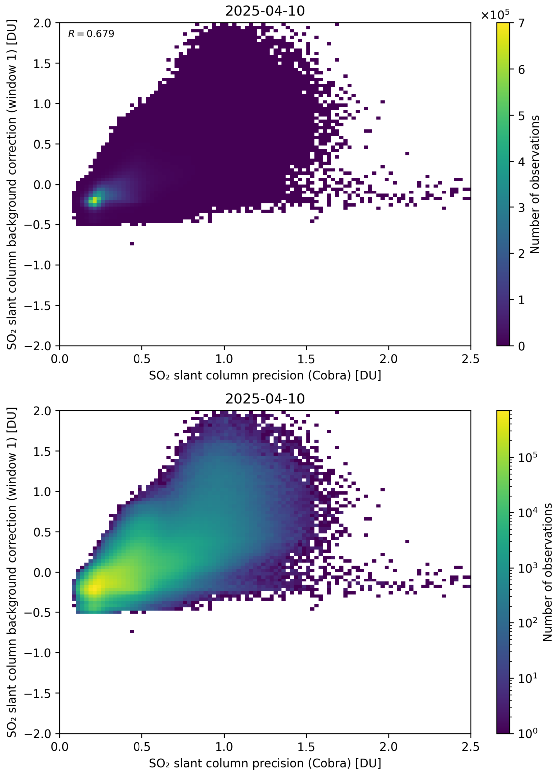
Figure 199: Scatter density plot of “SO 2 slant column precision (Cobra)” against “SO 2 slant column background correction (window 1)” for 2025-04-09 to 2025-04-11.
