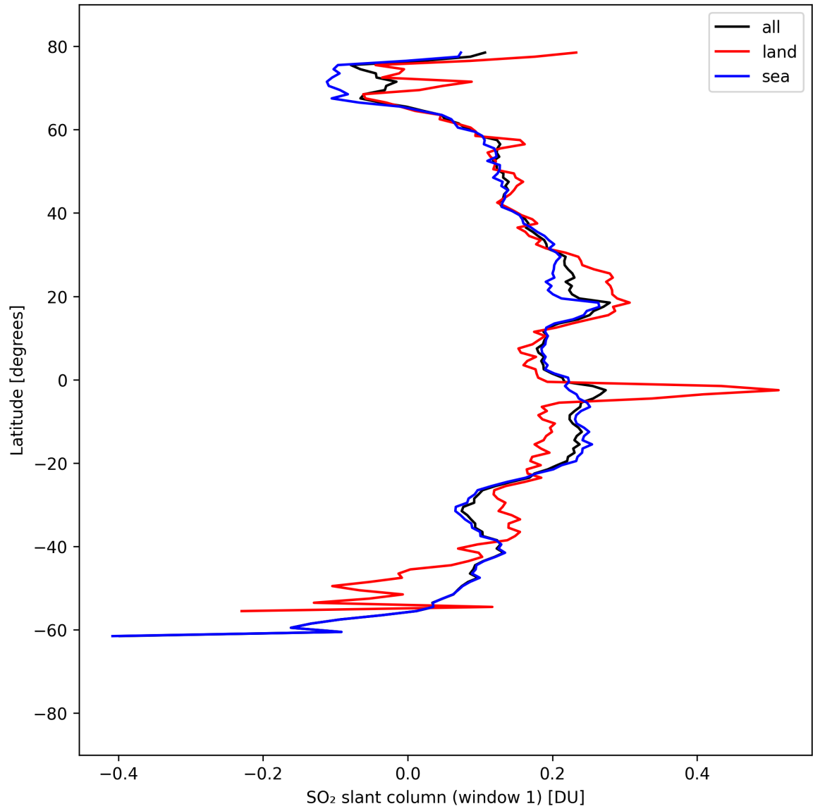
Figure 37: Zonal average of “SO 2 slant column (window 1)” for 2025-04-09 to 2025-04-11.
