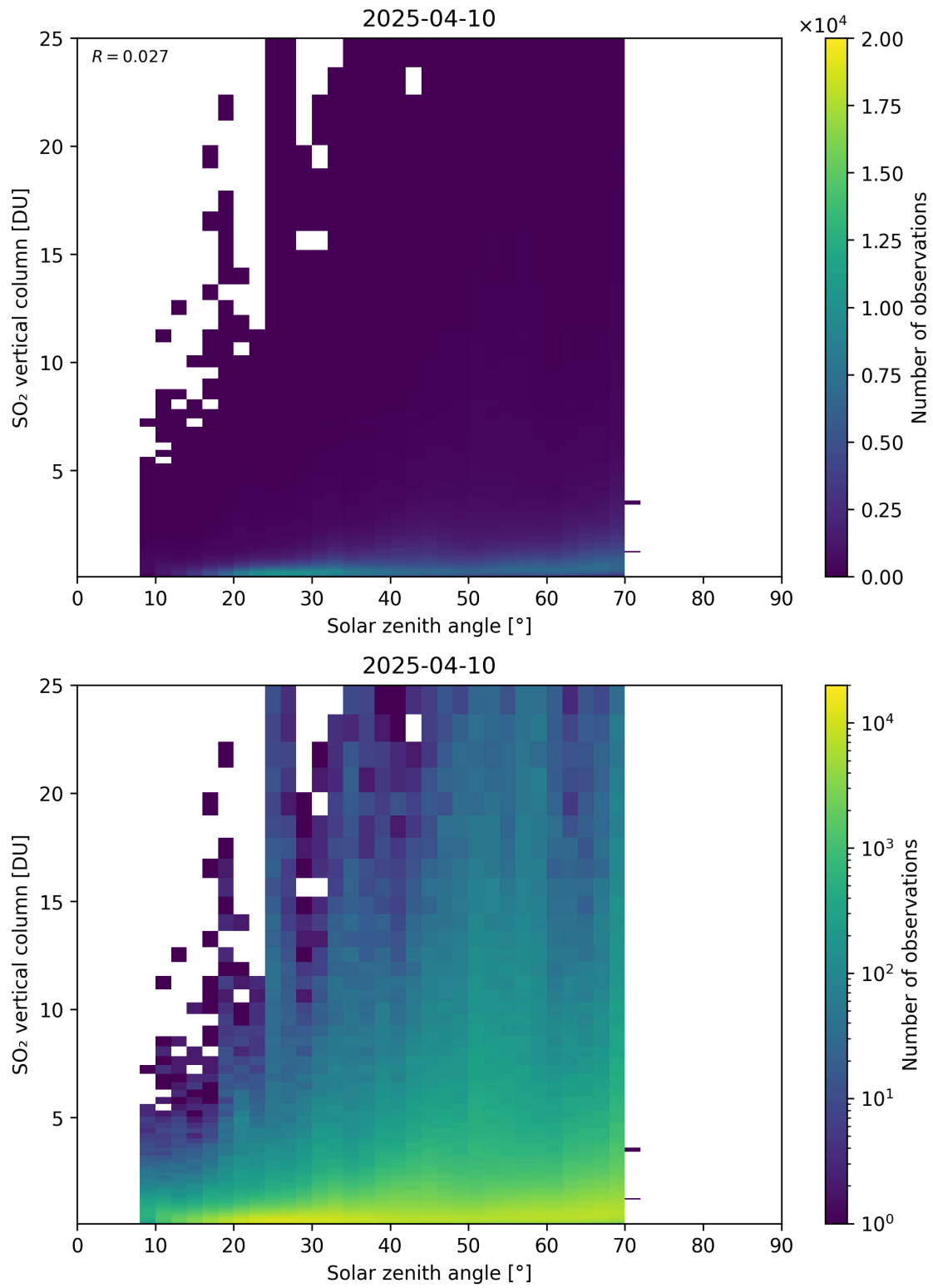
Figure 191: Scatter density plot of “Solar zenith angle” against “SO 2 vertical column” for 2025-04-09 to 2025-04-11.
