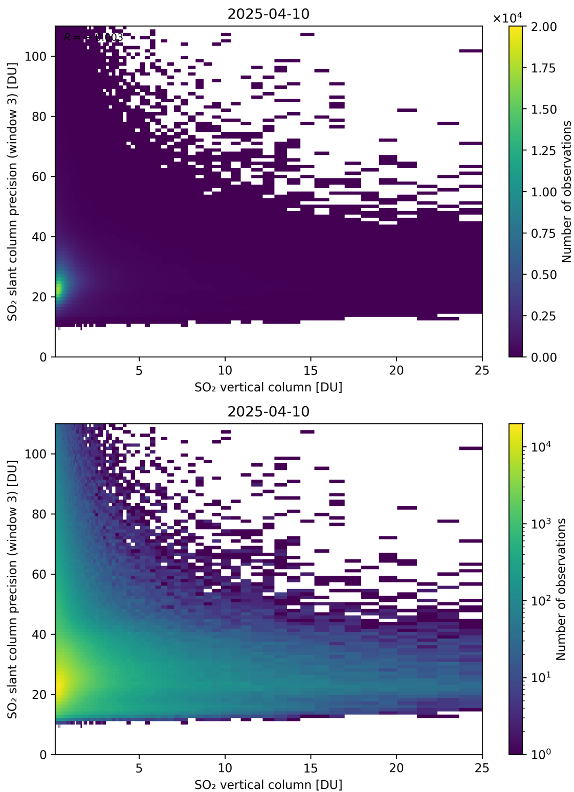
Figure 358: Scatter density plot of “SO 2 vertical column” against “SO 2 slant column precision (window 3)” for 2025-04-09 to 2025-04-11.
