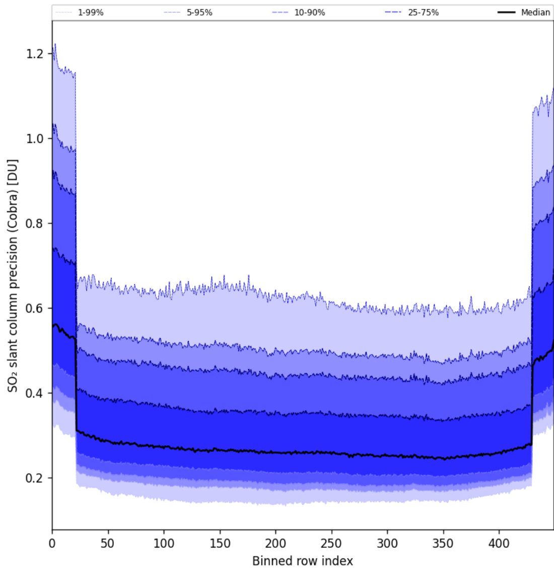
Figure 88: Along track statistics of “SO 2 slant column precision (Cobra)” for 2025-04-09 to 2025-04-11
