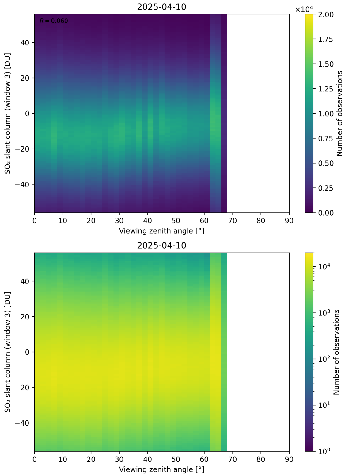
Figure 379: Scatter density plot of “Viewing zenith angle” against “SO 2 slant column (window 3)” for 2025-04-09 to 2025-04-11.
