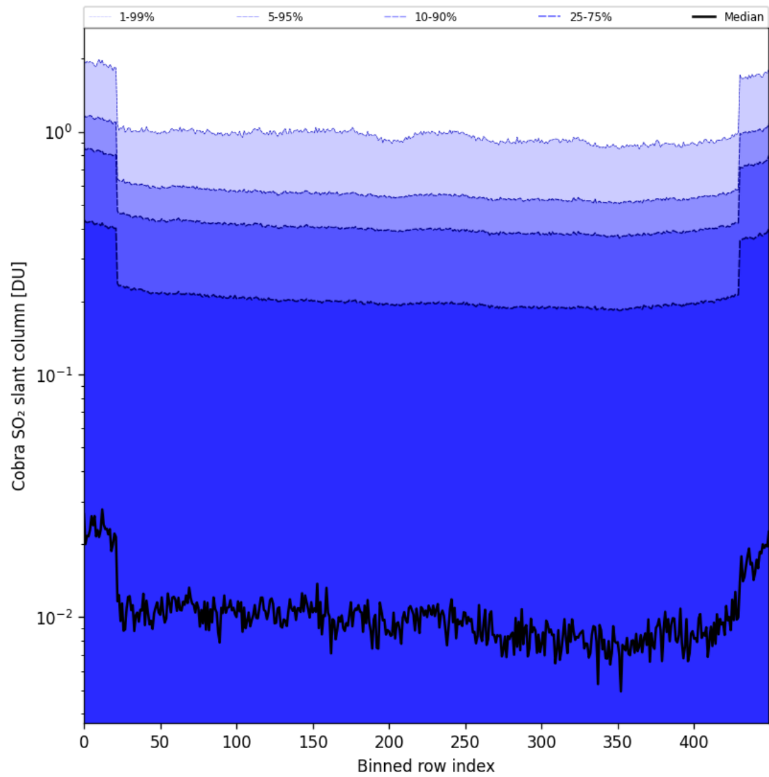
Figure 87: Along track statistics of "Cobra SO 2 slant column" for 2025-04-09 to 2025-04-11
