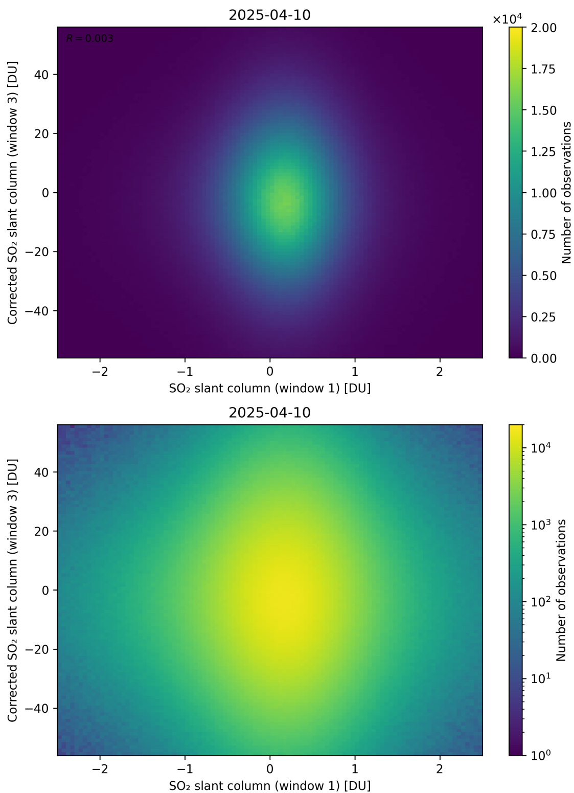
Figure 284: Scatter density plot of “SO 2 slant column (window 1)” against “Corrected SO 2 slant column (window 3)” for 2025-04-09 to 2025-04-11.
