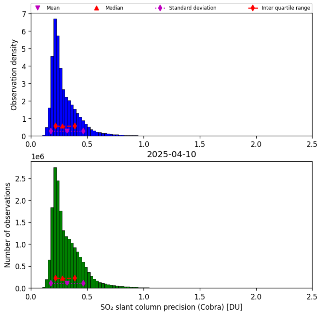
Figure 62: Histogram of “SO 2 slant column precision (Cobra)” for 2025-04-09 to 2025-04-11
