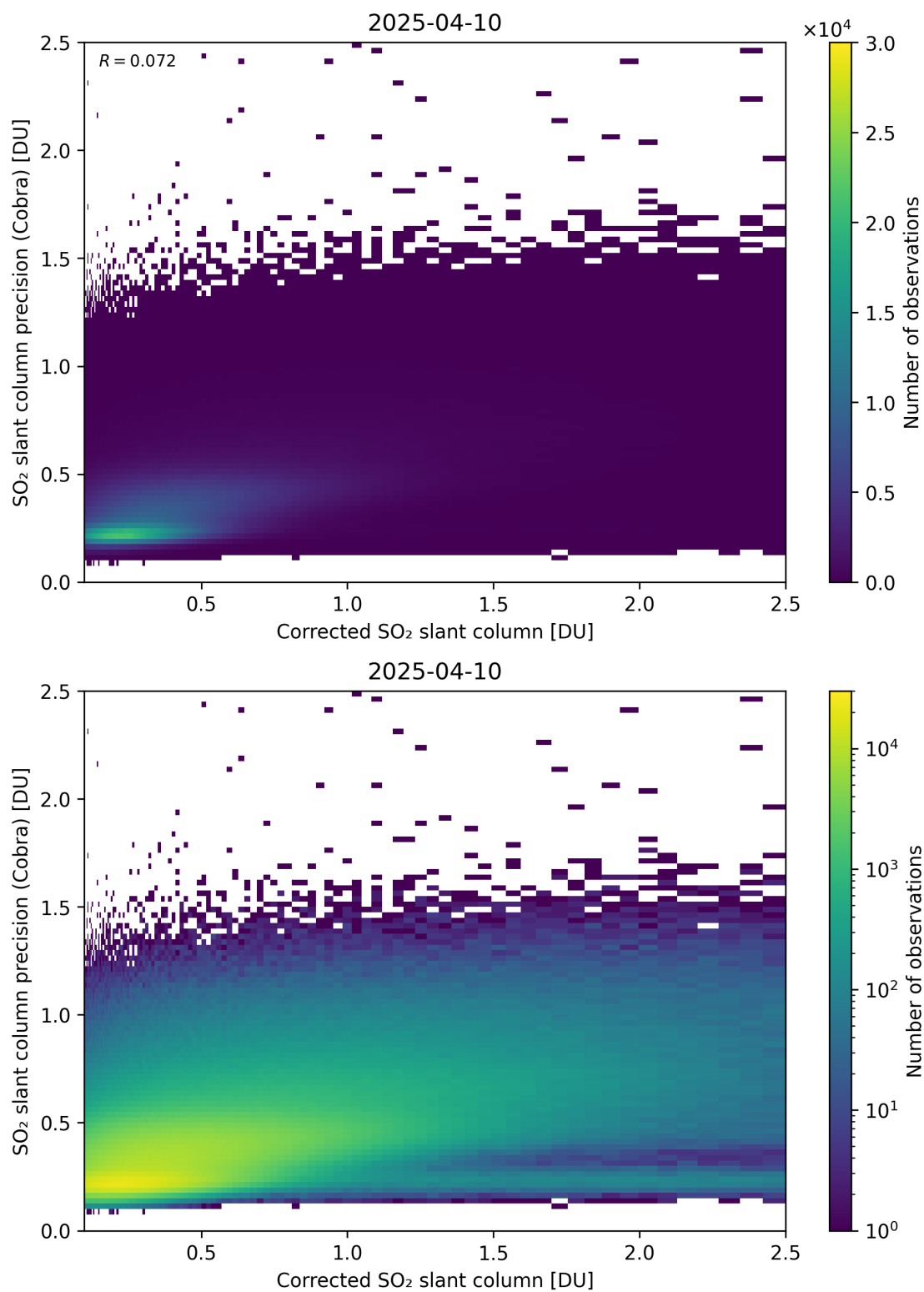
Figure 234: Scatter density plot of “Corrected SO 2 slant column” against “SO 2 slant column precision (Cobra)” for 2025-04-09 to 2025-04-11.
