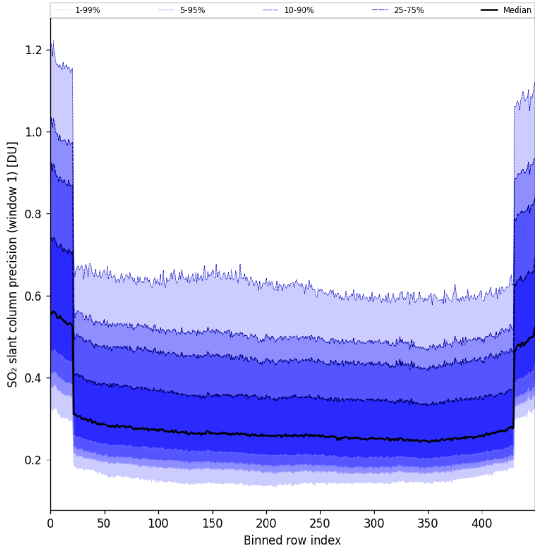
Figure 90: Along track statistics of “SO 2 slant column precision (window 1)” for 2025-04-09 to 2025-04-11
