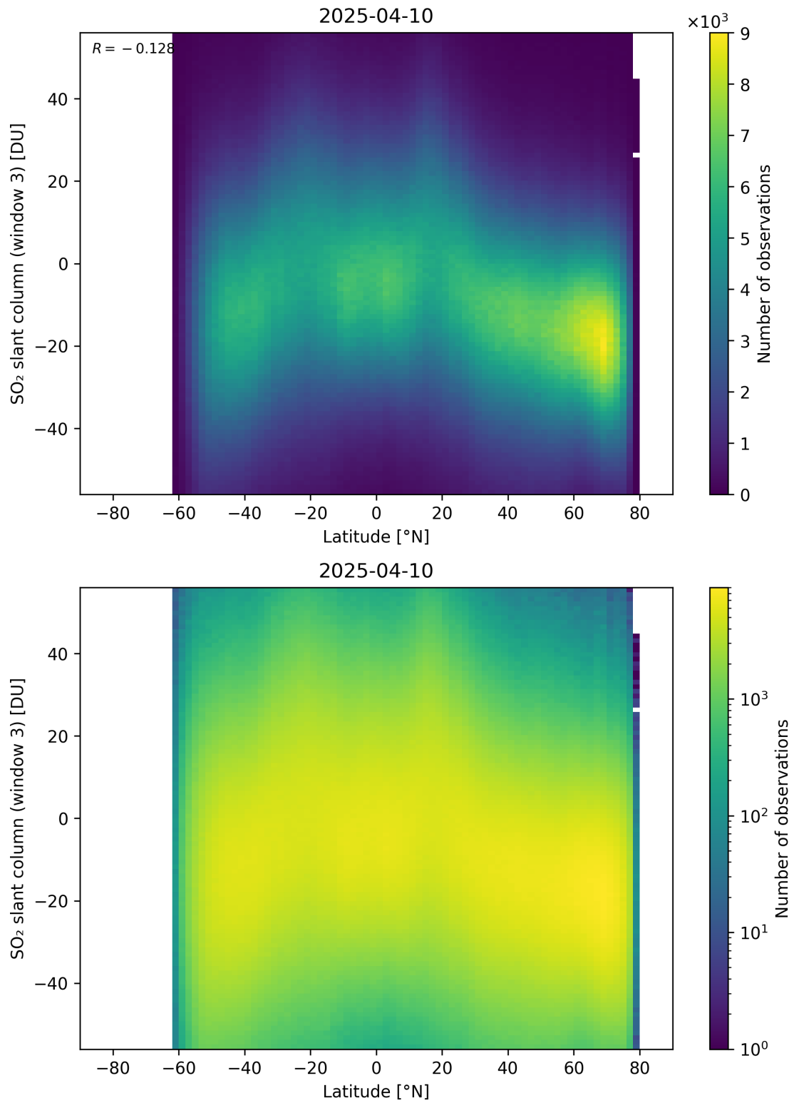
Figure 165: Scatter density plot of “Latitude” against “SO 2 slant column (window 3)” for 2025-04-09 to 2025-04-11.
