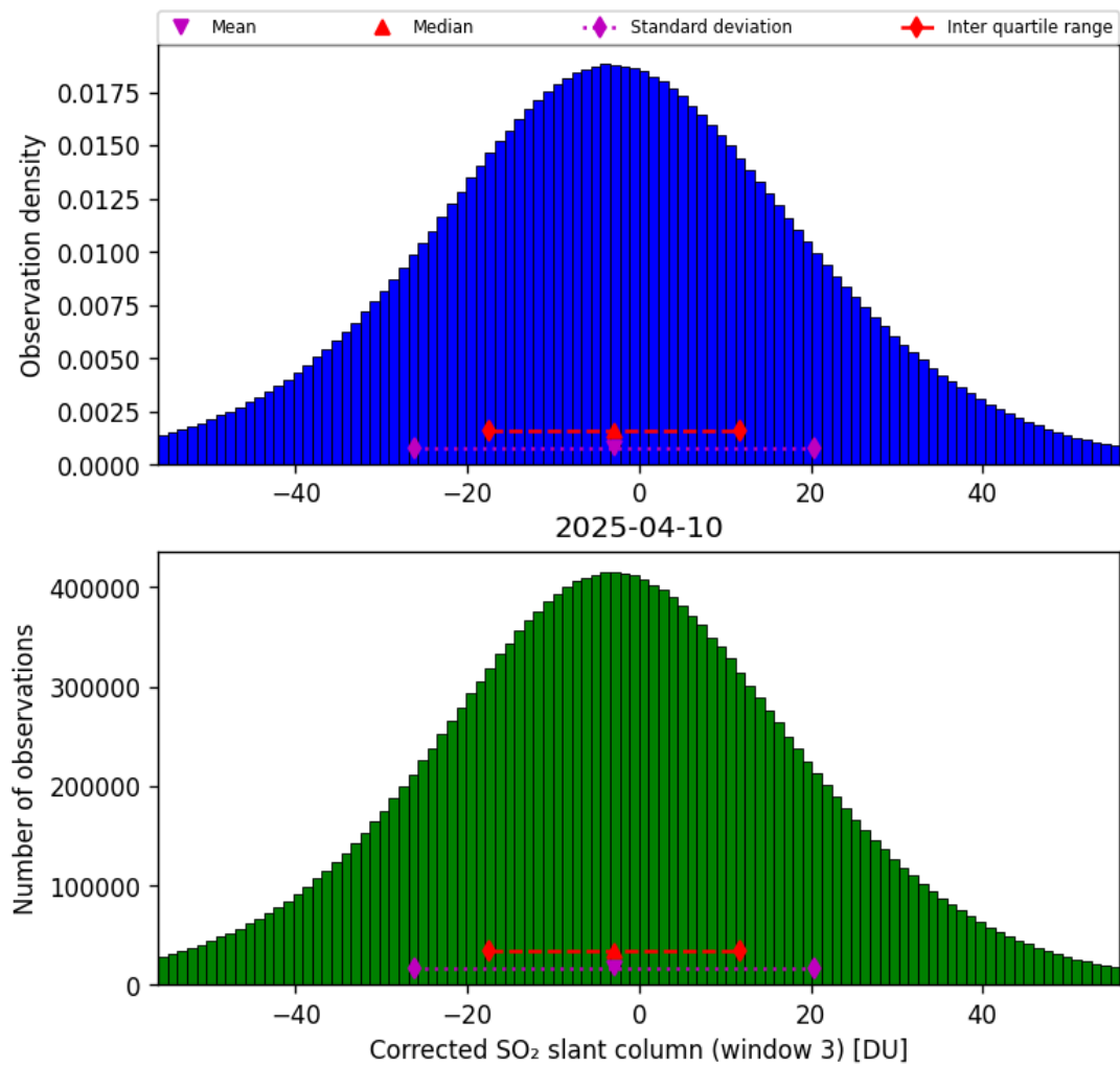
Figure 73: Histogram of “Corrected SO 2 slant column (window 3)” for 2025-04-09 to 2025-04-11
