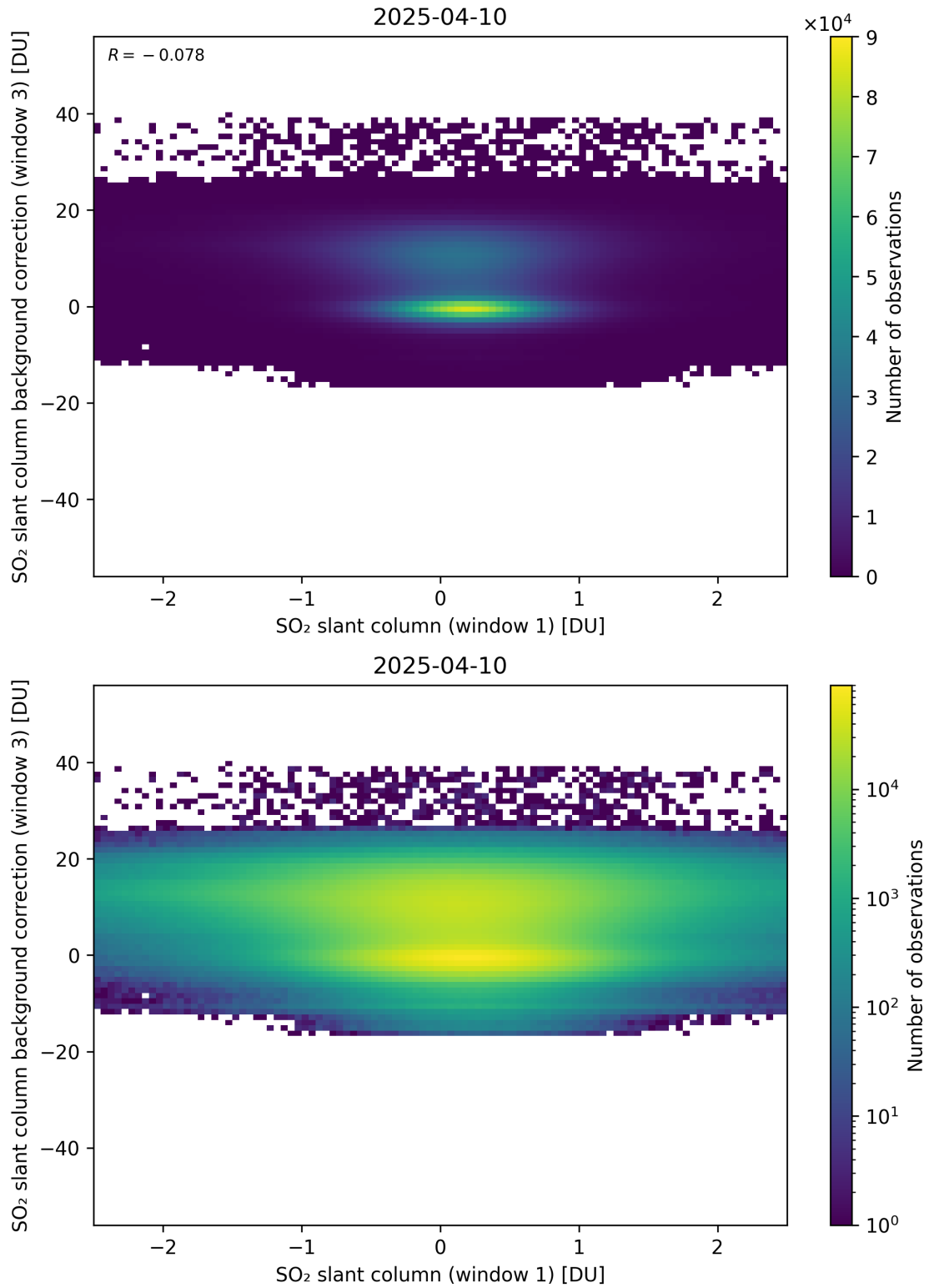
Figure 264: Scatter density plot of “SO 2 slant column (window 1)” against “SO 2 slant column background correction (window 3)” for 2025-04-09 to 2025-04-11.
