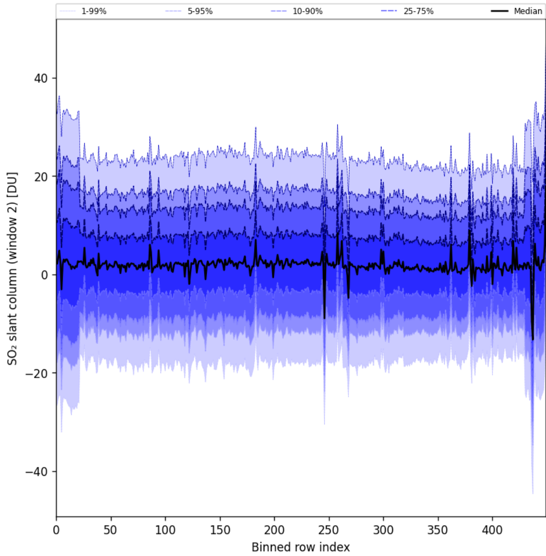
Figure 93: Along track statistics of “SO 2 slant column (window 2)” for 2025-04-09 to 2025-04-11
