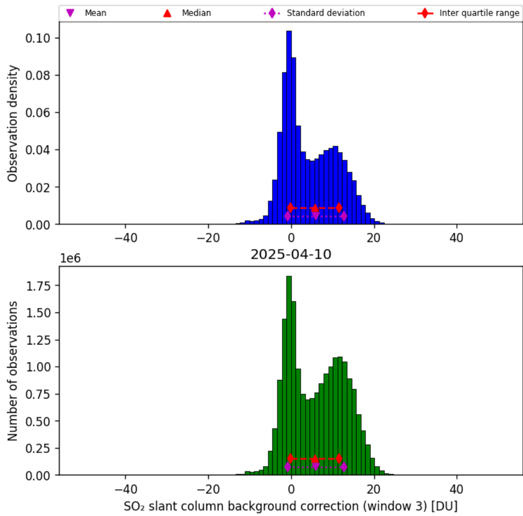
Figure 74: Histogram of “SO 2 slant column background correction (window 3)” for 2025-04-09 to 2025-04-11
