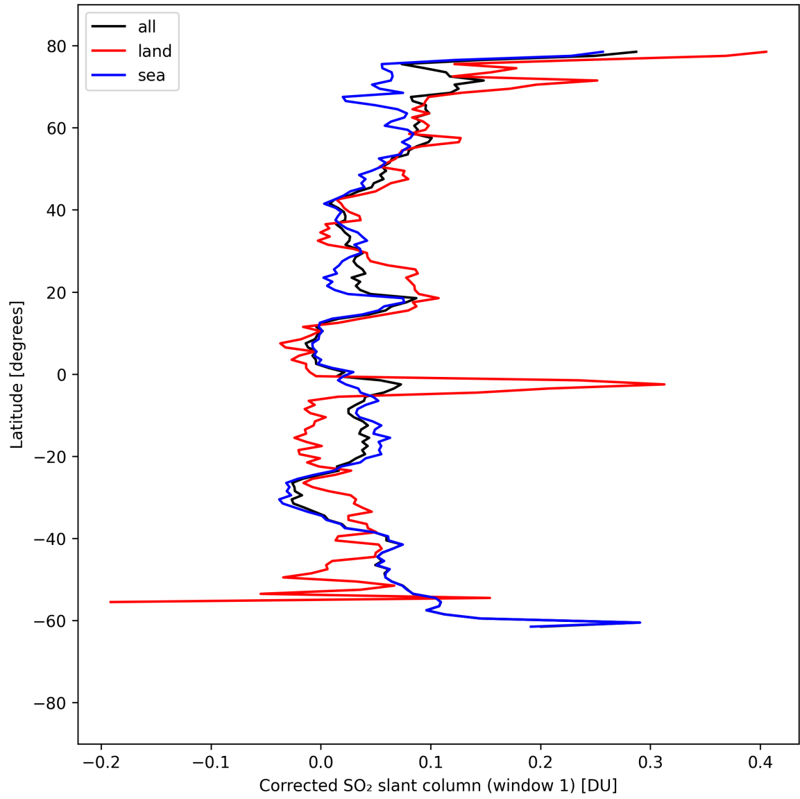
Figure 39: Zonal average of “Corrected SO 2 slant column (window 1)” for 2025-04-09 to 2025-04-11.
