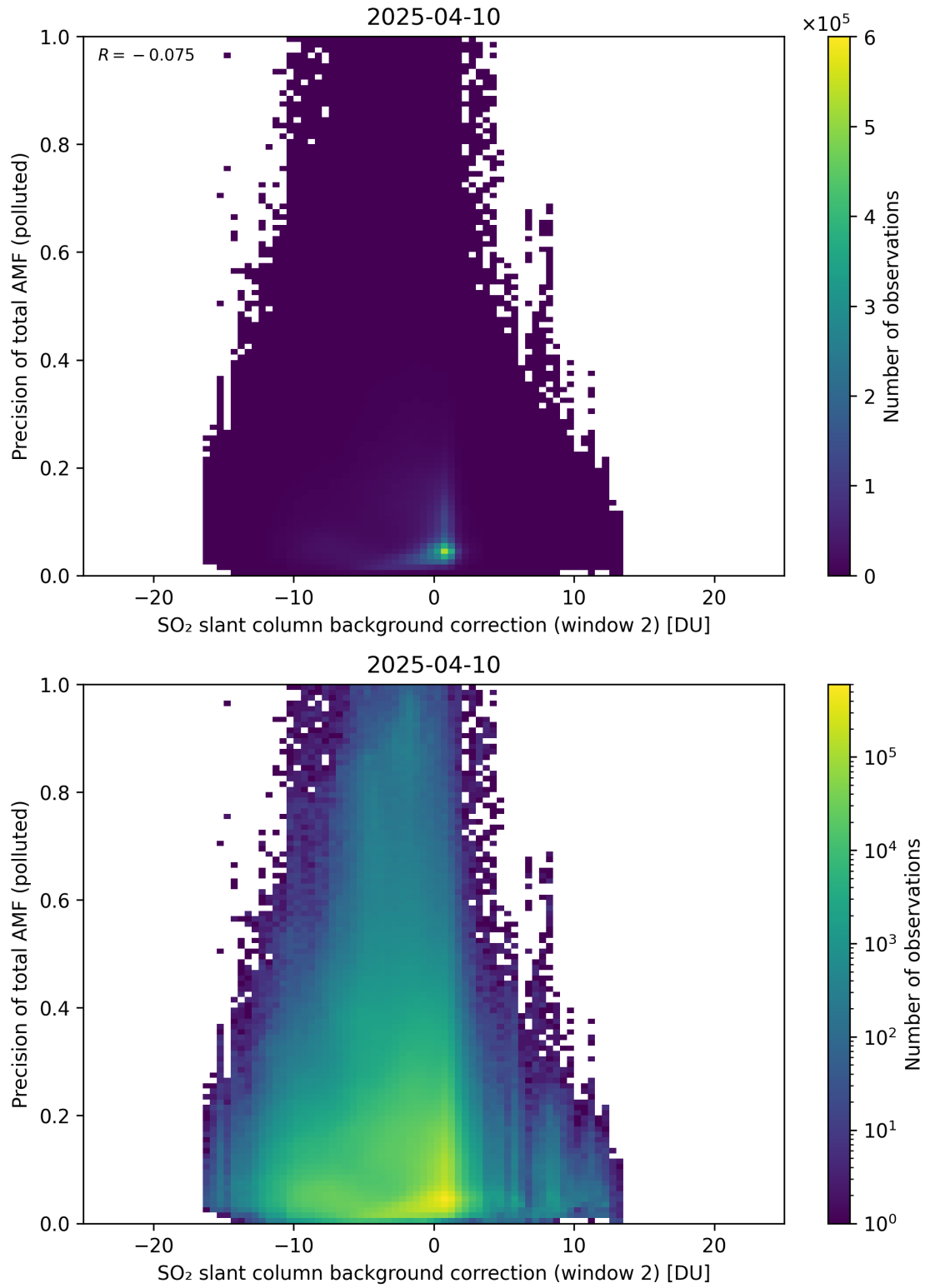
Figure 131: Scatter density plot of “SO 2 slant column background correction (window 2)” against “Precision of total AMF (polluted)” for 2025-04-09 to 2025-04-11.
