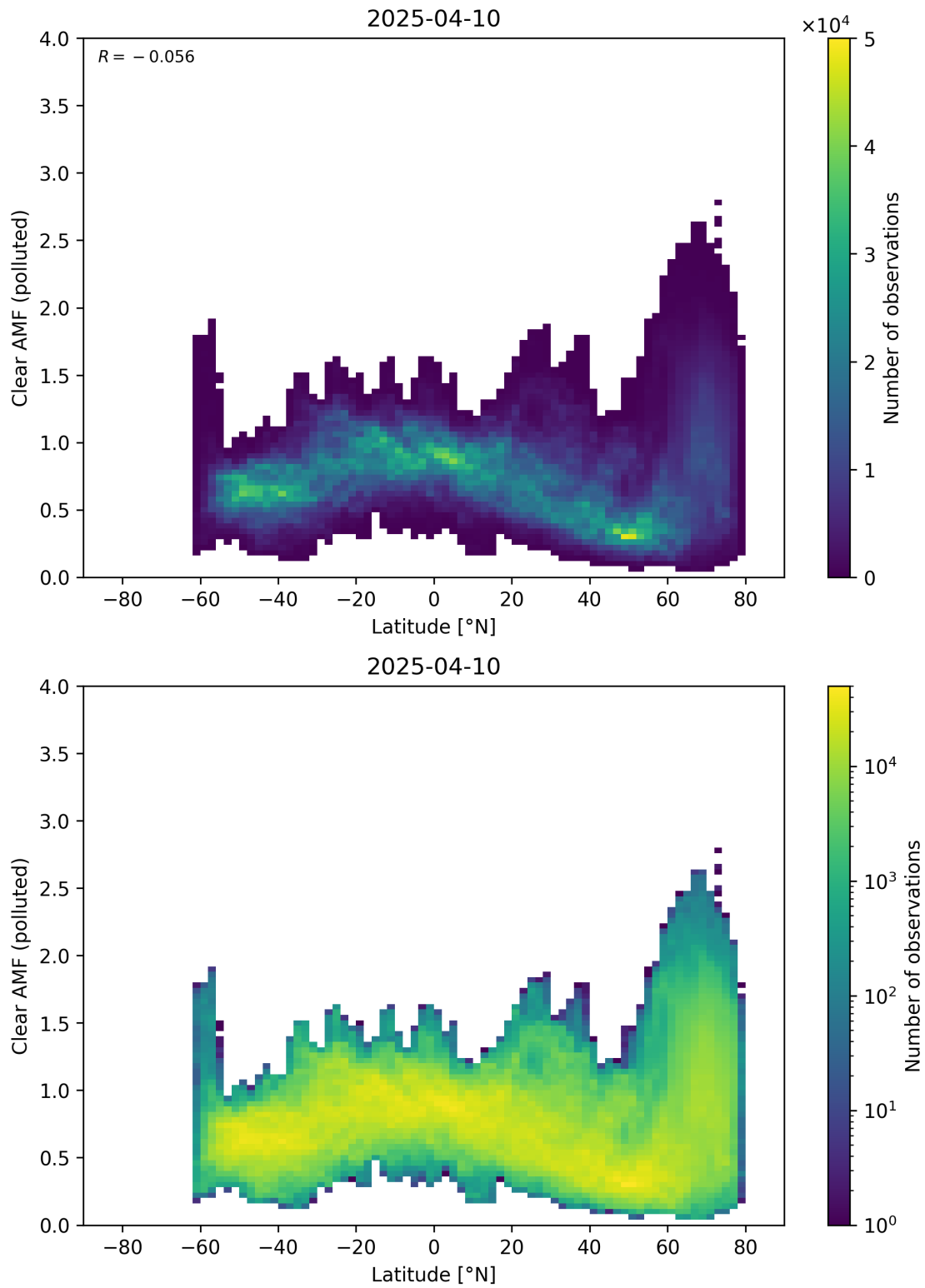
Figure 156: Scatter density plot of “Latitude” against “Clear AMF (polluted)” for 2025-04-09 to 2025-04-11.
