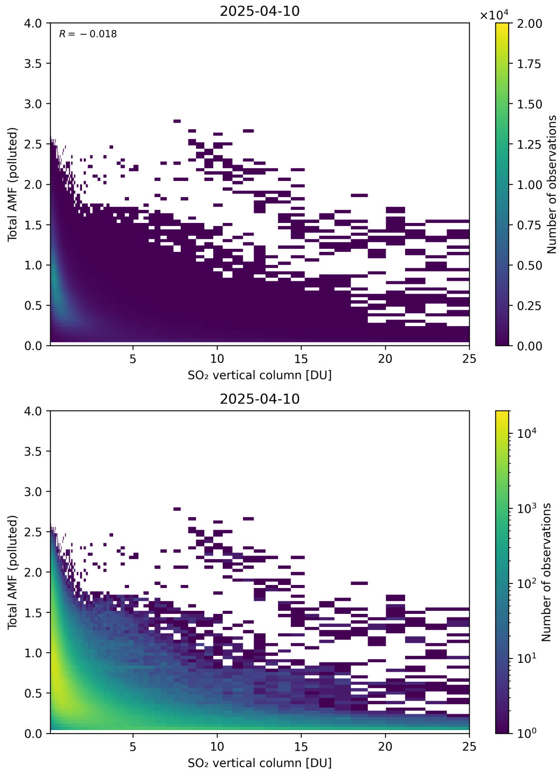
Figure 359: Scatter density plot of “SO 2 vertical column” against “Total AMF (polluted)” for 2025-04-09 to 2025-04-11.
