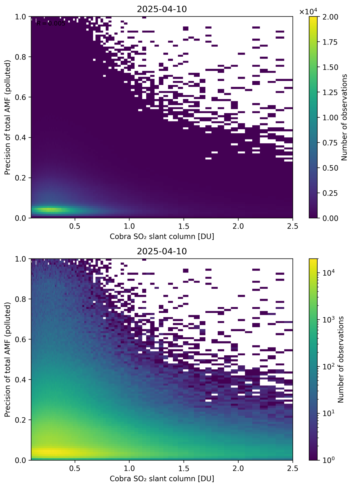
Figure 225: Scatter density plot of “Cobra SO 2 slant column” against “Precision of total AMF (polluted)” for 2025-04-09 to 2025-04-11.
