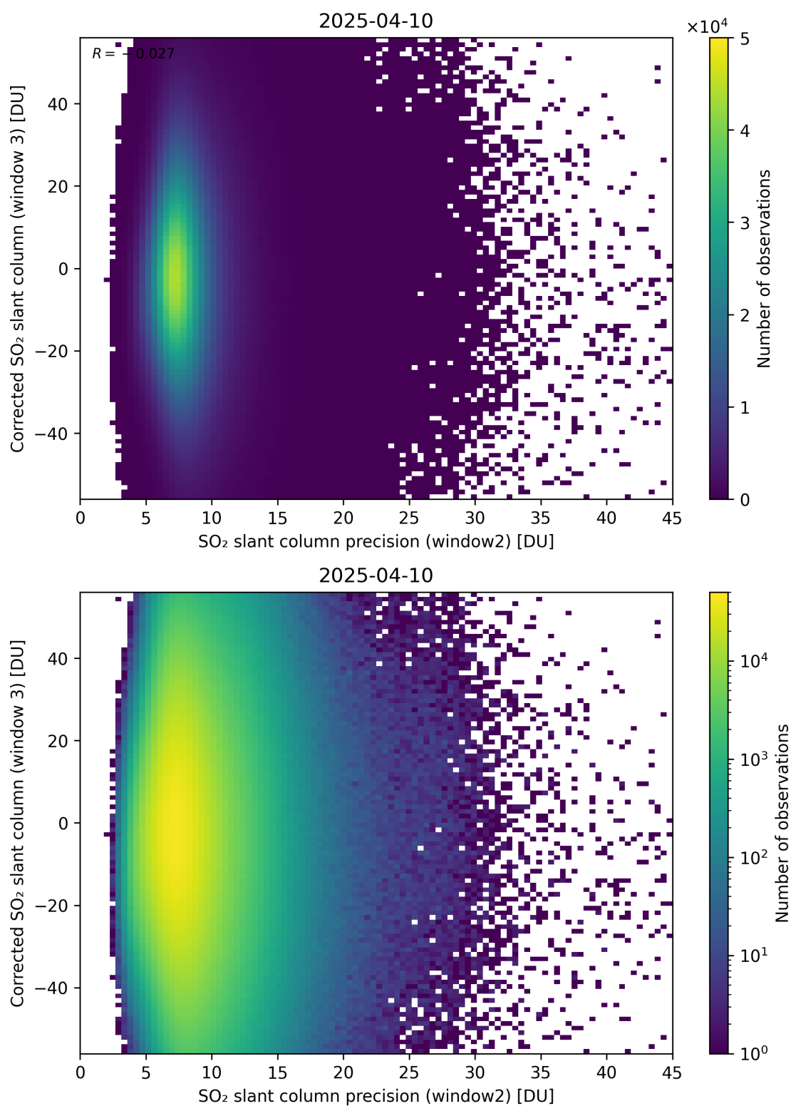
Figure 298: Scatter density plot of “SO 2 slant column precision (window2)” against “Corrected SO 2 slant column (window 3)” for 2025-04-09 to 2025-04-11.
