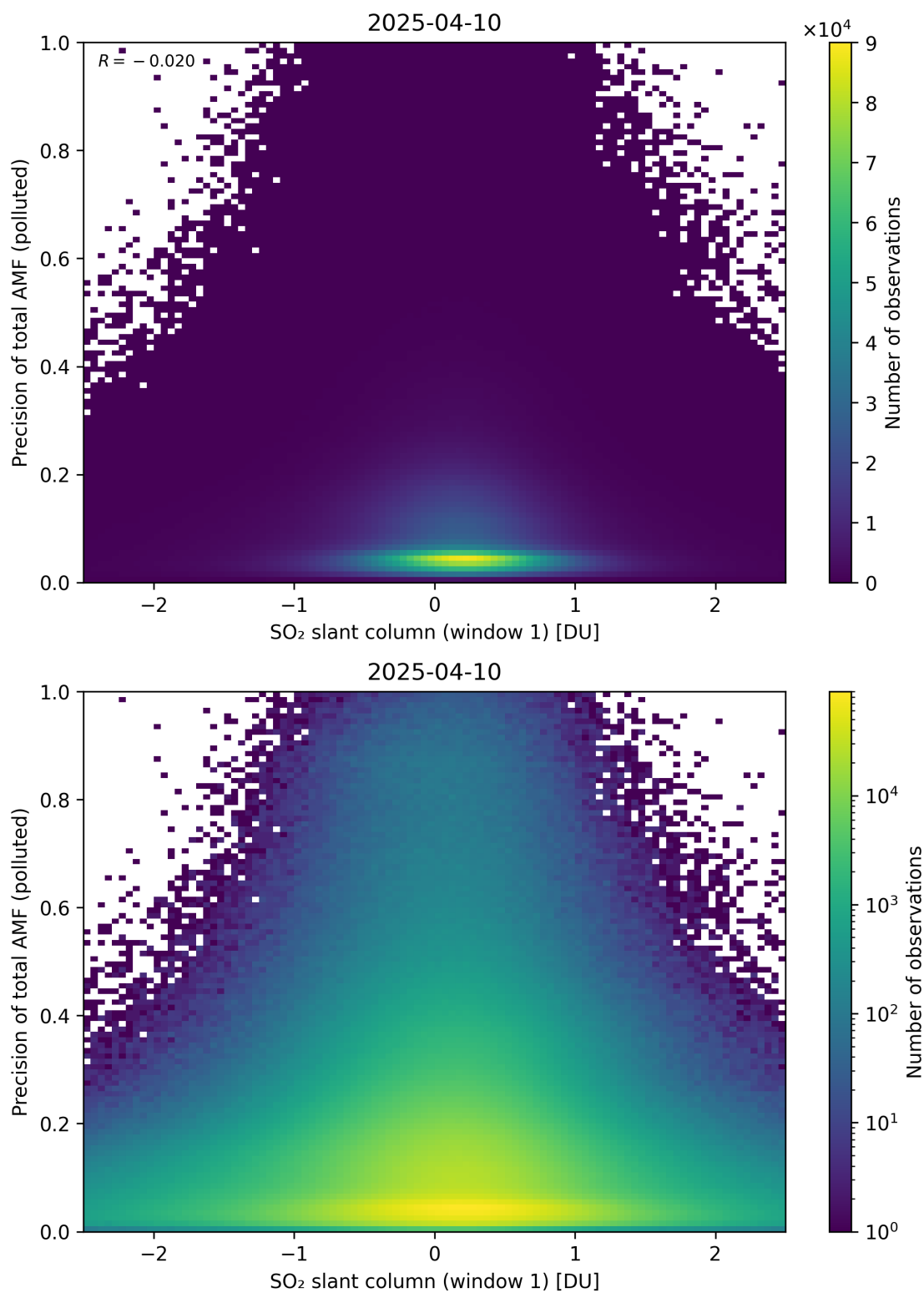
Figure 290: Scatter density plot of “SO 2 slant column (window 1)” against “Precision of total AMF (polluted)” for 2025-04-09 to 2025-04-11.
