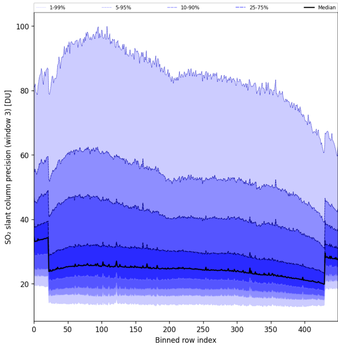
Figure 98: Along track statistics of “SO 2 slant column precision (window 3)” for 2025-04-09 to 2025-04-11
