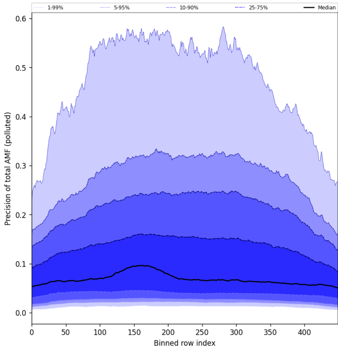
Figure 106: Along track statistics of “Precision of total AMF (polluted)” for 2025-04-09 to 2025-04-11
