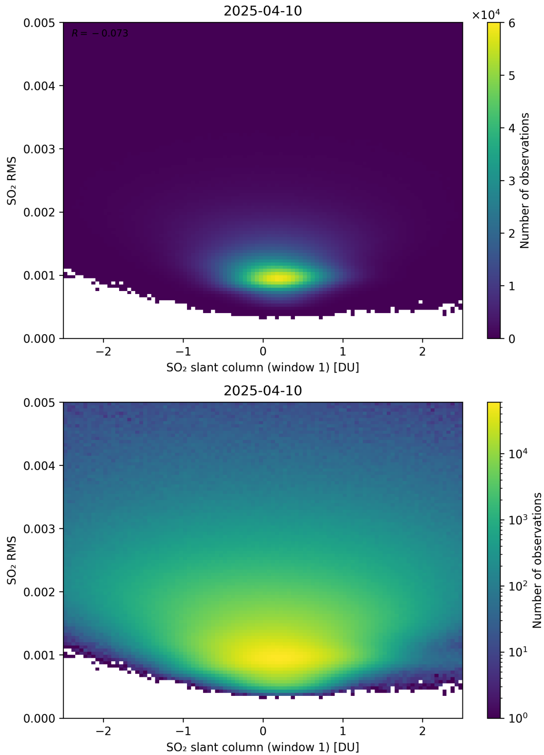
Figure 267: Scatter density plot of “SO 2 slant column (window 1)” against “SO 2 RMS” for 2025-04-09 to 2025-04-11.
