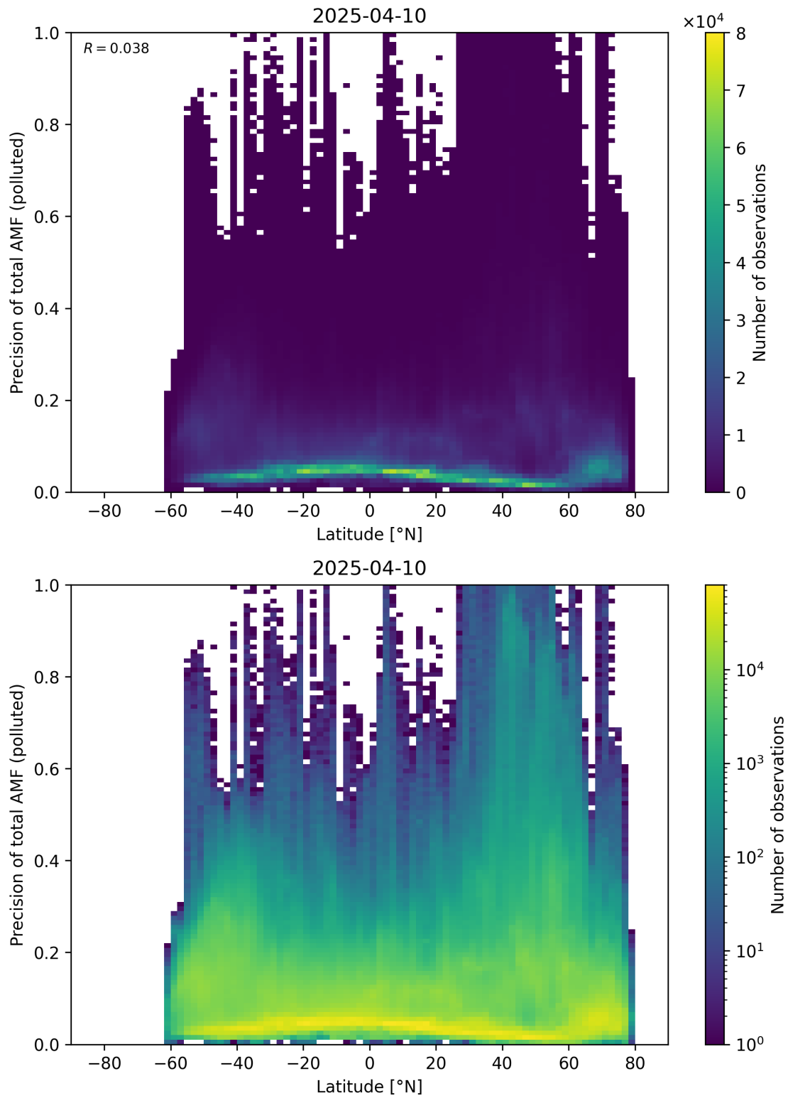
Figure 168: Scatter density plot of “Latitude” against “Precision of total AMF (polluted)” for 2025-04-09 to 2025-04-11.
