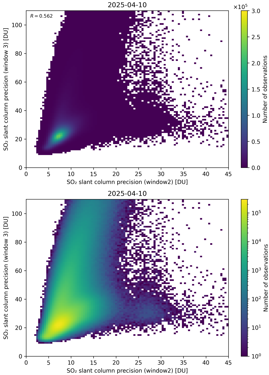
Figure 300: Scatter density plot of “SO 2 slant column precision (window2)” against “SO 2 slant column precision (window 3)” for 2025-04-09 to 2025-04-11.
