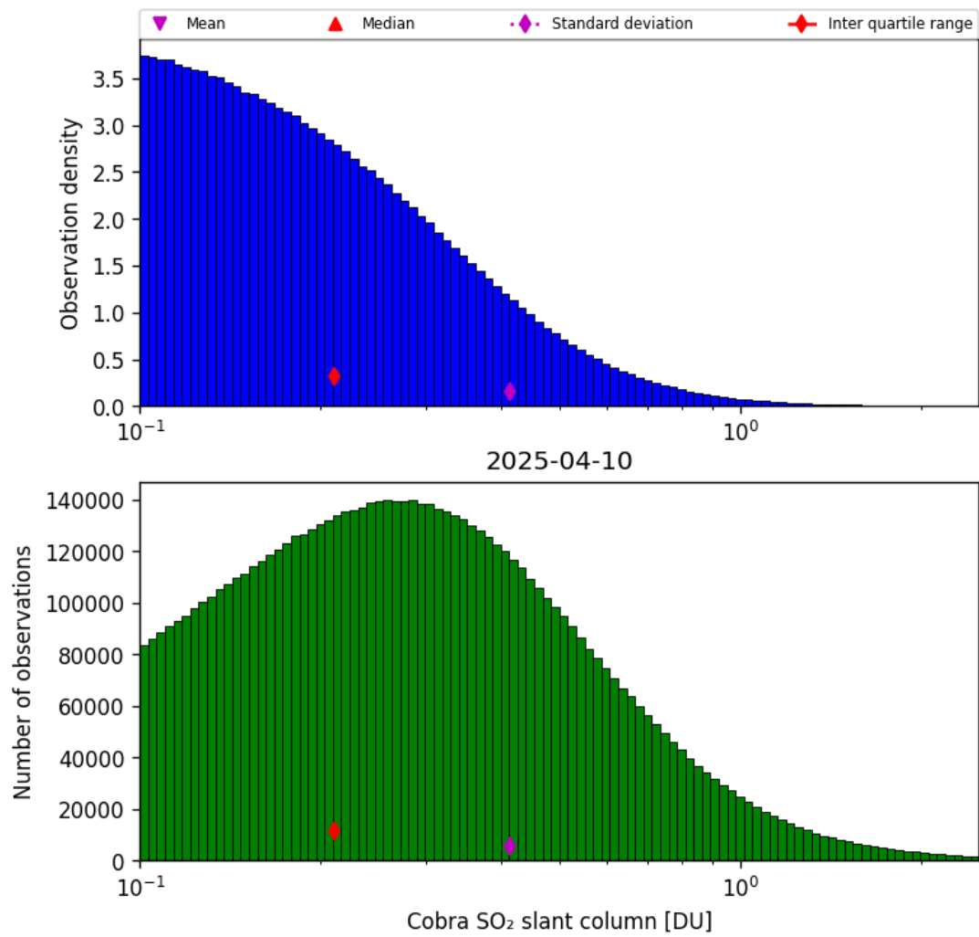
Figure 61: Histogram of “Cobra SO 2 slant column” for 2025-04-09 to 2025-04-11
