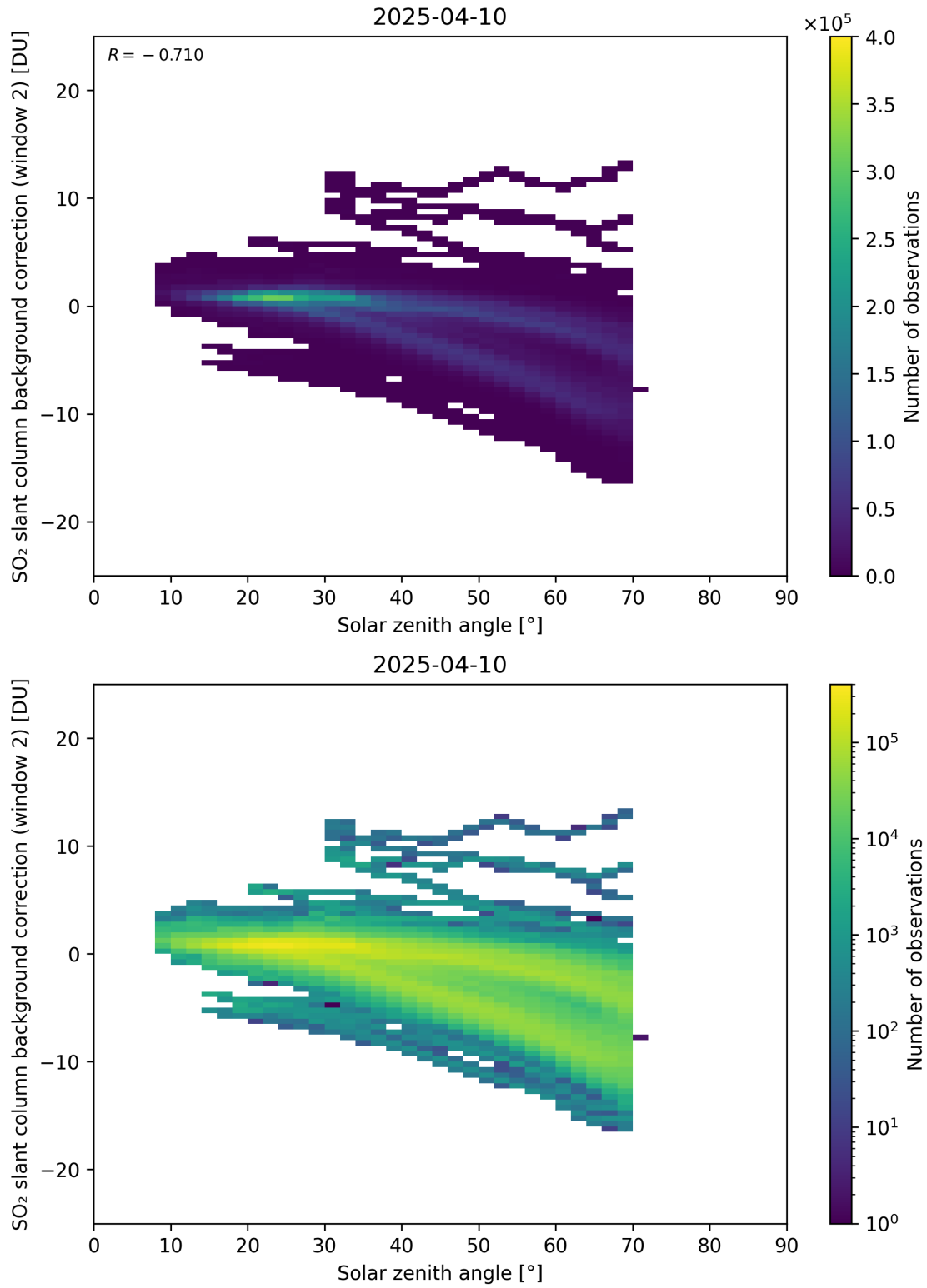
Figure 172: Scatter density plot of “Solar zenith angle” against “SO 2 slant column background correction (window 2)” for 2025-04-09 to 2025-04-11.
