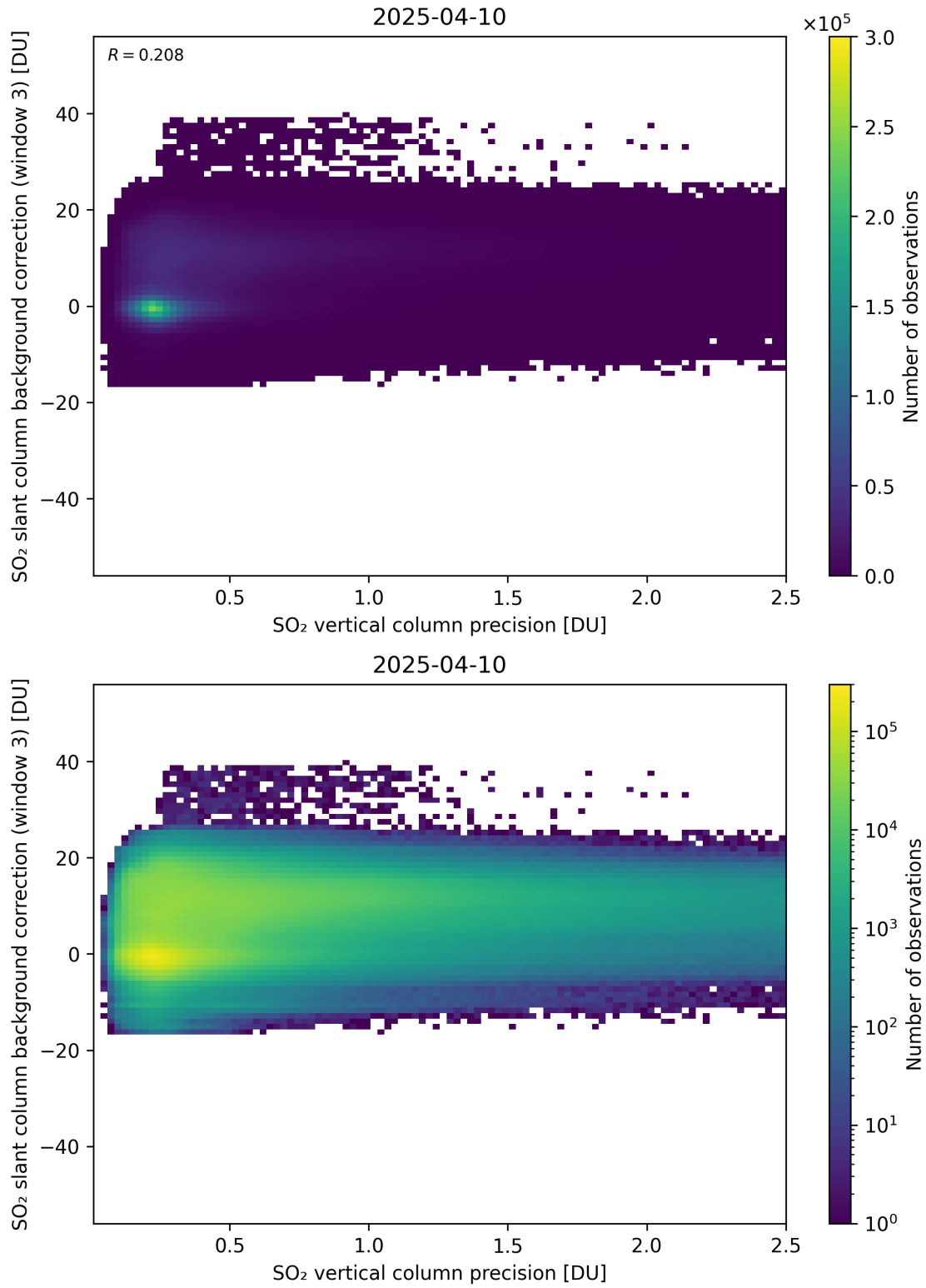
Figure 331: Scatter density plot of “SO 2 vertical column precision” against “SO 2 slant column background correction (window 3)” for 2025-04-09 to 2025-04-11.
