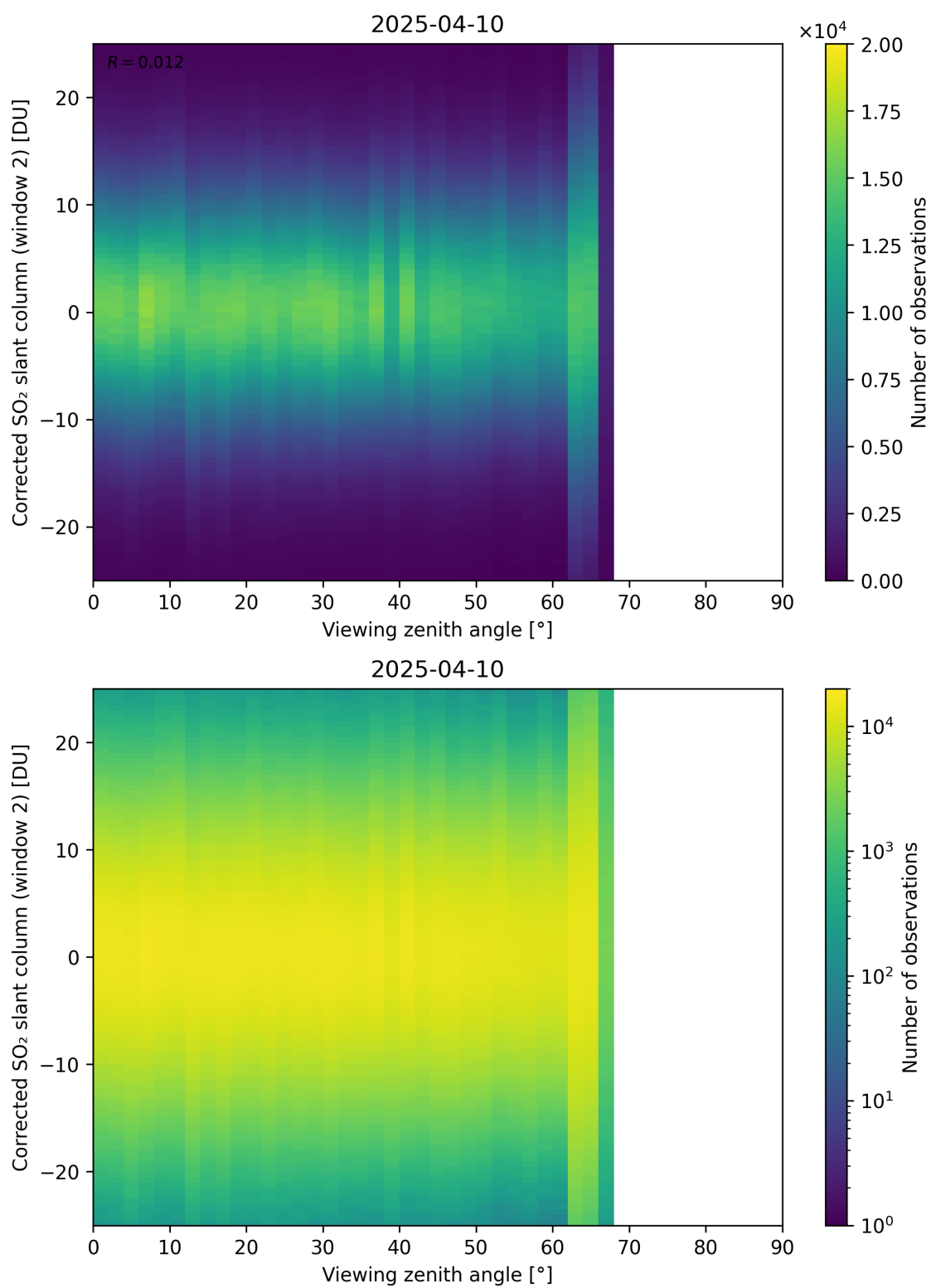
Figure 374: Scatter density plot of “Viewing zenith angle” against “Corrected SO 2 slant column (window 2)” for 2025-04-09 to 2025-04-11.
