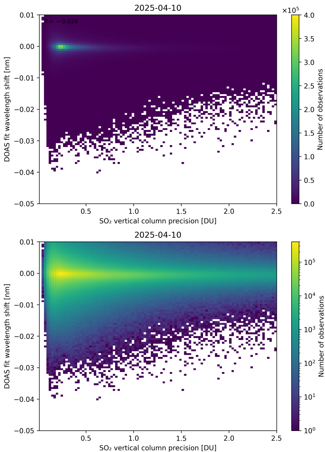
Figure 332: Scatter density plot of “SO 2 vertical column precision” against “DOAS fit wavelength shift” for 2025-04-09 to 2025-04-11.
