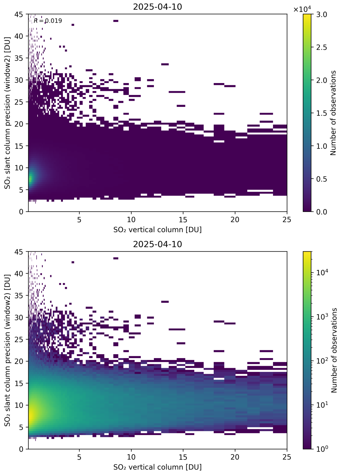
Figure 356: Scatter density plot of “SO 2 vertical column” against “SO 2 slant column precision (window2)” for 2025-04-09 to 2025-04-11.
