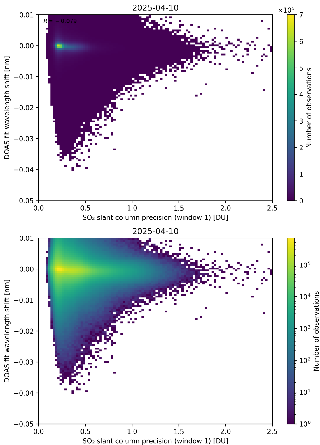
Figure 271: Scatter density plot of “SO 2 slant column precision (window 1)” against “DOAS fit wavelength shift” for 2025-04-09 to 2025-04-11.
