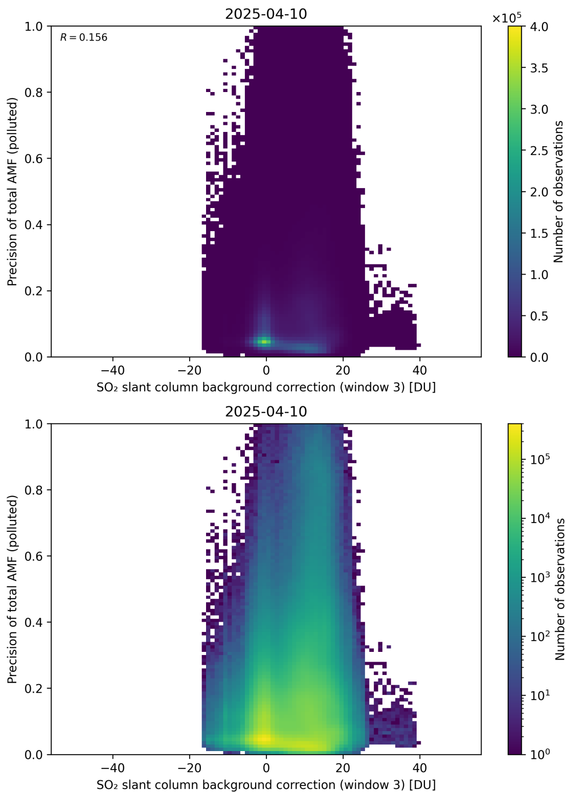
Figure 137: Scatter density plot of “SO 2 slant column background correction (window 3)” against “Precision of total AMF (polluted)” for 2025-04-09 to 2025-04-11.
