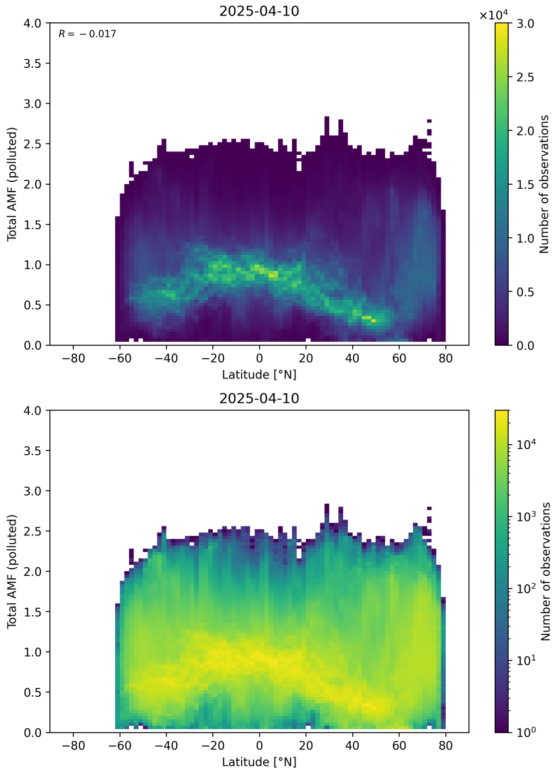
Figure 167: Scatter density plot of “Latitude” against “Total AMF (polluted)” for 2025-04-09 to 2025-04-11.
