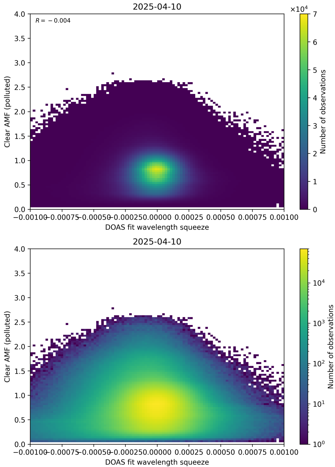
Figure 144: Scatter density plot of “DOAS fit wavelength squeeze” against “Clear AMF (polluted)” for 2025-04-09 to 2025-04-11.
