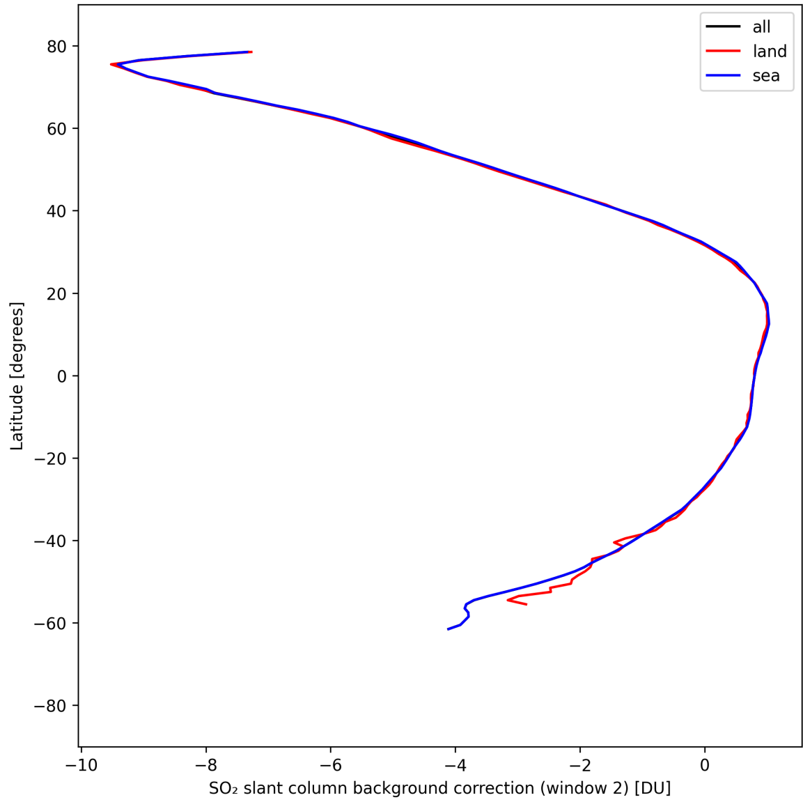
Figure 44: Zonal average of “SO 2 slant column background correction (window 2)” for 2025-04-09 to 2025-04-11.
