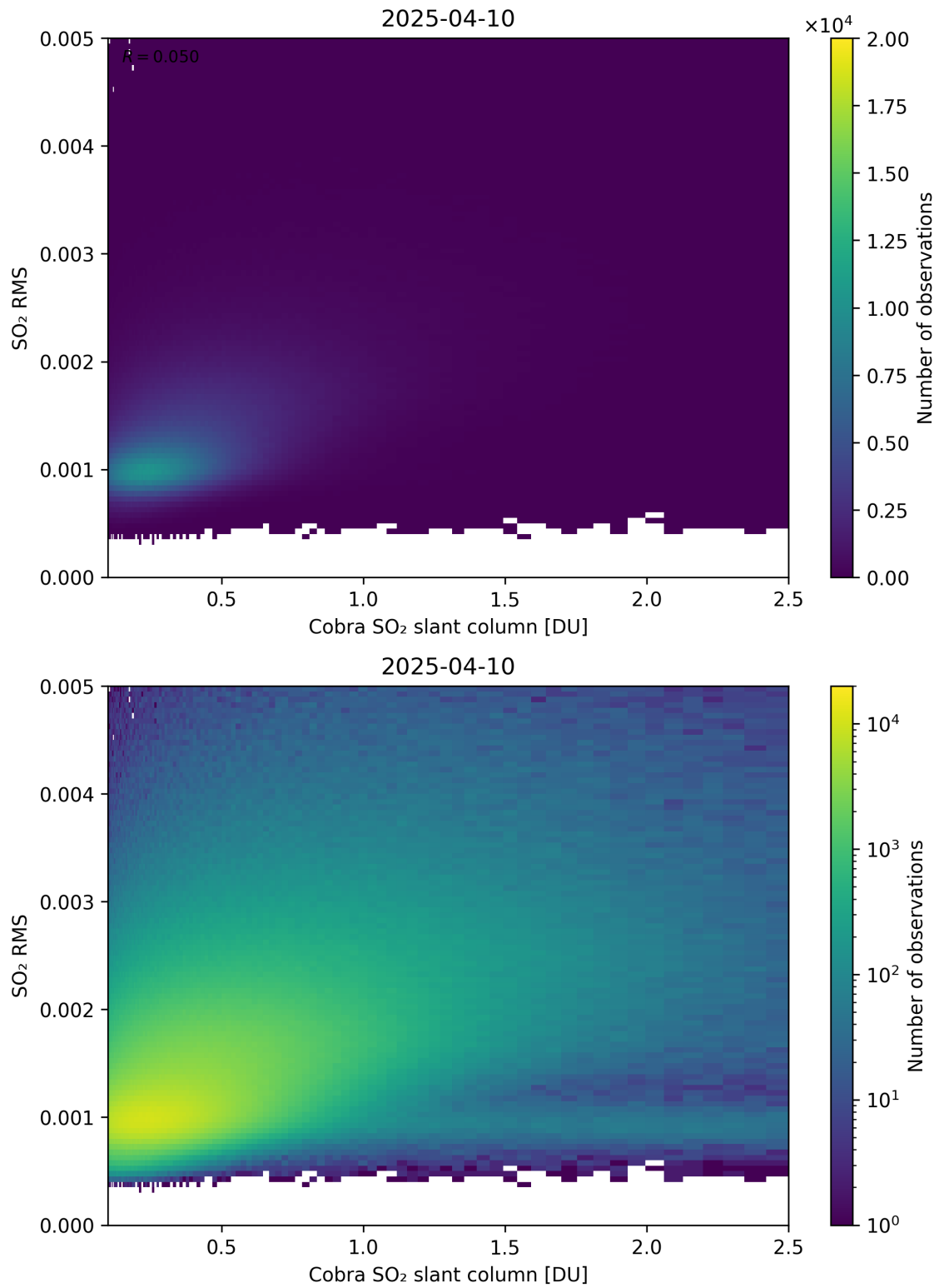
Figure 198: Scatter density plot of “Cobra SO 2 slant column” against “SO 2 RMS” for 2025-04-09 to 2025-04-11.
