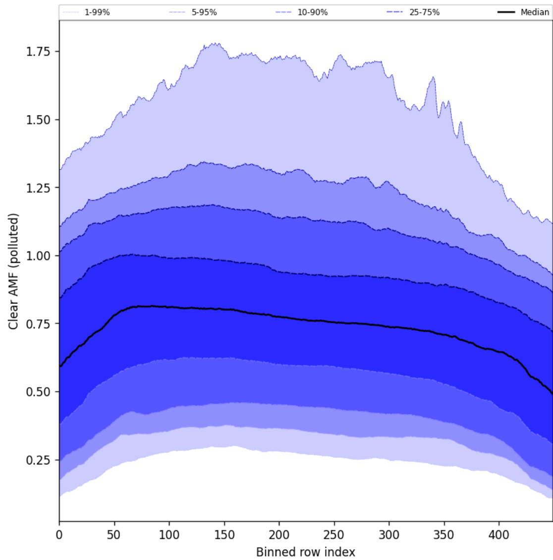
Figure 107: Along track statistics of “Clear AMF (polluted)” for 2025-04-09 to 2025-04-11
