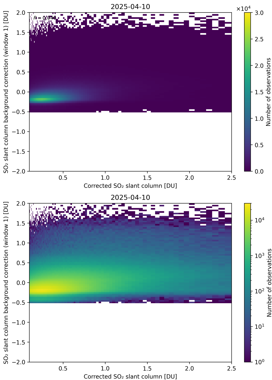
Figure 226: Scatter density plot of “Corrected SO 2 slant column” against “SO 2 slant column background correction (window 1)” for 2025-04-09 to 2025-04-11.
