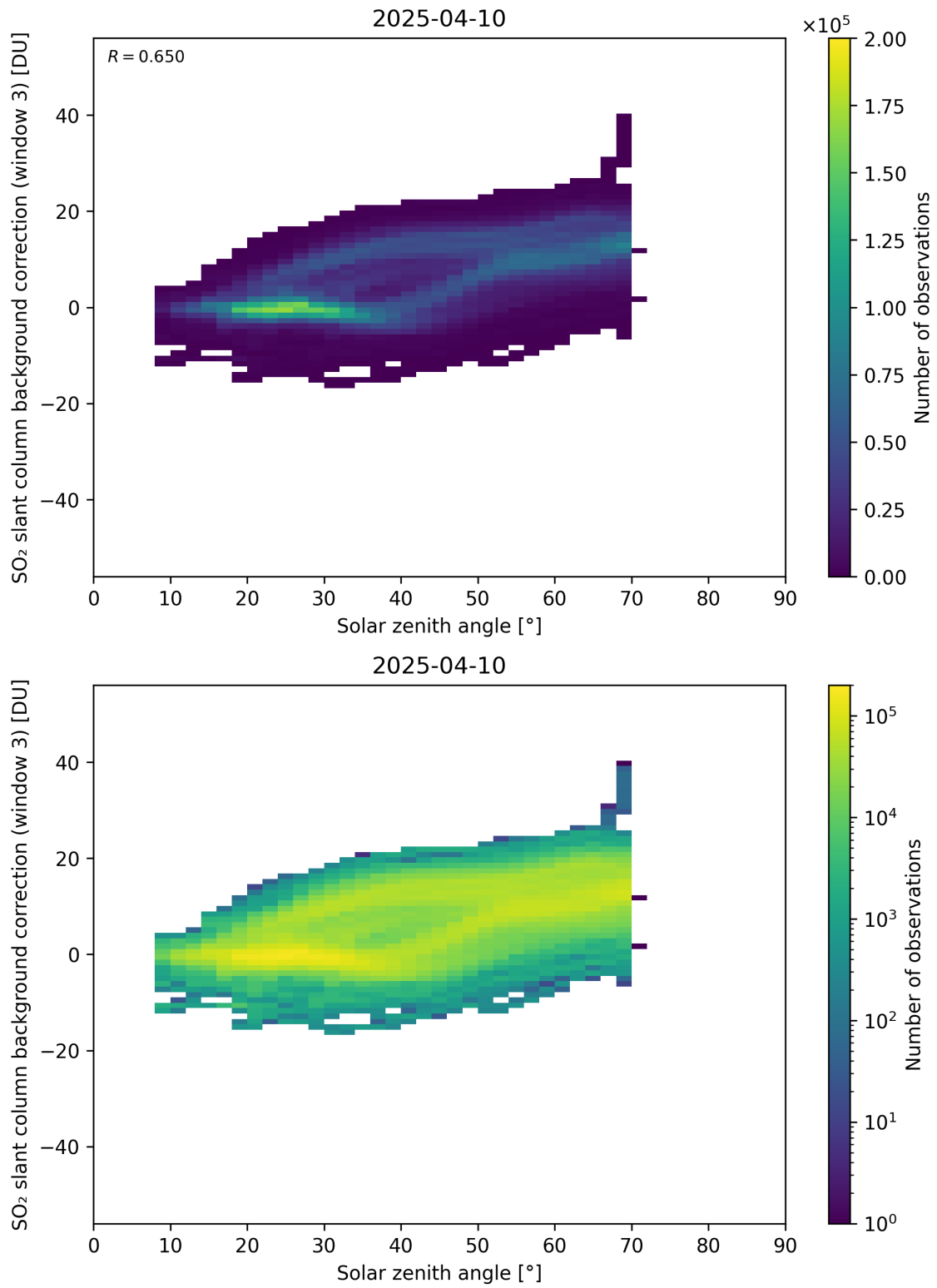
Figure 173: Scatter density plot of “Solar zenith angle” against “SO 2 slant column background correction (window 3)” for 2025-04-09 to 2025-04-11.
