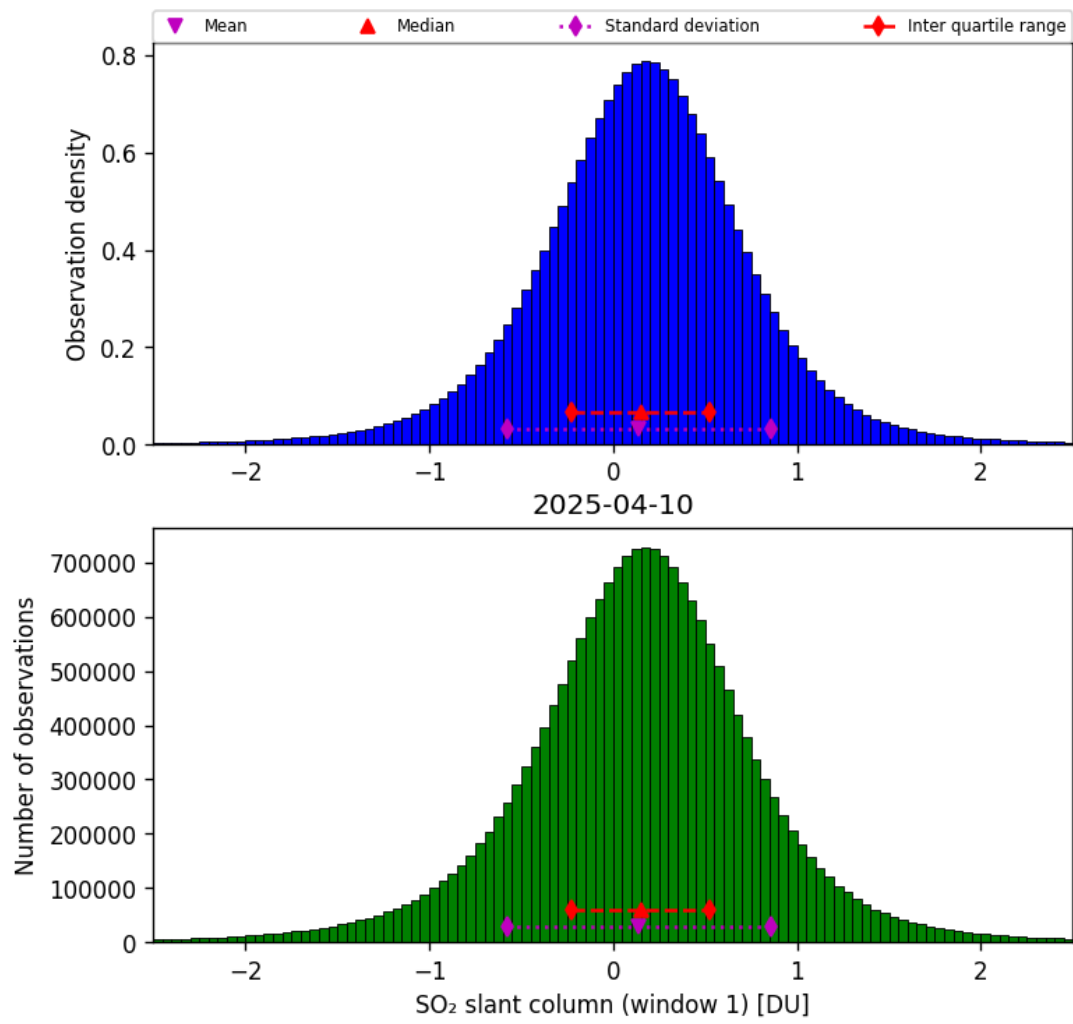
Figure 63: Histogram of “SO 2 slant column (window 1)” for 2025-04-09 to 2025-04-11
