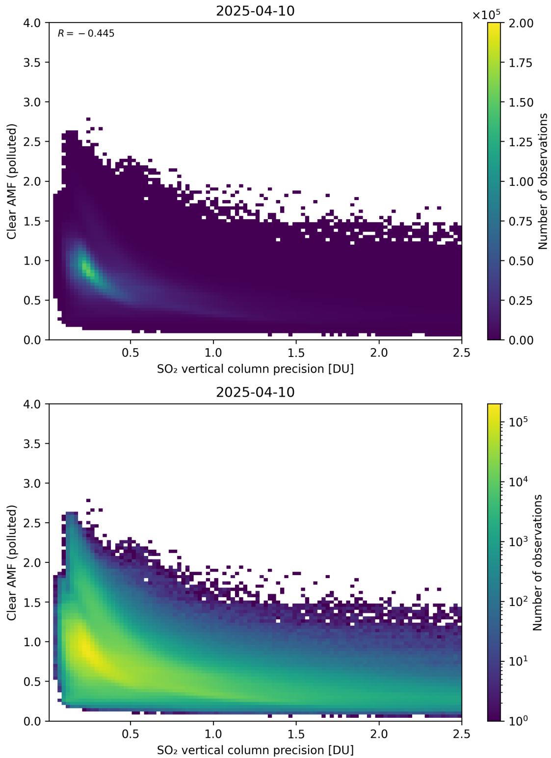
Figure 335: Scatter density plot of “SO 2 vertical column precision” against “Clear AMF (polluted)” for 2025-04-09 to 2025-04-11.
