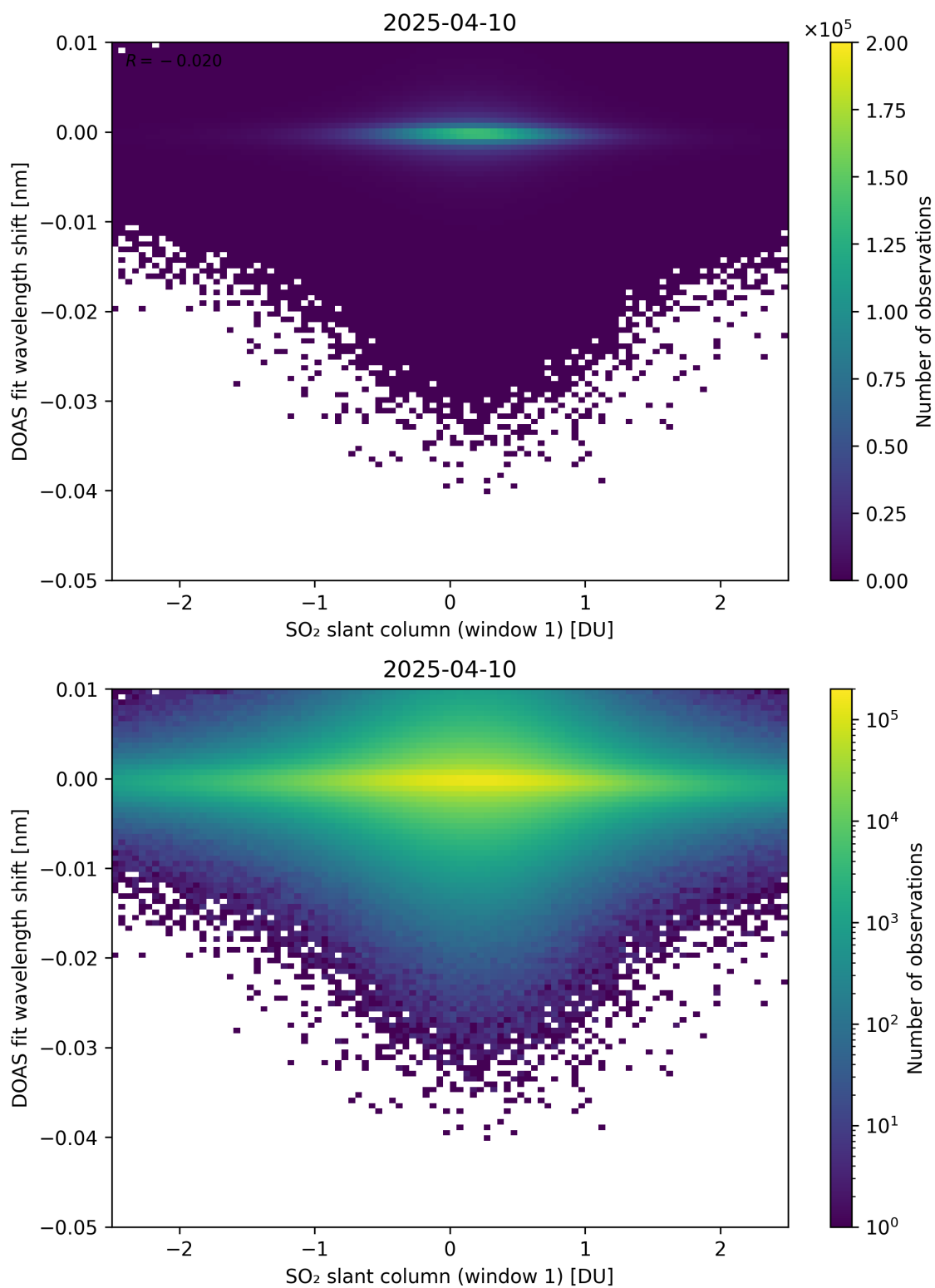
Figure 265: Scatter density plot of “SO 2 slant column (window 1)” against “DOAS fit wavelength shift” for 2025-04-09 to 2025-04-11.
