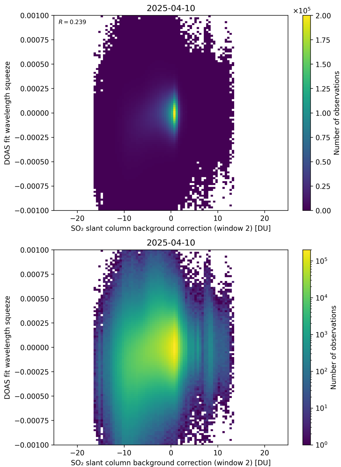
Figure 124: Scatter density plot of “SO 2 slant column background correction (window 2)” against “DOAS fit wavelength squeeze” for 2025-04-09 to 2025-04-11.
