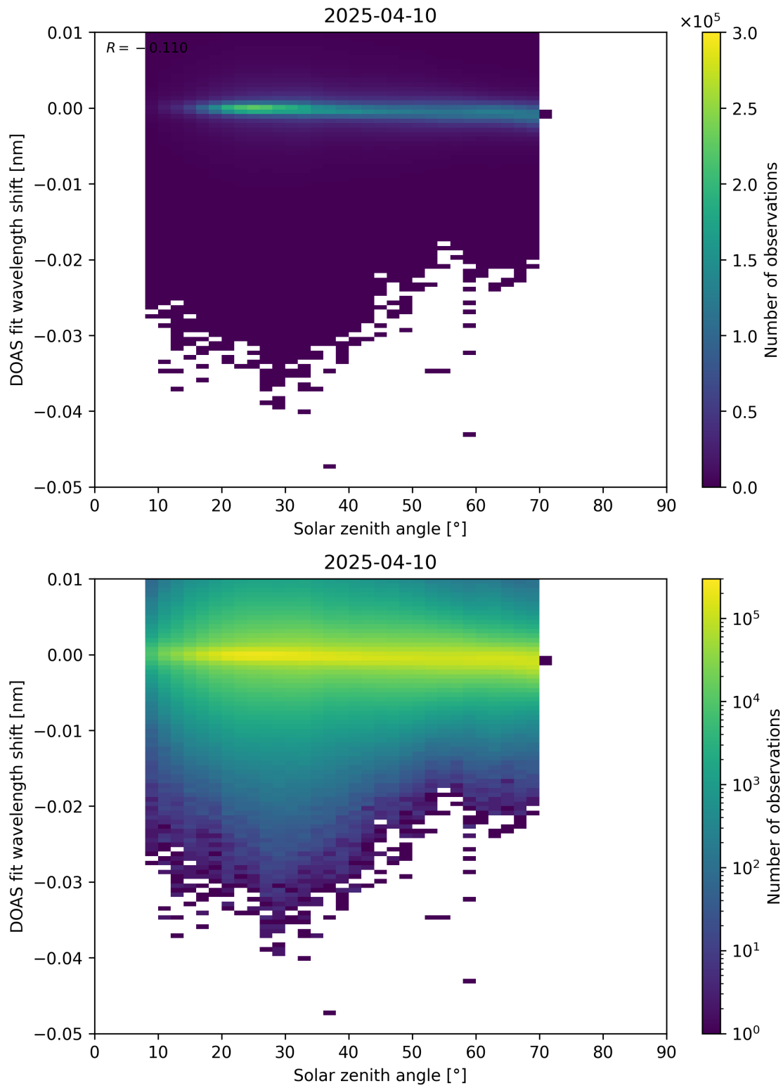
Figure 174: Scatter density plot of “Solar zenith angle” against “DOAS fit wavelength shift” for 2025-04-09 to 2025-04-11.
