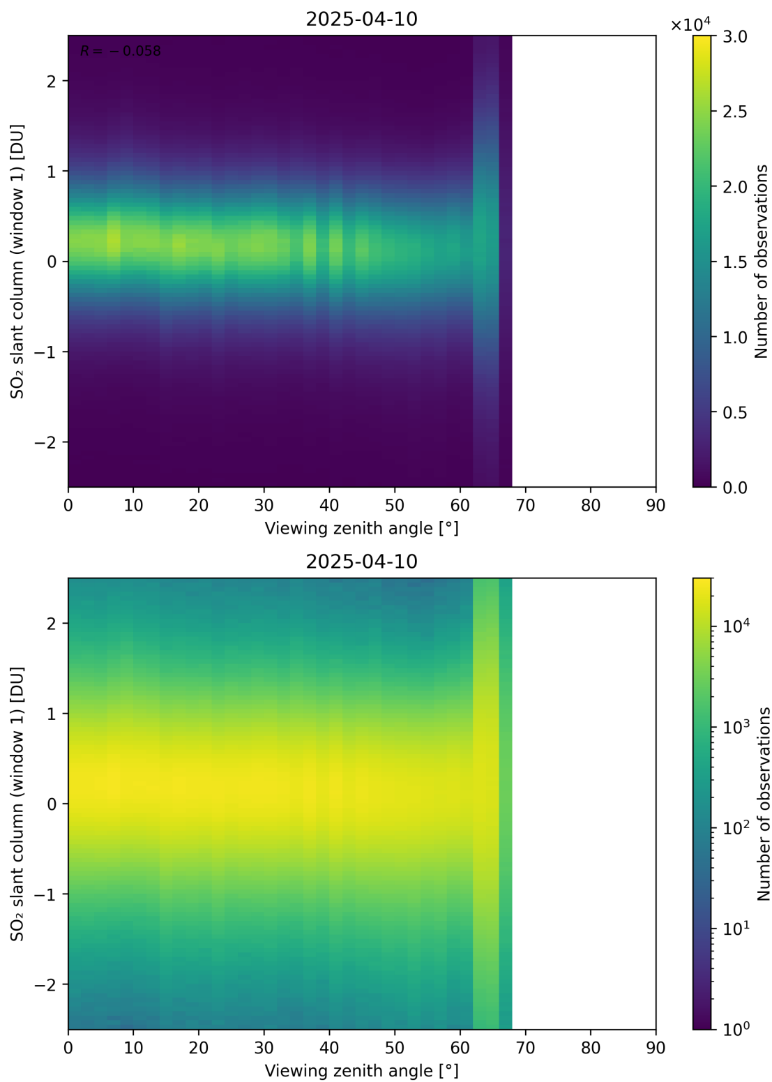
Figure 376: Scatter density plot of “Viewing zenith angle” against “SO 2 slant column (window 1)” for 2025-04-09 to 2025-04-11.
