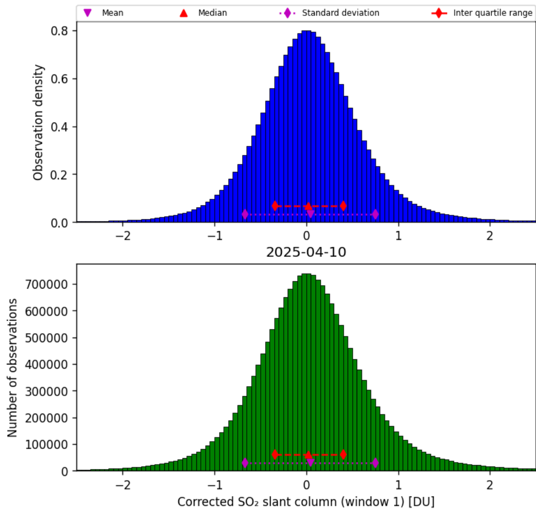
Figure 65: Histogram of “Corrected SO 2 slant column (window 1)” for 2025-04-09 to 2025-04-11
