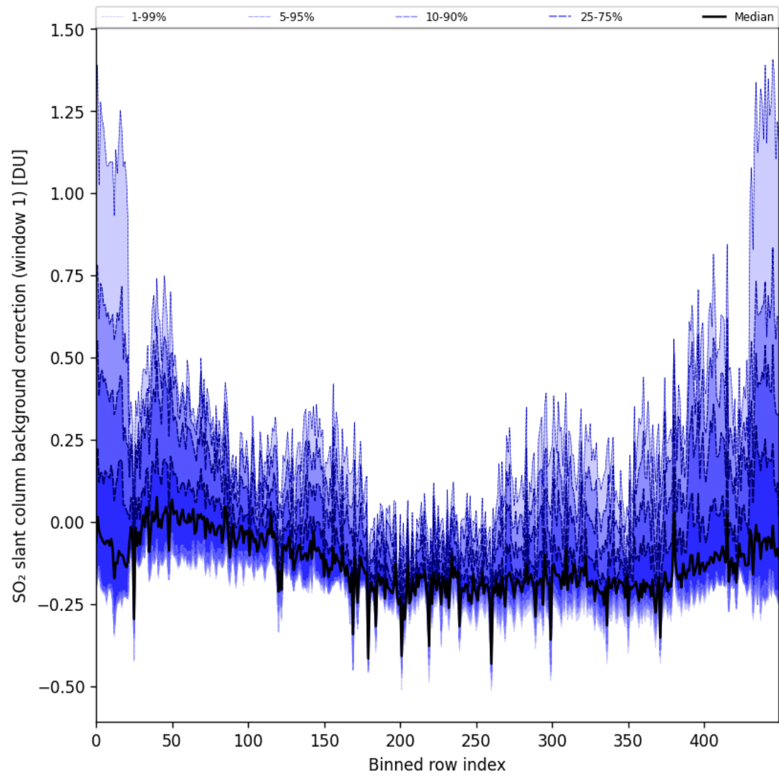
Figure 92: Along track statistics of “SO 2 slant column background correction (window 1)” for 2025-04-09 to 2025-04-11
