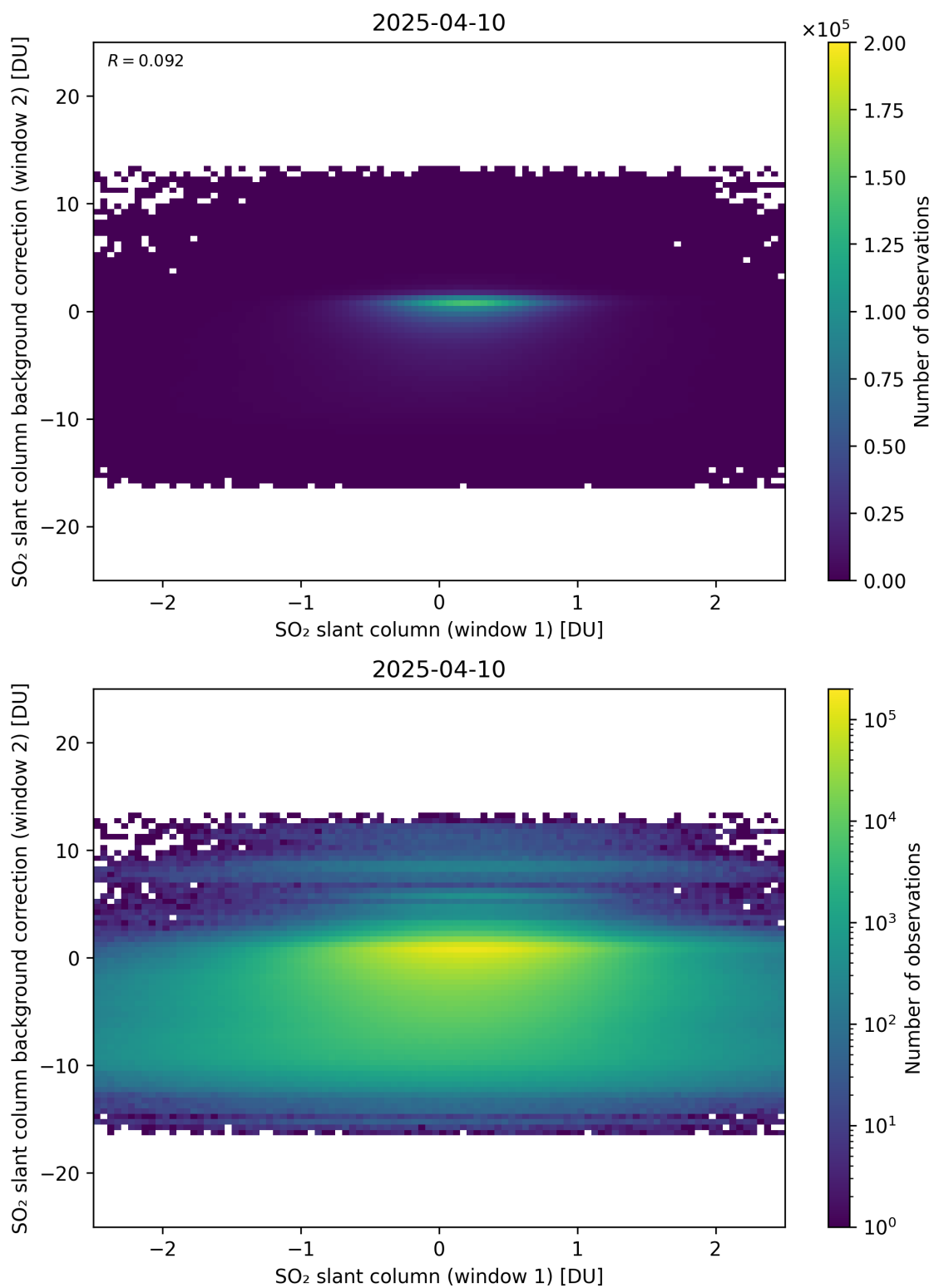
Figure 263: Scatter density plot of “SO 2 slant column (window 1)” against “SO 2 slant column background correction (window 2)” for 2025-04-09 to 2025-04-11.
