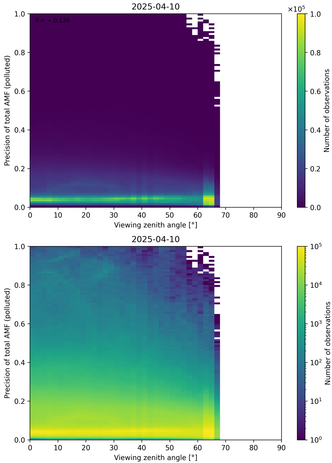
Figure 382: Scatter density plot of “Viewing zenith angle” against “Precision of total AMF (polluted)” for 2025-04-09 to 2025-04-11.
