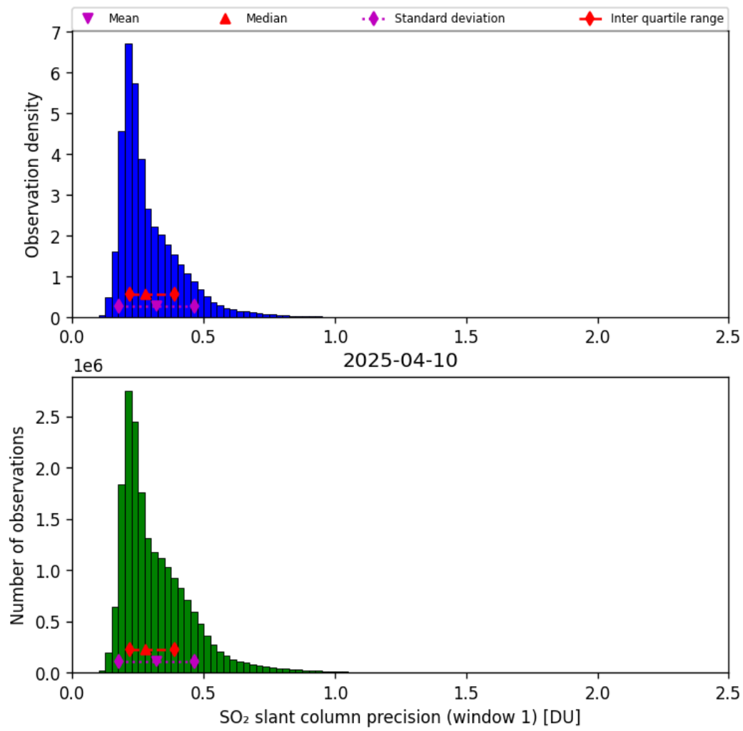
Figure 64: Histogram of “SO 2 slant column precision (window 1)” for 2025-04-09 to 2025-04-11
