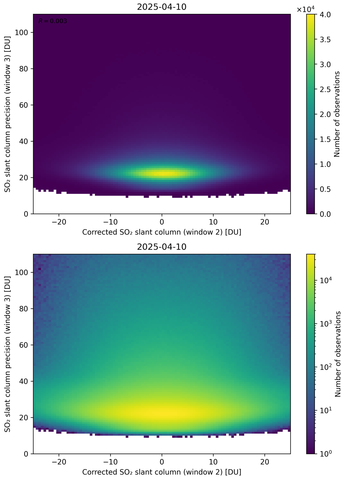
Figure 252: Scatter density plot of “Corrected SO 2 slant column (window 2)” against “SO 2 slant column precision (window 3)” for 2025-04-09 to 2025-04-11.
