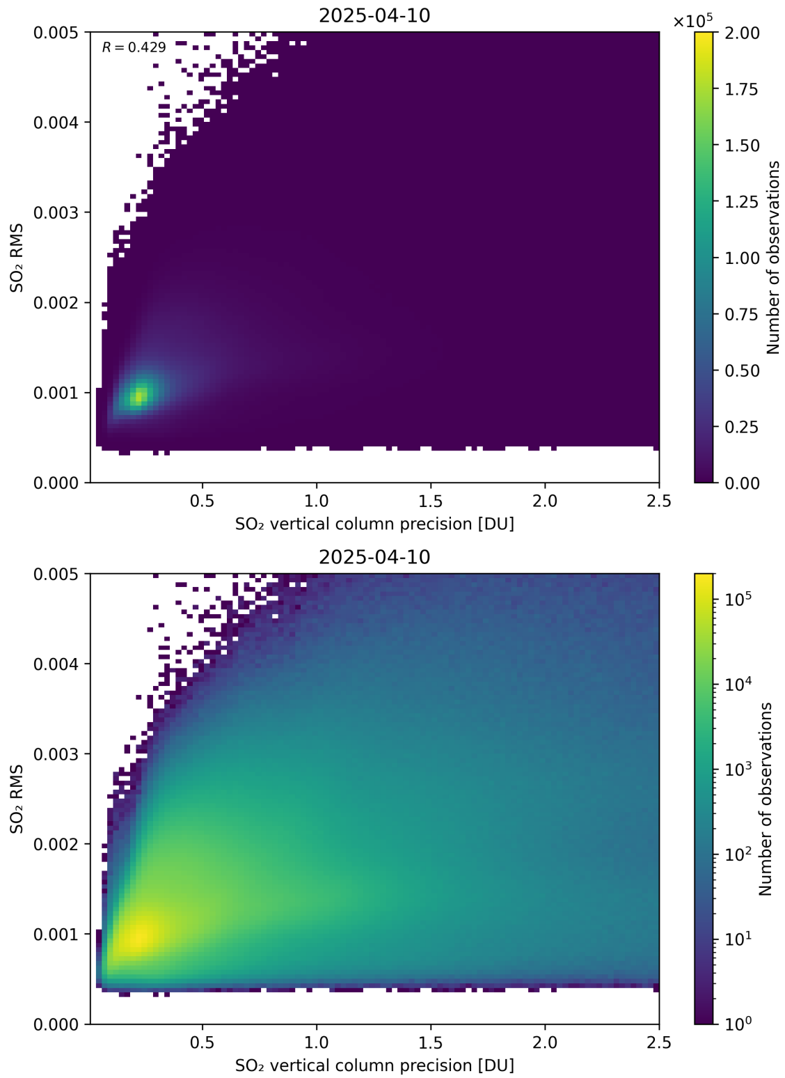
Figure 334: Scatter density plot of “SO 2 vertical column precision” against “SO 2 RMS” for 2025-04-09 to 2025-04-11.
