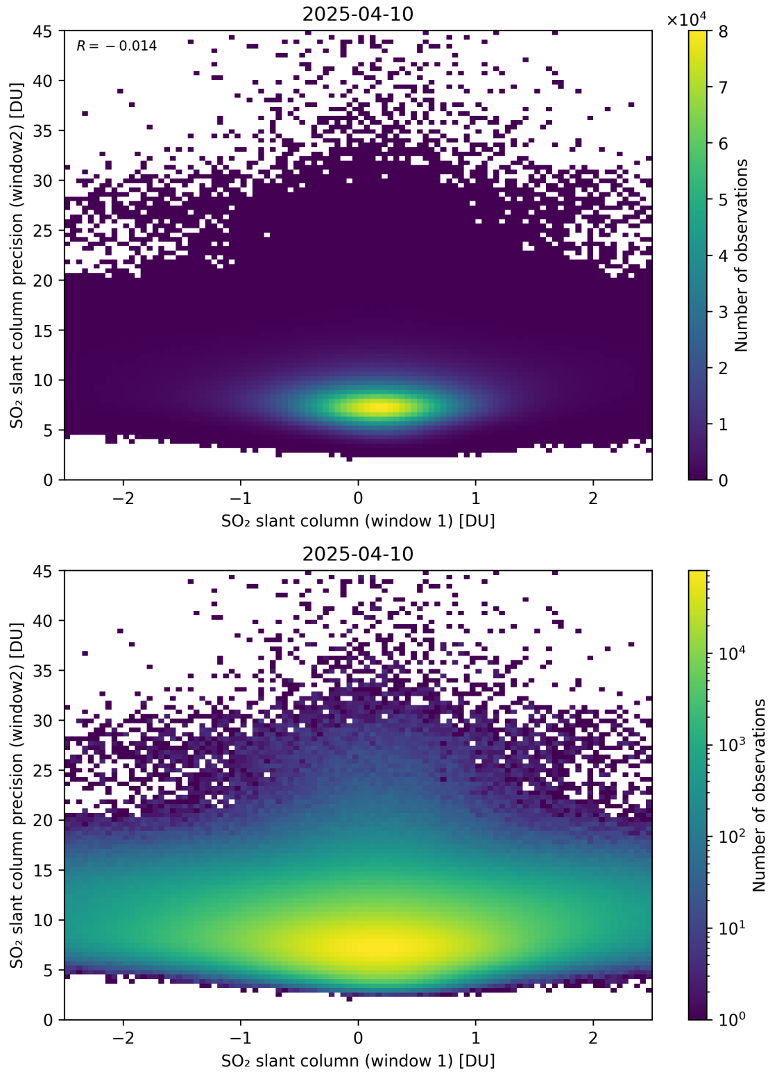
Figure 286: Scatter density plot of “SO 2 slant column (window 1)” against “SO 2 slant column precision (window2)” for 2025-04-09 to 2025-04-11.
