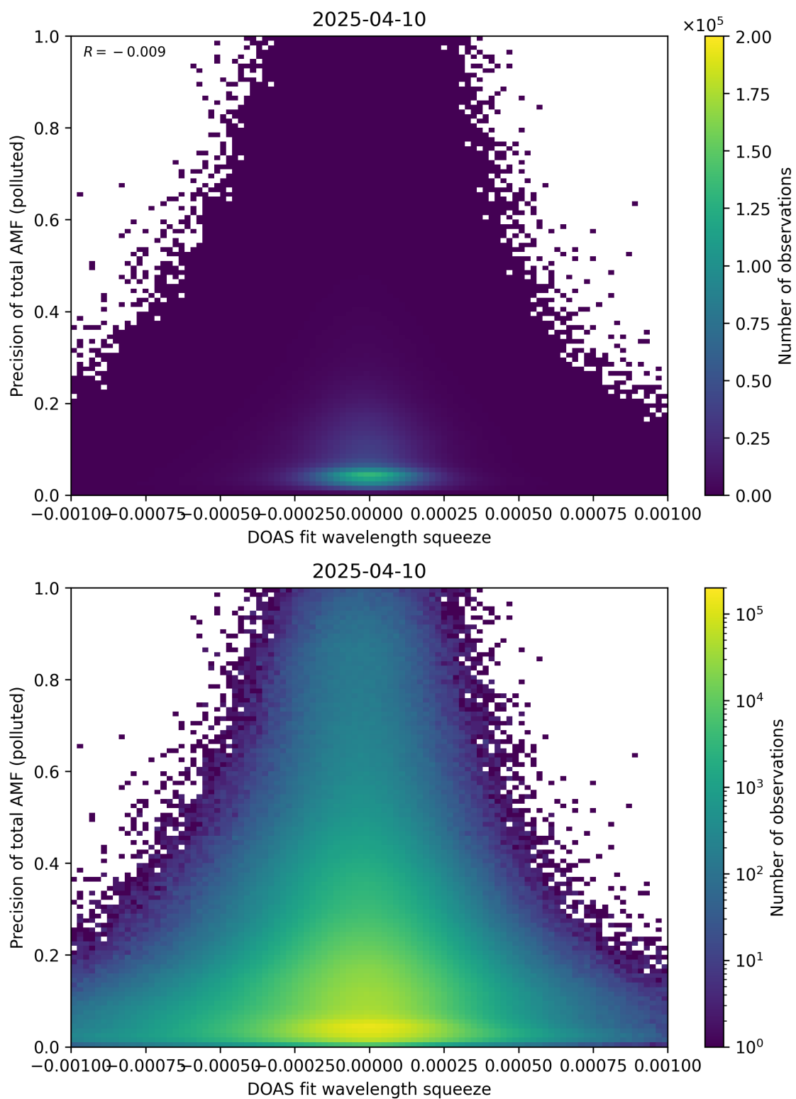
Figure 146: Scatter density plot of “DOAS fit wavelength squeeze” against “Precision of total AMF (polluted)” for 2025-04-09 to 2025-04-11.
