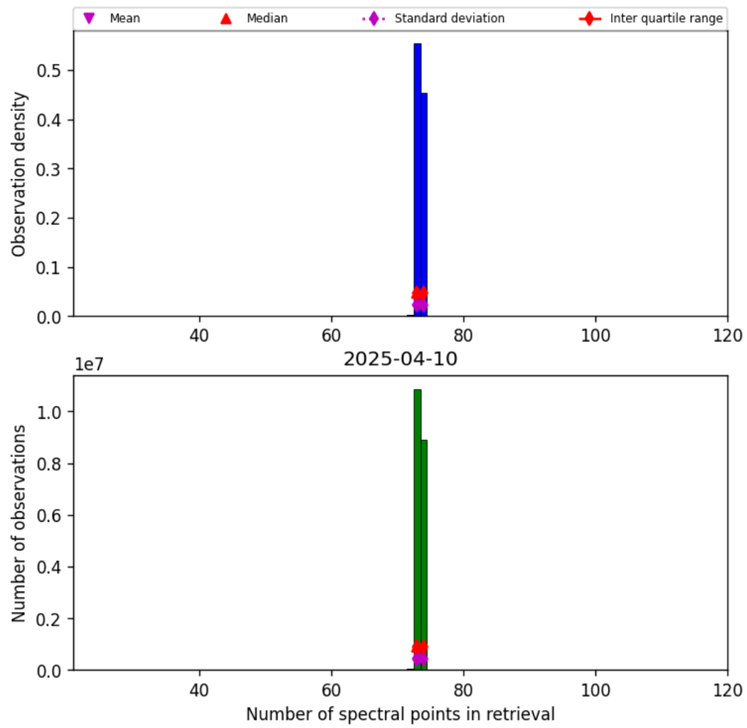
Figure 82: Histogram of “Number of spectral points in retrieval” for 2025-04-09 to 2025-04-11
