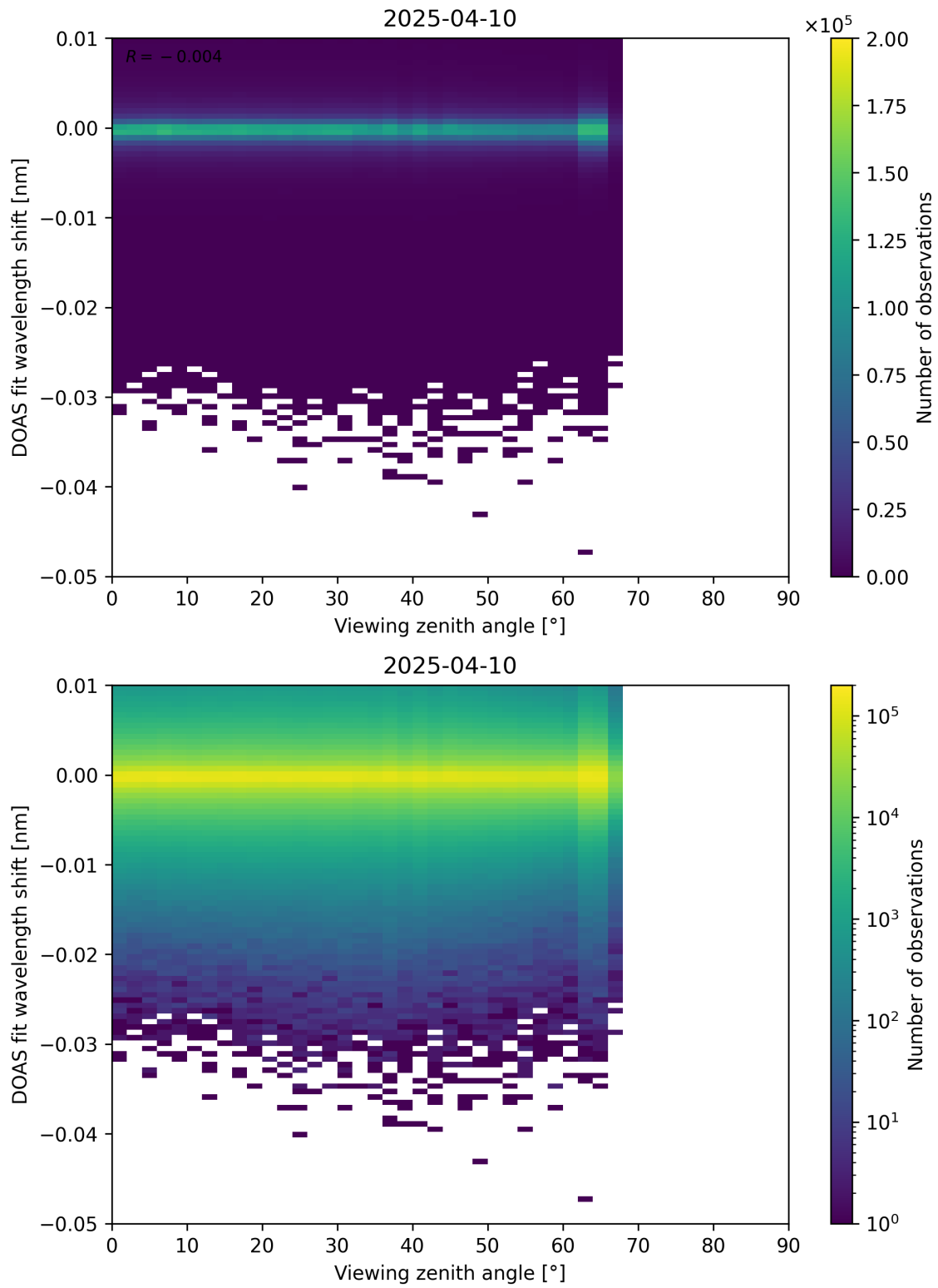
Figure 365: Scatter density plot of “Viewing zenith angle” against “DOAS fit wavelength shift” for 2025-04-09 to 2025-04-11.
