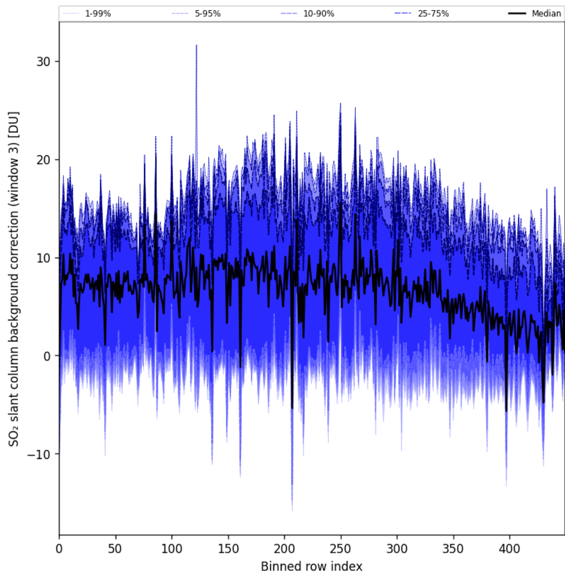
Figure 100: Along track statistics of “SO 2 slant column background correction (window 3)” for 2025-04-09 to 2025-04-11
