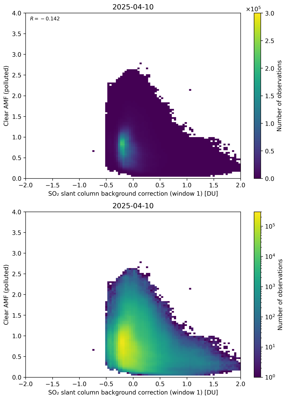
Figure 114: Scatter density plot of “SO 2 slant column background correction (window 1)” against “Clear AMF (polluted)” for 2025-04-09 to 2025-04-11.
