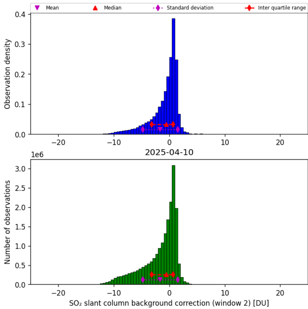
Figure 70: Histogram of “SO 2 slant column background correction (window 2)” for 2025-04-09 to 2025-04-11
