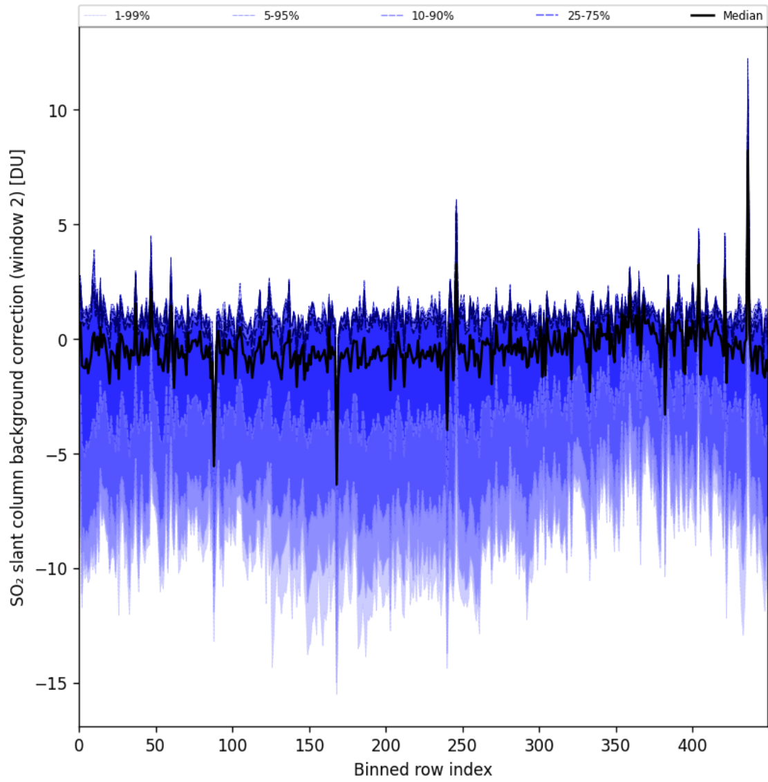
Figure 96: Along track statistics of “SO 2 slant column background correction (window 2)” for 2025-04-09 to 2025-04-11
