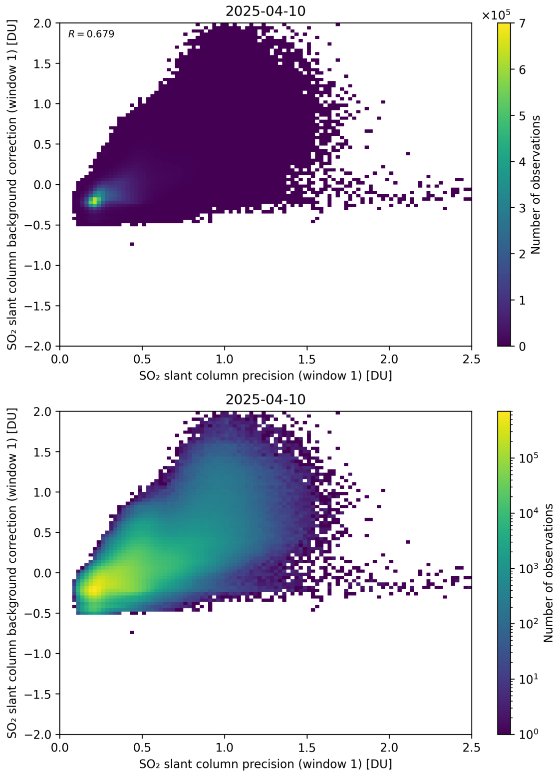
Figure 268: Scatter density plot of “SO 2 slant column precision (window 1)” against “SO 2 slant column background correction (window 1)” for 2025-04-09 to 2025-04-11.
