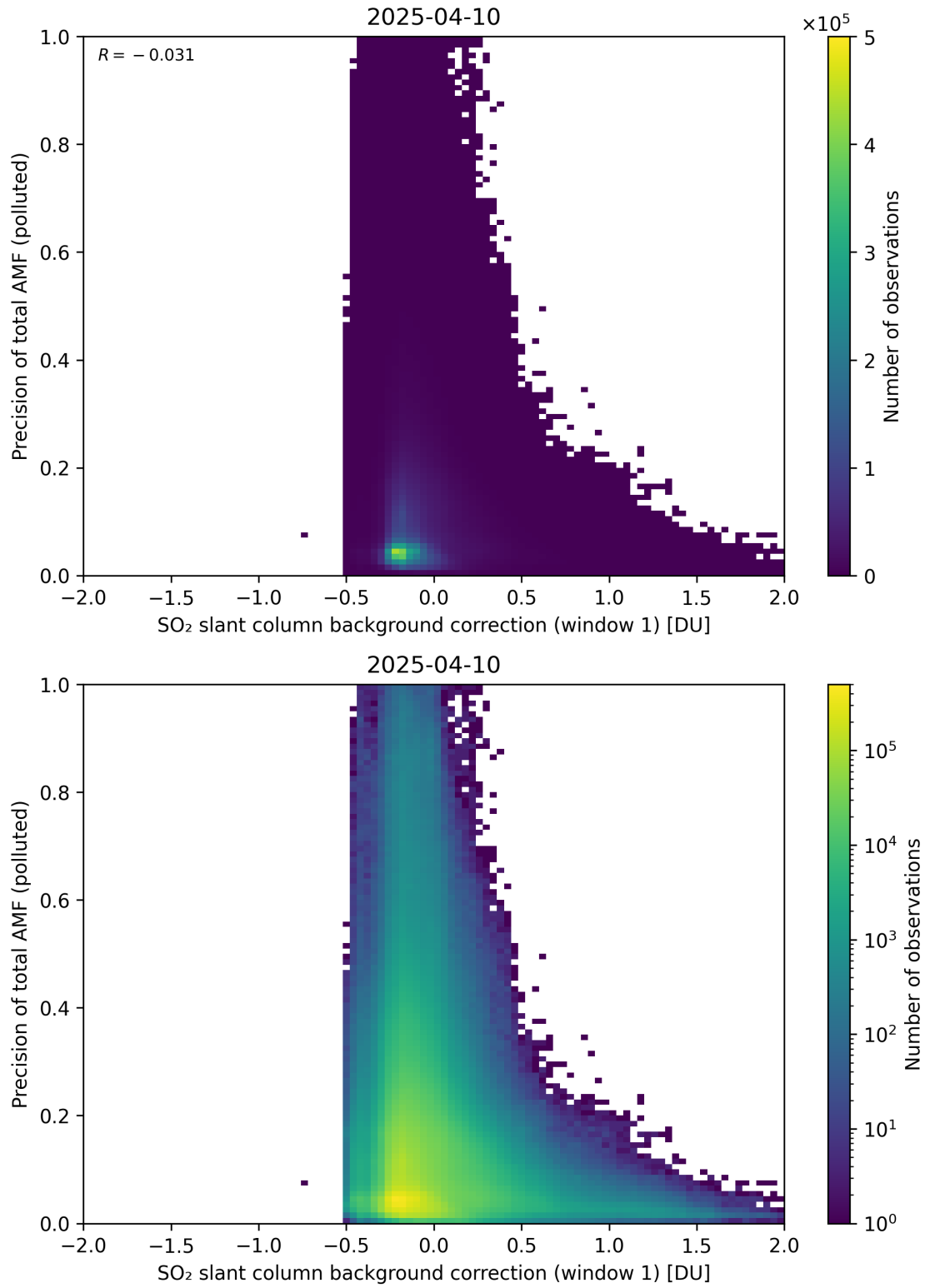
Figure 121: Scatter density plot of “SO 2 slant column background correction (window 1)” against “Precision of total AMF (polluted)” for 2025-04-09 to 2025-04-11.
