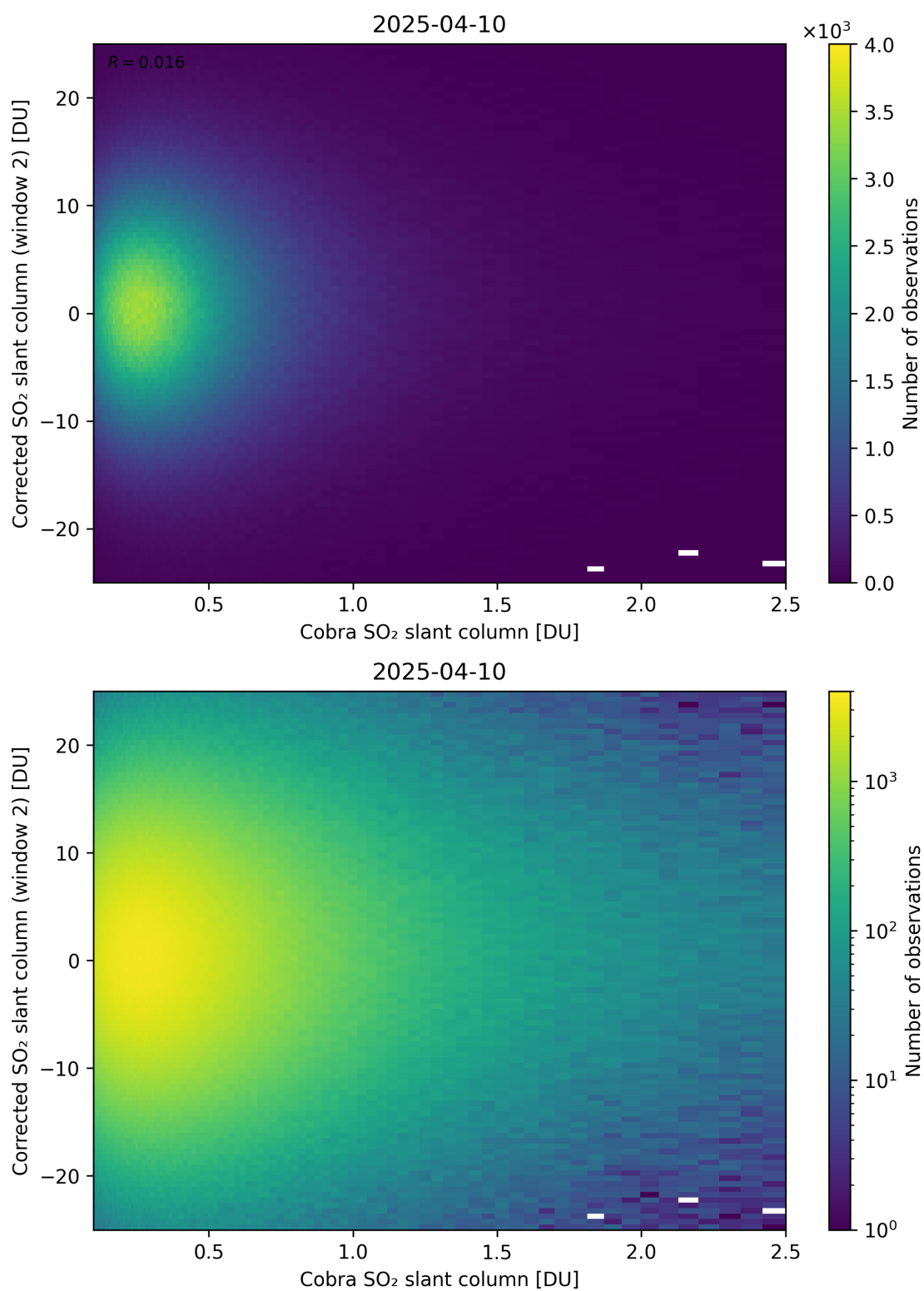
Figure 217: Scatter density plot of “Cobra SO 2 slant column” against “Corrected SO 2 slant column (window 2)” for 2025-04-09 to 2025-04-11.
