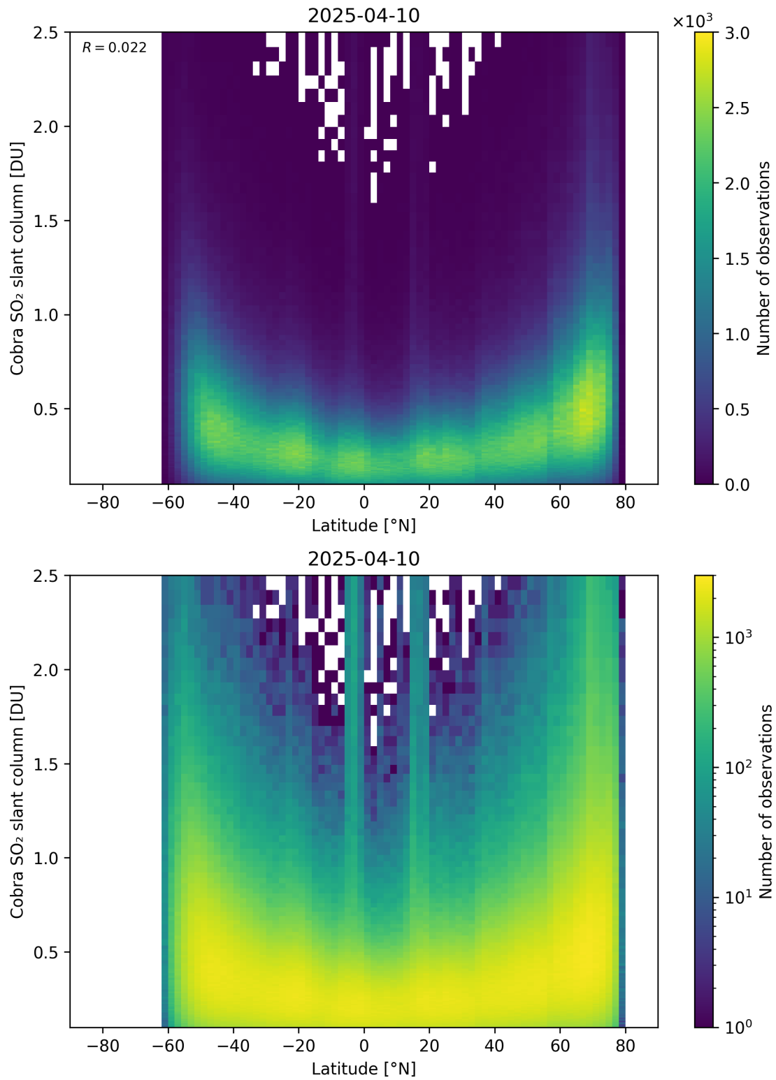
Figure 157: Scatter density plot of “Latitude” against “Cobra SO 2 slant column” for 2025-04-09 to 2025-04-11.
