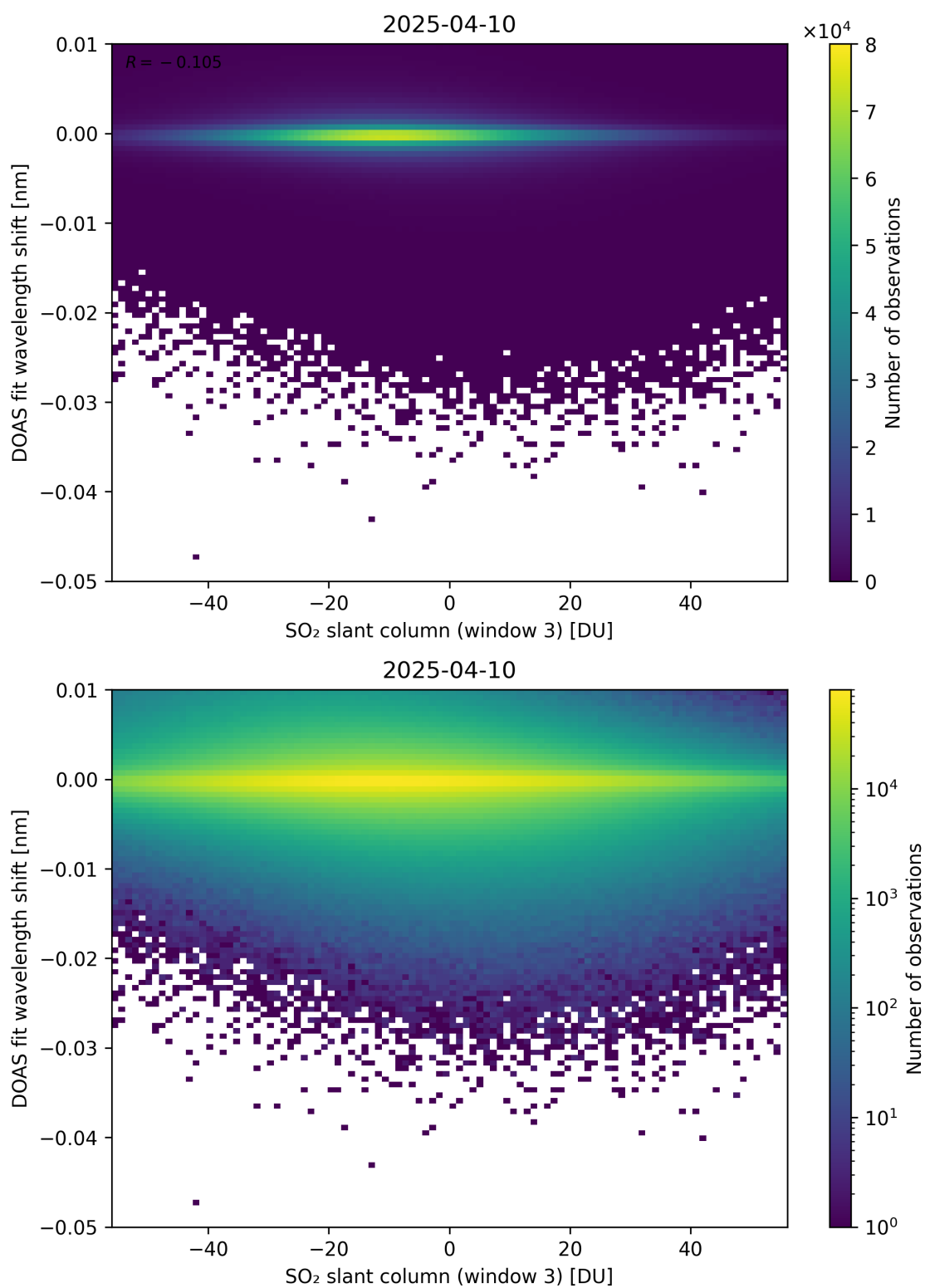
Figure 304: Scatter density plot of “SO 2 slant column (window 3)” against “DOAS fit wavelength shift” for 2025-04-09 to 2025-04-11.
