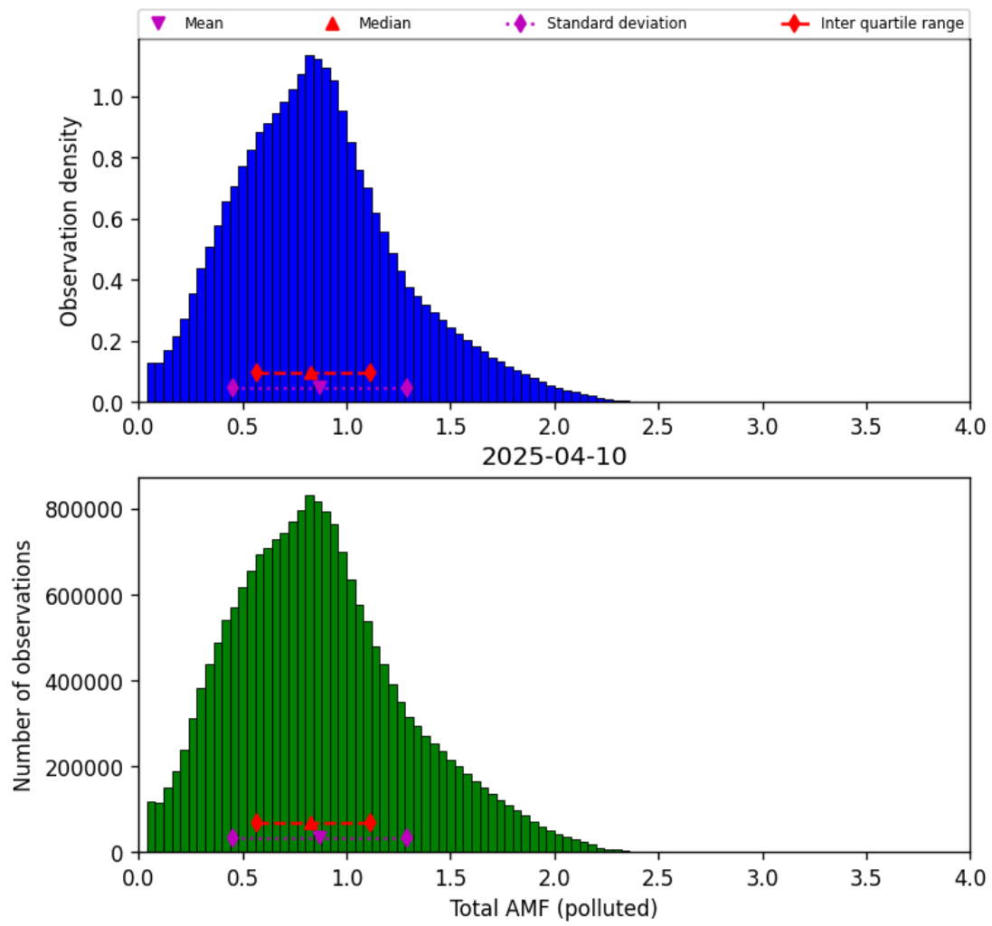
Figure 79: Histogram of “Total AMF (polluted)” for 2025-04-09 to 2025-04-11
