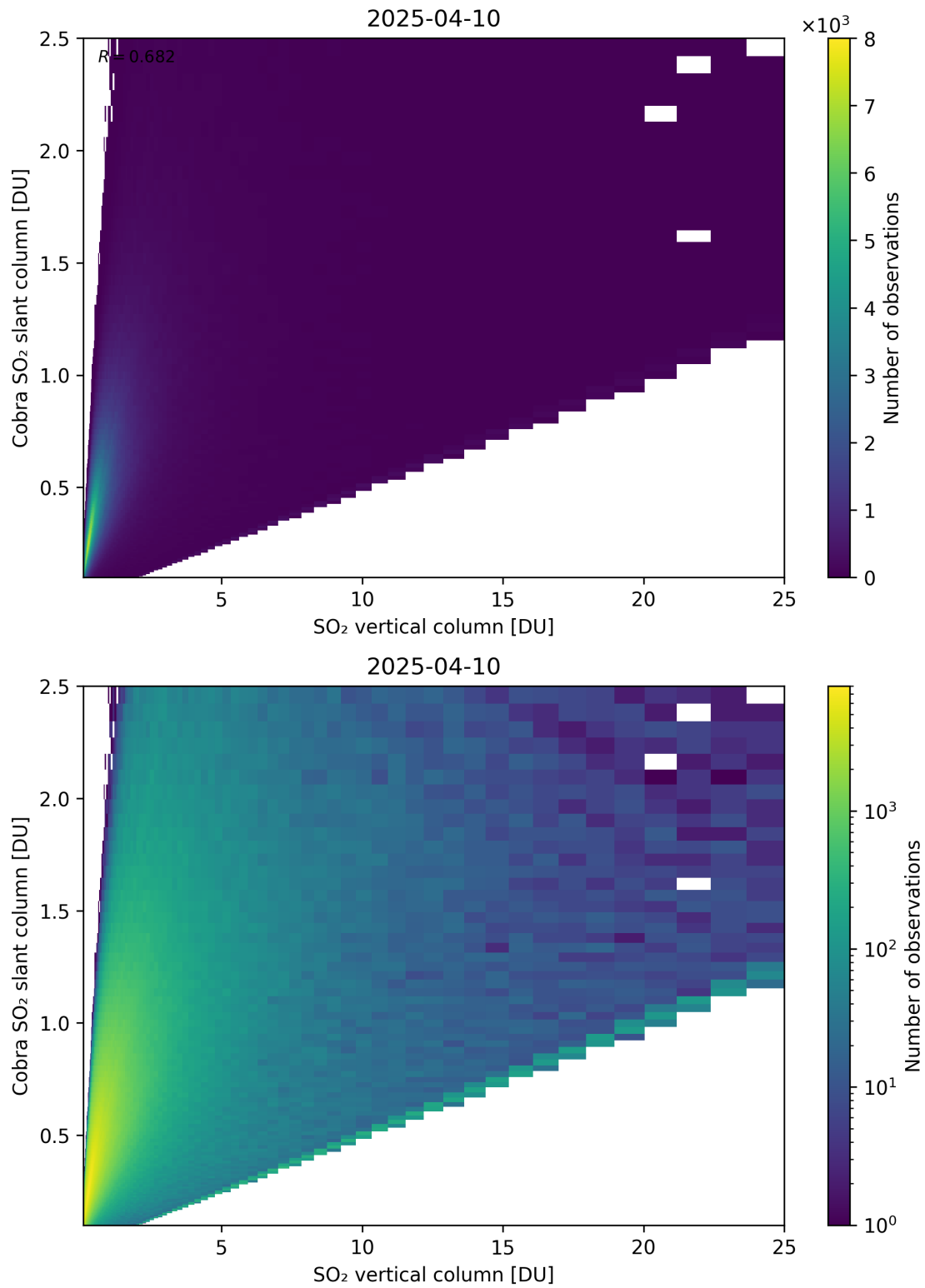
Figure 349: Scatter density plot of “SO 2 vertical column” against “Cobra SO 2 slant column” for 2025-04-09 to 2025-04-11.
