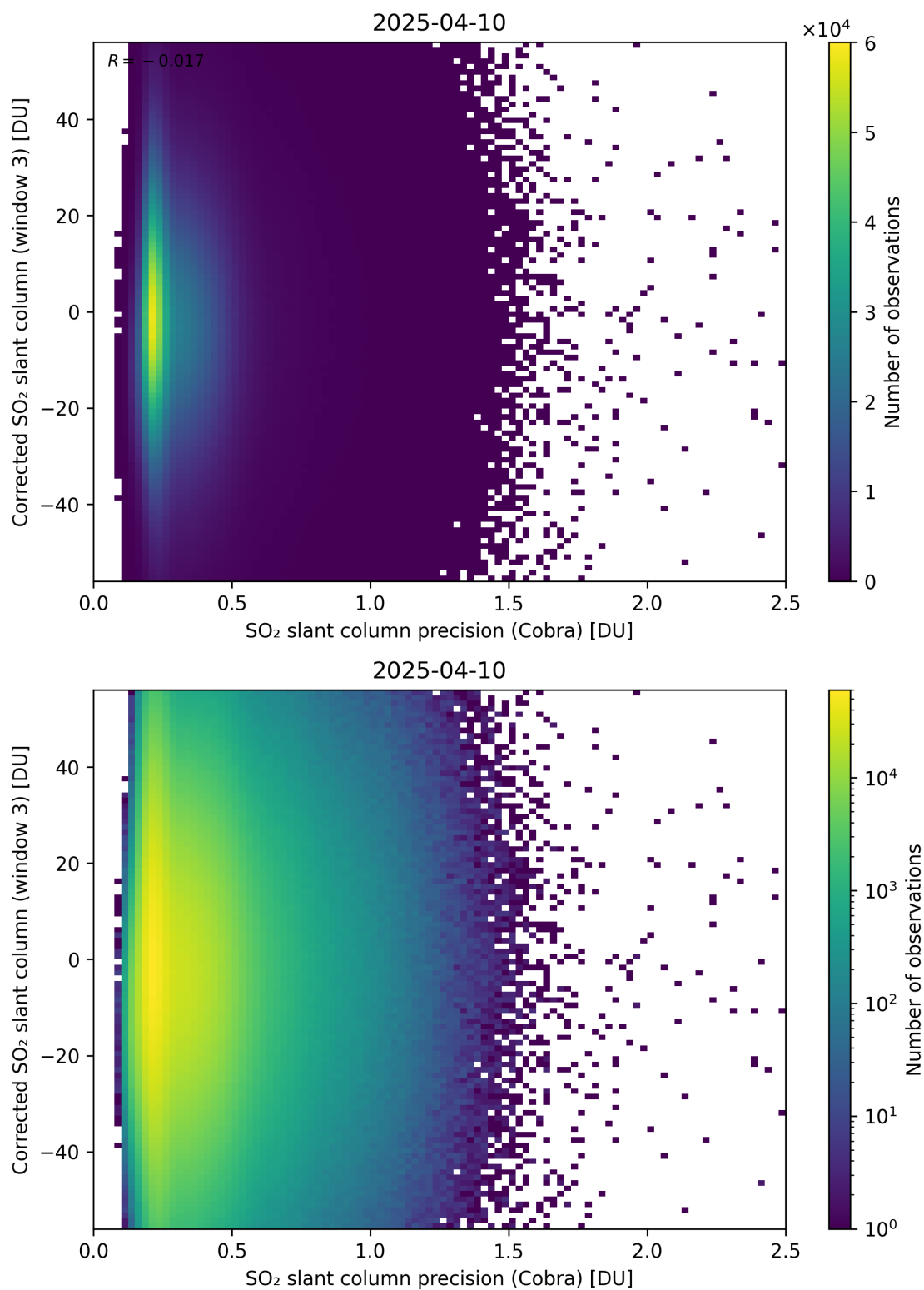
Figure 207: Scatter density plot of “SO 2 slant column precision (Cobra)” against “Corrected SO 2 slant column (window 3)” for 2025-04-09 to 2025-04-11.
