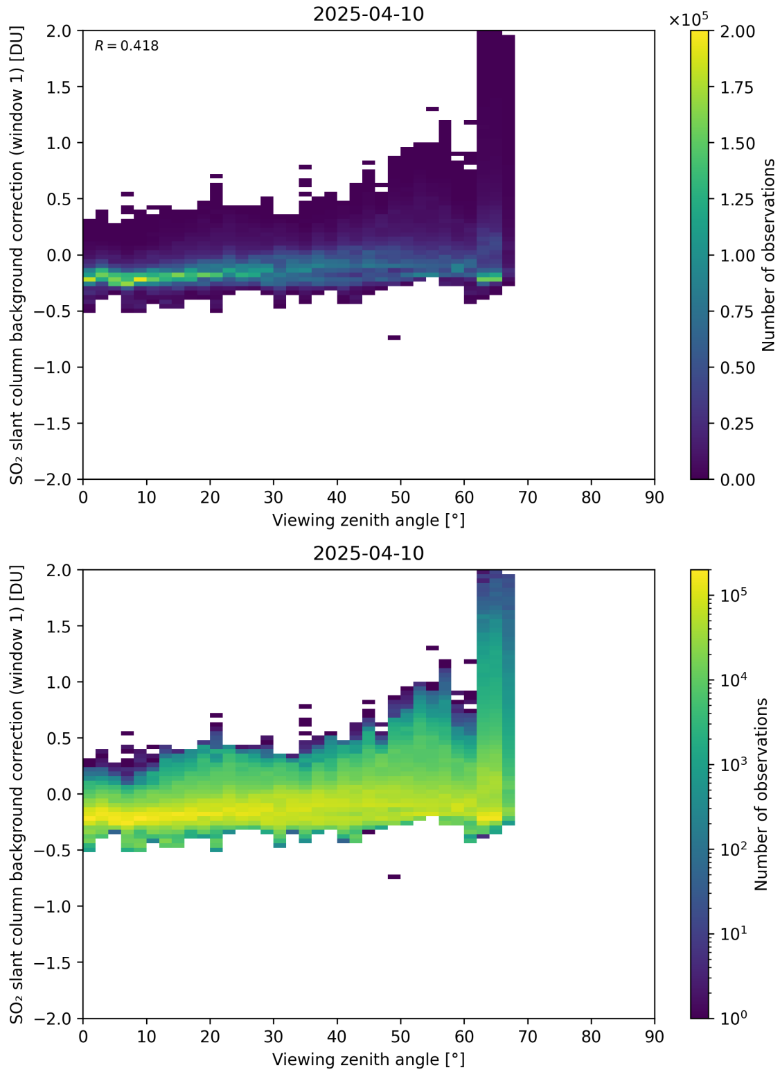
Figure 362: Scatter density plot of “Viewing zenith angle” against “SO 2 slant column background correction (window 1)” for 2025-04-09 to 2025-04-11.
