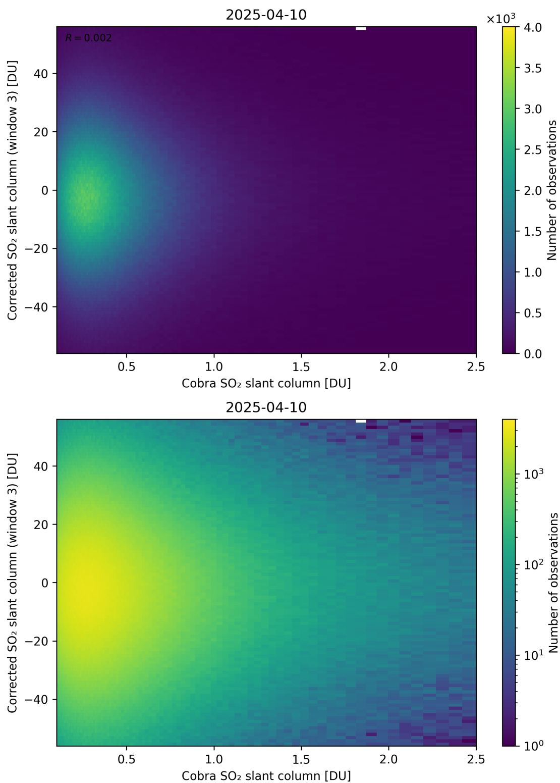
Figure 218: Scatter density plot of “Cobra SO 2 slant column” against “Corrected SO 2 slant column (window 3)” for 2025-04-09 to 2025-04-11.
