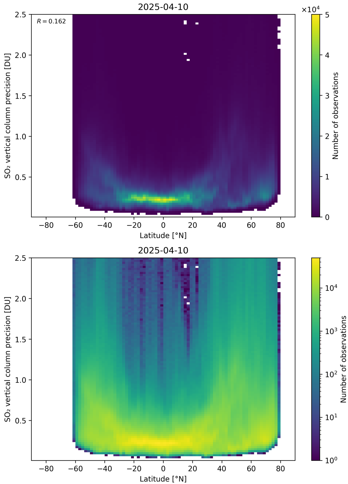
Figure 170: Scatter density plot of “Latitude” against “SO 2 vertical column precision” for 2025-04-09 to 2025-04-11.
