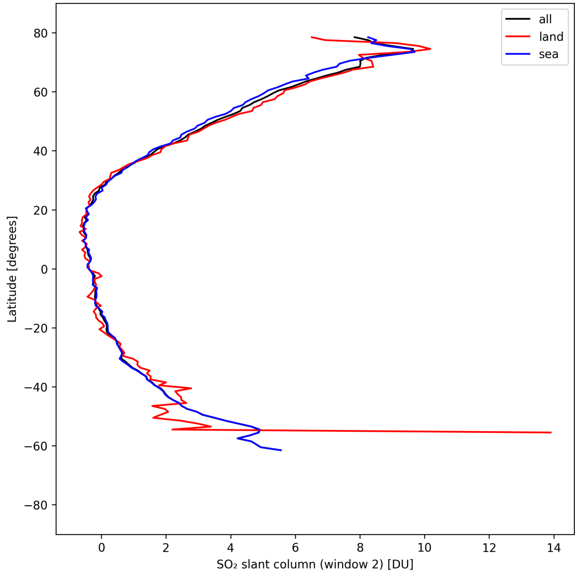
Figure 41: Zonal average of “SO 2 slant column (window 2)” for 2025-04-09 to 2025-04-11.
