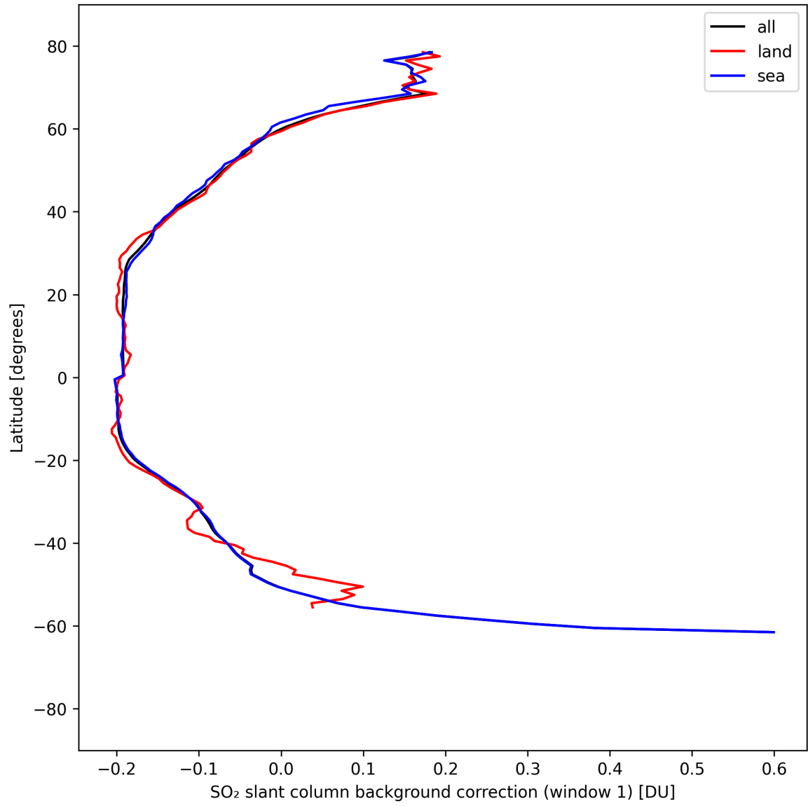
Figure 40: Zonal average of “SO 2 slant column background correction (window 1)” for 2025-04-09 to 2025-04-11.
