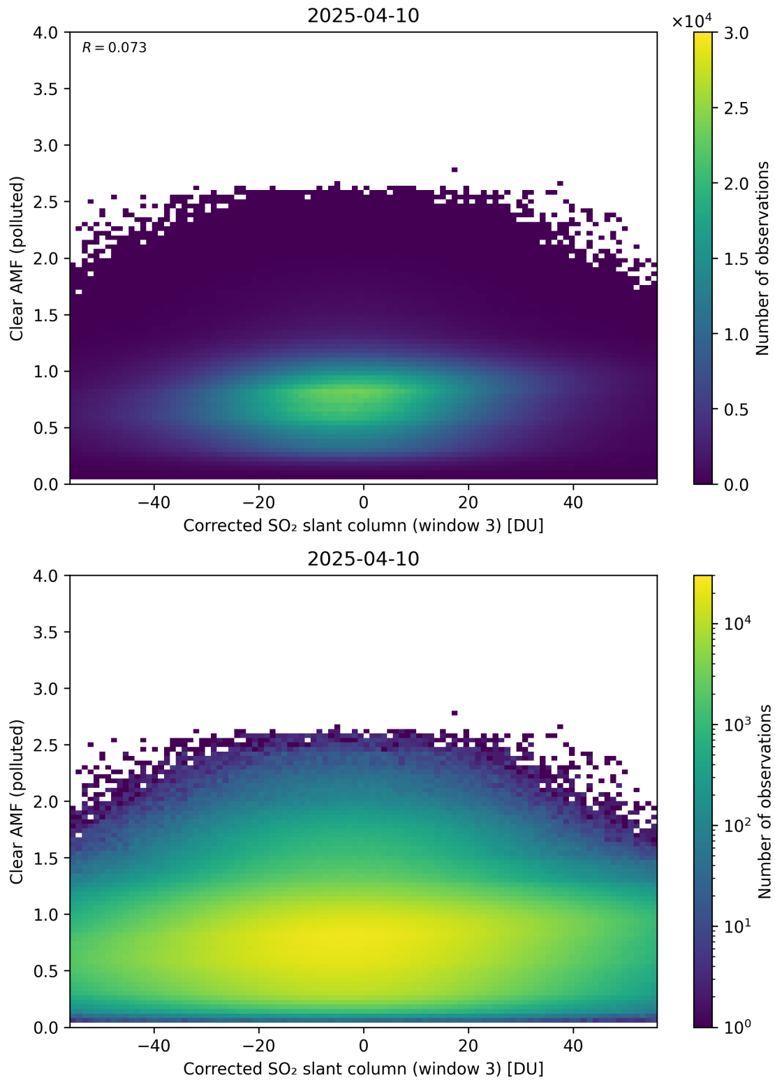
Figure 259: Scatter density plot of “Corrected SO 2 slant column (window 3)” against “Clear AMF (polluted)” for 2025-04-09 to 2025-04-11.
