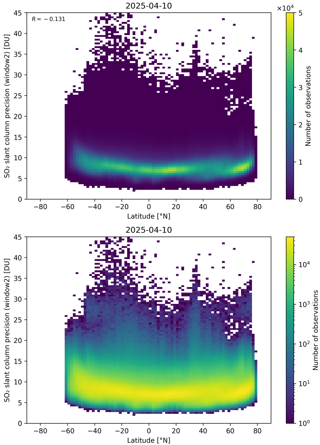
Figure 164: Scatter density plot of “Latitude” against “SO 2 slant column precision (window2)” for 2025-04-09 to 2025-04-11.
