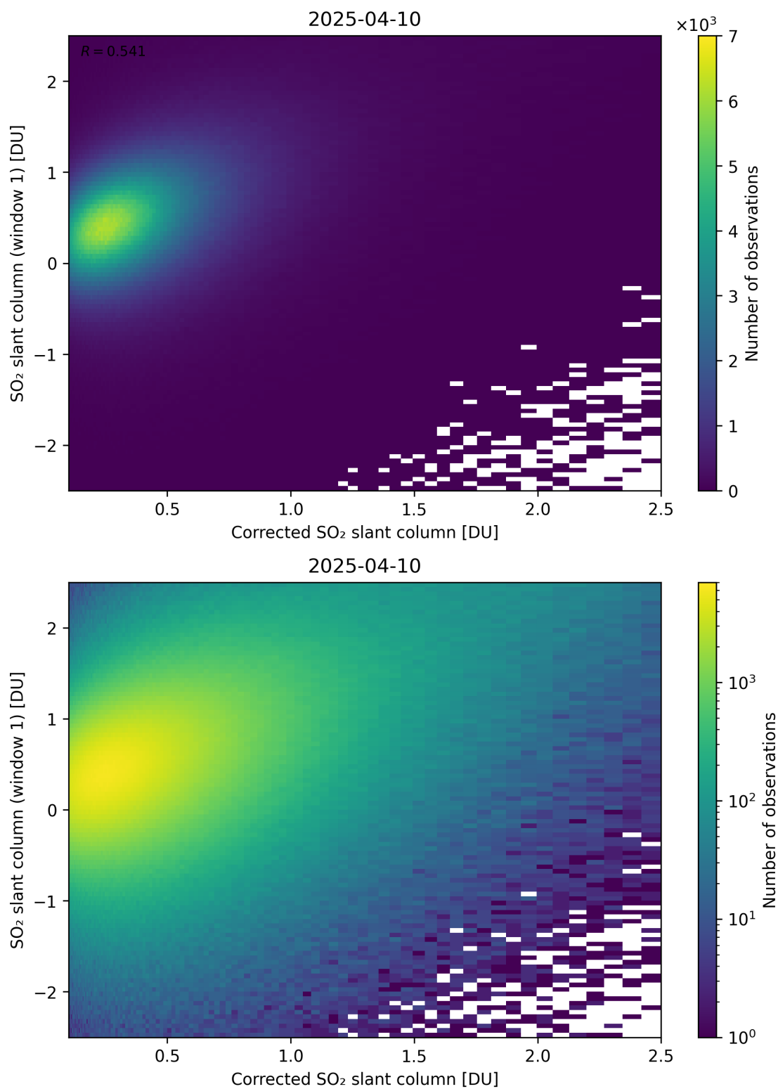
Figure 237: Scatter density plot of “Corrected SO 2 slant column” against “SO 2 slant column (window 1)” for 2025-04-09 to 2025-04-11.
