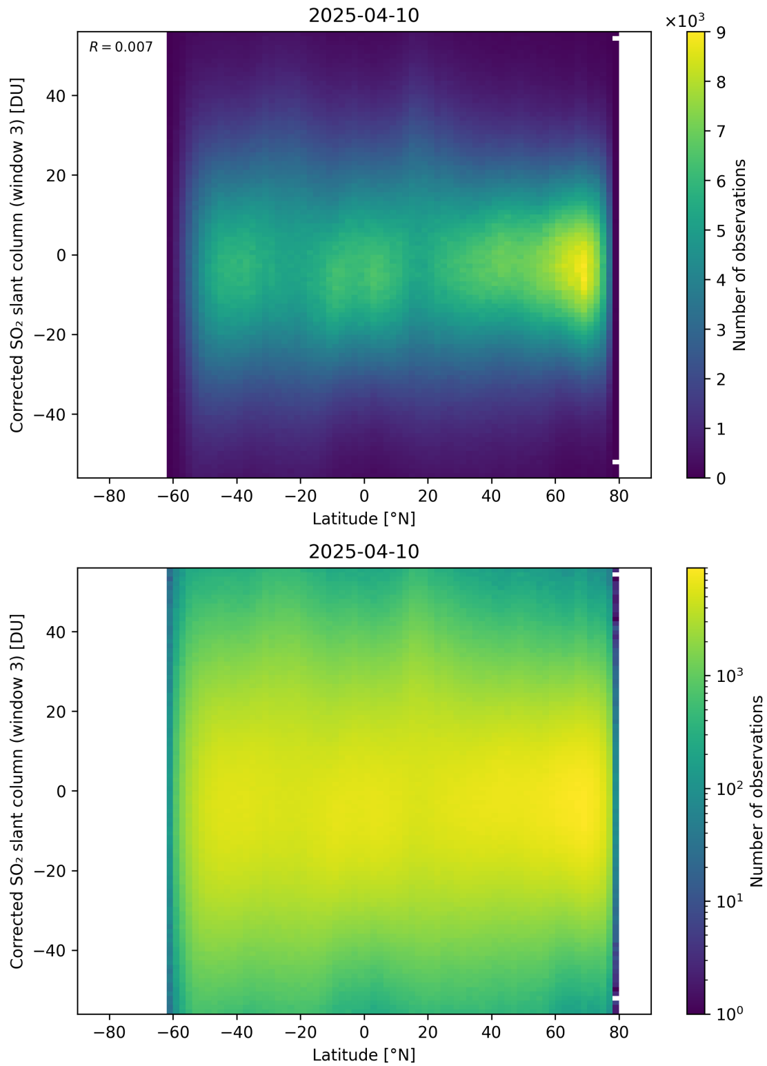
Figure 161: Scatter density plot of “Latitude” against “Corrected SO 2 slant column (window 3)” for 2025-04-09 to 2025-04-11.
