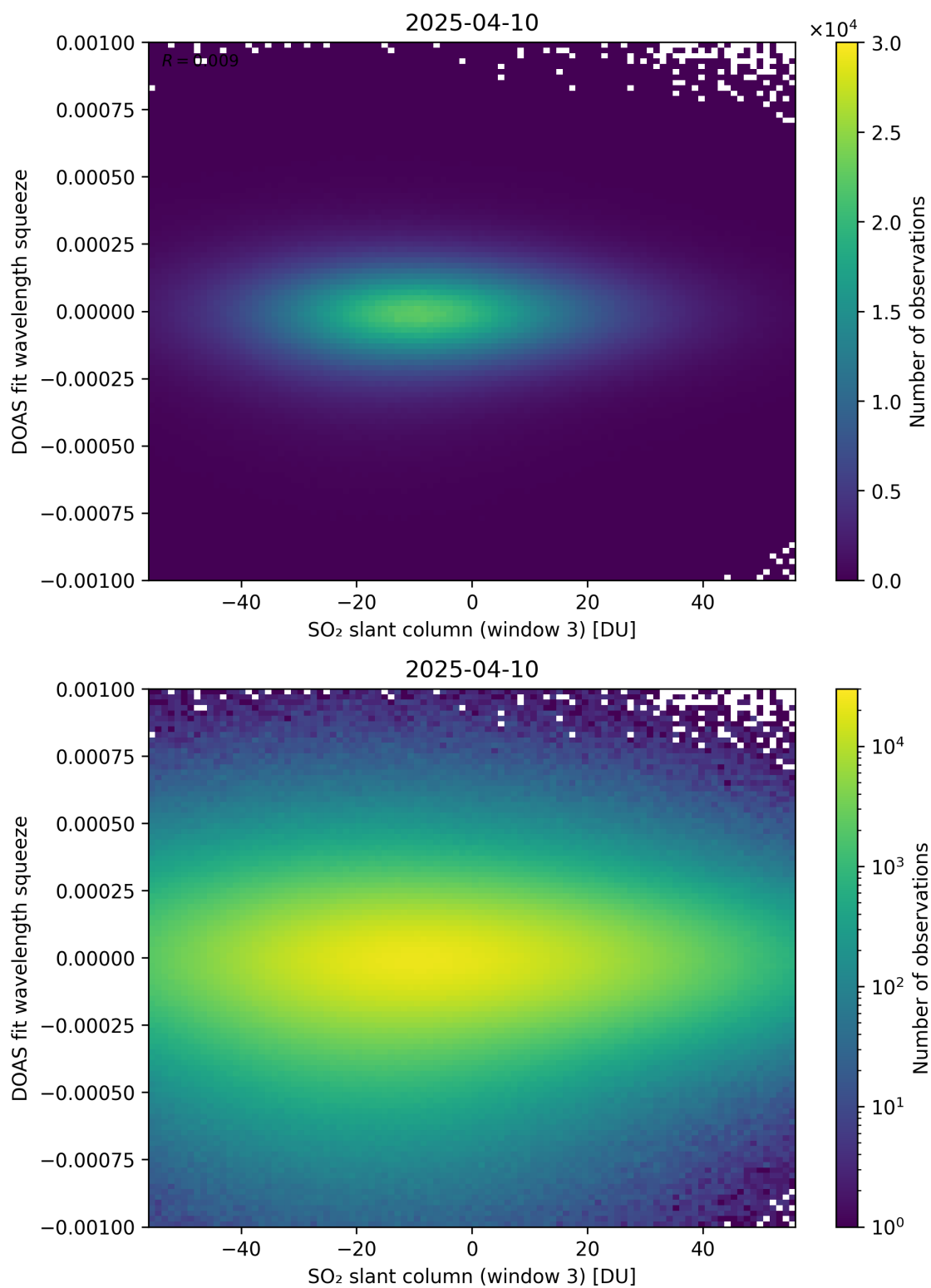
Figure 305: Scatter density plot of “SO 2 slant column (window 3)” against “DOAS fit wavelength squeeze” for 2025-04-09 to 2025-04-11.
