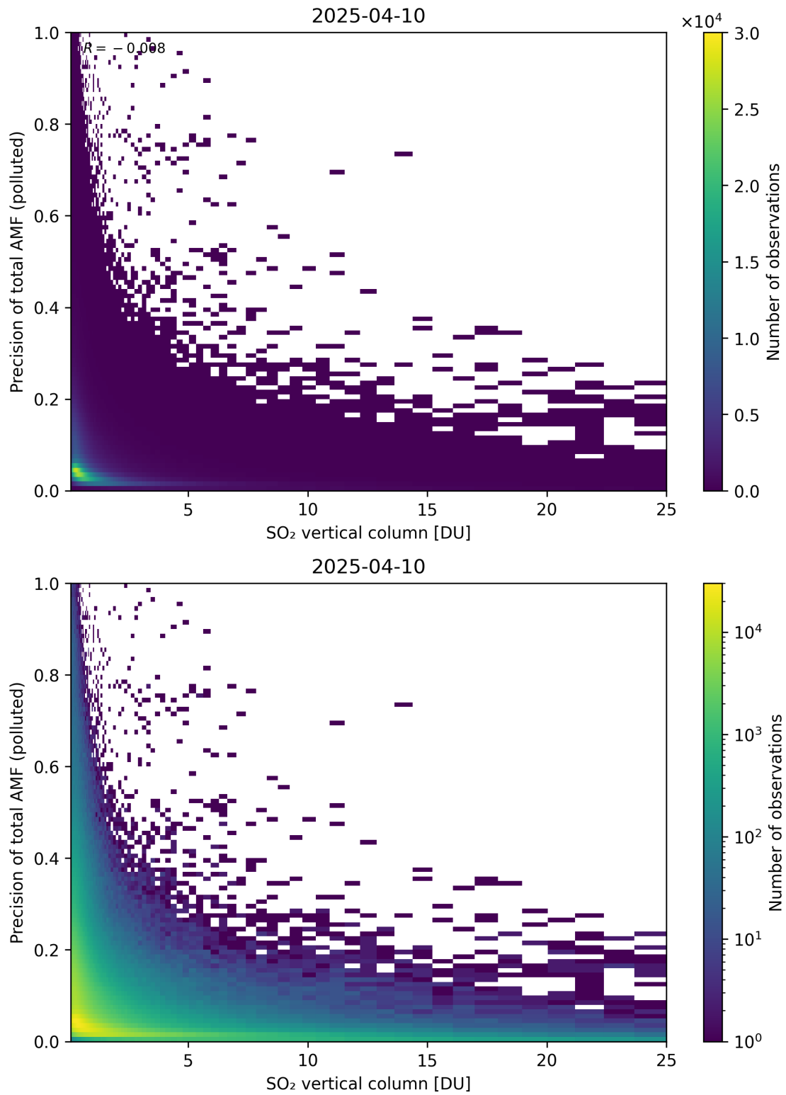
Figure 360: Scatter density plot of “SO 2 vertical column” against “Precision of total AMF (polluted)” for 2025-04-09 to 2025-04-11.
