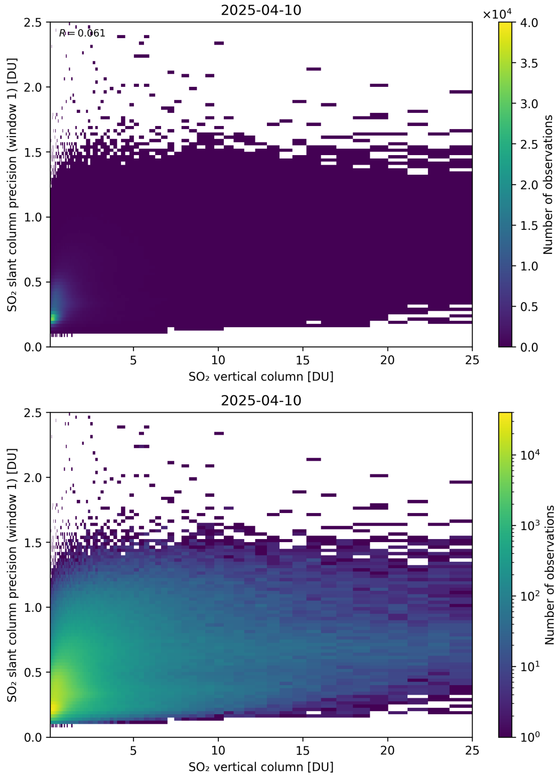
Figure 355: Scatter density plot of “SO 2 vertical column” against “SO 2 slant column precision (window 1)” for 2025-04-09 to 2025-04-11.
