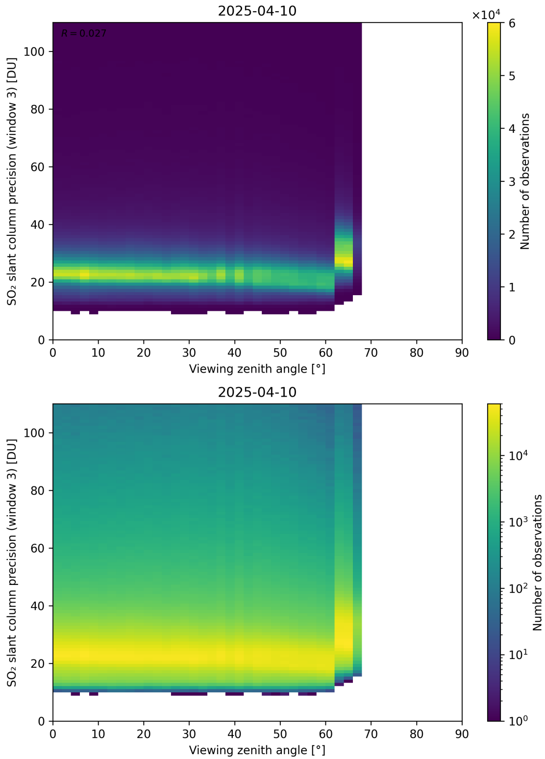
Figure 380: Scatter density plot of “Viewing zenith angle” against “SO 2 slant column precision (window 3)” for 2025-04-09 to 2025-04-11.
