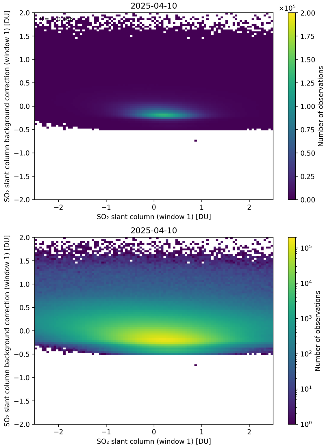
Figure 262: Scatter density plot of “SO 2 slant column (window 1)” against “SO 2 slant column background correction (window 1)” for 2025-04-09 to 2025-04-11.
