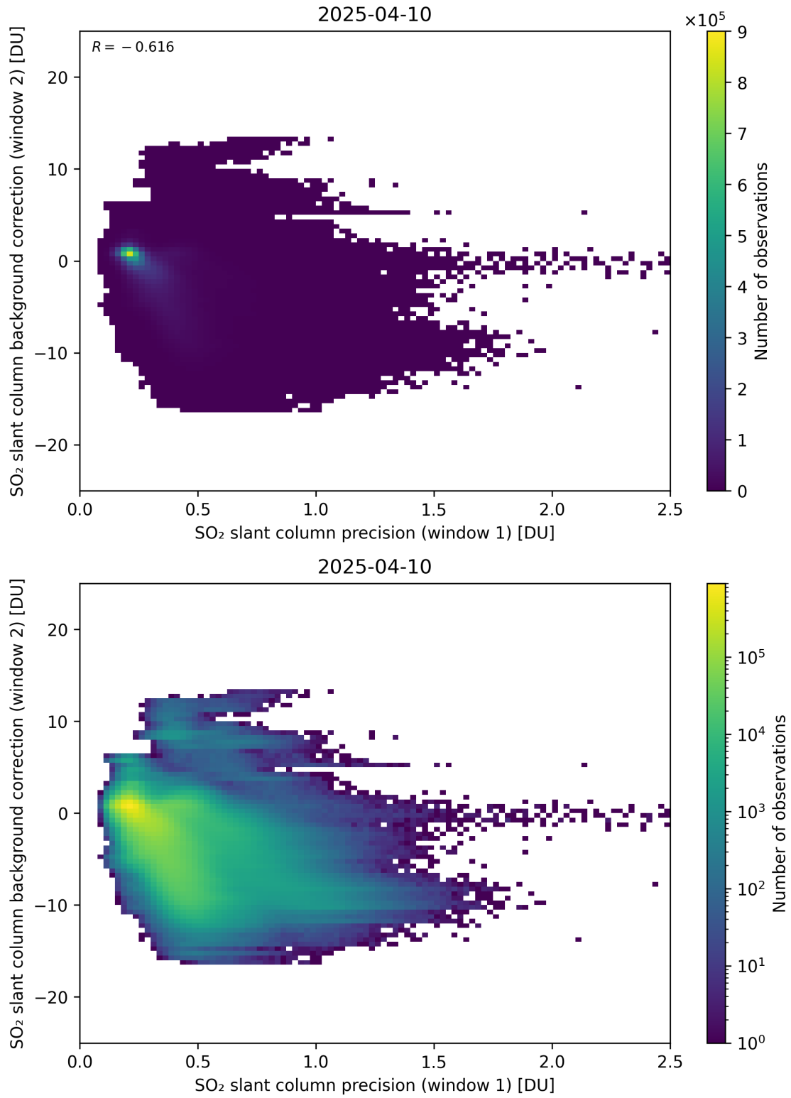
Figure 269: Scatter density plot of “SO 2 slant column precision (window 1)” against “SO 2 slant column background correction (window 2)” for 2025-04-09 to 2025-04-11.
