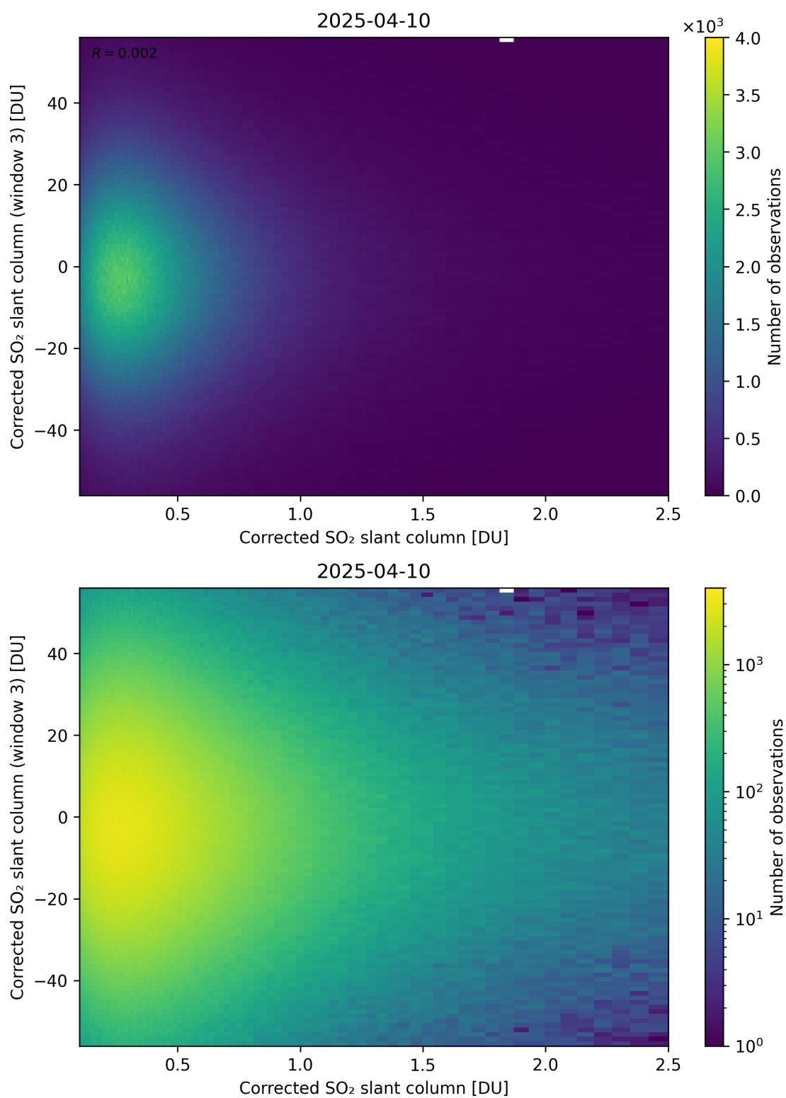
Figure 236: Scatter density plot of “Corrected SO 2 slant column” against “Corrected SO 2 slant column (window 3)” for 2025-04-09 to 2025-04-11.
