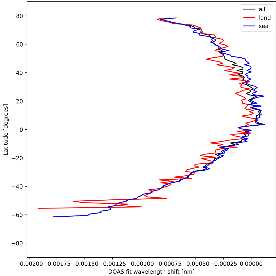
Figure 50: Zonal average of “DOAS fit wavelength shift” for 2025-04-09 to 2025-04-11.
