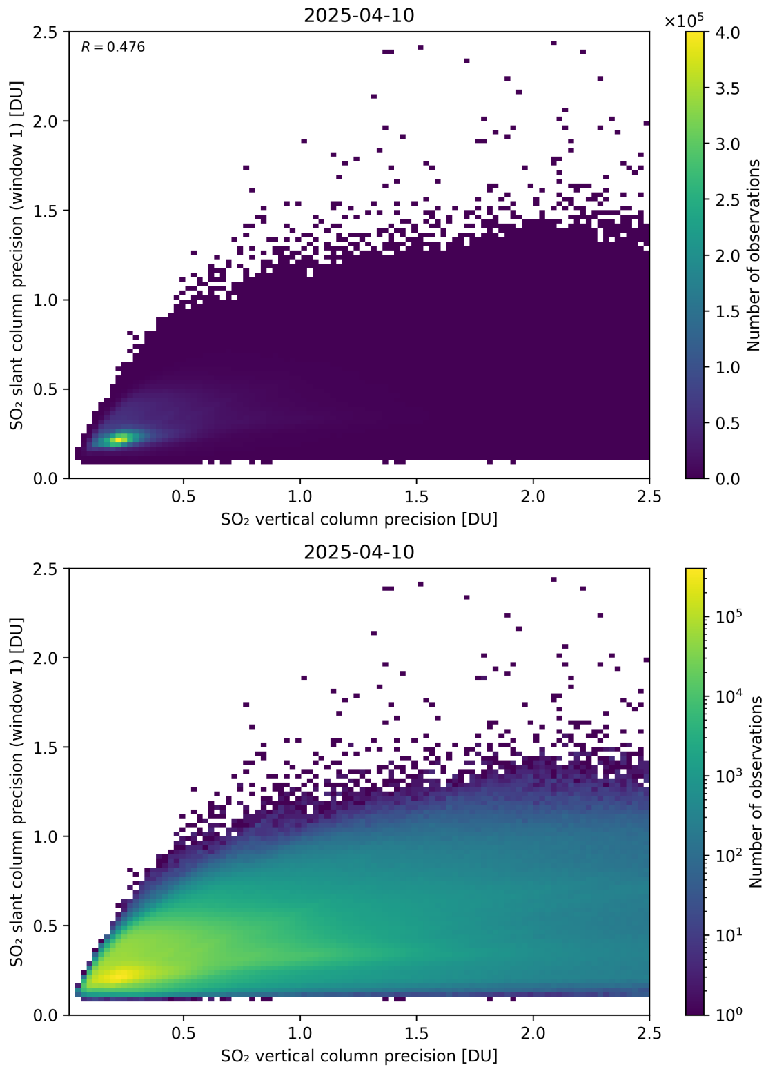
Figure 342: Scatter density plot of “SO 2 vertical column precision” against “SO 2 slant column precision (window 1)” for 2025-04-09 to 2025-04-11.
