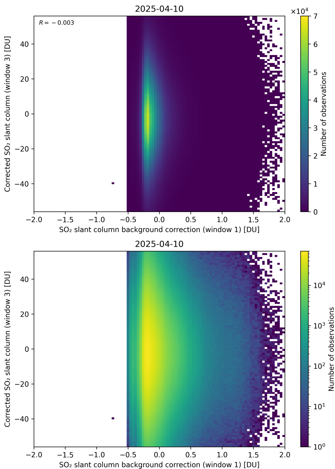
Figure 116: Scatter density plot of “SO 2 slant column background correction (window 1)” against “Corrected SO 2 slant column (window 3)” for 2025-04-09 to 2025-04-11.
