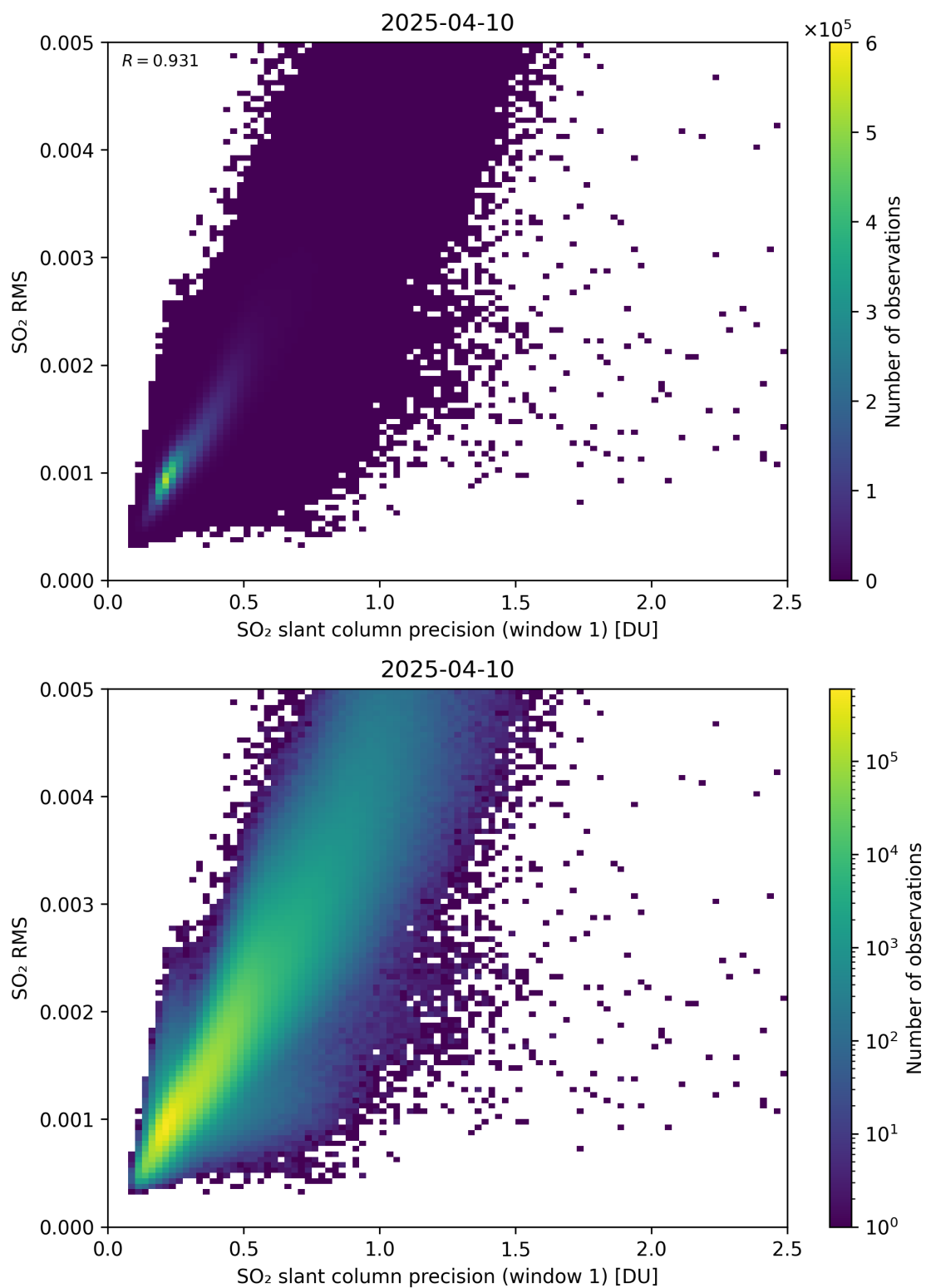
Figure 273: Scatter density plot of “SO 2 slant column precision (window 1)” against “SO 2 RMS” for 2025-04-09 to 2025-04-11.
