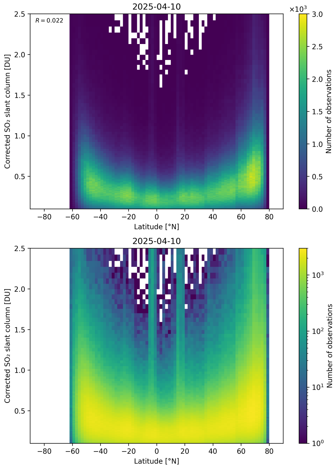
Figure 159: Scatter density plot of “Latitude” against “Corrected SO 2 slant column” for 2025-04-09 to 2025-04-11.
