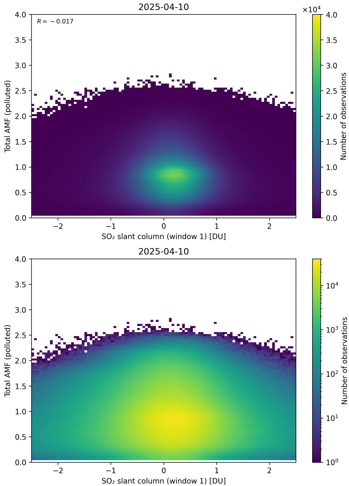
Figure 289: Scatter density plot of “SO 2 slant column (window 1)” against “Total AMF (polluted)” for 2025-04-09 to 2025-04-11.
