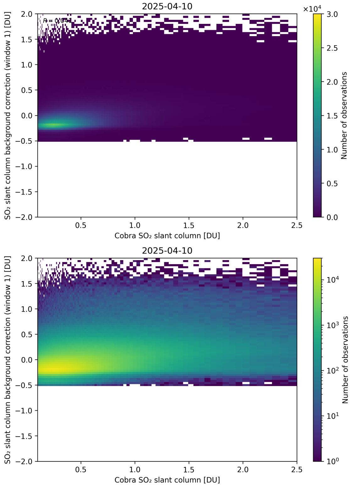
Figure 193: Scatter density plot of “Cobra SO 2 slant column” against “SO 2 slant column background correction (window 1)” for 2025-04-09 to 2025-04-11.
