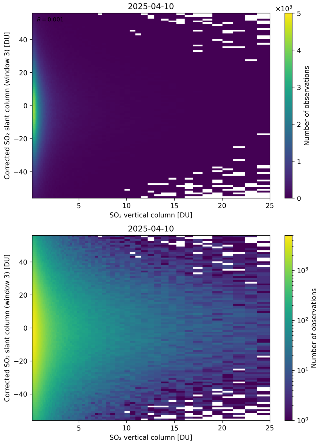
Figure 353: Scatter density plot of “SO 2 vertical column” against “Corrected SO 2 slant column (window 3)” for 2025-04-09 to 2025-04-11.
