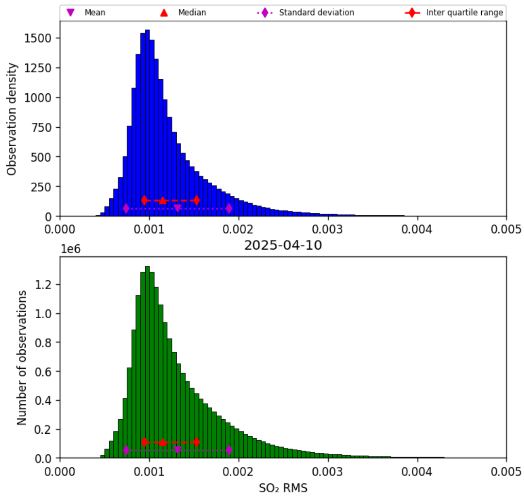
Figure 78: Histogram of “SO 2 RMS” for 2025-04-09 to 2025-04-11
