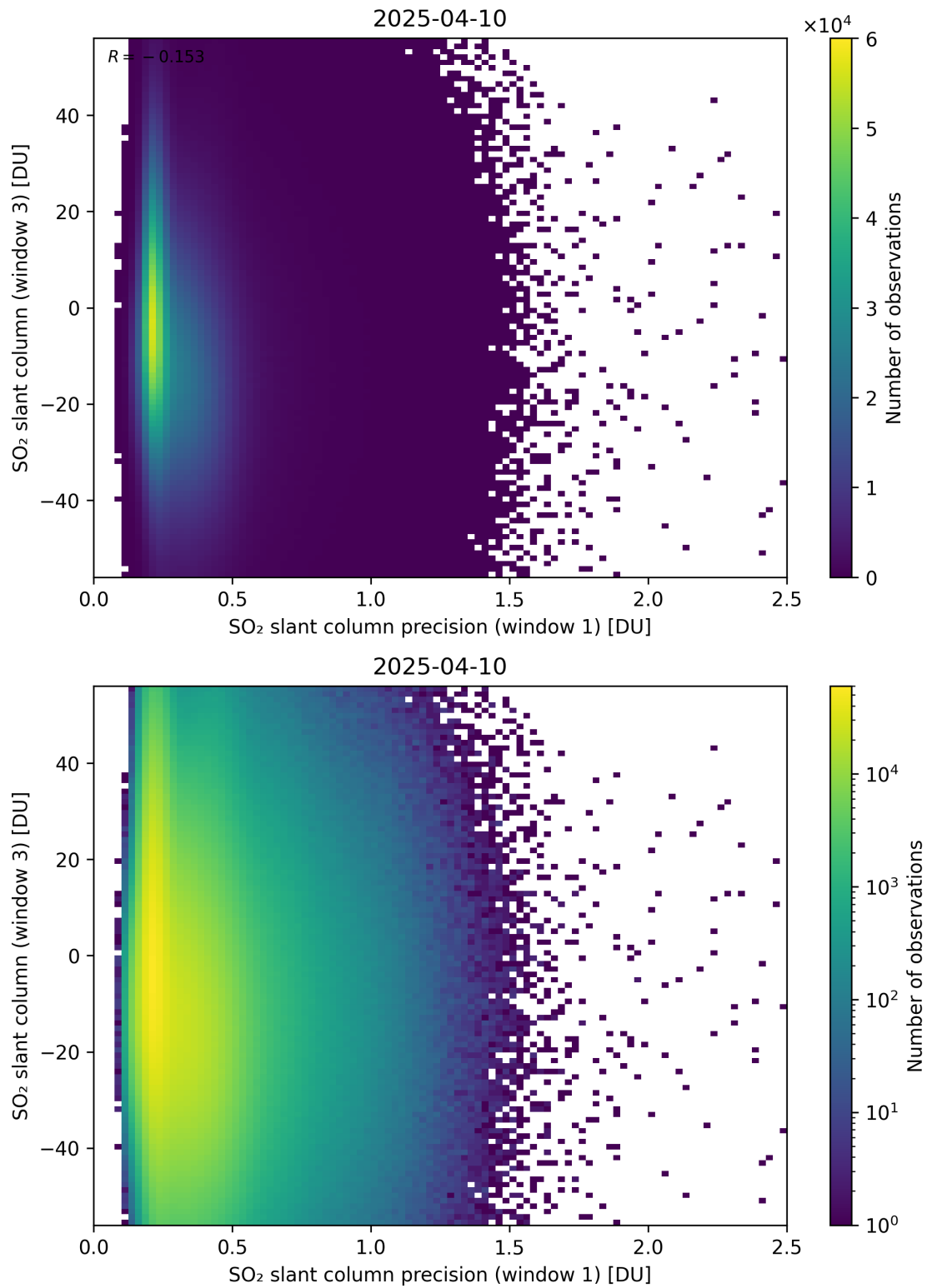
Figure 278: Scatter density plot of “SO 2 slant column precision (window 1)” against “SO 2 slant column (window 3)” for 2025-04-09 to 2025-04-11.
