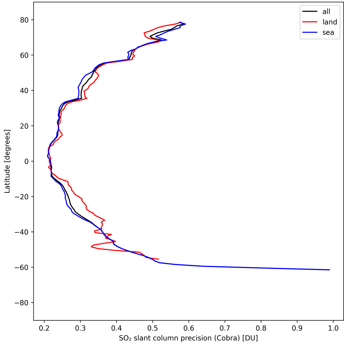
Figure 36: Zonal average of “SO 2 slant column precision (Cobra)” for 2025-04-09 to 2025-04-11.
