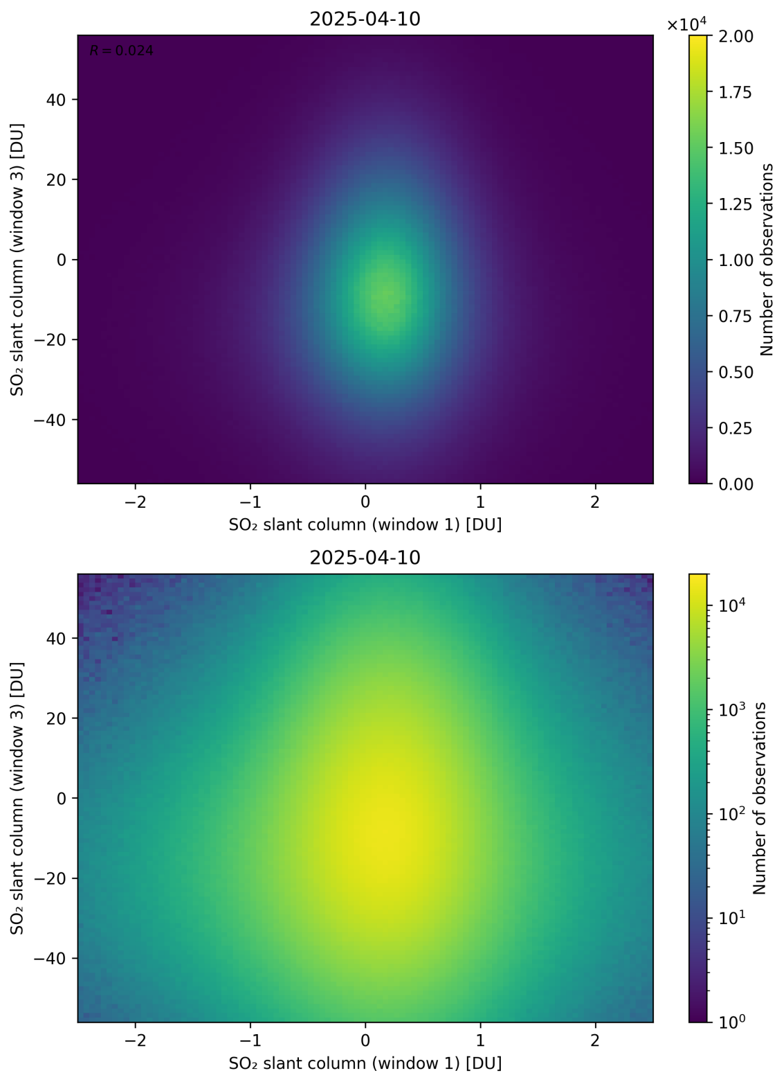
Figure 287: Scatter density plot of “SO 2 slant column (window 1)” against “SO 2 slant column (window 3)” for 2025-04-09 to 2025-04-11.
