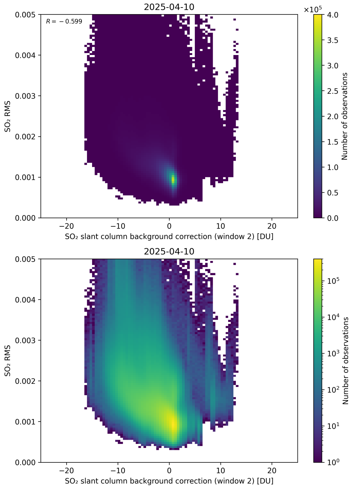
Figure 125: Scatter density plot of “SO 2 slant column background correction (window 2)” against “SO 2 RMS” for 2025-04-09 to 2025-04-11.
