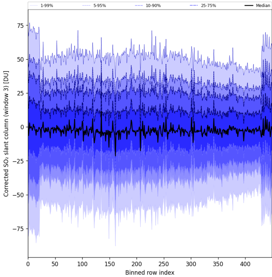
Figure 99: Along track statistics of “Corrected SO 2 slant column (window 3)” for 2025-04-09 to 2025-04-11
