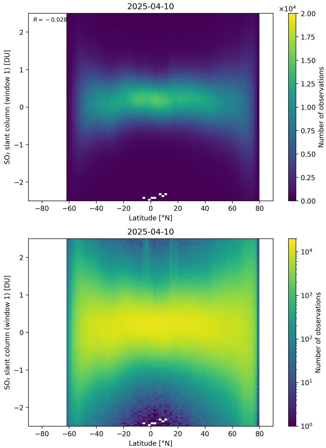
Figure 162: Scatter density plot of “Latitude” against “SO 2 slant column (window 1)” for 2025-04-09 to 2025-04-11.
