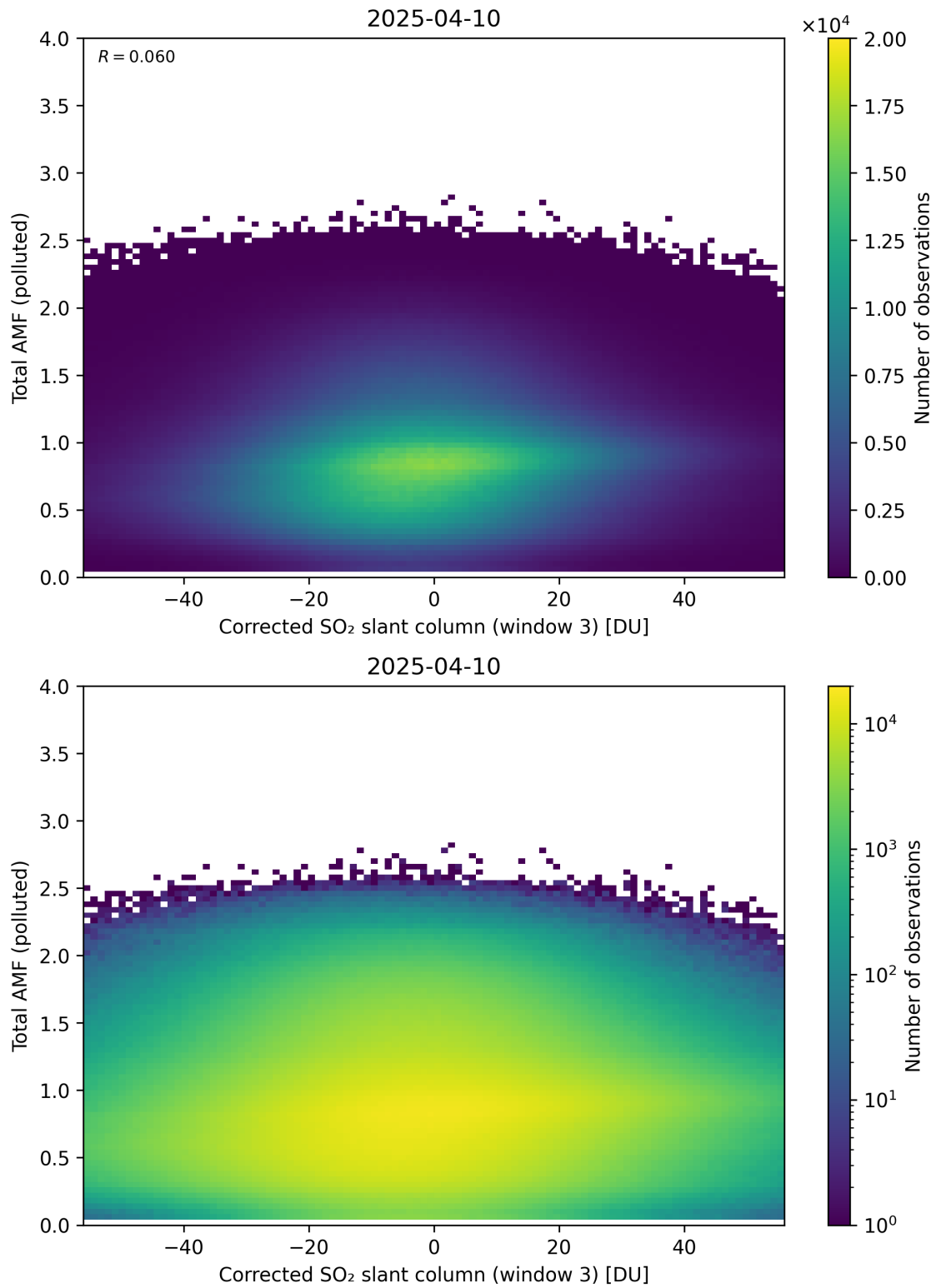
Figure 260: Scatter density plot of “Corrected SO 2 slant column (window 3)” against “Total AMF (polluted)” for 2025-04-09 to 2025-04-11.
