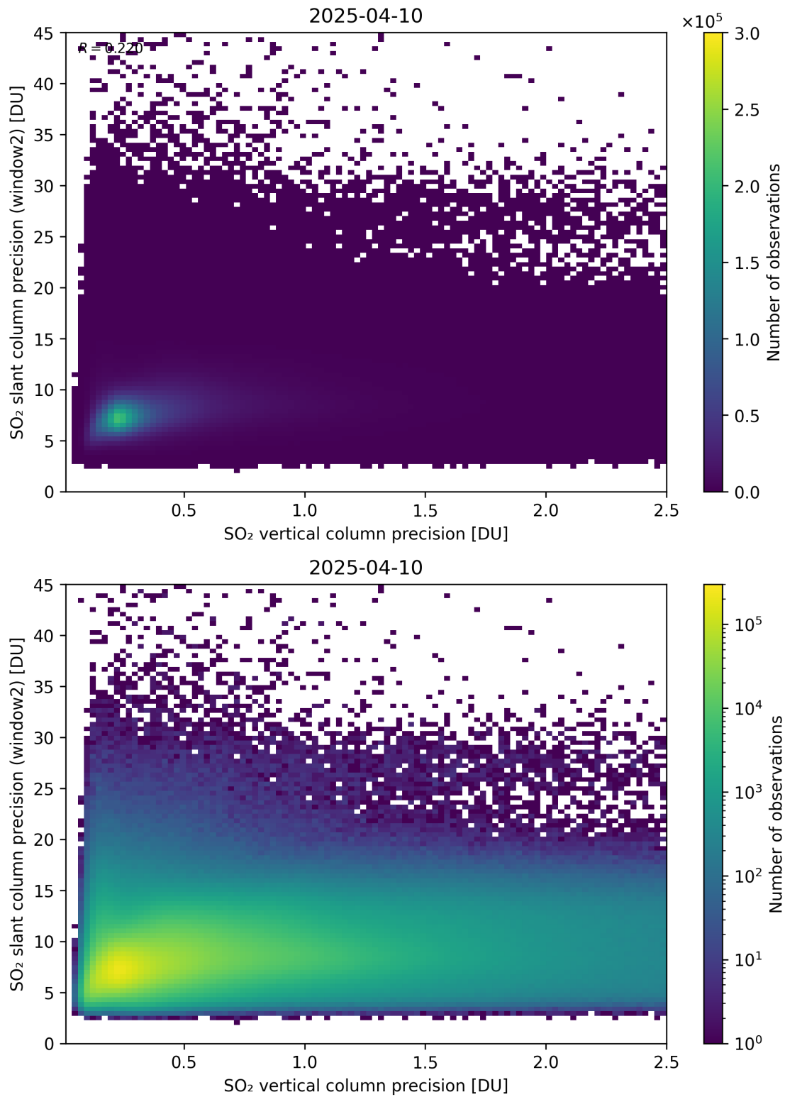
Figure 343: Scatter density plot of “SO 2 vertical column precision” against “SO 2 slant column precision (window2)” for 2025-04-09 to 2025-04-11.
