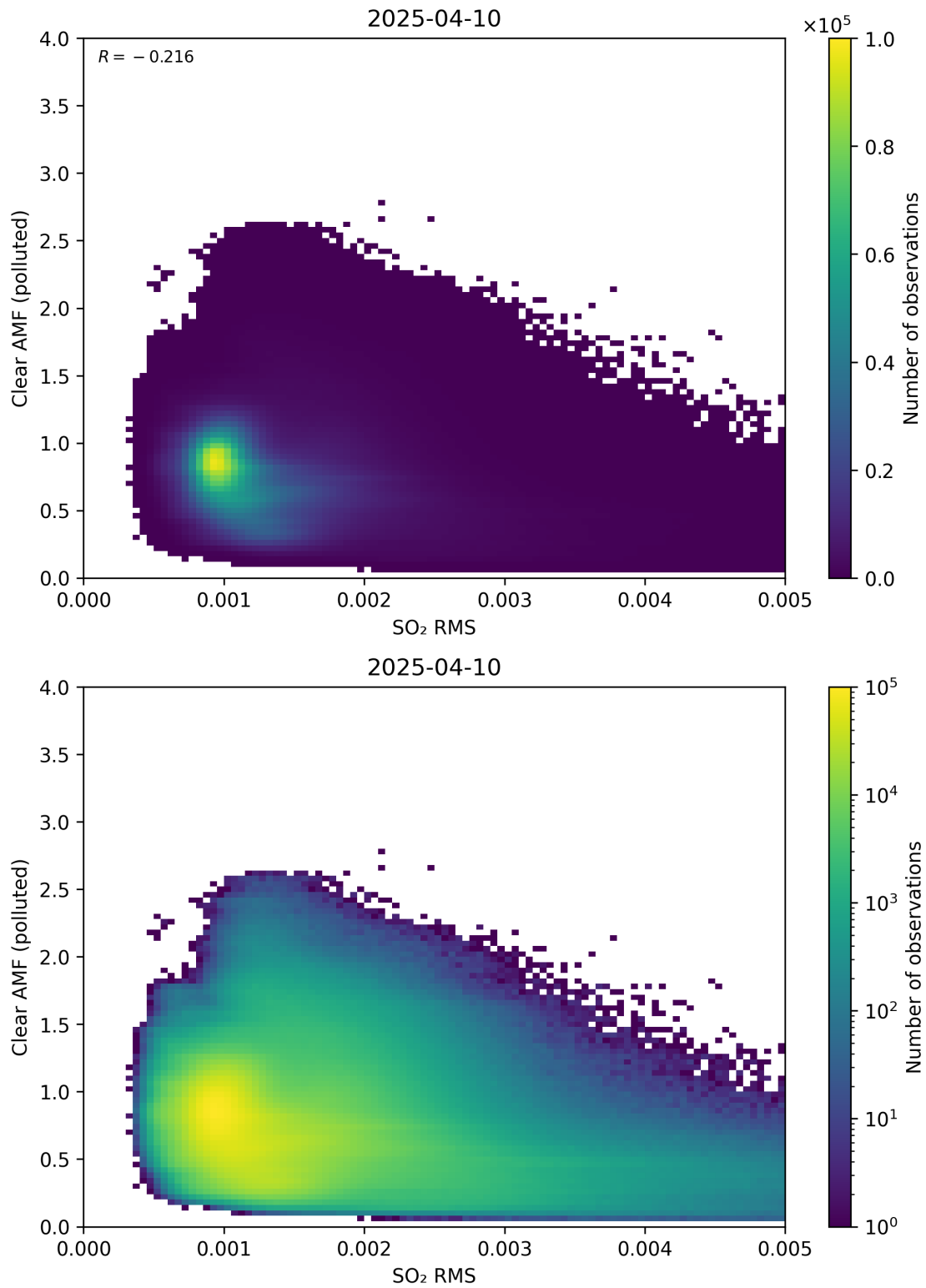
Figure 147: Scatter density plot of “SO 2 RMS” against “Clear AMF (polluted)” for 2025-04-09 to 2025-04-11.
