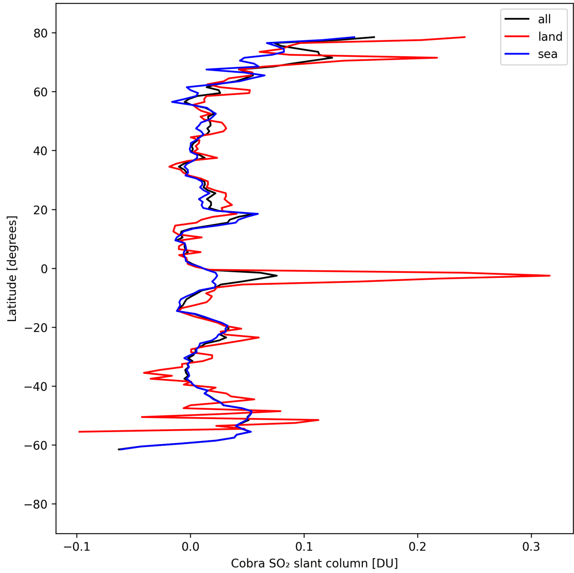
Figure 35: Zonal average of “Cobra SO 2 slant column” for 2025-04-09 to 2025-04-11.
