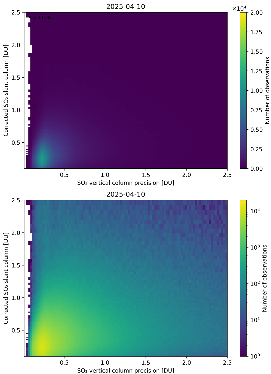
Figure 338: Scatter density plot of “SO 2 vertical column precision” against “Corrected SO 2 slant column” for 2025-04-09 to 2025-04-11.
