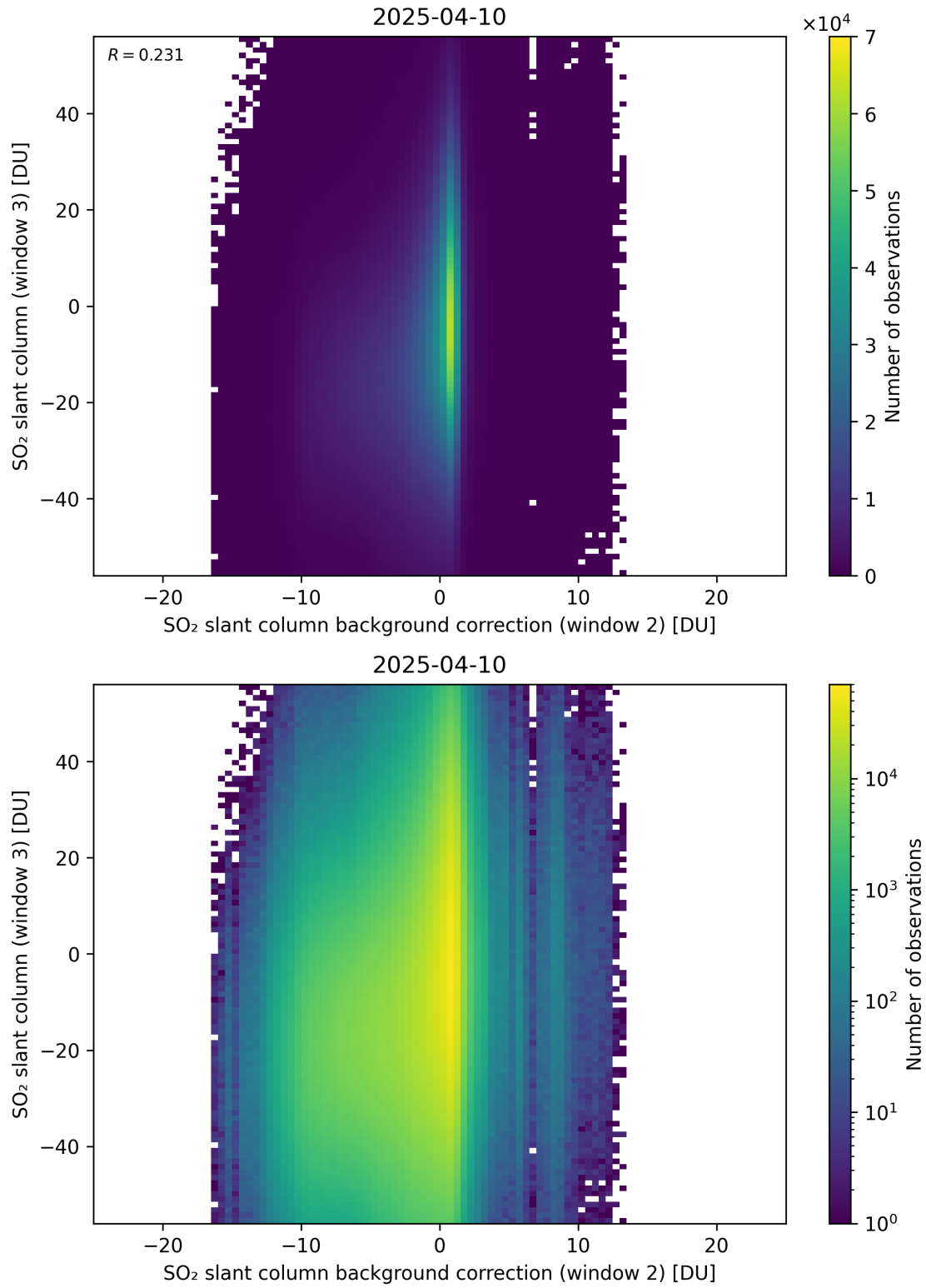
Figure 128: Scatter density plot of “SO 2 slant column background correction (window 2)” against “SO 2 slant column (window 3)” for 2025-04-09 to 2025-04-11.
