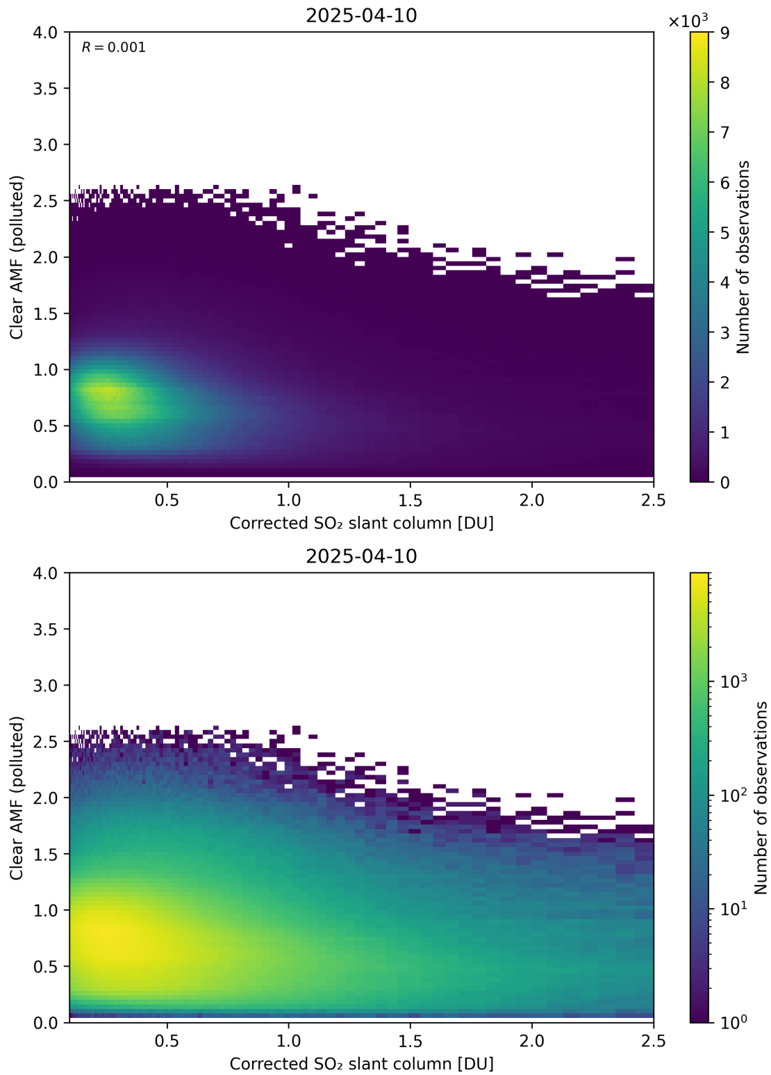
Figure 232: Scatter density plot of “Corrected SO 2 slant column” against “Clear AMF (polluted)” for 2025-04-09 to 2025-04-11.
