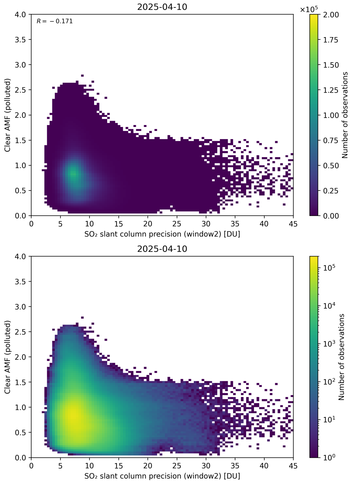
Figure 296: Scatter density plot of “SO 2 slant column precision (window2)” against “Clear AMF (polluted)” for 2025-04-09 to 2025-04-11.
