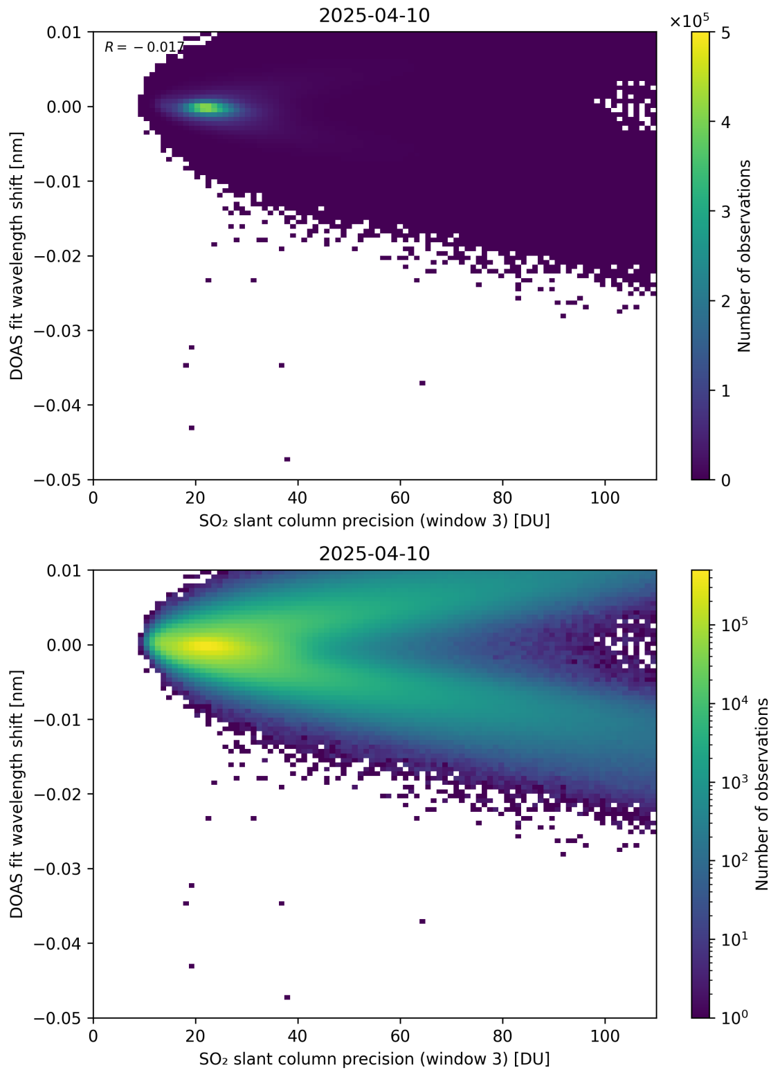
Figure 308: Scatter density plot of “SO 2 slant column precision (window 3)” against “DOAS fit wavelength shift” for 2025-04-09 to 2025-04-11.
