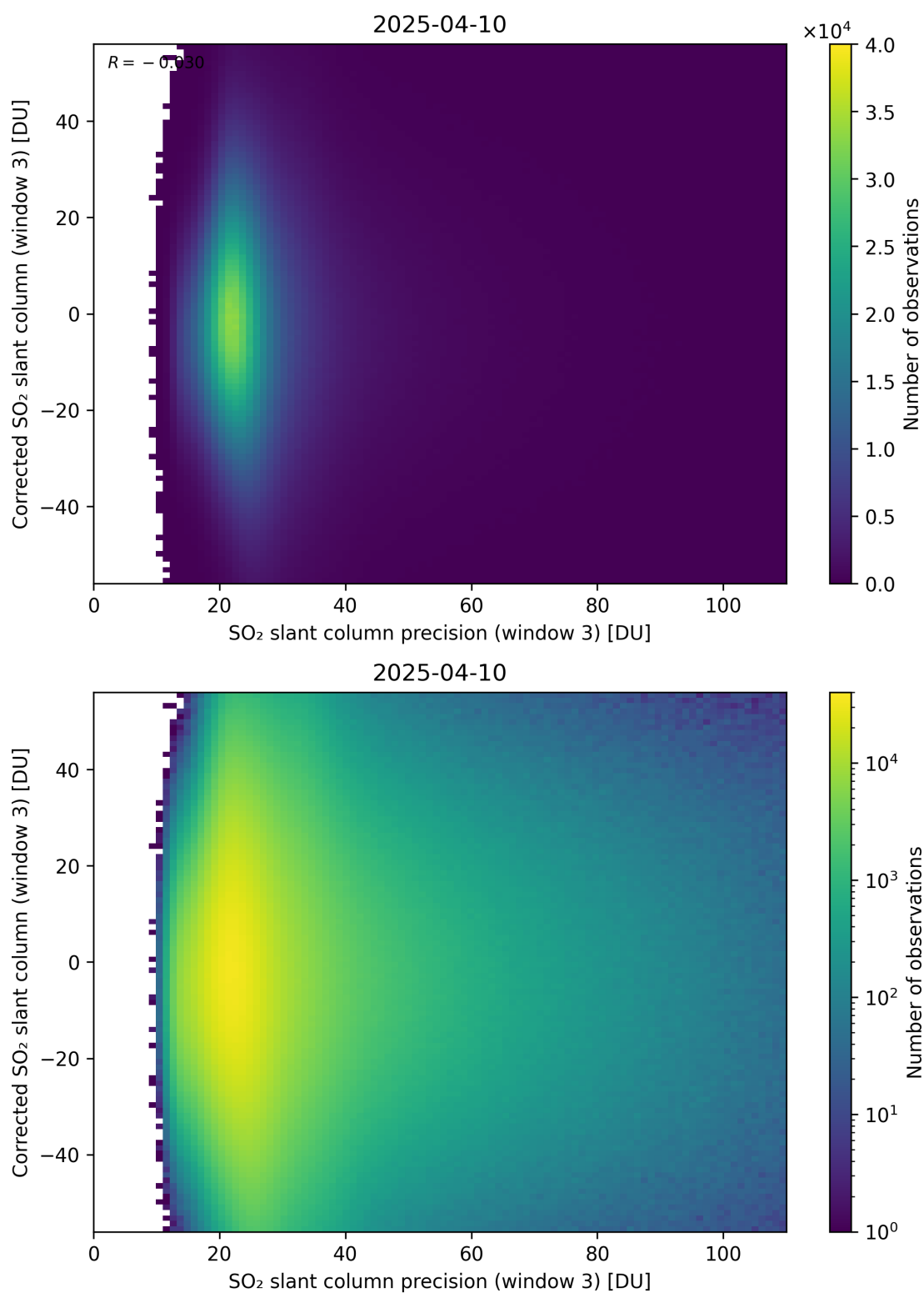
Figure 312: Scatter density plot of “SO 2 slant column precision (window 3)” against “Corrected SO 2 slant column (window 3)” for 2025-04-09 to 2025-04-11.
