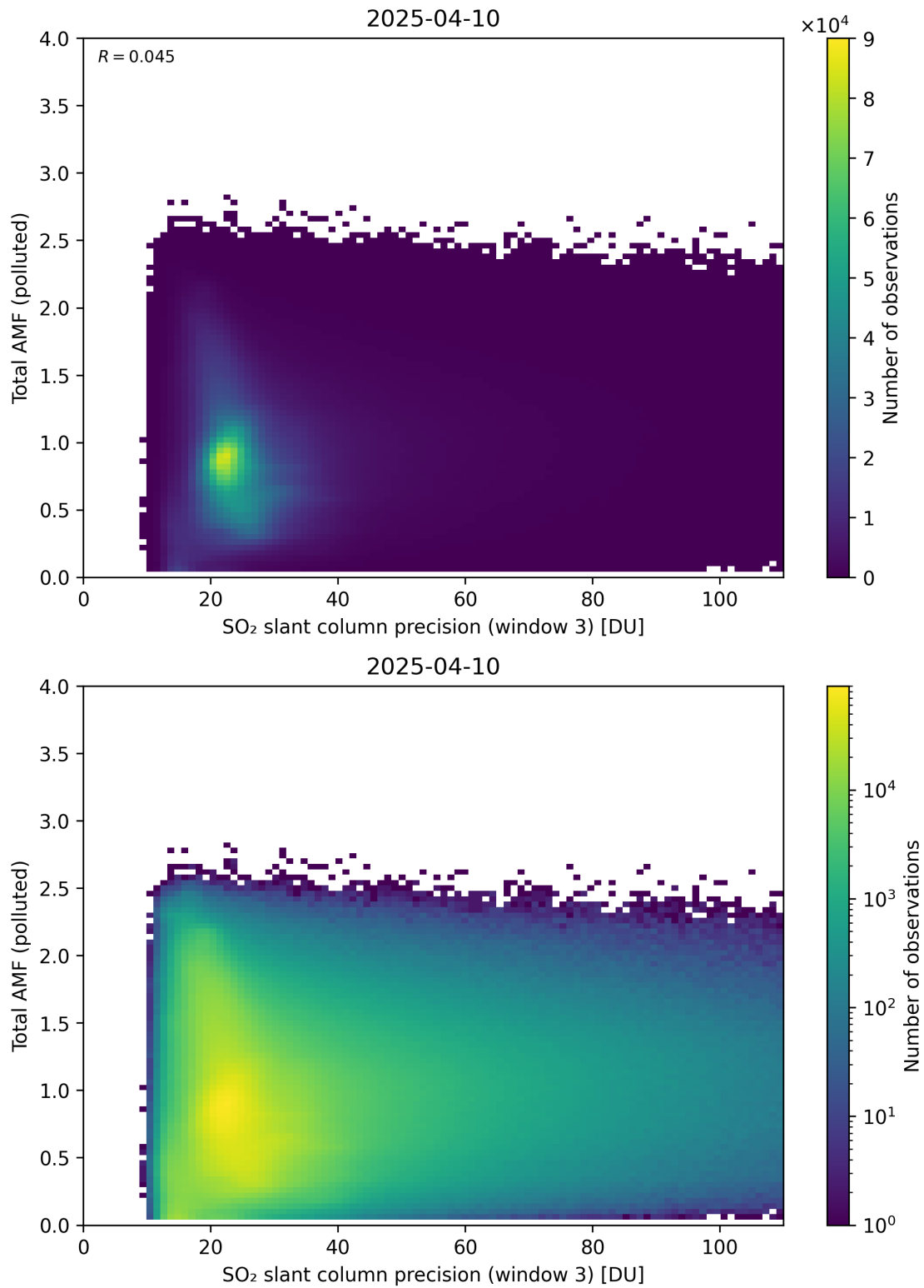
Figure 313: Scatter density plot of “SO 2 slant column precision (window 3)” against “Total AMF (polluted)” for 2025-04-09 to 2025-04-11.
