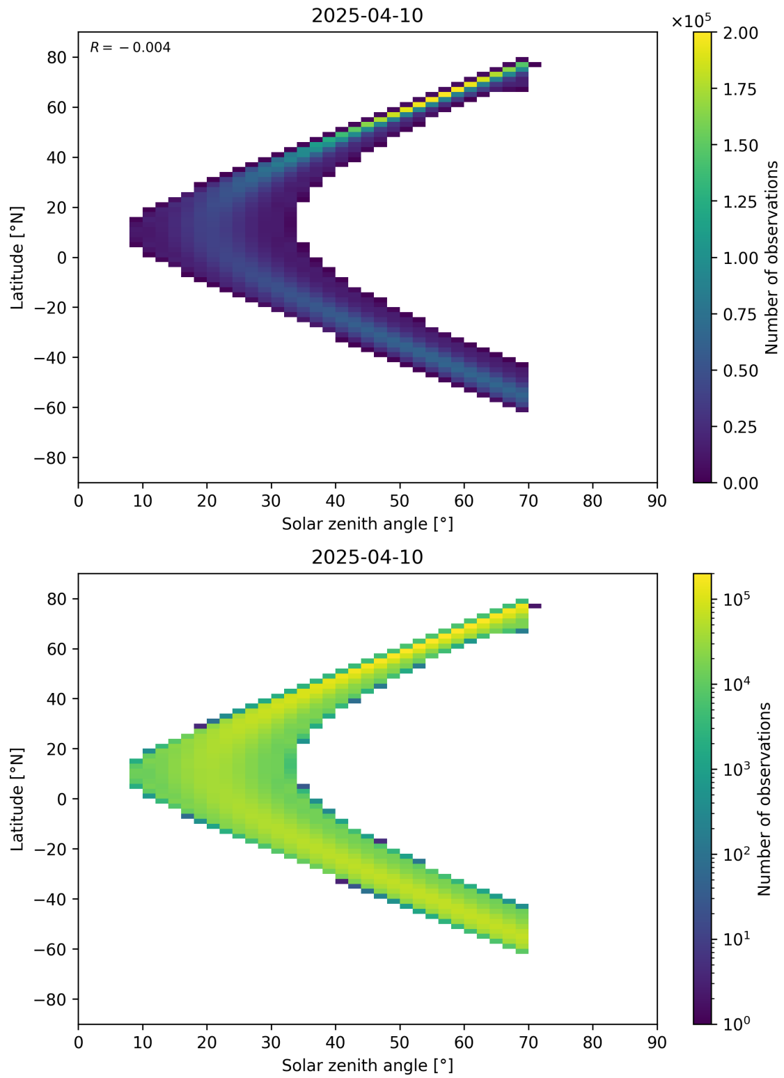
Figure 177: Scatter density plot of “Solar zenith angle” against “Latitude” for 2025-04-09 to 2025-04-11.
