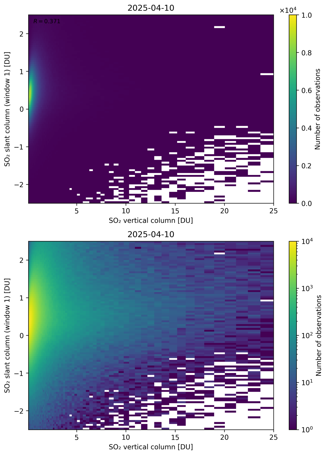
Figure 354: Scatter density plot of “SO 2 vertical column” against “SO 2 slant column (window 1)” for 2025-04-09 to 2025-04-11.
