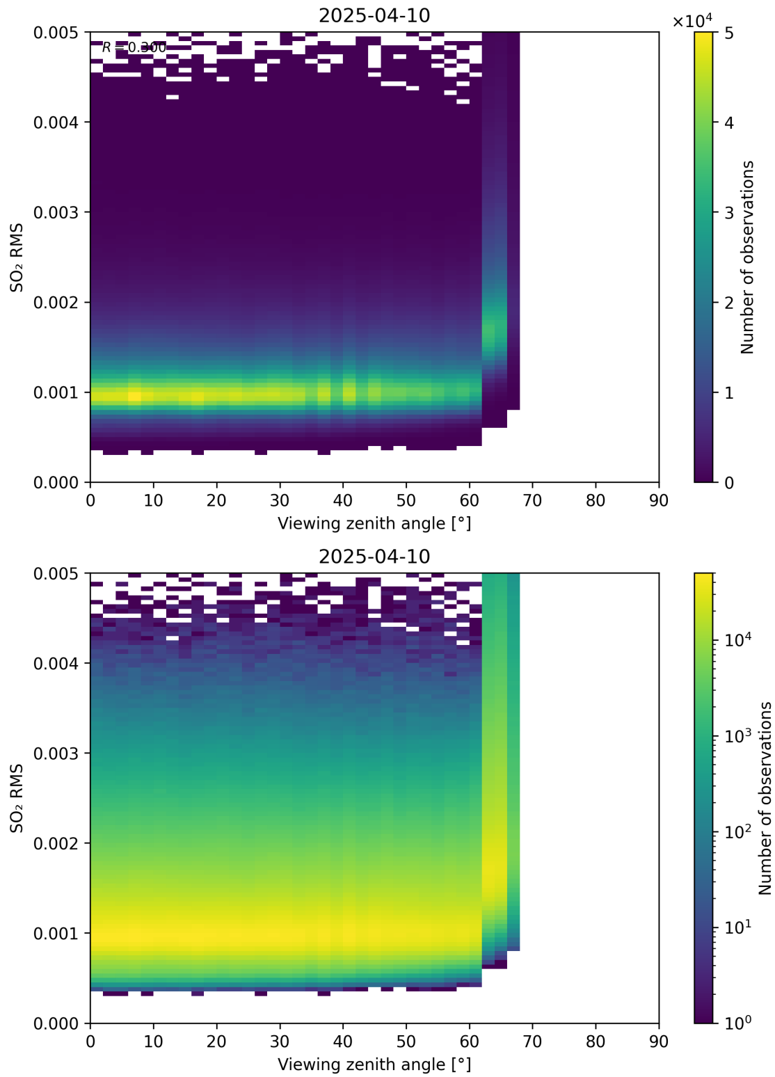
Figure 367: Scatter density plot of “Viewing zenith angle” against “SO 2 RMS” for 2025-04-09 to 2025-04-11.
