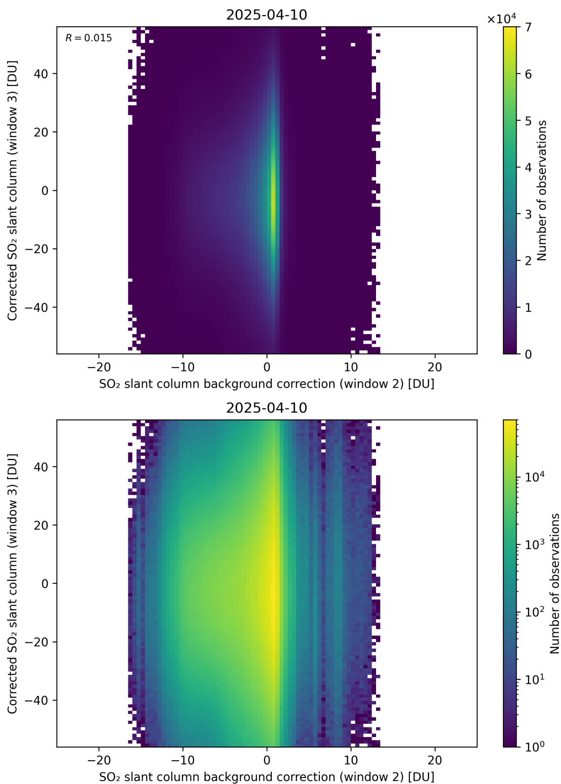
Figure 127: Scatter density plot of “SO 2 slant column background correction (window 2)” against “Corrected SO 2 slant column (window 3)” for 2025-04-09 to 2025-04-11.
