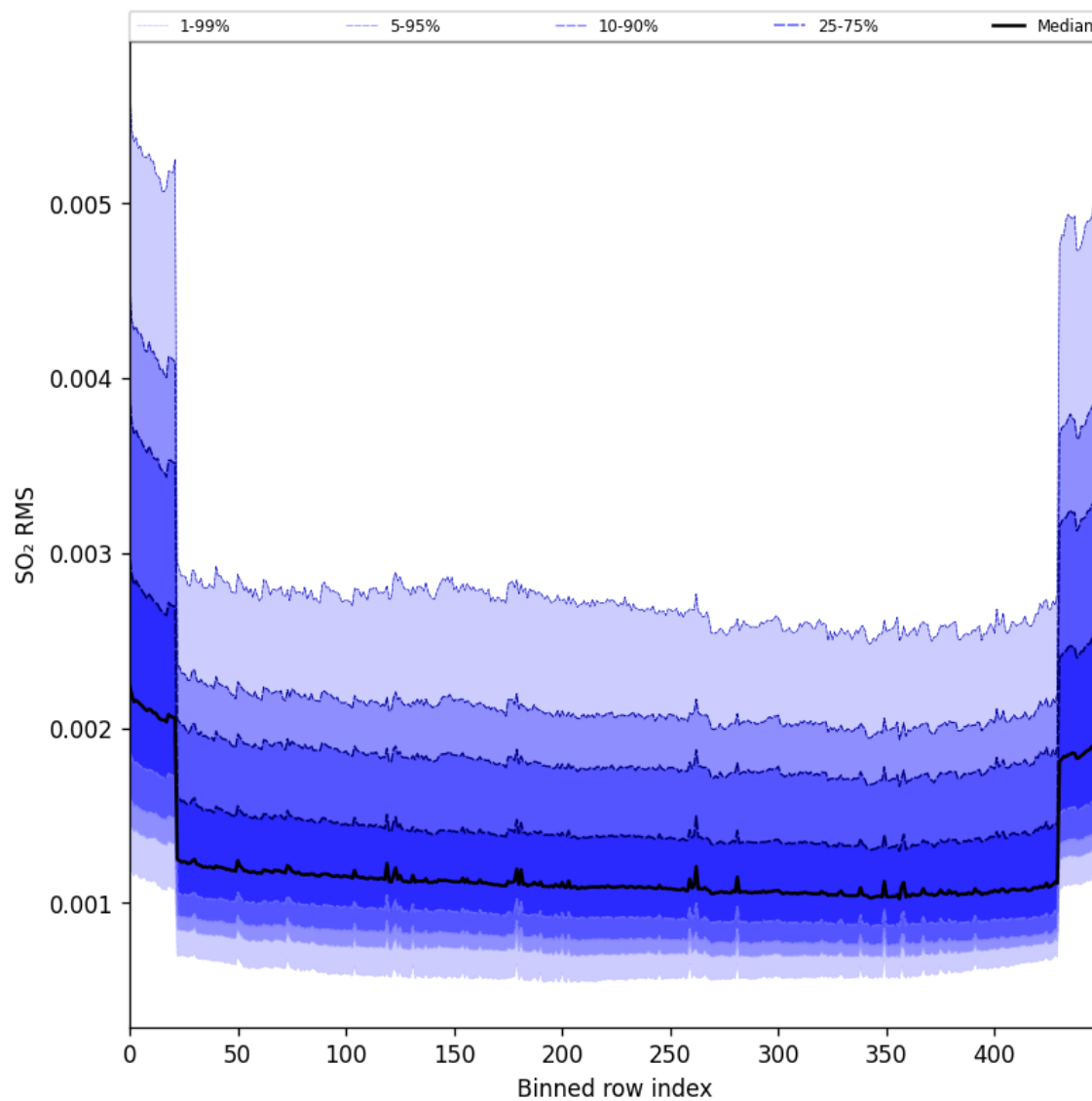
Figure 104: Along track statistics of “SO 2 RMS” for 2025-04-09 to 2025-04-11
