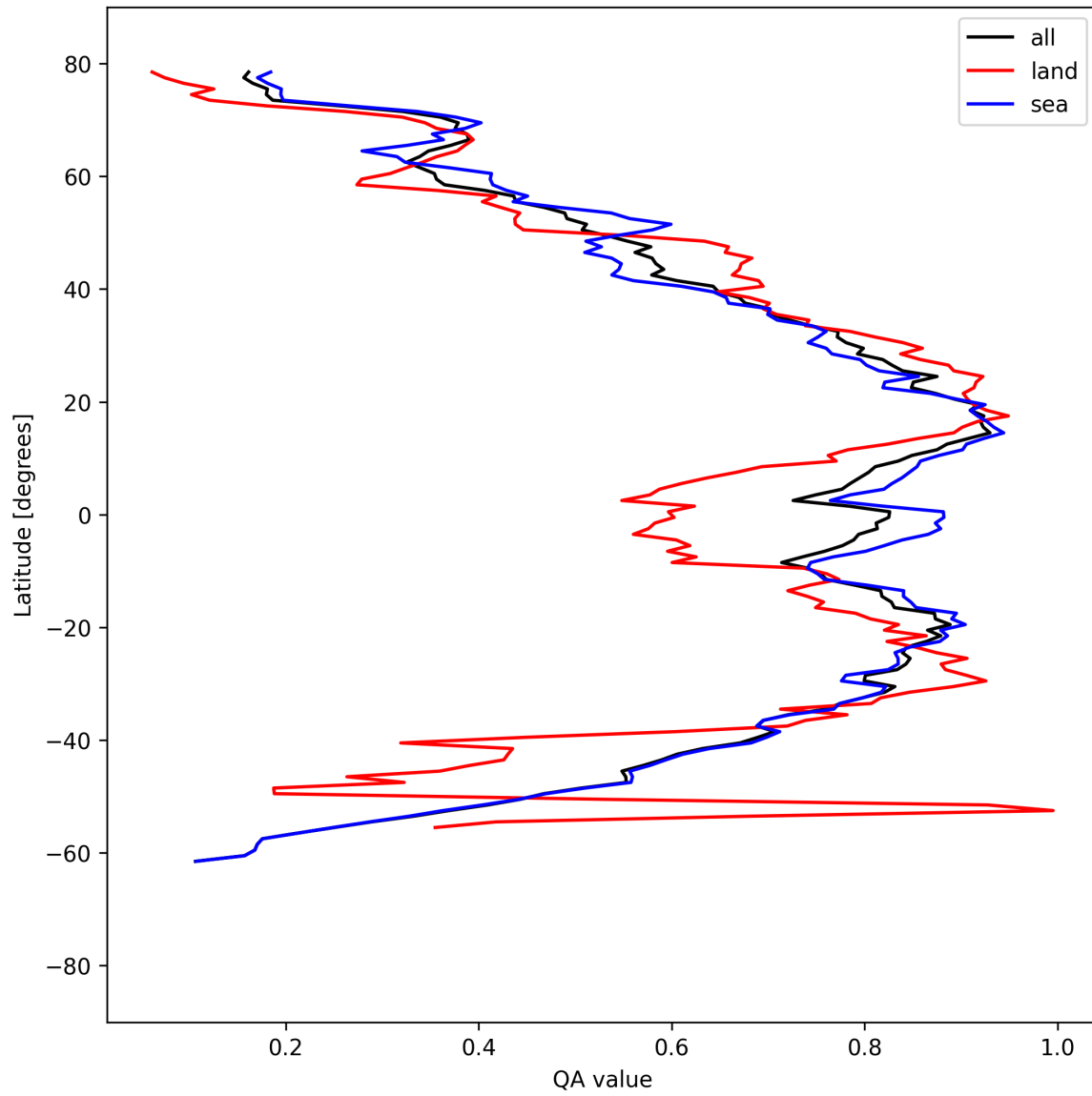
Figure 31: Zonal average of “QA value” for 2025-04-09 to 2025-04-11.
