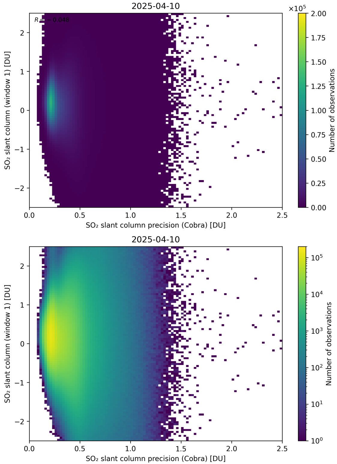
Figure 208: Scatter density plot of “SO 2 slant column precision (Cobra)” against “SO 2 slant column (window 1)” for 2025-04-09 to 2025-04-11.
