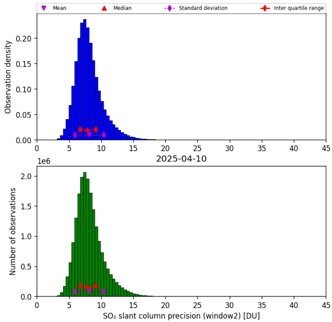
Figure 68: Histogram of “SO 2 slant column precision (window2)” for 2025-04-09 to 2025-04-11
