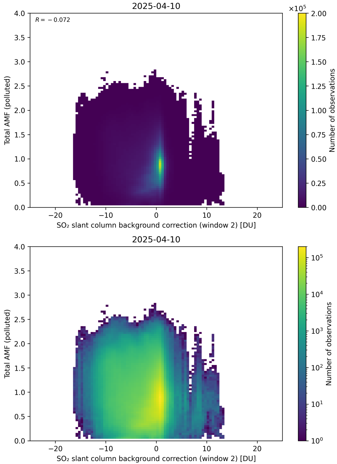
Figure 130: Scatter density plot of “SO 2 slant column background correction (window 2)” against “Total AMF (polluted)” for 2025-04-09 to 2025-04-11.
