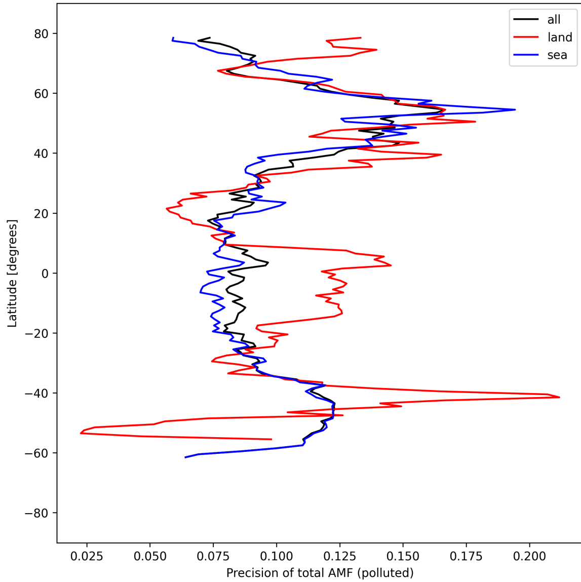
Figure 54: Zonal average of “Precision of total AMF (polluted)” for 2025-04-09 to 2025-04-11.
