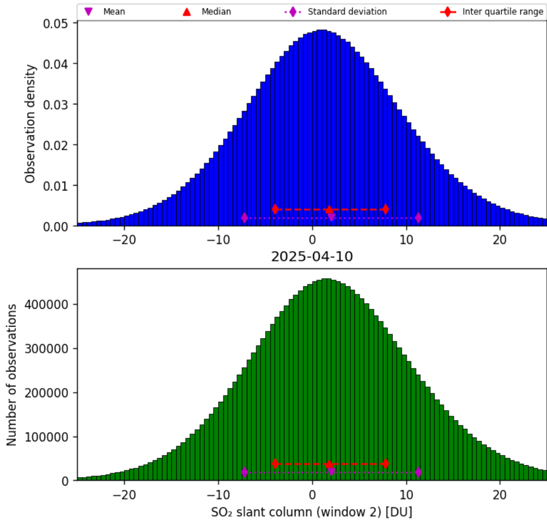
Figure 67: Histogram of “SO 2 slant column (window 2)” for 2025-04-09 to 2025-04-11
