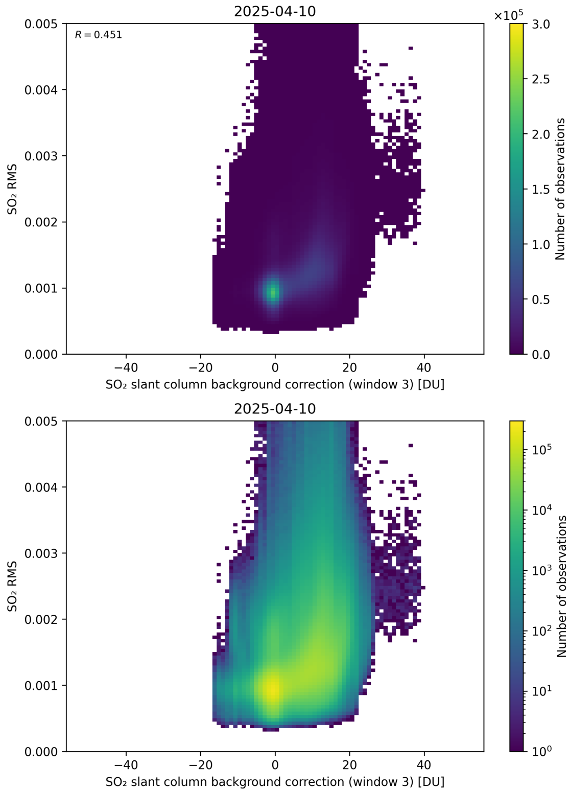
Figure 134: Scatter density plot of “SO 2 slant column background correction (window 3)” against “SO 2 RMS” for 2025-04-09 to 2025-04-11.
