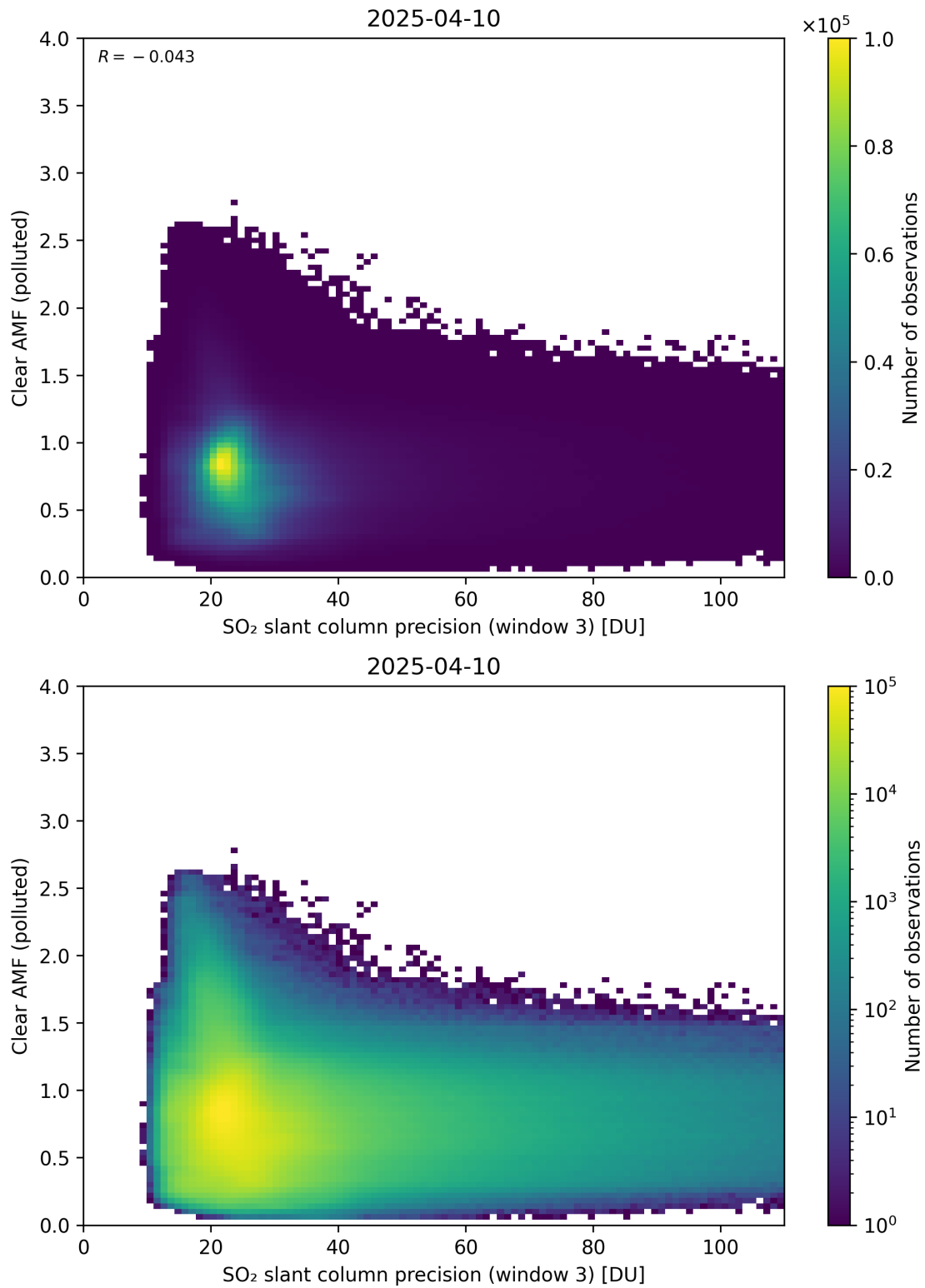
Figure 311: Scatter density plot of “SO 2 slant column precision (window 3)” against “Clear AMF (polluted)” for 2025-04-09 to 2025-04-11.
