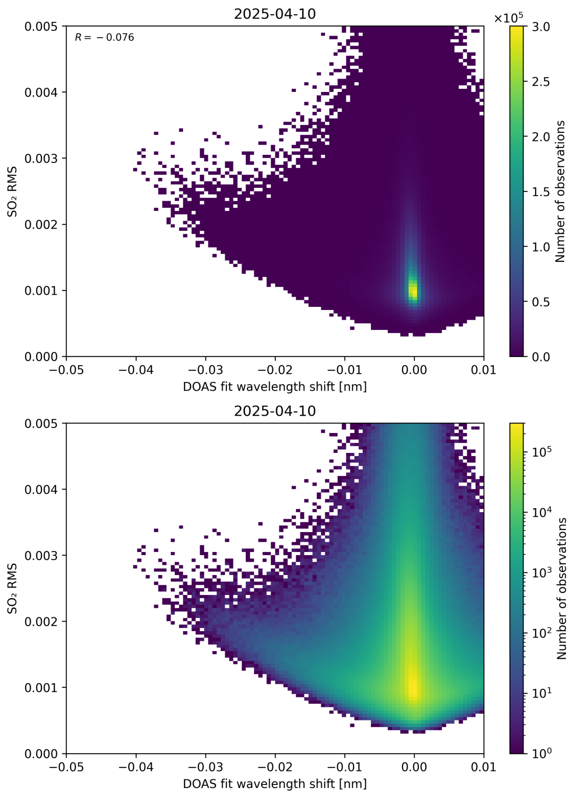
Figure 139: Scatter density plot of “DOAS fit wavelength shift” against “SO 2 RMS” for 2025-04-09 to 2025-04-11.
