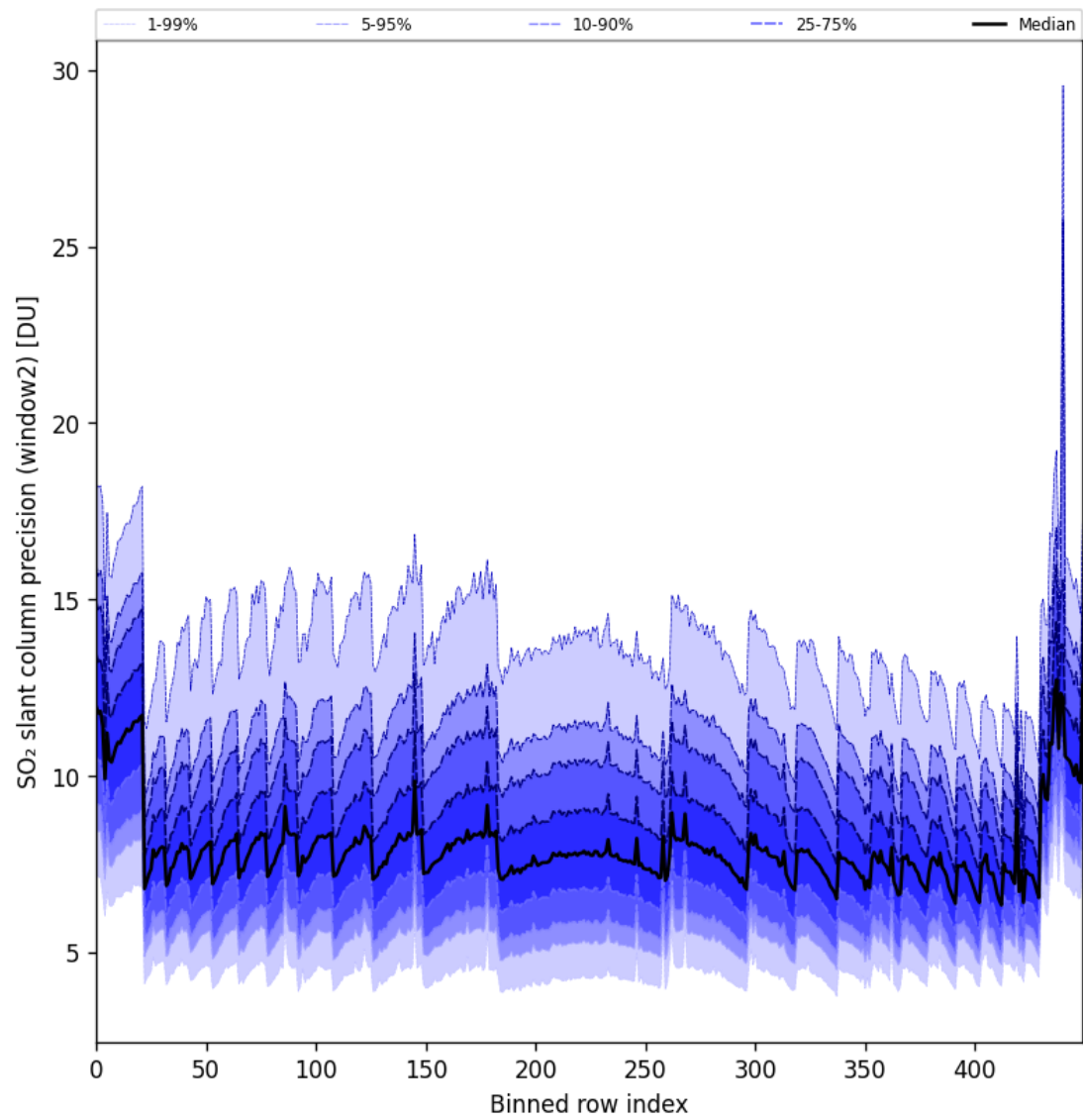
Figure 94: Along track statistics of “SO 2 slant column precision (window2)” for 2025-04-09 to 2025-04-11
