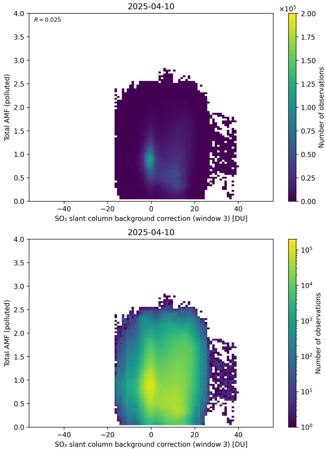
Figure 136: Scatter density plot of “SO 2 slant column background correction (window 3)” against “Total AMF (polluted)” for 2025-04-09 to 2025-04-11.
