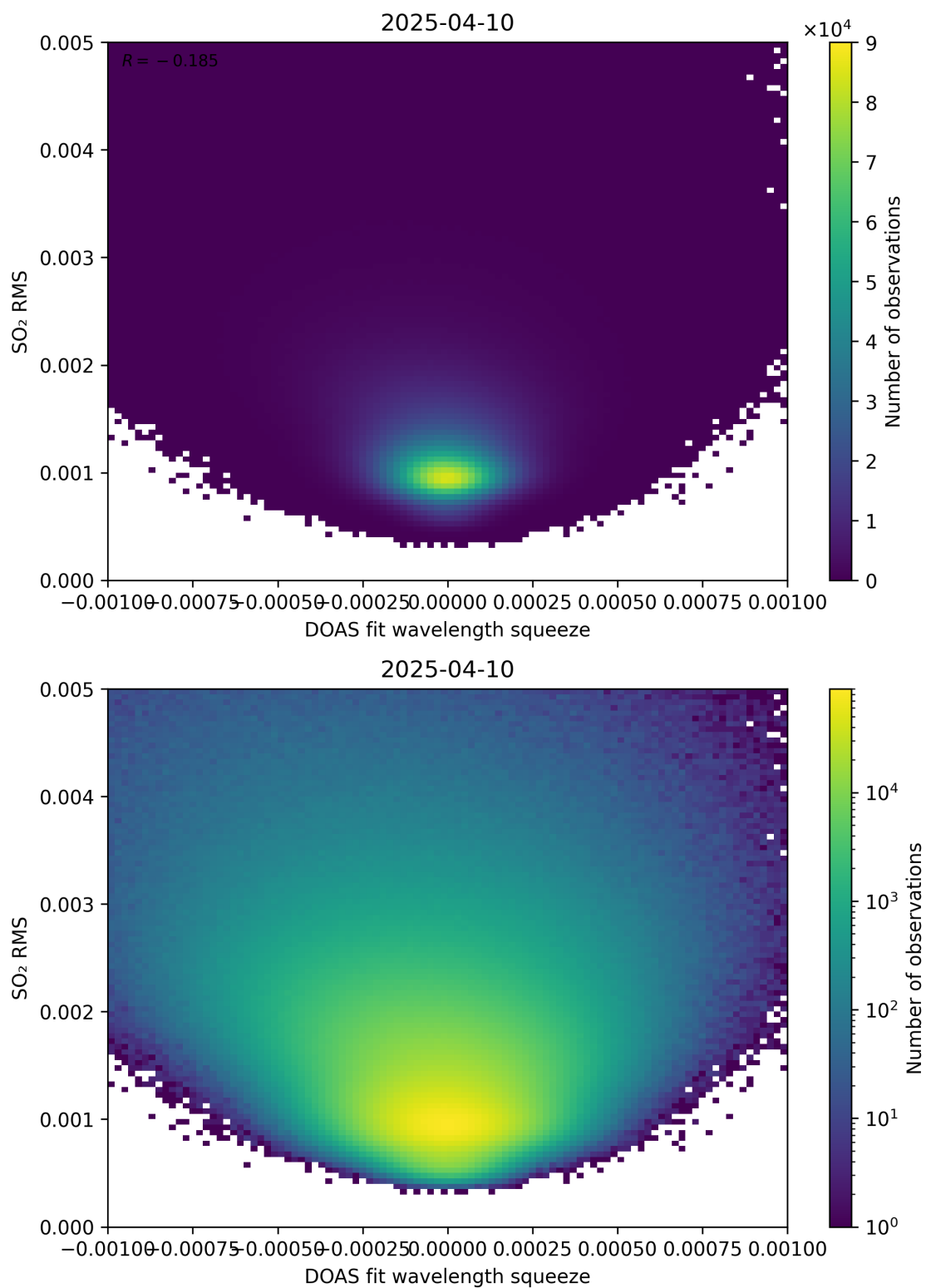
Figure 143: Scatter density plot of “DOAS fit wavelength squeeze” against “SO 2 RMS” for 2025-04-09 to 2025-04-11.
