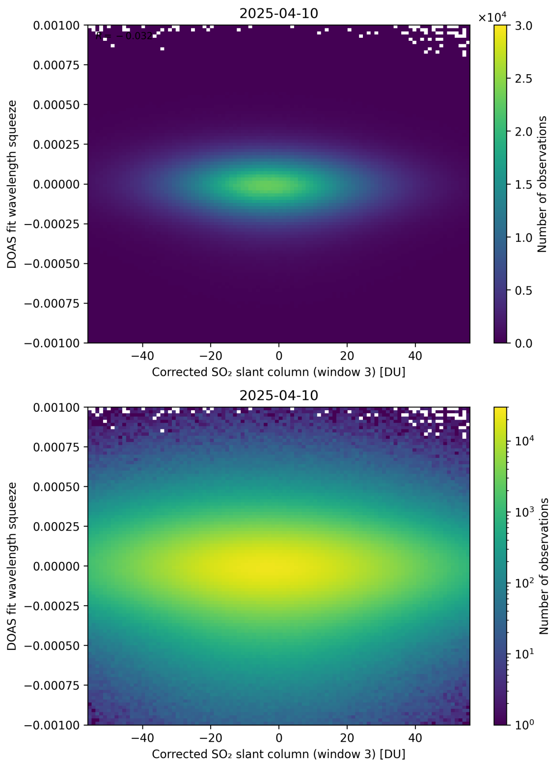
Figure 257: Scatter density plot of “Corrected SO 2 slant column (window 3)” against “DOAS fit wavelength squeeze” for 2025-04-09 to 2025-04-11.
