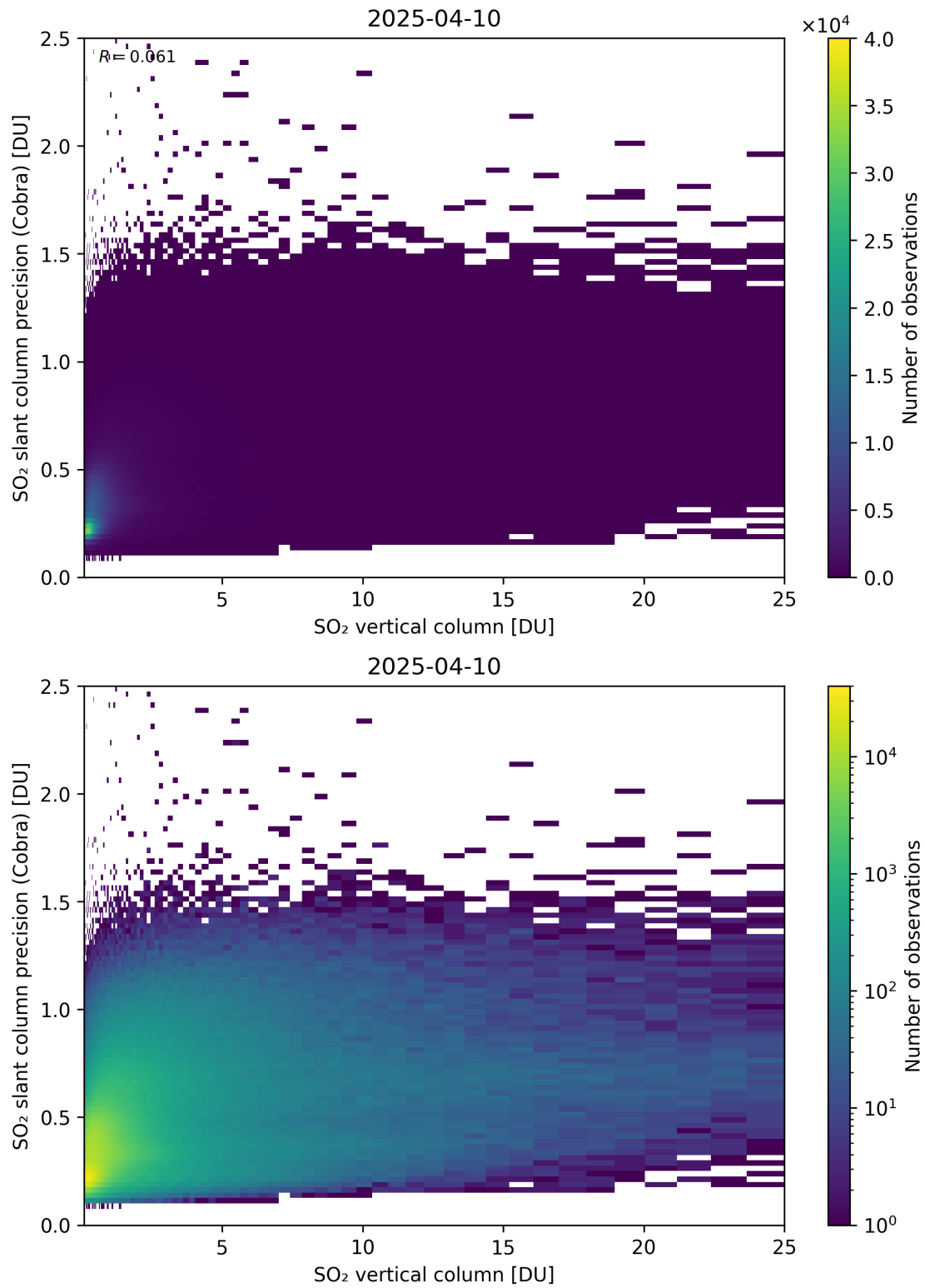
Figure 350: Scatter density plot of “SO 2 vertical column” against “SO 2 slant column precision (Cobra)” for 2025-04-09 to 2025-04-11.
