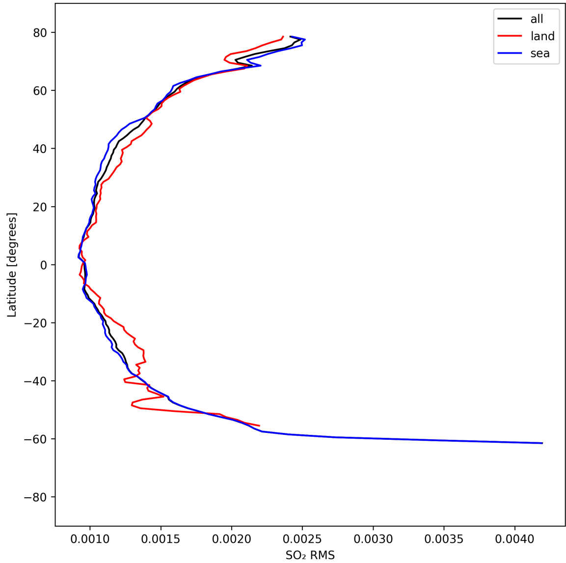
Figure 52: Zonal average of “SO 2 RMS” for 2025-04-09 to 2025-04-11.
