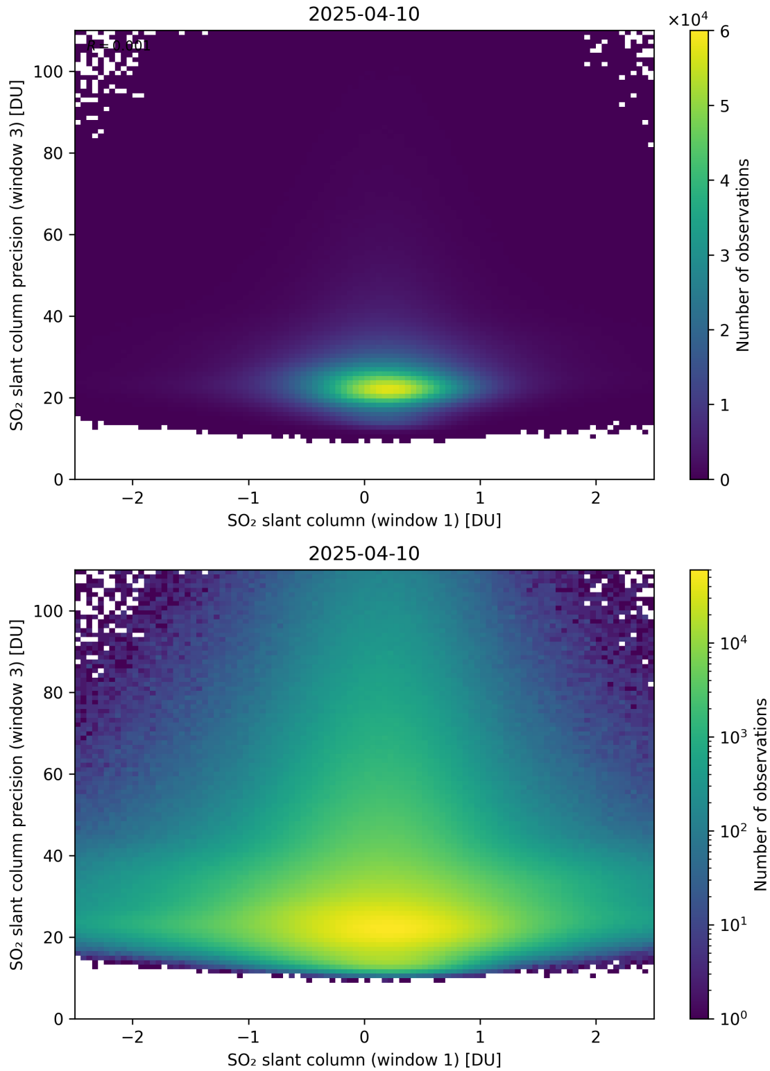
Figure 288: Scatter density plot of “SO 2 slant column (window 1)” against “SO 2 slant column precision (window 3)” for 2025-04-09 to 2025-04-11.
