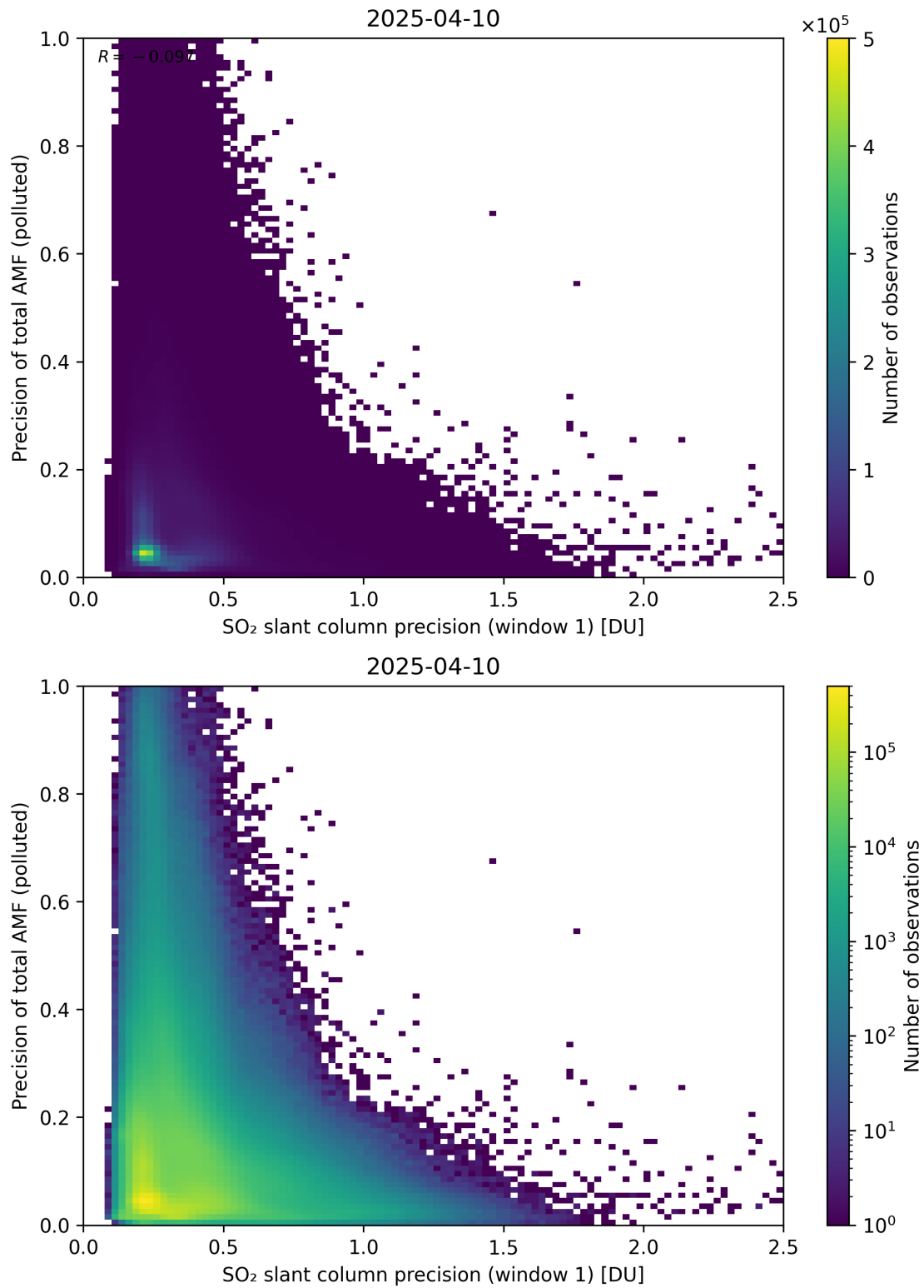
Figure 281: Scatter density plot of “SO 2 slant column precision (window 1)” against “Precision of total AMF (polluted)” for 2025-04-09 to 2025-04-11.
