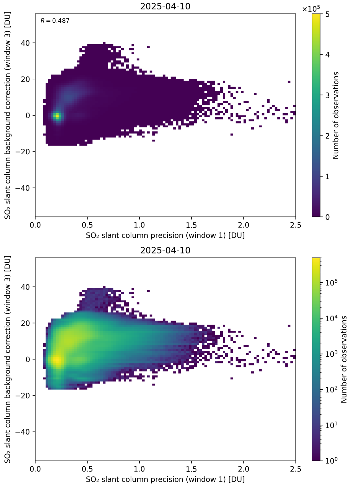
Figure 270: Scatter density plot of “SO 2 slant column precision (window 1)” against “SO 2 slant column background correction (window 3)” for 2025-04-09 to 2025-04-11.
