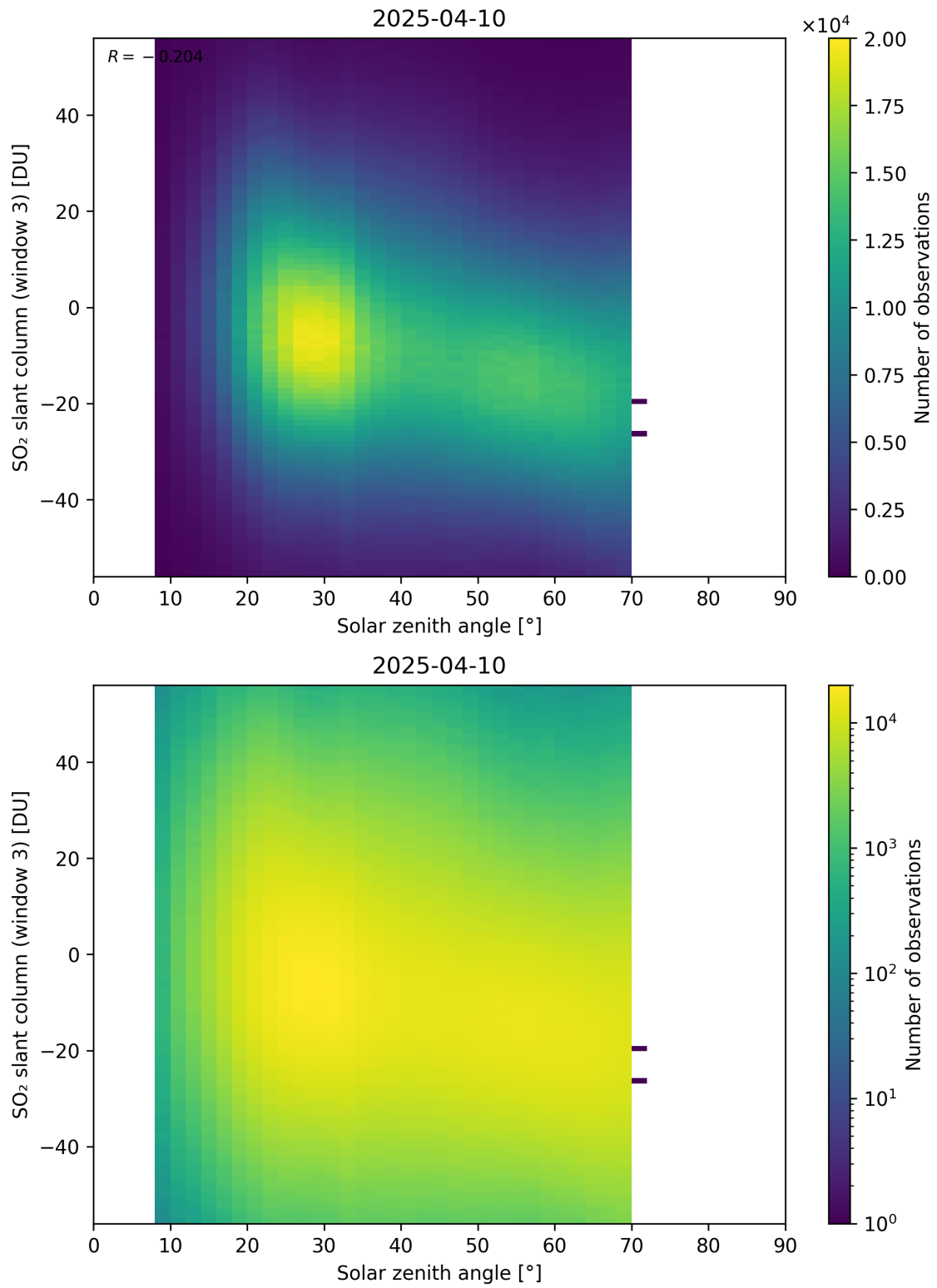
Figure 187: Scatter density plot of “Solar zenith angle” against “SO 2 slant column (window 3)” for 2025-04-09 to 2025-04-11.
