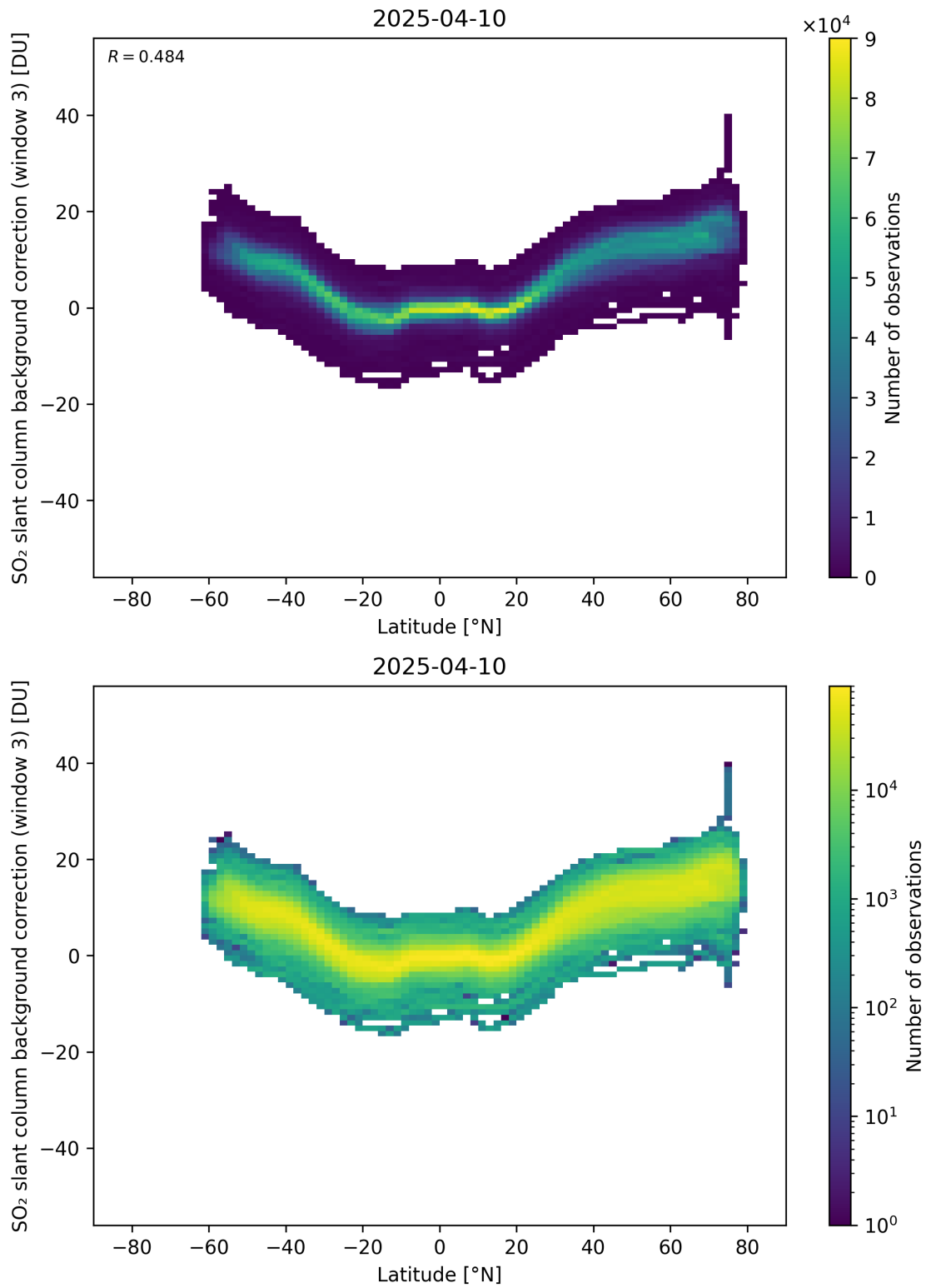
Figure 152: Scatter density plot of “Latitude” against “SO 2 slant column background correction (window 3)” for 2025-04-09 to 2025-04-11.
