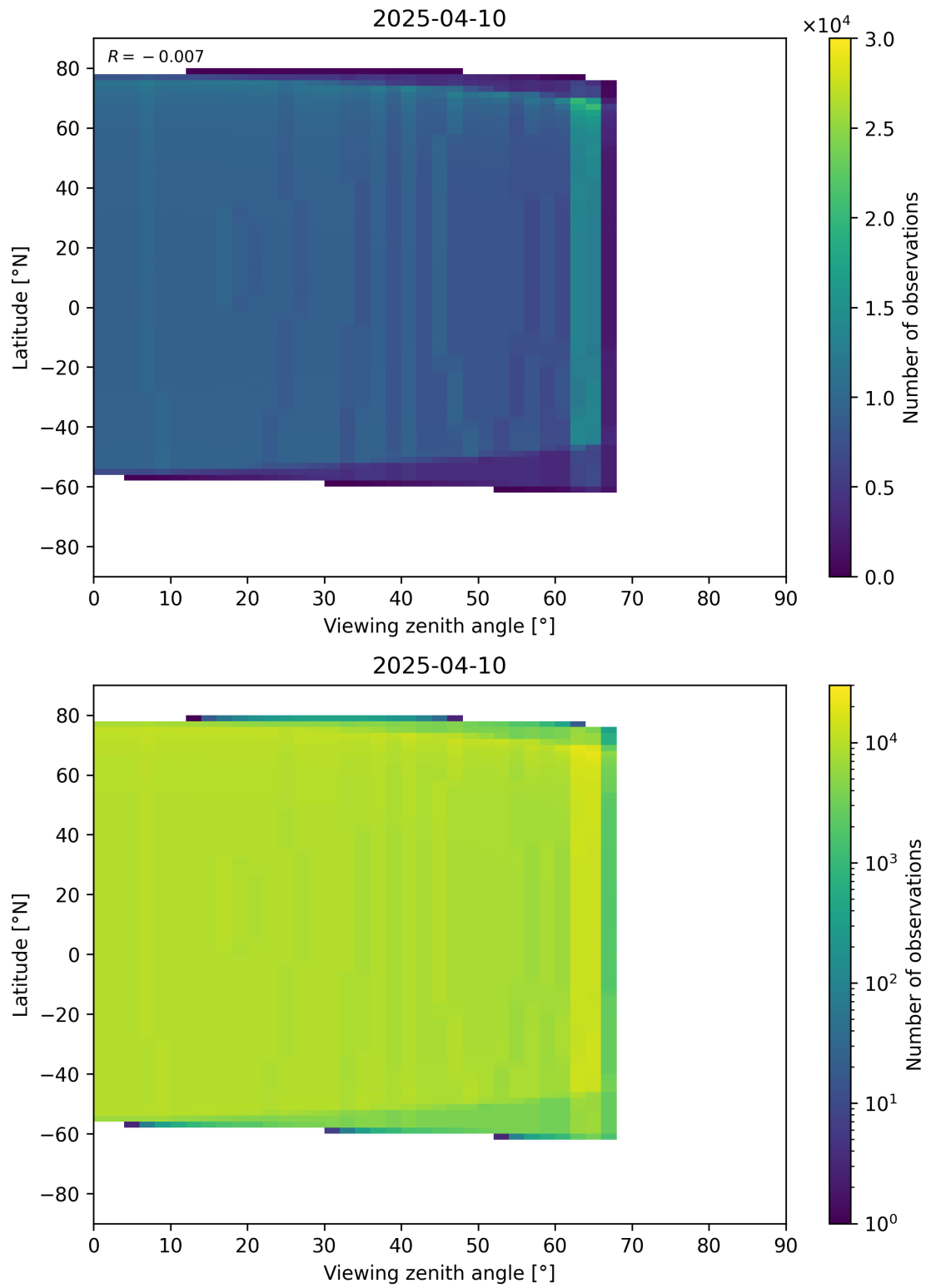
Figure 368: Scatter density plot of “Viewing zenith angle” against “Latitude” for 2025-04-09 to 2025-04-11.
