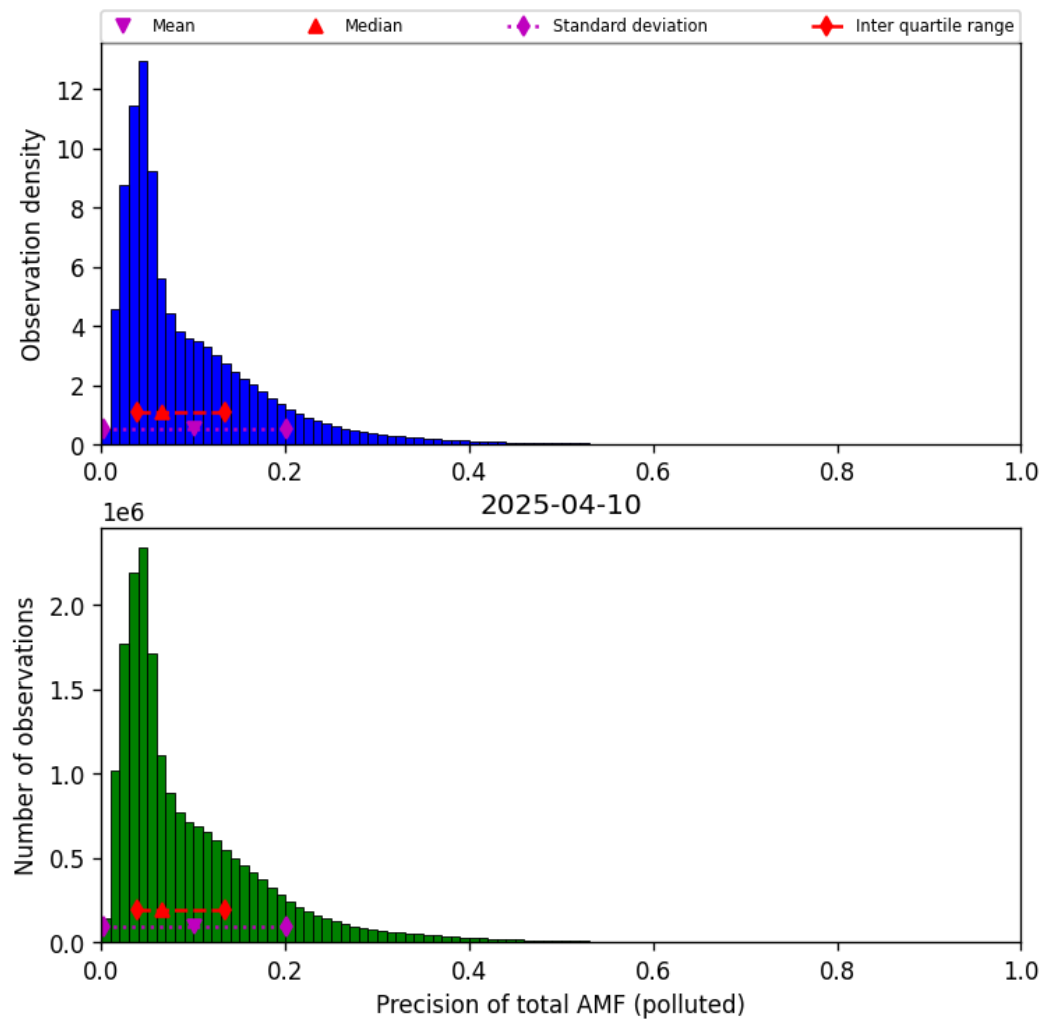
Figure 80: Histogram of “Precision of total AMF (polluted)” for 2025-04-09 to 2025-04-11
