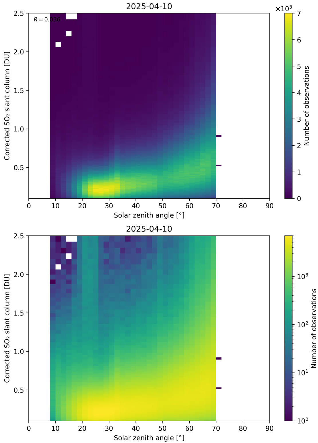
Figure 181: Scatter density plot of “Solar zenith angle” against “Corrected SO 2 slant column” for 2025-04-09 to 2025-04-11.
