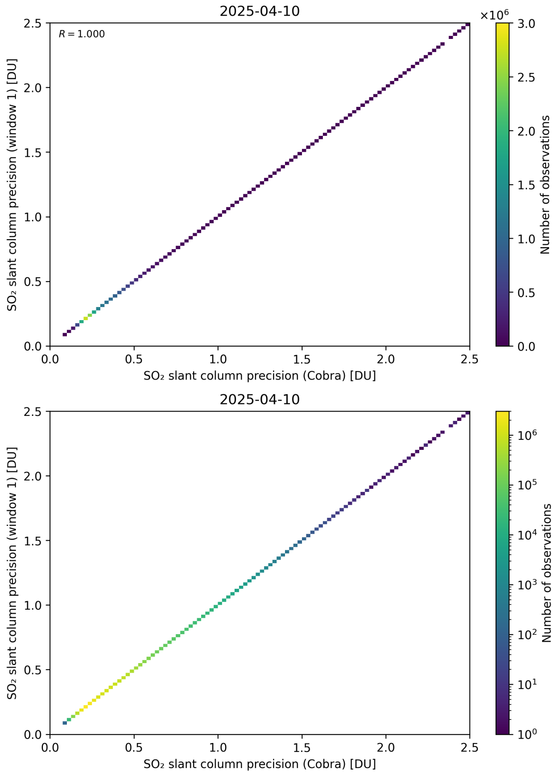
Figure 209: Scatter density plot of “SO 2 slant column precision (Cobra)” against “SO 2 slant column precision (window 1)” for 2025-04-09 to 2025-04-11.
