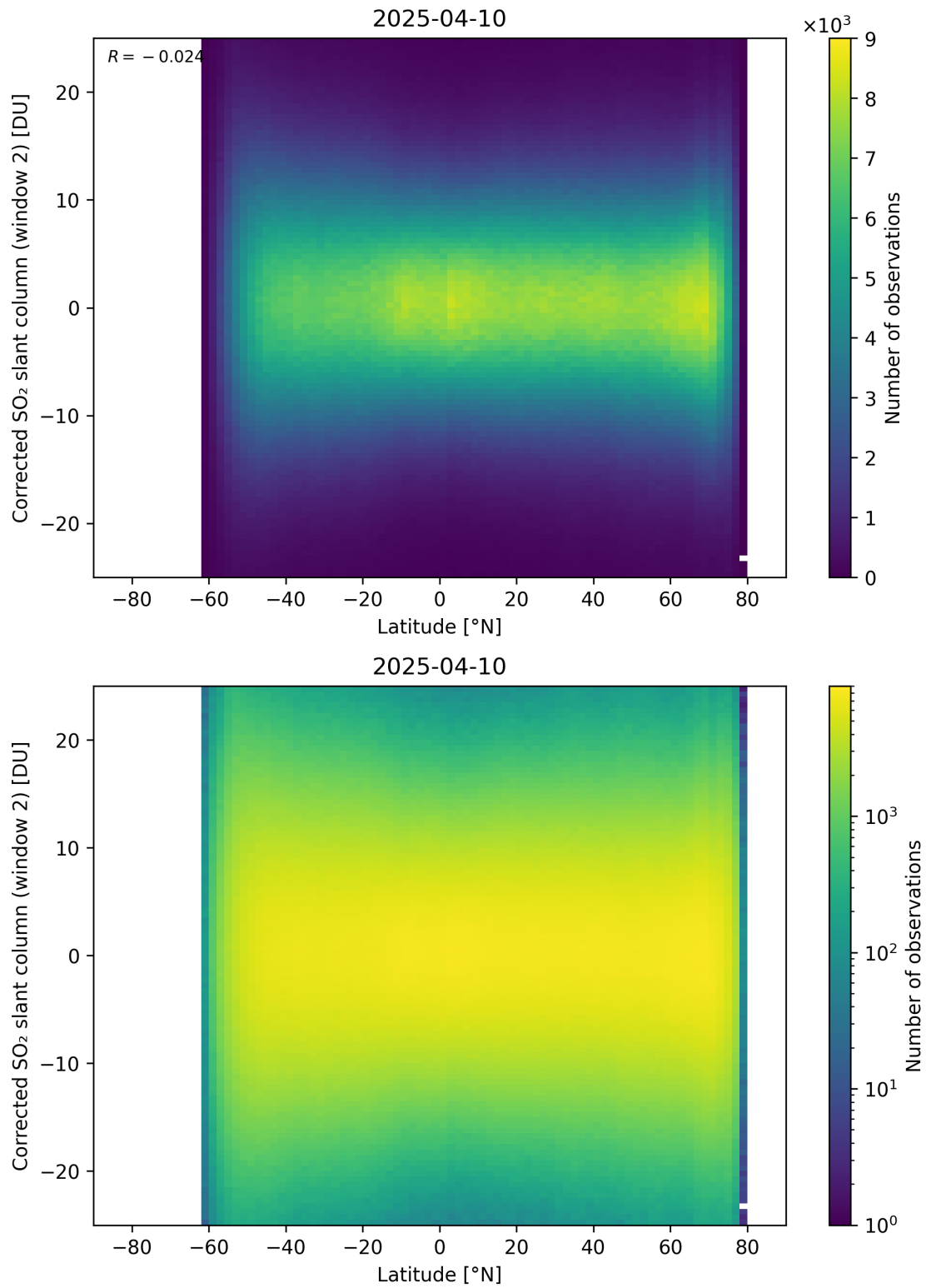
Figure 160: Scatter density plot of “Latitude” against “Corrected SO 2 slant column (window 2)” for 2025-04-09 to 2025-04-11.
