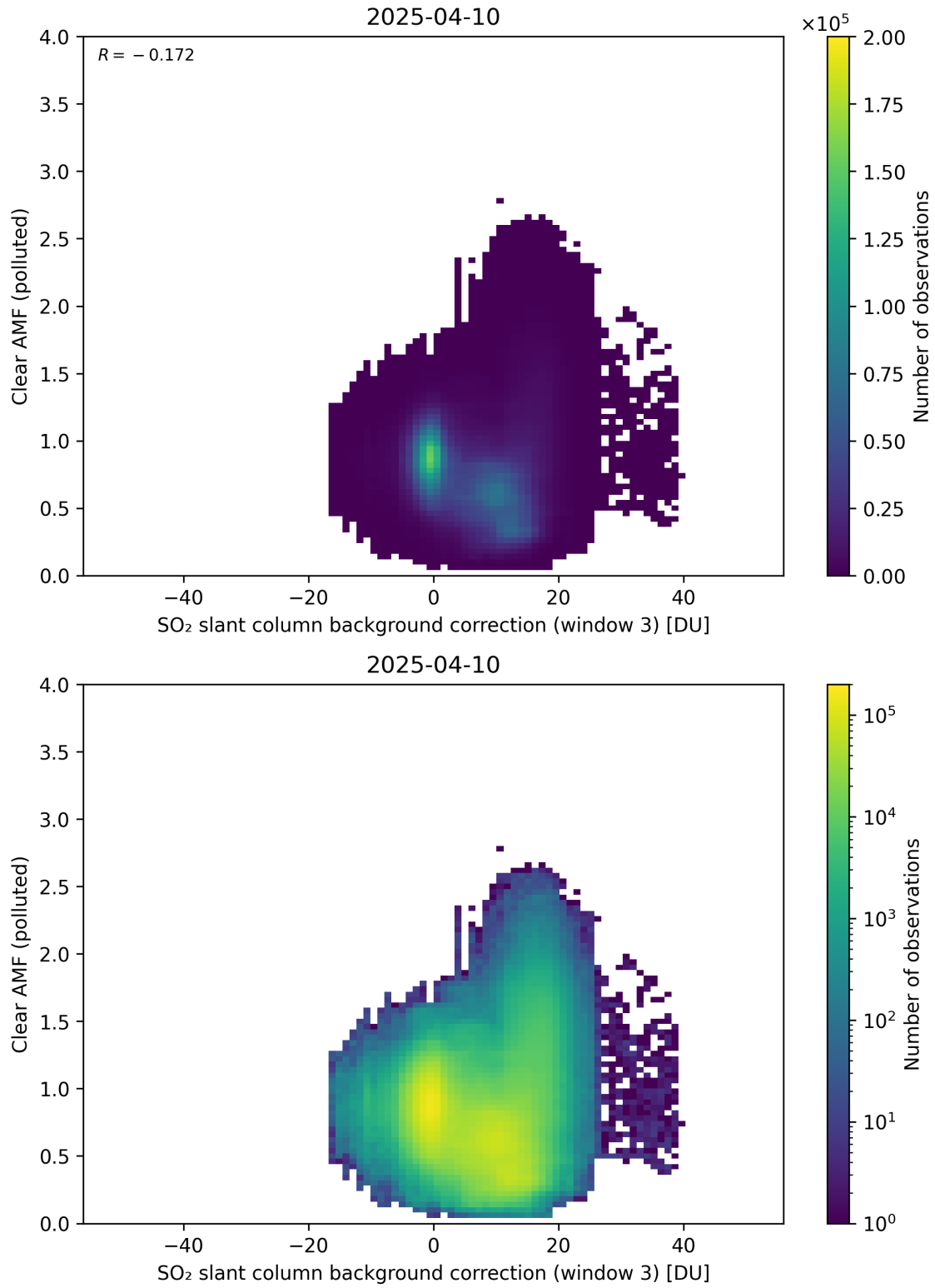
Figure 135: Scatter density plot of “SO 2 slant column background correction (window 3)” against “Clear AMF (polluted)” for 2025-04-09 to 2025-04-11.
