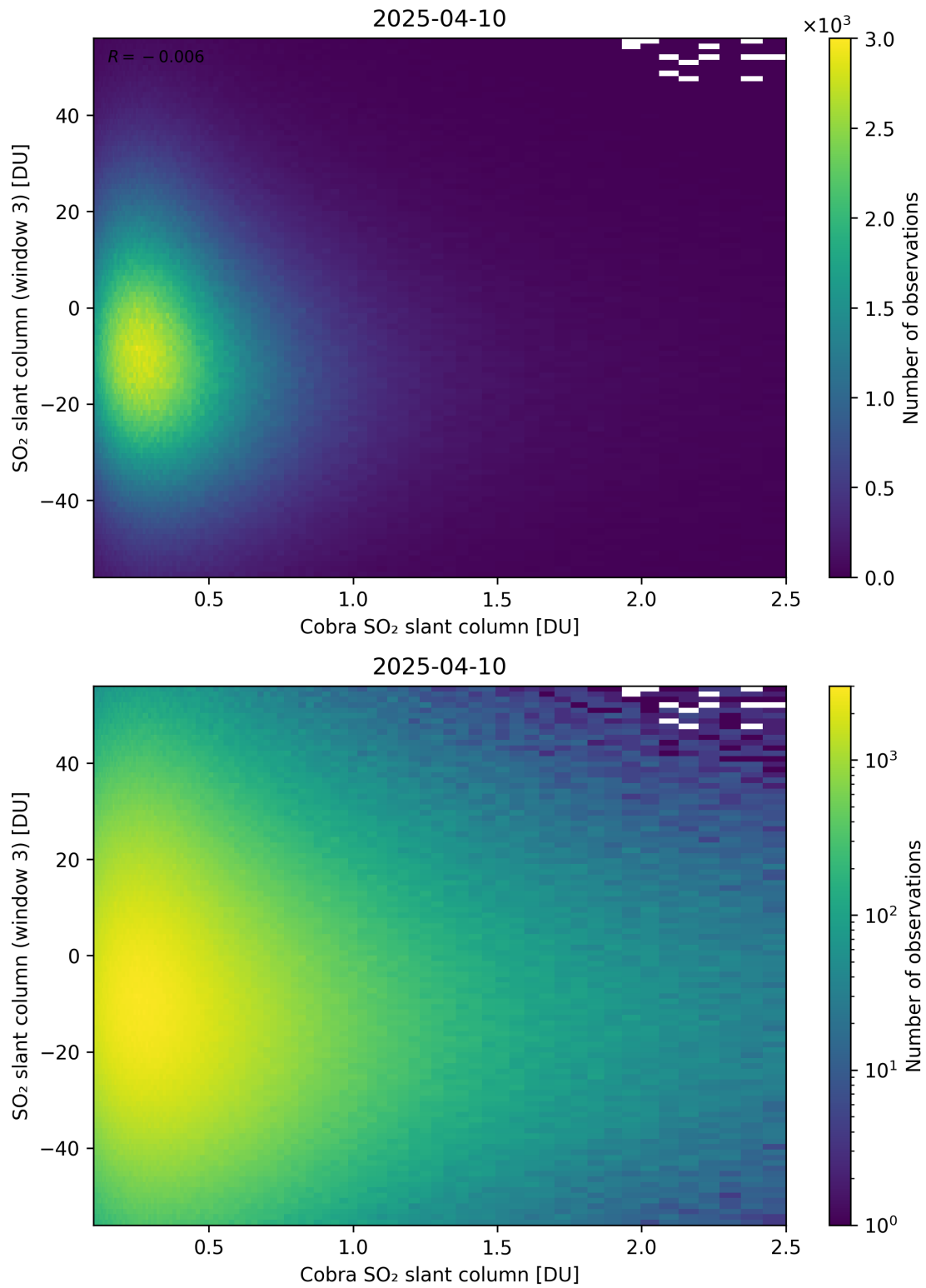
Figure 222: Scatter density plot of “Cobra SO 2 slant column” against “SO 2 slant column (window 3)” for 2025-04-09 to 2025-04-11.
