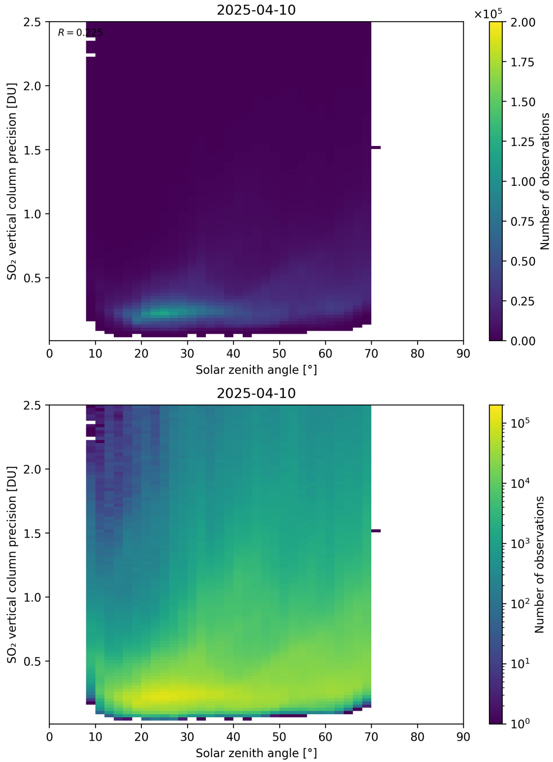
Figure 192: Scatter density plot of “Solar zenith angle” against “SO 2 vertical column precision” for 2025-04-09 to 2025-04-11.
