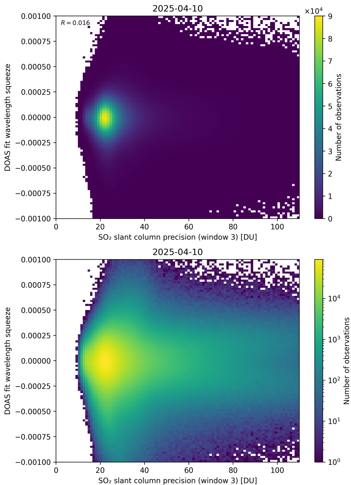
Figure 309: Scatter density plot of “SO 2 slant column precision (window 3)” against “DOAS fit wavelength squeeze” for 2025-04-09 to 2025-04-11.
