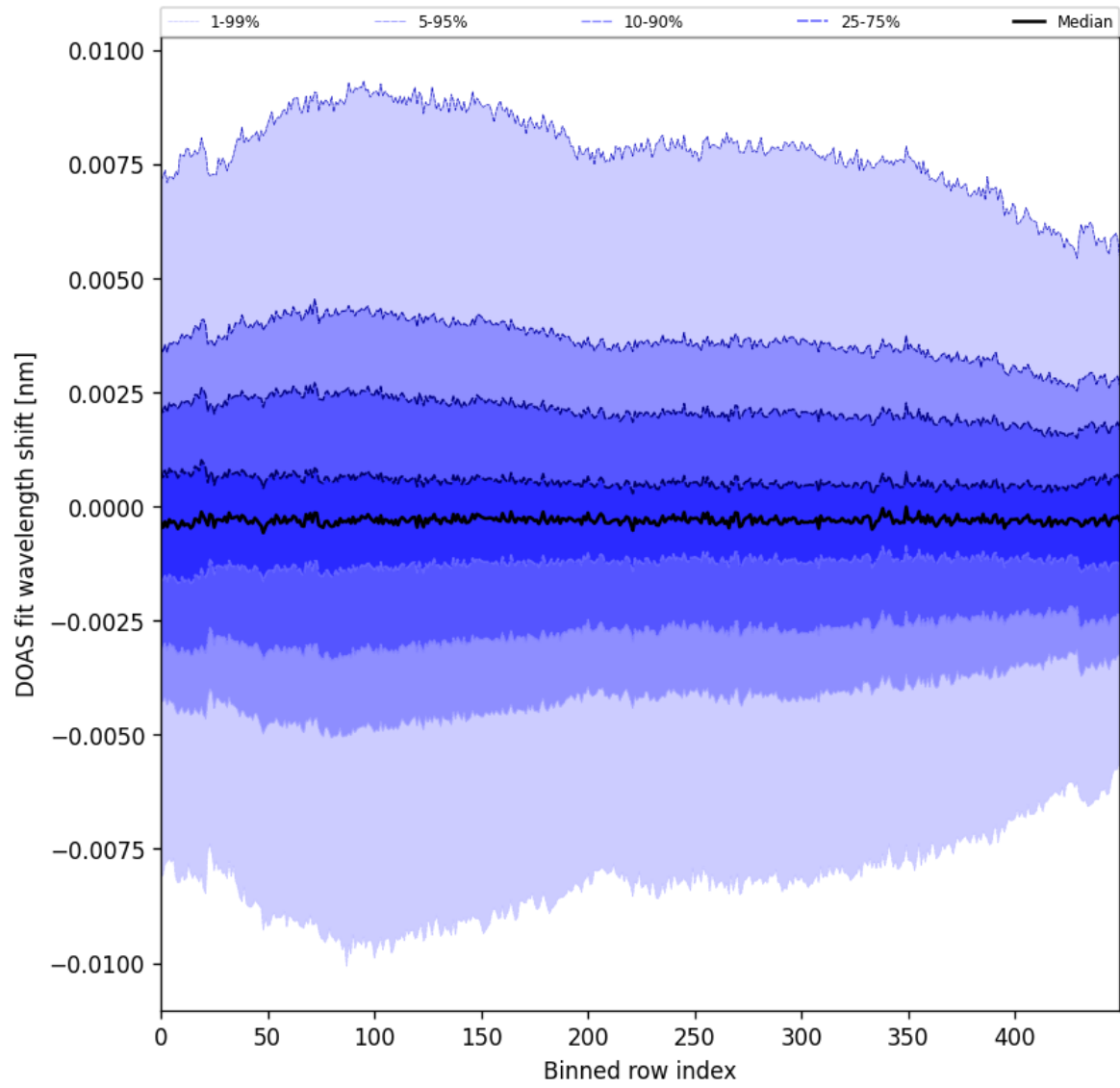
Figure 102: Along track statistics of “DOAS fit wavelength shift” for 2025-04-09 to 2025-04-11
