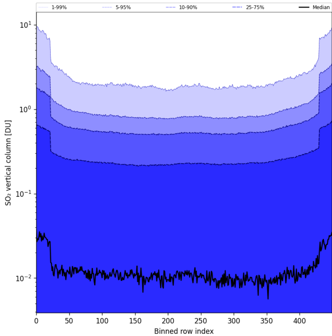
Figure 84: Along track statistics of “SO 2 vertical column” for 2025-04-09 to 2025-04-11
