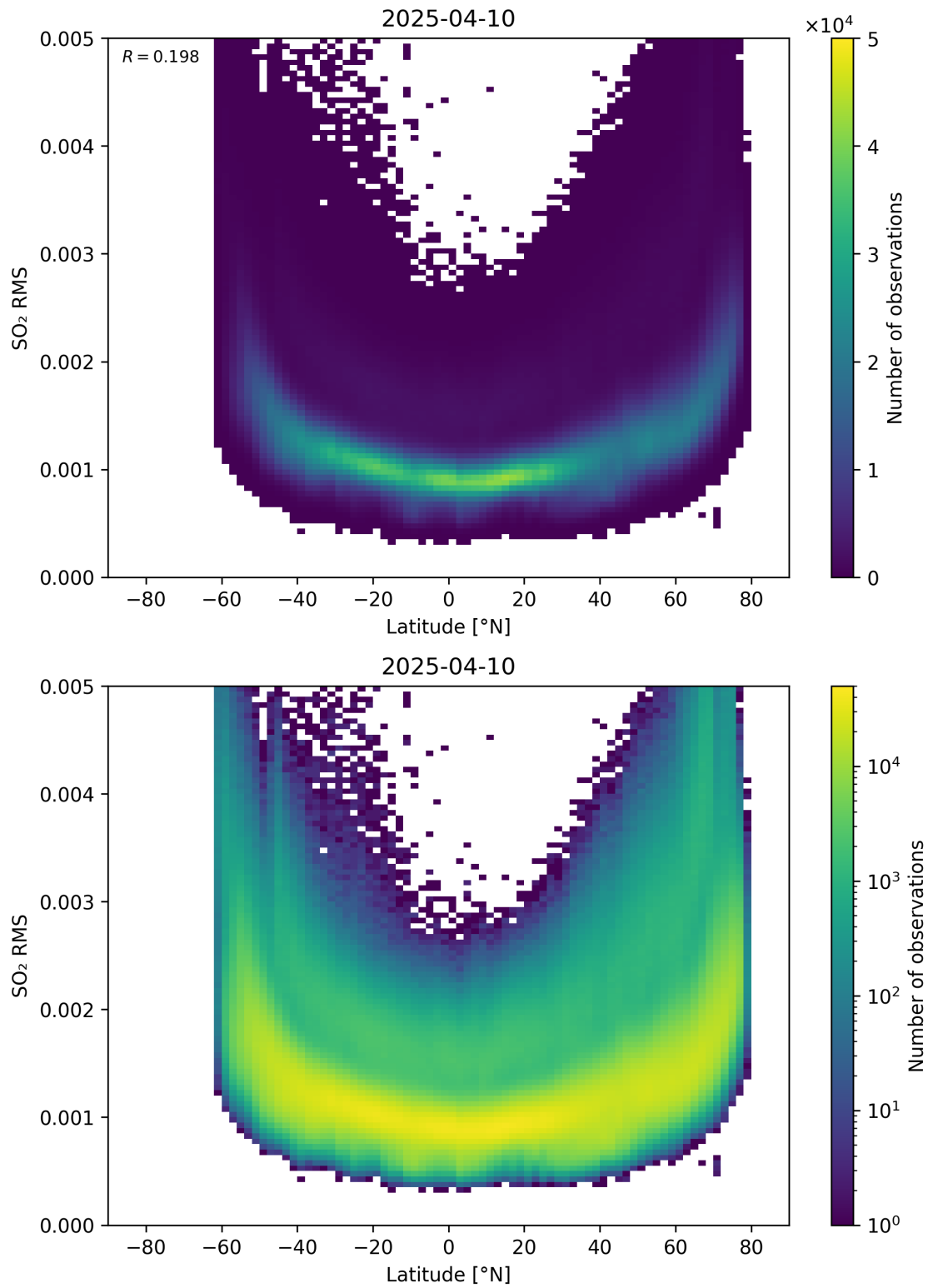
Figure 155: Scatter density plot of “Latitude” against “SO 2 RMS” for 2025-04-09 to 2025-04-11.
