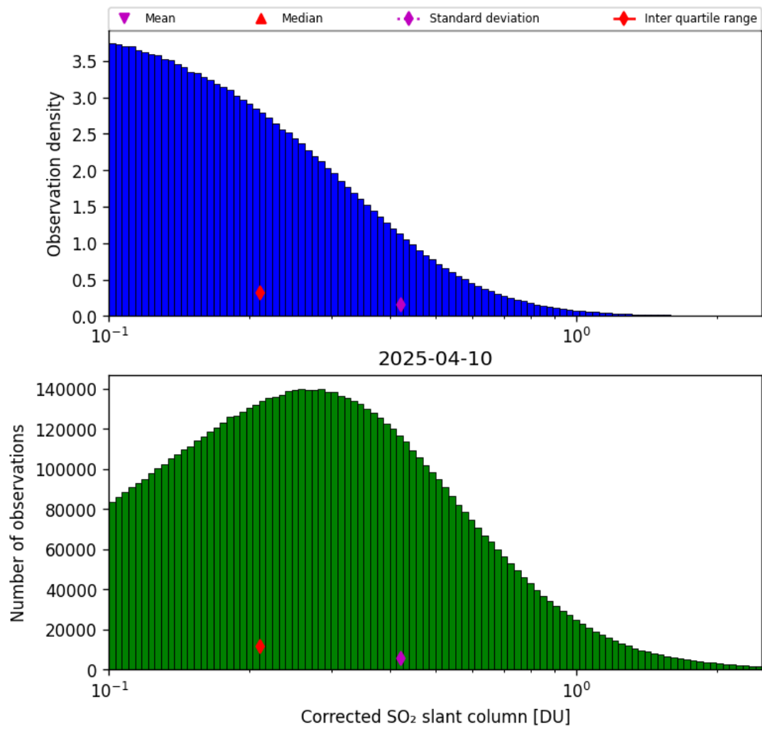
Figure 60: Histogram of "Corrected SO 2 slant column" for 2025-04-09 to 2025-04-11
