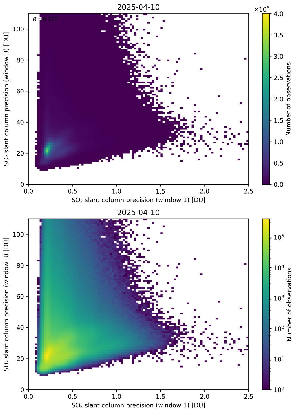
Figure 279: Scatter density plot of “SO 2 slant column precision (window 1)” against “SO 2 slant column precision (window 3)” for 2025-04-09 to 2025-04-11.
