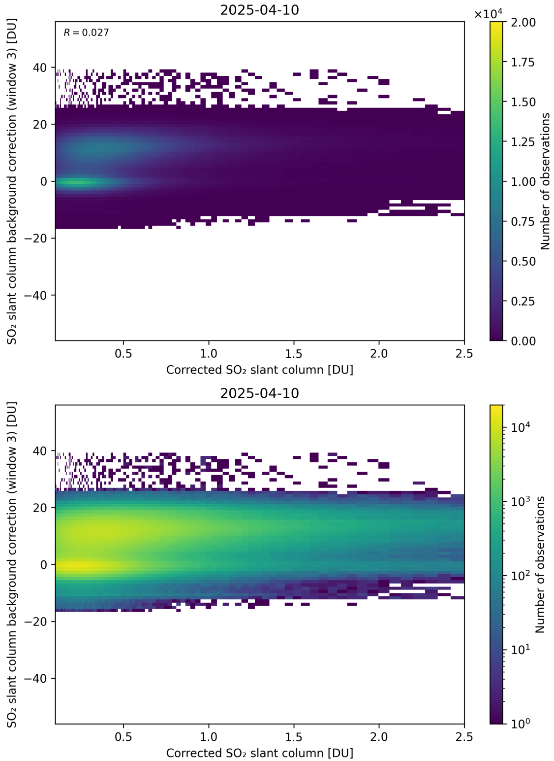
Figure 228: Scatter density plot of “Corrected SO 2 slant column” against “SO 2 slant column background correction (window 3)” for 2025-04-09 to 2025-04-11.
