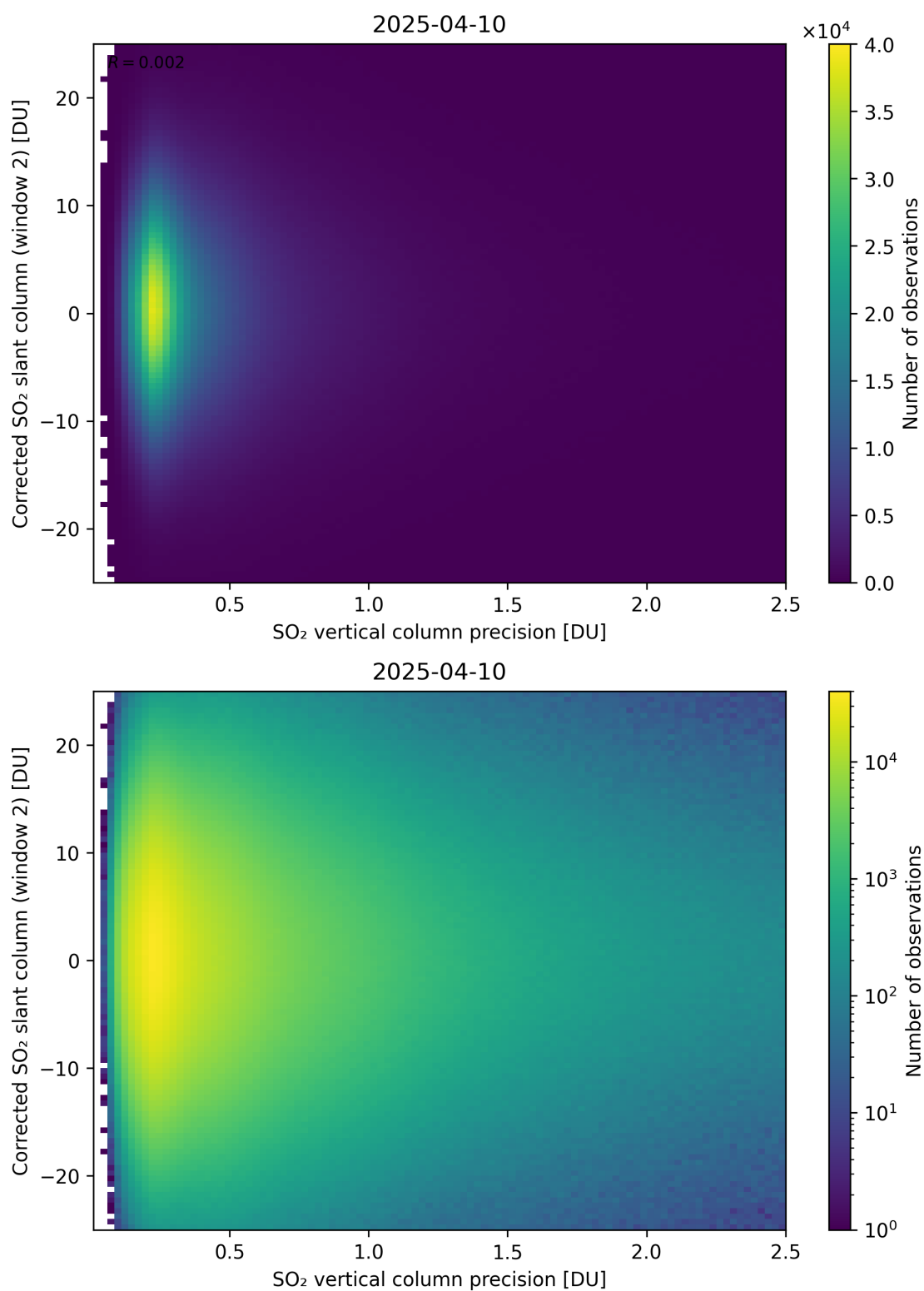
Figure 339: Scatter density plot of “SO 2 vertical column precision” against “Corrected SO 2 slant column (window 2)” for 2025-04-09 to 2025-04-11.
