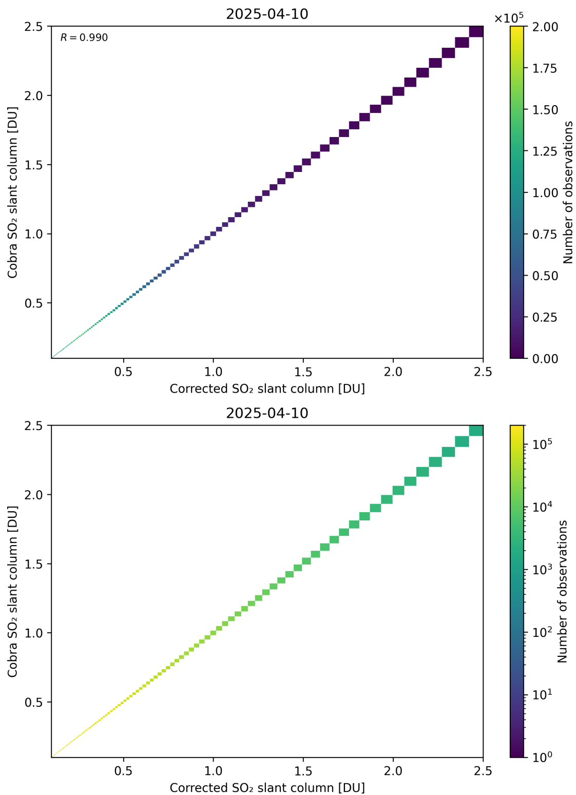
Figure 233: Scatter density plot of “Corrected SO 2 slant column” against “Cobra SO 2 slant column” for 2025-04-09 to 2025-04-11.
