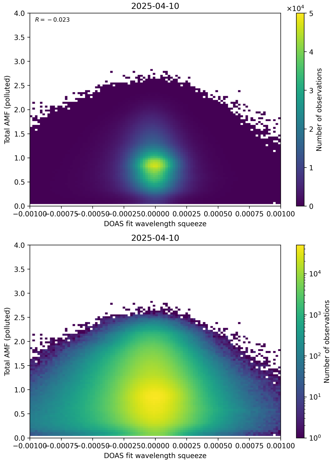
Figure 145: Scatter density plot of “DOAS fit wavelength squeeze” against “Total AMF (polluted)” for 2025-04-09 to 2025-04-11.
