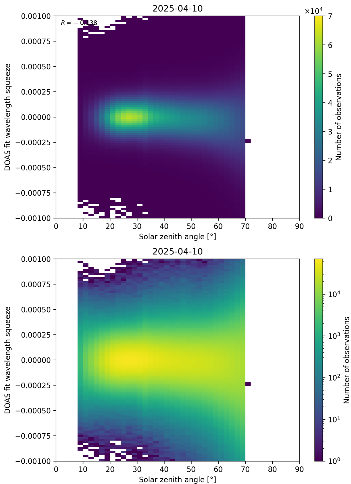
Figure 175: Scatter density plot of “Solar zenith angle” against “DOAS fit wavelength squeeze” for 2025-04-09 to 2025-04-11.
