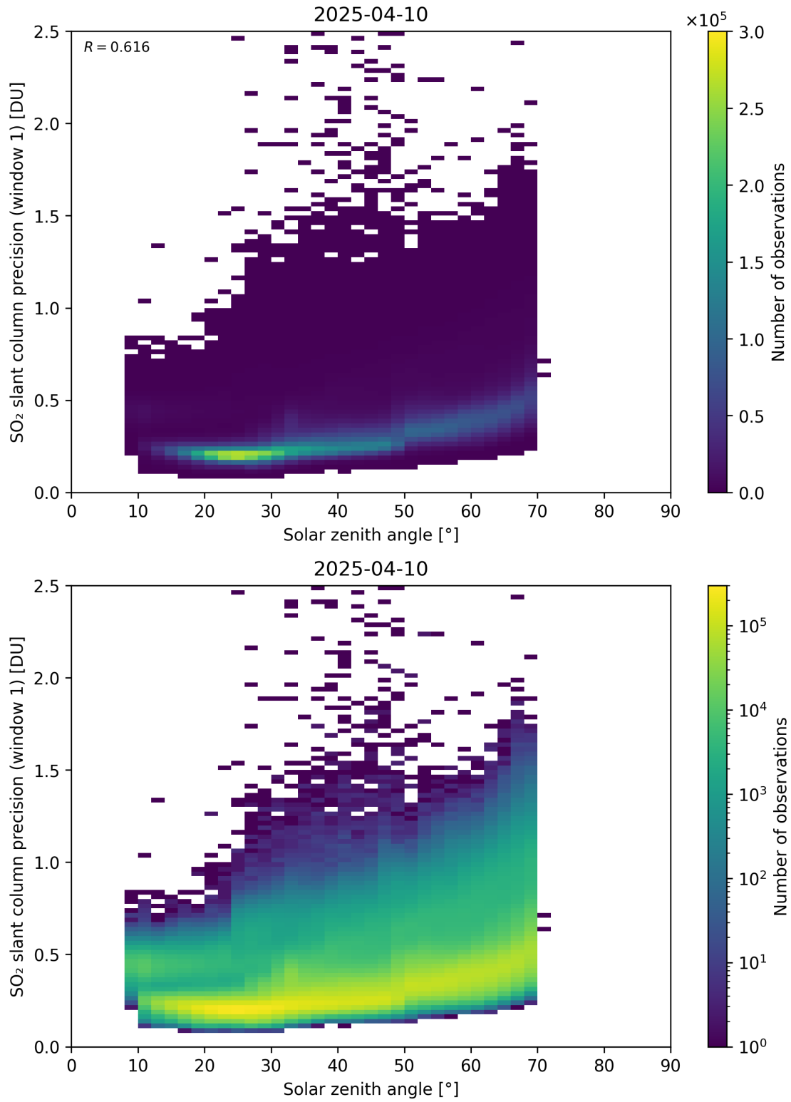
Figure 185: Scatter density plot of “Solar zenith angle” against “SO 2 slant column precision (window 1)” for 2025-04-09 to 2025-04-11.
