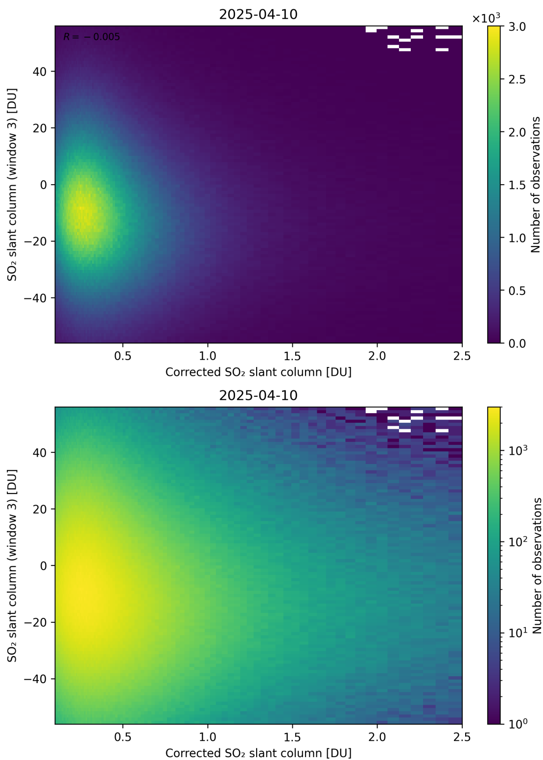
Figure 240: Scatter density plot of “Corrected SO 2 slant column” against “SO 2 slant column (window 3)” for 2025-04-09 to 2025-04-11.
