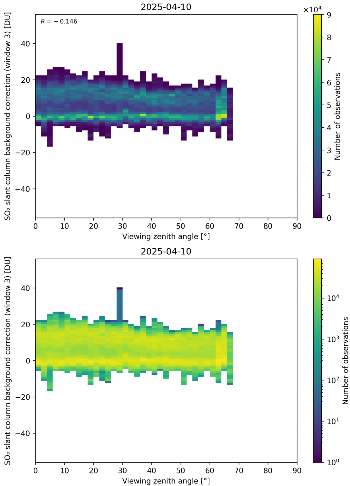
Figure 364: Scatter density plot of “Viewing zenith angle” against “SO 2 slant column background correction (window 3)” for 2025-04-09 to 2025-04-11.
