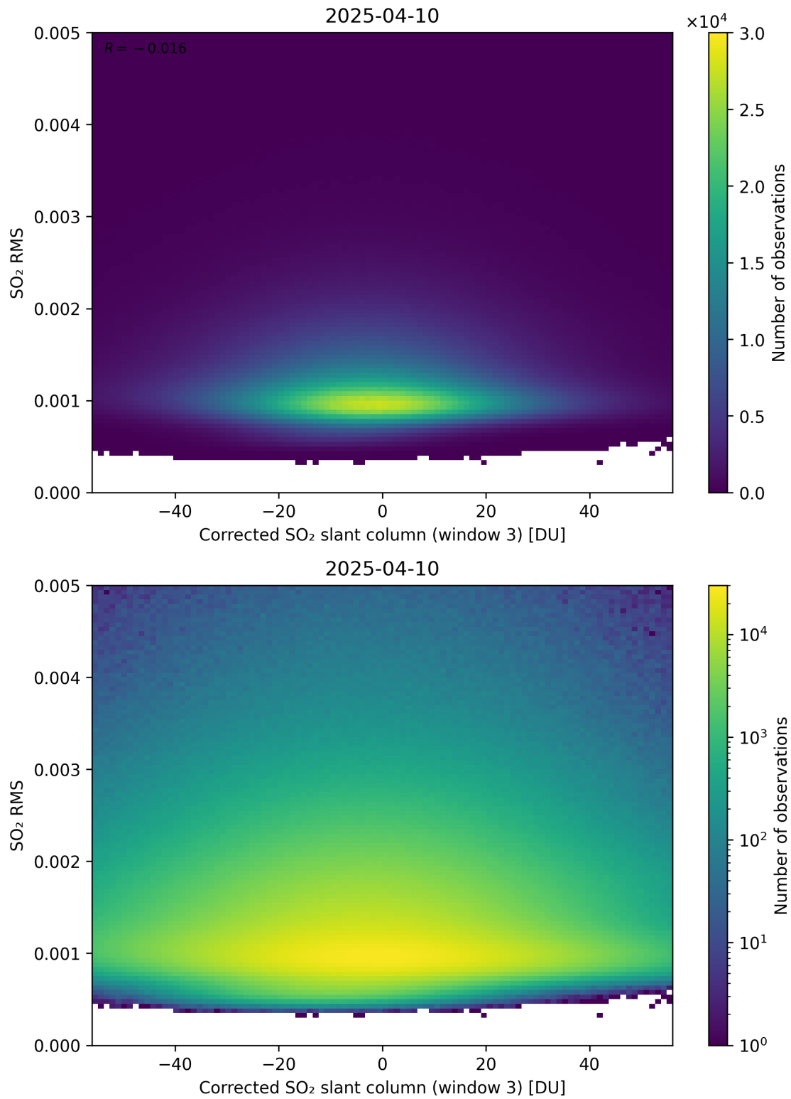
Figure 258: Scatter density plot of “Corrected SO 2 slant column (window 3)” against “SO 2 RMS” for 2025-04-09 to 2025-04-11.
