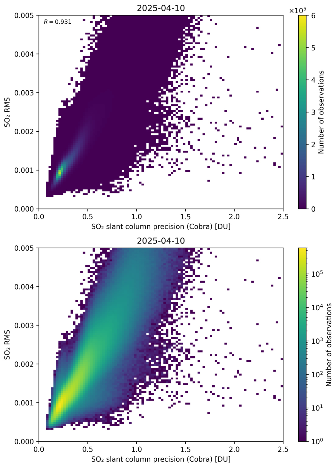
Figure 204: Scatter density plot of “SO 2 slant column precision (Cobra)” against “SO 2 RMS” for 2025-04-09 to 2025-04-11.
