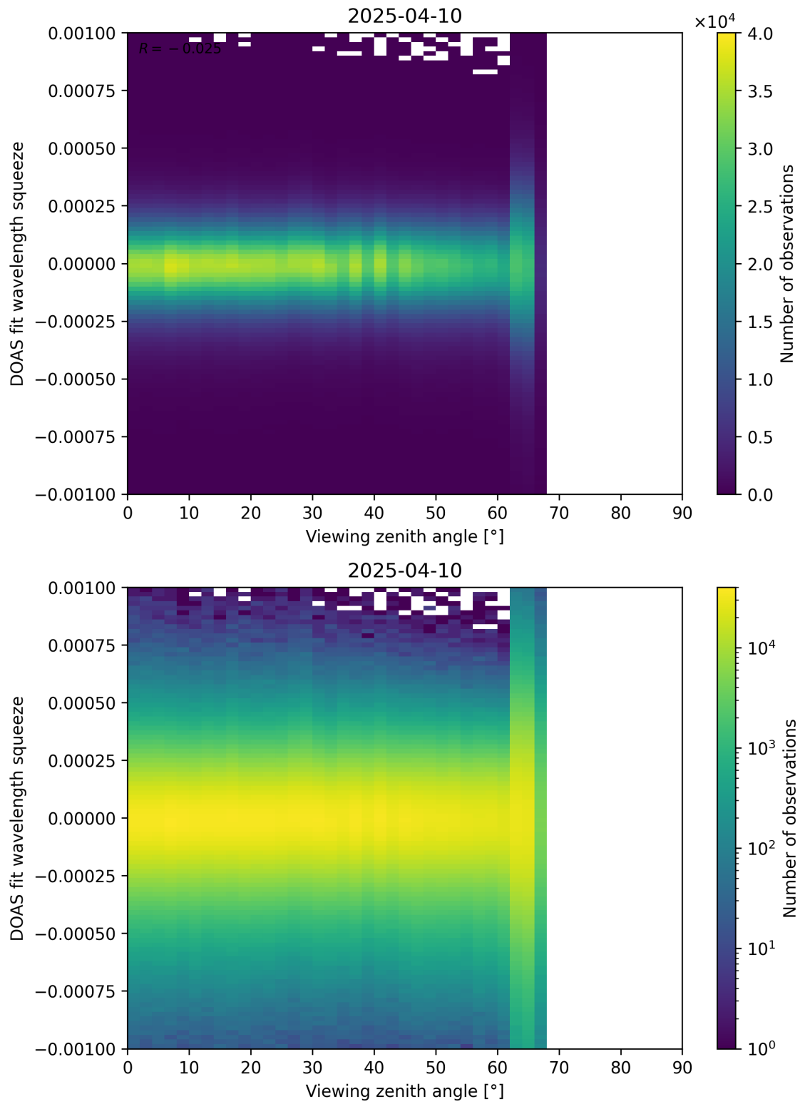
Figure 366: Scatter density plot of “Viewing zenith angle” against “DOAS fit wavelength squeeze” for 2025-04-09 to 2025-04-11.
