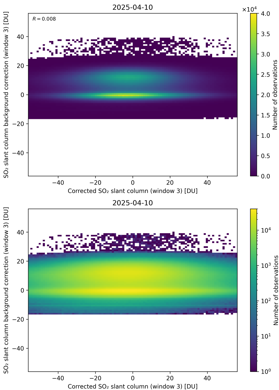
Figure 255: Scatter density plot of “Corrected SO 2 slant column (window 3)” against “SO 2 slant column background correction (window 3)” for 2025-04-09 to 2025-04-11.
