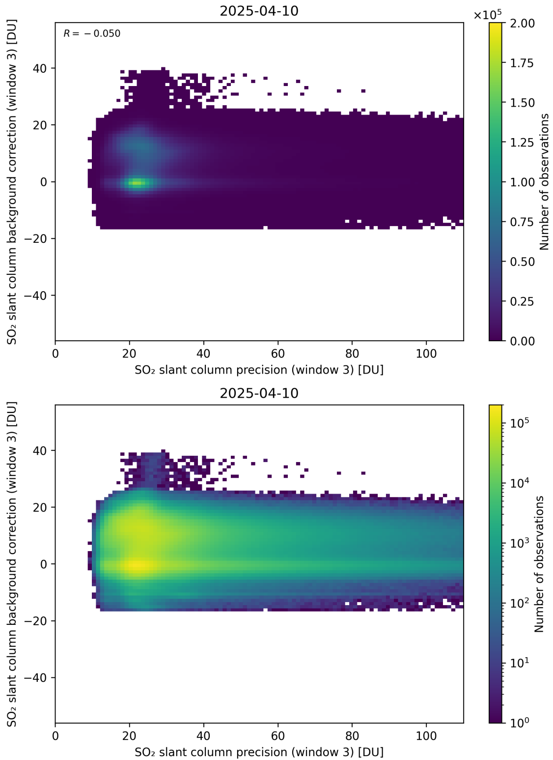
Figure 307: Scatter density plot of “SO 2 slant column precision (window 3)” against “SO 2 slant column background correction (window 3)” for 2025-04-09 to 2025-04-11.
