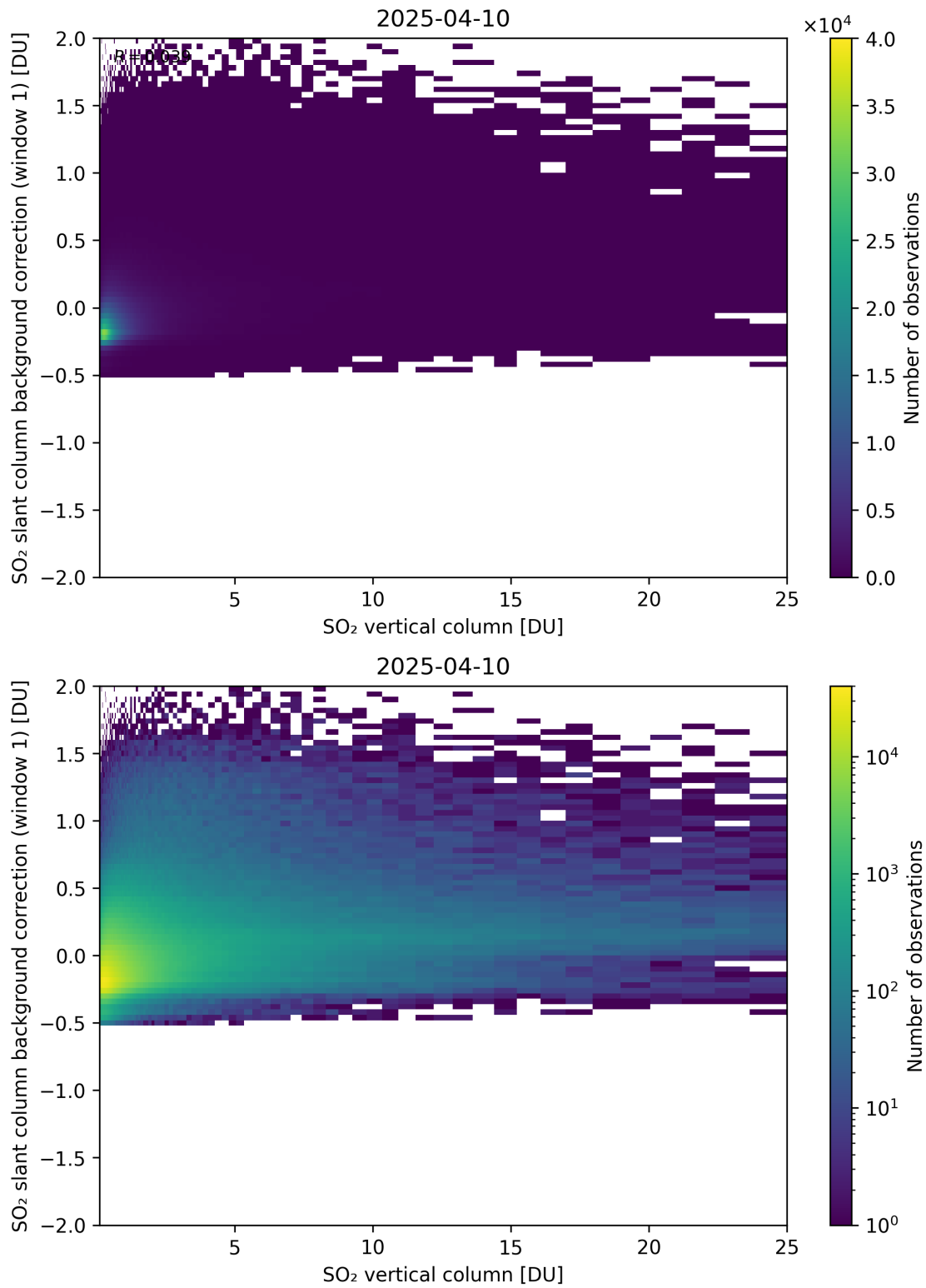
Figure 323: Scatter density plot of “SO 2 vertical column” against “SO 2 slant column background correction (window 1)” for 2025-04-09 to 2025-04-11.
