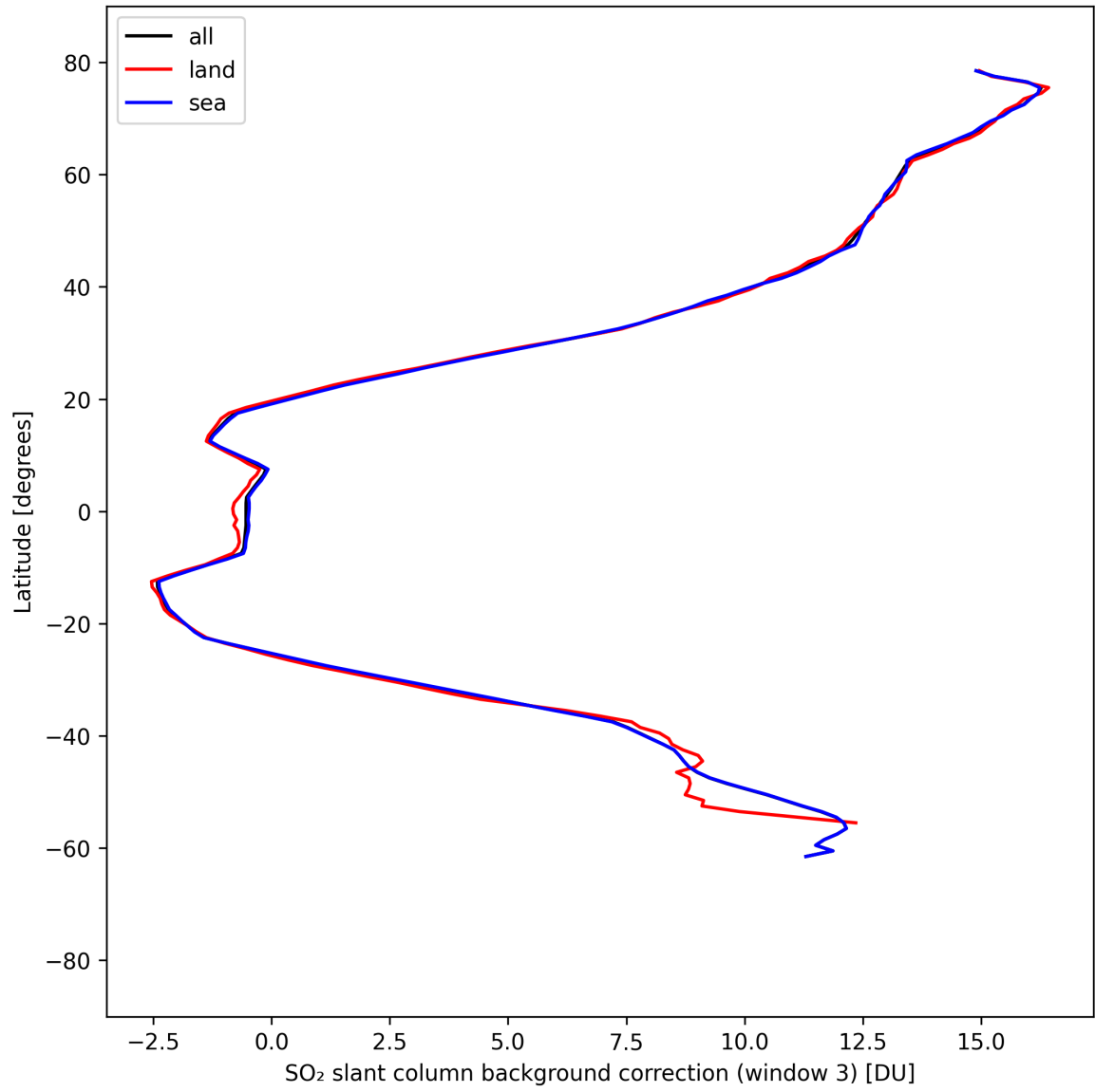
Figure 48: Zonal average of “SO 2 slant column background correction (window 3)” for 2025-04-09 to 2025-04-11.
