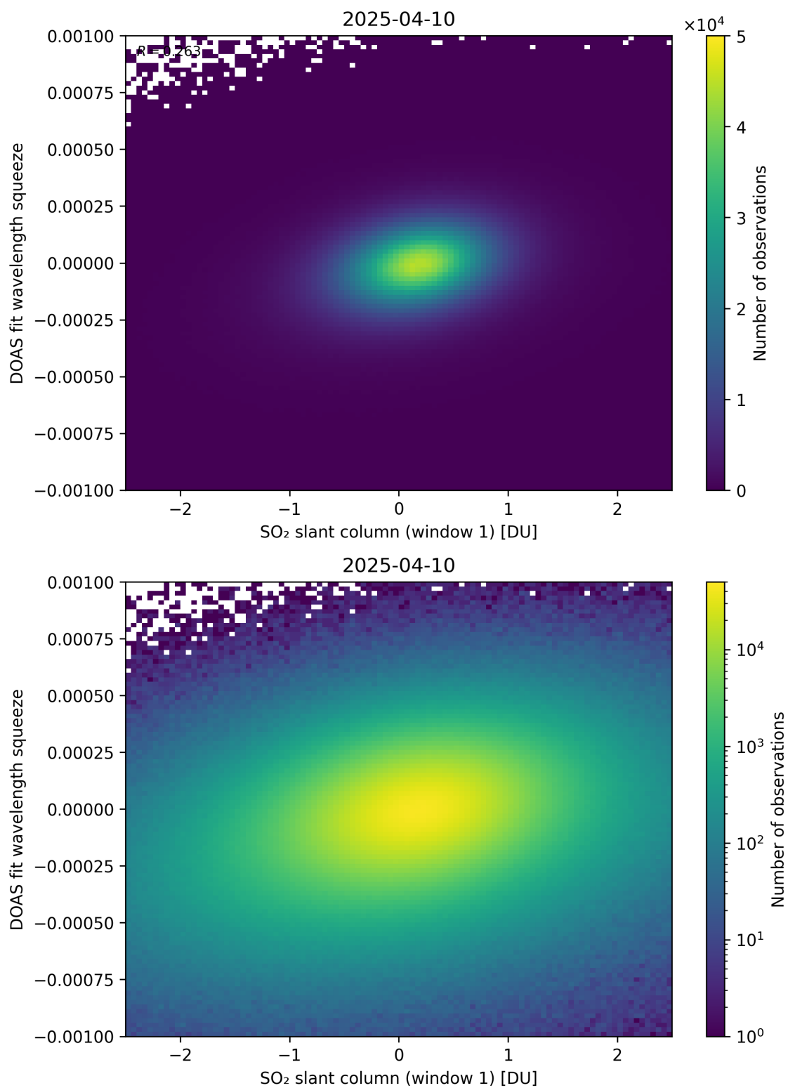
Figure 266: Scatter density plot of “SO 2 slant column (window 1)” against “DOAS fit wavelength squeeze” for 2025-04-09 to 2025-04-11.
