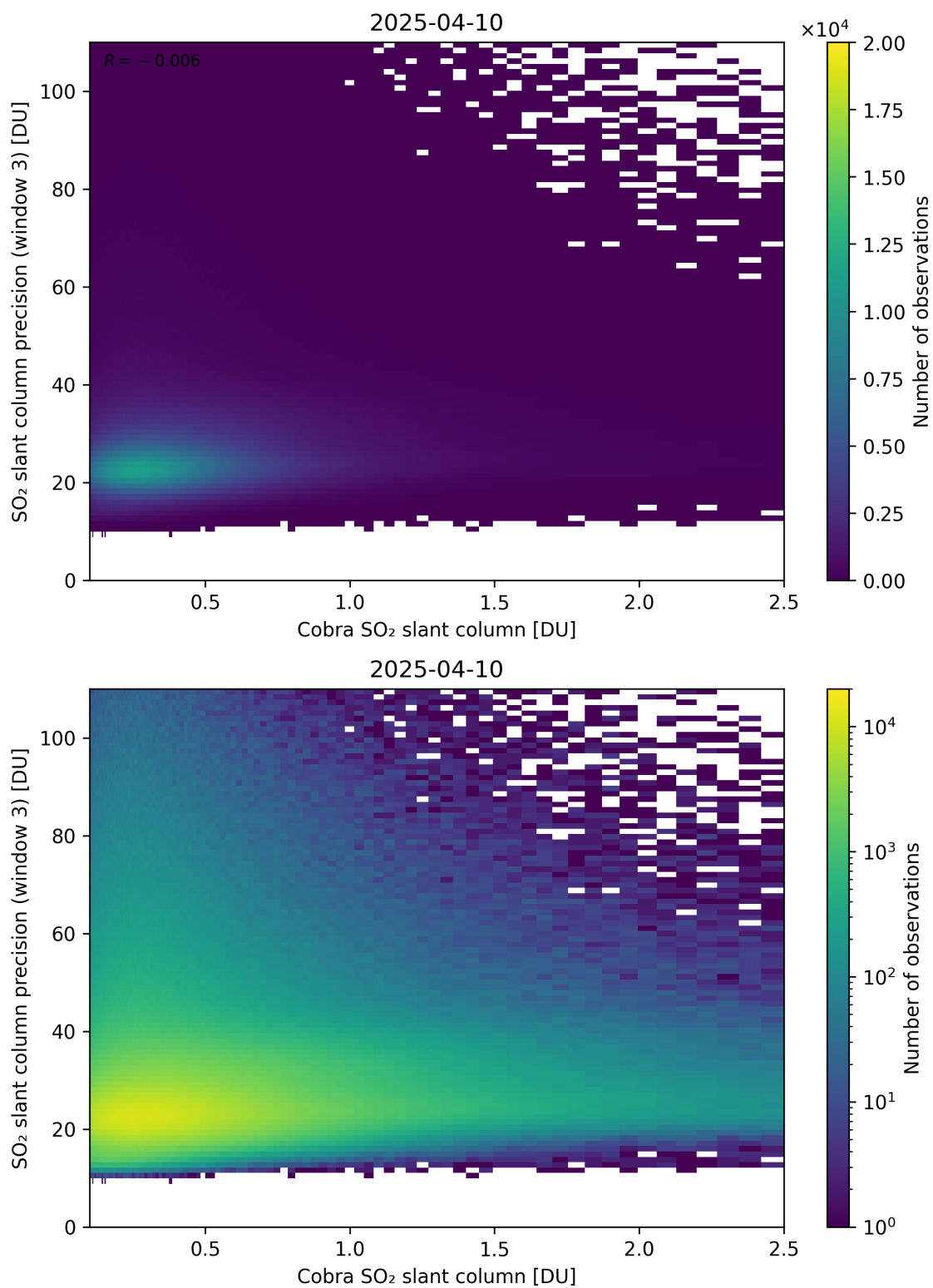
Figure 223: Scatter density plot of “Cobra SO 2 slant column” against “SO 2 slant column precision (window 3)” for 2025-04-09 to 2025-04-11.
