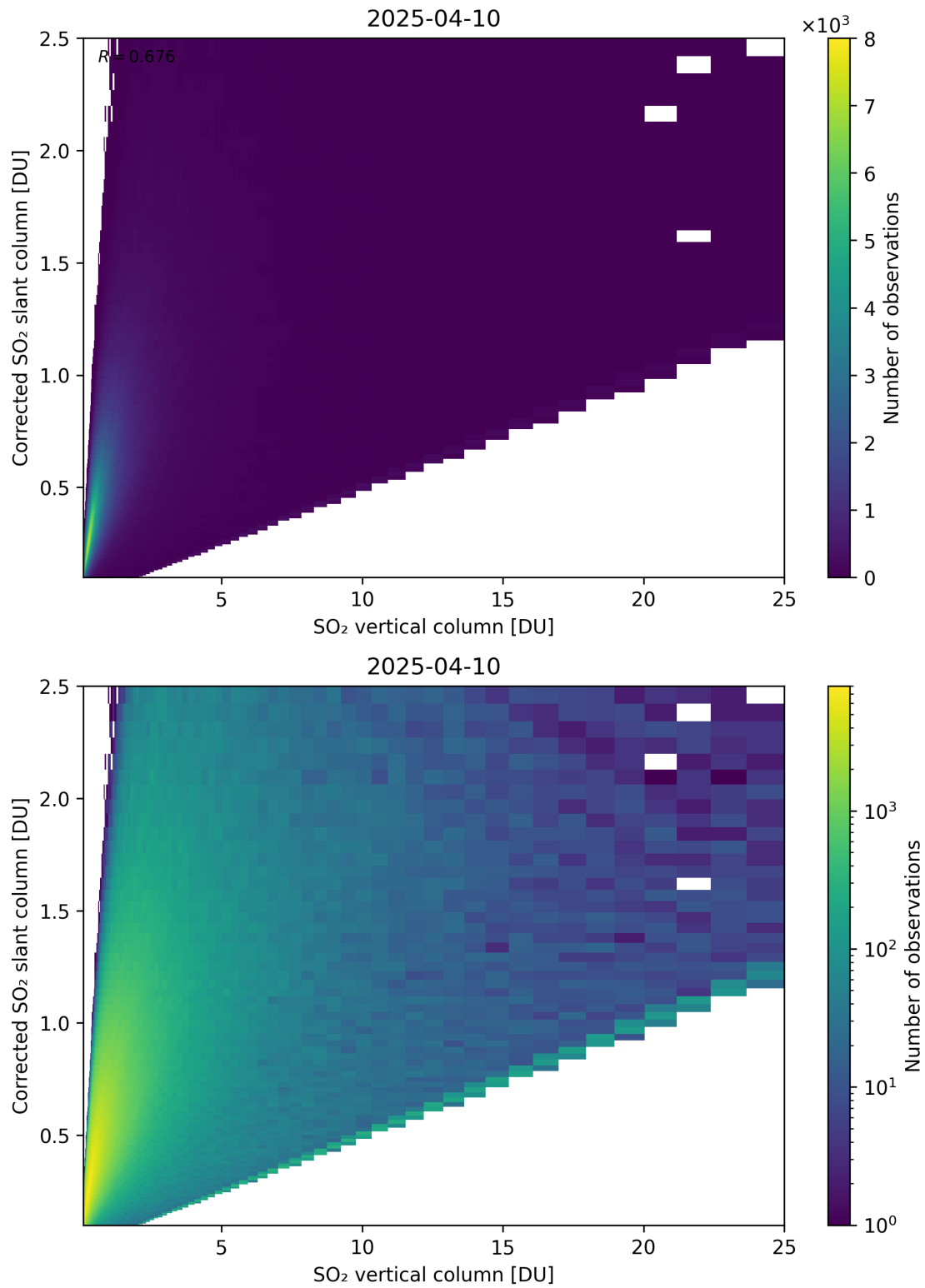
Figure 351: Scatter density plot of “SO 2 vertical column” against “Corrected SO 2 slant column” for 2025-04-09 to 2025-04-11.
