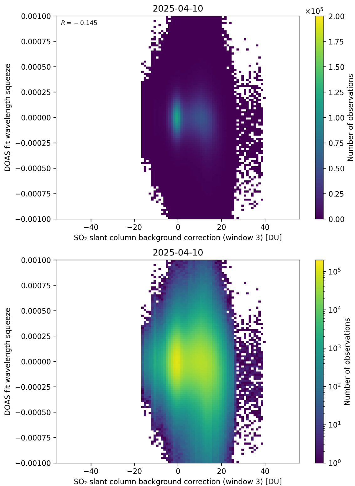
Figure 133: Scatter density plot of “SO 2 slant column background correction (window 3)” against “DOAS fit wavelength squeeze” for 2025-04-09 to 2025-04-11.
