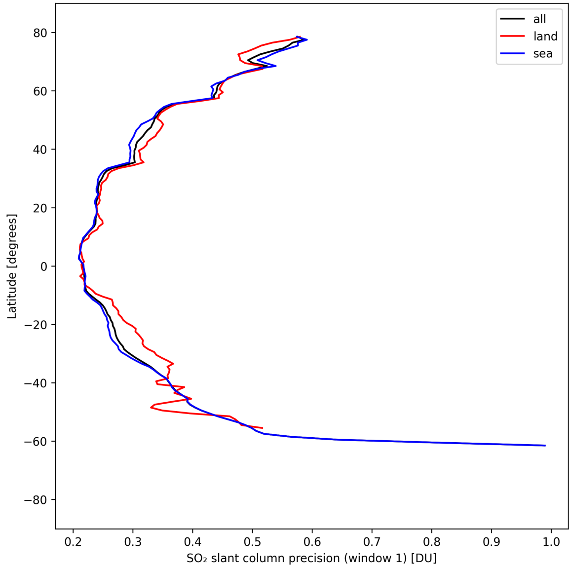
Figure 38: Zonal average of “SO 2 slant column precision (window 1)” for 2025-04-09 to 2025-04-11.
