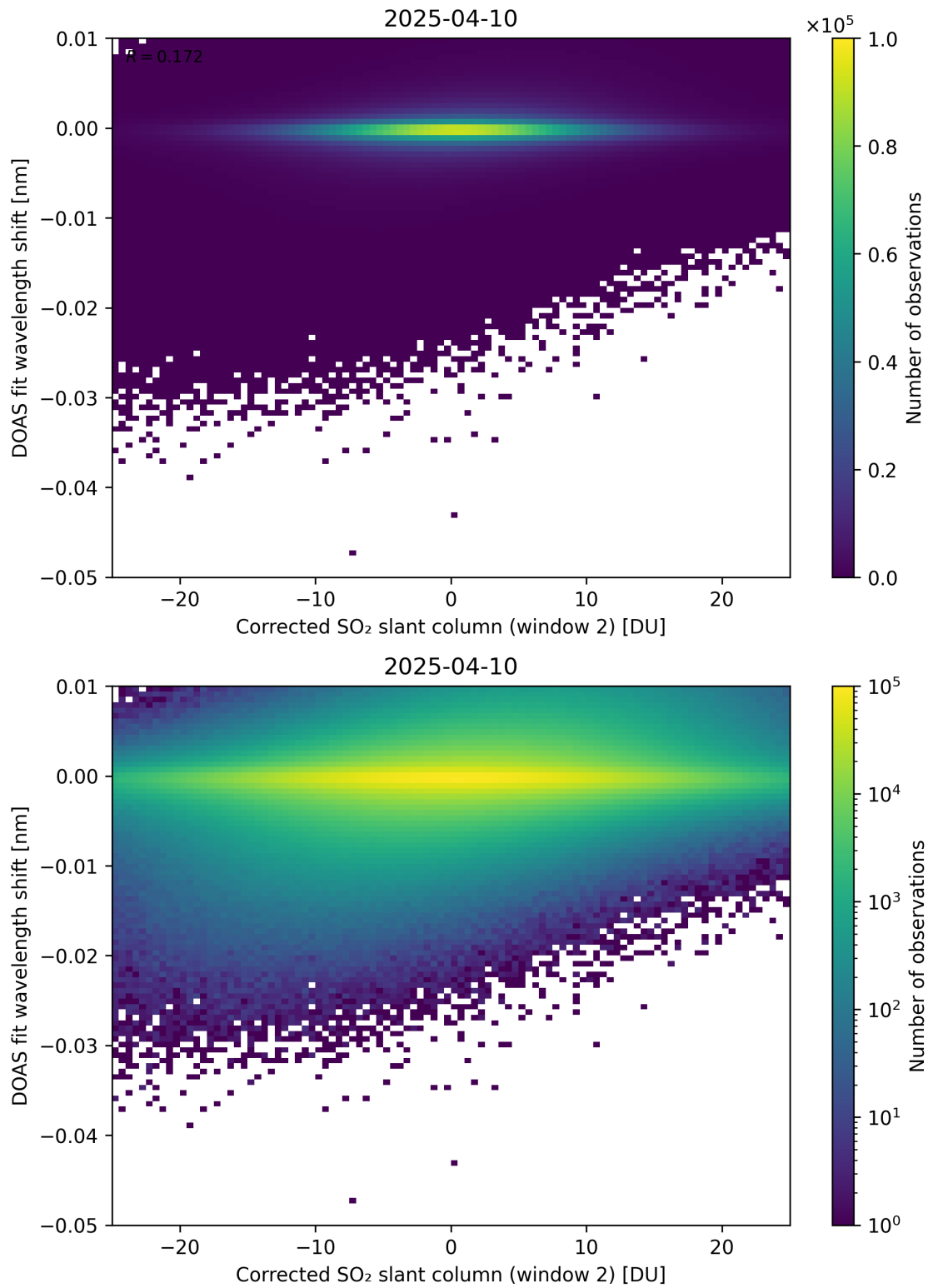
Figure 246: Scatter density plot of “Corrected SO 2 slant column (window 2)” against “DOAS fit wavelength shift” for 2025-04-09 to 2025-04-11.
