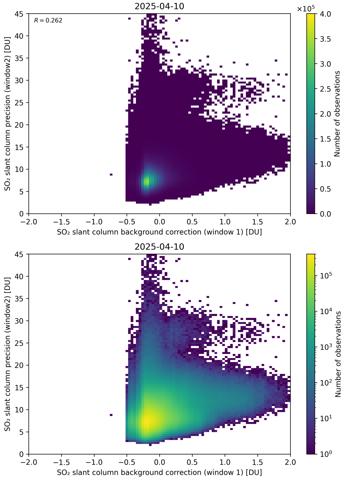
Figure 117: Scatter density plot of “SO 2 slant column background correction (window 1)” against “SO 2 slant column precision (window2)” for 2025-04-09 to 2025-04-11.
