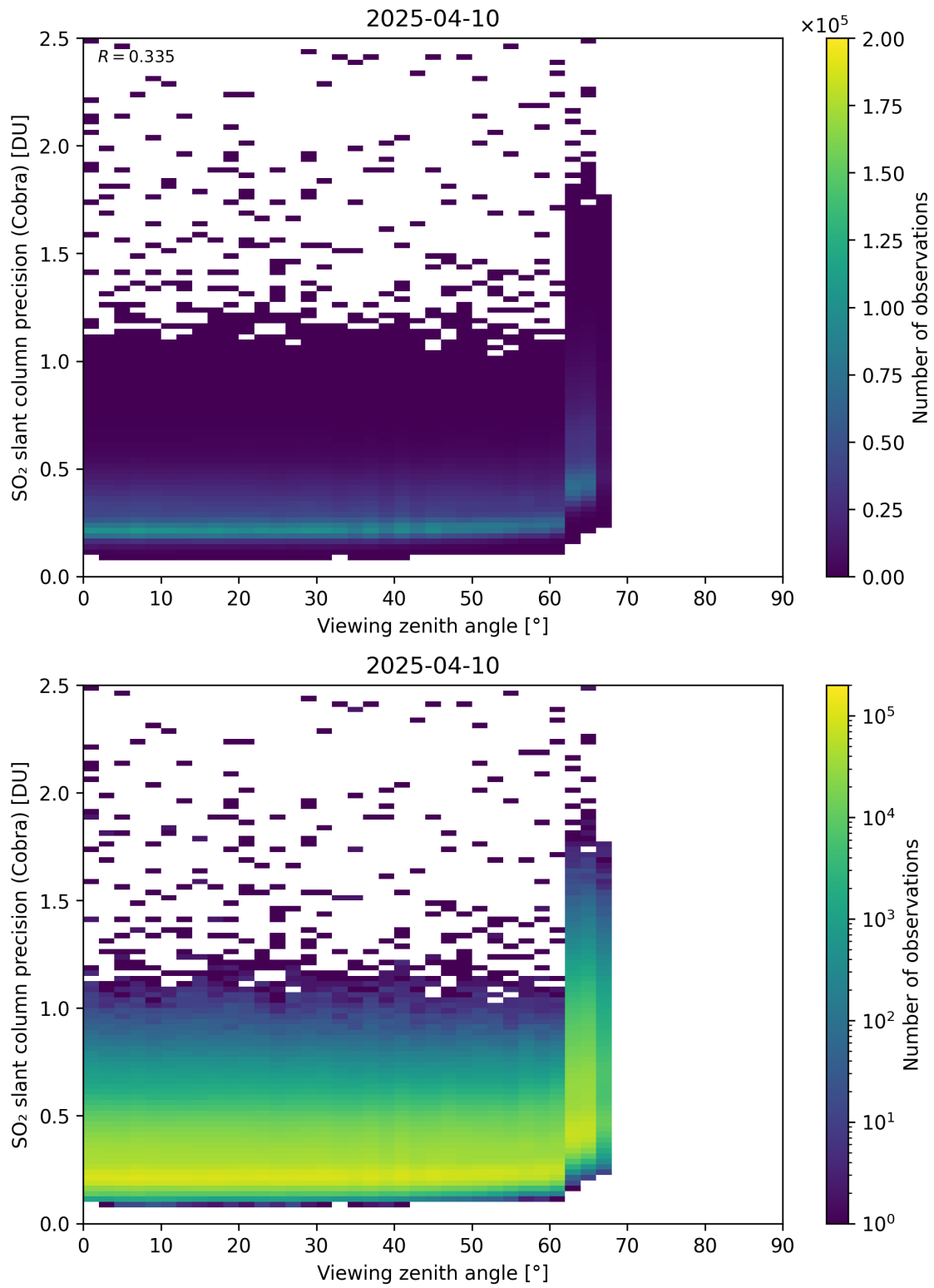
Figure 372: Scatter density plot of “Viewing zenith angle” against “SO 2 slant column precision (Cobra)” for 2025-04-09 to 2025-04-11.
