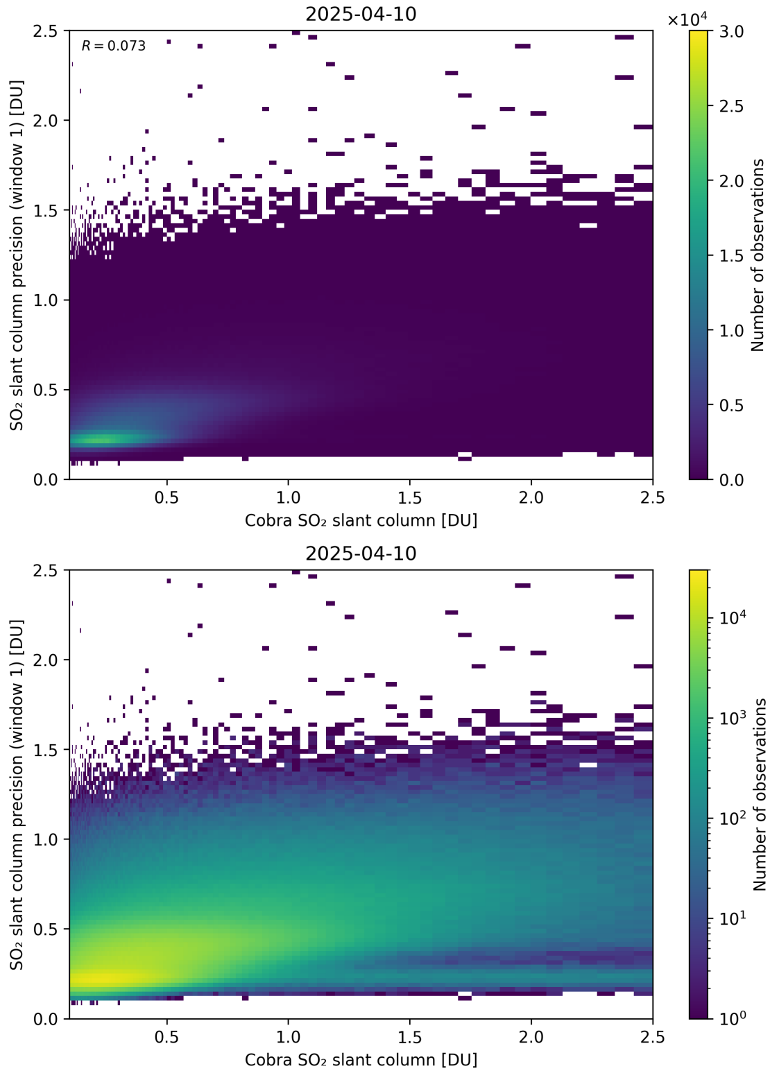
Figure 220: Scatter density plot of “Cobra SO 2 slant column” against “SO 2 slant column precision (window 1)” for 2025-04-09 to 2025-04-11.
