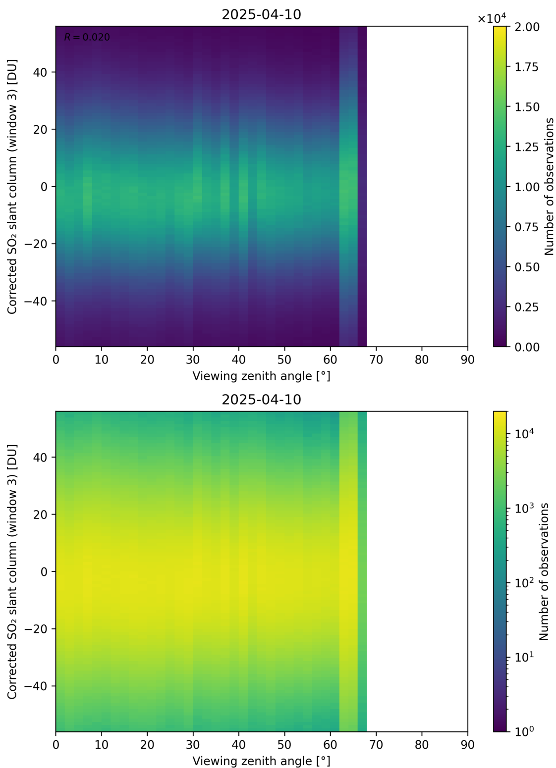
Figure 375: Scatter density plot of “Viewing zenith angle” against “Corrected SO 2 slant column (window 3)” for 2025-04-09 to 2025-04-11.
