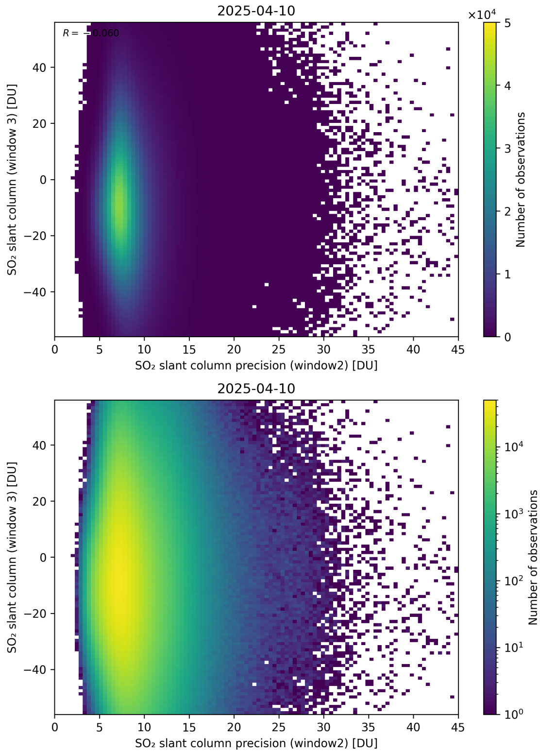
Figure 299: Scatter density plot of “SO 2 slant column precision (window2)” against “SO 2 slant column (window 3)” for 2025-04-09 to 2025-04-11.
