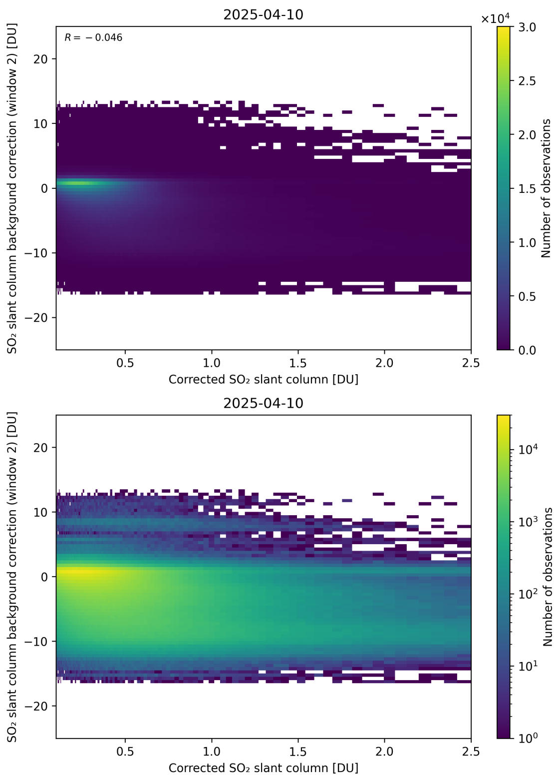
Figure 227: Scatter density plot of “Corrected SO 2 slant column” against “SO 2 slant column background correction (window 2)” for 2025-04-09 to 2025-04-11.
