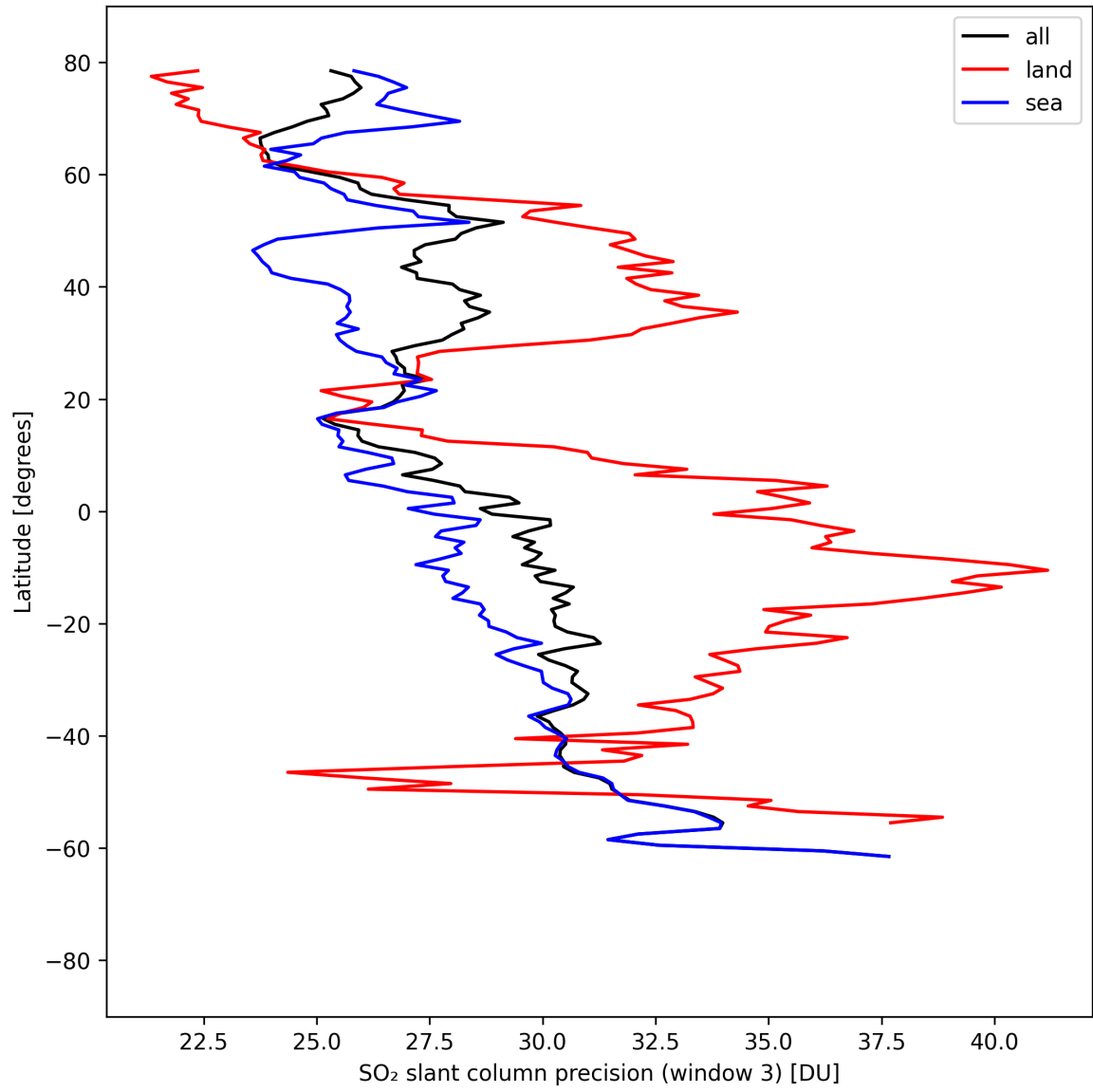
Figure 46: Zonal average of “SO 2 slant column precision (window 3)” for 2025-04-09 to 2025-04-11.
