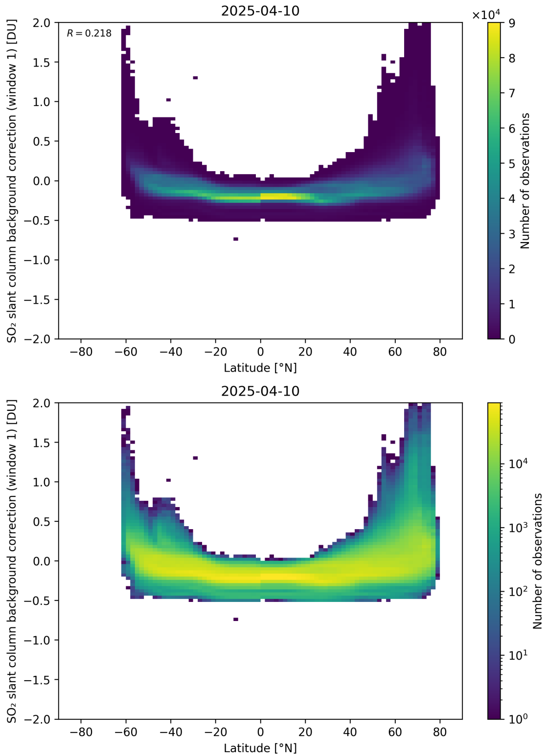
Figure 150: Scatter density plot of “Latitude” against “SO 2 slant column background correction (window 1)” for 2025-04-09 to 2025-04-11.
