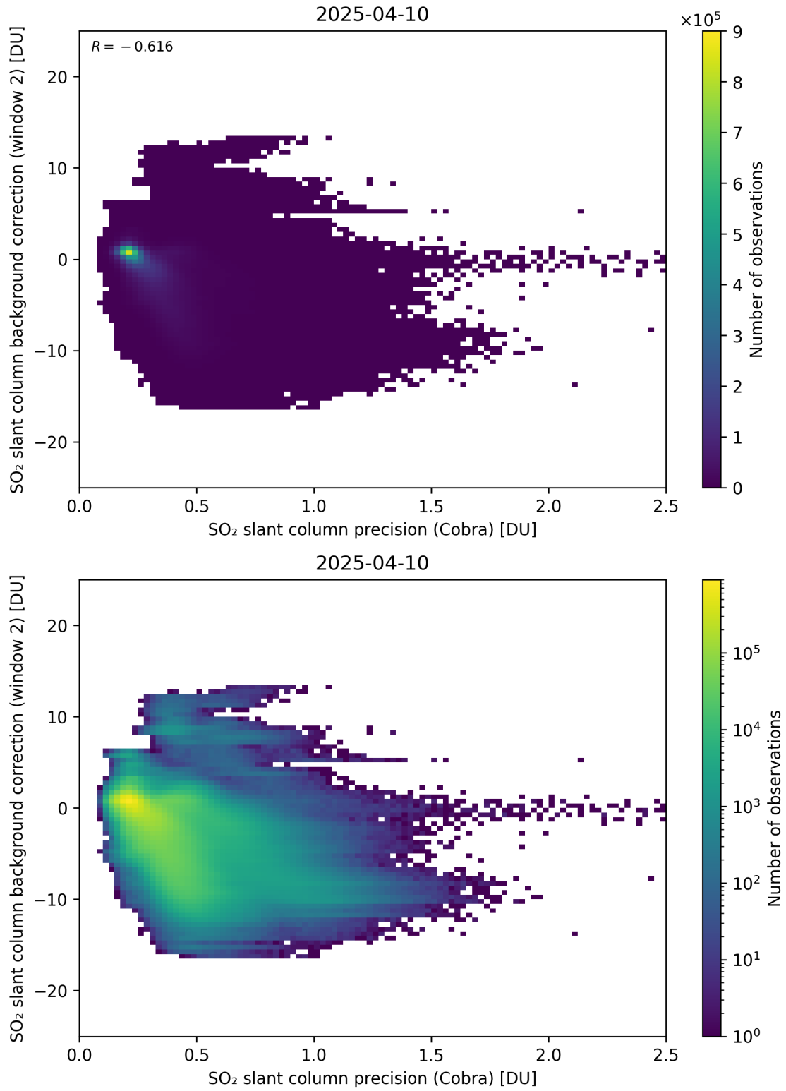
Figure 200: Scatter density plot of “SO 2 slant column precision (Cobra)” against “SO 2 slant column background correction (window 2)” for 2025-04-09 to 2025-04-11.
