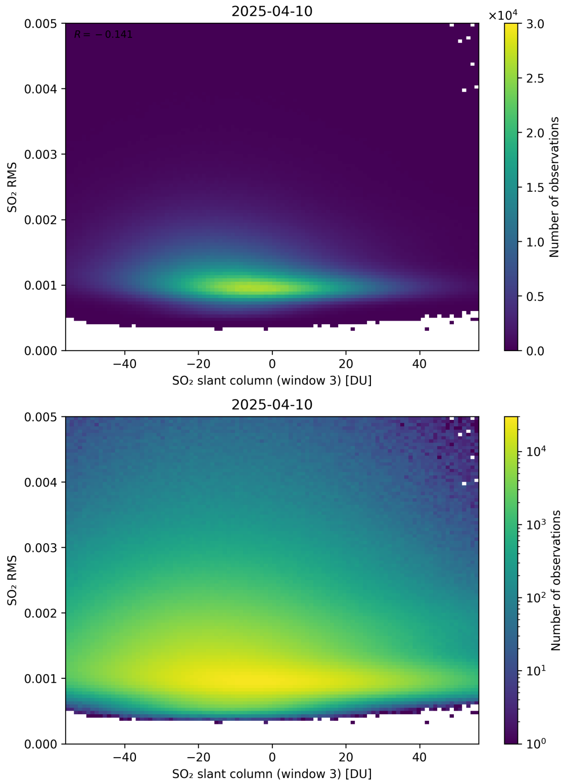
Figure 306: Scatter density plot of “SO 2 slant column (window 3)” against “SO 2 RMS” for 2025-04-09 to 2025-04-11.
