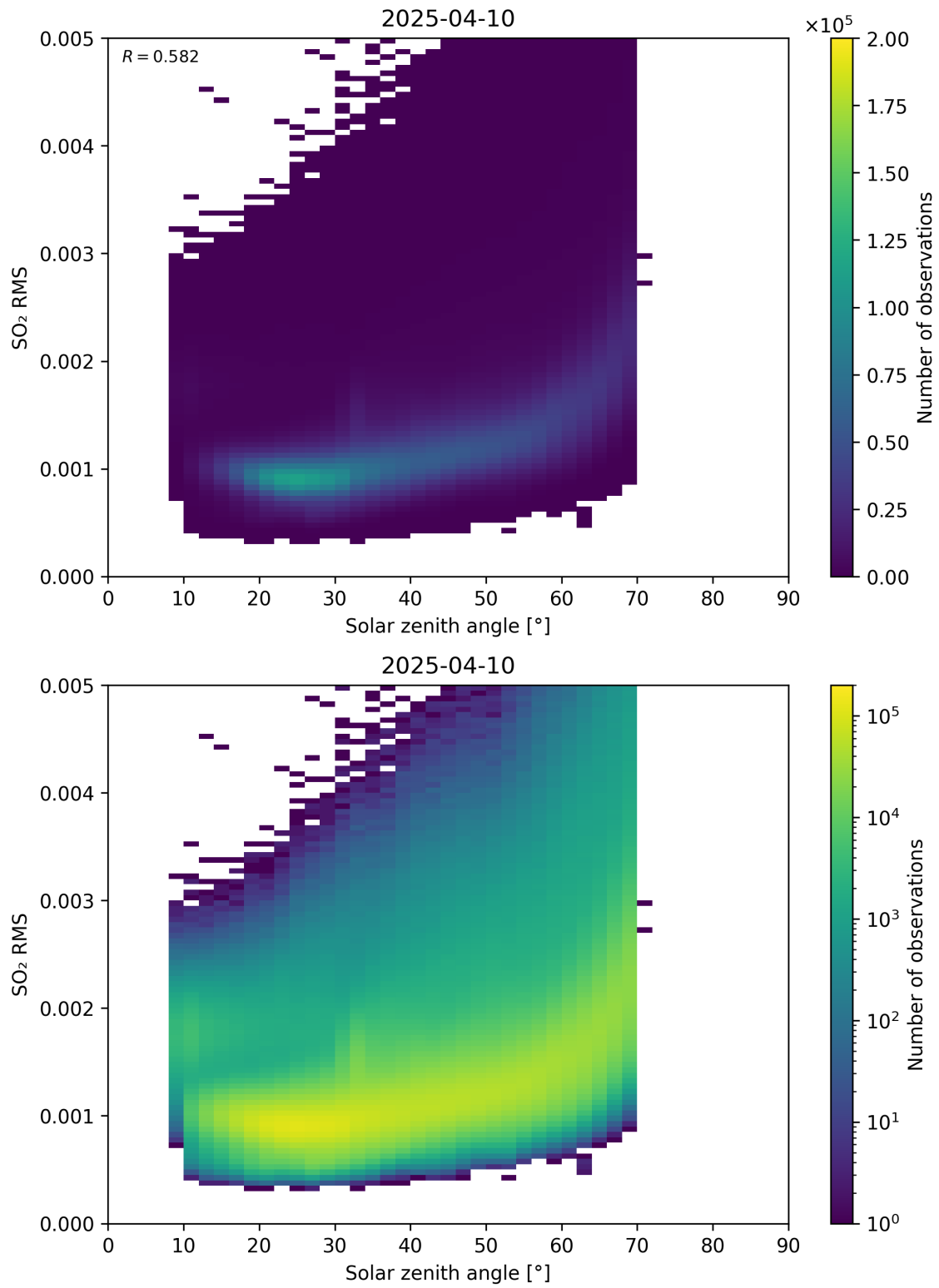
Figure 176: Scatter density plot of “Solar zenith angle” against “SO 2 RMS” for 2025-04-09 to 2025-04-11.
