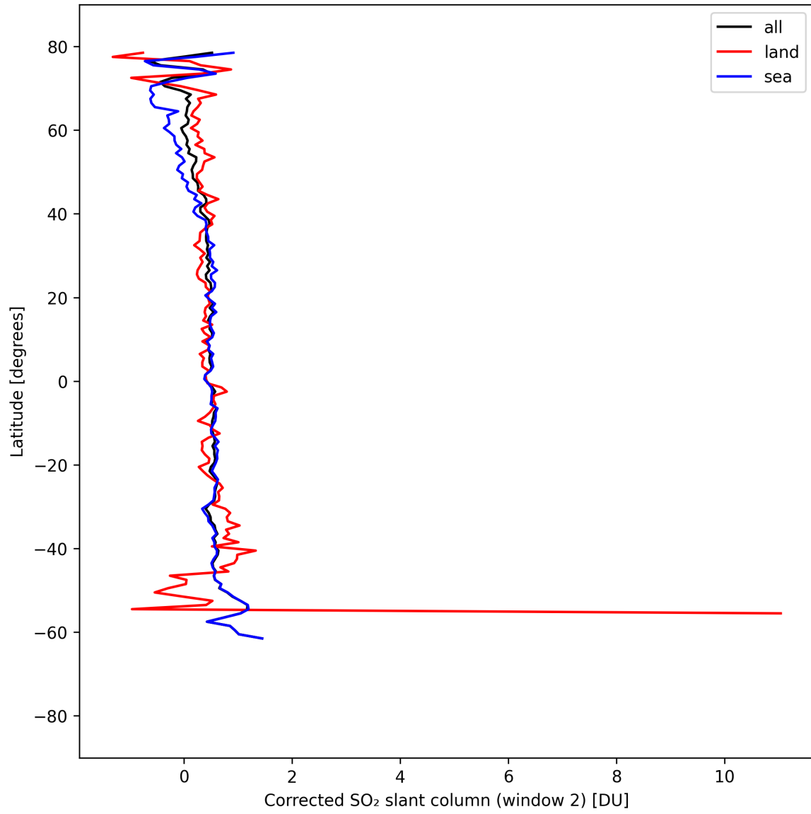
Figure 43: Zonal average of “Corrected SO 2 slant column (window 2)” for 2025-04-09 to 2025-04-11.
