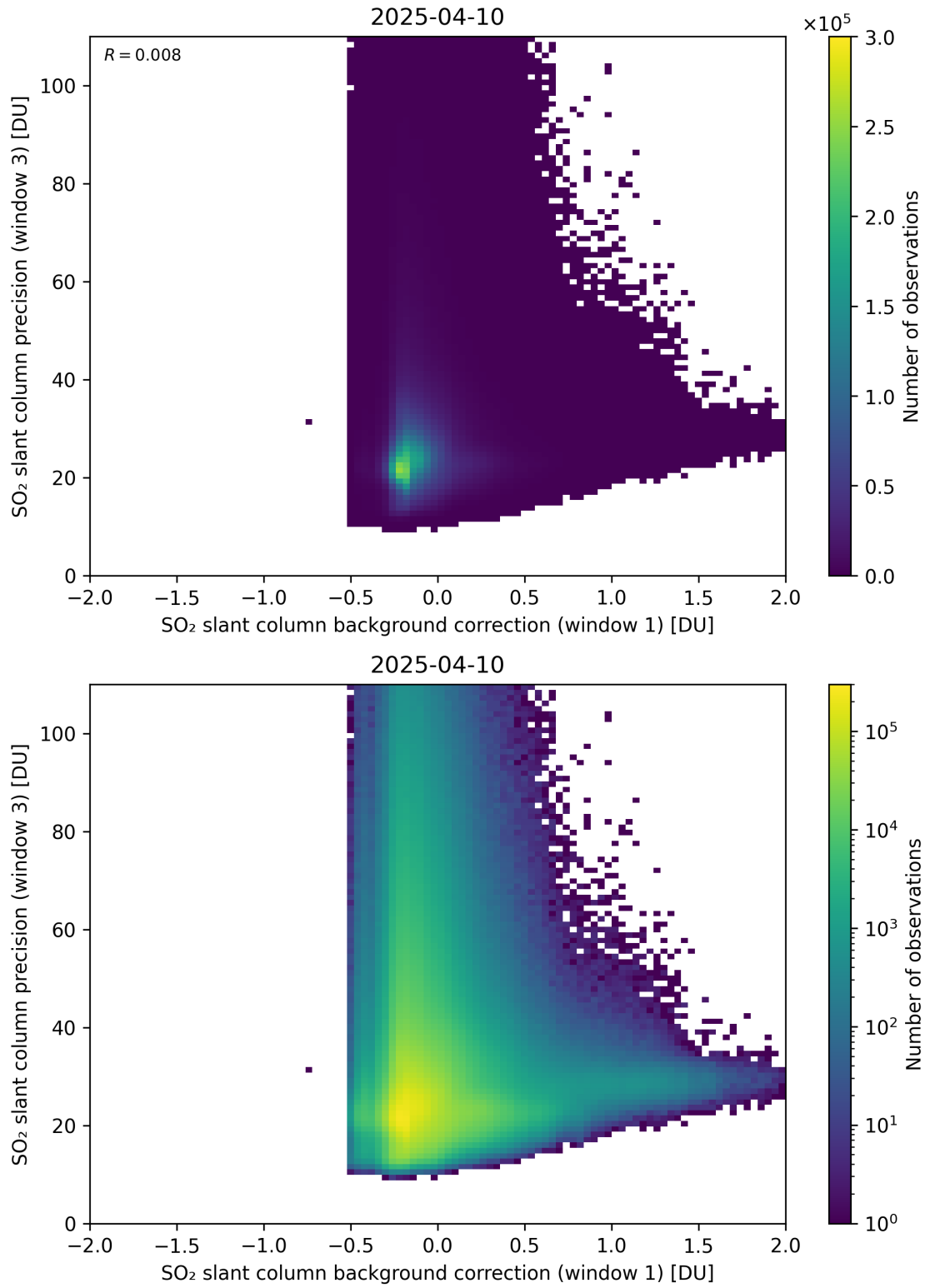
Figure 119: Scatter density plot of “SO 2 slant column background correction (window 1)” against “SO 2 slant column precision (window 3)” for 2025-04-09 to 2025-04-11.
