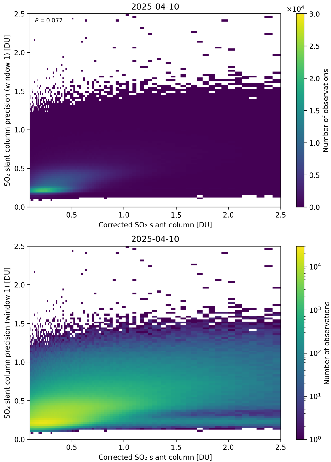
Figure 238: Scatter density plot of “Corrected SO 2 slant column” against “SO 2 slant column precision (window 1)” for 2025-04-09 to 2025-04-11.
