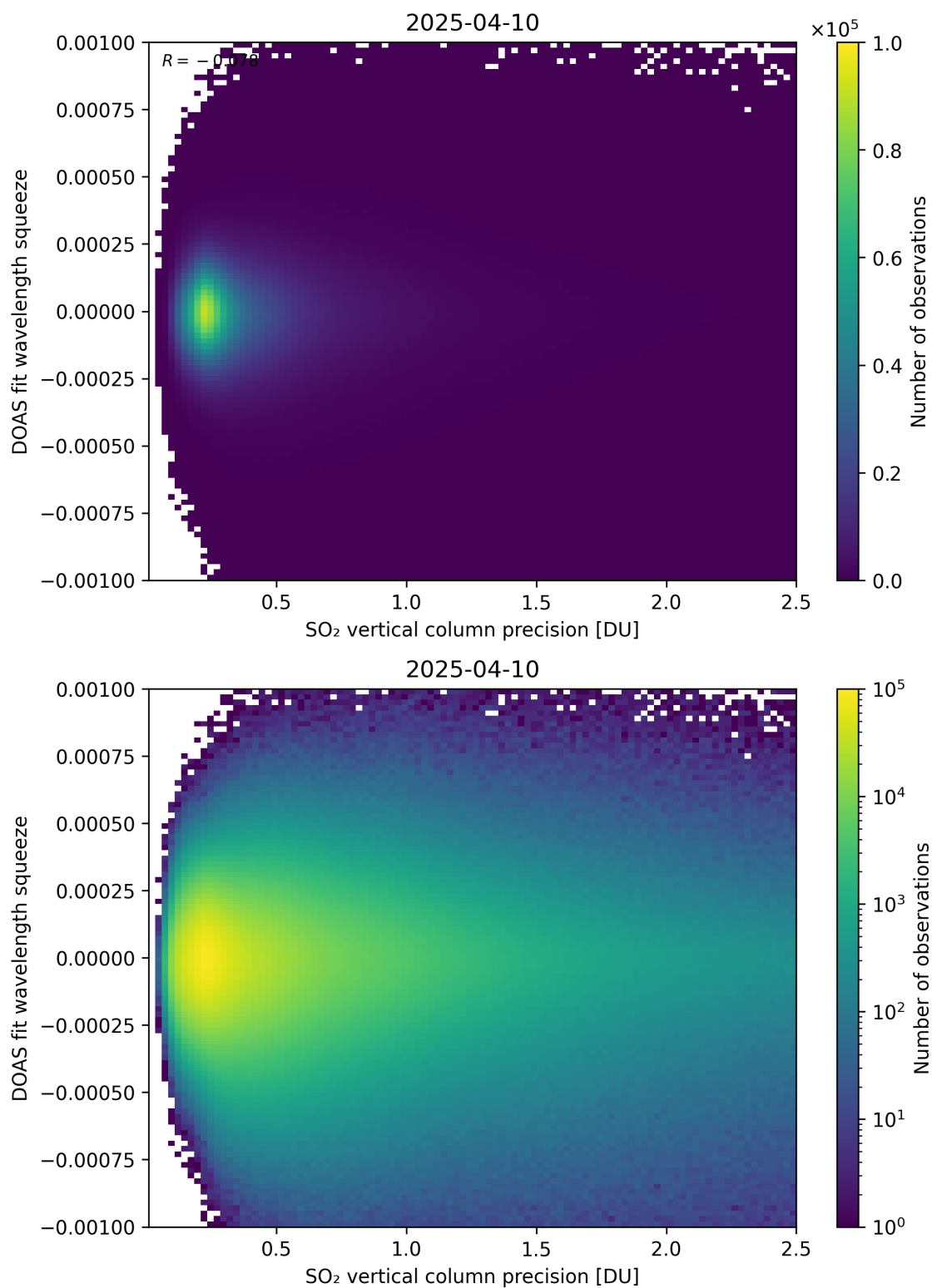
Figure 333: Scatter density plot of “SO 2 vertical column precision” against “DOAS fit wavelength squeeze” for 2025-04-09 to 2025-04-11.
