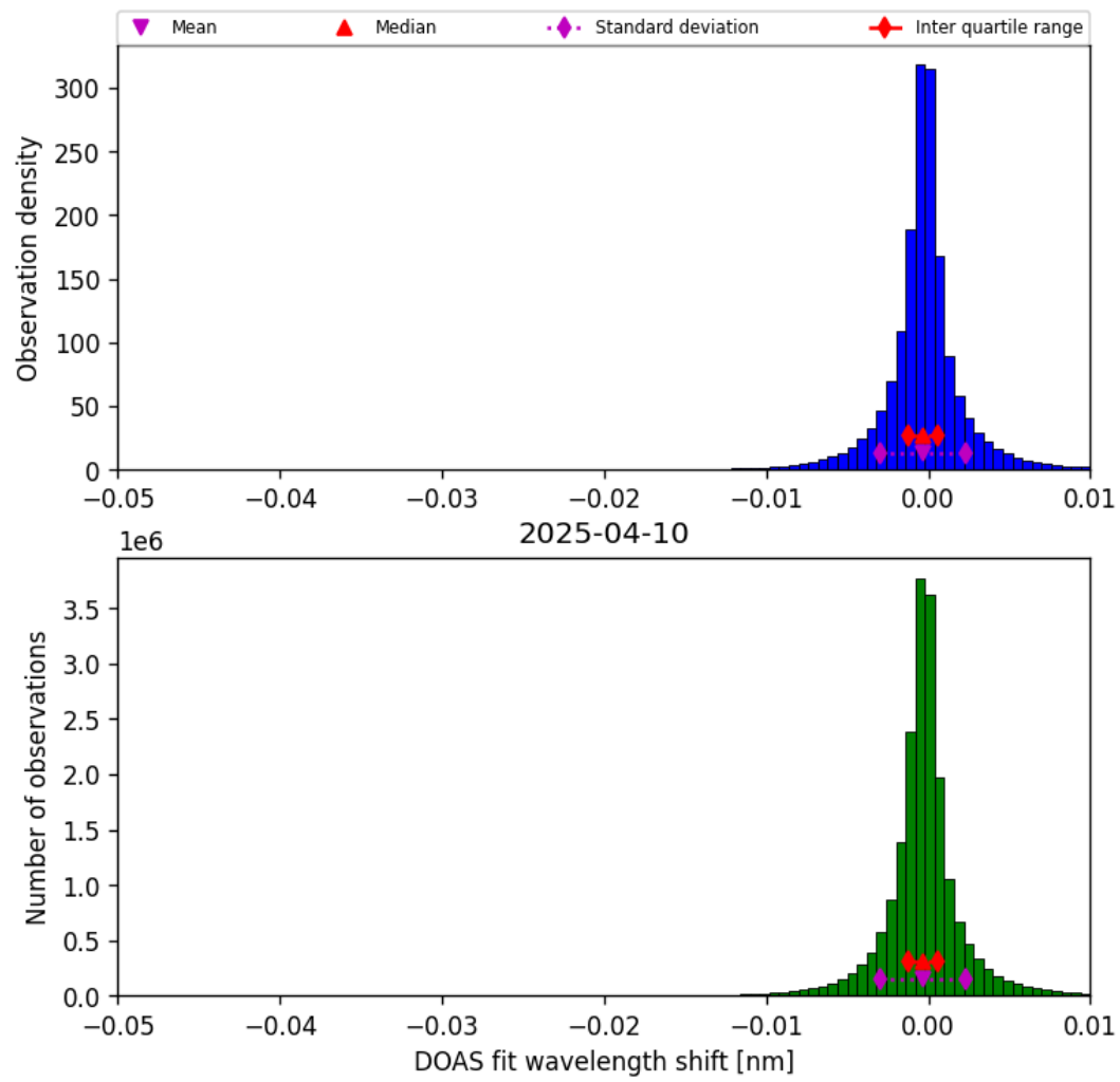
Figure 76: Histogram of “DOAS fit wavelength shift” for 2025-04-09 to 2025-04-11
