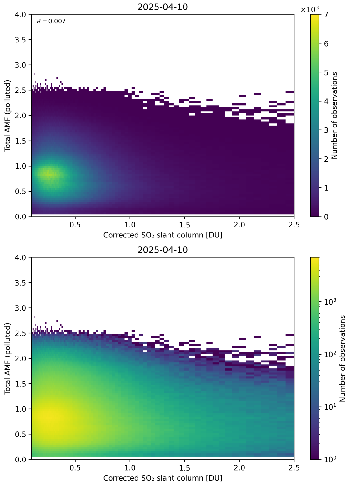
Figure 242: Scatter density plot of “Corrected SO 2 slant column” against “Total AMF (polluted)” for 2025-04-09 to 2025-04-11.
