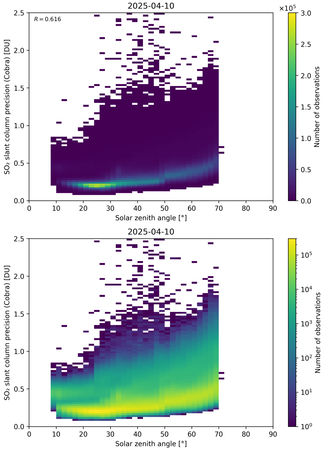
Figure 180: Scatter density plot of “Solar zenith angle” against “SO 2 slant column precision (Cobra)” for 2025-04-09 to 2025-04-11.
