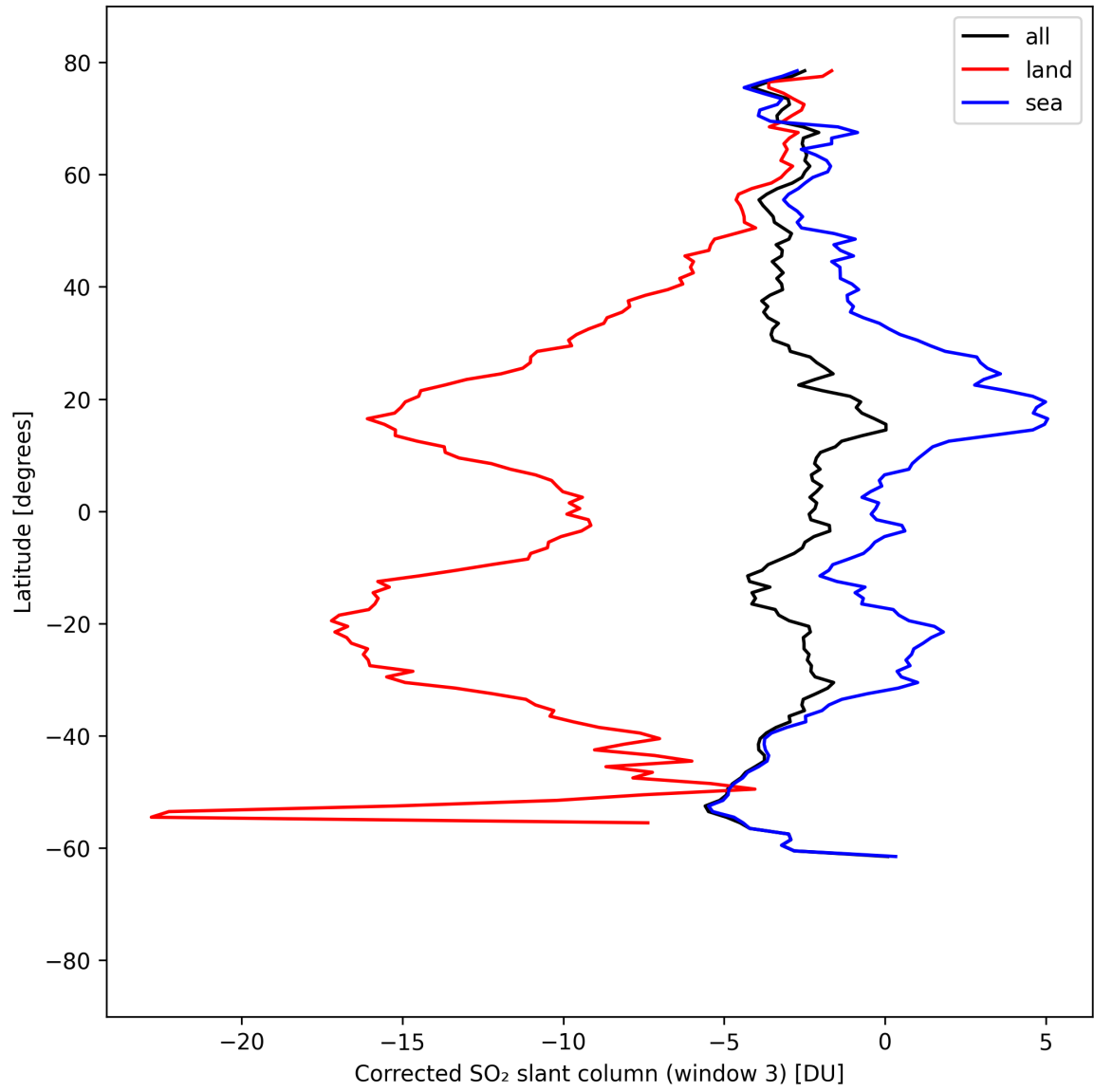
Figure 47: Zonal average of “Corrected SO 2 slant column (window 3)” for 2025-04-09 to 2025-04-11.
