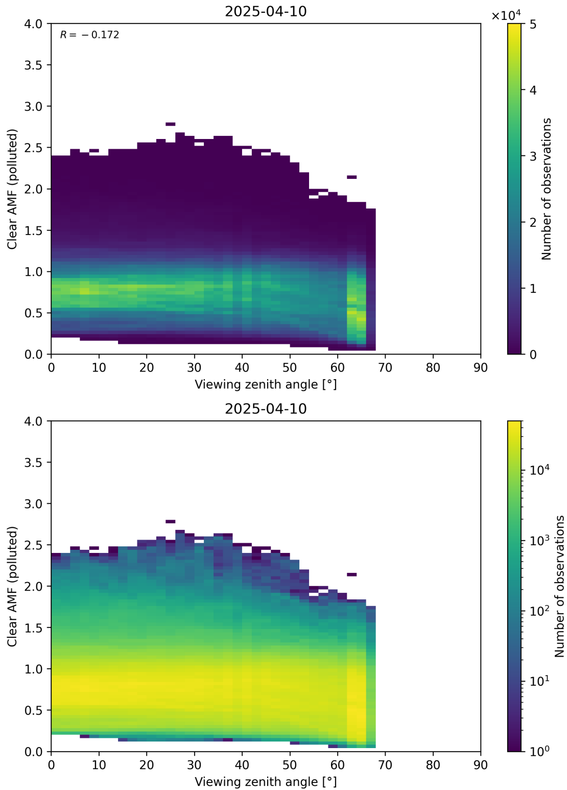
Figure 370: Scatter density plot of “Viewing zenith angle” against “Clear AMF (polluted)” for 2025-04-09 to 2025-04-11.
