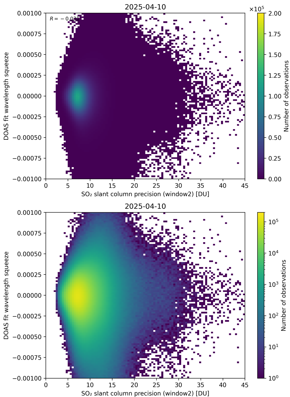
Figure 294: Scatter density plot of “SO 2 slant column precision (window2)” against “DOAS fit wavelength squeeze” for 2025-04-09 to 2025-04-11.
