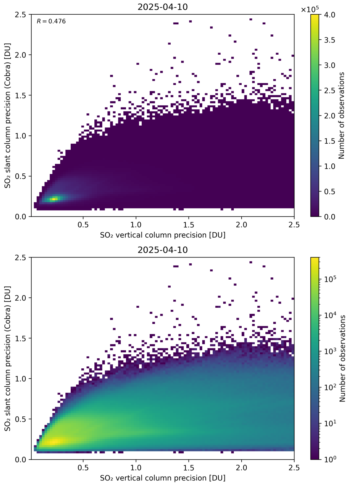
Figure 337: Scatter density plot of “SO 2 vertical column precision” against “SO 2 slant column precision (Cobra)” for 2025-04-09 to 2025-04-11.
