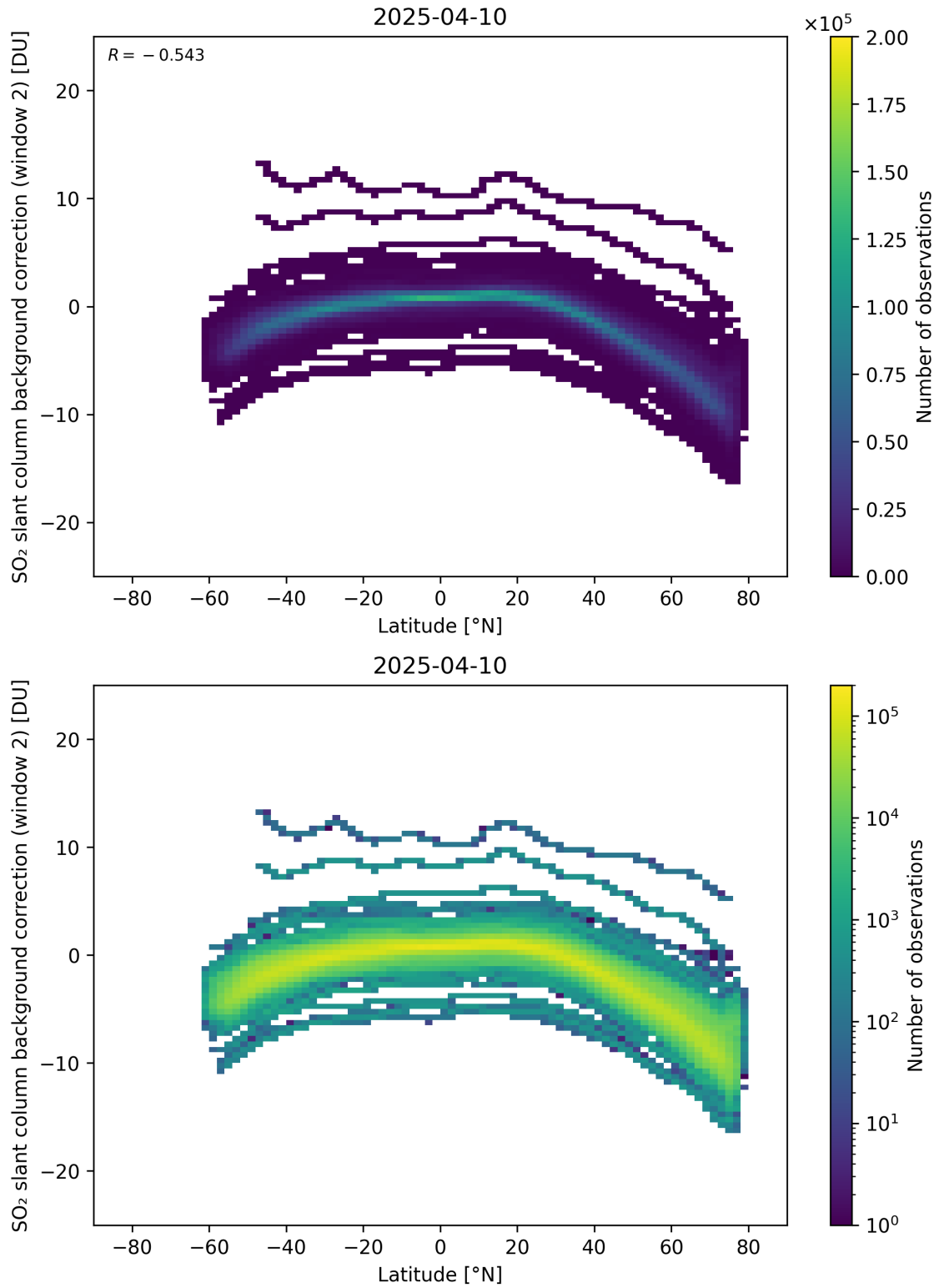
Figure 151: Scatter density plot of “Latitude” against “SO 2 slant column background correction (window 2)” for 2025-04-09 to 2025-04-11.
