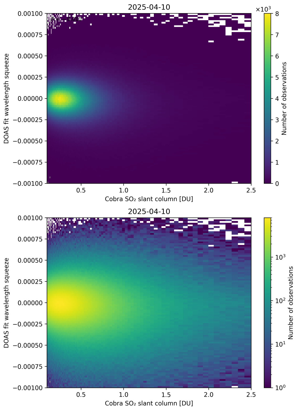
Figure 197: Scatter density plot of “Cobra SO 2 slant column” against “DOAS fit wavelength squeeze” for 2025-04-09 to 2025-04-11.
