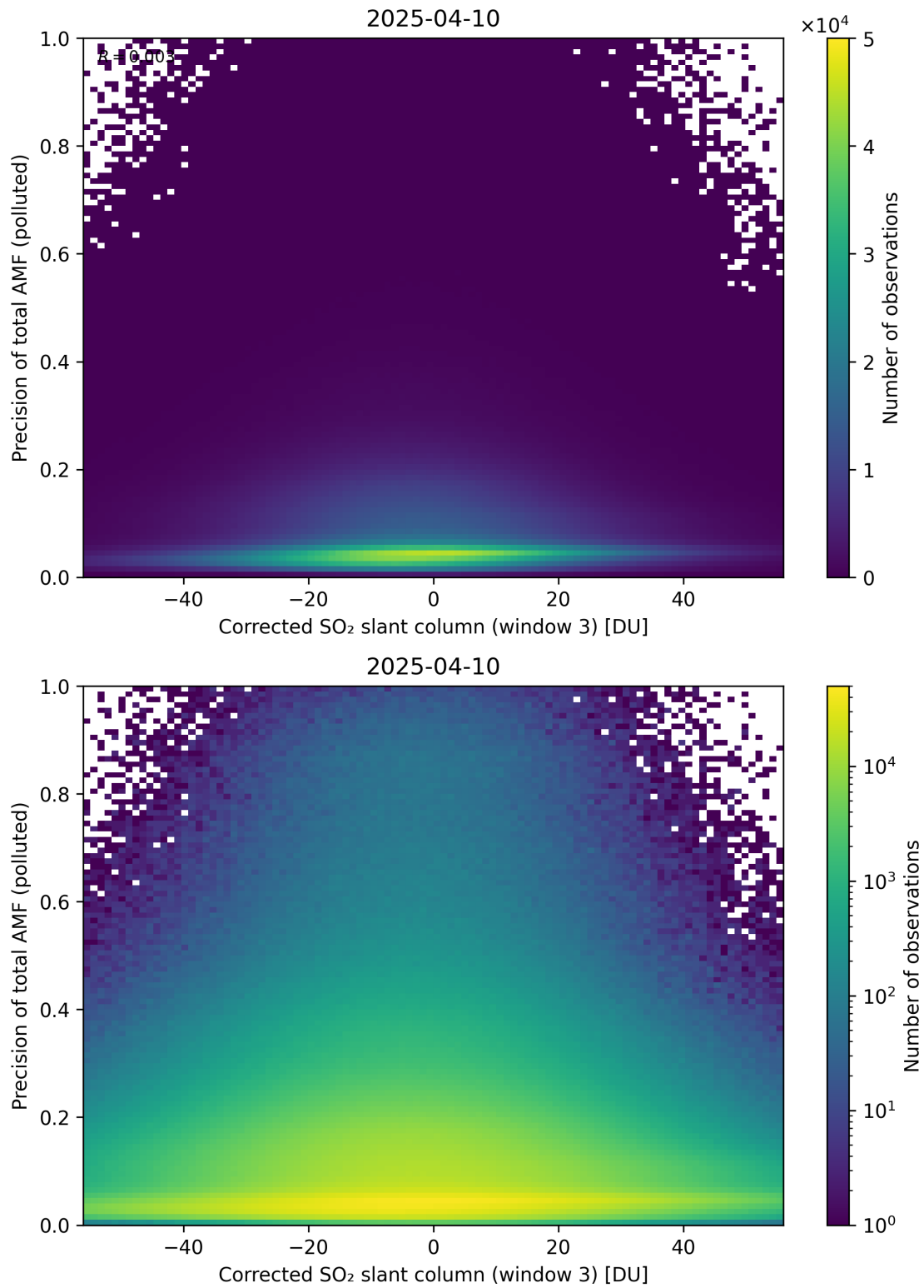
Figure 261: Scatter density plot of “Corrected SO 2 slant column (window 3)” against “Precision of total AMF (polluted)” for 2025-04-09 to 2025-04-11.
