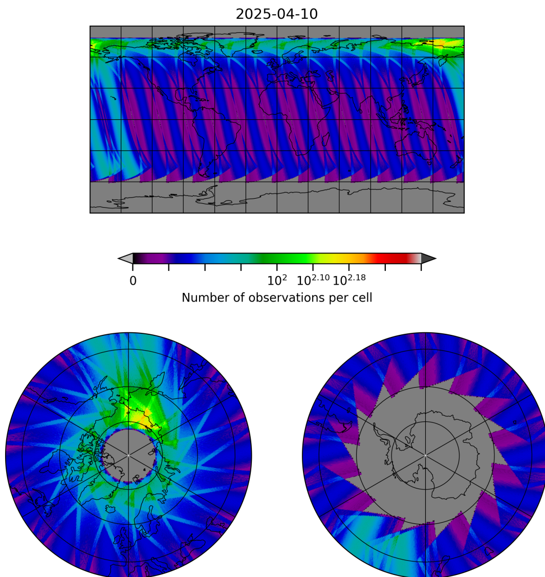
Figure 30: Map of the number of observations for 2025-04-09 to 2025-04-11
