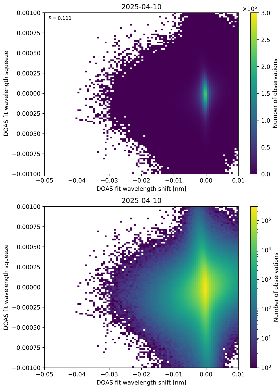
Figure 138: Scatter density plot of “DOAS fit wavelength shift” against “DOAS fit wavelength squeeze” for 2025-04-09 to 2025-04-11.
