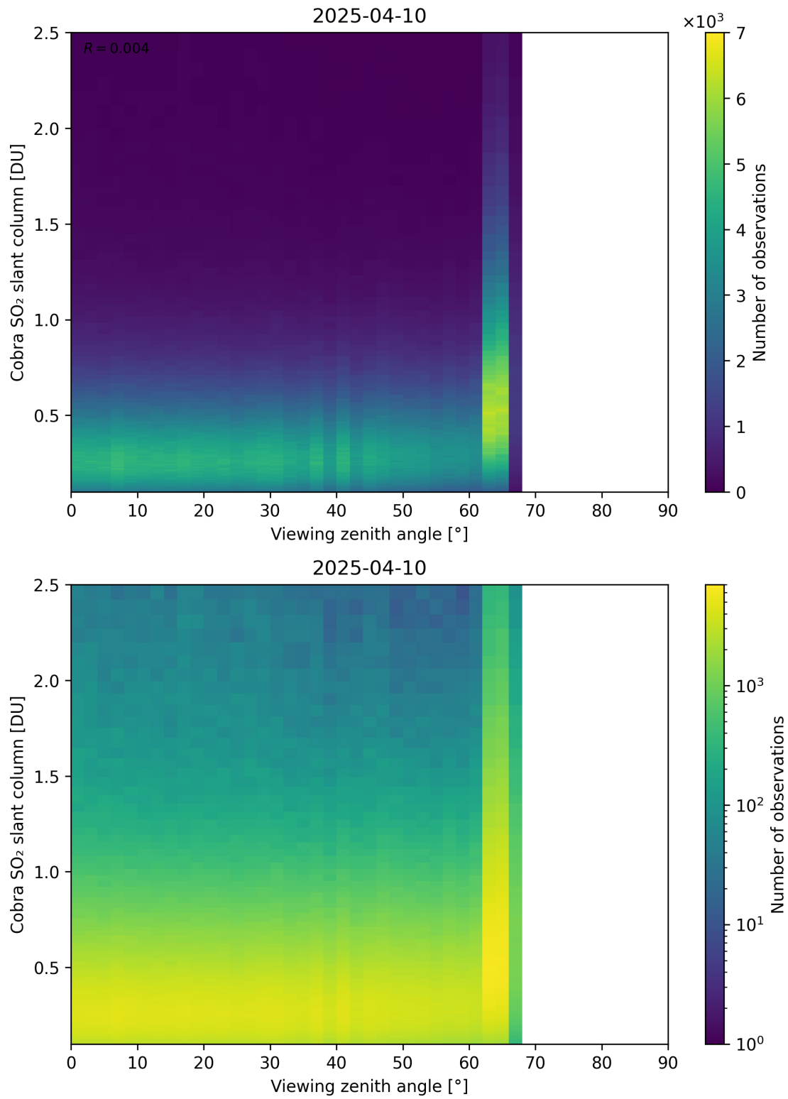
Figure 371: Scatter density plot of “Viewing zenith angle” against “Cobra SO 2 slant column” for 2025-04-09 to 2025-04-11.
