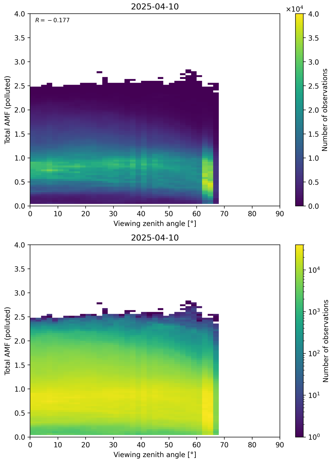
Figure 381: Scatter density plot of “Viewing zenith angle” against “Total AMF (polluted)” for 2025-04-09 to 2025-04-11.
