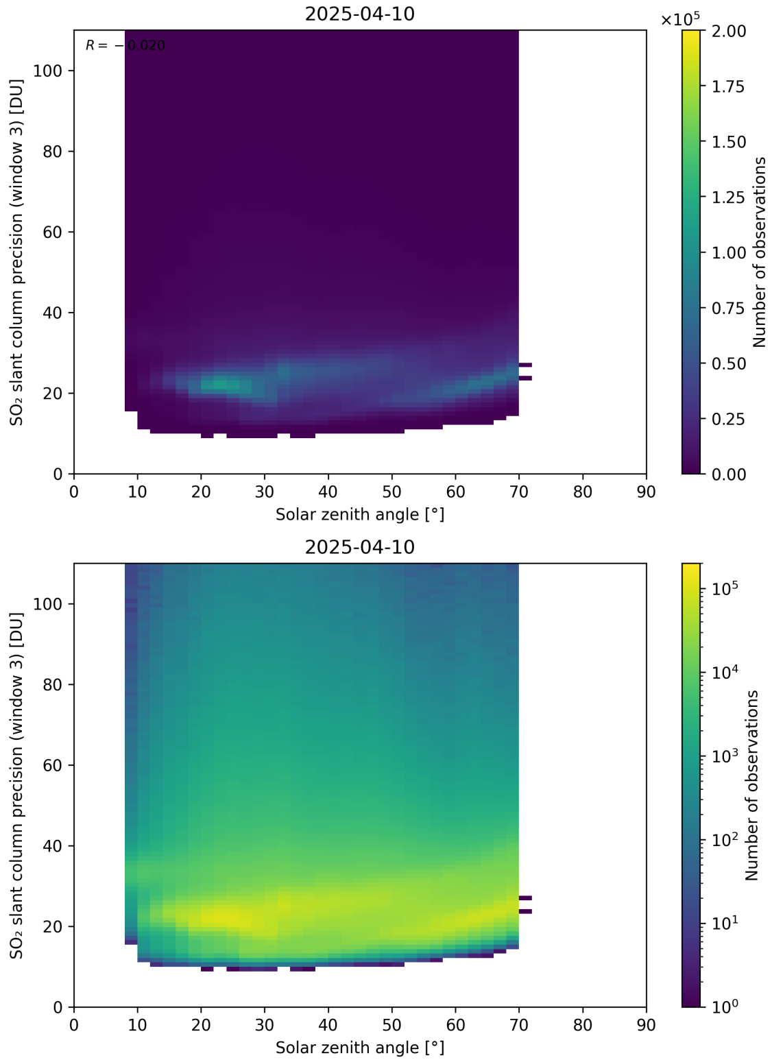
Figure 188: Scatter density plot of “Solar zenith angle” against “SO 2 slant column precision (window 3)” for 2025-04-09 to 2025-04-11.
