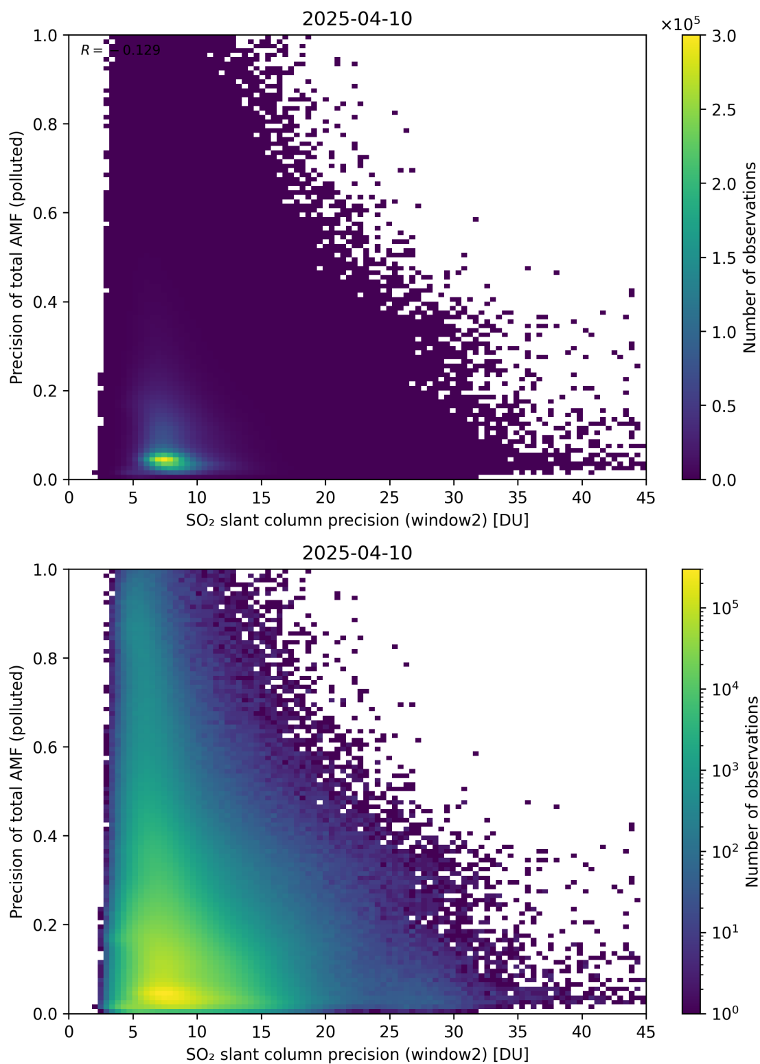
Figure 302: Scatter density plot of “SO 2 slant column precision (window2)” against “Precision of total AMF (polluted)” for 2025-04-09 to 2025-04-11.
