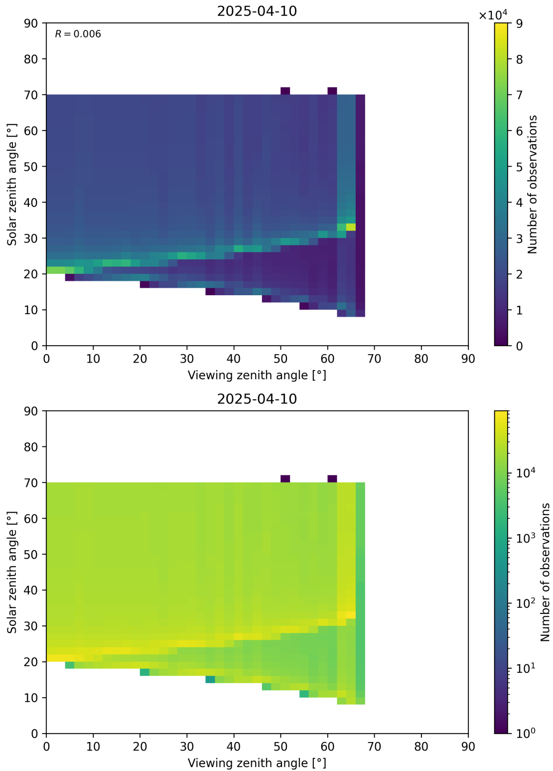
Figure 369: Scatter density plot of “Viewing zenith angle” against “Solar zenith angle” for 2025-04-09 to 2025-04-11.
