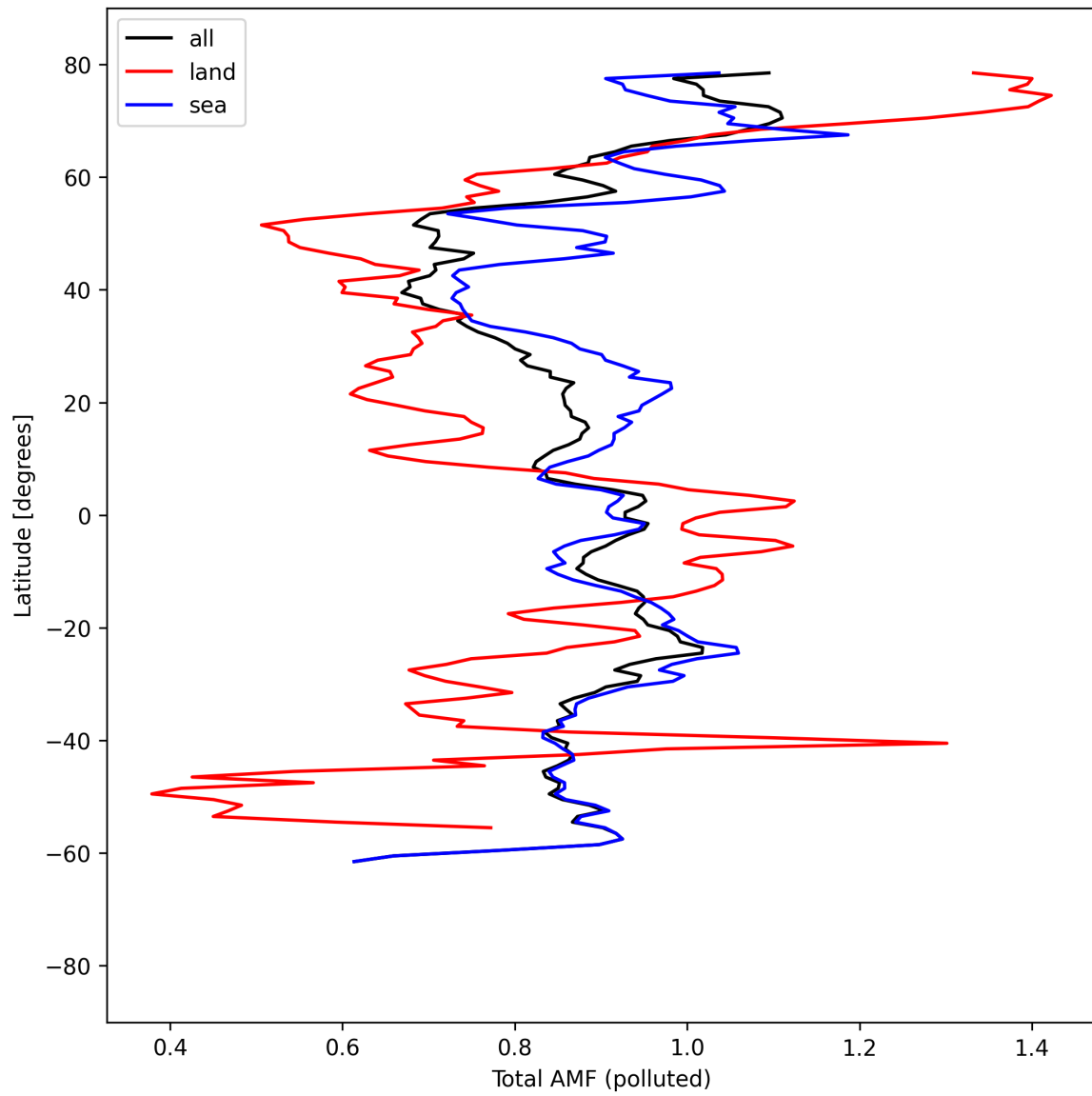
Figure 53: Zonal average of “Total AMF (polluted)” for 2025-04-09 to 2025-04-11.
