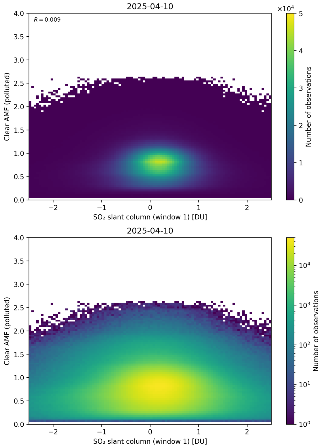
Figure 282: Scatter density plot of “SO 2 slant column (window 1)” against “Clear AMF (polluted)” for 2025-04-09 to 2025-04-11.
