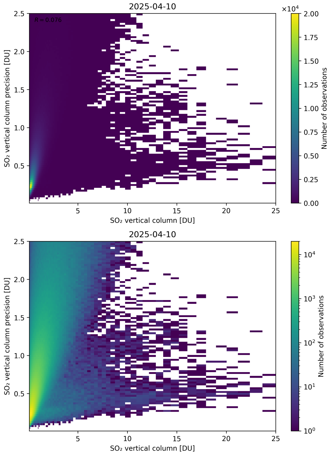
Figure 361: Scatter density plot of “SO 2 vertical column” against “SO 2 vertical column precision” for 2025-04-09 to 2025-04-11.
