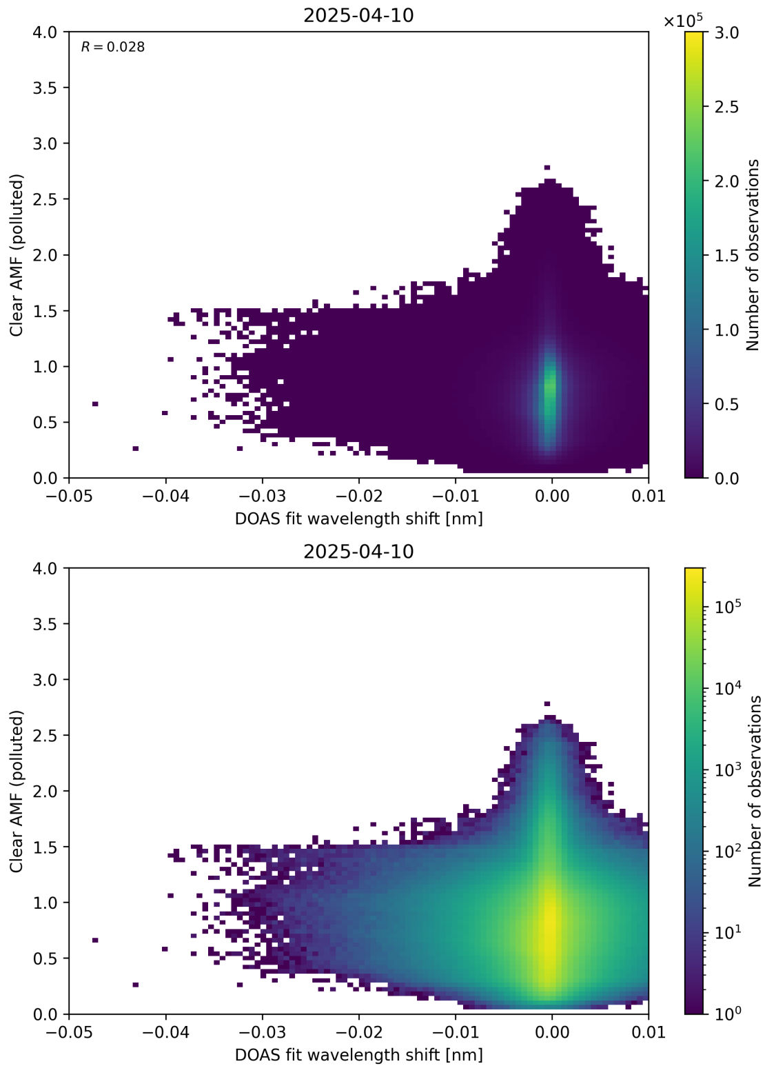
Figure 140: Scatter density plot of “DOAS fit wavelength shift” against “Clear AMF (polluted)” for 2025-04-09 to 2025-04-11.
