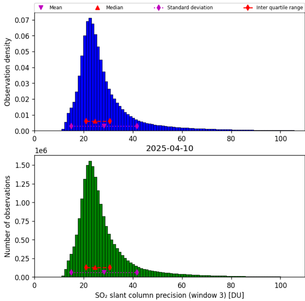
Figure 72: Histogram of “SO 2 slant column precision (window 3)” for 2025-04-09 to 2025-04-11
