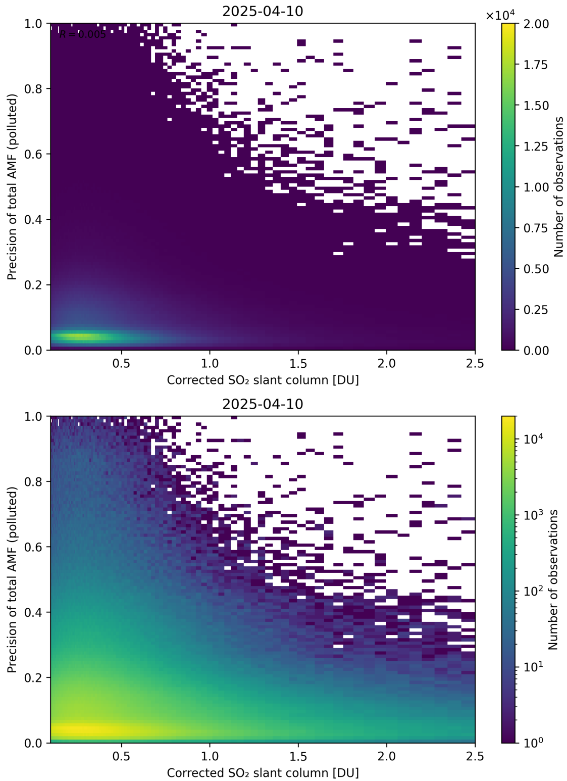
Figure 243: Scatter density plot of “Corrected SO 2 slant column” against “Precision of total AMF (polluted)” for 2025-04-09 to 2025-04-11.
