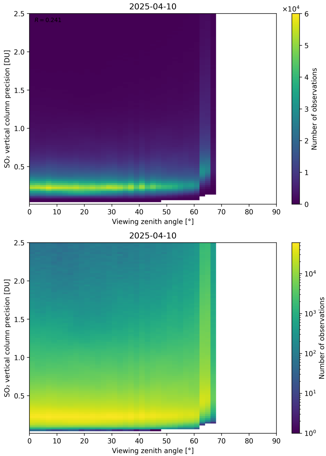
Figure 384: Scatter density plot of “Viewing zenith angle” against “SO 2 vertical column precision” for 2025-04-09 to 2025-04-11.
