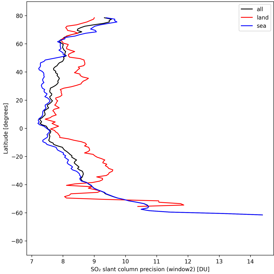
Figure 42: Zonal average of “SO 2 slant column precision (window2)” for 2025-04-09 to 2025-04-11.
