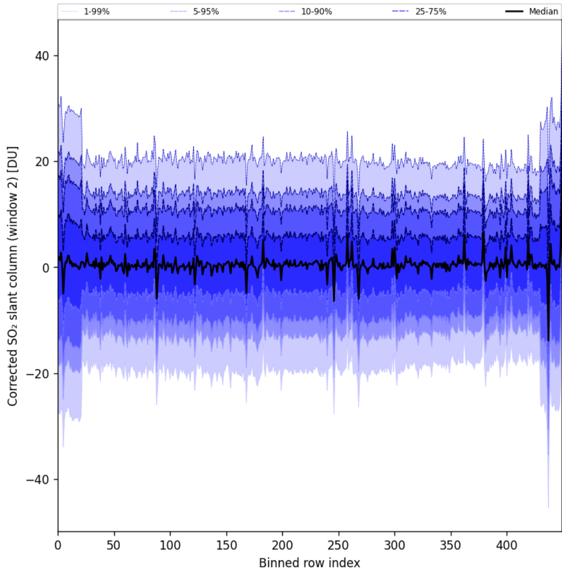
Figure 95: Along track statistics of “Corrected SO 2 slant column (window 2)” for 2025-04-09 to 2025-04-11
