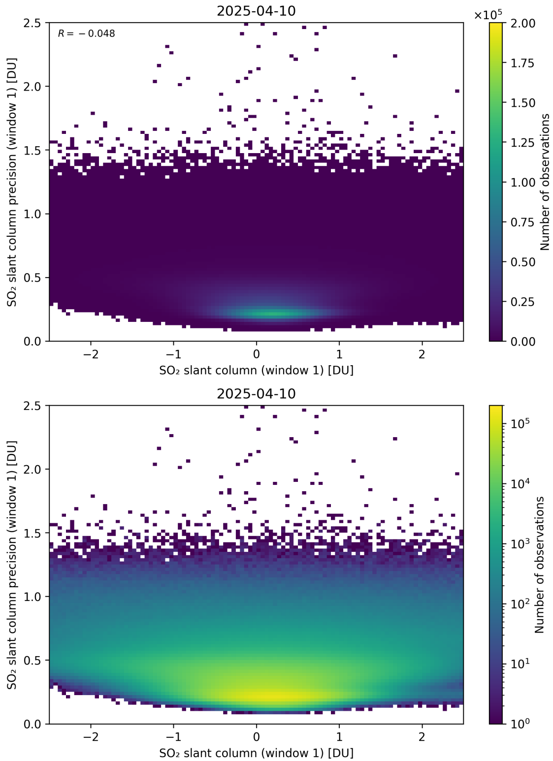
Figure 285: Scatter density plot of “SO 2 slant column (window 1)” against “SO 2 slant column precision (window 1)” for 2025-04-09 to 2025-04-11.
