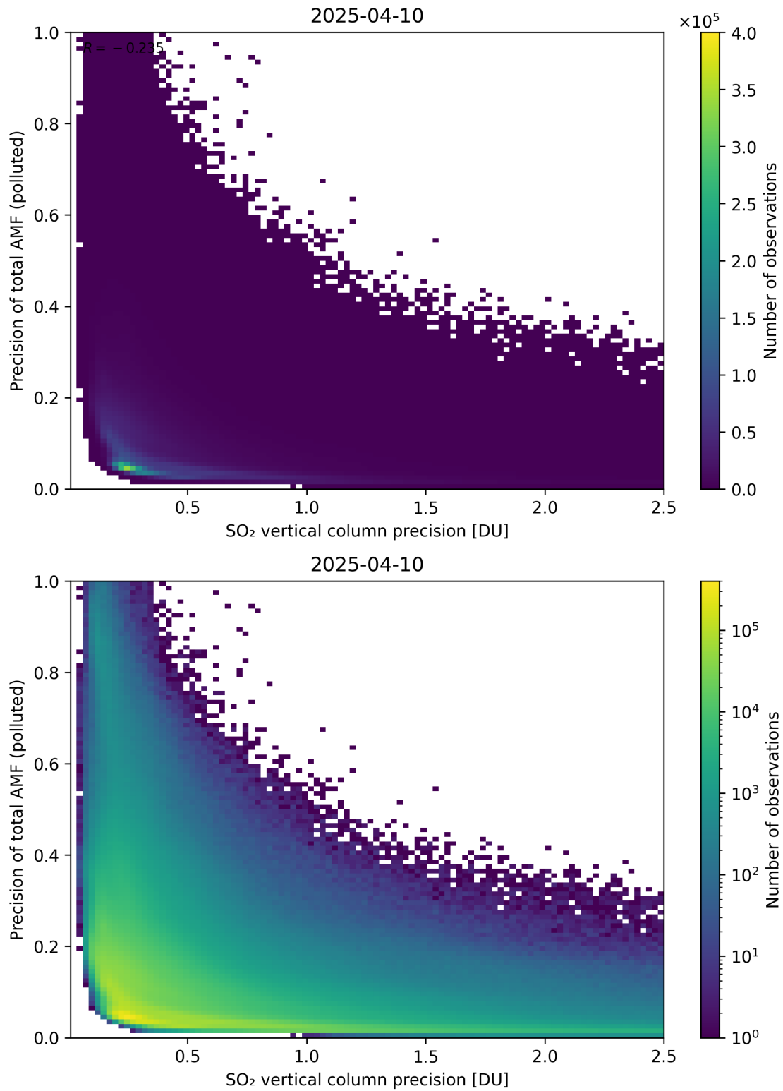
Figure 347: Scatter density plot of “SO 2 vertical column precision” against “Precision of total AMF (polluted)” for 2025-04-09 to 2025-04-11.
