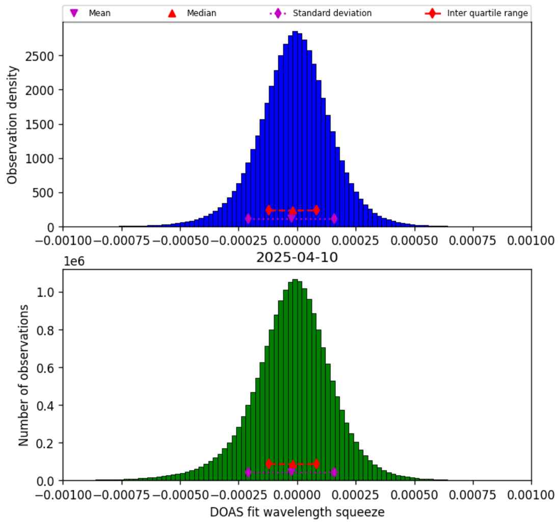
Figure 77: Histogram of “DOAS fit wavelength squeeze” for 2025-04-09 to 2025-04-11
