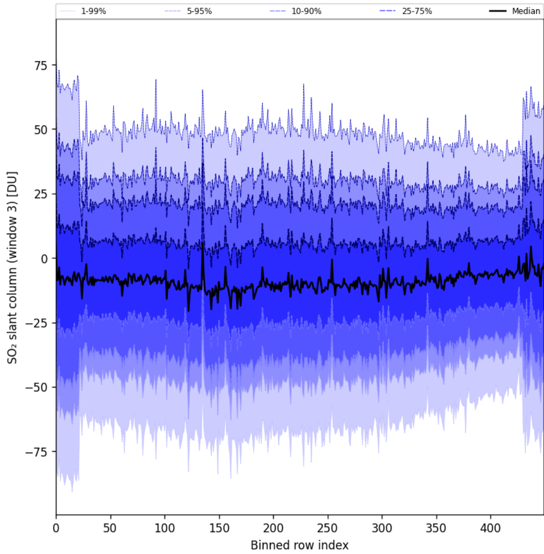
Figure 97: Along track statistics of “SO 2 slant column (window 3)” for 2025-04-09 to 2025-04-11
