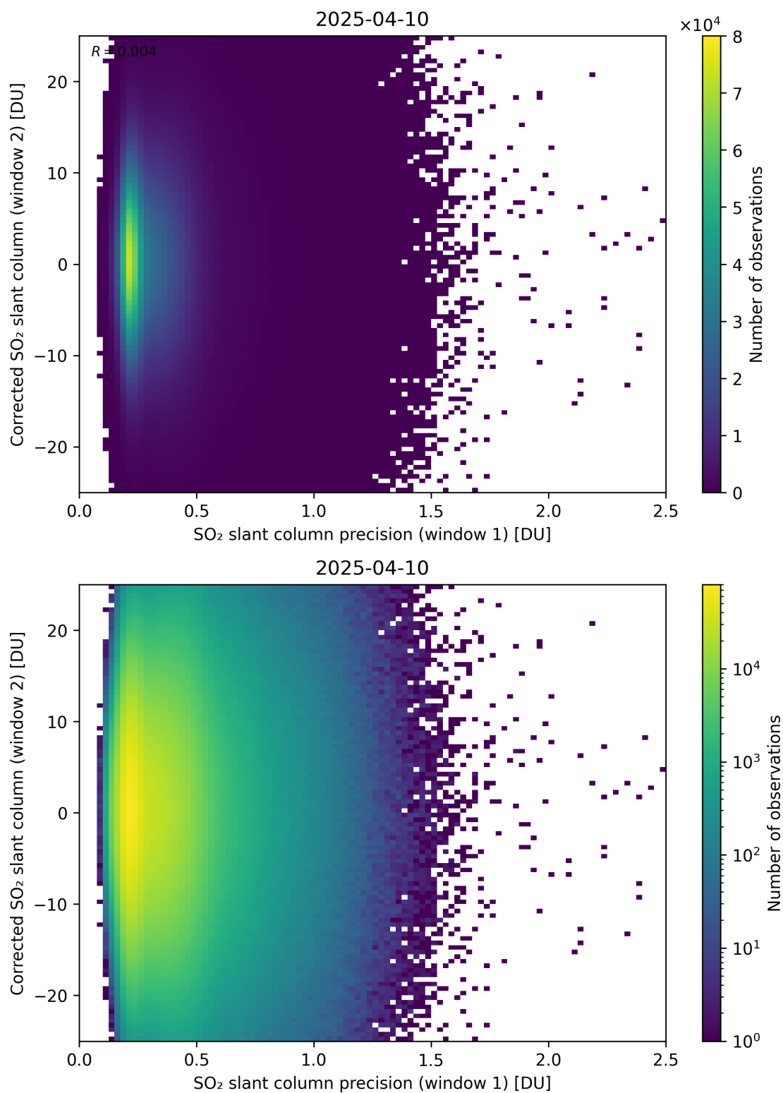
Figure 275: Scatter density plot of “SO 2 slant column precision (window 1)” against “Corrected SO 2 slant column (window 2)” for 2025-04-09 to 2025-04-11.
