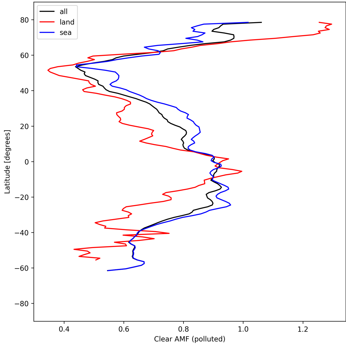
Figure 55: Zonal average of “Clear AMF (polluted)” for 2025-04-09 to 2025-04-11.
