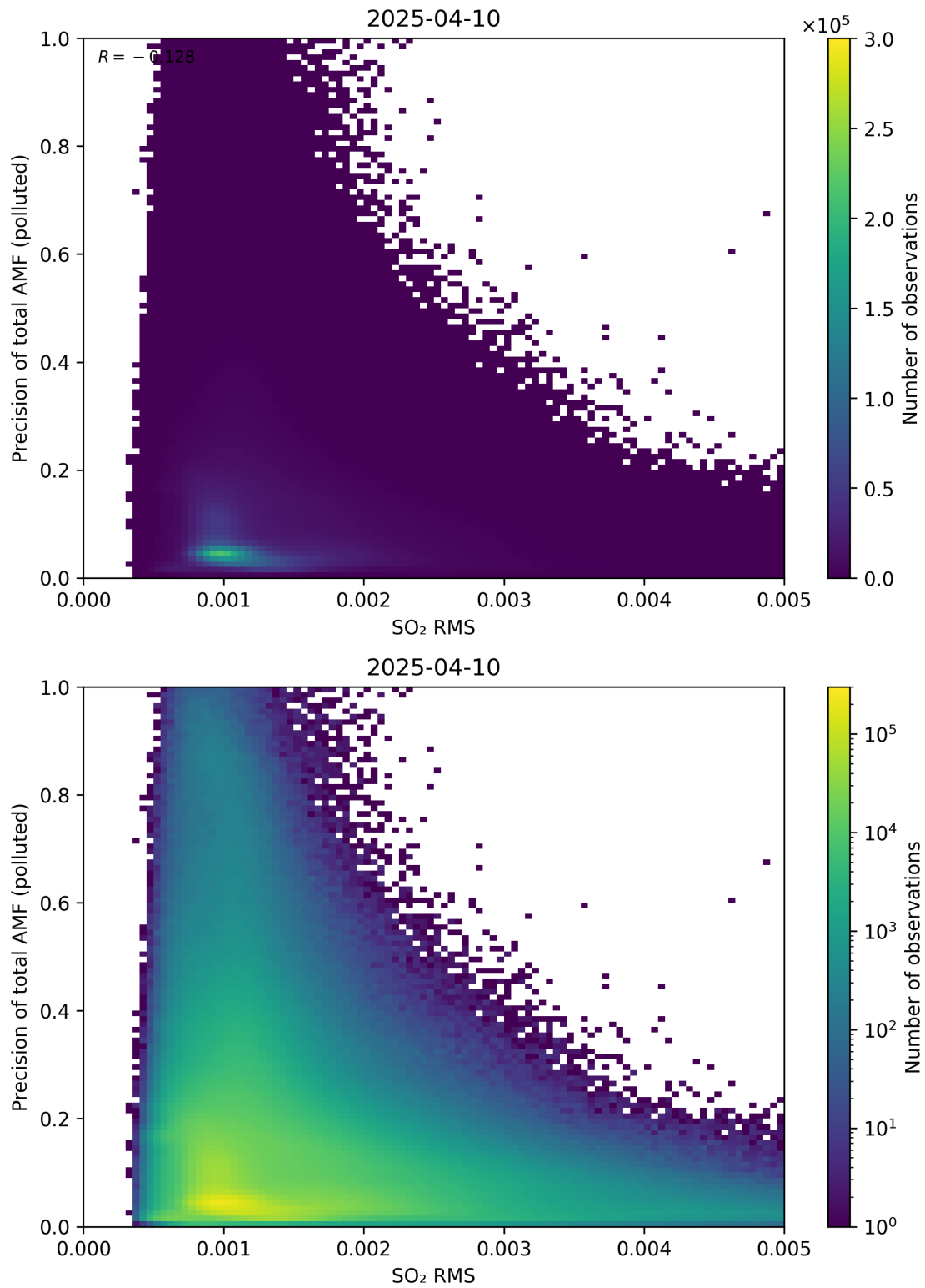
Figure 149: Scatter density plot of “SO 2 RMS” against “Precision of total AMF (polluted)” for 2025-04-09 to 2025-04-11.
