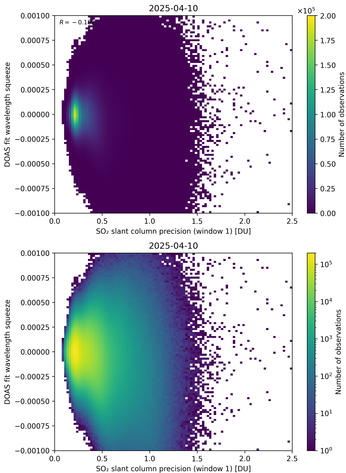
Figure 272: Scatter density plot of “SO 2 slant column precision (window 1)” against “DOAS fit wavelength squeeze” for 2025-04-09 to 2025-04-11.
