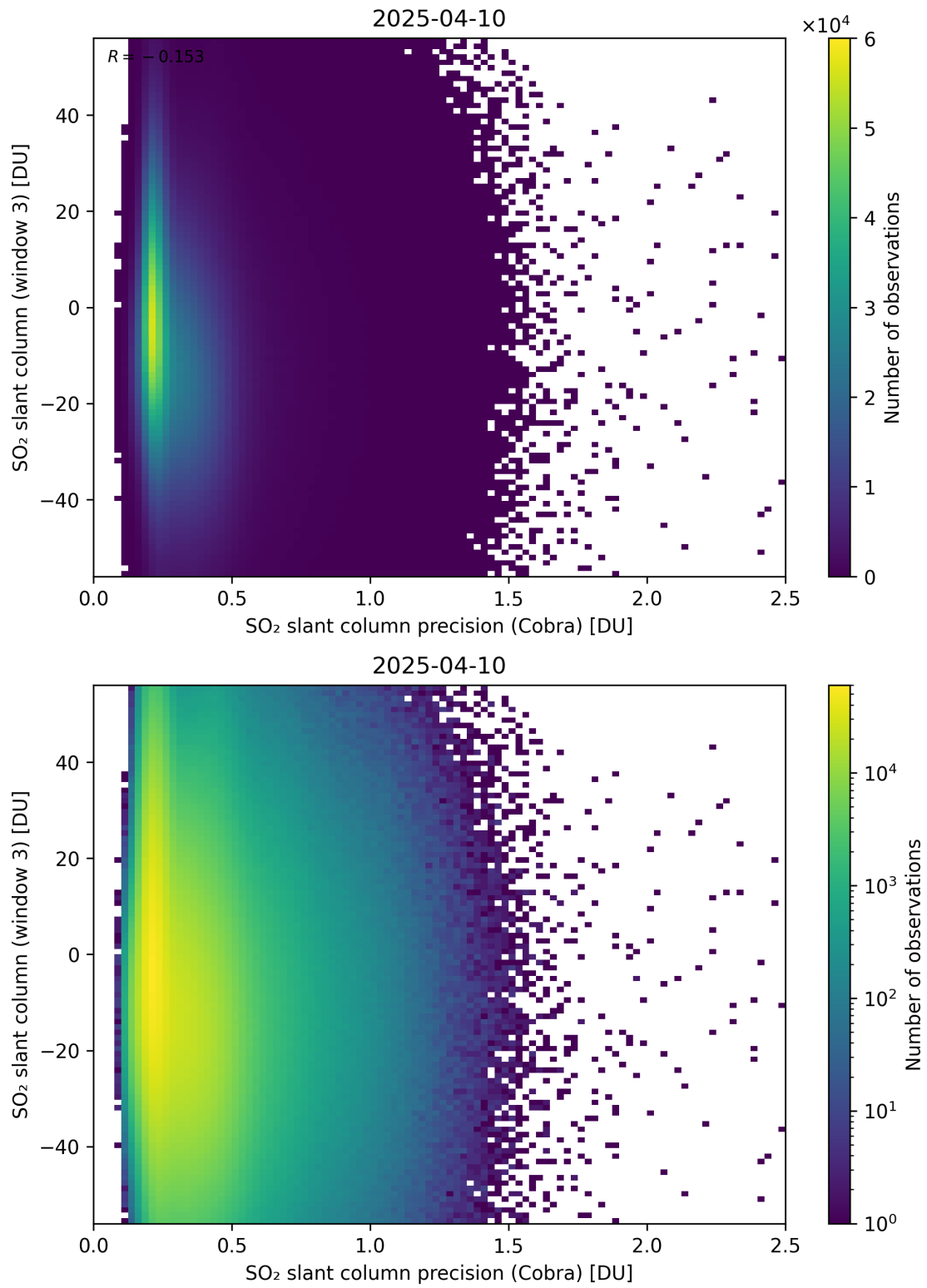
Figure 211: Scatter density plot of “SO 2 slant column precision (Cobra)” against “SO 2 slant column (window 3)” for 2025-04-09 to 2025-04-11.
