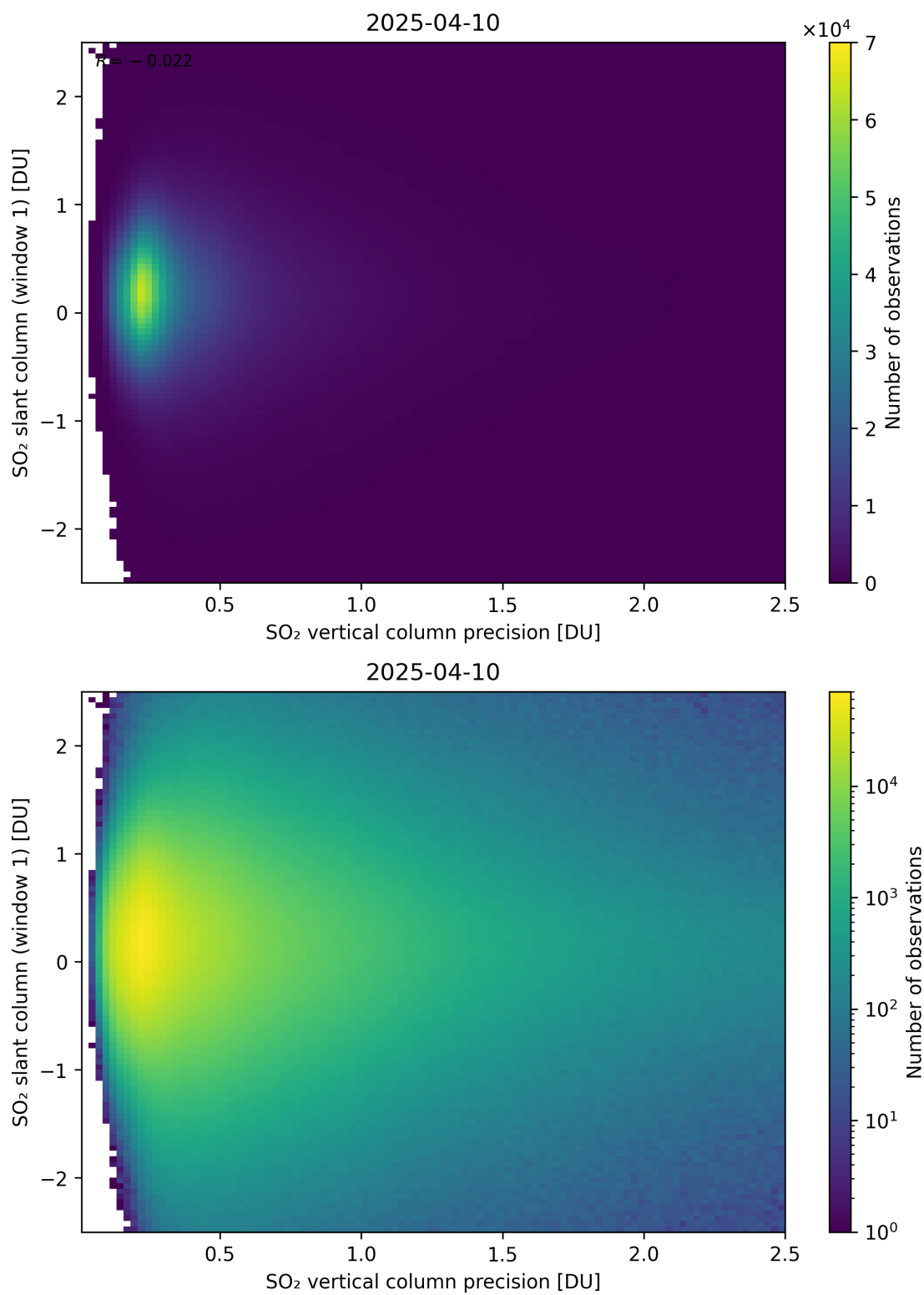
Figure 341: Scatter density plot of “SO 2 vertical column precision” against “SO 2 slant column (window 1)” for 2025-04-09 to 2025-04-11.
