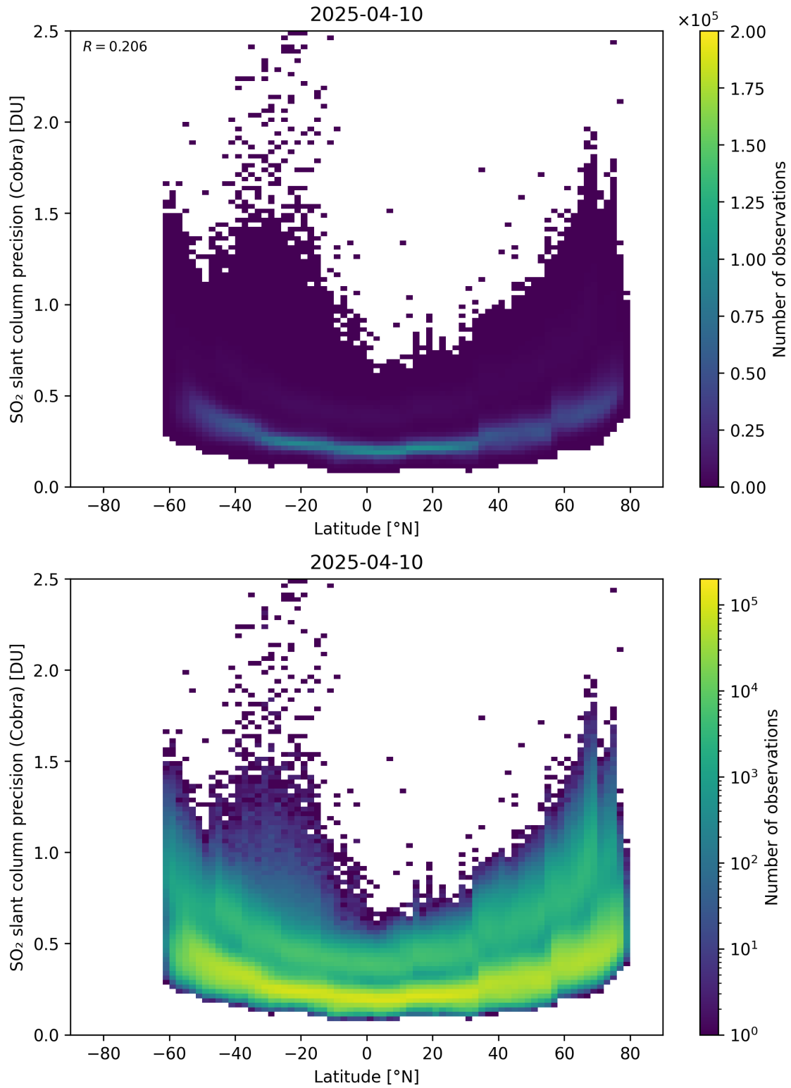
Figure 158: Scatter density plot of “Latitude” against “SO 2 slant column precision (Cobra)” for 2025-04-09 to 2025-04-11.
