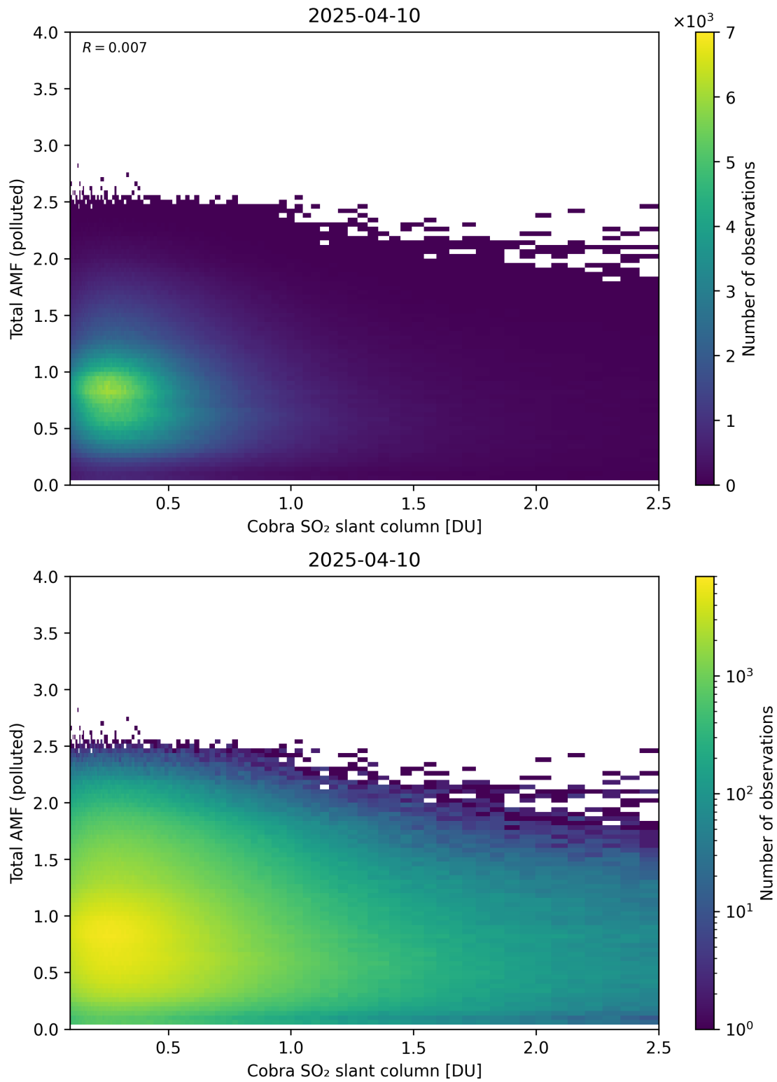
Figure 224: Scatter density plot of “Cobra SO 2 slant column” against “Total AMF (polluted)” for 2025-04-09 to 2025-04-11.
