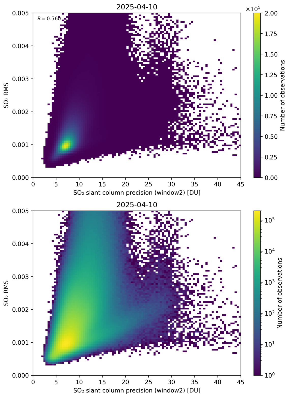
Figure 295: Scatter density plot of “SO 2 slant column precision (window2)” against “SO 2 RMS” for 2025-04-09 to 2025-04-11.
