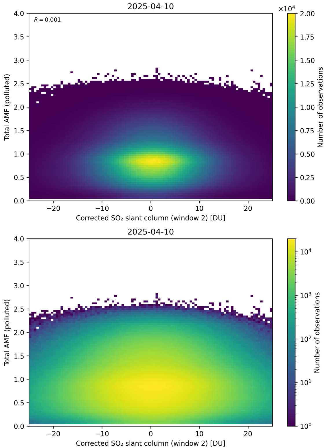
Figure 253: Scatter density plot of “Corrected SO 2 slant column (window 2)” against “Total AMF (polluted)” for 2025-04-09 to 2025-04-11.
