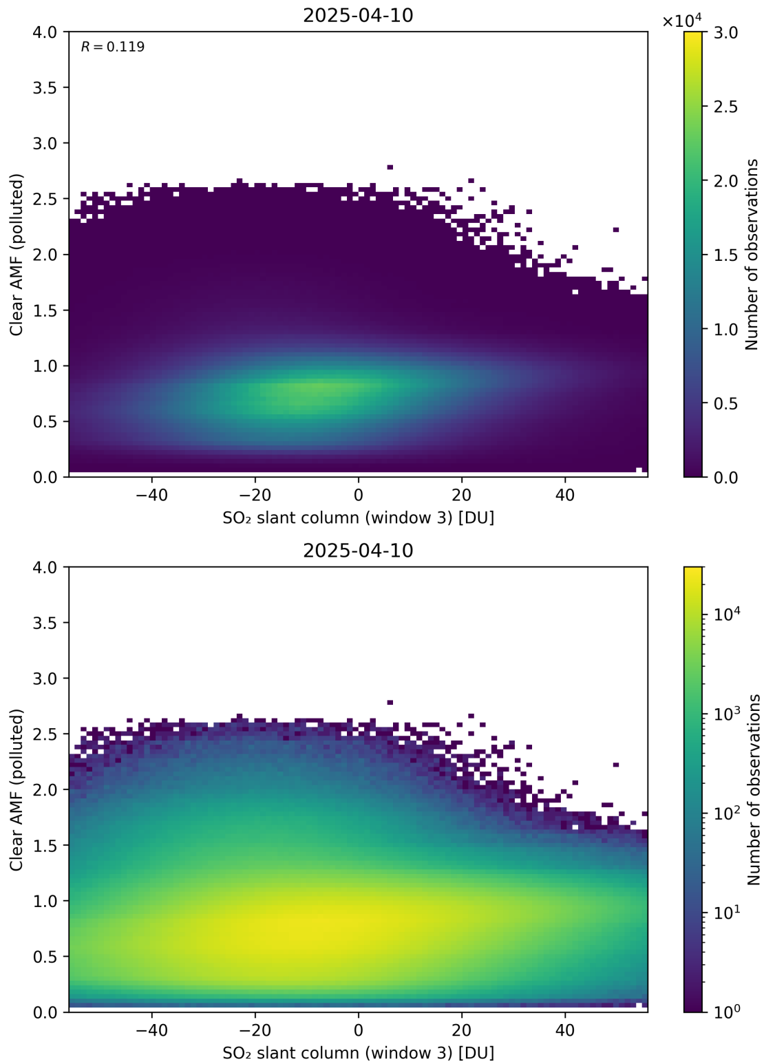
Figure 315: Scatter density plot of “SO 2 slant column (window 3)” against “Clear AMF (polluted)” for 2025-04-09 to 2025-04-11.
