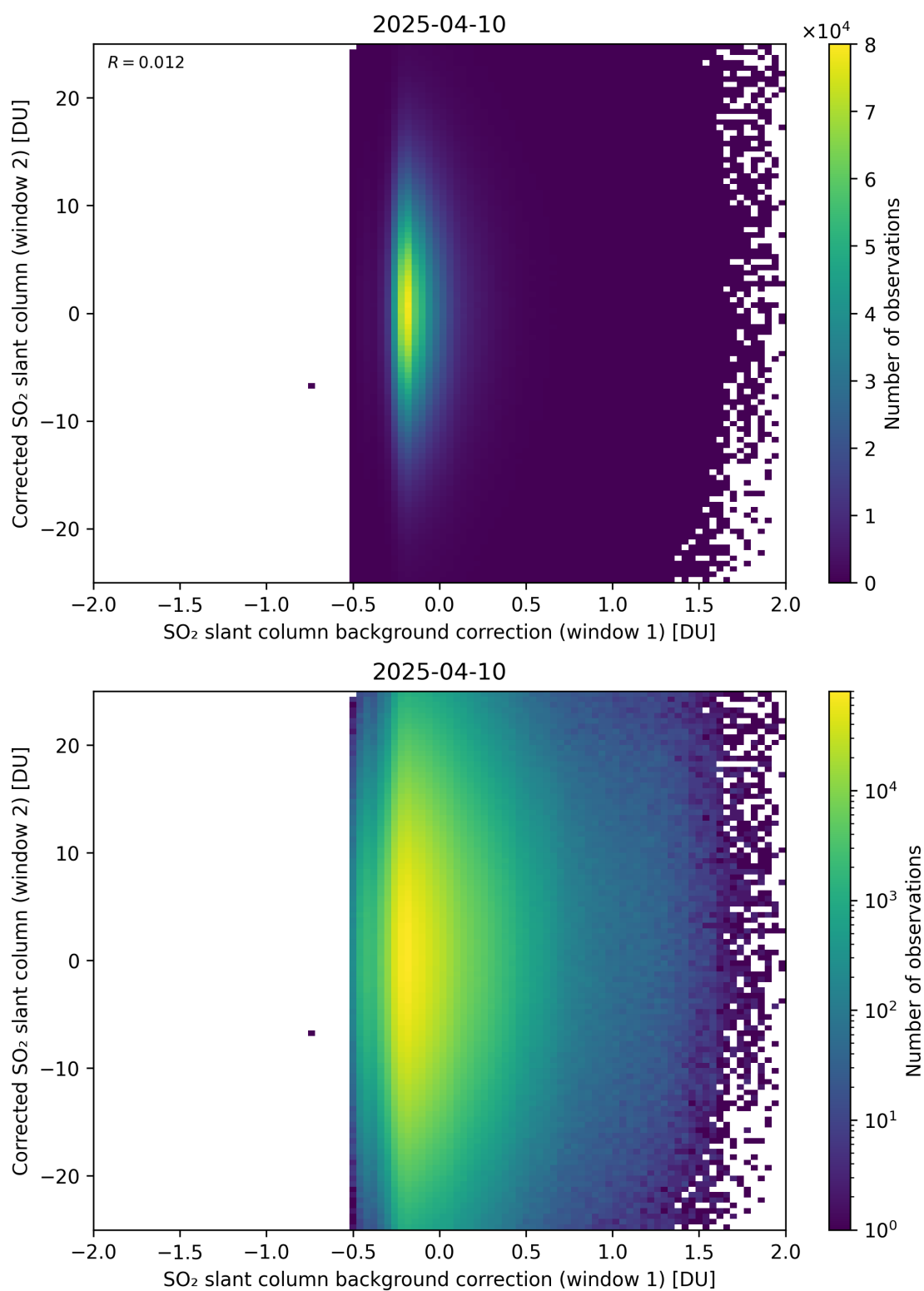
Figure 115: Scatter density plot of “SO 2 slant column background correction (window 1)” against “Corrected SO 2 slant column (window 2)” for 2025-04-09 to 2025-04-11.
