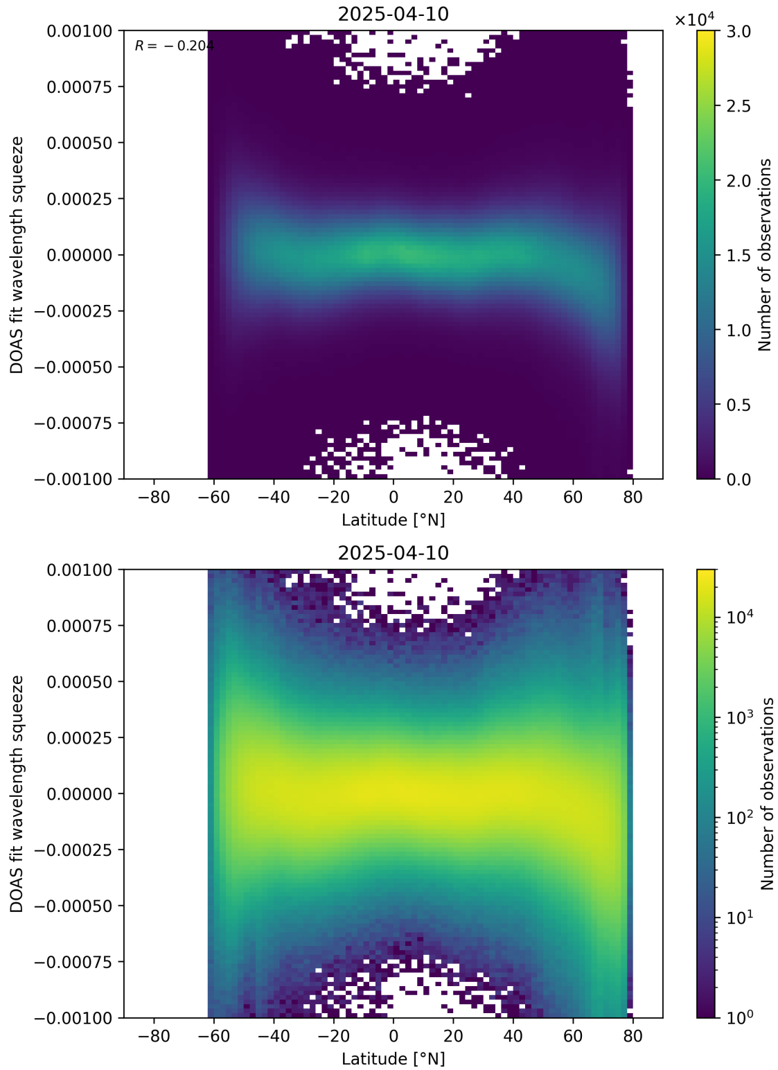
Figure 154: Scatter density plot of “Latitude” against “DOAS fit wavelength squeeze” for 2025-04-09 to 2025-04-11.
