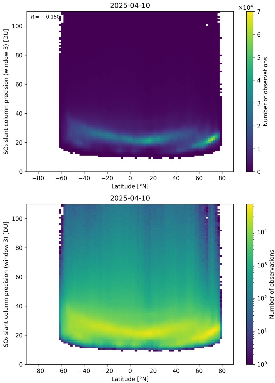
Figure 166: Scatter density plot of “Latitude” against “SO 2 slant column precision (window 3)” for 2025-04-09 to 2025-04-11.
