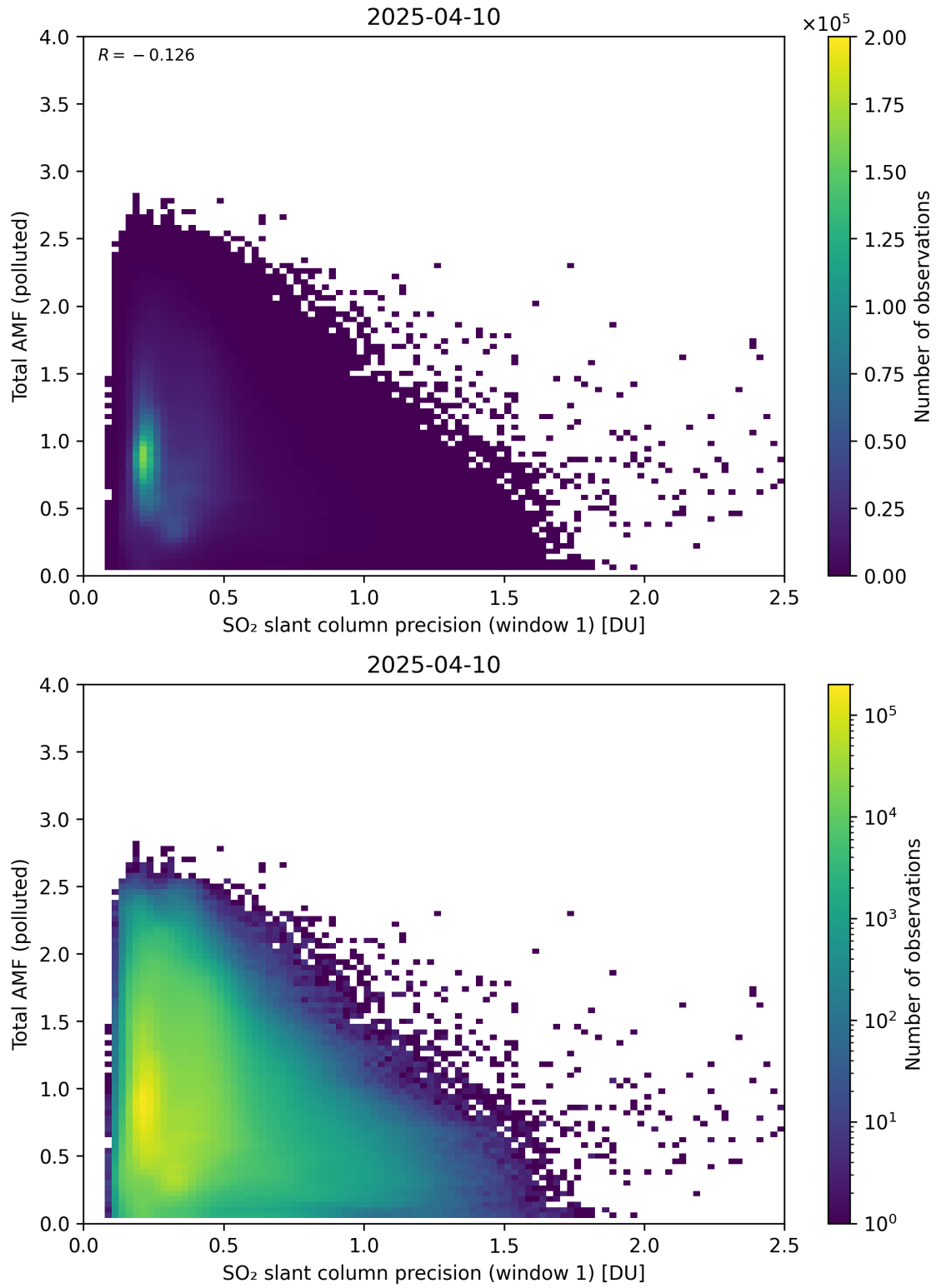
Figure 280: Scatter density plot of “SO 2 slant column precision (window 1)” against “Total AMF (polluted)” for 2025-04-09 to 2025-04-11.
