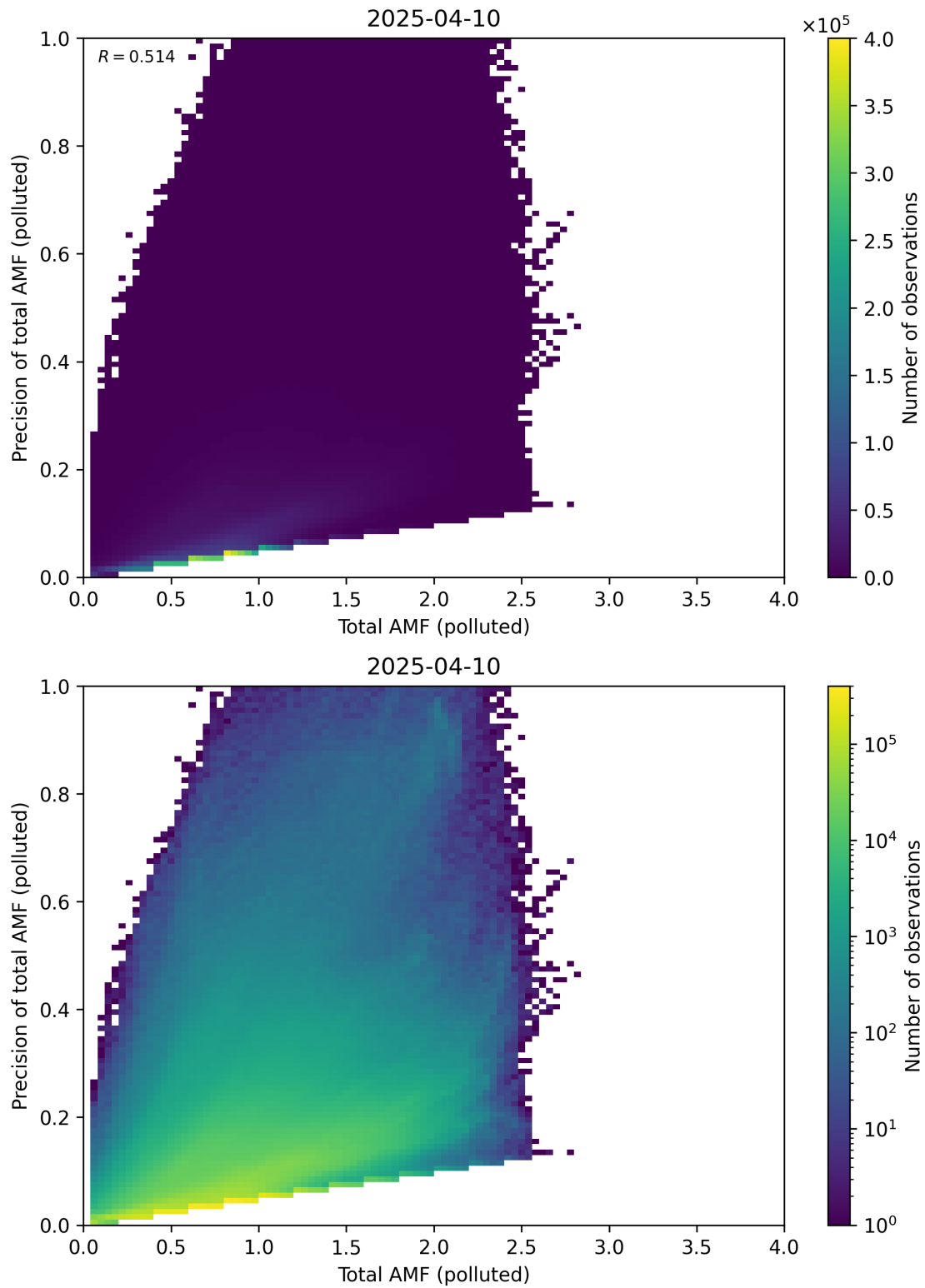
Figure 322: Scatter density plot of “Total AMF (polluted)” against “Precision of total AMF (polluted)” for 2025-04-09 to 2025-04-11.
