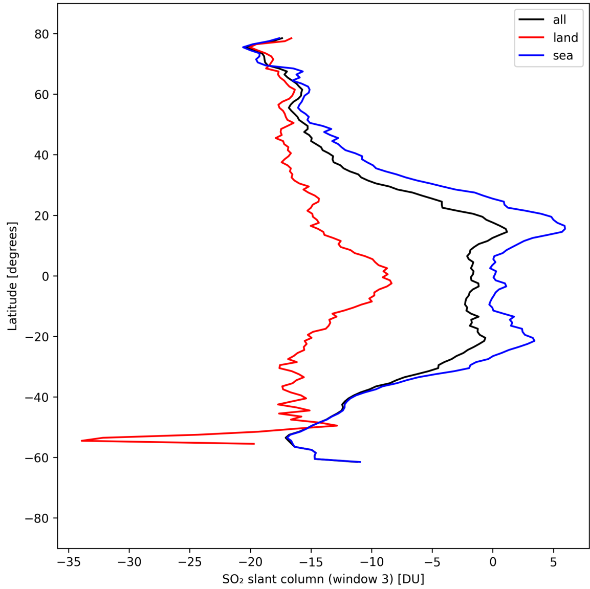
Figure 45: Zonal average of “SO 2 slant column (window 3)” for 2025-04-09 to 2025-04-11.
