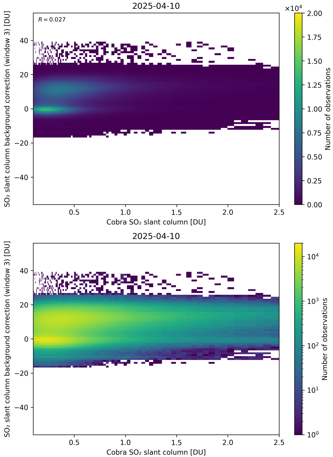
Figure 195: Scatter density plot of “Cobra SO 2 slant column” against “SO 2 slant column background correction (window 3)” for 2025-04-09 to 2025-04-11.
