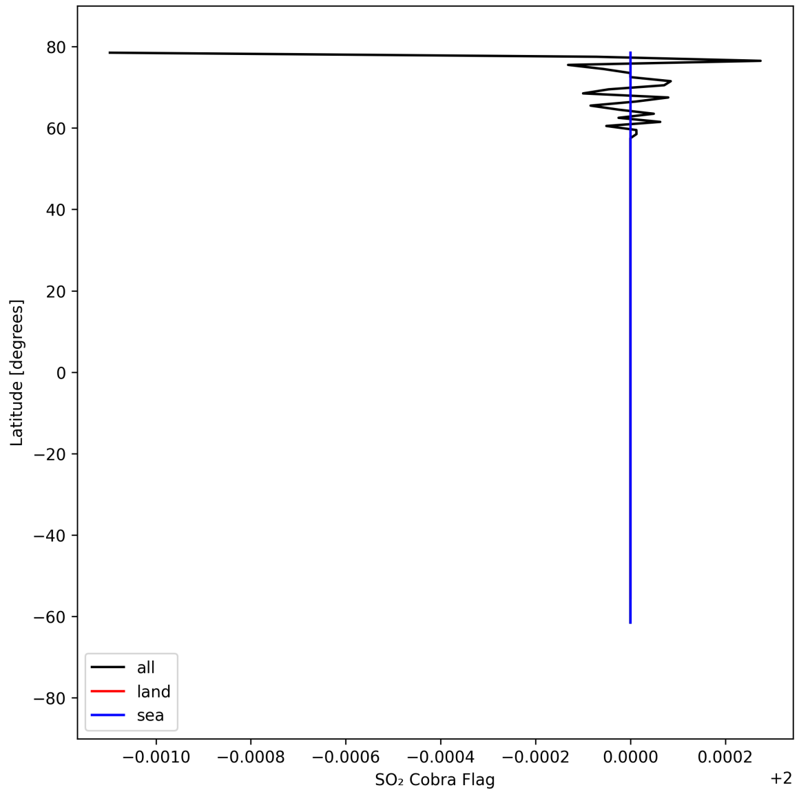
Figure 49: Zonal average of "SO 2 Cobra Flag" for 2025-04-09 to 2025-04-11.
