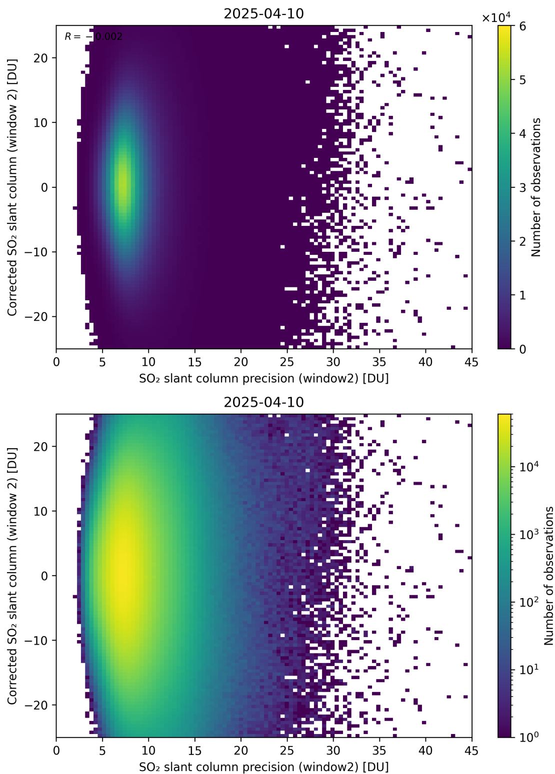
Figure 297: Scatter density plot of “SO 2 slant column precision (window2)” against “Corrected SO 2 slant column (window 2)” for 2025-04-09 to 2025-04-11.
