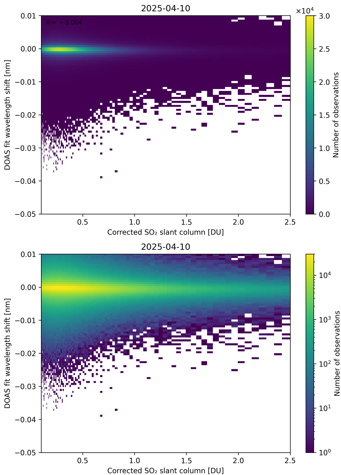
Figure 229: Scatter density plot of “Corrected SO 2 slant column” against “DOAS fit wavelength shift” for 2025-04-09 to 2025-04-11.
