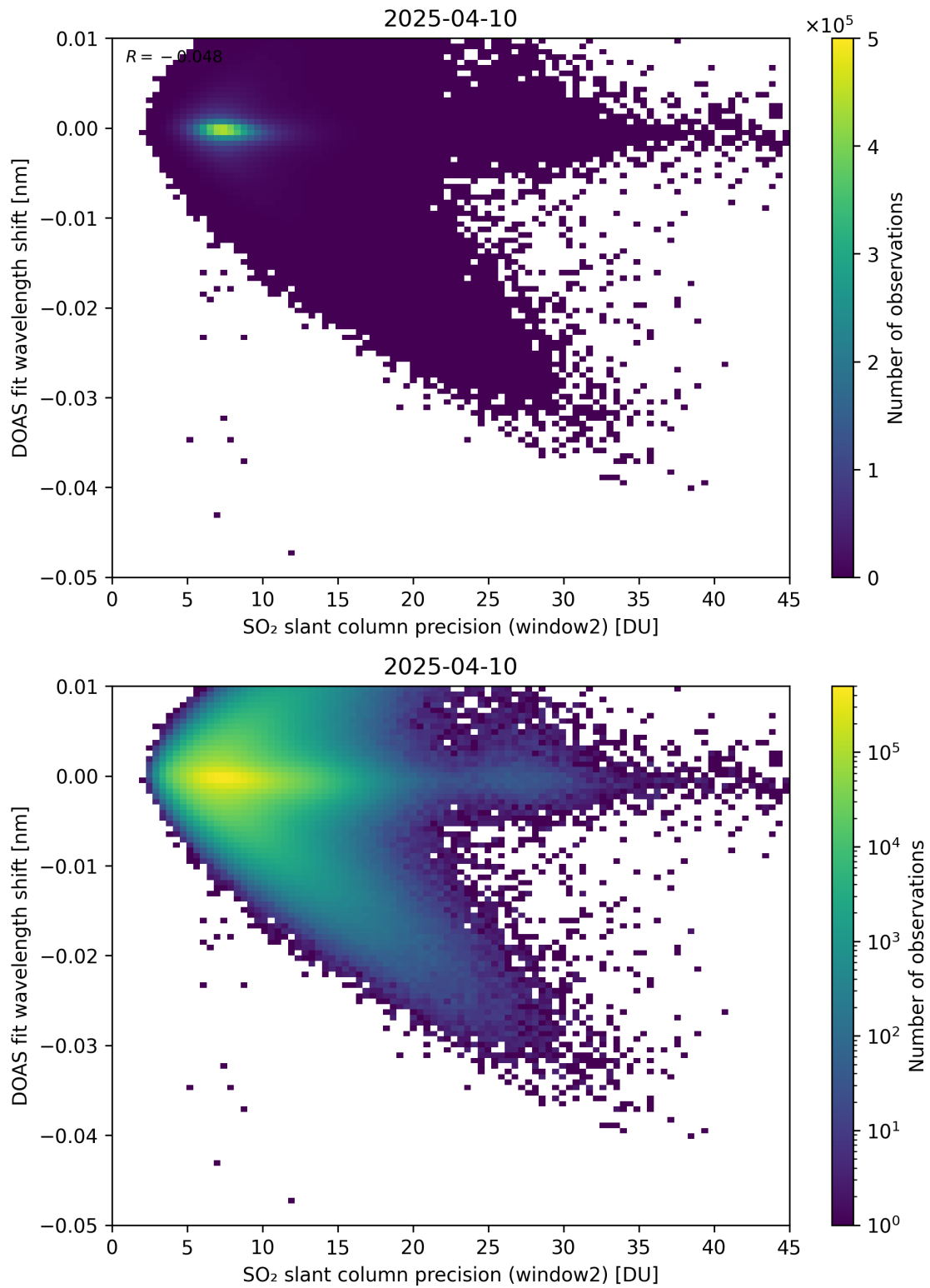
Figure 293: Scatter density plot of “SO 2 slant column precision (window2)” against “DOAS fit wavelength shift” for 2025-04-09 to 2025-04-11.
