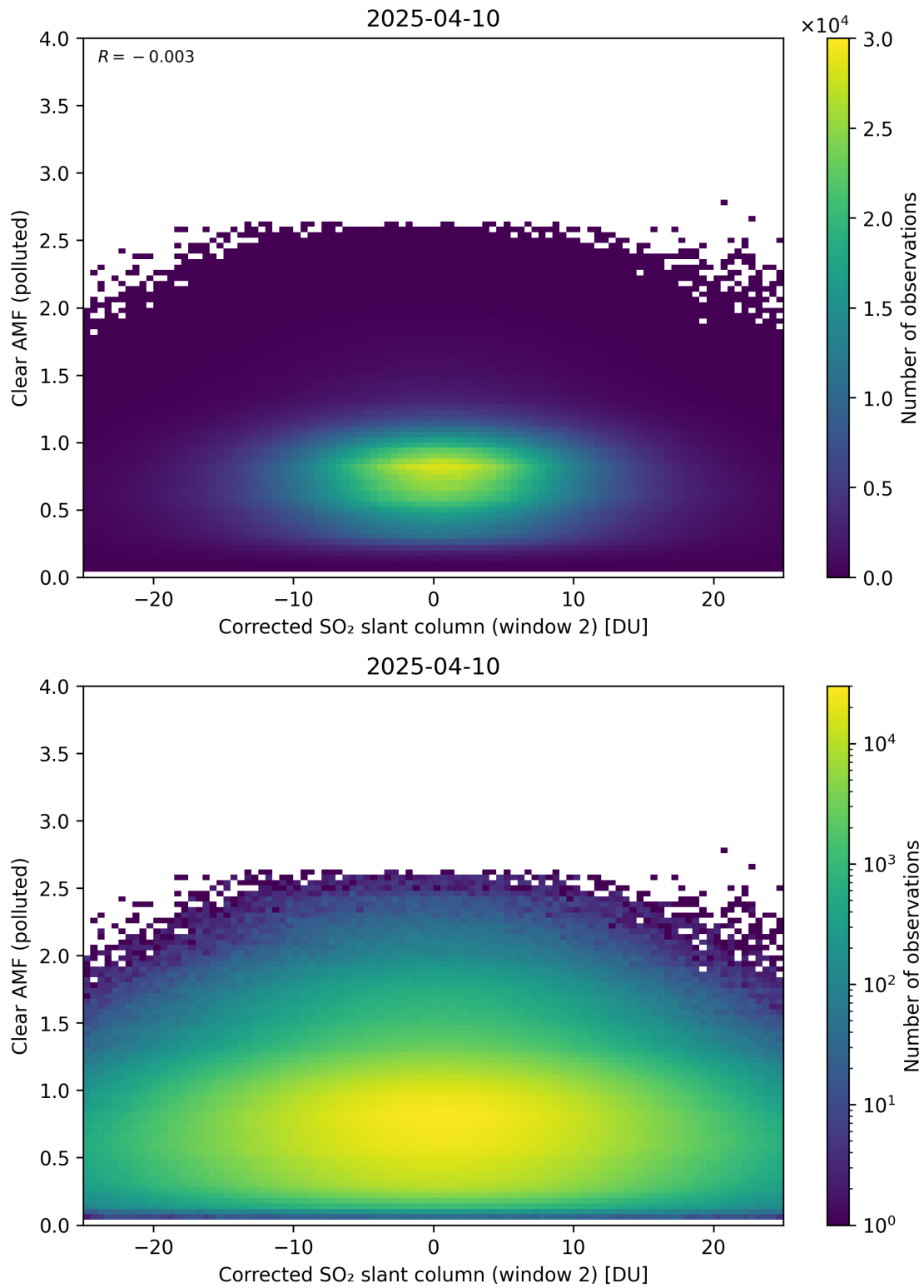
Figure 249: Scatter density plot of “Corrected SO 2 slant column (window 2)” against “Clear AMF (polluted)” for 2025-04-09 to 2025-04-11.
