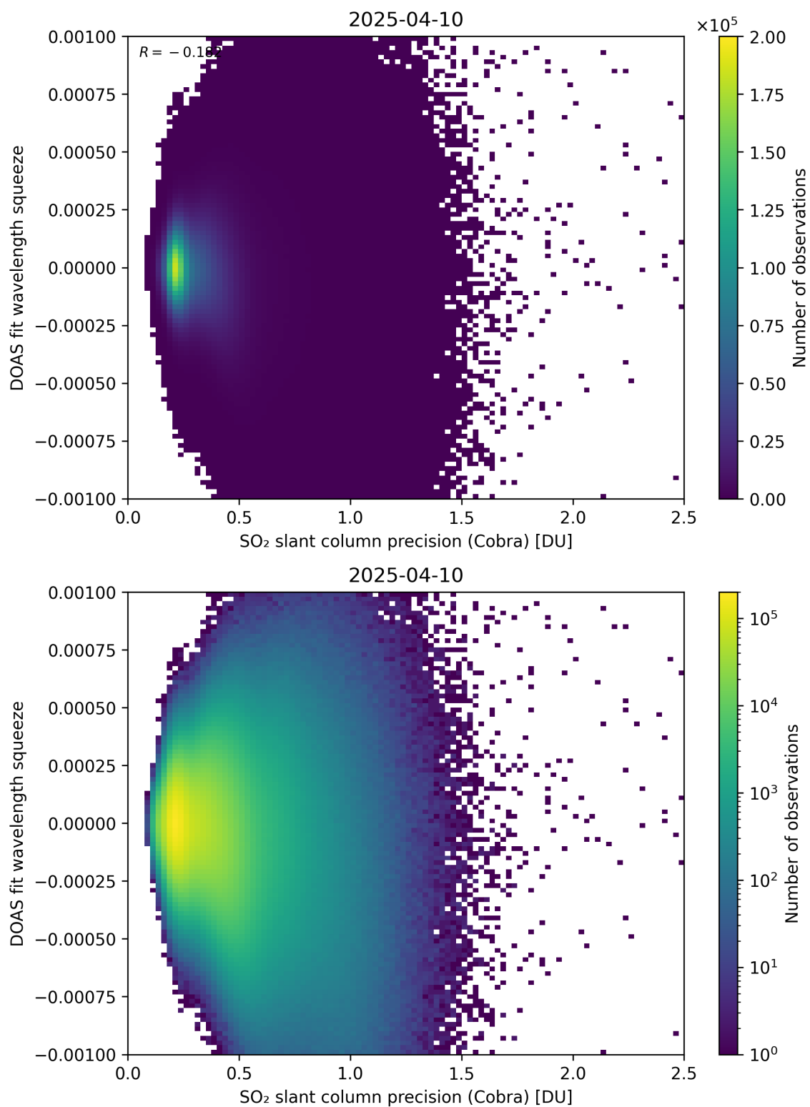
Figure 203: Scatter density plot of “SO 2 slant column precision (Cobra)” against “DOAS fit wavelength squeeze” for 2025-04-09 to 2025-04-11.
