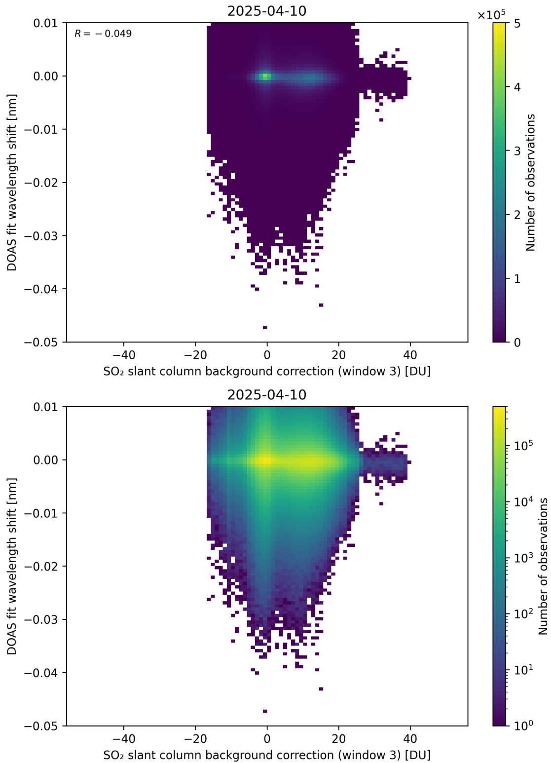
Figure 132: Scatter density plot of “SO 2 slant column background correction (window 3)” against “DOAS fit wavelength shift” for 2025-04-09 to 2025-04-11.
