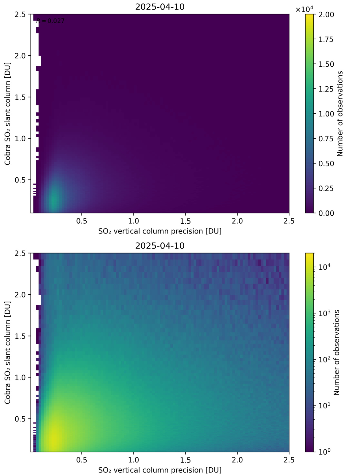
Figure 336: Scatter density plot of “SO 2 vertical column precision” against “Cobra SO 2 slant column” for 2025-04-09 to 2025-04-11.
