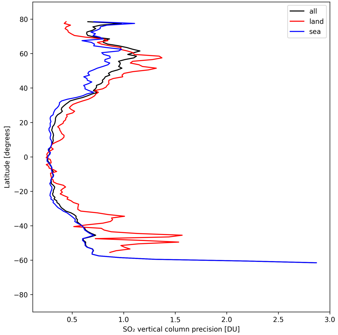
Figure 33: Zonal average of “SO 2 vertical column precision” for 2025-04-09 to 2025-04-11.
