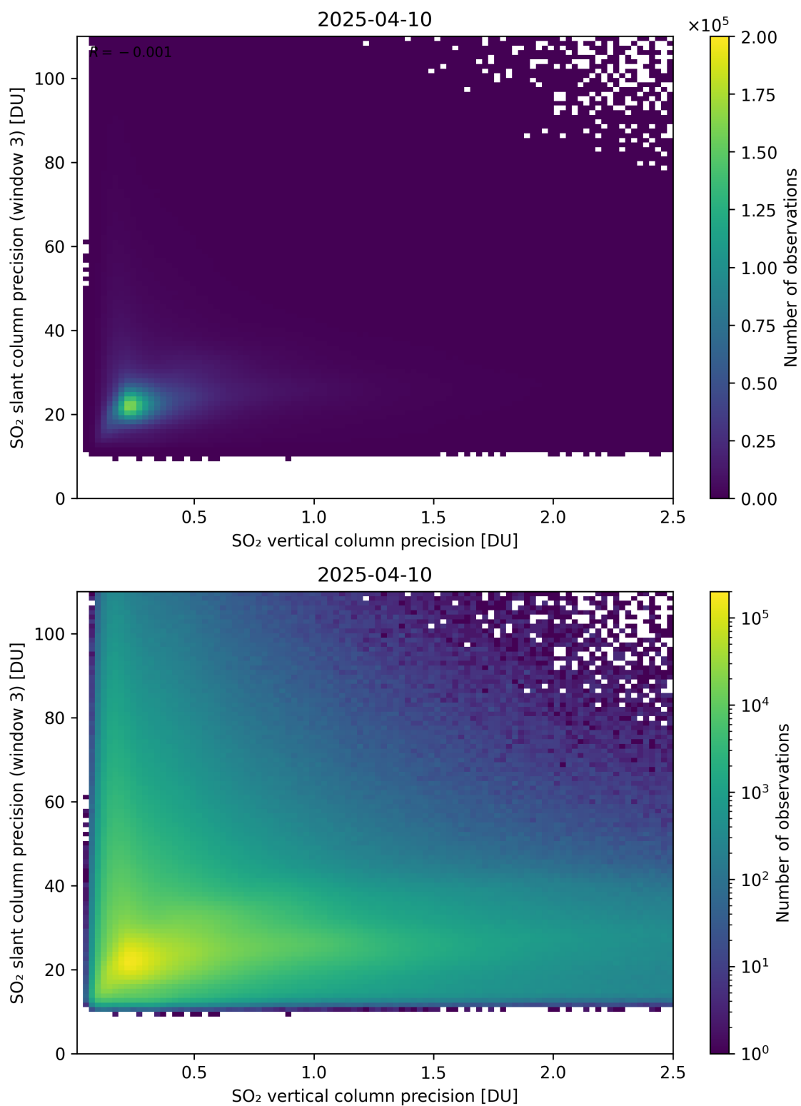
Figure 345: Scatter density plot of “SO 2 vertical column precision” against “SO 2 slant column precision (window 3)” for 2025-04-09 to 2025-04-11.
