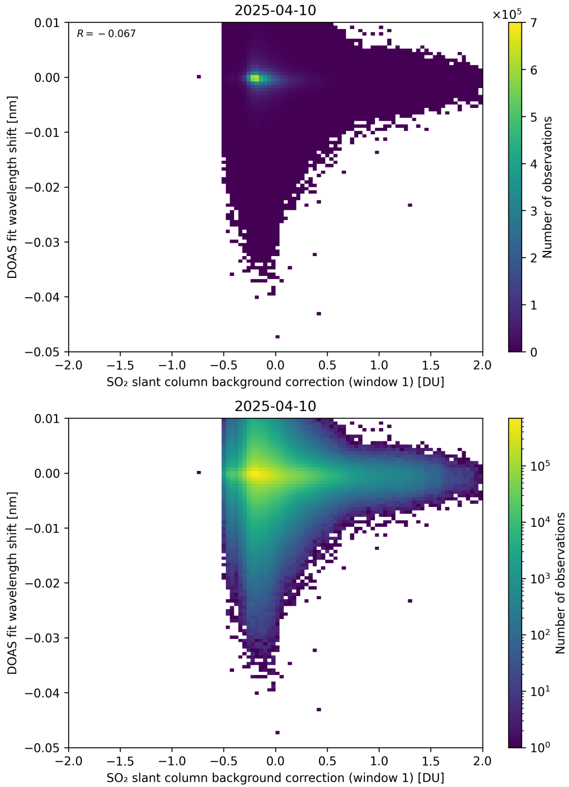
Figure 111: Scatter density plot of “SO 2 slant column background correction (window 1)” against “DOAS fit wavelength shift” for 2025-04-09 to 2025-04-11.
