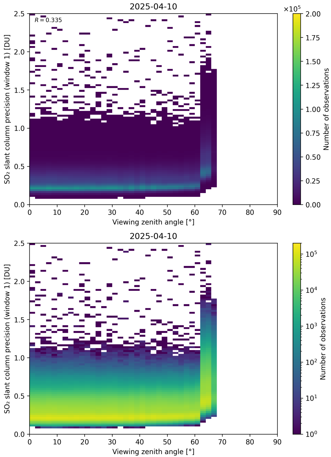
Figure 377: Scatter density plot of “Viewing zenith angle” against “SO 2 slant column precision (window 1)” for 2025-04-09 to 2025-04-11.
