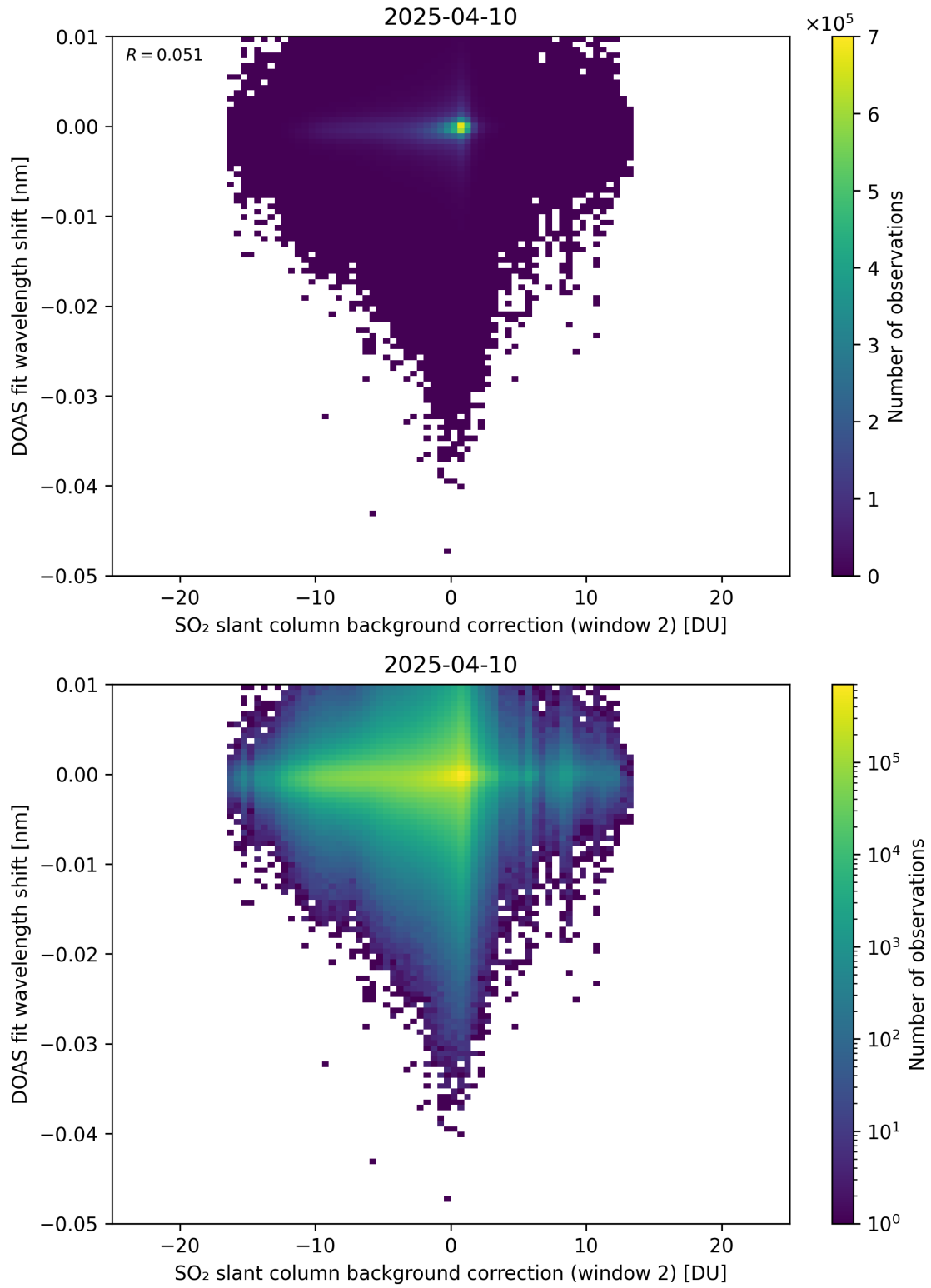
Figure 123: Scatter density plot of “SO 2 slant column background correction (window 2)” against “DOAS fit wavelength shift” for 2025-04-09 to 2025-04-11.
