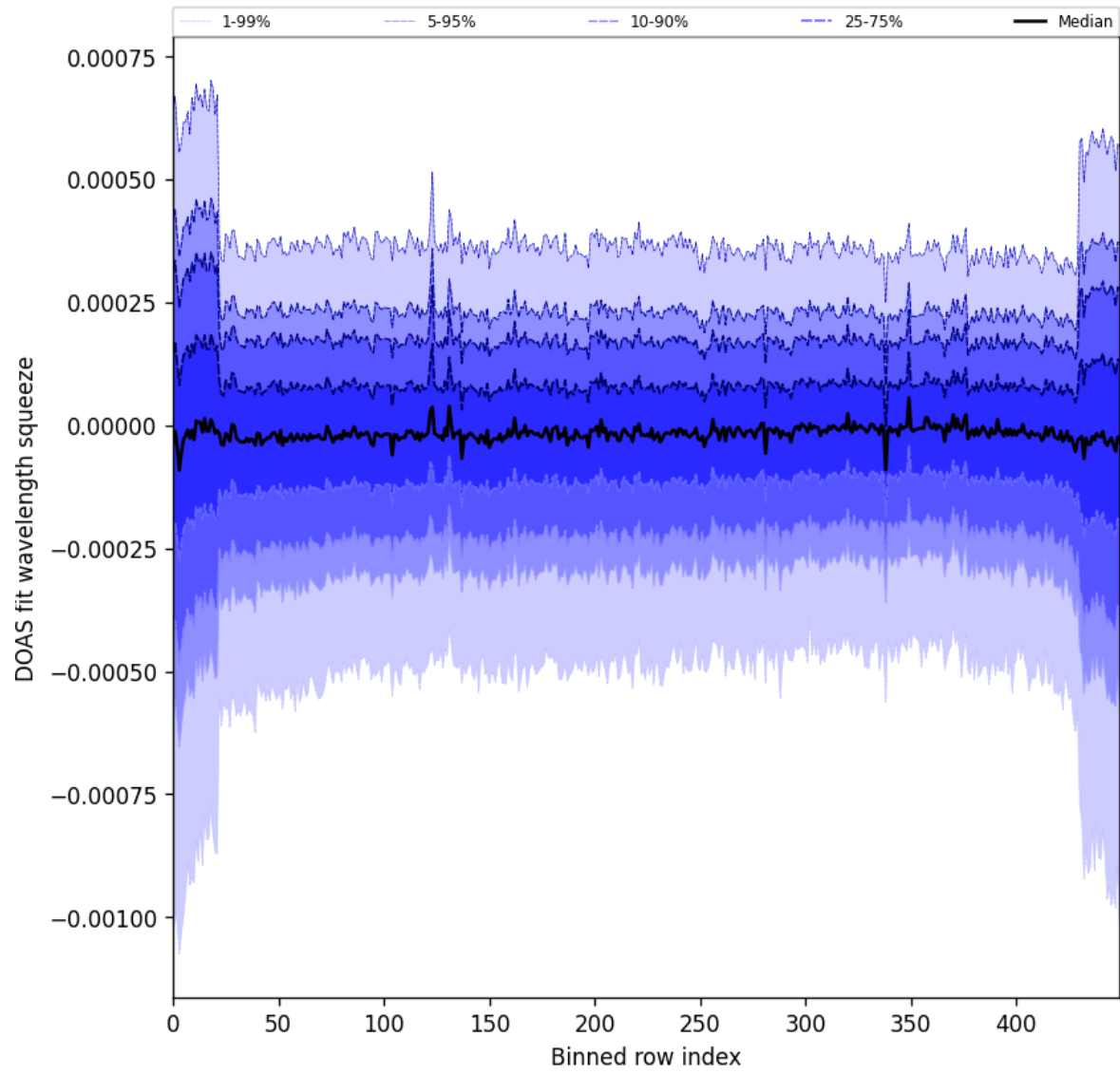
Figure 103: Along track statistics of “DOAS fit wavelength squeeze” for 2025-04-09 to 2025-04-11
