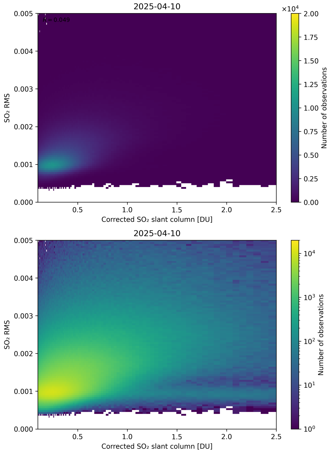
Figure 231: Scatter density plot of “Corrected SO 2 slant column” against “SO 2 RMS” for 2025-04-09 to 2025-04-11.
