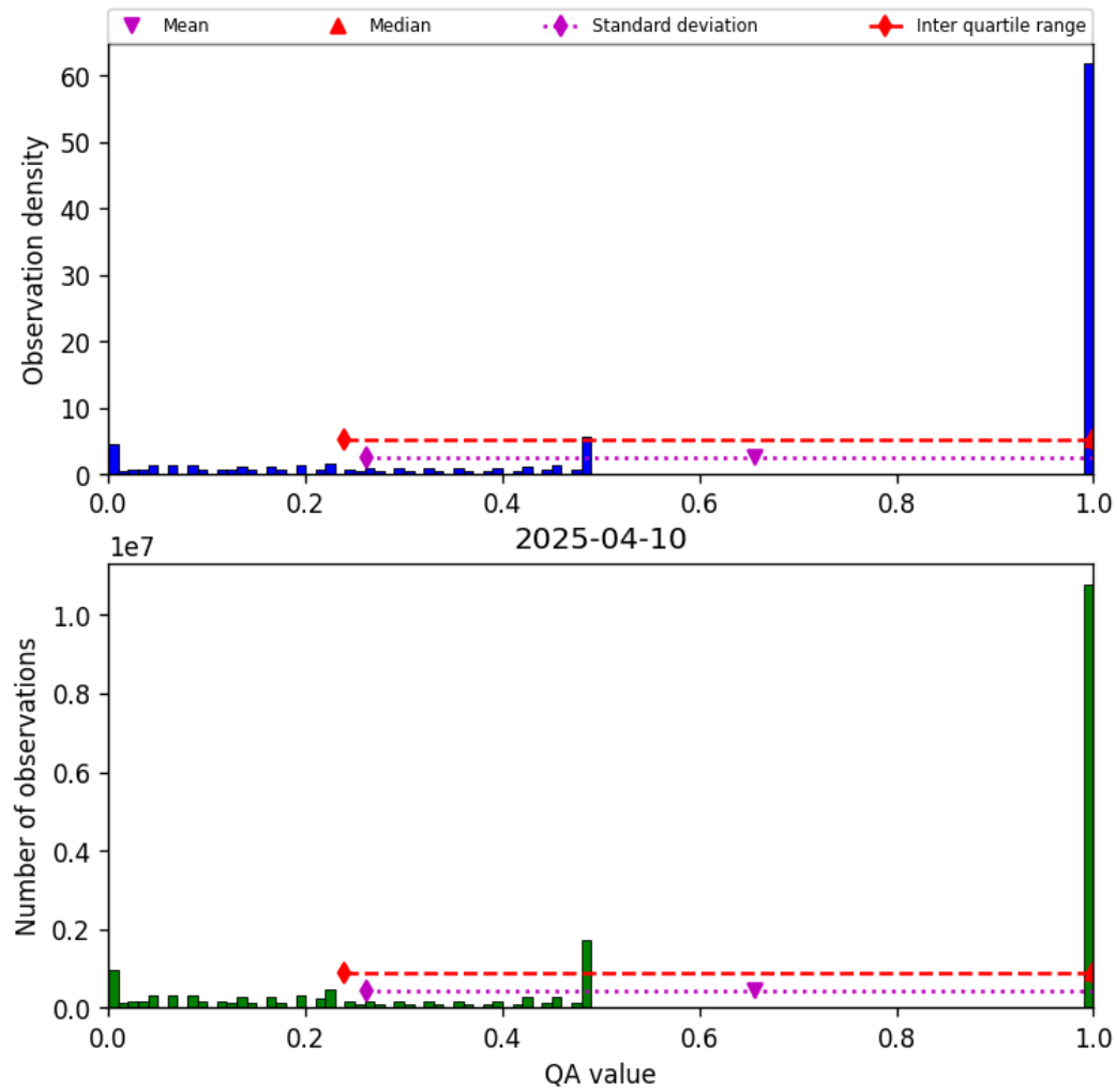
Figure 57: Histogram of “QA value” for 2025-04-09 to 2025-04-11
