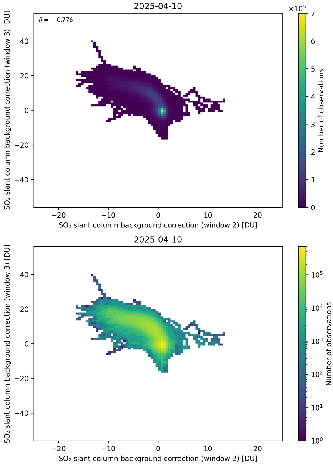
Figure 122: Scatter density plot of “SO 2 slant column background correction (window 2)” against “SO 2 slant column background correction (window 3)” for 2025-04-09 to 2025-04-11.
