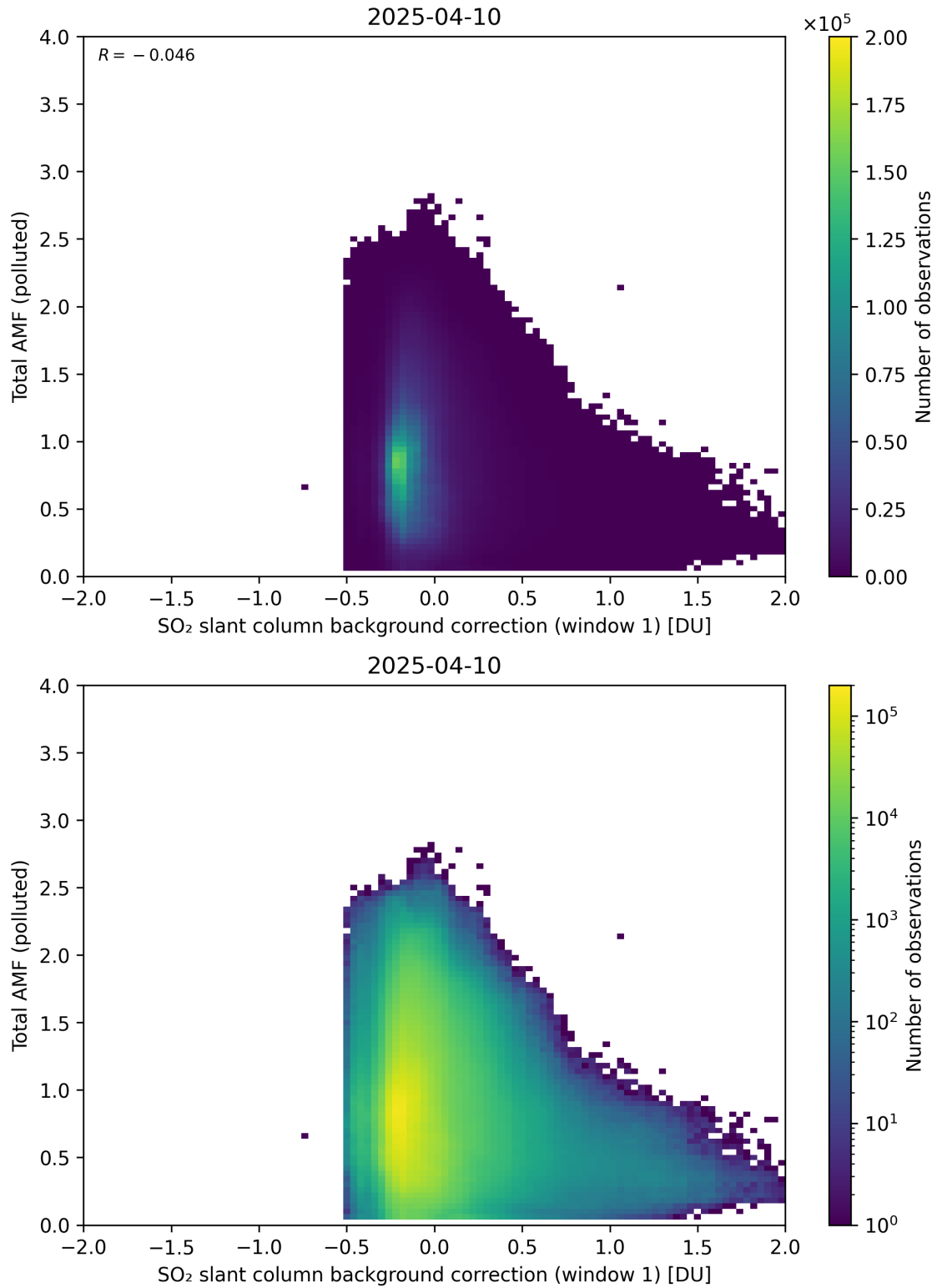
Figure 120: Scatter density plot of “SO 2 slant column background correction (window 1)” against “Total AMF (polluted)” for 2025-04-09 to 2025-04-11.
