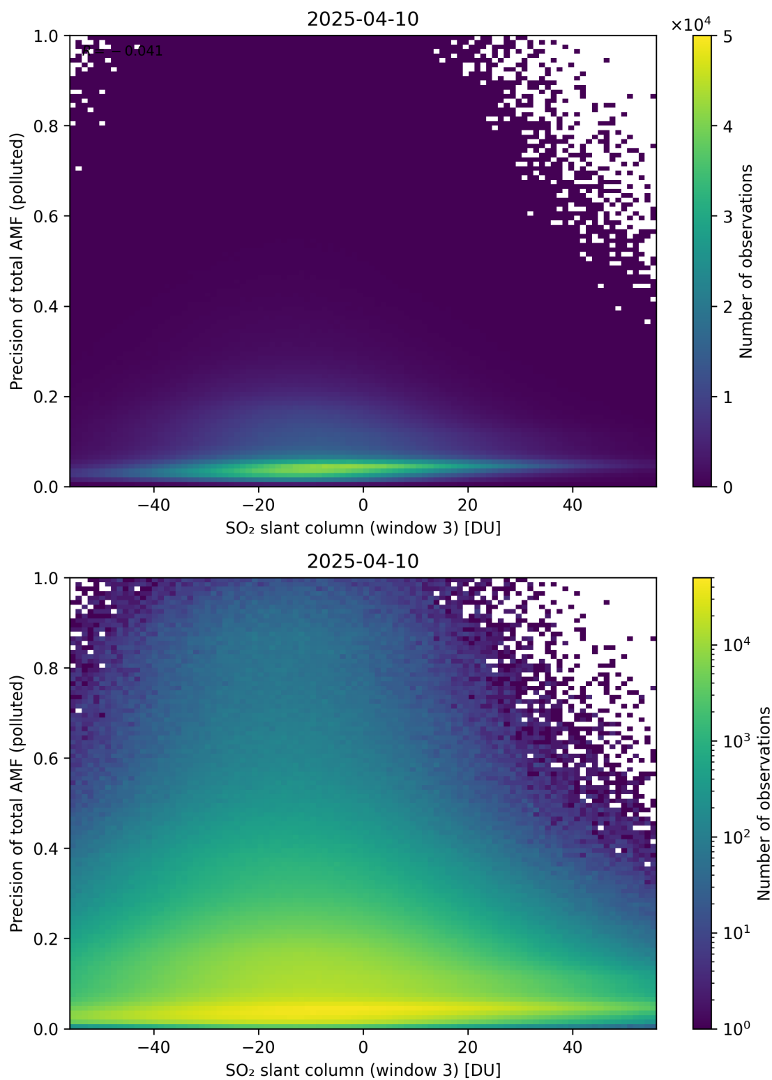
Figure 319: Scatter density plot of “SO 2 slant column (window 3)” against “Precision of total AMF (polluted)” for 2025-04-09 to 2025-04-11.
