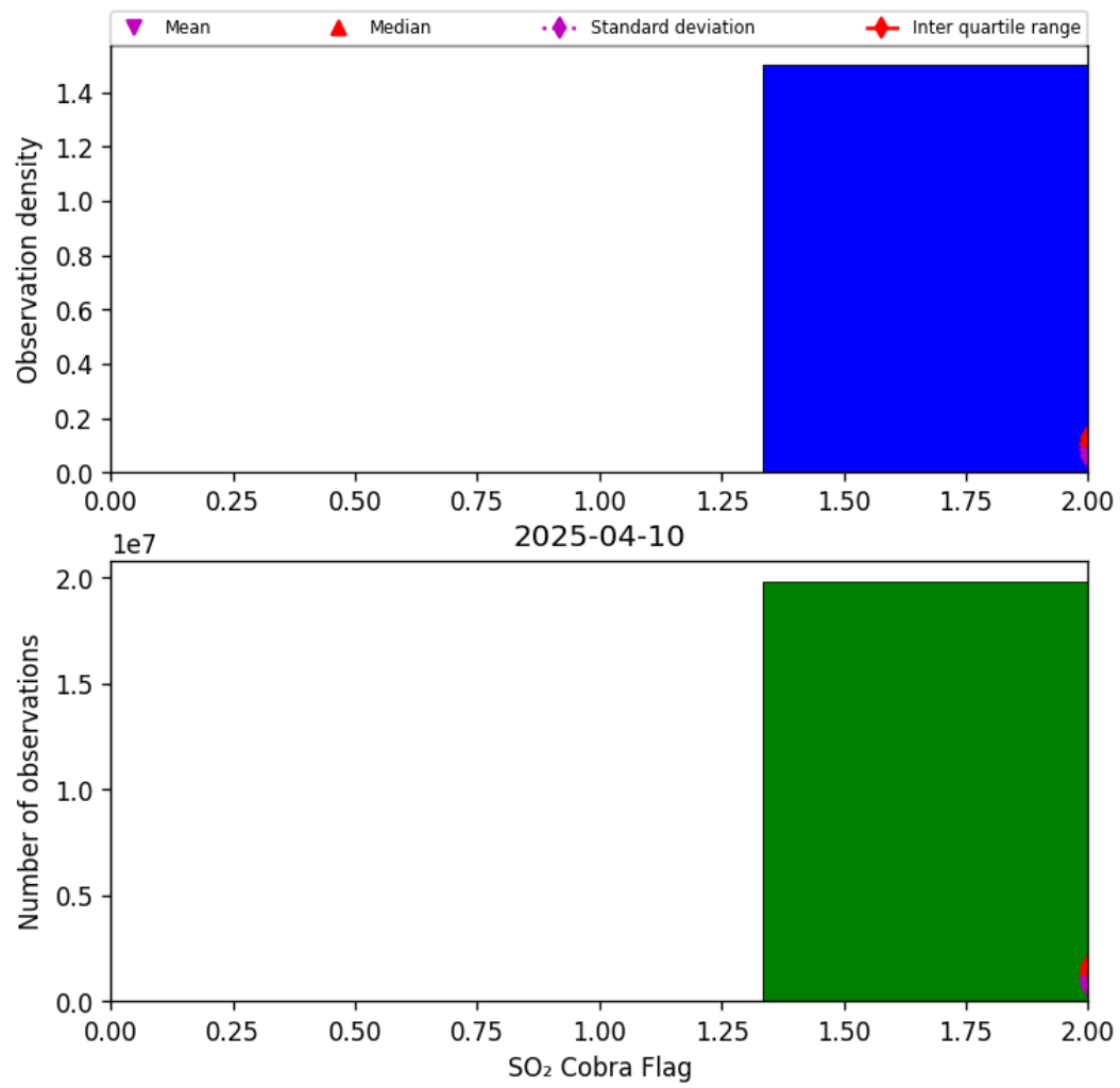
Figure 75: Histogram of “SO 2 Cobra Flag” for 2025-04-09 to 2025-04-11
