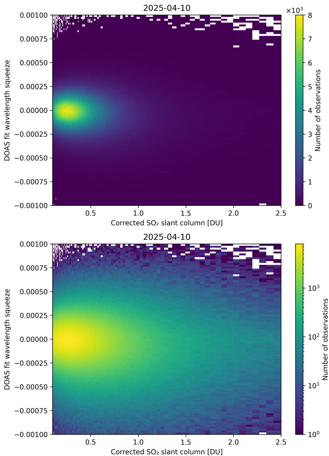
Figure 230: Scatter density plot of “Corrected SO 2 slant column” against “DOAS fit wavelength squeeze” for 2025-04-09 to 2025-04-11.
