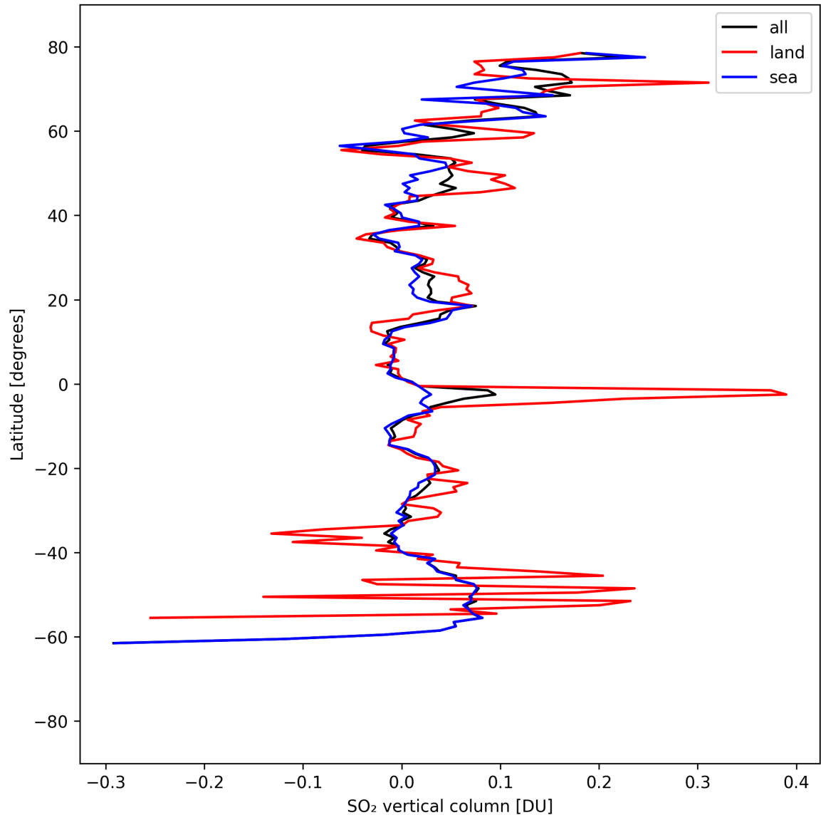
Figure 32: Zonal average of “SO 2 vertical column” for 2025-04-09 to 2025-04-11.
