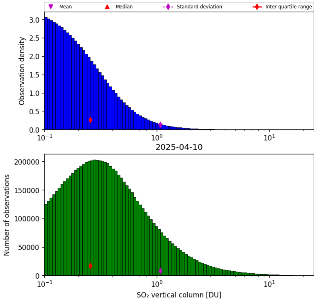
Figure 58: Histogram of “SO 2 vertical column” for 2025-04-09 to 2025-04-11
