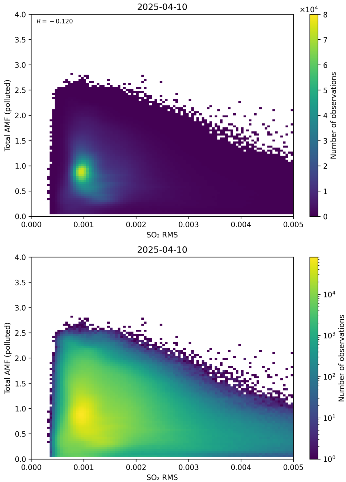
Figure 148: Scatter density plot of “SO 2 RMS” against “Total AMF (polluted)” for 2025-04-09 to 2025-04-11.
