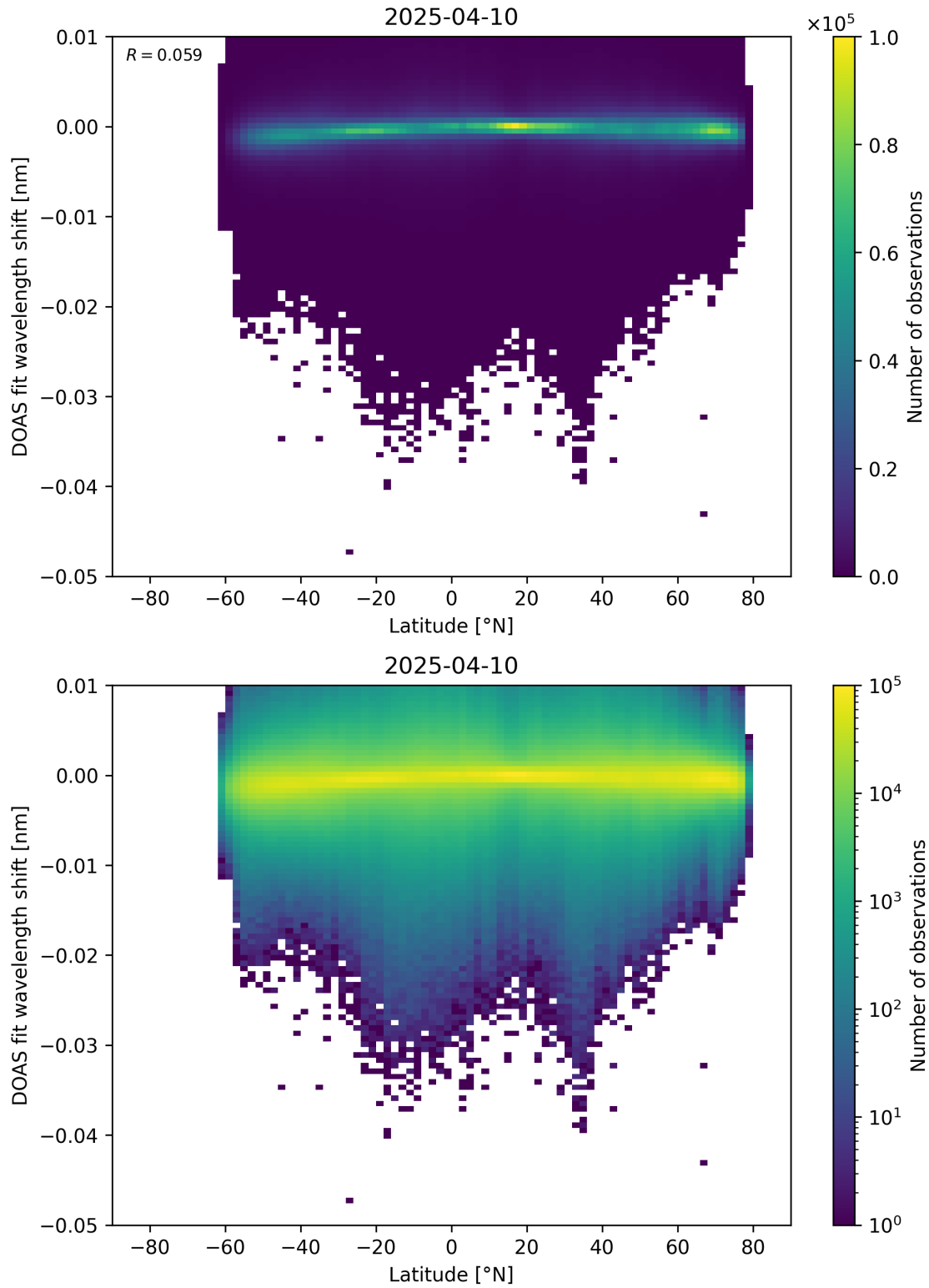
Figure 153: Scatter density plot of “Latitude” against “DOAS fit wavelength shift” for 2025-04-09 to 2025-04-11.
