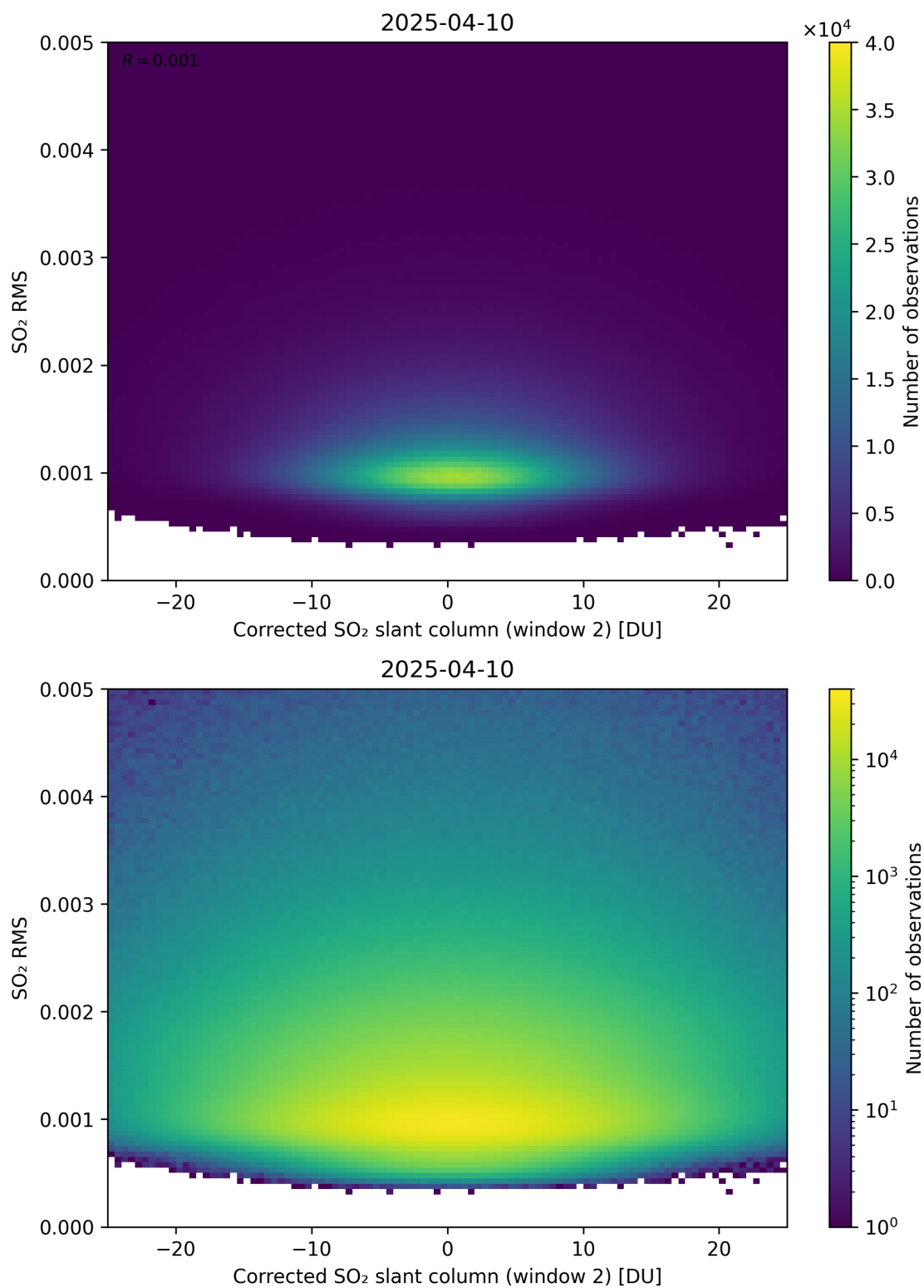
Figure 248: Scatter density plot of “Corrected SO 2 slant column (window 2)” against “SO 2 RMS” for 2025-04-09 to 2025-04-11.
