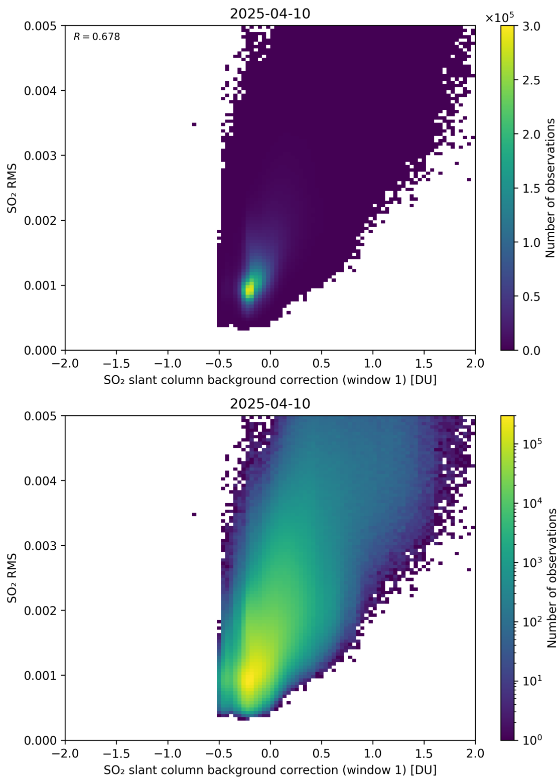
Figure 113: Scatter density plot of “SO 2 slant column background correction (window 1)” against “SO 2 RMS” for 2025-04-09 to 2025-04-11.
