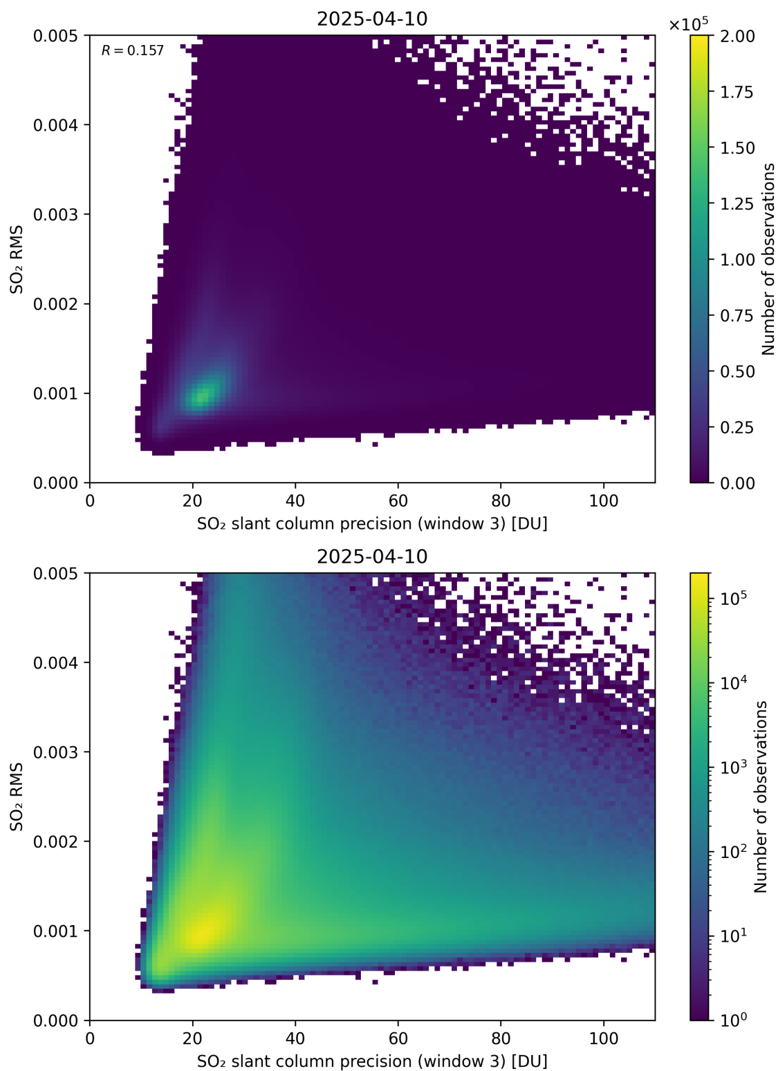
Figure 310: Scatter density plot of “SO 2 slant column precision (window 3)” against “SO 2 RMS” for 2025-04-09 to 2025-04-11.
