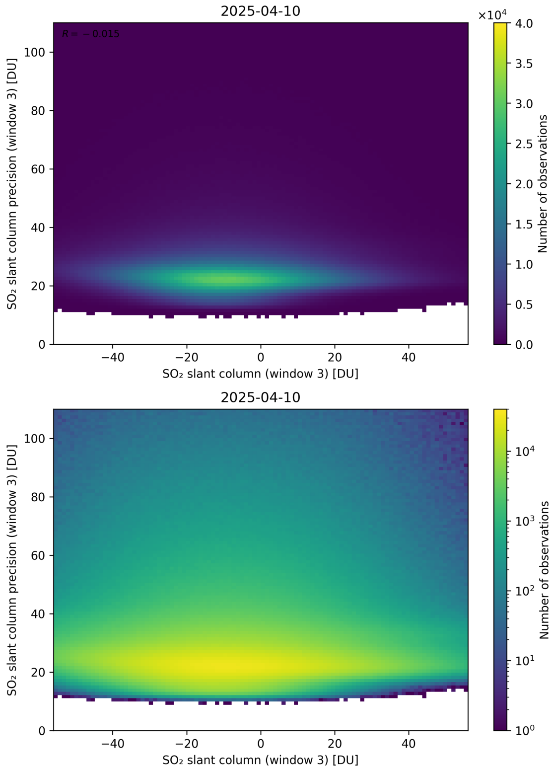
Figure 317: Scatter density plot of “SO 2 slant column (window 3)” against “SO 2 slant column precision (window 3)” for 2025-04-09 to 2025-04-11.
