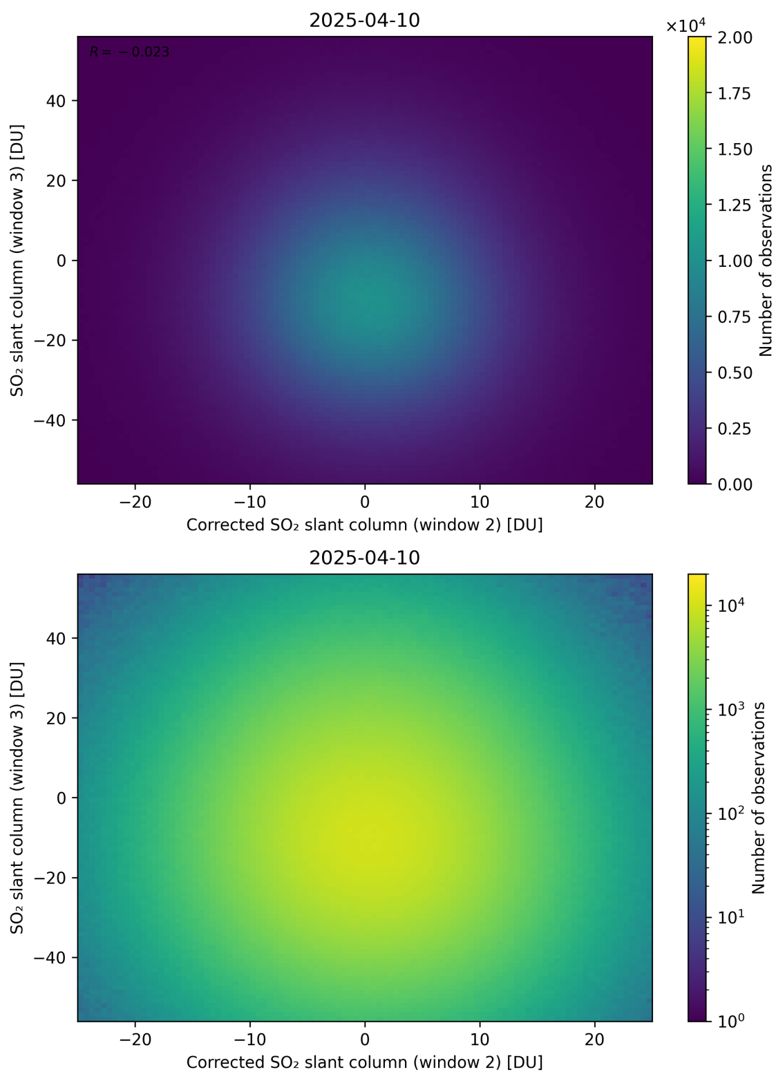
Figure 251: Scatter density plot of “Corrected SO 2 slant column (window 2)” against “SO 2 slant column (window 3)” for 2025-04-09 to 2025-04-11.
