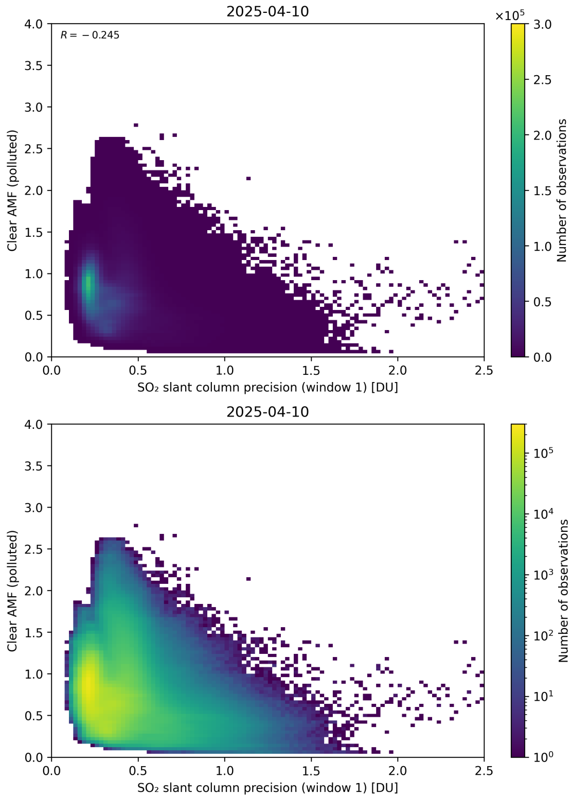
Figure 274: Scatter density plot of “SO 2 slant column precision (window 1)” against “Clear AMF (polluted)” for 2025-04-09 to 2025-04-11.
