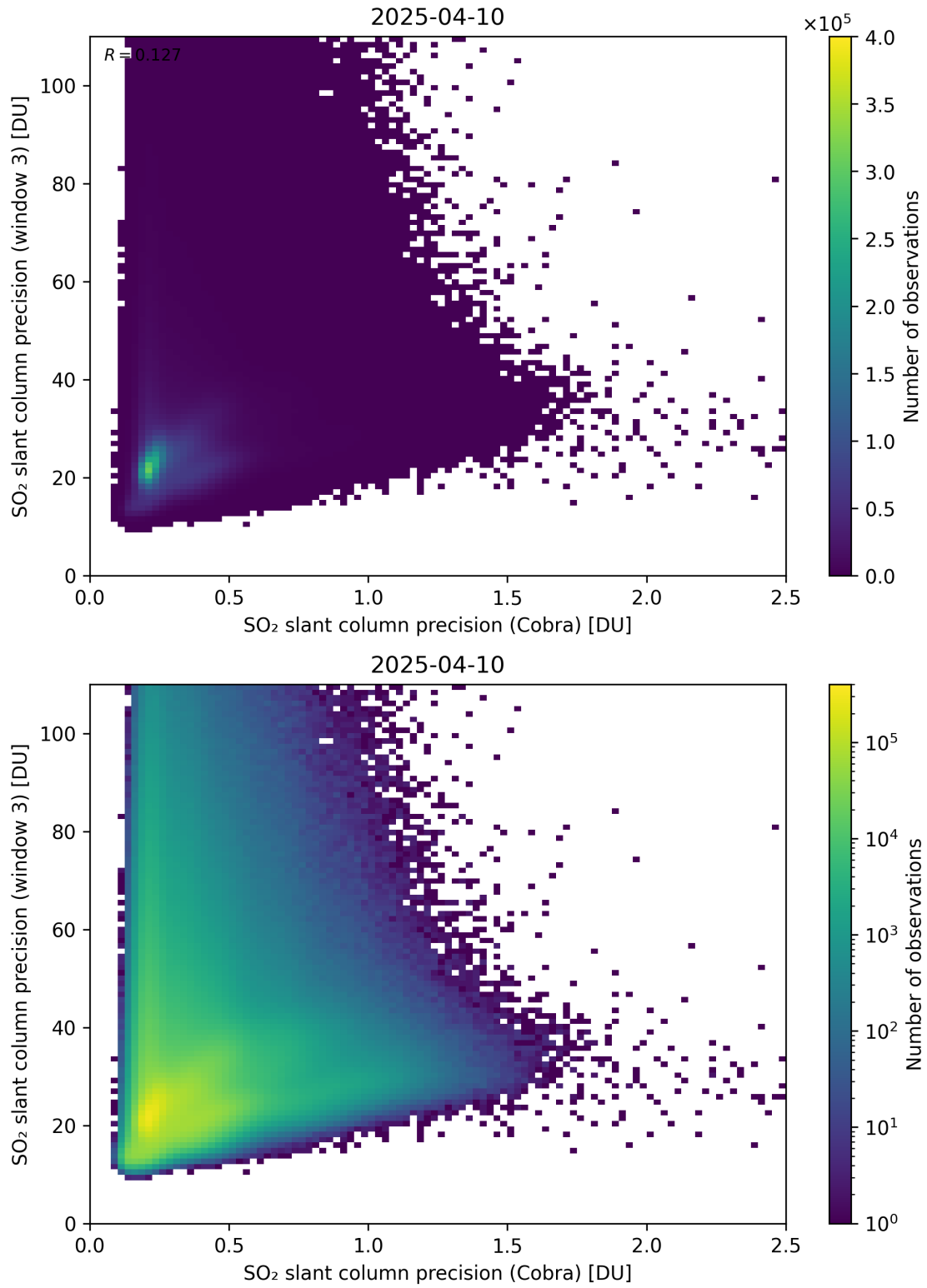
Figure 212: Scatter density plot of “SO 2 slant column precision (Cobra)” against “SO 2 slant column precision (window 3)” for 2025-04-09 to 2025-04-11.
