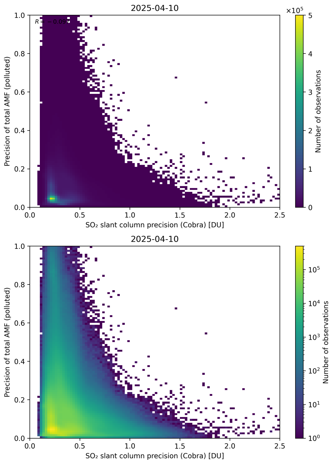
Figure 214: Scatter density plot of “SO 2 slant column precision (Cobra)” against “Precision of total AMF (polluted)” for 2025-04-09 to 2025-04-11.
