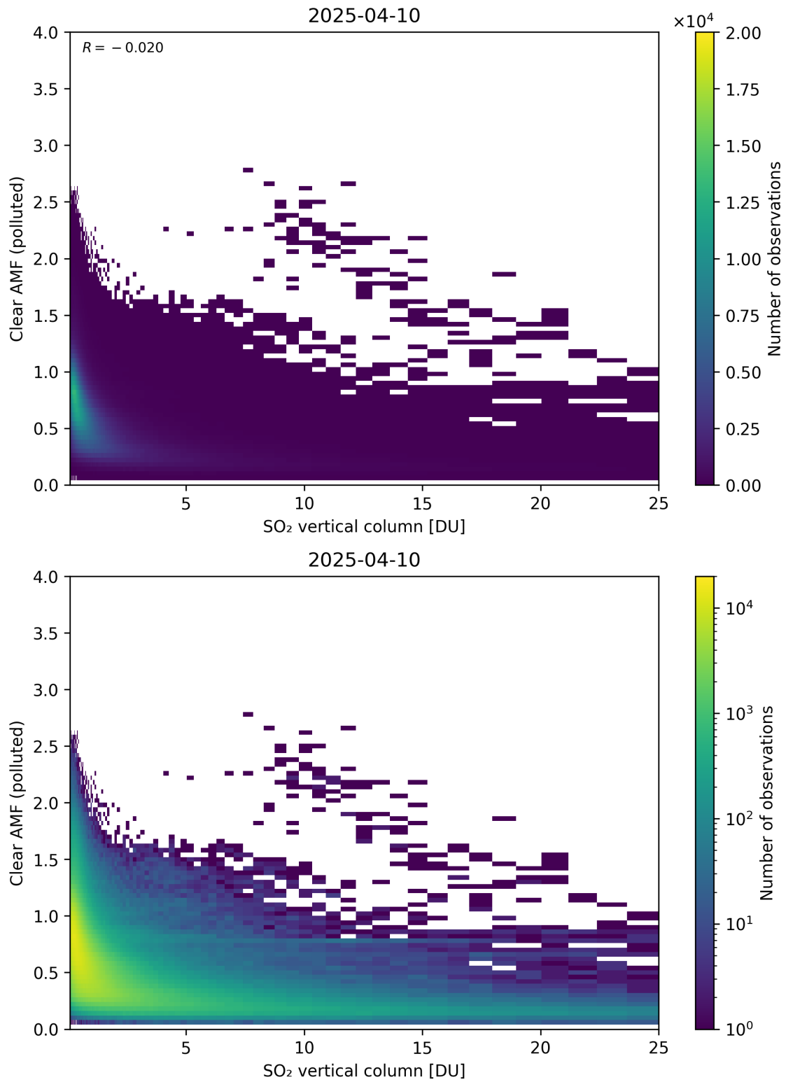
Figure 348: Scatter density plot of “SO 2 vertical column” against “Clear AMF (polluted)” for 2025-04-09 to 2025-04-11.
