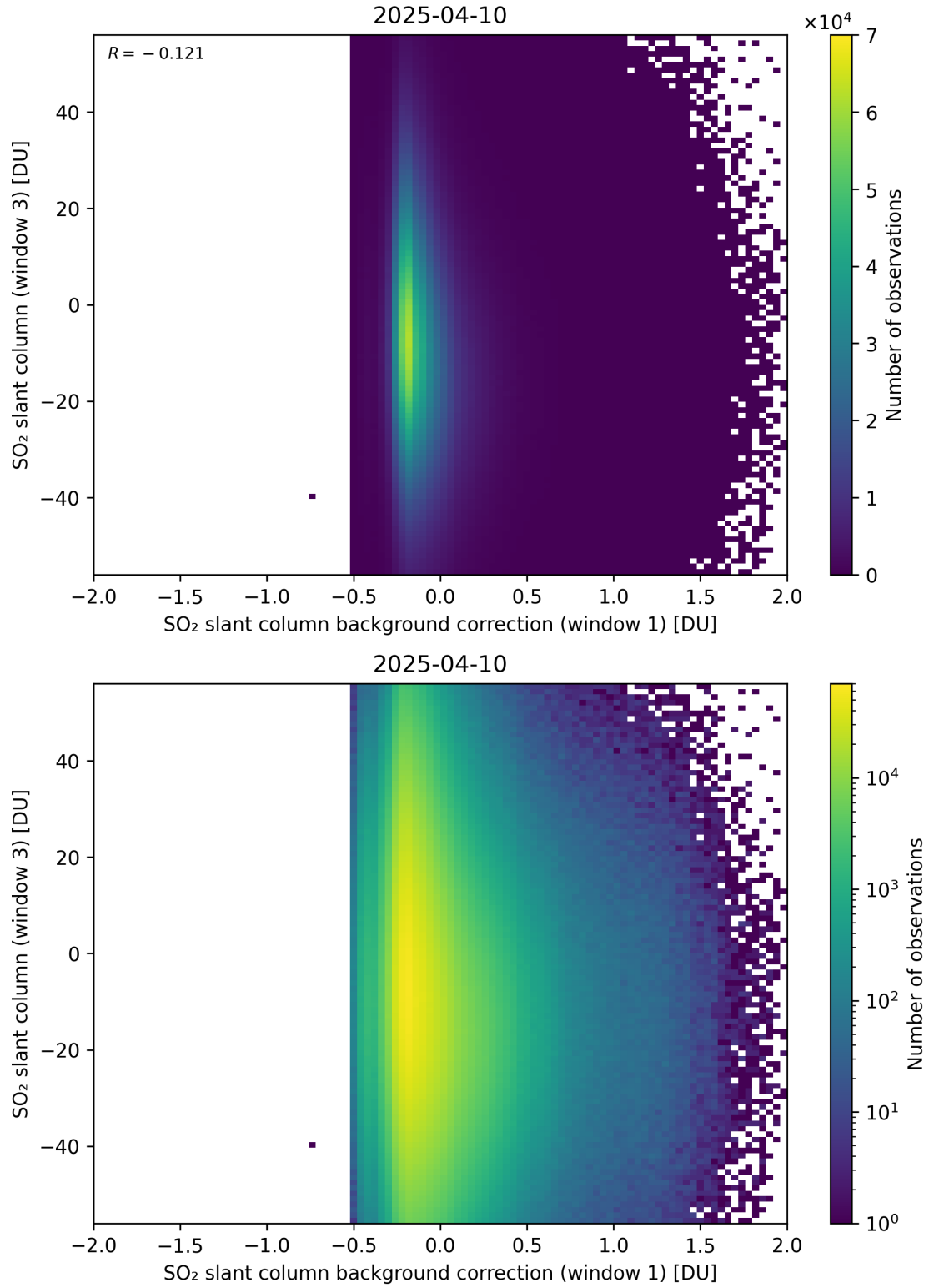
Figure 118: Scatter density plot of “SO 2 slant column background correction (window 1)” against “SO 2 slant column (window 3)” for 2025-04-09 to 2025-04-11.
