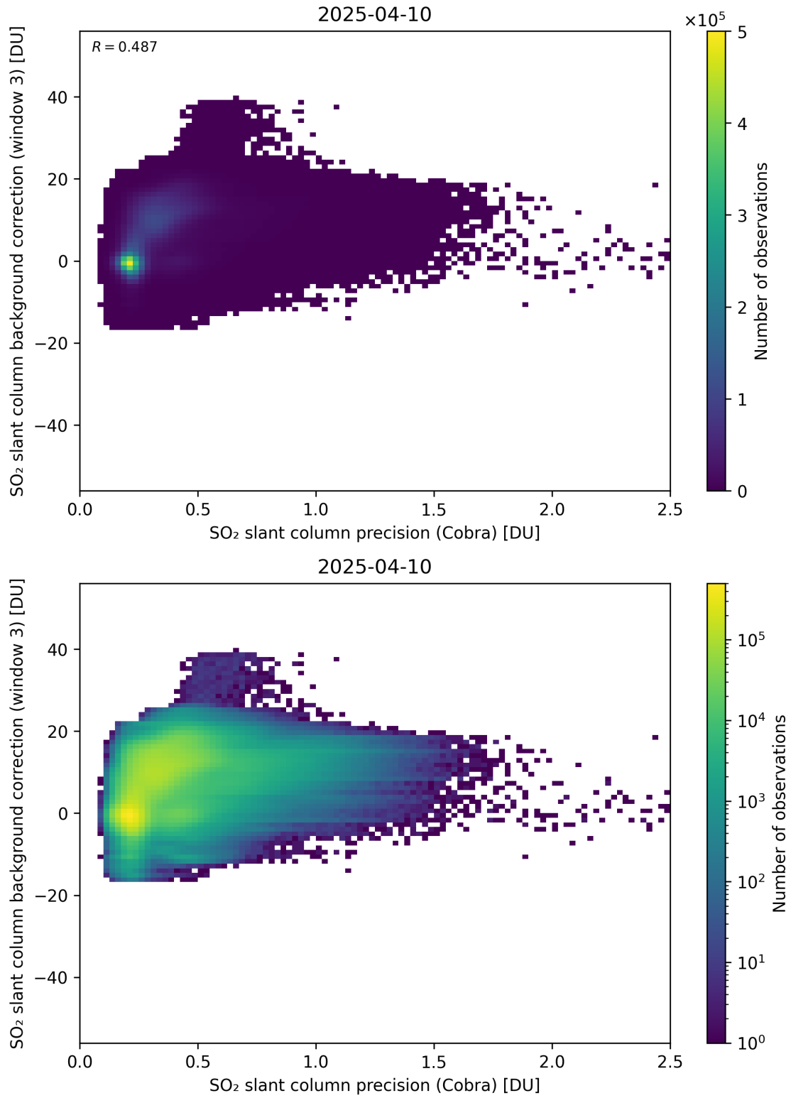
Figure 201: Scatter density plot of “SO 2 slant column precision (Cobra)” against “SO 2 slant column background correction (window 3)” for 2025-04-09 to 2025-04-11.
