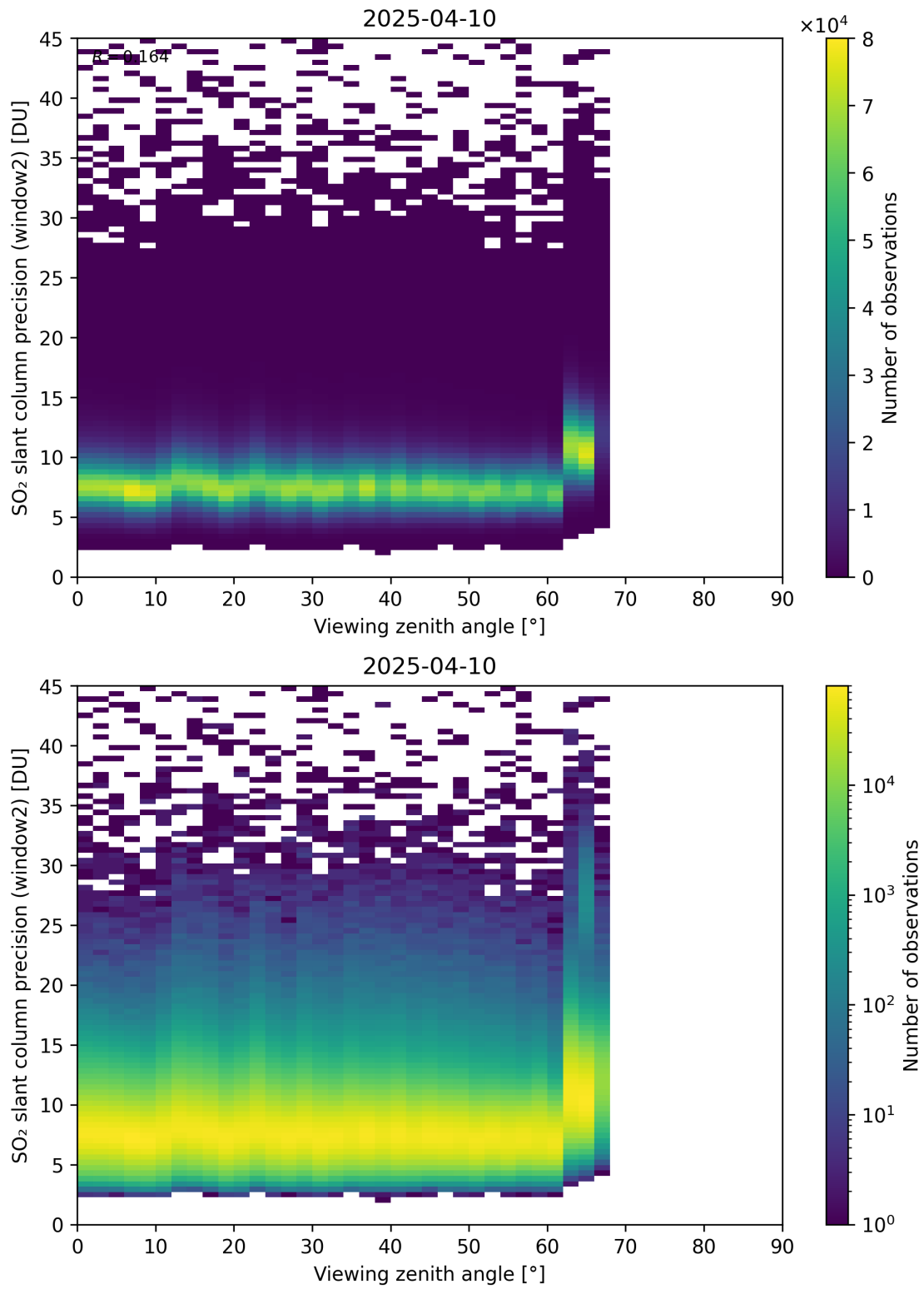
Figure 378: Scatter density plot of “Viewing zenith angle” against “SO 2 slant column precision (window2)” for 2025-04-09 to 2025-04-11.
