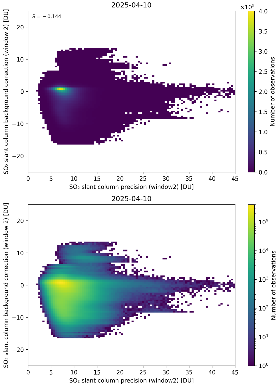
Figure 291: Scatter density plot of “SO 2 slant column precision (window2)” against “SO 2 slant column background correction (window 2)” for 2025-04-09 to 2025-04-11.
