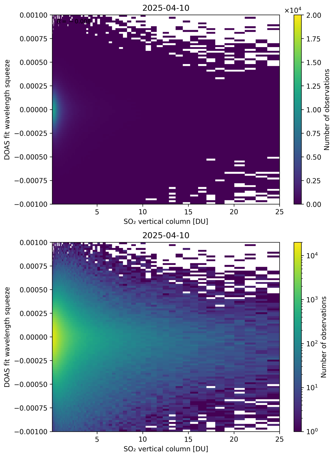
Figure 327: Scatter density plot of “SO 2 vertical column” against “DOAS fit wavelength squeeze” for 2025-04-09 to 2025-04-11.
