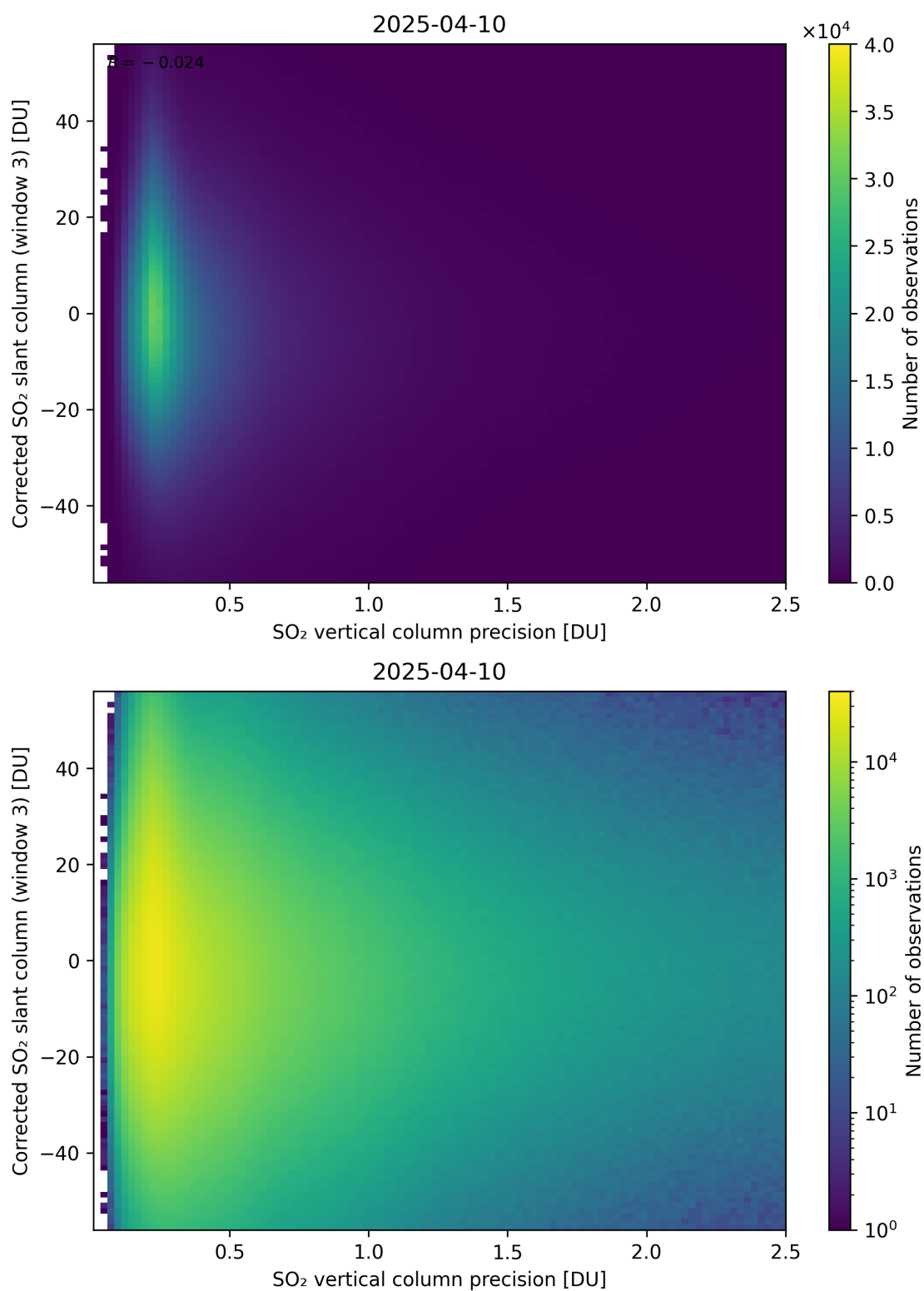
Figure 340: Scatter density plot of “SO 2 vertical column precision” against “Corrected SO 2 slant column (window 3)” for 2025-04-09 to 2025-04-11.
