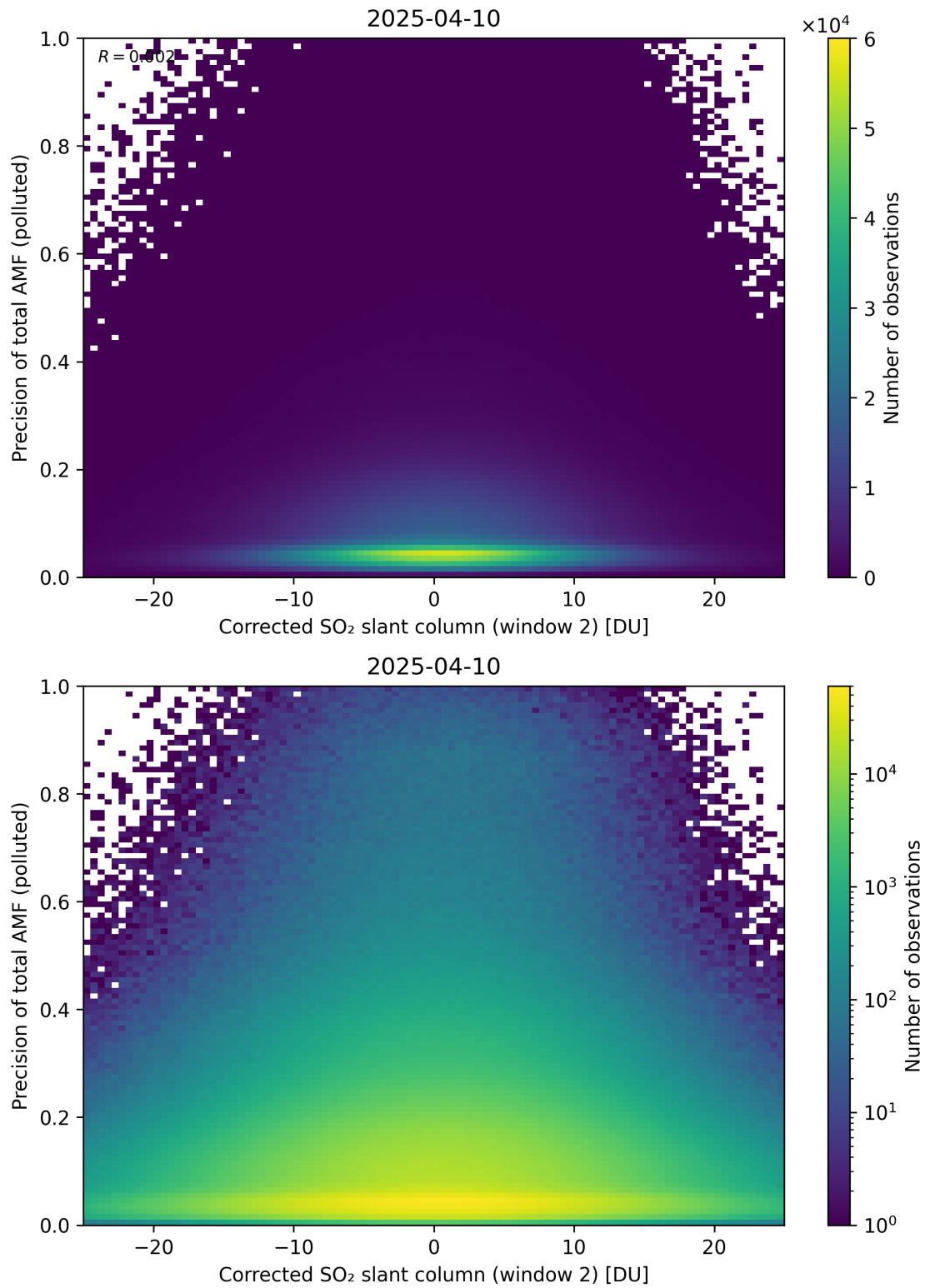
Figure 254: Scatter density plot of “Corrected SO 2 slant column (window 2)” against “Precision of total AMF (polluted)” for 2025-04-09 to 2025-04-11.
