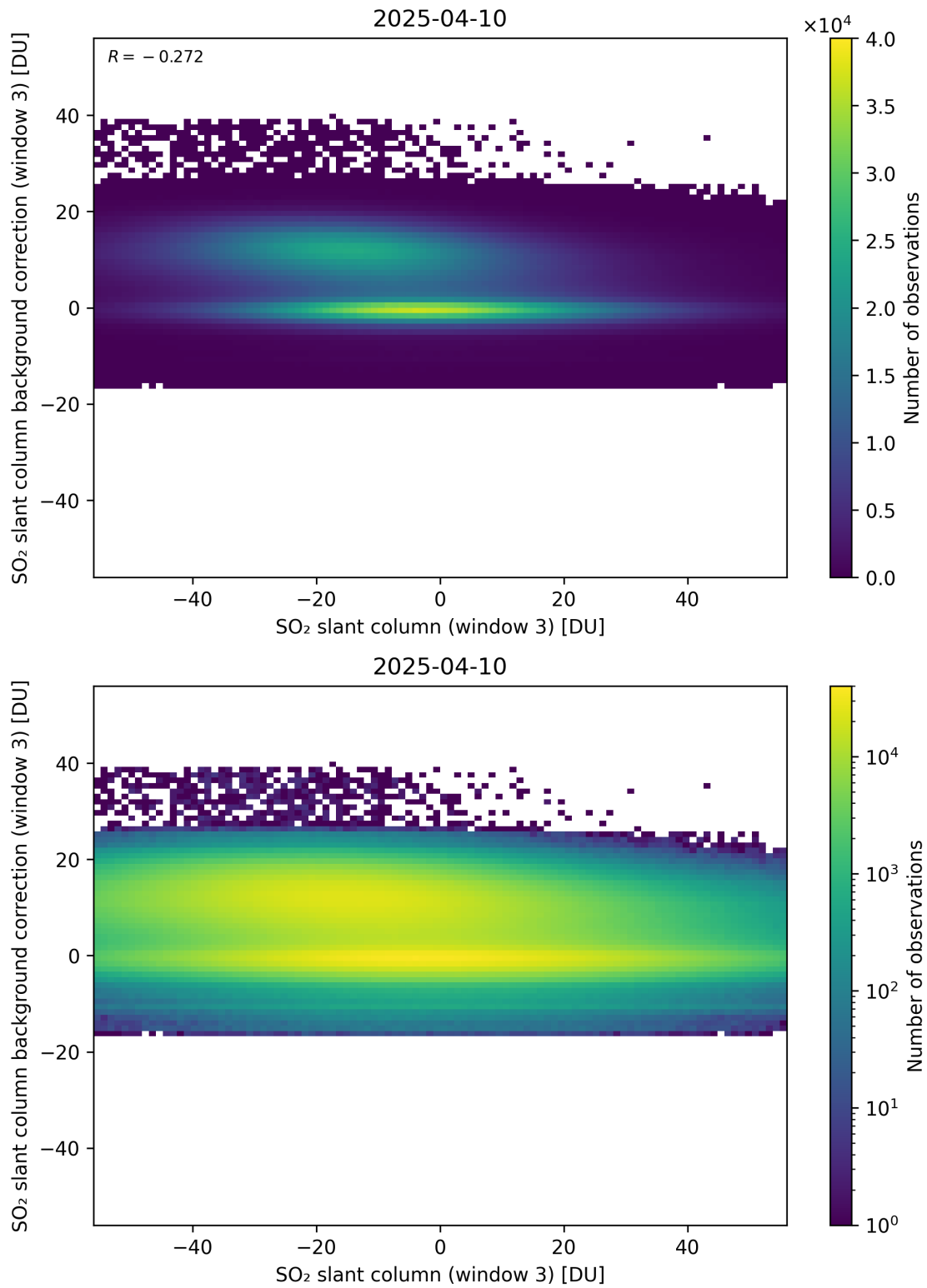
Figure 303: Scatter density plot of “SO 2 slant column (window 3)” against “SO 2 slant column background correction (window 3)” for 2025-04-09 to 2025-04-11.
