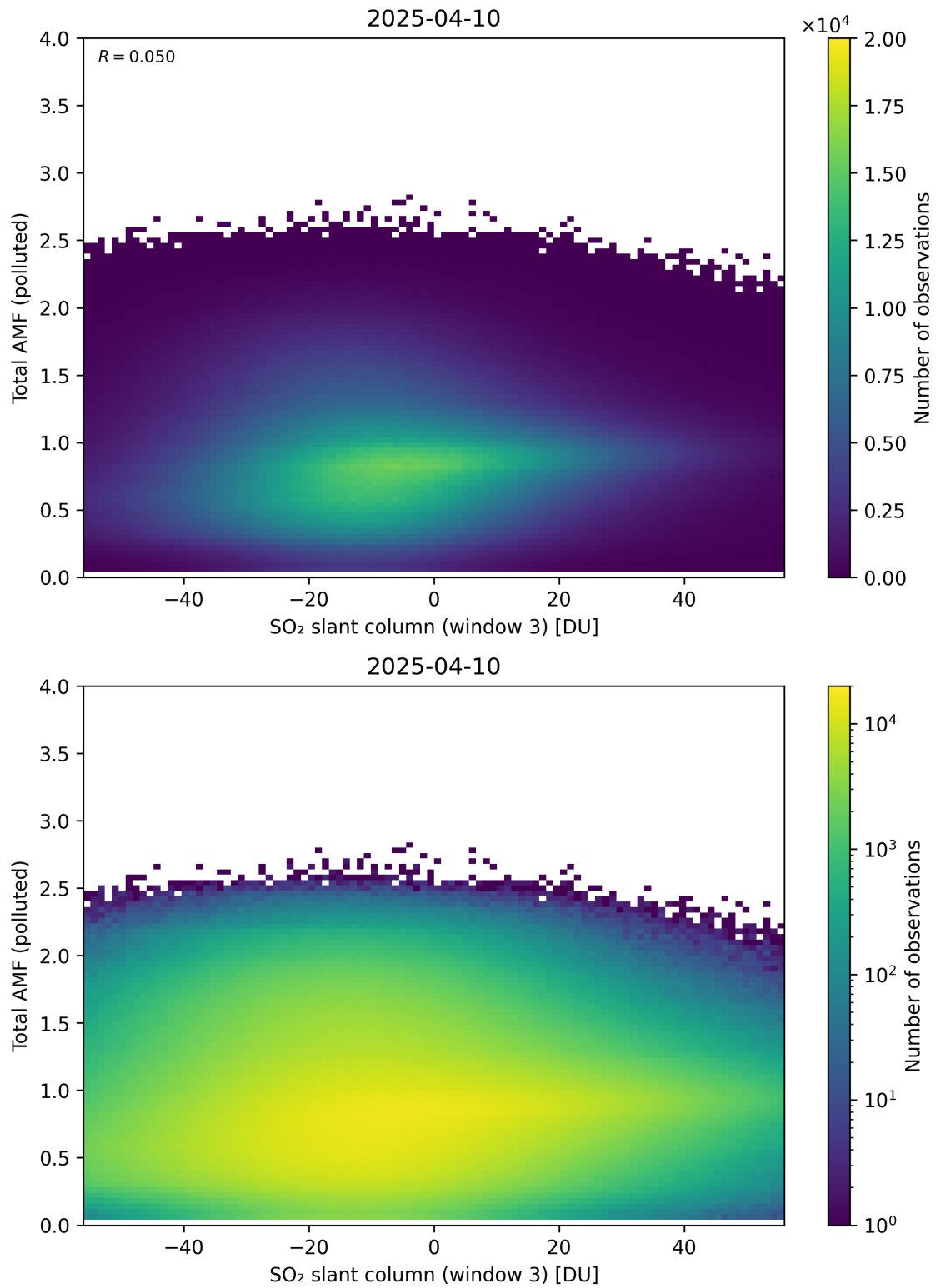
Figure 318: Scatter density plot of “SO 2 slant column (window 3)” against “Total AMF (polluted)” for 2025-04-09 to 2025-04-11.
