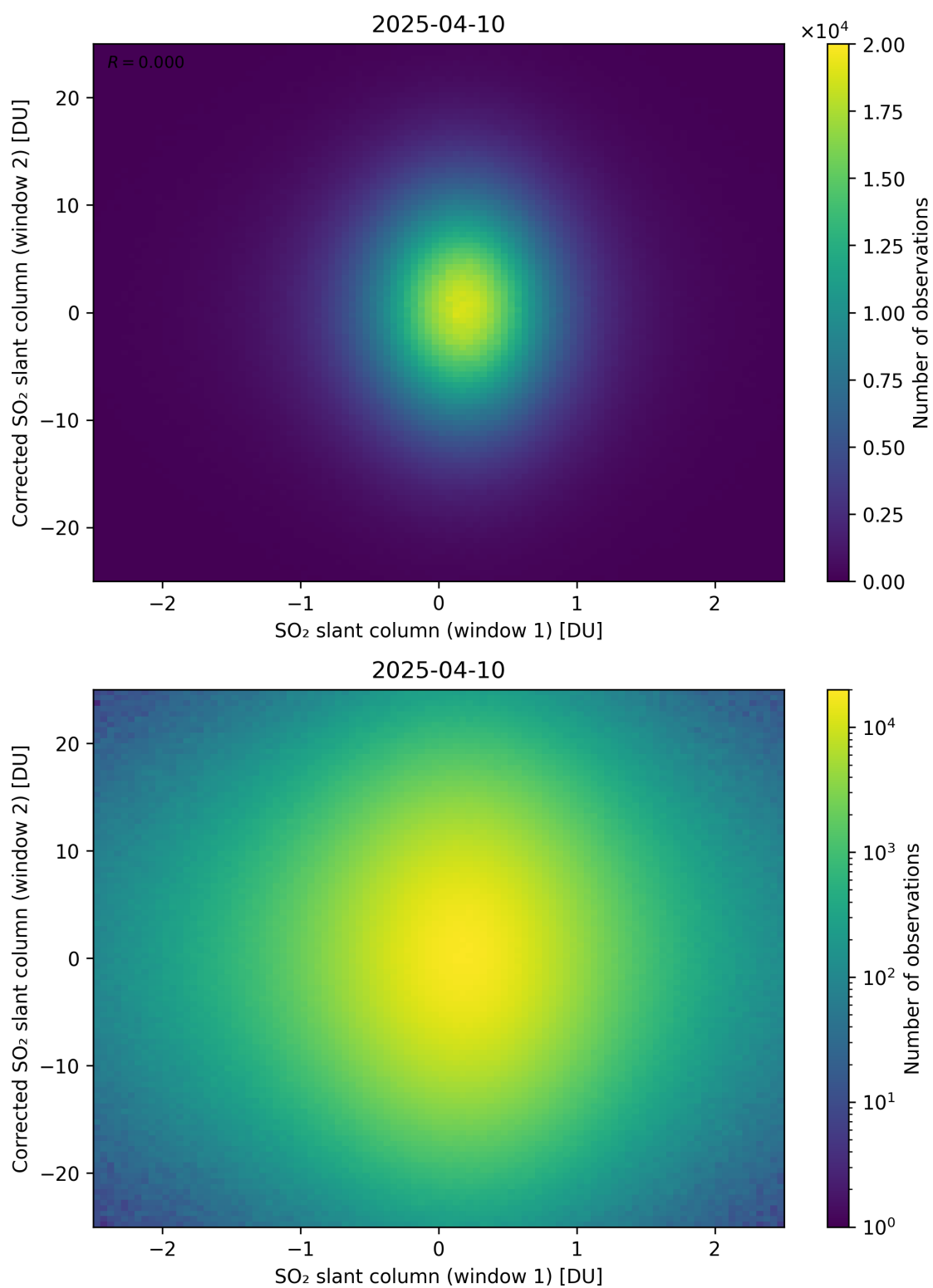
Figure 283: Scatter density plot of “SO 2 slant column (window 1)” against “Corrected SO 2 slant column (window 2)” for 2025-04-09 to 2025-04-11.
