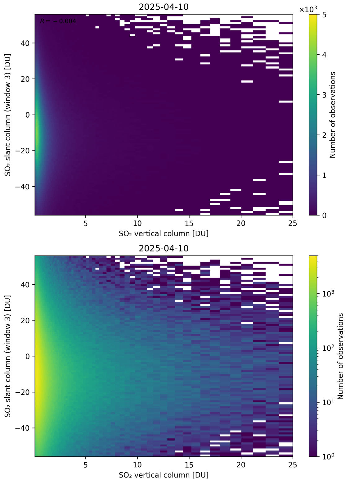
Figure 357: Scatter density plot of “SO 2 vertical column” against “SO 2 slant column (window 3)” for 2025-04-09 to 2025-04-11.
