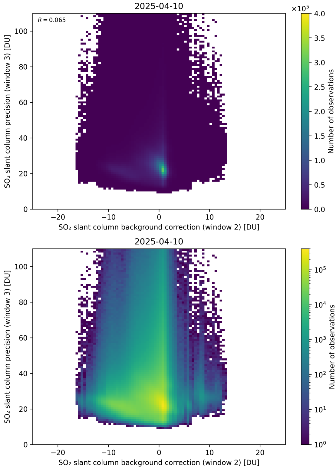
Figure 129: Scatter density plot of “SO 2 slant column background correction (window 2)” against “SO 2 slant column precision (window 3)” for 2025-04-09 to 2025-04-11.
