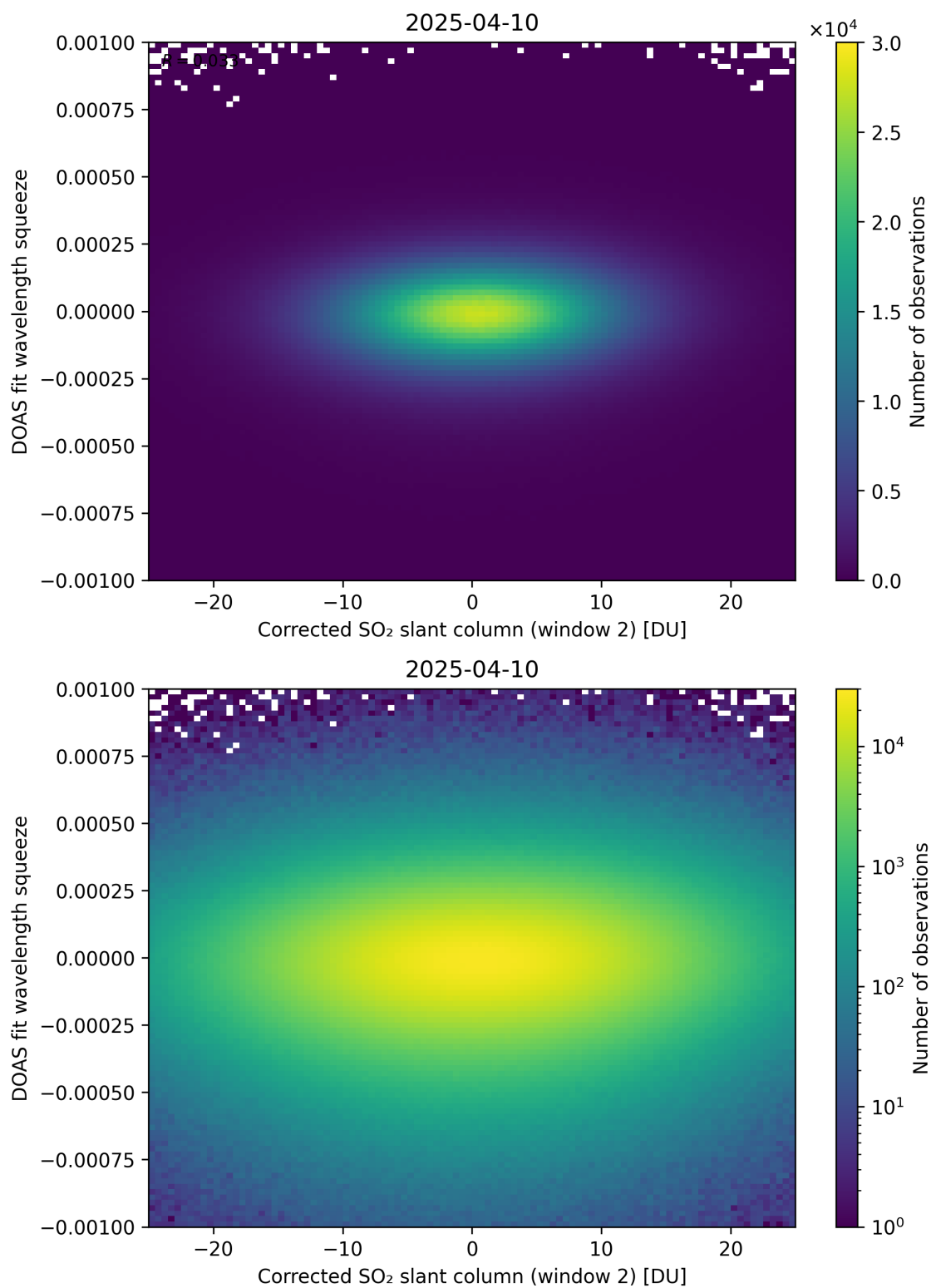
Figure 247: Scatter density plot of “Corrected SO 2 slant column (window 2)” against “DOAS fit wavelength squeeze” for 2025-04-09 to 2025-04-11.
