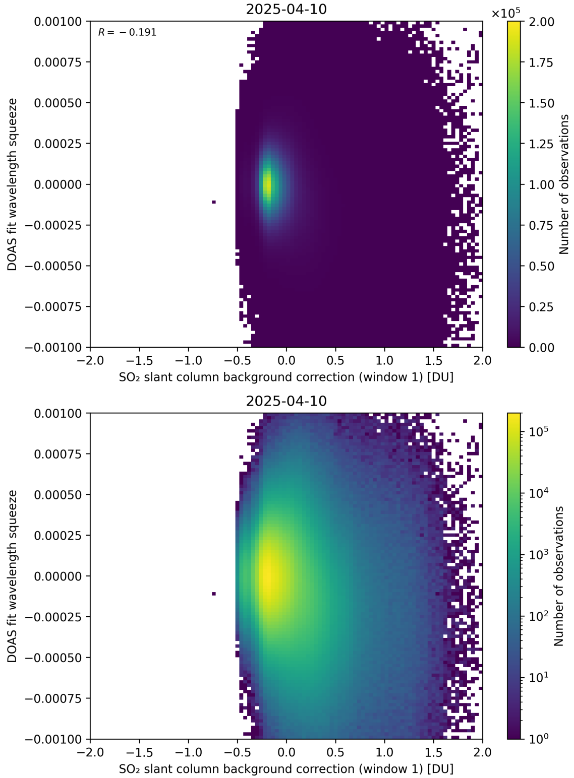
Figure 112: Scatter density plot of “SO 2 slant column background correction (window 1)” against “DOAS fit wavelength squeeze” for 2025-04-09 to 2025-04-11.
