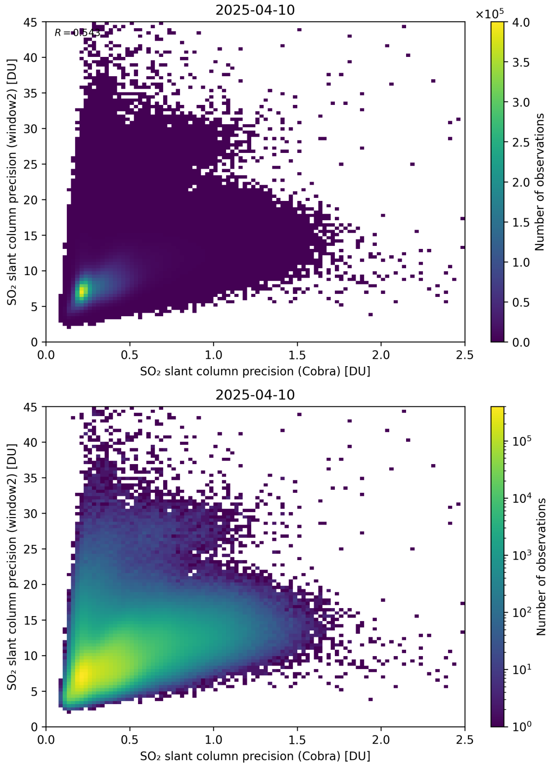
Figure 210: Scatter density plot of “SO 2 slant column precision (Cobra)” against “SO 2 slant column precision (window2)” for 2025-04-09 to 2025-04-11.
