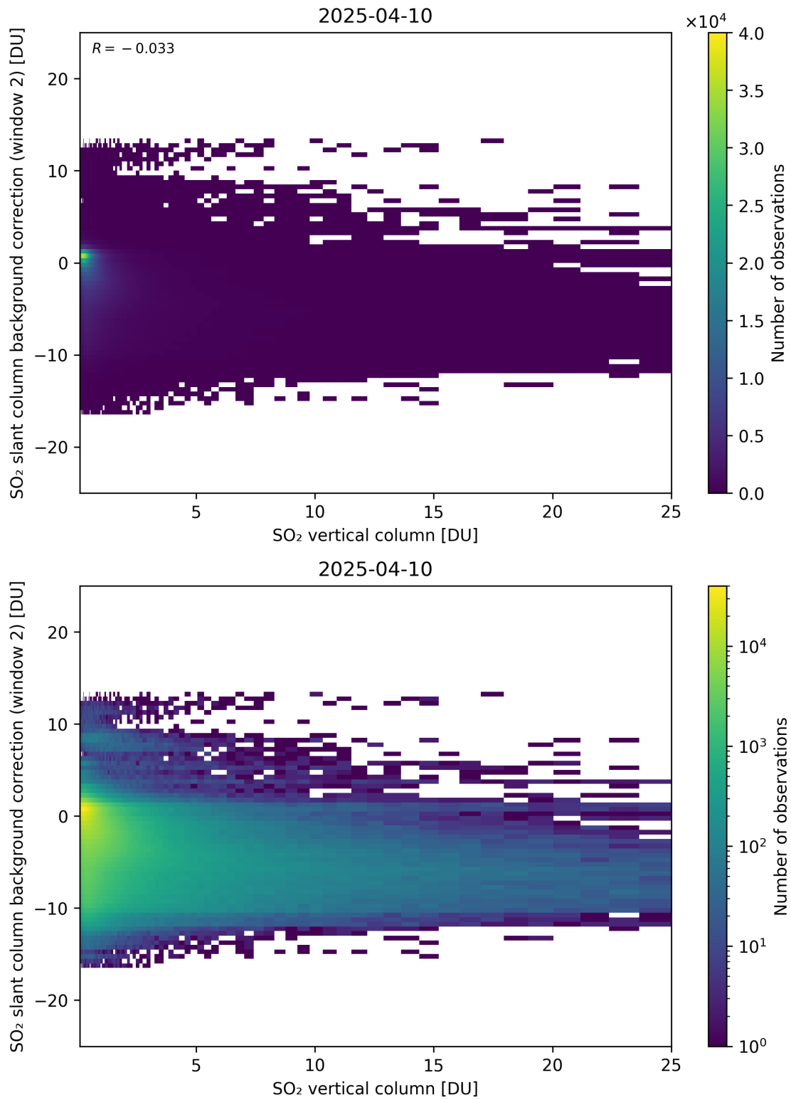
Figure 324: Scatter density plot of “SO 2 vertical column” against “SO 2 slant column background correction (window 2)” for 2025-04-09 to 2025-04-11.
