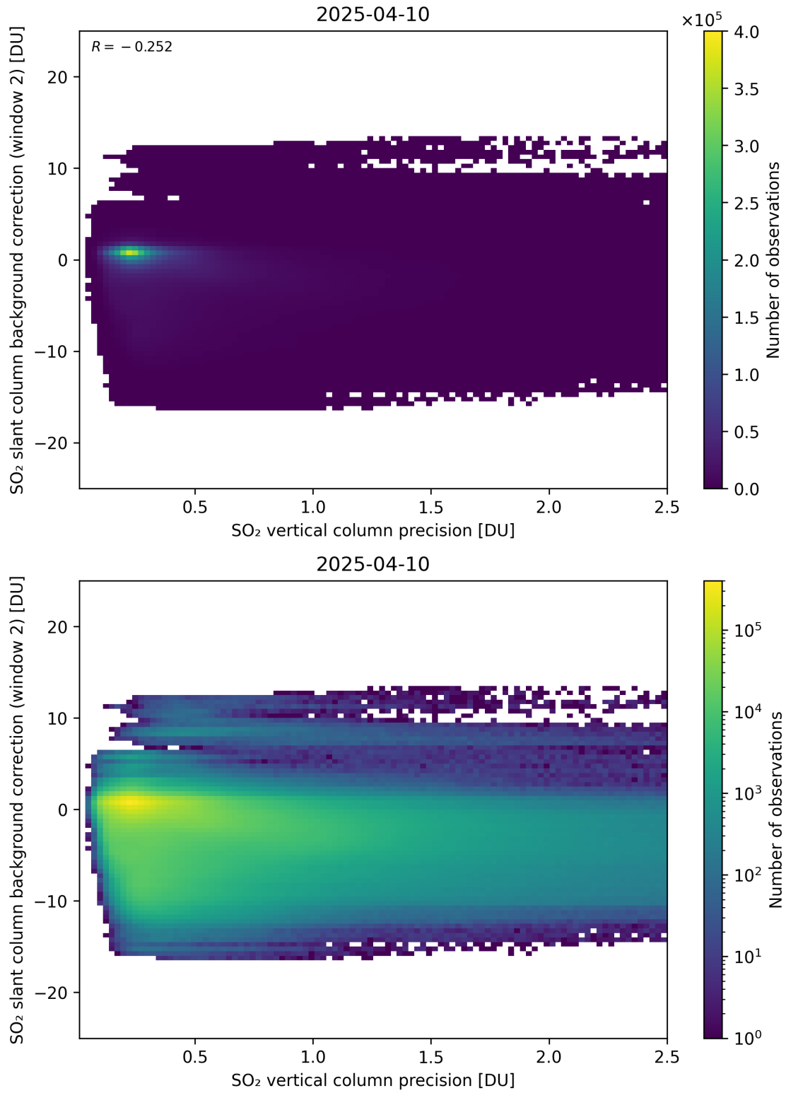
Figure 330: Scatter density plot of “SO 2 vertical column precision” against “SO 2 slant column background correction (window 2)” for 2025-04-09 to 2025-04-11.
