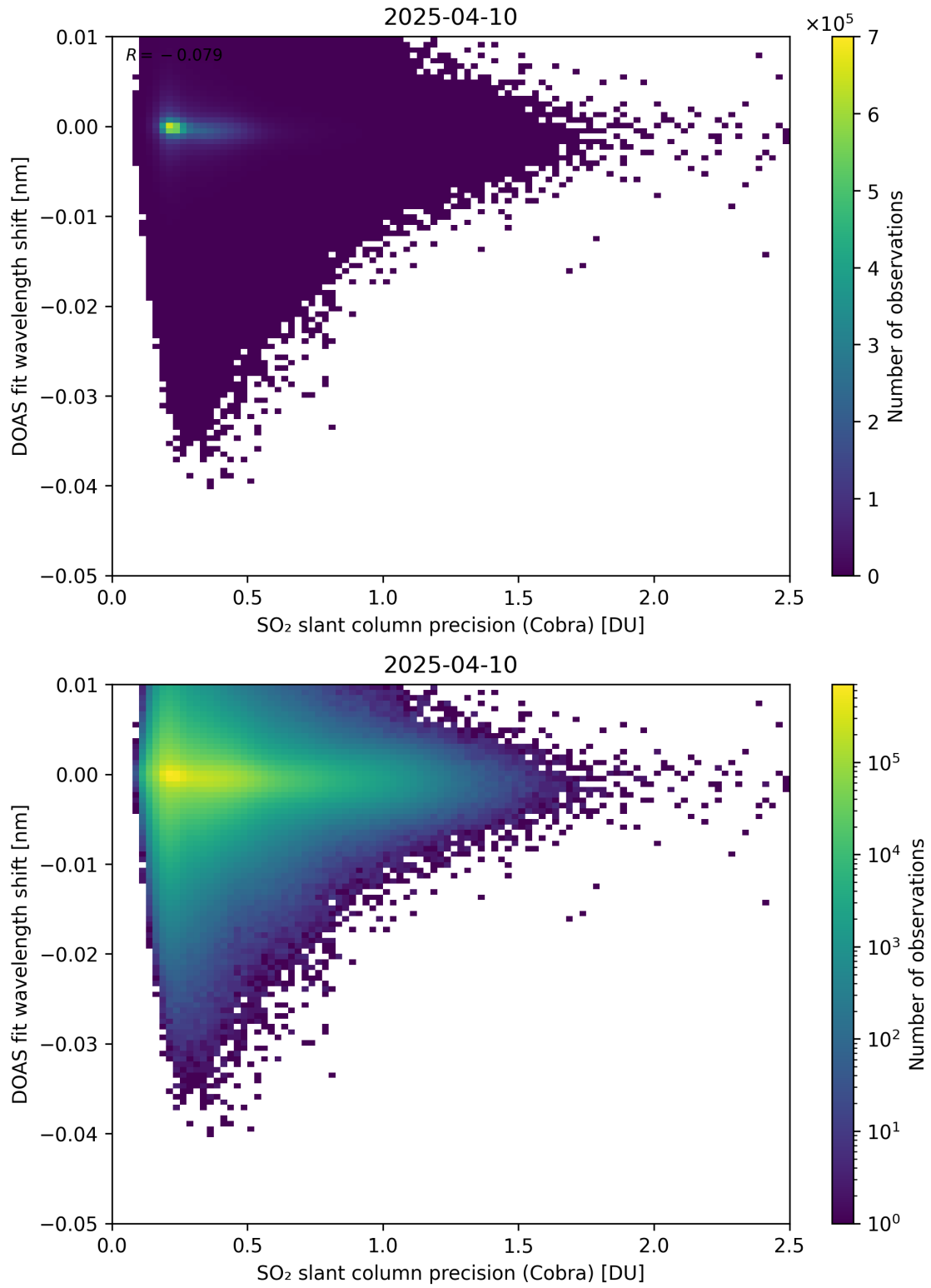
Figure 202: Scatter density plot of “SO 2 slant column precision (Cobra)” against “DOAS fit wavelength shift” for 2025-04-09 to 2025-04-11.
