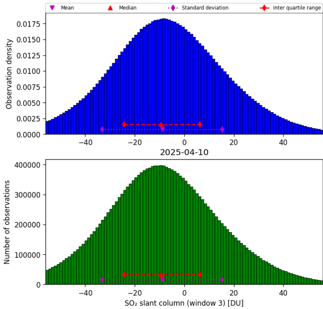
Figure 71: Histogram of “SO 2 slant column (window 3)” for 2025-04-09 to 2025-04-11
