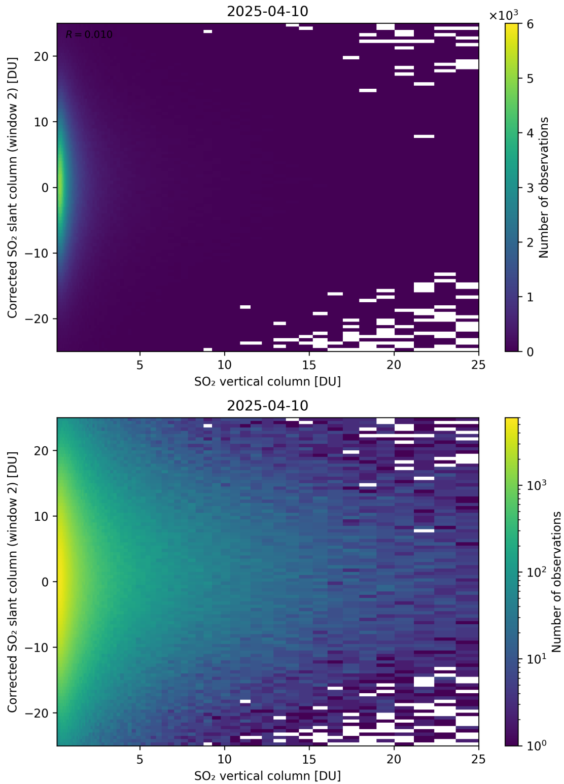
Figure 352: Scatter density plot of “SO 2 vertical column” against “Corrected SO 2 slant column (window 2)” for 2025-04-09 to 2025-04-11.
