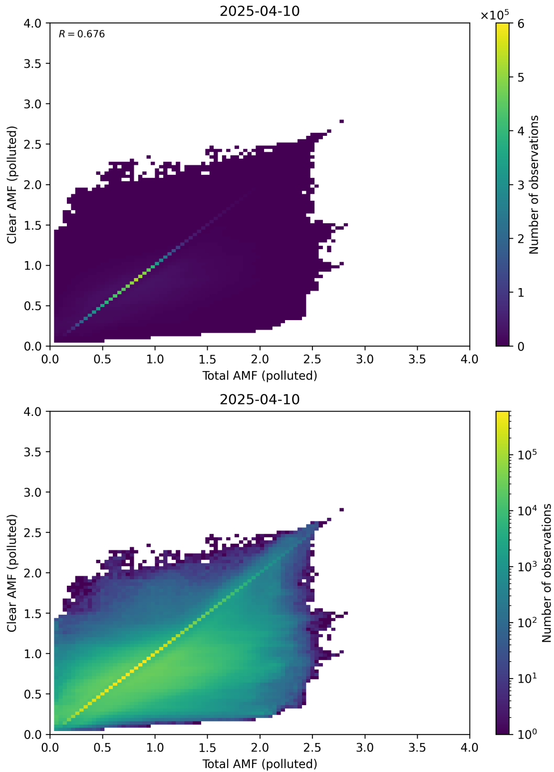
Figure 321: Scatter density plot of “Total AMF (polluted)” against “Clear AMF (polluted)” for 2025-04-09 to 2025-04-11.
