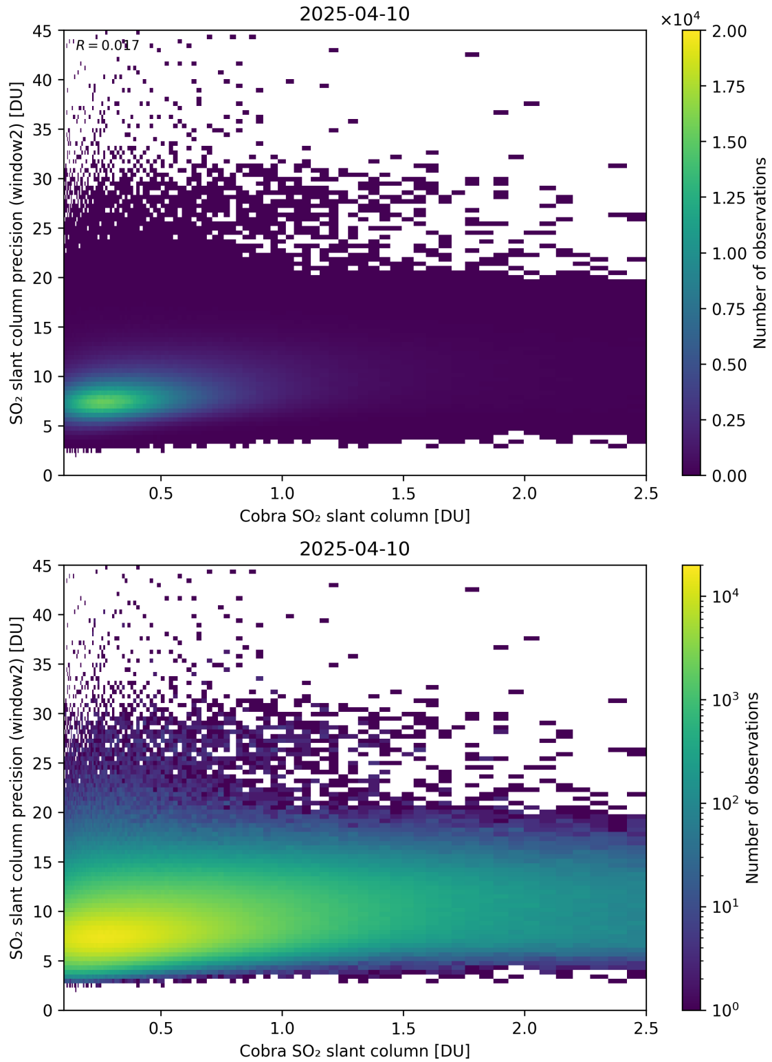
Figure 221: Scatter density plot of “Cobra SO 2 slant column” against “SO 2 slant column precision (window2)” for 2025-04-09 to 2025-04-11.
