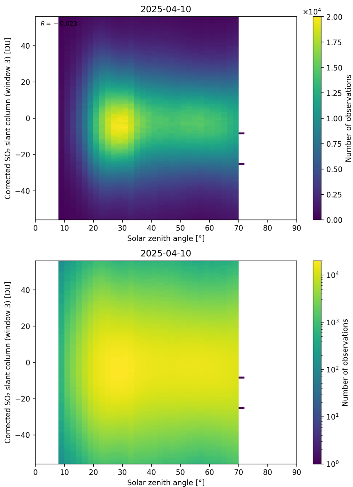
Figure 183: Scatter density plot of “Solar zenith angle” against “Corrected SO 2 slant column (window 3)” for 2025-04-09 to 2025-04-11.
