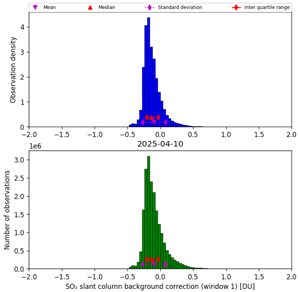
Figure 66: Histogram of “SO 2 slant column background correction (window 1)” for 2025-04-09 to 2025-04-11
