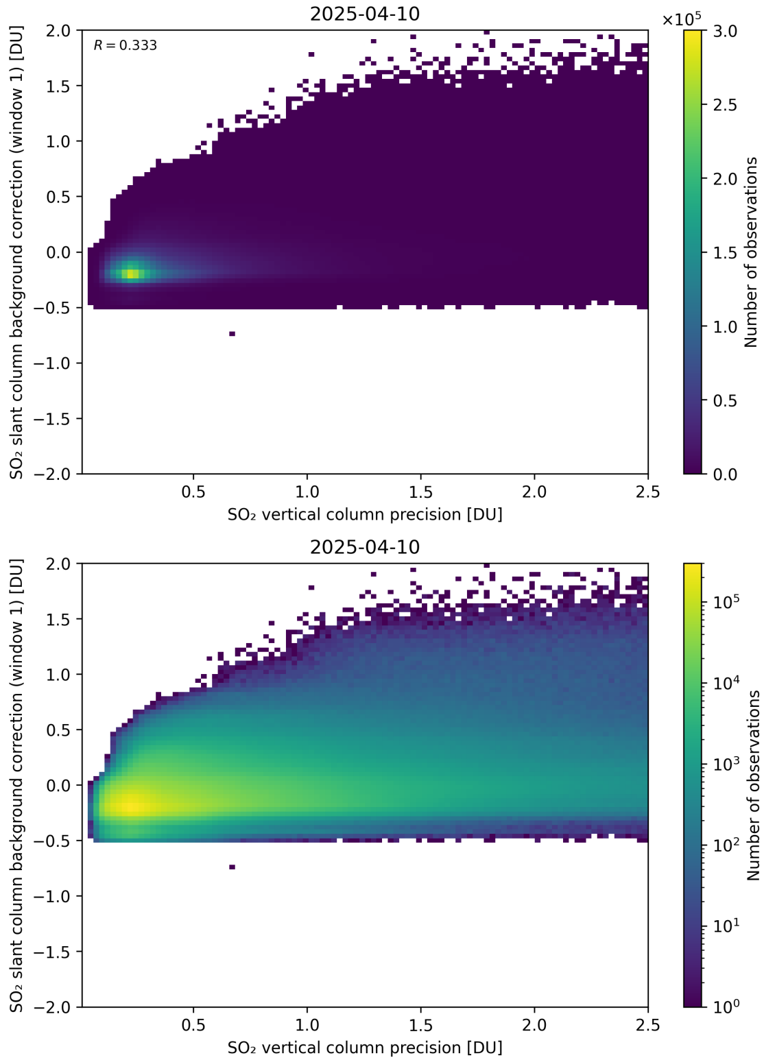
Figure 329: Scatter density plot of “SO 2 vertical column precision” against “SO 2 slant column background correction (window 1)” for 2025-04-09 to 2025-04-11.
