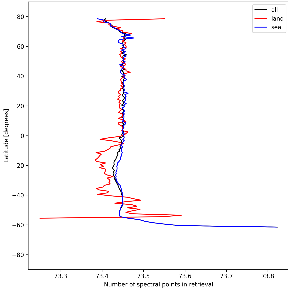
Figure 56: Zonal average of “Number of spectral points in retrieval” for 2025-04-09 to 2025-04-11.
