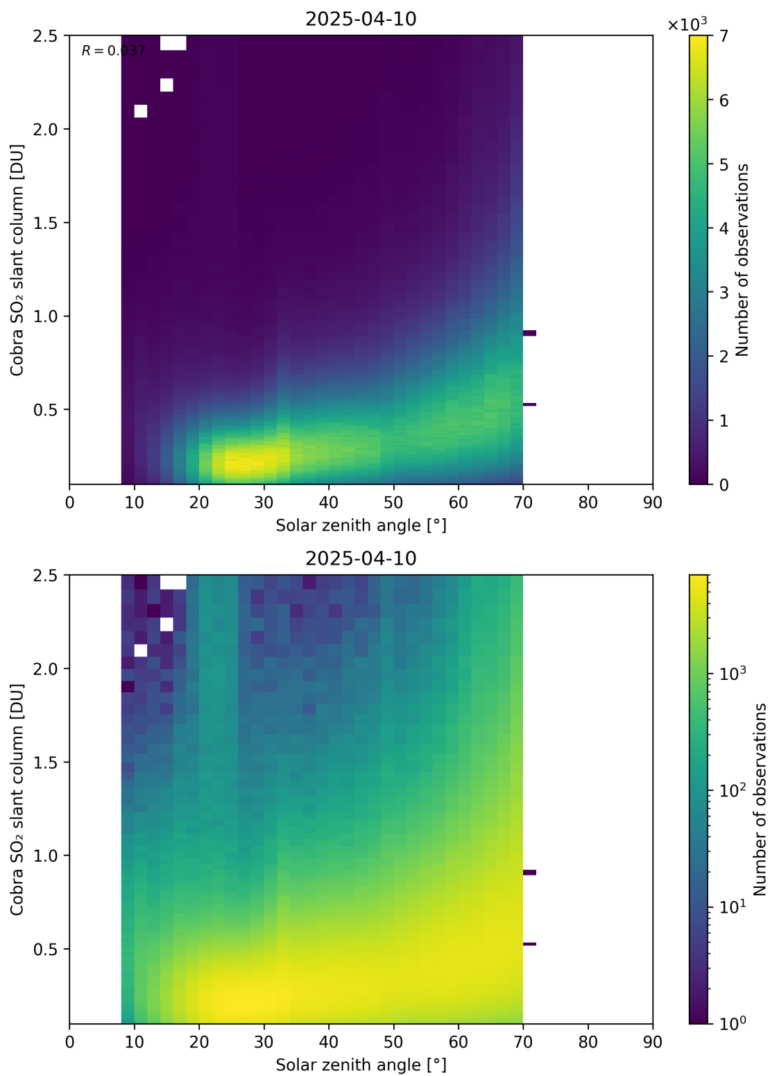
Figure 179: Scatter density plot of “Solar zenith angle” against “Cobra SO 2 slant column” for 2025-04-09 to 2025-04-11.
