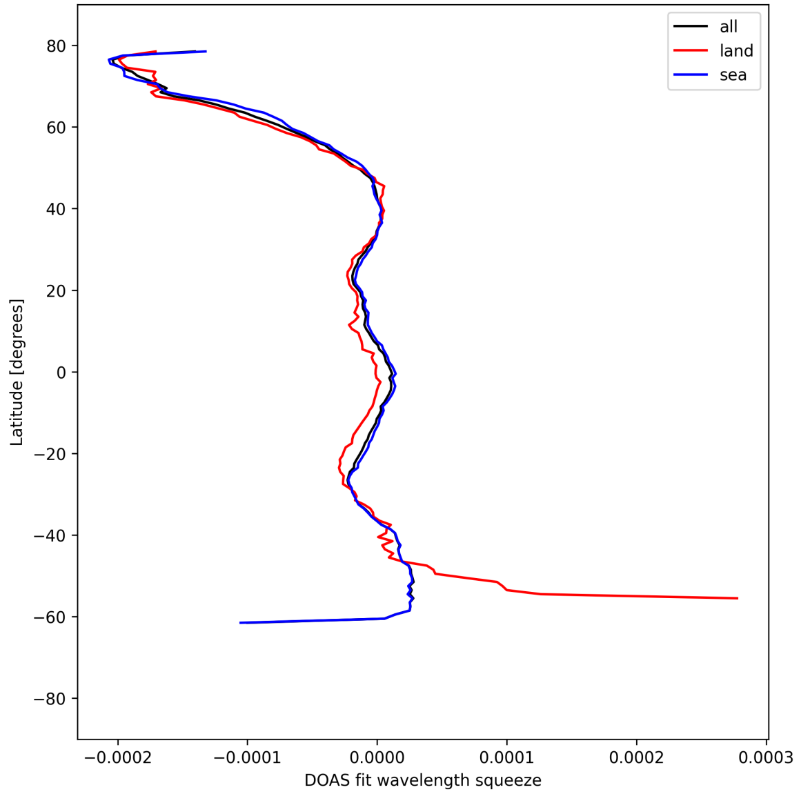
Figure 51: Zonal average of “DOAS fit wavelength squeeze” for 2025-04-09 to 2025-04-11.
