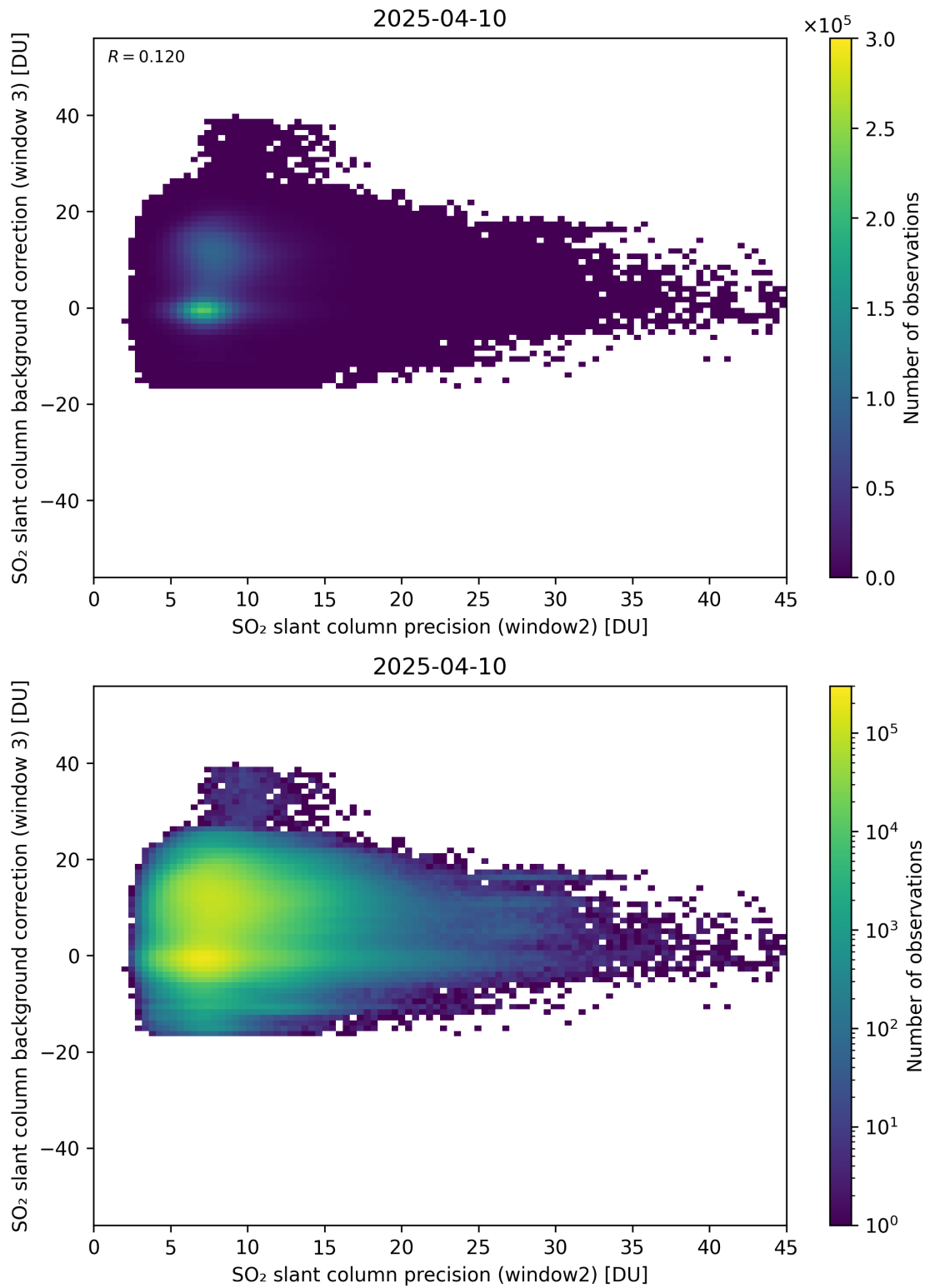
Figure 292: Scatter density plot of “SO 2 slant column precision (window2)” against “SO 2 slant column background correction (window 3)” for 2025-04-09 to 2025-04-11.
