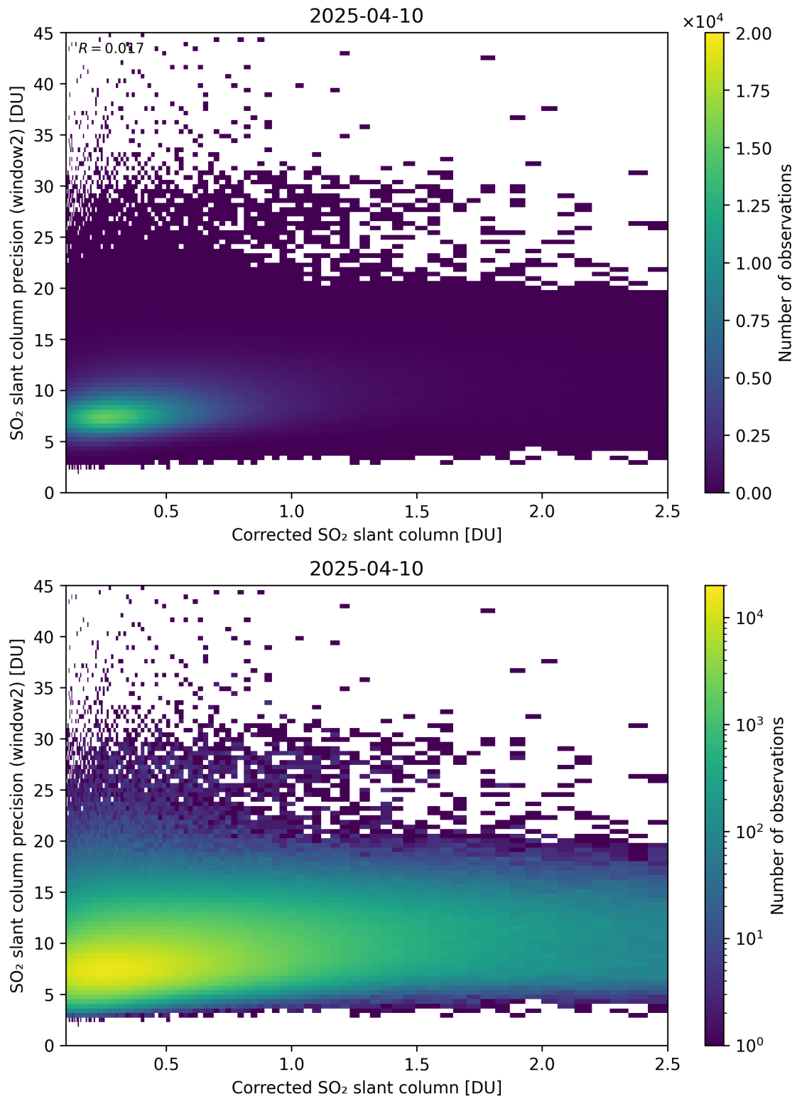
Figure 239: Scatter density plot of “Corrected SO 2 slant column” against “SO 2 slant column precision (window2)” for 2025-04-09 to 2025-04-11.
