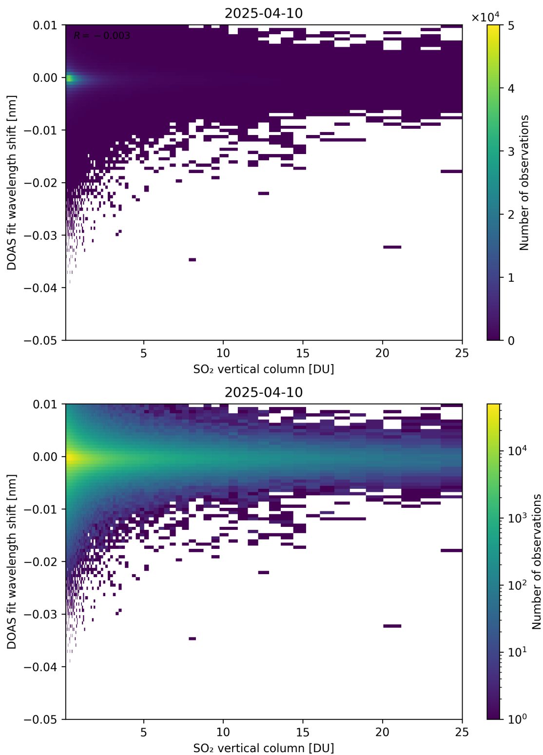
Figure 326: Scatter density plot of “SO 2 vertical column” against “DOAS fit wavelength shift” for 2025-04-09 to 2025-04-11.
