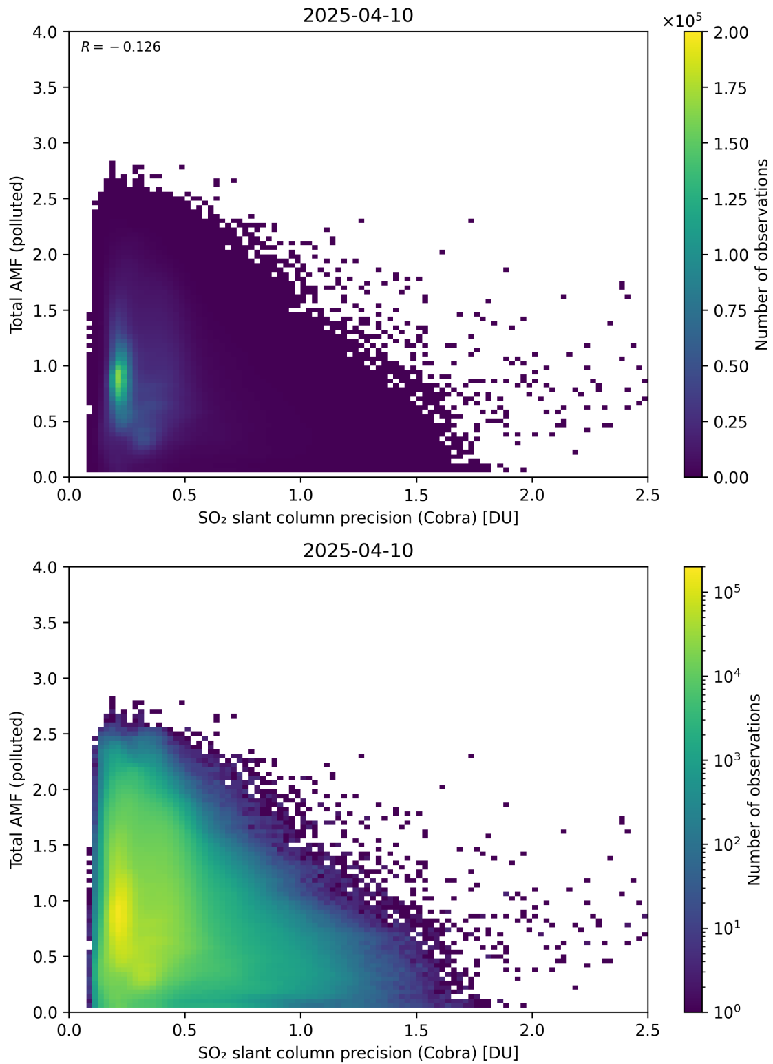
Figure 213: Scatter density plot of “SO 2 slant column precision (Cobra)” against “Total AMF (polluted)” for 2025-04-09 to 2025-04-11.
