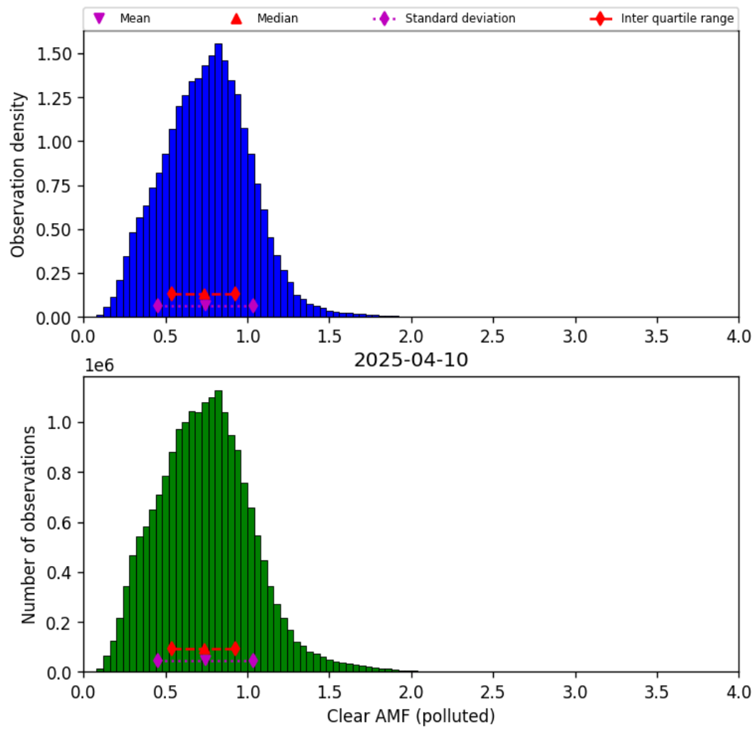
Figure 81: Histogram of “Clear AMF (polluted)” for 2025-04-09 to 2025-04-11
