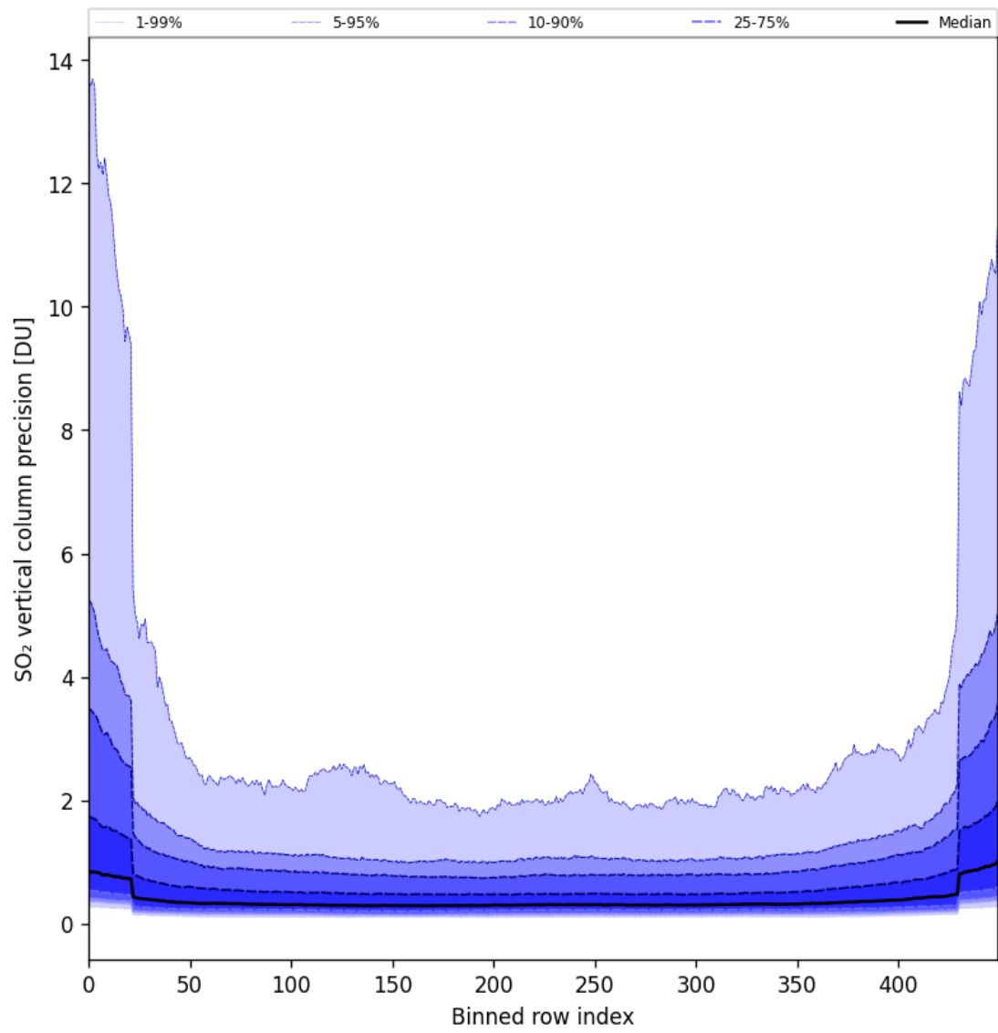
Figure 85: Along track statistics of “SO 2 vertical column precision” for 2025-04-09 to 2025-04-11
