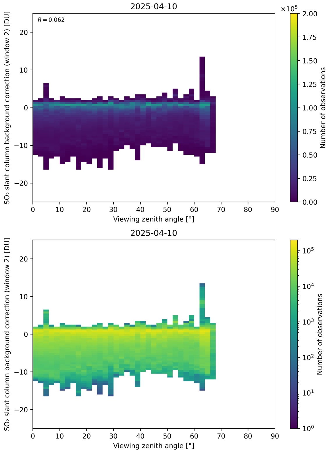
Figure 363: Scatter density plot of “Viewing zenith angle” against “SO 2 slant column background correction (window 2)” for 2025-04-09 to 2025-04-11.
