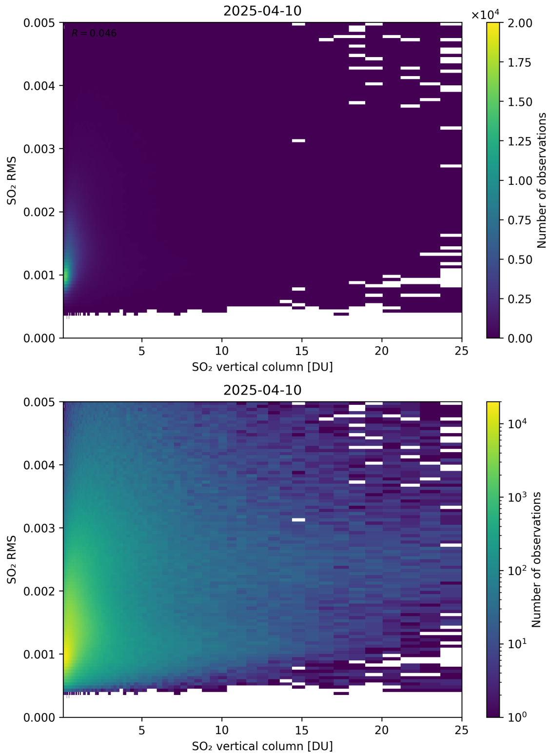
Figure 328: Scatter density plot of “SO 2 vertical column” against “SO 2 RMS” for 2025-04-09 to 2025-04-11.
