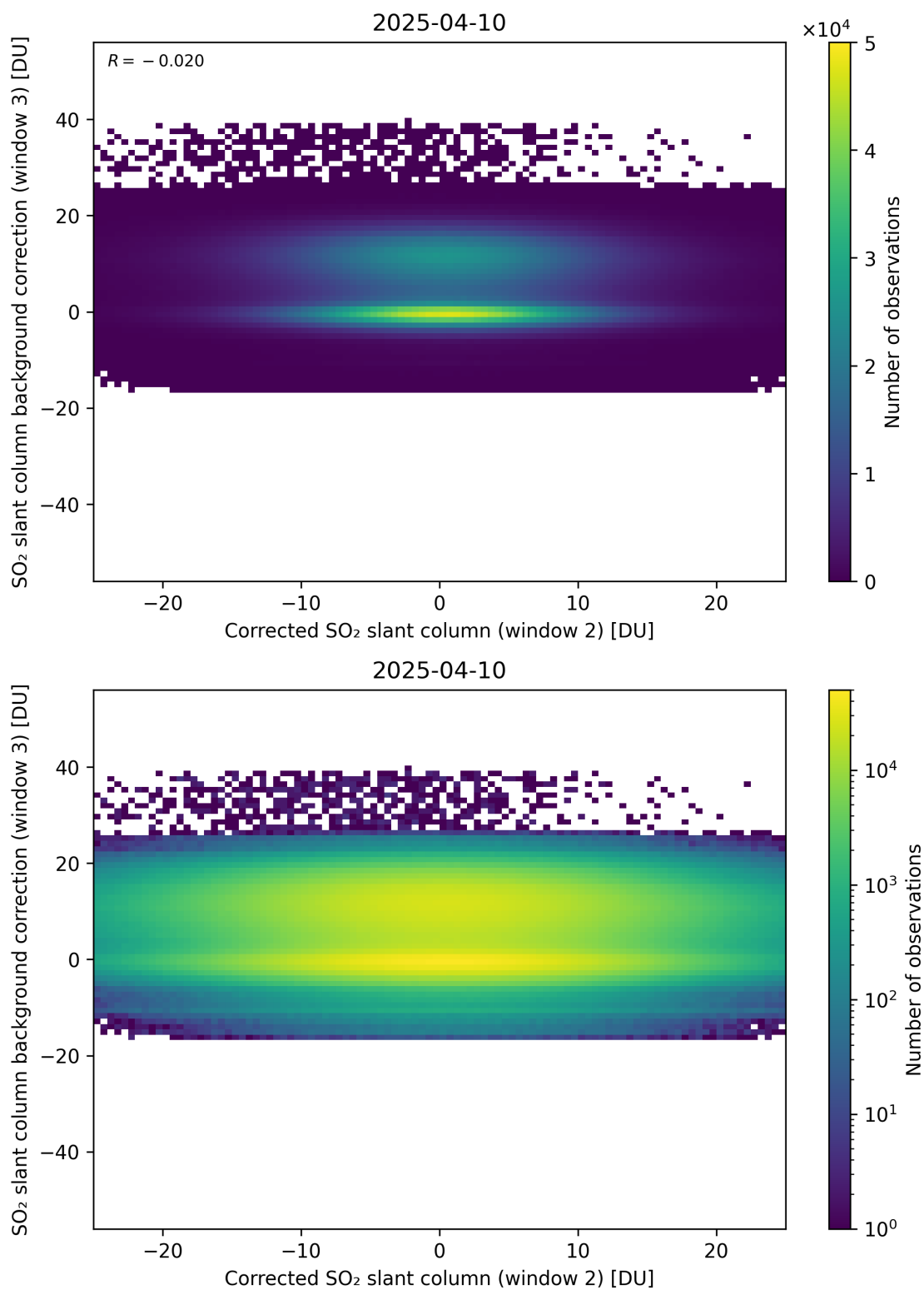
Figure 245: Scatter density plot of “Corrected SO 2 slant column (window 2)” against “SO 2 slant column background correction (window 3)” for 2025-04-09 to 2025-04-11.
