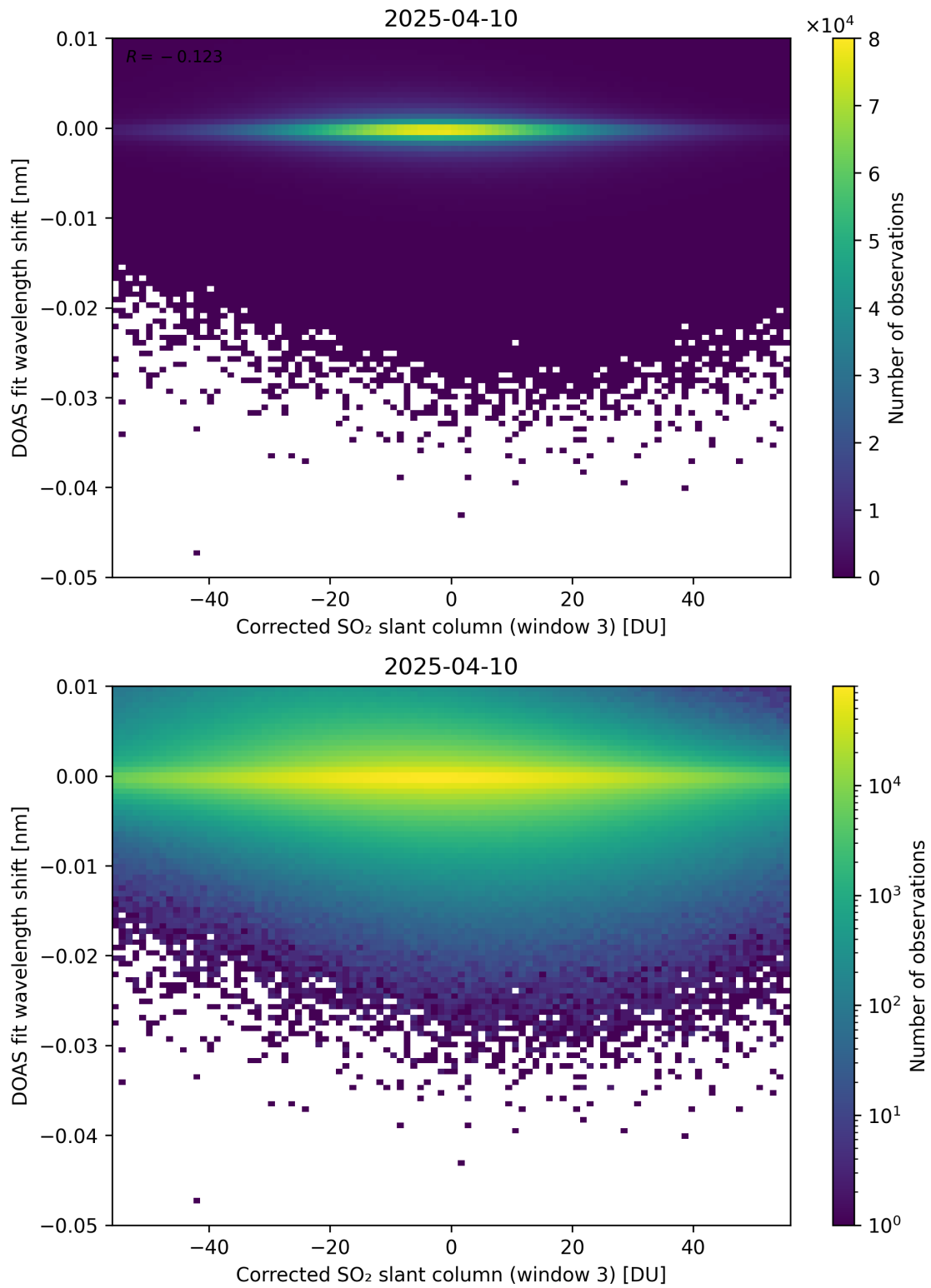
Figure 256: Scatter density plot of “Corrected SO 2 slant column (window 3)” against “DOAS fit wavelength shift” for 2025-04-09 to 2025-04-11.
