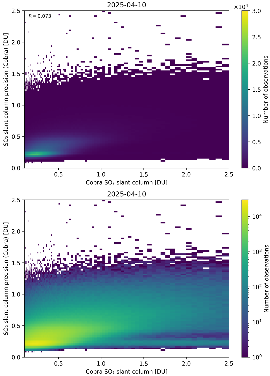
Figure 216: Scatter density plot of “Cobra SO 2 slant column” against “SO 2 slant column precision (Cobra)” for 2025-04-09 to 2025-04-11.
