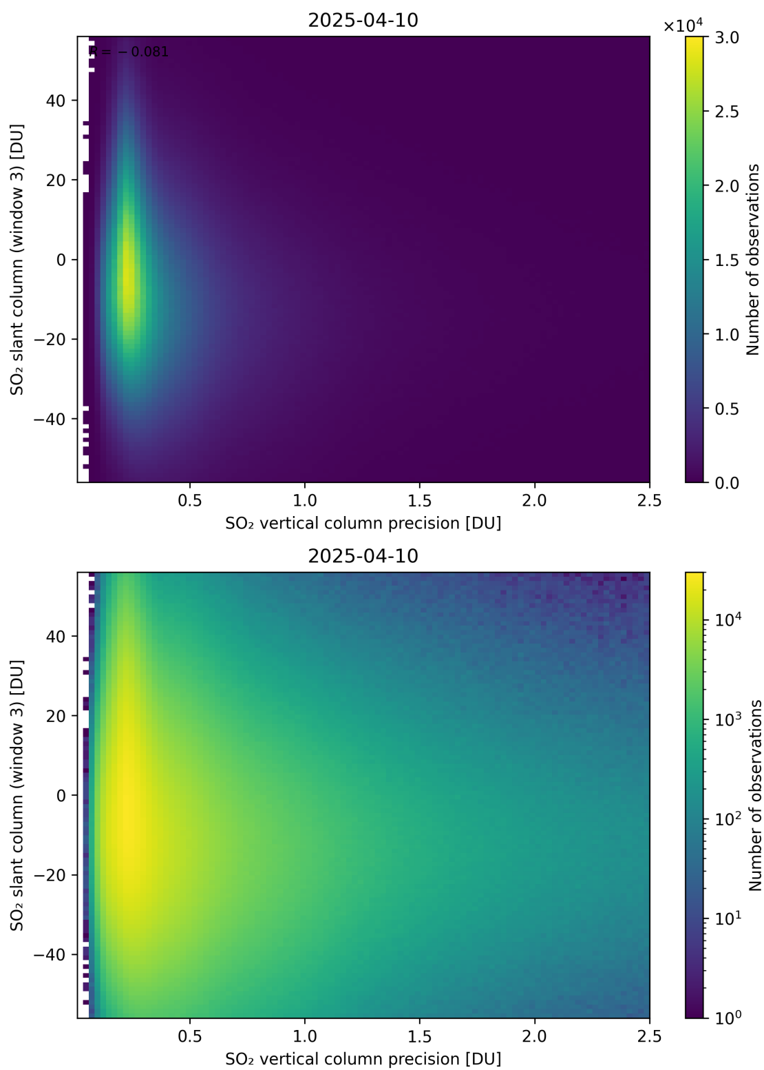
Figure 344: Scatter density plot of “SO 2 vertical column precision” against “SO 2 slant column (window 3)” for 2025-04-09 to 2025-04-11.
