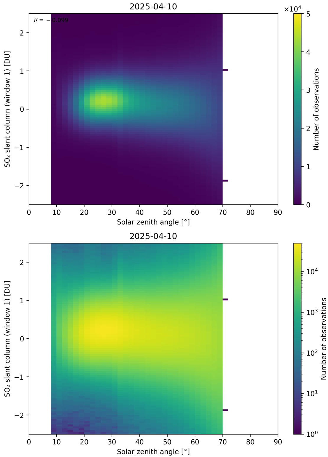
Figure 184: Scatter density plot of “Solar zenith angle” against “SO 2 slant column (window 1)” for 2025-04-09 to 2025-04-11.
