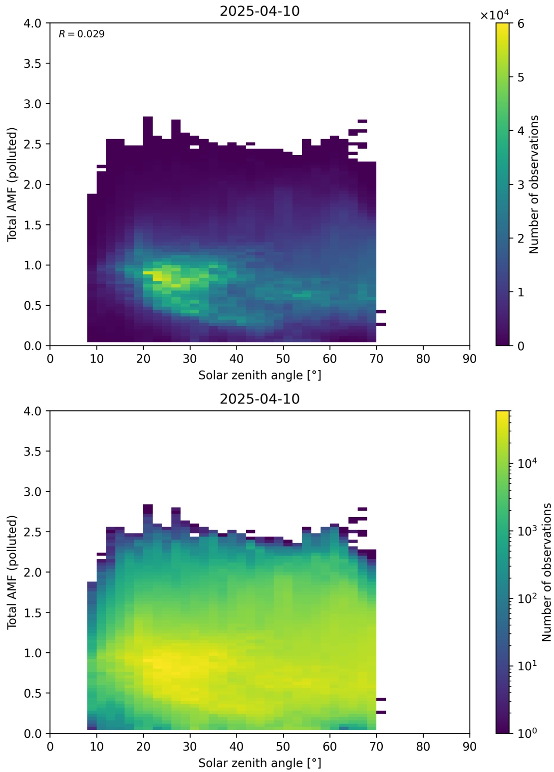
Figure 189: Scatter density plot of “Solar zenith angle” against “Total AMF (polluted)” for 2025-04-09 to 2025-04-11.
