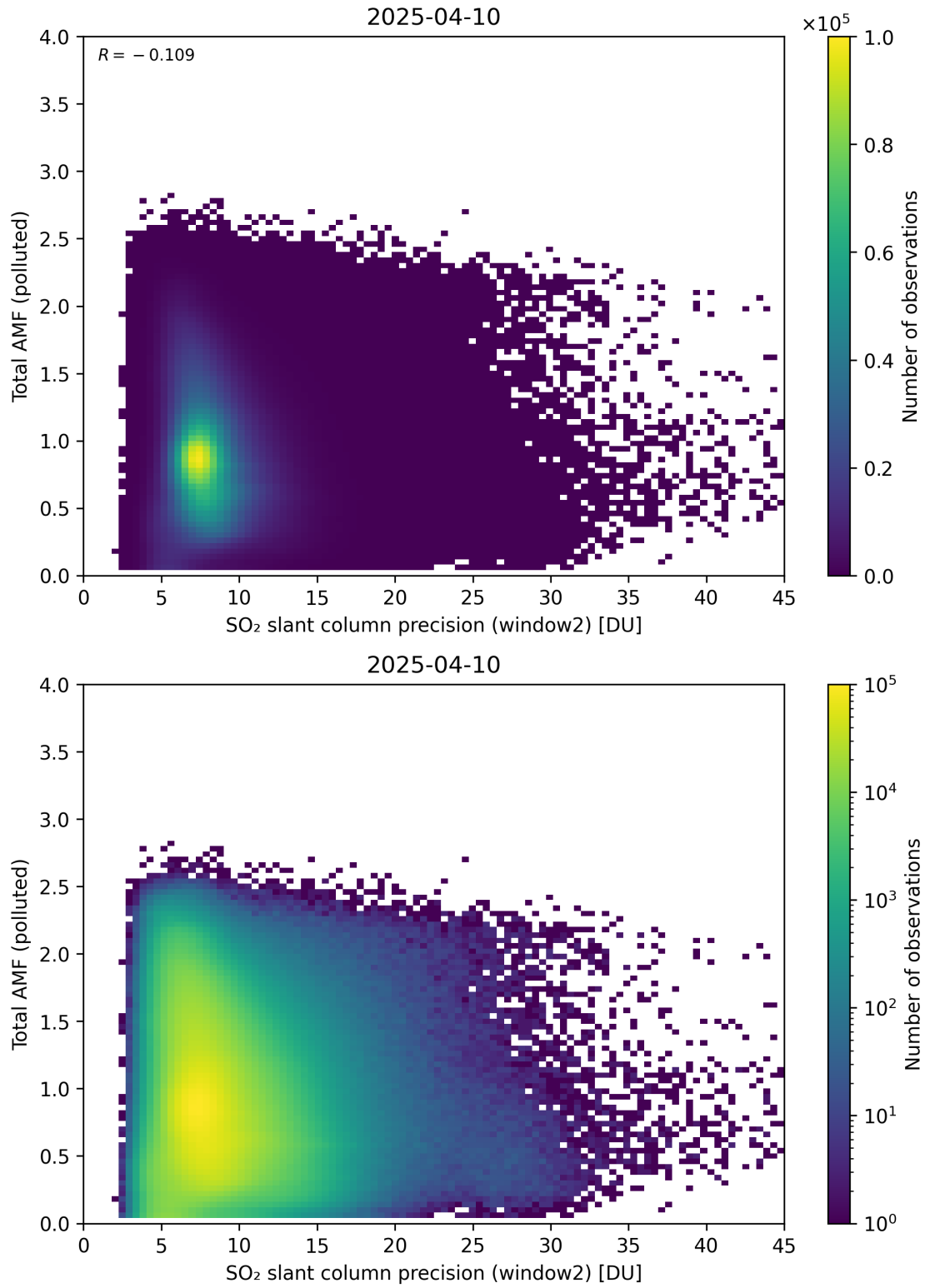
Figure 301: Scatter density plot of “SO 2 slant column precision (window2)” against “Total AMF (polluted)” for 2025-04-09 to 2025-04-11.
