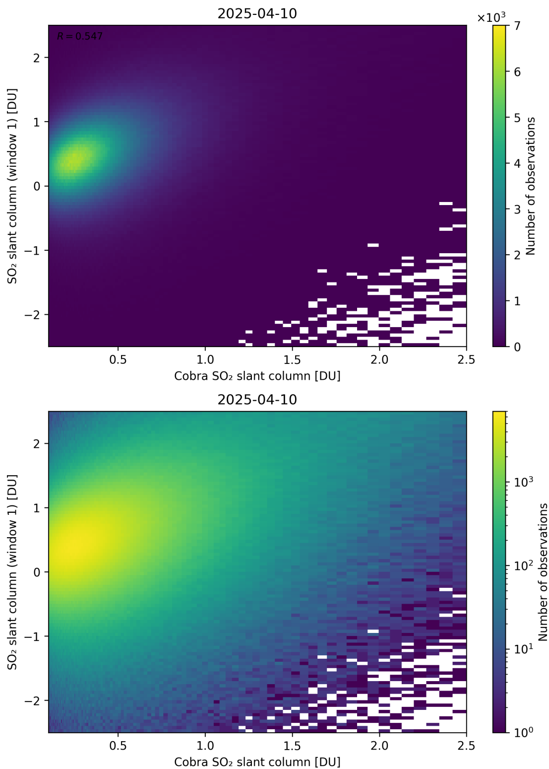
Figure 219: Scatter density plot of “Cobra SO 2 slant column” against “SO 2 slant column (window 1)” for 2025-04-09 to 2025-04-11.
