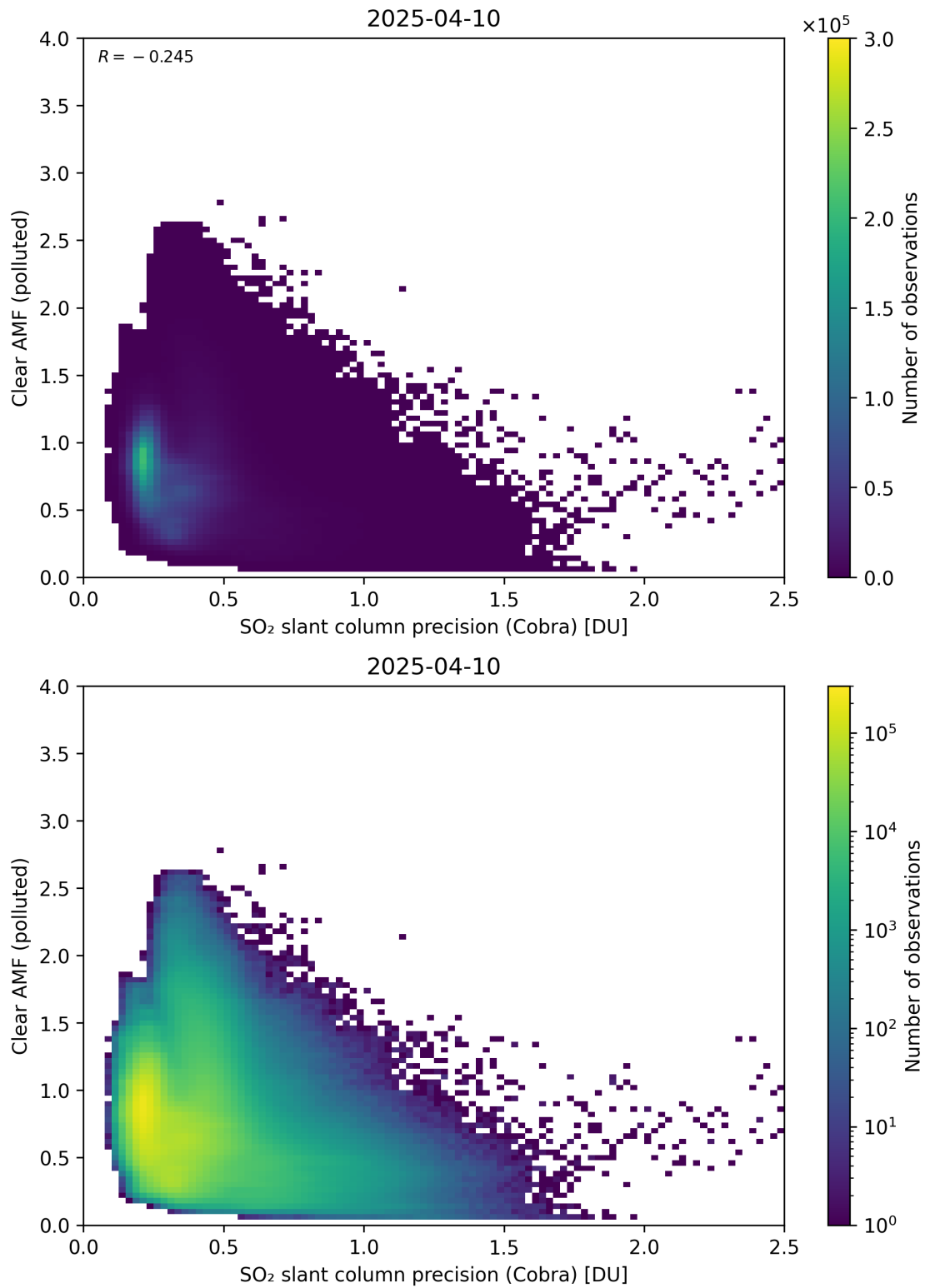
Figure 205: Scatter density plot of “SO 2 slant column precision (Cobra)” against “Clear AMF (polluted)” for 2025-04-09 to 2025-04-11.
