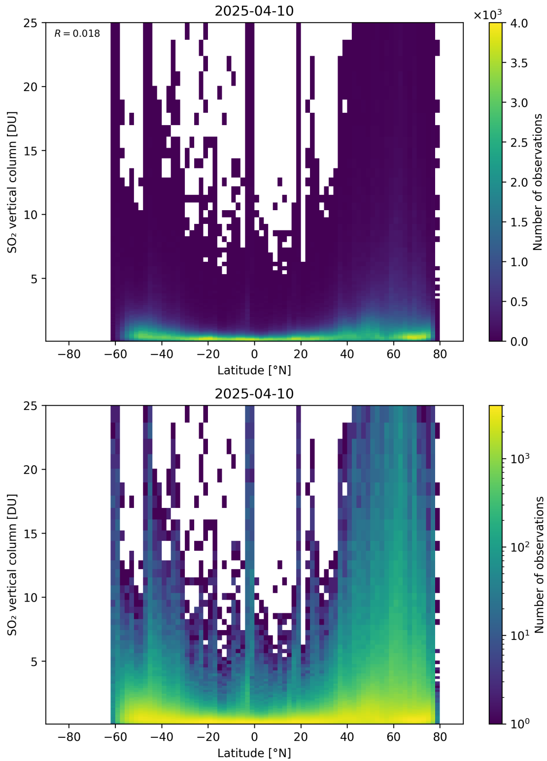
Figure 169: Scatter density plot of “Latitude” against “SO 2 vertical column” for 2025-04-09 to 2025-04-11.
