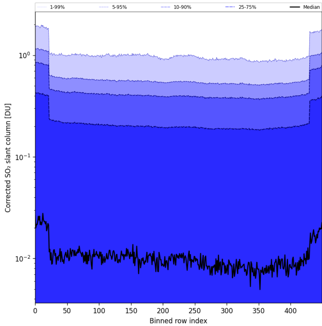
Figure 86: Along track statistics of “Corrected SO 2 slant column” for 2025-04-09 to 2025-04-11
