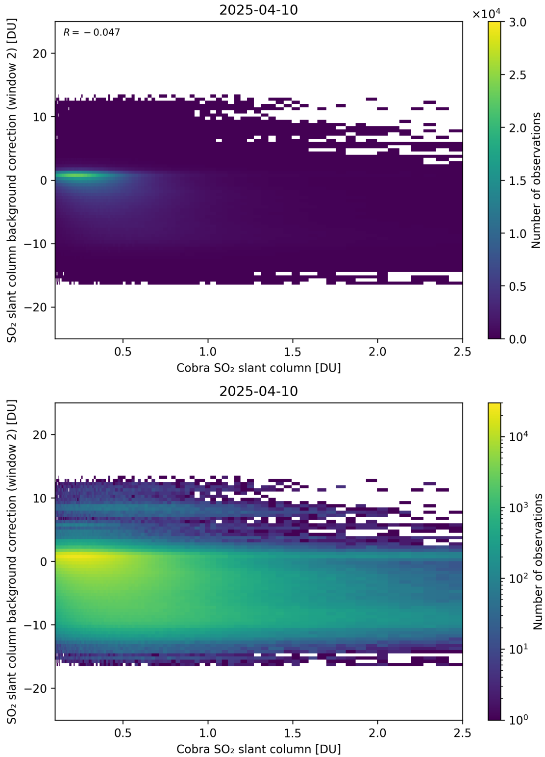
Figure 194: Scatter density plot of “Cobra SO 2 slant column” against “SO 2 slant column background correction (window 2)” for 2025-04-09 to 2025-04-11.
