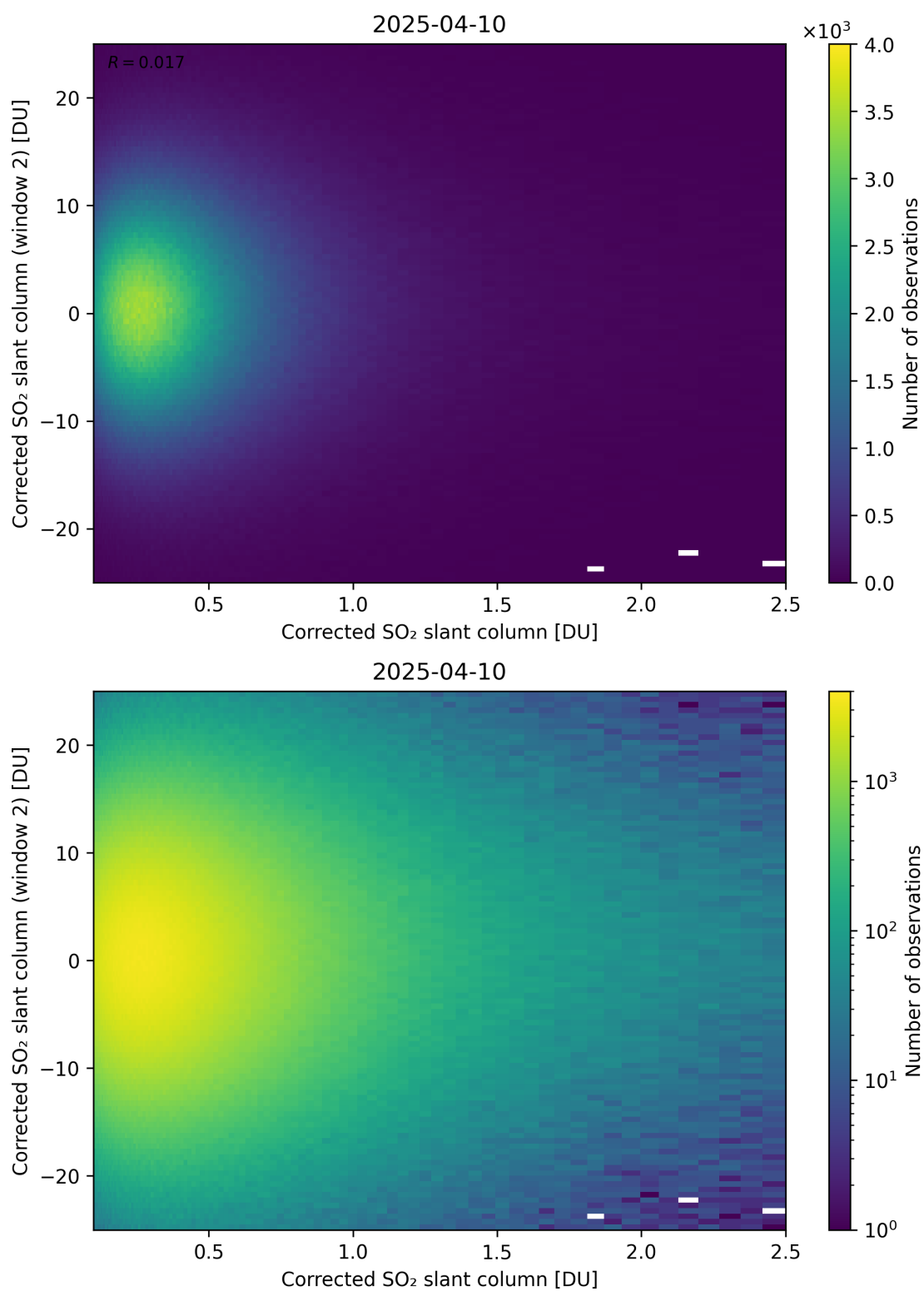
Figure 235: Scatter density plot of “Corrected SO 2 slant column” against “Corrected SO 2 slant column (window 2)” for 2025-04-09 to 2025-04-11.
