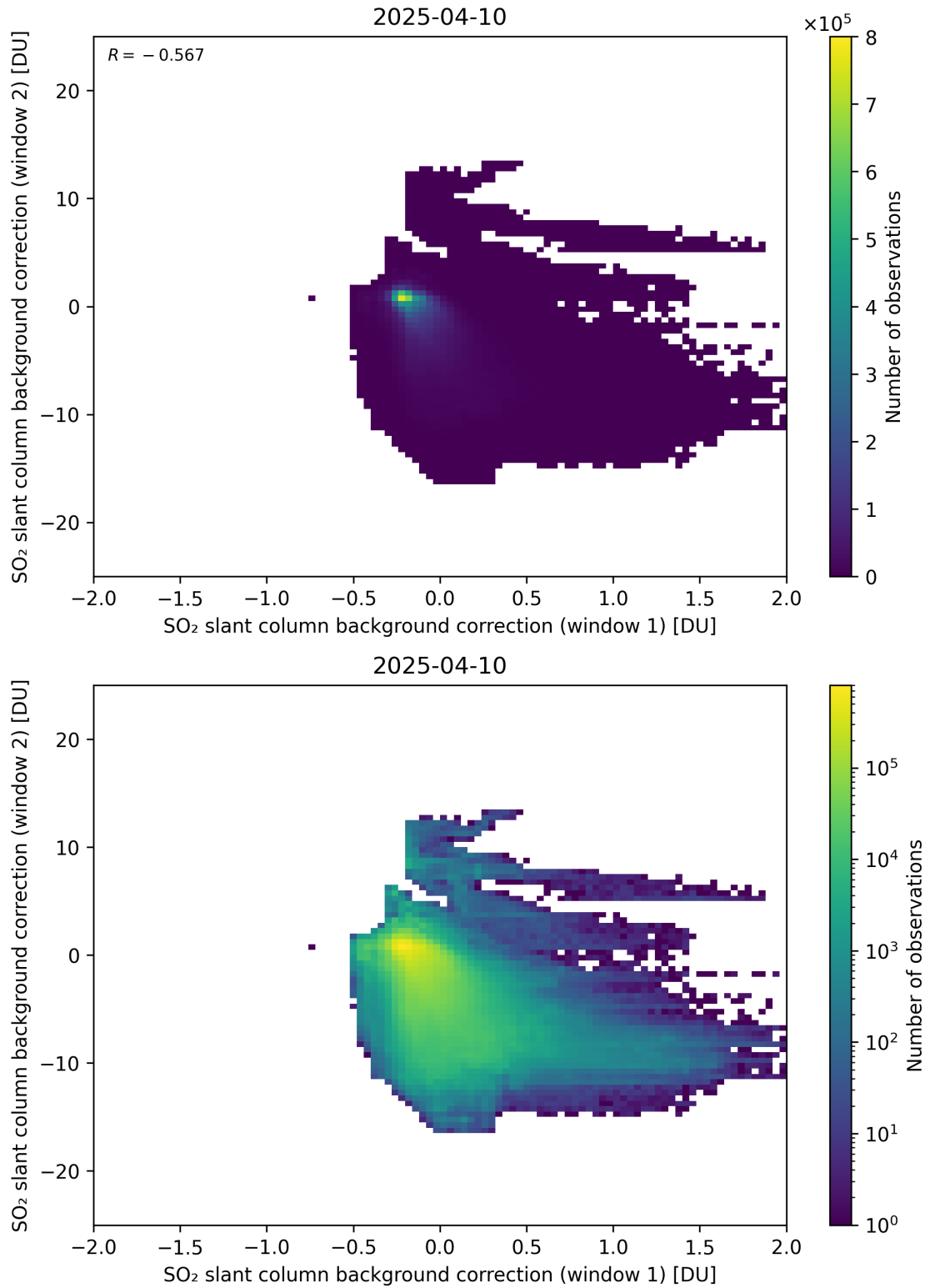
Figure 109: Scatter density plot of “SO 2 slant column background correction (window 1)” against “SO 2 slant column background correction (window 2)” for 2025-04-09 to 2025-04-11.
