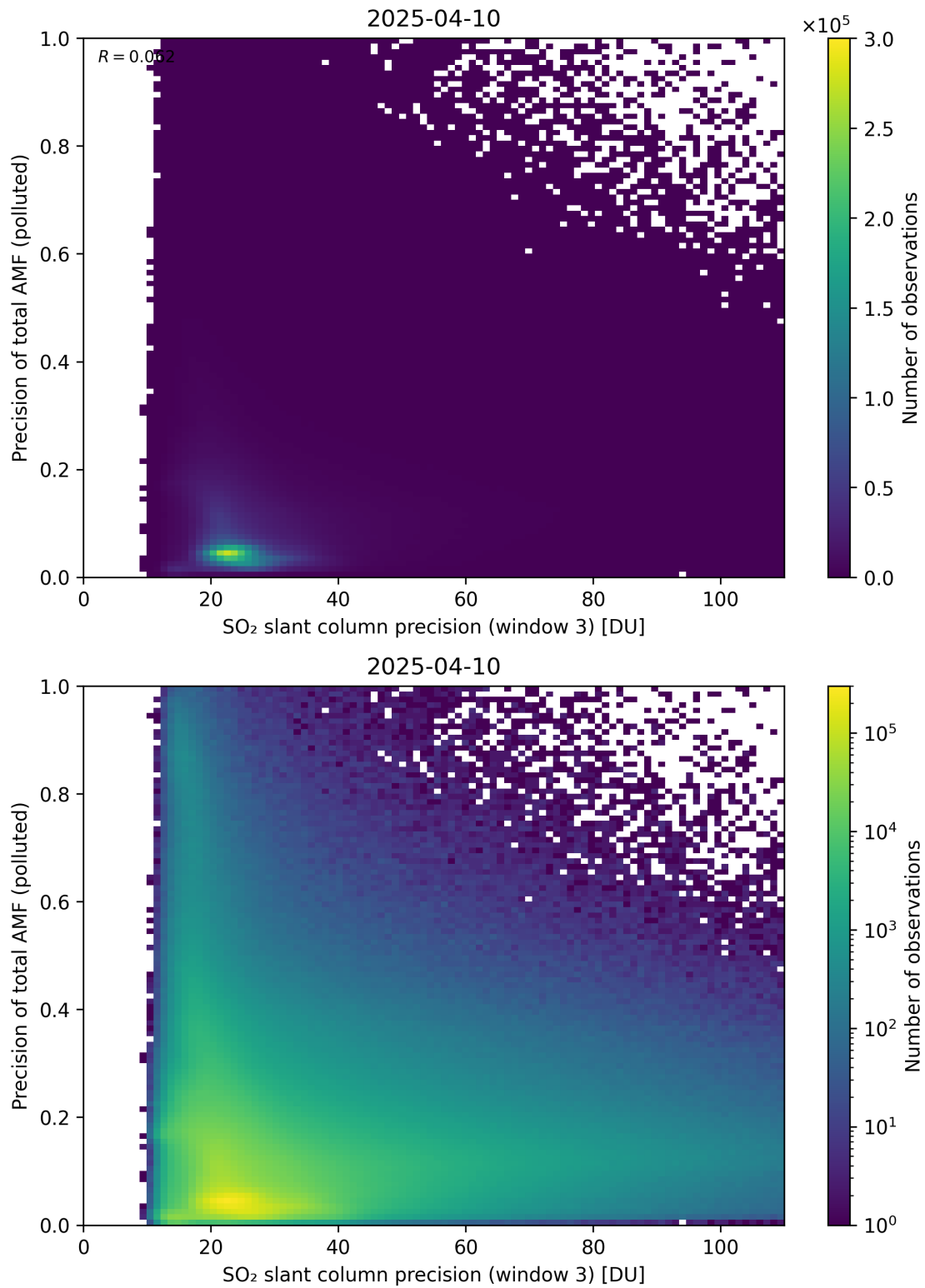
Figure 314: Scatter density plot of “SO 2 slant column precision (window 3)” against “Precision of total AMF (polluted)” for 2025-04-09 to 2025-04-11.
