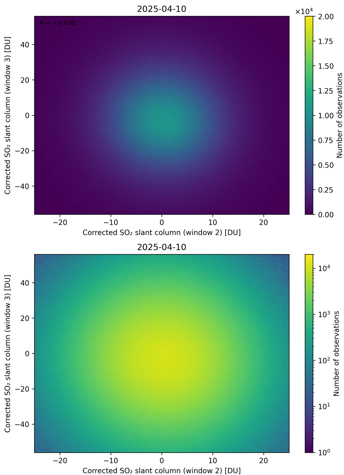
Figure 250: Scatter density plot of “Corrected SO 2 slant column (window 2)” against “Corrected SO 2 slant column (window 3)” for 2025-04-09 to 2025-04-11.
