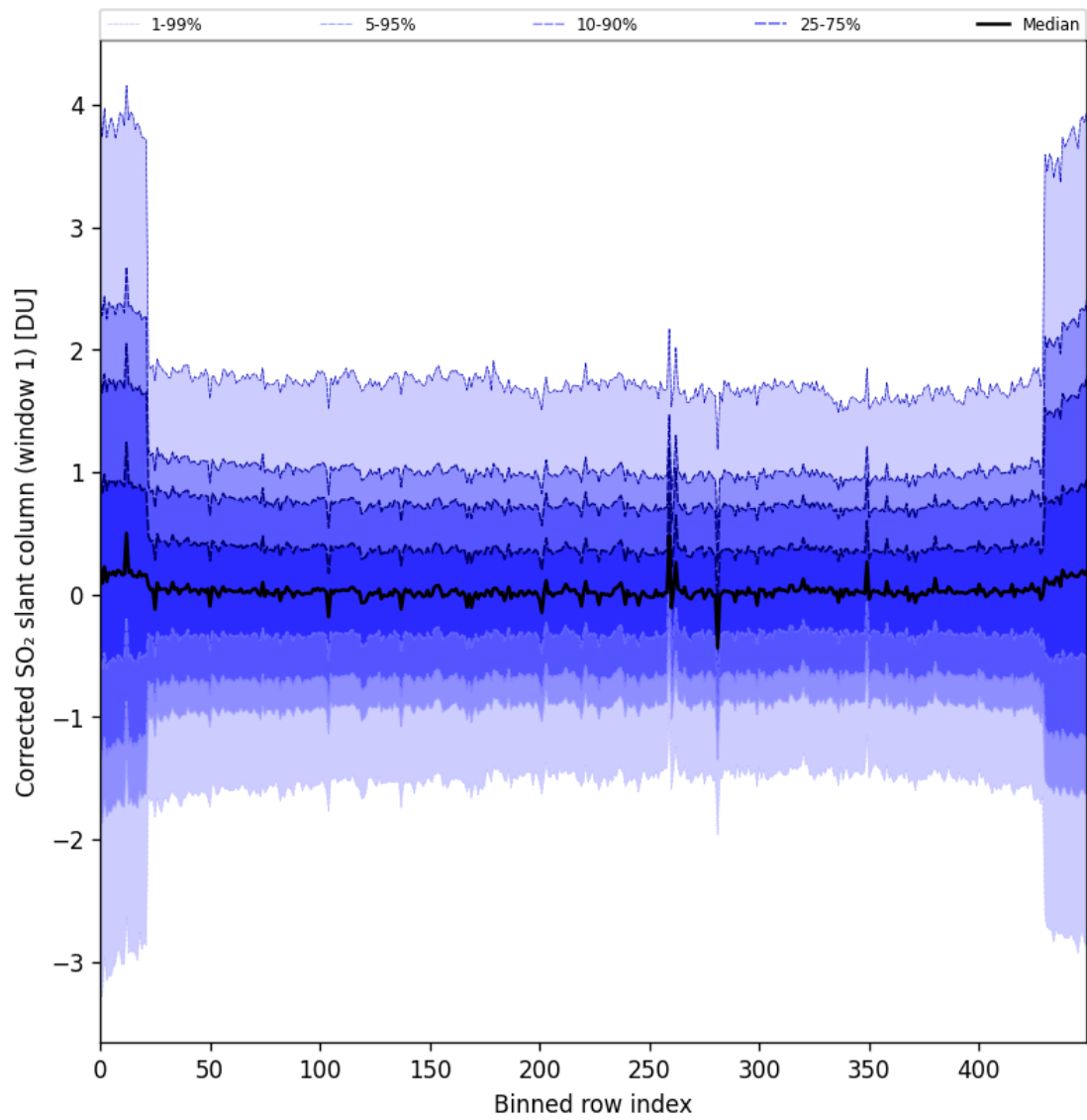
Figure 91: Along track statistics of “Corrected SO 2 slant column (window 1)” for 2025-04-09 to 2025-04-11
