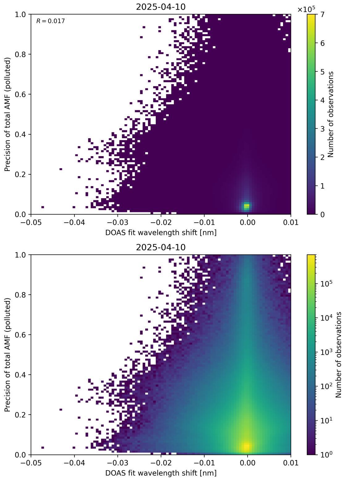
Figure 142: Scatter density plot of “DOAS fit wavelength shift” against “Precision of total AMF (polluted)” for 2025-04-09 to 2025-04-11.
