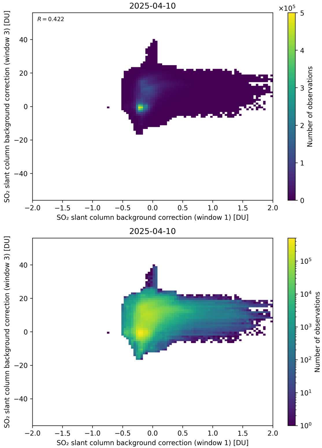
Figure 110: Scatter density plot of “SO 2 slant column background correction (window 1)” against “SO 2 slant column background correction (window 3)” for 2025-04-09 to 2025-04-11.
