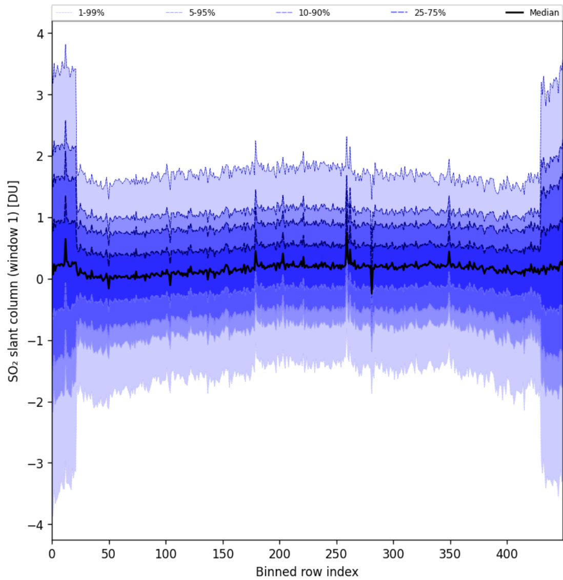
Figure 89: Along track statistics of “SO 2 slant column (window 1)” for 2025-04-09 to 2025-04-11
