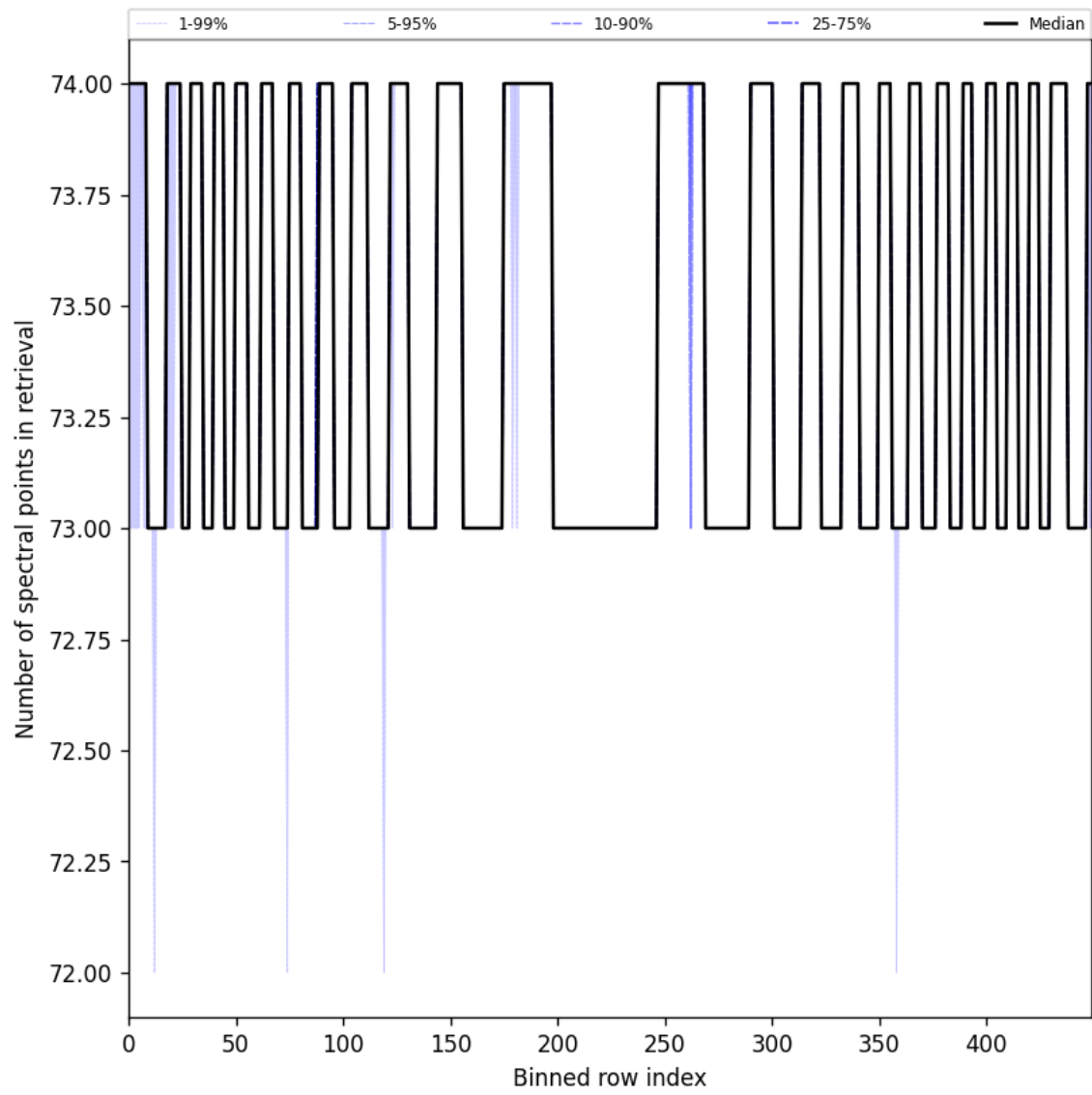
Figure 108: Along track statistics of “Number of spectral points in retrieval” for 2025-04-09 to 2025-04-11
