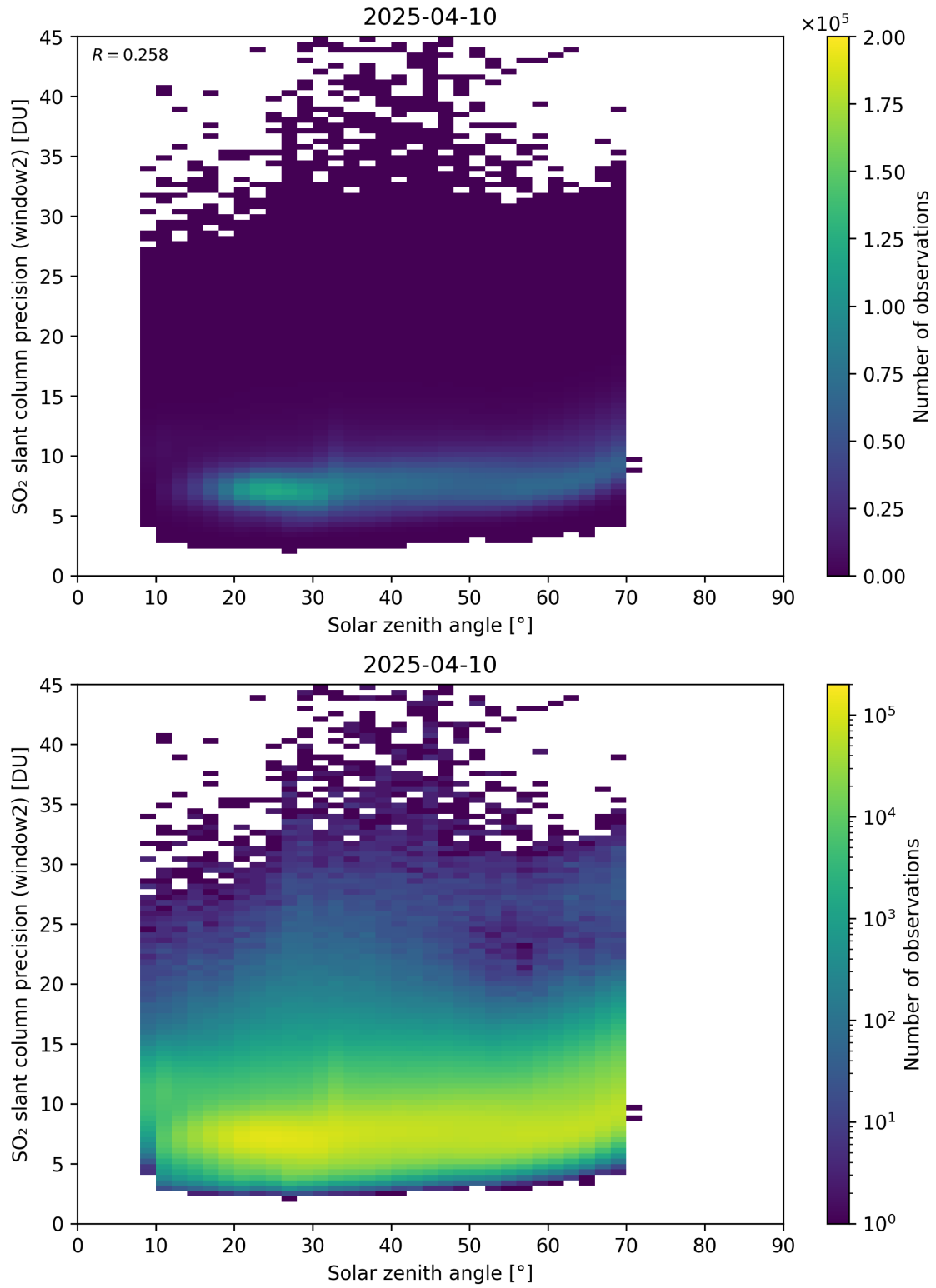
Figure 186: Scatter density plot of “Solar zenith angle” against “SO 2 slant column precision (window2)” for 2025-04-09 to 2025-04-11.
