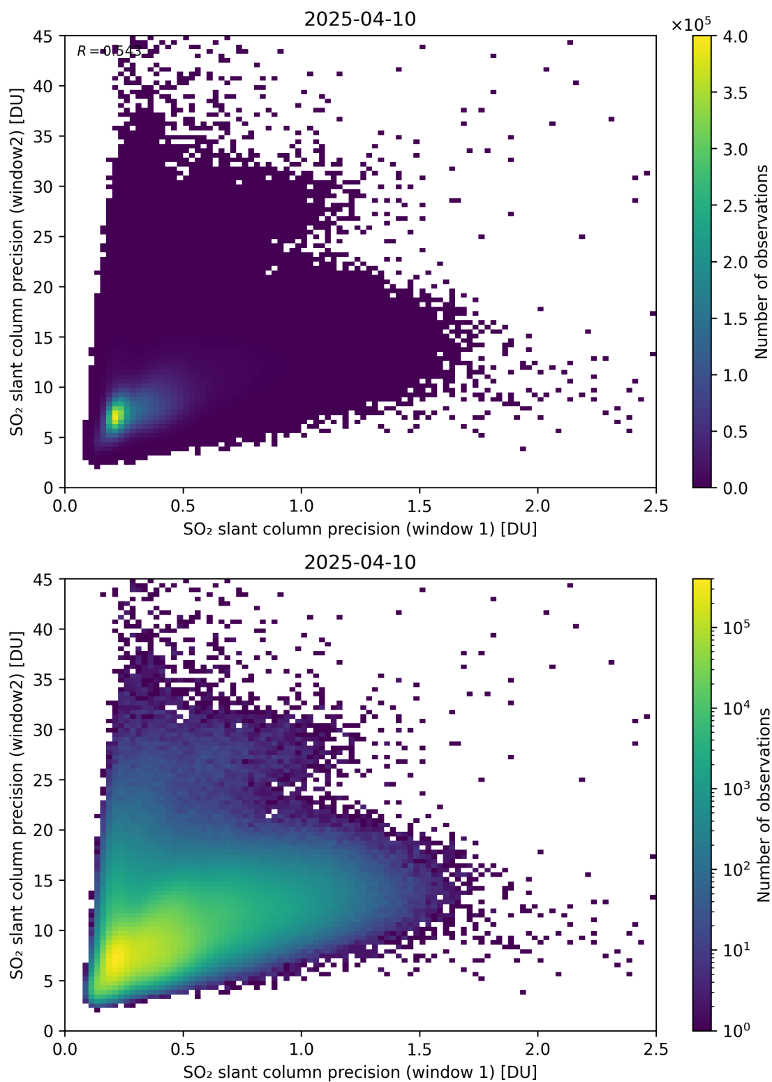
Figure 277: Scatter density plot of “SO 2 slant column precision (window 1)” against “SO 2 slant column precision (window2)” for 2025-04-09 to 2025-04-11.
