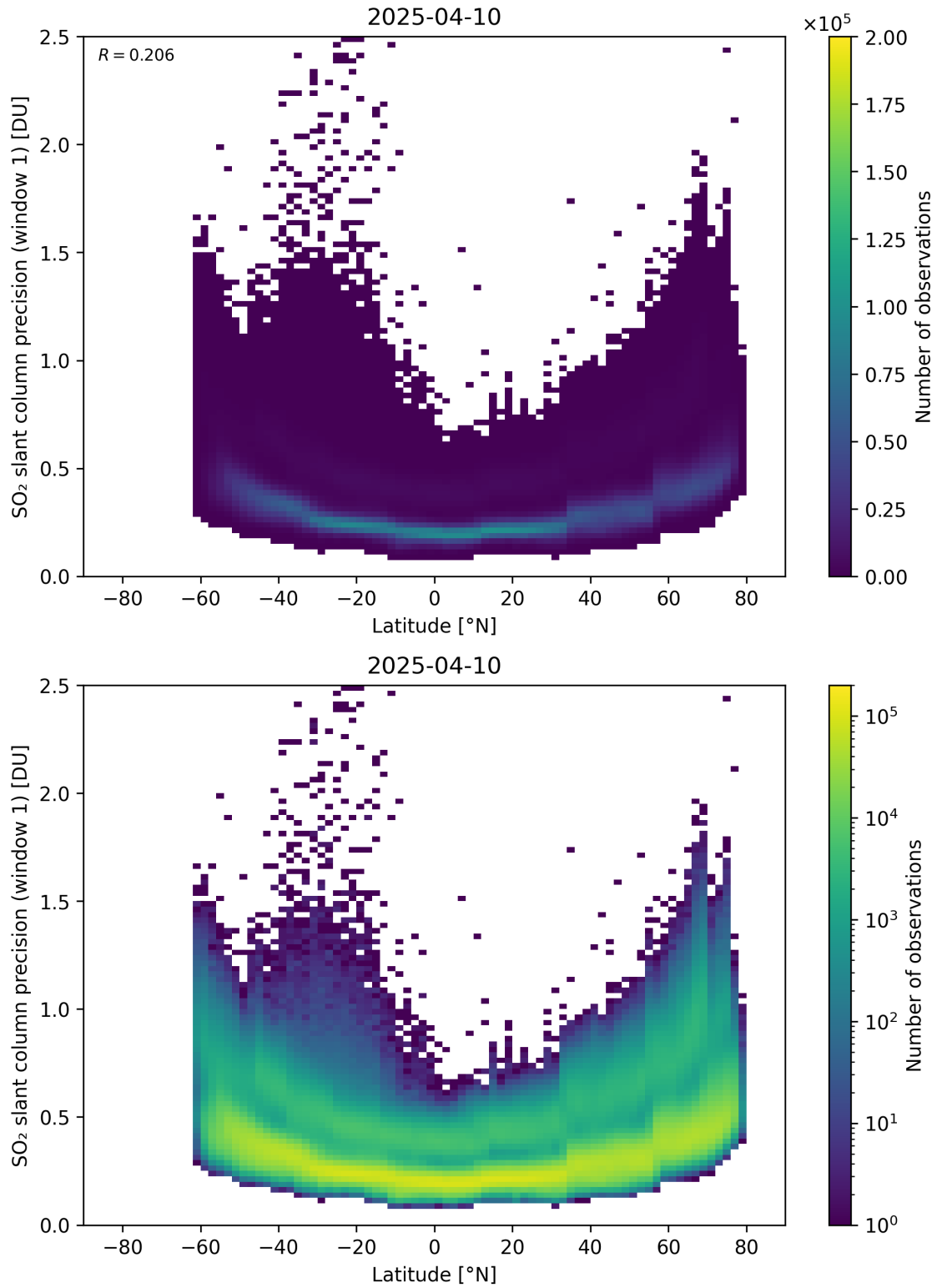
Figure 163: Scatter density plot of “Latitude” against “SO 2 slant column precision (window 1)” for 2025-04-09 to 2025-04-11.
