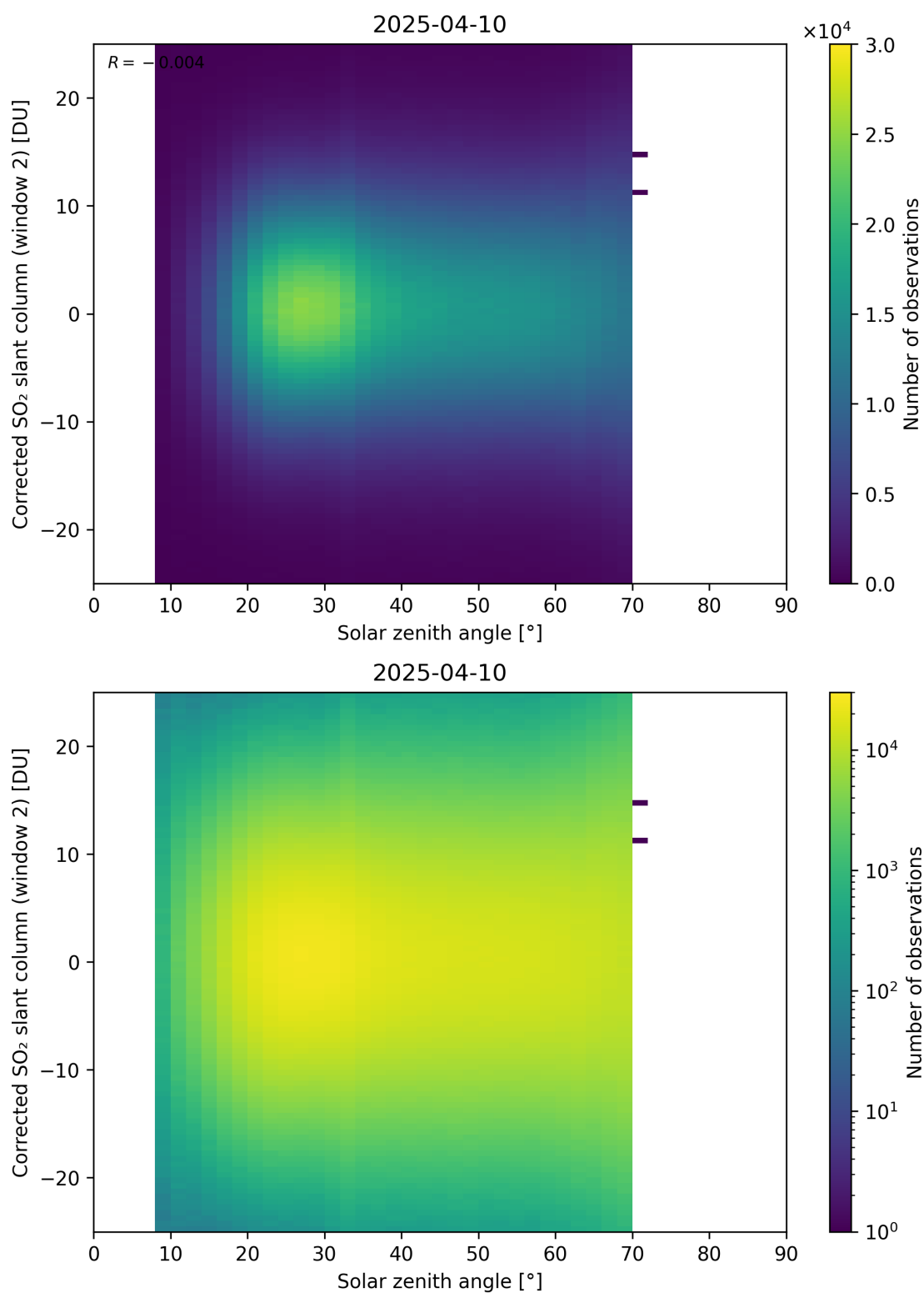
Figure 182: Scatter density plot of “Solar zenith angle” against “Corrected SO 2 slant column (window 2)” for 2025-04-09 to 2025-04-11.
