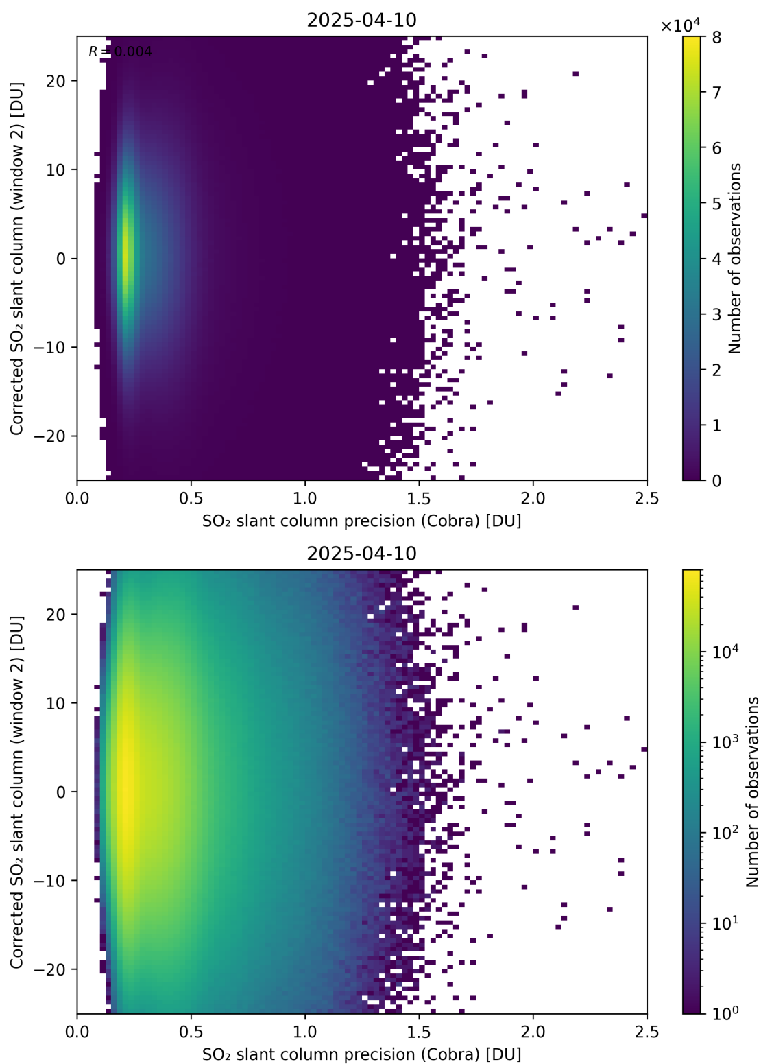
Figure 206: Scatter density plot of “SO 2 slant column precision (Cobra)” against “Corrected SO 2 slant column (window 2)” for 2025-04-09 to 2025-04-11.
