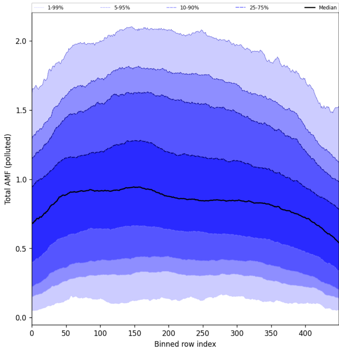
Figure 105: Along track statistics of “Total AMF (polluted)” for 2025-04-09 to 2025-04-11
