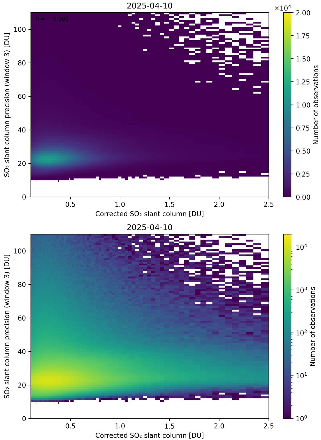
Figure 241: Scatter density plot of “Corrected SO 2 slant column” against “SO 2 slant column precision (window 3)” for 2025-04-09 to 2025-04-11.
