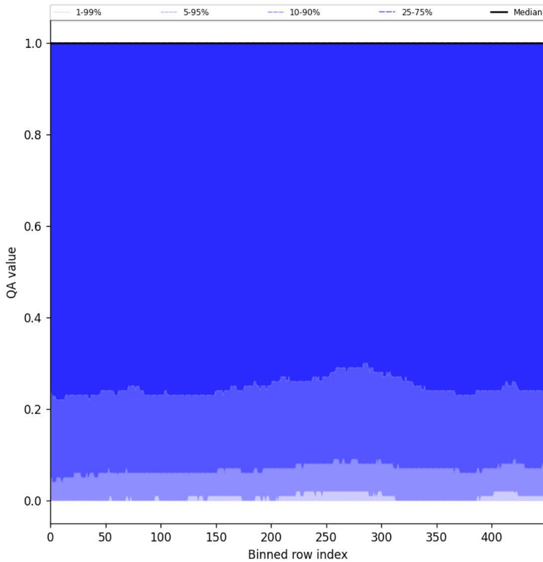
Figure 83: Along track statistics of “QA value” for 2025-04-09 to 2025-04-11
