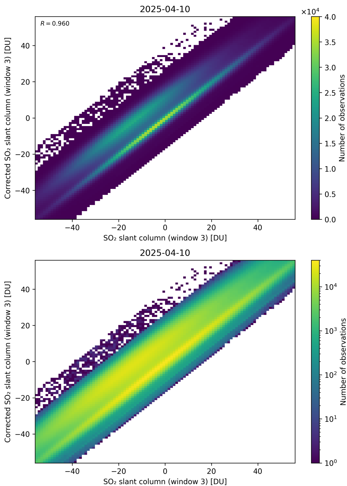
Figure 316: Scatter density plot of “SO 2 slant column (window 3)” against “Corrected SO 2 slant column (window 3)” for 2025-04-09 to 2025-04-11.
