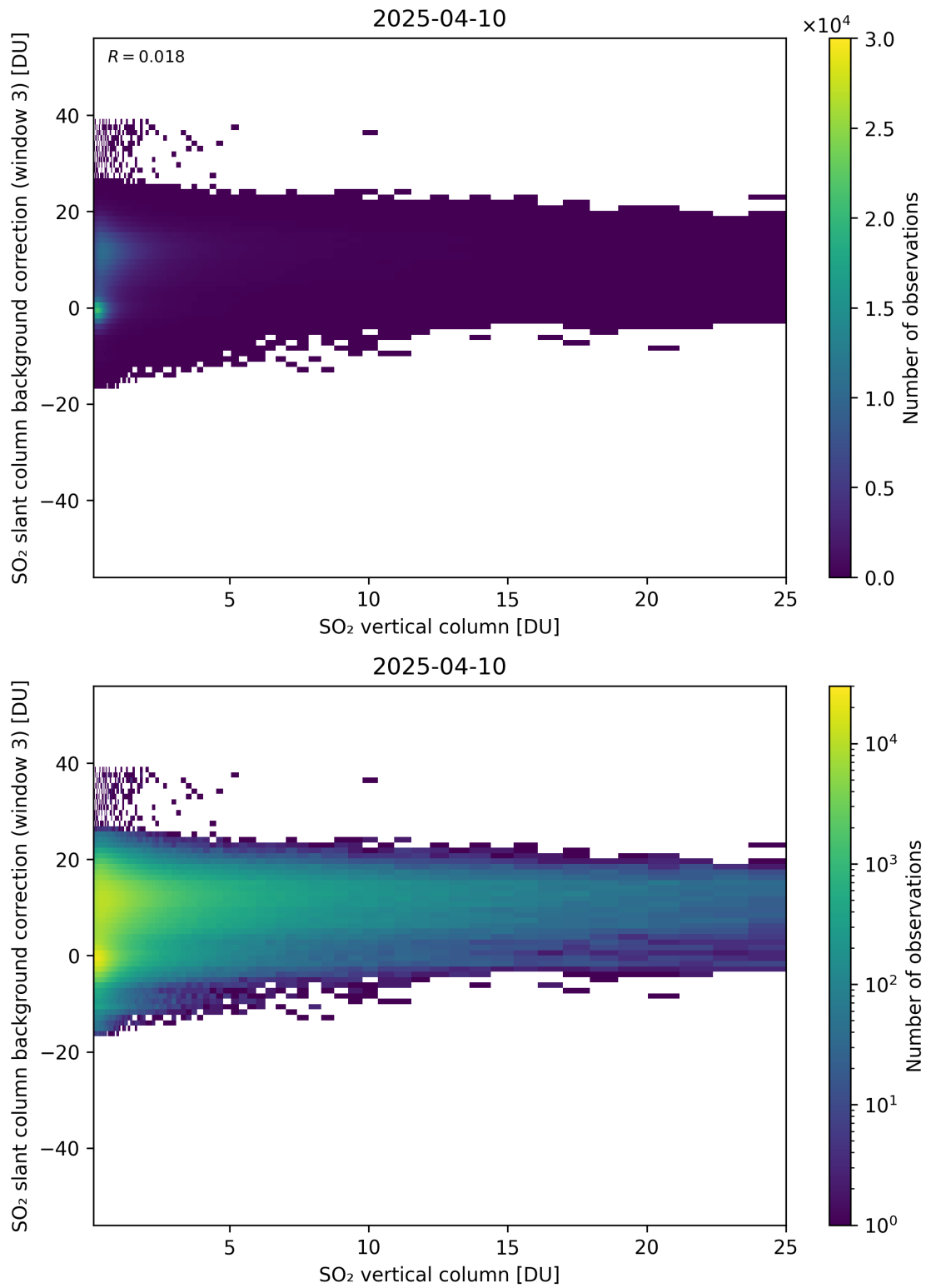
Figure 325: Scatter density plot of “SO 2 vertical column” against “SO 2 slant column background correction (window 3)” for 2025-04-09 to 2025-04-11.
