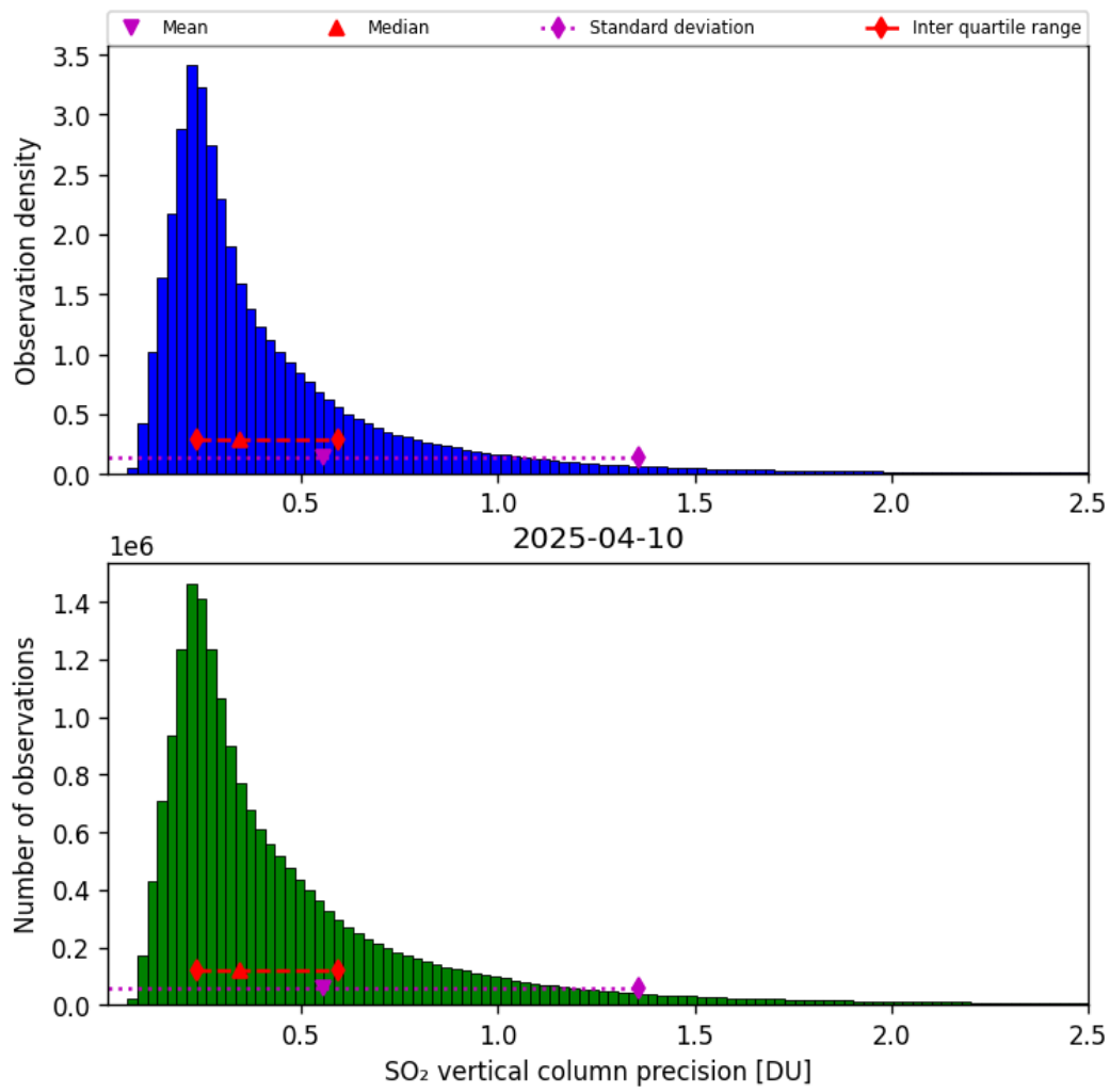
Figure 59: Histogram of “SO 2 vertical column precision” for 2025-04-09 to 2025-04-11
