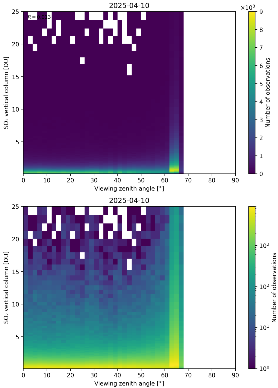
Figure 383: Scatter density plot of “Viewing zenith angle” against “SO 2 vertical column” for 2025-04-09 to 2025-04-11.
