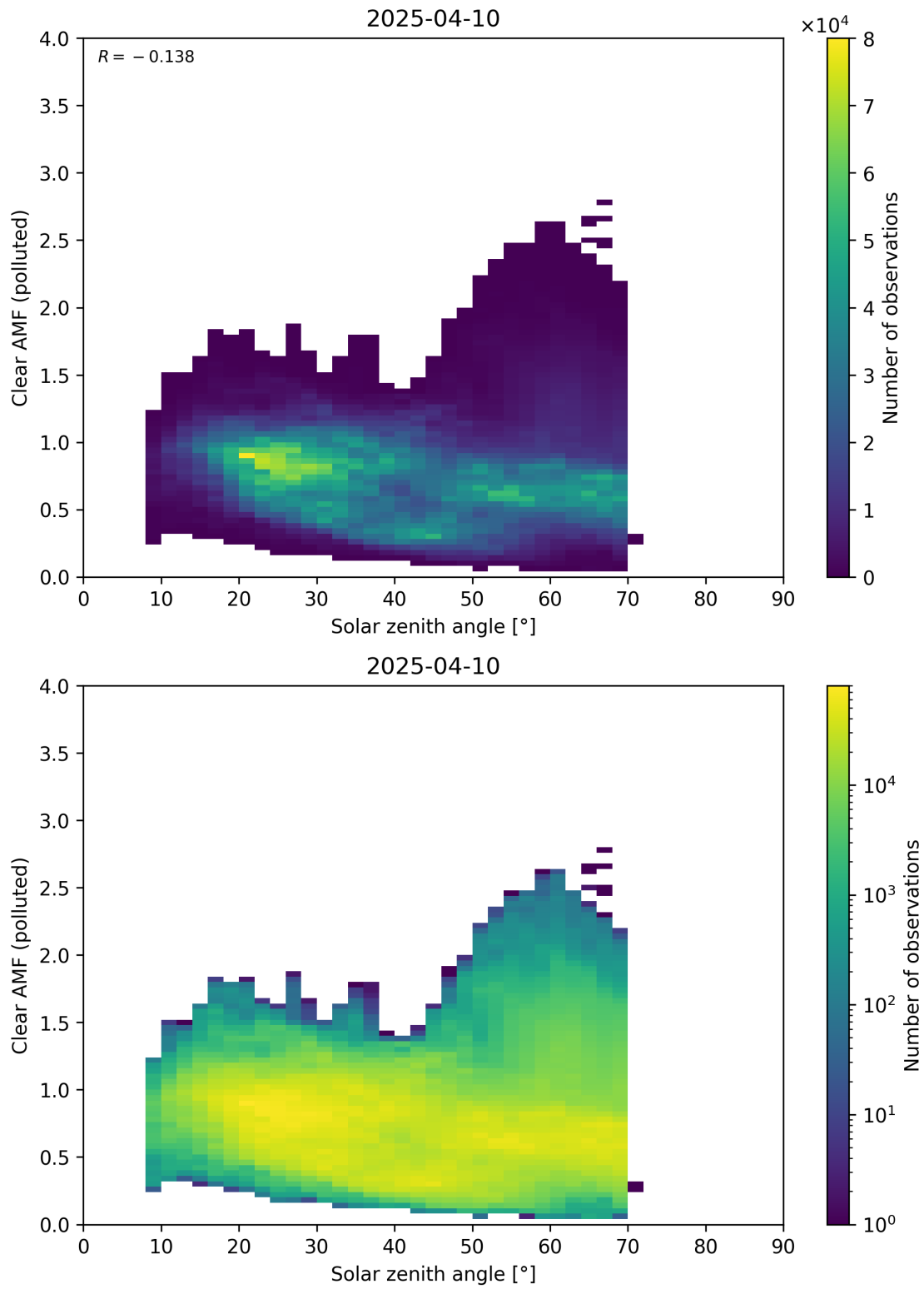
Figure 178: Scatter density plot of “Solar zenith angle” against “Clear AMF (polluted)” for 2025-04-09 to 2025-04-11.
