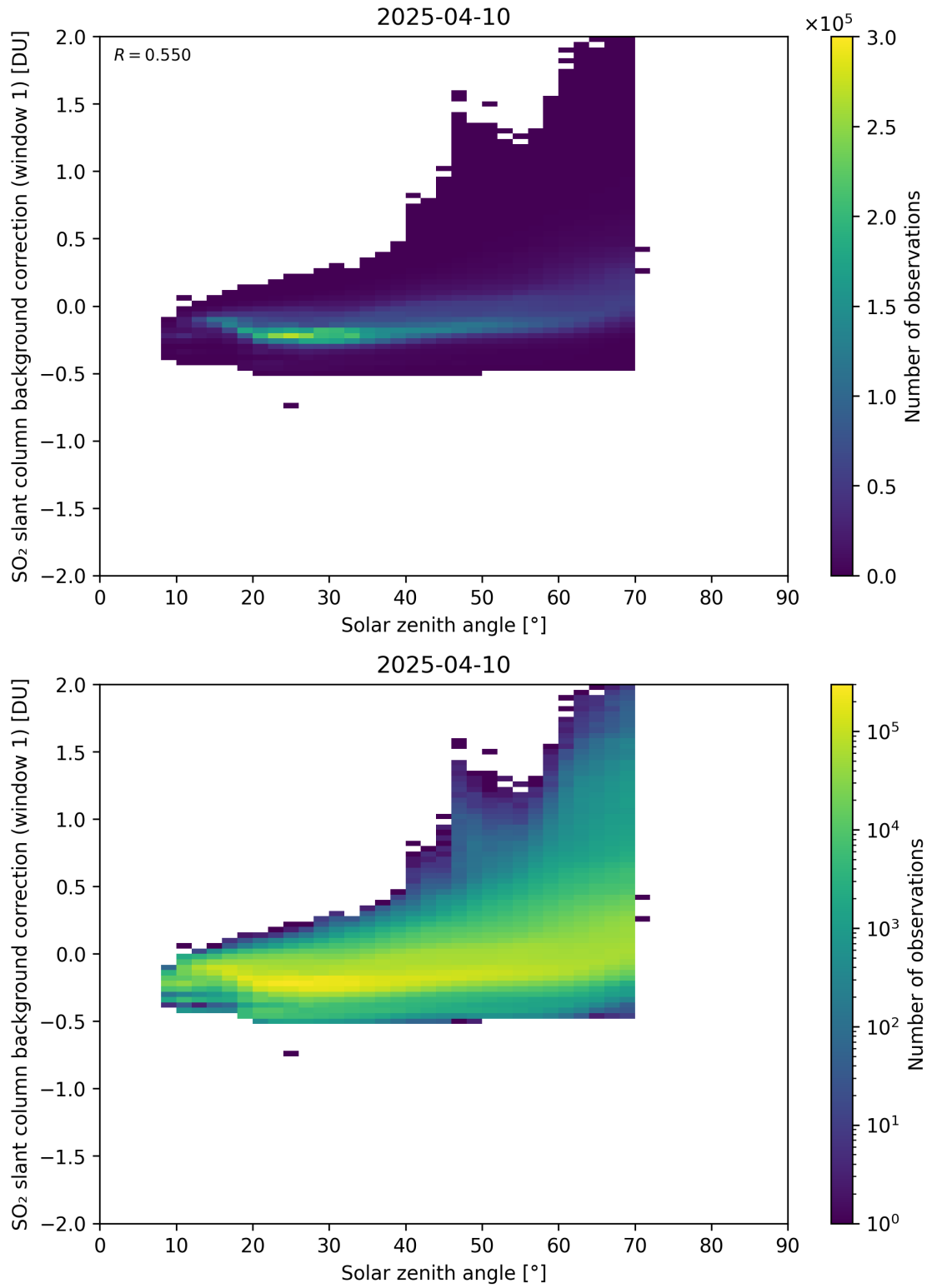
Figure 171: Scatter density plot of “Solar zenith angle” against “SO 2 slant column background correction (window 1)” for 2025-04-09 to 2025-04-11.
