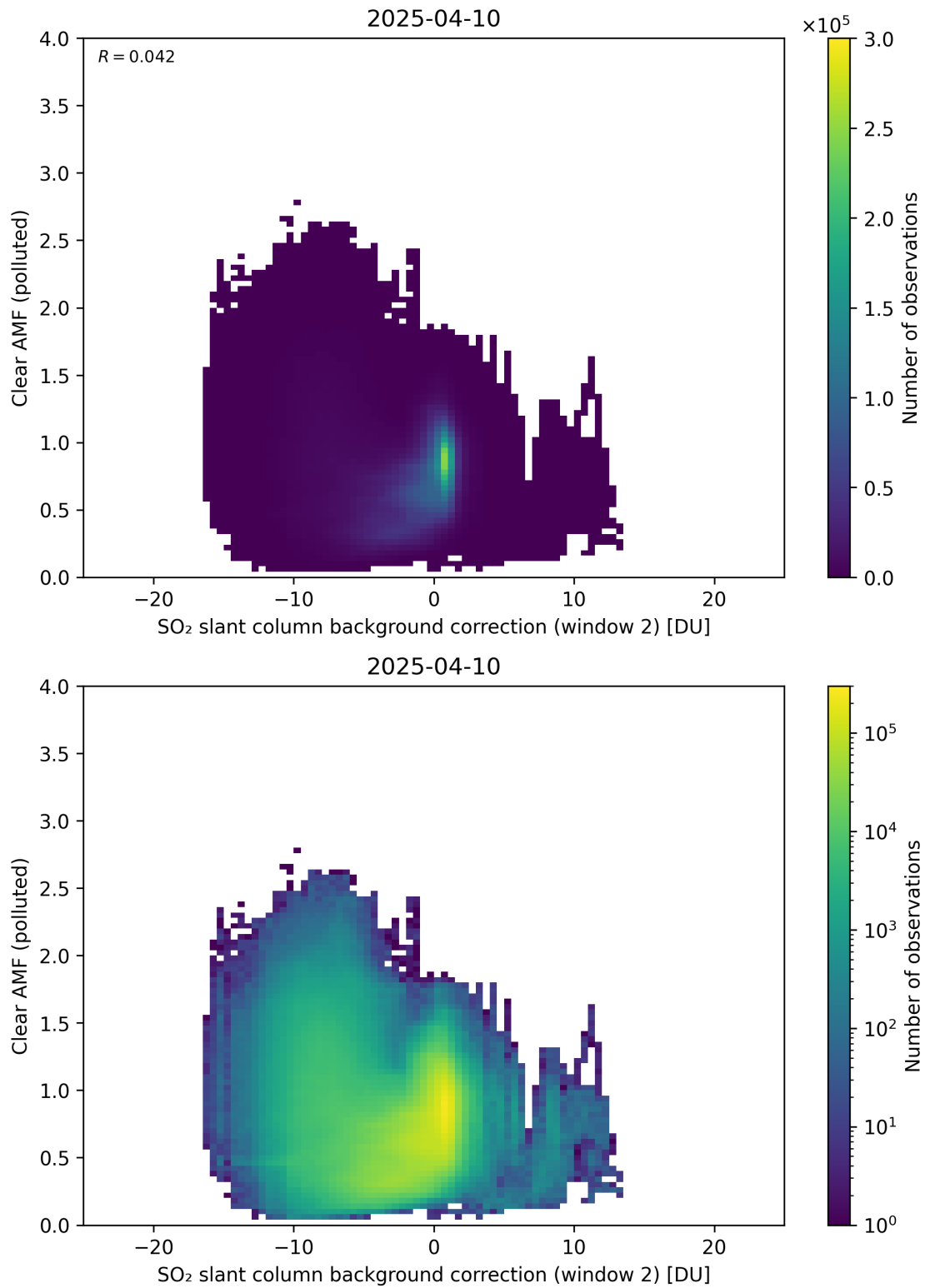
Figure 126: Scatter density plot of “SO 2 slant column background correction (window 2)” against “Clear AMF (polluted)” for 2025-04-09 to 2025-04-11.
