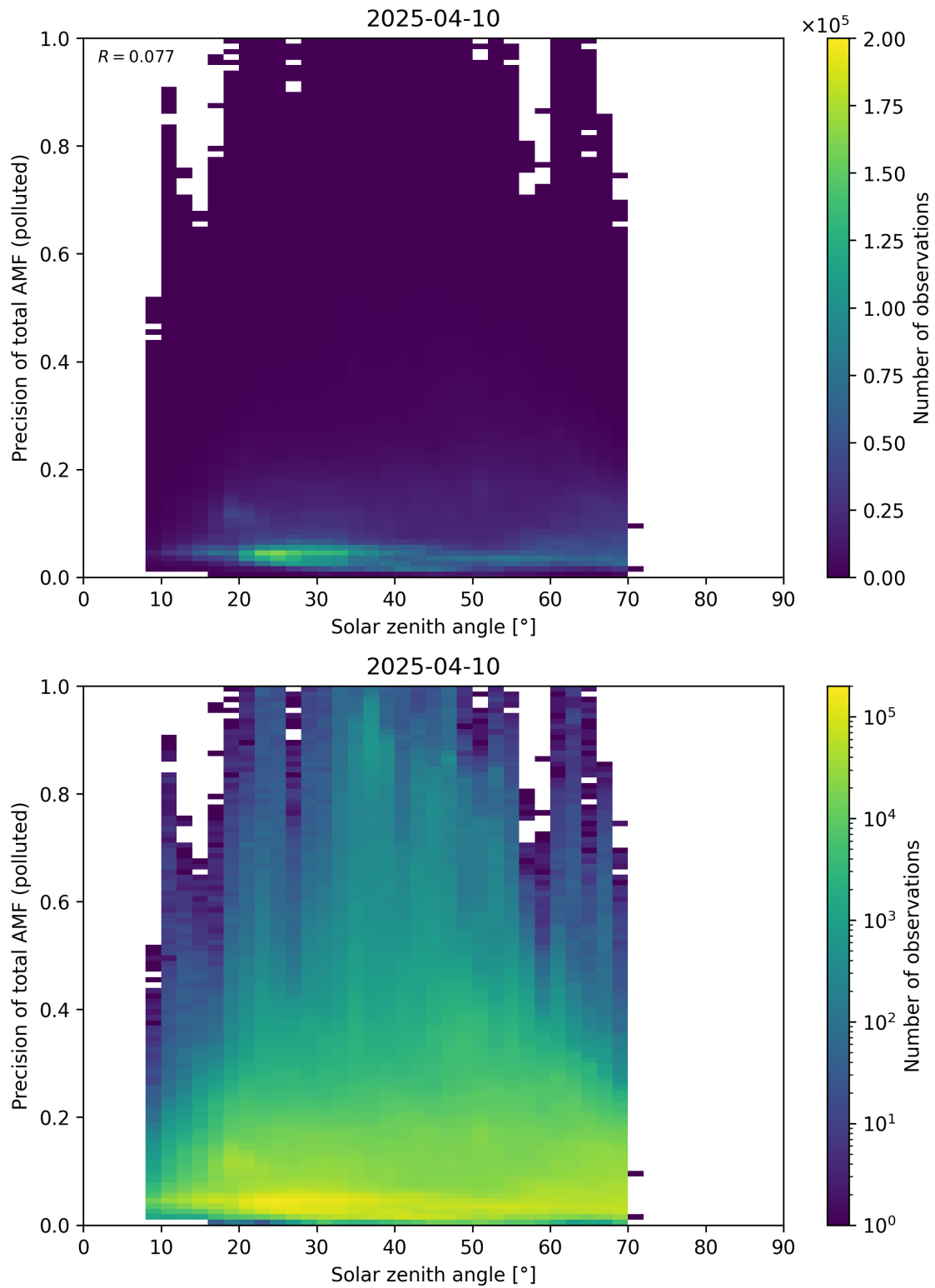
Figure 190: Scatter density plot of “Solar zenith angle” against “Precision of total AMF (polluted)” for 2025-04-09 to 2025-04-11.
