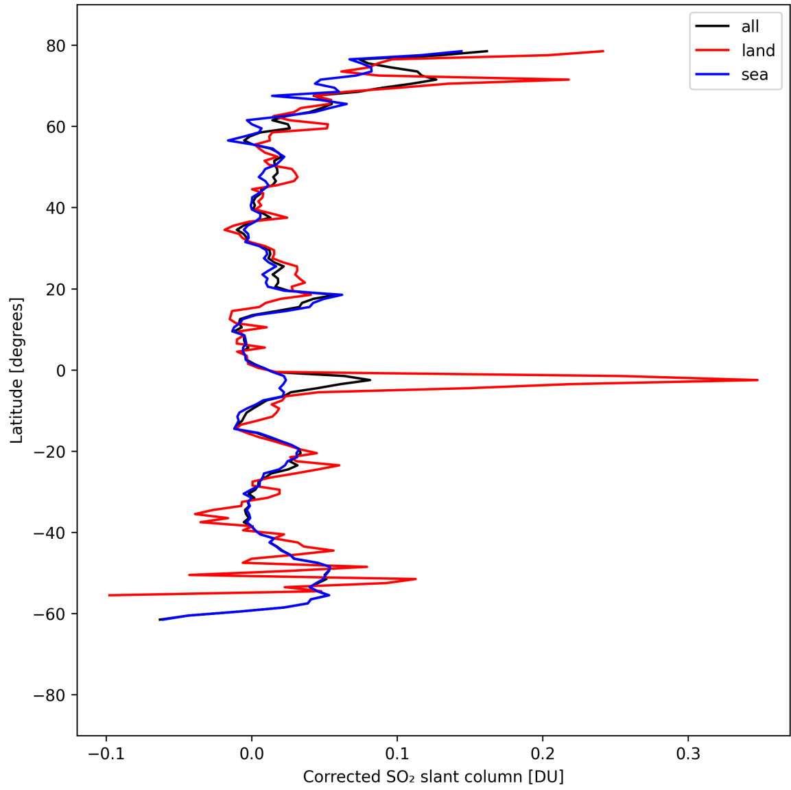
Figure 34: Zonal average of “Corrected SO 2 slant column” for 2025-04-09 to 2025-04-11.
