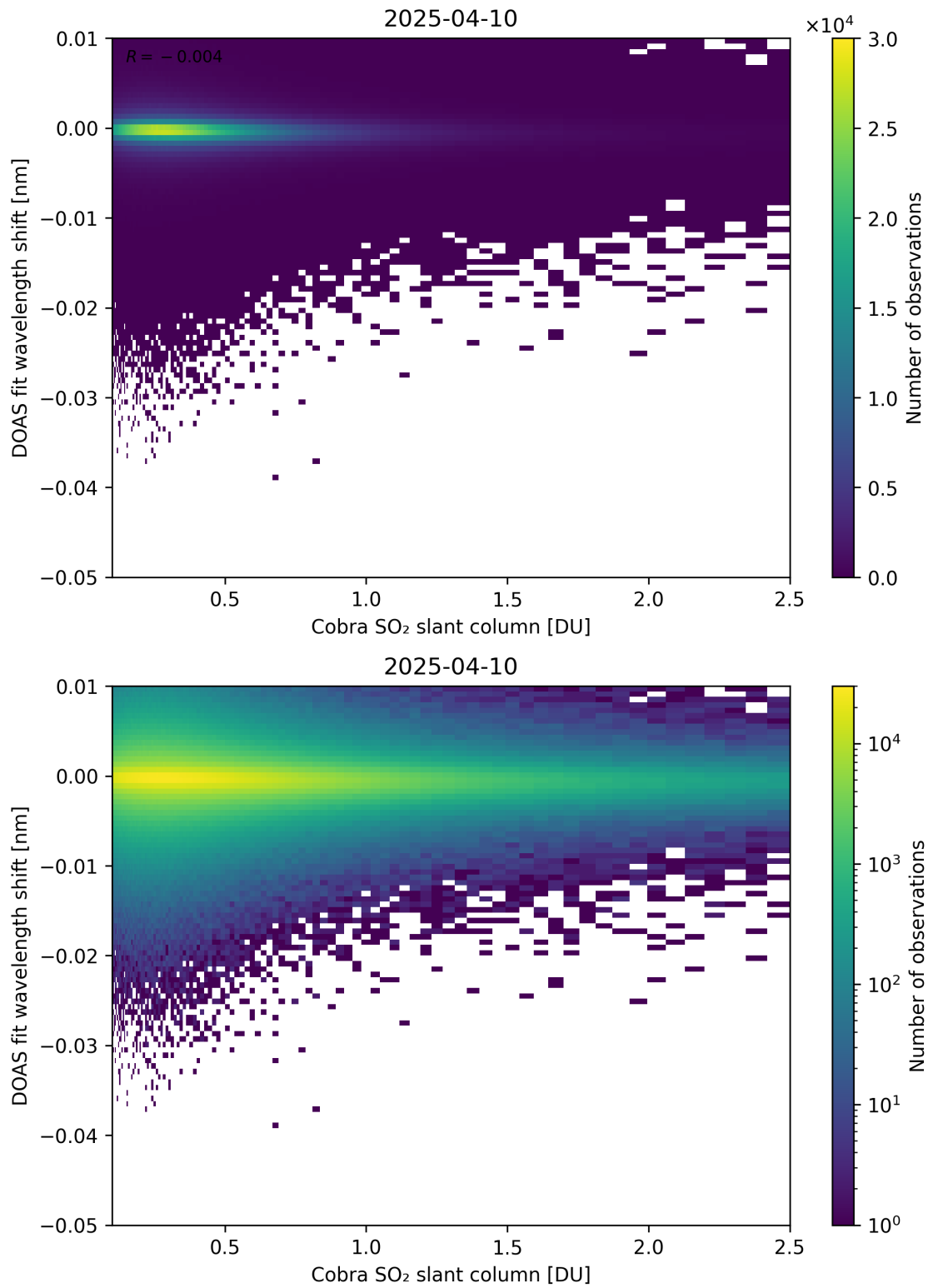
Figure 196: Scatter density plot of “Cobra SO 2 slant column” against “DOAS fit wavelength shift” for 2025-04-09 to 2025-04-11.
