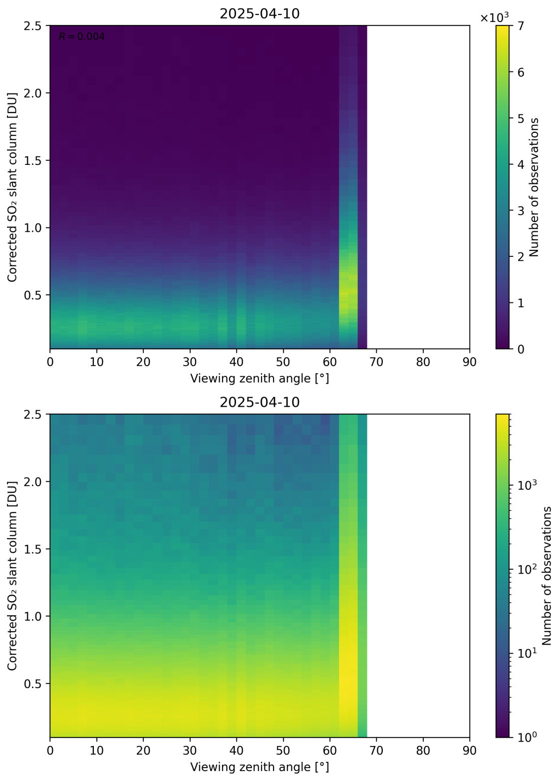
Figure 373: Scatter density plot of “Viewing zenith angle” against “Corrected SO 2 slant column” for 2025-04-09 to 2025-04-11.
