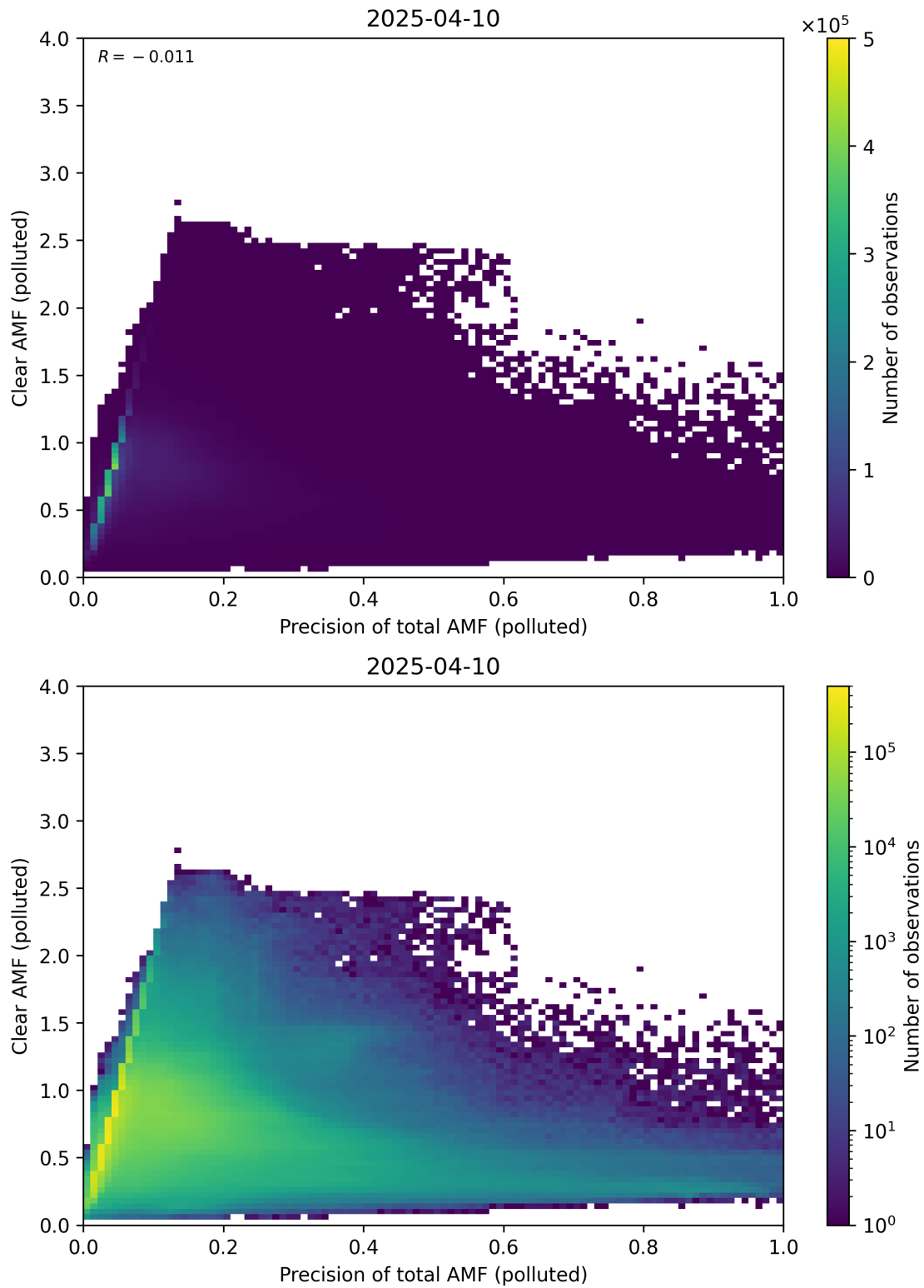
Figure 320: Scatter density plot of “Precision of total AMF (polluted)” against “Clear AMF (polluted)” for 2025-04-09 to 2025-04-11.
