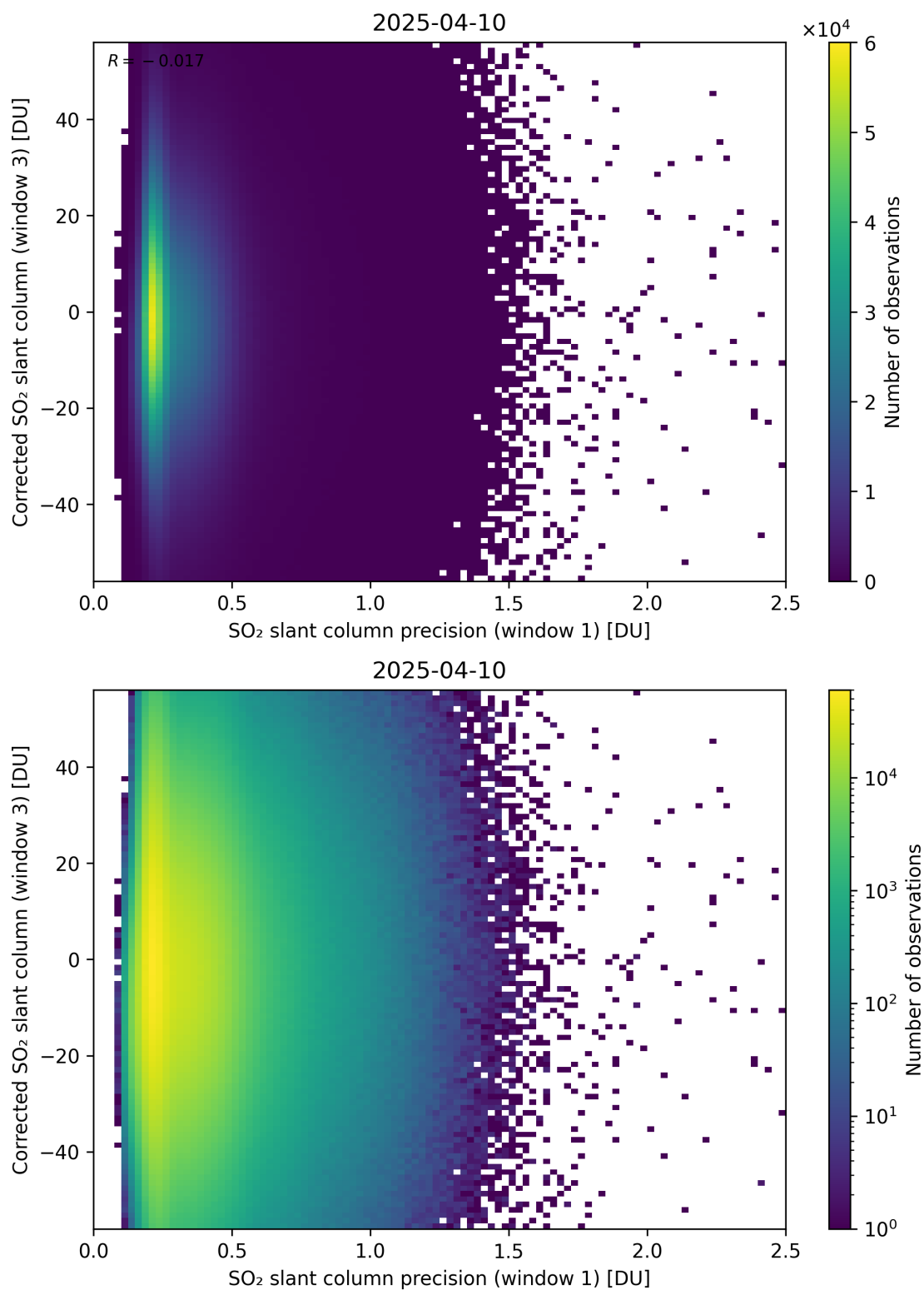
Figure 276: Scatter density plot of “SO 2 slant column precision (window 1)” against “Corrected SO 2 slant column (window 3)” for 2025-04-09 to 2025-04-11.
