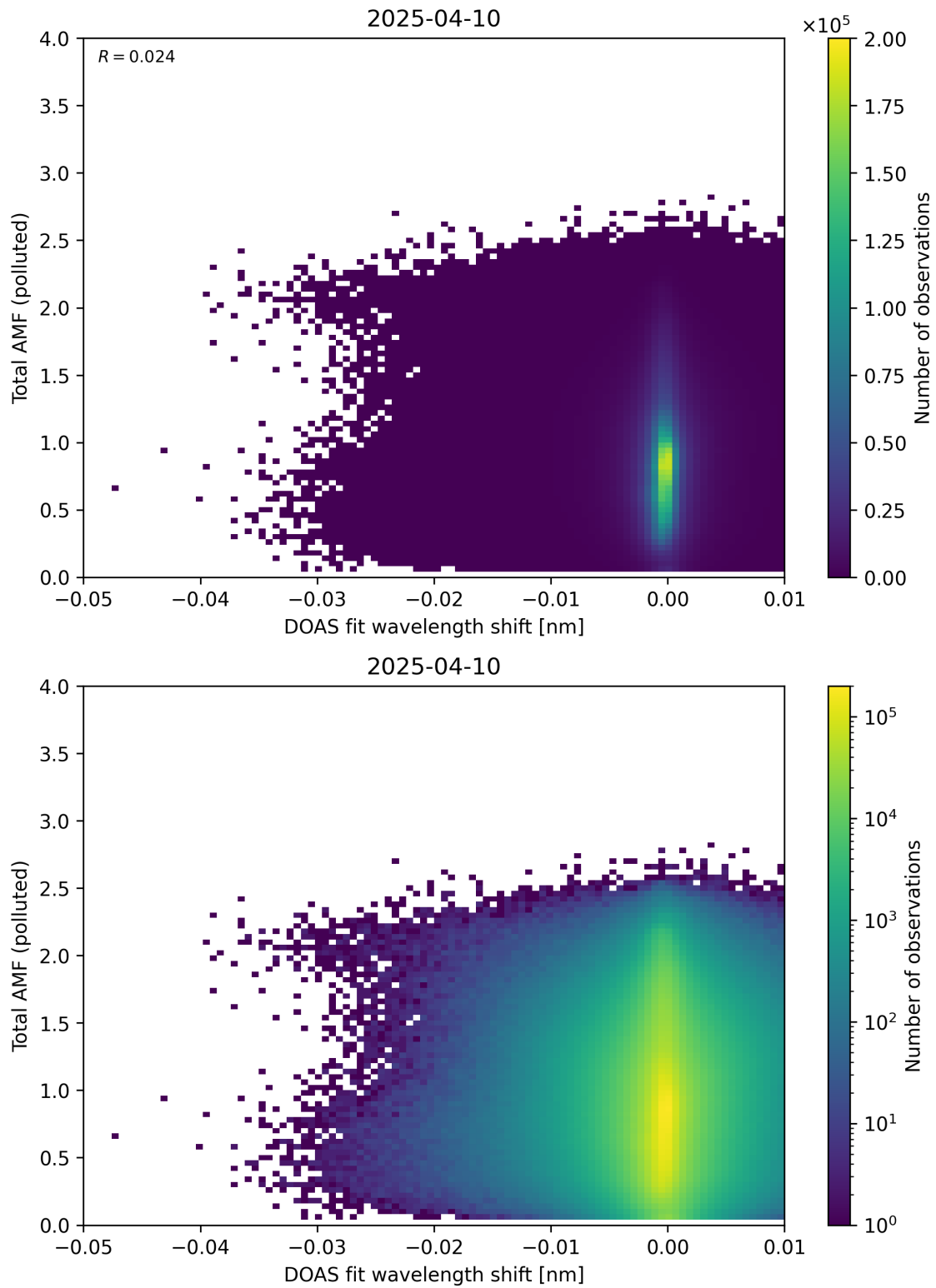
Figure 141: Scatter density plot of “DOAS fit wavelength shift” against “Total AMF (polluted)” for 2025-04-09 to 2025-04-11.
