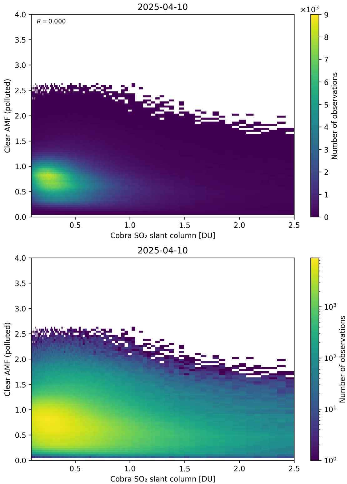
Figure 215: Scatter density plot of “Cobra SO 2 slant column” against “Clear AMF (polluted)” for 2025-04-09 to 2025-04-11.
