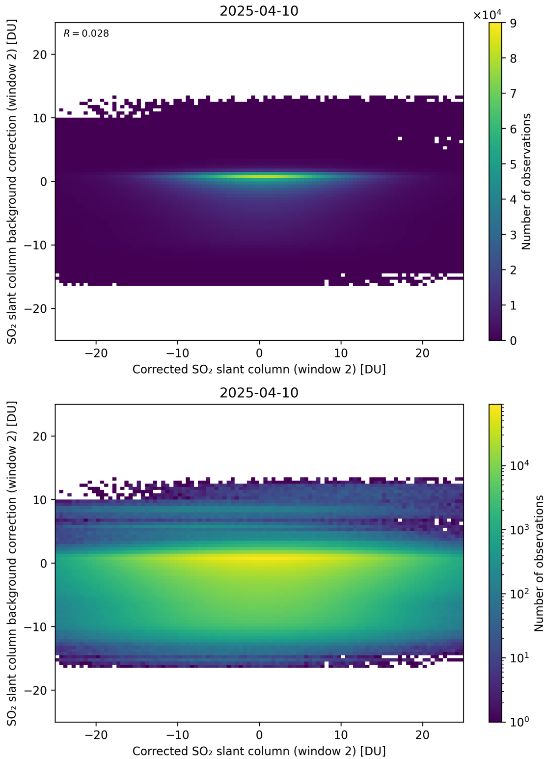
Figure 244: Scatter density plot of “Corrected SO 2 slant column (window 2)” against “SO 2 slant column background correction (window 2)” for 2025-04-09 to 2025-04-11.
