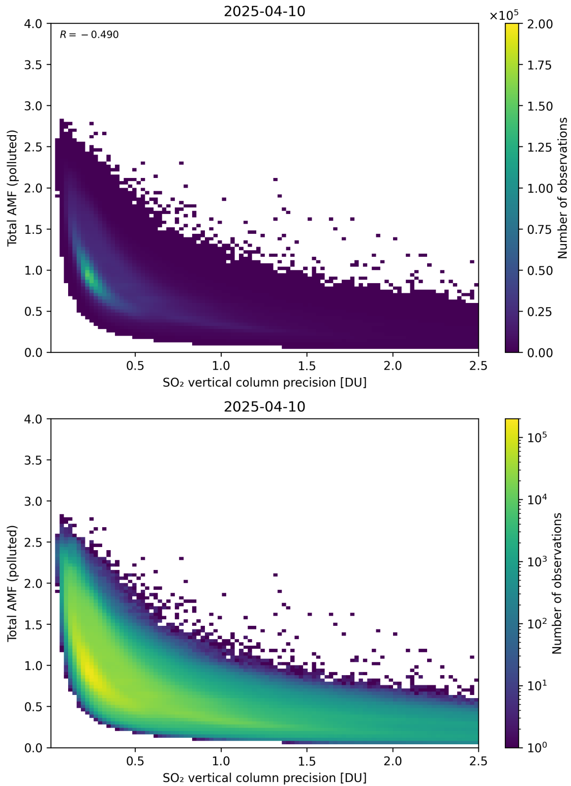
Figure 346: Scatter density plot of “SO 2 vertical column precision” against “Total AMF (polluted)” for 2025-04-09 to 2025-04-11.
