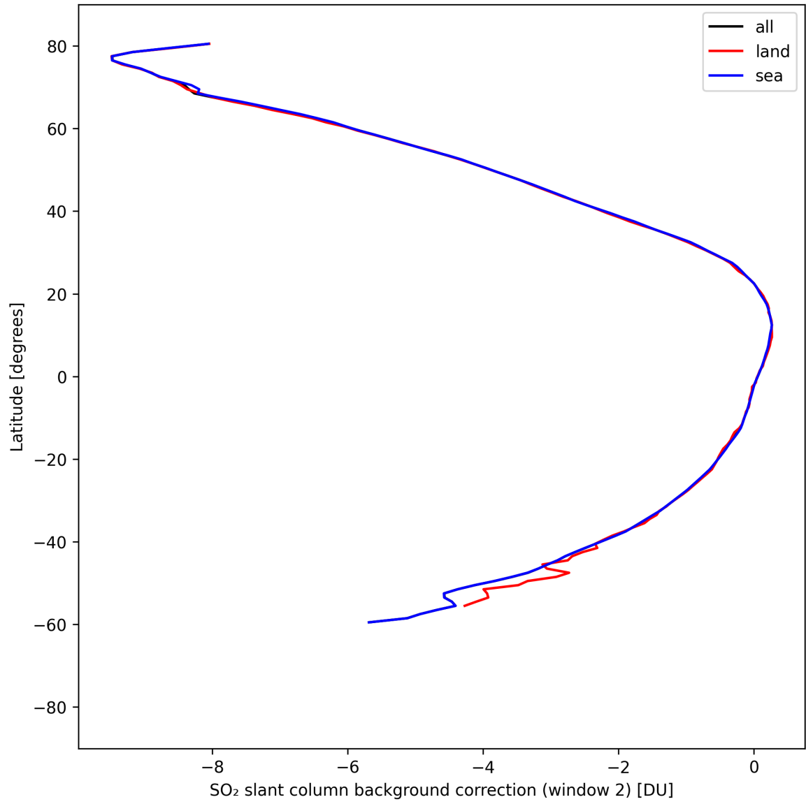
Figure 44: Zonal average of “SO 2 slant column background correction (window 2)” for 2025-04-15 to 2025-04-17.
