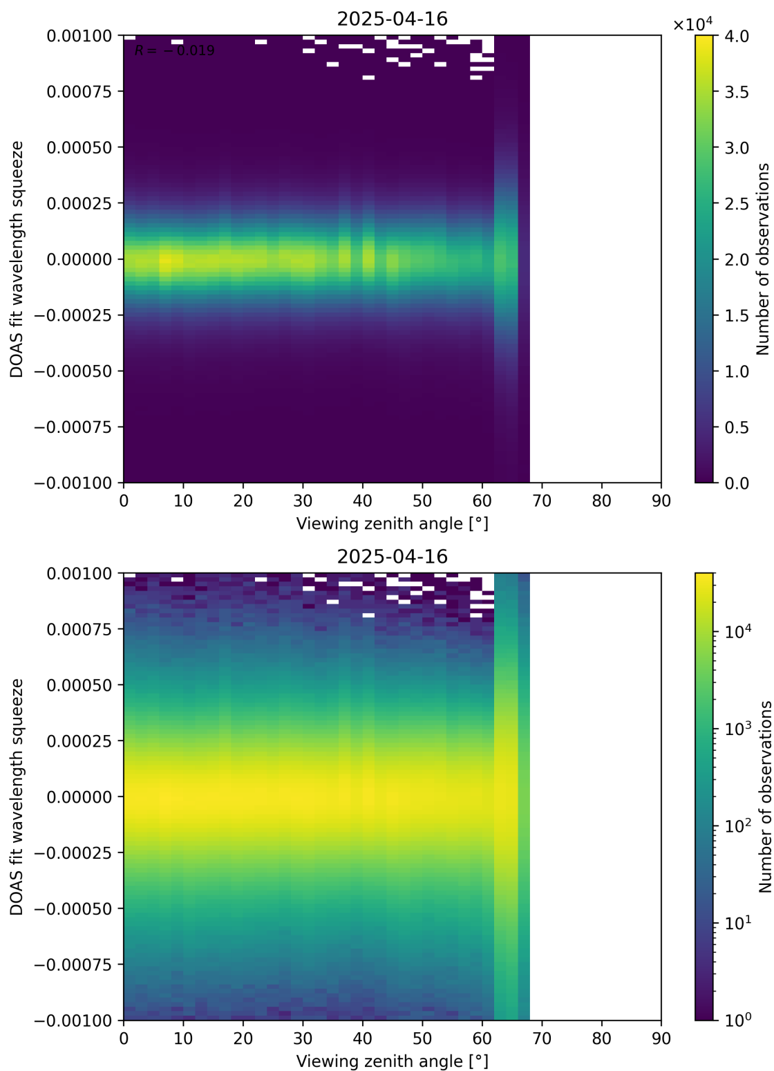
Figure 366: Scatter density plot of “Viewing zenith angle” against “DOAS fit wavelength squeeze” for 2025-04-15 to 2025-04-17.
