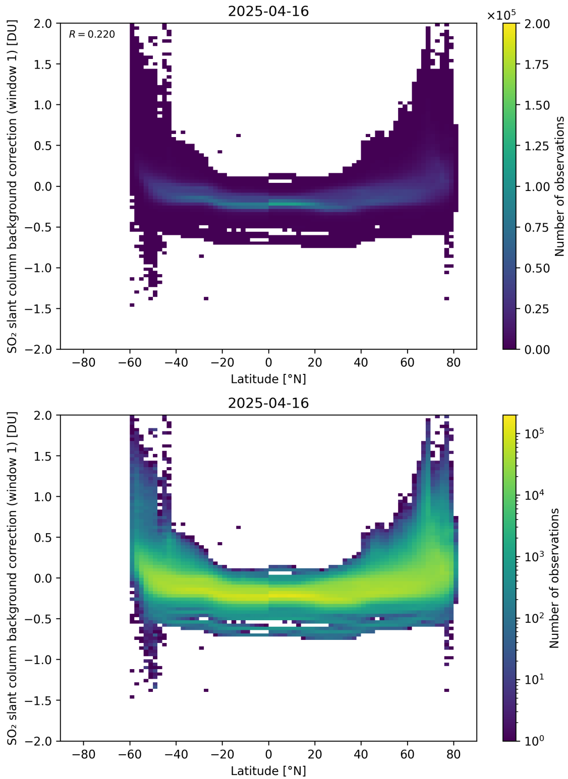
Figure 150: Scatter density plot of “Latitude” against “SO 2 slant column background correction (window 1)” for 2025-04-15 to 2025-04-17.
