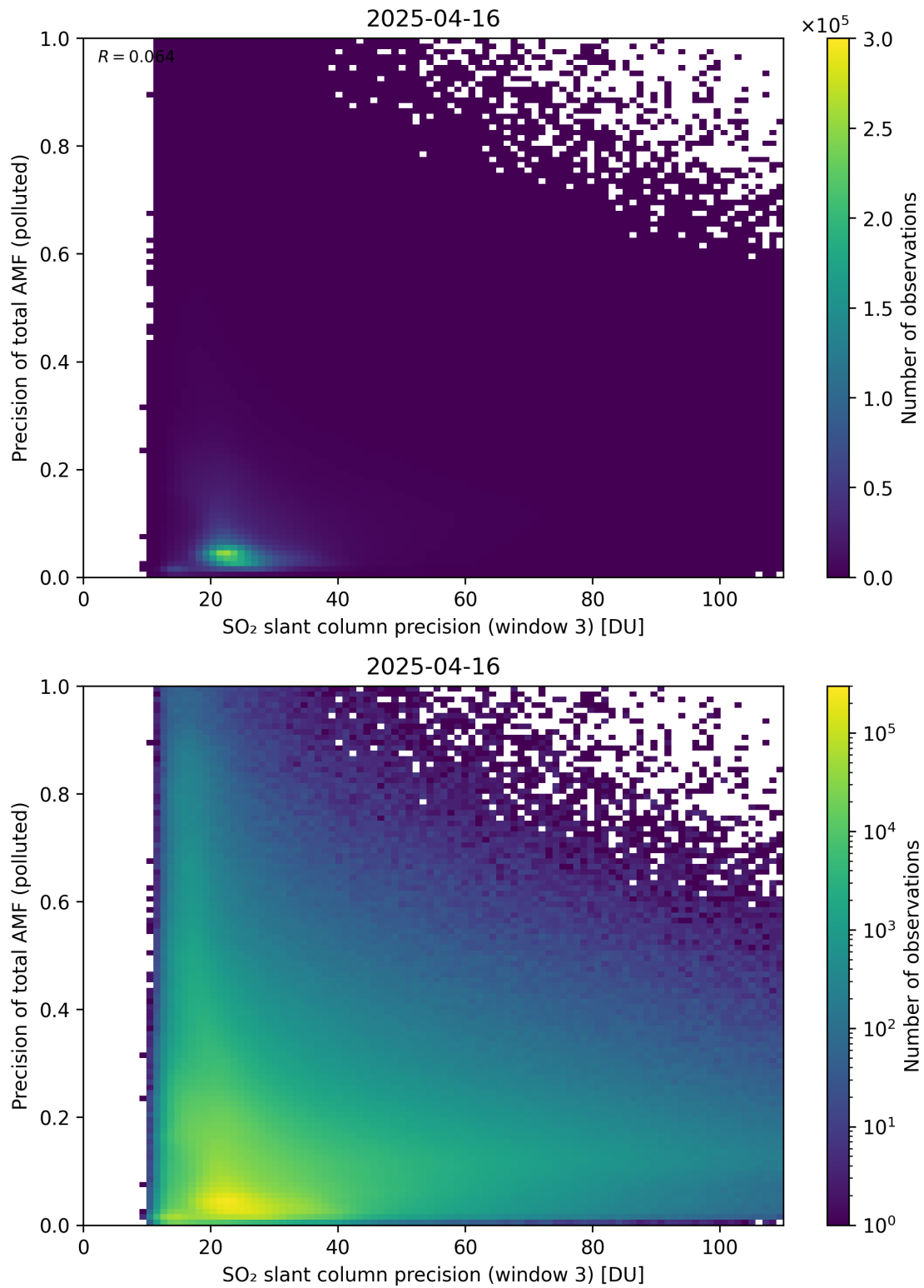
Figure 314: Scatter density plot of “SO 2 slant column precision (window 3)” against “Precision of total AMF (polluted)” for 2025-04-15 to 2025-04-17.
