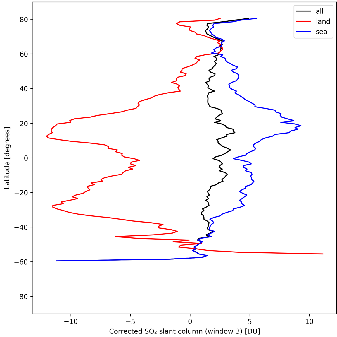
Figure 47: Zonal average of “Corrected SO 2 slant column (window 3)” for 2025-04-15 to 2025-04-17.
