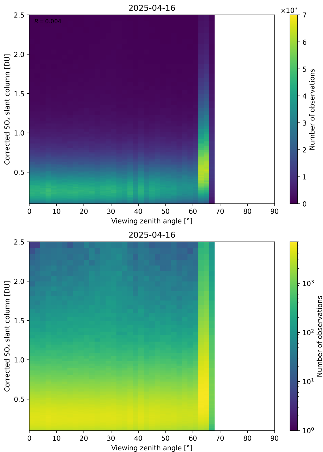
Figure 373: Scatter density plot of “Viewing zenith angle” against “Corrected SO 2 slant column” for 2025-04-15 to 2025-04-17.
