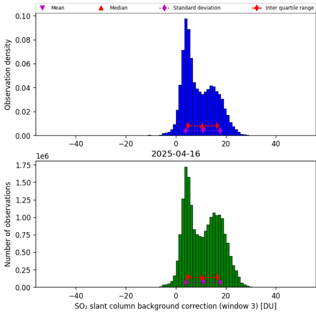
Figure 74: Histogram of “SO 2 slant column background correction (window 3)” for 2025-04-15 to 2025-04-17
