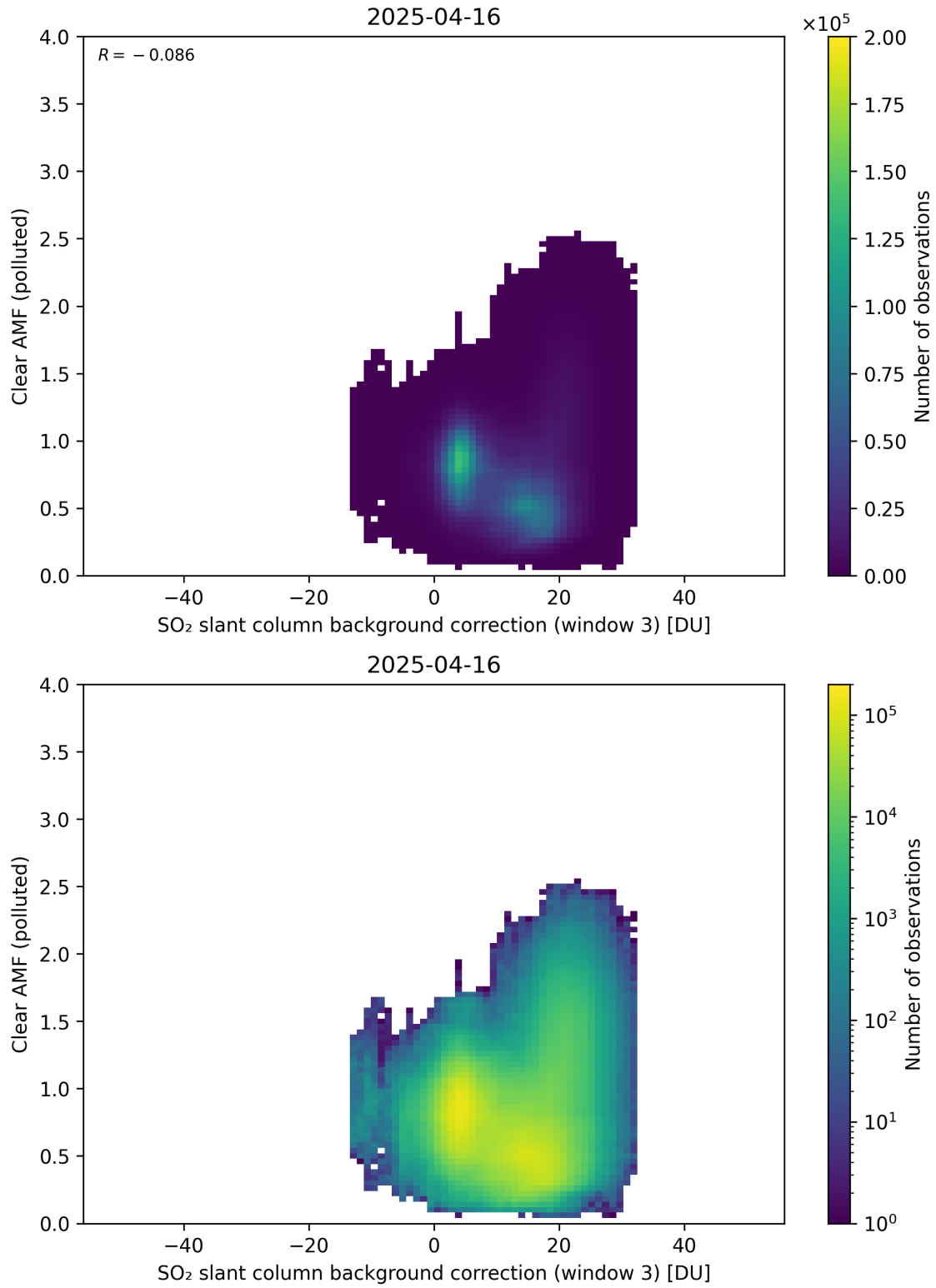
Figure 135: Scatter density plot of “SO 2 slant column background correction (window 3)” against “Clear AMF (polluted)” for 2025-04-15 to 2025-04-17.
