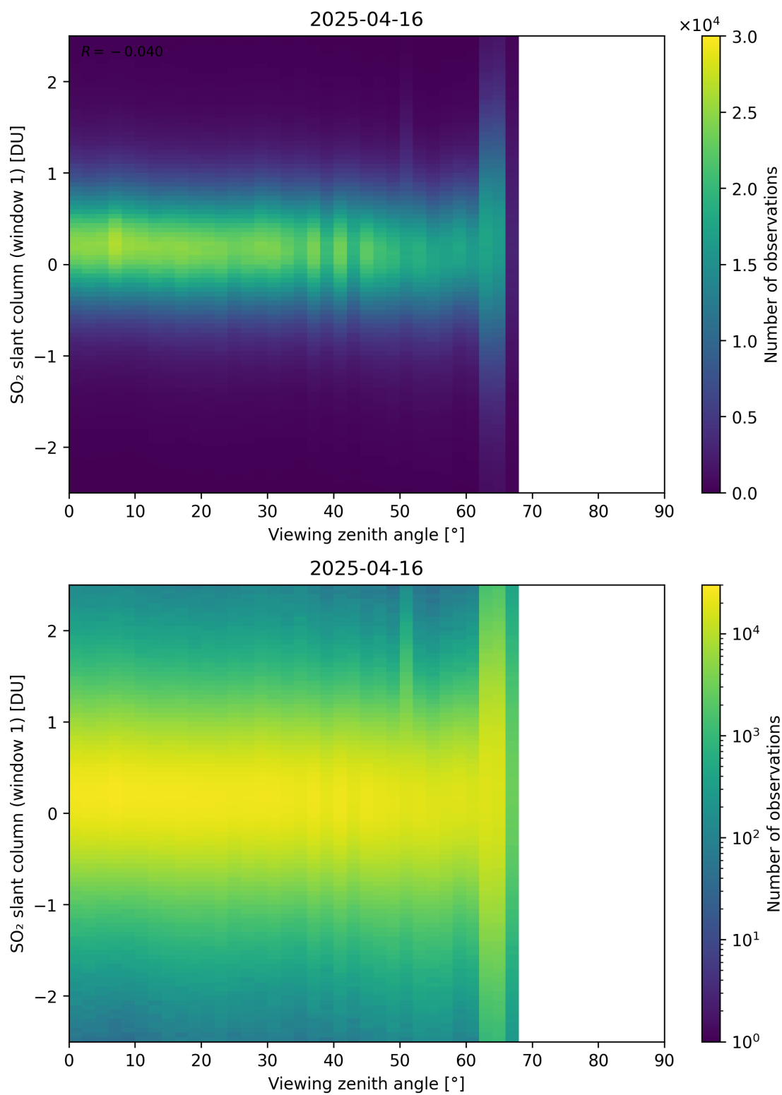
Figure 376: Scatter density plot of “Viewing zenith angle” against “SO 2 slant column (window 1)” for 2025-04-15 to 2025-04-17.
