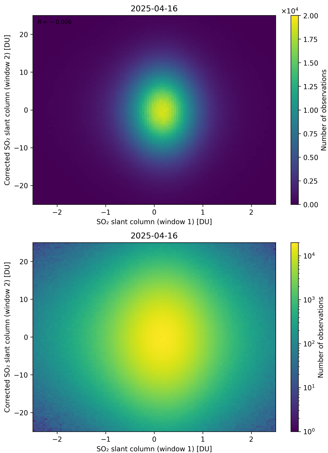
Figure 283: Scatter density plot of “SO 2 slant column (window 1)” against “Corrected SO 2 slant column (window 2)” for 2025-04-15 to 2025-04-17.
