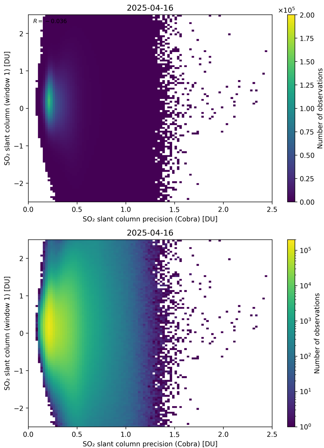
Figure 208: Scatter density plot of “SO 2 slant column precision (Cobra)” against “SO 2 slant column (window 1)” for 2025-04-15 to 2025-04-17.
