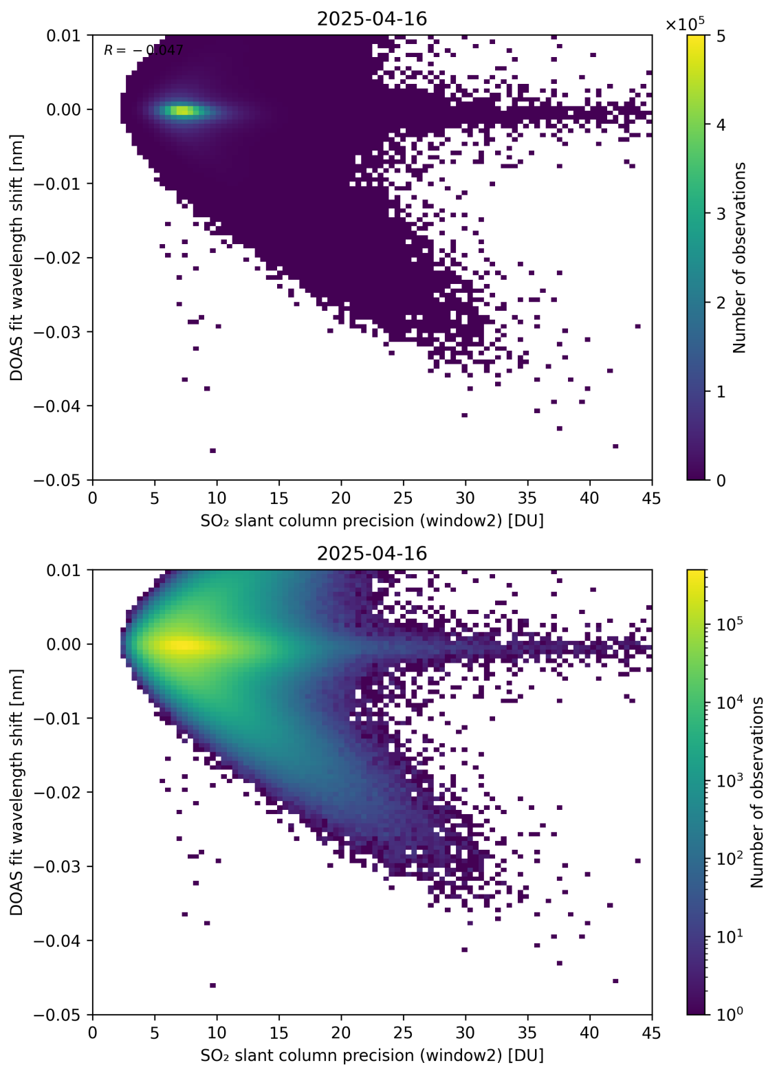
Figure 293: Scatter density plot of “SO 2 slant column precision (window2)” against “DOAS fit wavelength shift” for 2025-04-15 to 2025-04-17.
