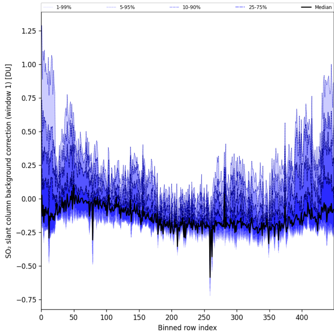
Figure 92: Along track statistics of “SO 2 slant column background correction (window 1)” for 2025-04-15 to 2025-04-17
