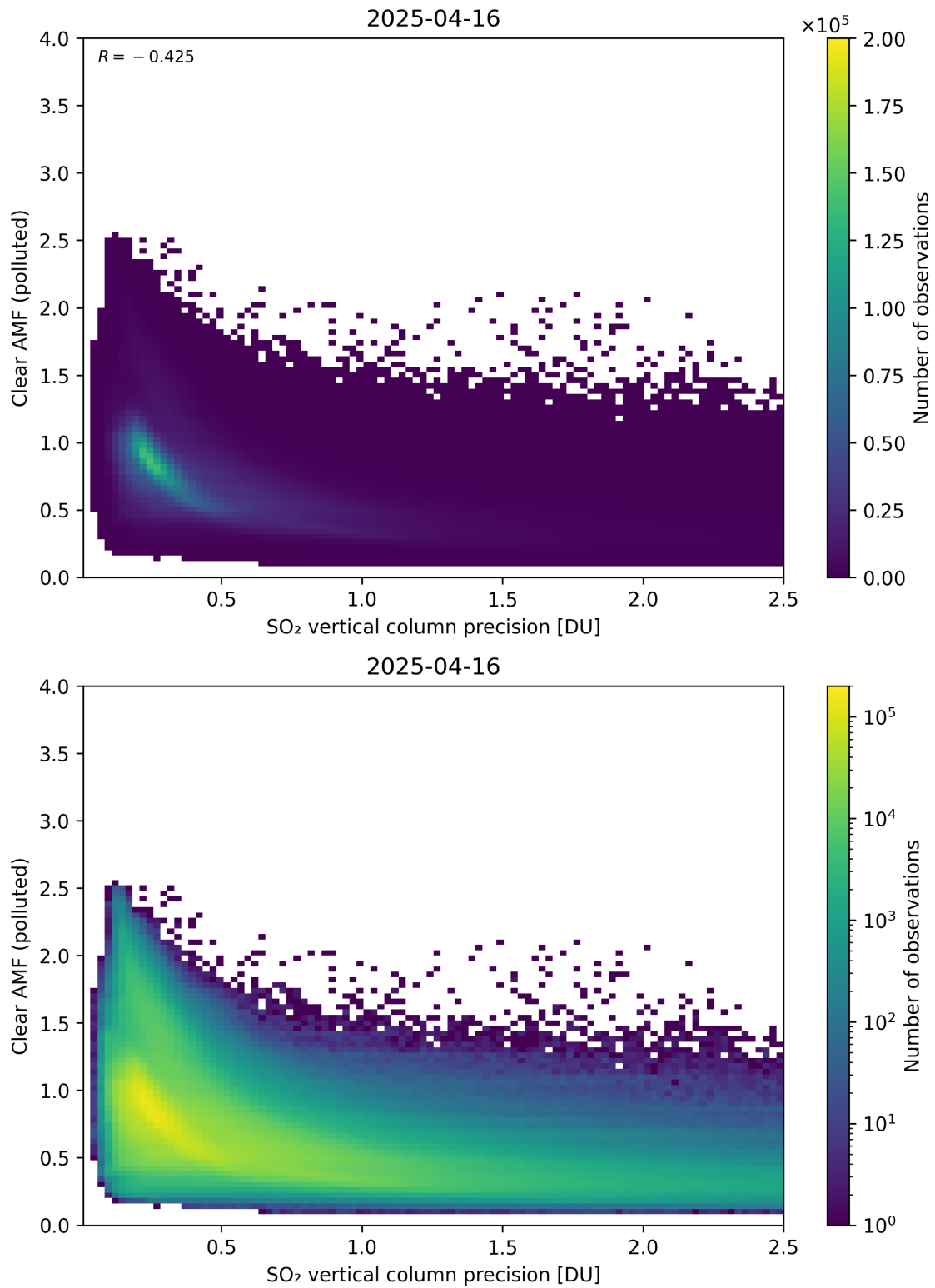
Figure 335: Scatter density plot of “SO 2 vertical column precision” against “Clear AMF (polluted)” for 2025-04-15 to 2025-04-17.
