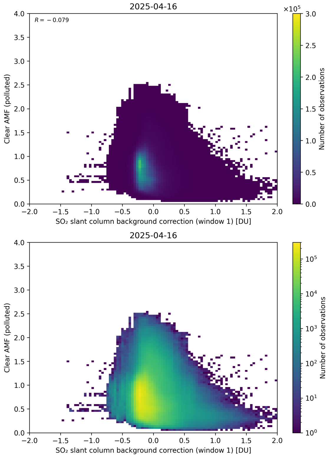
Figure 114: Scatter density plot of “SO 2 slant column background correction (window 1)” against “Clear AMF (polluted)” for 2025-04-15 to 2025-04-17.
