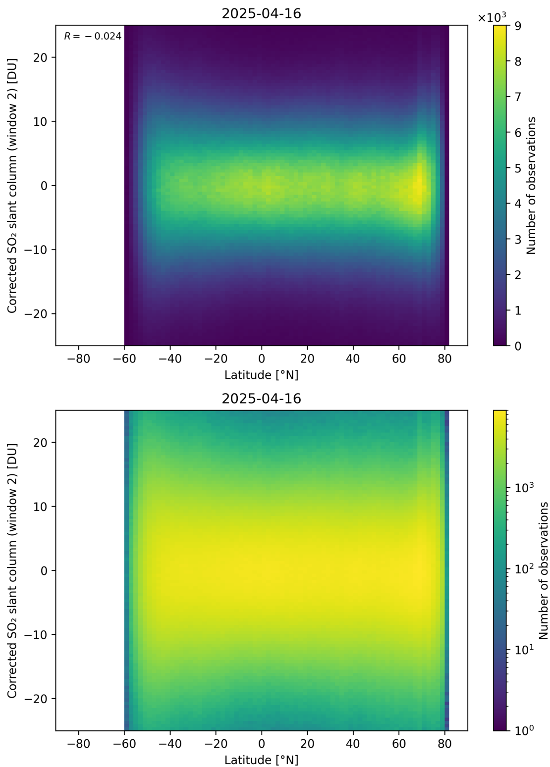
Figure 160: Scatter density plot of “Latitude” against “Corrected SO 2 slant column (window 2)” for 2025-04-15 to 2025-04-17.
