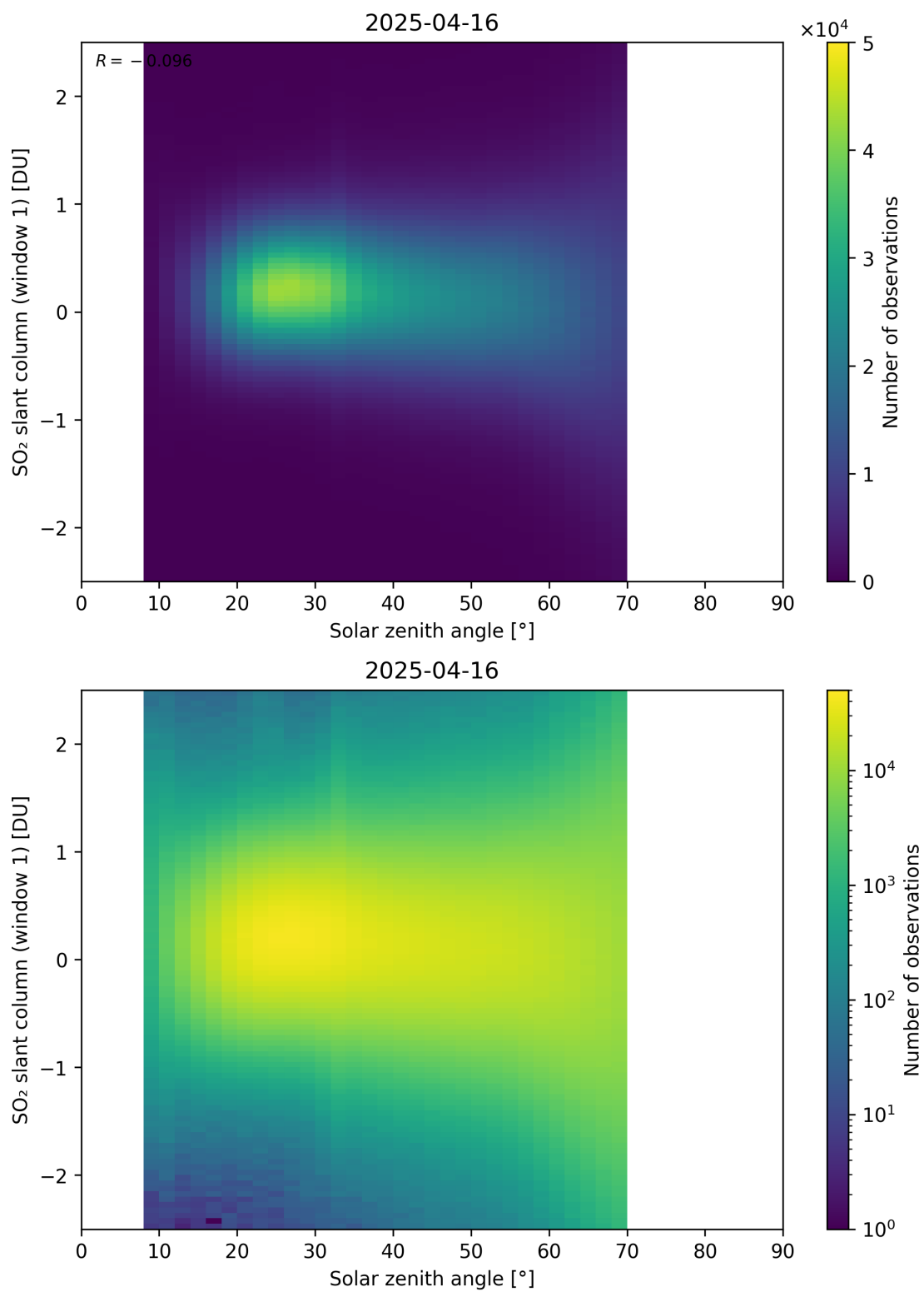
Figure 184: Scatter density plot of “Solar zenith angle” against “SO 2 slant column (window 1)” for 2025-04-15 to 2025-04-17.
