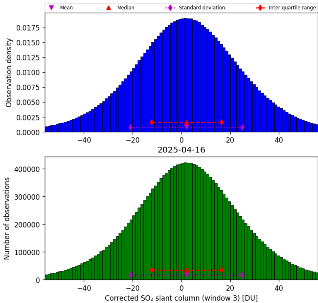
Figure 73: Histogram of “Corrected SO 2 slant column (window 3)” for 2025-04-15 to 2025-04-17
