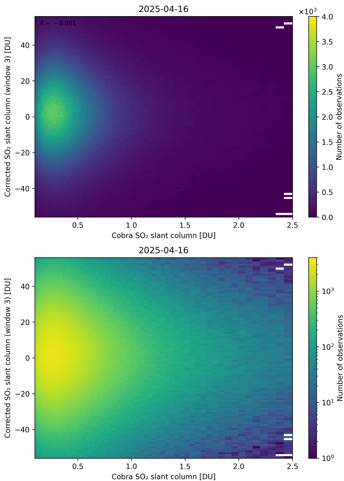
Figure 218: Scatter density plot of “Cobra SO 2 slant column” against “Corrected SO 2 slant column (window 3)” for 2025-04-15 to 2025-04-17.
