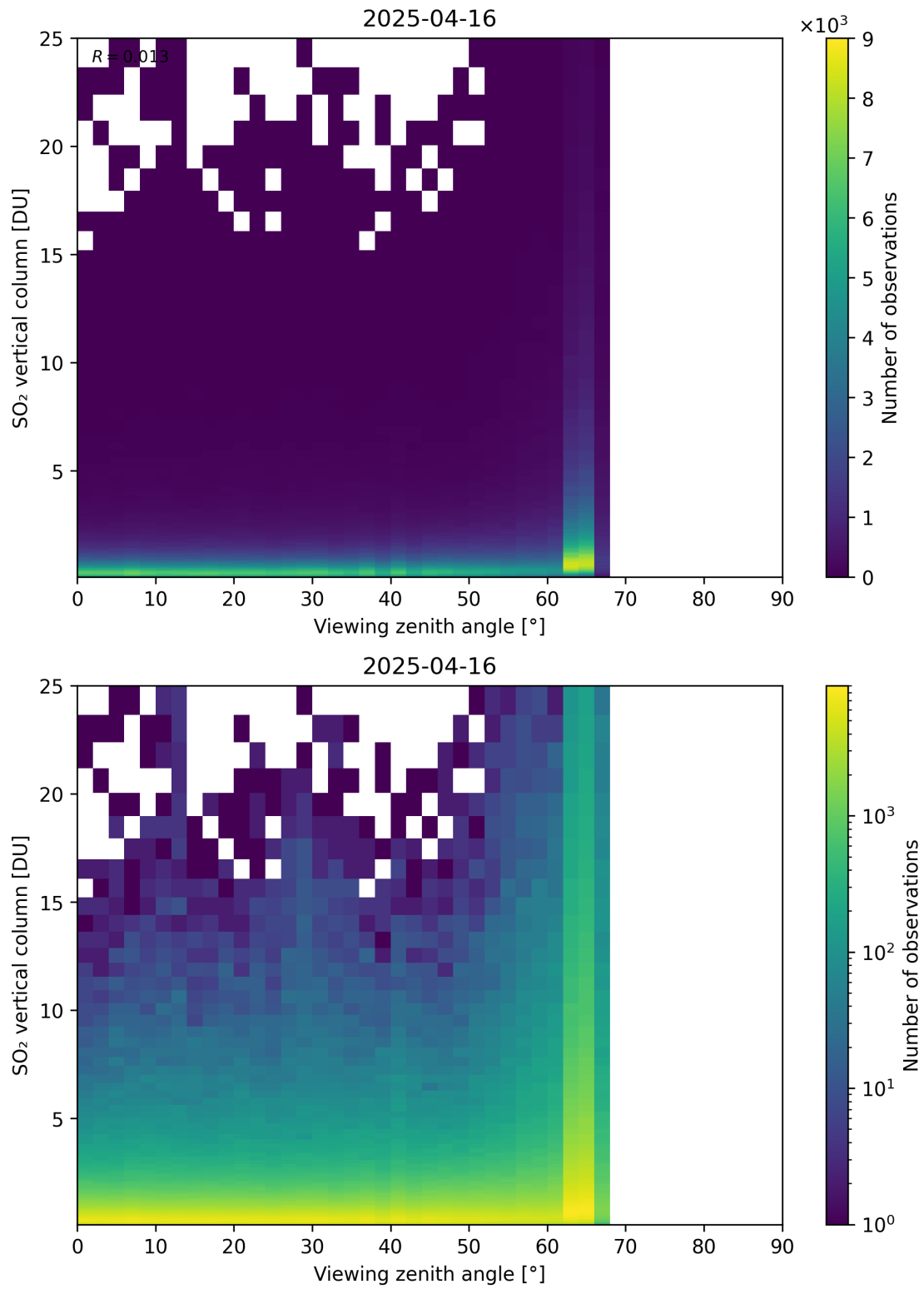
Figure 383: Scatter density plot of “Viewing zenith angle” against “SO 2 vertical column” for 2025-04-15 to 2025-04-17.
