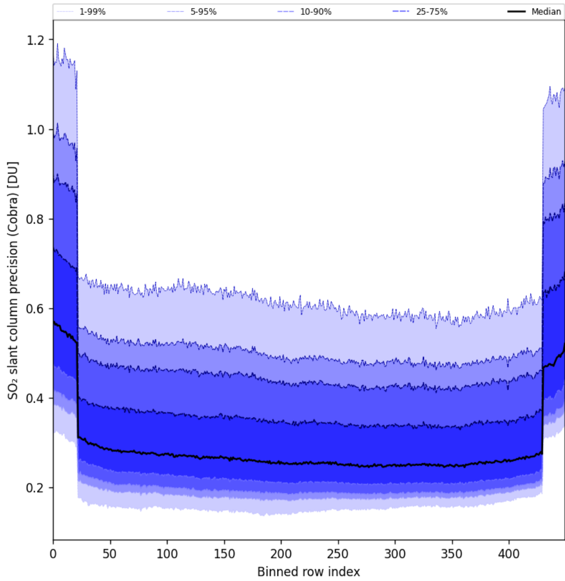
Figure 88: Along track statistics of “SO 2 slant column precision (Cobra)” for 2025-04-15 to 2025-04-17
