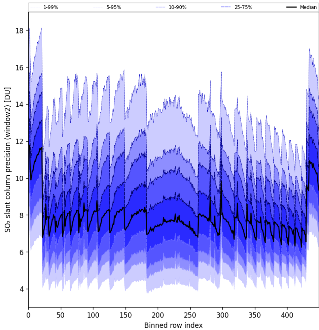
Figure 94: Along track statistics of “SO 2 slant column precision (window2)” for 2025-04-15 to 2025-04-17
