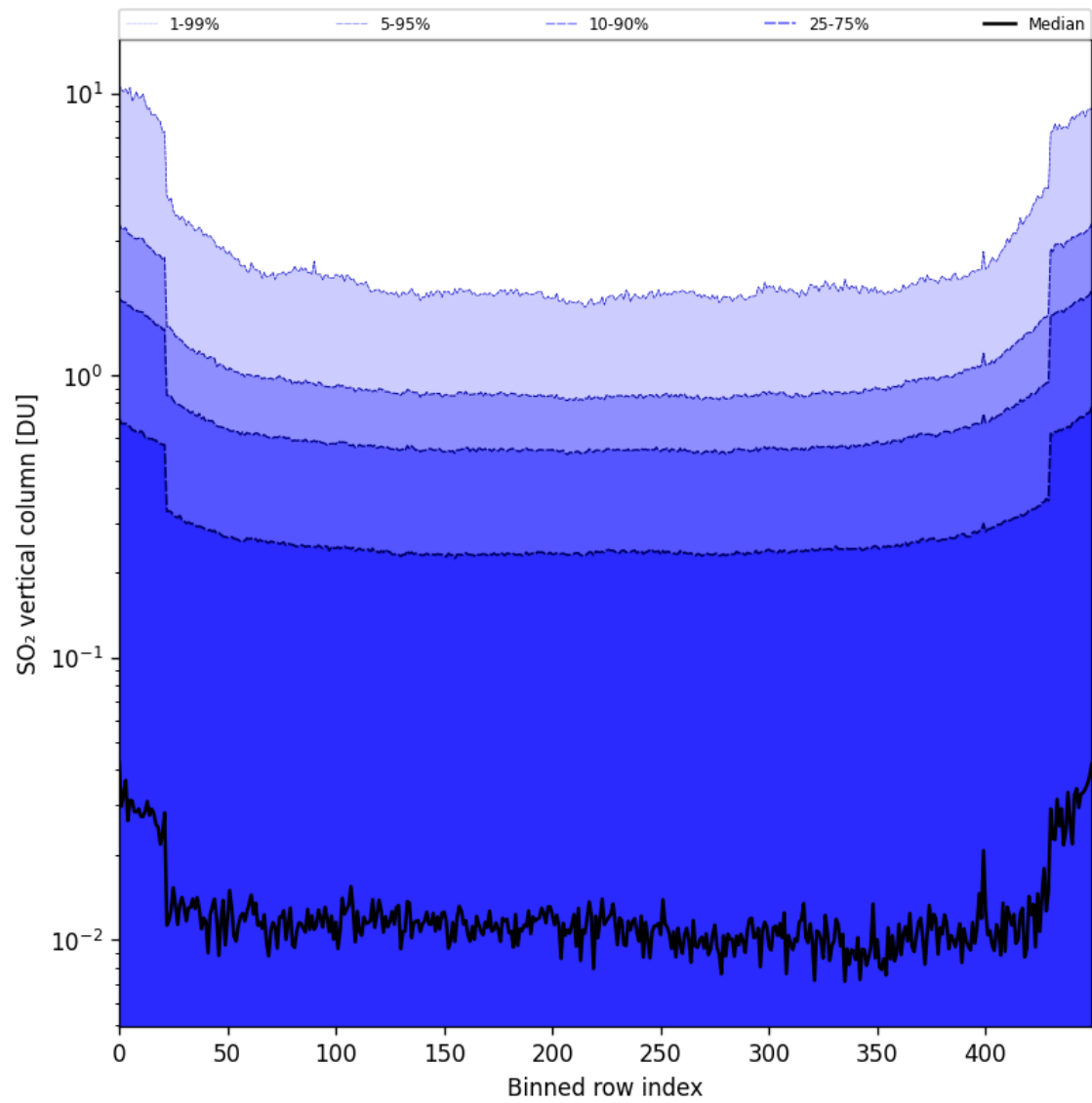
Figure 84: Along track statistics of “SO 2 vertical column” for 2025-04-15 to 2025-04-17
