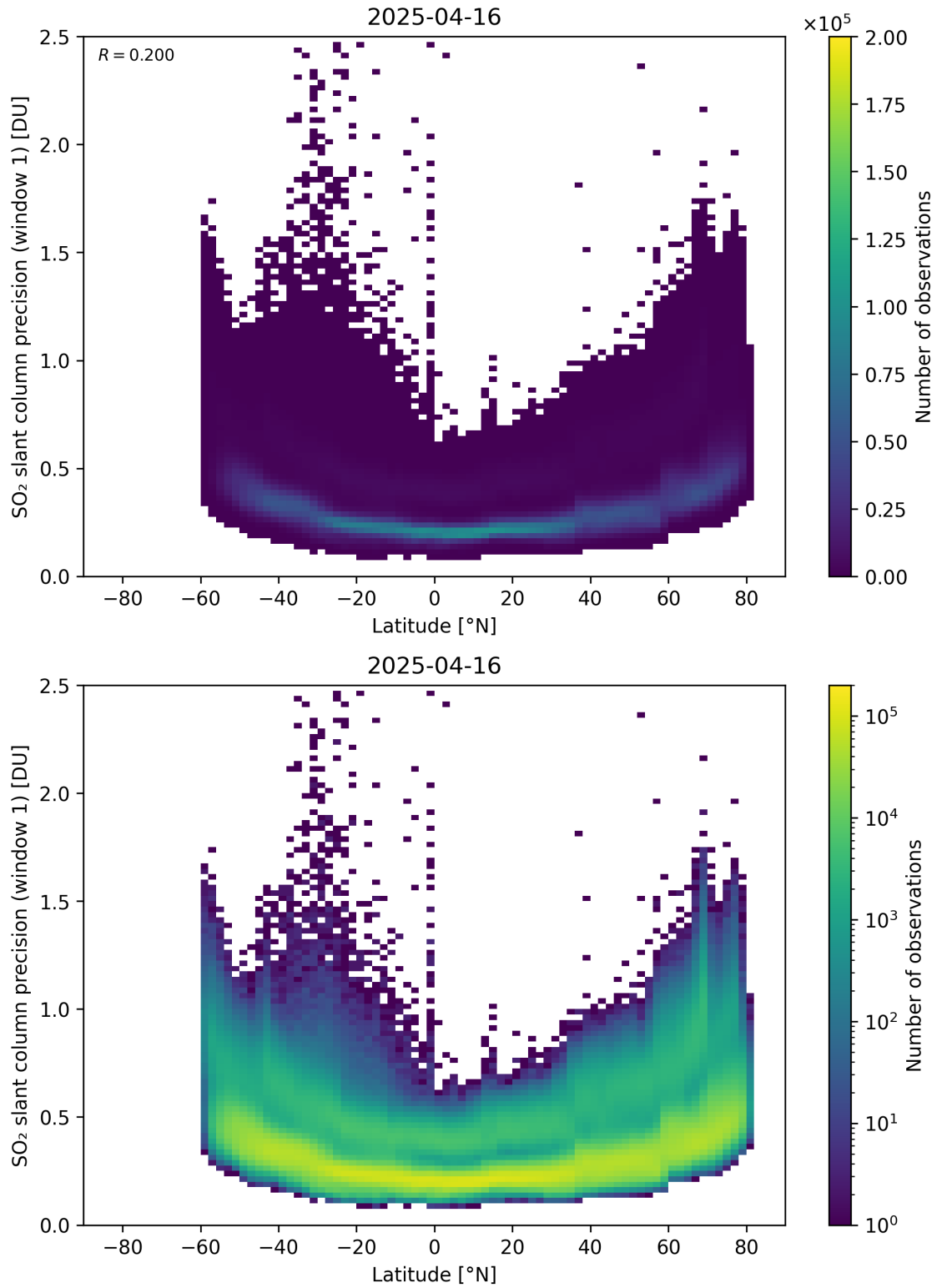
Figure 163: Scatter density plot of “Latitude” against “SO 2 slant column precision (window 1)” for 2025-04-15 to 2025-04-17.
