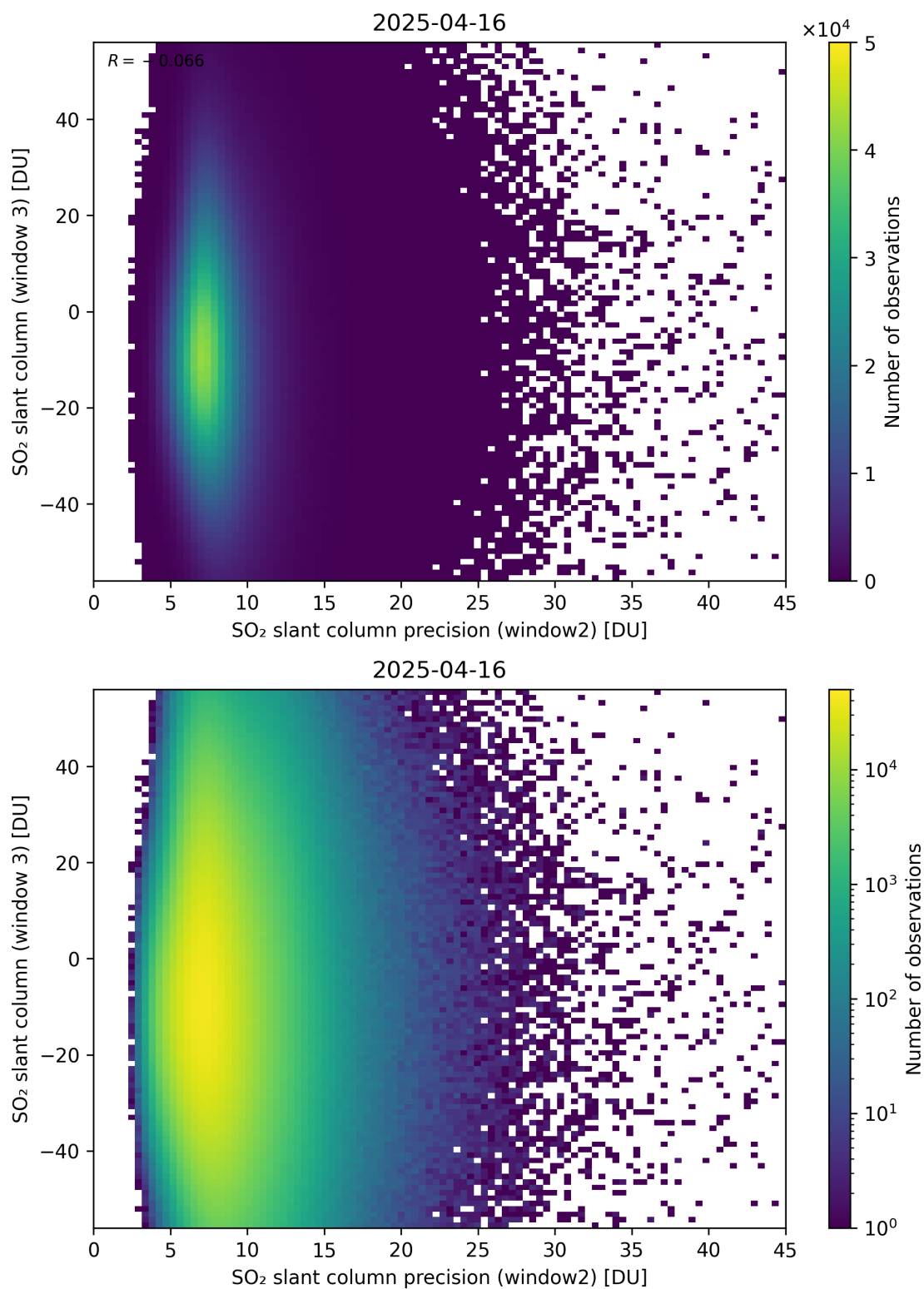
Figure 299: Scatter density plot of “SO 2 slant column precision (window2)” against “SO 2 slant column (window 3)” for 2025-04-15 to 2025-04-17.
