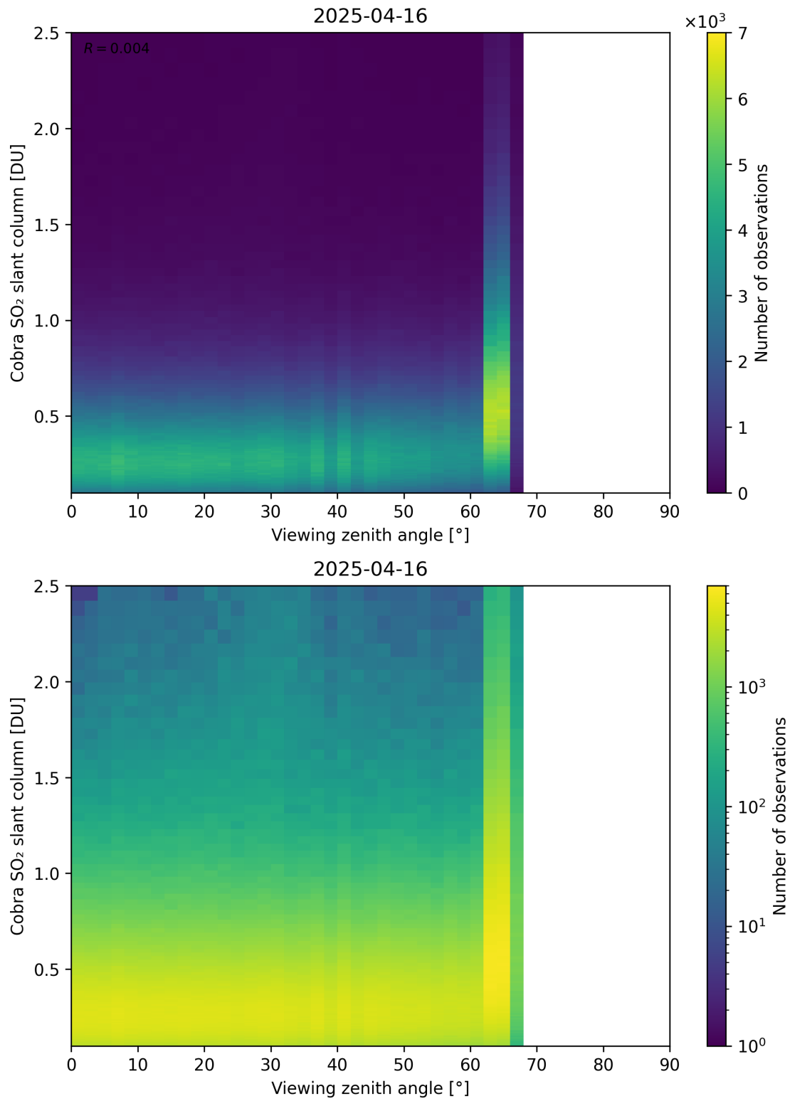
Figure 371: Scatter density plot of “Viewing zenith angle” against “Cobra SO 2 slant column” for 2025-04-15 to 2025-04-17.
