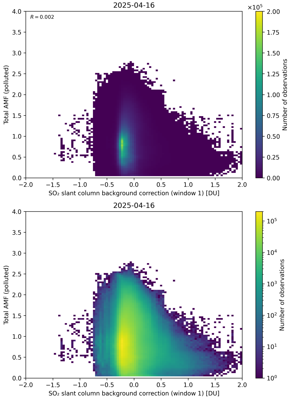
Figure 120: Scatter density plot of “SO 2 slant column background correction (window 1)” against “Total AMF (polluted)” for 2025-04-15 to 2025-04-17.
