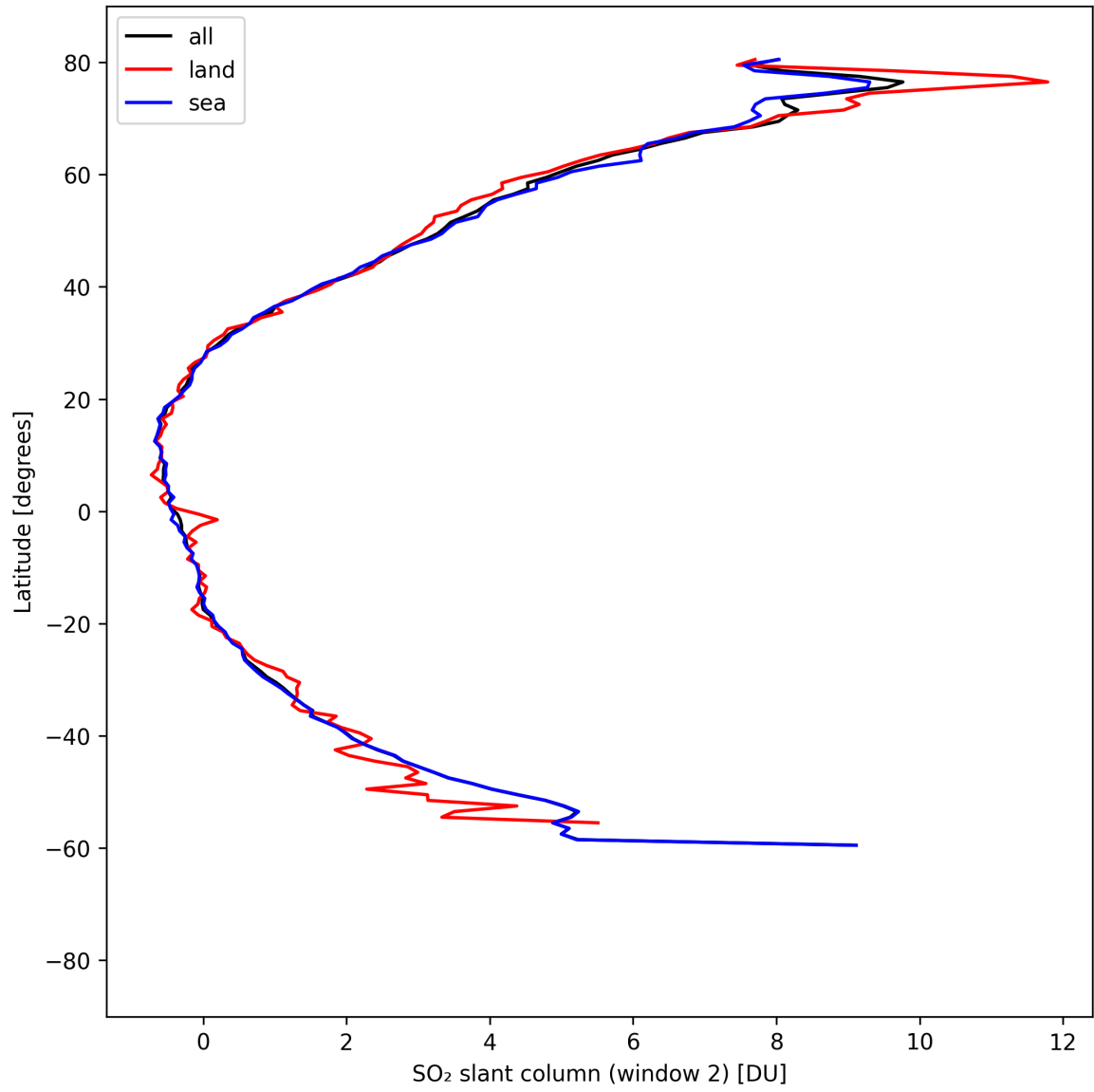
Figure 41: Zonal average of “SO 2 slant column (window 2)” for 2025-04-15 to 2025-04-17.
