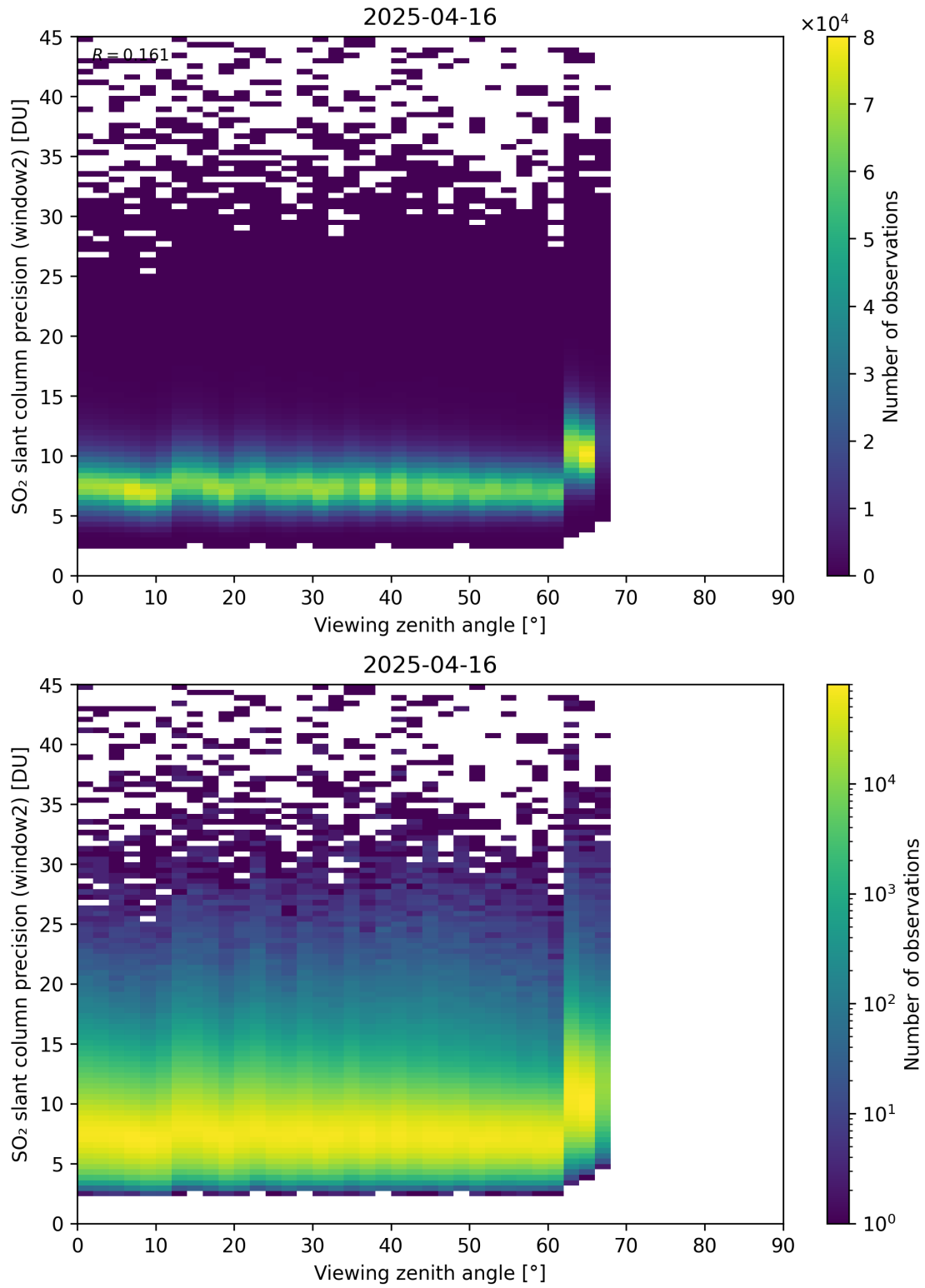
Figure 378: Scatter density plot of “Viewing zenith angle” against “SO 2 slant column precision (window2)” for 2025-04-15 to 2025-04-17.
