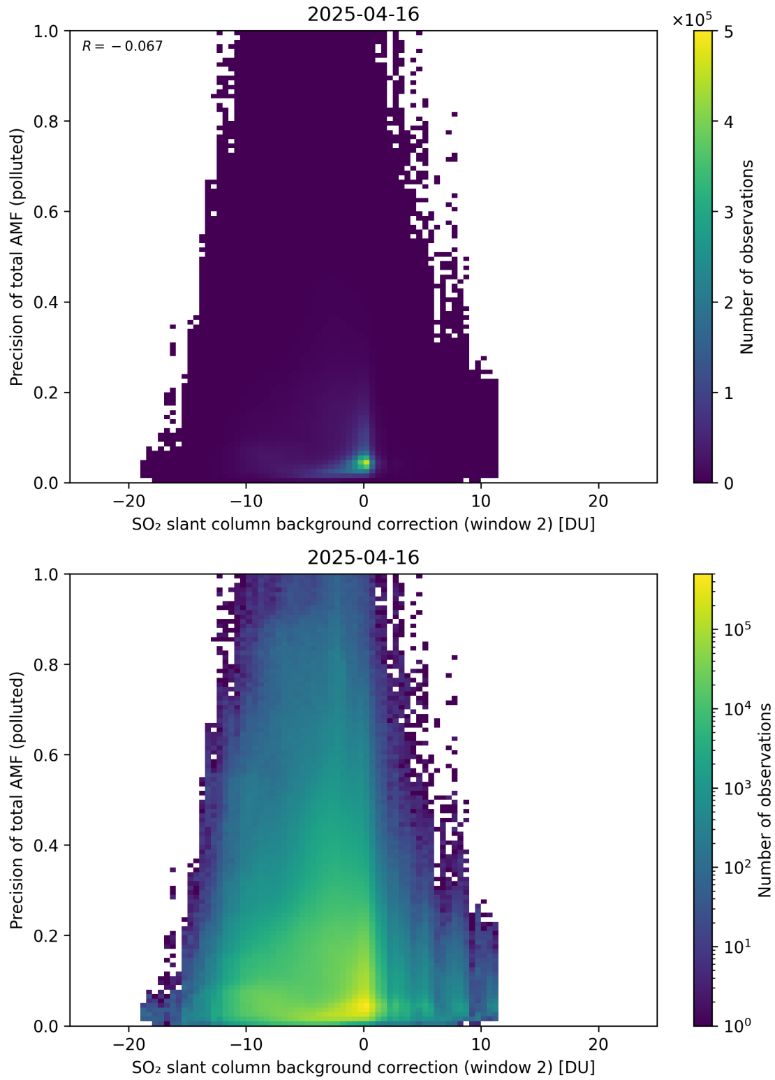
Figure 131: Scatter density plot of “SO 2 slant column background correction (window 2)” against “Precision of total AMF (polluted)” for 2025-04-15 to 2025-04-17.
