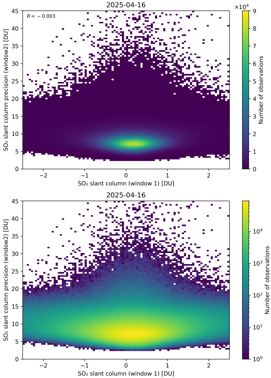
Figure 286: Scatter density plot of “SO 2 slant column (window 1)” against “SO 2 slant column precision (window2)” for 2025-04-15 to 2025-04-17.
