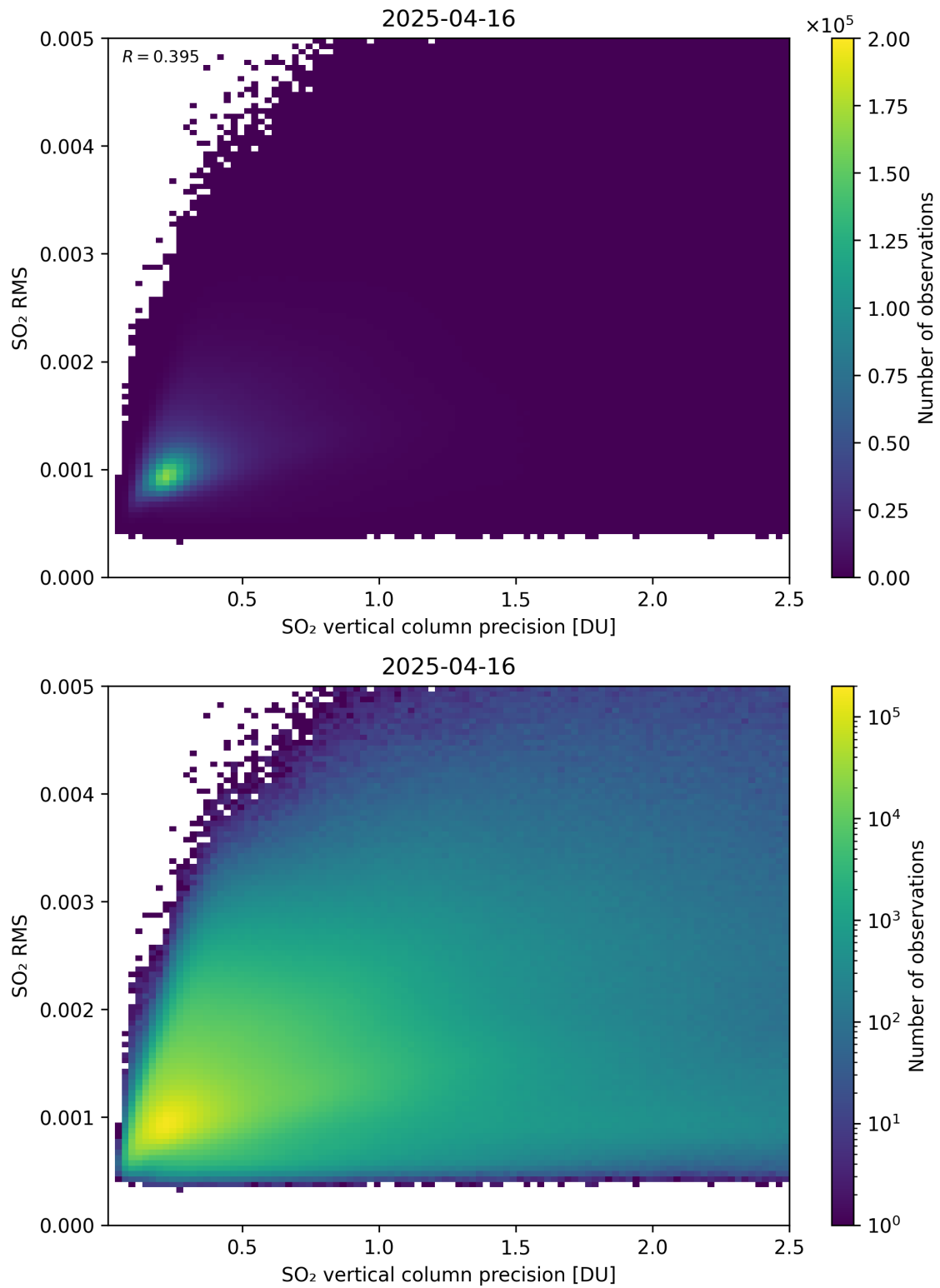
Figure 334: Scatter density plot of “SO 2 vertical column precision” against “SO 2 RMS” for 2025-04-15 to 2025-04-17.
