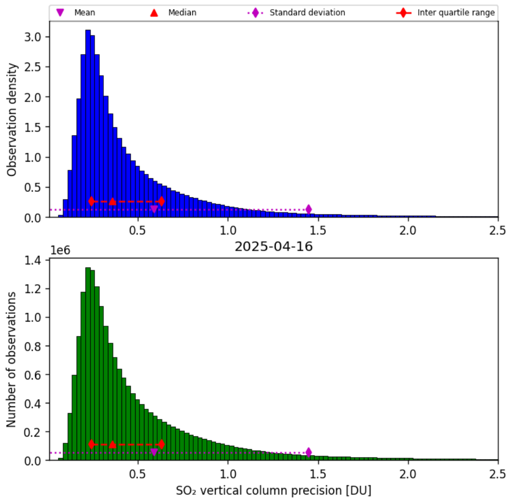
Figure 59: Histogram of “SO 2 vertical column precision” for 2025-04-15 to 2025-04-17
