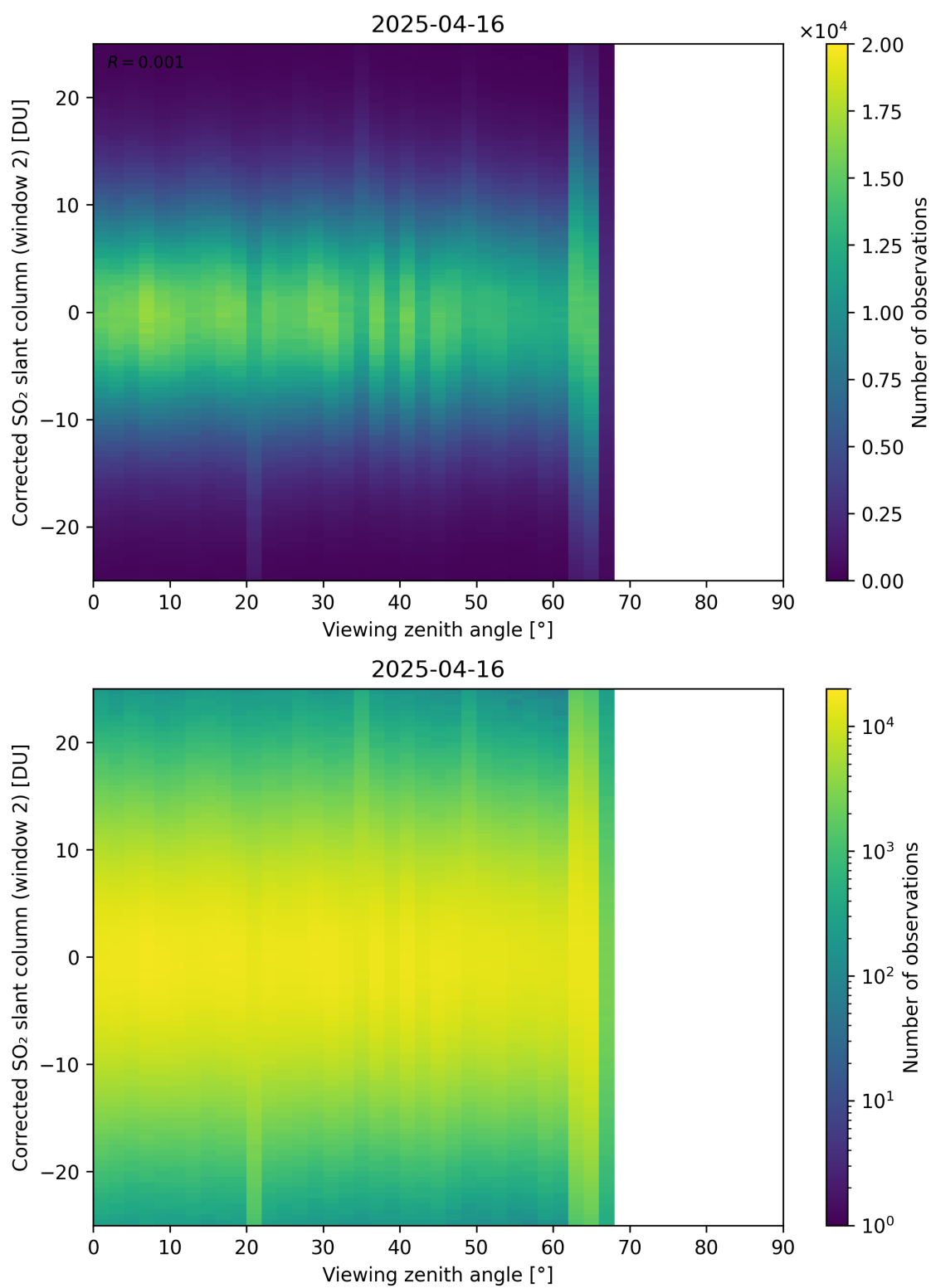
Figure 374: Scatter density plot of “Viewing zenith angle” against “Corrected SO 2 slant column (window 2)” for 2025-04-15 to 2025-04-17.
