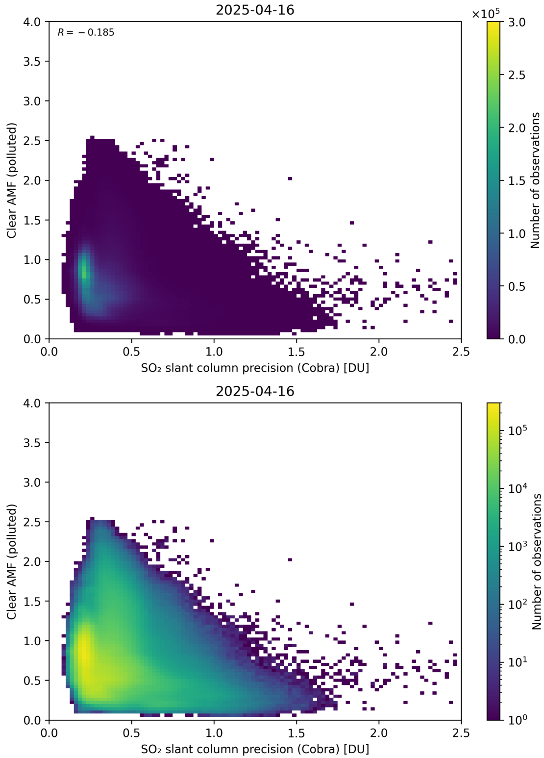
Figure 205: Scatter density plot of “SO 2 slant column precision (Cobra)” against “Clear AMF (polluted)” for 2025-04-15 to 2025-04-17.
