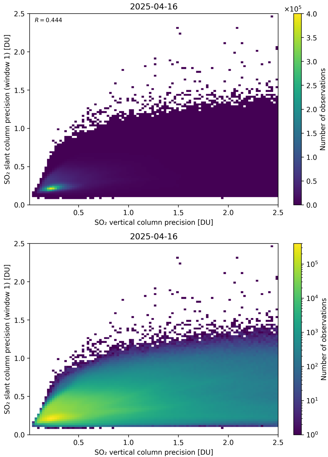
Figure 342: Scatter density plot of “SO 2 vertical column precision” against “SO 2 slant column precision (window 1)” for 2025-04-15 to 2025-04-17.
