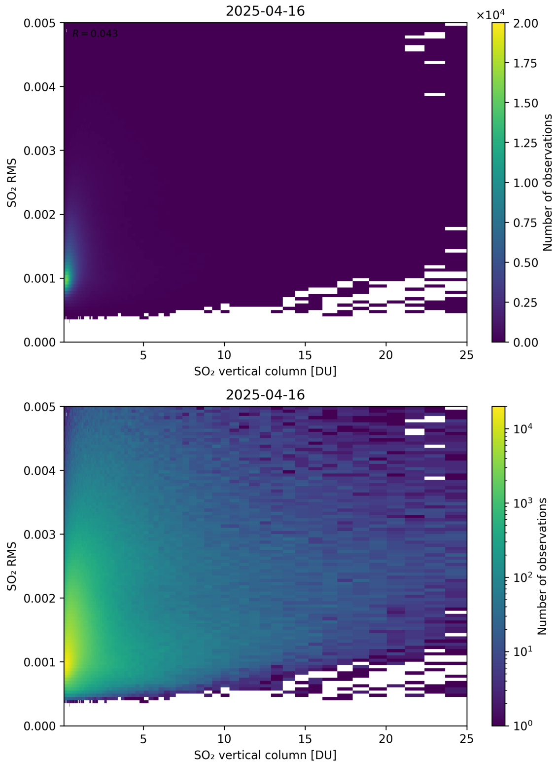
Figure 328: Scatter density plot of “SO 2 vertical column” against “SO 2 RMS” for 2025-04-15 to 2025-04-17.
