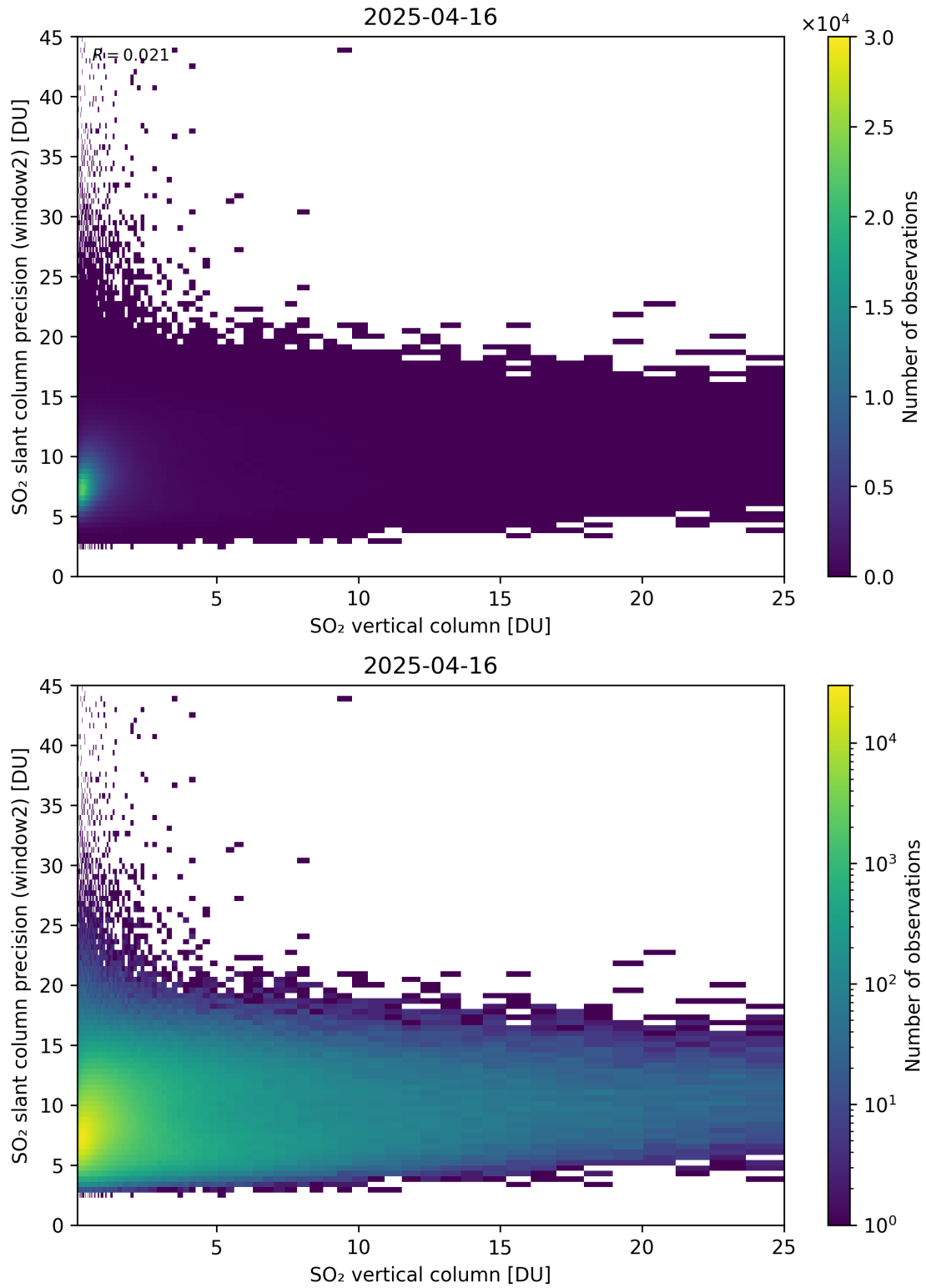
Figure 356: Scatter density plot of “SO 2 vertical column” against “SO 2 slant column precision (window2)” for 2025-04-15 to 2025-04-17.
