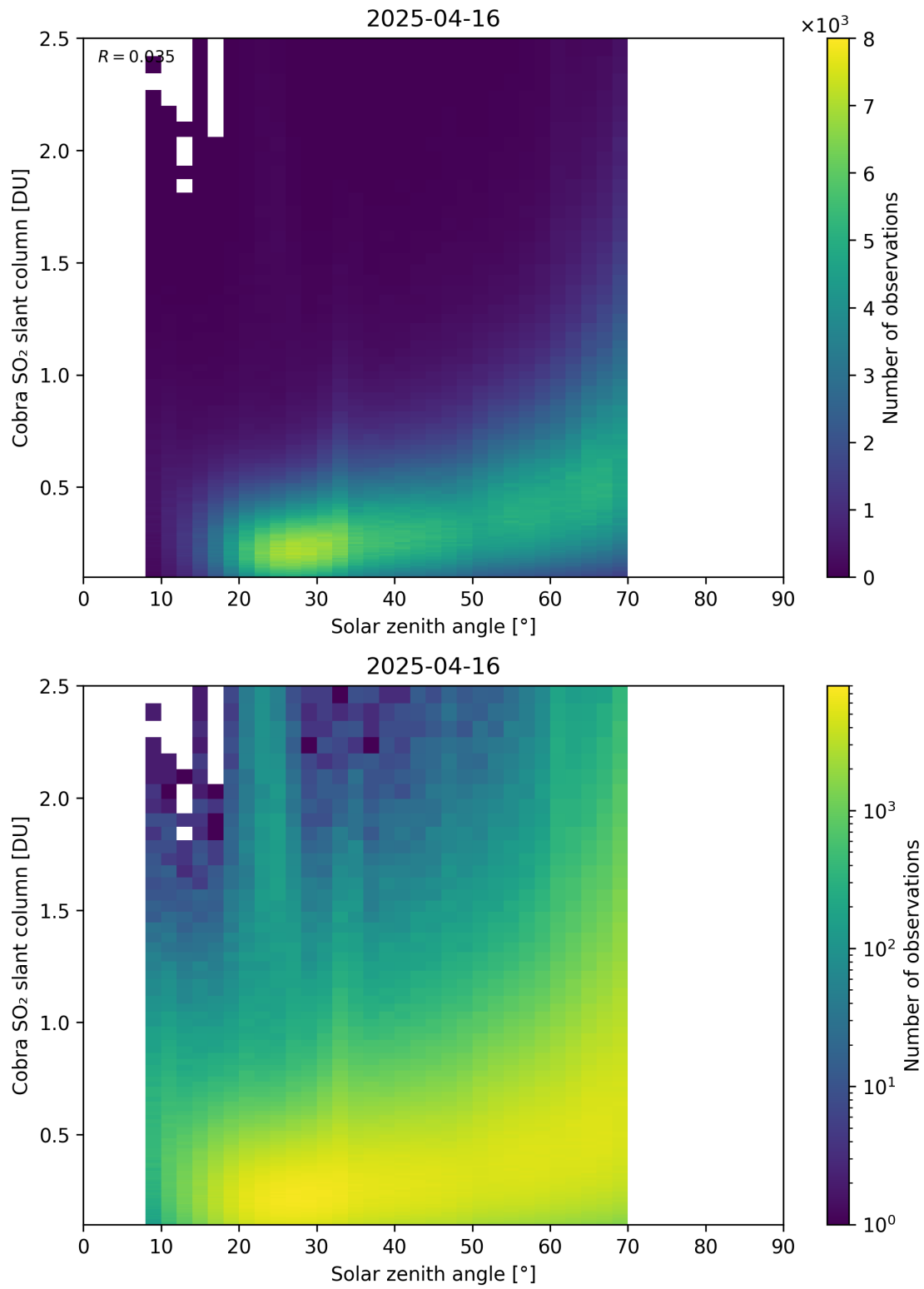
Figure 179: Scatter density plot of “Solar zenith angle” against “Cobra SO 2 slant column” for 2025-04-15 to 2025-04-17.
