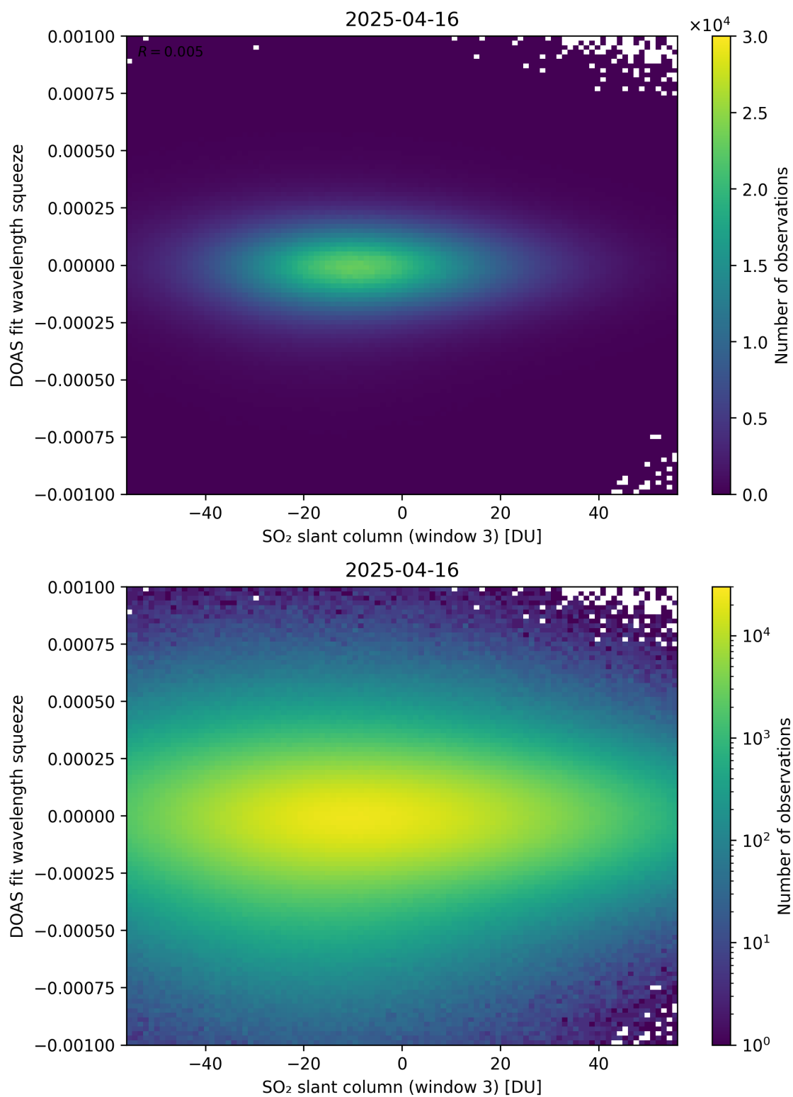
Figure 305: Scatter density plot of “SO 2 slant column (window 3)” against “DOAS fit wavelength squeeze” for 2025-04-15 to 2025-04-17.
