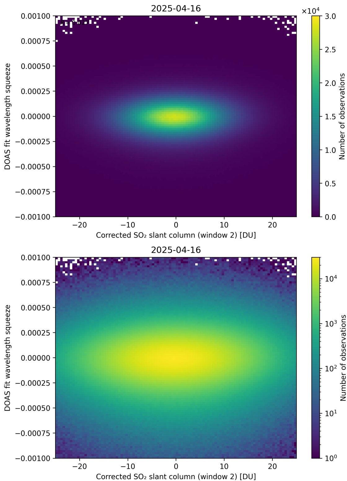
Figure 247: Scatter density plot of “Corrected SO 2 slant column (window 2)” against “DOAS fit wavelength squeeze” for 2025-04-15 to 2025-04-17.
