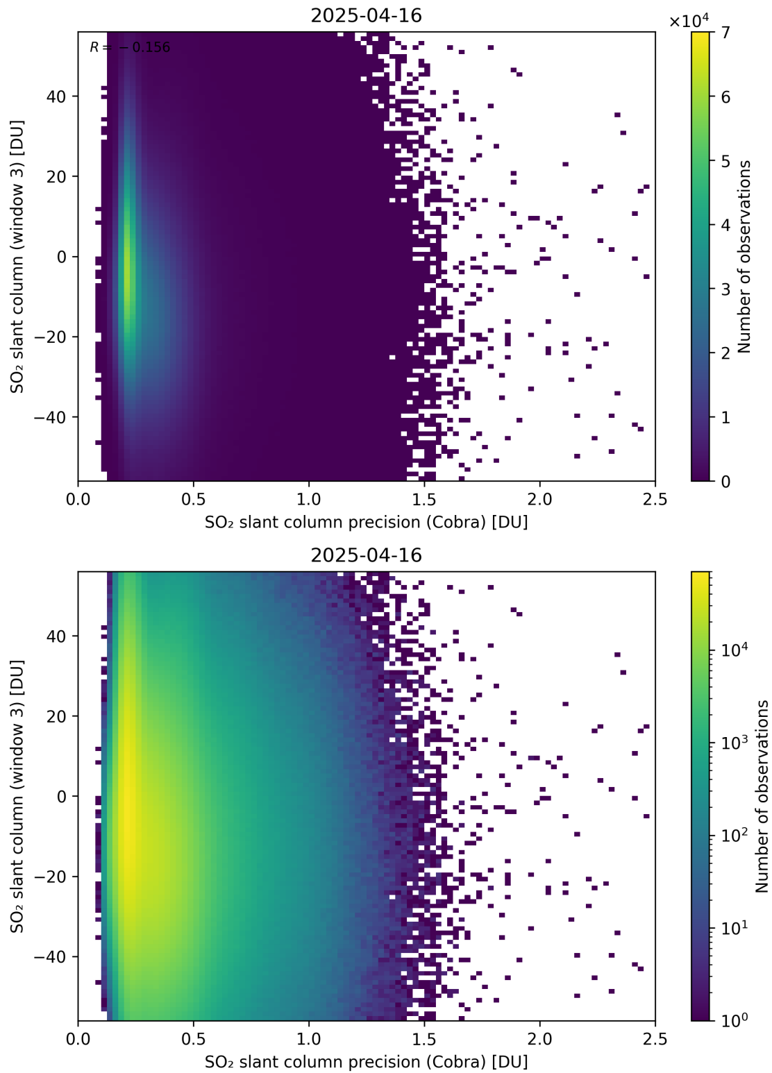
Figure 211: Scatter density plot of “SO 2 slant column precision (Cobra)” against “SO 2 slant column (window 3)” for 2025-04-15 to 2025-04-17.
