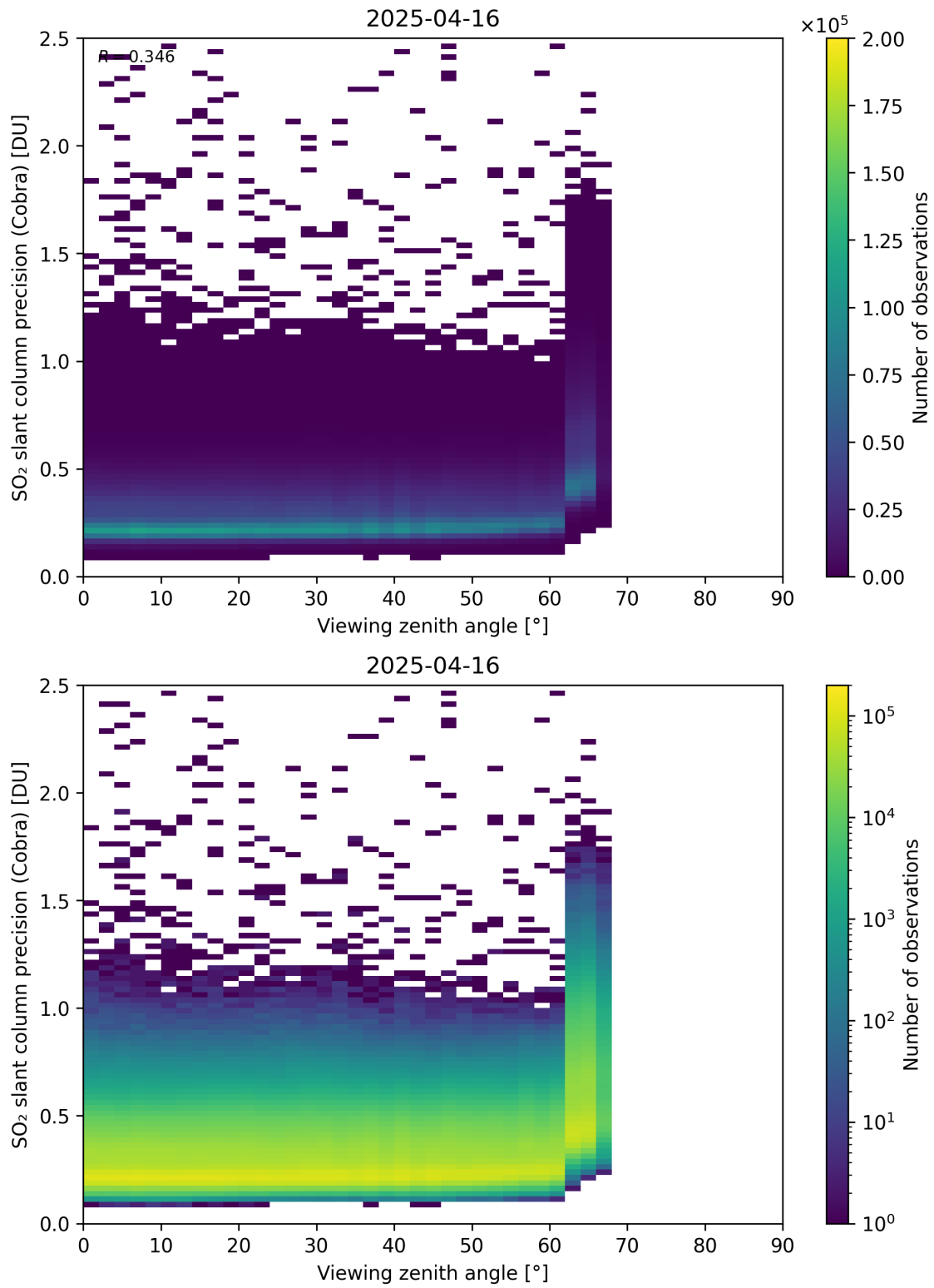
Figure 372: Scatter density plot of “Viewing zenith angle” against “SO 2 slant column precision (Cobra)” for 2025-04-15 to 2025-04-17.
