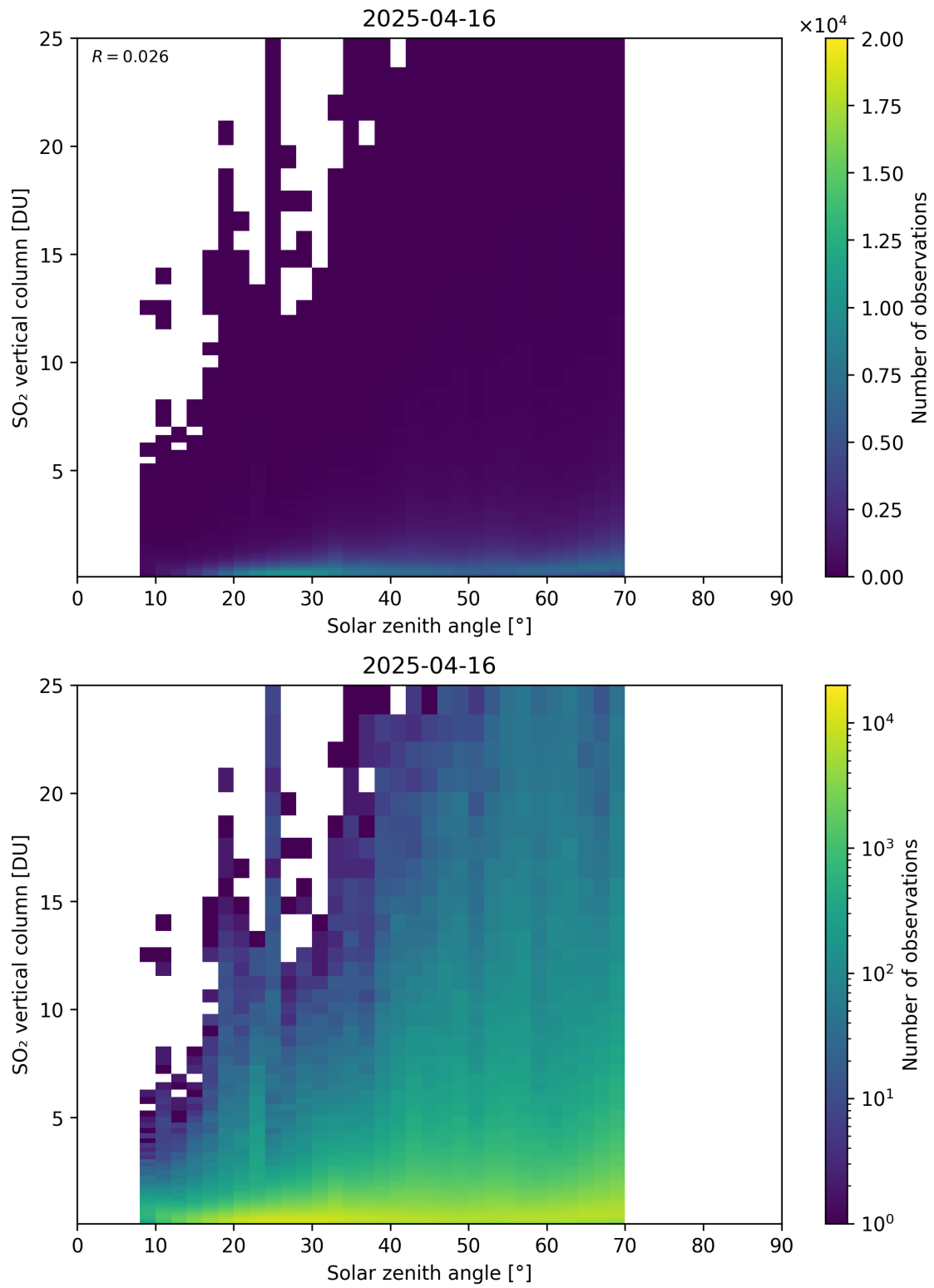
Figure 191: Scatter density plot of “Solar zenith angle” against “SO 2 vertical column” for 2025-04-15 to 2025-04-17.
