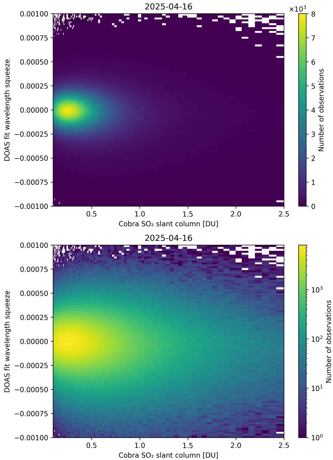
Figure 197: Scatter density plot of “Cobra SO 2 slant column” against “DOAS fit wavelength squeeze” for 2025-04-15 to 2025-04-17.
