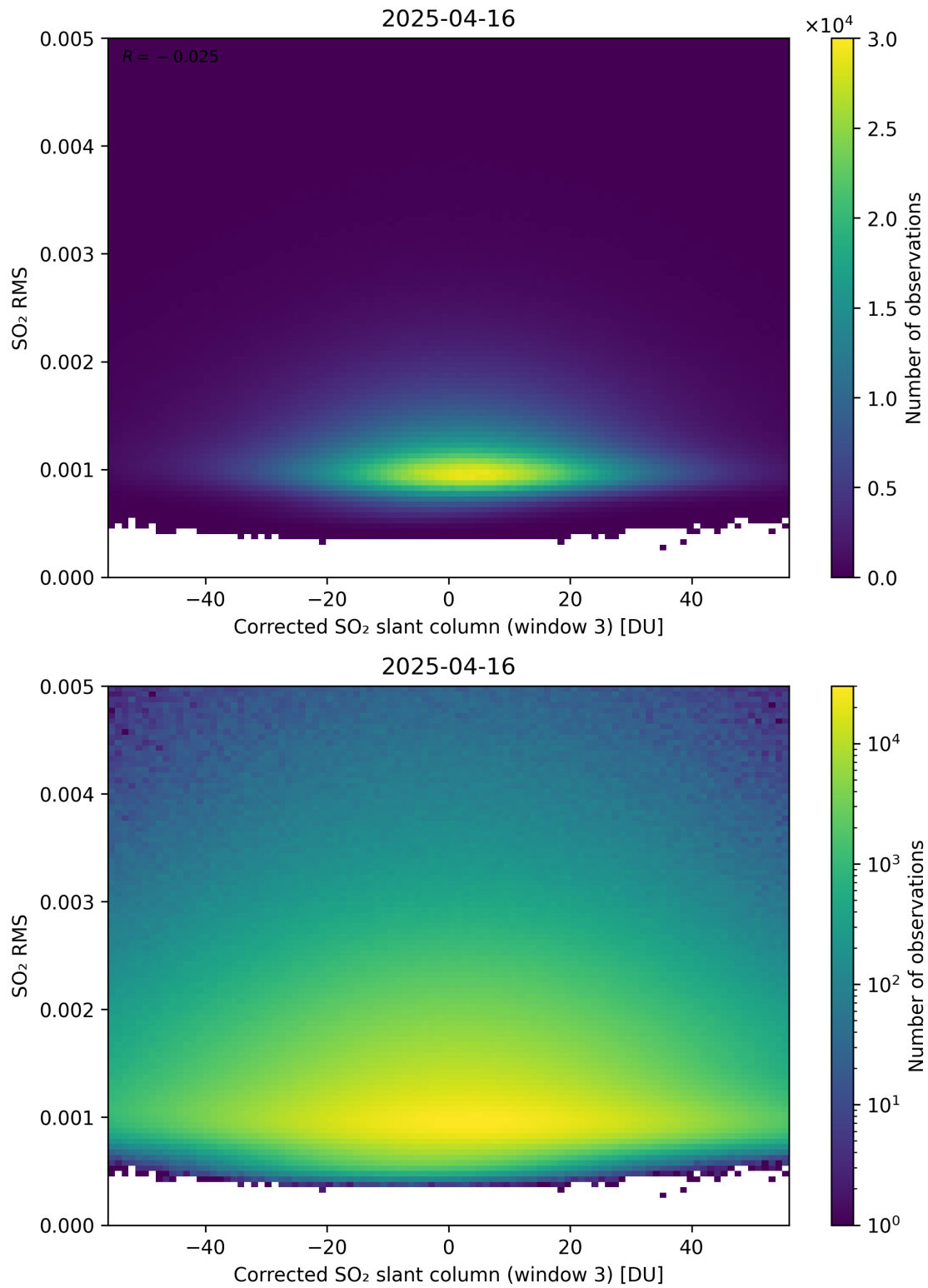
Figure 258: Scatter density plot of “Corrected SO 2 slant column (window 3)” against “SO 2 RMS” for 2025-04-15 to 2025-04-17.
