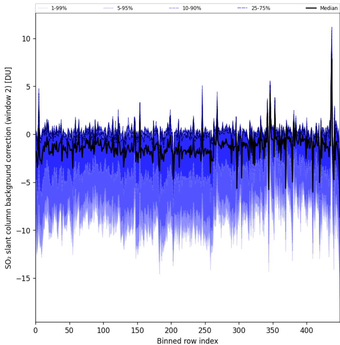
Figure 96: Along track statistics of “SO 2 slant column background correction (window 2)” for 2025-04-15 to 2025-04-17
