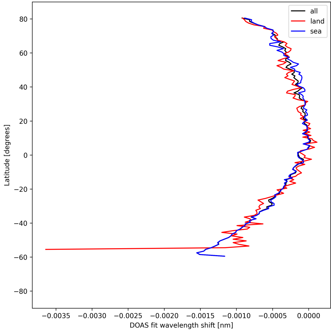
Figure 50: Zonal average of “DOAS fit wavelength shift” for 2025-04-15 to 2025-04-17.
