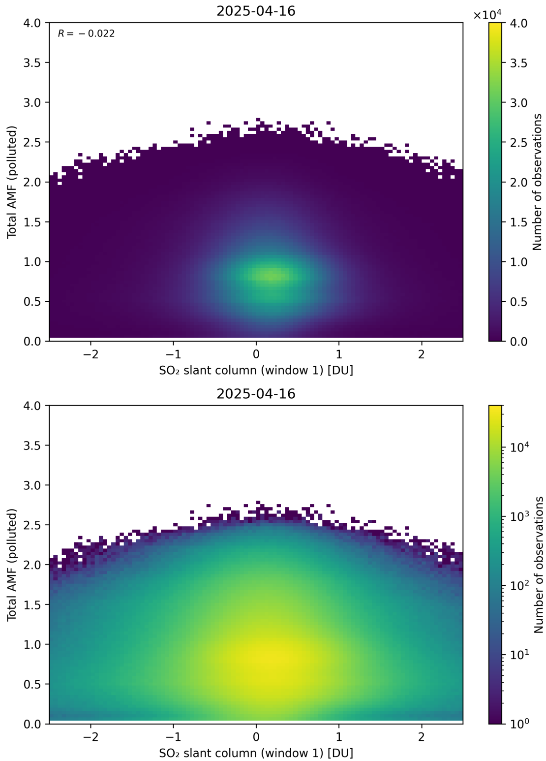
Figure 289: Scatter density plot of “SO 2 slant column (window 1)” against “Total AMF (polluted)” for 2025-04-15 to 2025-04-17.
