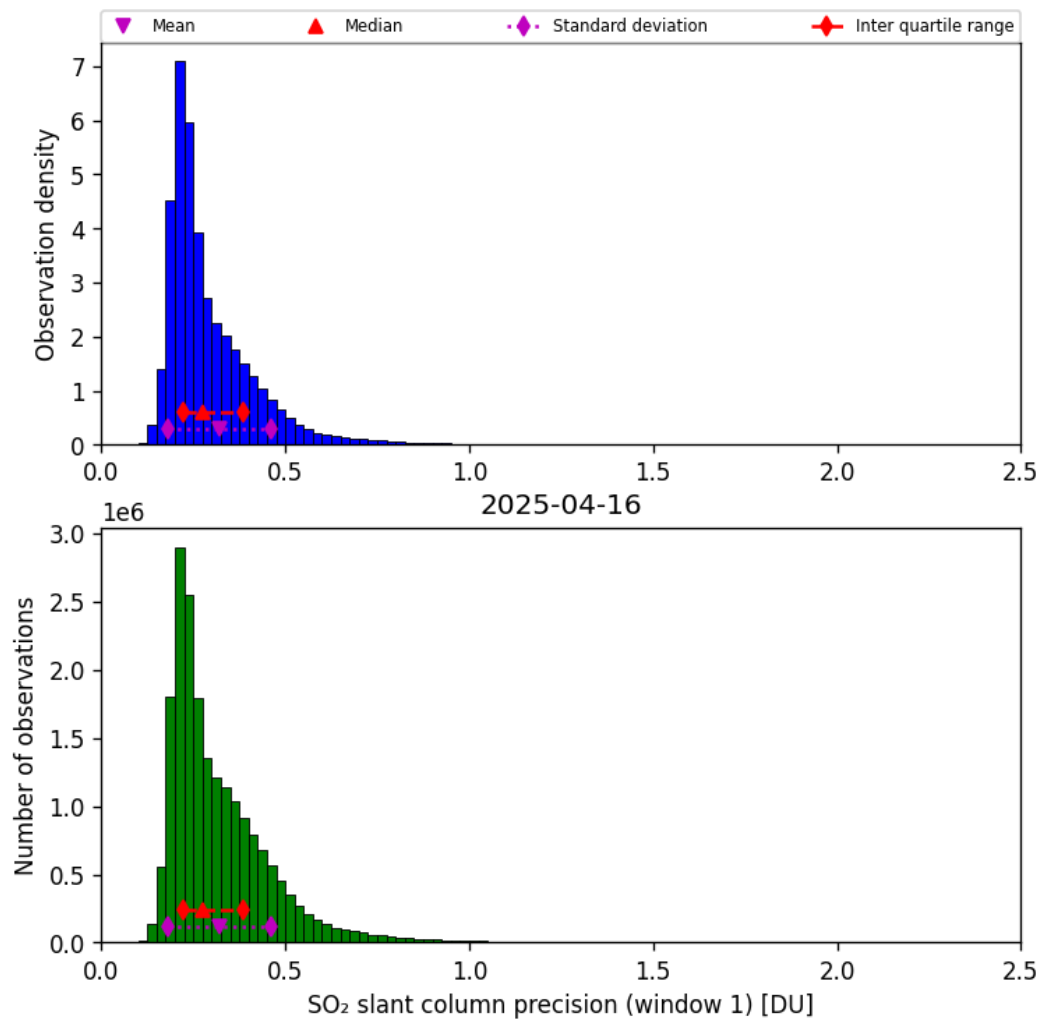
Figure 64: Histogram of “SO 2 slant column precision (window 1)” for 2025-04-15 to 2025-04-17
