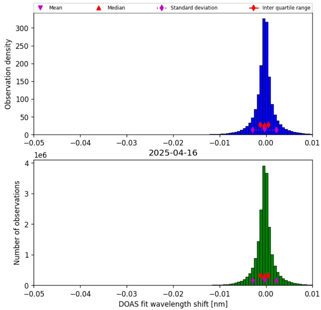
Figure 76: Histogram of “DOAS fit wavelength shift” for 2025-04-15 to 2025-04-17
