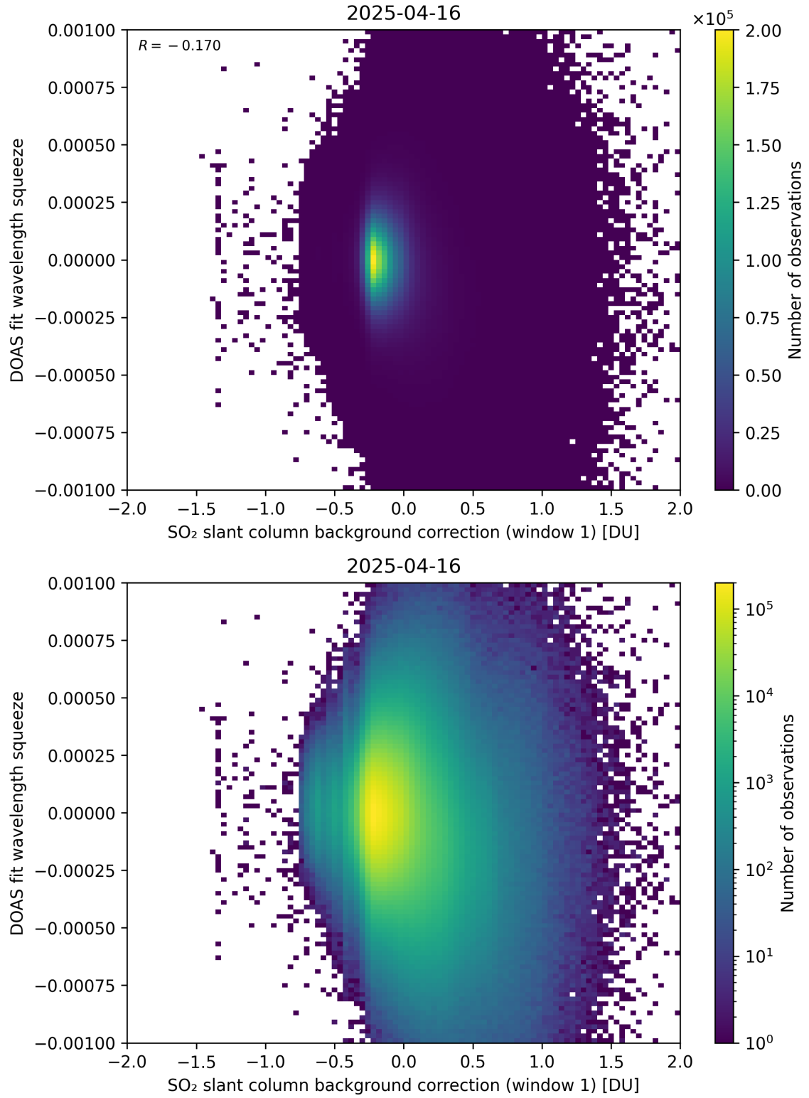
Figure 112: Scatter density plot of “SO 2 slant column background correction (window 1)” against “DOAS fit wavelength squeeze” for 2025-04-15 to 2025-04-17.
