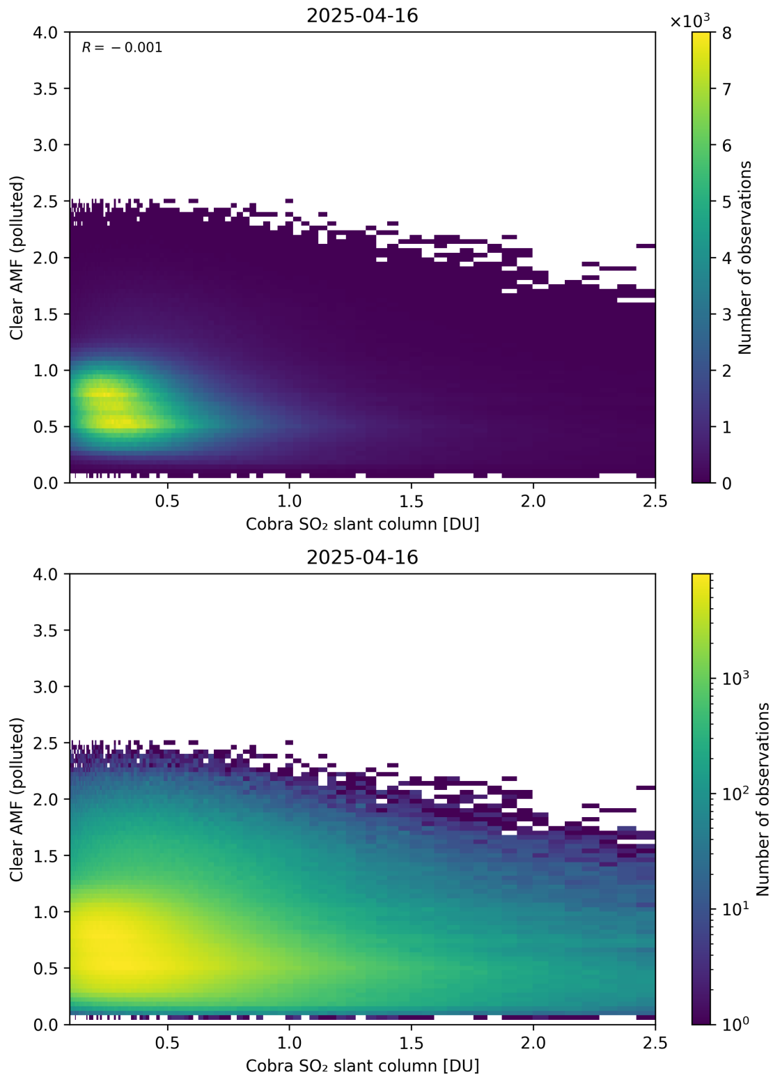
Figure 215: Scatter density plot of “Cobra SO 2 slant column” against “Clear AMF (polluted)” for 2025-04-15 to 2025-04-17.
