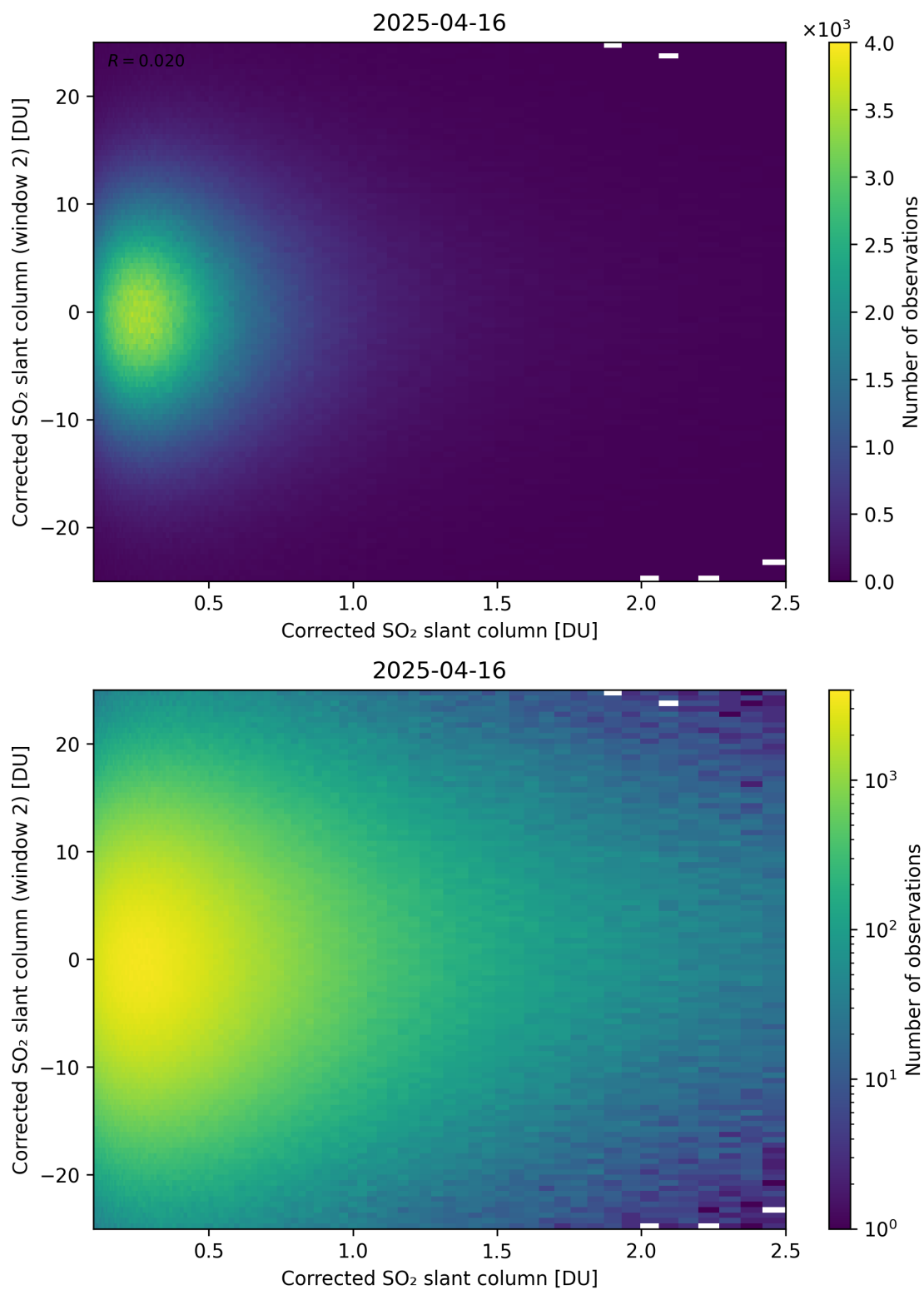
Figure 235: Scatter density plot of “Corrected SO 2 slant column” against “Corrected SO 2 slant column (window 2)” for 2025-04-15 to 2025-04-17.
