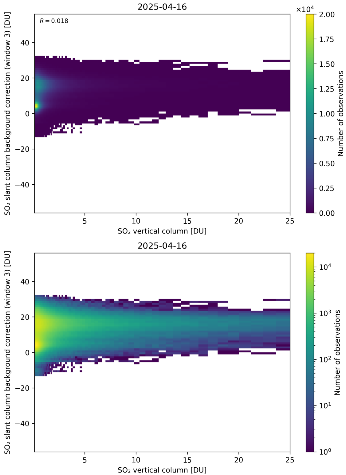
Figure 325: Scatter density plot of “SO 2 vertical column” against “SO 2 slant column background correction (window 3)” for 2025-04-15 to 2025-04-17.
