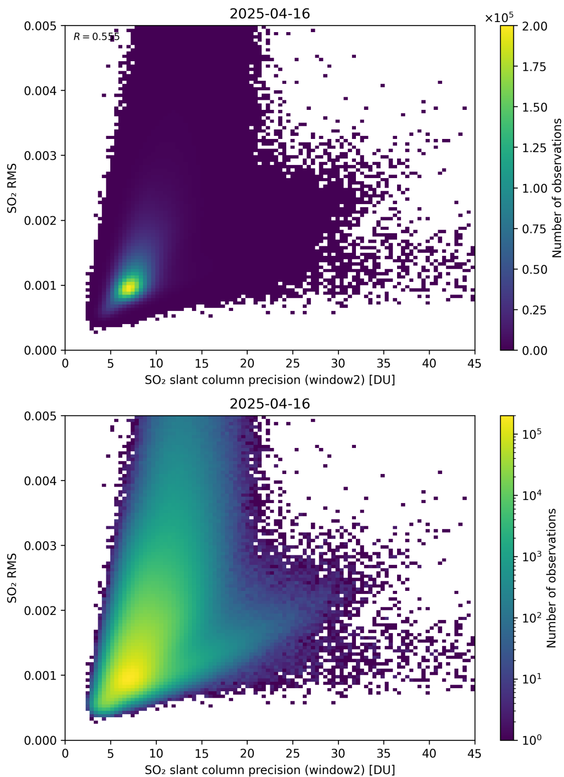
Figure 295: Scatter density plot of “SO 2 slant column precision (window2)” against “SO 2 RMS” for 2025-04-15 to 2025-04-17.
