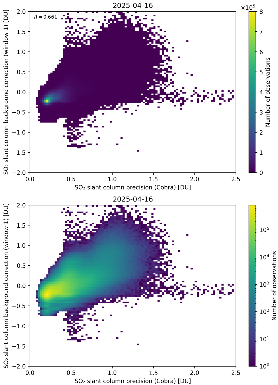
Figure 199: Scatter density plot of “SO 2 slant column precision (Cobra)” against “SO 2 slant column background correction (window 1)” for 2025-04-15 to 2025-04-17.
