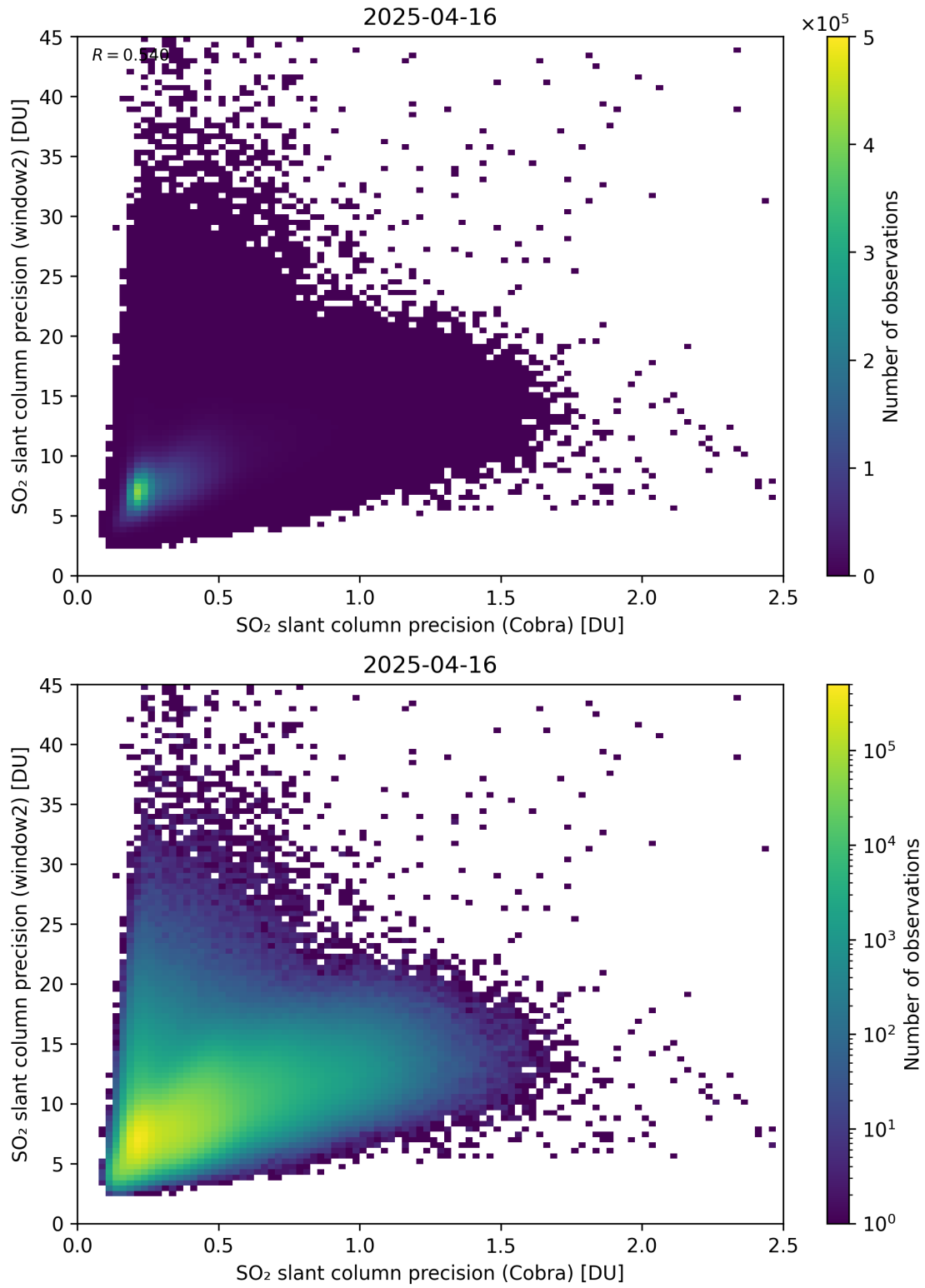
Figure 210: Scatter density plot of “SO 2 slant column precision (Cobra)” against “SO 2 slant column precision (window2)” for 2025-04-15 to 2025-04-17.
