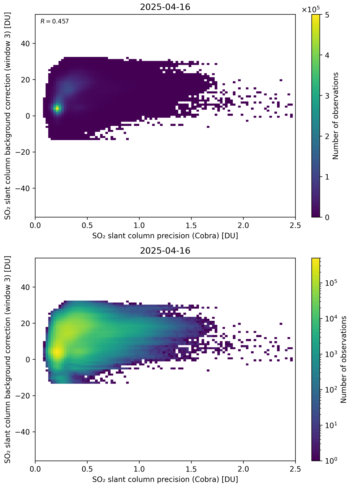
Figure 201: Scatter density plot of “SO 2 slant column precision (Cobra)” against “SO 2 slant column background correction (window 3)” for 2025-04-15 to 2025-04-17.
