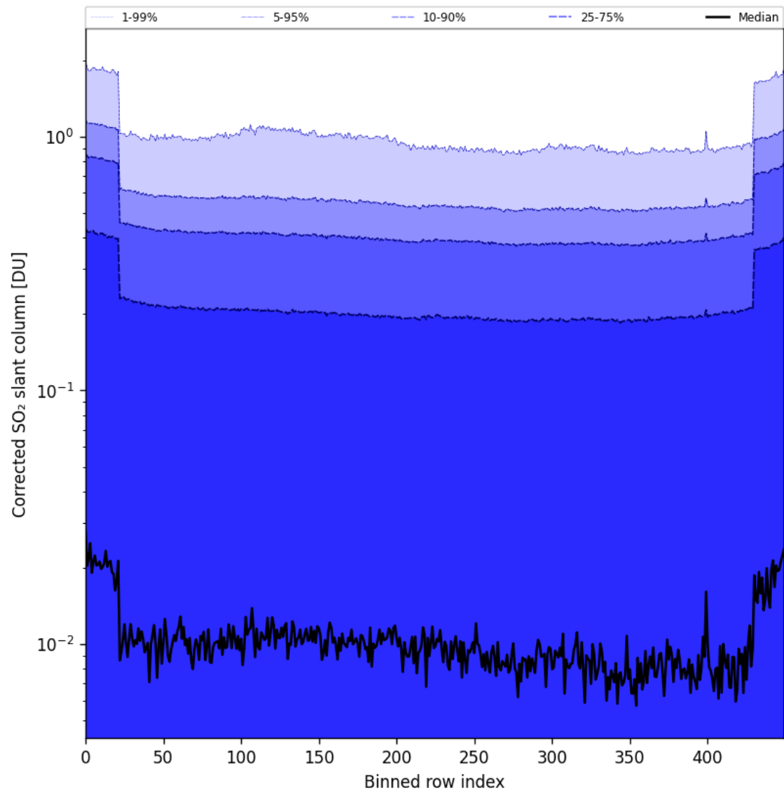
Figure 86: Along track statistics of “Corrected SO 2 slant column” for 2025-04-15 to 2025-04-17
