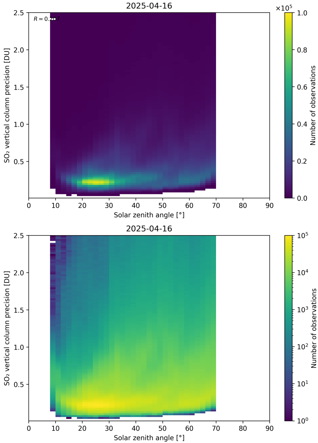
Figure 192: Scatter density plot of “Solar zenith angle” against “SO 2 vertical column precision” for 2025-04-15 to 2025-04-17.
