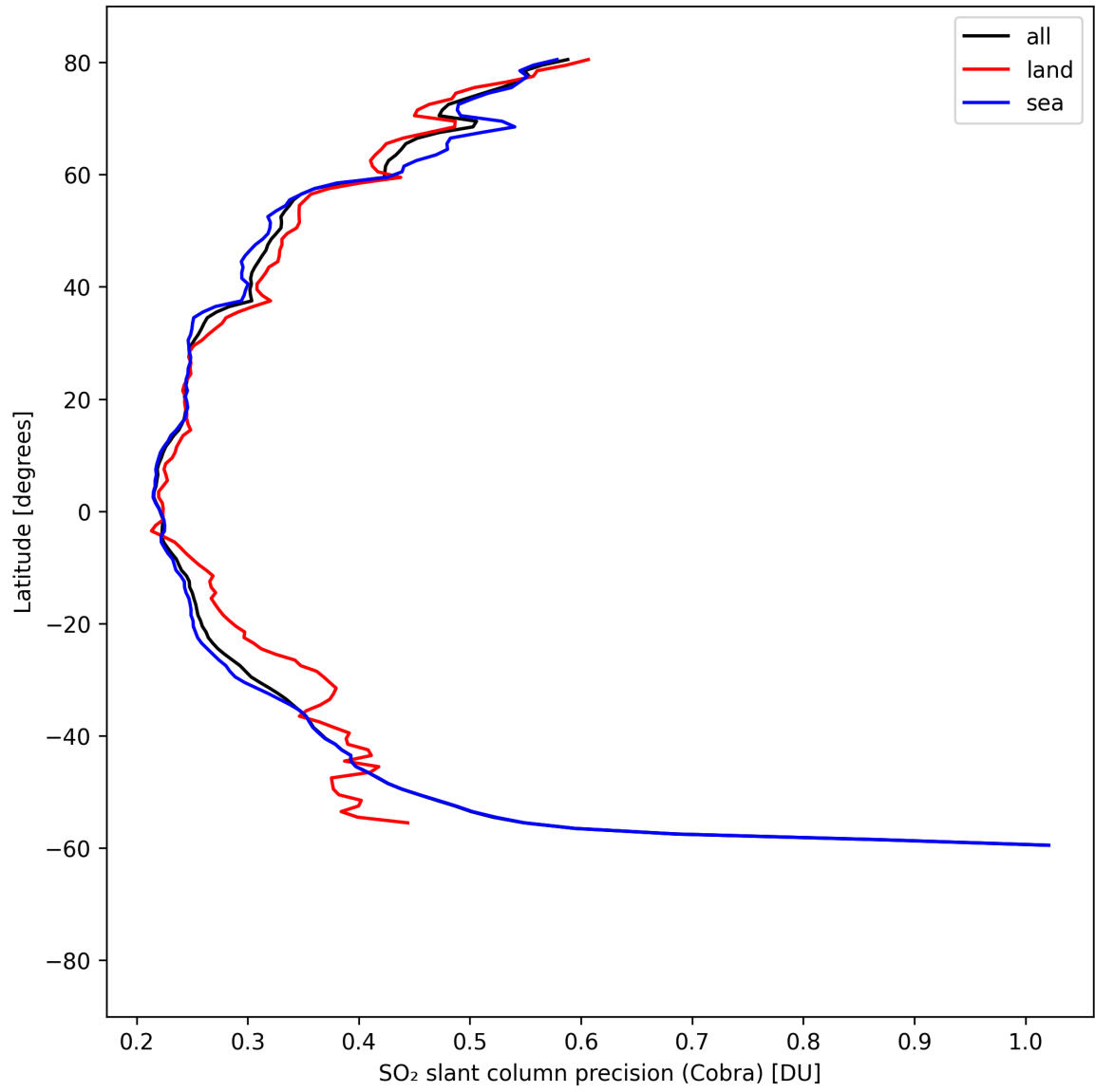
Figure 36: Zonal average of “SO 2 slant column precision (Cobra)” for 2025-04-15 to 2025-04-17.
