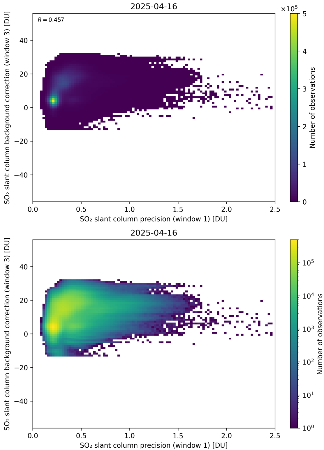
Figure 270: Scatter density plot of “SO 2 slant column precision (window 1)” against “SO 2 slant column background correction (window 3)” for 2025-04-15 to 2025-04-17.
