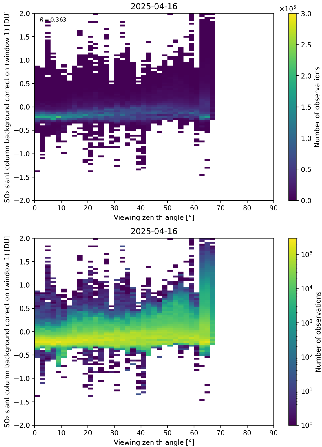
Figure 362: Scatter density plot of “Viewing zenith angle” against “SO 2 slant column background correction (window 1)” for 2025-04-15 to 2025-04-17.
