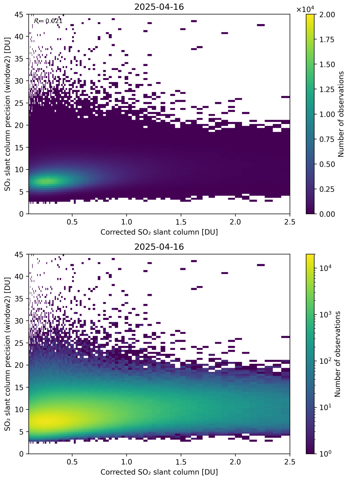
Figure 239: Scatter density plot of “Corrected SO 2 slant column” against “SO 2 slant column precision (window2)” for 2025-04-15 to 2025-04-17.
