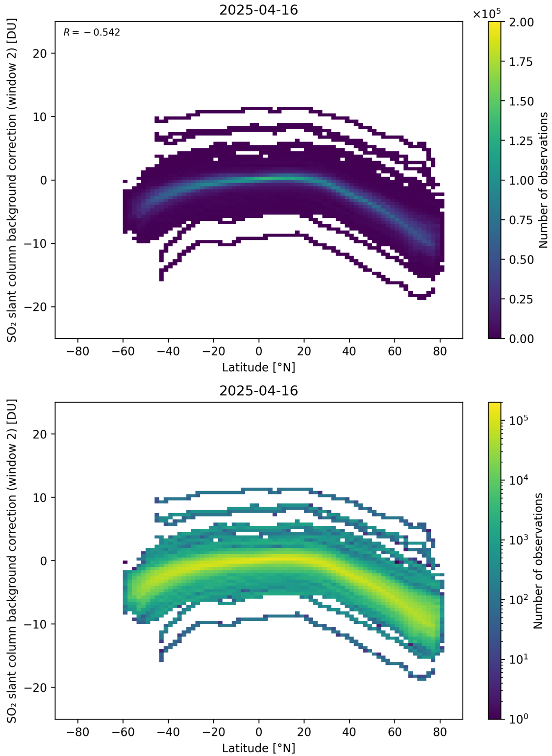
Figure 151: Scatter density plot of “Latitude” against “SO 2 slant column background correction (window 2)” for 2025-04-15 to 2025-04-17.
