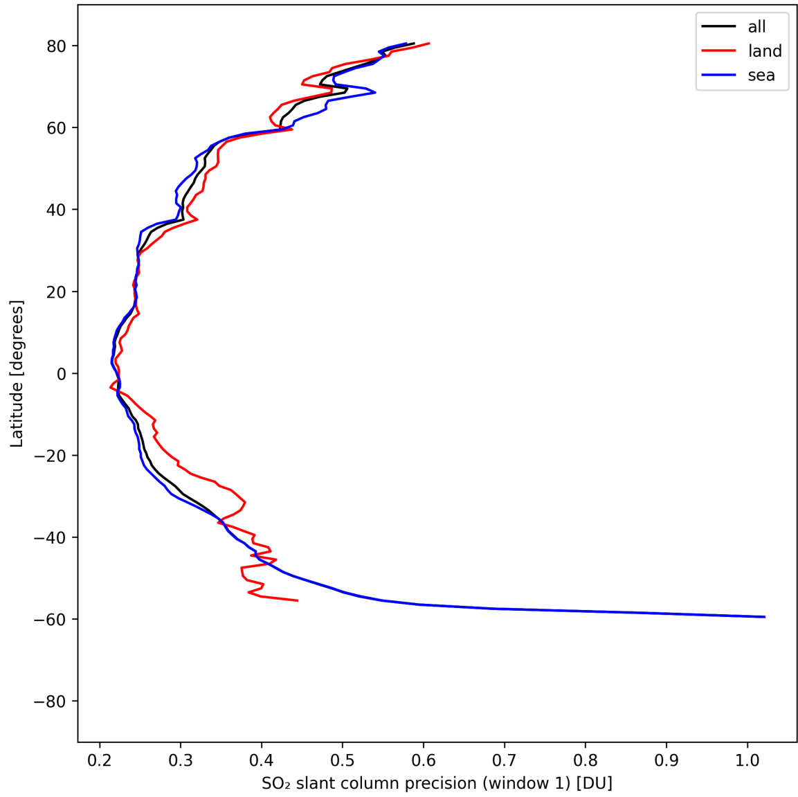
Figure 38: Zonal average of “SO 2 slant column precision (window 1)” for 2025-04-15 to 2025-04-17.
