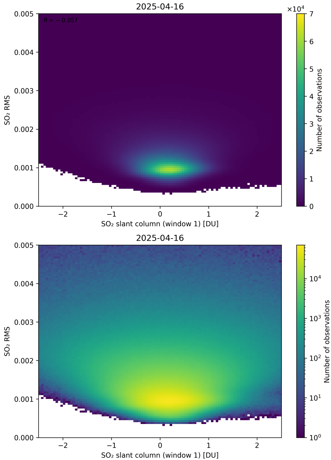
Figure 267: Scatter density plot of “SO 2 slant column (window 1)” against “SO 2 RMS” for 2025-04-15 to 2025-04-17.
