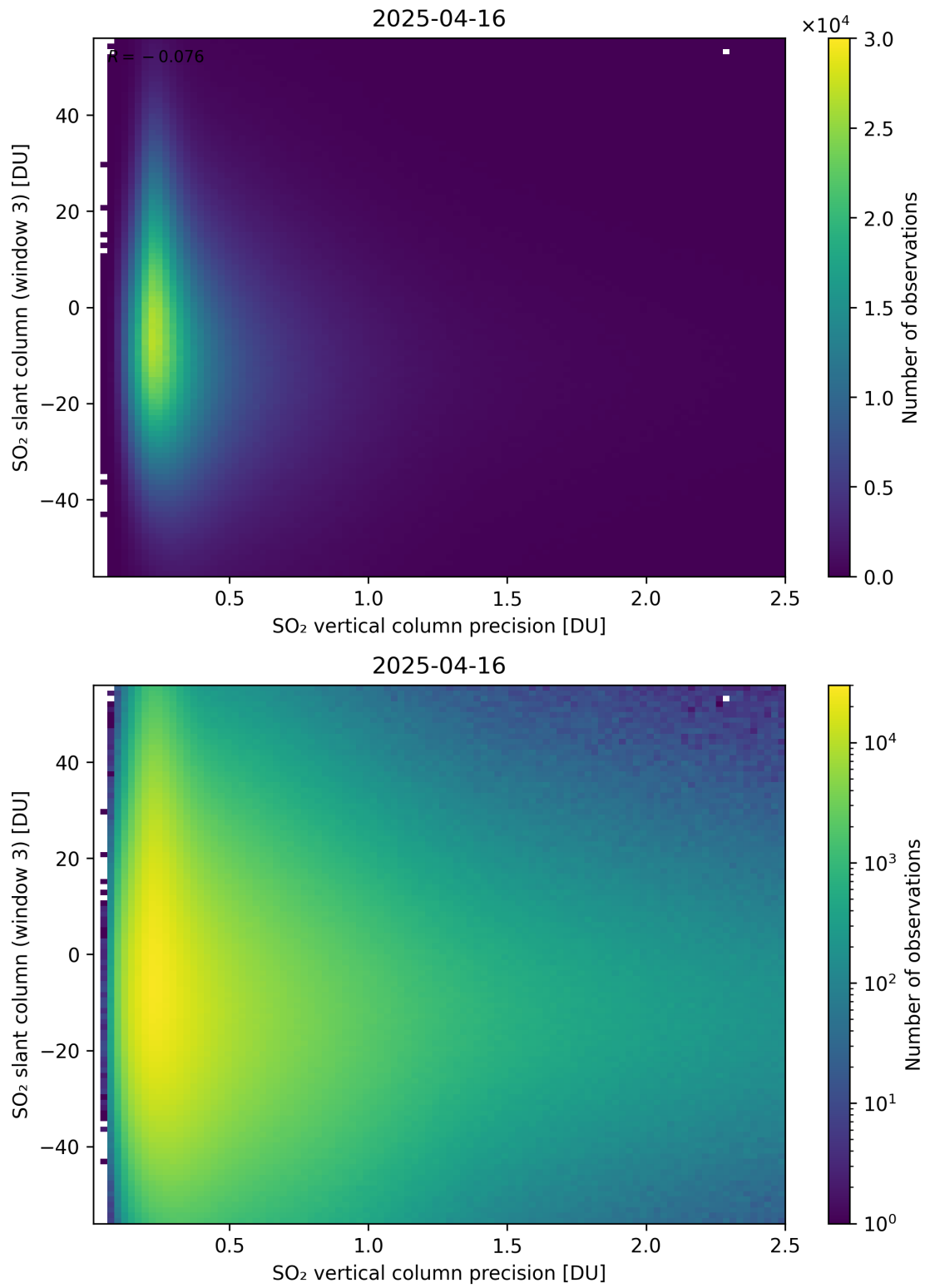
Figure 344: Scatter density plot of “SO 2 vertical column precision” against “SO 2 slant column (window 3)” for 2025-04-15 to 2025-04-17.
