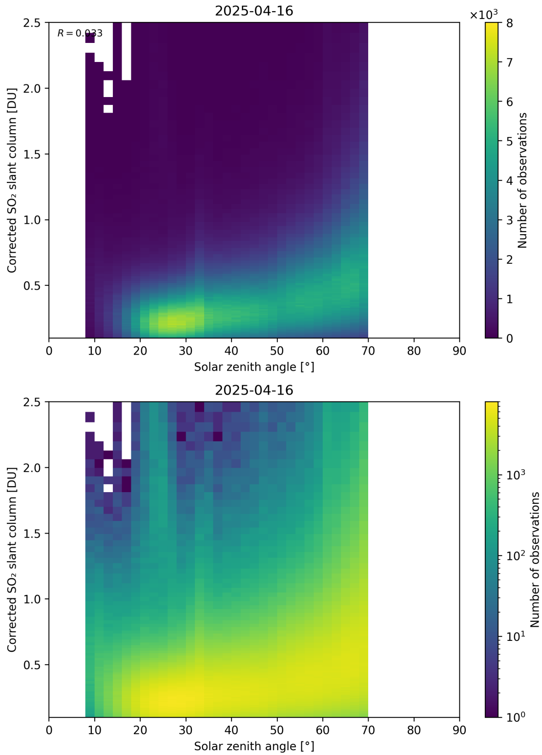
Figure 181: Scatter density plot of “Solar zenith angle” against “Corrected SO 2 slant column” for 2025-04-15 to 2025-04-17.
