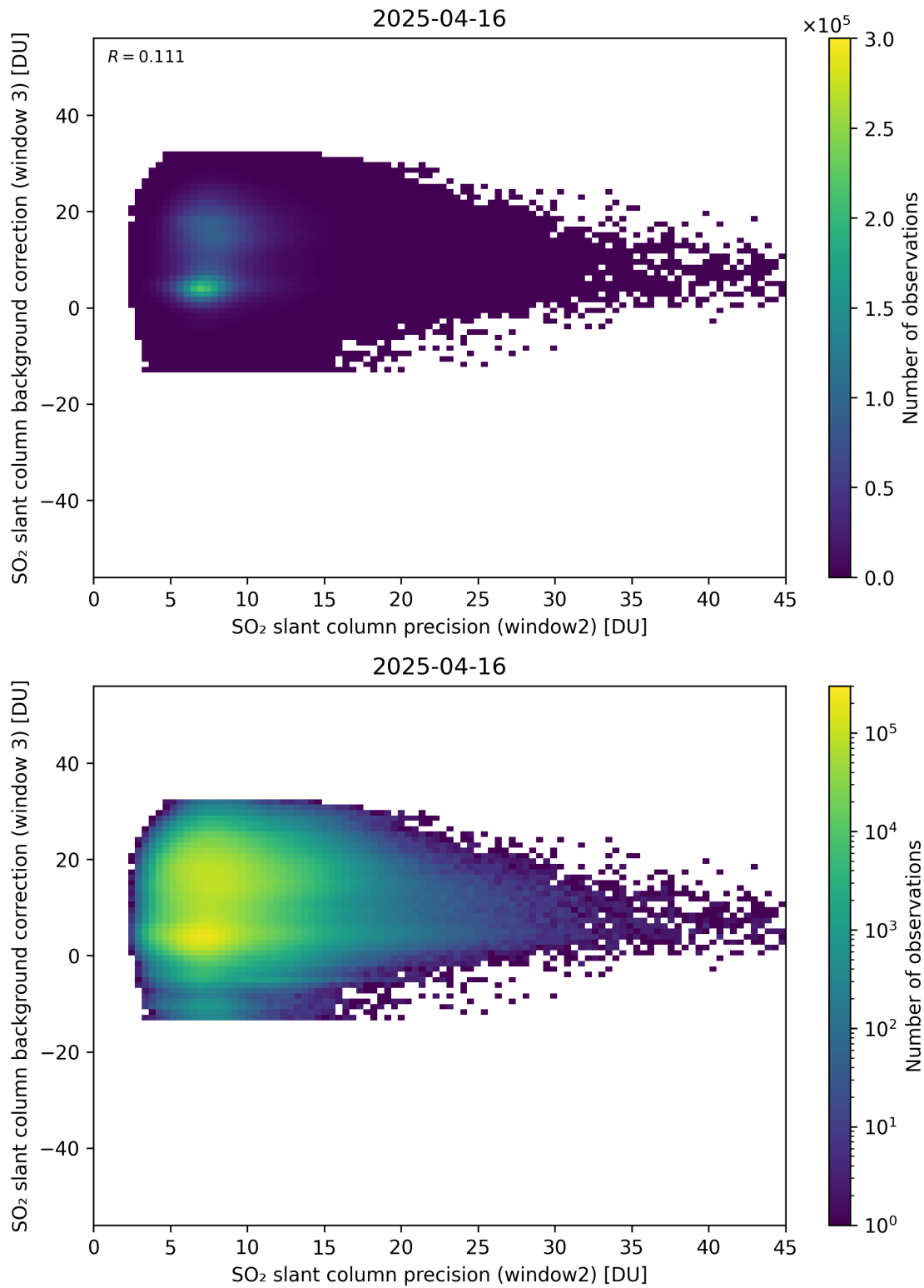
Figure 292: Scatter density plot of “SO 2 slant column precision (window2)” against “SO 2 slant column background correction (window 3)” for 2025-04-15 to 2025-04-17.
