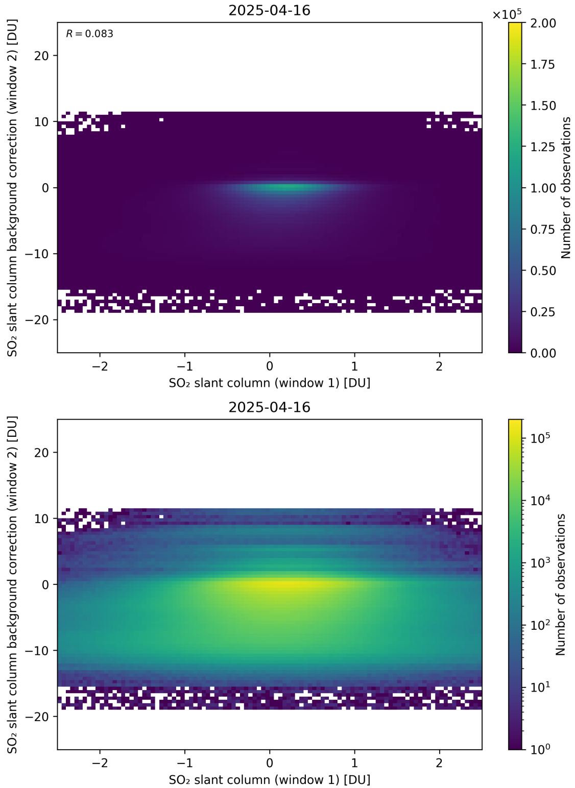
Figure 263: Scatter density plot of “SO 2 slant column (window 1)” against “SO 2 slant column background correction (window 2)” for 2025-04-15 to 2025-04-17.
