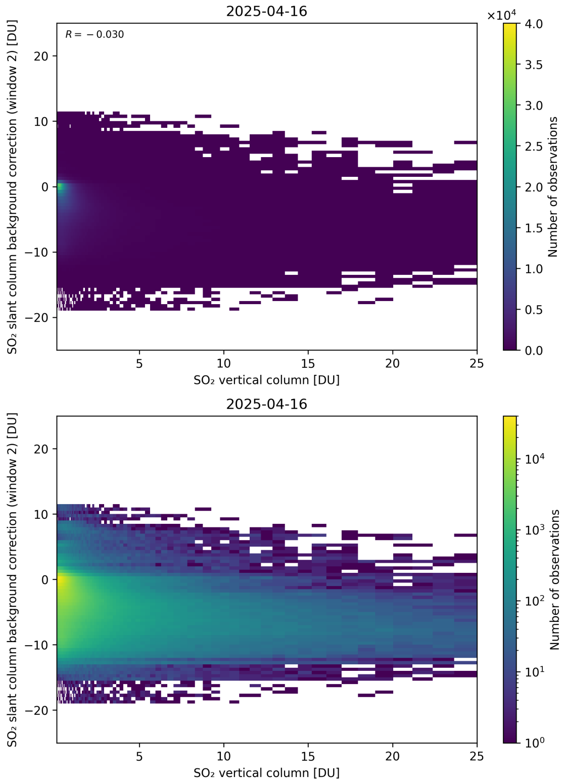
Figure 324: Scatter density plot of “SO 2 vertical column” against “SO 2 slant column background correction (window 2)” for 2025-04-15 to 2025-04-17.
