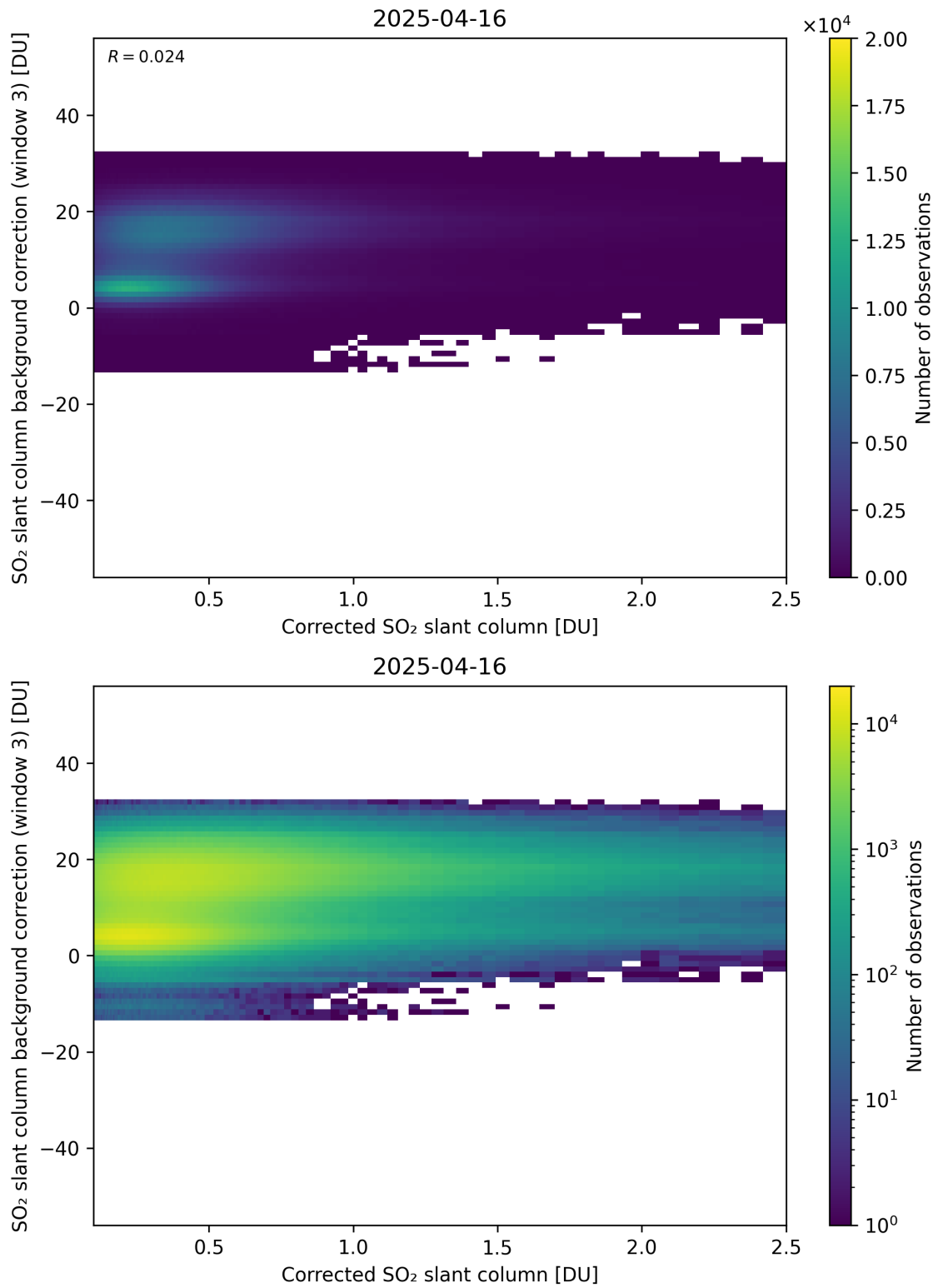
Figure 228: Scatter density plot of “Corrected SO 2 slant column” against “SO 2 slant column background correction (window 3)” for 2025-04-15 to 2025-04-17.
