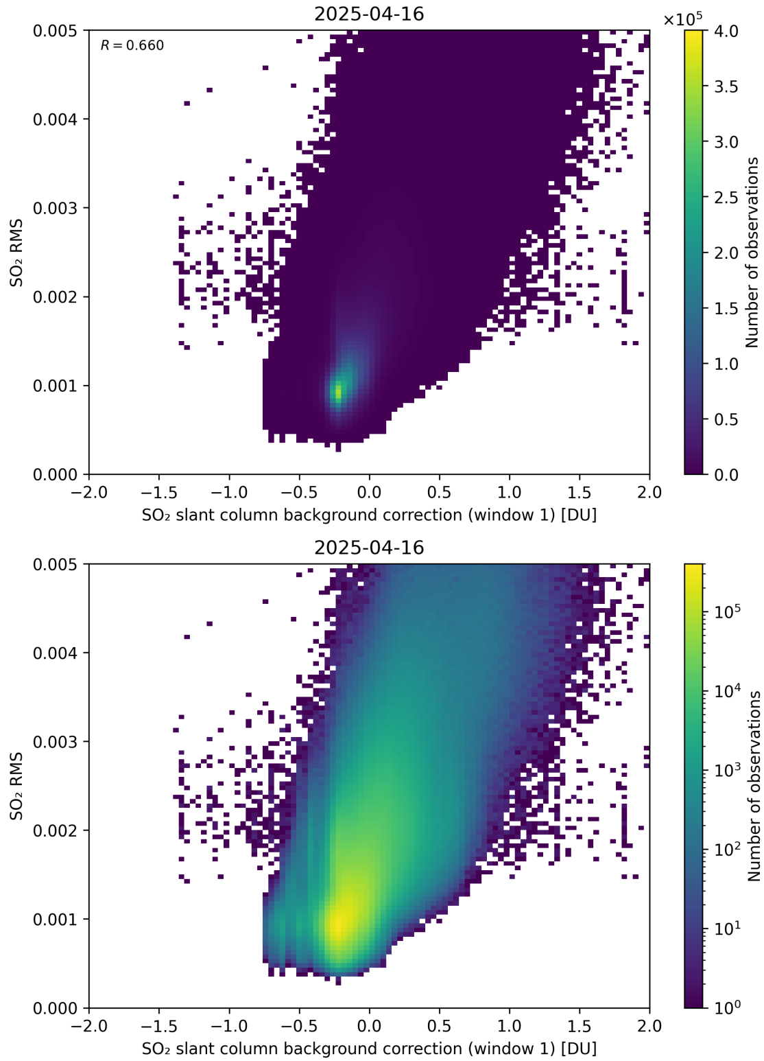
Figure 113: Scatter density plot of “SO 2 slant column background correction (window 1)” against “SO 2 RMS” for 2025-04-15 to 2025-04-17.
