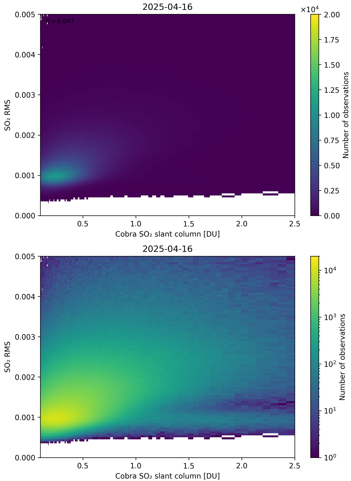
Figure 198: Scatter density plot of “Cobra SO 2 slant column” against “SO 2 RMS” for 2025-04-15 to 2025-04-17.
