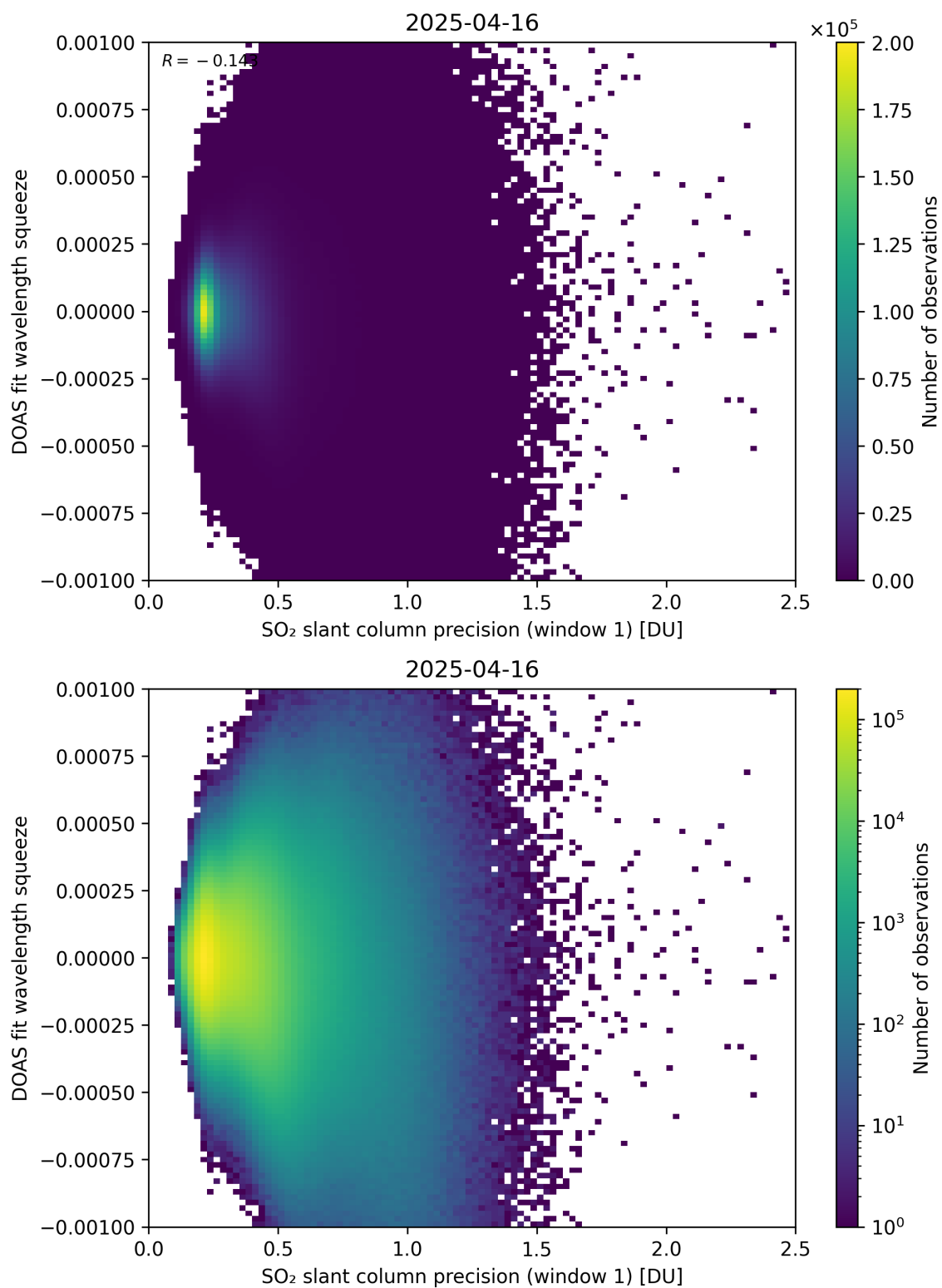
Figure 272: Scatter density plot of “SO 2 slant column precision (window 1)” against “DOAS fit wavelength squeeze” for 2025-04-15 to 2025-04-17.
