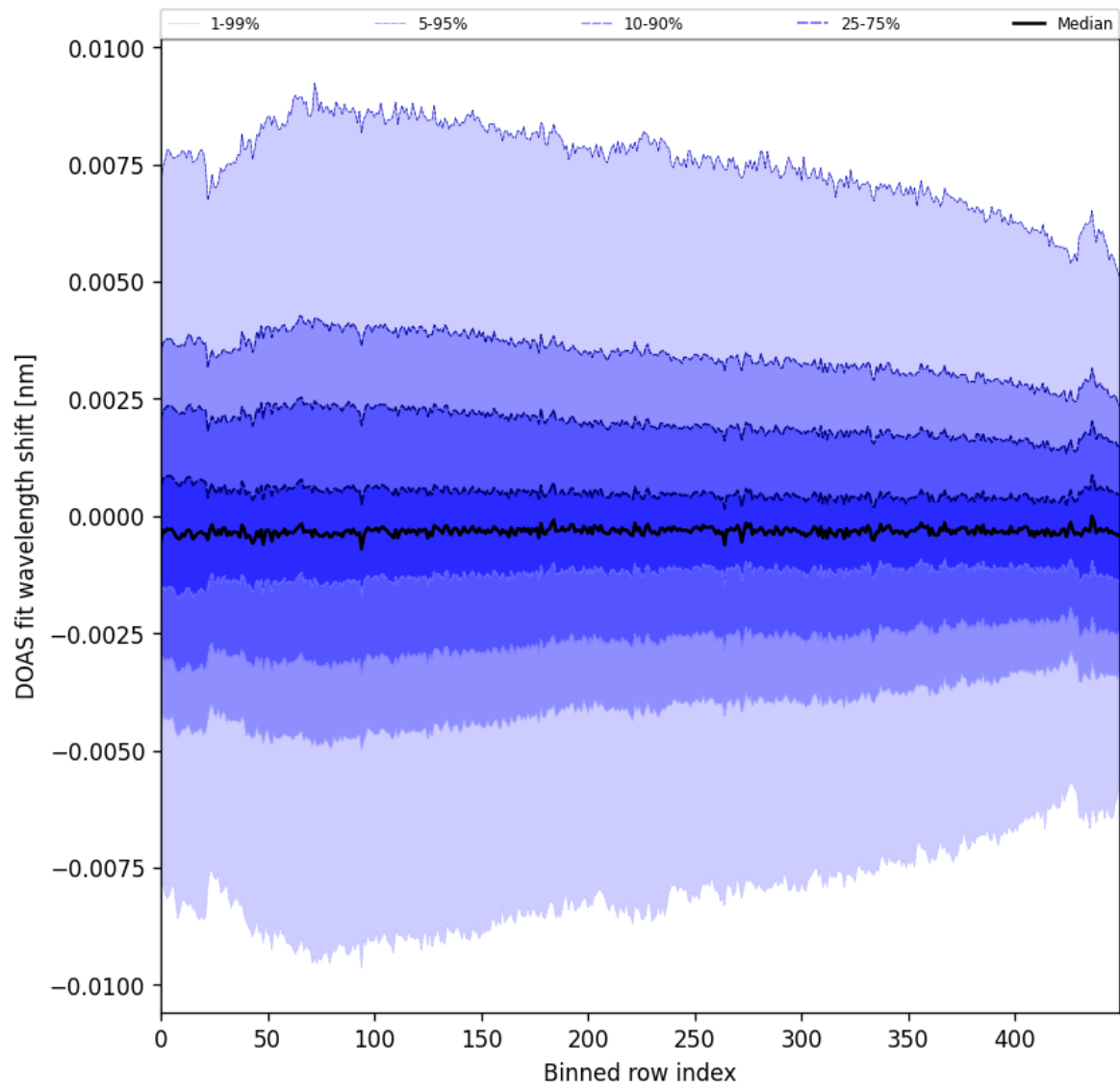
Figure 102: Along track statistics of “DOAS fit wavelength shift” for 2025-04-15 to 2025-04-17
