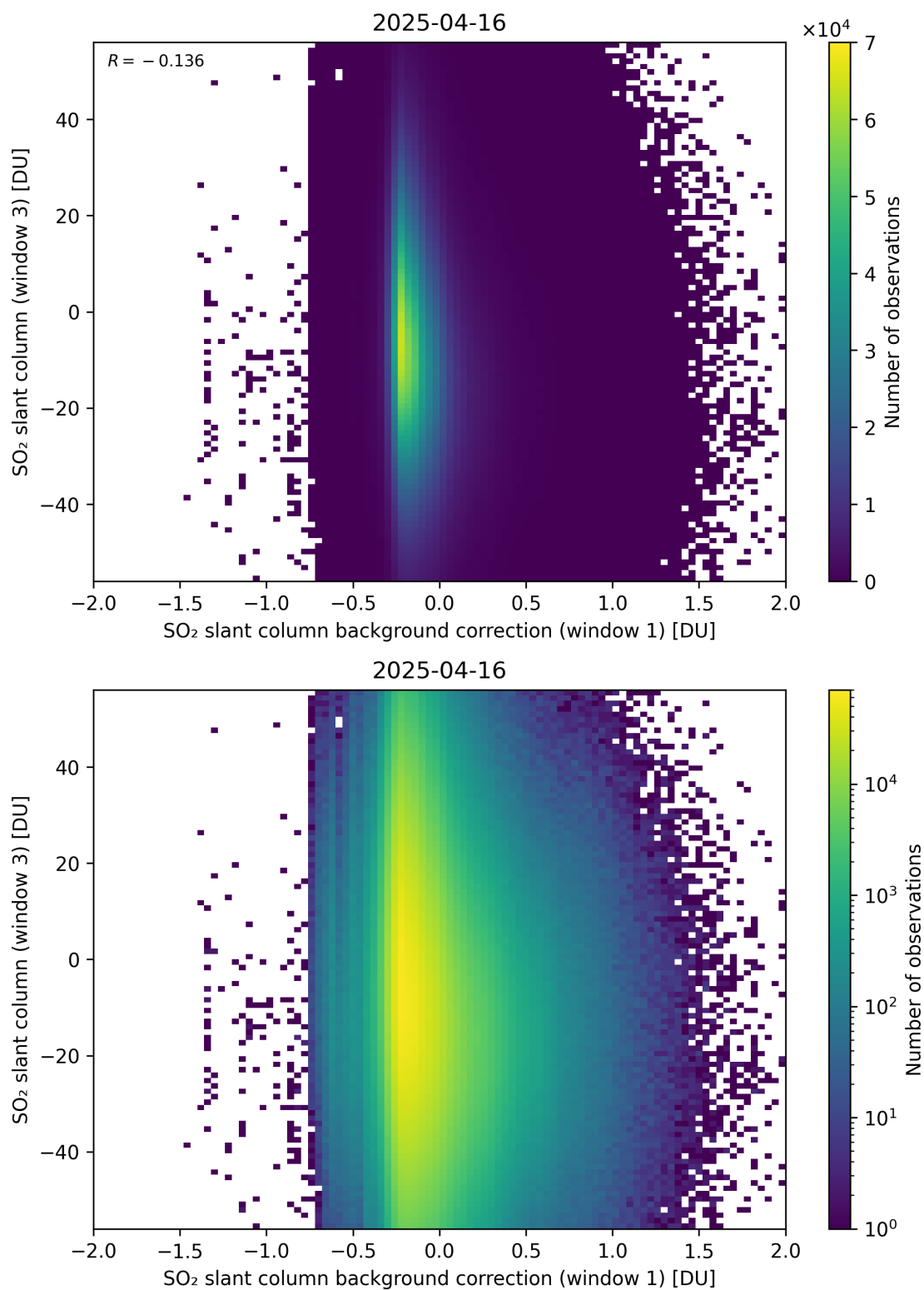
Figure 118: Scatter density plot of “SO 2 slant column background correction (window 1)” against “SO 2 slant column (window 3)” for 2025-04-15 to 2025-04-17.
