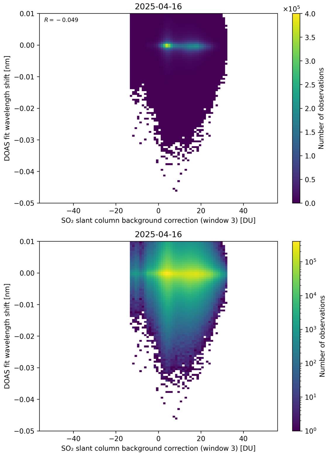
Figure 132: Scatter density plot of “SO 2 slant column background correction (window 3)” against “DOAS fit wavelength shift” for 2025-04-15 to 2025-04-17.
