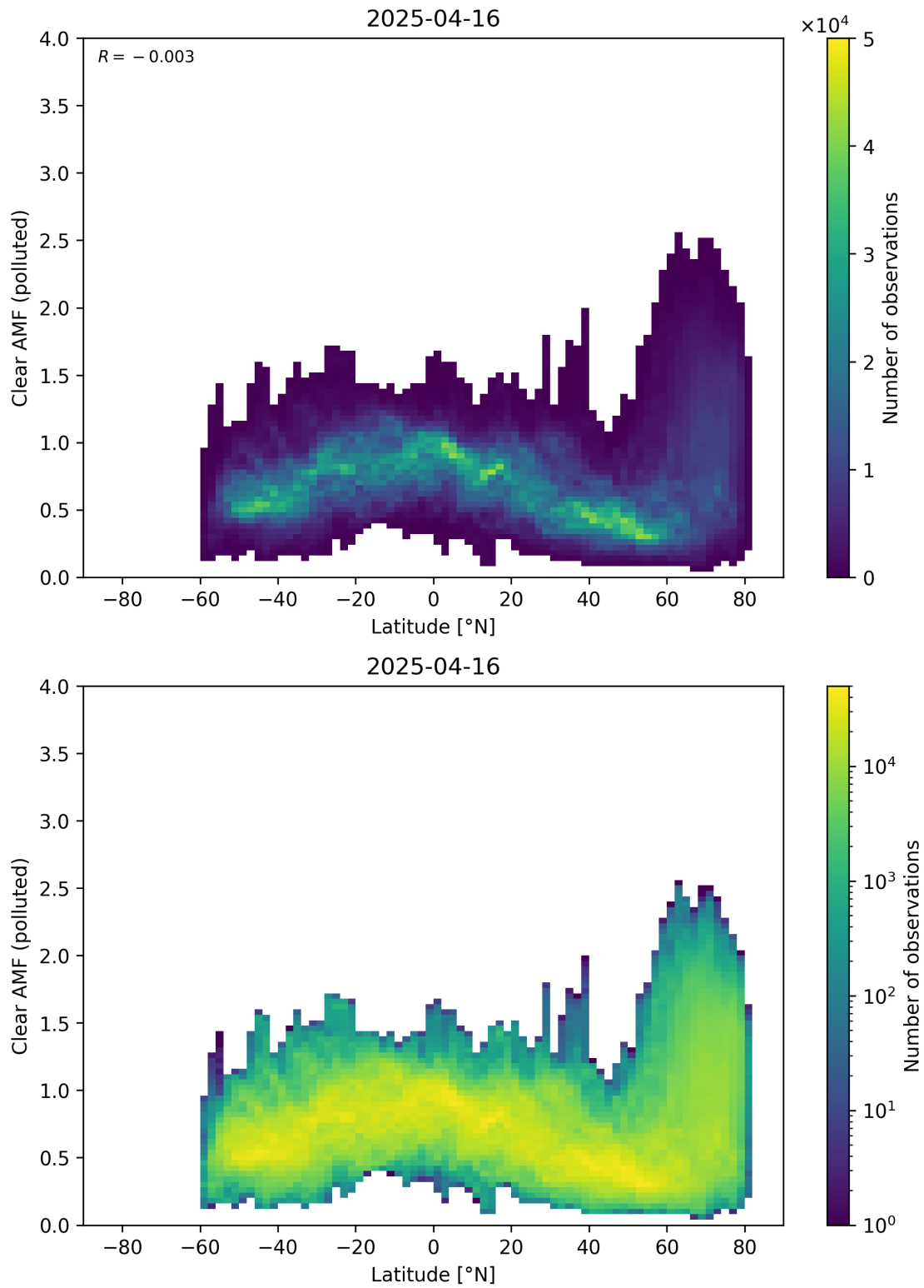
Figure 156: Scatter density plot of “Latitude” against “Clear AMF (polluted)” for 2025-04-15 to 2025-04-17.
