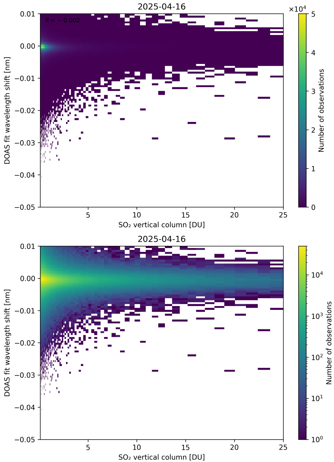
Figure 326: Scatter density plot of “SO 2 vertical column” against “DOAS fit wavelength shift” for 2025-04-15 to 2025-04-17.
