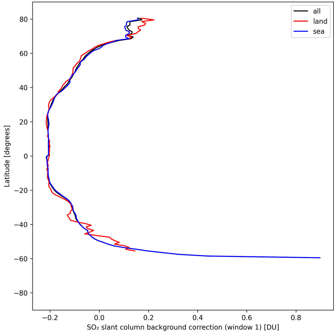
Figure 40: Zonal average of "SO 2 slant column background correction (window 1)" for 2025-04-15 to 2025-04-17.
