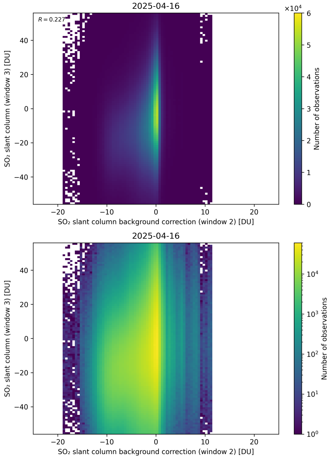
Figure 128: Scatter density plot of “SO 2 slant column background correction (window 2)” against “SO 2 slant column (window 3)” for 2025-04-15 to 2025-04-17.
