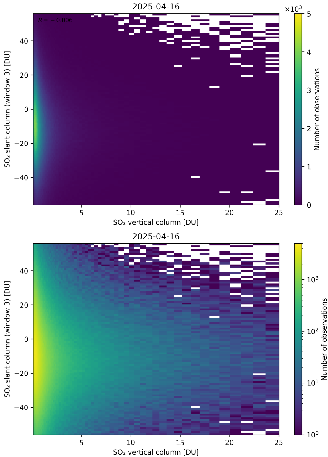
Figure 357: Scatter density plot of “SO 2 vertical column” against “SO 2 slant column (window 3)” for 2025-04-15 to 2025-04-17.
