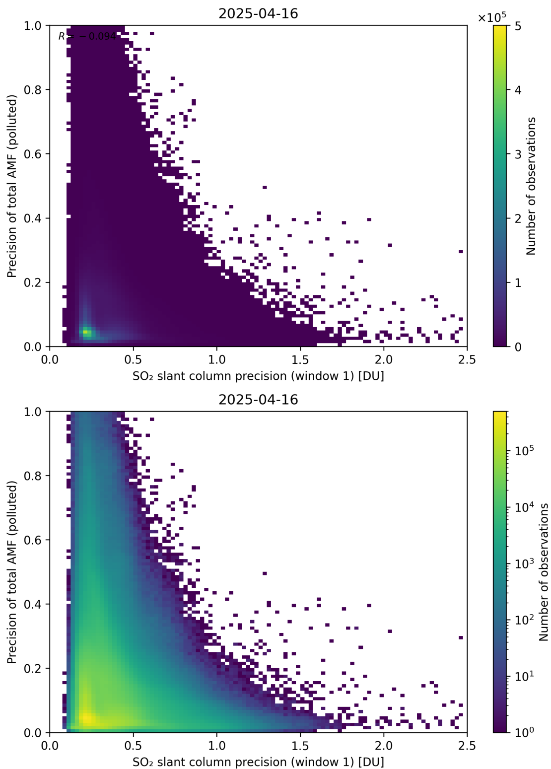
Figure 281: Scatter density plot of “SO 2 slant column precision (window 1)” against “Precision of total AMF (polluted)” for 2025-04-15 to 2025-04-17.
