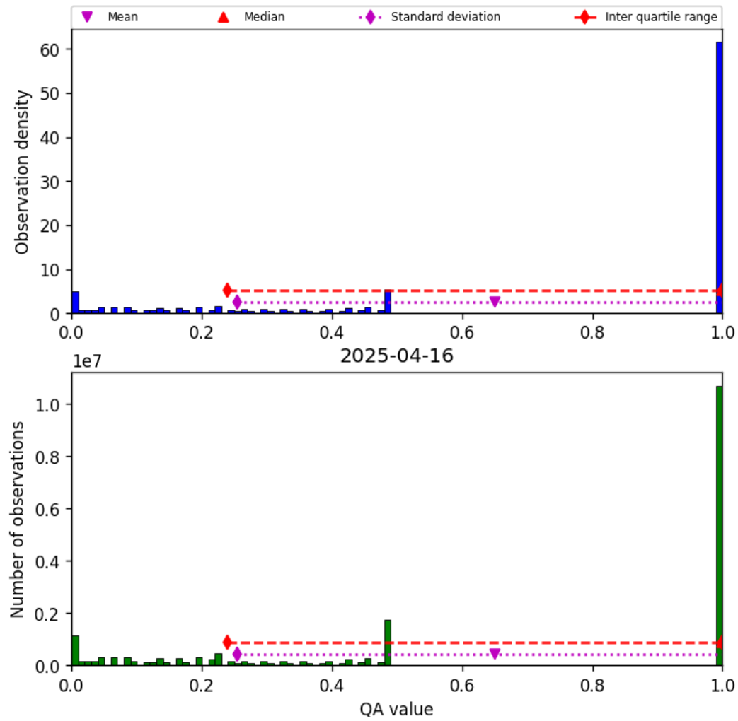
Figure 57: Histogram of “QA value” for 2025-04-15 to 2025-04-17
