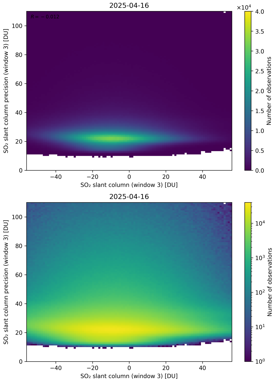
Figure 317: Scatter density plot of “SO 2 slant column (window 3)” against “SO 2 slant column precision (window 3)” for 2025-04-15 to 2025-04-17.
