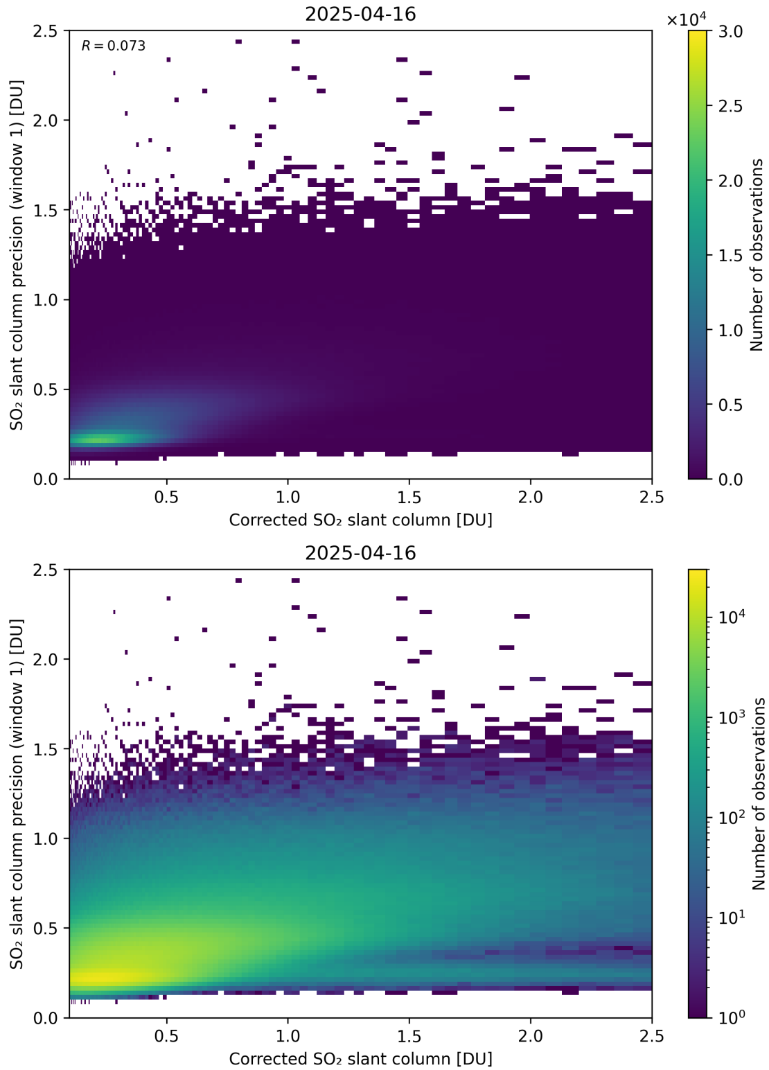
Figure 238: Scatter density plot of “Corrected SO 2 slant column” against “SO 2 slant column precision (window 1)” for 2025-04-15 to 2025-04-17.
