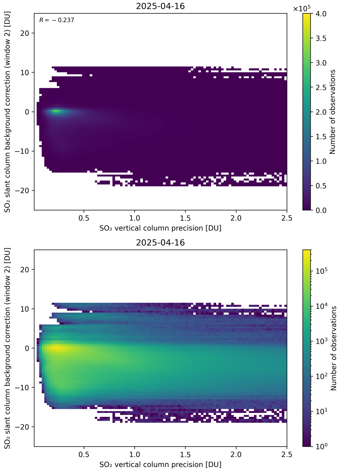
Figure 330: Scatter density plot of “SO 2 vertical column precision” against “SO 2 slant column background correction (window 2)” for 2025-04-15 to 2025-04-17.
