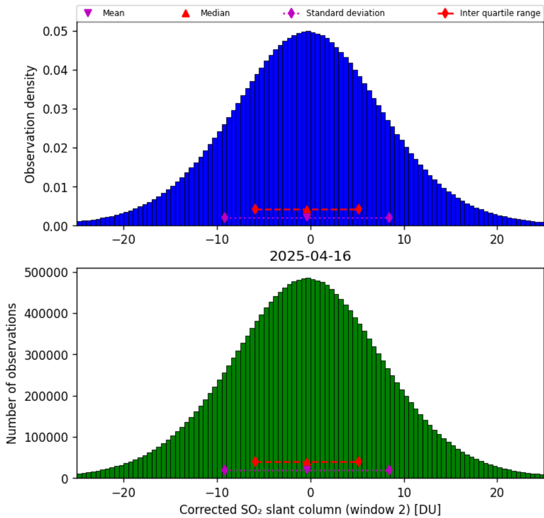
Figure 69: Histogram of “Corrected SO 2 slant column (window 2)” for 2025-04-15 to 2025-04-17
