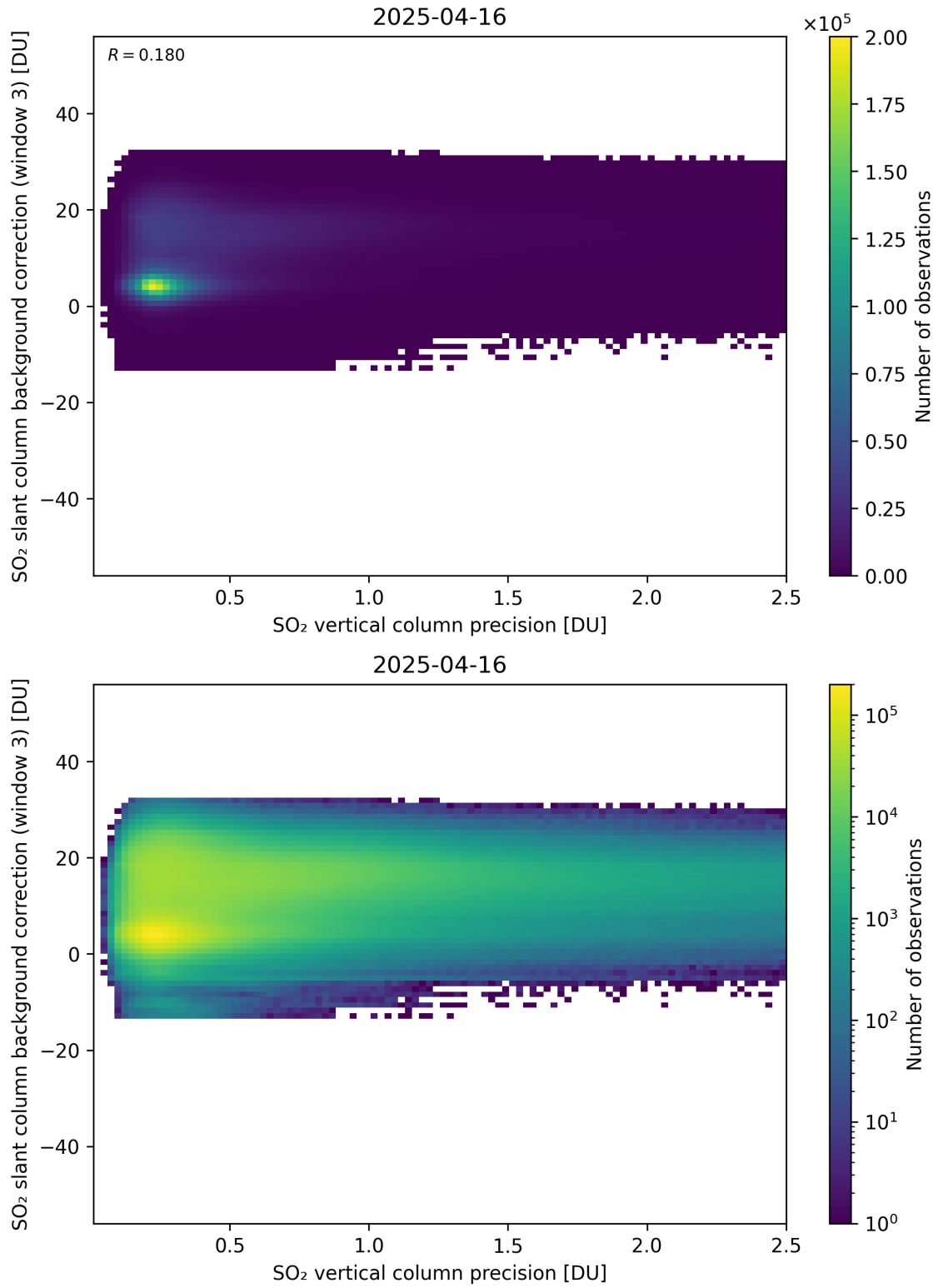
Figure 331: Scatter density plot of “SO 2 vertical column precision” against “SO 2 slant column background correction (window 3)” for 2025-04-15 to 2025-04-17.
