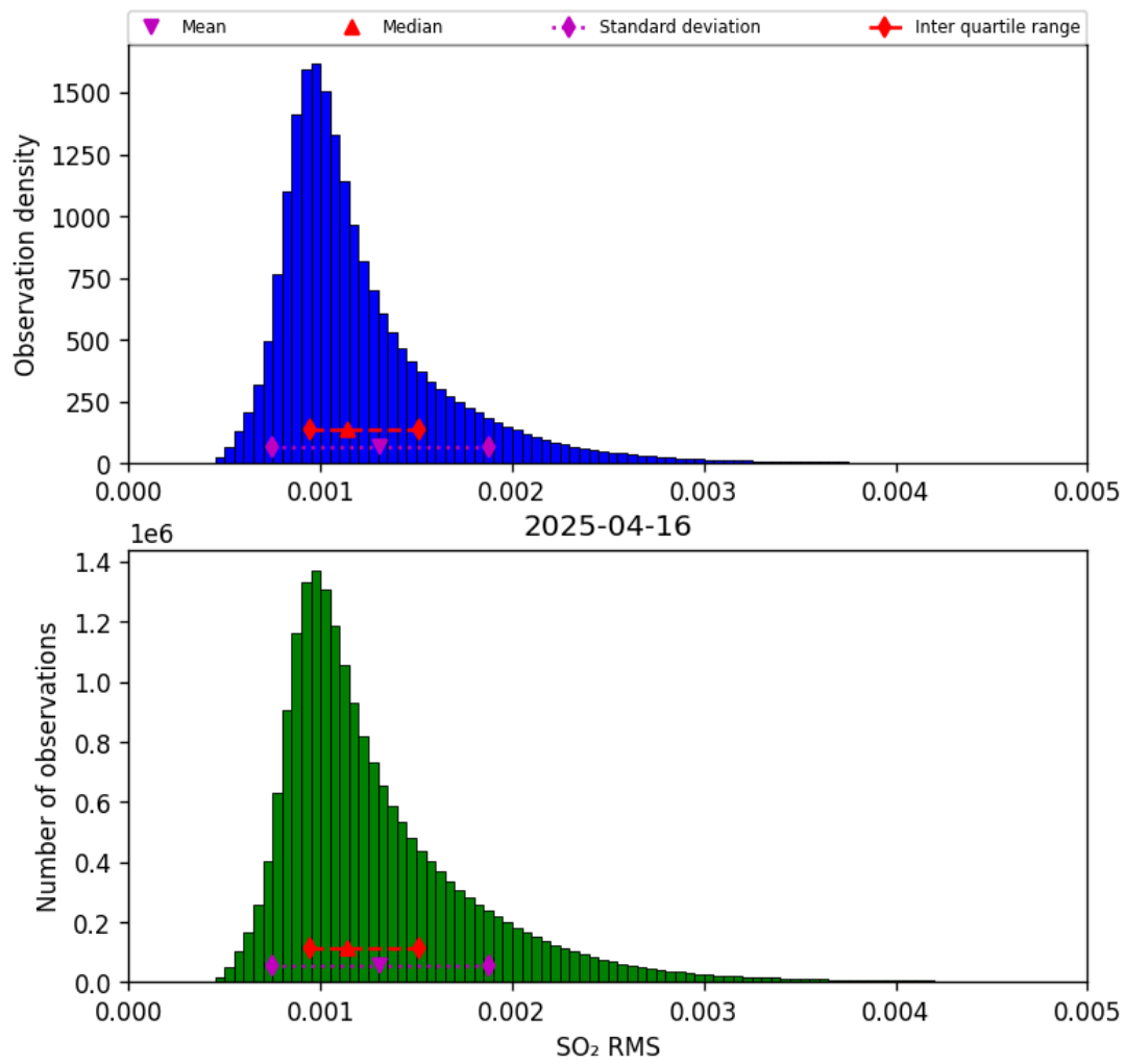
Figure 78: Histogram of “SO 2 RMS” for 2025-04-15 to 2025-04-17
