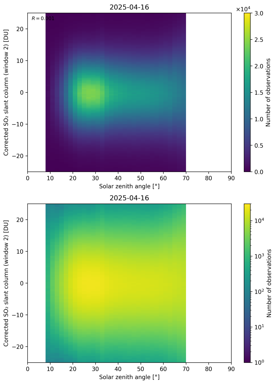
Figure 182: Scatter density plot of “Solar zenith angle” against “Corrected SO 2 slant column (window 2)” for 2025-04-15 to 2025-04-17.
