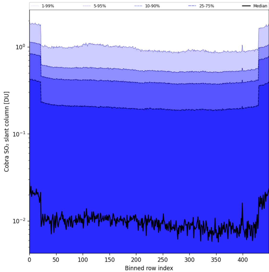
Figure 87: Along track statistics of “Cobra SO 2 slant column” for 2025-04-15 to 2025-04-17
