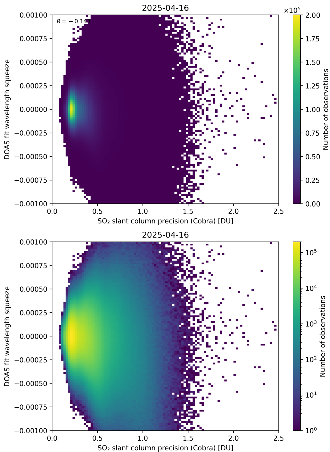
Figure 203: Scatter density plot of “SO 2 slant column precision (Cobra)” against “DOAS fit wavelength squeeze” for 2025-04-15 to 2025-04-17.
