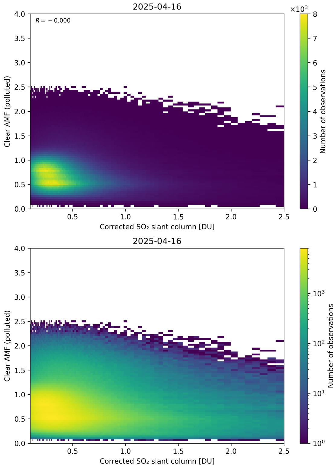
Figure 232: Scatter density plot of “Corrected SO 2 slant column” against “Clear AMF (polluted)” for 2025-04-15 to 2025-04-17.
