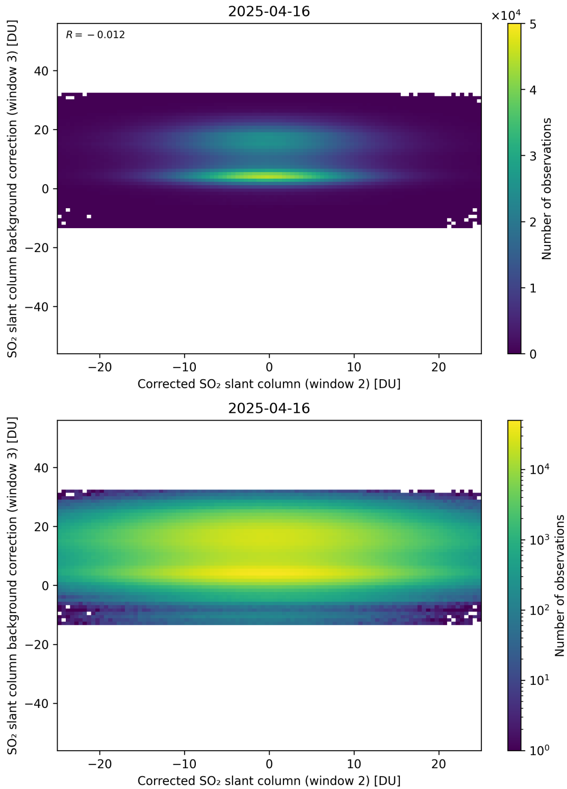
Figure 245: Scatter density plot of “Corrected SO 2 slant column (window 2)” against “SO 2 slant column background correction (window 3)” for 2025-04-15 to 2025-04-17.
