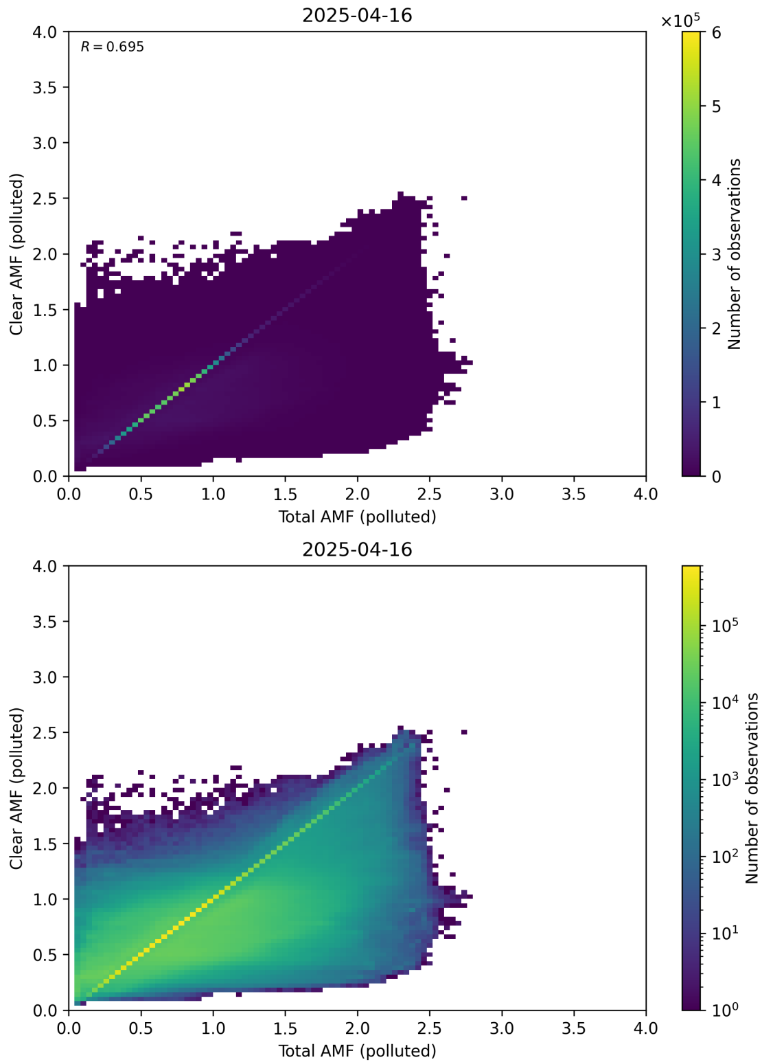
Figure 321: Scatter density plot of “Total AMF (polluted)” against “Clear AMF (polluted)” for 2025-04-15 to 2025-04-17.
