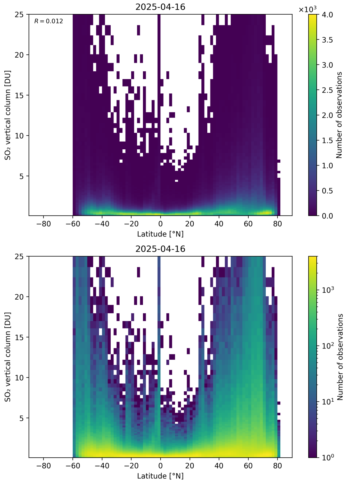
Figure 169: Scatter density plot of “Latitude” against “SO 2 vertical column” for 2025-04-15 to 2025-04-17.
