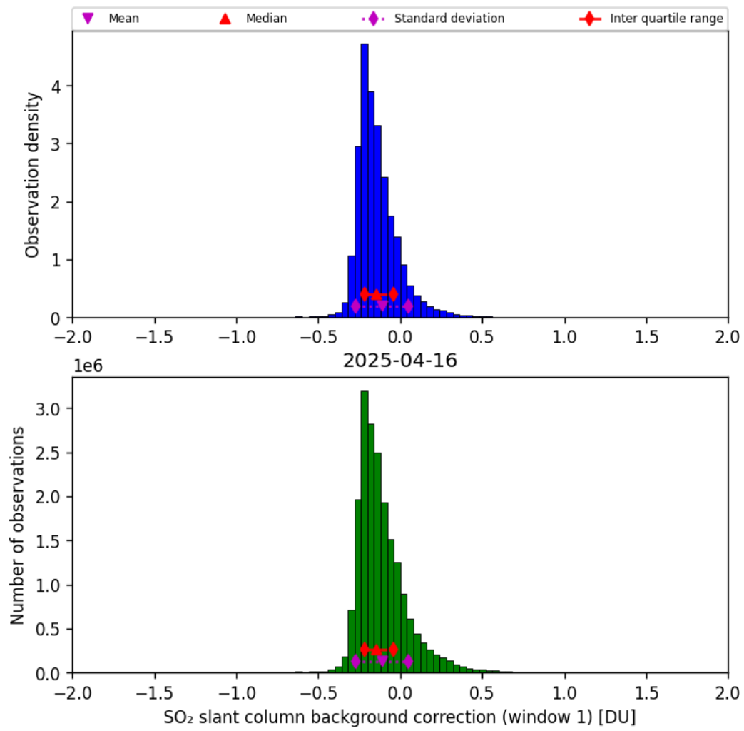
Figure 66: Histogram of “SO 2 slant column background correction (window 1)” for 2025-04-15 to 2025-04-17
