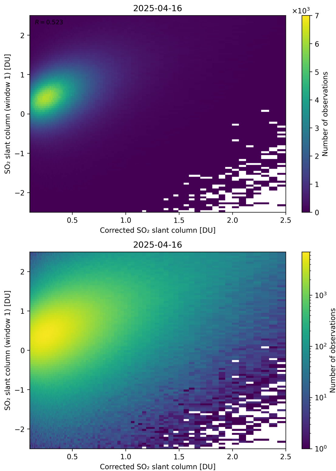
Figure 237: Scatter density plot of “Corrected SO 2 slant column” against “SO 2 slant column (window 1)” for 2025-04-15 to 2025-04-17.
