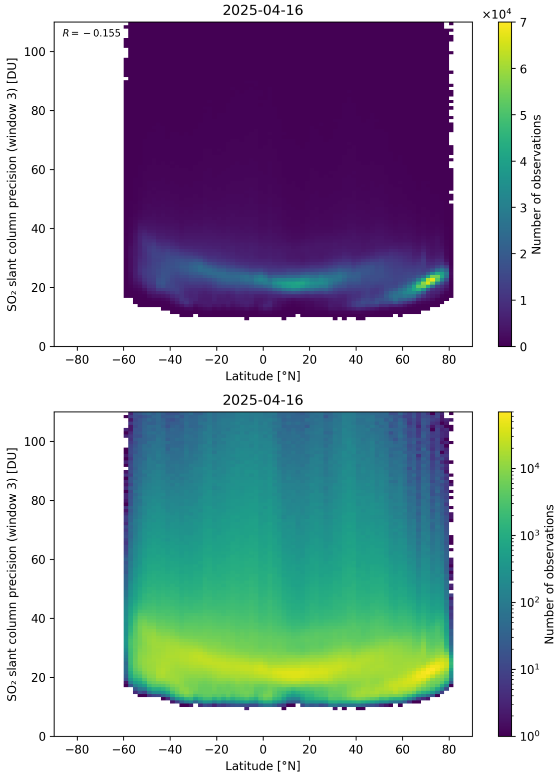
Figure 166: Scatter density plot of “Latitude” against “SO 2 slant column precision (window 3)” for 2025-04-15 to 2025-04-17.
