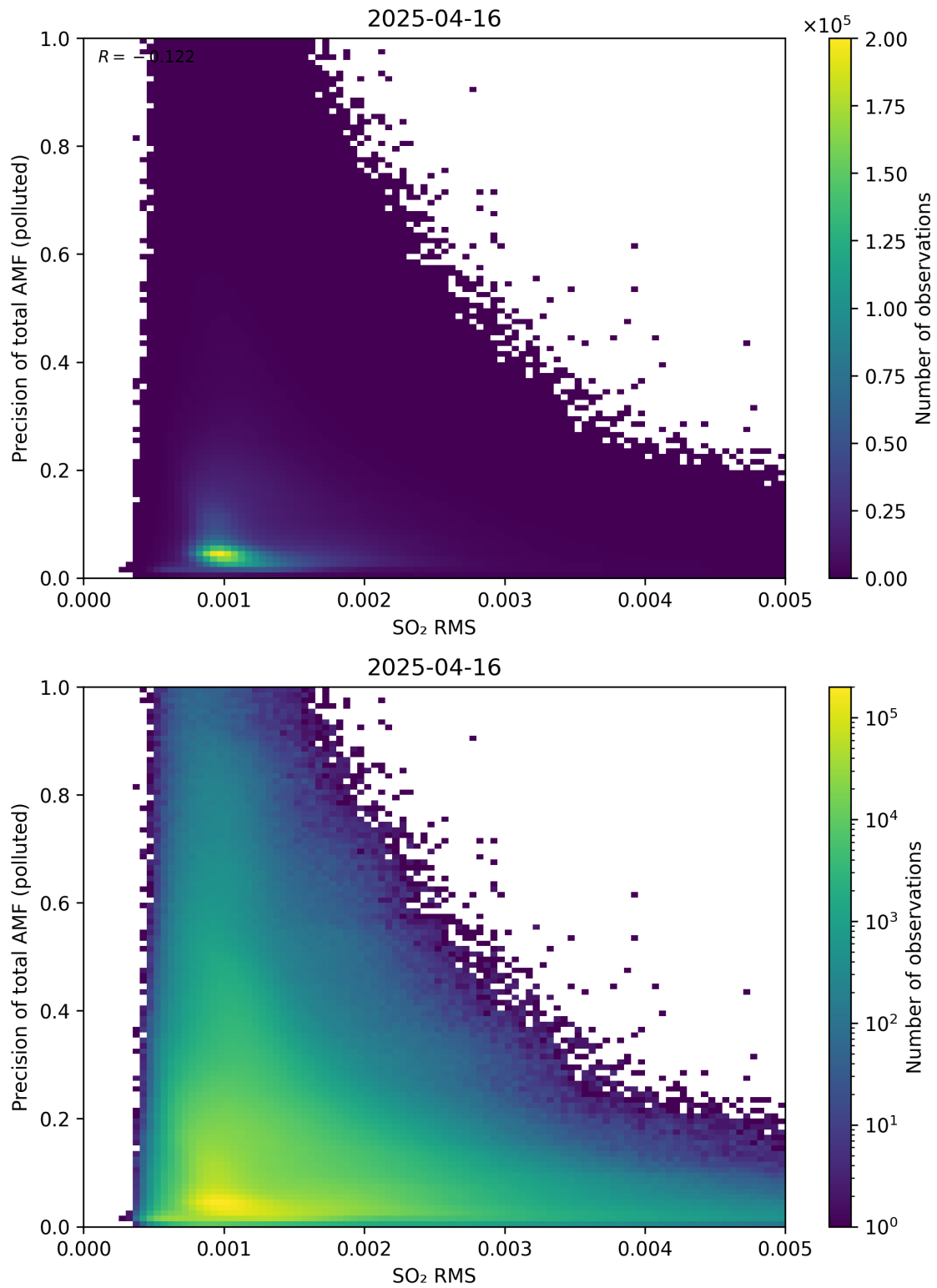
Figure 149: Scatter density plot of “SO 2 RMS” against “Precision of total AMF (polluted)” for 2025-04-15 to 2025-04-17.
