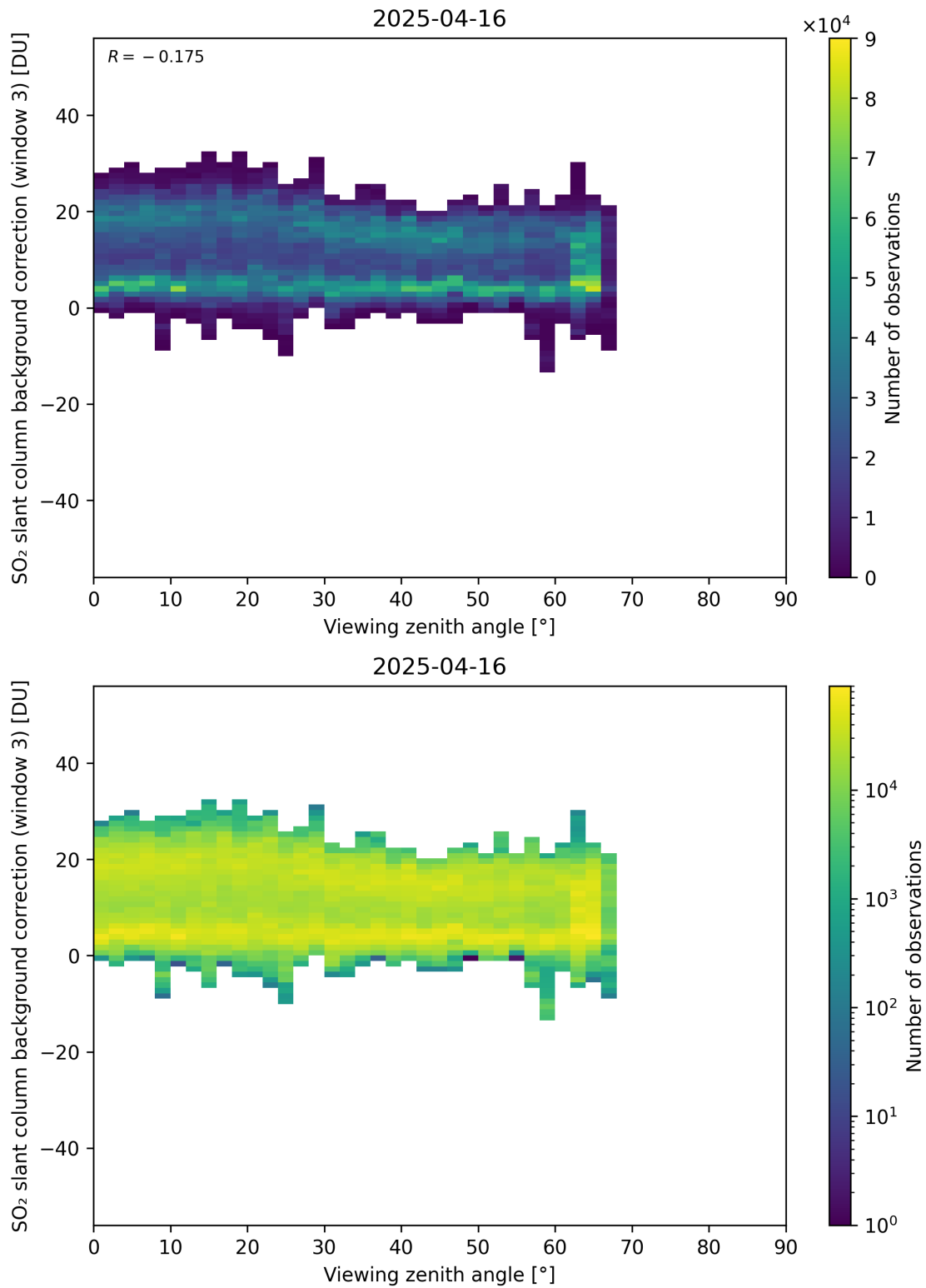
Figure 364: Scatter density plot of “Viewing zenith angle” against “SO 2 slant column background correction (window 3)” for 2025-04-15 to 2025-04-17.
