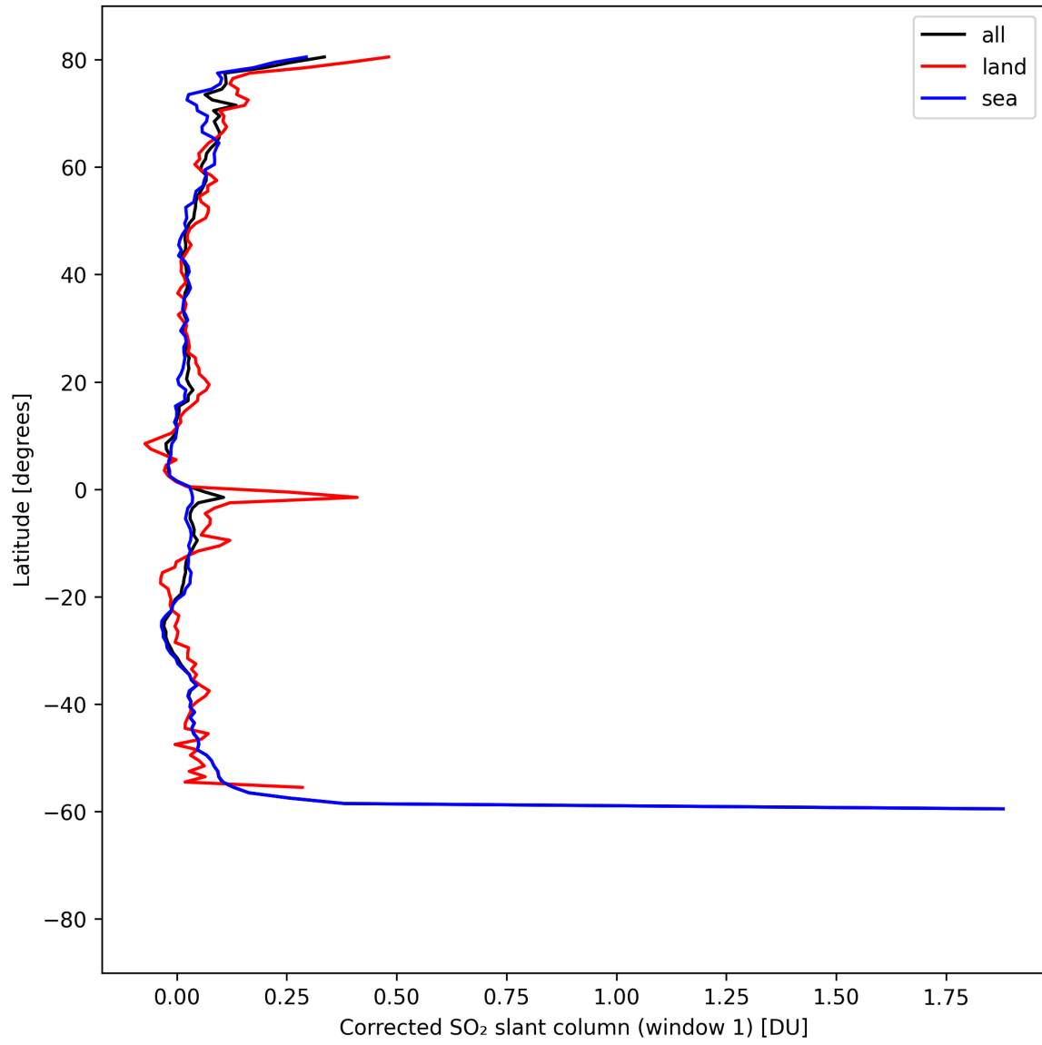
Figure 39: Zonal average of “Corrected SO 2 slant column (window 1)” for 2025-04-15 to 2025-04-17.
