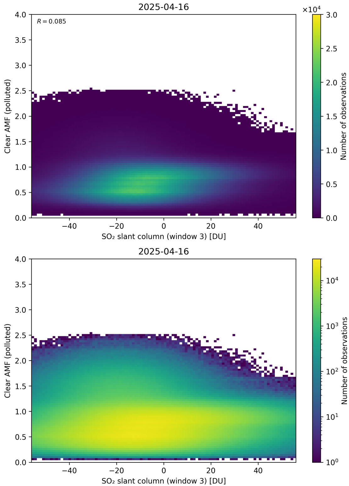
Figure 315: Scatter density plot of “SO 2 slant column (window 3)” against “Clear AMF (polluted)” for 2025-04-15 to 2025-04-17.
