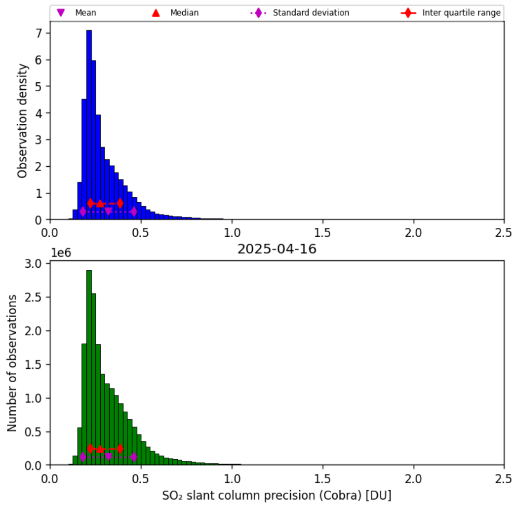
Figure 62: Histogram of “SO 2 slant column precision (Cobra)” for 2025-04-15 to 2025-04-17
