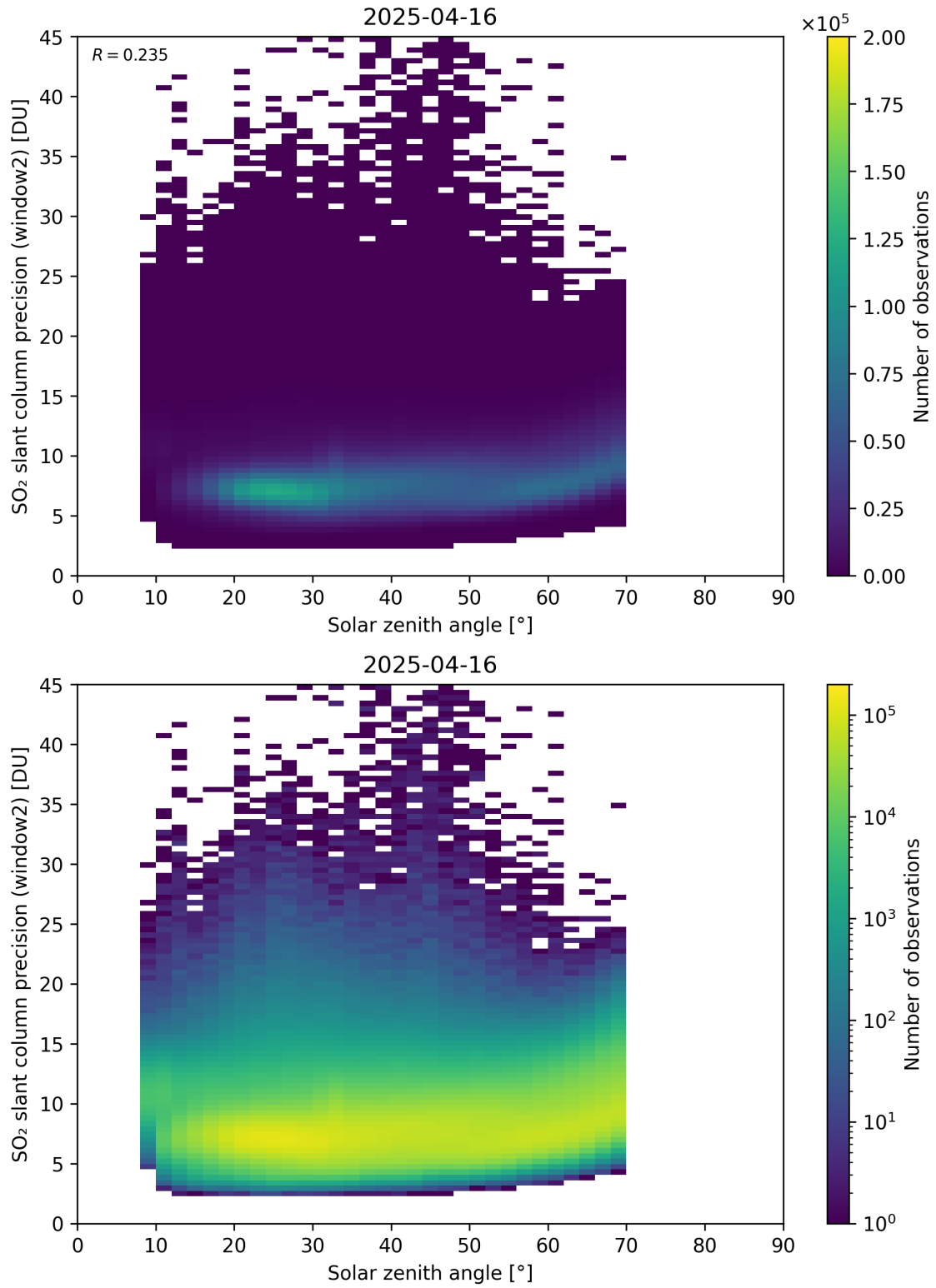
Figure 186: Scatter density plot of “Solar zenith angle” against “SO 2 slant column precision (window2)” for 2025-04-15 to 2025-04-17.
