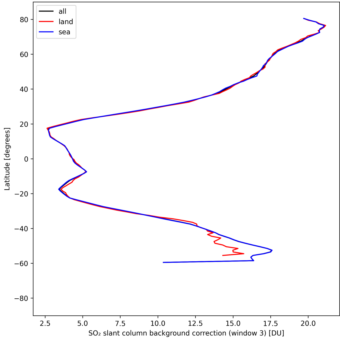
Figure 48: Zonal average of “SO 2 slant column background correction (window 3)” for 2025-04-15 to 2025-04-17.
