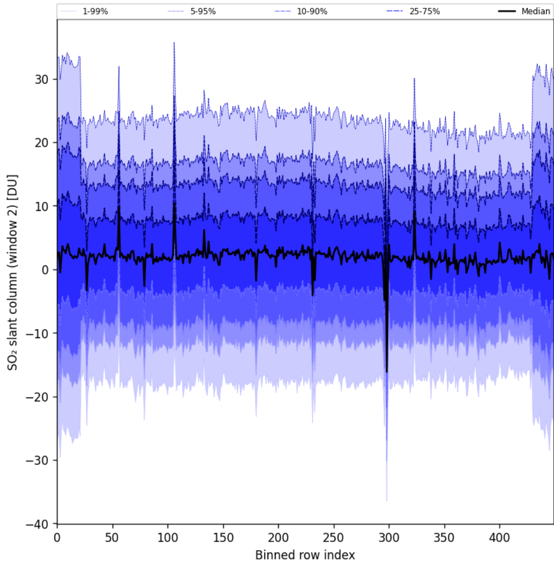
Figure 93: Along track statistics of “SO 2 slant column (window 2)” for 2025-04-15 to 2025-04-17
