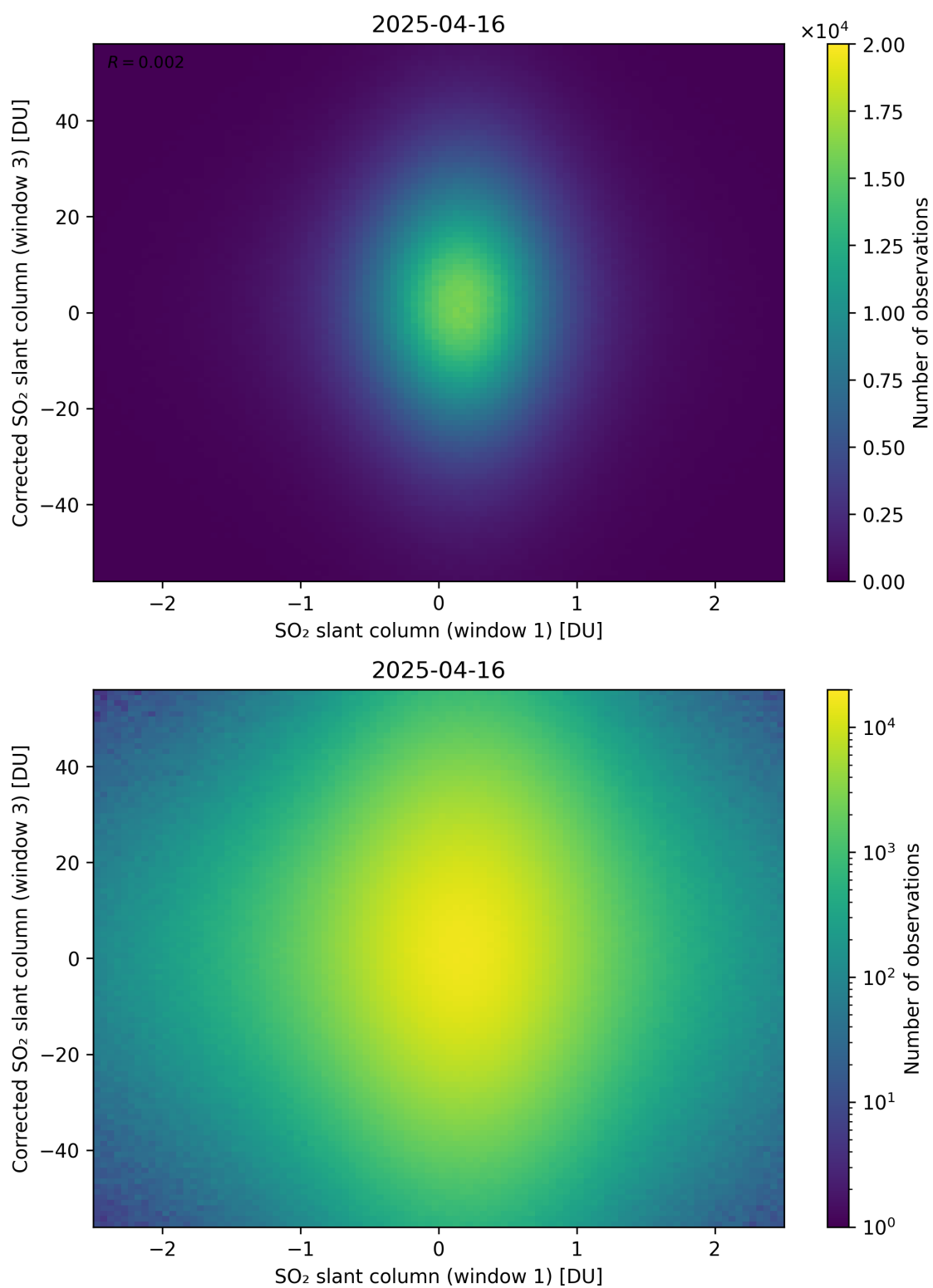
Figure 284: Scatter density plot of “SO 2 slant column (window 1)” against “Corrected SO 2 slant column (window 3)” for 2025-04-15 to 2025-04-17.
