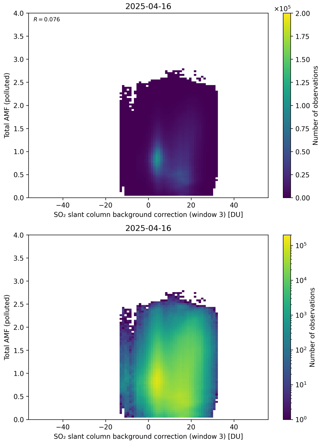
Figure 136: Scatter density plot of “SO 2 slant column background correction (window 3)” against “Total AMF (polluted)” for 2025-04-15 to 2025-04-17.
