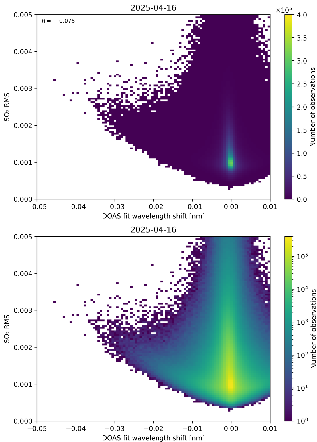
Figure 139: Scatter density plot of “DOAS fit wavelength shift” against “SO 2 RMS” for 2025-04-15 to 2025-04-17.
