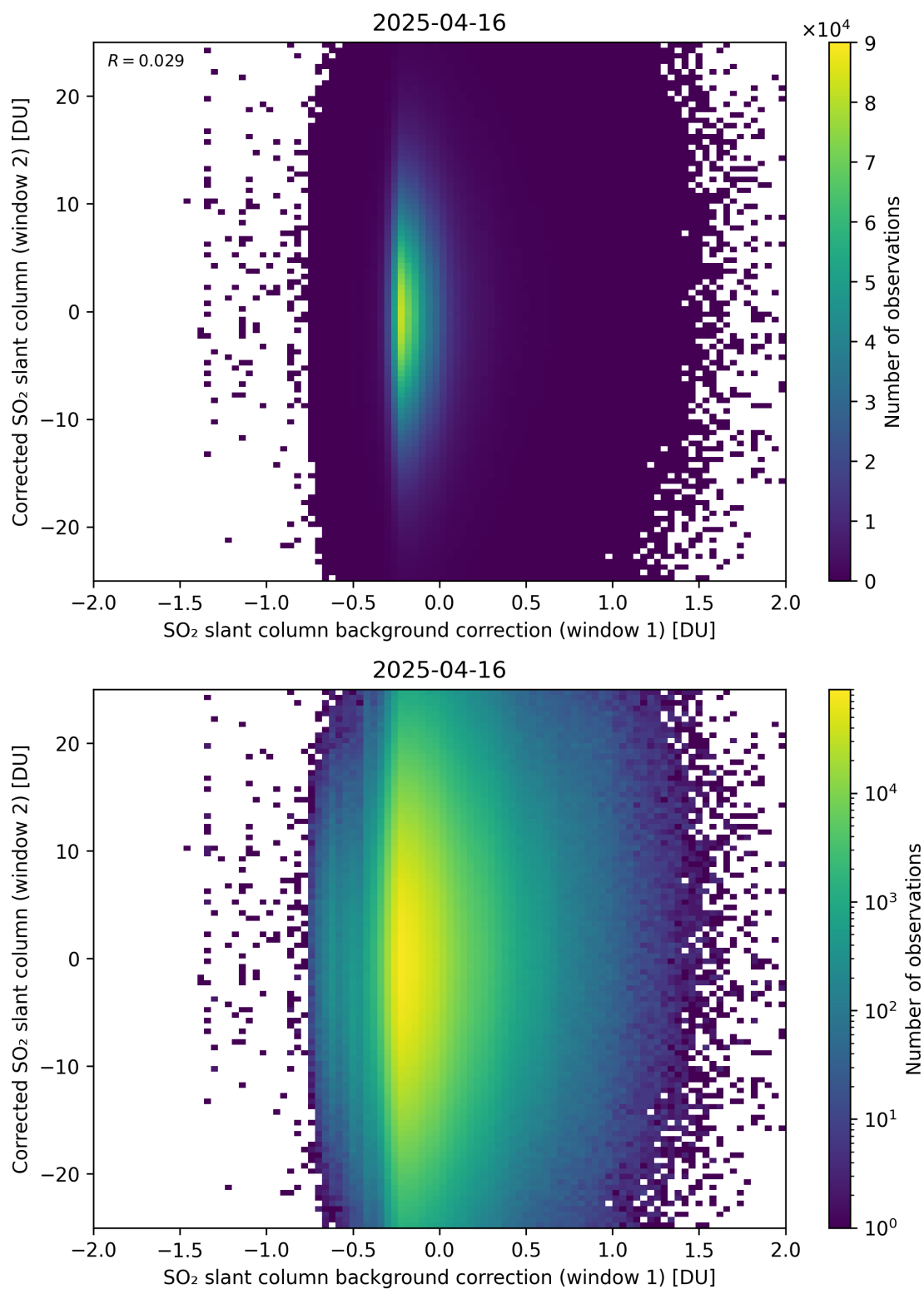
Figure 115: Scatter density plot of “SO 2 slant column background correction (window 1)” against “Corrected SO 2 slant column (window 2)” for 2025-04-15 to 2025-04-17.
