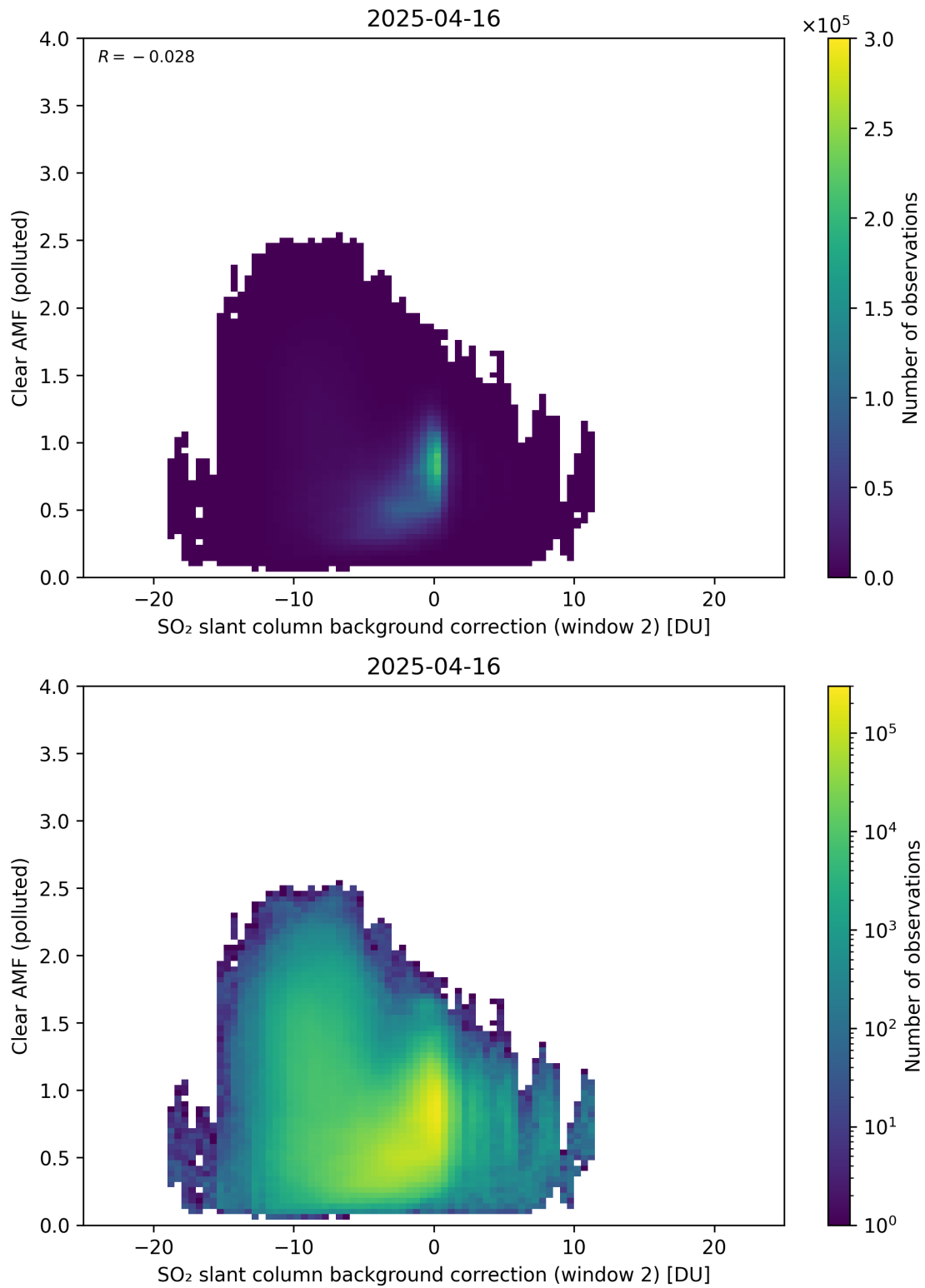
Figure 126: Scatter density plot of “SO 2 slant column background correction (window 2)” against “Clear AMF (polluted)” for 2025-04-15 to 2025-04-17.
