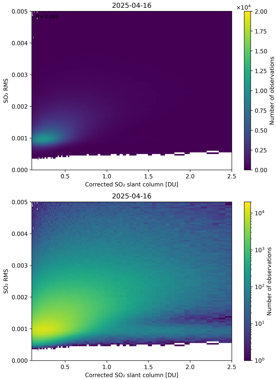
Figure 231: Scatter density plot of “Corrected SO 2 slant column” against “SO 2 RMS” for 2025-04-15 to 2025-04-17.
