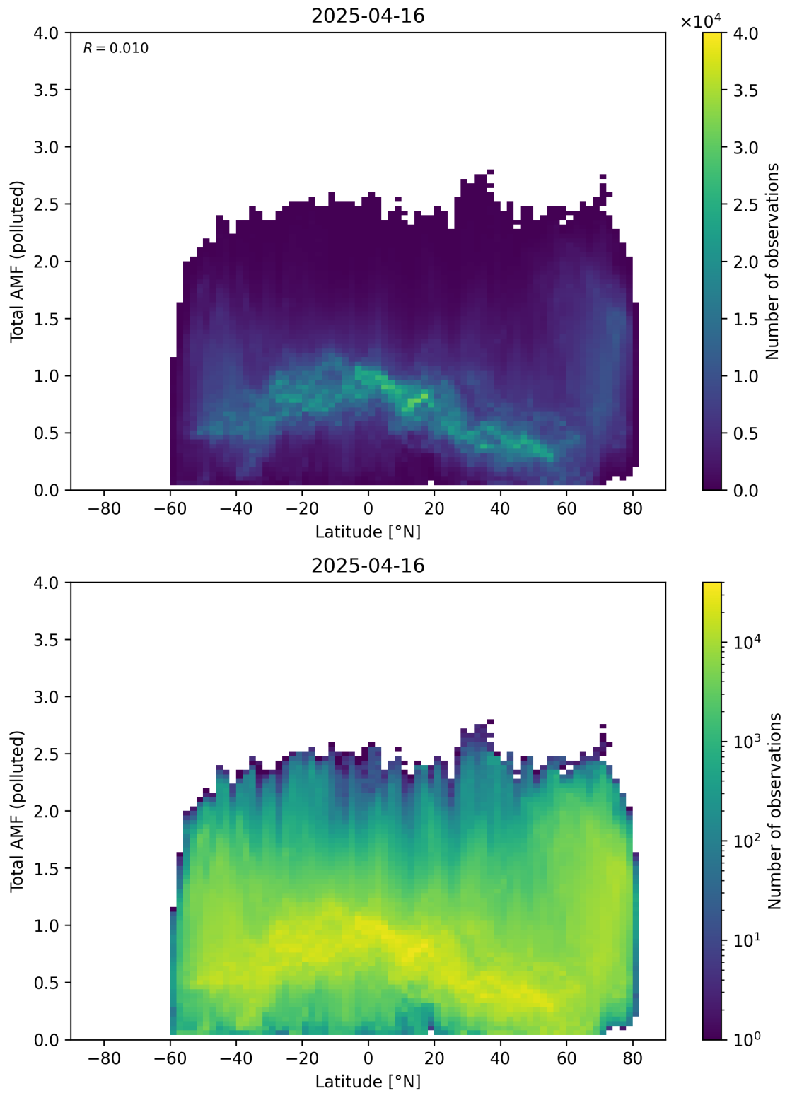
Figure 167: Scatter density plot of “Latitude” against “Total AMF (polluted)” for 2025-04-15 to 2025-04-17.
