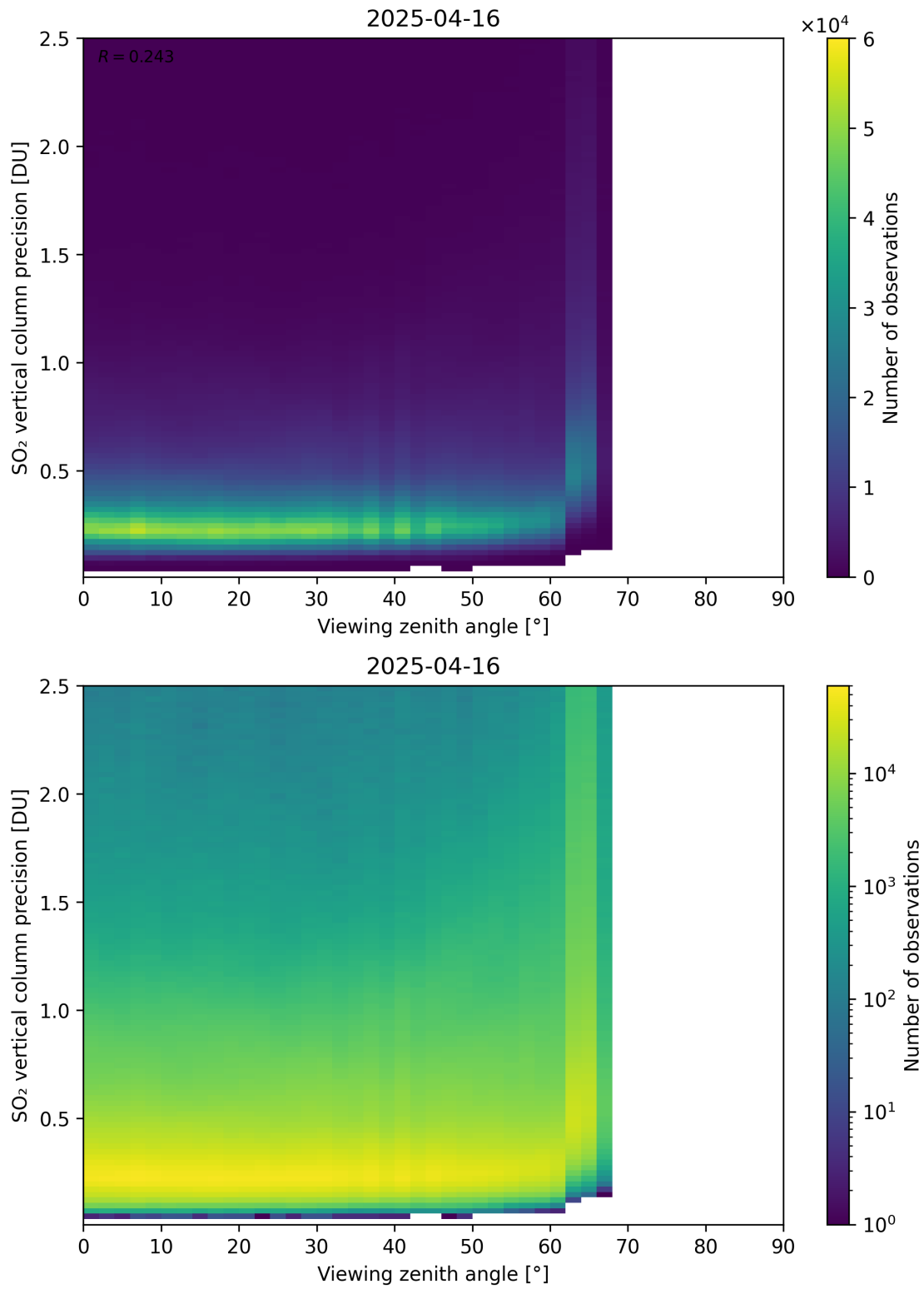
Figure 384: Scatter density plot of “Viewing zenith angle” against “SO 2 vertical column precision” for 2025-04-15 to 2025-04-17.
