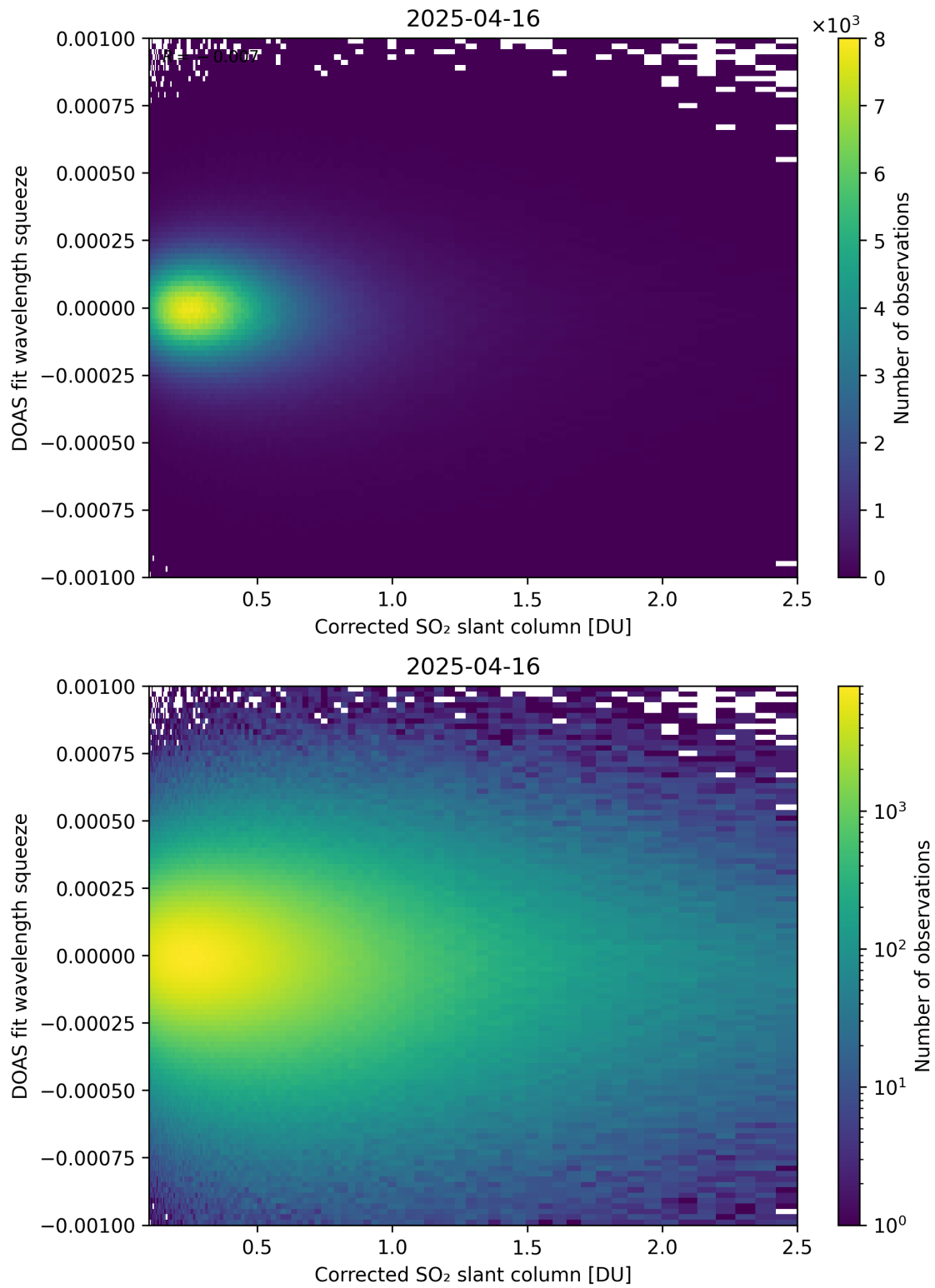
Figure 230: Scatter density plot of “Corrected SO 2 slant column” against “DOAS fit wavelength squeeze” for 2025-04-15 to 2025-04-17.
