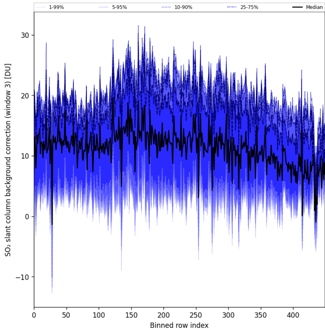
Figure 100: Along track statistics of “SO 2 slant column background correction (window 3)” for 2025-04-15 to 2025-04-17
