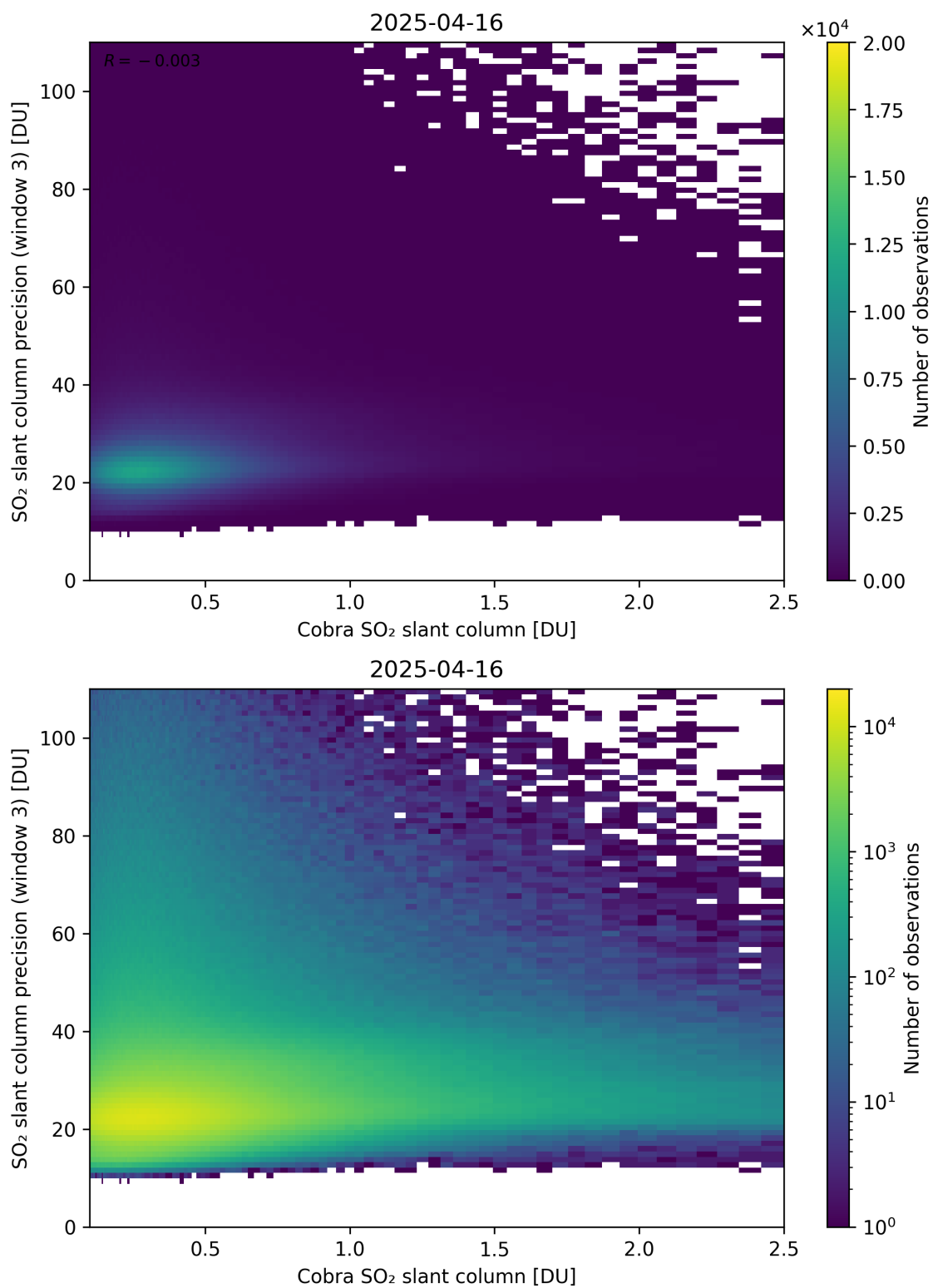
Figure 223: Scatter density plot of “Cobra SO 2 slant column” against “SO 2 slant column precision (window 3)” for 2025-04-15 to 2025-04-17.
