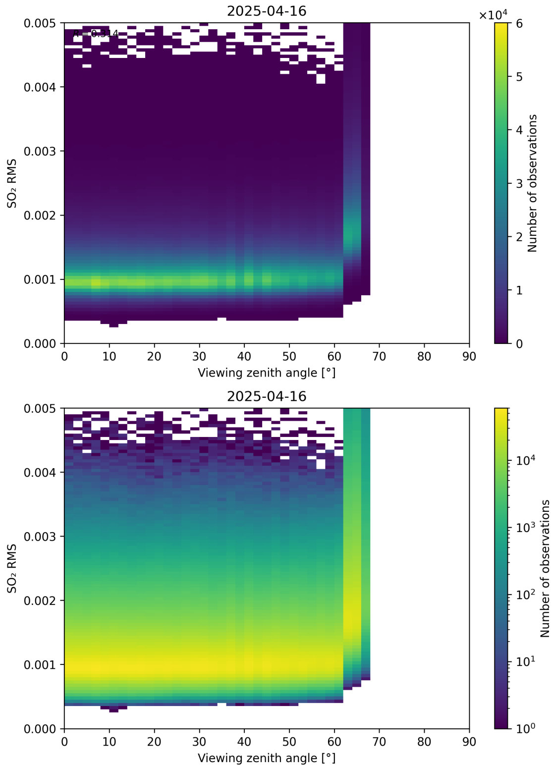
Figure 367: Scatter density plot of “Viewing zenith angle” against “SO 2 RMS” for 2025-04-15 to 2025-04-17.
