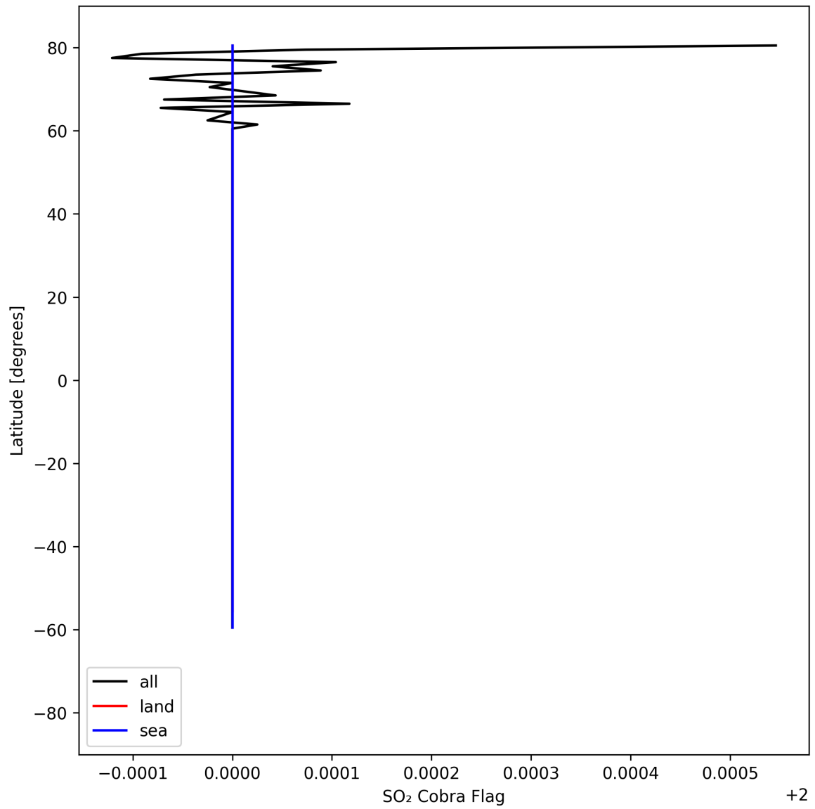
Figure 49: Zonal average of "SO 2 Cobra Flag" for 2025-04-15 to 2025-04-17.
