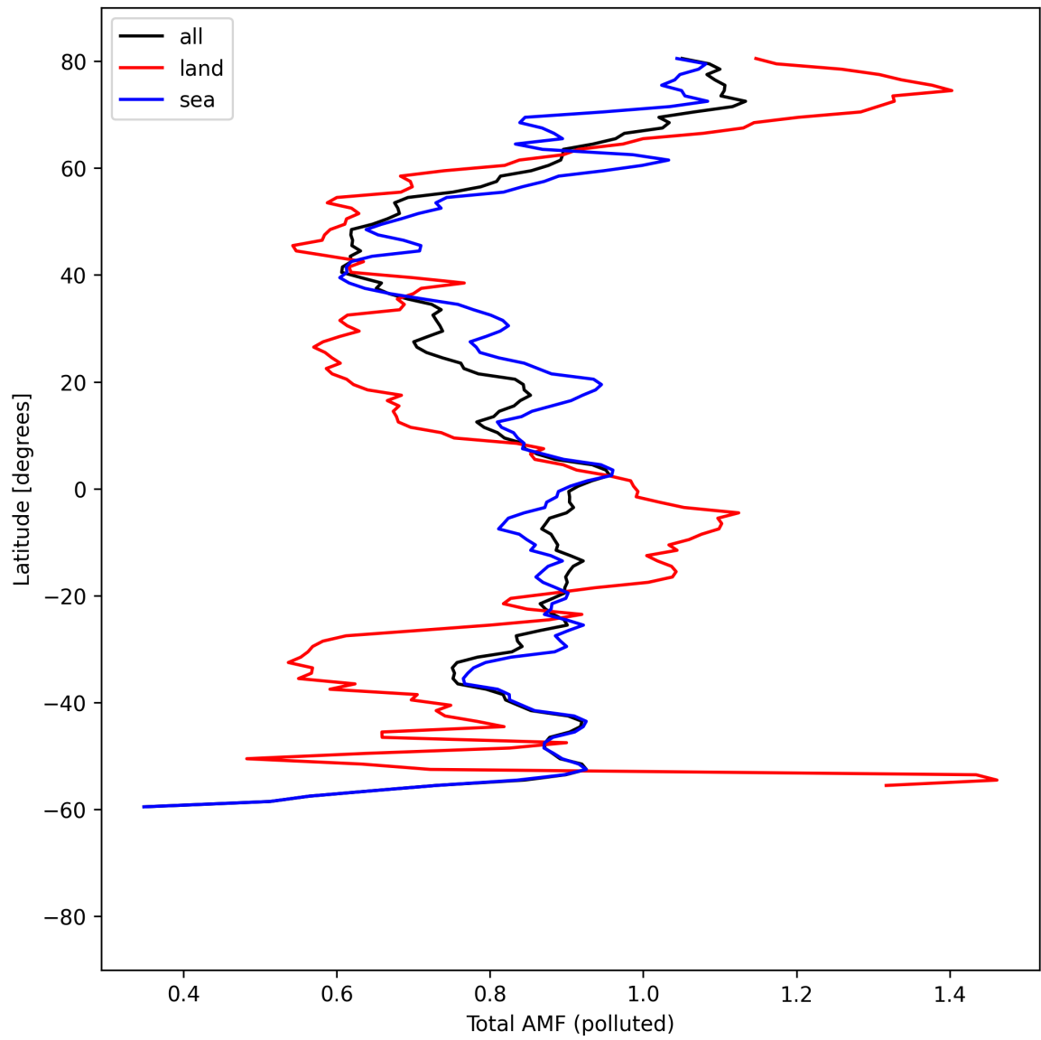
Figure 53: Zonal average of “Total AMF (polluted)” for 2025-04-15 to 2025-04-17.
