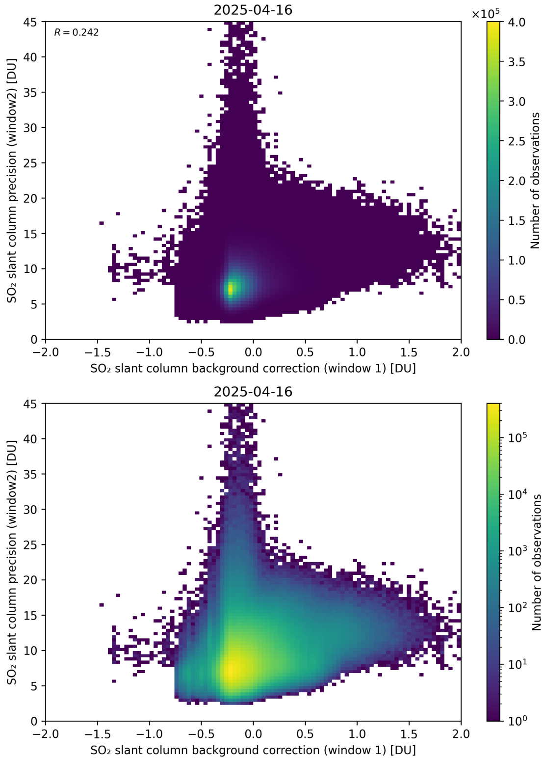
Figure 117: Scatter density plot of “SO 2 slant column background correction (window 1)” against “SO 2 slant column precision (window2)” for 2025-04-15 to 2025-04-17.
