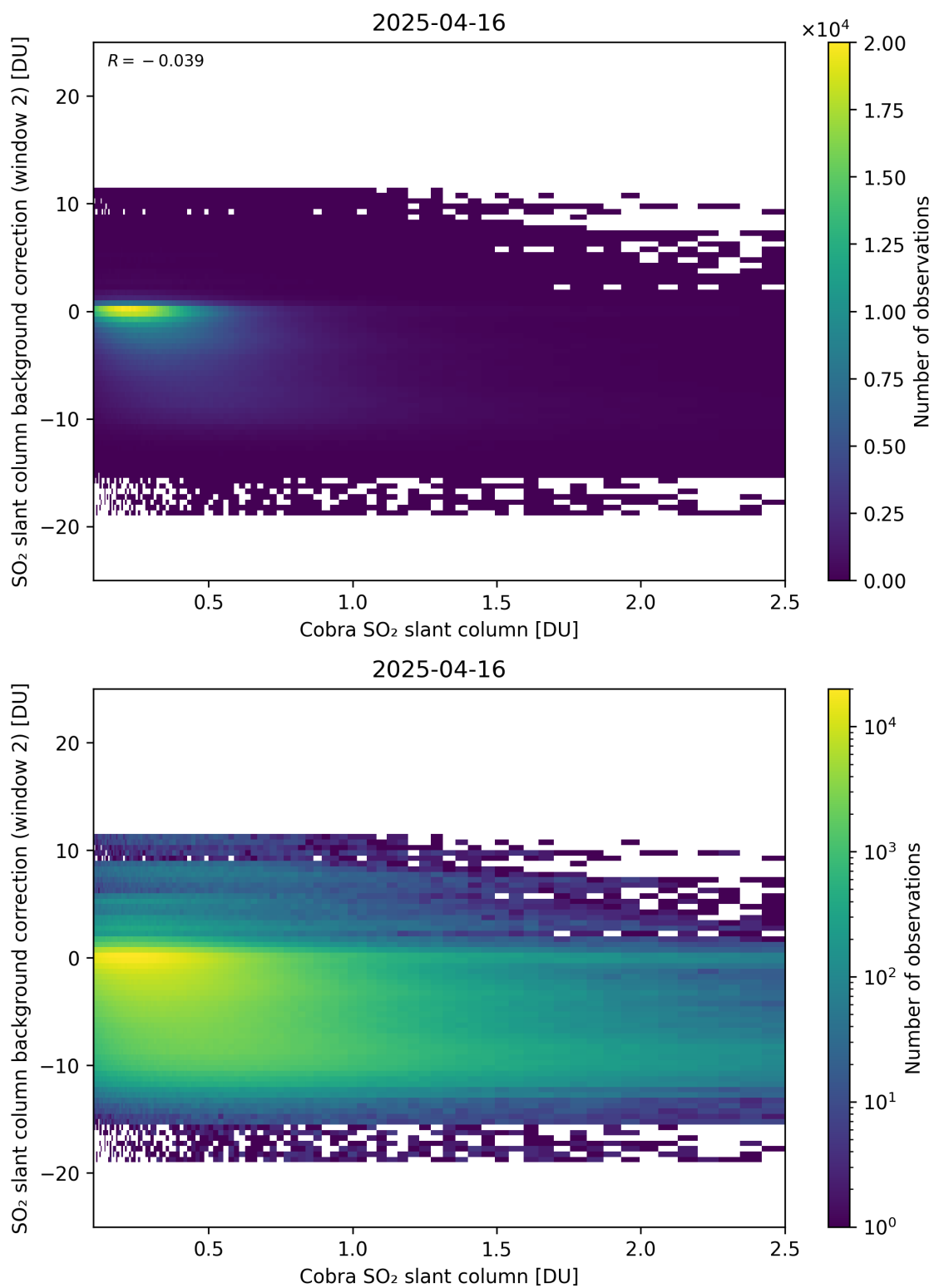
Figure 194: Scatter density plot of “Cobra SO 2 slant column” against “SO 2 slant column background correction (window 2)” for 2025-04-15 to 2025-04-17.
