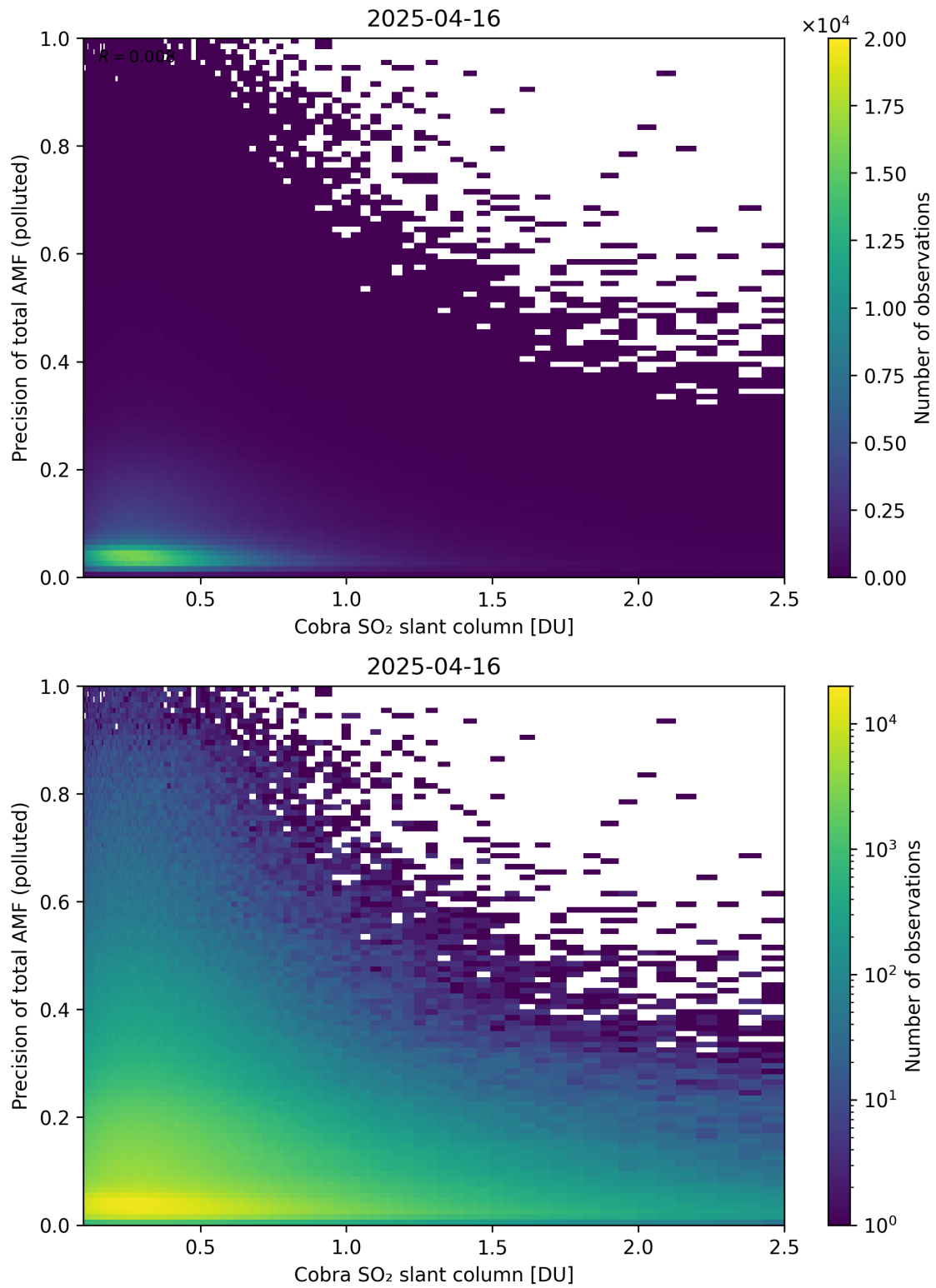
Figure 225: Scatter density plot of “Cobra SO 2 slant column” against “Precision of total AMF (polluted)” for 2025-04-15 to 2025-04-17.
