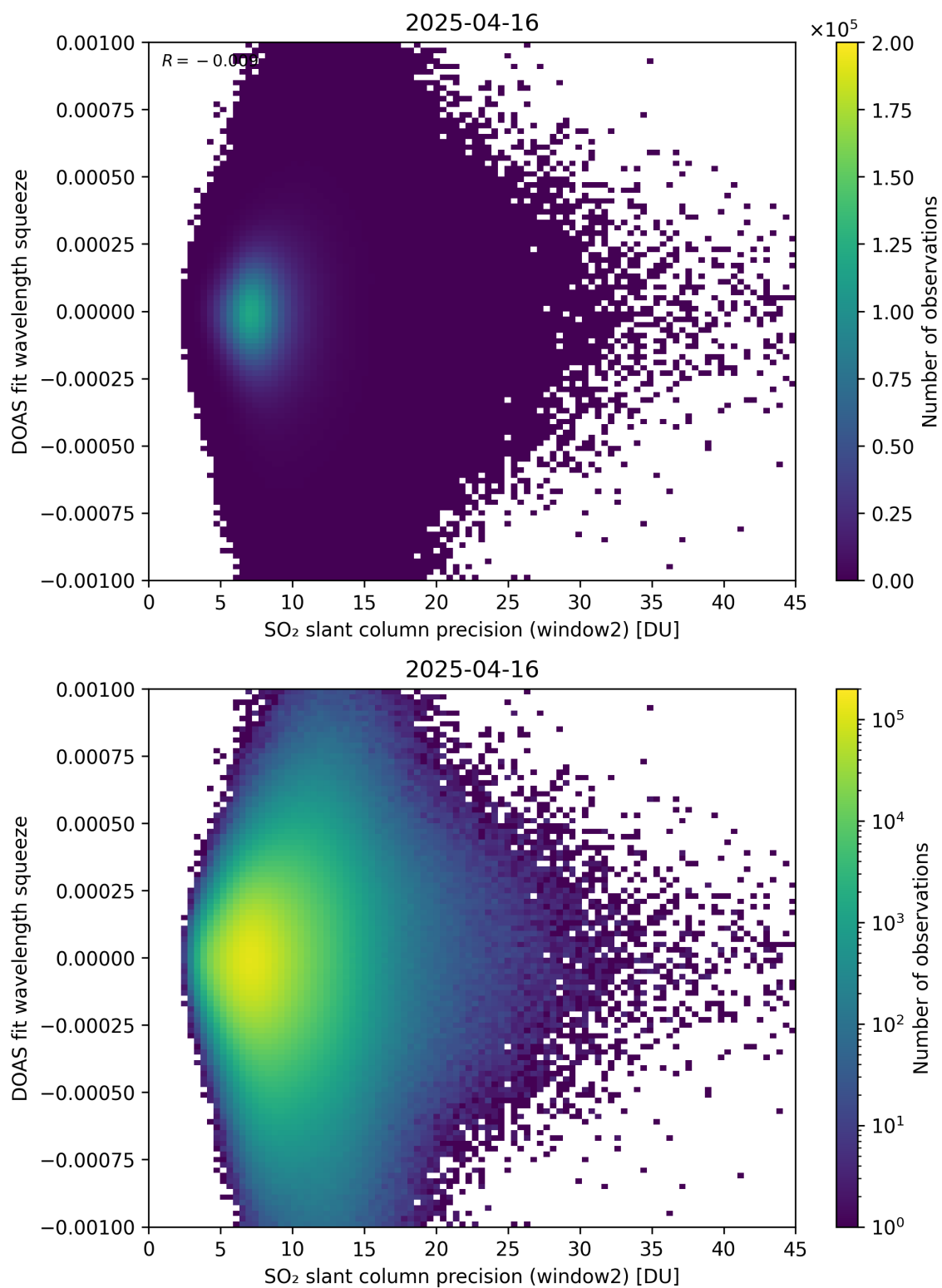
Figure 294: Scatter density plot of “SO 2 slant column precision (window2)” against “DOAS fit wavelength squeeze” for 2025-04-15 to 2025-04-17.
