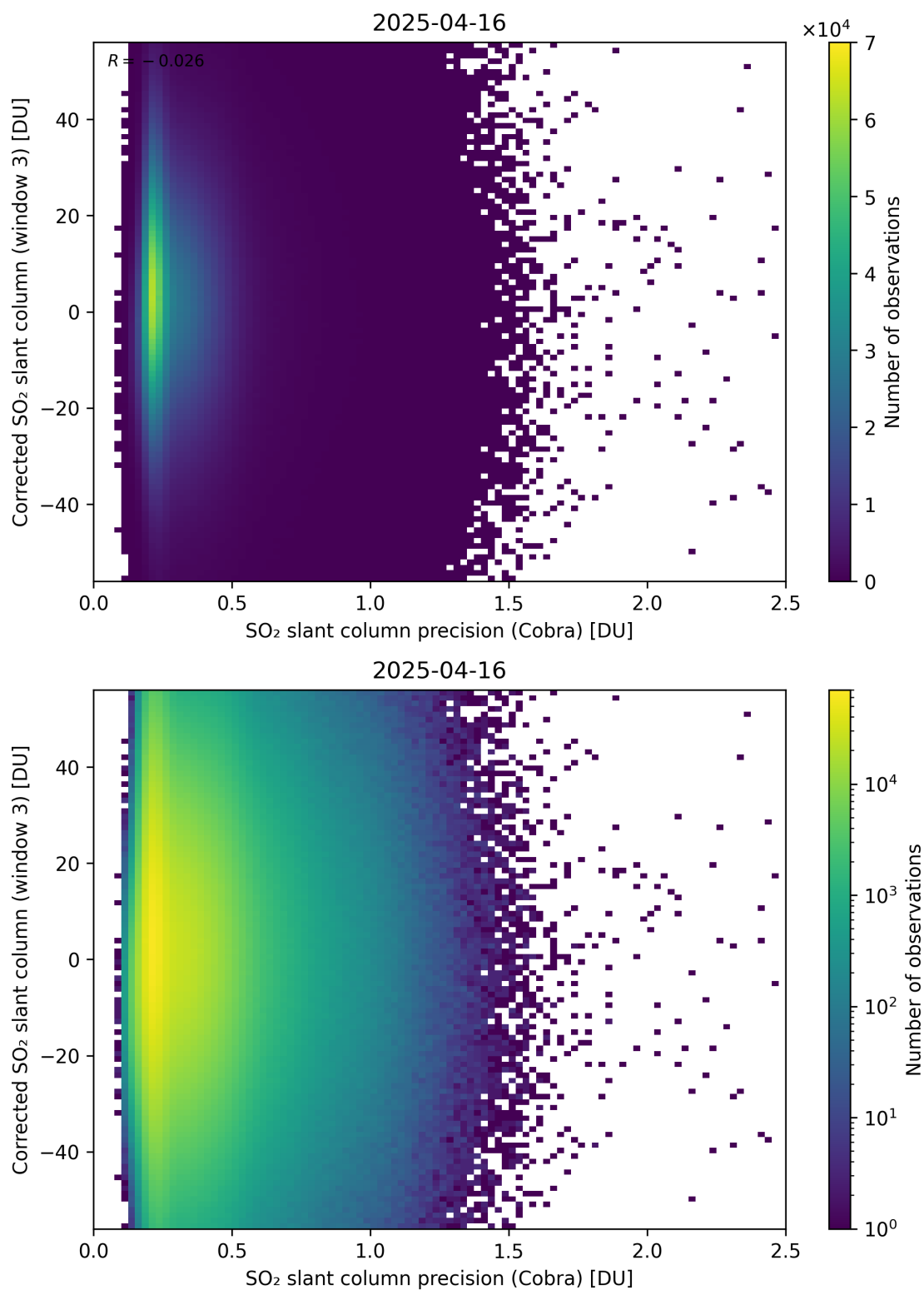
Figure 207: Scatter density plot of “SO 2 slant column precision (Cobra)” against “Corrected SO 2 slant column (window 3)” for 2025-04-15 to 2025-04-17.
