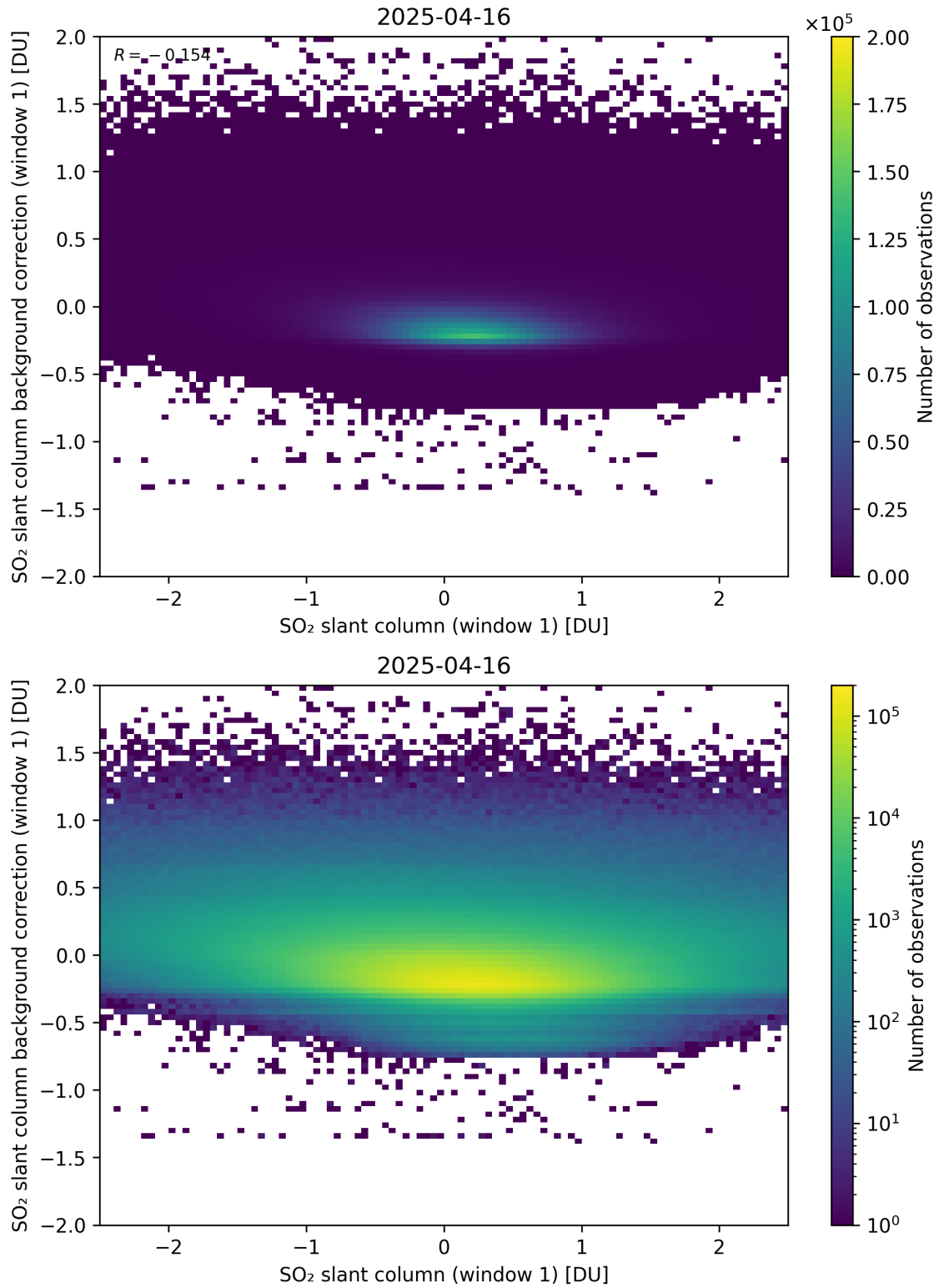
Figure 262: Scatter density plot of “SO 2 slant column (window 1)” against “SO 2 slant column background correction (window 1)” for 2025-04-15 to 2025-04-17.
