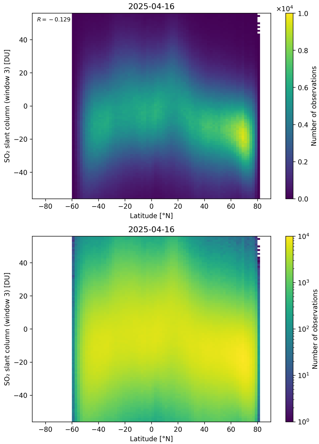
Figure 165: Scatter density plot of “Latitude” against “SO 2 slant column (window 3)” for 2025-04-15 to 2025-04-17.
