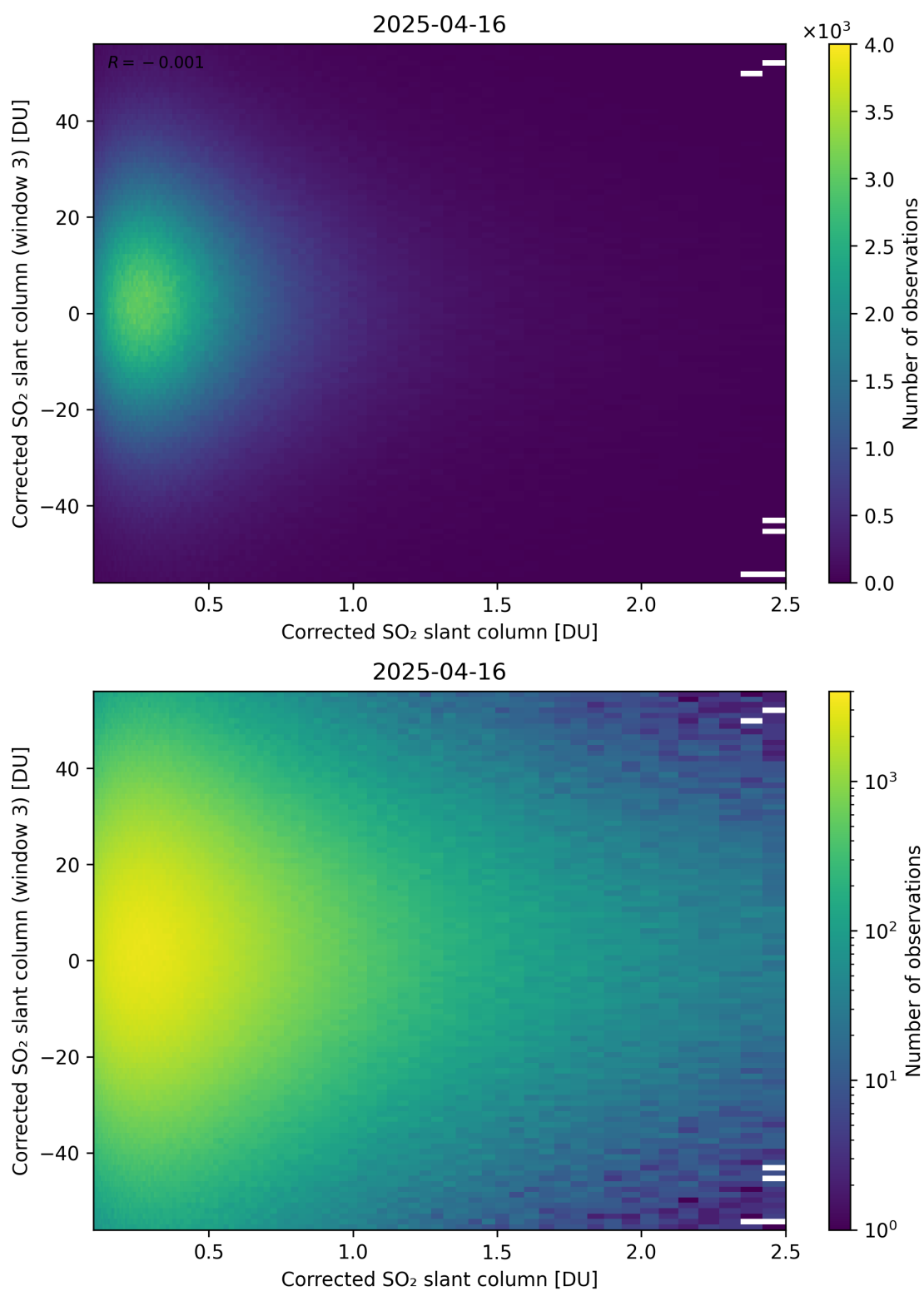
Figure 236: Scatter density plot of “Corrected SO 2 slant column” against “Corrected SO 2 slant column (window 3)” for 2025-04-15 to 2025-04-17.
