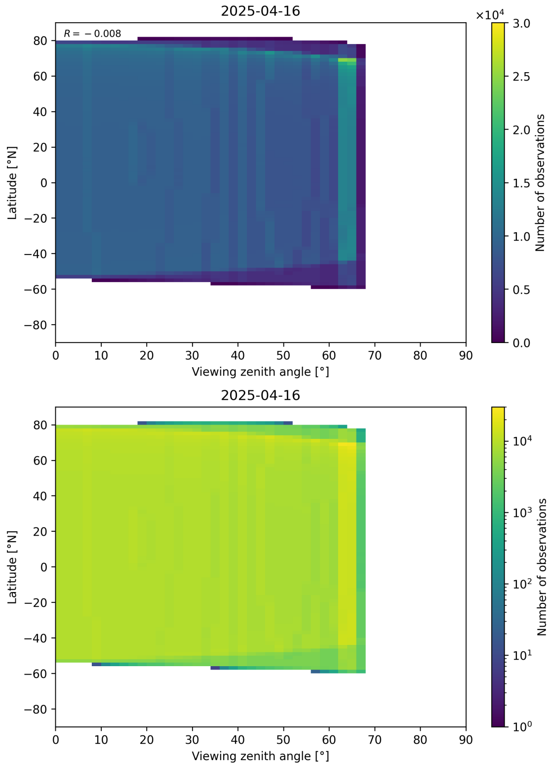
Figure 368: Scatter density plot of “Viewing zenith angle” against “Latitude” for 2025-04-15 to 2025-04-17.
