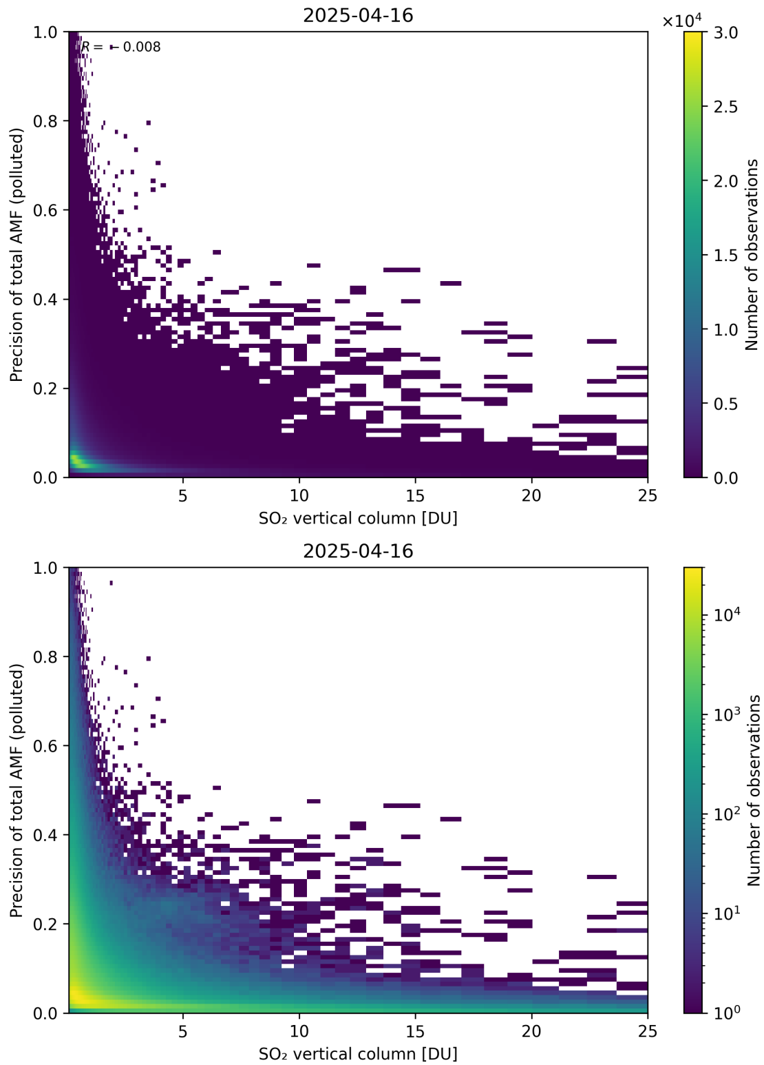
Figure 360: Scatter density plot of “SO 2 vertical column” against “Precision of total AMF (polluted)” for 2025-04-15 to 2025-04-17.
