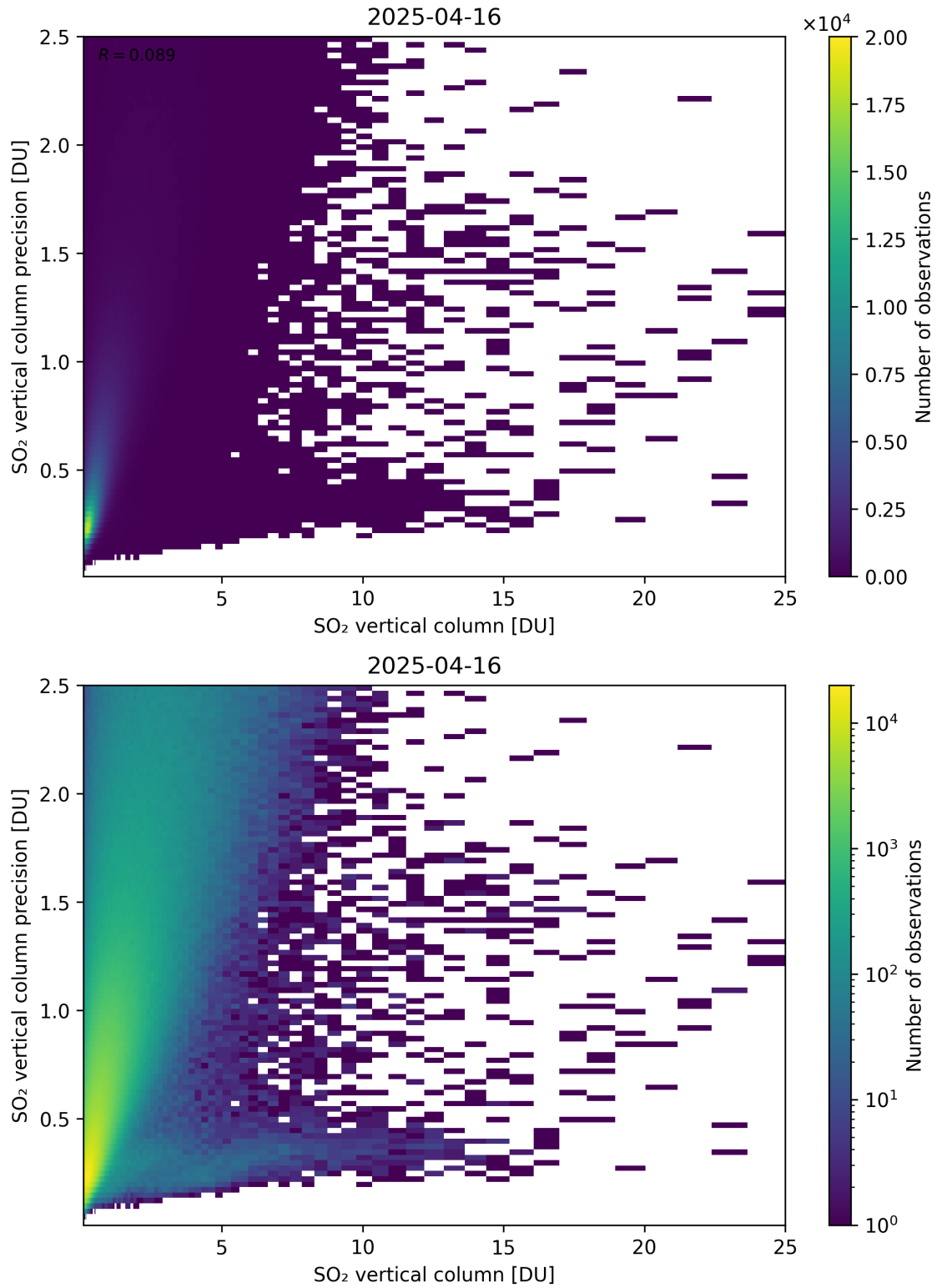
Figure 361: Scatter density plot of “SO 2 vertical column” against “SO 2 vertical column precision” for 2025-04-15 to 2025-04-17.
