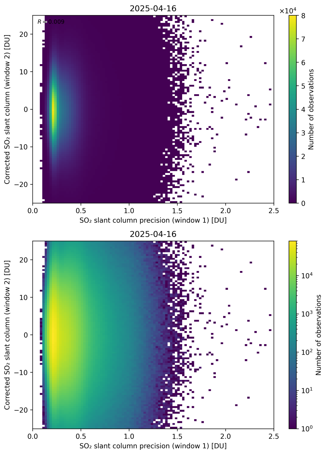
Figure 275: Scatter density plot of “SO 2 slant column precision (window 1)” against “Corrected SO 2 slant column (window 2)” for 2025-04-15 to 2025-04-17.
