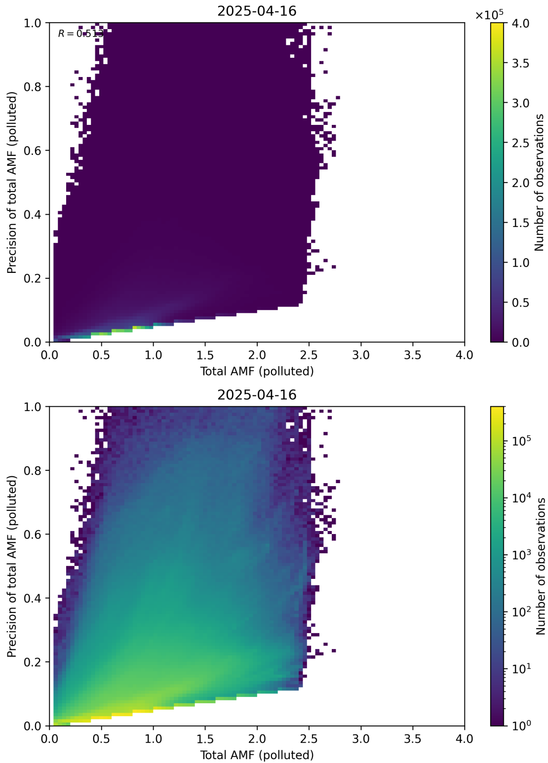
Figure 322: Scatter density plot of “Total AMF (polluted)” against “Precision of total AMF (polluted)” for 2025-04-15 to 2025-04-17.
