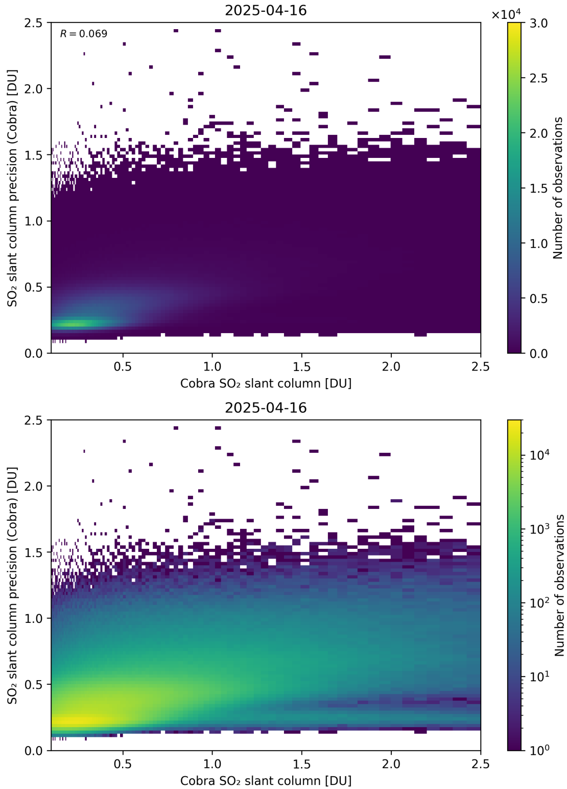
Figure 216: Scatter density plot of “Cobra SO 2 slant column” against “SO 2 slant column precision (Cobra)” for 2025-04-15 to 2025-04-17.
