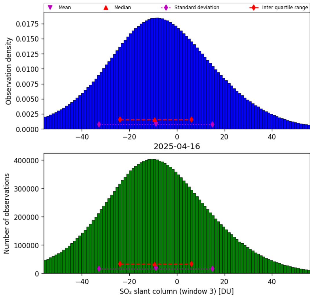
Figure 71: Histogram of “SO 2 slant column (window 3)” for 2025-04-15 to 2025-04-17
