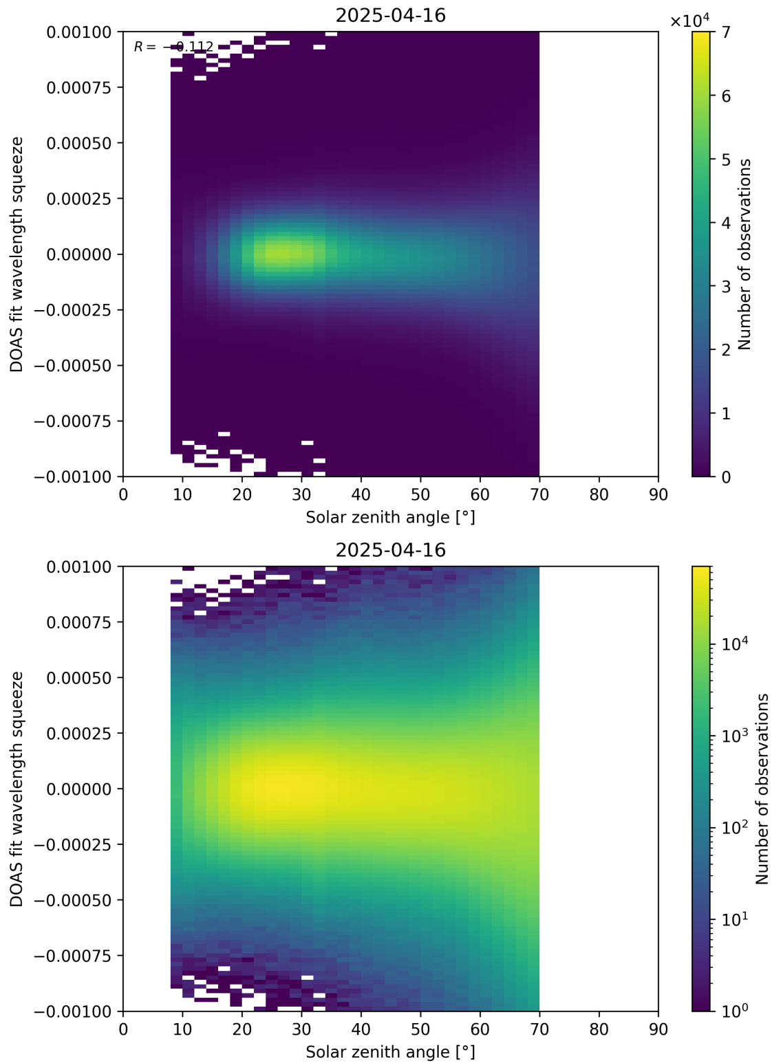
Figure 175: Scatter density plot of “Solar zenith angle” against “DOAS fit wavelength squeeze” for 2025-04-15 to 2025-04-17.
