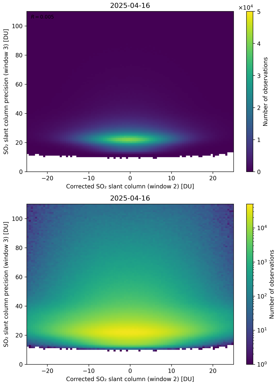
Figure 252: Scatter density plot of “Corrected SO 2 slant column (window 2)” against “SO 2 slant column precision (window 3)” for 2025-04-15 to 2025-04-17.
