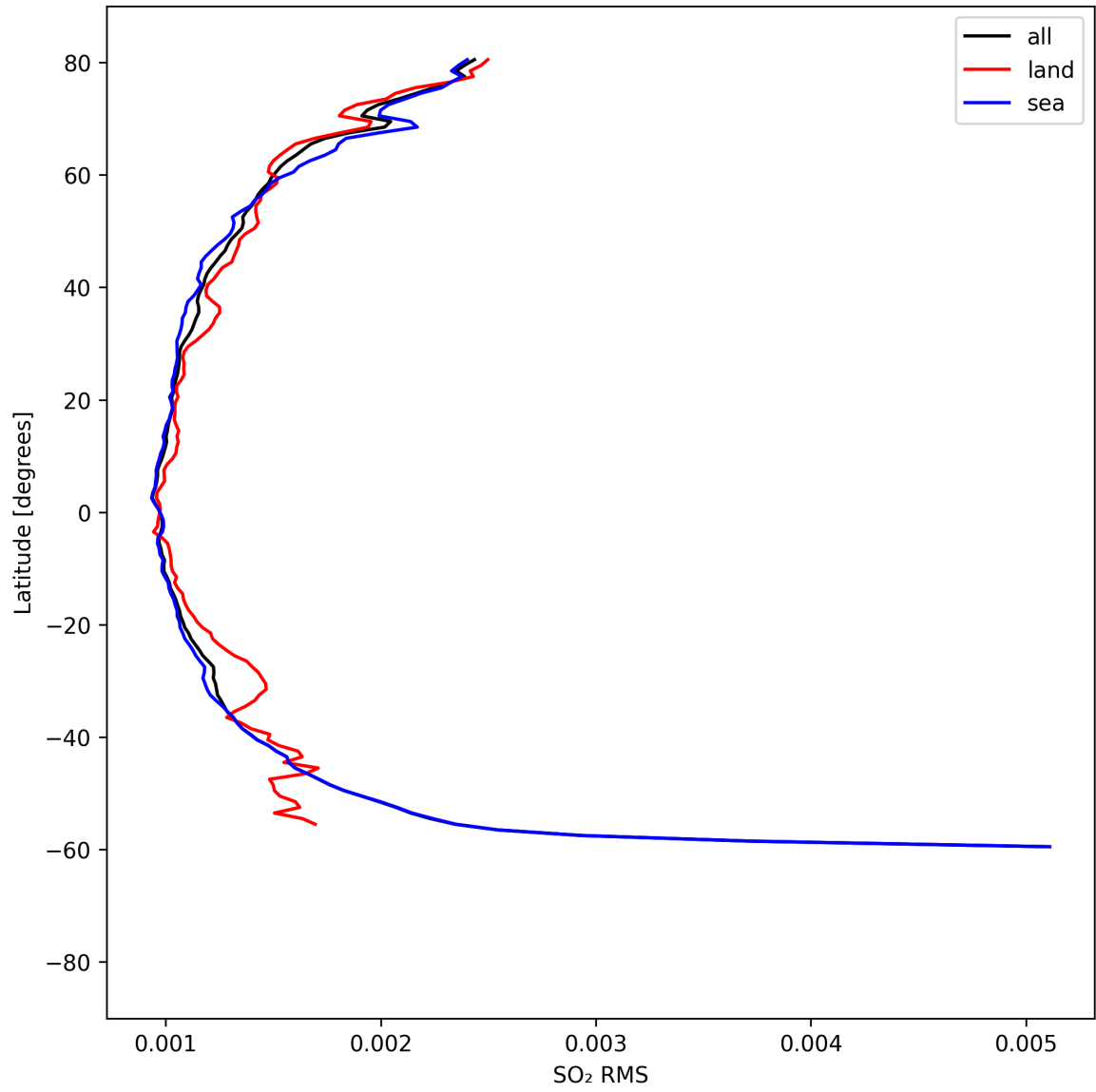
Figure 52: Zonal average of “SO 2 RMS” for 2025-04-15 to 2025-04-17.
