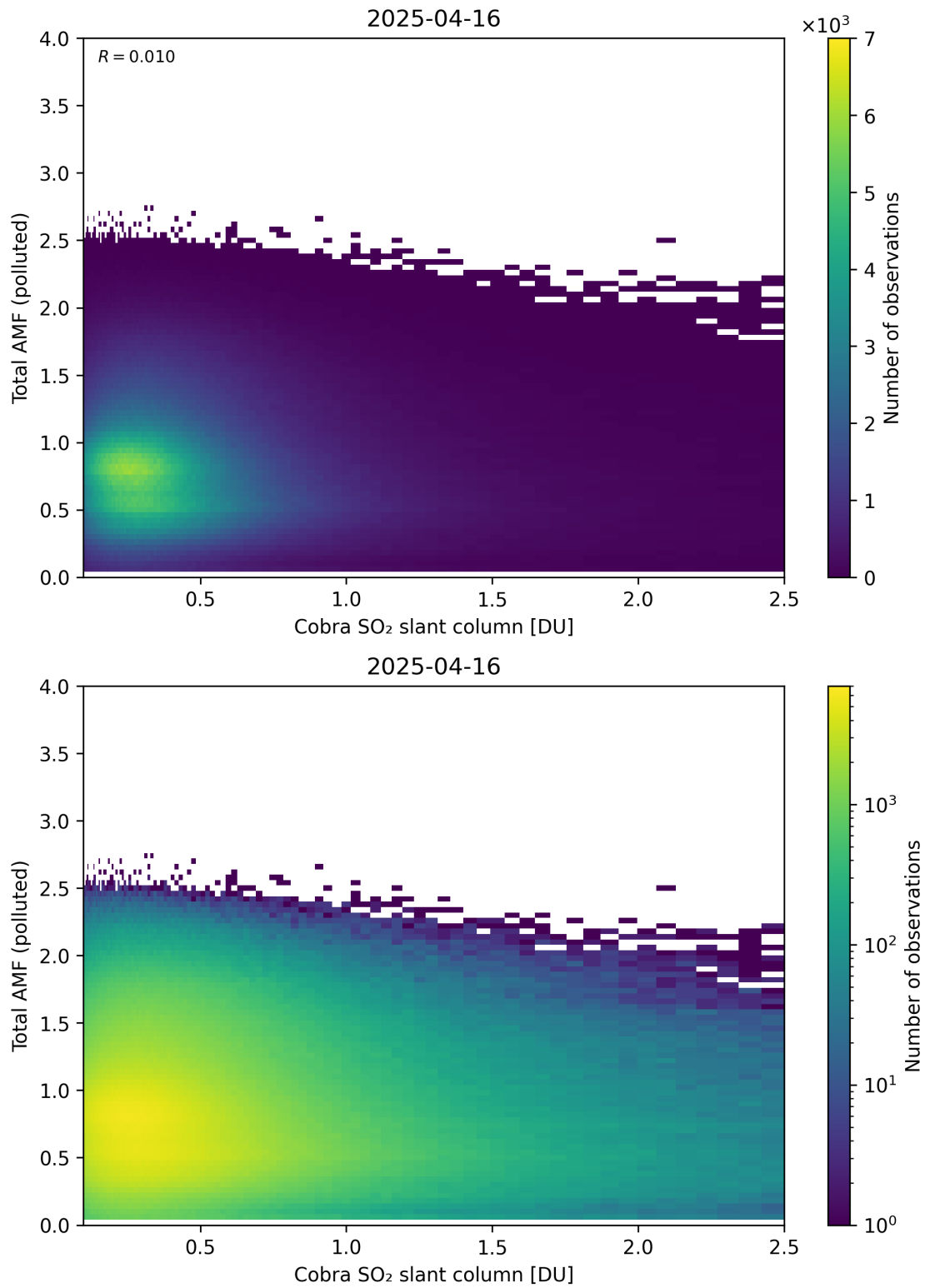
Figure 224: Scatter density plot of “Cobra SO 2 slant column” against “Total AMF (polluted)” for 2025-04-15 to 2025-04-17.
