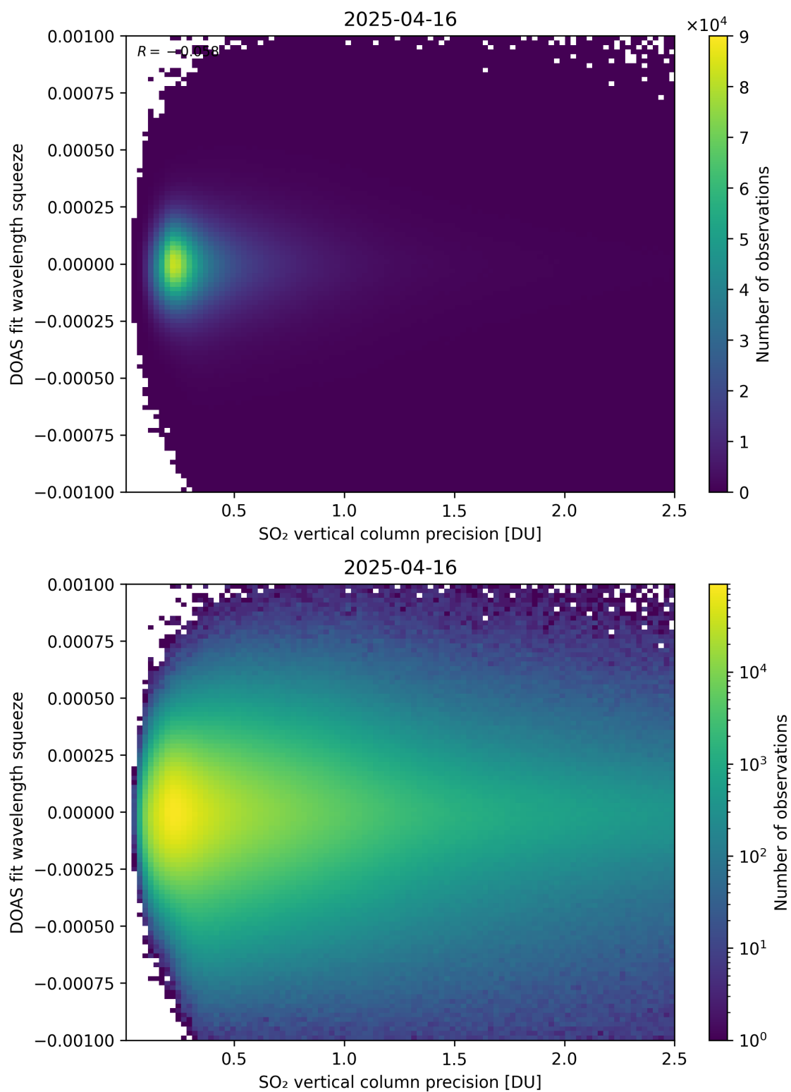
Figure 333: Scatter density plot of “SO 2 vertical column precision” against “DOAS fit wavelength squeeze” for 2025-04-15 to 2025-04-17.
