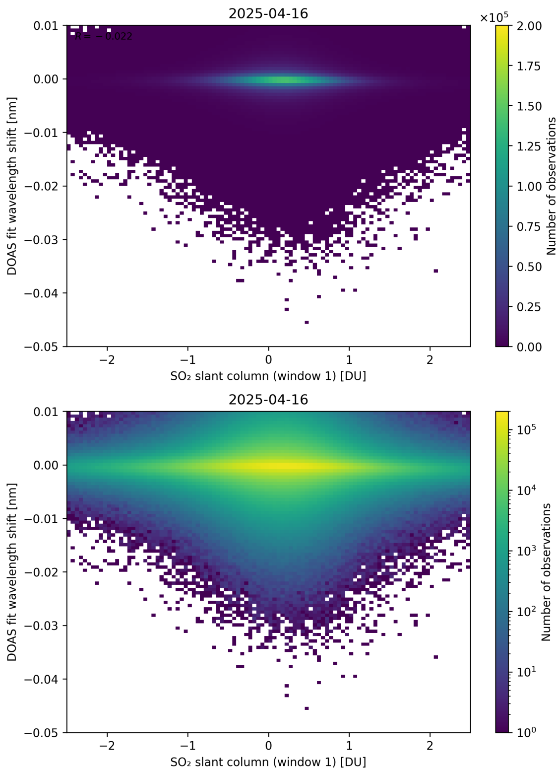
Figure 265: Scatter density plot of “SO 2 slant column (window 1)” against “DOAS fit wavelength shift” for 2025-04-15 to 2025-04-17.
