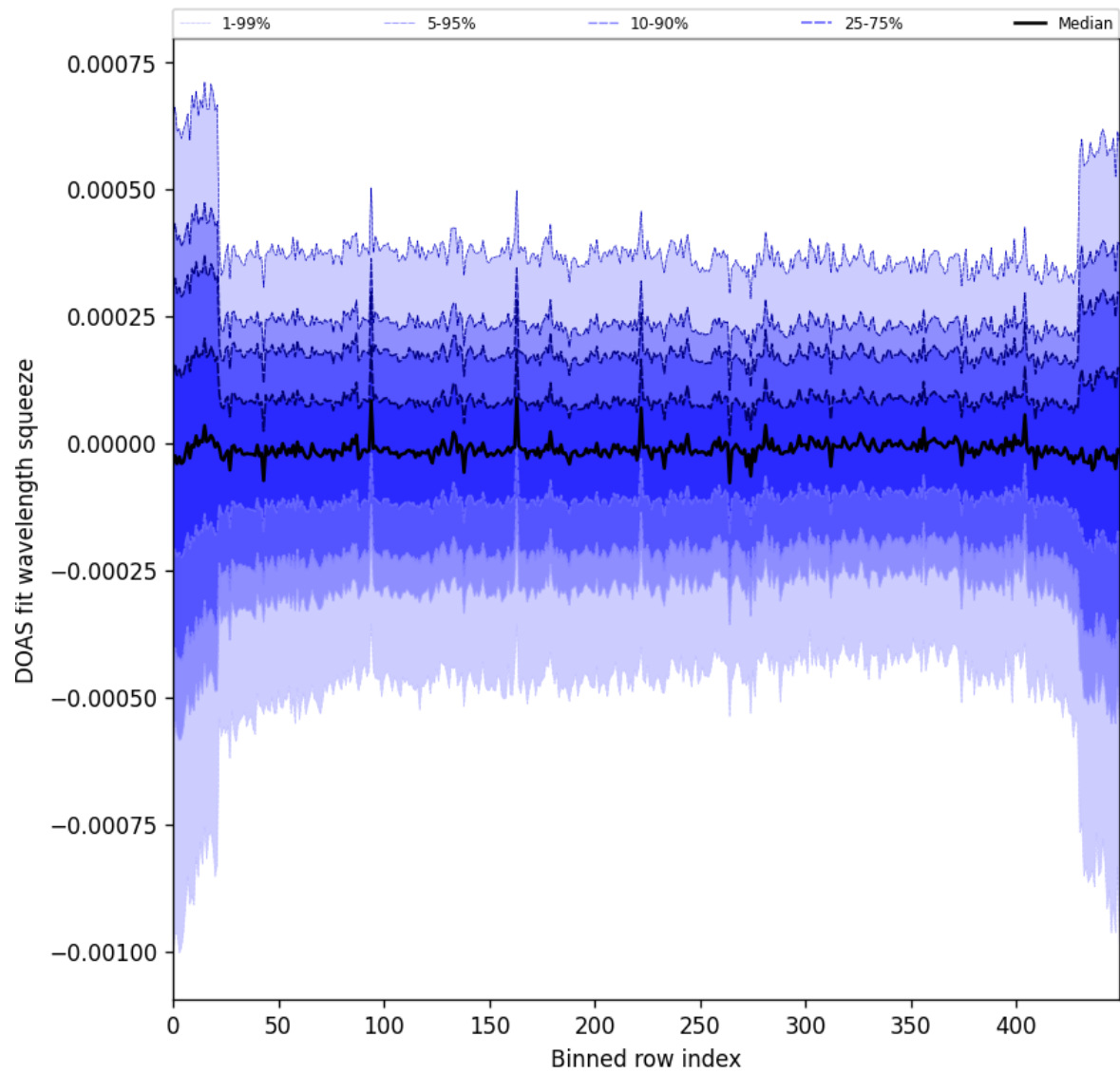
Figure 103: Along track statistics of “DOAS fit wavelength squeeze” for 2025-04-15 to 2025-04-17
