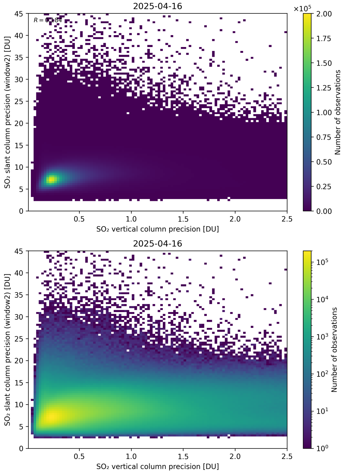
Figure 343: Scatter density plot of “SO 2 vertical column precision” against “SO 2 slant column precision (window2)” for 2025-04-15 to 2025-04-17.
