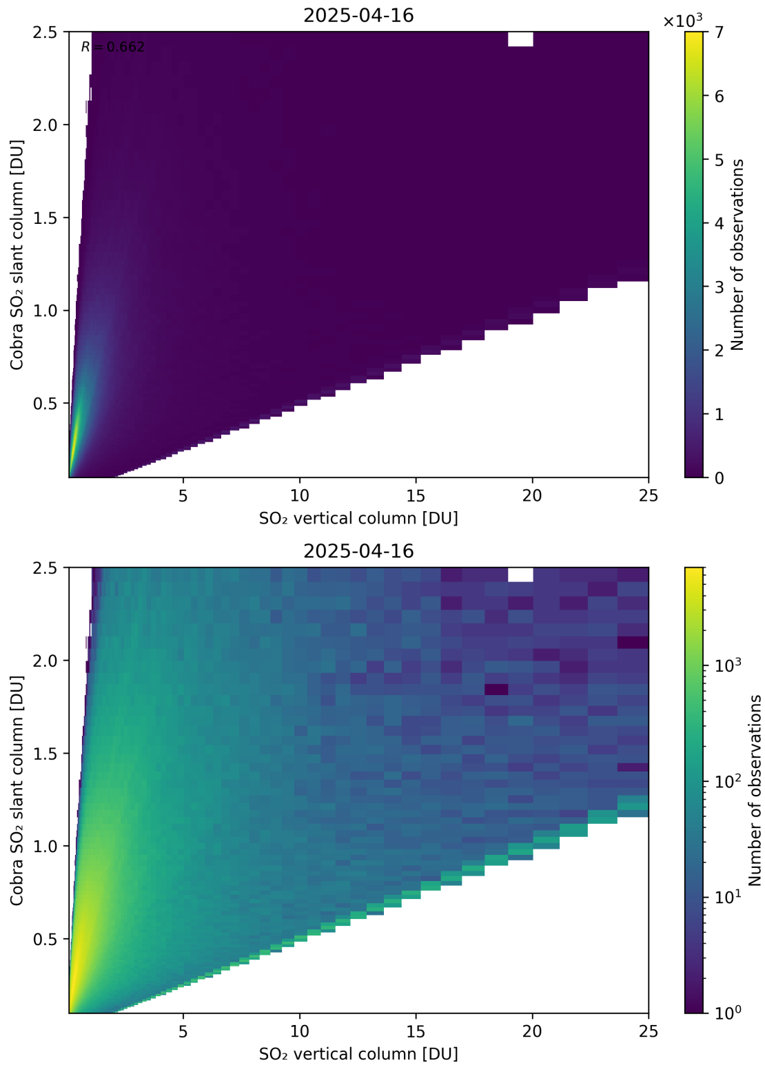
Figure 349: Scatter density plot of “SO 2 vertical column” against “Cobra SO 2 slant column” for 2025-04-15 to 2025-04-17.
