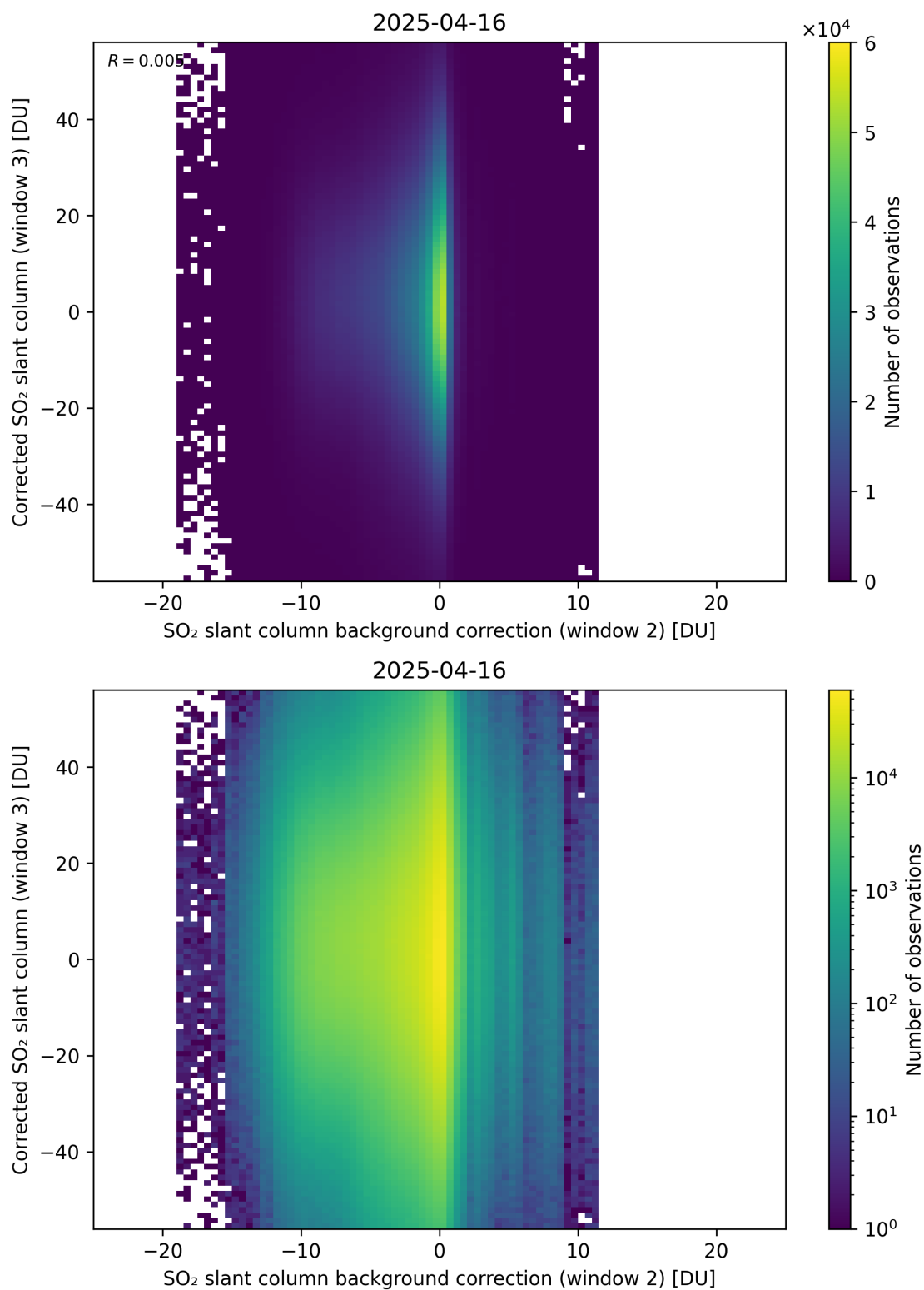
Figure 127: Scatter density plot of “SO 2 slant column background correction (window 2)” against “Corrected SO 2 slant column (window 3)” for 2025-04-15 to 2025-04-17.
