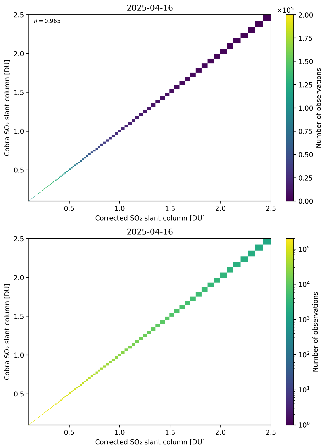
Figure 233: Scatter density plot of “Corrected SO 2 slant column” against “Cobra SO 2 slant column” for 2025-04-15 to 2025-04-17.
