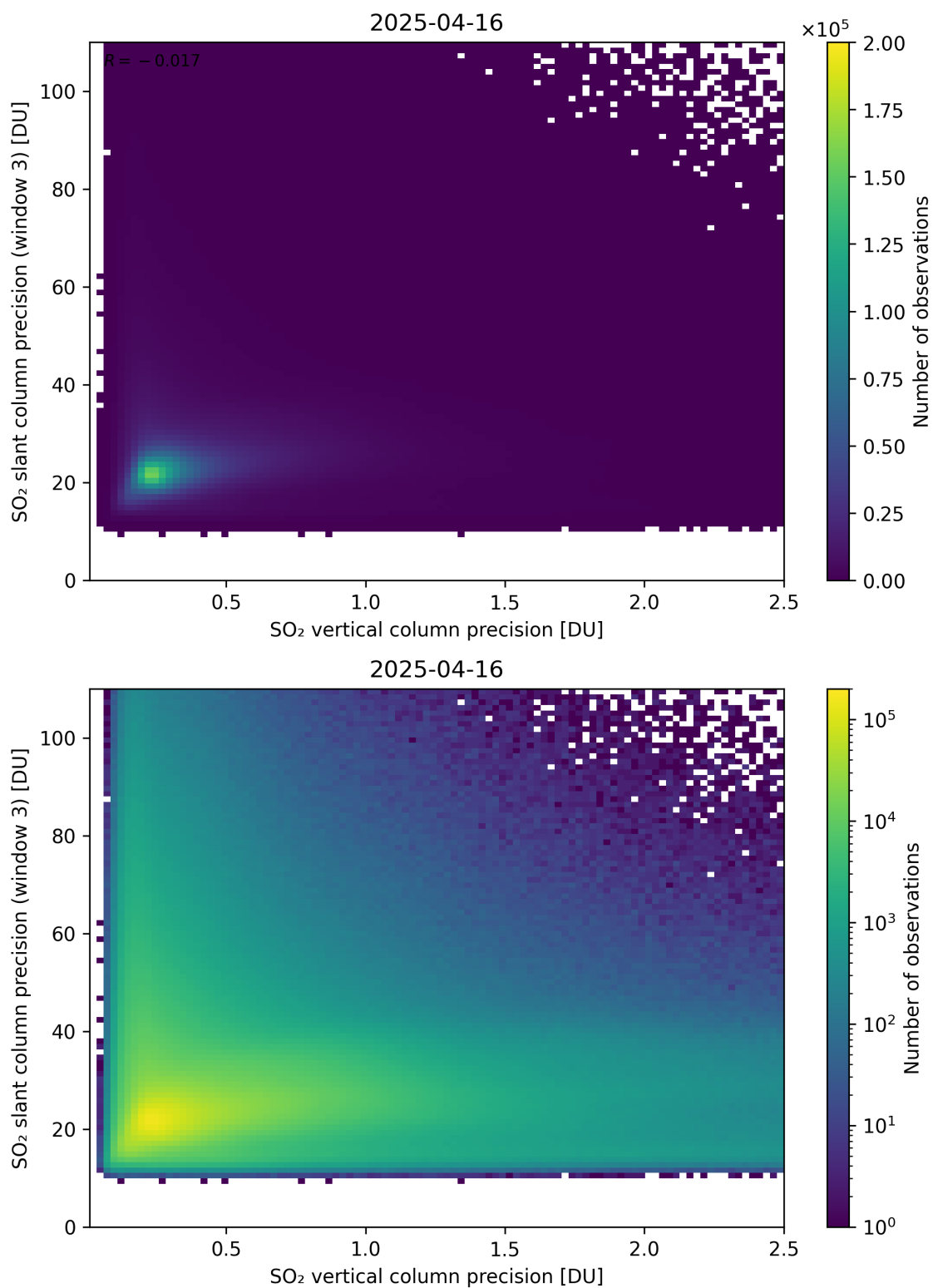
Figure 345: Scatter density plot of “SO 2 vertical column precision” against “SO 2 slant column precision (window 3)” for 2025-04-15 to 2025-04-17.
