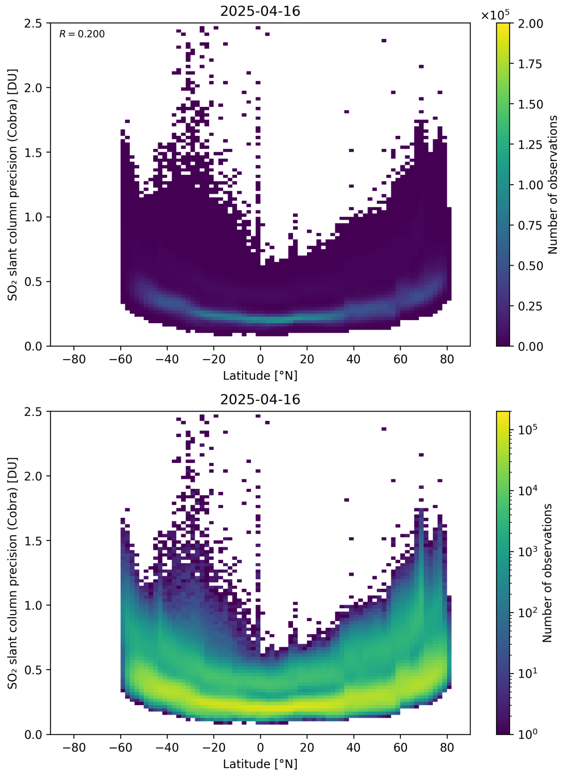
Figure 158: Scatter density plot of “Latitude” against “SO 2 slant column precision (Cobra)” for 2025-04-15 to 2025-04-17.
