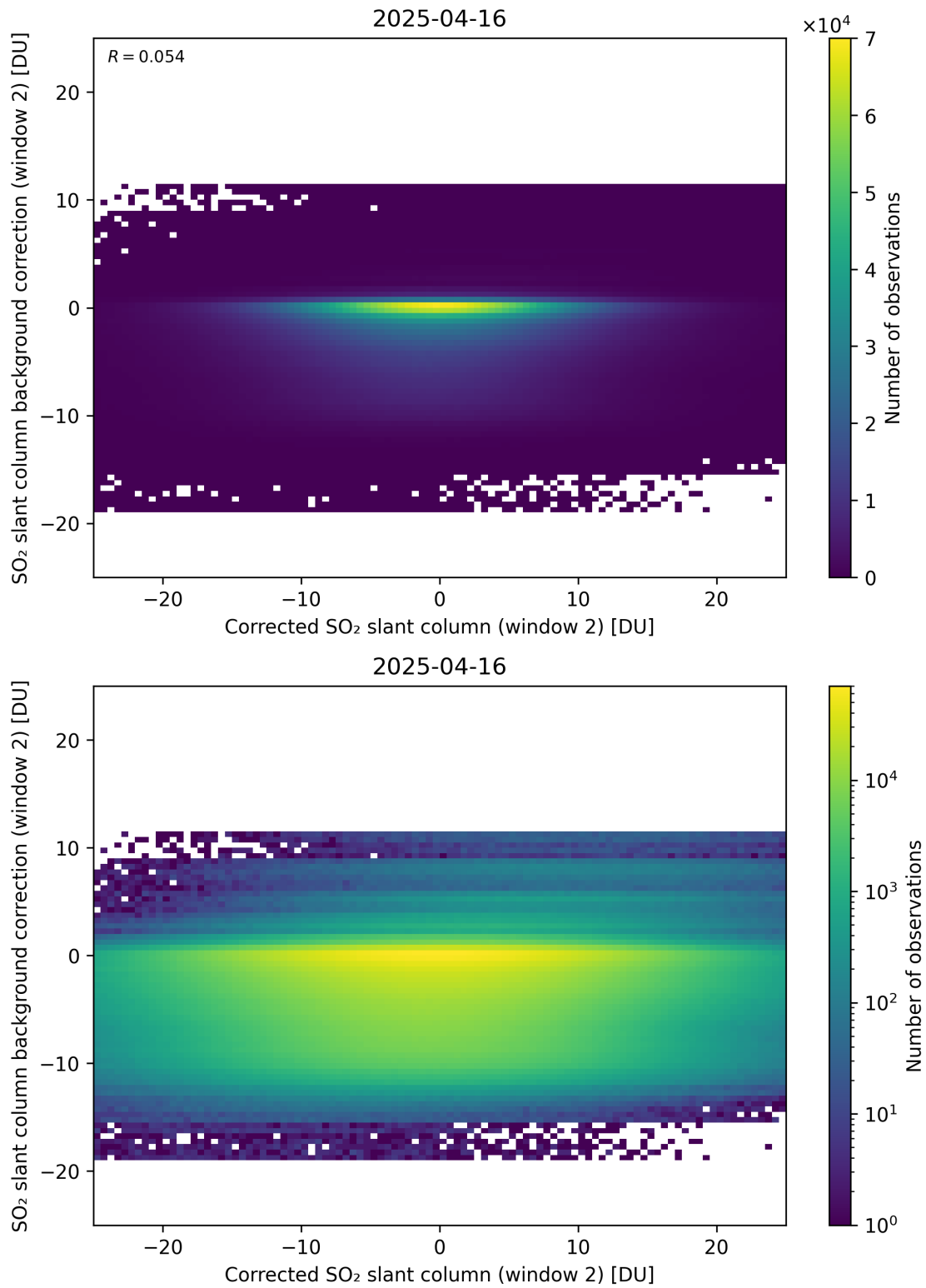
Figure 244: Scatter density plot of “Corrected SO 2 slant column (window 2)” against “SO 2 slant column background correction (window 2)” for 2025-04-15 to 2025-04-17.
