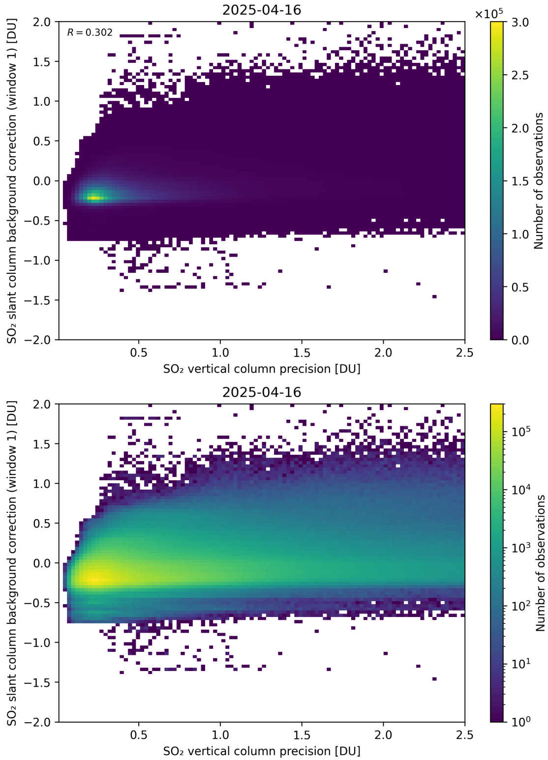
Figure 329: Scatter density plot of “SO 2 vertical column precision” against “SO 2 slant column background correction (window 1)” for 2025-04-15 to 2025-04-17.
