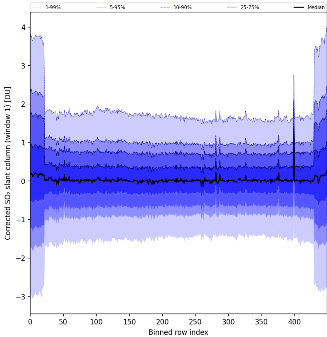
Figure 91: Along track statistics of “Corrected SO 2 slant column (window 1)” for 2025-04-15 to 2025-04-17
