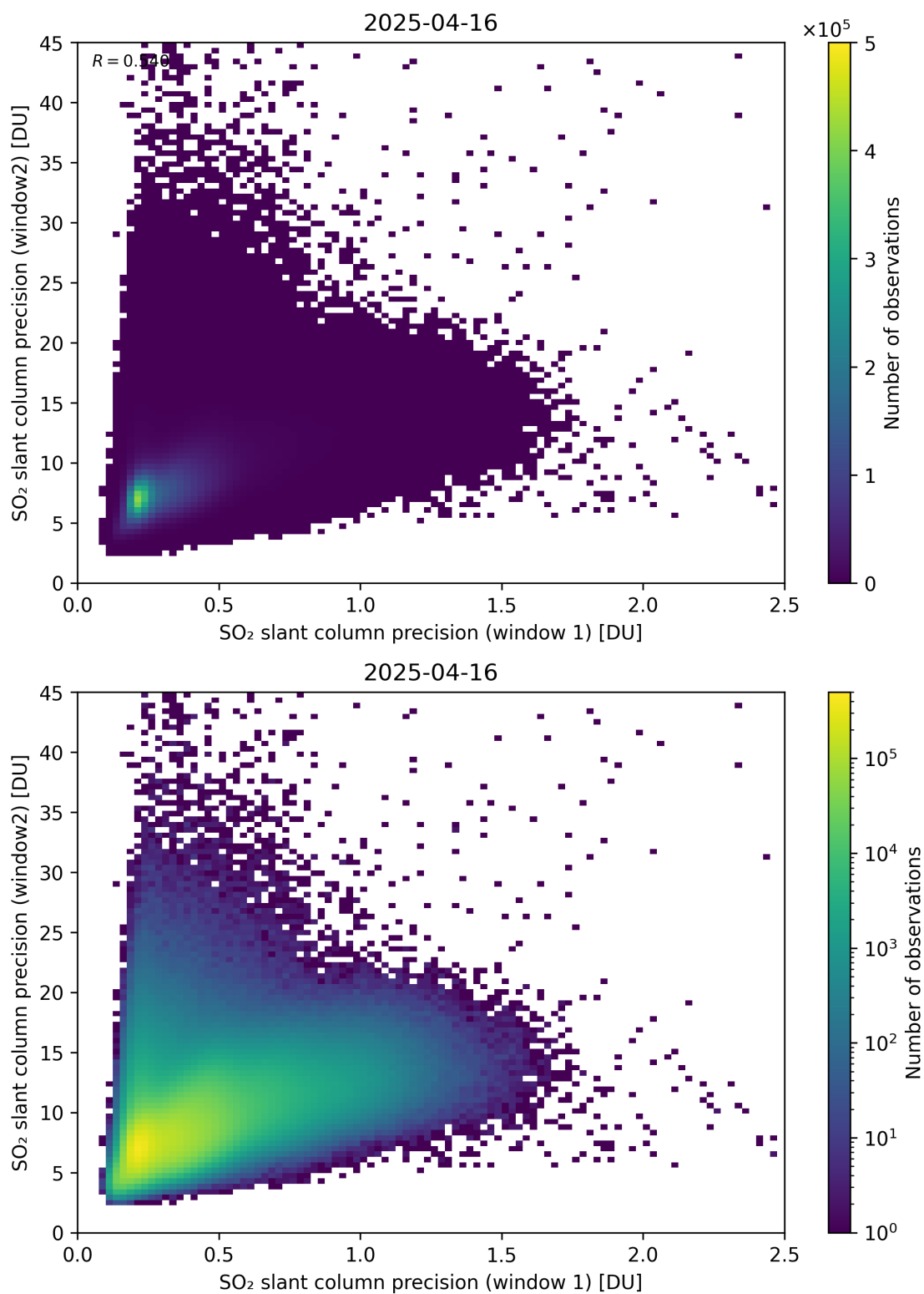
Figure 277: Scatter density plot of “SO 2 slant column precision (window 1)” against “SO 2 slant column precision (window 2)” for 2025-04-15 to 2025-04-17.
