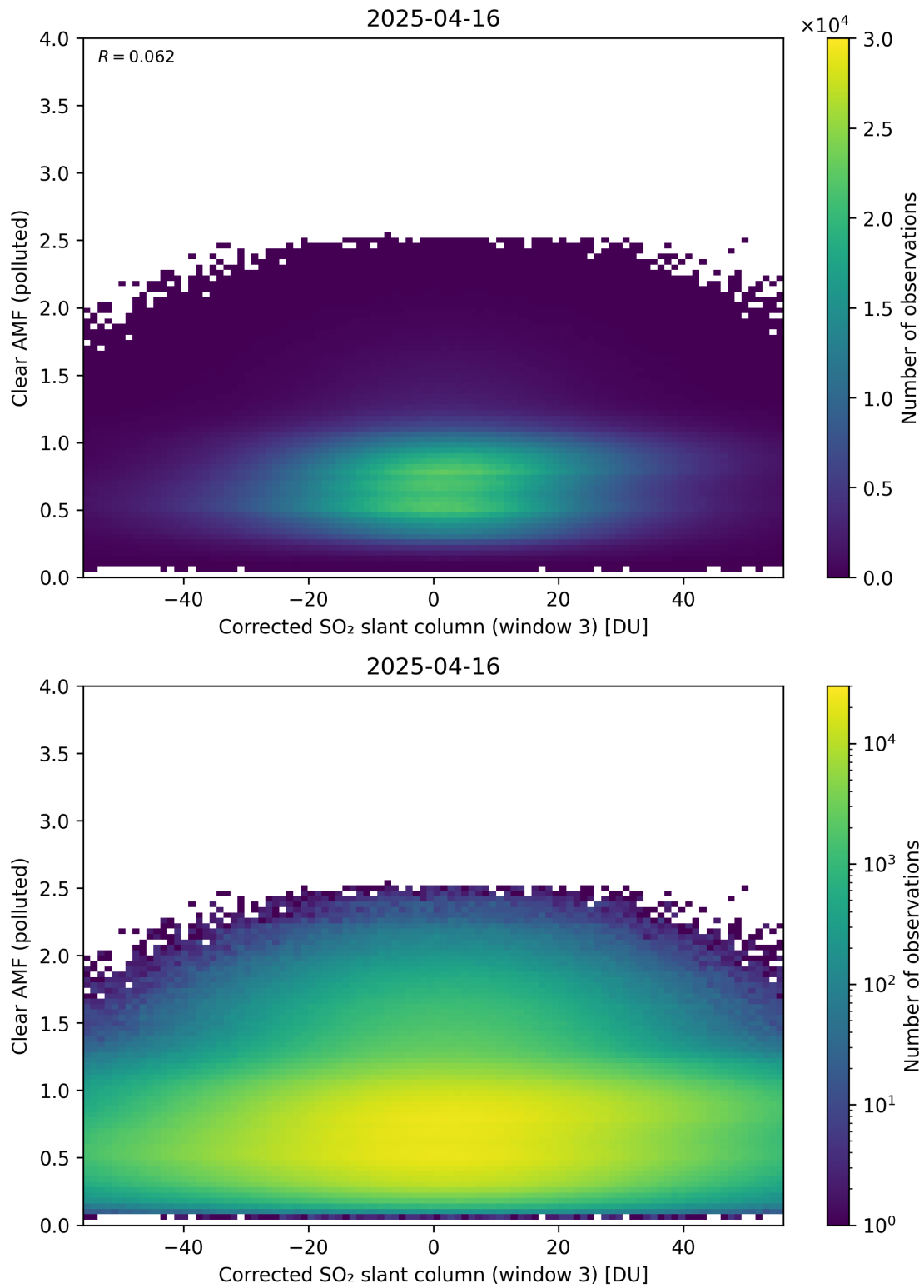
Figure 259: Scatter density plot of “Corrected SO 2 slant column (window 3)” against “Clear AMF (polluted)” for 2025-04-15 to 2025-04-17.
