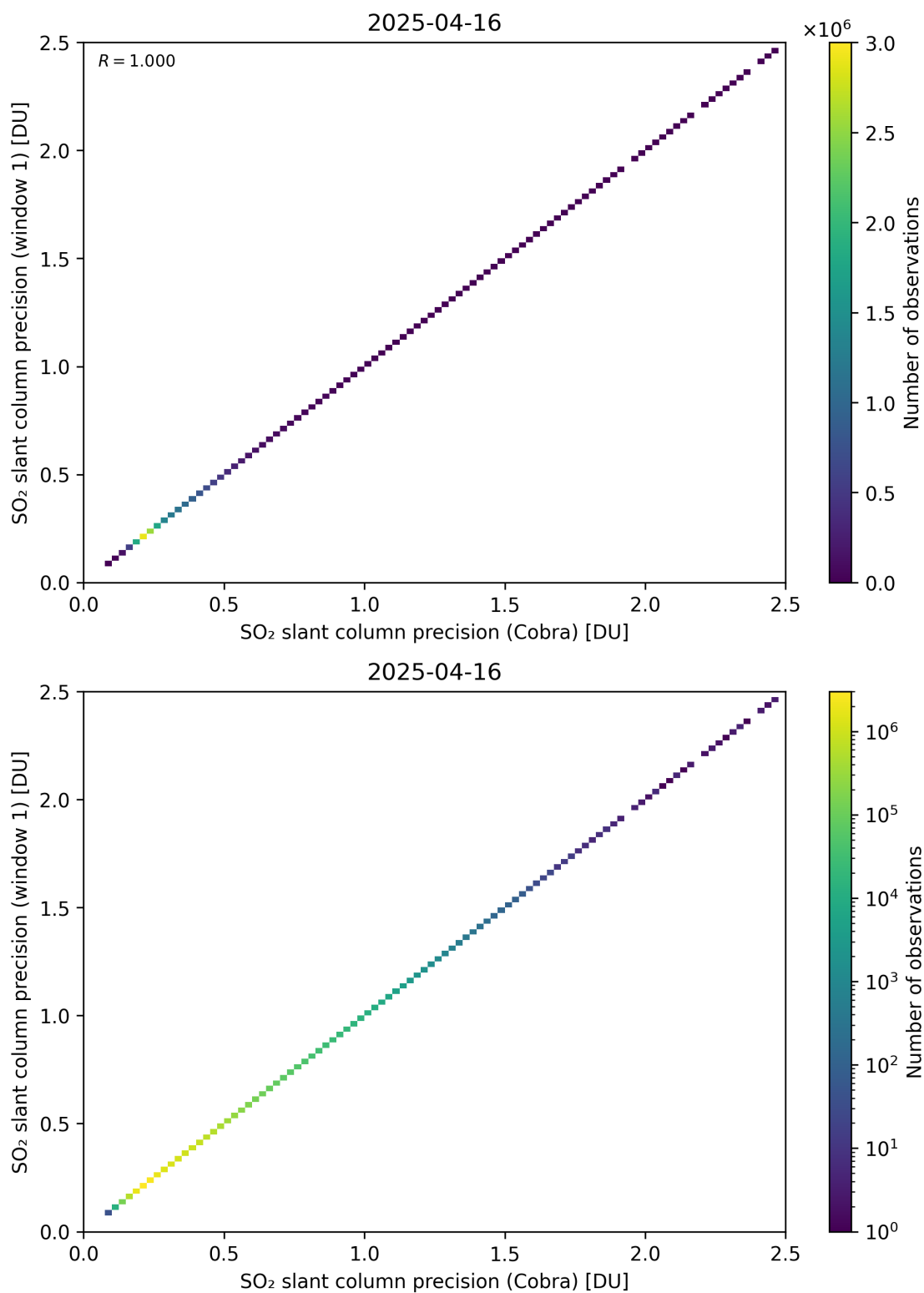
Figure 209: Scatter density plot of “SO 2 slant column precision (Cobra)” against “SO 2 slant column precision (window 1)” for 2025-04-15 to 2025-04-17.
