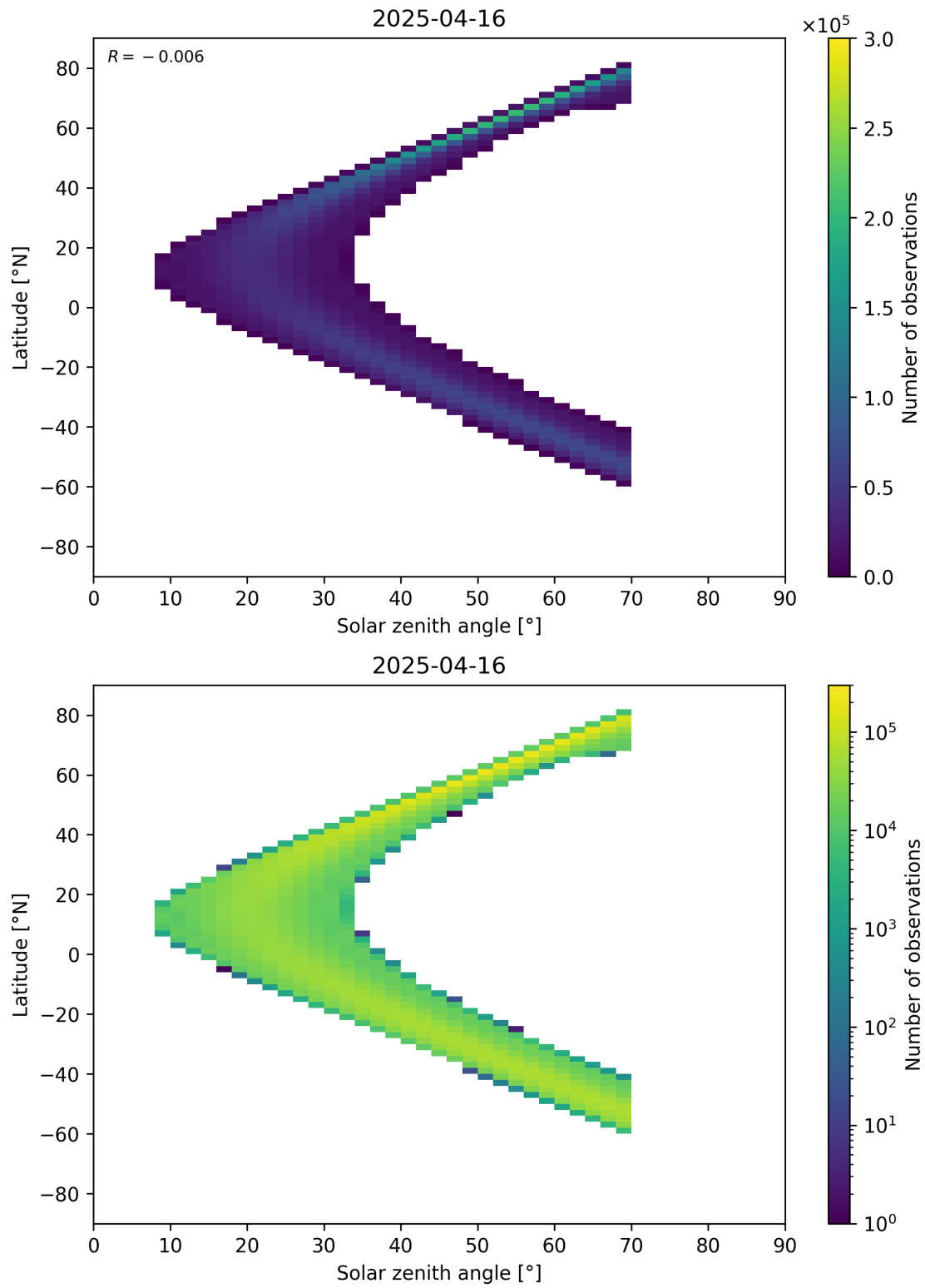
Figure 177: Scatter density plot of “Solar zenith angle” against “Latitude” for 2025-04-15 to 2025-04-17.
