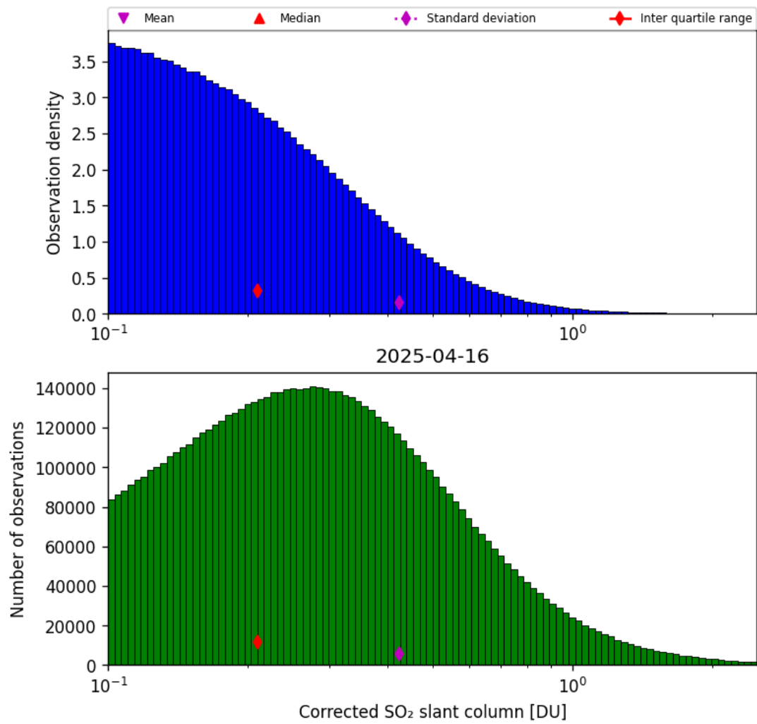
Figure 60: Histogram of “Corrected SO 2 slant column” for 2025-04-15 to 2025-04-17
