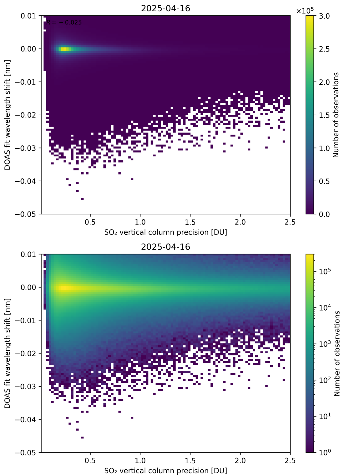
Figure 332: Scatter density plot of “SO 2 vertical column precision” against “DOAS fit wavelength shift” for 2025-04-15 to 2025-04-17.
