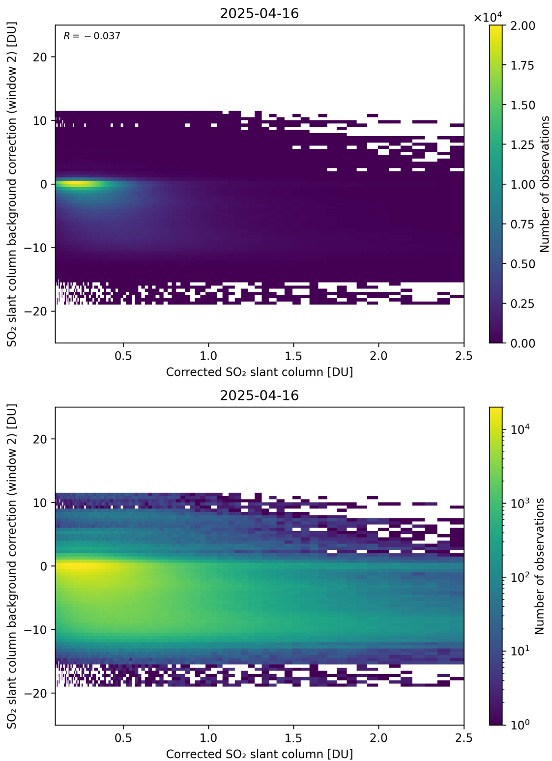
Figure 227: Scatter density plot of “Corrected SO 2 slant column” against “SO 2 slant column background correction (window 2)” for 2025-04-15 to 2025-04-17.
