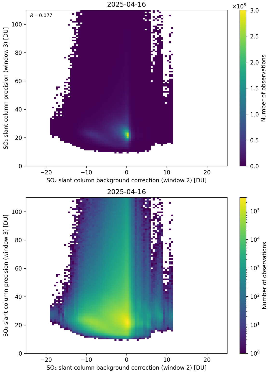
Figure 129: Scatter density plot of “SO 2 slant column background correction (window 2)” against “SO 2 slant column precision (window 3)” for 2025-04-15 to 2025-04-17.
