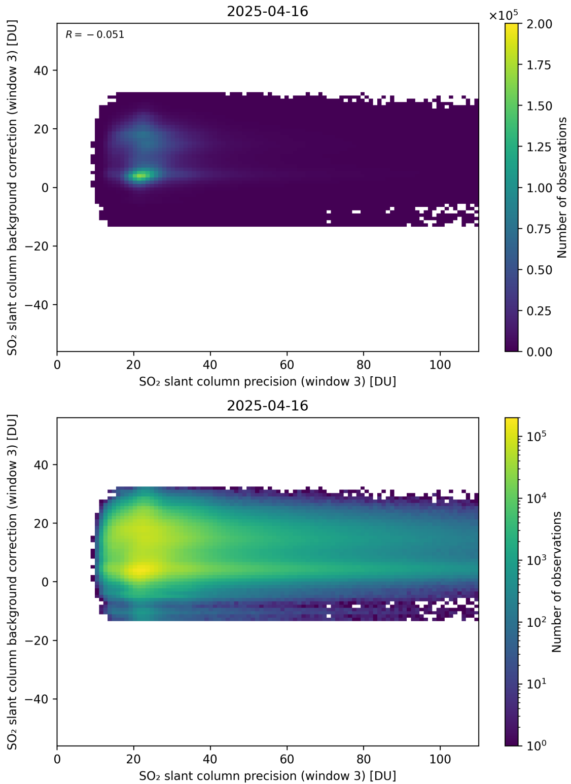
Figure 307: Scatter density plot of “SO 2 slant column precision (window 3)” against “SO 2 slant column background correction (window 3)” for 2025-04-15 to 2025-04-17.
