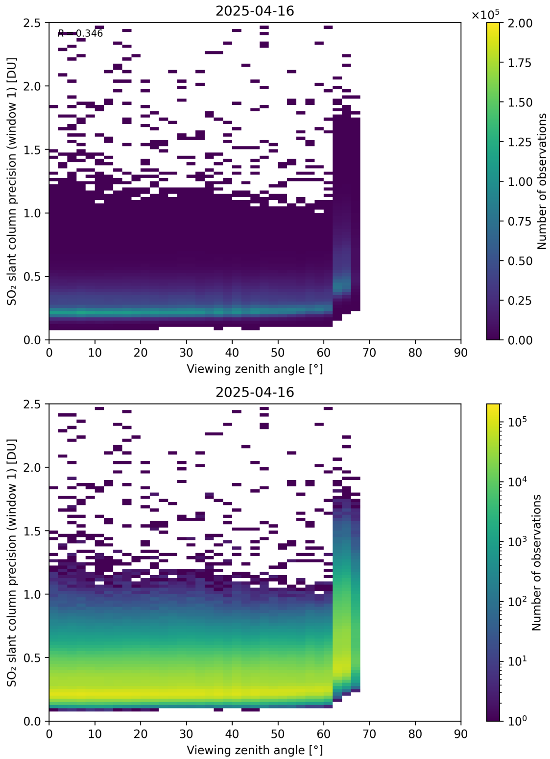
Figure 377: Scatter density plot of “Viewing zenith angle” against “SO 2 slant column precision (window 1)” for 2025-04-15 to 2025-04-17.
