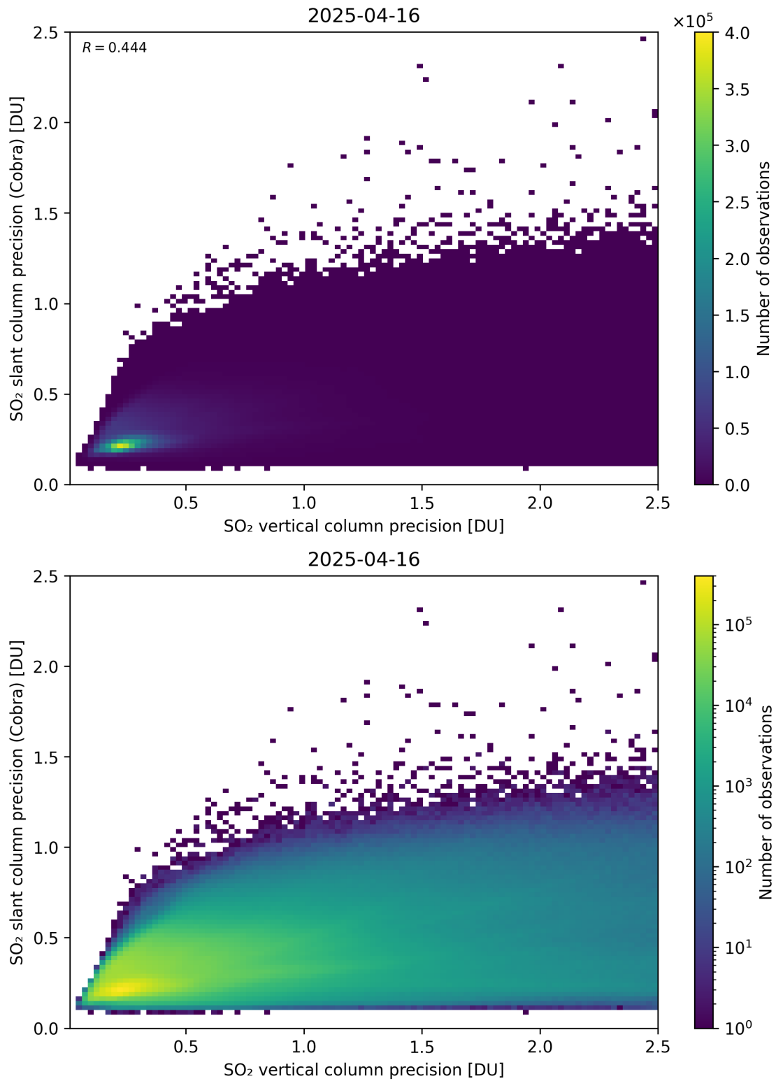
Figure 337: Scatter density plot of “SO 2 vertical column precision” against “SO 2 slant column precision (Cobra)” for 2025-04-15 to 2025-04-17.
