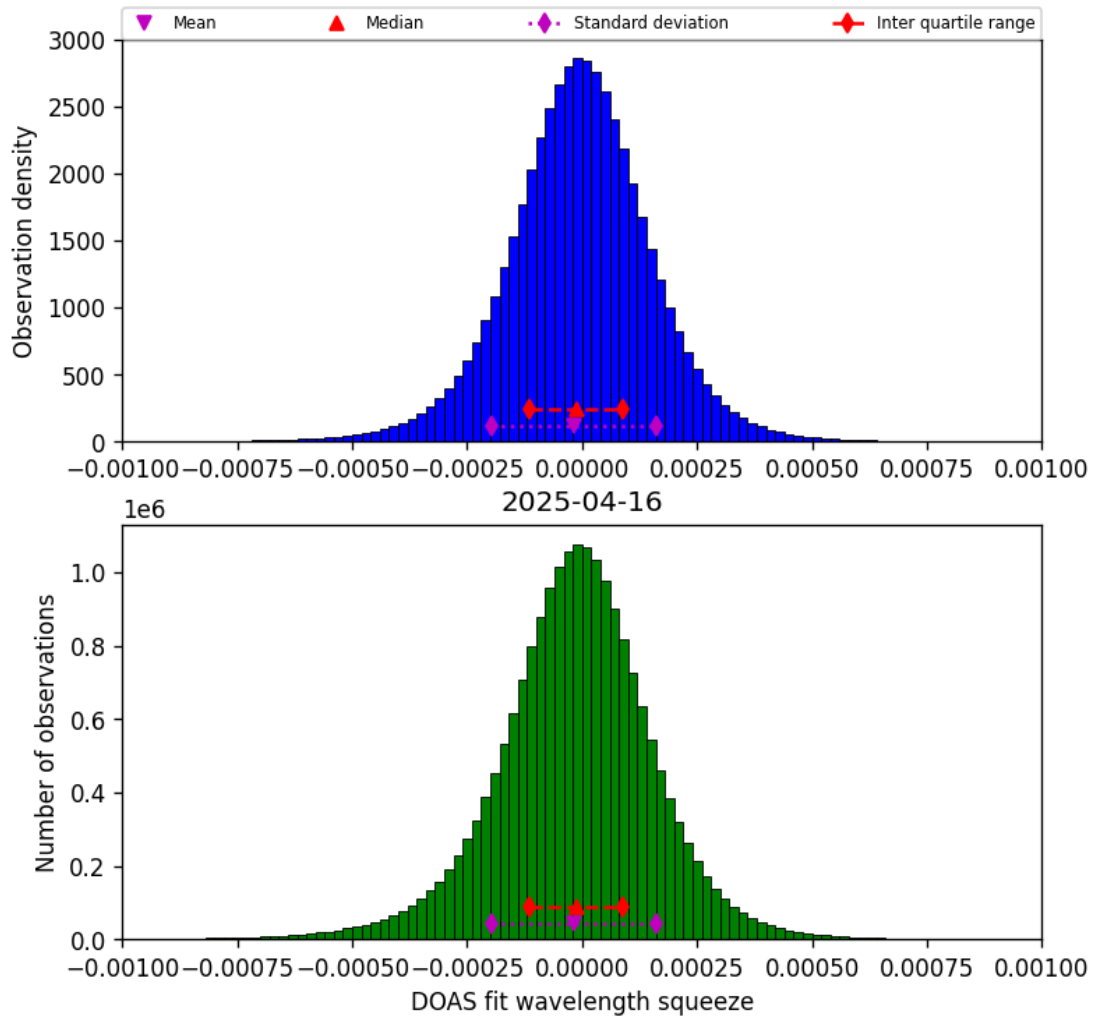
Figure 77: Histogram of “DOAS fit wavelength squeeze” for 2025-04-15 to 2025-04-17
