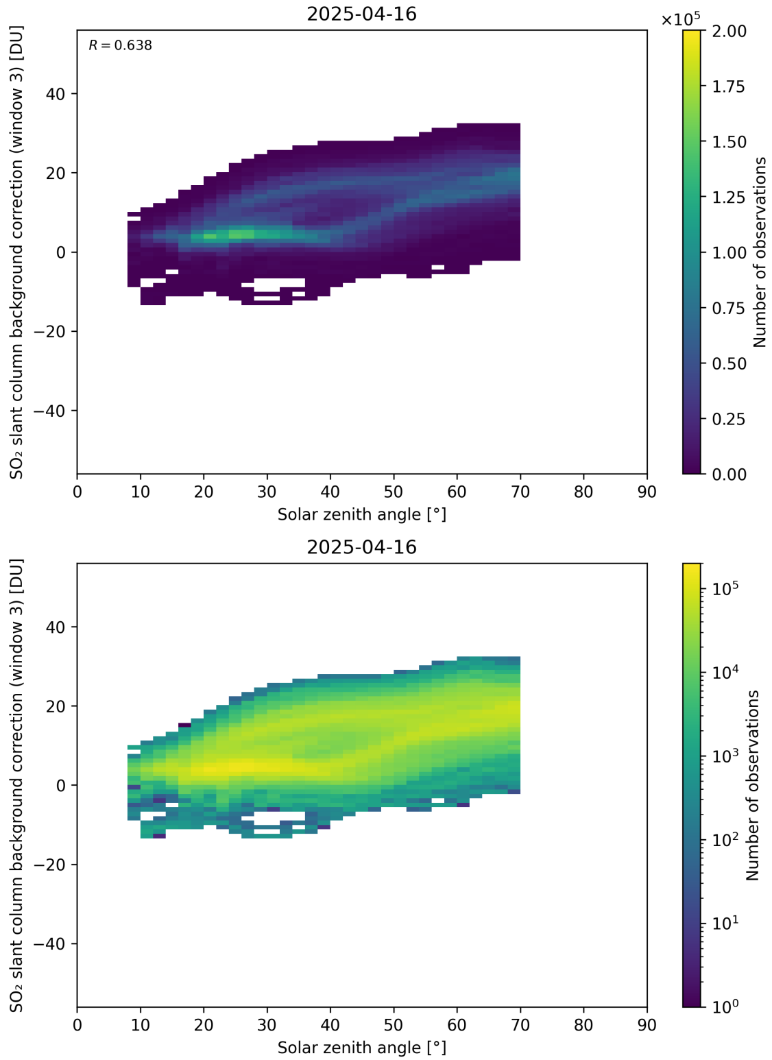
Figure 173: Scatter density plot of “Solar zenith angle” against “SO 2 slant column background correction (window 3)” for 2025-04-15 to 2025-04-17.
