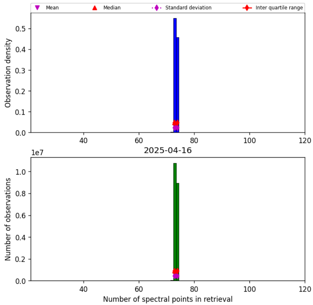
Figure 82: Histogram of “Number of spectral points in retrieval” for 2025-04-15 to 2025-04-17
