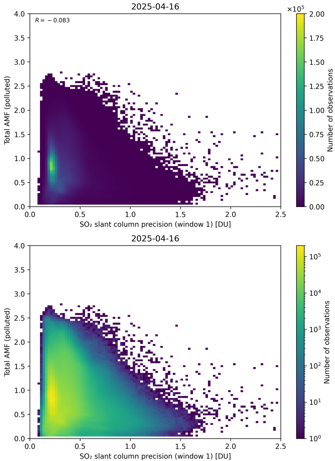
Figure 280: Scatter density plot of “SO 2 slant column precision (window 1)” against “Total AMF (polluted)” for 2025-04-15 to 2025-04-17.
