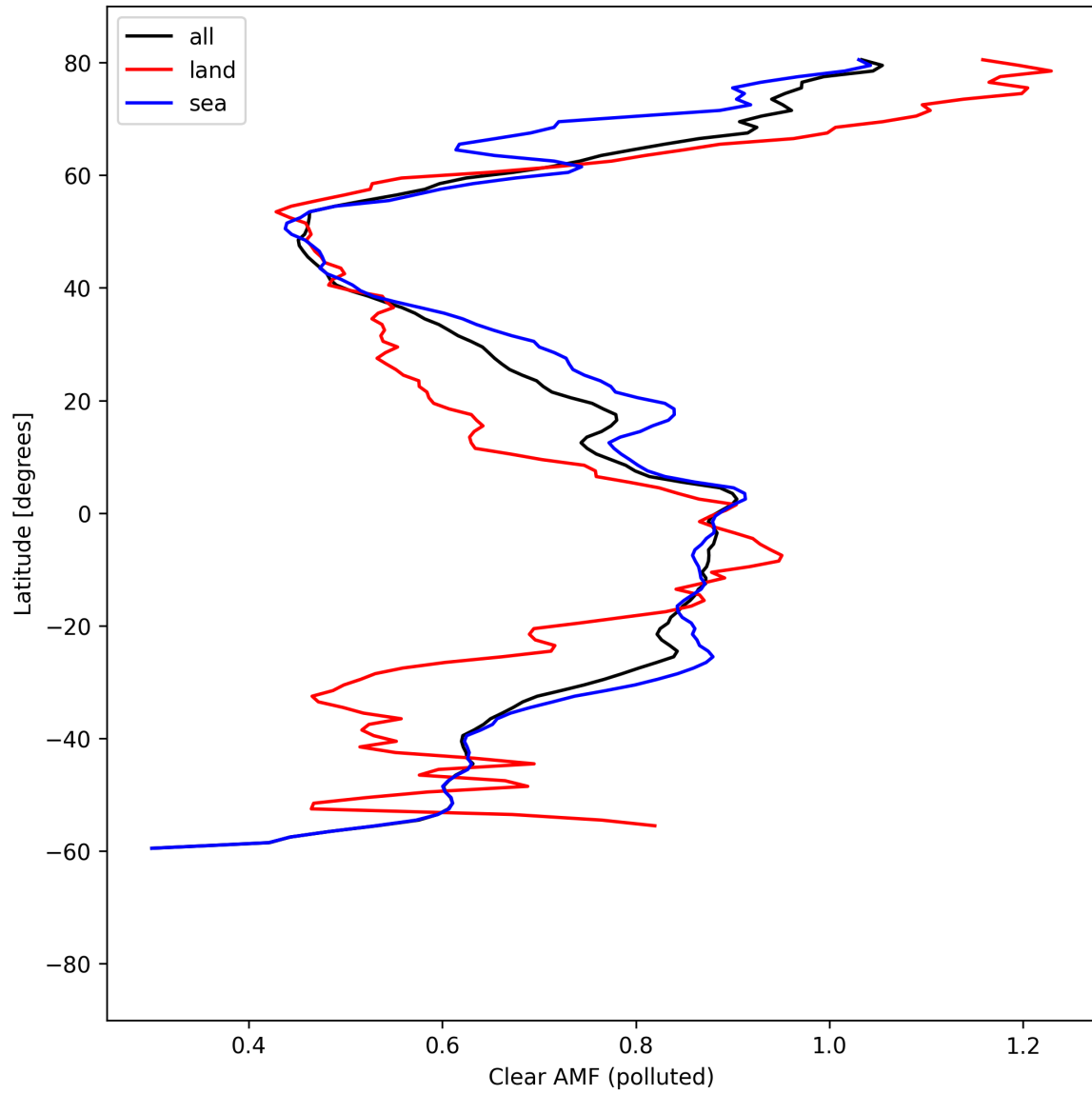
Figure 55: Zonal average of “Clear AMF (polluted)” for 2025-04-15 to 2025-04-17.
