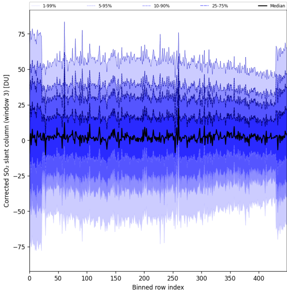
Figure 99: Along track statistics of “Corrected SO 2 slant column (window 3)” for 2025-04-15 to 2025-04-17
