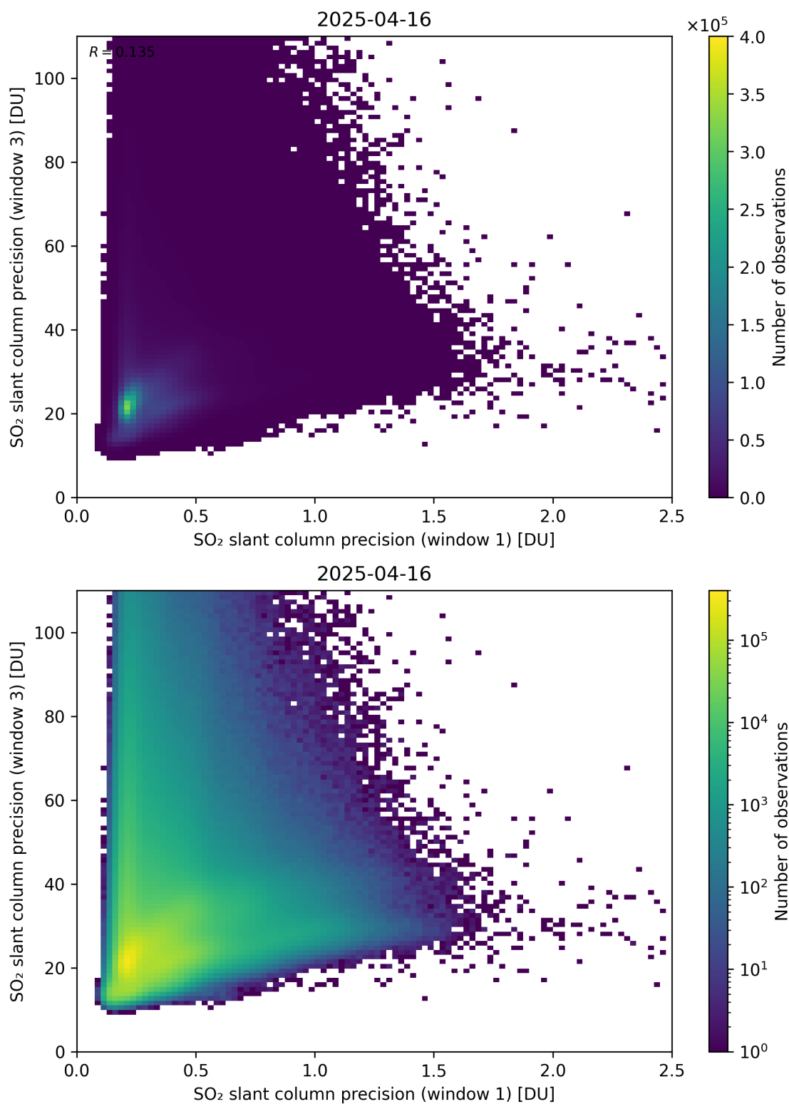
Figure 279: Scatter density plot of “SO 2 slant column precision (window 1)” against “SO 2 slant column precision (window 3)” for 2025-04-15 to 2025-04-17.
