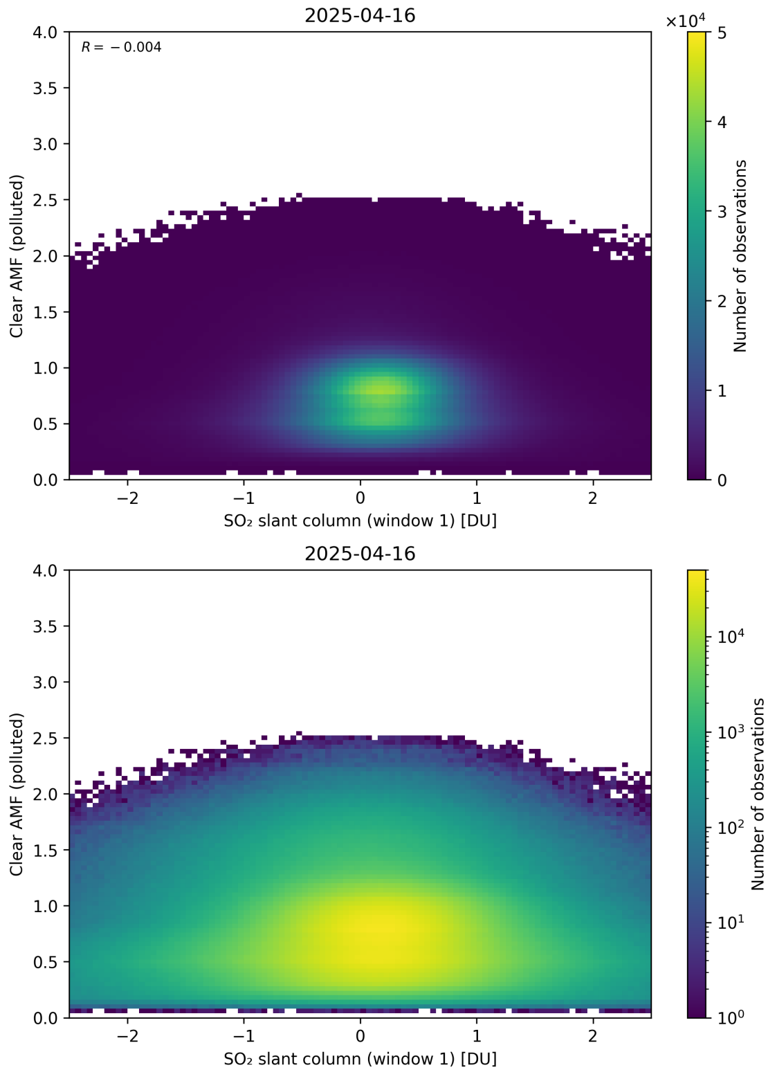
Figure 282: Scatter density plot of “SO 2 slant column (window 1)” against “Clear AMF (polluted)” for 2025-04-15 to 2025-04-17.
