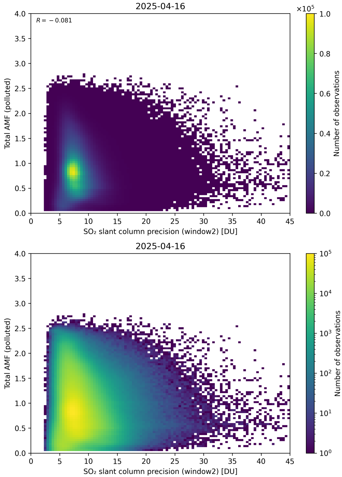
Figure 301: Scatter density plot of “SO 2 slant column precision (window2)” against “Total AMF (polluted)” for 2025-04-15 to 2025-04-17.
