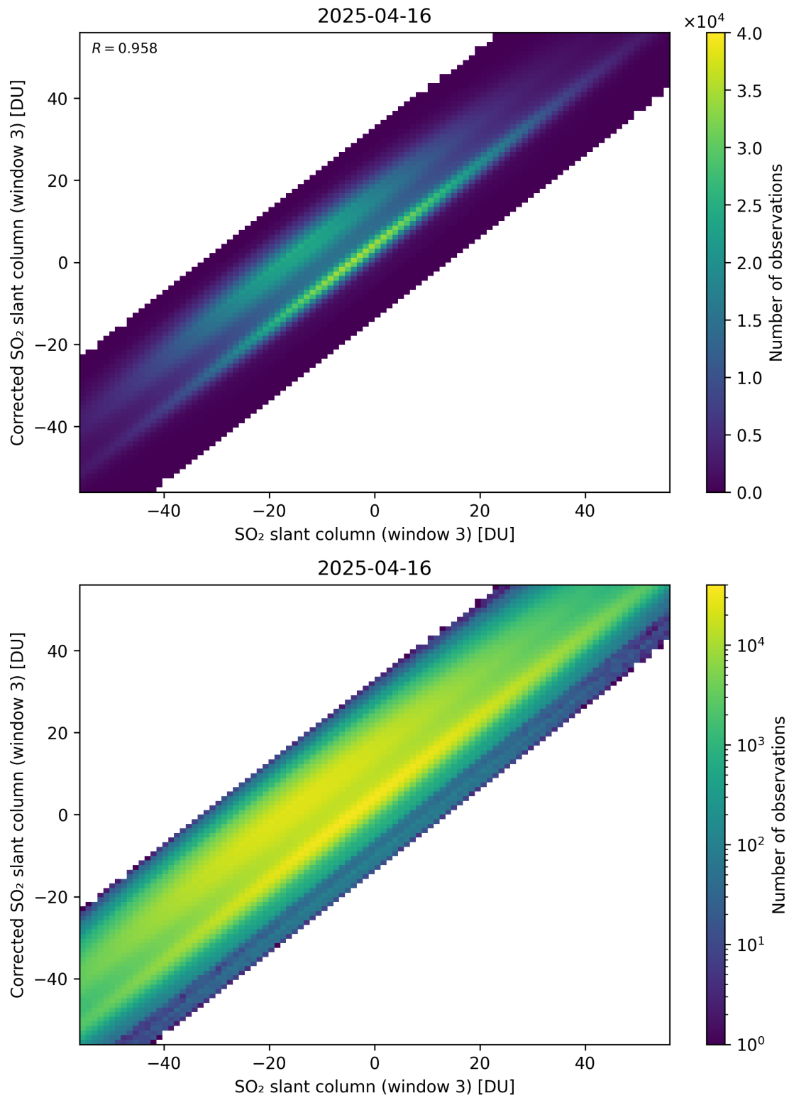
Figure 316: Scatter density plot of “SO 2 slant column (window 3)” against “Corrected SO 2 slant column (window 3)” for 2025-04-15 to 2025-04-17.
