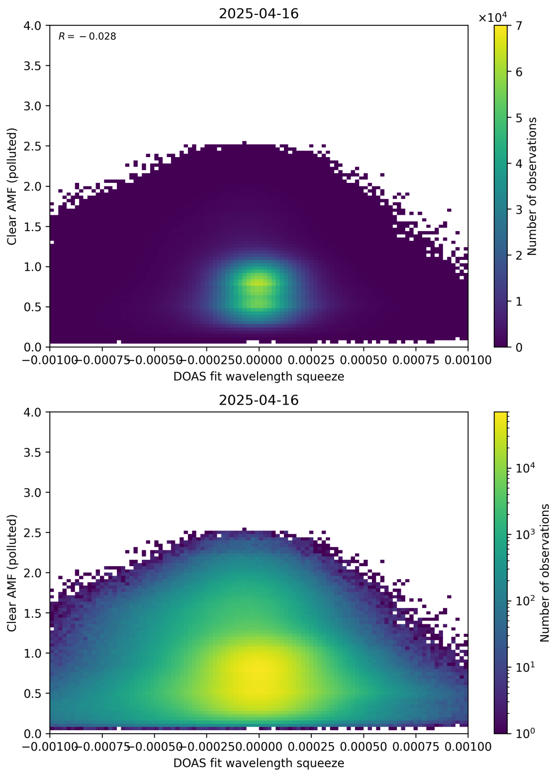
Figure 144: Scatter density plot of “DOAS fit wavelength squeeze” against “Clear AMF (polluted)” for 2025-04-15 to 2025-04-17.
