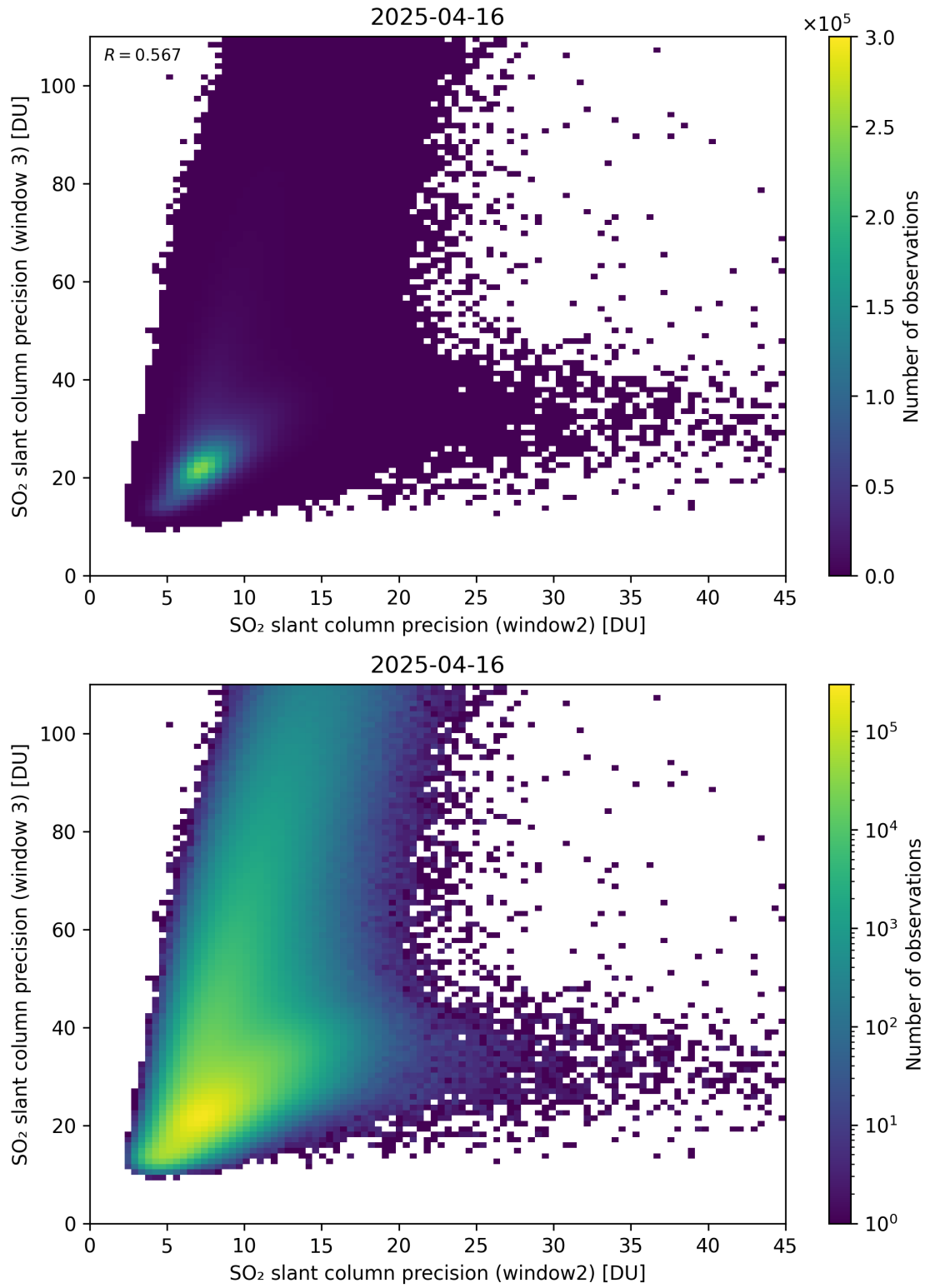
Figure 300: Scatter density plot of “SO 2 slant column precision (window2)” against “SO 2 slant column precision (window 3)” for 2025-04-15 to 2025-04-17.
