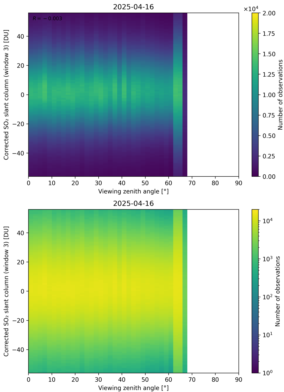
Figure 375: Scatter density plot of “Viewing zenith angle” against “Corrected SO 2 slant column (window 3)” for 2025-04-15 to 2025-04-17.
