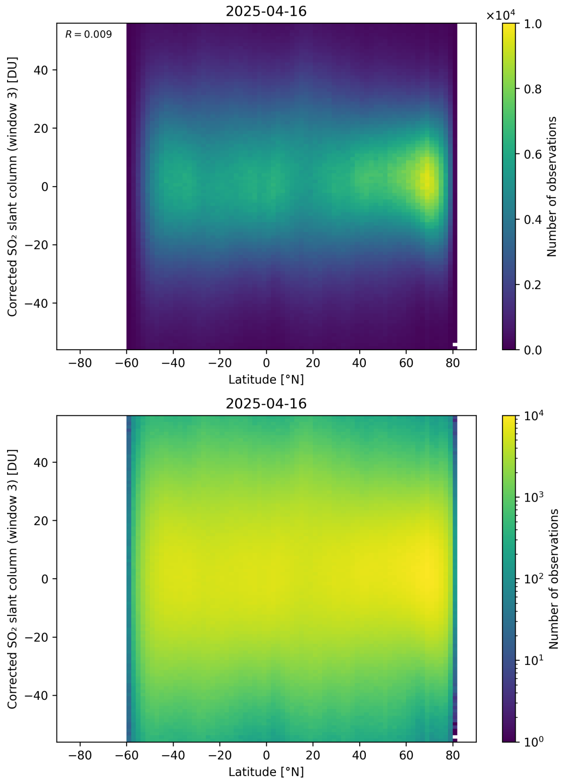
Figure 161: Scatter density plot of “Latitude” against “Corrected SO 2 slant column (window 3)” for 2025-04-15 to 2025-04-17.
