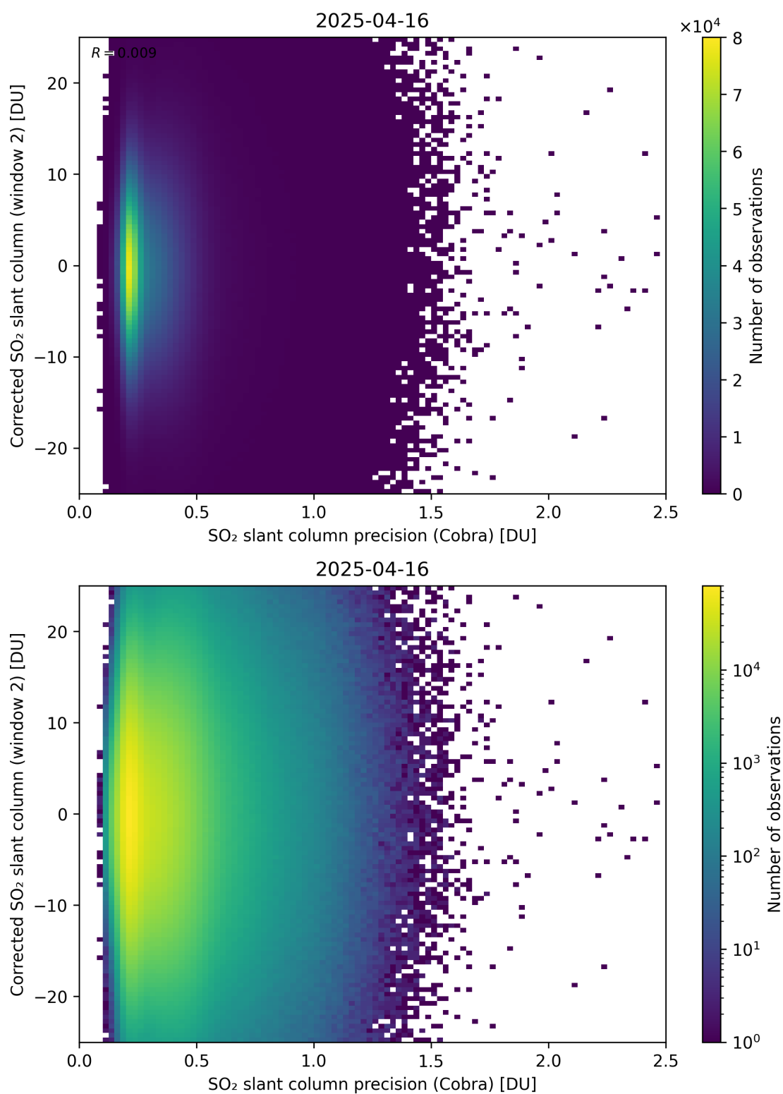
Figure 206: Scatter density plot of “SO 2 slant column precision (Cobra)” against “Corrected SO 2 slant column (window 2)” for 2025-04-15 to 2025-04-17.
