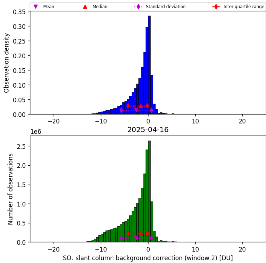
Figure 70: Histogram of “SO 2 slant column background correction (window 2)” for 2025-04-15 to 2025-04-17
