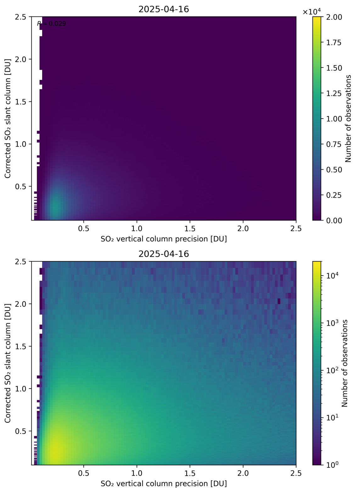
Figure 338: Scatter density plot of “SO 2 vertical column precision” against “Corrected SO 2 slant column” for 2025-04-15 to 2025-04-17.
