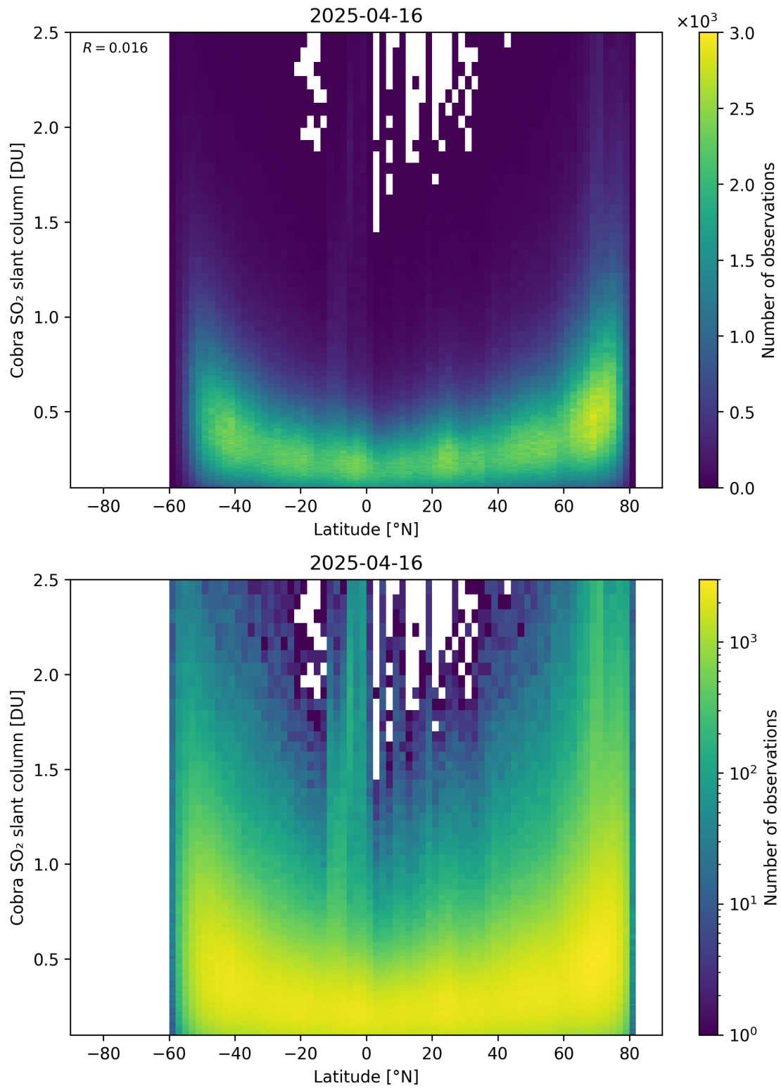
Figure 157: Scatter density plot of “Latitude” against “Cobra SO 2 slant column” for 2025-04-15 to 2025-04-17.
