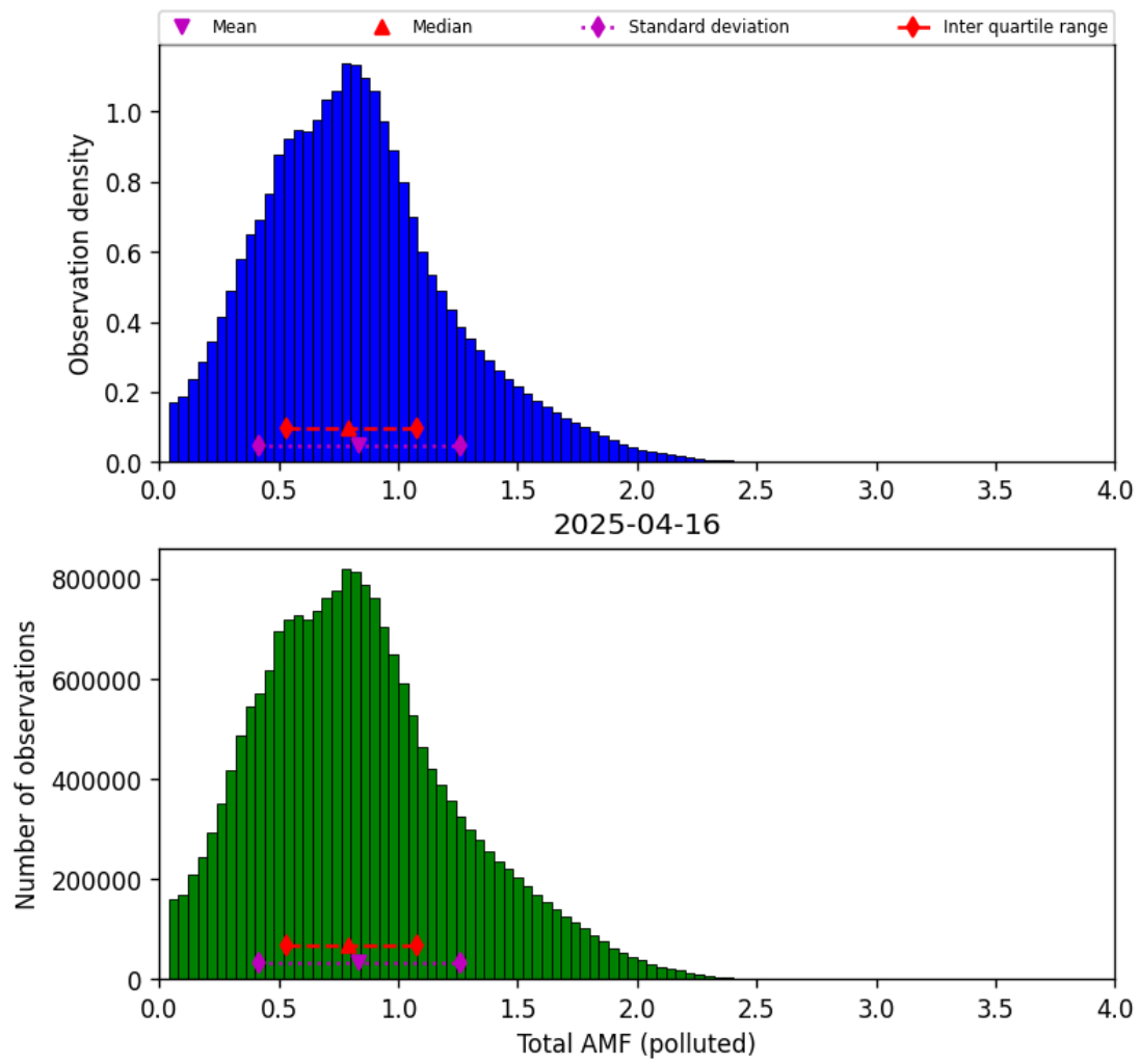
Figure 79: Histogram of “Total AMF (polluted)” for 2025-04-15 to 2025-04-17
