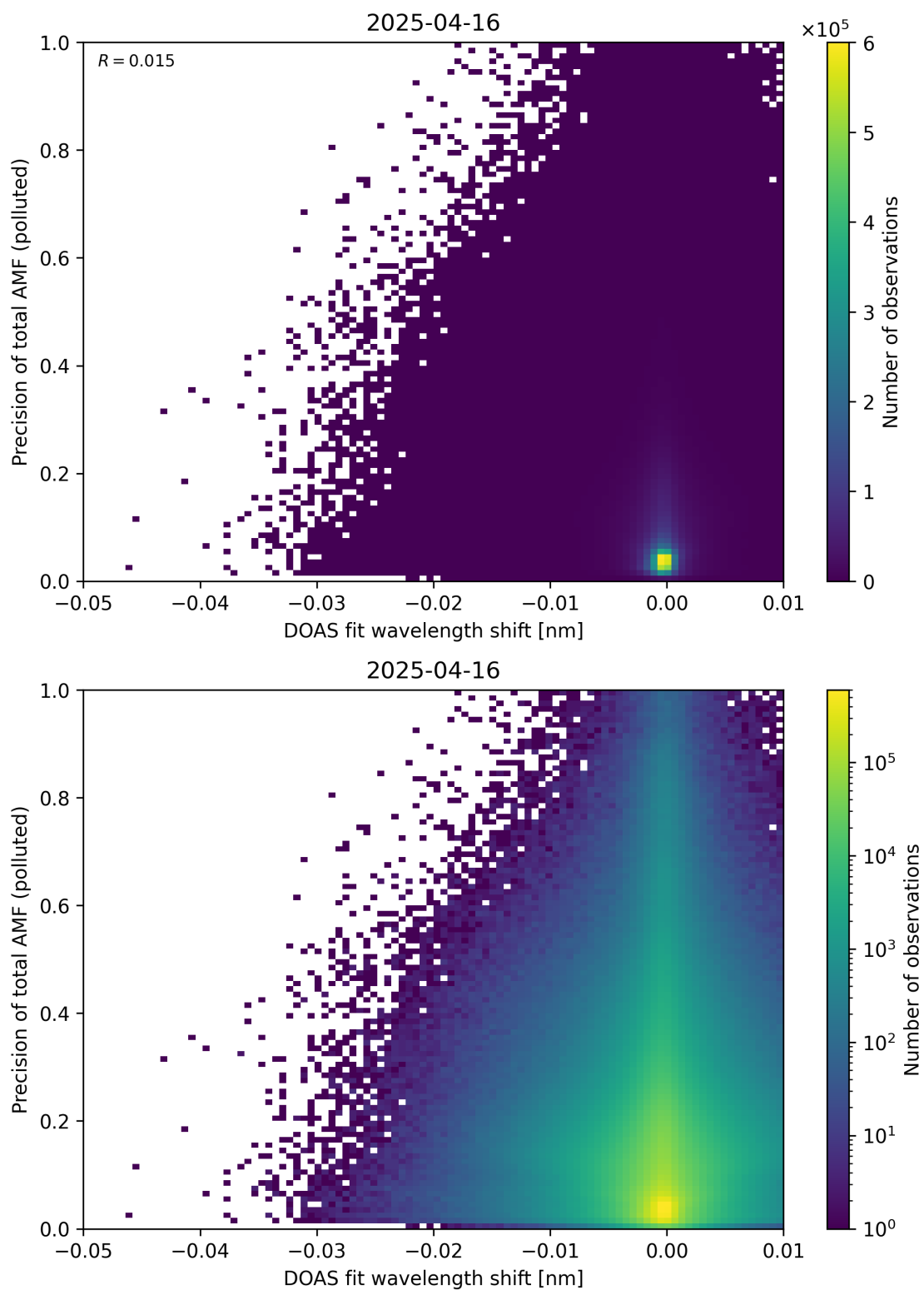
Figure 142: Scatter density plot of “DOAS fit wavelength shift” against “Precision of total AMF (polluted)” for 2025-04-15 to 2025-04-17.
