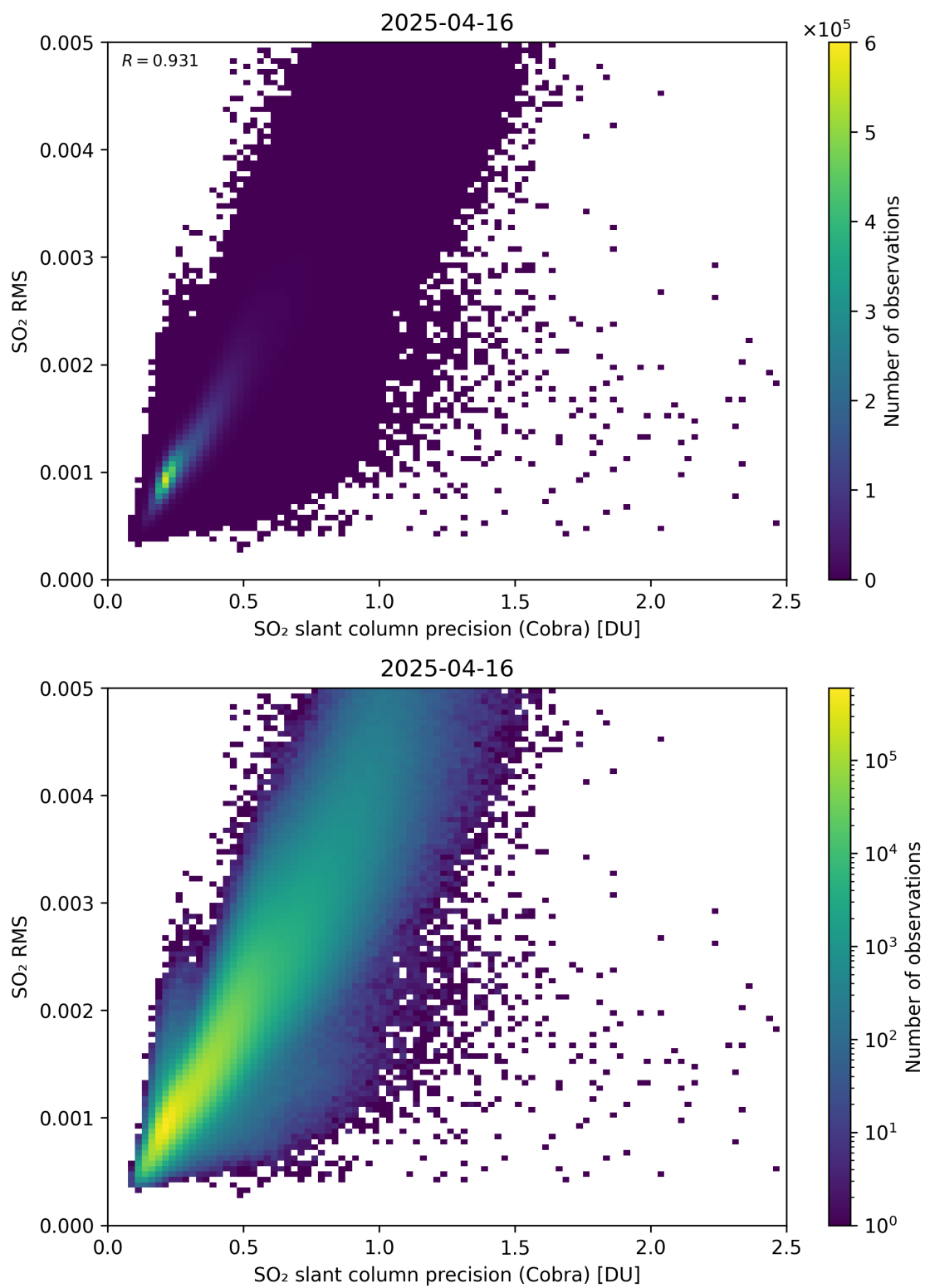
Figure 204: Scatter density plot of “SO 2 slant column precision (Cobra)” against “SO 2 RMS” for 2025-04-15 to 2025-04-17.
