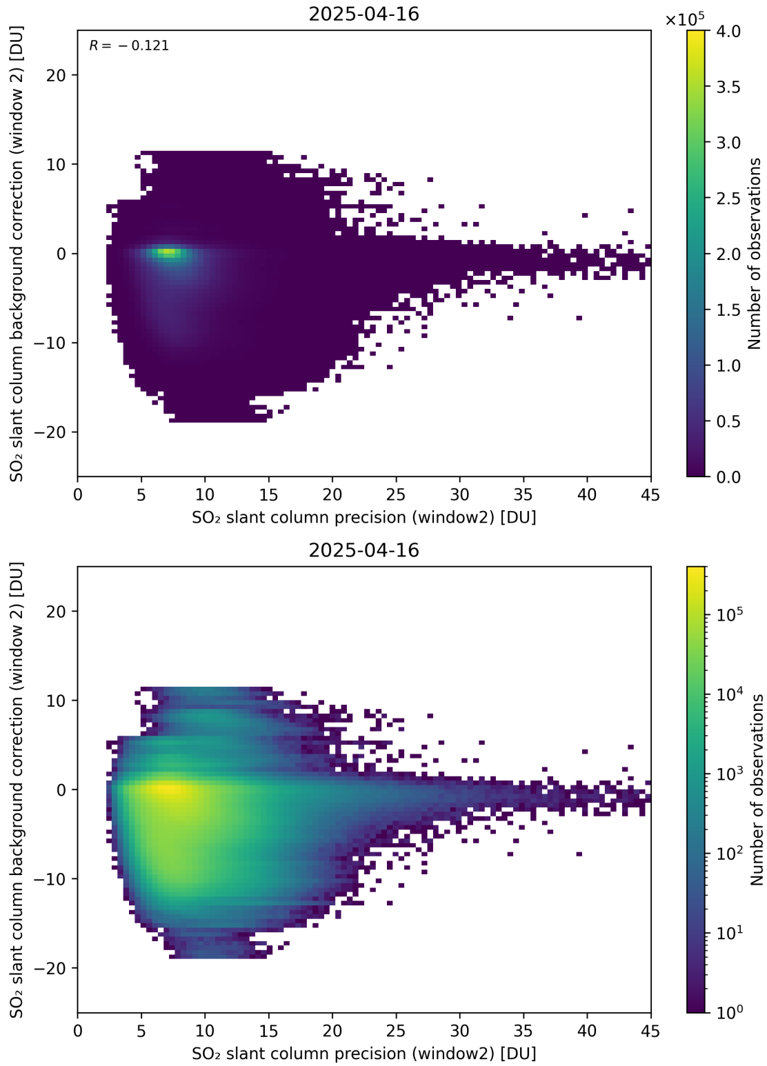
Figure 291: Scatter density plot of “SO 2 slant column precision (window2)” against “SO 2 slant column background correction (window 2)” for 2025-04-15 to 2025-04-17.
