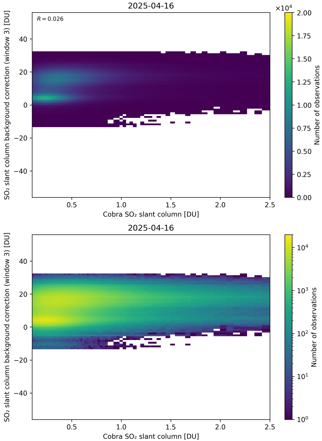
Figure 195: Scatter density plot of “Cobra SO 2 slant column” against “SO 2 slant column background correction (window 3)” for 2025-04-15 to 2025-04-17.
