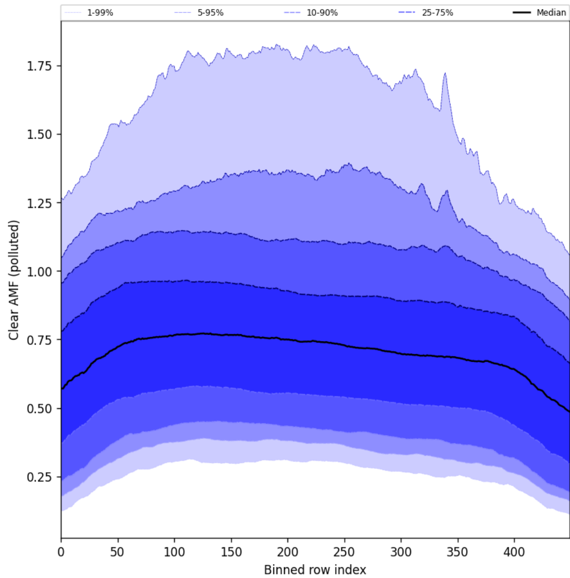
Figure 107: Along track statistics of “Clear AMF (polluted)” for 2025-04-15 to 2025-04-17
