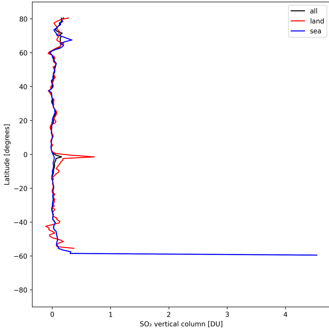
Figure 32: Zonal average of “SO 2 vertical column” for 2025-04-15 to 2025-04-17.
