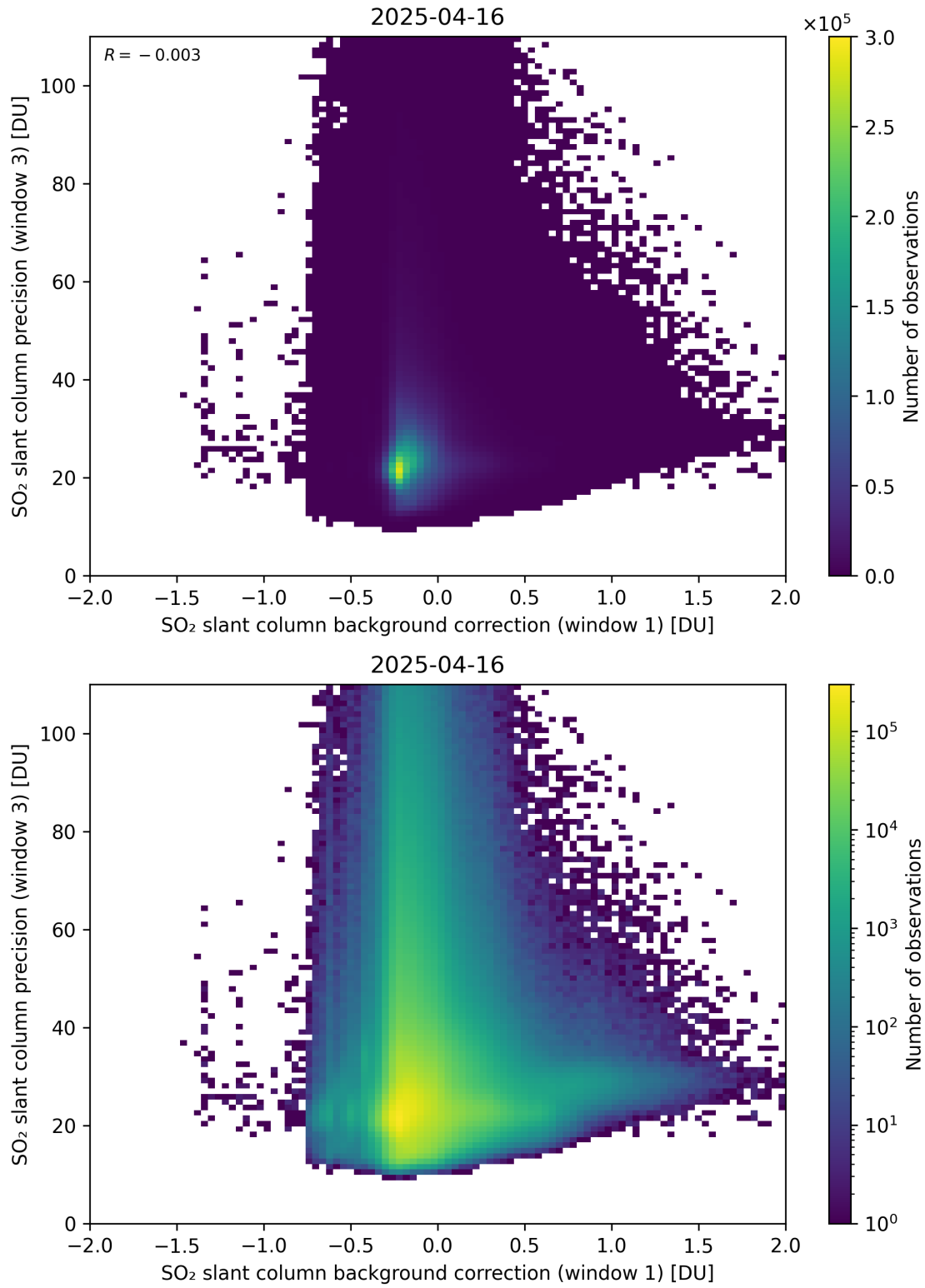
Figure 119: Scatter density plot of “SO 2 slant column background correction (window 1)” against “SO 2 slant column precision (window 3)” for 2025-04-15 to 2025-04-17.
