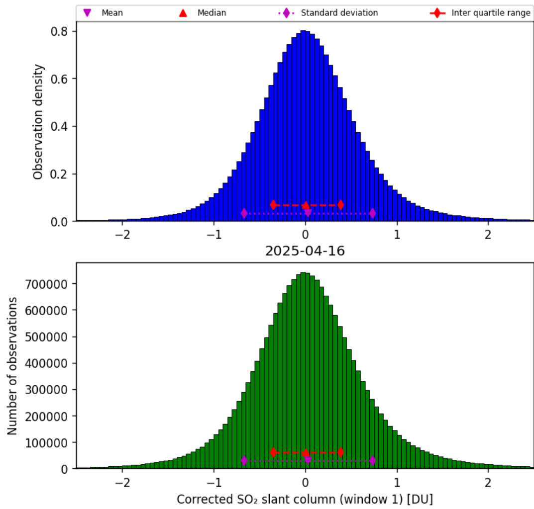
Figure 65: Histogram of “Corrected SO 2 slant column (window 1)” for 2025-04-15 to 2025-04-17
