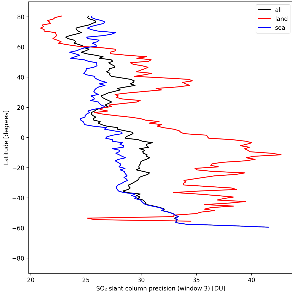
Figure 46: Zonal average of “SO 2 slant column precision (window 3)” for 2025-04-15 to 2025-04-17.
