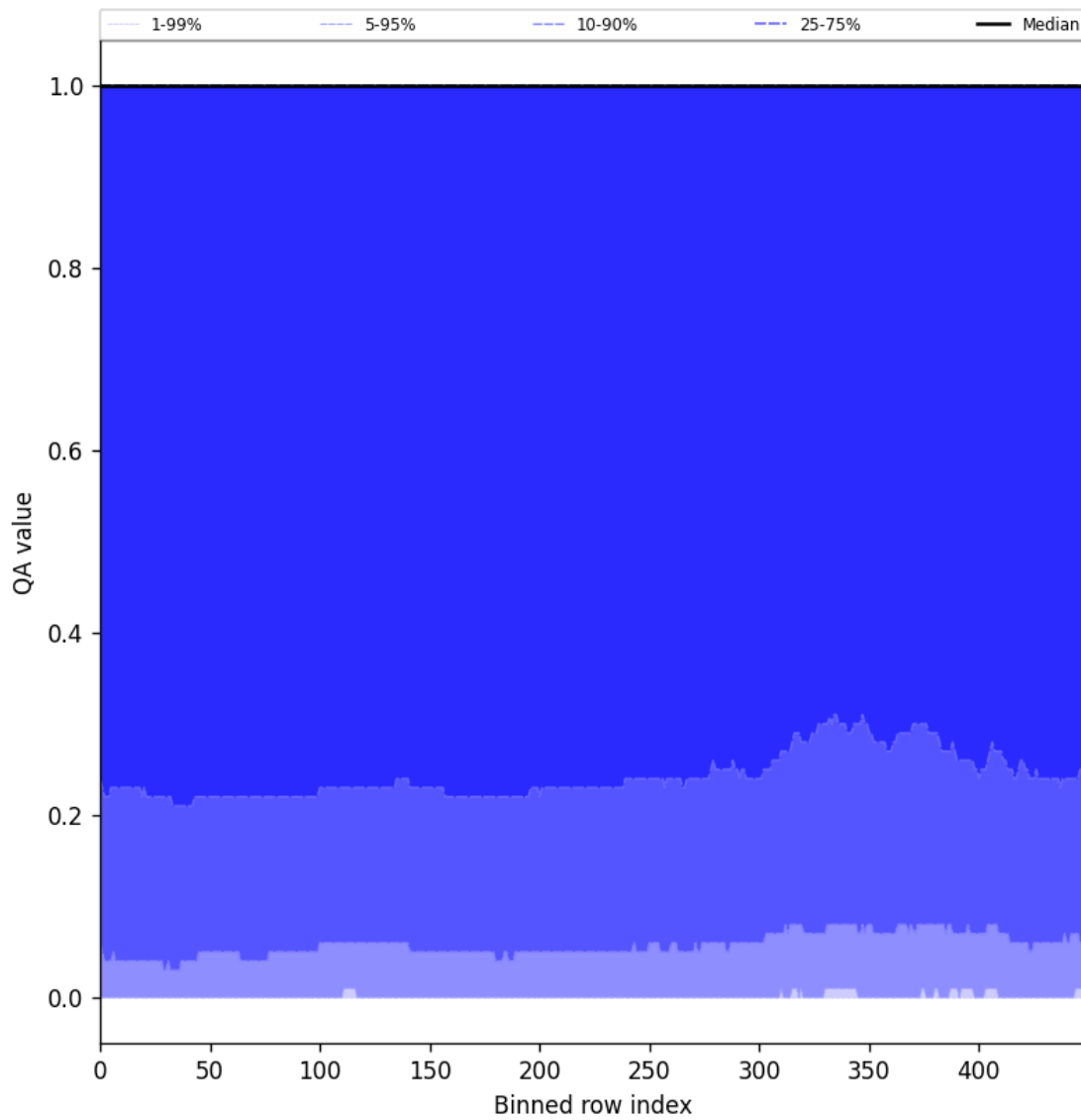
Figure 83: Along track statistics of “QA value” for 2025-04-15 to 2025-04-17
