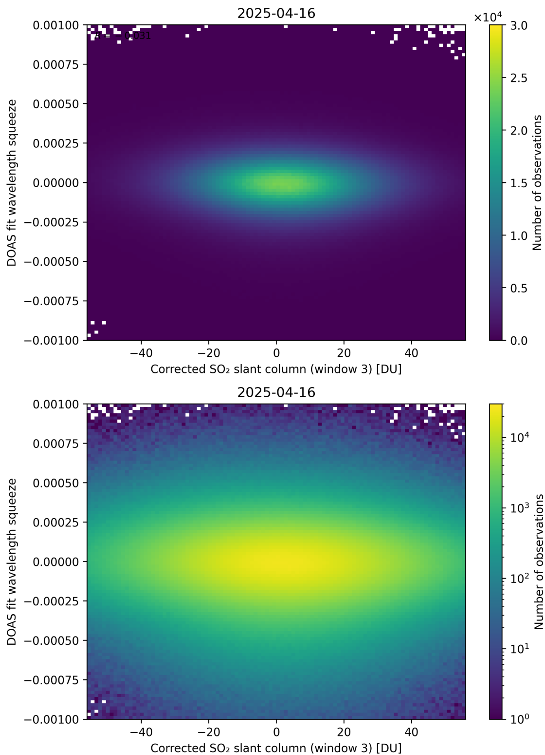
Figure 257: Scatter density plot of “Corrected SO 2 slant column (window 3)” against “DOAS fit wavelength squeeze” for 2025-04-15 to 2025-04-17.
