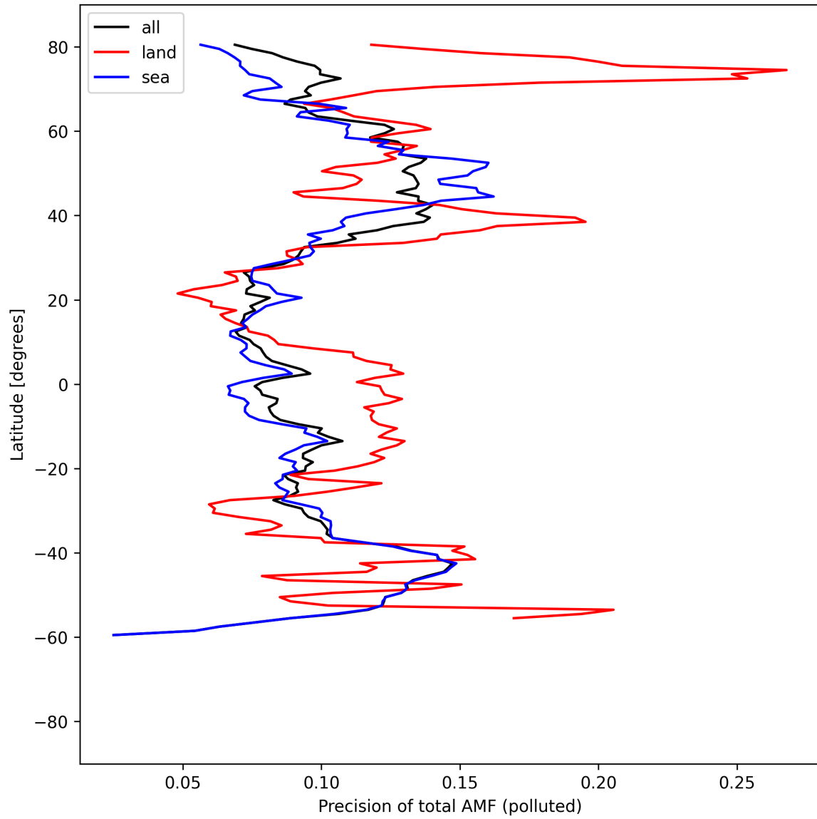
Figure 54: Zonal average of “Precision of total AMF (polluted)” for 2025-04-15 to 2025-04-17.
