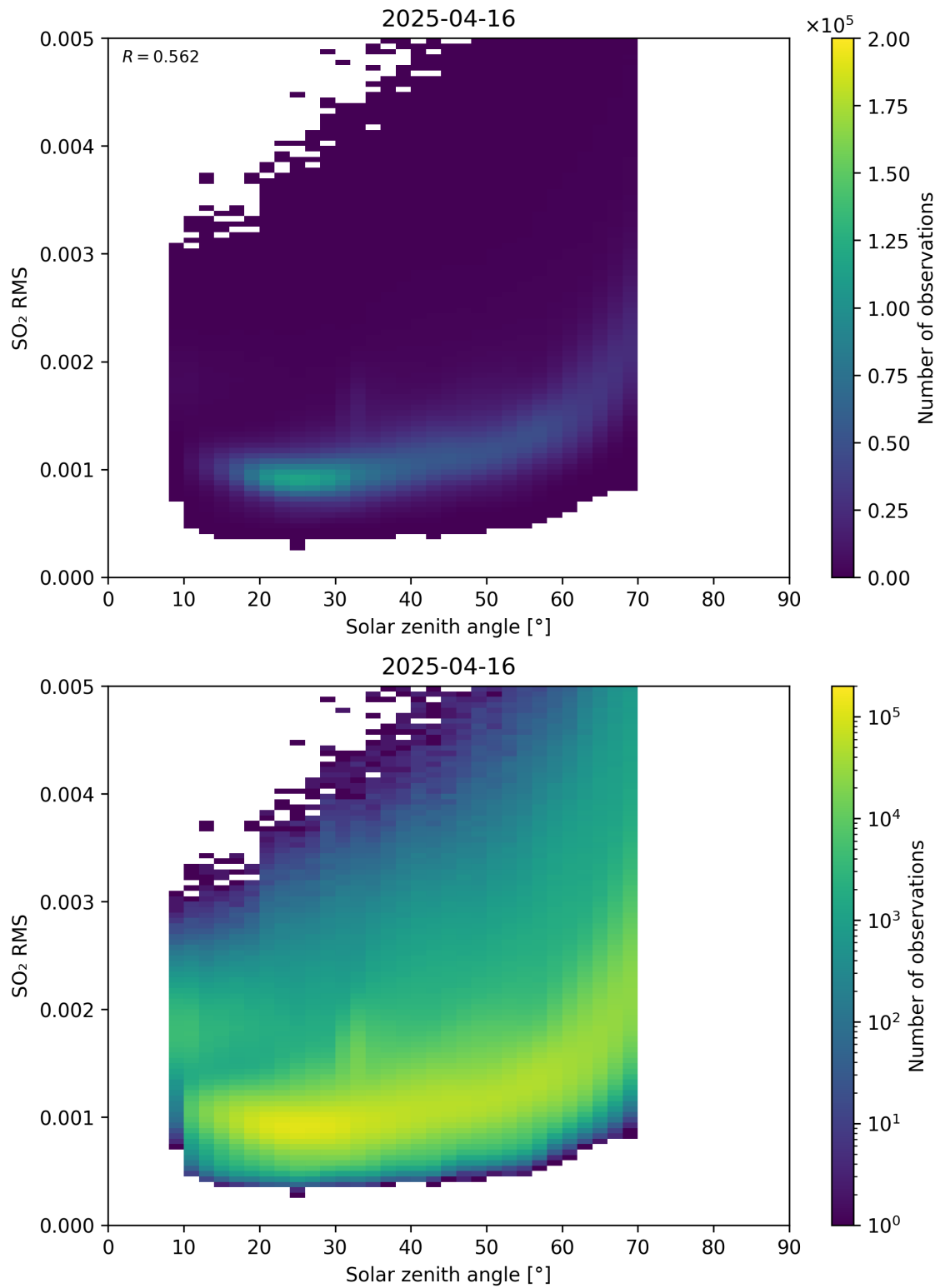
Figure 176: Scatter density plot of “Solar zenith angle” against “SO 2 RMS” for 2025-04-15 to 2025-04-17.
