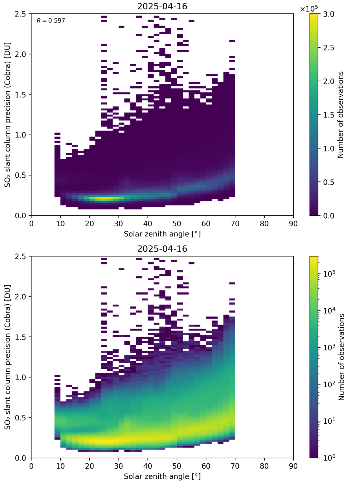
Figure 180: Scatter density plot of “Solar zenith angle” against “SO 2 slant column precision (Cobra)” for 2025-04-15 to 2025-04-17.
