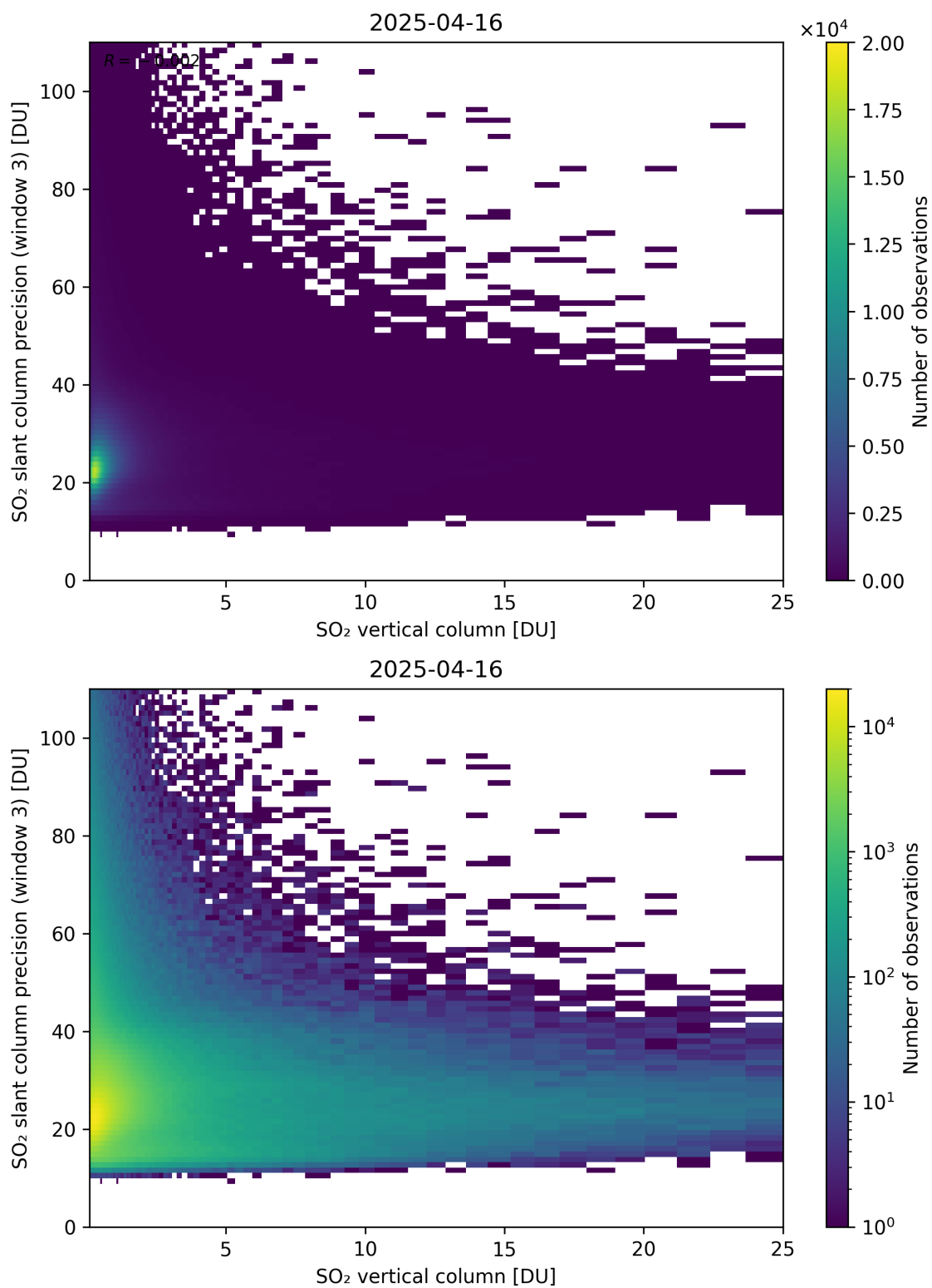
Figure 358: Scatter density plot of “SO 2 vertical column” against “SO 2 slant column precision (window 3)” for 2025-04-15 to 2025-04-17.
