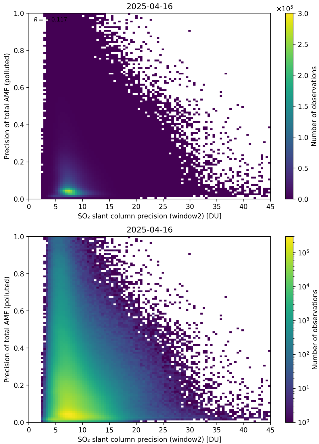
Figure 302: Scatter density plot of “SO 2 slant column precision (window2)” against “Precision of total AMF (polluted)” for 2025-04-15 to 2025-04-17.
