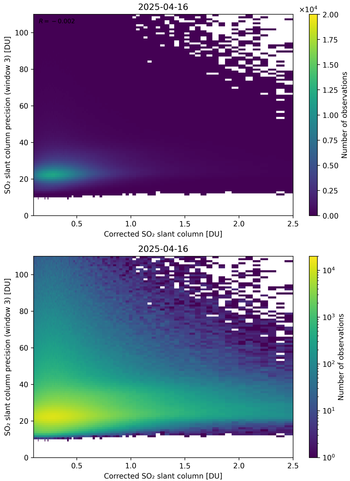
Figure 241: Scatter density plot of “Corrected SO 2 slant column” against “SO 2 slant column precision (window 3)” for 2025-04-15 to 2025-04-17.
