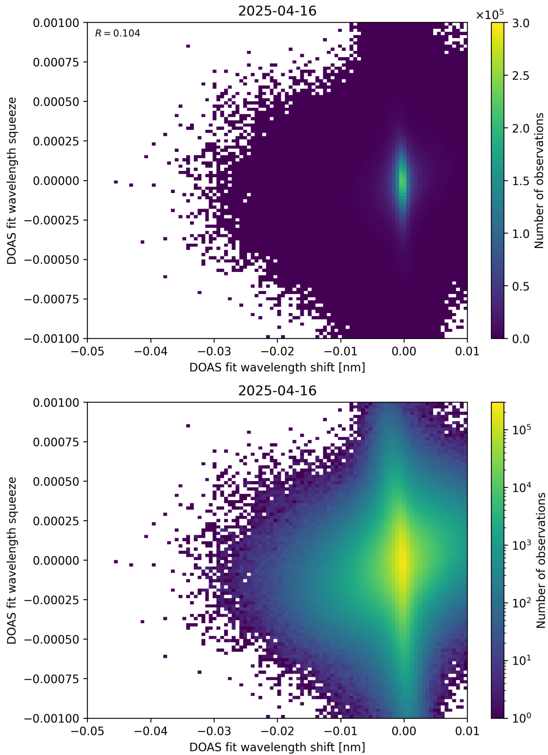
Figure 138: Scatter density plot of “DOAS fit wavelength shift” against “DOAS fit wavelength squeeze” for 2025-04-15 to 2025-04-17.
