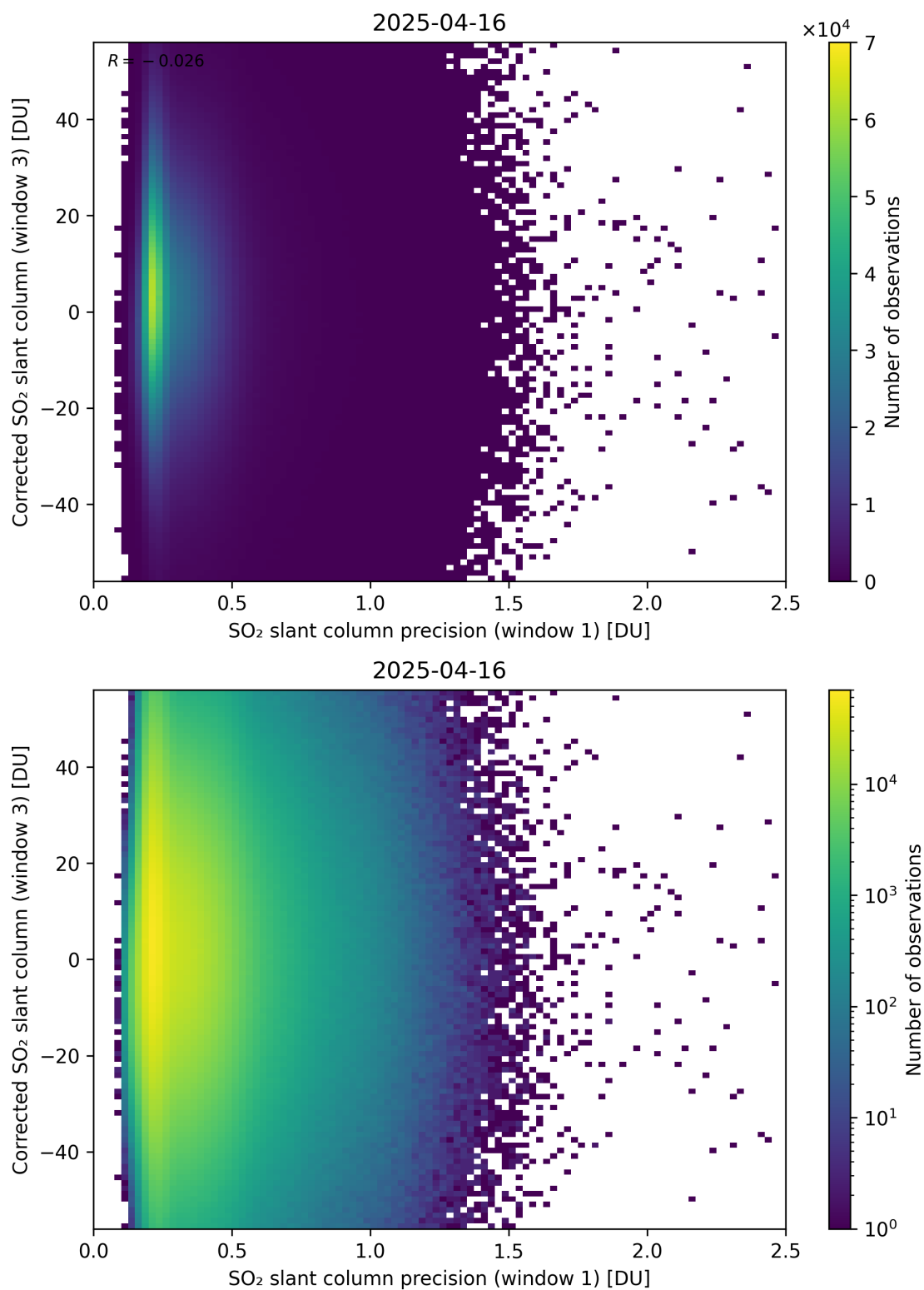
Figure 276: Scatter density plot of “SO 2 slant column precision (window 1)” against “Corrected SO 2 slant column (window 3)” for 2025-04-15 to 2025-04-17.
