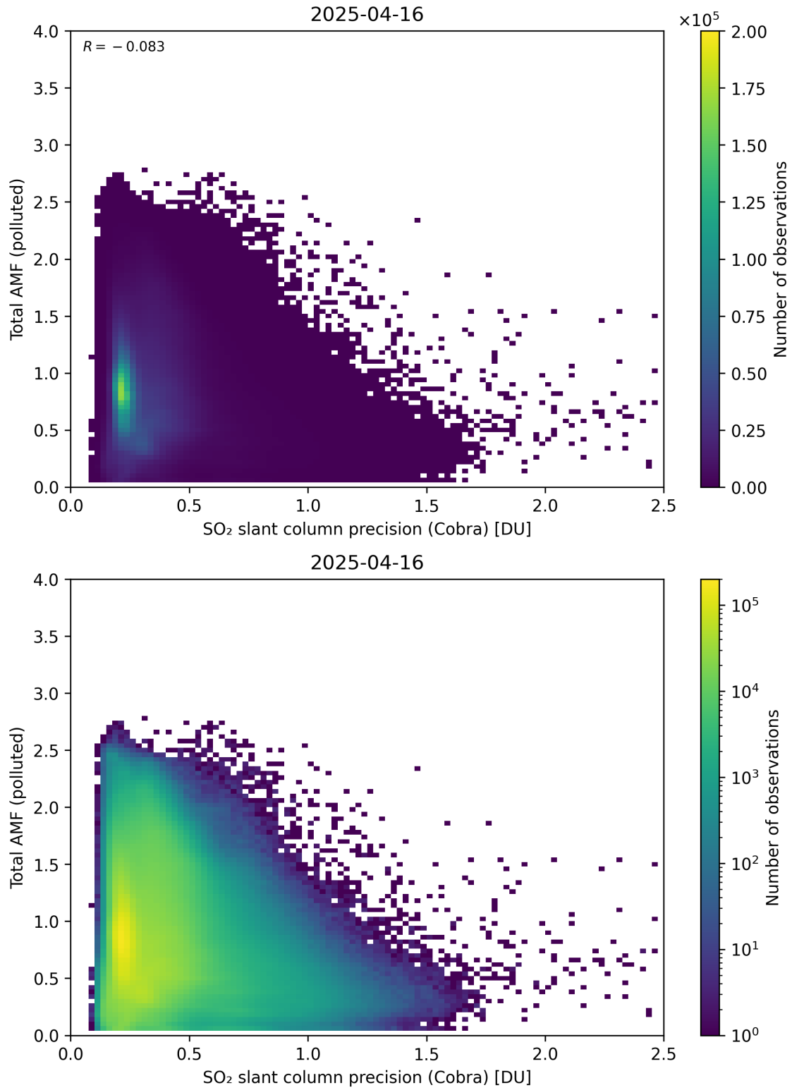
Figure 213: Scatter density plot of “SO 2 slant column precision (Cobra)” against “Total AMF (polluted)” for 2025-04-15 to 2025-04-17.
