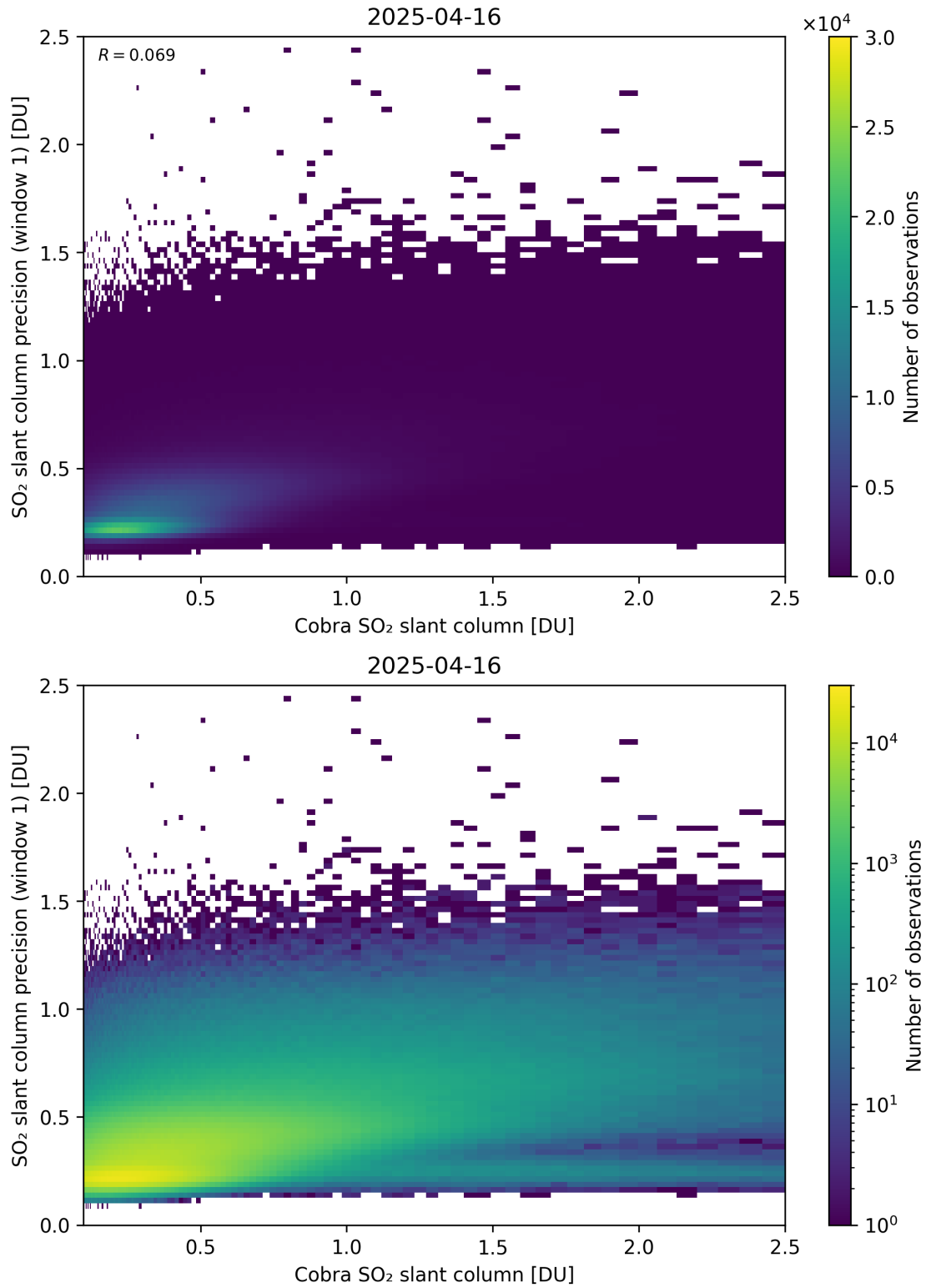
Figure 220: Scatter density plot of “Cobra SO 2 slant column” against “SO 2 slant column precision (window 1)” for 2025-04-15 to 2025-04-17.
