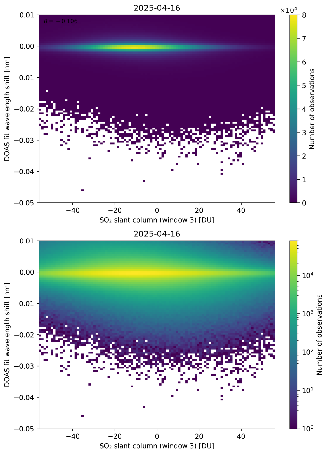
Figure 304: Scatter density plot of “SO 2 slant column (window 3)” against “DOAS fit wavelength shift” for 2025-04-15 to 2025-04-17.
