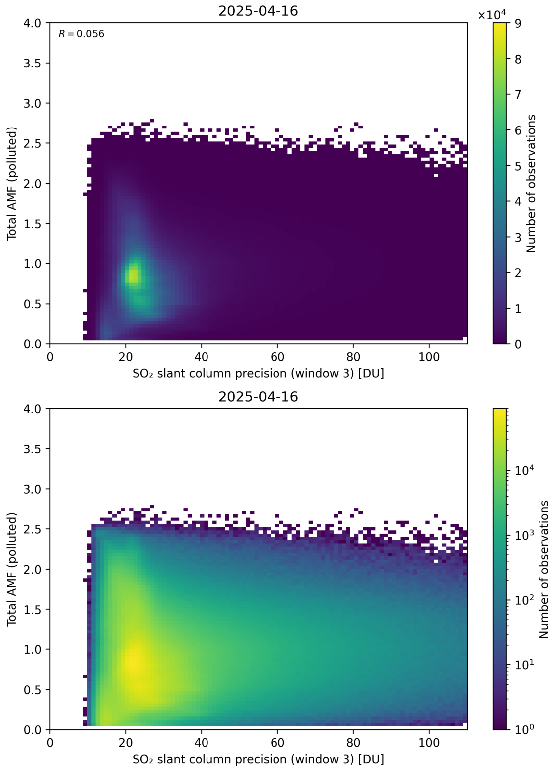
Figure 313: Scatter density plot of “SO 2 slant column precision (window 3)” against “Total AMF (polluted)” for 2025-04-15 to 2025-04-17.
