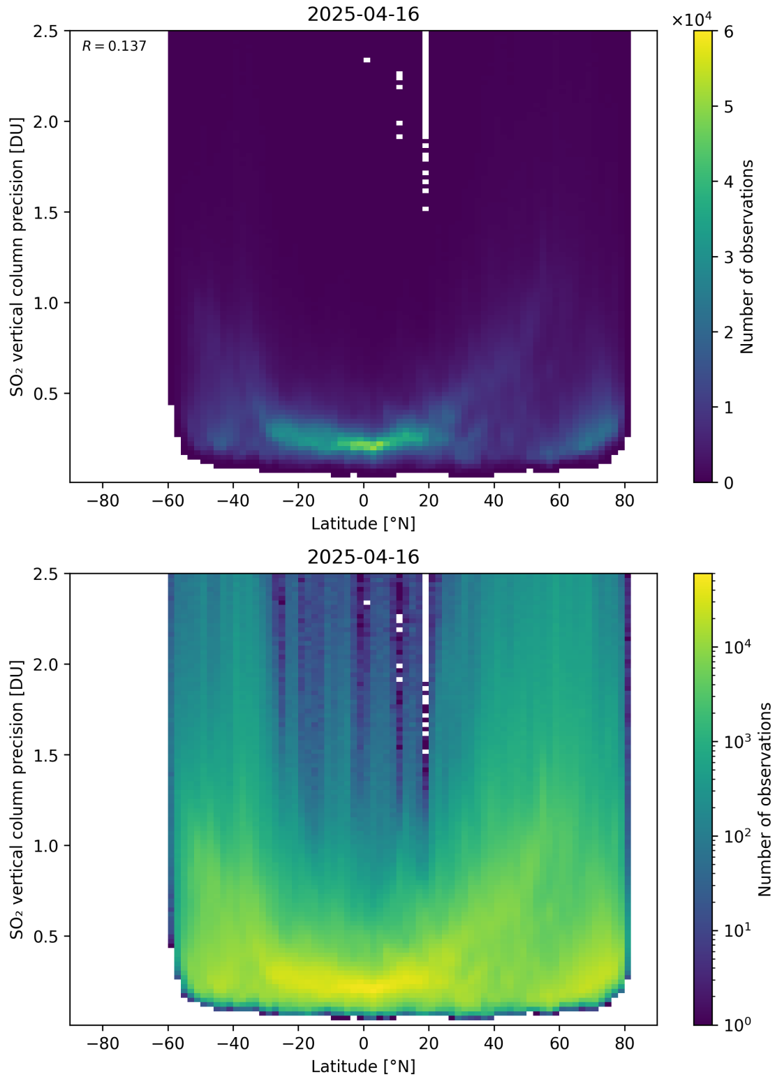
Figure 170: Scatter density plot of “Latitude” against “SO 2 vertical column precision” for 2025-04-15 to 2025-04-17.
