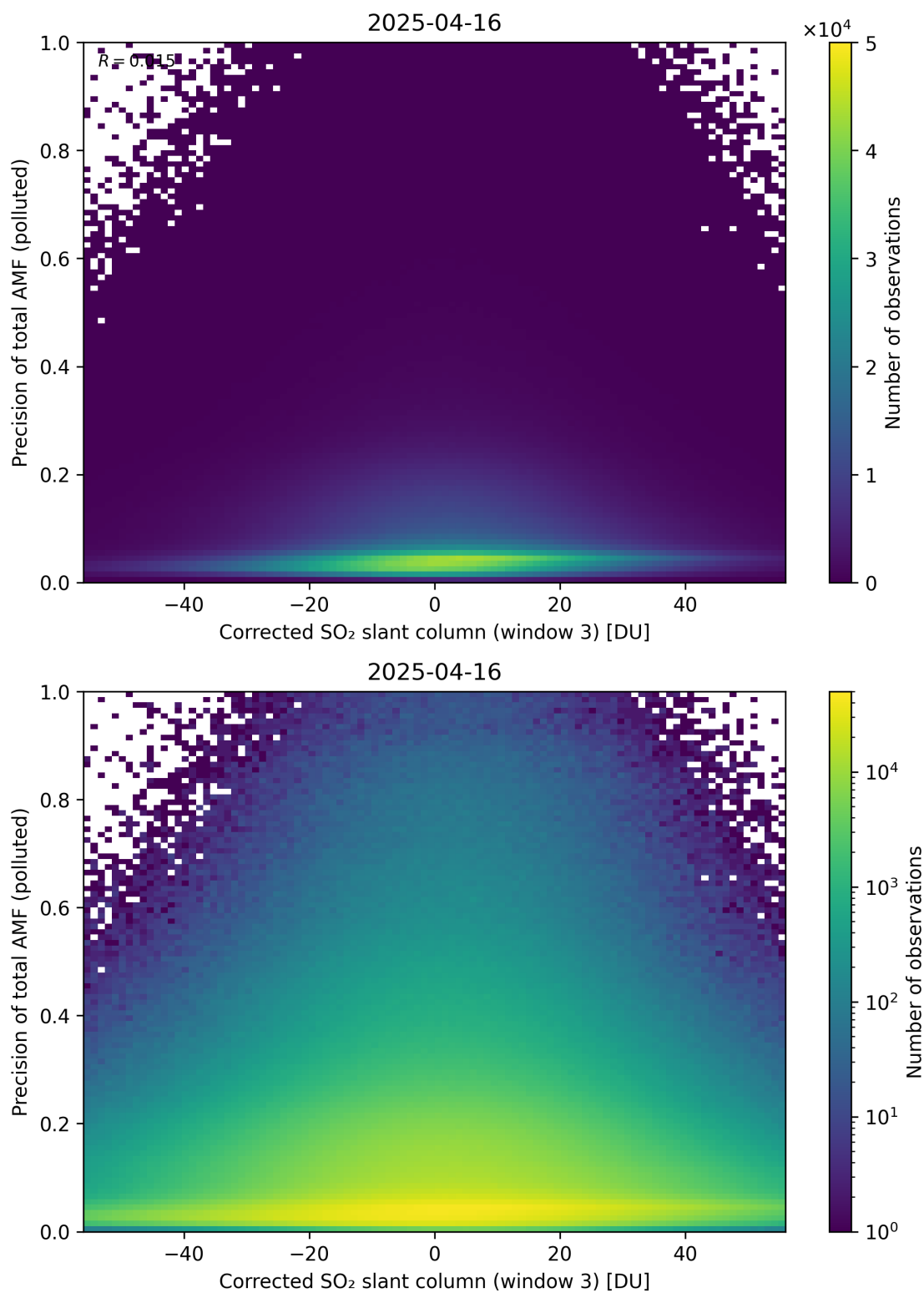
Figure 261: Scatter density plot of “Corrected SO 2 slant column (window 3)” against “Precision of total AMF (polluted)” for 2025-04-15 to 2025-04-17.
