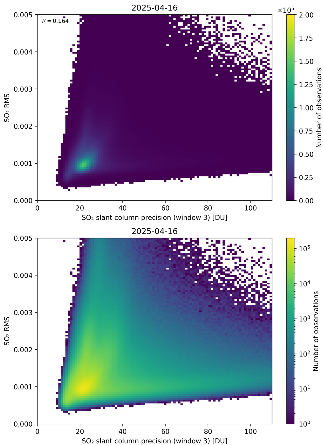
Figure 310: Scatter density plot of “SO 2 slant column precision (window 3)” against “SO 2 RMS” for 2025-04-15 to 2025-04-17.
