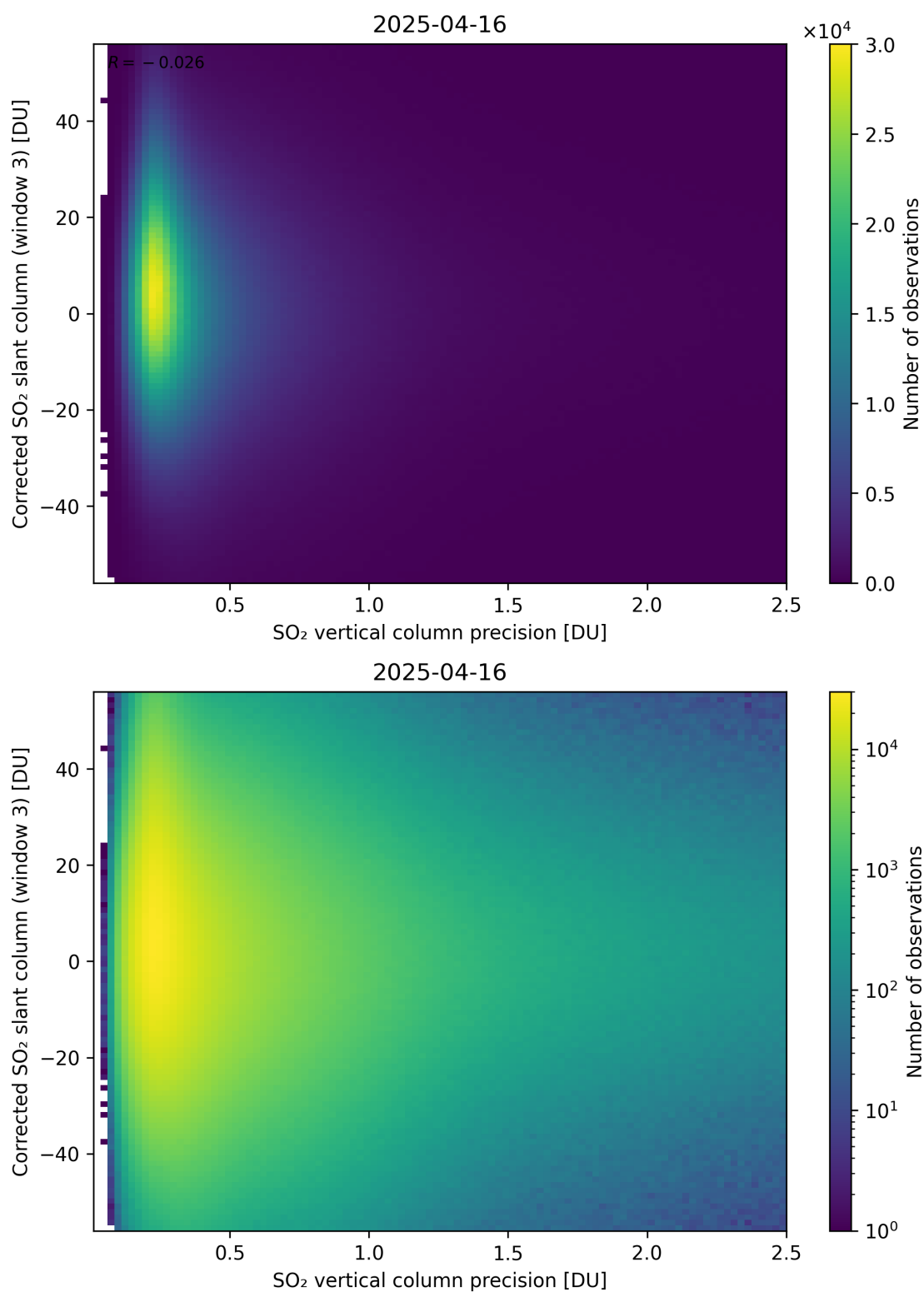
Figure 340: Scatter density plot of “SO 2 vertical column precision” against “Corrected SO 2 slant column (window 3)” for 2025-04-15 to 2025-04-17.
