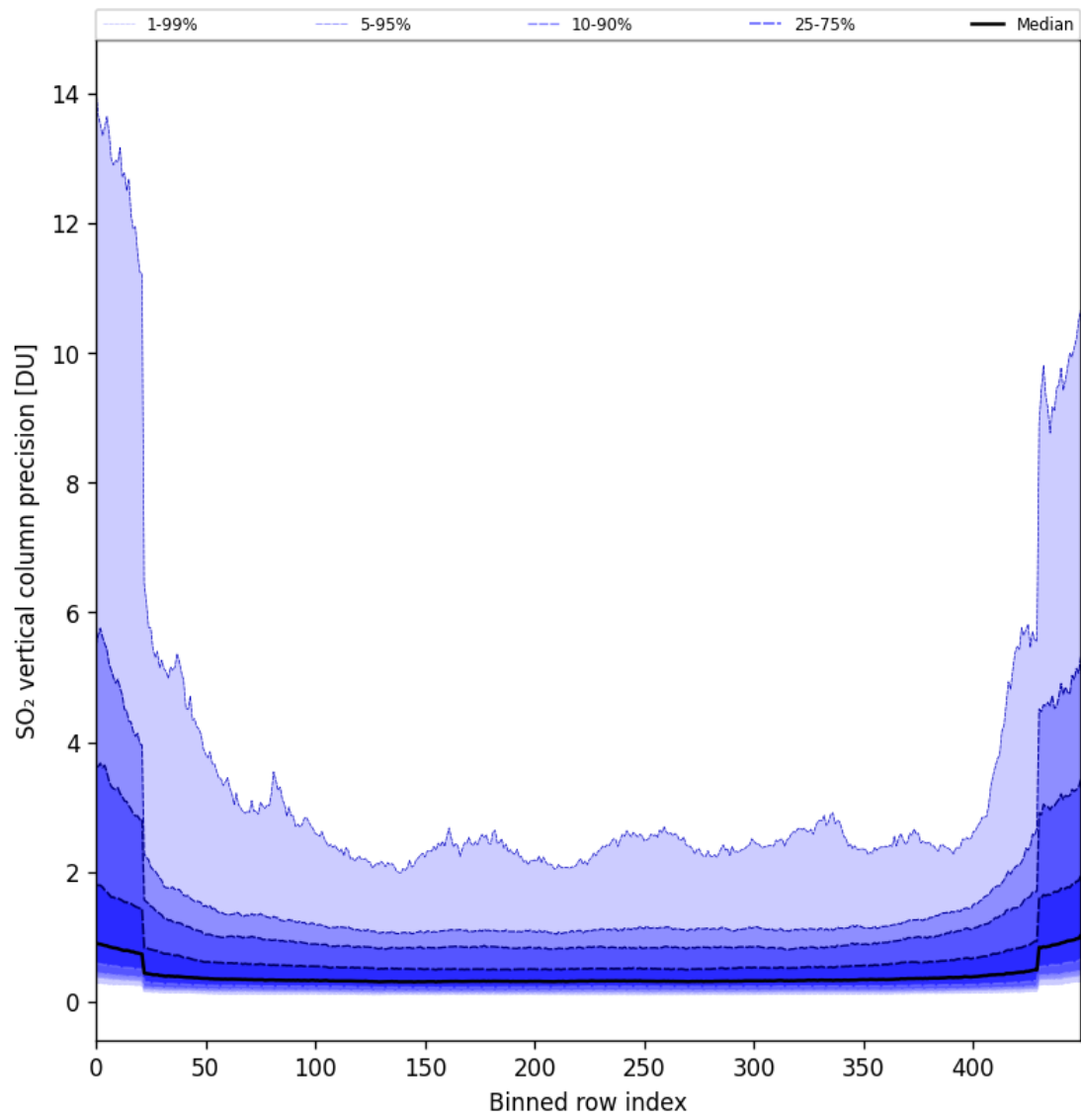
Figure 85: Along track statistics of “SO 2 vertical column precision” for 2025-04-15 to 2025-04-17
