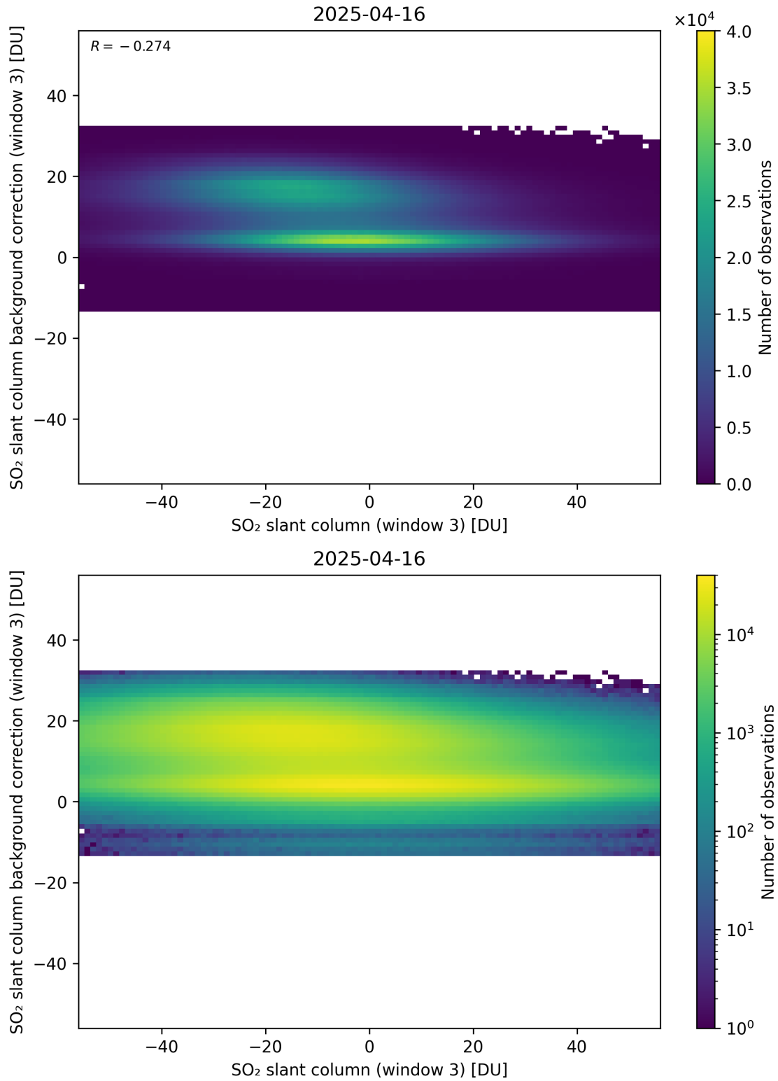
Figure 303: Scatter density plot of “SO 2 slant column (window 3)” against “SO 2 slant column background correction (window 3)” for 2025-04-15 to 2025-04-17.
