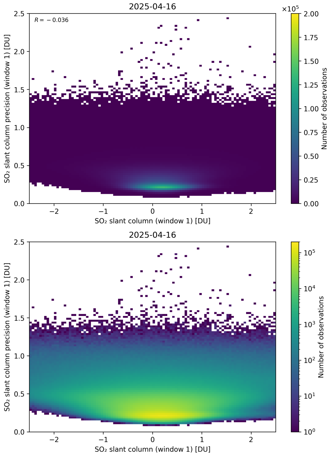
Figure 285: Scatter density plot of “SO 2 slant column (window 1)” against “SO 2 slant column precision (window 1)” for 2025-04-15 to 2025-04-17.
