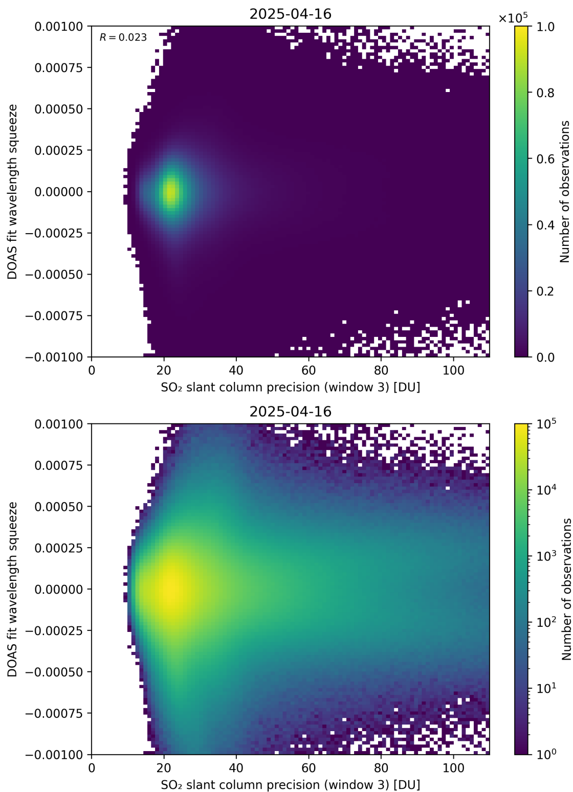
Figure 309: Scatter density plot of “SO 2 slant column precision (window 3)” against “DOAS fit wavelength squeeze” for 2025-04-15 to 2025-04-17.
