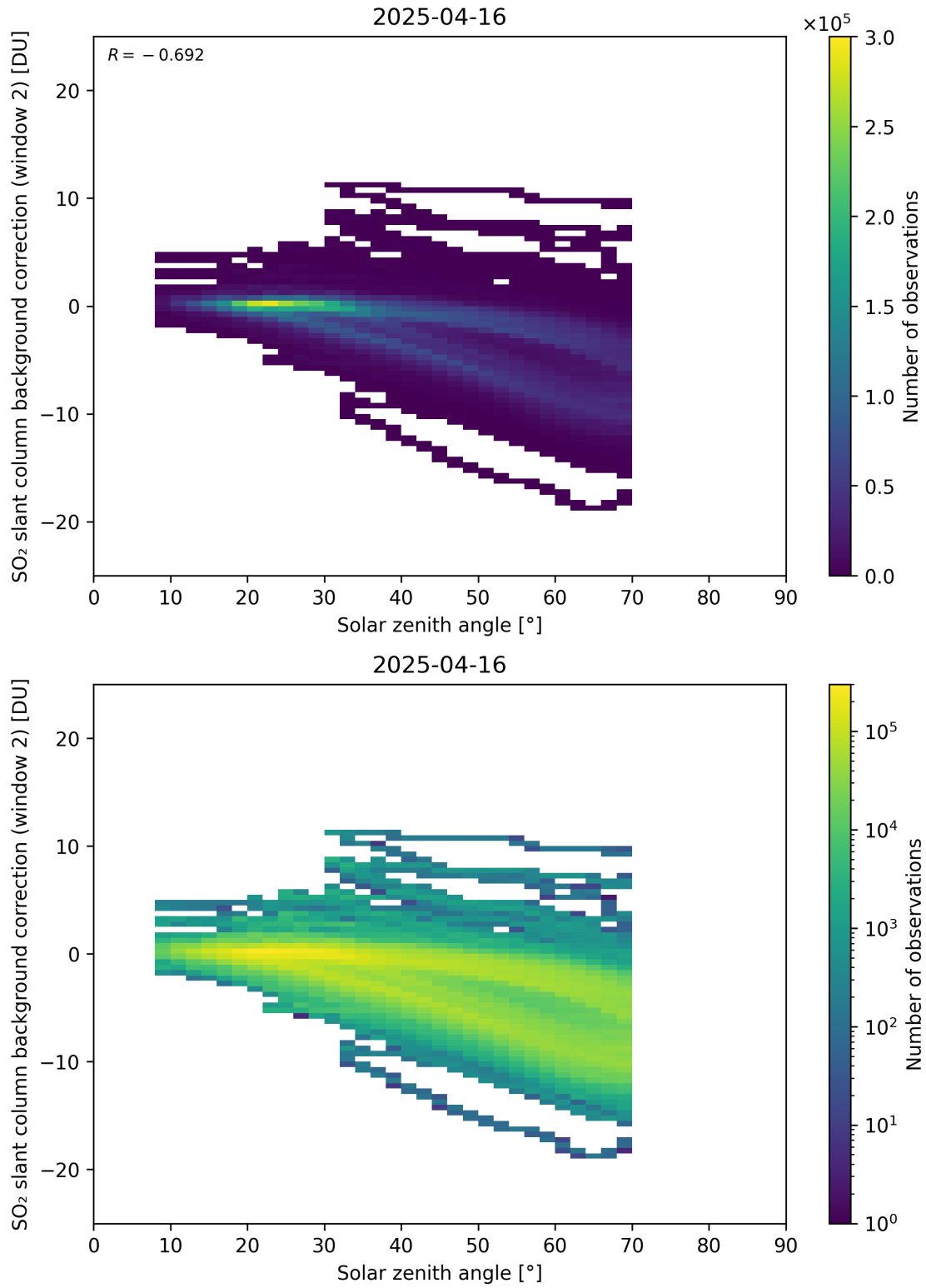
Figure 172: Scatter density plot of “Solar zenith angle” against “SO 2 slant column background correction (window 2)” for 2025-04-15 to 2025-04-17.
