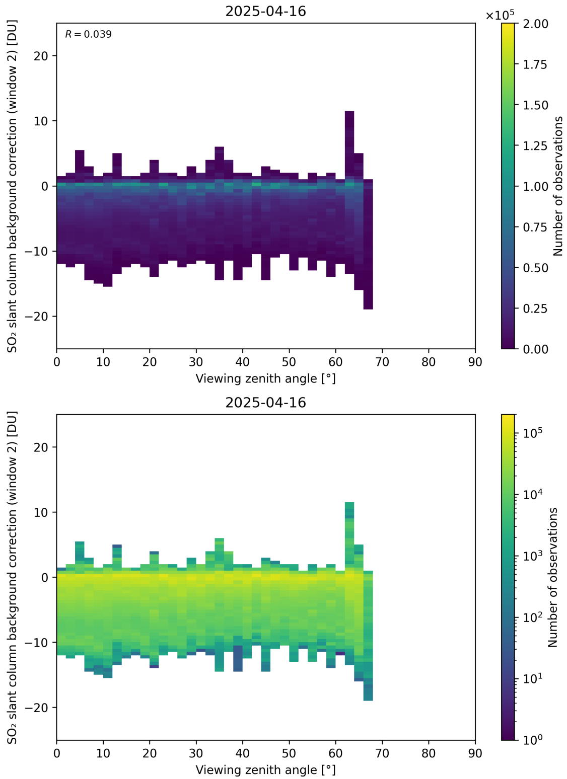
Figure 363: Scatter density plot of “Viewing zenith angle” against “SO 2 slant column background correction (window 2)” for 2025-04-15 to 2025-04-17.
