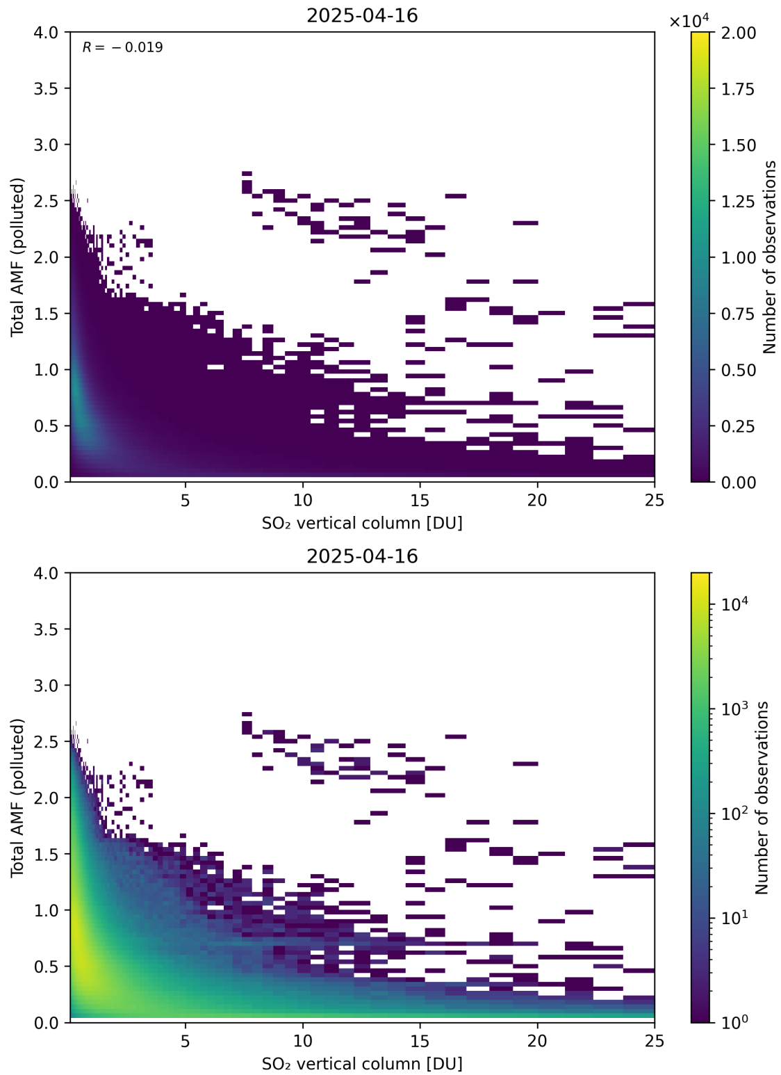
Figure 359: Scatter density plot of “SO 2 vertical column” against “Total AMF (polluted)” for 2025-04-15 to 2025-04-17.
