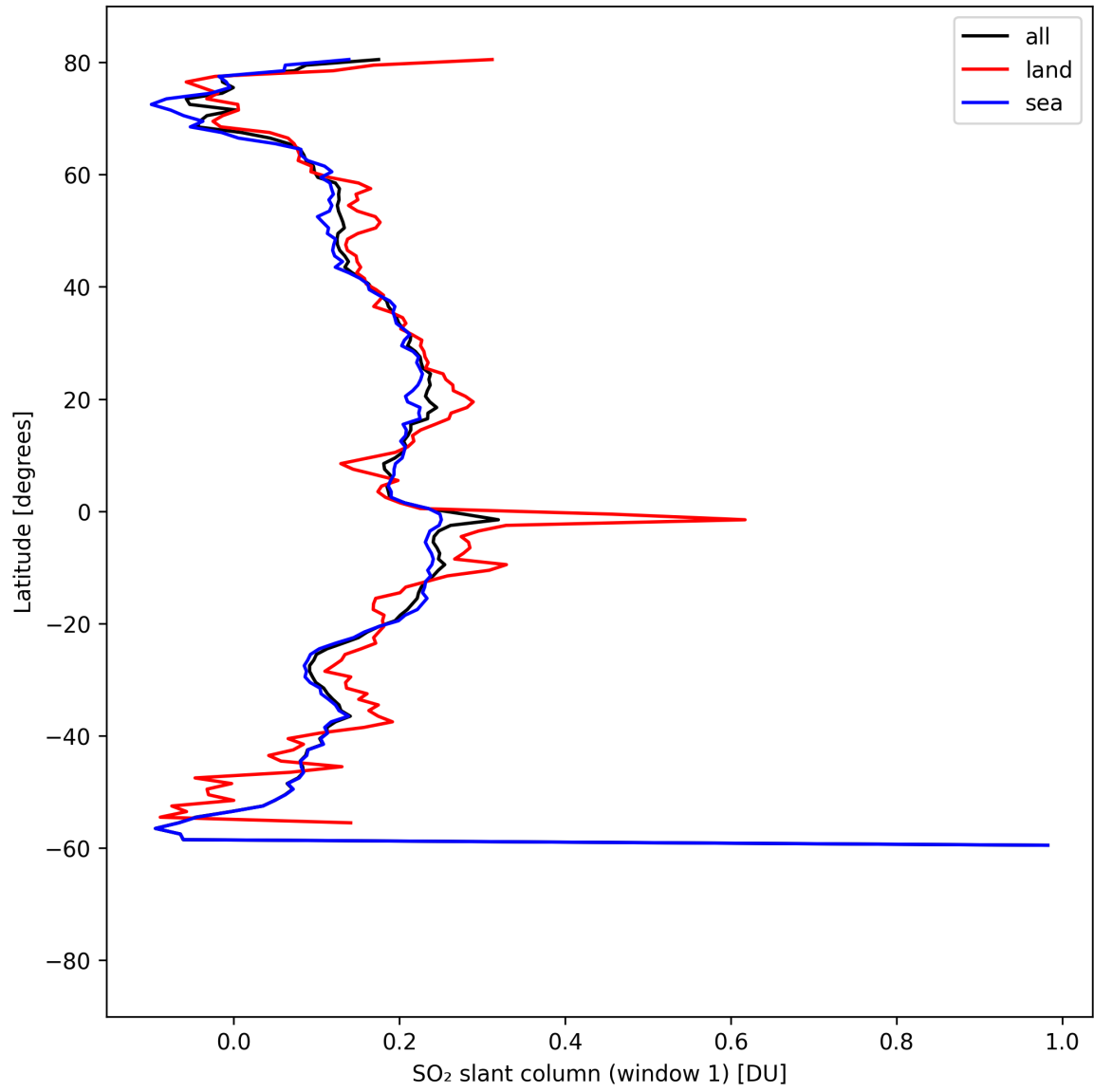
Figure 37: Zonal average of “SO 2 slant column (window 1)” for 2025-04-15 to 2025-04-17.
