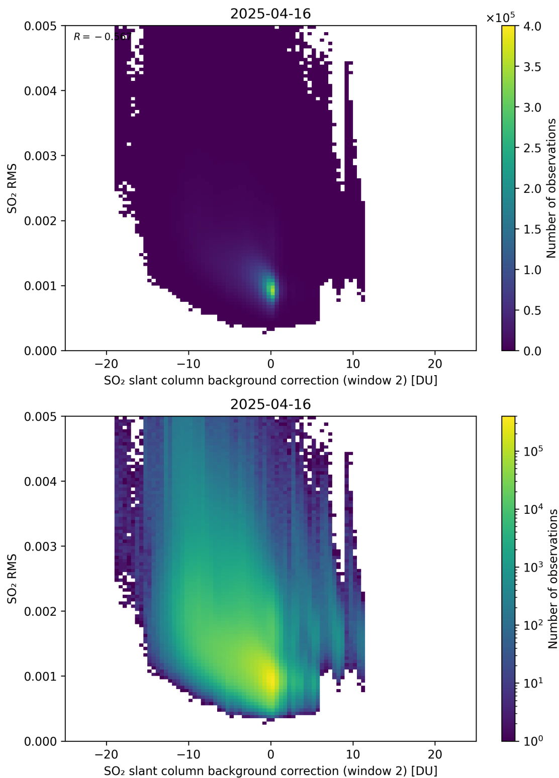
Figure 125: Scatter density plot of “SO 2 slant column background correction (window 2)” against “SO 2 RMS” for 2025-04-15 to 2025-04-17.
