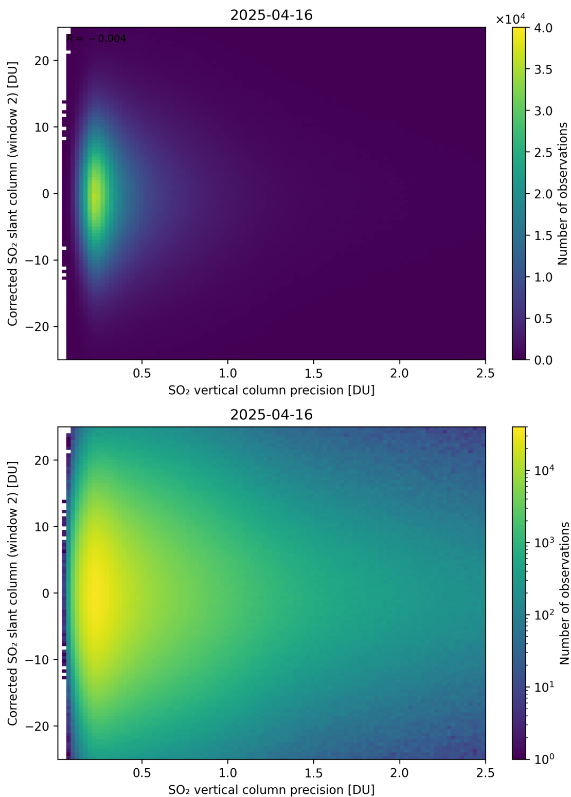
Figure 339: Scatter density plot of “SO 2 vertical column precision” against “Corrected SO 2 slant column (window 2)” for 2025-04-15 to 2025-04-17.
