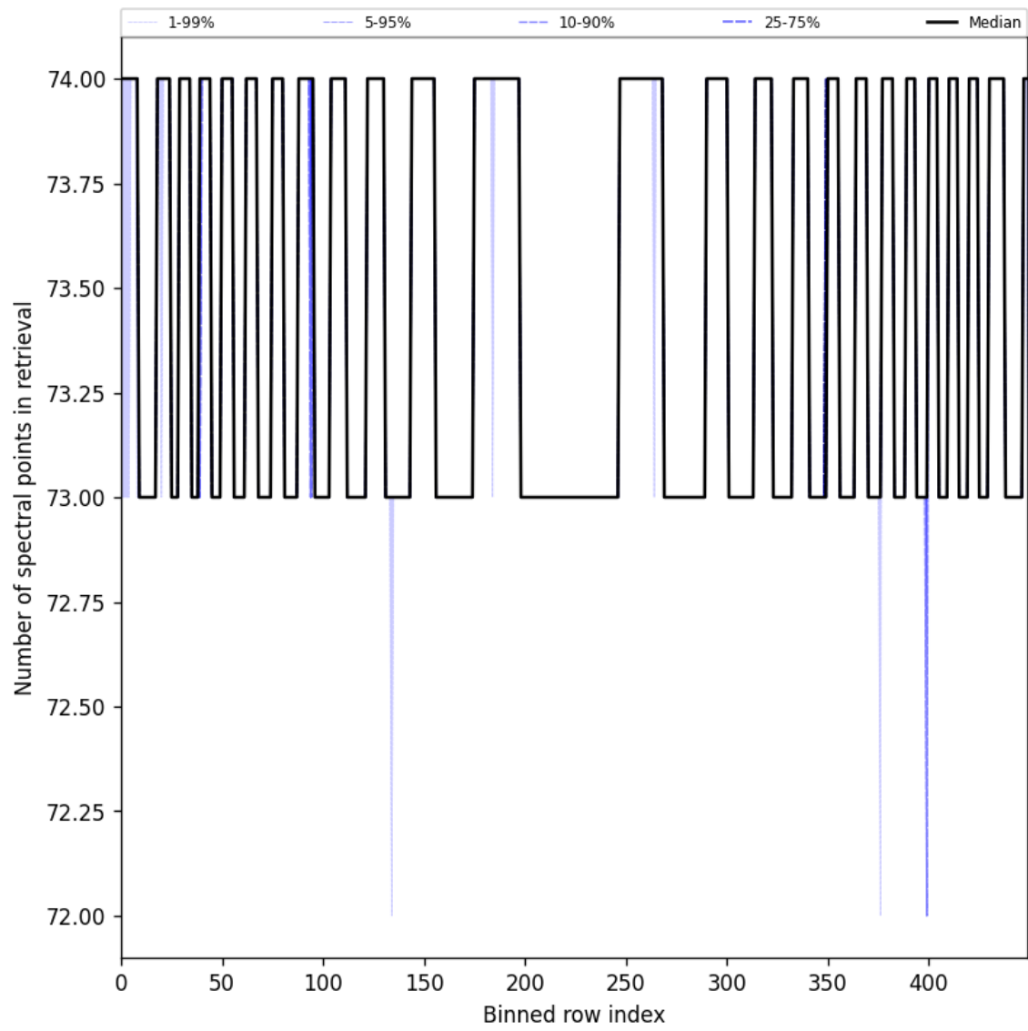
Figure 108: Along track statistics of “Number of spectral points in retrieval” for 2025-04-15 to 2025-04-17
