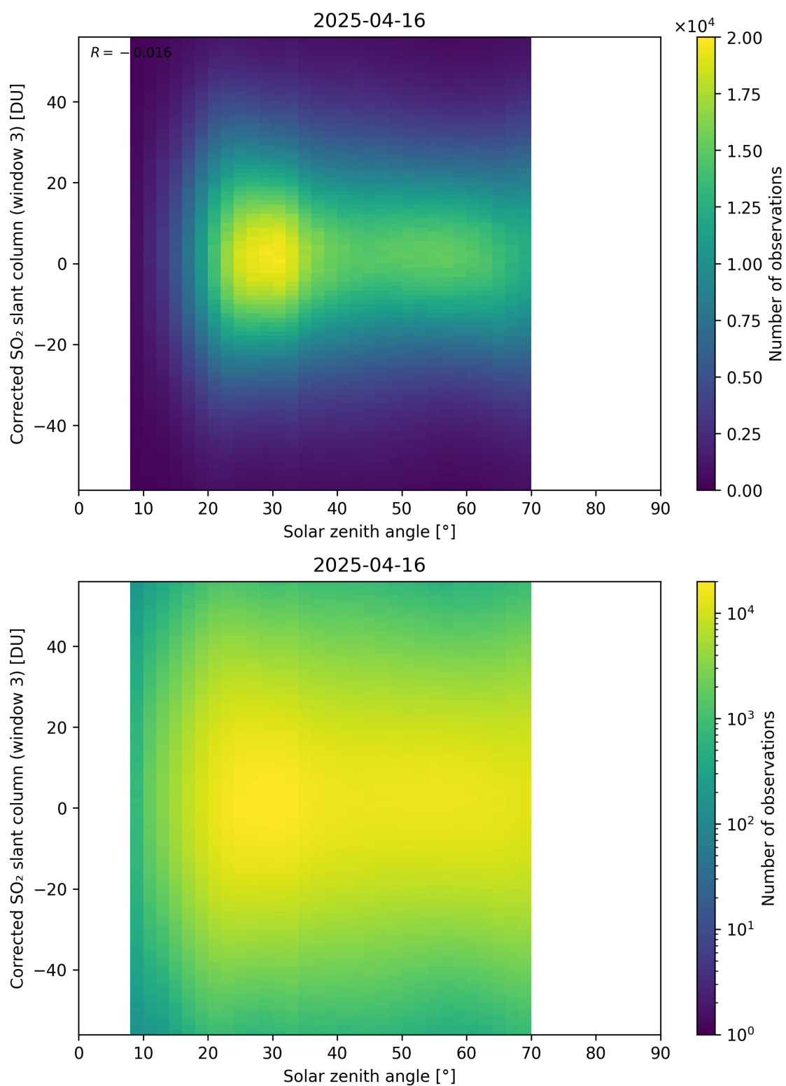
Figure 183: Scatter density plot of “Solar zenith angle” against “Corrected SO 2 slant column (window 3)” for 2025-04-15 to 2025-04-17.
