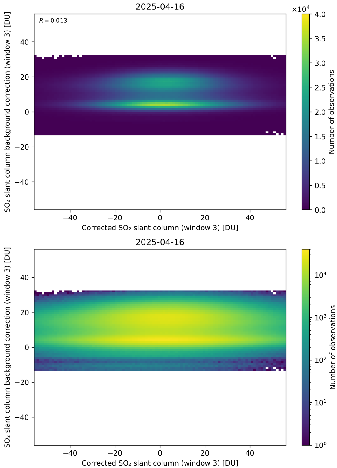
Figure 255: Scatter density plot of “Corrected SO 2 slant column (window 3)” against “SO 2 slant column background correction (window 3)” for 2025-04-15 to 2025-04-17.
