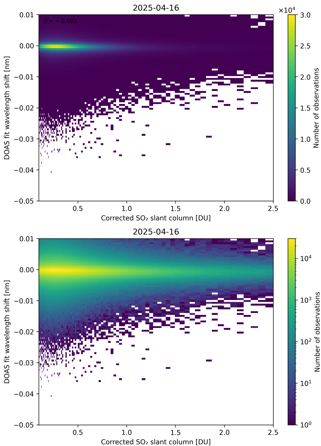
Figure 229: Scatter density plot of “Corrected SO 2 slant column” against “DOAS fit wavelength shift” for 2025-04-15 to 2025-04-17.
