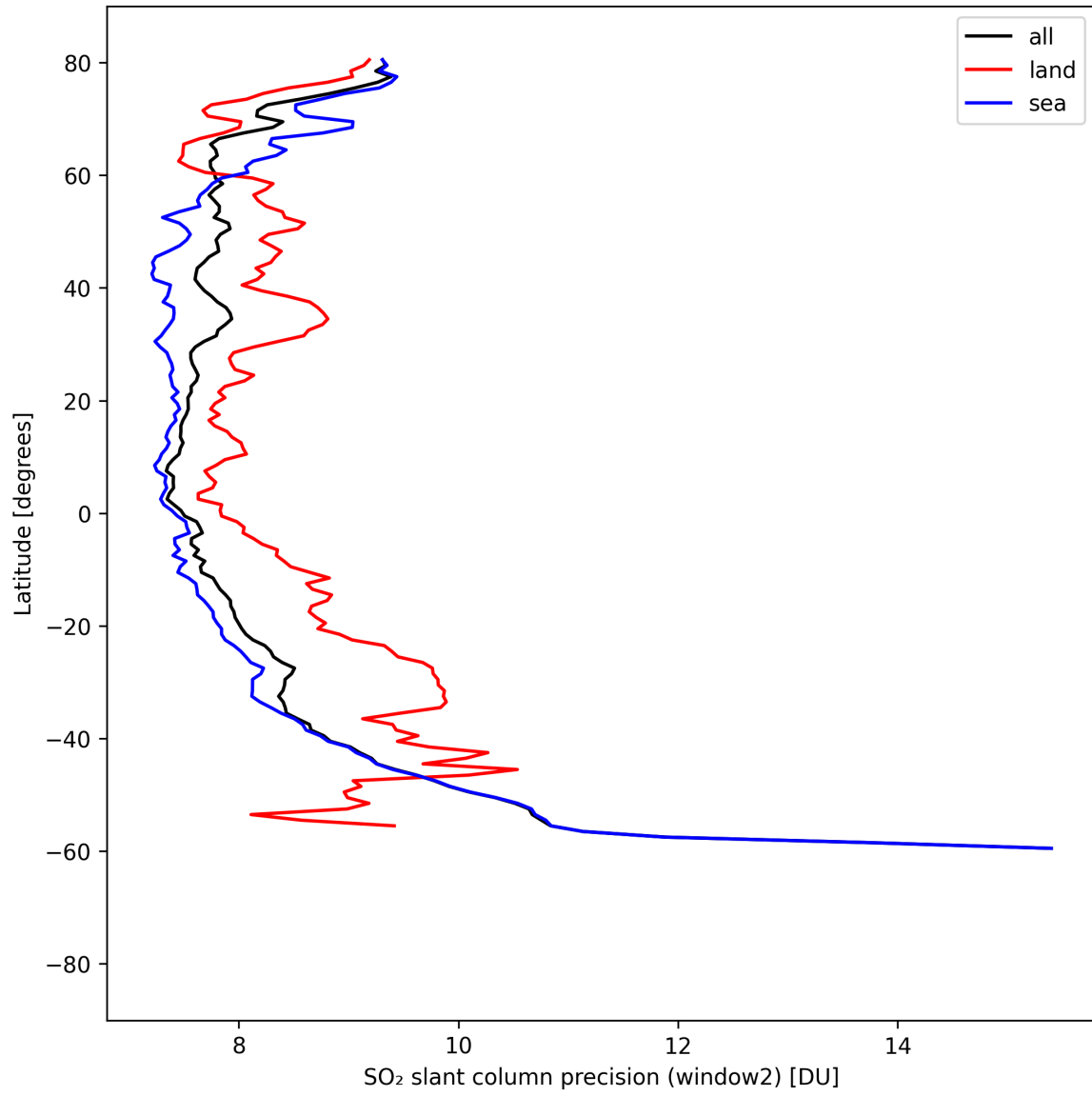
Figure 42: Zonal average of “SO 2 slant column precision (window2)” for 2025-04-15 to 2025-04-17.
