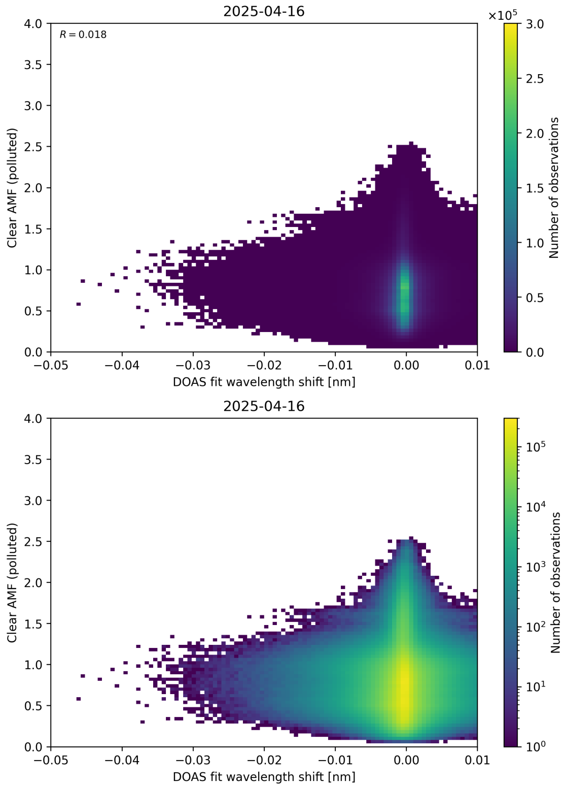
Figure 140: Scatter density plot of “DOAS fit wavelength shift” against “Clear AMF (polluted)” for 2025-04-15 to 2025-04-17.
