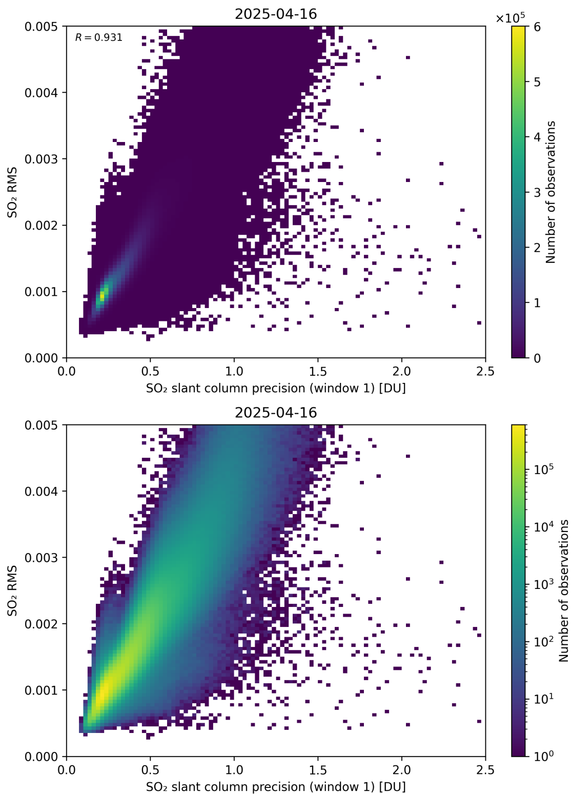
Figure 273: Scatter density plot of “SO 2 slant column precision (window 1)” against “SO 2 RMS” for 2025-04-15 to 2025-04-17.
