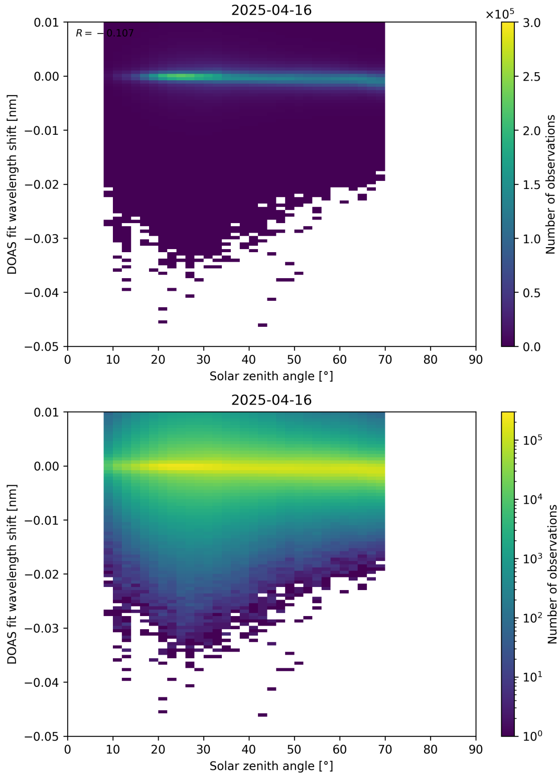
Figure 174: Scatter density plot of “Solar zenith angle” against “DOAS fit wavelength shift” for 2025-04-15 to 2025-04-17.
