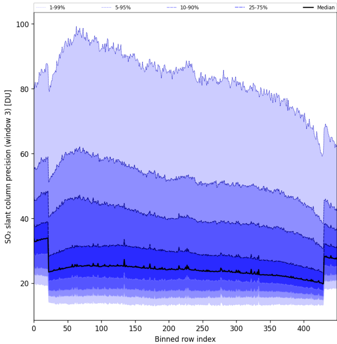
Figure 98: Along track statistics of “SO 2 slant column precision (window 3)” for 2025-04-15 to 2025-04-17
