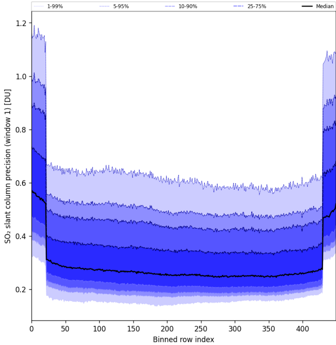
Figure 90: Along track statistics of “SO 2 slant column precision (window 1)” for 2025-04-15 to 2025-04-17
