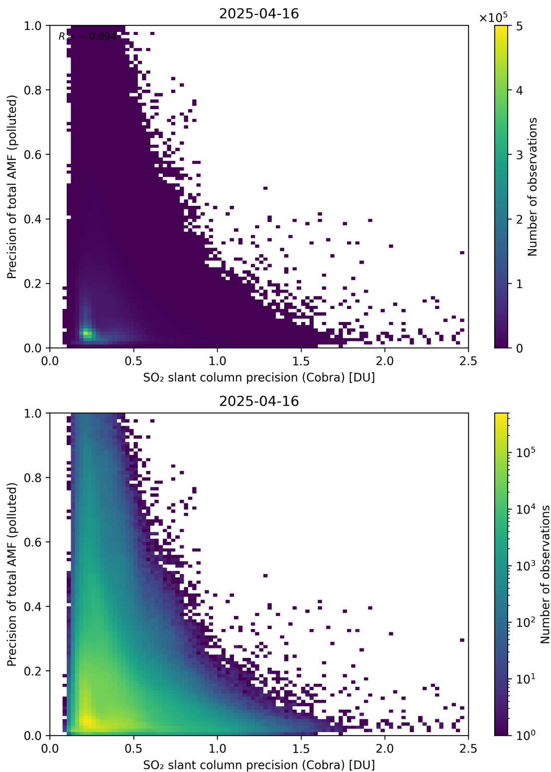
Figure 214: Scatter density plot of “SO 2 slant column precision (Cobra)” against “Precision of total AMF (polluted)” for 2025-04-15 to 2025-04-17.
