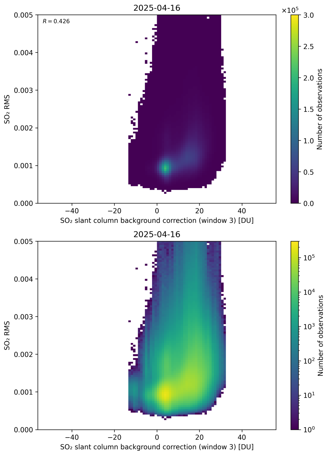
Figure 134: Scatter density plot of “SO 2 slant column background correction (window 3)” against “SO 2 RMS” for 2025-04-15 to 2025-04-17.
