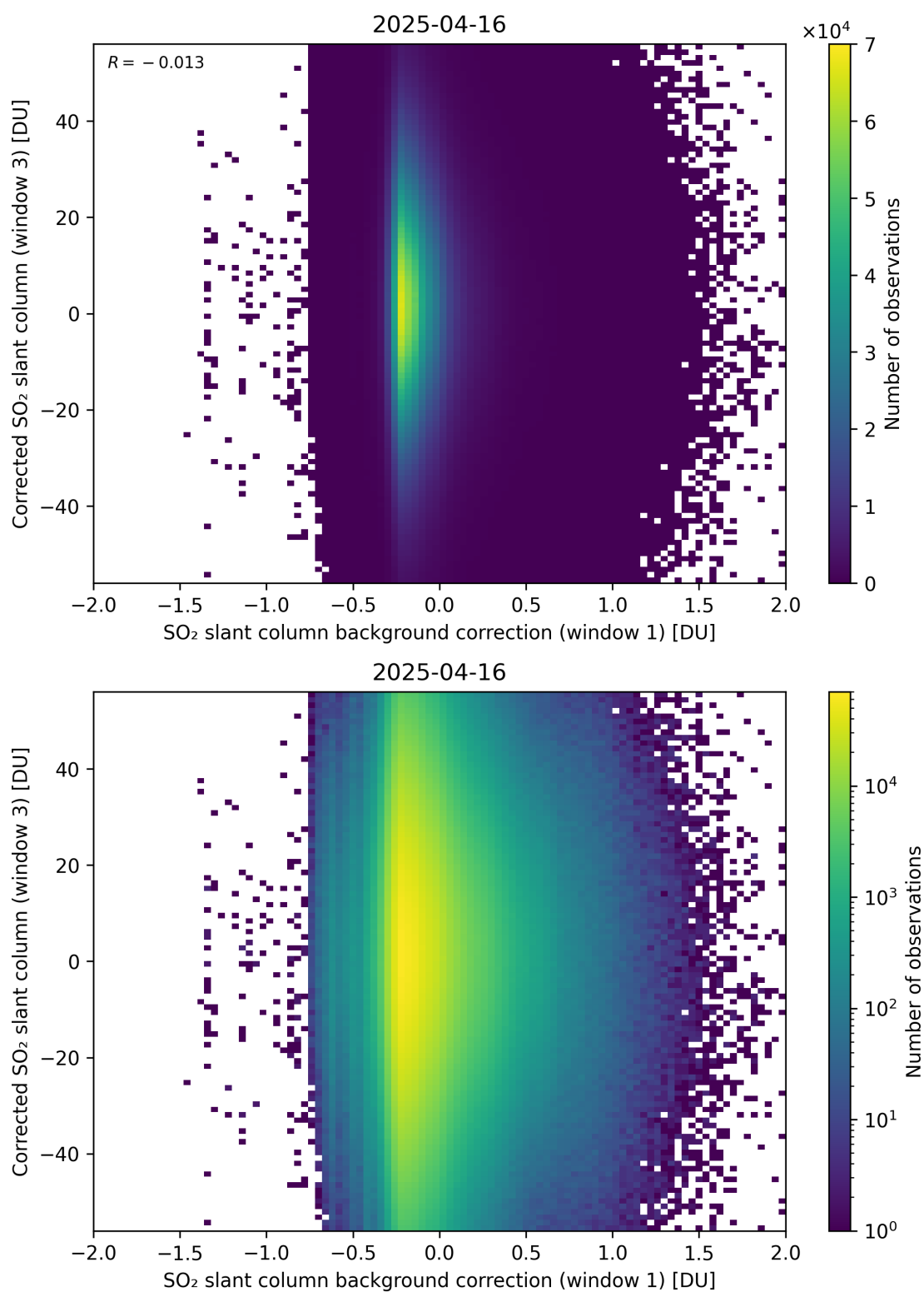
Figure 116: Scatter density plot of “SO 2 slant column background correction (window 1)” against “Corrected SO 2 slant column (window 3)” for 2025-04-15 to 2025-04-17.
