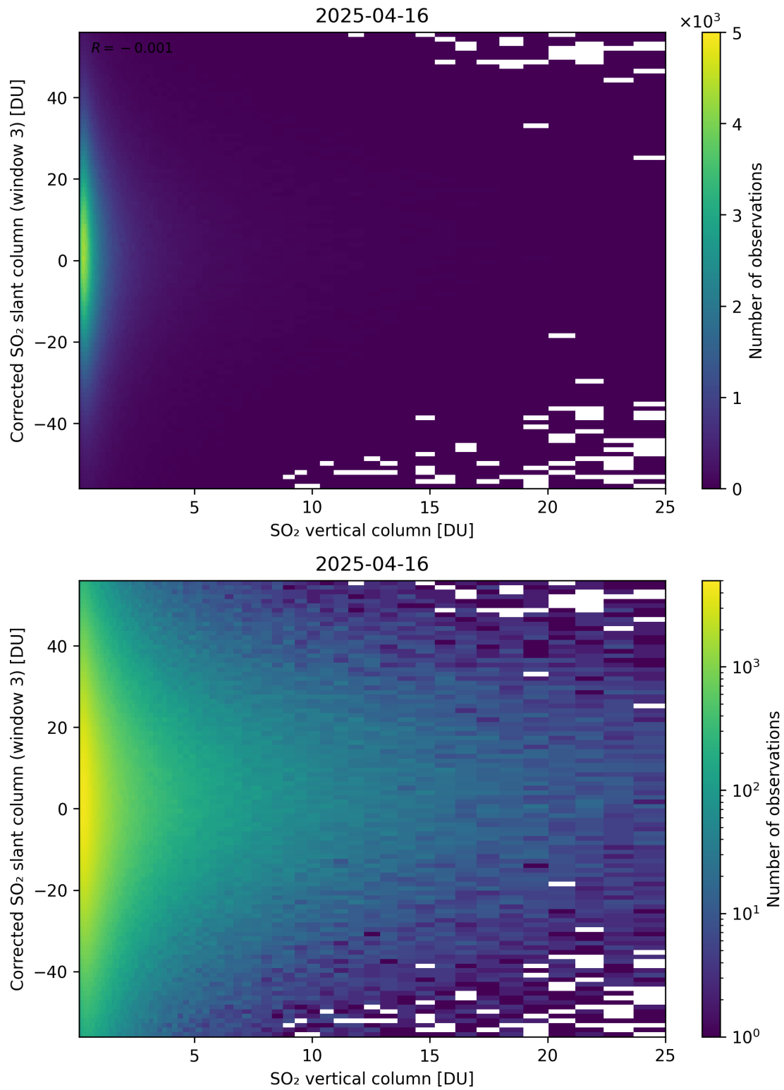
Figure 353: Scatter density plot of “SO 2 vertical column” against “Corrected SO 2 slant column (window 3)” for 2025-04-15 to 2025-04-17.
