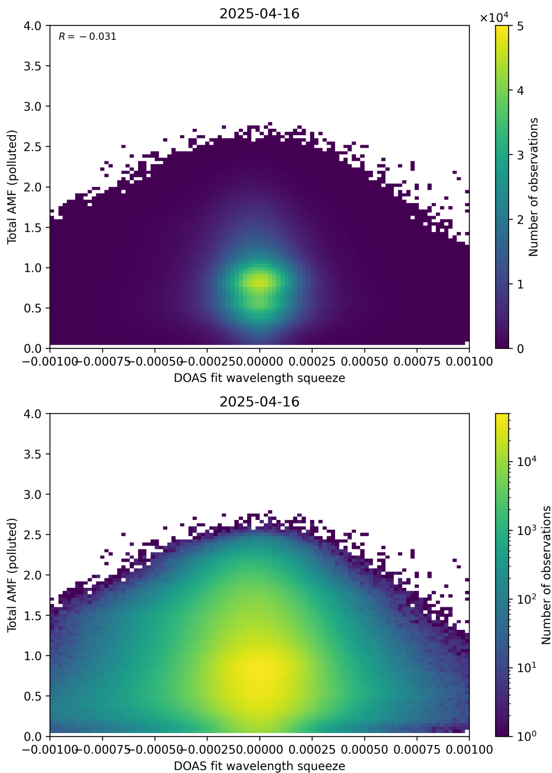
Figure 145: Scatter density plot of “DOAS fit wavelength squeeze” against “Total AMF (polluted)” for 2025-04-15 to 2025-04-17.
