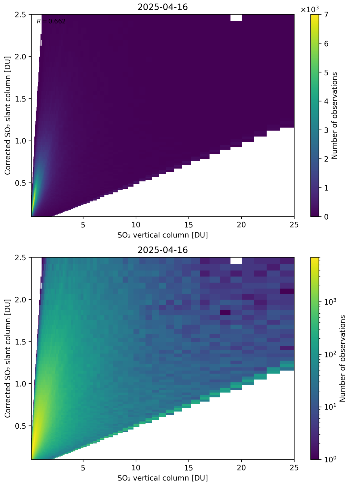
Figure 351: Scatter density plot of “SO 2 vertical column” against “Corrected SO 2 slant column” for 2025-04-15 to 2025-04-17.
