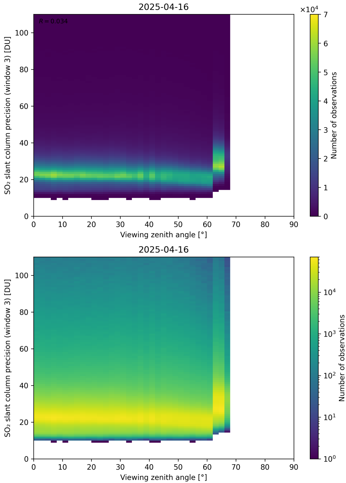
Figure 380: Scatter density plot of “Viewing zenith angle” against “SO 2 slant column precision (window 3)” for 2025-04-15 to 2025-04-17.
