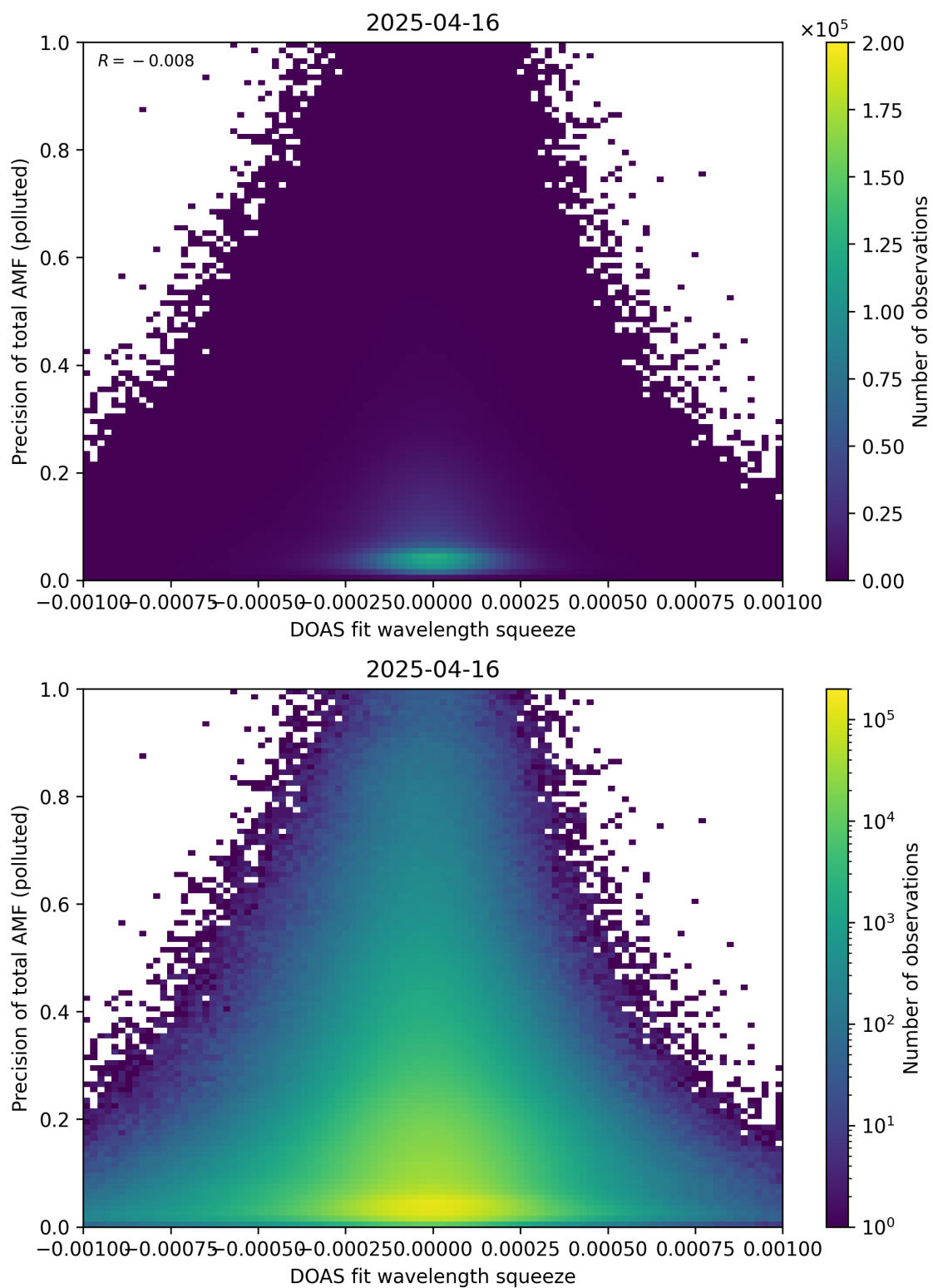
Figure 146: Scatter density plot of “DOAS fit wavelength squeeze” against “Precision of total AMF (polluted)” for 2025-04-15 to 2025-04-17.
