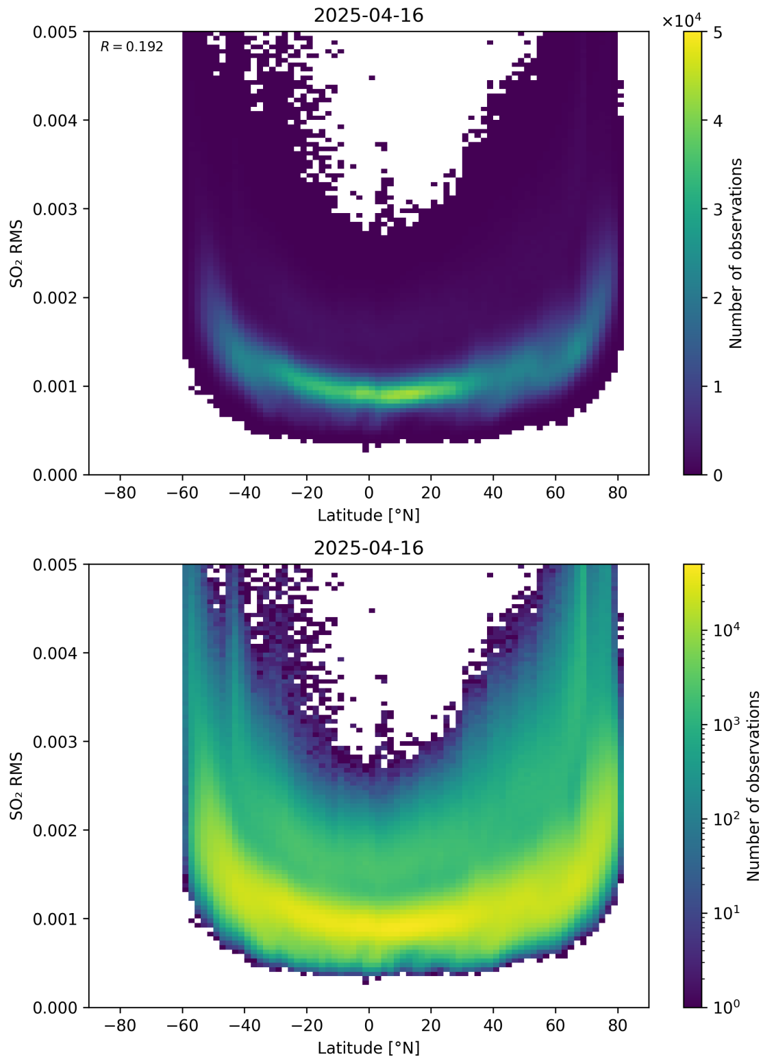
Figure 155: Scatter density plot of “Latitude” against “SO 2 RMS” for 2025-04-15 to 2025-04-17.
