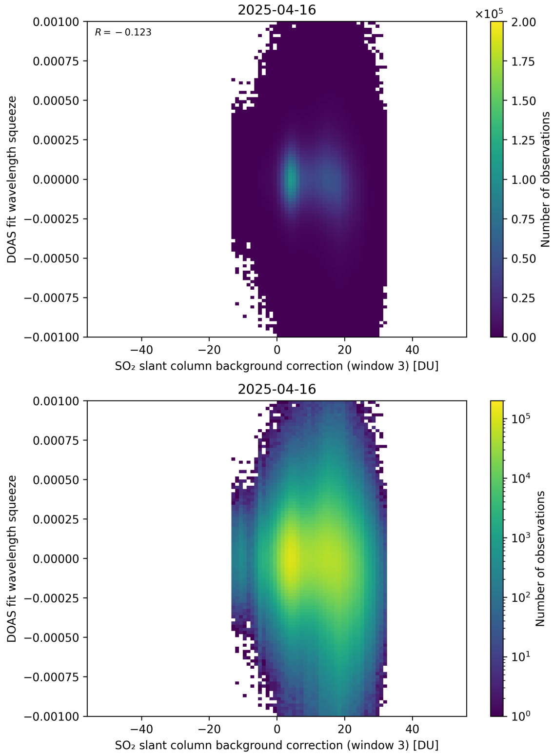
Figure 133: Scatter density plot of “SO 2 slant column background correction (window 3)” against “DOAS fit wavelength squeeze” for 2025-04-15 to 2025-04-17.
