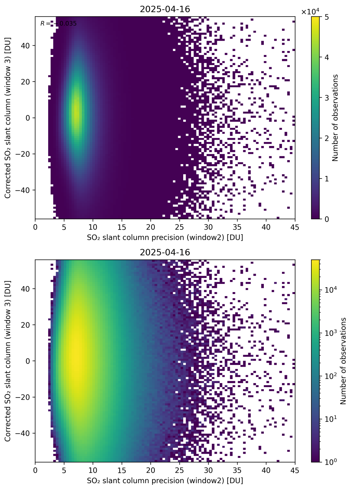
Figure 298: Scatter density plot of “SO 2 slant column precision (window2)” against “Corrected SO 2 slant column (window 3)” for 2025-04-15 to 2025-04-17.
