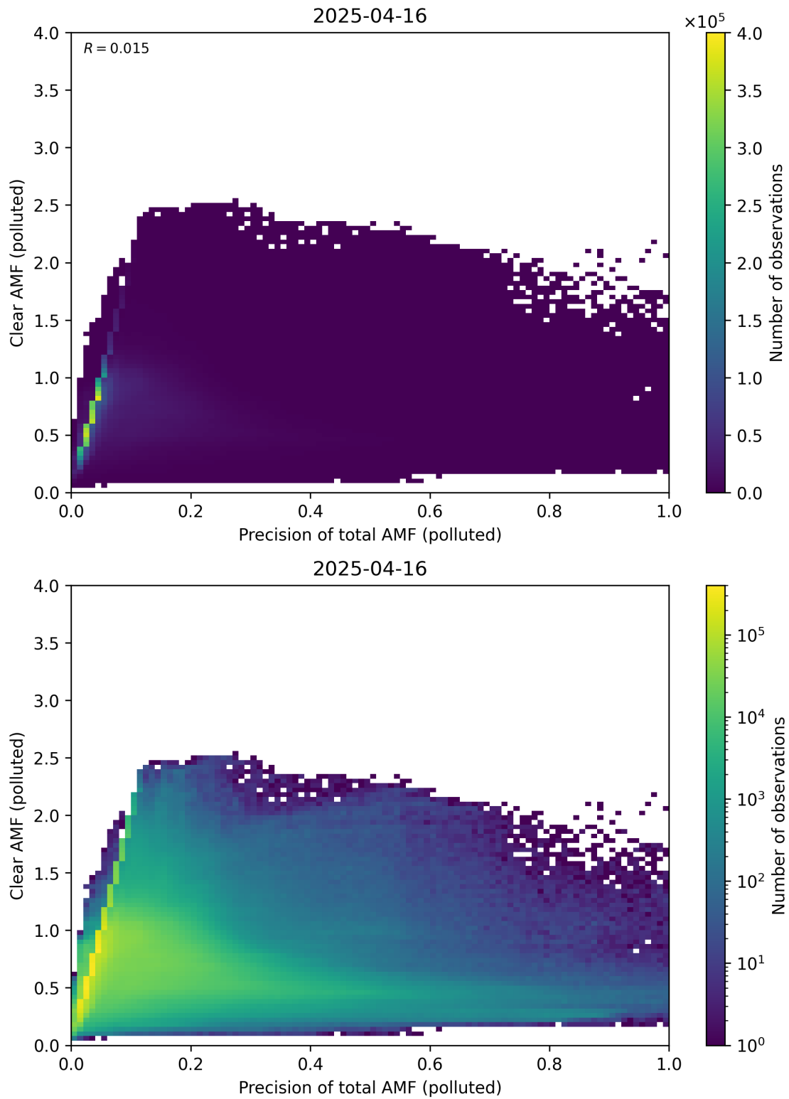
Figure 320: Scatter density plot of “Precision of total AMF (polluted)” against “Clear AMF (polluted)” for 2025-04-15 to 2025-04-17.
