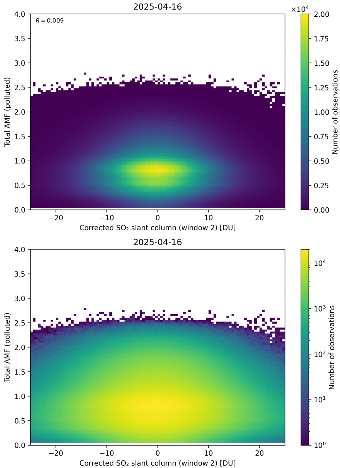
Figure 253: Scatter density plot of “Corrected SO 2 slant column (window 2)” against “Total AMF (polluted)” for 2025-04-15 to 2025-04-17.
