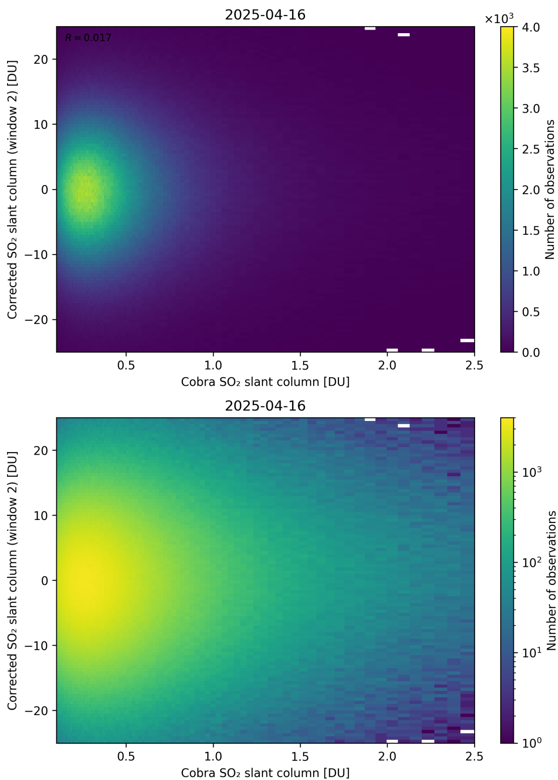
Figure 217: Scatter density plot of “Cobra SO 2 slant column” against “Corrected SO 2 slant column (window 2)” for 2025-04-15 to 2025-04-17.
