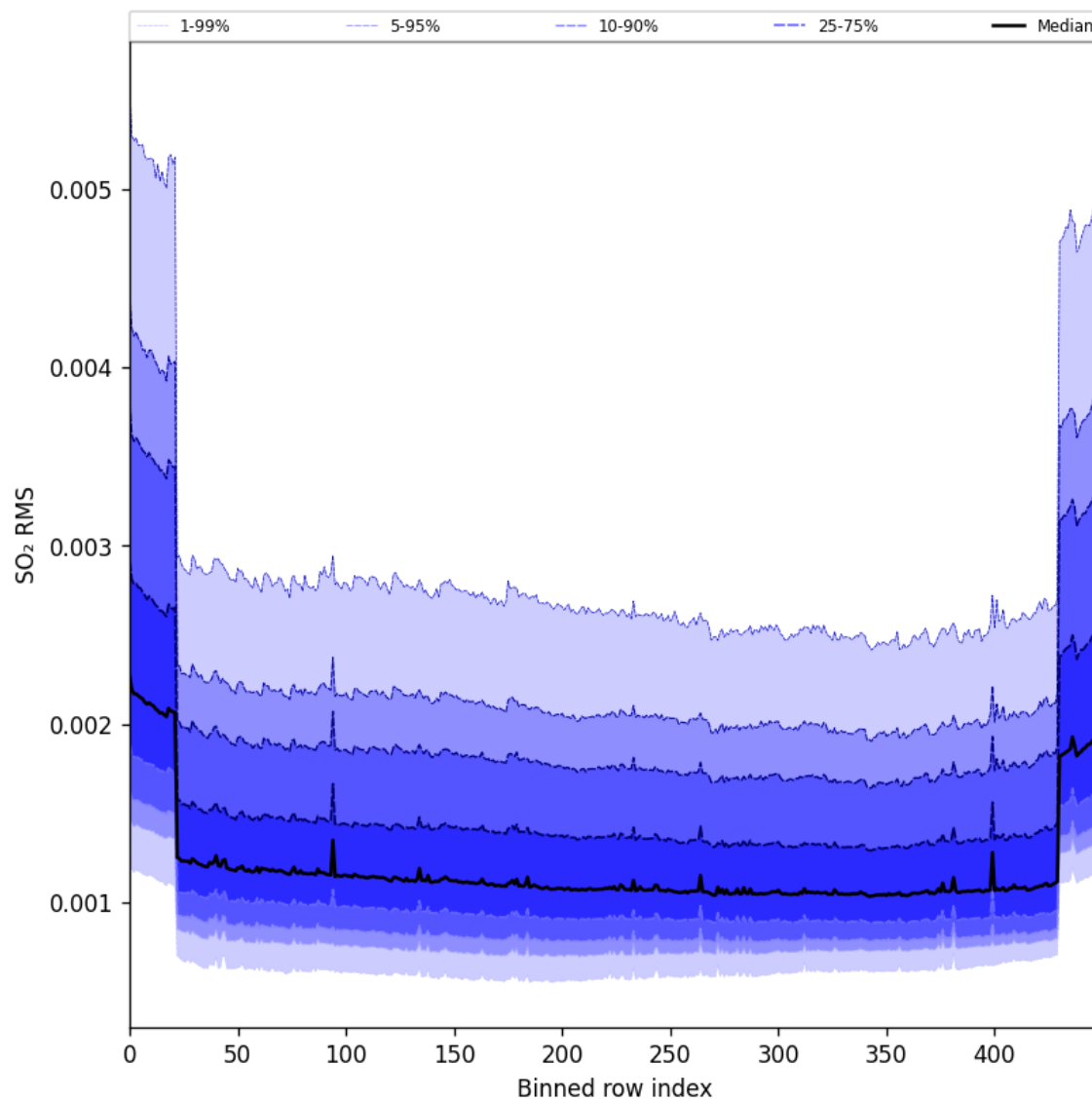
Figure 104: Along track statistics of “SO 2 RMS” for 2025-04-15 to 2025-04-17
