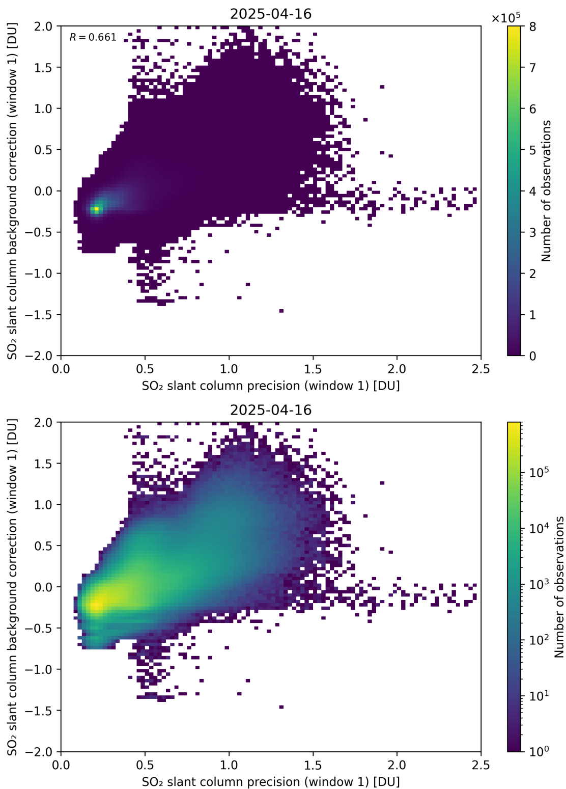
Figure 268: Scatter density plot of “SO 2 slant column precision (window 1)” against “SO 2 slant column background correction (window 1)” for 2025-04-15 to 2025-04-17.
