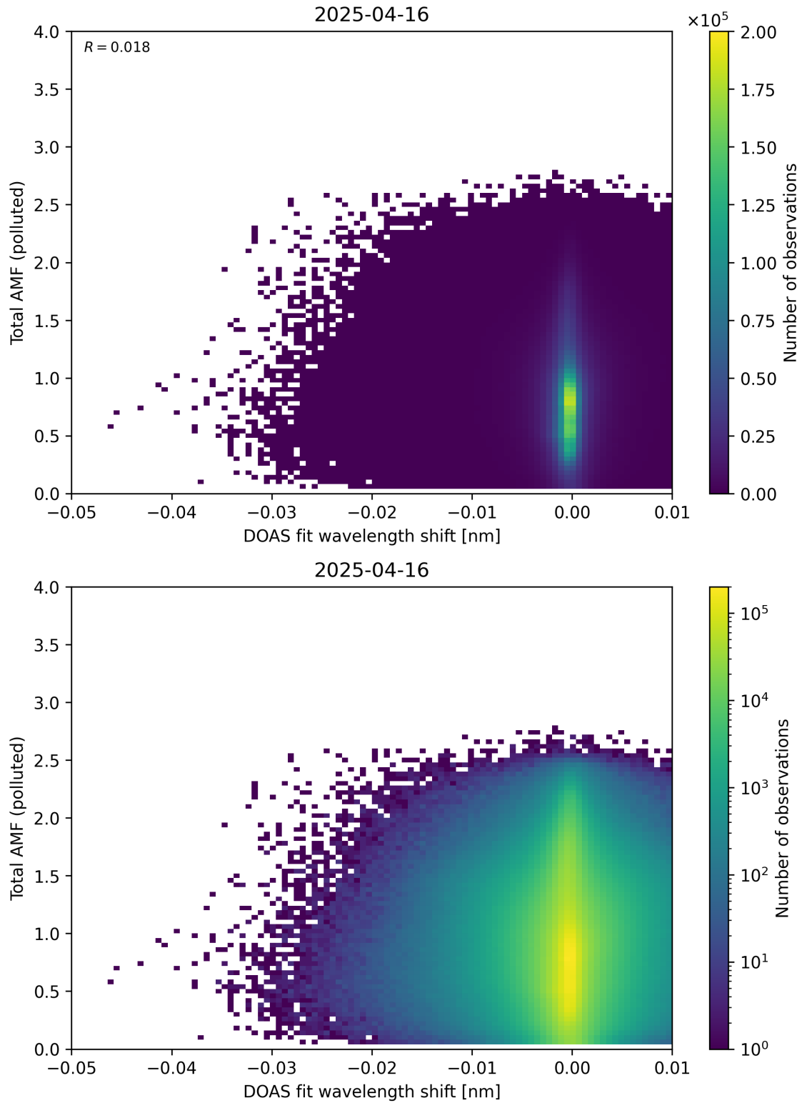
Figure 141: Scatter density plot of “DOAS fit wavelength shift” against “Total AMF (polluted)” for 2025-04-15 to 2025-04-17.
