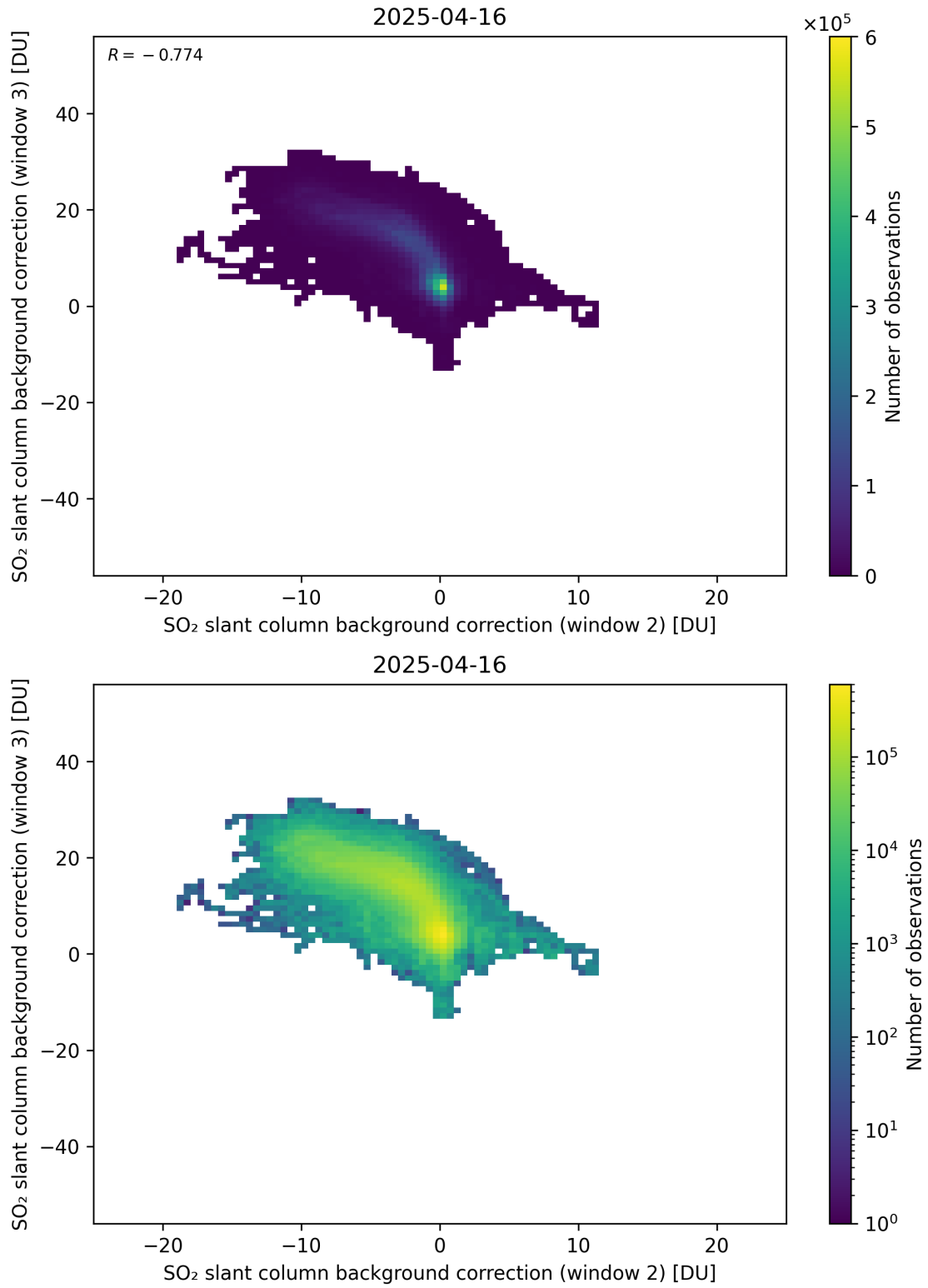
Figure 122: Scatter density plot of “SO 2 slant column background correction (window 2)” against “SO 2 slant column background correction (window 3)” for 2025-04-15 to 2025-04-17.
