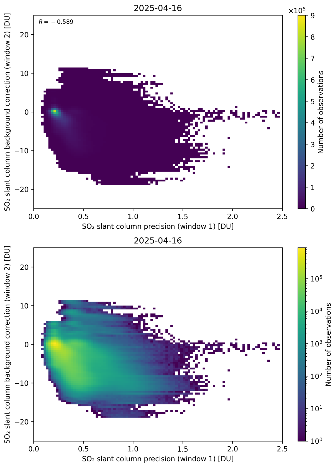
Figure 269: Scatter density plot of “SO 2 slant column precision (window 1)” against “SO 2 slant column background correction (window 2)” for 2025-04-15 to 2025-04-17.
