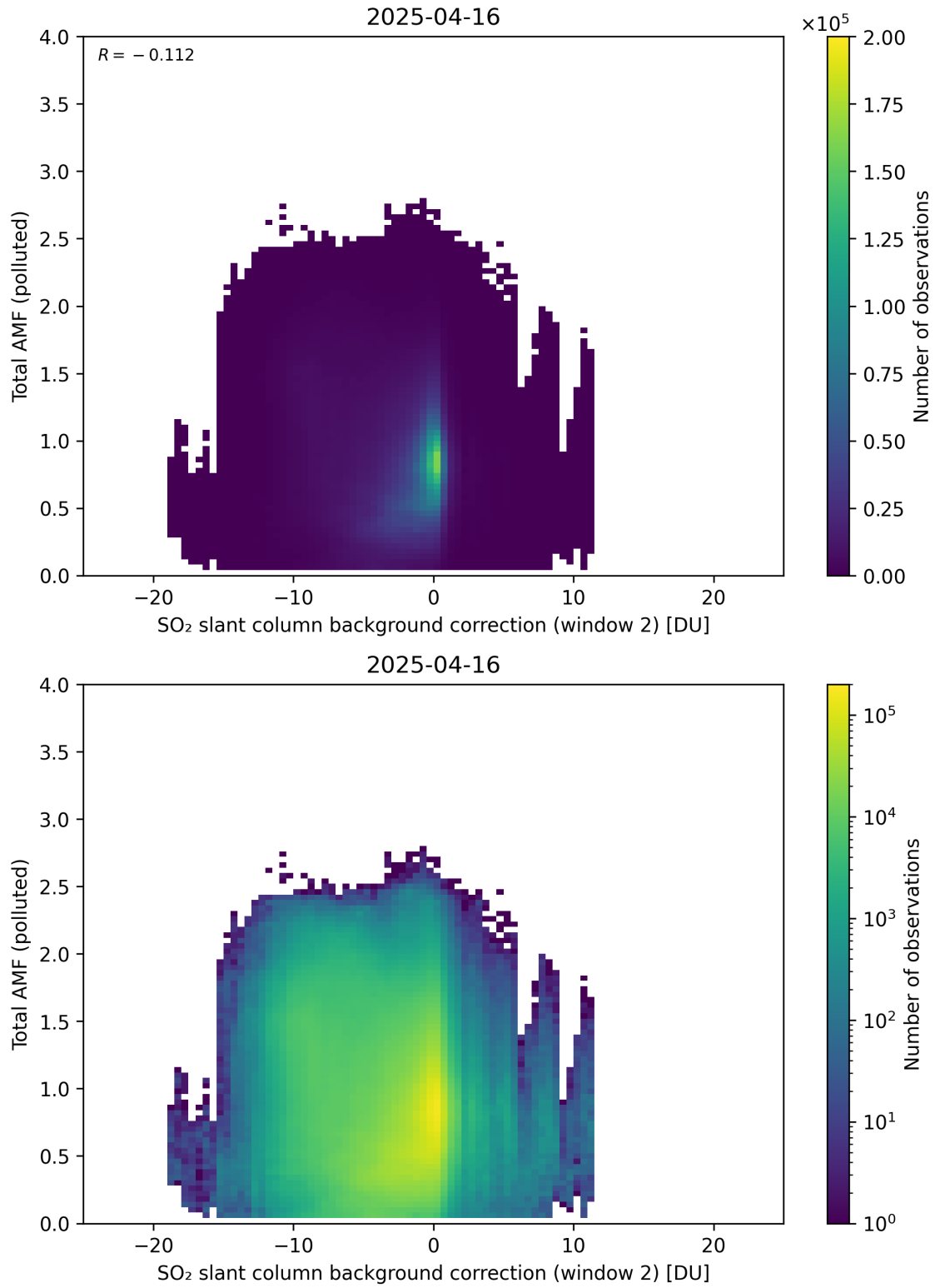
Figure 130: Scatter density plot of “SO 2 slant column background correction (window 2)” against “Total AMF (polluted)” for 2025-04-15 to 2025-04-17.
