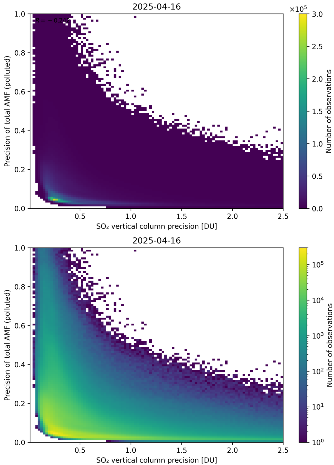
Figure 347: Scatter density plot of “SO 2 vertical column precision” against “Precision of total AMF (polluted)” for 2025-04-15 to 2025-04-17.
