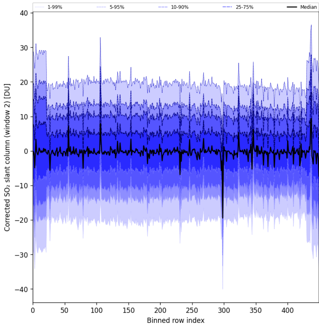
Figure 95: Along track statistics of “Corrected SO 2 slant column (window 2)” for 2025-04-15 to 2025-04-17
