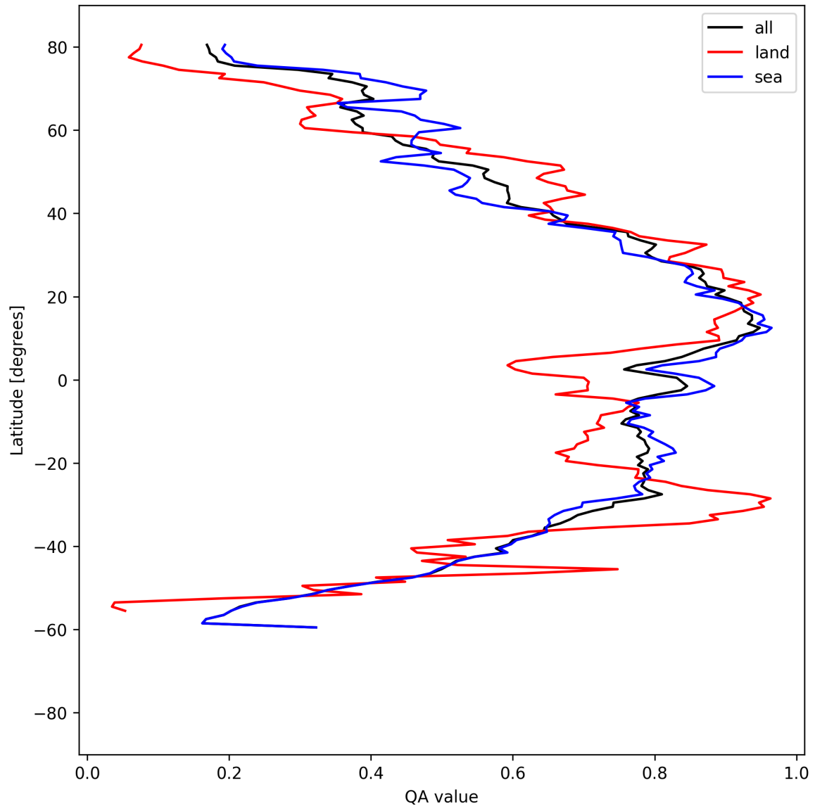
Figure 31: Zonal average of “QA value” for 2025-04-15 to 2025-04-17.
