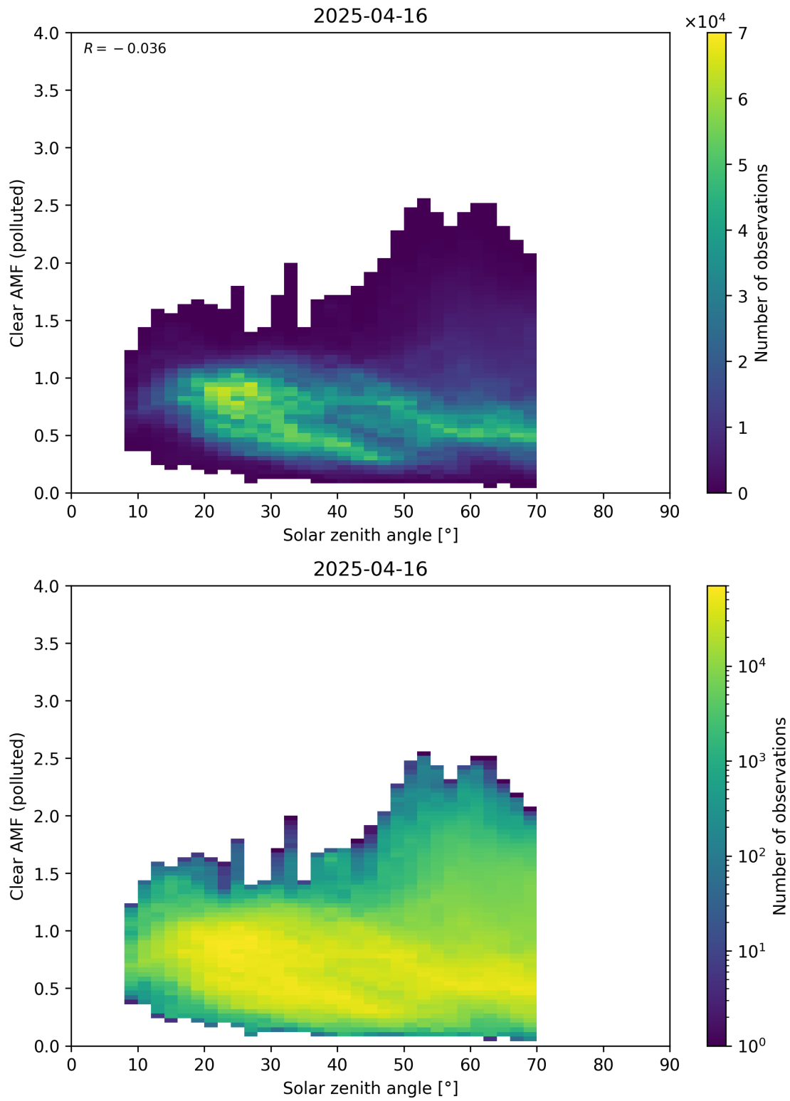
Figure 178: Scatter density plot of “Solar zenith angle” against “Clear AMF (polluted)” for 2025-04-15 to 2025-04-17.
