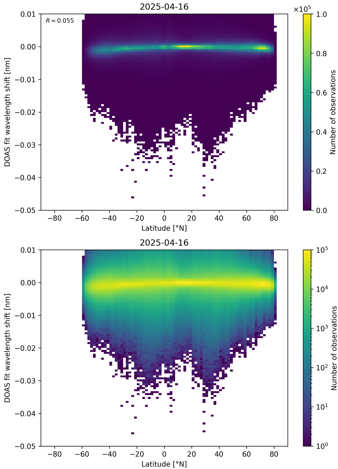
Figure 153: Scatter density plot of “Latitude” against “DOAS fit wavelength shift” for 2025-04-15 to 2025-04-17.
