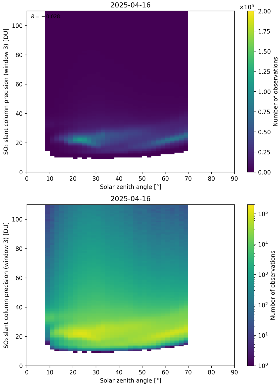
Figure 188: Scatter density plot of “Solar zenith angle” against “SO 2 slant column precision (window 3)” for 2025-04-15 to 2025-04-17.
