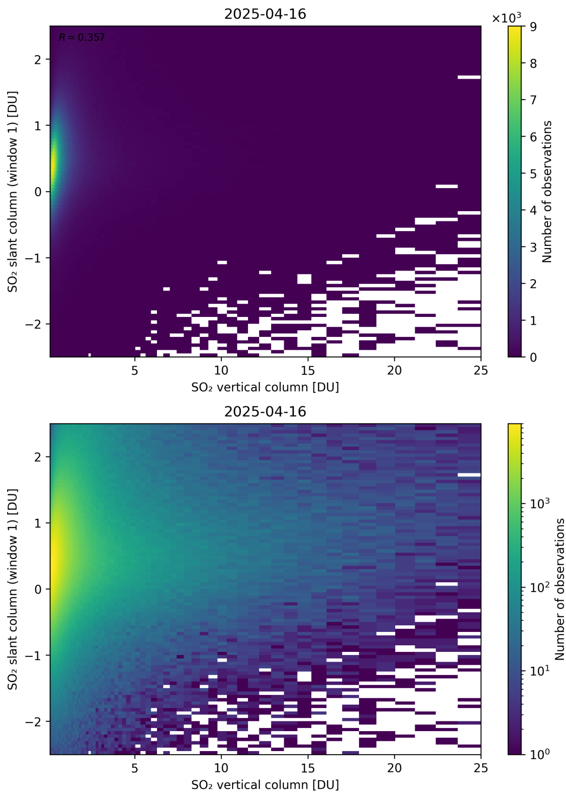
Figure 354: Scatter density plot of “SO 2 vertical column” against “SO 2 slant column (window 1)” for 2025-04-15 to 2025-04-17.
