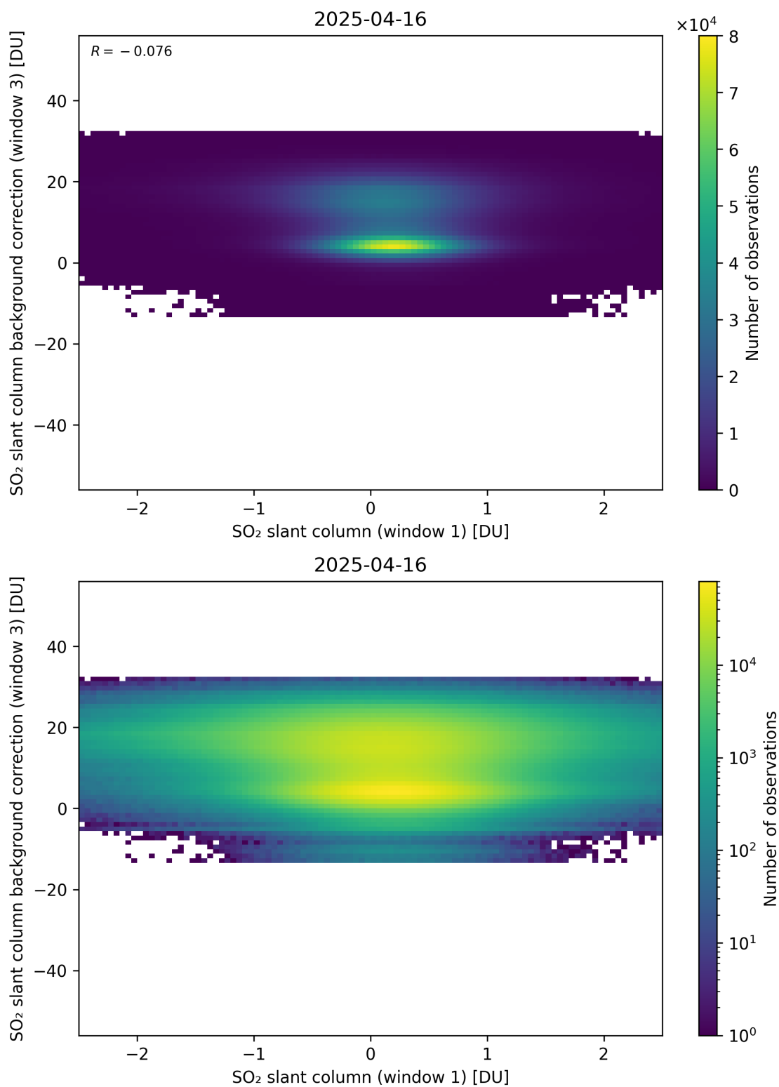
Figure 264: Scatter density plot of “SO 2 slant column (window 1)” against “SO 2 slant column background correction (window 3)” for 2025-04-15 to 2025-04-17.
