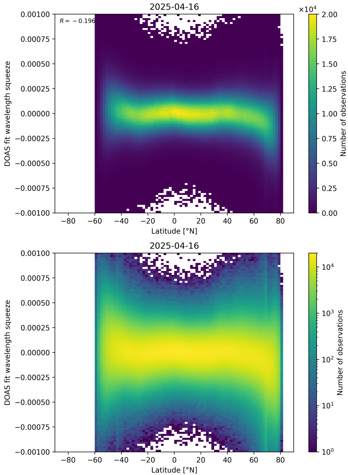
Figure 154: Scatter density plot of “Latitude” against “DOAS fit wavelength squeeze” for 2025-04-15 to 2025-04-17.
