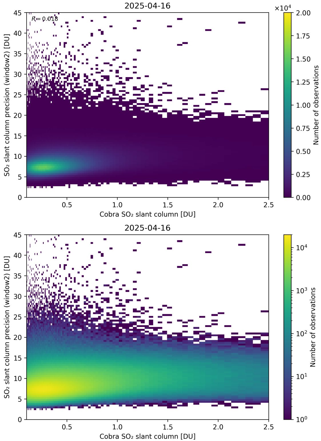
Figure 221: Scatter density plot of “Cobra SO 2 slant column” against “SO 2 slant column precision (window2)” for 2025-04-15 to 2025-04-17.
