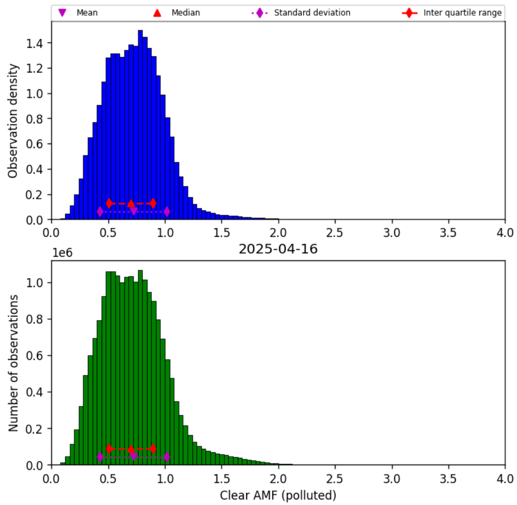
Figure 81: Histogram of “Clear AMF (polluted)” for 2025-04-15 to 2025-04-17
