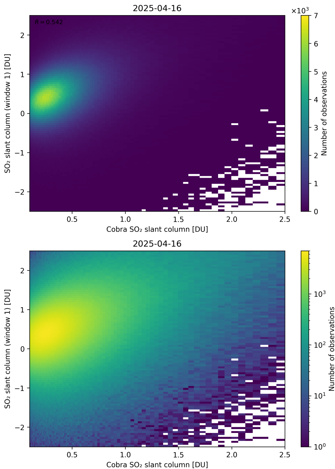
Figure 219: Scatter density plot of “Cobra SO 2 slant column” against “SO 2 slant column (window 1)” for 2025-04-15 to 2025-04-17.
