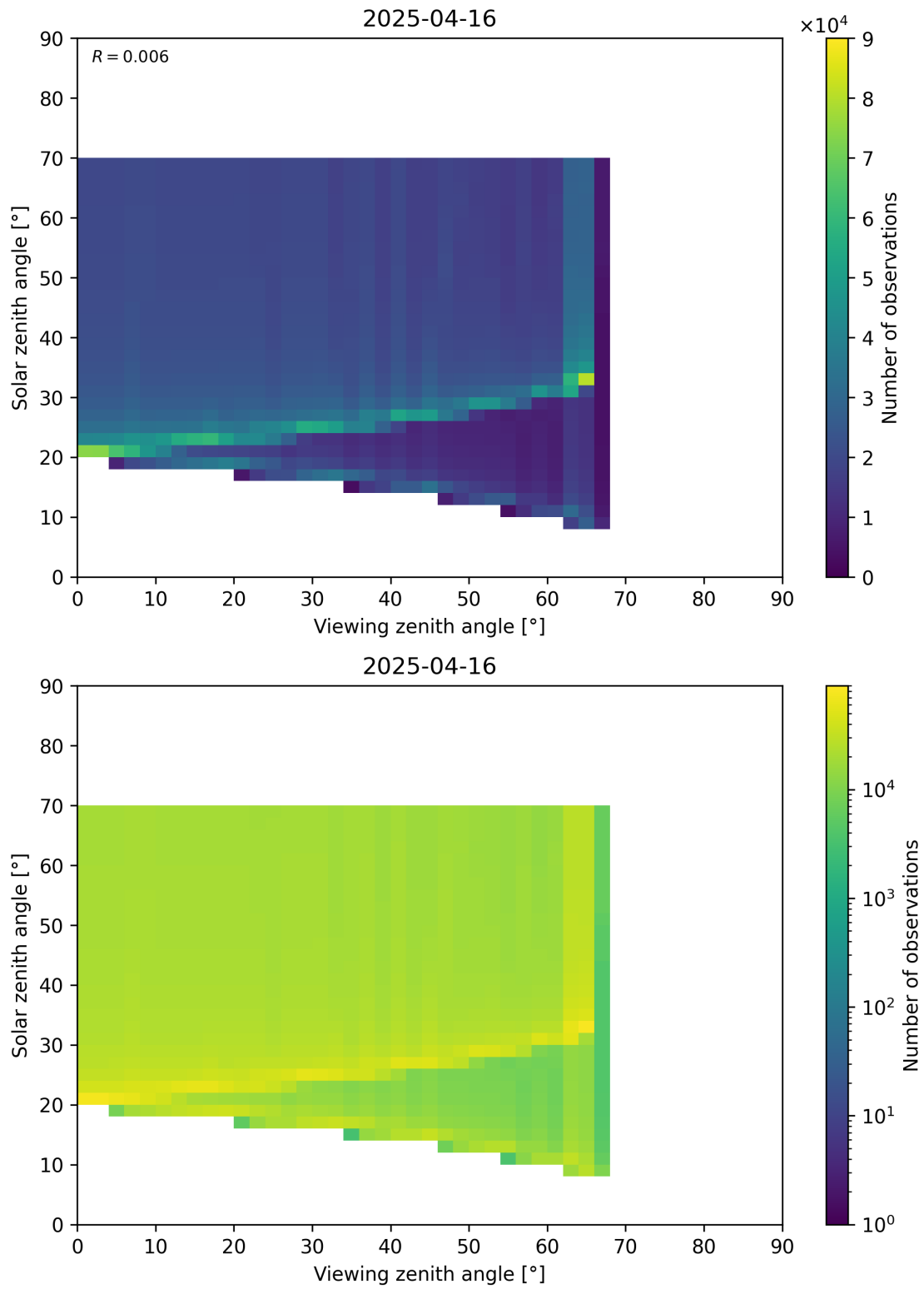
Figure 369: Scatter density plot of “Viewing zenith angle” against “Solar zenith angle” for 2025-04-15 to 2025-04-17.
