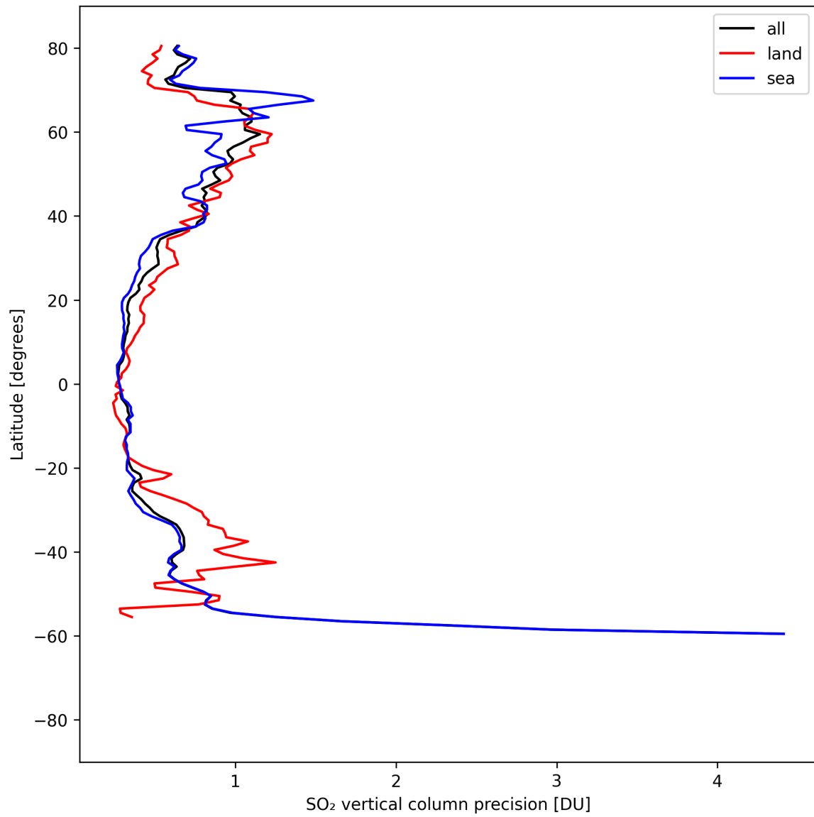
Figure 33: Zonal average of “SO 2 vertical column precision” for 2025-04-15 to 2025-04-17.
