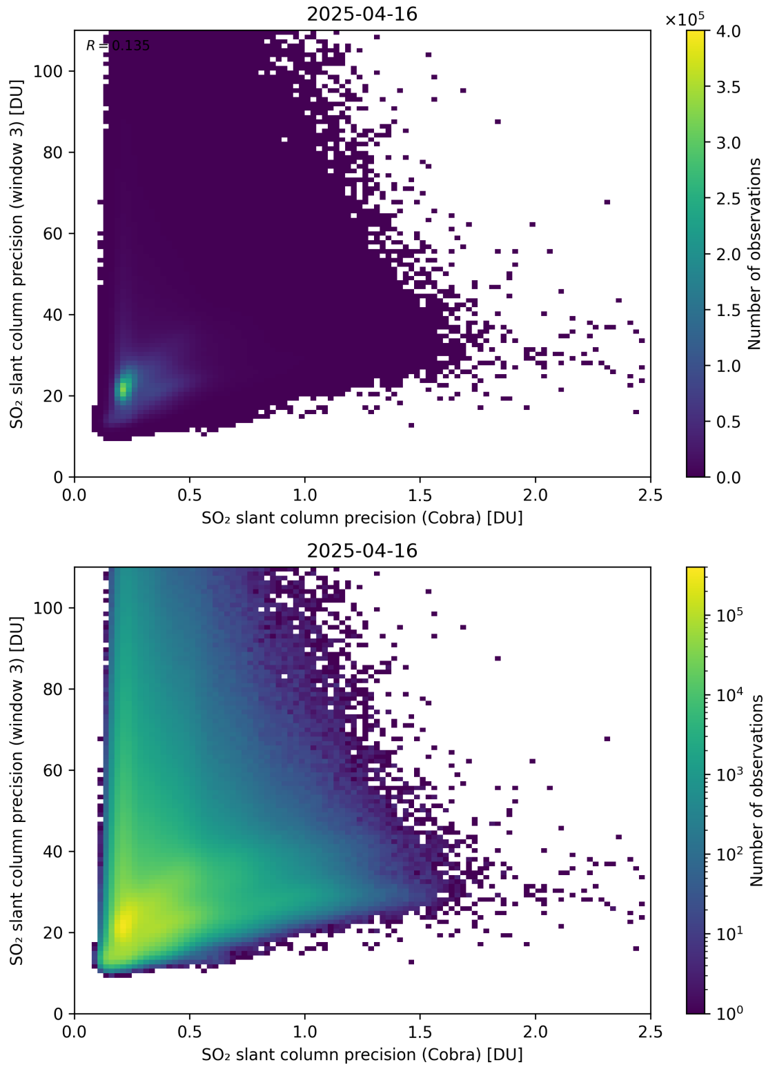
Figure 212: Scatter density plot of “SO 2 slant column precision (Cobra)” against “SO 2 slant column precision (window 3)” for 2025-04-15 to 2025-04-17.
