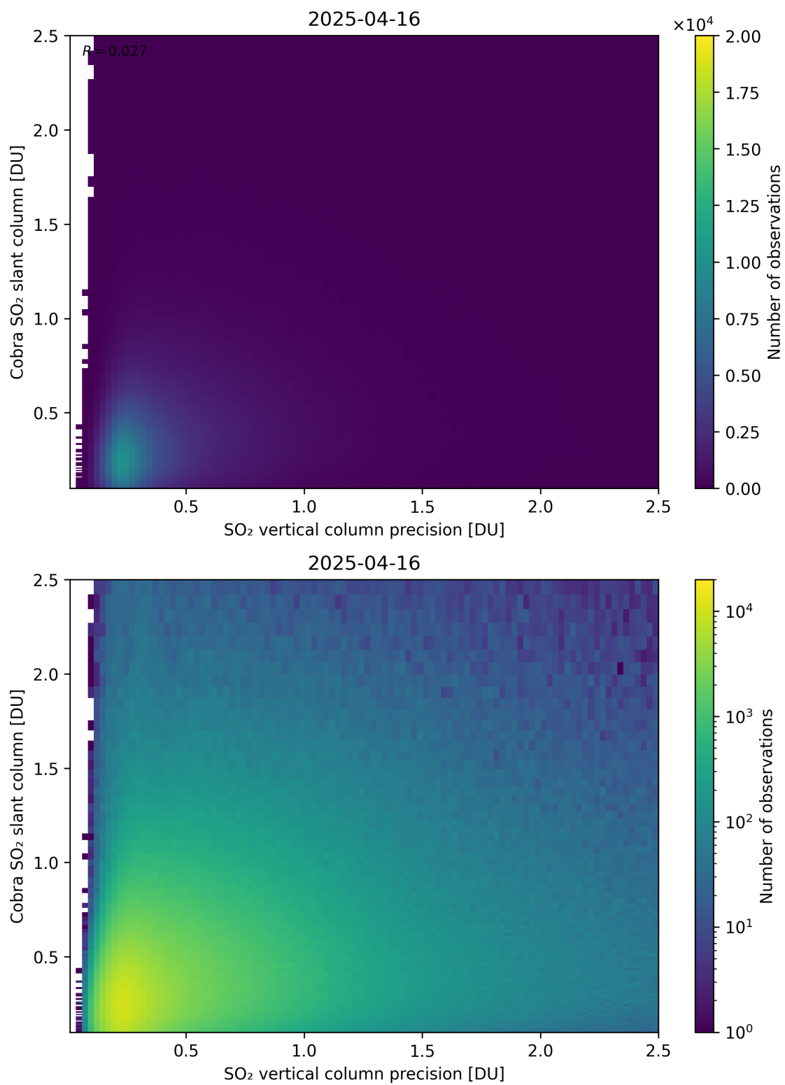
Figure 336: Scatter density plot of “SO 2 vertical column precision” against “Cobra SO 2 slant column” for 2025-04-15 to 2025-04-17.
