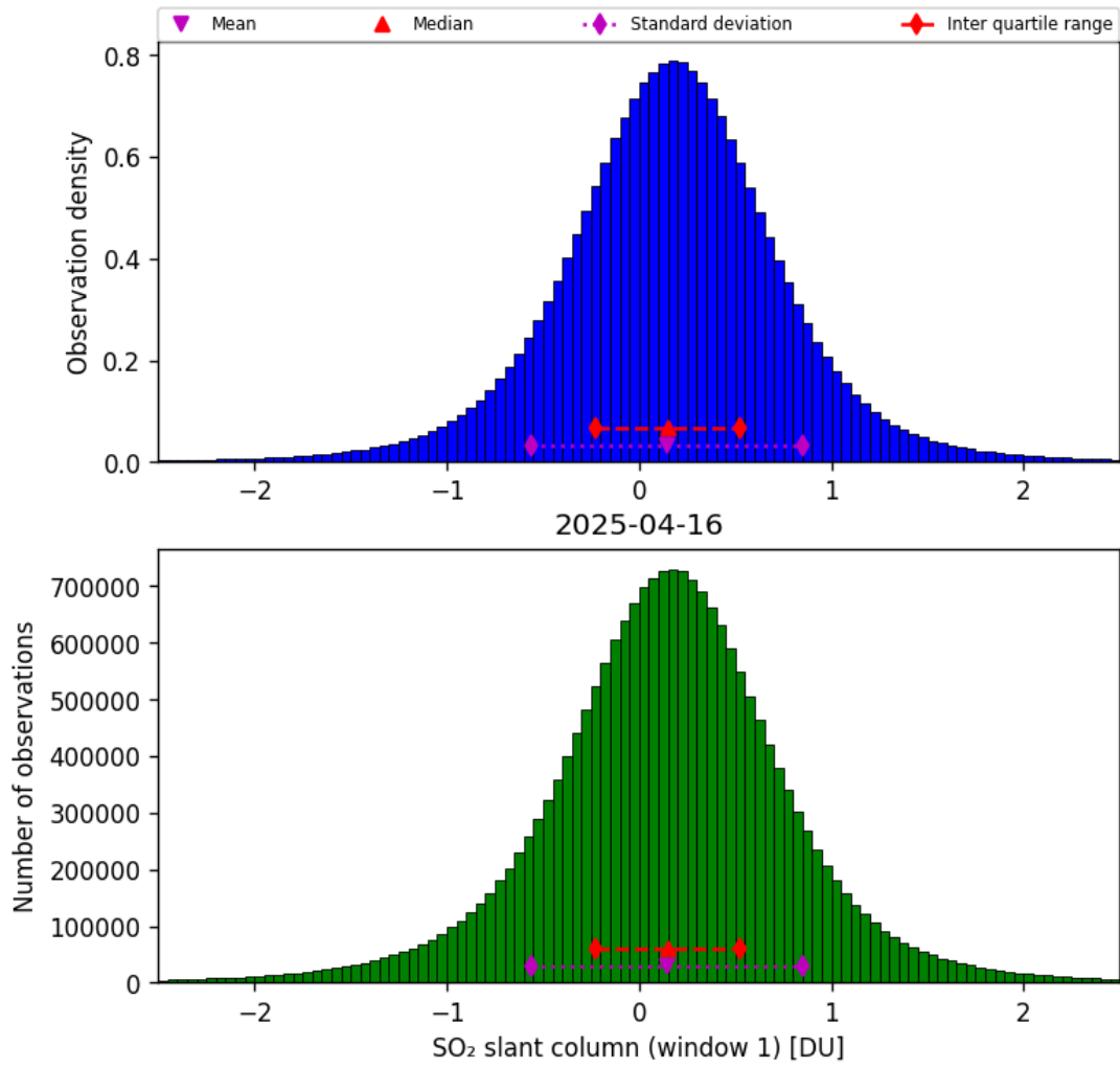
Figure 63: Histogram of “SO 2 slant column (window 1)” for 2025-04-15 to 2025-04-17
