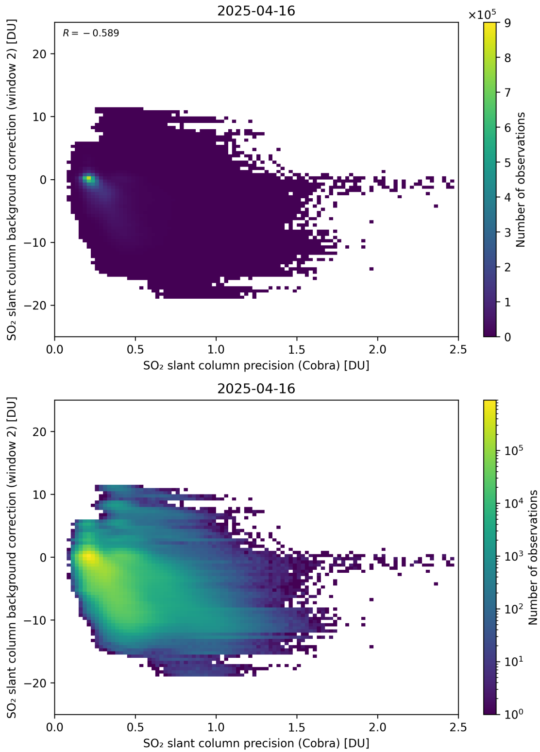
Figure 200: Scatter density plot of “SO 2 slant column precision (Cobra)” against “SO 2 slant column background correction (window 2)” for 2025-04-15 to 2025-04-17.
