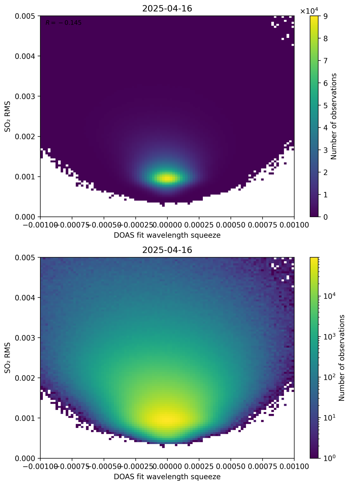
Figure 143: Scatter density plot of “DOAS fit wavelength squeeze” against “SO 2 RMS” for 2025-04-15 to 2025-04-17.
