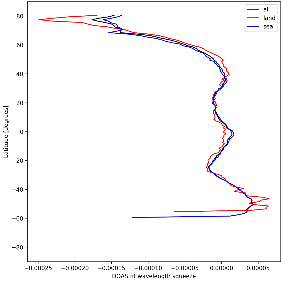
Figure 51: Zonal average of “DOAS fit wavelength squeeze” for 2025-04-15 to 2025-04-17.
