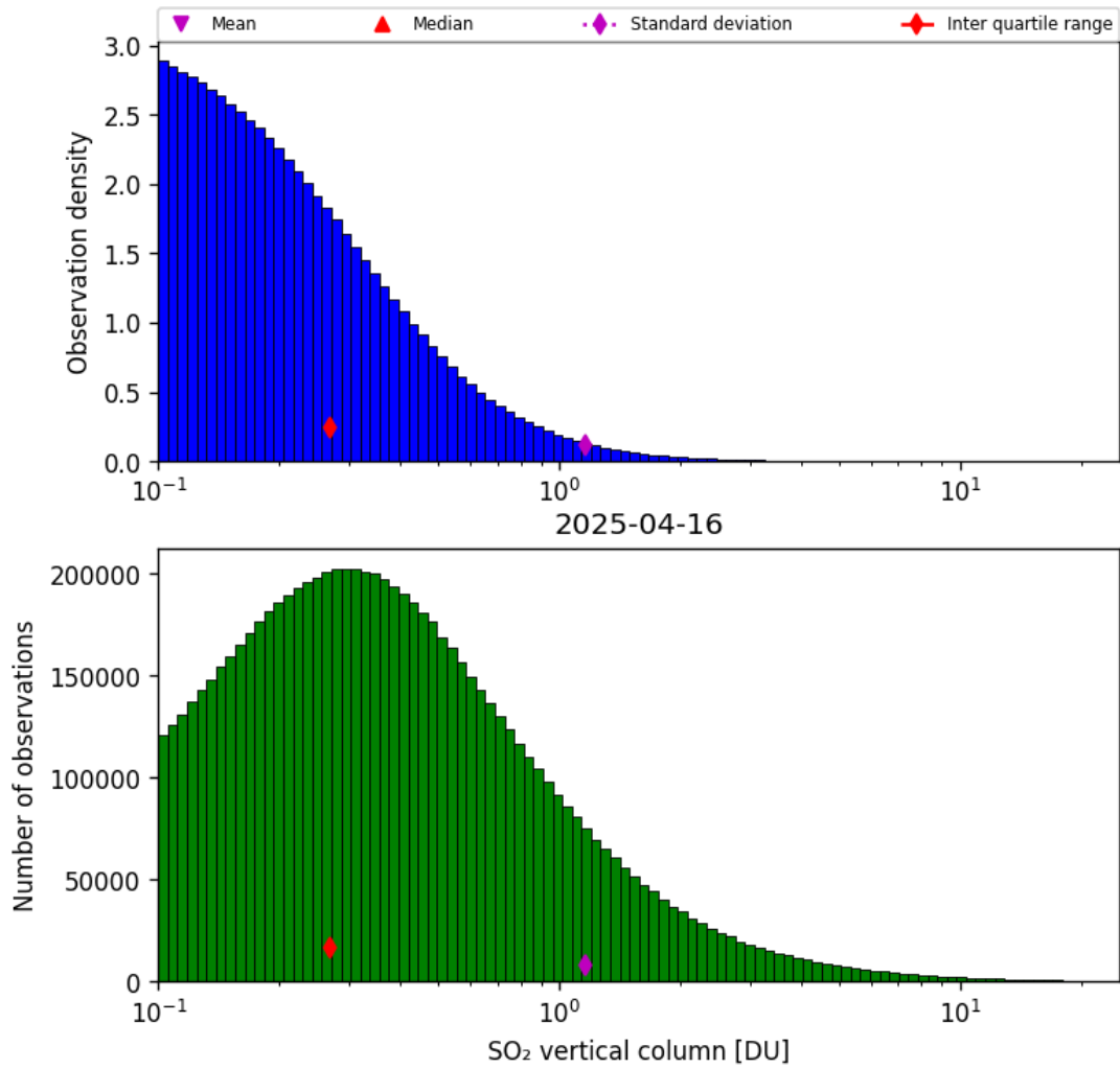
Figure 58: Histogram of “SO 2 vertical column” for 2025-04-15 to 2025-04-17
