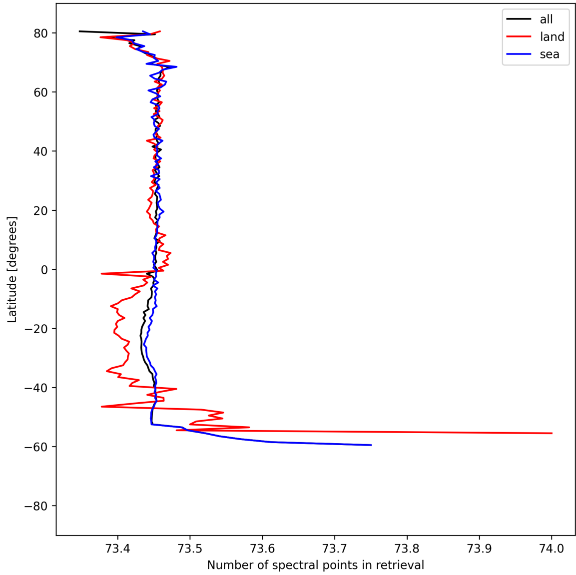
Figure 56: Zonal average of “Number of spectral points in retrieval” for 2025-04-15 to 2025-04-17.
