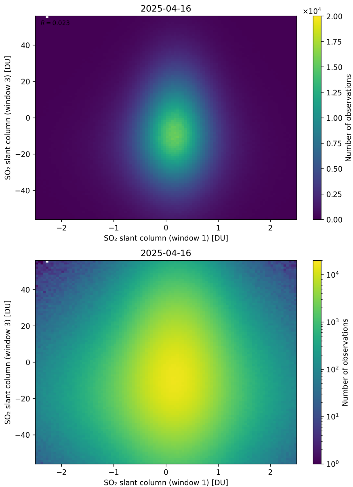
Figure 287: Scatter density plot of “SO 2 slant column (window 1)” against “SO 2 slant column (window 3)” for 2025-04-15 to 2025-04-17.
