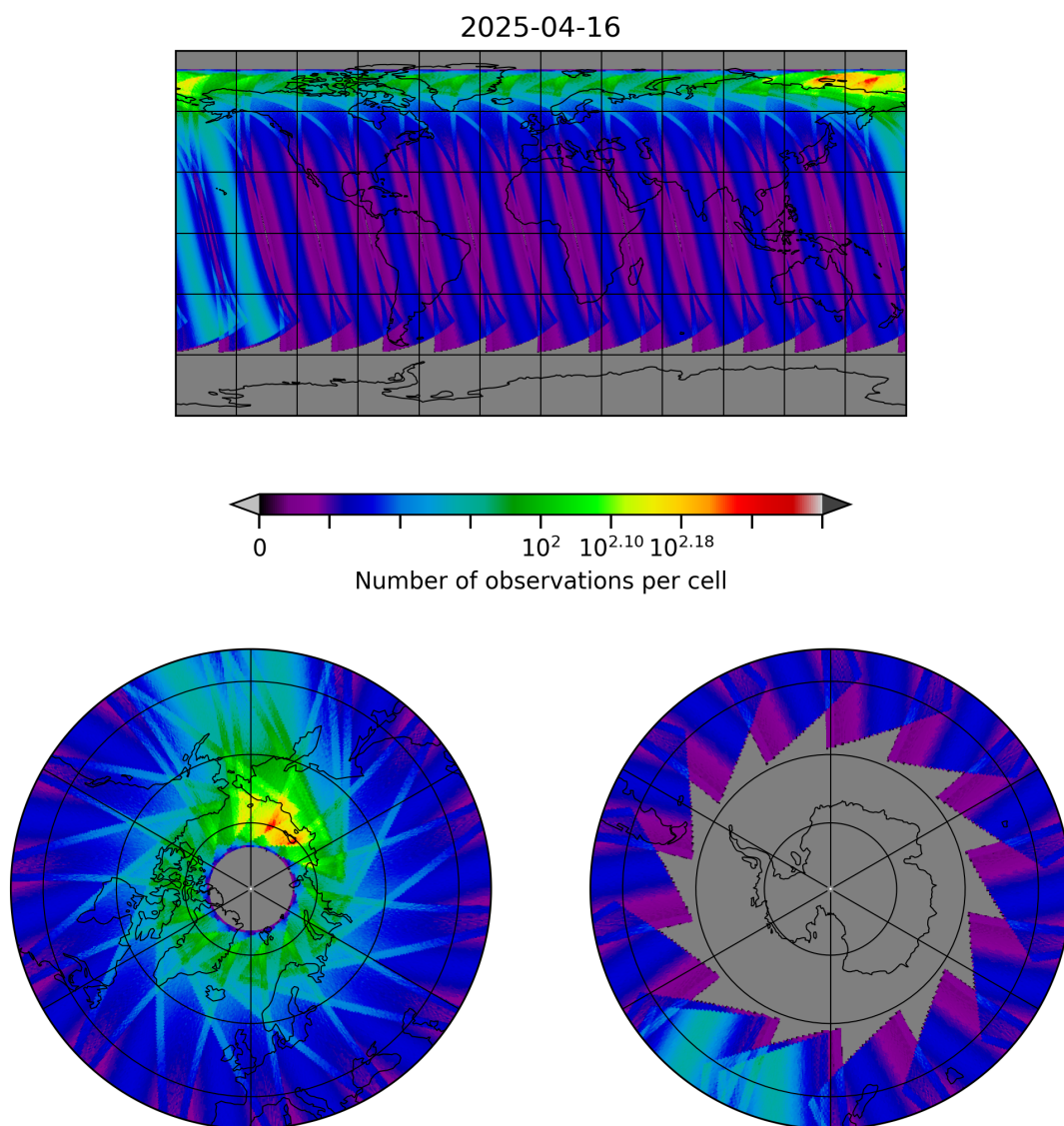
Figure 30: Map of the number of observations for 2025-04-15 to 2025-04-17
