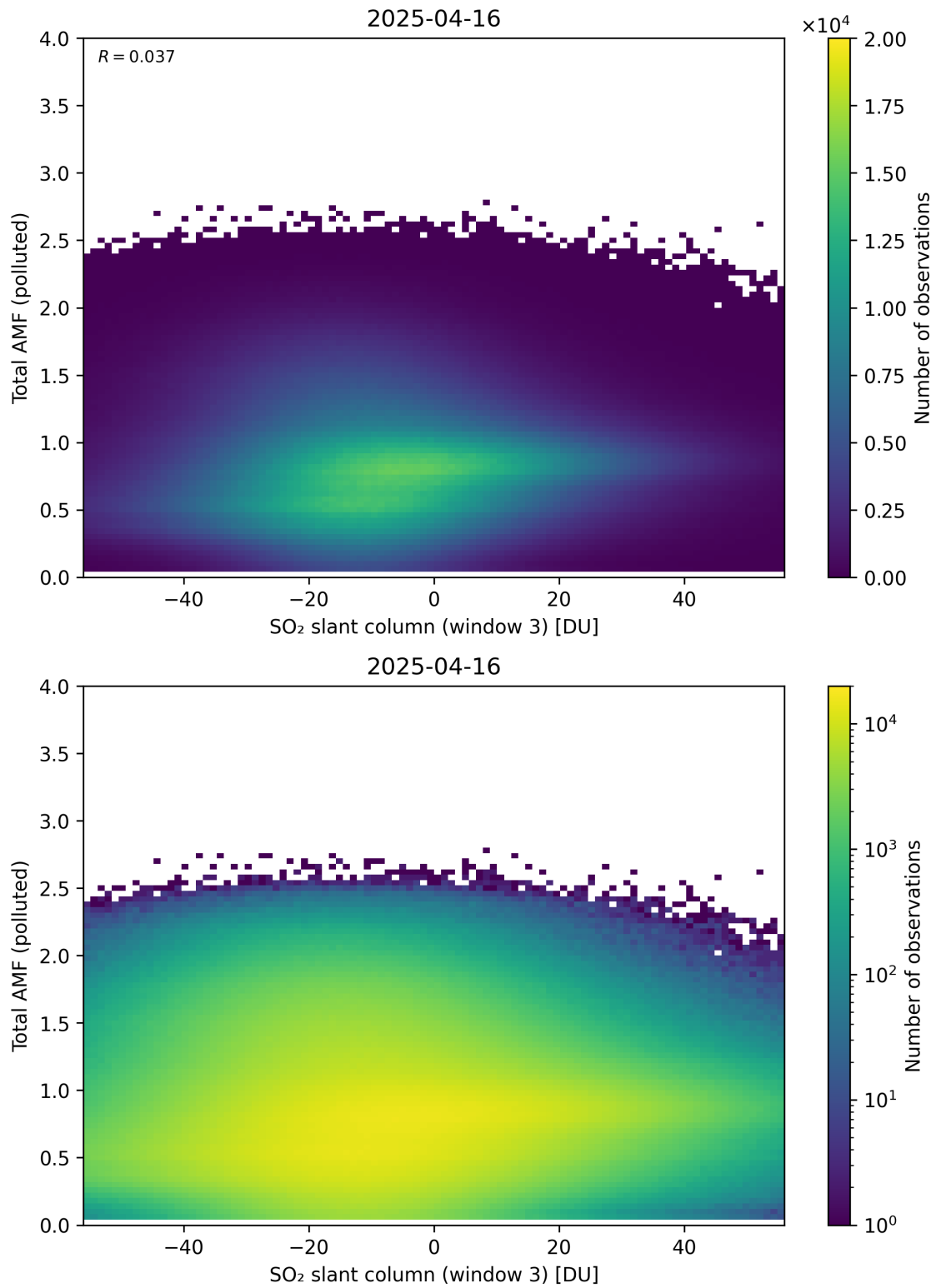
Figure 318: Scatter density plot of “SO 2 slant column (window 3)” against “Total AMF (polluted)” for 2025-04-15 to 2025-04-17.
