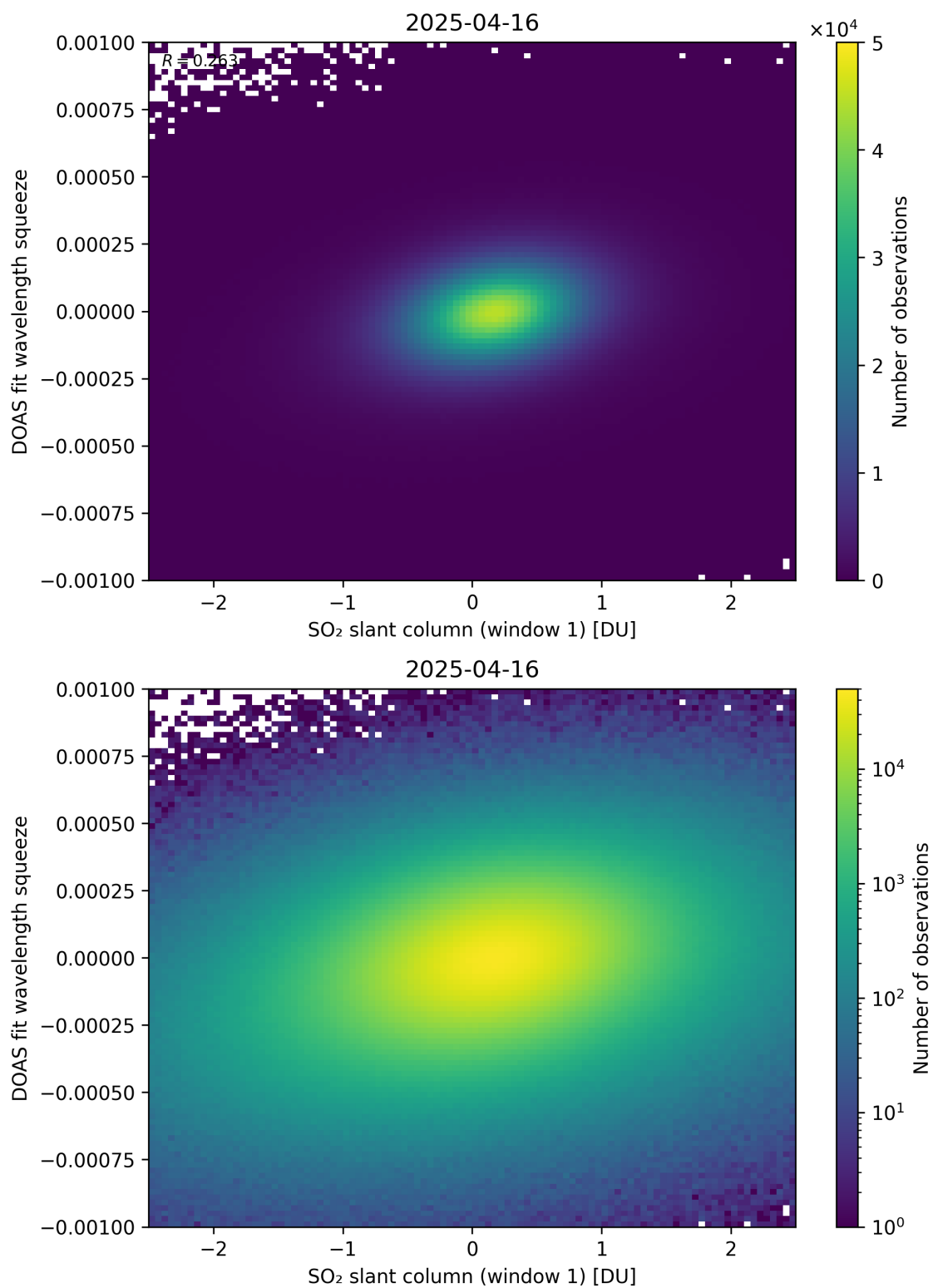
Figure 266: Scatter density plot of “SO 2 slant column (window 1)” against “DOAS fit wavelength squeeze” for 2025-04-15 to 2025-04-17.
