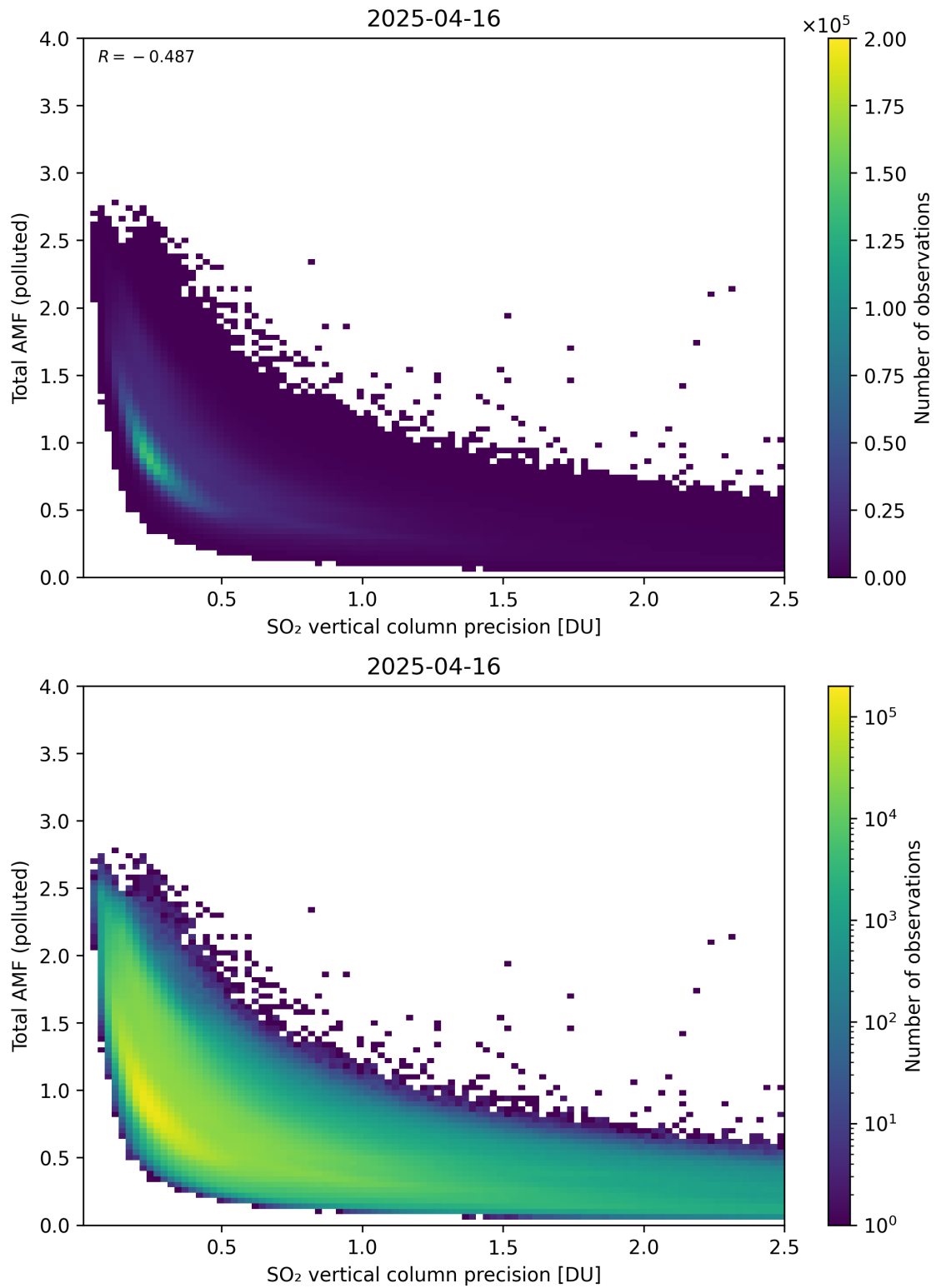
Figure 346: Scatter density plot of “SO 2 vertical column precision” against “Total AMF (polluted)” for 2025-04-15 to 2025-04-17.
