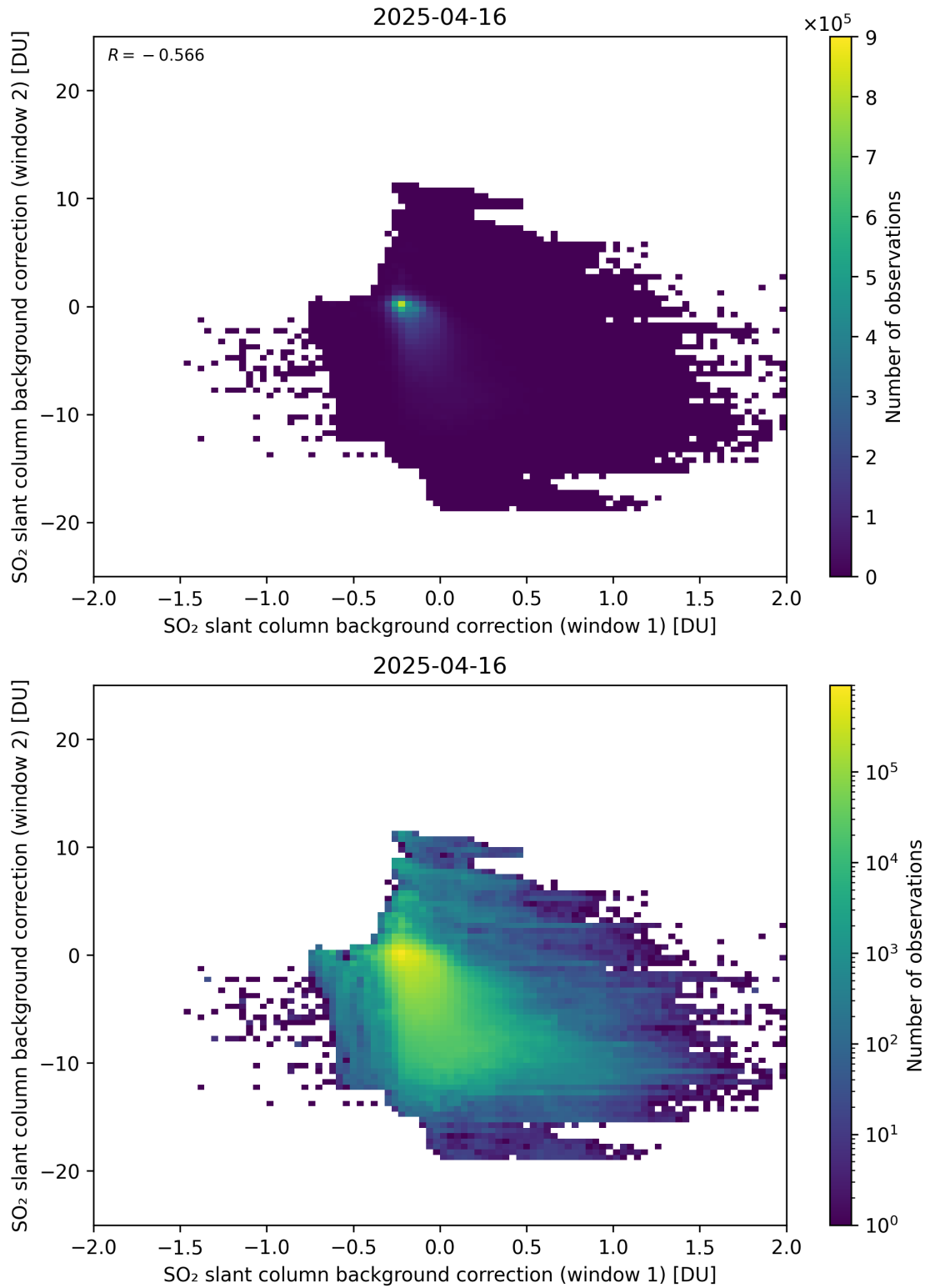
Figure 109: Scatter density plot of “SO 2 slant column background correction (window 1)” against “SO 2 slant column background correction (window 2)” for 2025-04-15 to 2025-04-17.
