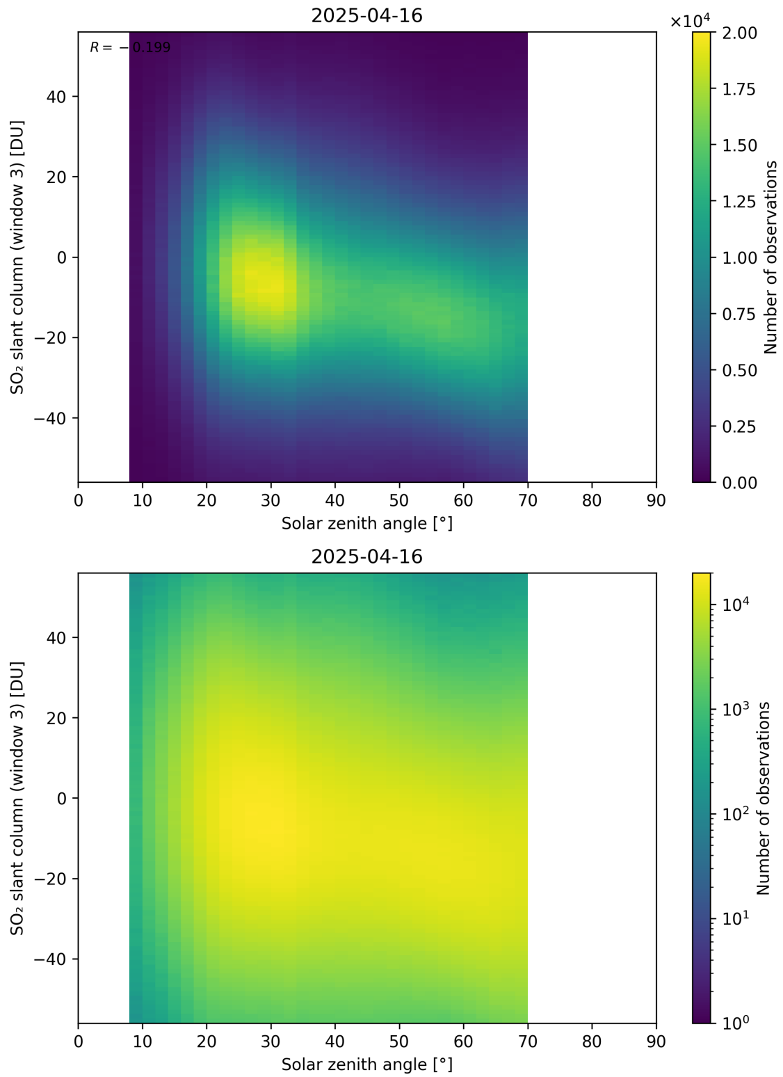
Figure 187: Scatter density plot of “Solar zenith angle” against “SO 2 slant column (window 3)” for 2025-04-15 to 2025-04-17.
