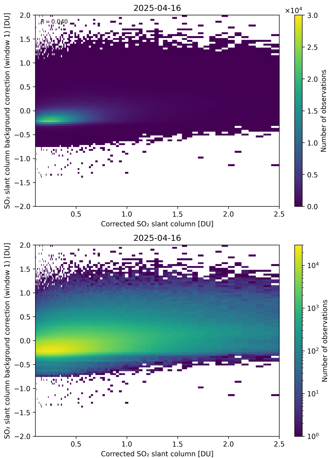
Figure 226: Scatter density plot of “Corrected SO 2 slant column” against “SO 2 slant column background correction (window 1)” for 2025-04-15 to 2025-04-17.
