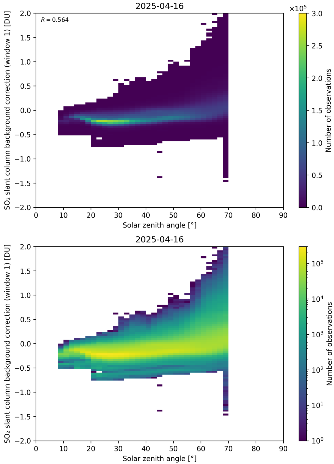
Figure 171: Scatter density plot of “Solar zenith angle” against “SO 2 slant column background correction (window 1)” for 2025-04-15 to 2025-04-17.
