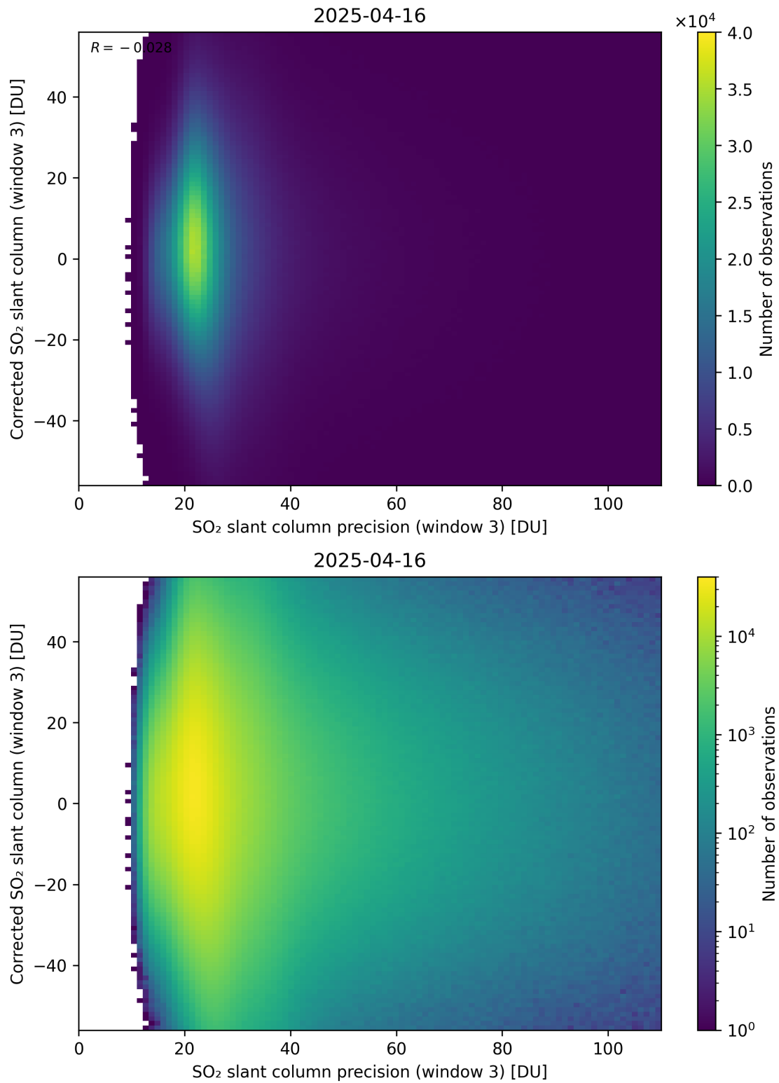
Figure 312: Scatter density plot of “SO 2 slant column precision (window 3)” against “Corrected SO 2 slant column (window 3)” for 2025-04-15 to 2025-04-17.
