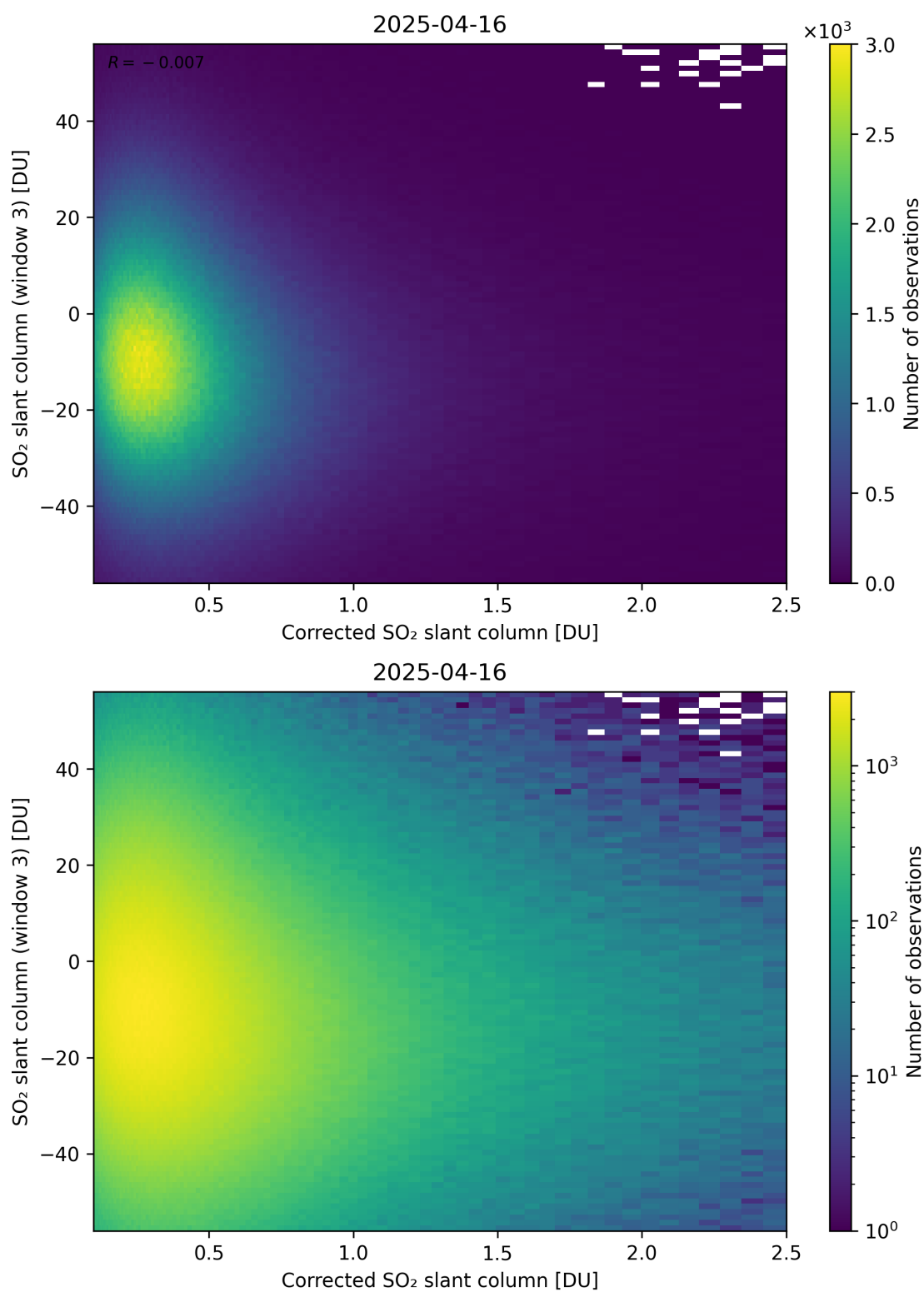
Figure 240: Scatter density plot of “Corrected SO 2 slant column” against “SO 2 slant column (window 3)” for 2025-04-15 to 2025-04-17.
