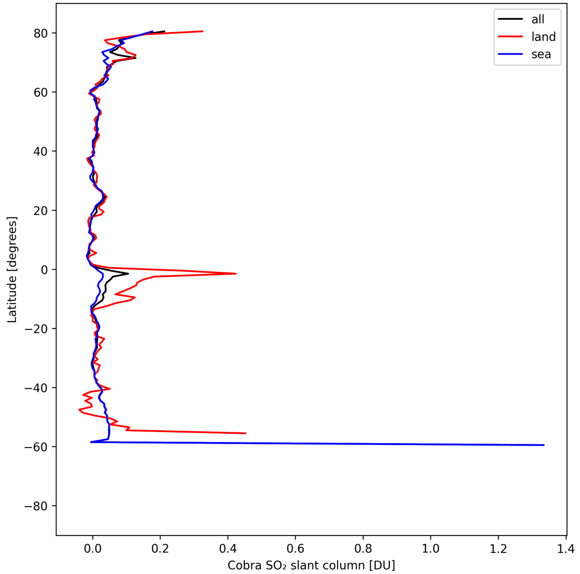
Figure 35: Zonal average of “Cobra SO 2 slant column” for 2025-04-15 to 2025-04-17.
