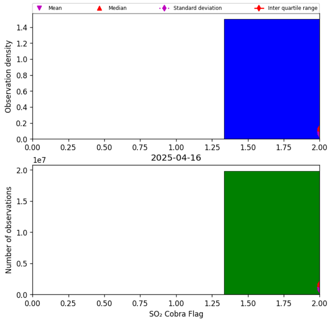
Figure 75: Histogram of “SO 2 Cobra Flag” for 2025-04-15 to 2025-04-17
