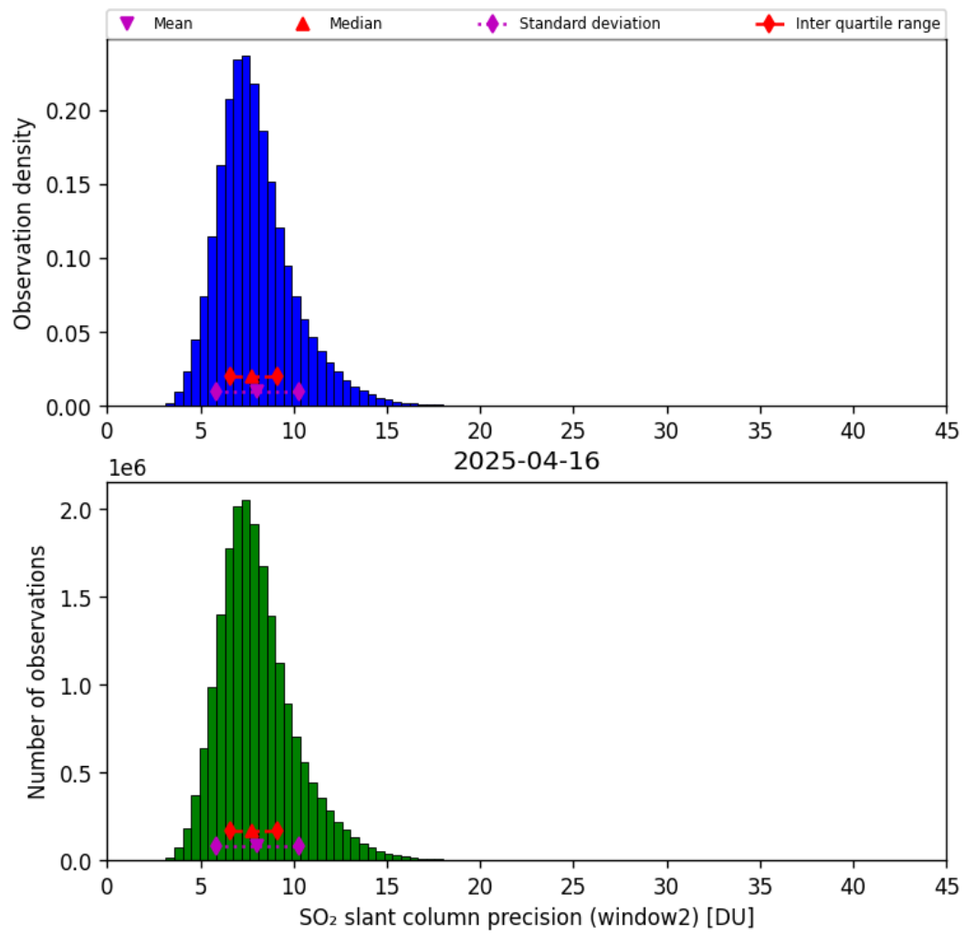
Figure 68: Histogram of “SO 2 slant column precision (window2)” for 2025-04-15 to 2025-04-17
