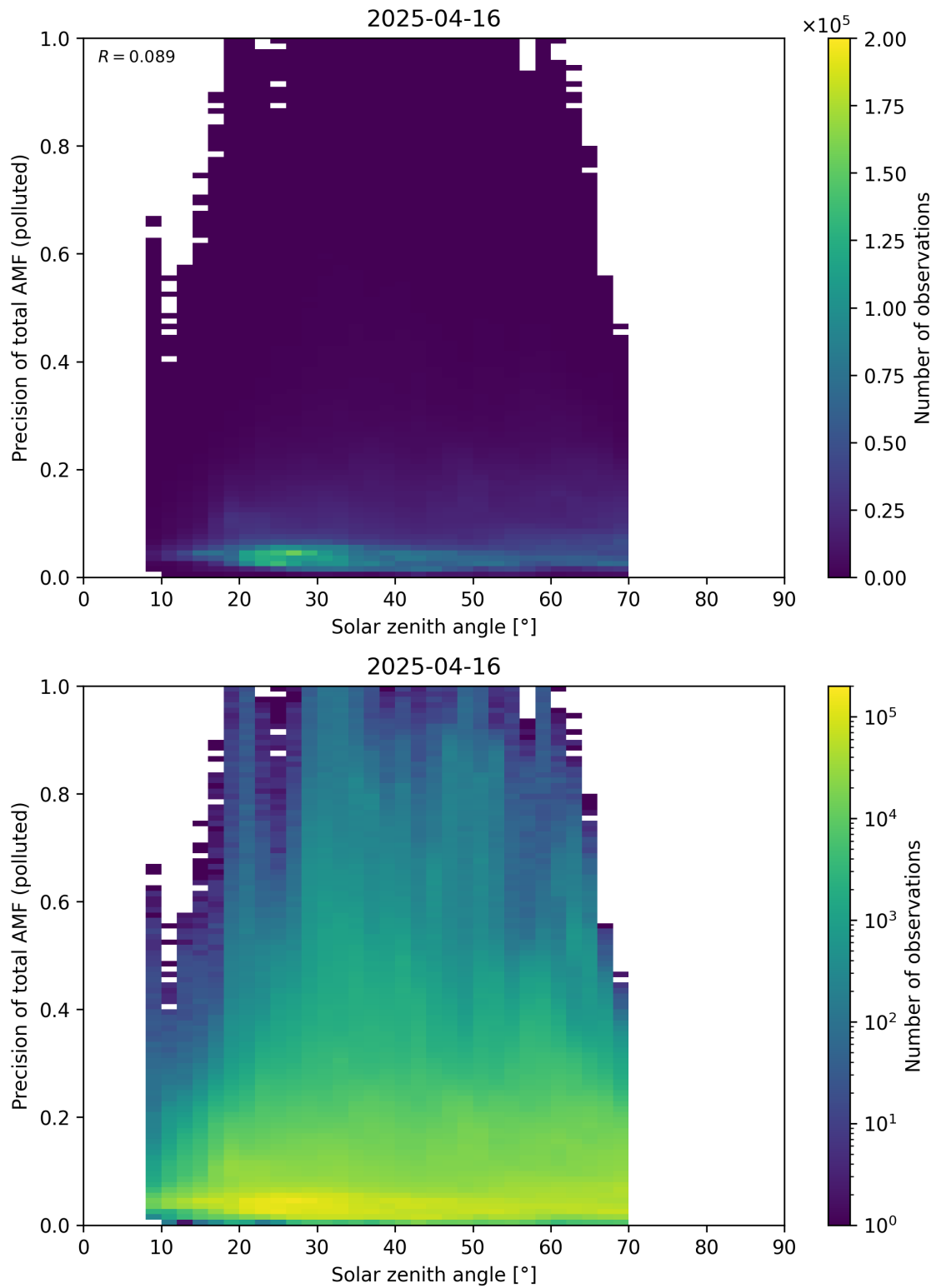
Figure 190: Scatter density plot of “Solar zenith angle” against “Precision of total AMF (polluted)” for 2025-04-15 to 2025-04-17.
