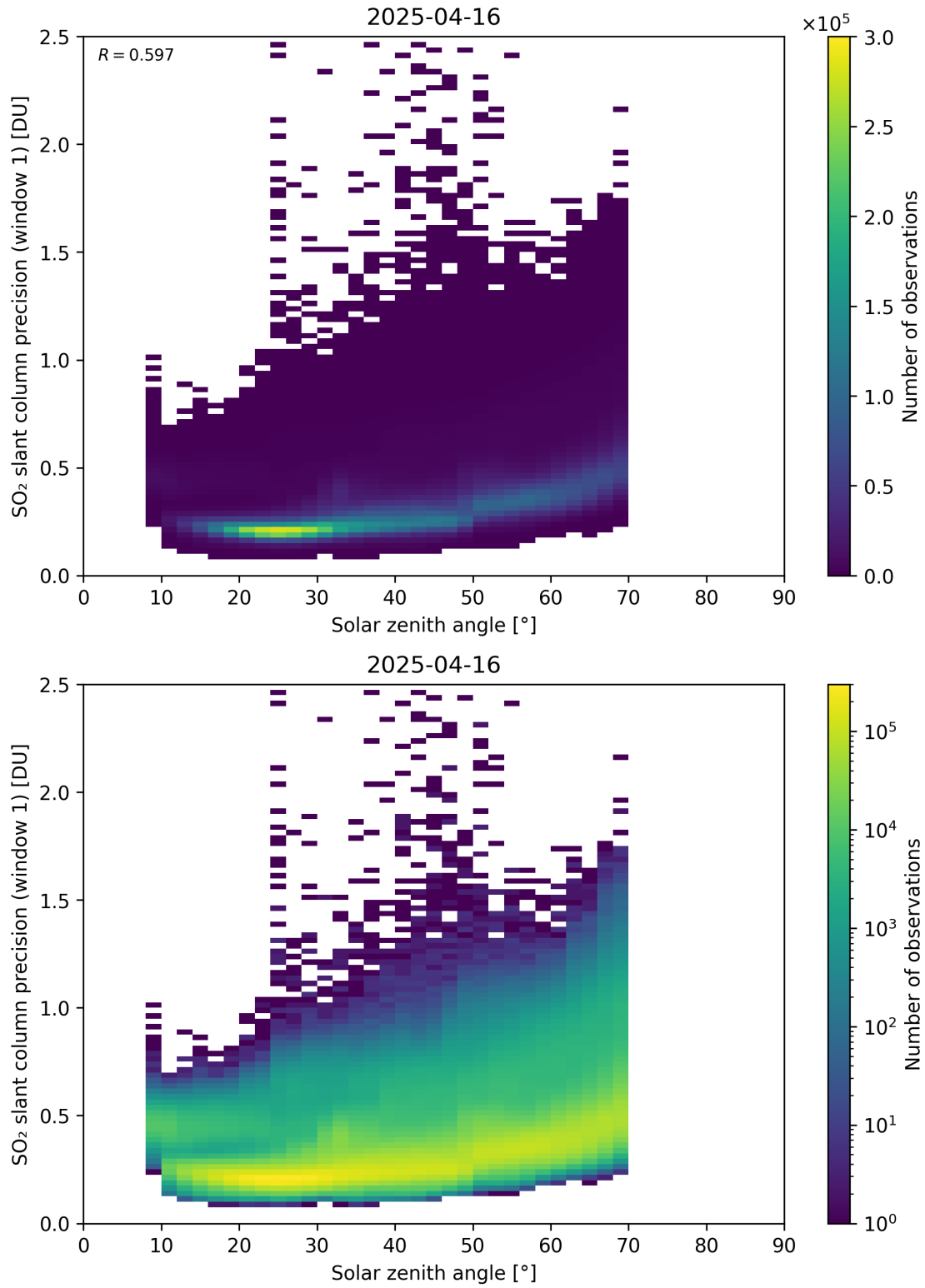
Figure 185: Scatter density plot of “Solar zenith angle” against “SO 2 slant column precision (window 1)” for 2025-04-15 to 2025-04-17.
