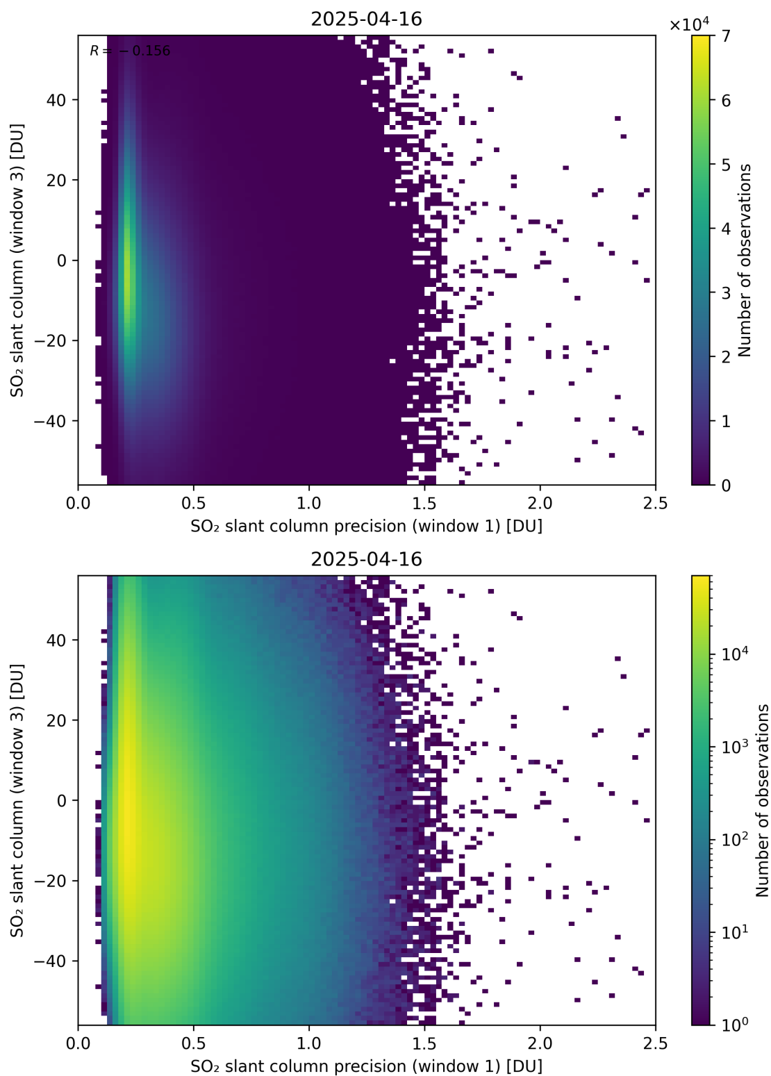
Figure 278: Scatter density plot of “SO 2 slant column precision (window 1)” against “SO 2 slant column (window 3)” for 2025-04-15 to 2025-04-17.
