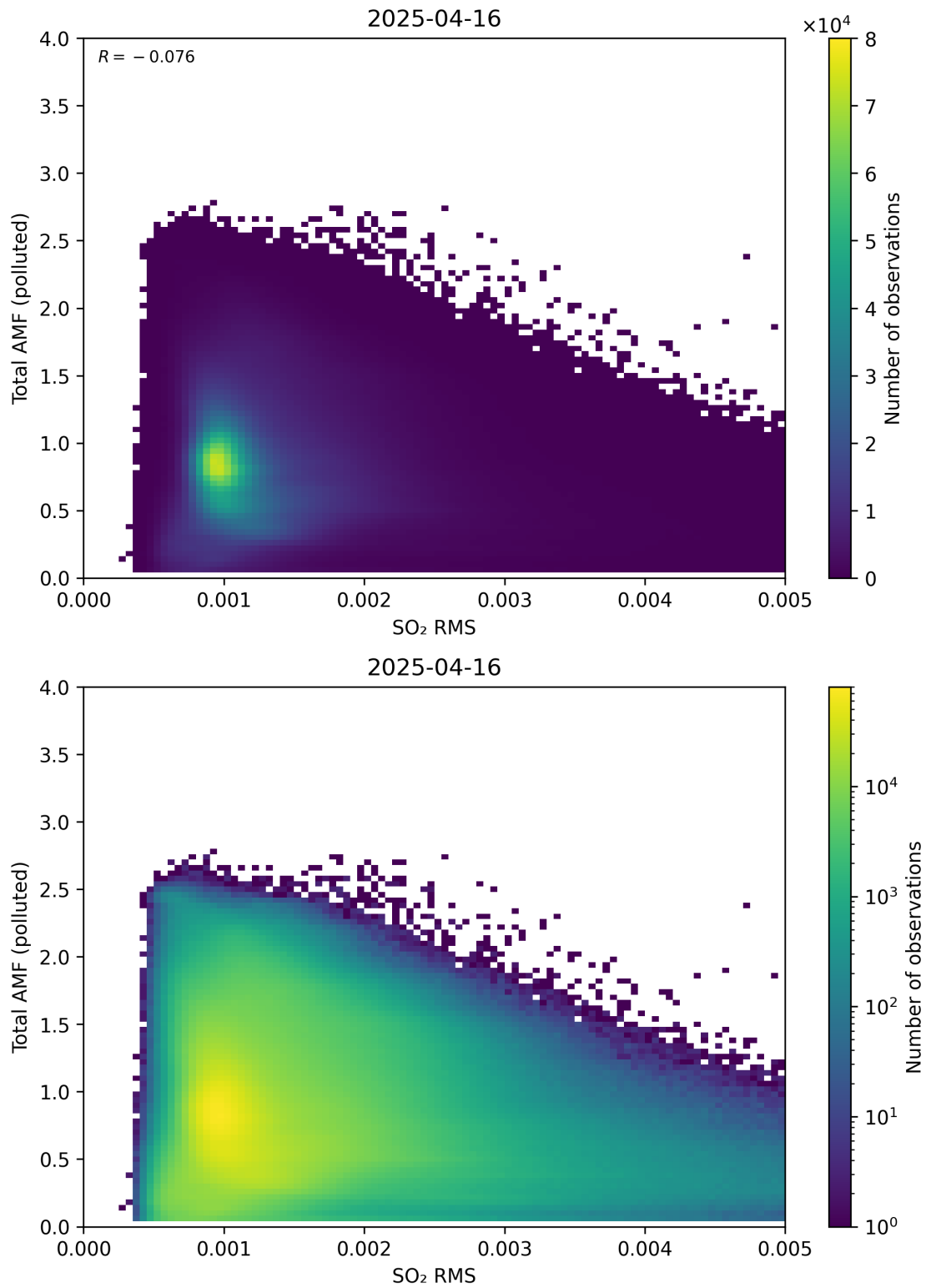
Figure 148: Scatter density plot of “SO 2 RMS” against “Total AMF (polluted)” for 2025-04-15 to 2025-04-17.
