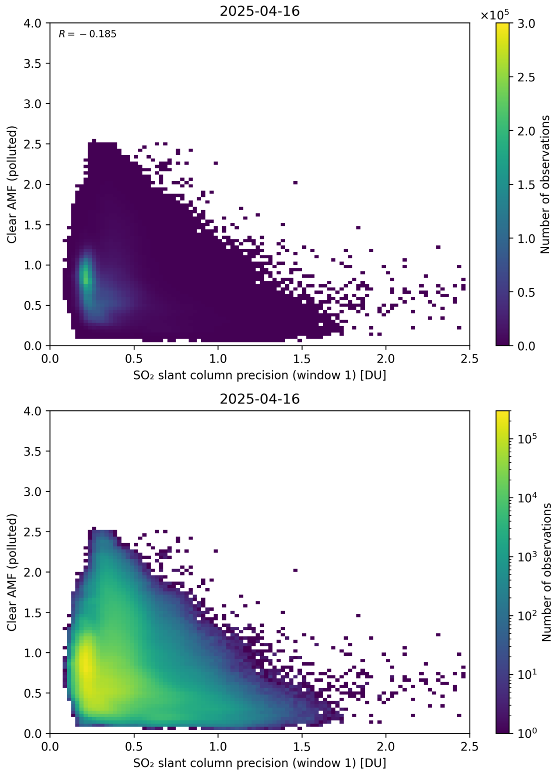
Figure 274: Scatter density plot of “SO 2 slant column precision (window 1)” against “Clear AMF (polluted)” for 2025-04-15 to 2025-04-17.
