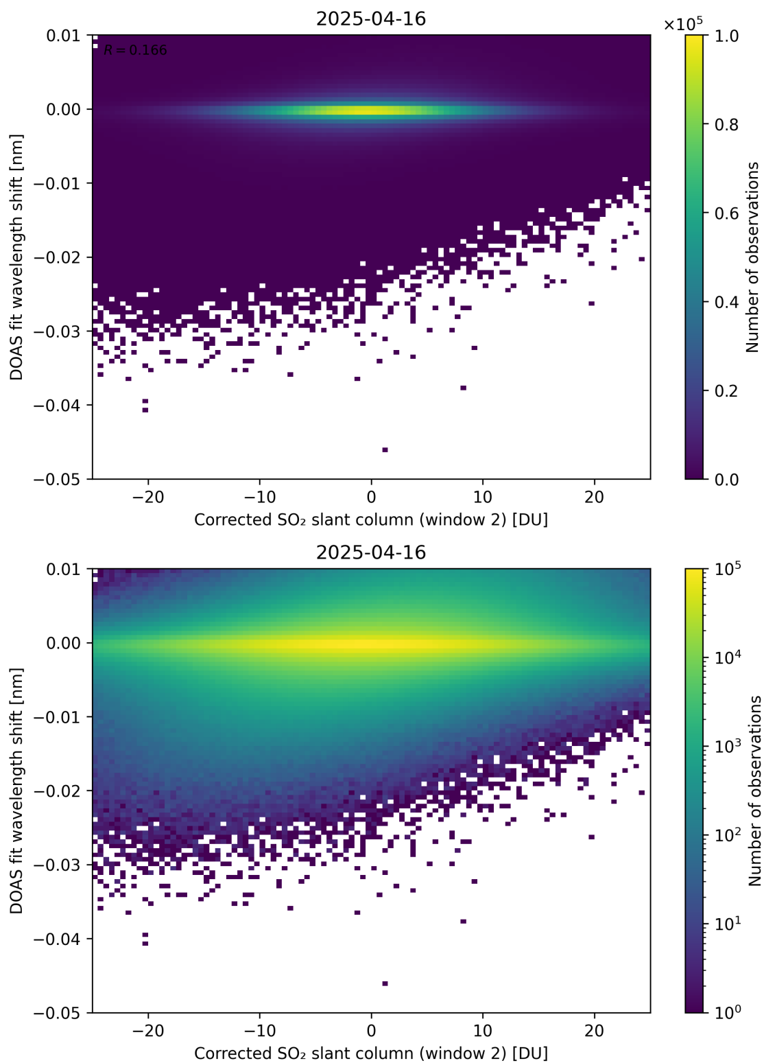
Figure 246: Scatter density plot of “Corrected SO 2 slant column (window 2)” against “DOAS fit wavelength shift” for 2025-04-15 to 2025-04-17.
