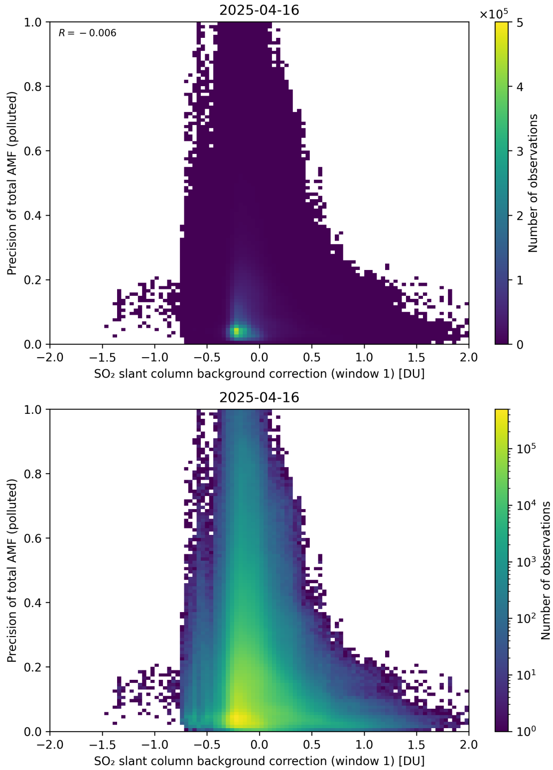
Figure 121: Scatter density plot of “SO 2 slant column background correction (window 1)” against “Precision of total AMF (polluted)” for 2025-04-15 to 2025-04-17.
