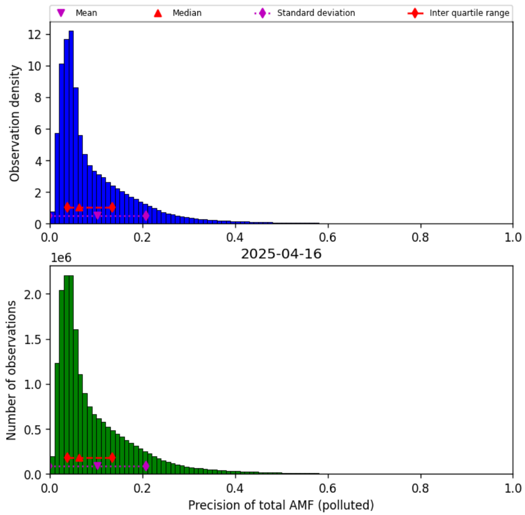
Figure 80: Histogram of “Precision of total AMF (polluted)” for 2025-04-15 to 2025-04-17
