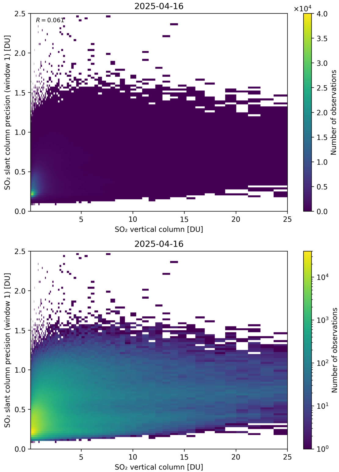
Figure 355: Scatter density plot of “SO 2 vertical column” against “SO 2 slant column precision (window 1)” for 2025-04-15 to 2025-04-17.
