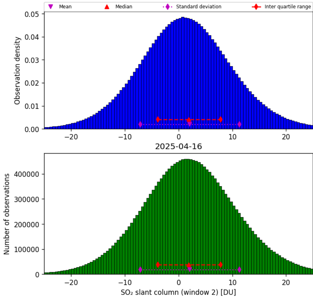
Figure 67: Histogram of “SO 2 slant column (window 2)” for 2025-04-15 to 2025-04-17
