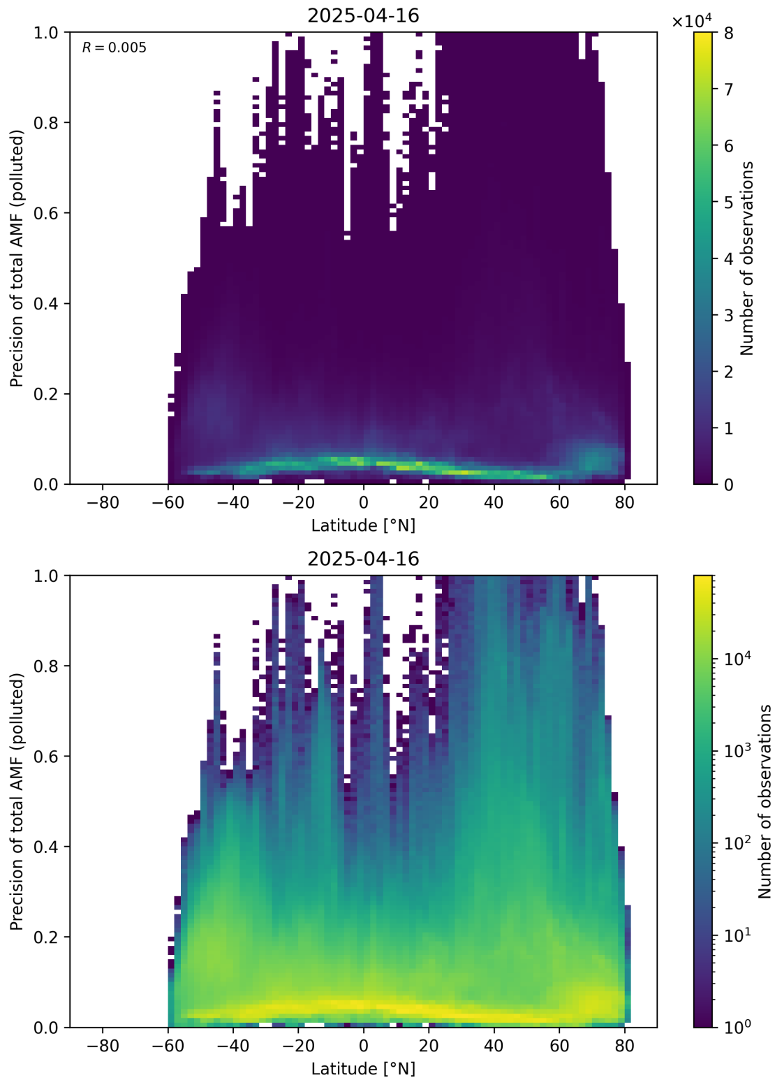
Figure 168: Scatter density plot of “Latitude” against “Precision of total AMF (polluted)” for 2025-04-15 to 2025-04-17.
