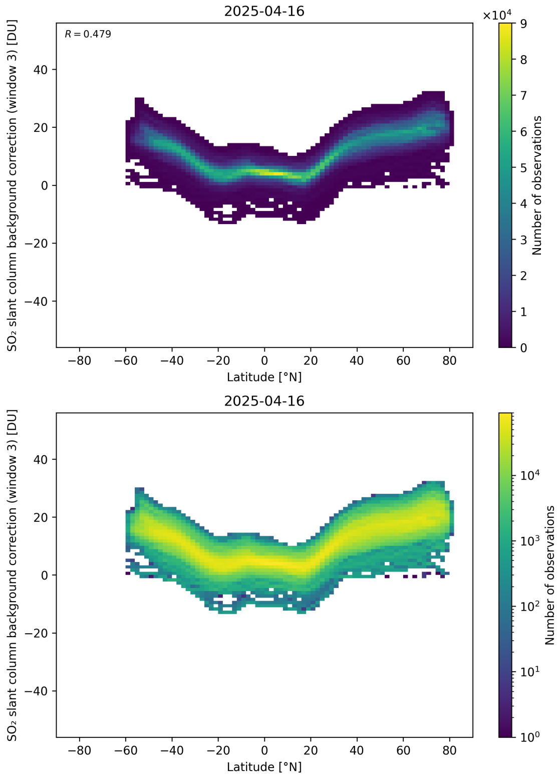
Figure 152: Scatter density plot of “Latitude” against “SO 2 slant column background correction (window 3)” for 2025-04-15 to 2025-04-17.
