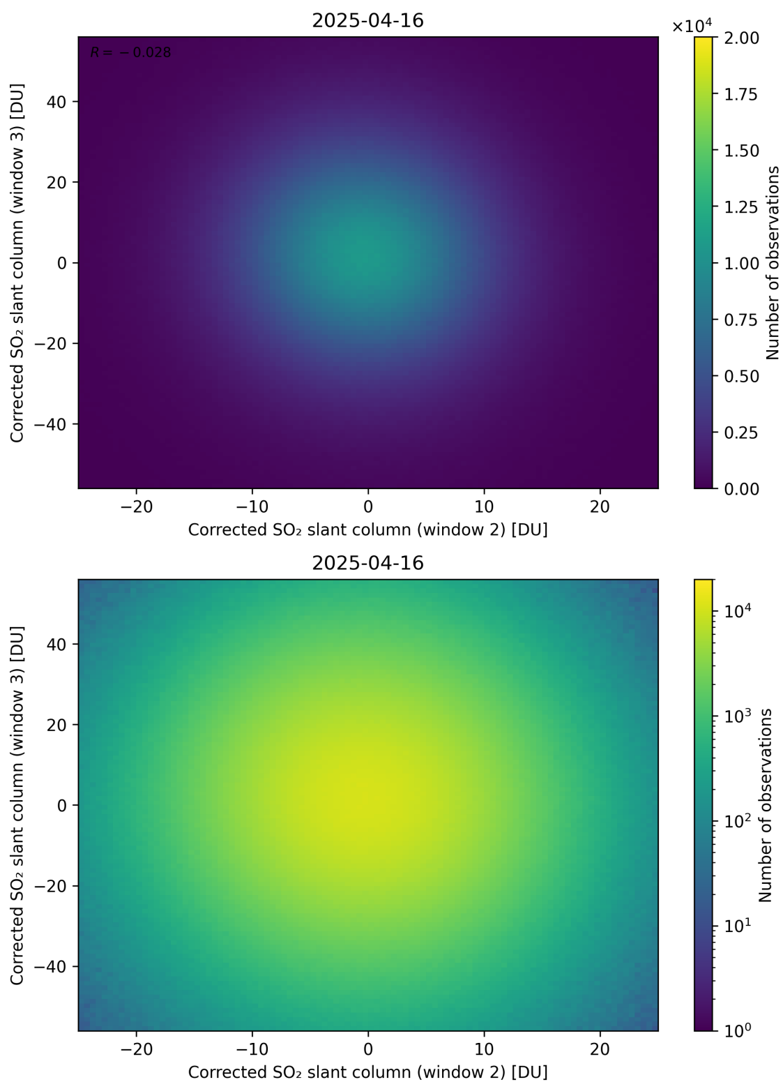
Figure 250: Scatter density plot of “Corrected SO 2 slant column (window 2)” against “Corrected SO 2 slant column (window 3)” for 2025-04-15 to 2025-04-17.
