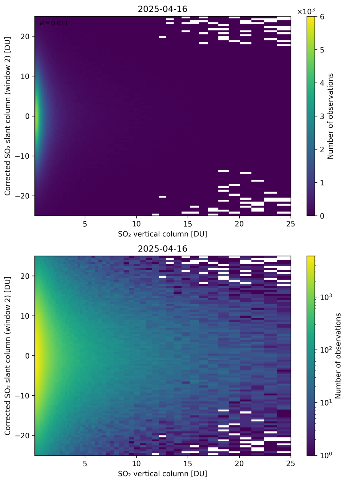
Figure 352: Scatter density plot of “SO 2 vertical column” against “Corrected SO 2 slant column (window 2)” for 2025-04-15 to 2025-04-17.
