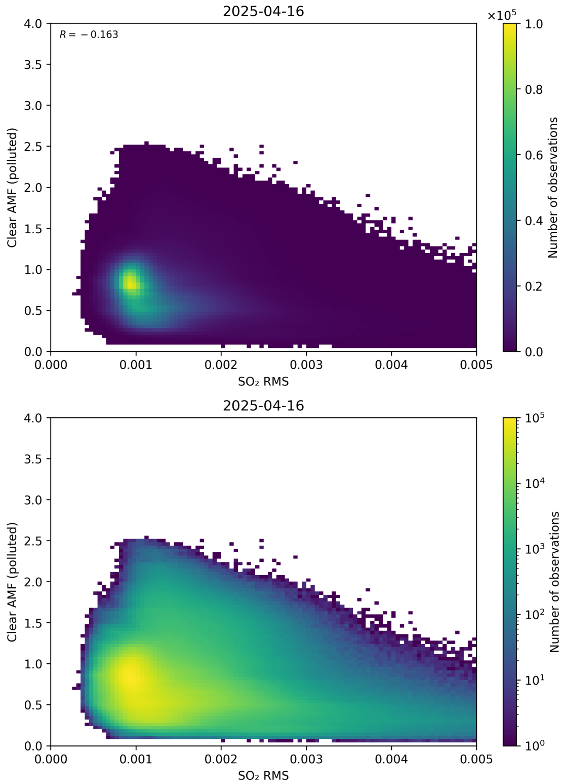
Figure 147: Scatter density plot of “SO 2 RMS” against “Clear AMF (polluted)” for 2025-04-15 to 2025-04-17.
