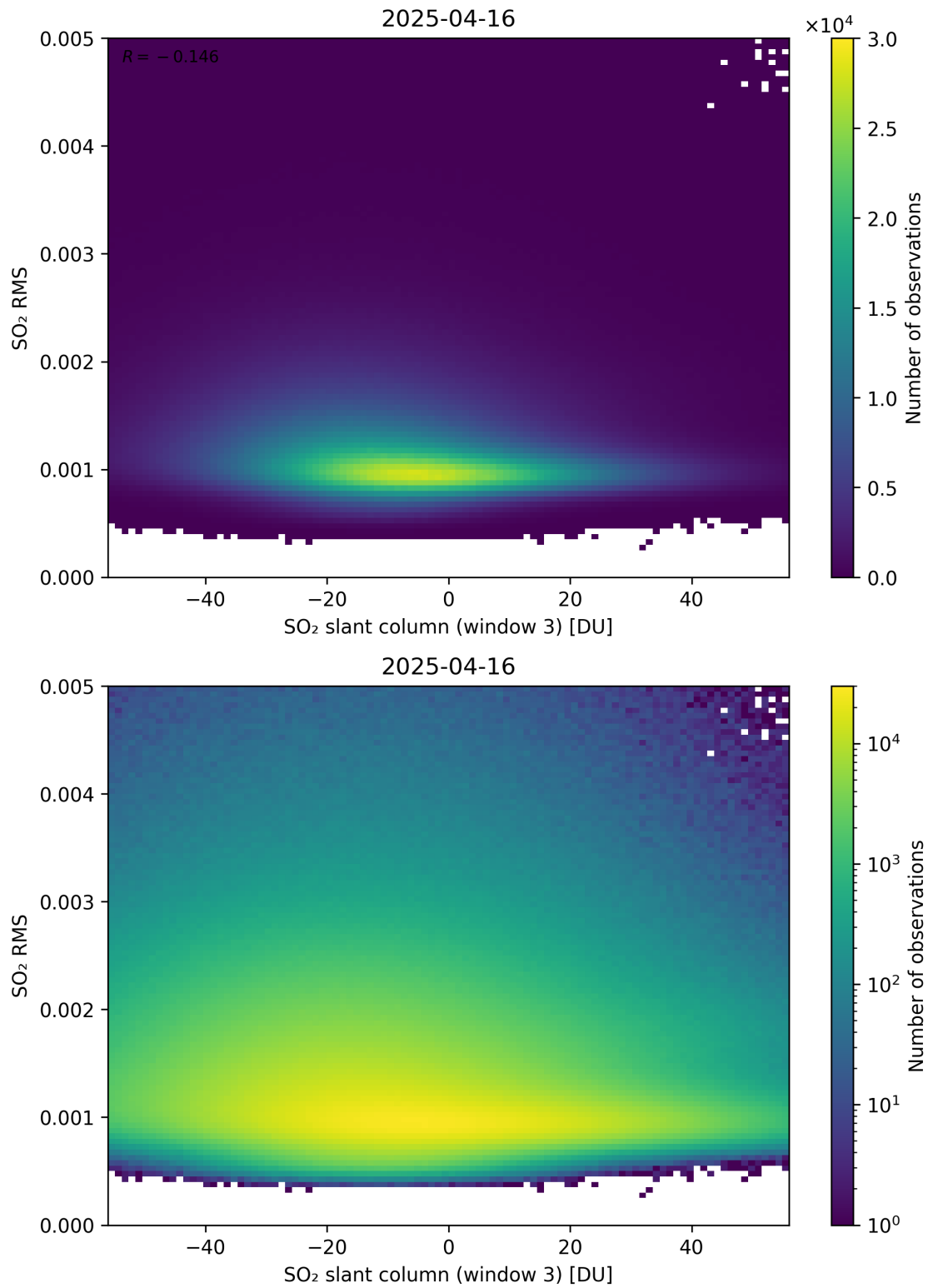
Figure 306: Scatter density plot of “SO 2 slant column (window 3)” against “SO 2 RMS” for 2025-04-15 to 2025-04-17.
