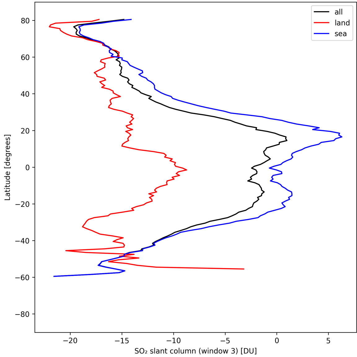
Figure 45: Zonal average of “SO 2 slant column (window 3)” for 2025-04-15 to 2025-04-17.
