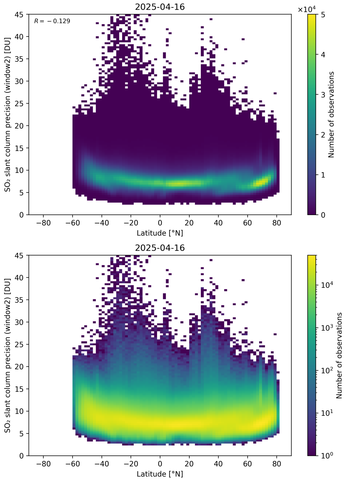
Figure 164: Scatter density plot of “Latitude” against “SO 2 slant column precision (window2)” for 2025-04-15 to 2025-04-17.
