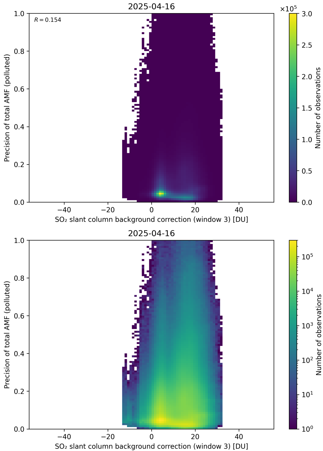
Figure 137: Scatter density plot of “SO 2 slant column background correction (window 3)” against “Precision of total AMF (polluted)” for 2025-04-15 to 2025-04-17.
