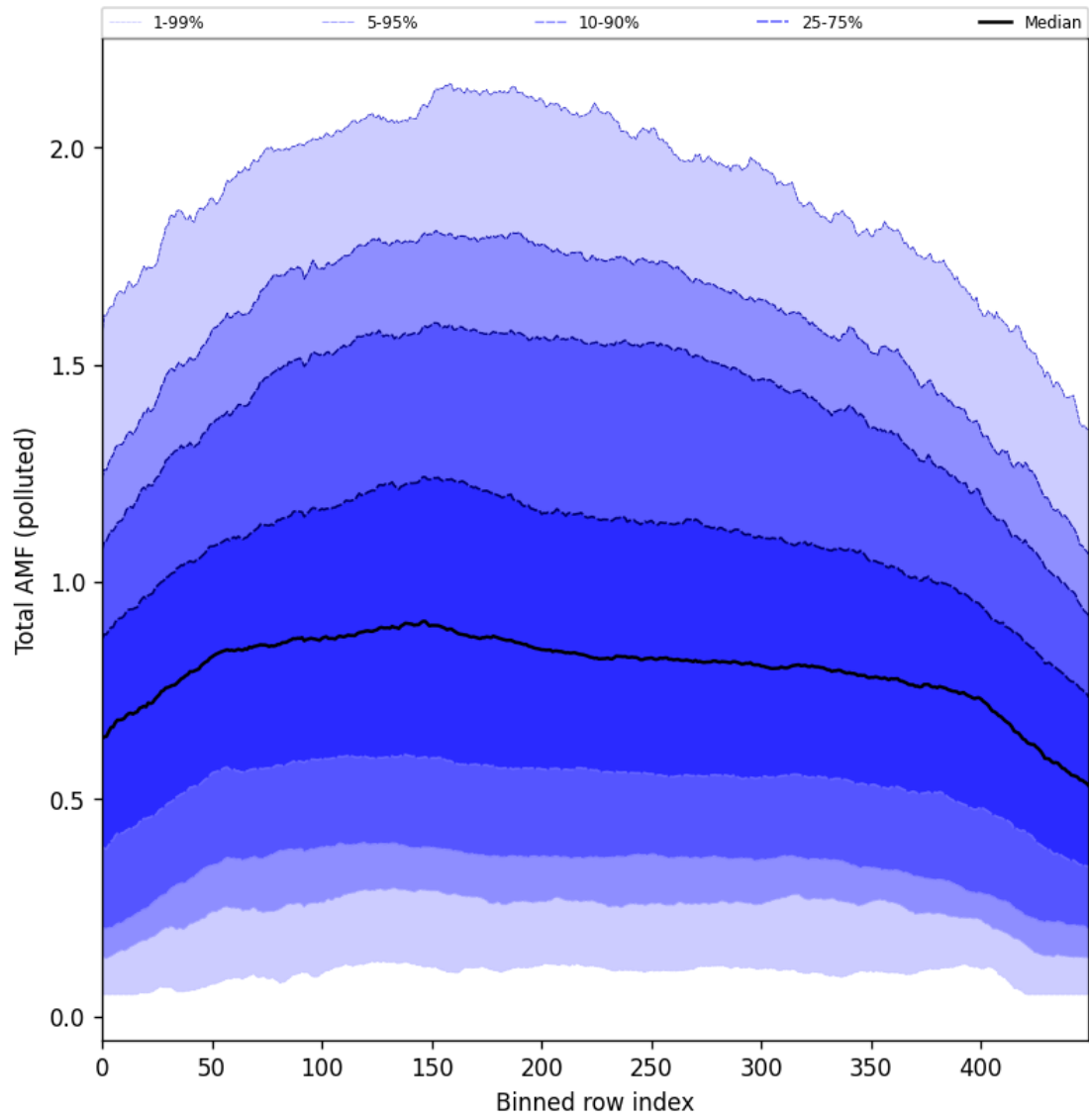
Figure 105: Along track statistics of “Total AMF (polluted)” for 2025-04-15 to 2025-04-17
