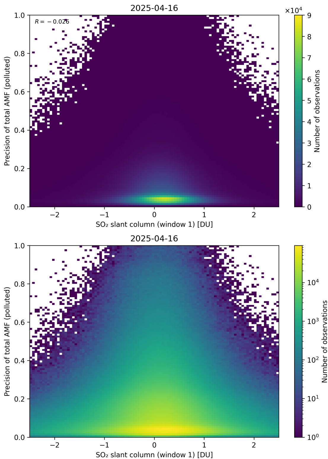
Figure 290: Scatter density plot of “SO 2 slant column (window 1)” against “Precision of total AMF (polluted)” for 2025-04-15 to 2025-04-17.
