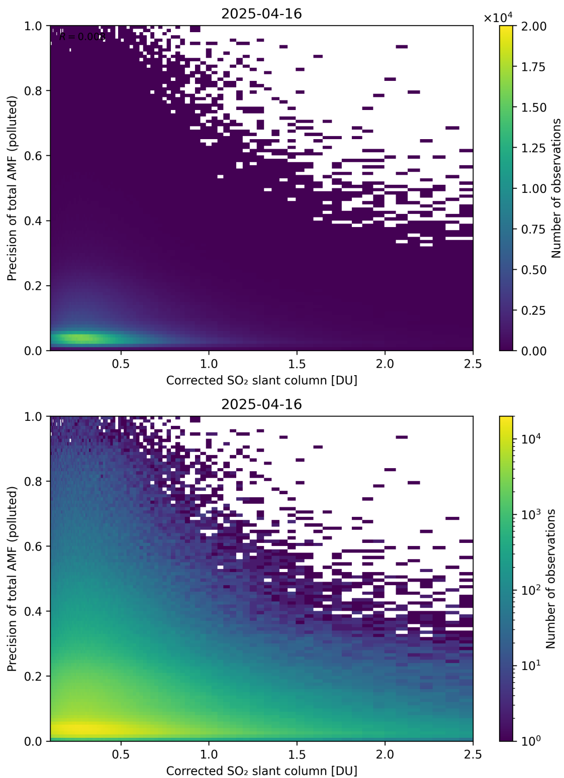
Figure 243: Scatter density plot of “Corrected SO 2 slant column” against “Precision of total AMF (polluted)” for 2025-04-15 to 2025-04-17.
