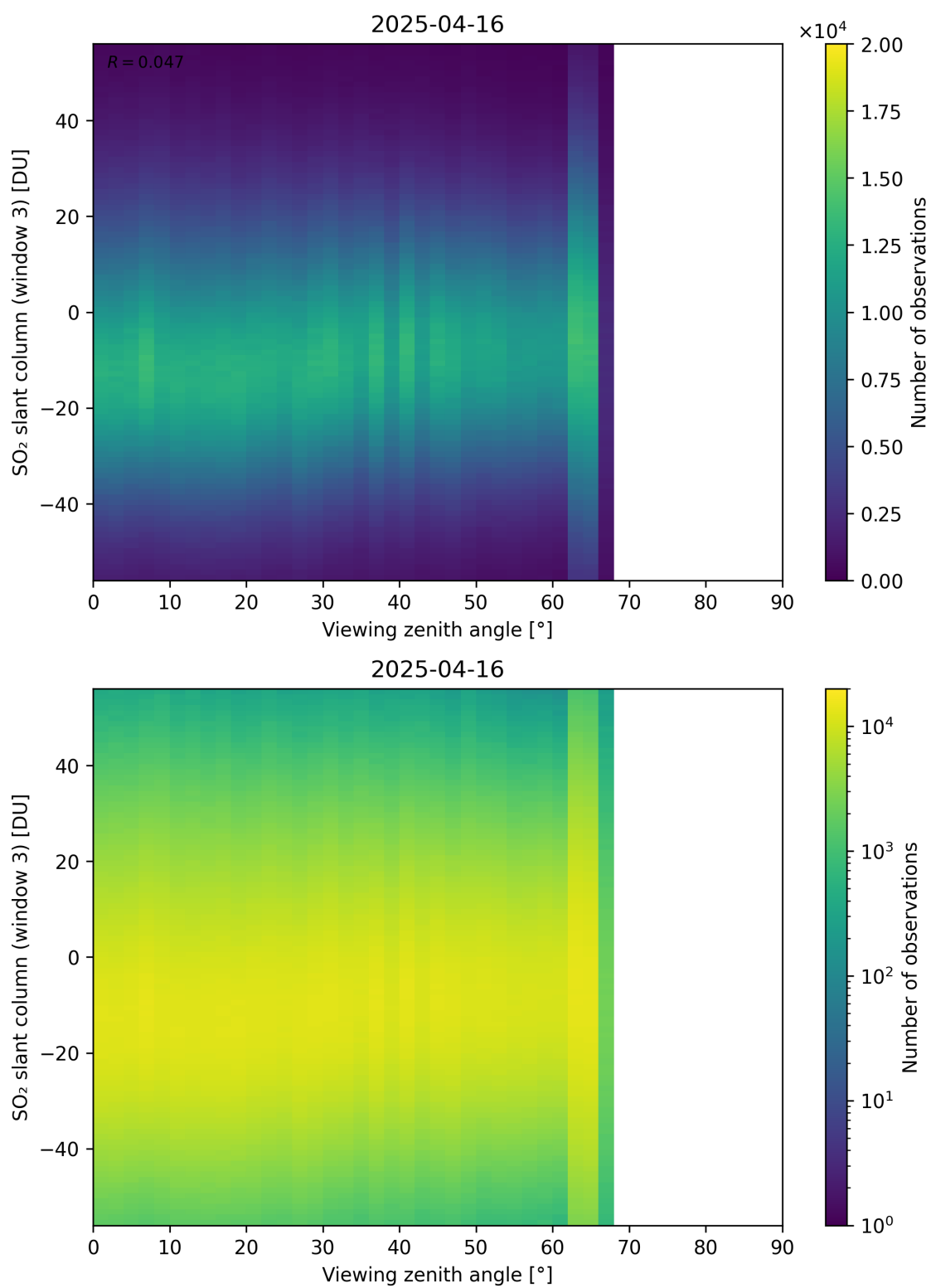
Figure 379: Scatter density plot of “Viewing zenith angle” against “SO 2 slant column (window 3)” for 2025-04-15 to 2025-04-17.
