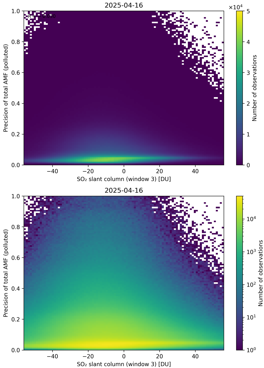
Figure 319: Scatter density plot of “SO 2 slant column (window 3)” against “Precision of total AMF (polluted)” for 2025-04-15 to 2025-04-17.
