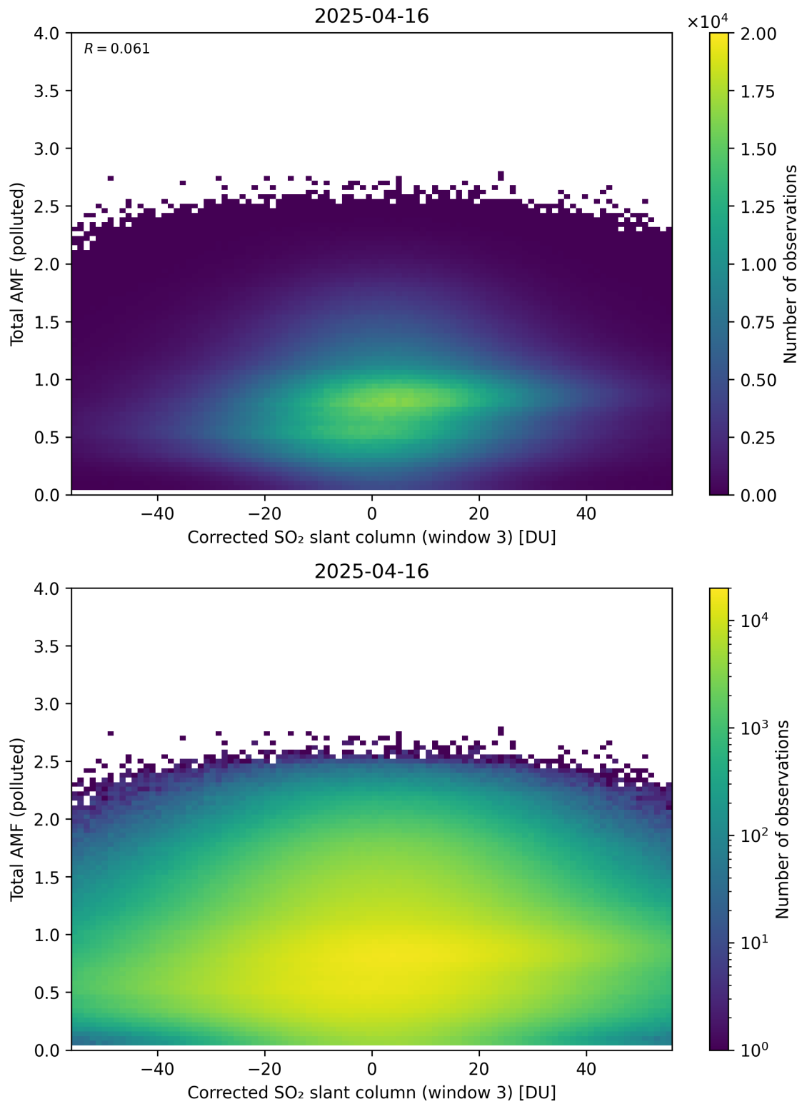
Figure 260: Scatter density plot of “Corrected SO 2 slant column (window 3)” against “Total AMF (polluted)” for 2025-04-15 to 2025-04-17.
