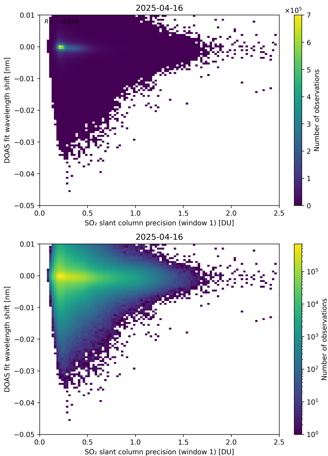
Figure 271: Scatter density plot of “SO 2 slant column precision (window 1)” against “DOAS fit wavelength shift” for 2025-04-15 to 2025-04-17.
