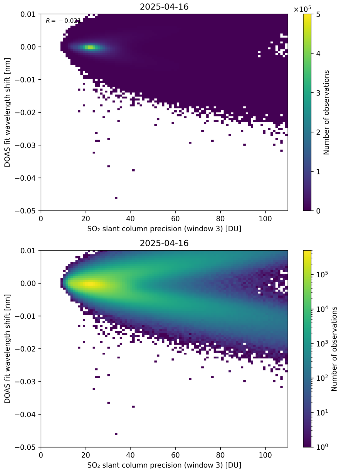
Figure 308: Scatter density plot of “SO 2 slant column precision (window 3)” against “DOAS fit wavelength shift” for 2025-04-15 to 2025-04-17.
