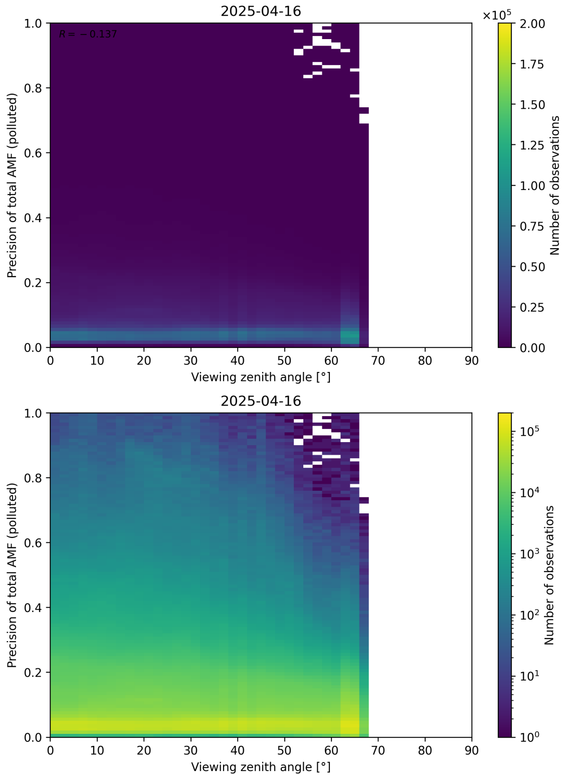
Figure 382: Scatter density plot of “Viewing zenith angle” against “Precision of total AMF (polluted)” for 2025-04-15 to 2025-04-17.
