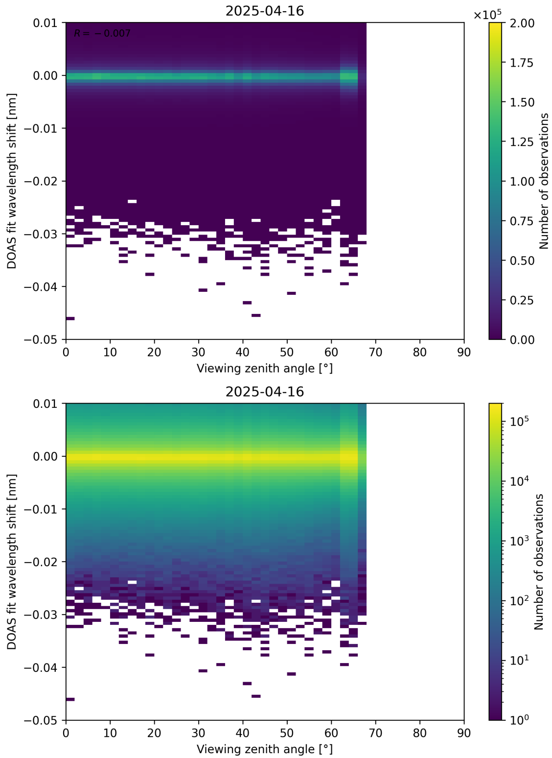
Figure 365: Scatter density plot of “Viewing zenith angle” against “DOAS fit wavelength shift” for 2025-04-15 to 2025-04-17.
