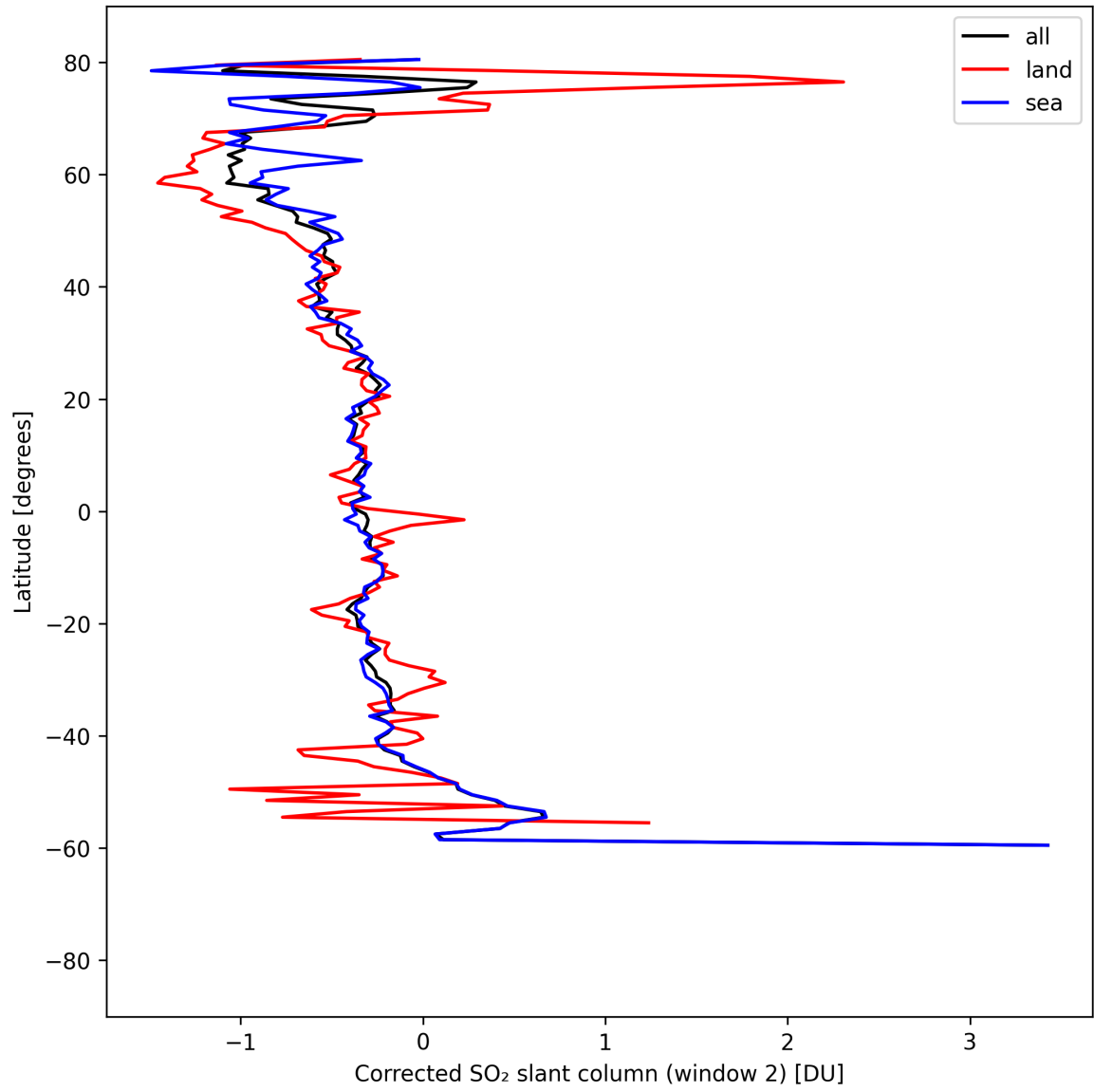
Figure 43: Zonal average of “Corrected SO 2 slant column (window 2)” for 2025-04-15 to 2025-04-17.
