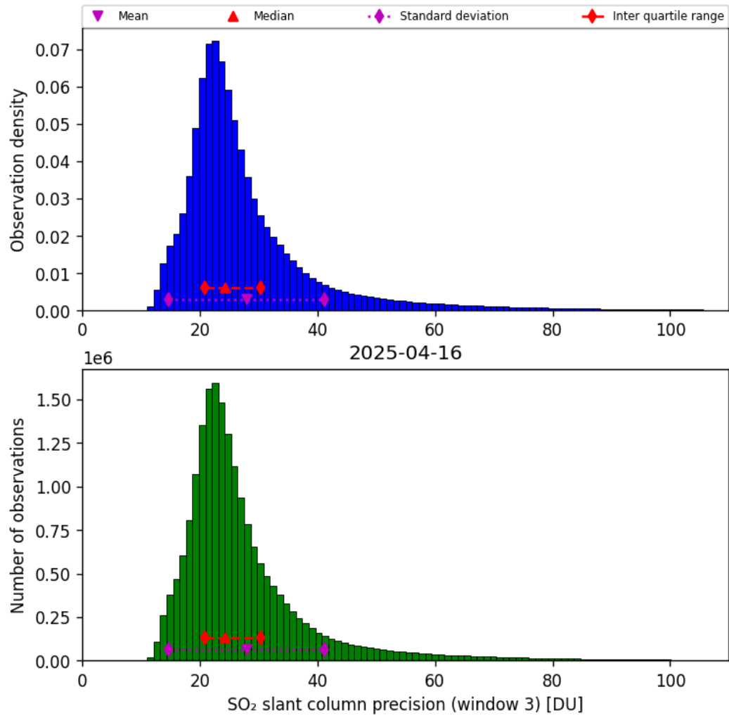
Figure 72: Histogram of “SO 2 slant column precision (window 3)” for 2025-04-15 to 2025-04-17
