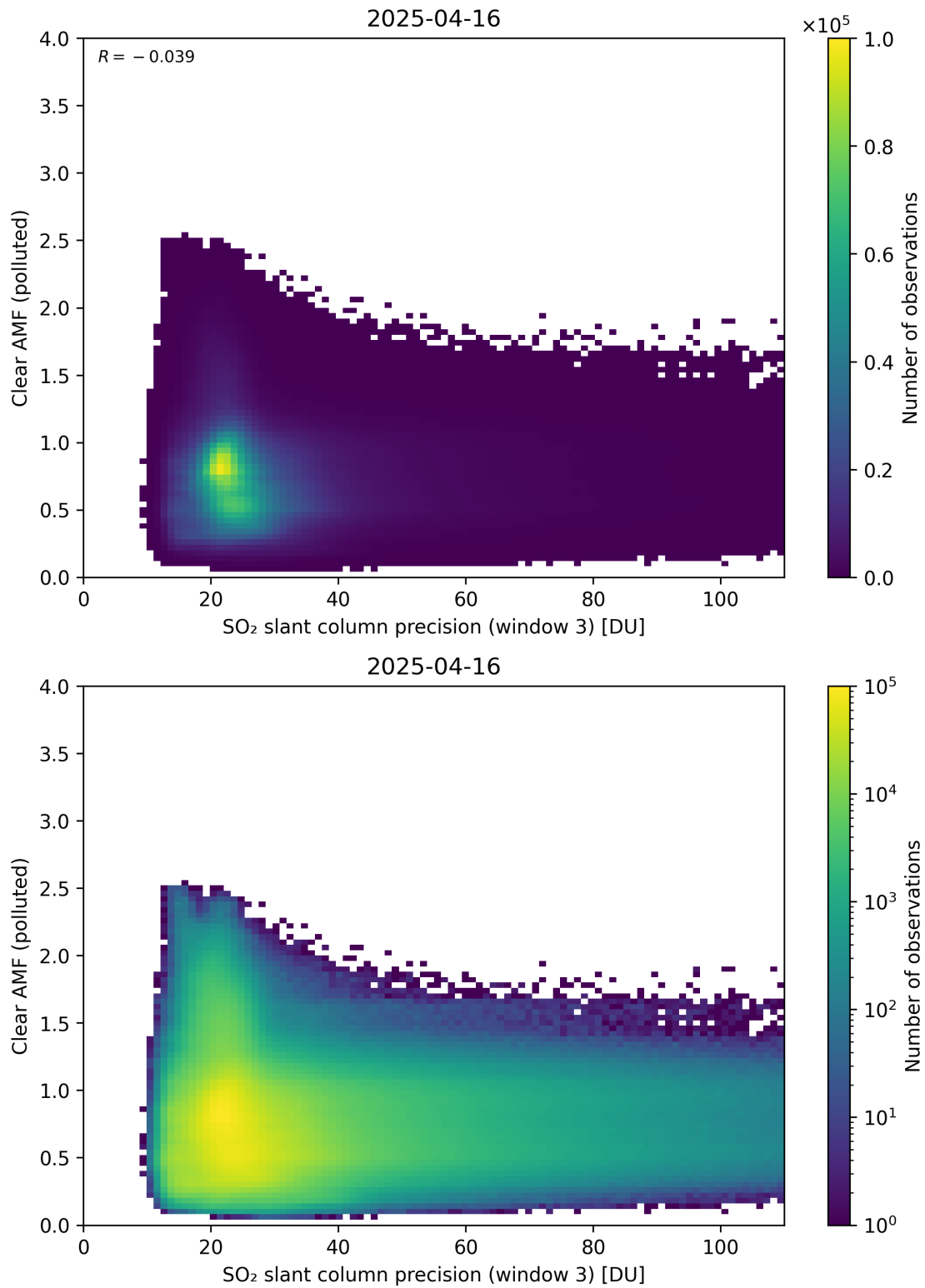
Figure 311: Scatter density plot of “SO 2 slant column precision (window 3)” against “Clear AMF (polluted)” for 2025-04-15 to 2025-04-17.
