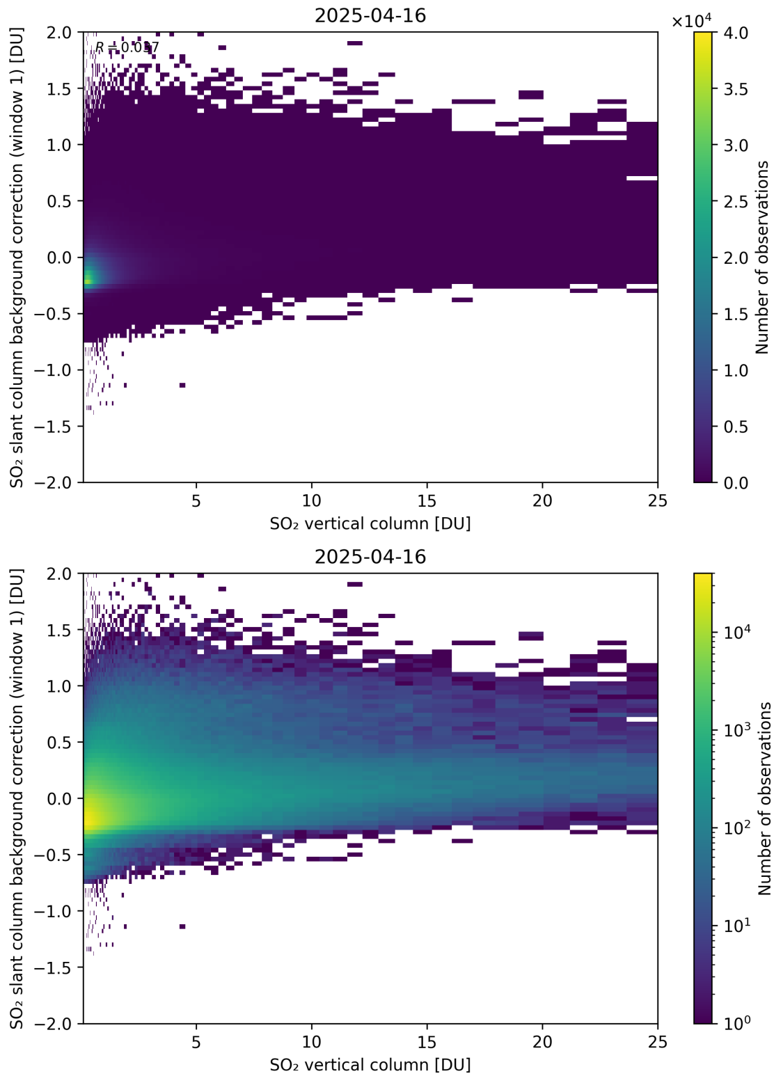
Figure 323: Scatter density plot of “SO 2 vertical column” against “SO 2 slant column background correction (window 1)” for 2025-04-15 to 2025-04-17.
