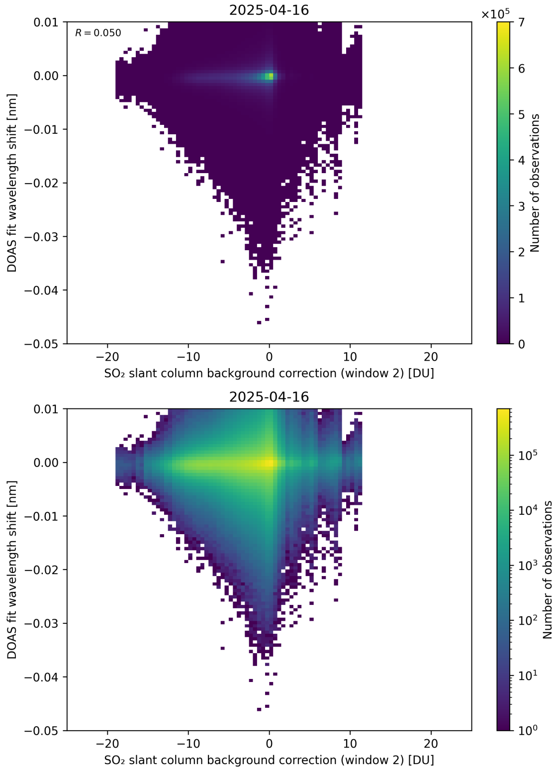
Figure 123: Scatter density plot of “SO 2 slant column background correction (window 2)” against “DOAS fit wavelength shift” for 2025-04-15 to 2025-04-17.
