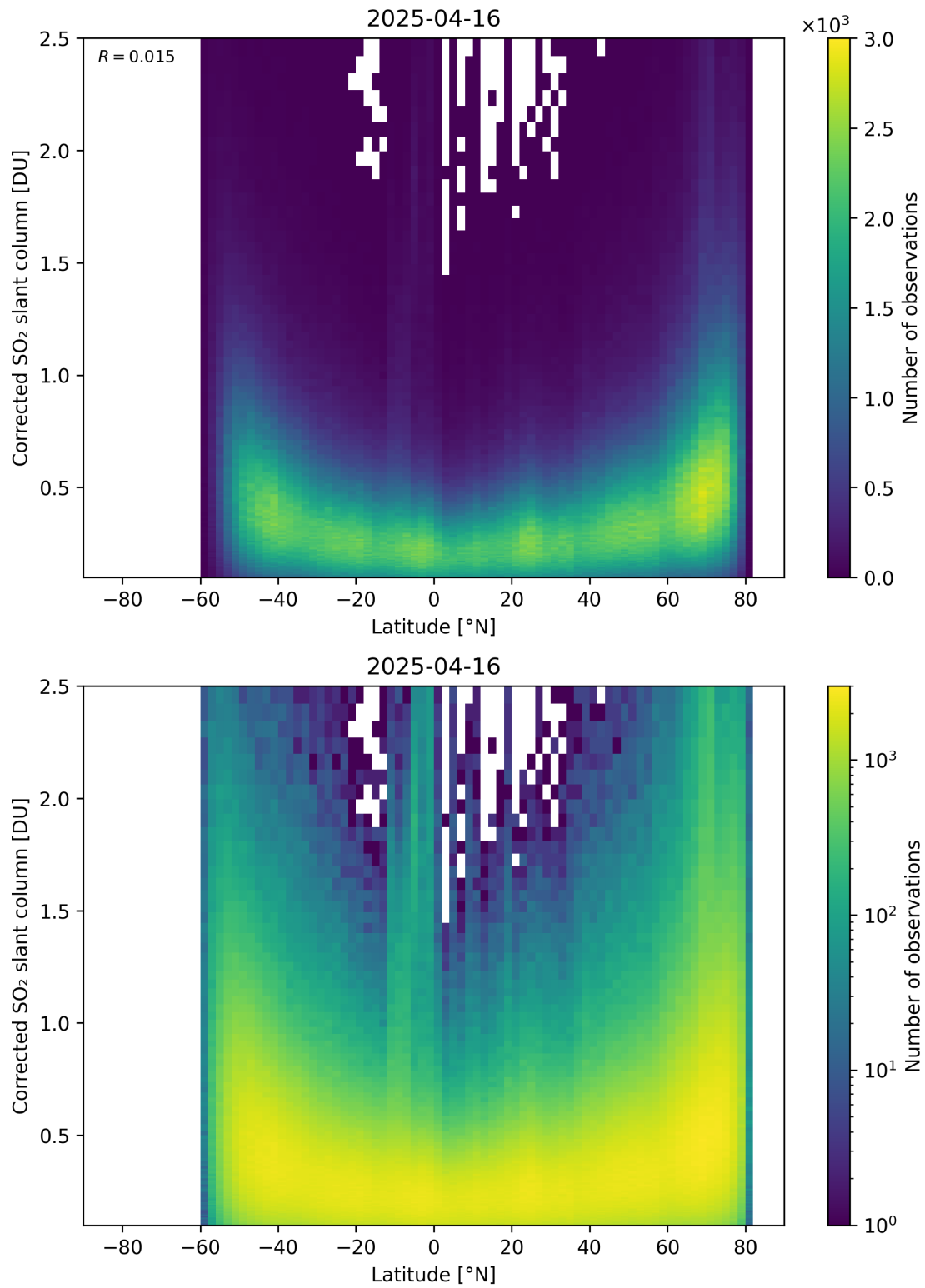
Figure 159: Scatter density plot of “Latitude” against “Corrected SO 2 slant column” for 2025-04-15 to 2025-04-17.
