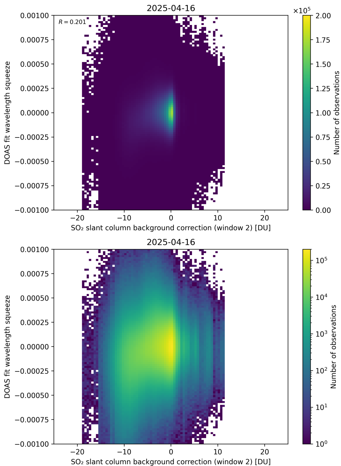
Figure 124: Scatter density plot of “SO 2 slant column background correction (window 2)” against “DOAS fit wavelength squeeze” for 2025-04-15 to 2025-04-17.
