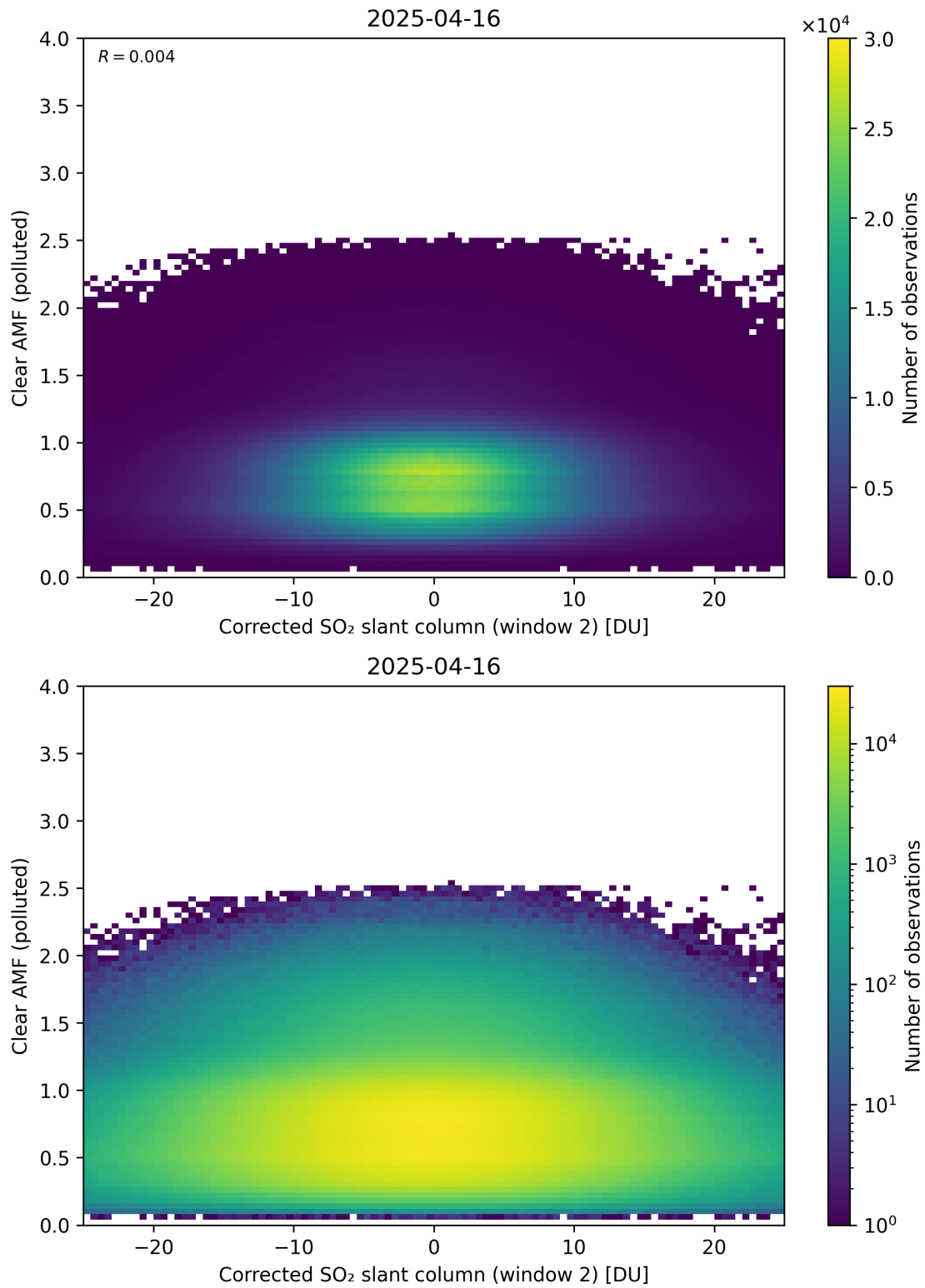
Figure 249: Scatter density plot of “Corrected SO 2 slant column (window 2)” against “Clear AMF (polluted)” for 2025-04-15 to 2025-04-17.
