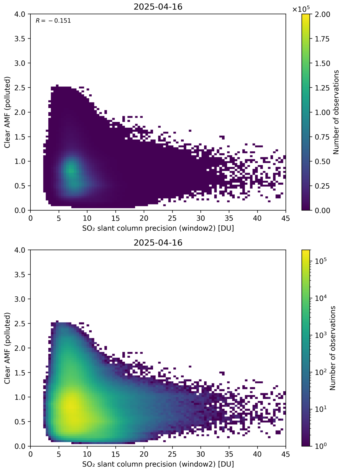
Figure 296: Scatter density plot of “SO 2 slant column precision (window2)” against “Clear AMF (polluted)” for 2025-04-15 to 2025-04-17.
