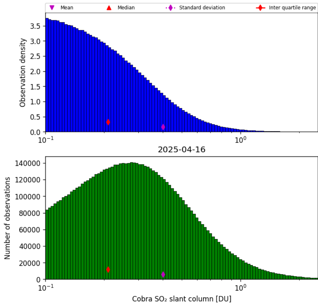
Figure 61: Histogram of “Cobra SO 2 slant column” for 2025-04-15 to 2025-04-17
