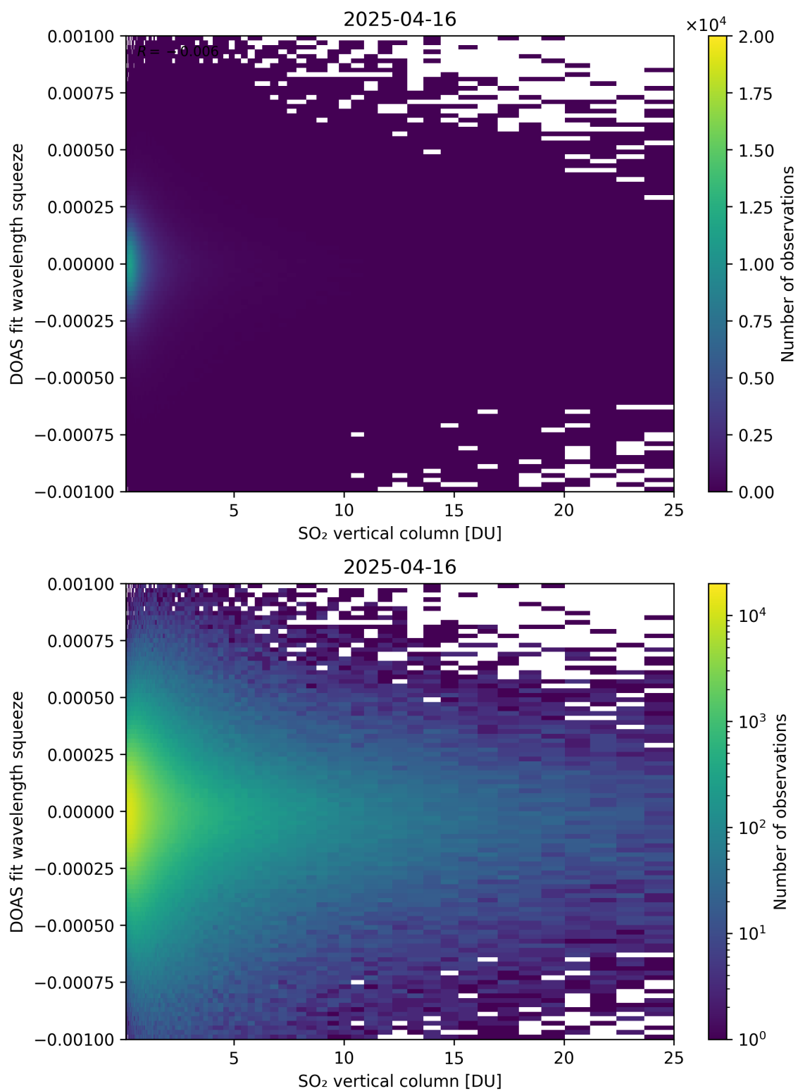
Figure 327: Scatter density plot of “SO 2 vertical column” against “DOAS fit wavelength squeeze” for 2025-04-15 to 2025-04-17.
