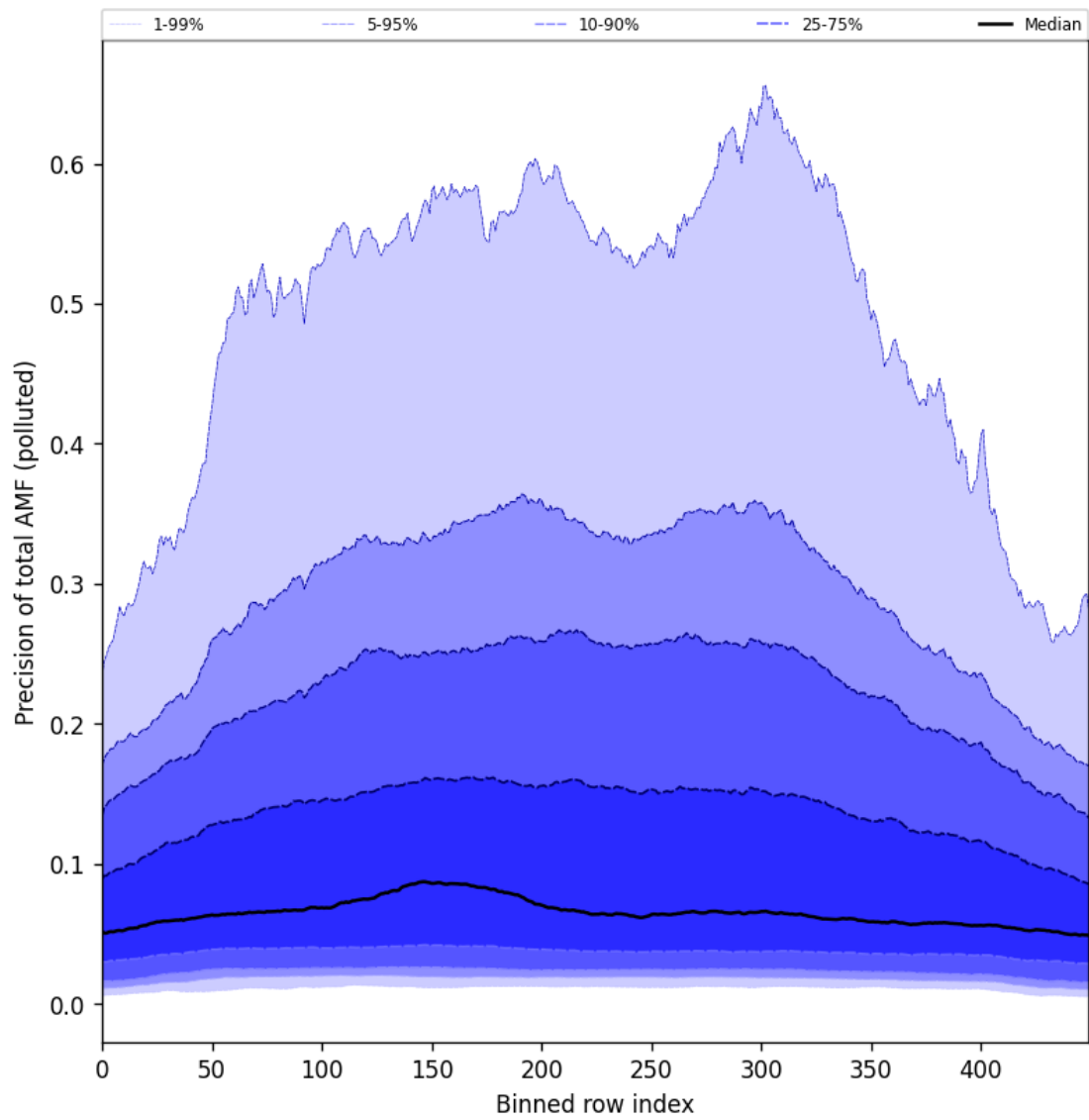
Figure 106: Along track statistics of “Precision of total AMF (polluted)” for 2025-04-15 to 2025-04-17
