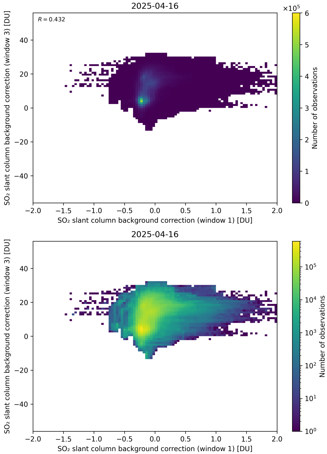
Figure 110: Scatter density plot of “SO 2 slant column background correction (window 1)” against “SO 2 slant column background correction (window 3)” for 2025-04-15 to 2025-04-17.
