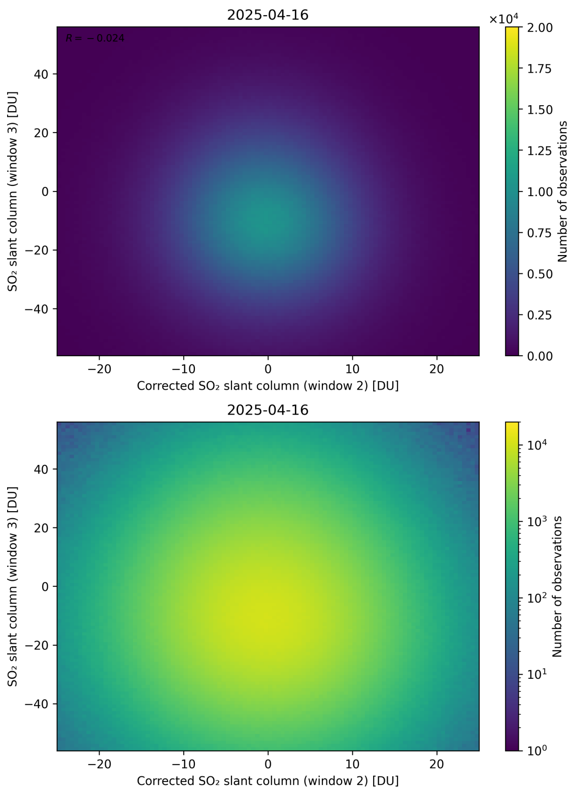
Figure 251: Scatter density plot of “Corrected SO 2 slant column (window 2)” against “SO 2 slant column (window 3)” for 2025-04-15 to 2025-04-17.
