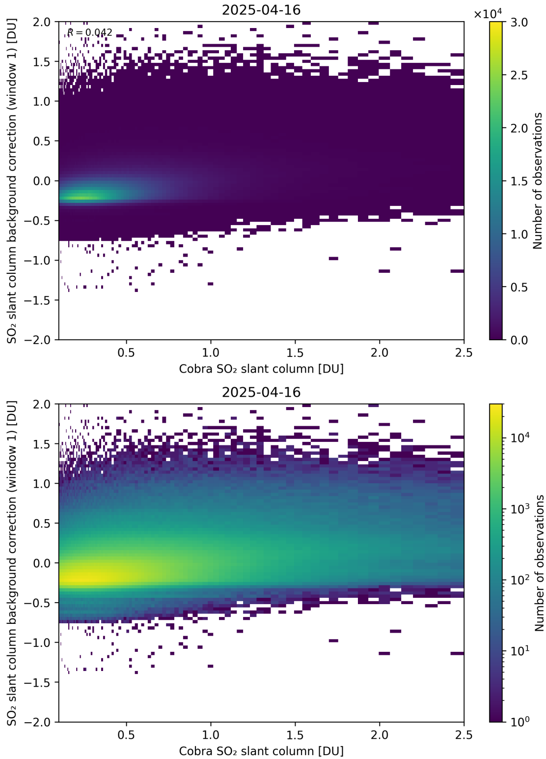
Figure 193: Scatter density plot of “Cobra SO 2 slant column” against “SO 2 slant column background correction (window 1)” for 2025-04-15 to 2025-04-17.
