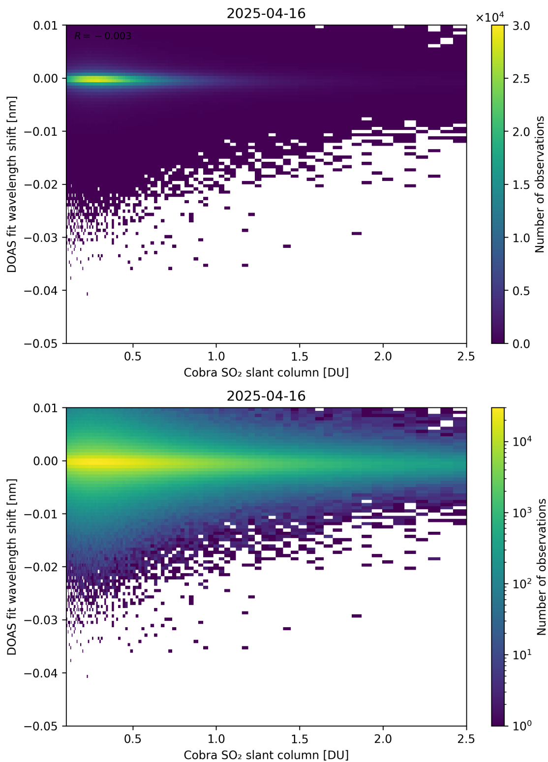
Figure 196: Scatter density plot of “Cobra SO 2 slant column” against “DOAS fit wavelength shift” for 2025-04-15 to 2025-04-17.
