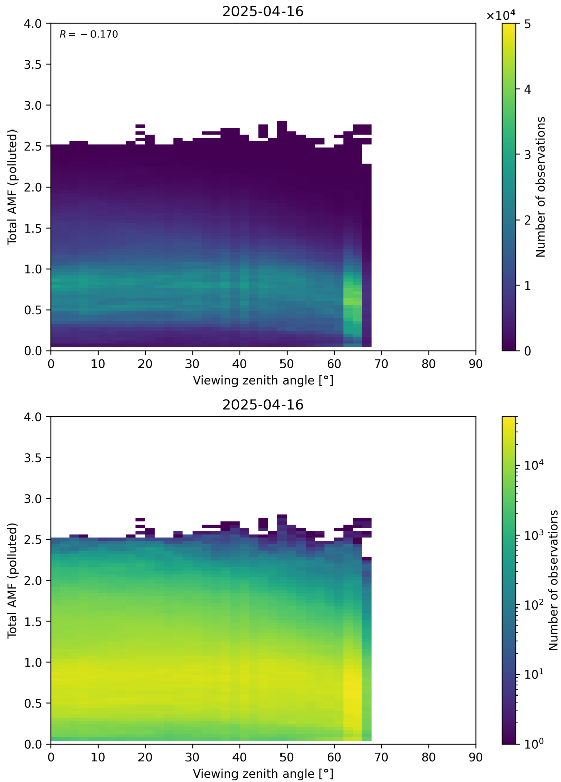
Figure 381: Scatter density plot of “Viewing zenith angle” against “Total AMF (polluted)” for 2025-04-15 to 2025-04-17.
