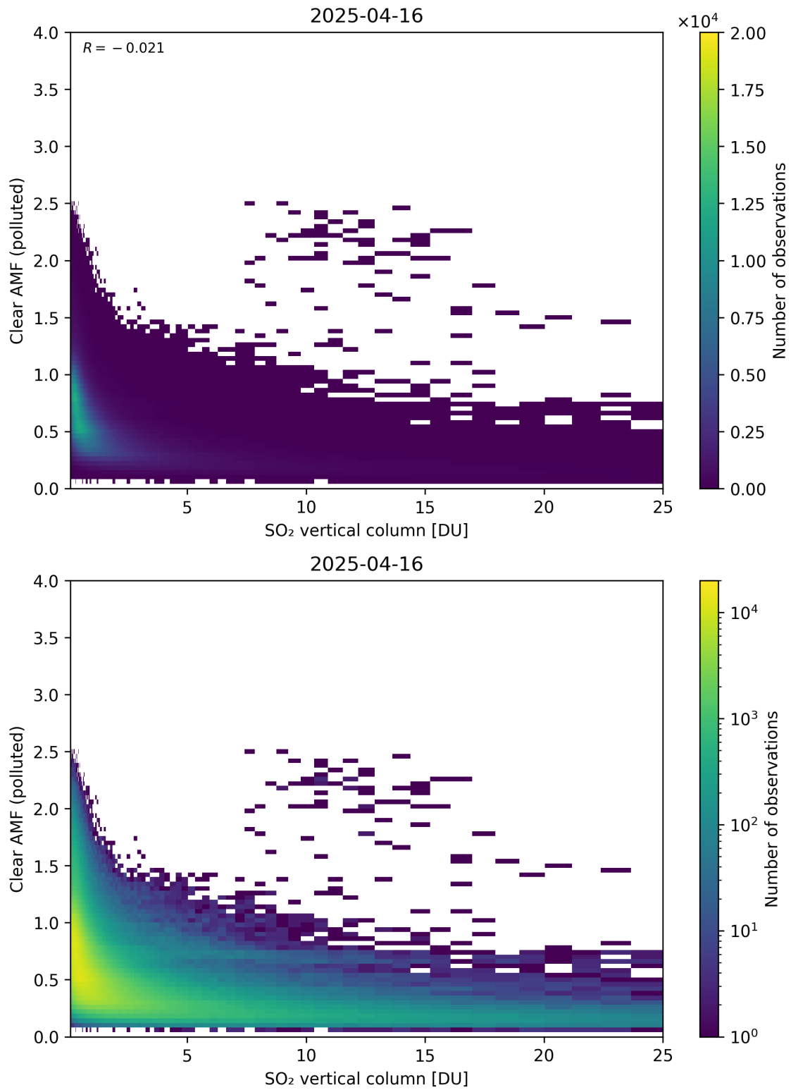
Figure 348: Scatter density plot of “SO 2 vertical column” against “Clear AMF (polluted)” for 2025-04-15 to 2025-04-17.
