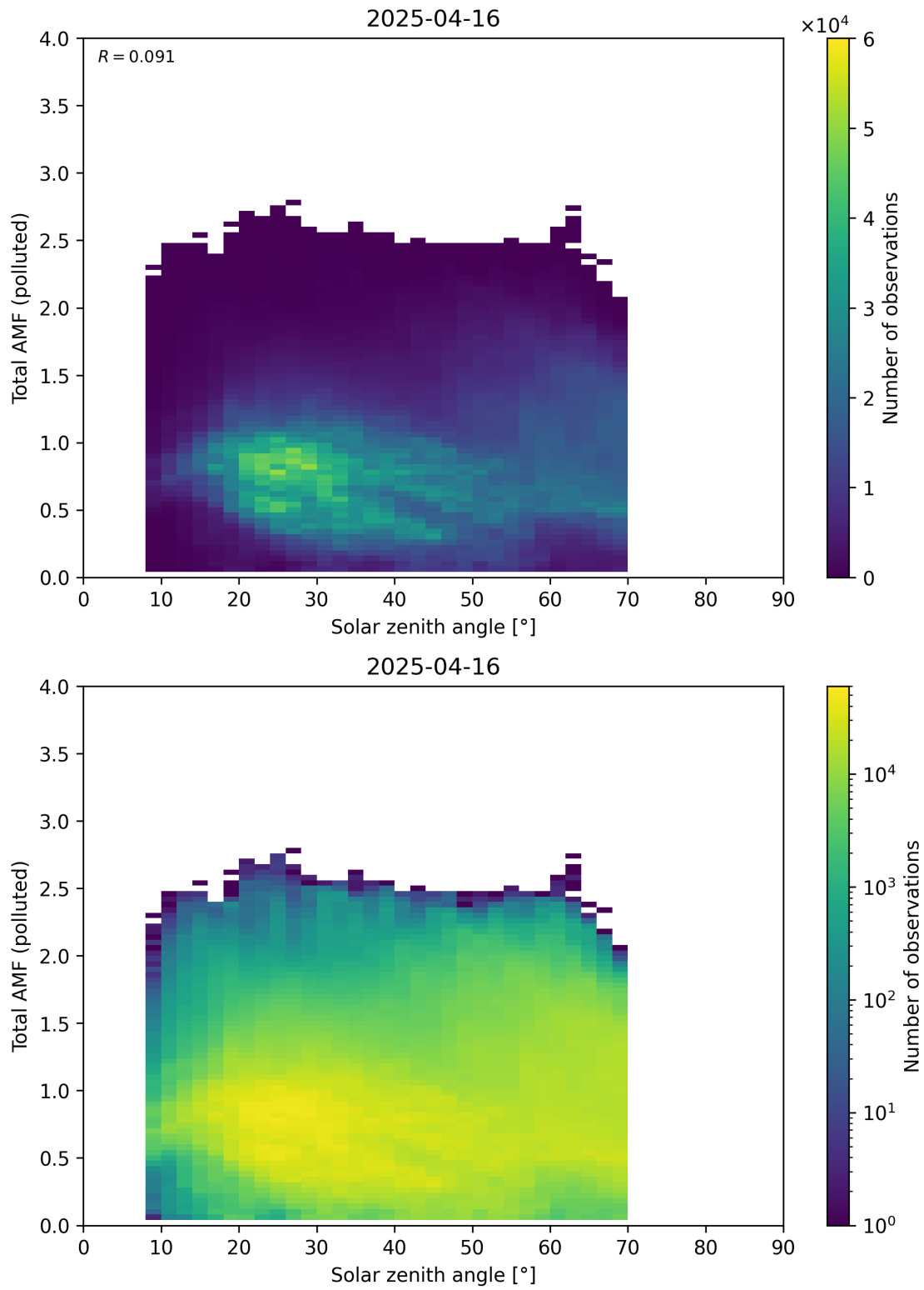
Figure 189: Scatter density plot of “Solar zenith angle” against “Total AMF (polluted)” for 2025-04-15 to 2025-04-17.
