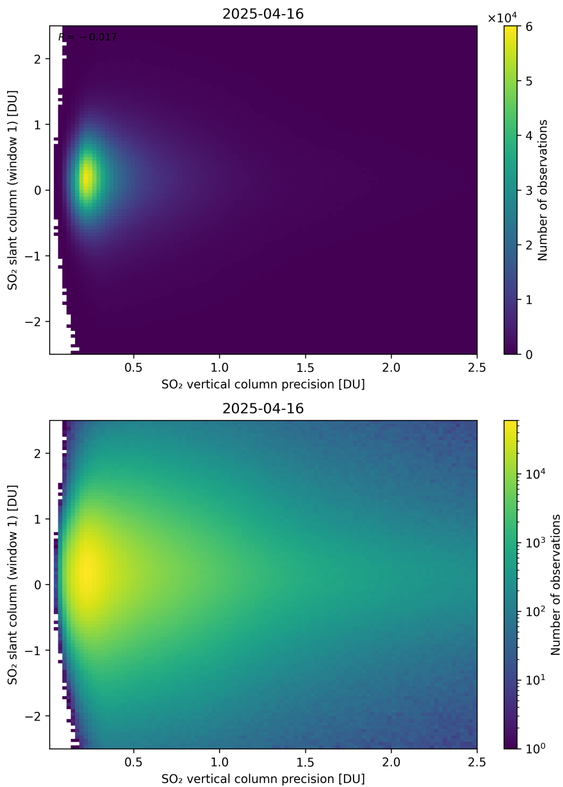
Figure 341: Scatter density plot of “SO 2 vertical column precision” against “SO 2 slant column (window 1)” for 2025-04-15 to 2025-04-17.
