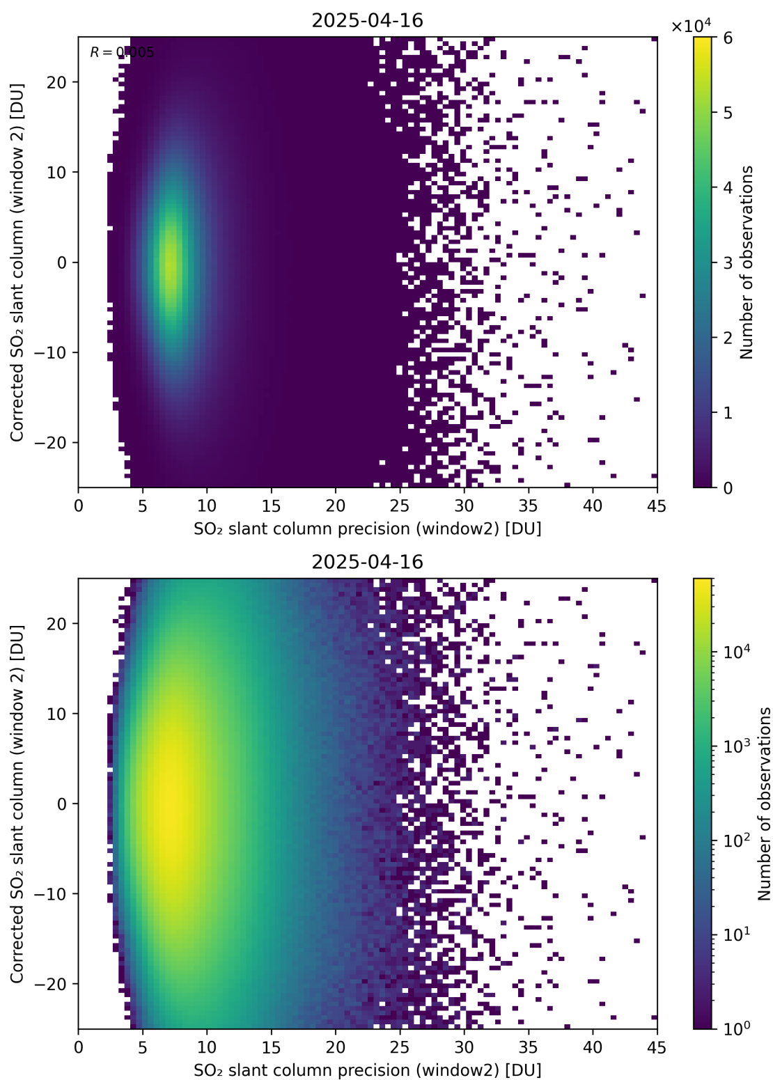
Figure 297: Scatter density plot of “SO 2 slant column precision (window2)” against “Corrected SO 2 slant column (window 2)” for 2025-04-15 to 2025-04-17.
