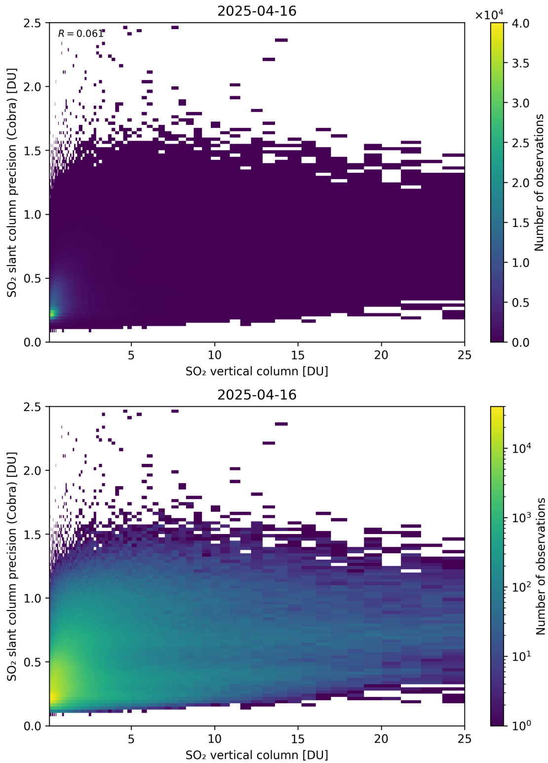
Figure 350: Scatter density plot of “SO 2 vertical column” against “SO 2 slant column precision (Cobra)” for 2025-04-15 to 2025-04-17.
