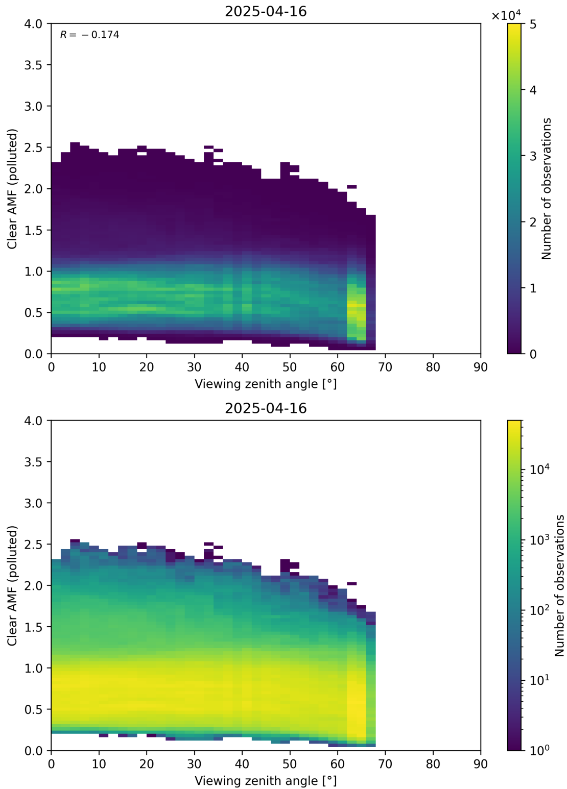
Figure 370: Scatter density plot of “Viewing zenith angle” against “Clear AMF (polluted)” for 2025-04-15 to 2025-04-17.
