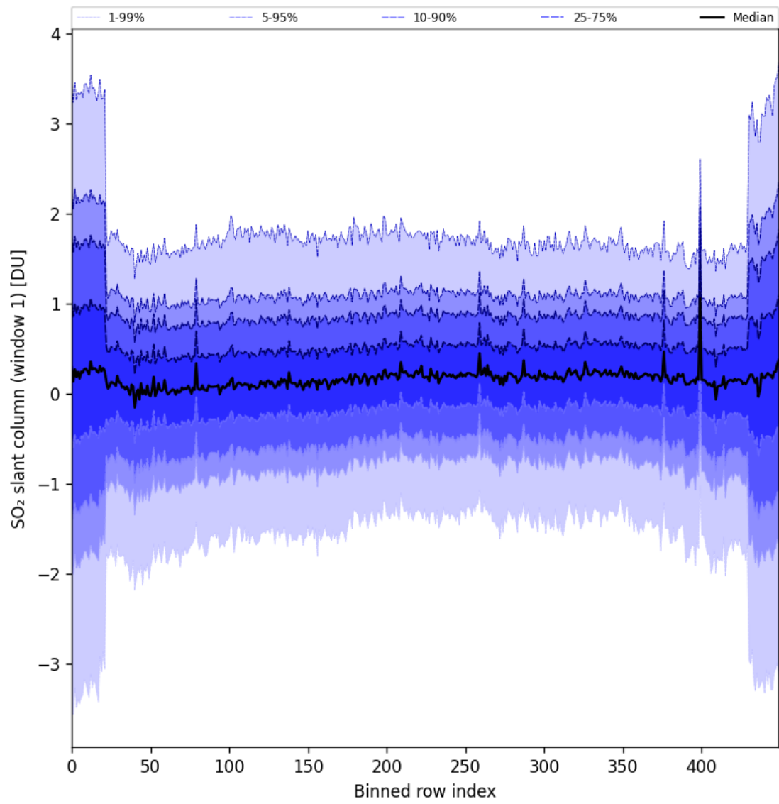
Figure 89: Along track statistics of “SO 2 slant column (window 1)” for 2025-04-15 to 2025-04-17
