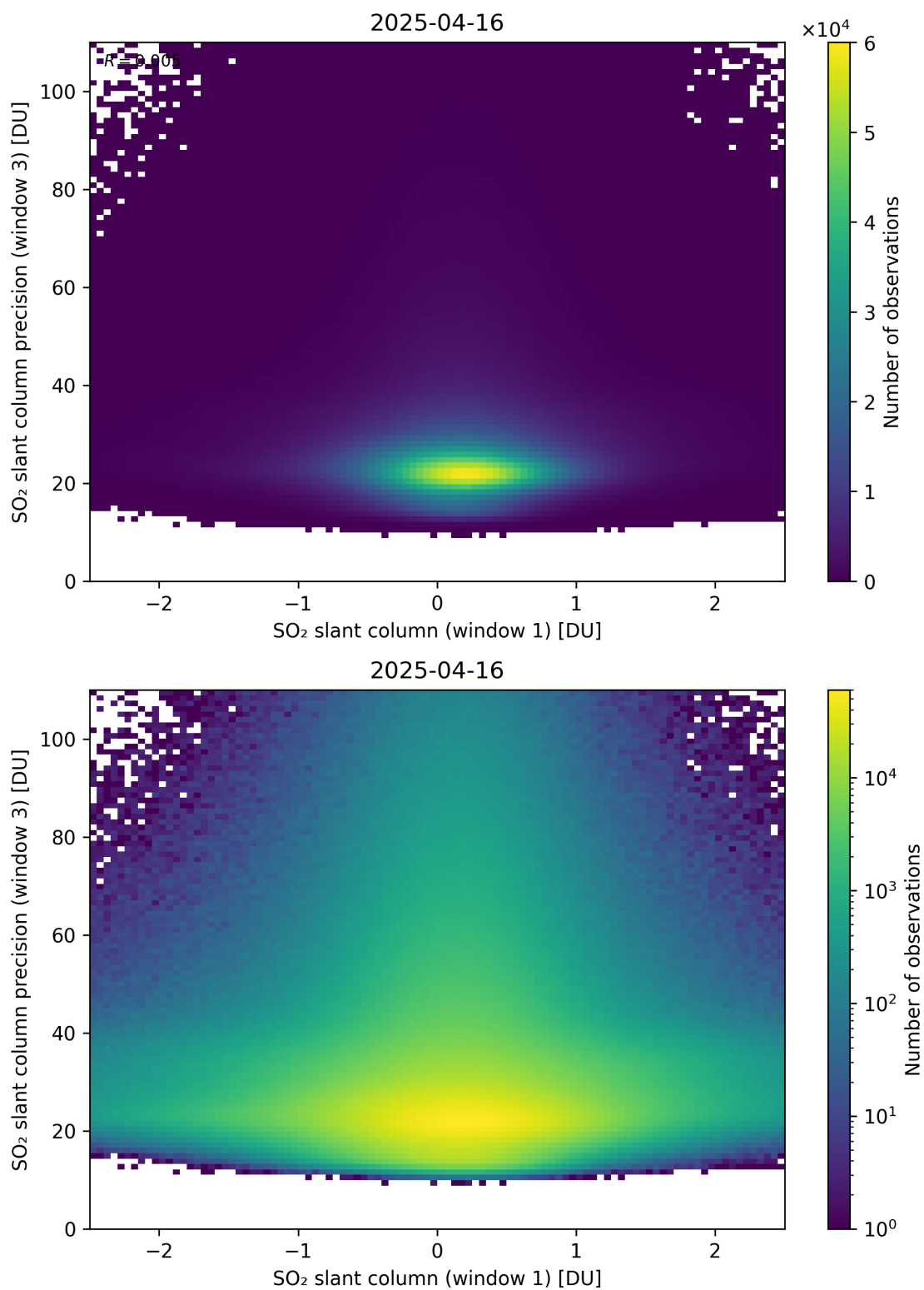
Figure 288: Scatter density plot of “SO 2 slant column (window 1)” against “SO 2 slant column precision (window 3)” for 2025-04-15 to 2025-04-17.
