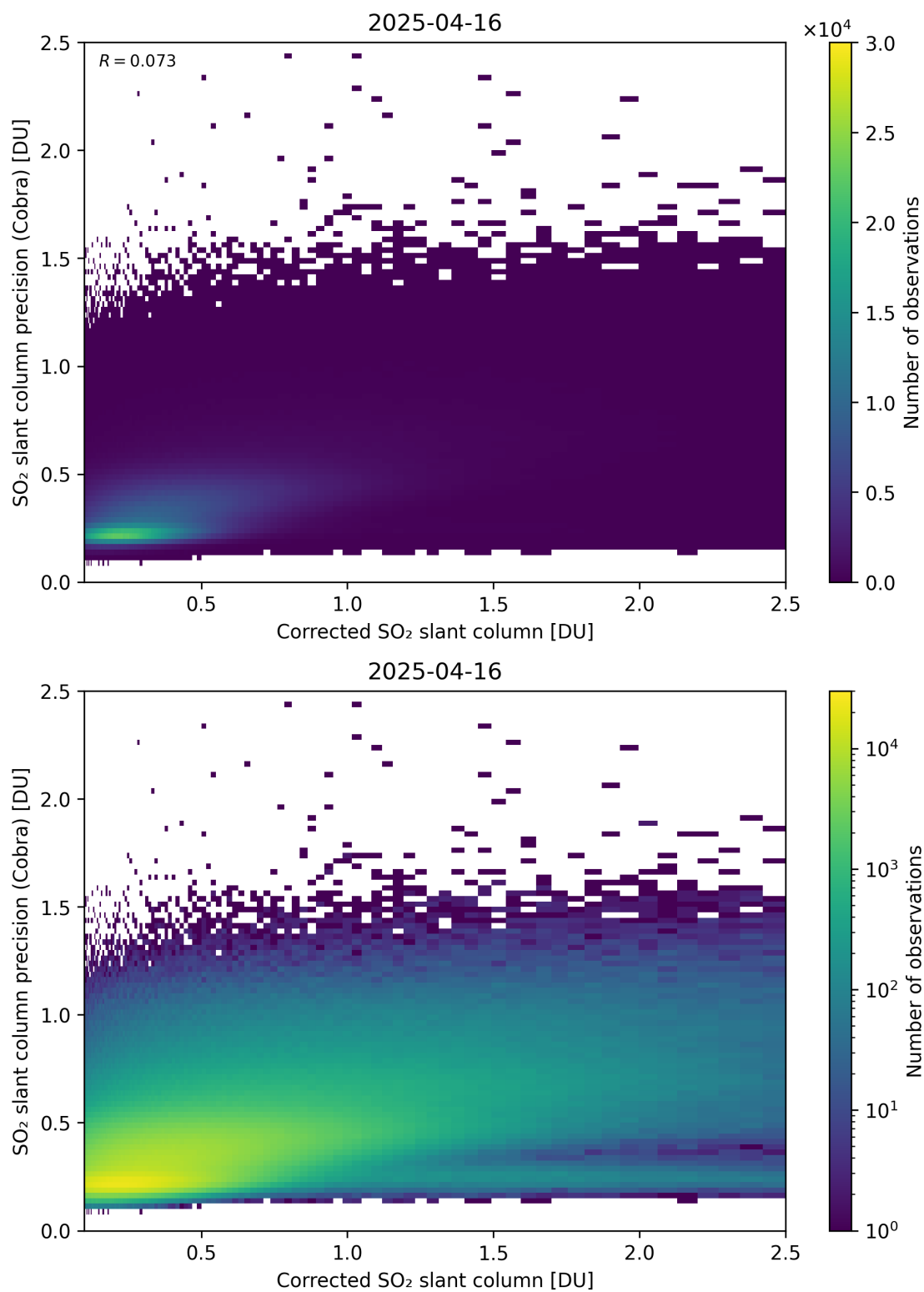
Figure 234: Scatter density plot of “Corrected SO 2 slant column” against “SO 2 slant column precision (Cobra)” for 2025-04-15 to 2025-04-17.
