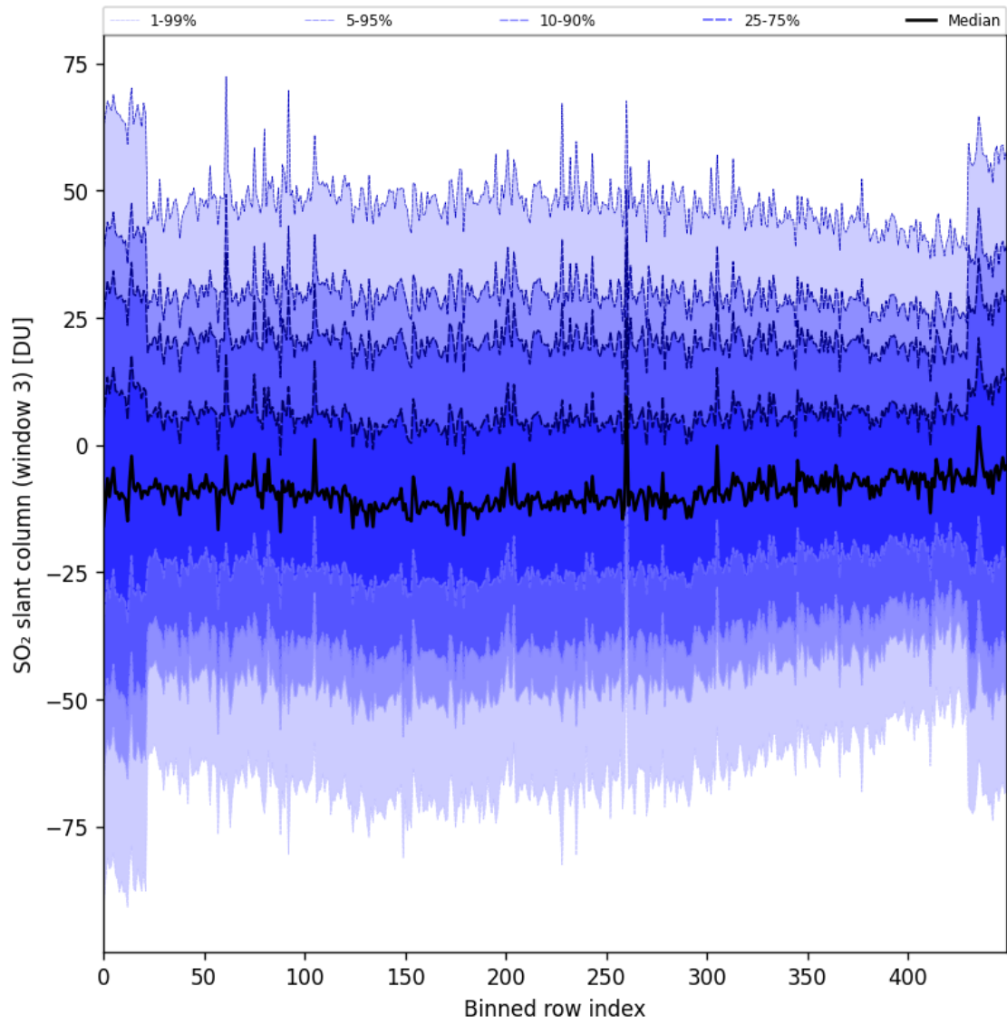
Figure 97: Along track statistics of “SO 2 slant column (window 3)” for 2025-04-15 to 2025-04-17
