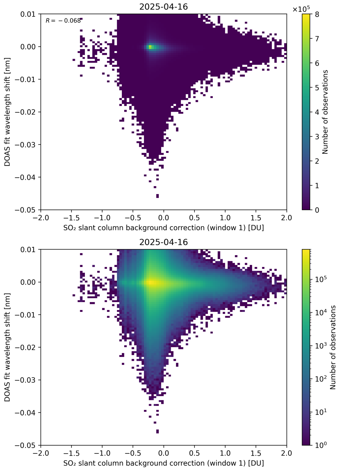
Figure 111: Scatter density plot of “SO 2 slant column background correction (window 1)” against “DOAS fit wavelength shift” for 2025-04-15 to 2025-04-17.
