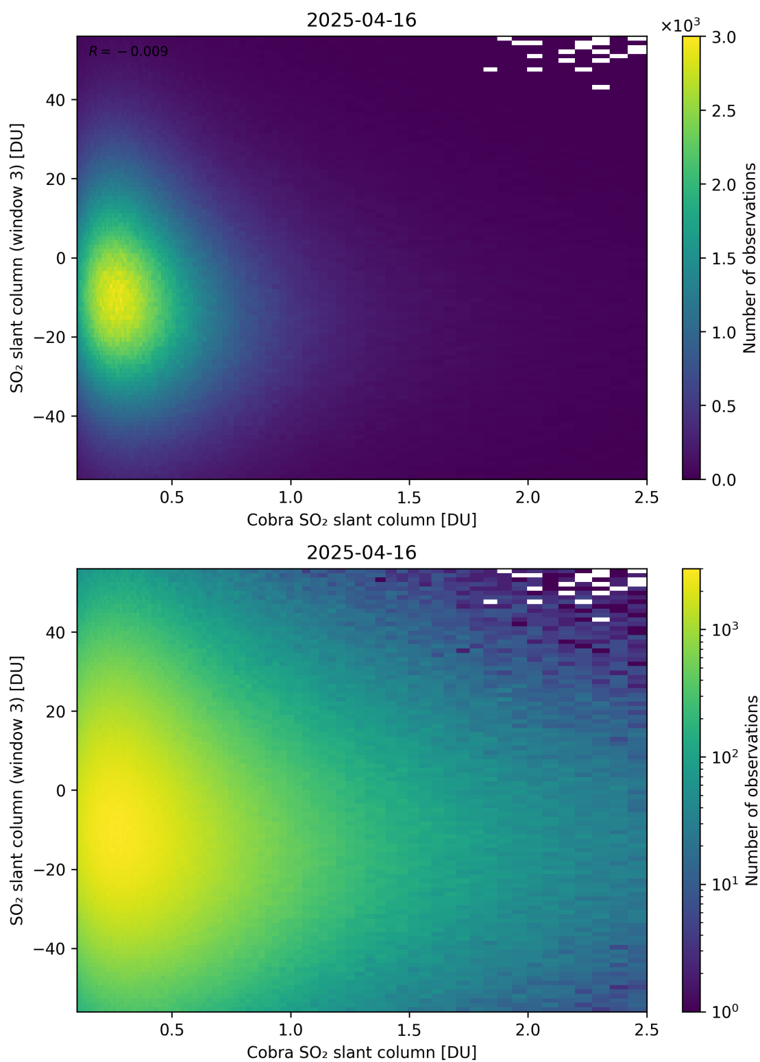
Figure 222: Scatter density plot of “Cobra SO 2 slant column” against “SO 2 slant column (window 3)” for 2025-04-15 to 2025-04-17.
