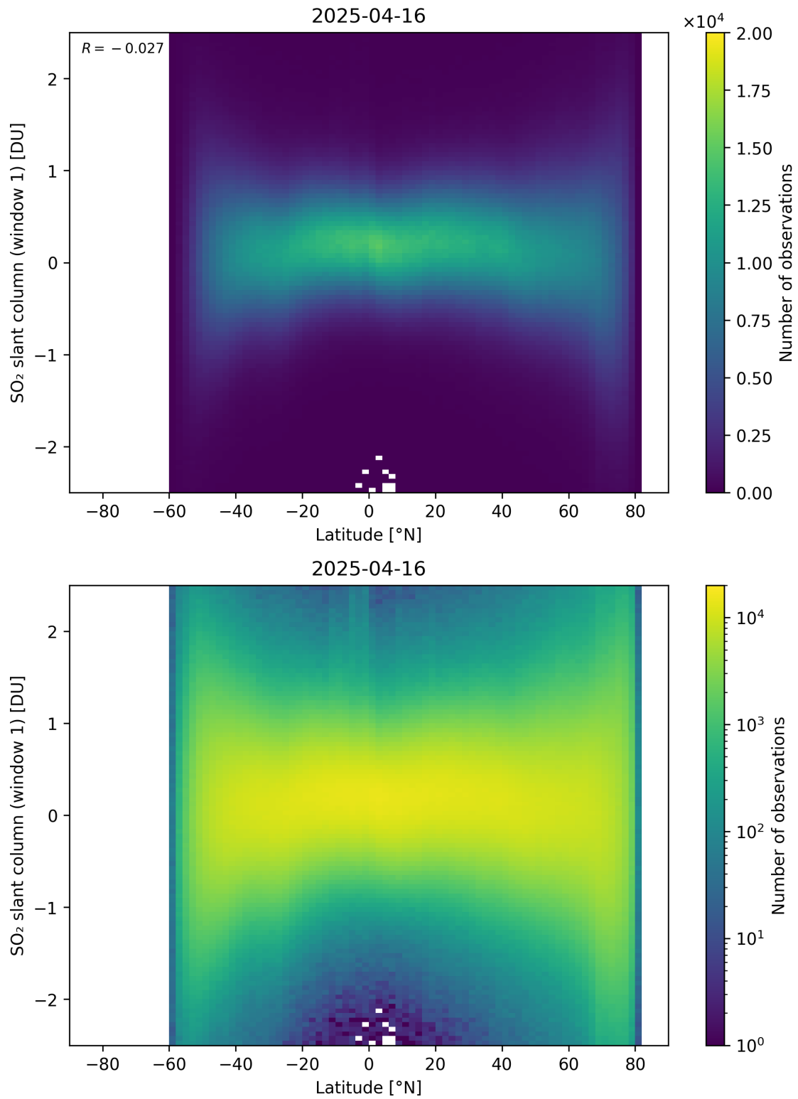
Figure 162: Scatter density plot of “Latitude” against “SO 2 slant column (window 1)” for 2025-04-15 to 2025-04-17.
