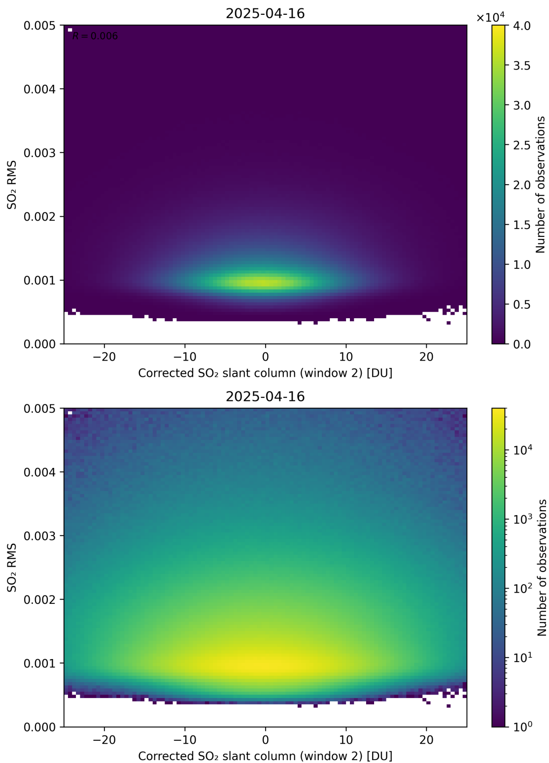
Figure 248: Scatter density plot of “Corrected SO 2 slant column (window 2)” against “SO 2 RMS” for 2025-04-15 to 2025-04-17.
