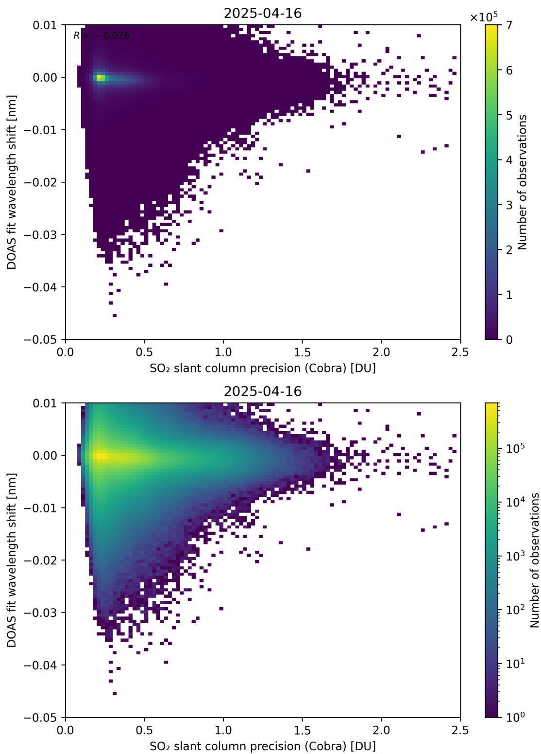
Figure 202: Scatter density plot of “SO 2 slant column precision (Cobra)” against “DOAS fit wavelength shift” for 2025-04-15 to 2025-04-17.
