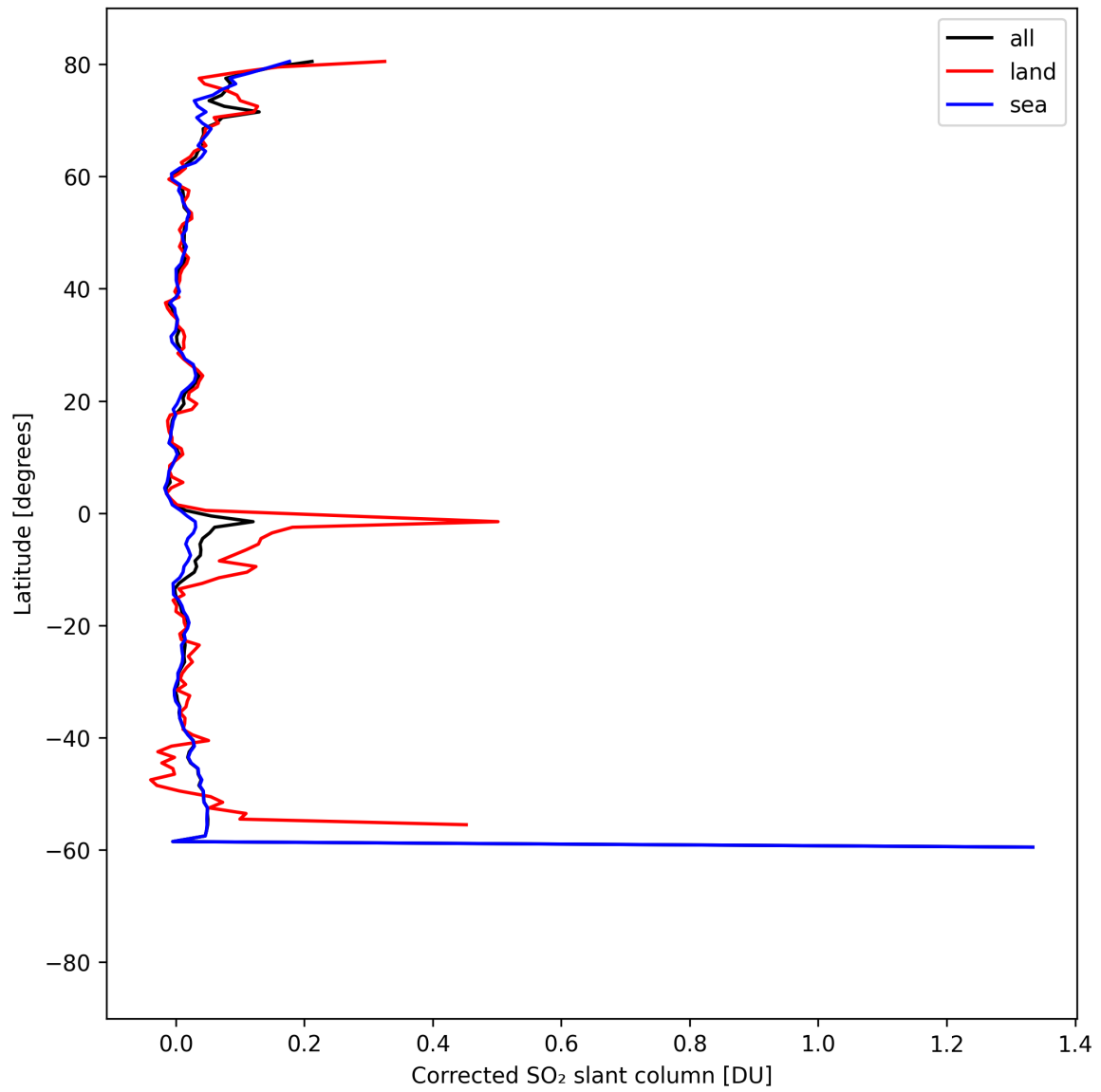
Figure 34: Zonal average of “Corrected SO 2 slant column” for 2025-04-15 to 2025-04-17.
