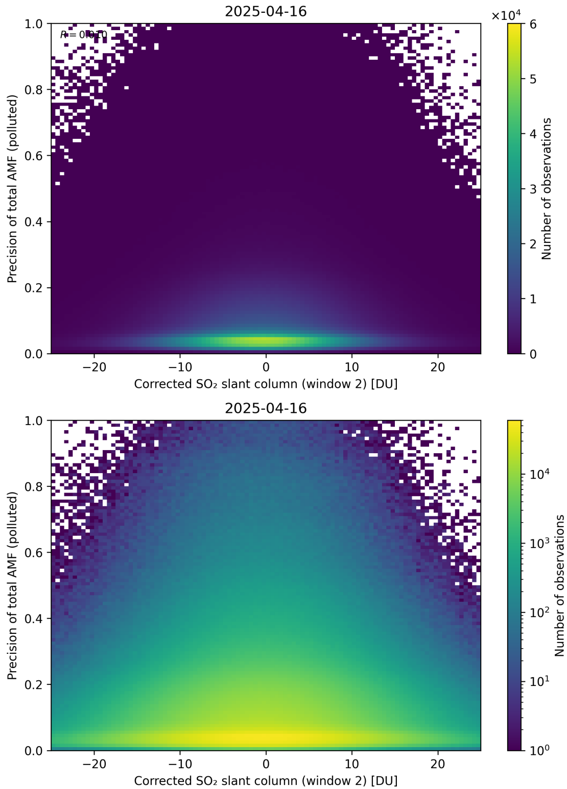
Figure 254: Scatter density plot of “Corrected SO 2 slant column (window 2)” against “Precision of total AMF (polluted)” for 2025-04-15 to 2025-04-17.
