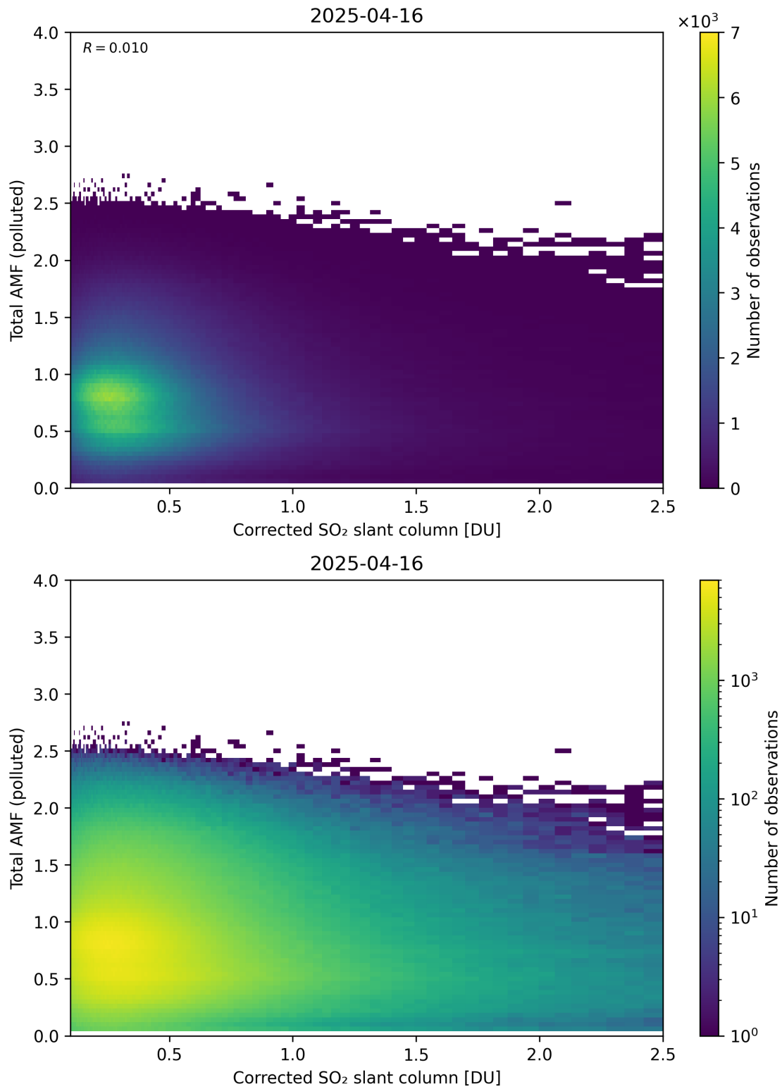
Figure 242: Scatter density plot of “Corrected SO 2 slant column” against “Total AMF (polluted)” for 2025-04-15 to 2025-04-17.
