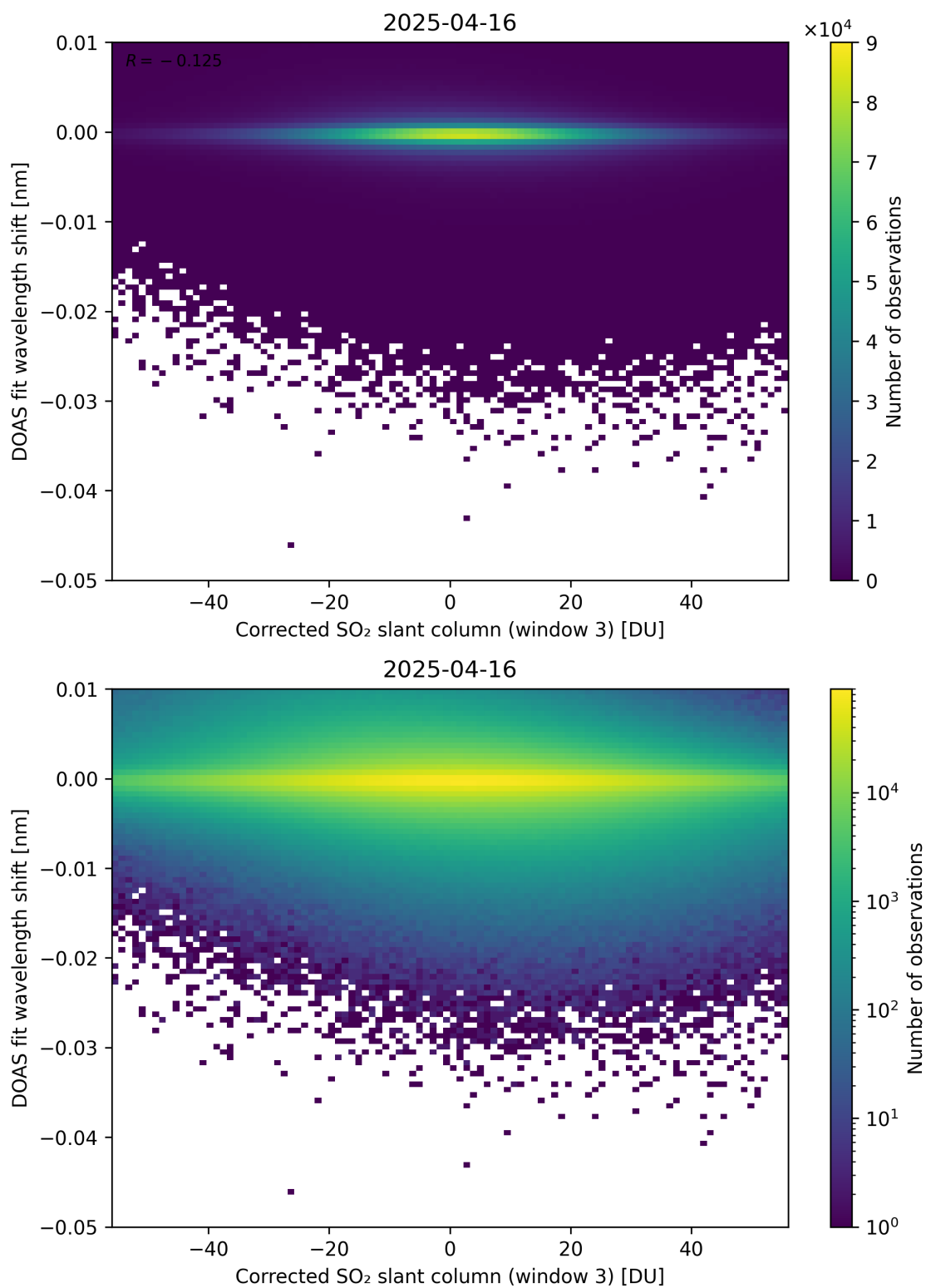
Figure 256: Scatter density plot of “Corrected SO 2 slant column (window 3)” against “DOAS fit wavelength shift” for 2025-04-15 to 2025-04-17.
