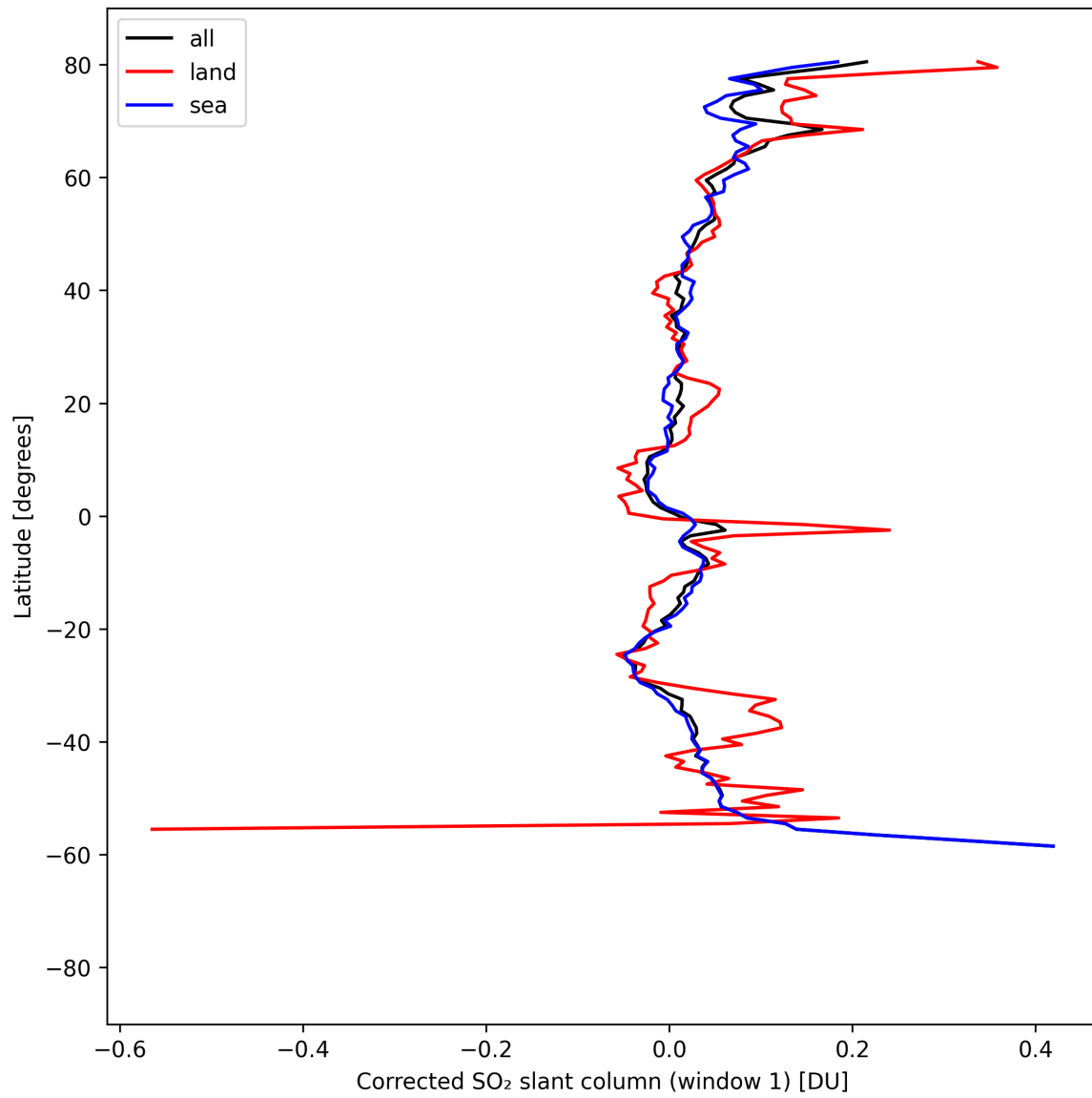
Figure 39: Zonal average of “Corrected SO 2 slant column (window 1)” for 2025-04-16 to 2025-04-18.
