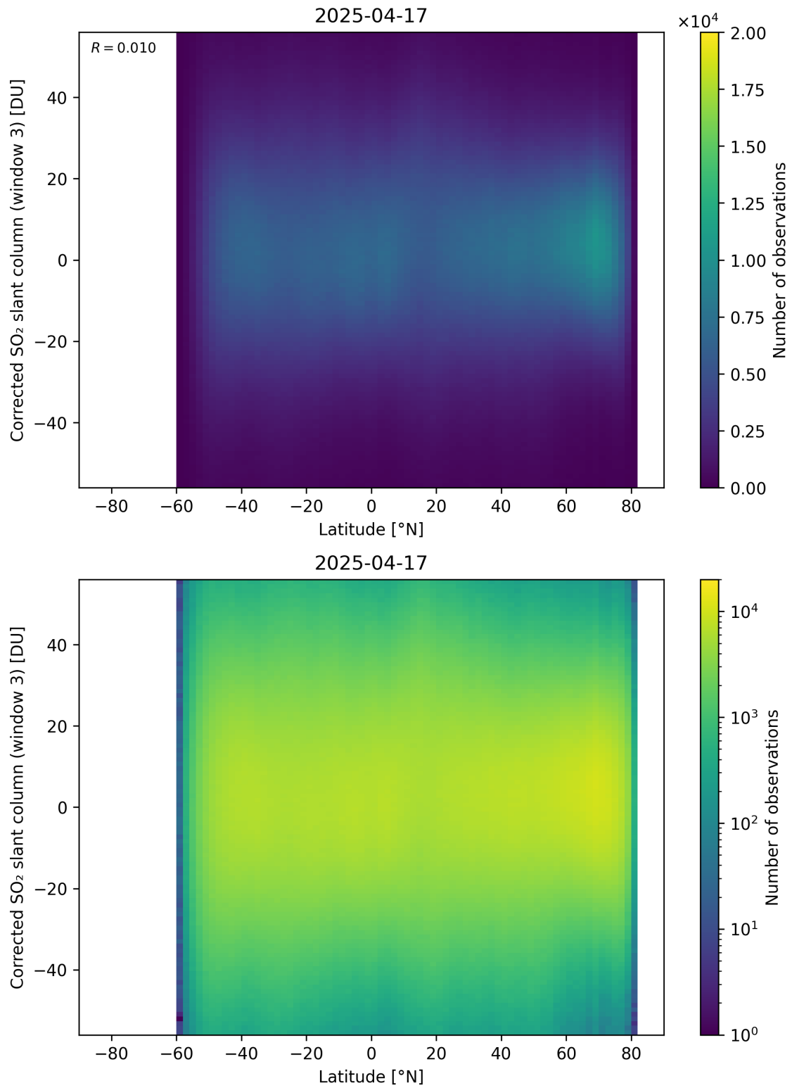
Figure 161: Scatter density plot of “Latitude” against “Corrected SO 2 slant column (window 3)” for 2025-04-16 to 2025-04-18.
