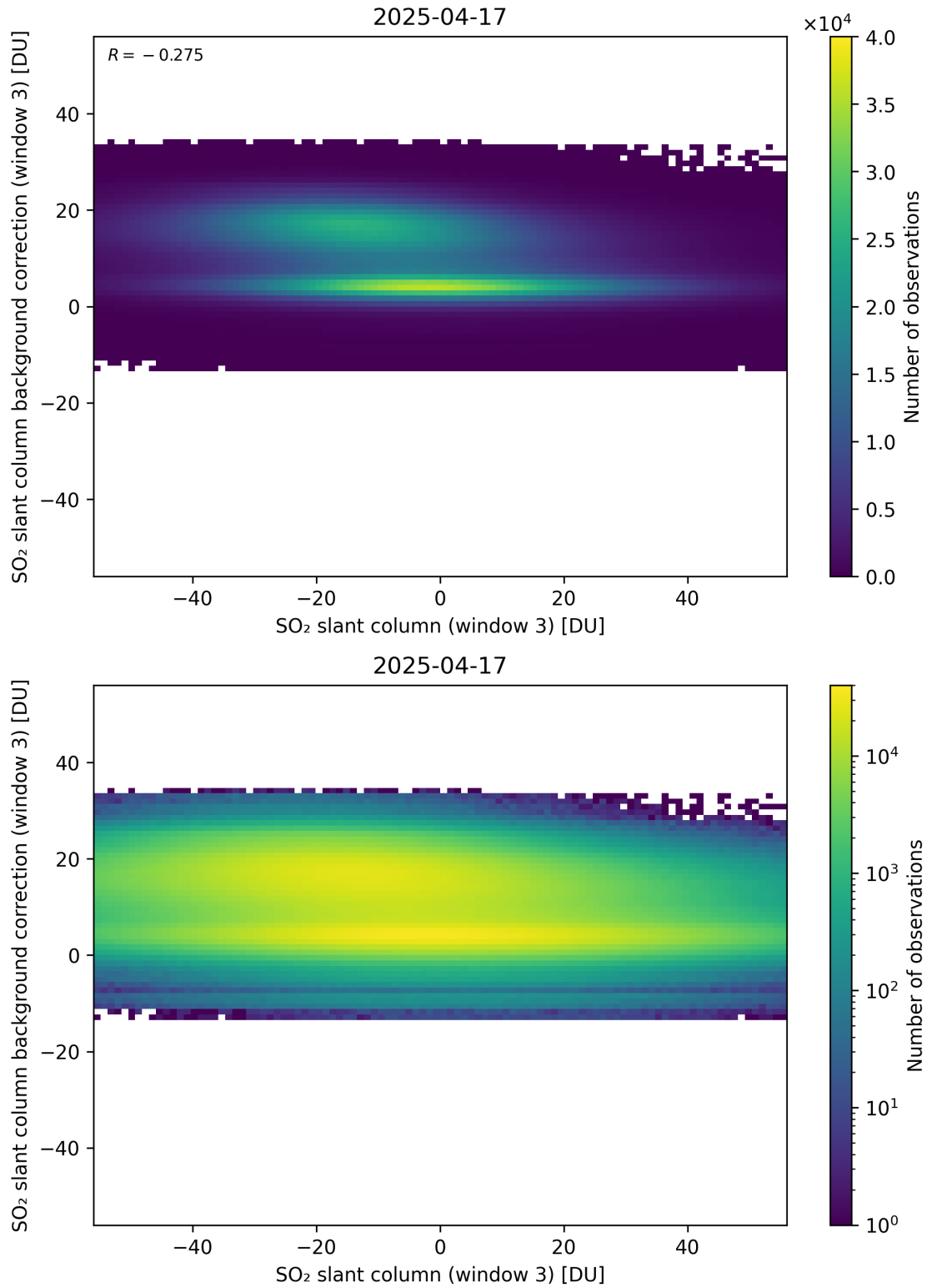
Figure 303: Scatter density plot of “SO 2 slant column (window 3)” against “SO 2 slant column background correction (window 3)” for 2025-04-16 to 2025-04-18.
