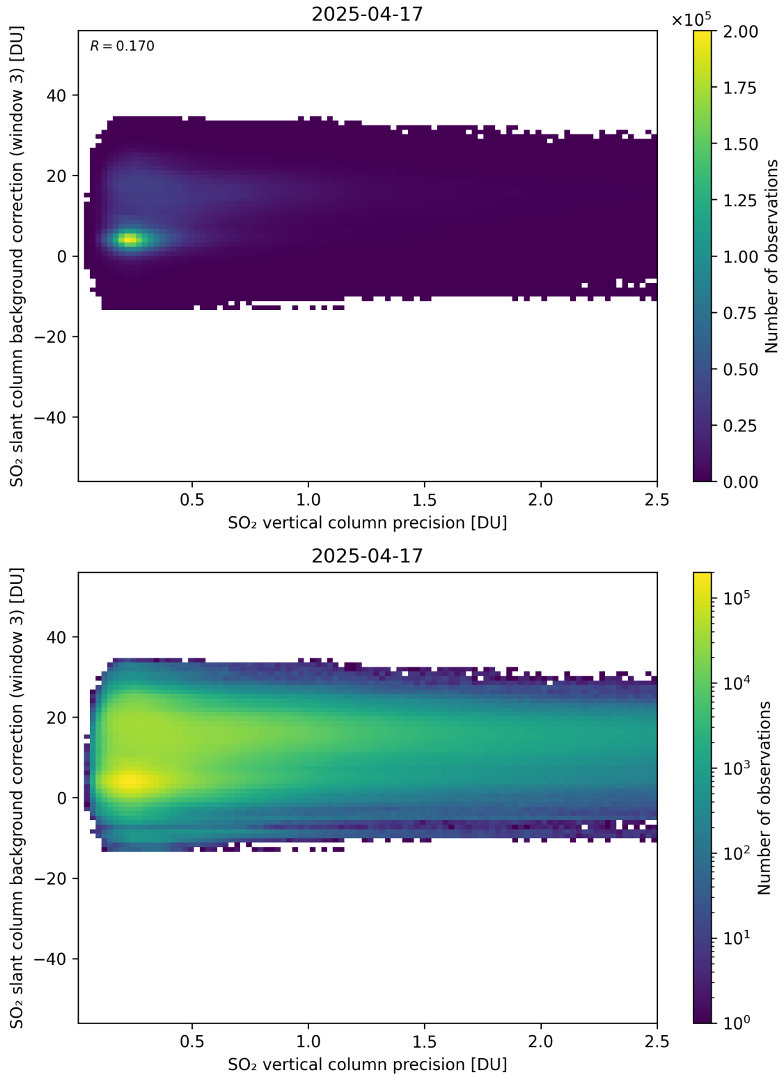
Figure 331: Scatter density plot of “SO 2 vertical column precision” against “SO 2 slant column background correction (window 3)” for 2025-04-16 to 2025-04-18.
