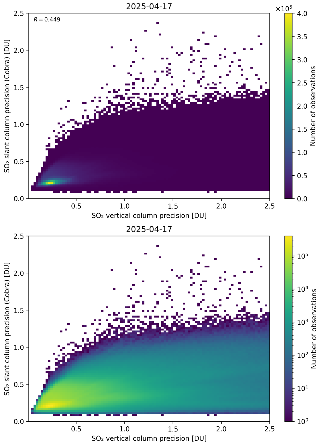
Figure 337: Scatter density plot of “SO 2 vertical column precision” against “SO 2 slant column precision (Cobra)” for 2025-04-16 to 2025-04-18.
