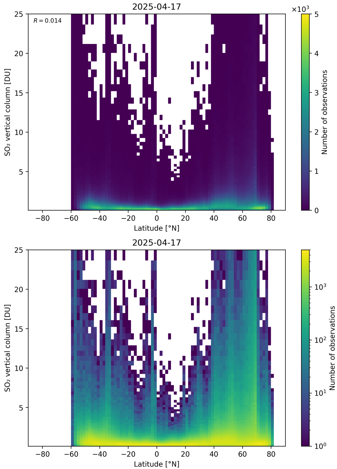
Figure 169: Scatter density plot of “Latitude” against “SO 2 vertical column” for 2025-04-16 to 2025-04-18.
