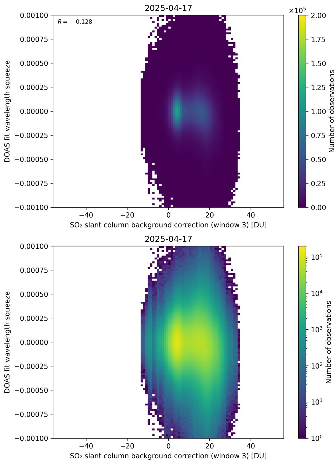
Figure 133: Scatter density plot of “SO 2 slant column background correction (window 3)” against “DOAS fit wavelength squeeze” for 2025-04-16 to 2025-04-18.
