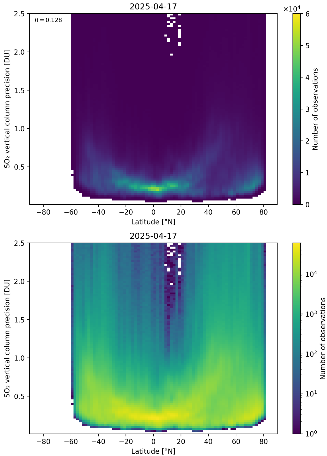
Figure 170: Scatter density plot of “Latitude” against “SO 2 vertical column precision” for 2025-04-16 to 2025-04-18.
