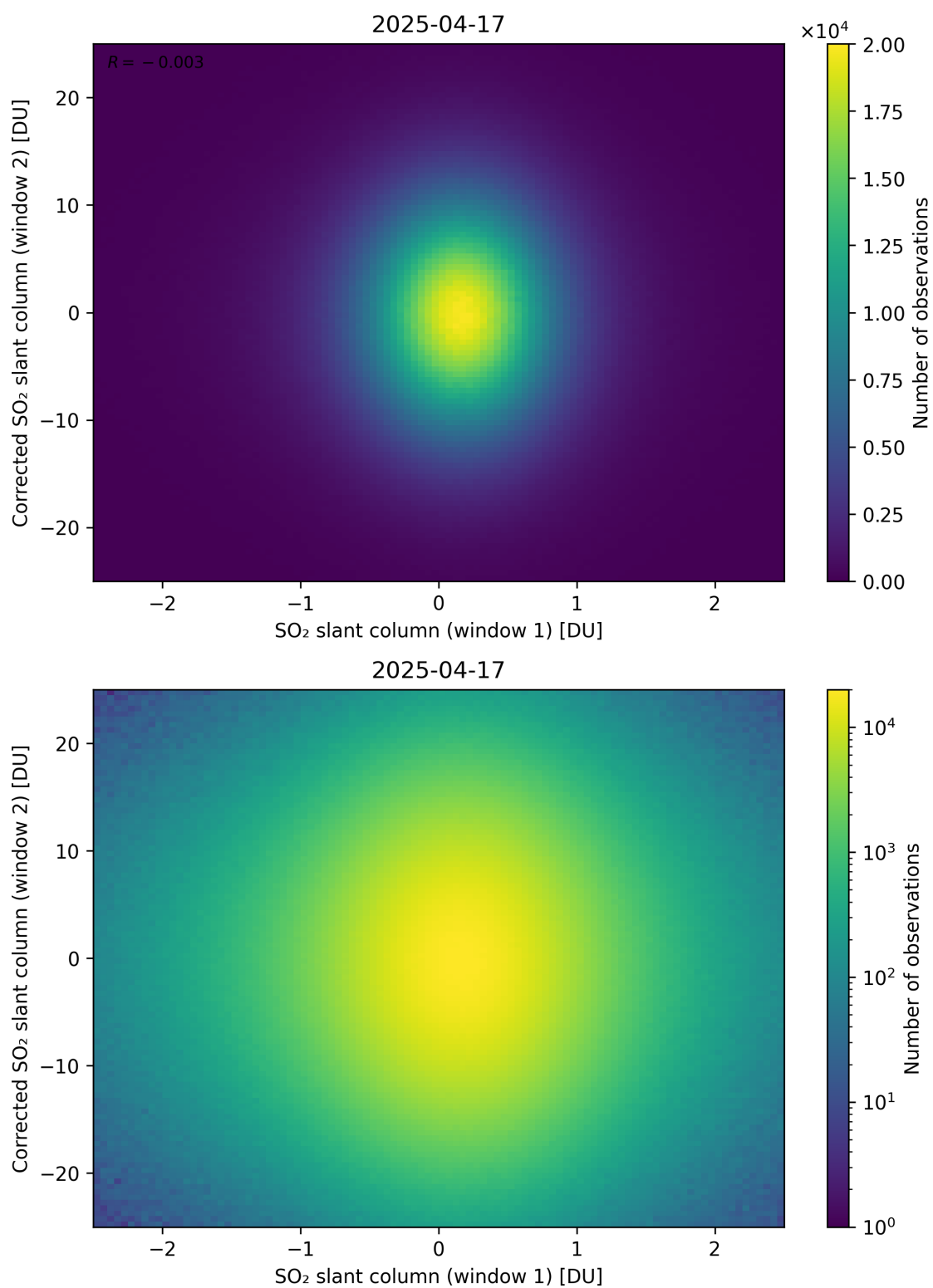
Figure 283: Scatter density plot of “SO 2 slant column (window 1)” against “Corrected SO 2 slant column (window 2)” for 2025-04-16 to 2025-04-18.
