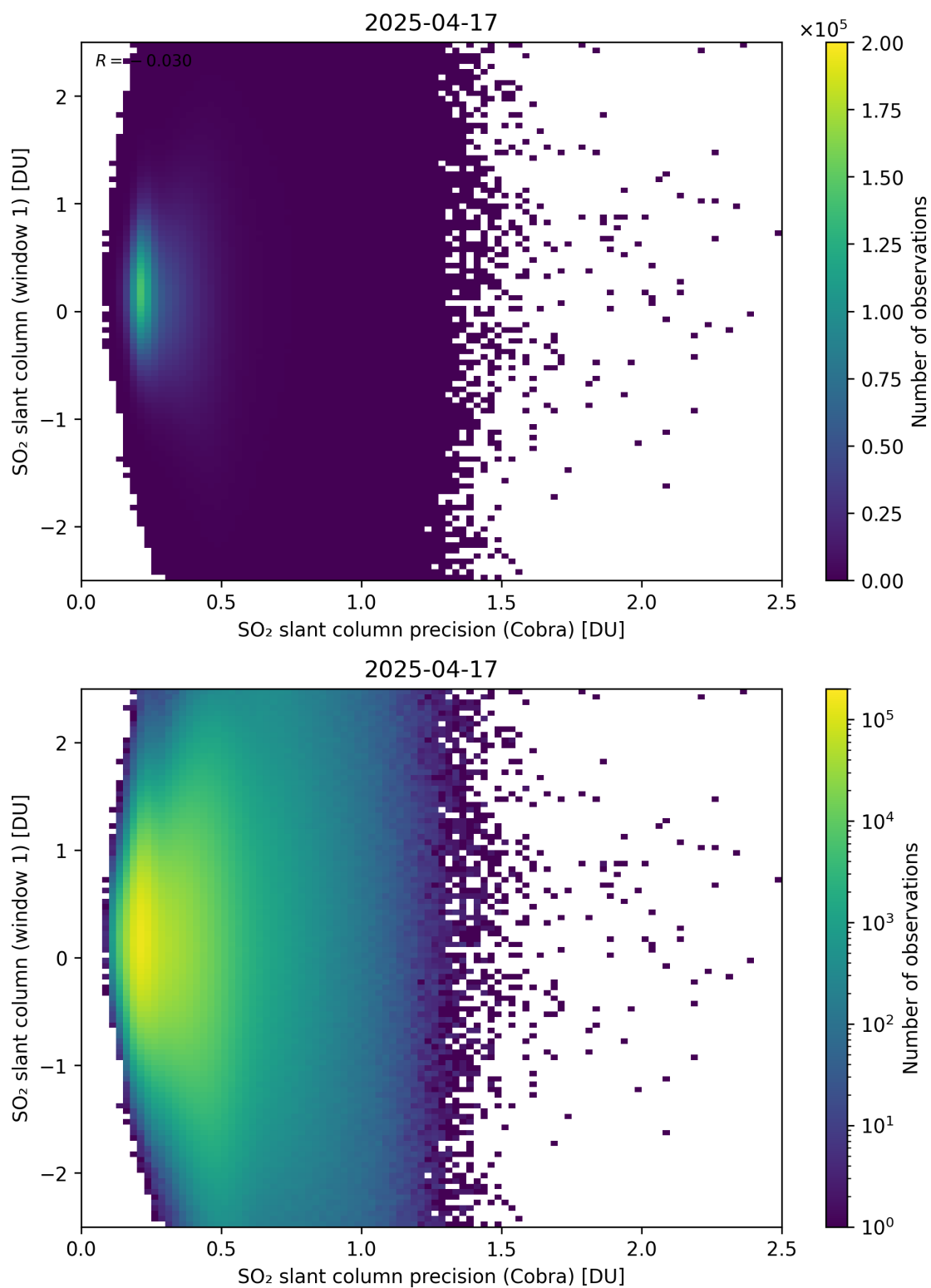
Figure 208: Scatter density plot of “SO 2 slant column precision (Cobra)” against “SO 2 slant column (window 1)” for 2025-04-16 to 2025-04-18.
