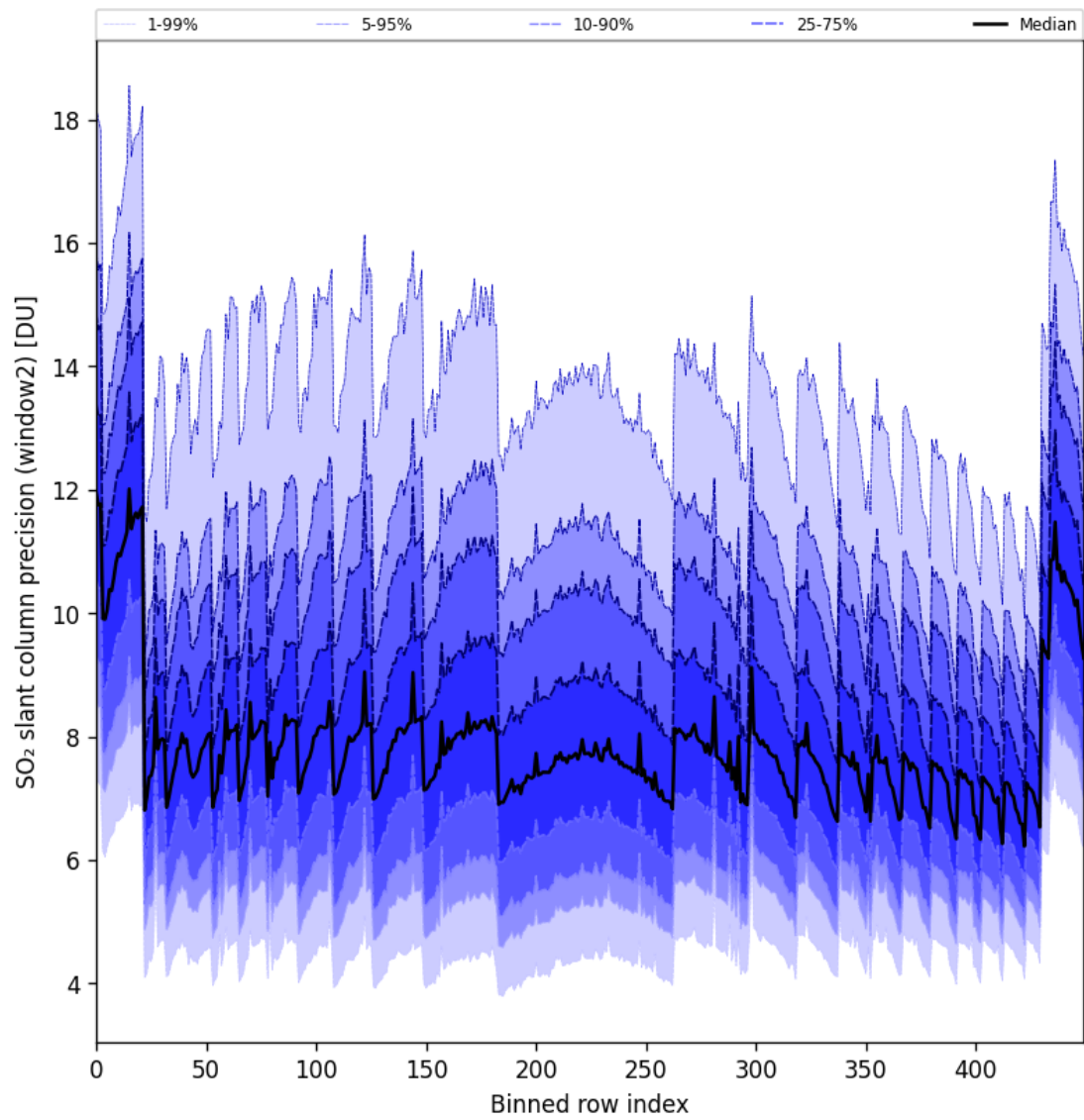
Figure 94: Along track statistics of “SO 2 slant column precision (window2)” for 2025-04-16 to 2025-04-18
