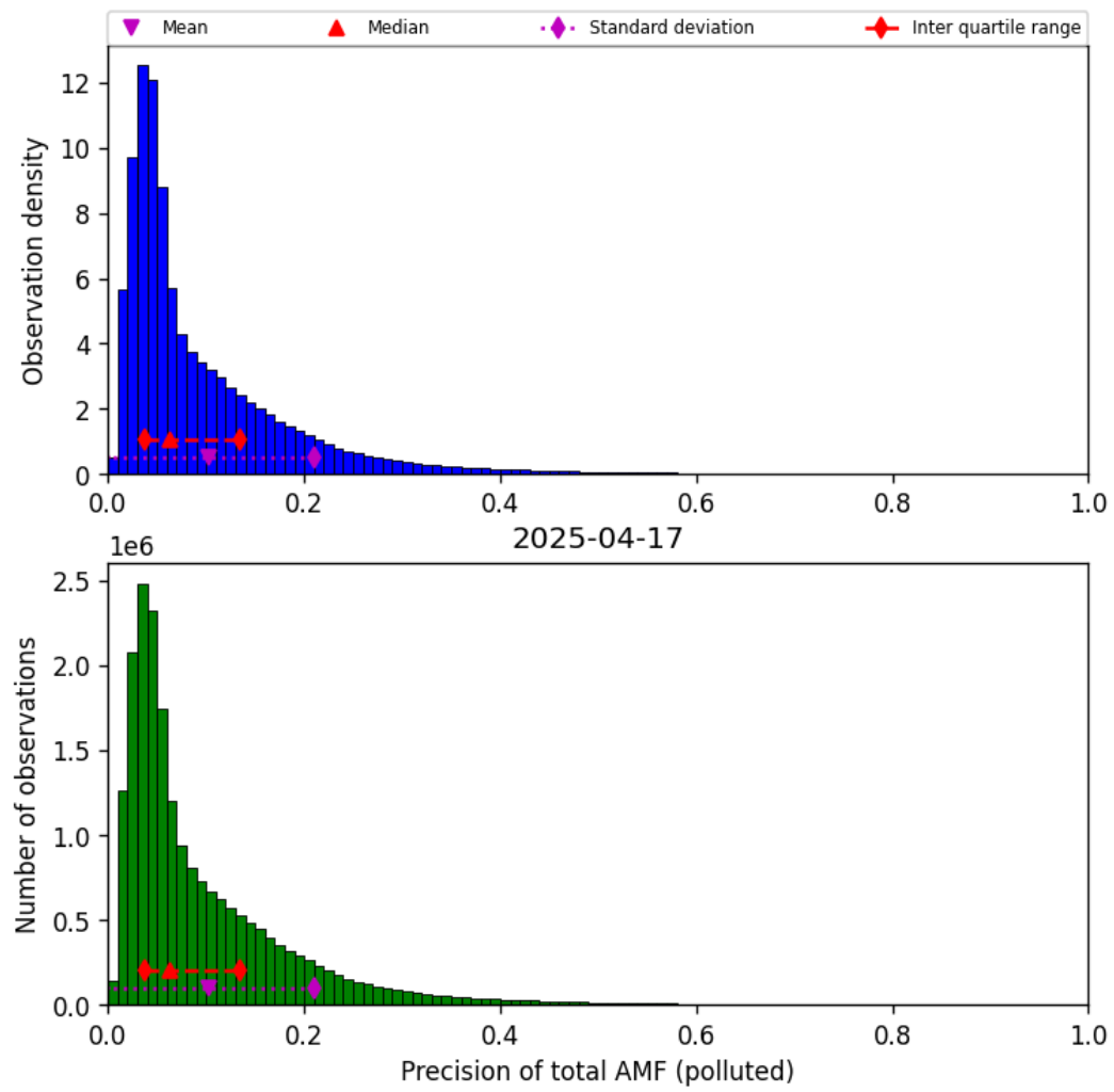
Figure 80: Histogram of “Precision of total AMF (polluted)” for 2025-04-16 to 2025-04-18
