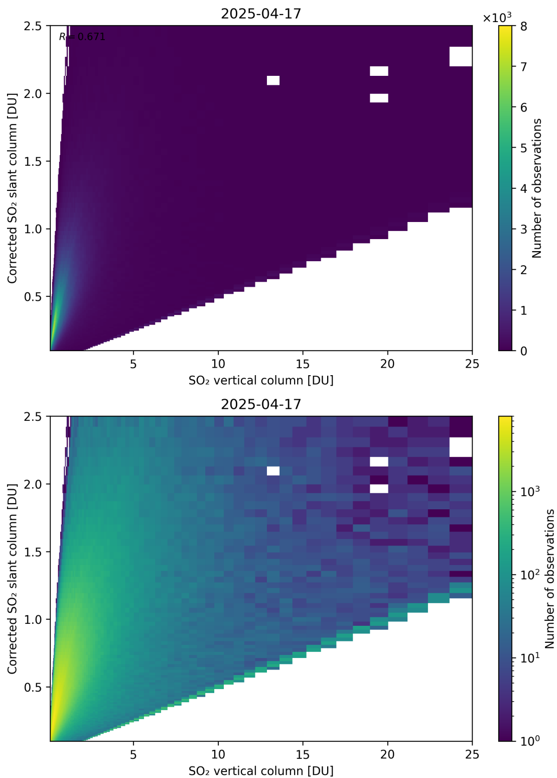
Figure 351: Scatter density plot of “SO 2 vertical column” against “Corrected SO 2 slant column” for 2025-04-16 to 2025-04-18.
