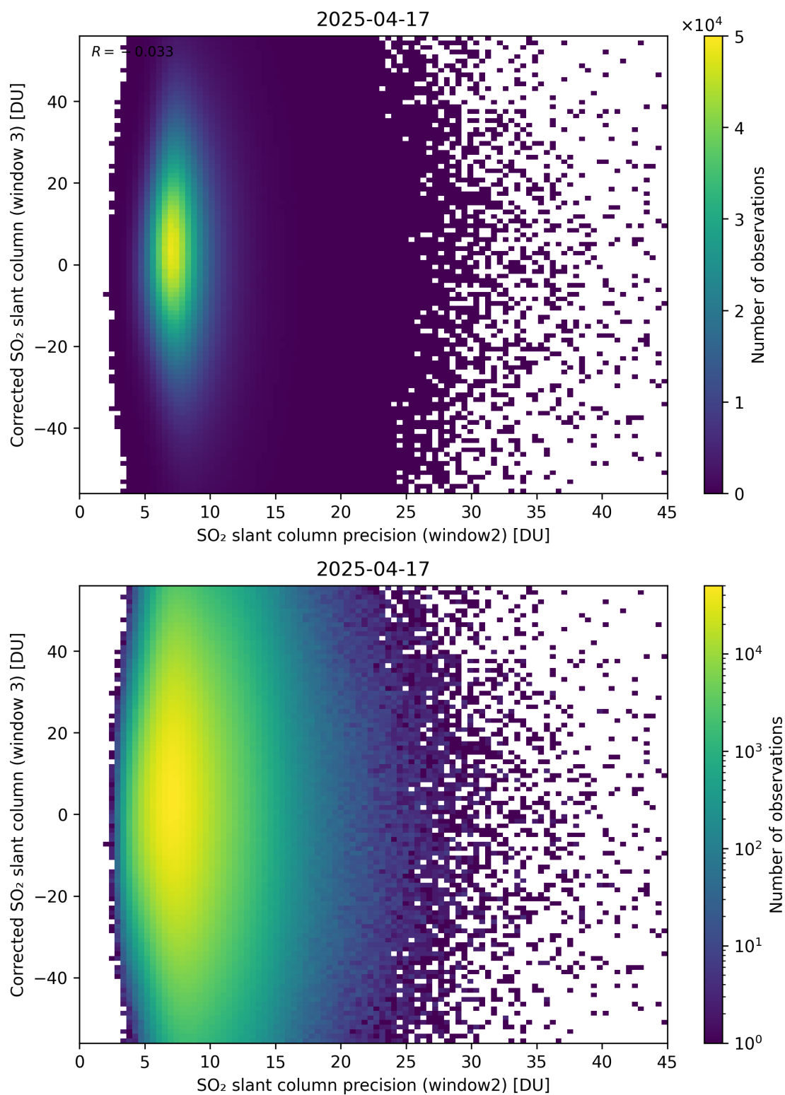
Figure 298: Scatter density plot of “SO 2 slant column precision (window2)” against “Corrected SO 2 slant column (window 3)” for 2025-04-16 to 2025-04-18.
