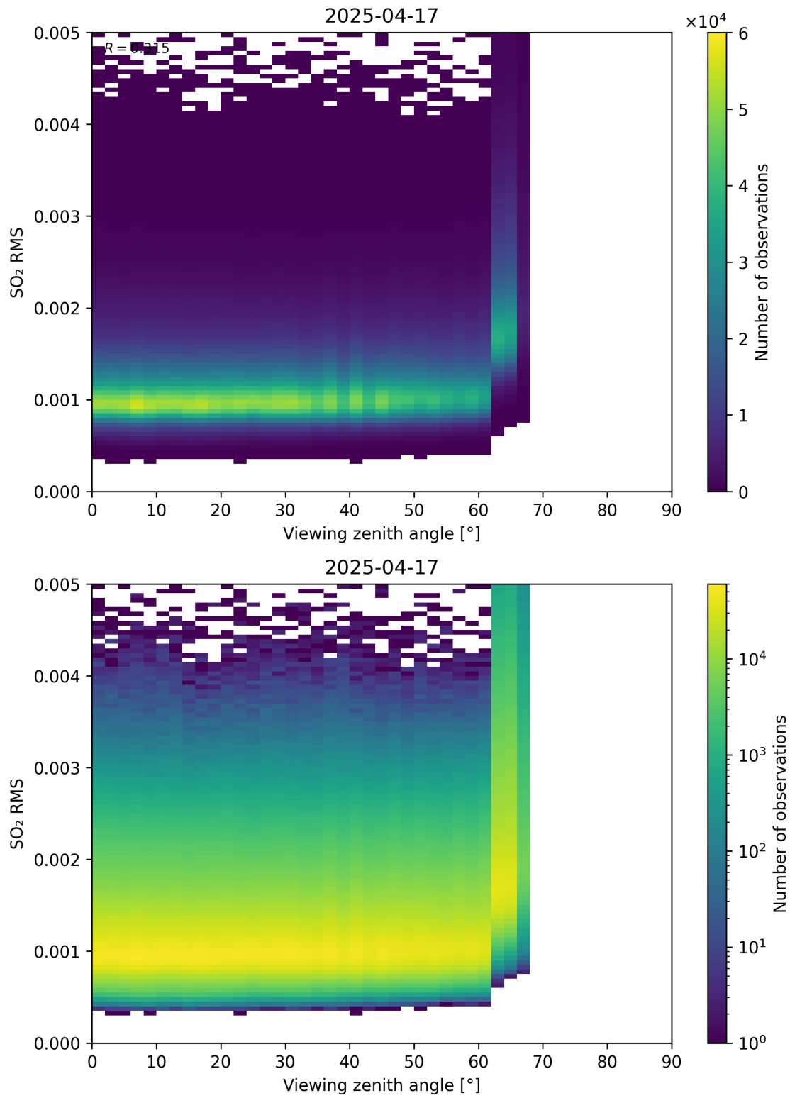
Figure 367: Scatter density plot of “Viewing zenith angle” against “SO 2 RMS” for 2025-04-16 to 2025-04-18.
