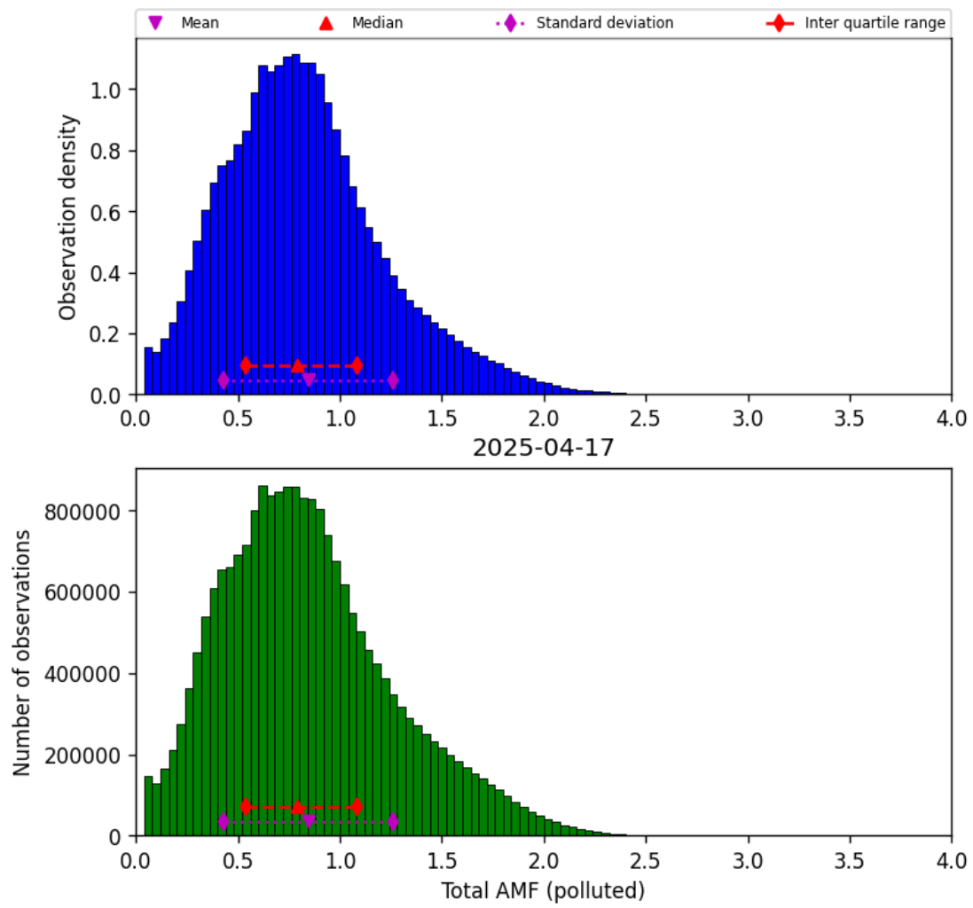
Figure 79: Histogram of “Total AMF (polluted)” for 2025-04-16 to 2025-04-18
