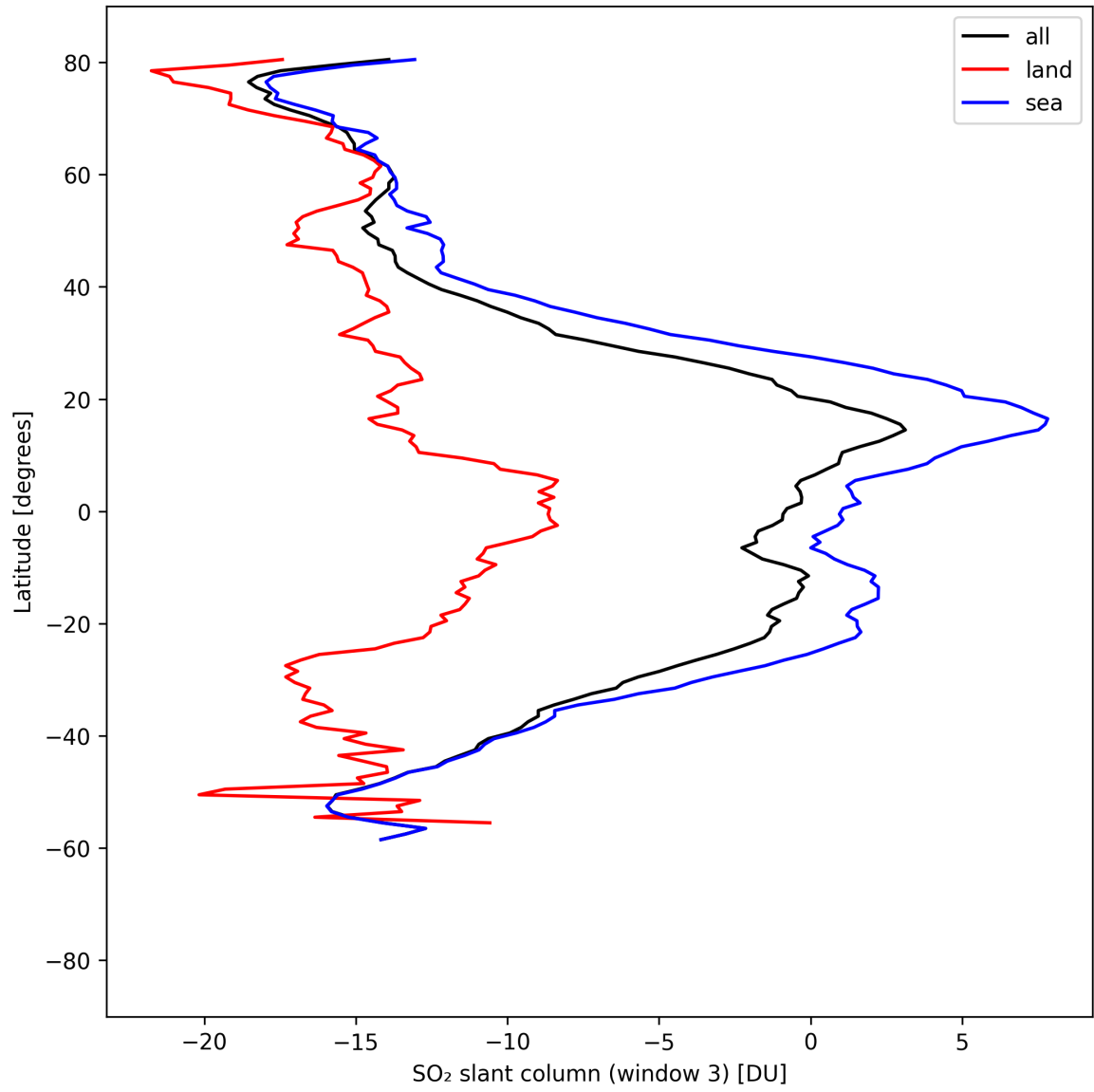
Figure 45: Zonal average of “SO 2 slant column (window 3)” for 2025-04-16 to 2025-04-18.
