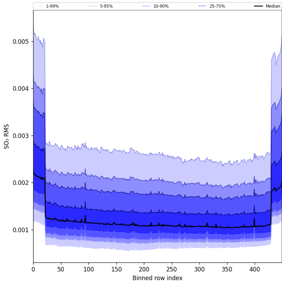
Figure 104: Along track statistics of “SO 2 RMS” for 2025-04-16 to 2025-04-18
