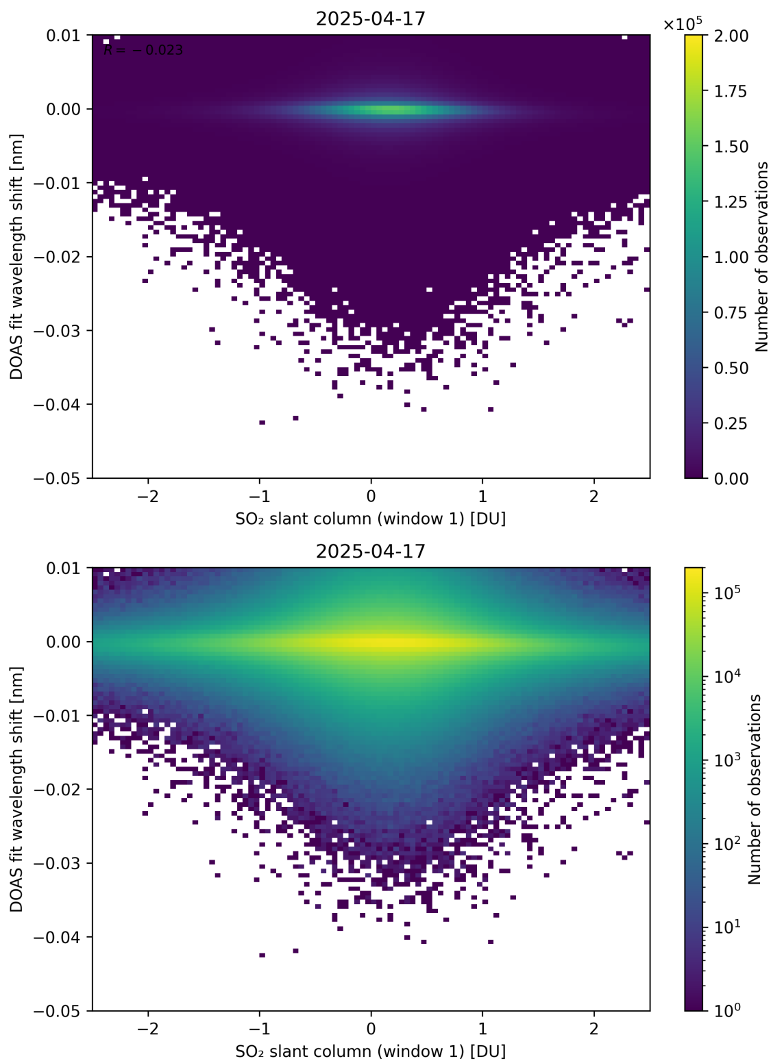
Figure 265: Scatter density plot of “SO 2 slant column (window 1)” against “DOAS fit wavelength shift” for 2025-04-16 to 2025-04-18.
