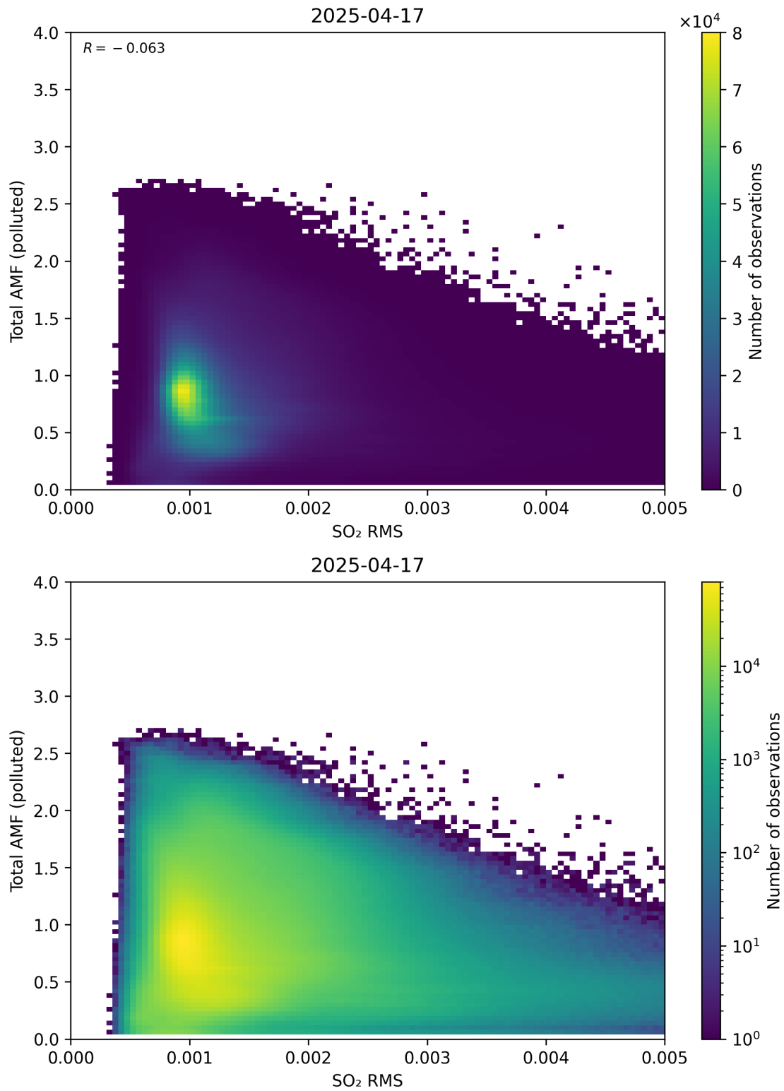
Figure 148: Scatter density plot of “SO 2 RMS” against “Total AMF (polluted)” for 2025-04-16 to 2025-04-18.
