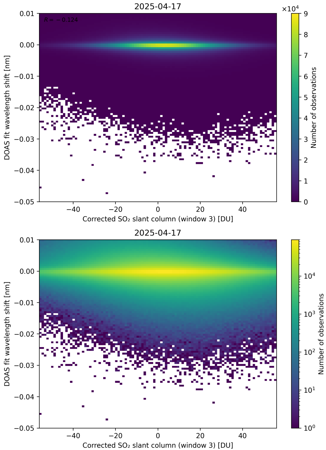
Figure 256: Scatter density plot of “Corrected SO 2 slant column (window 3)” against “DOAS fit wavelength shift” for 2025-04-16 to 2025-04-18.
