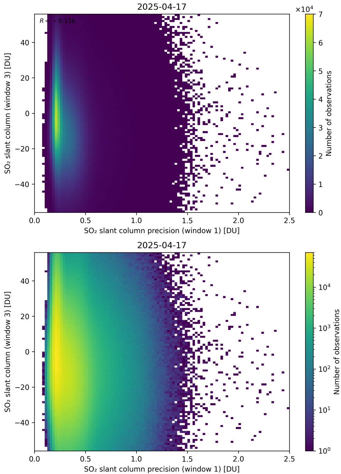
Figure 278: Scatter density plot of “SO 2 slant column precision (window 1)” against “SO 2 slant column (window 3)” for 2025-04-16 to 2025-04-18.
