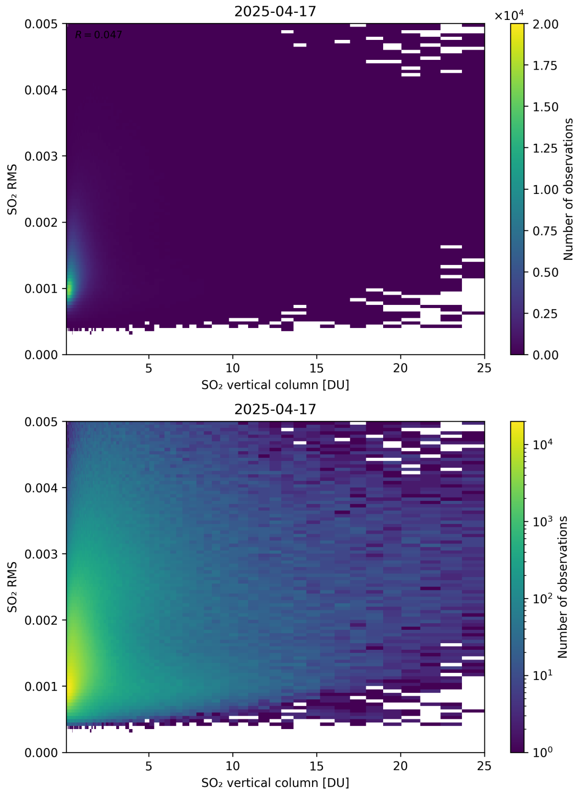
Figure 328: Scatter density plot of “SO 2 vertical column” against “SO 2 RMS” for 2025-04-16 to 2025-04-18.
