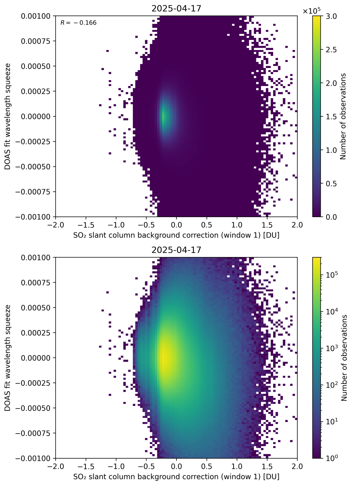
Figure 112: Scatter density plot of “SO 2 slant column background correction (window 1)” against “DOAS fit wavelength squeeze” for 2025-04-16 to 2025-04-18.
