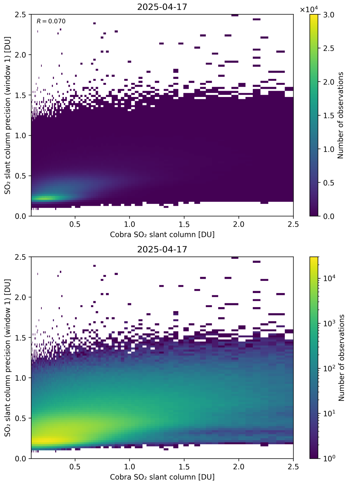
Figure 220: Scatter density plot of “Cobra SO 2 slant column” against “SO 2 slant column precision (window 1)” for 2025-04-16 to 2025-04-18.
