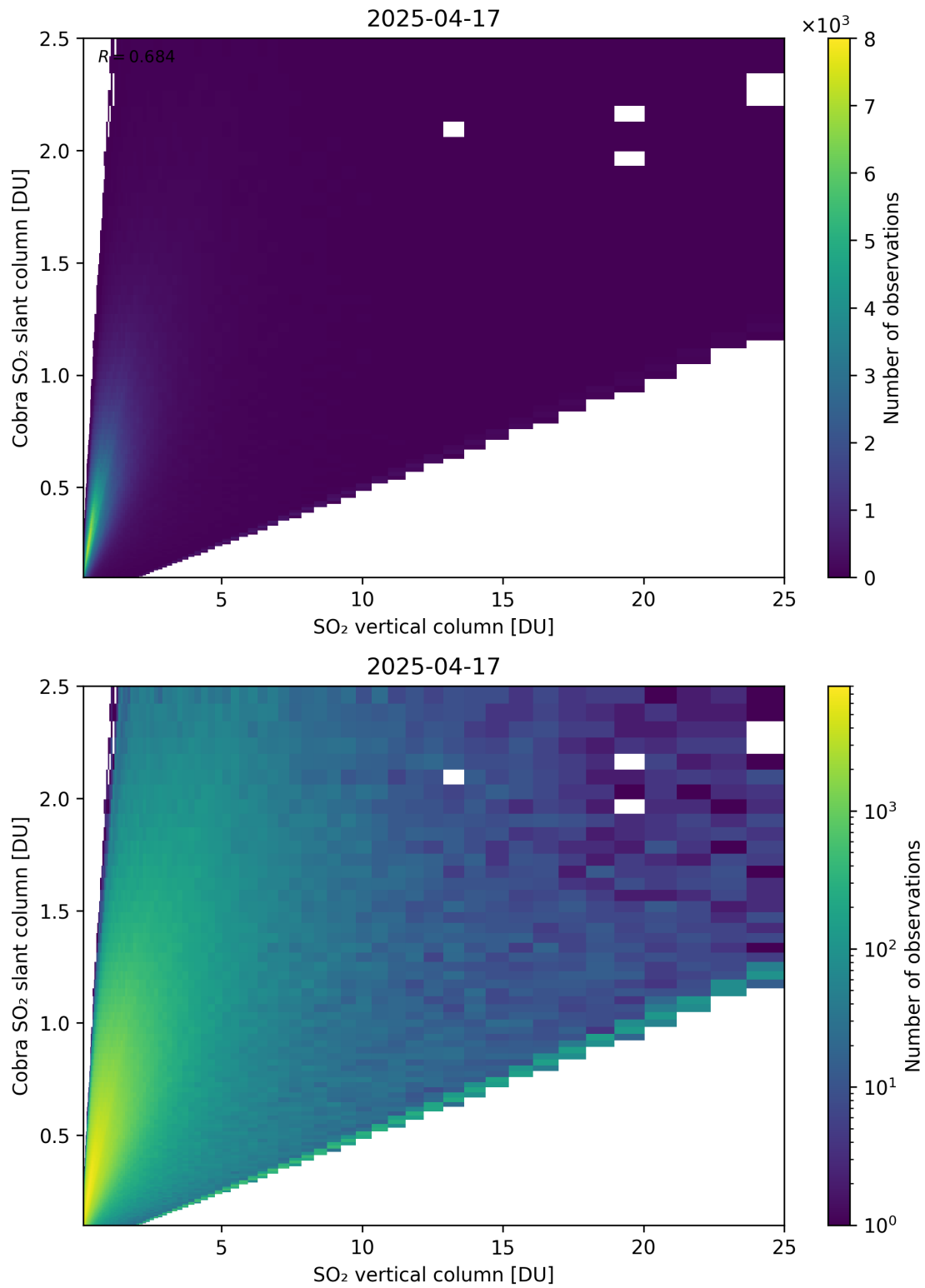
Figure 349: Scatter density plot of “SO 2 vertical column” against “Cobra SO 2 slant column” for 2025-04-16 to 2025-04-18.
