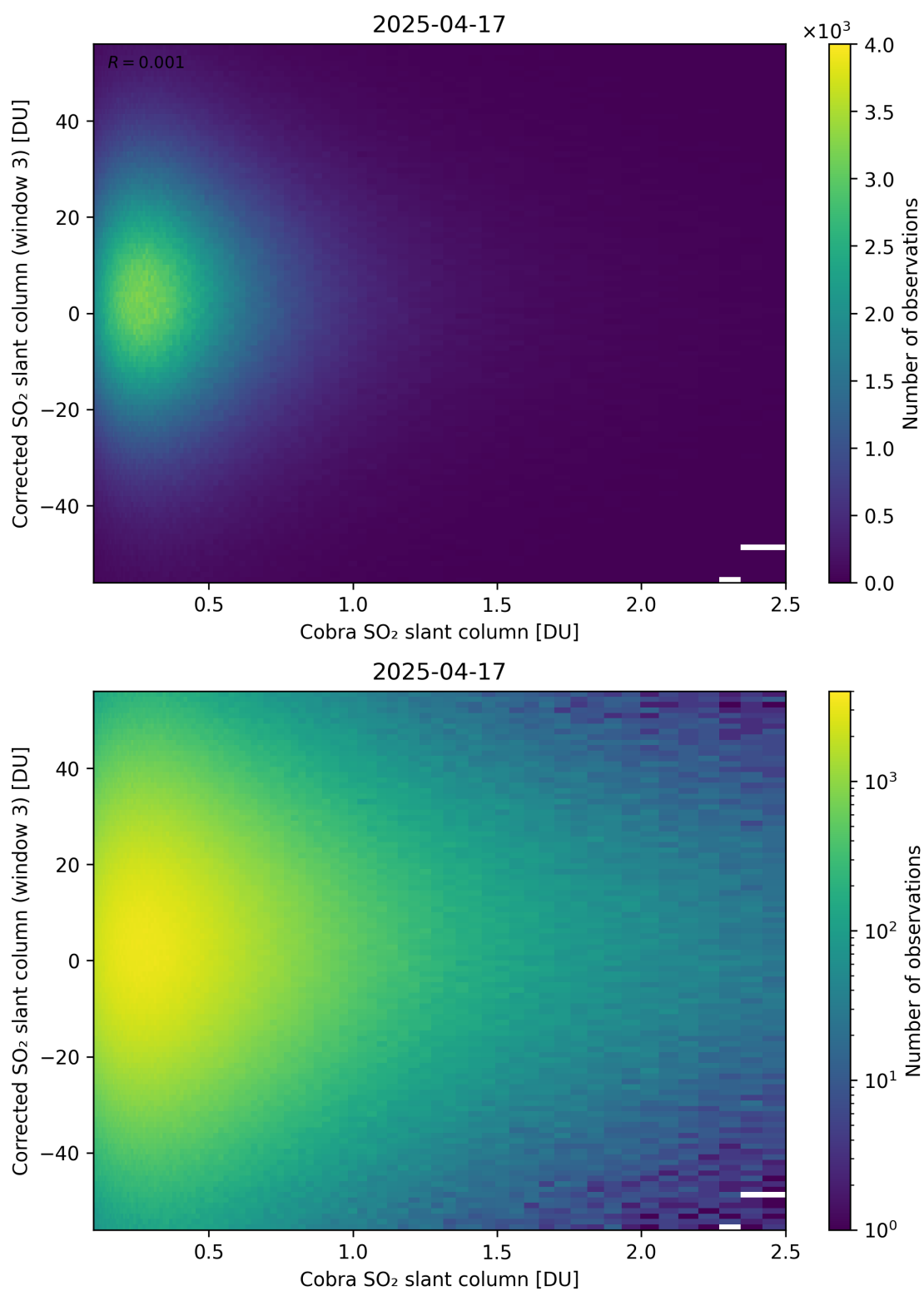
Figure 218: Scatter density plot of “Cobra SO 2 slant column” against “Corrected SO 2 slant column (window 3)” for 2025-04-16 to 2025-04-18.
