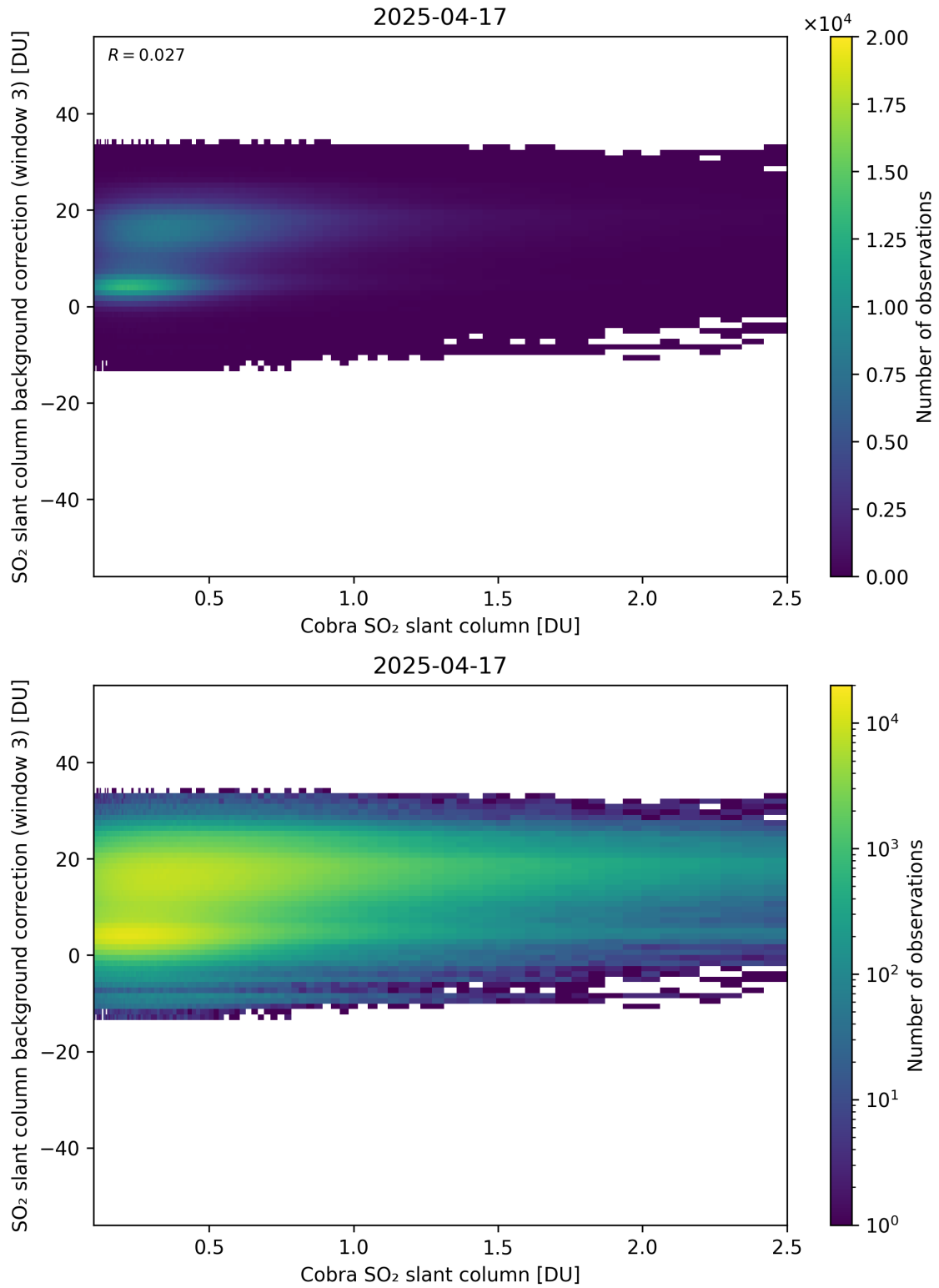
Figure 195: Scatter density plot of “Cobra SO 2 slant column” against “SO 2 slant column background correction (window 3)” for 2025-04-16 to 2025-04-18.
