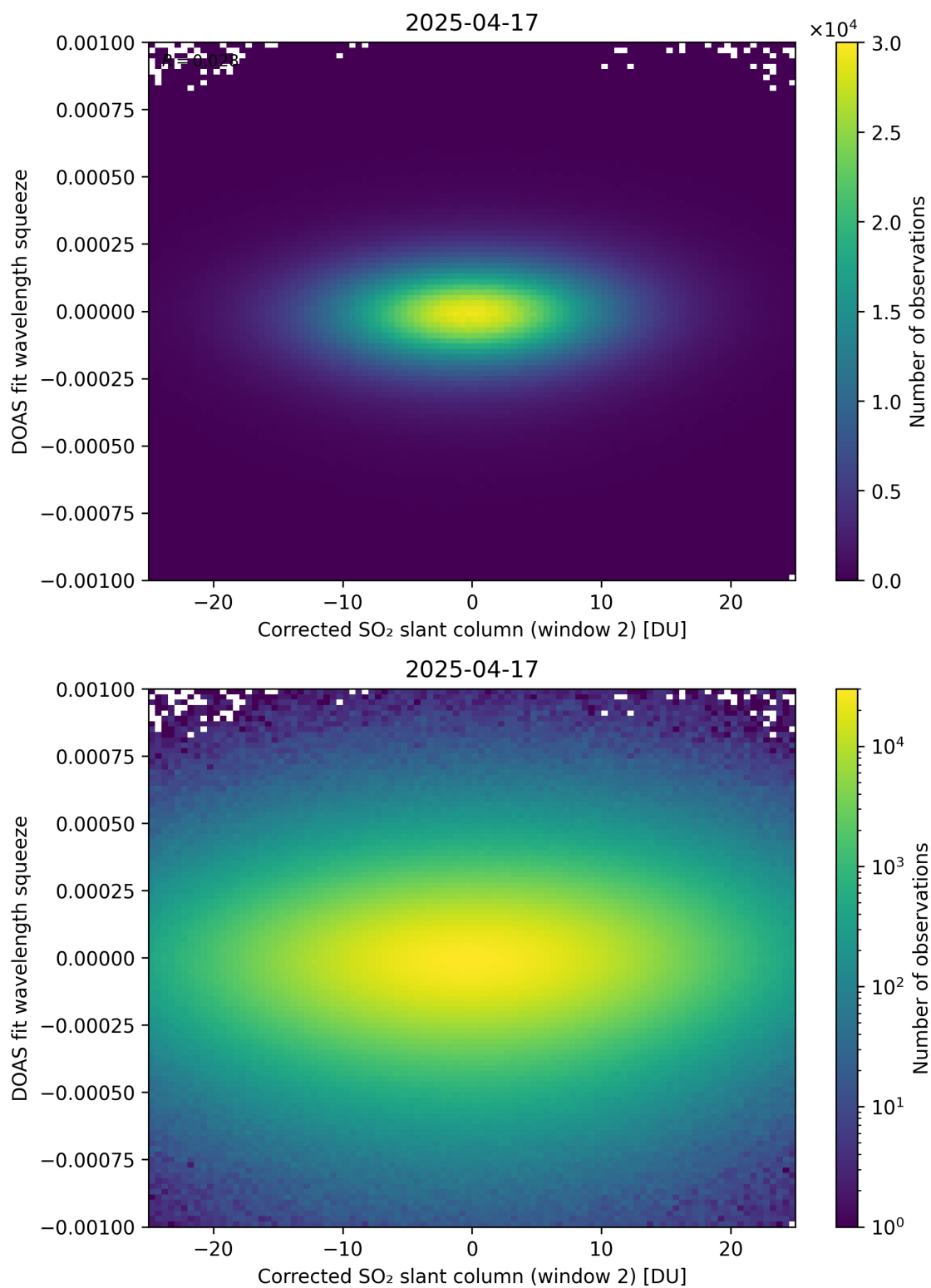
Figure 247: Scatter density plot of “Corrected SO 2 slant column (window 2)” against “DOAS fit wavelength squeeze” for 2025-04-16 to 2025-04-18.
