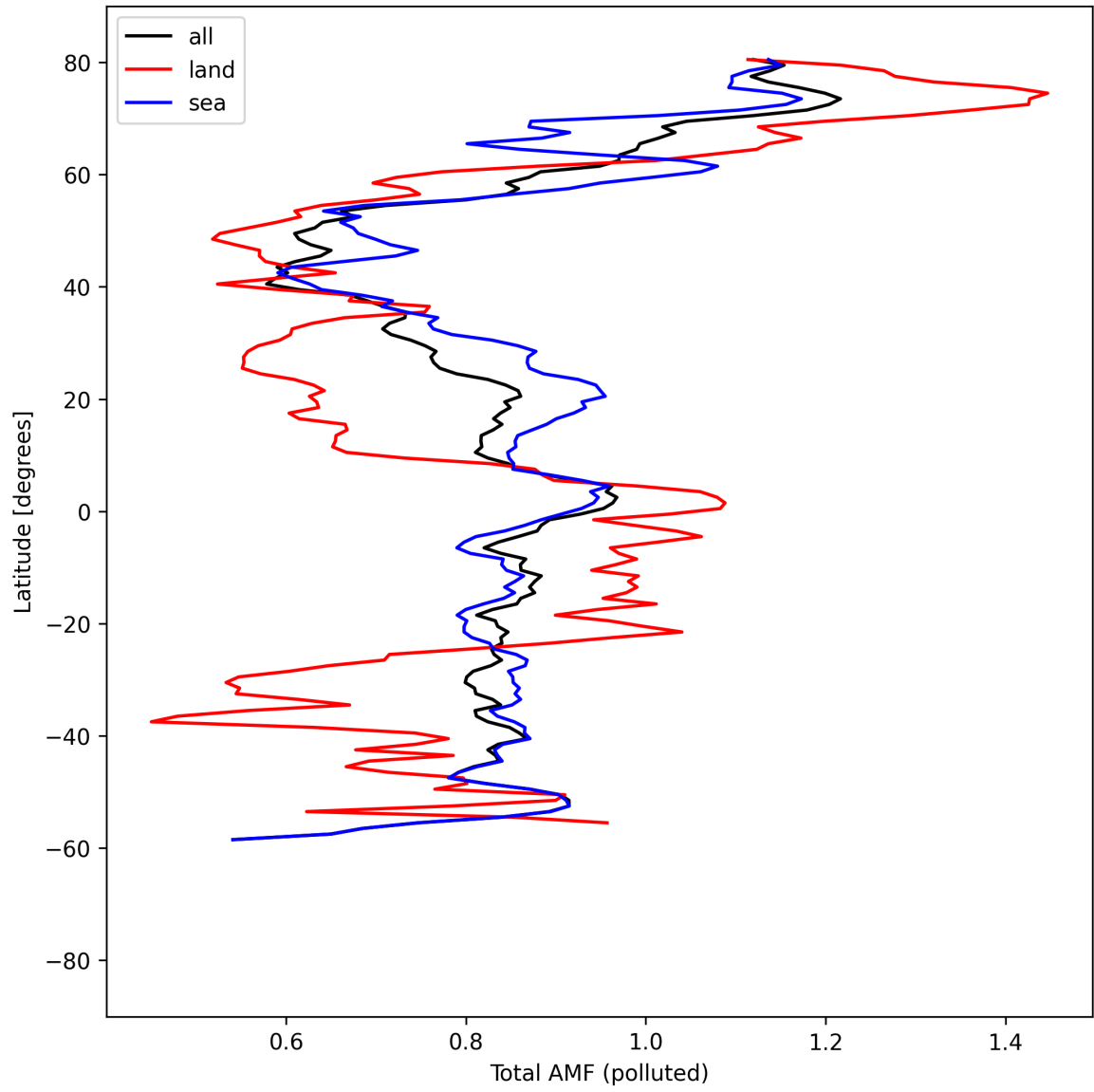
Figure 53: Zonal average of “Total AMF (polluted)” for 2025-04-16 to 2025-04-18.
