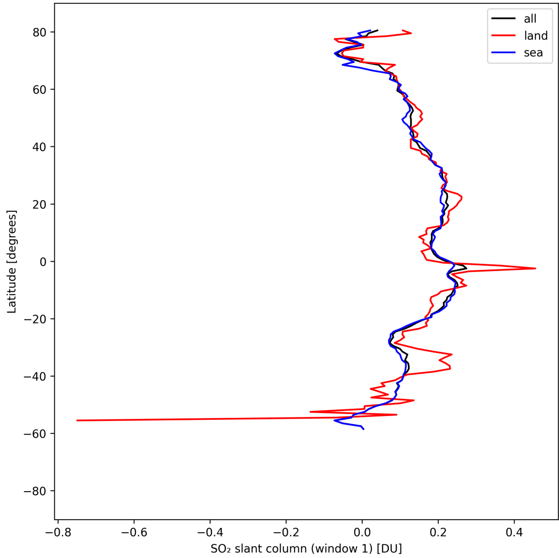
Figure 37: Zonal average of “SO 2 slant column (window 1)” for 2025-04-16 to 2025-04-18.
