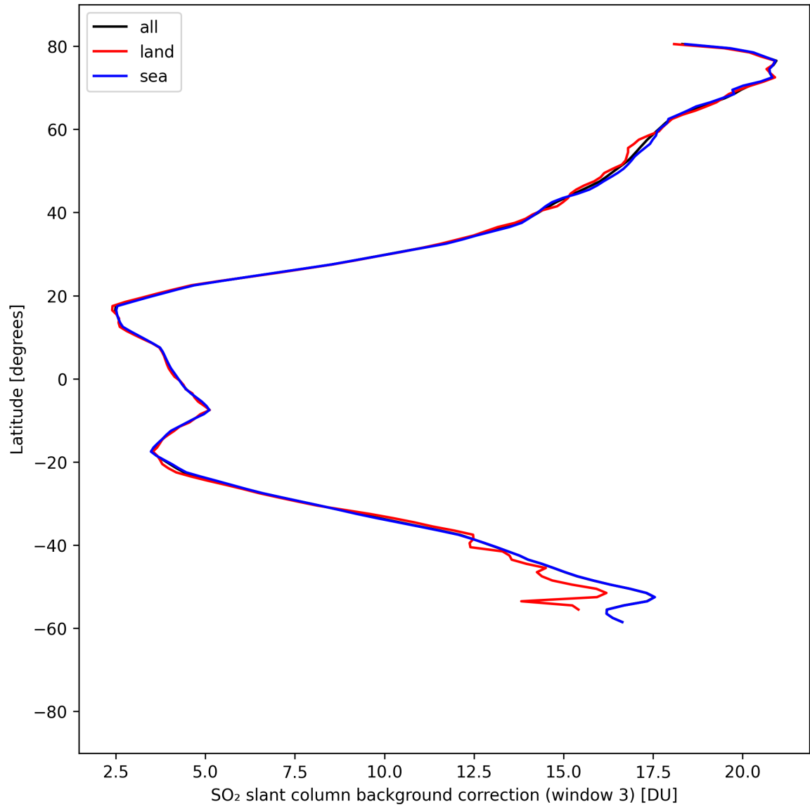
Figure 48: Zonal average of “SO 2 slant column background correction (window 3)” for 2025-04-16 to 2025-04-18.
