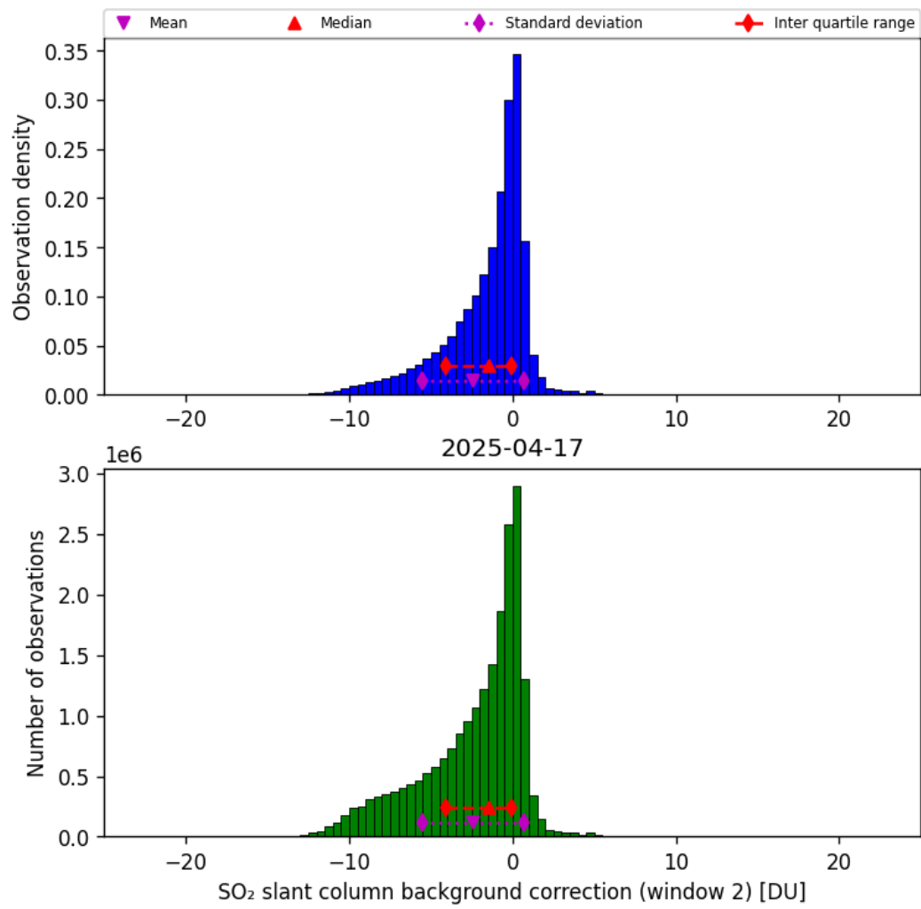
Figure 70: Histogram of “SO 2 slant column background correction (window 2)” for 2025-04-16 to 2025-04-18
