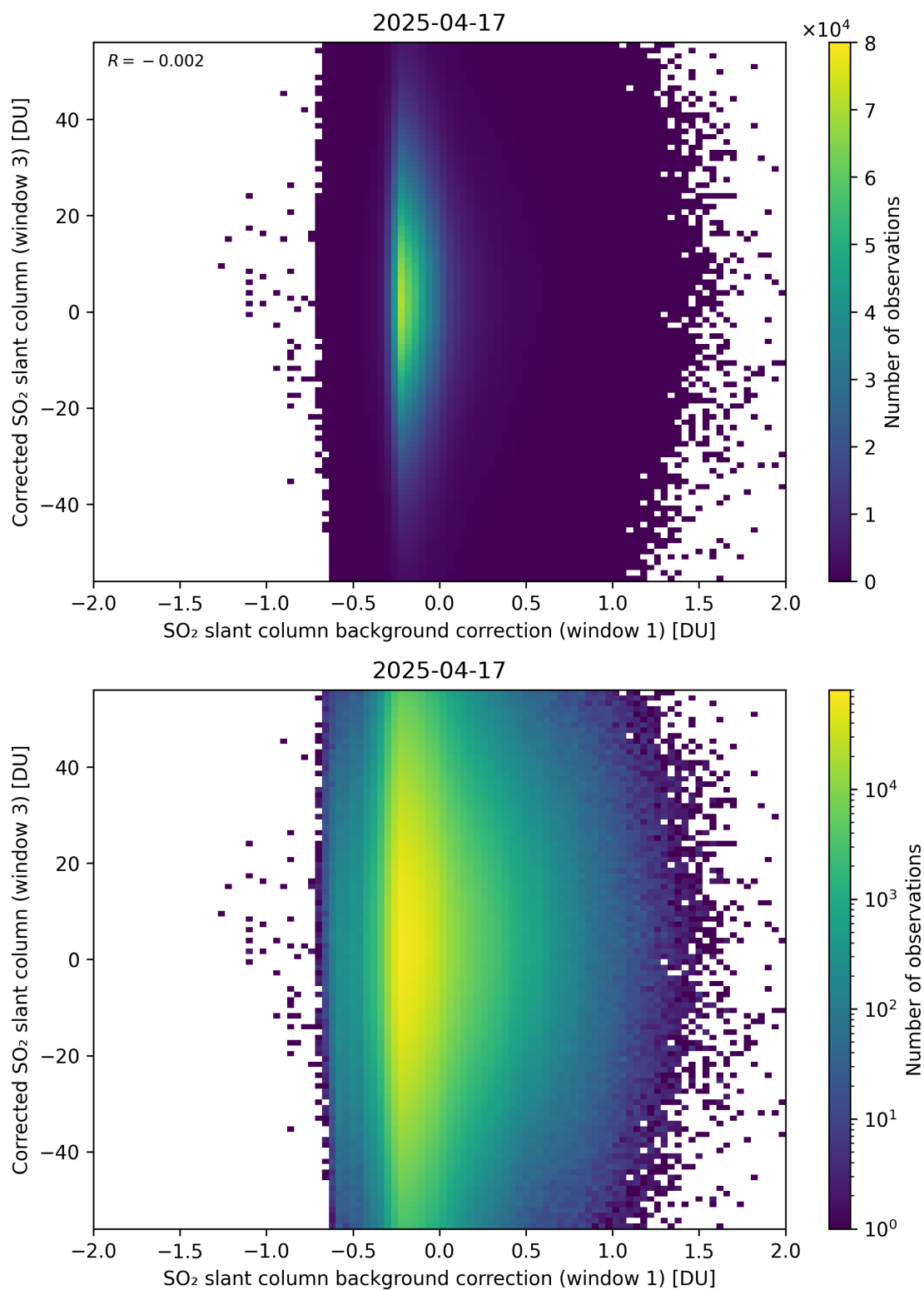
Figure 116: Scatter density plot of “SO 2 slant column background correction (window 1)” against “Corrected SO 2 slant column (window 3)” for 2025-04-16 to 2025-04-18.
