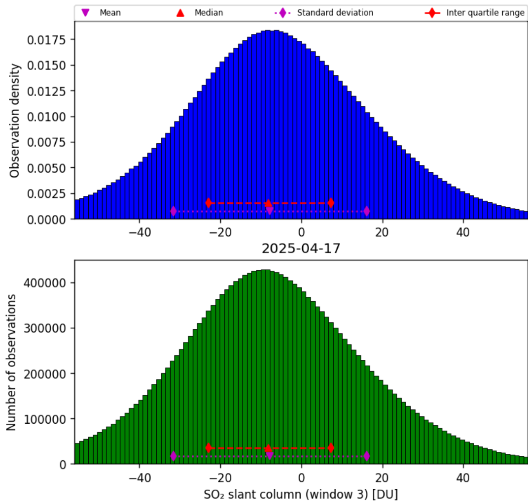
Figure 71: Histogram of “SO 2 slant column (window 3)” for 2025-04-16 to 2025-04-18
