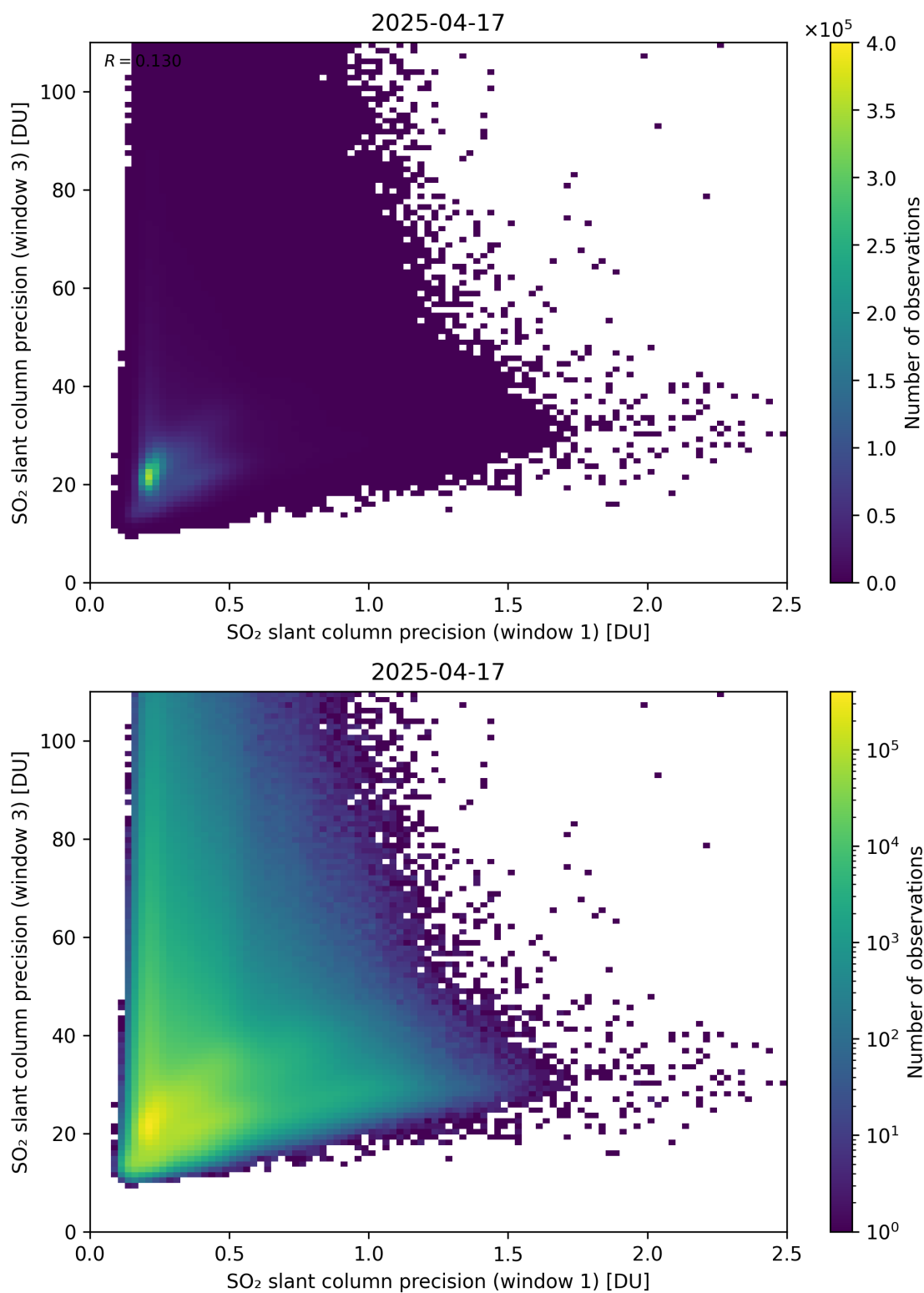
Figure 279: Scatter density plot of “SO 2 slant column precision (window 1)” against “SO 2 slant column precision (window 3)” for 2025-04-16 to 2025-04-18.
