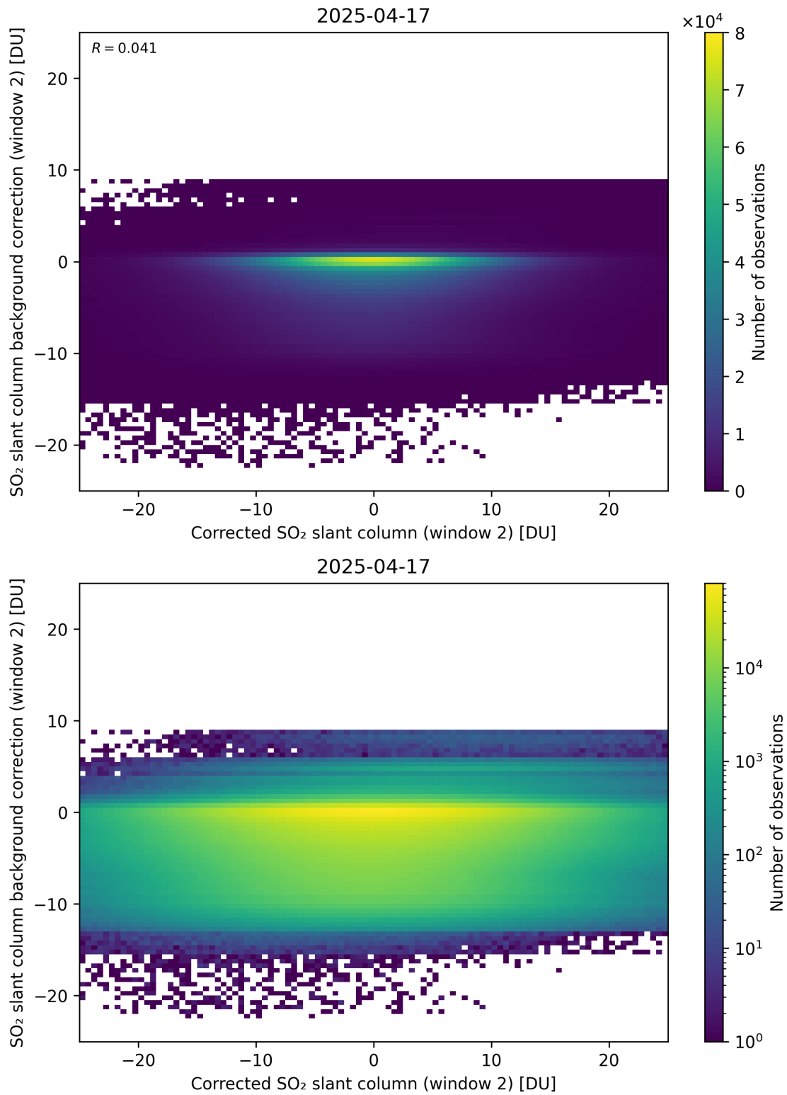
Figure 244: Scatter density plot of “Corrected SO 2 slant column (window 2)” against “SO 2 slant column background correction (window 2)” for 2025-04-16 to 2025-04-18.
