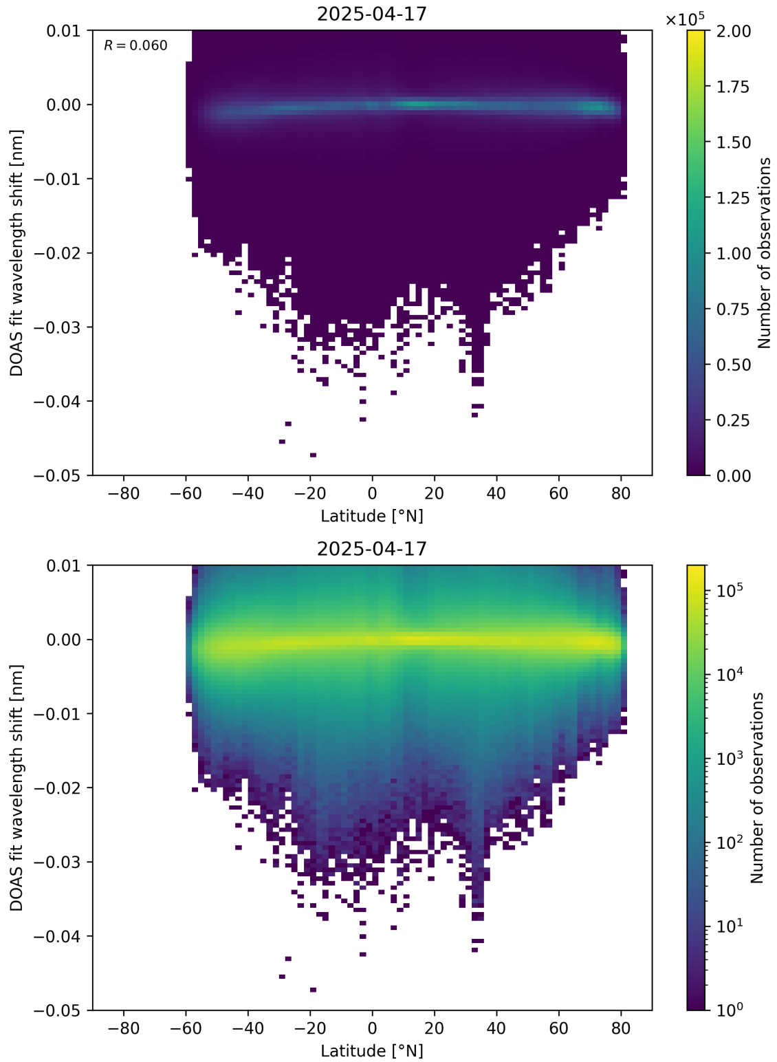
Figure 153: Scatter density plot of “Latitude” against “DOAS fit wavelength shift” for 2025-04-16 to 2025-04-18.
