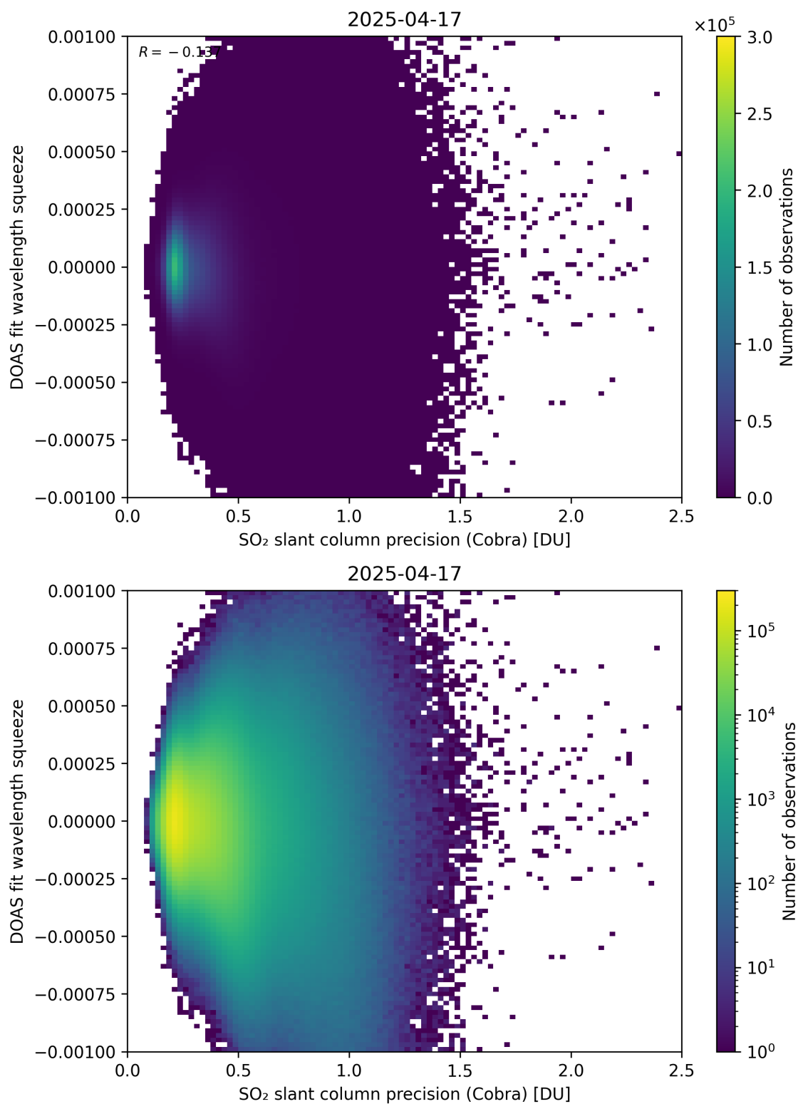
Figure 203: Scatter density plot of “SO 2 slant column precision (Cobra)” against “DOAS fit wavelength squeeze” for 2025-04-16 to 2025-04-18.
