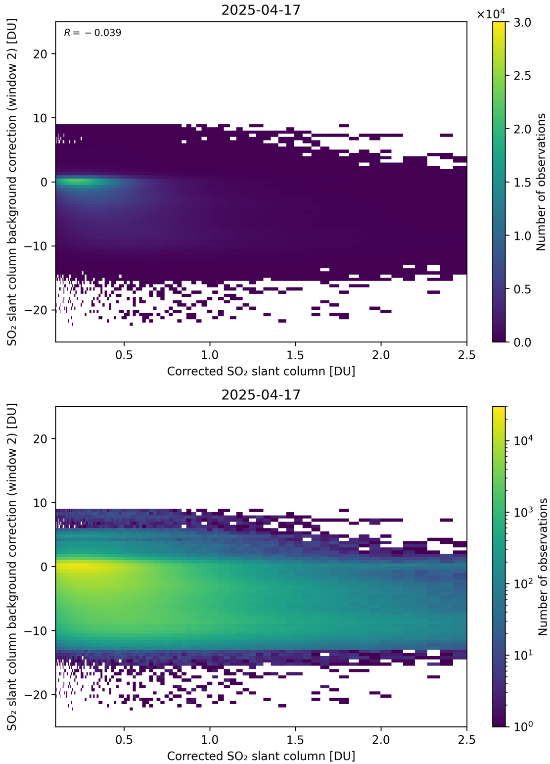
Figure 227: Scatter density plot of “Corrected SO 2 slant column” against “SO 2 slant column background correction (window 2)” for 2025-04-16 to 2025-04-18.
