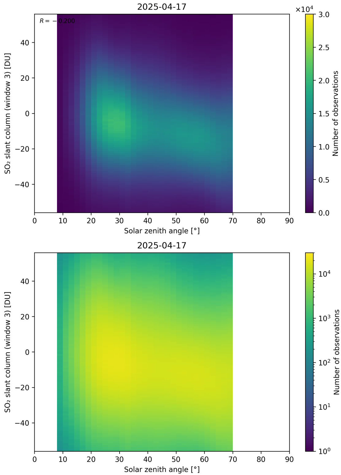
Figure 187: Scatter density plot of “Solar zenith angle” against “SO 2 slant column (window 3)” for 2025-04-16 to 2025-04-18.
