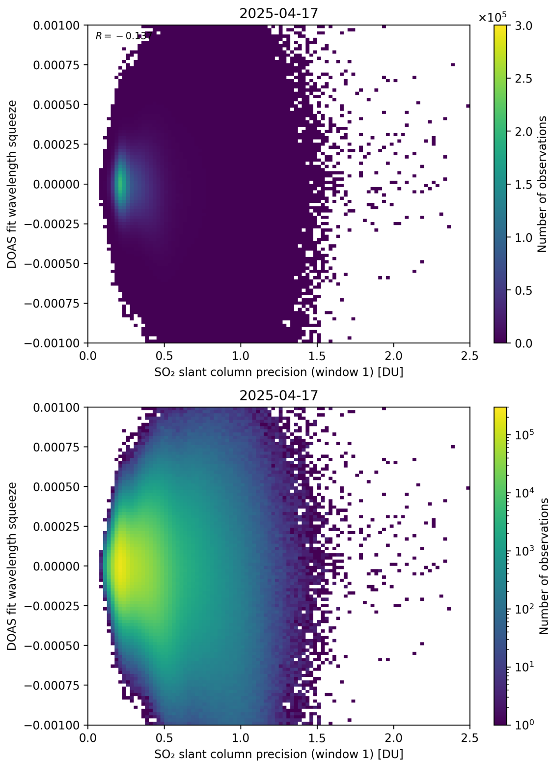
Figure 272: Scatter density plot of “SO 2 slant column precision (window 1)” against “DOAS fit wavelength squeeze” for 2025-04-16 to 2025-04-18.
