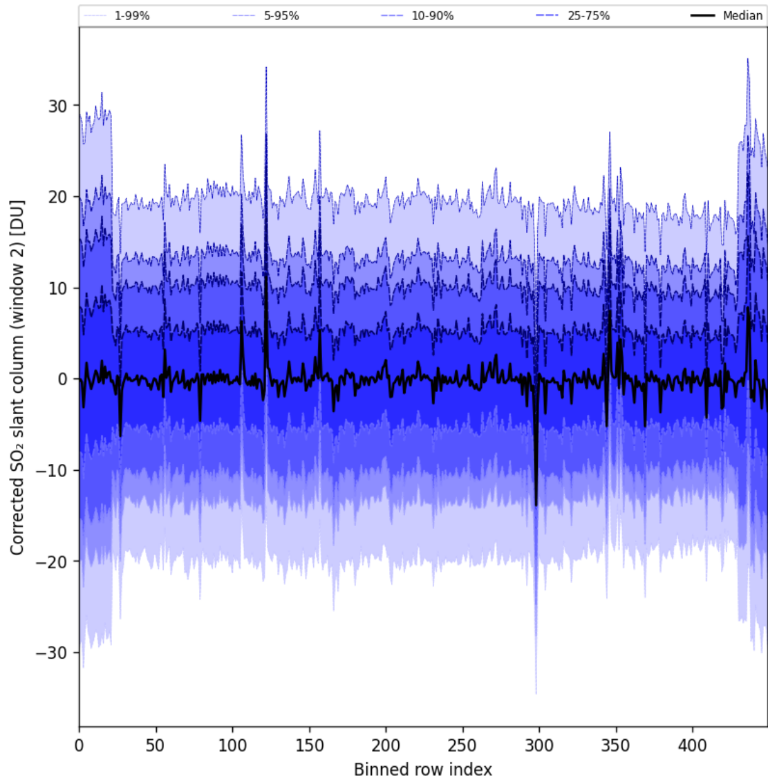
Figure 95: Along track statistics of “Corrected SO 2 slant column (window 2)” for 2025-04-16 to 2025-04-18
