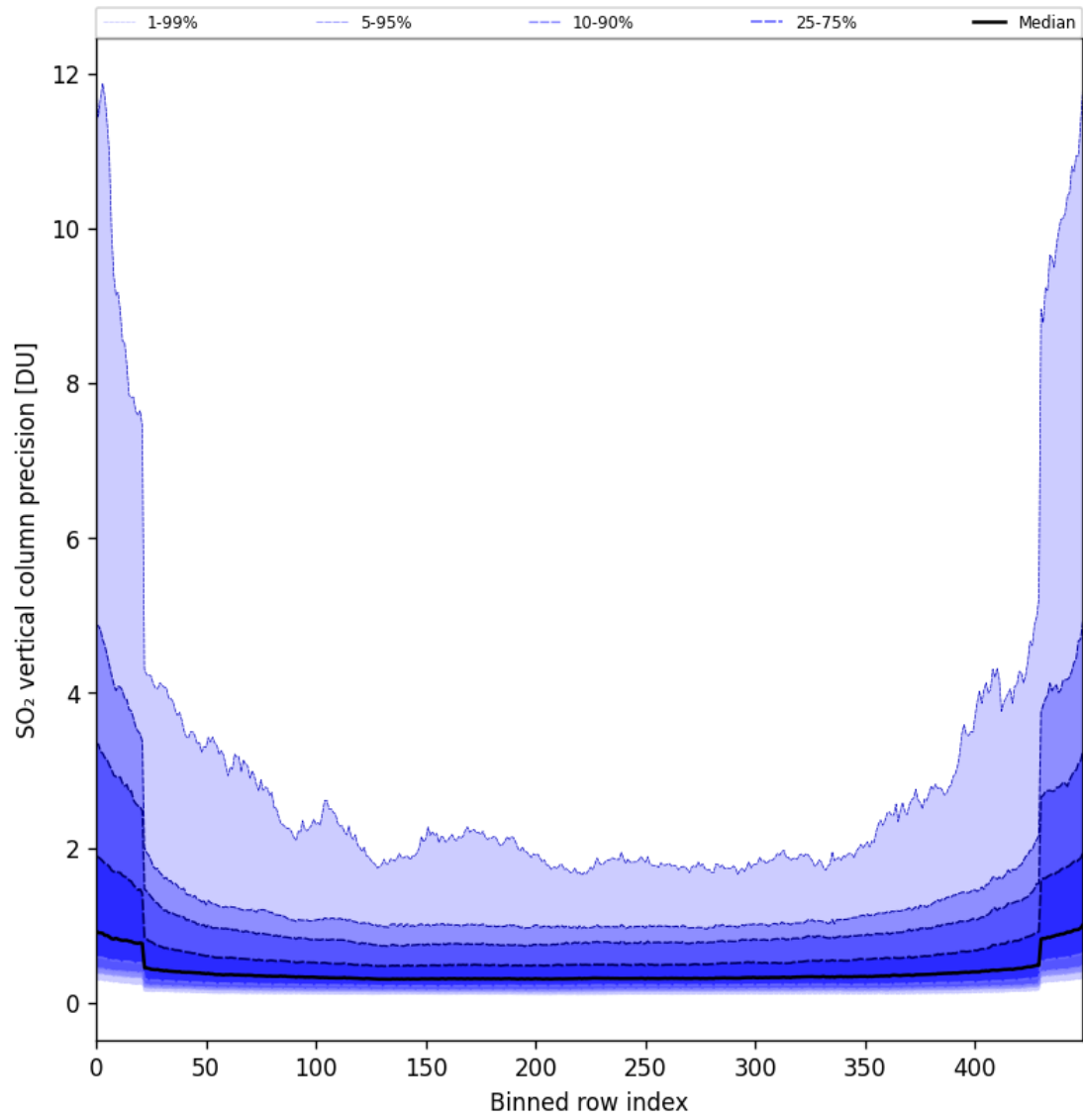
Figure 85: Along track statistics of “SO 2 vertical column precision” for 2025-04-16 to 2025-04-18
