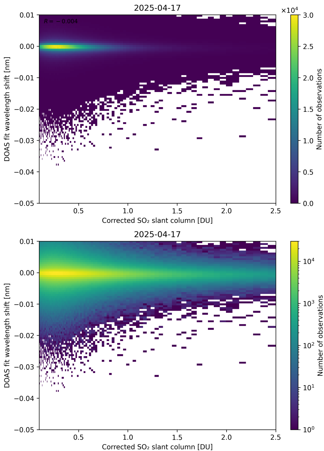
Figure 229: Scatter density plot of “Corrected SO 2 slant column” against “DOAS fit wavelength shift” for 2025-04-16 to 2025-04-18.
