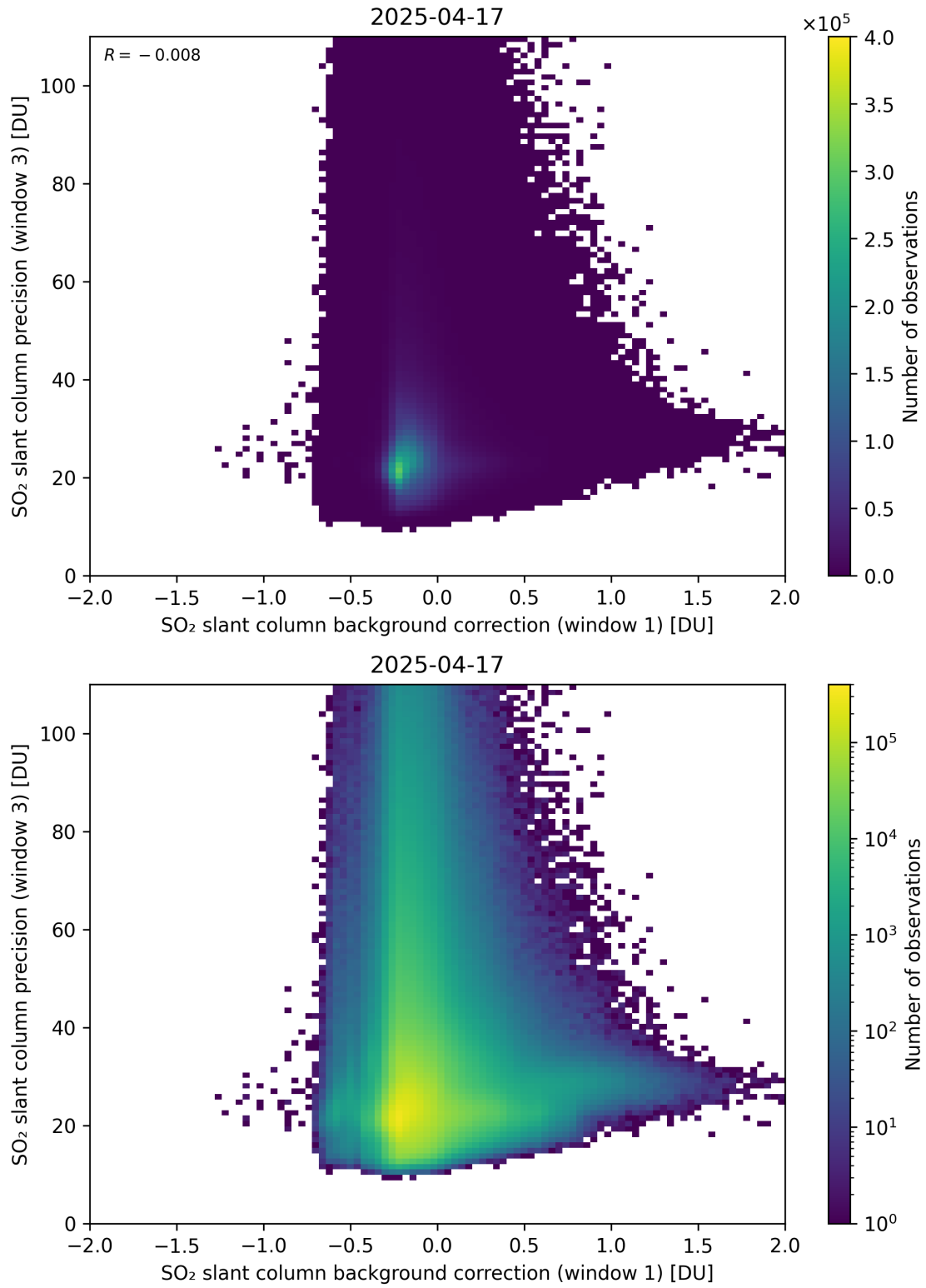
Figure 119: Scatter density plot of “SO 2 slant column background correction (window 1)” against “SO 2 slant column precision (window 3)” for 2025-04-16 to 2025-04-18.
