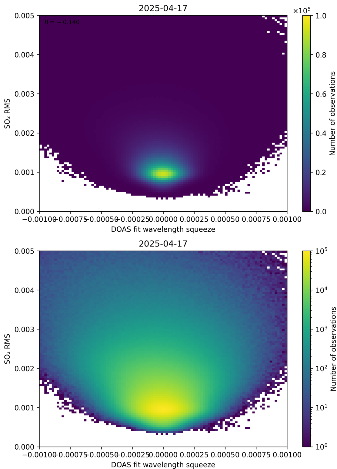
Figure 143: Scatter density plot of “DOAS fit wavelength squeeze” against “SO 2 RMS” for 2025-04-16 to 2025-04-18.
