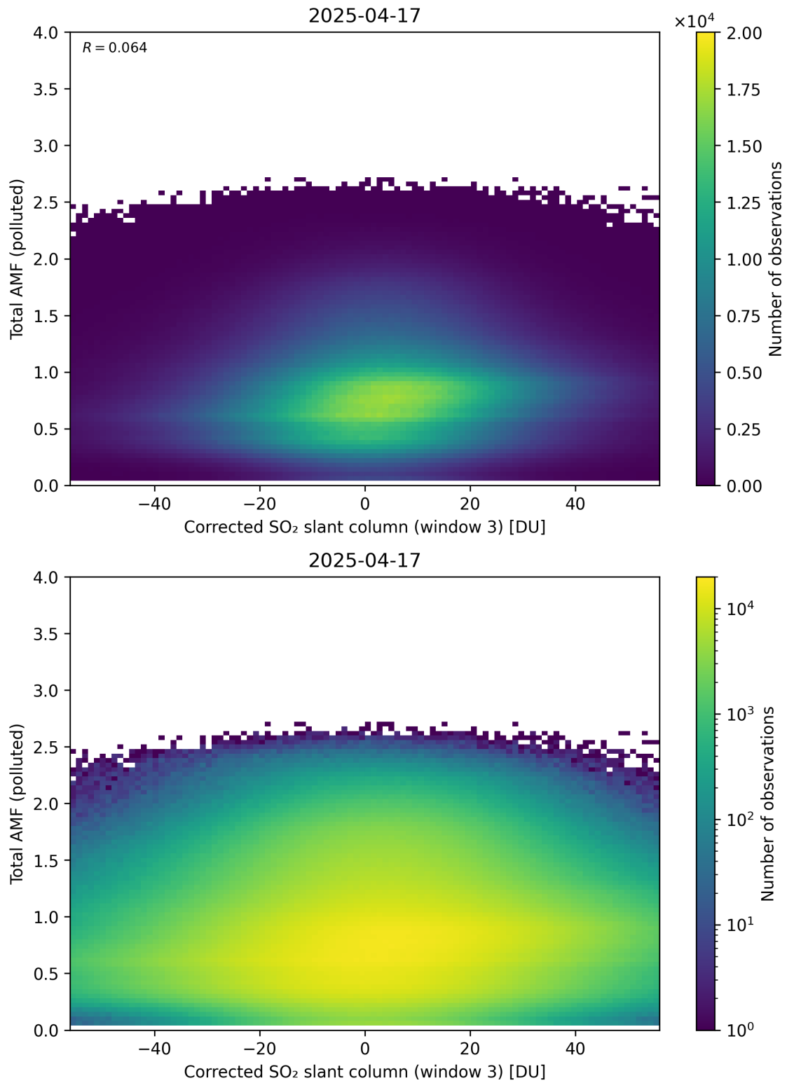
Figure 260: Scatter density plot of “Corrected SO 2 slant column (window 3)” against “Total AMF (polluted)” for 2025-04-16 to 2025-04-18.
