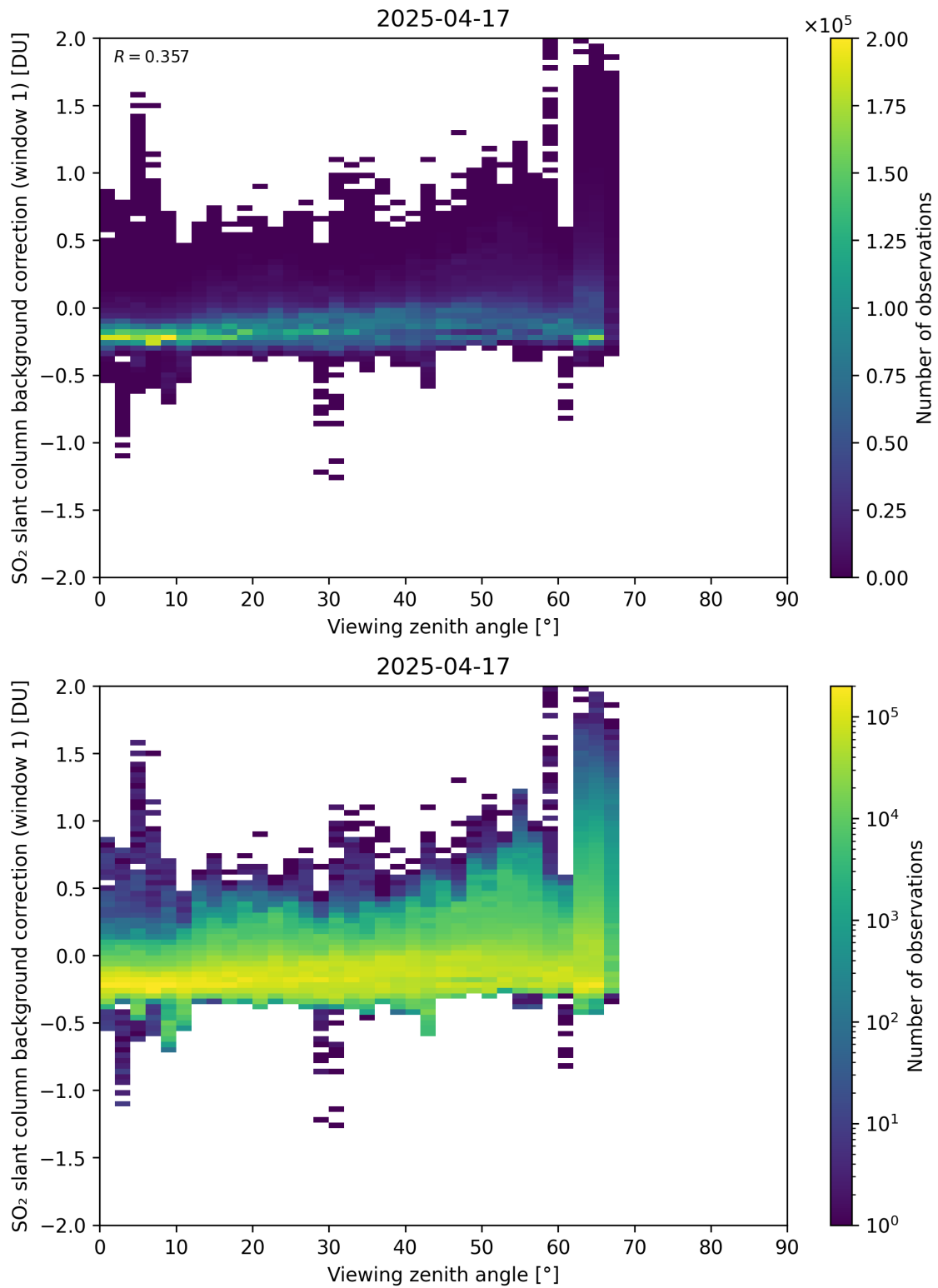
Figure 362: Scatter density plot of “Viewing zenith angle” against “SO 2 slant column background correction (window 1)” for 2025-04-16 to 2025-04-18.
