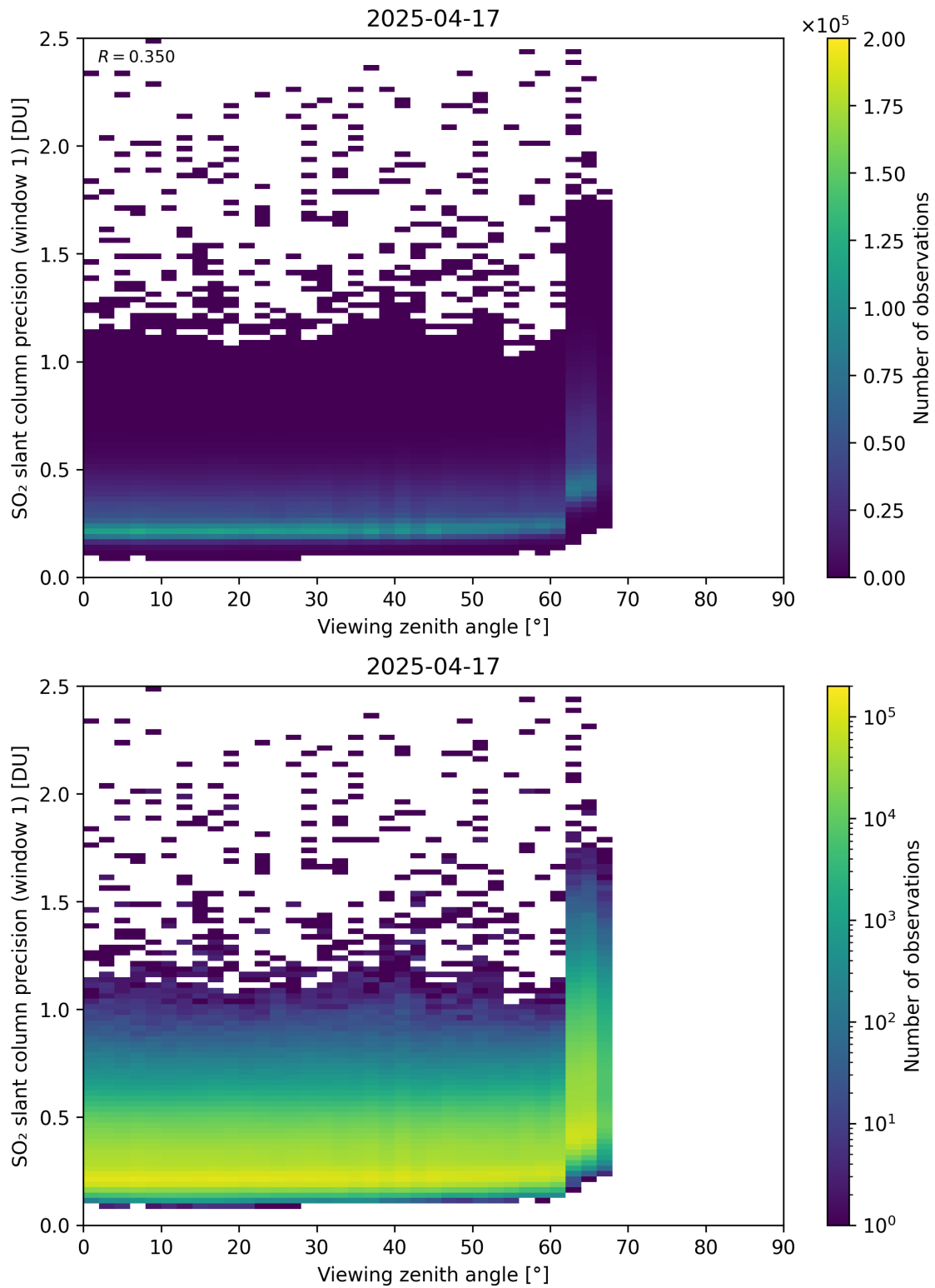
Figure 377: Scatter density plot of “Viewing zenith angle” against “SO 2 slant column precision (window 1)” for 2025-04-16 to 2025-04-18.
