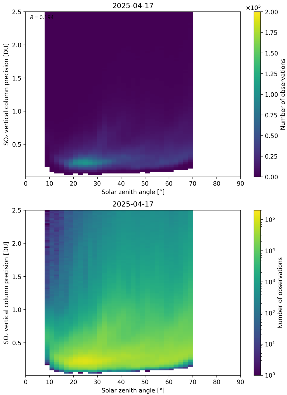
Figure 192: Scatter density plot of “Solar zenith angle” against “SO 2 vertical column precision” for 2025-04-16 to 2025-04-18.
