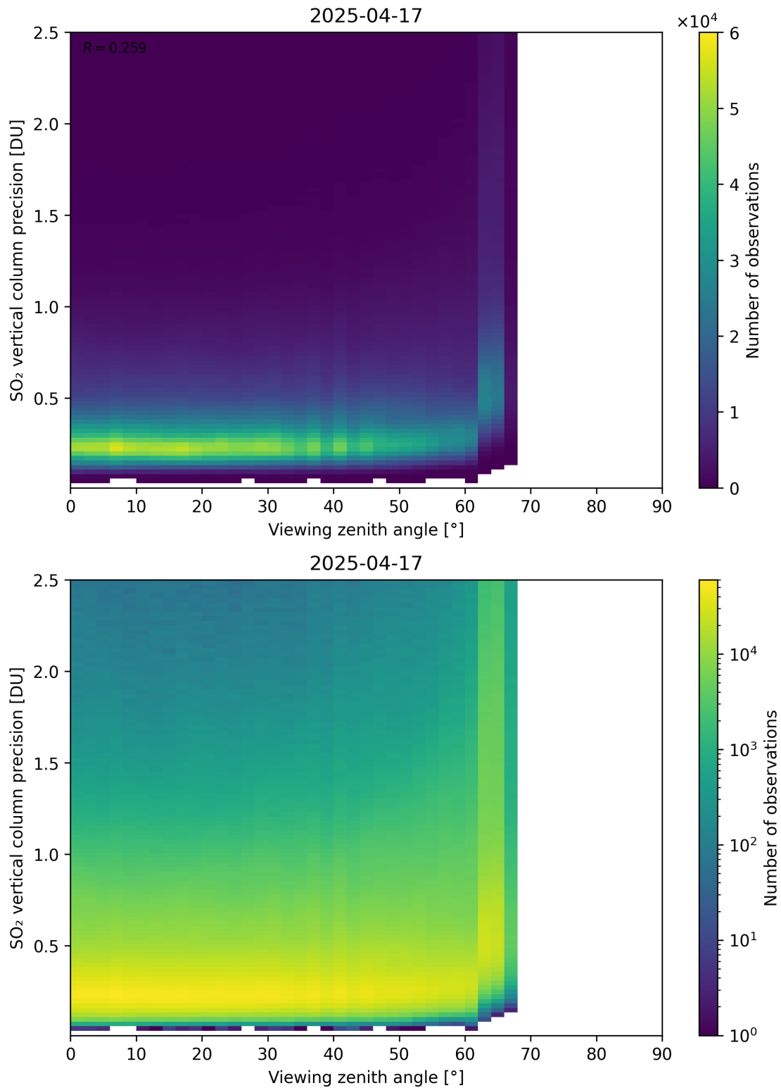
Figure 384: Scatter density plot of “Viewing zenith angle” against “SO 2 vertical column precision” for 2025-04-16 to 2025-04-18.
