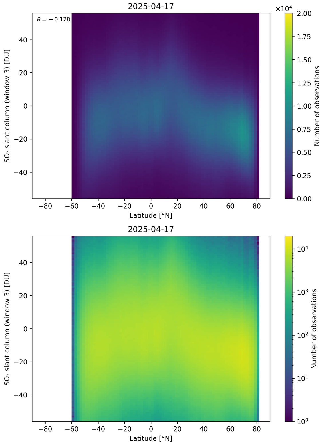
Figure 165: Scatter density plot of “Latitude” against “SO 2 slant column (window 3)” for 2025-04-16 to 2025-04-18.
