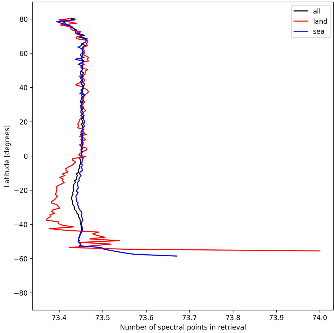
Figure 56: Zonal average of “Number of spectral points in retrieval” for 2025-04-16 to 2025-04-18.
