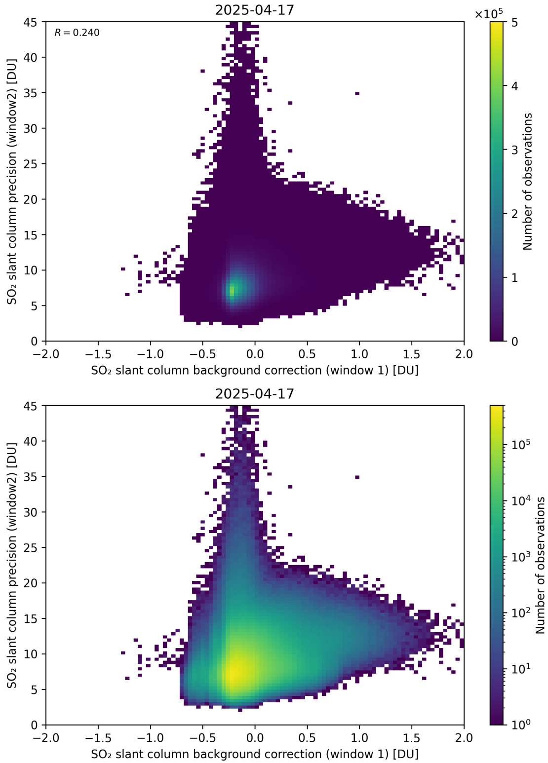
Figure 117: Scatter density plot of “SO 2 slant column background correction (window 1)” against “SO 2 slant column precision (window2)” for 2025-04-16 to 2025-04-18.
