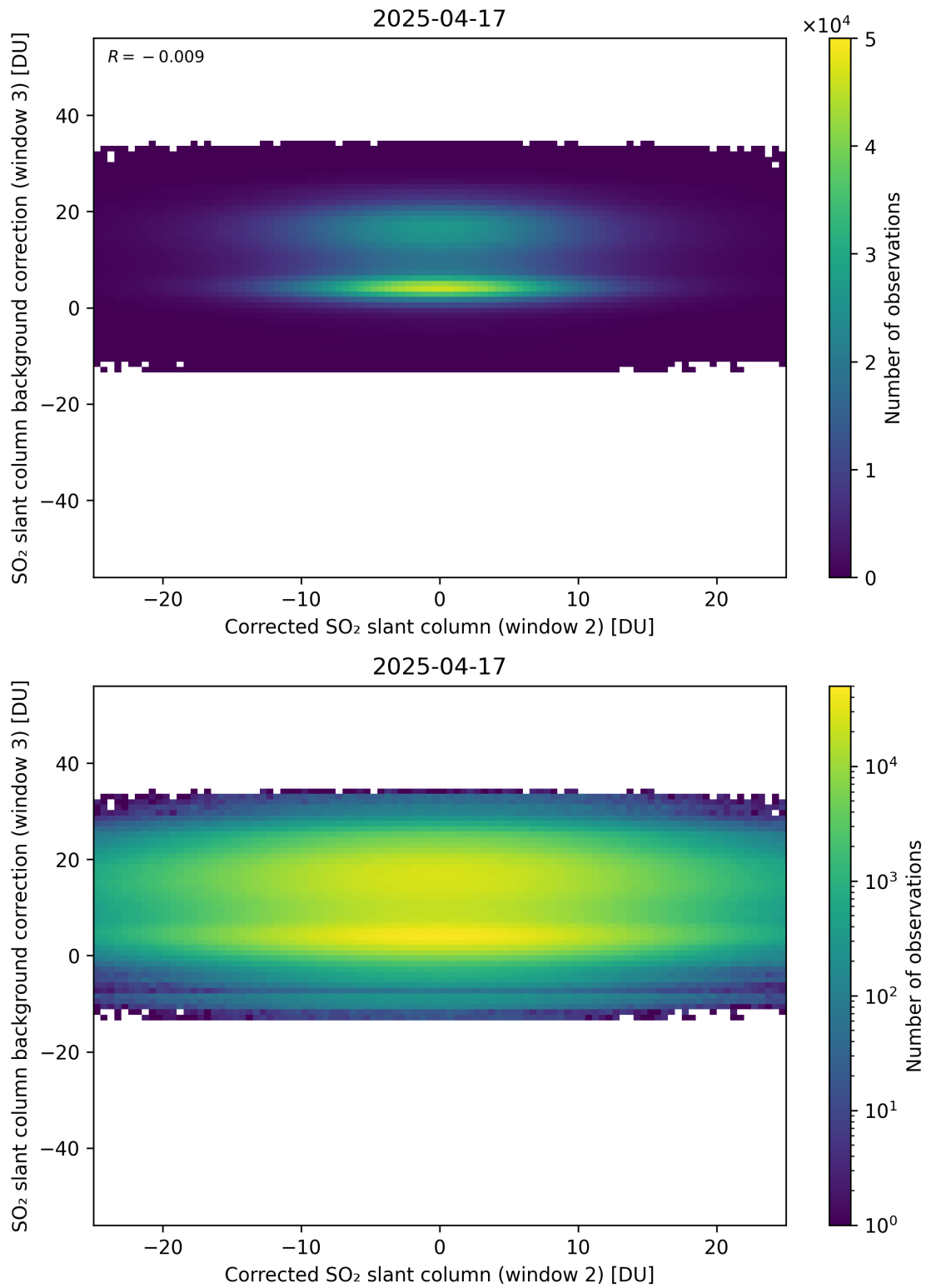
Figure 245: Scatter density plot of “Corrected SO 2 slant column (window 2)” against “SO 2 slant column background correction (window 3)” for 2025-04-16 to 2025-04-18.
