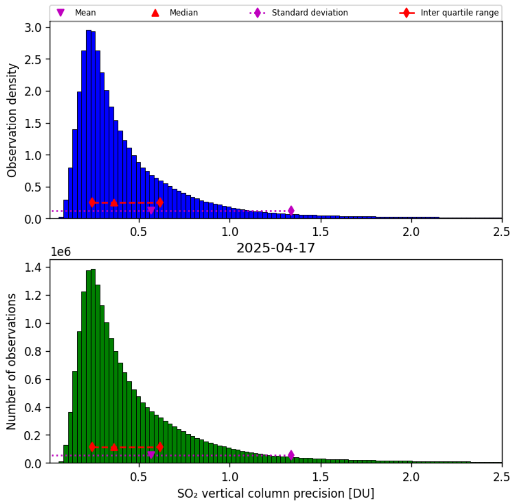
Figure 59: Histogram of “SO 2 vertical column precision” for 2025-04-16 to 2025-04-18
