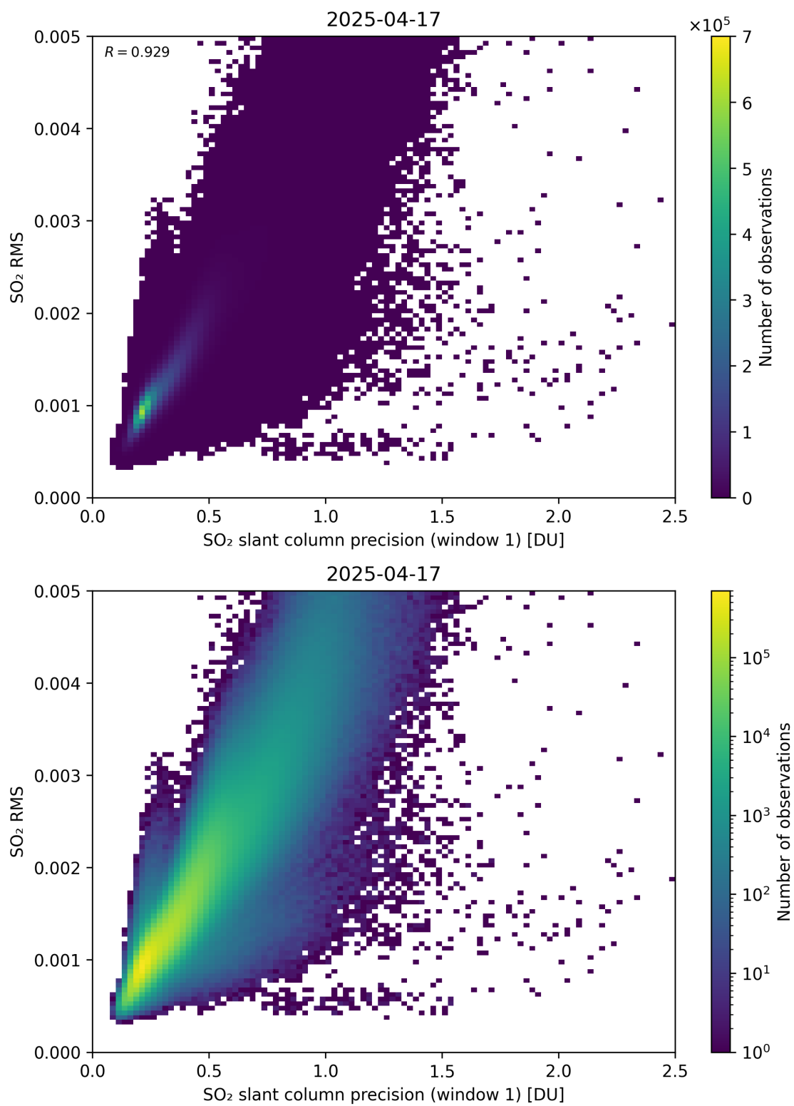
Figure 273: Scatter density plot of “SO 2 slant column precision (window 1)” against “SO 2 RMS” for 2025-04-16 to 2025-04-18.
