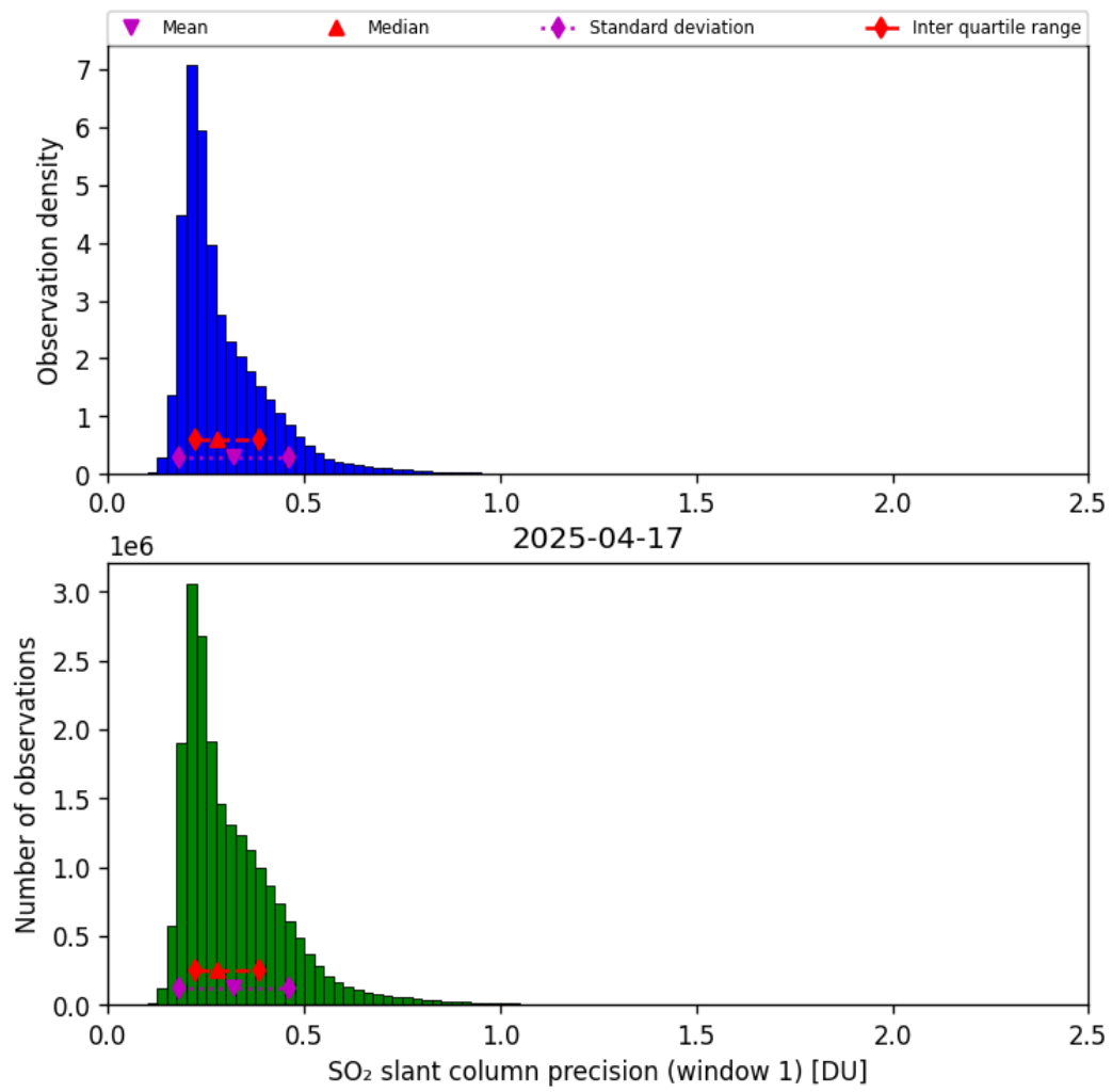
Figure 64: Histogram of “SO 2 slant column precision (window 1)” for 2025-04-16 to 2025-04-18
