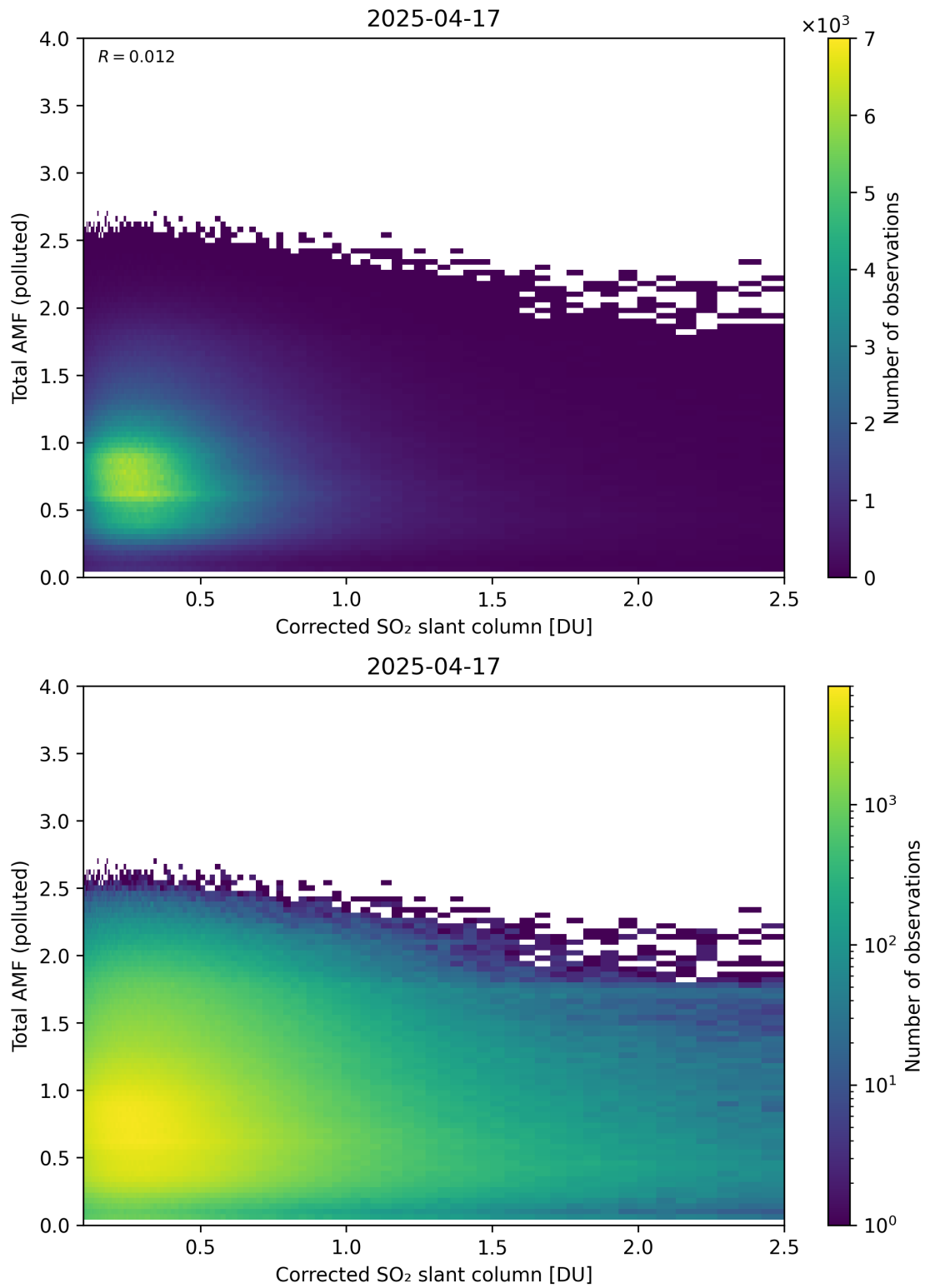
Figure 242: Scatter density plot of “Corrected SO 2 slant column” against “Total AMF (polluted)” for 2025-04-16 to 2025-04-18.
