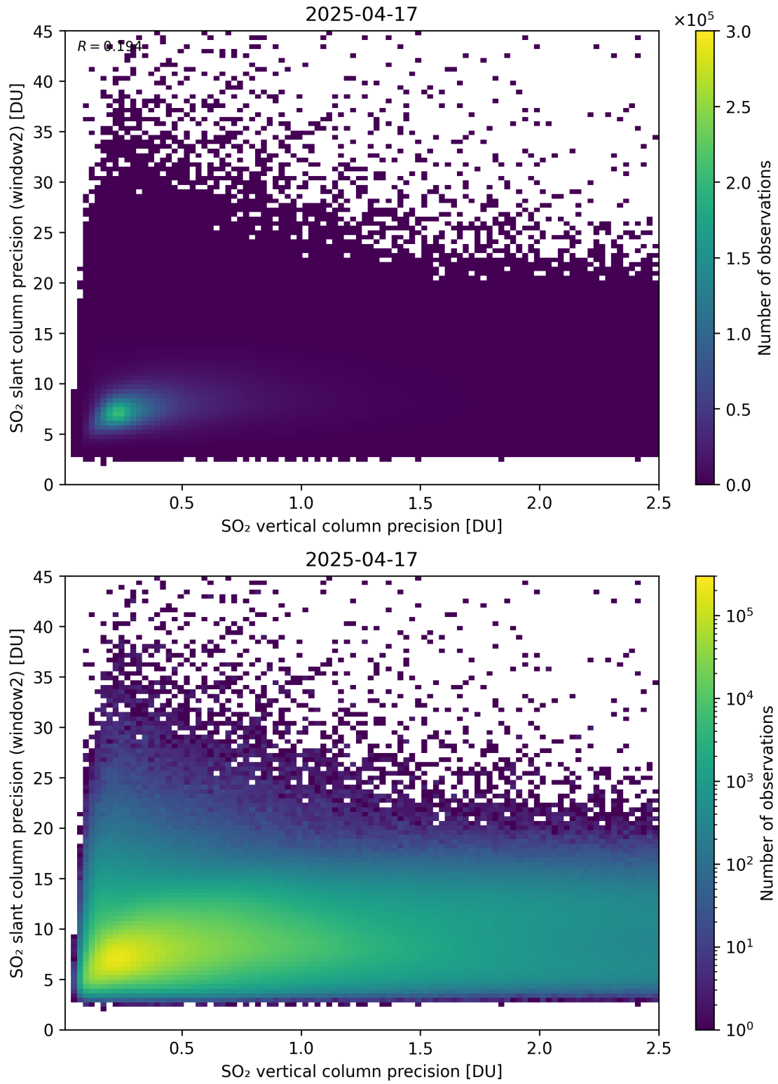
Figure 343: Scatter density plot of “SO 2 vertical column precision” against “SO 2 slant column precision (window2)” for 2025-04-16 to 2025-04-18.
