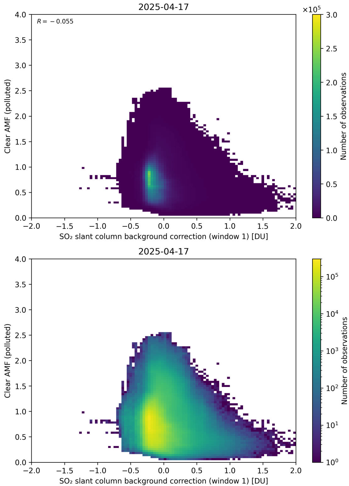
Figure 114: Scatter density plot of “SO 2 slant column background correction (window 1)” against “Clear AMF (polluted)” for 2025-04-16 to 2025-04-18.
