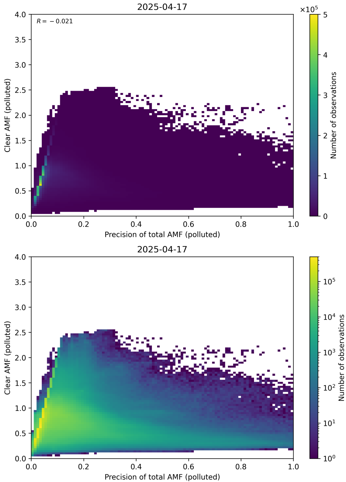
Figure 320: Scatter density plot of “Precision of total AMF (polluted)” against “Clear AMF (polluted)” for 2025-04-16 to 2025-04-18.
