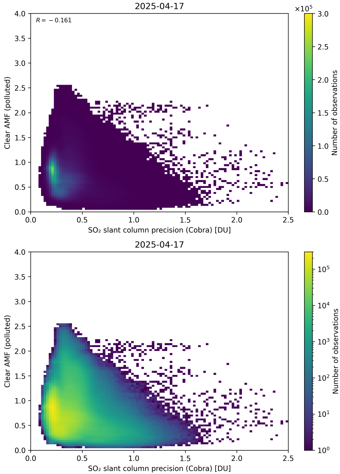
Figure 205: Scatter density plot of “SO 2 slant column precision (Cobra)” against “Clear AMF (polluted)” for 2025-04-16 to 2025-04-18.
