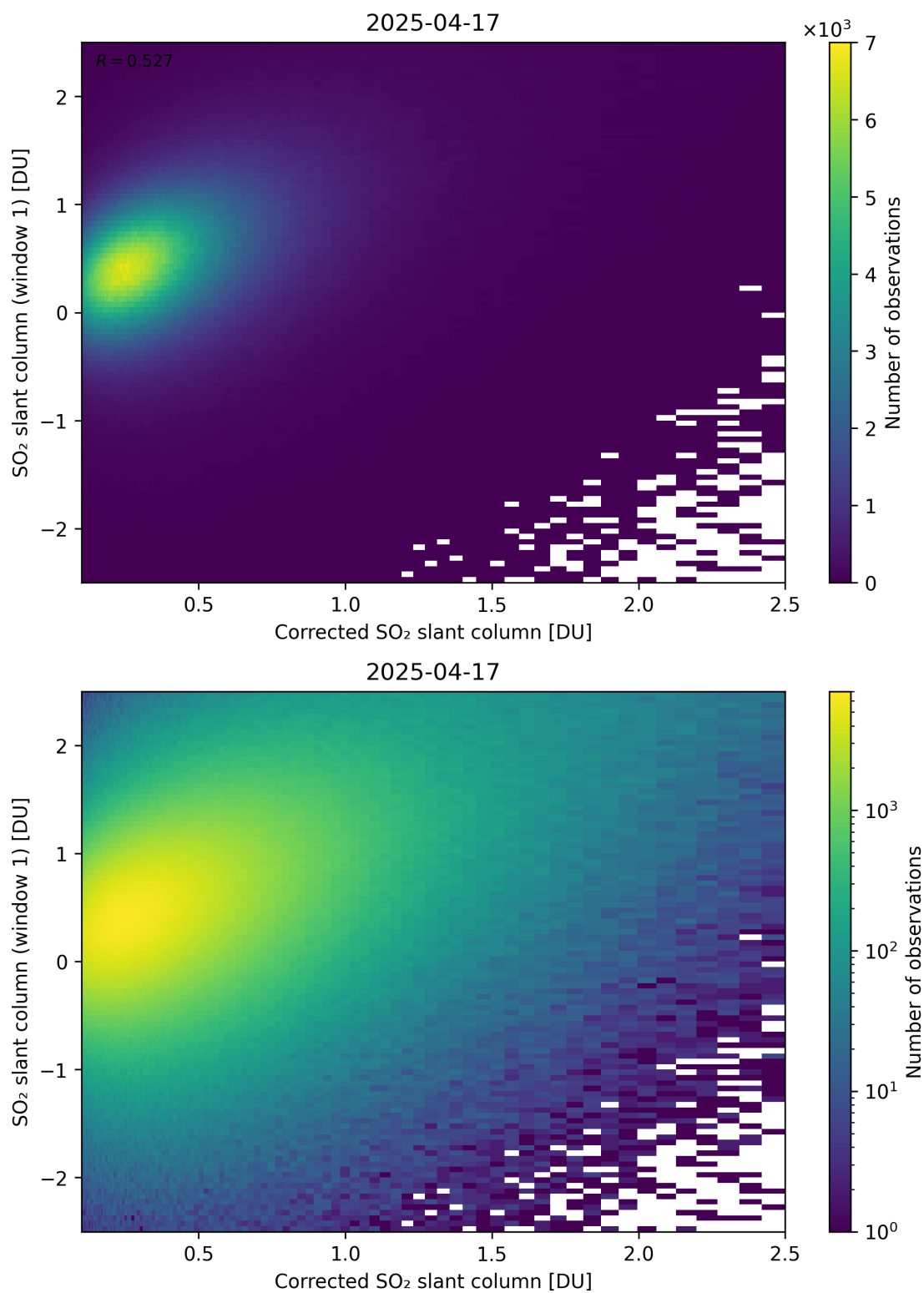
Figure 237: Scatter density plot of “Corrected SO 2 slant column” against “SO 2 slant column (window 1)” for 2025-04-16 to 2025-04-18.
