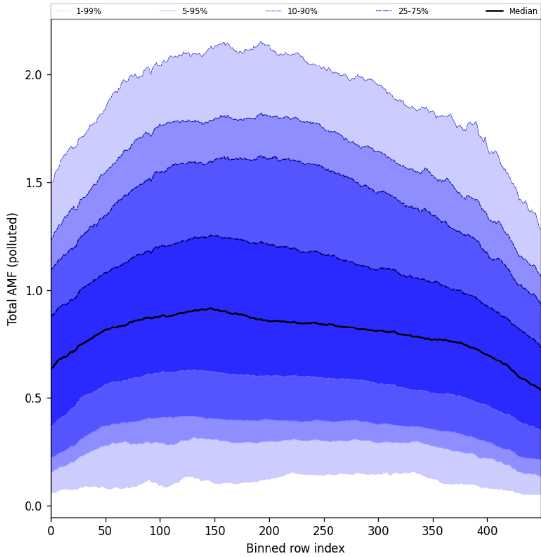
Figure 105: Along track statistics of “Total AMF (polluted)” for 2025-04-16 to 2025-04-18
