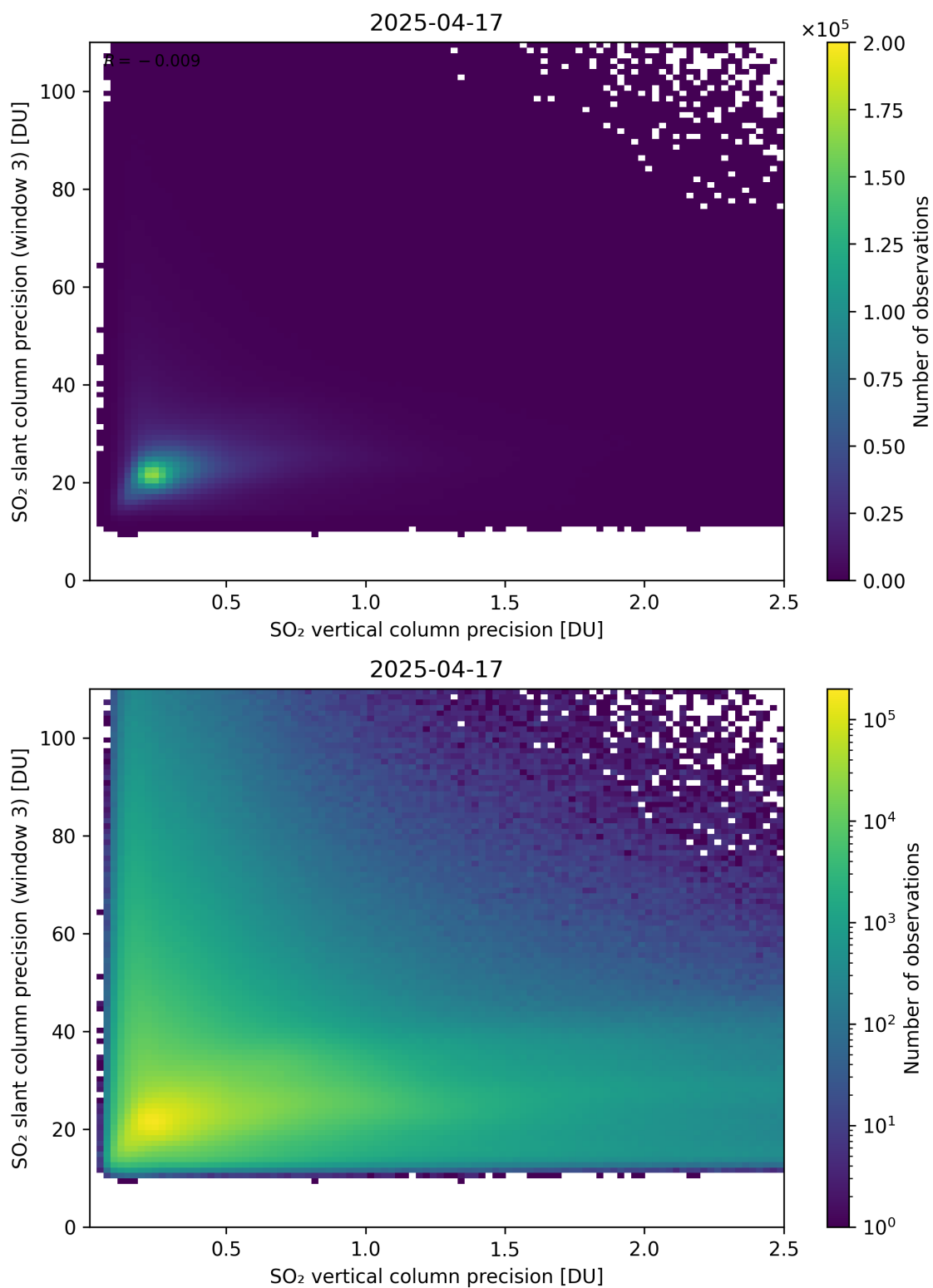
Figure 345: Scatter density plot of “SO 2 vertical column precision” against “SO 2 slant column precision (window 3)” for 2025-04-16 to 2025-04-18.
