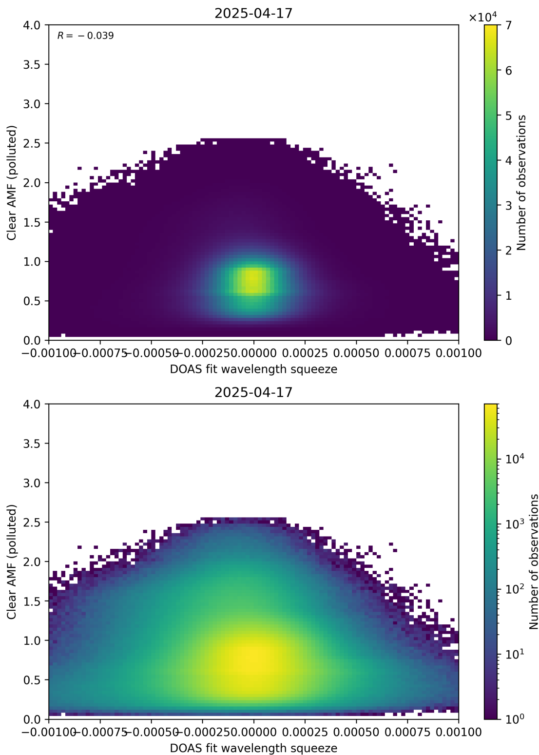
Figure 144: Scatter density plot of “DOAS fit wavelength squeeze” against “Clear AMF (polluted)” for 2025-04-16 to 2025-04-18.
