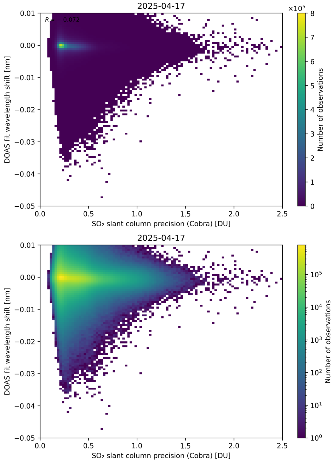
Figure 202: Scatter density plot of “SO 2 slant column precision (Cobra)” against “DOAS fit wavelength shift” for 2025-04-16 to 2025-04-18.
