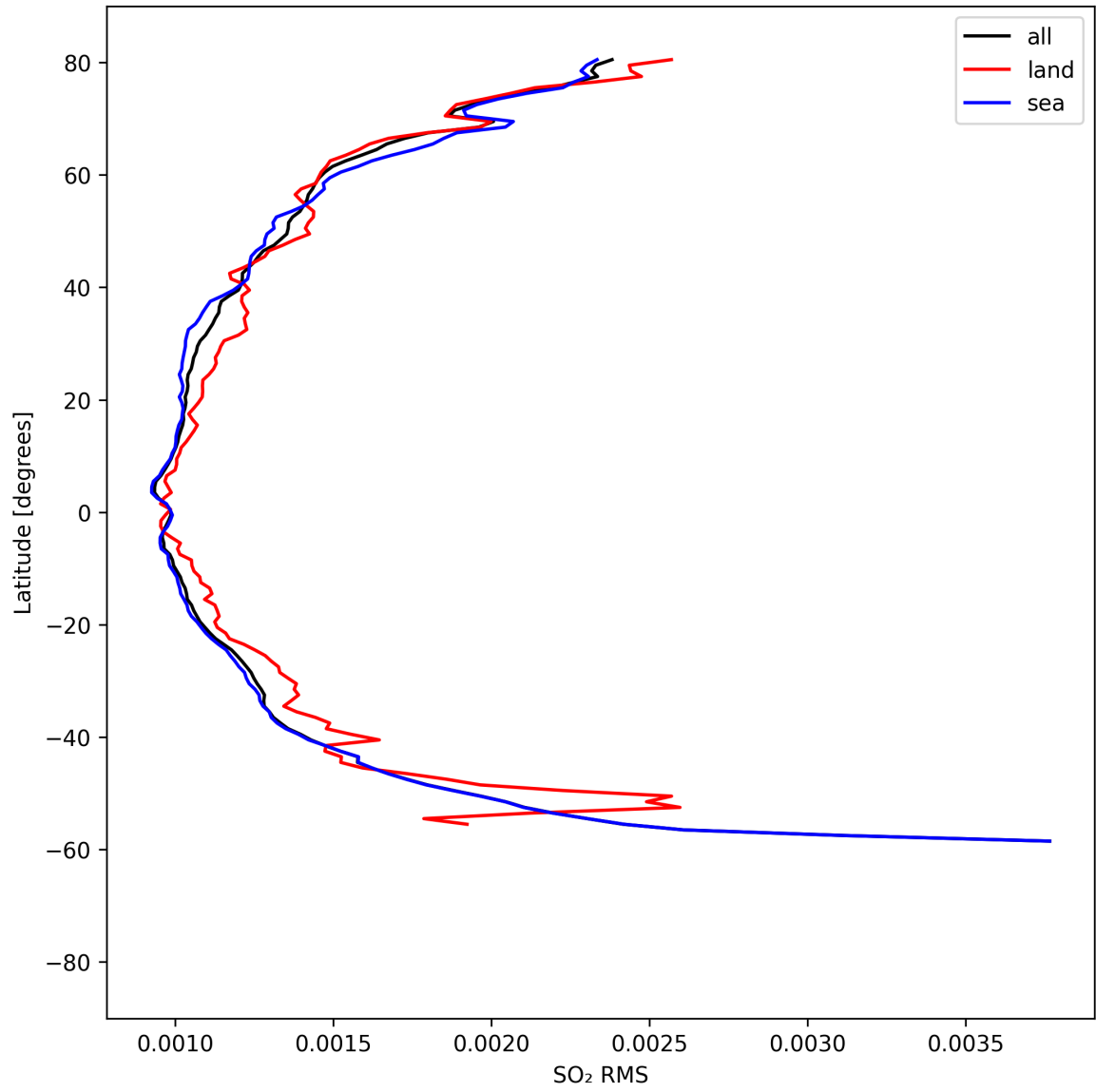
Figure 52: Zonal average of “SO 2 RMS” for 2025-04-16 to 2025-04-18.
