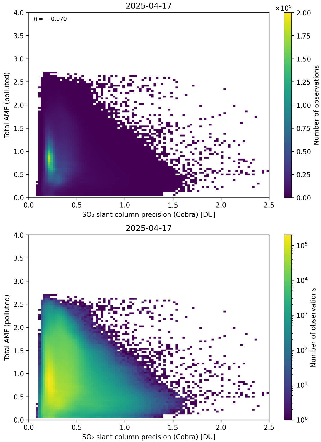
Figure 213: Scatter density plot of “SO 2 slant column precision (Cobra)” against “Total AMF (polluted)” for 2025-04-16 to 2025-04-18.
