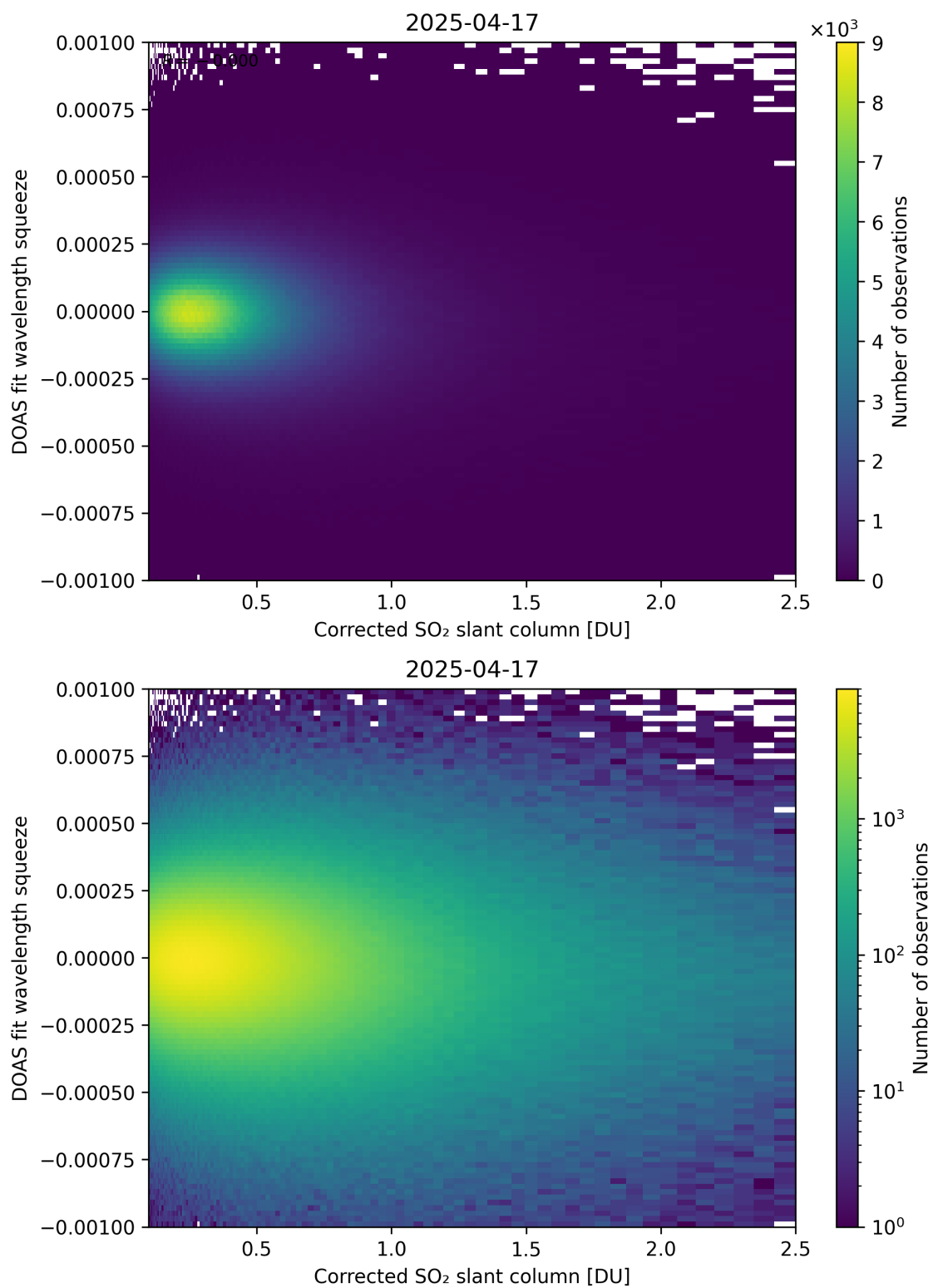
Figure 230: Scatter density plot of “Corrected SO 2 slant column” against “DOAS fit wavelength squeeze” for 2025-04-16 to 2025-04-18.
