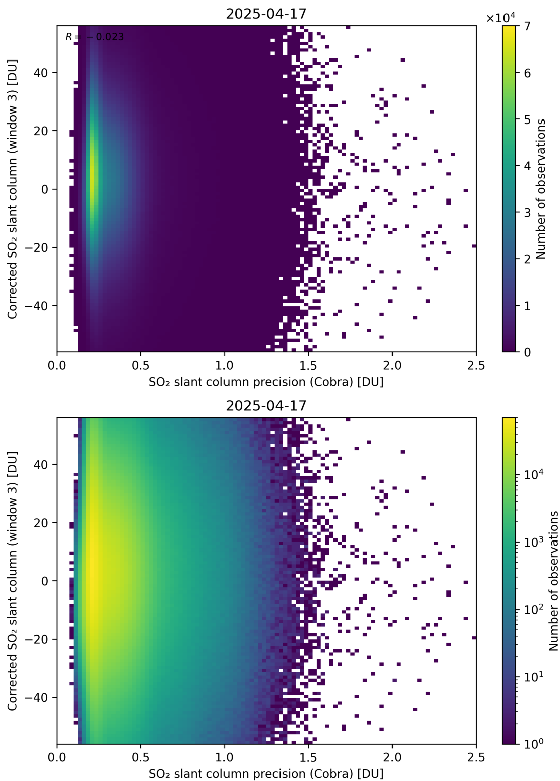
Figure 207: Scatter density plot of “SO 2 slant column precision (Cobra)” against “Corrected SO 2 slant column (window 3)” for 2025-04-16 to 2025-04-18.
