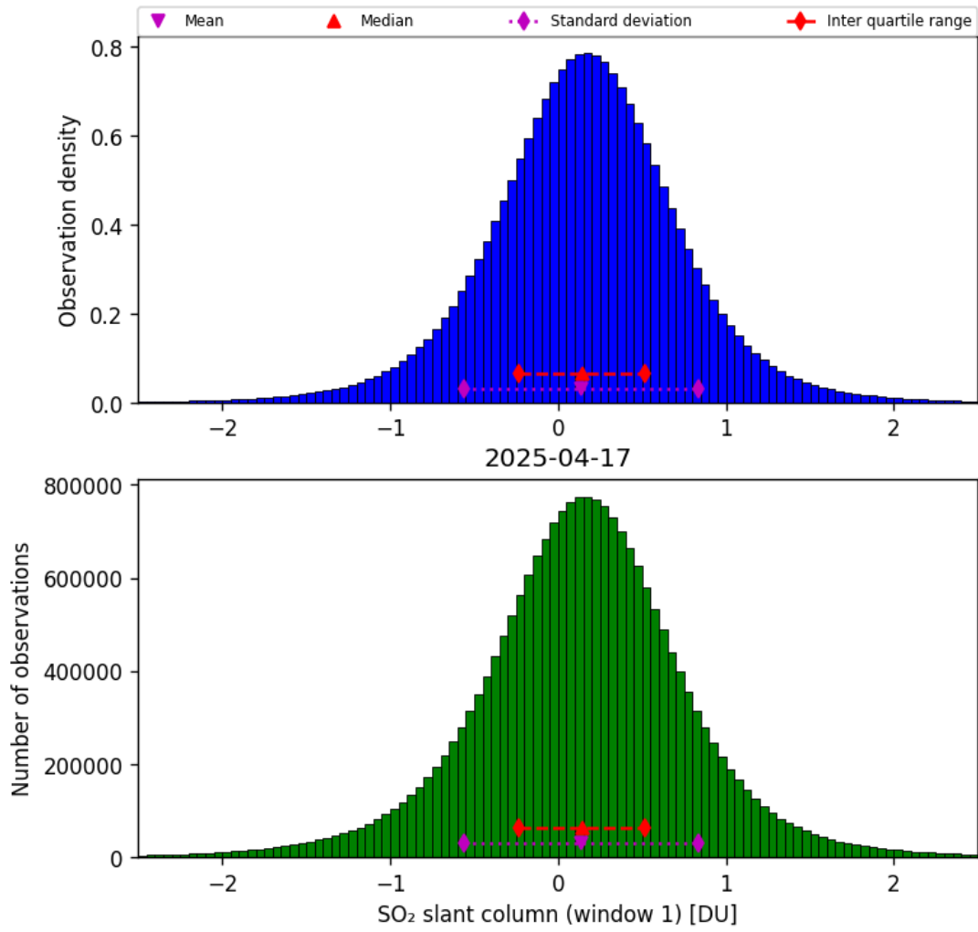
Figure 63: Histogram of “SO 2 slant column (window 1)” for 2025-04-16 to 2025-04-18
