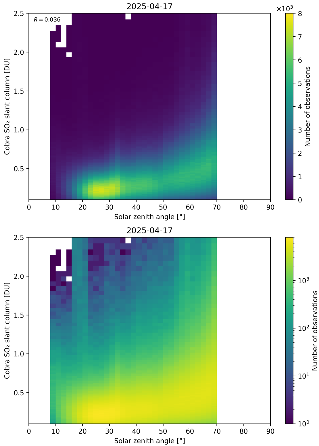
Figure 179: Scatter density plot of “Solar zenith angle” against “Cobra SO 2 slant column” for 2025-04-16 to 2025-04-18.
