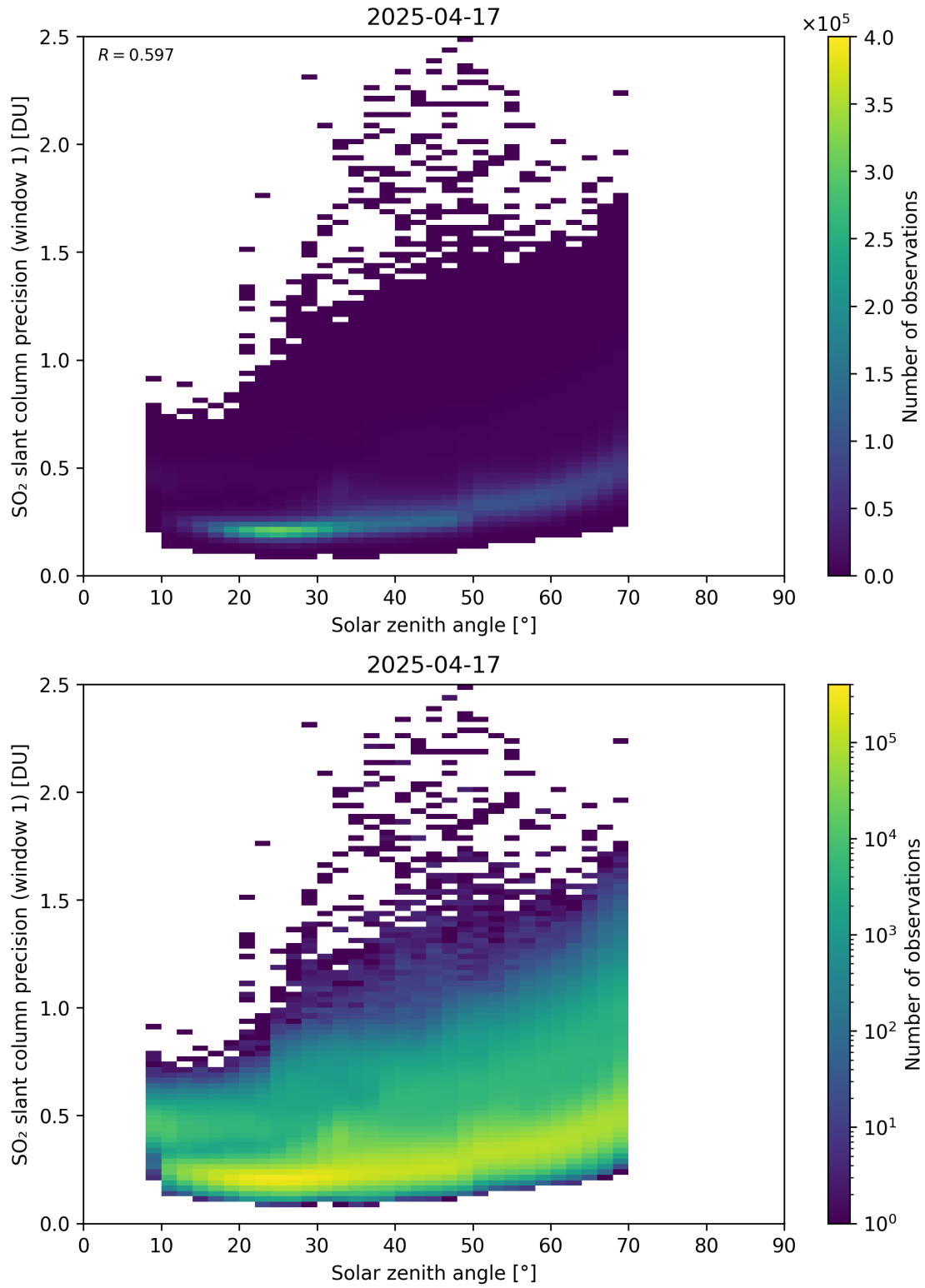
Figure 185: Scatter density plot of “Solar zenith angle” against “SO 2 slant column precision (window 1)” for 2025-04-16 to 2025-04-18.
