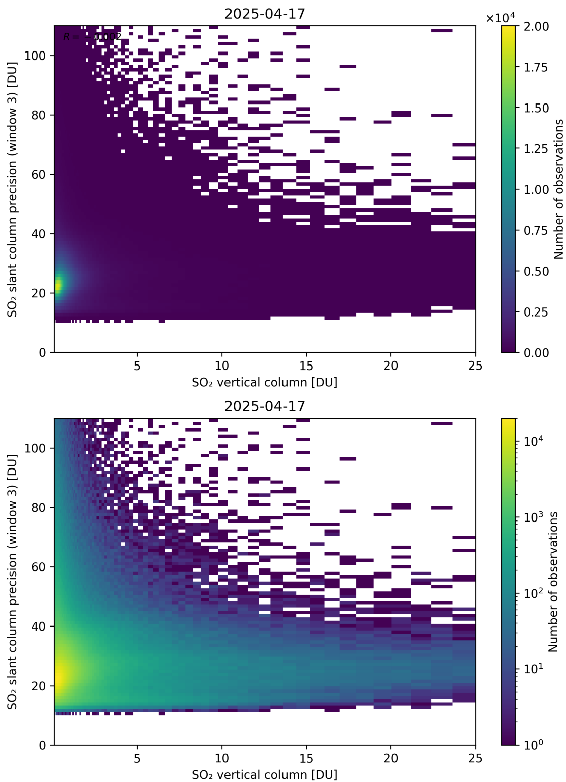
Figure 358: Scatter density plot of “SO 2 vertical column” against “SO 2 slant column precision (window 3)” for 2025-04-16 to 2025-04-18.
