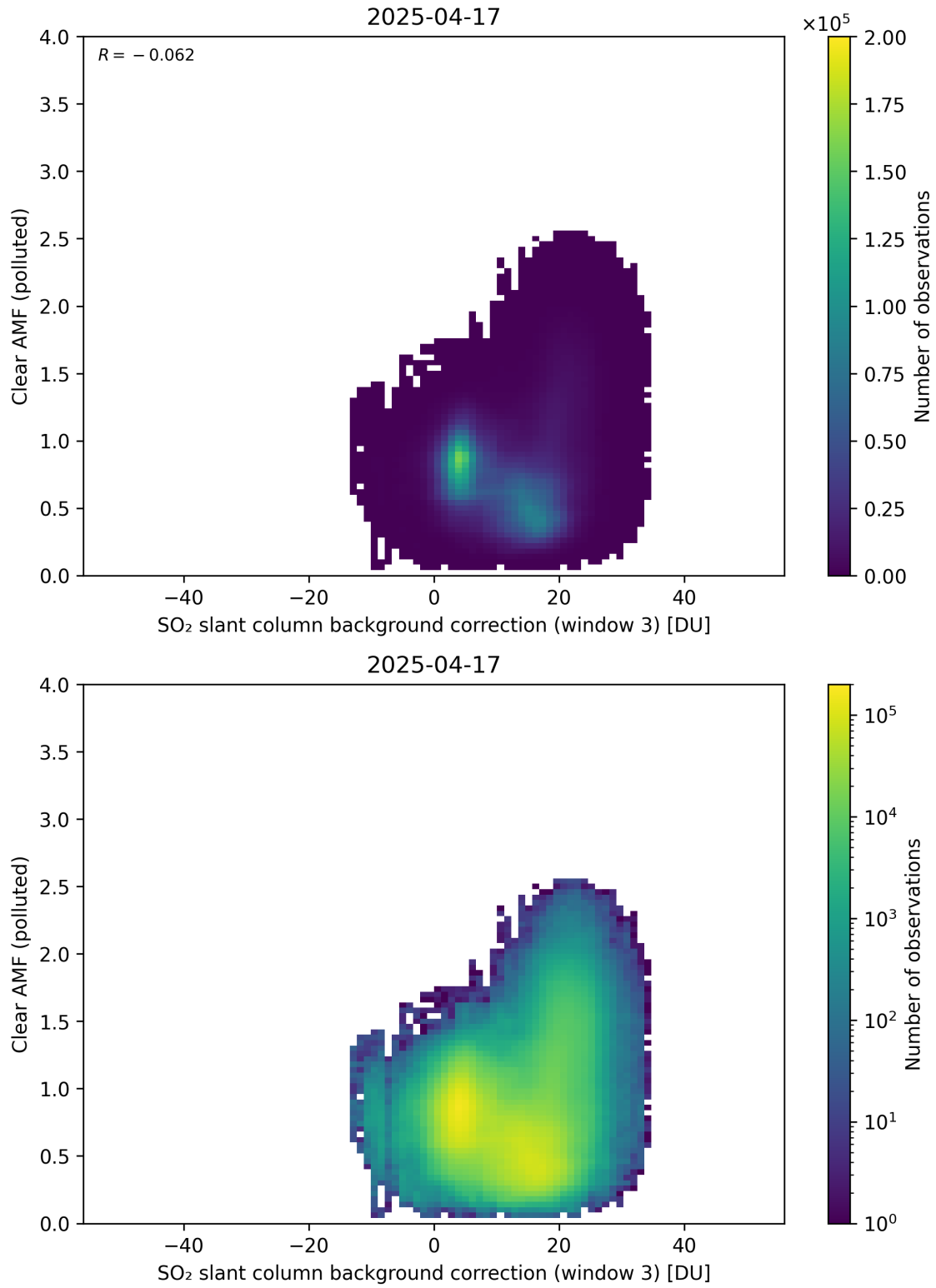
Figure 135: Scatter density plot of “SO 2 slant column background correction (window 3)” against “Clear AMF (polluted)” for 2025-04-16 to 2025-04-18.
