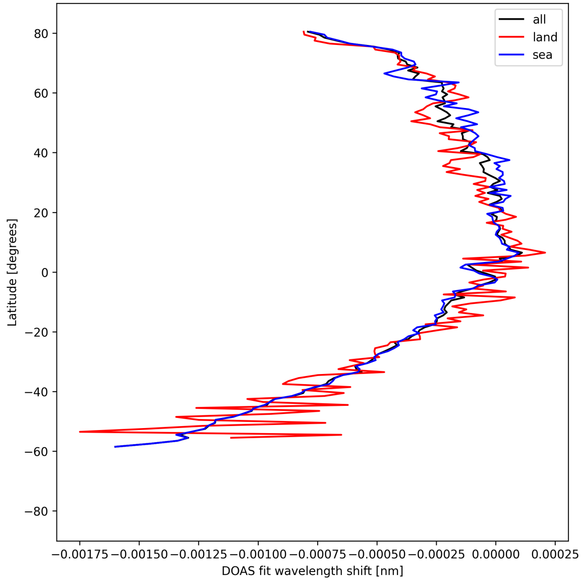
Figure 50: Zonal average of “DOAS fit wavelength shift” for 2025-04-16 to 2025-04-18.
