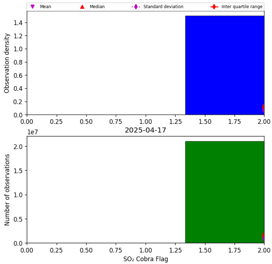
Figure 75: Histogram of “SO 2 Cobra Flag” for 2025-04-16 to 2025-04-18
