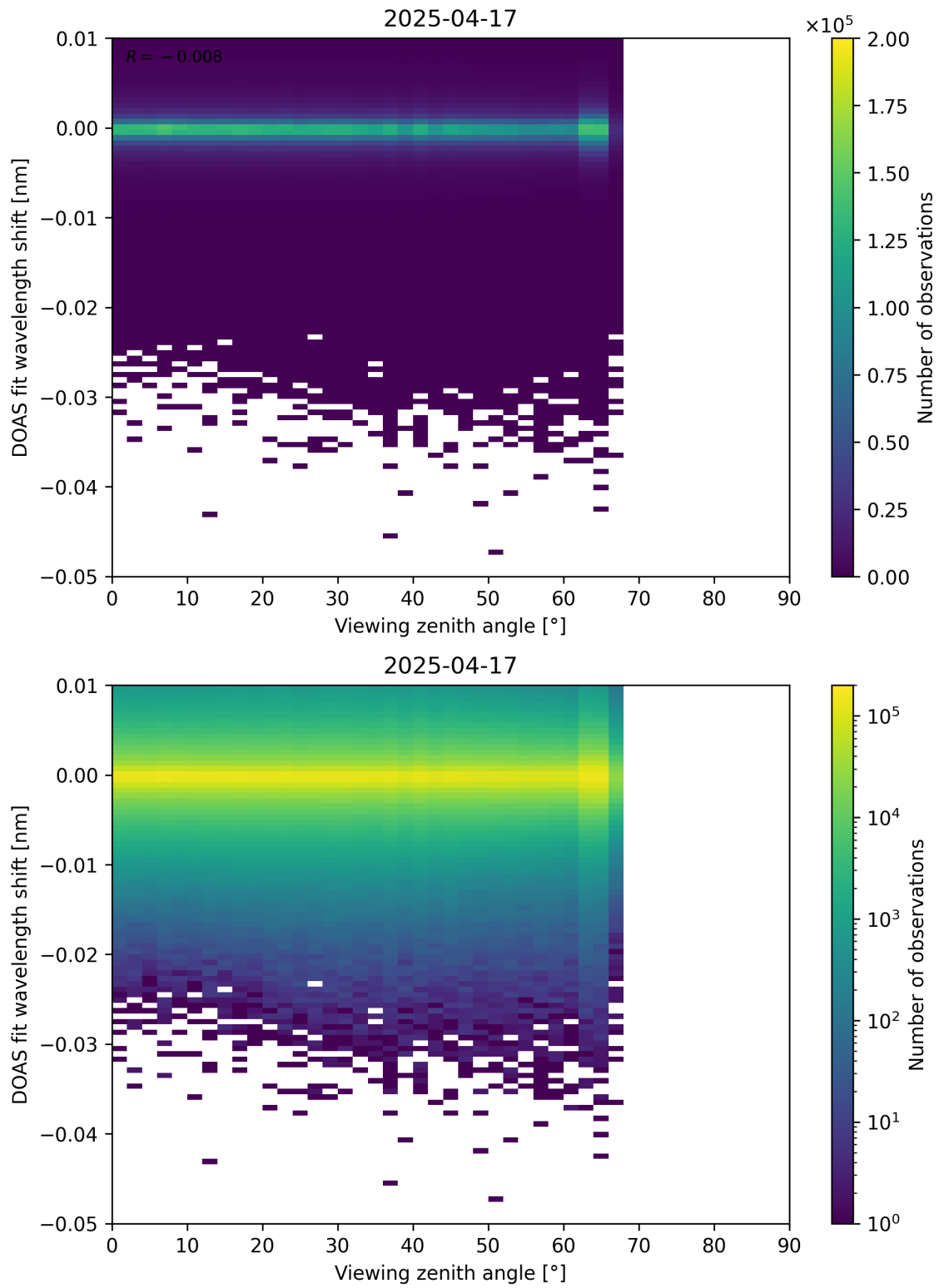
Figure 365: Scatter density plot of “Viewing zenith angle” against “DOAS fit wavelength shift” for 2025-04-16 to 2025-04-18.
