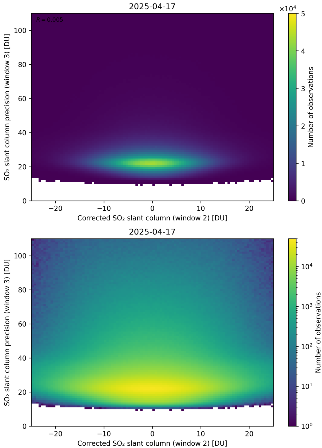
Figure 252: Scatter density plot of “Corrected SO 2 slant column (window 2)” against “SO 2 slant column precision (window 3)” for 2025-04-16 to 2025-04-18.
