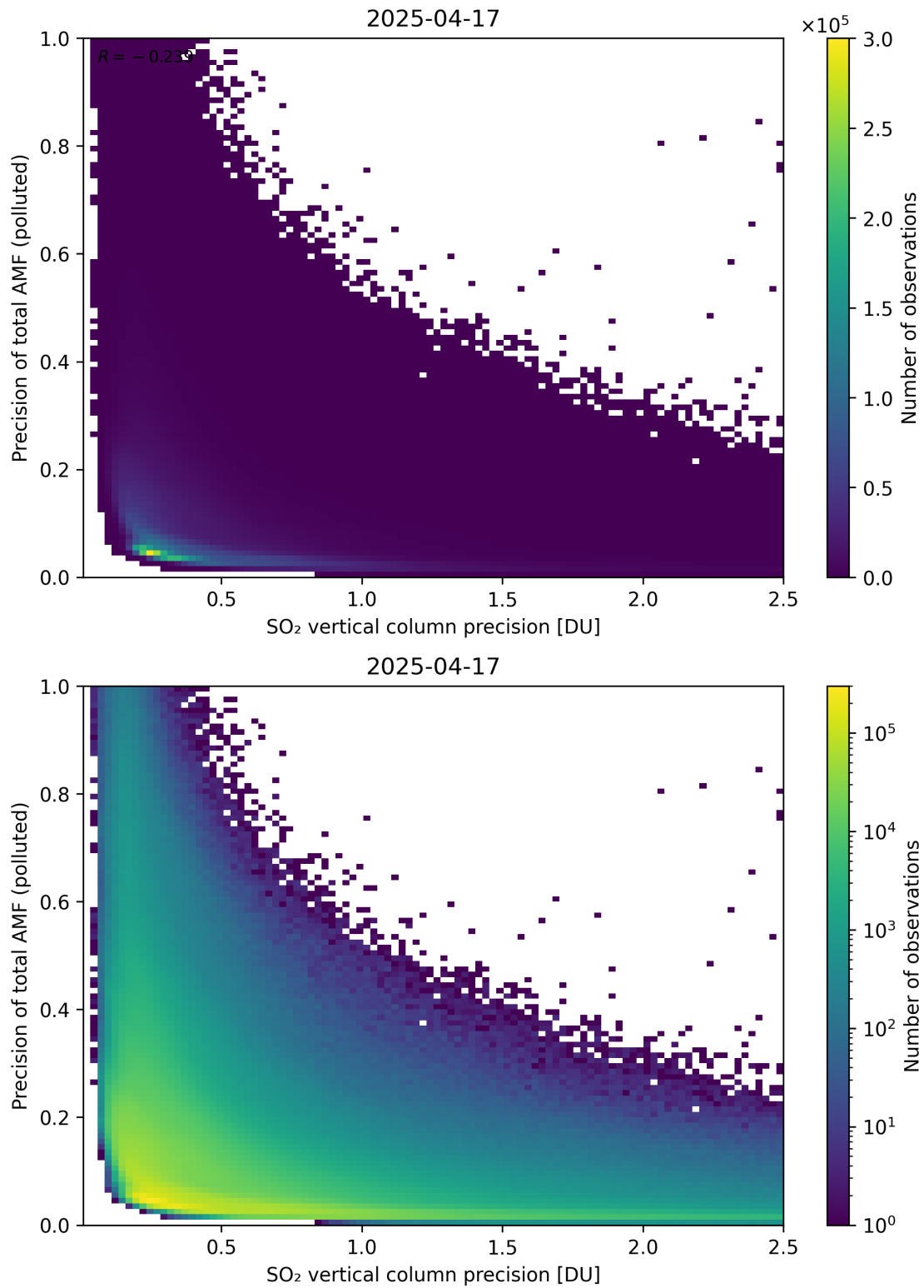
Figure 347: Scatter density plot of “SO 2 vertical column precision” against “Precision of total AMF (polluted)” for 2025-04-16 to 2025-04-18.
