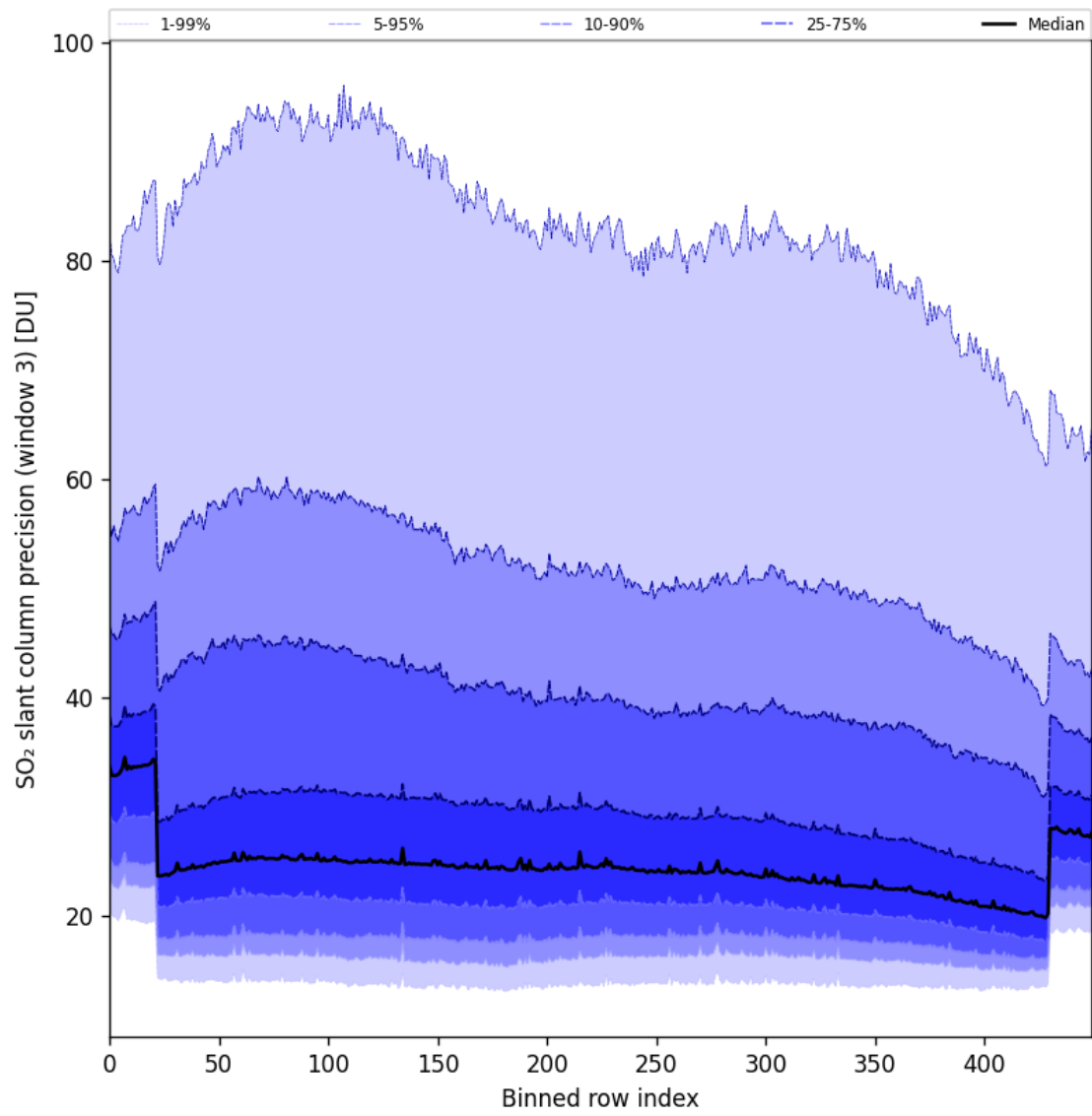
Figure 98: Along track statistics of “SO 2 slant column precision (window 3)” for 2025-04-16 to 2025-04-18
