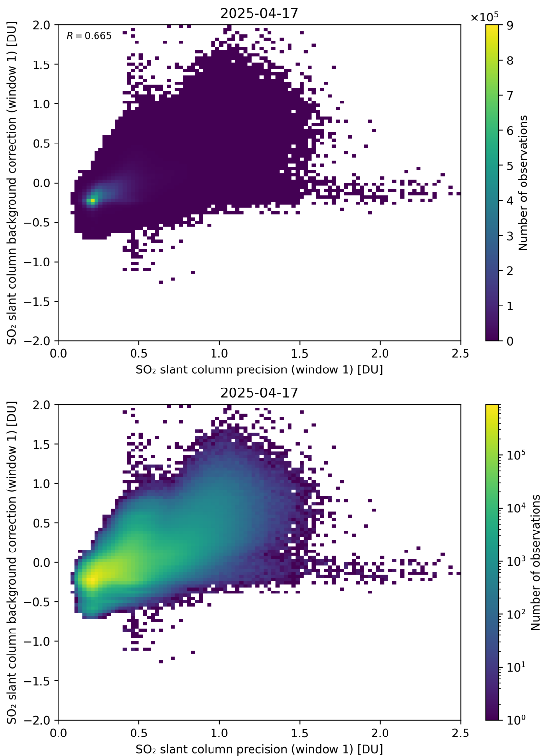
Figure 268: Scatter density plot of “SO 2 slant column precision (window 1)” against “SO 2 slant column background correction (window 1)” for 2025-04-16 to 2025-04-18.
