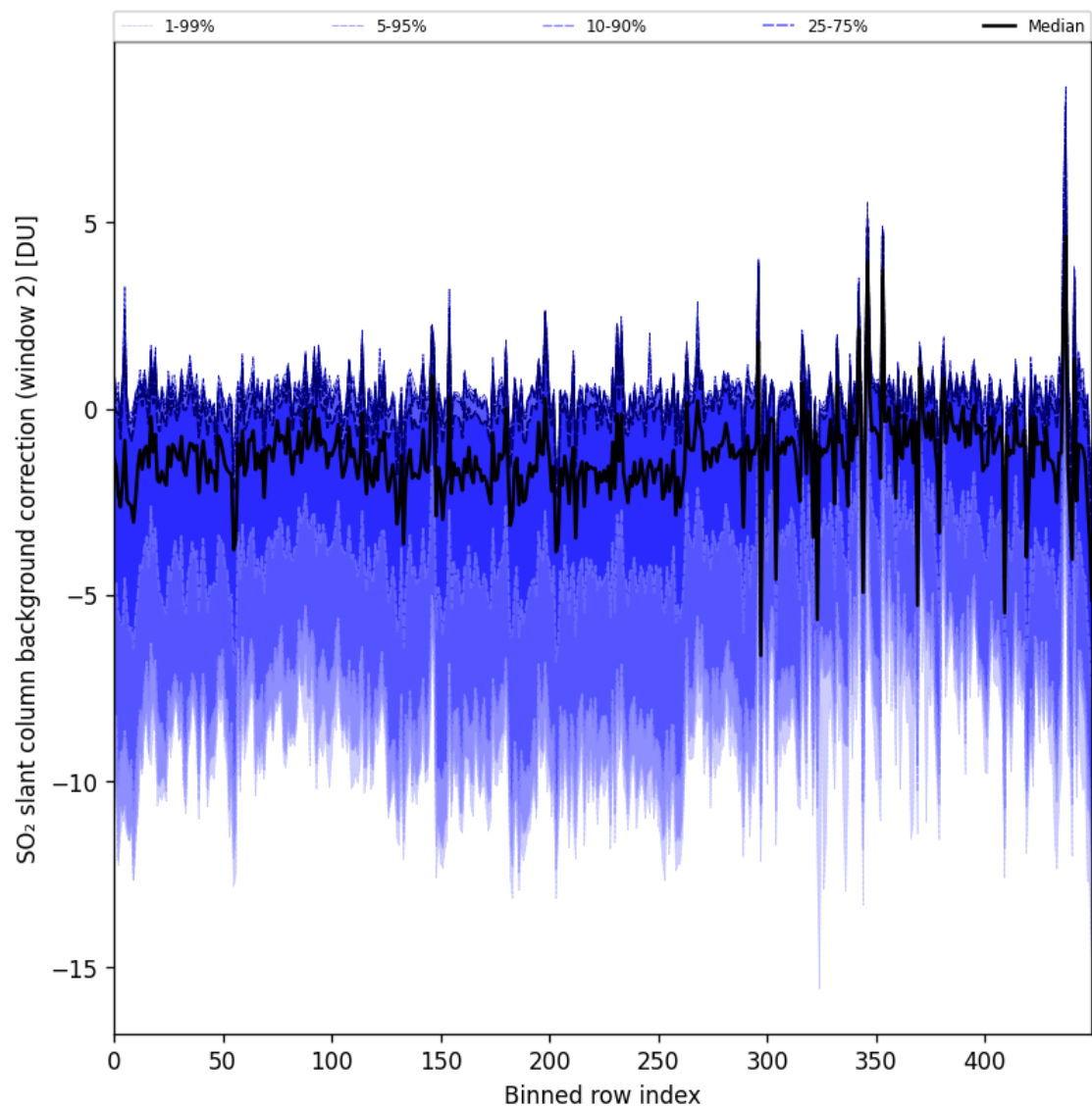
Figure 96: Along track statistics of “SO 2 slant column background correction (window 2)” for 2025-04-16 to 2025-04-18
