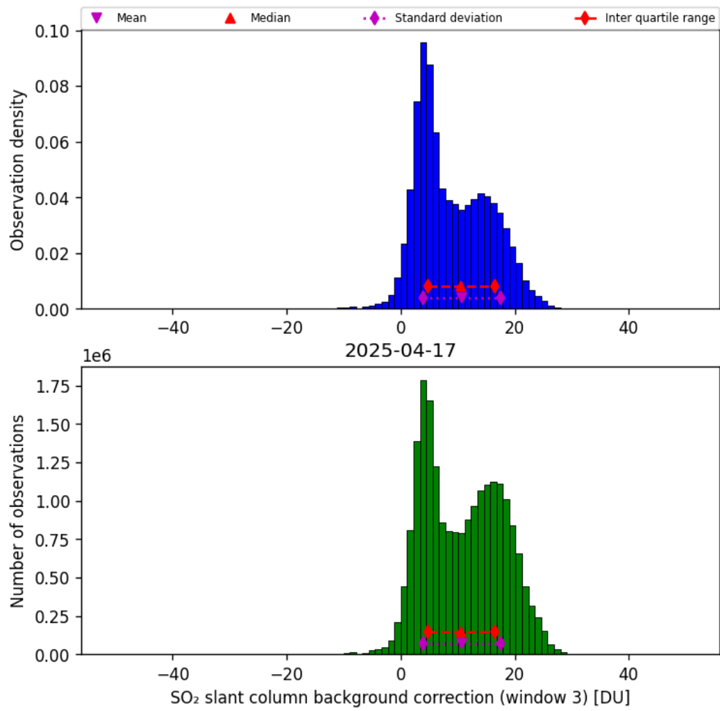
Figure 74: Histogram of “SO 2 slant column background correction (window 3)” for 2025-04-16 to 2025-04-18
