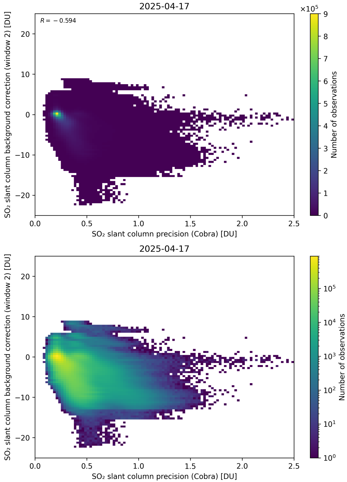
Figure 200: Scatter density plot of “SO 2 slant column precision (Cobra)” against “SO 2 slant column background correction (window 2)” for 2025-04-16 to 2025-04-18.
