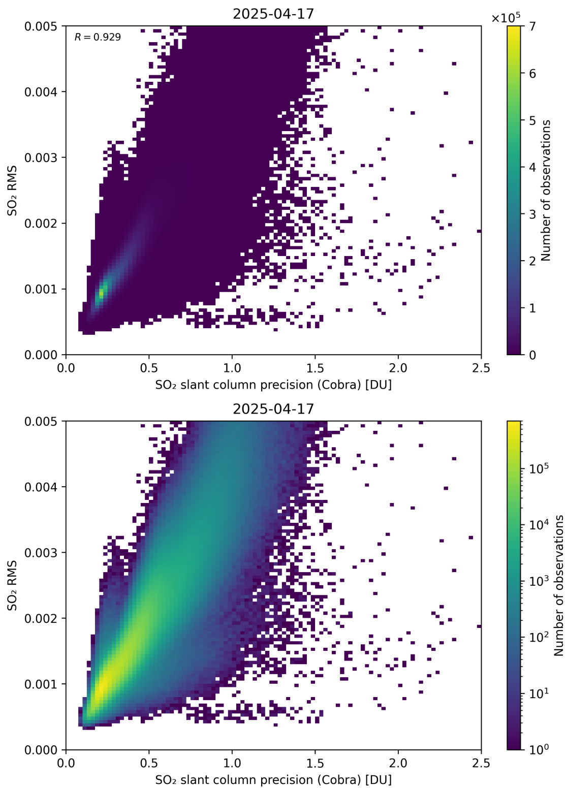
Figure 204: Scatter density plot of “SO 2 slant column precision (Cobra)” against “SO 2 RMS” for 2025-04-16 to 2025-04-18.
