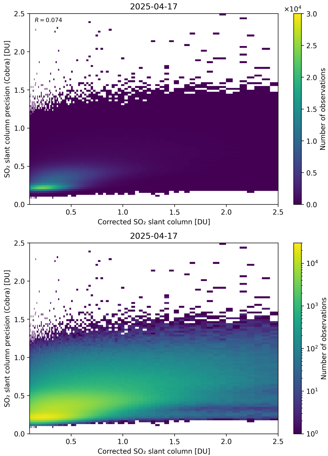
Figure 234: Scatter density plot of “Corrected SO 2 slant column” against “SO 2 slant column precision (Cobra)” for 2025-04-16 to 2025-04-18.
