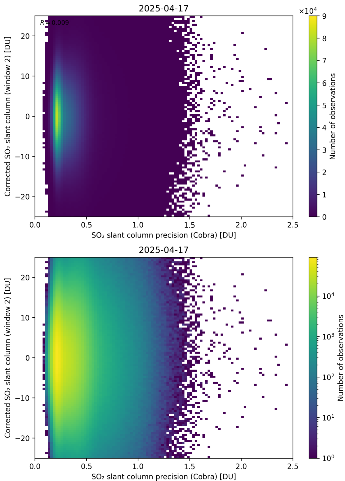
Figure 206: Scatter density plot of “SO 2 slant column precision (Cobra)” against “Corrected SO 2 slant column (window 2)” for 2025-04-16 to 2025-04-18.
