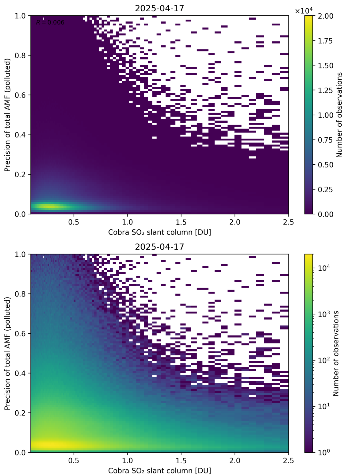
Figure 225: Scatter density plot of “Cobra SO 2 slant column” against “Precision of total AMF (polluted)” for 2025-04-16 to 2025-04-18.
