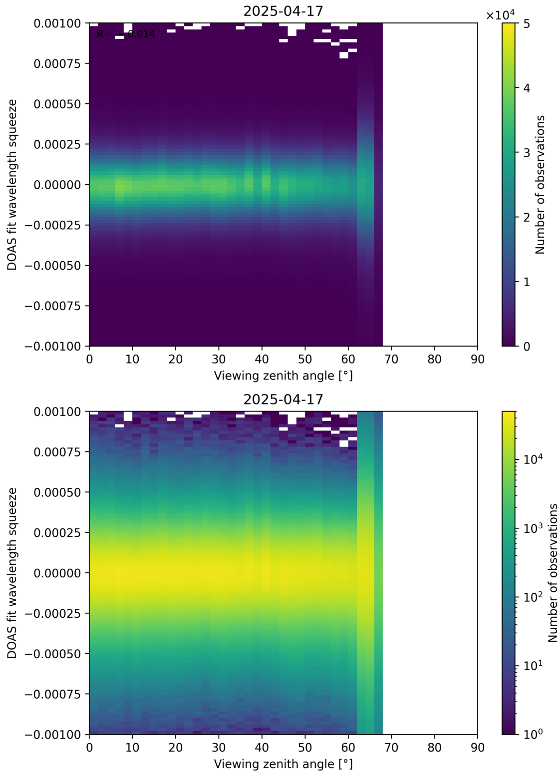
Figure 366: Scatter density plot of “Viewing zenith angle” against “DOAS fit wavelength squeeze” for 2025-04-16 to 2025-04-18.
