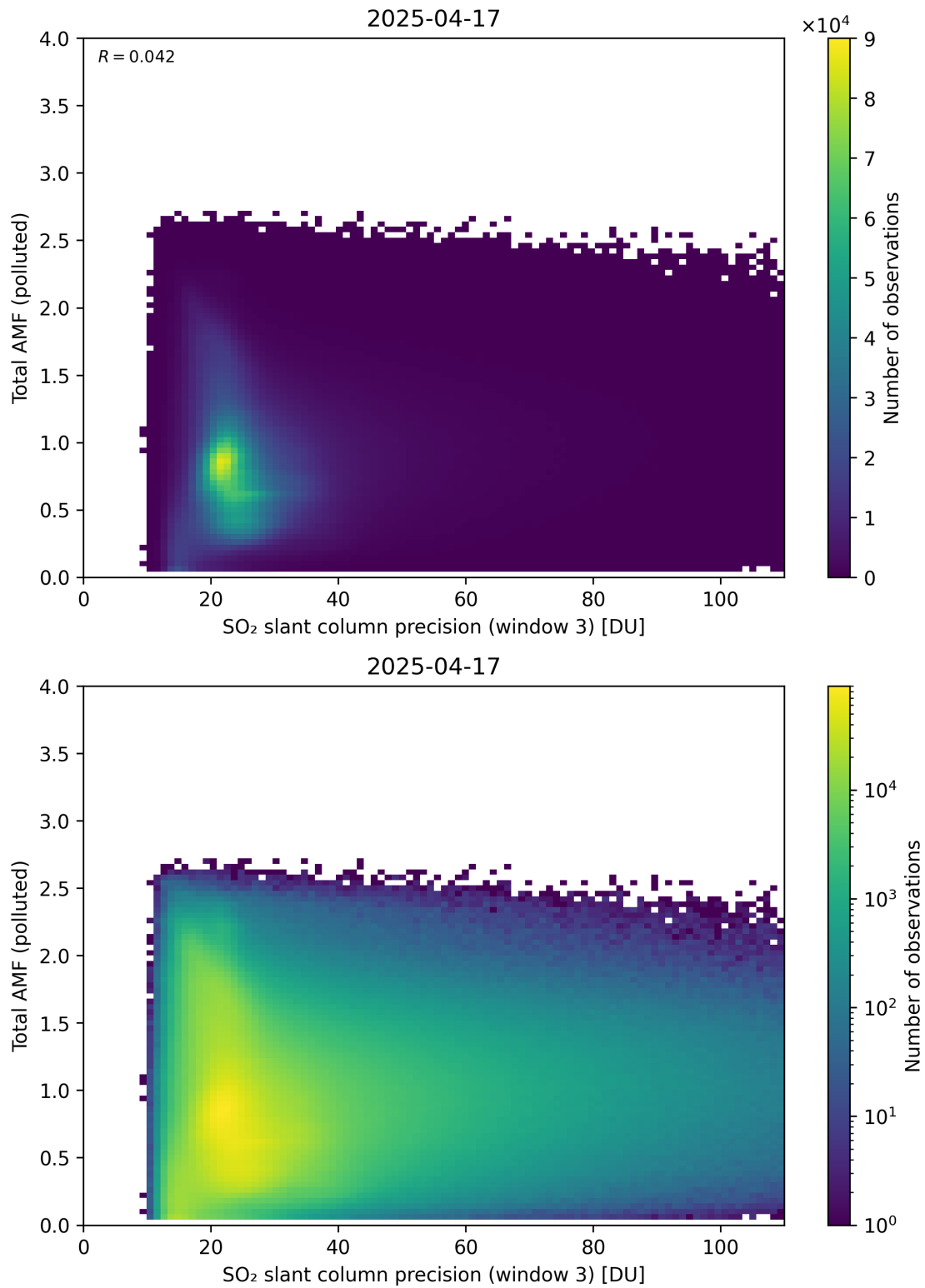
Figure 313: Scatter density plot of “SO 2 slant column precision (window 3)” against “Total AMF (polluted)” for 2025-04-16 to 2025-04-18.
