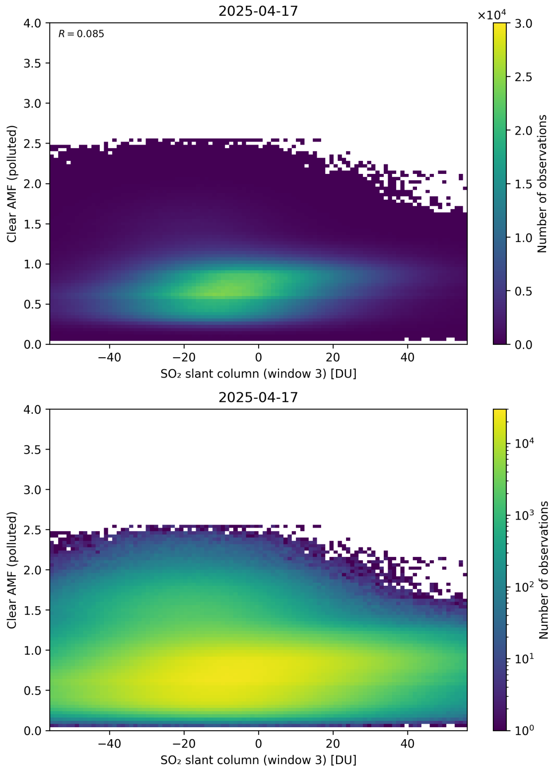
Figure 315: Scatter density plot of “SO 2 slant column (window 3)” against “Clear AMF (polluted)” for 2025-04-16 to 2025-04-18.
