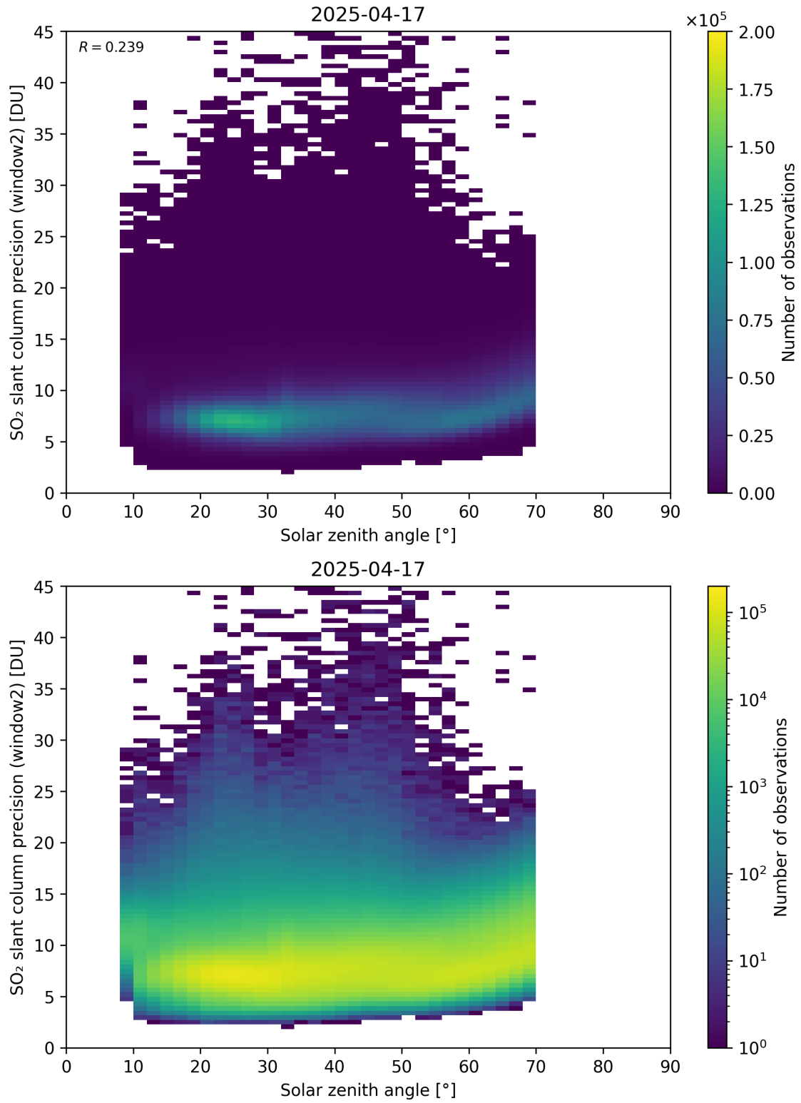
Figure 186: Scatter density plot of “Solar zenith angle” against “SO 2 slant column precision (window2)” for 2025-04-16 to 2025-04-18.
