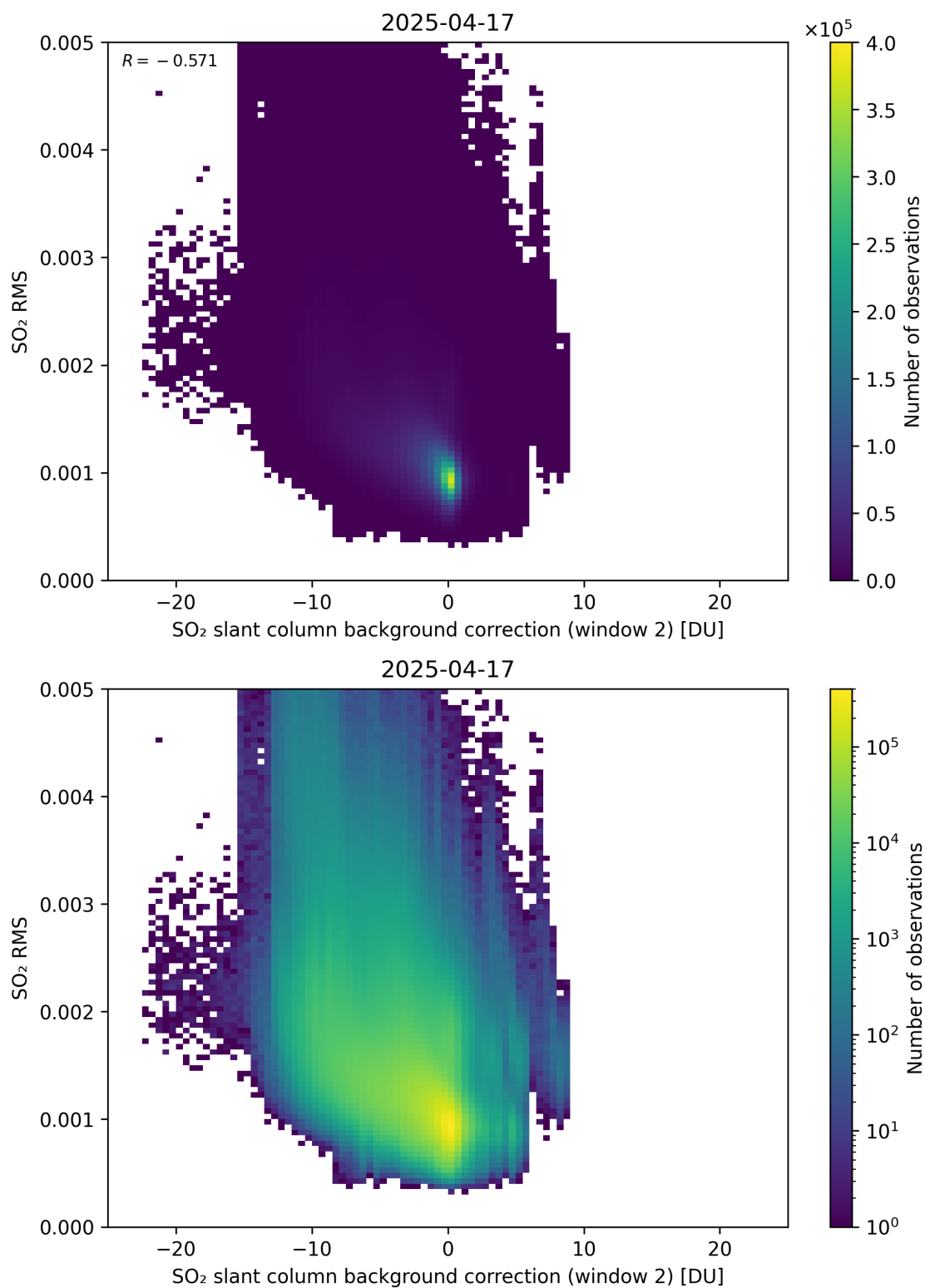
Figure 125: Scatter density plot of “SO 2 slant column background correction (window 2)” against “SO 2 RMS” for 2025-04-16 to 2025-04-18.
