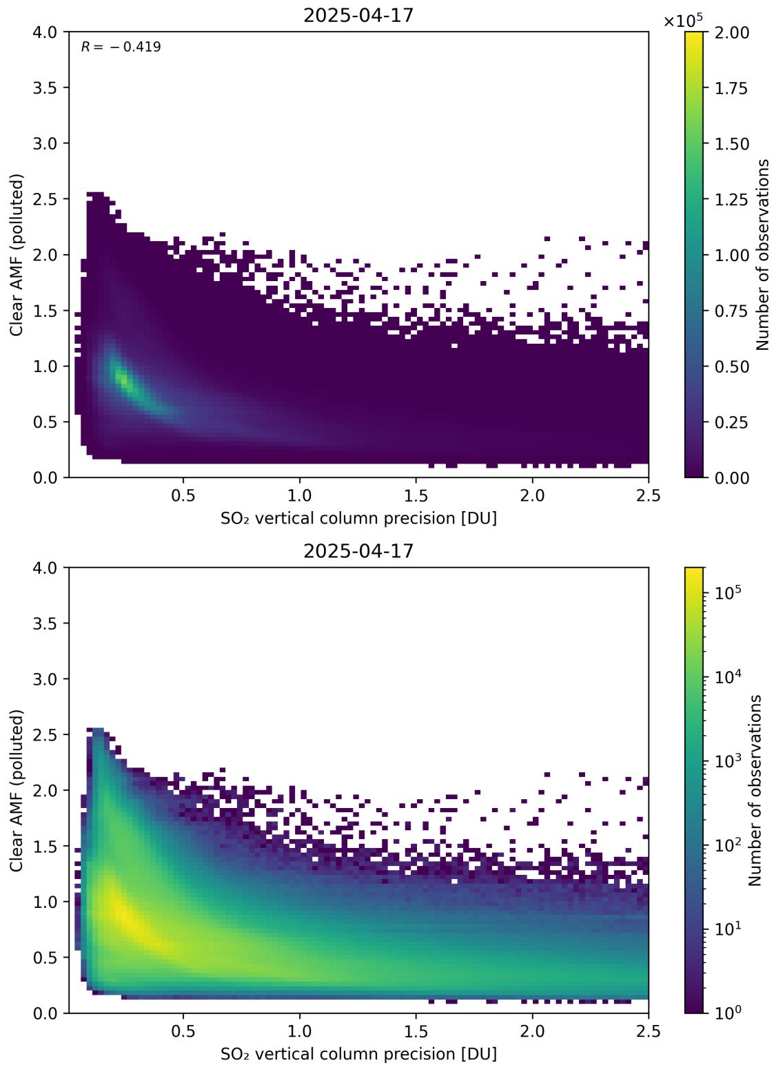
Figure 335: Scatter density plot of “SO 2 vertical column precision” against “Clear AMF (polluted)” for 2025-04-16 to 2025-04-18.
