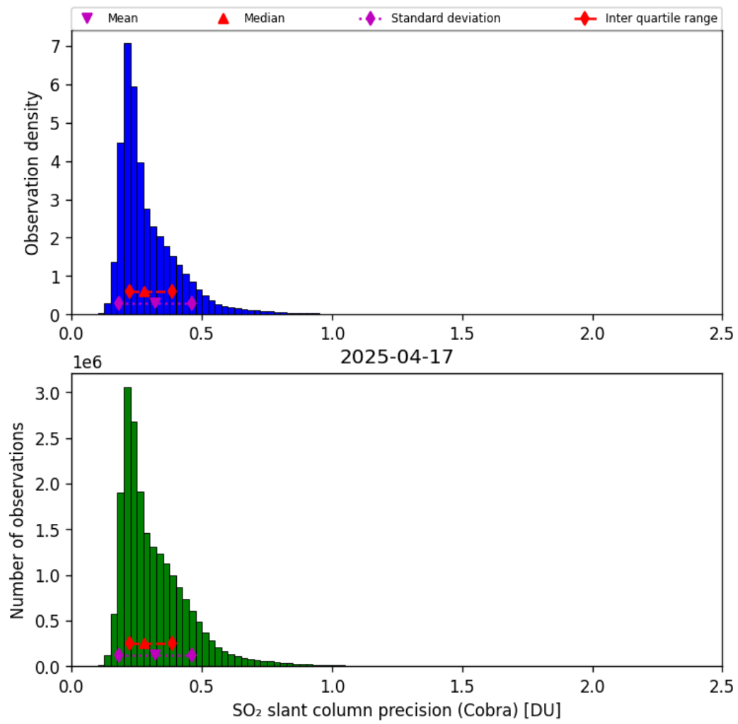
Figure 62: Histogram of “SO 2 slant column precision (Cobra)” for 2025-04-16 to 2025-04-18
