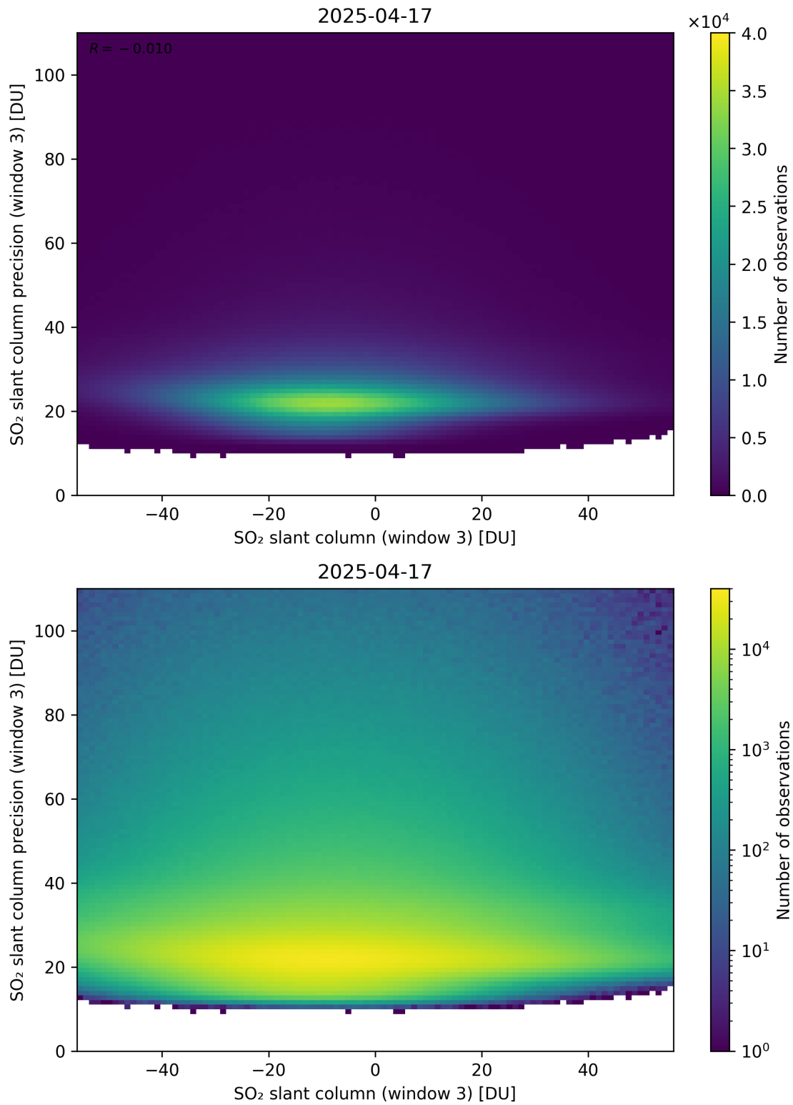
Figure 317: Scatter density plot of “SO 2 slant column (window 3)” against “SO 2 slant column precision (window 3)” for 2025-04-16 to 2025-04-18.
