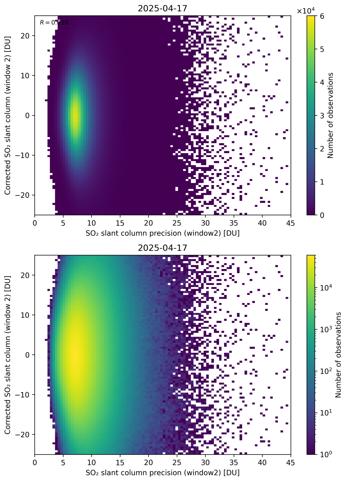
Figure 297: Scatter density plot of “SO 2 slant column precision (window2)” against “Corrected SO 2 slant column (window 2)” for 2025-04-16 to 2025-04-18.
