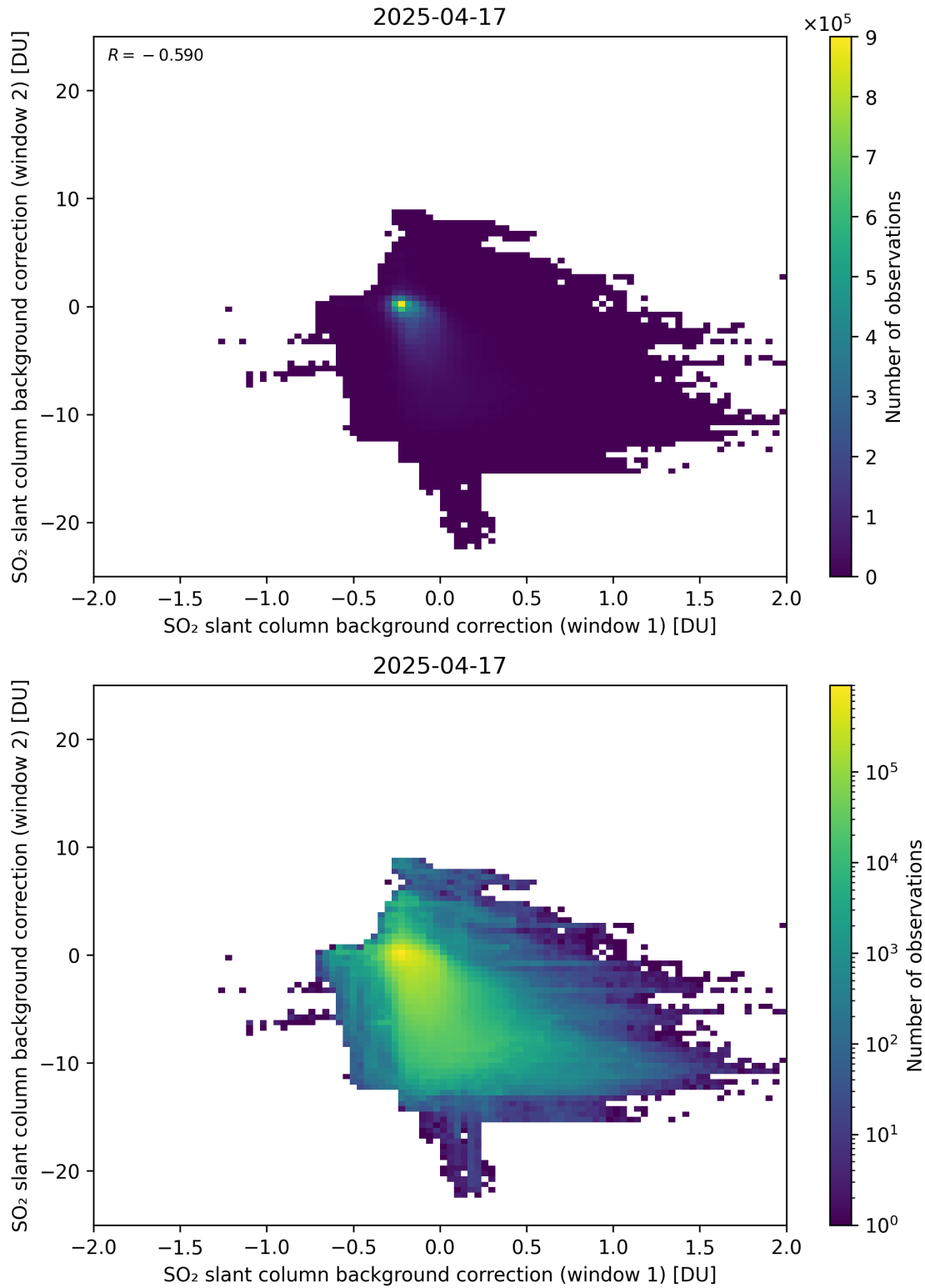
Figure 109: Scatter density plot of “SO 2 slant column background correction (window 1)” against “SO 2 slant column background correction (window 2)” for 2025-04-16 to 2025-04-18.
