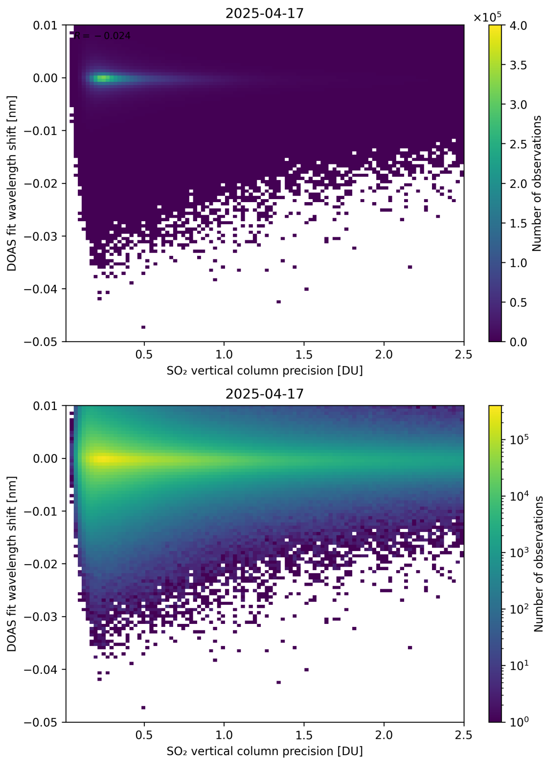
Figure 332: Scatter density plot of “SO 2 vertical column precision” against “DOAS fit wavelength shift” for 2025-04-16 to 2025-04-18.
