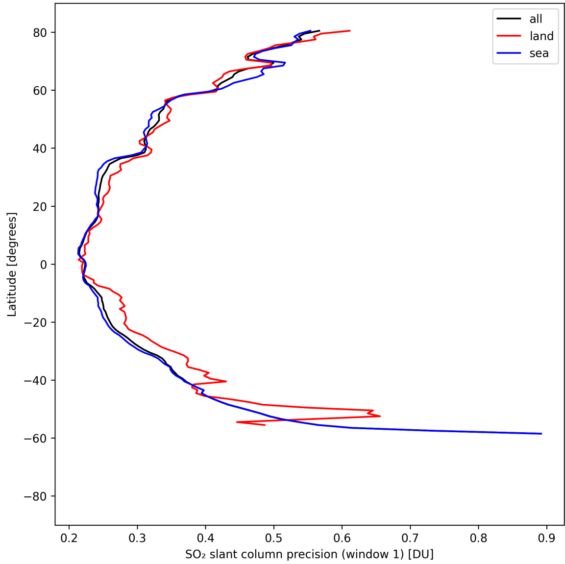
Figure 38: Zonal average of “SO 2 slant column precision (window 1)” for 2025-04-16 to 2025-04-18.
