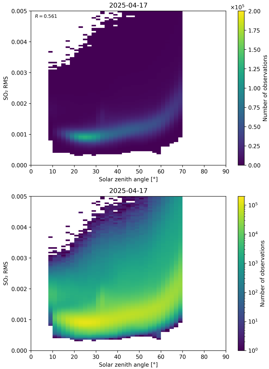
Figure 176: Scatter density plot of “Solar zenith angle” against “SO 2 RMS” for 2025-04-16 to 2025-04-18.
