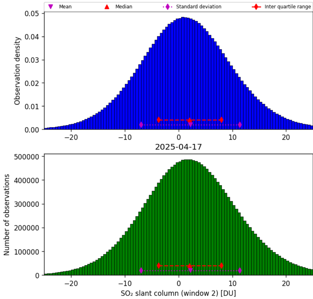
Figure 67: Histogram of “SO 2 slant column (window 2)” for 2025-04-16 to 2025-04-18
