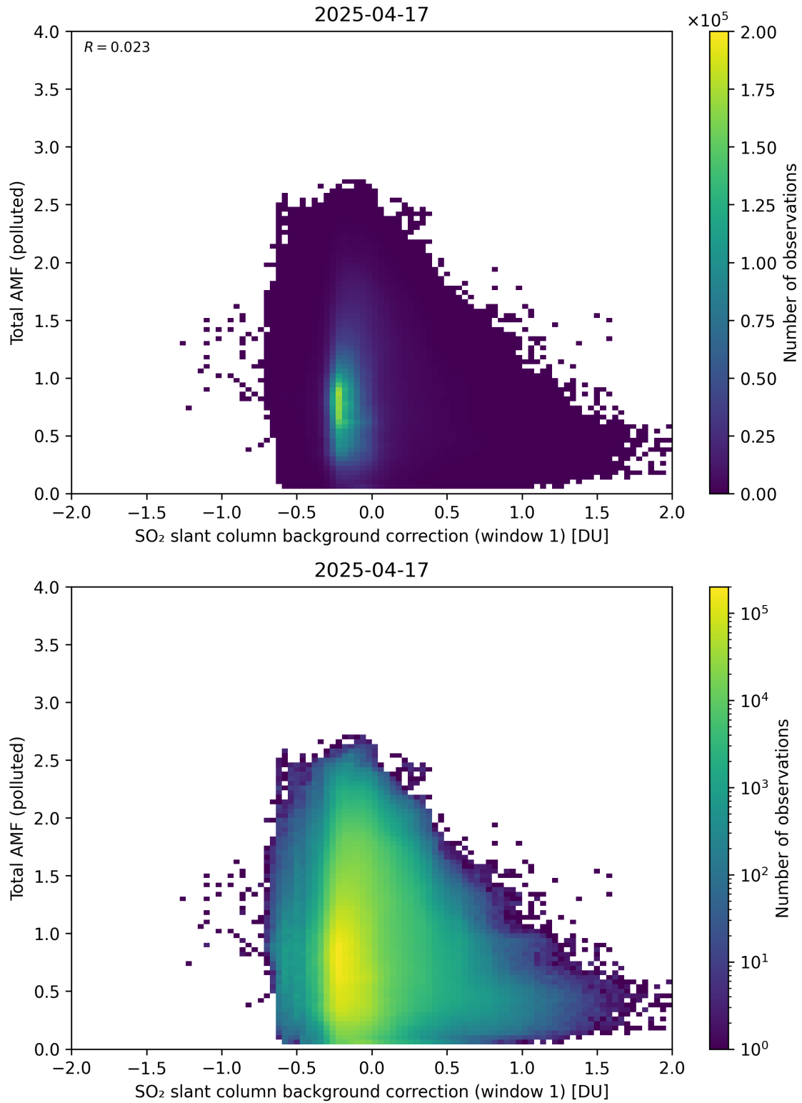
Figure 120: Scatter density plot of “SO 2 slant column background correction (window 1)” against “Total AMF (polluted)” for 2025-04-16 to 2025-04-18.
