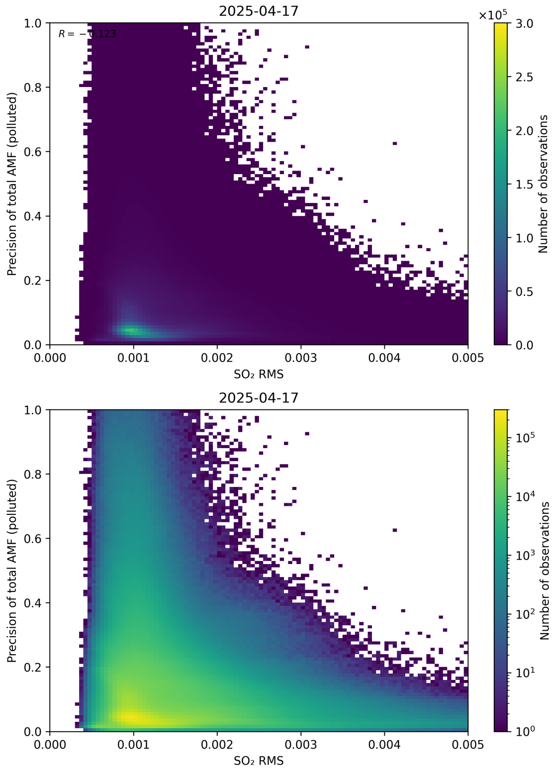
Figure 149: Scatter density plot of “SO 2 RMS” against “Precision of total AMF (polluted)” for 2025-04-16 to 2025-04-18.
