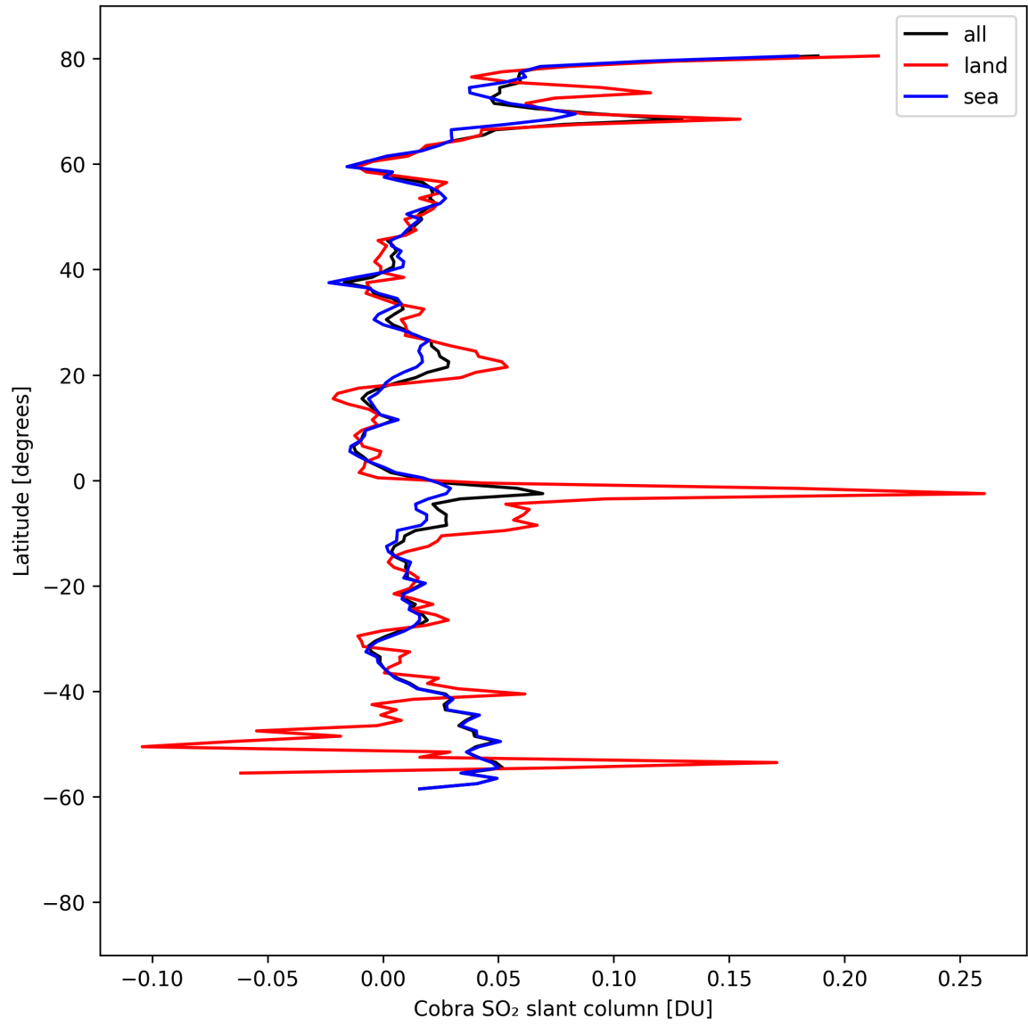
Figure 35: Zonal average of “Cobra SO 2 slant column” for 2025-04-16 to 2025-04-18.
