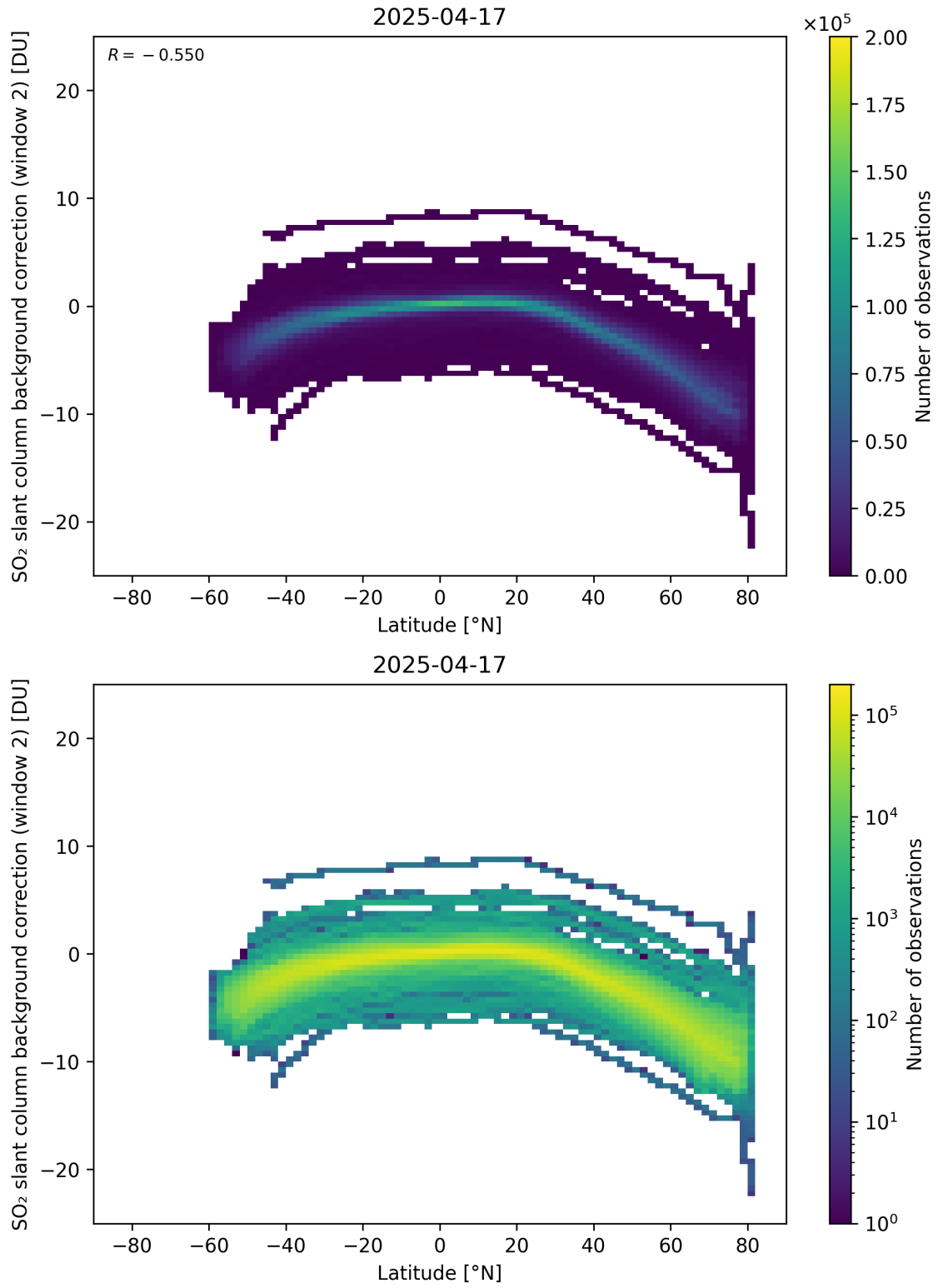
Figure 151: Scatter density plot of “Latitude” against “SO 2 slant column background correction (window 2)” for 2025-04-16 to 2025-04-18.
