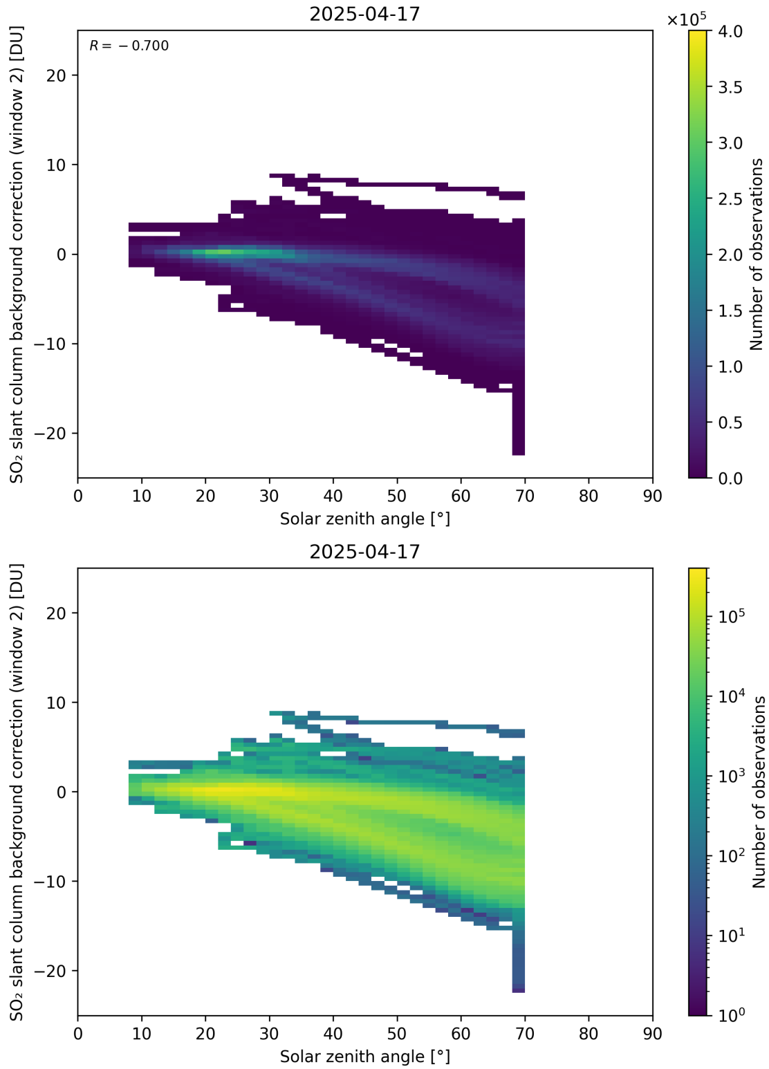
Figure 172: Scatter density plot of “Solar zenith angle” against “SO 2 slant column background correction (window 2)” for 2025-04-16 to 2025-04-18.
