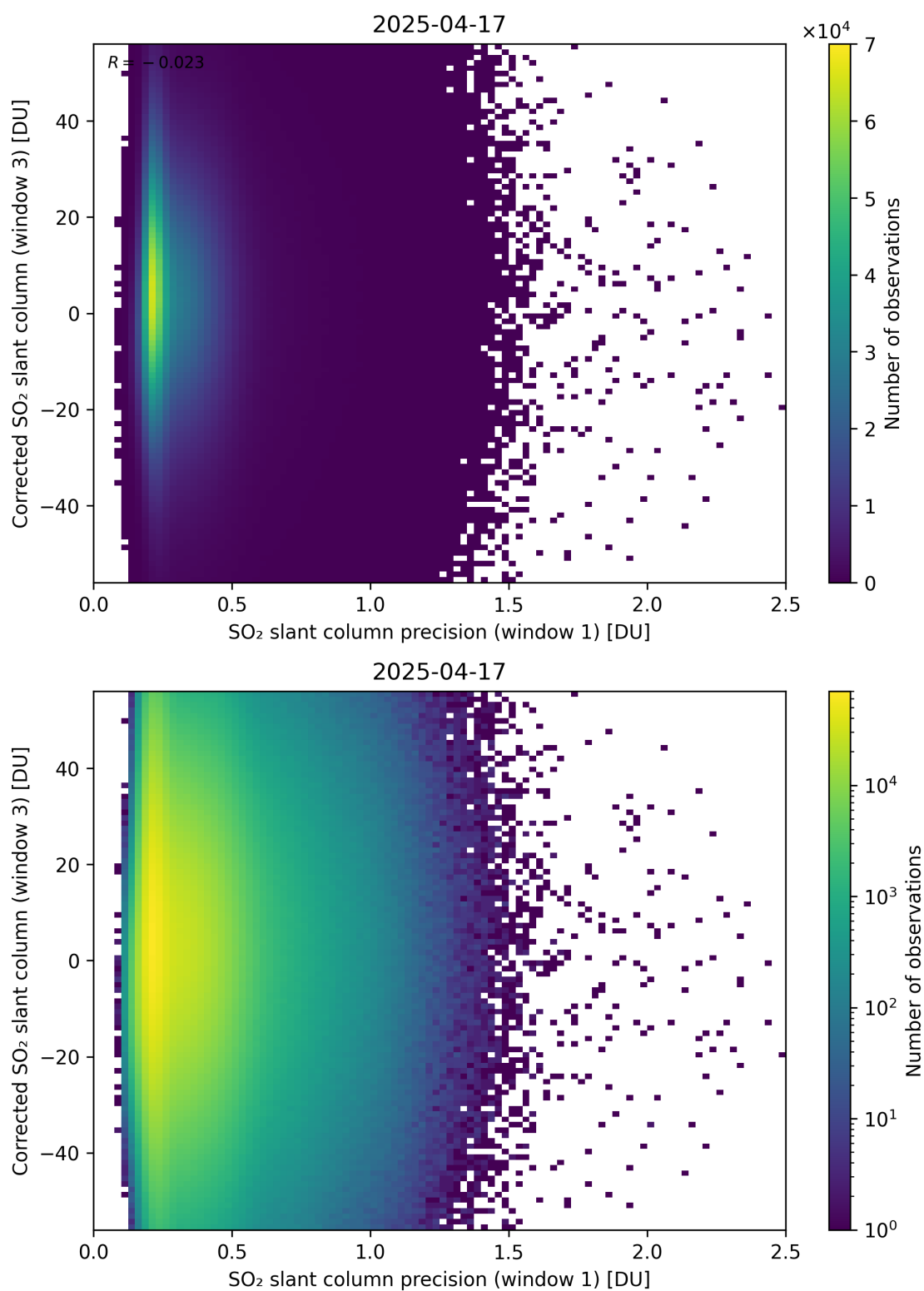
Figure 276: Scatter density plot of “SO 2 slant column precision (window 1)” against “Corrected SO 2 slant column (window 3)” for 2025-04-16 to 2025-04-18.
