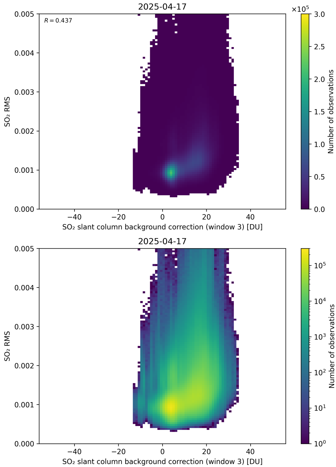
Figure 134: Scatter density plot of “SO 2 slant column background correction (window 3)” against “SO 2 RMS” for 2025-04-16 to 2025-04-18.
