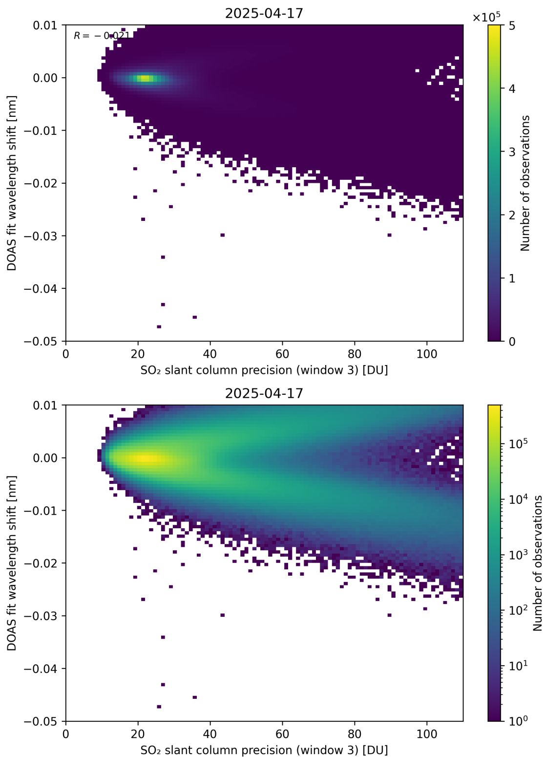
Figure 308: Scatter density plot of “SO 2 slant column precision (window 3)” against “DOAS fit wavelength shift” for 2025-04-16 to 2025-04-18.
