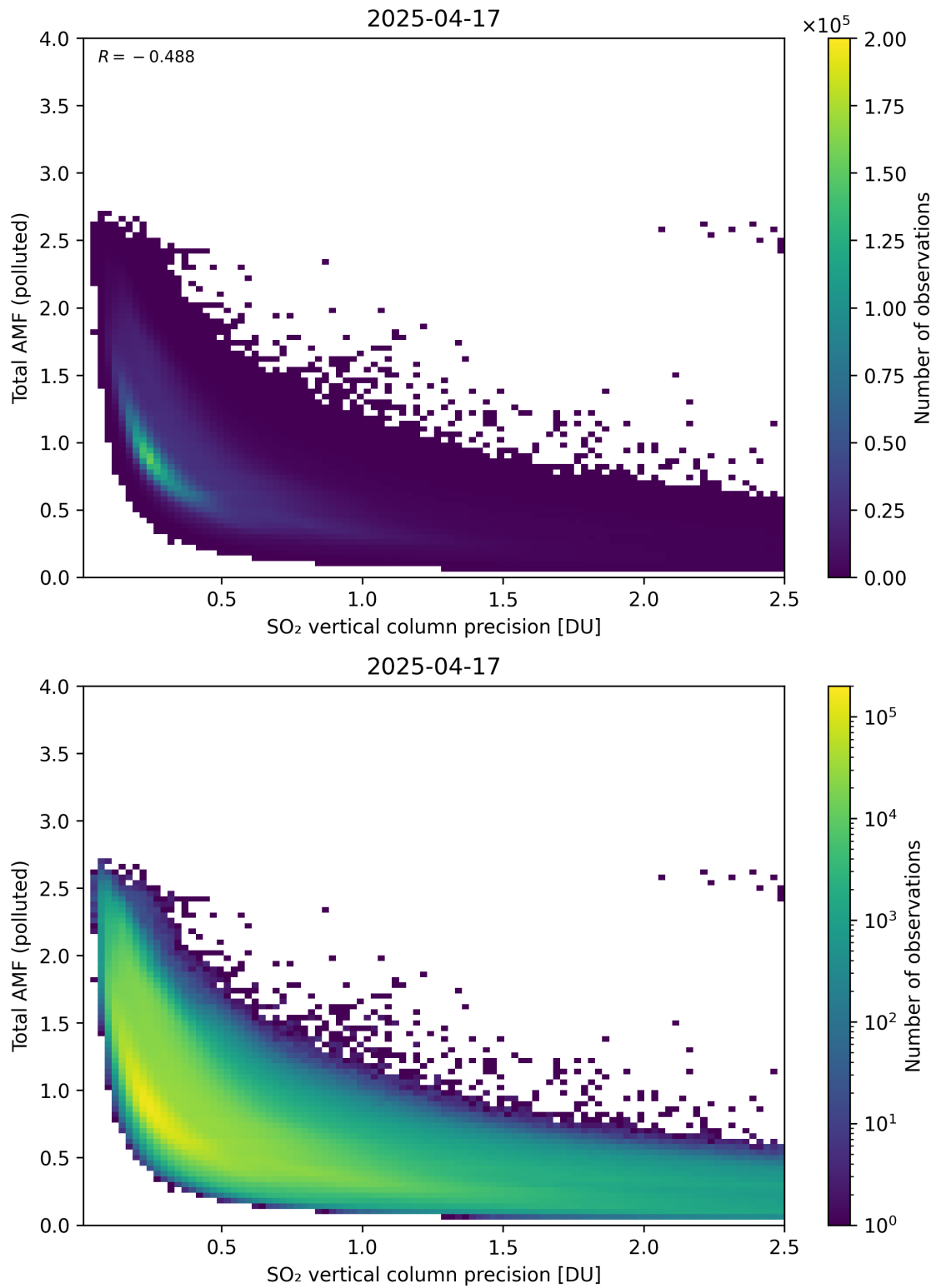
Figure 346: Scatter density plot of “SO 2 vertical column precision” against “Total AMF (polluted)” for 2025-04-16 to 2025-04-18.
