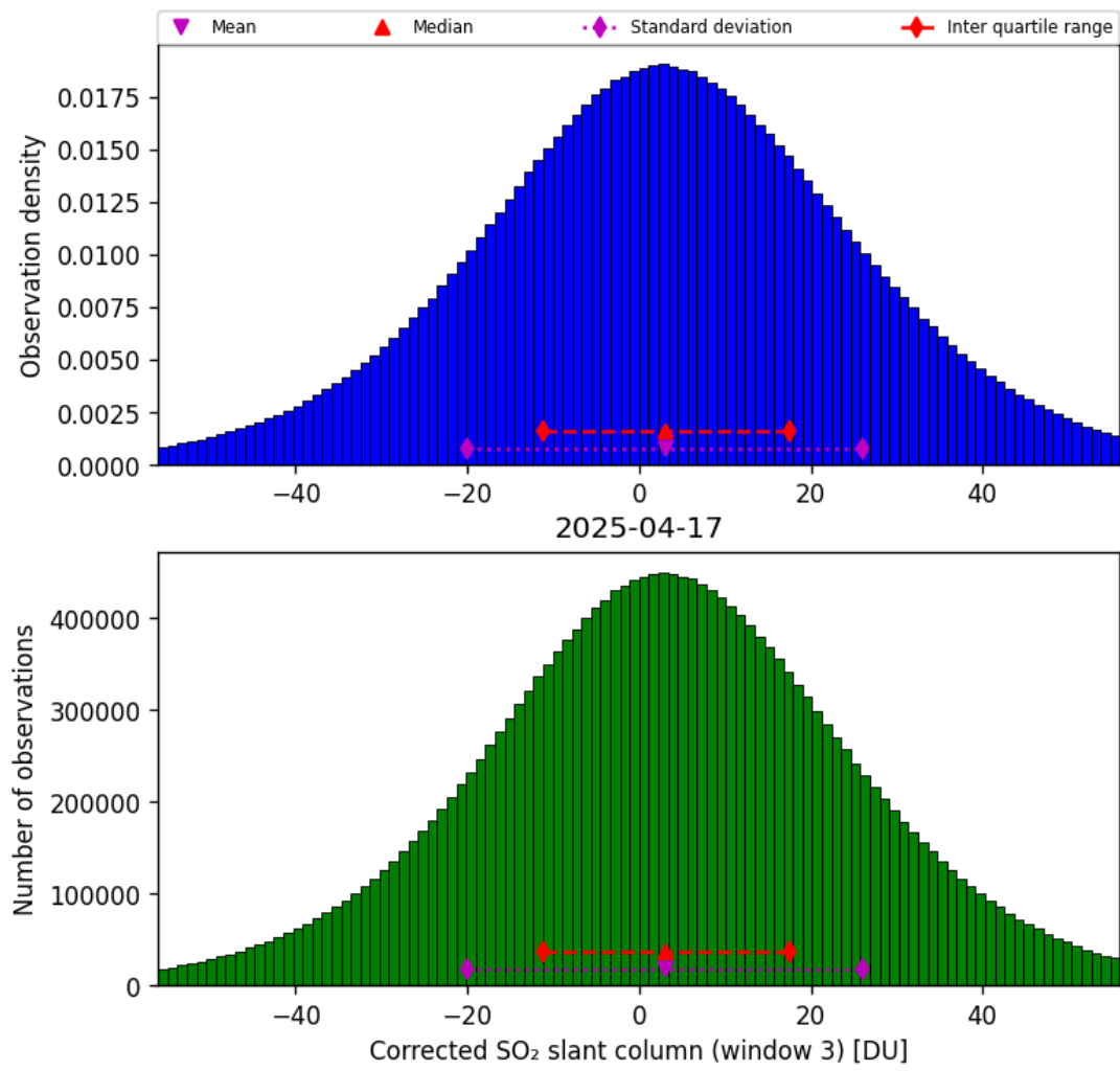
Figure 73: Histogram of “Corrected SO 2 slant column (window 3)” for 2025-04-16 to 2025-04-18
