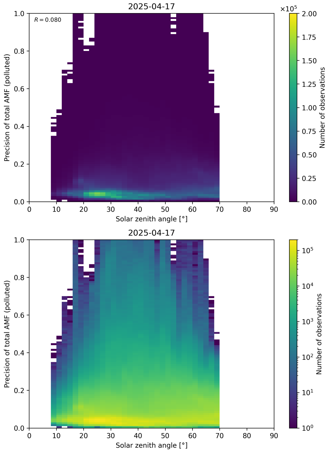
Figure 190: Scatter density plot of “Solar zenith angle” against “Precision of total AMF (polluted)” for 2025-04-16 to 2025-04-18.
