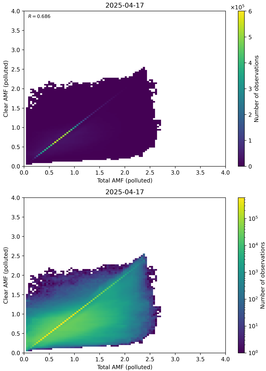
Figure 321: Scatter density plot of “Total AMF (polluted)” against “Clear AMF (polluted)” for 2025-04-16 to 2025-04-18.
