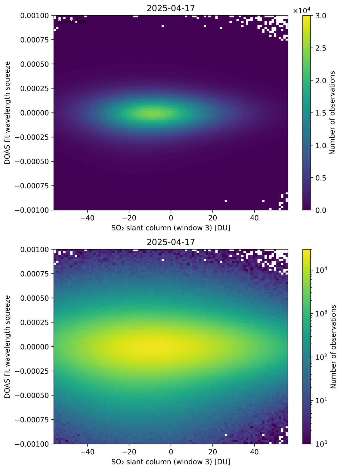
Figure 305: Scatter density plot of “SO 2 slant column (window 3)” against “DOAS fit wavelength squeeze” for 2025-04-16 to 2025-04-18.
