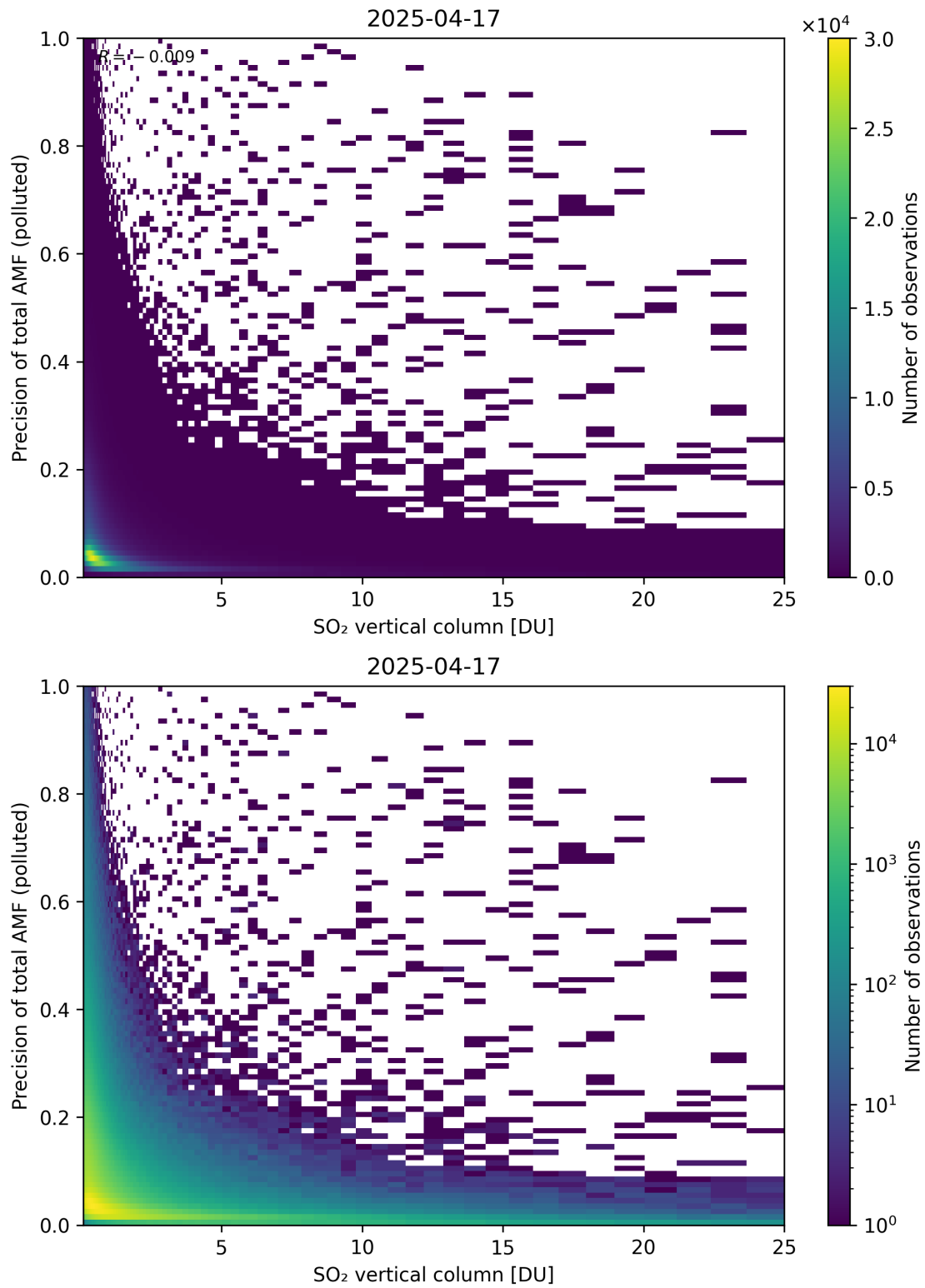
Figure 360: Scatter density plot of “SO 2 vertical column” against “Precision of total AMF (polluted)” for 2025-04-16 to 2025-04-18.
