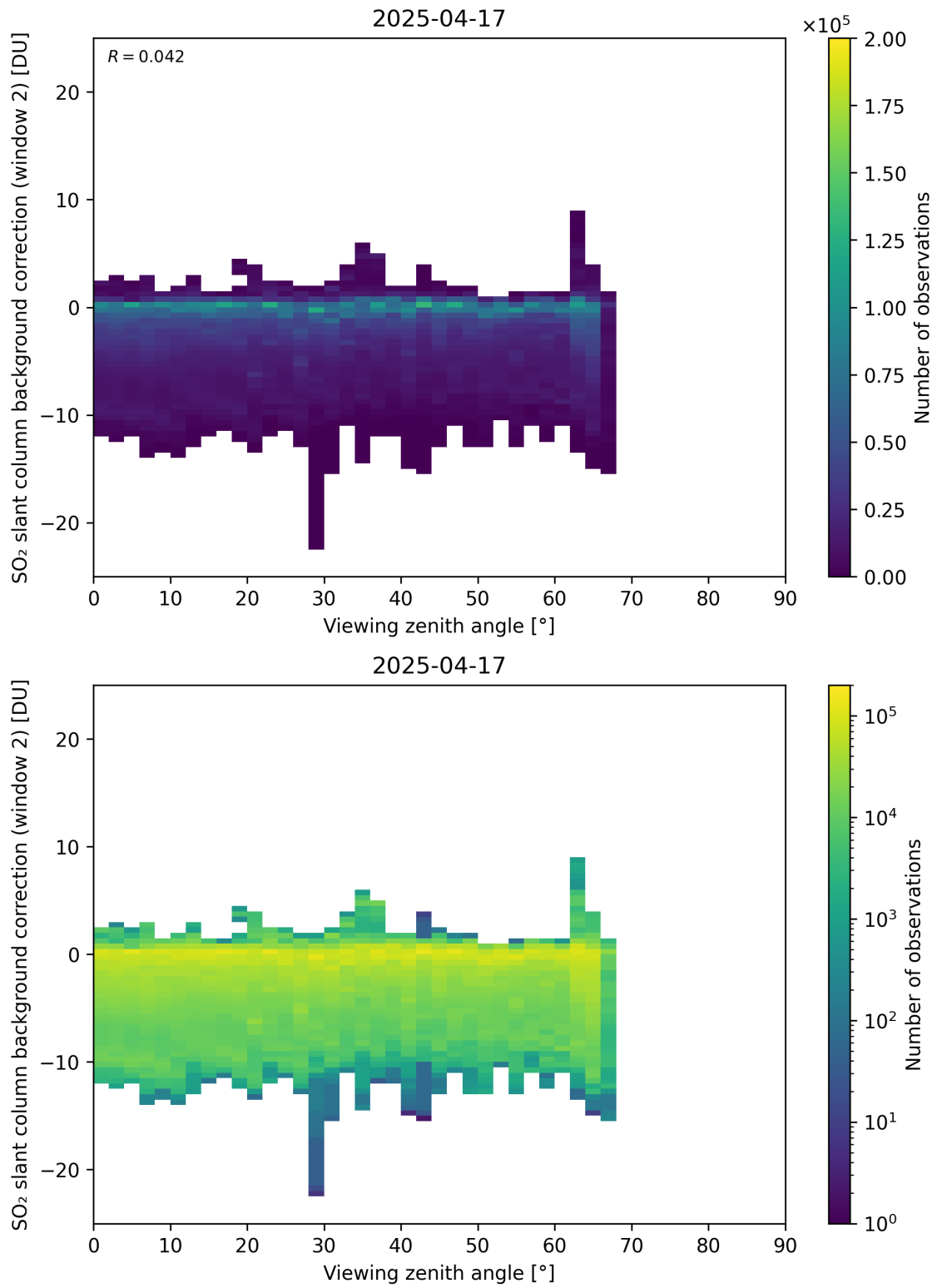
Figure 363: Scatter density plot of “Viewing zenith angle” against “SO 2 slant column background correction (window 2)” for 2025-04-16 to 2025-04-18.
