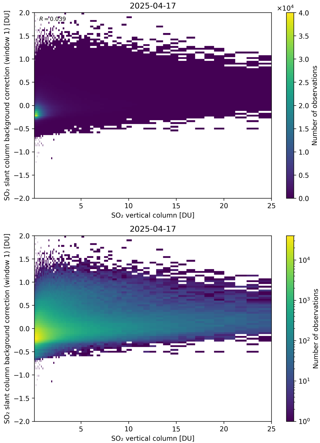
Figure 323: Scatter density plot of “SO 2 vertical column” against “SO 2 slant column background correction (window 1)” for 2025-04-16 to 2025-04-18.
