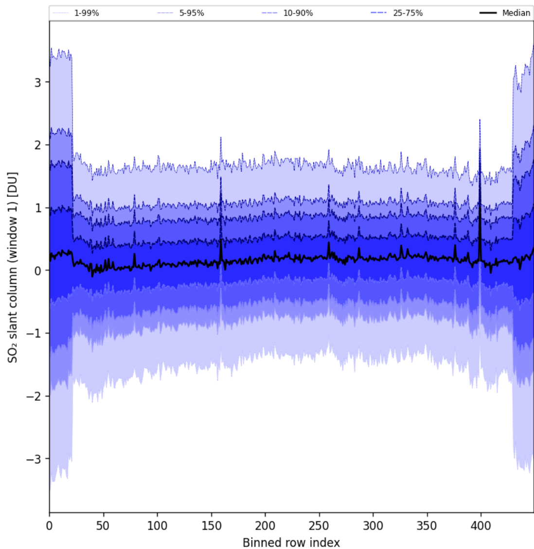
Figure 89: Along track statistics of “SO 2 slant column (window 1)” for 2025-04-16 to 2025-04-18
