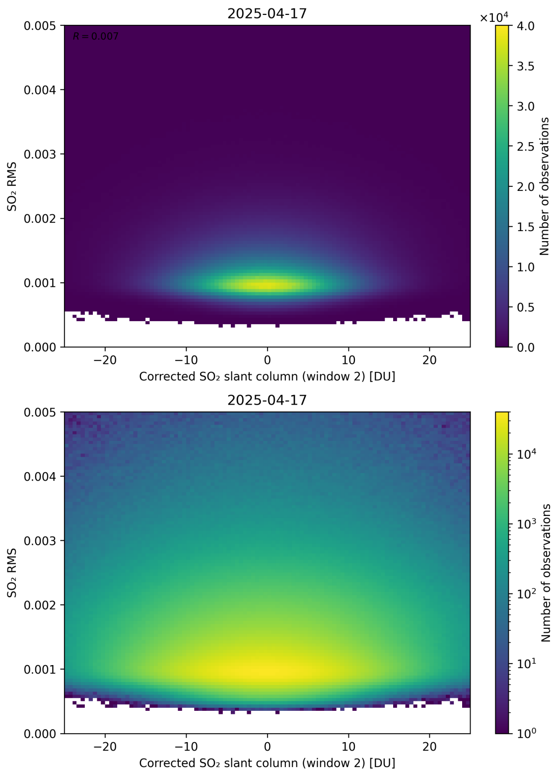
Figure 248: Scatter density plot of “Corrected SO 2 slant column (window 2)” against “SO 2 RMS” for 2025-04-16 to 2025-04-18.
