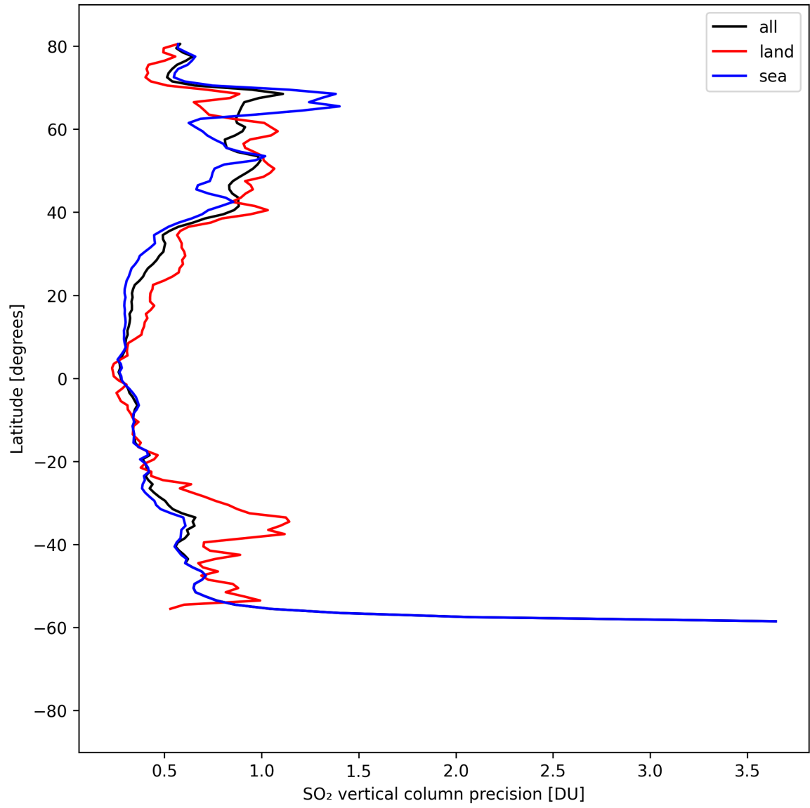
Figure 33: Zonal average of “SO 2 vertical column precision” for 2025-04-16 to 2025-04-18.
