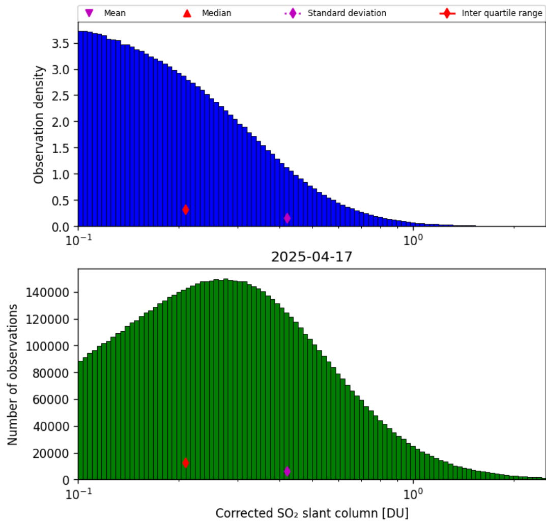
Figure 60: Histogram of “Corrected SO 2 slant column” for 2025-04-16 to 2025-04-18
