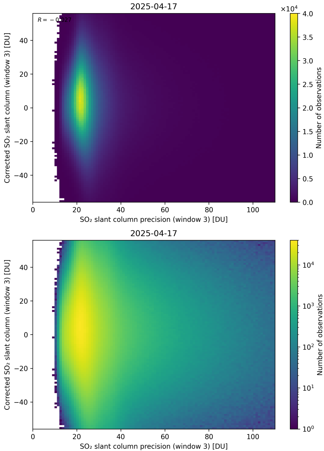
Figure 312: Scatter density plot of “SO 2 slant column precision (window 3)” against “Corrected SO 2 slant column (window 3)” for 2025-04-16 to 2025-04-18.
