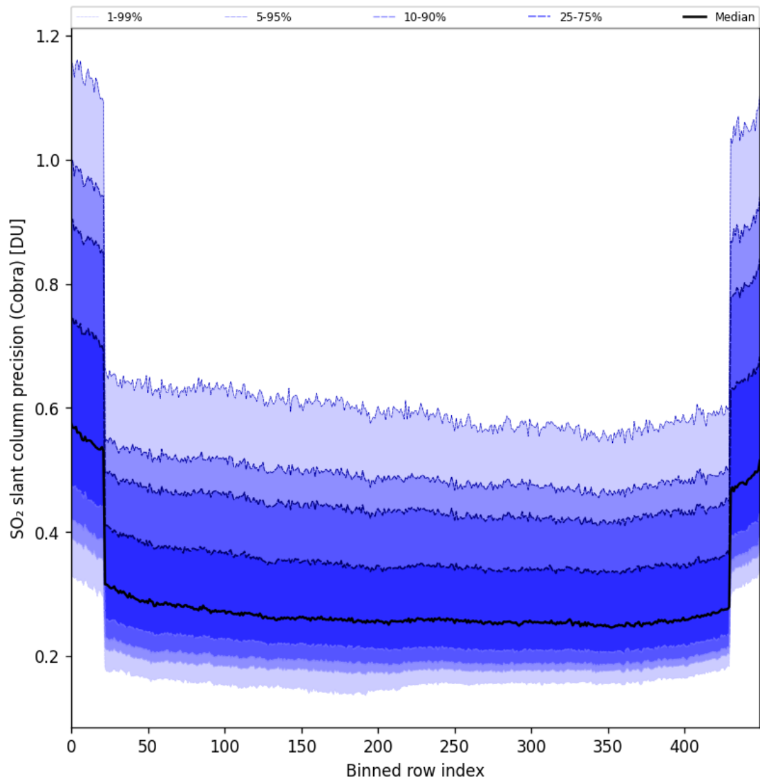
Figure 88: Along track statistics of “SO 2 slant column precision (Cobra)” for 2025-04-16 to 2025-04-18
