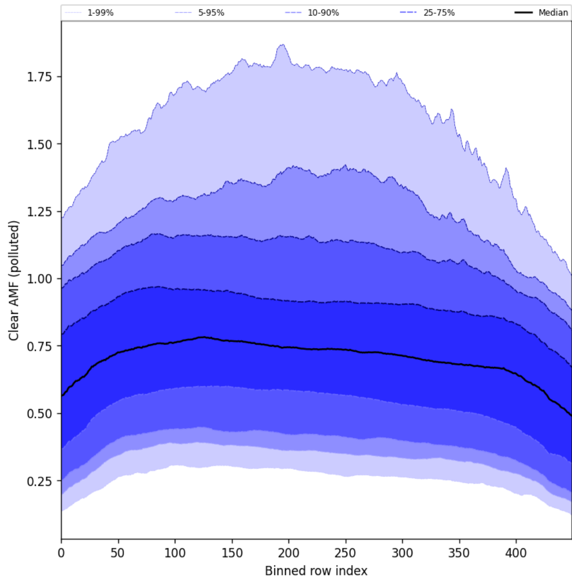
Figure 107: Along track statistics of “Clear AMF (polluted)” for 2025-04-16 to 2025-04-18
