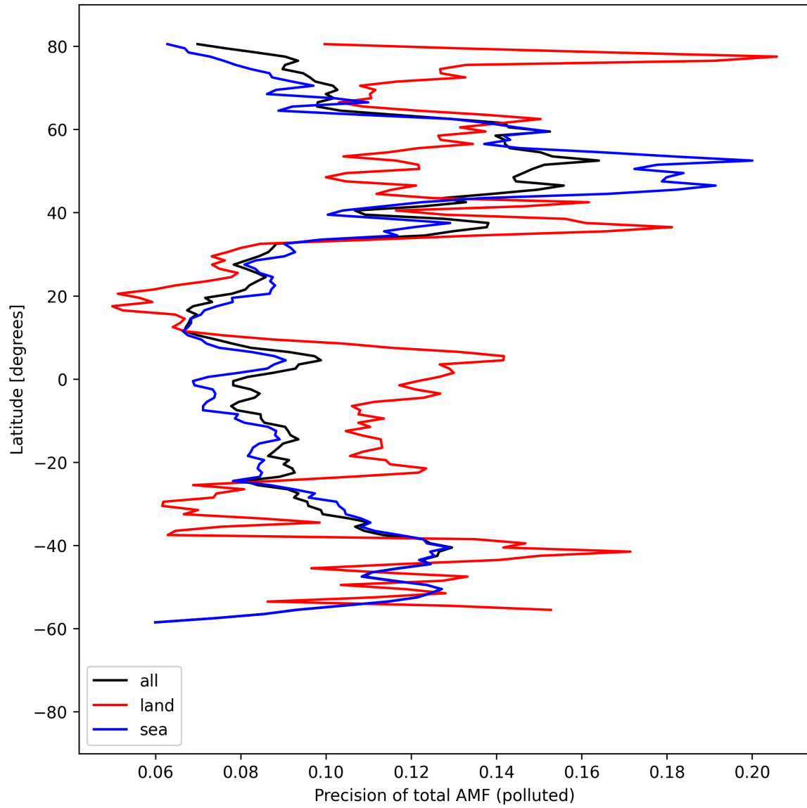
Figure 54: Zonal average of “Precision of total AMF (polluted)” for 2025-04-16 to 2025-04-18.
