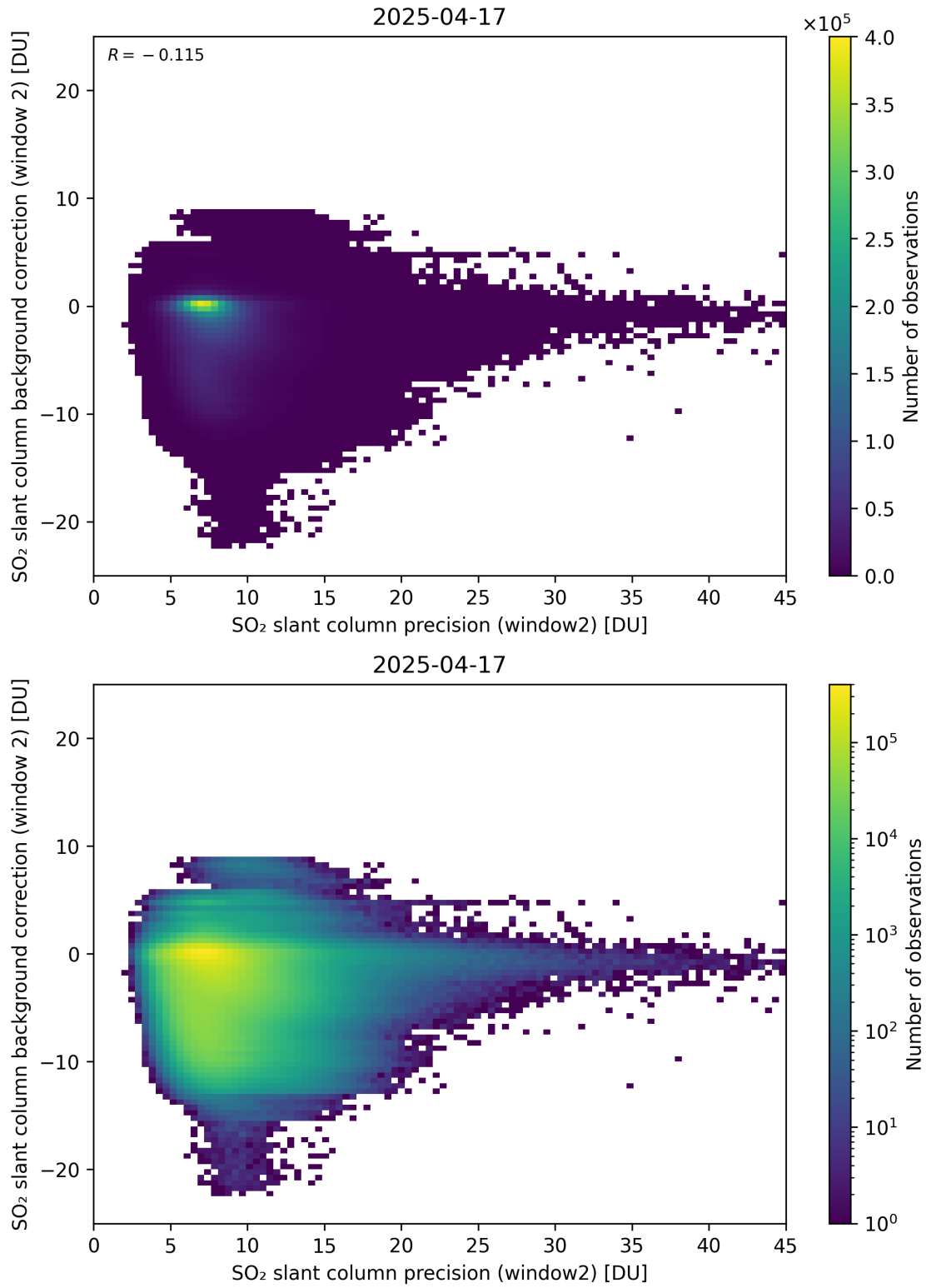
Figure 291: Scatter density plot of “SO 2 slant column precision (window2)” against “SO 2 slant column background correction (window 2)” for 2025-04-16 to 2025-04-18.
