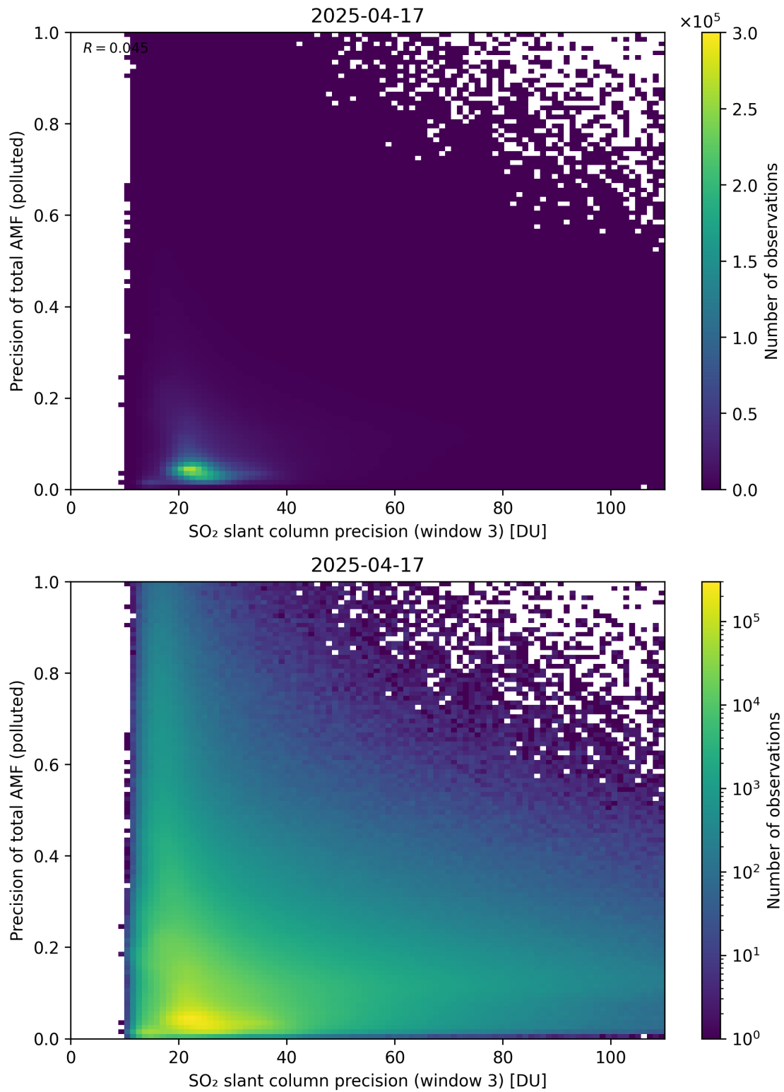
Figure 314: Scatter density plot of “SO 2 slant column precision (window 3)” against “Precision of total AMF (polluted)” for 2025-04-16 to 2025-04-18.
