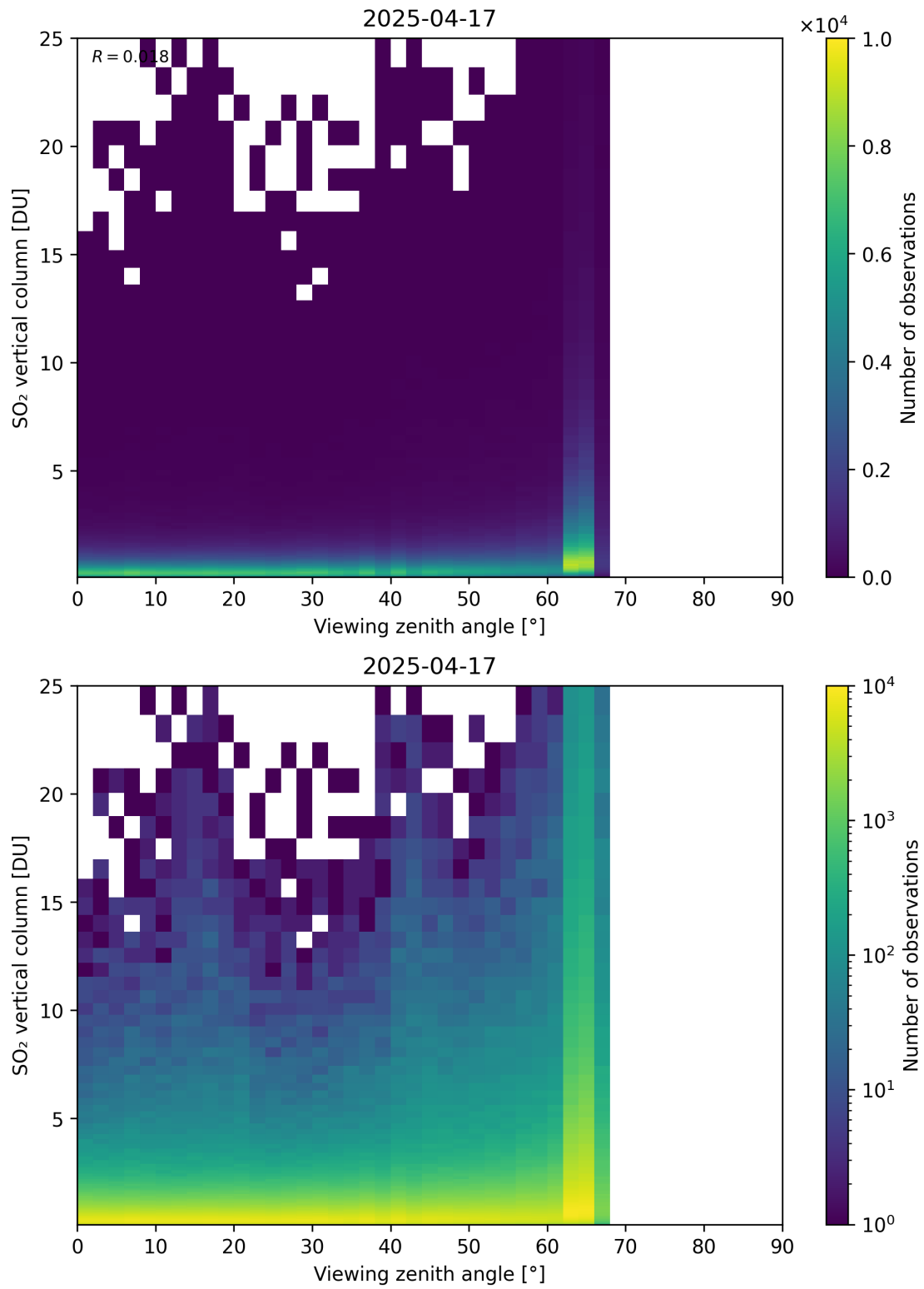
Figure 383: Scatter density plot of “Viewing zenith angle” against “SO 2 vertical column” for 2025-04-16 to 2025-04-18.
