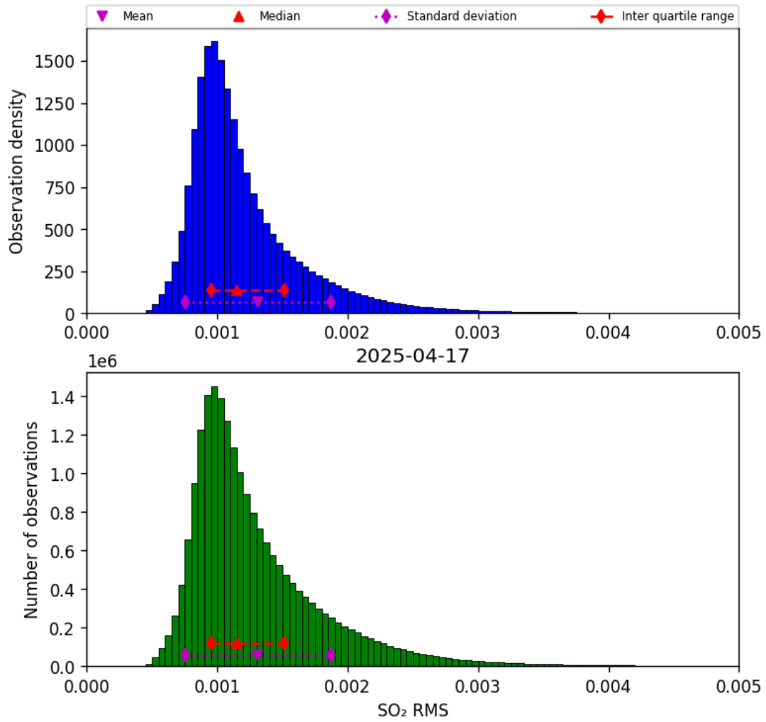
Figure 78: Histogram of “SO 2 RMS” for 2025-04-16 to 2025-04-18
