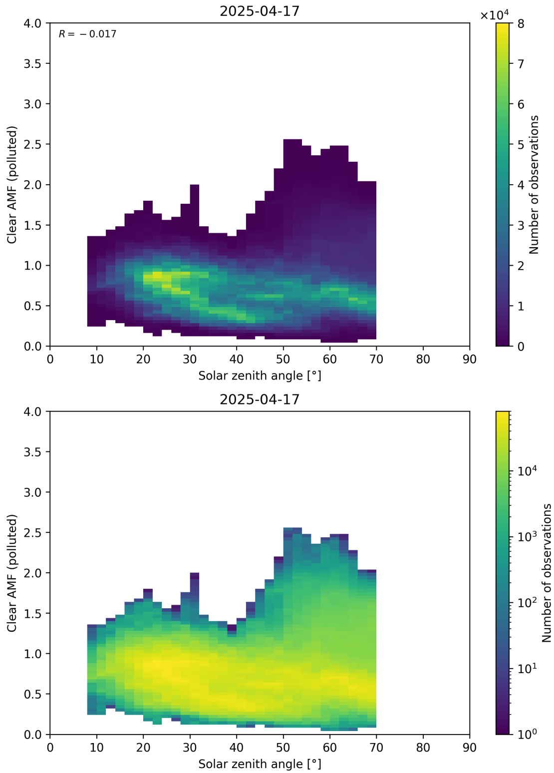
Figure 178: Scatter density plot of “Solar zenith angle” against “Clear AMF (polluted)” for 2025-04-16 to 2025-04-18.
