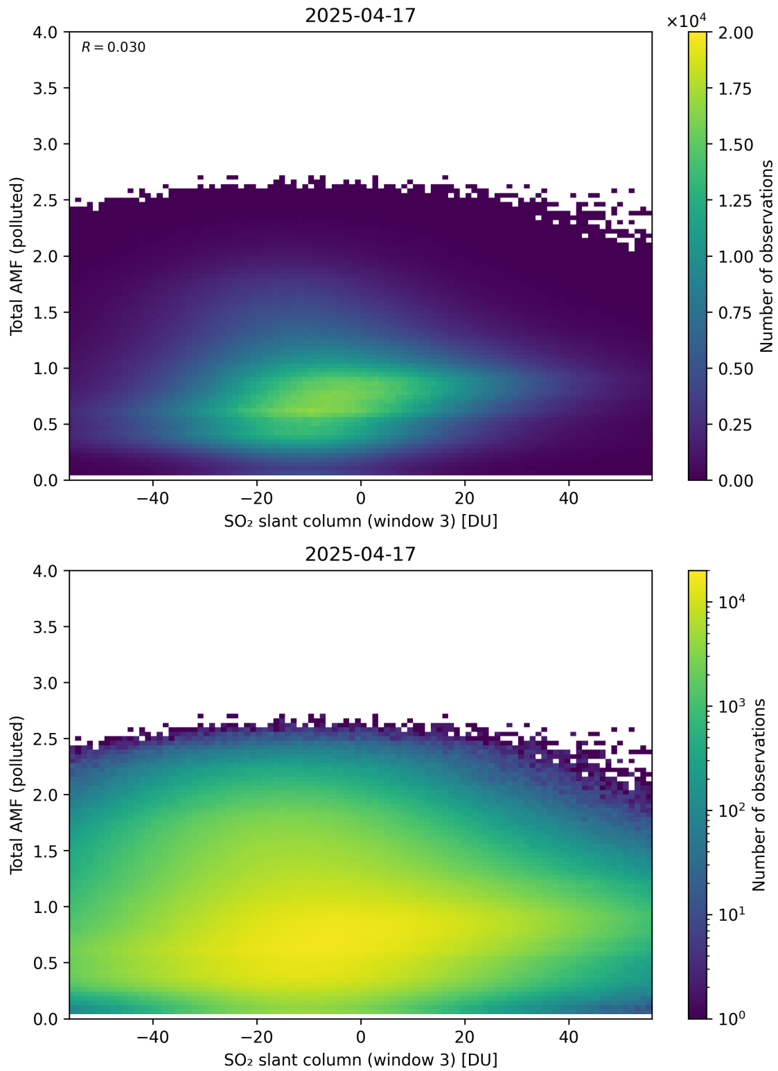
Figure 318: Scatter density plot of “SO 2 slant column (window 3)” against “Total AMF (polluted)” for 2025-04-16 to 2025-04-18.
