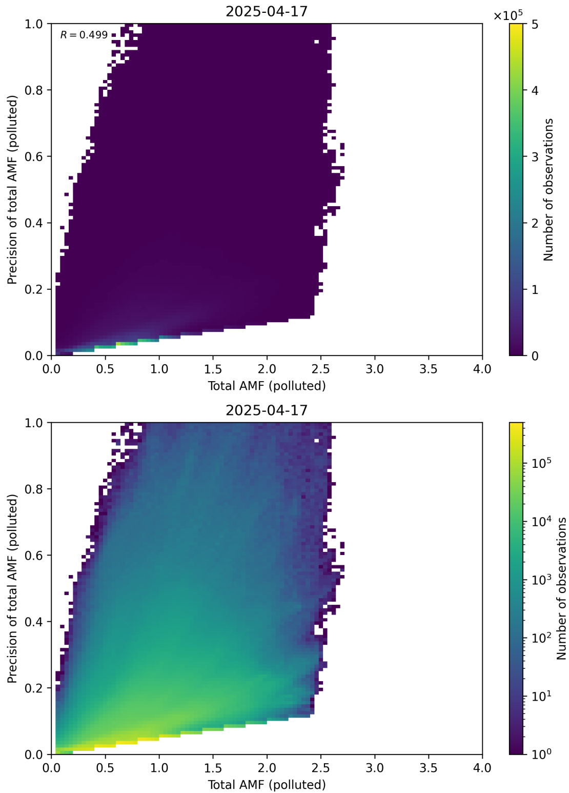
Figure 322: Scatter density plot of “Total AMF (polluted)” against “Precision of total AMF (polluted)” for 2025-04-16 to 2025-04-18.
