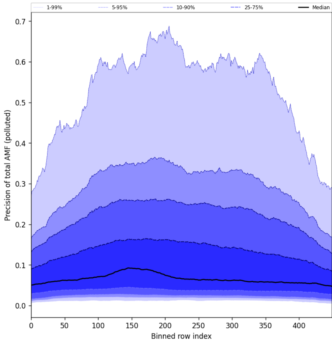
Figure 106: Along track statistics of “Precision of total AMF (polluted)” for 2025-04-16 to 2025-04-18
