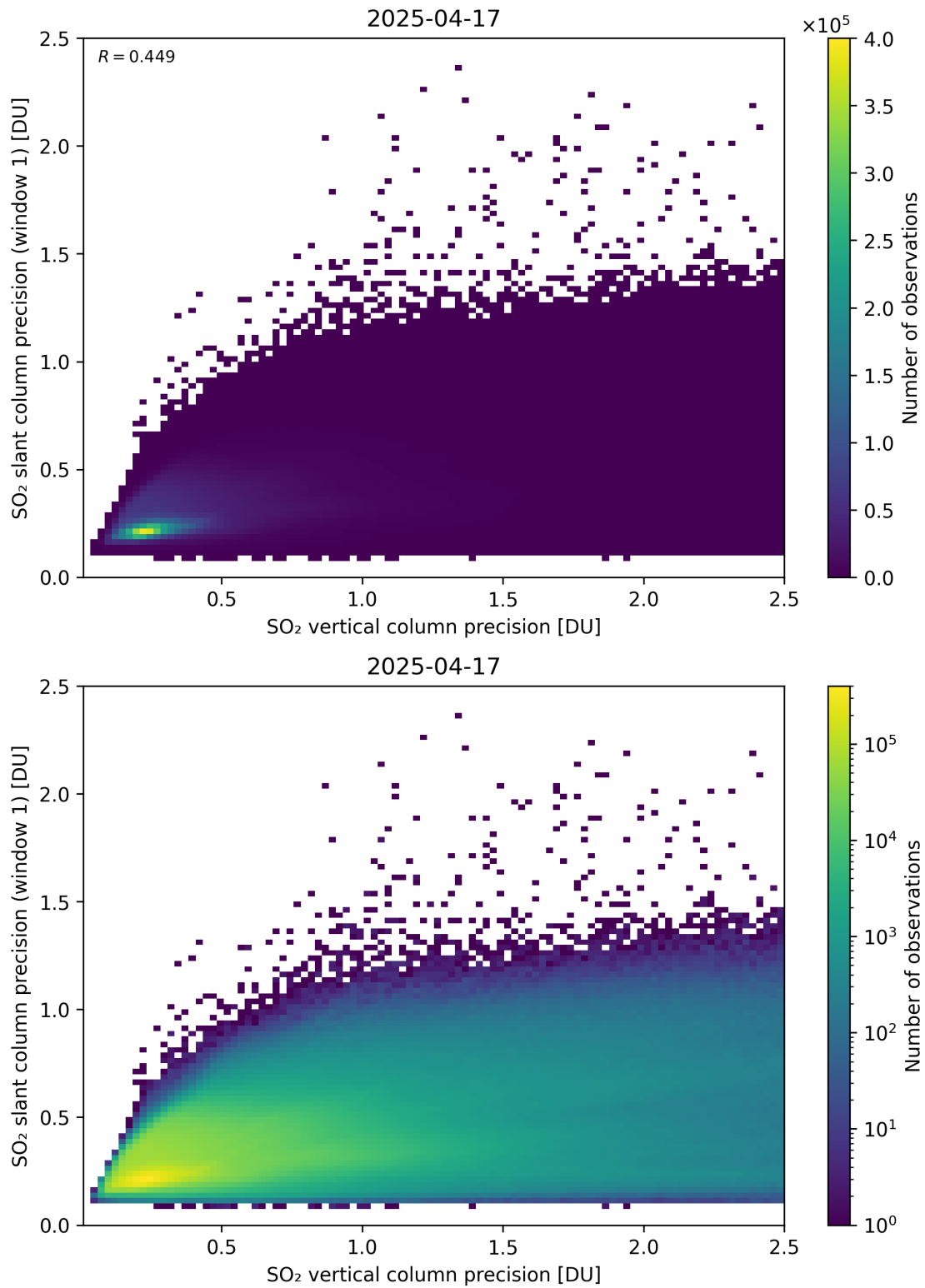
Figure 342: Scatter density plot of “SO 2 vertical column precision” against “SO 2 slant column precision (window 1)” for 2025-04-16 to 2025-04-18.
