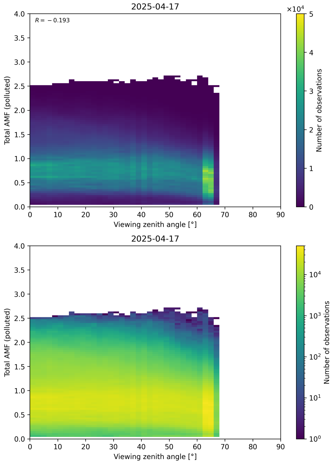
Figure 381: Scatter density plot of “Viewing zenith angle” against “Total AMF (polluted)” for 2025-04-16 to 2025-04-18.
