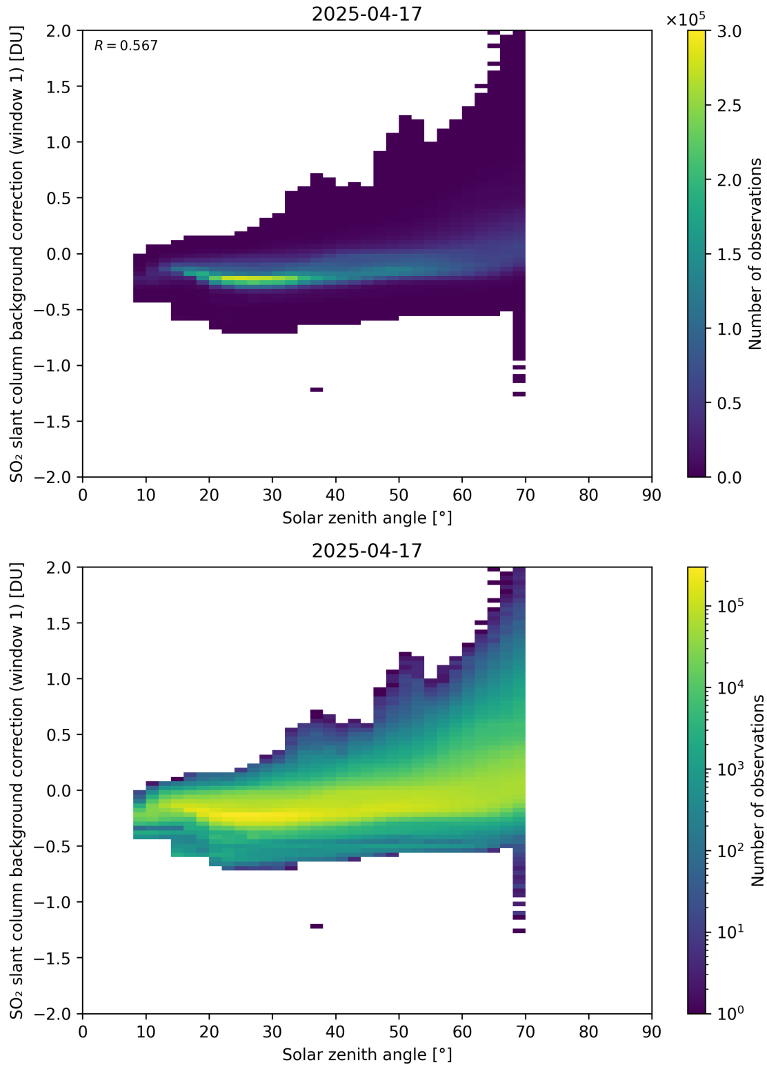
Figure 171: Scatter density plot of “Solar zenith angle” against “SO 2 slant column background correction (window 1)” for 2025-04-16 to 2025-04-18.
