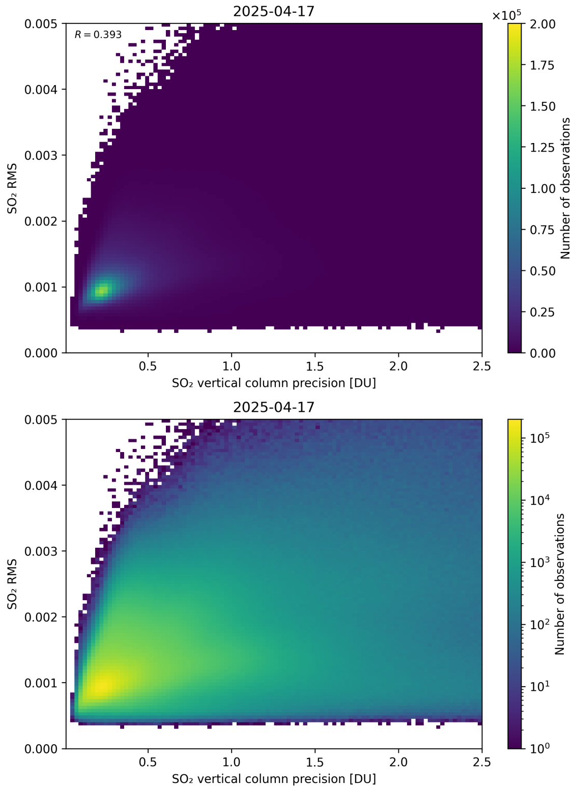
Figure 334: Scatter density plot of “SO 2 vertical column precision” against “SO 2 RMS” for 2025-04-16 to 2025-04-18.
