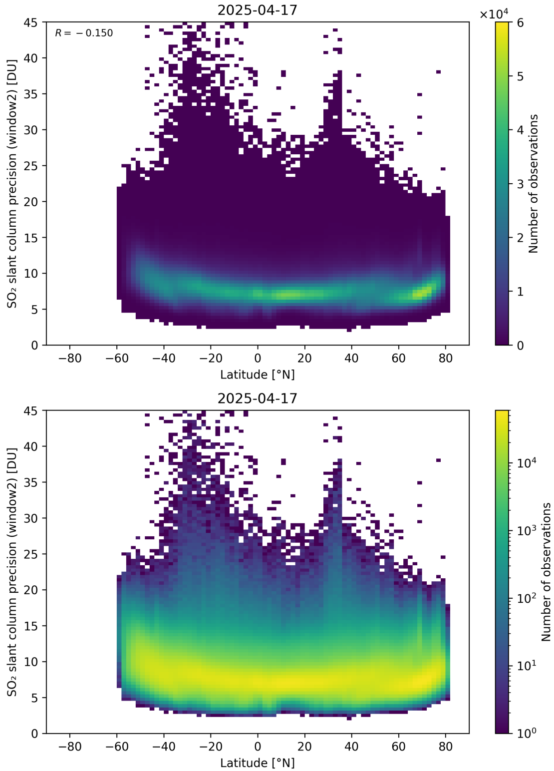
Figure 164: Scatter density plot of “Latitude” against “SO 2 slant column precision (window2)” for 2025-04-16 to 2025-04-18.
