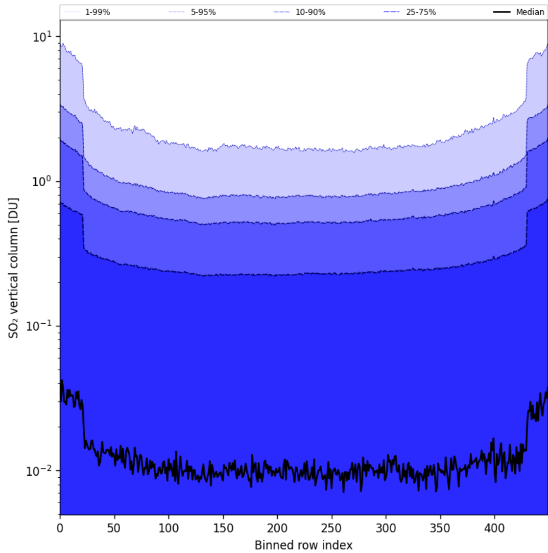
Figure 84: Along track statistics of “SO 2 vertical column” for 2025-04-16 to 2025-04-18
