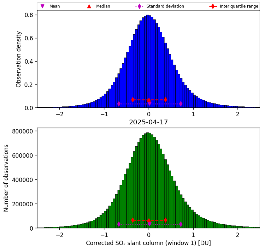
Figure 65: Histogram of “Corrected SO 2 slant column (window 1)” for 2025-04-16 to 2025-04-18
