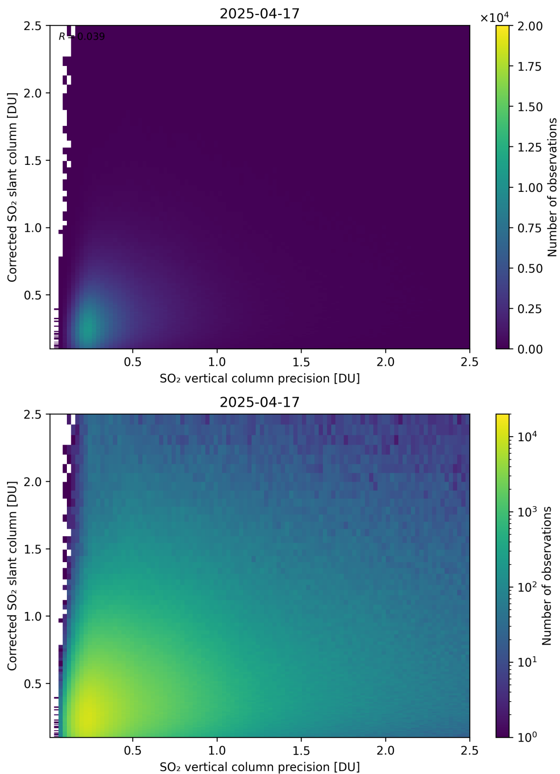
Figure 338: Scatter density plot of “SO 2 vertical column precision” against “Corrected SO 2 slant column” for 2025-04-16 to 2025-04-18.
