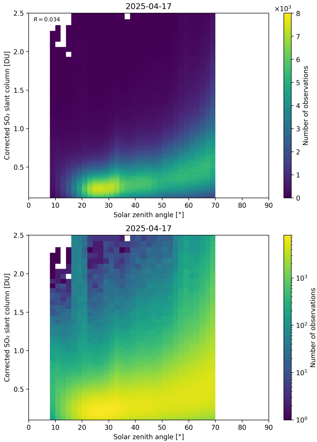
Figure 181: Scatter density plot of “Solar zenith angle” against “Corrected SO 2 slant column” for 2025-04-16 to 2025-04-18.
