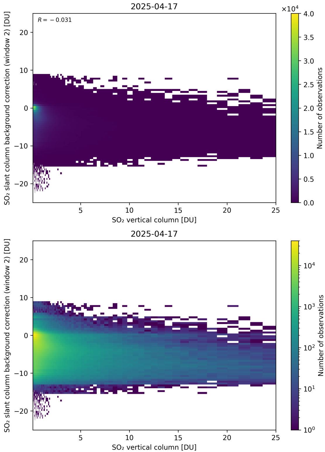
Figure 324: Scatter density plot of “SO 2 vertical column” against “SO 2 slant column background correction (window 2)” for 2025-04-16 to 2025-04-18.
