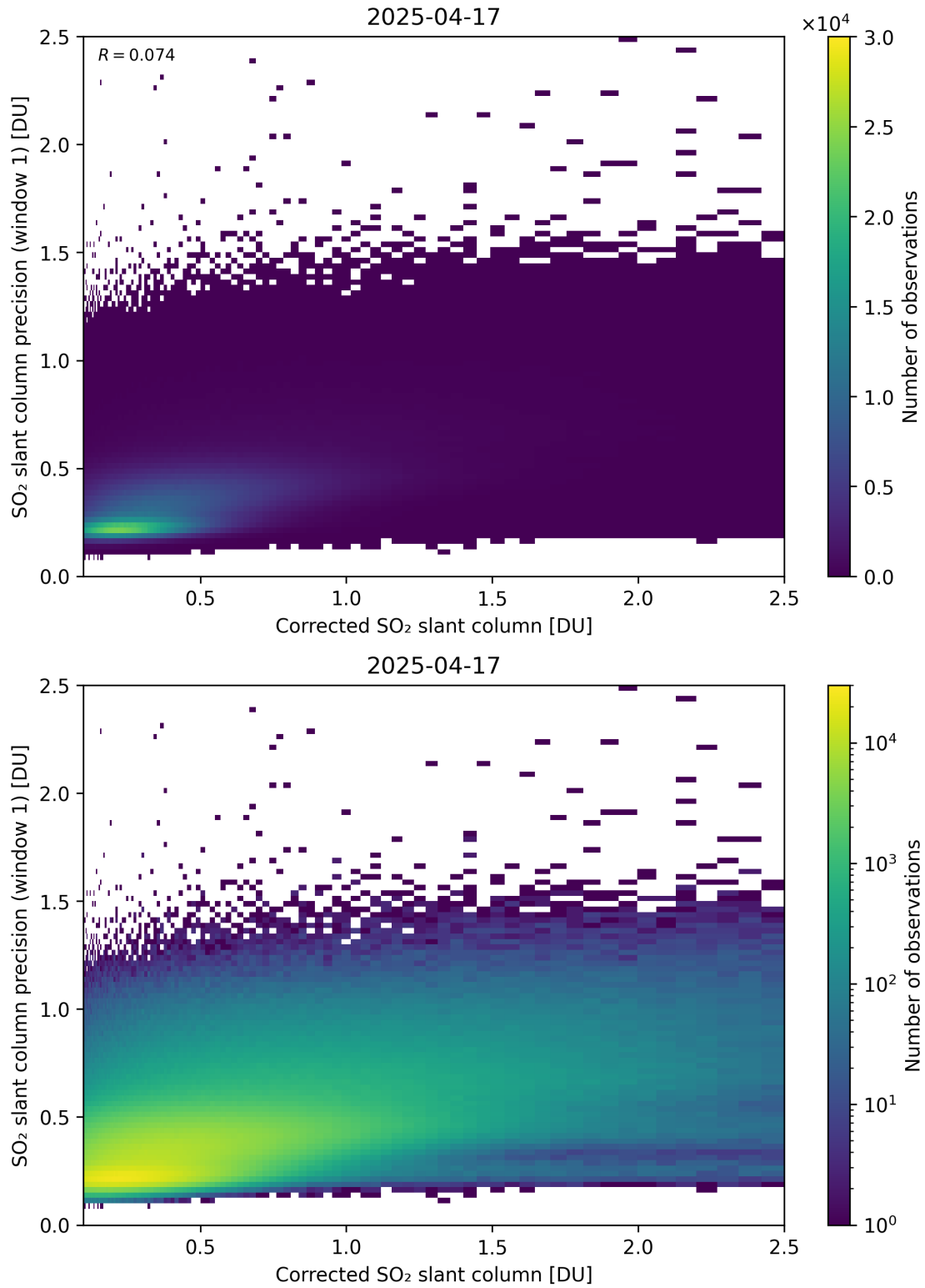
Figure 238: Scatter density plot of “Corrected SO 2 slant column” against “SO 2 slant column precision (window 1)” for 2025-04-16 to 2025-04-18.
