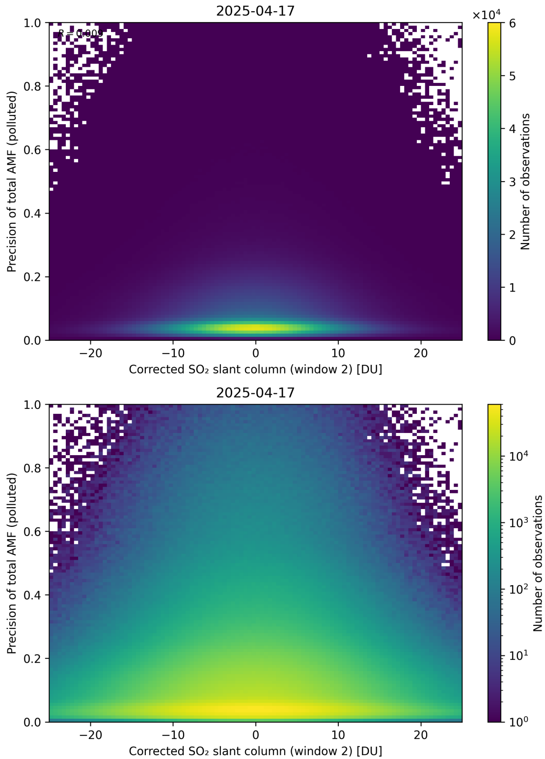
Figure 254: Scatter density plot of “Corrected SO 2 slant column (window 2)” against “Precision of total AMF (polluted)” for 2025-04-16 to 2025-04-18.
