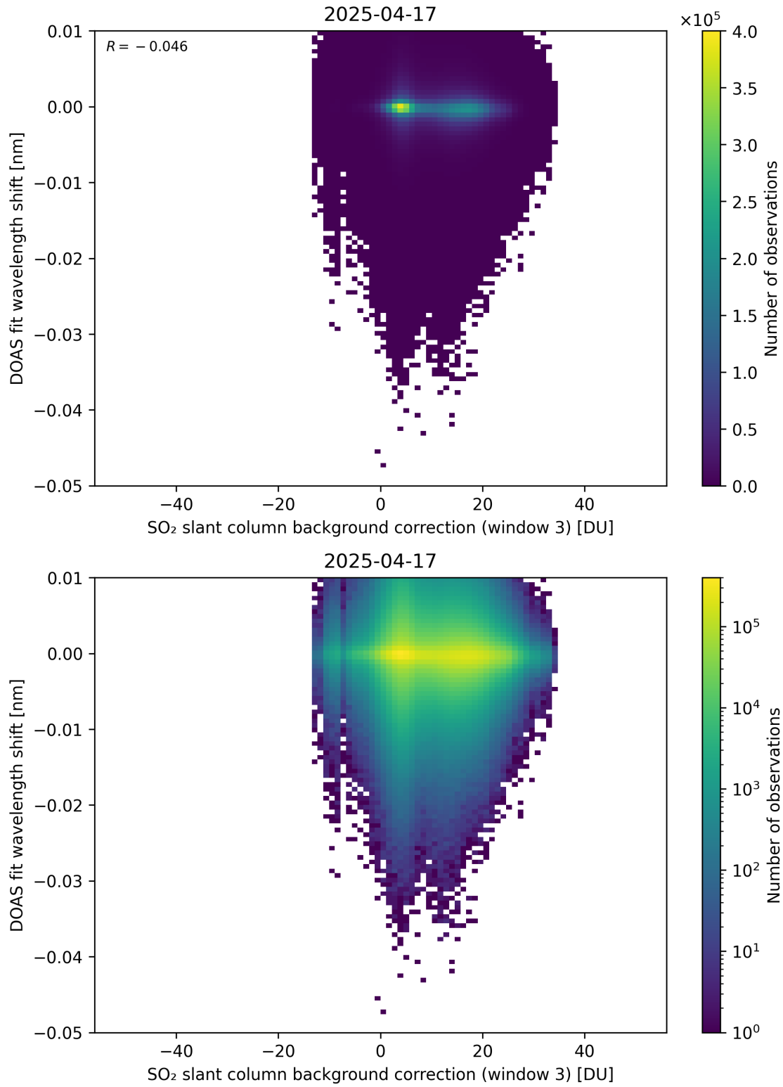
Figure 132: Scatter density plot of “SO 2 slant column background correction (window 3)” against “DOAS fit wavelength shift” for 2025-04-16 to 2025-04-18.
