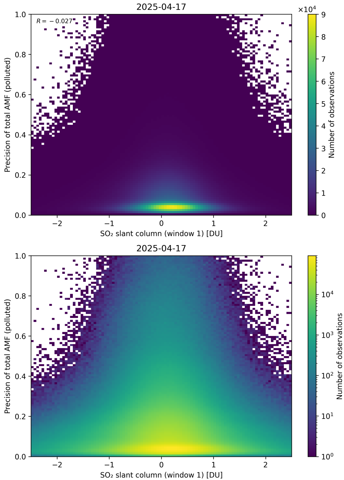
Figure 290: Scatter density plot of “SO 2 slant column (window 1)” against “Precision of total AMF (polluted)” for 2025-04-16 to 2025-04-18.
