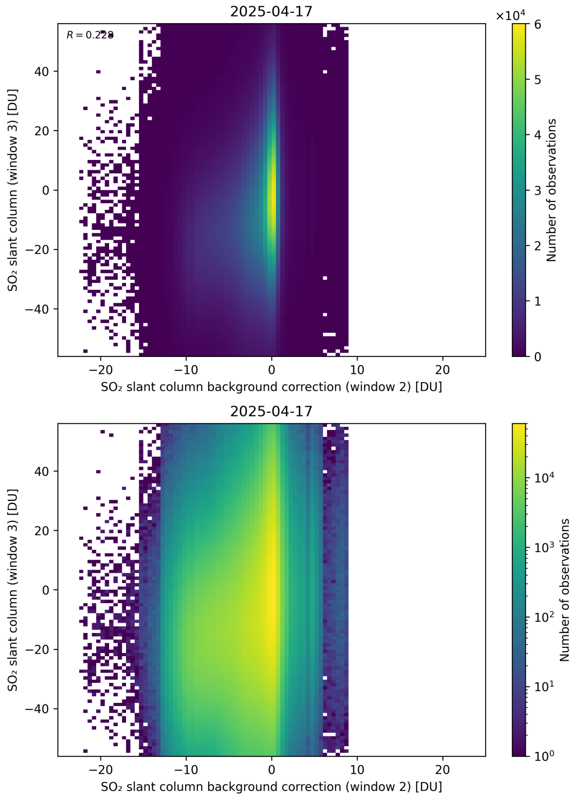
Figure 128: Scatter density plot of “SO 2 slant column background correction (window 2)” against “SO 2 slant column (window 3)” for 2025-04-16 to 2025-04-18.
