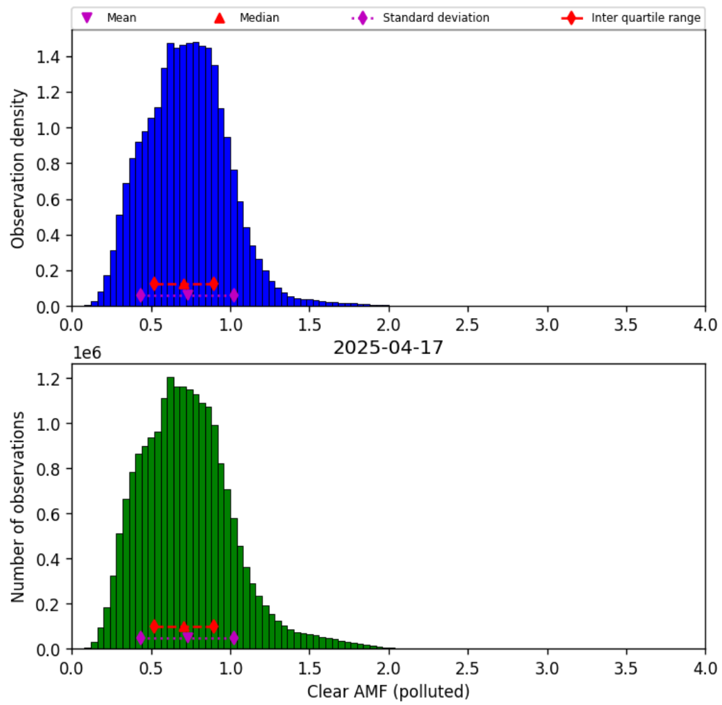
Figure 81: Histogram of “Clear AMF (polluted)” for 2025-04-16 to 2025-04-18
