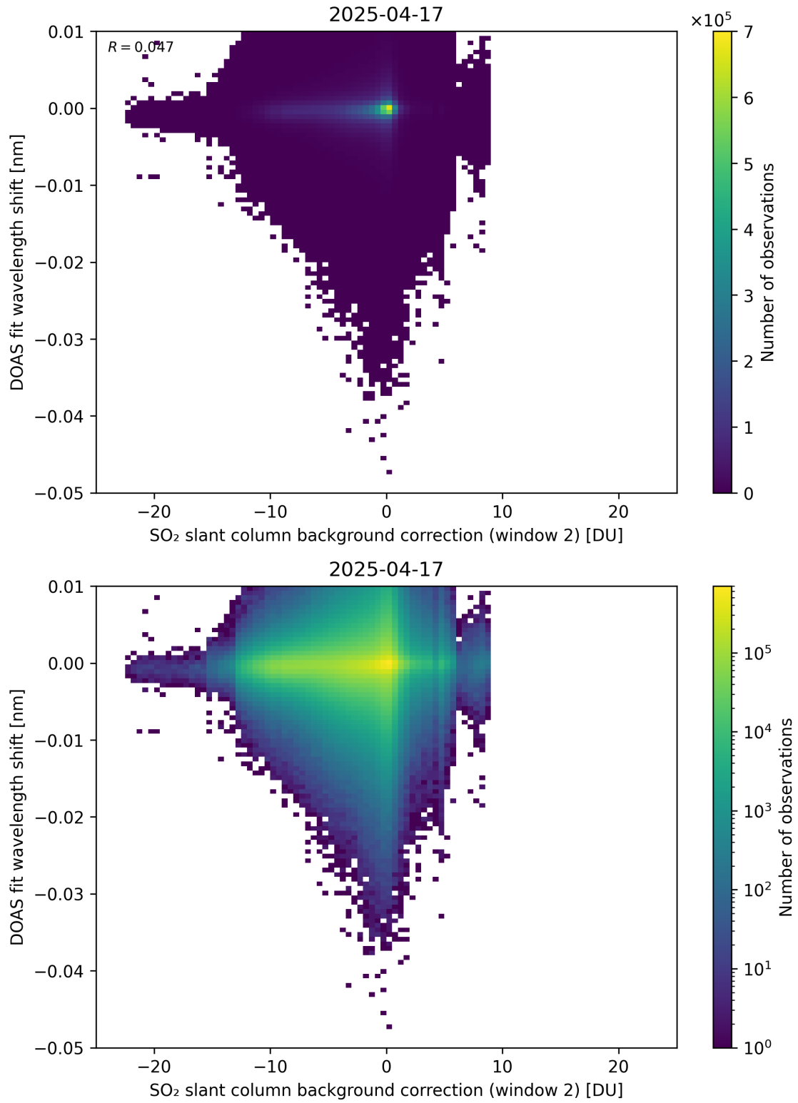
Figure 123: Scatter density plot of “SO 2 slant column background correction (window 2)” against “DOAS fit wavelength shift” for 2025-04-16 to 2025-04-18.
