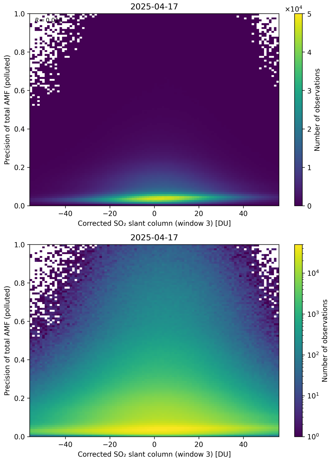
Figure 261: Scatter density plot of “Corrected SO 2 slant column (window 3)” against “Precision of total AMF (polluted)” for 2025-04-16 to 2025-04-18.
