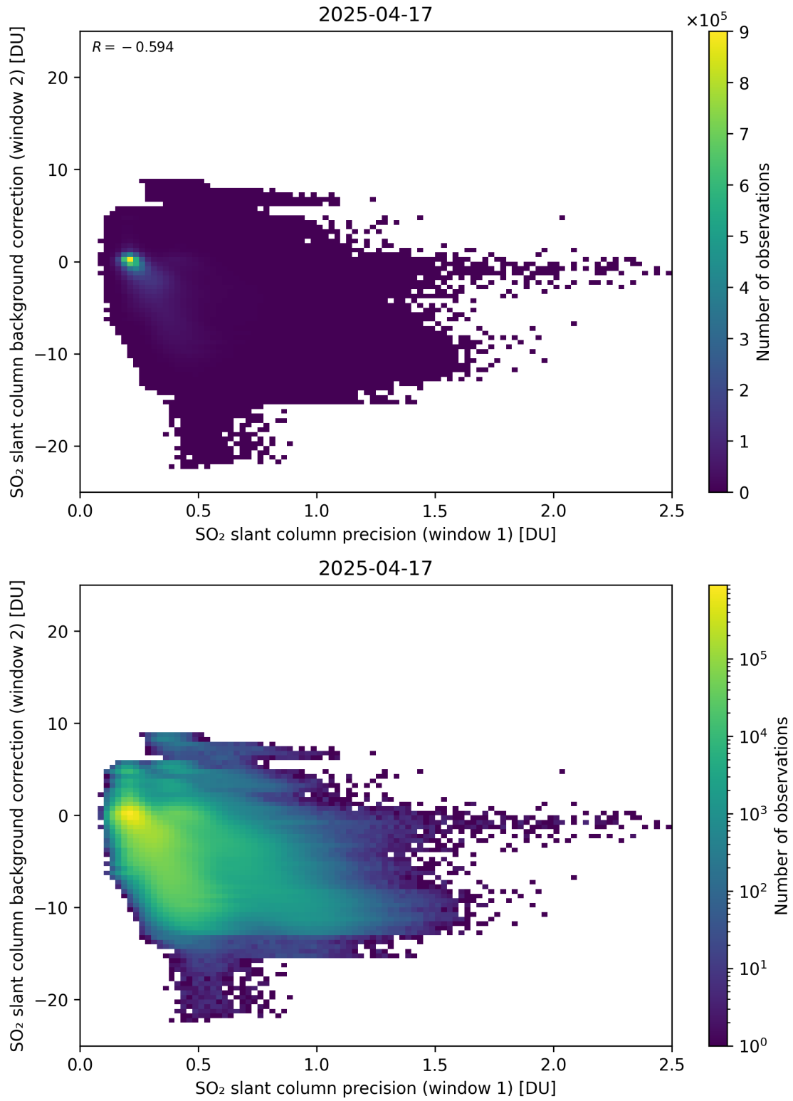
Figure 269: Scatter density plot of “SO 2 slant column precision (window 1)” against “SO 2 slant column background correction (window 2)” for 2025-04-16 to 2025-04-18.
