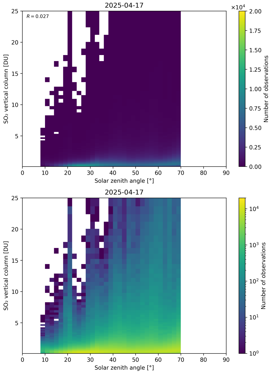
Figure 191: Scatter density plot of “Solar zenith angle” against “SO 2 vertical column” for 2025-04-16 to 2025-04-18.
