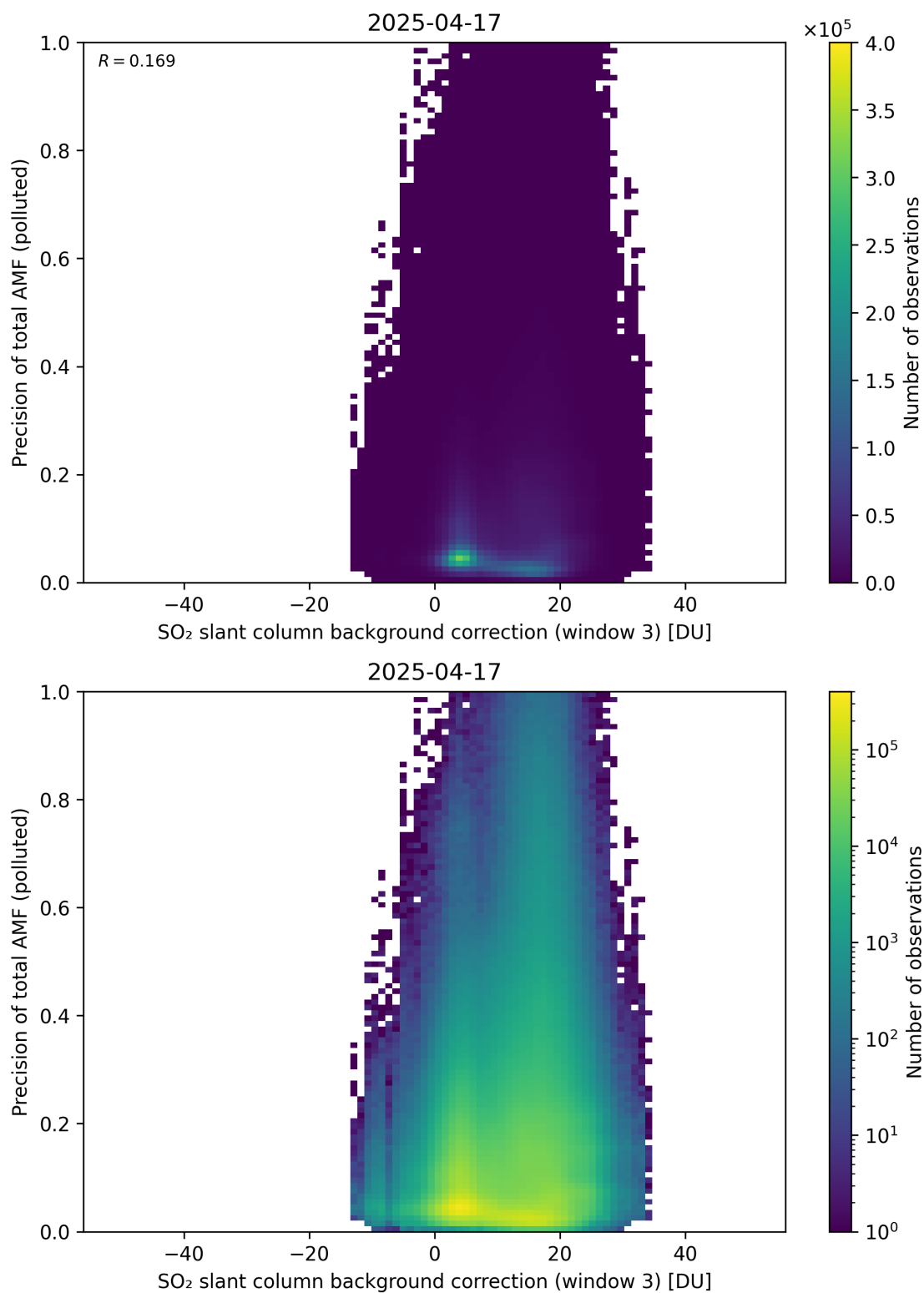
Figure 137: Scatter density plot of “SO 2 slant column background correction (window 3)” against “Precision of total AMF (polluted)” for 2025-04-16 to 2025-04-18.
