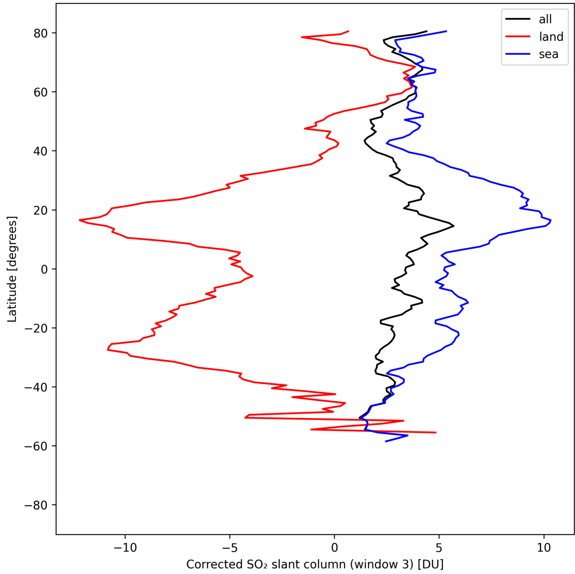
Figure 47: Zonal average of “Corrected SO 2 slant column (window 3)” for 2025-04-16 to 2025-04-18.
