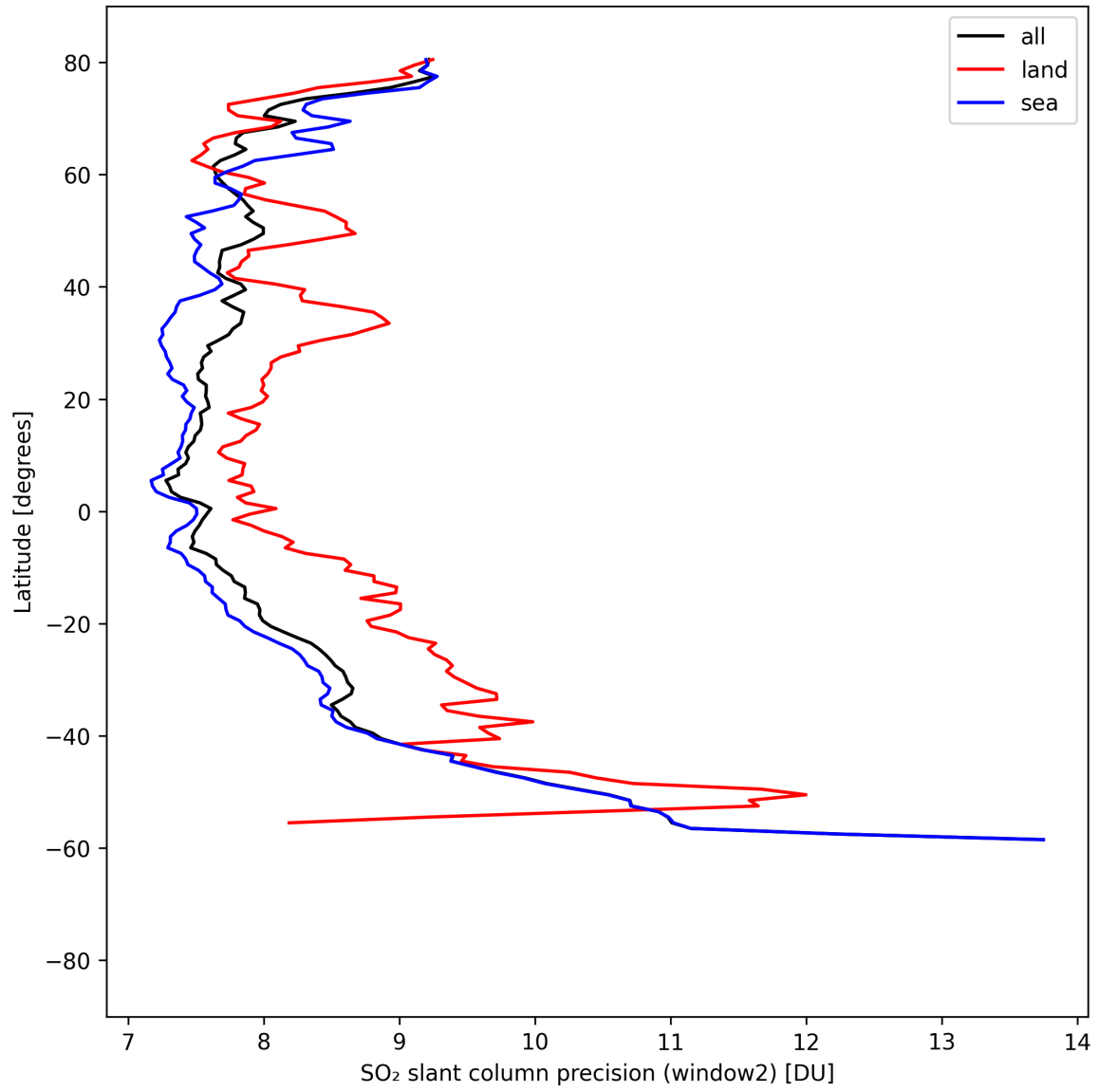
Figure 42: Zonal average of “SO 2 slant column precision (window2)” for 2025-04-16 to 2025-04-18.
