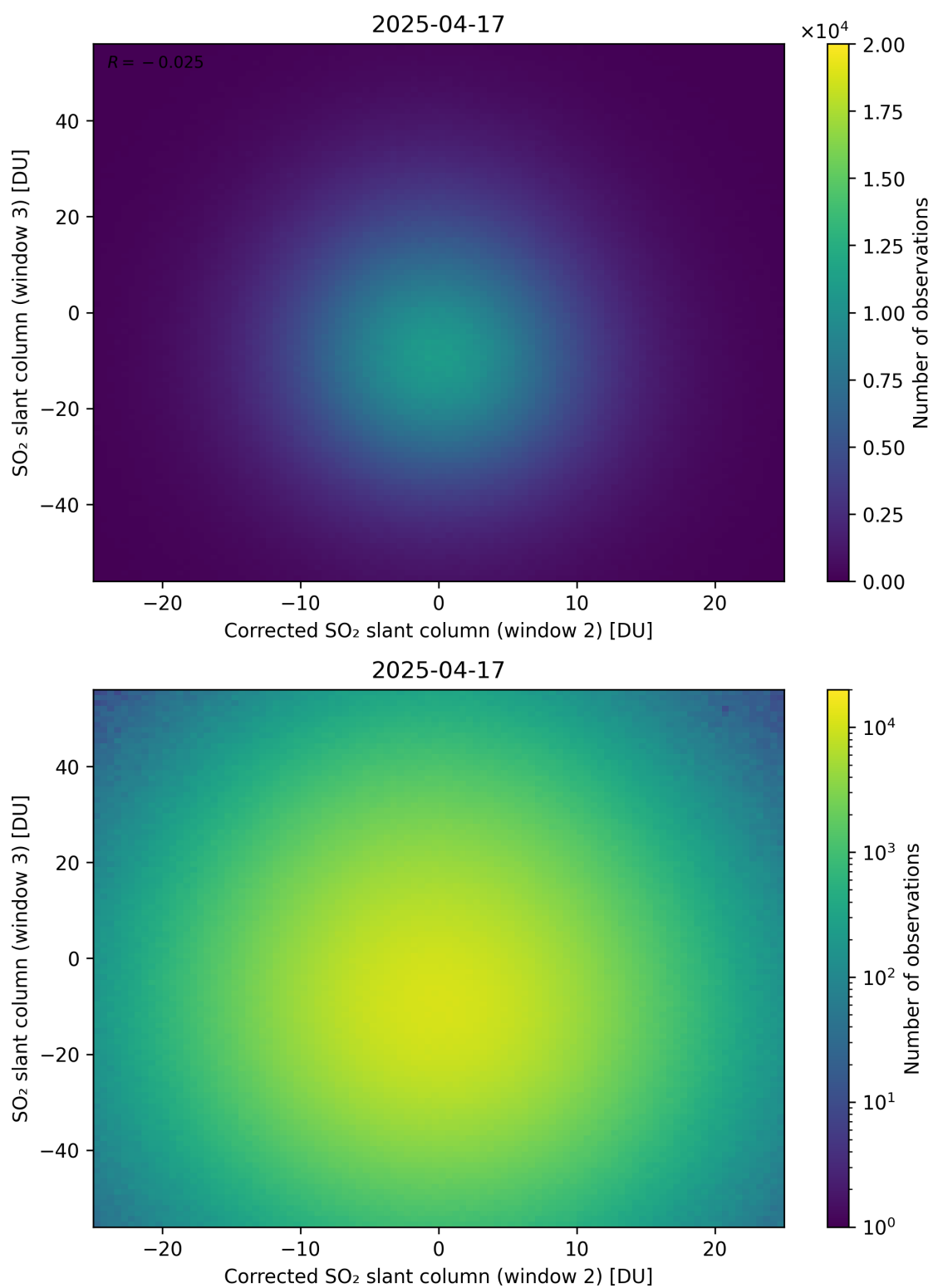
Figure 251: Scatter density plot of “Corrected SO 2 slant column (window 2)” against “SO 2 slant column (window 3)” for 2025-04-16 to 2025-04-18.
