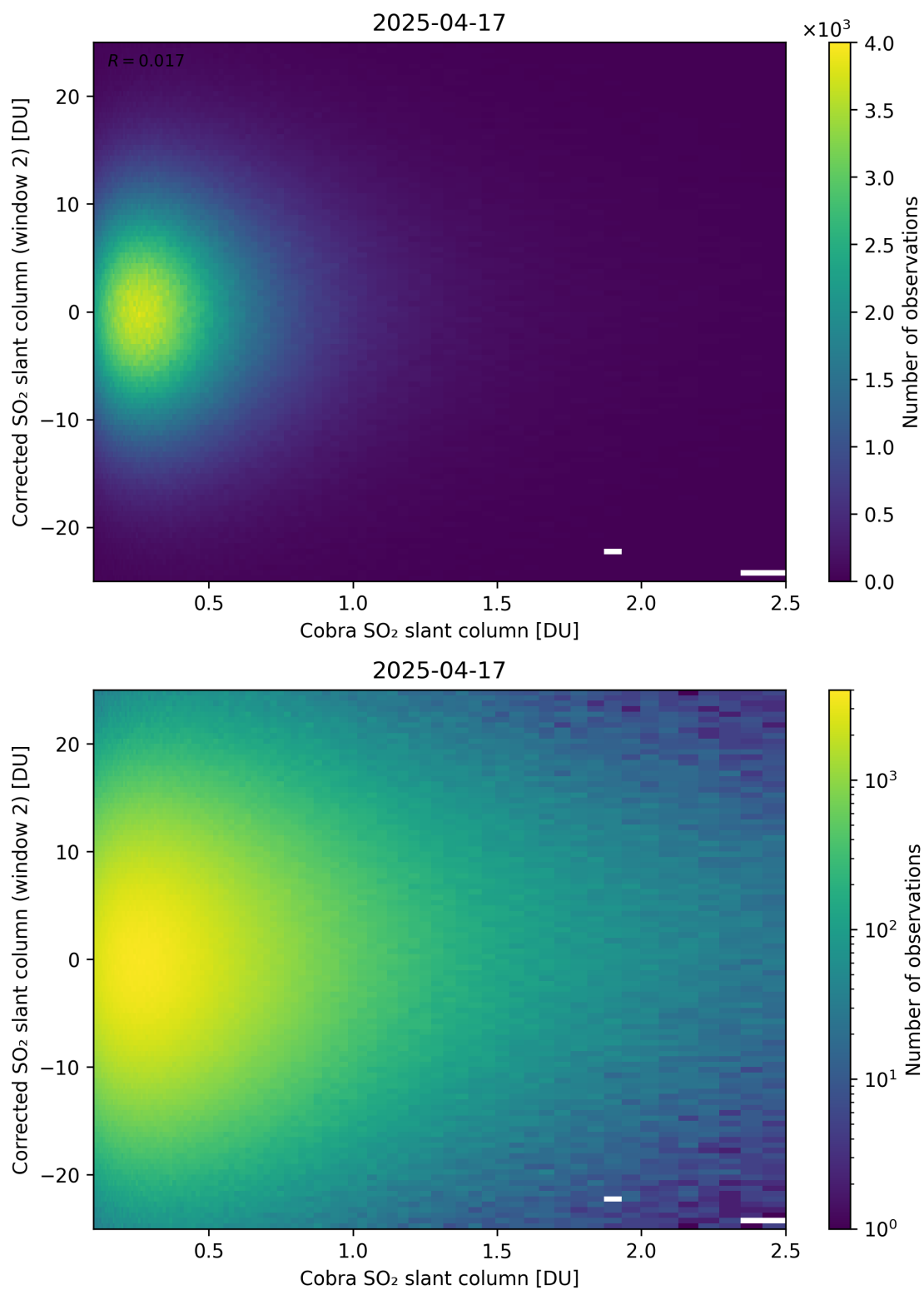
Figure 217: Scatter density plot of “Cobra SO 2 slant column” against “Corrected SO 2 slant column (window 2)” for 2025-04-16 to 2025-04-18.
