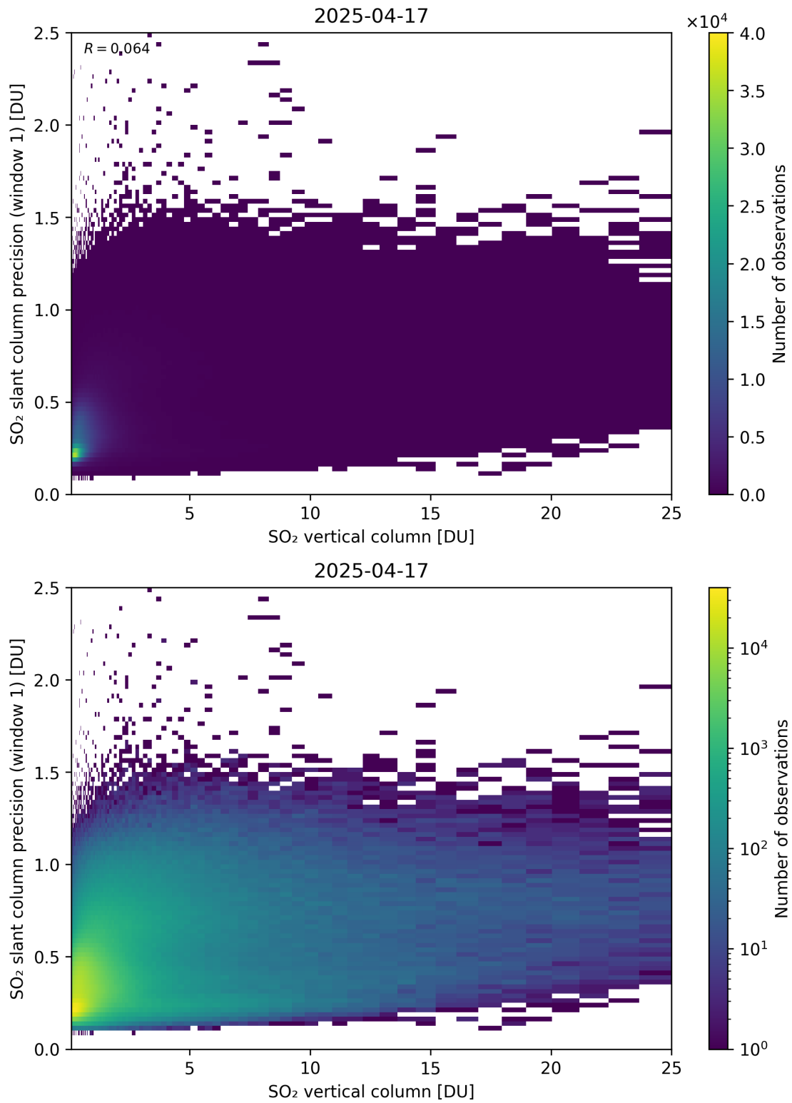
Figure 355: Scatter density plot of “SO 2 vertical column” against “SO 2 slant column precision (window 1)” for 2025-04-16 to 2025-04-18.
