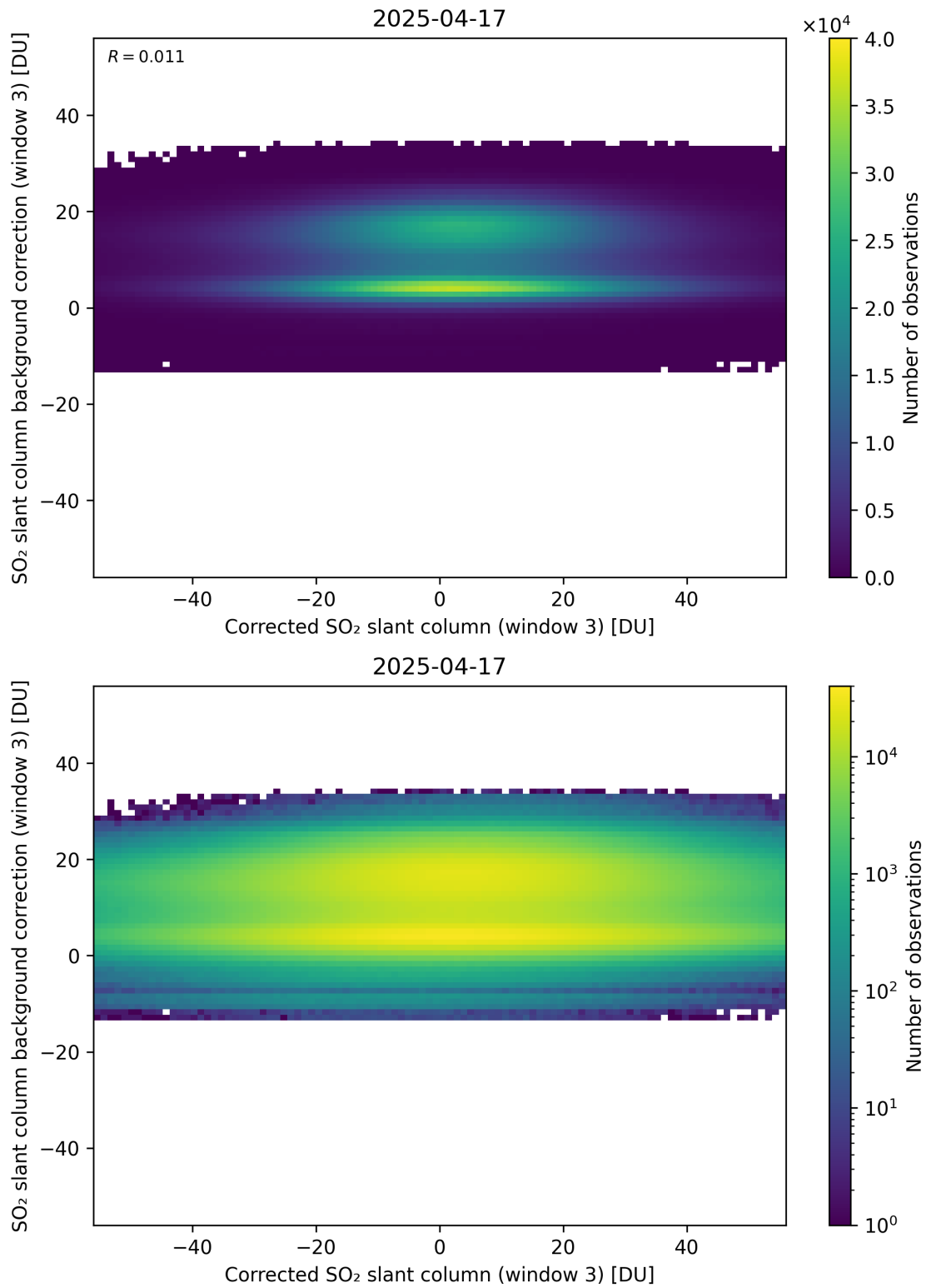
Figure 255: Scatter density plot of “Corrected SO 2 slant column (window 3)” against “SO 2 slant column background correction (window 3)” for 2025-04-16 to 2025-04-18.
