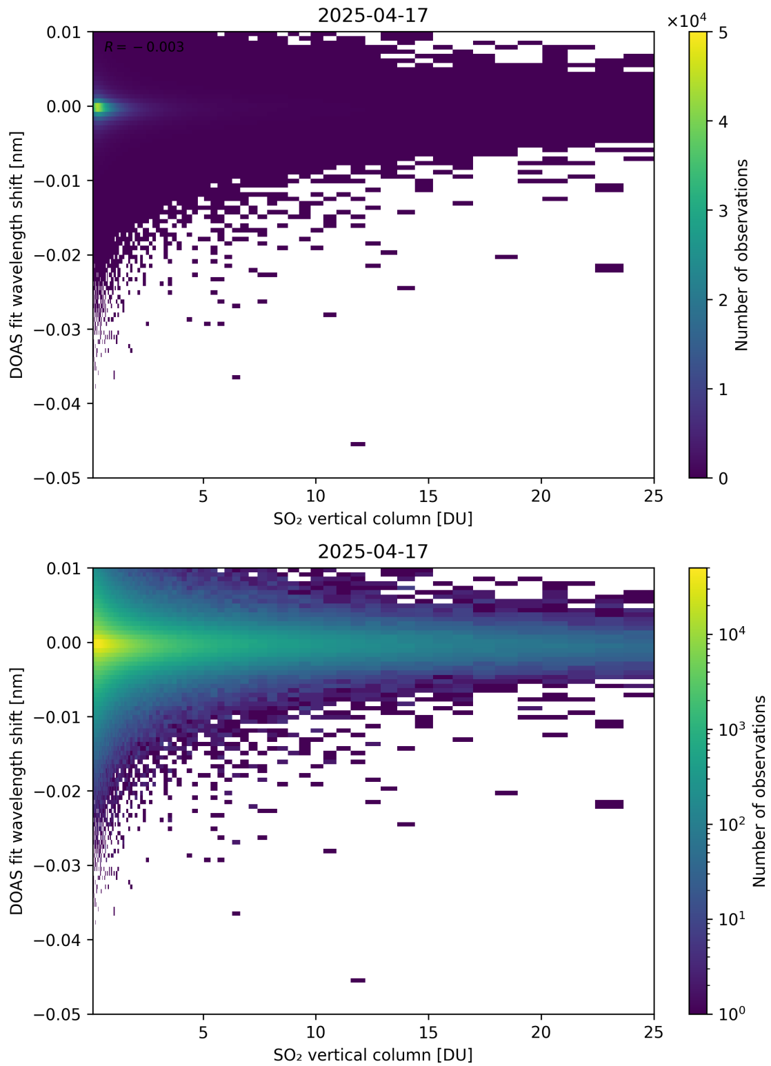
Figure 326: Scatter density plot of “SO 2 vertical column” against “DOAS fit wavelength shift” for 2025-04-16 to 2025-04-18.
