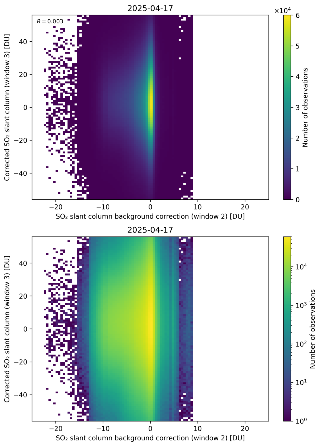
Figure 127: Scatter density plot of “SO 2 slant column background correction (window 2)” against “Corrected SO 2 slant column (window 3)” for 2025-04-16 to 2025-04-18.
