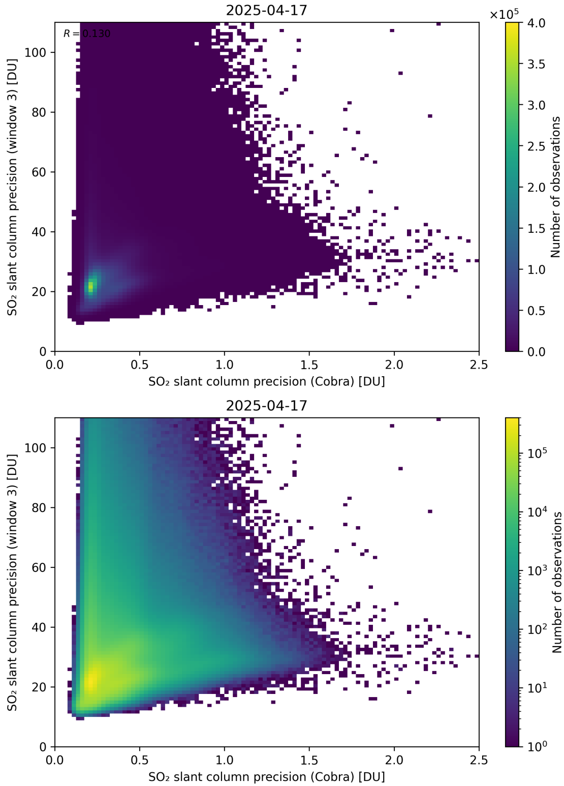
Figure 212: Scatter density plot of “SO 2 slant column precision (Cobra)” against “SO 2 slant column precision (window 3)” for 2025-04-16 to 2025-04-18.
