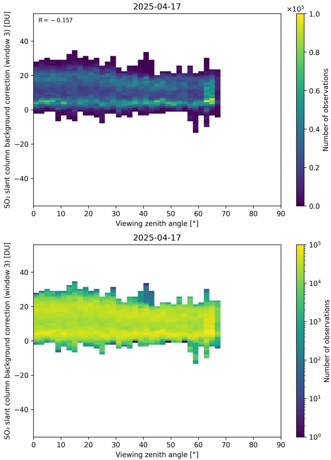
Figure 364: Scatter density plot of “Viewing zenith angle” against “SO 2 slant column background correction (window 3)” for 2025-04-16 to 2025-04-18.
