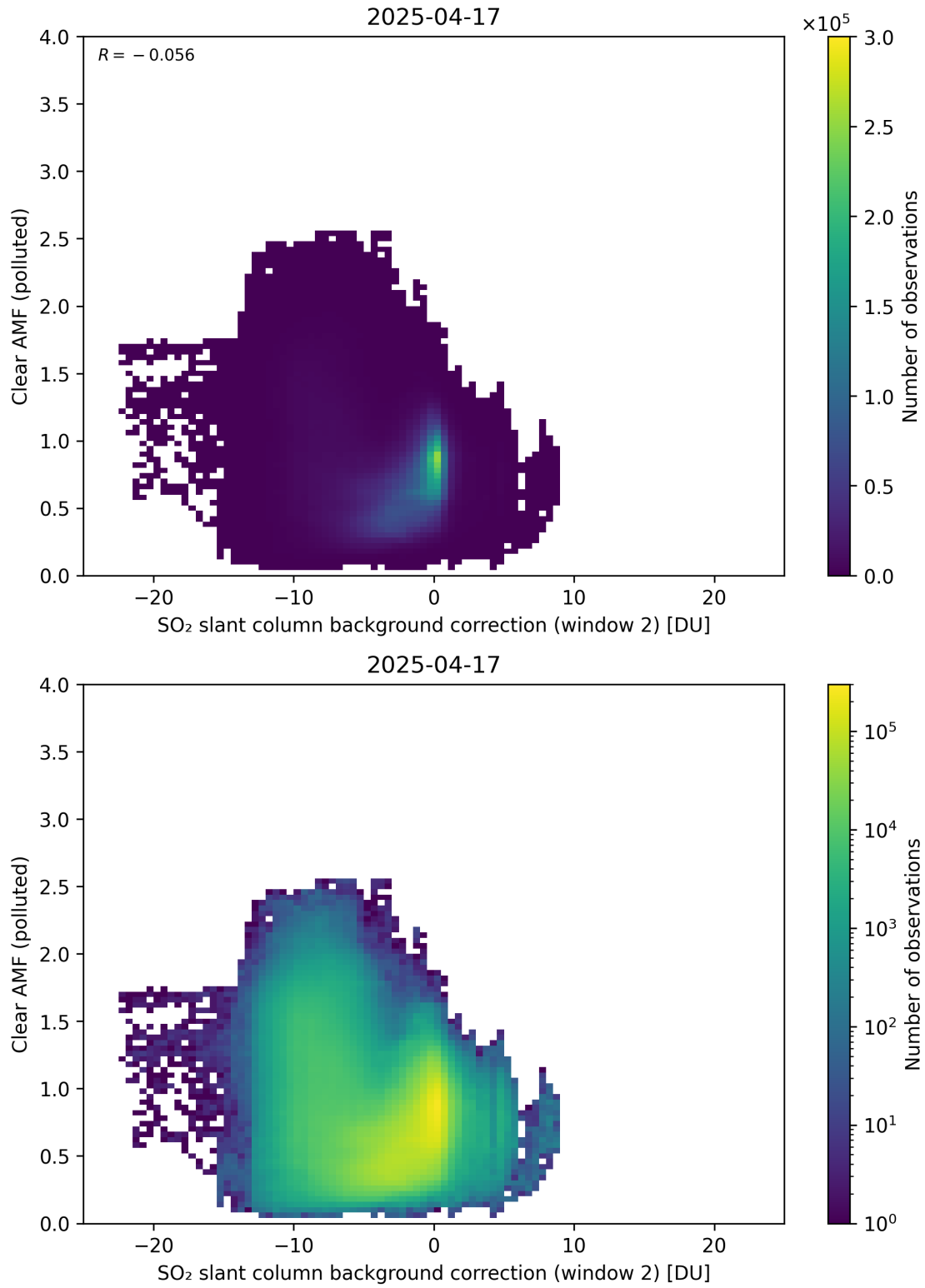
Figure 126: Scatter density plot of “SO 2 slant column background correction (window 2)” against “Clear AMF (polluted)” for 2025-04-16 to 2025-04-18.
