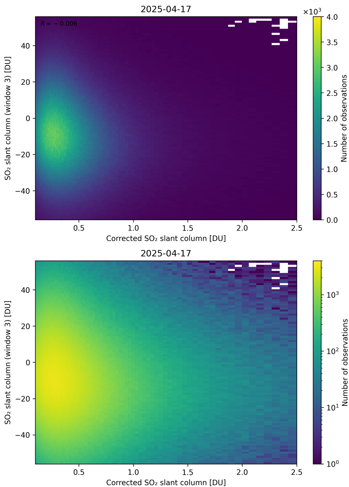
Figure 240: Scatter density plot of “Corrected SO 2 slant column” against “SO 2 slant column (window 3)” for 2025-04-16 to 2025-04-18.
