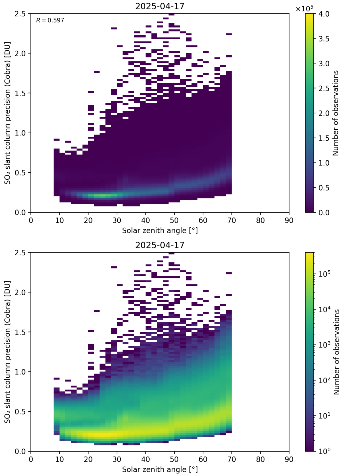
Figure 180: Scatter density plot of “Solar zenith angle” against “SO 2 slant column precision (Cobra)” for 2025-04-16 to 2025-04-18.
