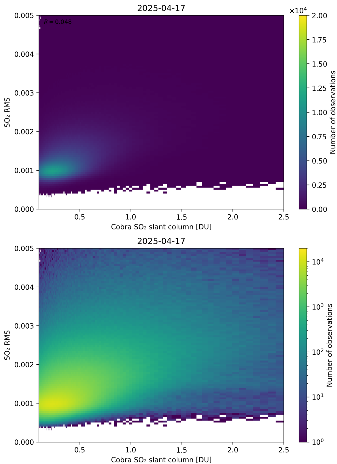
Figure 198: Scatter density plot of “Cobra SO 2 slant column” against “SO 2 RMS” for 2025-04-16 to 2025-04-18.
