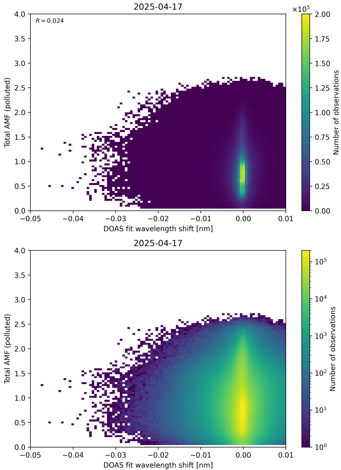
Figure 141: Scatter density plot of “DOAS fit wavelength shift” against “Total AMF (polluted)” for 2025-04-16 to 2025-04-18.
