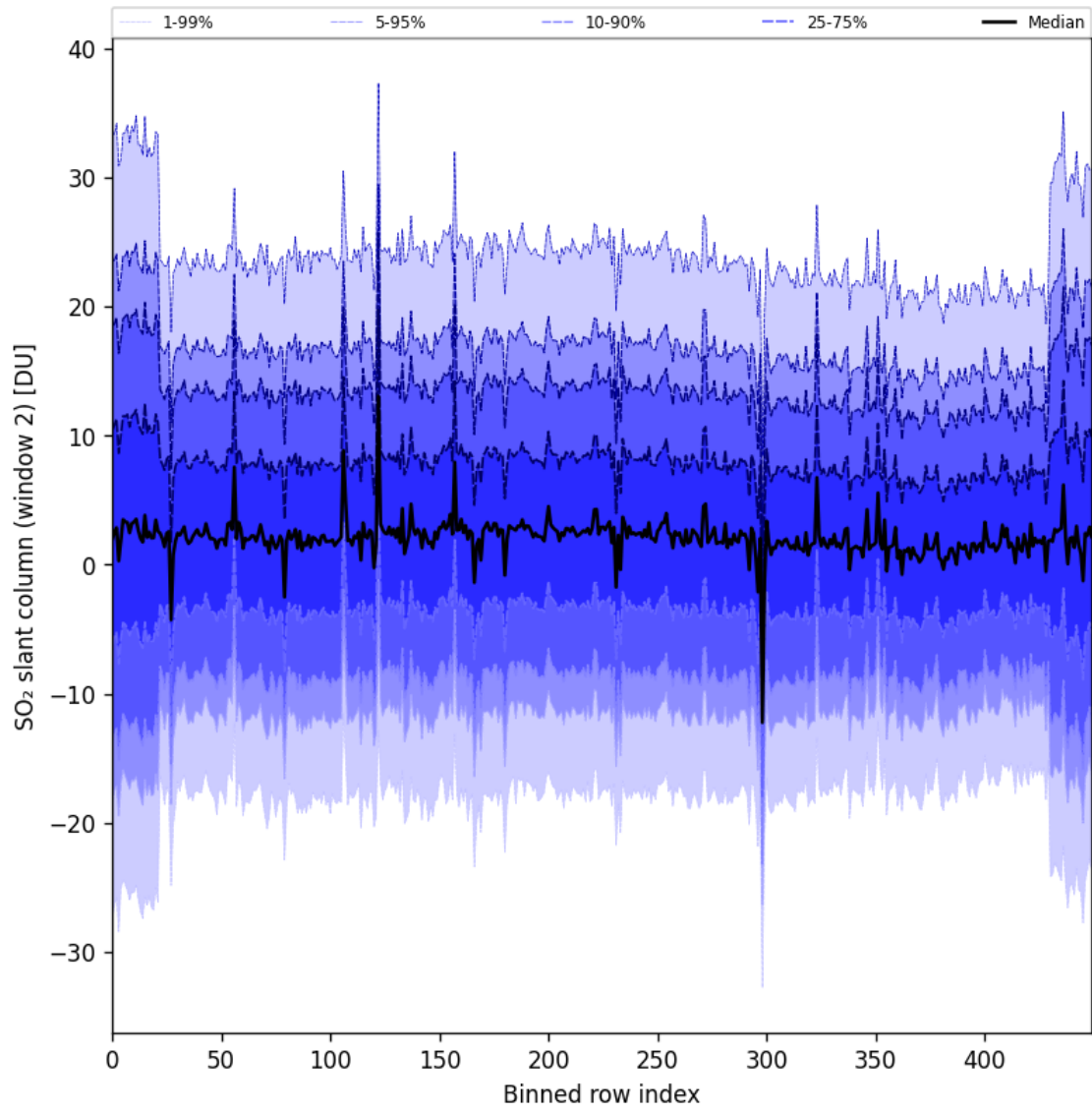
Figure 93: Along track statistics of “SO 2 slant column (window 2)” for 2025-04-16 to 2025-04-18
