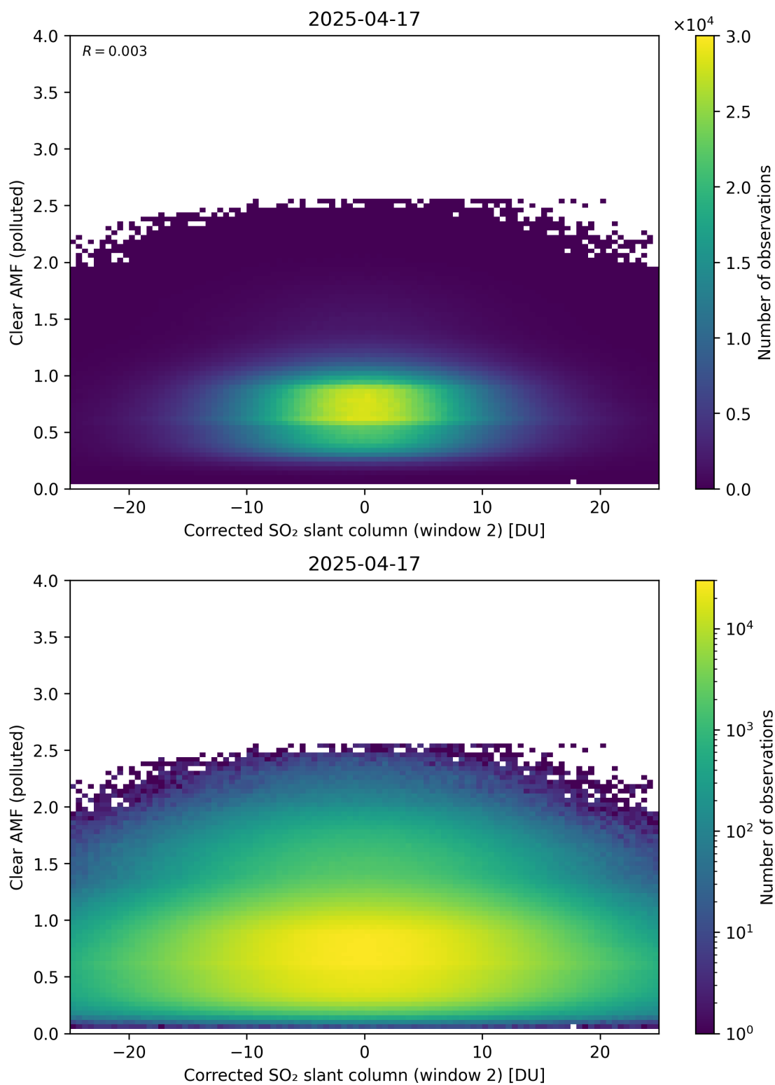
Figure 249: Scatter density plot of “Corrected SO 2 slant column (window 2)” against “Clear AMF (polluted)” for 2025-04-16 to 2025-04-18.
