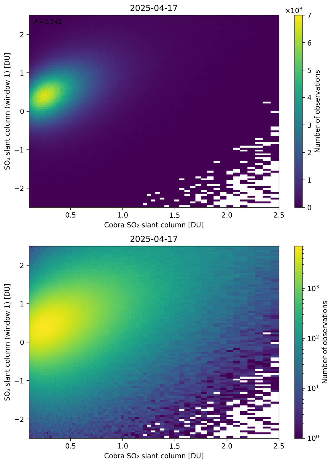
Figure 219: Scatter density plot of “Cobra SO 2 slant column” against “SO 2 slant column (window 1)” for 2025-04-16 to 2025-04-18.
