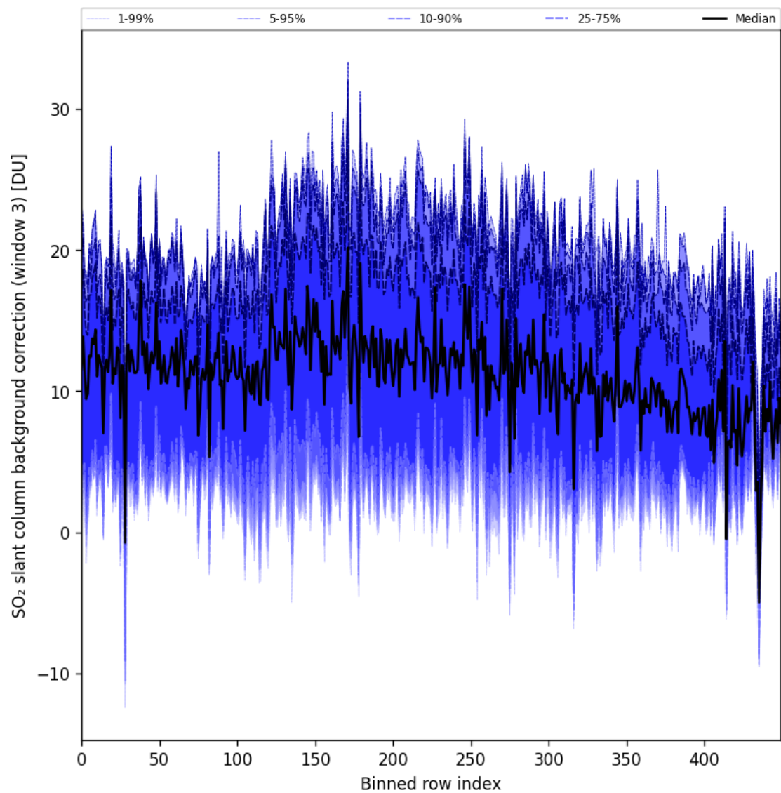
Figure 100: Along track statistics of “SO 2 slant column background correction (window 3)” for 2025-04-16 to 2025-04-18
