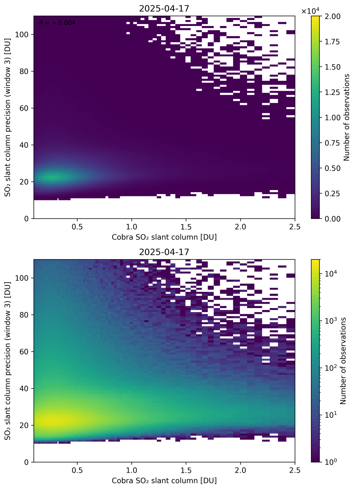
Figure 223: Scatter density plot of “Cobra SO 2 slant column” against “SO 2 slant column precision (window 3)” for 2025-04-16 to 2025-04-18.
