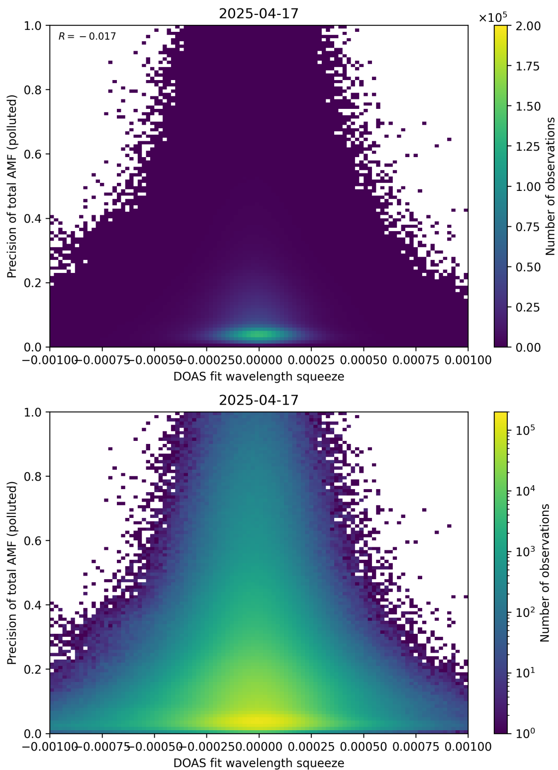
Figure 146: Scatter density plot of “DOAS fit wavelength squeeze” against “Precision of total AMF (polluted)” for 2025-04-16 to 2025-04-18.
