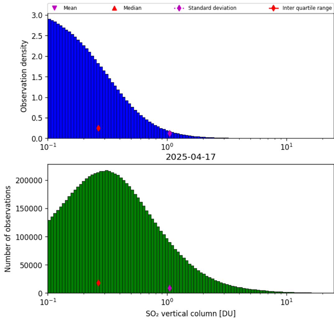
Figure 58: Histogram of “SO 2 vertical column” for 2025-04-16 to 2025-04-18
