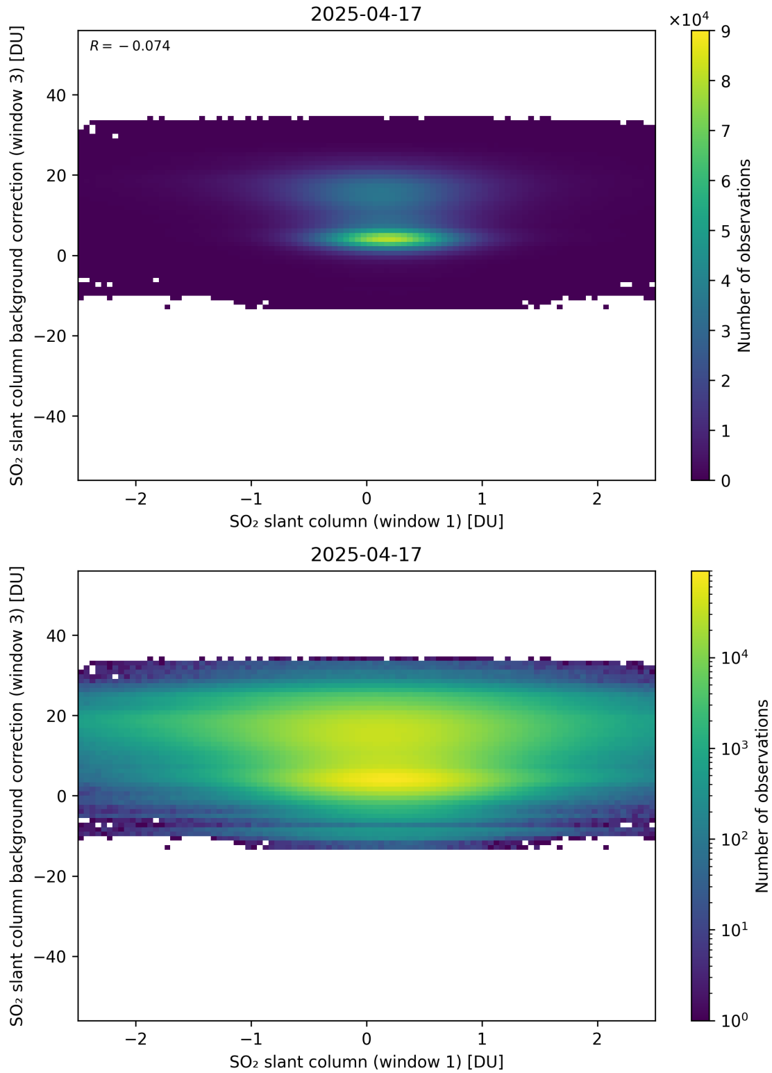
Figure 264: Scatter density plot of “SO 2 slant column (window 1)” against “SO 2 slant column background correction (window 3)” for 2025-04-16 to 2025-04-18.
