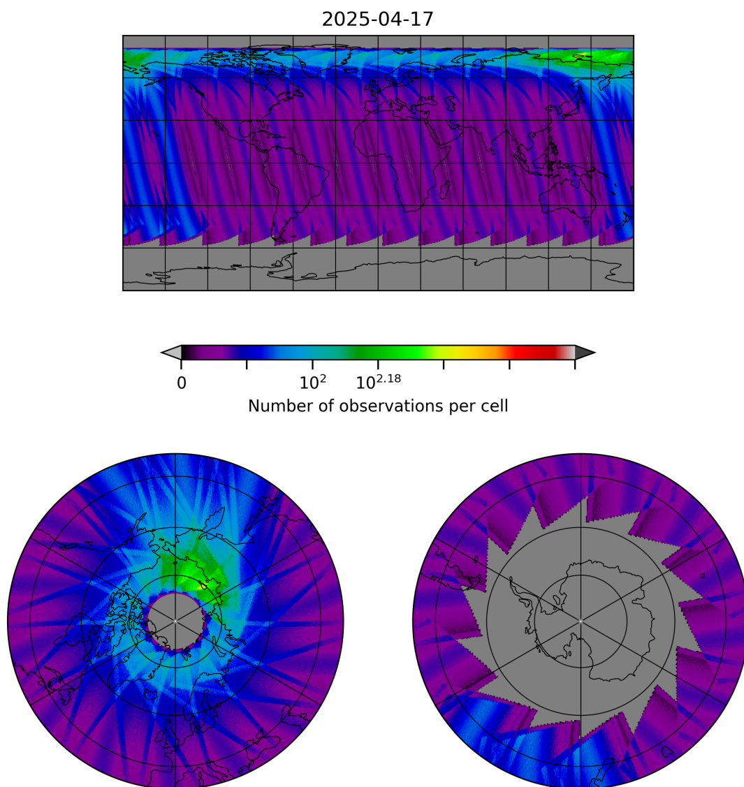
Figure 30: Map of the number of observations for 2025-04-16 to 2025-04-18
