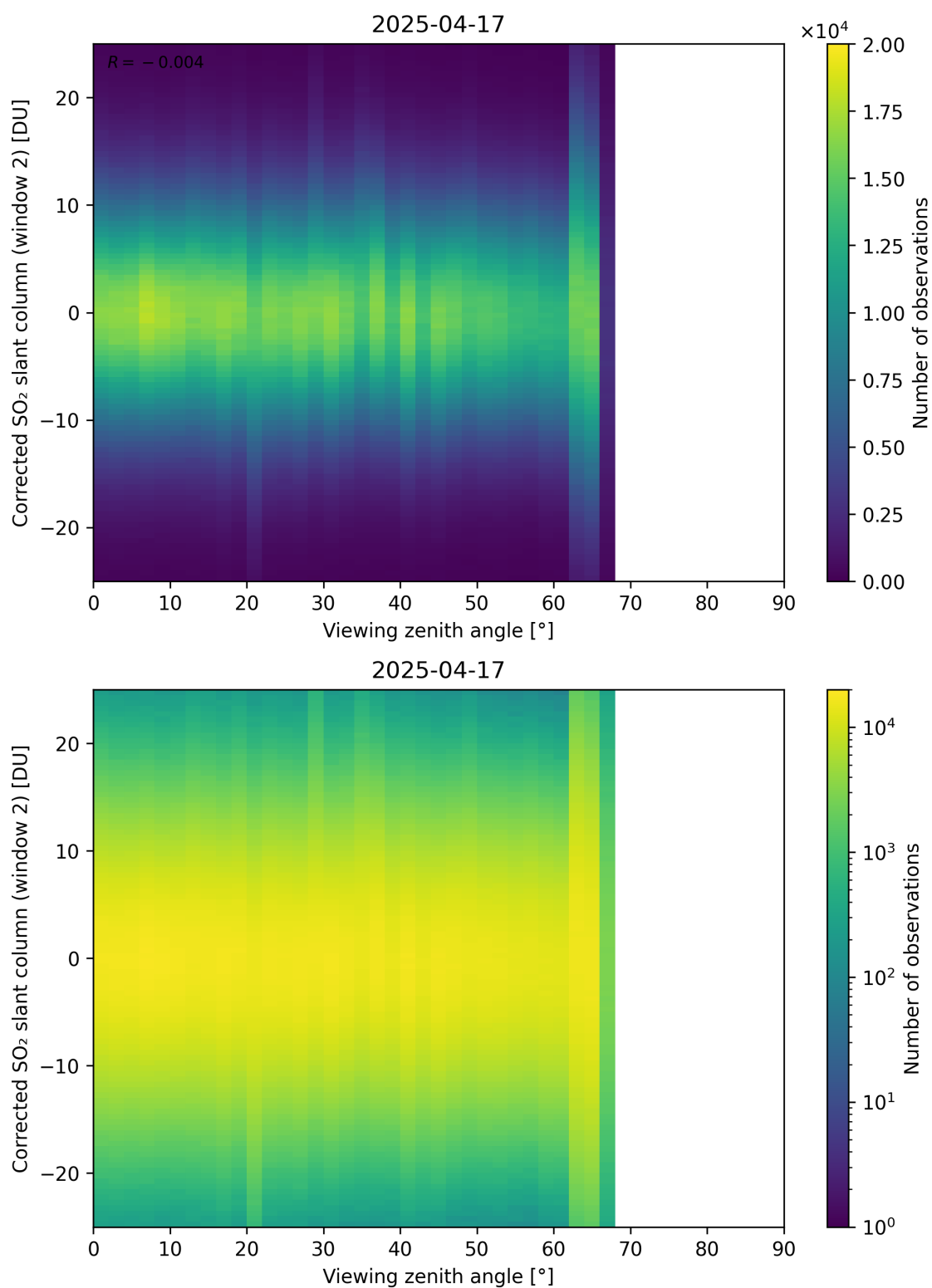
Figure 374: Scatter density plot of “Viewing zenith angle” against “Corrected SO 2 slant column (window 2)” for 2025-04-16 to 2025-04-18.
