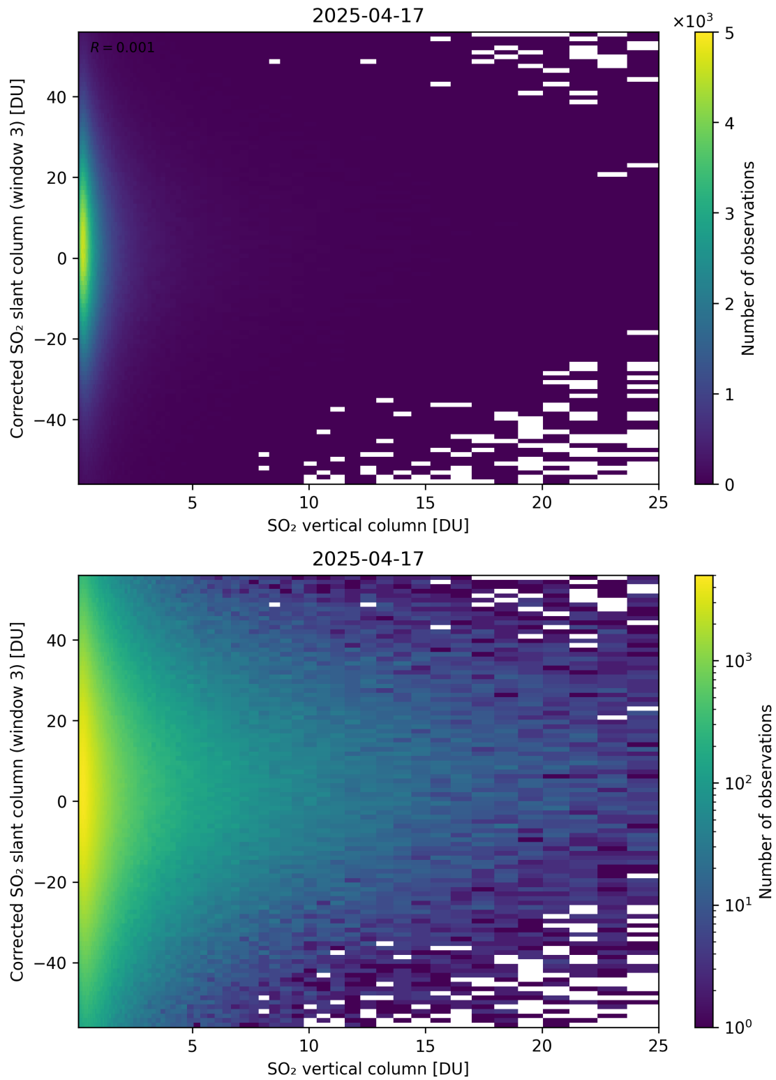
Figure 353: Scatter density plot of “SO 2 vertical column” against “Corrected SO 2 slant column (window 3)” for 2025-04-16 to 2025-04-18.
