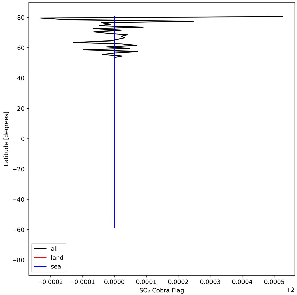
Figure 49: Zonal average of "SO 2 Cobra Flag" for 2025-04-16 to 2025-04-18.
