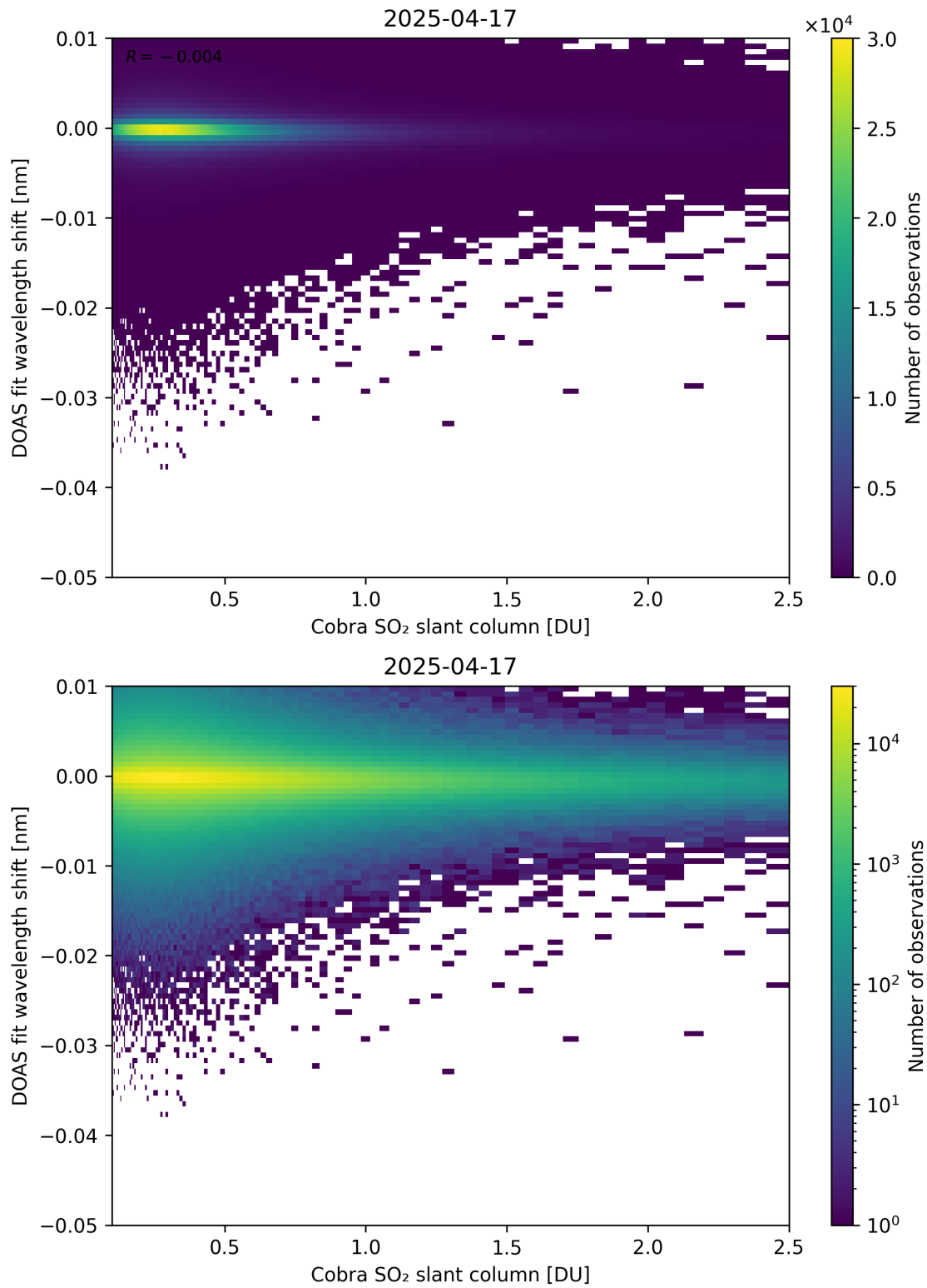
Figure 196: Scatter density plot of “Cobra SO 2 slant column” against “DOAS fit wavelength shift” for 2025-04-16 to 2025-04-18.
