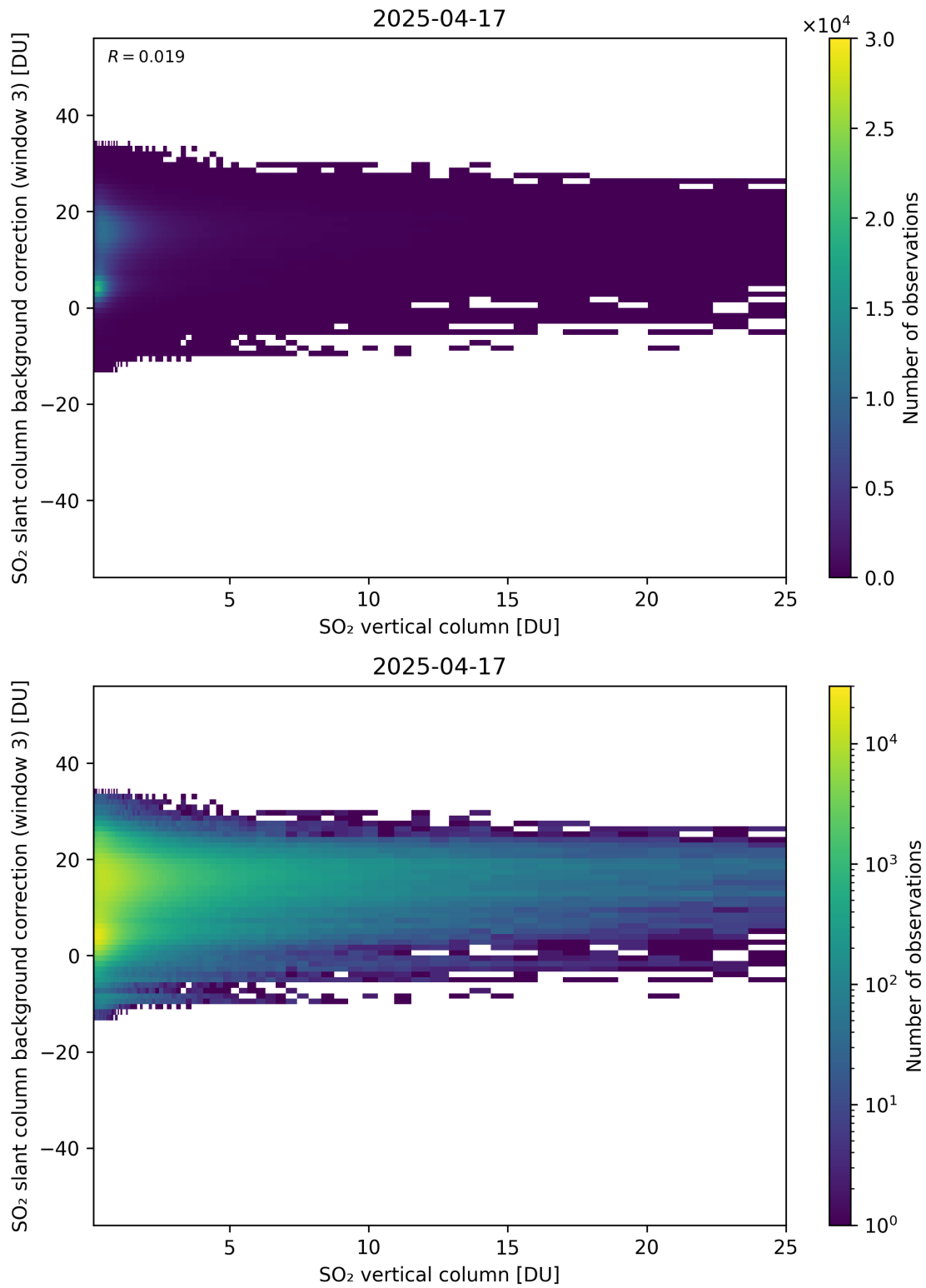
Figure 325: Scatter density plot of “SO 2 vertical column” against “SO 2 slant column background correction (window 3)” for 2025-04-16 to 2025-04-18.
