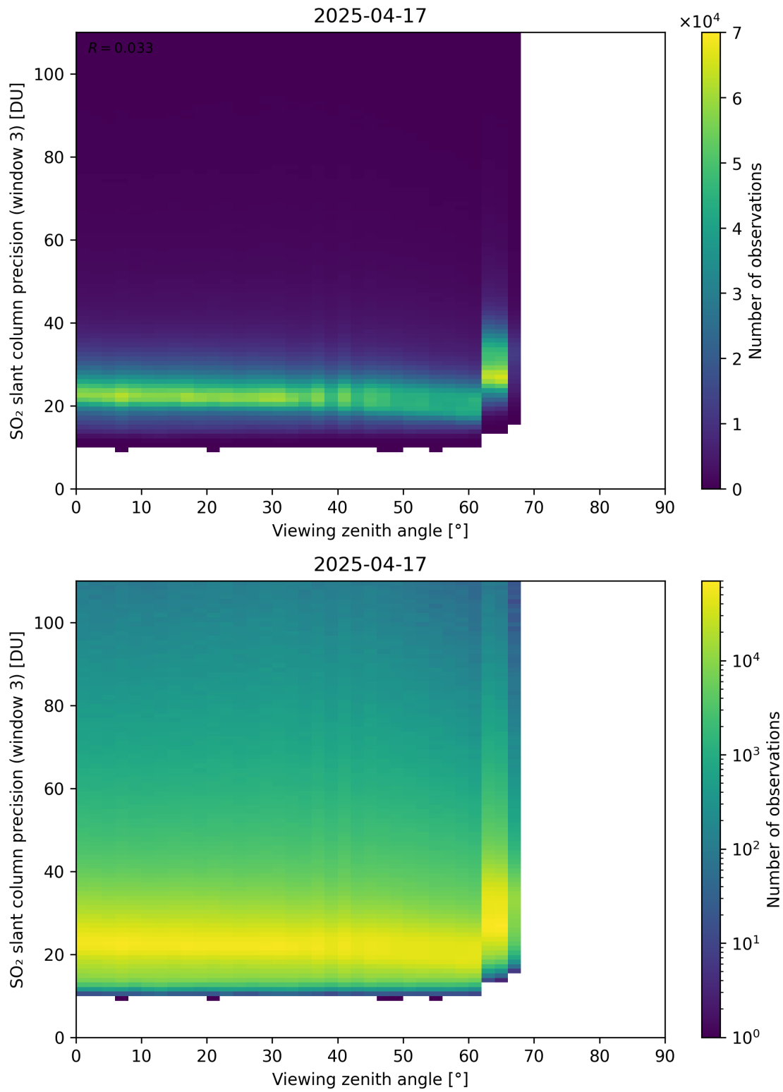
Figure 380: Scatter density plot of “Viewing zenith angle” against “SO 2 slant column precision (window 3)” for 2025-04-16 to 2025-04-18.
