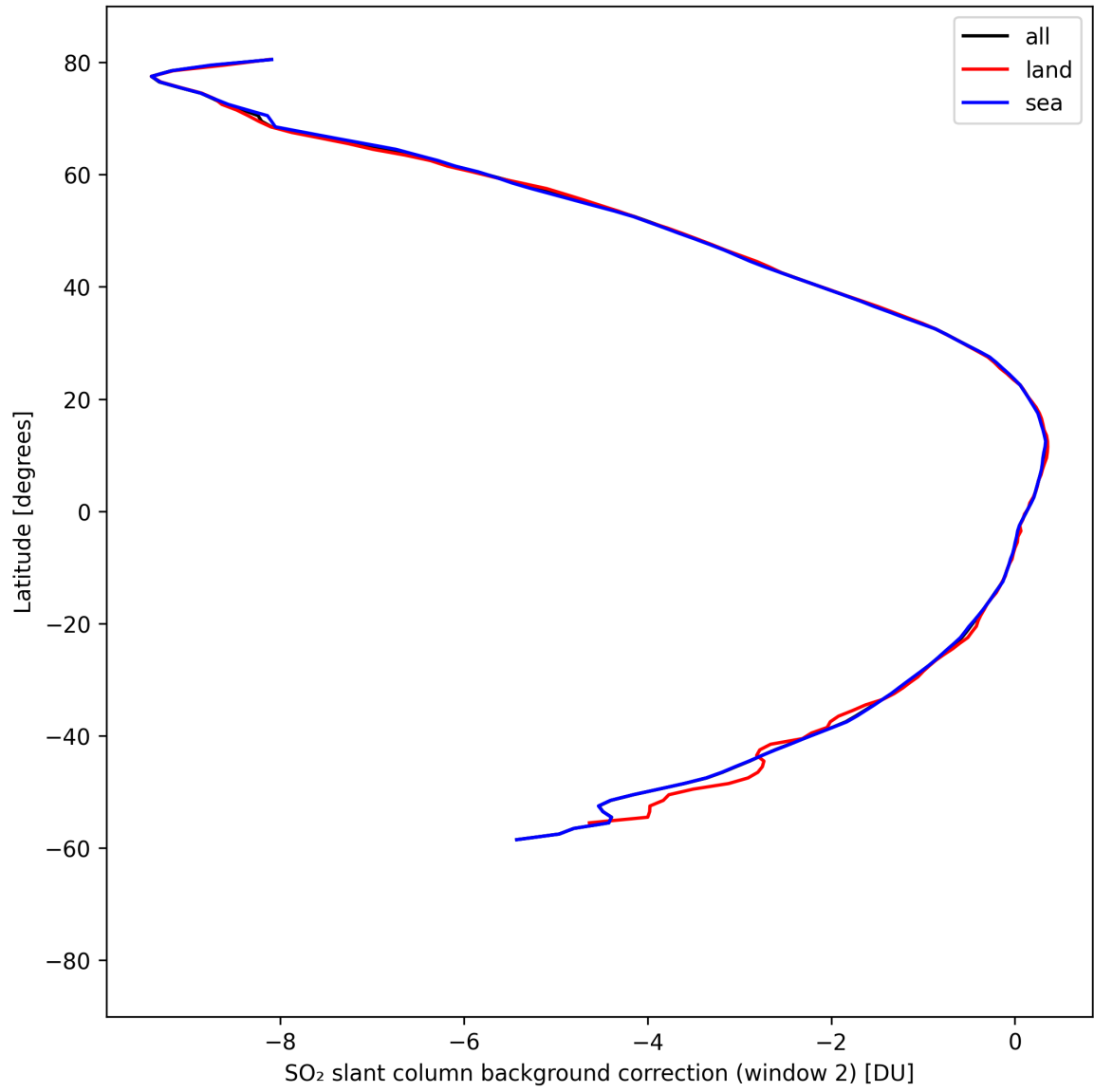
Figure 44: Zonal average of “SO 2 slant column background correction (window 2)” for 2025-04-16 to 2025-04-18.
