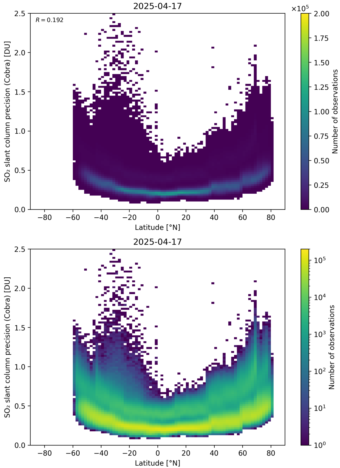
Figure 158: Scatter density plot of “Latitude” against “SO 2 slant column precision (Cobra)” for 2025-04-16 to 2025-04-18.
