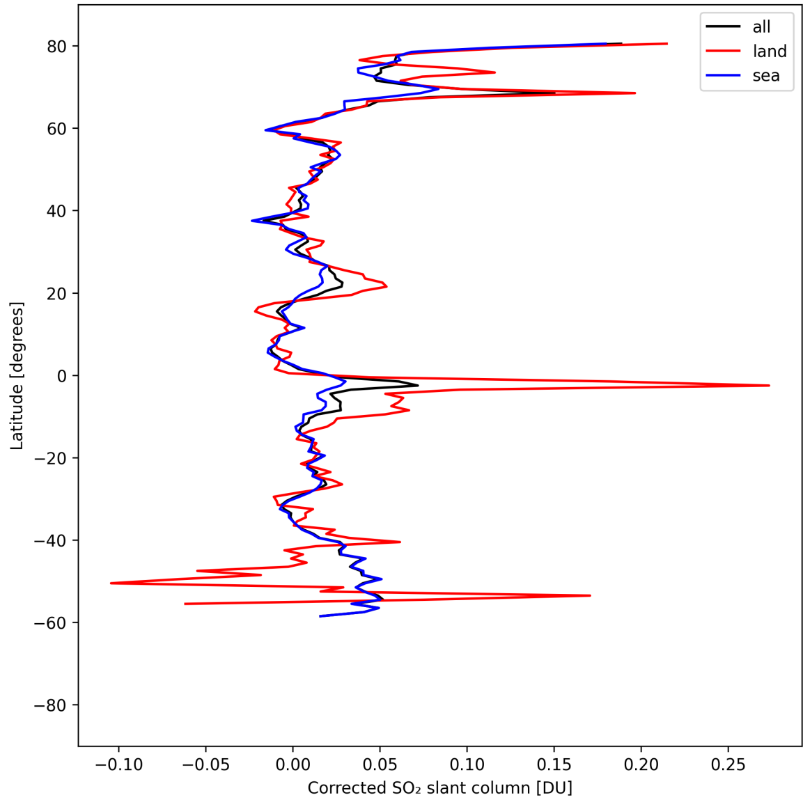
Figure 34: Zonal average of “Corrected SO 2 slant column” for 2025-04-16 to 2025-04-18.
