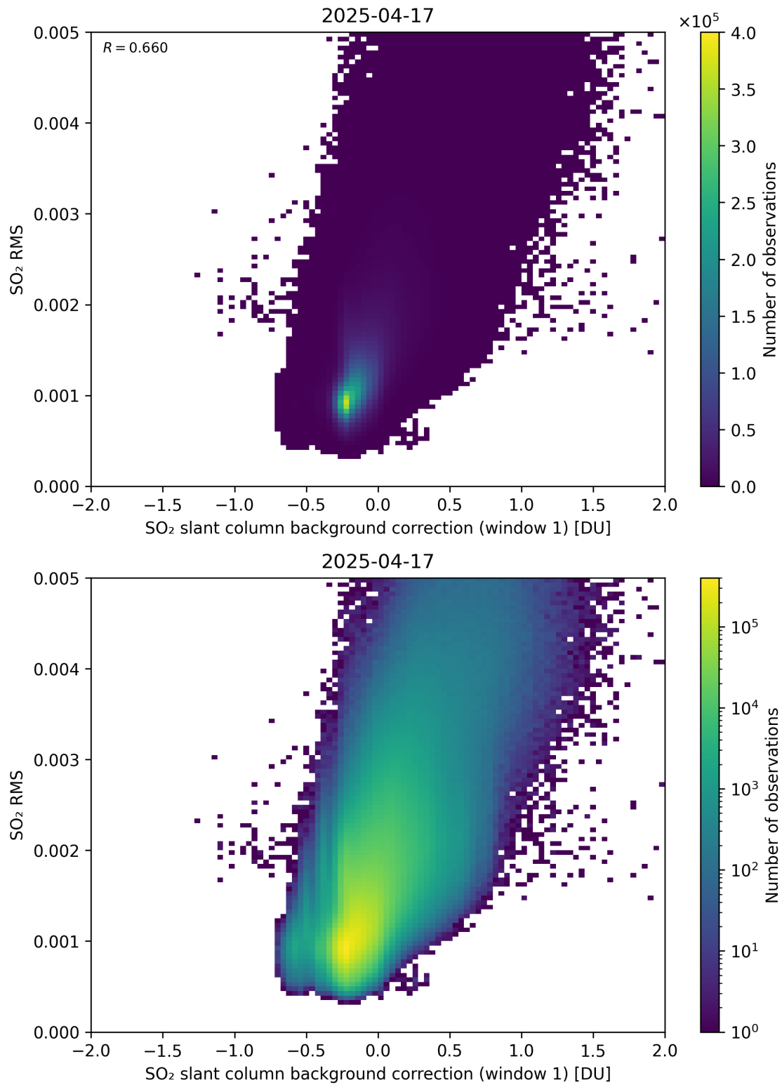
Figure 113: Scatter density plot of “SO 2 slant column background correction (window 1)” against “SO 2 RMS” for 2025-04-16 to 2025-04-18.
