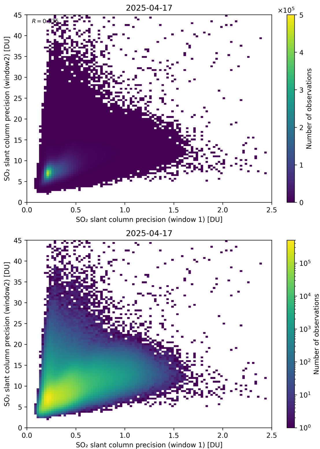
Figure 277: Scatter density plot of “SO 2 slant column precision (window 1)” against “SO 2 slant column precision (window2)” for 2025-04-16 to 2025-04-18.
