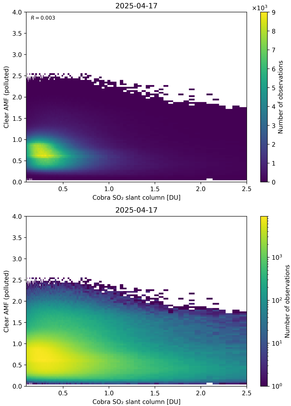
Figure 215: Scatter density plot of “Cobra SO 2 slant column” against “Clear AMF (polluted)” for 2025-04-16 to 2025-04-18.
