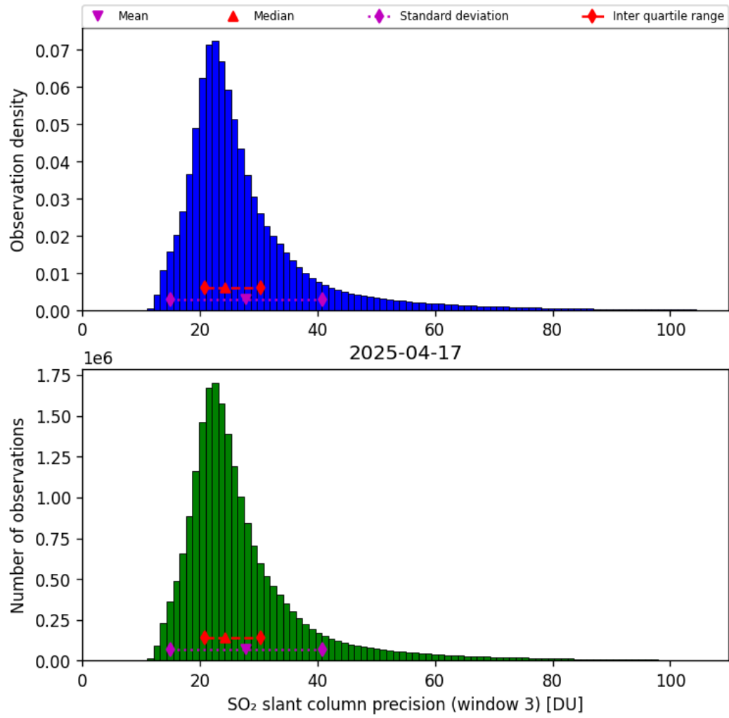
Figure 72: Histogram of “SO 2 slant column precision (window 3)” for 2025-04-16 to 2025-04-18
