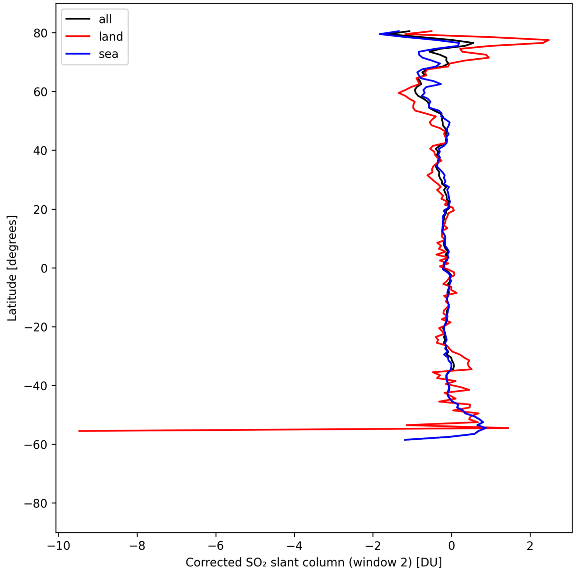
Figure 43: Zonal average of “Corrected SO 2 slant column (window 2)” for 2025-04-16 to 2025-04-18.
