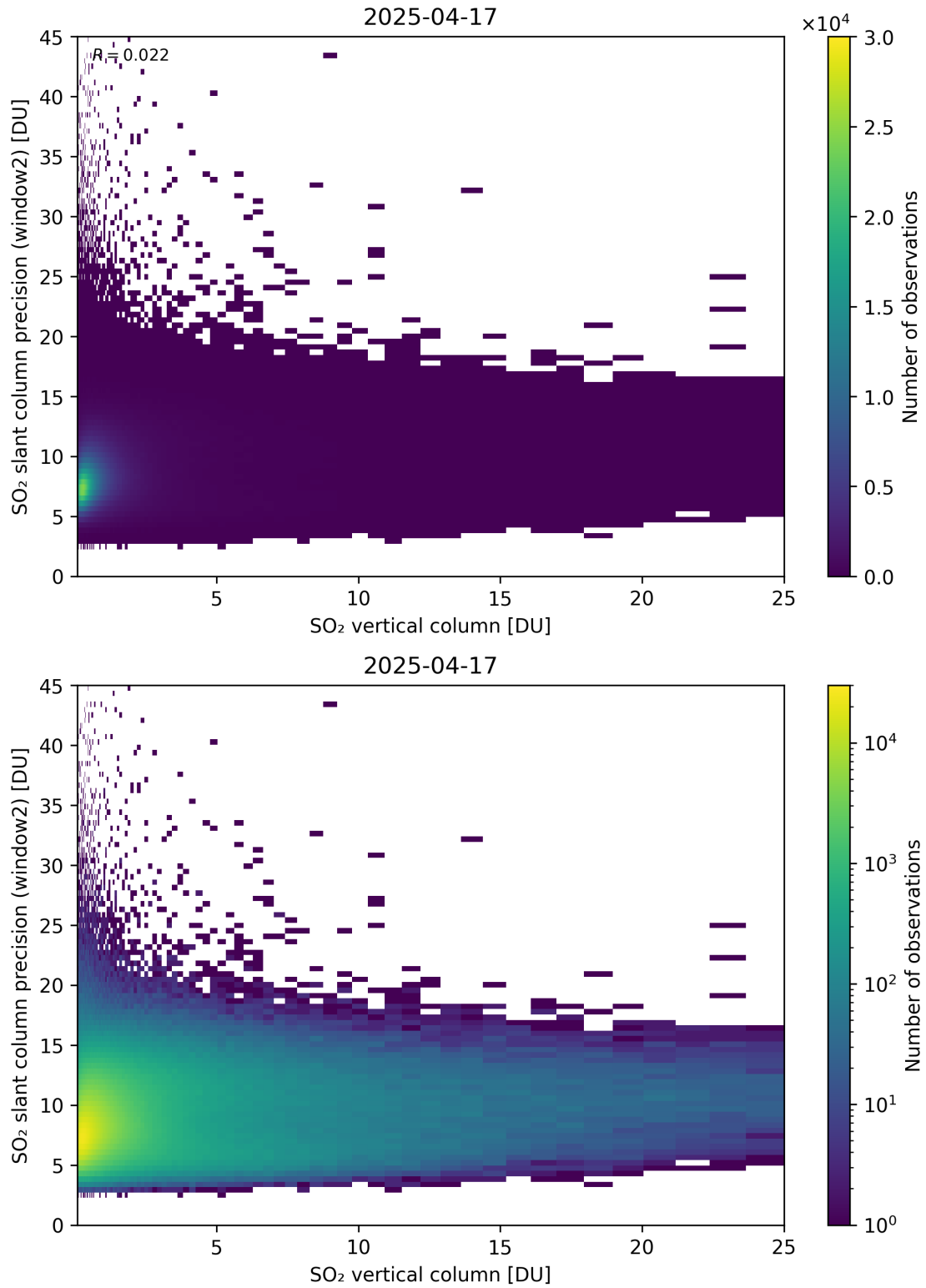
Figure 356: Scatter density plot of “SO 2 vertical column” against “SO 2 slant column precision (window2)” for 2025-04-16 to 2025-04-18.
