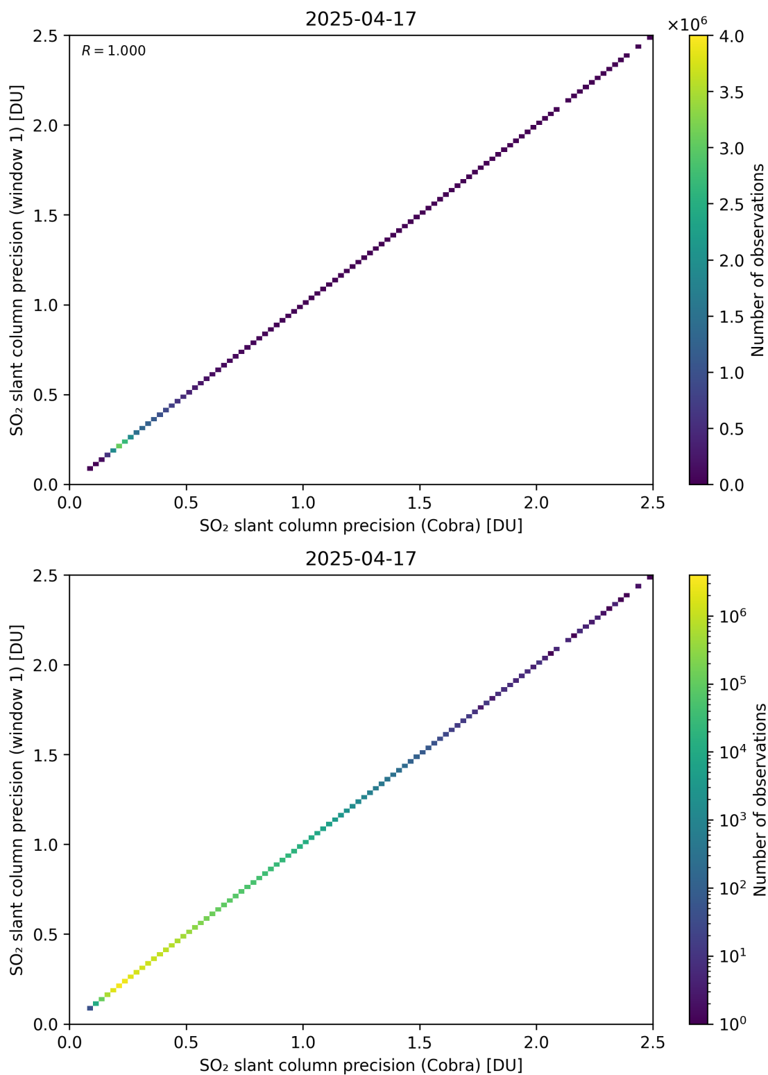
Figure 209: Scatter density plot of “SO 2 slant column precision (Cobra)” against “SO 2 slant column precision (window 1)” for 2025-04-16 to 2025-04-18.
