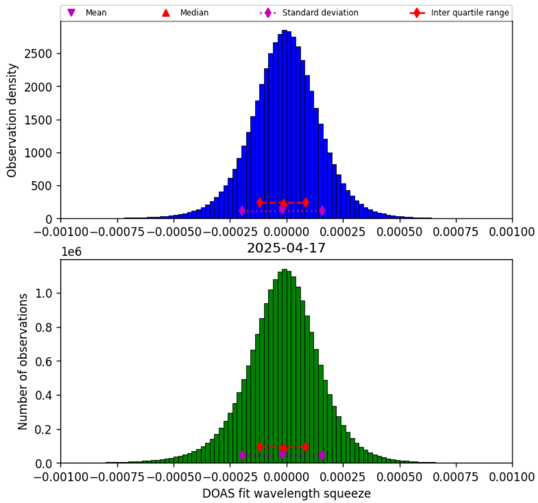
Figure 77: Histogram of “DOAS fit wavelength squeeze” for 2025-04-16 to 2025-04-18
