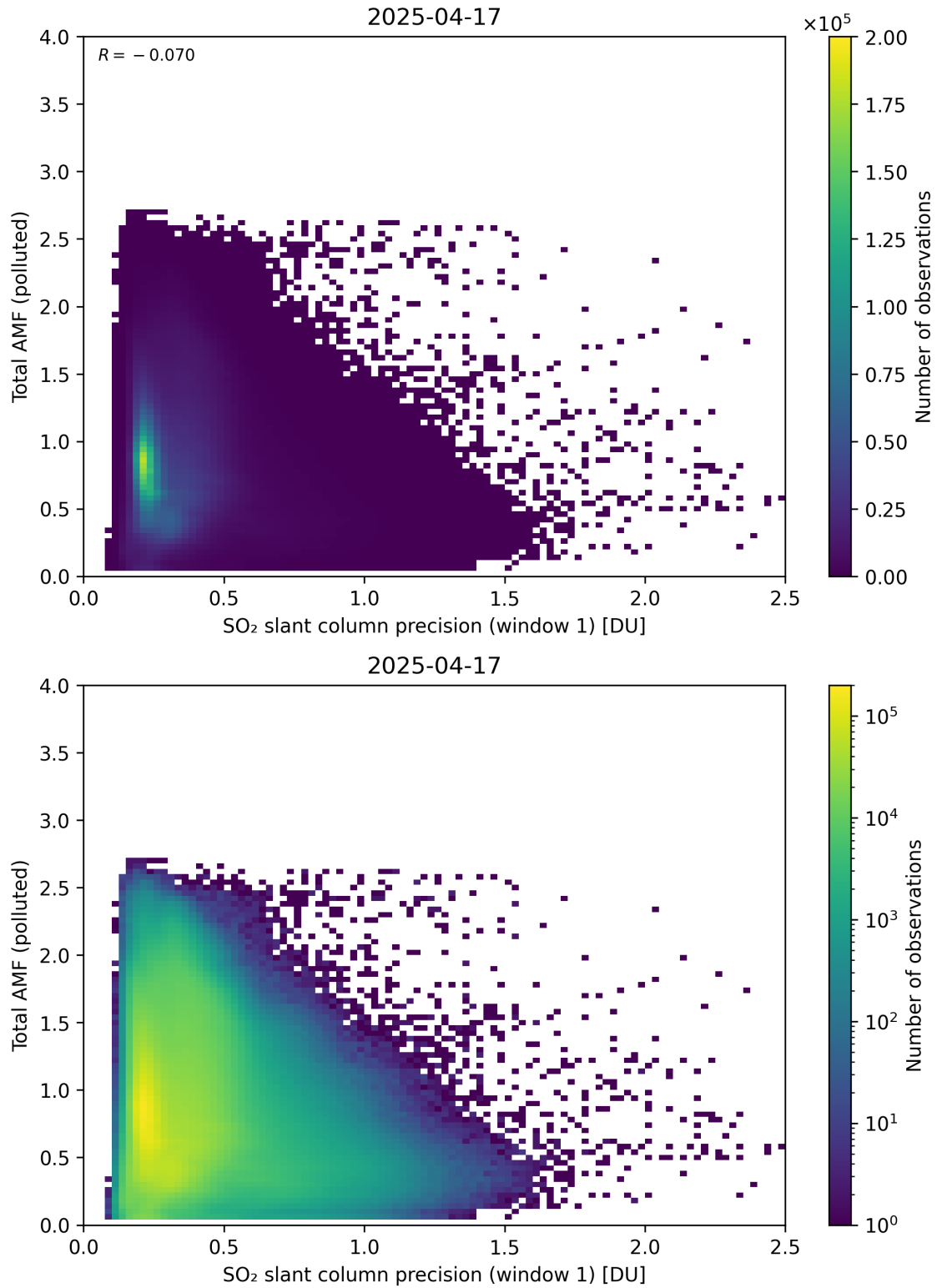
Figure 280: Scatter density plot of “SO 2 slant column precision (window 1)” against “Total AMF (polluted)” for 2025-04-16 to 2025-04-18.
