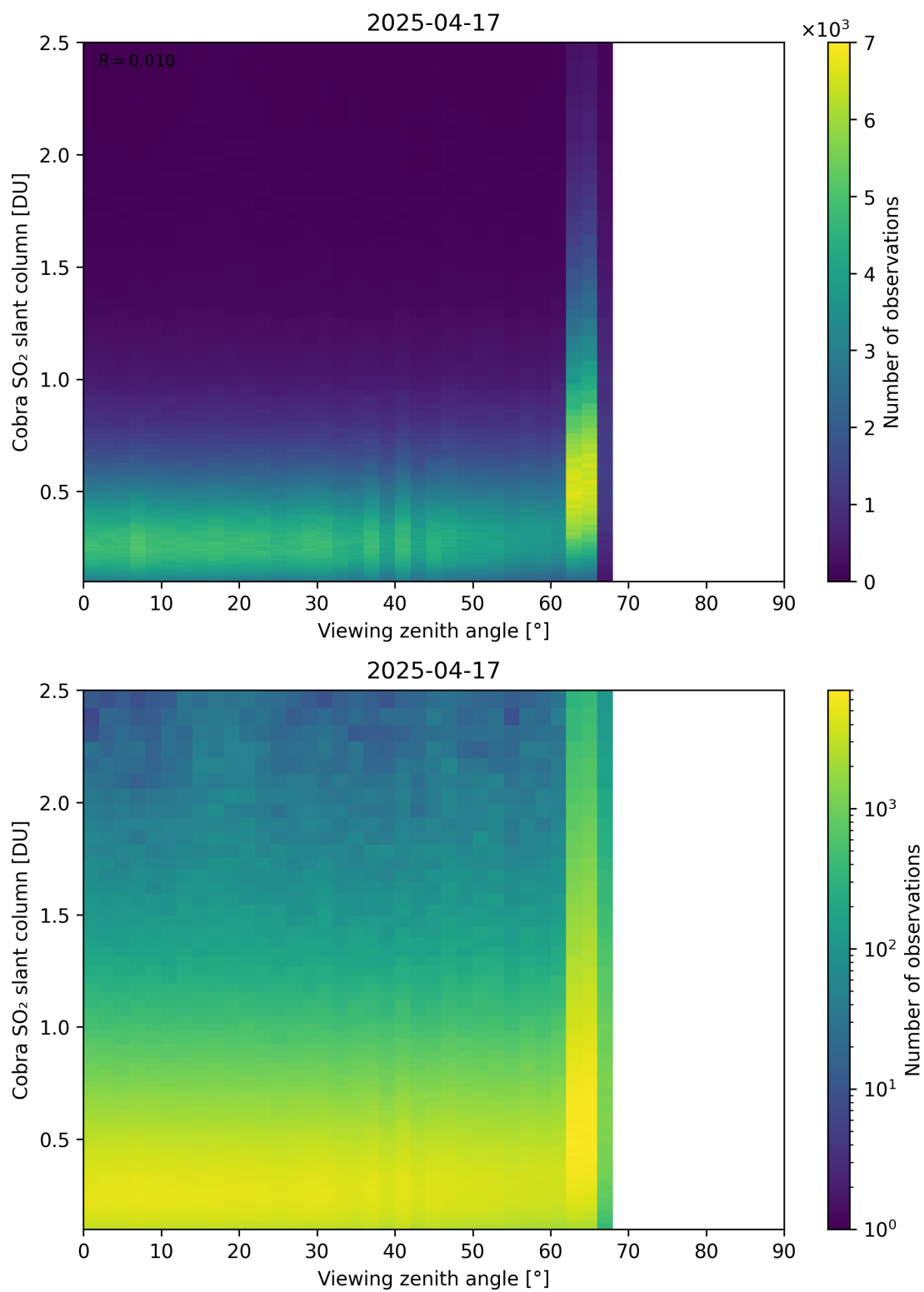
Figure 371: Scatter density plot of “Viewing zenith angle” against “Cobra SO 2 slant column” for 2025-04-16 to 2025-04-18.
