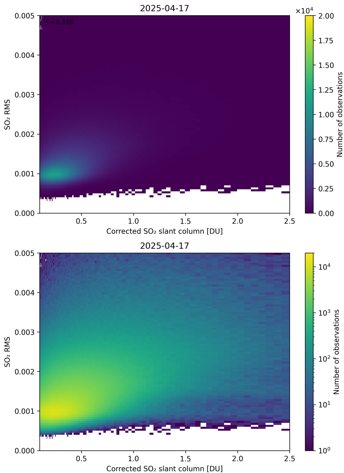
Figure 231: Scatter density plot of “Corrected SO 2 slant column” against “SO 2 RMS” for 2025-04-16 to 2025-04-18.
