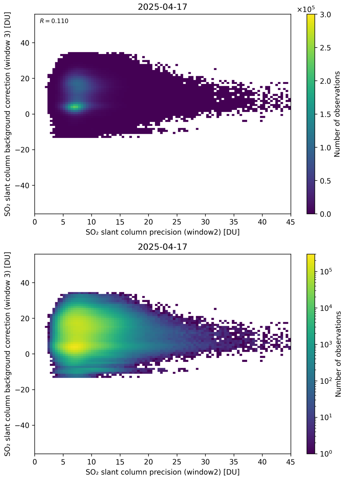
Figure 292: Scatter density plot of “SO 2 slant column precision (window2)” against “SO 2 slant column background correction (window 3)” for 2025-04-16 to 2025-04-18.
