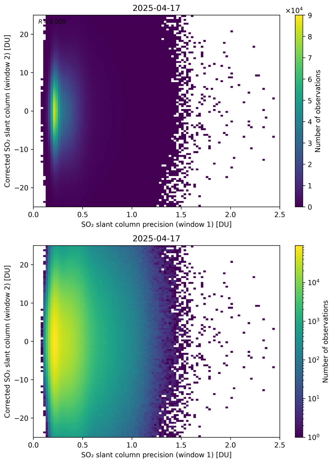
Figure 275: Scatter density plot of “SO 2 slant column precision (window 1)” against “Corrected SO 2 slant column (window 2)” for 2025-04-16 to 2025-04-18.
