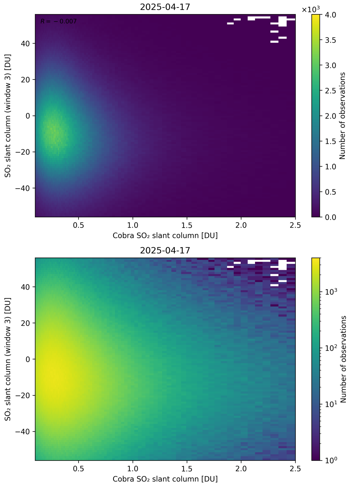
Figure 222: Scatter density plot of “Cobra SO 2 slant column” against “SO 2 slant column (window 3)” for 2025-04-16 to 2025-04-18.
