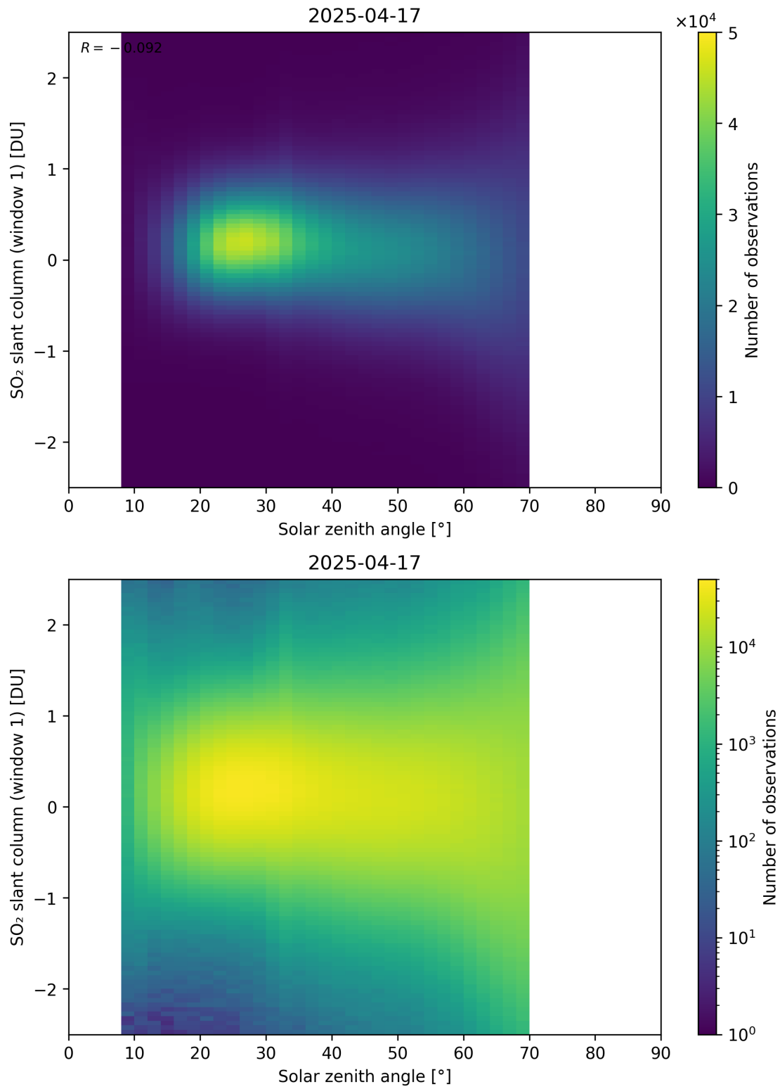
Figure 184: Scatter density plot of “Solar zenith angle” against “SO 2 slant column (window 1)” for 2025-04-16 to 2025-04-18.
