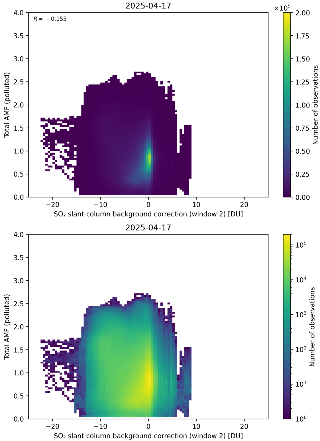
Figure 130: Scatter density plot of “SO 2 slant column background correction (window 2)” against “Total AMF (polluted)” for 2025-04-16 to 2025-04-18.
