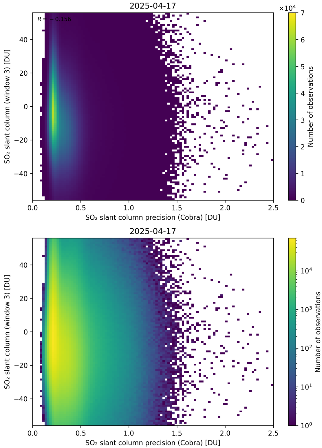
Figure 211: Scatter density plot of “SO 2 slant column precision (Cobra)” against “SO 2 slant column (window 3)” for 2025-04-16 to 2025-04-18.
