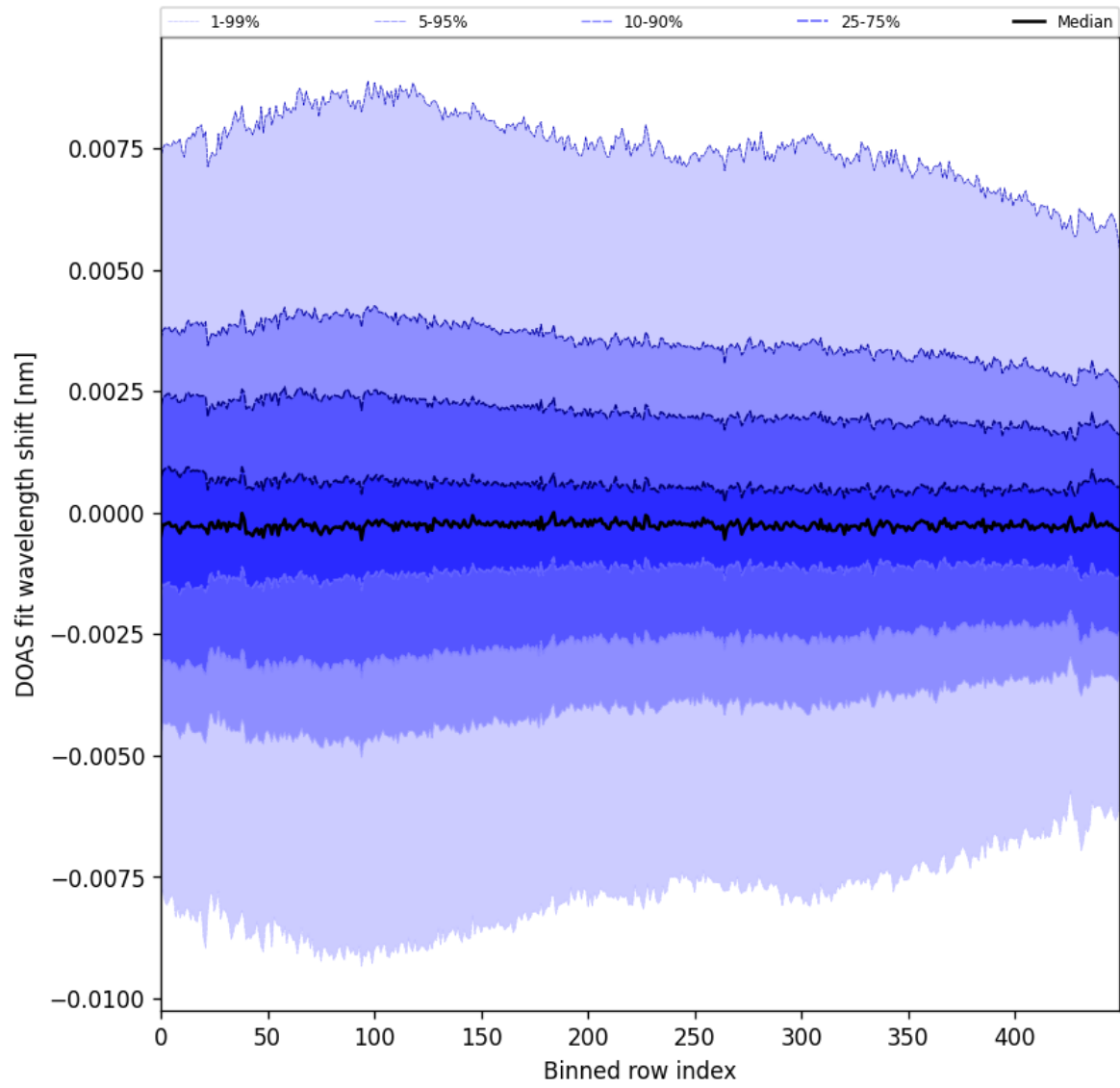
Figure 102: Along track statistics of “DOAS fit wavelength shift” for 2025-04-16 to 2025-04-18
