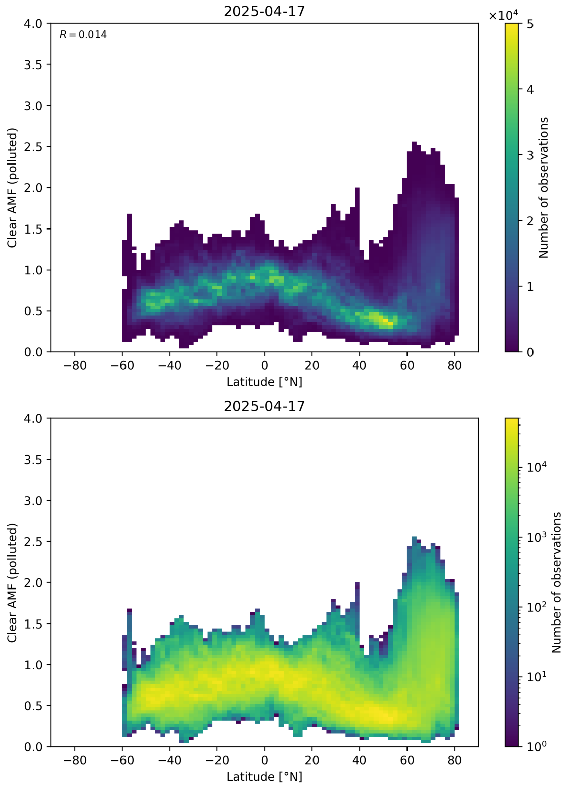
Figure 156: Scatter density plot of “Latitude” against “Clear AMF (polluted)” for 2025-04-16 to 2025-04-18.
