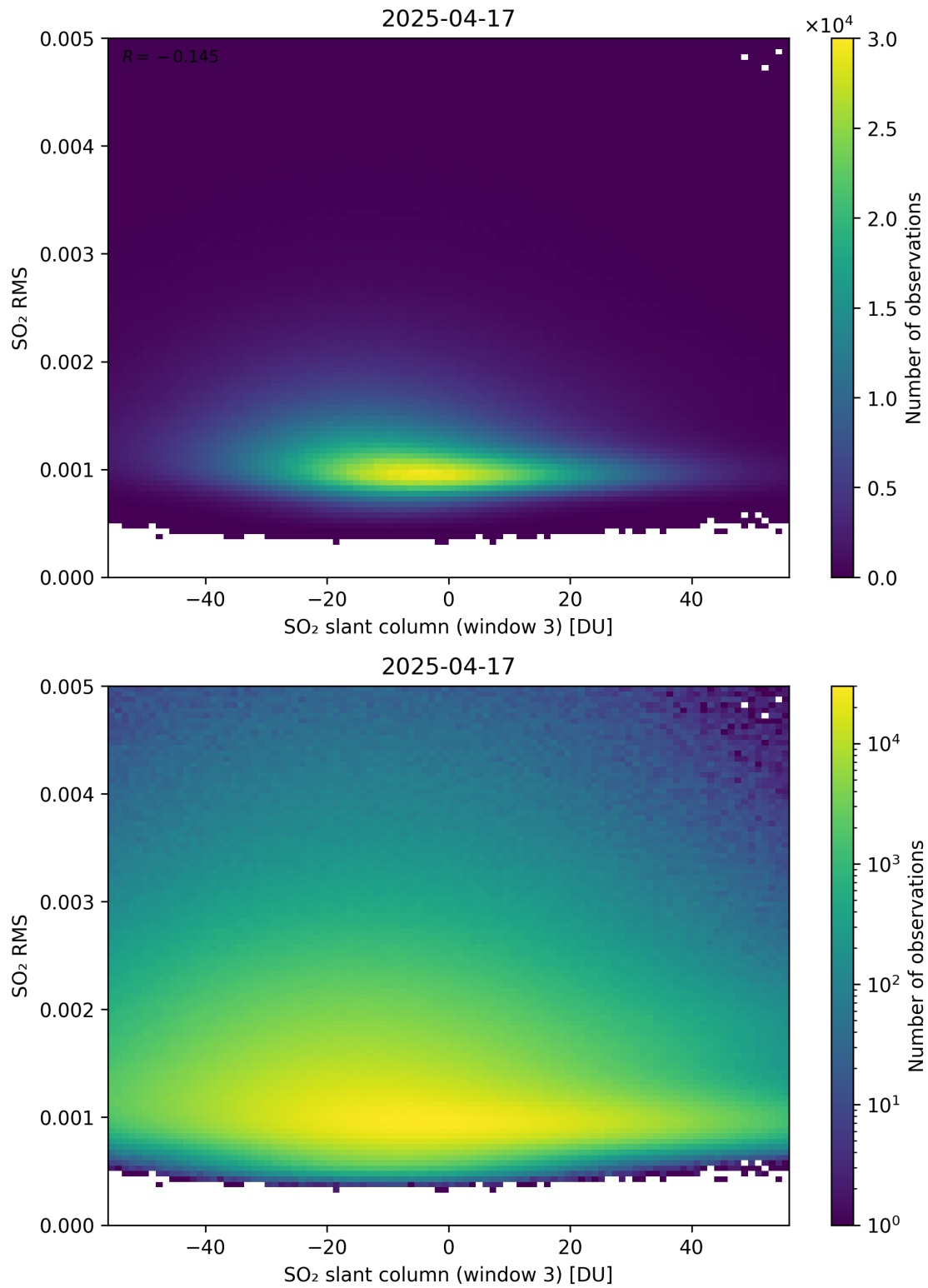
Figure 306: Scatter density plot of “SO 2 slant column (window 3)” against “SO 2 RMS” for 2025-04-16 to 2025-04-18.
