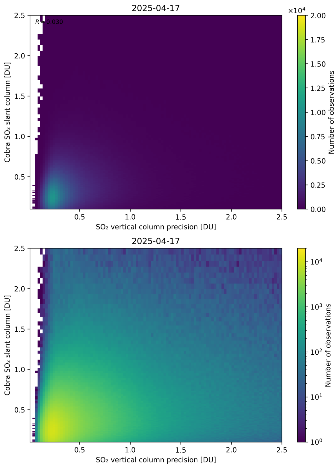
Figure 336: Scatter density plot of “SO 2 vertical column precision” against “Cobra SO 2 slant column” for 2025-04-16 to 2025-04-18.
