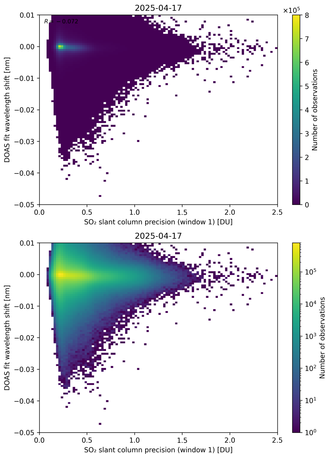
Figure 271: Scatter density plot of “SO 2 slant column precision (window 1)” against “DOAS fit wavelength shift” for 2025-04-16 to 2025-04-18.
