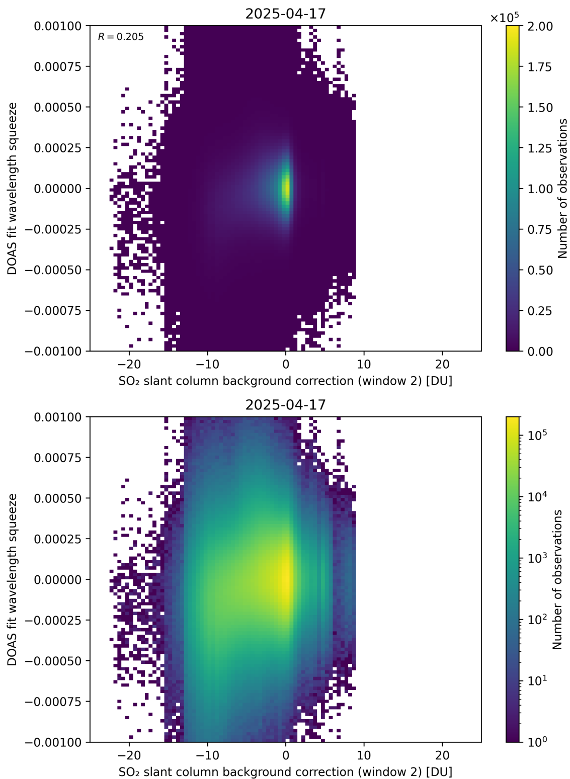
Figure 124: Scatter density plot of “SO 2 slant column background correction (window 2)” against “DOAS fit wavelength squeeze” for 2025-04-16 to 2025-04-18.
