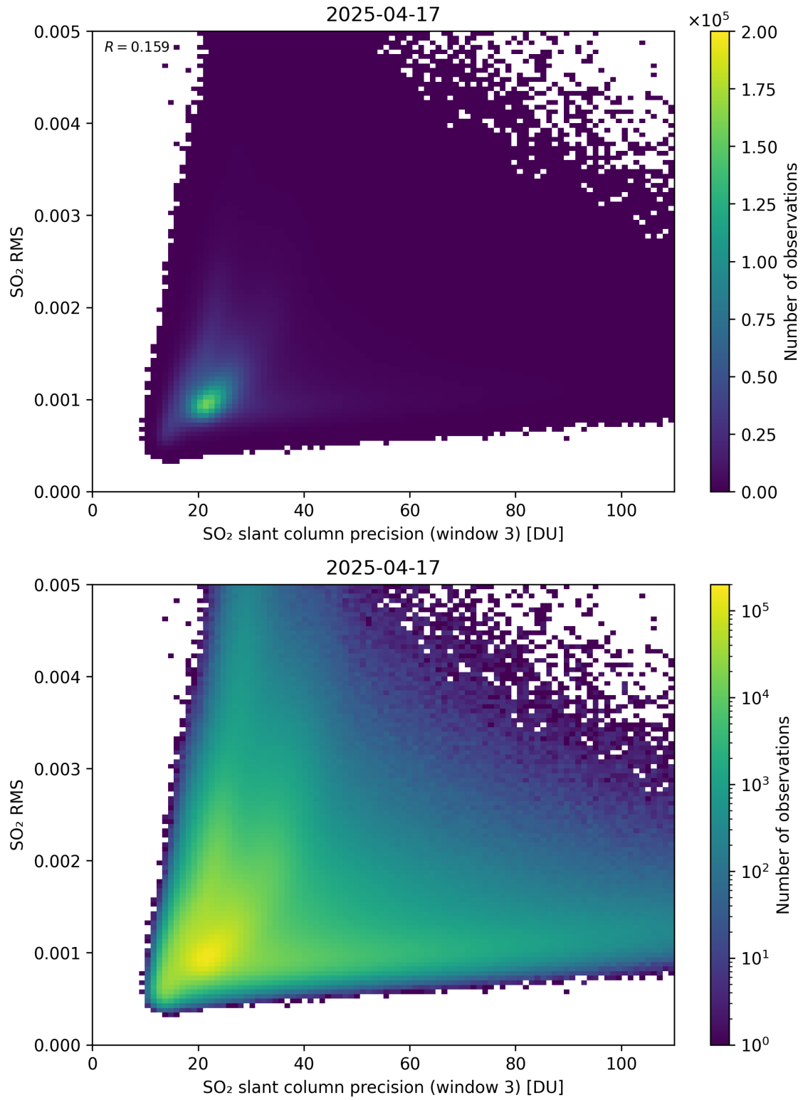
Figure 310: Scatter density plot of “SO 2 slant column precision (window 3)” against “SO 2 RMS” for 2025-04-16 to 2025-04-18.
