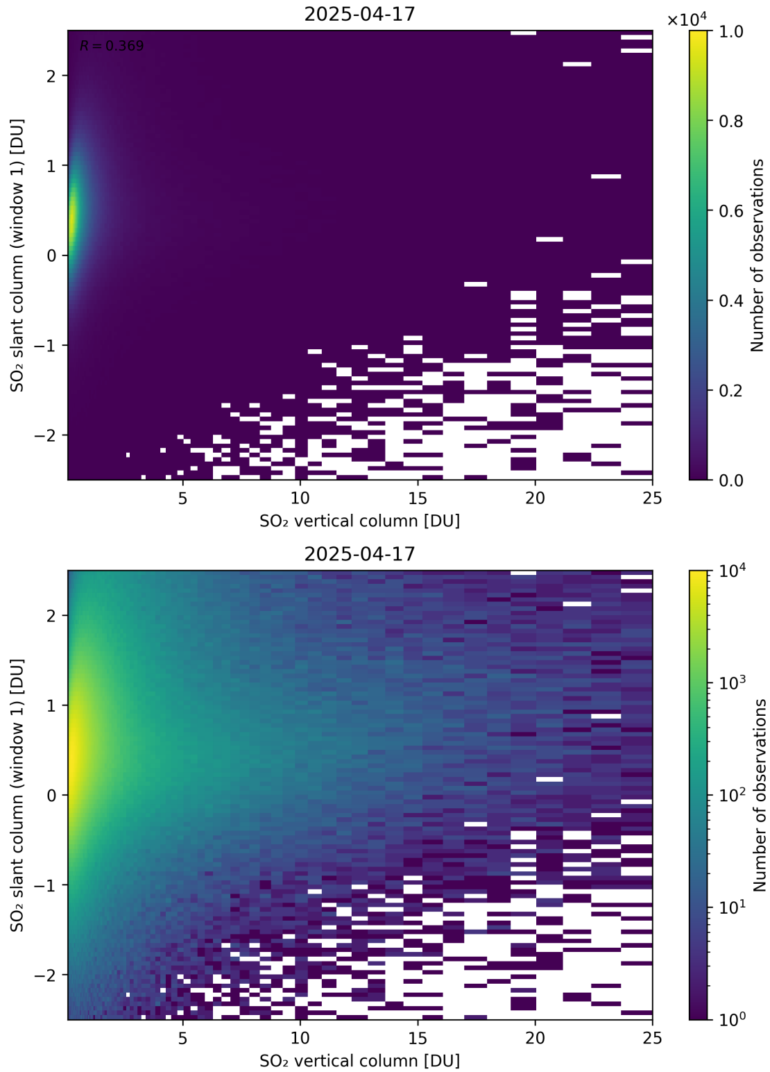
Figure 354: Scatter density plot of “SO 2 vertical column” against “SO 2 slant column (window 1)” for 2025-04-16 to 2025-04-18.
