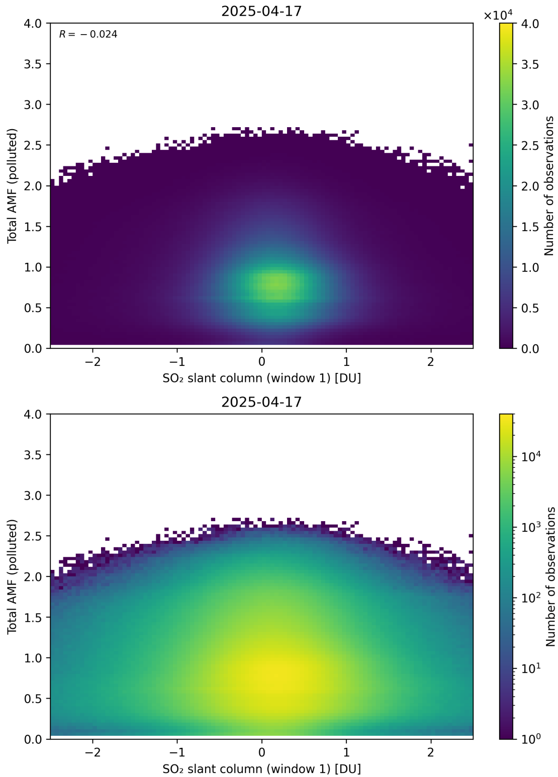
Figure 289: Scatter density plot of “SO 2 slant column (window 1)” against “Total AMF (polluted)” for 2025-04-16 to 2025-04-18.
