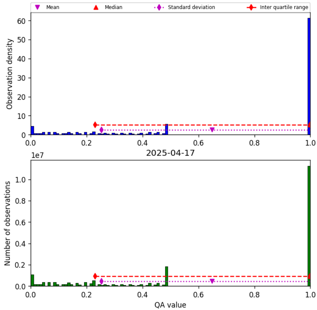
Figure 57: Histogram of “QA value” for 2025-04-16 to 2025-04-18
