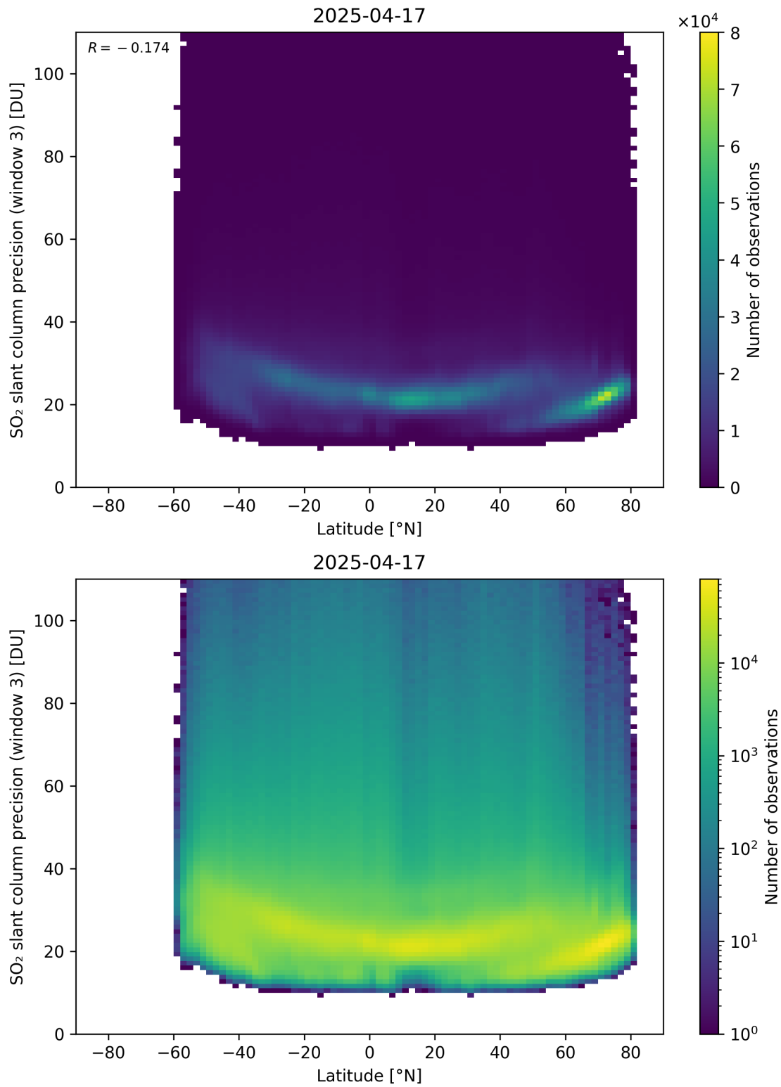
Figure 166: Scatter density plot of “Latitude” against “SO 2 slant column precision (window 3)” for 2025-04-16 to 2025-04-18.
