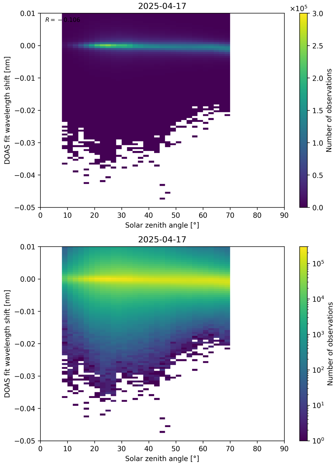
Figure 174: Scatter density plot of “Solar zenith angle” against “DOAS fit wavelength shift” for 2025-04-16 to 2025-04-18.
