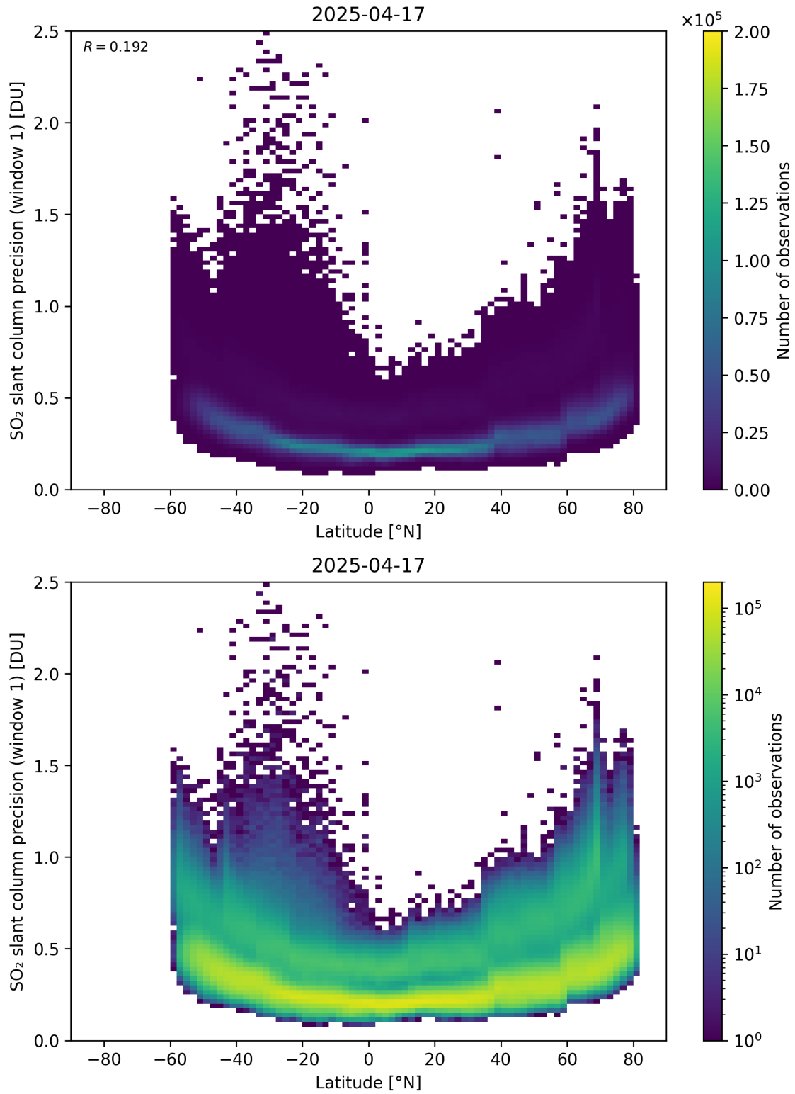
Figure 163: Scatter density plot of “Latitude” against “SO 2 slant column precision (window 1)” for 2025-04-16 to 2025-04-18.
