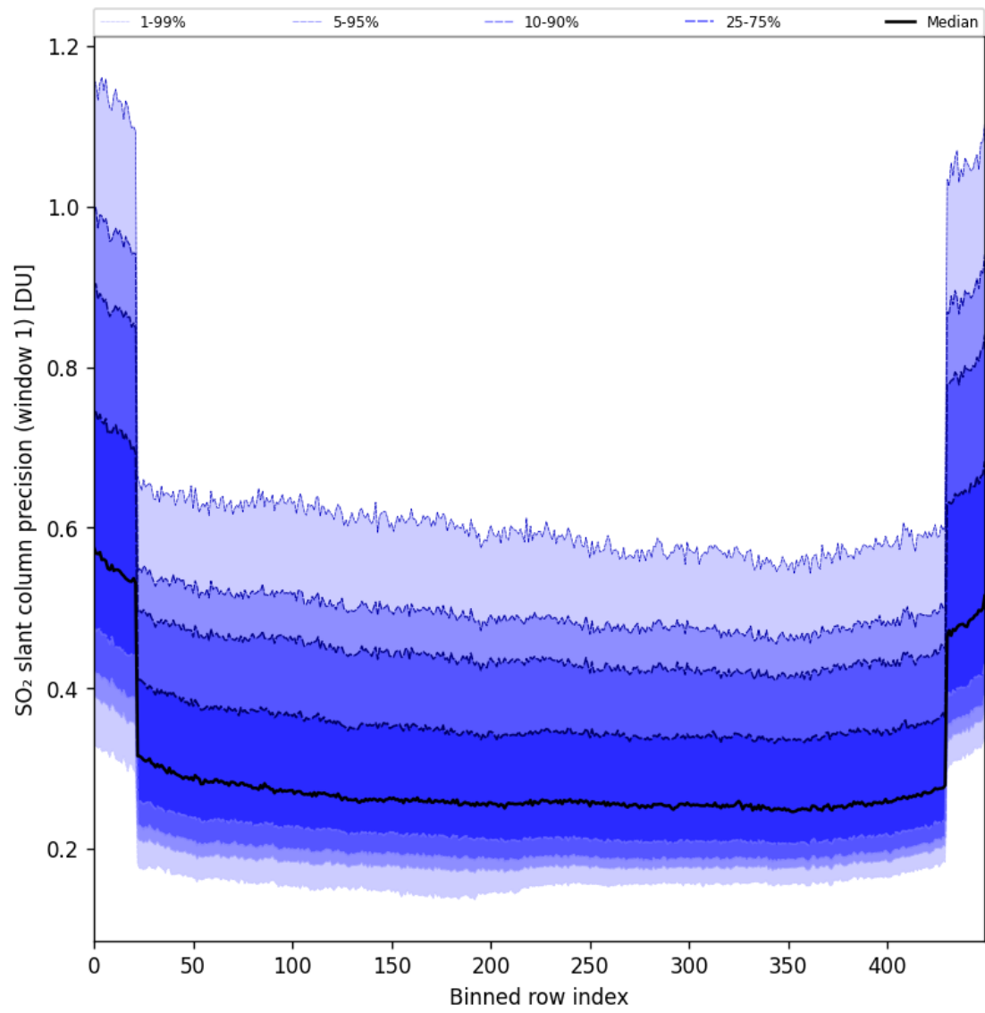
Figure 90: Along track statistics of “SO 2 slant column precision (window 1)” for 2025-04-16 to 2025-04-18
