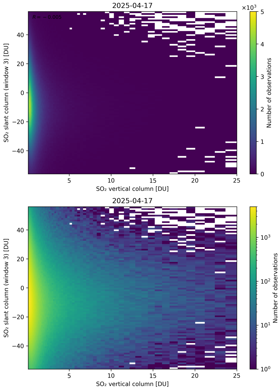
Figure 357: Scatter density plot of “SO 2 vertical column” against “SO 2 slant column (window 3)” for 2025-04-16 to 2025-04-18.
