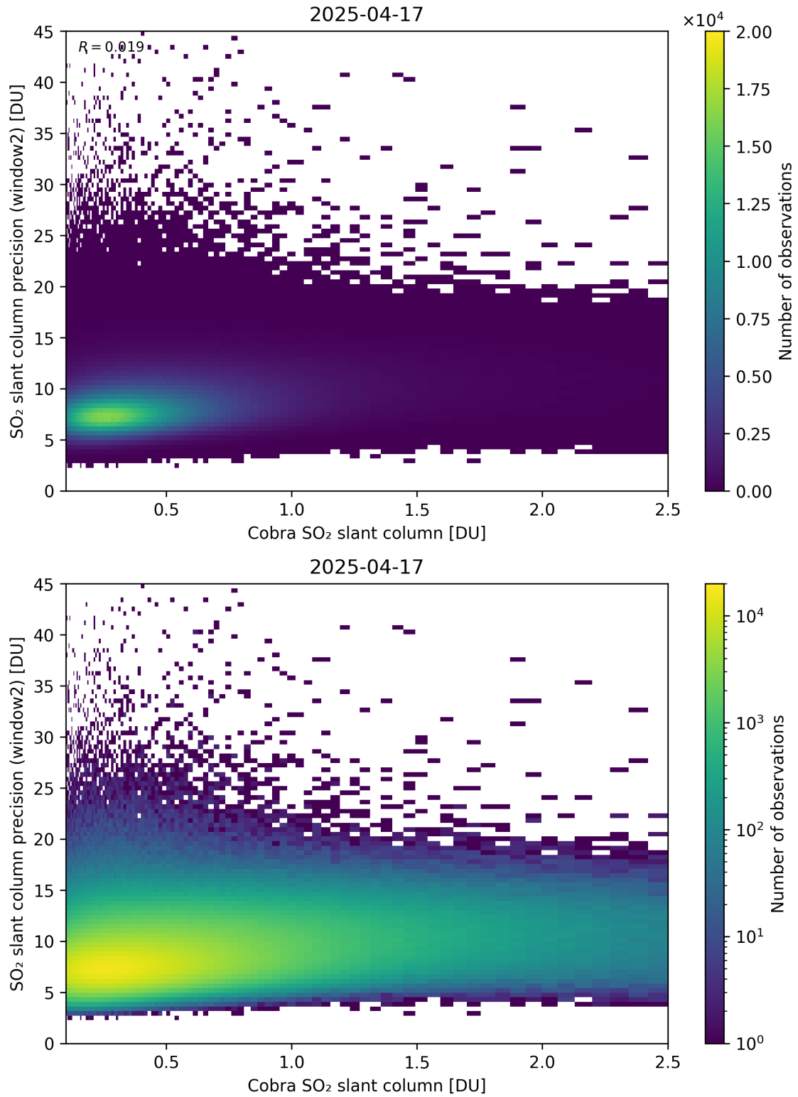
Figure 221: Scatter density plot of “Cobra SO 2 slant column” against “SO 2 slant column precision (window2)” for 2025-04-16 to 2025-04-18.
