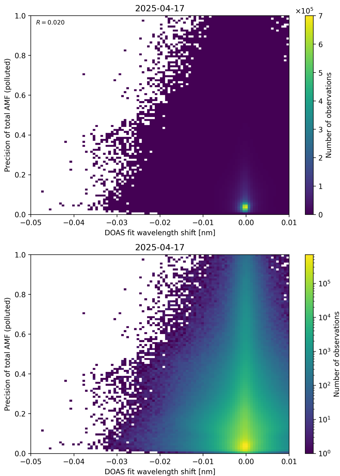
Figure 142: Scatter density plot of “DOAS fit wavelength shift” against “Precision of total AMF (polluted)” for 2025-04-16 to 2025-04-18.
