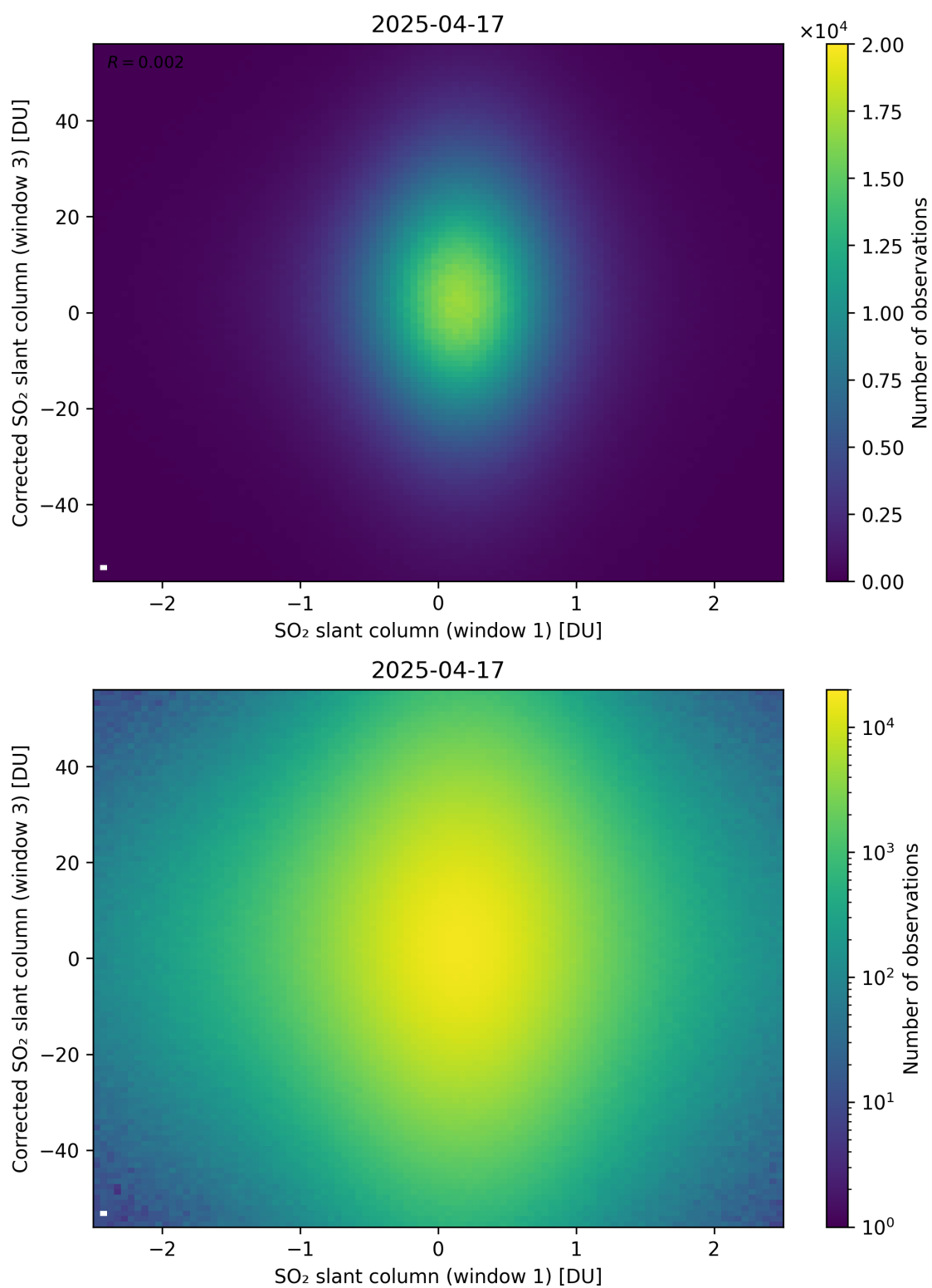
Figure 284: Scatter density plot of “SO 2 slant column (window 1)” against “Corrected SO 2 slant column (window 3)” for 2025-04-16 to 2025-04-18.
