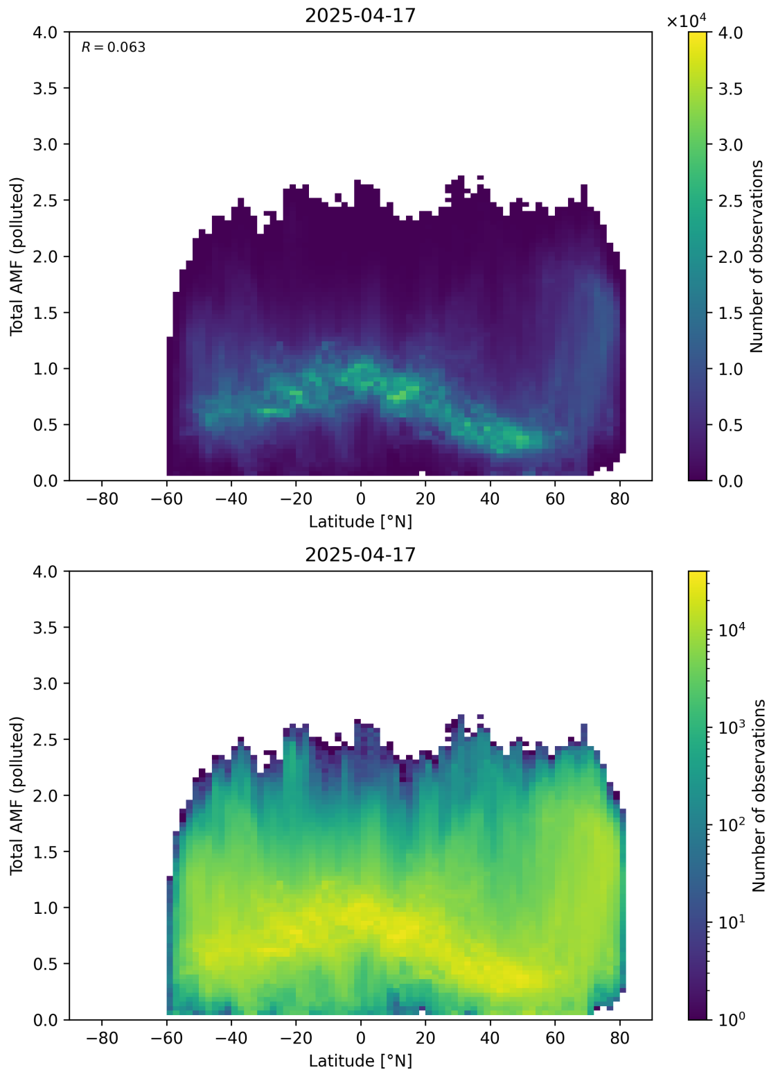
Figure 167: Scatter density plot of “Latitude” against “Total AMF (polluted)” for 2025-04-16 to 2025-04-18.
