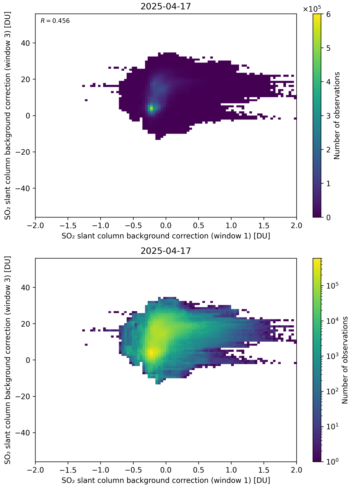
Figure 110: Scatter density plot of “SO 2 slant column background correction (window 1)” against “SO 2 slant column background correction (window 3)” for 2025-04-16 to 2025-04-18.
