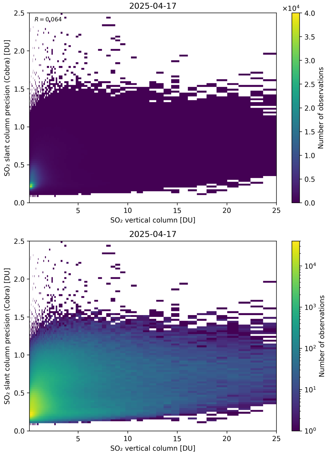
Figure 350: Scatter density plot of “SO 2 vertical column” against “SO 2 slant column precision (Cobra)” for 2025-04-16 to 2025-04-18.
