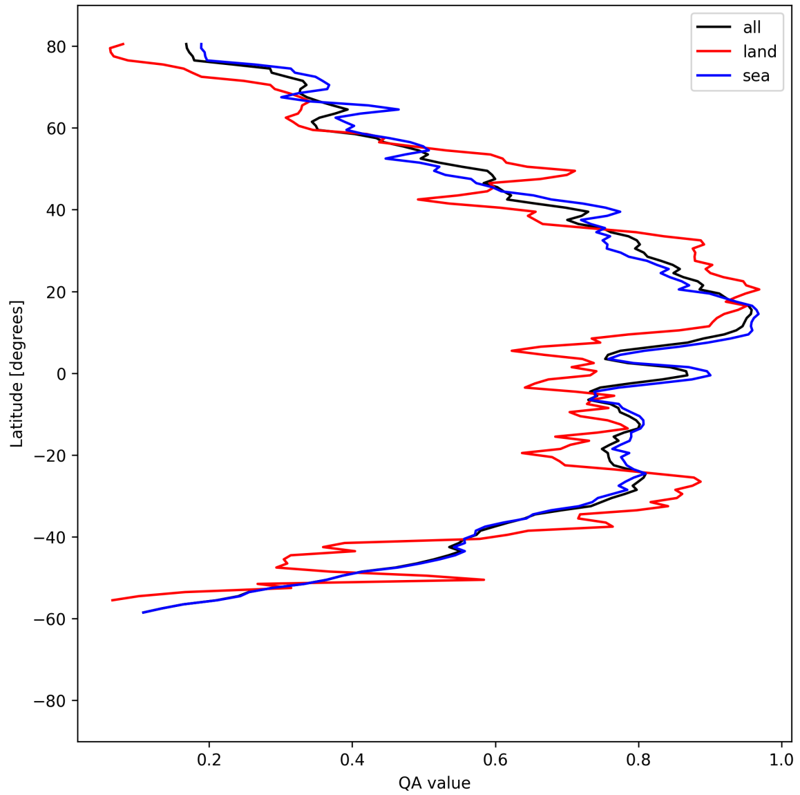
Figure 31: Zonal average of “QA value” for 2025-04-16 to 2025-04-18.
