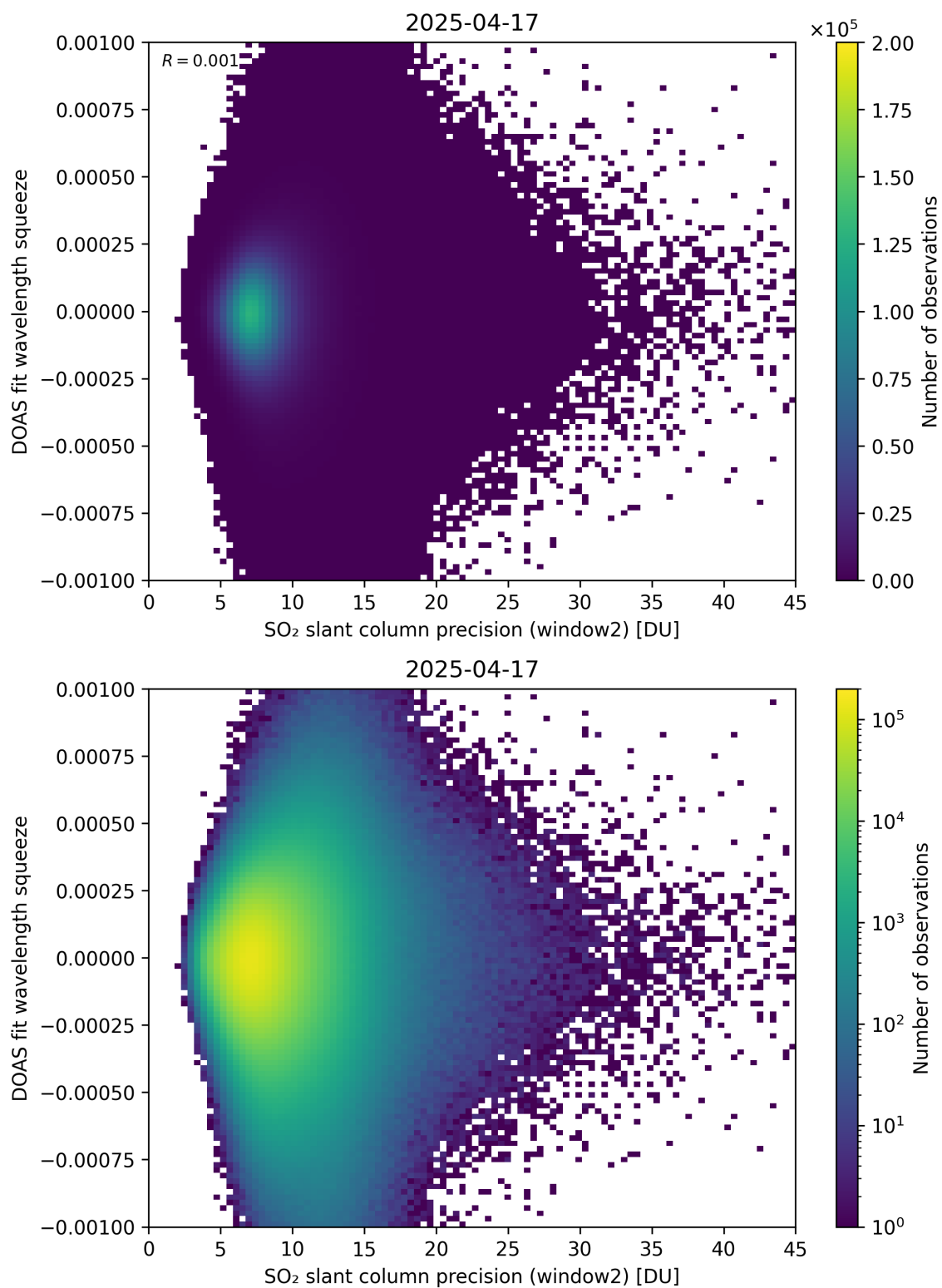
Figure 294: Scatter density plot of “SO 2 slant column precision (window2)” against “DOAS fit wavelength squeeze” for 2025-04-16 to 2025-04-18.
