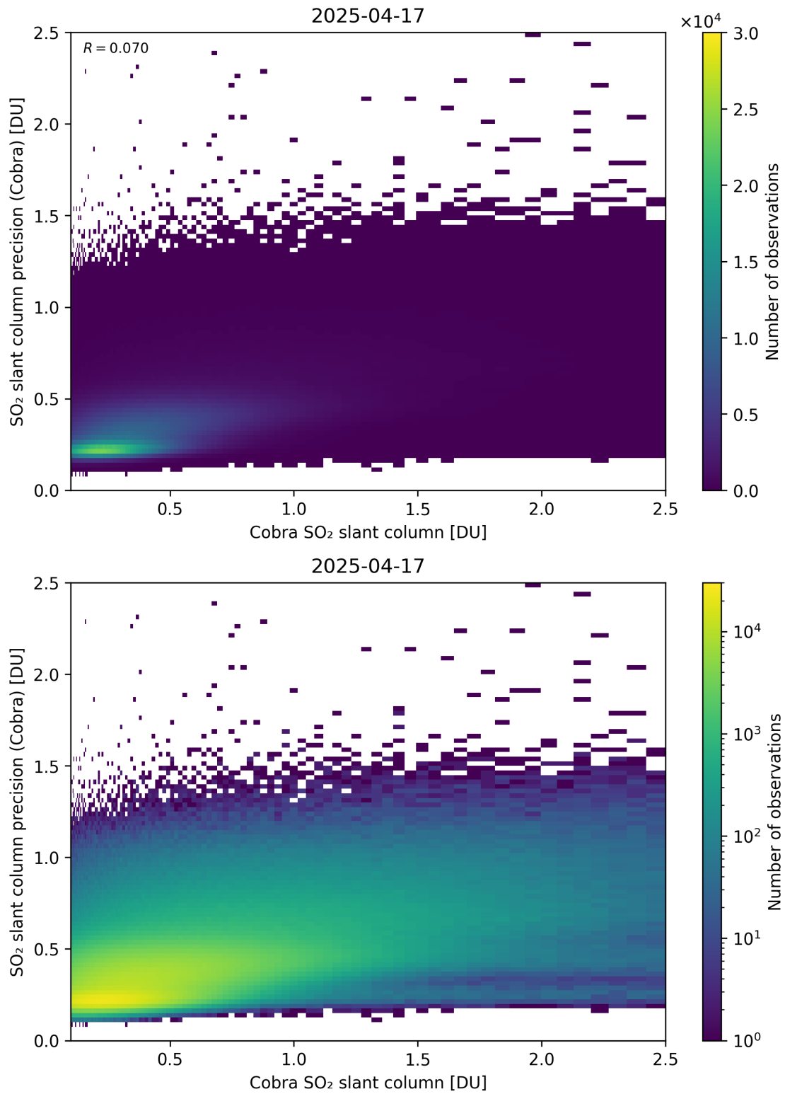
Figure 216: Scatter density plot of “Cobra SO 2 slant column” against “SO 2 slant column precision (Cobra)” for 2025-04-16 to 2025-04-18.
