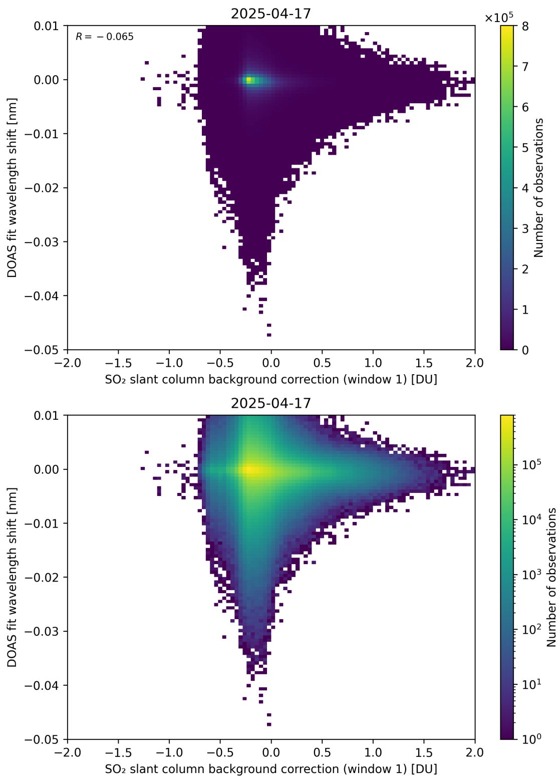
Figure 111: Scatter density plot of “SO 2 slant column background correction (window 1)” against “DOAS fit wavelength shift” for 2025-04-16 to 2025-04-18.
