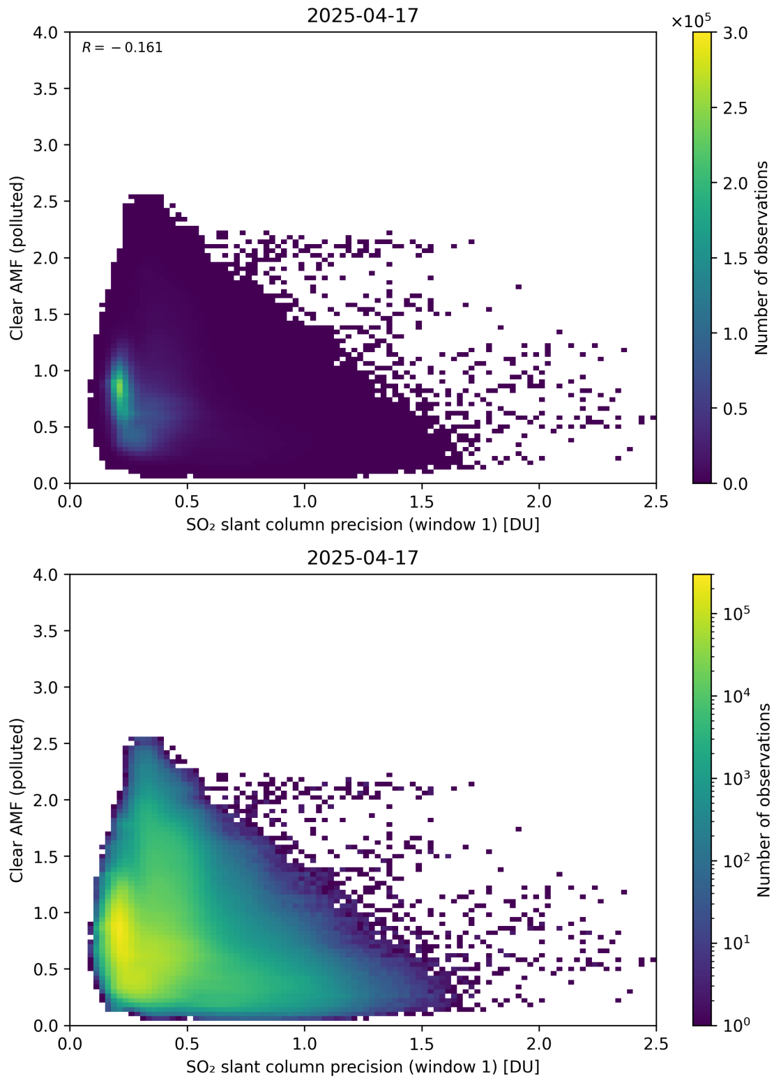
Figure 274: Scatter density plot of “SO 2 slant column precision (window 1)” against “Clear AMF (polluted)” for 2025-04-16 to 2025-04-18.
