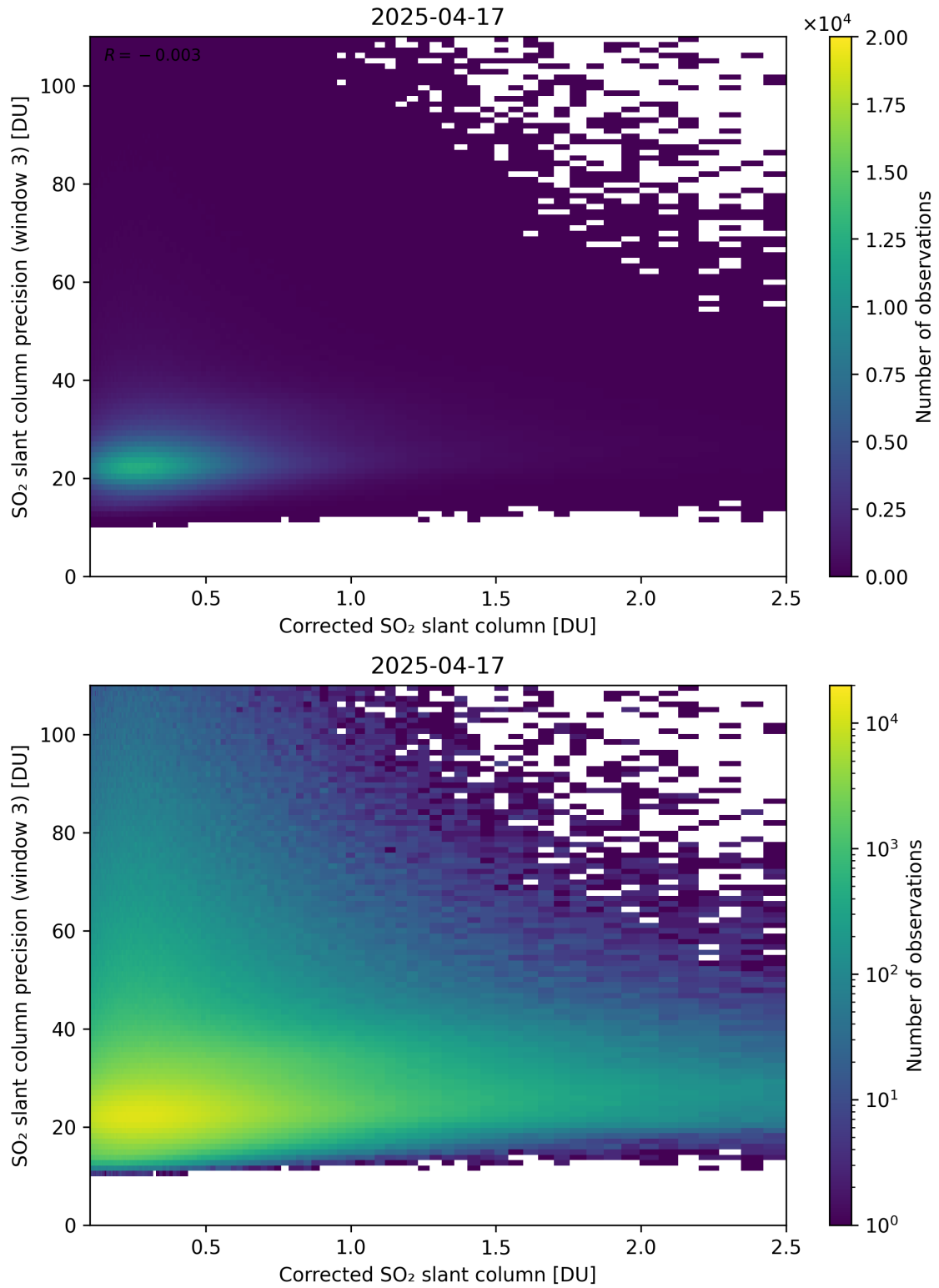
Figure 241: Scatter density plot of “Corrected SO 2 slant column” against “SO 2 slant column precision (window 3)” for 2025-04-16 to 2025-04-18.
