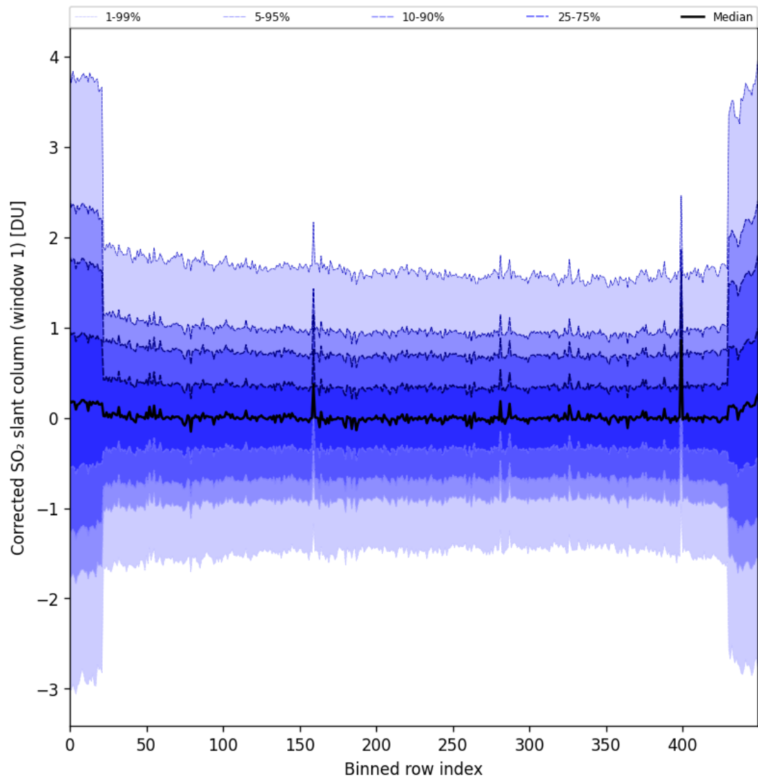
Figure 91: Along track statistics of “Corrected SO 2 slant column (window 1)” for 2025-04-16 to 2025-04-18
