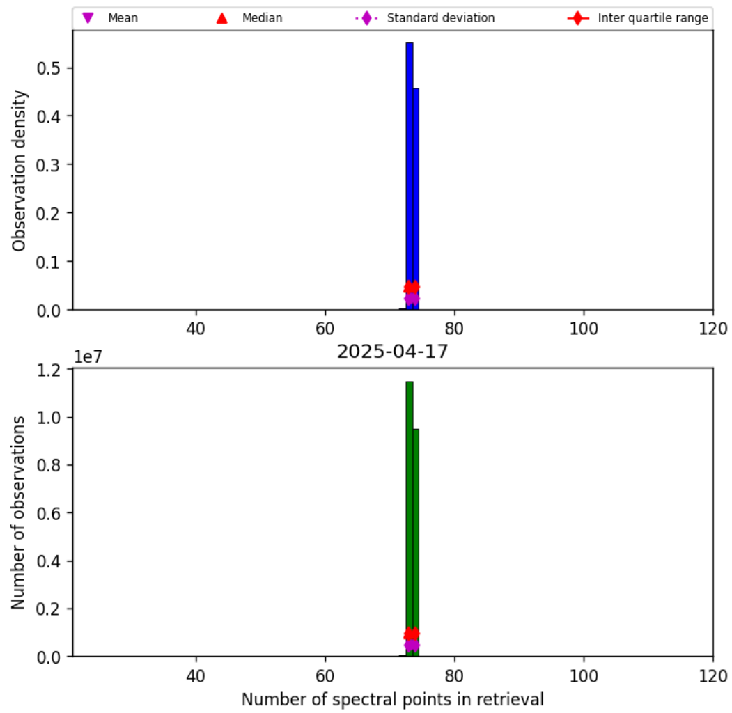
Figure 82: Histogram of “Number of spectral points in retrieval” for 2025-04-16 to 2025-04-18
