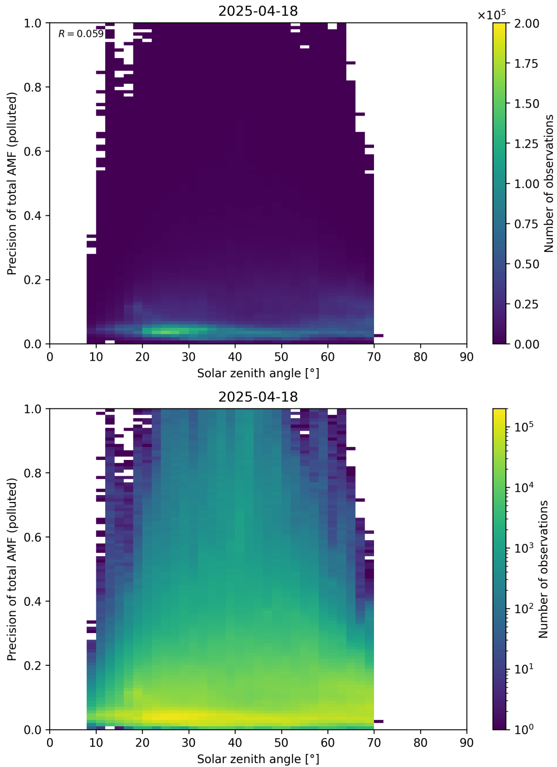
Figure 190: Scatter density plot of “Solar zenith angle” against “Precision of total AMF (polluted)” for 2025-04-18 to 2025-04-19.
