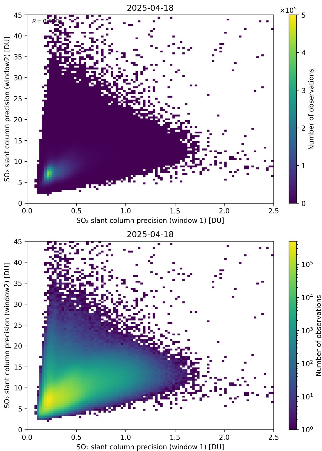
Figure 277: Scatter density plot of “SO 2 slant column precision (window 1)” against “SO 2 slant column precision (window2)” for 2025-04-18 to 2025-04-19.
