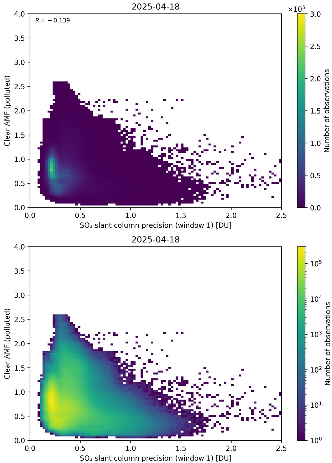
Figure 274: Scatter density plot of “SO 2 slant column precision (window 1)” against “Clear AMF (polluted)” for 2025-04-18 to 2025-04-19.
