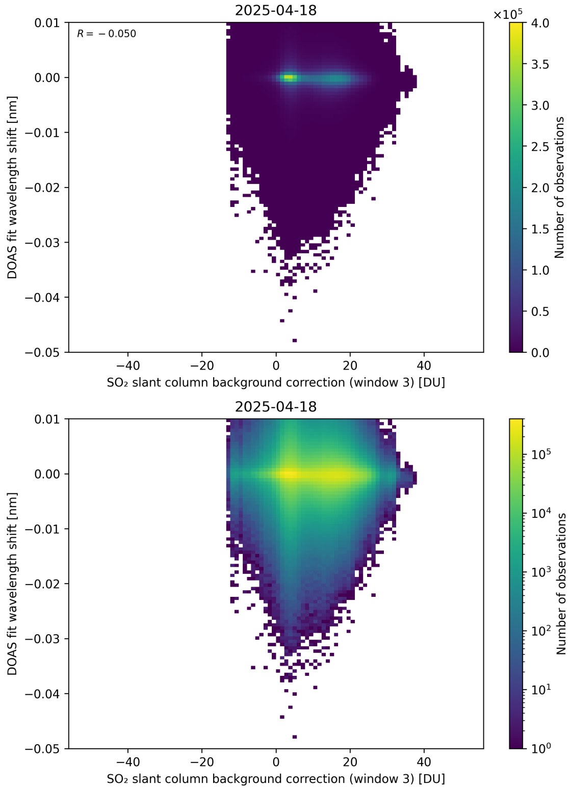
Figure 132: Scatter density plot of “SO 2 slant column background correction (window 3)” against “DOAS fit wavelength shift” for 2025-04-18 to 2025-04-19.
