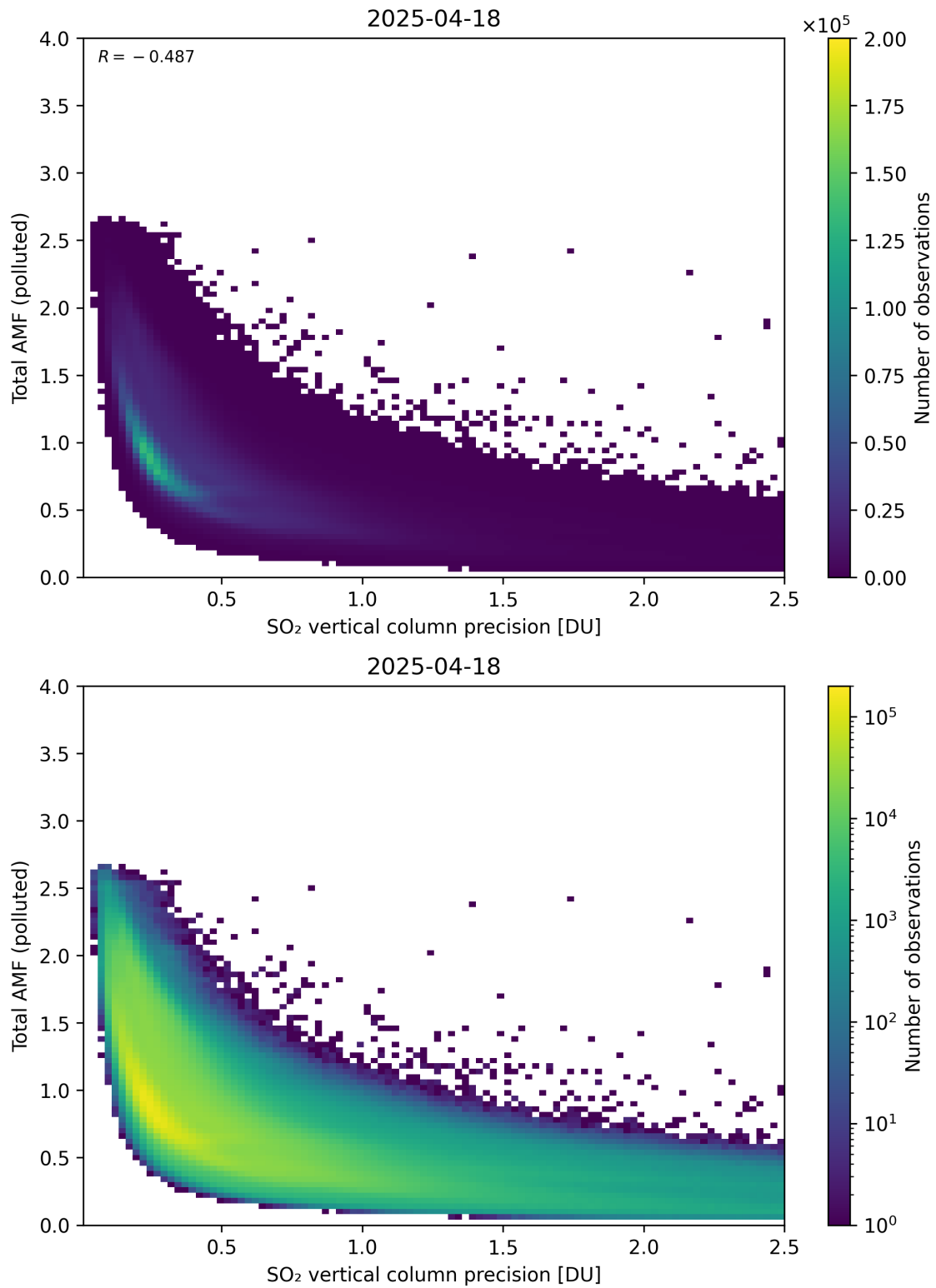
Figure 346: Scatter density plot of “SO 2 vertical column precision” against “Total AMF (polluted)” for 2025-04-18 to 2025-04-19.
