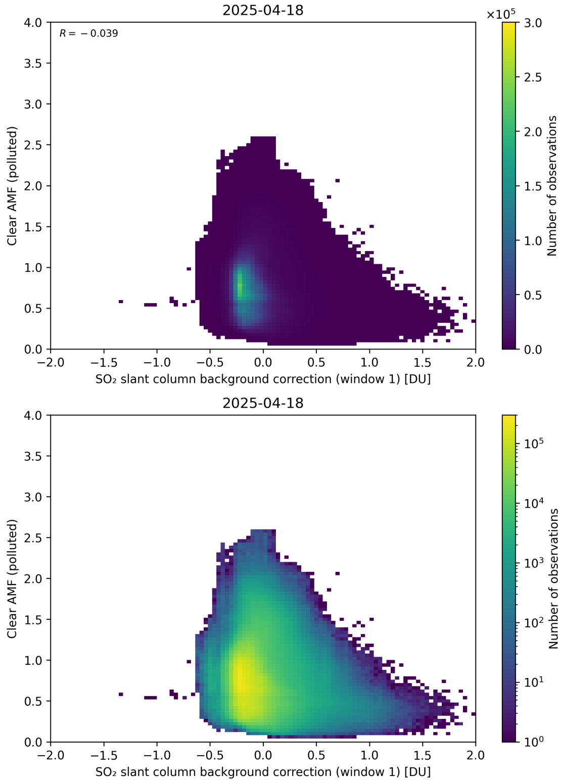
Figure 114: Scatter density plot of “SO 2 slant column background correction (window 1)” against “Clear AMF (polluted)” for 2025-04-18 to 2025-04-19.
