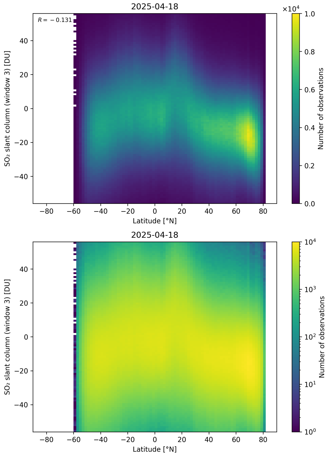
Figure 165: Scatter density plot of “Latitude” against “SO 2 slant column (window 3)” for 2025-04-18 to 2025-04-19.
