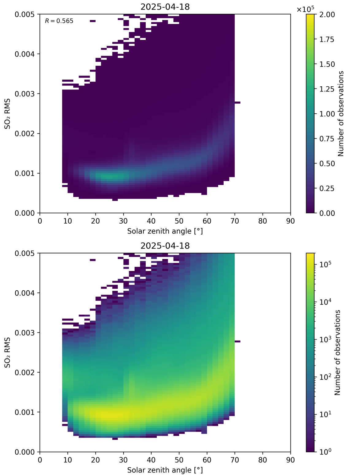
Figure 176: Scatter density plot of “Solar zenith angle” against “SO 2 RMS” for 2025-04-18 to 2025-04-19.
