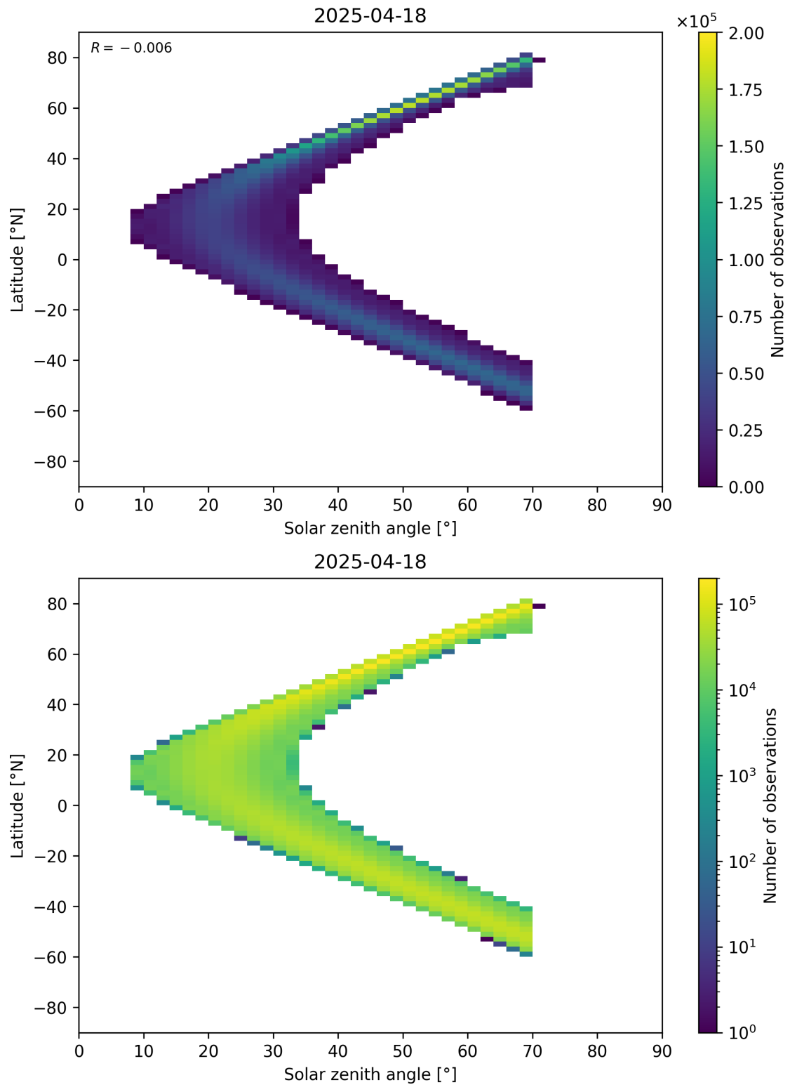
Figure 177: Scatter density plot of “Solar zenith angle” against “Latitude” for 2025-04-18 to 2025-04-19.
