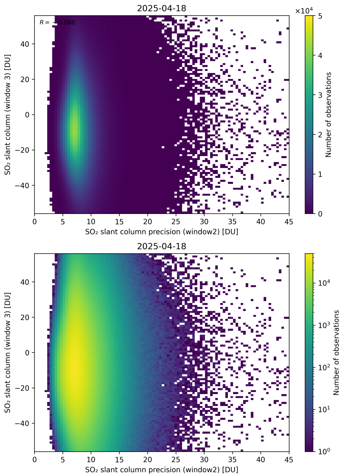
Figure 299: Scatter density plot of “SO 2 slant column precision (window2)” against “SO 2 slant column (window 3)” for 2025-04-18 to 2025-04-19.
