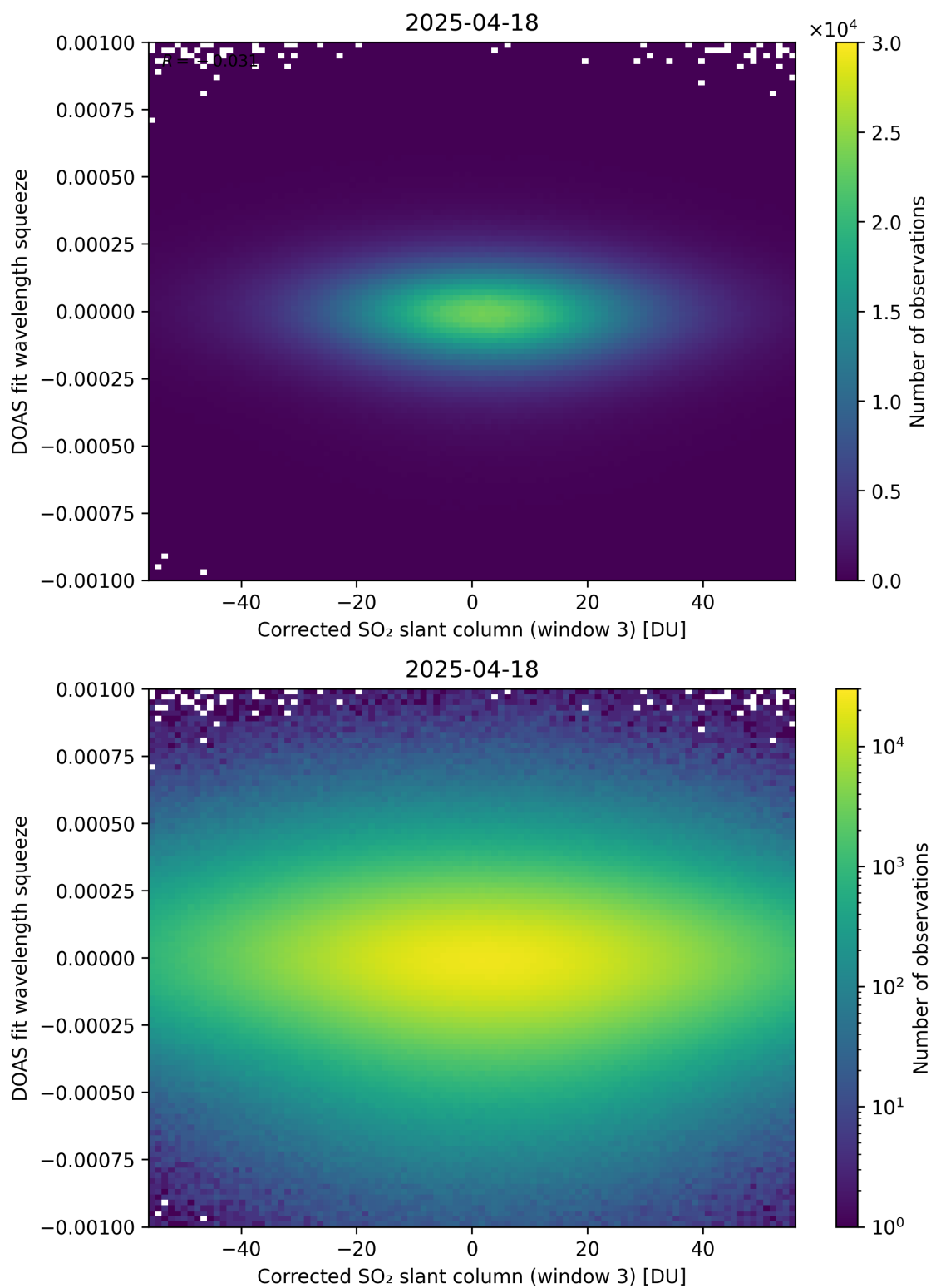
Figure 257: Scatter density plot of “Corrected SO 2 slant column (window 3)” against “DOAS fit wavelength squeeze” for 2025-04-18 to 2025-04-19.
