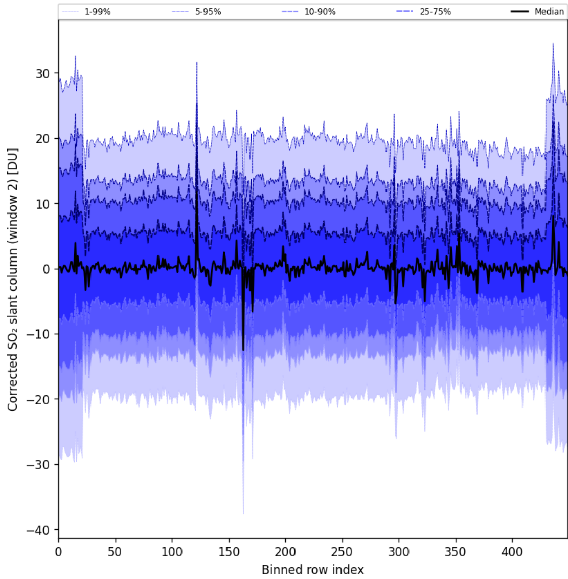
Figure 95: Along track statistics of “Corrected SO 2 slant column (window 2)” for 2025-04-18 to 2025-04-19
