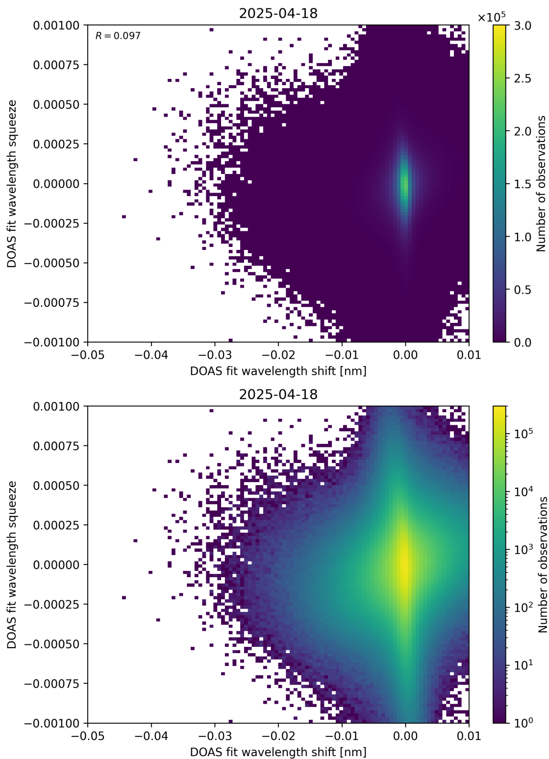
Figure 138: Scatter density plot of “DOAS fit wavelength shift” against “DOAS fit wavelength squeeze” for 2025-04-18 to 2025-04-19.
