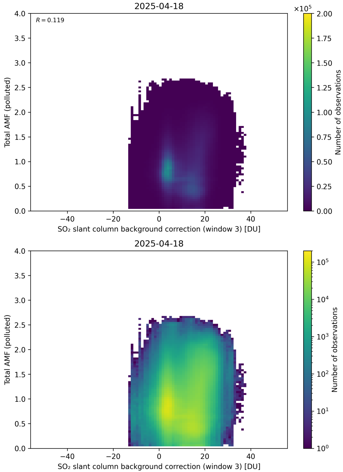
Figure 136: Scatter density plot of “SO 2 slant column background correction (window 3)” against “Total AMF (polluted)” for 2025-04-18 to 2025-04-19.
