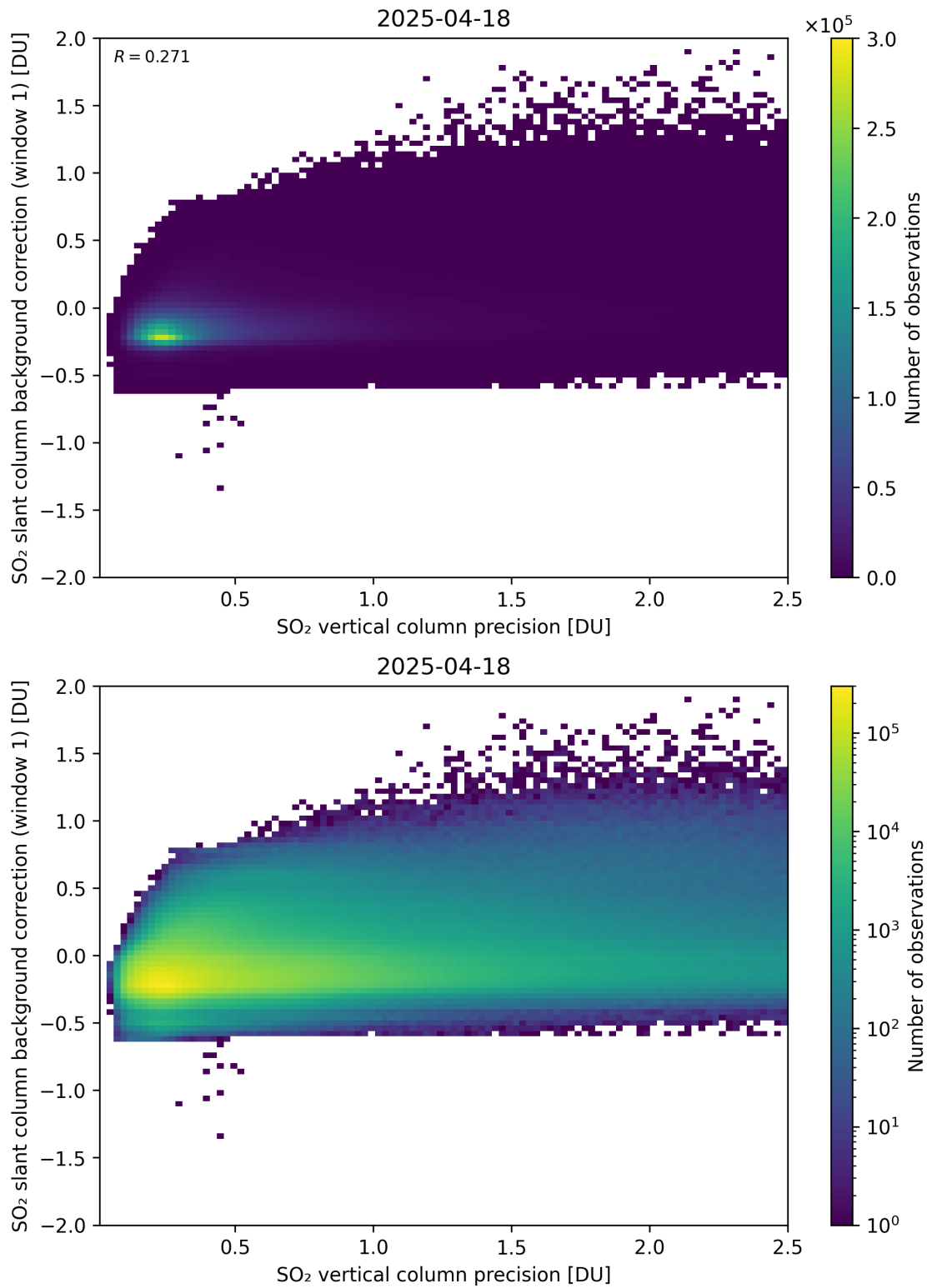
Figure 329: Scatter density plot of “SO 2 vertical column precision” against “SO 2 slant column background correction (window 1)” for 2025-04-18 to 2025-04-19.
