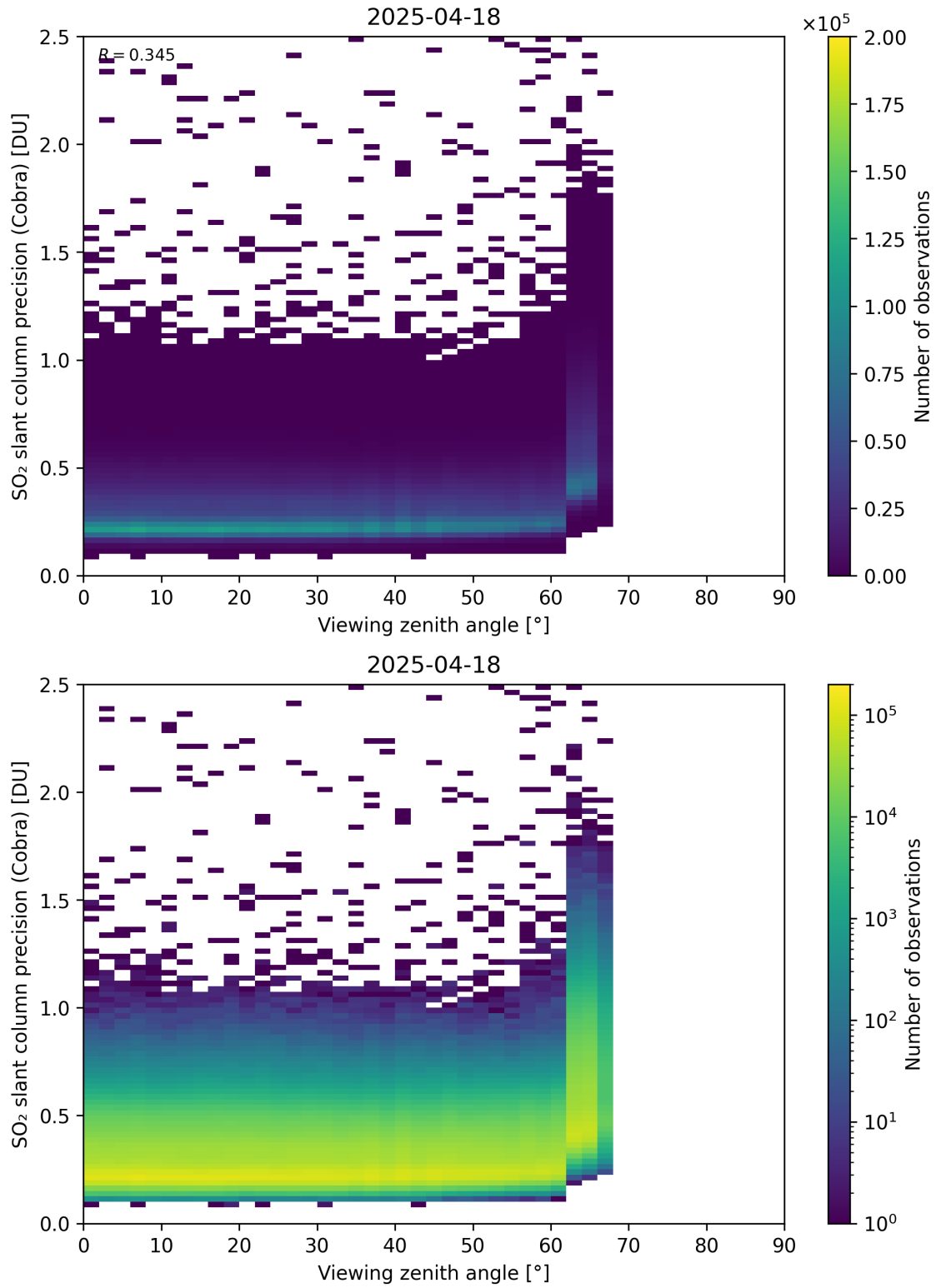
Figure 372: Scatter density plot of “Viewing zenith angle” against “SO 2 slant column precision (Cobra)” for 2025-04-18 to 2025-04-19.
