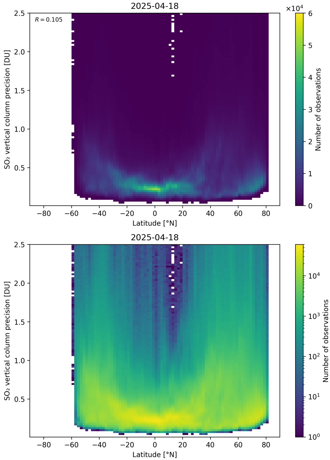
Figure 170: Scatter density plot of “Latitude” against “SO 2 vertical column precision” for 2025-04-18 to 2025-04-19.
