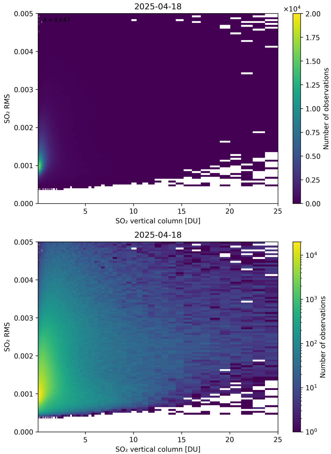
Figure 328: Scatter density plot of “SO 2 vertical column” against “SO 2 RMS” for 2025-04-18 to 2025-04-19.
