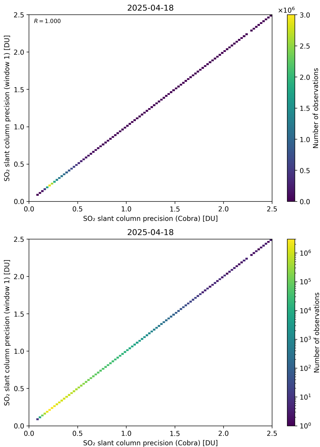
Figure 209: Scatter density plot of “SO 2 slant column precision (Cobra)” against “SO 2 slant column precision (window 1)” for 2025-04-18 to 2025-04-19.
