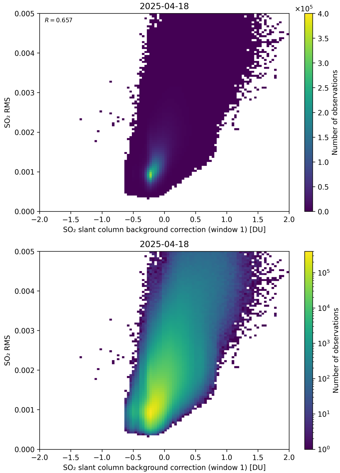
Figure 113: Scatter density plot of “SO 2 slant column background correction (window 1)” against “SO 2 RMS” for 2025-04-18 to 2025-04-19.
