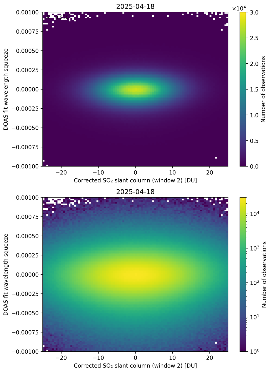
Figure 247: Scatter density plot of “Corrected SO 2 slant column (window 2)” against “DOAS fit wavelength squeeze” for 2025-04-18 to 2025-04-19.
