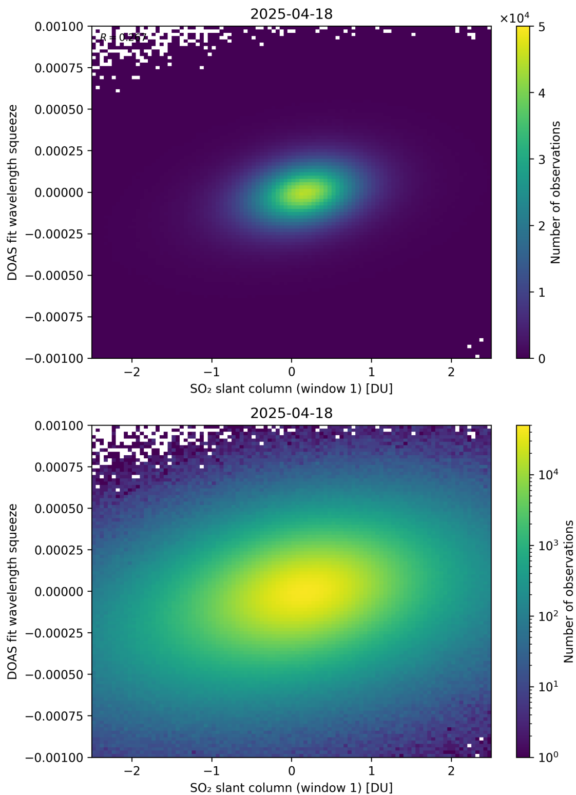
Figure 266: Scatter density plot of “SO 2 slant column (window 1)” against “DOAS fit wavelength squeeze” for 2025-04-18 to 2025-04-19.
