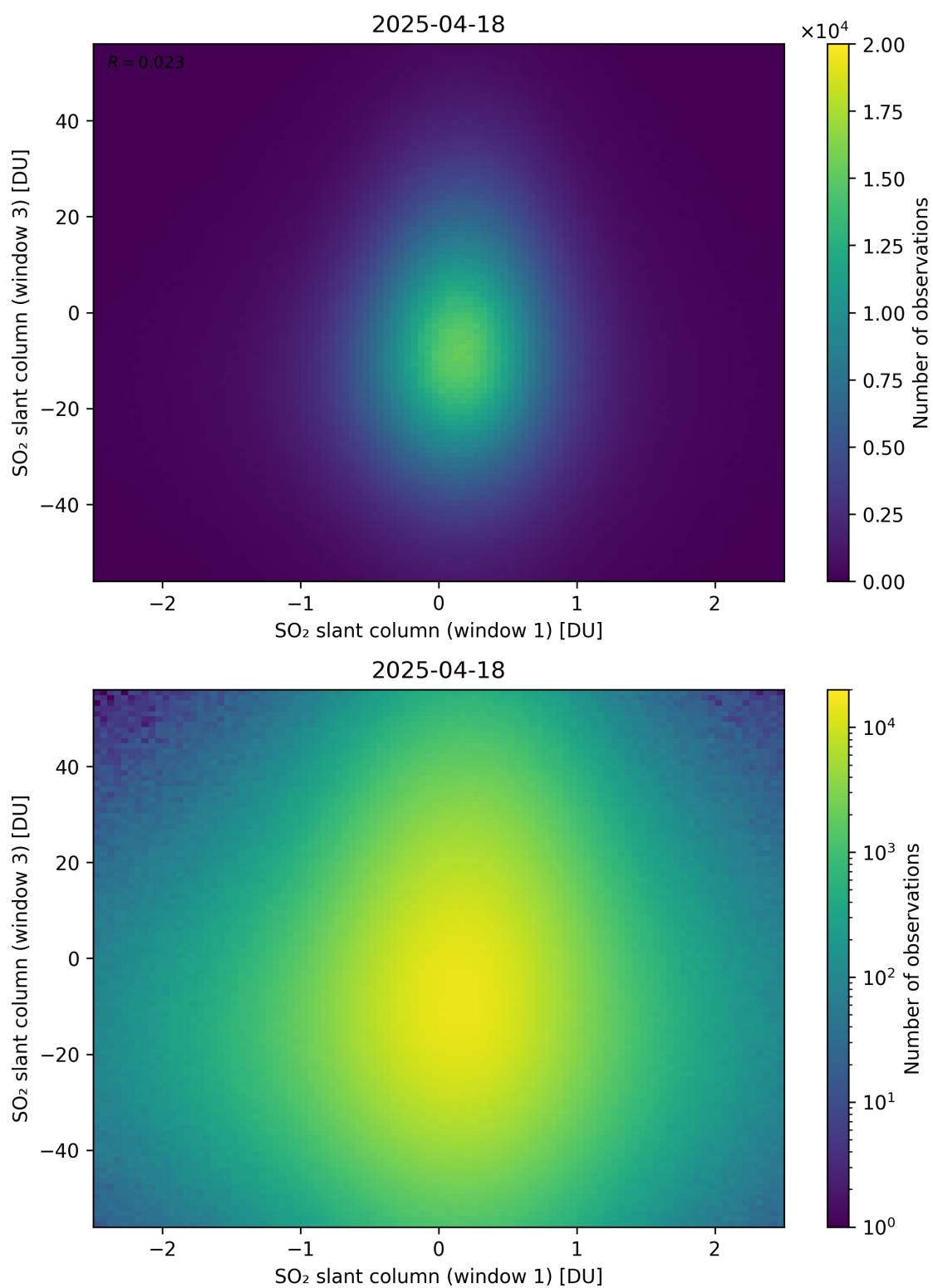
Figure 287: Scatter density plot of “SO 2 slant column (window 1)” against “SO 2 slant column (window 3)” for 2025-04-18 to 2025-04-19.
