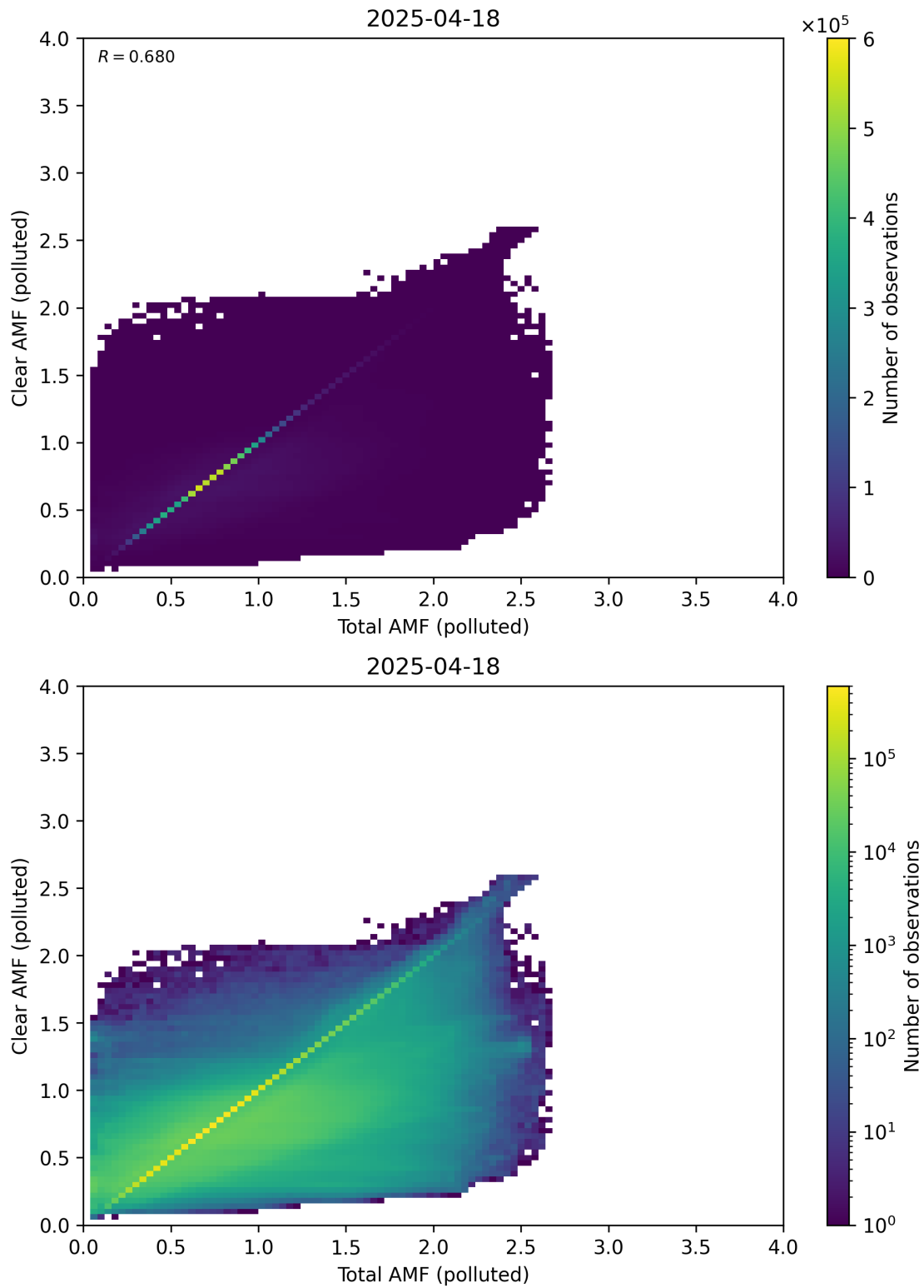
Figure 321: Scatter density plot of “Total AMF (polluted)” against “Clear AMF (polluted)” for 2025-04-18 to 2025-04-19.
