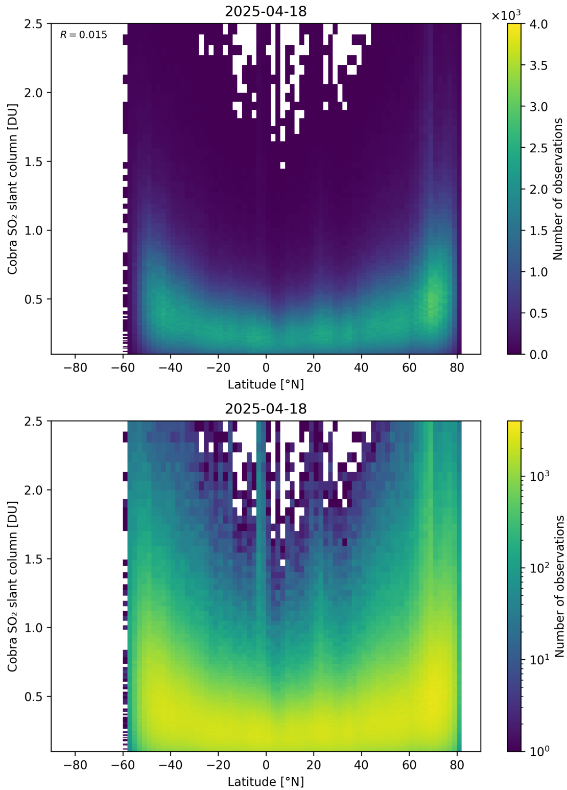
Figure 157: Scatter density plot of “Latitude” against “Cobra SO 2 slant column” for 2025-04-18 to 2025-04-19.
