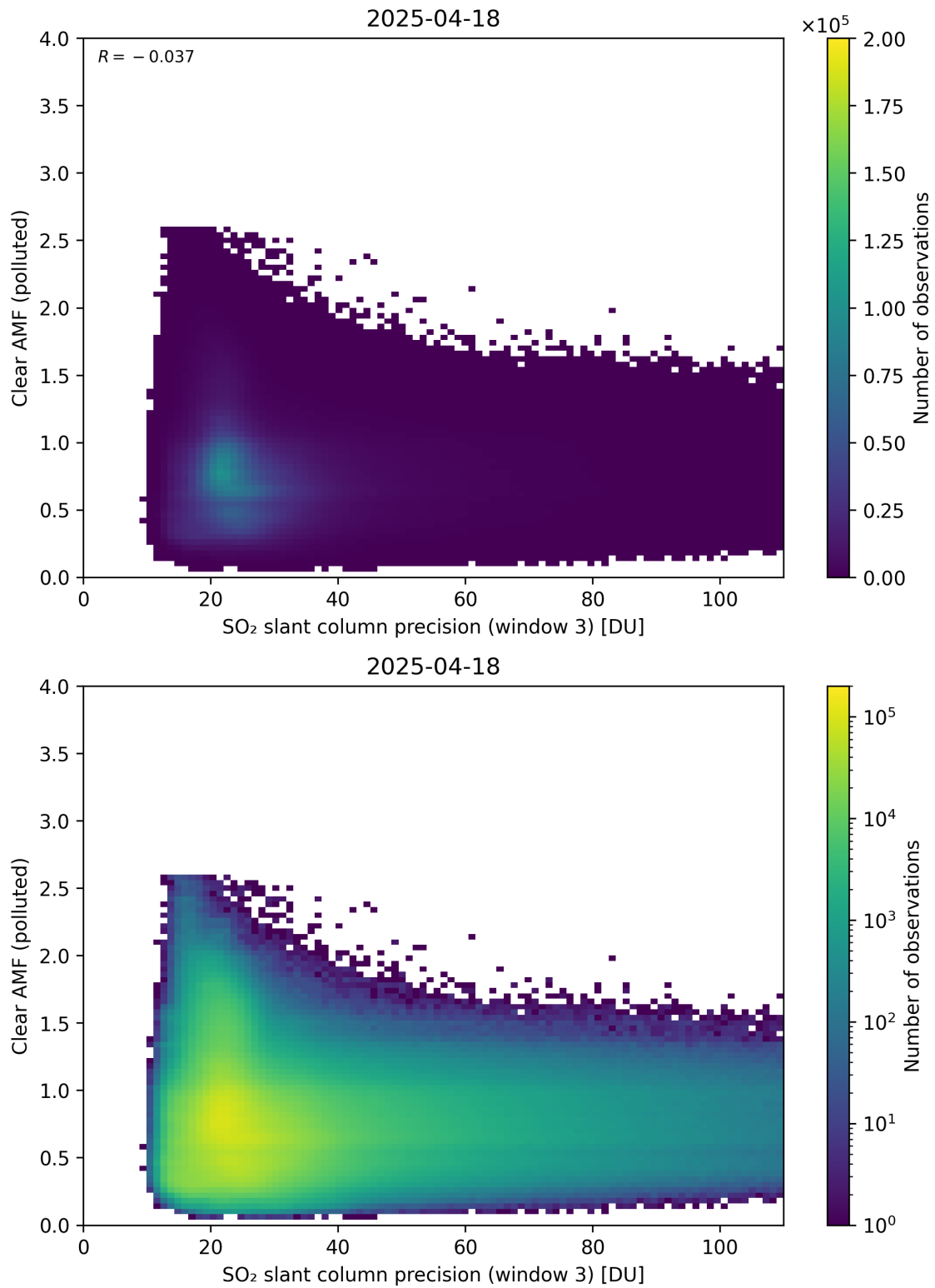
Figure 311: Scatter density plot of “SO 2 slant column precision (window 3)” against “Clear AMF (polluted)” for 2025-04-18 to 2025-04-19.
