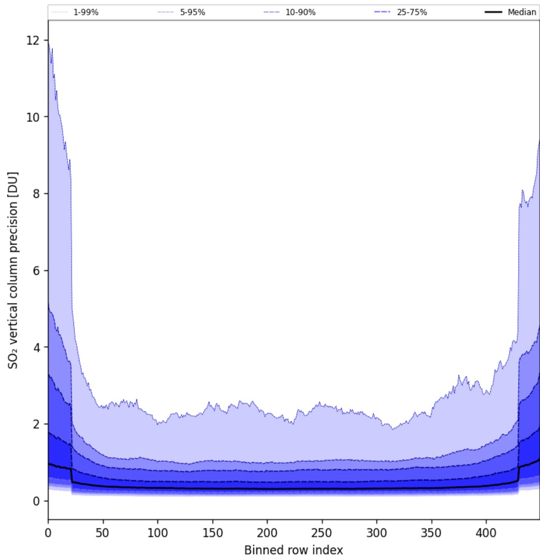
Figure 85: Along track statistics of “SO 2 vertical column precision” for 2025-04-18 to 2025-04-19
