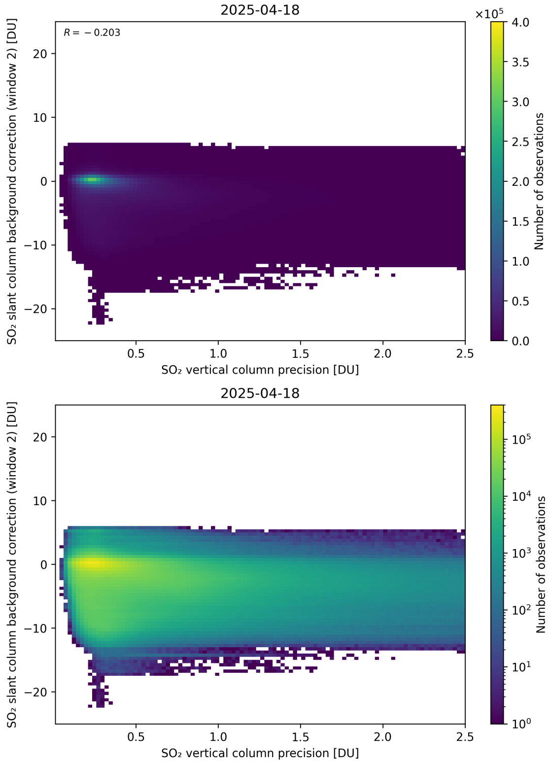
Figure 330: Scatter density plot of “SO 2 vertical column precision” against “SO 2 slant column background correction (window 2)” for 2025-04-18 to 2025-04-19.
