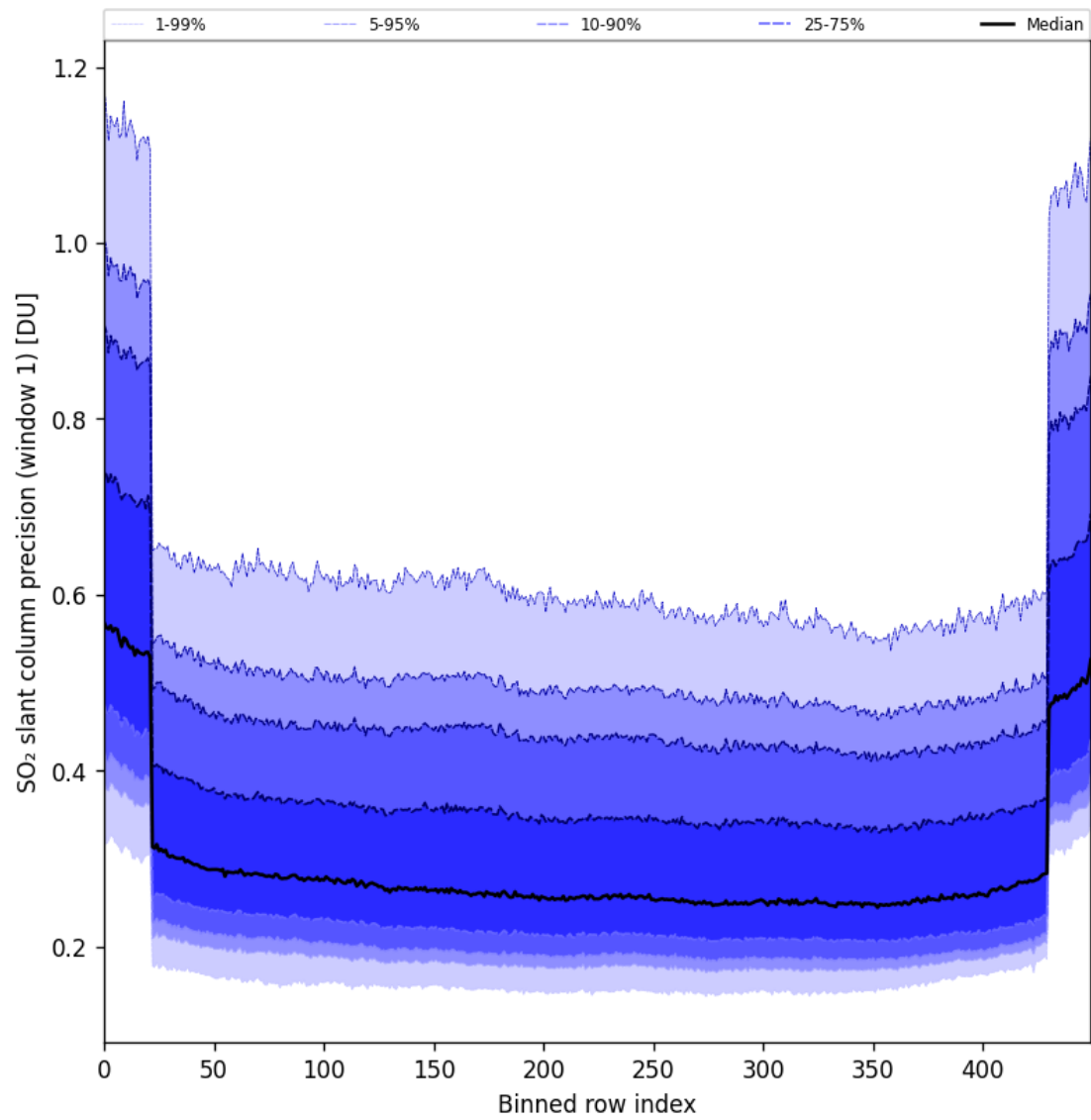
Figure 90: Along track statistics of “SO 2 slant column precision (window 1)” for 2025-04-18 to 2025-04-19
