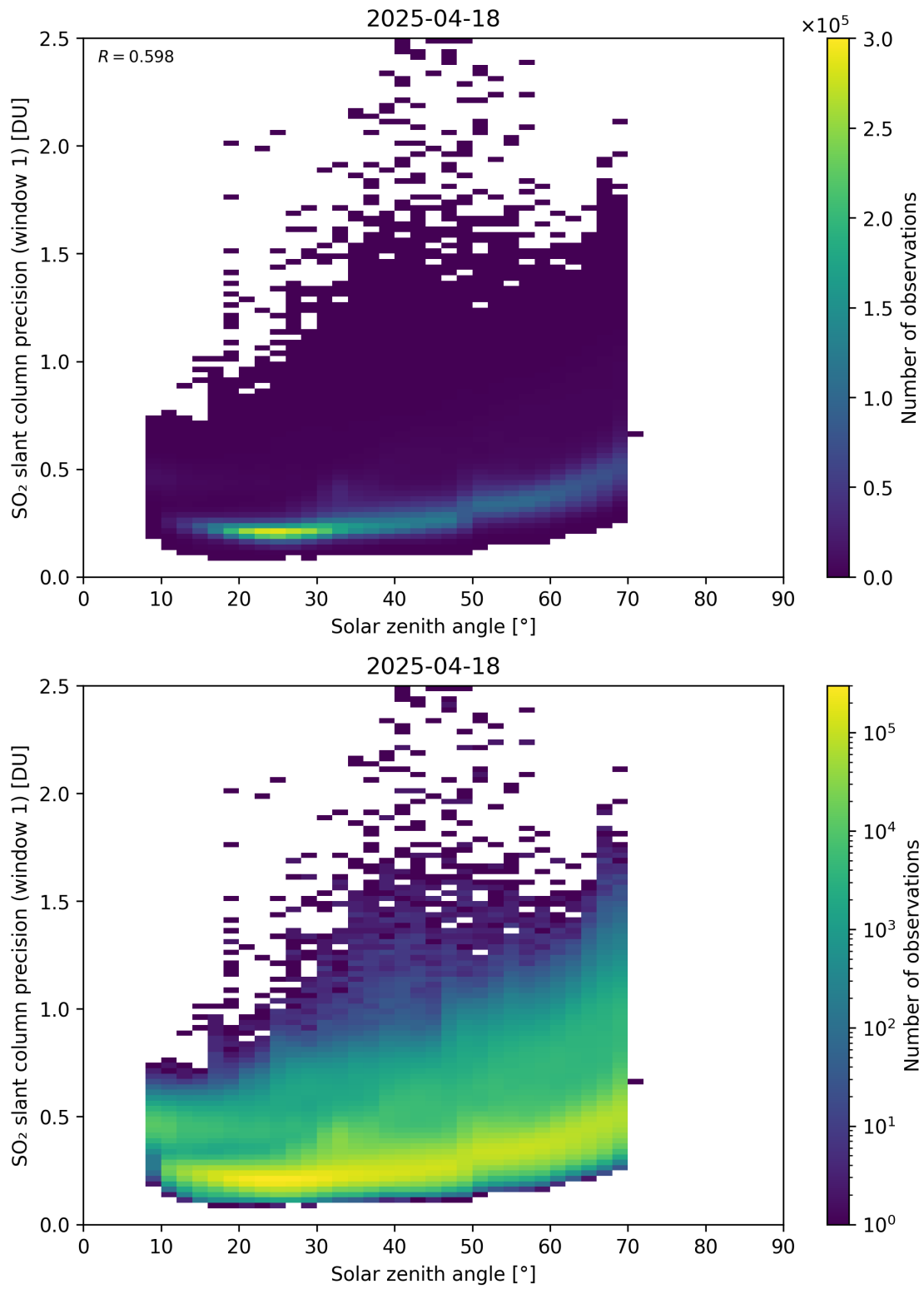
Figure 185: Scatter density plot of “Solar zenith angle” against “SO 2 slant column precision (window 1)” for 2025-04-18 to 2025-04-19.
