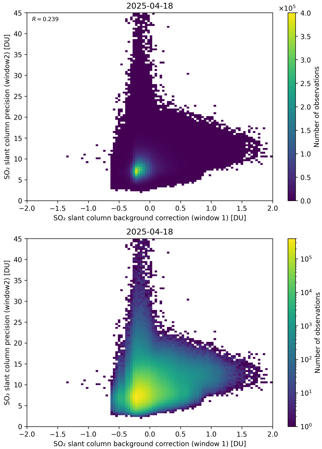
Figure 117: Scatter density plot of “SO 2 slant column background correction (window 1)” against “SO 2 slant column precision (window2)” for 2025-04-18 to 2025-04-19.
