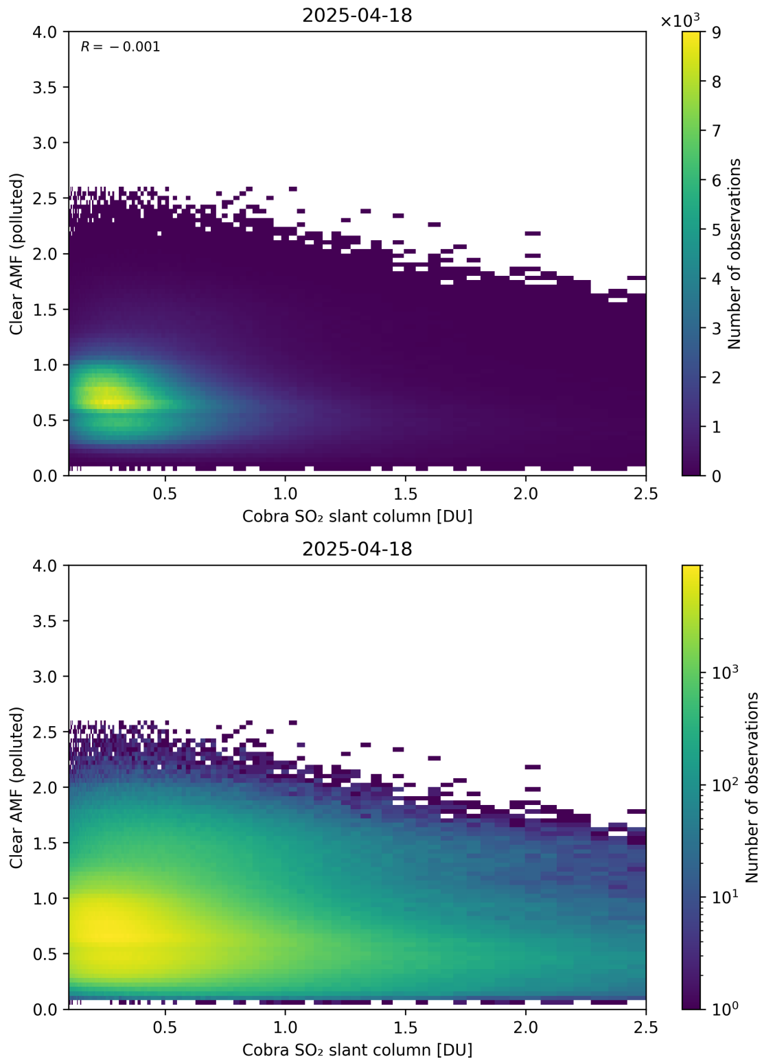
Figure 215: Scatter density plot of “Cobra SO 2 slant column” against “Clear AMF (polluted)” for 2025-04-18 to 2025-04-19.
