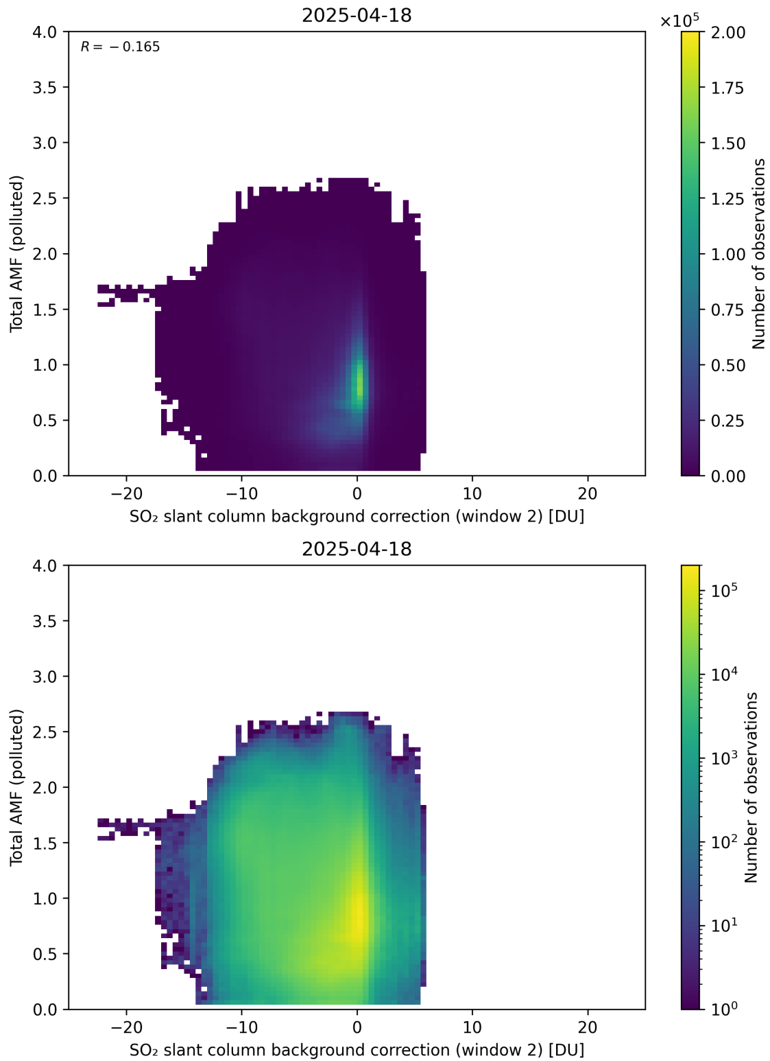
Figure 130: Scatter density plot of “SO 2 slant column background correction (window 2)” against “Total AMF (polluted)” for 2025-04-18 to 2025-04-19.
