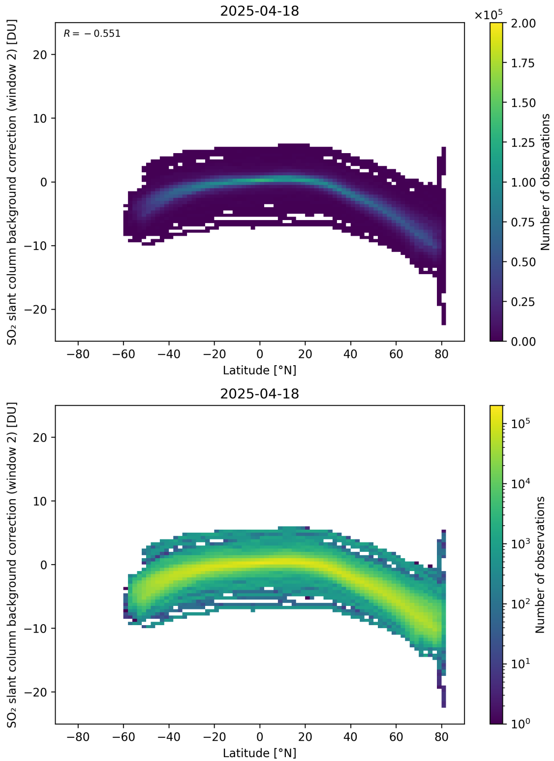
Figure 151: Scatter density plot of “Latitude” against “SO 2 slant column background correction (window 2)” for 2025-04-18 to 2025-04-19.
