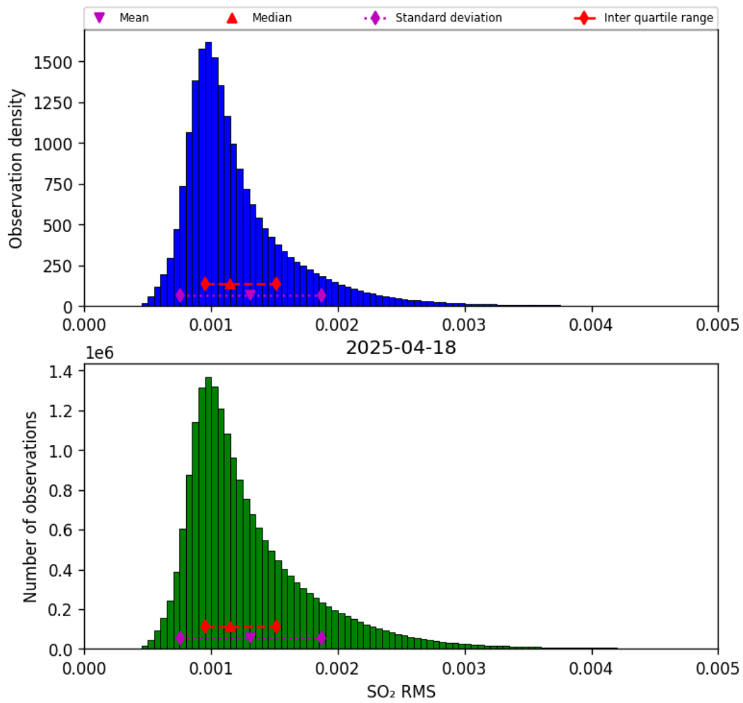
Figure 78: Histogram of “SO 2 RMS” for 2025-04-18 to 2025-04-19
