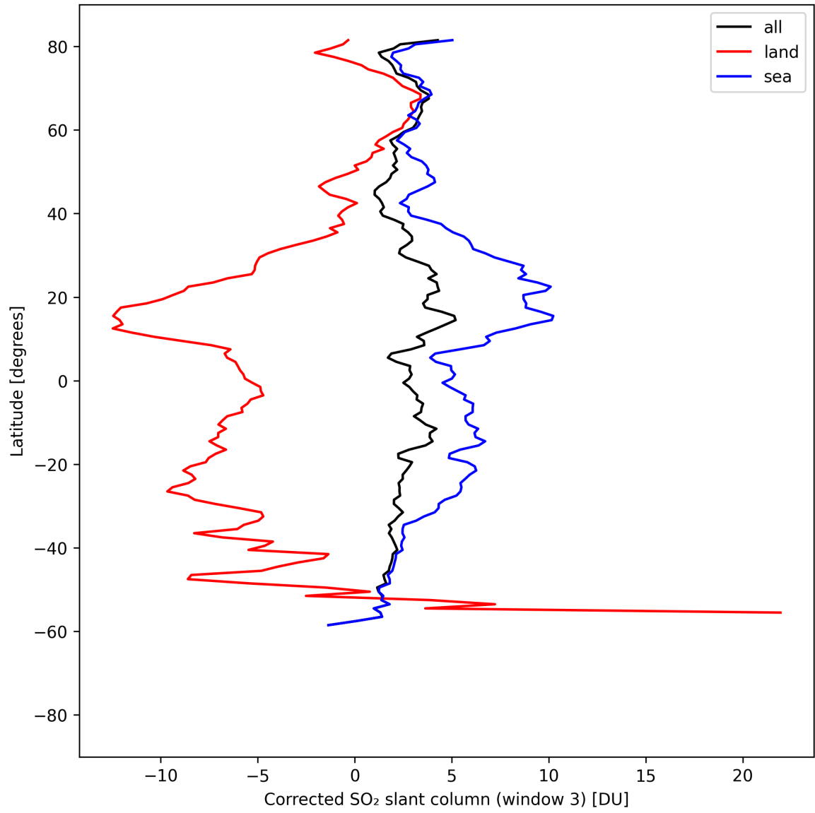
Figure 47: Zonal average of “Corrected SO 2 slant column (window 3)” for 2025-04-18 to 2025-04-19.
