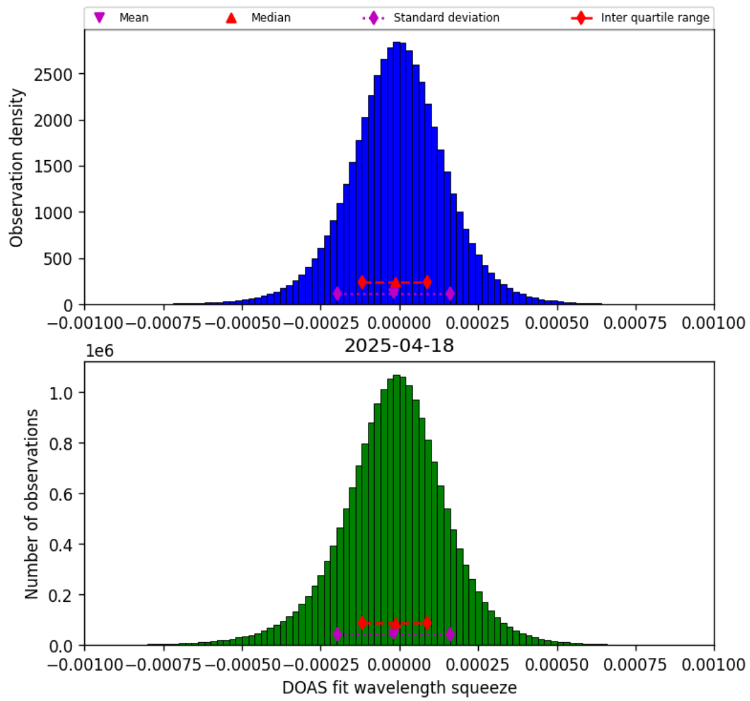
Figure 77: Histogram of “DOAS fit wavelength squeeze” for 2025-04-18 to 2025-04-19
