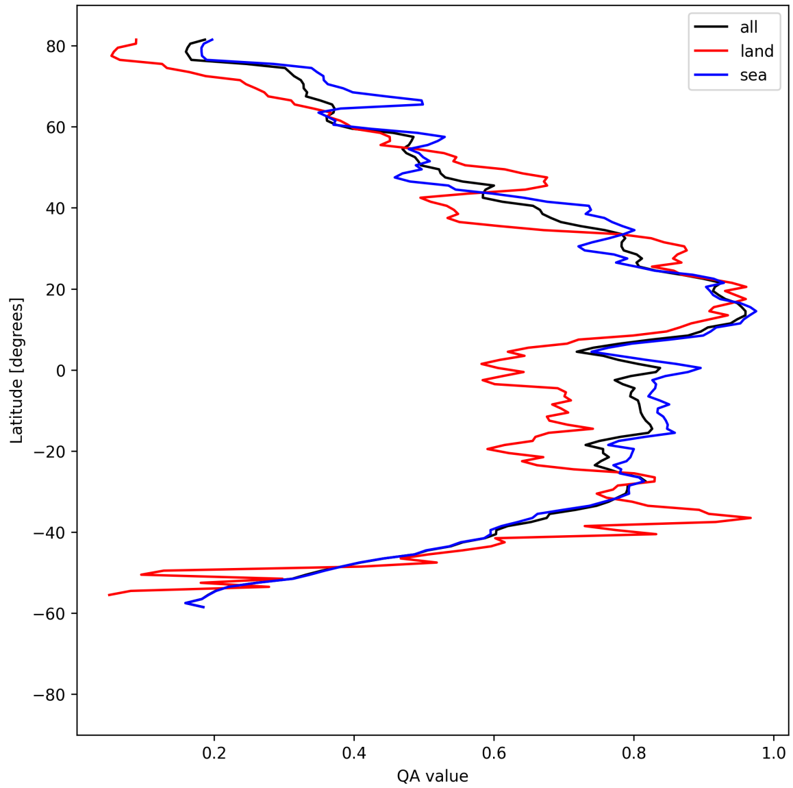
Figure 31: Zonal average of “QA value” for 2025-04-18 to 2025-04-19.
