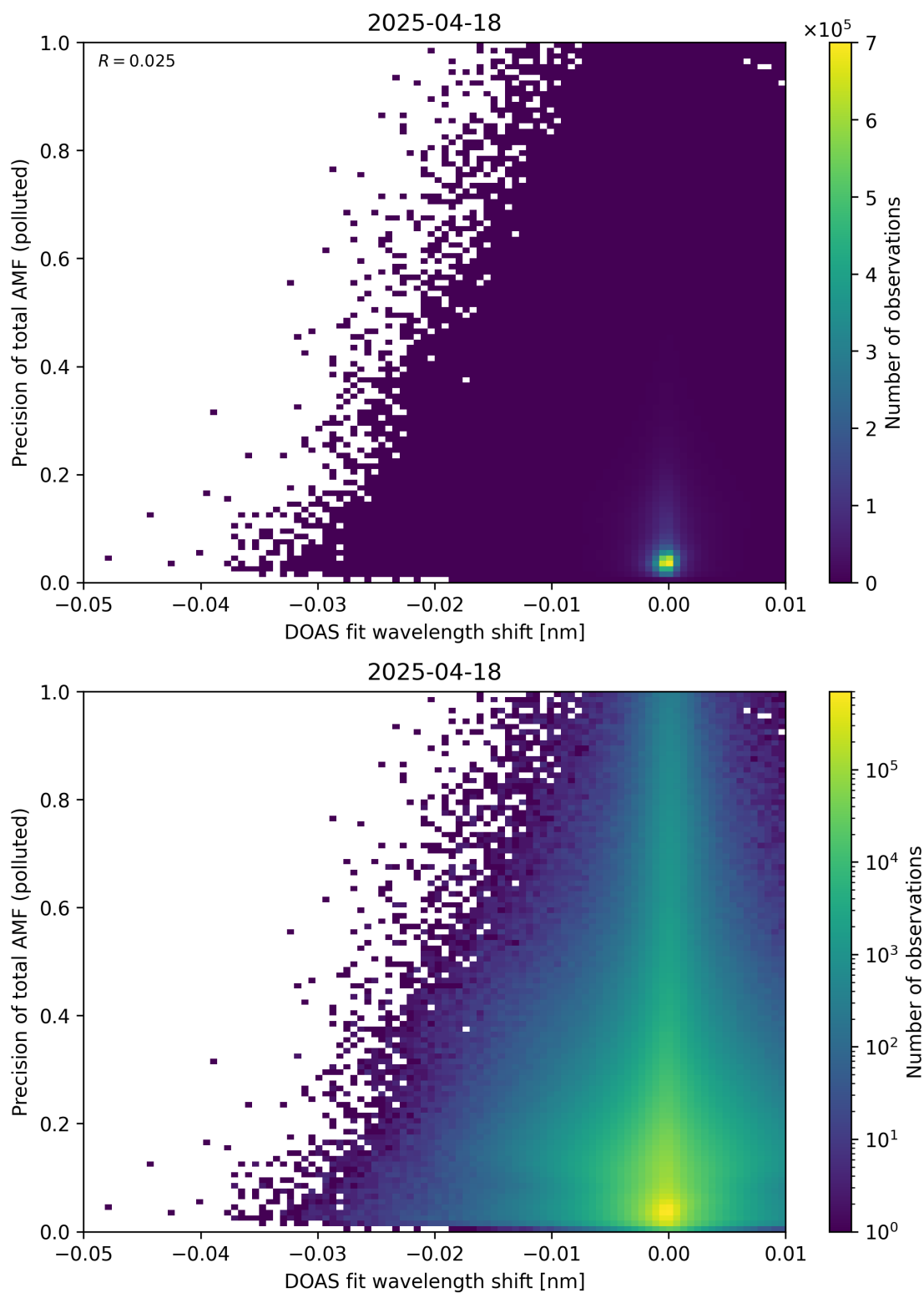
Figure 142: Scatter density plot of “DOAS fit wavelength shift” against “Precision of total AMF (polluted)” for 2025-04-18 to 2025-04-19.
