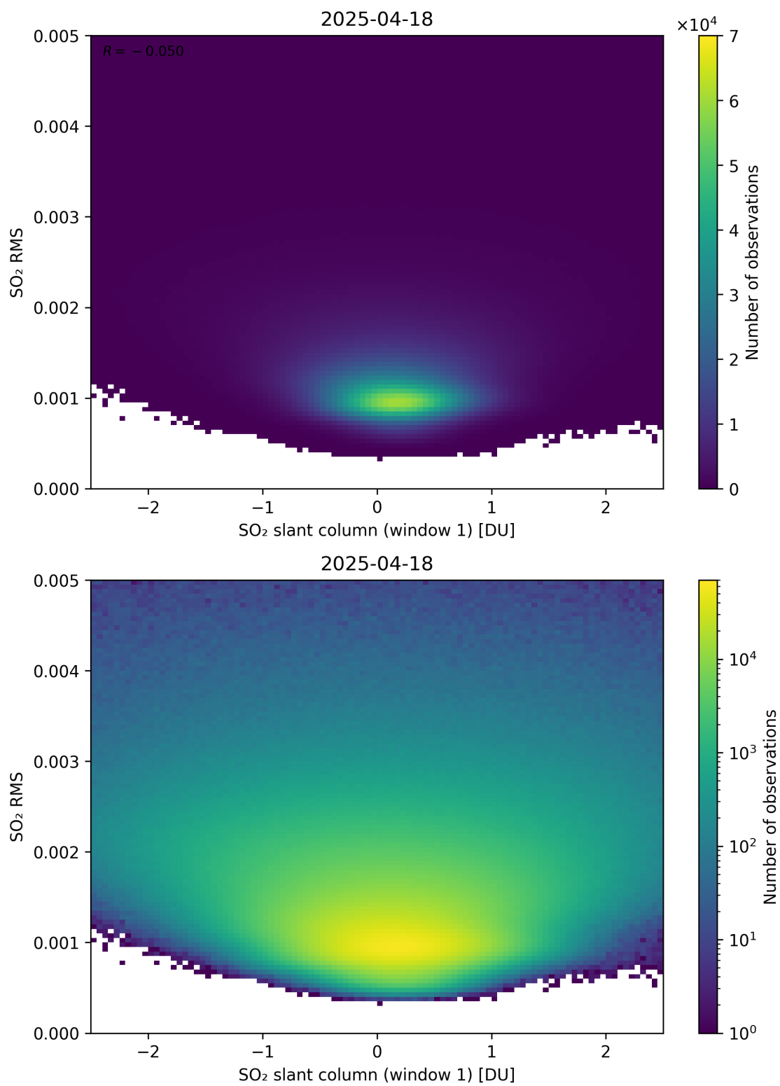
Figure 267: Scatter density plot of “SO 2 slant column (window 1)” against “SO 2 RMS” for 2025-04-18 to 2025-04-19.
