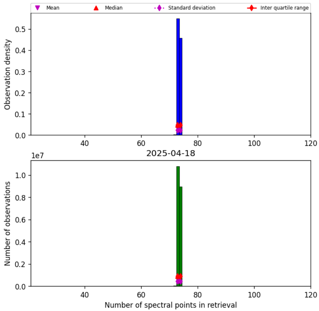
Figure 82: Histogram of “Number of spectral points in retrieval” for 2025-04-18 to 2025-04-19
