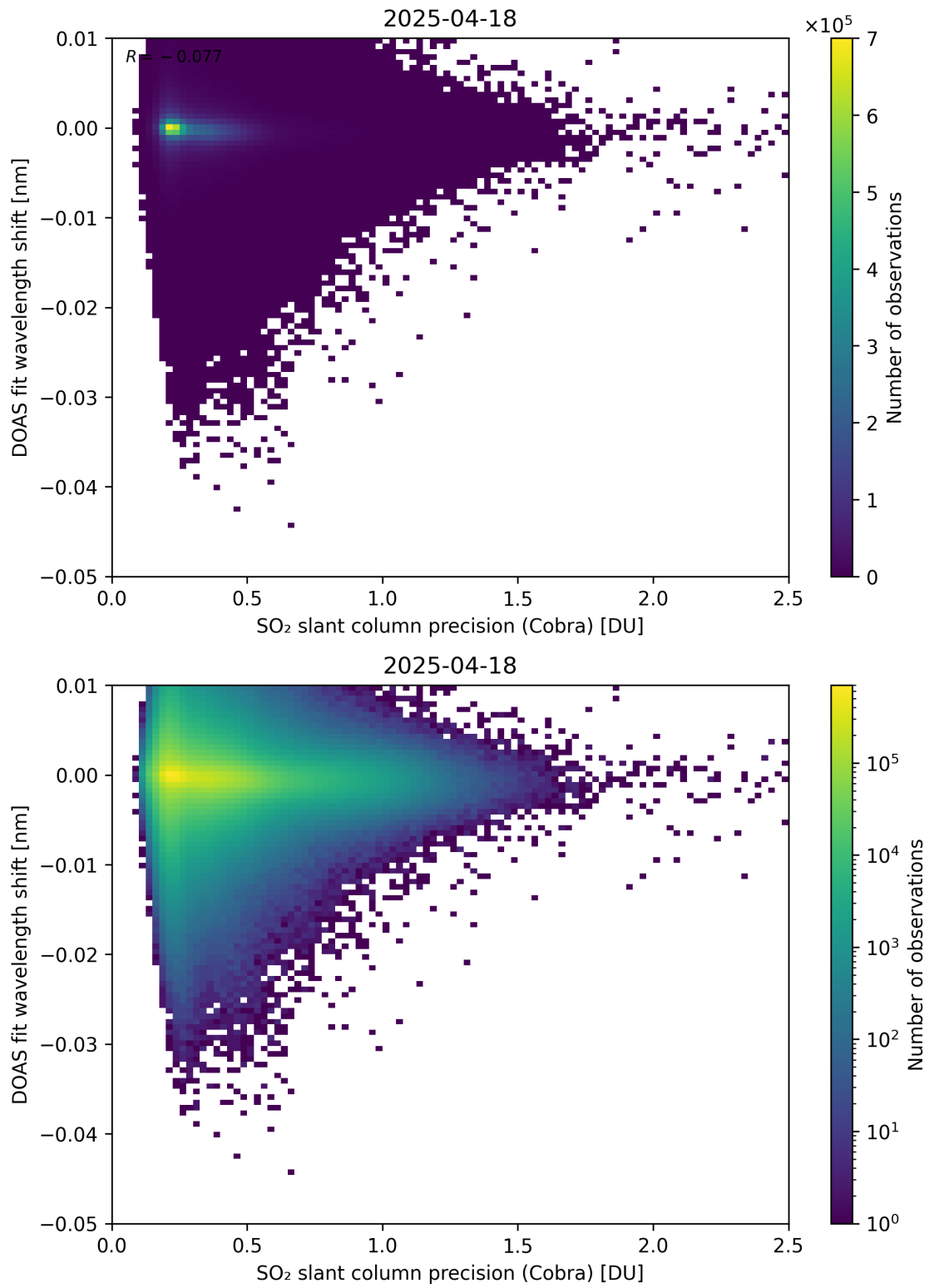
Figure 202: Scatter density plot of “SO 2 slant column precision (Cobra)” against “DOAS fit wavelength shift” for 2025-04-18 to 2025-04-19.
