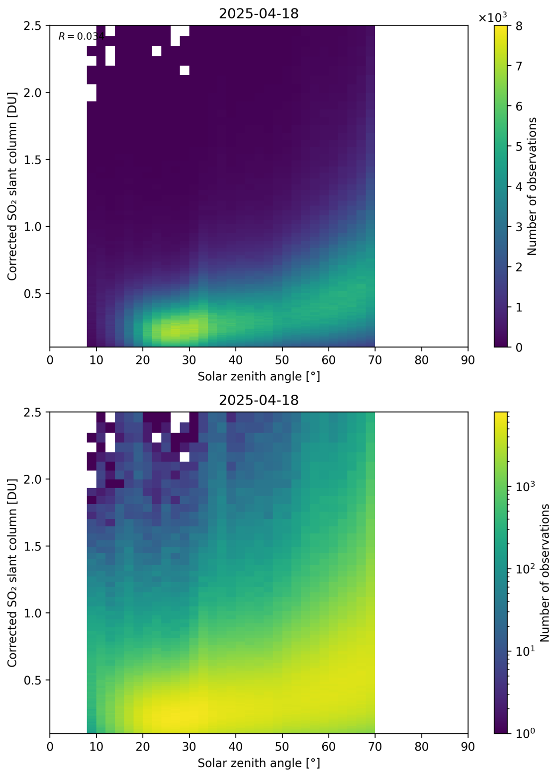
Figure 181: Scatter density plot of “Solar zenith angle” against “Corrected SO 2 slant column” for 2025-04-18 to 2025-04-19.
