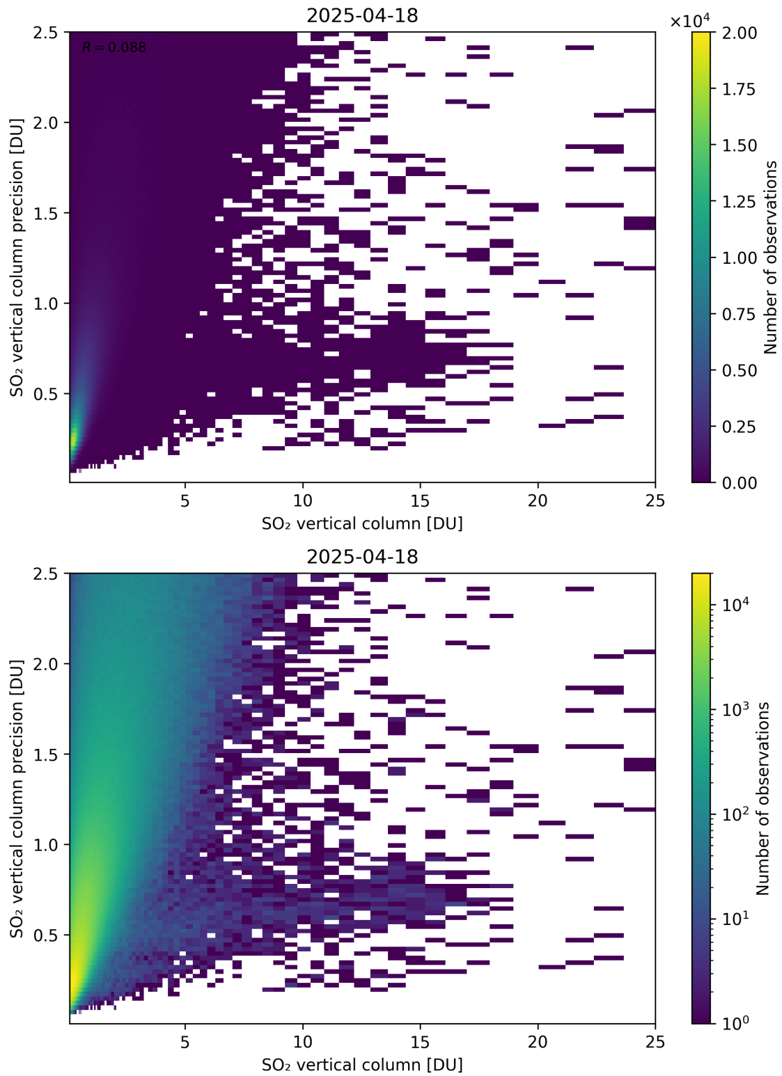
Figure 361: Scatter density plot of “SO 2 vertical column” against “SO 2 vertical column precision” for 2025-04-18 to 2025-04-19.
