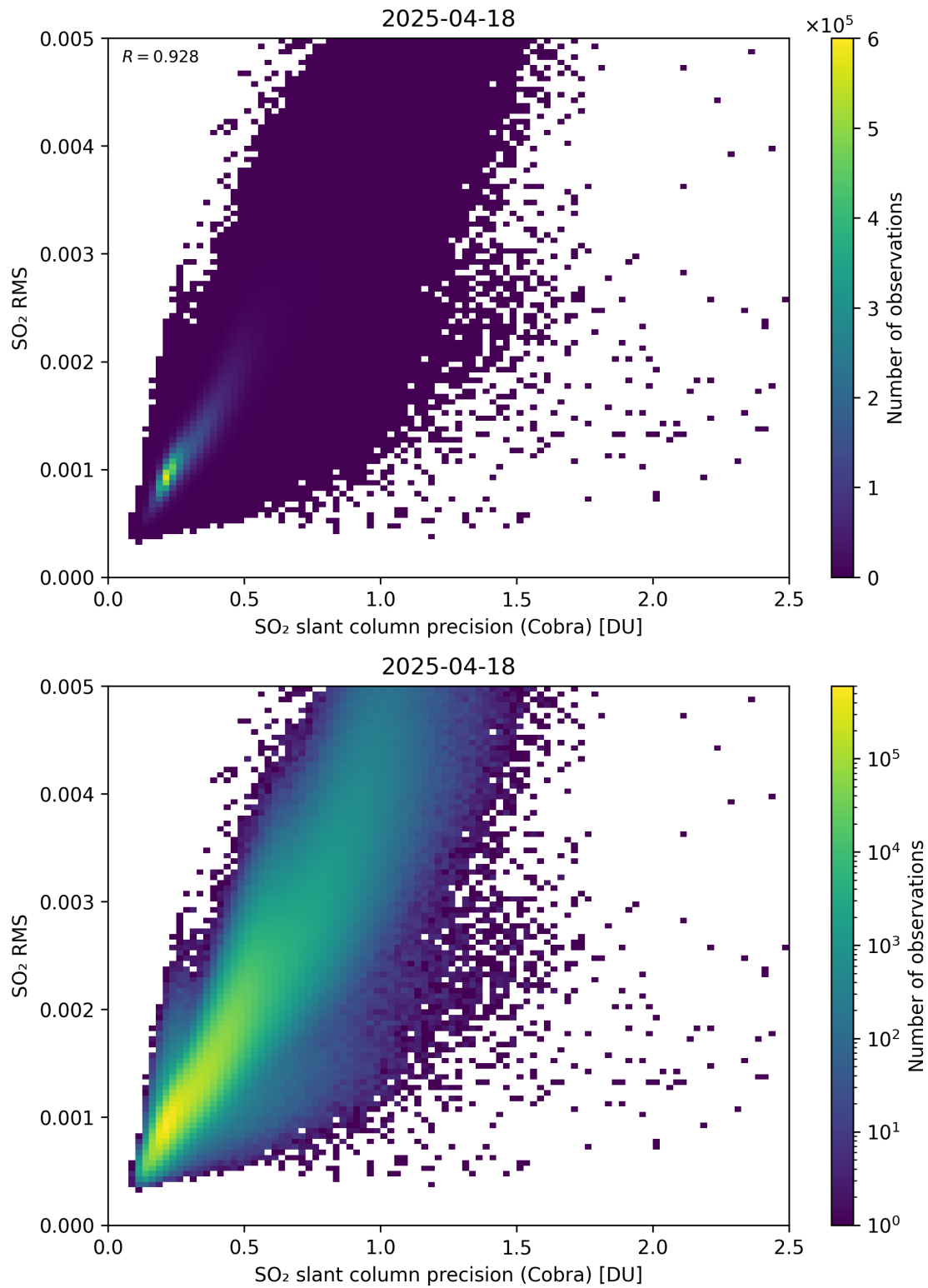
Figure 204: Scatter density plot of “SO 2 slant column precision (Cobra)” against “SO 2 RMS” for 2025-04-18 to 2025-04-19.
