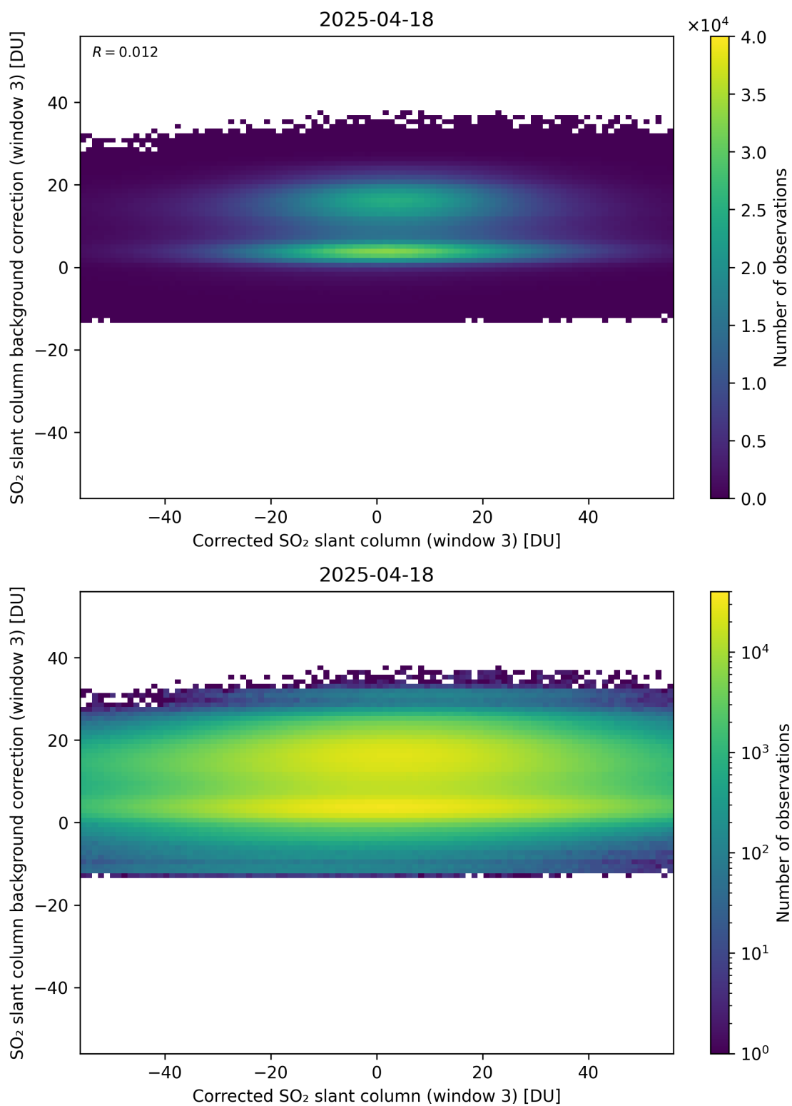
Figure 255: Scatter density plot of “Corrected SO 2 slant column (window 3)” against “SO 2 slant column background correction (window 3)” for 2025-04-18 to 2025-04-19.
