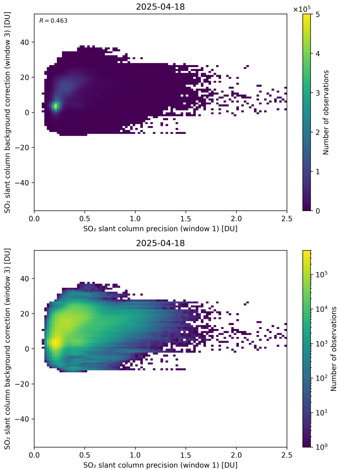
Figure 270: Scatter density plot of “SO 2 slant column precision (window 1)” against “SO 2 slant column background correction (window 3)” for 2025-04-18 to 2025-04-19.
