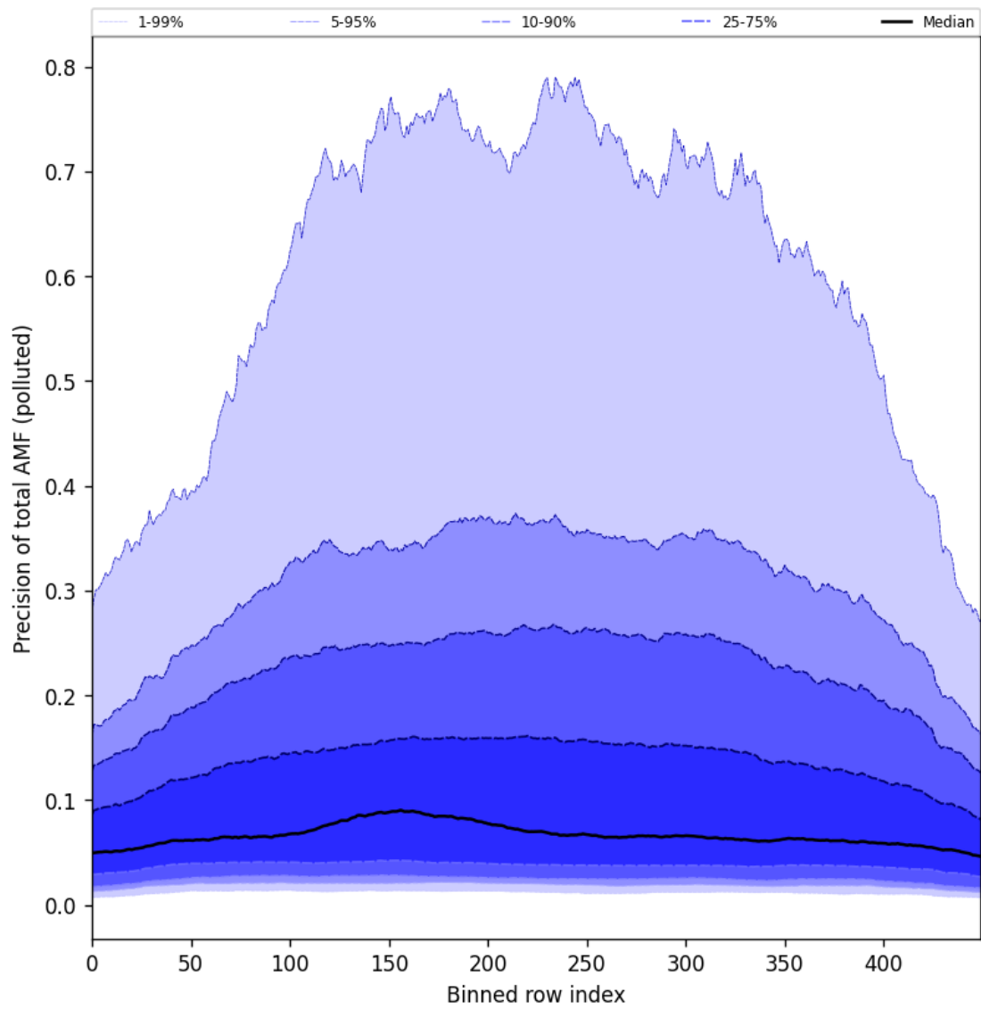
Figure 106: Along track statistics of “Precision of total AMF (polluted)” for 2025-04-18 to 2025-04-19
