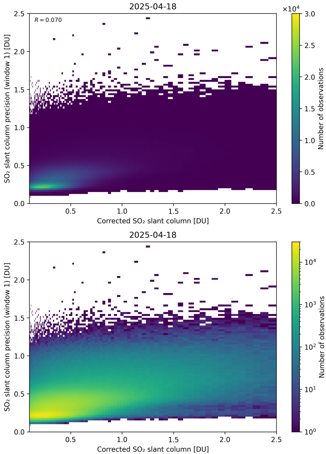
Figure 238: Scatter density plot of “Corrected SO 2 slant column” against “SO 2 slant column precision (window 1)” for 2025-04-18 to 2025-04-19.
