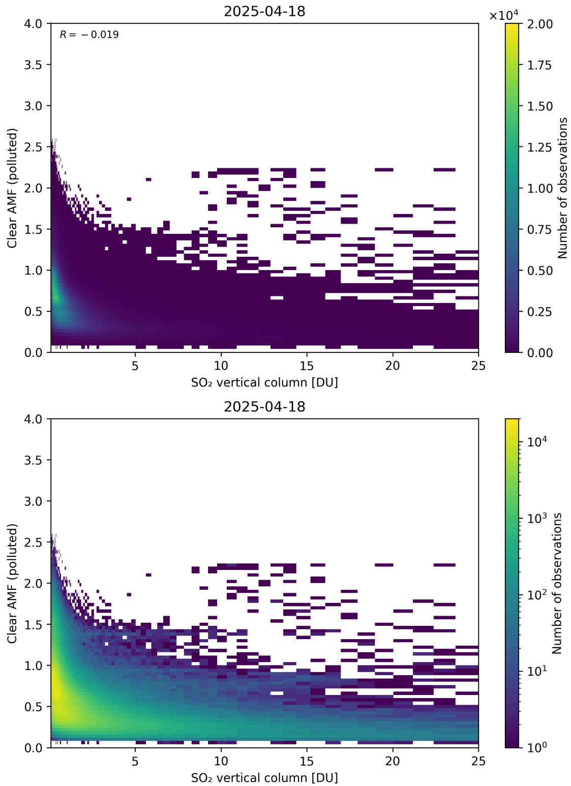
Figure 348: Scatter density plot of “SO 2 vertical column” against “Clear AMF (polluted)” for 2025-04-18 to 2025-04-19.
