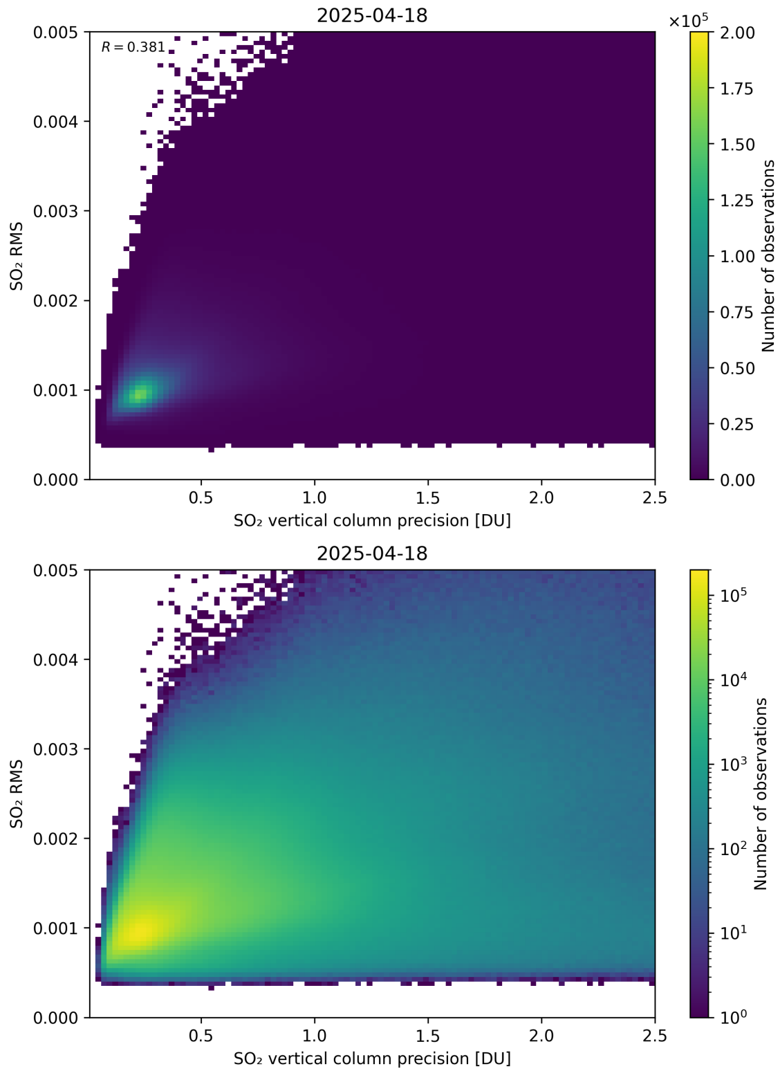
Figure 334: Scatter density plot of “SO 2 vertical column precision” against “SO 2 RMS” for 2025-04-18 to 2025-04-19.
