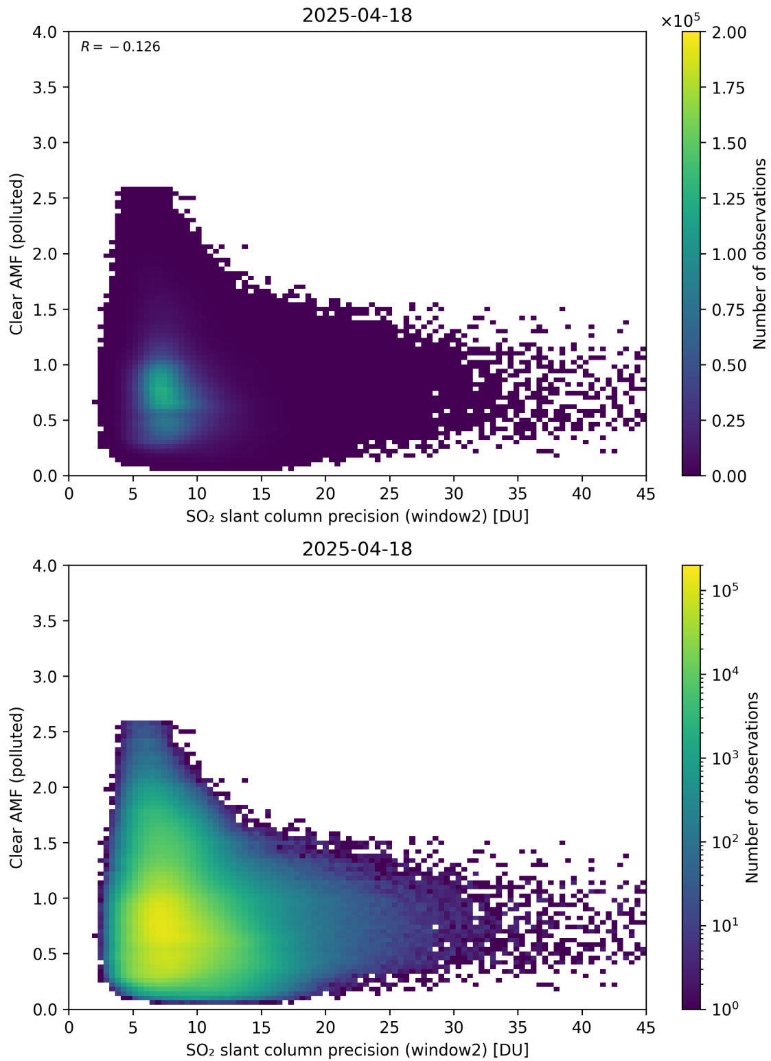
Figure 296: Scatter density plot of “SO 2 slant column precision (window2)” against “Clear AMF (polluted)” for 2025-04-18 to 2025-04-19.
