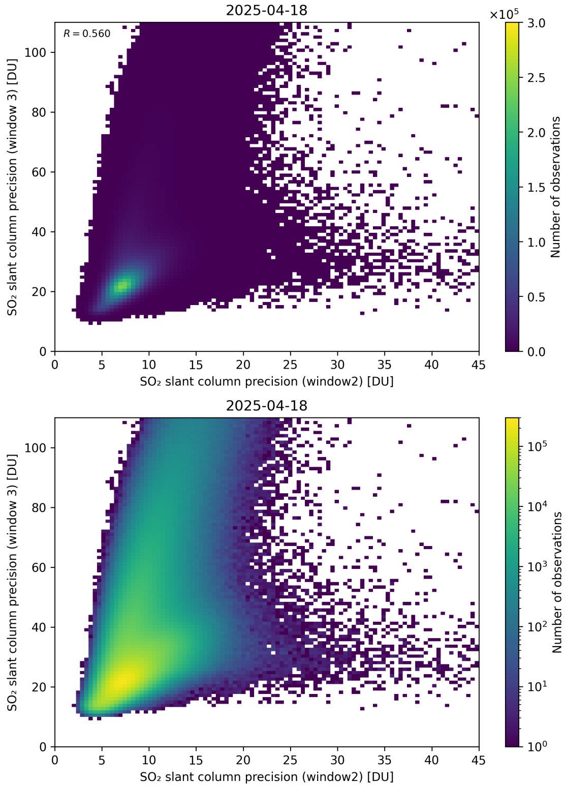
Figure 300: Scatter density plot of “SO 2 slant column precision (window2)” against “SO 2 slant column precision (window 3)” for 2025-04-18 to 2025-04-19.
