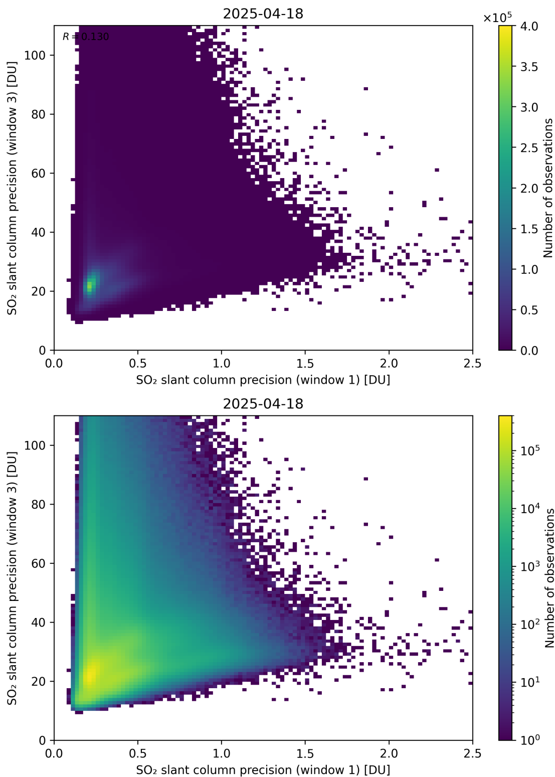
Figure 279: Scatter density plot of “SO 2 slant column precision (window 1)” against “SO 2 slant column precision (window 3)” for 2025-04-18 to 2025-04-19.
