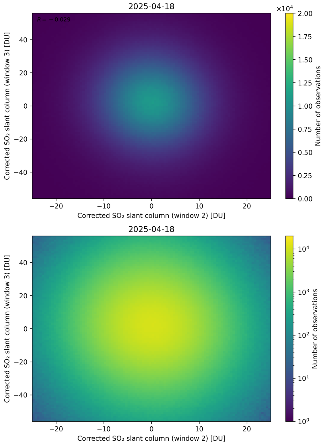
Figure 250: Scatter density plot of “Corrected SO 2 slant column (window 2)” against “Corrected SO 2 slant column (window 3)” for 2025-04-18 to 2025-04-19.
