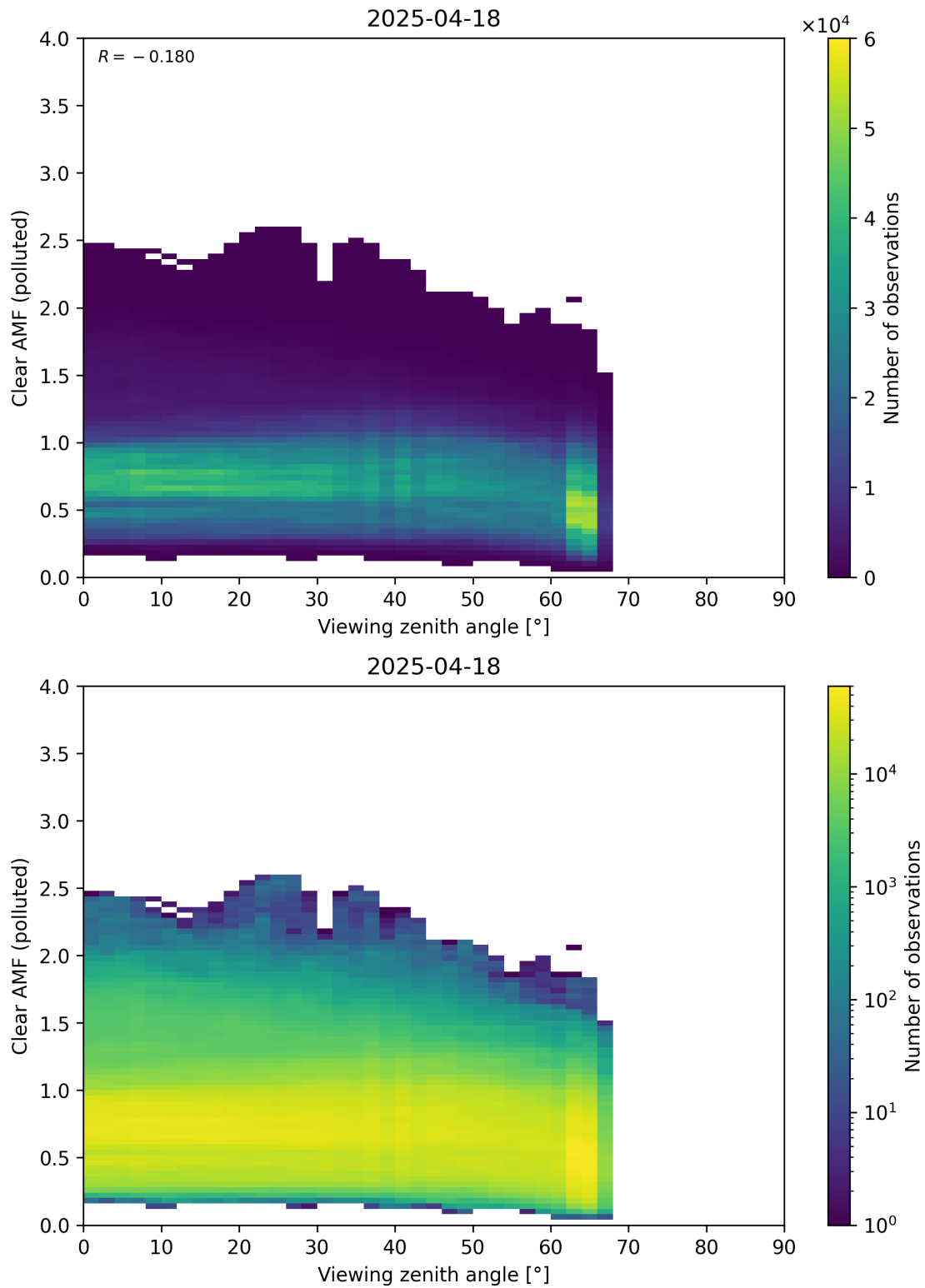
Figure 370: Scatter density plot of “Viewing zenith angle” against “Clear AMF (polluted)” for 2025-04-18 to 2025-04-19.
