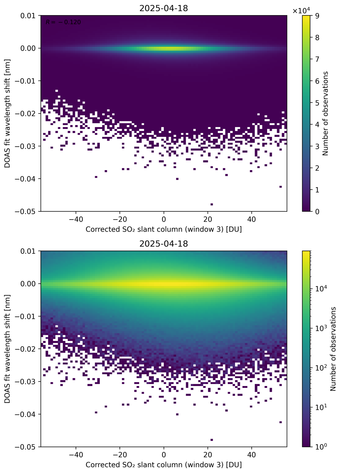
Figure 256: Scatter density plot of “Corrected SO 2 slant column (window 3)” against “DOAS fit wavelength shift” for 2025-04-18 to 2025-04-19.
