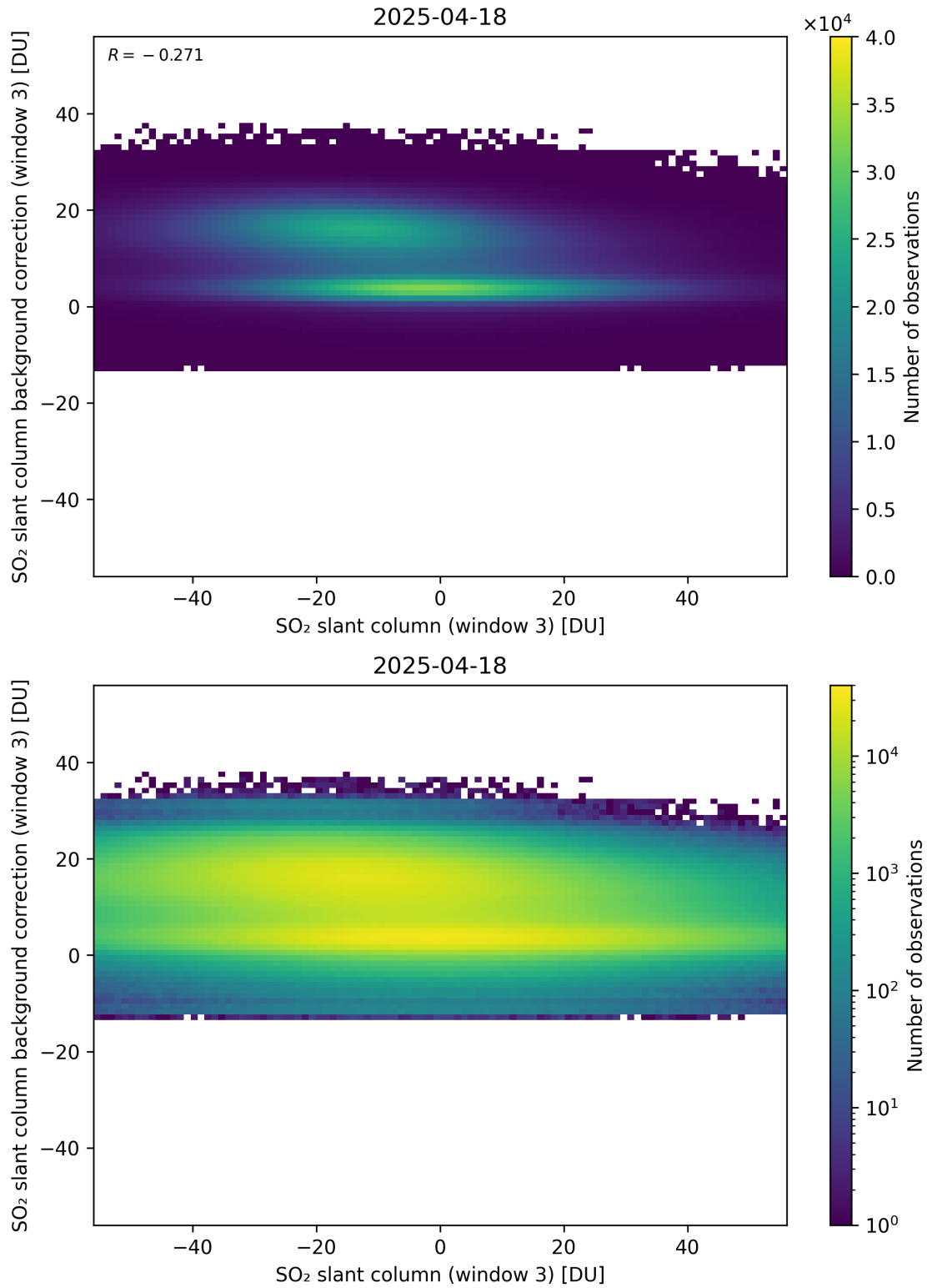
Figure 303: Scatter density plot of “SO 2 slant column (window 3)” against “SO 2 slant column background correction (window 3)” for 2025-04-18 to 2025-04-19.
