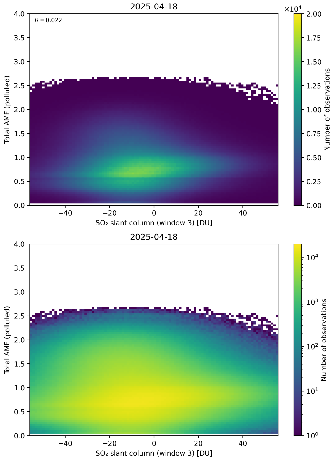
Figure 318: Scatter density plot of “SO 2 slant column (window 3)” against “Total AMF (polluted)” for 2025-04-18 to 2025-04-19.
