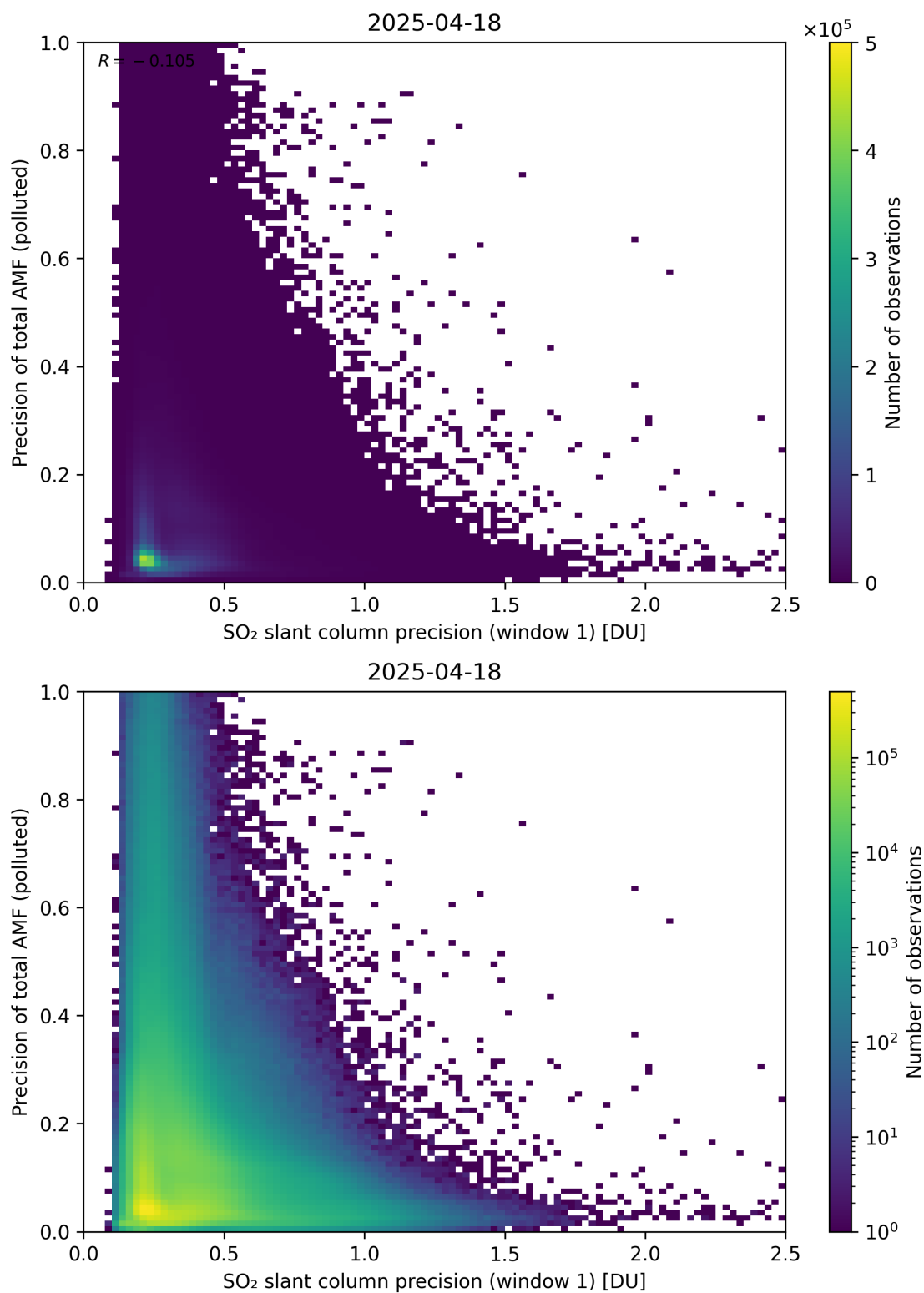
Figure 281: Scatter density plot of “SO 2 slant column precision (window 1)” against “Precision of total AMF (polluted)” for 2025-04-18 to 2025-04-19.
