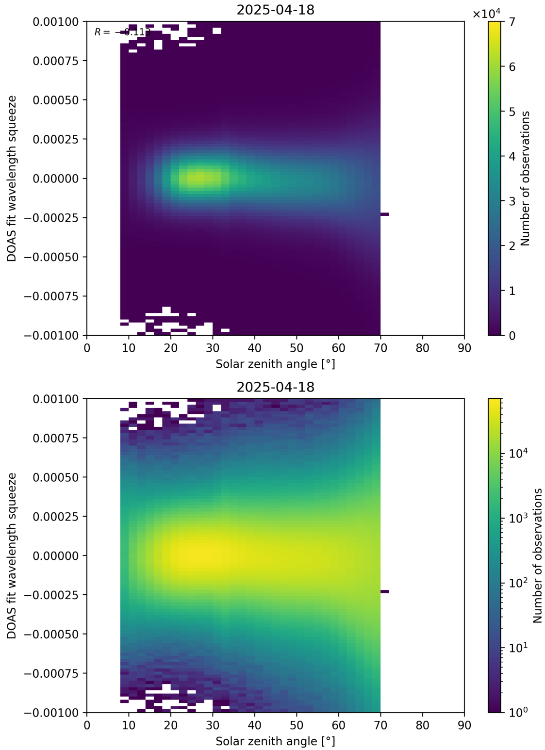
Figure 175: Scatter density plot of “Solar zenith angle” against “DOAS fit wavelength squeeze” for 2025-04-18 to 2025-04-19.
