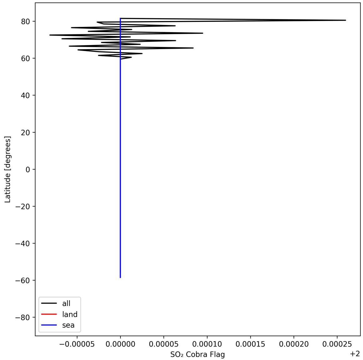
Figure 49: Zonal average of "SO 2 Cobra Flag" for 2025-04-18 to 2025-04-19.
