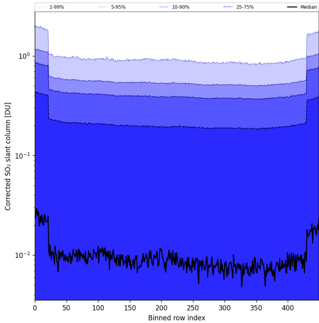
Figure 86: Along track statistics of “Corrected SO 2 slant column” for 2025-04-18 to 2025-04-19
