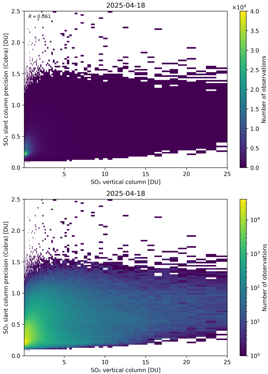
Figure 350: Scatter density plot of “SO 2 vertical column” against “SO 2 slant column precision (Cobra)” for 2025-04-18 to 2025-04-19.
