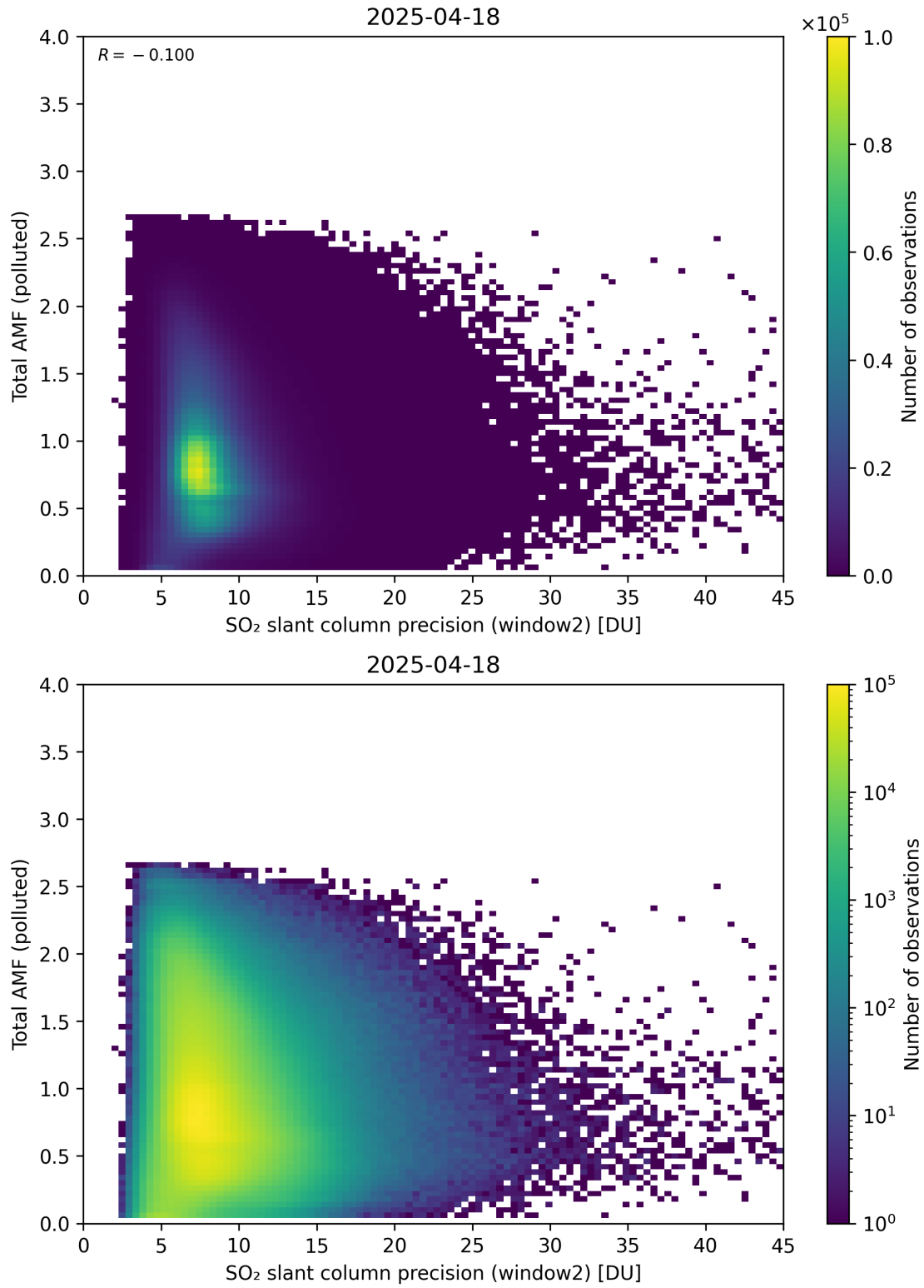
Figure 301: Scatter density plot of “SO 2 slant column precision (window2)” against “Total AMF (polluted)” for 2025-04-18 to 2025-04-19.
