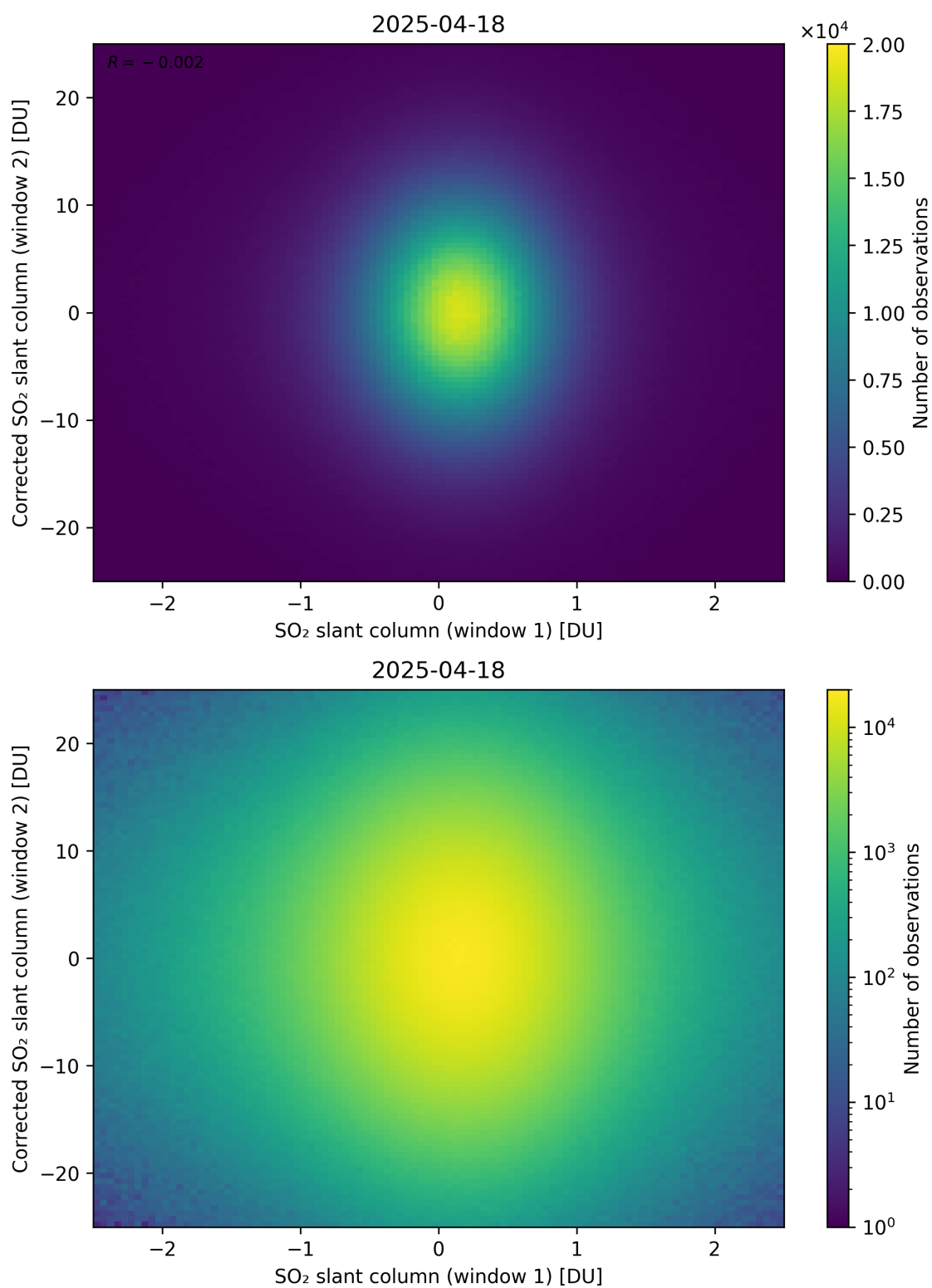
Figure 283: Scatter density plot of “SO 2 slant column (window 1)” against “Corrected SO 2 slant column (window 2)” for 2025-04-18 to 2025-04-19.
