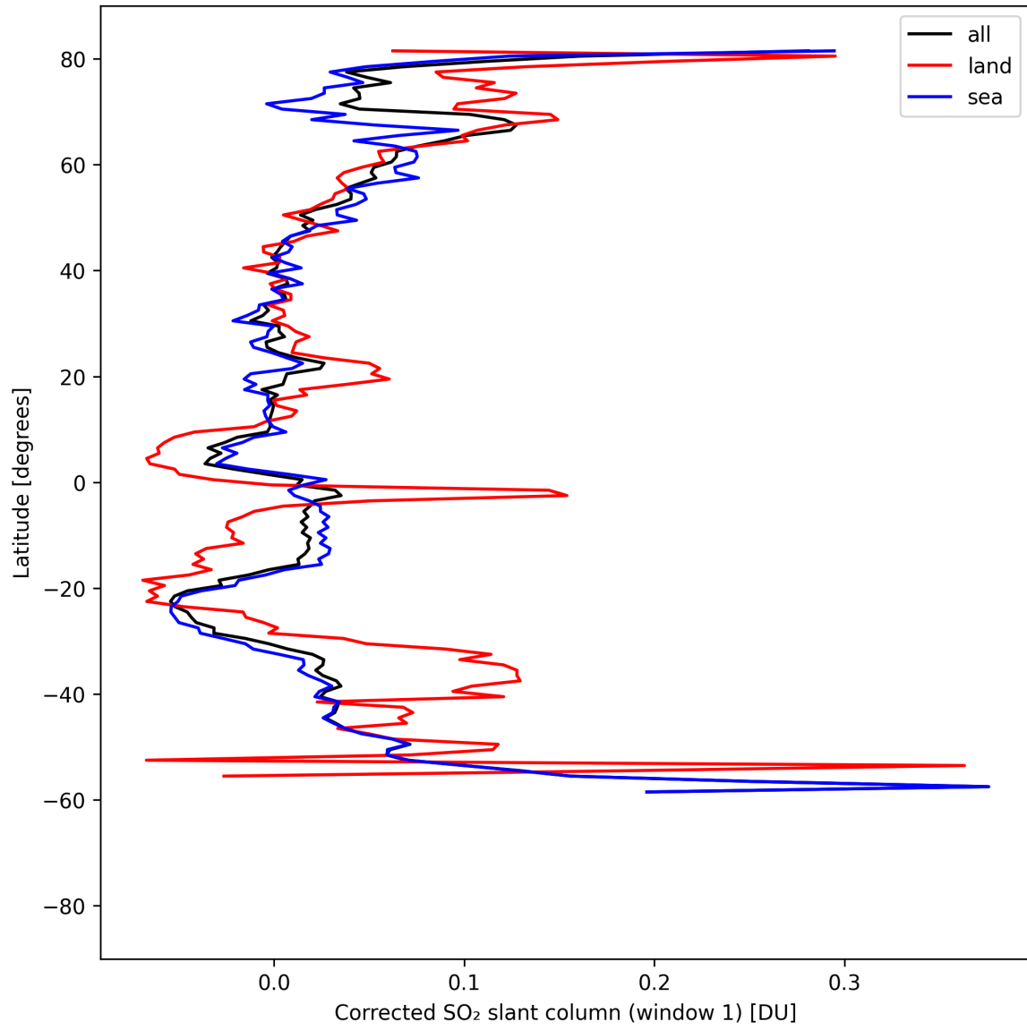
Figure 39: Zonal average of “Corrected SO 2 slant column (window 1)” for 2025-04-18 to 2025-04-19.
