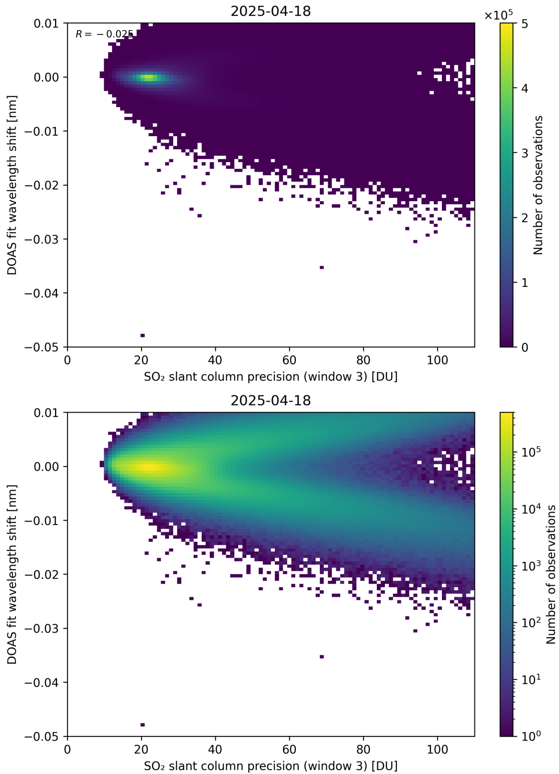
Figure 308: Scatter density plot of “SO 2 slant column precision (window 3)” against “DOAS fit wavelength shift” for 2025-04-18 to 2025-04-19.
