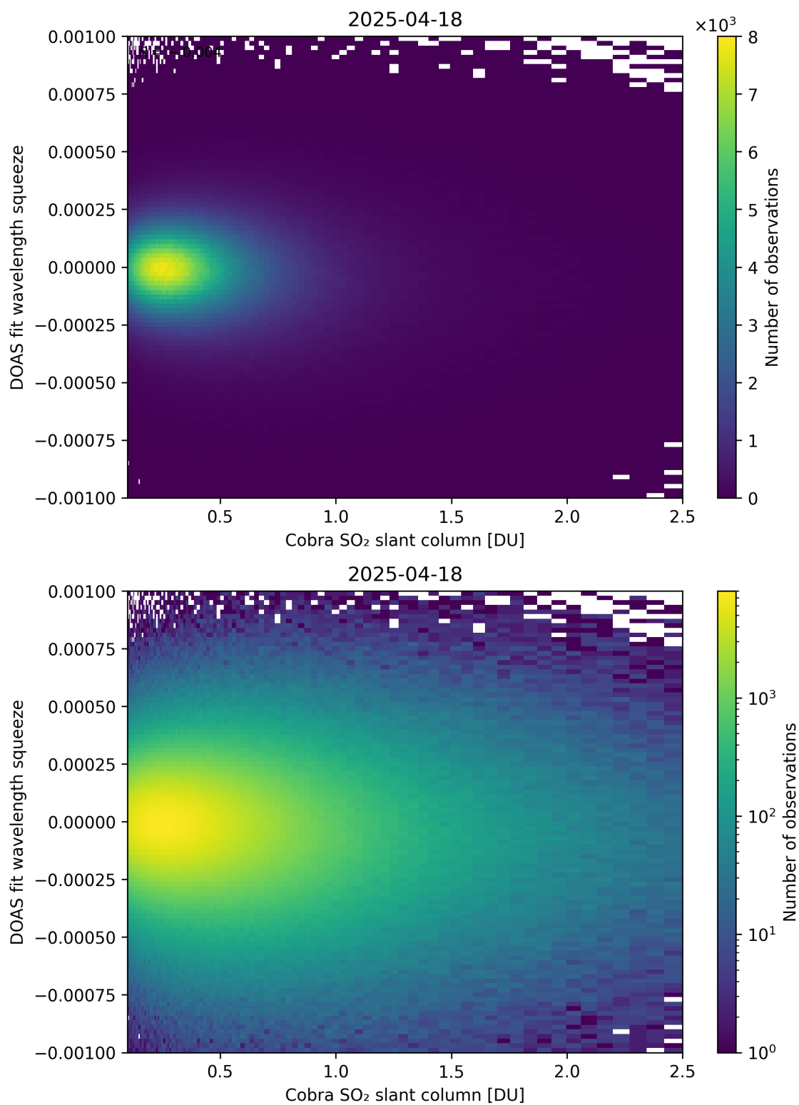
Figure 197: Scatter density plot of “Cobra SO 2 slant column” against “DOAS fit wavelength squeeze” for 2025-04-18 to 2025-04-19.
