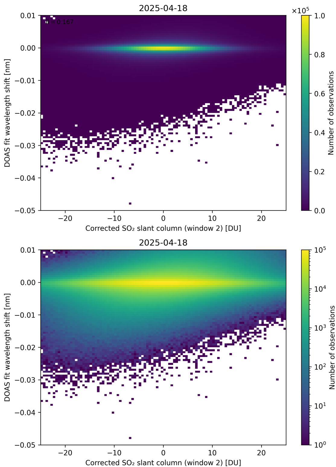
Figure 246: Scatter density plot of “Corrected SO 2 slant column (window 2)” against “DOAS fit wavelength shift” for 2025-04-18 to 2025-04-19.
