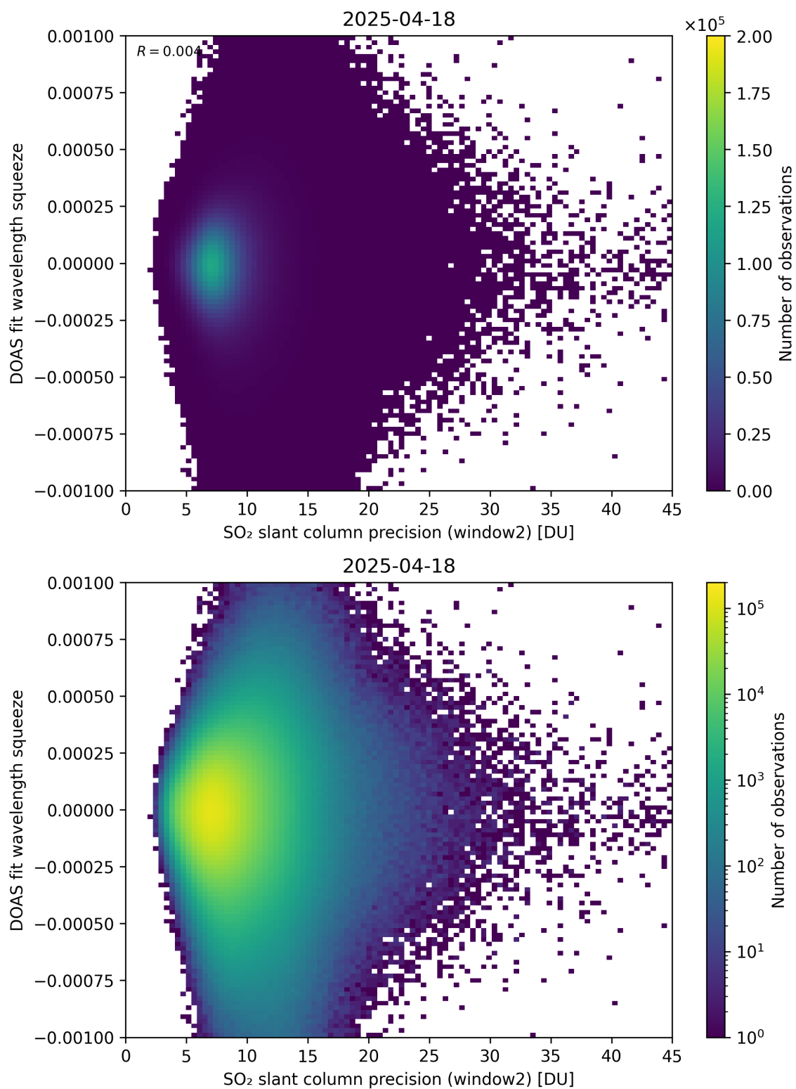
Figure 294: Scatter density plot of “SO 2 slant column precision (window2)” against “DOAS fit wavelength squeeze” for 2025-04-18 to 2025-04-19.
