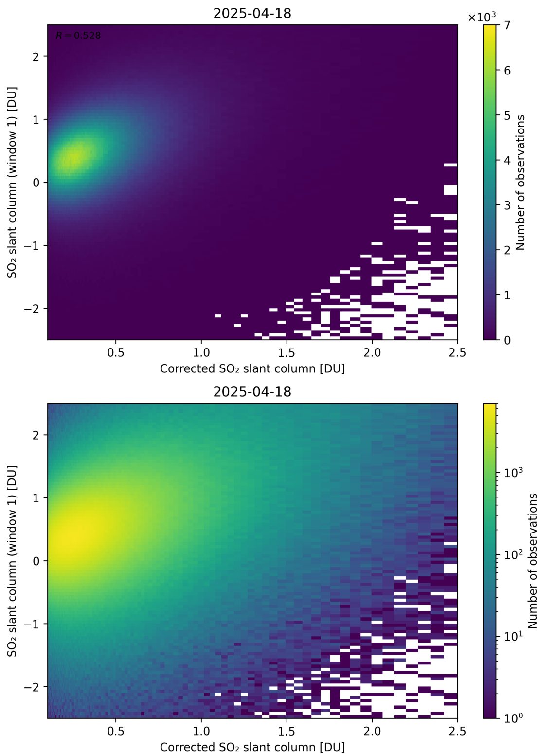
Figure 237: Scatter density plot of “Corrected SO 2 slant column” against “SO 2 slant column (window 1)” for 2025-04-18 to 2025-04-19.
