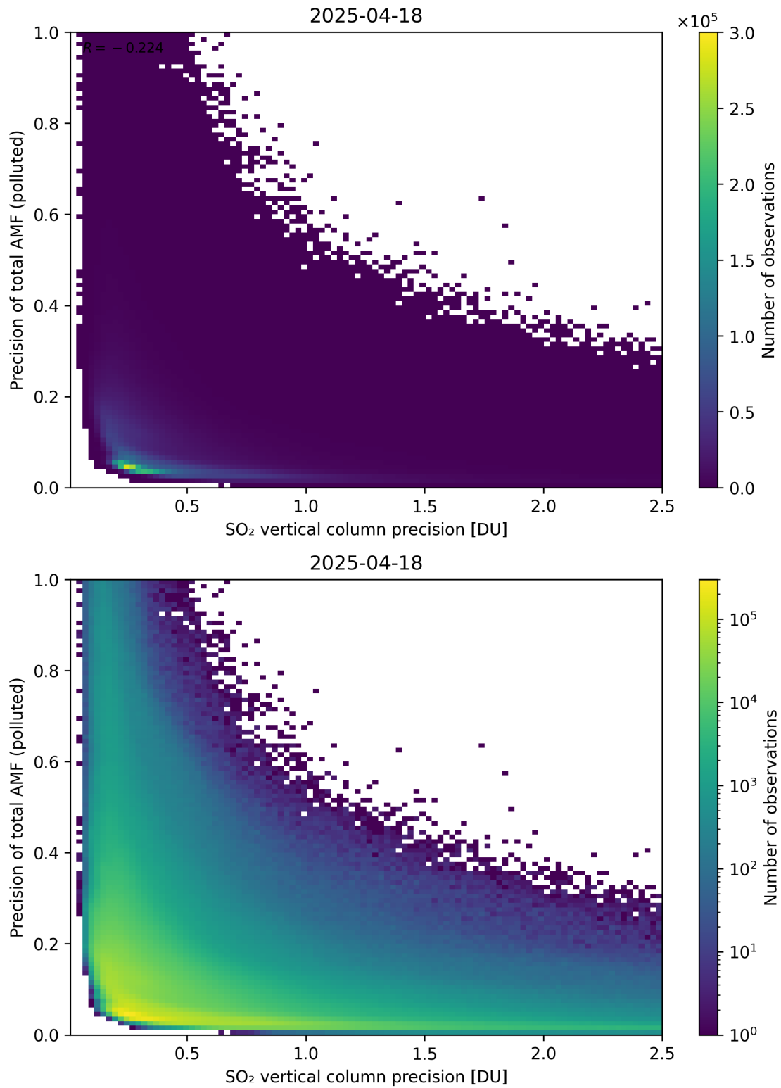
Figure 347: Scatter density plot of “SO 2 vertical column precision” against “Precision of total AMF (polluted)” for 2025-04-18 to 2025-04-19.
