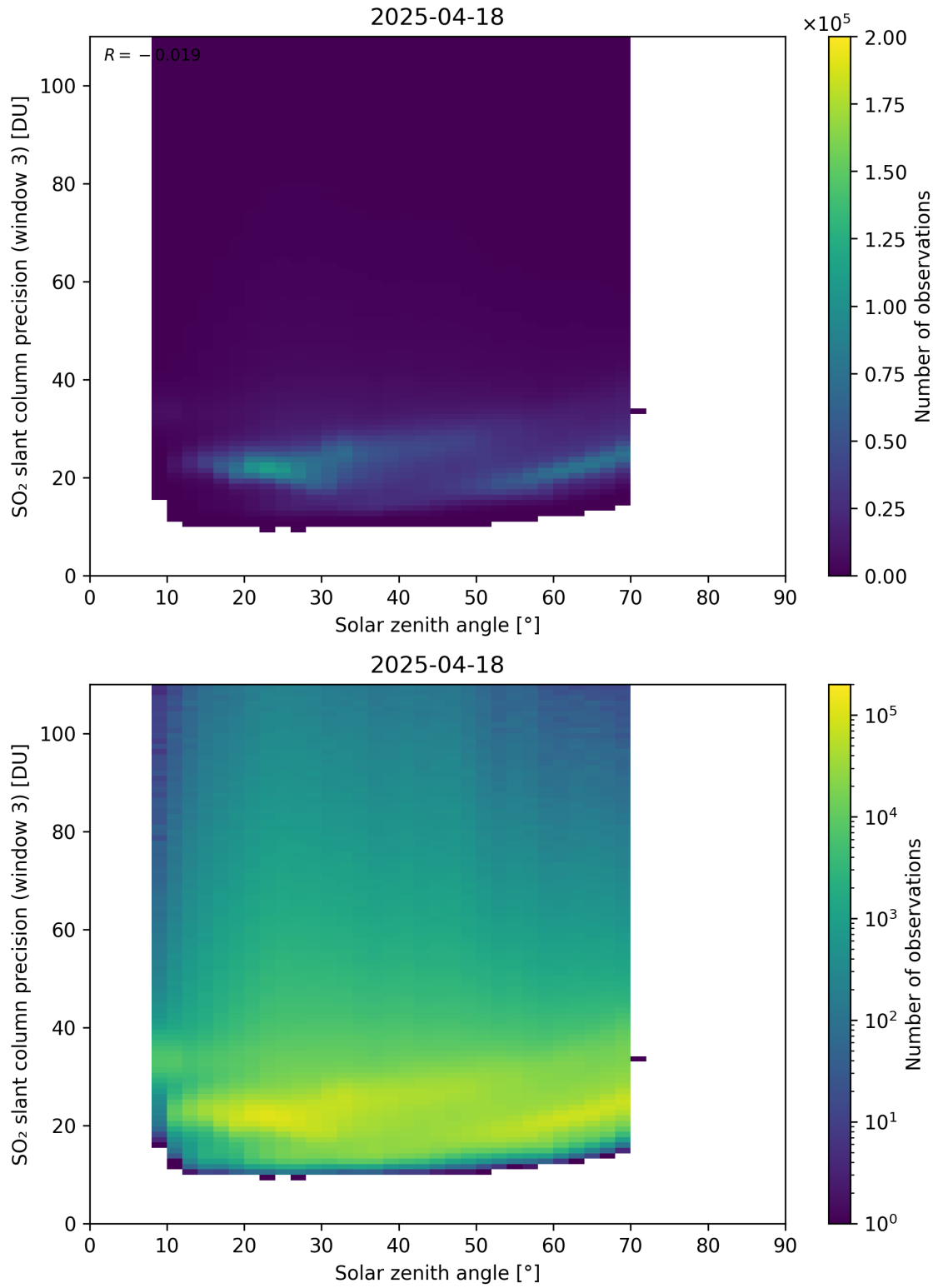
Figure 188: Scatter density plot of “Solar zenith angle” against “SO 2 slant column precision (window 3)” for 2025-04-18 to 2025-04-19.
