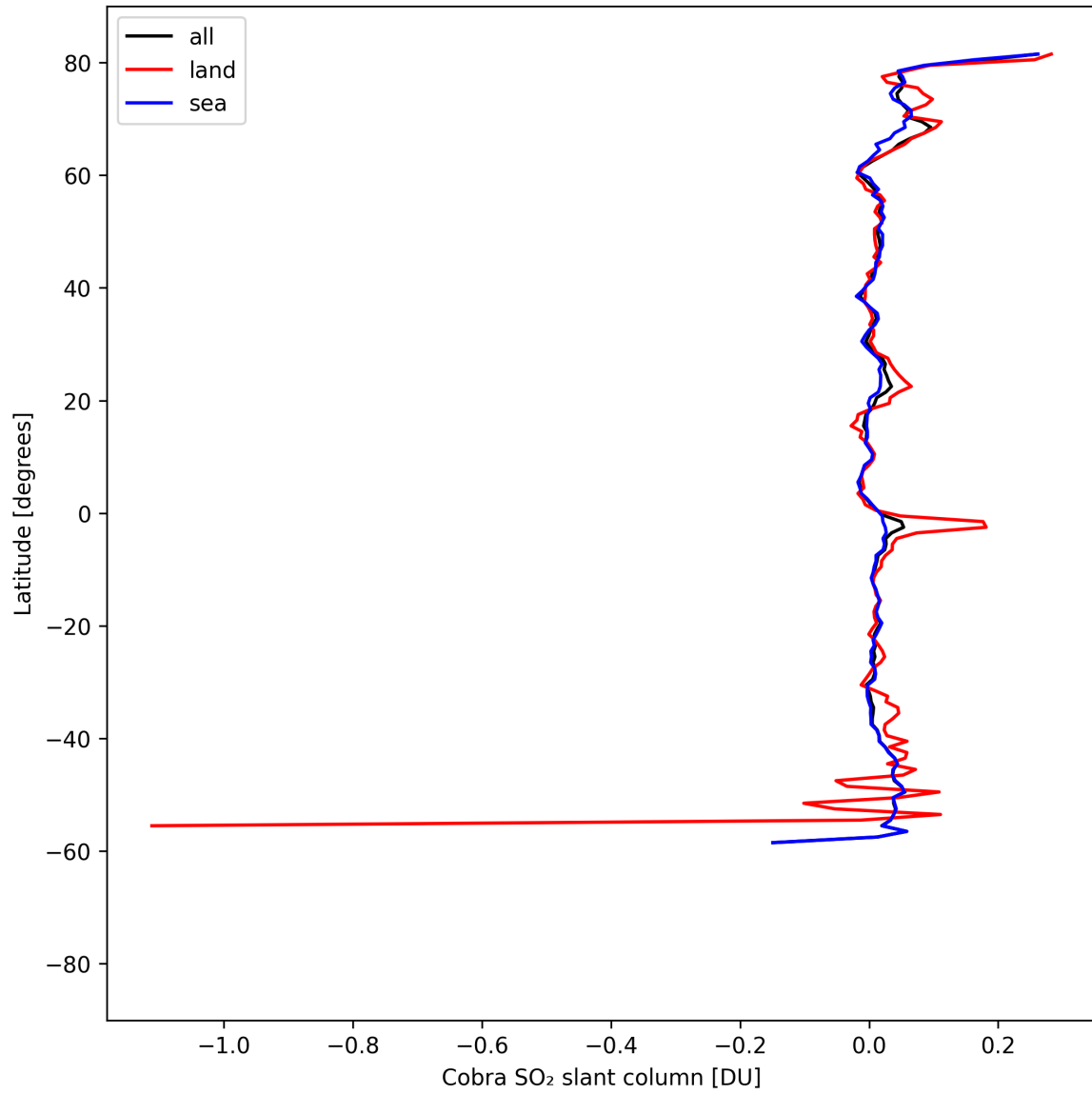
Figure 35: Zonal average of “Cobra SO 2 slant column” for 2025-04-18 to 2025-04-19.
