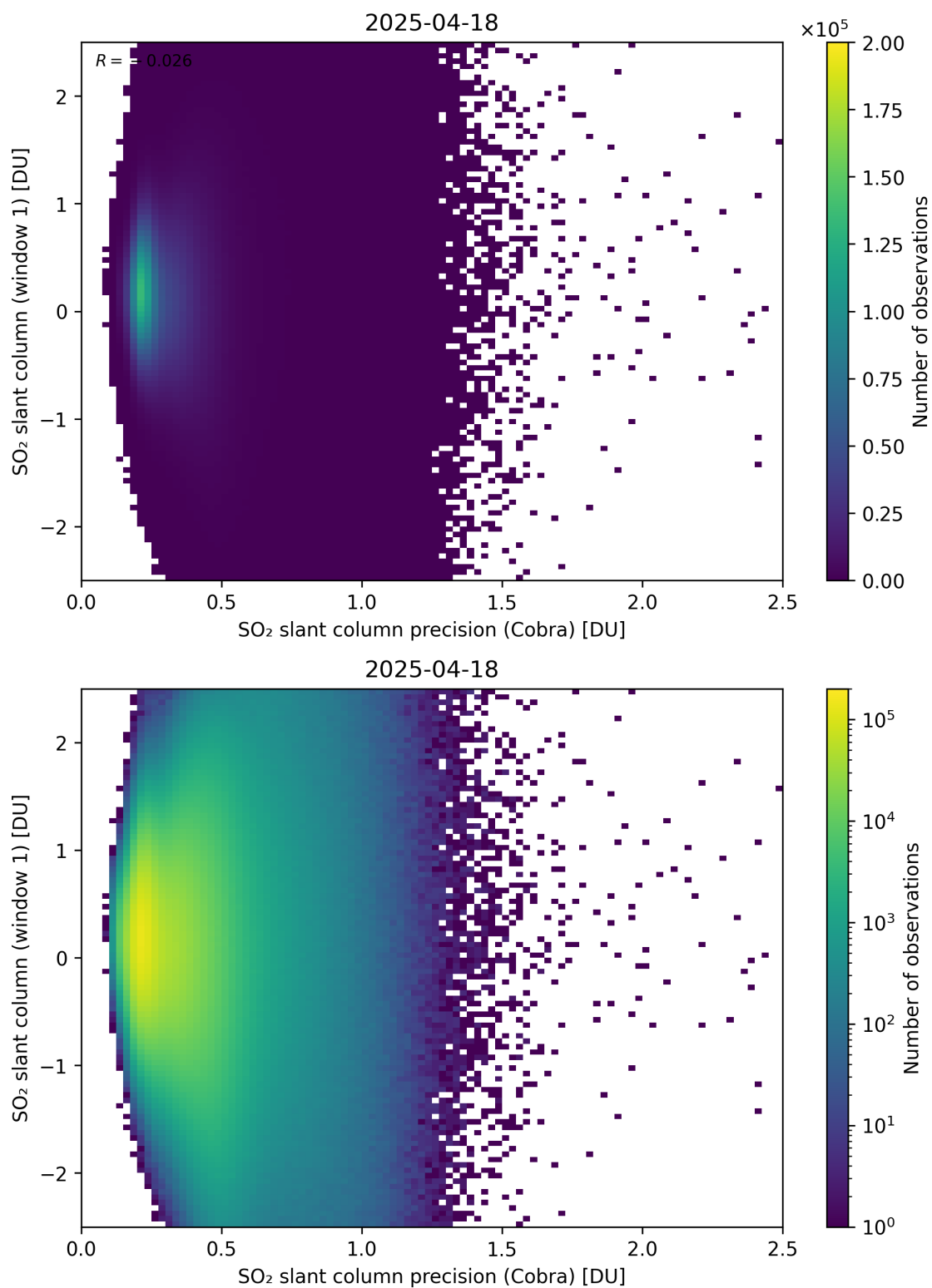
Figure 208: Scatter density plot of “SO 2 slant column precision (Cobra)” against “SO 2 slant column (window 1)” for 2025-04-18 to 2025-04-19.
