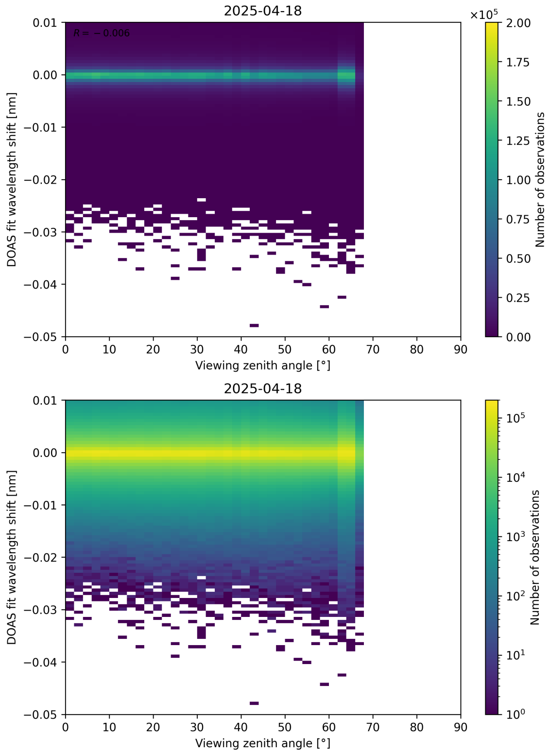
Figure 365: Scatter density plot of “Viewing zenith angle” against “DOAS fit wavelength shift” for 2025-04-18 to 2025-04-19.
