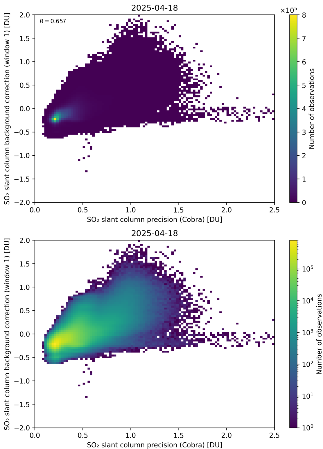
Figure 199: Scatter density plot of “SO 2 slant column precision (Cobra)” against “SO 2 slant column background correction (window 1)” for 2025-04-18 to 2025-04-19.
