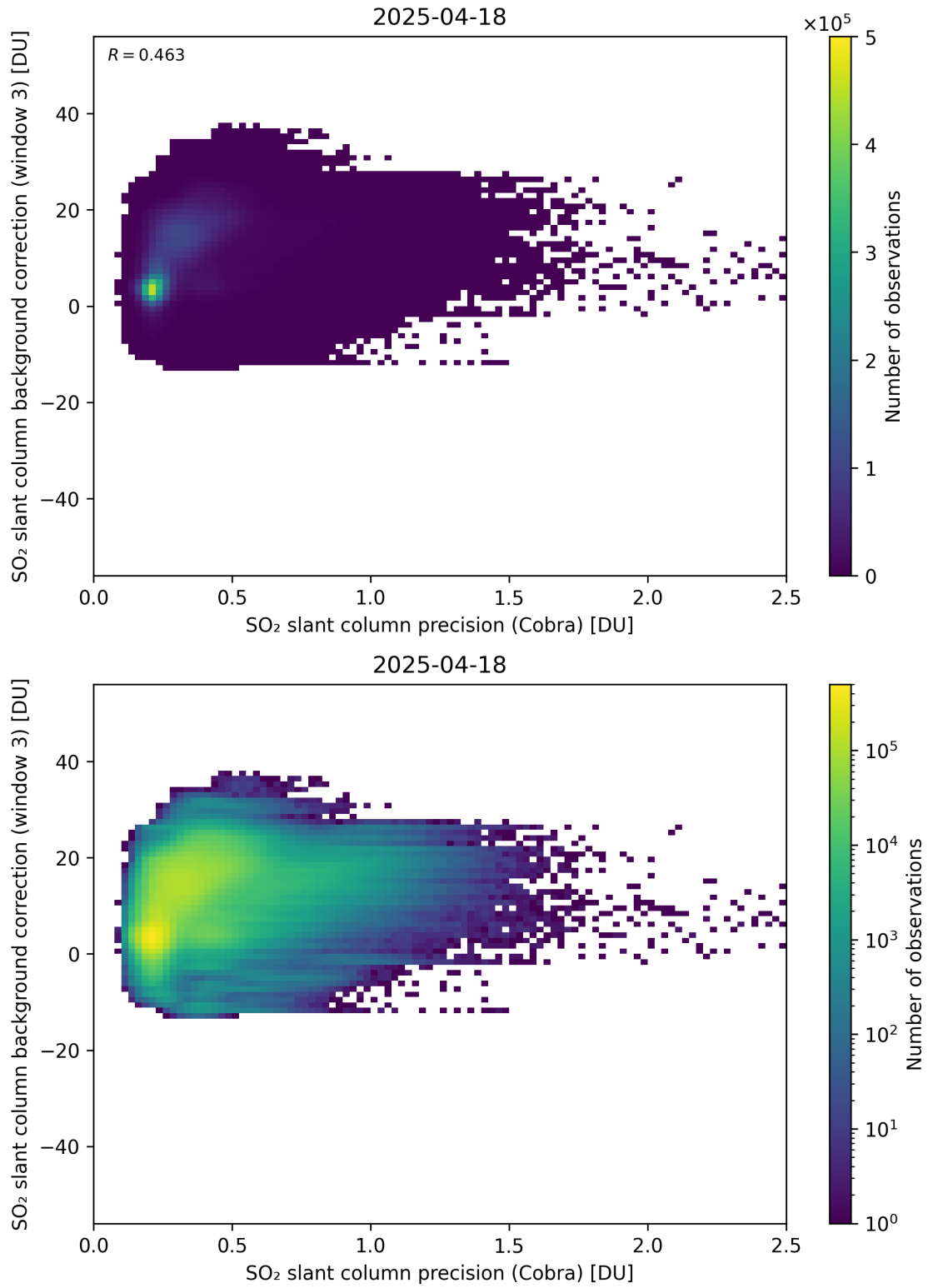
Figure 201: Scatter density plot of “SO 2 slant column precision (Cobra)” against “SO 2 slant column background correction (window 3)” for 2025-04-18 to 2025-04-19.
