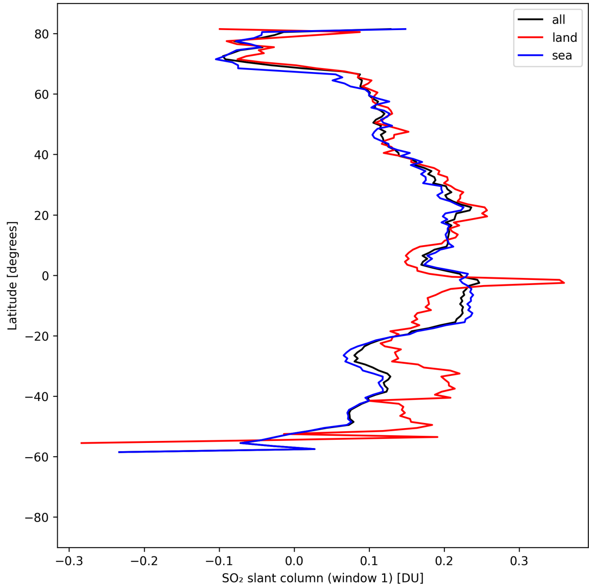
Figure 37: Zonal average of “SO 2 slant column (window 1)” for 2025-04-18 to 2025-04-19.
