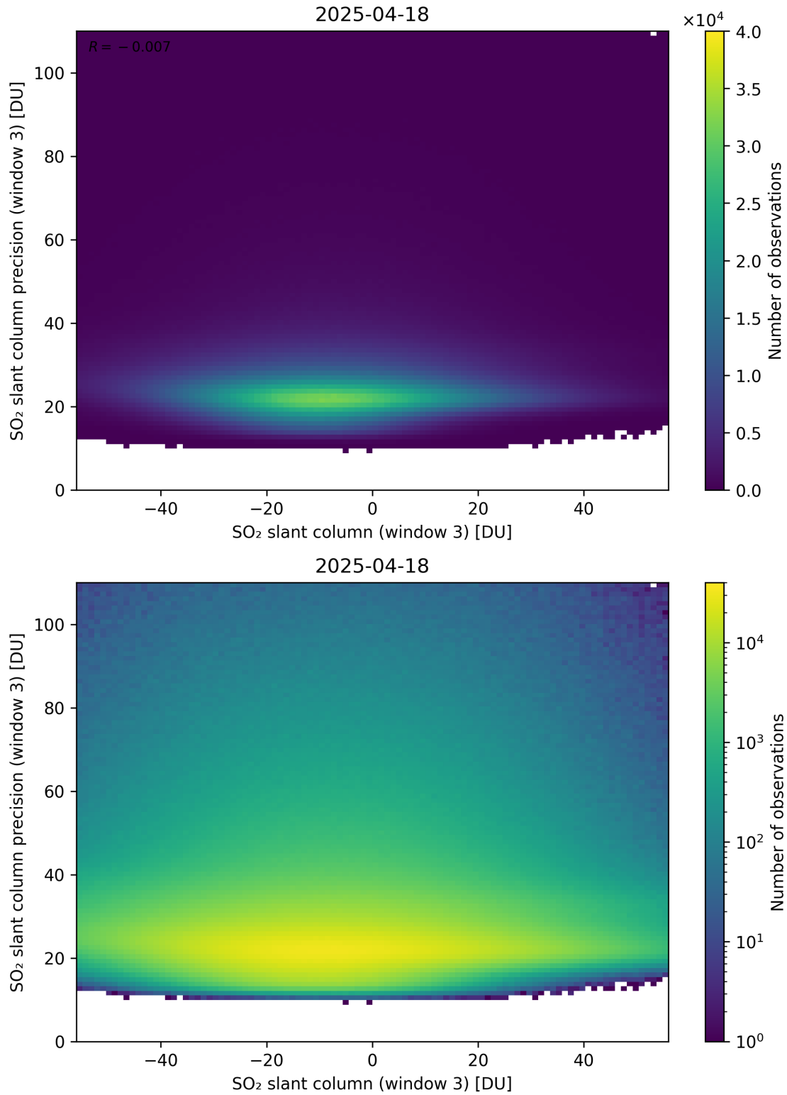
Figure 317: Scatter density plot of “SO 2 slant column (window 3)” against “SO 2 slant column precision (window 3)” for 2025-04-18 to 2025-04-19.
