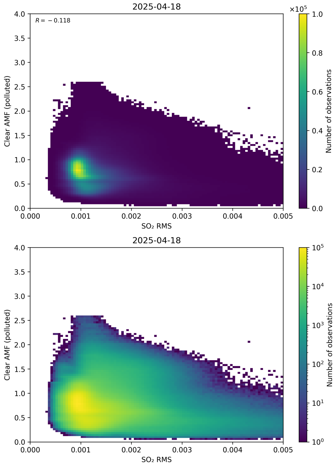
Figure 147: Scatter density plot of “SO 2 RMS” against “Clear AMF (polluted)” for 2025-04-18 to 2025-04-19.
