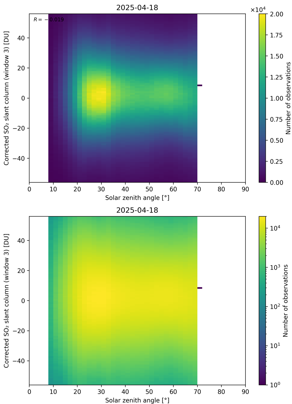
Figure 183: Scatter density plot of “Solar zenith angle” against “Corrected SO 2 slant column (window 3)” for 2025-04-18 to 2025-04-19.
