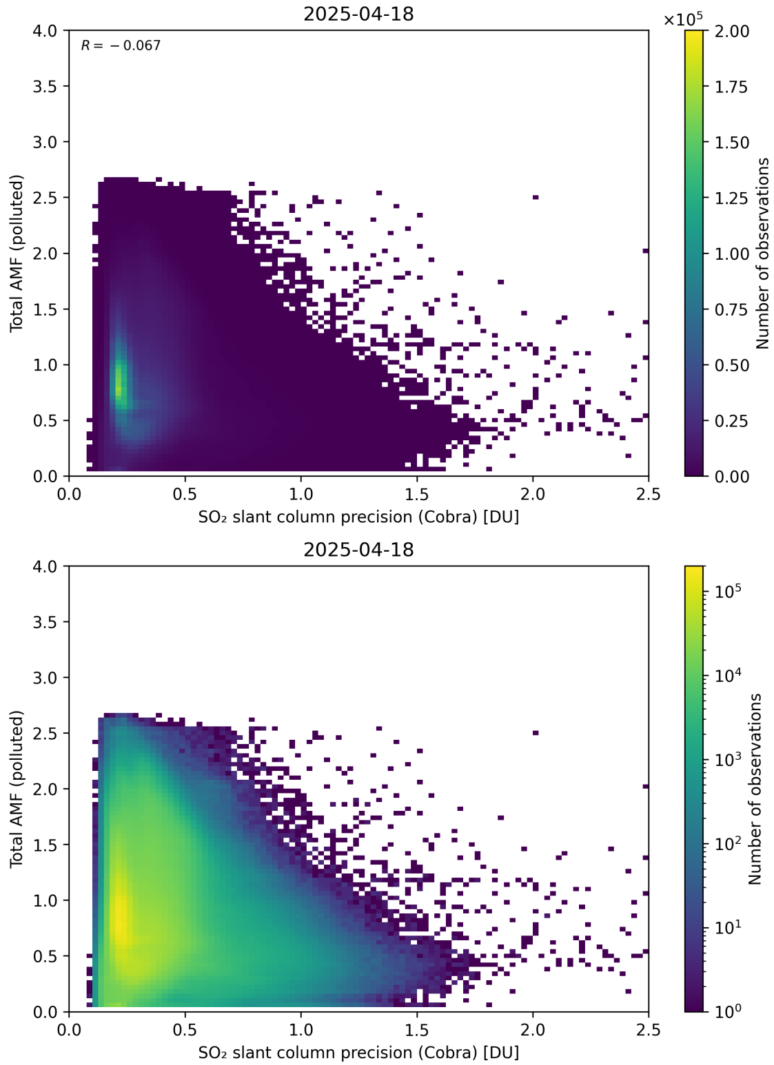
Figure 213: Scatter density plot of “SO 2 slant column precision (Cobra)” against “Total AMF (polluted)” for 2025-04-18 to 2025-04-19.
