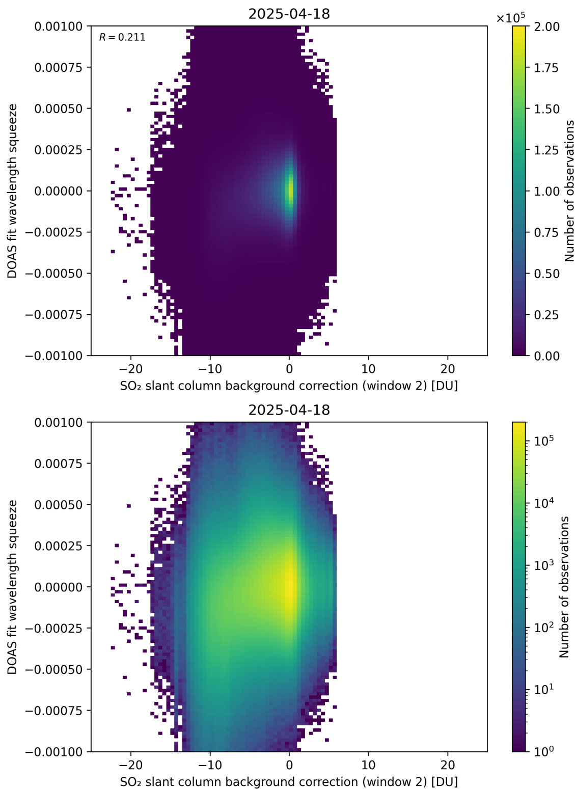
Figure 124: Scatter density plot of “SO 2 slant column background correction (window 2)” against “DOAS fit wavelength squeeze” for 2025-04-18 to 2025-04-19.
