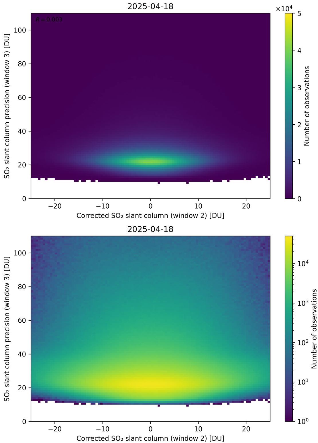
Figure 252: Scatter density plot of “Corrected SO 2 slant column (window 2)” against “SO 2 slant column precision (window 3)” for 2025-04-18 to 2025-04-19.
