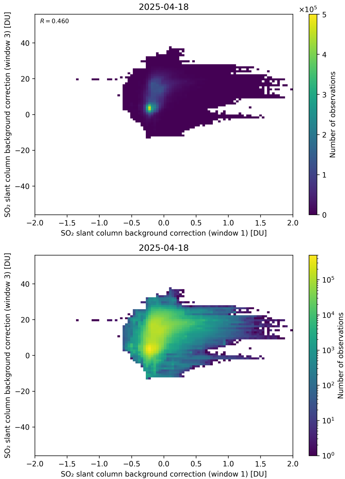
Figure 110: Scatter density plot of “SO 2 slant column background correction (window 1)” against “SO 2 slant column background correction (window 3)” for 2025-04-18 to 2025-04-19.
