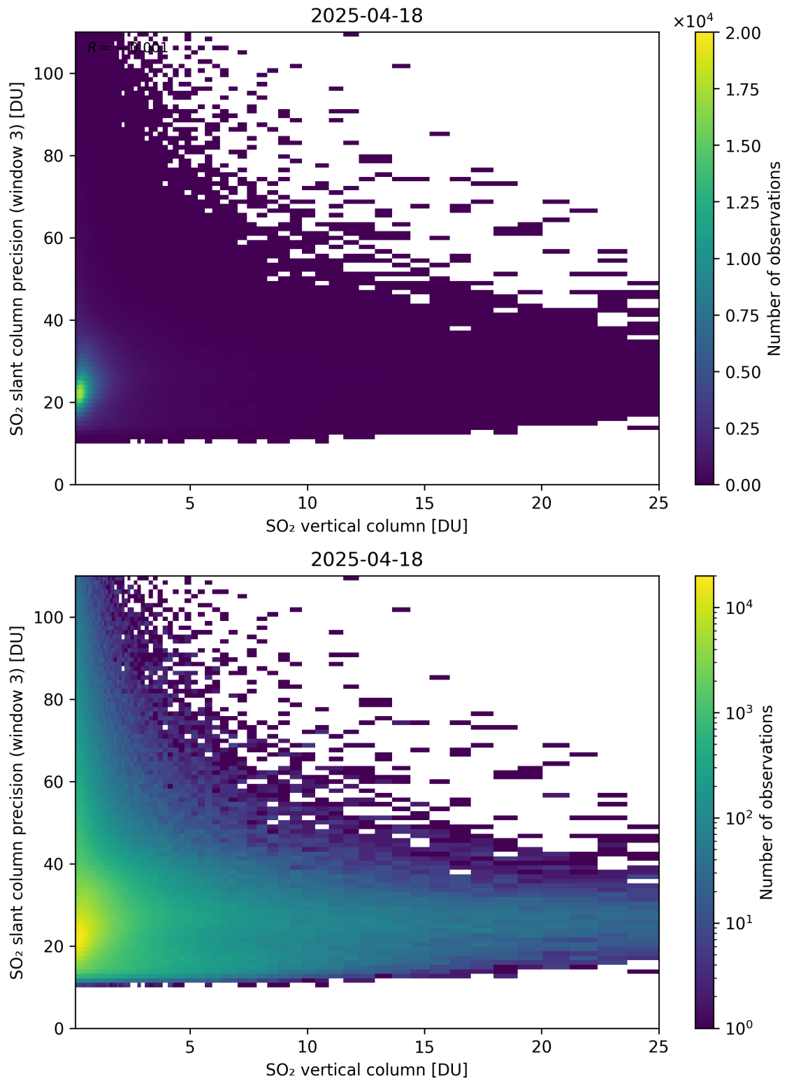
Figure 358: Scatter density plot of “SO 2 vertical column” against “SO 2 slant column precision (window 3)” for 2025-04-18 to 2025-04-19.
