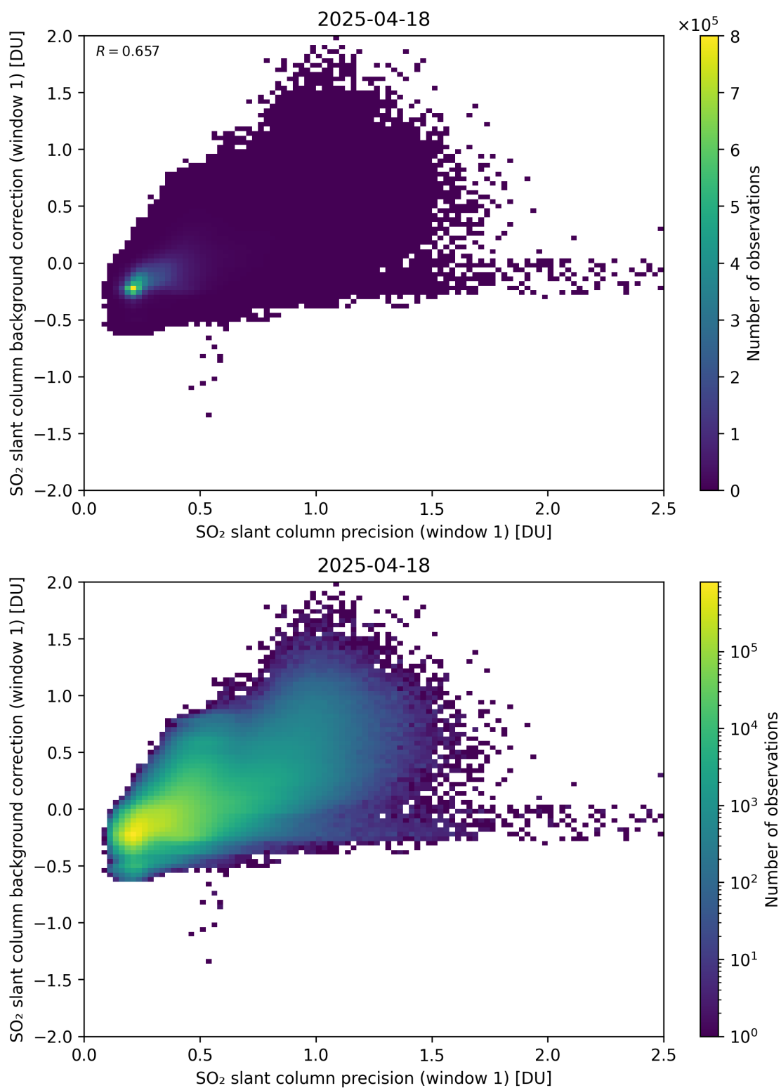
Figure 268: Scatter density plot of “SO 2 slant column precision (window 1)” against “SO 2 slant column background correction (window 1)” for 2025-04-18 to 2025-04-19.
