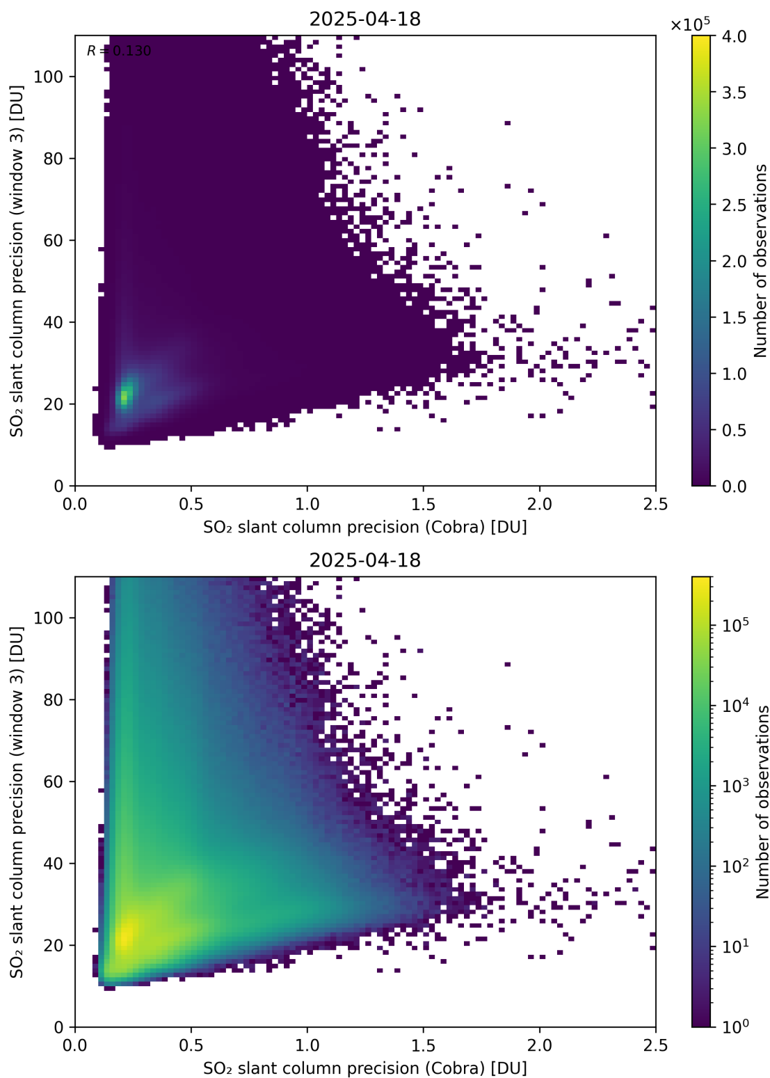
Figure 212: Scatter density plot of “SO 2 slant column precision (Cobra)” against “SO 2 slant column precision (window 3)” for 2025-04-18 to 2025-04-19.
