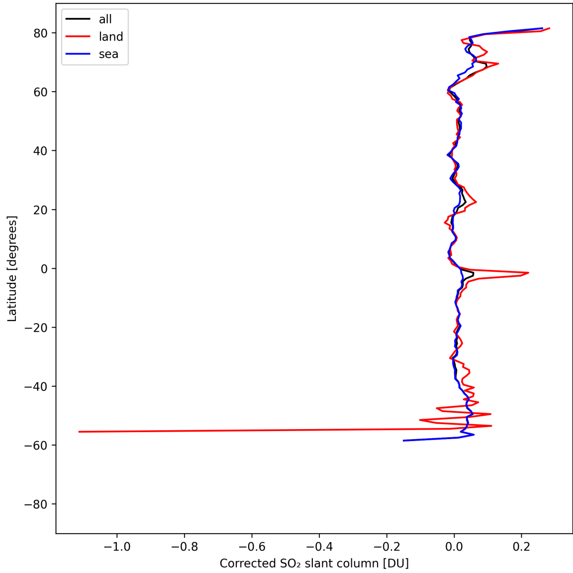
Figure 34: Zonal average of “Corrected SO 2 slant column” for 2025-04-18 to 2025-04-19.
