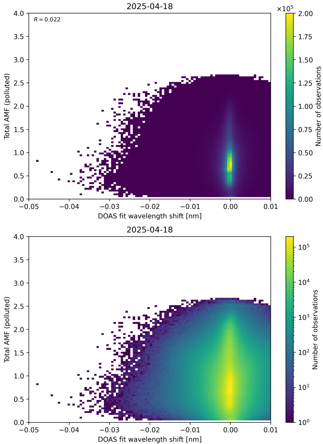
Figure 141: Scatter density plot of “DOAS fit wavelength shift” against “Total AMF (polluted)” for 2025-04-18 to 2025-04-19.
