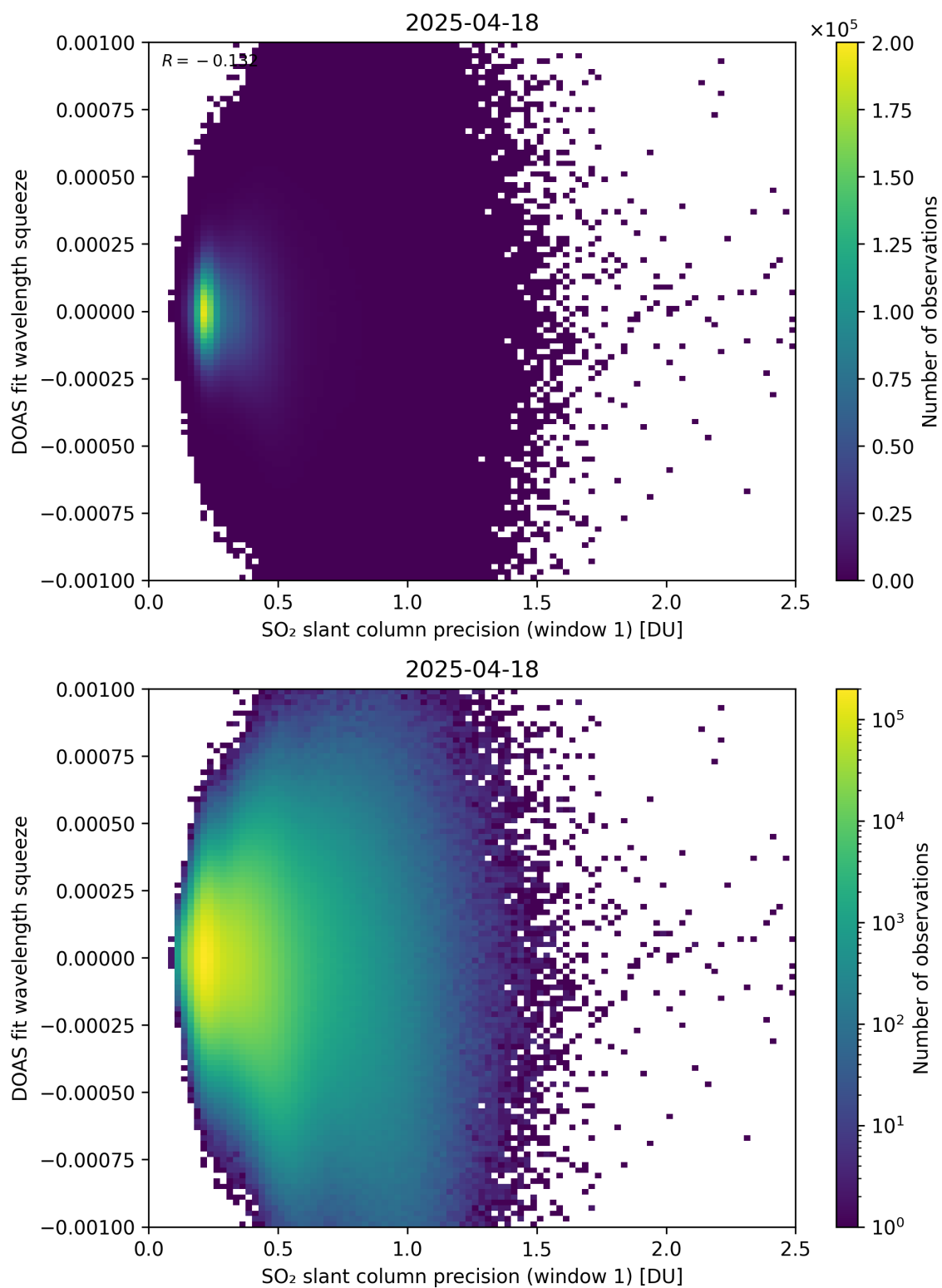
Figure 272: Scatter density plot of “SO 2 slant column precision (window 1)” against “DOAS fit wavelength squeeze” for 2025-04-18 to 2025-04-19.
