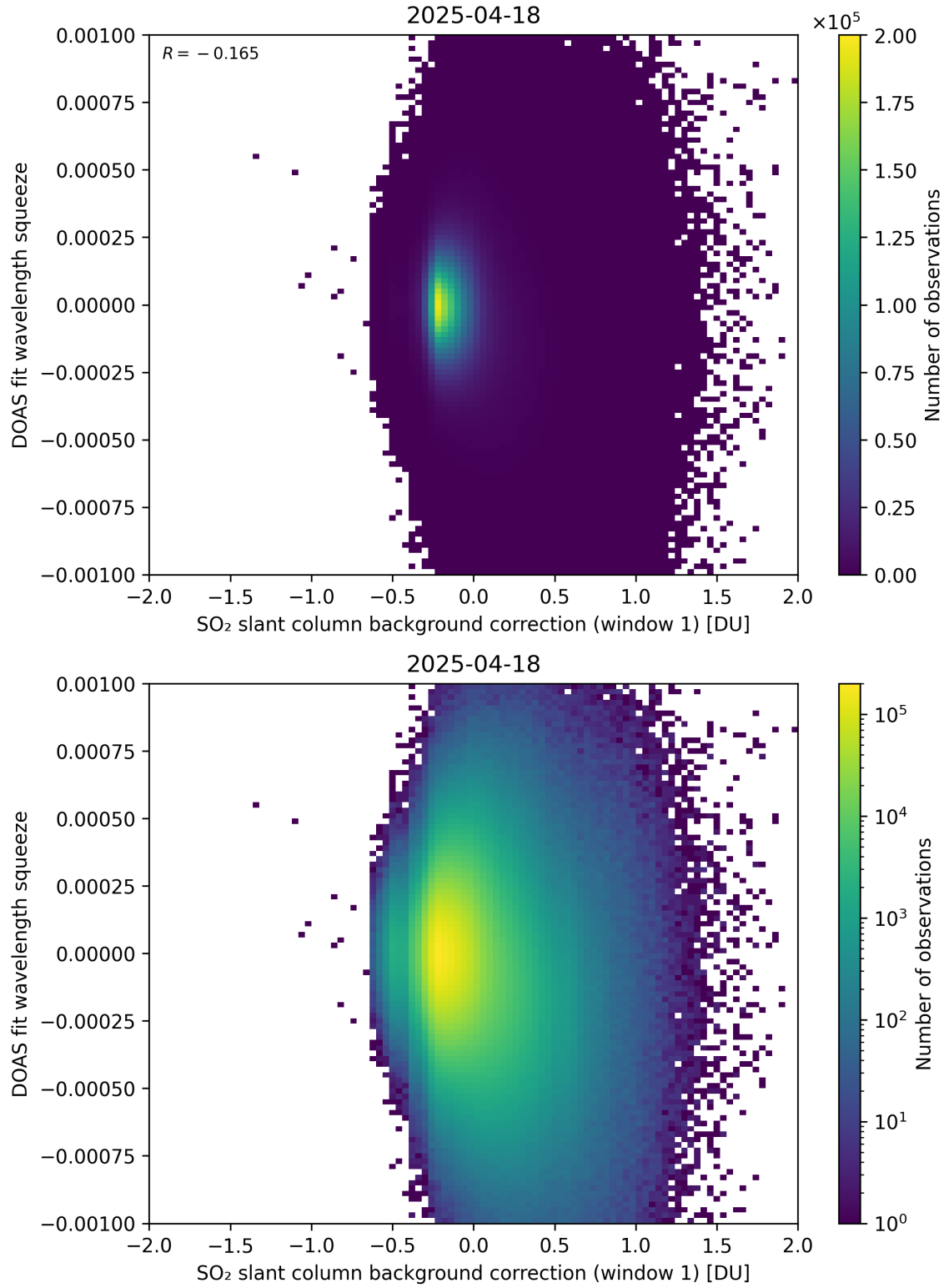
Figure 112: Scatter density plot of “SO 2 slant column background correction (window 1)” against “DOAS fit wavelength squeeze” for 2025-04-18 to 2025-04-19.
