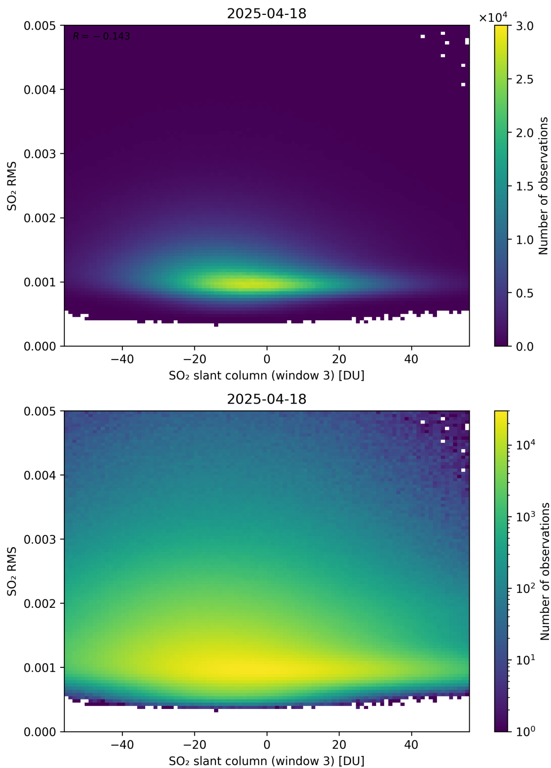
Figure 306: Scatter density plot of “SO 2 slant column (window 3)” against “SO 2 RMS” for 2025-04-18 to 2025-04-19.
