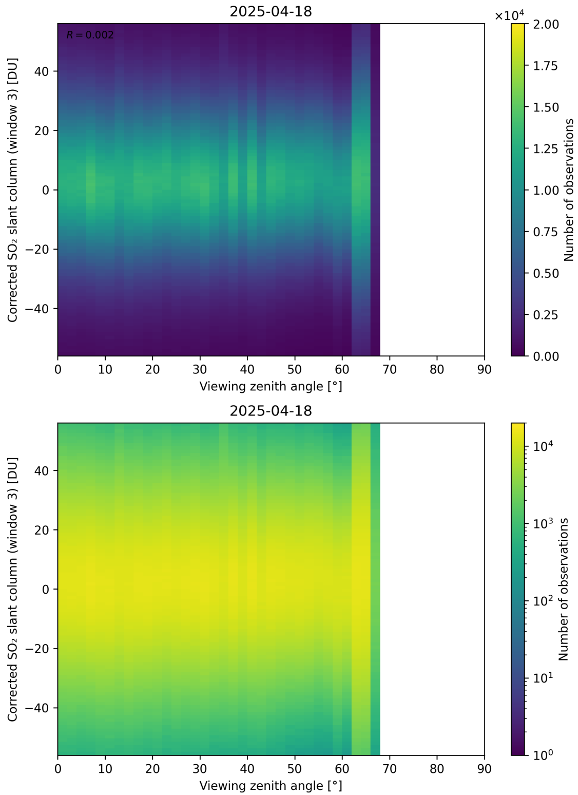
Figure 375: Scatter density plot of “Viewing zenith angle” against “Corrected SO 2 slant column (window 3)” for 2025-04-18 to 2025-04-19.
