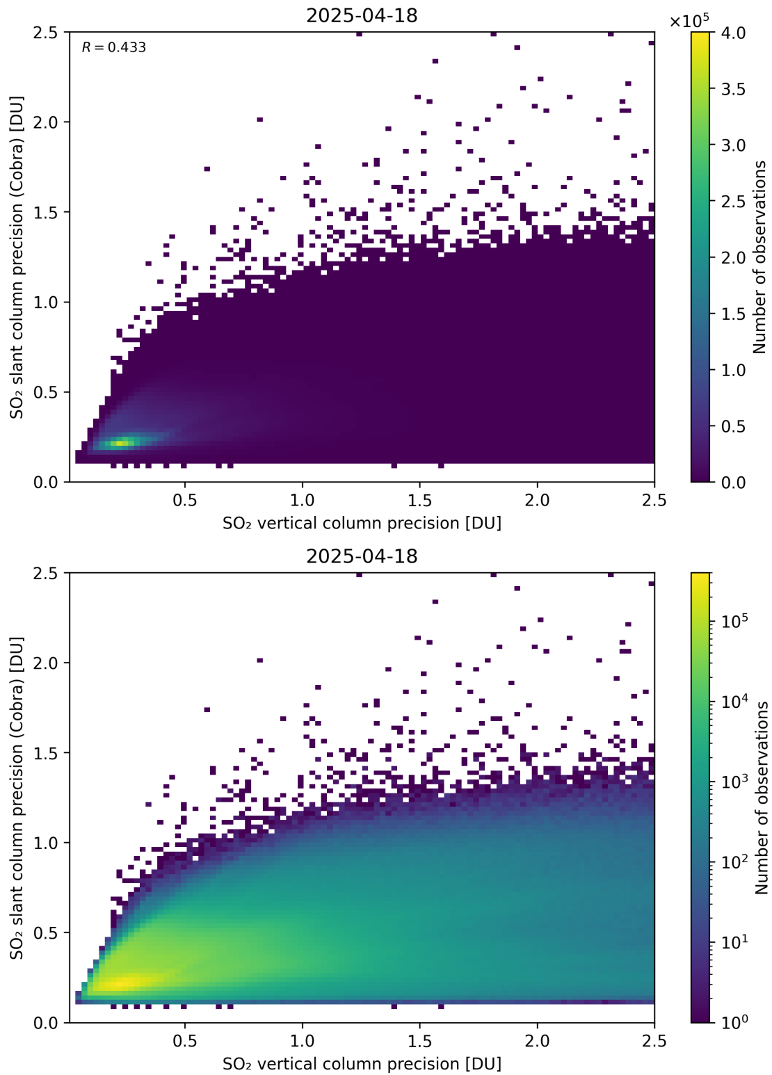
Figure 337: Scatter density plot of “SO 2 vertical column precision” against “SO 2 slant column precision (Cobra)” for 2025-04-18 to 2025-04-19.
