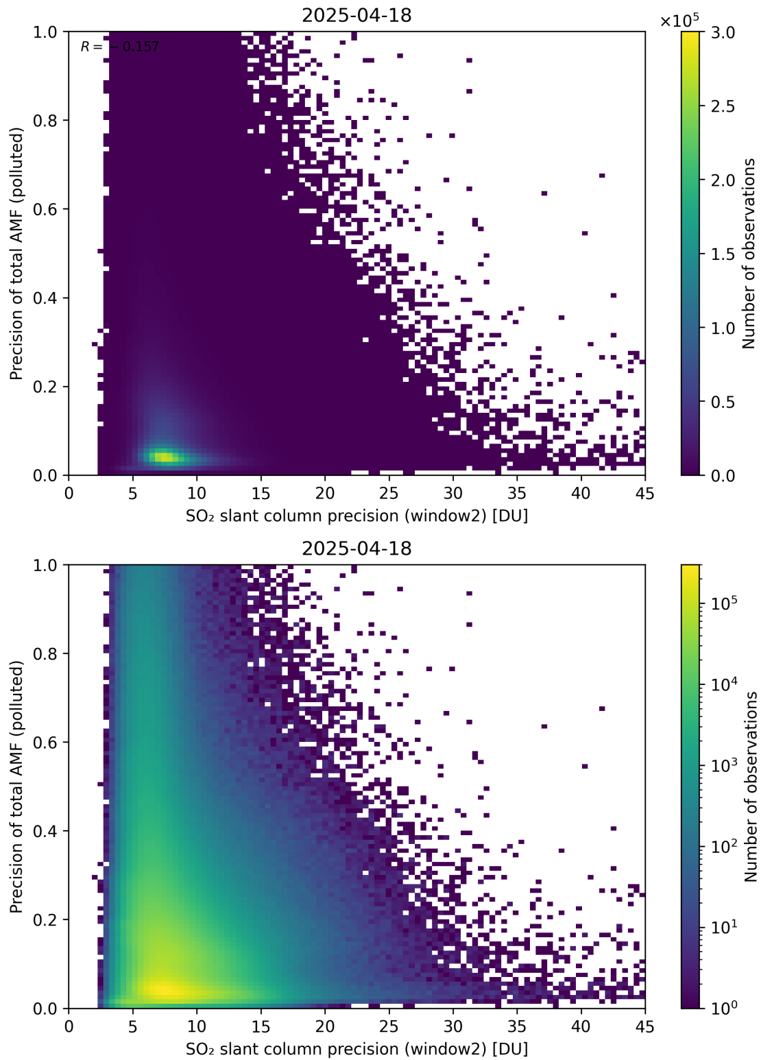
Figure 302: Scatter density plot of “SO 2 slant column precision (window2)” against “Precision of total AMF (polluted)” for 2025-04-18 to 2025-04-19.
