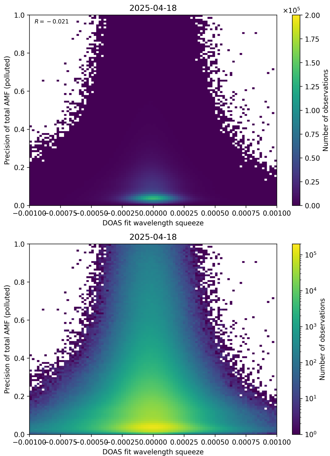
Figure 146: Scatter density plot of “DOAS fit wavelength squeeze” against “Precision of total AMF (polluted)” for 2025-04-18 to 2025-04-19.
