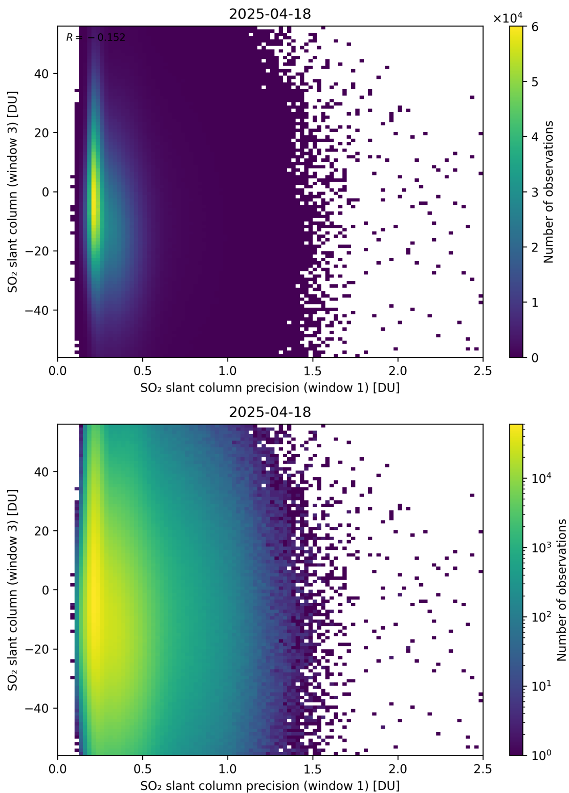
Figure 278: Scatter density plot of “SO 2 slant column precision (window 1)” against “SO 2 slant column (window 3)” for 2025-04-18 to 2025-04-19.
