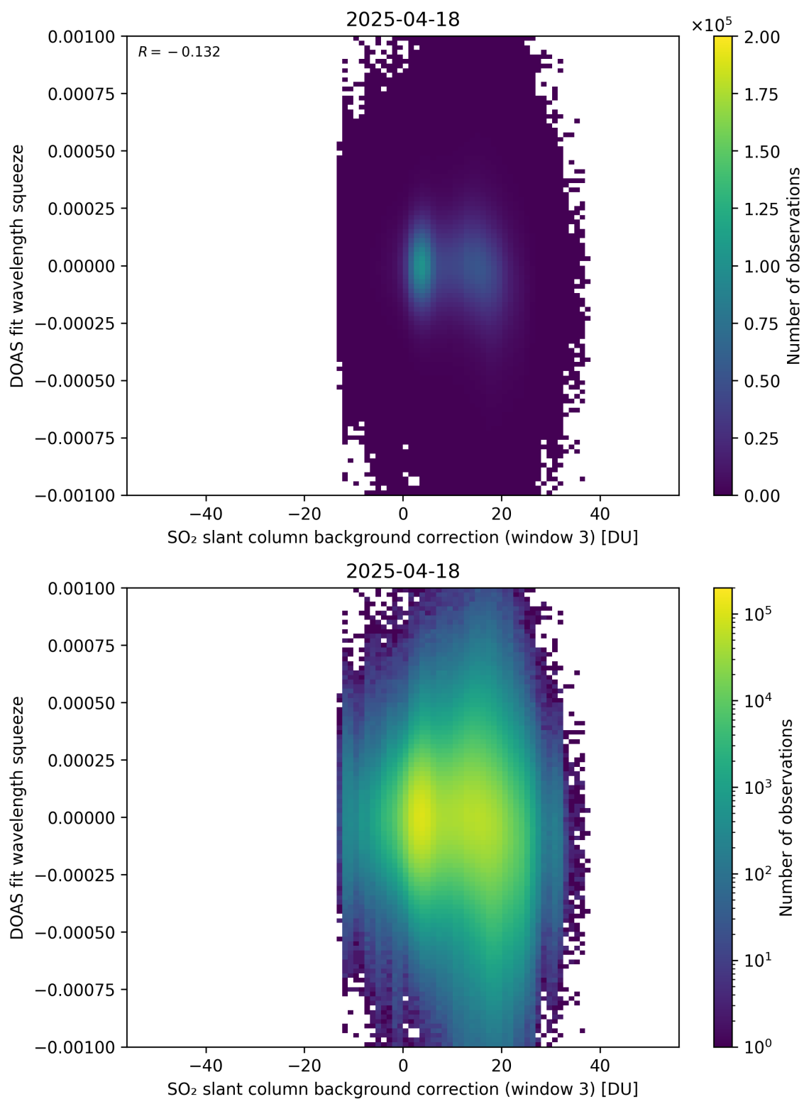
Figure 133: Scatter density plot of “SO 2 slant column background correction (window 3)” against “DOAS fit wavelength squeeze” for 2025-04-18 to 2025-04-19.
