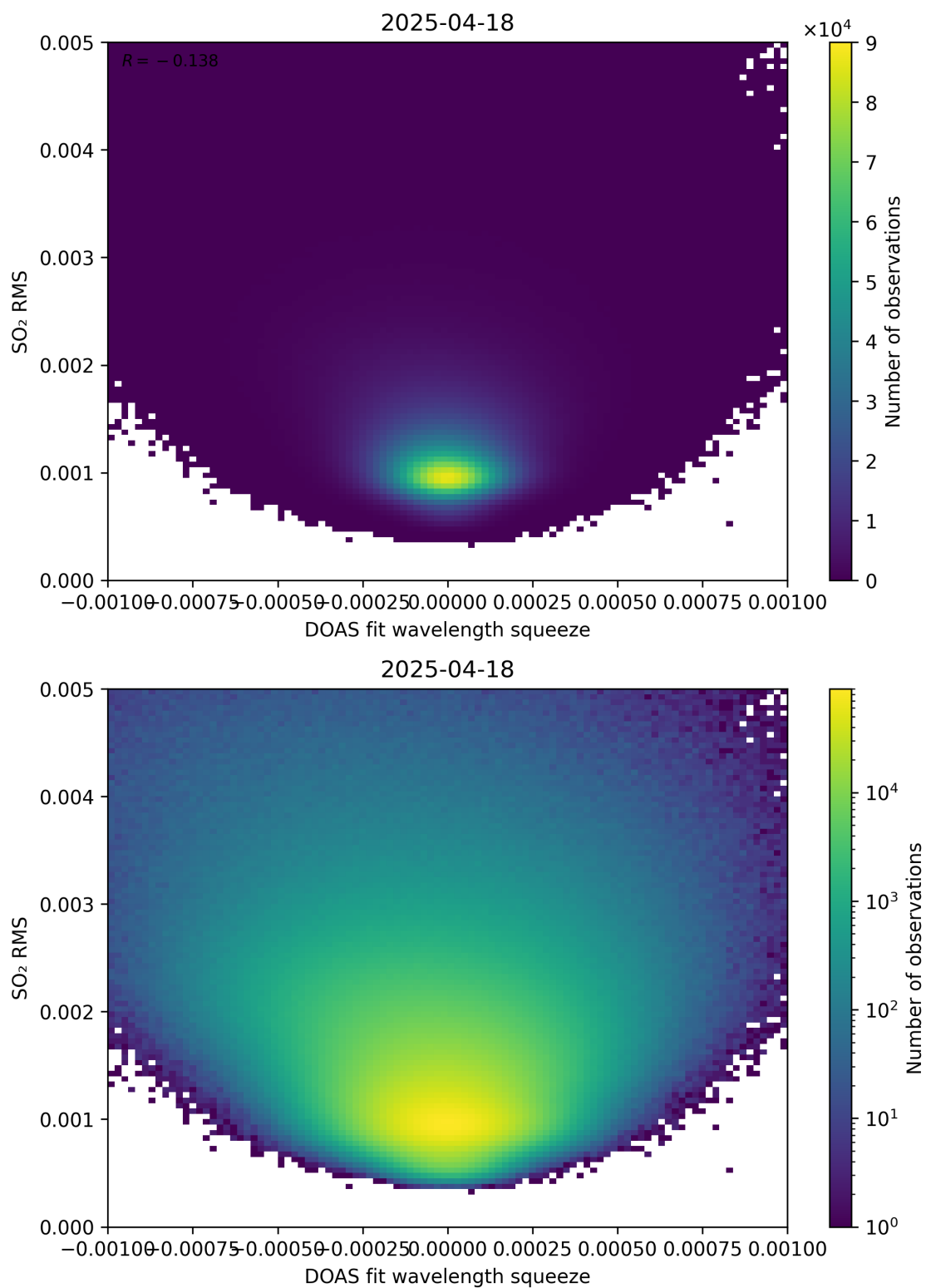
Figure 143: Scatter density plot of “DOAS fit wavelength squeeze” against “SO 2 RMS” for 2025-04-18 to 2025-04-19.
