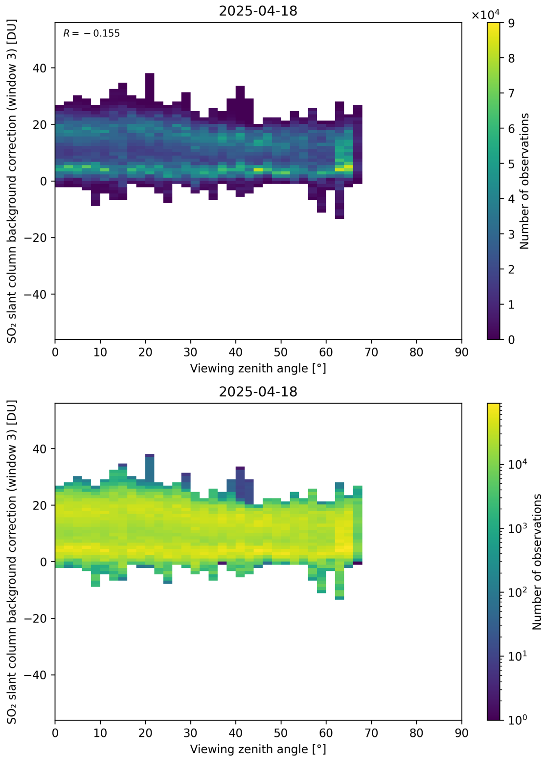
Figure 364: Scatter density plot of “Viewing zenith angle” against “SO 2 slant column background correction (window 3)” for 2025-04-18 to 2025-04-19.
