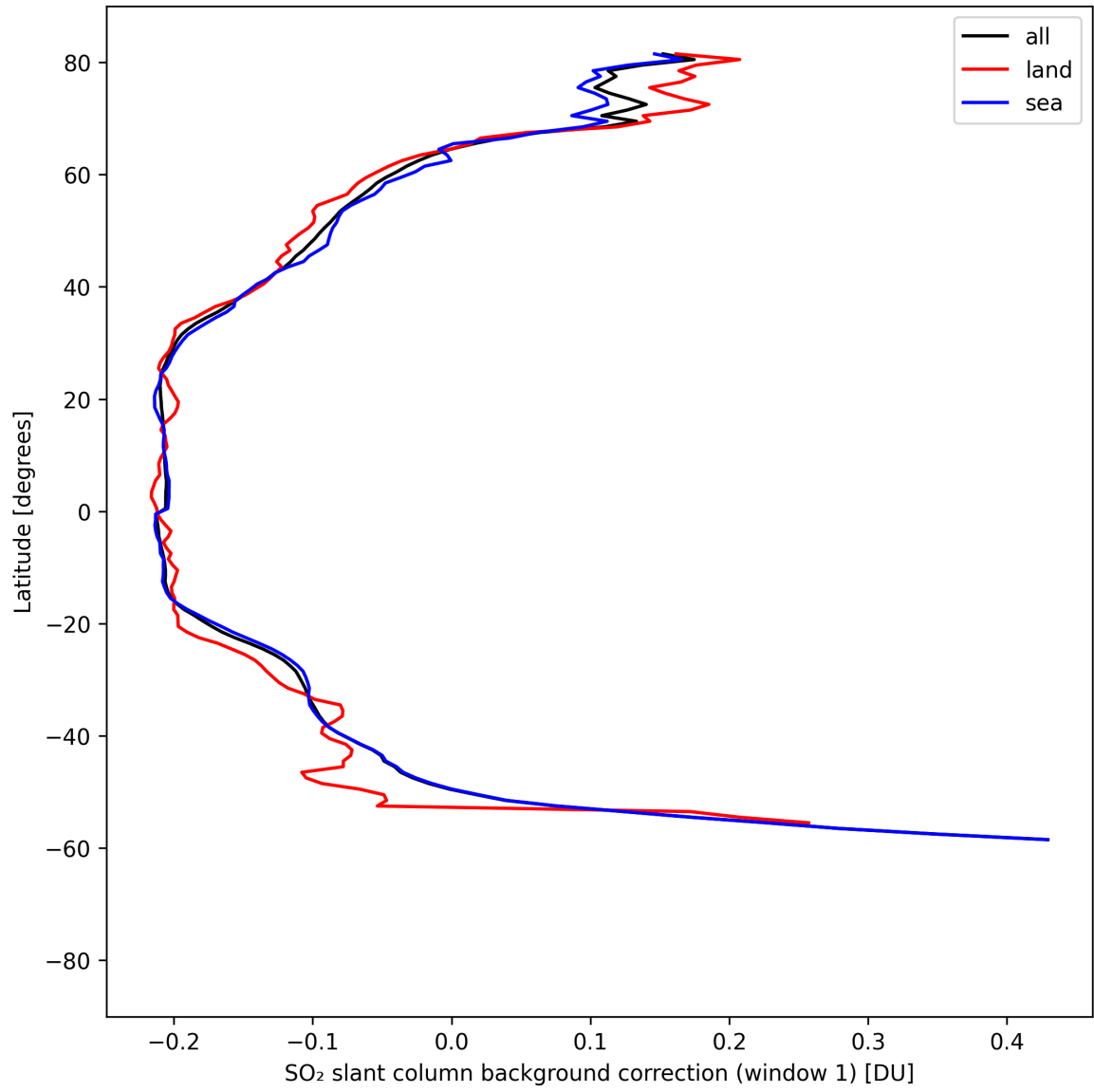
Figure 40: Zonal average of “SO 2 slant column background correction (window 1)” for 2025-04-18 to 2025-04-19.
