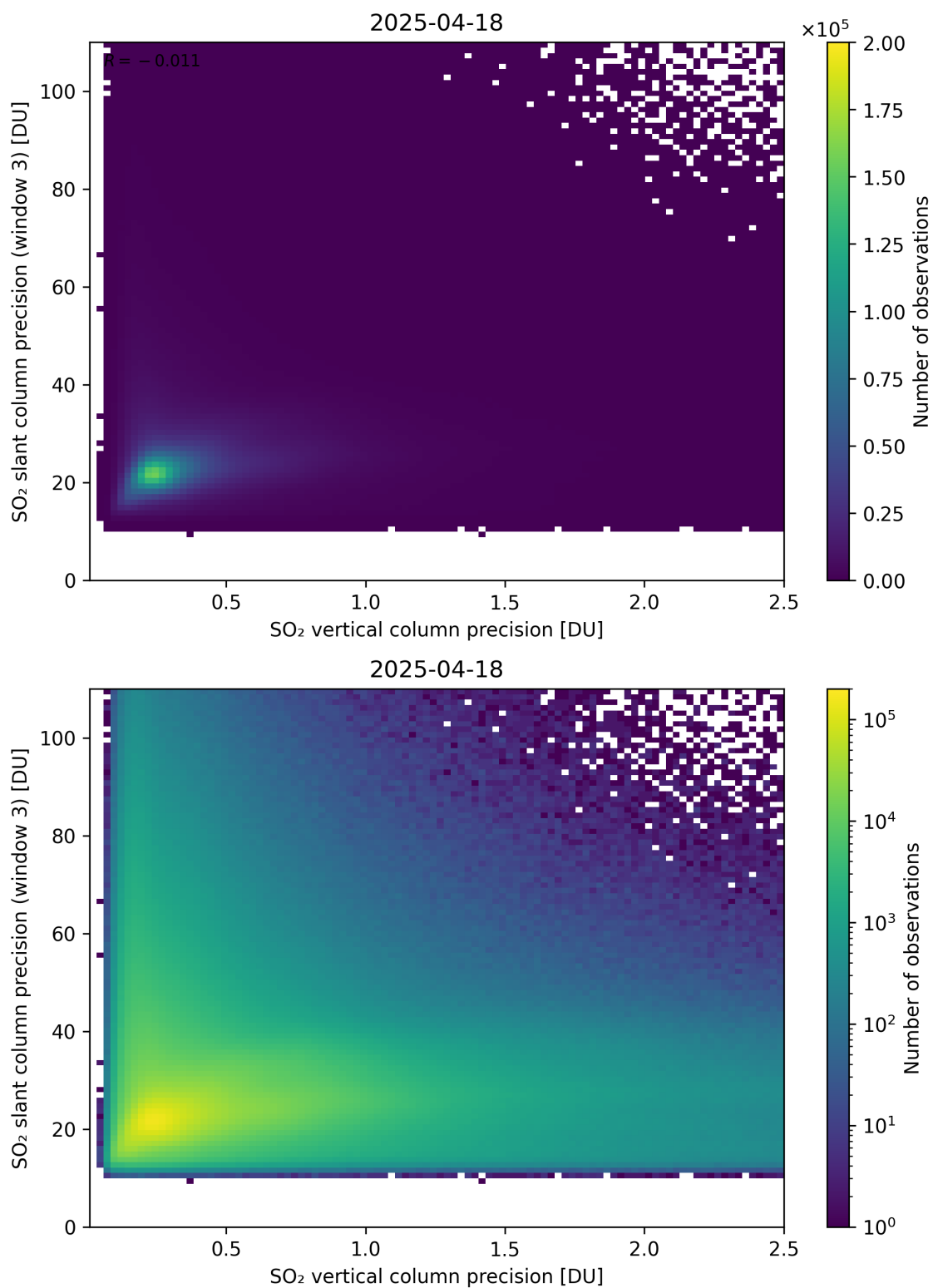
Figure 345: Scatter density plot of “SO 2 vertical column precision” against “SO 2 slant column precision (window 3)” for 2025-04-18 to 2025-04-19.
