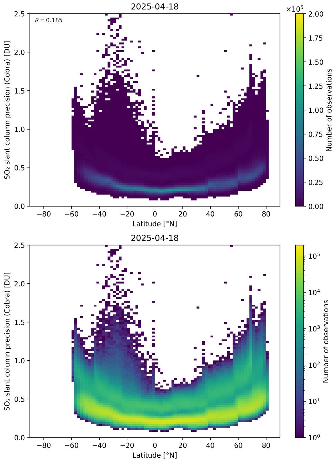
Figure 158: Scatter density plot of “Latitude” against “SO 2 slant column precision (Cobra)” for 2025-04-18 to 2025-04-19.
