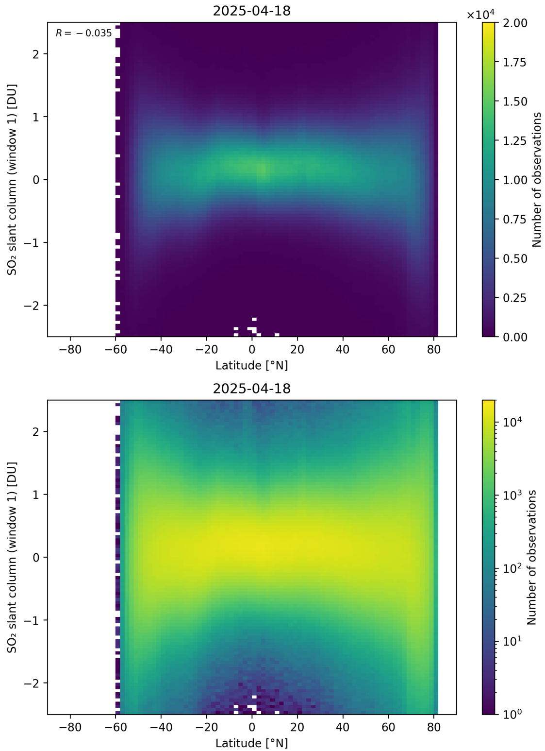
Figure 162: Scatter density plot of “Latitude” against “SO 2 slant column (window 1)” for 2025-04-18 to 2025-04-19.
