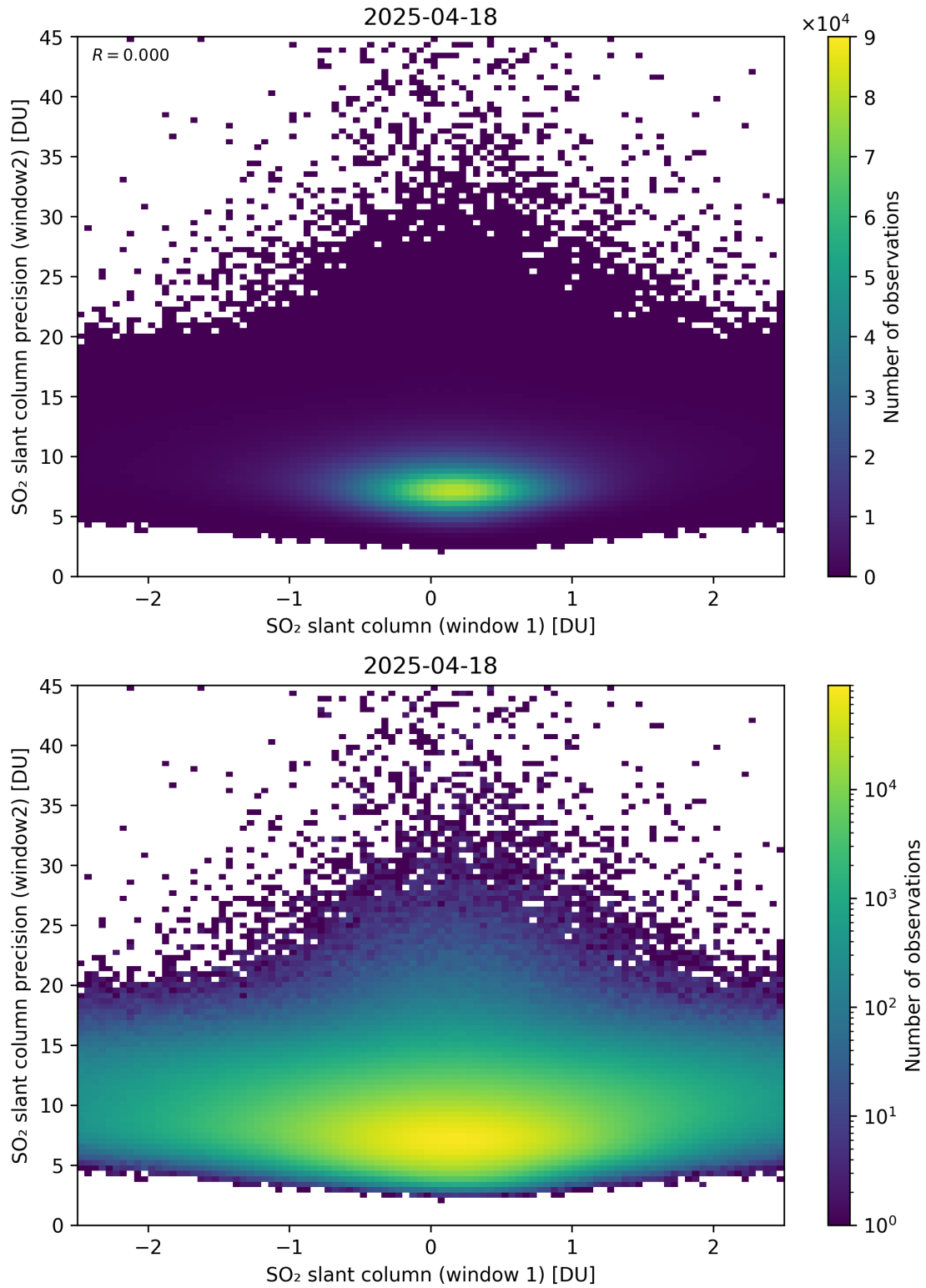
Figure 286: Scatter density plot of “SO 2 slant column (window 1)” against “SO 2 slant column precision (window2)” for 2025-04-18 to 2025-04-19.
