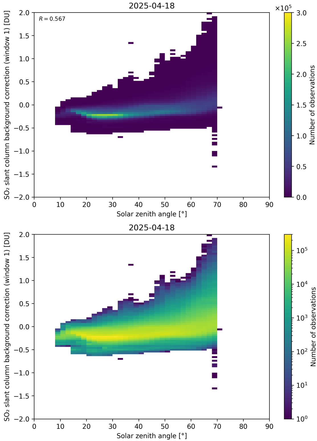
Figure 171: Scatter density plot of “Solar zenith angle” against “SO 2 slant column background correction (window 1)” for 2025-04-18 to 2025-04-19.
