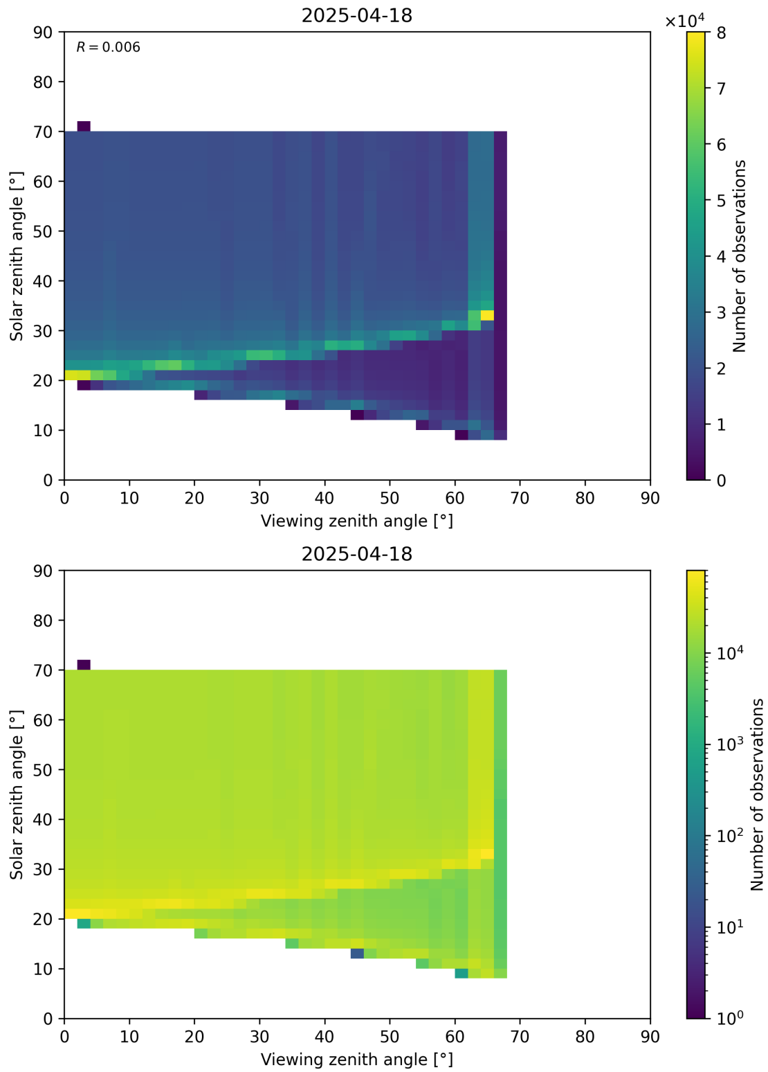
Figure 369: Scatter density plot of “Viewing zenith angle” against “Solar zenith angle” for 2025-04-18 to 2025-04-19.
