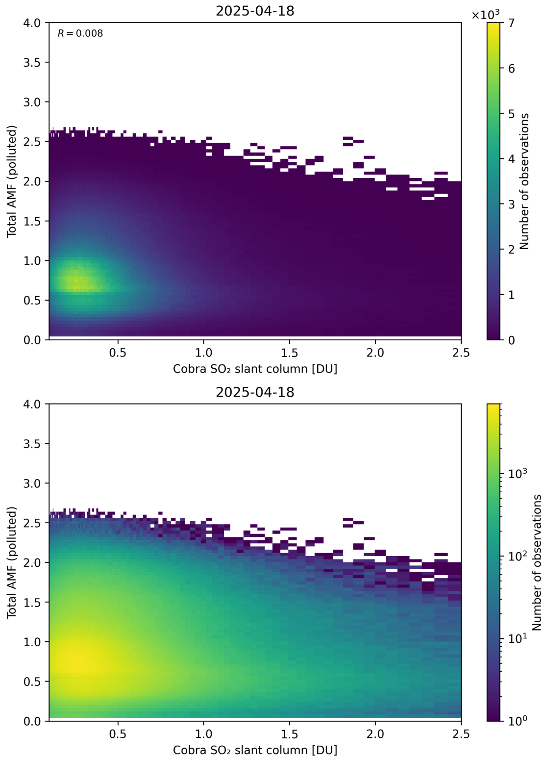
Figure 224: Scatter density plot of “Cobra SO 2 slant column” against “Total AMF (polluted)” for 2025-04-18 to 2025-04-19.
