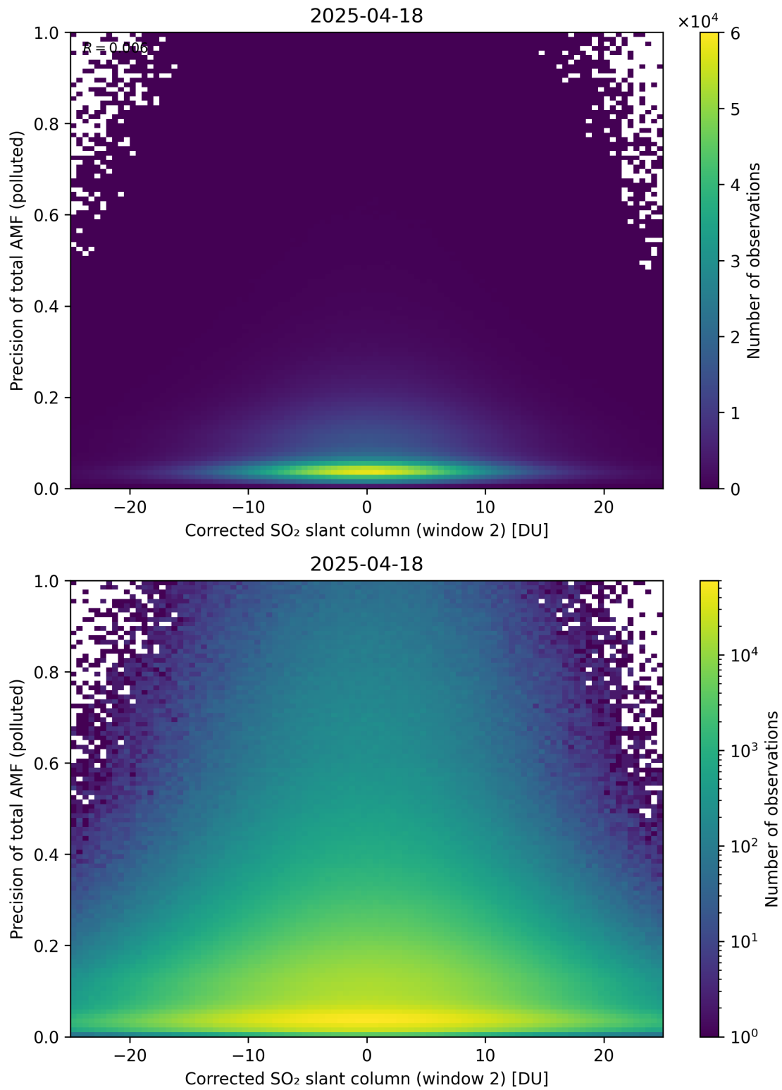
Figure 254: Scatter density plot of “Corrected SO 2 slant column (window 2)” against “Precision of total AMF (polluted)” for 2025-04-18 to 2025-04-19.
