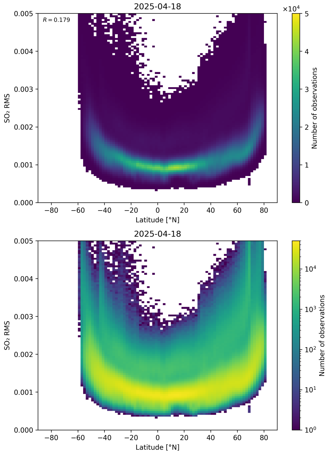
Figure 155: Scatter density plot of “Latitude” against “SO 2 RMS” for 2025-04-18 to 2025-04-19.
