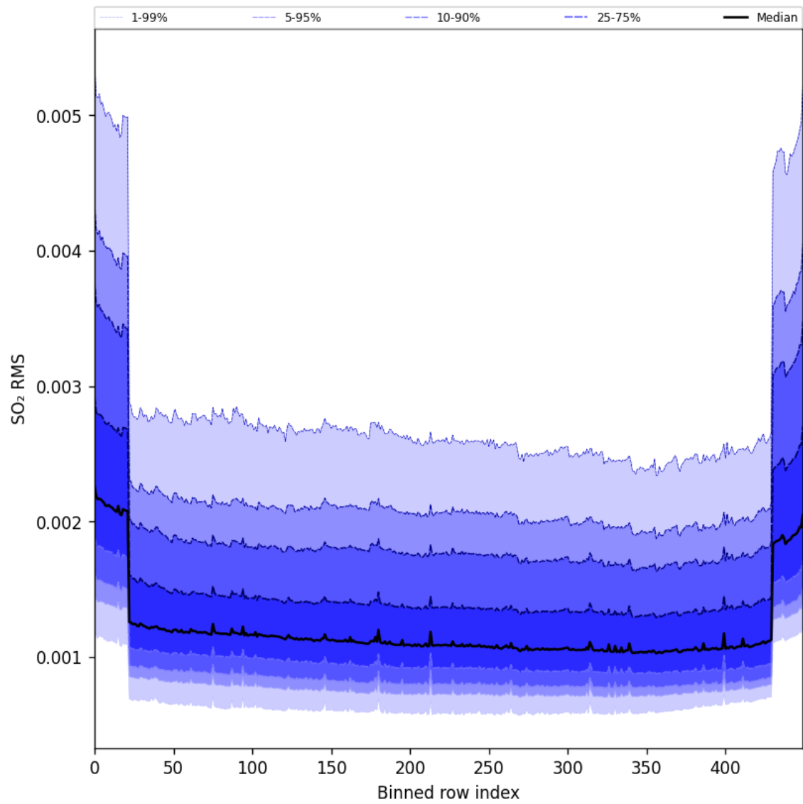
Figure 104: Along track statistics of “SO 2 RMS” for 2025-04-18 to 2025-04-19
