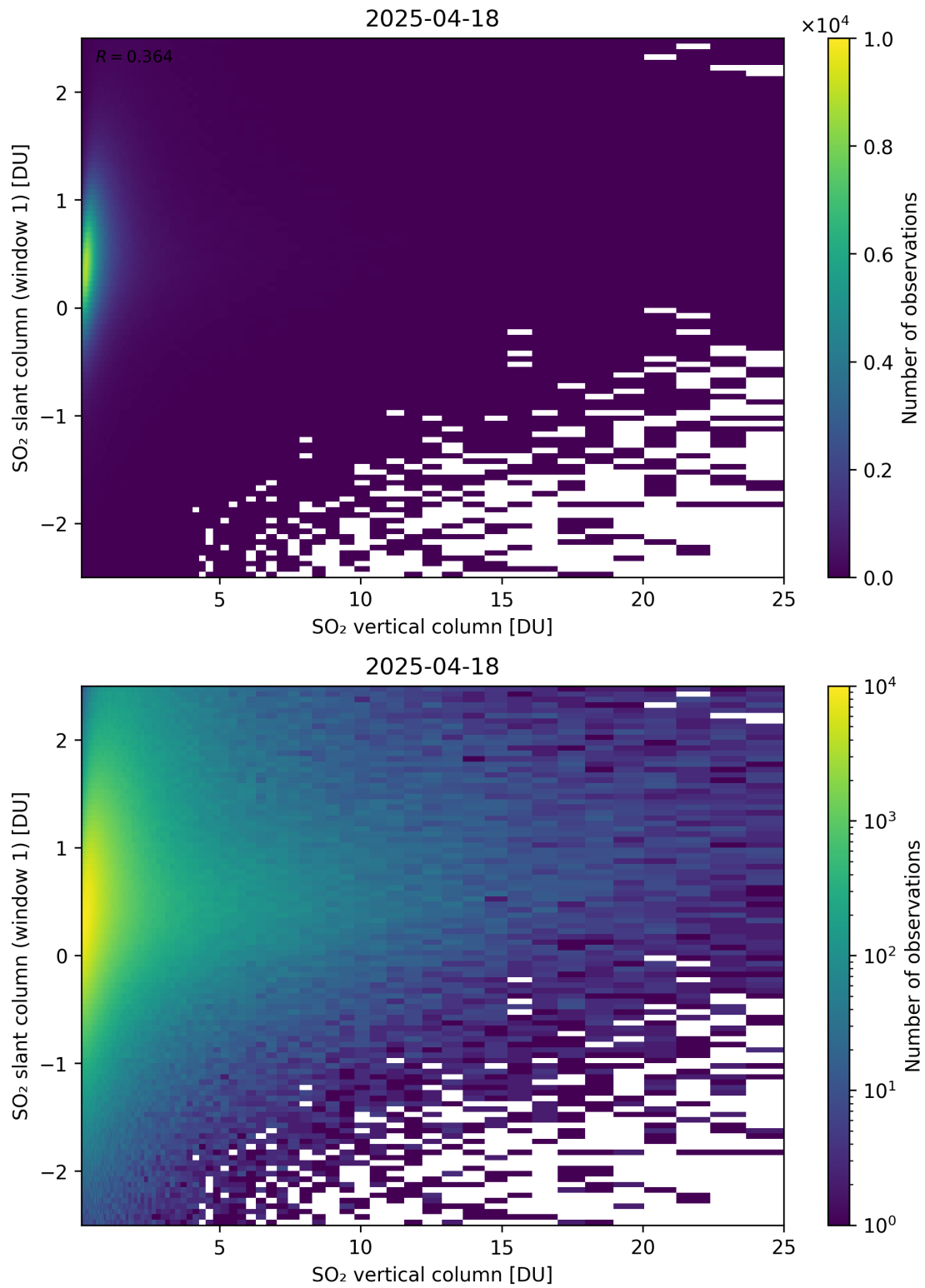
Figure 354: Scatter density plot of “SO 2 vertical column” against “SO 2 slant column (window 1)” for 2025-04-18 to 2025-04-19.
