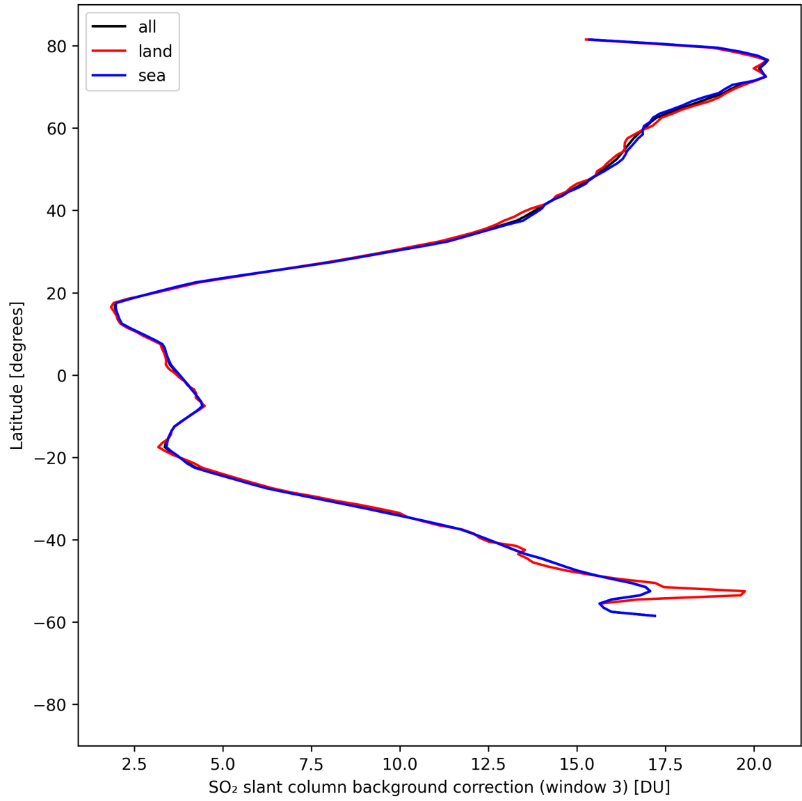
Figure 48: Zonal average of “SO 2 slant column background correction (window 3)” for 2025-04-18 to 2025-04-19.
