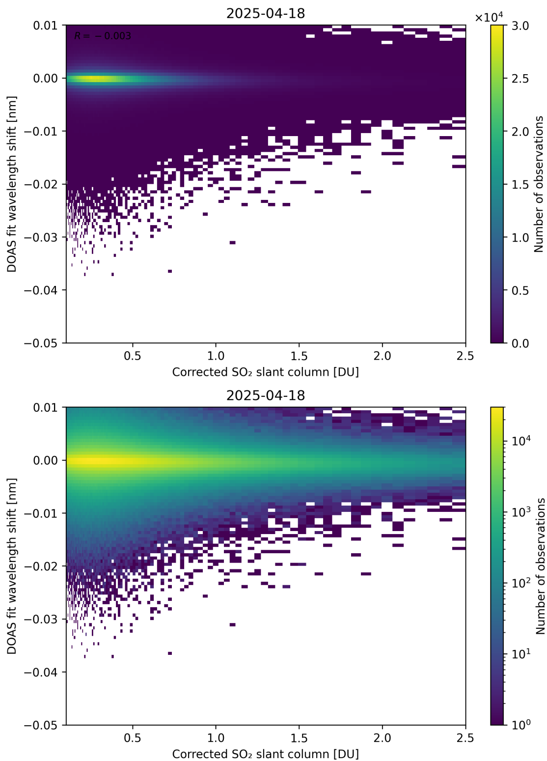
Figure 229: Scatter density plot of “Corrected SO 2 slant column” against “DOAS fit wavelength shift” for 2025-04-18 to 2025-04-19.
