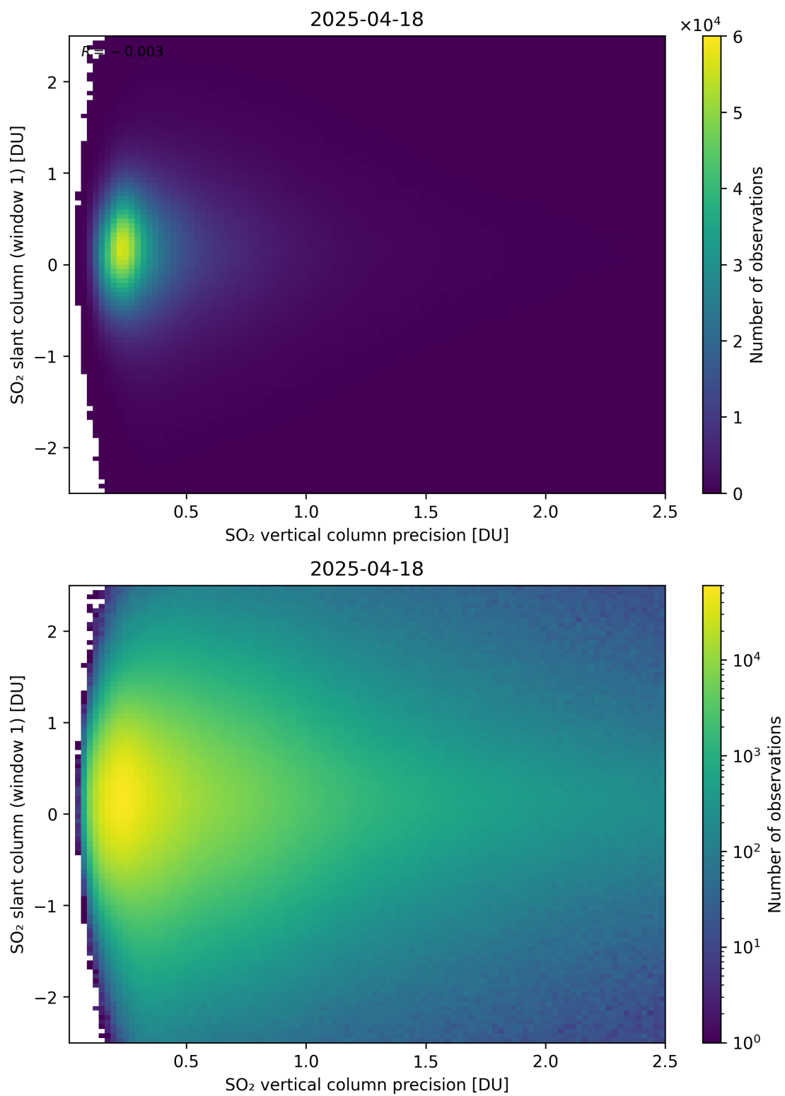
Figure 341: Scatter density plot of “SO 2 vertical column precision” against “SO 2 slant column (window 1)” for 2025-04-18 to 2025-04-19.
