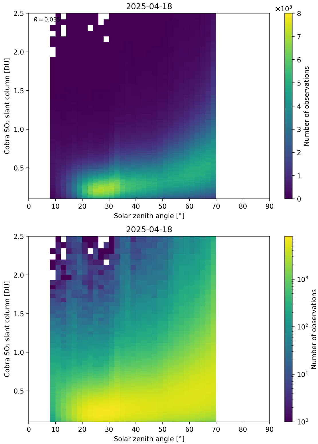
Figure 179: Scatter density plot of “Solar zenith angle” against “Cobra SO 2 slant column” for 2025-04-18 to 2025-04-19.
