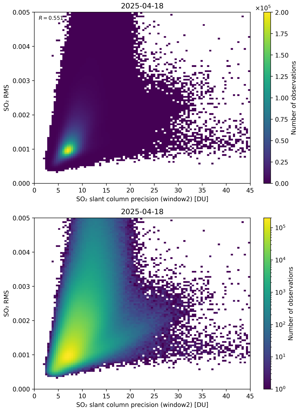
Figure 295: Scatter density plot of “SO 2 slant column precision (window2)” against “SO 2 RMS” for 2025-04-18 to 2025-04-19.
