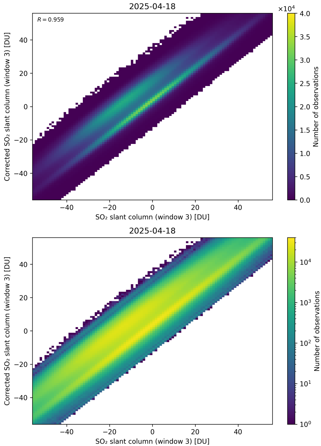
Figure 316: Scatter density plot of “SO 2 slant column (window 3)” against “Corrected SO 2 slant column (window 3)” for 2025-04-18 to 2025-04-19.
