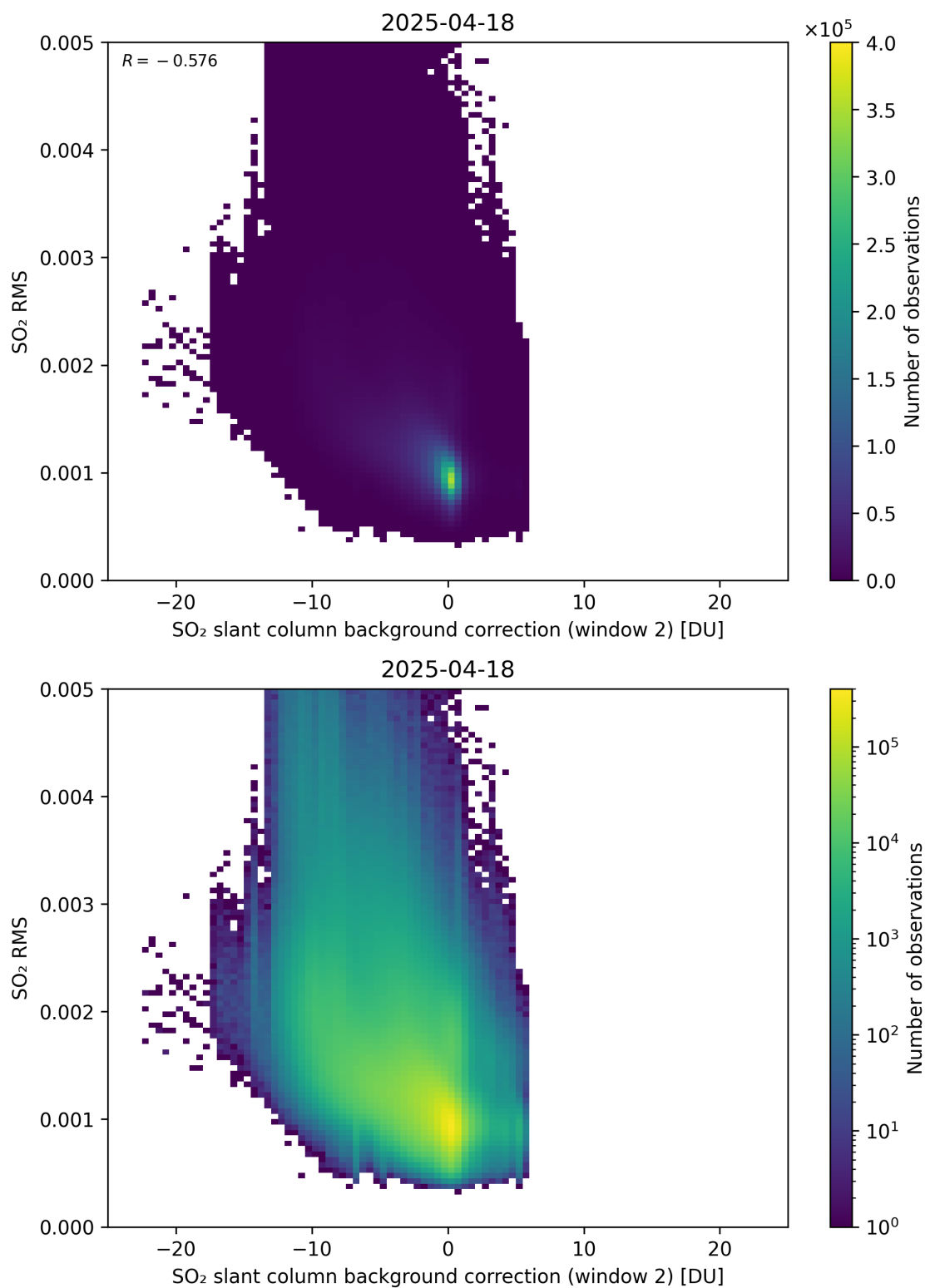
Figure 125: Scatter density plot of “SO 2 slant column background correction (window 2)” against “SO 2 RMS” for 2025-04-18 to 2025-04-19.
