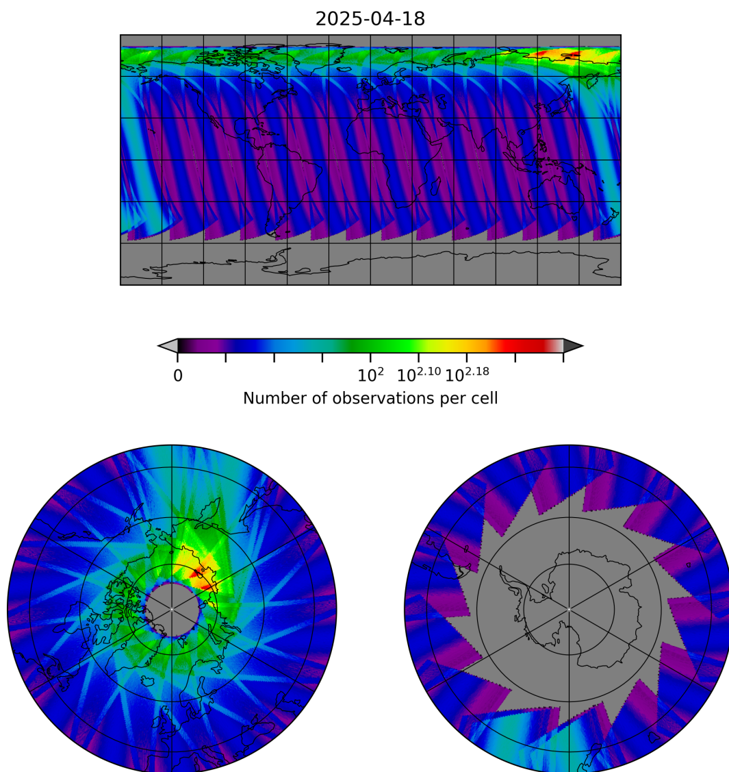
Figure 30: Map of the number of observations for 2025-04-18 to 2025-04-19
