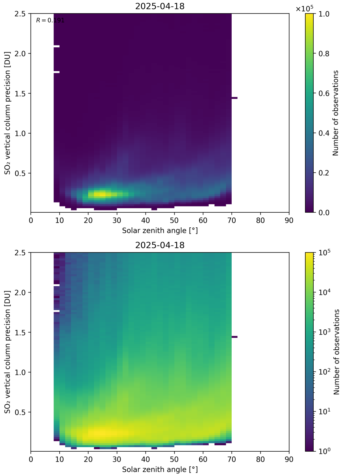
Figure 192: Scatter density plot of “Solar zenith angle” against “SO 2 vertical column precision” for 2025-04-18 to 2025-04-19.
