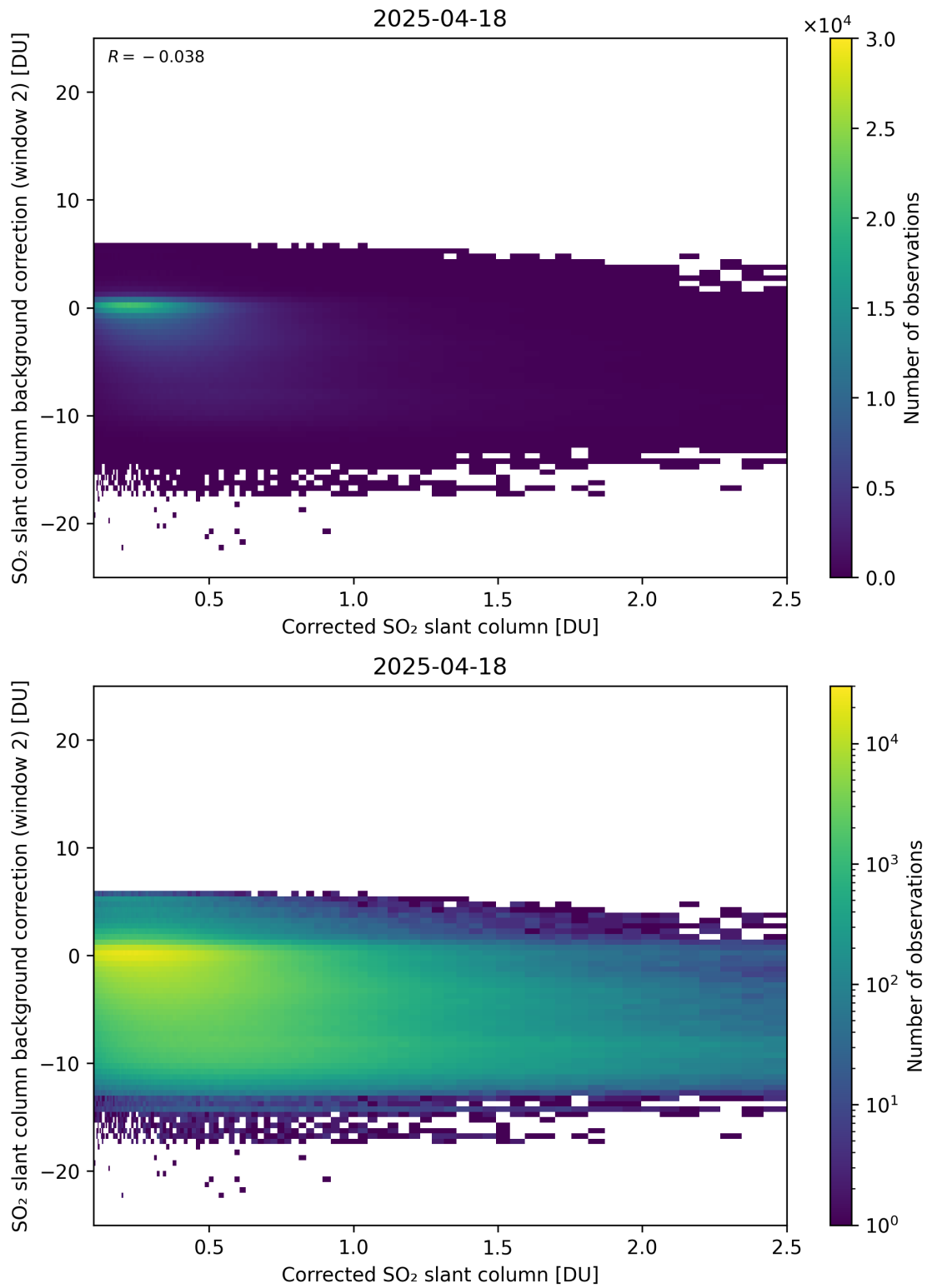
Figure 227: Scatter density plot of “Corrected SO 2 slant column” against “SO 2 slant column background correction (window 2)” for 2025-04-18 to 2025-04-19.
