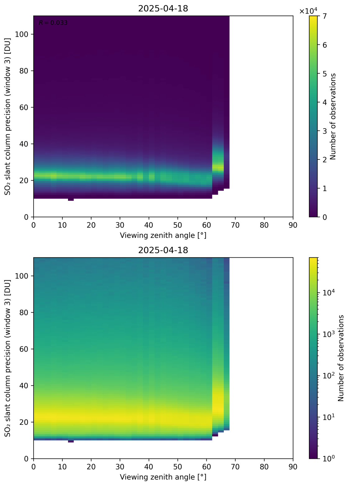
Figure 380: Scatter density plot of “Viewing zenith angle” against “SO 2 slant column precision (window 3)” for 2025-04-18 to 2025-04-19.
