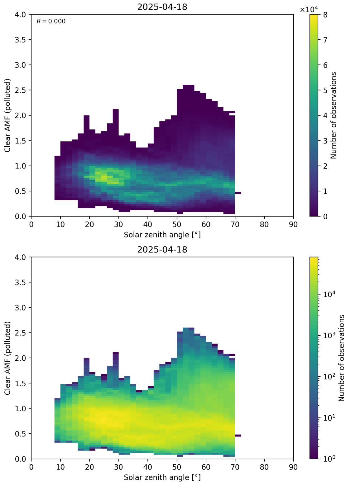
Figure 178: Scatter density plot of “Solar zenith angle” against “Clear AMF (polluted)” for 2025-04-18 to 2025-04-19.
