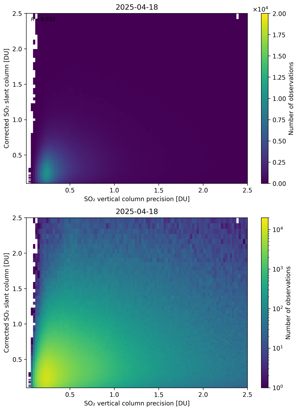
Figure 338: Scatter density plot of “SO 2 vertical column precision” against “Corrected SO 2 slant column” for 2025-04-18 to 2025-04-19.
