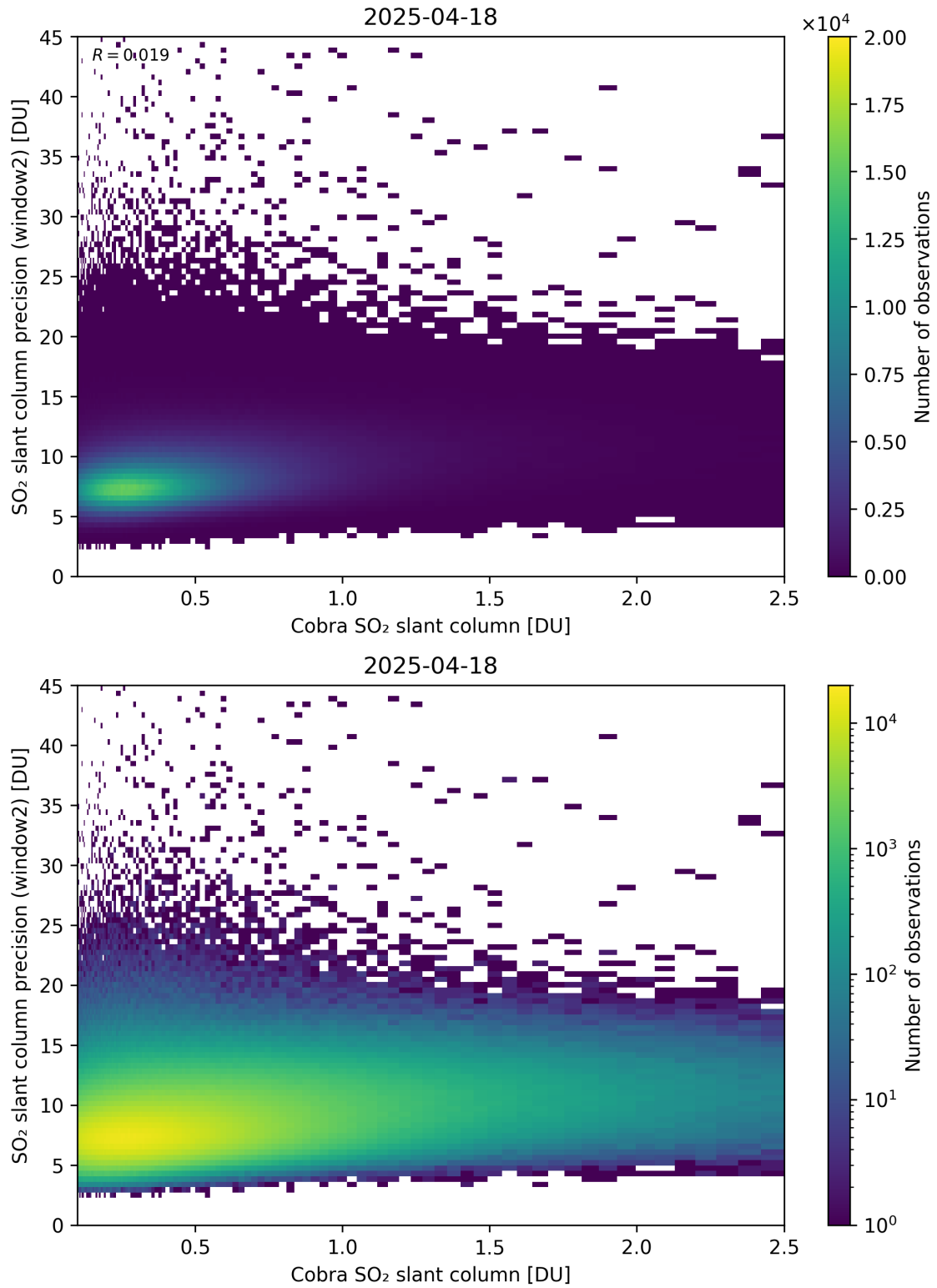
Figure 221: Scatter density plot of “Cobra SO 2 slant column” against “SO 2 slant column precision (window2)” for 2025-04-18 to 2025-04-19.
