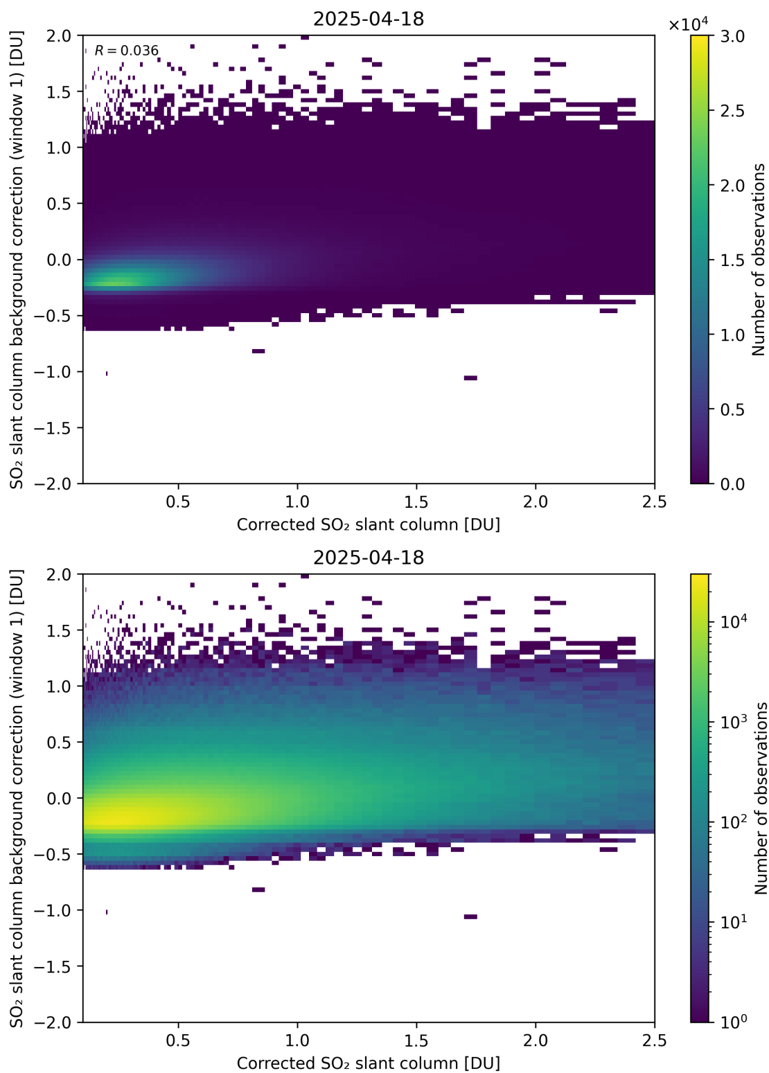
Figure 226: Scatter density plot of “Corrected SO 2 slant column” against “SO 2 slant column background correction (window 1)” for 2025-04-18 to 2025-04-19.
