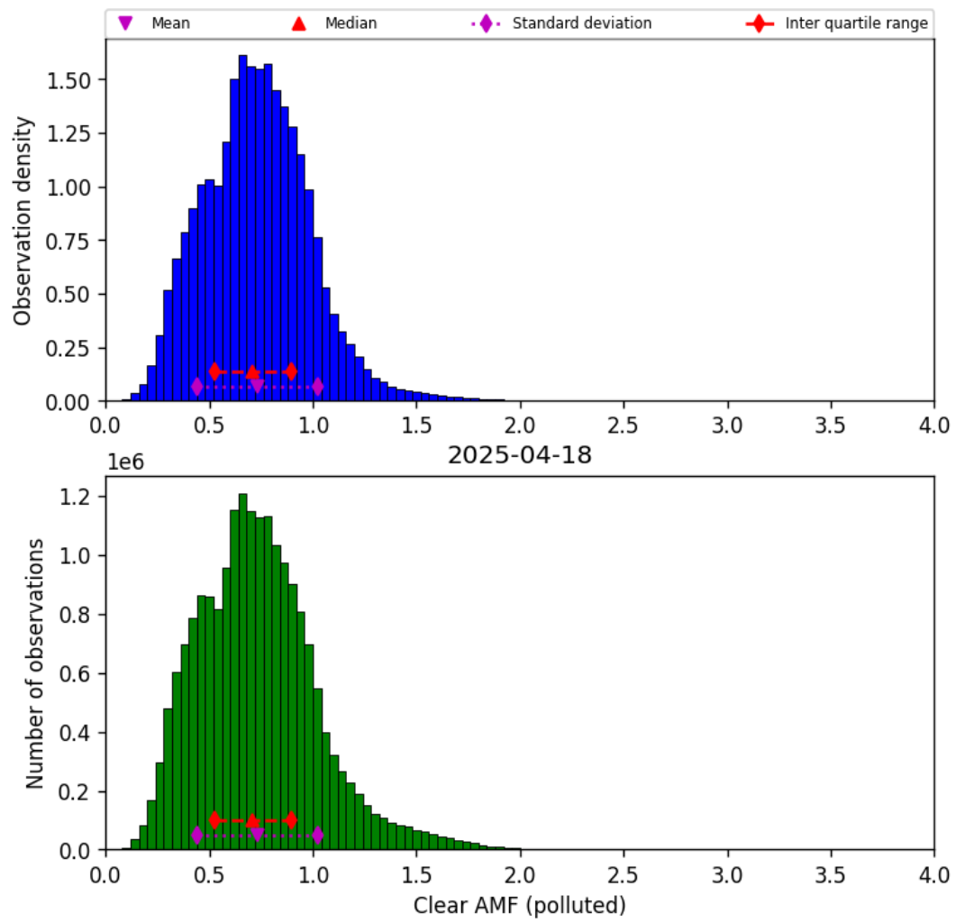
Figure 81: Histogram of “Clear AMF (polluted)” for 2025-04-18 to 2025-04-19
