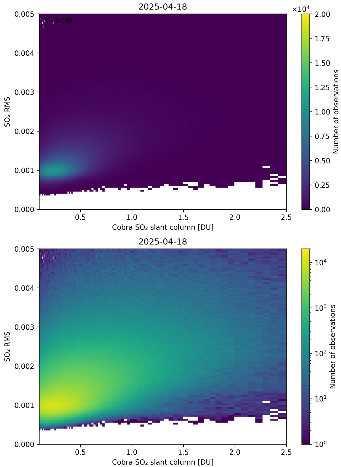
Figure 198: Scatter density plot of “Cobra SO 2 slant column” against “SO 2 RMS” for 2025-04-18 to 2025-04-19.
