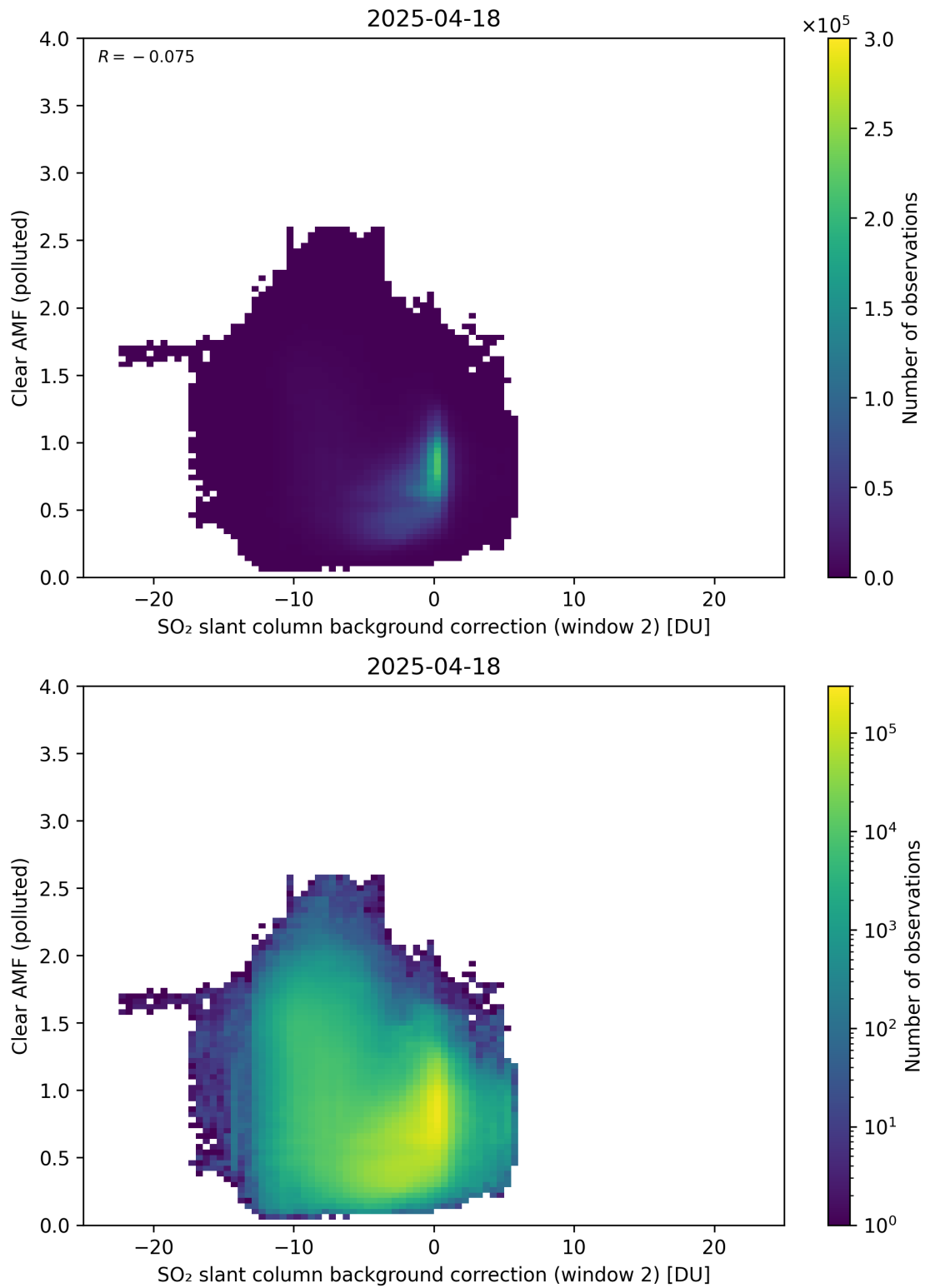
Figure 126: Scatter density plot of “SO 2 slant column background correction (window 2)” against “Clear AMF (polluted)” for 2025-04-18 to 2025-04-19.
