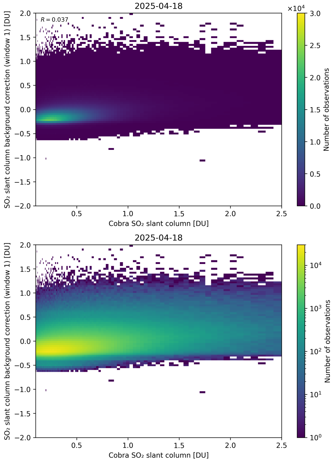
Figure 193: Scatter density plot of “Cobra SO 2 slant column” against “SO 2 slant column background correction (window 1)” for 2025-04-18 to 2025-04-19.
