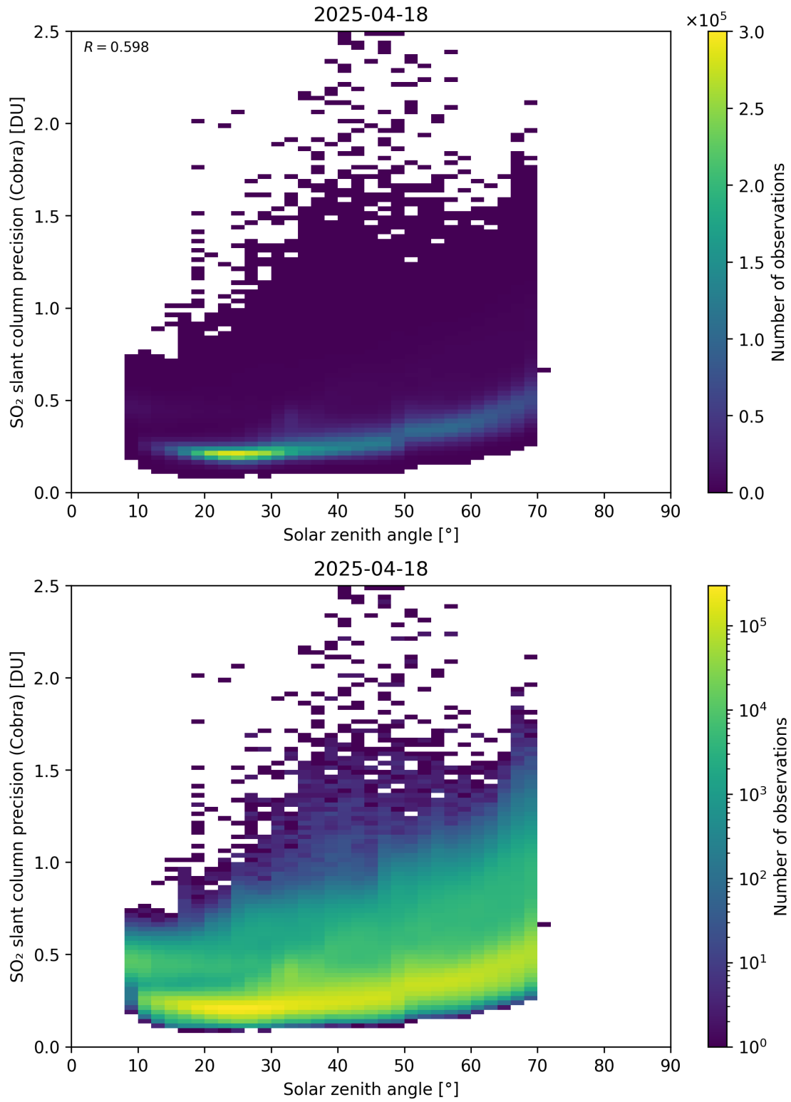
Figure 180: Scatter density plot of “Solar zenith angle” against “SO 2 slant column precision (Cobra)” for 2025-04-18 to 2025-04-19.
