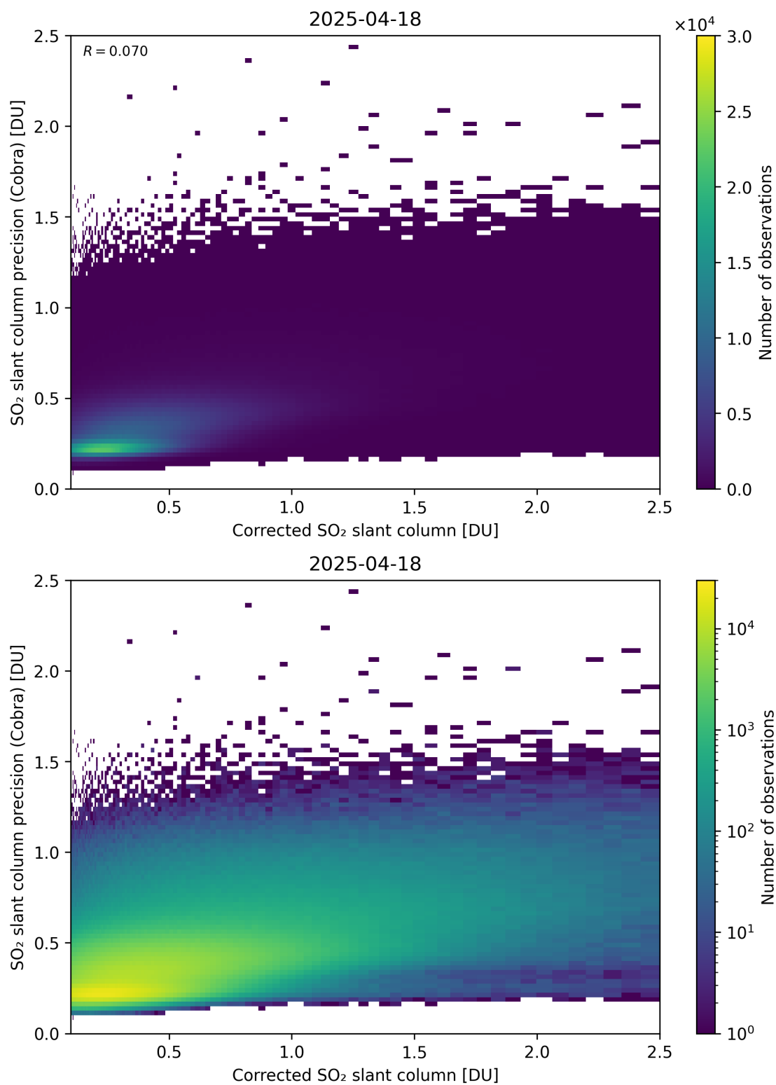
Figure 234: Scatter density plot of “Corrected SO 2 slant column” against “SO 2 slant column precision (Cobra)” for 2025-04-18 to 2025-04-19.
