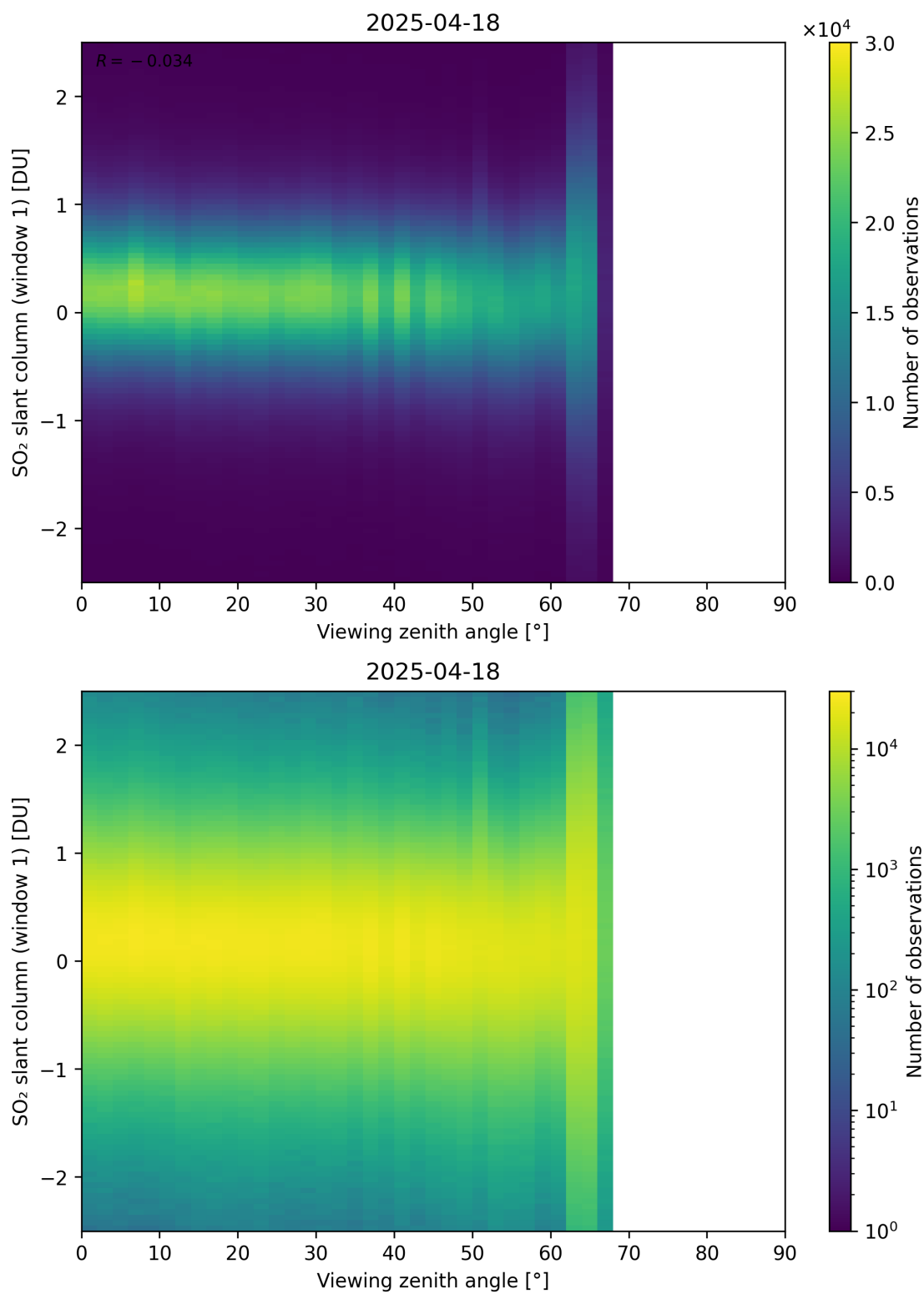
Figure 376: Scatter density plot of “Viewing zenith angle” against “SO 2 slant column (window 1)” for 2025-04-18 to 2025-04-19.
