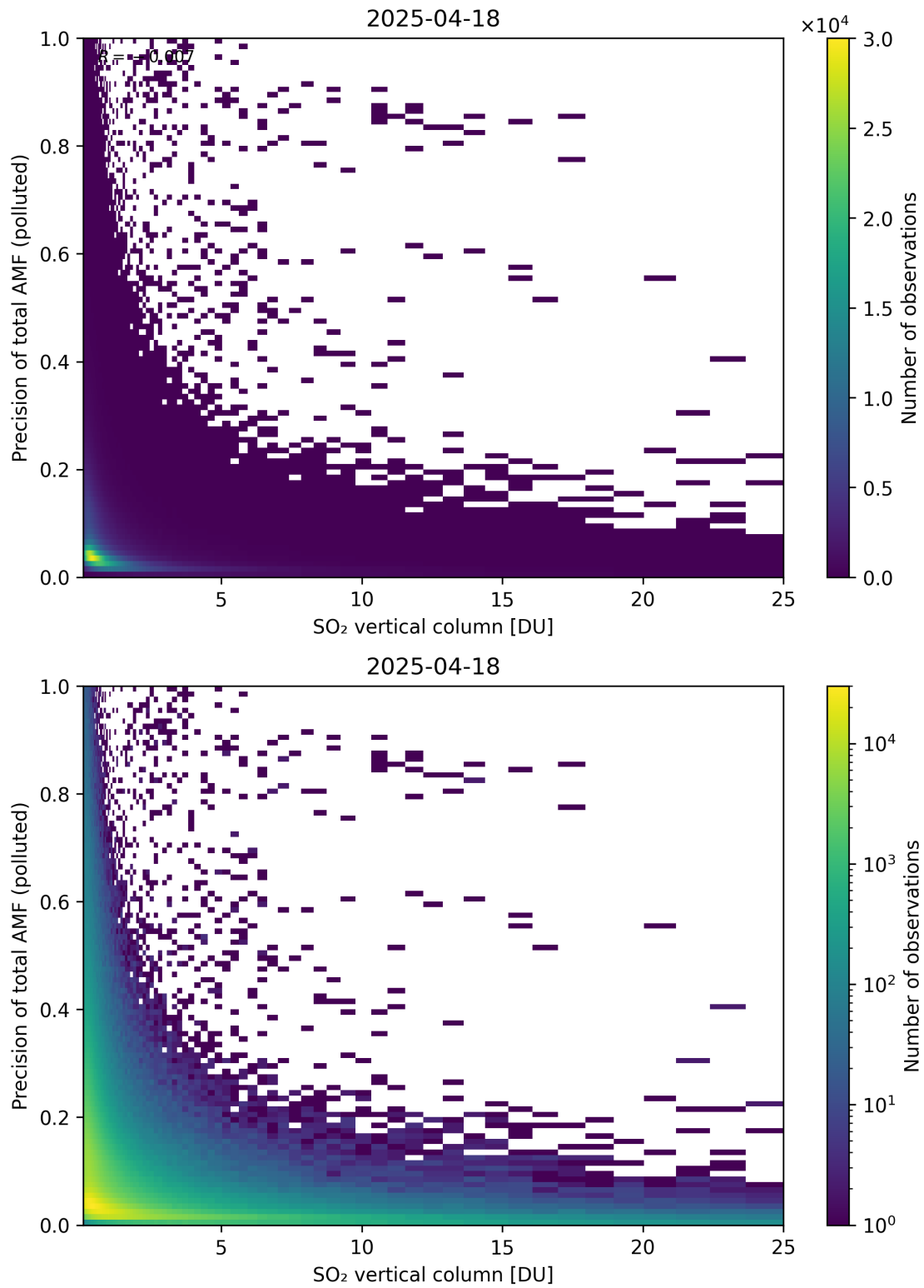
Figure 360: Scatter density plot of “SO 2 vertical column” against “Precision of total AMF (polluted)” for 2025-04-18 to 2025-04-19.
