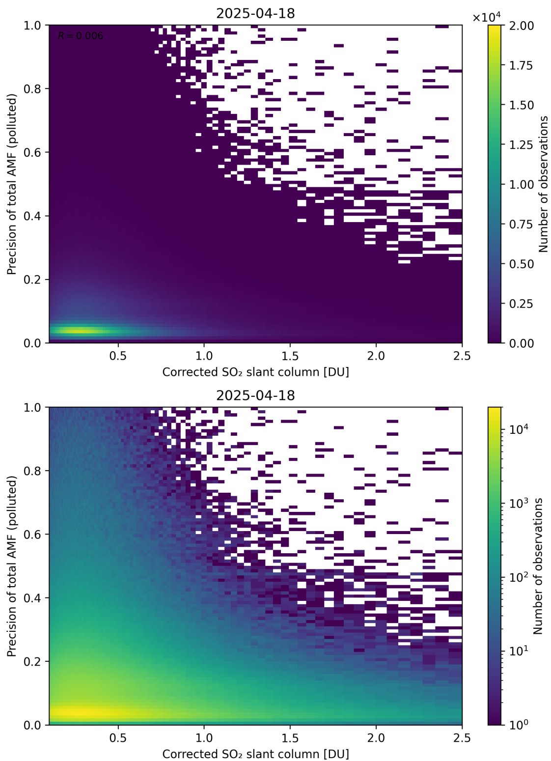
Figure 243: Scatter density plot of “Corrected SO 2 slant column” against “Precision of total AMF (polluted)” for 2025-04-18 to 2025-04-19.
