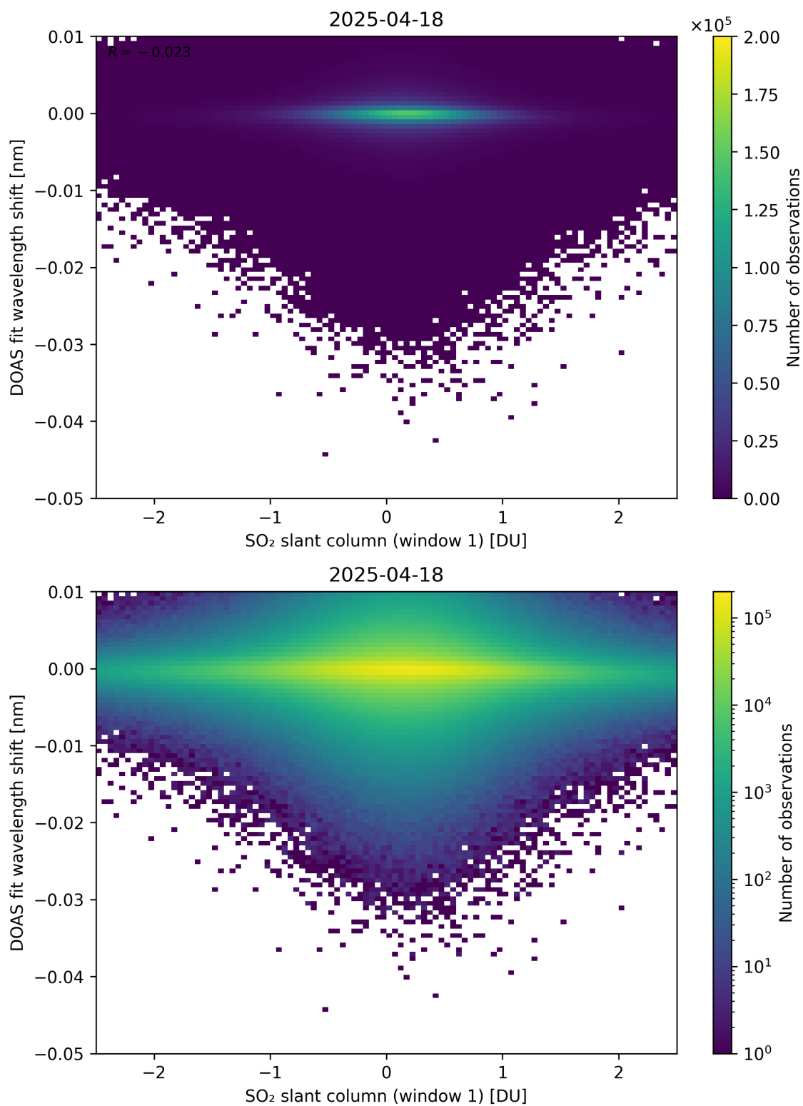
Figure 265: Scatter density plot of “SO 2 slant column (window 1)” against “DOAS fit wavelength shift” for 2025-04-18 to 2025-04-19.
