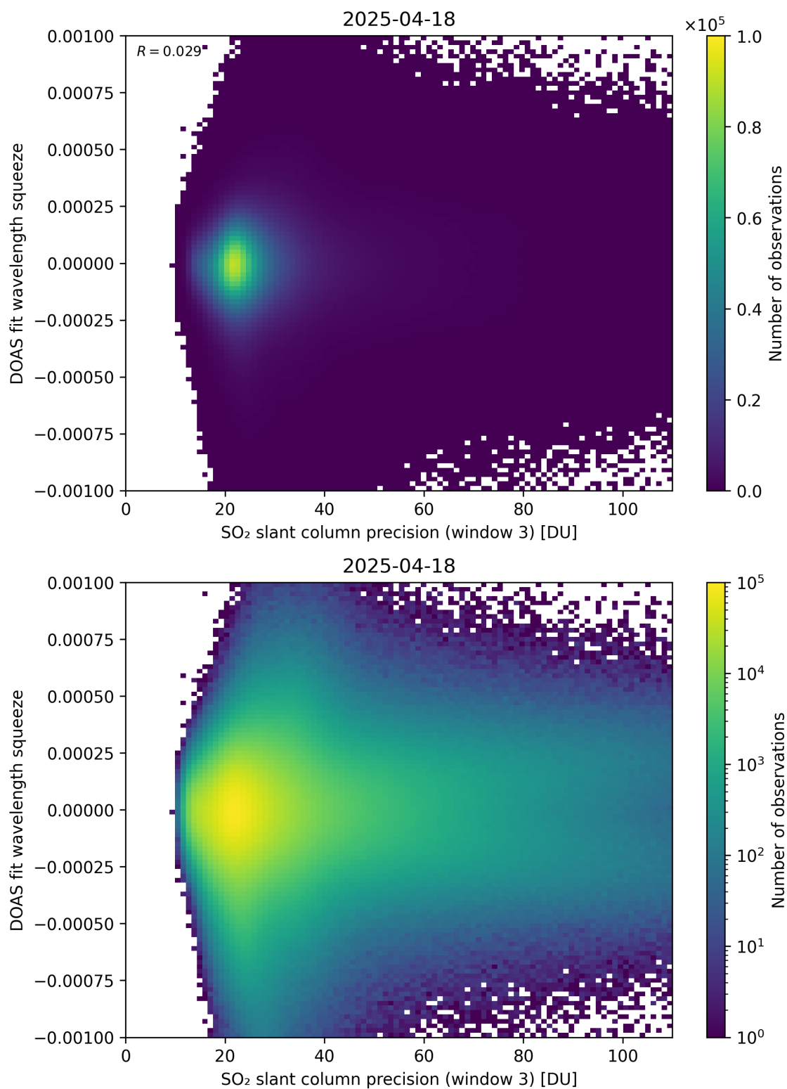
Figure 309: Scatter density plot of “SO 2 slant column precision (window 3)” against “DOAS fit wavelength squeeze” for 2025-04-18 to 2025-04-19.
