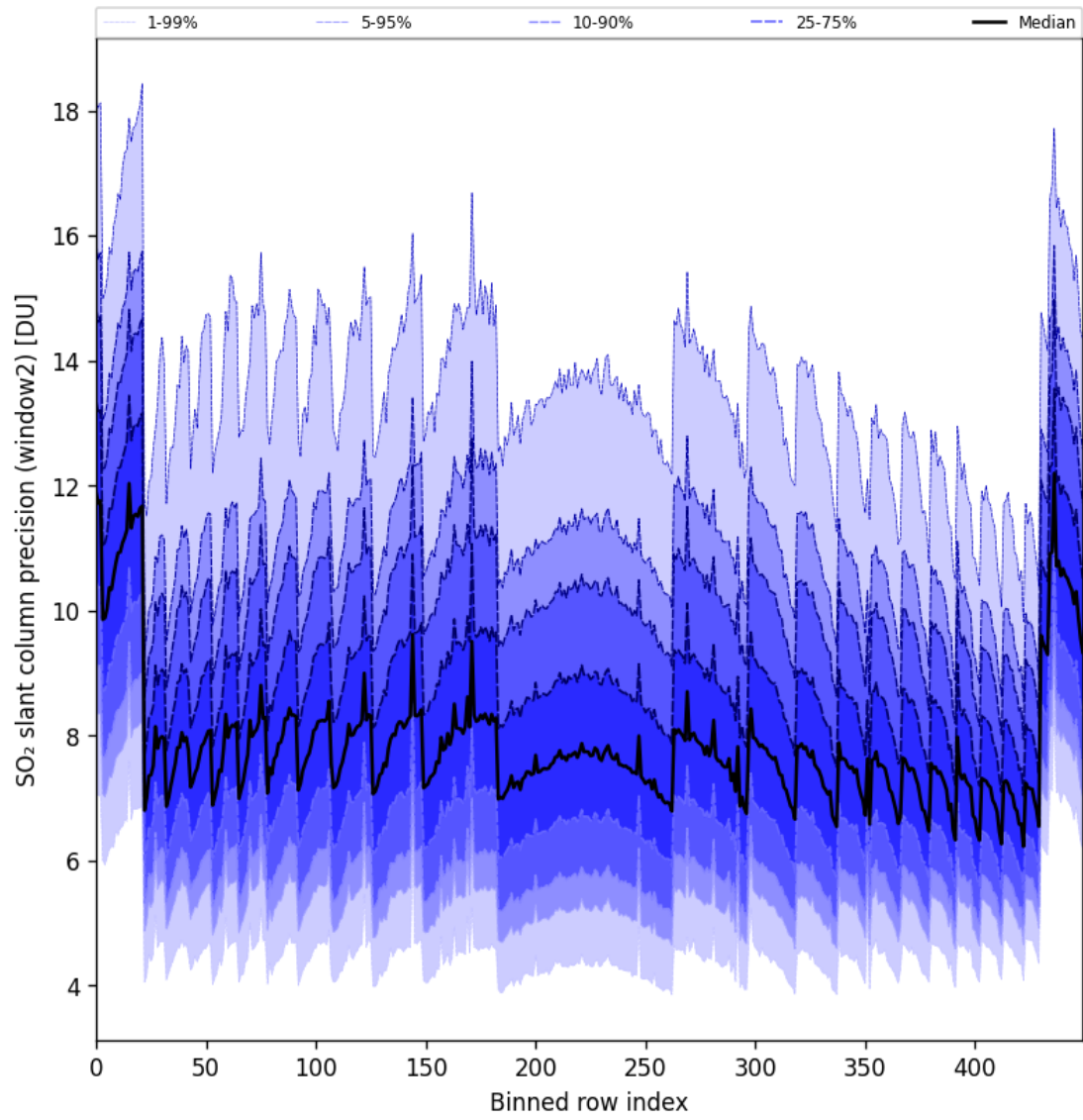
Figure 94: Along track statistics of “SO 2 slant column precision (window2)” for 2025-04-18 to 2025-04-19
