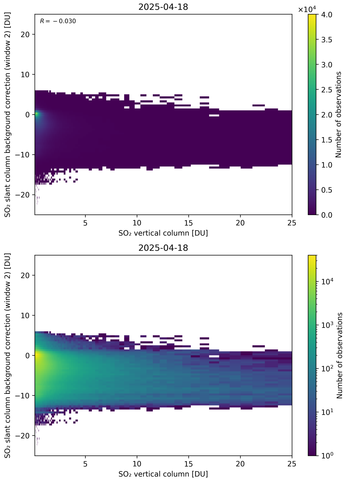
Figure 324: Scatter density plot of “SO 2 vertical column” against “SO 2 slant column background correction (window 2)” for 2025-04-18 to 2025-04-19.
