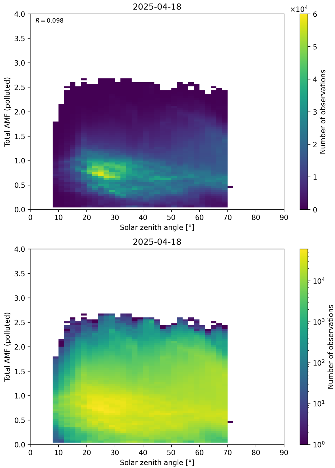
Figure 189: Scatter density plot of “Solar zenith angle” against “Total AMF (polluted)” for 2025-04-18 to 2025-04-19.
