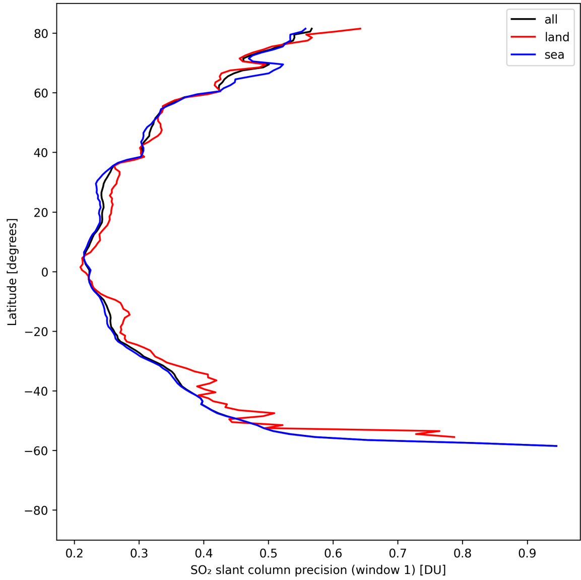
Figure 38: Zonal average of “SO 2 slant column precision (window 1)” for 2025-04-18 to 2025-04-19.
