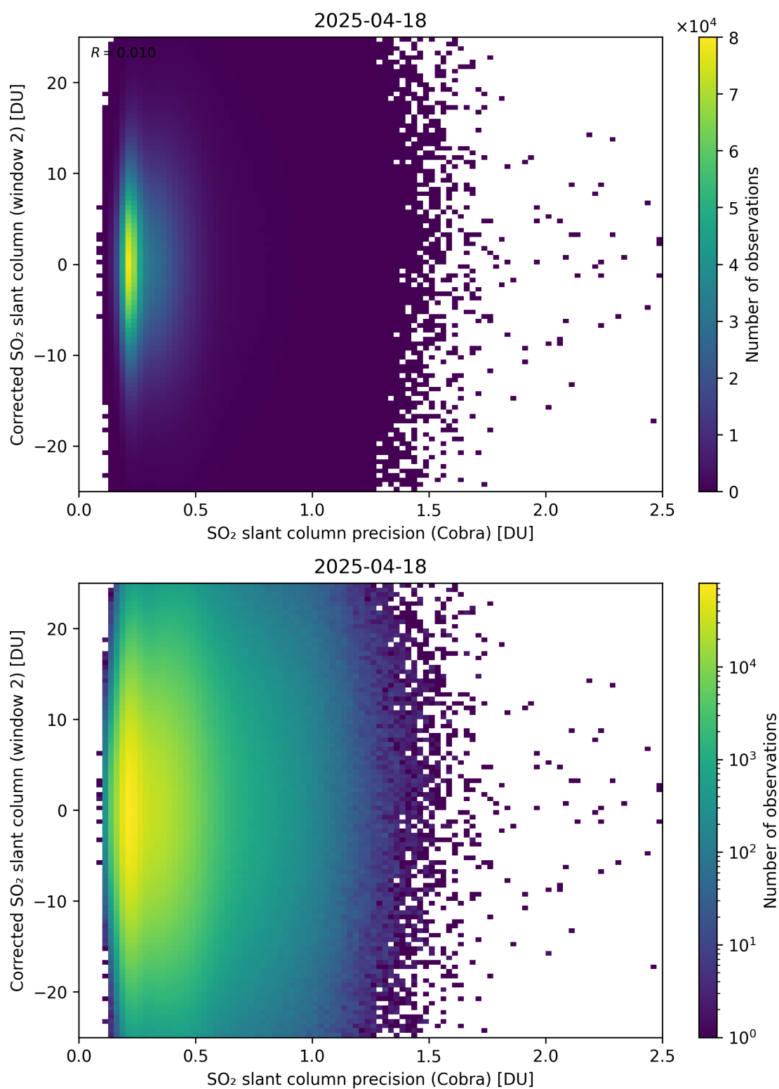
Figure 206: Scatter density plot of “SO 2 slant column precision (Cobra)” against “Corrected SO 2 slant column (window 2)” for 2025-04-18 to 2025-04-19.
