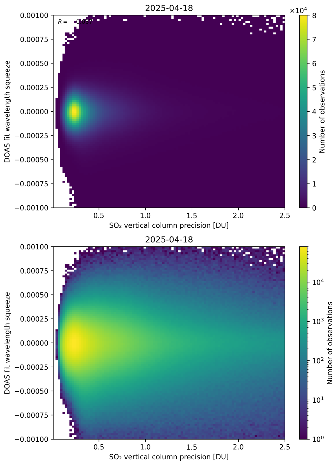
Figure 333: Scatter density plot of “SO 2 vertical column precision” against “DOAS fit wavelength squeeze” for 2025-04-18 to 2025-04-19.
