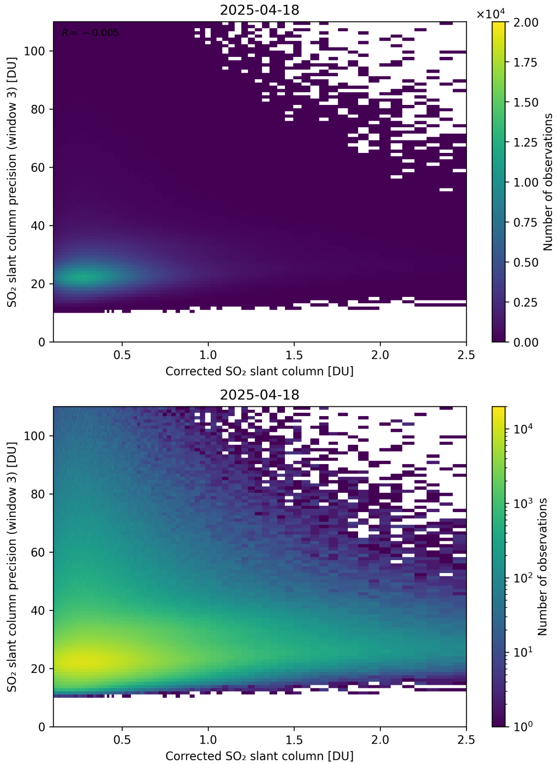
Figure 241: Scatter density plot of “Corrected SO 2 slant column” against “SO 2 slant column precision (window 3)” for 2025-04-18 to 2025-04-19.
