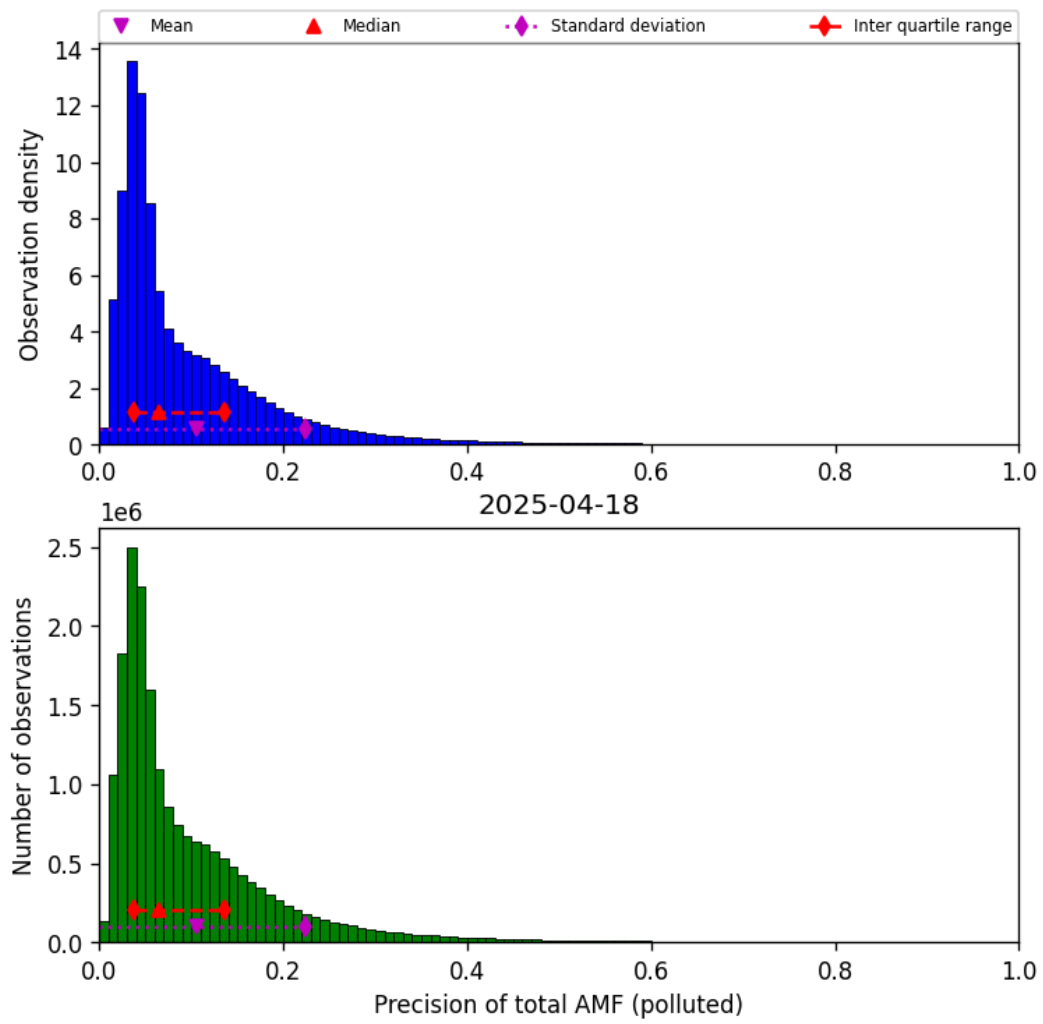
Figure 80: Histogram of “Precision of total AMF (polluted)” for 2025-04-18 to 2025-04-19
