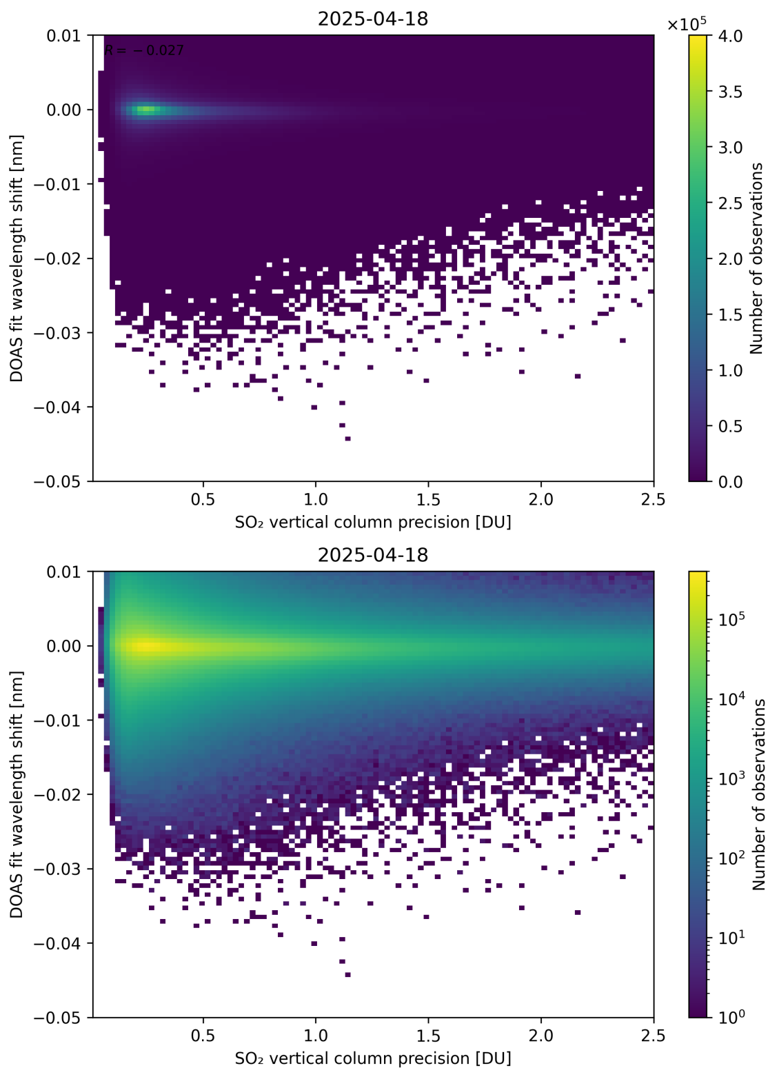
Figure 332: Scatter density plot of “SO 2 vertical column precision” against “DOAS fit wavelength shift” for 2025-04-18 to 2025-04-19.
