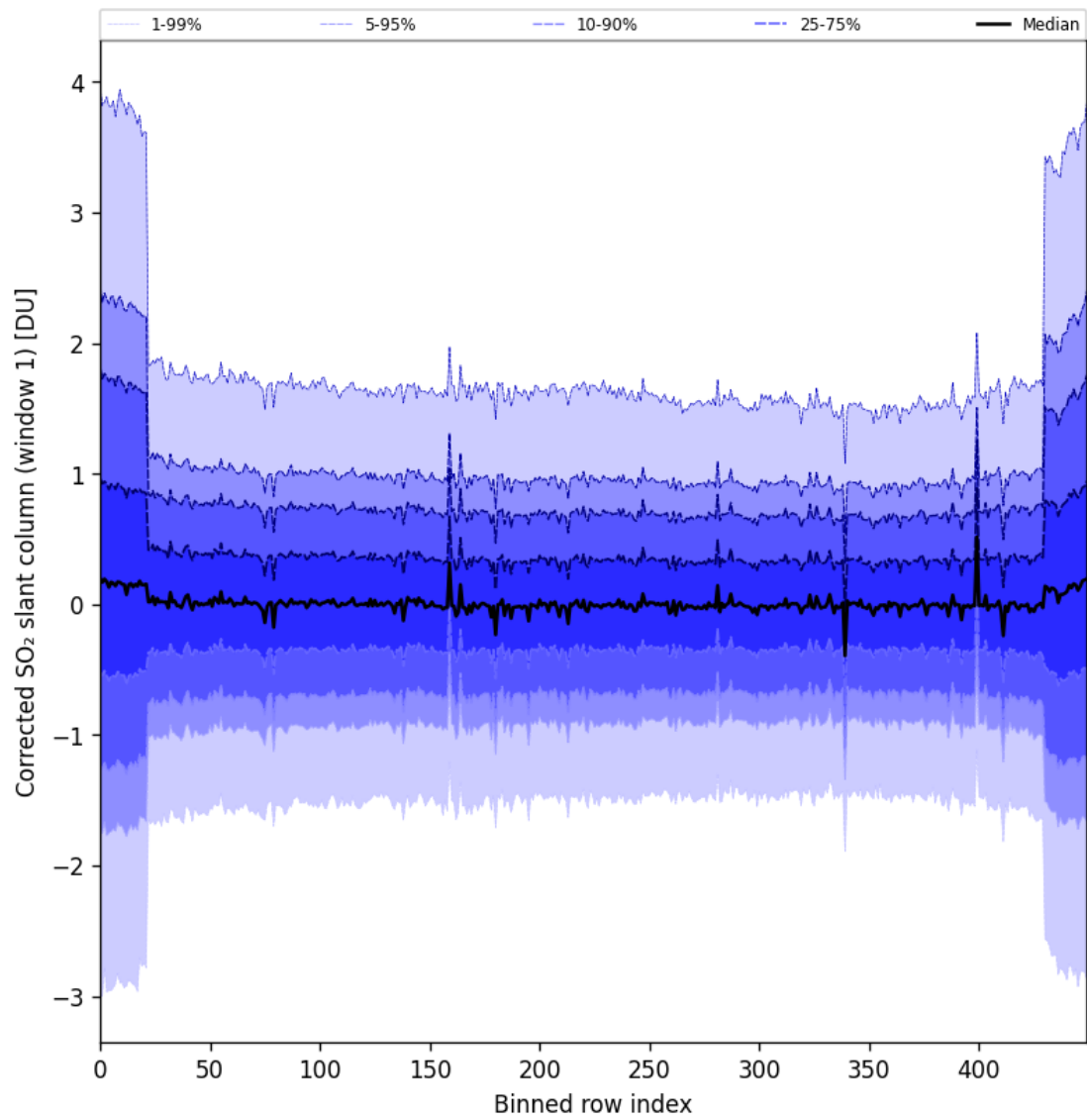
Figure 91: Along track statistics of “Corrected SO 2 slant column (window 1)” for 2025-04-18 to 2025-04-19
