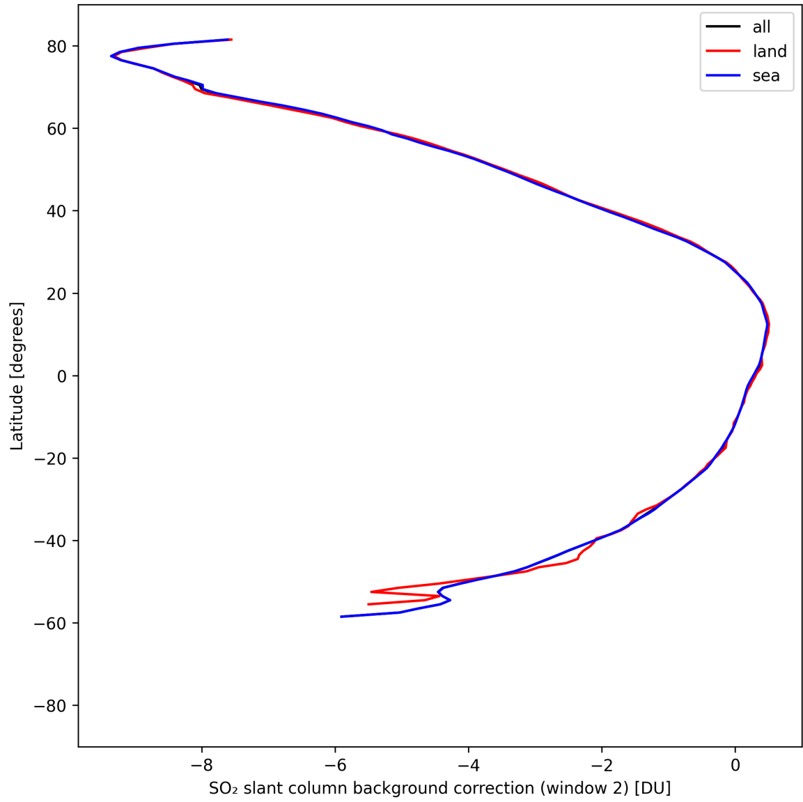
Figure 44: Zonal average of “SO 2 slant column background correction (window 2)” for 2025-04-18 to 2025-04-19.
