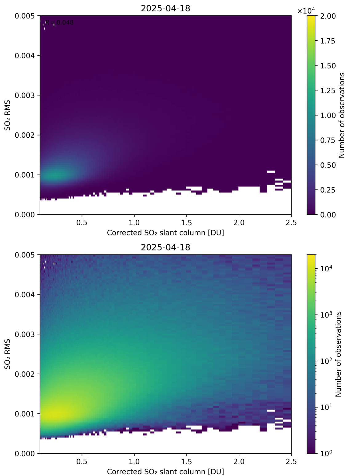
Figure 231: Scatter density plot of “Corrected SO 2 slant column” against “SO 2 RMS” for 2025-04-18 to 2025-04-19.
