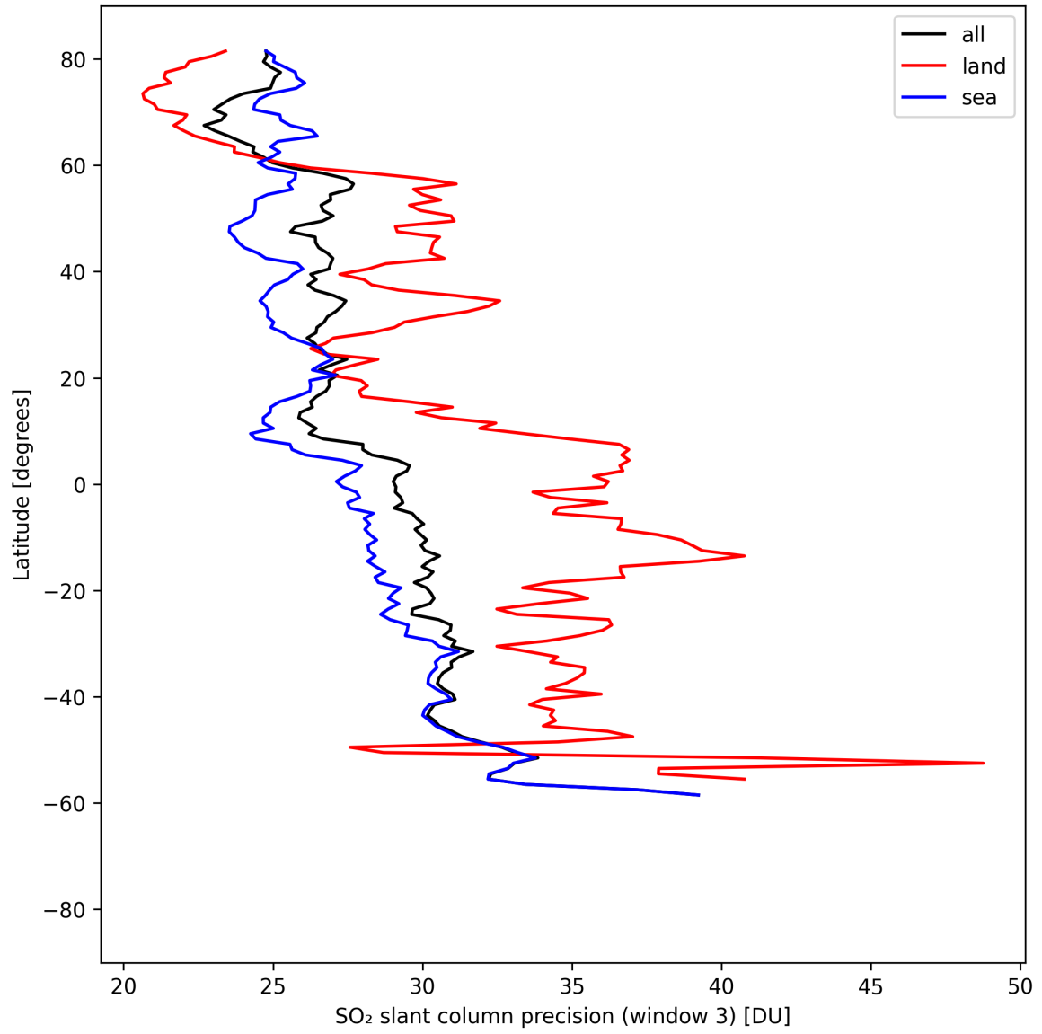
Figure 46: Zonal average of “SO 2 slant column precision (window 3)” for 2025-04-18 to 2025-04-19.
