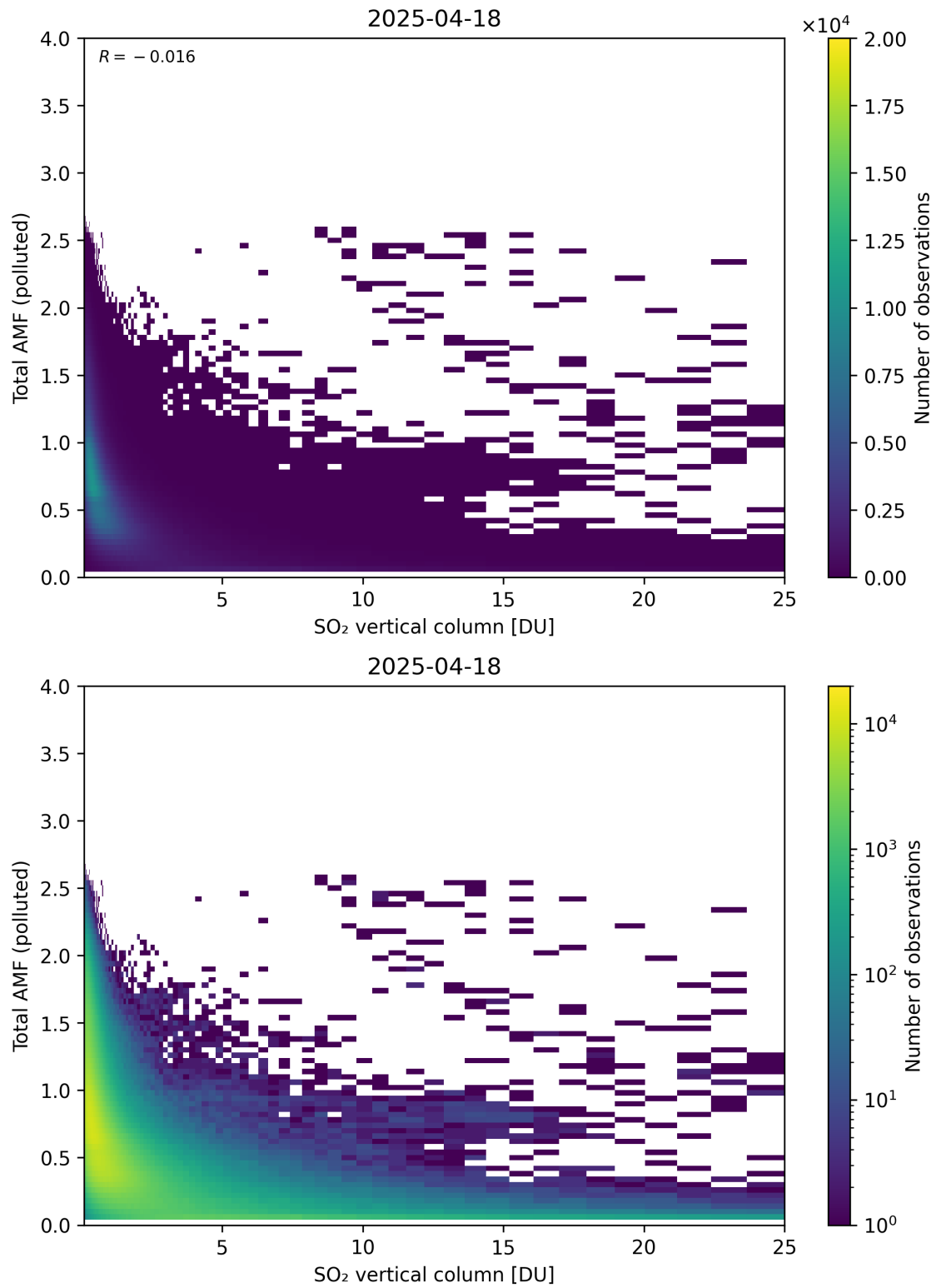
Figure 359: Scatter density plot of “SO 2 vertical column” against “Total AMF (polluted)” for 2025-04-18 to 2025-04-19.
