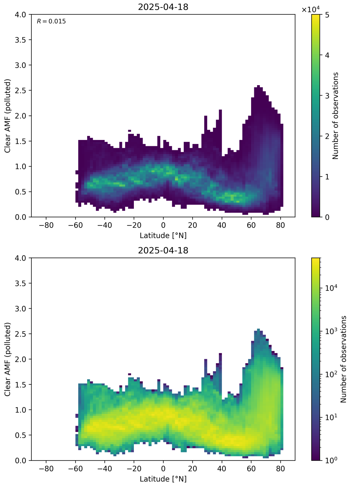
Figure 156: Scatter density plot of “Latitude” against “Clear AMF (polluted)” for 2025-04-18 to 2025-04-19.
