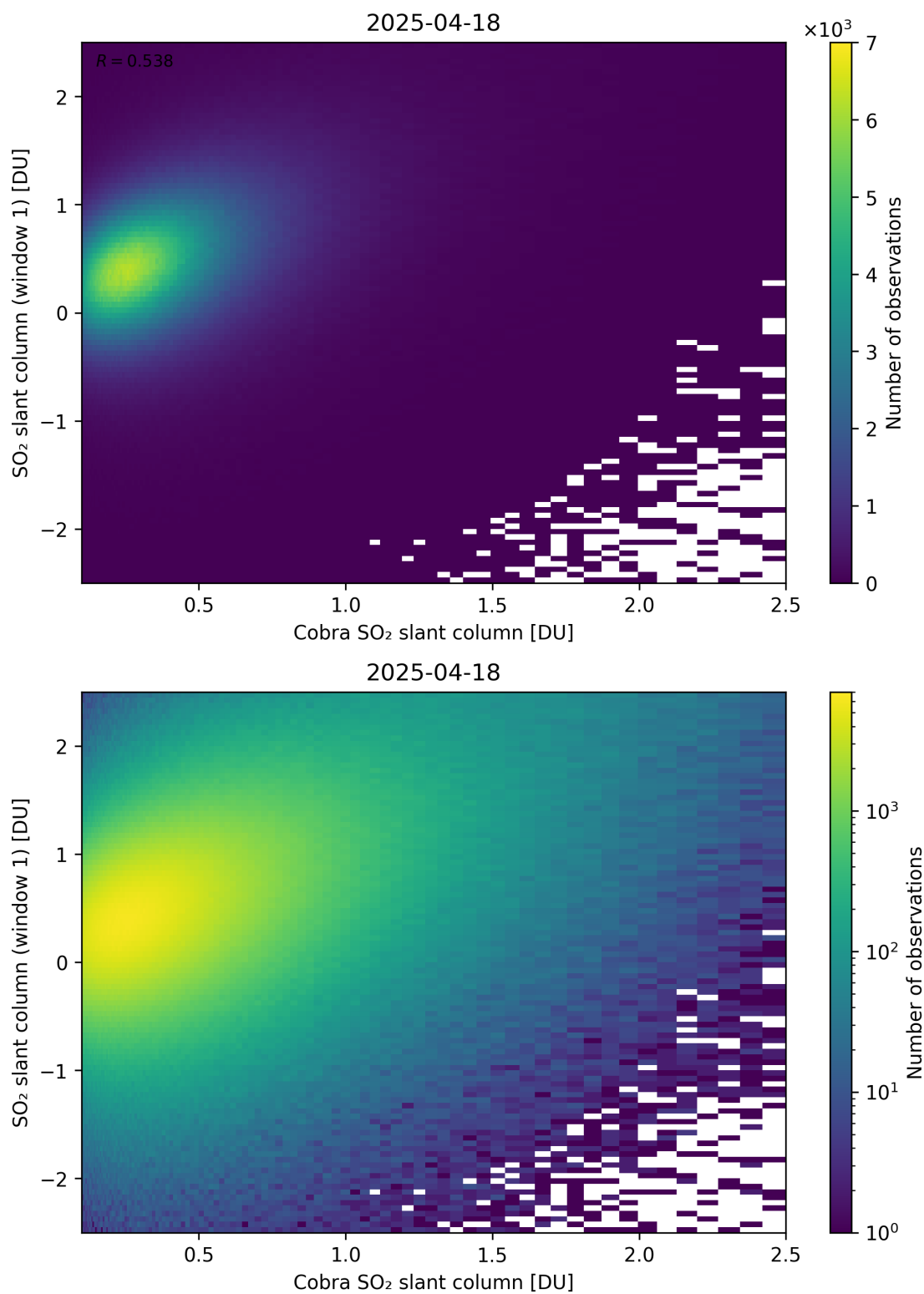
Figure 219: Scatter density plot of “Cobra SO 2 slant column” against “SO 2 slant column (window 1)” for 2025-04-18 to 2025-04-19.
