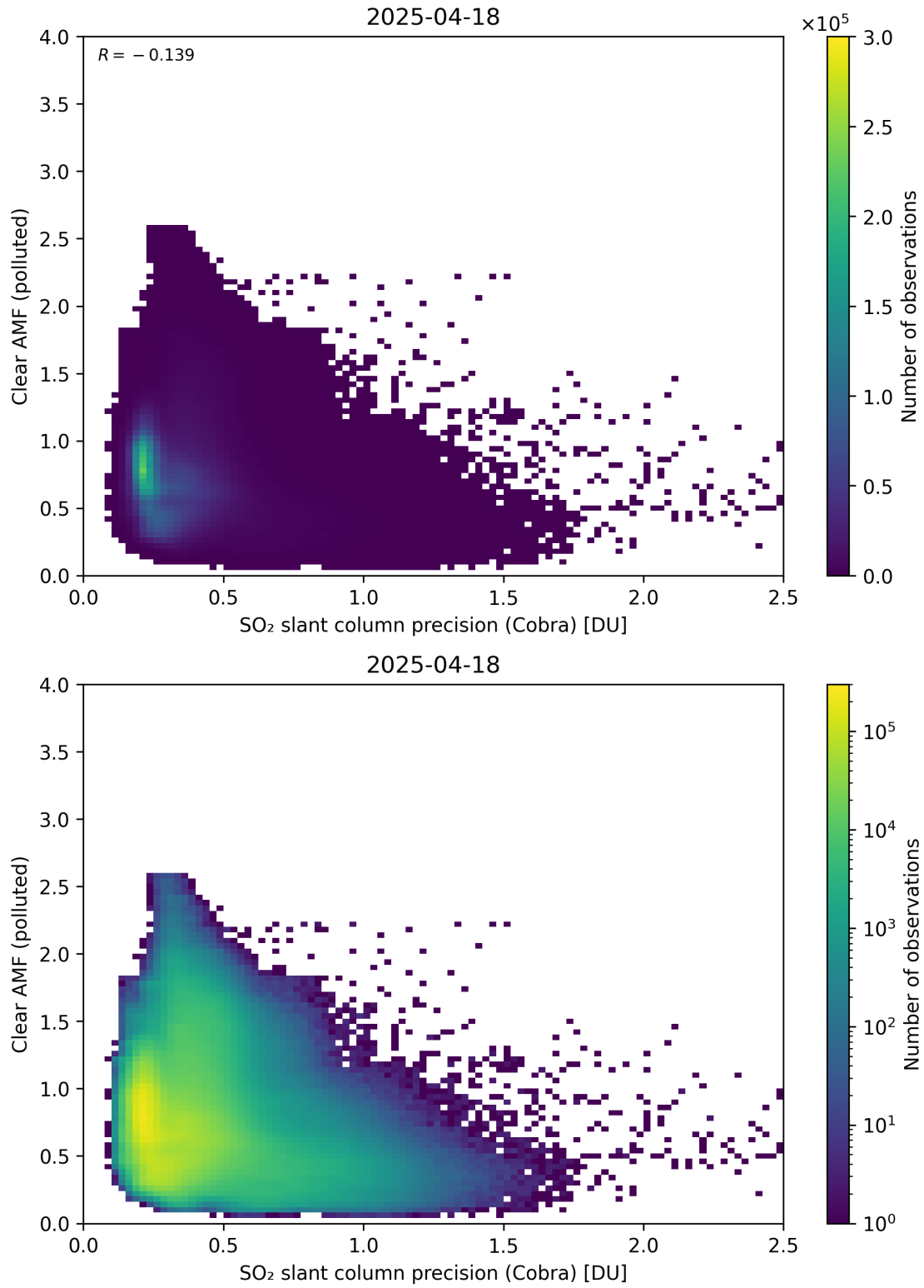
Figure 205: Scatter density plot of “SO 2 slant column precision (Cobra)” against “Clear AMF (polluted)” for 2025-04-18 to 2025-04-19.
