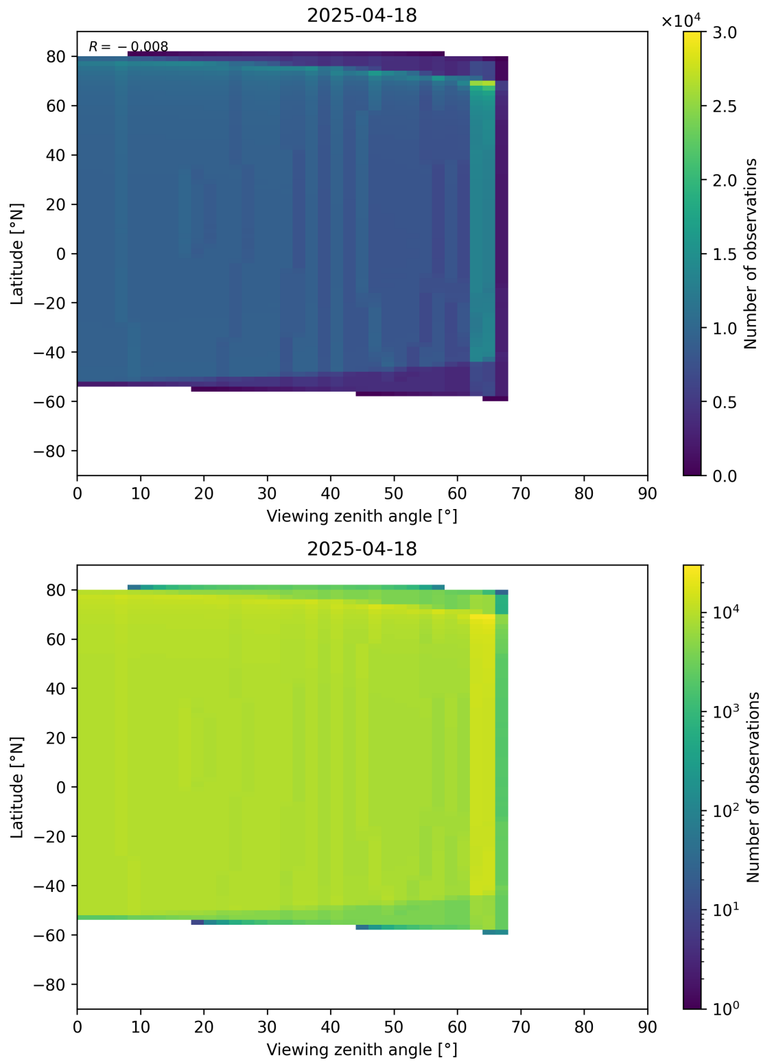
Figure 368: Scatter density plot of “Viewing zenith angle” against “Latitude” for 2025-04-18 to 2025-04-19.
