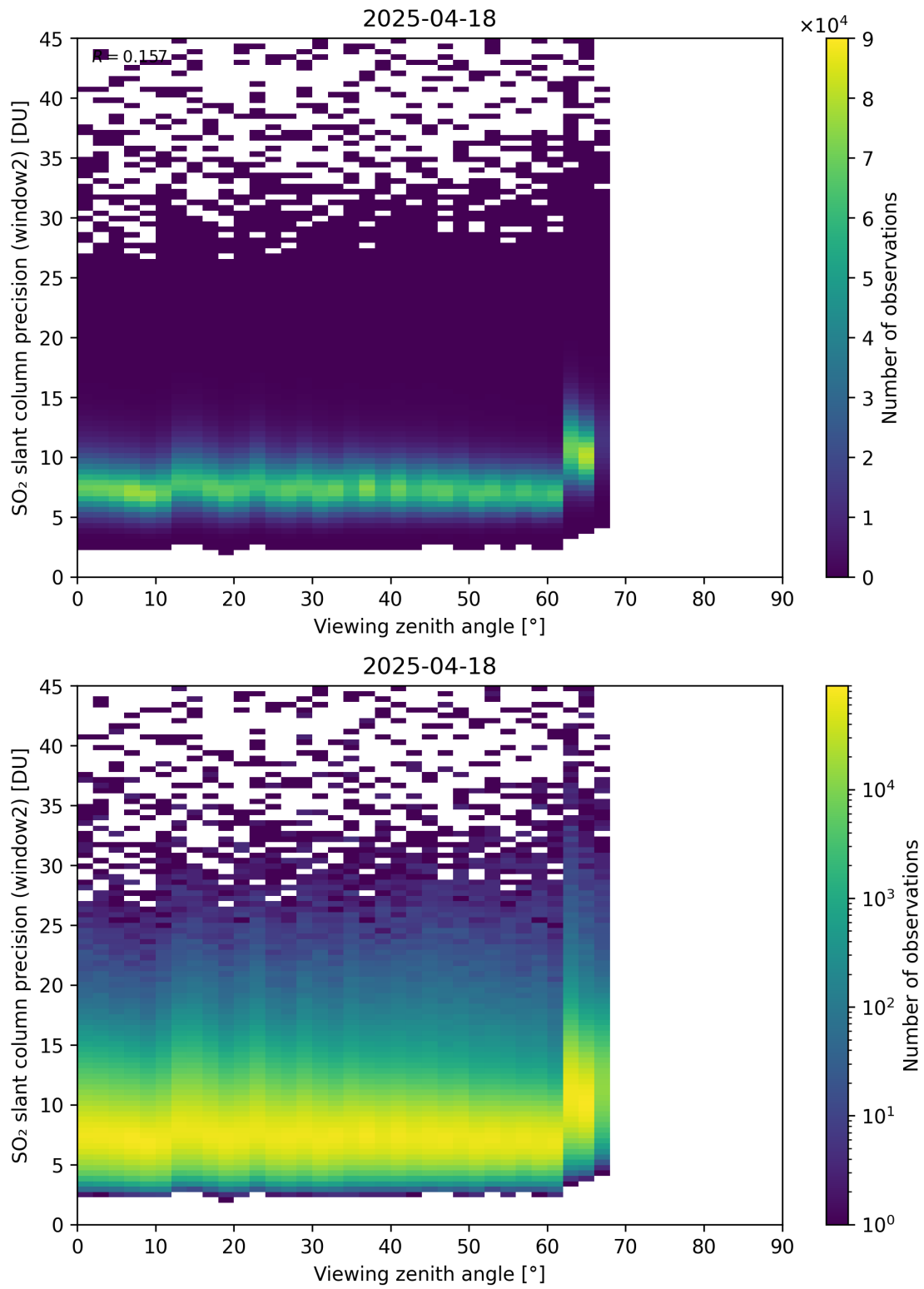
Figure 378: Scatter density plot of “Viewing zenith angle” against “SO 2 slant column precision (window2)” for 2025-04-18 to 2025-04-19.
