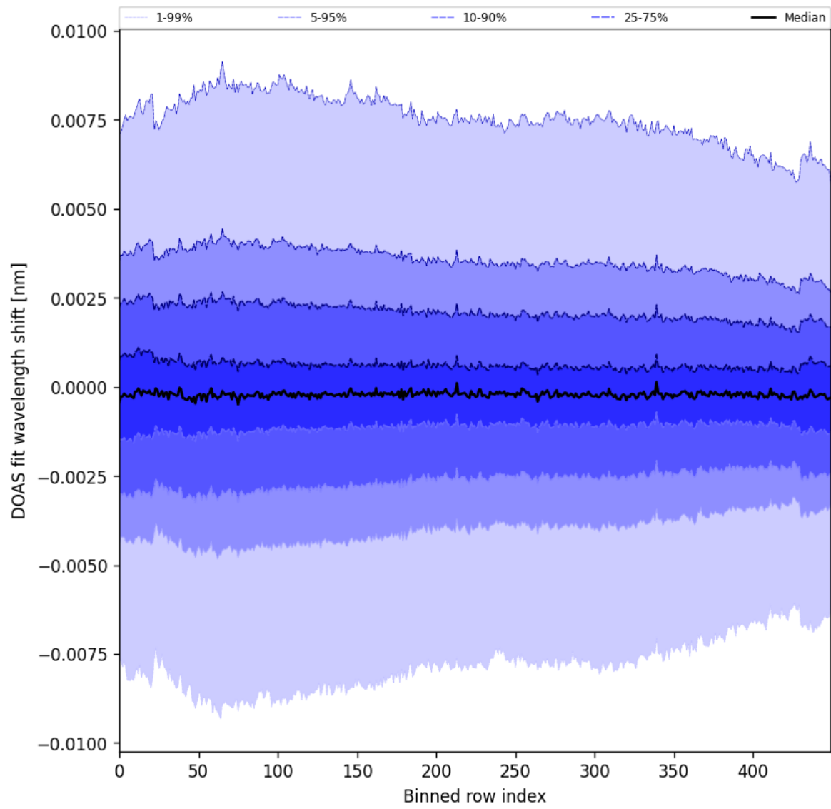
Figure 102: Along track statistics of “DOAS fit wavelength shift” for 2025-04-18 to 2025-04-19
