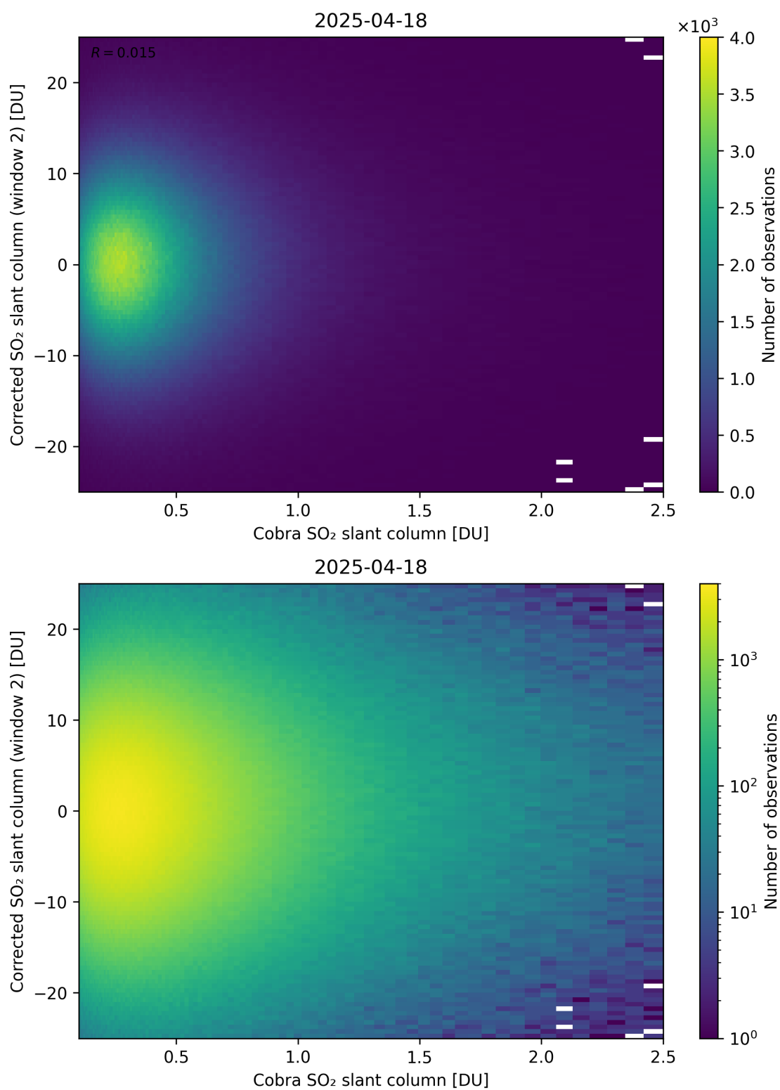
Figure 217: Scatter density plot of “Cobra SO 2 slant column” against “Corrected SO 2 slant column (window 2)” for 2025-04-18 to 2025-04-19.
