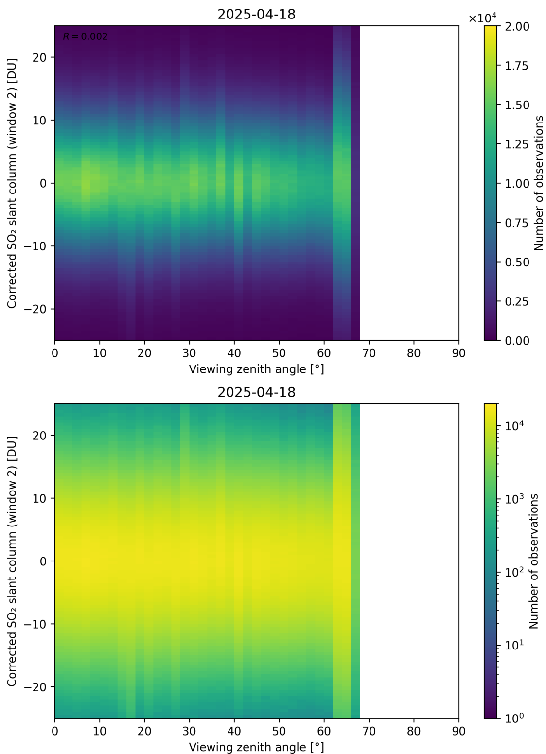
Figure 374: Scatter density plot of “Viewing zenith angle” against “Corrected SO 2 slant column (window 2)” for 2025-04-18 to 2025-04-19.
