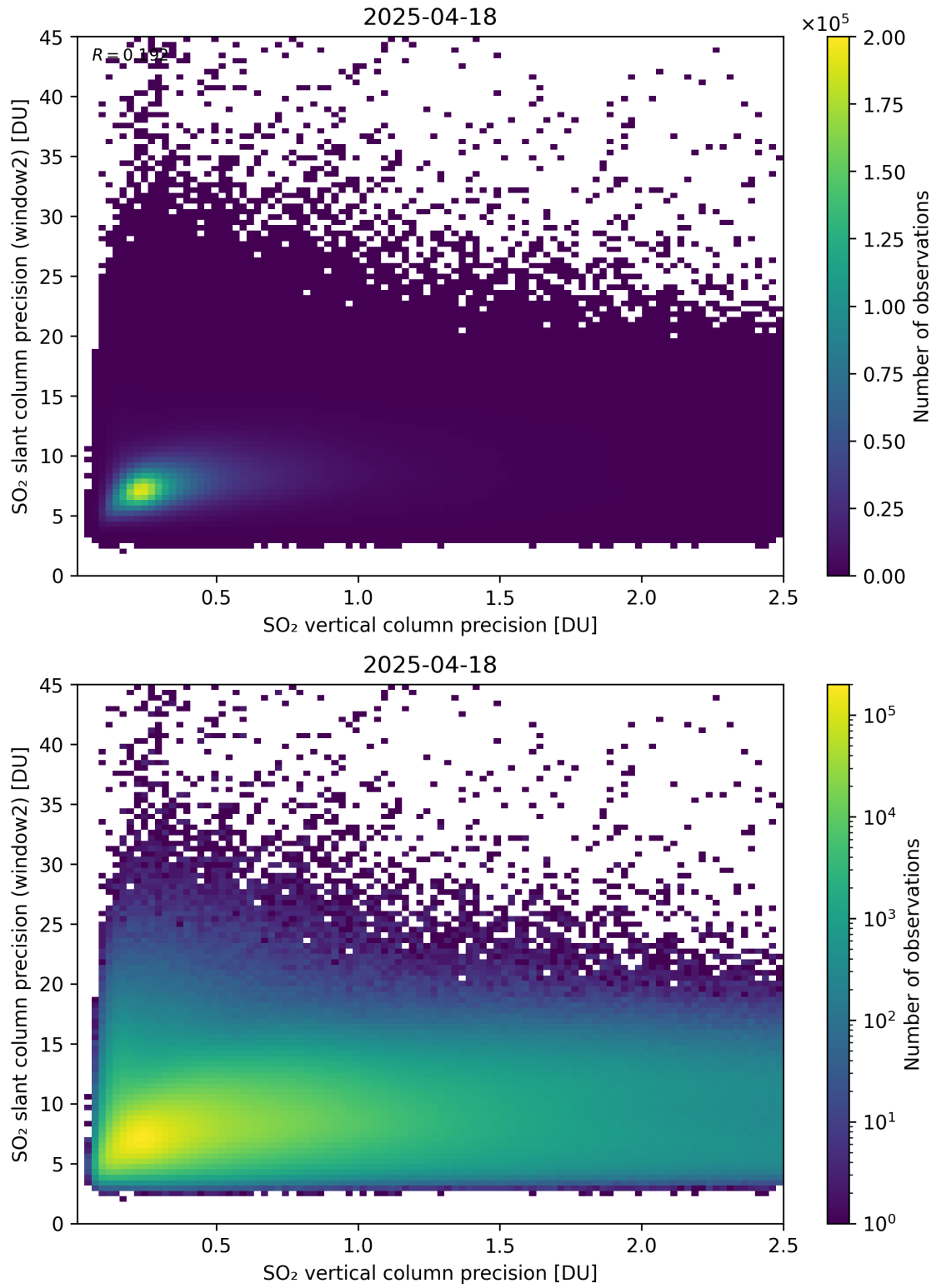
Figure 343: Scatter density plot of “SO 2 vertical column precision” against “SO 2 slant column precision (window2)” for 2025-04-18 to 2025-04-19.
