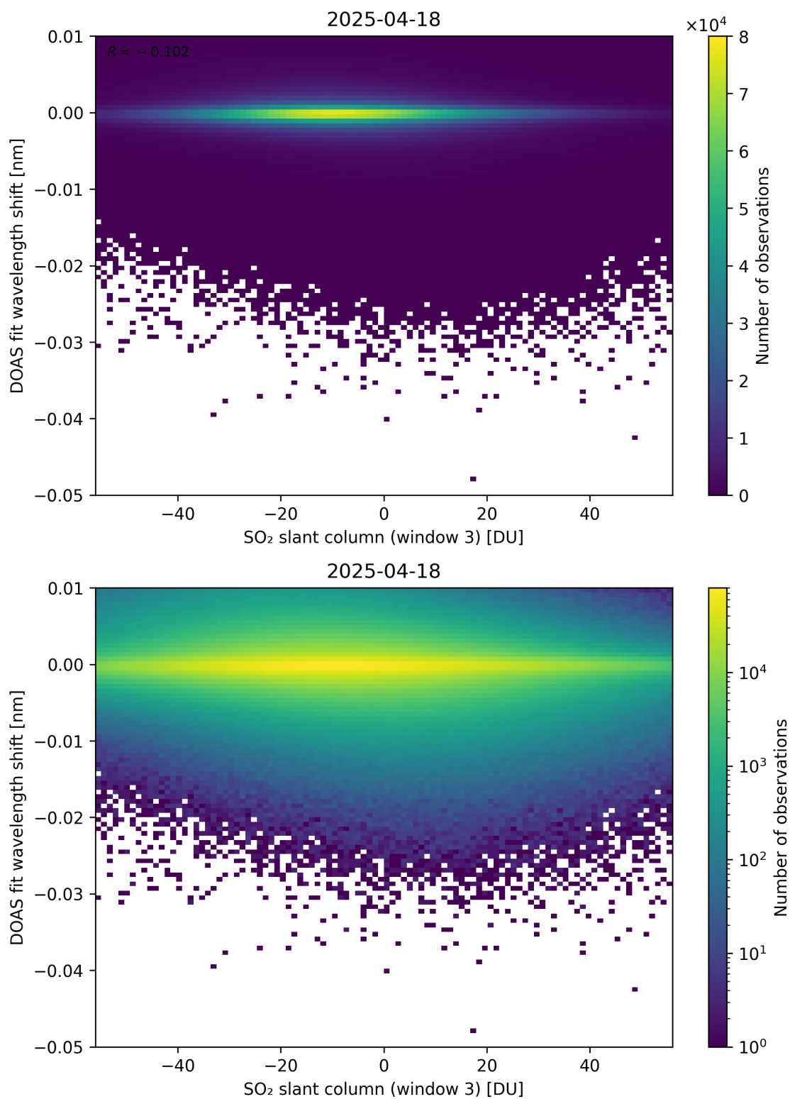
Figure 304: Scatter density plot of “SO 2 slant column (window 3)” against “DOAS fit wavelength shift” for 2025-04-18 to 2025-04-19.
