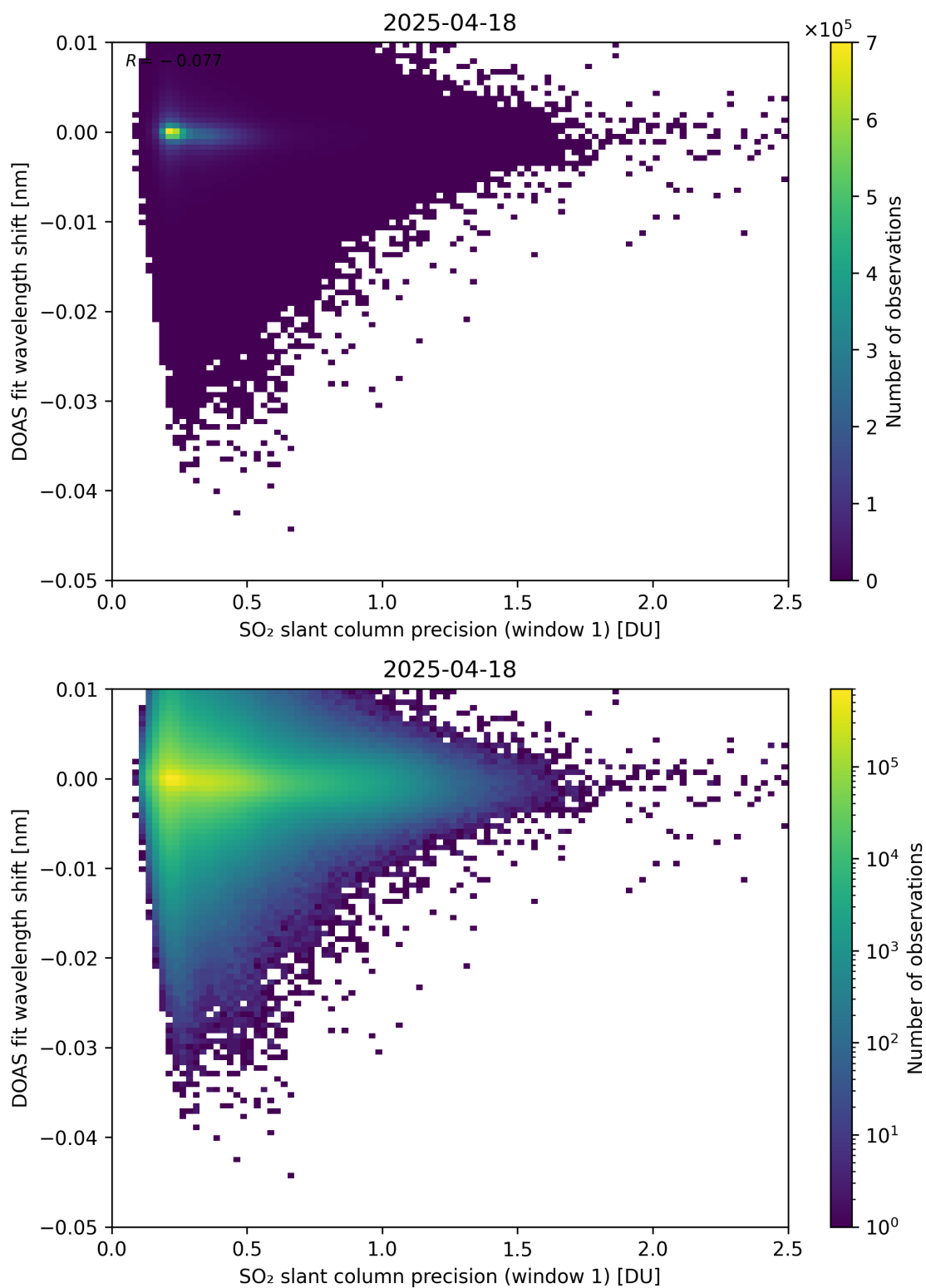
Figure 271: Scatter density plot of “SO 2 slant column precision (window 1)” against “DOAS fit wavelength shift” for 2025-04-18 to 2025-04-19.
