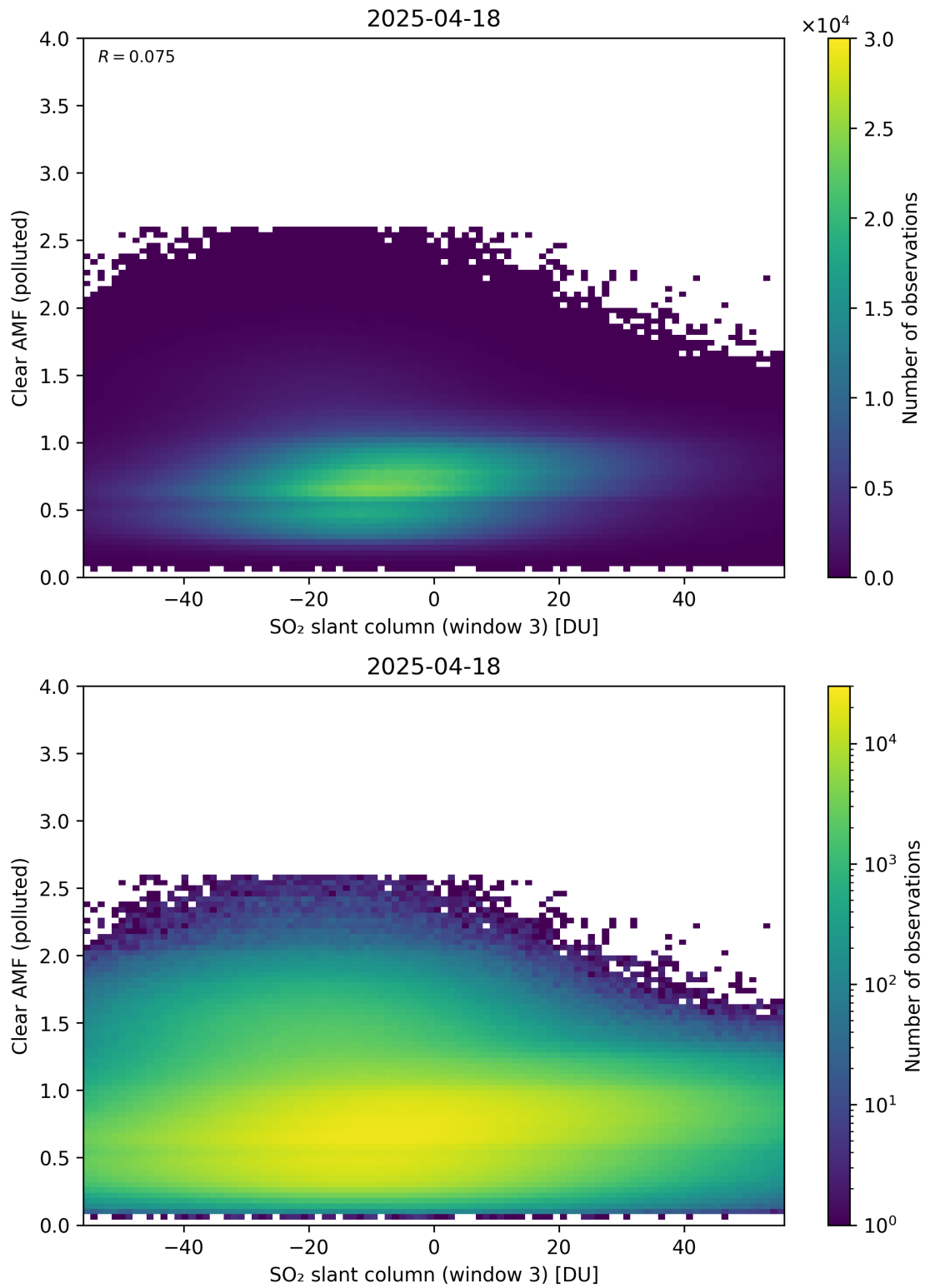
Figure 315: Scatter density plot of “SO 2 slant column (window 3)” against “Clear AMF (polluted)” for 2025-04-18 to 2025-04-19.
