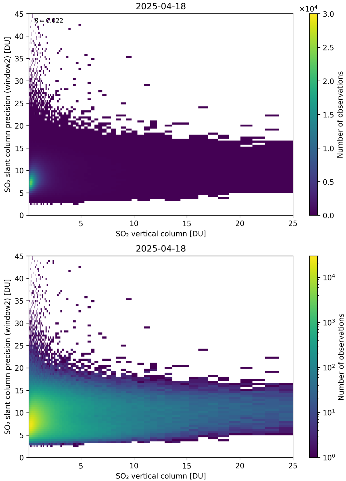
Figure 356: Scatter density plot of “SO 2 vertical column” against “SO 2 slant column precision (window2)” for 2025-04-18 to 2025-04-19.
