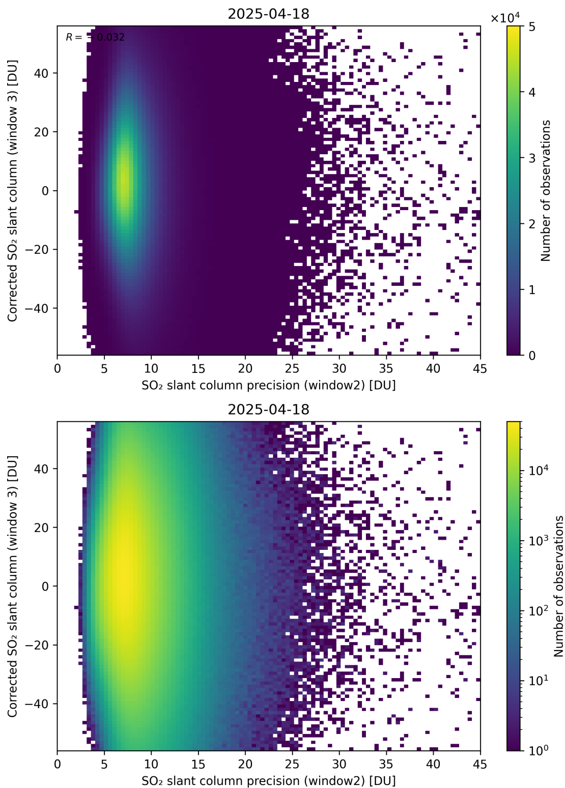
Figure 298: Scatter density plot of “SO 2 slant column precision (window2)” against “Corrected SO 2 slant column (window 3)” for 2025-04-18 to 2025-04-19.
