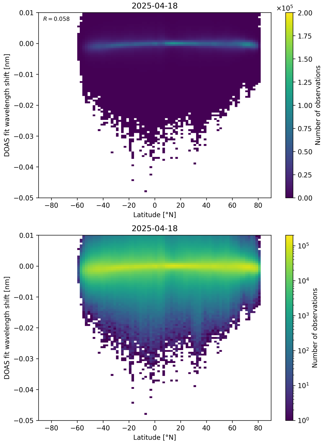
Figure 153: Scatter density plot of “Latitude” against “DOAS fit wavelength shift” for 2025-04-18 to 2025-04-19.
