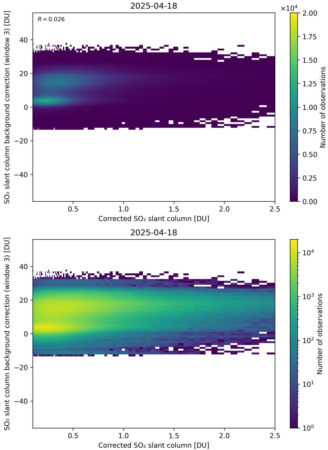
Figure 228: Scatter density plot of “Corrected SO 2 slant column” against “SO 2 slant column background correction (window 3)” for 2025-04-18 to 2025-04-19.
