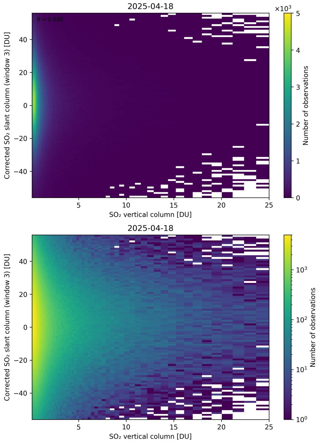
Figure 353: Scatter density plot of “SO 2 vertical column” against “Corrected SO 2 slant column (window 3)” for 2025-04-18 to 2025-04-19.
