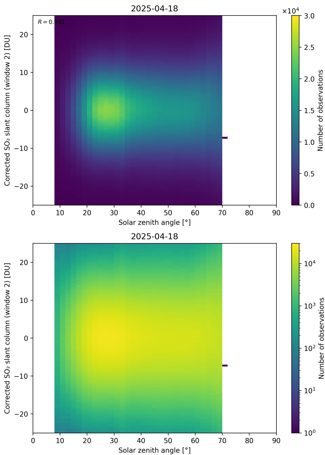
Figure 182: Scatter density plot of “Solar zenith angle” against “Corrected SO 2 slant column (window 2)” for 2025-04-18 to 2025-04-19.
