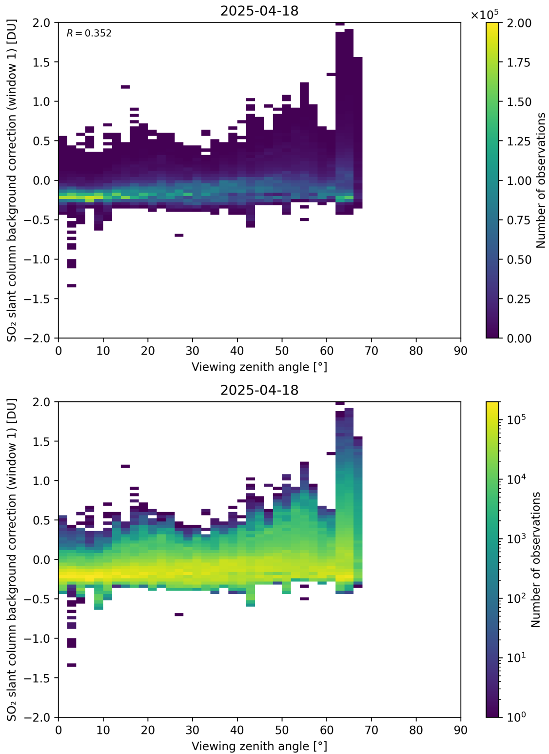
Figure 362: Scatter density plot of “Viewing zenith angle” against “SO 2 slant column background correction (window 1)” for 2025-04-18 to 2025-04-19.
