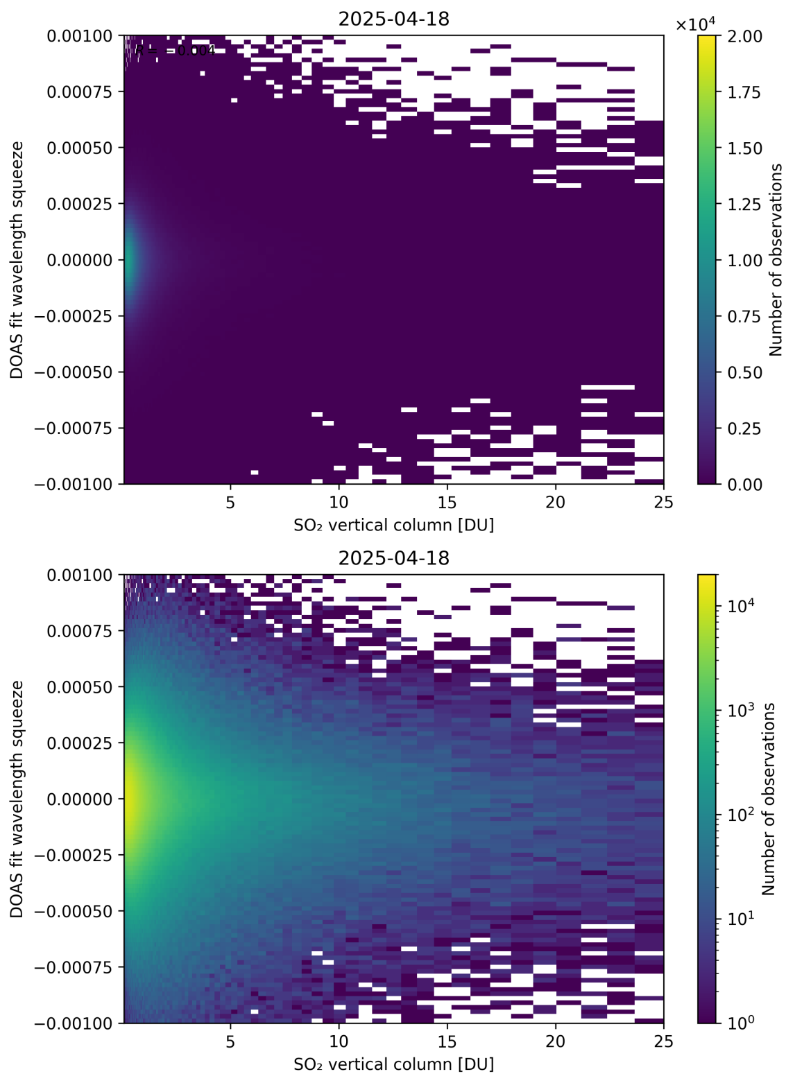
Figure 327: Scatter density plot of “SO 2 vertical column” against “DOAS fit wavelength squeeze” for 2025-04-18 to 2025-04-19.
