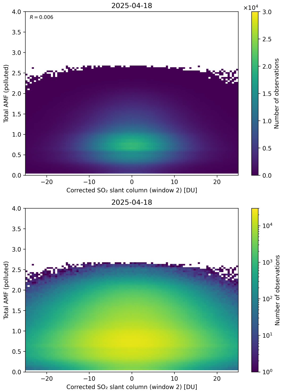
Figure 253: Scatter density plot of “Corrected SO 2 slant column (window 2)” against “Total AMF (polluted)” for 2025-04-18 to 2025-04-19.
