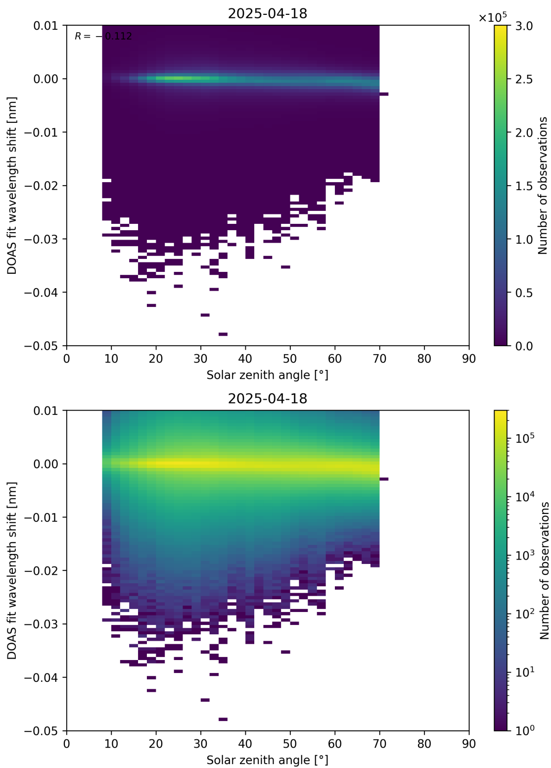
Figure 174: Scatter density plot of “Solar zenith angle” against “DOAS fit wavelength shift” for 2025-04-18 to 2025-04-19.
