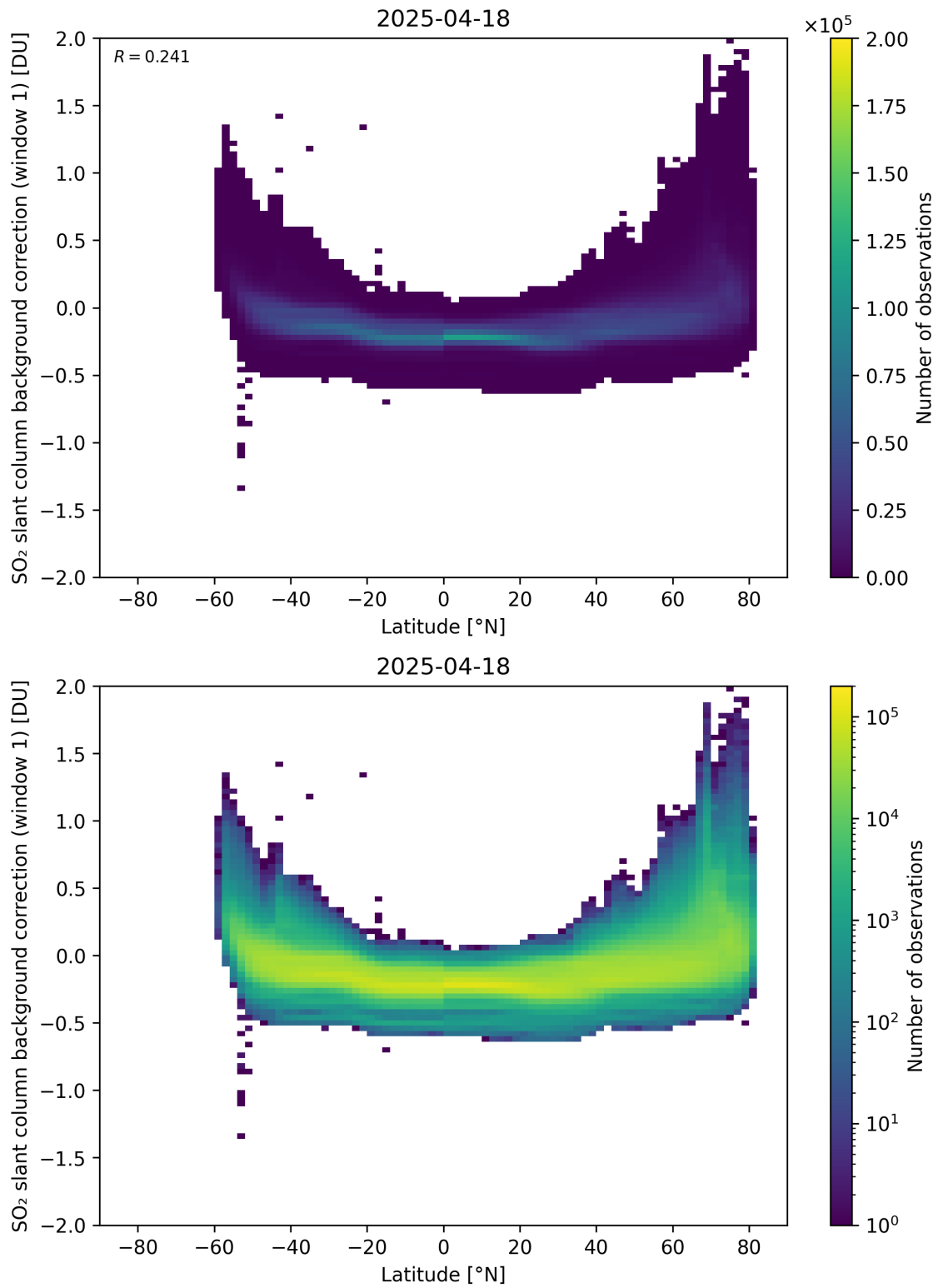
Figure 150: Scatter density plot of “Latitude” against “SO 2 slant column background correction (window 1)” for 2025-04-18 to 2025-04-19.
