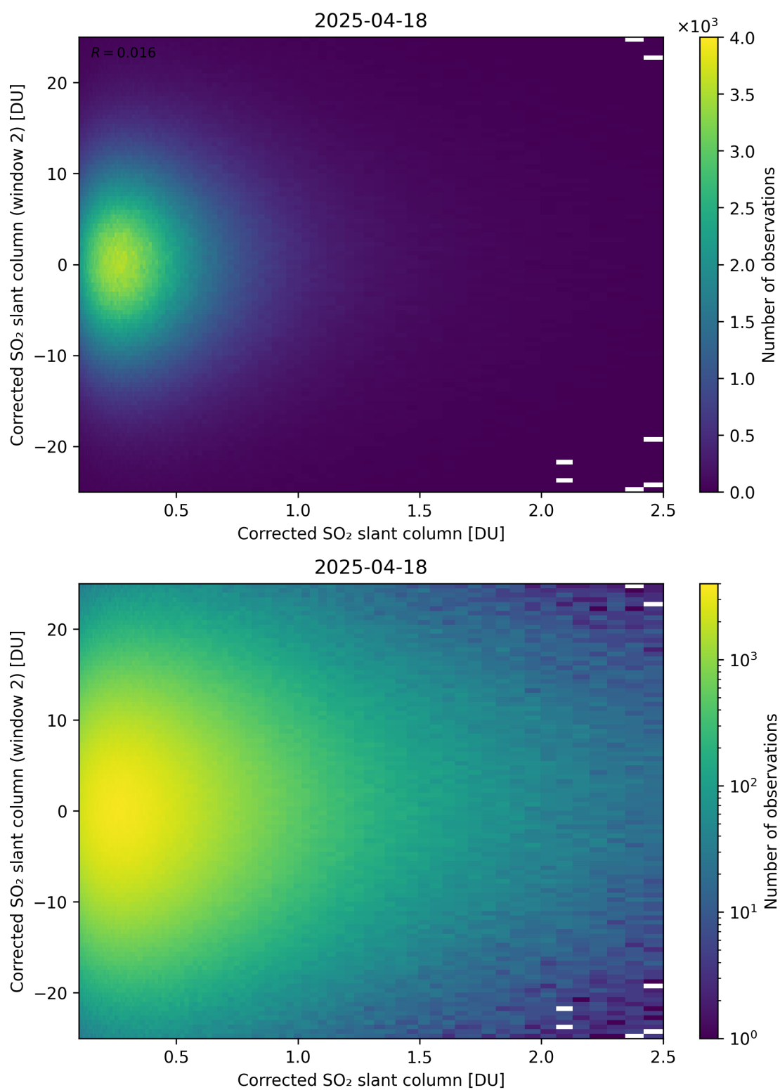
Figure 235: Scatter density plot of “Corrected SO 2 slant column” against “Corrected SO 2 slant column (window 2)” for 2025-04-18 to 2025-04-19.
