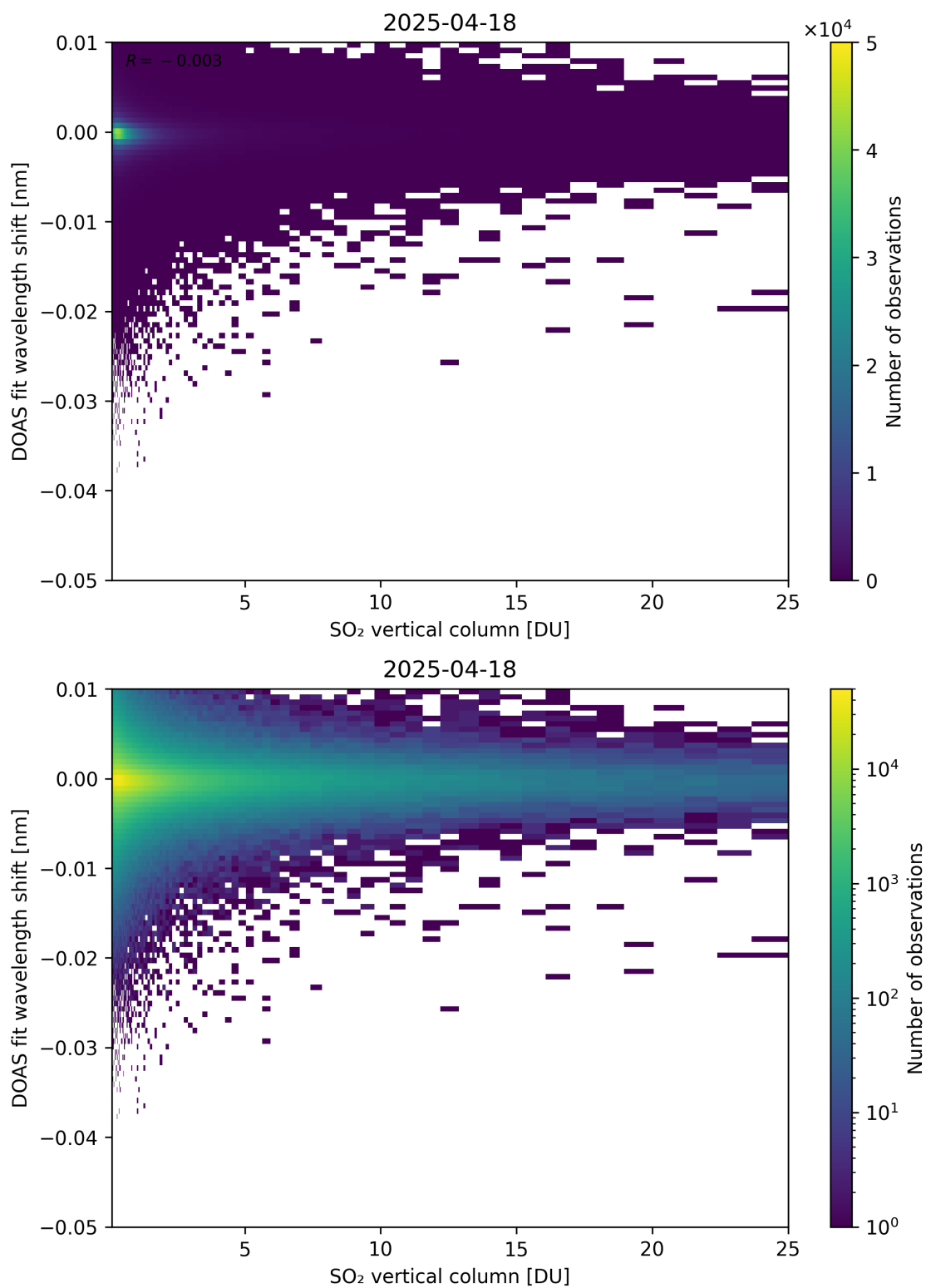
Figure 326: Scatter density plot of “SO 2 vertical column” against “DOAS fit wavelength shift” for 2025-04-18 to 2025-04-19.
