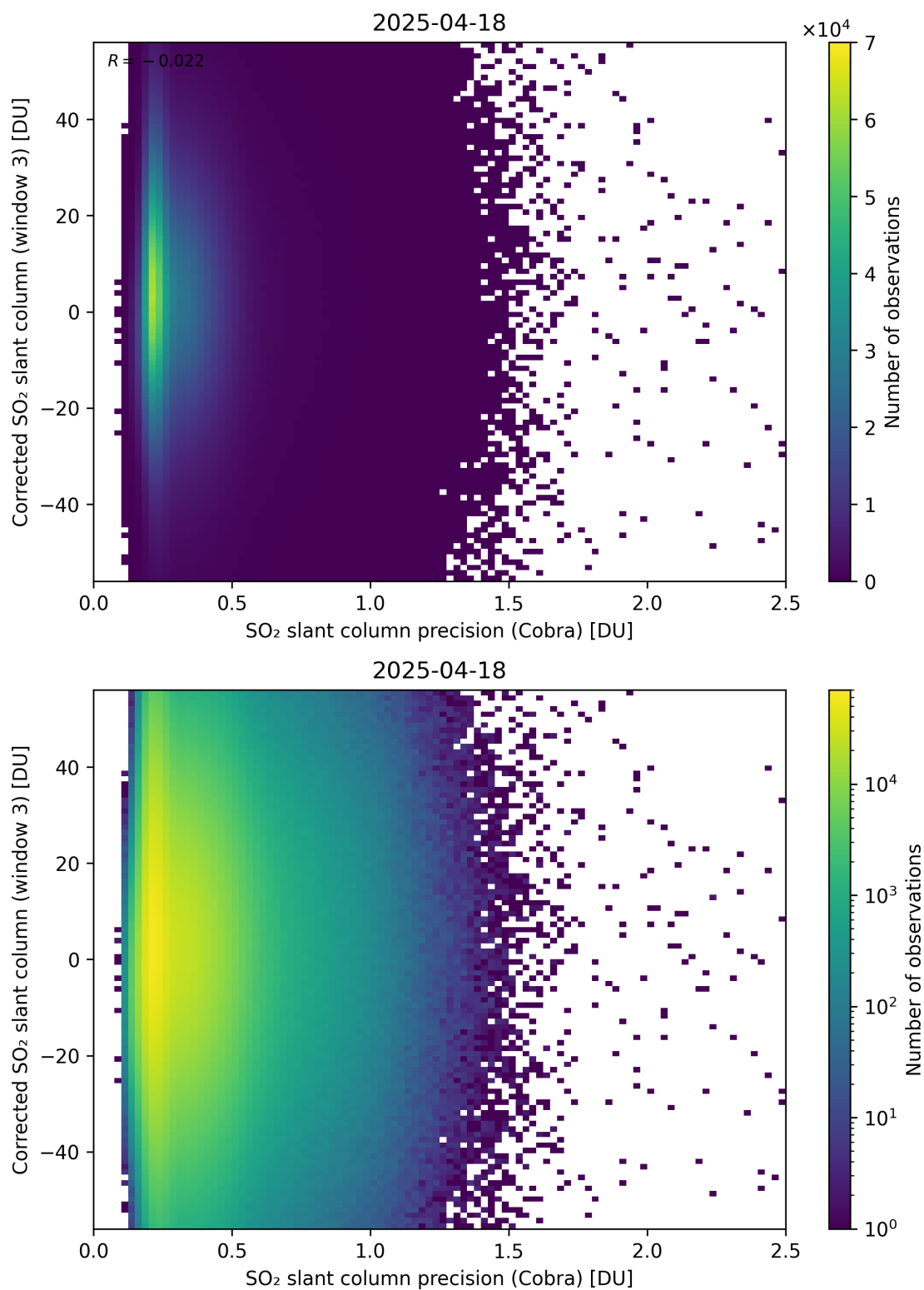
Figure 207: Scatter density plot of “SO 2 slant column precision (Cobra)” against “Corrected SO 2 slant column (window 3)” for 2025-04-18 to 2025-04-19.
