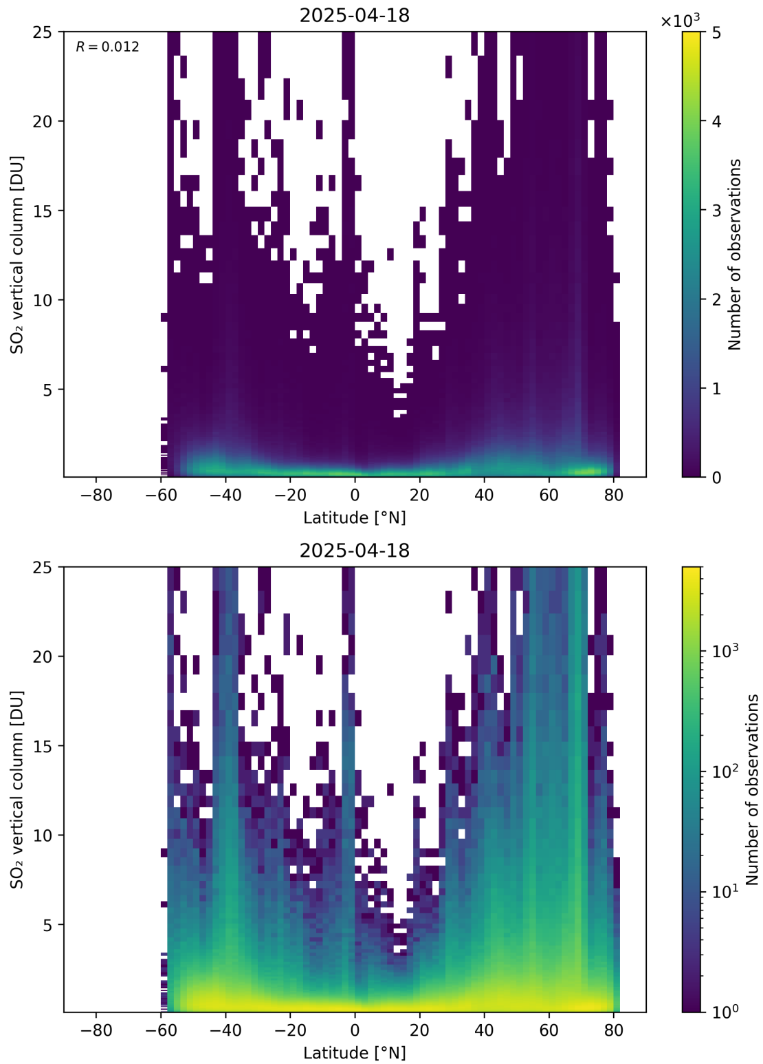
Figure 169: Scatter density plot of “Latitude” against “SO 2 vertical column” for 2025-04-18 to 2025-04-19.
