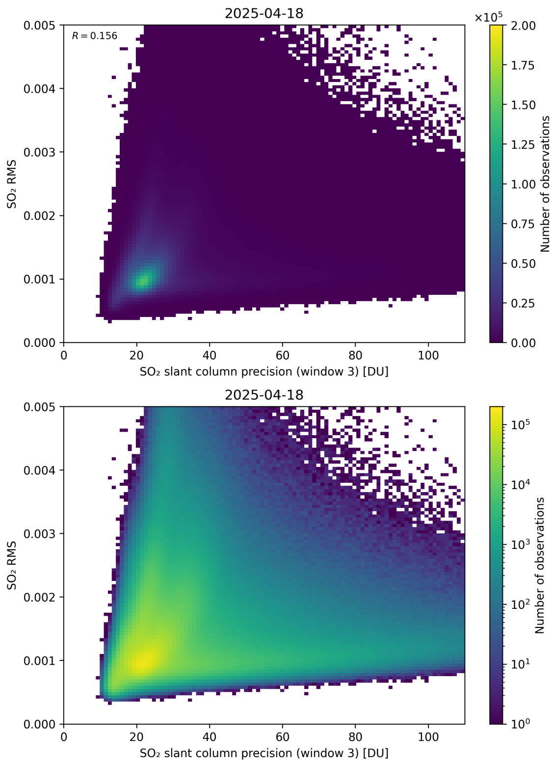
Figure 310: Scatter density plot of “SO 2 slant column precision (window 3)” against “SO 2 RMS” for 2025-04-18 to 2025-04-19.
