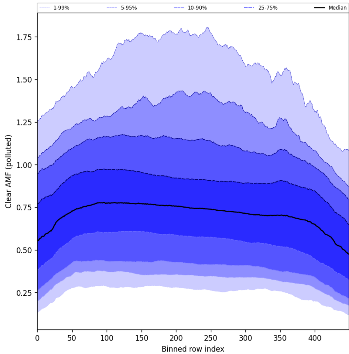
Figure 107: Along track statistics of “Clear AMF (polluted)” for 2025-04-18 to 2025-04-19
