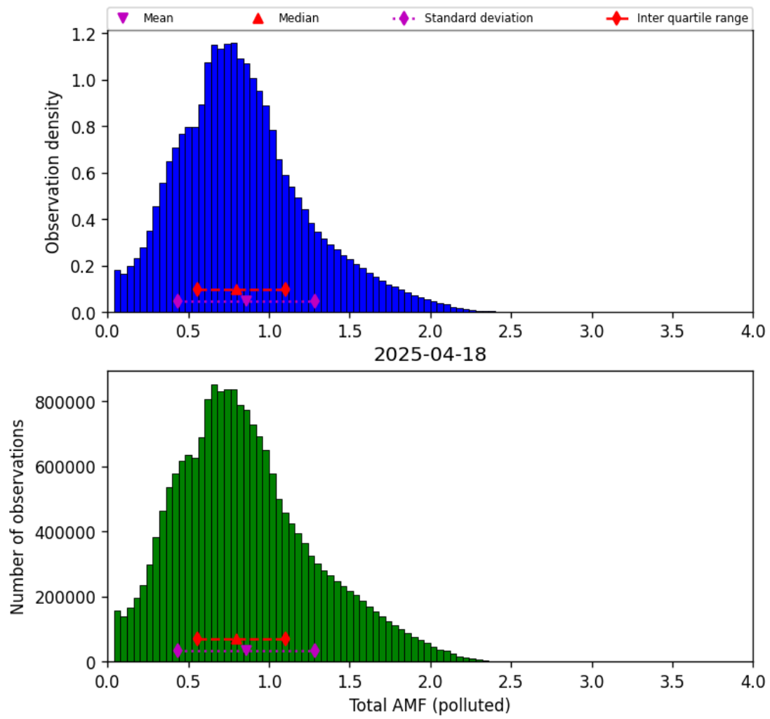
Figure 79: Histogram of “Total AMF (polluted)” for 2025-04-18 to 2025-04-19
