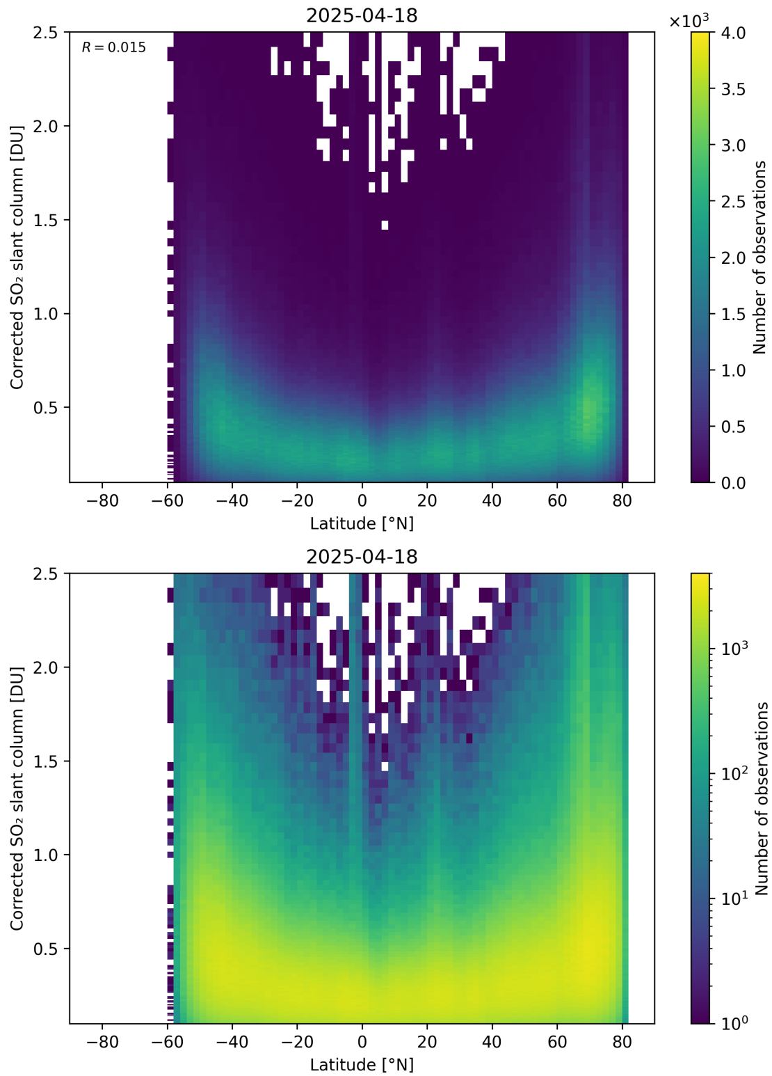
Figure 159: Scatter density plot of “Latitude” against “Corrected SO 2 slant column” for 2025-04-18 to 2025-04-19.
