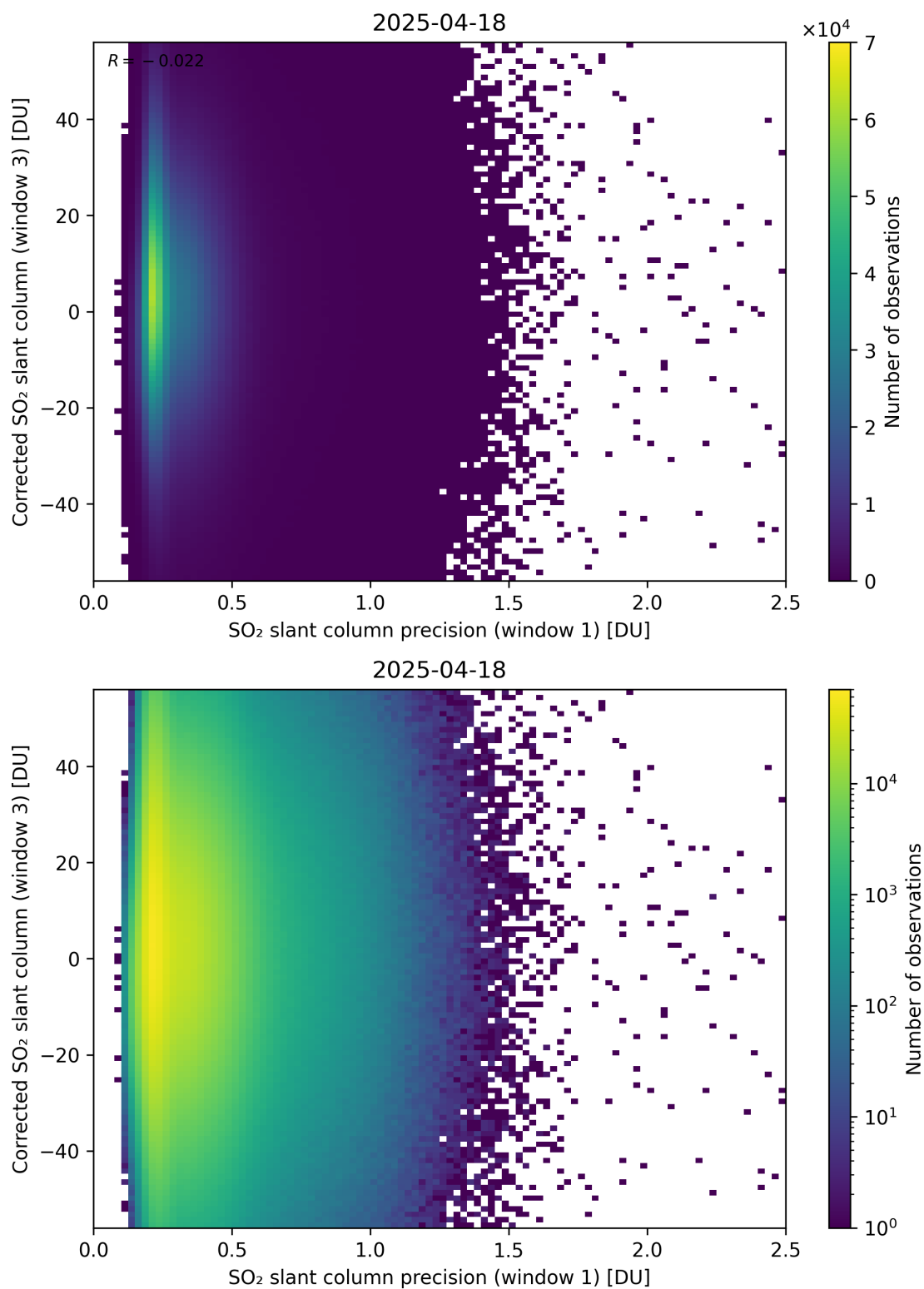
Figure 276: Scatter density plot of “SO 2 slant column precision (window 1)” against “Corrected SO 2 slant column (window 3)” for 2025-04-18 to 2025-04-19.
