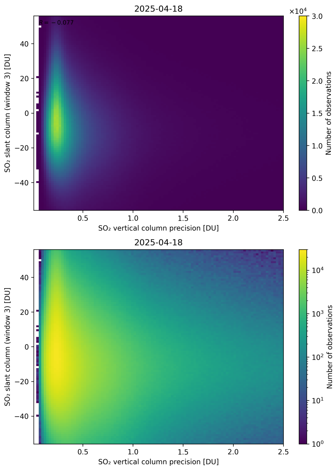
Figure 344: Scatter density plot of “SO 2 vertical column precision” against “SO 2 slant column (window 3)” for 2025-04-18 to 2025-04-19.
