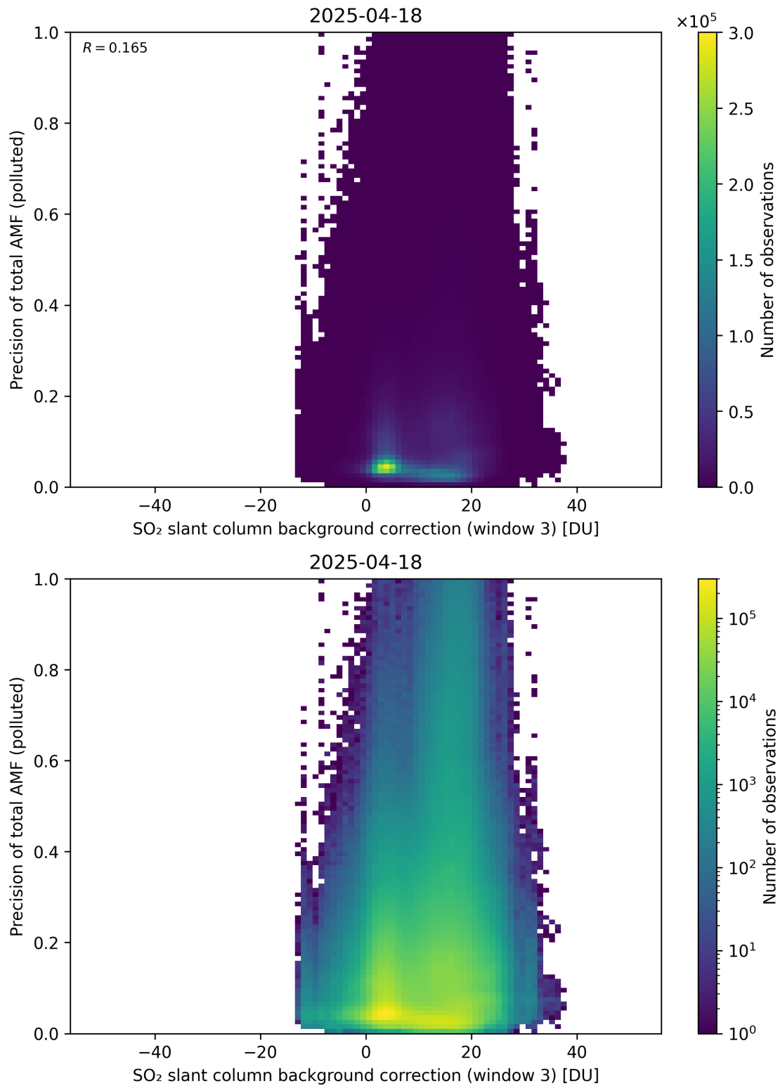
Figure 137: Scatter density plot of “SO 2 slant column background correction (window 3)” against “Precision of total AMF (polluted)” for 2025-04-18 to 2025-04-19.
