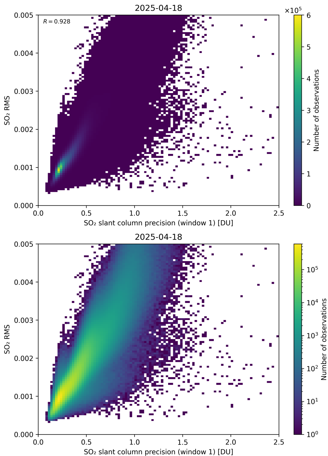
Figure 273: Scatter density plot of “SO 2 slant column precision (window 1)” against “SO 2 RMS” for 2025-04-18 to 2025-04-19.
