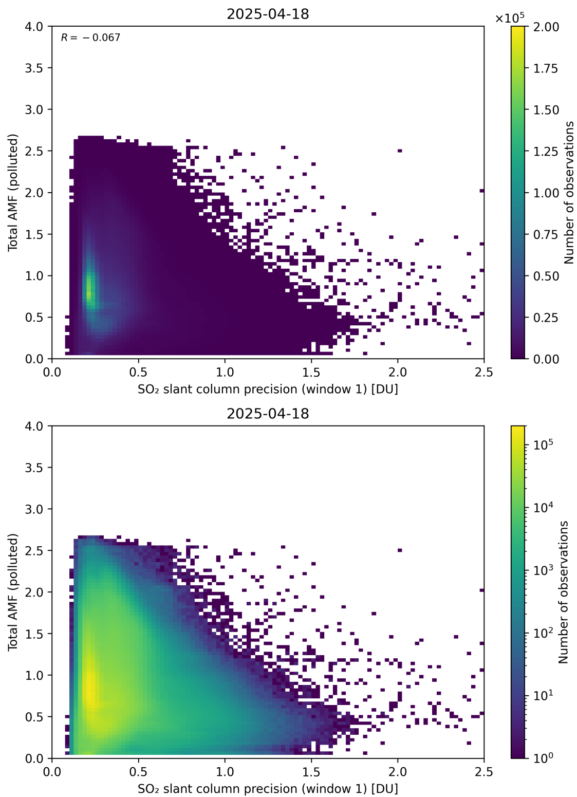
Figure 280: Scatter density plot of “SO 2 slant column precision (window 1)” against “Total AMF (polluted)” for 2025-04-18 to 2025-04-19.
