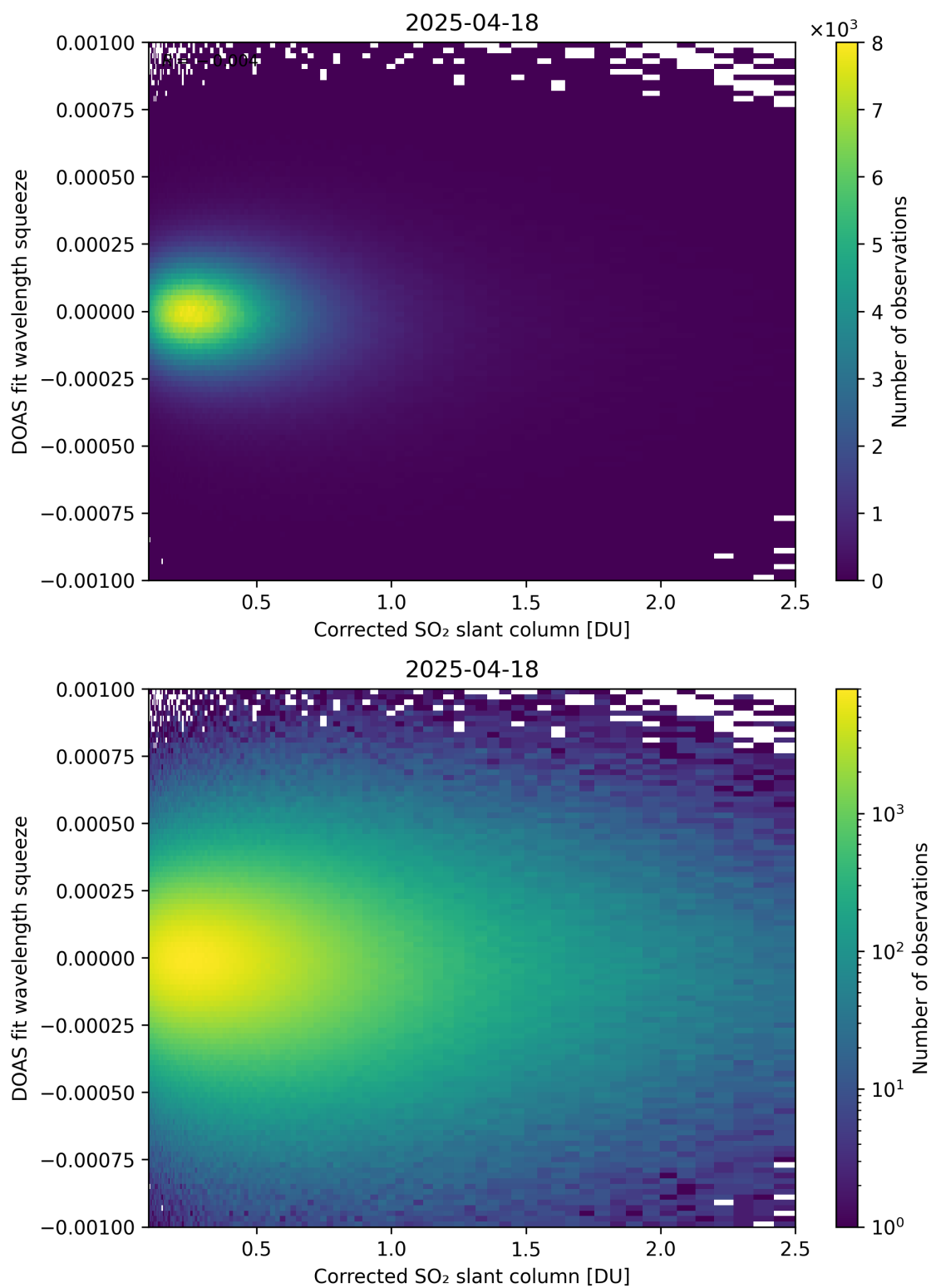
Figure 230: Scatter density plot of “Corrected SO 2 slant column” against “DOAS fit wavelength squeeze” for 2025-04-18 to 2025-04-19.
