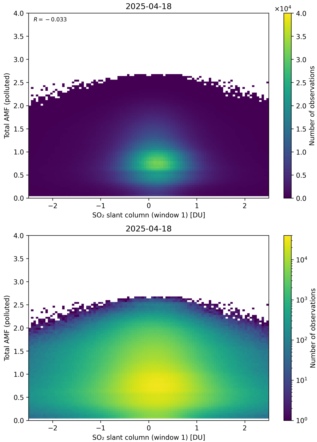
Figure 289: Scatter density plot of “SO 2 slant column (window 1)” against “Total AMF (polluted)” for 2025-04-18 to 2025-04-19.
