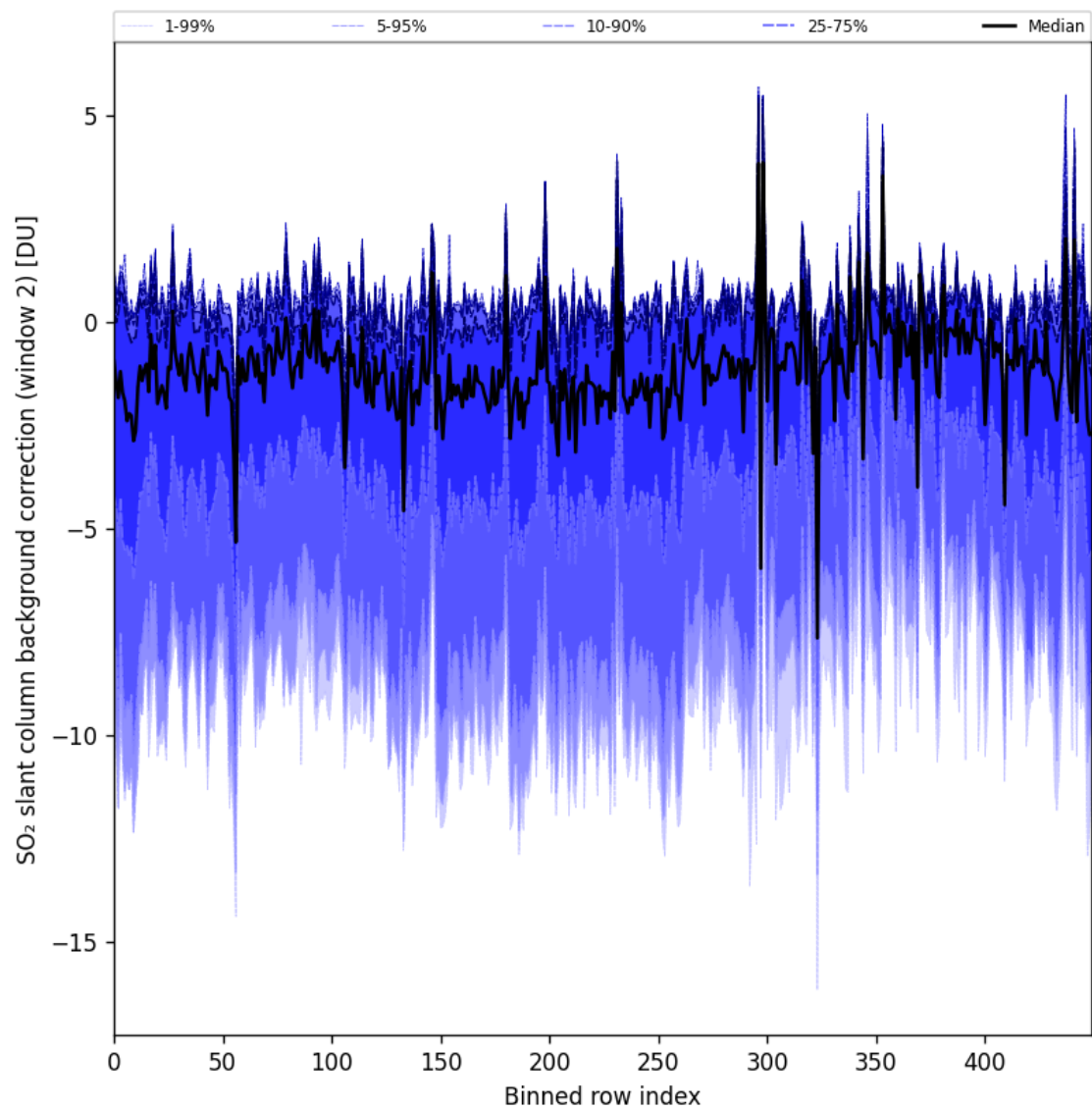
Figure 96: Along track statistics of “SO 2 slant column background correction (window 2)” for 2025-04-18 to 2025-04-19
