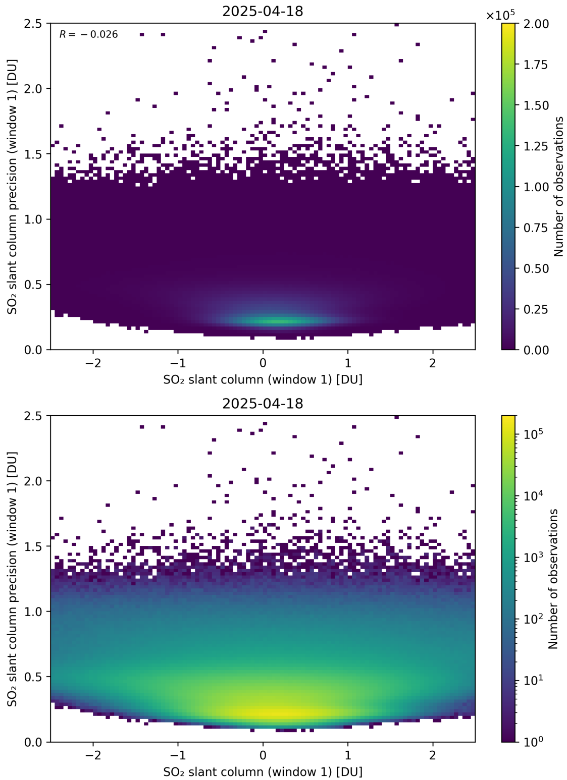
Figure 285: Scatter density plot of “SO 2 slant column (window 1)” against “SO 2 slant column precision (window 1)” for 2025-04-18 to 2025-04-19.
