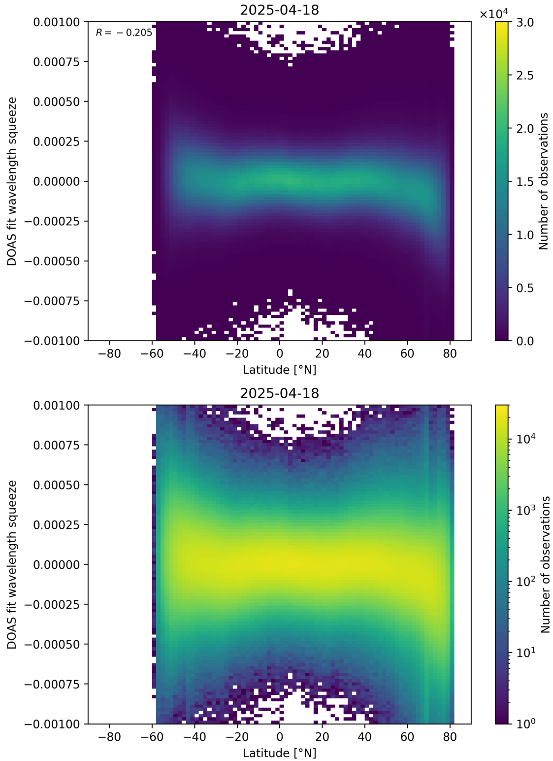
Figure 154: Scatter density plot of “Latitude” against “DOAS fit wavelength squeeze” for 2025-04-18 to 2025-04-19.
