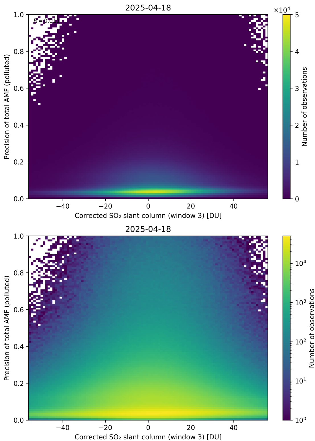
Figure 261: Scatter density plot of “Corrected SO 2 slant column (window 3)” against “Precision of total AMF (polluted)” for 2025-04-18 to 2025-04-19.
