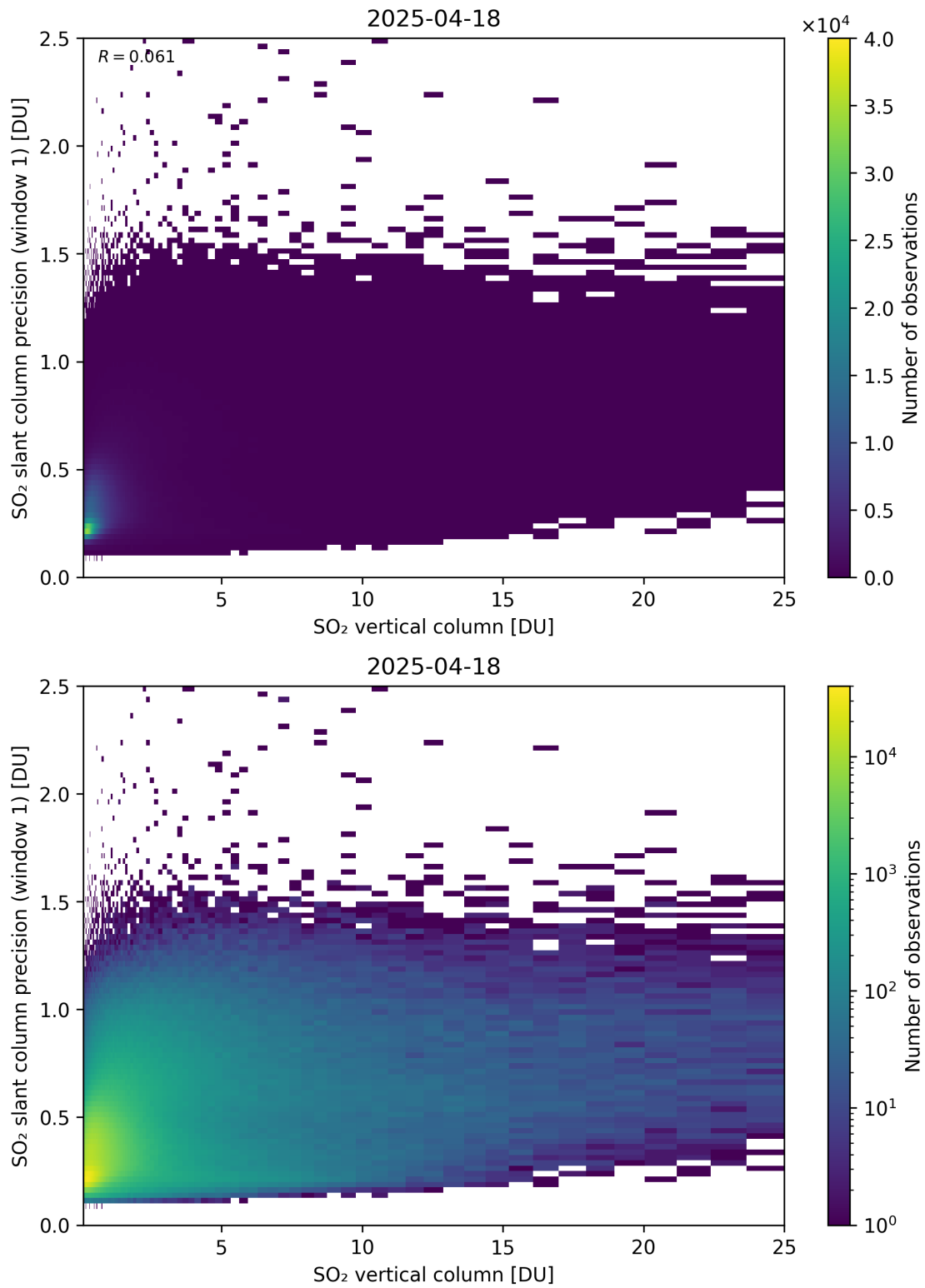
Figure 355: Scatter density plot of “SO 2 vertical column” against “SO 2 slant column precision (window 1)” for 2025-04-18 to 2025-04-19.
