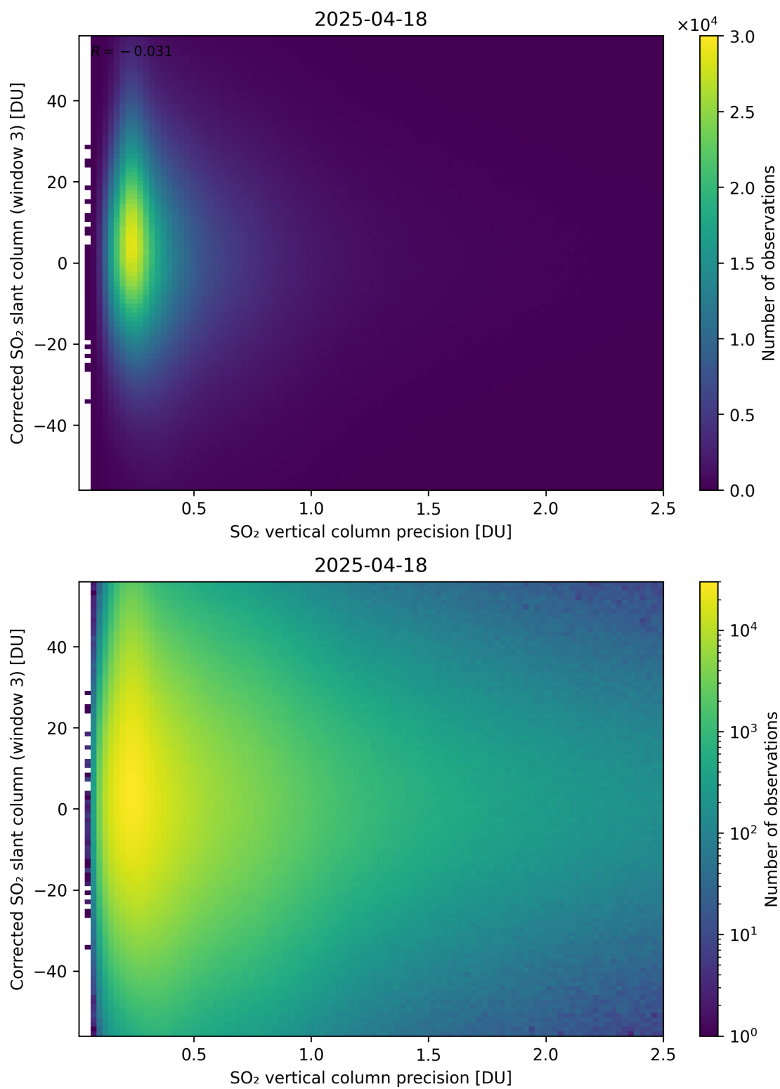
Figure 340: Scatter density plot of “SO 2 vertical column precision” against “Corrected SO 2 slant column (window 3)” for 2025-04-18 to 2025-04-19.
