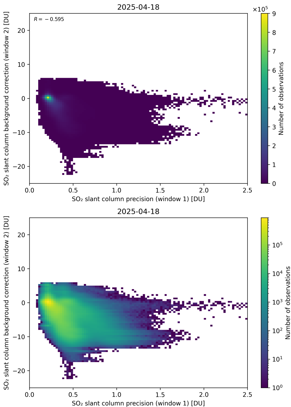
Figure 269: Scatter density plot of “SO 2 slant column precision (window 1)” against “SO 2 slant column background correction (window 2)” for 2025-04-18 to 2025-04-19.
