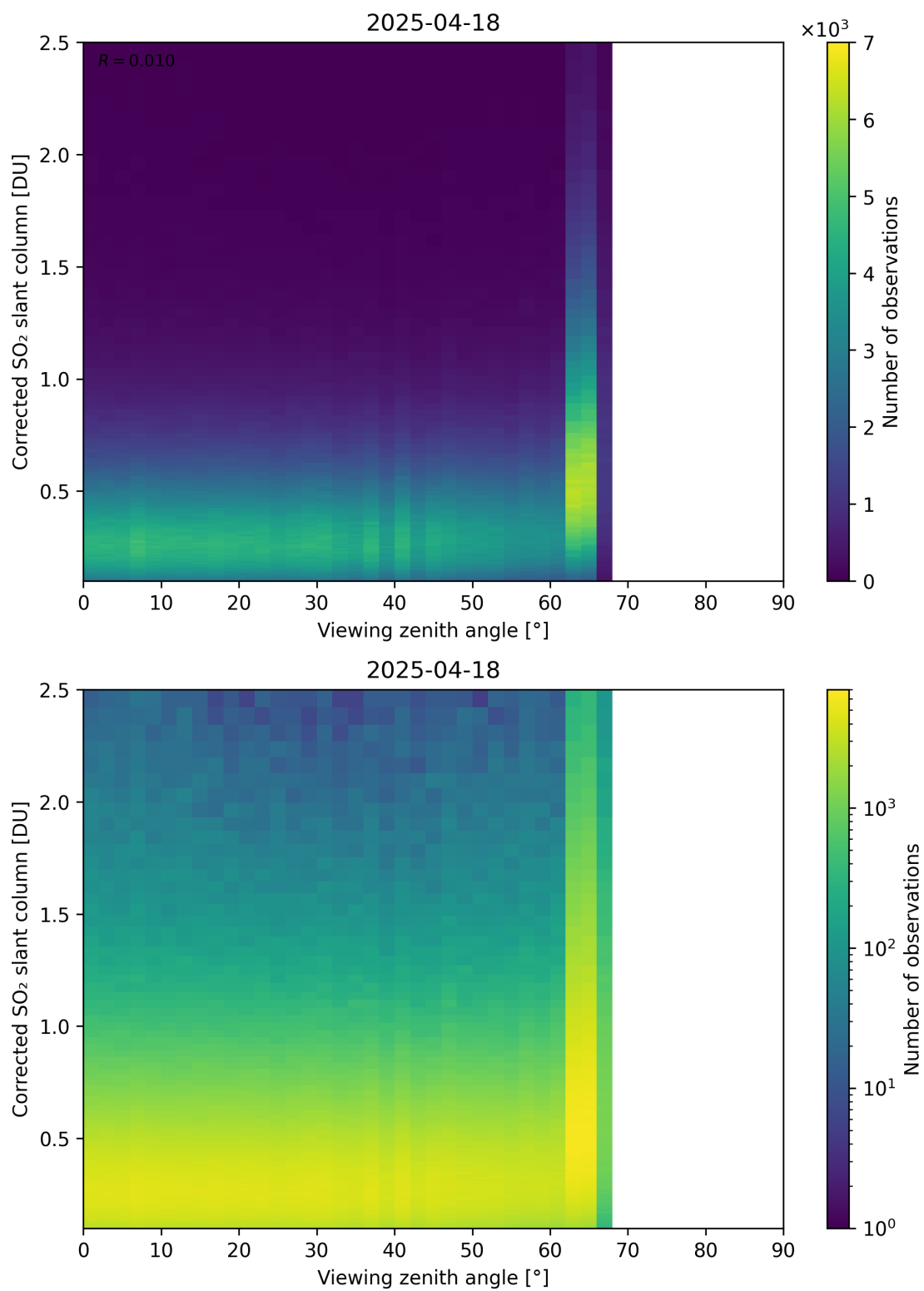
Figure 373: Scatter density plot of “Viewing zenith angle” against “Corrected SO 2 slant column” for 2025-04-18 to 2025-04-19.
