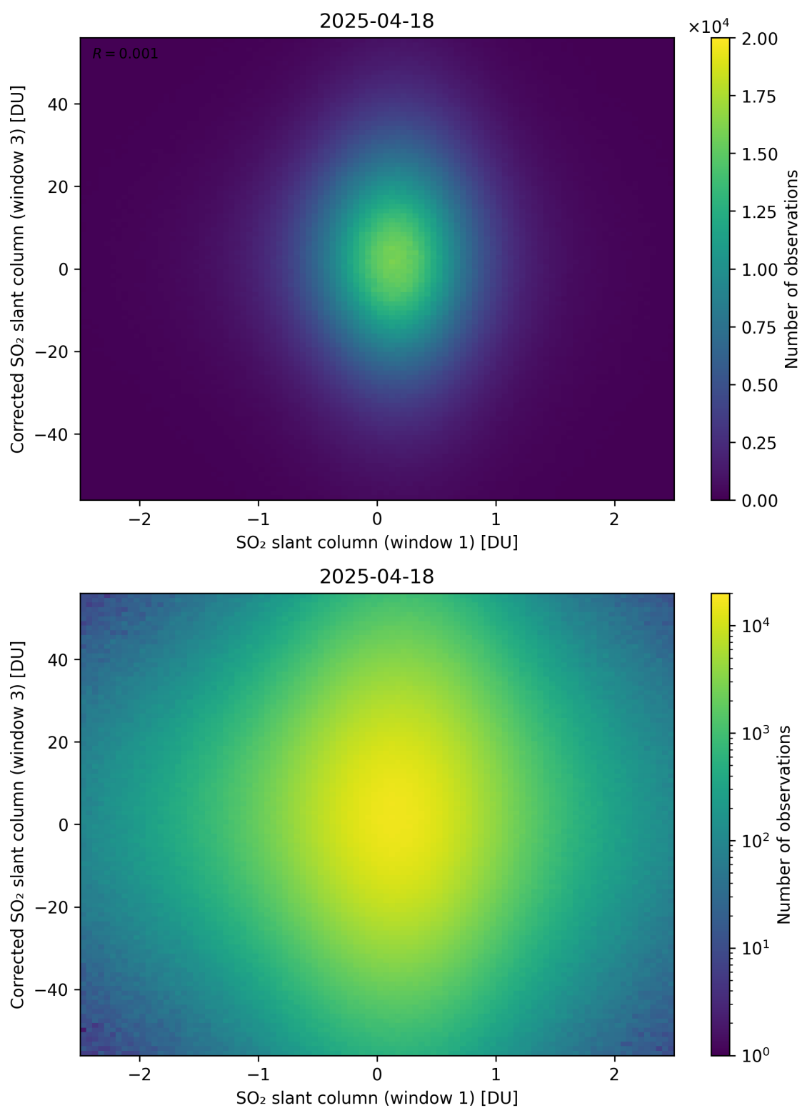
Figure 284: Scatter density plot of “SO 2 slant column (window 1)” against “Corrected SO 2 slant column (window 3)” for 2025-04-18 to 2025-04-19.
