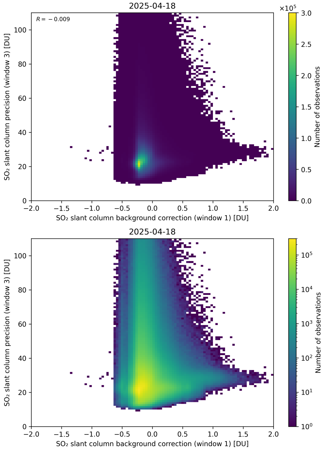
Figure 119: Scatter density plot of “SO 2 slant column background correction (window 1)” against “SO 2 slant column precision (window 3)” for 2025-04-18 to 2025-04-19.
