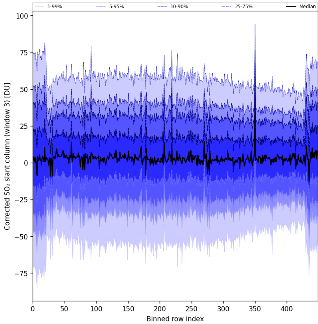
Figure 99: Along track statistics of “Corrected SO 2 slant column (window 3)” for 2025-04-18 to 2025-04-19
