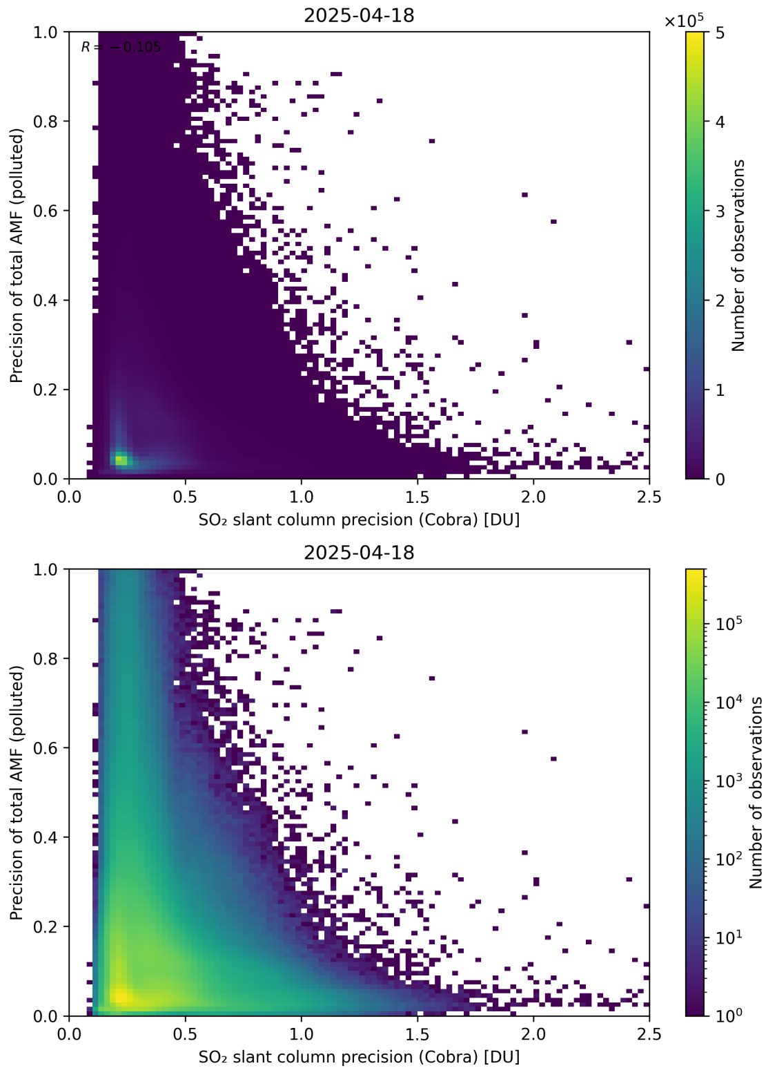
Figure 214: Scatter density plot of “SO 2 slant column precision (Cobra)” against “Precision of total AMF (polluted)” for 2025-04-18 to 2025-04-19.
