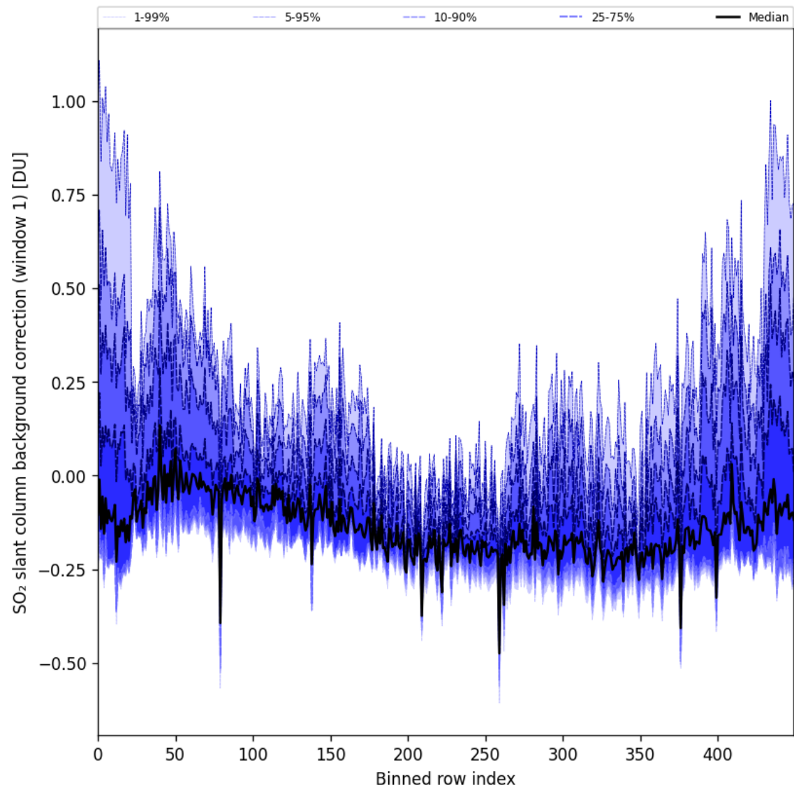
Figure 92: Along track statistics of “SO 2 slant column background correction (window 1)” for 2025-04-18 to 2025-04-19
