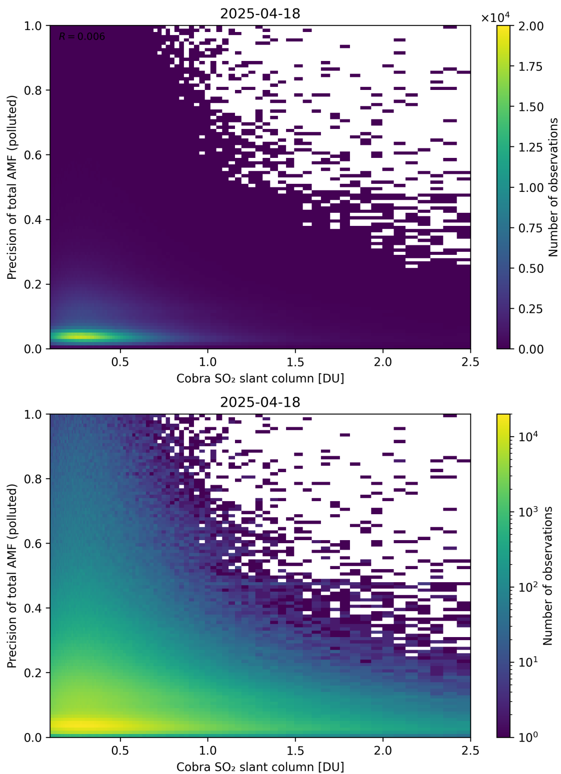
Figure 225: Scatter density plot of “Cobra SO 2 slant column” against “Precision of total AMF (polluted)” for 2025-04-18 to 2025-04-19.
