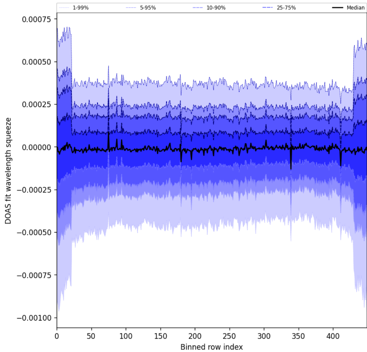
Figure 103: Along track statistics of “DOAS fit wavelength squeeze” for 2025-04-18 to 2025-04-19
