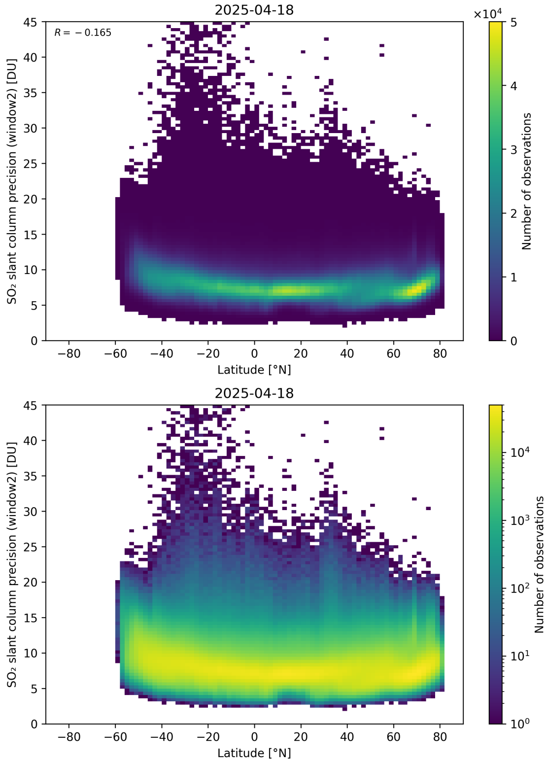
Figure 164: Scatter density plot of “Latitude” against “SO 2 slant column precision (window2)” for 2025-04-18 to 2025-04-19.
