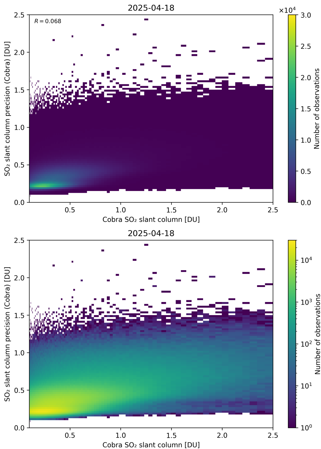
Figure 216: Scatter density plot of “Cobra SO 2 slant column” against “SO 2 slant column precision (Cobra)” for 2025-04-18 to 2025-04-19.
