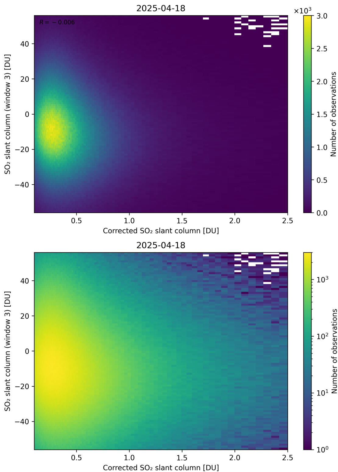
Figure 240: Scatter density plot of “Corrected SO 2 slant column” against “SO 2 slant column (window 3)” for 2025-04-18 to 2025-04-19.
