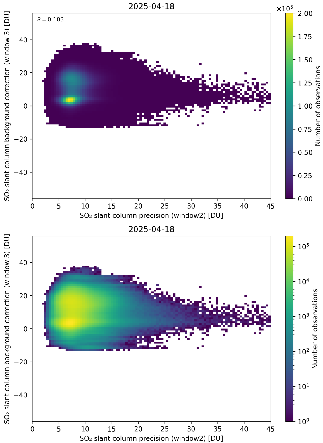
Figure 292: Scatter density plot of “SO 2 slant column precision (window2)” against “SO 2 slant column background correction (window 3)” for 2025-04-18 to 2025-04-19.
