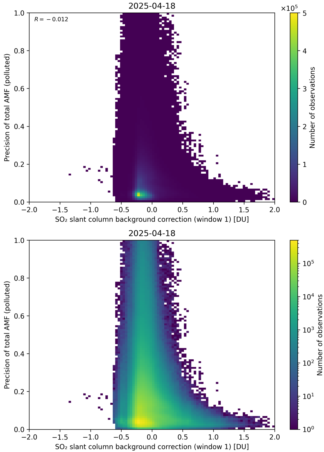
Figure 121: Scatter density plot of “SO 2 slant column background correction (window 1)” against “Precision of total AMF (polluted)” for 2025-04-18 to 2025-04-19.
