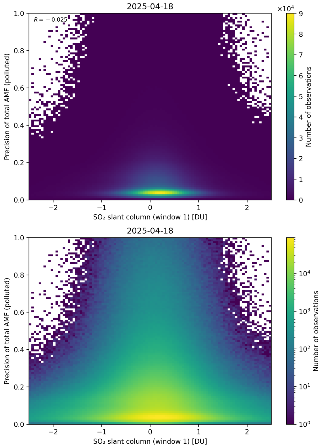
Figure 290: Scatter density plot of “SO 2 slant column (window 1)” against “Precision of total AMF (polluted)” for 2025-04-18 to 2025-04-19.
