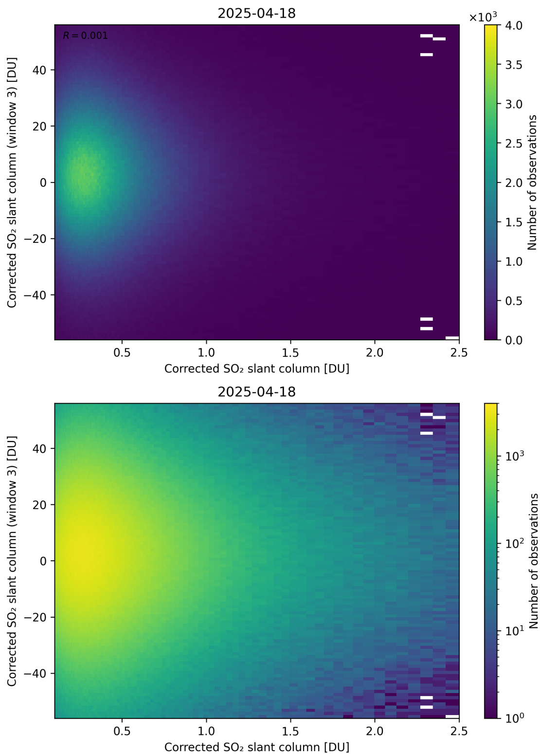
Figure 236: Scatter density plot of “Corrected SO 2 slant column” against “Corrected SO 2 slant column (window 3)” for 2025-04-18 to 2025-04-19.
