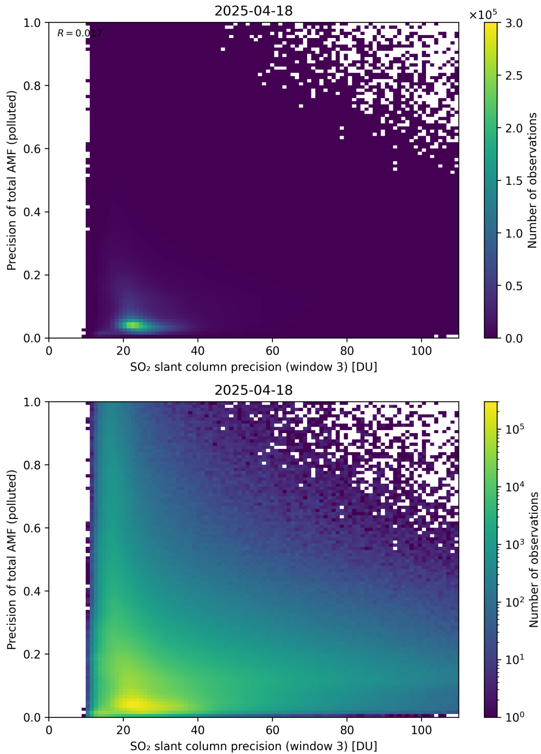
Figure 314: Scatter density plot of “SO 2 slant column precision (window 3)” against “Precision of total AMF (polluted)” for 2025-04-18 to 2025-04-19.
