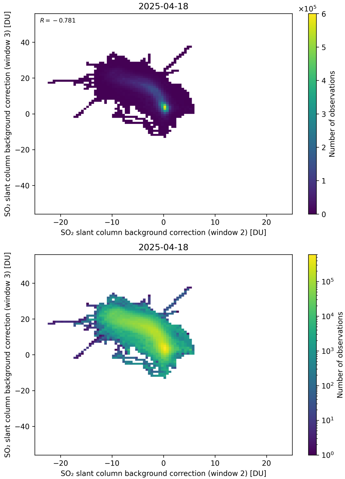
Figure 122: Scatter density plot of “SO 2 slant column background correction (window 2)” against “SO 2 slant column background correction (window 3)” for 2025-04-18 to 2025-04-19.
