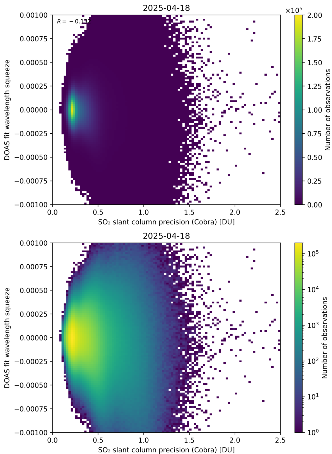
Figure 203: Scatter density plot of “SO 2 slant column precision (Cobra)” against “DOAS fit wavelength squeeze” for 2025-04-18 to 2025-04-19.
