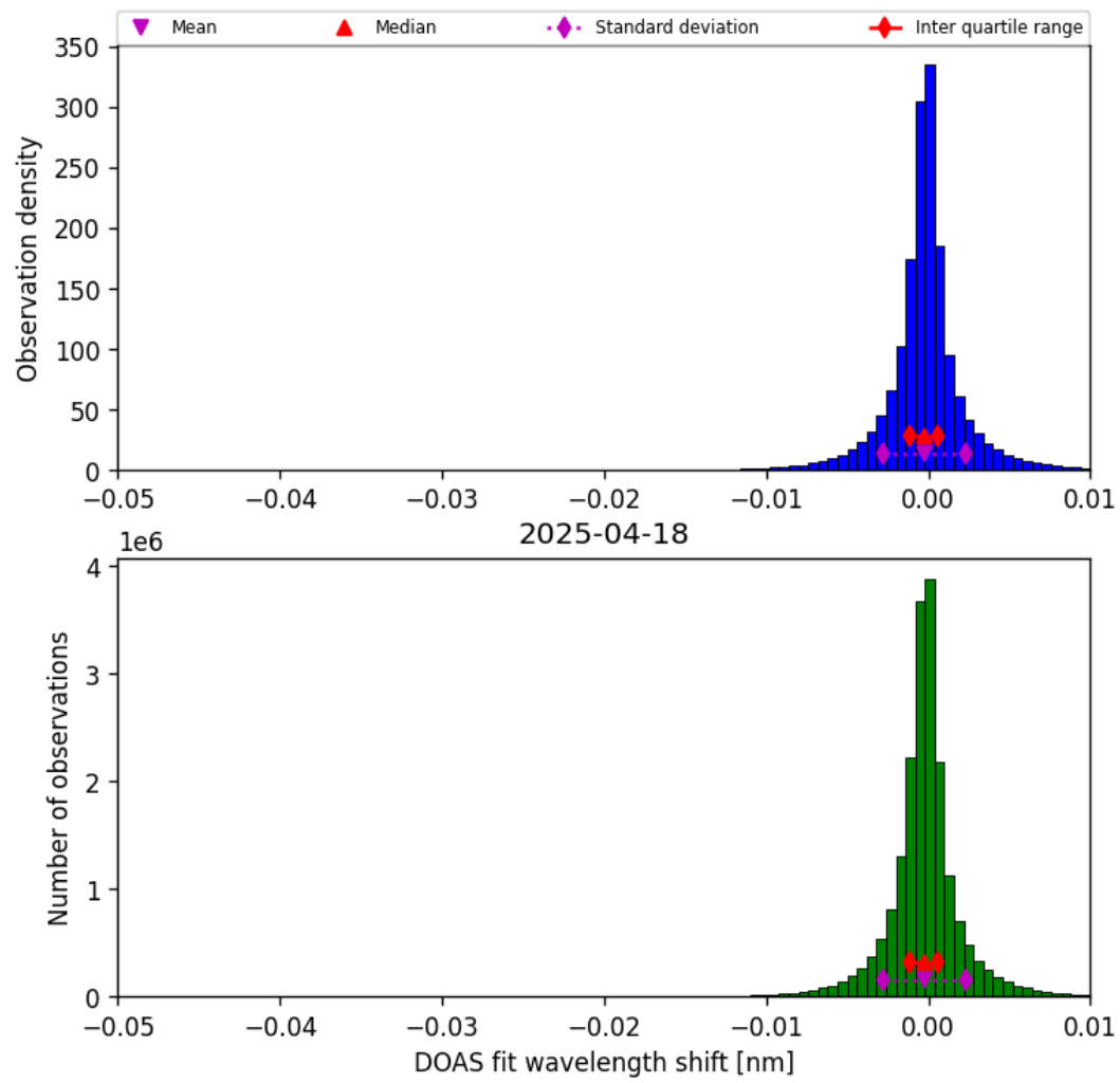
Figure 76: Histogram of “DOAS fit wavelength shift” for 2025-04-18 to 2025-04-19
