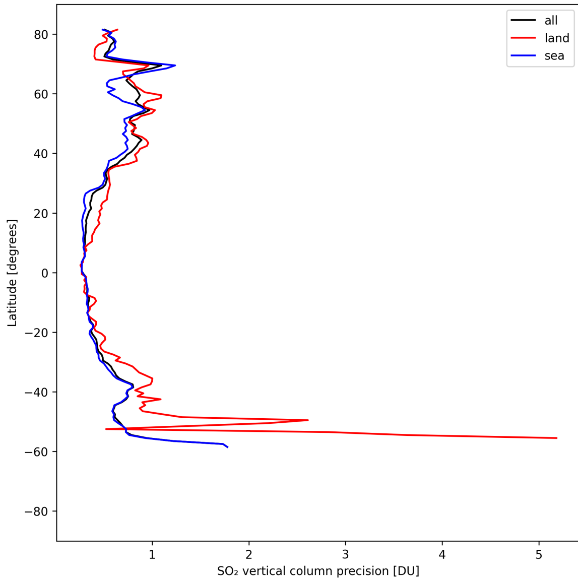
Figure 33: Zonal average of “SO 2 vertical column precision” for 2025-04-18 to 2025-04-19.
