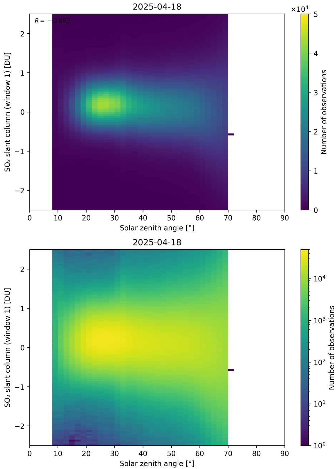
Figure 184: Scatter density plot of “Solar zenith angle” against “SO 2 slant column (window 1)” for 2025-04-18 to 2025-04-19.
