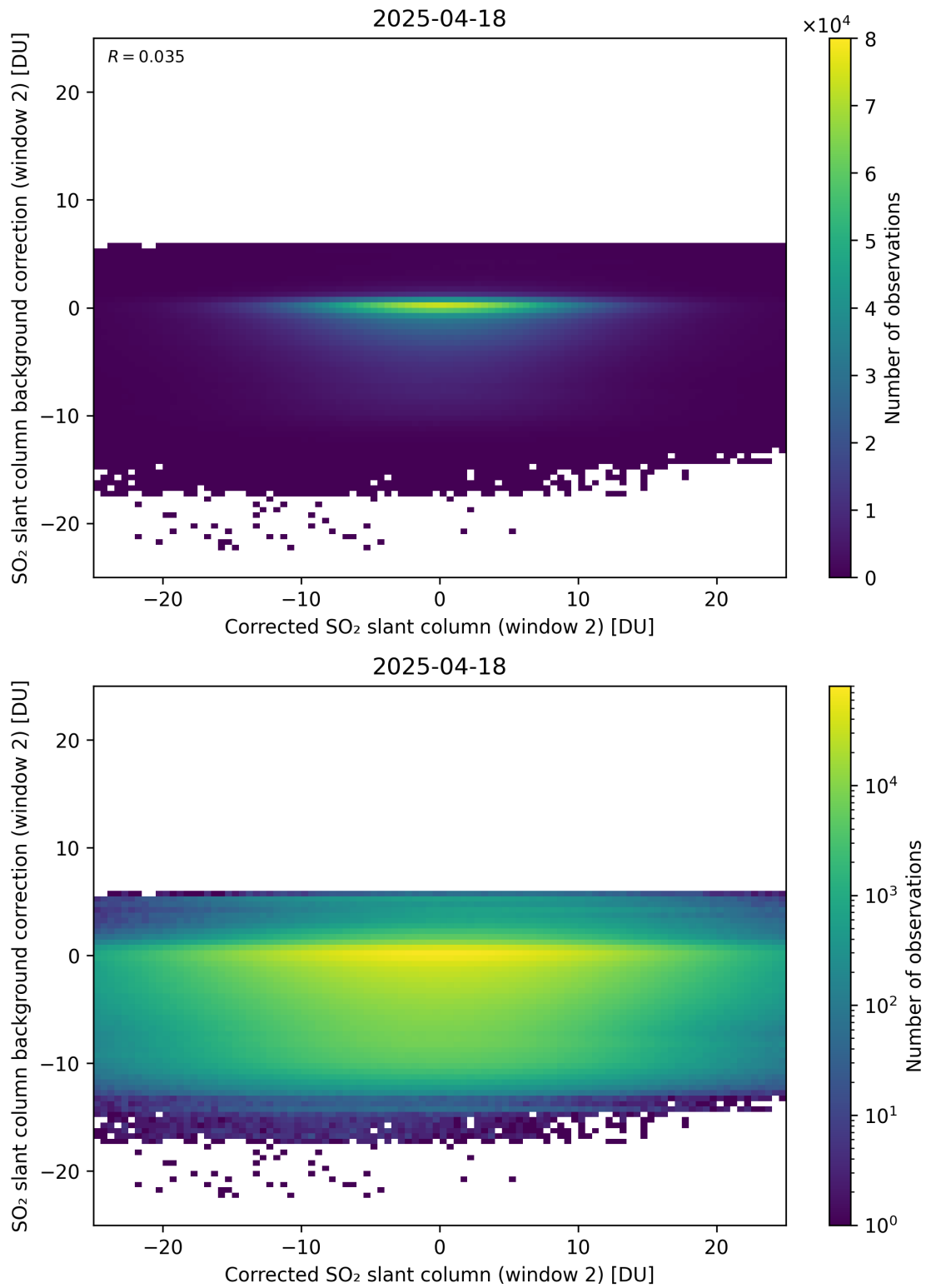
Figure 244: Scatter density plot of “Corrected SO 2 slant column (window 2)” against “SO 2 slant column background correction (window 2)” for 2025-04-18 to 2025-04-19.
