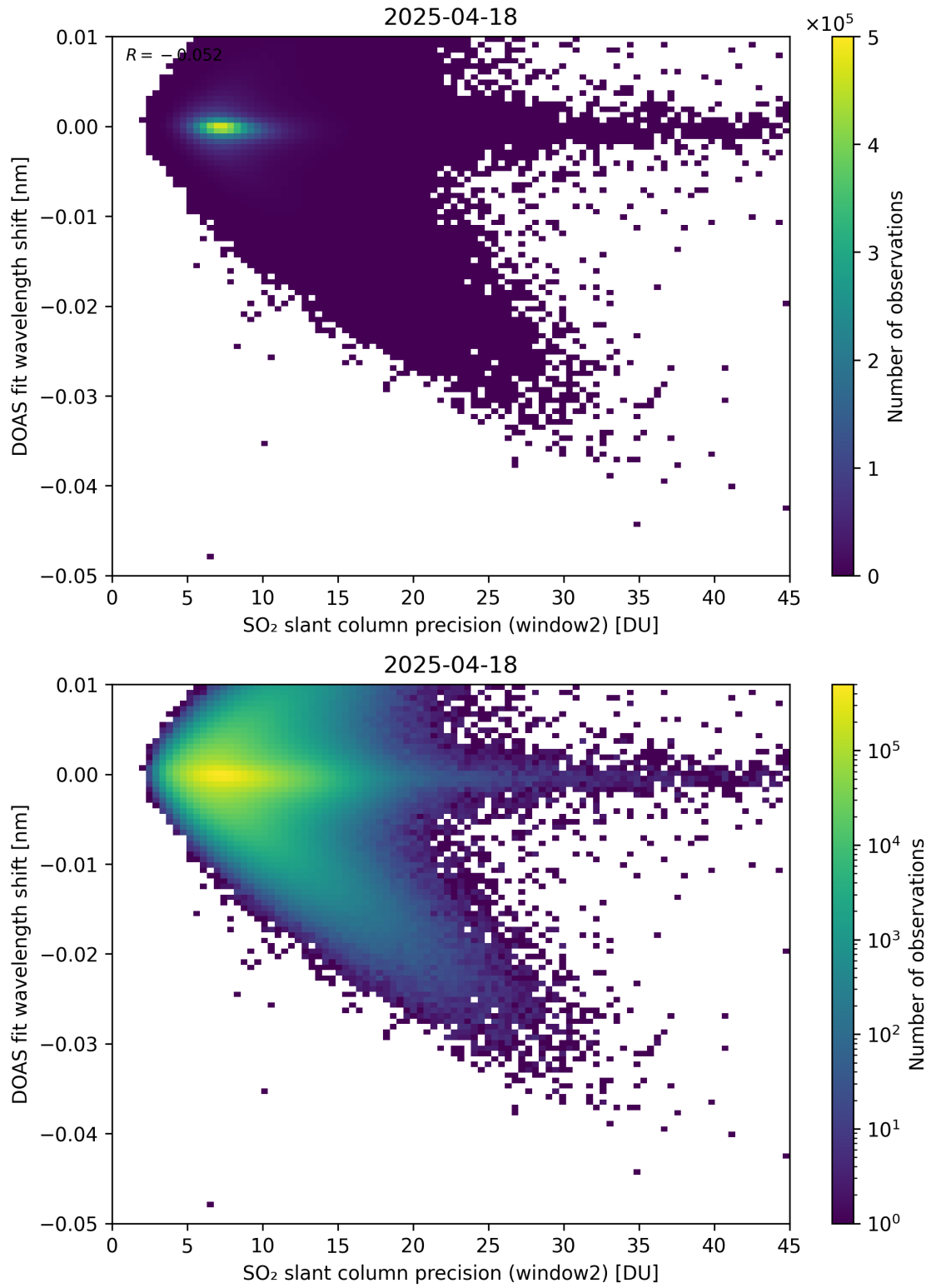
Figure 293: Scatter density plot of “SO 2 slant column precision (window2)” against “DOAS fit wavelength shift” for 2025-04-18 to 2025-04-19.
