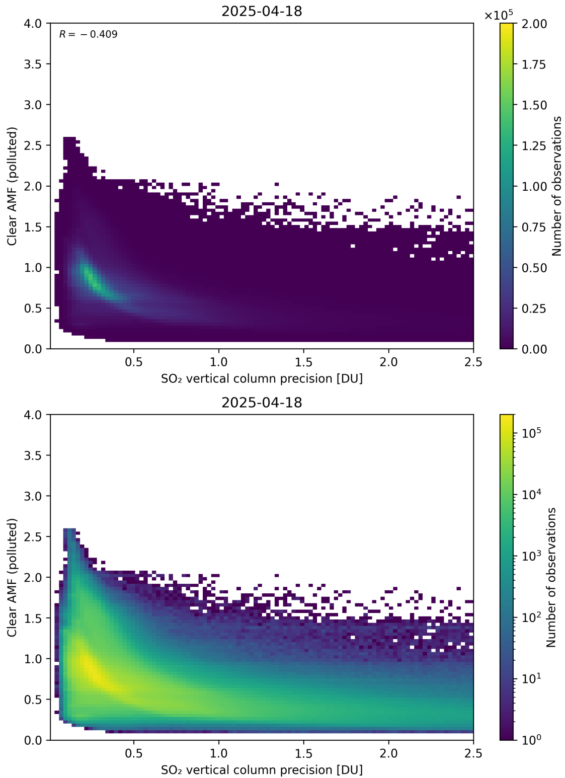
Figure 335: Scatter density plot of “SO 2 vertical column precision” against “Clear AMF (polluted)” for 2025-04-18 to 2025-04-19.
