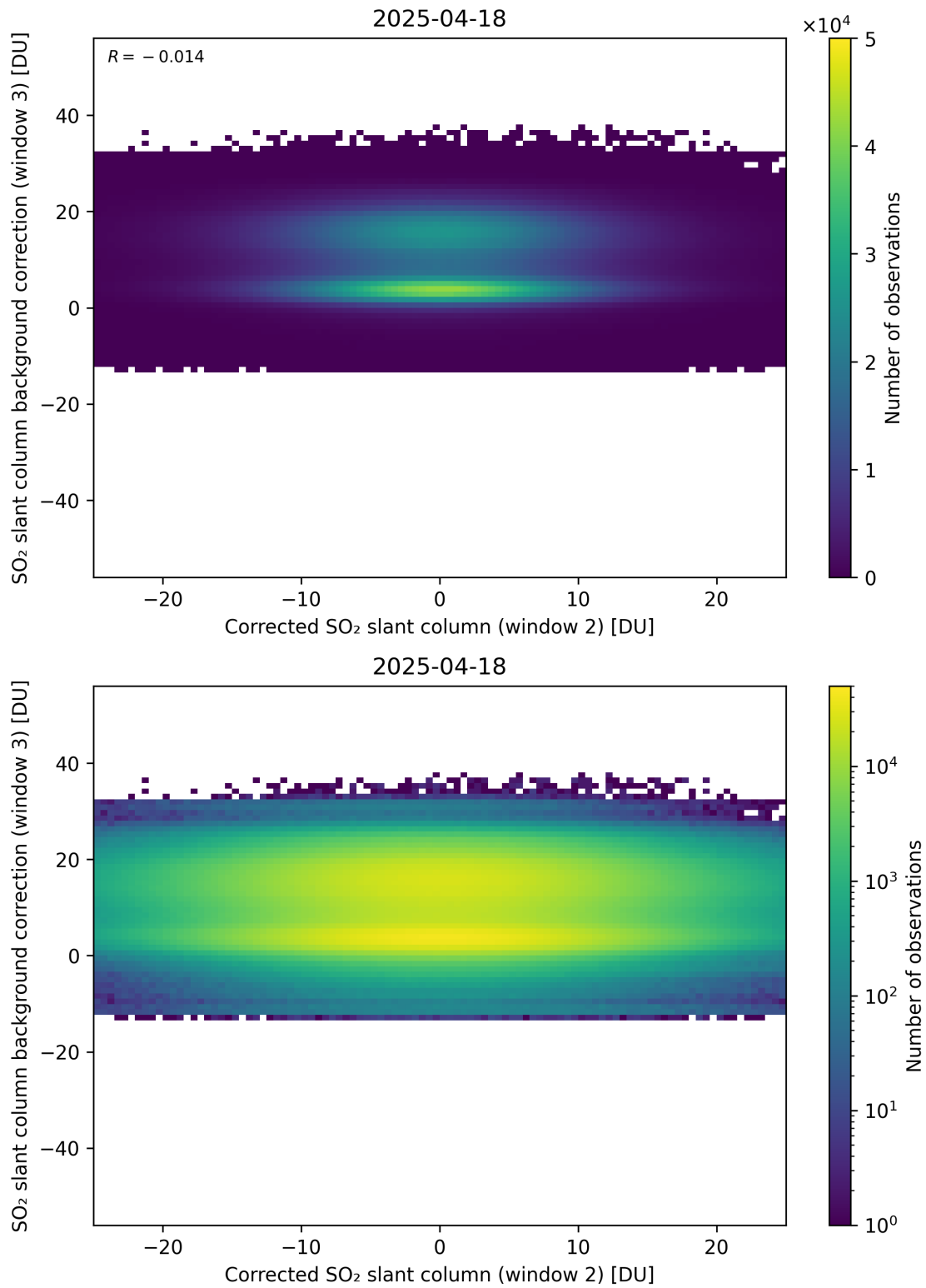
Figure 245: Scatter density plot of “Corrected SO 2 slant column (window 2)” against “SO 2 slant column background correction (window 3)” for 2025-04-18 to 2025-04-19.
