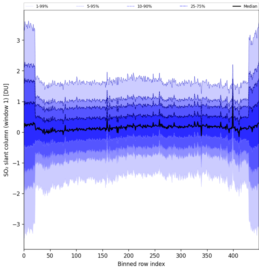
Figure 89: Along track statistics of “SO 2 slant column (window 1)” for 2025-04-18 to 2025-04-19
