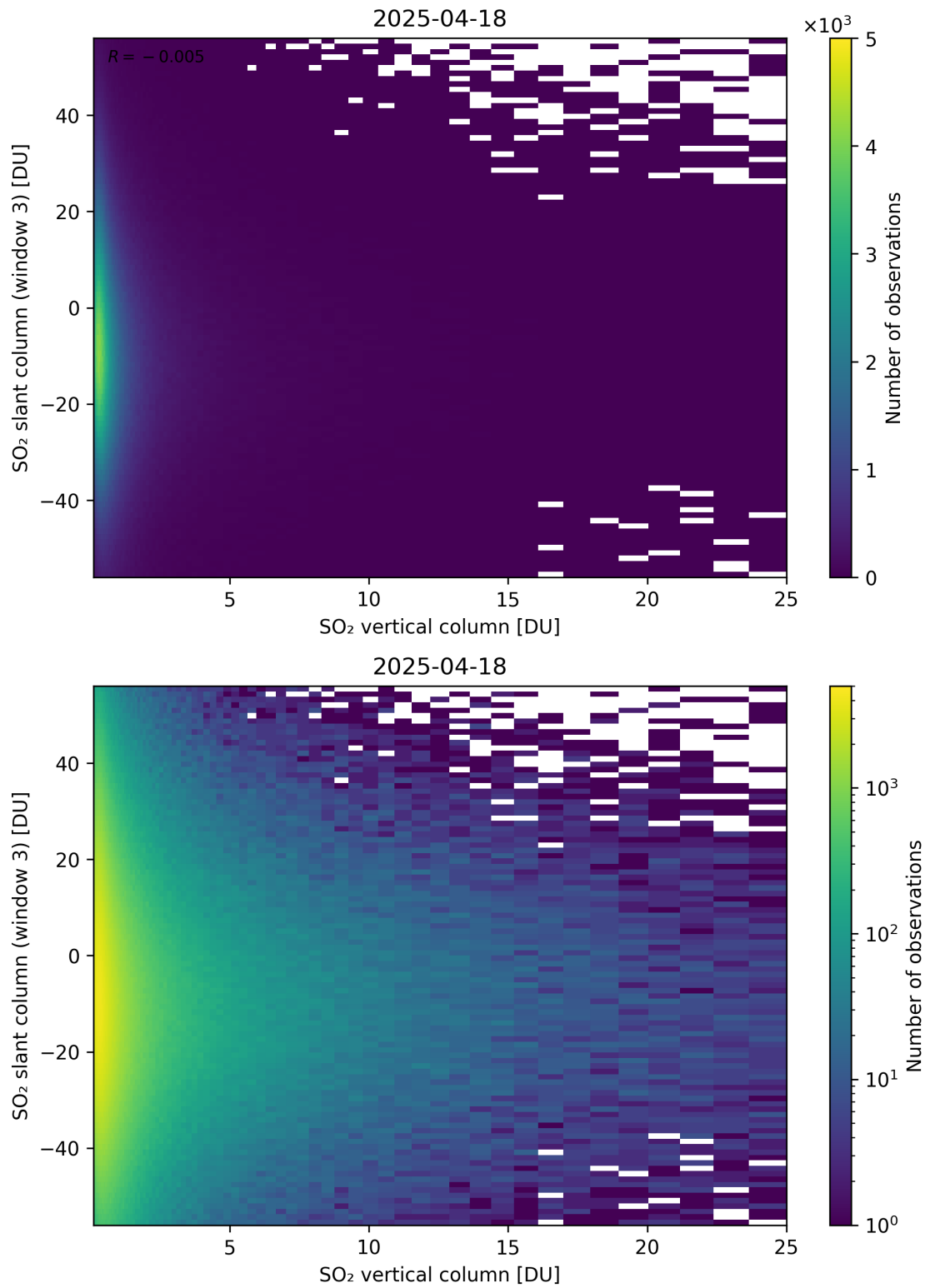
Figure 357: Scatter density plot of “SO 2 vertical column” against “SO 2 slant column (window 3)” for 2025-04-18 to 2025-04-19.
