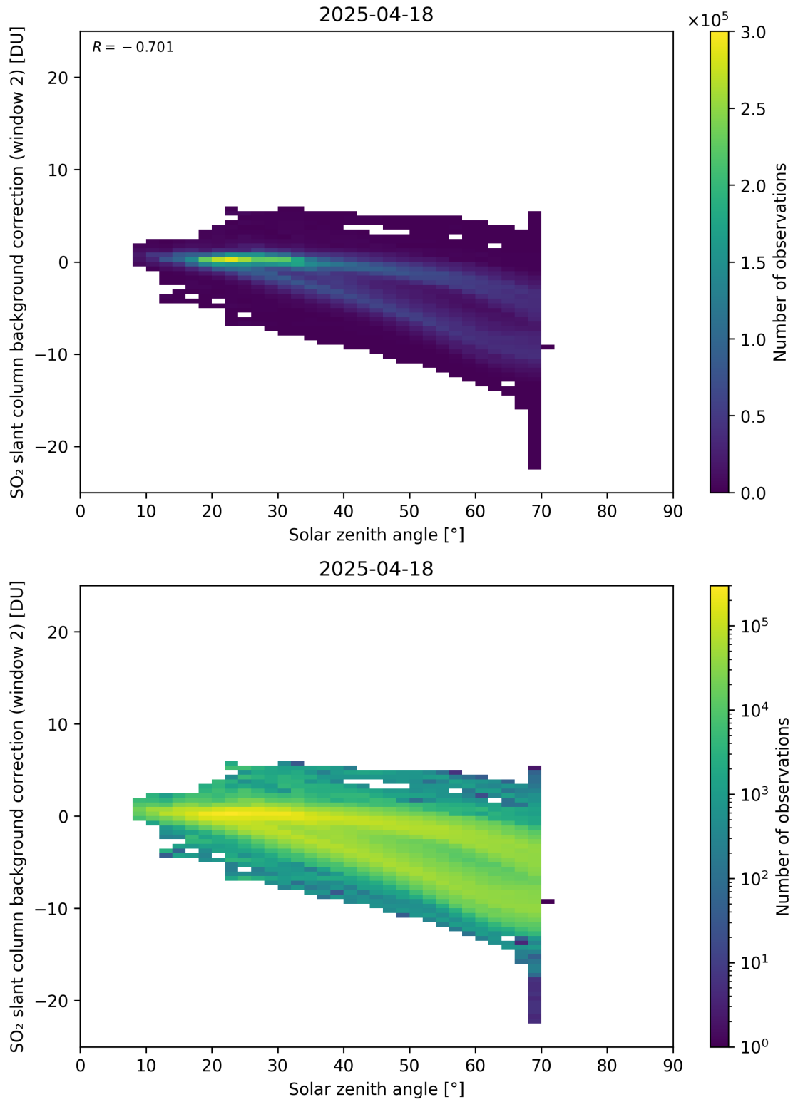
Figure 172: Scatter density plot of “Solar zenith angle” against “SO 2 slant column background correction (window 2)” for 2025-04-18 to 2025-04-19.
