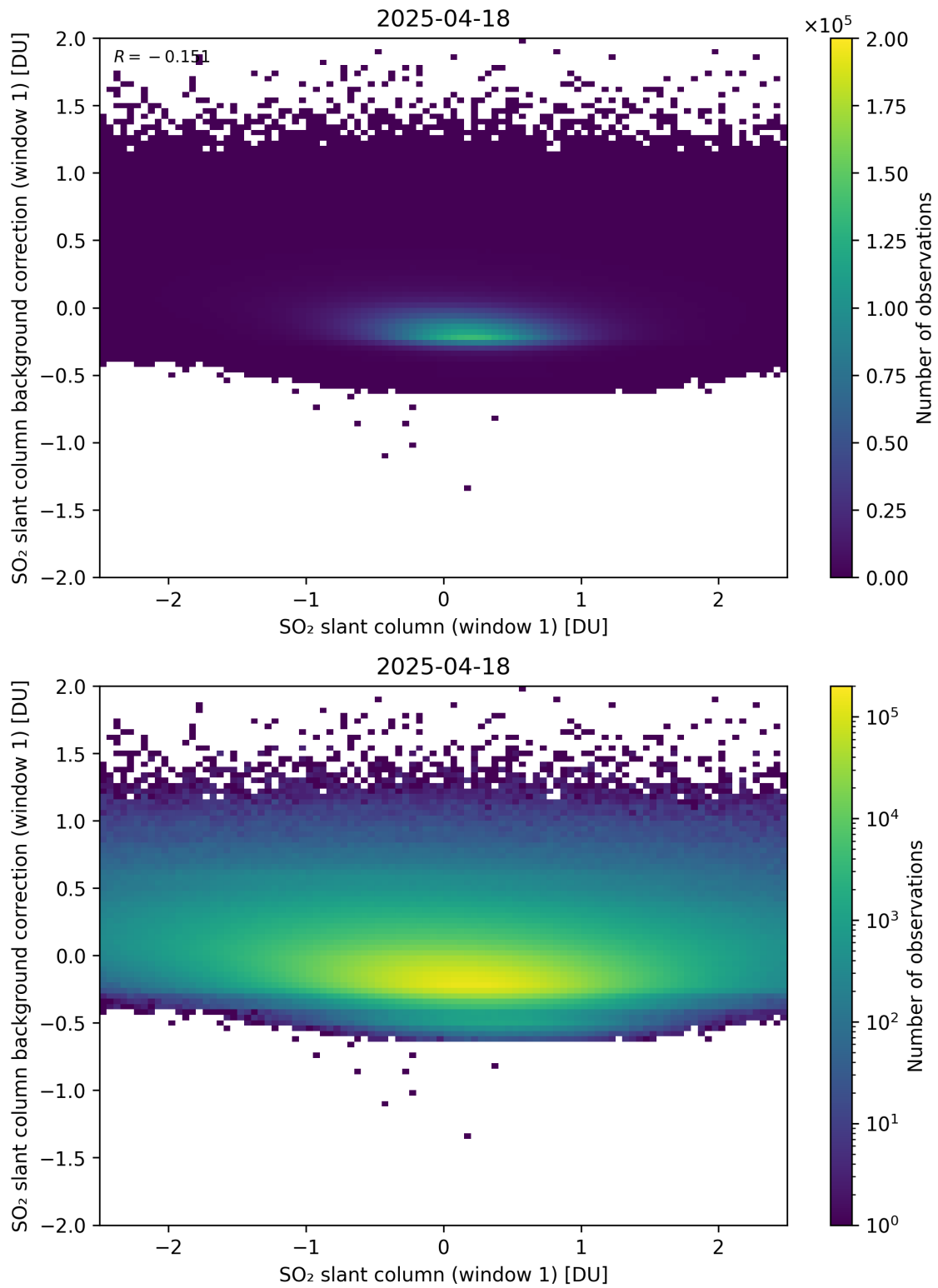
Figure 262: Scatter density plot of “SO 2 slant column (window 1)” against “SO 2 slant column background correction (window 1)” for 2025-04-18 to 2025-04-19.
