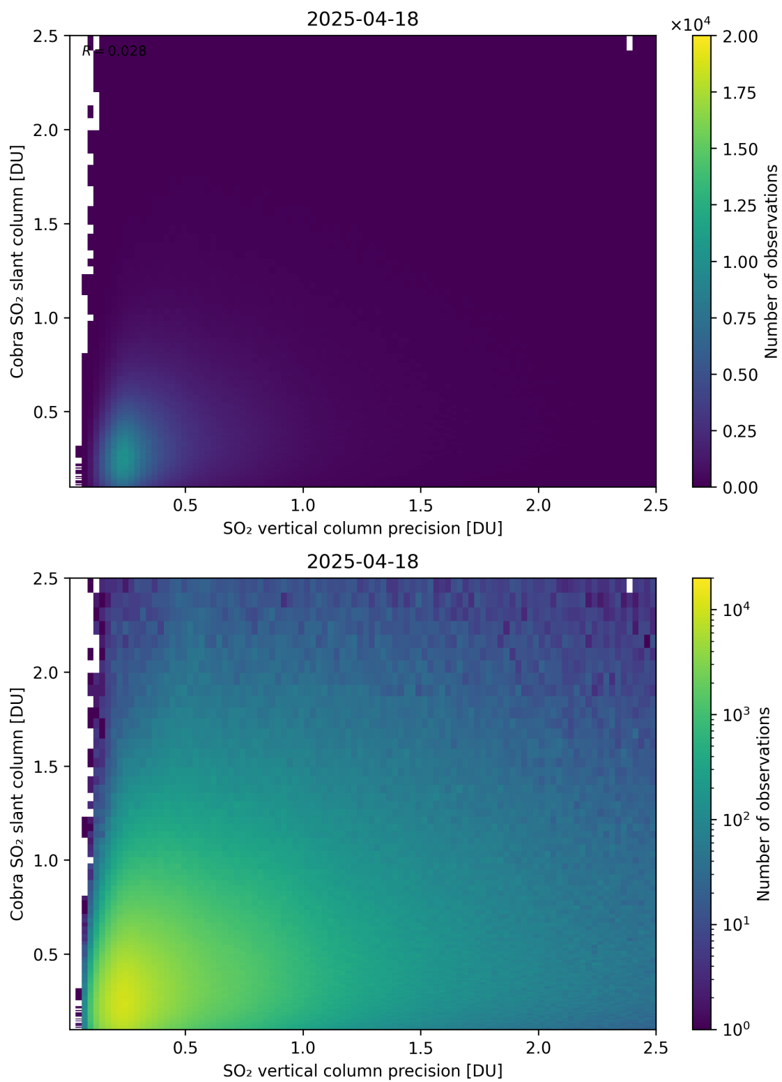
Figure 336: Scatter density plot of “SO 2 vertical column precision” against “Cobra SO 2 slant column” for 2025-04-18 to 2025-04-19.
