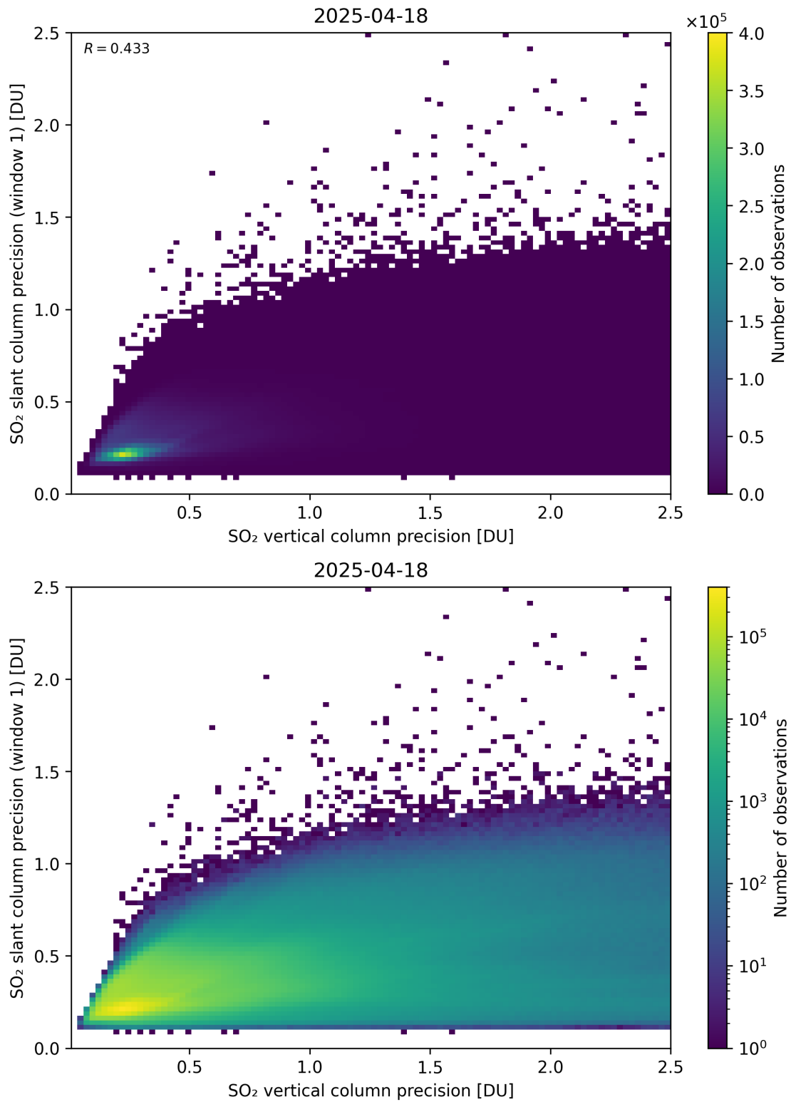
Figure 342: Scatter density plot of “SO 2 vertical column precision” against “SO 2 slant column precision (window 1)” for 2025-04-18 to 2025-04-19.
