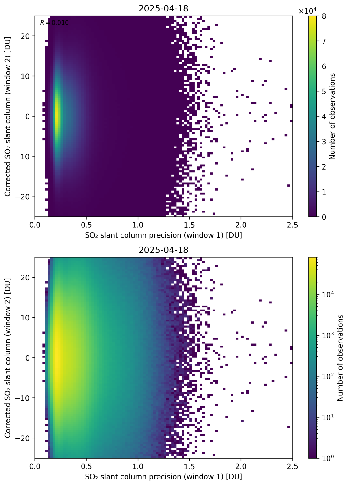
Figure 275: Scatter density plot of “SO 2 slant column precision (window 1)” against “Corrected SO 2 slant column (window 2)” for 2025-04-18 to 2025-04-19.
