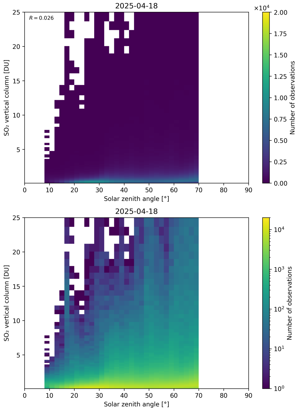
Figure 191: Scatter density plot of “Solar zenith angle” against “SO 2 vertical column” for 2025-04-18 to 2025-04-19.
