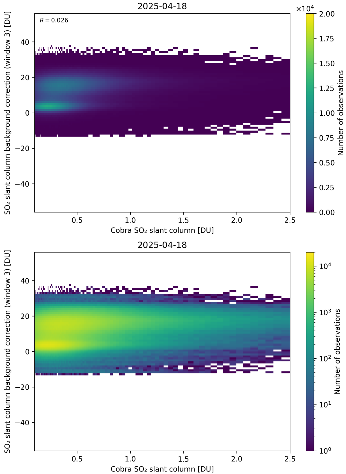
Figure 195: Scatter density plot of “Cobra SO 2 slant column” against “SO 2 slant column background correction (window 3)” for 2025-04-18 to 2025-04-19.
