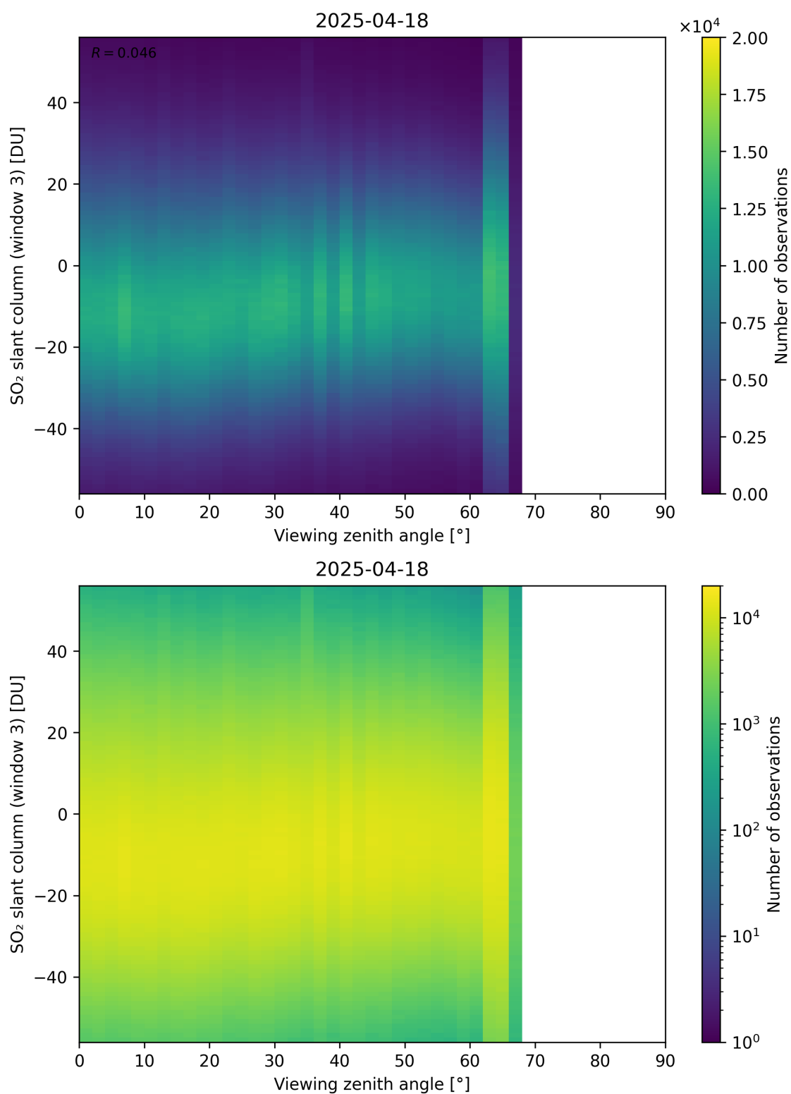
Figure 379: Scatter density plot of “Viewing zenith angle” against “SO 2 slant column (window 3)” for 2025-04-18 to 2025-04-19.
