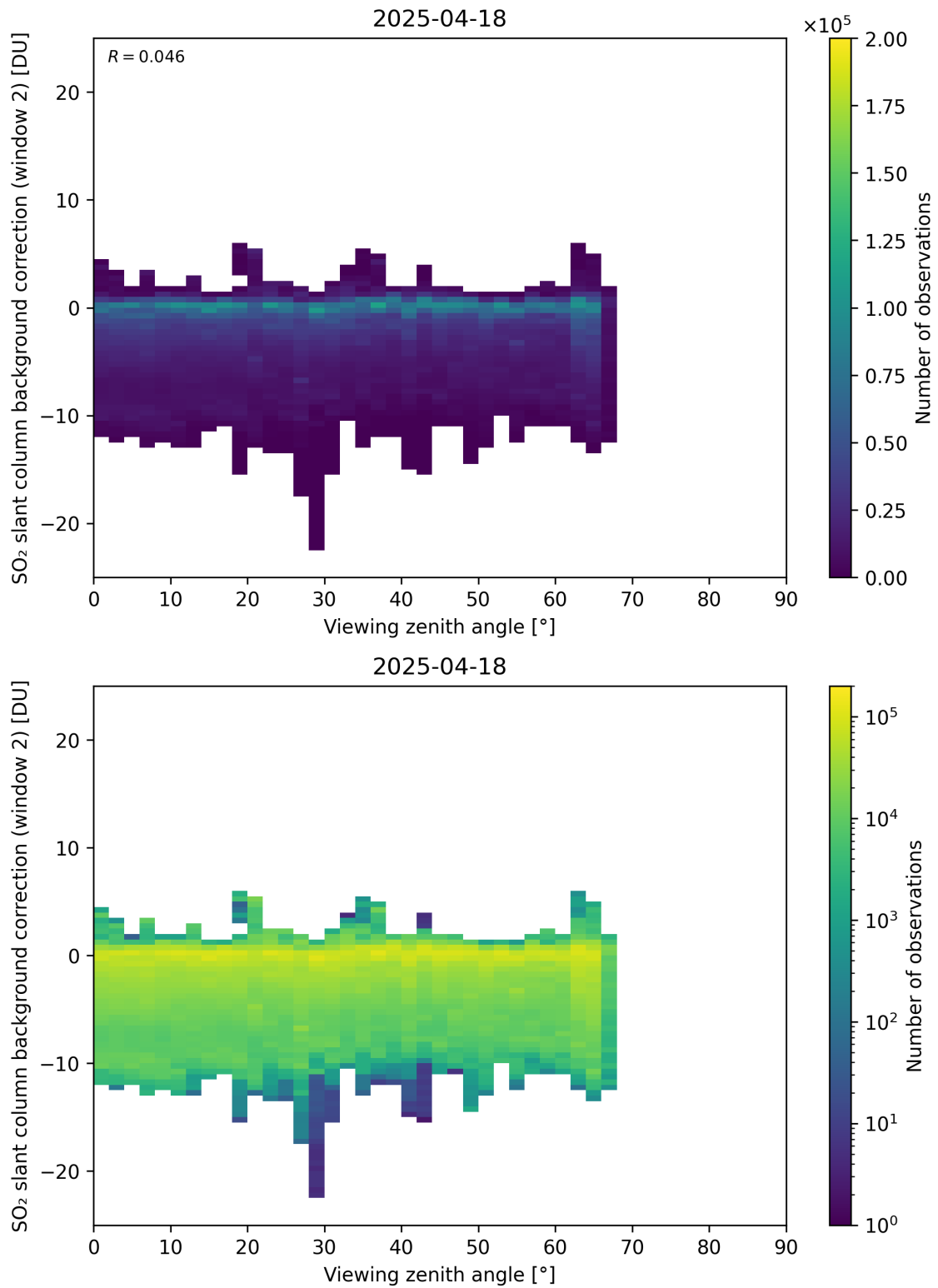
Figure 363: Scatter density plot of “Viewing zenith angle” against “SO 2 slant column background correction (window 2)” for 2025-04-18 to 2025-04-19.
