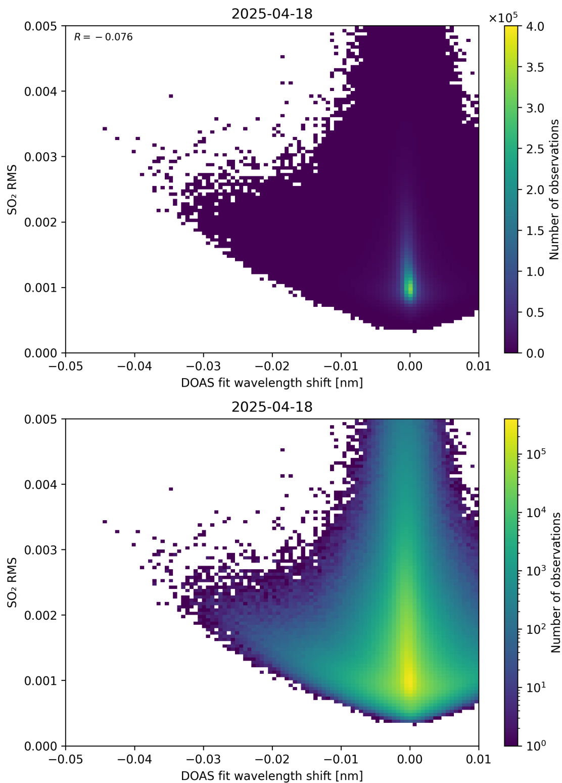
Figure 139: Scatter density plot of “DOAS fit wavelength shift” against “SO 2 RMS” for 2025-04-18 to 2025-04-19.
