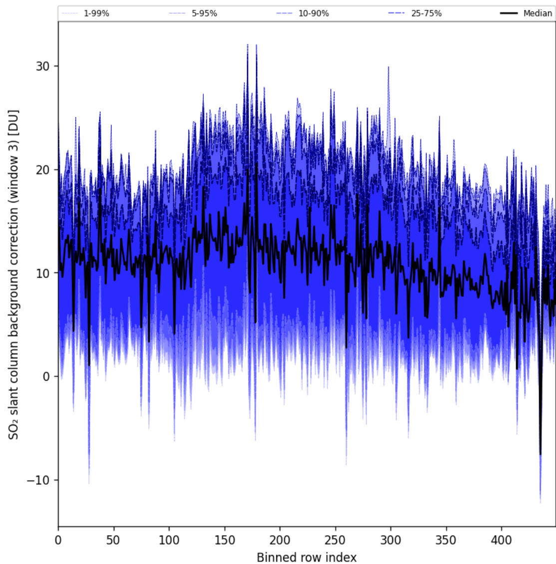
Figure 100: Along track statistics of “SO 2 slant column background correction (window 3)” for 2025-04-18 to 2025-04-19
