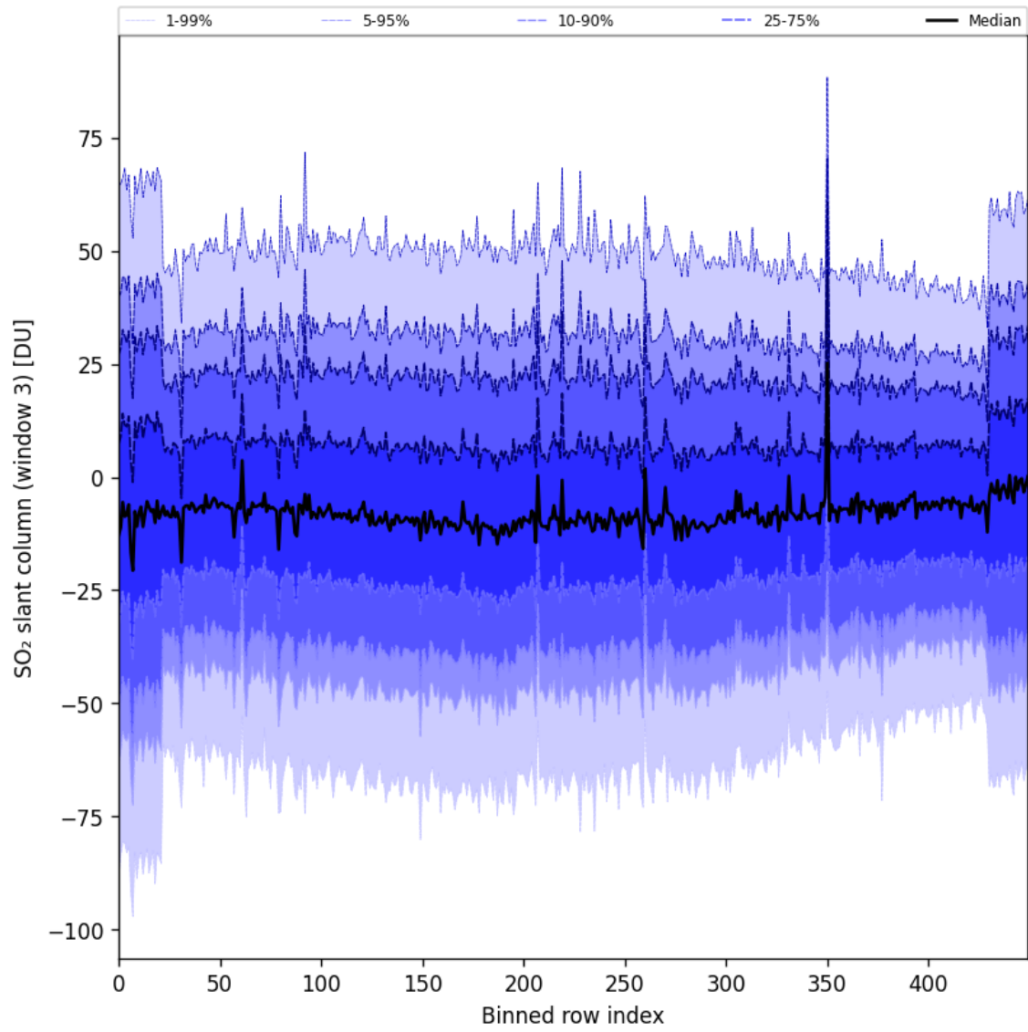
Figure 97: Along track statistics of “SO 2 slant column (window 3)” for 2025-04-18 to 2025-04-19
