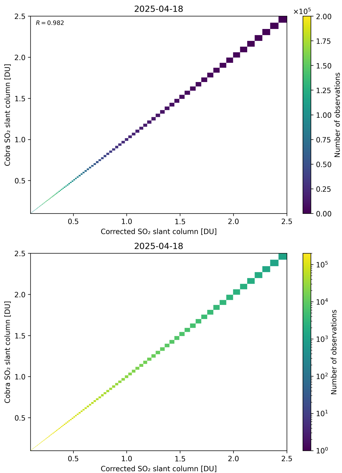
Figure 233: Scatter density plot of “Corrected SO 2 slant column” against “Cobra SO 2 slant column” for 2025-04-18 to 2025-04-19.
