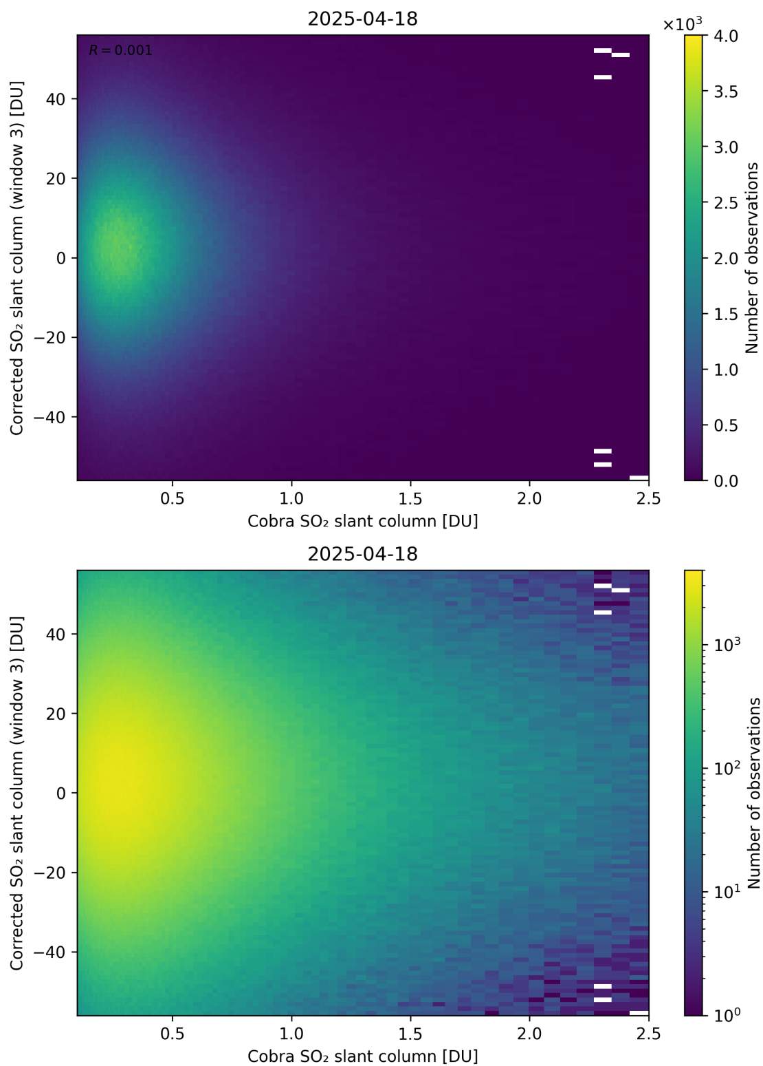
Figure 218: Scatter density plot of “Cobra SO 2 slant column” against “Corrected SO 2 slant column (window 3)” for 2025-04-18 to 2025-04-19.
