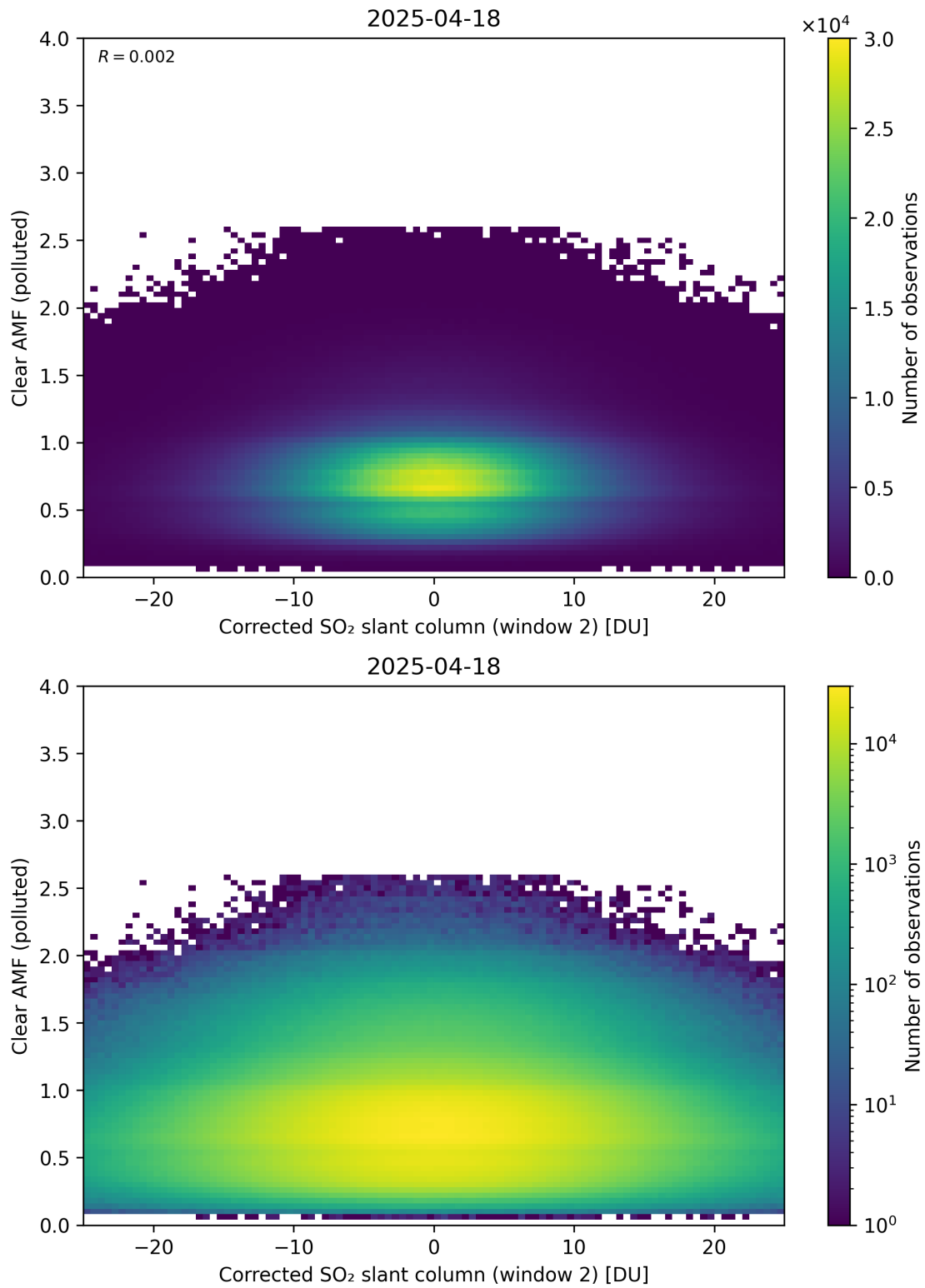
Figure 249: Scatter density plot of “Corrected SO 2 slant column (window 2)” against “Clear AMF (polluted)” for 2025-04-18 to 2025-04-19.
