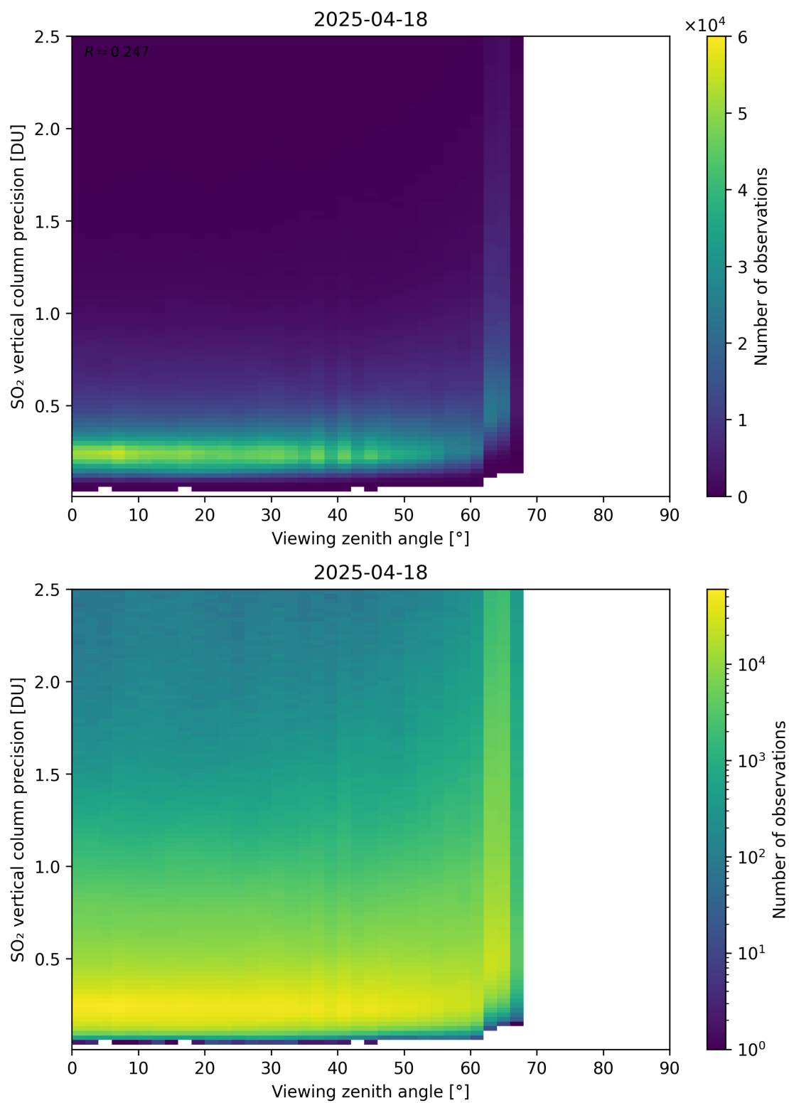
Figure 384: Scatter density plot of “Viewing zenith angle” against “SO 2 vertical column precision” for 2025-04-18 to 2025-04-19.
