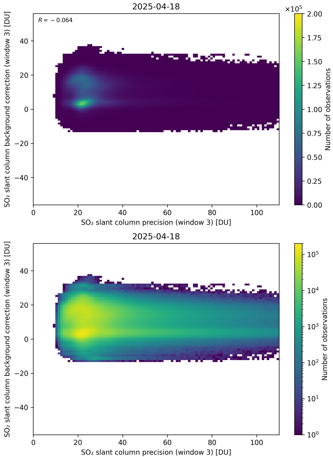
Figure 307: Scatter density plot of “SO 2 slant column precision (window 3)” against “SO 2 slant column background correction (window 3)” for 2025-04-18 to 2025-04-19.
