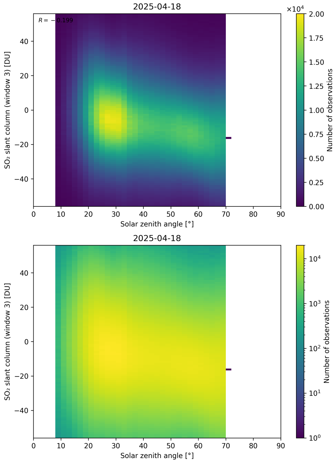
Figure 187: Scatter density plot of “Solar zenith angle” against “SO 2 slant column (window 3)” for 2025-04-18 to 2025-04-19.
