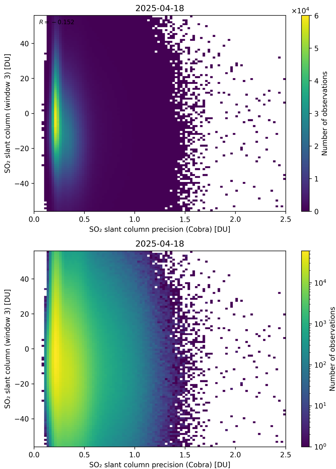
Figure 211: Scatter density plot of “SO 2 slant column precision (Cobra)” against “SO 2 slant column (window 3)” for 2025-04-18 to 2025-04-19.
