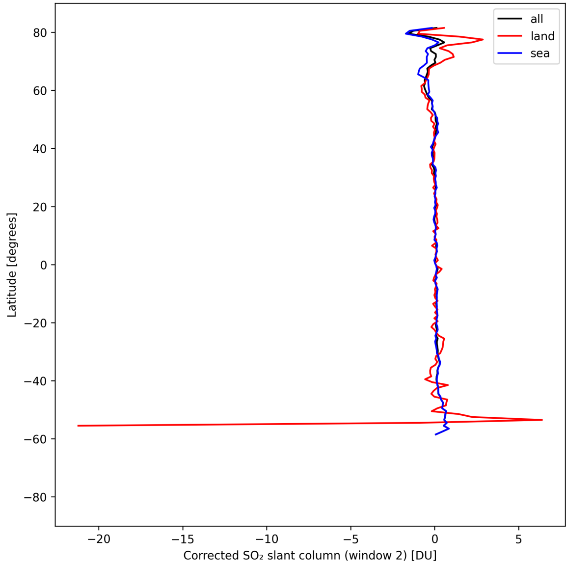
Figure 43: Zonal average of “Corrected SO 2 slant column (window 2)” for 2025-04-18 to 2025-04-19.
