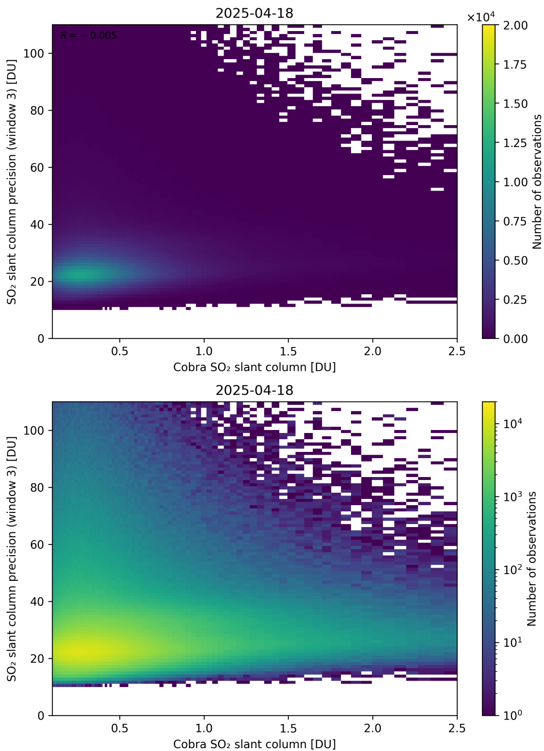
Figure 223: Scatter density plot of “Cobra SO 2 slant column” against “SO 2 slant column precision (window 3)” for 2025-04-18 to 2025-04-19.
