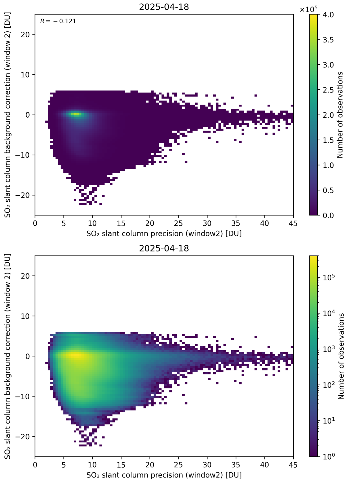
Figure 291: Scatter density plot of “SO 2 slant column precision (window2)” against “SO 2 slant column background correction (window 2)” for 2025-04-18 to 2025-04-19.
