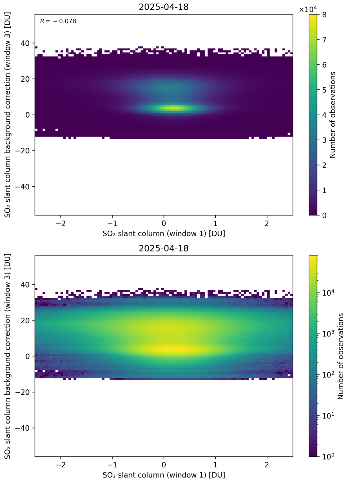
Figure 264: Scatter density plot of “SO 2 slant column (window 1)” against “SO 2 slant column background correction (window 3)” for 2025-04-18 to 2025-04-19.
