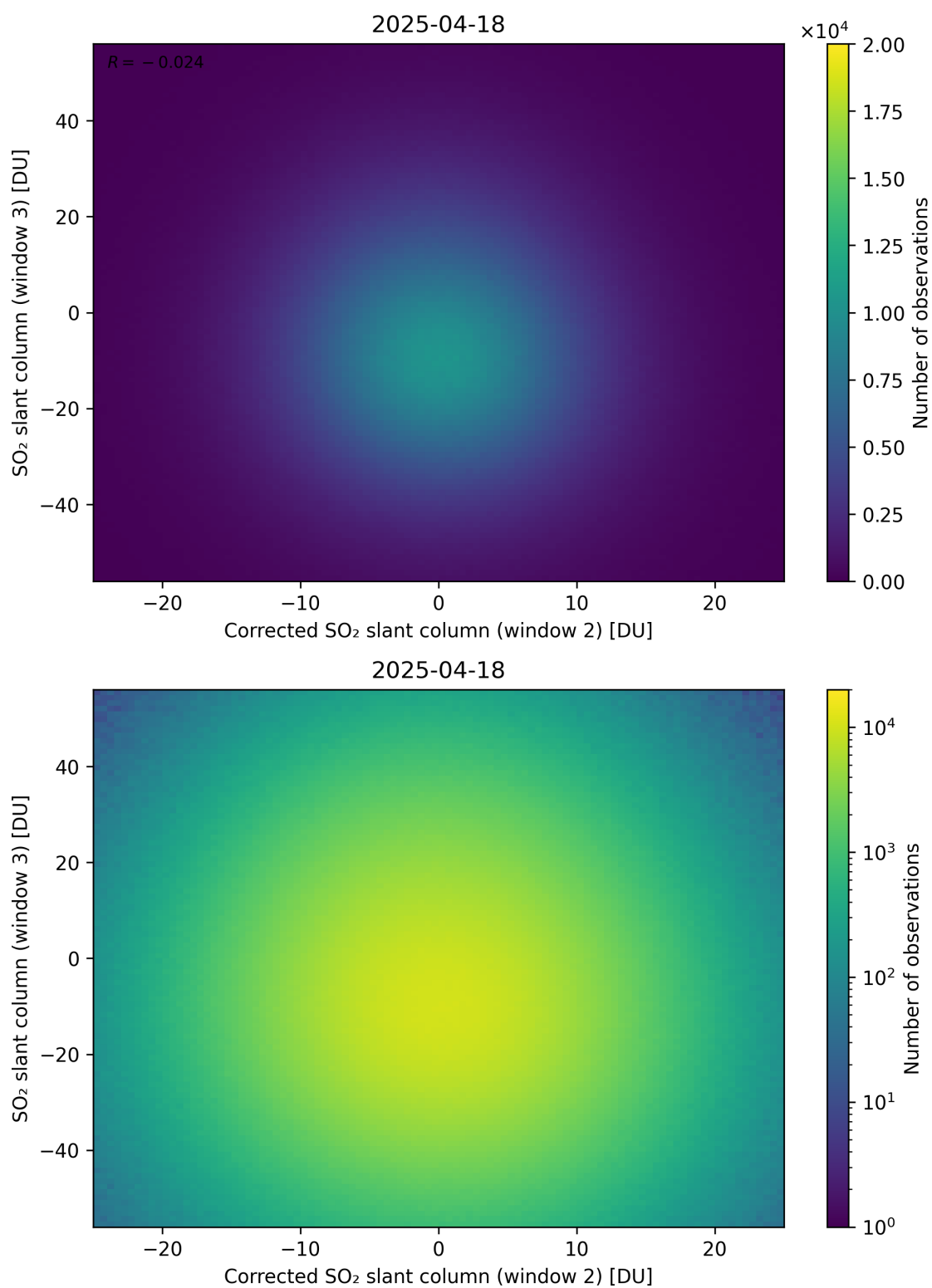
Figure 251: Scatter density plot of “Corrected SO 2 slant column (window 2)” against “SO 2 slant column (window 3)” for 2025-04-18 to 2025-04-19.
