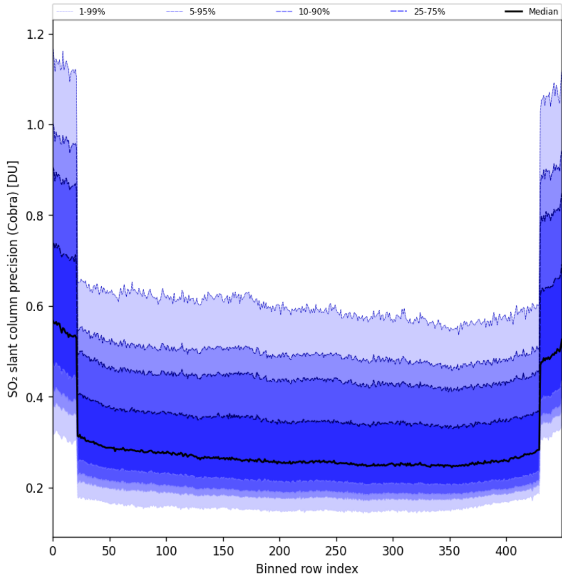
Figure 88: Along track statistics of “SO 2 slant column precision (Cobra)” for 2025-04-18 to 2025-04-19
