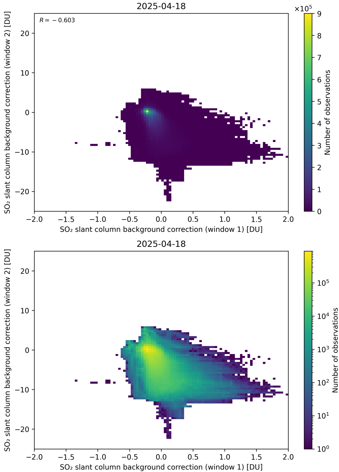
Figure 109: Scatter density plot of “SO 2 slant column background correction (window 1)” against “SO 2 slant column background correction (window 2)” for 2025-04-18 to 2025-04-19.
