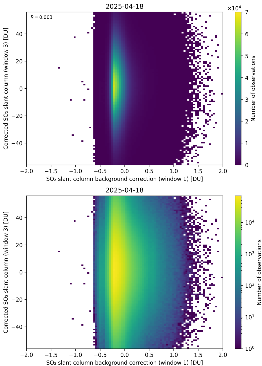
Figure 116: Scatter density plot of “SO 2 slant column background correction (window 1)” against “Corrected SO 2 slant column (window 3)” for 2025-04-18 to 2025-04-19.
