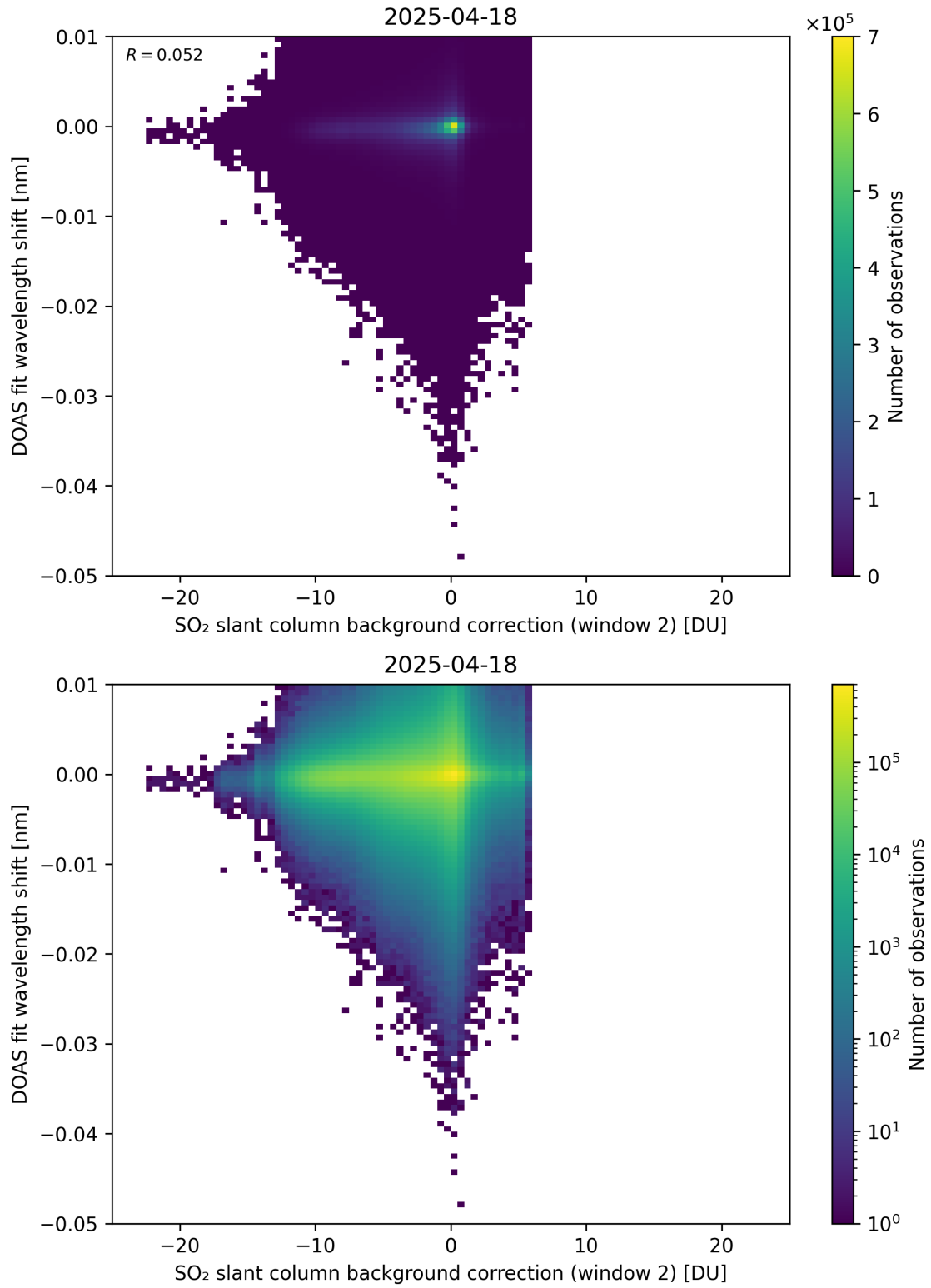
Figure 123: Scatter density plot of “SO 2 slant column background correction (window 2)” against “DOAS fit wavelength shift” for 2025-04-18 to 2025-04-19.
