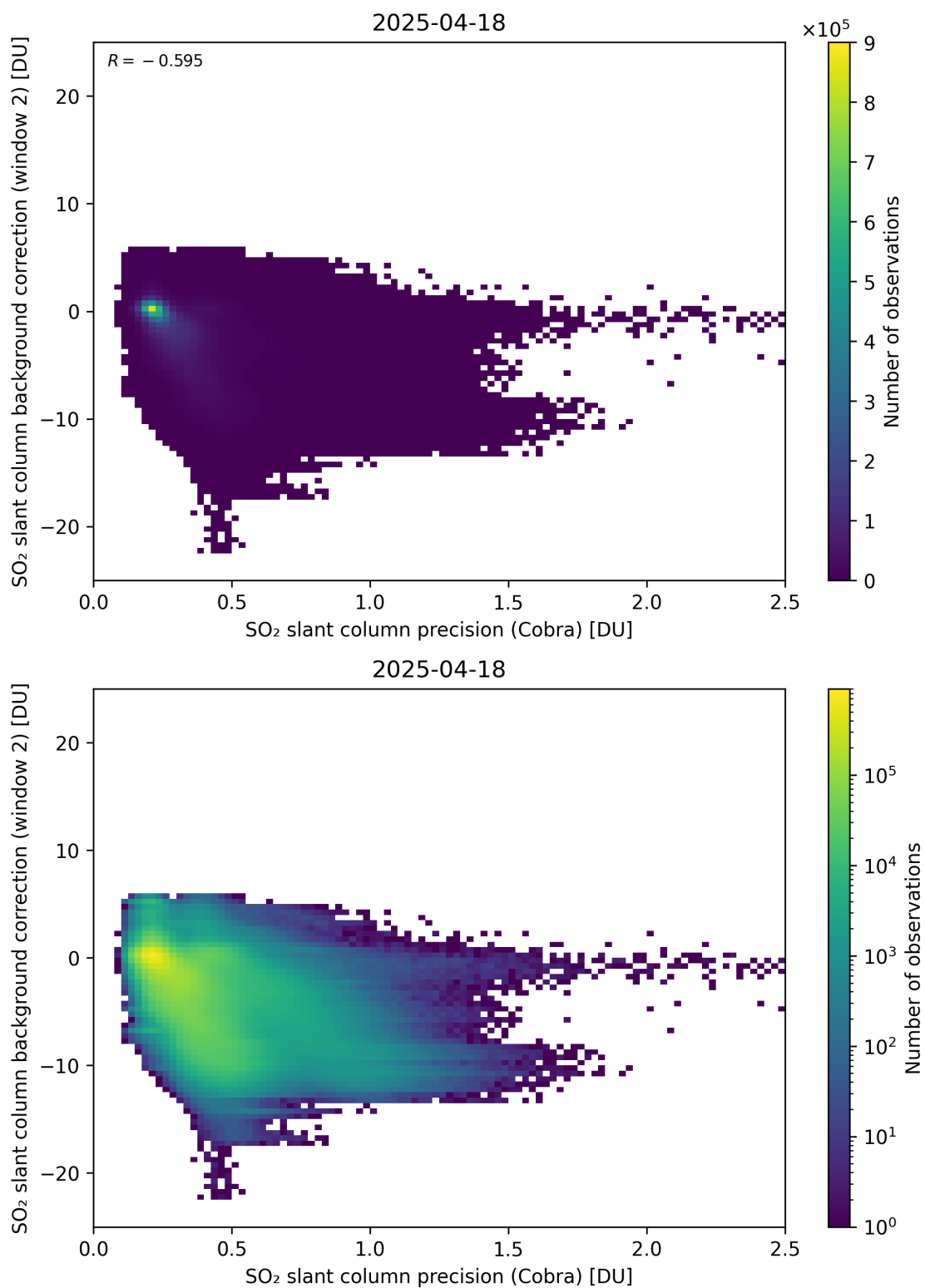
Figure 200: Scatter density plot of “SO 2 slant column precision (Cobra)” against “SO 2 slant column background correction (window 2)” for 2025-04-18 to 2025-04-19.
