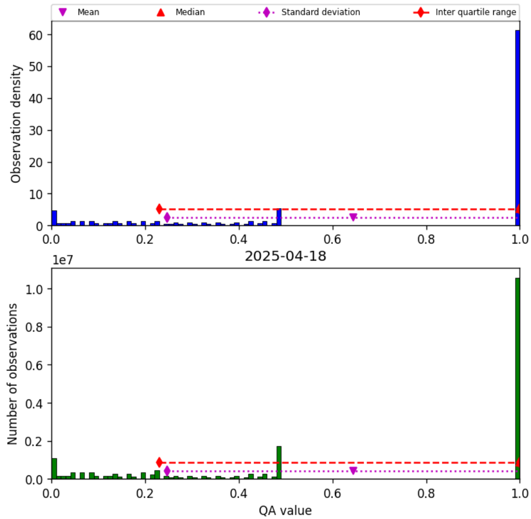
Figure 57: Histogram of “QA value” for 2025-04-18 to 2025-04-19
