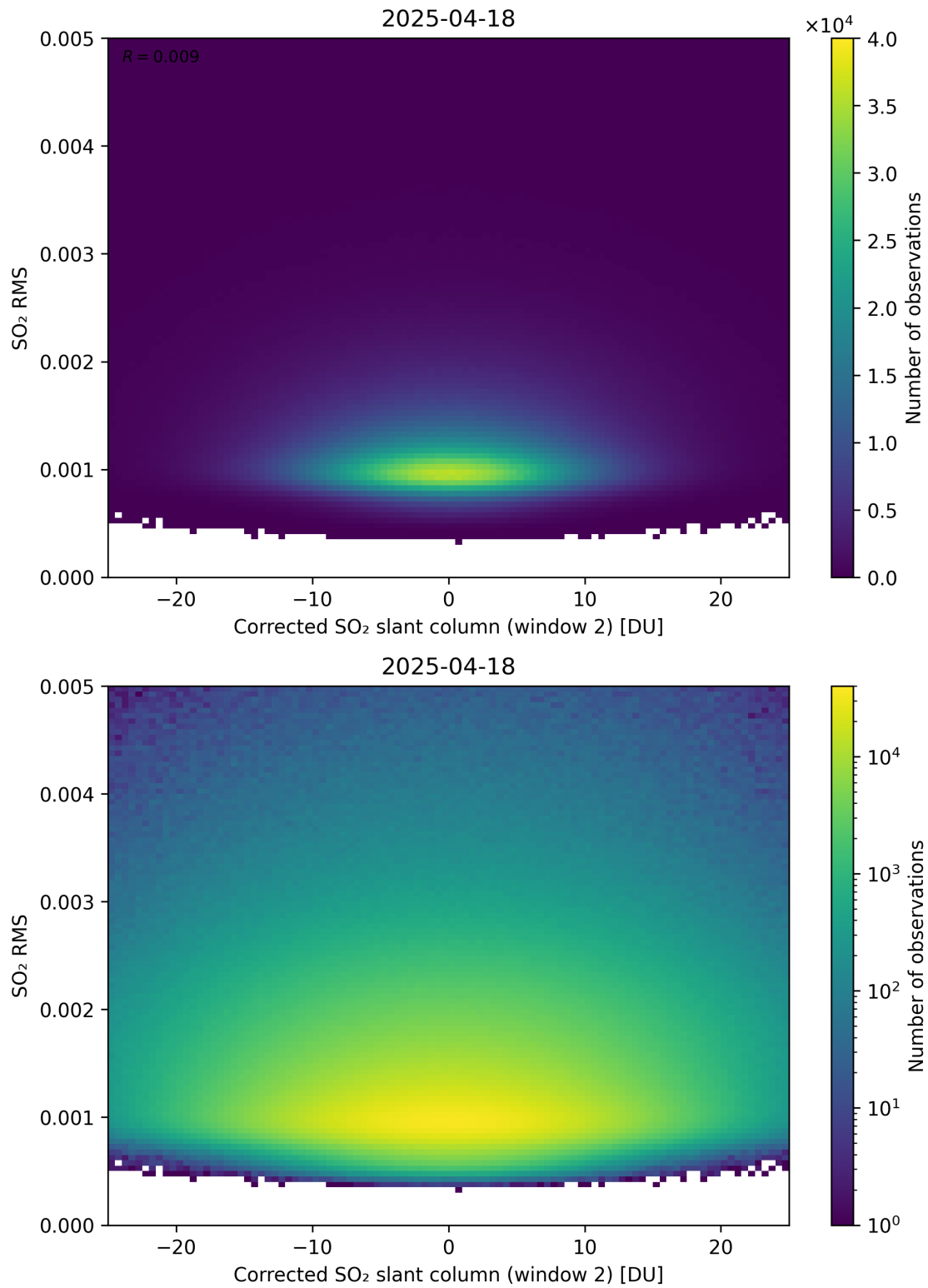
Figure 248: Scatter density plot of “Corrected SO 2 slant column (window 2)” against “SO 2 RMS” for 2025-04-18 to 2025-04-19.
