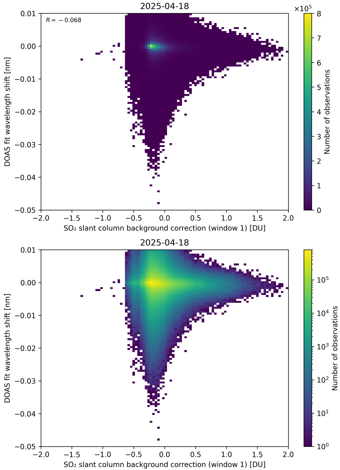
Figure 111: Scatter density plot of “SO 2 slant column background correction (window 1)” against “DOAS fit wavelength shift” for 2025-04-18 to 2025-04-19.
