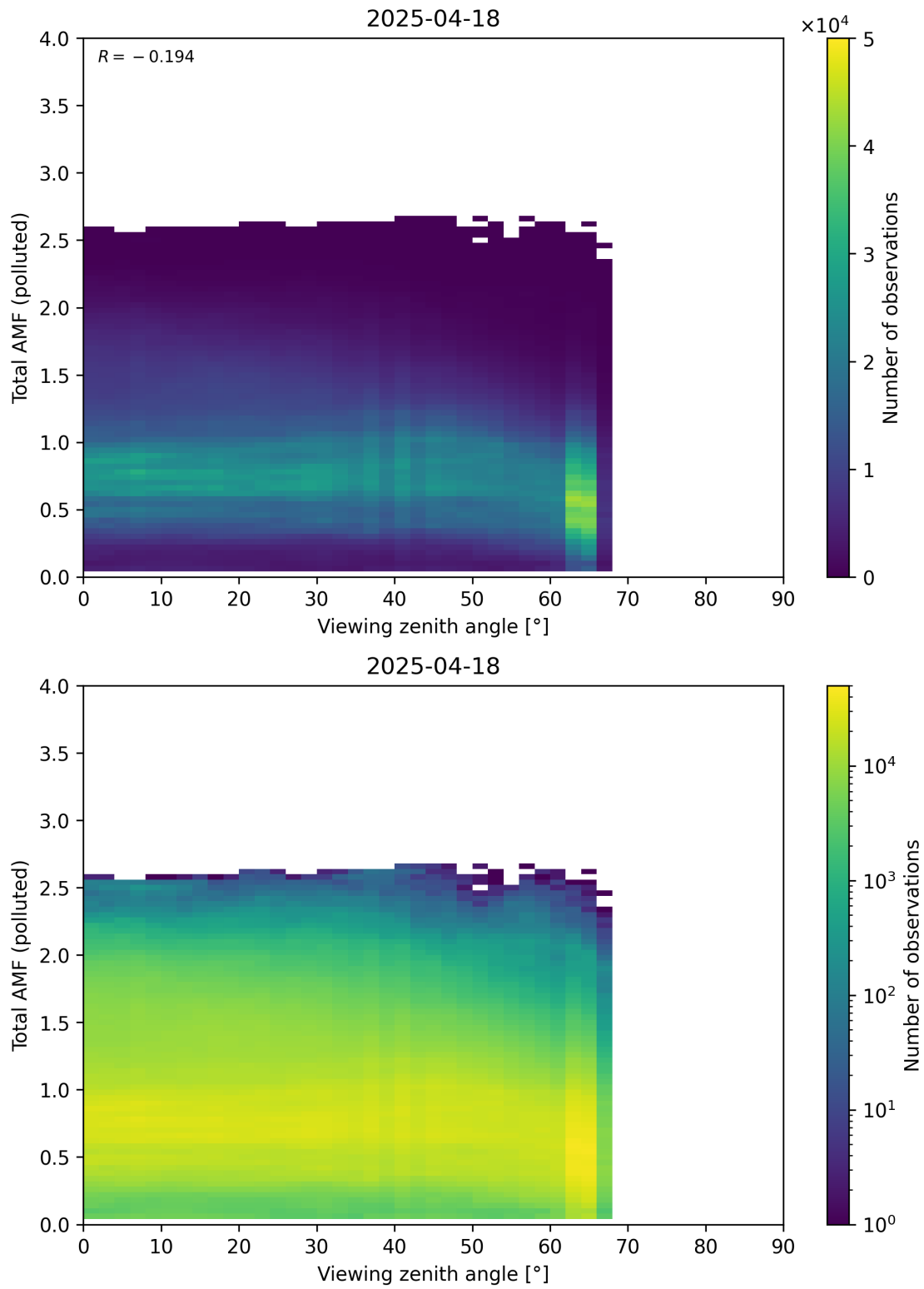
Figure 381: Scatter density plot of “Viewing zenith angle” against “Total AMF (polluted)” for 2025-04-18 to 2025-04-19.
