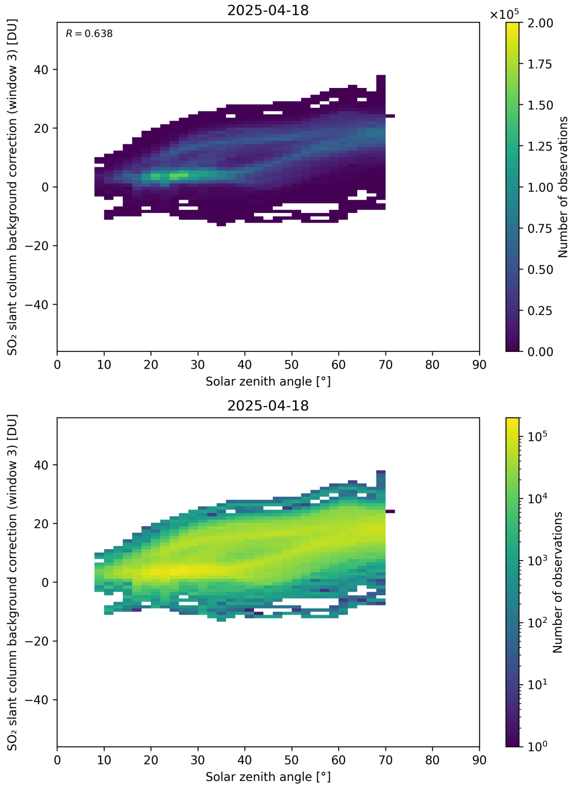
Figure 173: Scatter density plot of “Solar zenith angle” against “SO 2 slant column background correction (window 3)” for 2025-04-18 to 2025-04-19.
