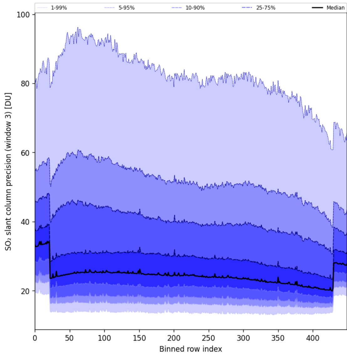
Figure 98: Along track statistics of “SO 2 slant column precision (window 3)” for 2025-04-18 to 2025-04-19
