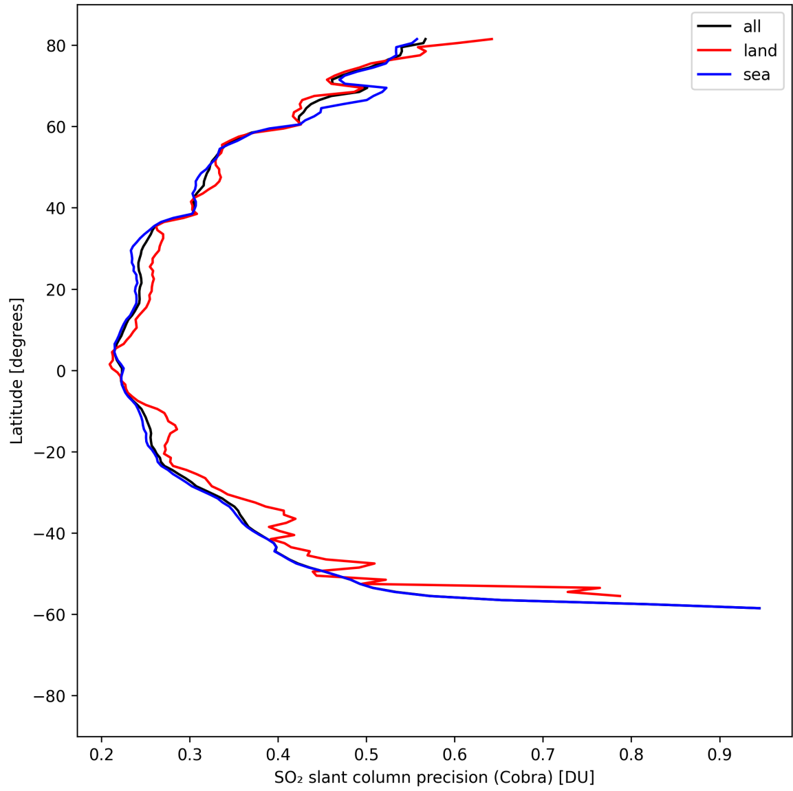
Figure 36: Zonal average of “SO 2 slant column precision (Cobra)” for 2025-04-18 to 2025-04-19.
