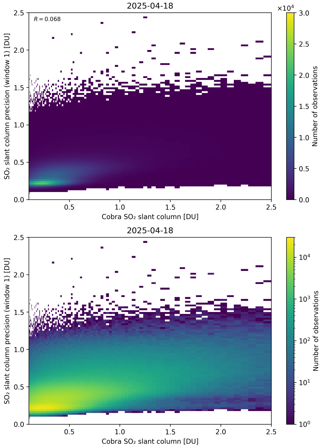
Figure 220: Scatter density plot of “Cobra SO 2 slant column” against “SO 2 slant column precision (window 1)” for 2025-04-18 to 2025-04-19.
