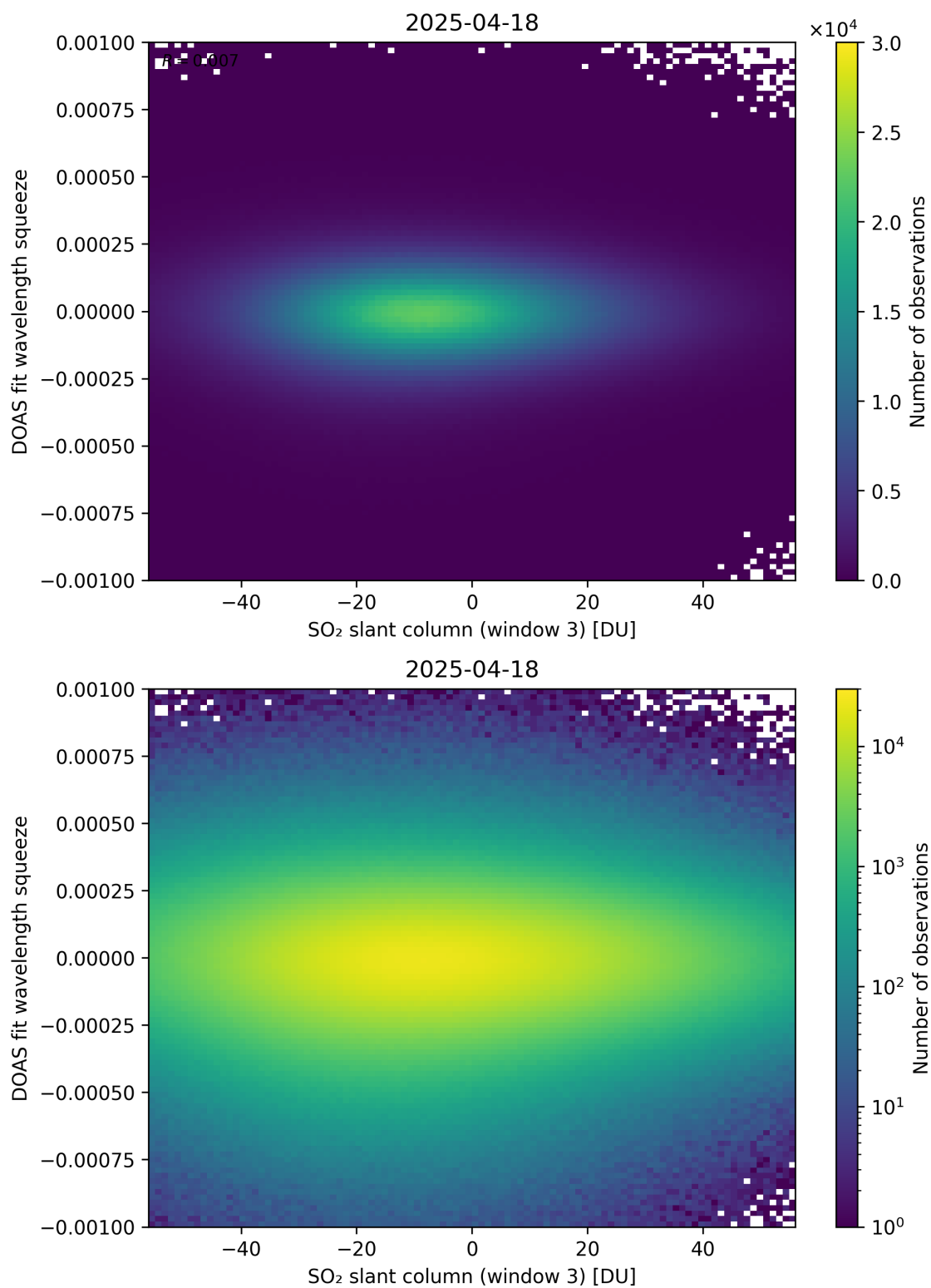
Figure 305: Scatter density plot of “SO 2 slant column (window 3)” against “DOAS fit wavelength squeeze” for 2025-04-18 to 2025-04-19.
