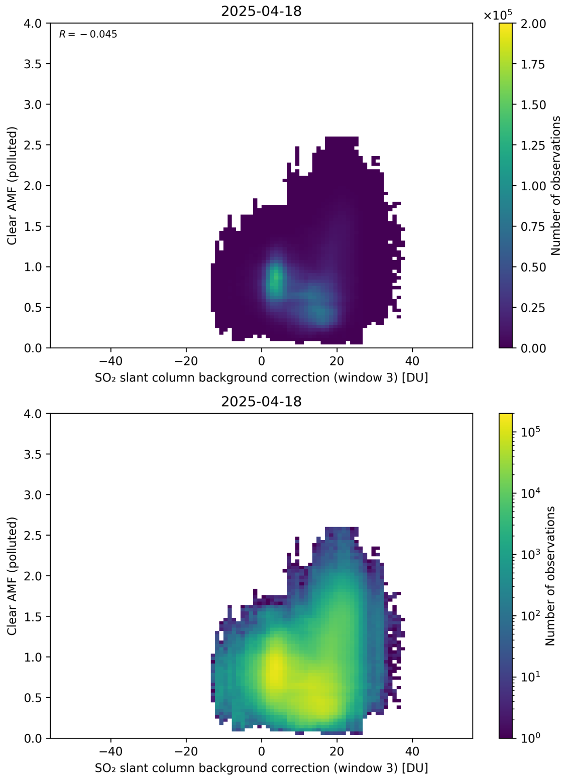
Figure 135: Scatter density plot of “SO 2 slant column background correction (window 3)” against “Clear AMF (polluted)” for 2025-04-18 to 2025-04-19.
