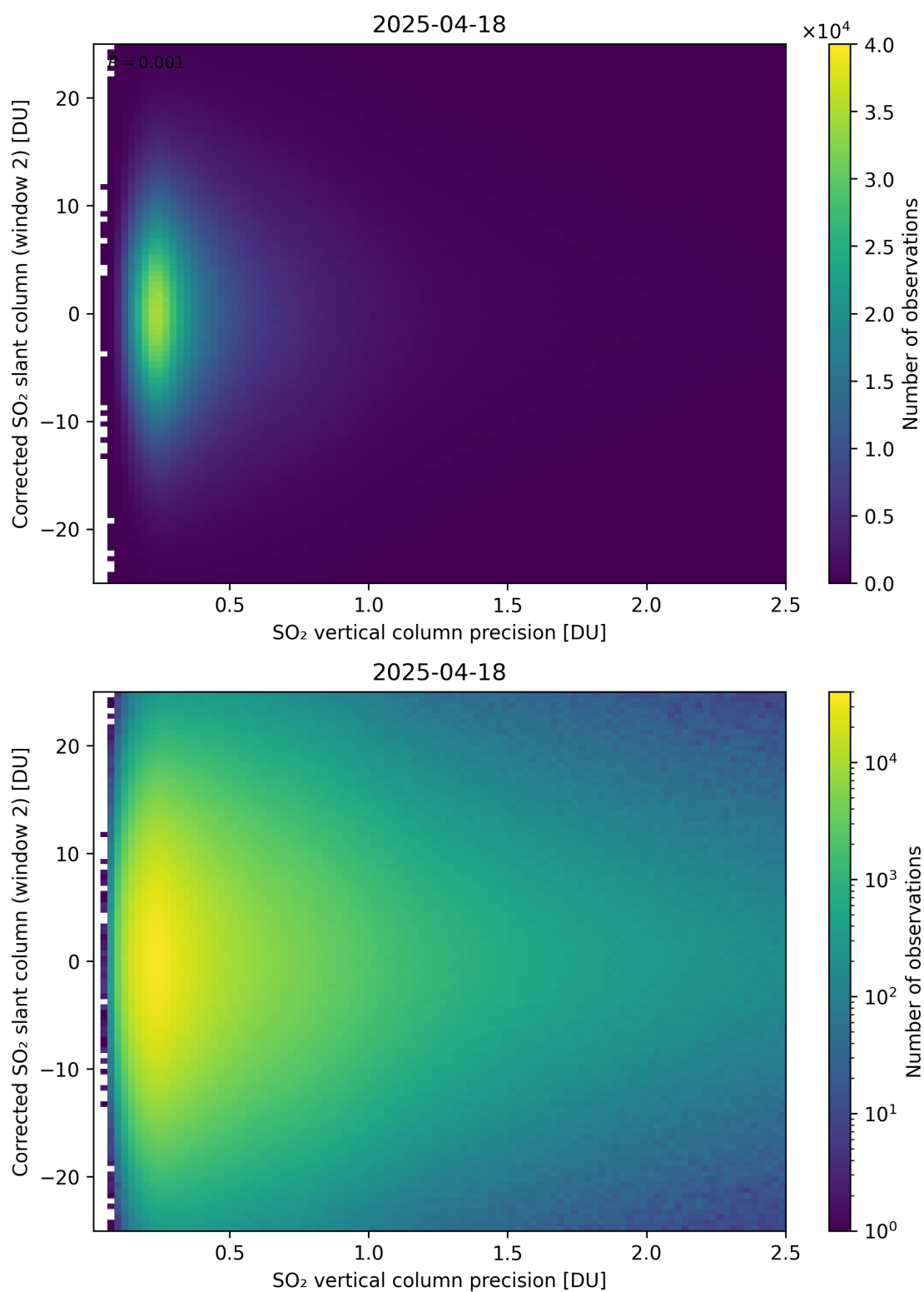
Figure 339: Scatter density plot of “SO 2 vertical column precision” against “Corrected SO 2 slant column (window 2)” for 2025-04-18 to 2025-04-19.
