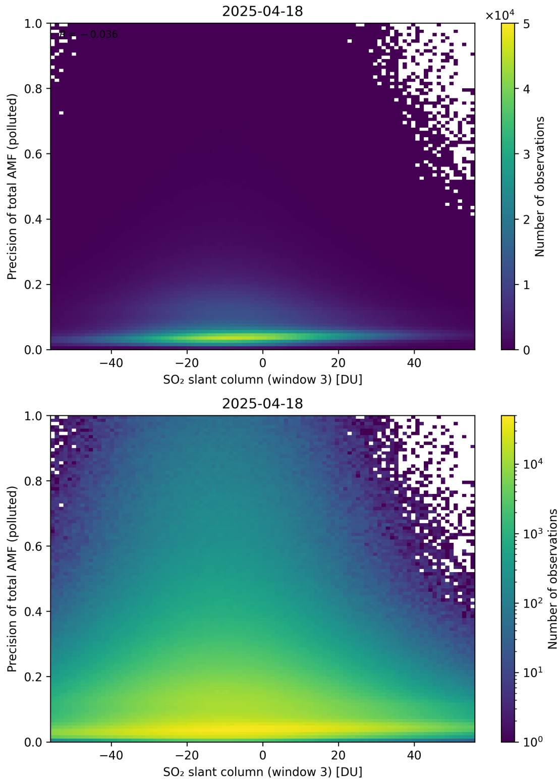
Figure 319: Scatter density plot of “SO 2 slant column (window 3)” against “Precision of total AMF (polluted)” for 2025-04-18 to 2025-04-19.
