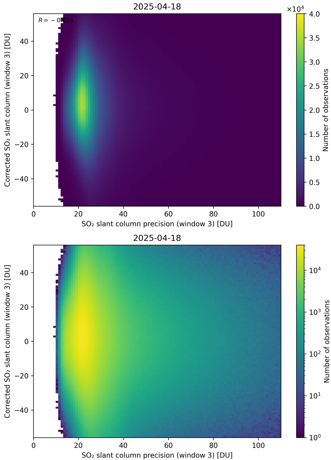
Figure 312: Scatter density plot of “SO 2 slant column precision (window 3)” against “Corrected SO 2 slant column (window 3)” for 2025-04-18 to 2025-04-19.
