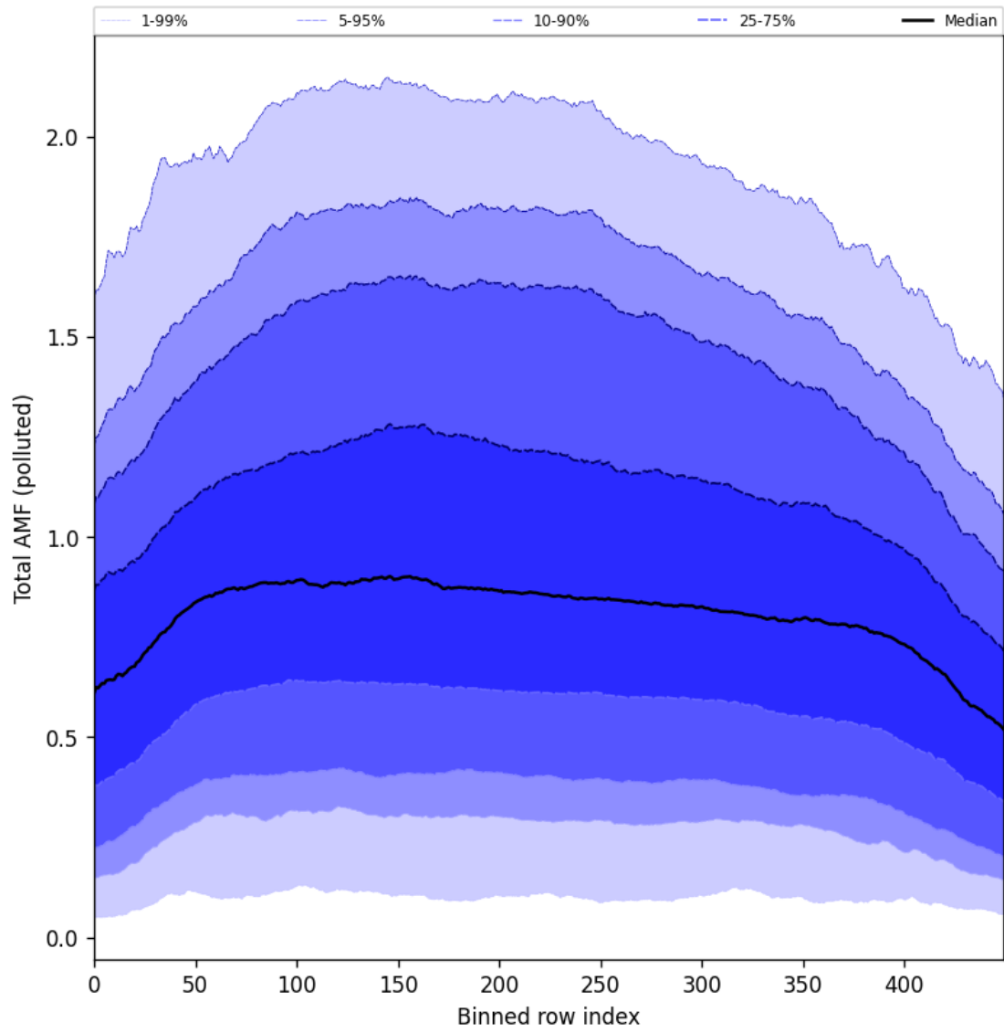
Figure 105: Along track statistics of “Total AMF (polluted)” for 2025-04-18 to 2025-04-19
