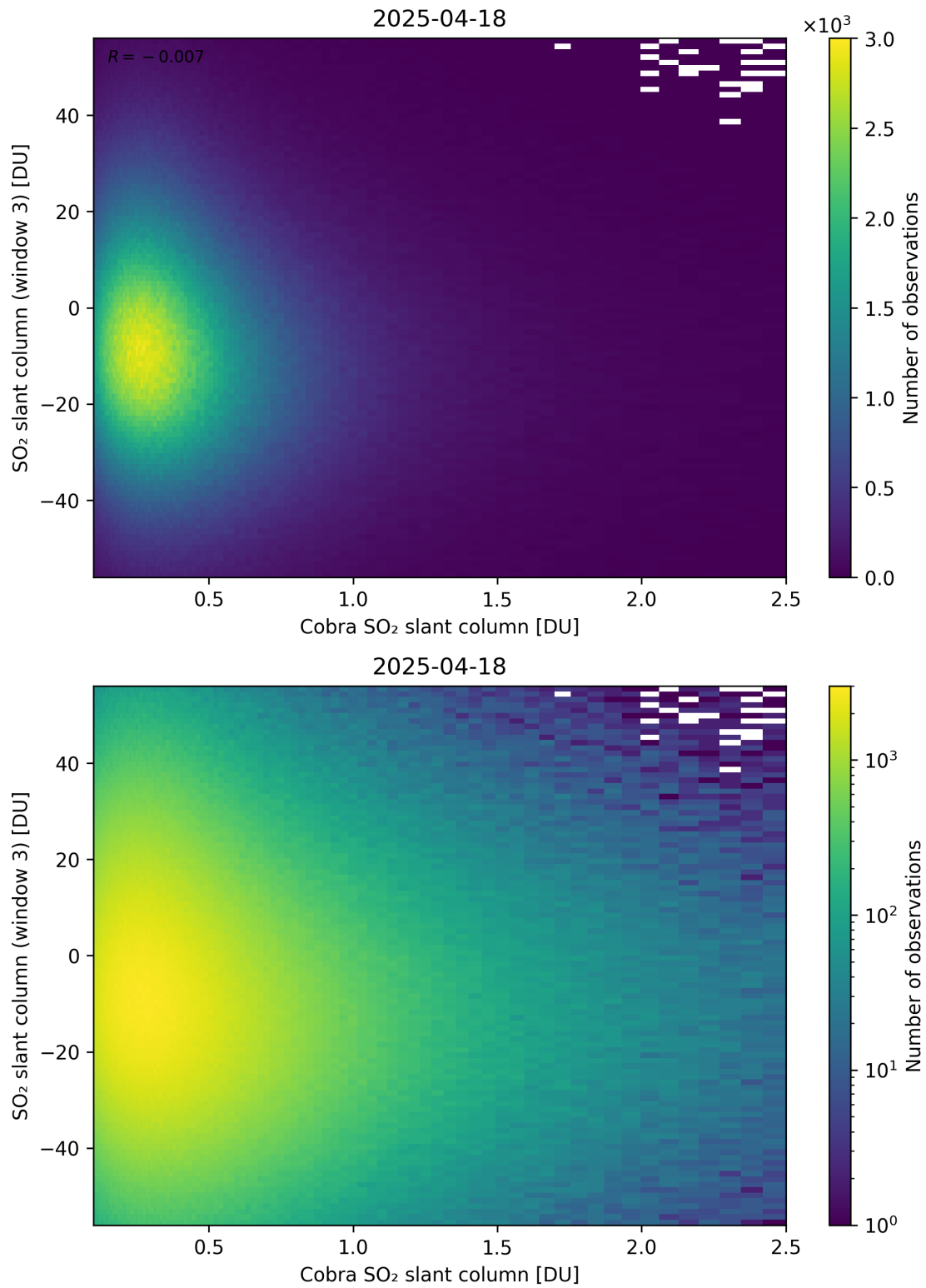
Figure 222: Scatter density plot of “Cobra SO 2 slant column” against “SO 2 slant column (window 3)” for 2025-04-18 to 2025-04-19.
