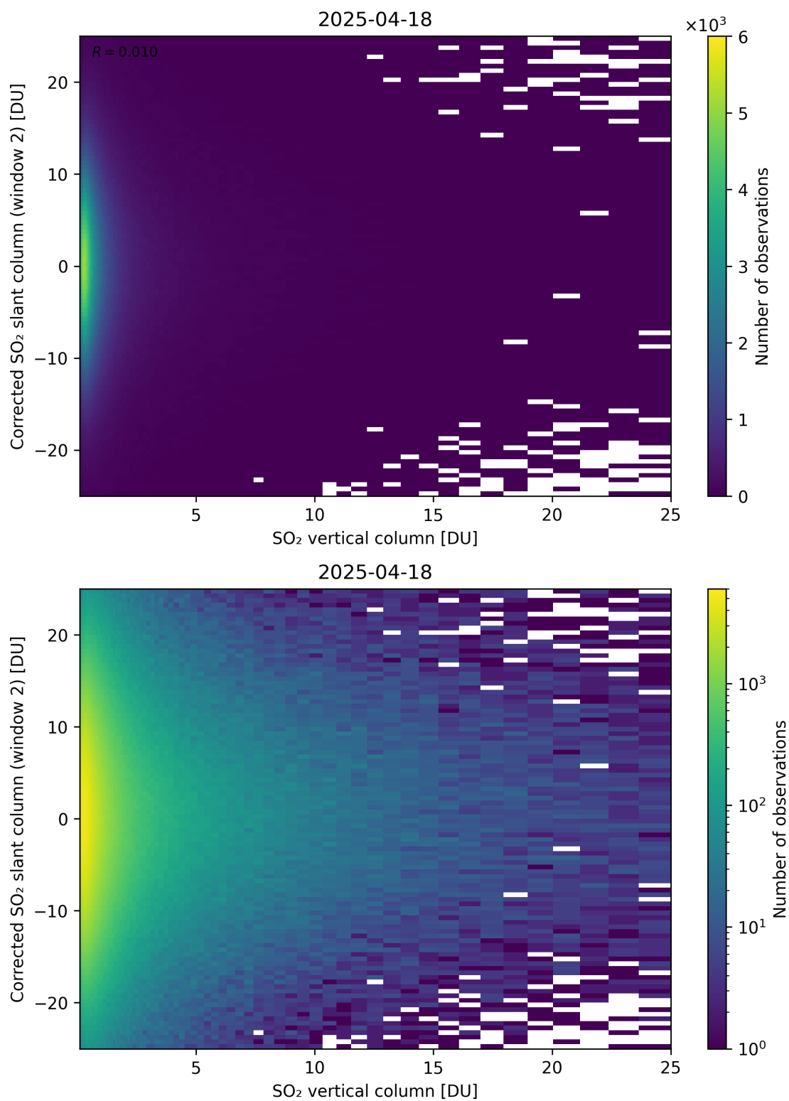
Figure 352: Scatter density plot of “SO 2 vertical column” against “Corrected SO 2 slant column (window 2)” for 2025-04-18 to 2025-04-19.
