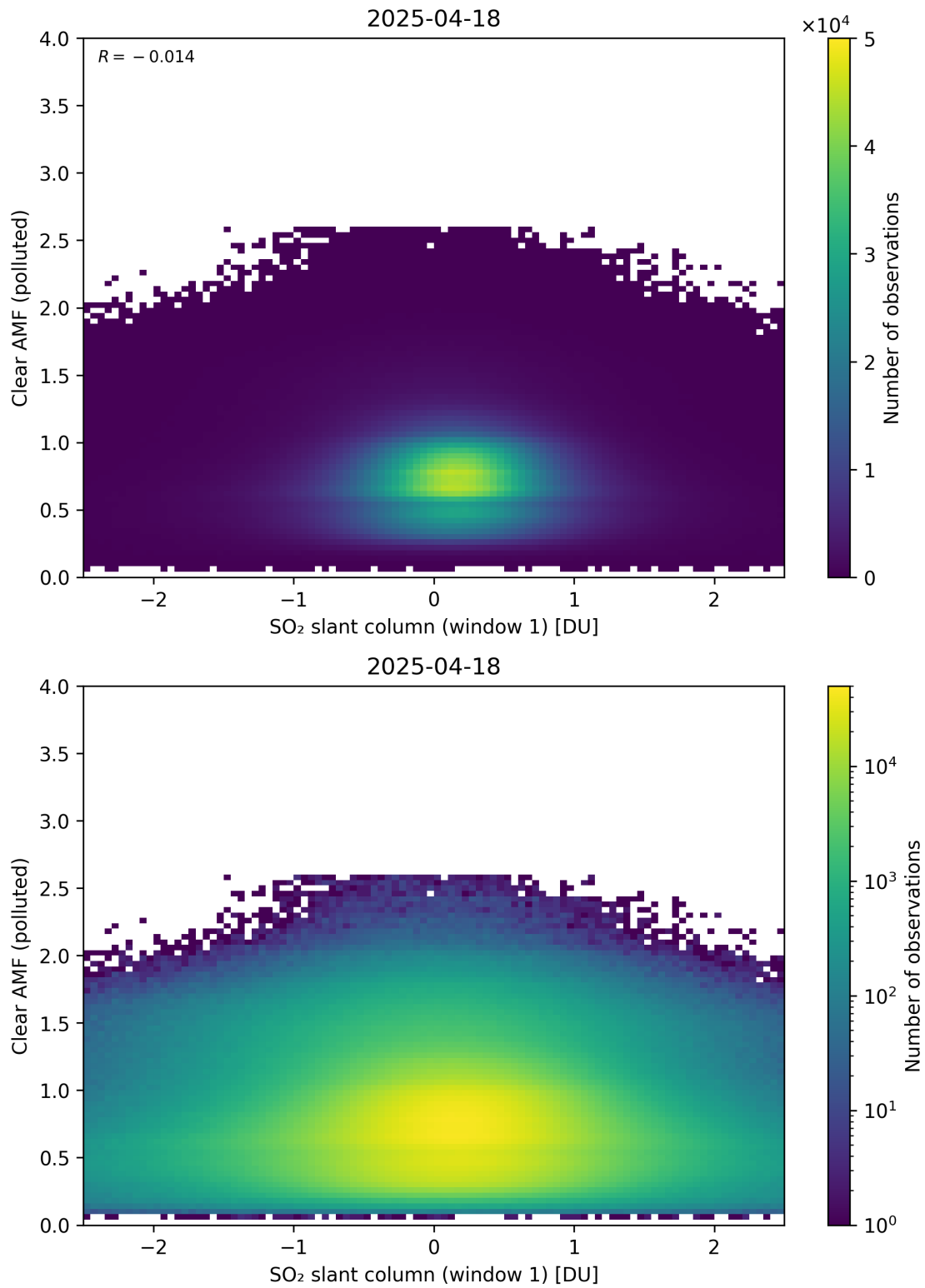
Figure 282: Scatter density plot of “SO 2 slant column (window 1)” against “Clear AMF (polluted)” for 2025-04-18 to 2025-04-19.
