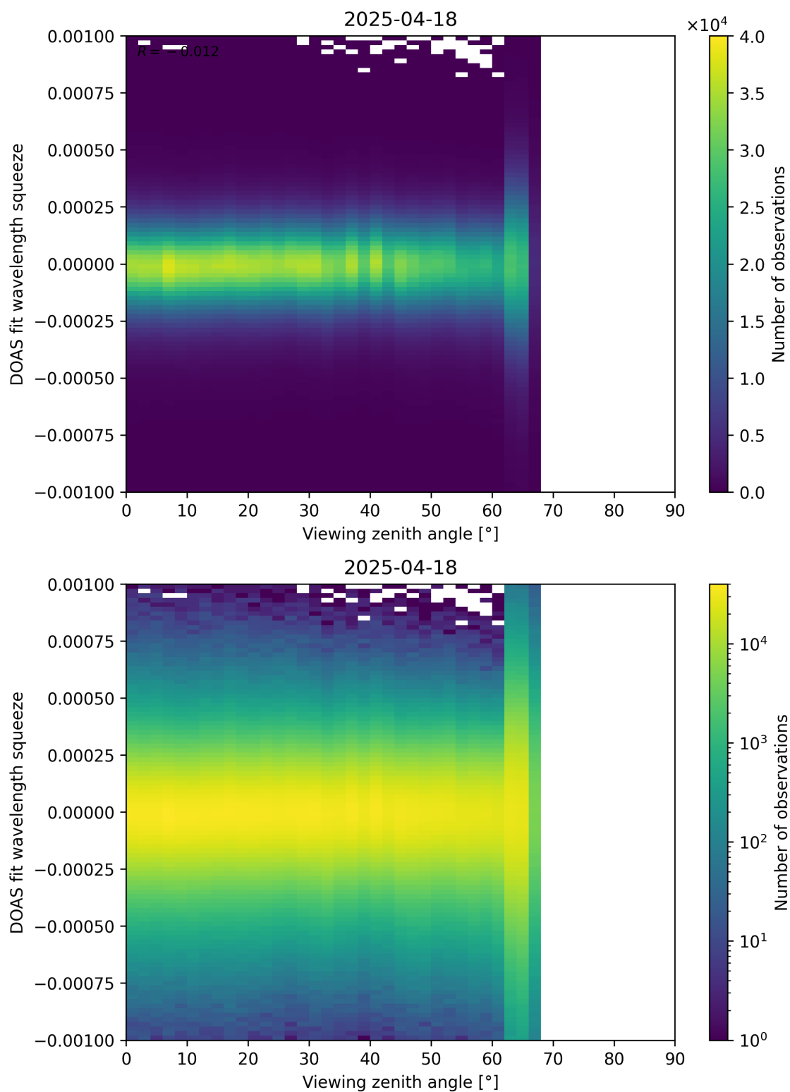
Figure 366: Scatter density plot of “Viewing zenith angle” against “DOAS fit wavelength squeeze” for 2025-04-18 to 2025-04-19.
