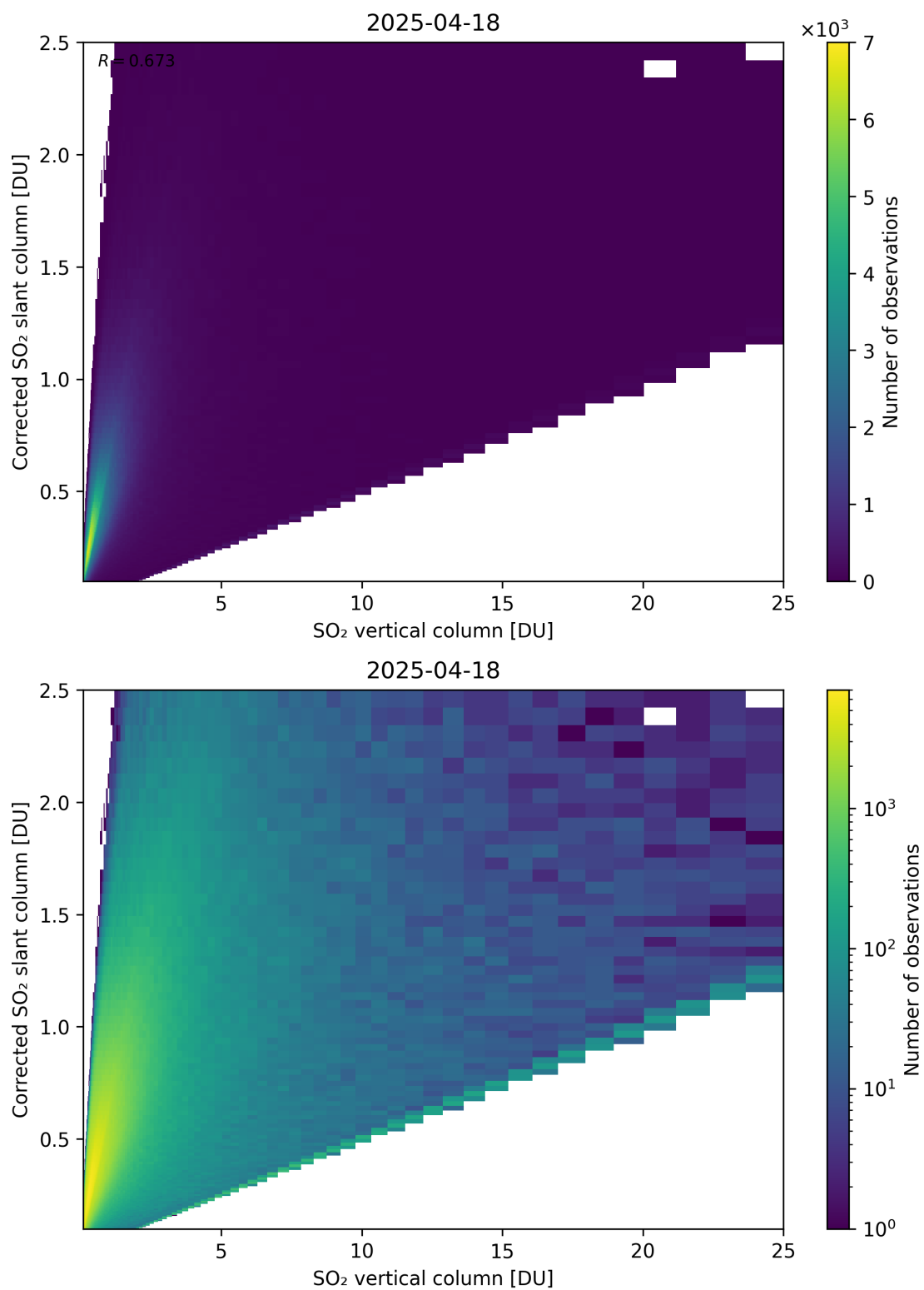
Figure 351: Scatter density plot of “SO 2 vertical column” against “Corrected SO 2 slant column” for 2025-04-18 to 2025-04-19.
