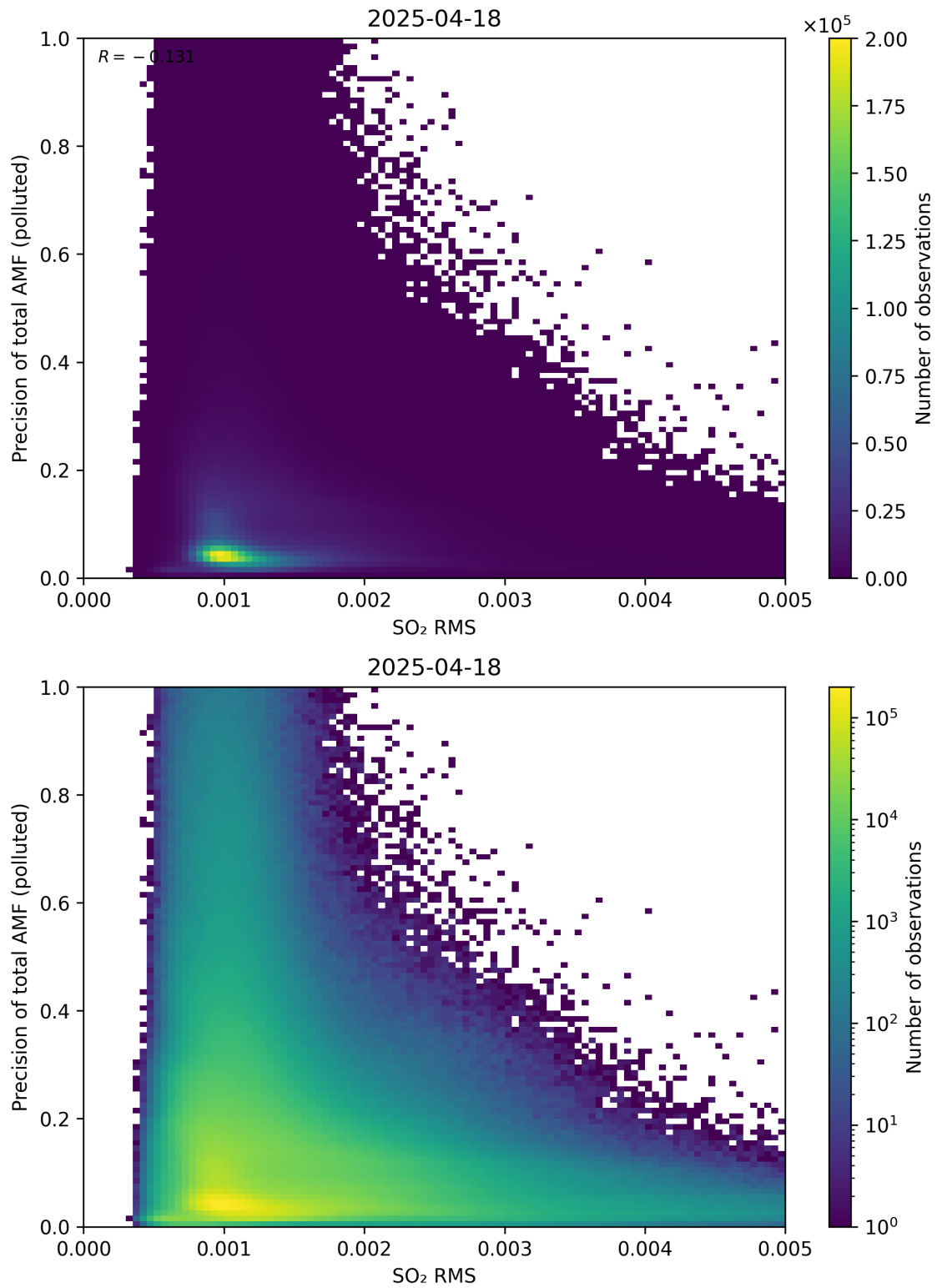
Figure 149: Scatter density plot of “SO 2 RMS” against “Precision of total AMF (polluted)” for 2025-04-18 to 2025-04-19.
