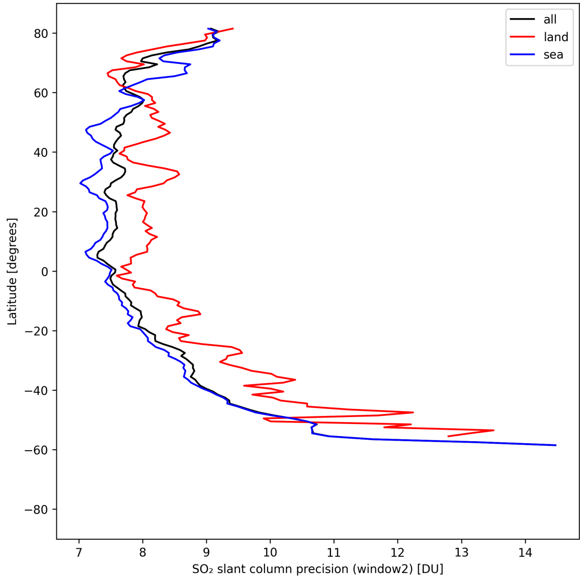
Figure 42: Zonal average of “SO 2 slant column precision (window2)” for 2025-04-18 to 2025-04-19.
