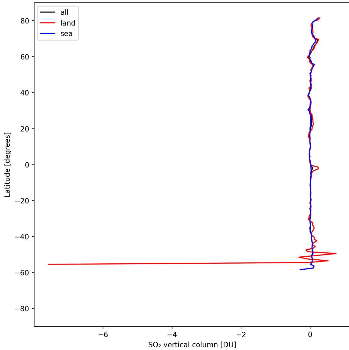
Figure 32: Zonal average of “SO 2 vertical column” for 2025-04-18 to 2025-04-19.
