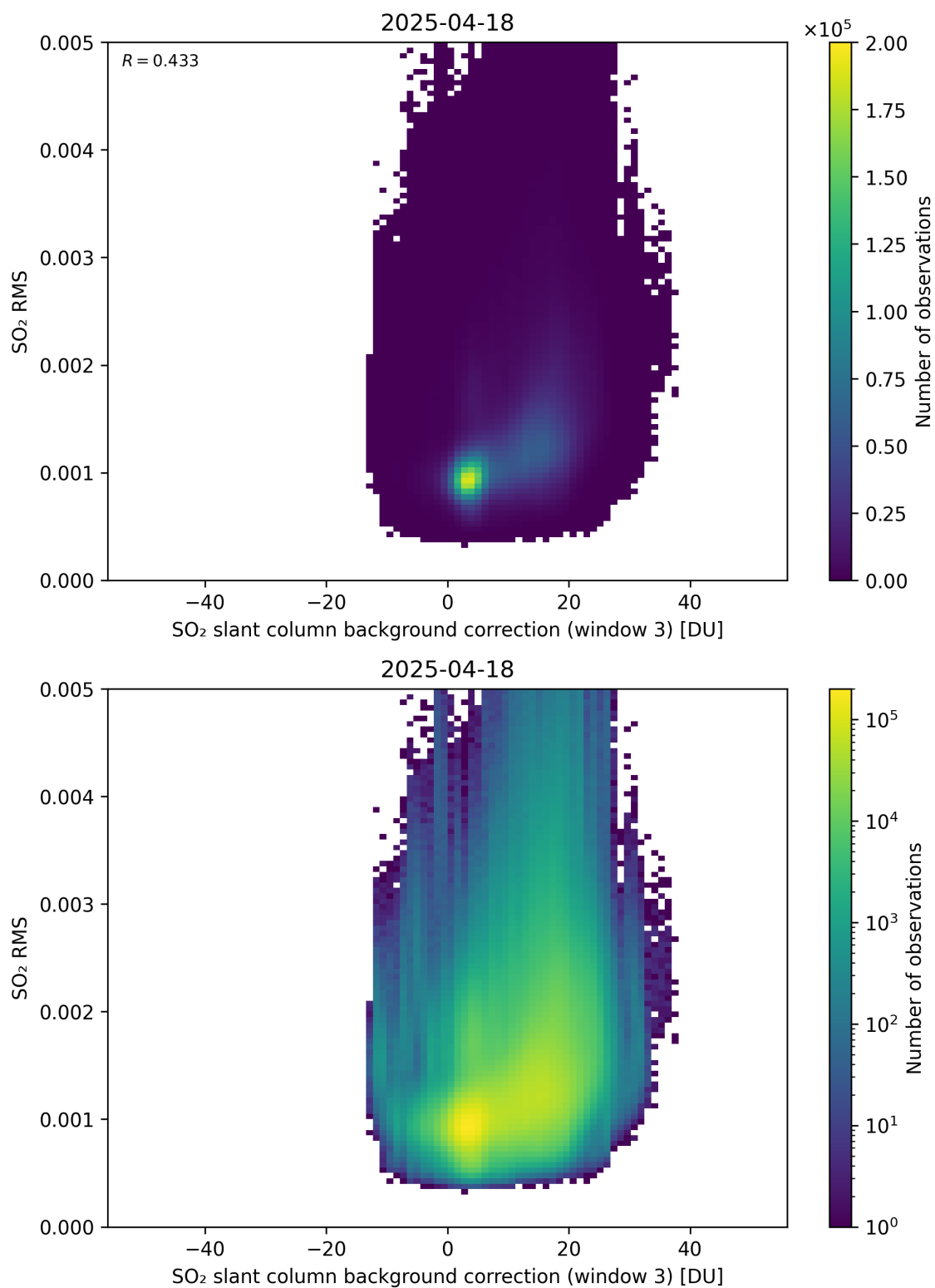
Figure 134: Scatter density plot of “SO 2 slant column background correction (window 3)” against “SO 2 RMS” for 2025-04-18 to 2025-04-19.
