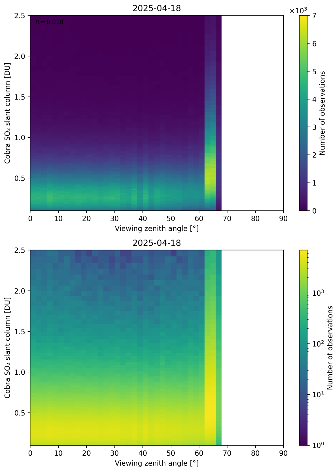
Figure 371: Scatter density plot of “Viewing zenith angle” against “Cobra SO 2 slant column” for 2025-04-18 to 2025-04-19.
