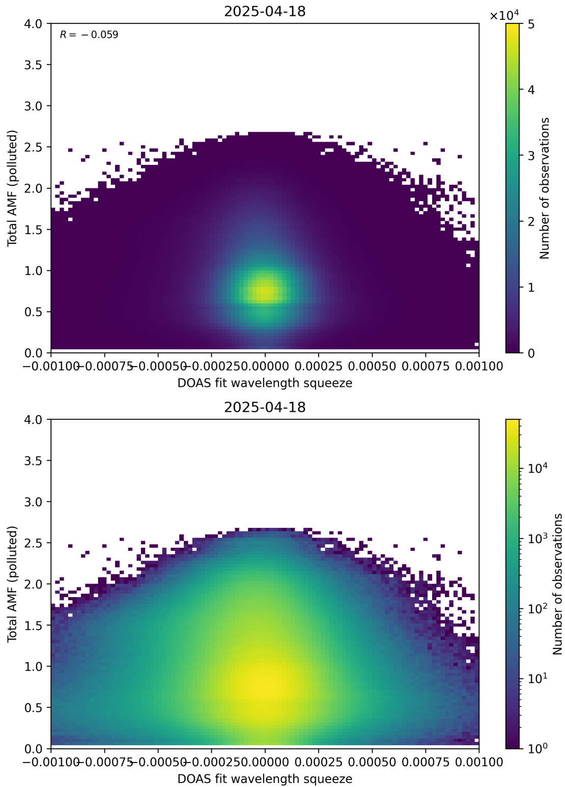
Figure 145: Scatter density plot of “DOAS fit wavelength squeeze” against “Total AMF (polluted)” for 2025-04-18 to 2025-04-19.
