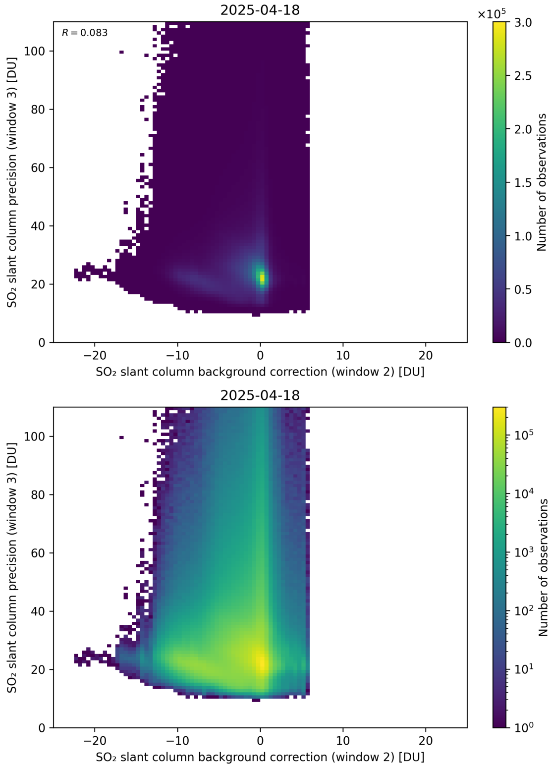
Figure 129: Scatter density plot of “SO 2 slant column background correction (window 2)” against “SO 2 slant column precision (window 3)” for 2025-04-18 to 2025-04-19.
