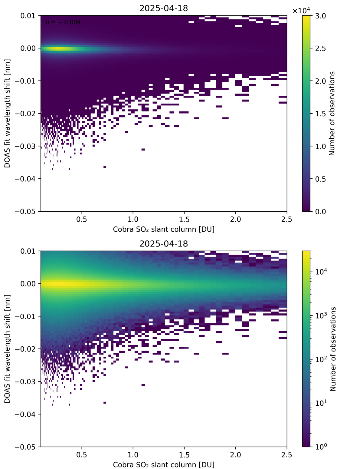
Figure 196: Scatter density plot of “Cobra SO 2 slant column” against “DOAS fit wavelength shift” for 2025-04-18 to 2025-04-19.
