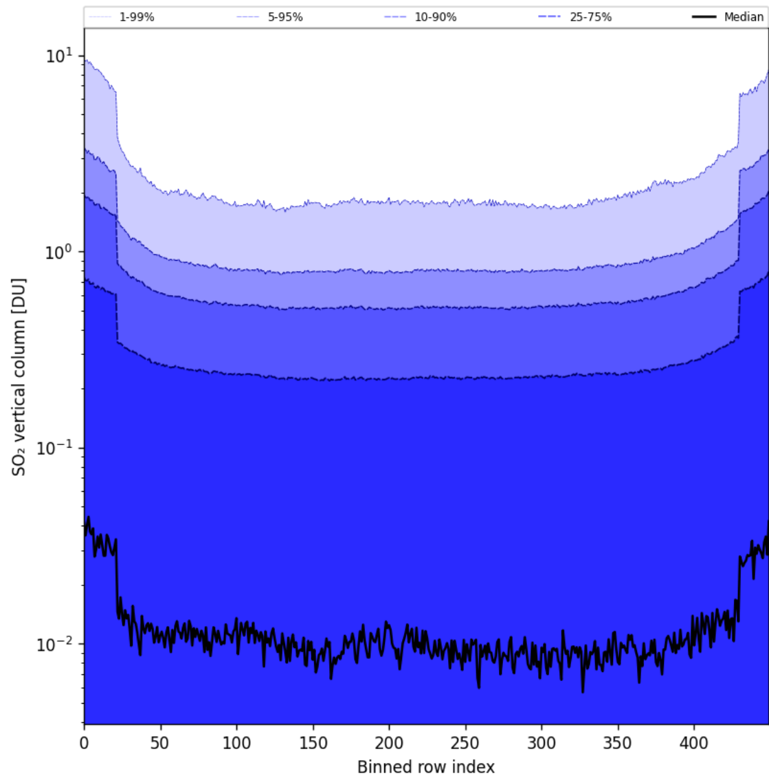
Figure 84: Along track statistics of “SO 2 vertical column” for 2025-04-18 to 2025-04-19
