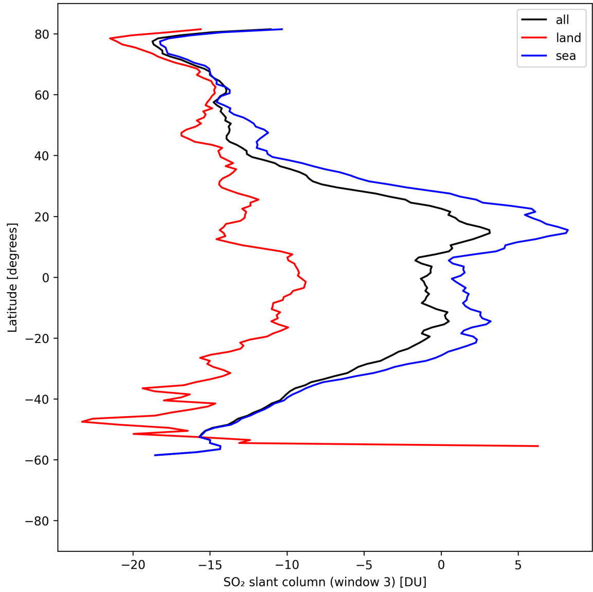
Figure 45: Zonal average of “SO 2 slant column (window 3)” for 2025-04-18 to 2025-04-19.
