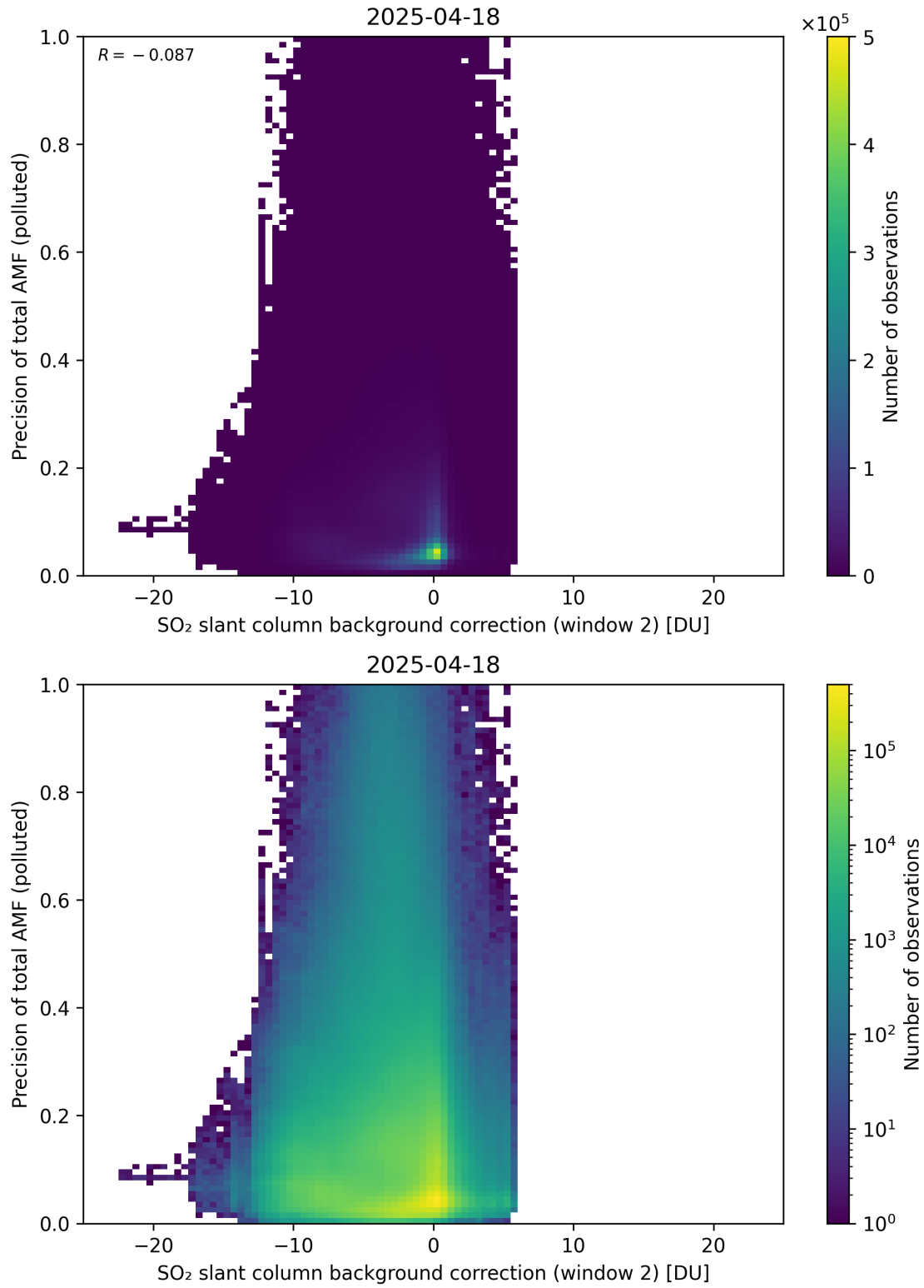
Figure 131: Scatter density plot of “SO 2 slant column background correction (window 2)” against “Precision of total AMF (polluted)” for 2025-04-18 to 2025-04-19.
