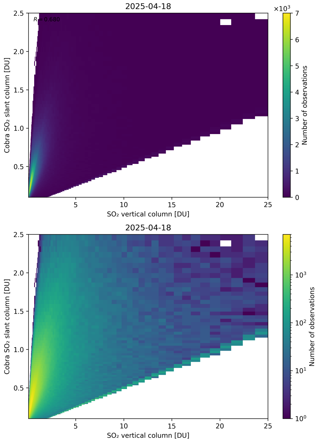
Figure 349: Scatter density plot of “SO 2 vertical column” against “Cobra SO 2 slant column” for 2025-04-18 to 2025-04-19.
