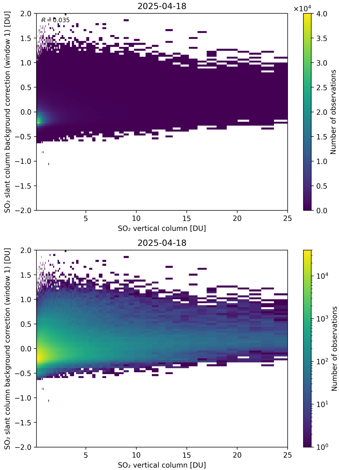
Figure 323: Scatter density plot of “SO 2 vertical column” against “SO 2 slant column background correction (window 1)” for 2025-04-18 to 2025-04-19.
