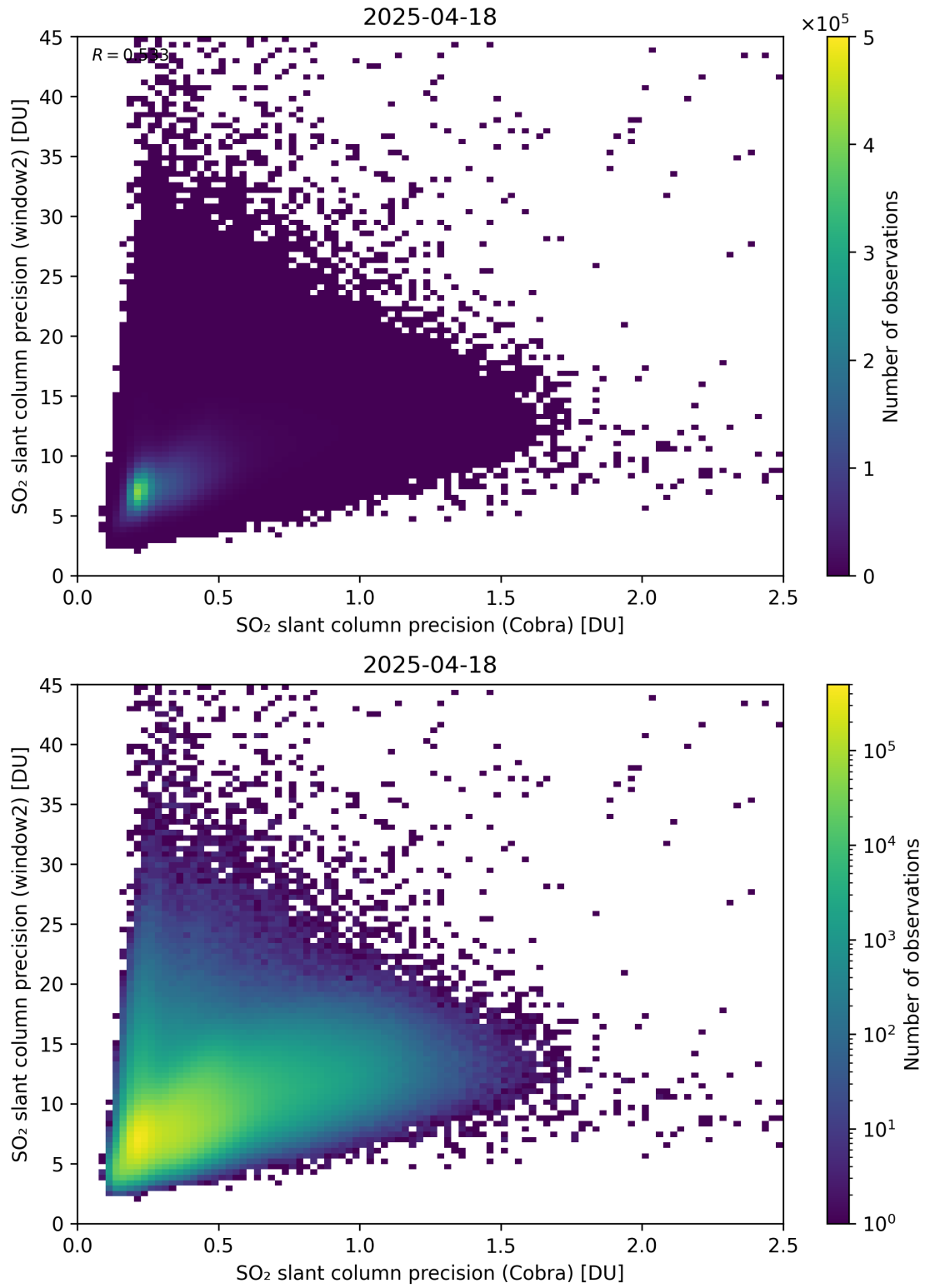
Figure 210: Scatter density plot of “SO 2 slant column precision (Cobra)” against “SO 2 slant column precision (window2)” for 2025-04-18 to 2025-04-19.
