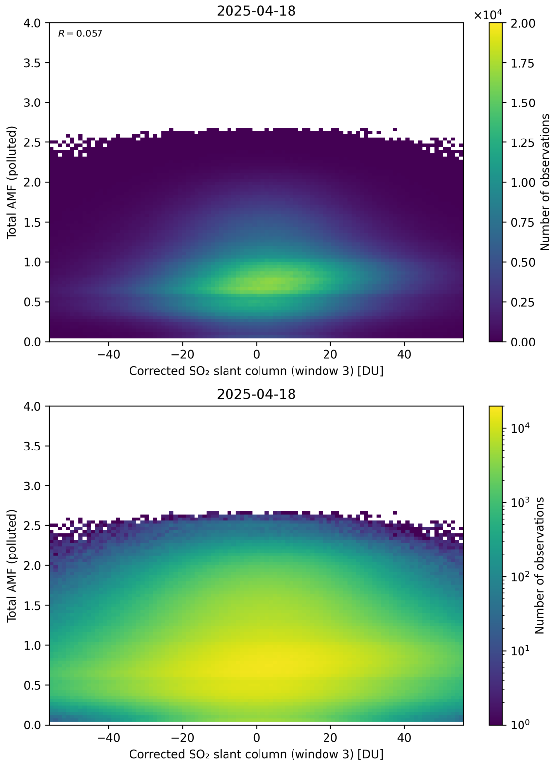
Figure 260: Scatter density plot of “Corrected SO 2 slant column (window 3)” against “Total AMF (polluted)” for 2025-04-18 to 2025-04-19.
