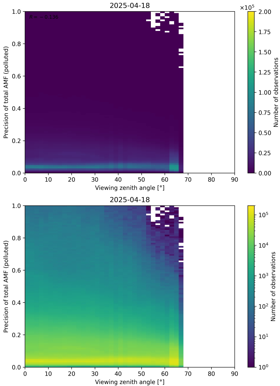
Figure 382: Scatter density plot of “Viewing zenith angle” against “Precision of total AMF (polluted)” for 2025-04-18 to 2025-04-19.
