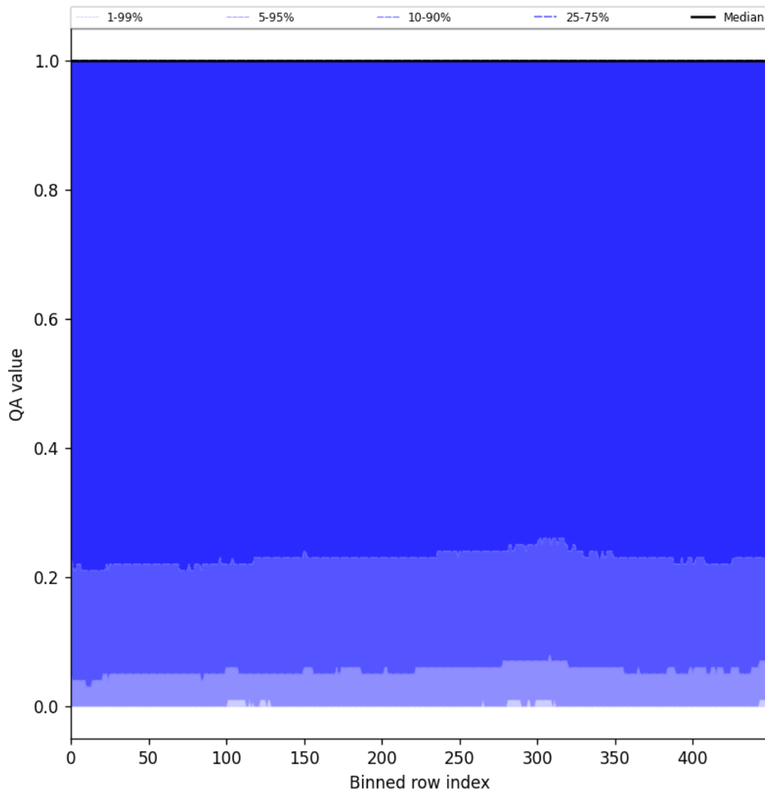
Figure 83: Along track statistics of “QA value” for 2025-04-18 to 2025-04-19
