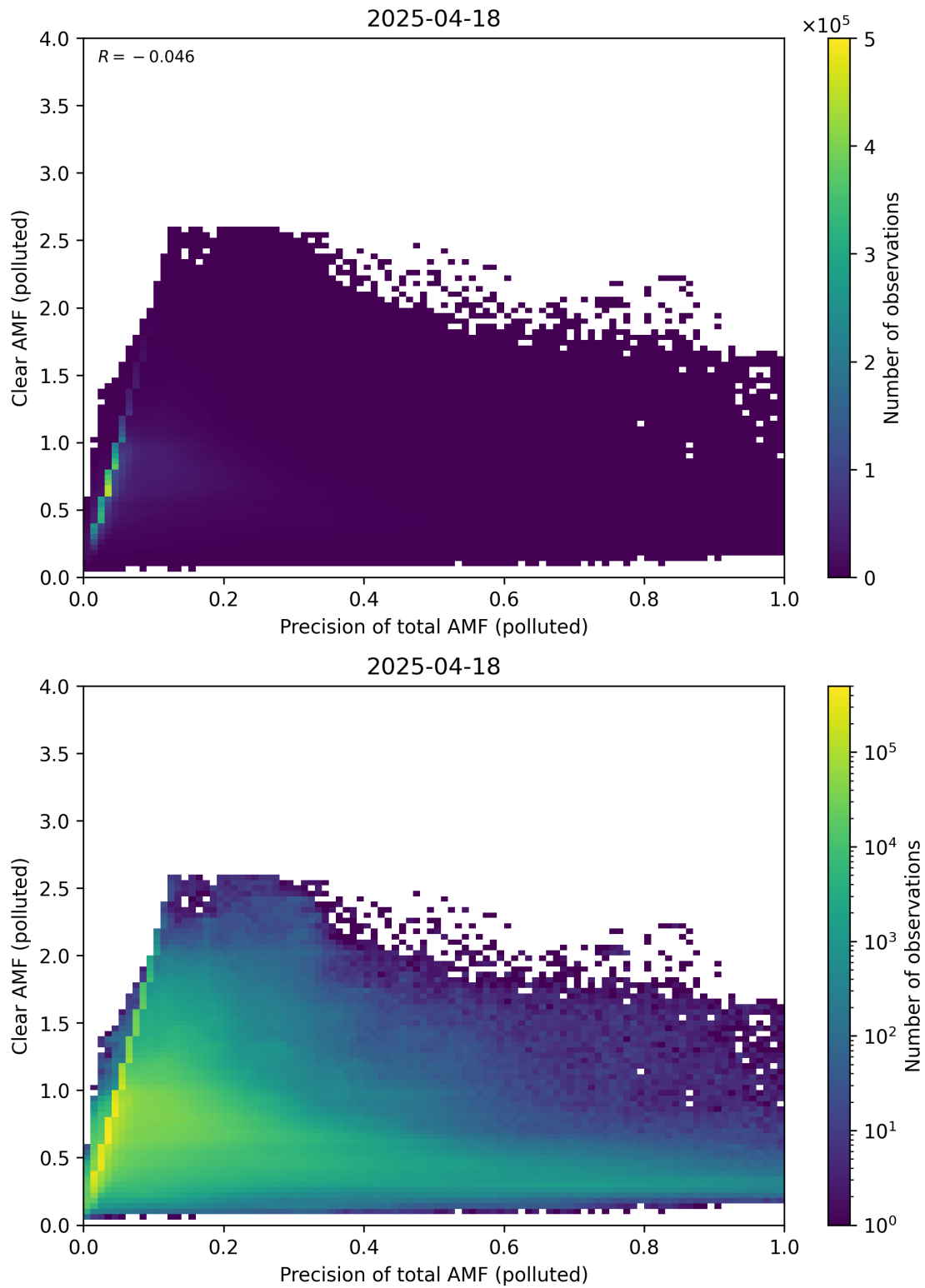
Figure 320: Scatter density plot of “Precision of total AMF (polluted)” against “Clear AMF (polluted)” for 2025-04-18 to 2025-04-19.
