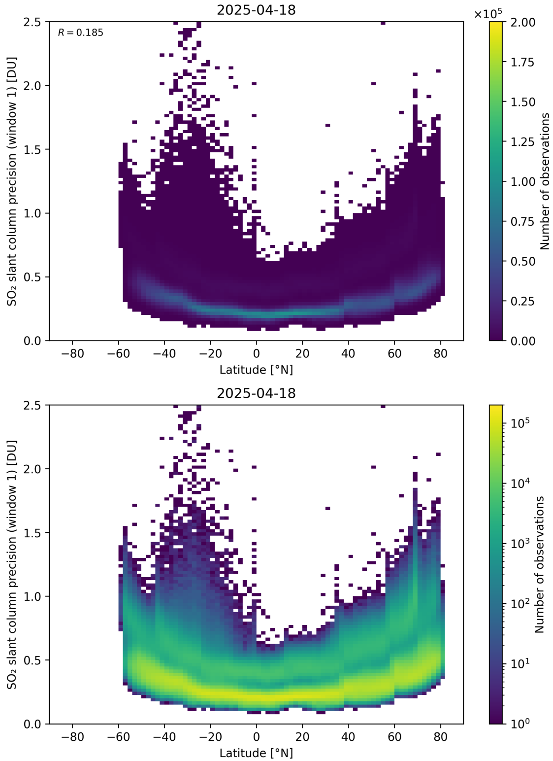
Figure 163: Scatter density plot of “Latitude” against “SO 2 slant column precision (window 1)” for 2025-04-18 to 2025-04-19.
