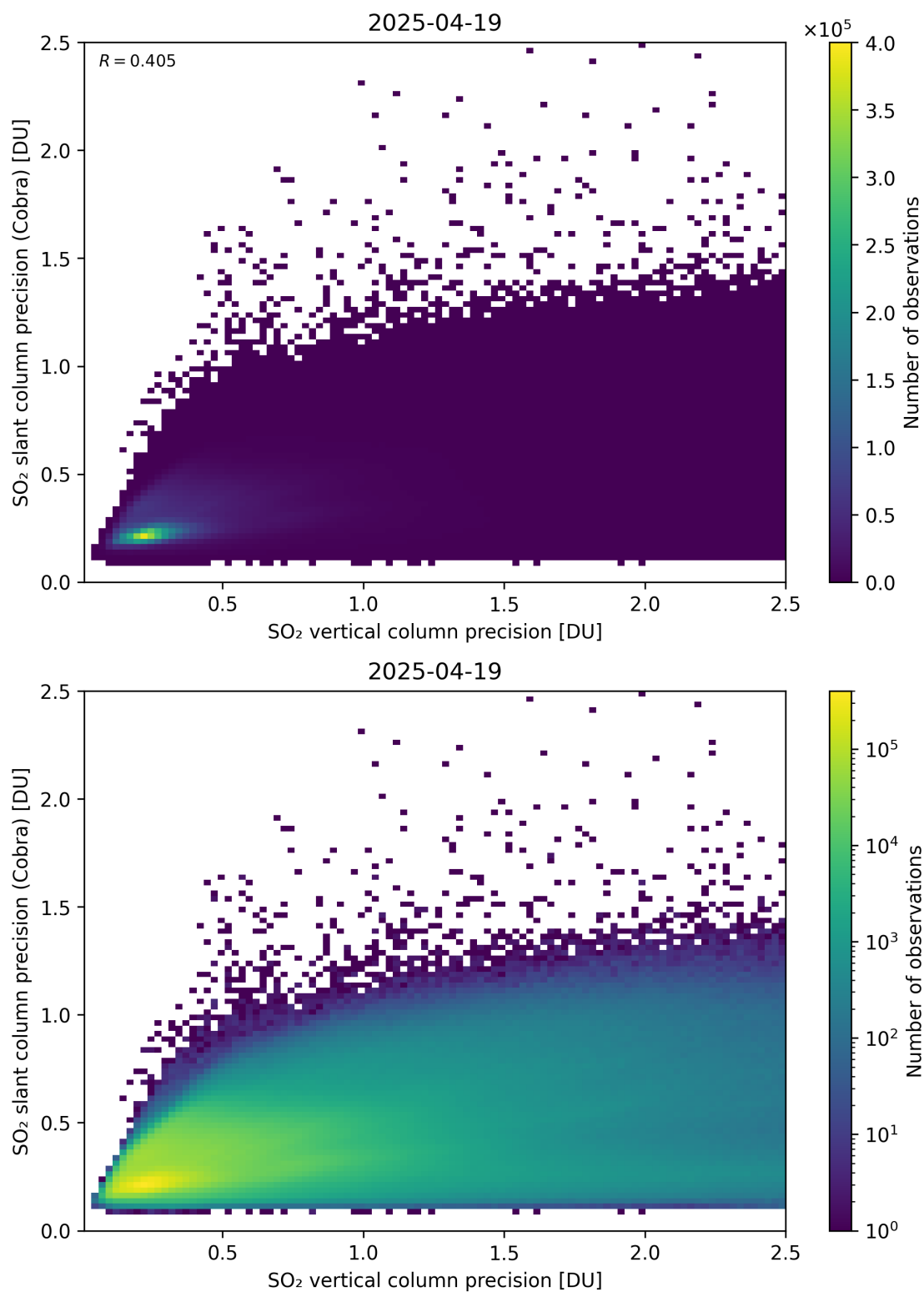
Figure 337: Scatter density plot of “SO 2 vertical column precision” against “SO 2 slant column precision (Cobra)” for 2025-04-19 to 2025-04-20.
