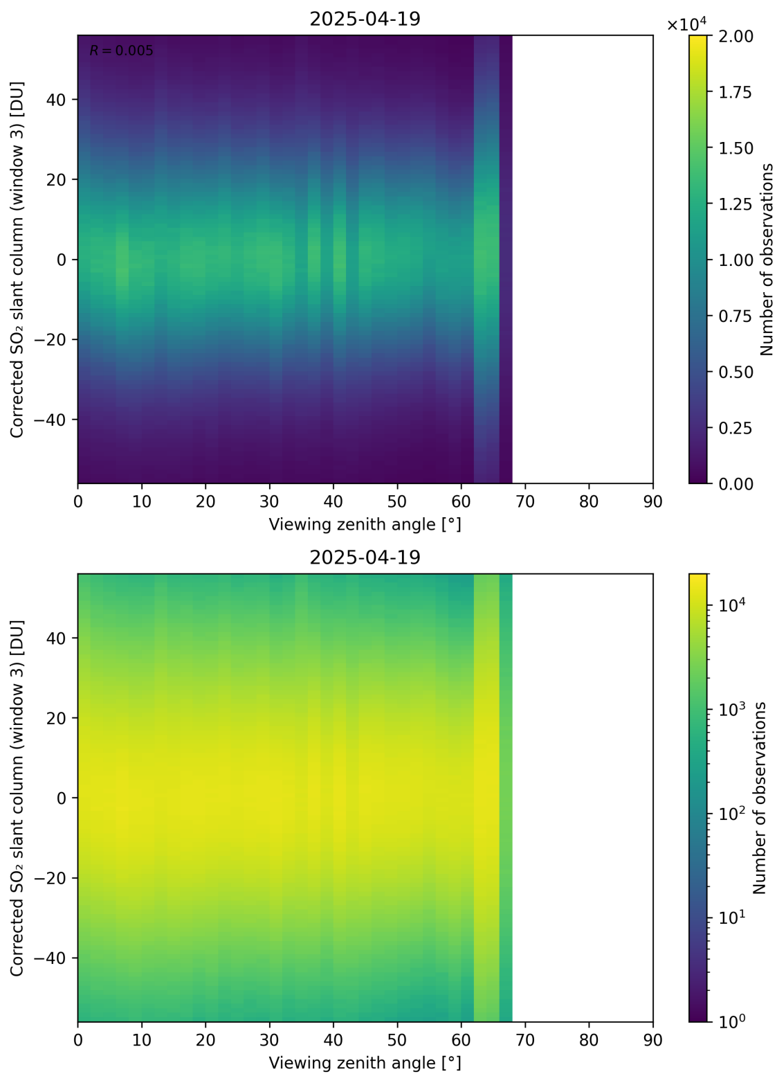
Figure 375: Scatter density plot of “Viewing zenith angle” against “Corrected SO 2 slant column (window 3)” for 2025-04-19 to 2025-04-20.
