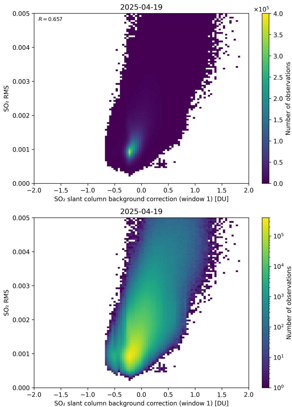
Figure 113: Scatter density plot of “SO 2 slant column background correction (window 1)” against “SO 2 RMS” for 2025-04-19 to 2025-04-20.
