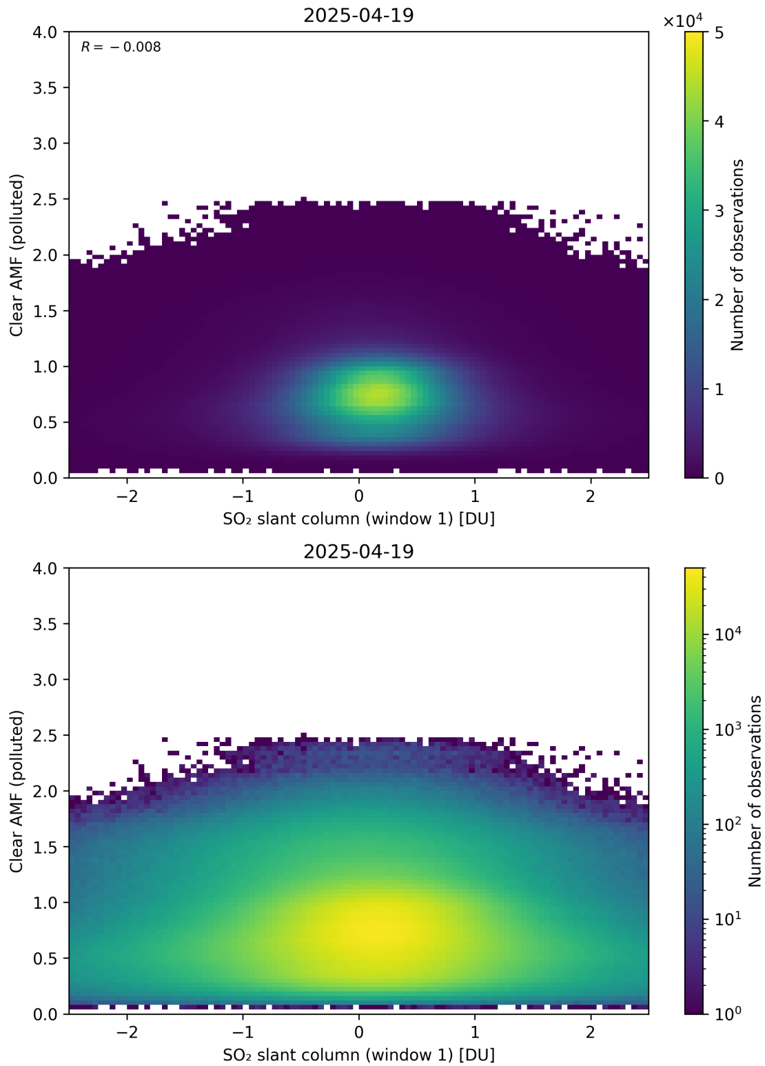
Figure 282: Scatter density plot of “SO 2 slant column (window 1)” against “Clear AMF (polluted)” for 2025-04-19 to 2025-04-20.
