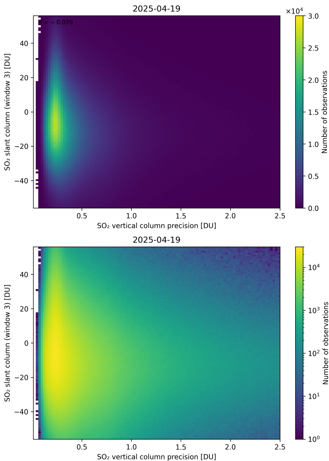
Figure 344: Scatter density plot of “SO 2 vertical column precision” against “SO 2 slant column (window 3)” for 2025-04-19 to 2025-04-20.
