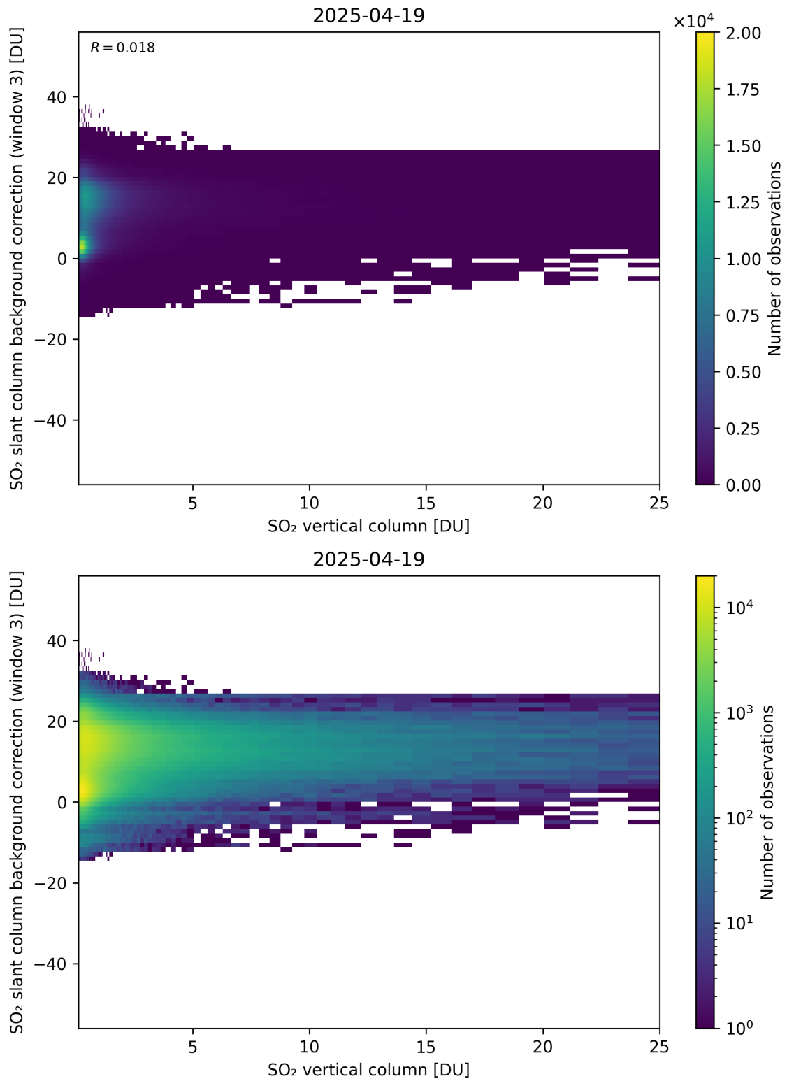
Figure 325: Scatter density plot of “SO 2 vertical column” against “SO 2 slant column background correction (window 3)” for 2025-04-19 to 2025-04-20.
