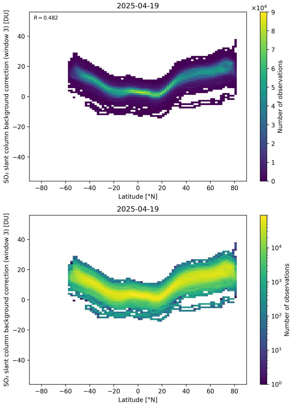
Figure 152: Scatter density plot of “Latitude” against “SO 2 slant column background correction (window 3)” for 2025-04-19 to 2025-04-20.
