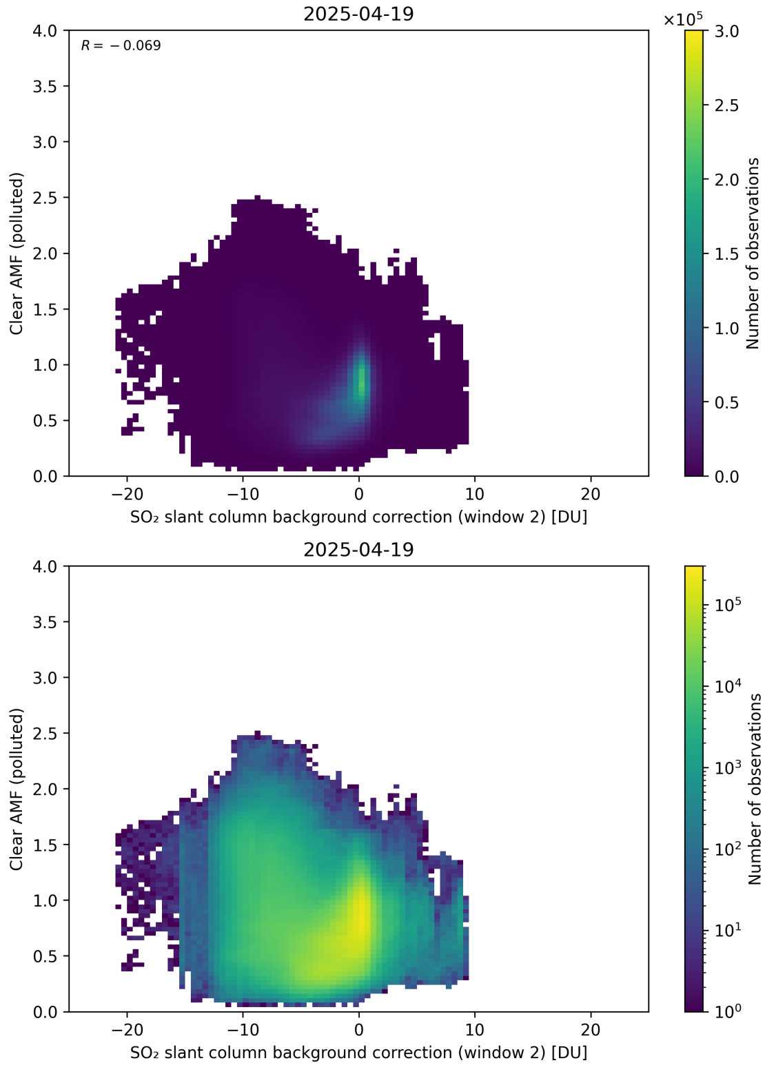
Figure 126: Scatter density plot of “SO 2 slant column background correction (window 2)” against “Clear AMF (polluted)” for 2025-04-19 to 2025-04-20.
