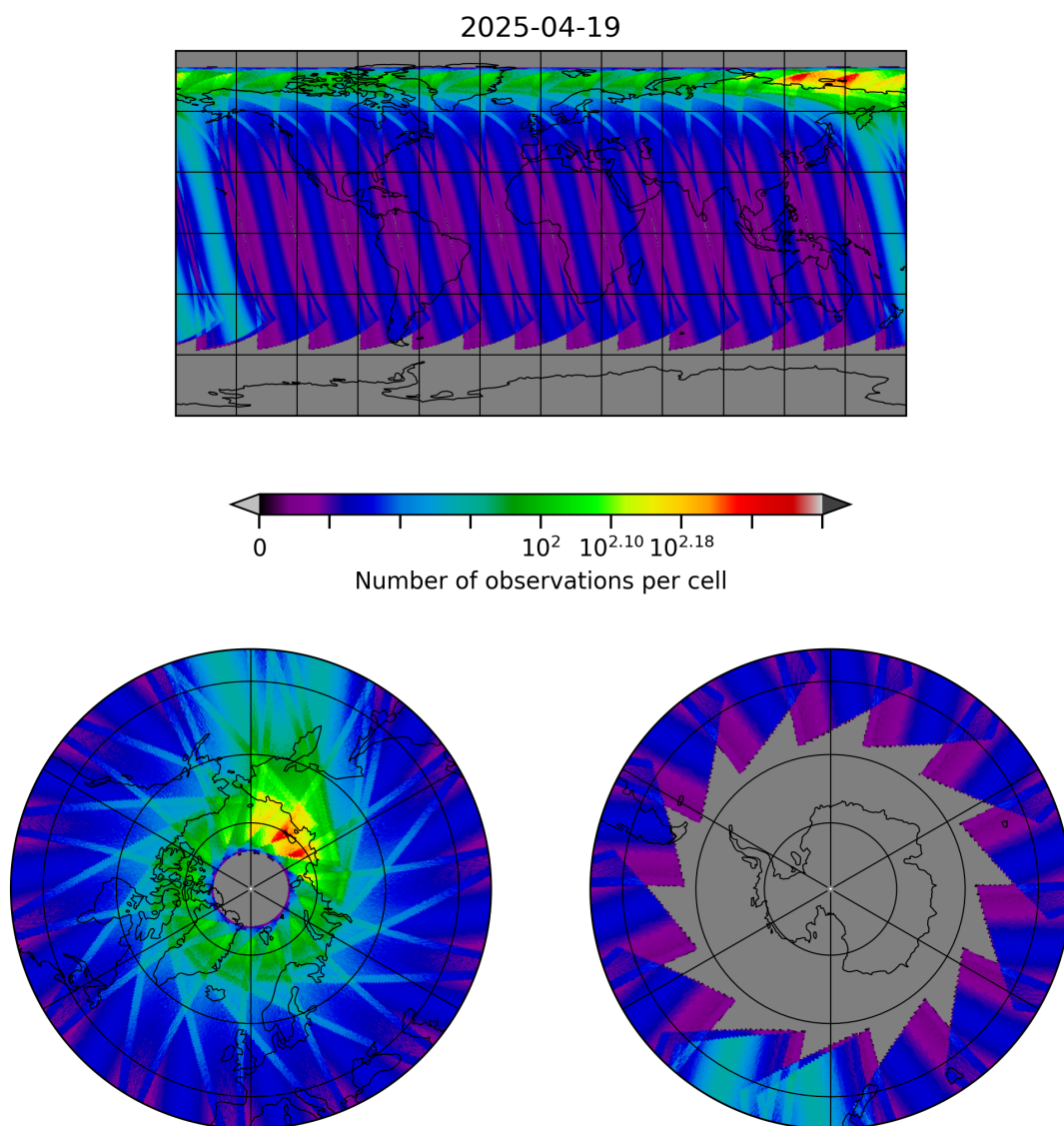
Figure 30: Map of the number of observations for 2025-04-19 to 2025-04-20
