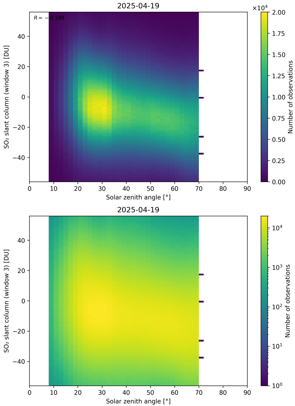
Figure 187: Scatter density plot of “Solar zenith angle” against “SO 2 slant column (window 3)” for 2025-04-19 to 2025-04-20.
