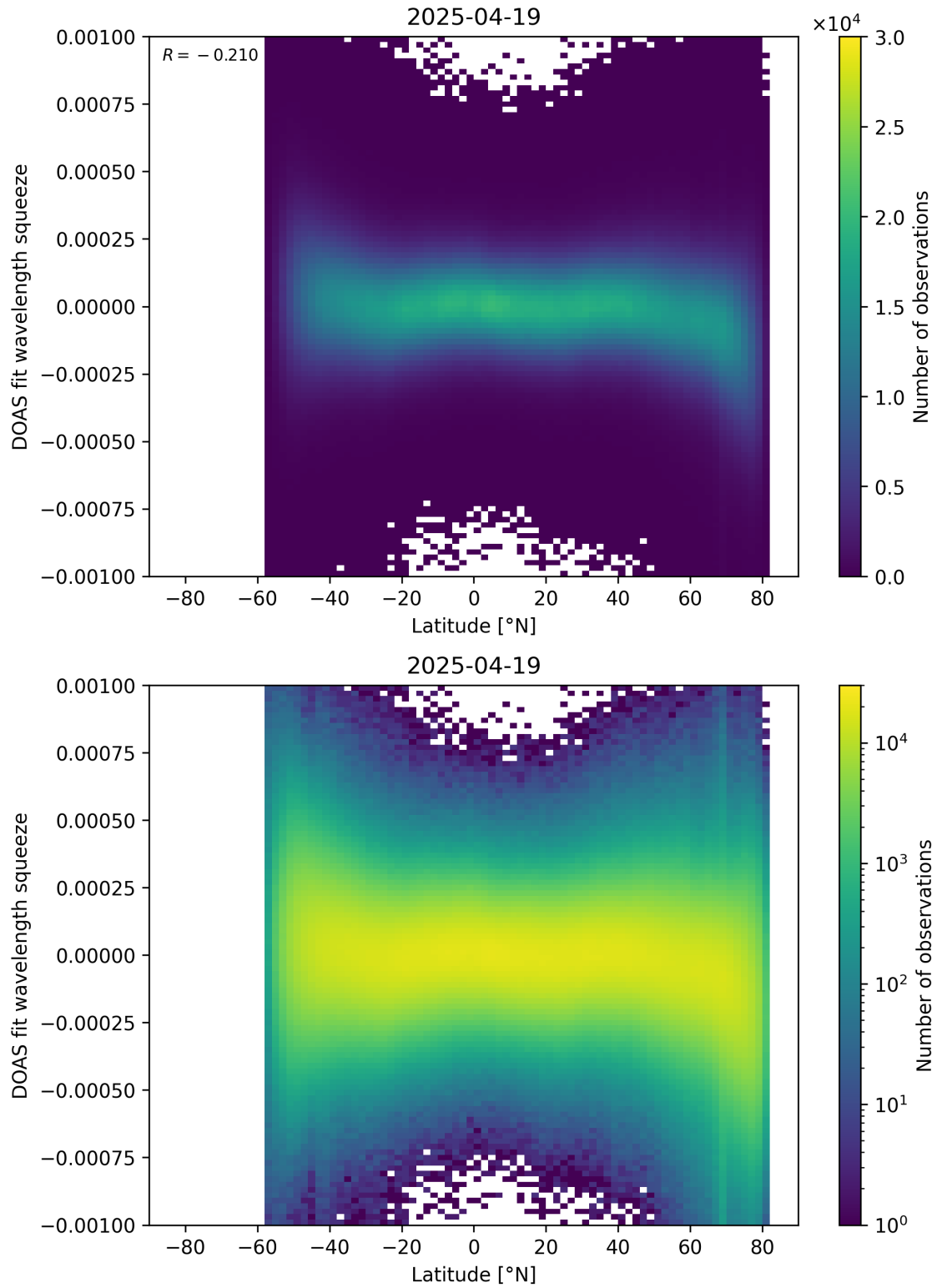
Figure 154: Scatter density plot of “Latitude” against “DOAS fit wavelength squeeze” for 2025-04-19 to 2025-04-20.
