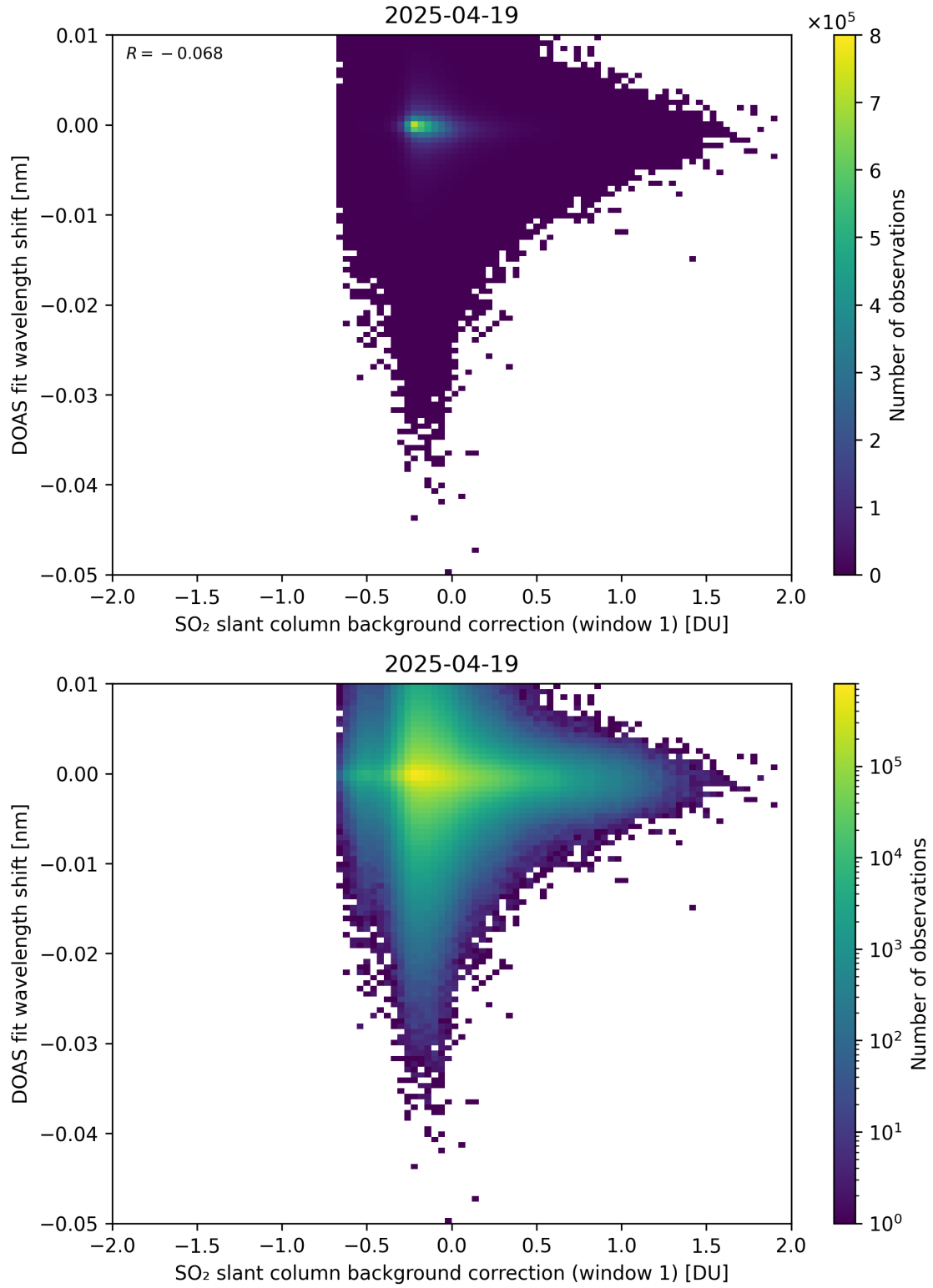
Figure 111: Scatter density plot of “SO 2 slant column background correction (window 1)” against “DOAS fit wavelength shift” for 2025-04-19 to 2025-04-20.
