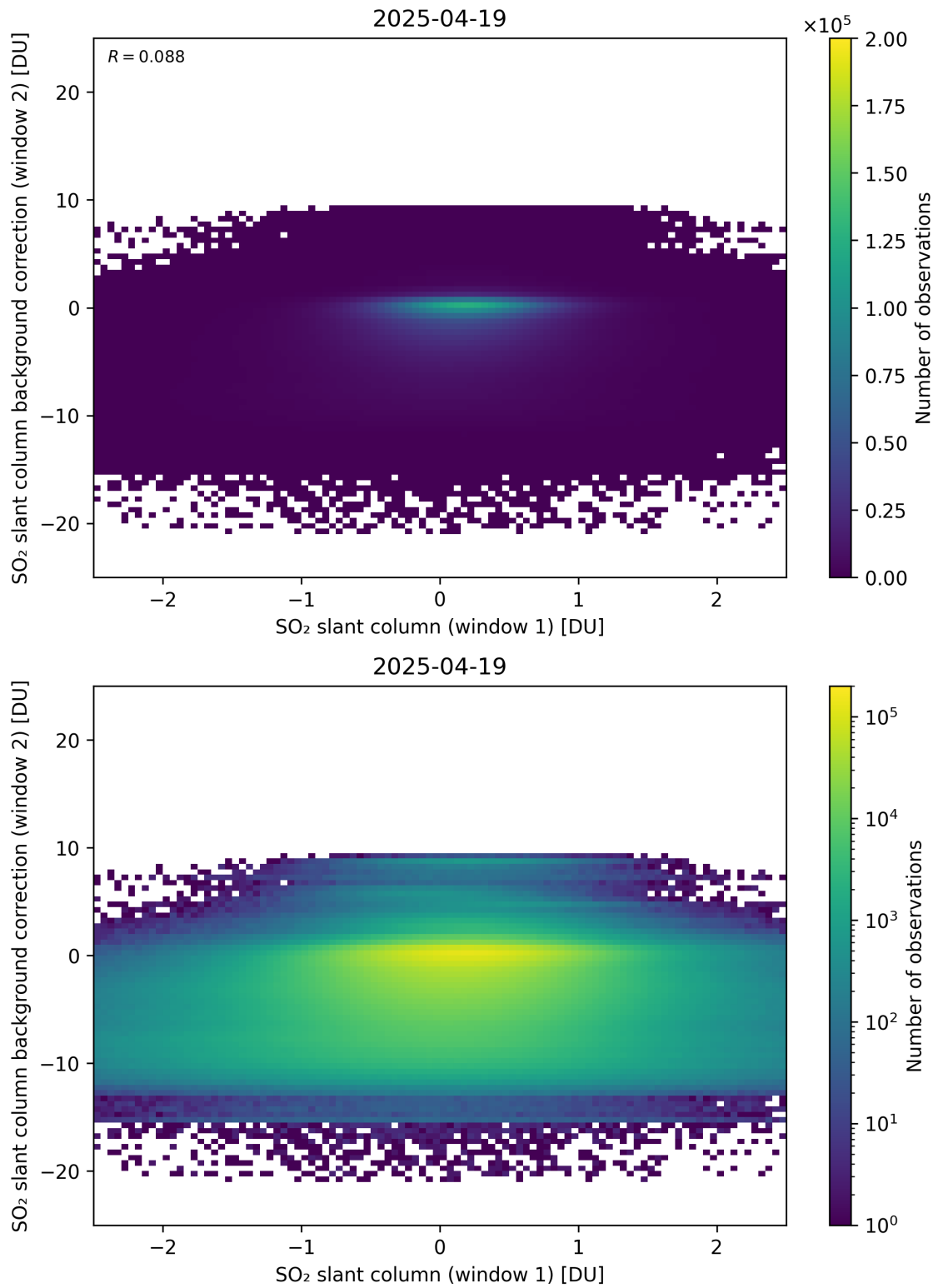
Figure 263: Scatter density plot of “SO 2 slant column (window 1)” against “SO 2 slant column background correction (window 2)” for 2025-04-19 to 2025-04-20.
