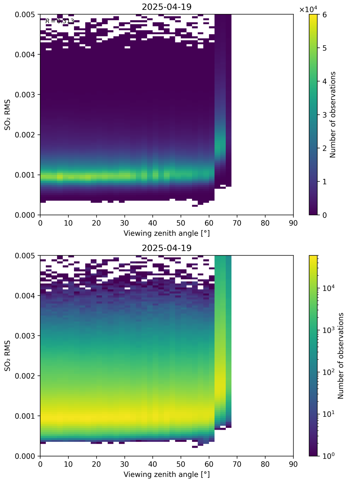
Figure 367: Scatter density plot of “Viewing zenith angle” against “SO 2 RMS” for 2025-04-19 to 2025-04-20.
