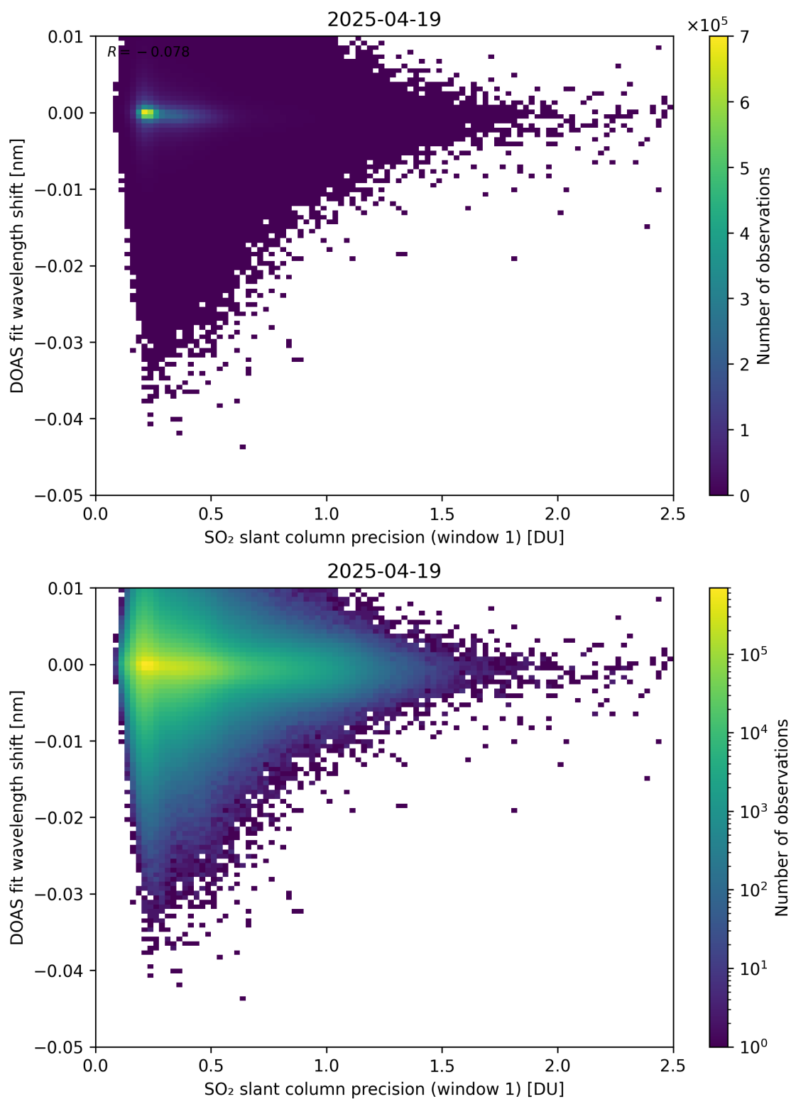
Figure 271: Scatter density plot of “SO 2 slant column precision (window 1)” against “DOAS fit wavelength shift” for 2025-04-19 to 2025-04-20.
