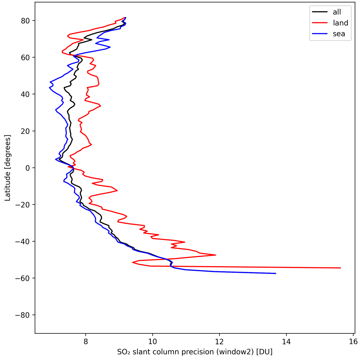
Figure 42: Zonal average of “SO 2 slant column precision (window2)” for 2025-04-19 to 2025-04-20.
