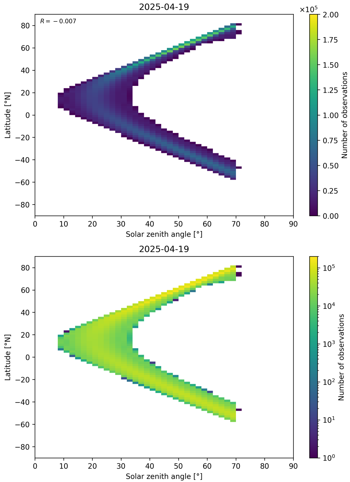
Figure 177: Scatter density plot of “Solar zenith angle” against “Latitude” for 2025-04-19 to 2025-04-20.
