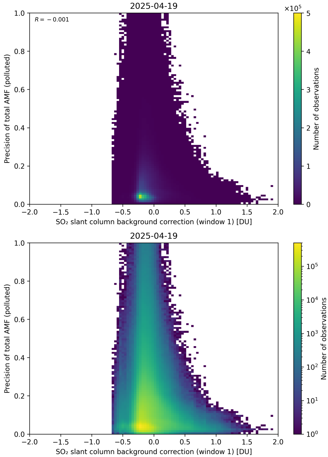
Figure 121: Scatter density plot of “SO 2 slant column background correction (window 1)” against “Precision of total AMF (polluted)” for 2025-04-19 to 2025-04-20.
