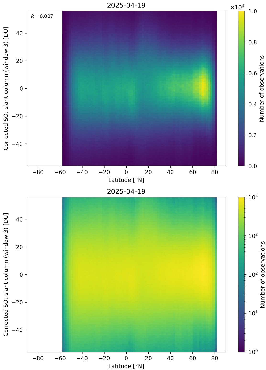
Figure 161: Scatter density plot of “Latitude” against “Corrected SO 2 slant column (window 3)” for 2025-04-19 to 2025-04-20.
