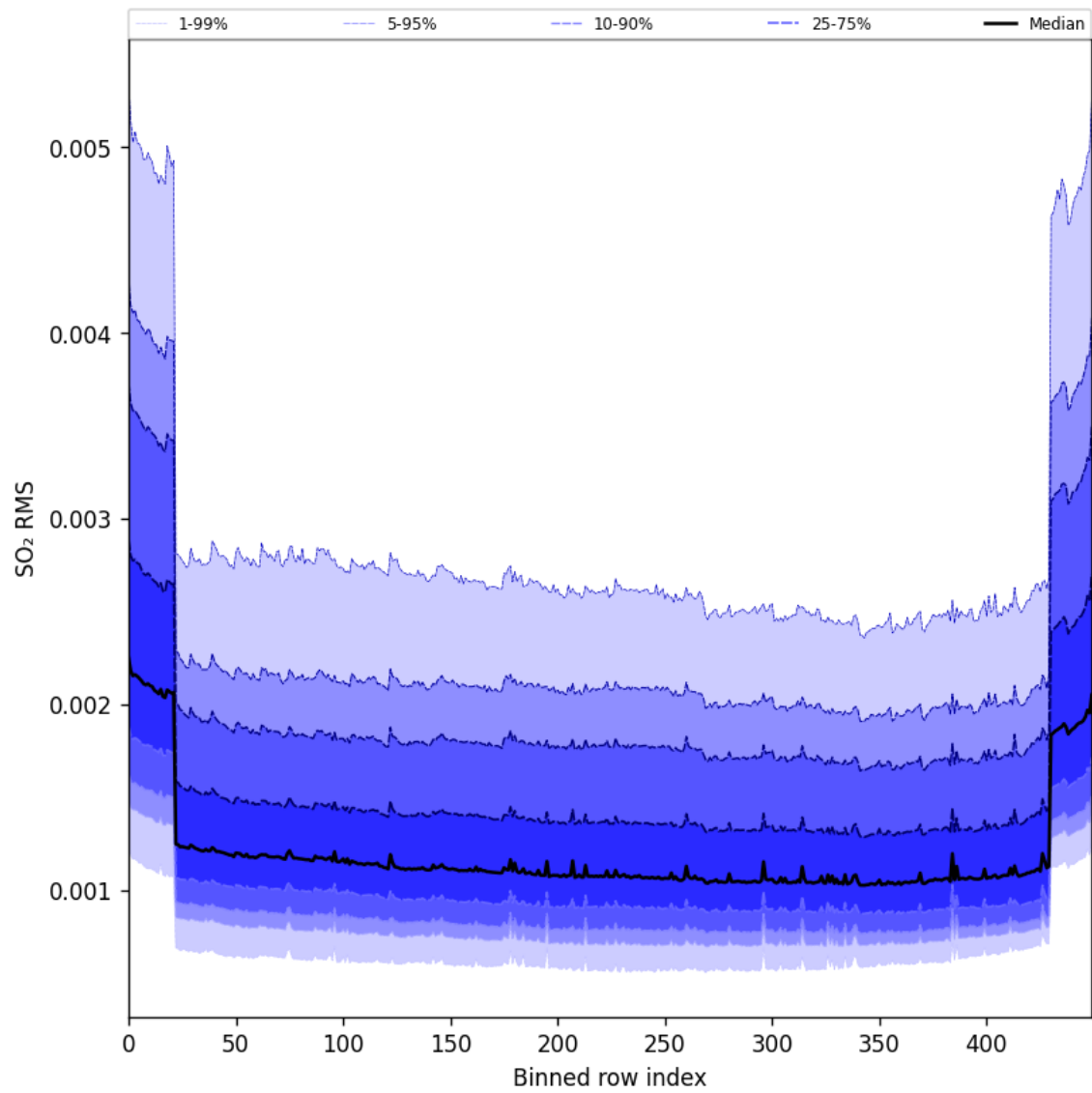
Figure 104: Along track statistics of “SO 2 RMS” for 2025-04-19 to 2025-04-20
