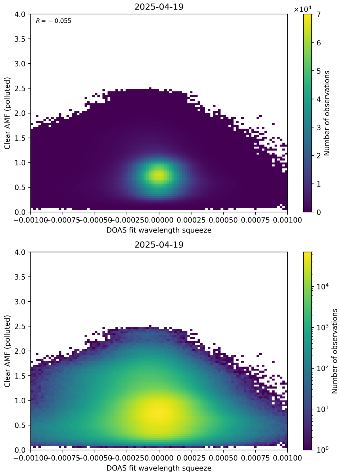
Figure 144: Scatter density plot of “DOAS fit wavelength squeeze” against “Clear AMF (polluted)” for 2025-04-19 to 2025-04-20.
