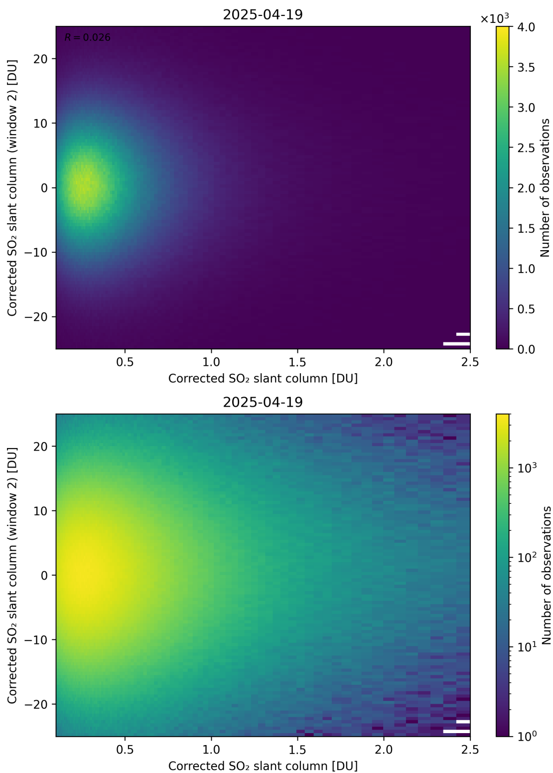
Figure 235: Scatter density plot of “Corrected SO 2 slant column” against “Corrected SO 2 slant column (window 2)” for 2025-04-19 to 2025-04-20.
