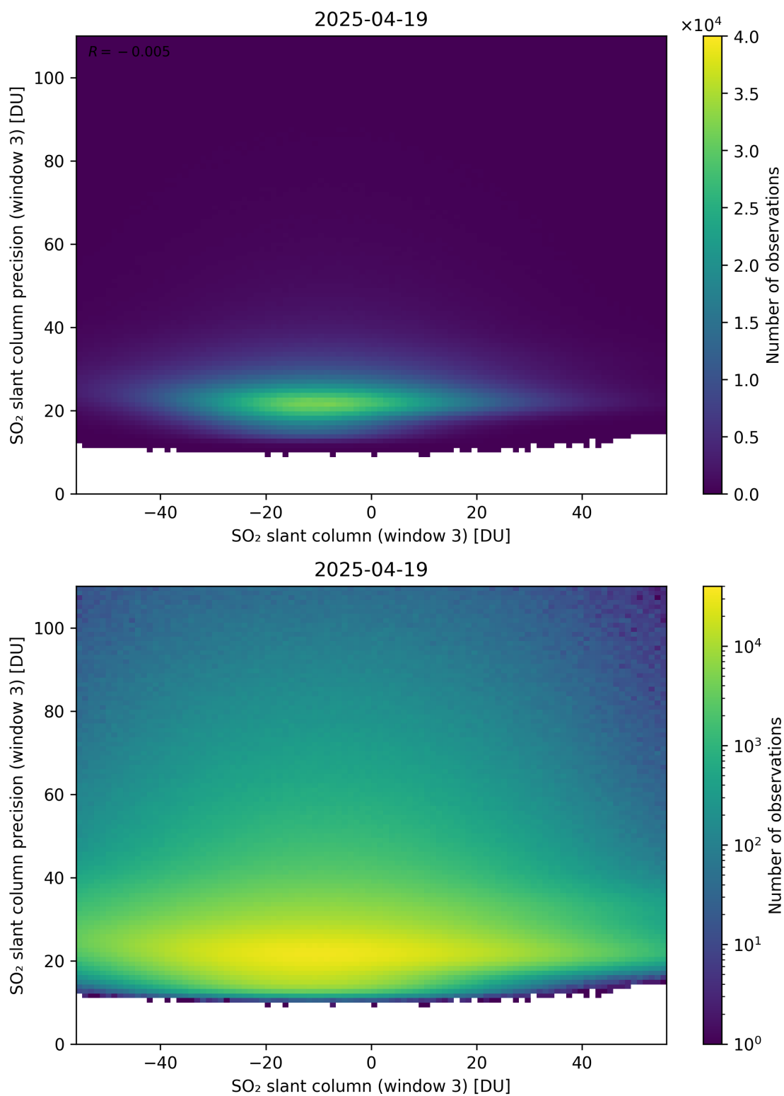
Figure 317: Scatter density plot of “SO 2 slant column (window 3)” against “SO 2 slant column precision (window 3)” for 2025-04-19 to 2025-04-20.
