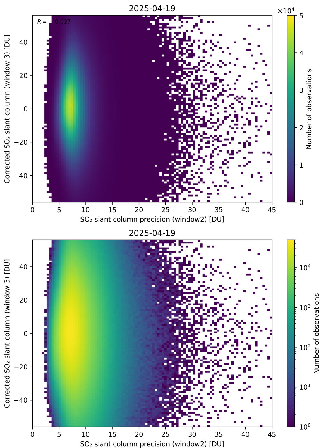
Figure 298: Scatter density plot of “SO 2 slant column precision (window2)” against “Corrected SO 2 slant column (window 3)” for 2025-04-19 to 2025-04-20.
