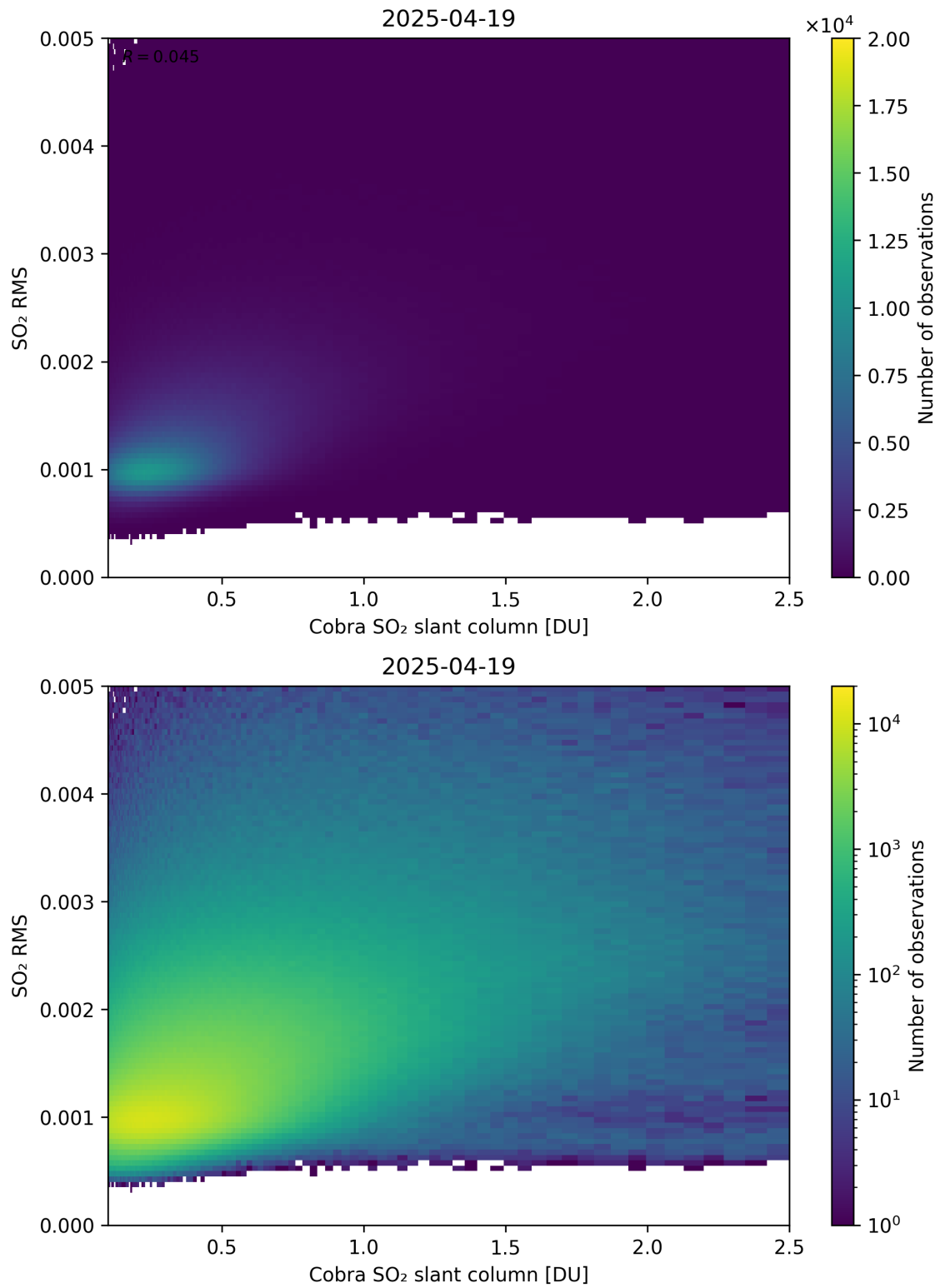
Figure 198: Scatter density plot of “Cobra SO 2 slant column” against “SO 2 RMS” for 2025-04-19 to 2025-04-20.
