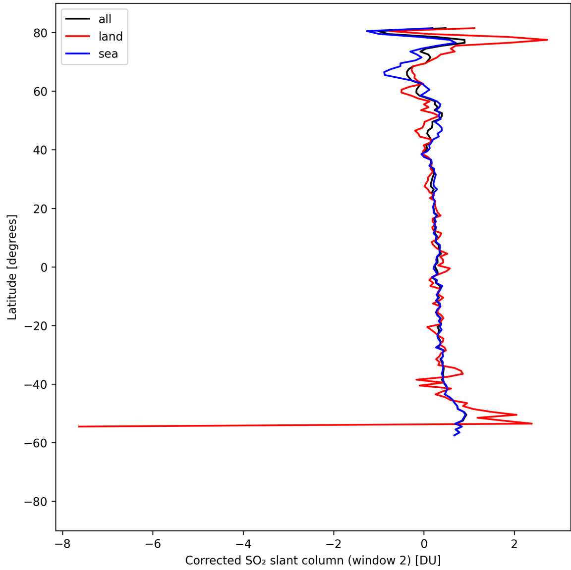
Figure 43: Zonal average of “Corrected SO 2 slant column (window 2)” for 2025-04-19 to 2025-04-20.
