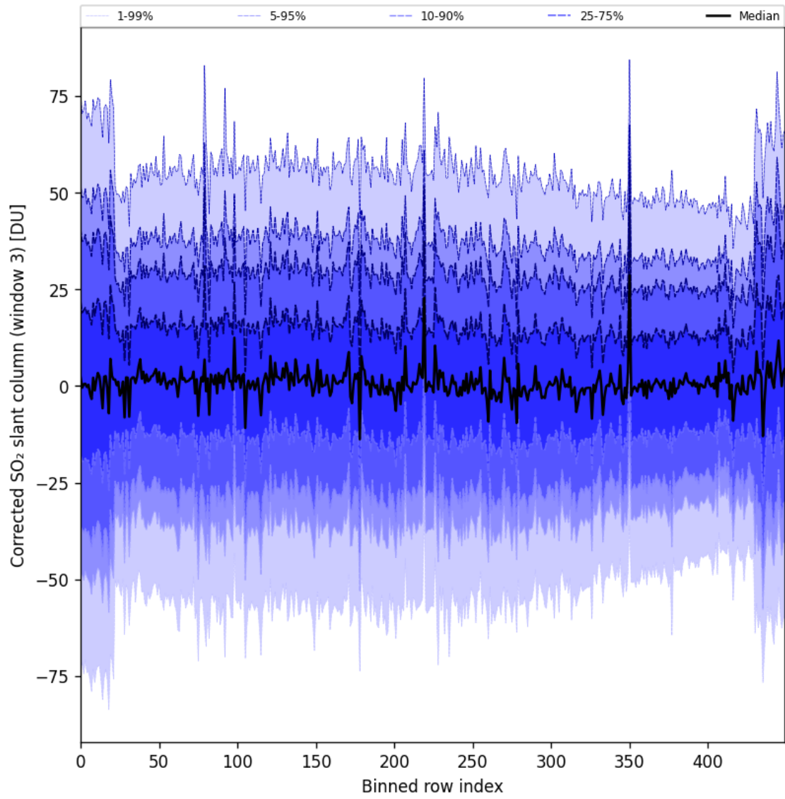
Figure 99: Along track statistics of “Corrected SO 2 slant column (window 3)” for 2025-04-19 to 2025-04-20
