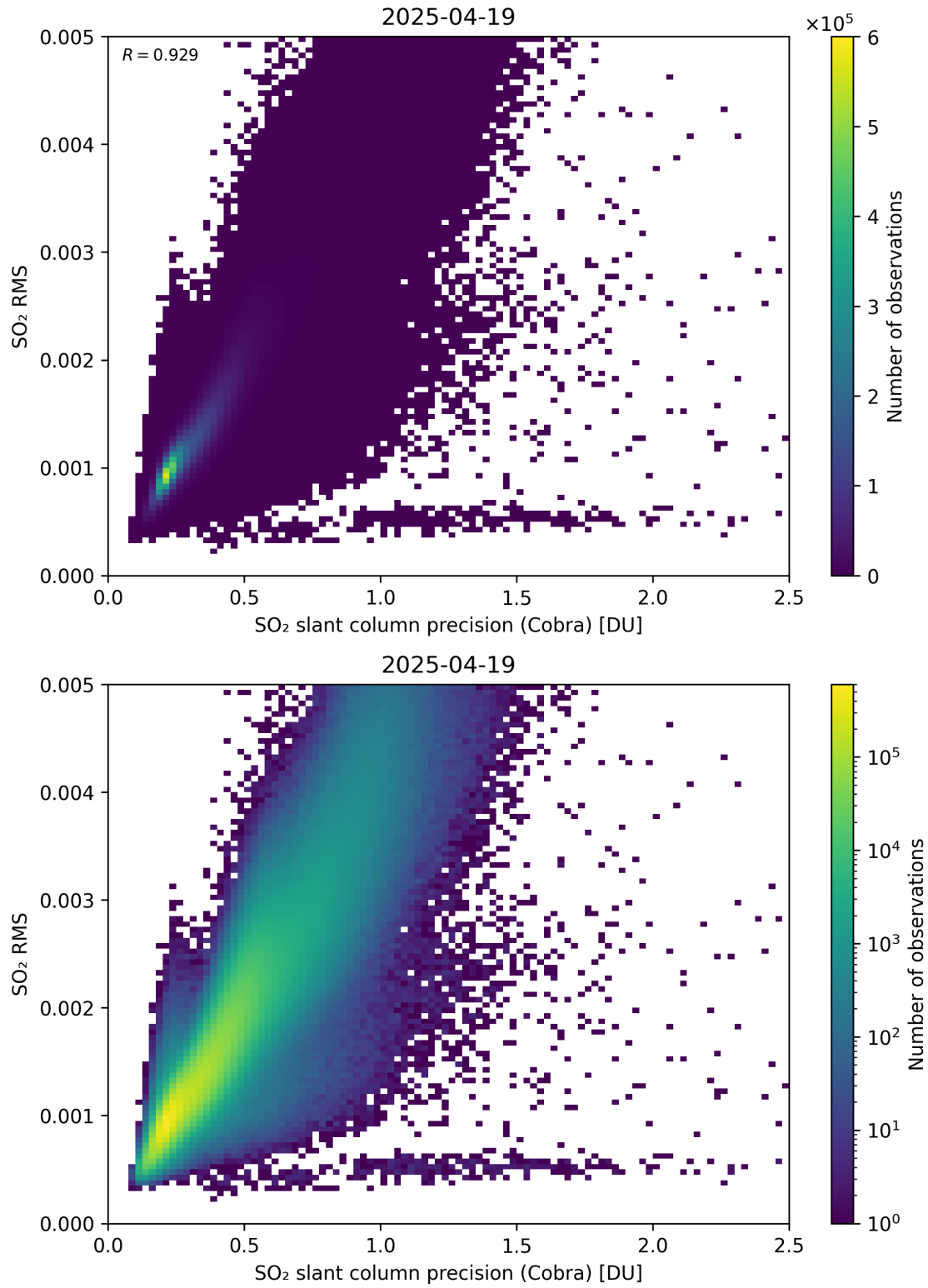
Figure 204: Scatter density plot of “SO 2 slant column precision (Cobra)” against “SO 2 RMS” for 2025-04-19 to 2025-04-20.
