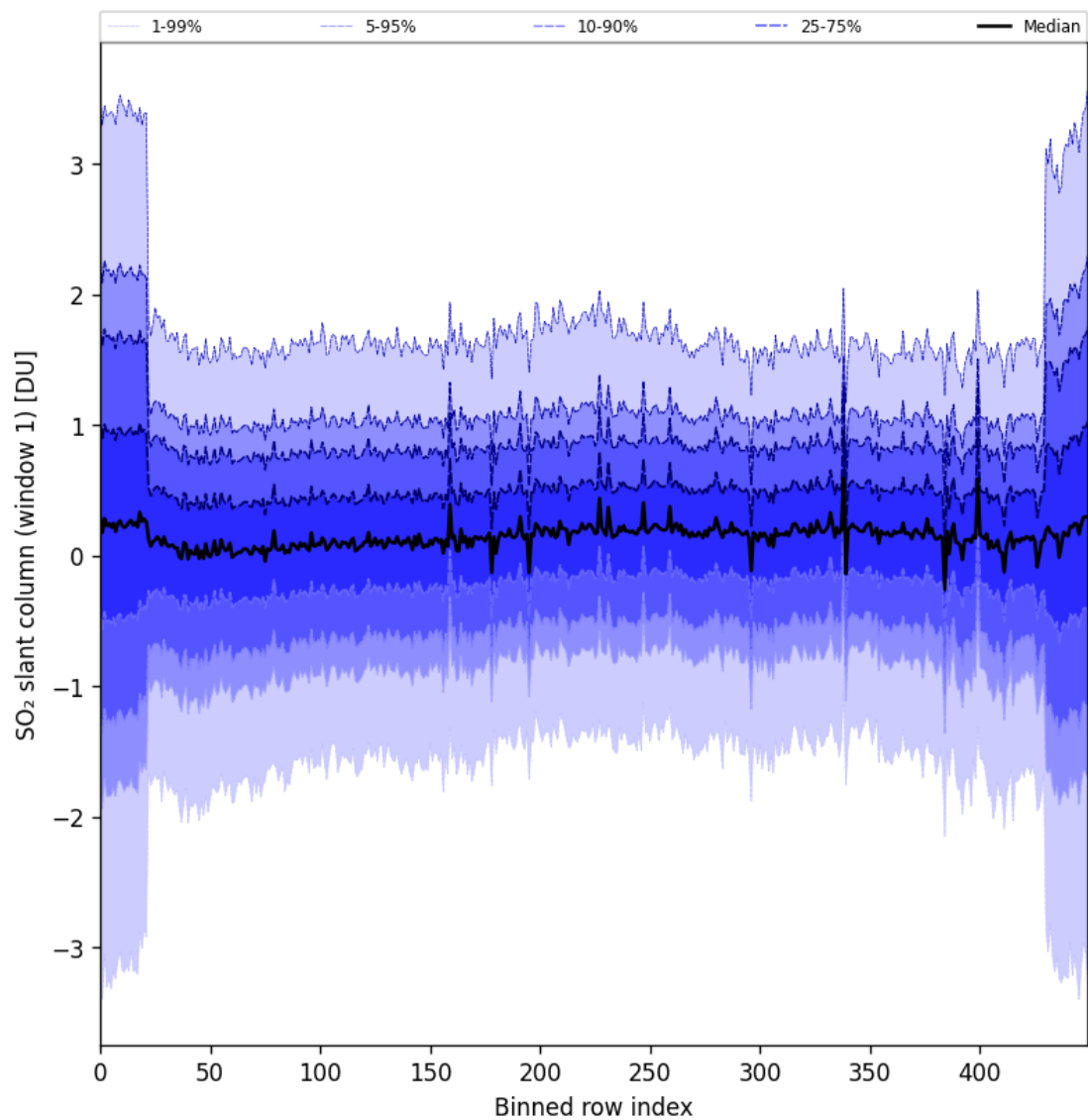
Figure 89: Along track statistics of “SO 2 slant column (window 1)” for 2025-04-19 to 2025-04-20
