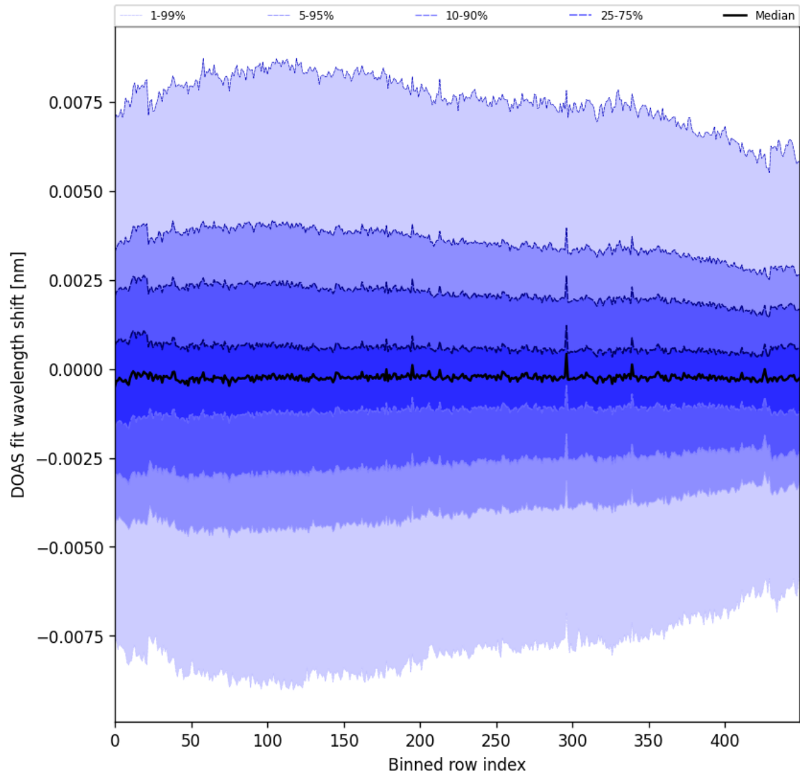
Figure 102: Along track statistics of “DOAS fit wavelength shift” for 2025-04-19 to 2025-04-20
