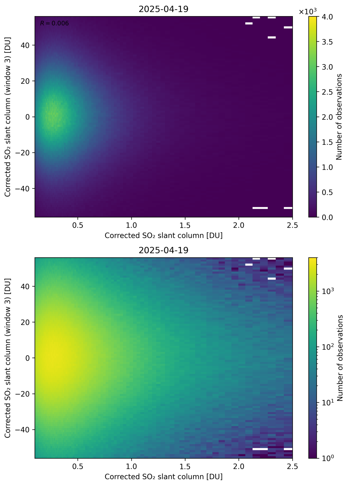
Figure 236: Scatter density plot of “Corrected SO 2 slant column” against “Corrected SO 2 slant column (window 3)” for 2025-04-19 to 2025-04-20.
