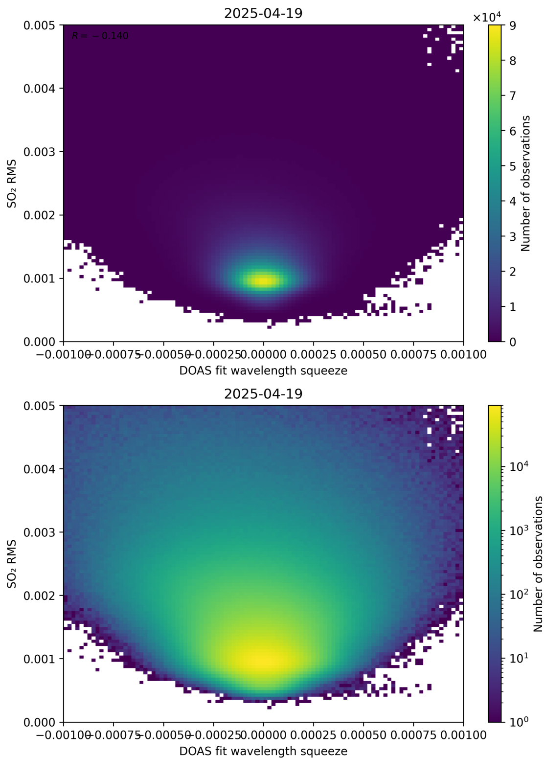
Figure 143: Scatter density plot of “DOAS fit wavelength squeeze” against “SO 2 RMS” for 2025-04-19 to 2025-04-20.
