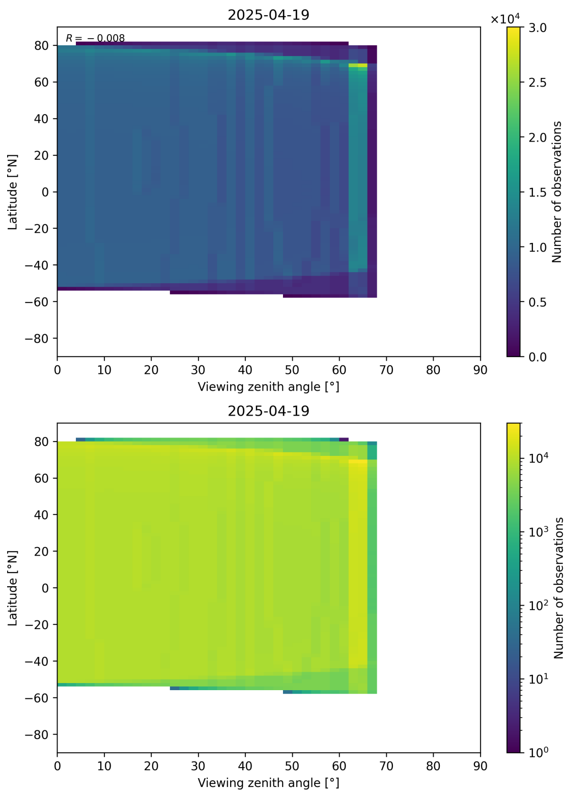
Figure 368: Scatter density plot of “Viewing zenith angle” against “Latitude” for 2025-04-19 to 2025-04-20.
