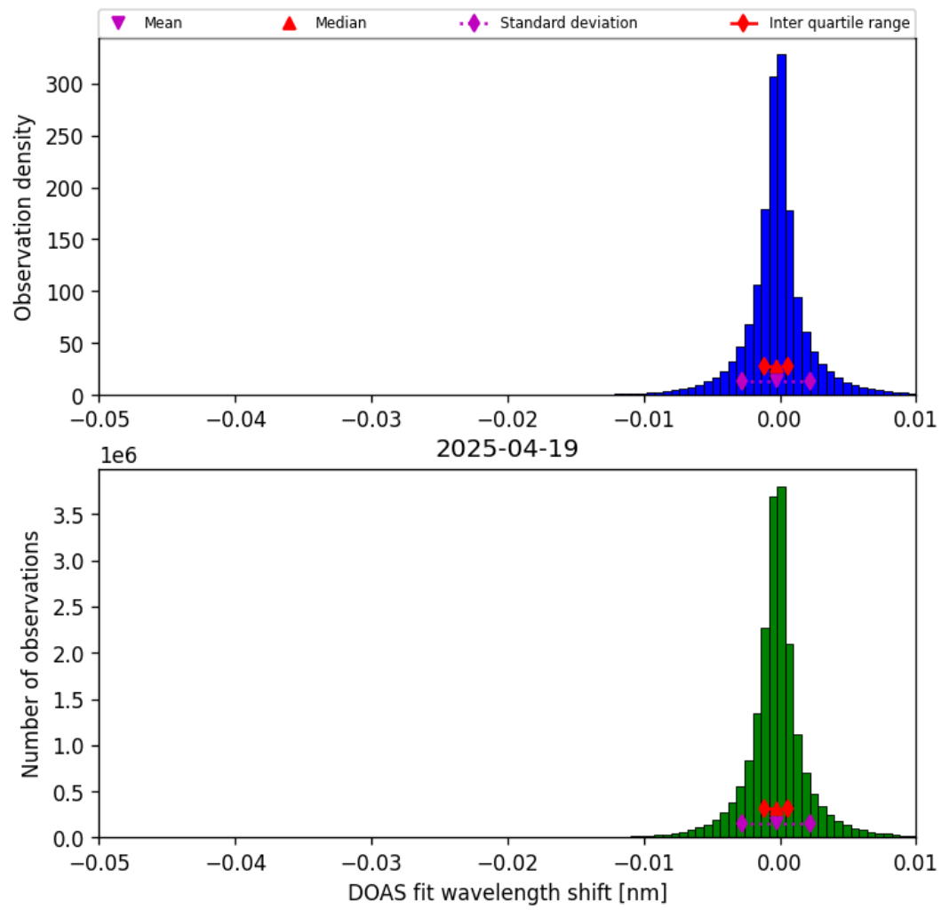
Figure 76: Histogram of “DOAS fit wavelength shift” for 2025-04-19 to 2025-04-20
