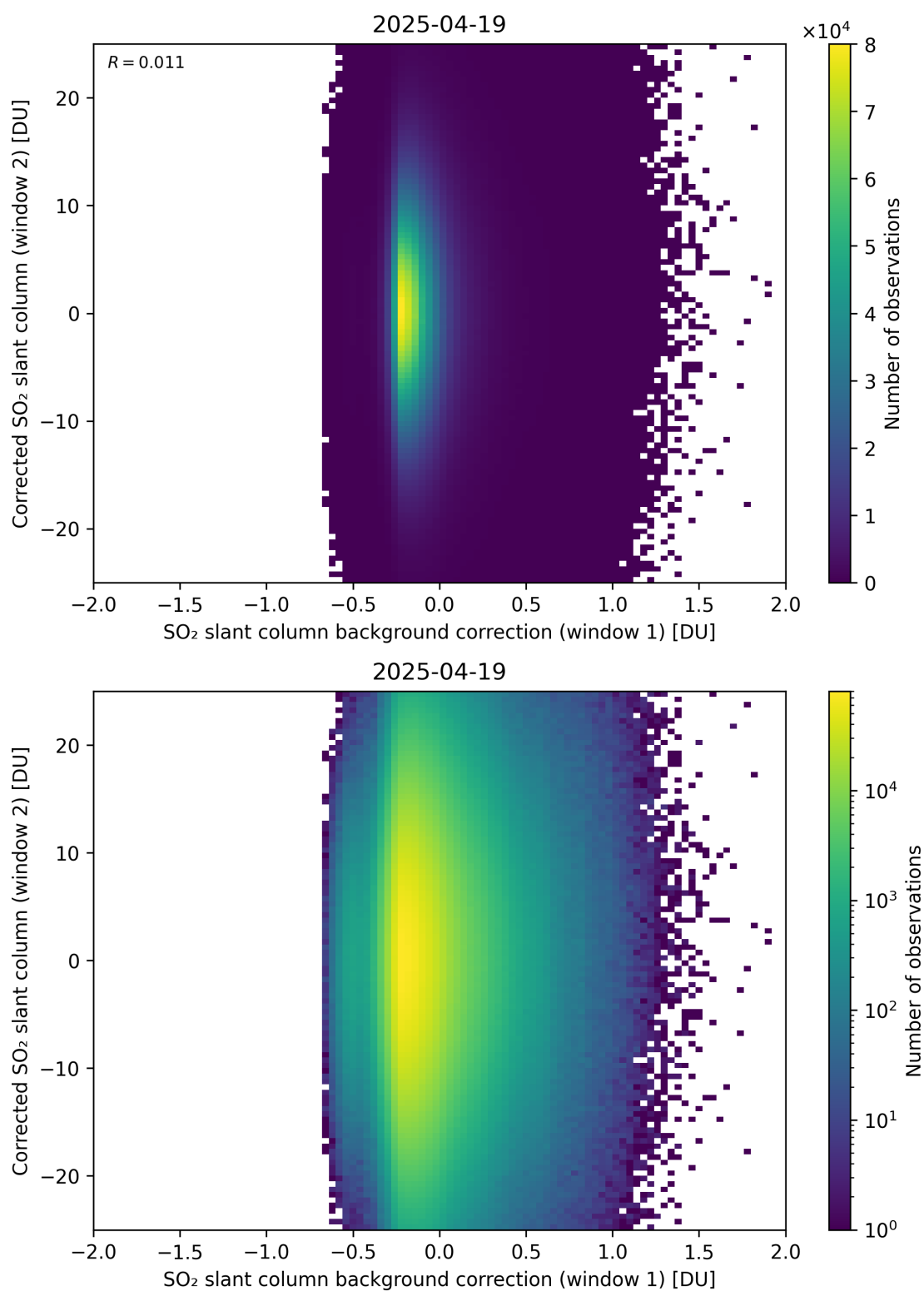
Figure 115: Scatter density plot of “SO 2 slant column background correction (window 1)” against “Corrected SO 2 slant column (window 2)” for 2025-04-19 to 2025-04-20.
