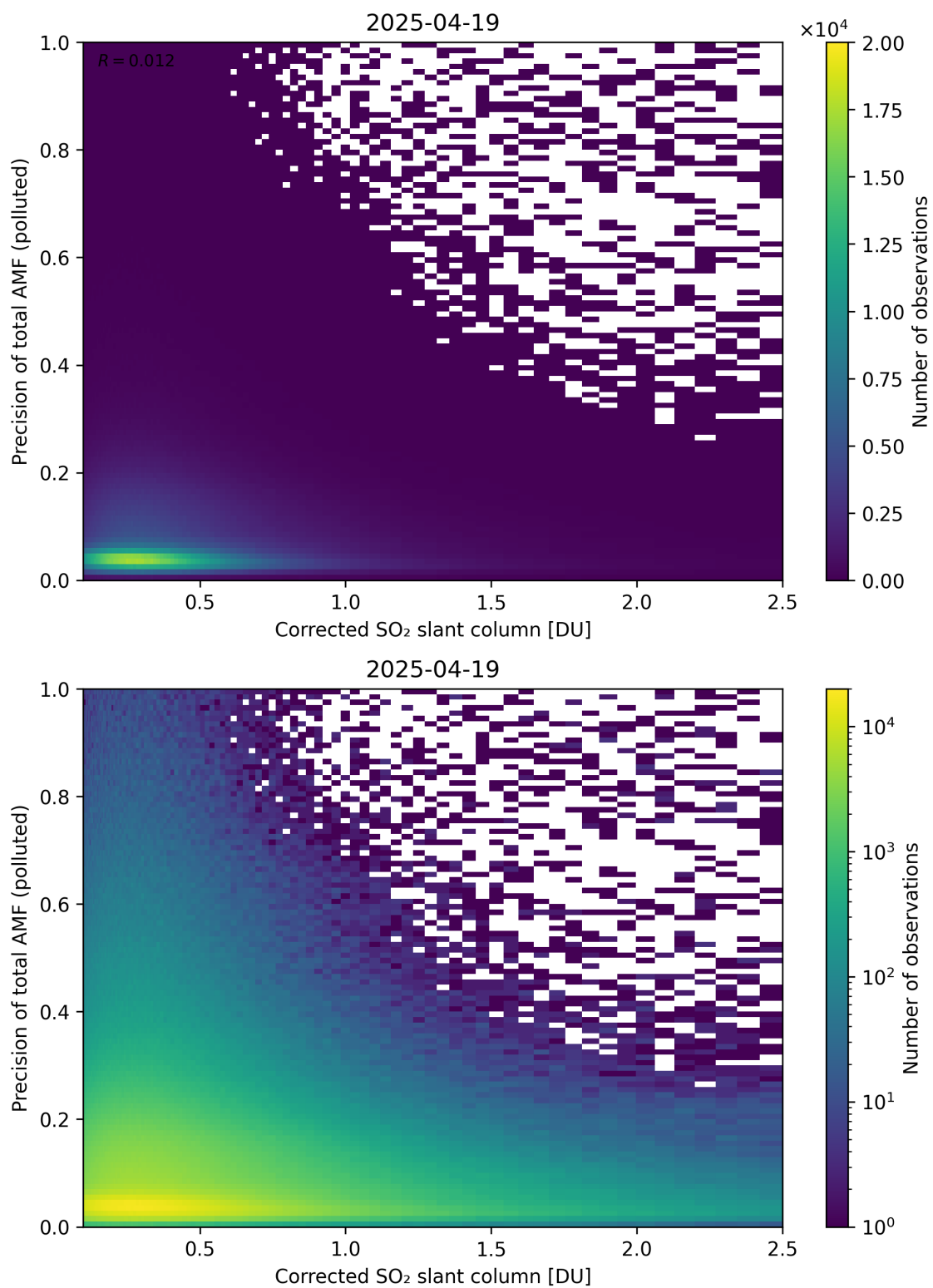
Figure 243: Scatter density plot of “Corrected SO 2 slant column” against “Precision of total AMF (polluted)” for 2025-04-19 to 2025-04-20.
