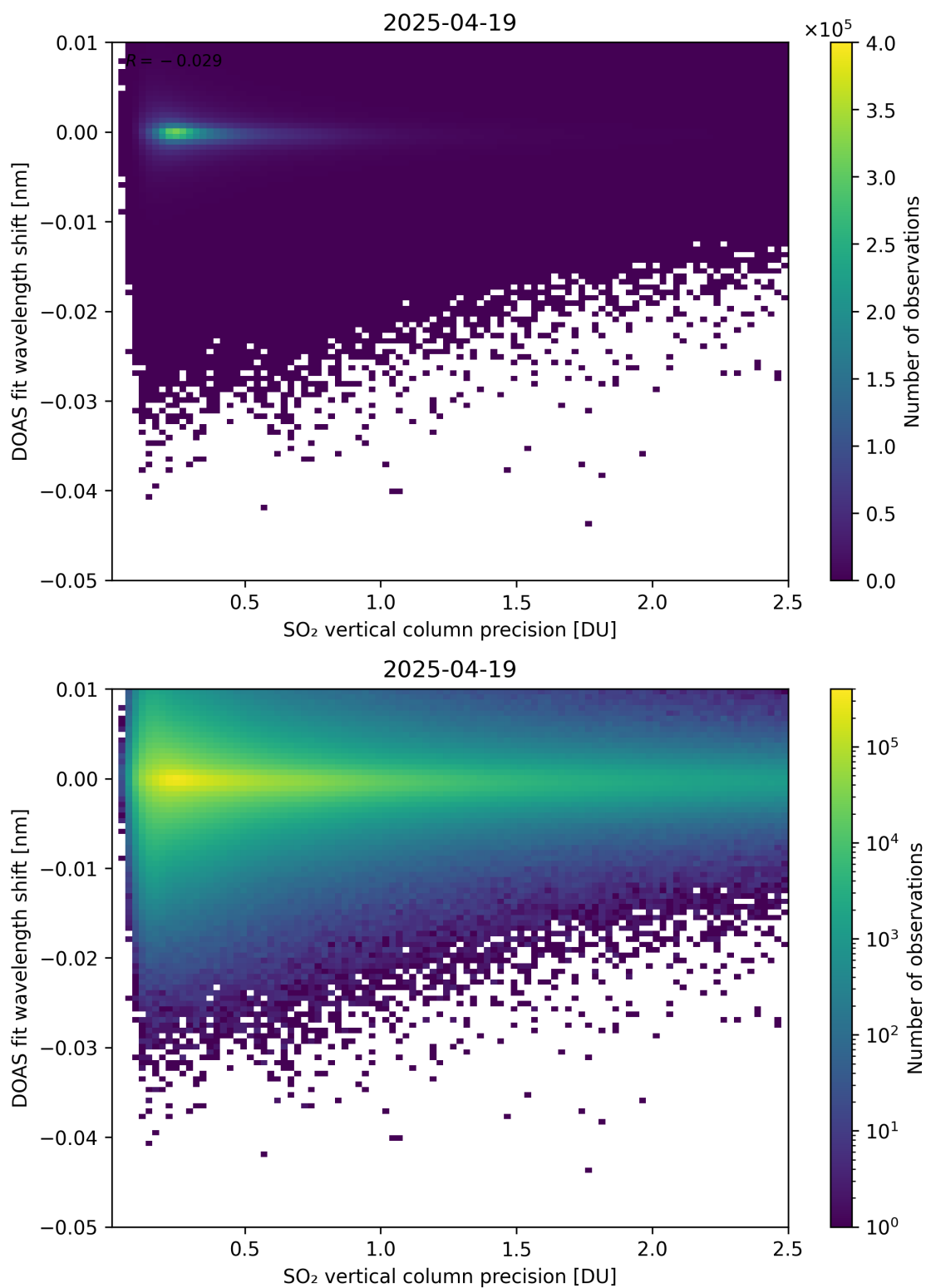
Figure 332: Scatter density plot of “SO 2 vertical column precision” against “DOAS fit wavelength shift” for 2025-04-19 to 2025-04-20.
