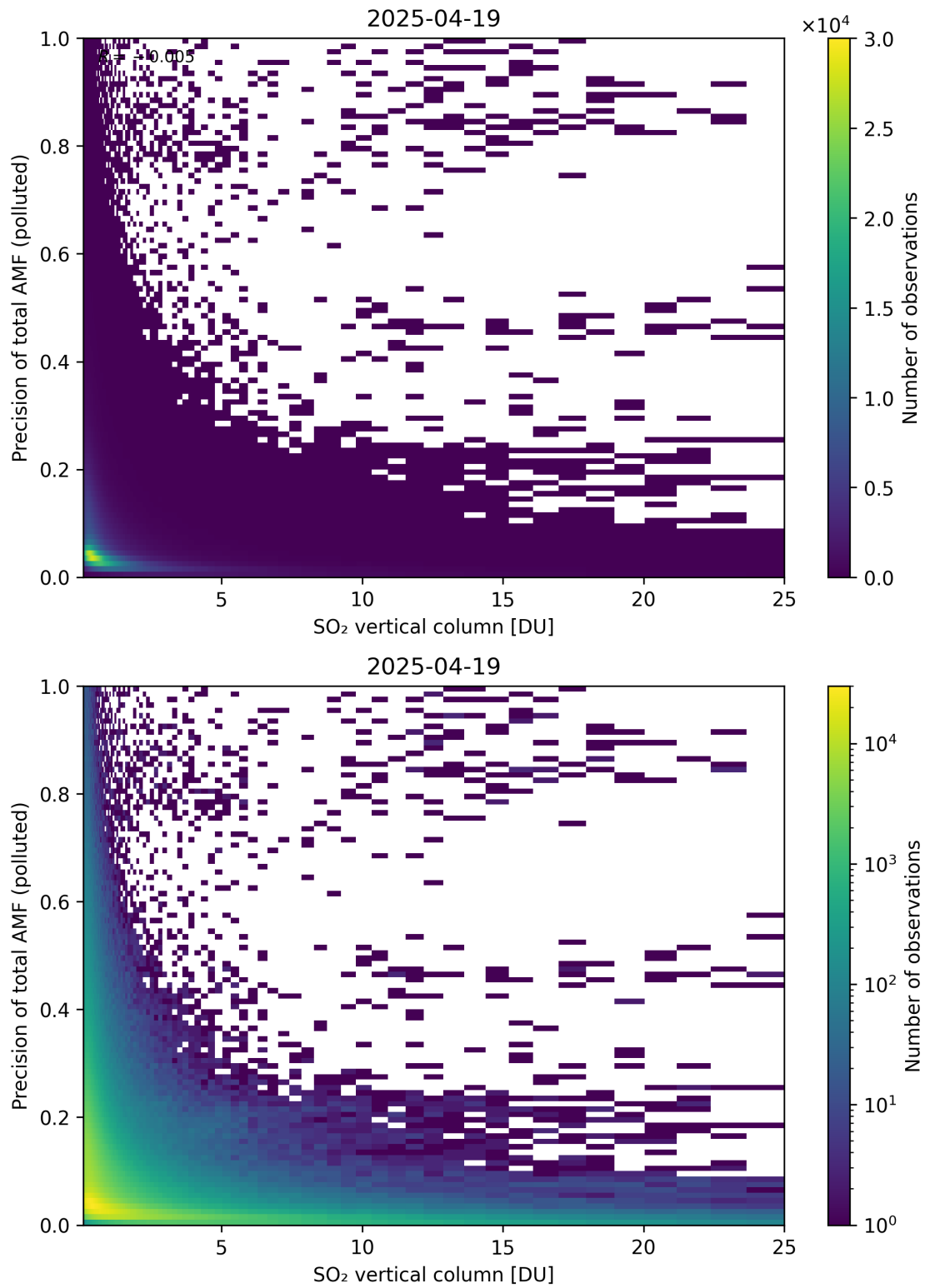
Figure 360: Scatter density plot of “SO 2 vertical column” against “Precision of total AMF (polluted)” for 2025-04-19 to 2025-04-20.
