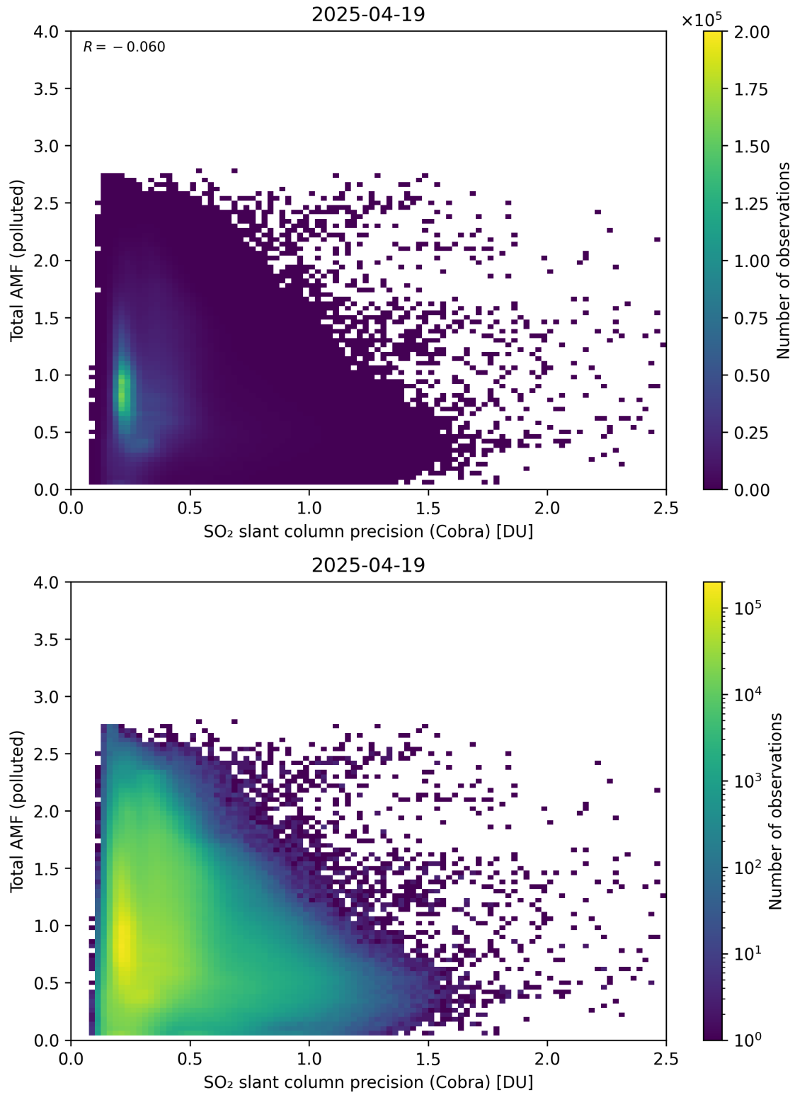
Figure 213: Scatter density plot of “SO 2 slant column precision (Cobra)” against “Total AMF (polluted)” for 2025-04-19 to 2025-04-20.
