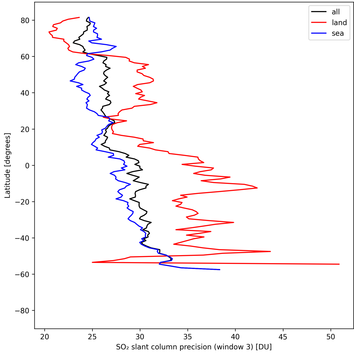
Figure 46: Zonal average of “SO 2 slant column precision (window 3)” for 2025-04-19 to 2025-04-20.
