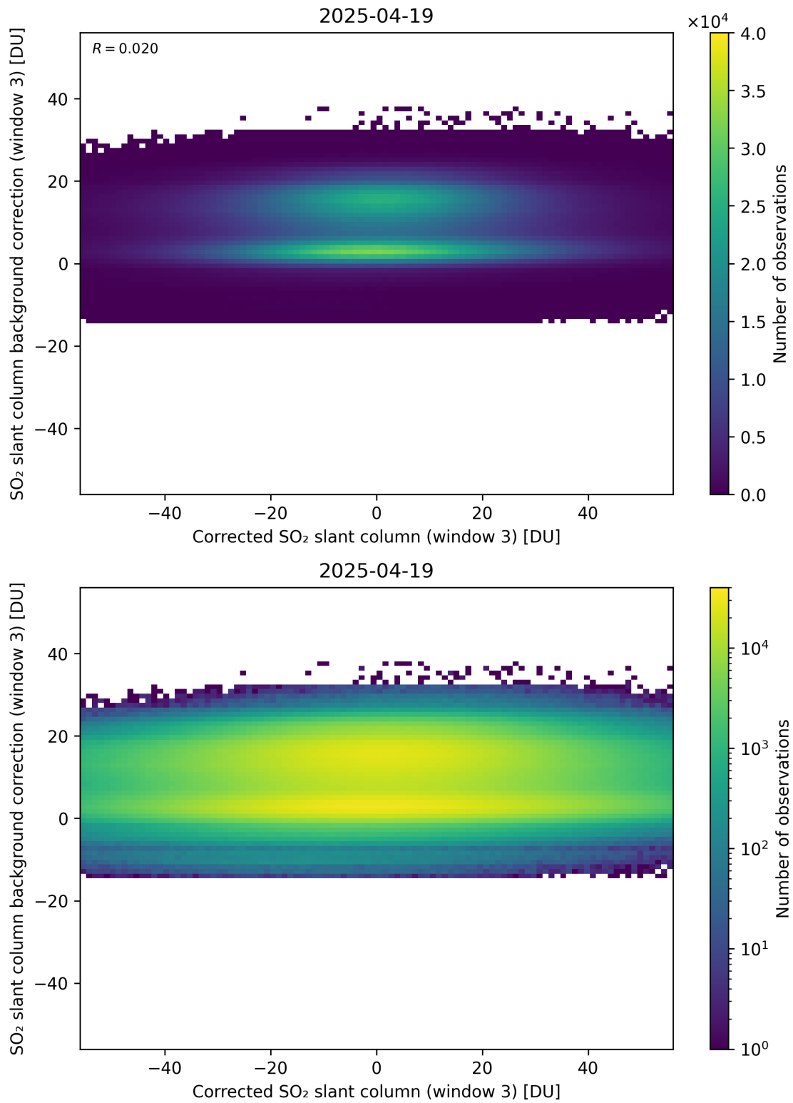
Figure 255: Scatter density plot of “Corrected SO 2 slant column (window 3)” against “SO 2 slant column background correction (window 3)” for 2025-04-19 to 2025-04-20.
