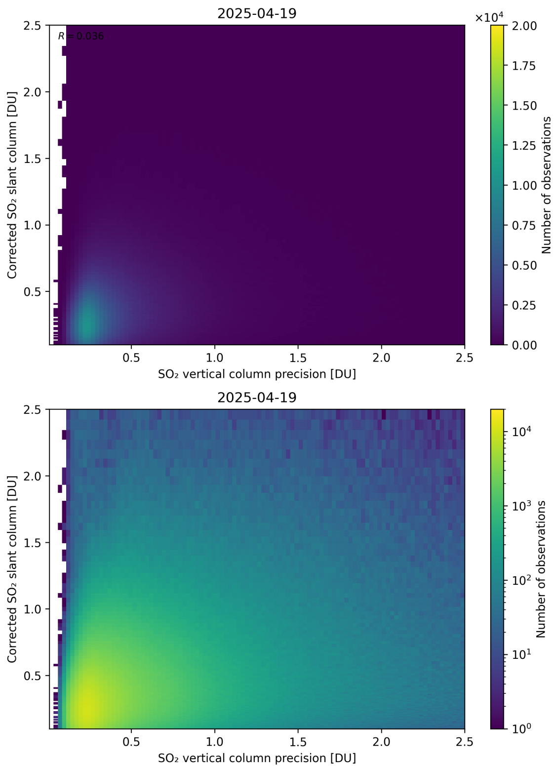
Figure 338: Scatter density plot of “SO 2 vertical column precision” against “Corrected SO 2 slant column” for 2025-04-19 to 2025-04-20.
