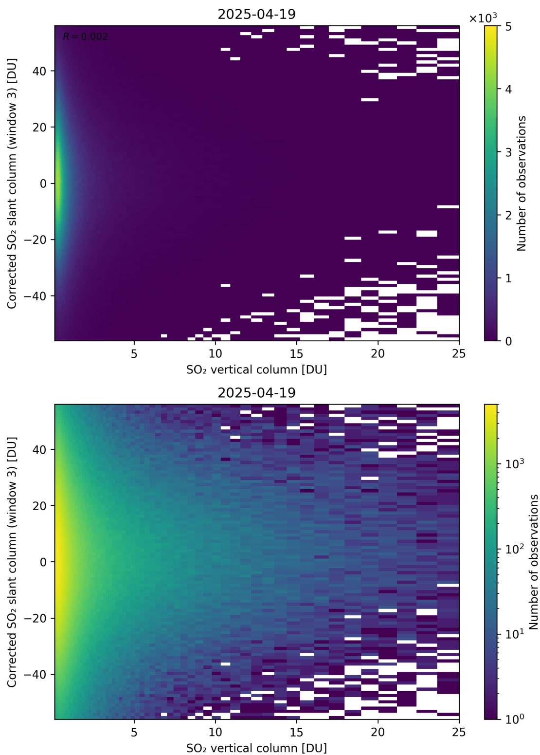
Figure 353: Scatter density plot of “SO 2 vertical column” against “Corrected SO 2 slant column (window 3)” for 2025-04-19 to 2025-04-20.
