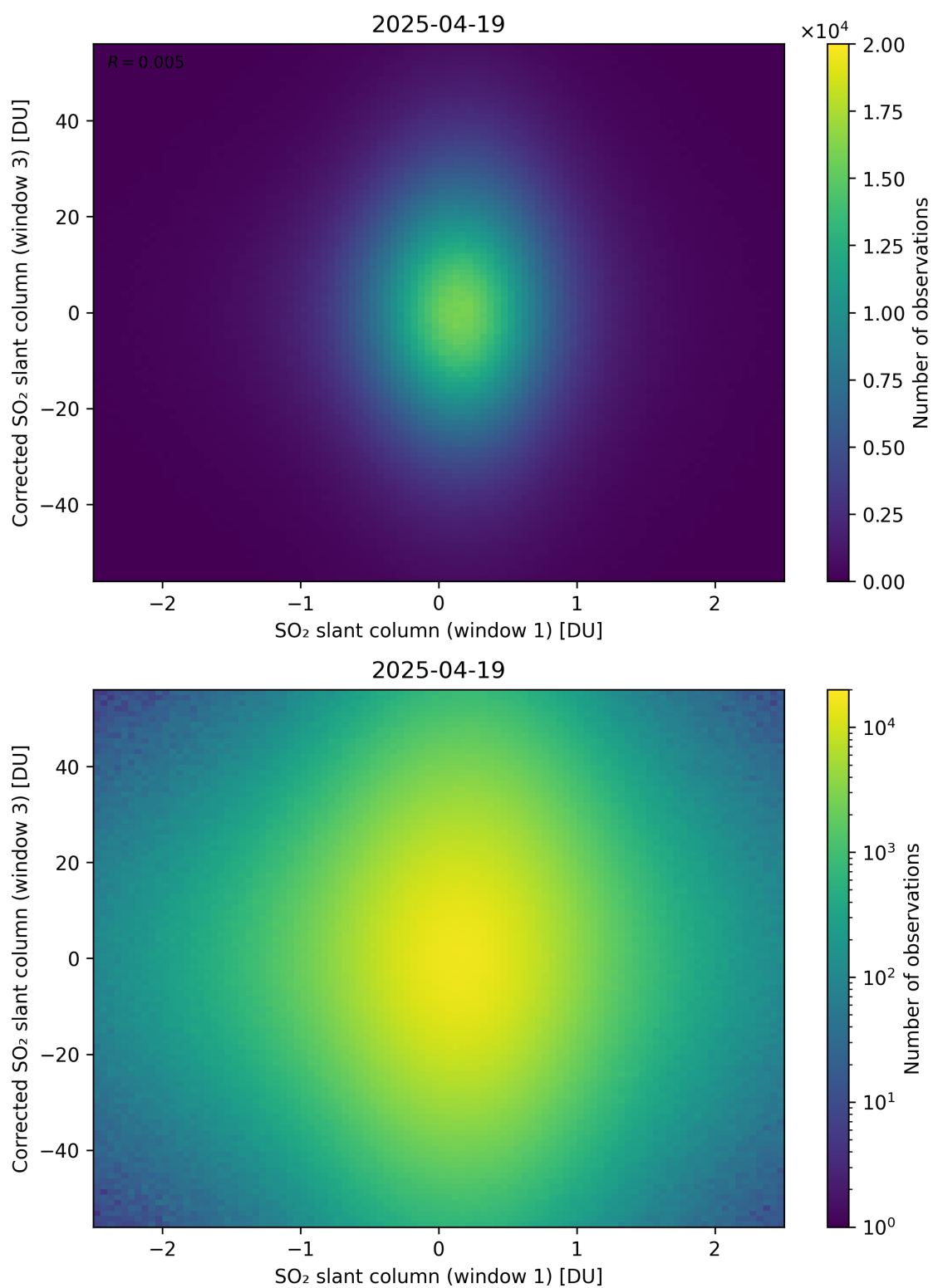
Figure 284: Scatter density plot of “SO 2 slant column (window 1)” against “Corrected SO 2 slant column (window 3)” for 2025-04-19 to 2025-04-20.
