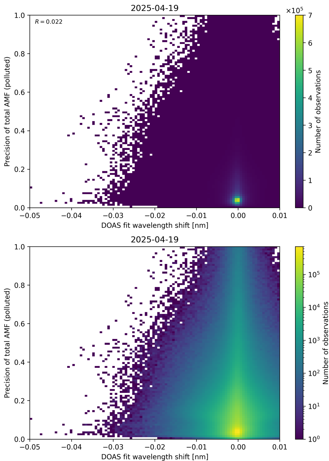
Figure 142: Scatter density plot of “DOAS fit wavelength shift” against “Precision of total AMF (polluted)” for 2025-04-19 to 2025-04-20.
