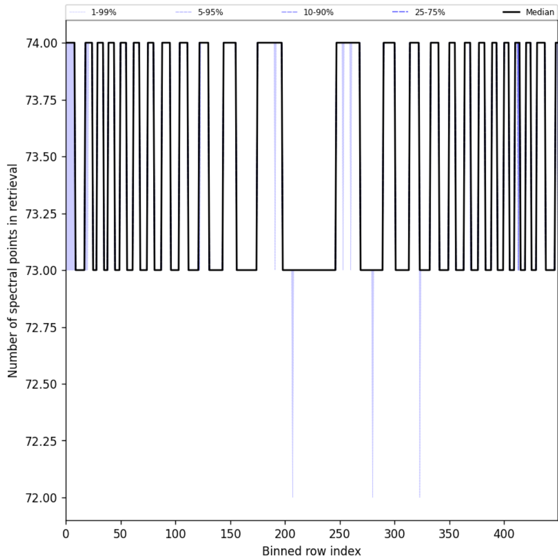
Figure 108: Along track statistics of “Number of spectral points in retrieval” for 2025-04-19 to 2025-04-20
