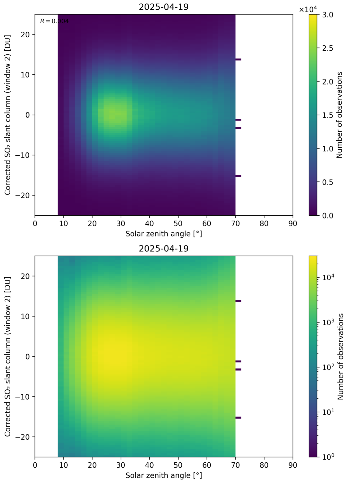
Figure 182: Scatter density plot of “Solar zenith angle” against “Corrected SO 2 slant column (window 2)” for 2025-04-19 to 2025-04-20.
