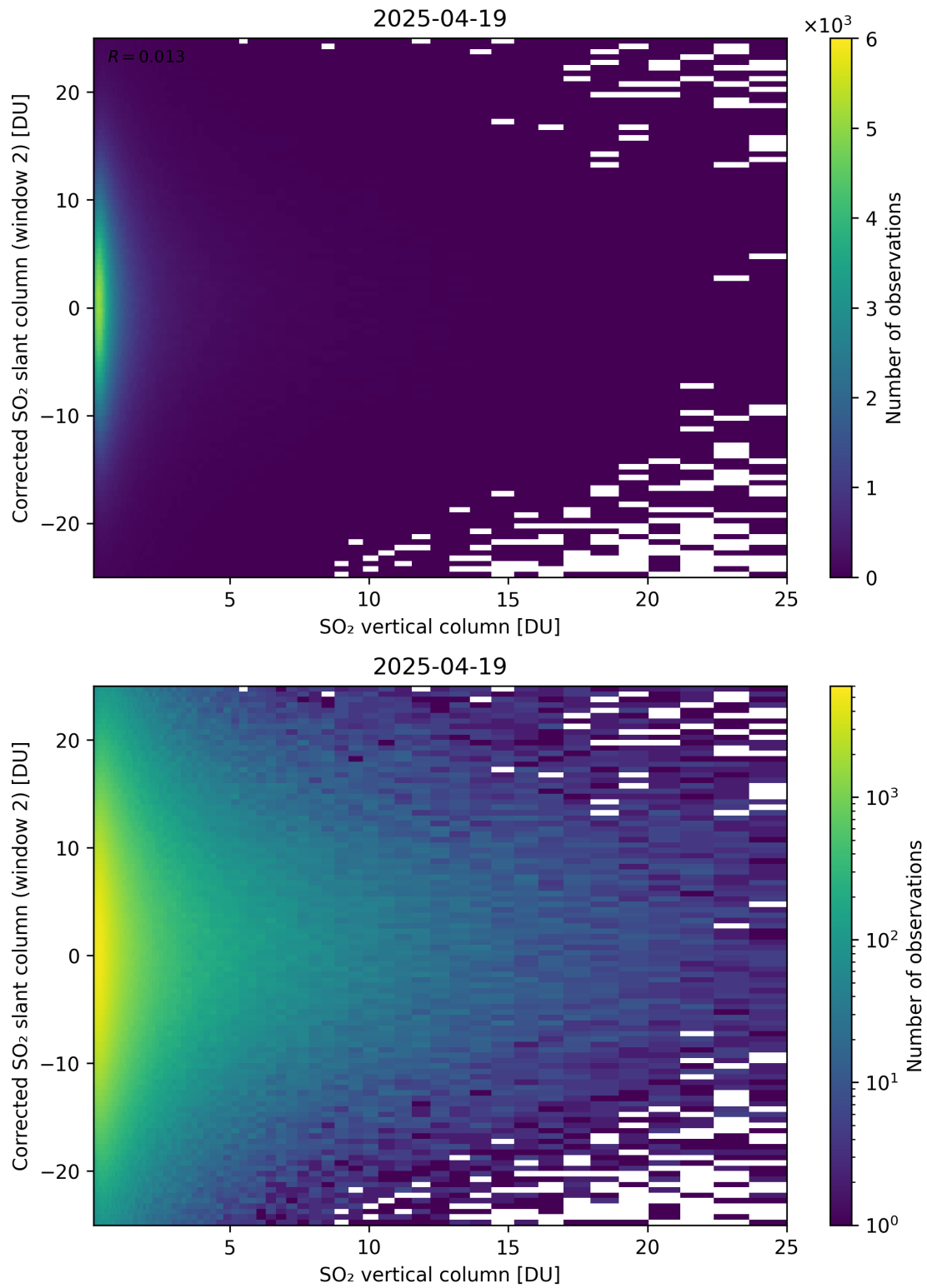
Figure 352: Scatter density plot of “SO 2 vertical column” against “Corrected SO 2 slant column (window 2)” for 2025-04-19 to 2025-04-20.
