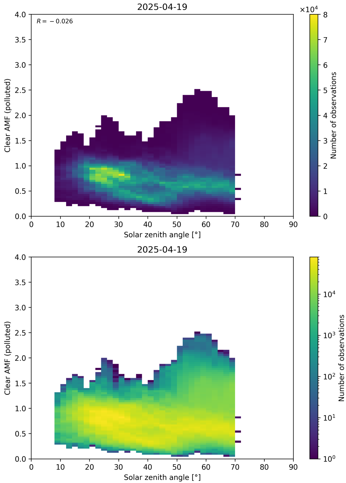
Figure 178: Scatter density plot of “Solar zenith angle” against “Clear AMF (polluted)” for 2025-04-19 to 2025-04-20.
