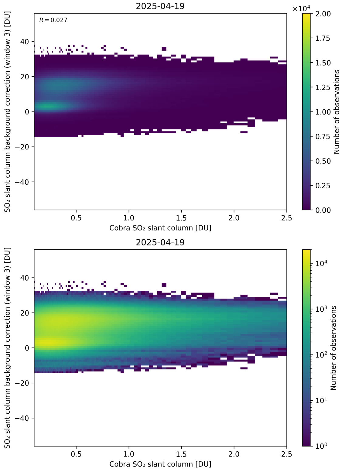
Figure 195: Scatter density plot of “Cobra SO 2 slant column” against “SO 2 slant column background correction (window 3)” for 2025-04-19 to 2025-04-20.
