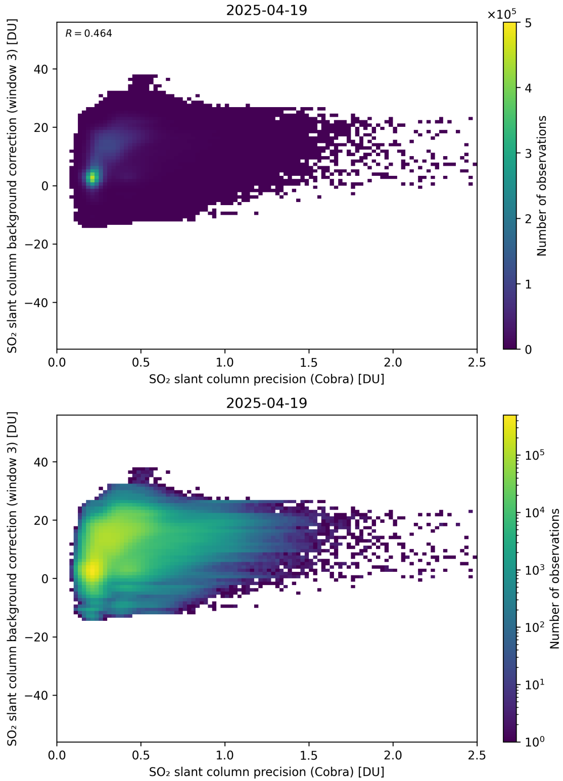
Figure 201: Scatter density plot of “SO 2 slant column precision (Cobra)” against “SO 2 slant column background correction (window 3)” for 2025-04-19 to 2025-04-20.
