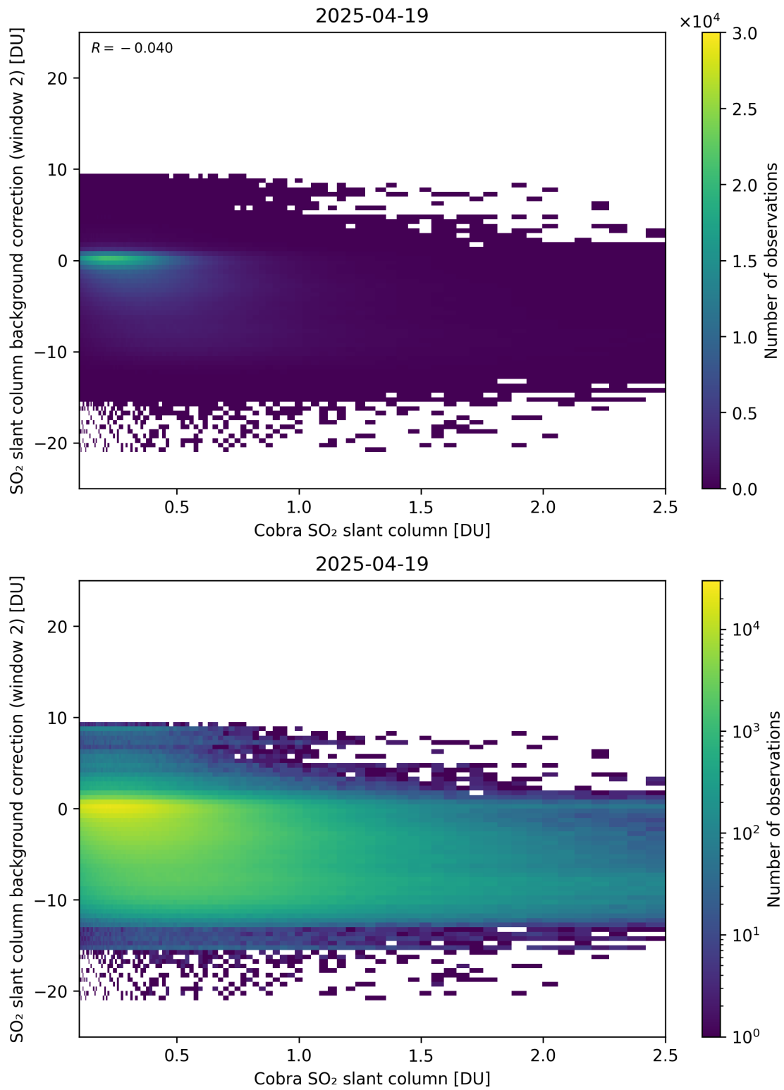
Figure 194: Scatter density plot of “Cobra SO 2 slant column” against “SO 2 slant column background correction (window 2)” for 2025-04-19 to 2025-04-20.
