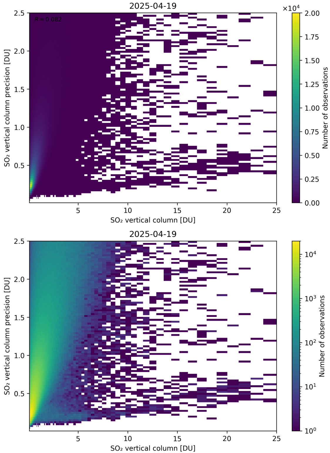
Figure 361: Scatter density plot of “SO 2 vertical column” against “SO 2 vertical column precision” for 2025-04-19 to 2025-04-20.
