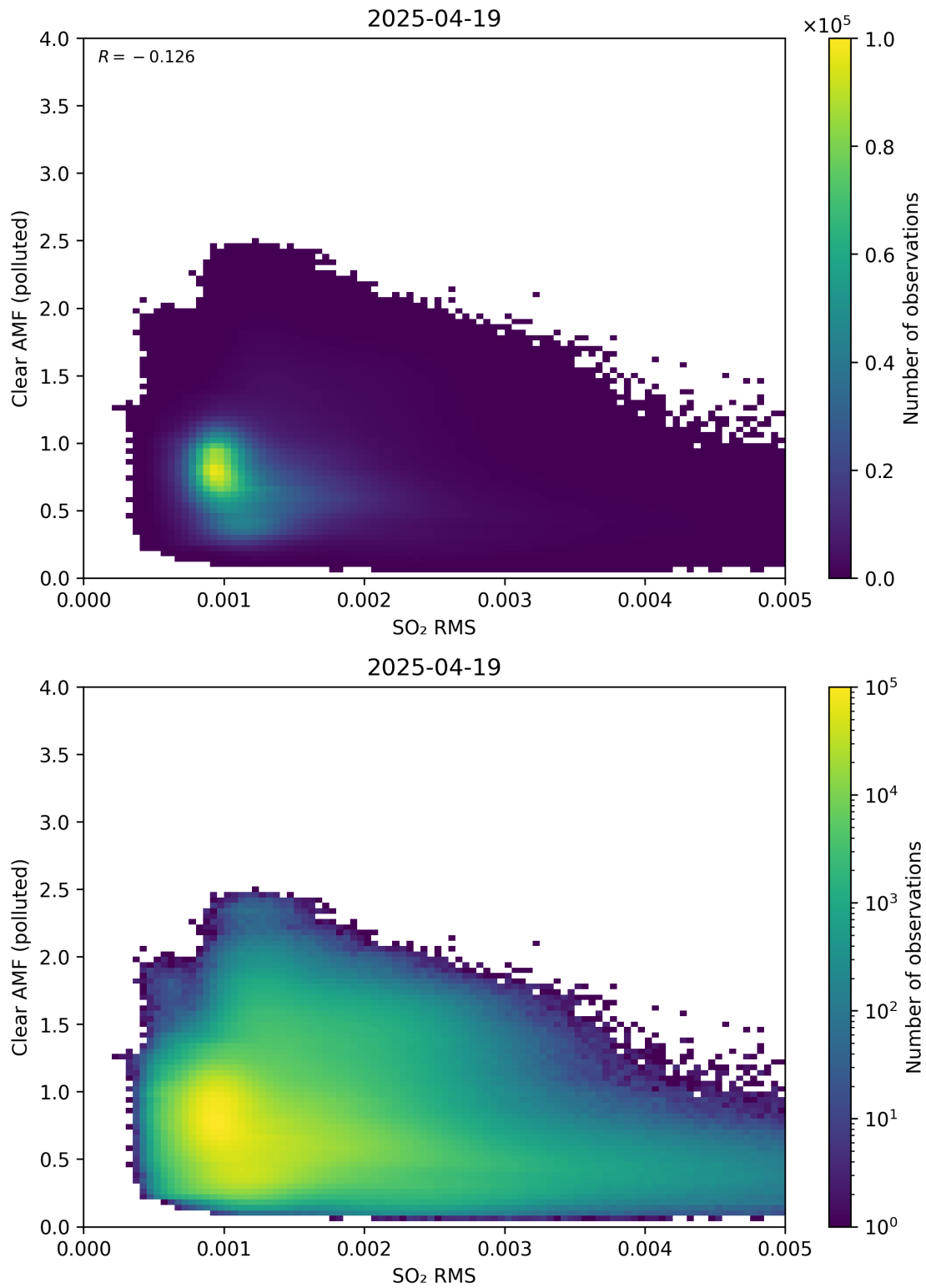
Figure 147: Scatter density plot of “SO 2 RMS” against “Clear AMF (polluted)” for 2025-04-19 to 2025-04-20.
