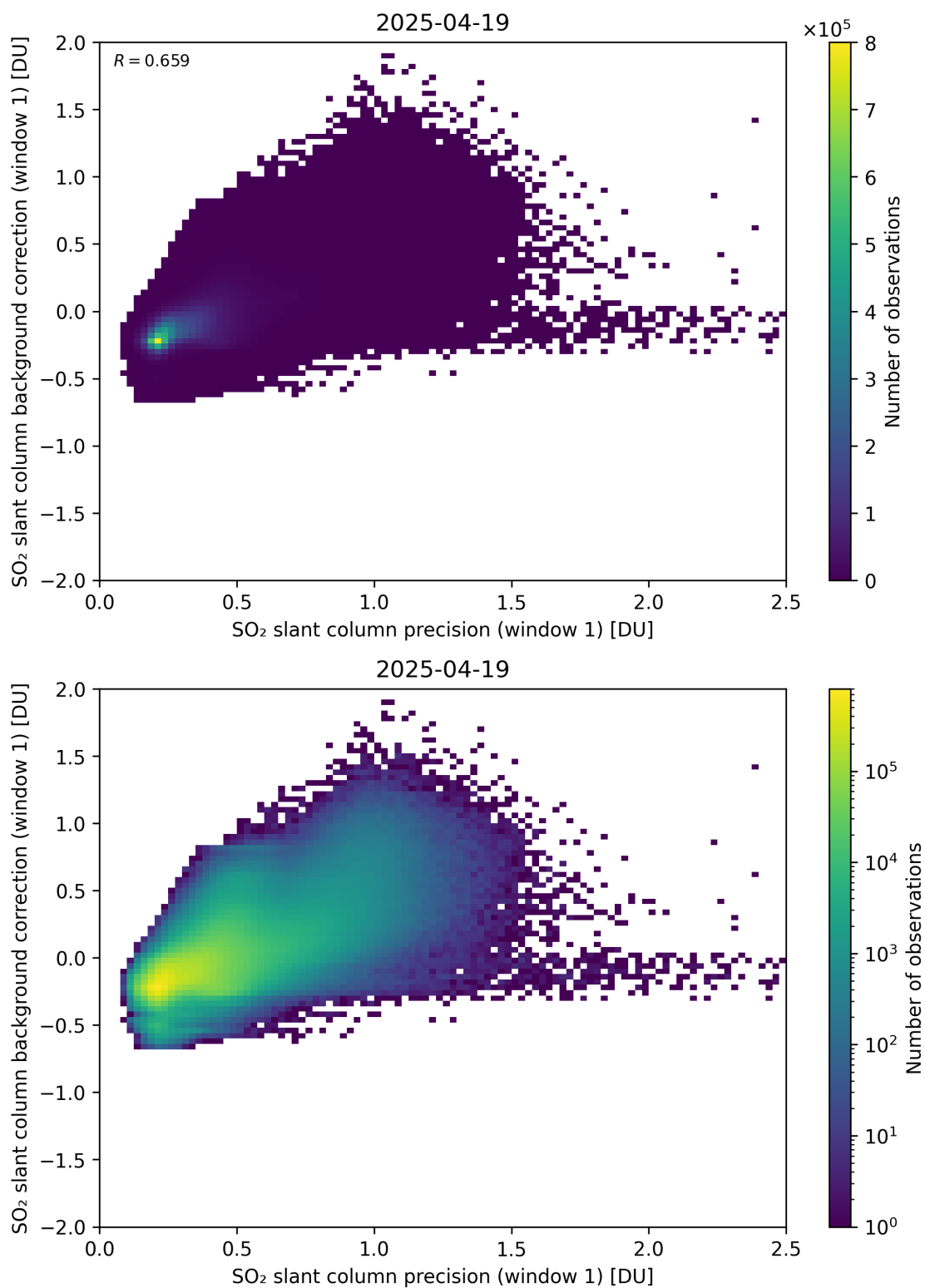
Figure 268: Scatter density plot of “SO 2 slant column precision (window 1)” against “SO 2 slant column background correction (window 1)” for 2025-04-19 to 2025-04-20.
