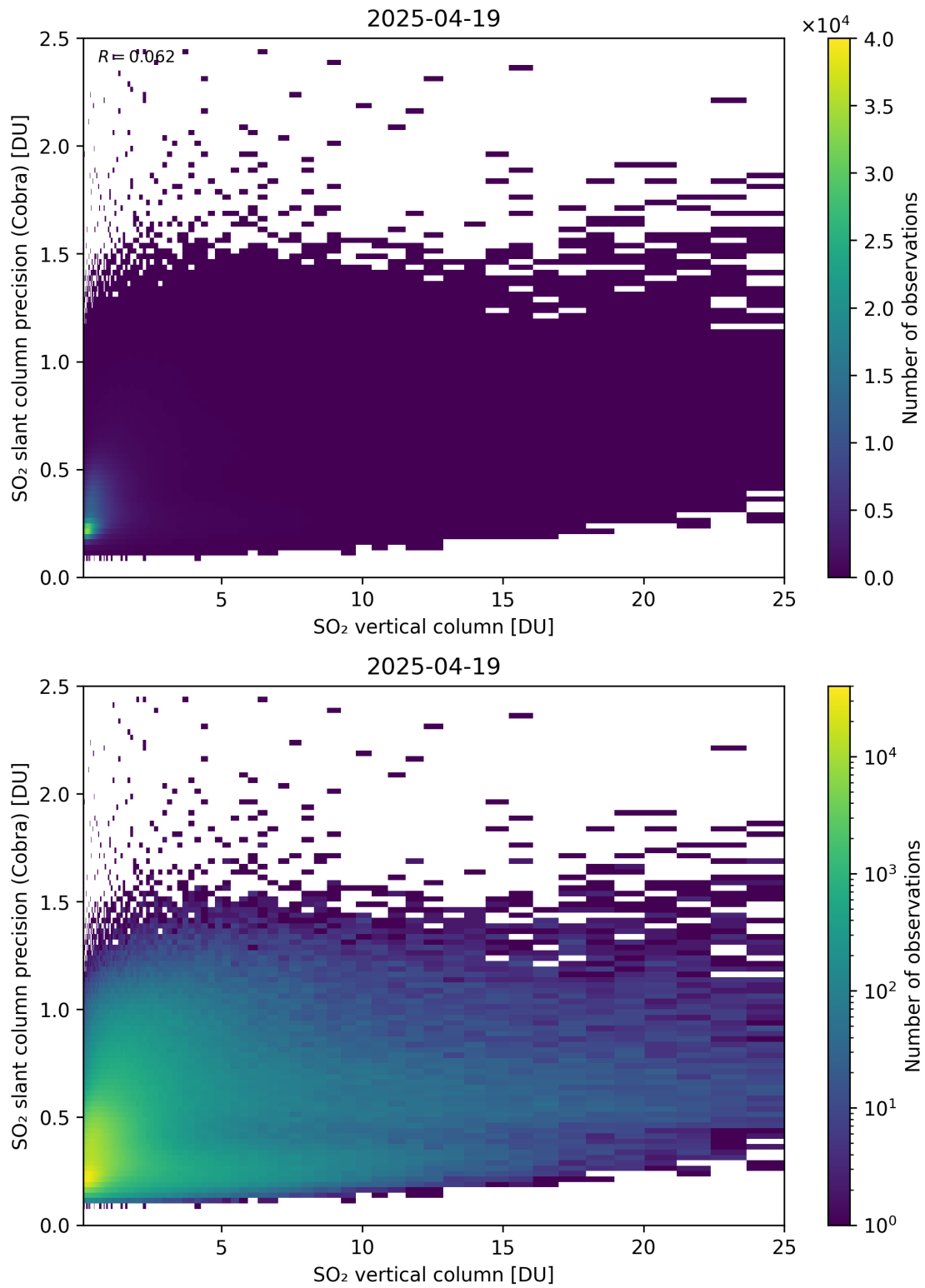
Figure 350: Scatter density plot of “SO 2 vertical column” against “SO 2 slant column precision (Cobra)” for 2025-04-19 to 2025-04-20.
