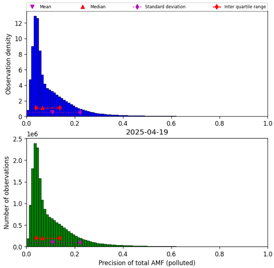
Figure 80: Histogram of “Precision of total AMF (polluted)” for 2025-04-19 to 2025-04-20
