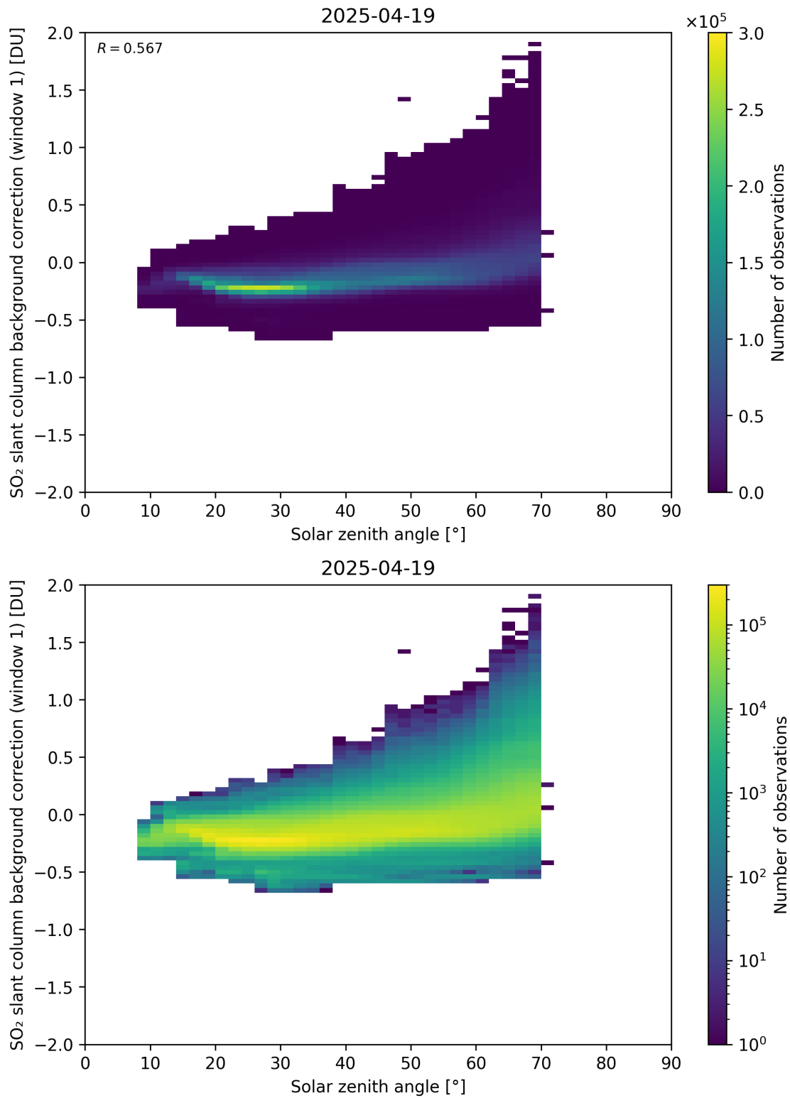
Figure 171: Scatter density plot of “Solar zenith angle” against “SO 2 slant column background correction (window 1)” for 2025-04-19 to 2025-04-20.
