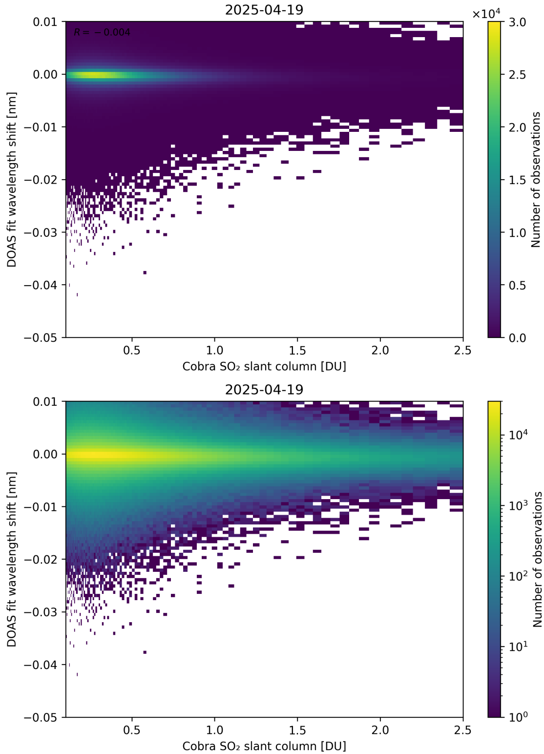
Figure 196: Scatter density plot of “Cobra SO 2 slant column” against “DOAS fit wavelength shift” for 2025-04-19 to 2025-04-20.
