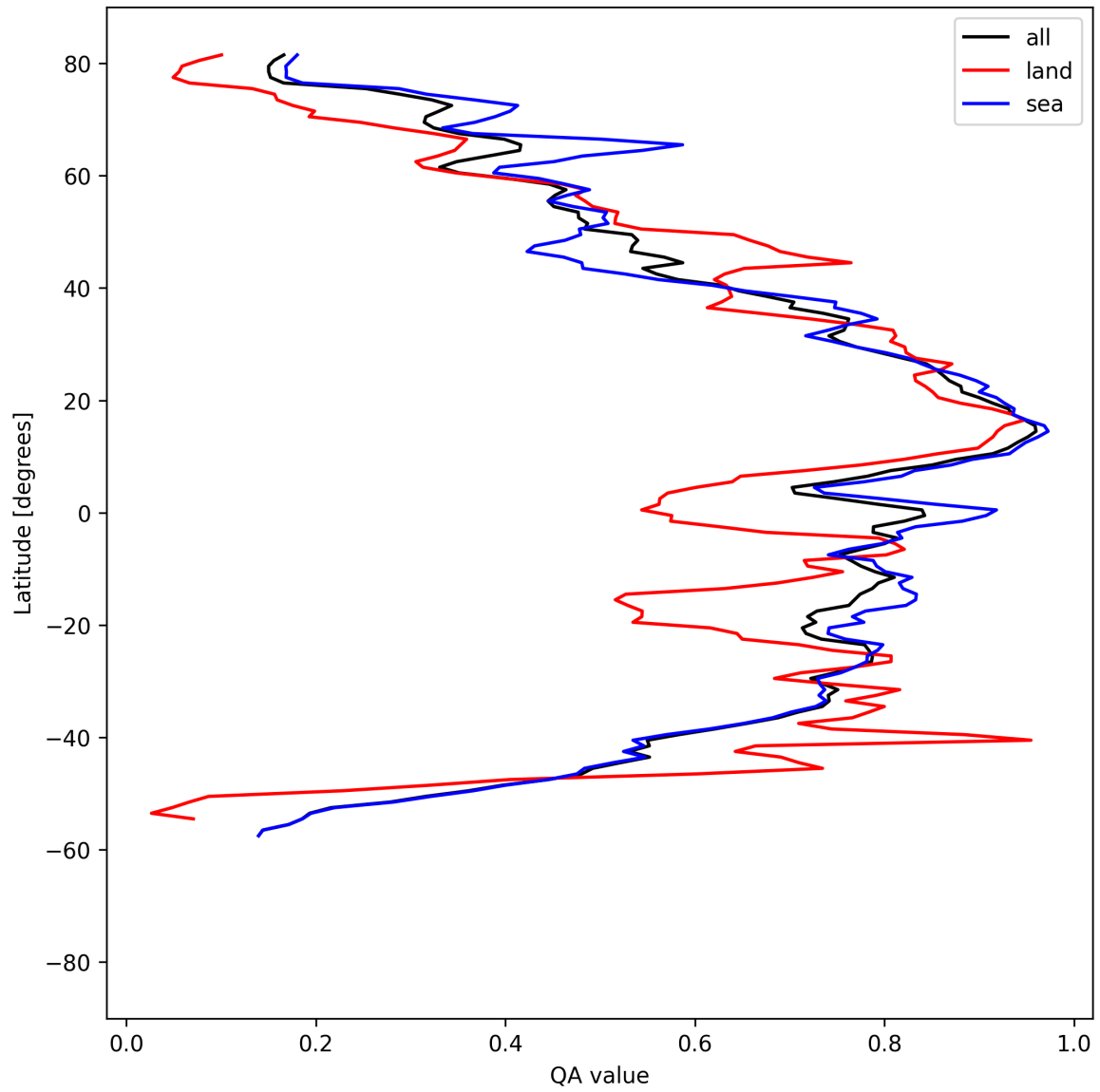
Figure 31: Zonal average of “QA value” for 2025-04-19 to 2025-04-20.
