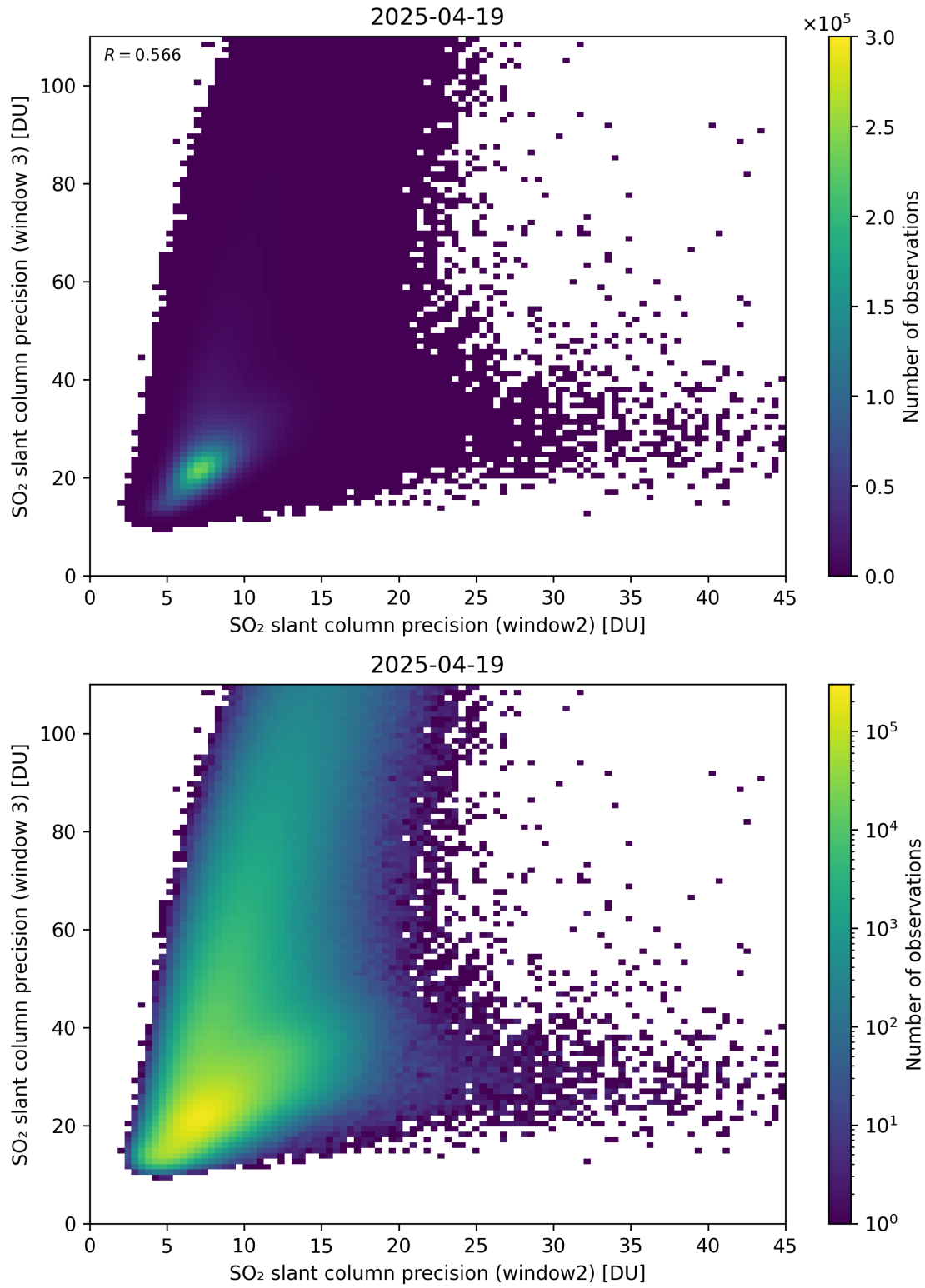
Figure 300: Scatter density plot of “SO 2 slant column precision (window2)” against “SO 2 slant column precision (window 3)” for 2025-04-19 to 2025-04-20.
