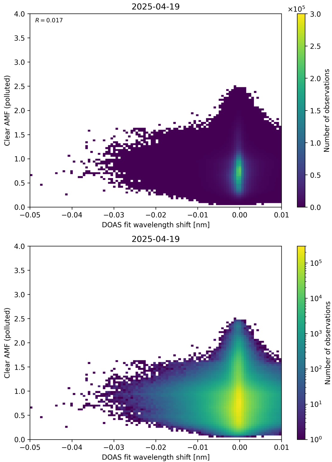
Figure 140: Scatter density plot of “DOAS fit wavelength shift” against “Clear AMF (polluted)” for 2025-04-19 to 2025-04-20.
