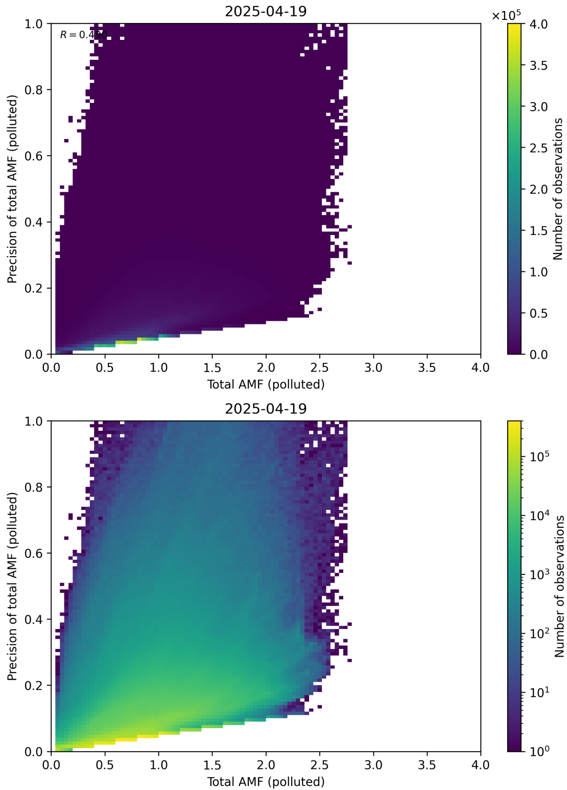
Figure 322: Scatter density plot of “Total AMF (polluted)” against “Precision of total AMF (polluted)” for 2025-04-19 to 2025-04-20.
