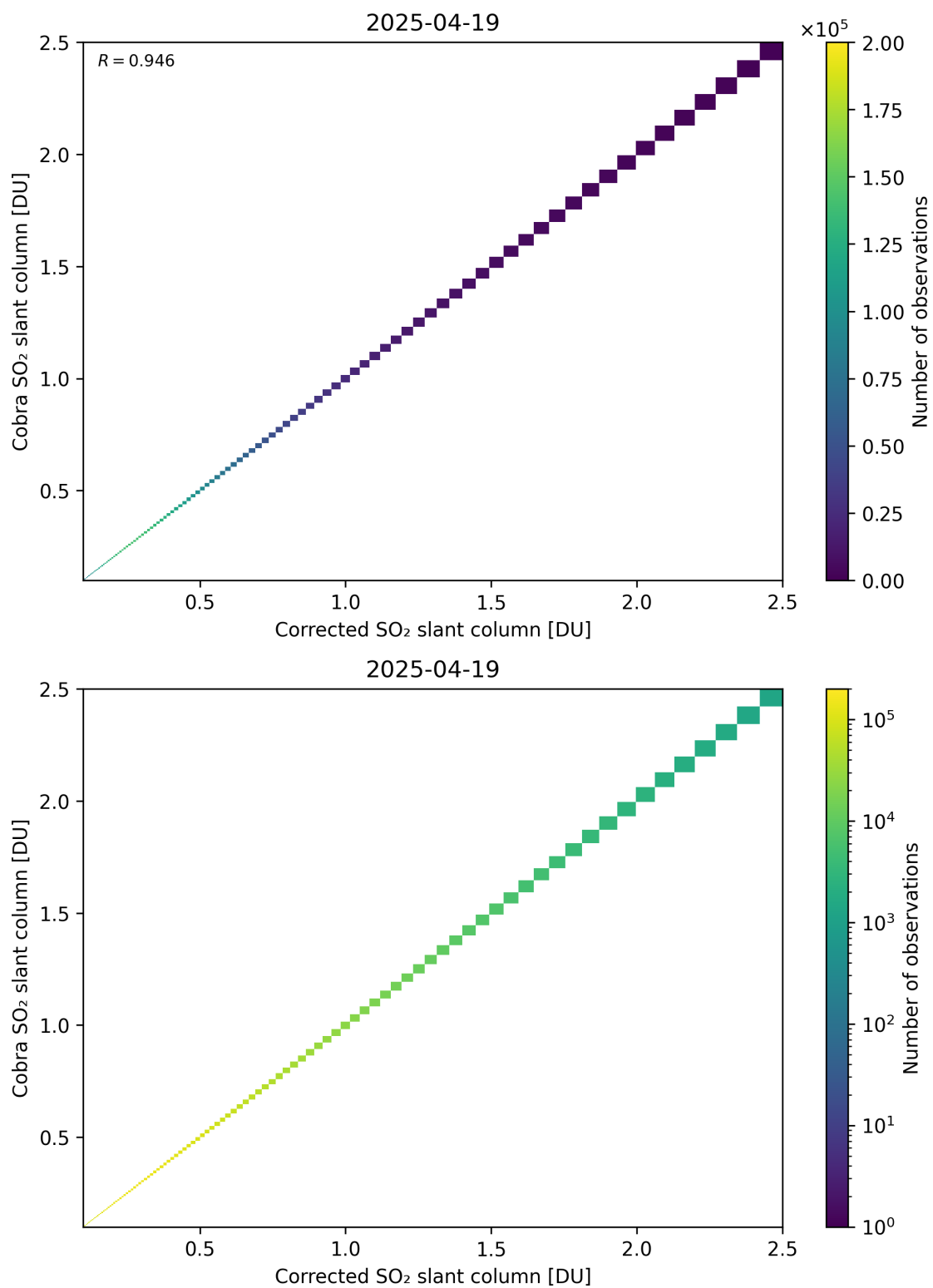
Figure 233: Scatter density plot of “Corrected SO 2 slant column” against “Cobra SO 2 slant column” for 2025-04-19 to 2025-04-20.
