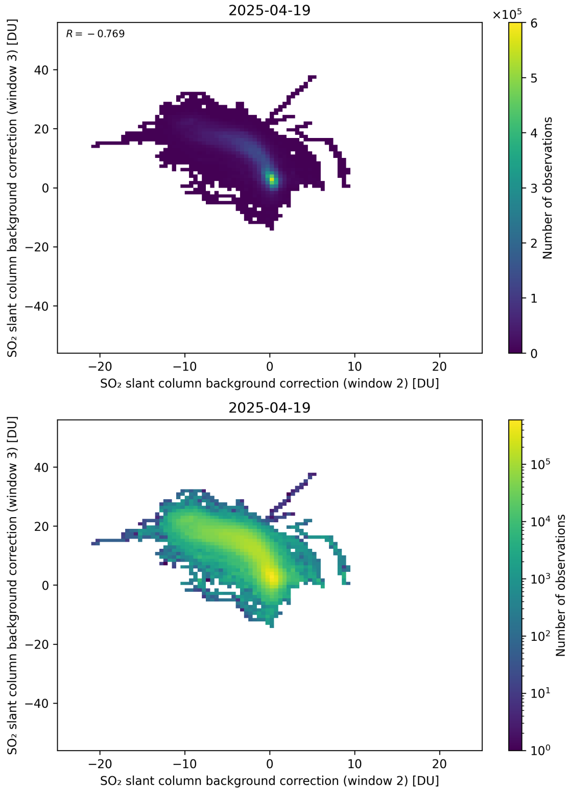
Figure 122: Scatter density plot of “SO 2 slant column background correction (window 2)” against “SO 2 slant column background correction (window 3)” for 2025-04-19 to 2025-04-20.
