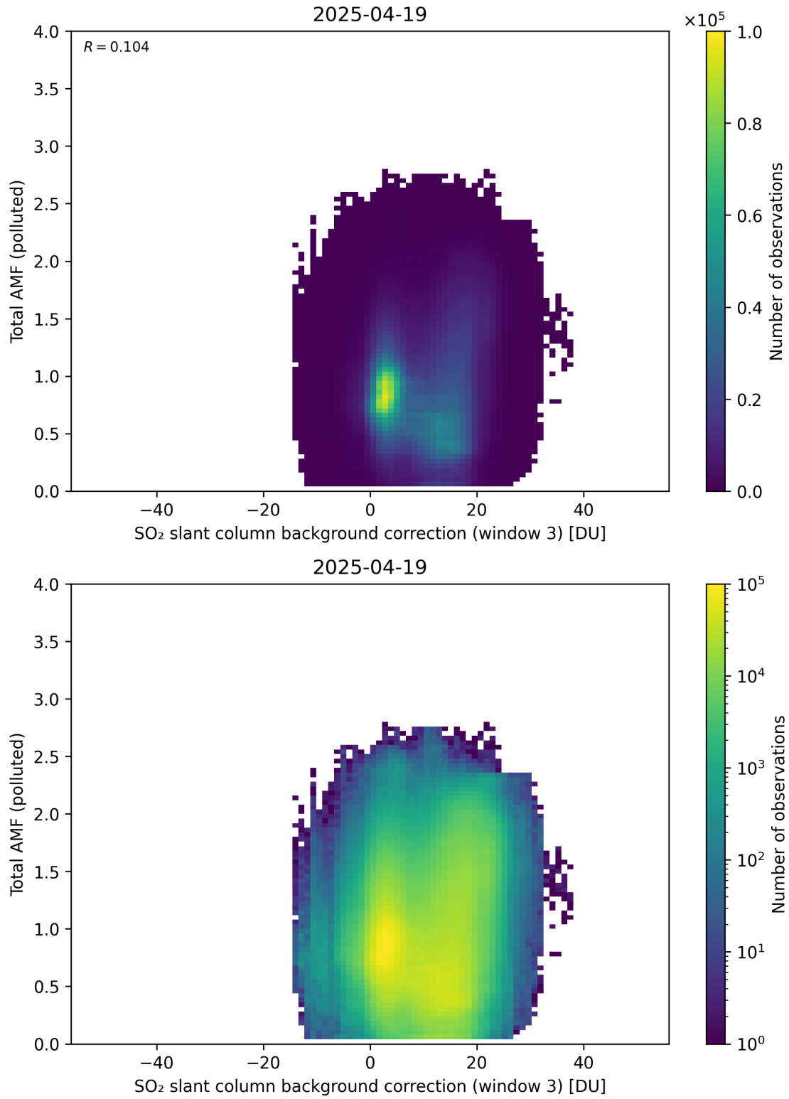
Figure 136: Scatter density plot of “SO 2 slant column background correction (window 3)” against “Total AMF (polluted)” for 2025-04-19 to 2025-04-20.
