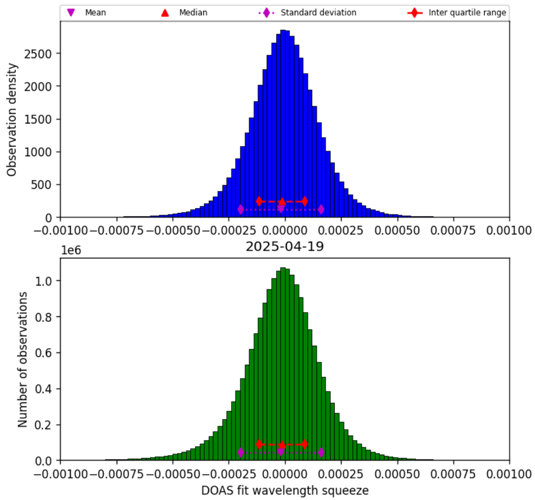
Figure 77: Histogram of “DOAS fit wavelength squeeze” for 2025-04-19 to 2025-04-20
