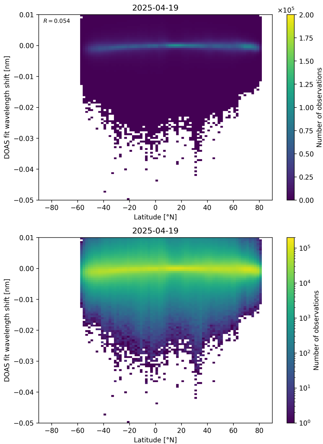
Figure 153: Scatter density plot of “Latitude” against “DOAS fit wavelength shift” for 2025-04-19 to 2025-04-20.
