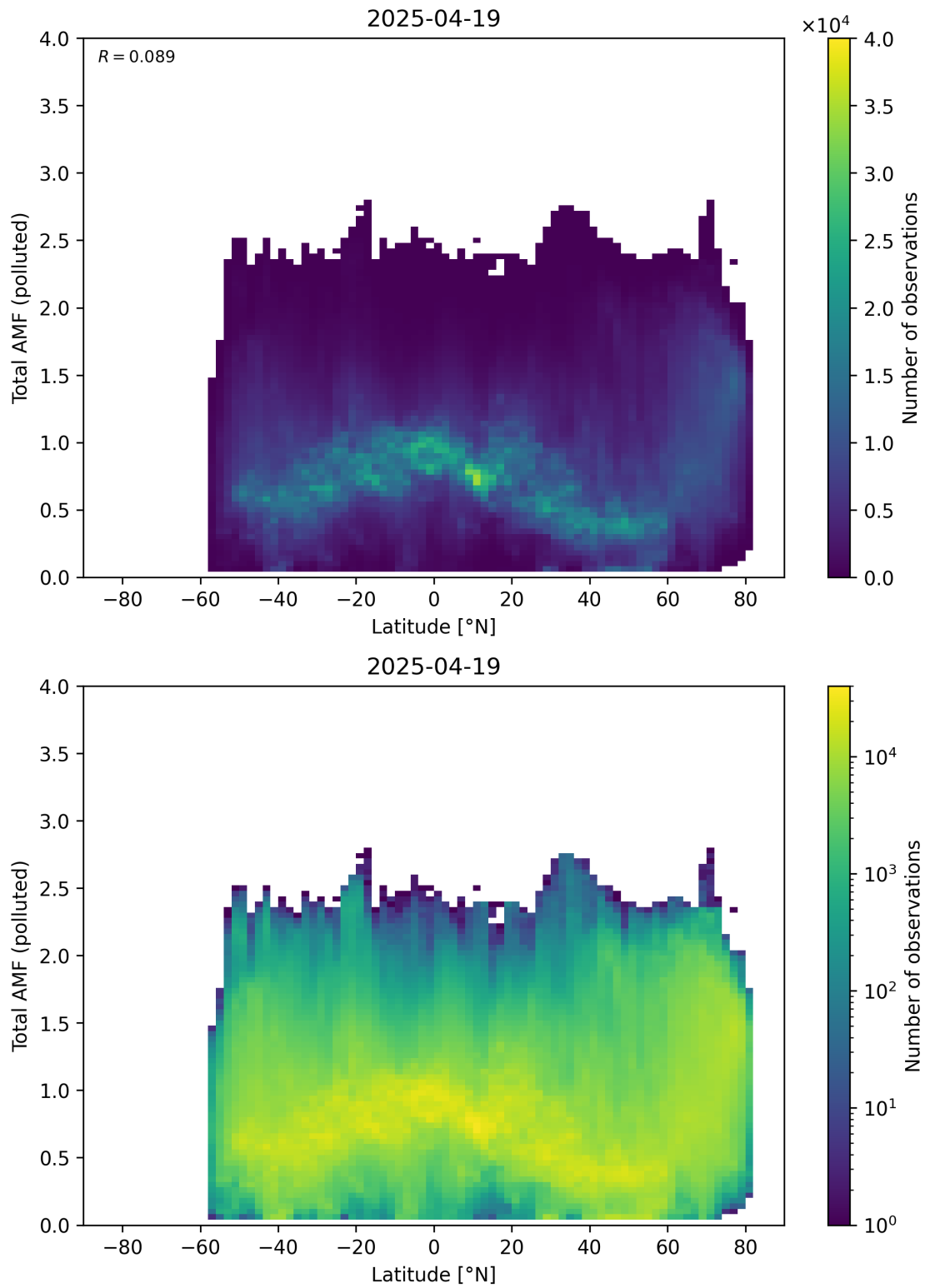
Figure 167: Scatter density plot of “Latitude” against “Total AMF (polluted)” for 2025-04-19 to 2025-04-20.
