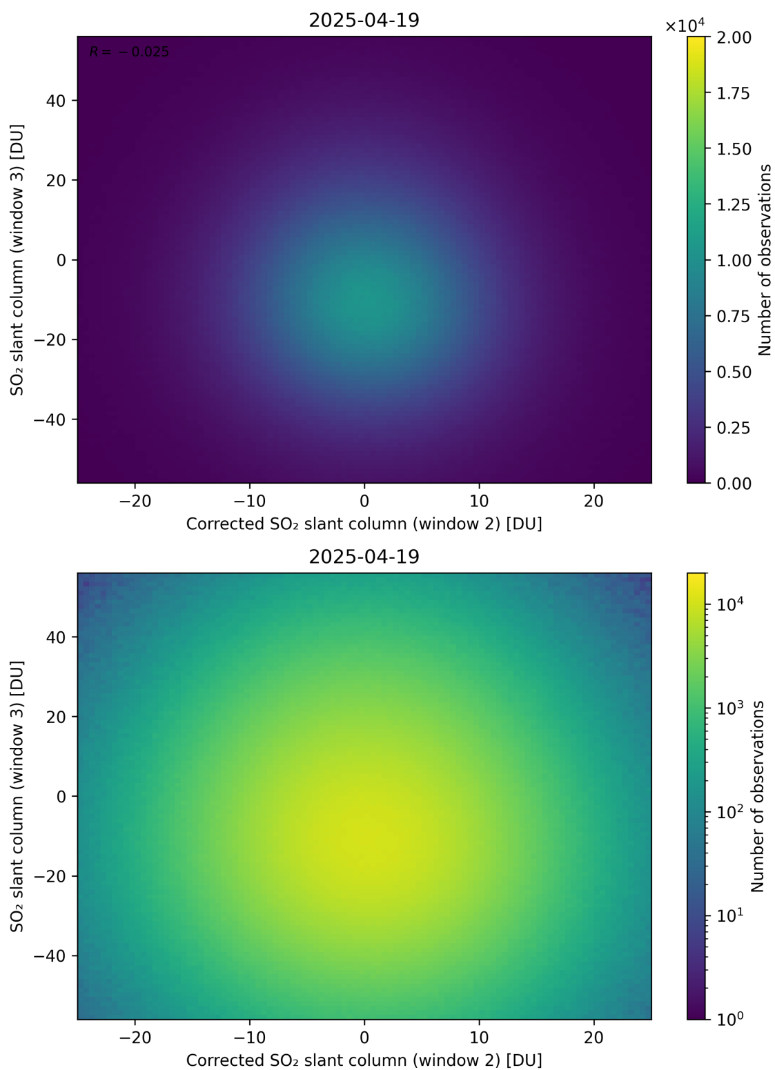
Figure 251: Scatter density plot of “Corrected SO 2 slant column (window 2)” against “SO 2 slant column (window 3)” for 2025-04-19 to 2025-04-20.
