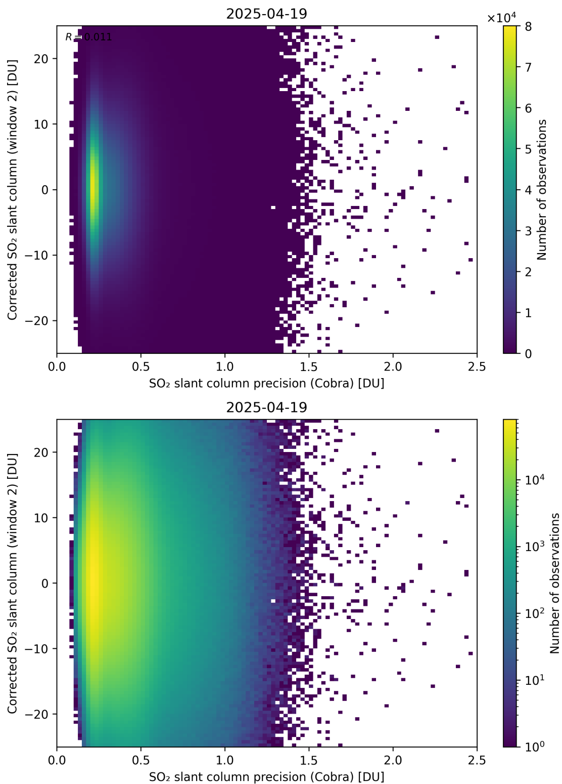
Figure 206: Scatter density plot of “SO 2 slant column precision (Cobra)” against “Corrected SO 2 slant column (window 2)” for 2025-04-19 to 2025-04-20.
