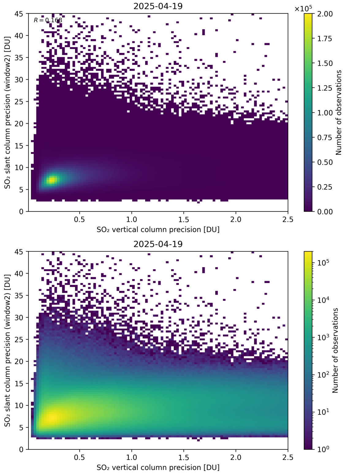
Figure 343: Scatter density plot of “SO 2 vertical column precision” against “SO 2 slant column precision (window2)” for 2025-04-19 to 2025-04-20.
