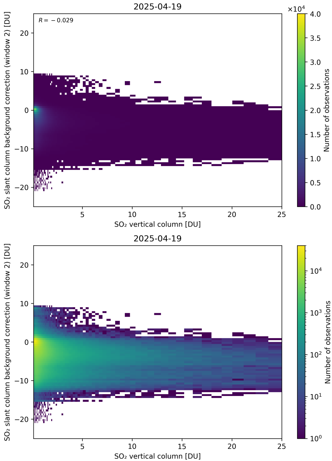
Figure 324: Scatter density plot of “SO 2 vertical column” against “SO 2 slant column background correction (window 2)” for 2025-04-19 to 2025-04-20.
