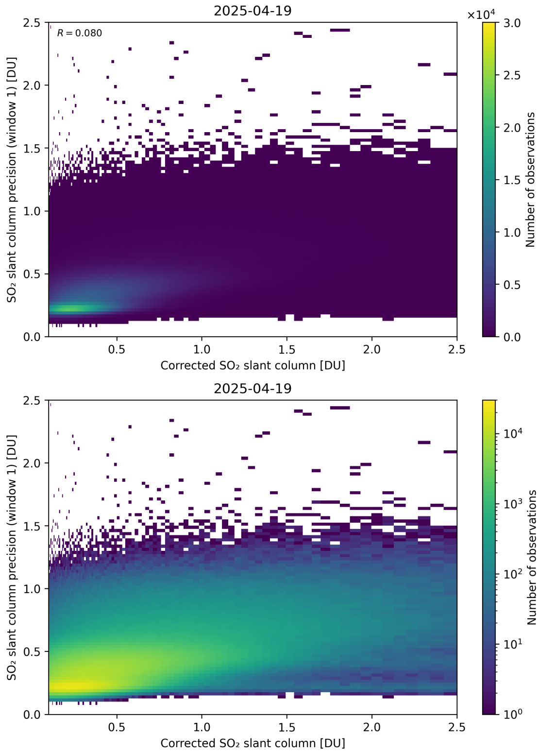
Figure 238: Scatter density plot of “Corrected SO 2 slant column” against “SO 2 slant column precision (window 1)” for 2025-04-19 to 2025-04-20.
