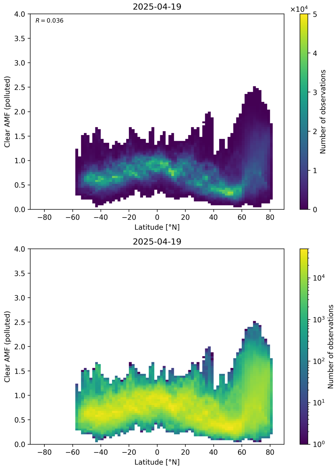
Figure 156: Scatter density plot of “Latitude” against “Clear AMF (polluted)” for 2025-04-19 to 2025-04-20.
