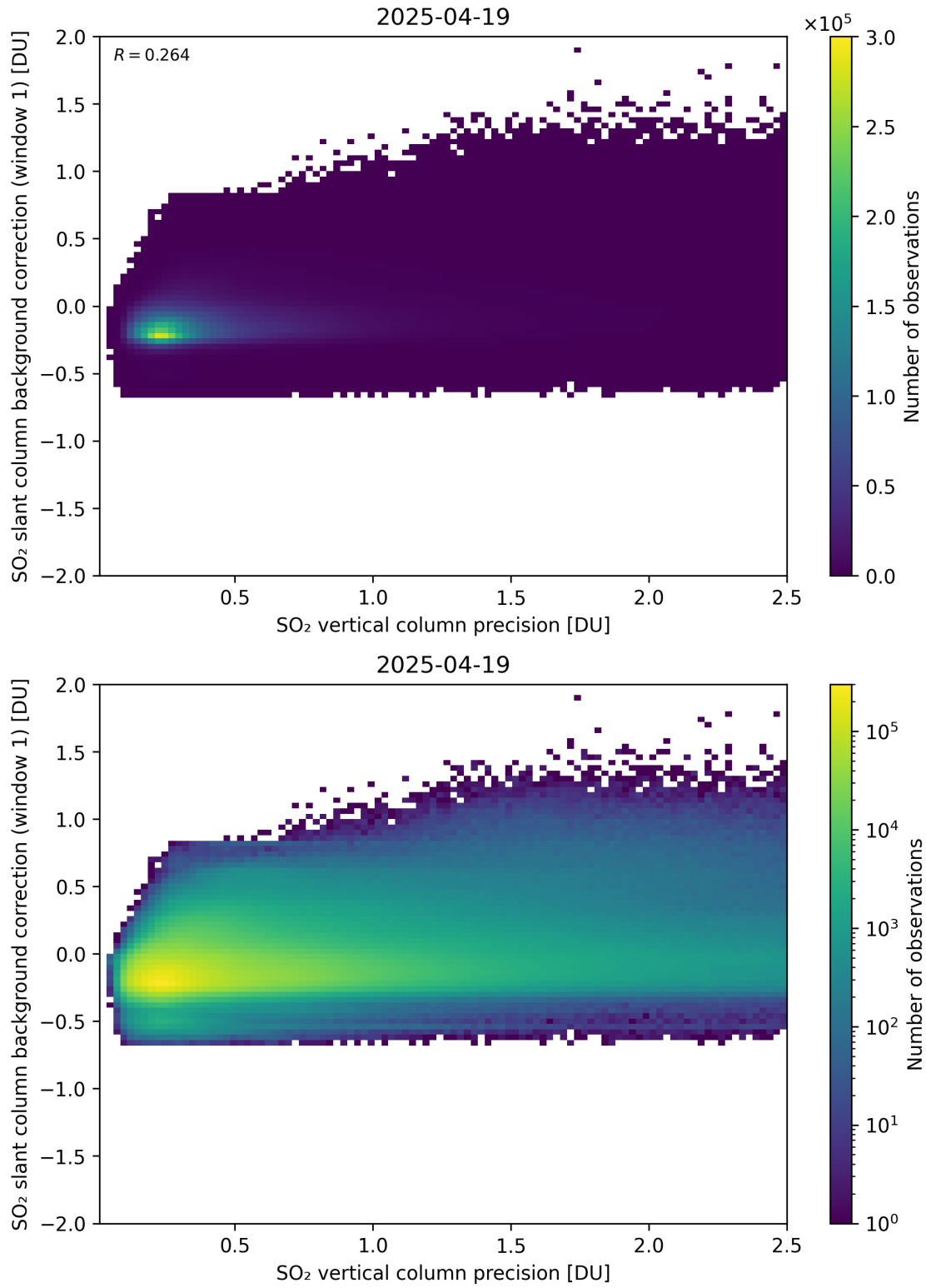
Figure 329: Scatter density plot of “SO 2 vertical column precision” against “SO 2 slant column background correction (window 1)” for 2025-04-19 to 2025-04-20.
