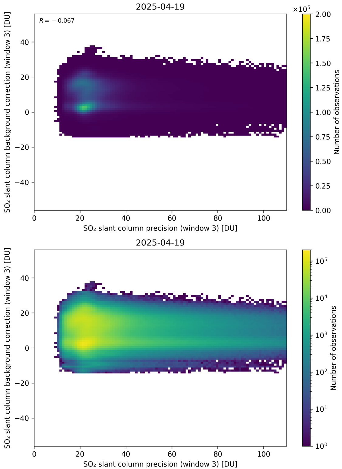
Figure 307: Scatter density plot of “SO 2 slant column precision (window 3)” against “SO 2 slant column background correction (window 3)” for 2025-04-19 to 2025-04-20.
