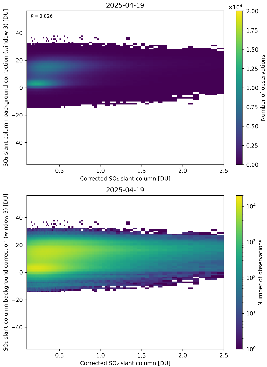
Figure 228: Scatter density plot of “Corrected SO 2 slant column” against “SO 2 slant column background correction (window 3)” for 2025-04-19 to 2025-04-20.
