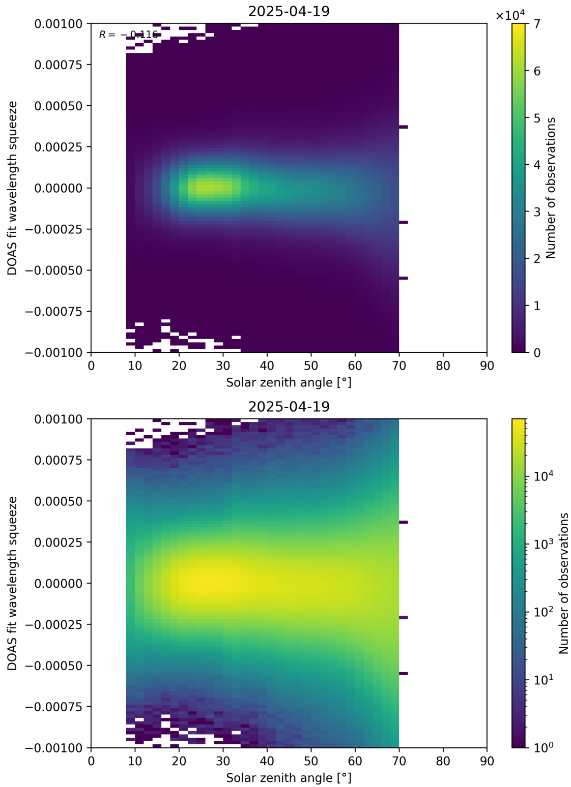
Figure 175: Scatter density plot of “Solar zenith angle” against “DOAS fit wavelength squeeze” for 2025-04-19 to 2025-04-20.
