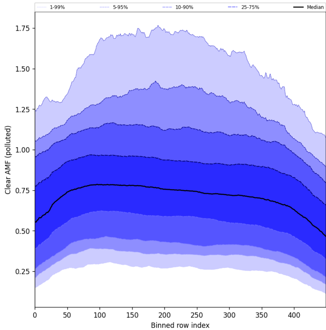
Figure 107: Along track statistics of “Clear AMF (polluted)” for 2025-04-19 to 2025-04-20
