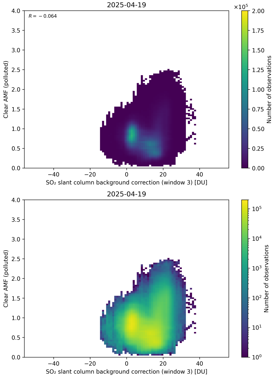
Figure 135: Scatter density plot of “SO 2 slant column background correction (window 3)” against “Clear AMF (polluted)” for 2025-04-19 to 2025-04-20.
