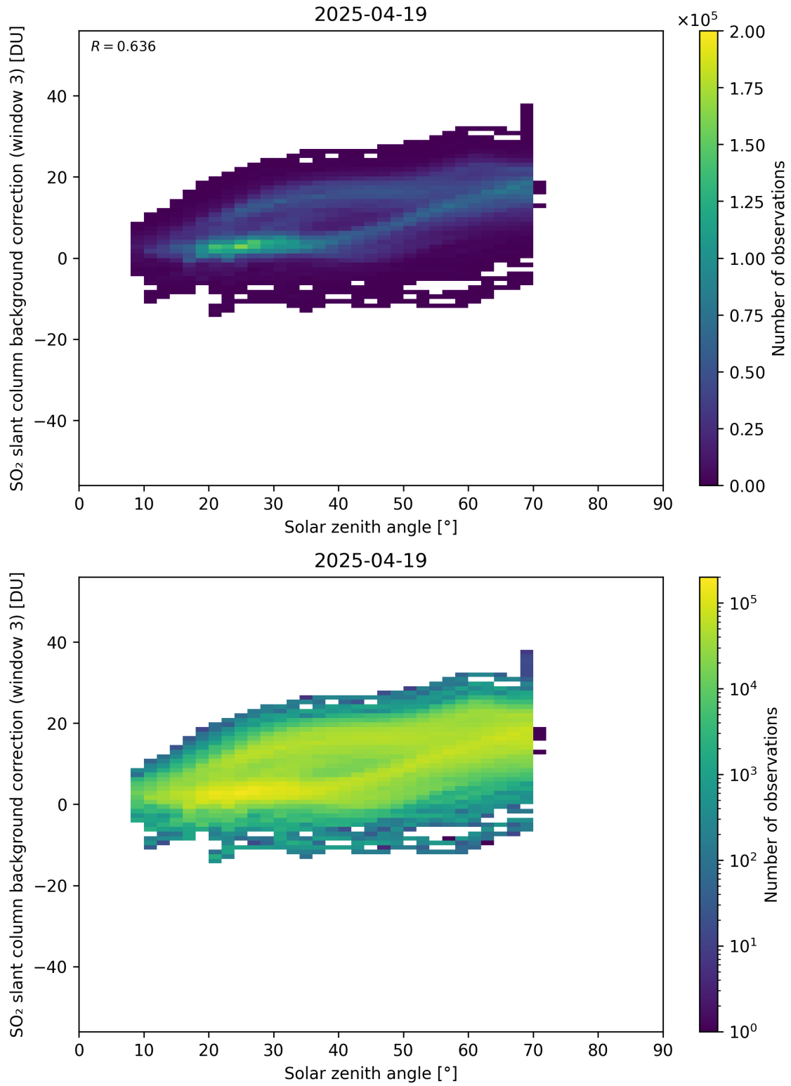
Figure 173: Scatter density plot of “Solar zenith angle” against “SO 2 slant column background correction (window 3)” for 2025-04-19 to 2025-04-20.
