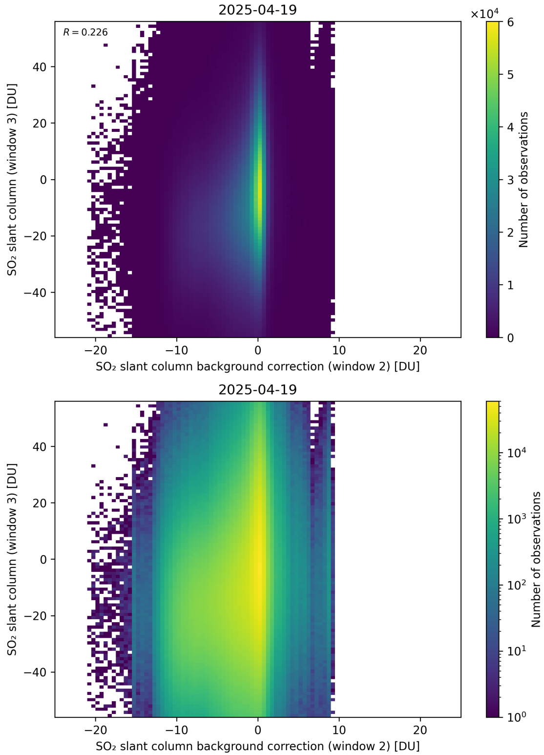
Figure 128: Scatter density plot of “SO 2 slant column background correction (window 2)” against “SO 2 slant column (window 3)” for 2025-04-19 to 2025-04-20.
