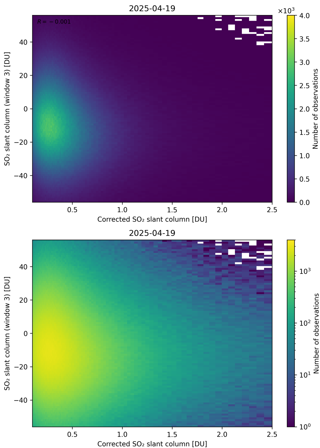
Figure 240: Scatter density plot of “Corrected SO 2 slant column” against “SO 2 slant column (window 3)” for 2025-04-19 to 2025-04-20.
