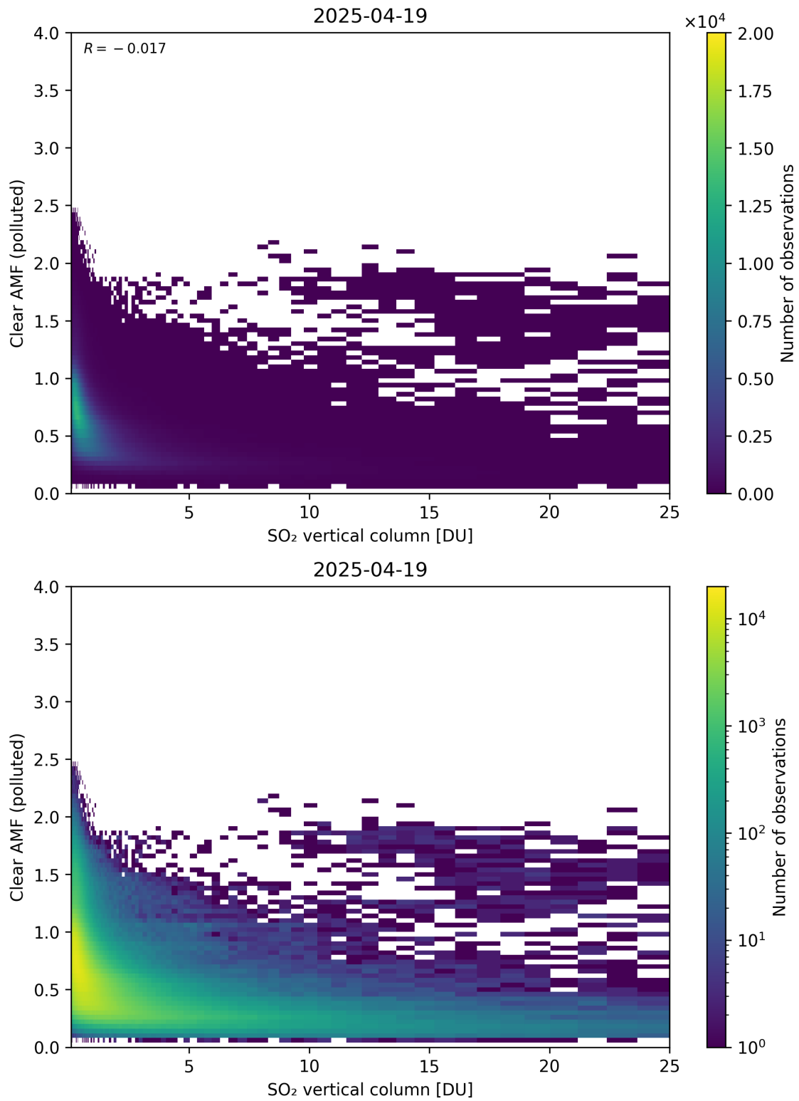
Figure 348: Scatter density plot of “SO 2 vertical column” against “Clear AMF (polluted)” for 2025-04-19 to 2025-04-20.
