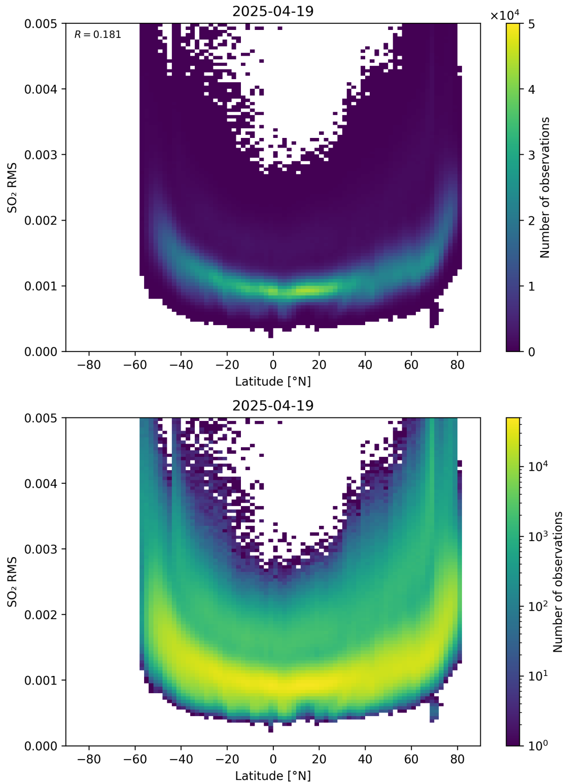
Figure 155: Scatter density plot of “Latitude” against “SO 2 RMS” for 2025-04-19 to 2025-04-20.
