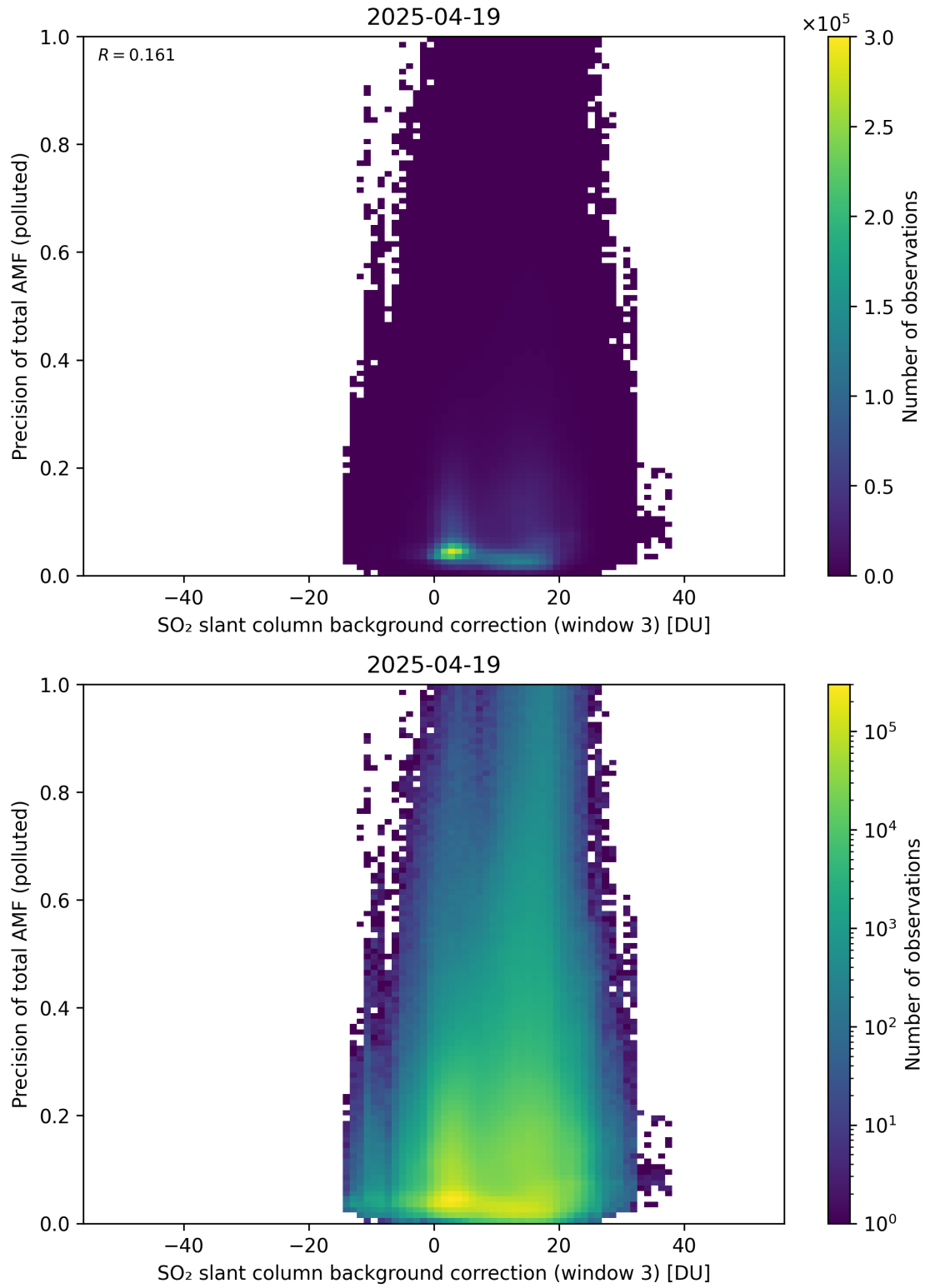
Figure 137: Scatter density plot of “SO 2 slant column background correction (window 3)” against “Precision of total AMF (polluted)” for 2025-04-19 to 2025-04-20.
