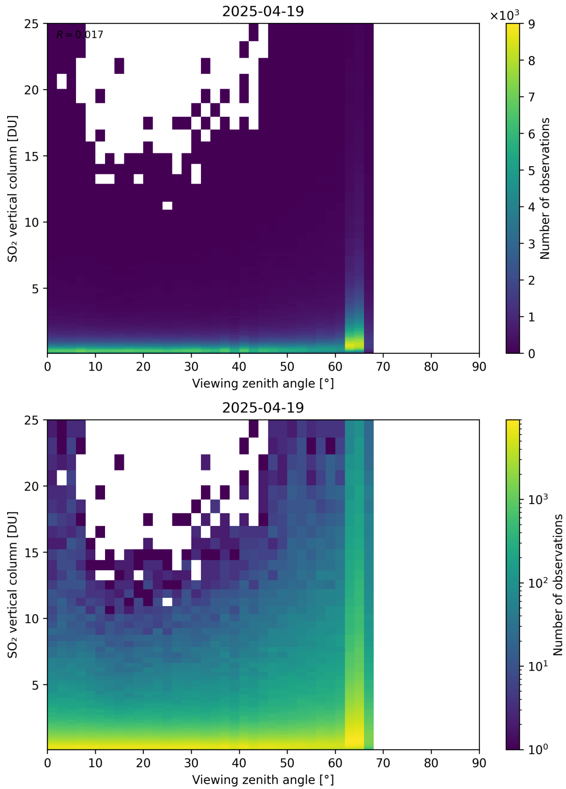
Figure 383: Scatter density plot of “Viewing zenith angle” against “SO 2 vertical column” for 2025-04-19 to 2025-04-20.
