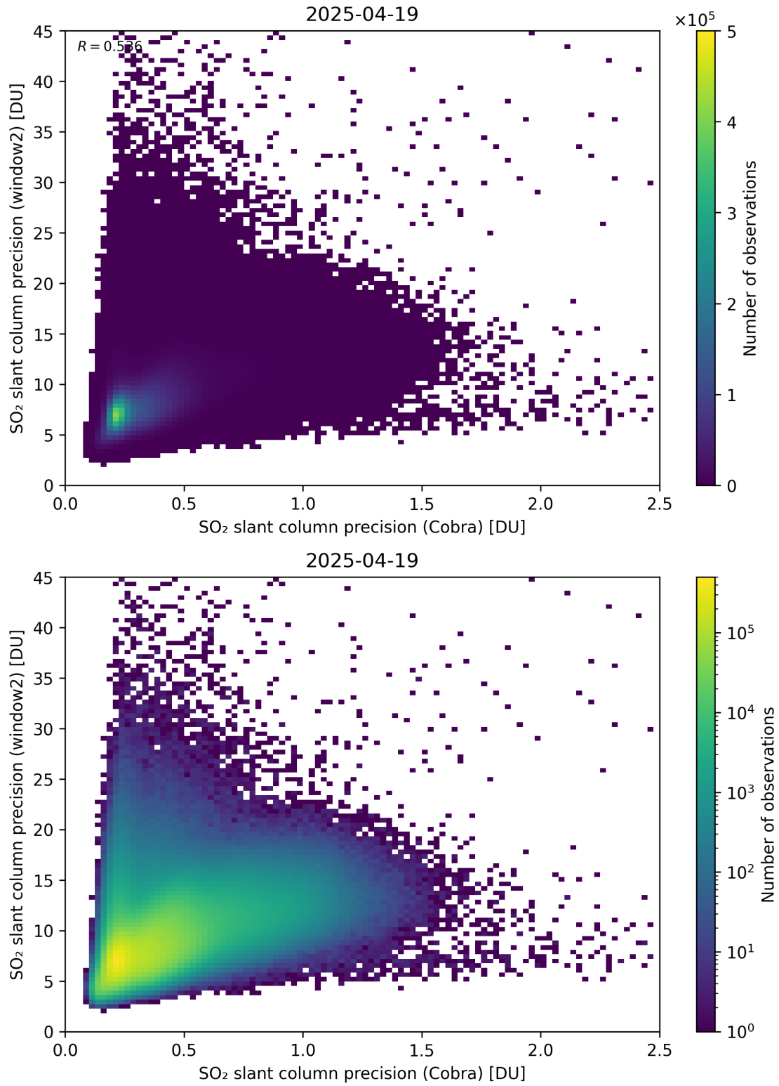
Figure 210: Scatter density plot of “SO 2 slant column precision (Cobra)” against “SO 2 slant column precision (window2)” for 2025-04-19 to 2025-04-20.
