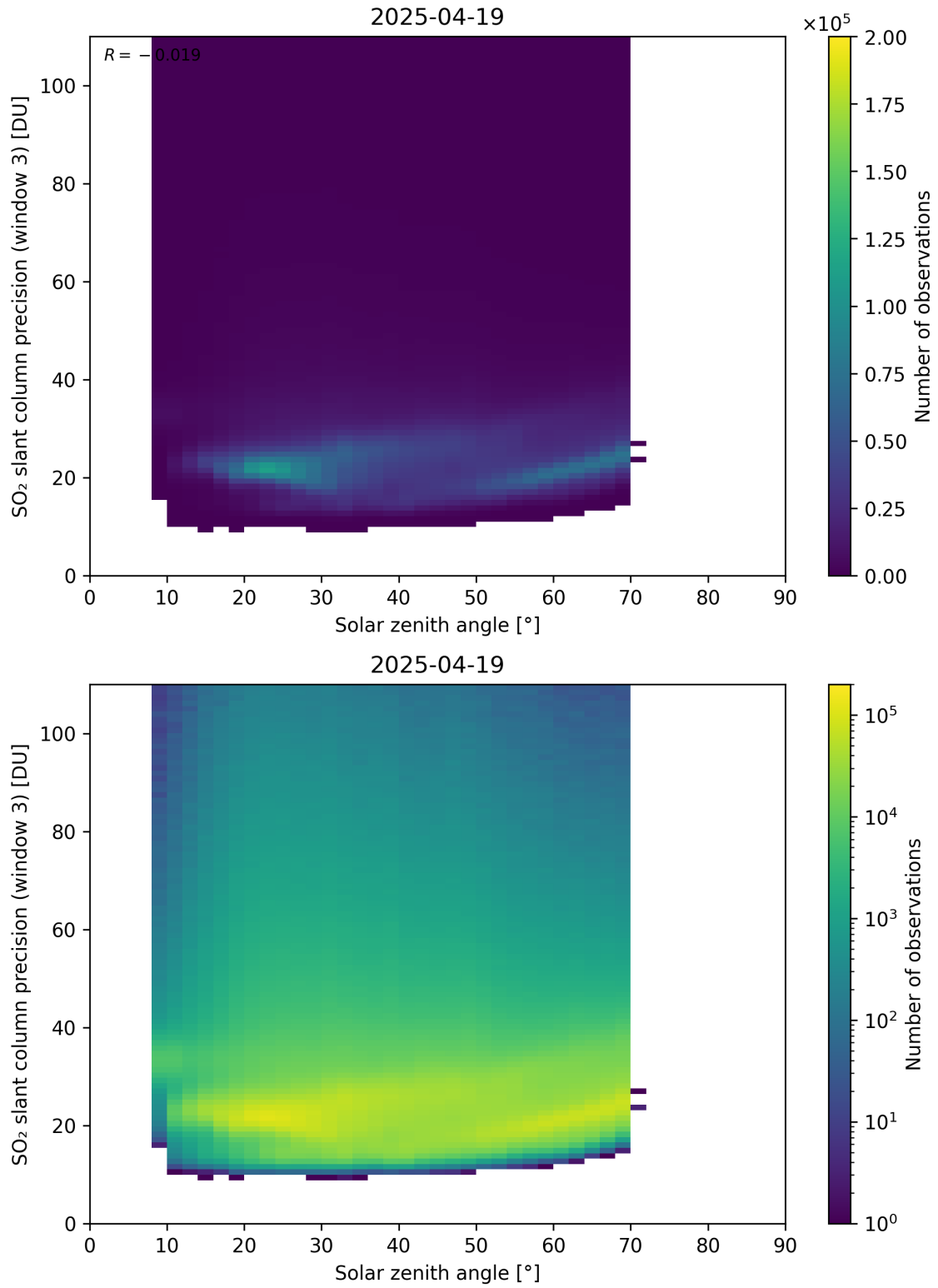
Figure 188: Scatter density plot of “Solar zenith angle” against “SO 2 slant column precision (window 3)” for 2025-04-19 to 2025-04-20.
