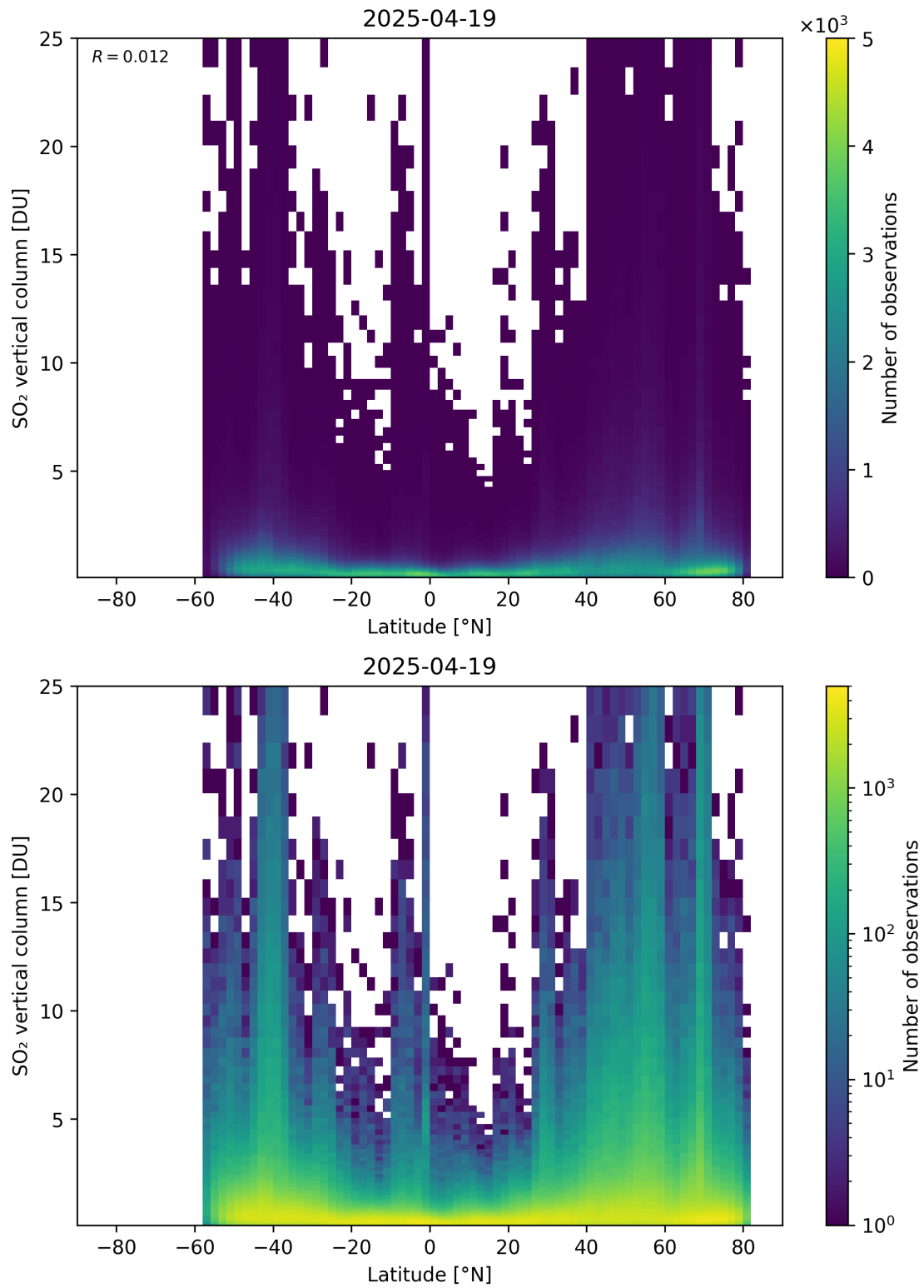
Figure 169: Scatter density plot of “Latitude” against “SO 2 vertical column” for 2025-04-19 to 2025-04-20.
