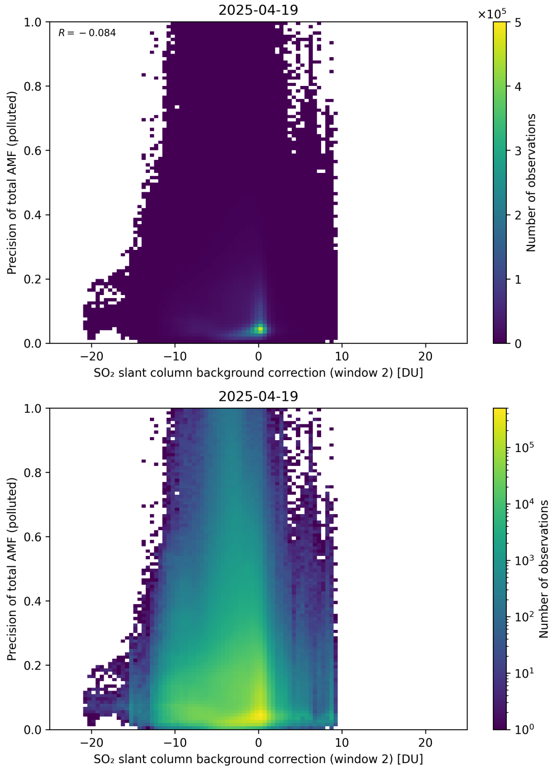
Figure 131: Scatter density plot of “SO 2 slant column background correction (window 2)” against “Precision of total AMF (polluted)” for 2025-04-19 to 2025-04-20.
