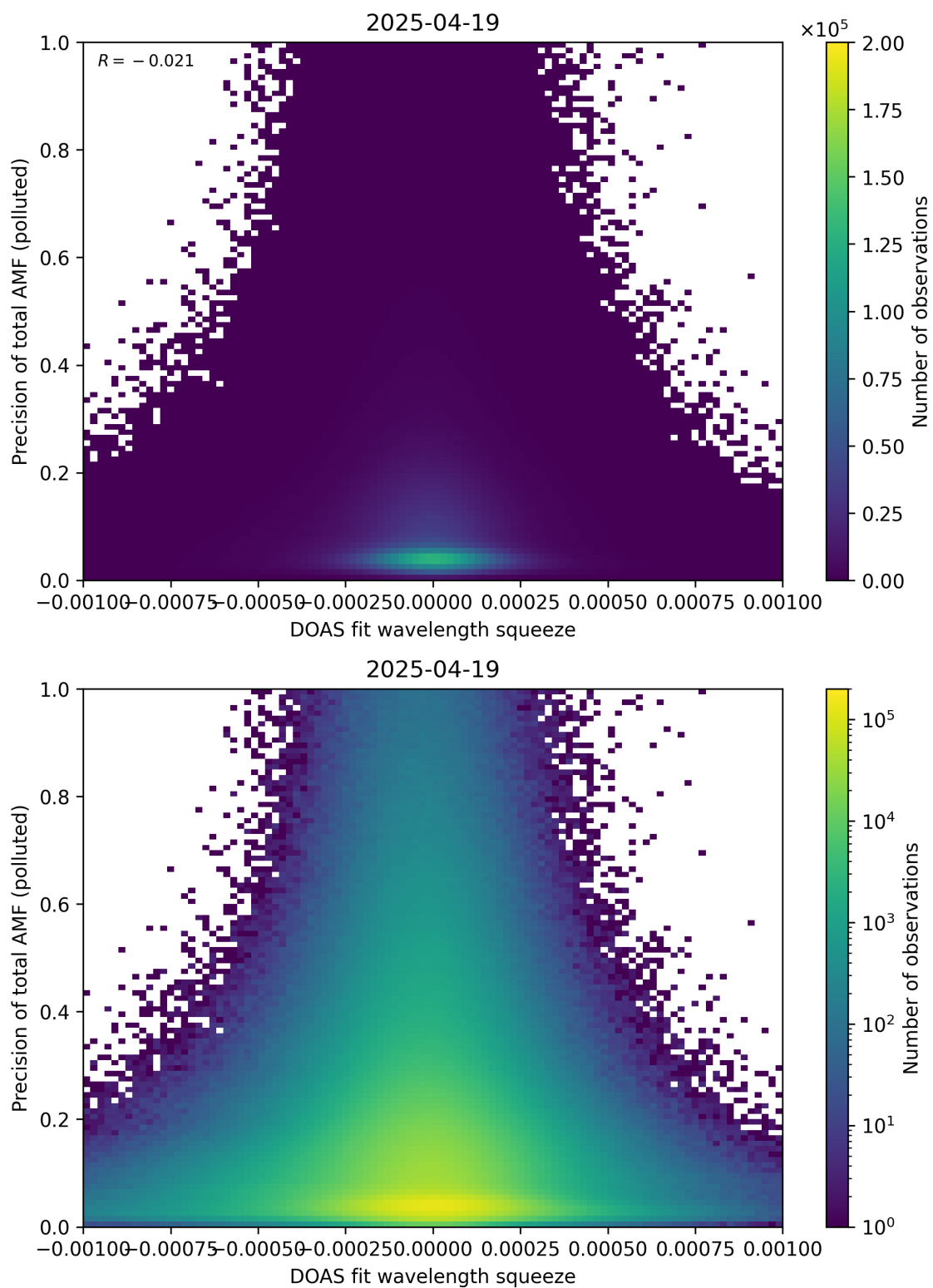
Figure 146: Scatter density plot of “DOAS fit wavelength squeeze” against “Precision of total AMF (polluted)” for 2025-04-19 to 2025-04-20.
