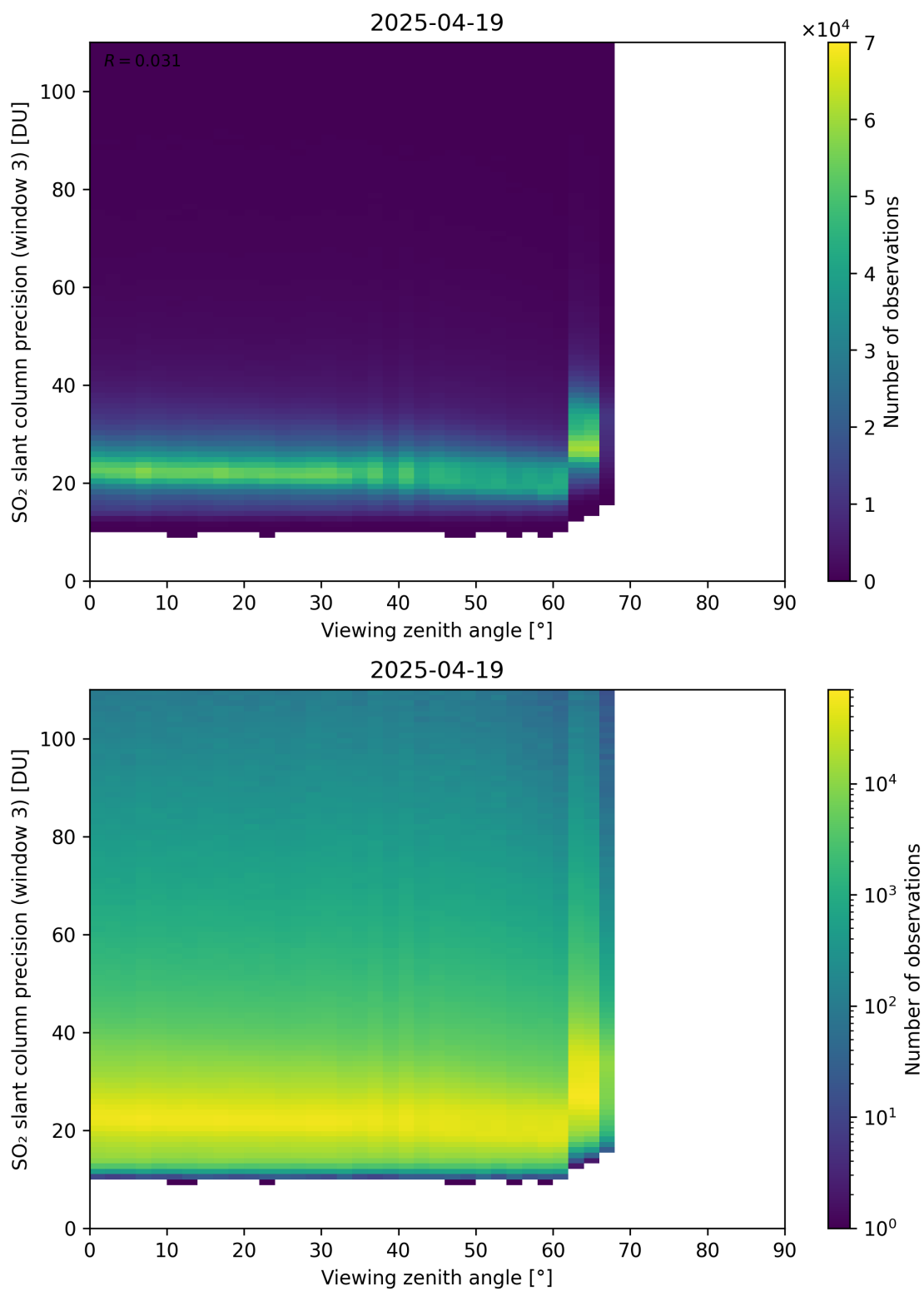
Figure 380: Scatter density plot of “Viewing zenith angle” against “SO 2 slant column precision (window 3)” for 2025-04-19 to 2025-04-20.
