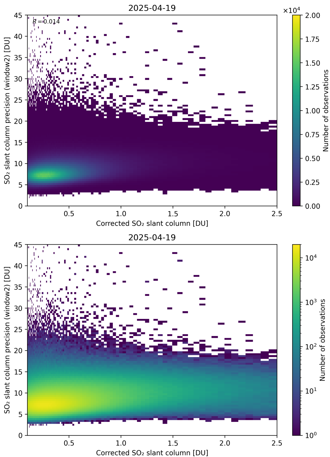
Figure 239: Scatter density plot of “Corrected SO 2 slant column” against “SO 2 slant column precision (window2)” for 2025-04-19 to 2025-04-20.
