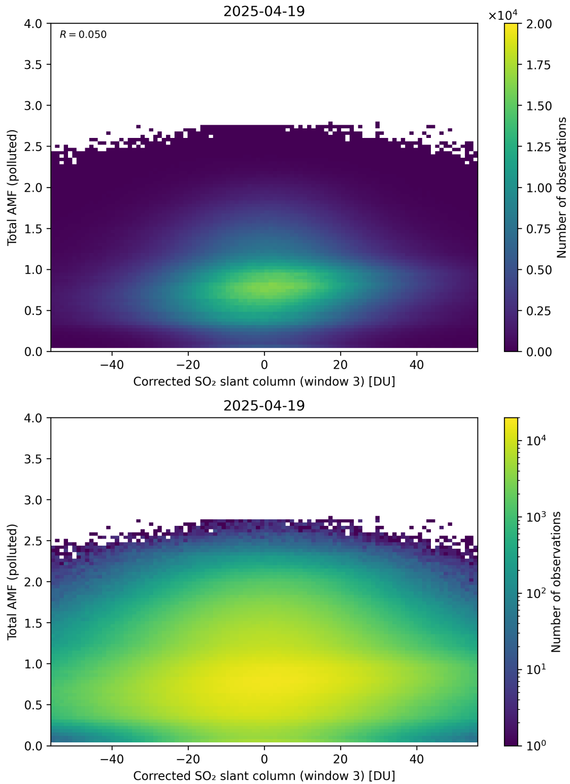
Figure 260: Scatter density plot of “Corrected SO 2 slant column (window 3)” against “Total AMF (polluted)” for 2025-04-19 to 2025-04-20.
