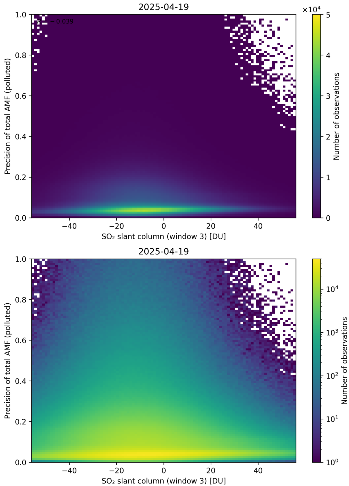
Figure 319: Scatter density plot of “SO 2 slant column (window 3)” against “Precision of total AMF (polluted)” for 2025-04-19 to 2025-04-20.
