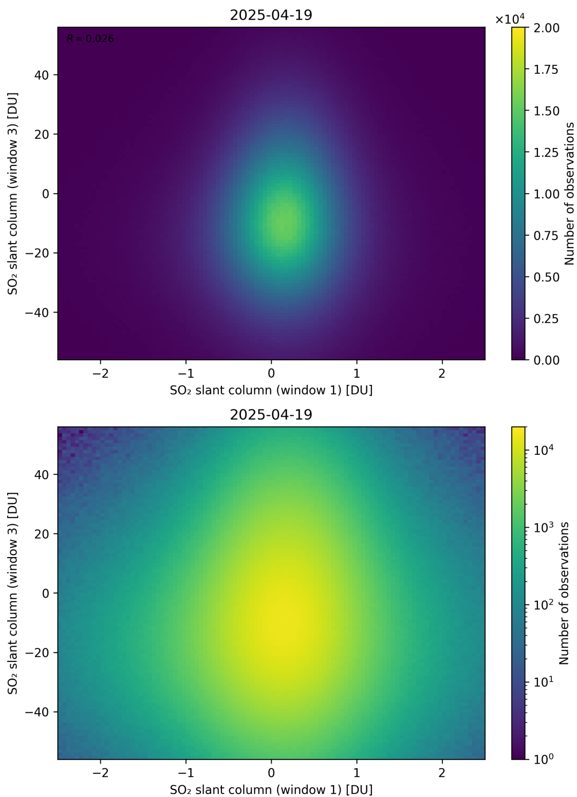
Figure 287: Scatter density plot of “SO 2 slant column (window 1)” against “SO 2 slant column (window 3)” for 2025-04-19 to 2025-04-20.
