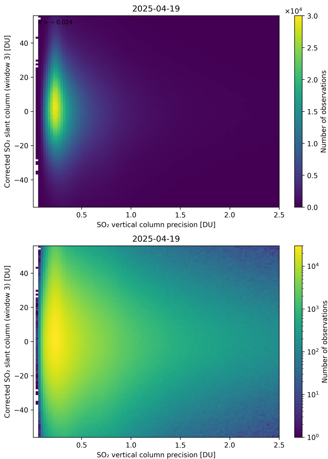
Figure 340: Scatter density plot of “SO 2 vertical column precision” against “Corrected SO 2 slant column (window 3)” for 2025-04-19 to 2025-04-20.
