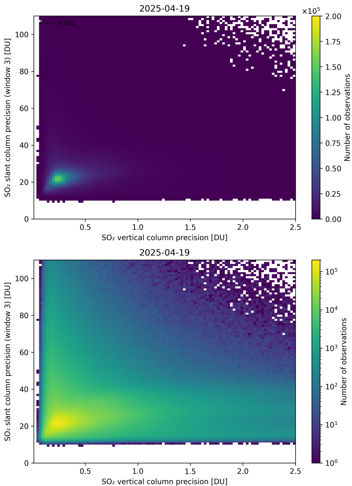
Figure 345: Scatter density plot of “SO 2 vertical column precision” against “SO 2 slant column precision (window 3)” for 2025-04-19 to 2025-04-20.
