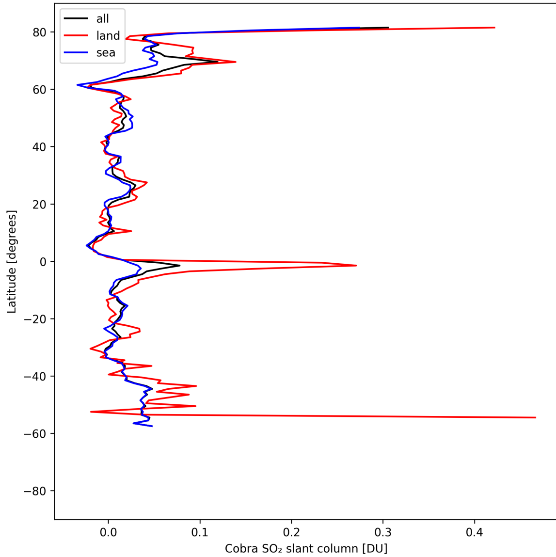
Figure 35: Zonal average of “Cobra SO 2 slant column” for 2025-04-19 to 2025-04-20.
