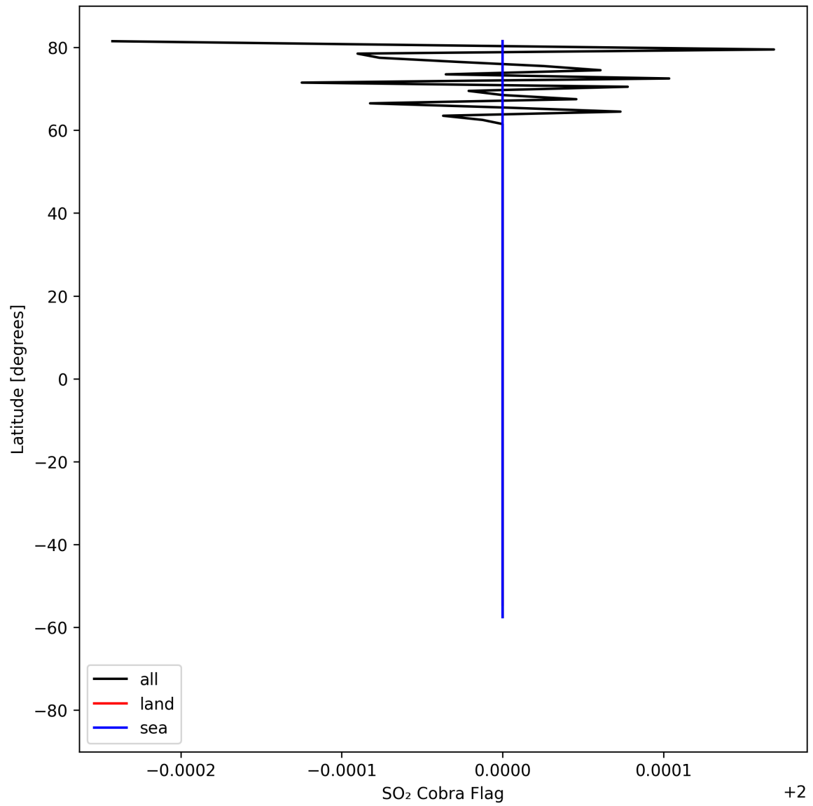
Figure 49: Zonal average of “SO 2 Cobra Flag” for 2025-04-19 to 2025-04-20.
