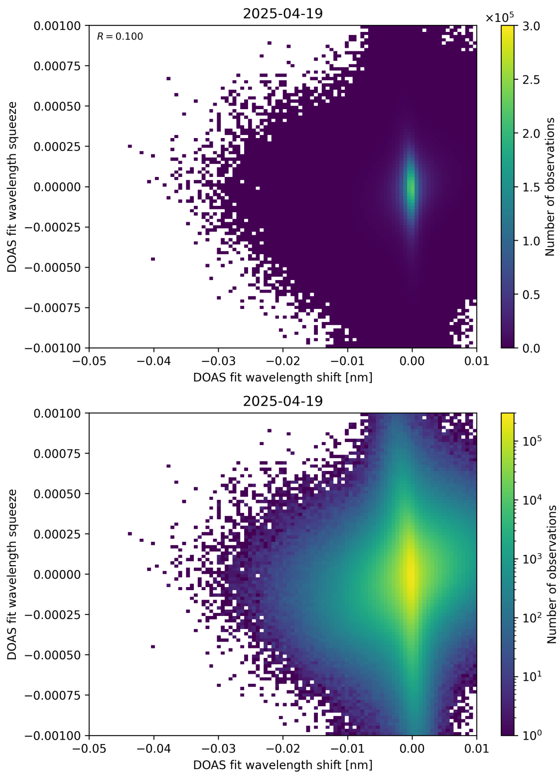
Figure 138: Scatter density plot of “DOAS fit wavelength shift” against “DOAS fit wavelength squeeze” for 2025-04-19 to 2025-04-20.
