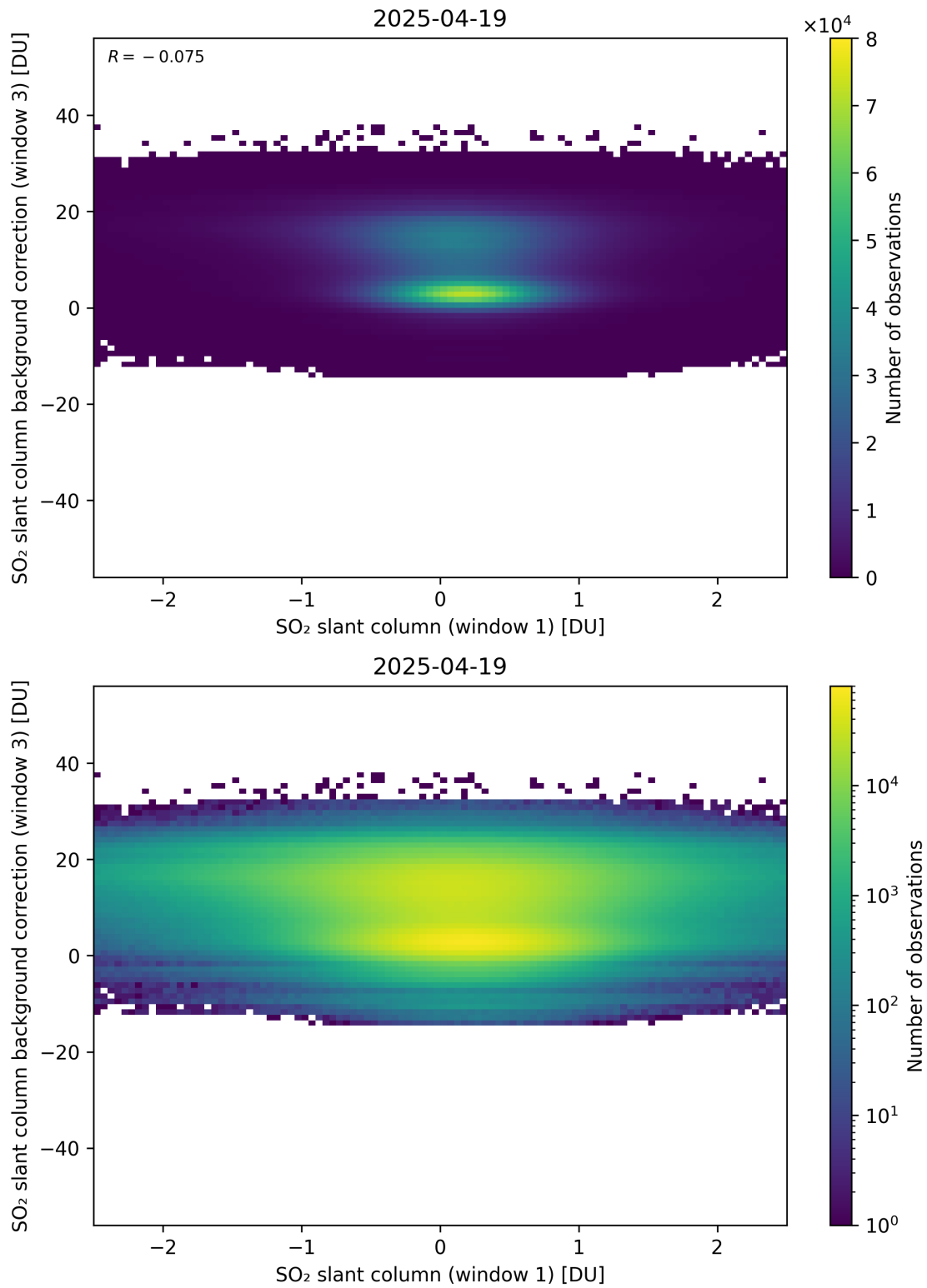
Figure 264: Scatter density plot of “SO 2 slant column (window 1)” against “SO 2 slant column background correction (window 3)” for 2025-04-19 to 2025-04-20.
