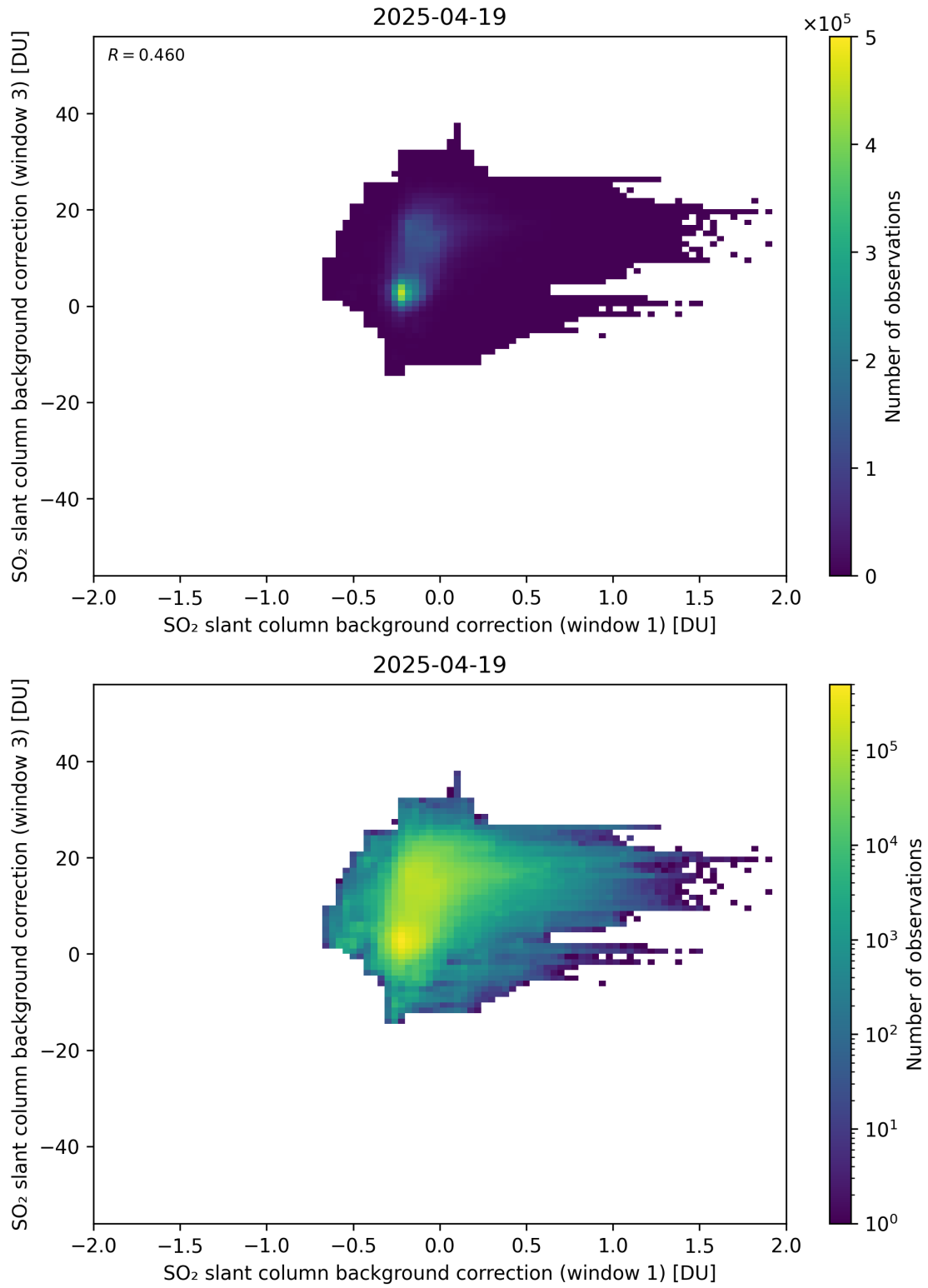
Figure 110: Scatter density plot of “SO 2 slant column background correction (window 1)” against “SO 2 slant column background correction (window 3)” for 2025-04-19 to 2025-04-20.
