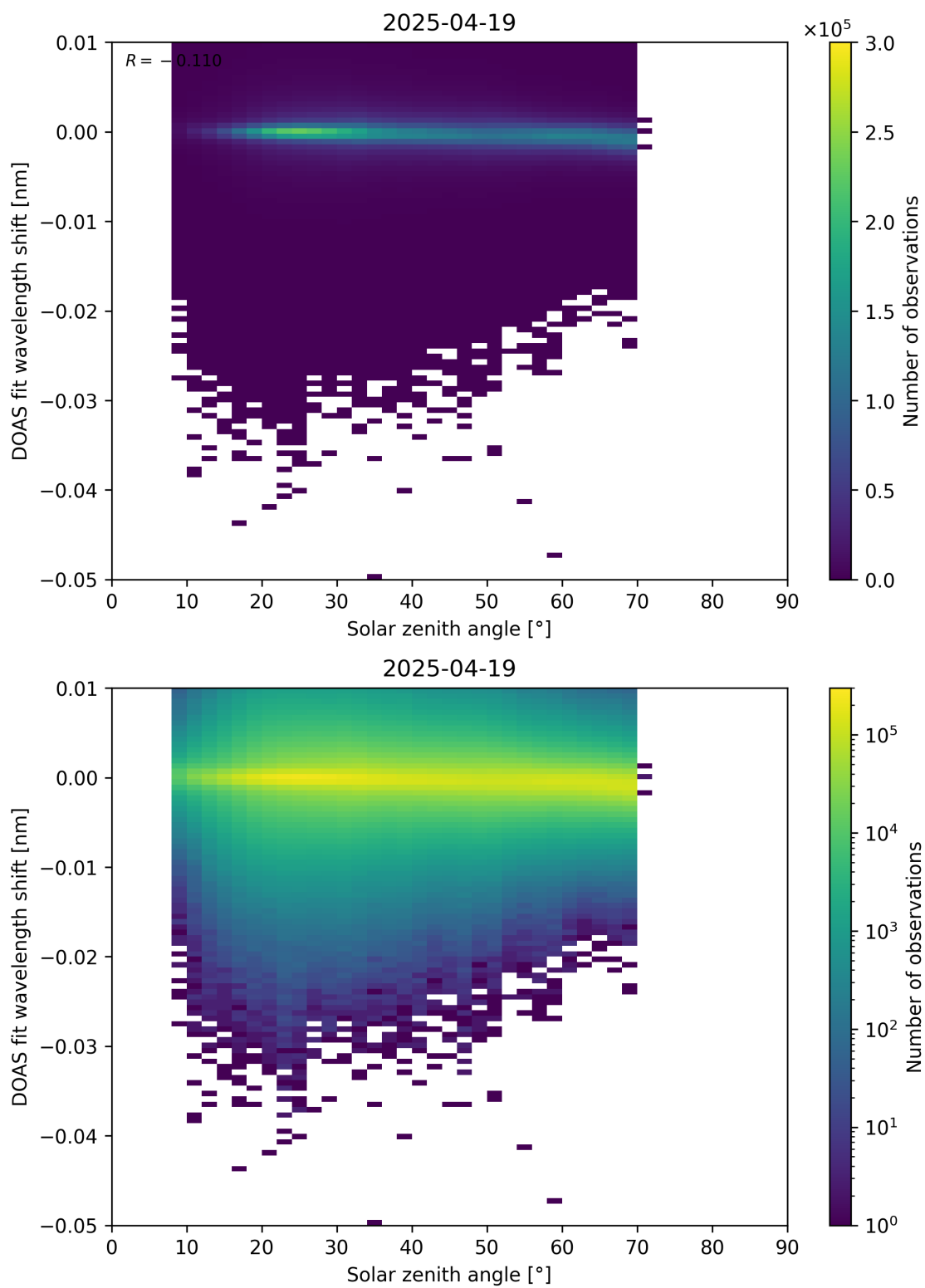
Figure 174: Scatter density plot of “Solar zenith angle” against “DOAS fit wavelength shift” for 2025-04-19 to 2025-04-20.
