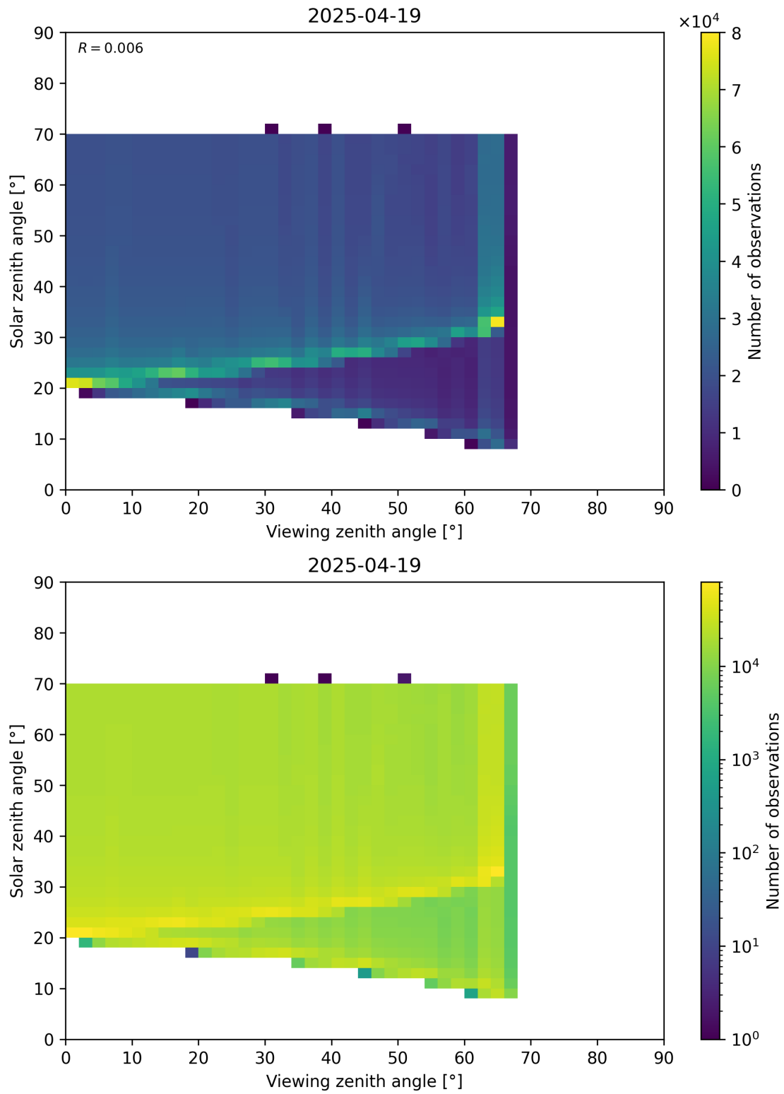
Figure 369: Scatter density plot of “Viewing zenith angle” against “Solar zenith angle” for 2025-04-19 to 2025-04-20.
