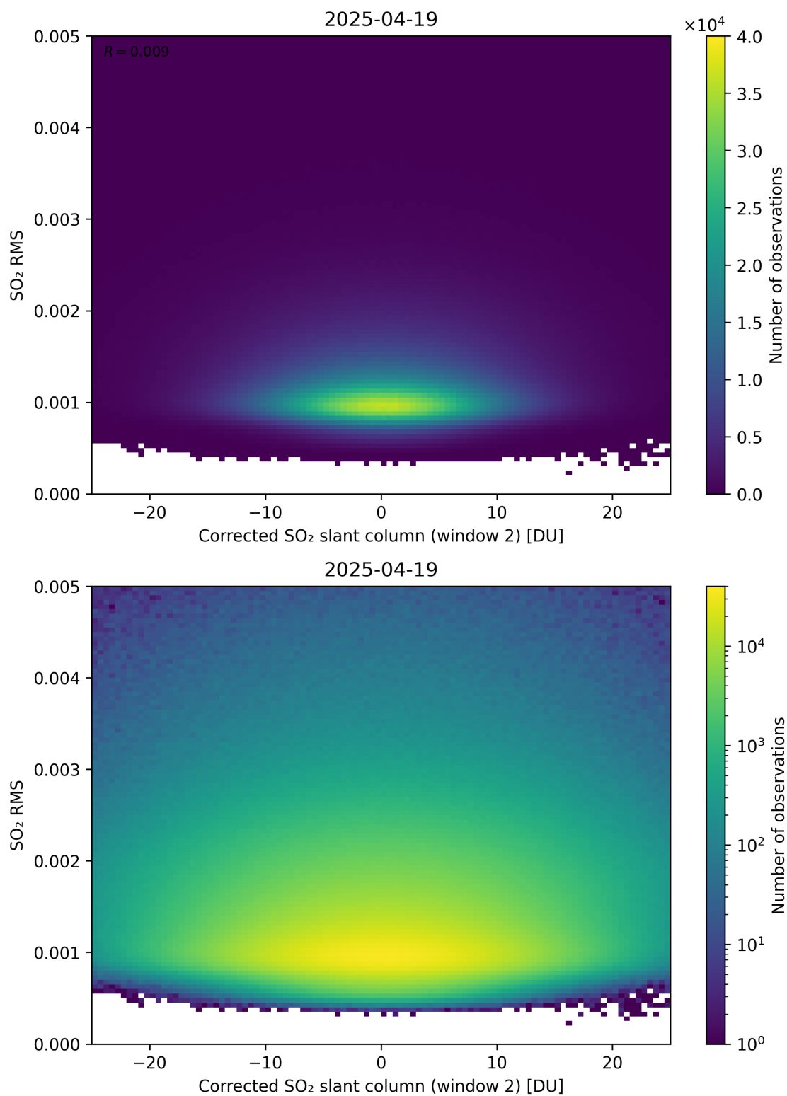
Figure 248: Scatter density plot of “Corrected SO 2 slant column (window 2)” against “SO 2 RMS” for 2025-04-19 to 2025-04-20.
