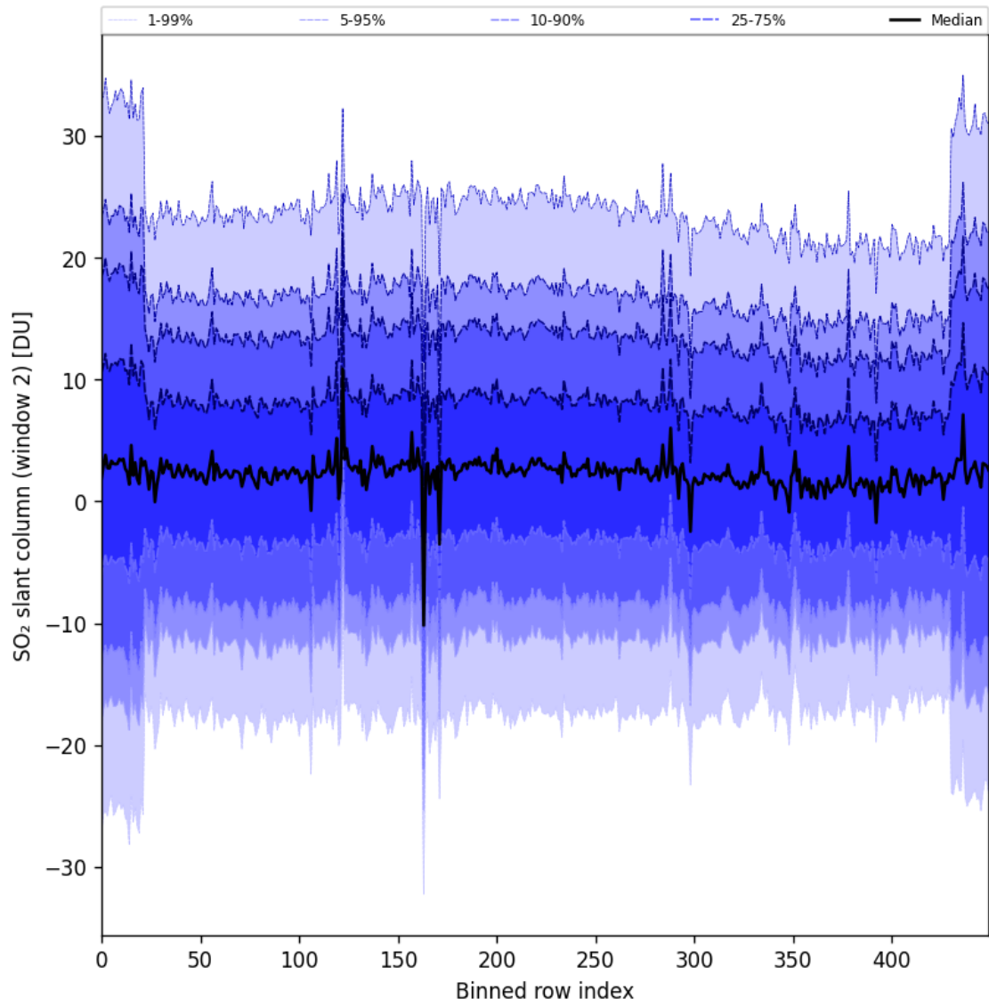
Figure 93: Along track statistics of “SO 2 slant column (window 2)” for 2025-04-19 to 2025-04-20
