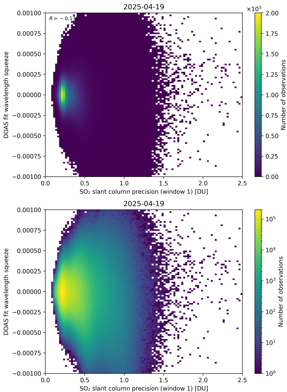
Figure 272: Scatter density plot of “SO 2 slant column precision (window 1)” against “DOAS fit wavelength squeeze” for 2025-04-19 to 2025-04-20.
