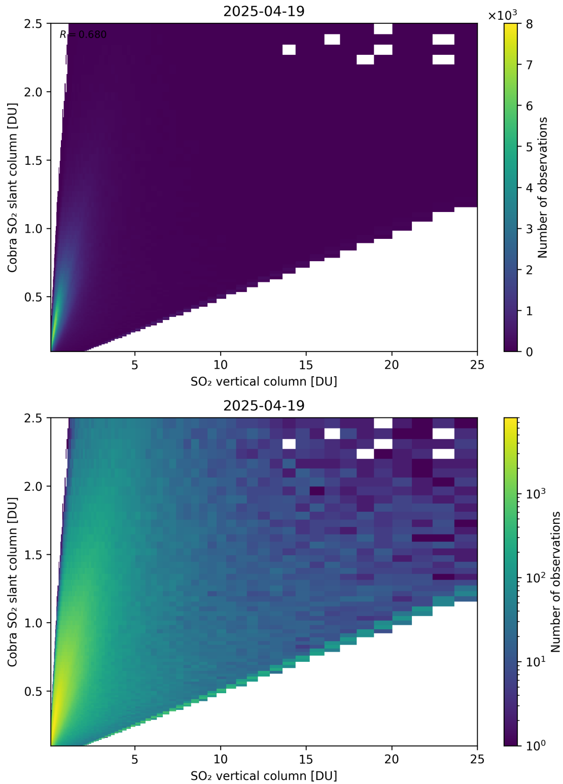
Figure 349: Scatter density plot of “SO 2 vertical column” against “Cobra SO 2 slant column” for 2025-04-19 to 2025-04-20.
