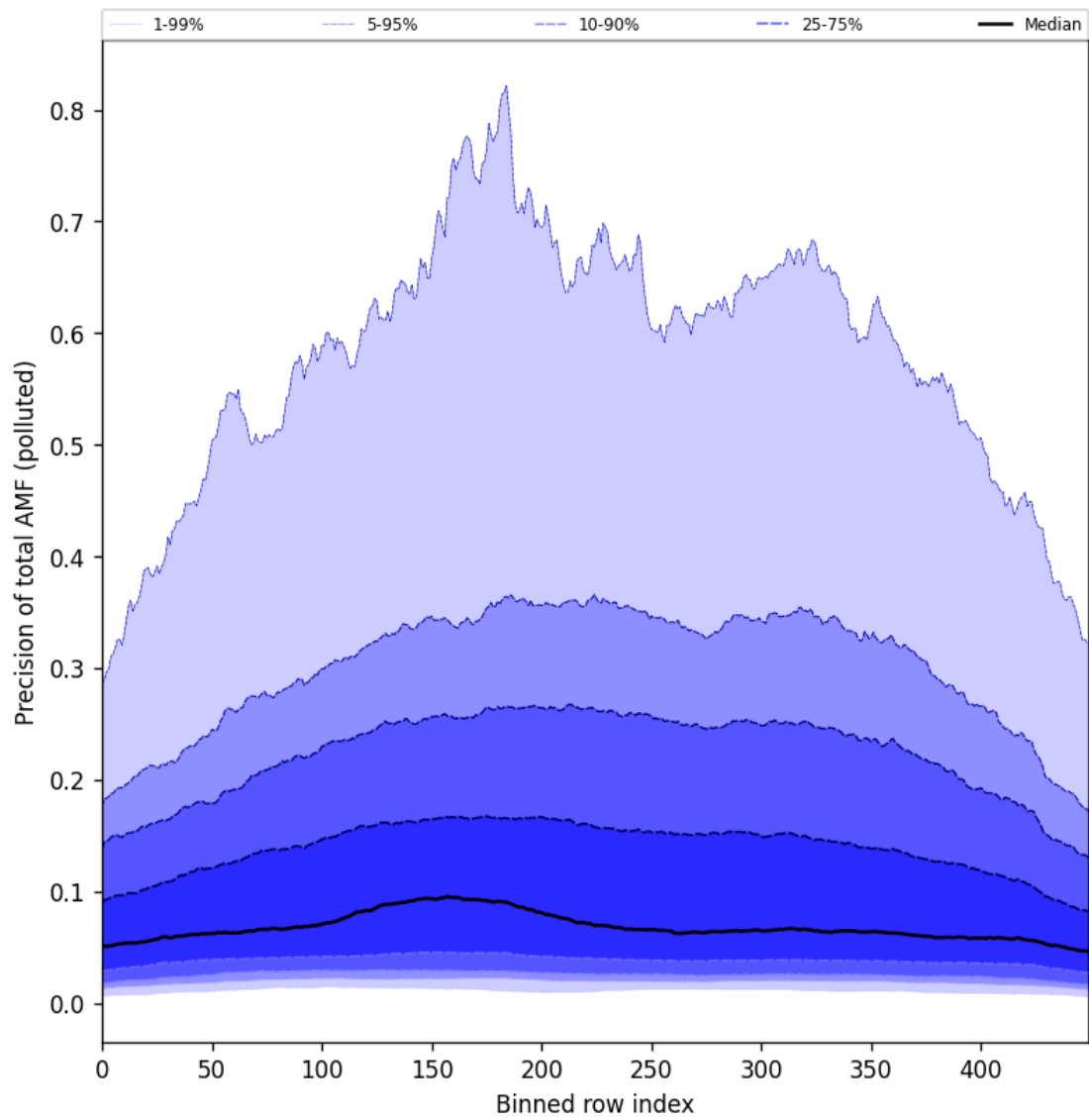
Figure 106: Along track statistics of “Precision of total AMF (polluted)” for 2025-04-19 to 2025-04-20
