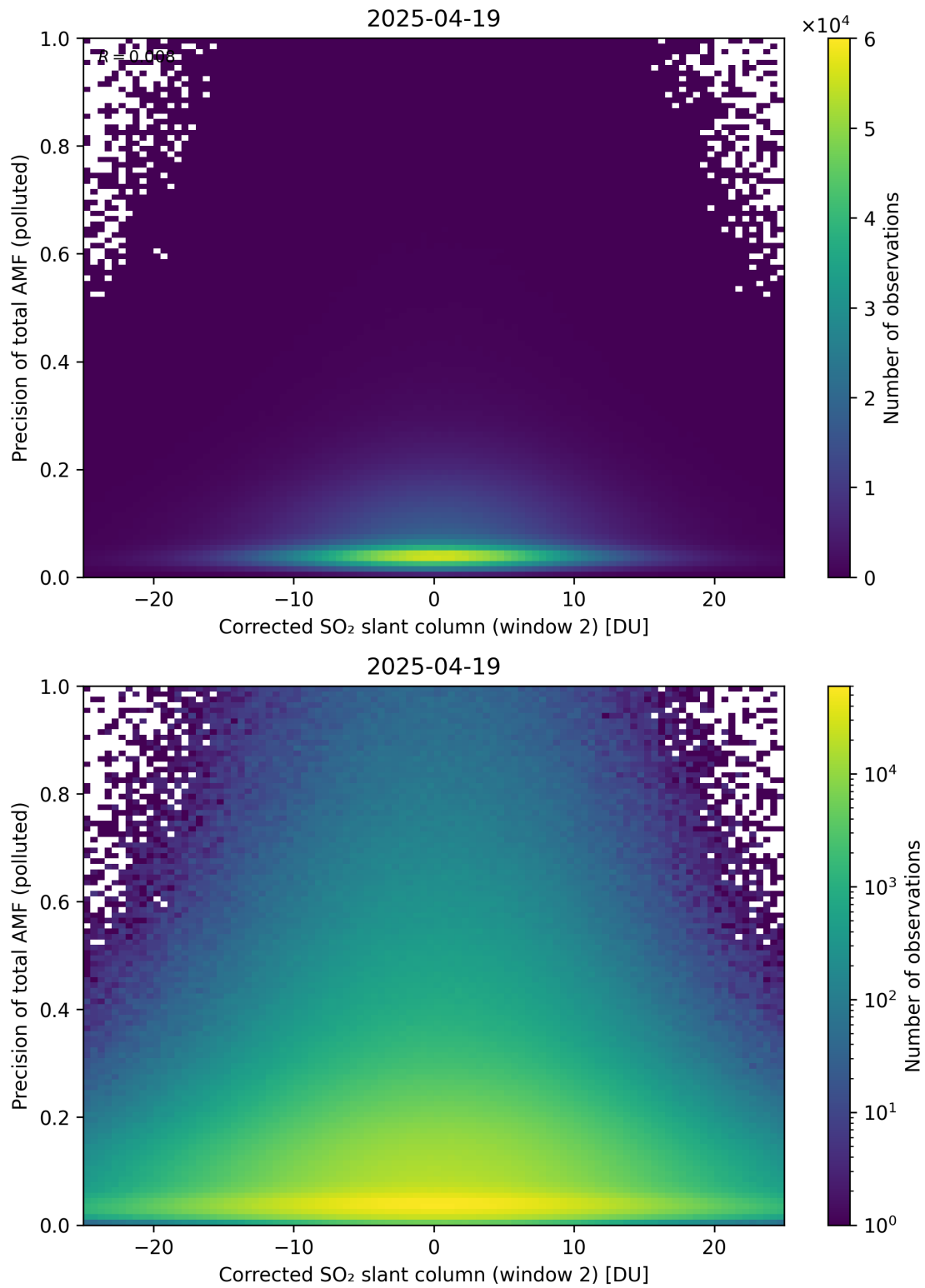
Figure 254: Scatter density plot of “Corrected SO 2 slant column (window 2)” against “Precision of total AMF (polluted)” for 2025-04-19 to 2025-04-20.
