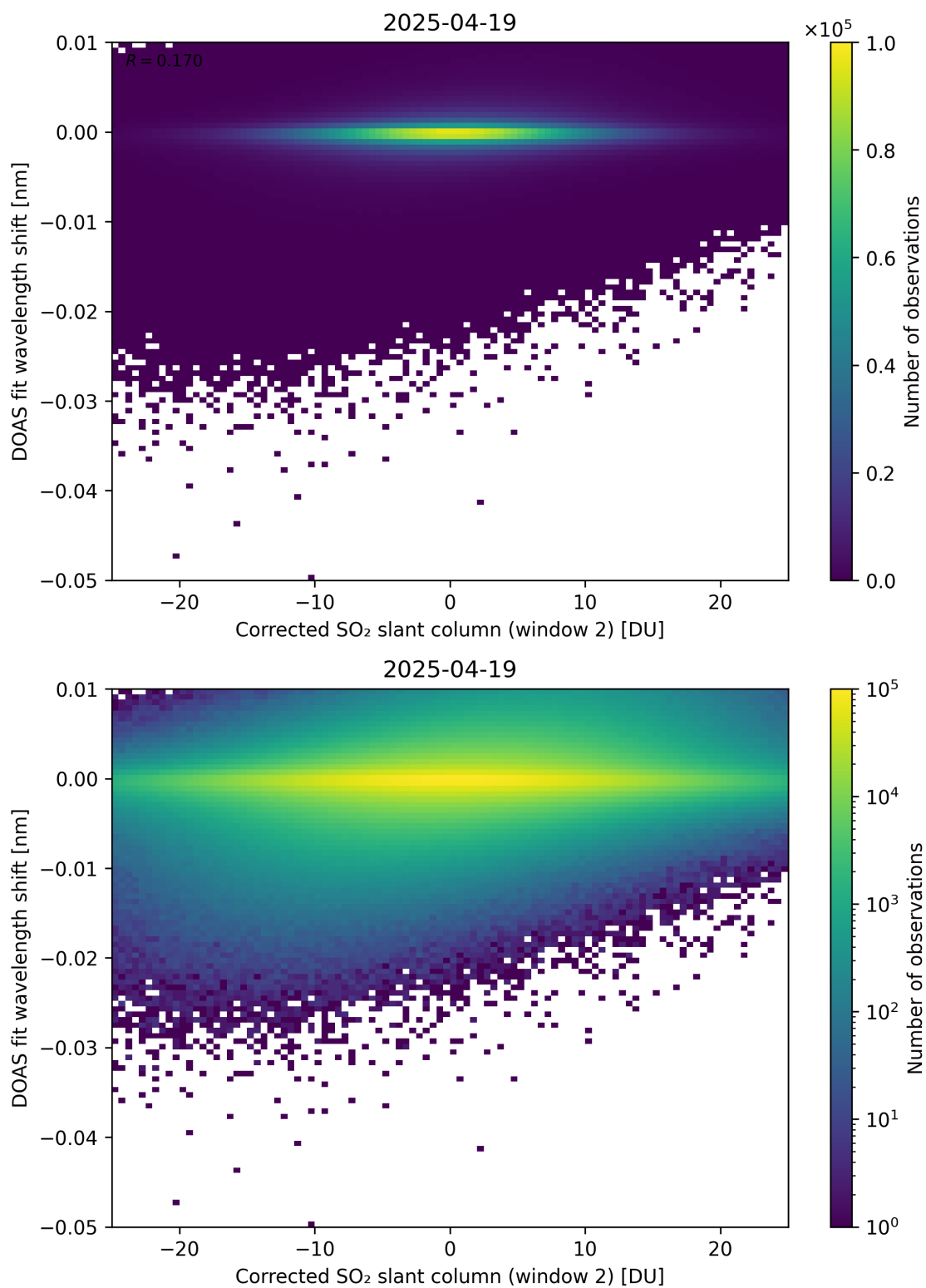
Figure 246: Scatter density plot of “Corrected SO 2 slant column (window 2)” against “DOAS fit wavelength shift” for 2025-04-19 to 2025-04-20.
