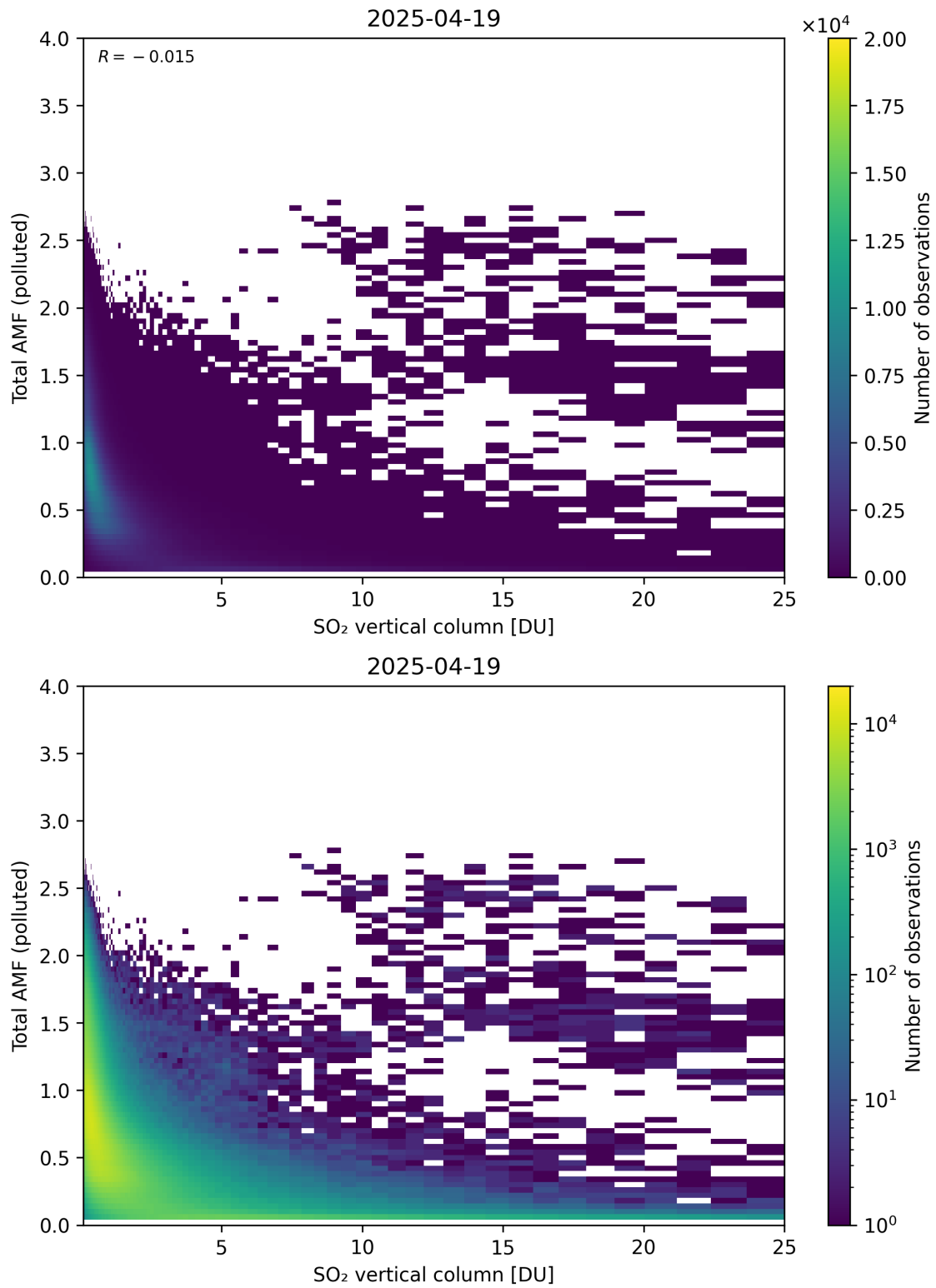
Figure 359: Scatter density plot of “SO 2 vertical column” against “Total AMF (polluted)” for 2025-04-19 to 2025-04-20.
