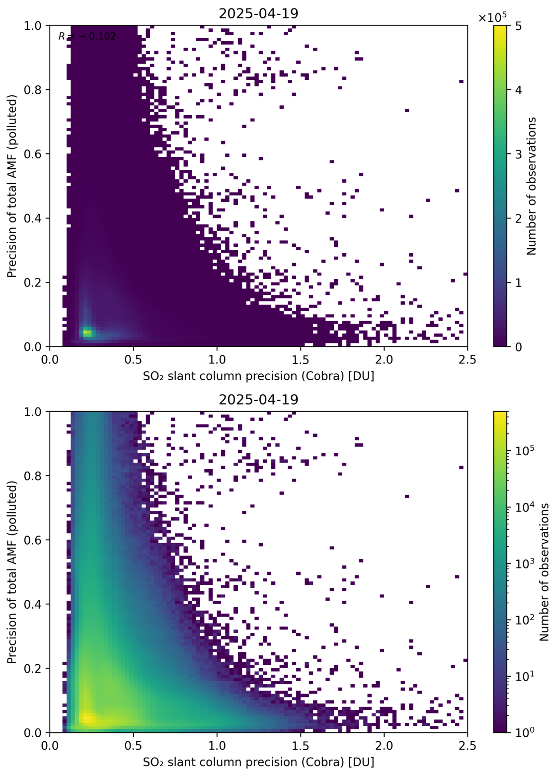
Figure 214: Scatter density plot of “SO 2 slant column precision (Cobra)” against “Precision of total AMF (polluted)” for 2025-04-19 to 2025-04-20.
