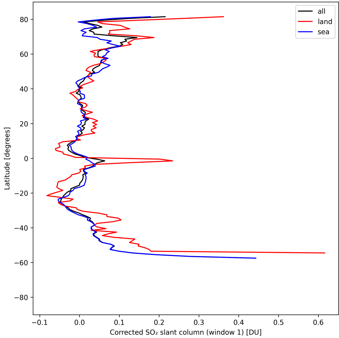
Figure 39: Zonal average of “Corrected SO 2 slant column (window 1)” for 2025-04-19 to 2025-04-20.
