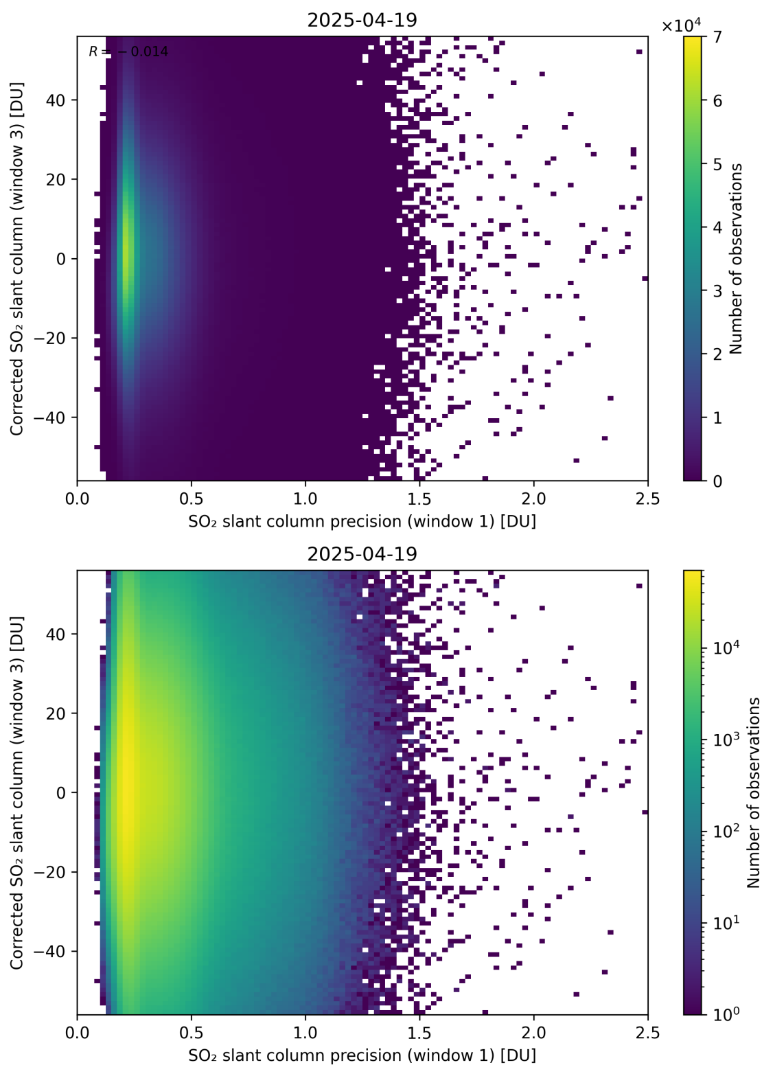
Figure 276: Scatter density plot of “SO 2 slant column precision (window 1)” against “Corrected SO 2 slant column (window 3)” for 2025-04-19 to 2025-04-20.
