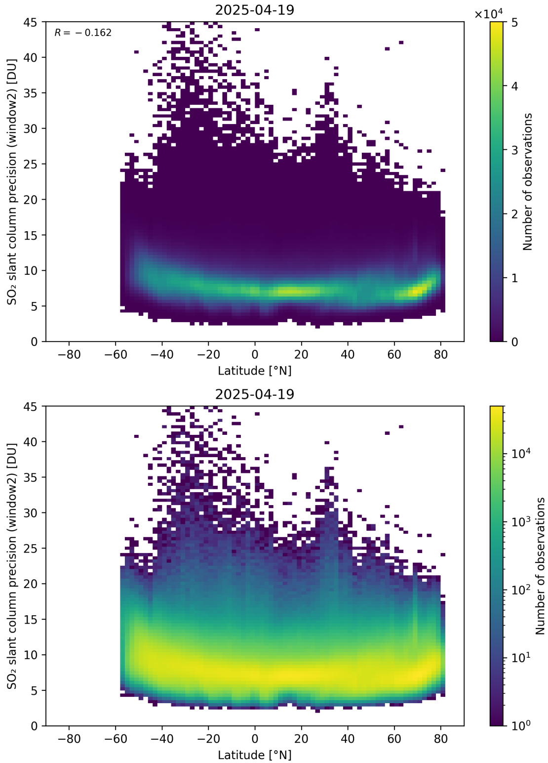
Figure 164: Scatter density plot of “Latitude” against “SO 2 slant column precision (window2)” for 2025-04-19 to 2025-04-20.
