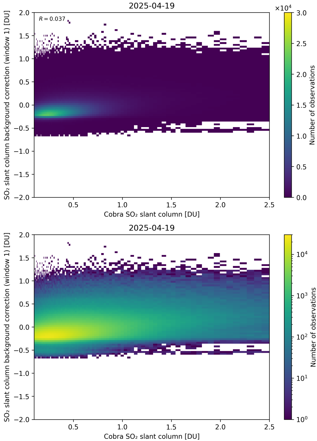
Figure 193: Scatter density plot of “Cobra SO 2 slant column” against “SO 2 slant column background correction (window 1)” for 2025-04-19 to 2025-04-20.
