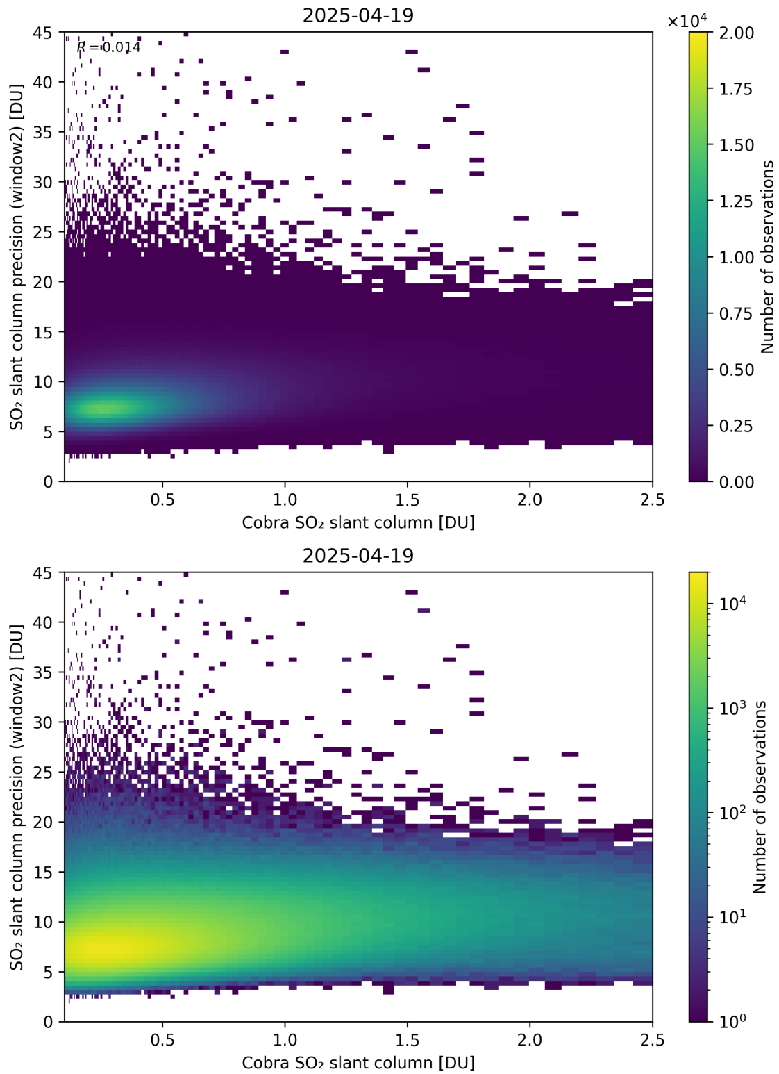
Figure 221: Scatter density plot of “Cobra SO 2 slant column” against “SO 2 slant column precision (window2)” for 2025-04-19 to 2025-04-20.
