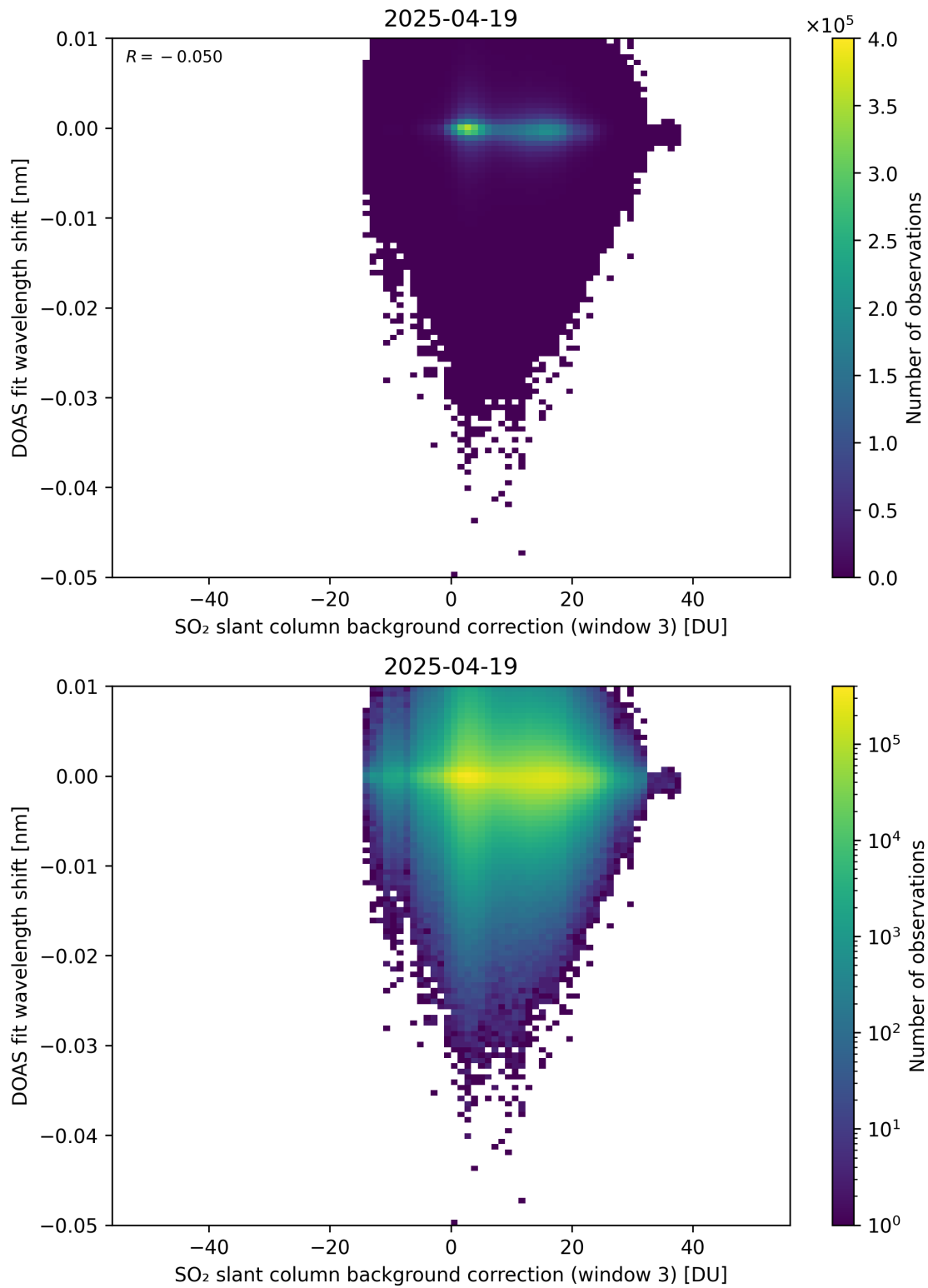
Figure 132: Scatter density plot of “SO 2 slant column background correction (window 3)” against “DOAS fit wavelength shift” for 2025-04-19 to 2025-04-20.
