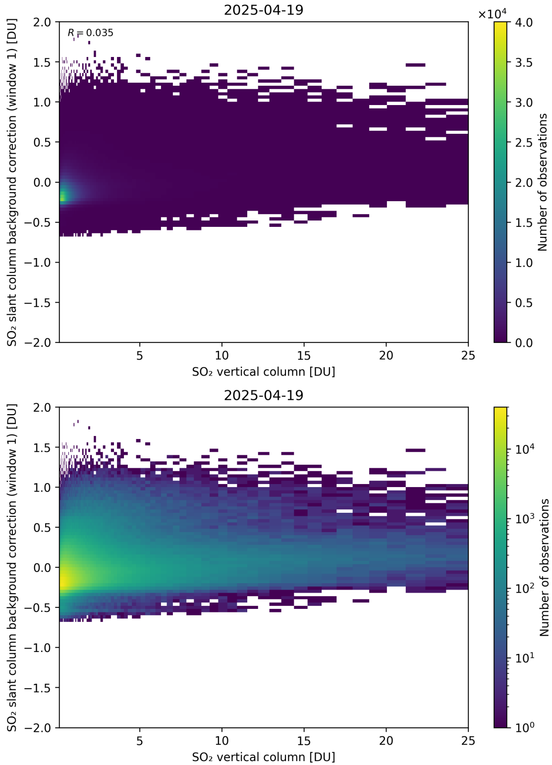
Figure 323: Scatter density plot of “SO 2 vertical column” against “SO 2 slant column background correction (window 1)” for 2025-04-19 to 2025-04-20.
