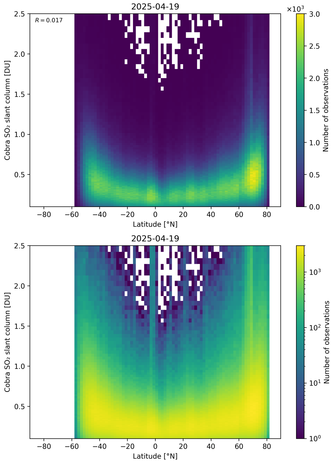
Figure 157: Scatter density plot of “Latitude” against “Cobra SO 2 slant column” for 2025-04-19 to 2025-04-20.
