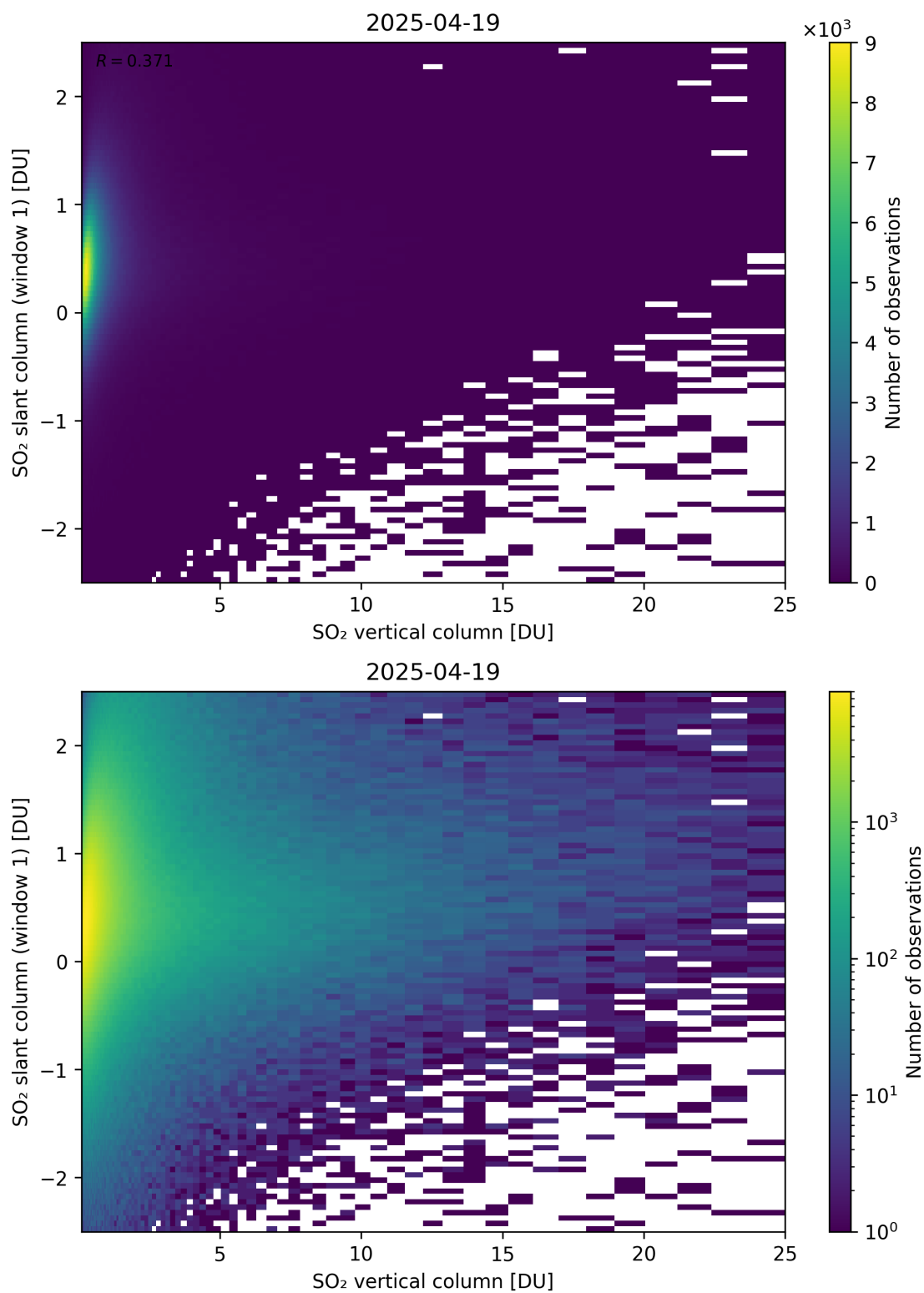
Figure 354: Scatter density plot of “SO 2 vertical column” against “SO 2 slant column (window 1)” for 2025-04-19 to 2025-04-20.
