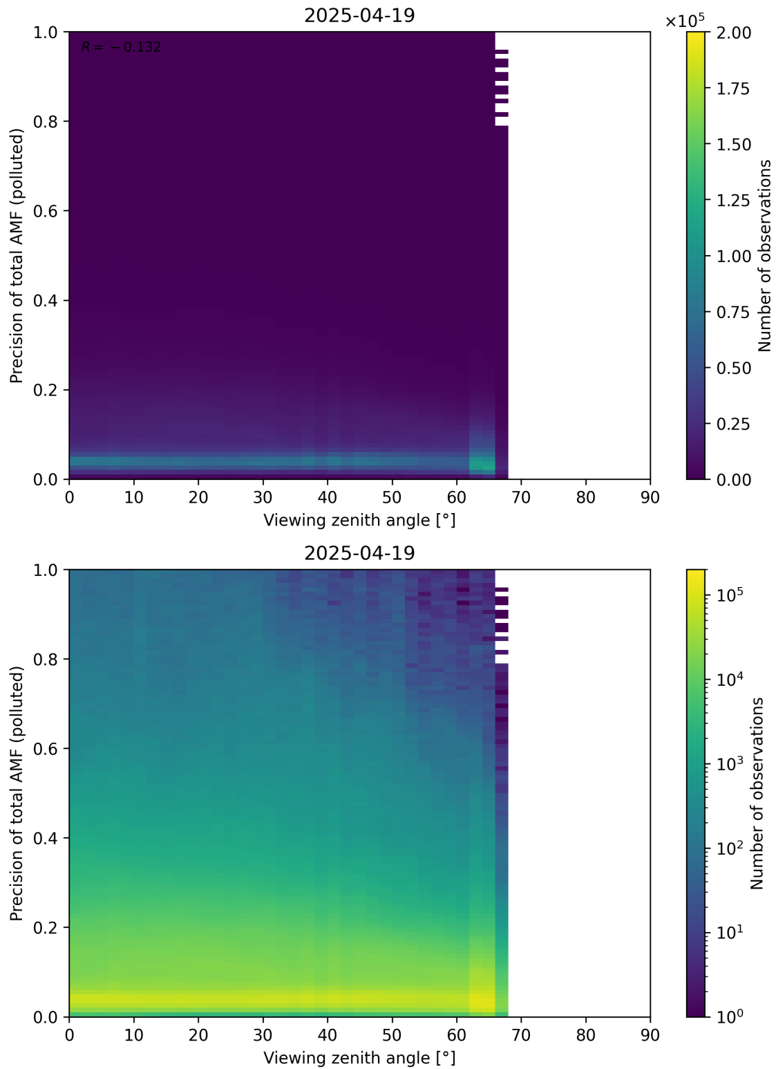
Figure 382: Scatter density plot of “Viewing zenith angle” against “Precision of total AMF (polluted)” for 2025-04-19 to 2025-04-20.
