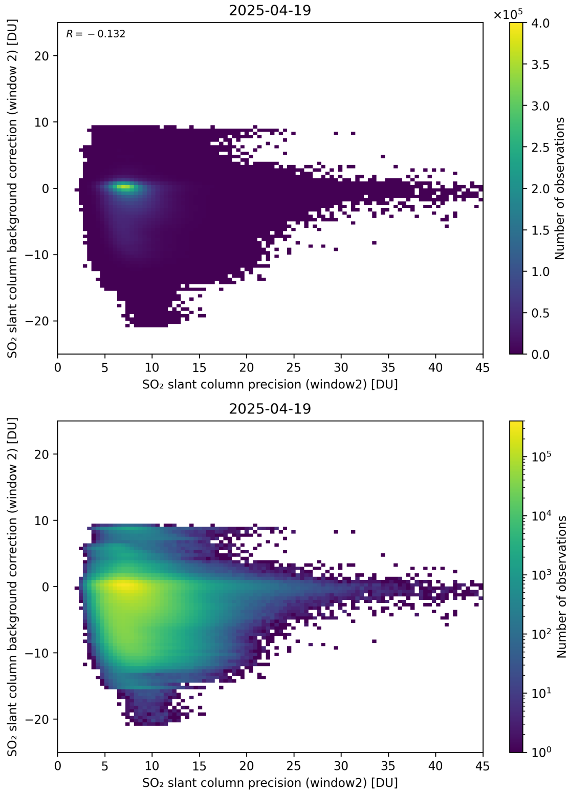
Figure 291: Scatter density plot of “SO 2 slant column precision (window2)” against “SO 2 slant column background correction (window 2)” for 2025-04-19 to 2025-04-20.
