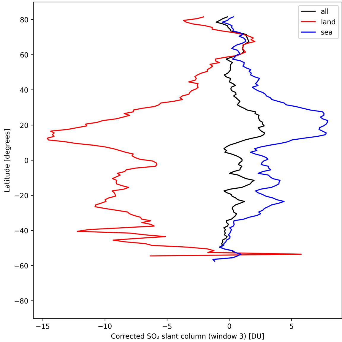
Figure 47: Zonal average of “Corrected SO 2 slant column (window 3)” for 2025-04-19 to 2025-04-20.
