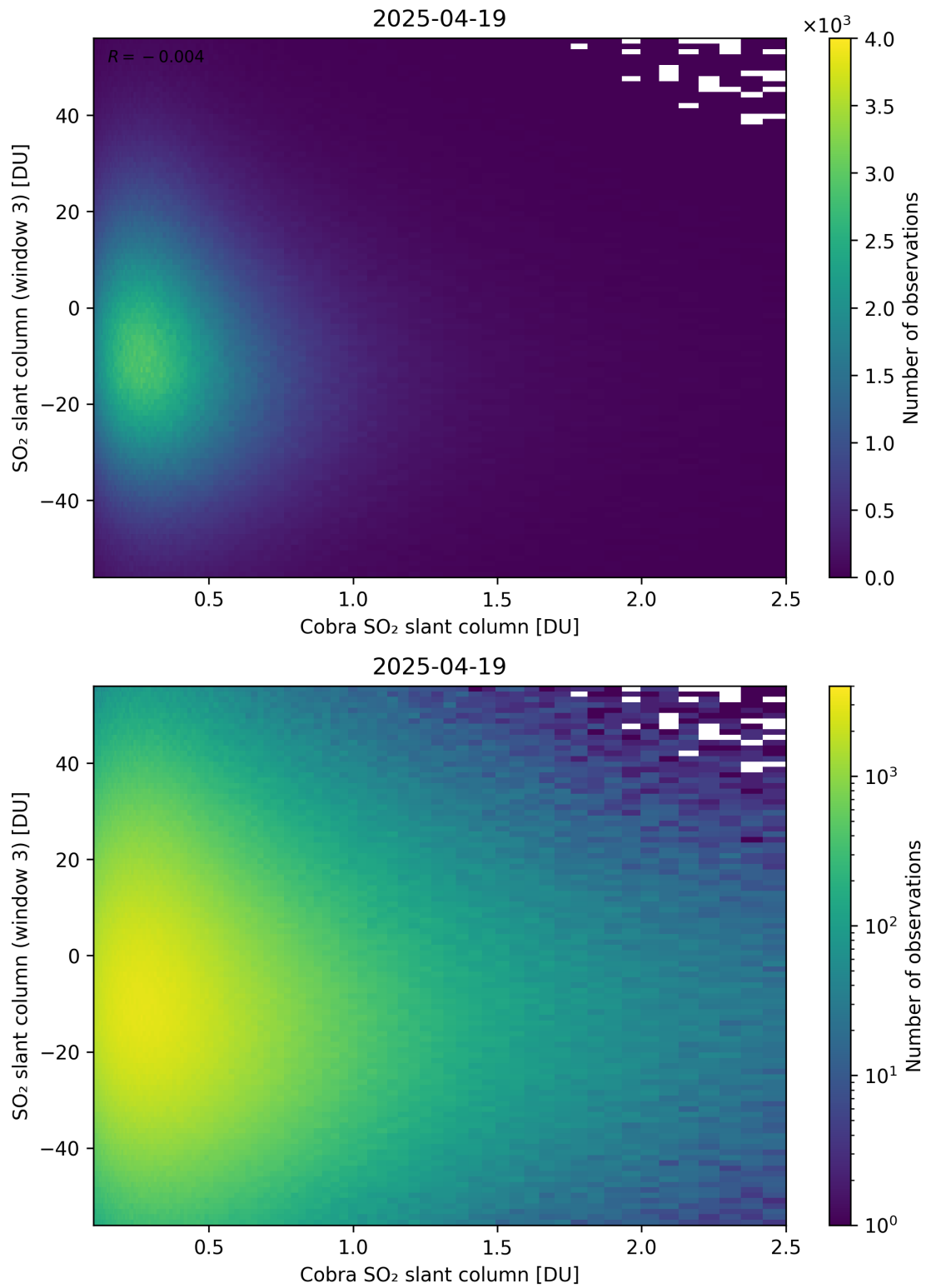
Figure 222: Scatter density plot of “Cobra SO 2 slant column” against “SO 2 slant column (window 3)” for 2025-04-19 to 2025-04-20.
