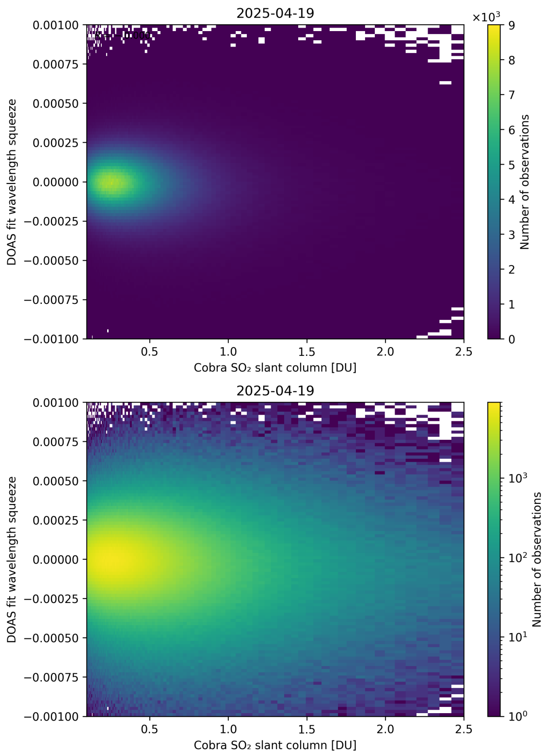
Figure 197: Scatter density plot of “Cobra SO 2 slant column” against “DOAS fit wavelength squeeze” for 2025-04-19 to 2025-04-20.
