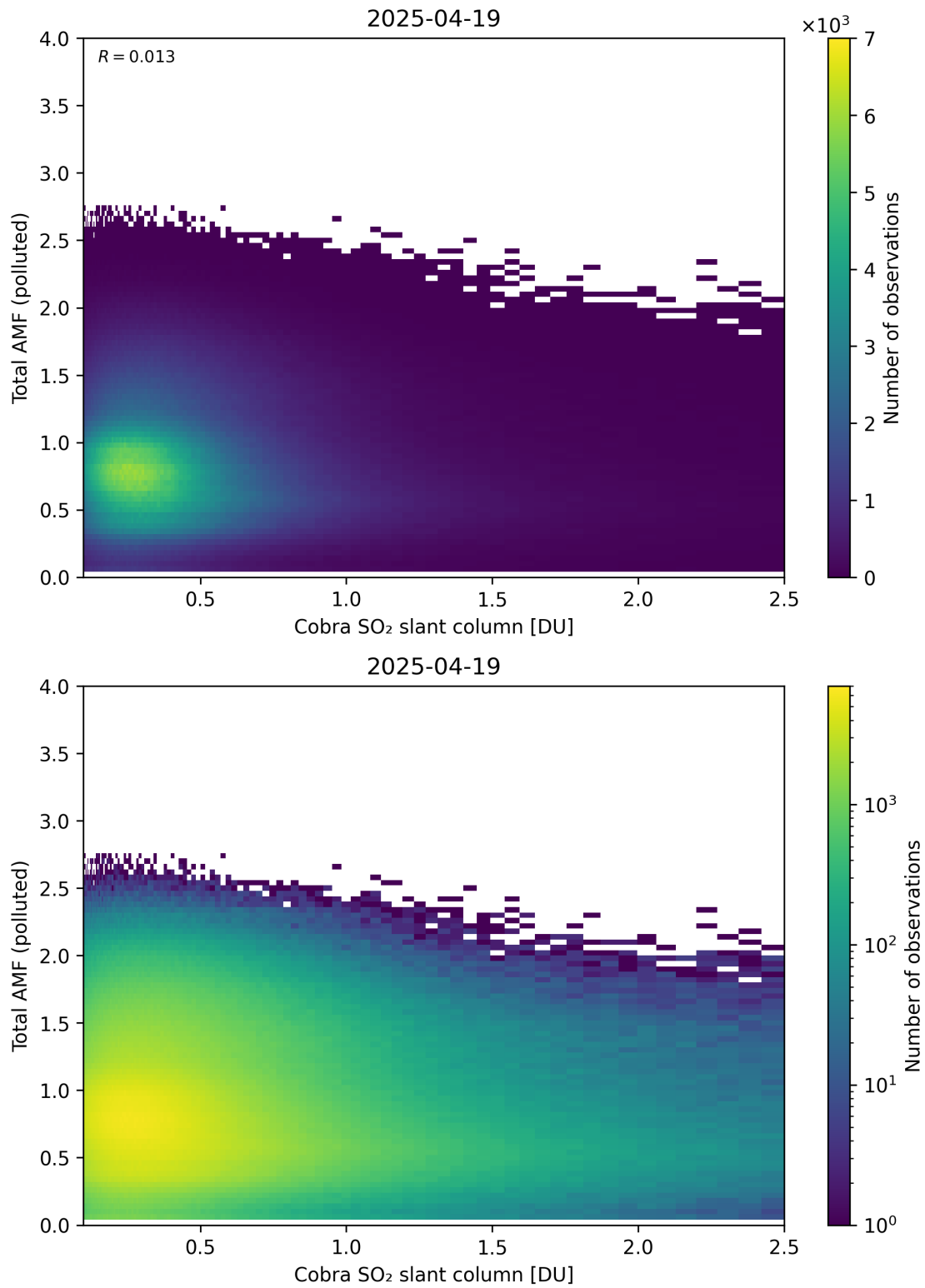
Figure 224: Scatter density plot of “Cobra SO 2 slant column” against “Total AMF (polluted)” for 2025-04-19 to 2025-04-20.
