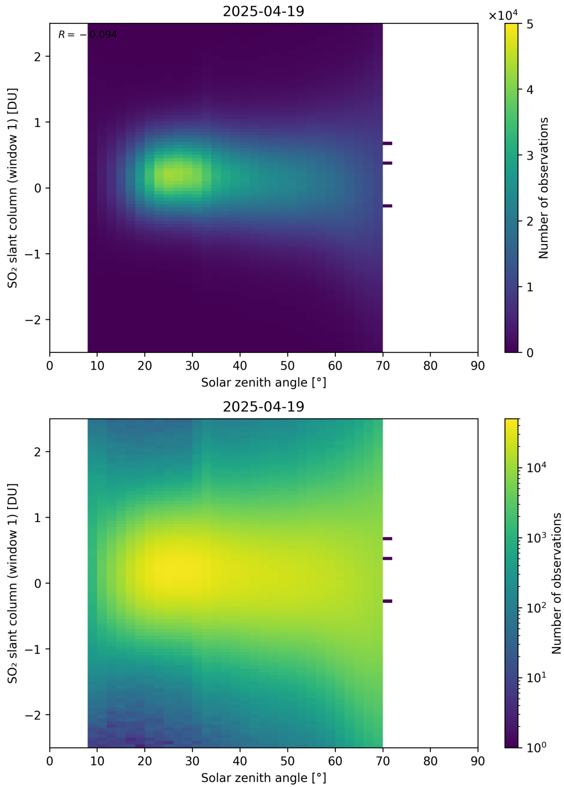
Figure 184: Scatter density plot of “Solar zenith angle” against “SO 2 slant column (window 1)” for 2025-04-19 to 2025-04-20.
