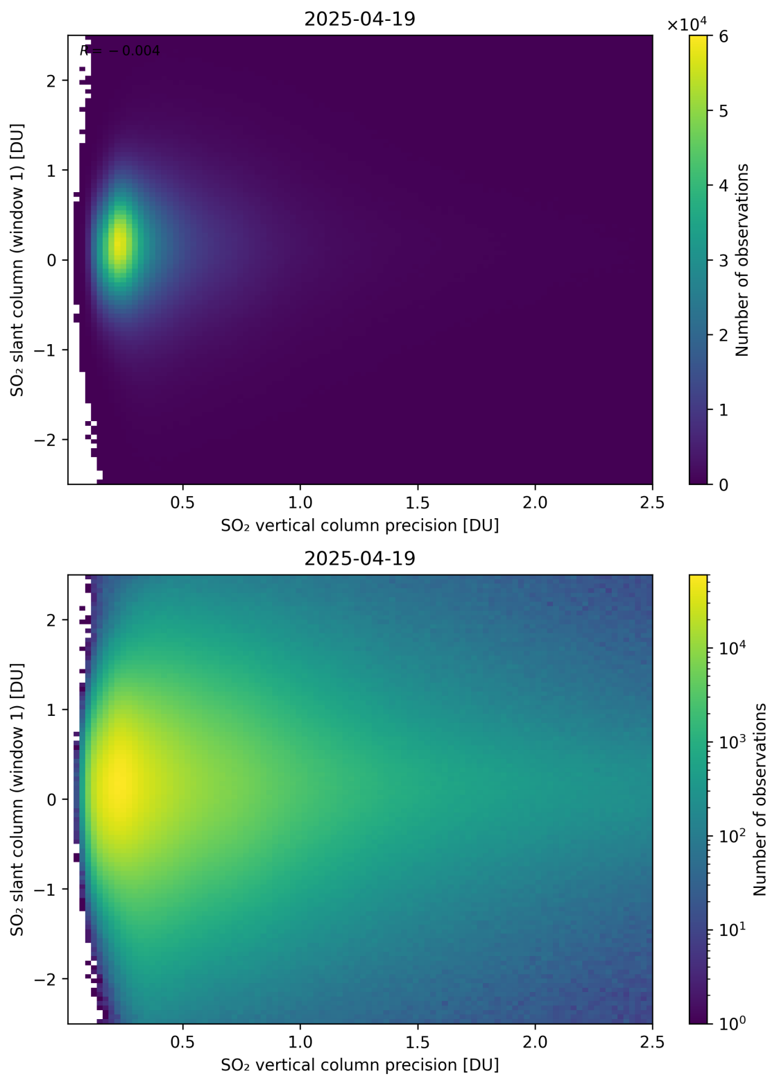
Figure 341: Scatter density plot of “SO 2 vertical column precision” against “SO 2 slant column (window 1)” for 2025-04-19 to 2025-04-20.
