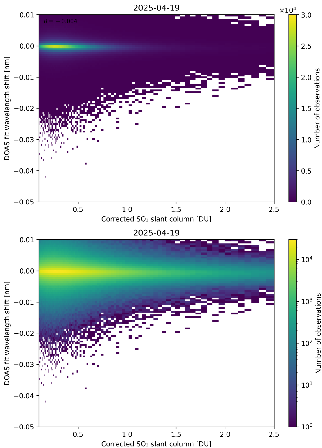
Figure 229: Scatter density plot of “Corrected SO 2 slant column” against “DOAS fit wavelength shift” for 2025-04-19 to 2025-04-20.
