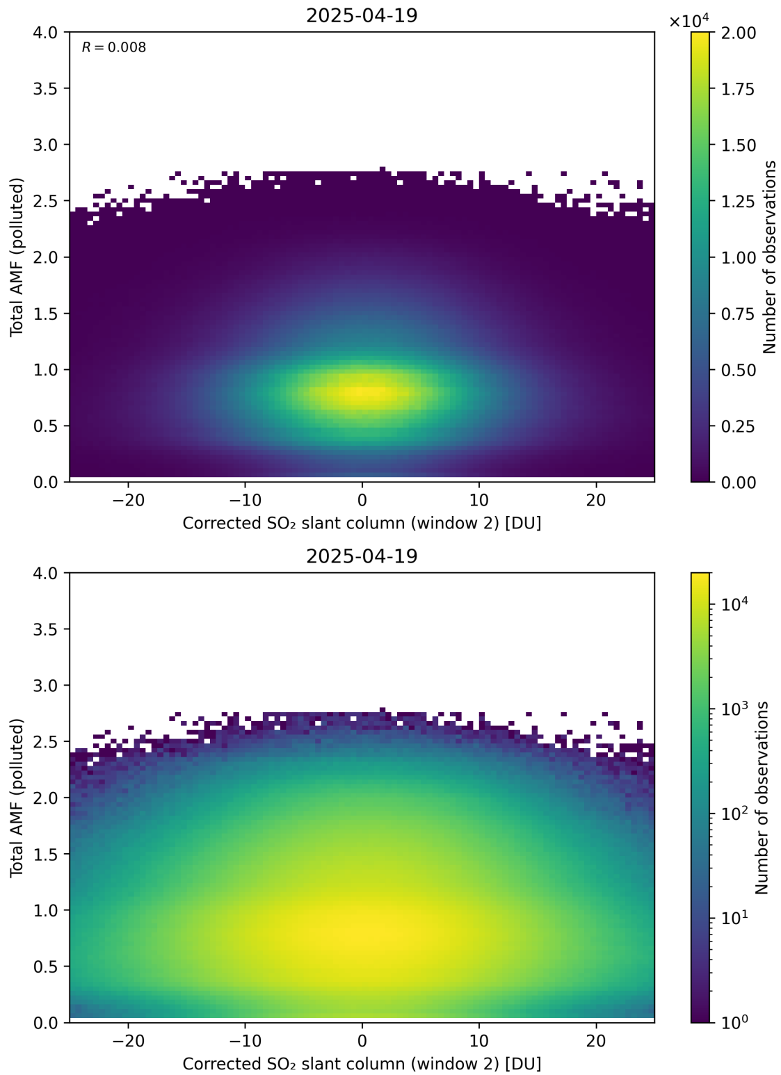
Figure 253: Scatter density plot of “Corrected SO 2 slant column (window 2)” against “Total AMF (polluted)” for 2025-04-19 to 2025-04-20.
