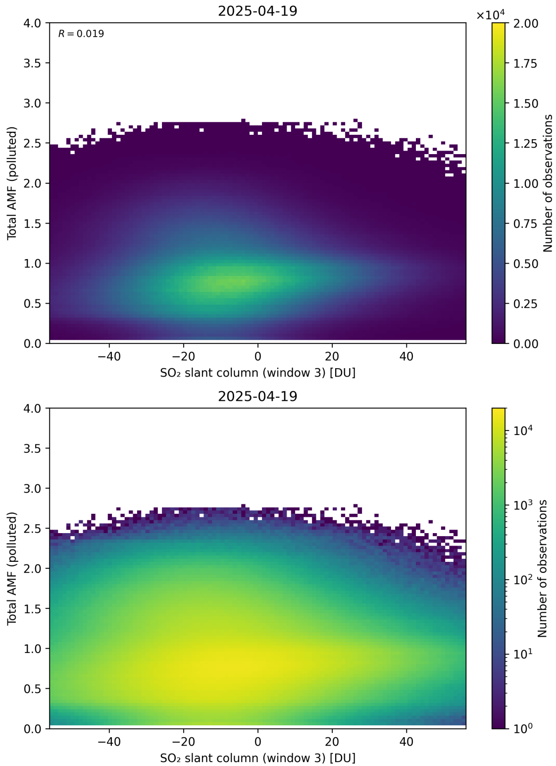
Figure 318: Scatter density plot of “SO 2 slant column (window 3)” against “Total AMF (polluted)” for 2025-04-19 to 2025-04-20.
