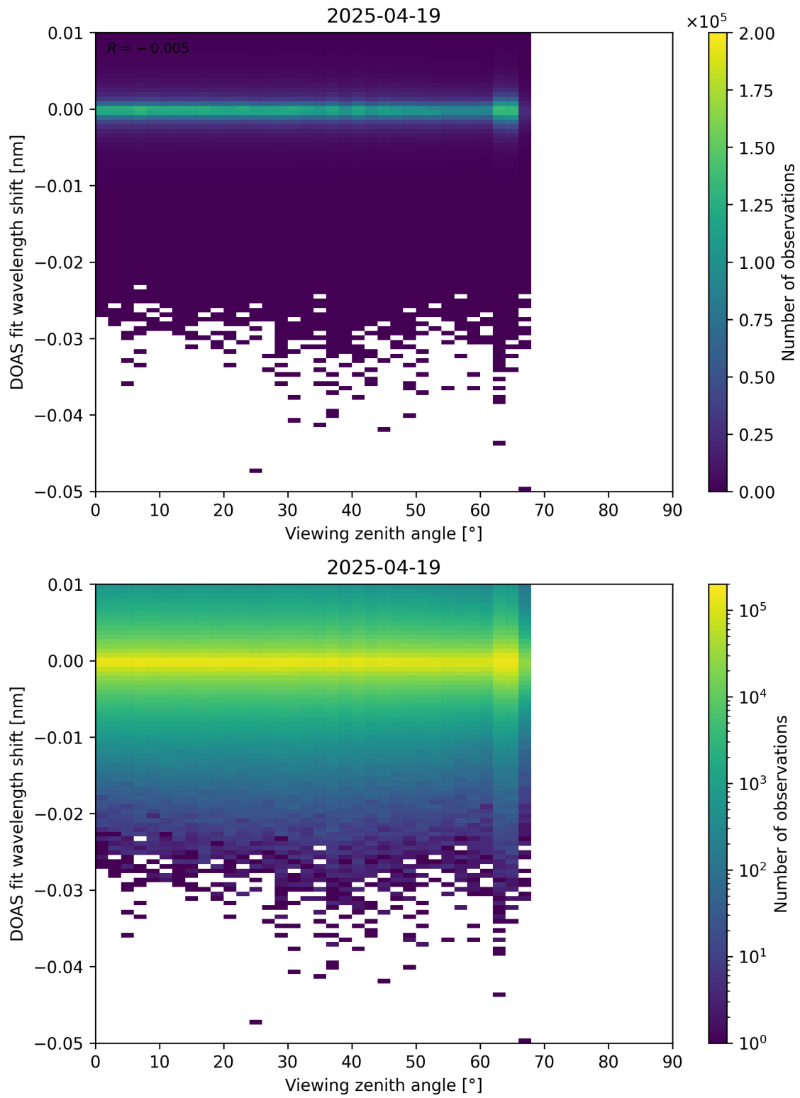
Figure 365: Scatter density plot of “Viewing zenith angle” against “DOAS fit wavelength shift” for 2025-04-19 to 2025-04-20.
