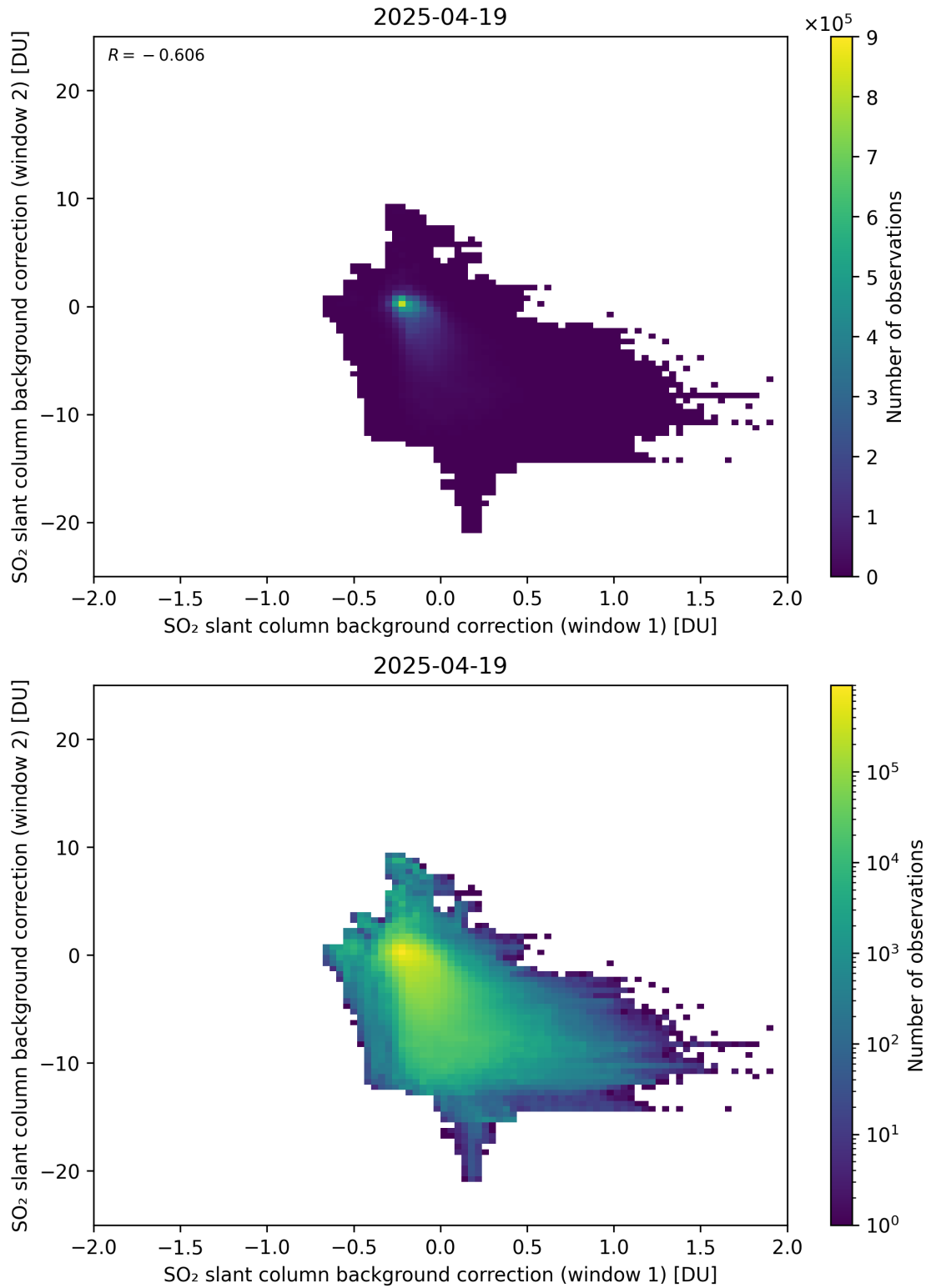
Figure 109: Scatter density plot of “SO 2 slant column background correction (window 1)” against “SO 2 slant column background correction (window 2)” for 2025-04-19 to 2025-04-20.
