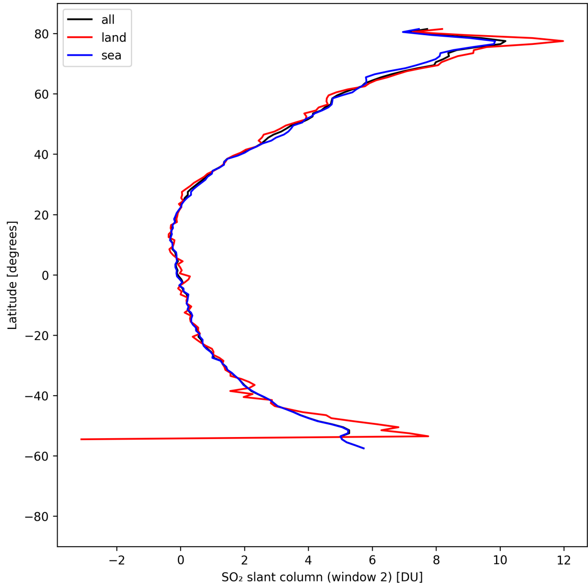
Figure 41: Zonal average of “SO 2 slant column (window 2)” for 2025-04-19 to 2025-04-20.
