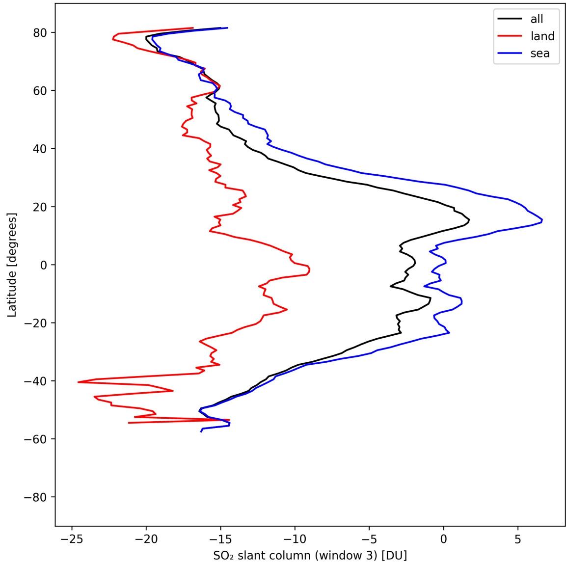
Figure 45: Zonal average of “SO 2 slant column (window 3)” for 2025-04-19 to 2025-04-20.
