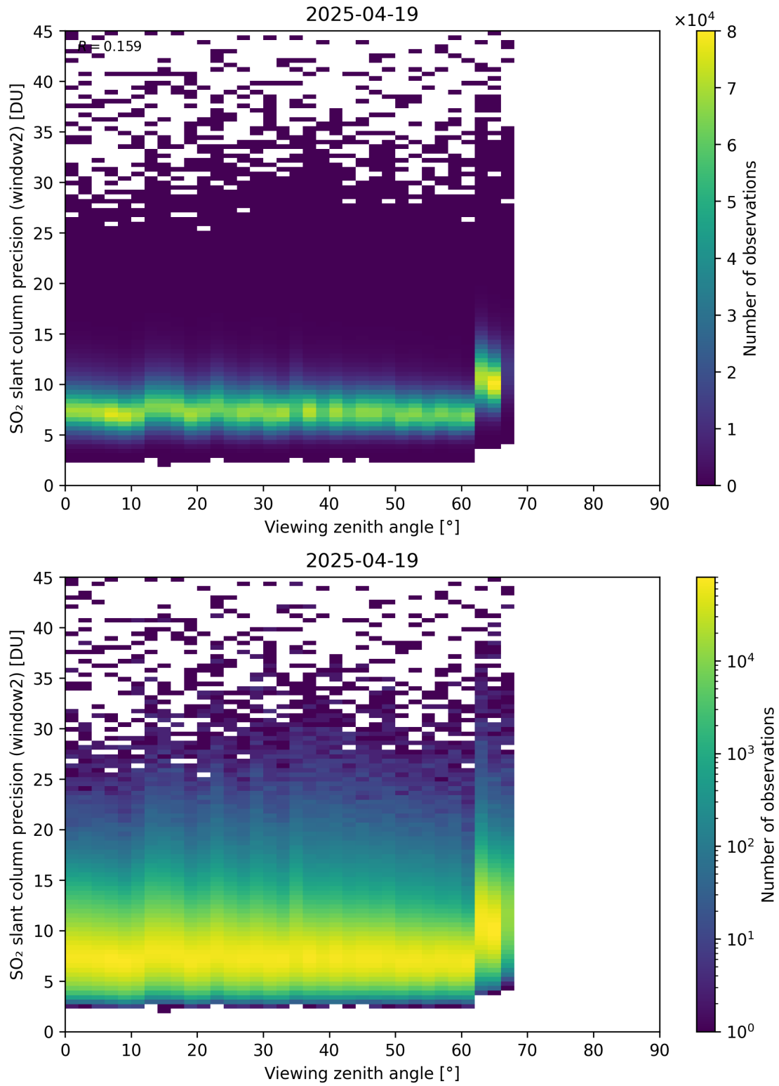
Figure 378: Scatter density plot of “Viewing zenith angle” against “SO 2 slant column precision (window2)” for 2025-04-19 to 2025-04-20.
