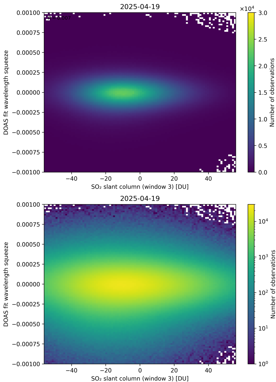
Figure 305: Scatter density plot of “SO 2 slant column (window 3)” against “DOAS fit wavelength squeeze” for 2025-04-19 to 2025-04-20.
