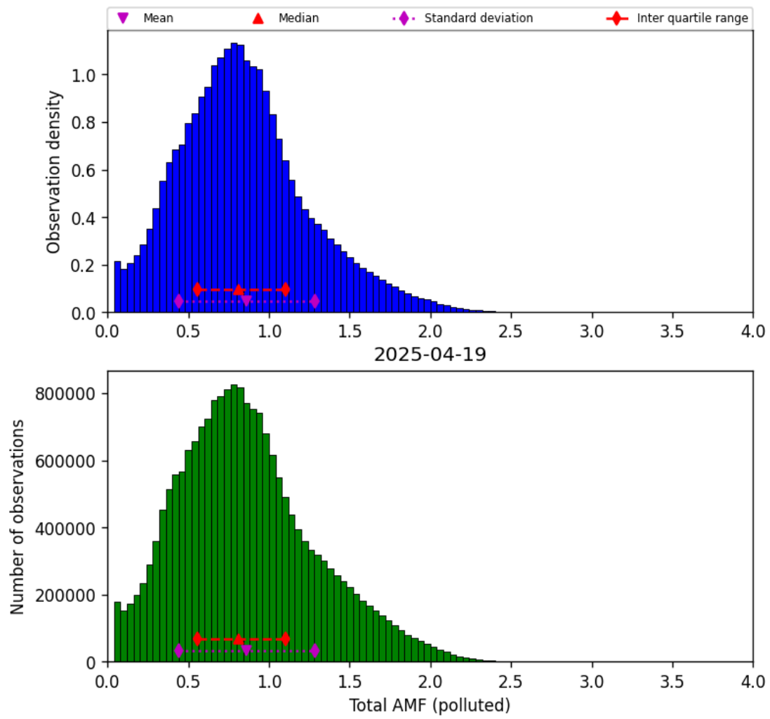
Figure 79: Histogram of “Total AMF (polluted)” for 2025-04-19 to 2025-04-20
