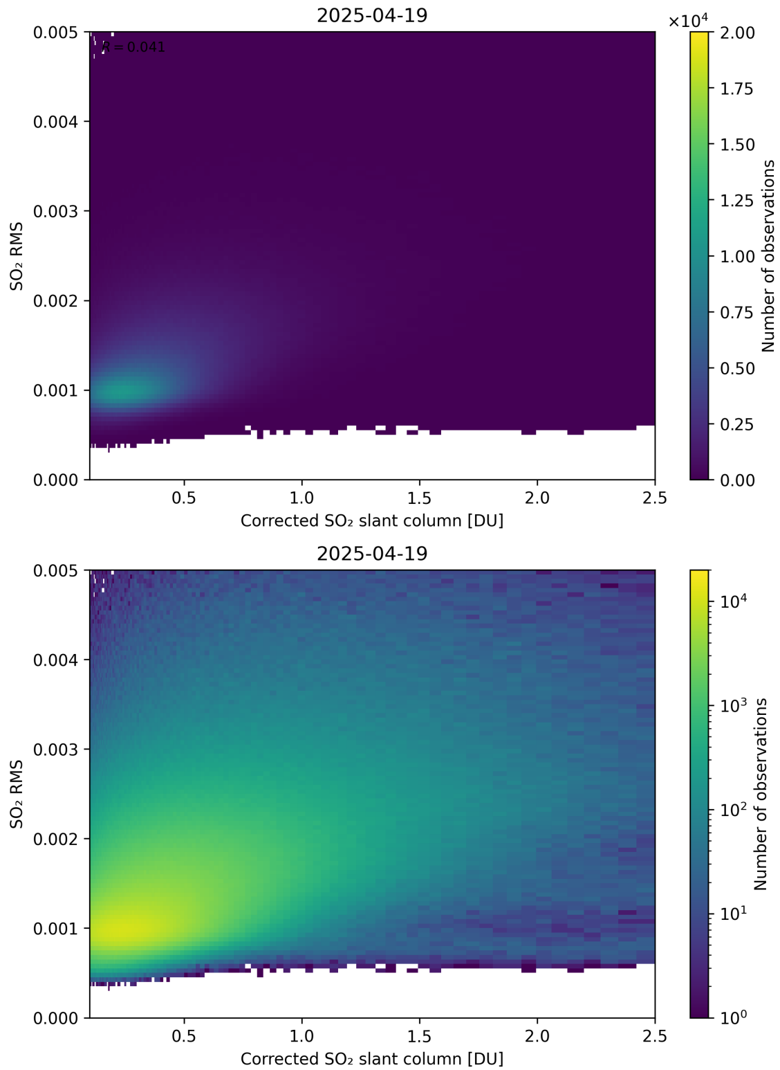
Figure 231: Scatter density plot of “Corrected SO 2 slant column” against “SO 2 RMS” for 2025-04-19 to 2025-04-20.
