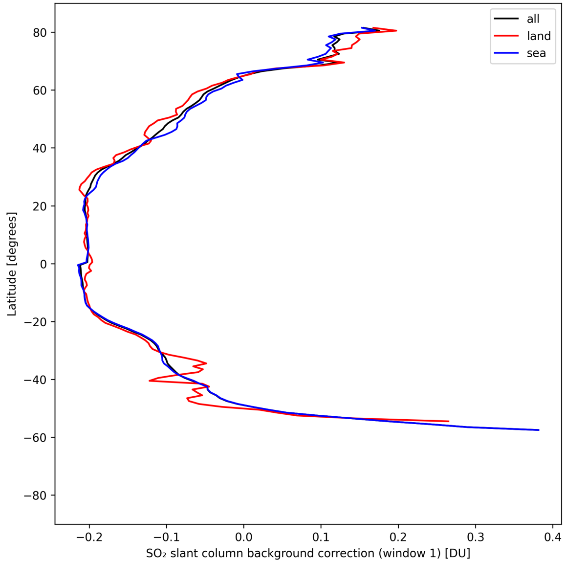
Figure 40: Zonal average of “SO 2 slant column background correction (window 1)” for 2025-04-19 to 2025-04-20.
