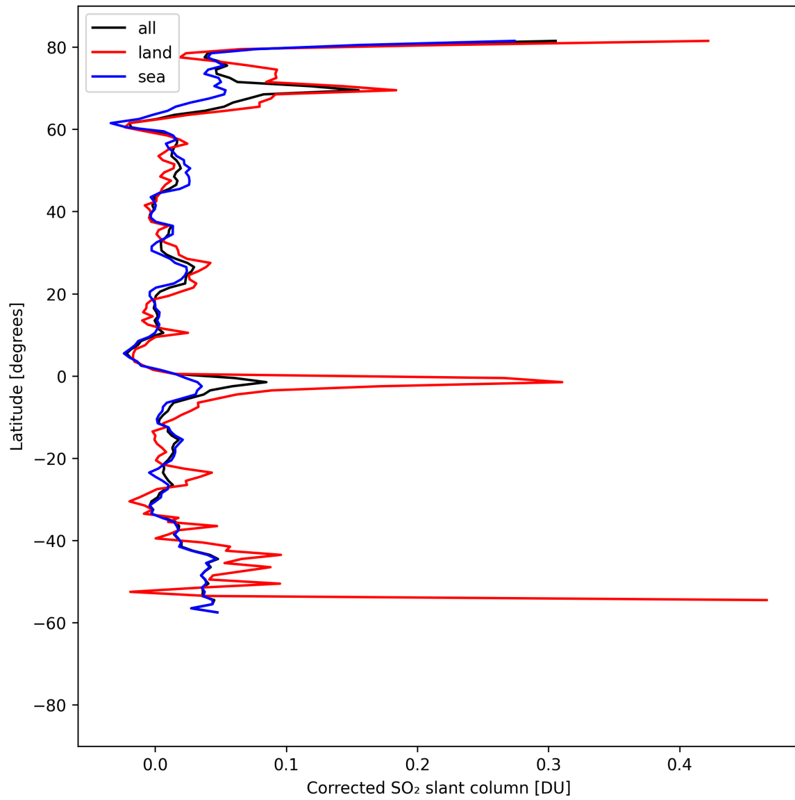
Figure 34: Zonal average of “Corrected SO 2 slant column” for 2025-04-19 to 2025-04-20.
