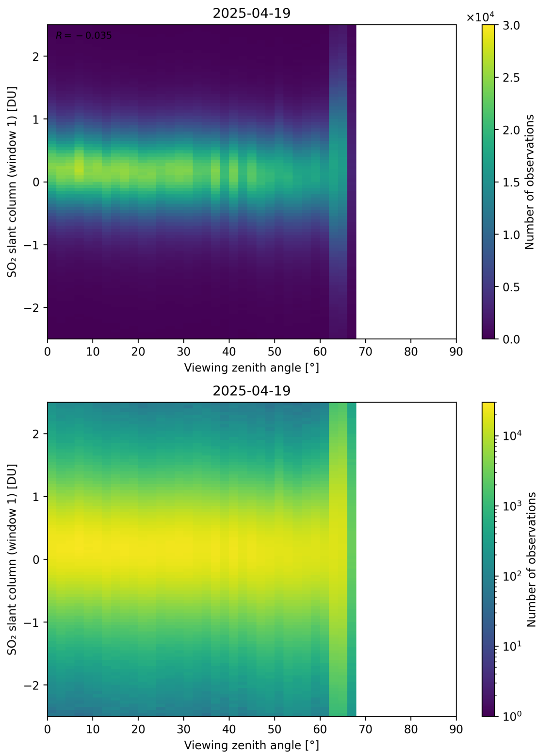
Figure 376: Scatter density plot of “Viewing zenith angle” against “SO 2 slant column (window 1)” for 2025-04-19 to 2025-04-20.
