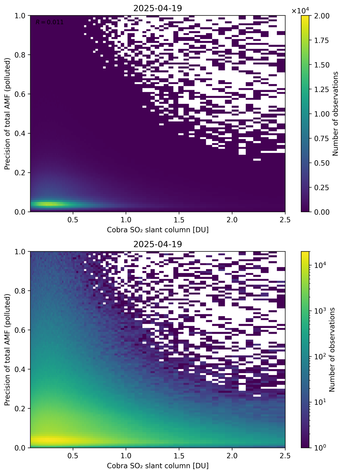
Figure 225: Scatter density plot of “Cobra SO 2 slant column” against “Precision of total AMF (polluted)” for 2025-04-19 to 2025-04-20.
