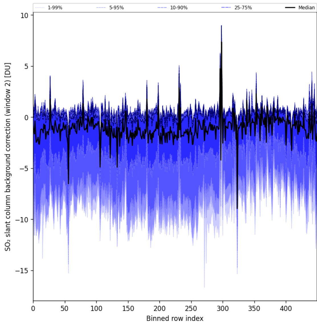
Figure 96: Along track statistics of “SO 2 slant column background correction (window 2)” for 2025-04-19 to 2025-04-20
