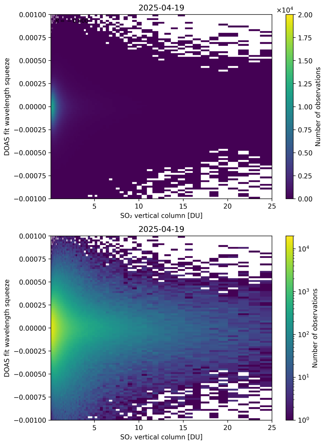
Figure 327: Scatter density plot of “SO 2 vertical column” against “DOAS fit wavelength squeeze” for 2025-04-19 to 2025-04-20.
