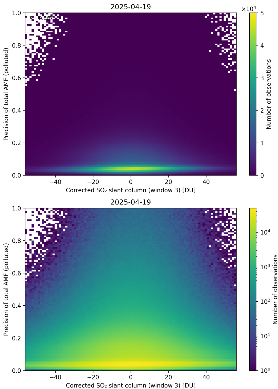
Figure 261: Scatter density plot of “Corrected SO 2 slant column (window 3)” against “Precision of total AMF (polluted)” for 2025-04-19 to 2025-04-20.
