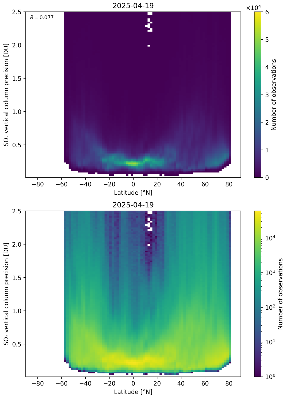
Figure 170: Scatter density plot of “Latitude” against “SO 2 vertical column precision” for 2025-04-19 to 2025-04-20.
