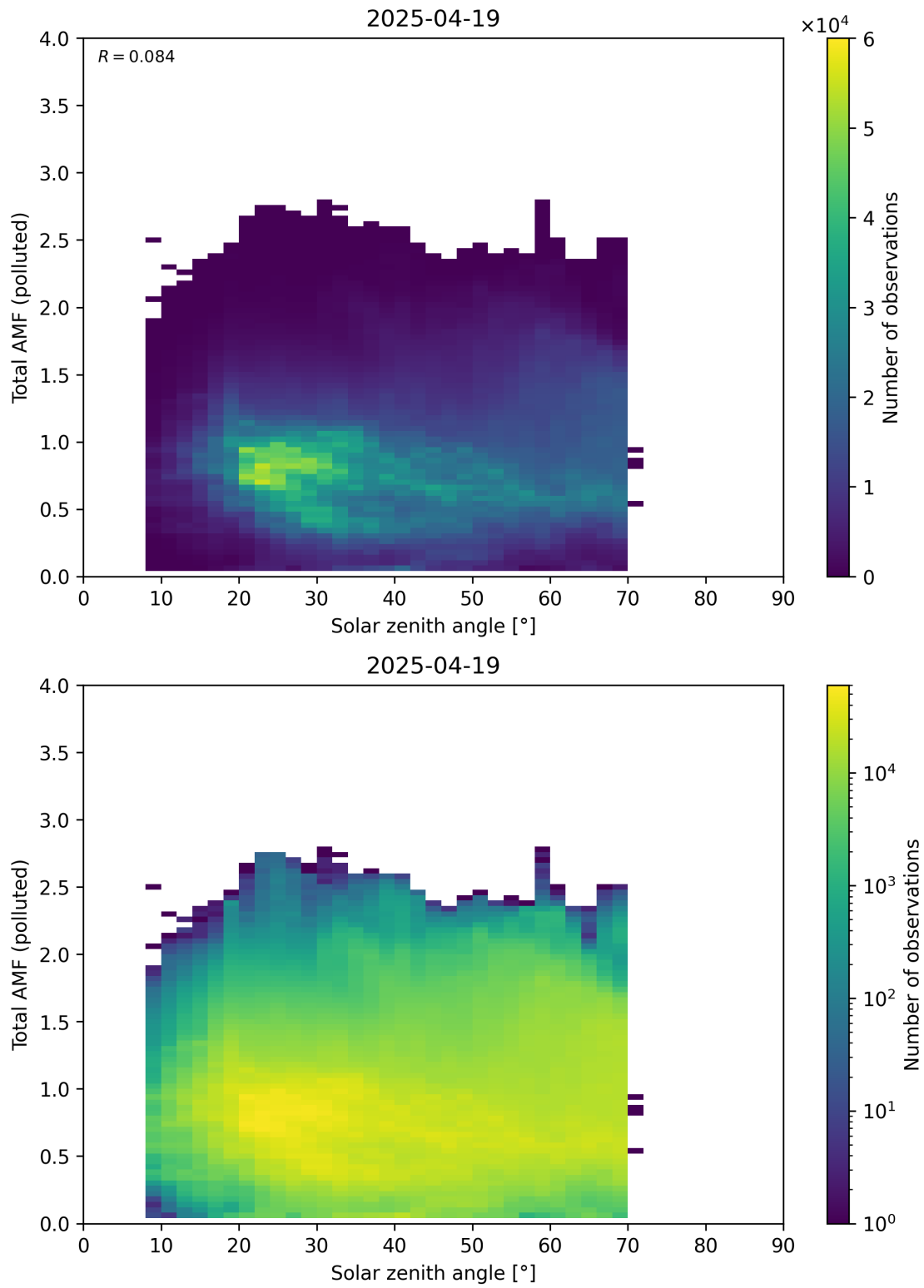
Figure 189: Scatter density plot of “Solar zenith angle” against “Total AMF (polluted)” for 2025-04-19 to 2025-04-20.
