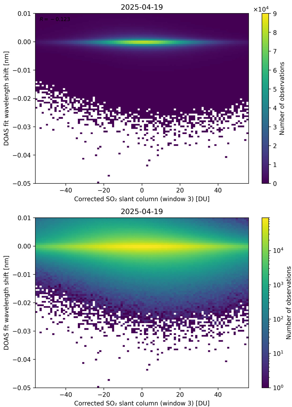
Figure 256: Scatter density plot of “Corrected SO 2 slant column (window 3)” against “DOAS fit wavelength shift” for 2025-04-19 to 2025-04-20.
