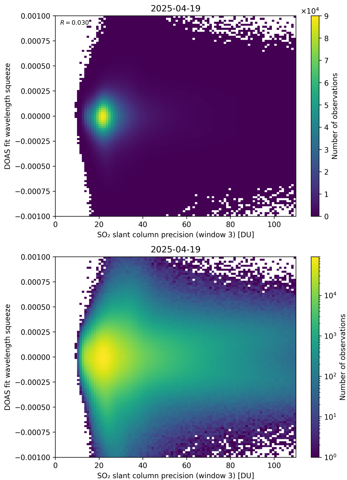
Figure 309: Scatter density plot of “SO 2 slant column precision (window 3)” against “DOAS fit wavelength squeeze” for 2025-04-19 to 2025-04-20.
