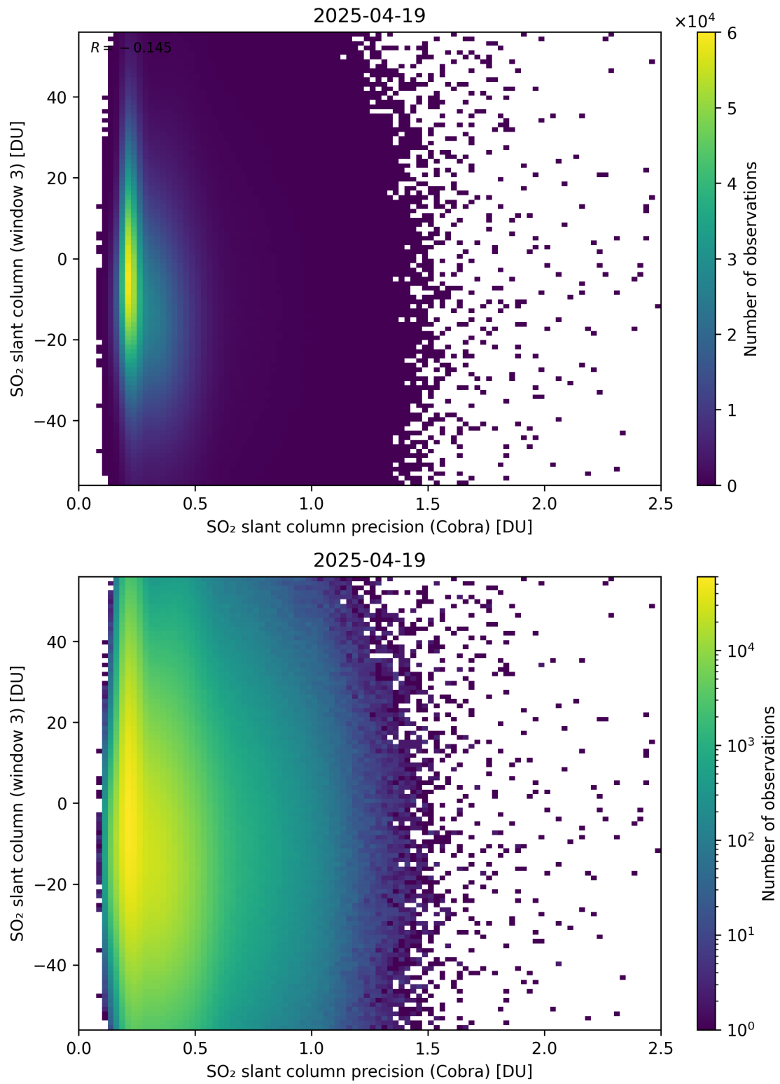
Figure 211: Scatter density plot of “SO 2 slant column precision (Cobra)” against “SO 2 slant column (window 3)” for 2025-04-19 to 2025-04-20.
