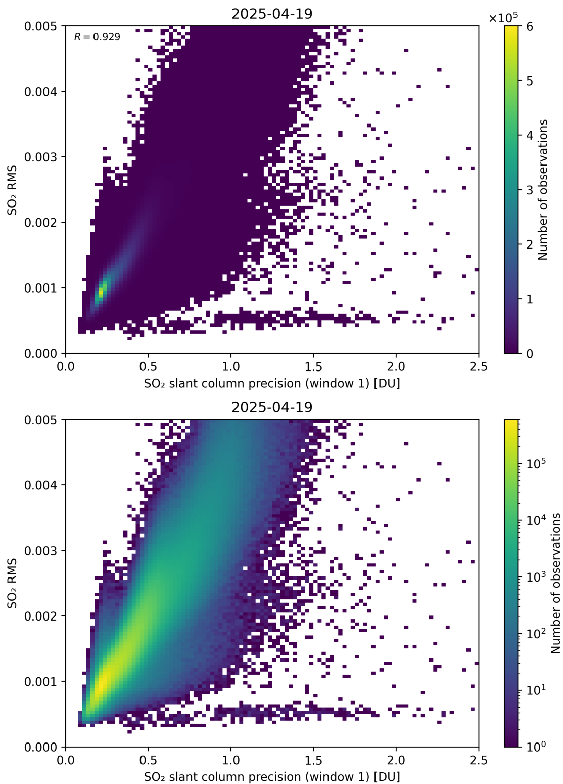
Figure 273: Scatter density plot of “SO 2 slant column precision (window 1)” against “SO 2 RMS” for 2025-04-19 to 2025-04-20.
