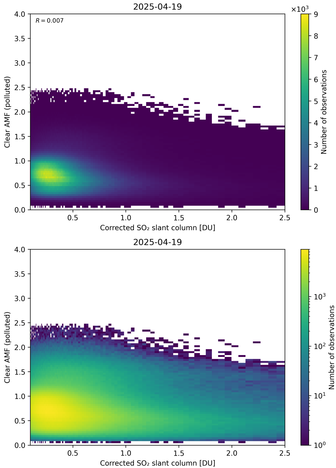
Figure 232: Scatter density plot of “Corrected SO 2 slant column” against “Clear AMF (polluted)” for 2025-04-19 to 2025-04-20.
