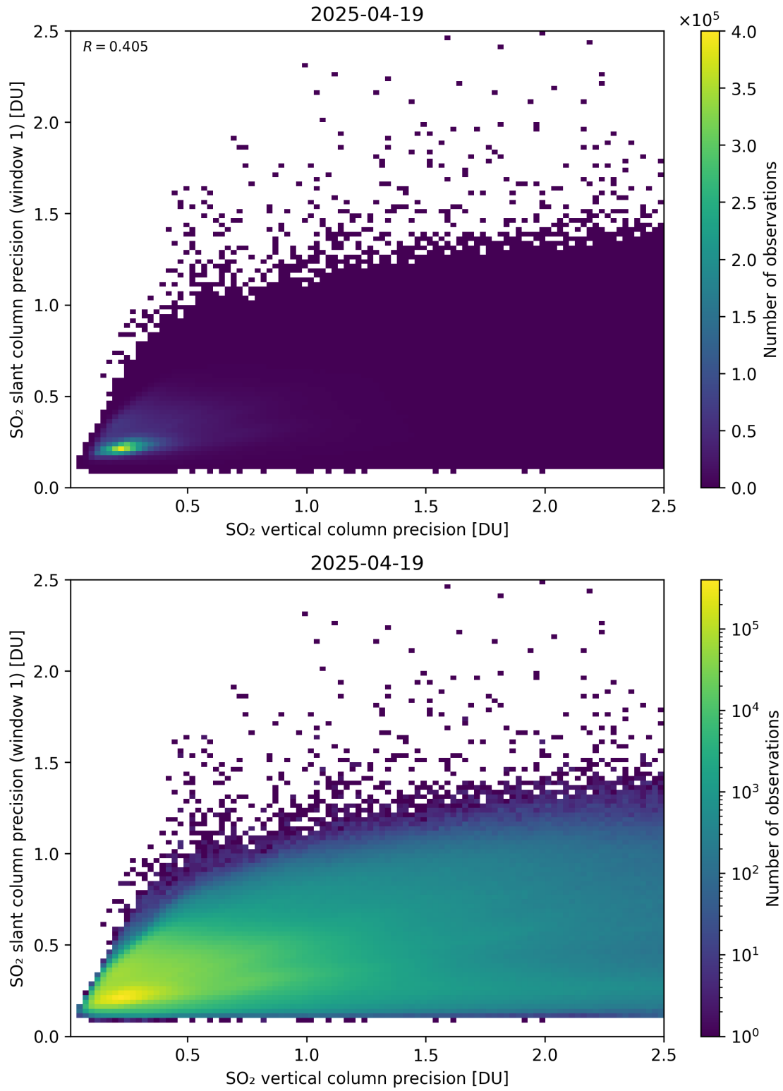
Figure 342: Scatter density plot of “SO 2 vertical column precision” against “SO 2 slant column precision (window 1)” for 2025-04-19 to 2025-04-20.
