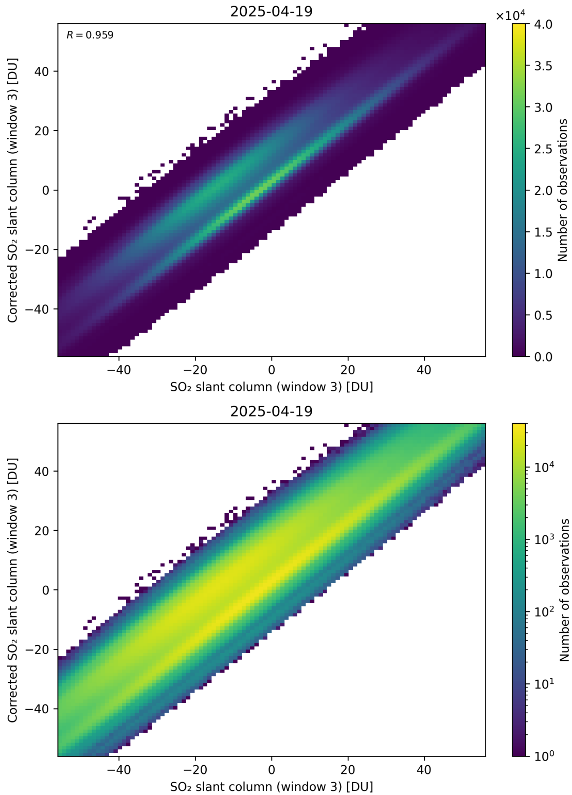
Figure 316: Scatter density plot of “SO 2 slant column (window 3)” against “Corrected SO 2 slant column (window 3)” for 2025-04-19 to 2025-04-20.
