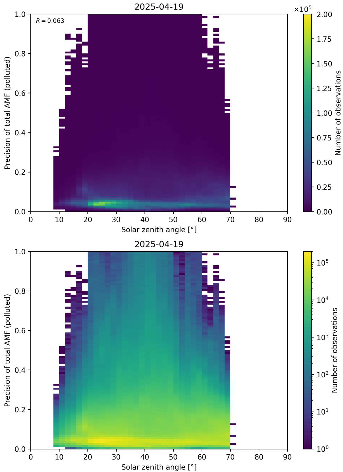
Figure 190: Scatter density plot of “Solar zenith angle” against “Precision of total AMF (polluted)” for 2025-04-19 to 2025-04-20.
