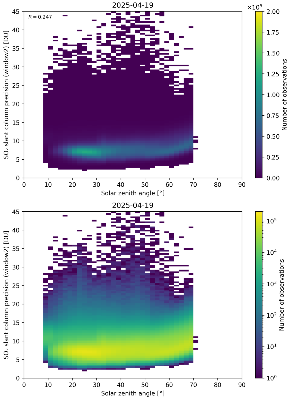
Figure 186: Scatter density plot of “Solar zenith angle” against “SO 2 slant column precision (window2)” for 2025-04-19 to 2025-04-20.
