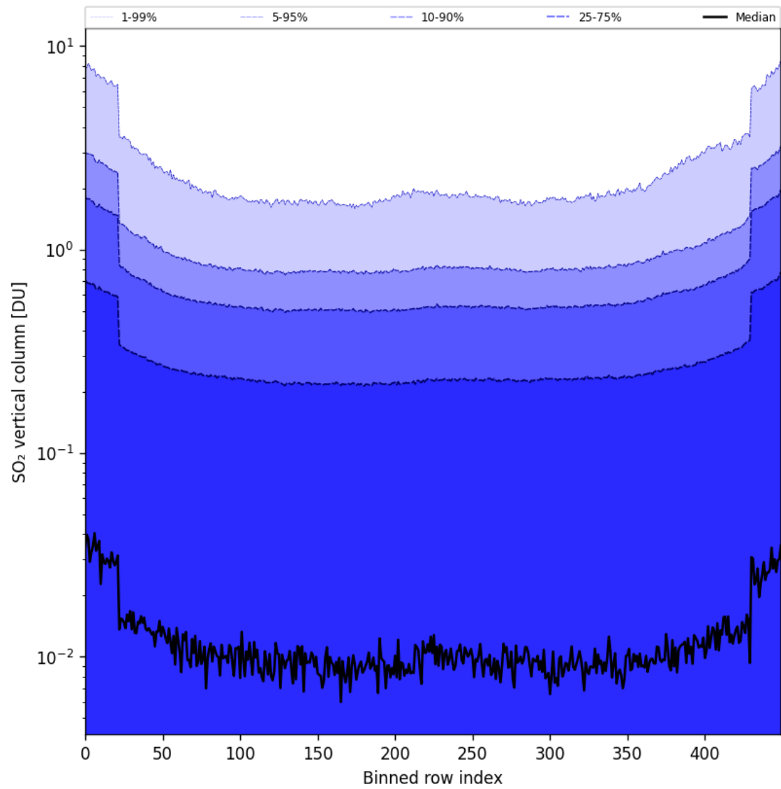
Figure 84: Along track statistics of “SO 2 vertical column” for 2025-04-19 to 2025-04-20
