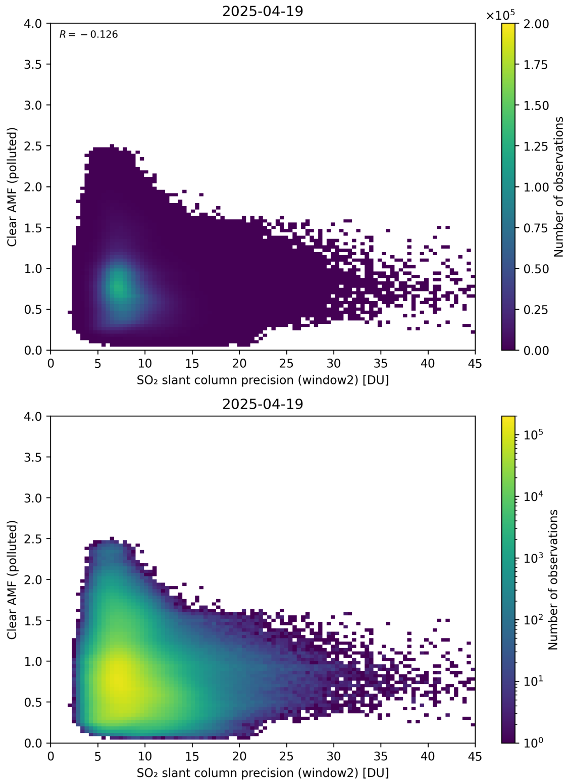
Figure 296: Scatter density plot of “SO 2 slant column precision (window2)” against “Clear AMF (polluted)” for 2025-04-19 to 2025-04-20.
