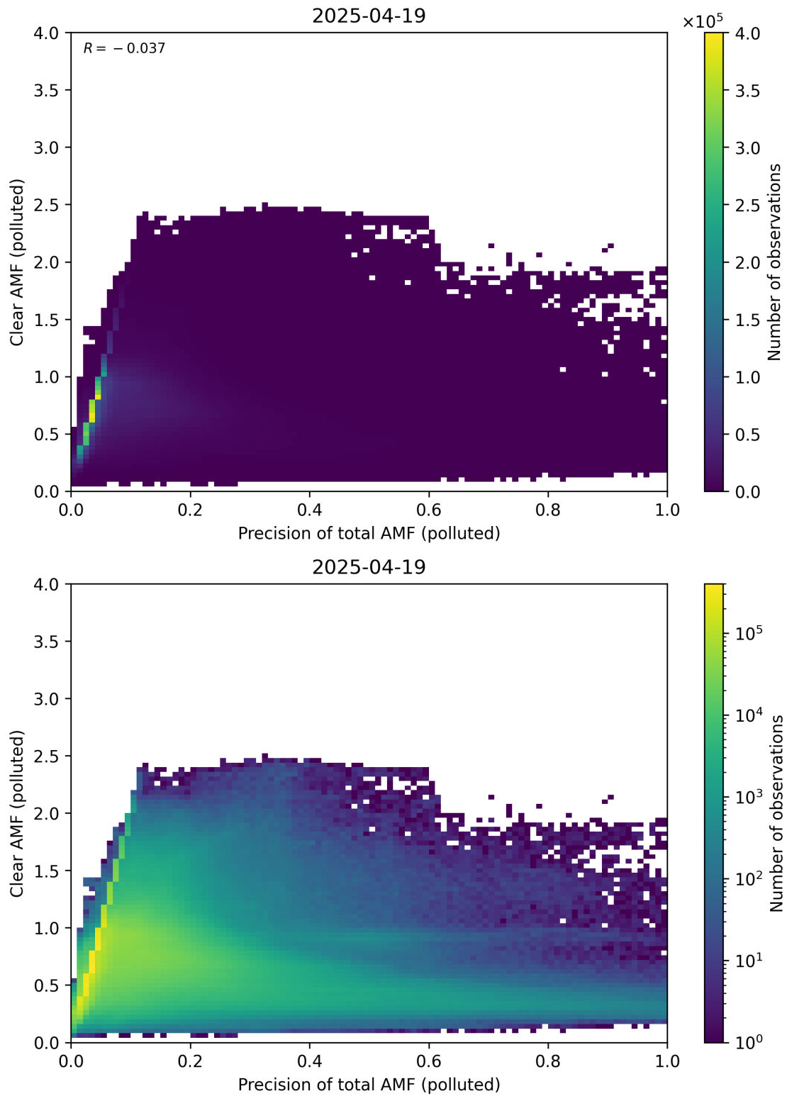
Figure 320: Scatter density plot of “Precision of total AMF (polluted)” against “Clear AMF (polluted)” for 2025-04-19 to 2025-04-20.
