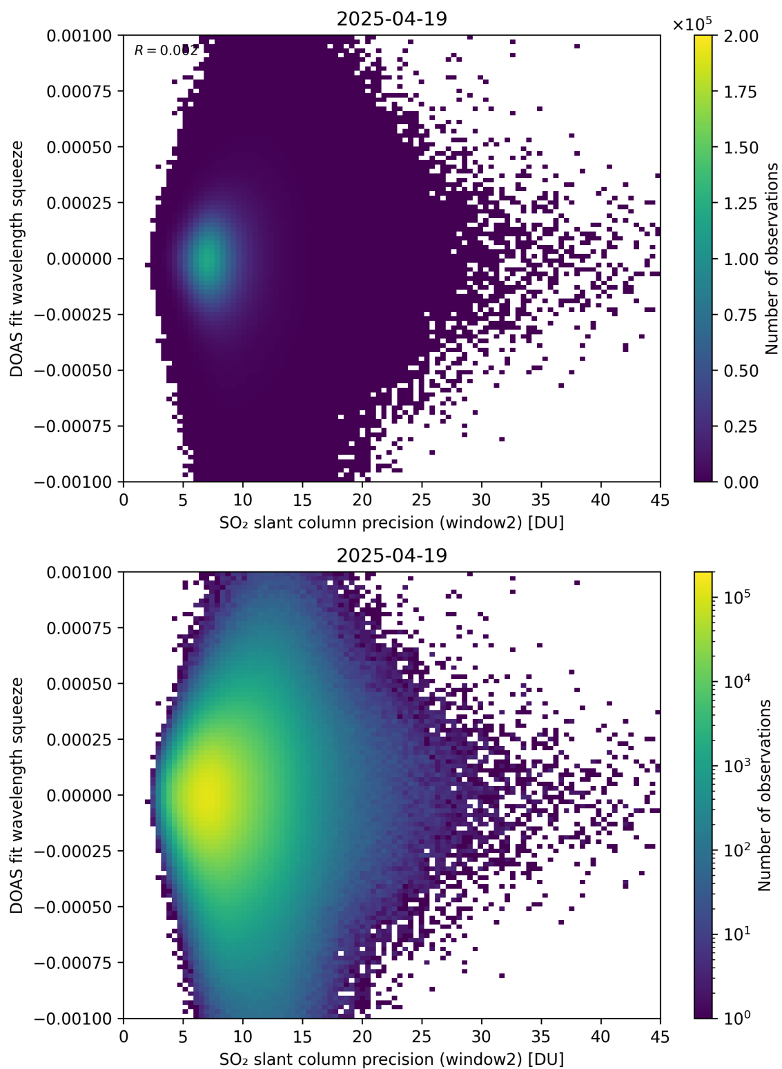
Figure 294: Scatter density plot of “SO 2 slant column precision (window2)” against “DOAS fit wavelength squeeze” for 2025-04-19 to 2025-04-20.
