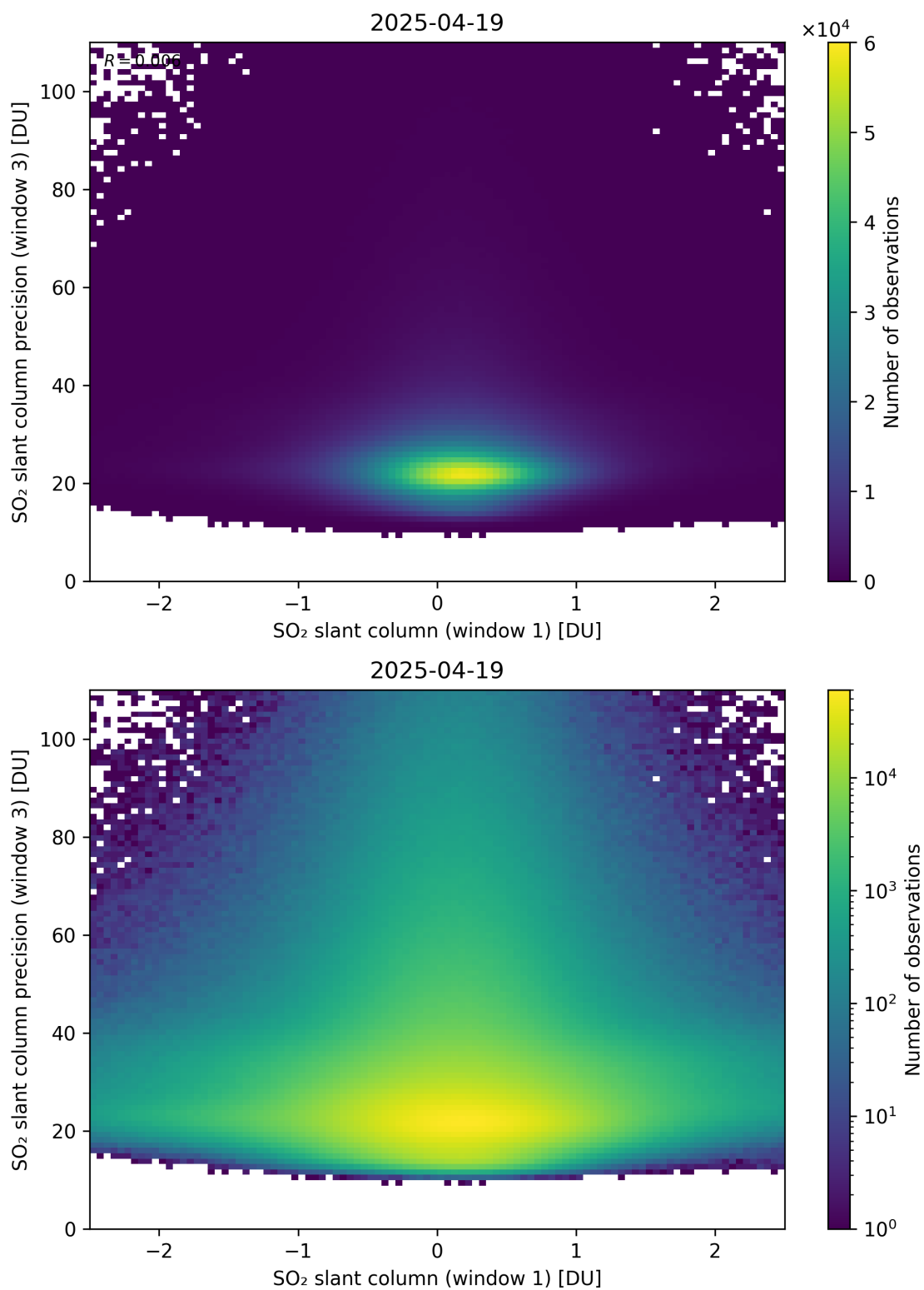
Figure 288: Scatter density plot of “SO 2 slant column (window 1)” against “SO 2 slant column precision (window 3)” for 2025-04-19 to 2025-04-20.
