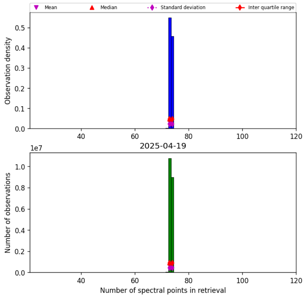
Figure 82: Histogram of “Number of spectral points in retrieval” for 2025-04-19 to 2025-04-20
