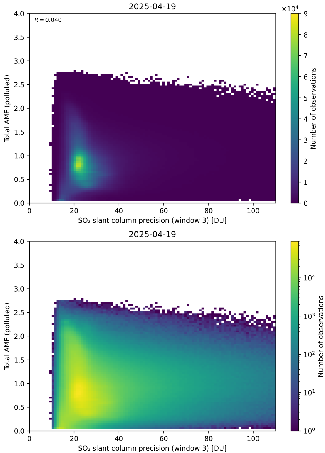
Figure 313: Scatter density plot of “SO 2 slant column precision (window 3)” against “Total AMF (polluted)” for 2025-04-19 to 2025-04-20.
