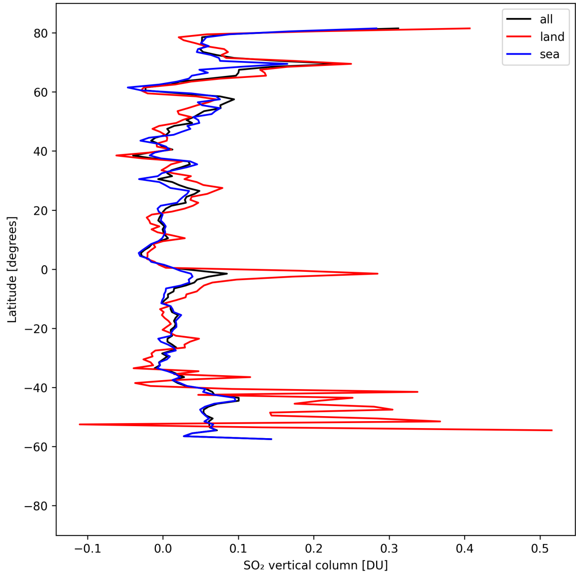
Figure 32: Zonal average of “SO 2 vertical column” for 2025-04-19 to 2025-04-20.
