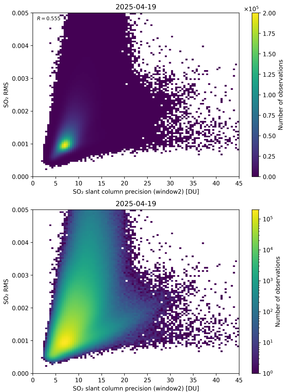
Figure 295: Scatter density plot of “SO 2 slant column precision (window2)” against “SO 2 RMS” for 2025-04-19 to 2025-04-20.
