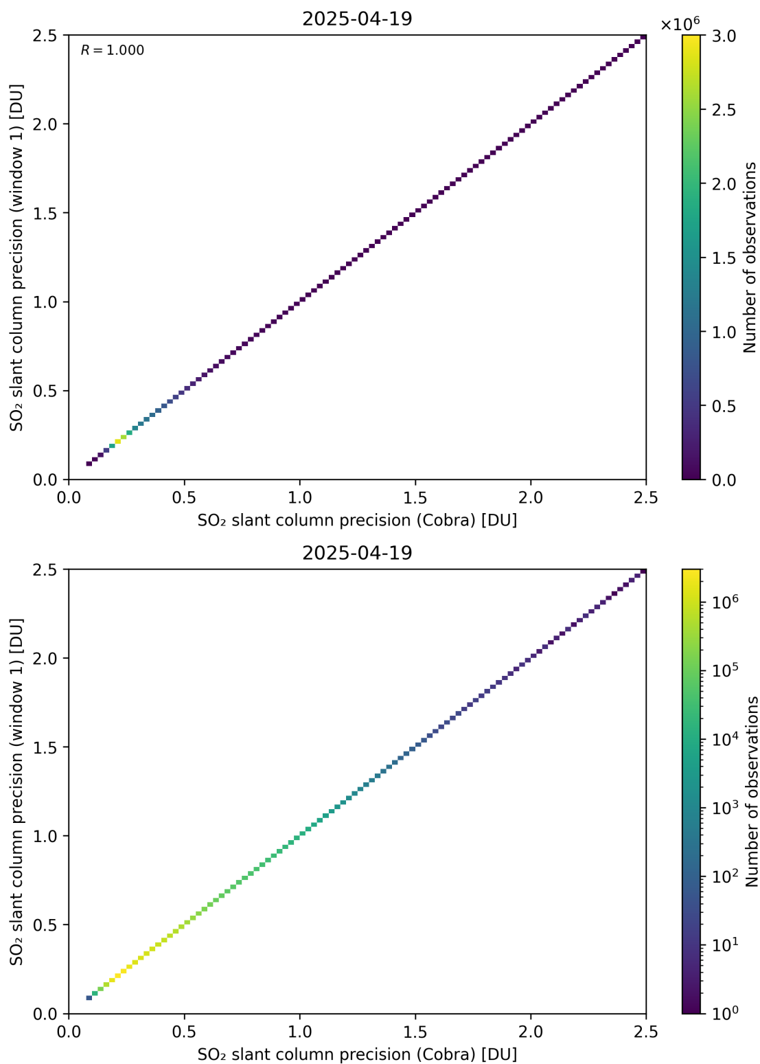
Figure 209: Scatter density plot of “SO 2 slant column precision (Cobra)” against “SO 2 slant column precision (window 1)” for 2025-04-19 to 2025-04-20.
