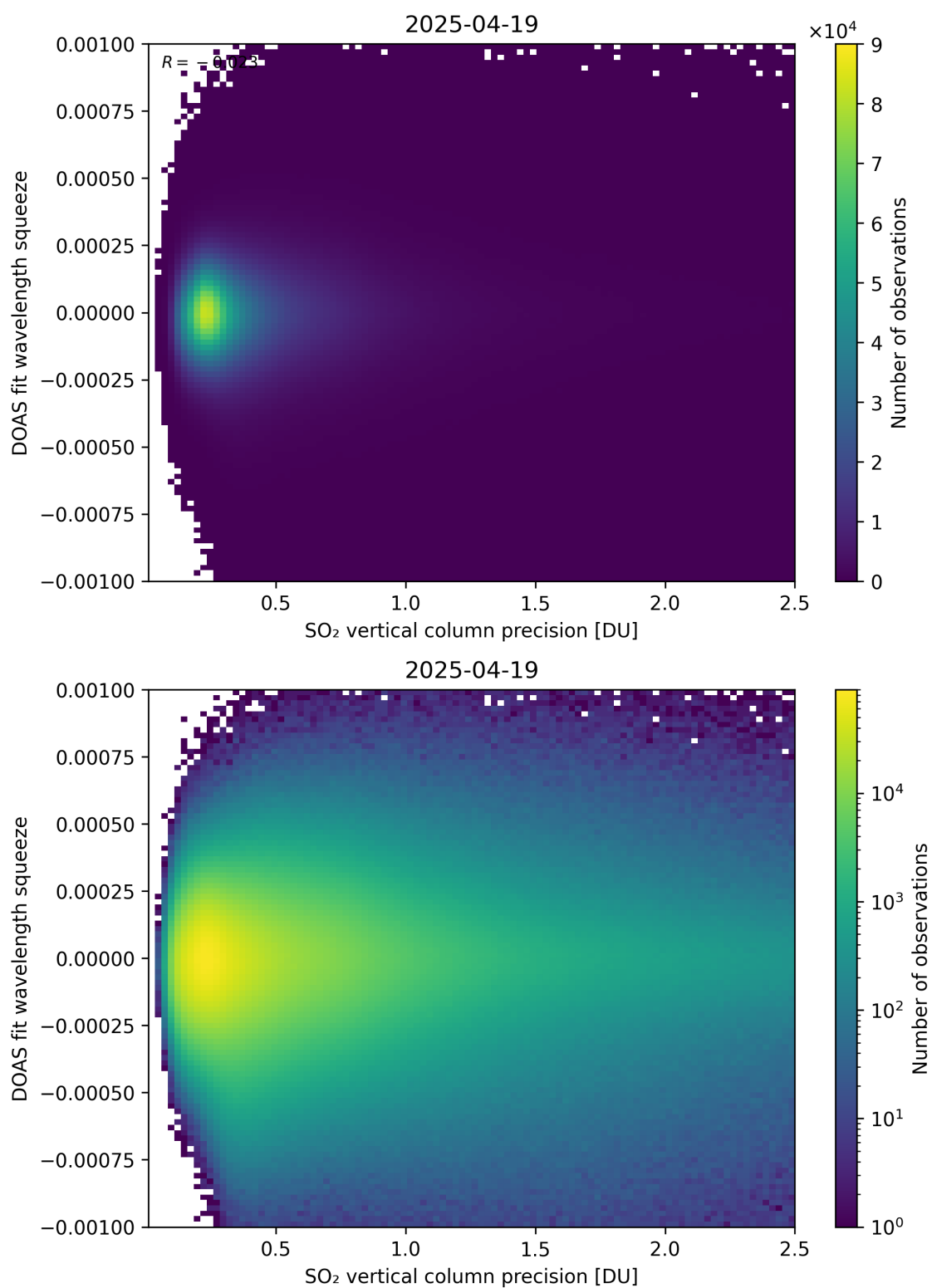
Figure 333: Scatter density plot of “SO 2 vertical column precision” against “DOAS fit wavelength squeeze” for 2025-04-19 to 2025-04-20.
