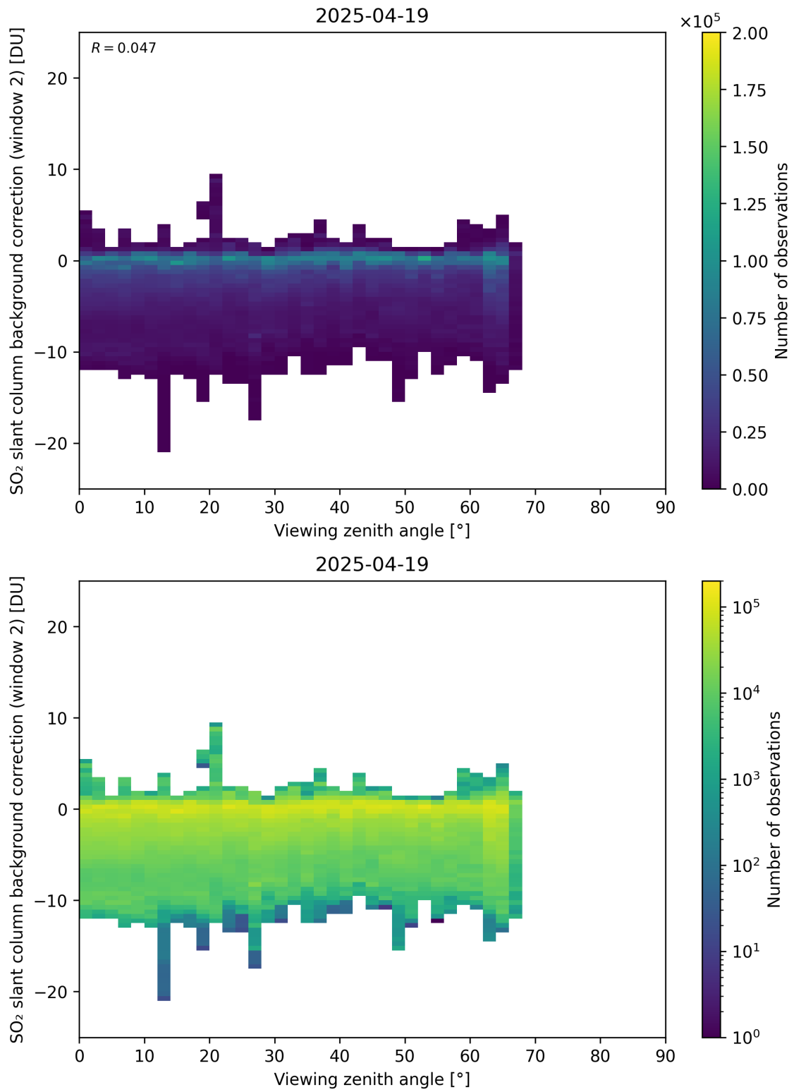
Figure 363: Scatter density plot of “Viewing zenith angle” against “SO 2 slant column background correction (window 2)” for 2025-04-19 to 2025-04-20.
