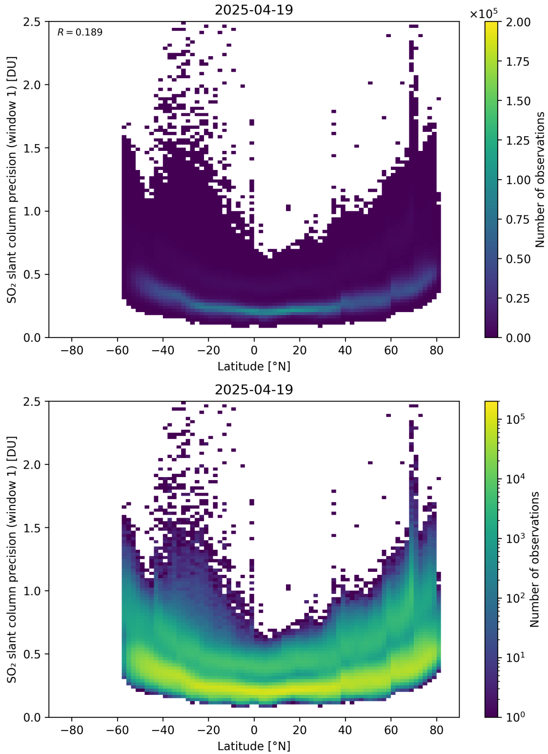
Figure 163: Scatter density plot of “Latitude” against “SO 2 slant column precision (window 1)” for 2025-04-19 to 2025-04-20.
