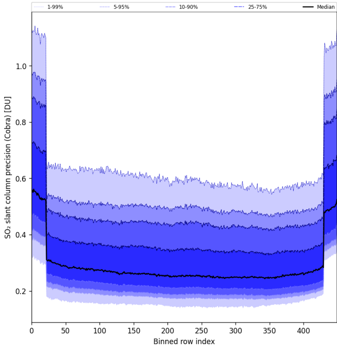
Figure 88: Along track statistics of “SO 2 slant column precision (Cobra)” for 2025-04-19 to 2025-04-20
