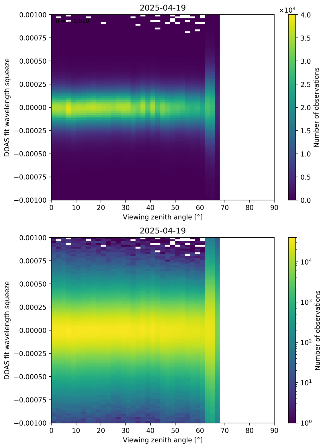
Figure 366: Scatter density plot of “Viewing zenith angle” against “DOAS fit wavelength squeeze” for 2025-04-19 to 2025-04-20.
