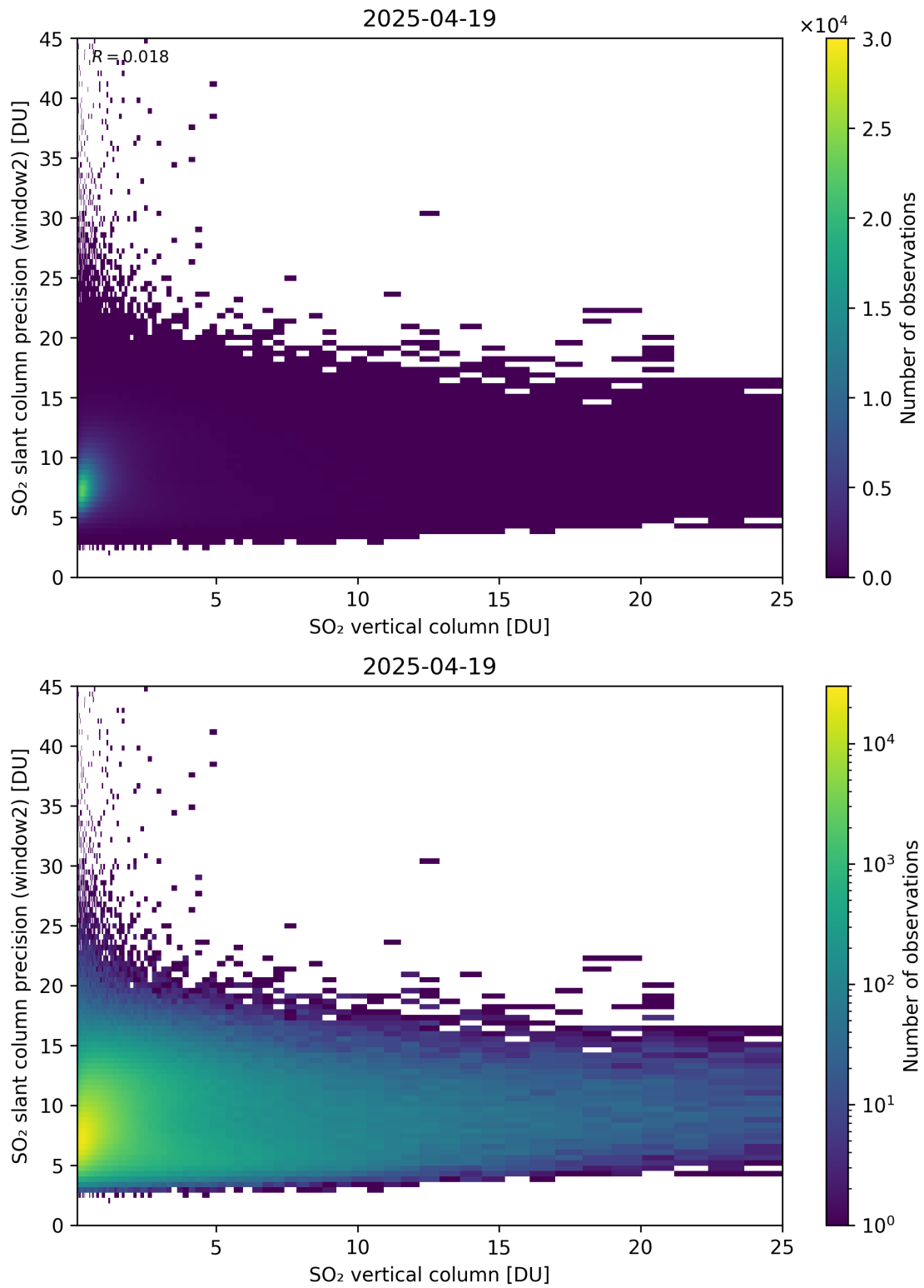
Figure 356: Scatter density plot of “SO 2 vertical column” against “SO 2 slant column precision (window2)” for 2025-04-19 to 2025-04-20.
