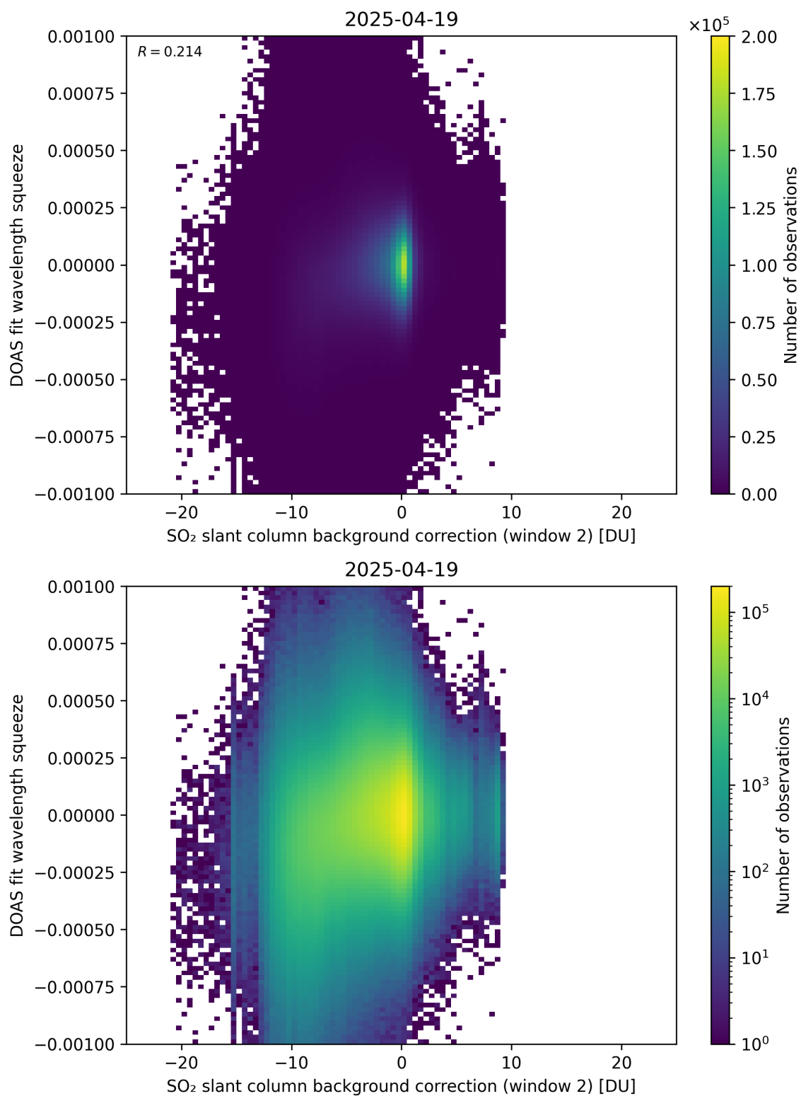
Figure 124: Scatter density plot of “SO 2 slant column background correction (window 2)” against “DOAS fit wavelength squeeze” for 2025-04-19 to 2025-04-20.
