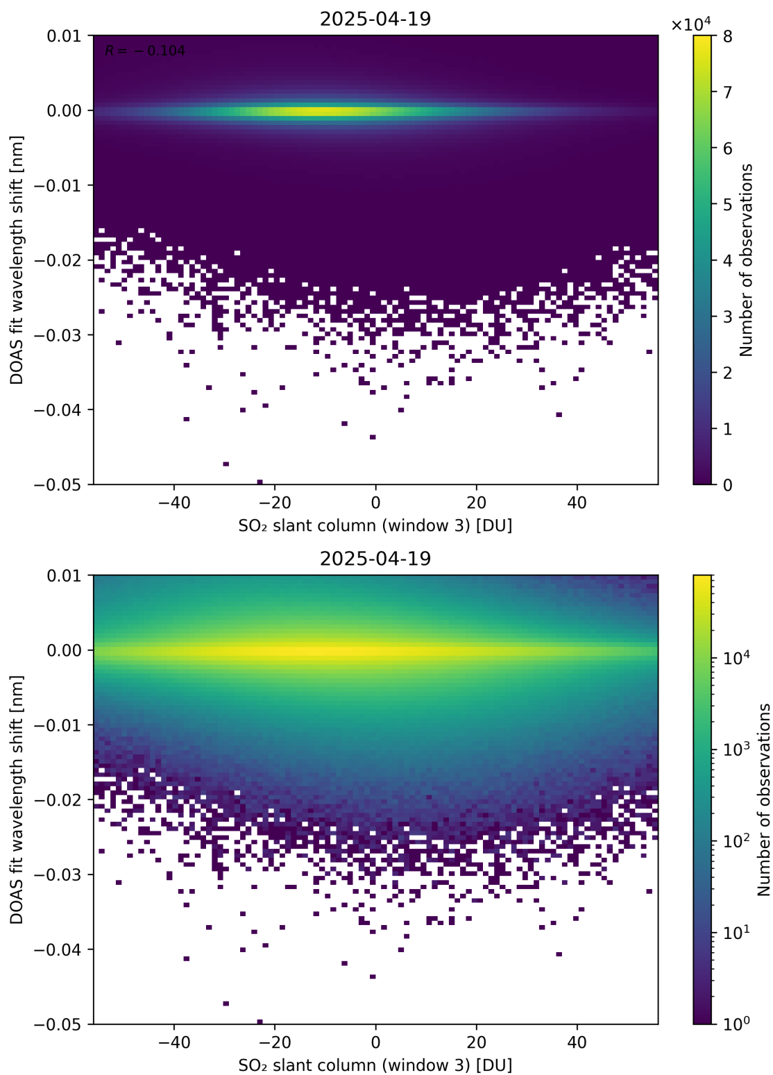
Figure 304: Scatter density plot of “SO 2 slant column (window 3)” against “DOAS fit wavelength shift” for 2025-04-19 to 2025-04-20.
