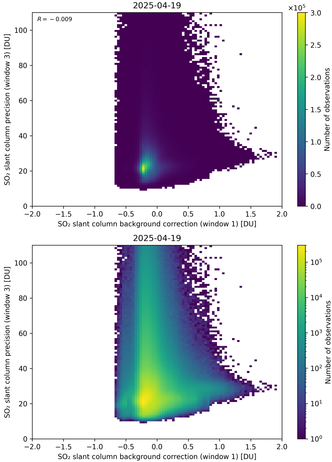
Figure 119: Scatter density plot of “SO 2 slant column background correction (window 1)” against “SO 2 slant column precision (window 3)” for 2025-04-19 to 2025-04-20.
