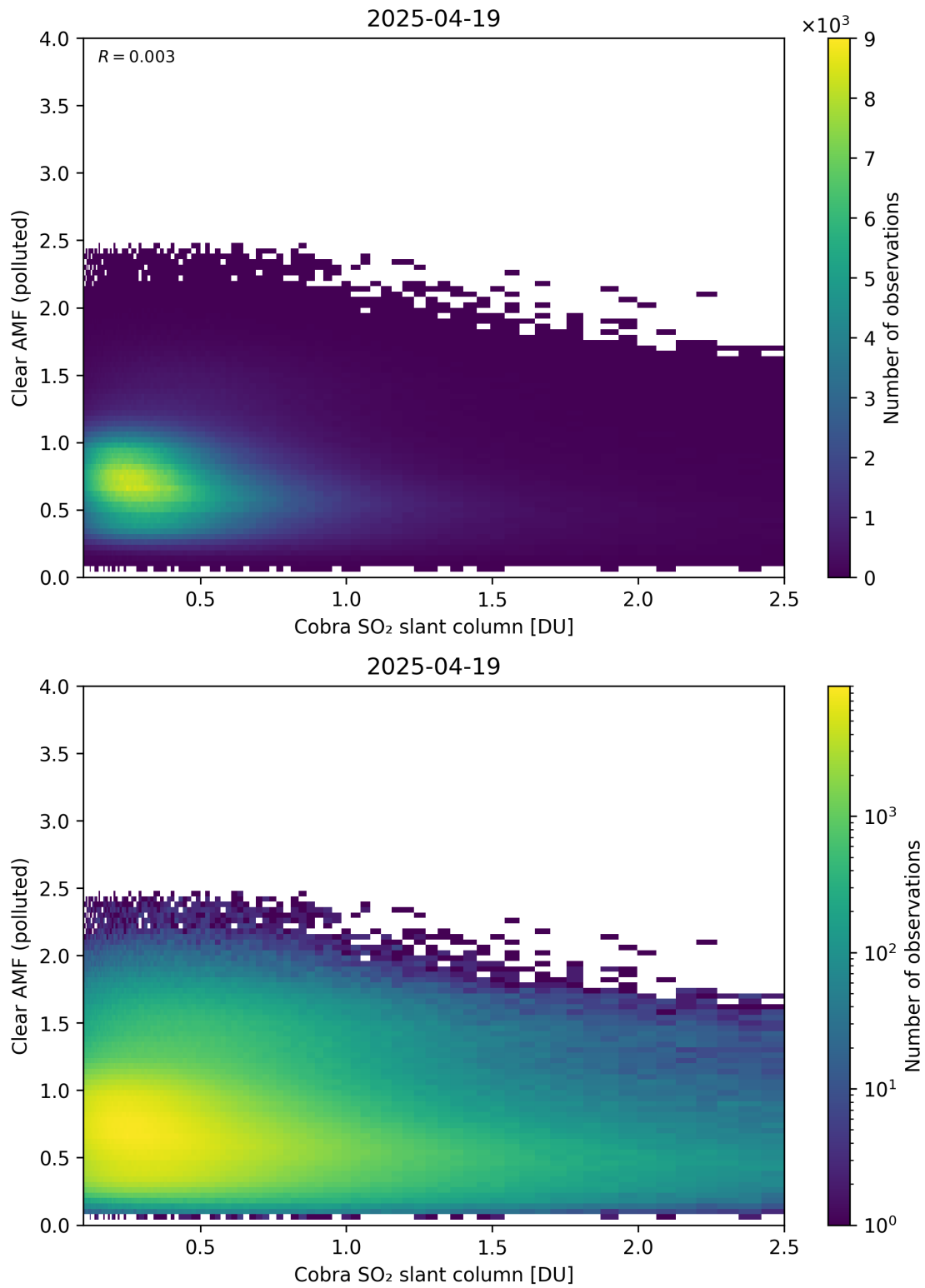
Figure 215: Scatter density plot of “Cobra SO 2 slant column” against “Clear AMF (polluted)” for 2025-04-19 to 2025-04-20.
