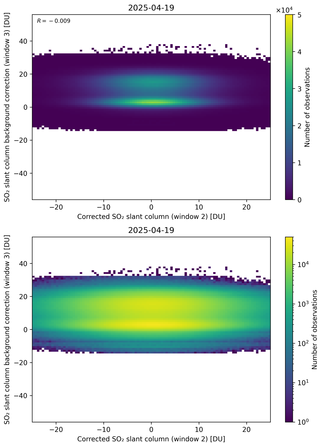
Figure 245: Scatter density plot of “Corrected SO 2 slant column (window 2)” against “SO 2 slant column background correction (window 3)” for 2025-04-19 to 2025-04-20.
