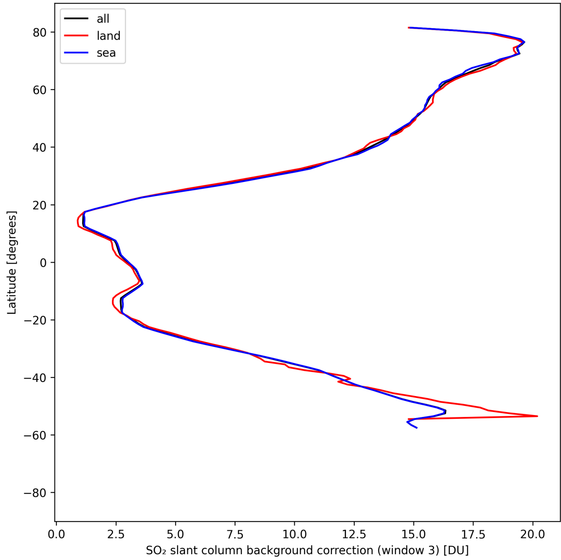
Figure 48: Zonal average of “SO 2 slant column background correction (window 3)” for 2025-04-19 to 2025-04-20.
