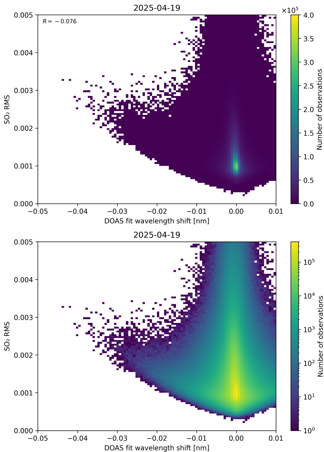
Figure 139: Scatter density plot of “DOAS fit wavelength shift” against “SO 2 RMS” for 2025-04-19 to 2025-04-20.
