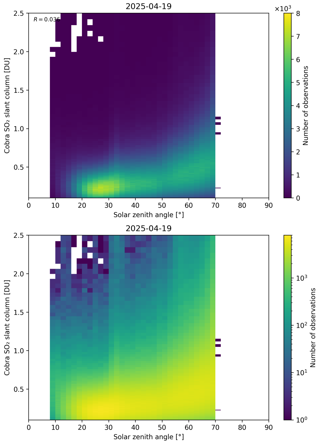
Figure 179: Scatter density plot of “Solar zenith angle” against “Cobra SO 2 slant column” for 2025-04-19 to 2025-04-20.
