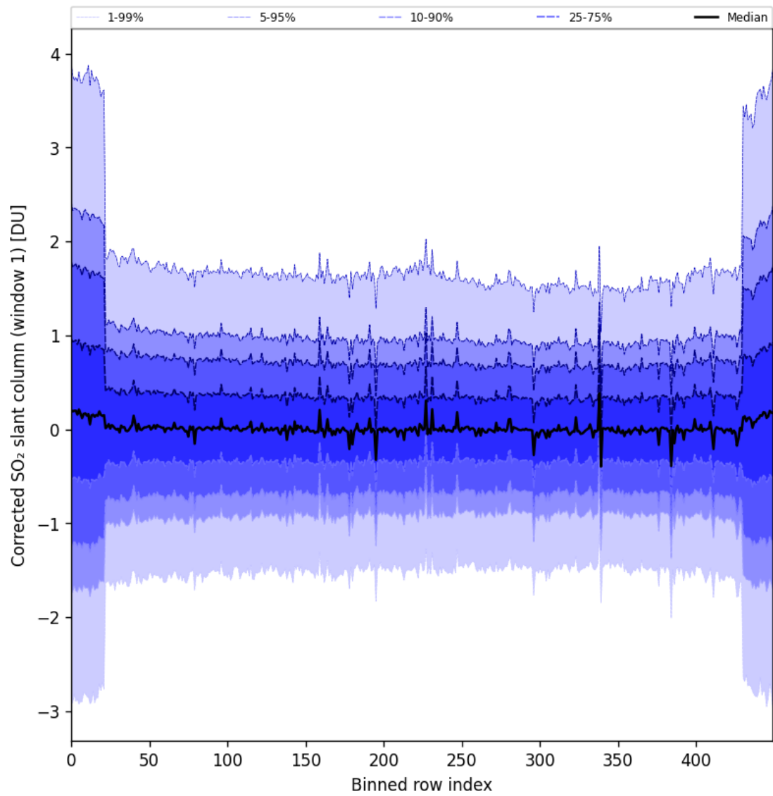
Figure 91: Along track statistics of “Corrected SO 2 slant column (window 1)” for 2025-04-19 to 2025-04-20
