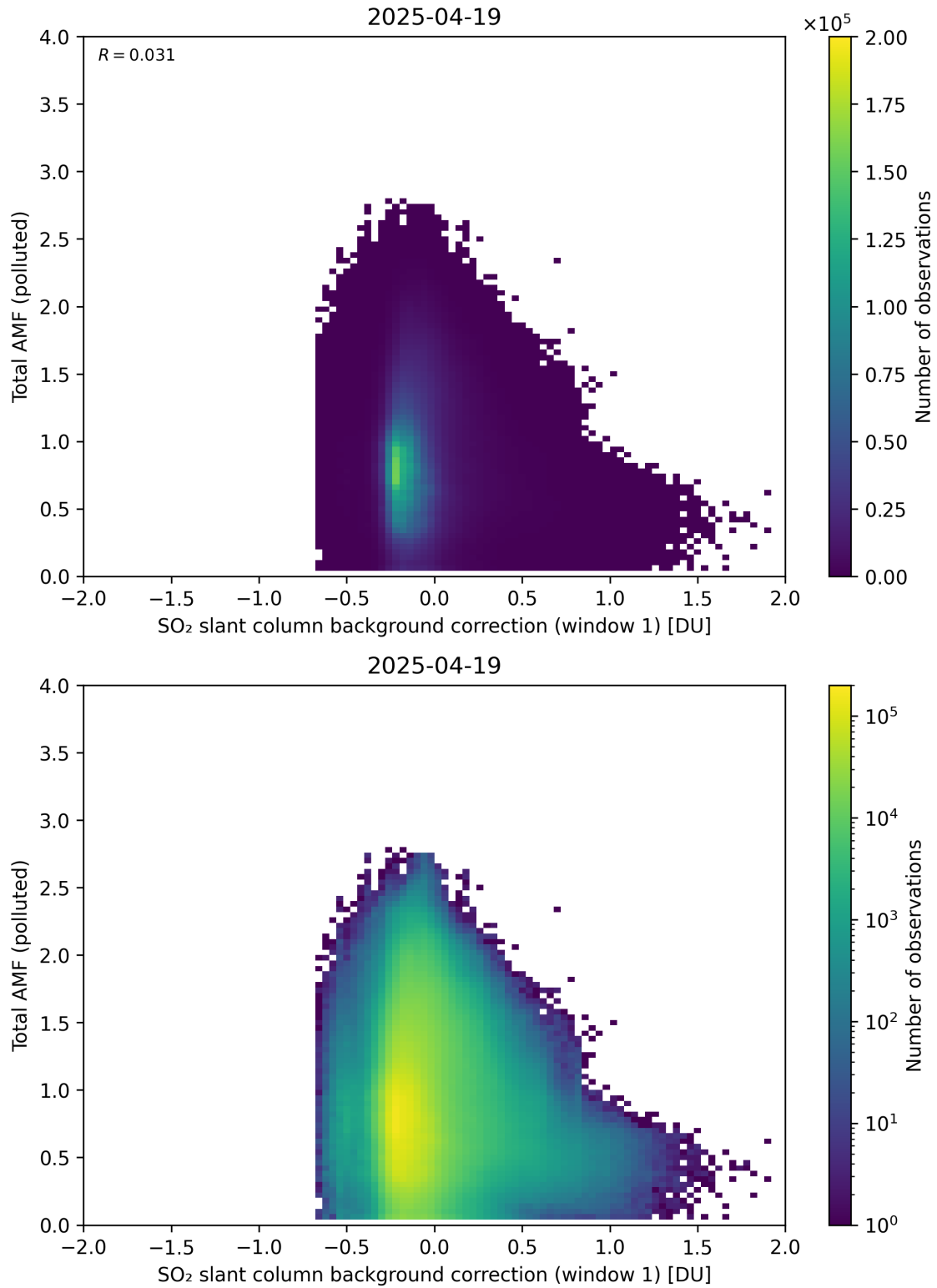
Figure 120: Scatter density plot of “SO 2 slant column background correction (window 1)” against “Total AMF (polluted)” for 2025-04-19 to 2025-04-20.
