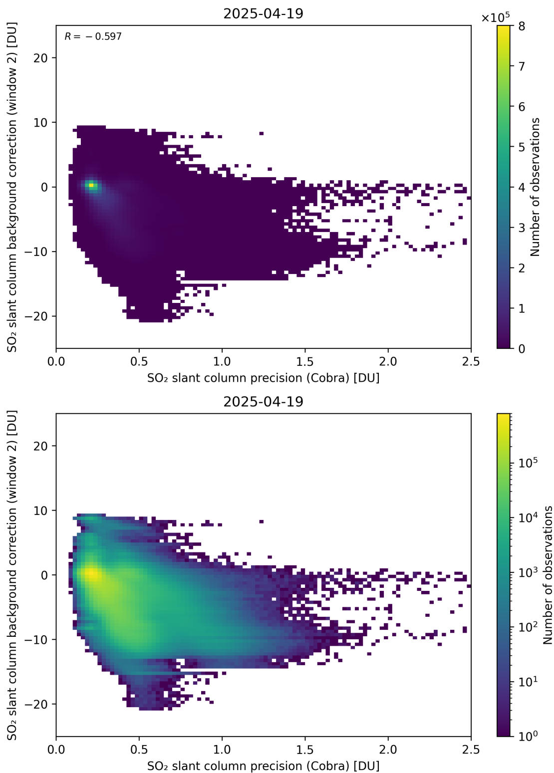
Figure 200: Scatter density plot of “SO 2 slant column precision (Cobra)” against “SO 2 slant column background correction (window 2)” for 2025-04-19 to 2025-04-20.
