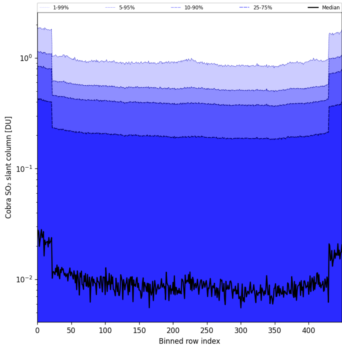
Figure 87: Along track statistics of “Cobra SO 2 slant column” for 2025-04-19 to 2025-04-20
