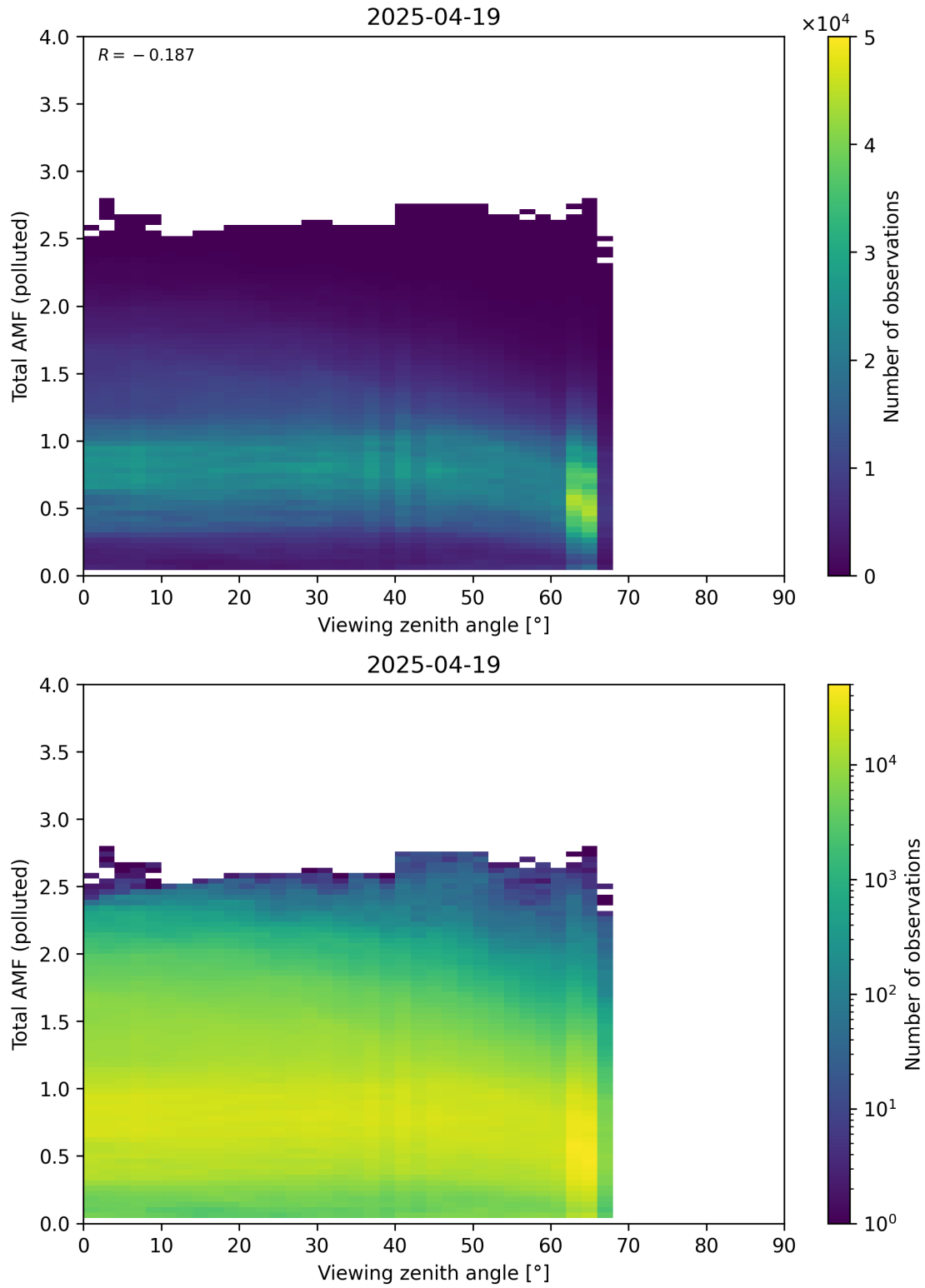
Figure 381: Scatter density plot of “Viewing zenith angle” against “Total AMF (polluted)” for 2025-04-19 to 2025-04-20.
