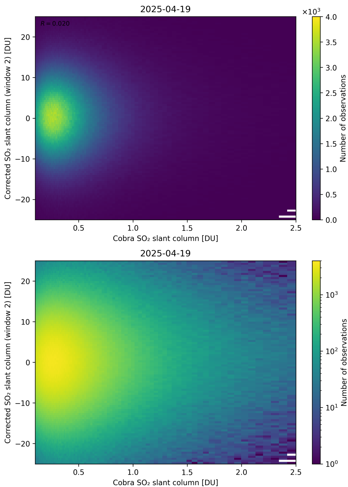
Figure 217: Scatter density plot of “Cobra SO 2 slant column” against “Corrected SO 2 slant column (window 2)” for 2025-04-19 to 2025-04-20.
