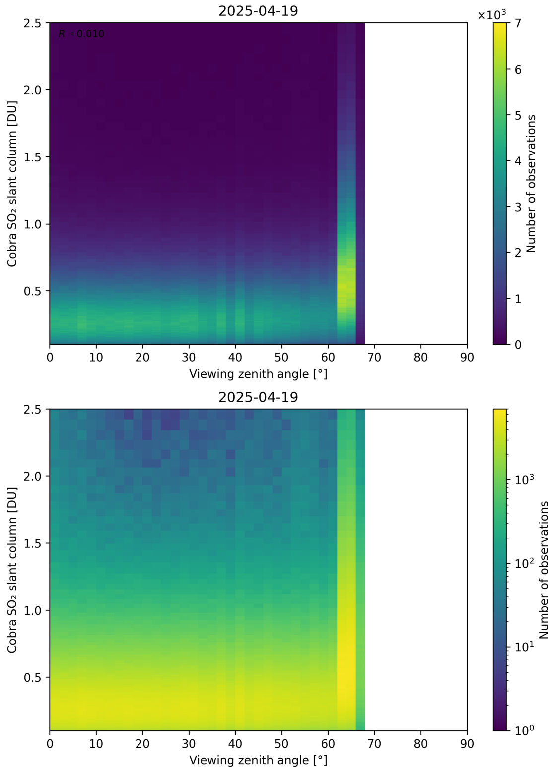
Figure 371: Scatter density plot of “Viewing zenith angle” against “Cobra SO 2 slant column” for 2025-04-19 to 2025-04-20.
