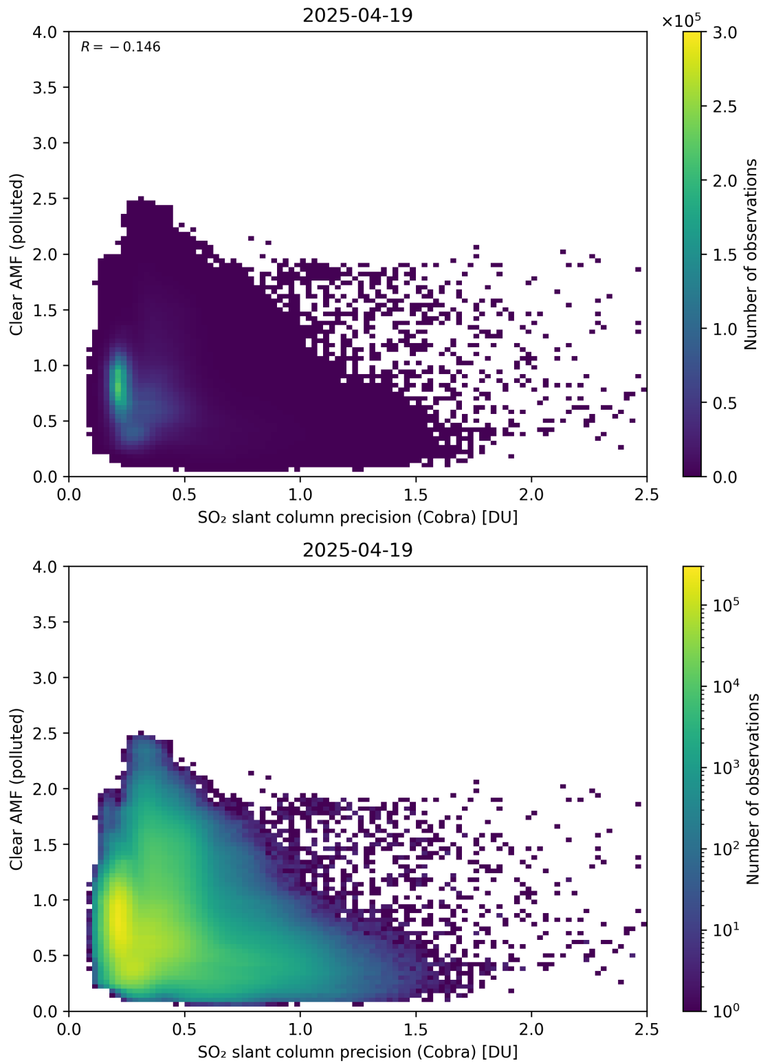
Figure 205: Scatter density plot of “SO 2 slant column precision (Cobra)” against “Clear AMF (polluted)” for 2025-04-19 to 2025-04-20.
