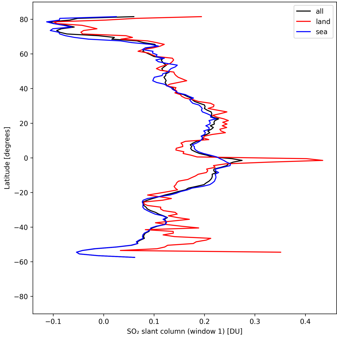
Figure 37: Zonal average of “SO 2 slant column (window 1)” for 2025-04-19 to 2025-04-20.
