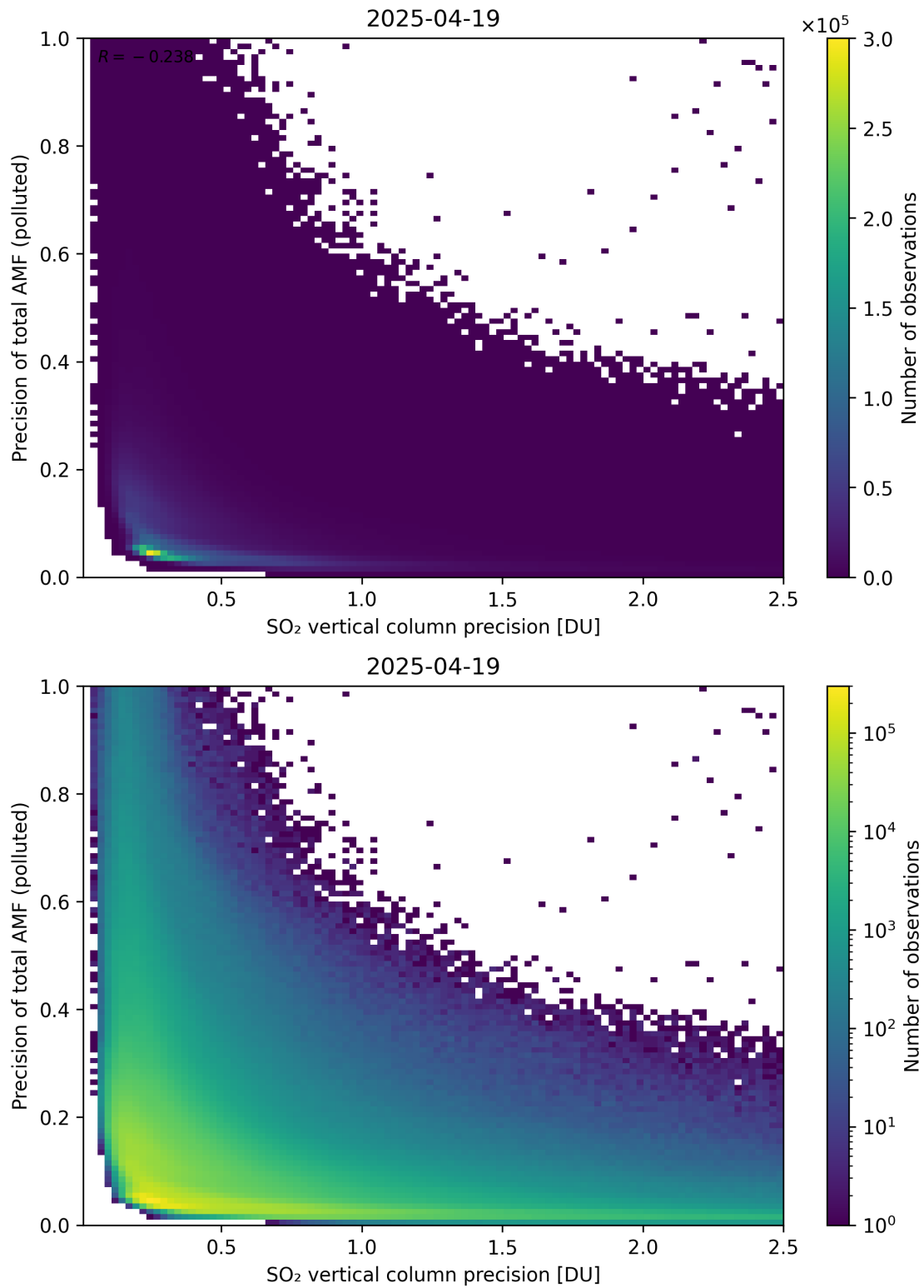
Figure 347: Scatter density plot of “SO 2 vertical column precision” against “Precision of total AMF (polluted)” for 2025-04-19 to 2025-04-20.
