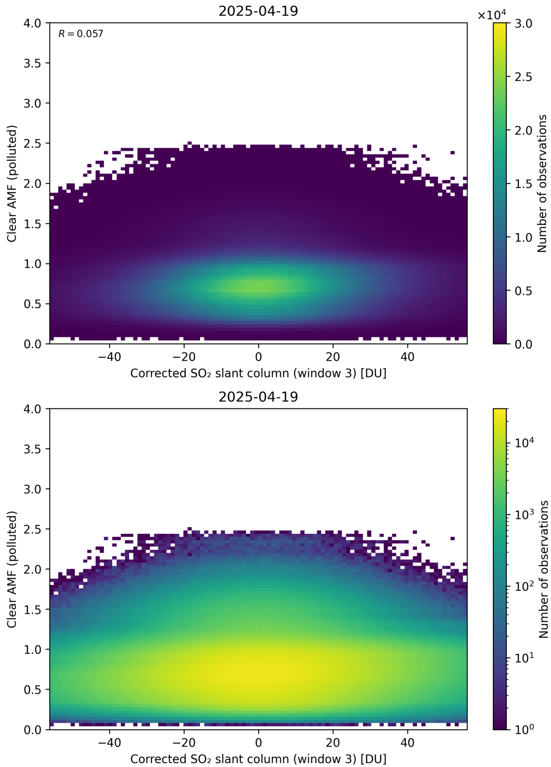
Figure 259: Scatter density plot of “Corrected SO 2 slant column (window 3)” against “Clear AMF (polluted)” for 2025-04-19 to 2025-04-20.
