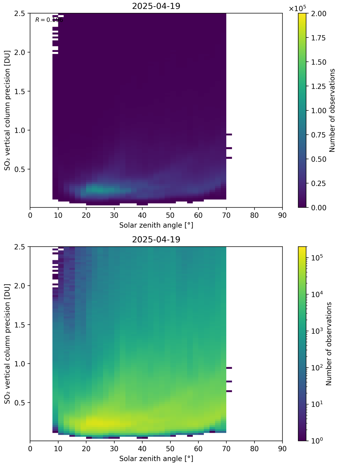
Figure 192: Scatter density plot of “Solar zenith angle” against “SO 2 vertical column precision” for 2025-04-19 to 2025-04-20.
