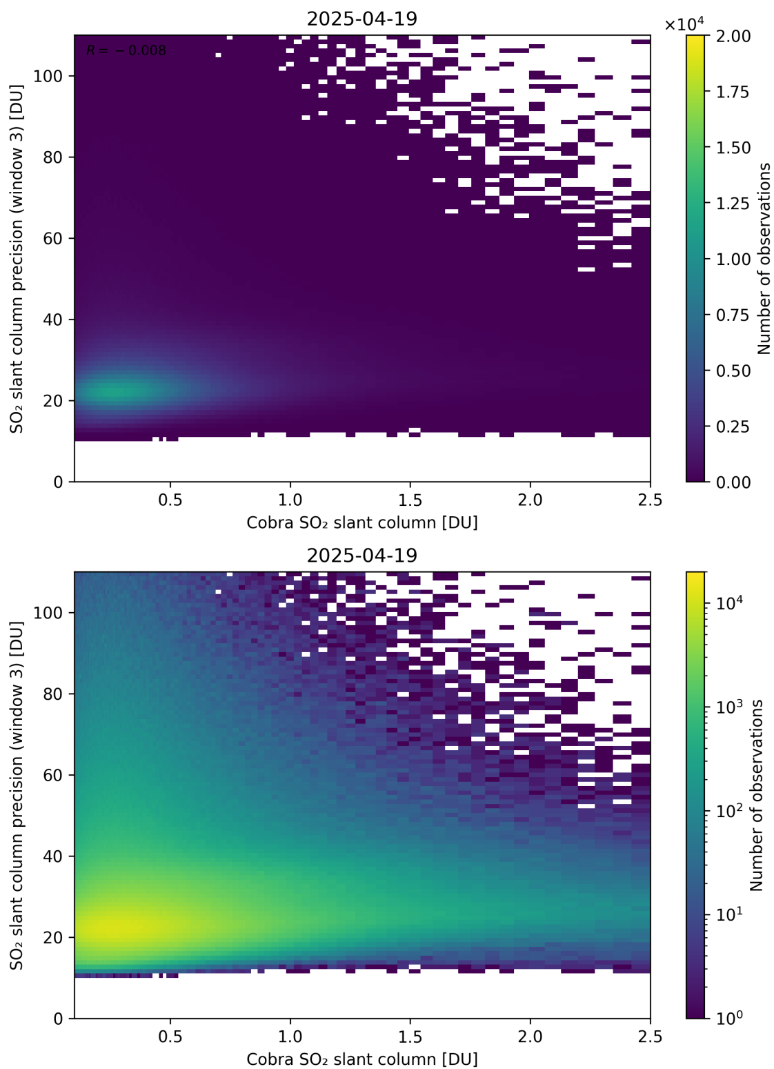
Figure 223: Scatter density plot of “Cobra SO 2 slant column” against “SO 2 slant column precision (window 3)” for 2025-04-19 to 2025-04-20.
