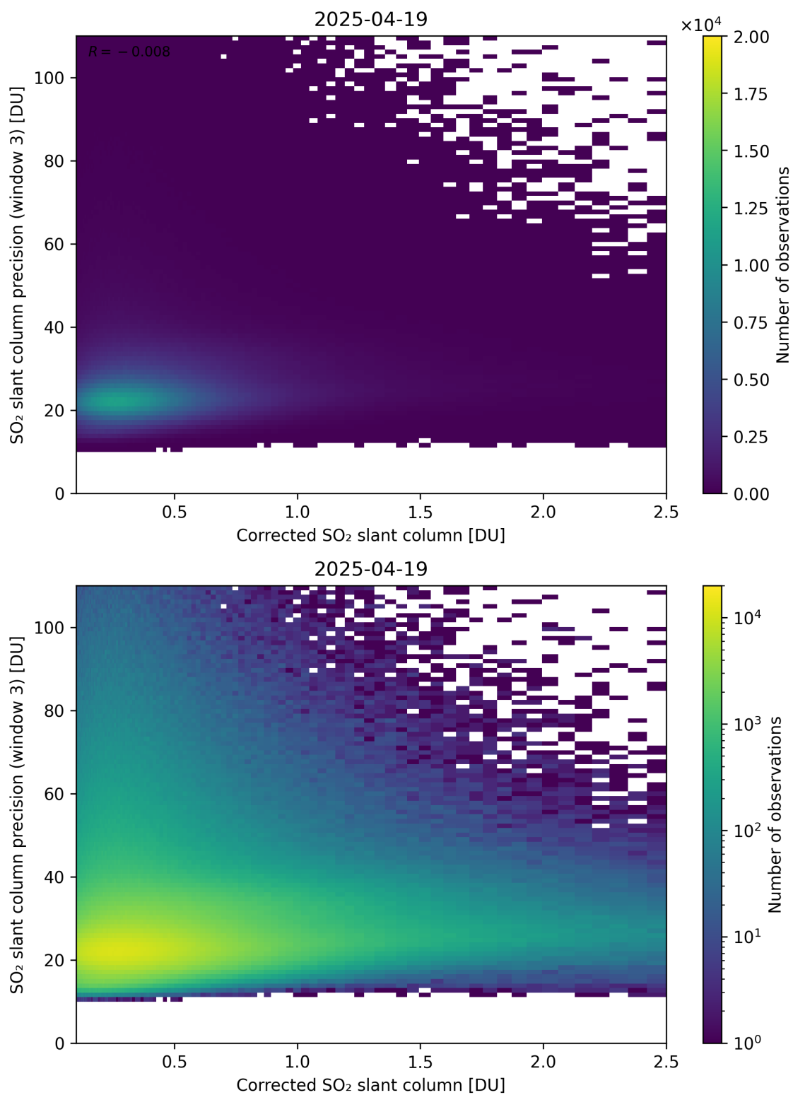
Figure 241: Scatter density plot of “Corrected SO 2 slant column” against “SO 2 slant column precision (window 3)” for 2025-04-19 to 2025-04-20.
