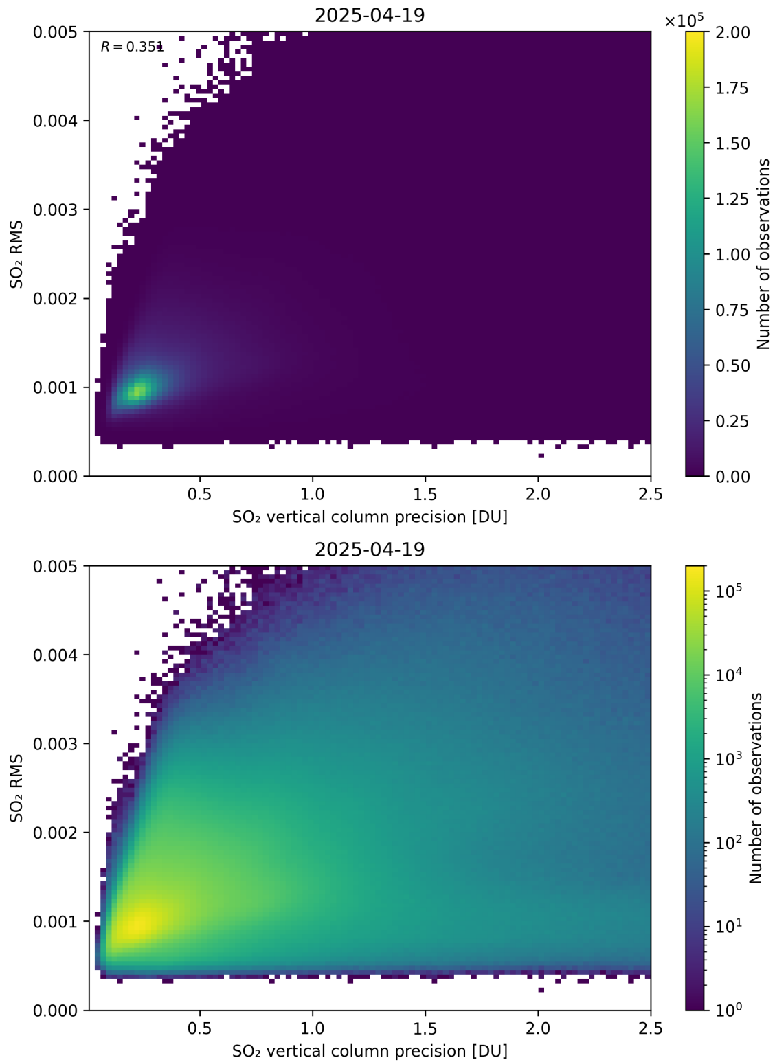
Figure 334: Scatter density plot of “SO 2 vertical column precision” against “SO 2 RMS” for 2025-04-19 to 2025-04-20.
