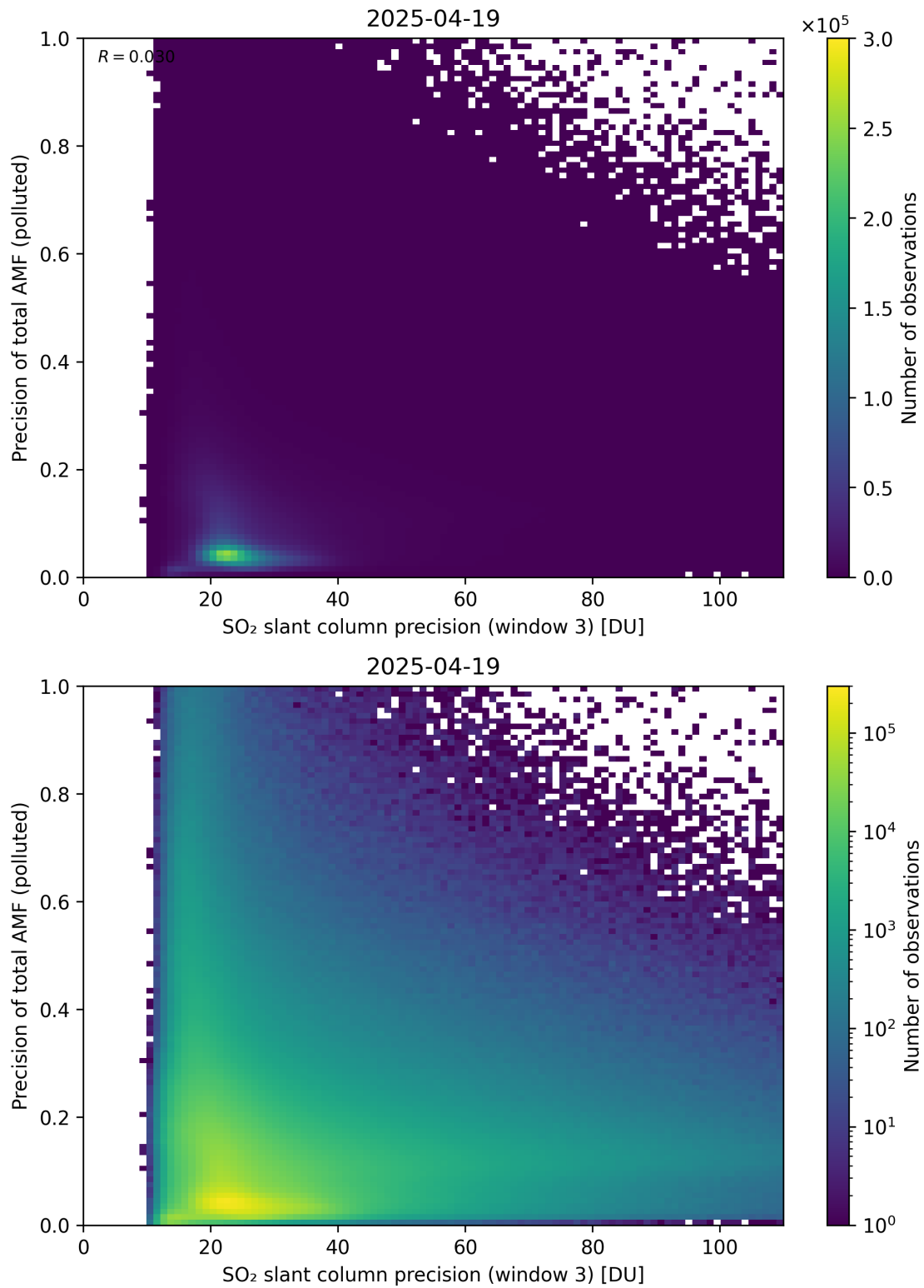
Figure 314: Scatter density plot of “SO 2 slant column precision (window 3)” against “Precision of total AMF (polluted)” for 2025-04-19 to 2025-04-20.
