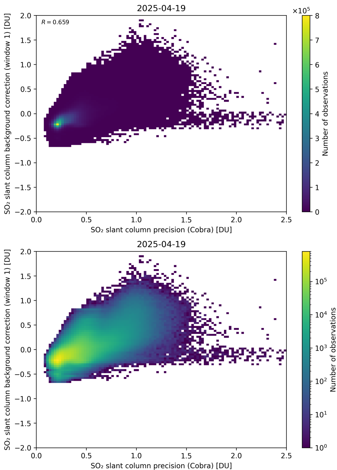
Figure 199: Scatter density plot of “SO 2 slant column precision (Cobra)” against “SO 2 slant column background correction (window 1)” for 2025-04-19 to 2025-04-20.
