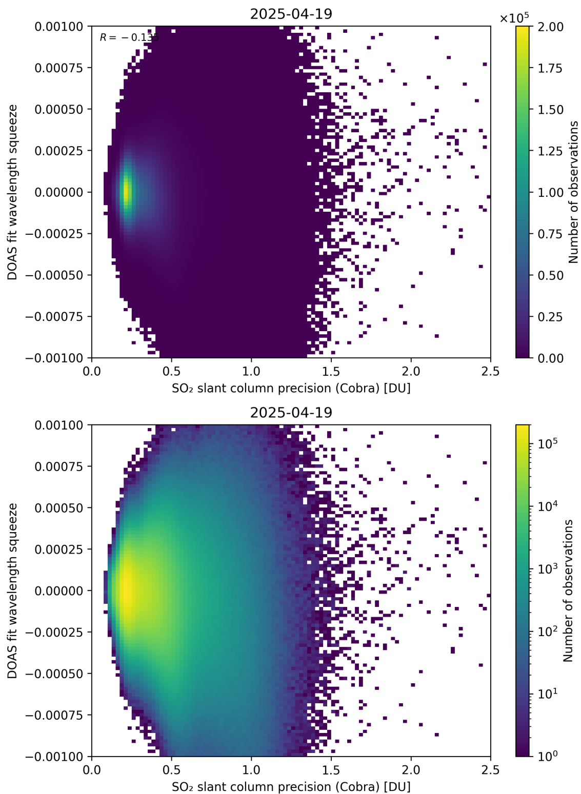
Figure 203: Scatter density plot of “SO 2 slant column precision (Cobra)” against “DOAS fit wavelength squeeze” for 2025-04-19 to 2025-04-20.
