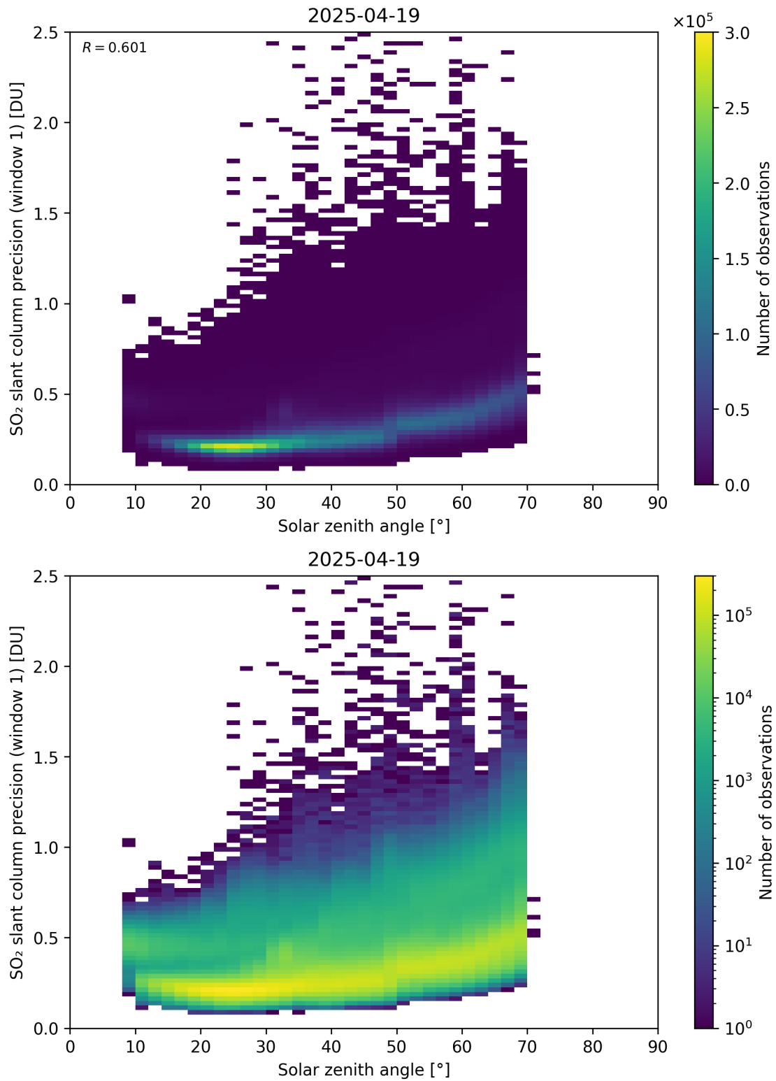
Figure 185: Scatter density plot of “Solar zenith angle” against “SO 2 slant column precision (window 1)” for 2025-04-19 to 2025-04-20.
