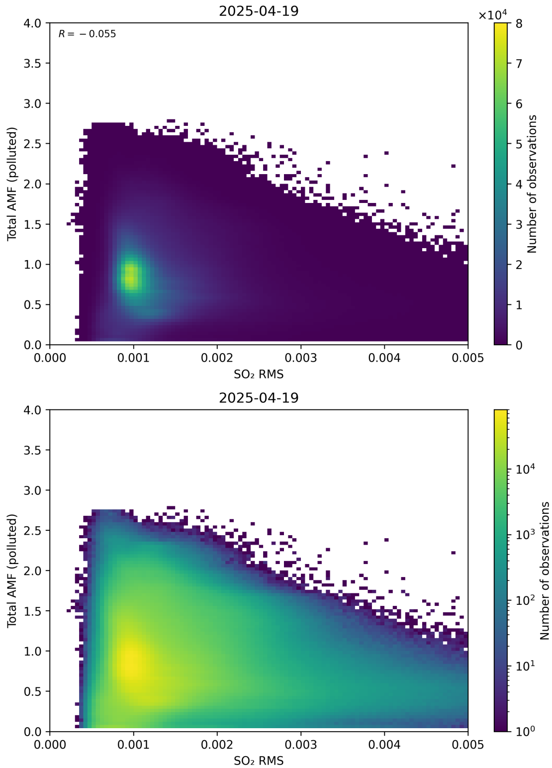
Figure 148: Scatter density plot of “SO 2 RMS” against “Total AMF (polluted)” for 2025-04-19 to 2025-04-20.
