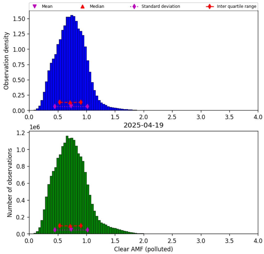
Figure 81: Histogram of "Clear AMF (polluted)" for 2025-04-19 to 2025-04-20
