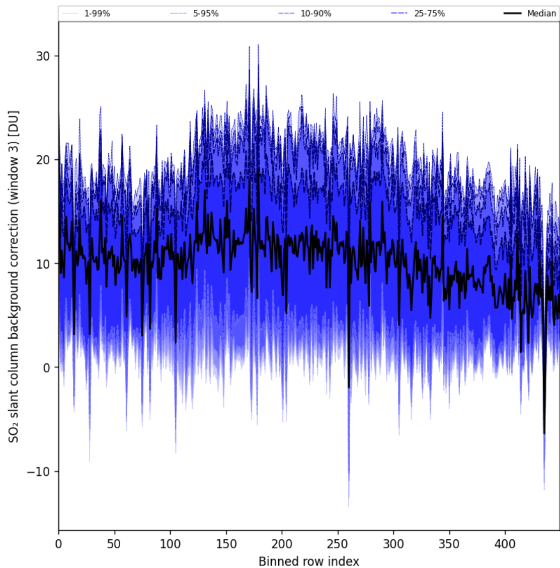
Figure 100: Along track statistics of “SO 2 slant column background correction (window 3)” for 2025-04-19 to 2025-04-20
