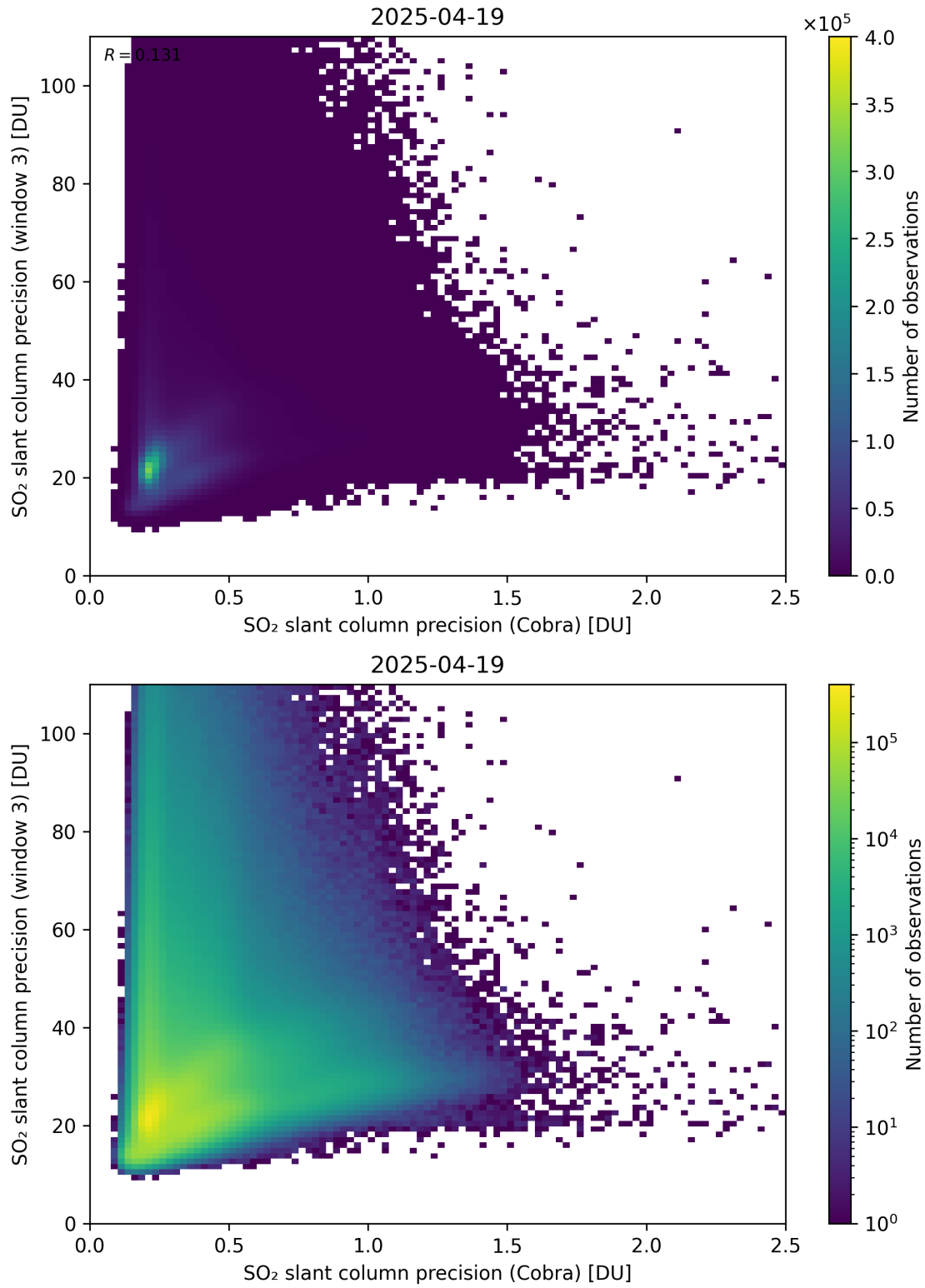
Figure 212: Scatter density plot of “SO 2 slant column precision (Cobra)” against “SO 2 slant column precision (window 3)” for 2025-04-19 to 2025-04-20.
