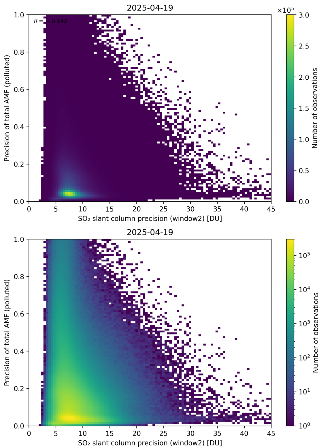
Figure 302: Scatter density plot of “SO 2 slant column precision (window2)” against “Precision of total AMF (polluted)” for 2025-04-19 to 2025-04-20.
