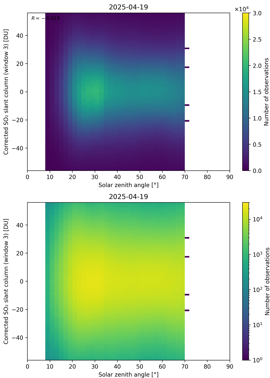
Figure 183: Scatter density plot of “Solar zenith angle” against “Corrected SO 2 slant column (window 3)” for 2025-04-19 to 2025-04-20.
