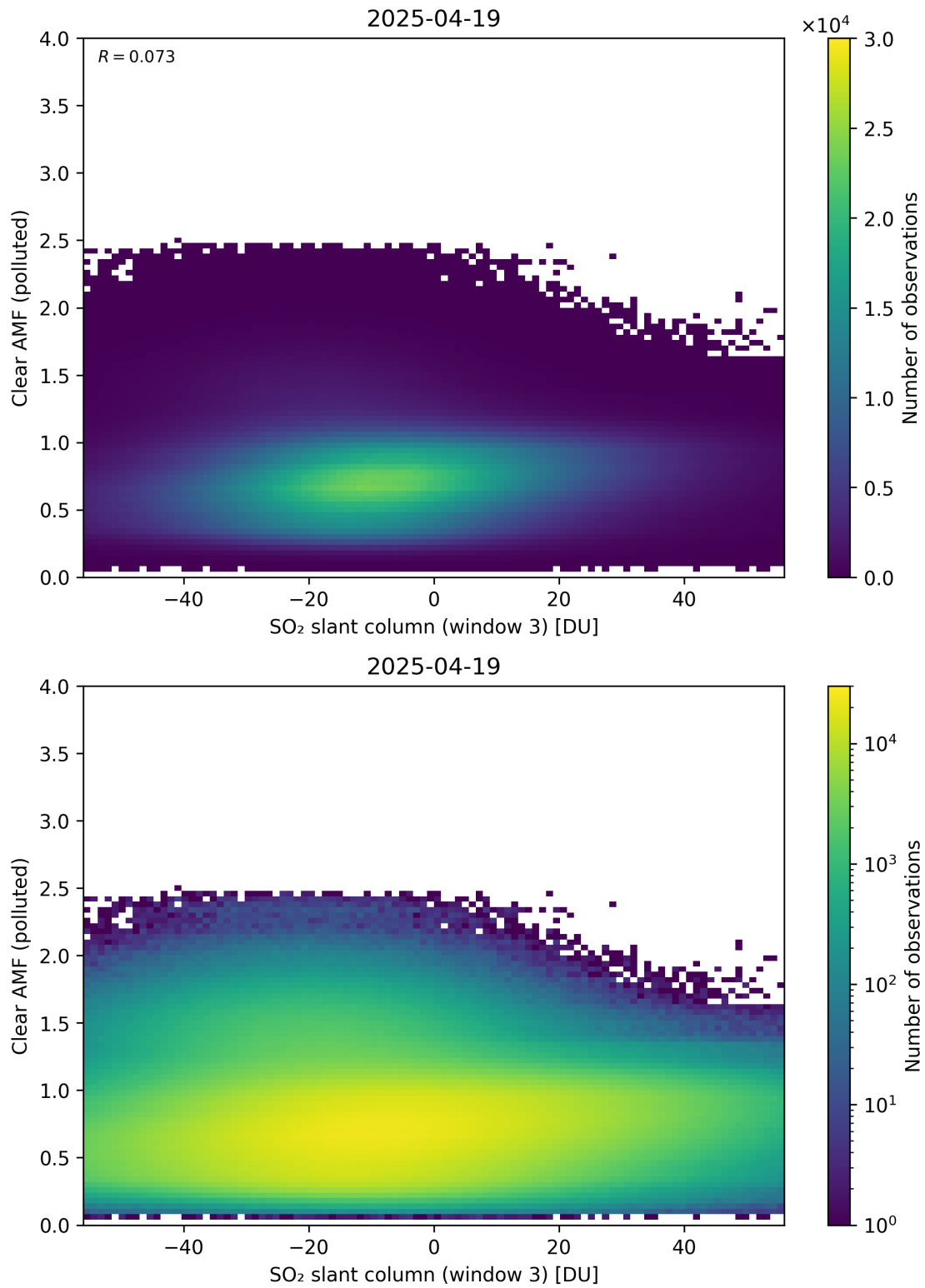
Figure 315: Scatter density plot of “SO 2 slant column (window 3)” against “Clear AMF (polluted)” for 2025-04-19 to 2025-04-20.
