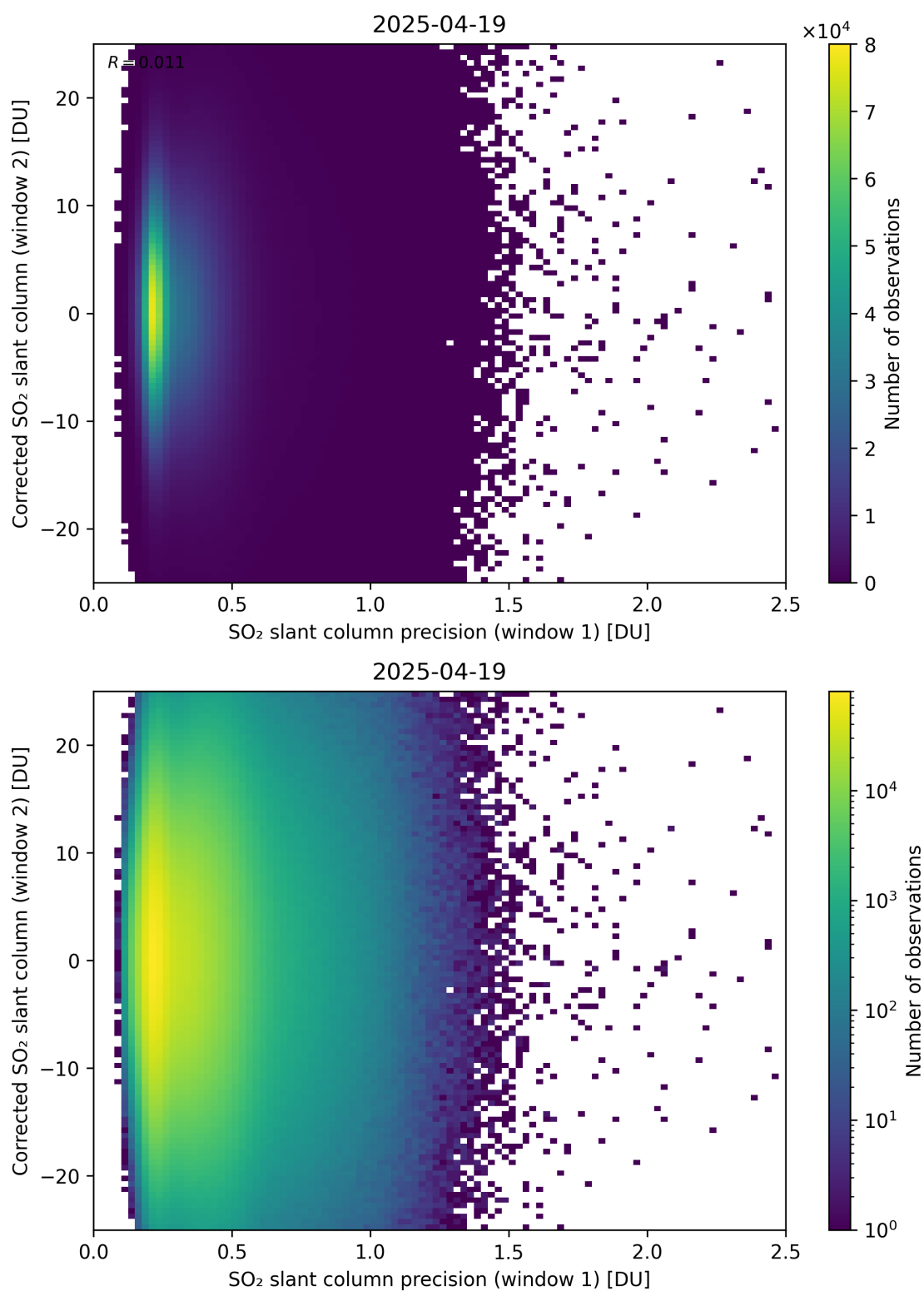
Figure 275: Scatter density plot of “SO 2 slant column precision (window 1)” against “Corrected SO 2 slant column (window 2)” for 2025-04-19 to 2025-04-20.
