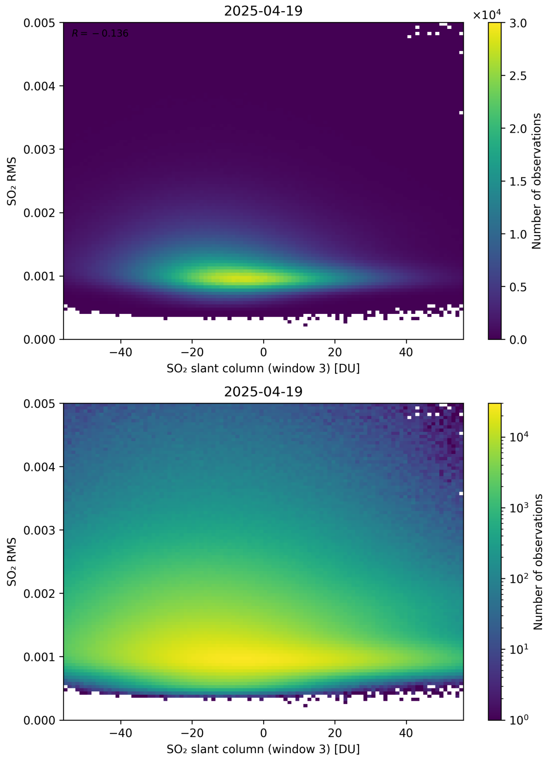
Figure 306: Scatter density plot of “SO 2 slant column (window 3)” against “SO 2 RMS” for 2025-04-19 to 2025-04-20.
