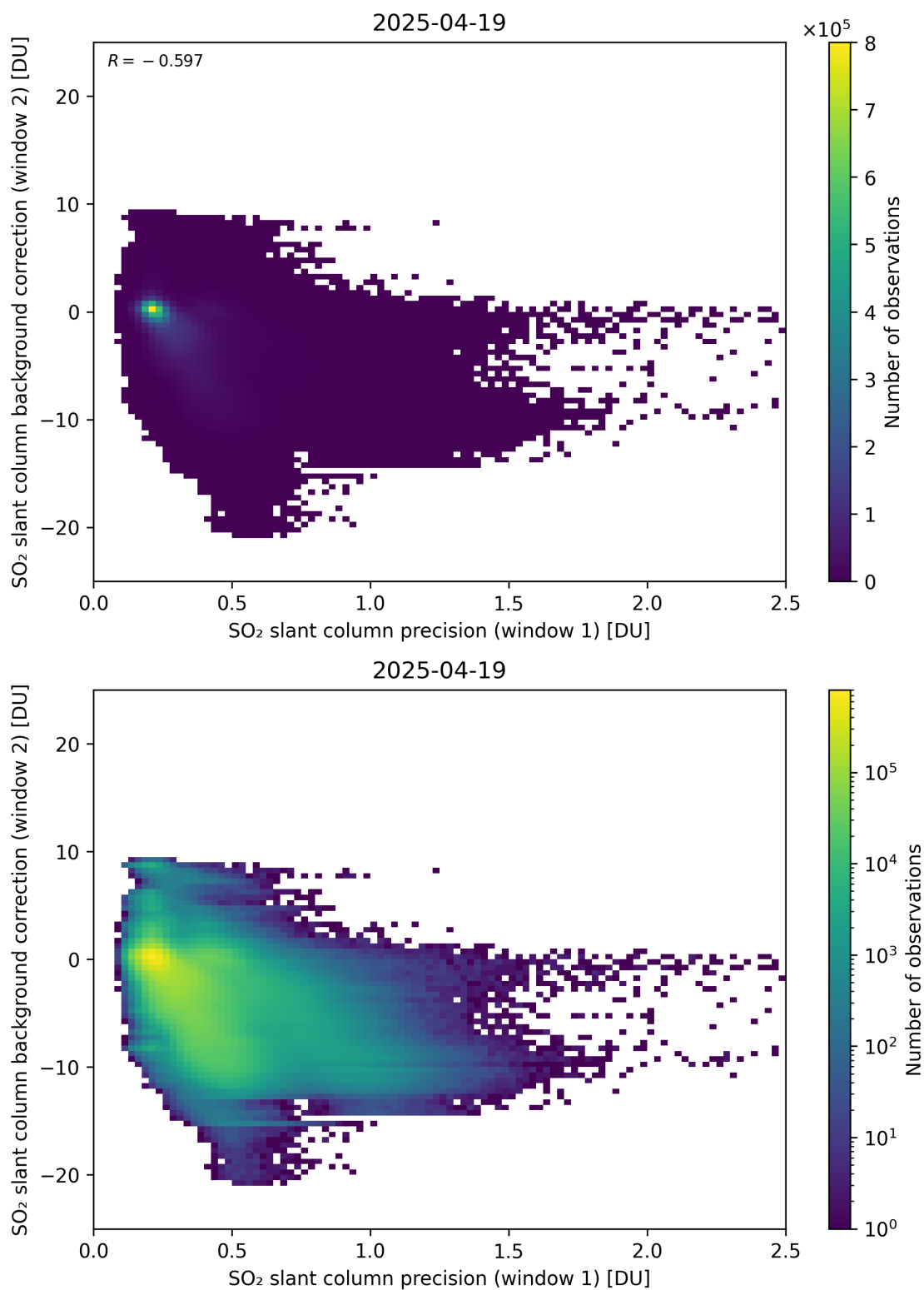
Figure 269: Scatter density plot of “SO 2 slant column precision (window 1)” against “SO 2 slant column background correction (window 2)” for 2025-04-19 to 2025-04-20.
