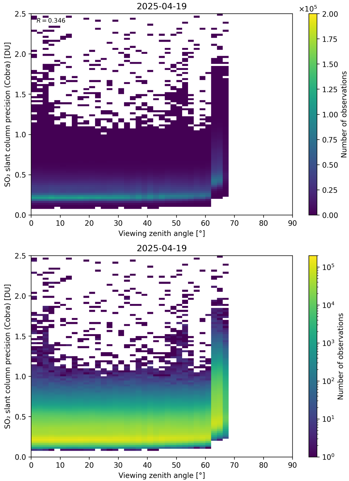
Figure 372: Scatter density plot of “Viewing zenith angle” against “SO 2 slant column precision (Cobra)” for 2025-04-19 to 2025-04-20.
