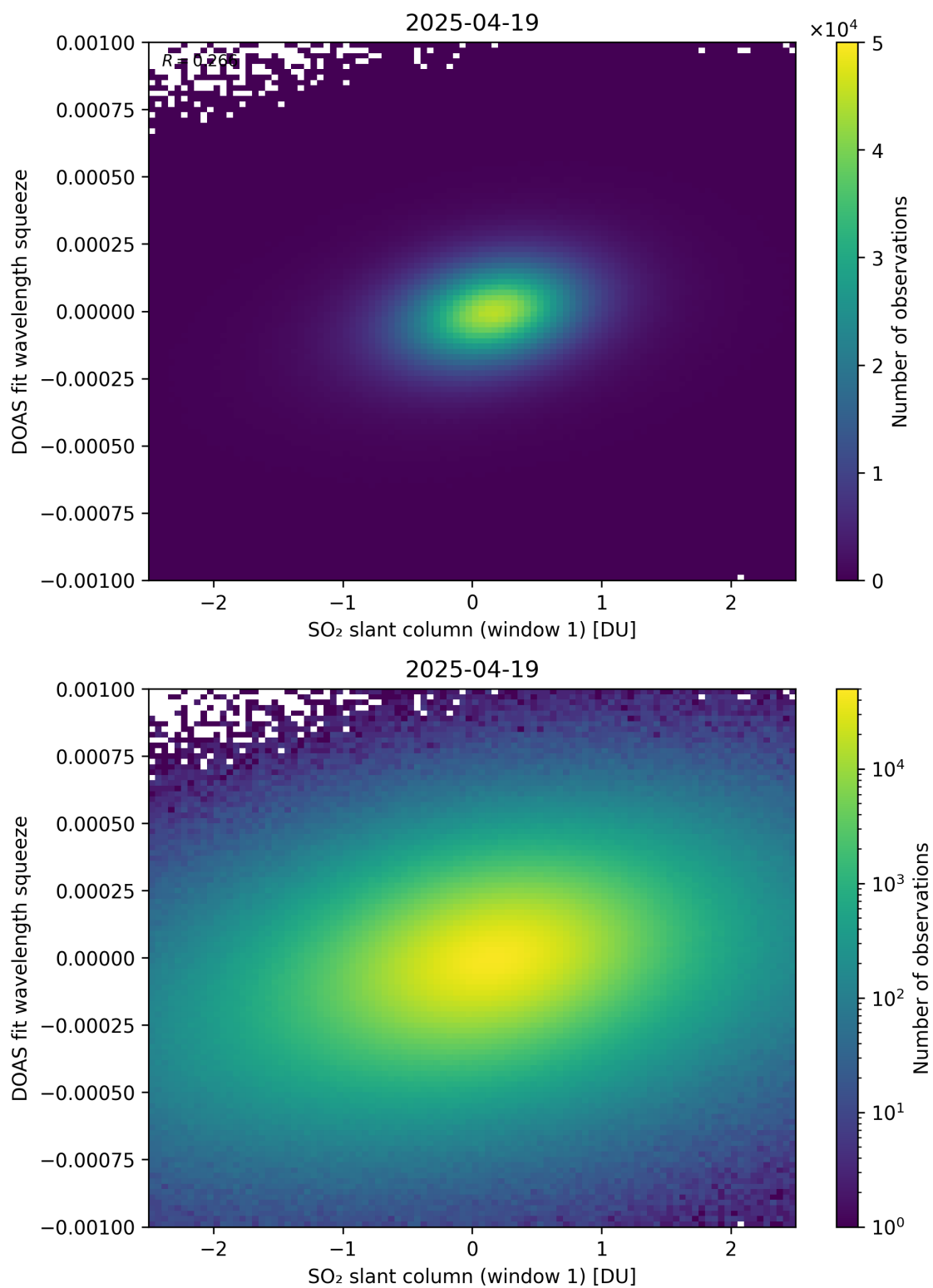
Figure 266: Scatter density plot of “SO 2 slant column (window 1)” against “DOAS fit wavelength squeeze” for 2025-04-19 to 2025-04-20.
