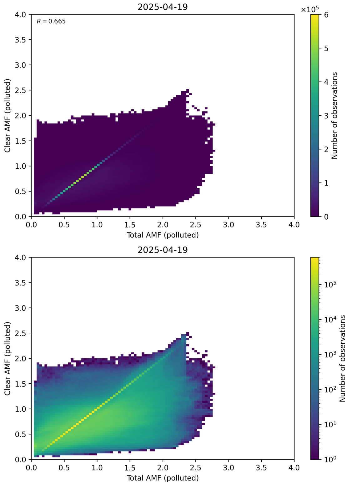
Figure 321: Scatter density plot of “Total AMF (polluted)” against “Clear AMF (polluted)” for 2025-04-19 to 2025-04-20.
