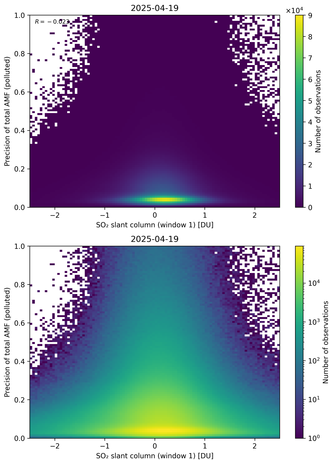
Figure 290: Scatter density plot of “SO 2 slant column (window 1)” against “Precision of total AMF (polluted)” for 2025-04-19 to 2025-04-20.
