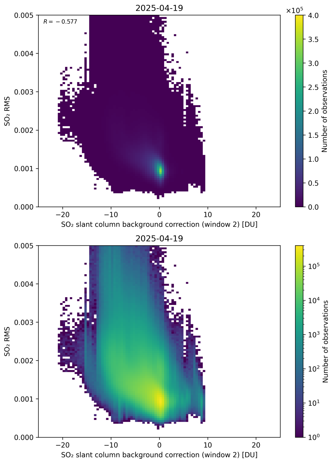
Figure 125: Scatter density plot of “SO 2 slant column background correction (window 2)” against “SO 2 RMS” for 2025-04-19 to 2025-04-20.
