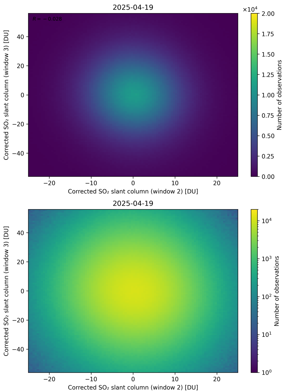
Figure 250: Scatter density plot of “Corrected SO 2 slant column (window 2)” against “Corrected SO 2 slant column (window 3)” for 2025-04-19 to 2025-04-20.
