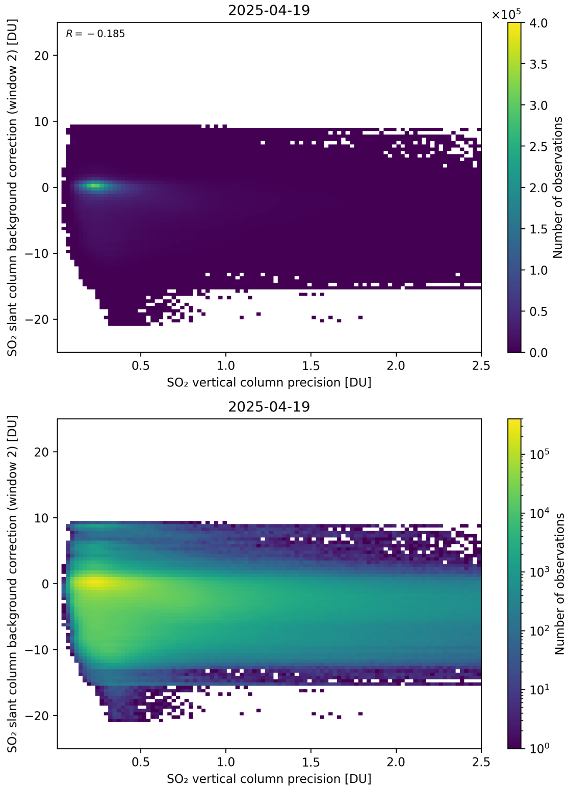
Figure 330: Scatter density plot of “SO 2 vertical column precision” against “SO 2 slant column background correction (window 2)” for 2025-04-19 to 2025-04-20.
