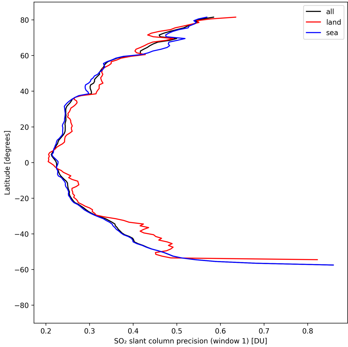
Figure 38: Zonal average of “SO 2 slant column precision (window 1)” for 2025-04-19 to 2025-04-20.
