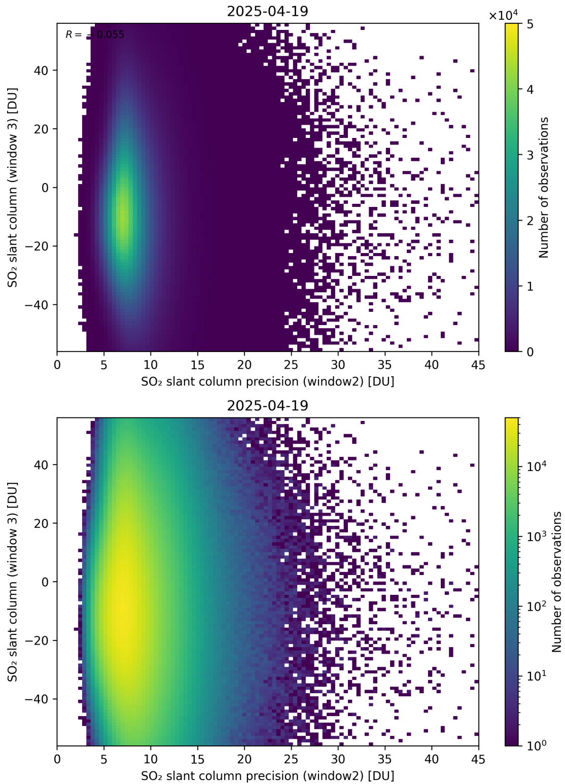
Figure 299: Scatter density plot of “SO 2 slant column precision (window2)” against “SO 2 slant column (window 3)” for 2025-04-19 to 2025-04-20.
