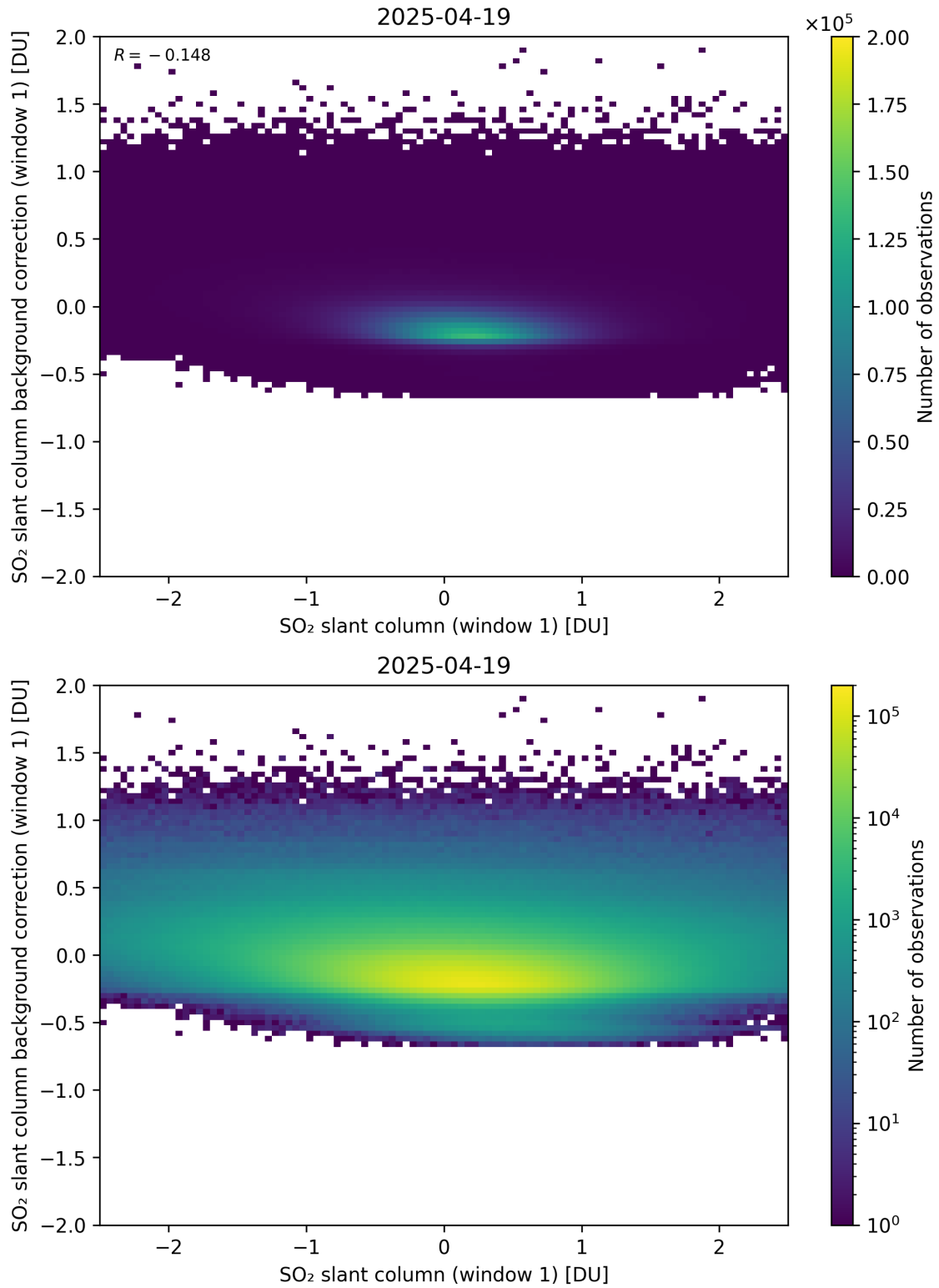
Figure 262: Scatter density plot of “SO 2 slant column (window 1)” against “SO 2 slant column background correction (window 1)” for 2025-04-19 to 2025-04-20.
