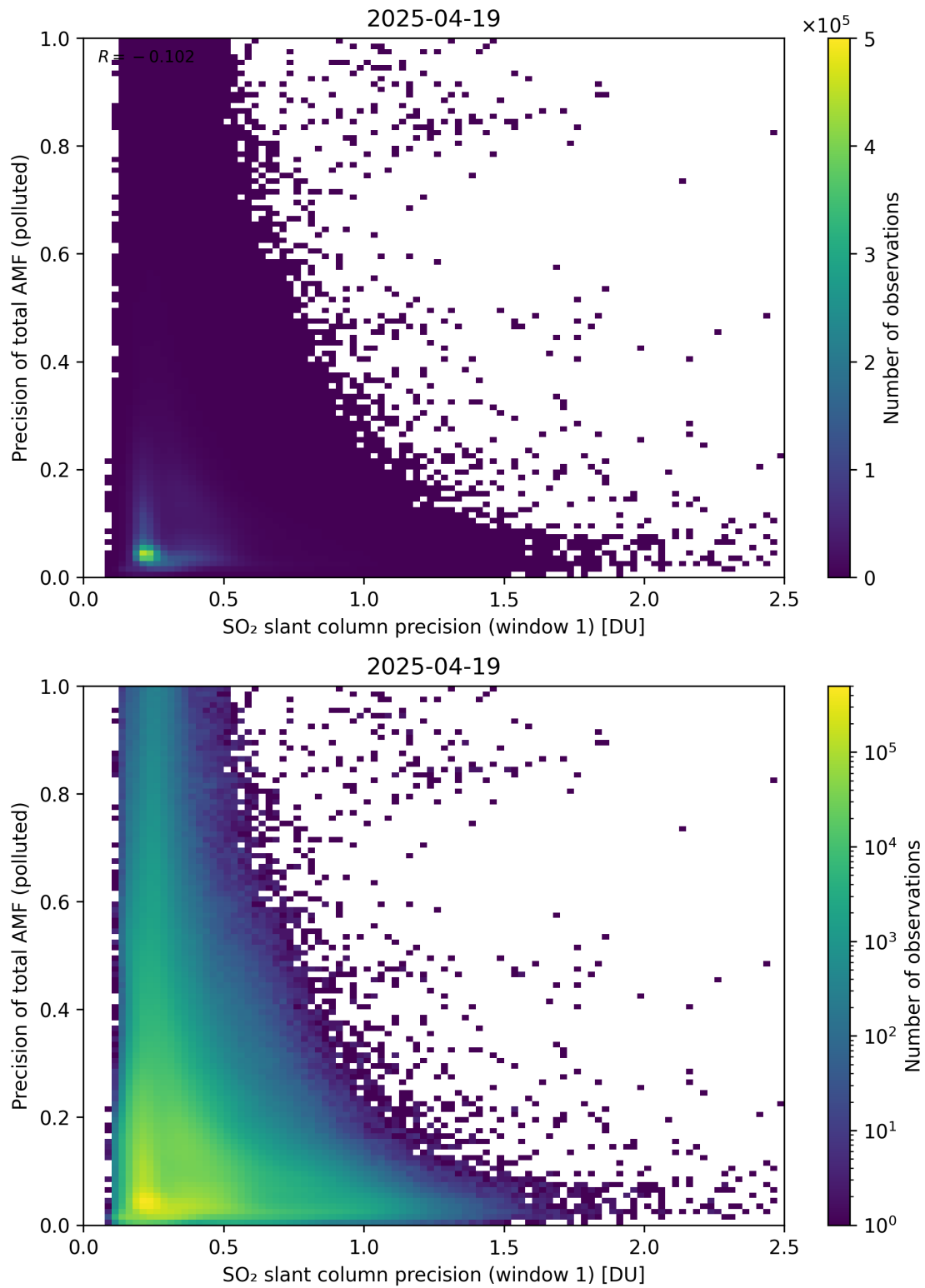
Figure 281: Scatter density plot of “SO 2 slant column precision (window 1)” against “Precision of total AMF (polluted)” for 2025-04-19 to 2025-04-20.
