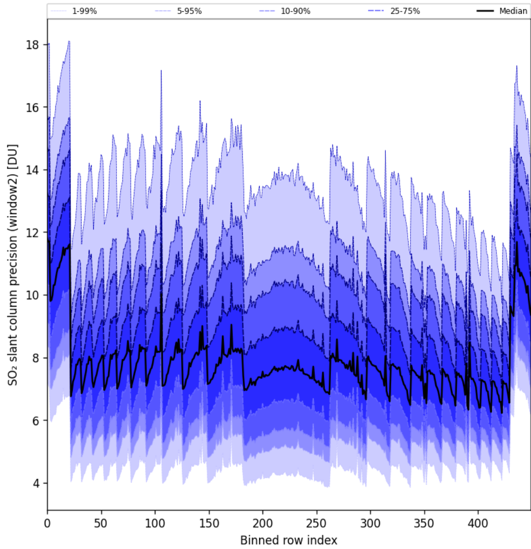
Figure 94: Along track statistics of “SO 2 slant column precision (window2)” for 2025-04-19 to 2025-04-20
