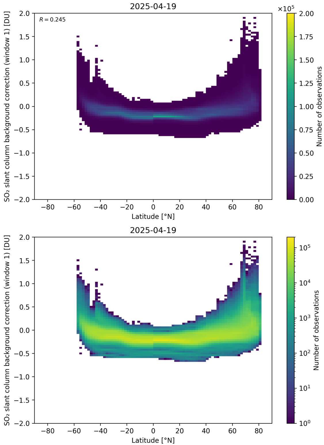
Figure 150: Scatter density plot of “Latitude” against “SO 2 slant column background correction (window 1)” for 2025-04-19 to 2025-04-20.
