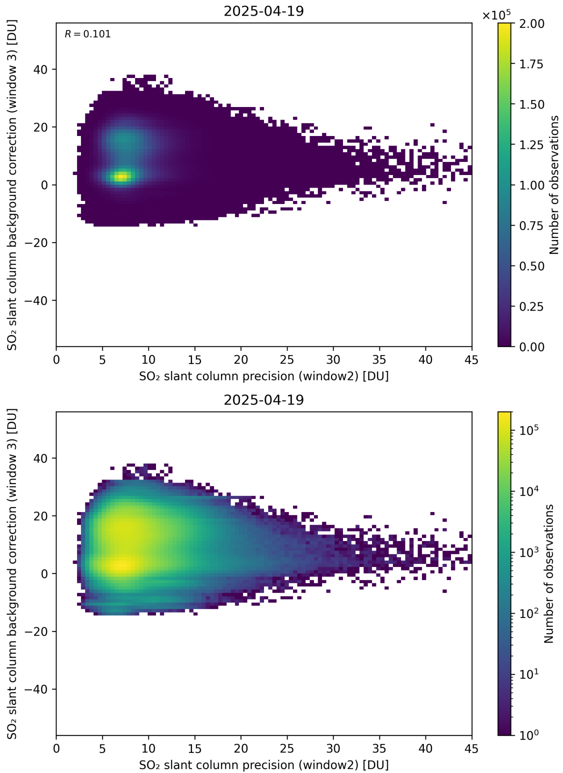
Figure 292: Scatter density plot of “SO 2 slant column precision (window2)” against “SO 2 slant column background correction (window 3)” for 2025-04-19 to 2025-04-20.
