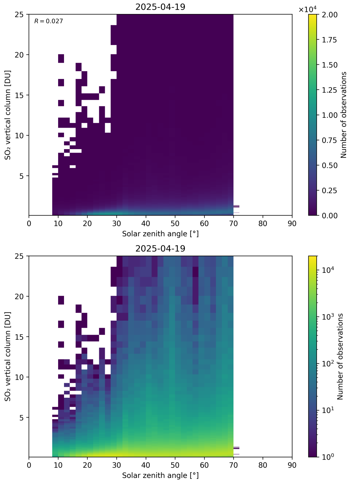
Figure 191: Scatter density plot of “Solar zenith angle” against “SO 2 vertical column” for 2025-04-19 to 2025-04-20.
