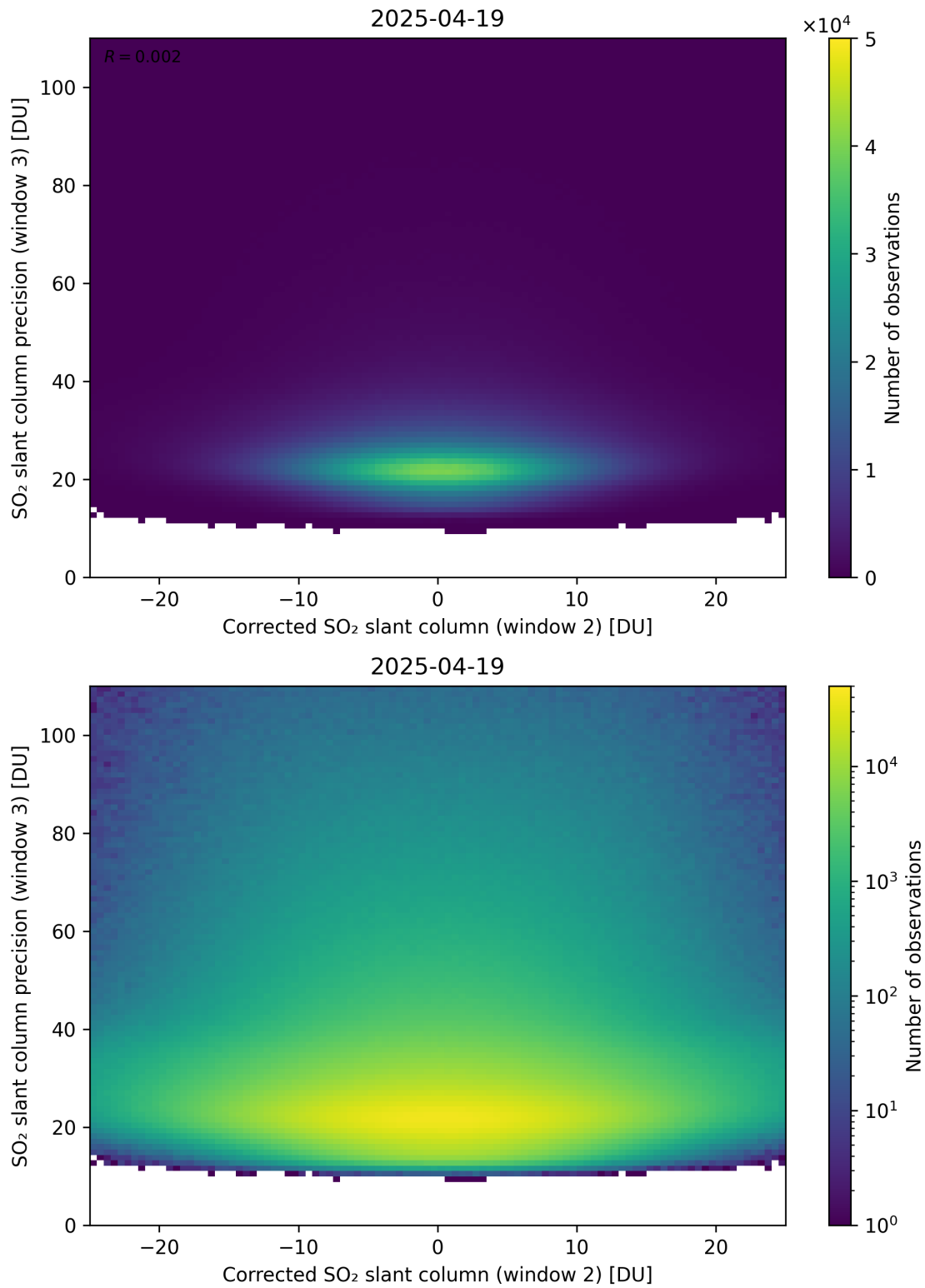
Figure 252: Scatter density plot of “Corrected SO 2 slant column (window 2)” against “SO 2 slant column precision (window 3)” for 2025-04-19 to 2025-04-20.
