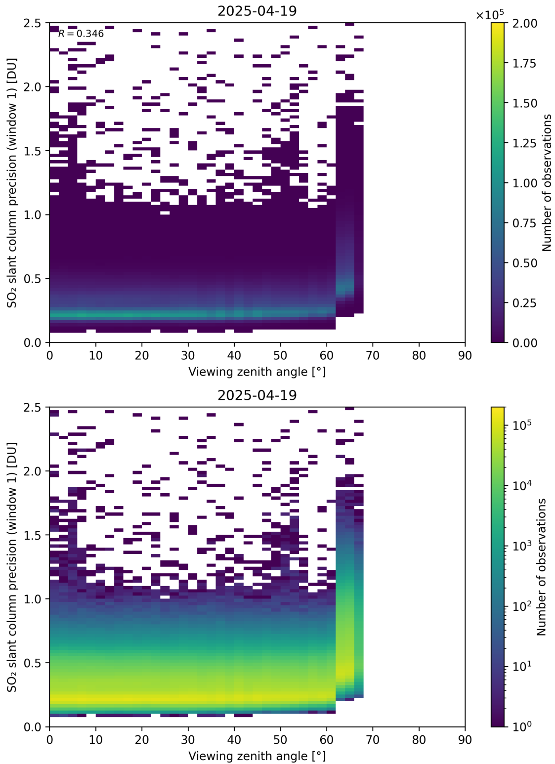
Figure 377: Scatter density plot of “Viewing zenith angle” against “SO 2 slant column precision (window 1)” for 2025-04-19 to 2025-04-20.
