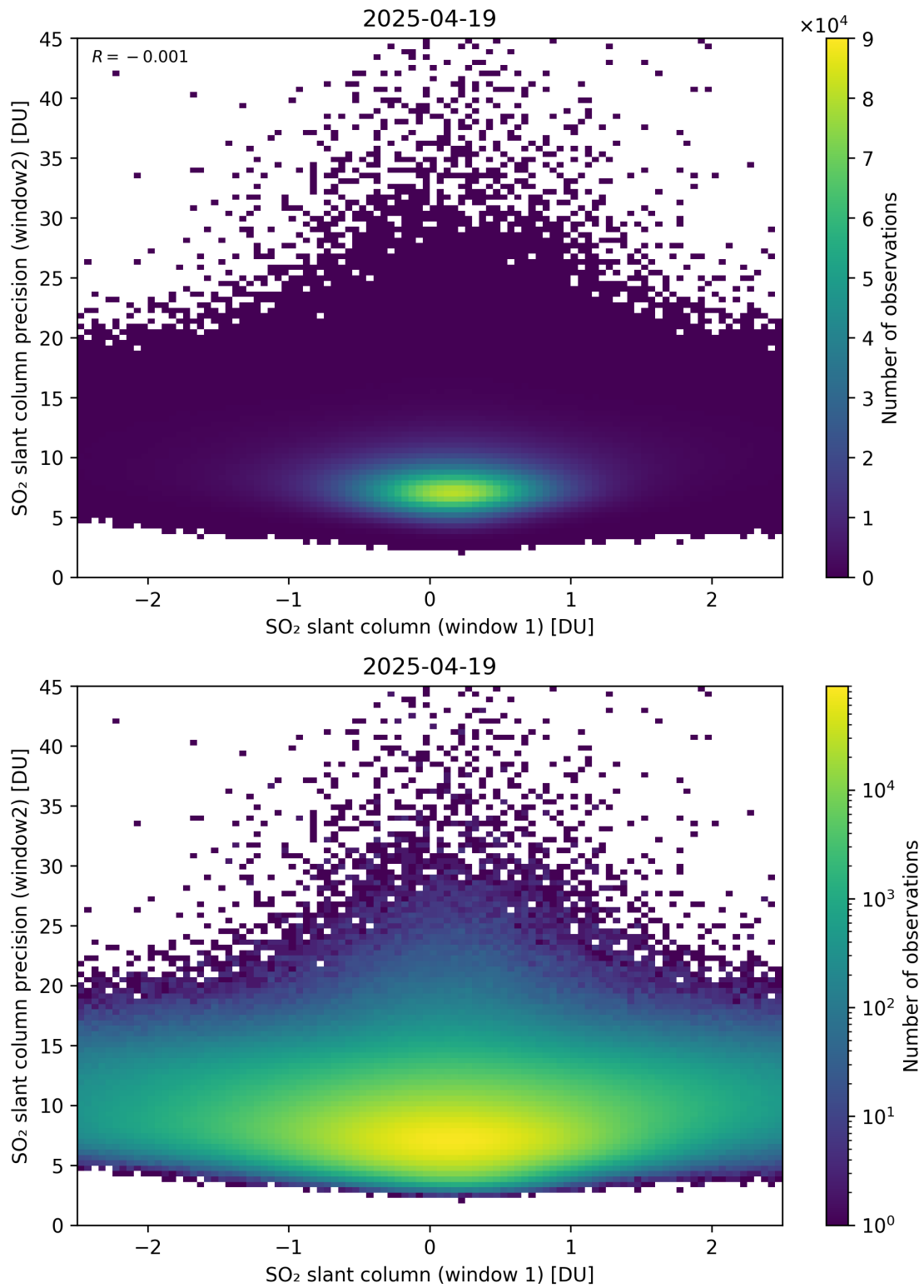
Figure 286: Scatter density plot of “SO 2 slant column (window 1)” against “SO 2 slant column precision (window2)” for 2025-04-19 to 2025-04-20.
