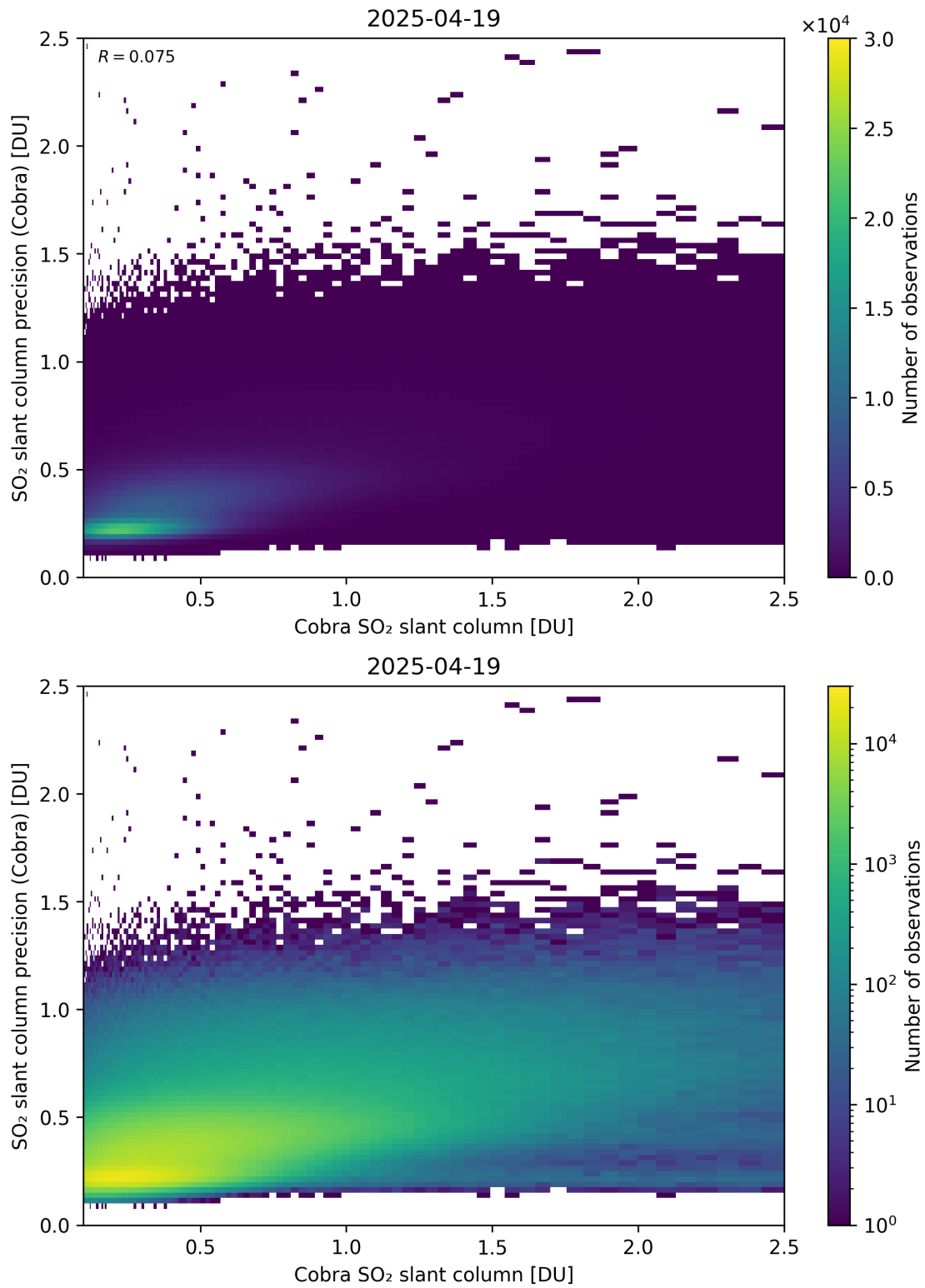
Figure 216: Scatter density plot of “Cobra SO 2 slant column” against “SO 2 slant column precision (Cobra)” for 2025-04-19 to 2025-04-20.
