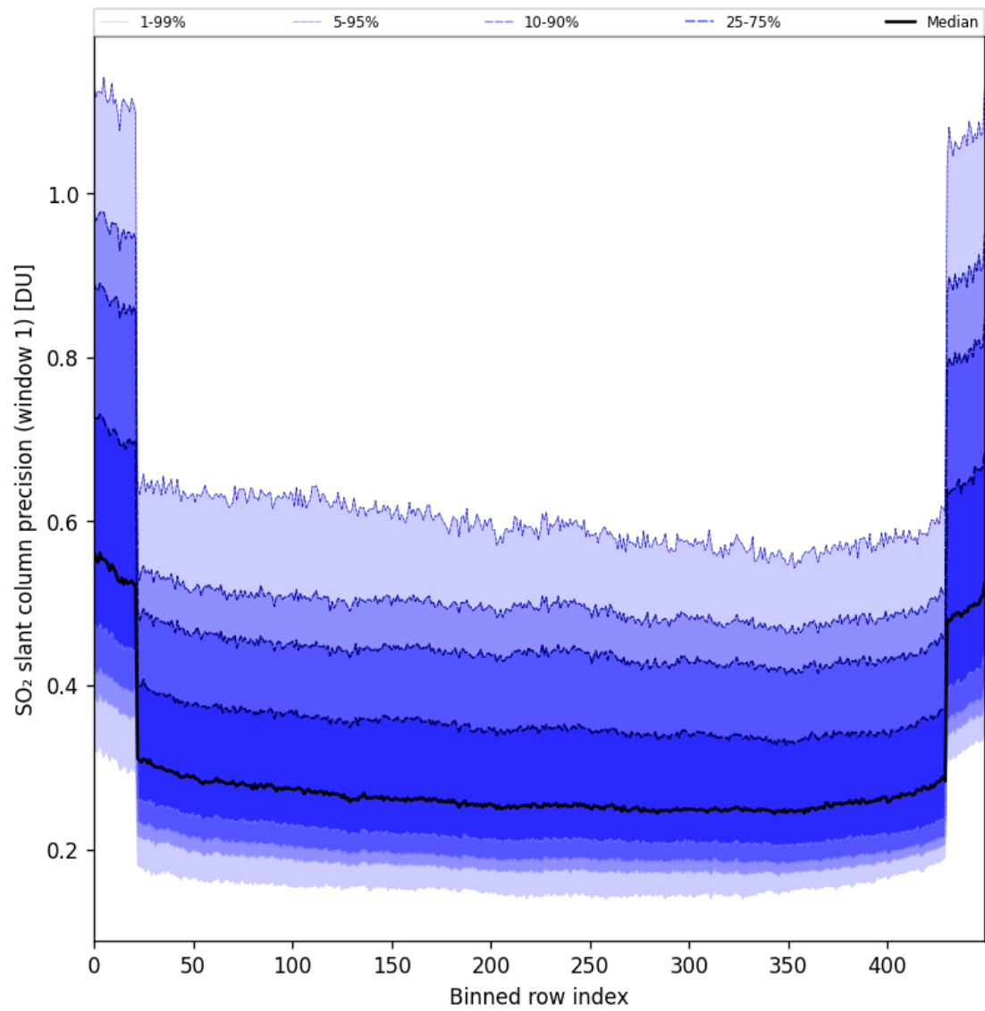
Figure 90: Along track statistics of “SO 2 slant column precision (window 1)” for 2025-04-19 to 2025-04-20
