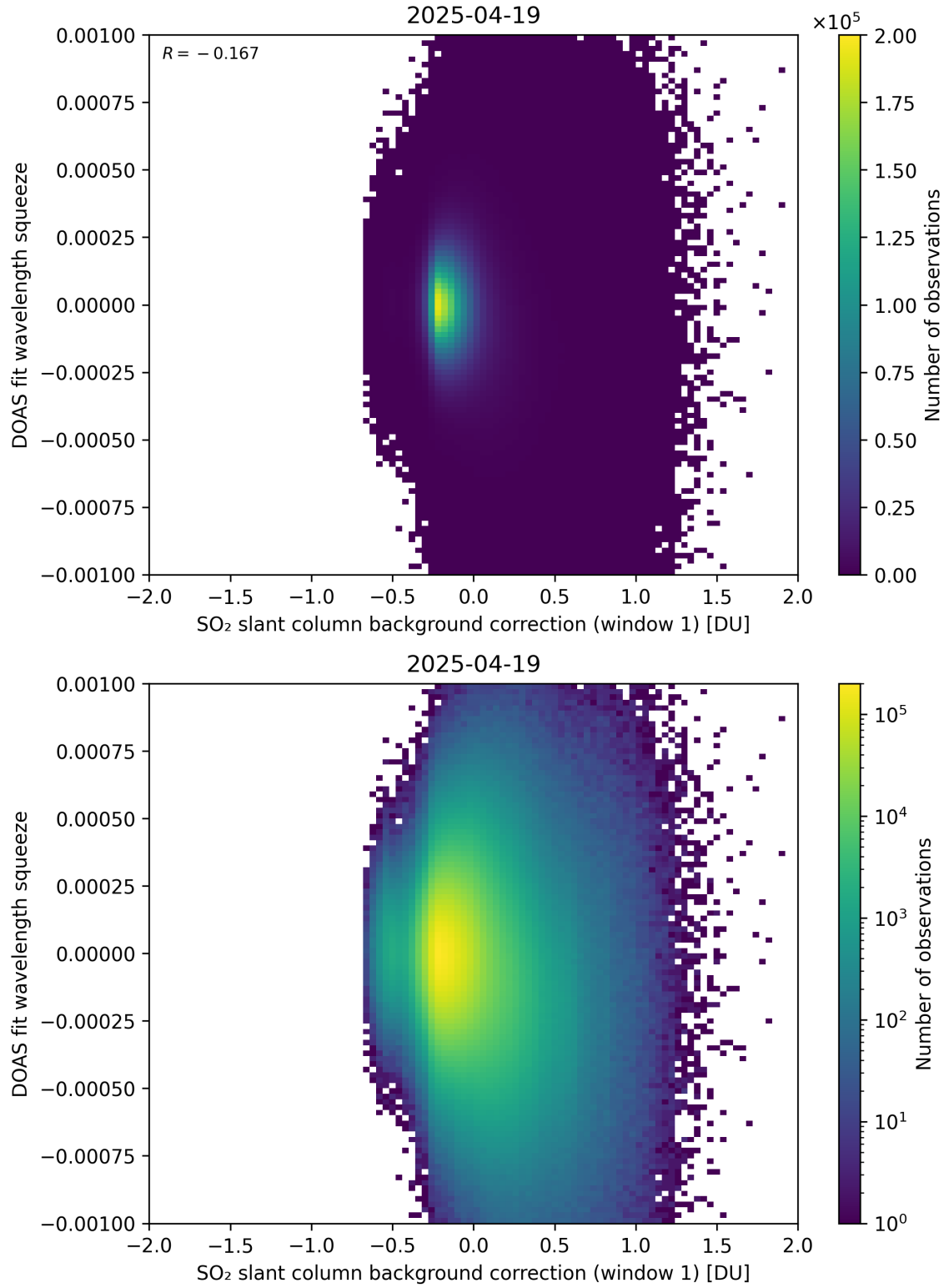
Figure 112: Scatter density plot of “SO 2 slant column background correction (window 1)” against “DOAS fit wavelength squeeze” for 2025-04-19 to 2025-04-20.
