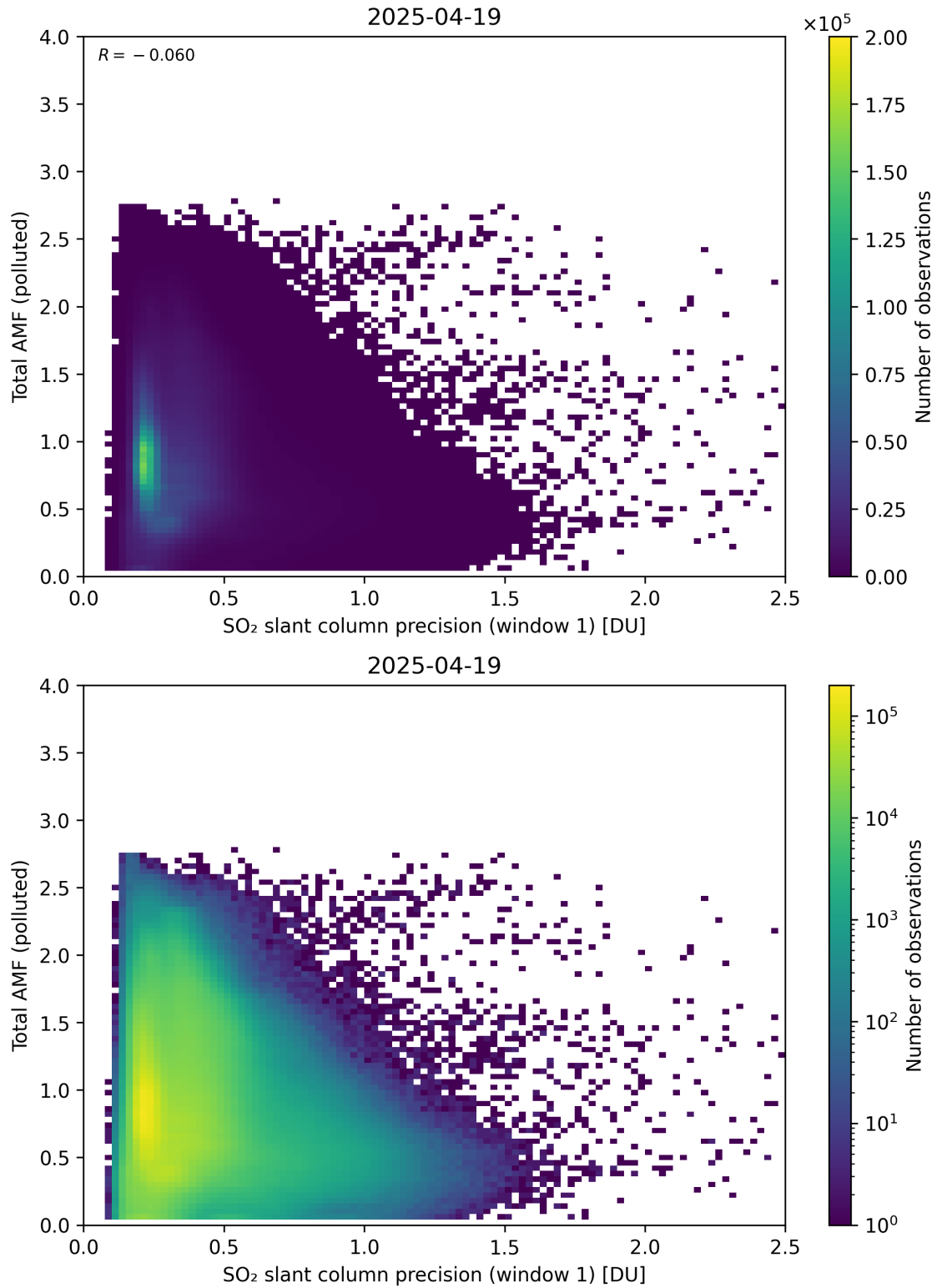
Figure 280: Scatter density plot of “SO 2 slant column precision (window 1)” against “Total AMF (polluted)” for 2025-04-19 to 2025-04-20.
