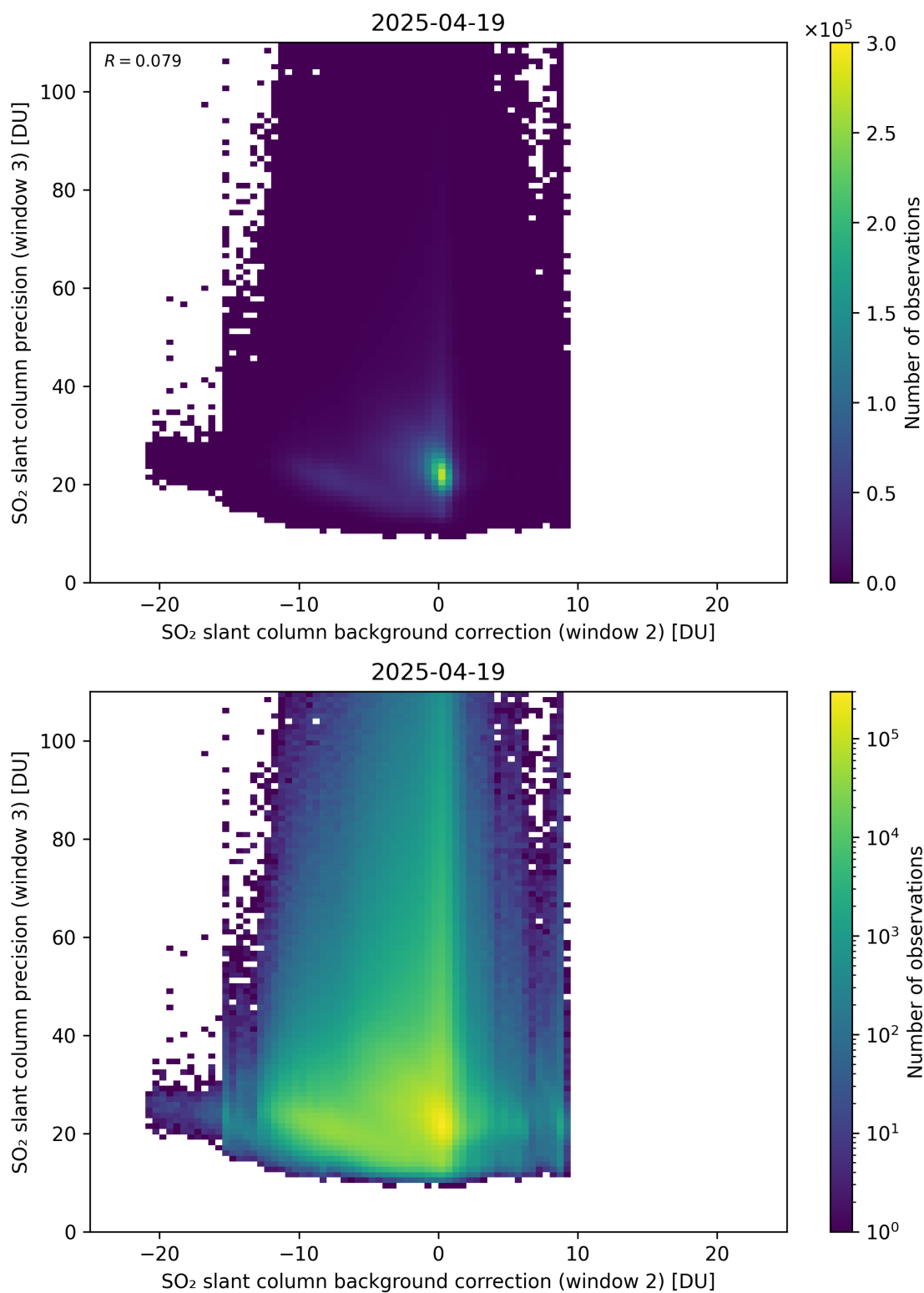
Figure 129: Scatter density plot of “SO 2 slant column background correction (window 2)” against “SO 2 slant column precision (window 3)” for 2025-04-19 to 2025-04-20.
