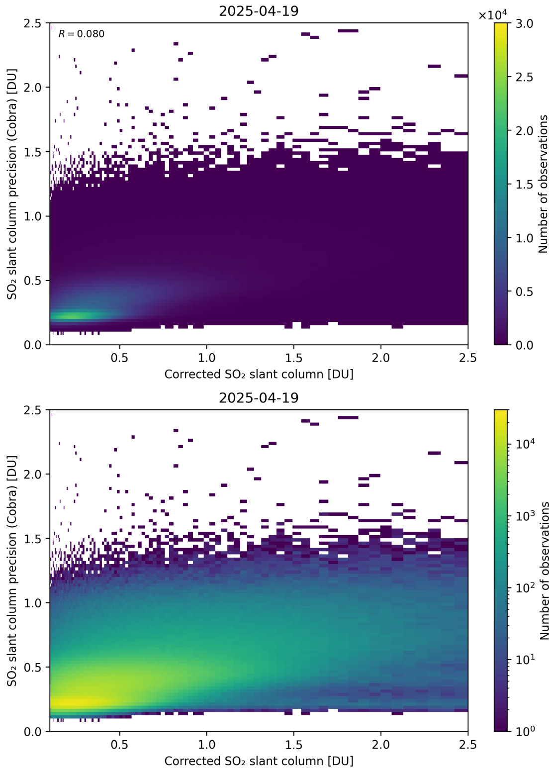
Figure 234: Scatter density plot of “Corrected SO 2 slant column” against “SO 2 slant column precision (Cobra)” for 2025-04-19 to 2025-04-20.
