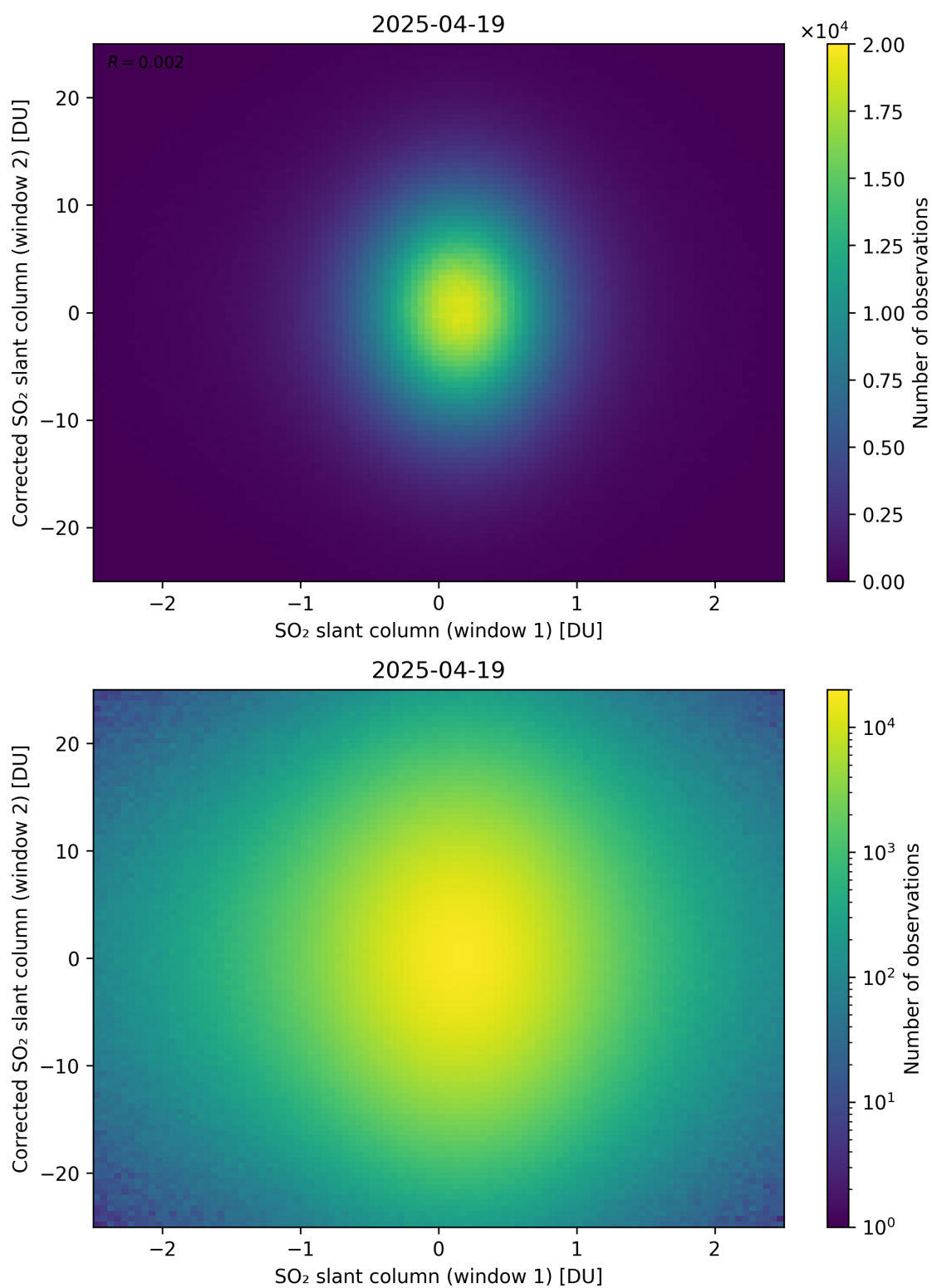
Figure 283: Scatter density plot of “SO 2 slant column (window 1)” against “Corrected SO 2 slant column (window 2)” for 2025-04-19 to 2025-04-20.
