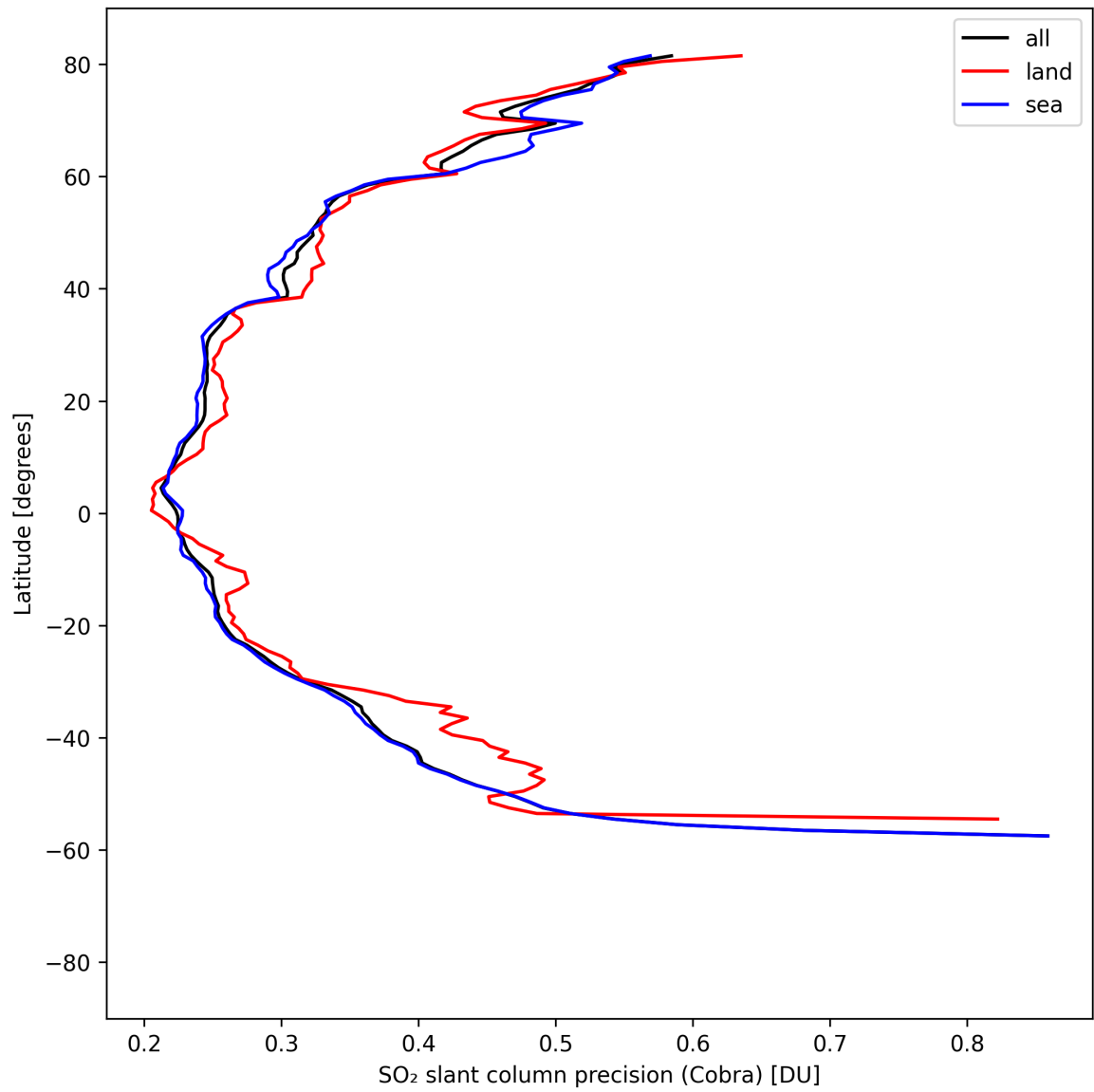
Figure 36: Zonal average of “SO 2 slant column precision (Cobra)” for 2025-04-19 to 2025-04-20.
