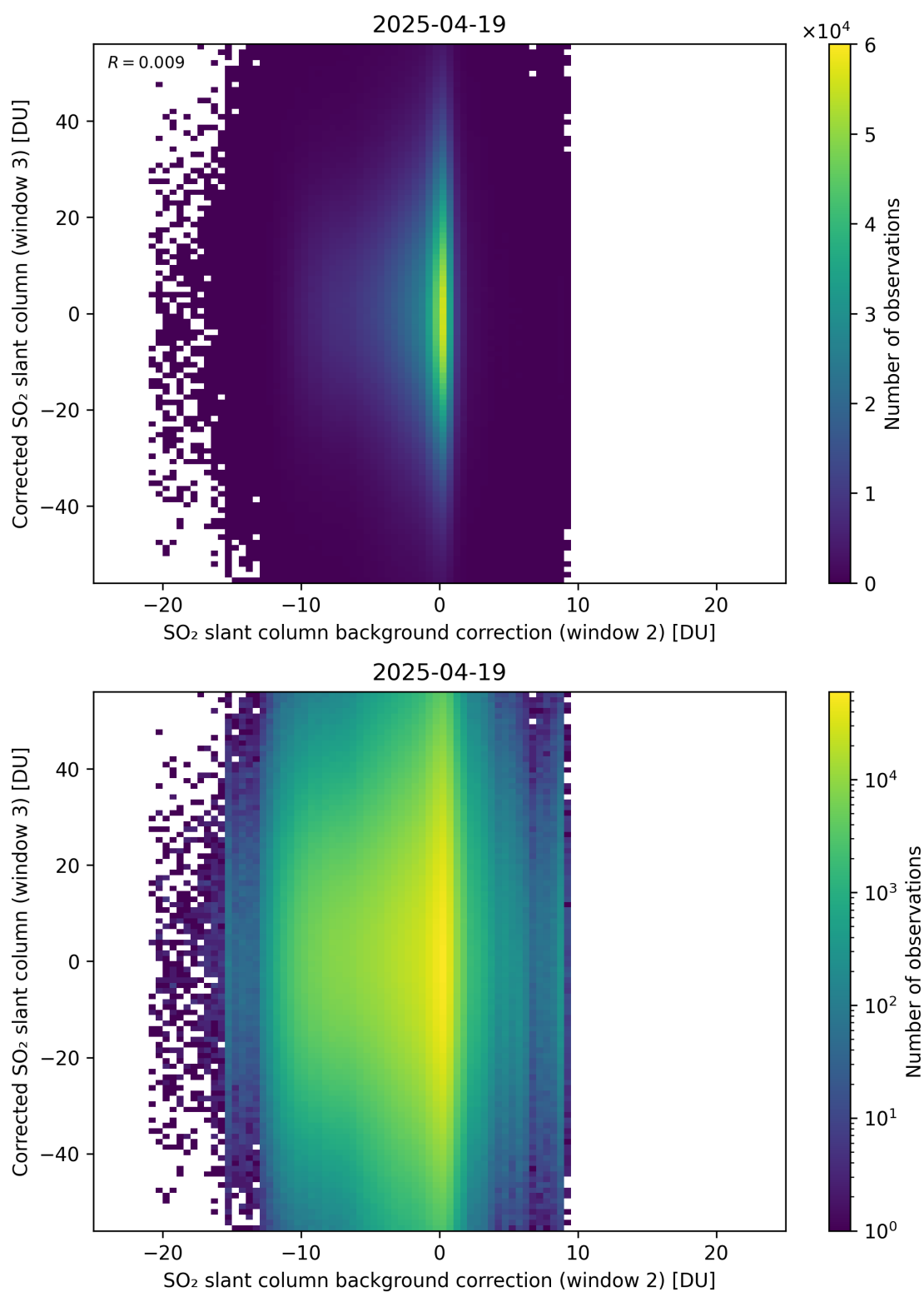
Figure 127: Scatter density plot of “SO 2 slant column background correction (window 2)” against “Corrected SO 2 slant column (window 3)” for 2025-04-19 to 2025-04-20.
