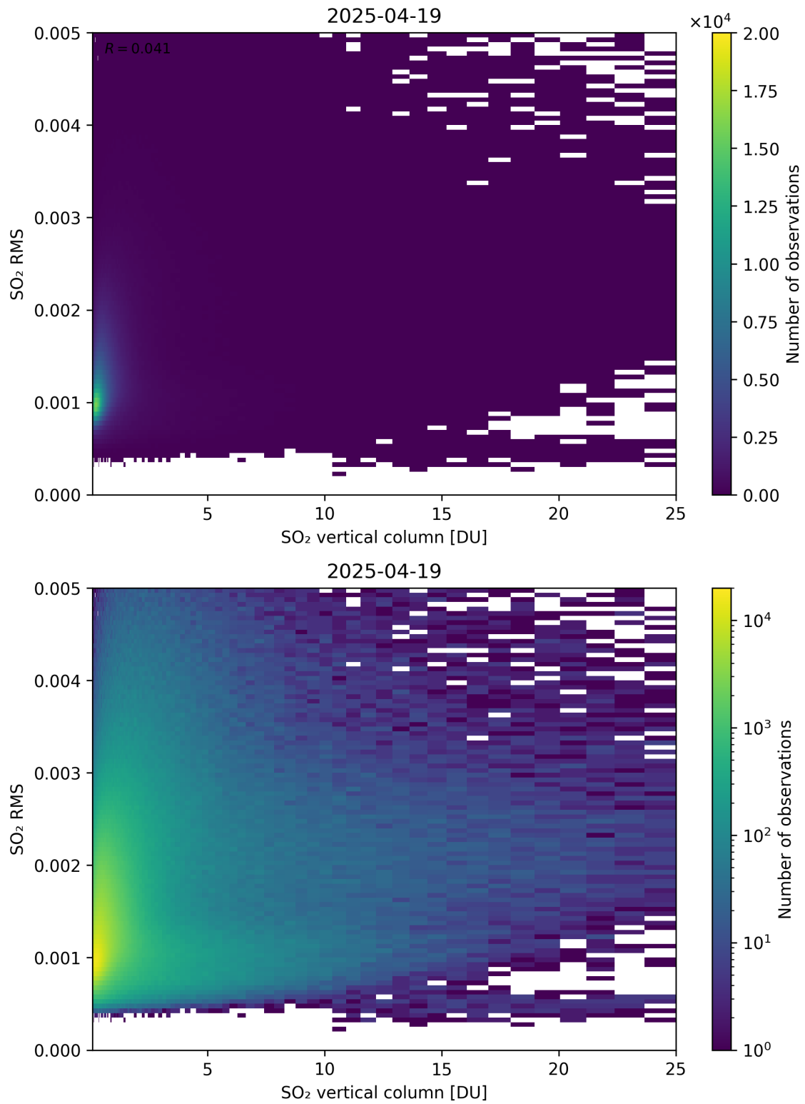
Figure 328: Scatter density plot of “SO 2 vertical column” against “SO 2 RMS” for 2025-04-19 to 2025-04-20.
