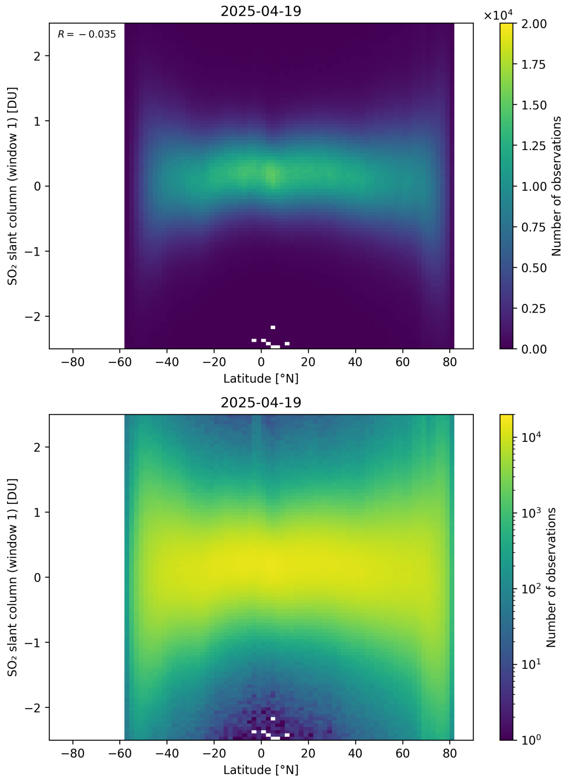
Figure 162: Scatter density plot of “Latitude” against “SO 2 slant column (window 1)” for 2025-04-19 to 2025-04-20.
