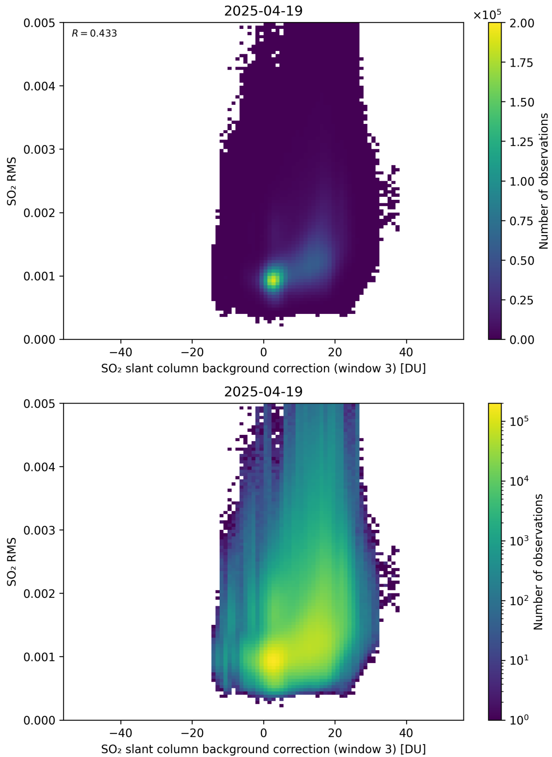
Figure 134: Scatter density plot of “SO 2 slant column background correction (window 3)” against “SO 2 RMS” for 2025-04-19 to 2025-04-20.
