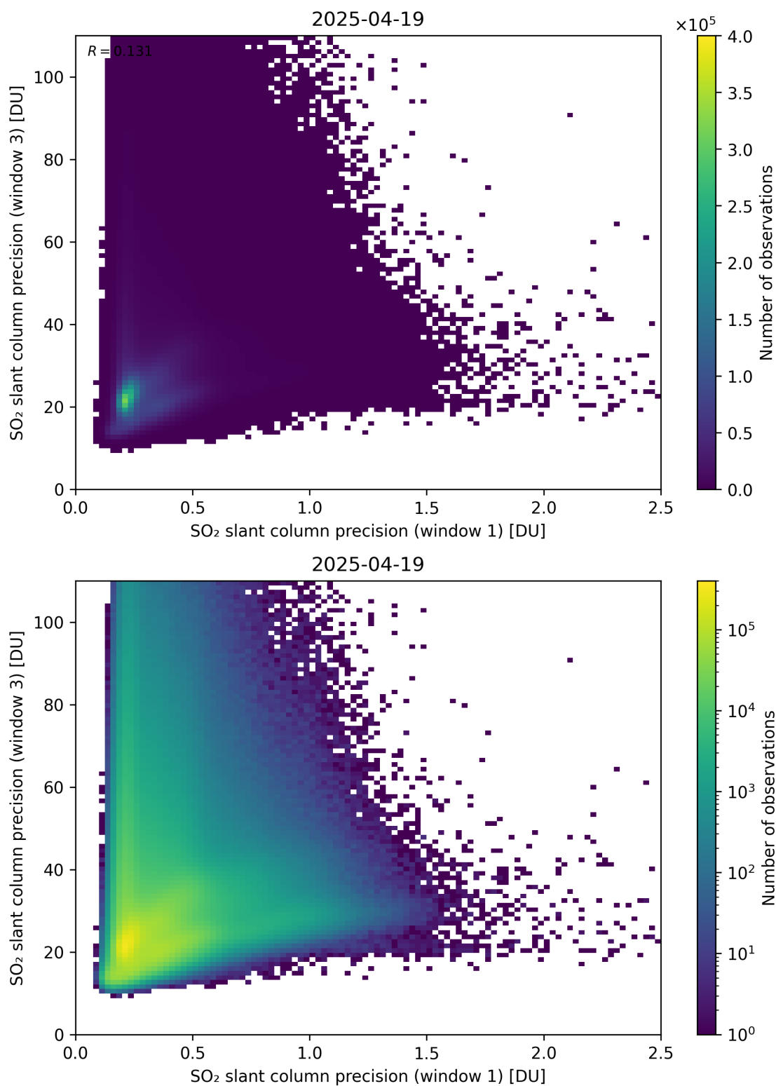
Figure 279: Scatter density plot of “SO 2 slant column precision (window 1)” against “SO 2 slant column precision (window 3)” for 2025-04-19 to 2025-04-20.
