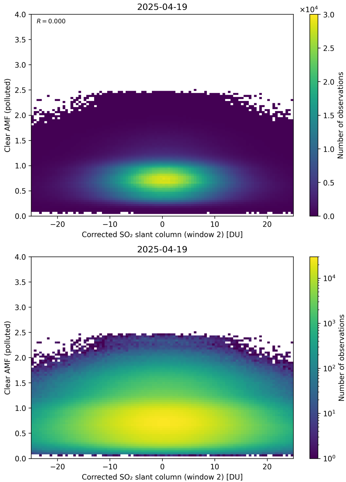
Figure 249: Scatter density plot of “Corrected SO 2 slant column (window 2)” against “Clear AMF (polluted)” for 2025-04-19 to 2025-04-20.
