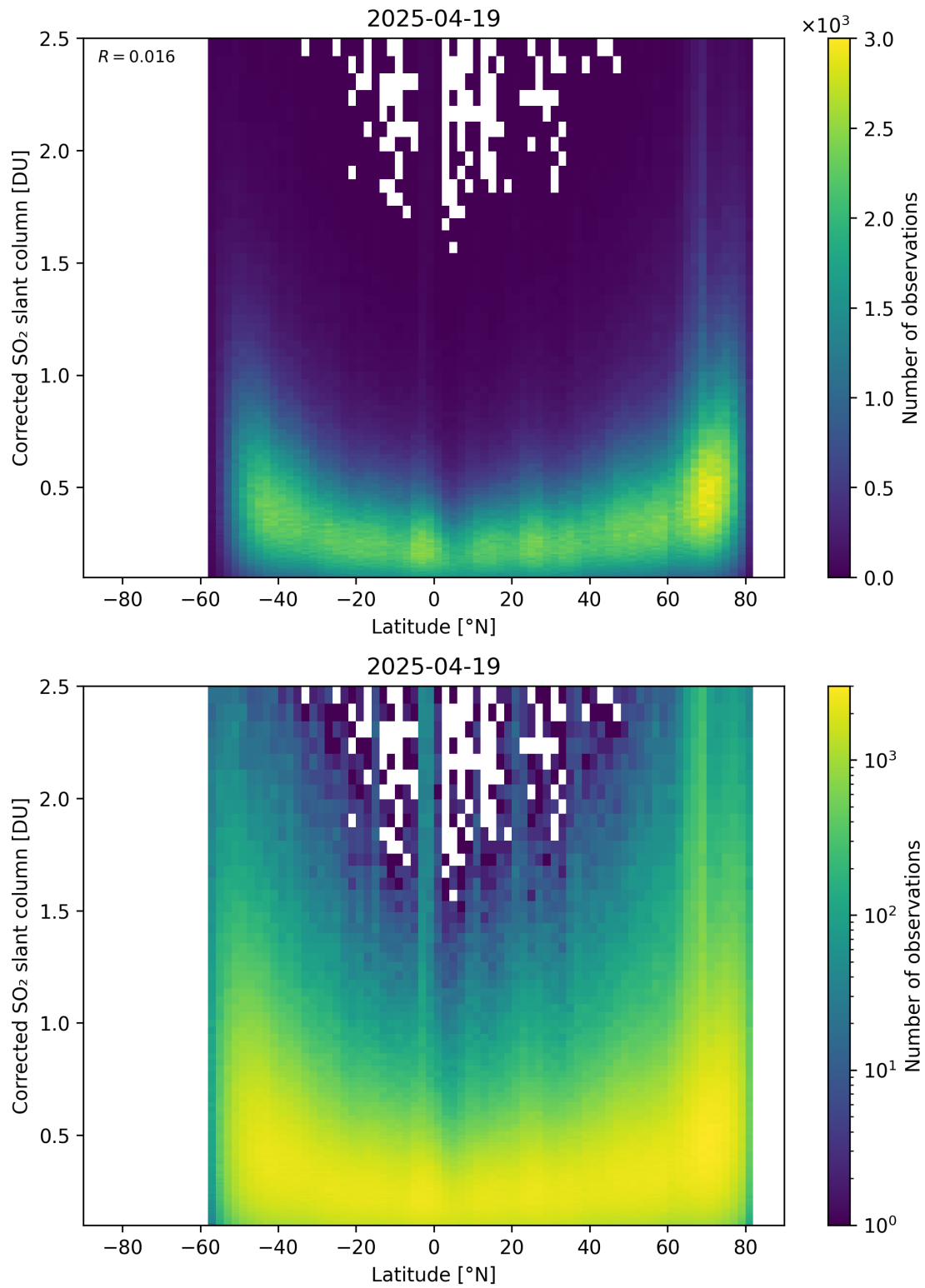
Figure 159: Scatter density plot of “Latitude” against “Corrected SO 2 slant column” for 2025-04-19 to 2025-04-20.
