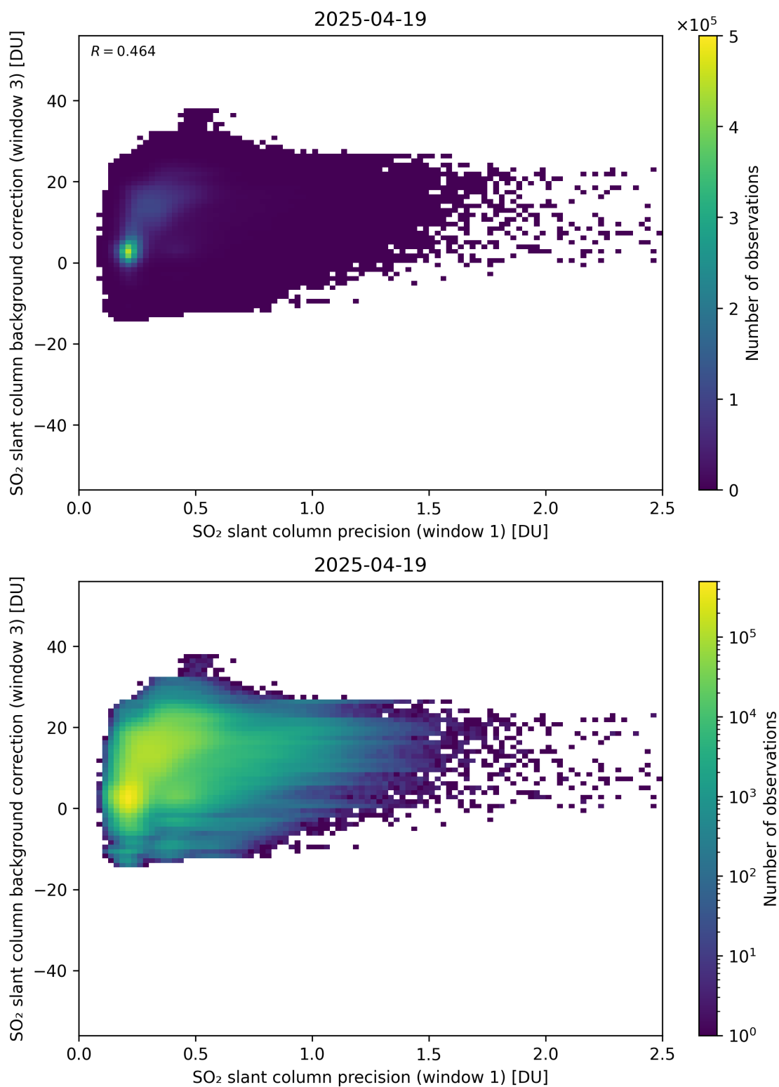
Figure 270: Scatter density plot of “SO 2 slant column precision (window 1)” against “SO 2 slant column background correction (window 3)” for 2025-04-19 to 2025-04-20.
