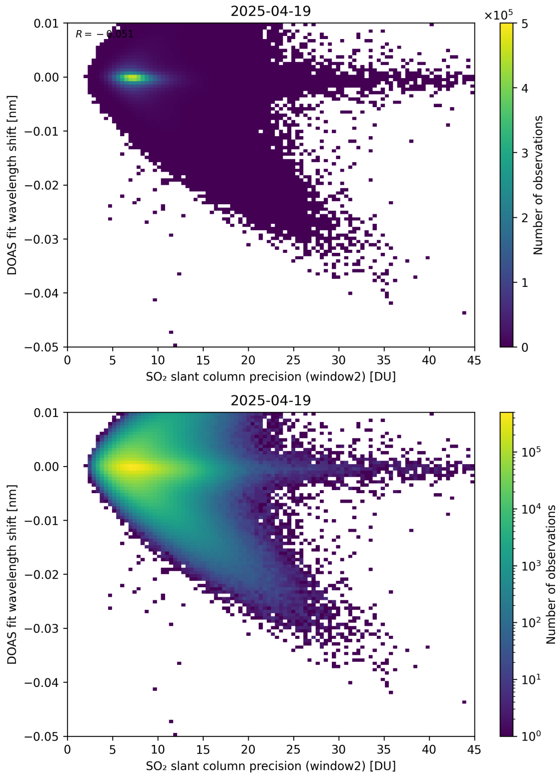
Figure 293: Scatter density plot of “SO 2 slant column precision (window2)” against “DOAS fit wavelength shift” for 2025-04-19 to 2025-04-20.
