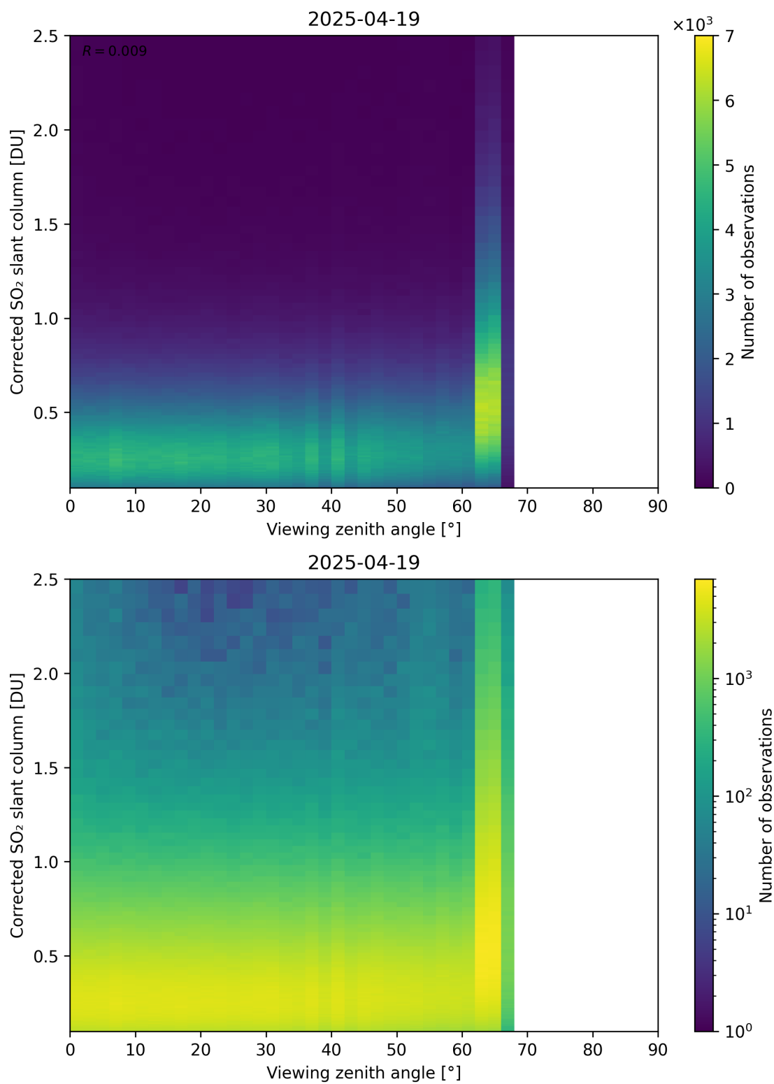
Figure 373: Scatter density plot of “Viewing zenith angle” against “Corrected SO 2 slant column” for 2025-04-19 to 2025-04-20.
