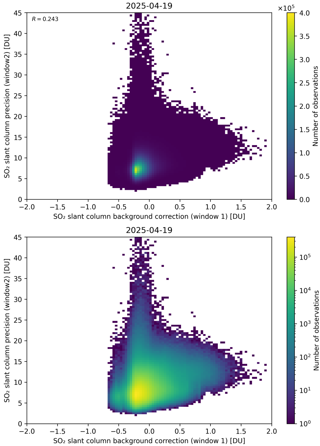
Figure 117: Scatter density plot of “SO 2 slant column background correction (window 1)” against “SO 2 slant column precision (window2)” for 2025-04-19 to 2025-04-20.
