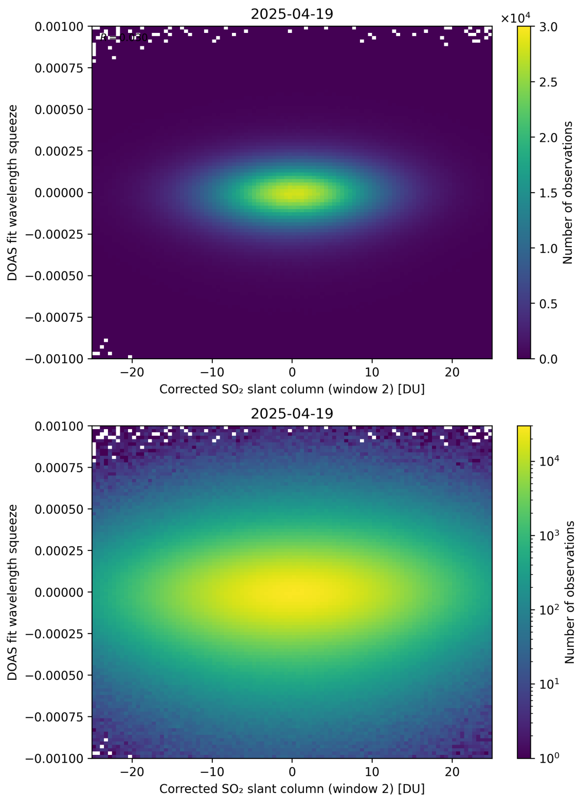
Figure 247: Scatter density plot of “Corrected SO 2 slant column (window 2)” against “DOAS fit wavelength squeeze” for 2025-04-19 to 2025-04-20.
