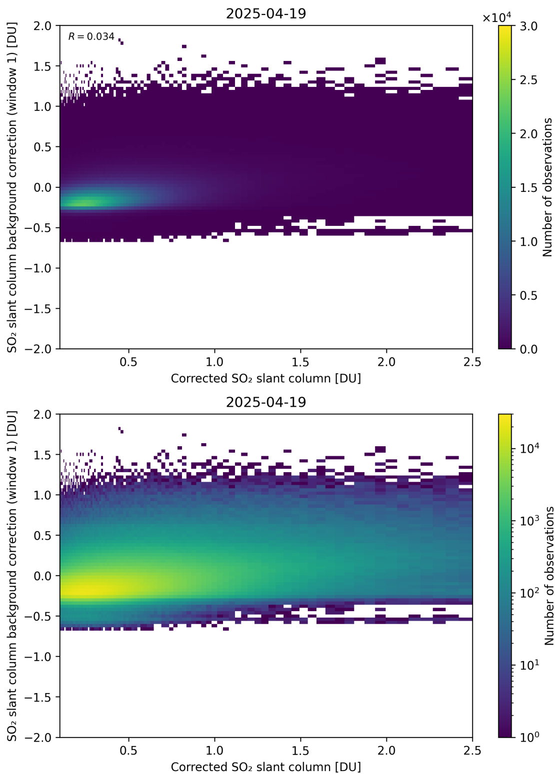
Figure 226: Scatter density plot of “Corrected SO 2 slant column” against “SO 2 slant column background correction (window 1)” for 2025-04-19 to 2025-04-20.
