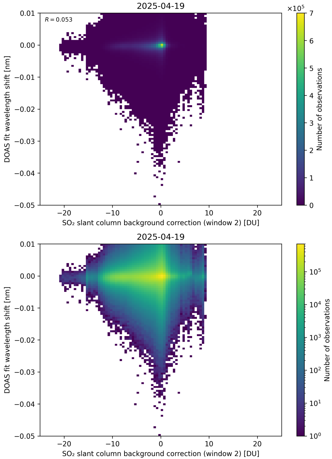
Figure 123: Scatter density plot of “SO 2 slant column background correction (window 2)” against “DOAS fit wavelength shift” for 2025-04-19 to 2025-04-20.
