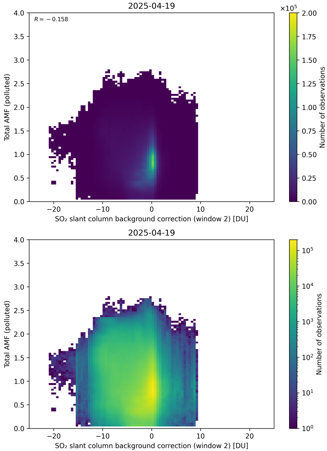
Figure 130: Scatter density plot of “SO 2 slant column background correction (window 2)” against “Total AMF (polluted)” for 2025-04-19 to 2025-04-20.
