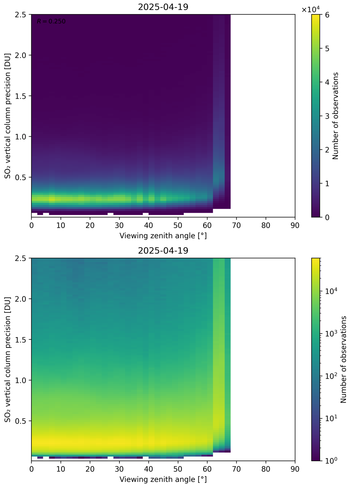
Figure 384: Scatter density plot of “Viewing zenith angle” against “SO 2 vertical column precision” for 2025-04-19 to 2025-04-20.
