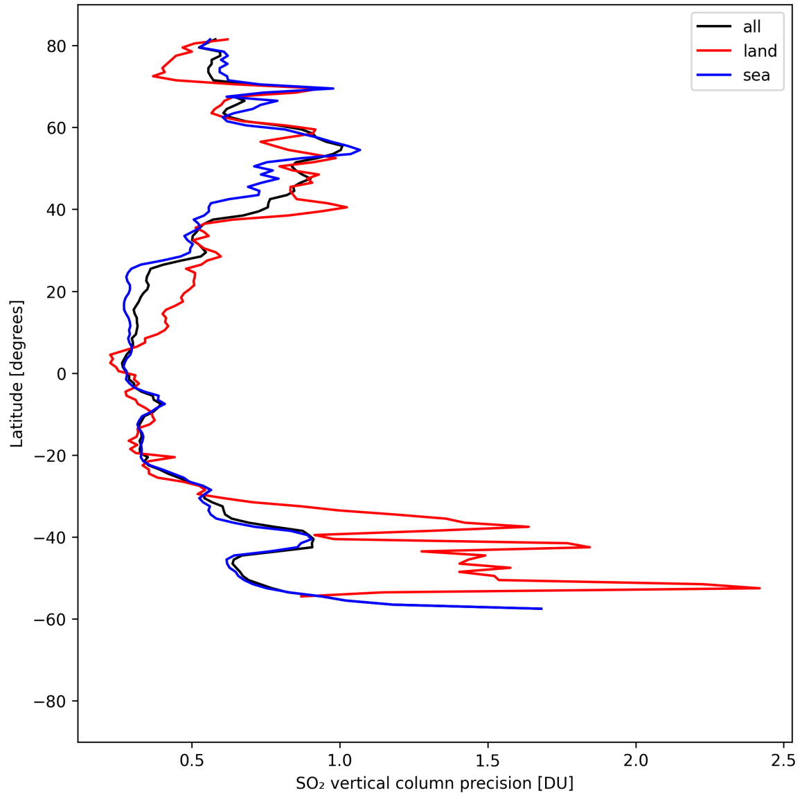
Figure 33: Zonal average of “SO 2 vertical column precision” for 2025-04-19 to 2025-04-20.
