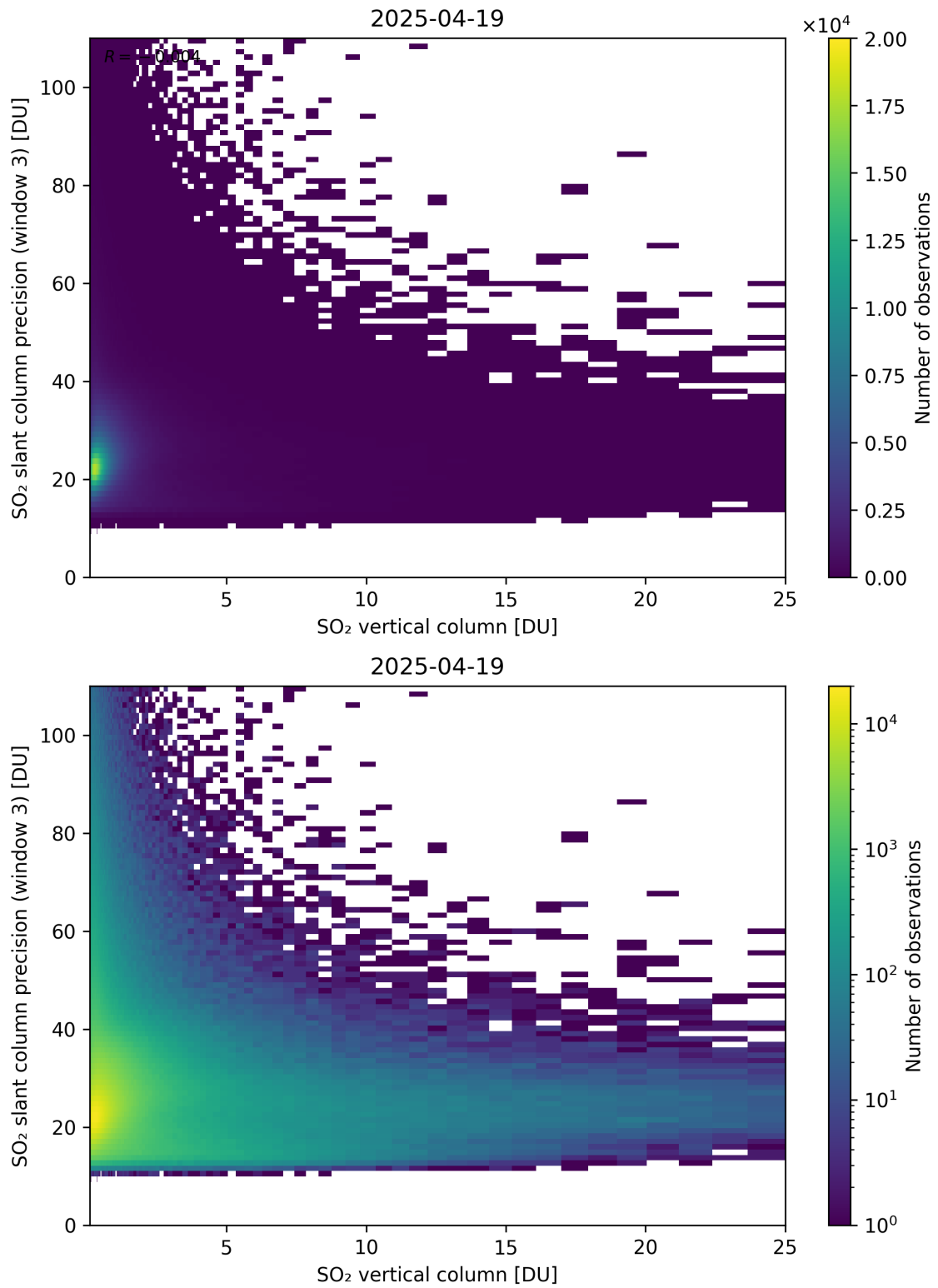
Figure 358: Scatter density plot of “SO 2 vertical column” against “SO 2 slant column precision (window 3)” for 2025-04-19 to 2025-04-20.
