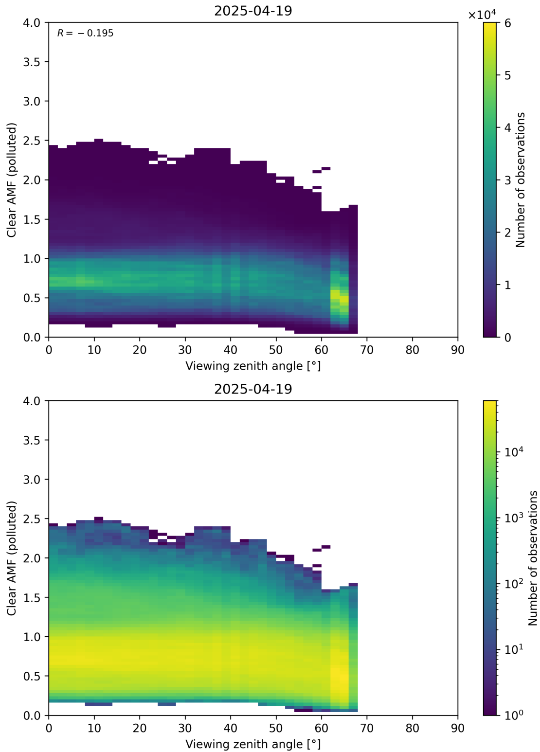
Figure 370: Scatter density plot of “Viewing zenith angle” against “Clear AMF (polluted)” for 2025-04-19 to 2025-04-20.
