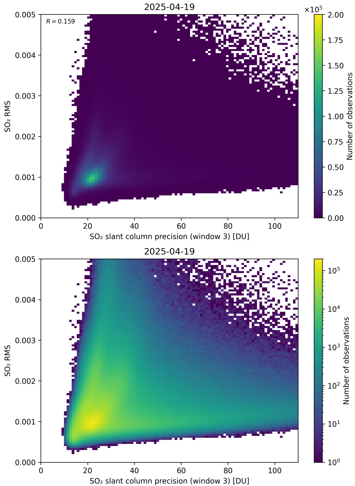
Figure 310: Scatter density plot of “SO 2 slant column precision (window 3)” against “SO 2 RMS” for 2025-04-19 to 2025-04-20.
