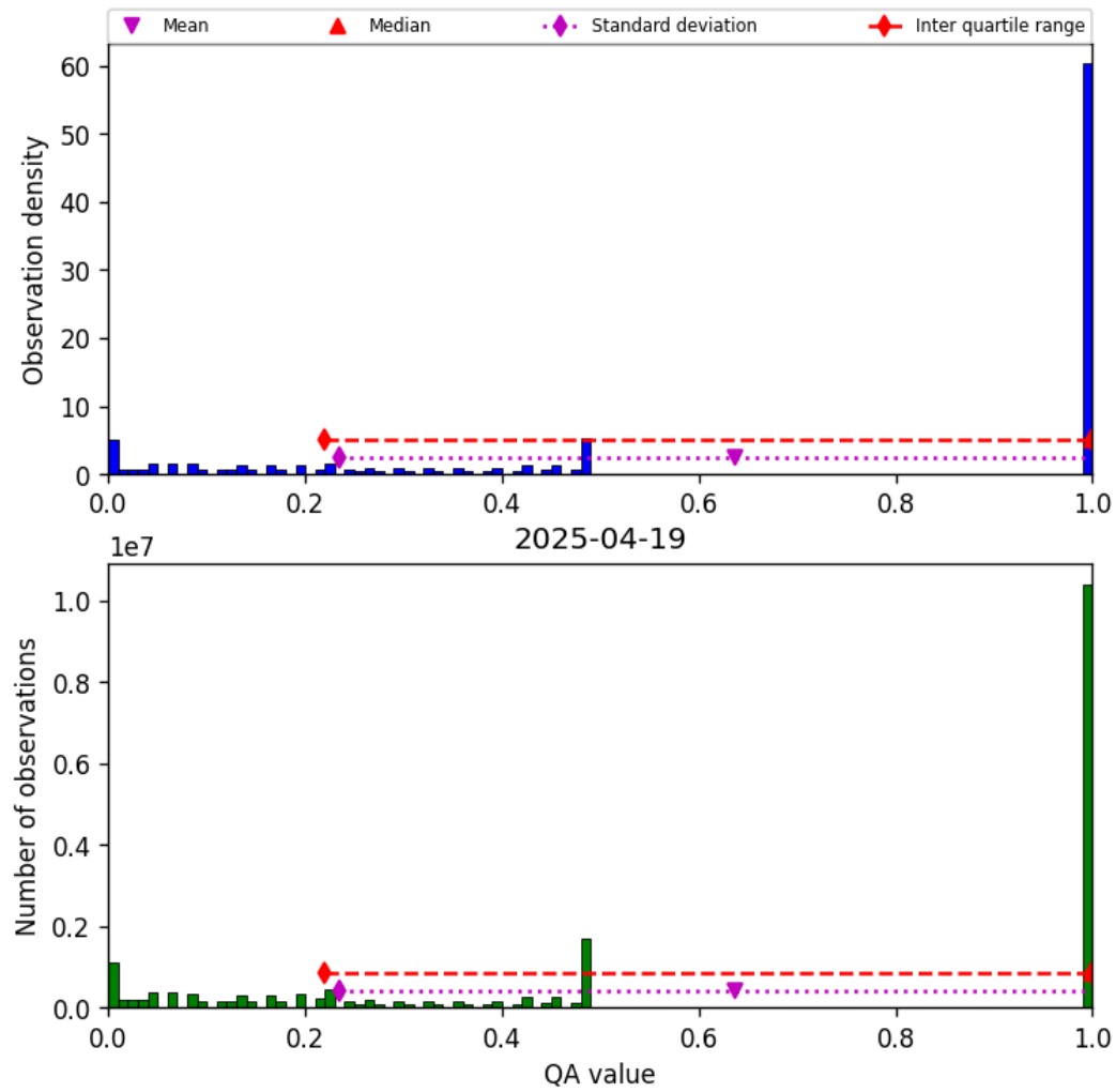
Figure 57: Histogram of “QA value” for 2025-04-19 to 2025-04-20
