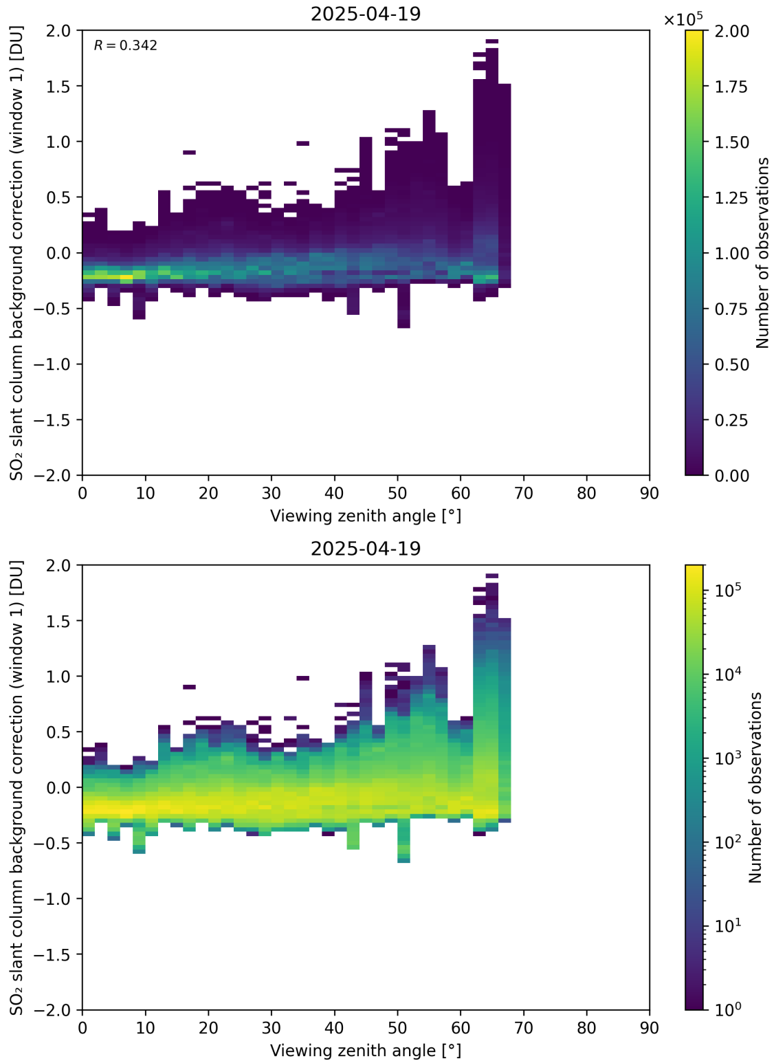
Figure 362: Scatter density plot of “Viewing zenith angle” against “SO 2 slant column background correction (window 1)” for 2025-04-19 to 2025-04-20.
