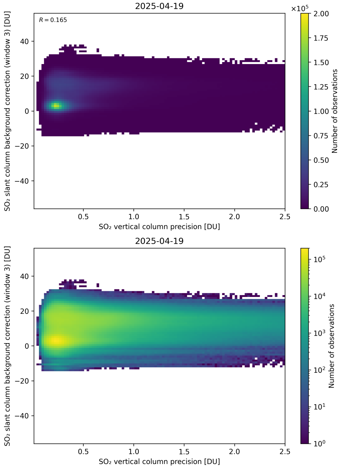
Figure 331: Scatter density plot of “SO 2 vertical column precision” against “SO 2 slant column background correction (window 3)” for 2025-04-19 to 2025-04-20.
