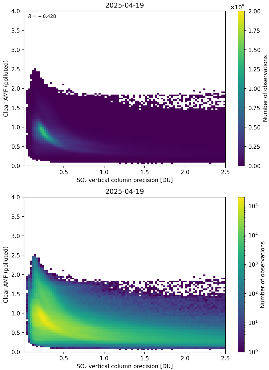
Figure 335: Scatter density plot of “SO 2 vertical column precision” against “Clear AMF (polluted)” for 2025-04-19 to 2025-04-20.
