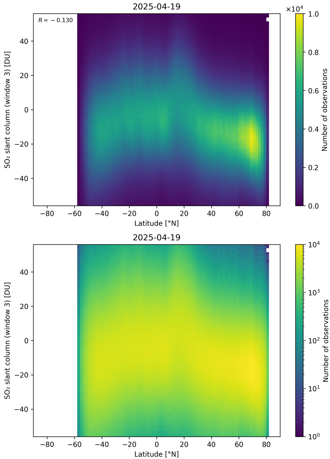
Figure 165: Scatter density plot of “Latitude” against “SO 2 slant column (window 3)” for 2025-04-19 to 2025-04-20.
