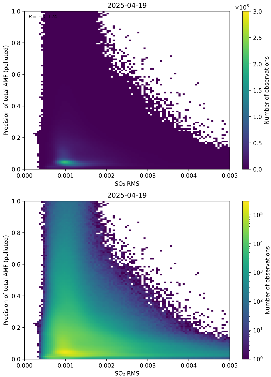
Figure 149: Scatter density plot of “SO 2 RMS” against “Precision of total AMF (polluted)” for 2025-04-19 to 2025-04-20.
