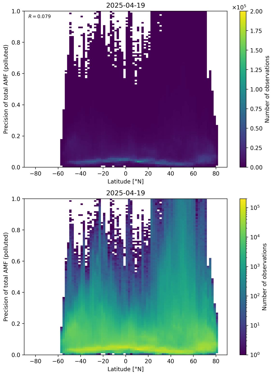
Figure 168: Scatter density plot of “Latitude” against “Precision of total AMF (polluted)” for 2025-04-19 to 2025-04-20.
