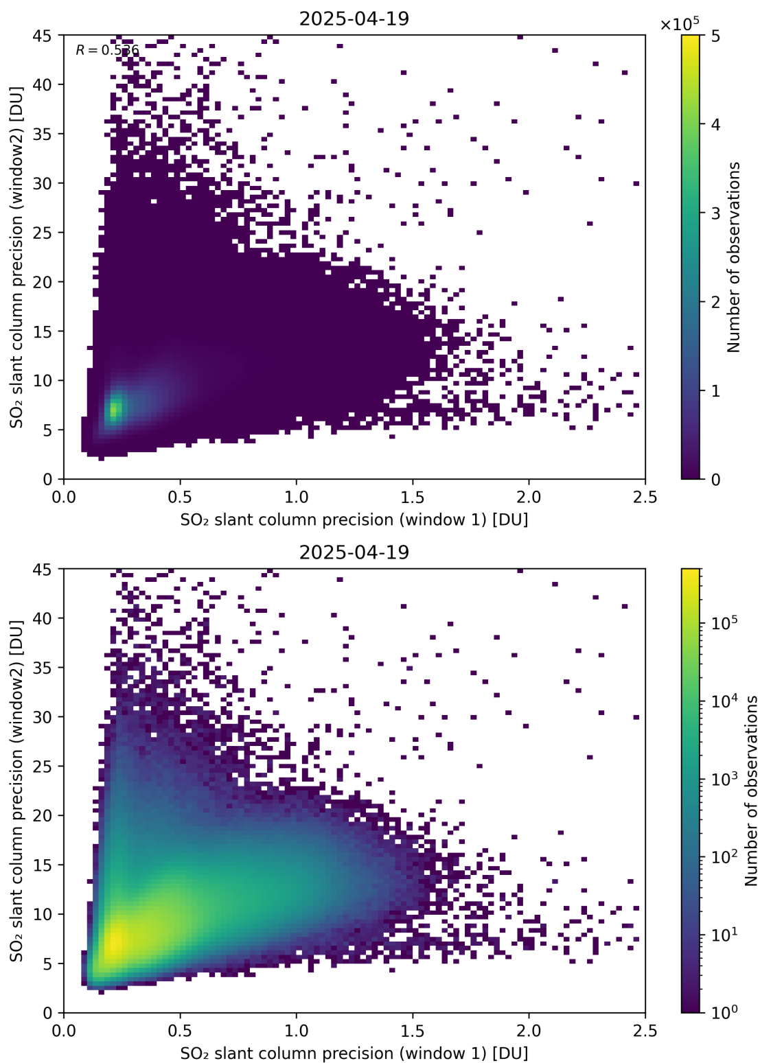
Figure 277: Scatter density plot of “SO 2 slant column precision (window 1)” against “SO 2 slant column precision (window2)” for 2025-04-19 to 2025-04-20.
