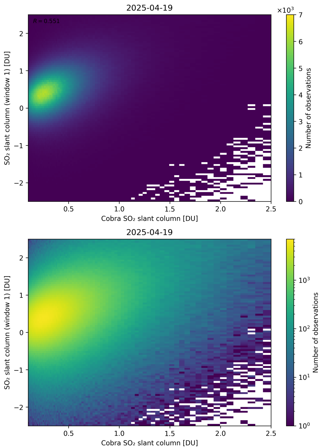
Figure 219: Scatter density plot of “Cobra SO 2 slant column” against “SO 2 slant column (window 1)” for 2025-04-19 to 2025-04-20.
