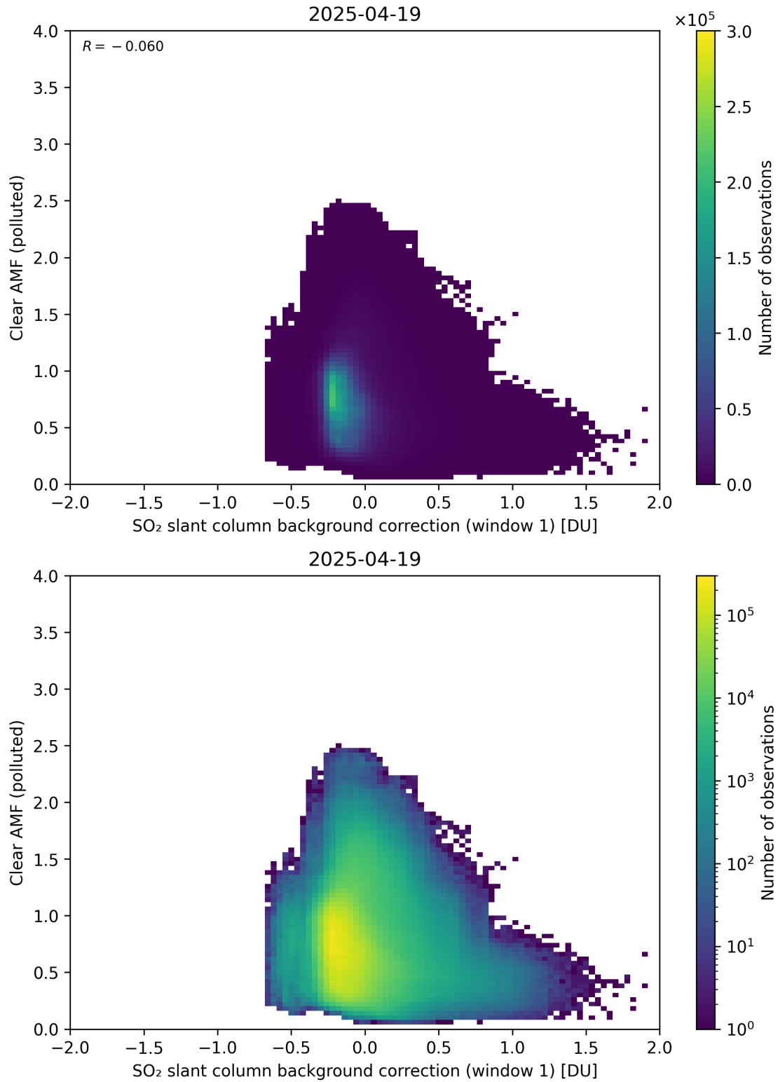
Figure 114: Scatter density plot of “SO 2 slant column background correction (window 1)” against “Clear AMF (polluted)” for 2025-04-19 to 2025-04-20.
