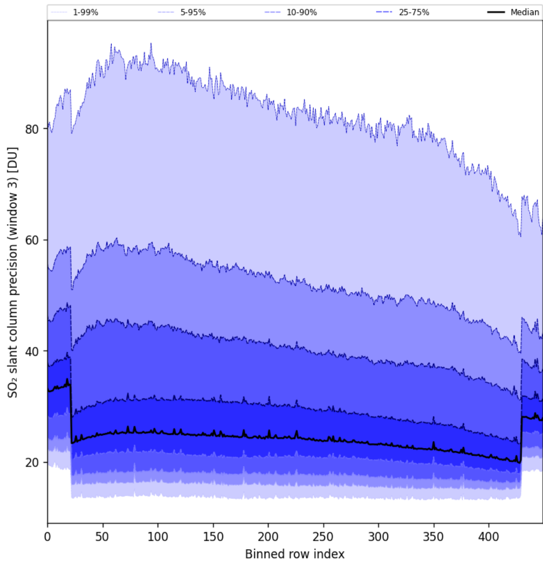
Figure 98: Along track statistics of “SO 2 slant column precision (window 3)” for 2025-04-19 to 2025-04-20
