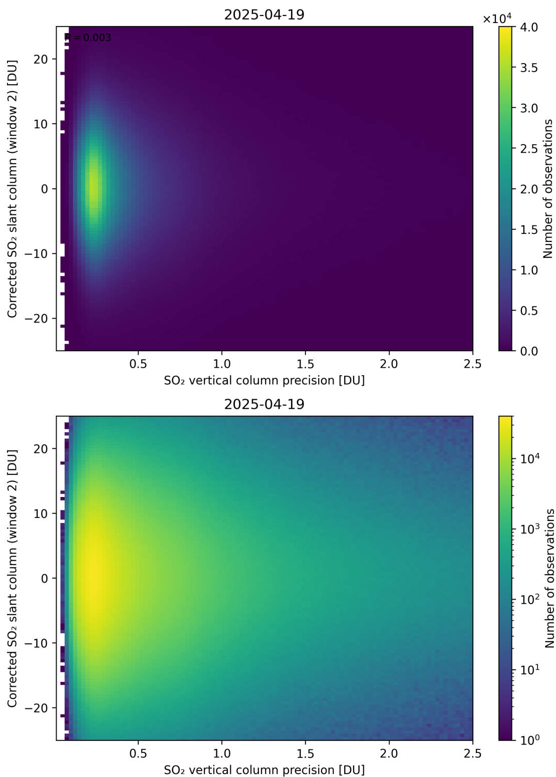
Figure 339: Scatter density plot of “SO 2 vertical column precision” against “Corrected SO 2 slant column (window 2)” for 2025-04-19 to 2025-04-20.
