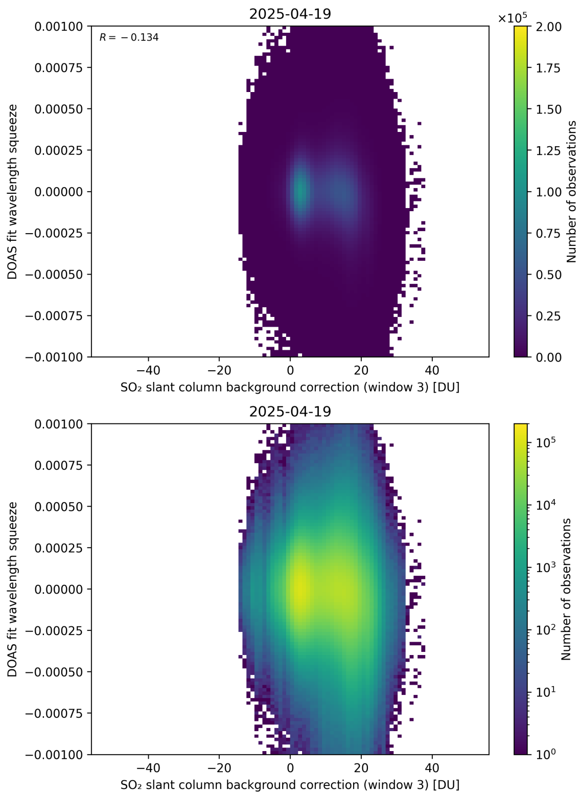
Figure 133: Scatter density plot of “SO 2 slant column background correction (window 3)” against “DOAS fit wavelength squeeze” for 2025-04-19 to 2025-04-20.
