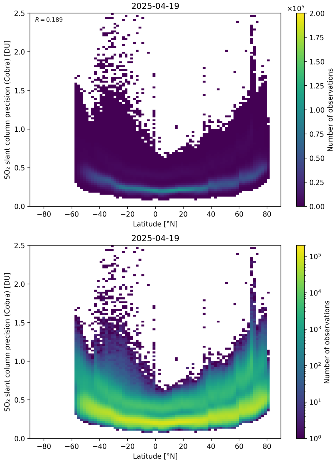
Figure 158: Scatter density plot of “Latitude” against “SO 2 slant column precision (Cobra)” for 2025-04-19 to 2025-04-20.
