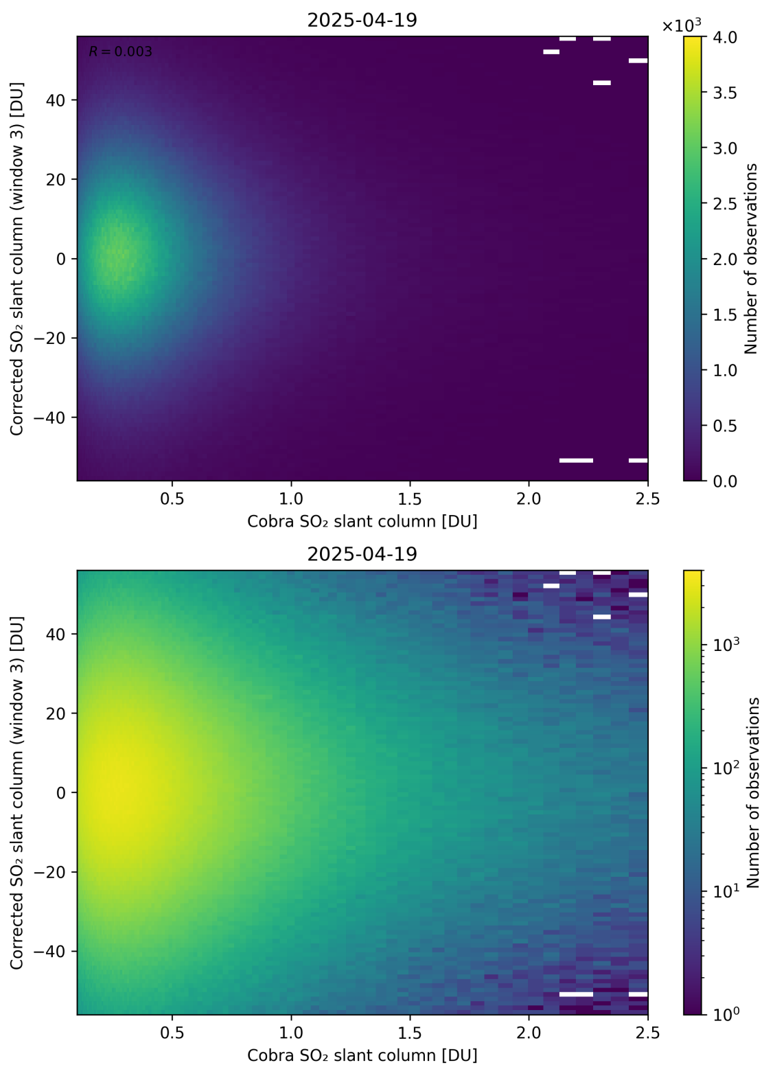
Figure 218: Scatter density plot of “Cobra SO 2 slant column” against “Corrected SO 2 slant column (window 3)” for 2025-04-19 to 2025-04-20.
