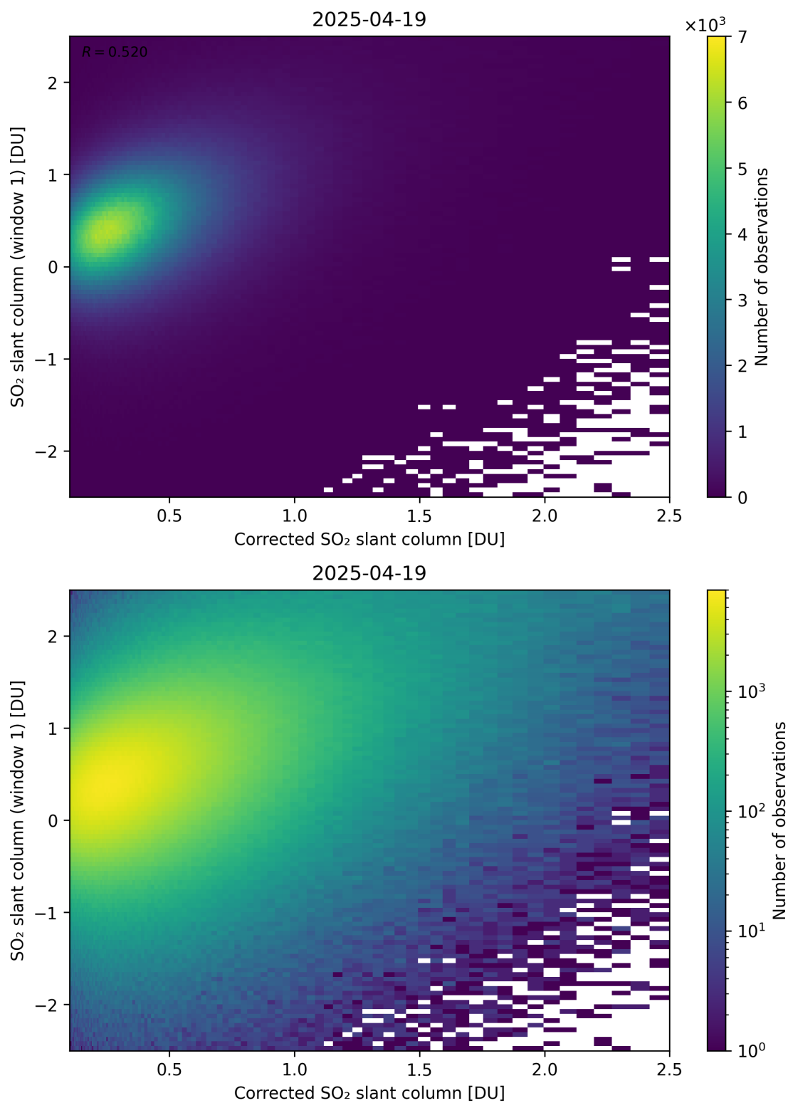
Figure 237: Scatter density plot of “Corrected SO 2 slant column” against “SO 2 slant column (window 1)” for 2025-04-19 to 2025-04-20.
