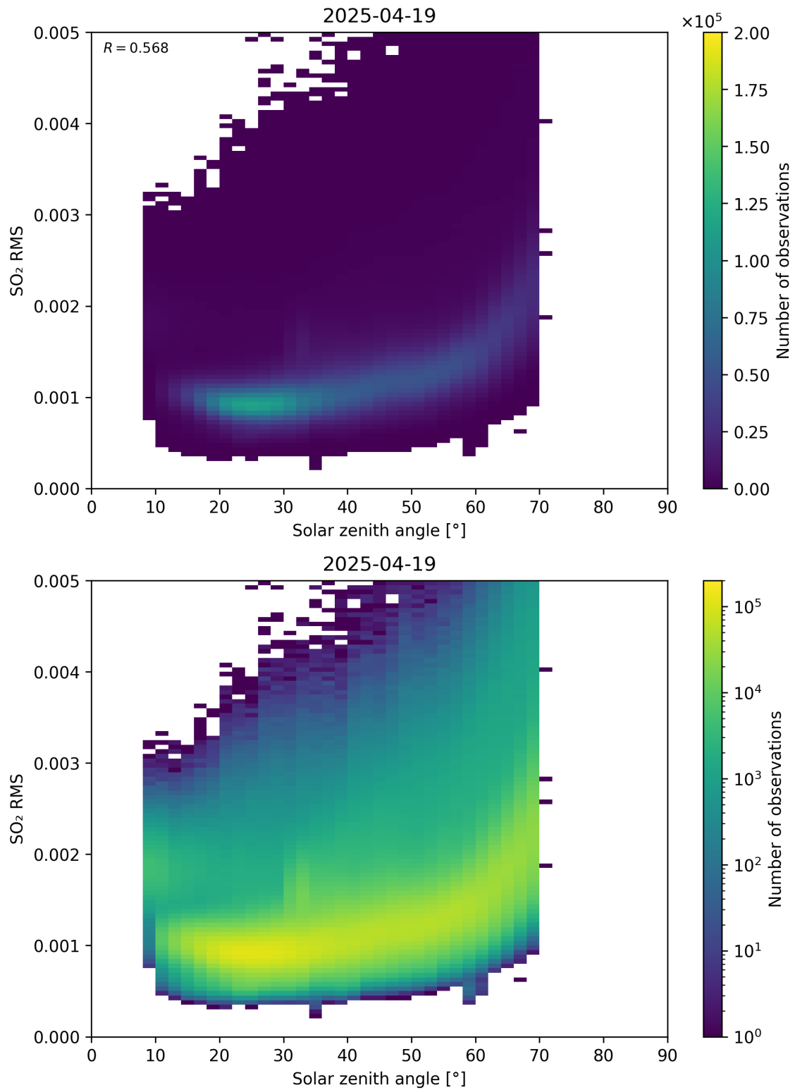
Figure 176: Scatter density plot of “Solar zenith angle” against “SO 2 RMS” for 2025-04-19 to 2025-04-20.
