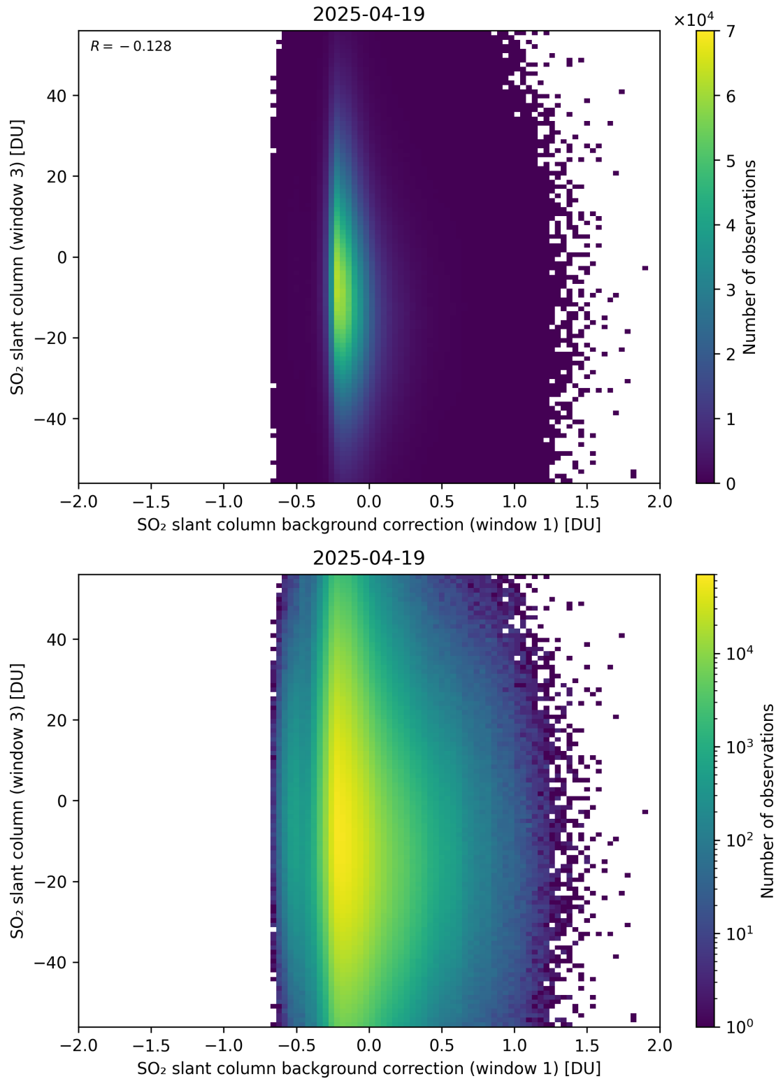
Figure 118: Scatter density plot of “SO 2 slant column background correction (window 1)” against “SO 2 slant column (window 3)” for 2025-04-19 to 2025-04-20.
