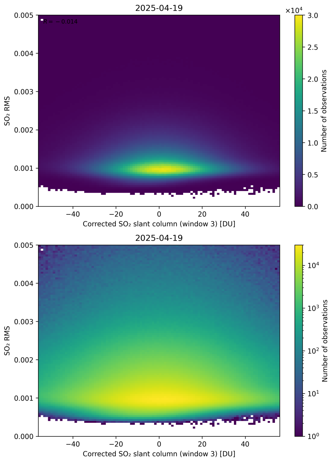
Figure 258: Scatter density plot of “Corrected SO 2 slant column (window 3)” against “SO 2 RMS” for 2025-04-19 to 2025-04-20.
