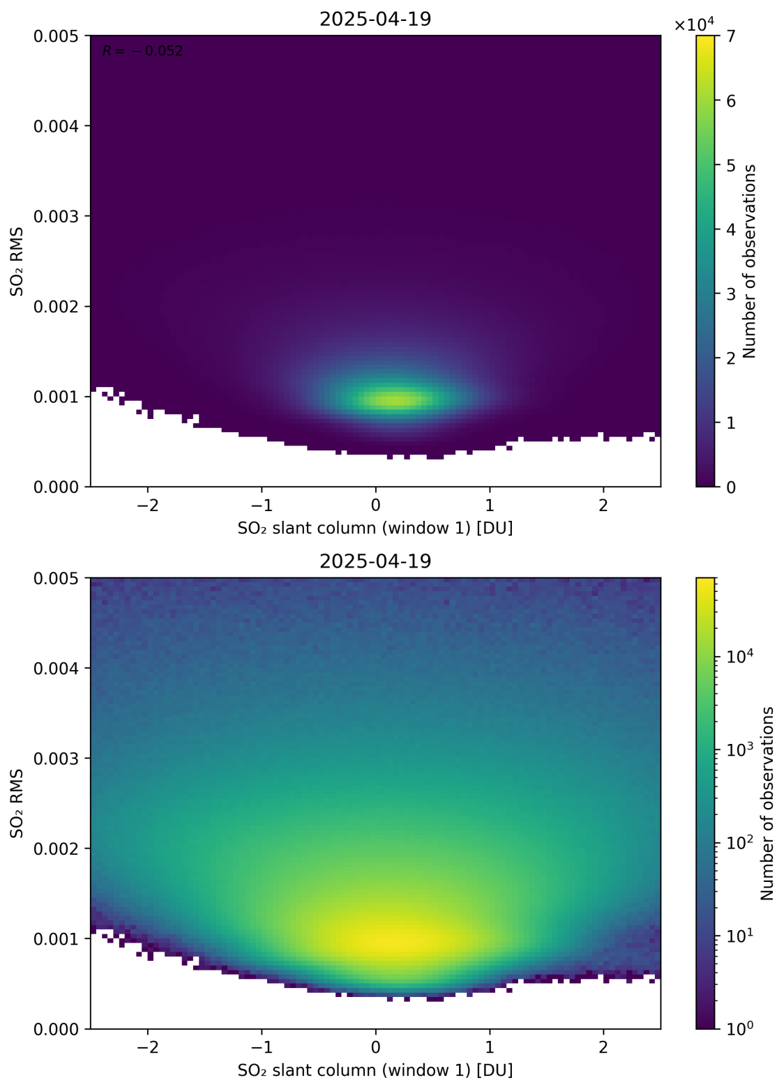
Figure 267: Scatter density plot of “SO 2 slant column (window 1)” against “SO 2 RMS” for 2025-04-19 to 2025-04-20.
