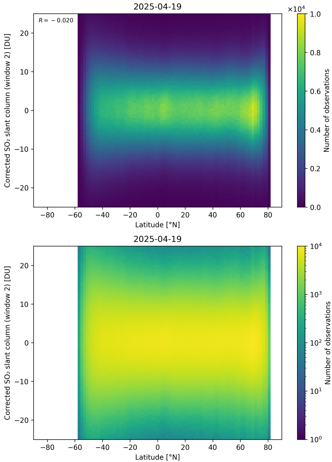
Figure 160: Scatter density plot of “Latitude” against “Corrected SO 2 slant column (window 2)” for 2025-04-19 to 2025-04-20.
