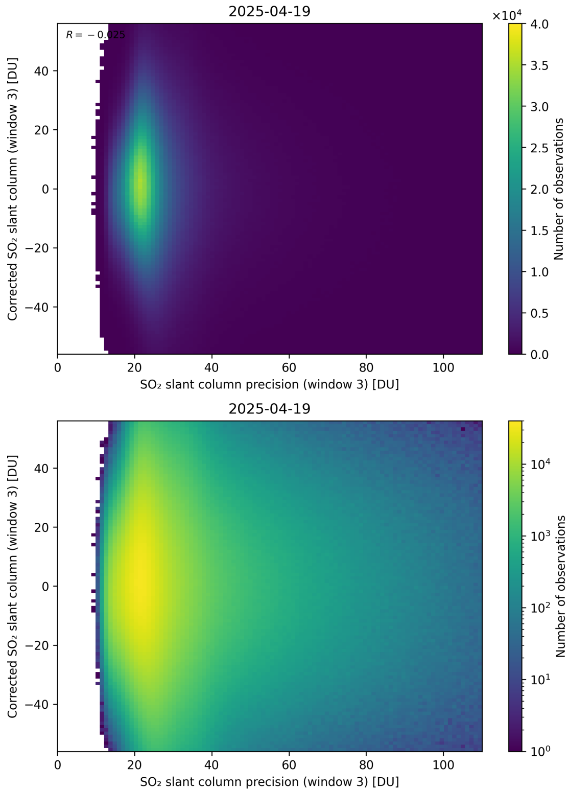
Figure 312: Scatter density plot of “SO 2 slant column precision (window 3)” against “Corrected SO 2 slant column (window 3)” for 2025-04-19 to 2025-04-20.
