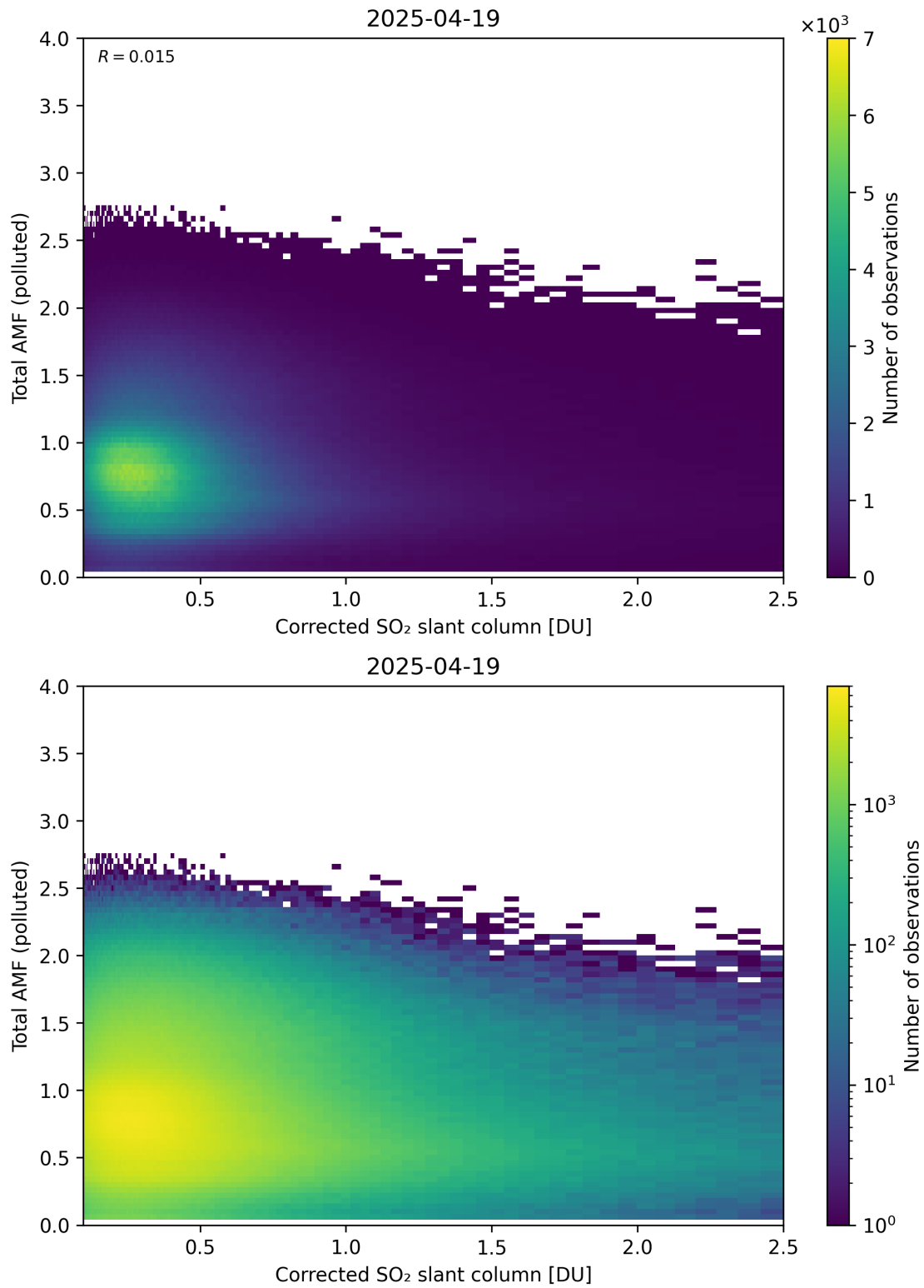
Figure 242: Scatter density plot of “Corrected SO 2 slant column” against “Total AMF (polluted)” for 2025-04-19 to 2025-04-20.
