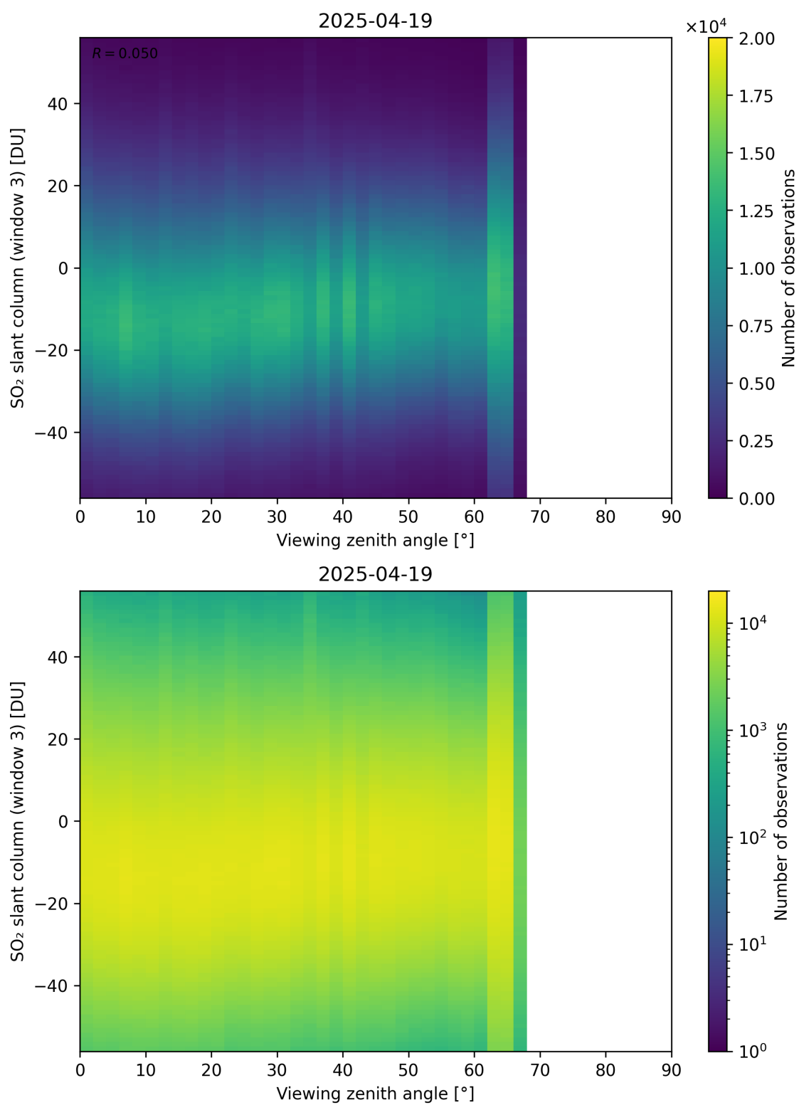
Figure 379: Scatter density plot of “Viewing zenith angle” against “SO 2 slant column (window 3)” for 2025-04-19 to 2025-04-20.
