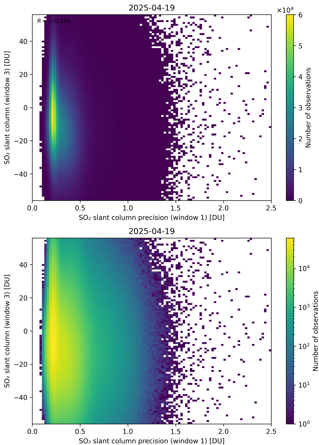
Figure 278: Scatter density plot of “SO 2 slant column precision (window 1)” against “SO 2 slant column (window 3)” for 2025-04-19 to 2025-04-20.
