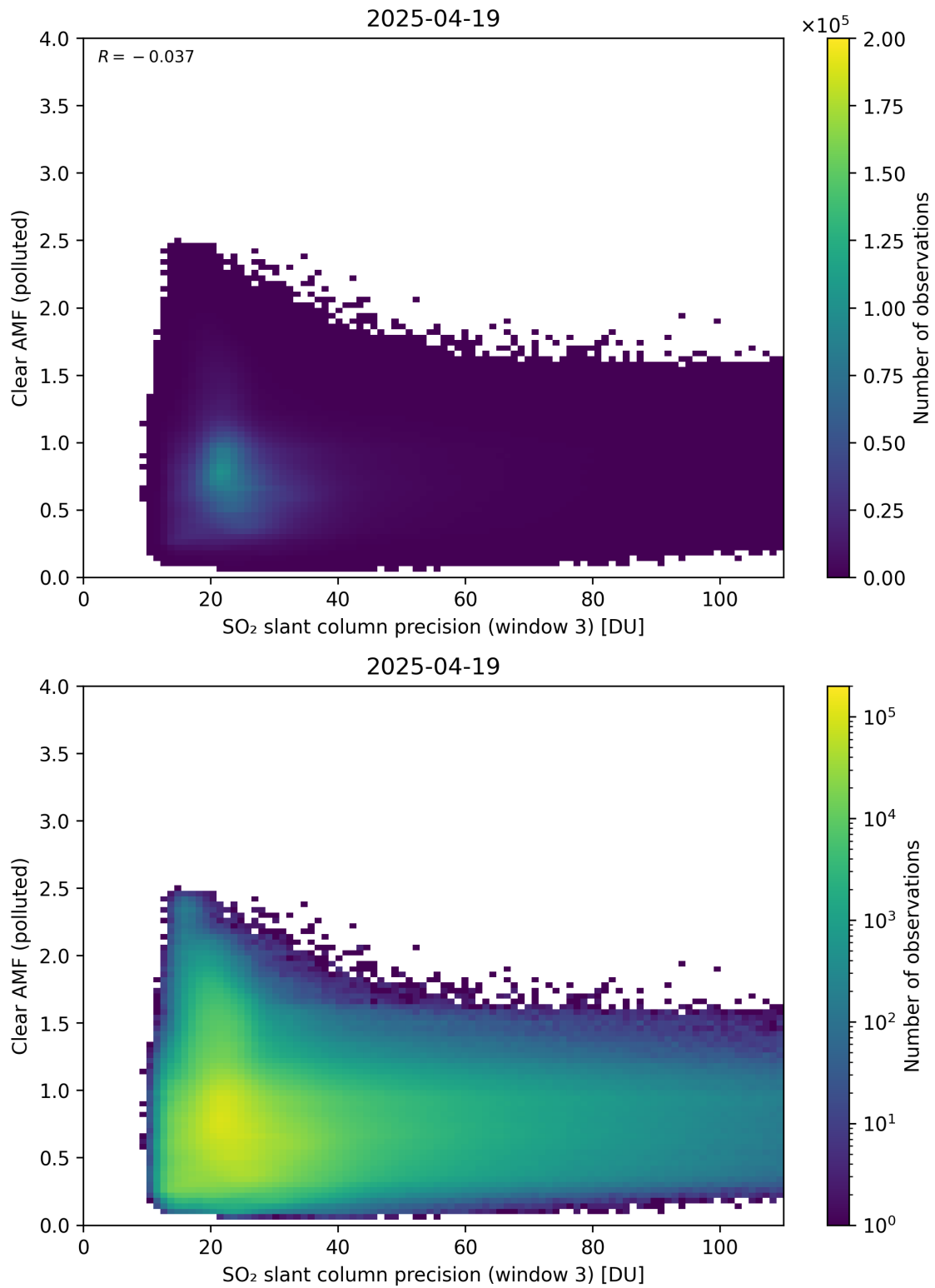
Figure 311: Scatter density plot of “SO 2 slant column precision (window 3)” against “Clear AMF (polluted)” for 2025-04-19 to 2025-04-20.
