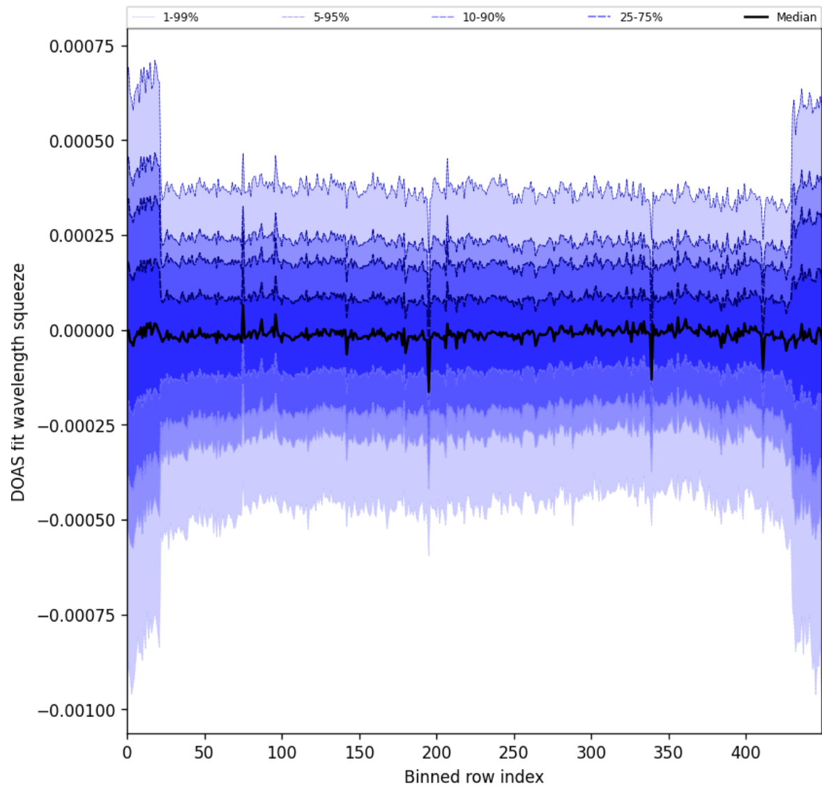
Figure 103: Along track statistics of “DOAS fit wavelength squeeze” for 2025-04-19 to 2025-04-20
