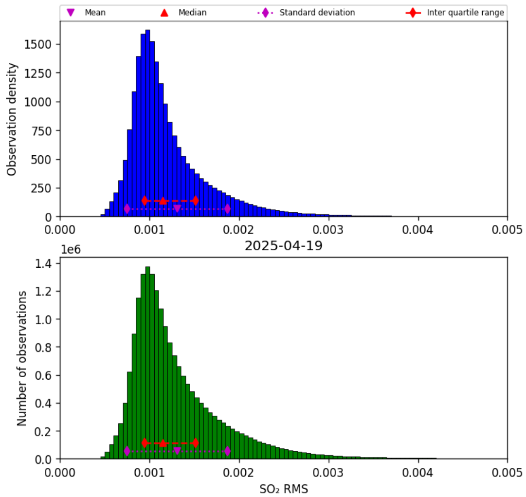
Figure 78: Histogram of “SO 2 RMS” for 2025-04-19 to 2025-04-20
