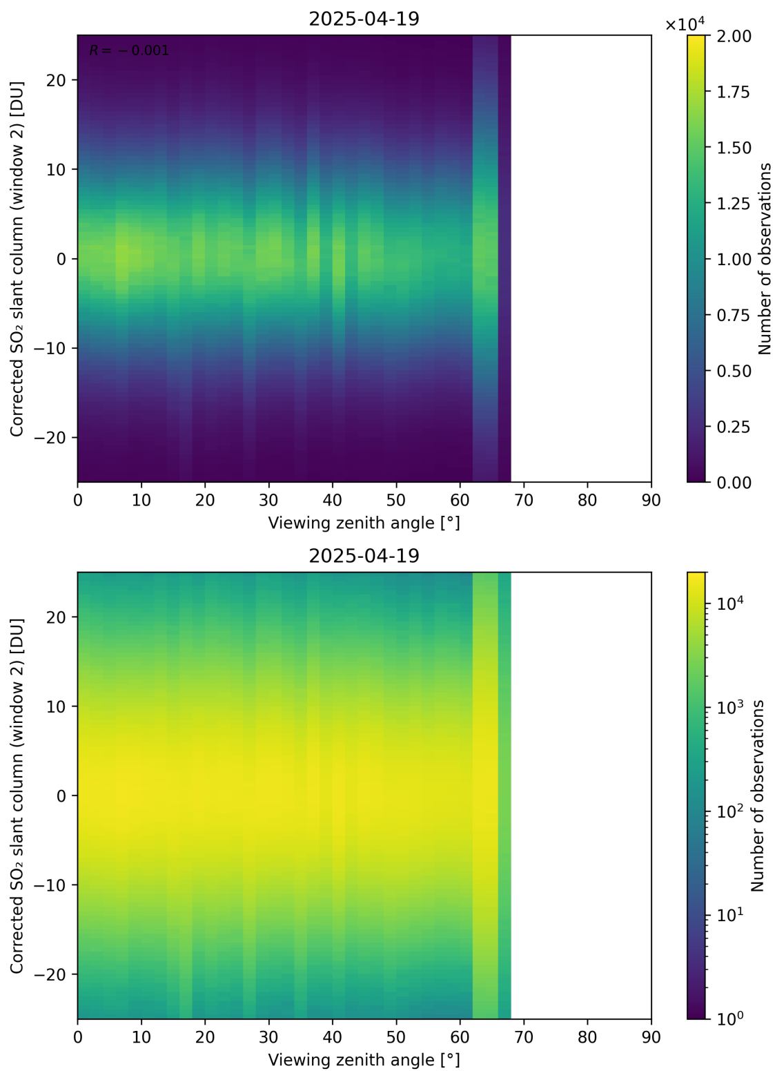
Figure 374: Scatter density plot of “Viewing zenith angle” against “Corrected SO 2 slant column (window 2)” for 2025-04-19 to 2025-04-20.
