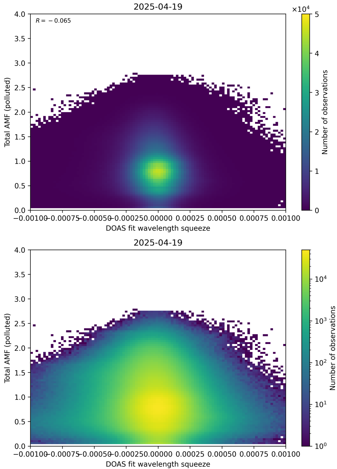
Figure 145: Scatter density plot of “DOAS fit wavelength squeeze” against “Total AMF (polluted)” for 2025-04-19 to 2025-04-20.
