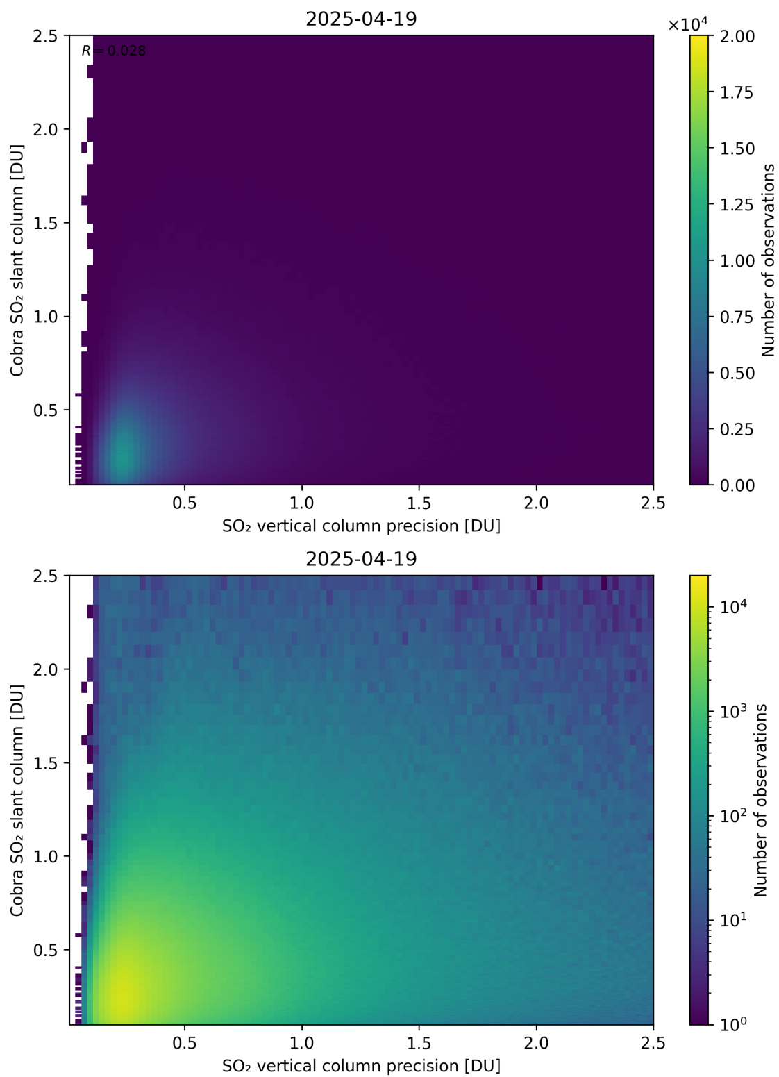
Figure 336: Scatter density plot of “SO 2 vertical column precision” against “Cobra SO 2 slant column” for 2025-04-19 to 2025-04-20.
