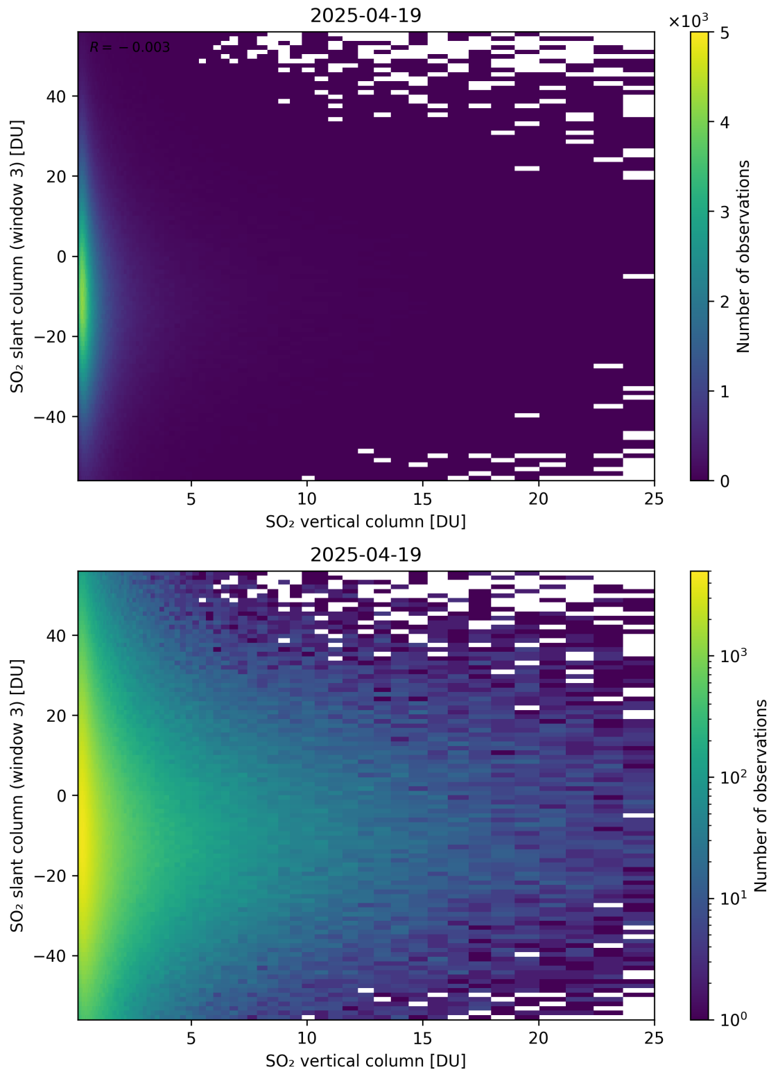
Figure 357: Scatter density plot of “SO 2 vertical column” against “SO 2 slant column (window 3)” for 2025-04-19 to 2025-04-20.
