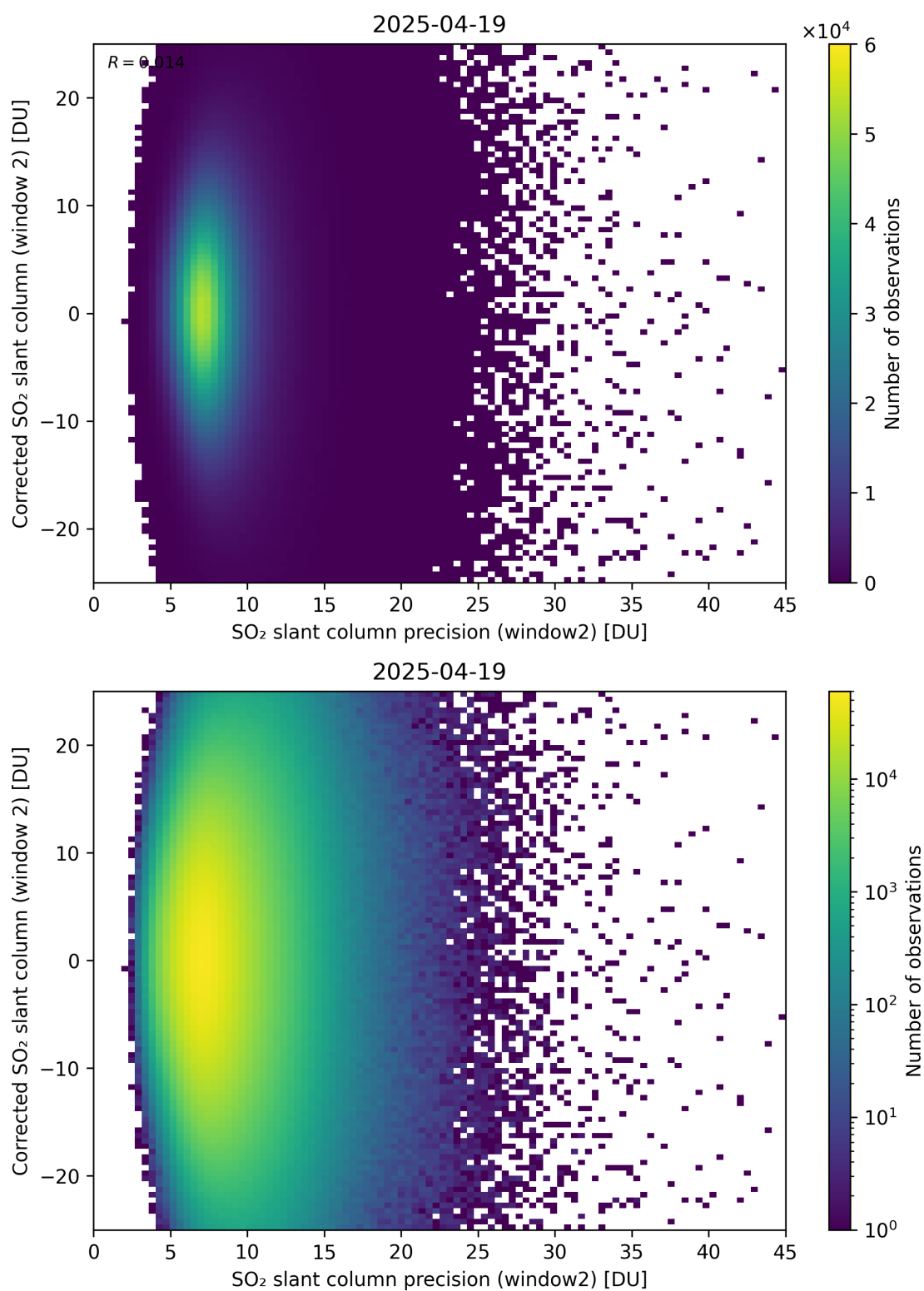
Figure 297: Scatter density plot of “SO 2 slant column precision (window2)” against “Corrected SO 2 slant column (window 2)” for 2025-04-19 to 2025-04-20.
