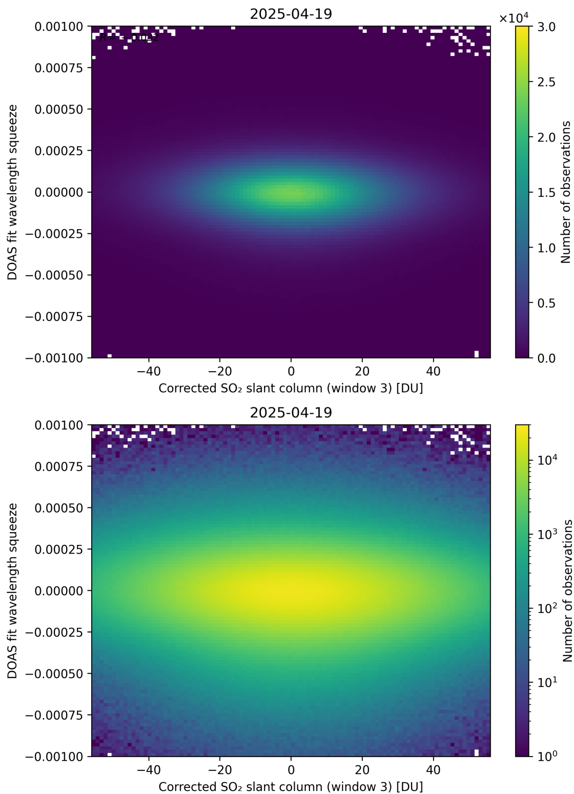
Figure 257: Scatter density plot of “Corrected SO 2 slant column (window 3)” against “DOAS fit wavelength squeeze” for 2025-04-19 to 2025-04-20.
