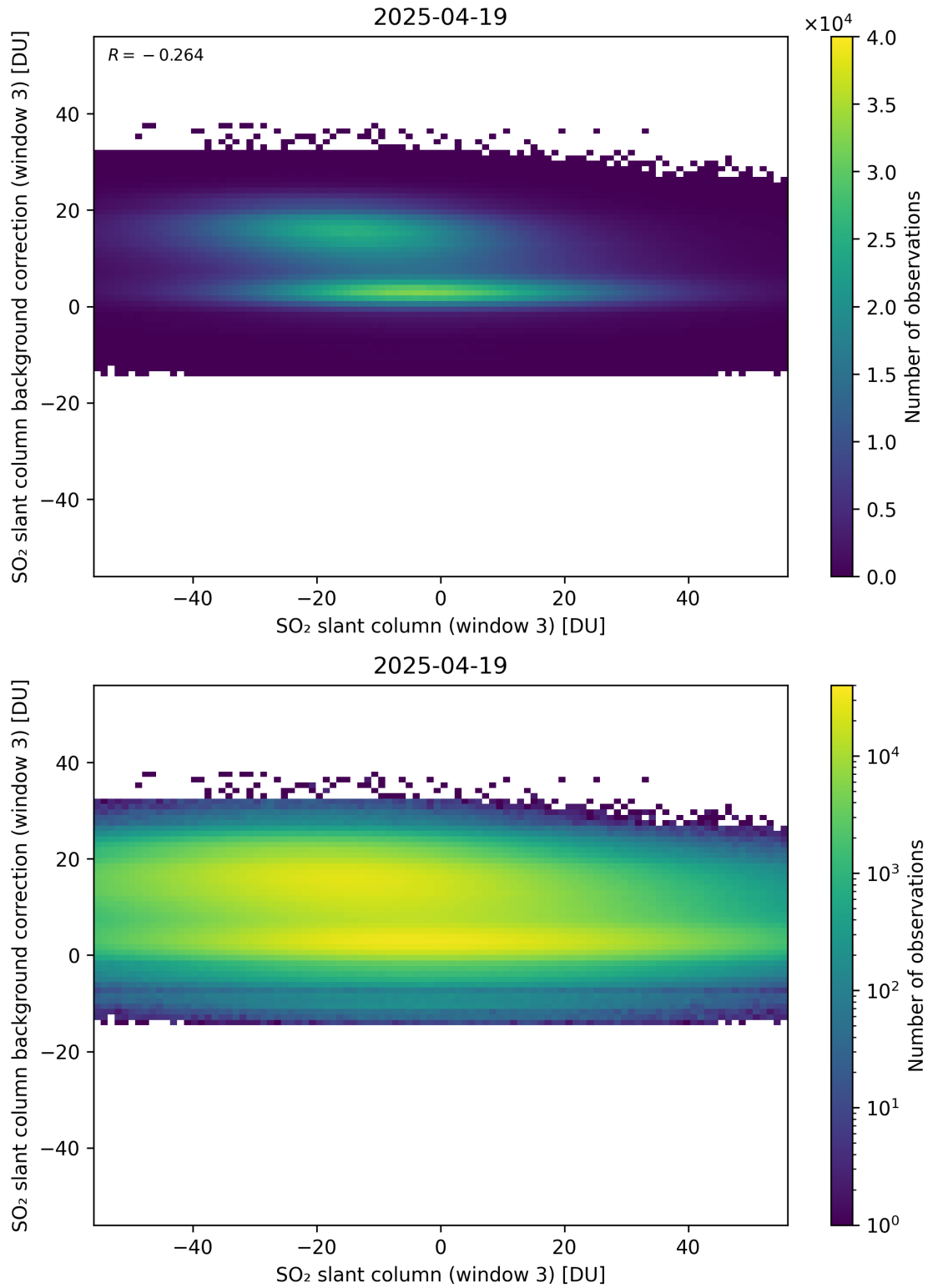
Figure 303: Scatter density plot of “SO 2 slant column (window 3)” against “SO 2 slant column background correction (window 3)” for 2025-04-19 to 2025-04-20.
