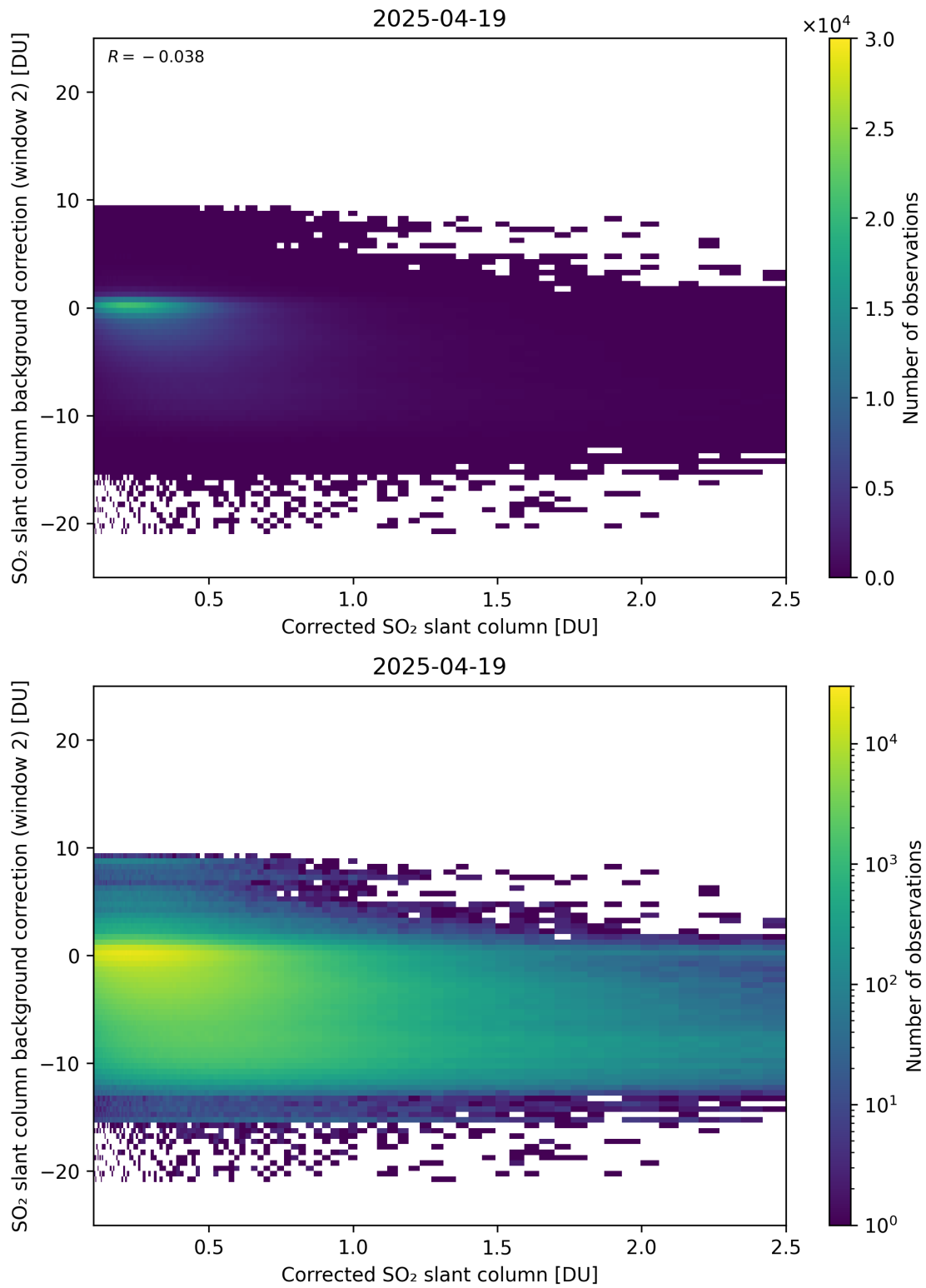
Figure 227: Scatter density plot of “Corrected SO 2 slant column” against “SO 2 slant column background correction (window 2)” for 2025-04-19 to 2025-04-20.
