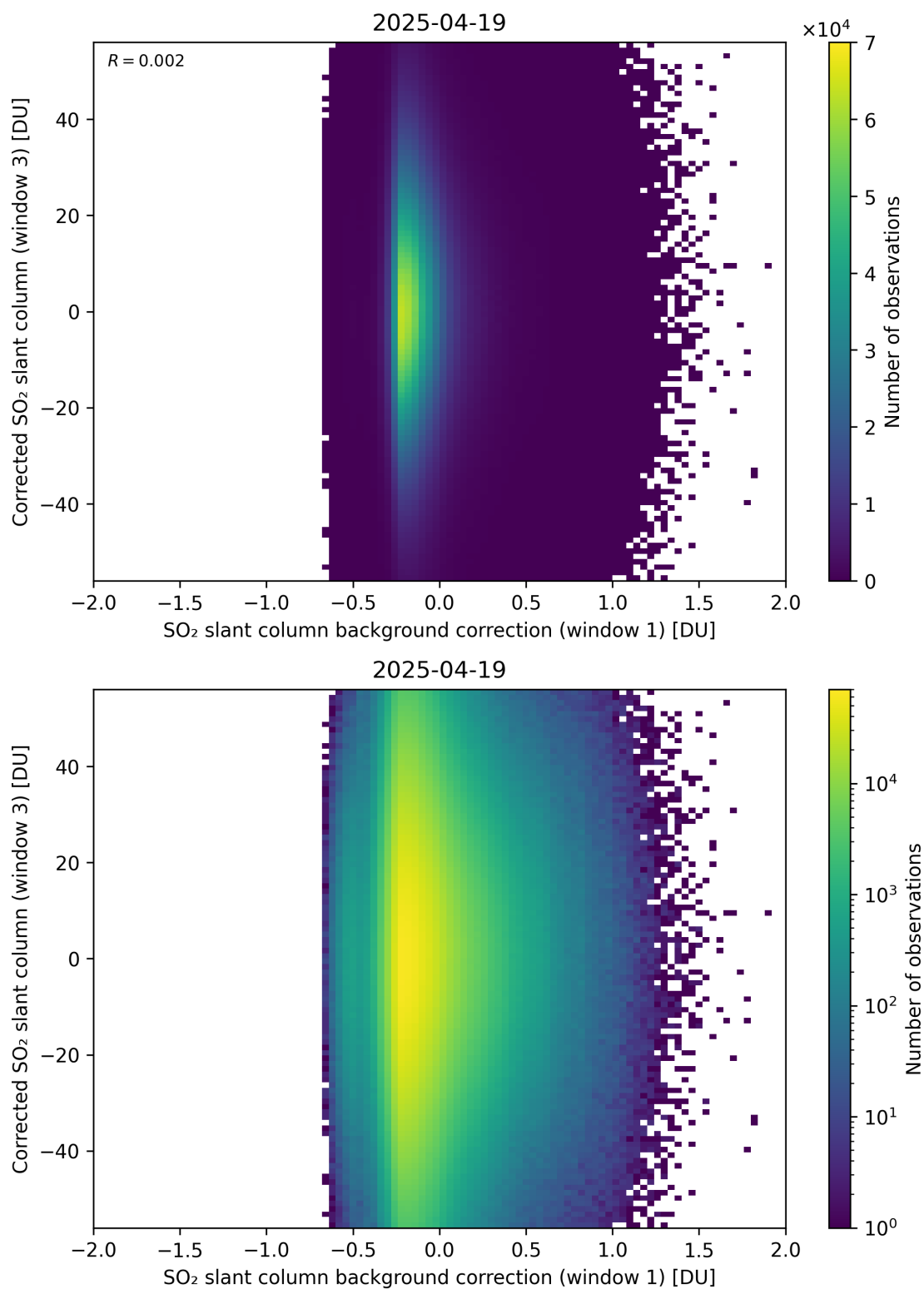
Figure 116: Scatter density plot of “SO 2 slant column background correction (window 1)” against “Corrected SO 2 slant column (window 3)” for 2025-04-19 to 2025-04-20.
