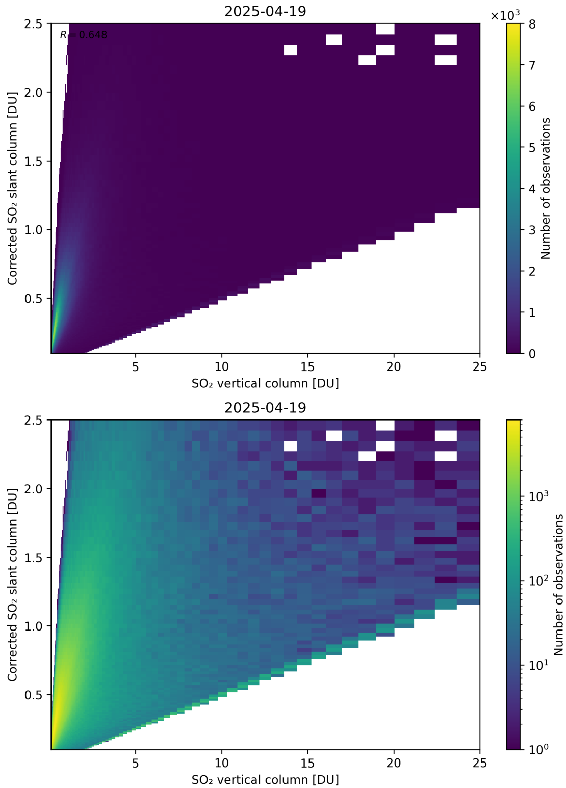
Figure 351: Scatter density plot of “SO 2 vertical column” against “Corrected SO 2 slant column” for 2025-04-19 to 2025-04-20.
