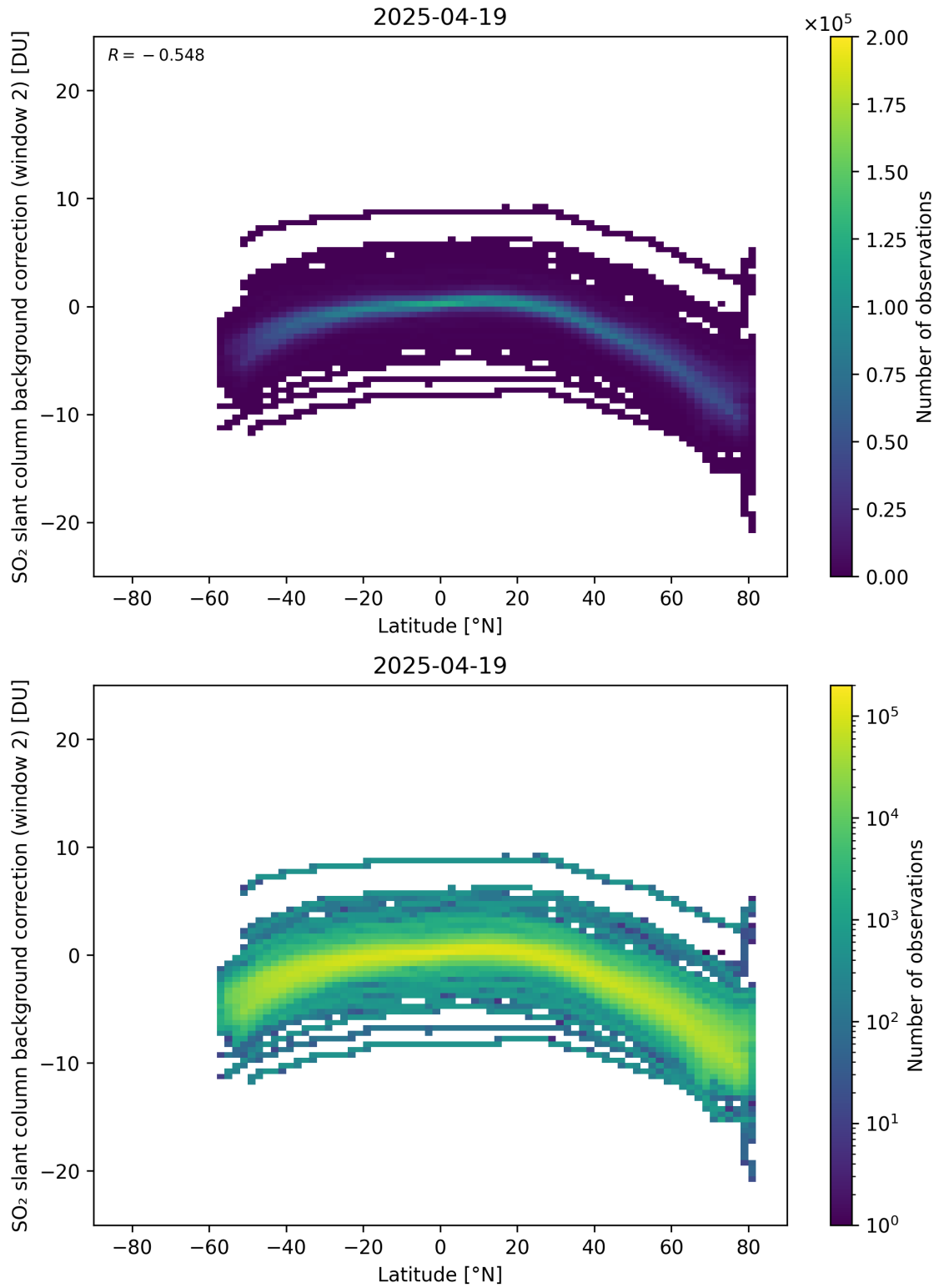
Figure 151: Scatter density plot of “Latitude” against “SO 2 slant column background correction (window 2)” for 2025-04-19 to 2025-04-20.
