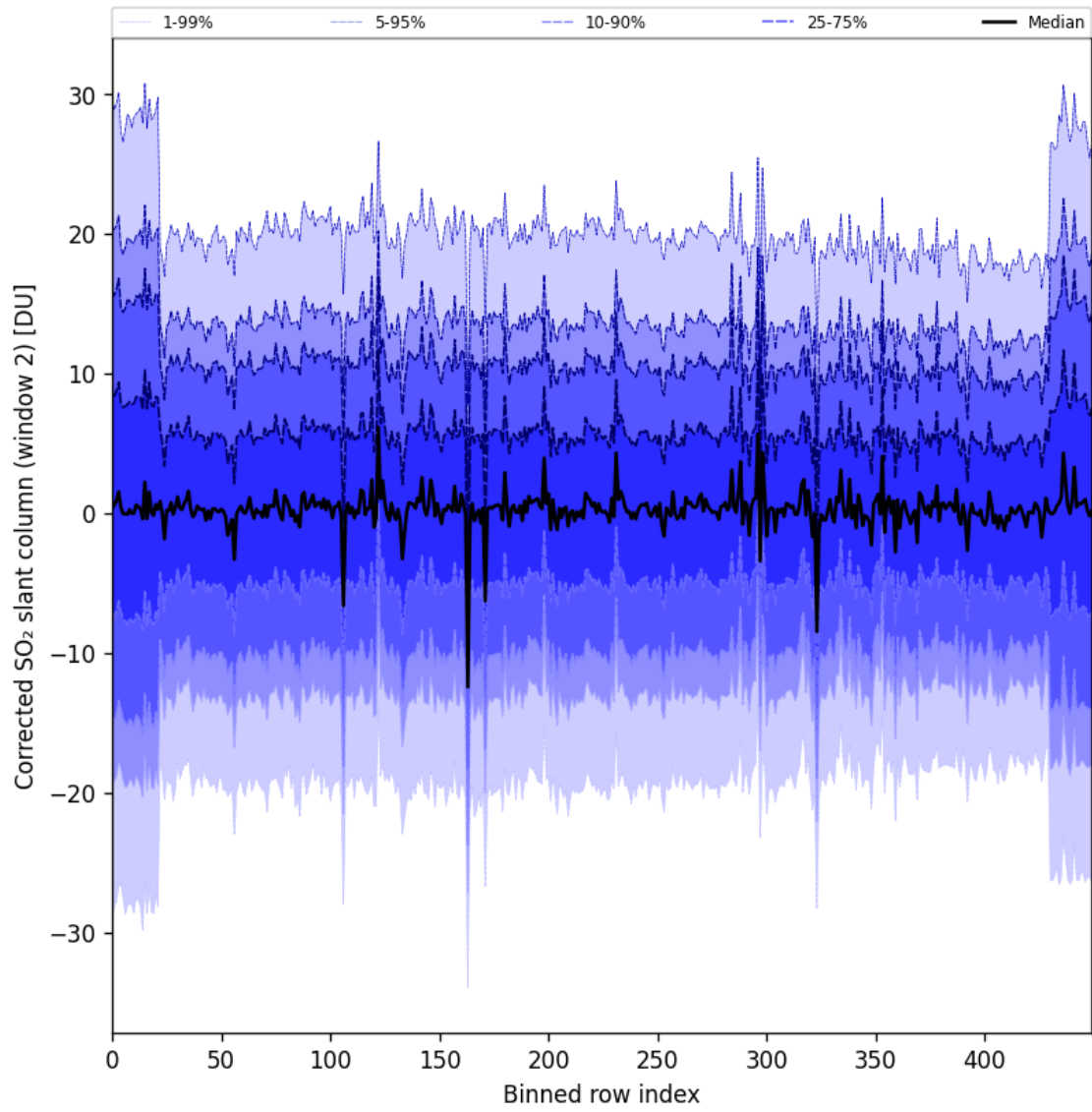
Figure 95: Along track statistics of “Corrected SO 2 slant column (window 2)” for 2025-04-19 to 2025-04-20
