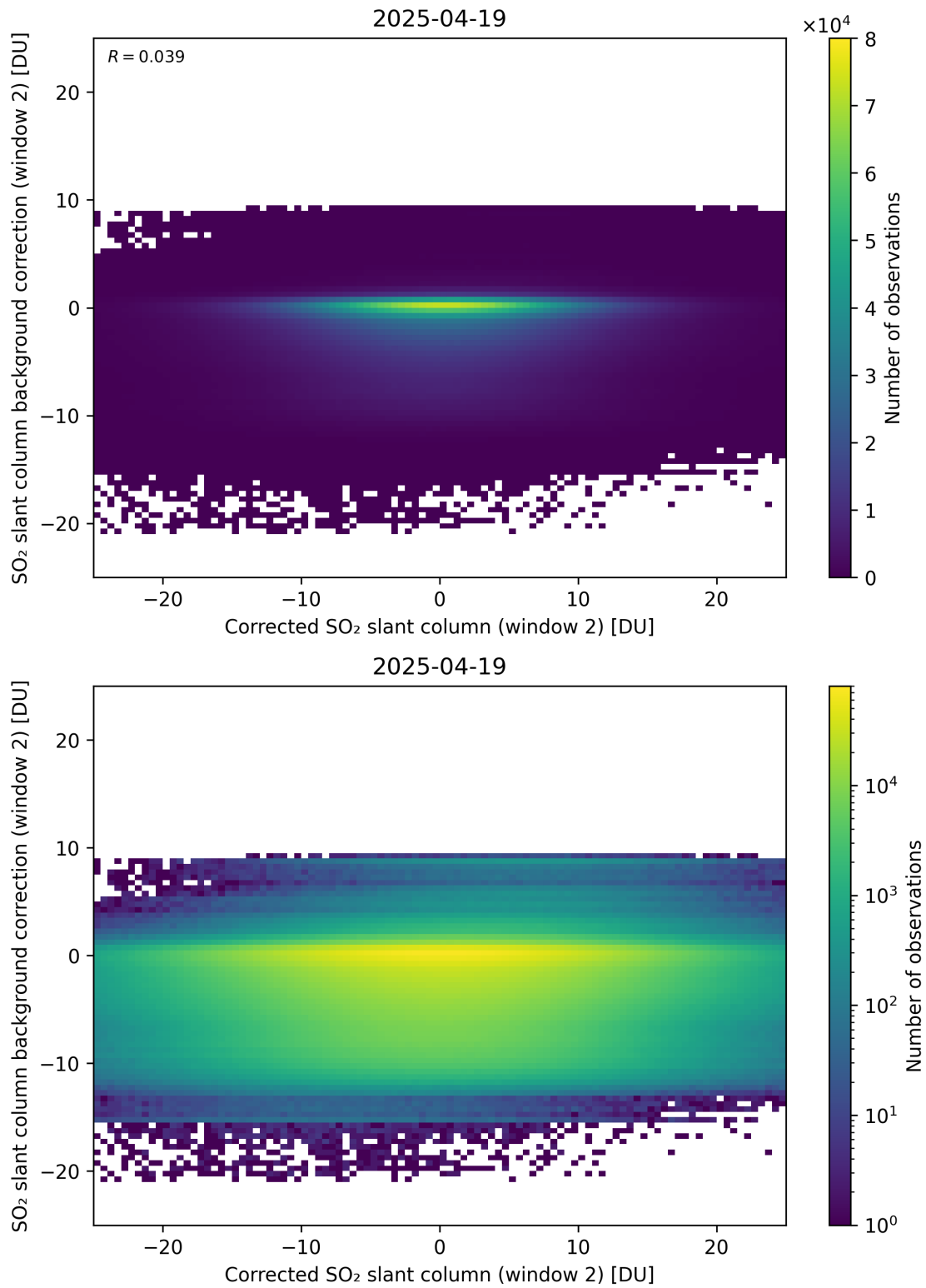
Figure 244: Scatter density plot of “Corrected SO 2 slant column (window 2)” against “SO 2 slant column background correction (window 2)” for 2025-04-19 to 2025-04-20.
