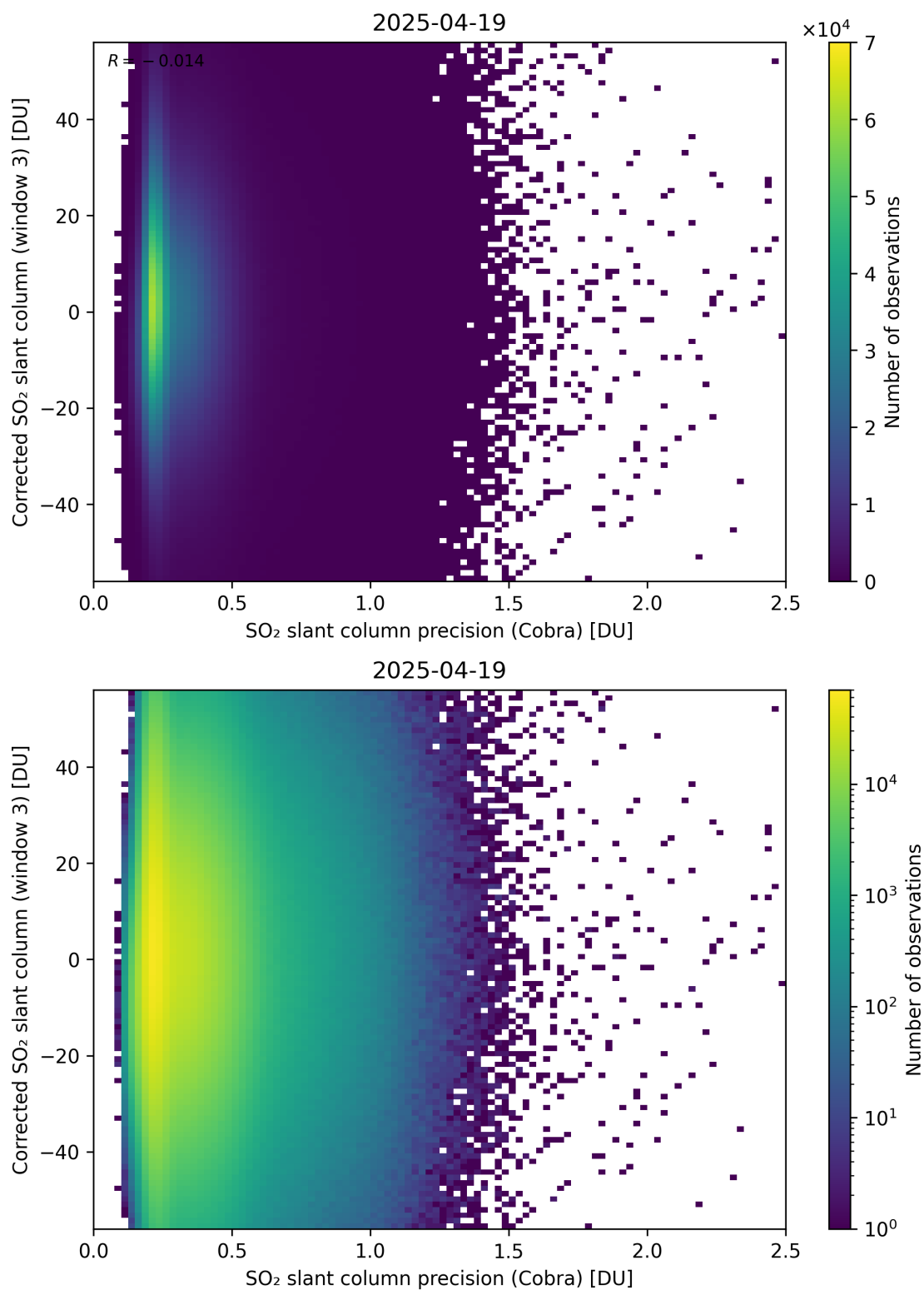
Figure 207: Scatter density plot of “SO 2 slant column precision (Cobra)” against “Corrected SO 2 slant column (window 3)” for 2025-04-19 to 2025-04-20.
