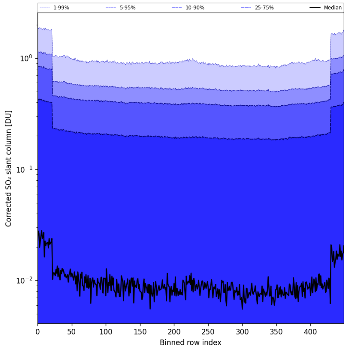
Figure 86: Along track statistics of “Corrected SO 2 slant column” for 2025-04-19 to 2025-04-20
