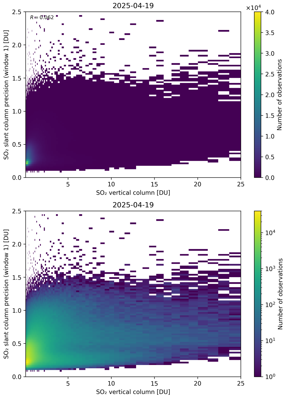
Figure 355: Scatter density plot of “SO 2 vertical column” against “SO 2 slant column precision (window 1)” for 2025-04-19 to 2025-04-20.
