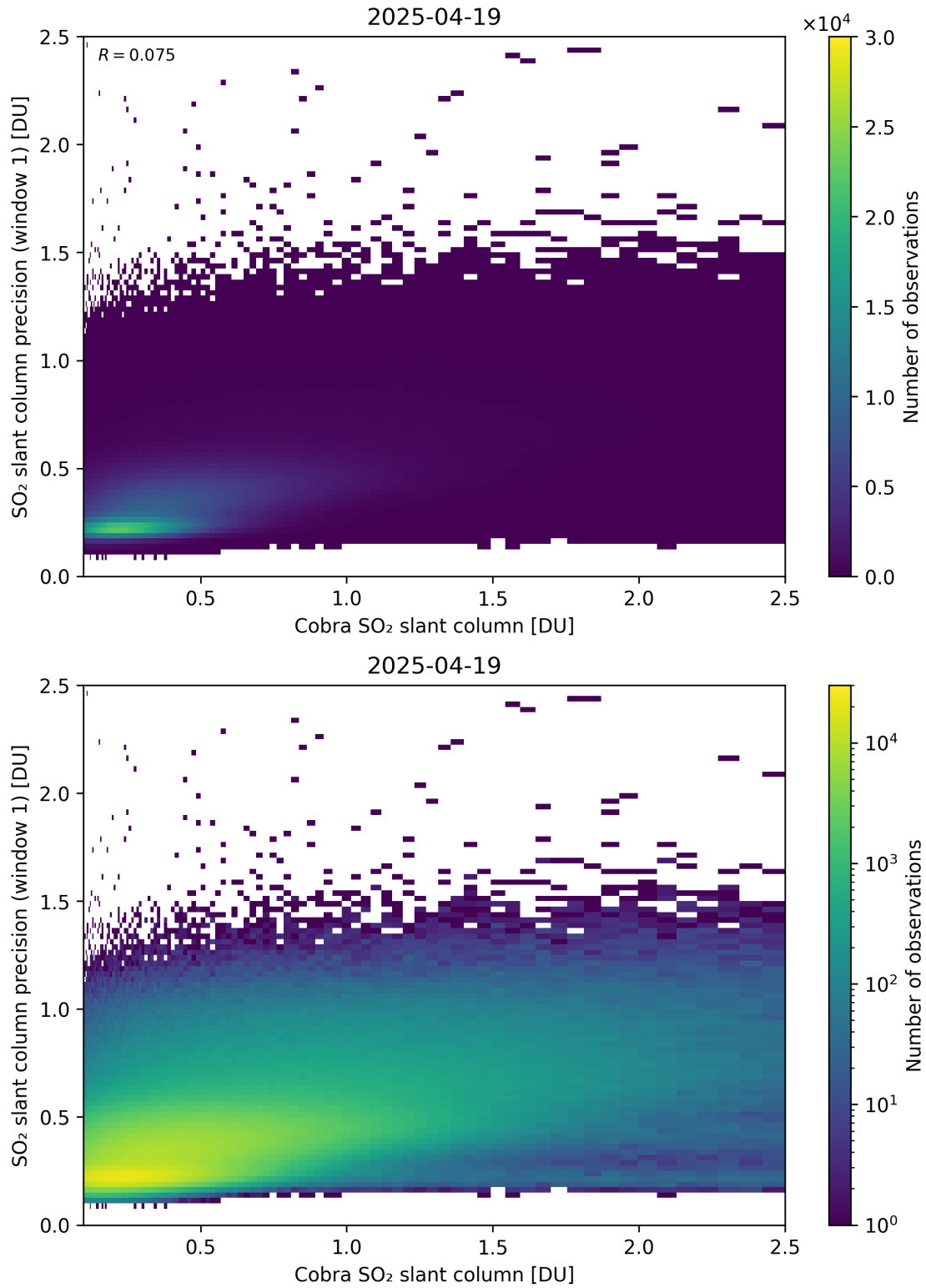
Figure 220: Scatter density plot of “Cobra SO 2 slant column” against “SO 2 slant column precision (window 1)” for 2025-04-19 to 2025-04-20.
