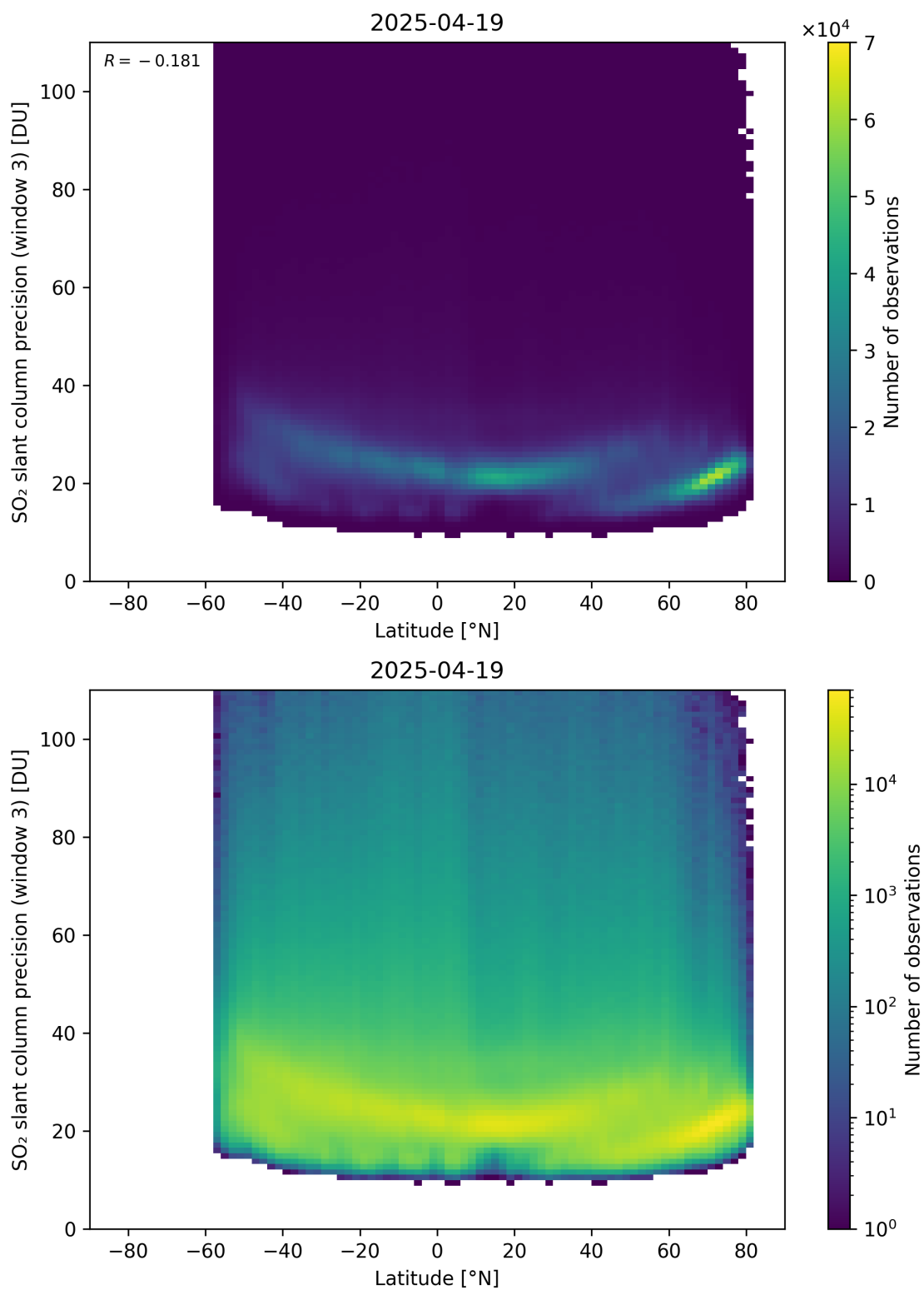
Figure 166: Scatter density plot of “Latitude” against “SO 2 slant column precision (window 3)” for 2025-04-19 to 2025-04-20.
