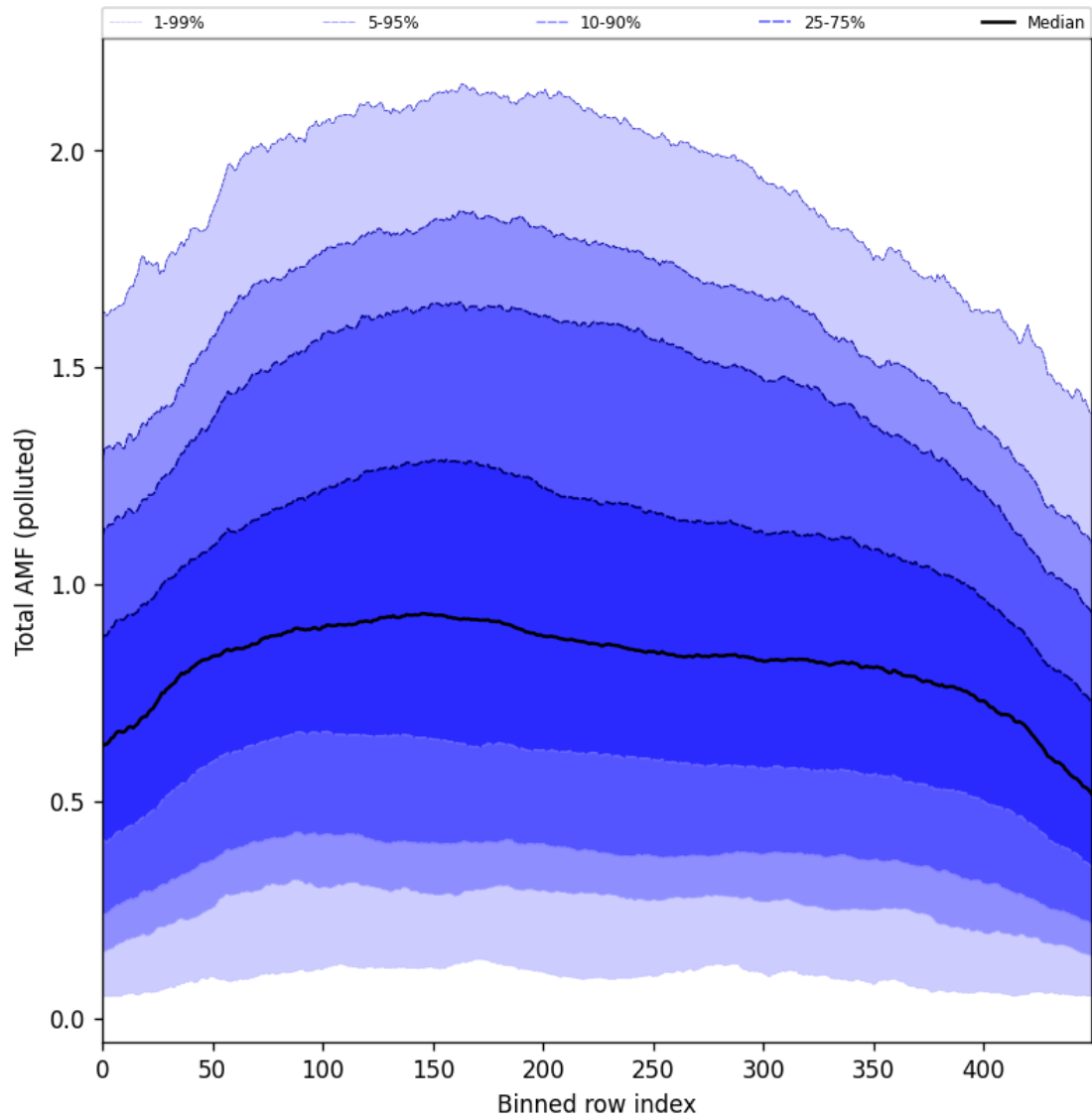
Figure 105: Along track statistics of “Total AMF (polluted)” for 2025-04-19 to 2025-04-20
