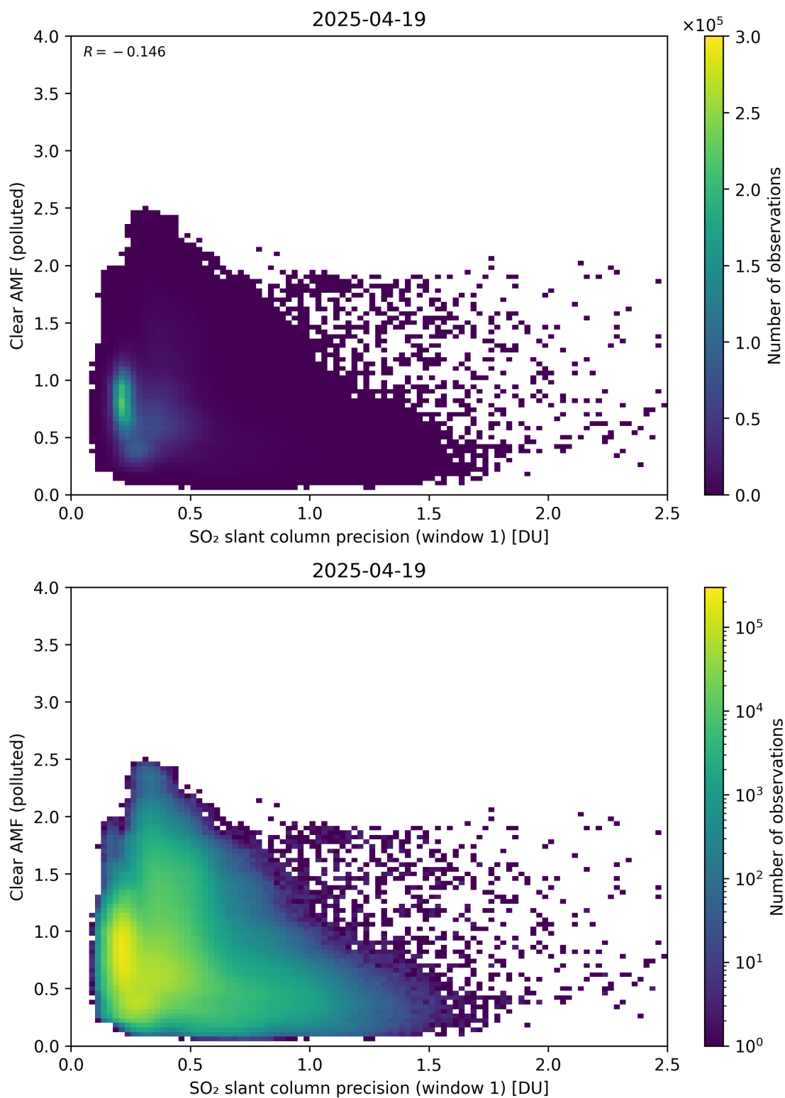
Figure 274: Scatter density plot of “SO 2 slant column precision (window 1)” against “Clear AMF (polluted)” for 2025-04-19 to 2025-04-20.
