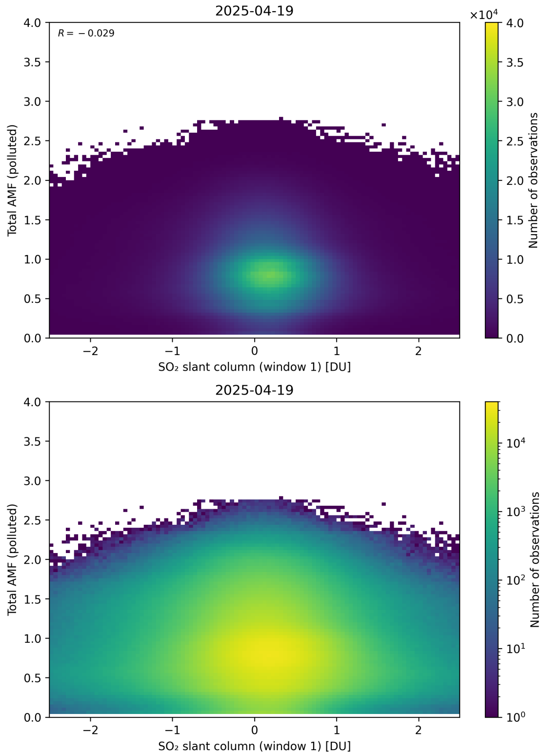
Figure 289: Scatter density plot of “SO 2 slant column (window 1)” against “Total AMF (polluted)” for 2025-04-19 to 2025-04-20.
