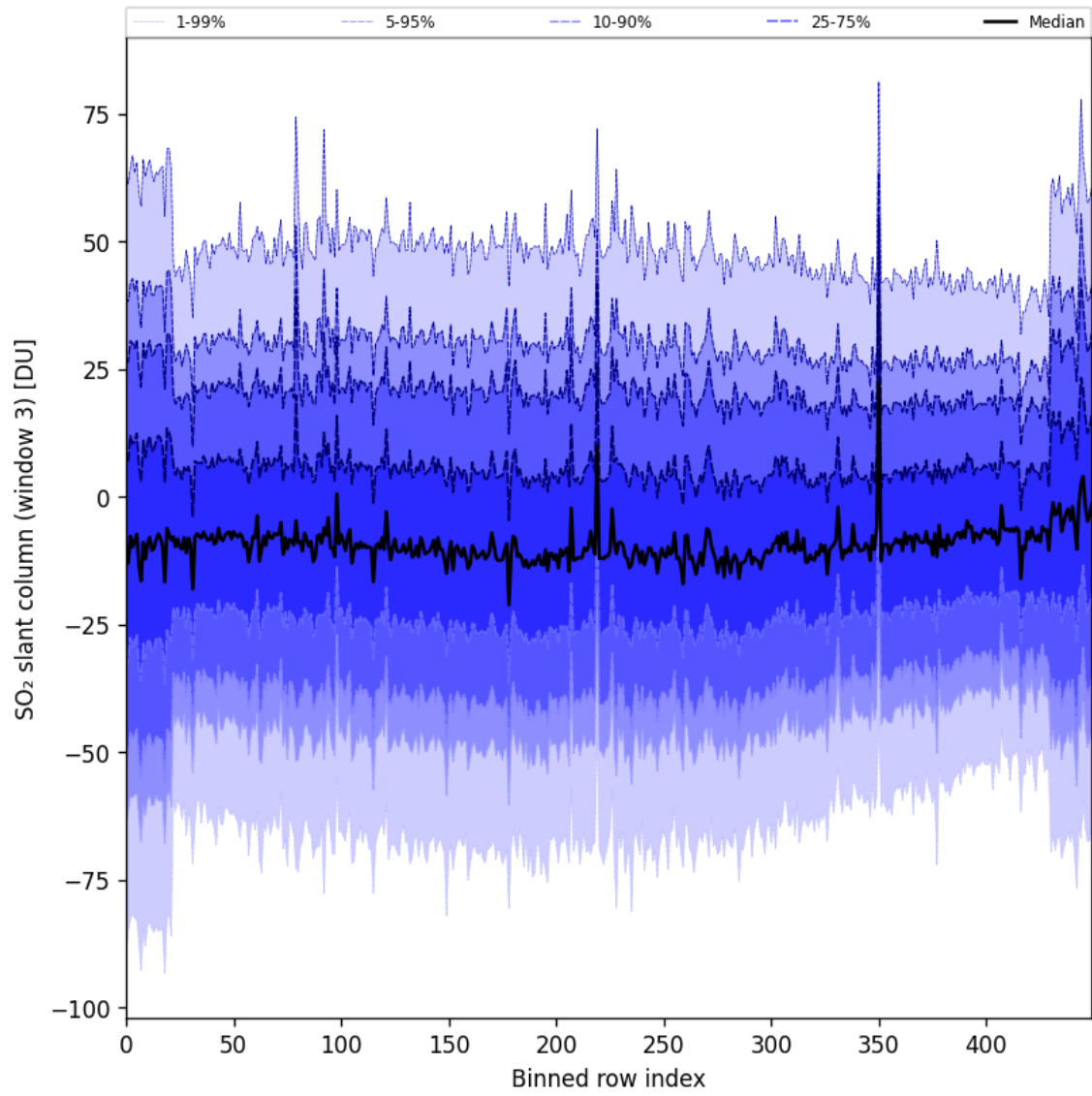
Figure 97: Along track statistics of “SO 2 slant column (window 3)” for 2025-04-19 to 2025-04-20
