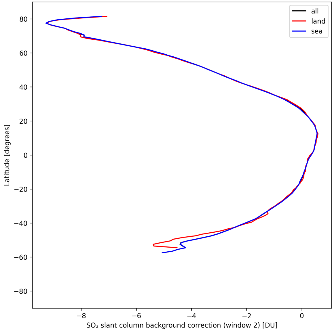
Figure 44: Zonal average of “SO 2 slant column background correction (window 2)” for 2025-04-19 to 2025-04-20.
