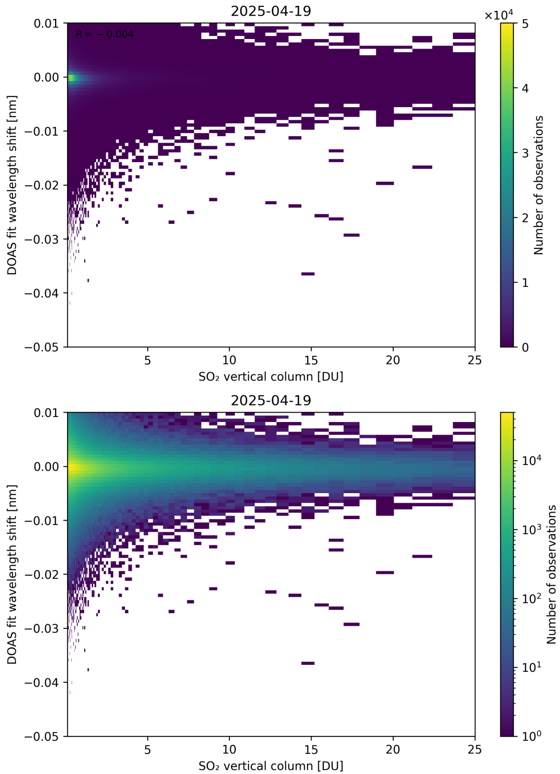
Figure 326: Scatter density plot of “SO 2 vertical column” against “DOAS fit wavelength shift” for 2025-04-19 to 2025-04-20.
