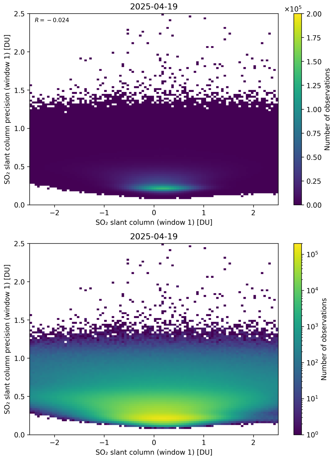
Figure 285: Scatter density plot of “SO 2 slant column (window 1)” against “SO 2 slant column precision (window 1)” for 2025-04-19 to 2025-04-20.
