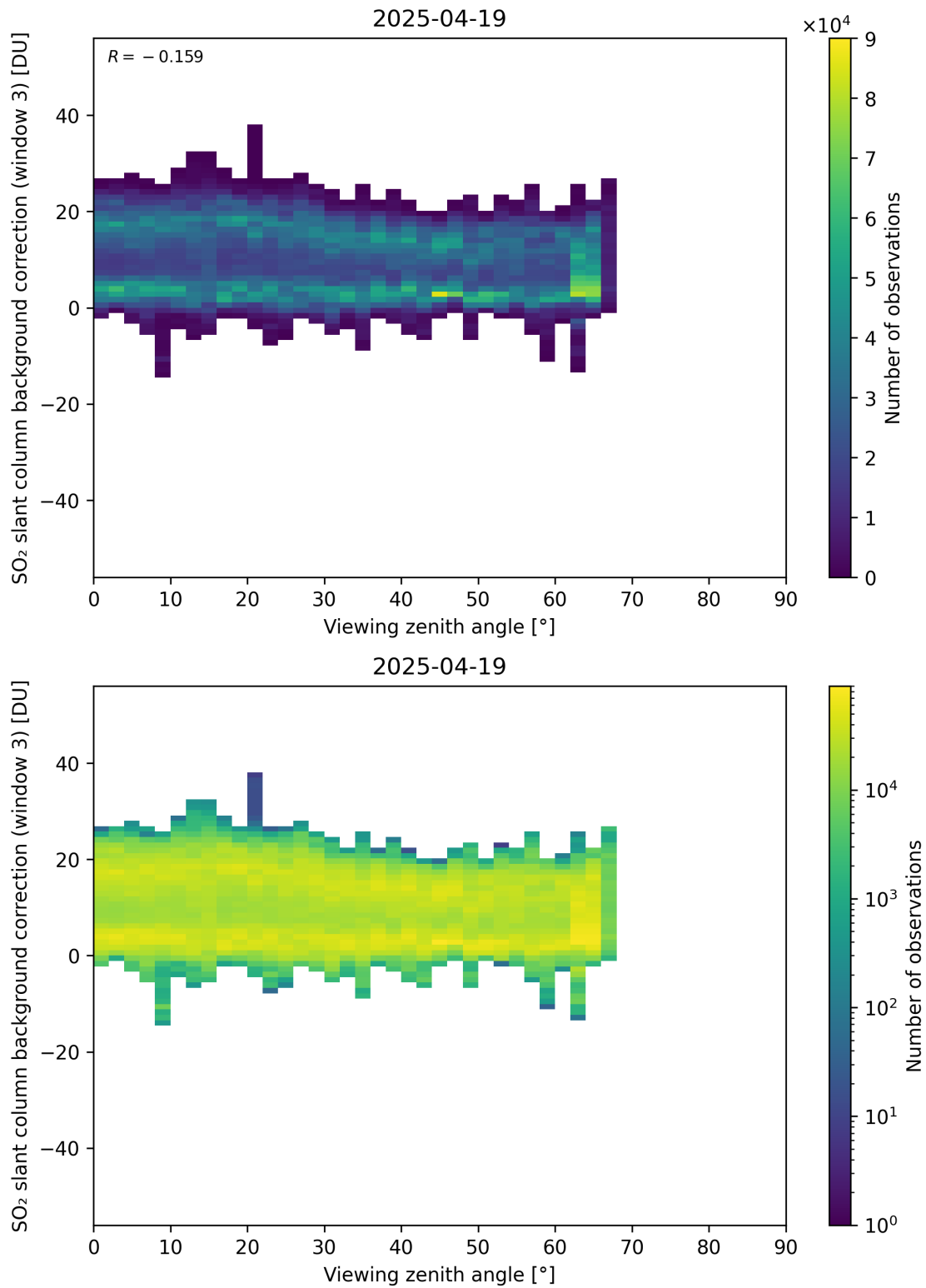
Figure 364: Scatter density plot of “Viewing zenith angle” against “SO 2 slant column background correction (window 3)” for 2025-04-19 to 2025-04-20.
