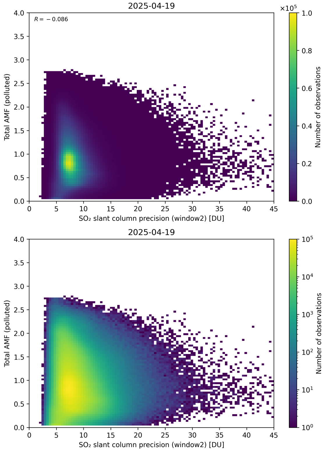
Figure 301: Scatter density plot of “SO 2 slant column precision (window2)” against “Total AMF (polluted)” for 2025-04-19 to 2025-04-20.
