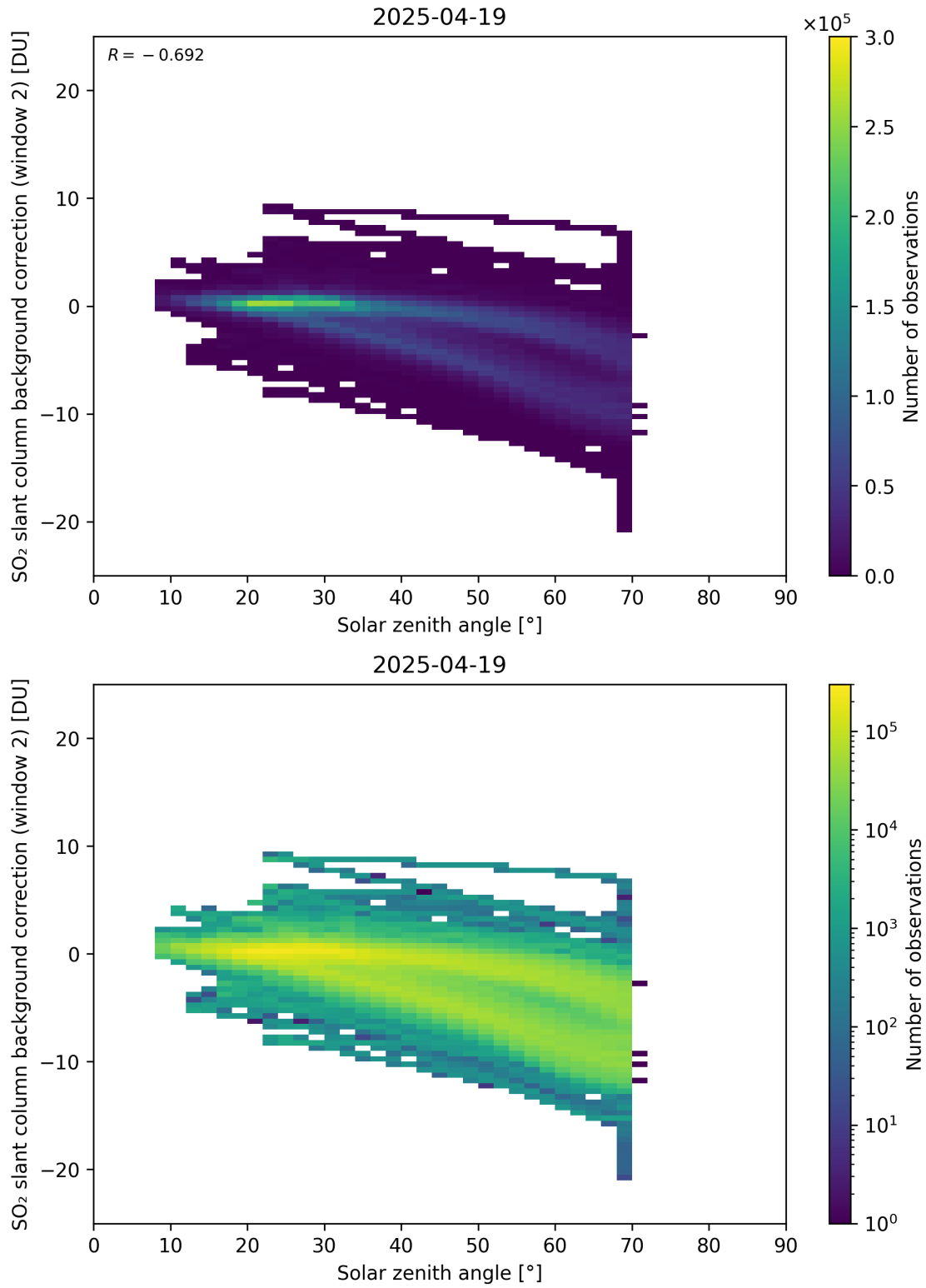
Figure 172: Scatter density plot of “Solar zenith angle” against “SO 2 slant column background correction (window 2)” for 2025-04-19 to 2025-04-20.
