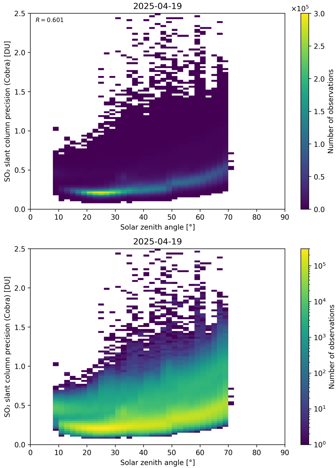
Figure 180: Scatter density plot of “Solar zenith angle” against “SO 2 slant column precision (Cobra)” for 2025-04-19 to 2025-04-20.
