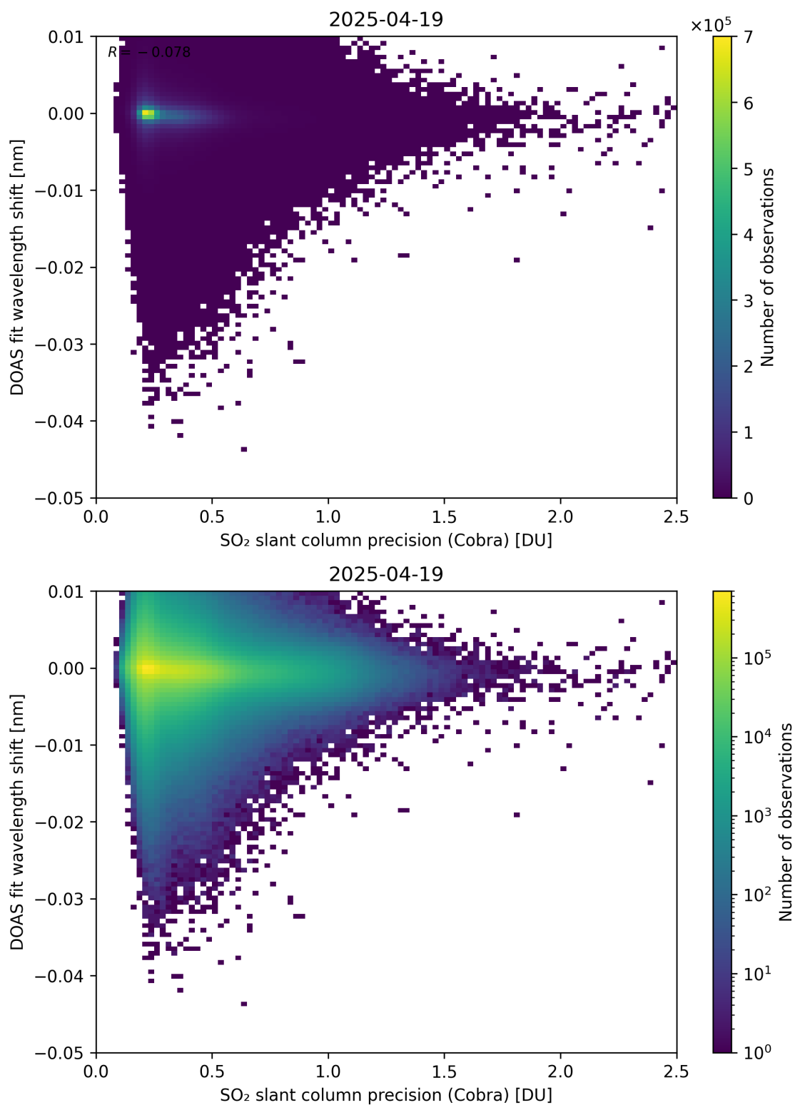
Figure 202: Scatter density plot of “SO 2 slant column precision (Cobra)” against “DOAS fit wavelength shift” for 2025-04-19 to 2025-04-20.
