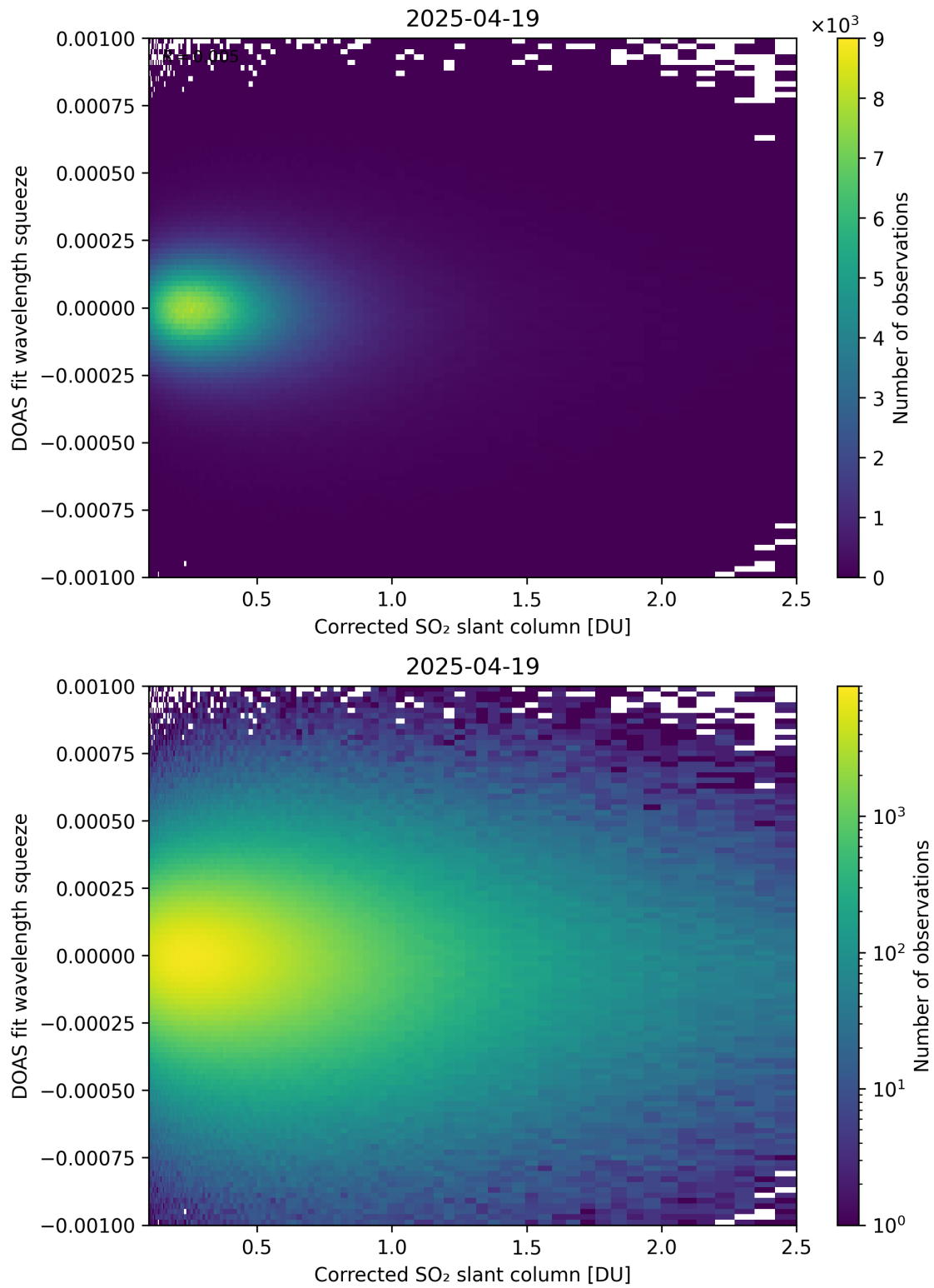
Figure 230: Scatter density plot of "Corrected SO 2 slant column" against "DOAS fit wavelength squeeze" for 2025-04-19 to 2025-04-20.
