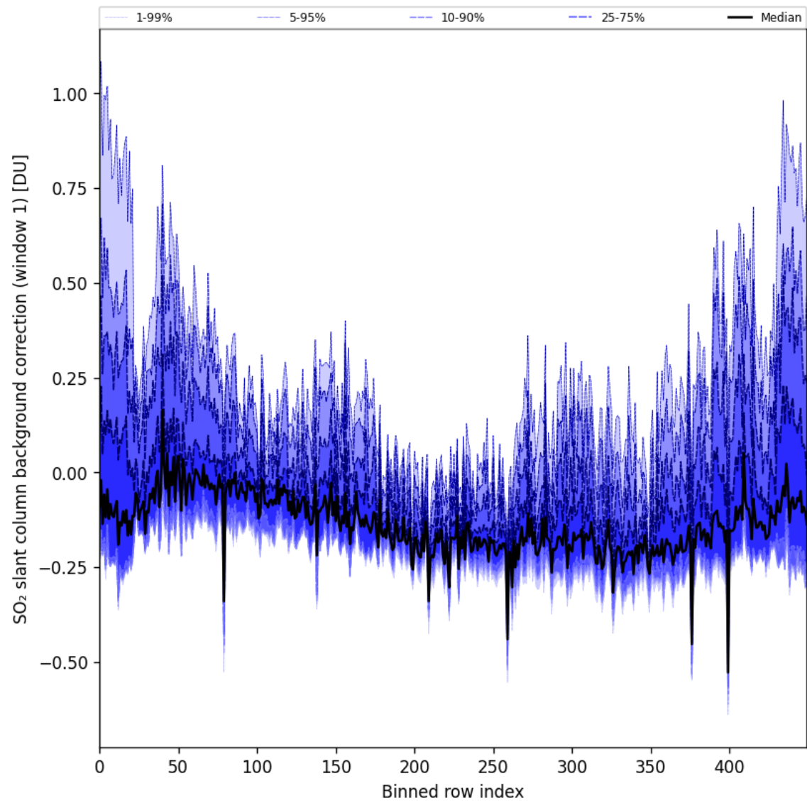
Figure 92: Along track statistics of “SO 2 slant column background correction (window 1)” for 2025-04-19 to 2025-04-20
