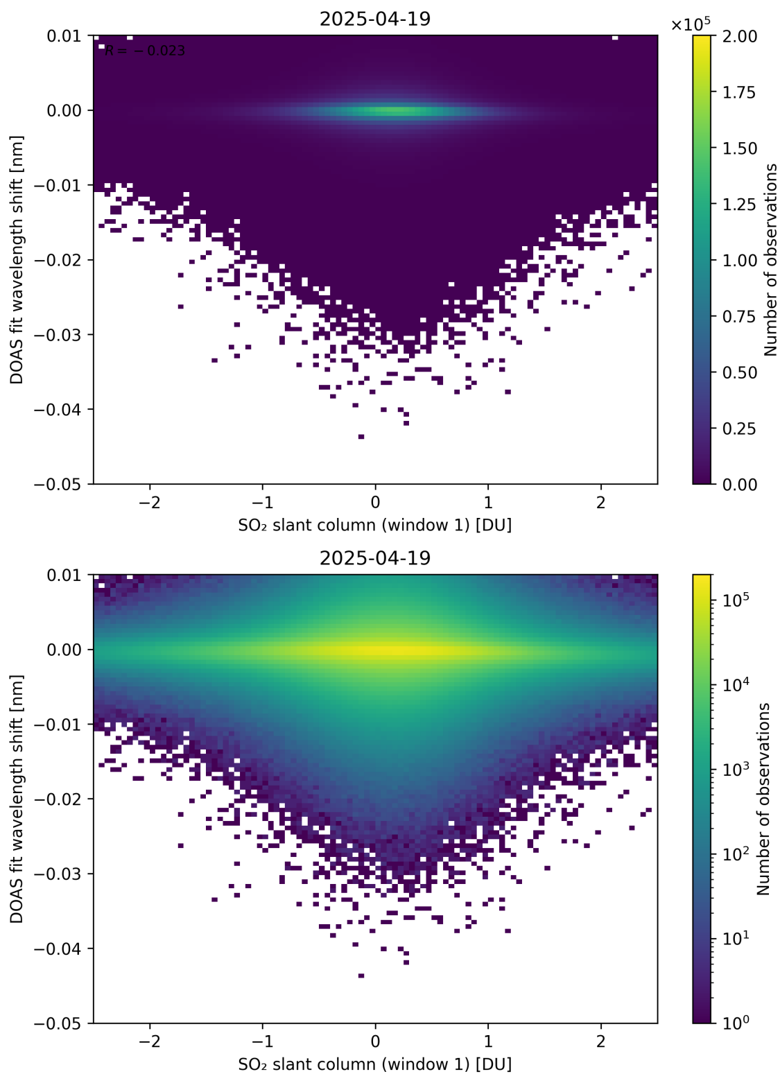
Figure 265: Scatter density plot of “SO 2 slant column (window 1)” against “DOAS fit wavelength shift” for 2025-04-19 to 2025-04-20.
