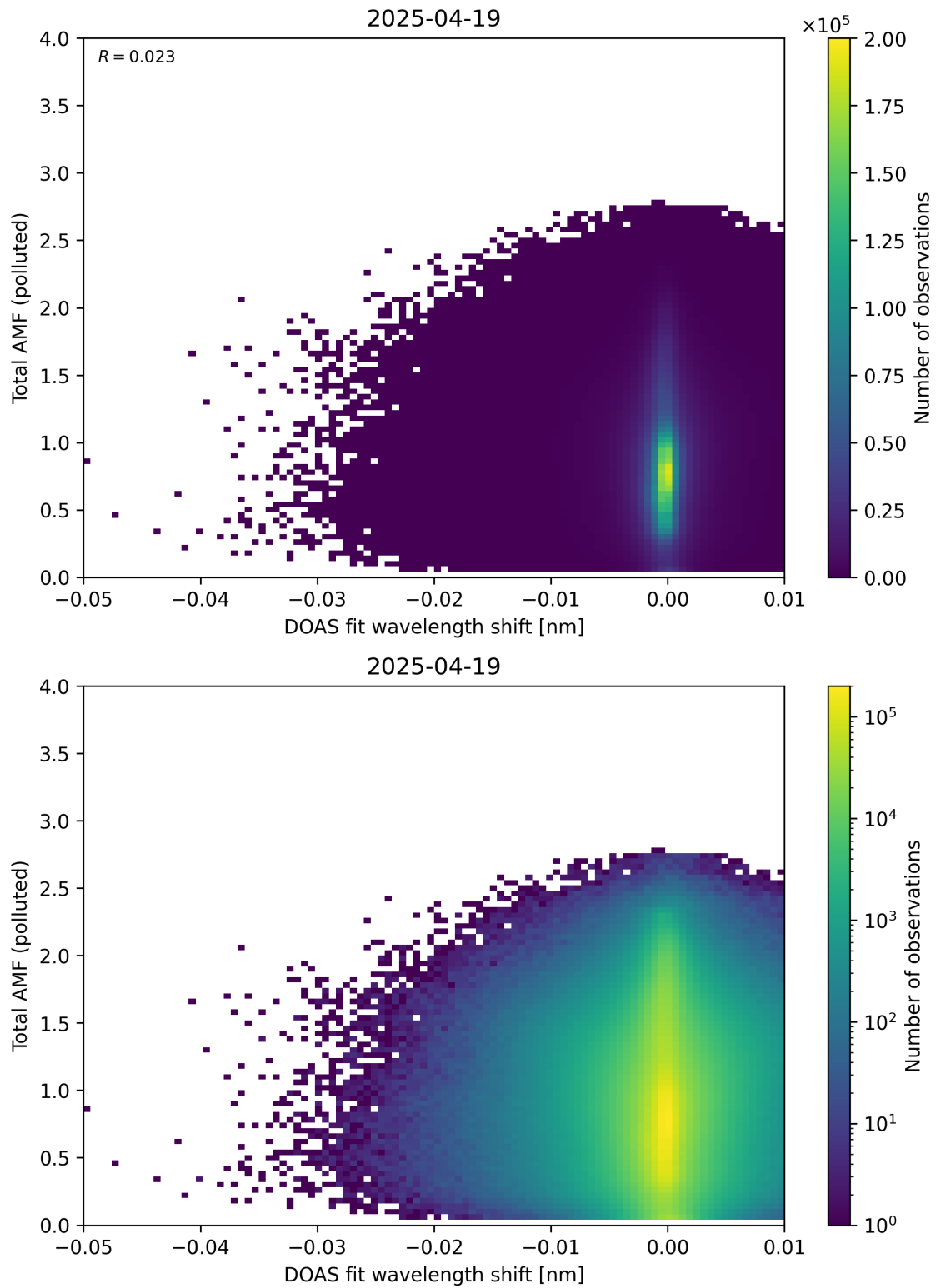
Figure 141: Scatter density plot of “DOAS fit wavelength shift” against “Total AMF (polluted)” for 2025-04-19 to 2025-04-20.
