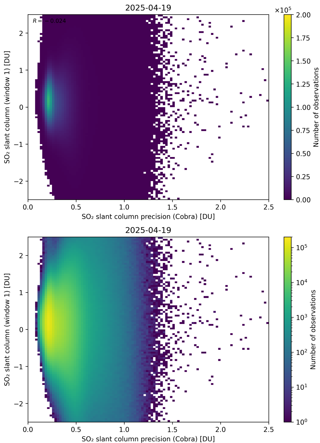
Figure 208: Scatter density plot of “SO 2 slant column precision (Cobra)” against “SO 2 slant column (window 1)” for 2025-04-19 to 2025-04-20.
