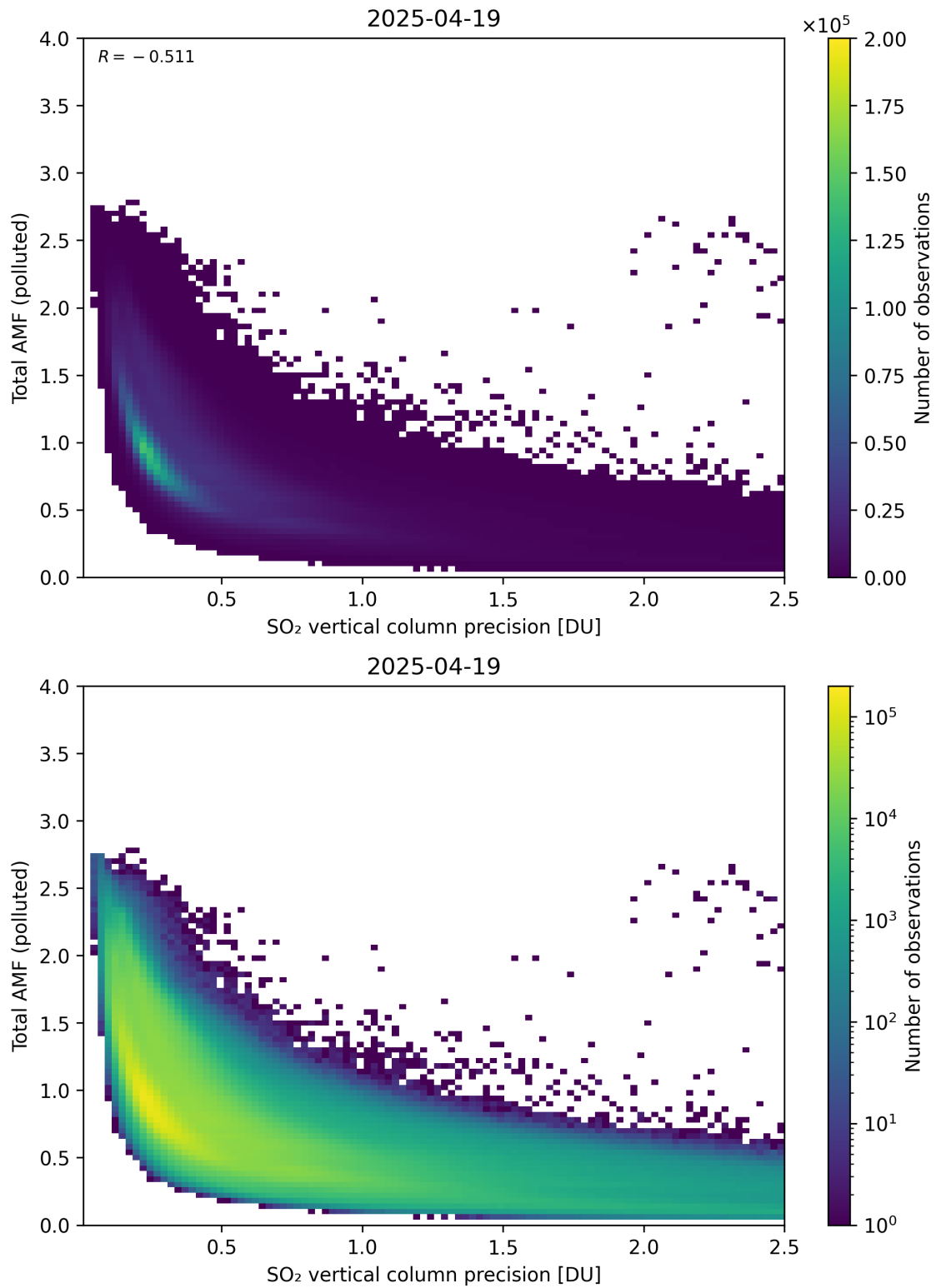
Figure 346: Scatter density plot of “SO 2 vertical column precision” against “Total AMF (polluted)” for 2025-04-19 to 2025-04-20.
