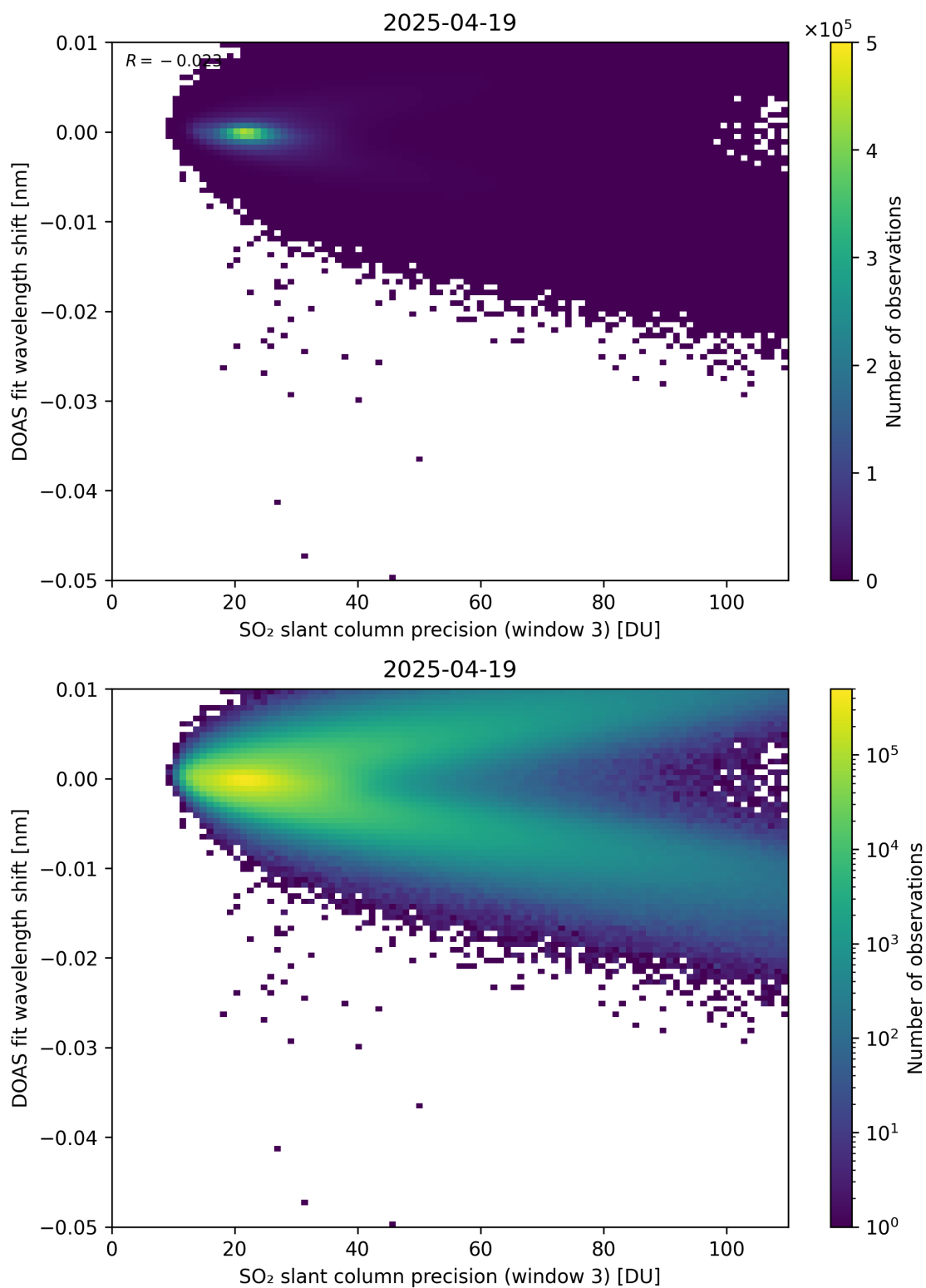
Figure 308: Scatter density plot of “SO 2 slant column precision (window 3)” against “DOAS fit wavelength shift” for 2025-04-19 to 2025-04-20.
