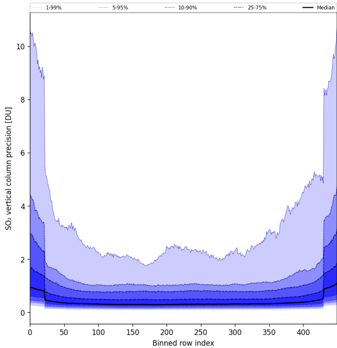
Figure 85: Along track statistics of “SO 2 vertical column precision” for 2025-04-19 to 2025-04-20
