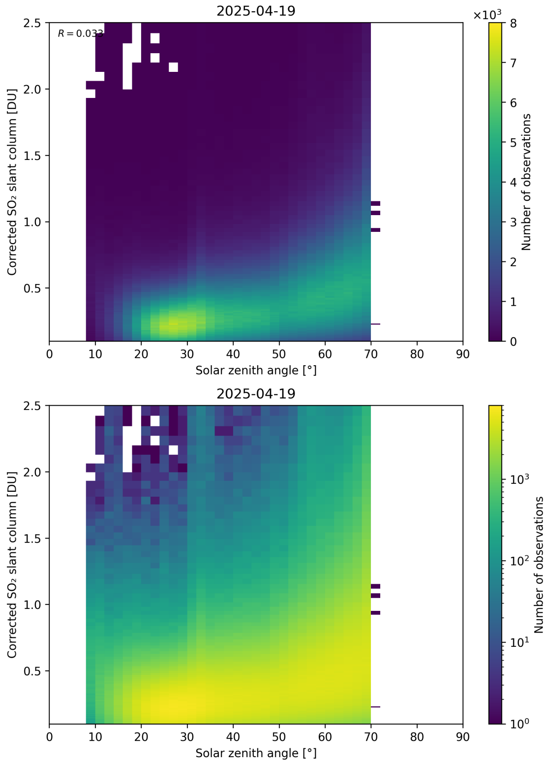
Figure 181: Scatter density plot of “Solar zenith angle” against “Corrected SO 2 slant column” for 2025-04-19 to 2025-04-20.
