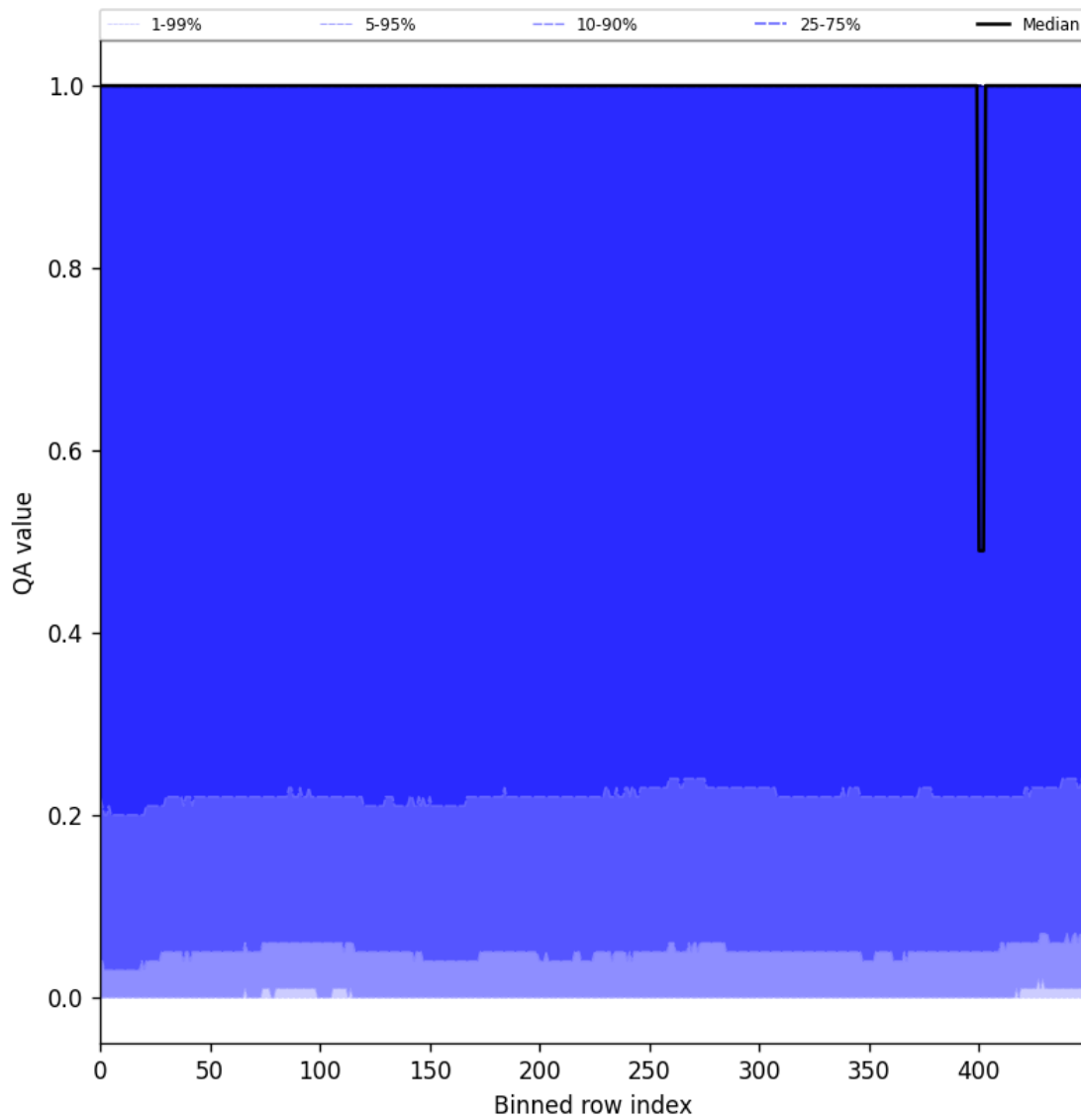
Figure 83: Along track statistics of “QA value” for 2025-04-19 to 2025-04-20
