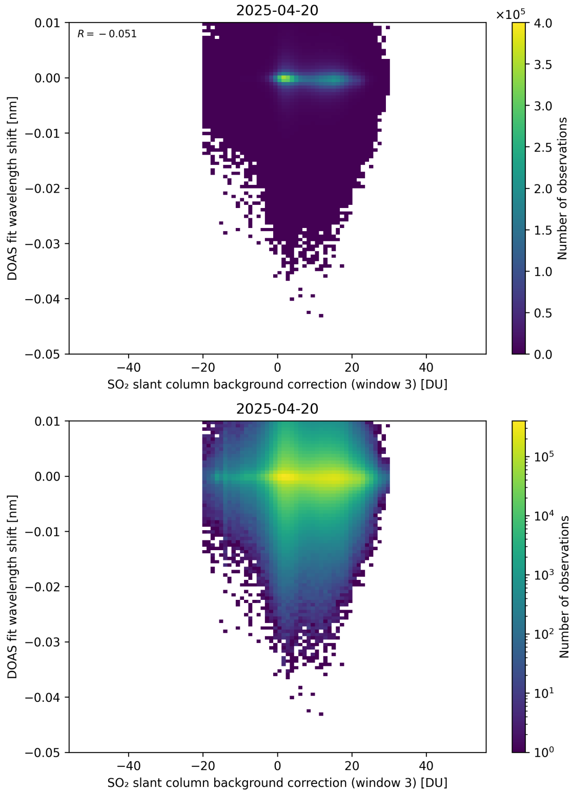
Figure 132: Scatter density plot of “SO 2 slant column background correction (window 3)” against “DOAS fit wavelength shift” for 2025-04-19 to 2025-04-21.
