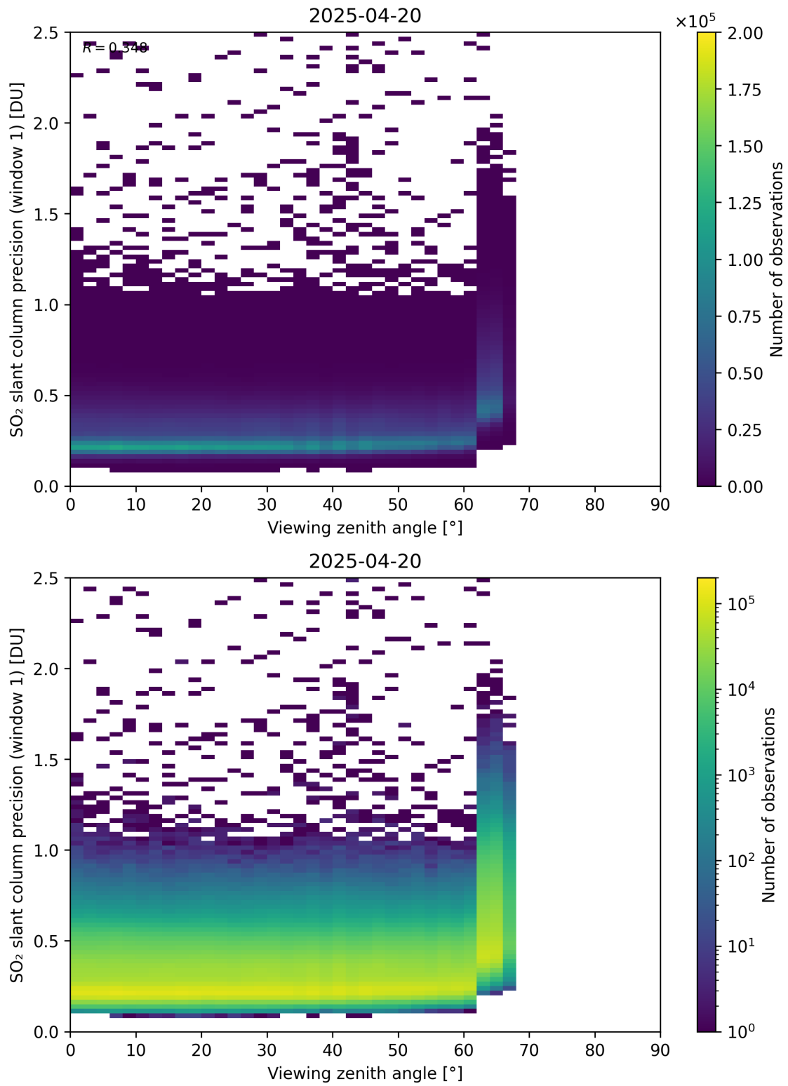
Figure 377: Scatter density plot of “Viewing zenith angle” against “SO 2 slant column precision (window 1)” for 2025-04-19 to 2025-04-21.
