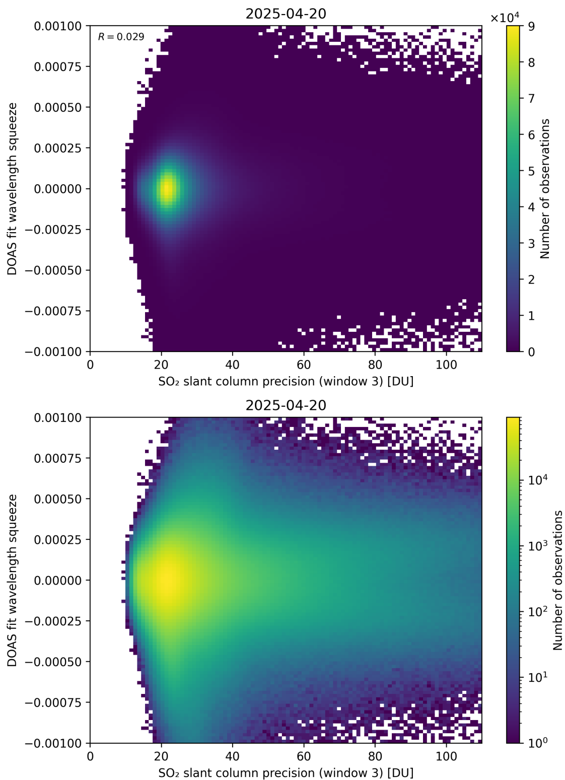
Figure 309: Scatter density plot of “SO 2 slant column precision (window 3)” against “DOAS fit wavelength squeeze” for 2025-04-19 to 2025-04-21.
