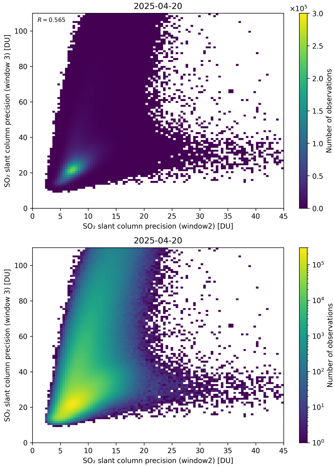
Figure 300: Scatter density plot of “SO 2 slant column precision (window2)” against “SO 2 slant column precision (window 3)” for 2025-04-19 to 2025-04-21.
