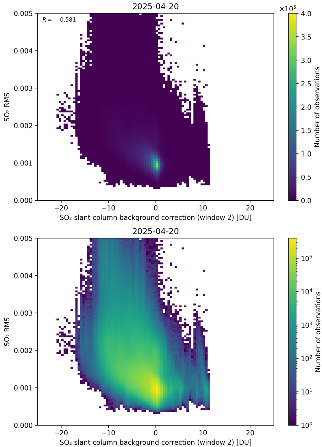
Figure 125: Scatter density plot of “SO 2 slant column background correction (window 2)” against “SO 2 RMS” for 2025-04-19 to 2025-04-21.
