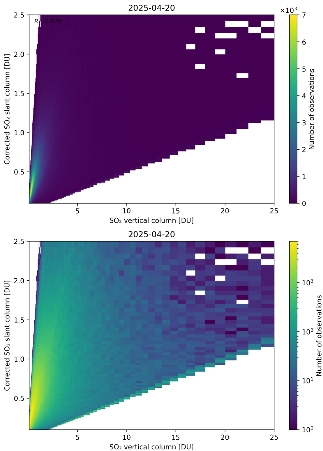
Figure 351: Scatter density plot of “SO 2 vertical column” against “Corrected SO 2 slant column” for 2025-04-19 to 2025-04-21.
