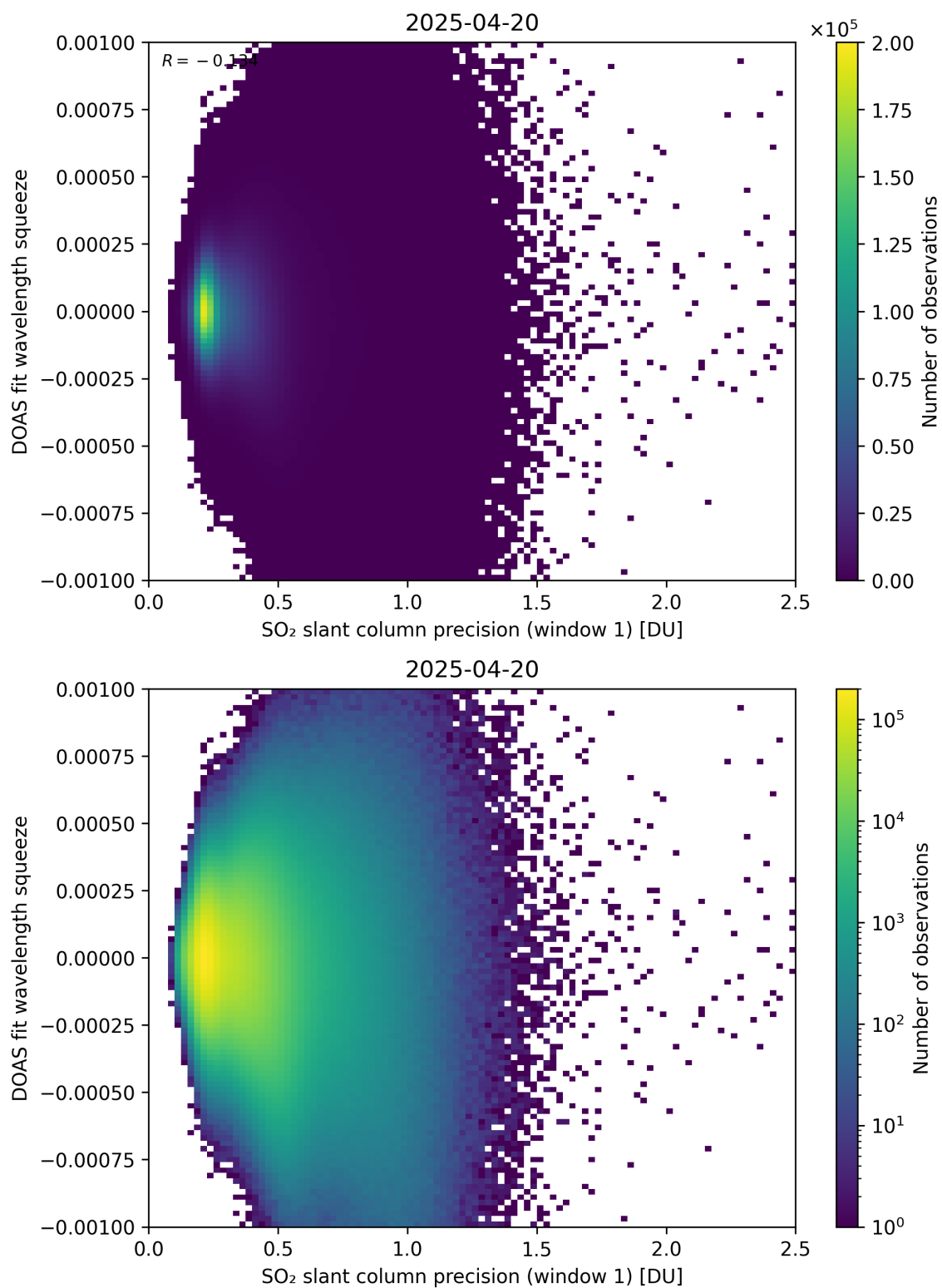
Figure 272: Scatter density plot of “SO 2 slant column precision (window 1)” against “DOAS fit wavelength squeeze” for 2025-04-19 to 2025-04-21.
