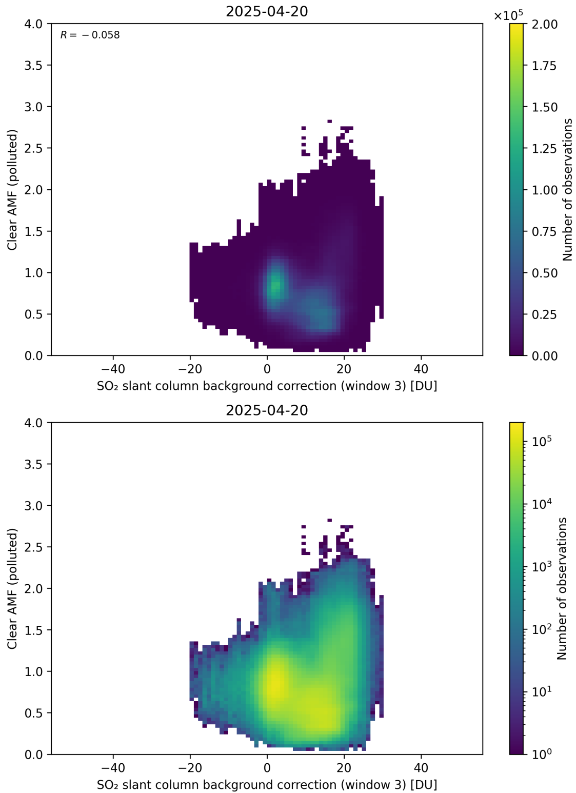
Figure 135: Scatter density plot of “SO 2 slant column background correction (window 3)” against “Clear AMF (polluted)” for 2025-04-19 to 2025-04-21.
