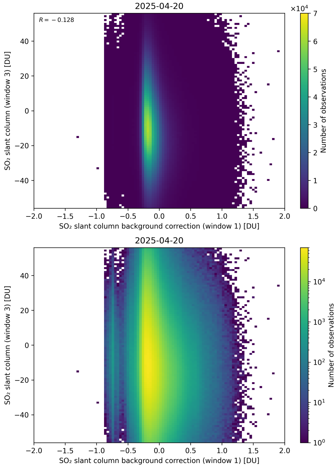
Figure 118: Scatter density plot of “SO 2 slant column background correction (window 1)” against “SO 2 slant column (window 3)” for 2025-04-19 to 2025-04-21.
