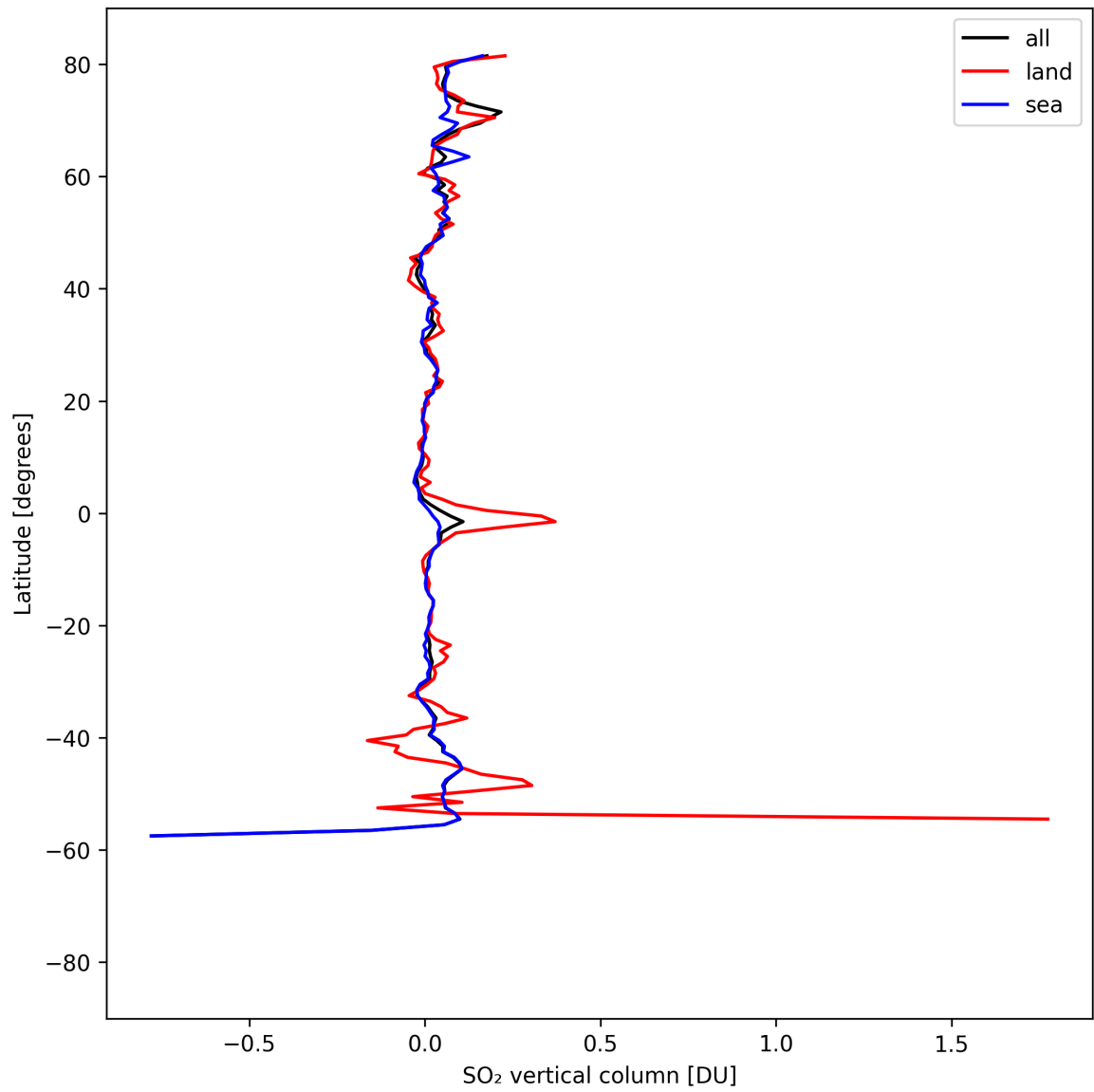
Figure 32: Zonal average of “SO 2 vertical column” for 2025-04-19 to 2025-04-21.
