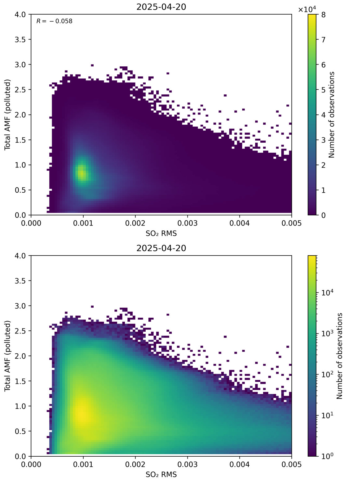
Figure 148: Scatter density plot of “SO 2 RMS” against “Total AMF (polluted)” for 2025-04-19 to 2025-04-21.
