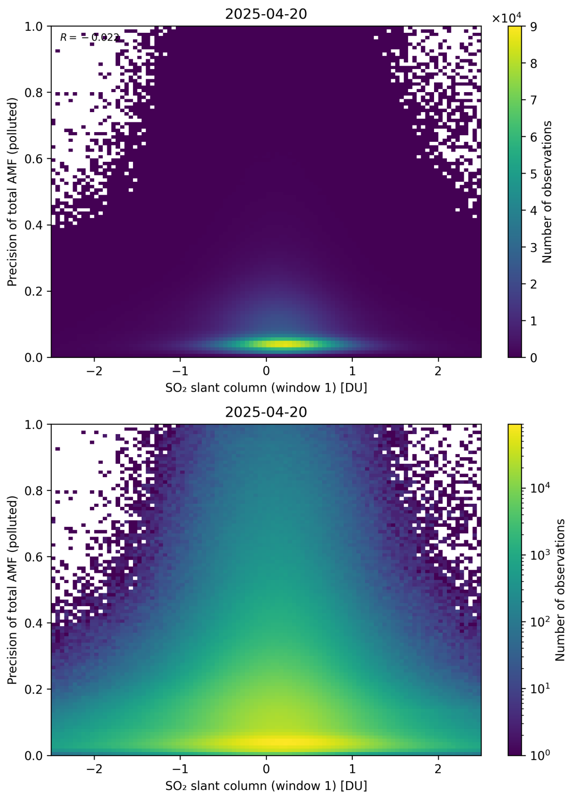
Figure 290: Scatter density plot of “SO 2 slant column (window 1)” against “Precision of total AMF (polluted)” for 2025-04-19 to 2025-04-21.
