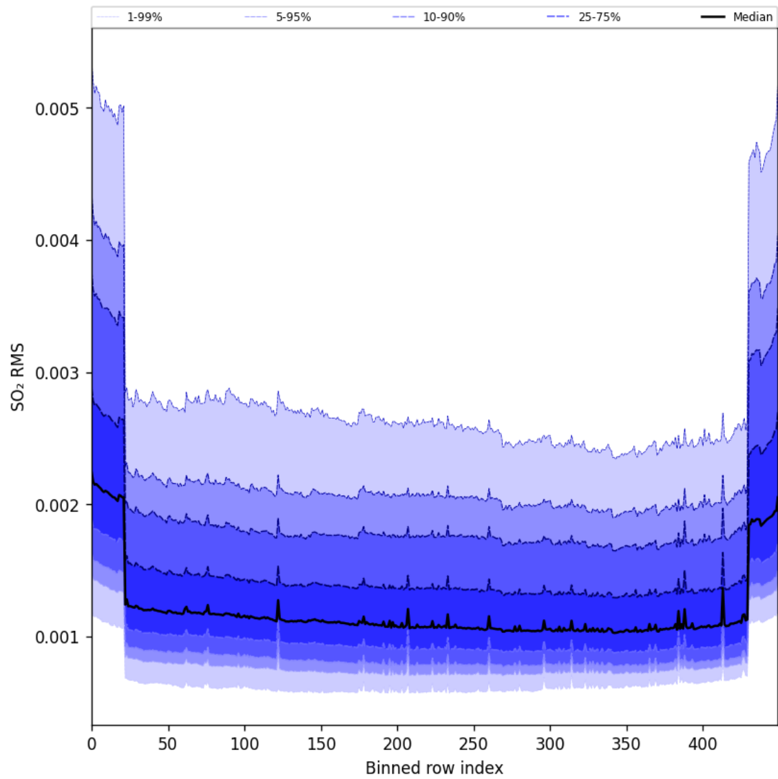
Figure 104: Along track statistics of “SO 2 RMS” for 2025-04-19 to 2025-04-21
