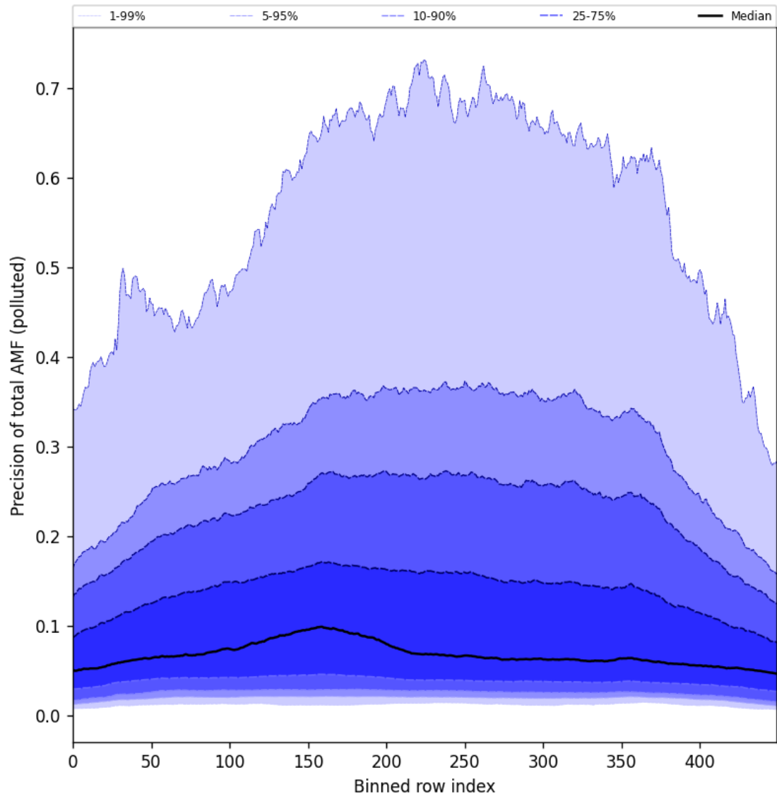
Figure 106: Along track statistics of “Precision of total AMF (polluted)” for 2025-04-19 to 2025-04-21
