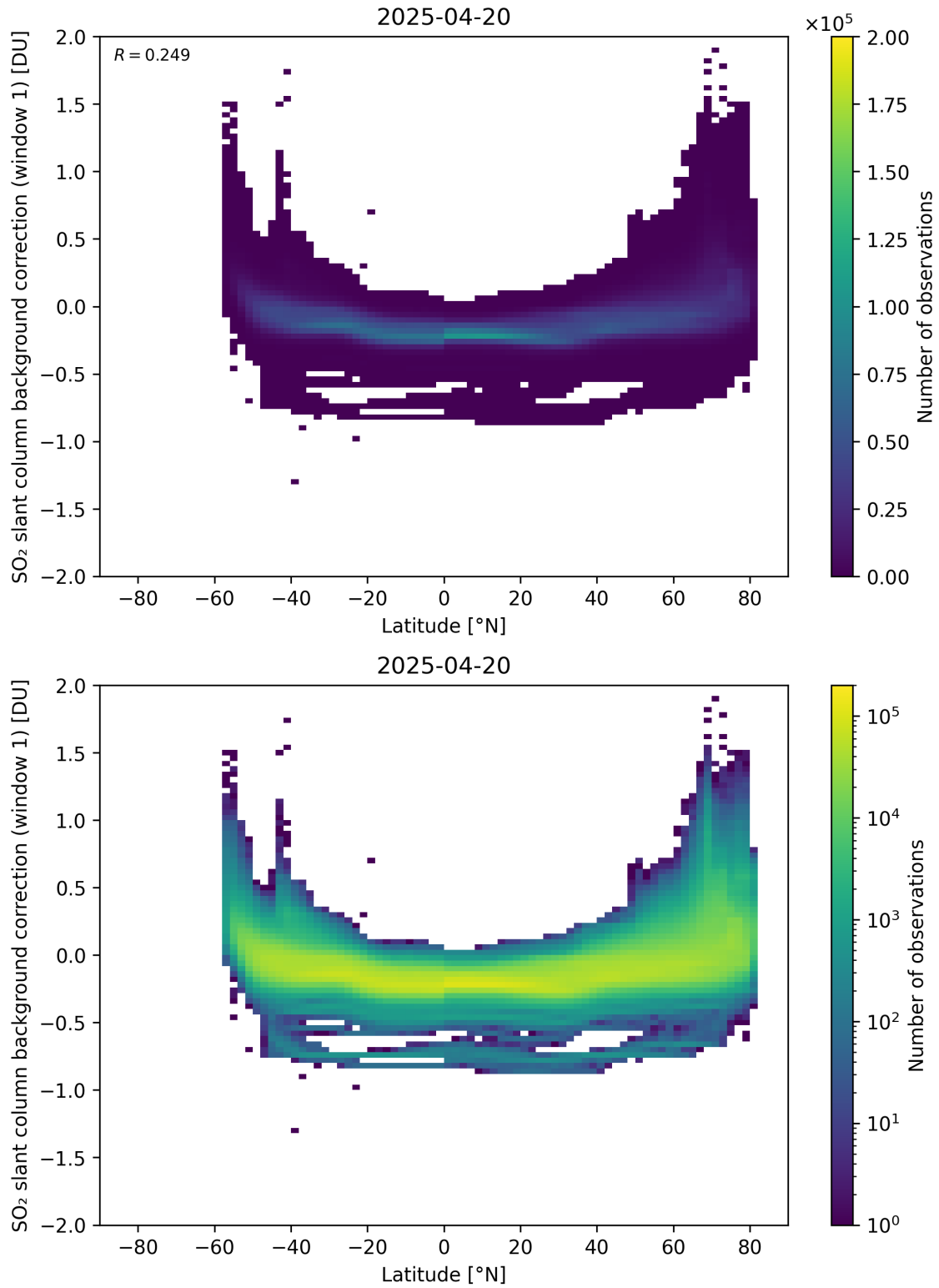
Figure 150: Scatter density plot of “Latitude” against “SO 2 slant column background correction (window 1)” for 2025-04-19 to 2025-04-21.
