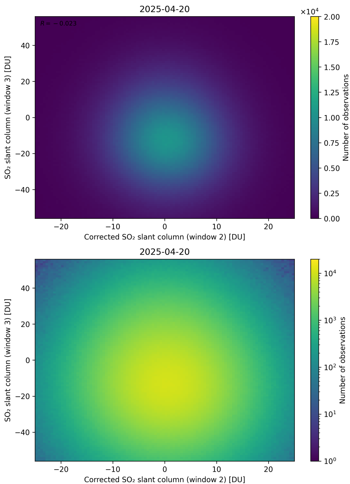
Figure 251: Scatter density plot of “Corrected SO 2 slant column (window 2)” against “SO 2 slant column (window 3)” for 2025-04-19 to 2025-04-21.
