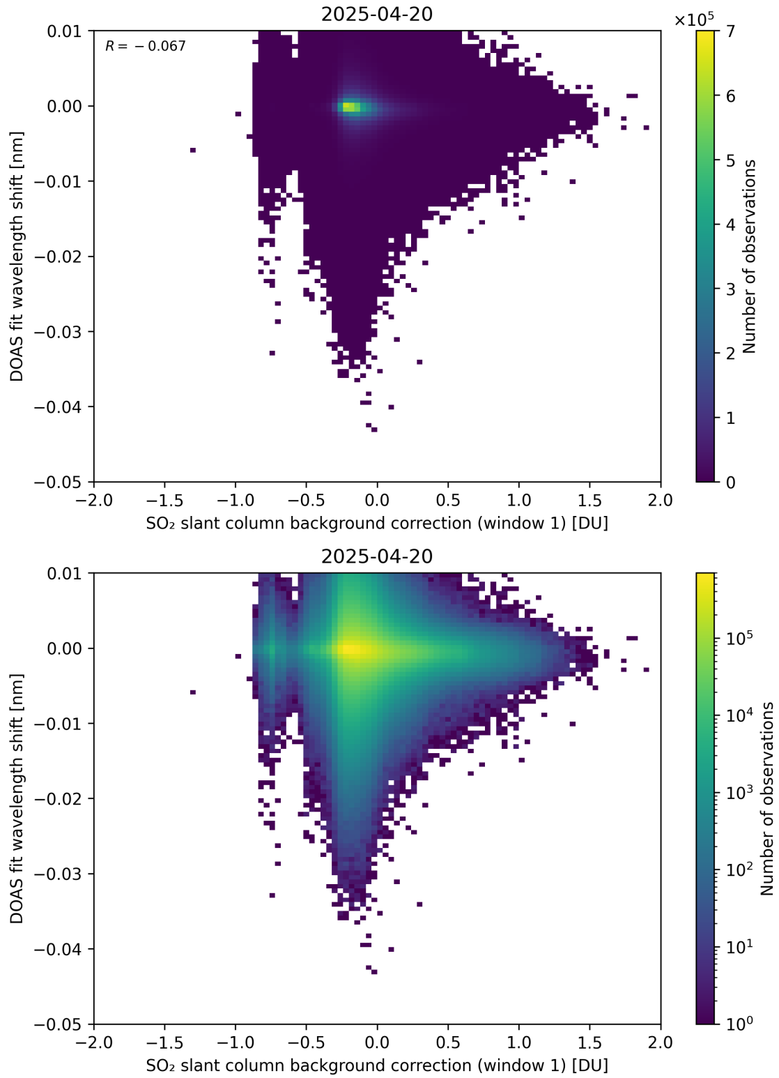
Figure 111: Scatter density plot of “SO 2 slant column background correction (window 1)” against “DOAS fit wavelength shift” for 2025-04-19 to 2025-04-21.
