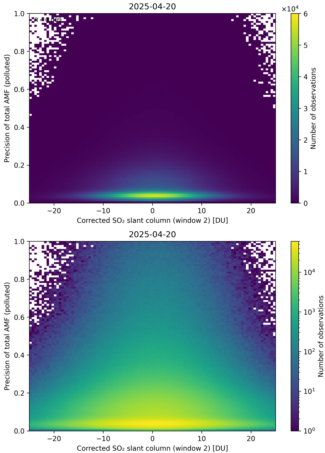
Figure 254: Scatter density plot of “Corrected SO 2 slant column (window 2)” against “Precision of total AMF (polluted)” for 2025-04-19 to 2025-04-21.
