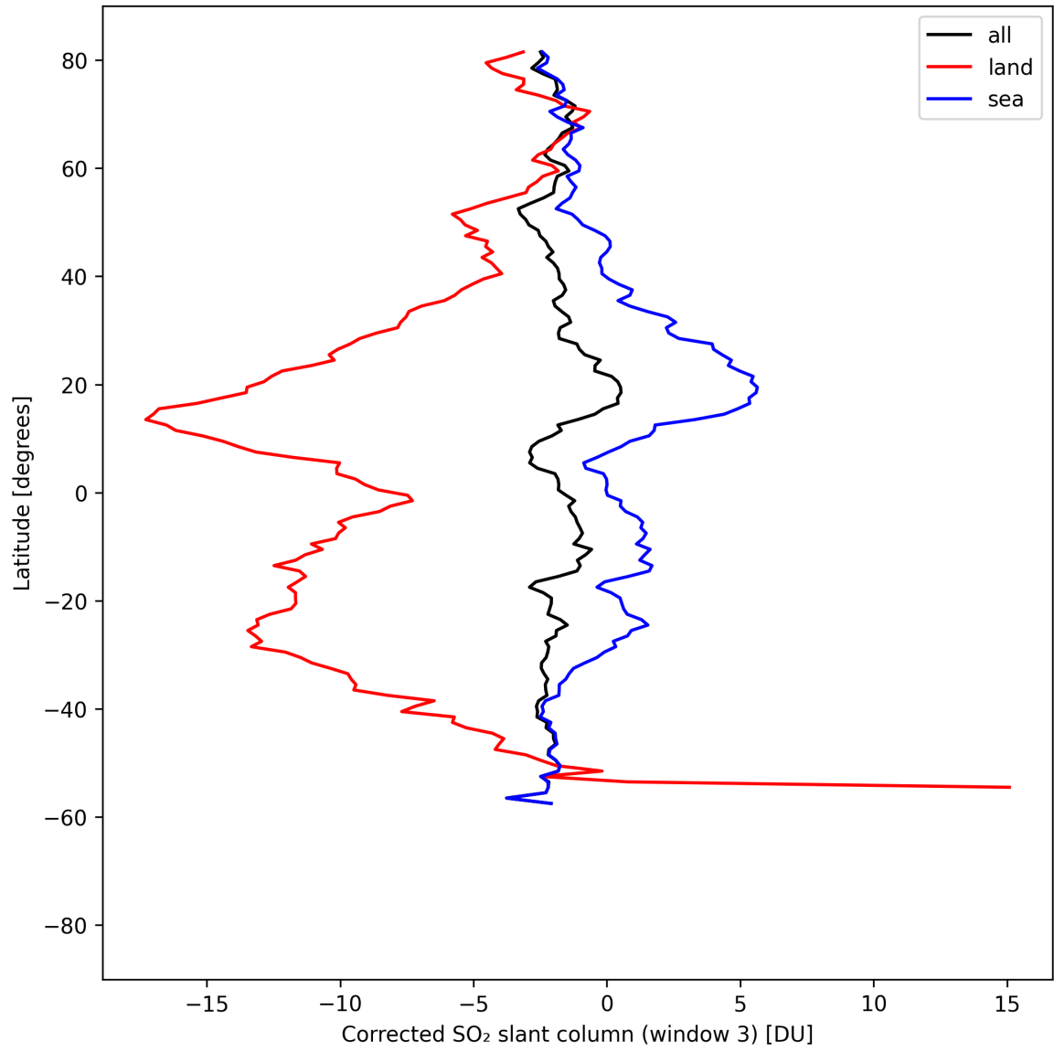
Figure 47: Zonal average of “Corrected SO 2 slant column (window 3)” for 2025-04-19 to 2025-04-21.
