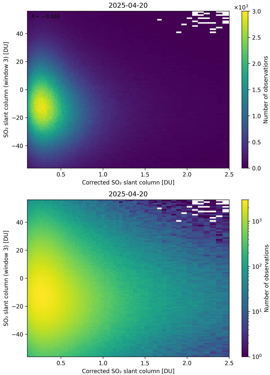
Figure 240: Scatter density plot of “Corrected SO 2 slant column” against “SO 2 slant column (window 3)” for 2025-04-19 to 2025-04-21.
