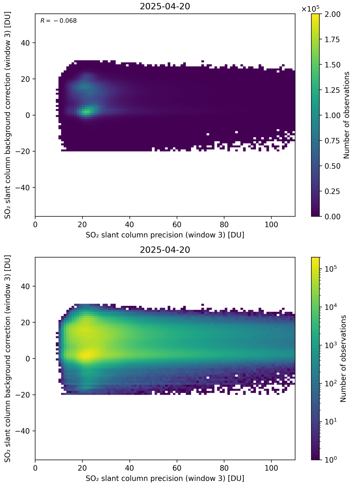
Figure 307: Scatter density plot of “SO 2 slant column precision (window 3)” against “SO 2 slant column background correction (window 3)” for 2025-04-19 to 2025-04-21.
