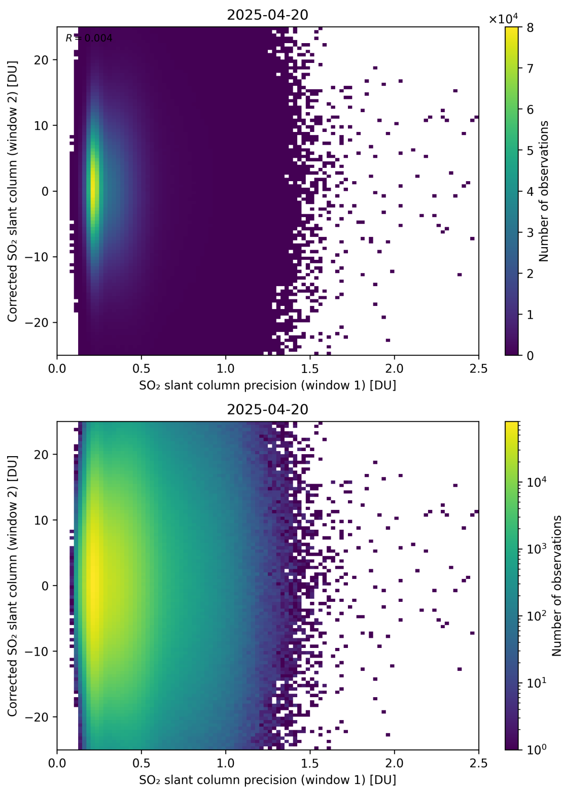
Figure 275: Scatter density plot of “SO 2 slant column precision (window 1)” against “Corrected SO 2 slant column (window 2)” for 2025-04-19 to 2025-04-21.
