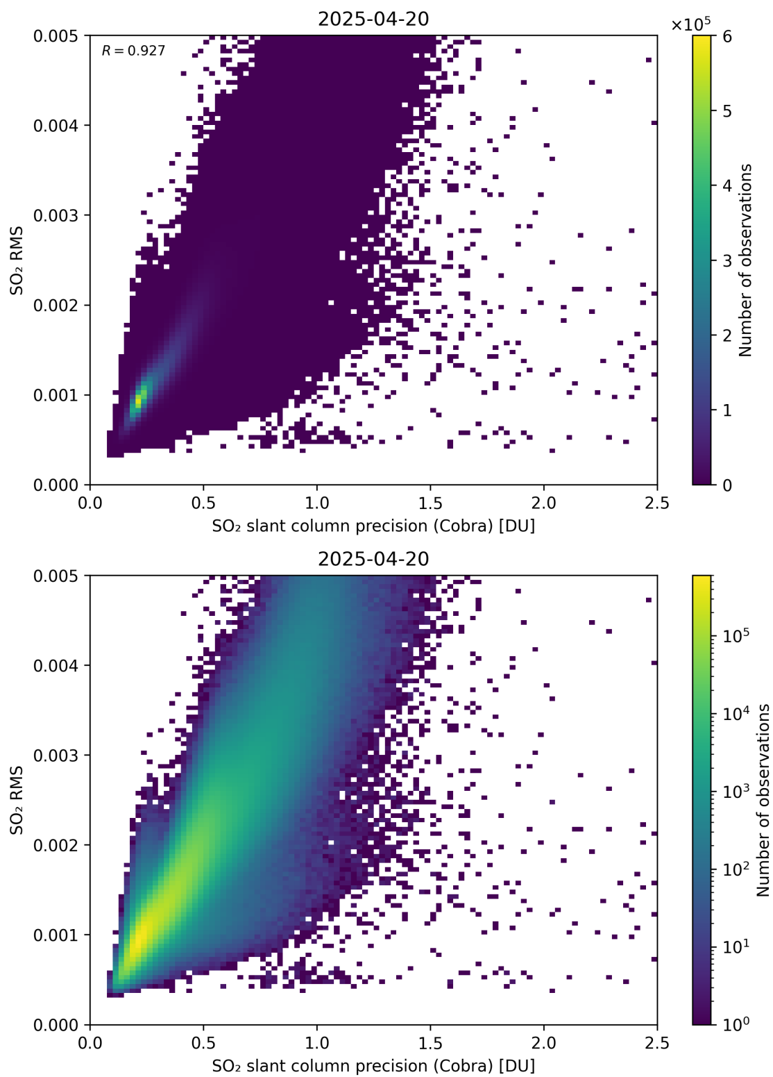
Figure 204: Scatter density plot of “SO 2 slant column precision (Cobra)” against “SO 2 RMS” for 2025-04-19 to 2025-04-21.
