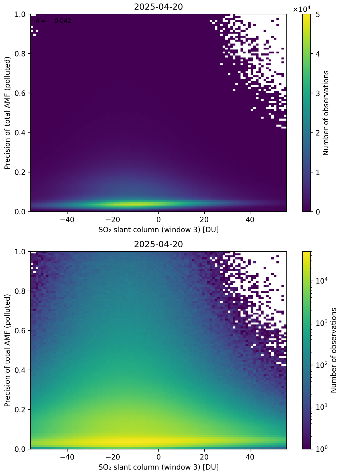
Figure 319: Scatter density plot of “SO 2 slant column (window 3)” against “Precision of total AMF (polluted)” for 2025-04-19 to 2025-04-21.
