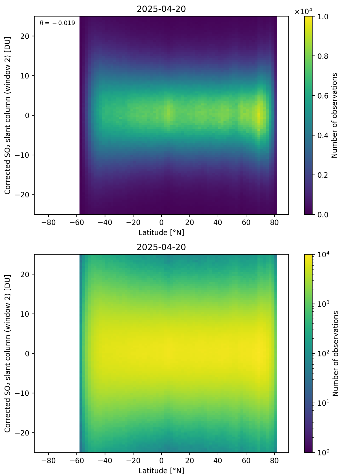
Figure 160: Scatter density plot of “Latitude” against “Corrected SO 2 slant column (window 2)” for 2025-04-19 to 2025-04-21.
