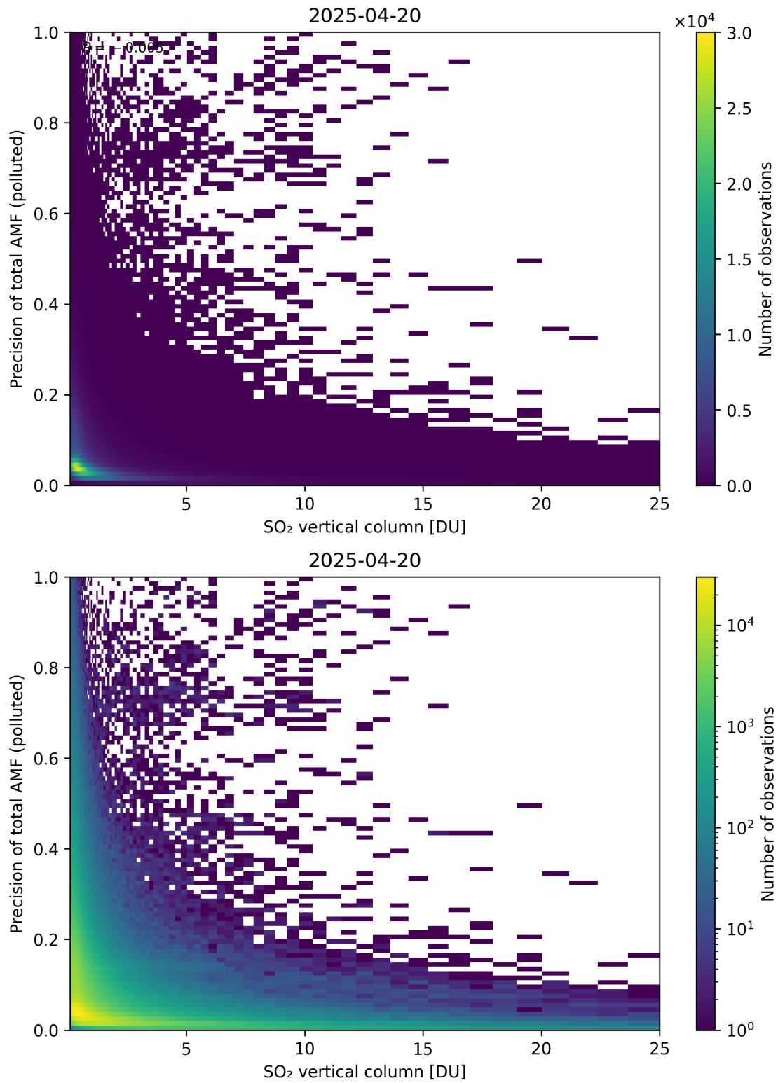
Figure 360: Scatter density plot of “SO 2 vertical column” against “Precision of total AMF (polluted)” for 2025-04-19 to 2025-04-21.
