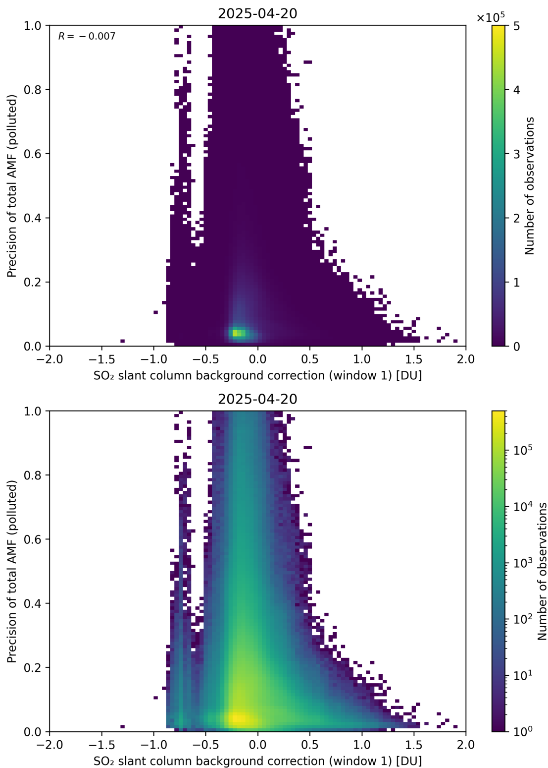
Figure 121: Scatter density plot of “SO 2 slant column background correction (window 1)” against “Precision of total AMF (polluted)” for 2025-04-19 to 2025-04-21.
