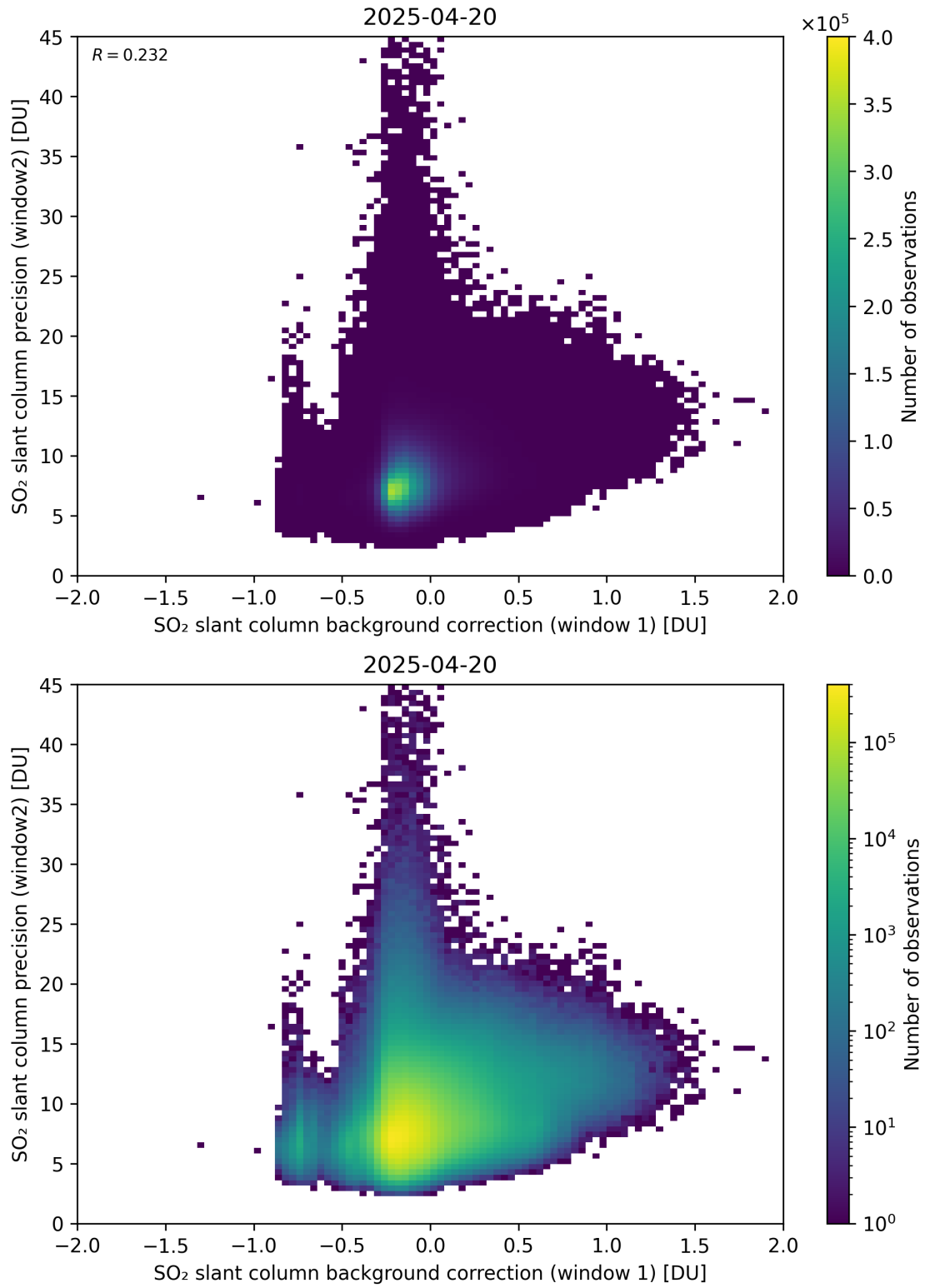
Figure 117: Scatter density plot of “SO 2 slant column background correction (window 1)” against “SO 2 slant column precision (window2)” for 2025-04-19 to 2025-04-21.
