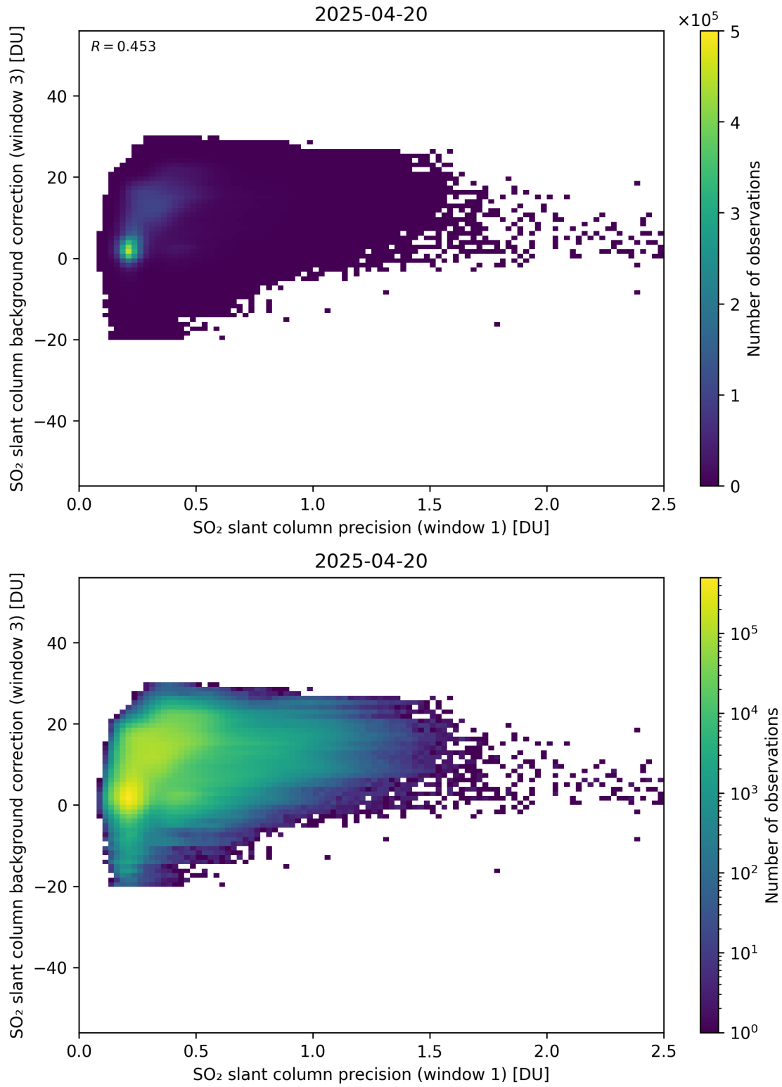
Figure 270: Scatter density plot of “SO 2 slant column precision (window 1)” against “SO 2 slant column background correction (window 3)” for 2025-04-19 to 2025-04-21.
