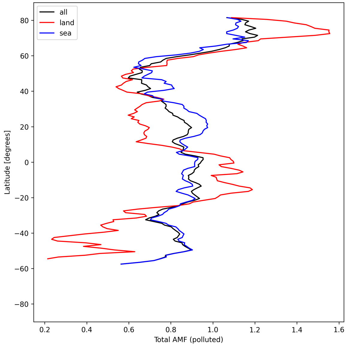
Figure 53: Zonal average of “Total AMF (polluted)” for 2025-04-19 to 2025-04-21.
