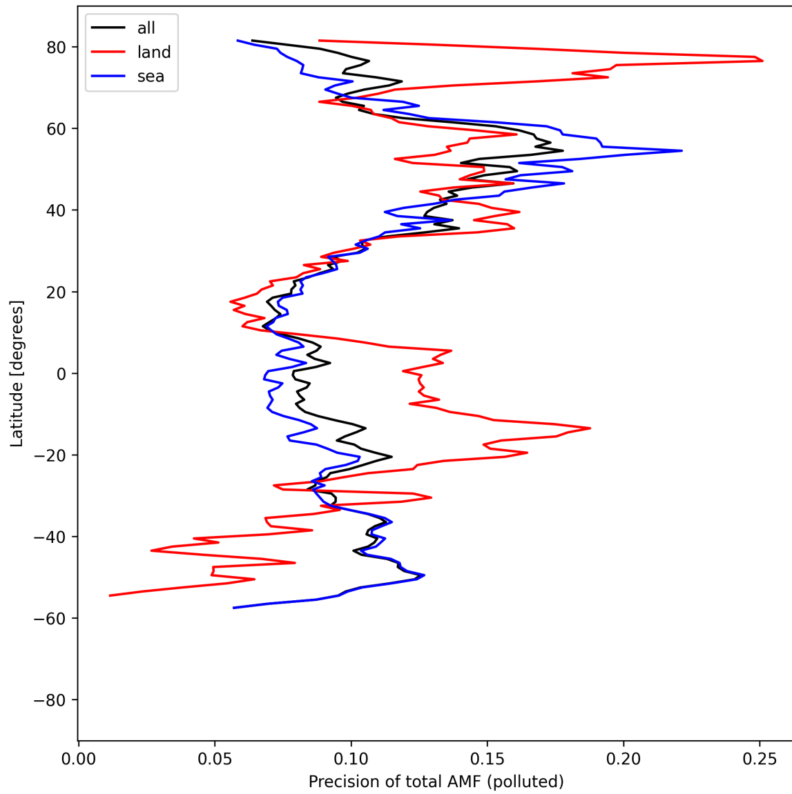
Figure 54: Zonal average of “Precision of total AMF (polluted)” for 2025-04-19 to 2025-04-21.
