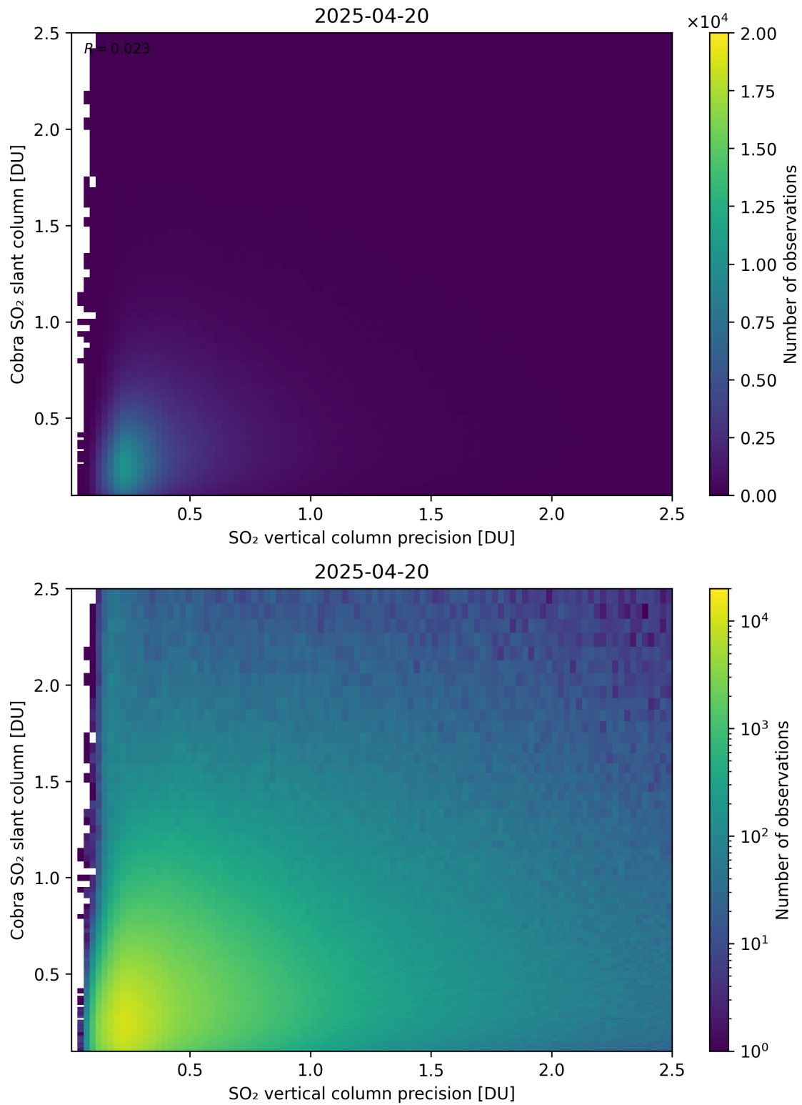
Figure 336: Scatter density plot of “SO 2 vertical column precision” against “Cobra SO 2 slant column” for 2025-04-19 to 2025-04-21.
