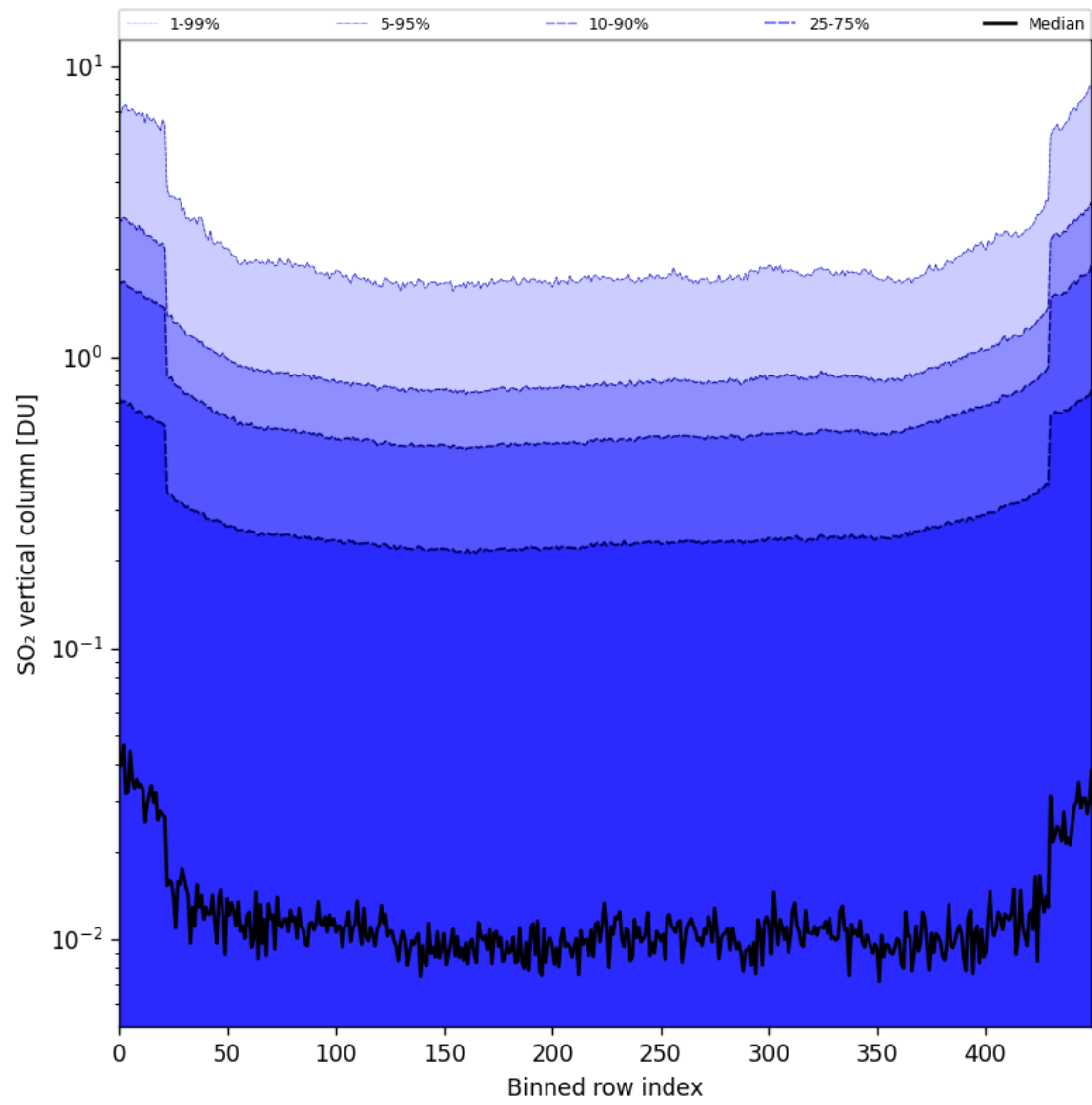
Figure 84: Along track statistics of “SO 2 vertical column” for 2025-04-19 to 2025-04-21
