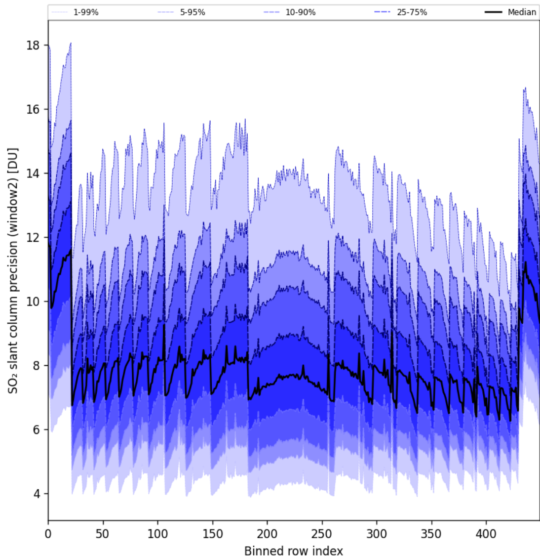
Figure 94: Along track statistics of “SO 2 slant column precision (window2)” for 2025-04-19 to 2025-04-21
