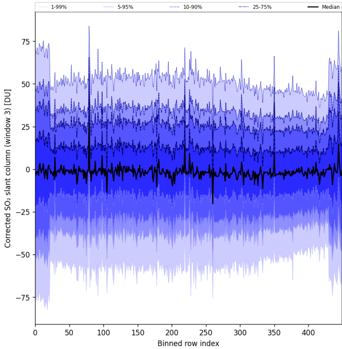
Figure 99: Along track statistics of “Corrected SO 2 slant column (window 3)” for 2025-04-19 to 2025-04-21
