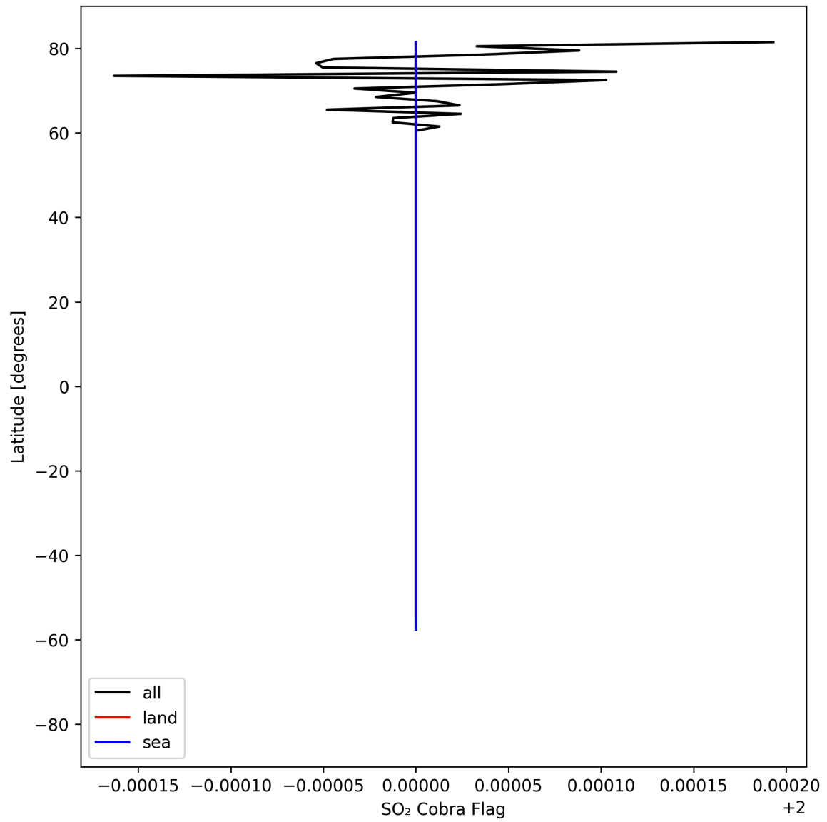
Figure 49: Zonal average of "SO 2 Cobra Flag" for 2025-04-19 to 2025-04-21.
