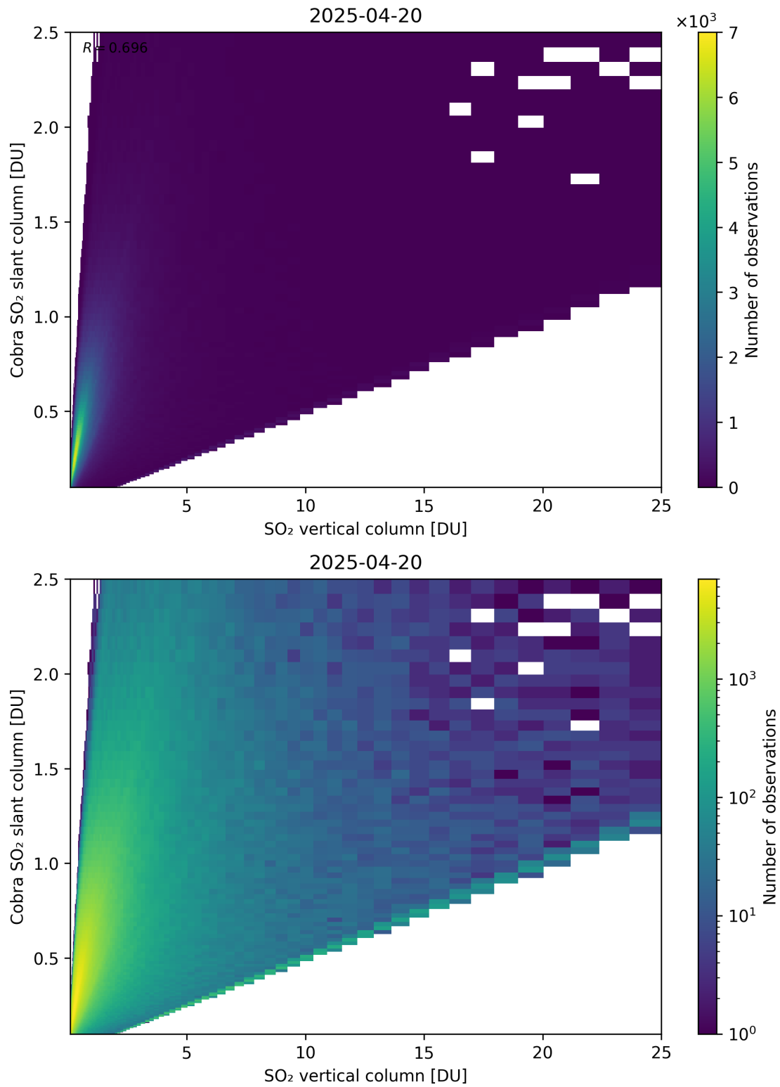
Figure 349: Scatter density plot of “SO 2 vertical column” against “Cobra SO 2 slant column” for 2025-04-19 to 2025-04-21.
