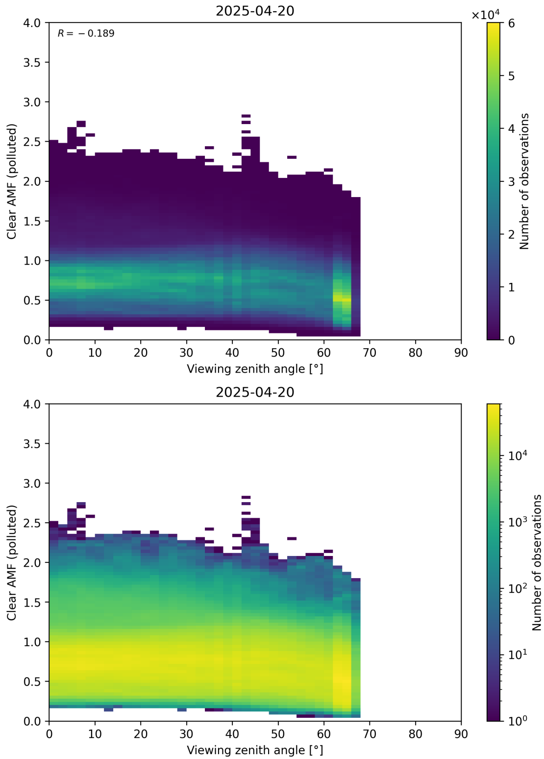
Figure 370: Scatter density plot of “Viewing zenith angle” against “Clear AMF (polluted)” for 2025-04-19 to 2025-04-21.
