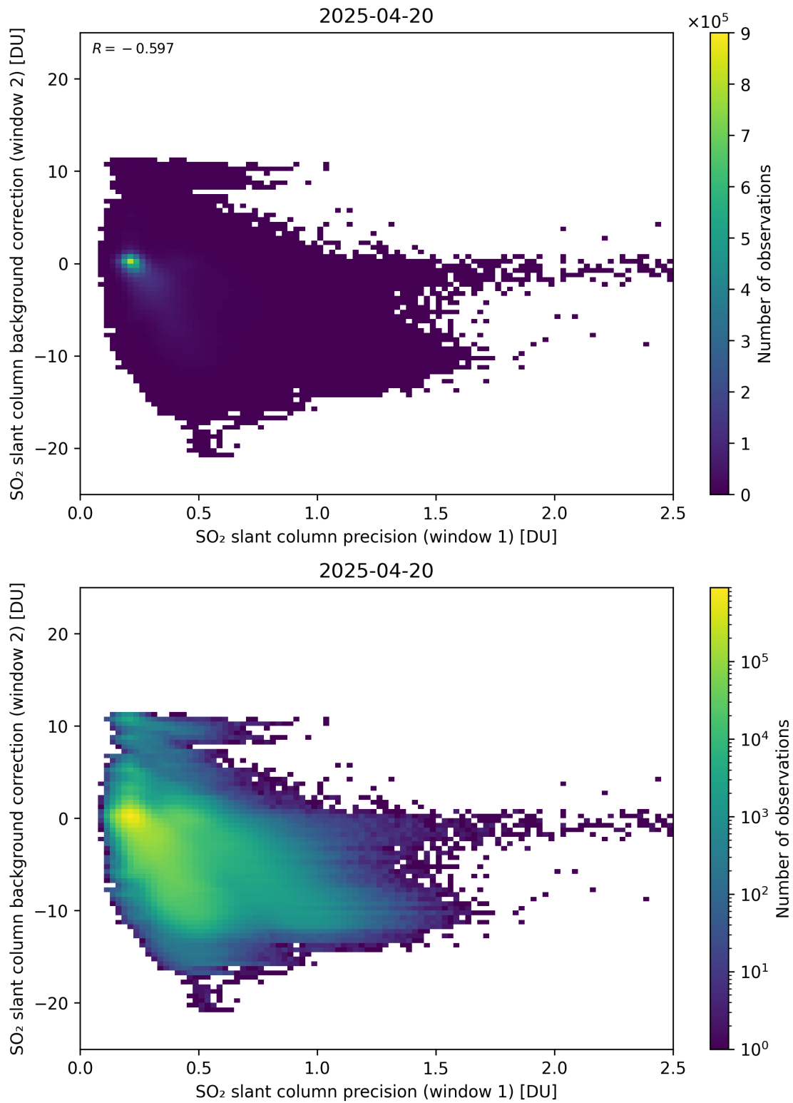
Figure 269: Scatter density plot of “SO 2 slant column precision (window 1)” against “SO 2 slant column background correction (window 2)” for 2025-04-19 to 2025-04-21.
