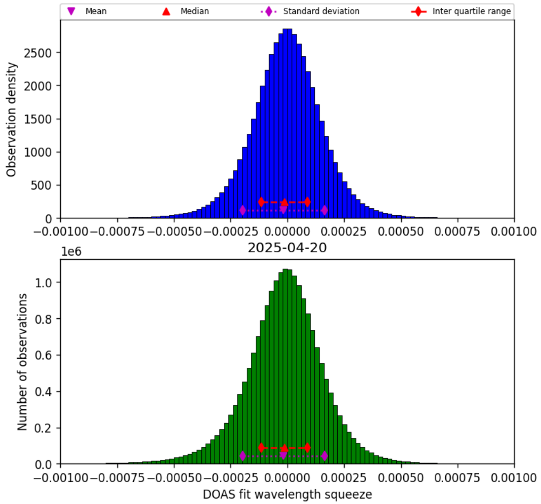
Figure 77: Histogram of “DOAS fit wavelength squeeze” for 2025-04-19 to 2025-04-21
