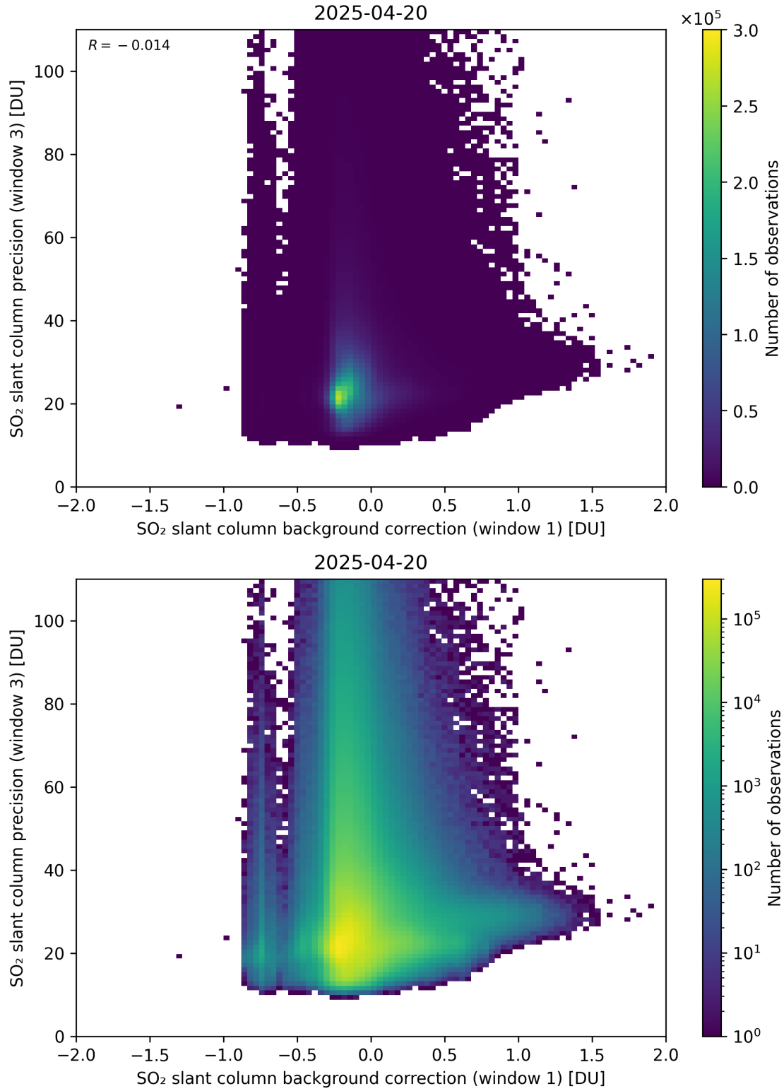
Figure 119: Scatter density plot of “SO 2 slant column background correction (window 1)” against “SO 2 slant column precision (window 3)” for 2025-04-19 to 2025-04-21.
