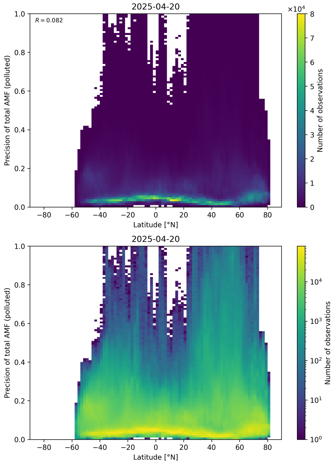
Figure 168: Scatter density plot of “Latitude” against “Precision of total AMF (polluted)” for 2025-04-19 to 2025-04-21.
