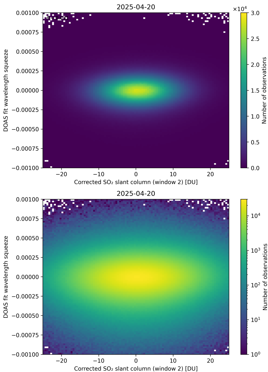
Figure 247: Scatter density plot of “Corrected SO 2 slant column (window 2)” against “DOAS fit wavelength squeeze” for 2025-04-19 to 2025-04-21.
