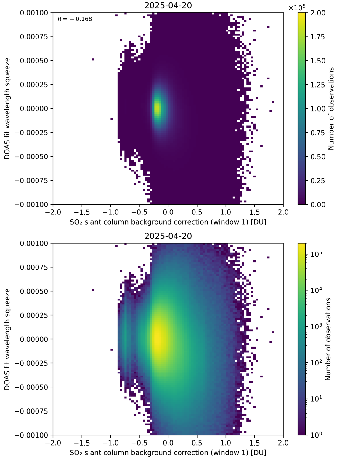
Figure 112: Scatter density plot of “SO 2 slant column background correction (window 1)” against “DOAS fit wavelength squeeze” for 2025-04-19 to 2025-04-21.
