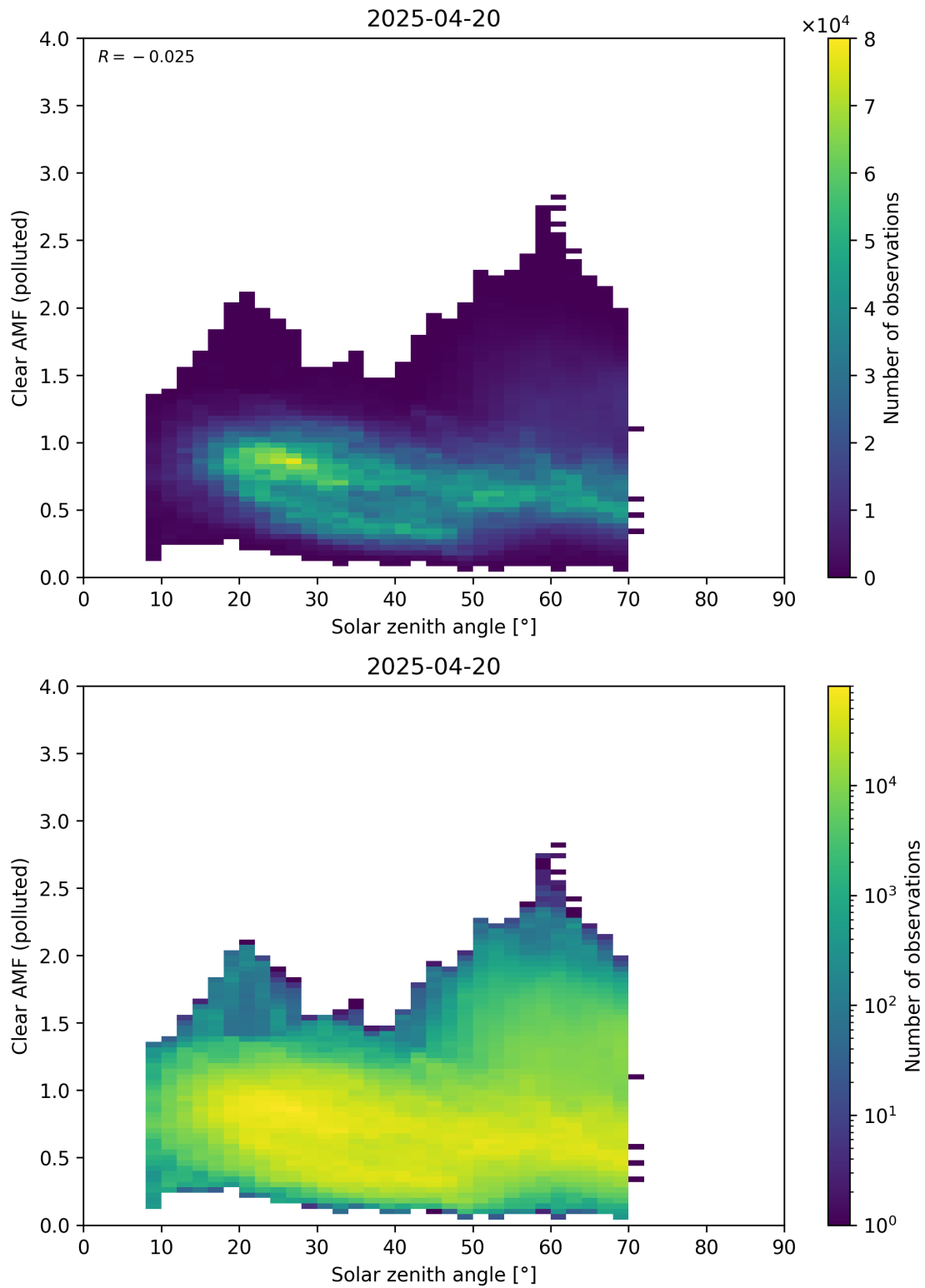
Figure 178: Scatter density plot of “Solar zenith angle” against “Clear AMF (polluted)” for 2025-04-19 to 2025-04-21.
