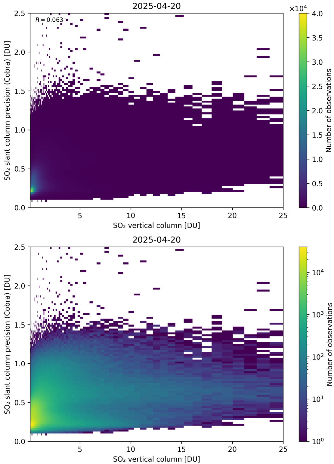
Figure 350: Scatter density plot of “SO 2 vertical column” against “SO 2 slant column precision (Cobra)” for 2025-04-19 to 2025-04-21.
