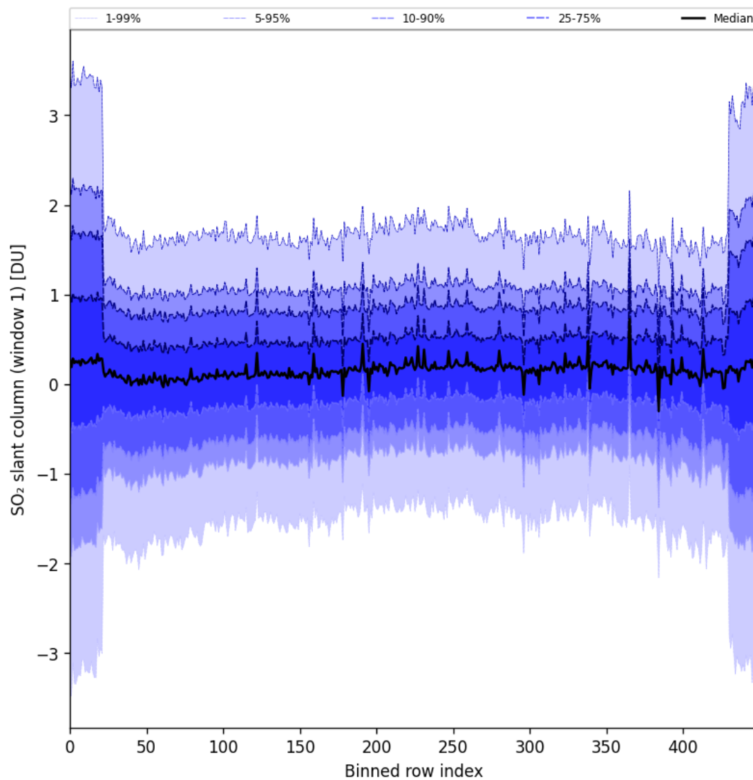
Figure 89: Along track statistics of “SO 2 slant column (window 1)” for 2025-04-19 to 2025-04-21
