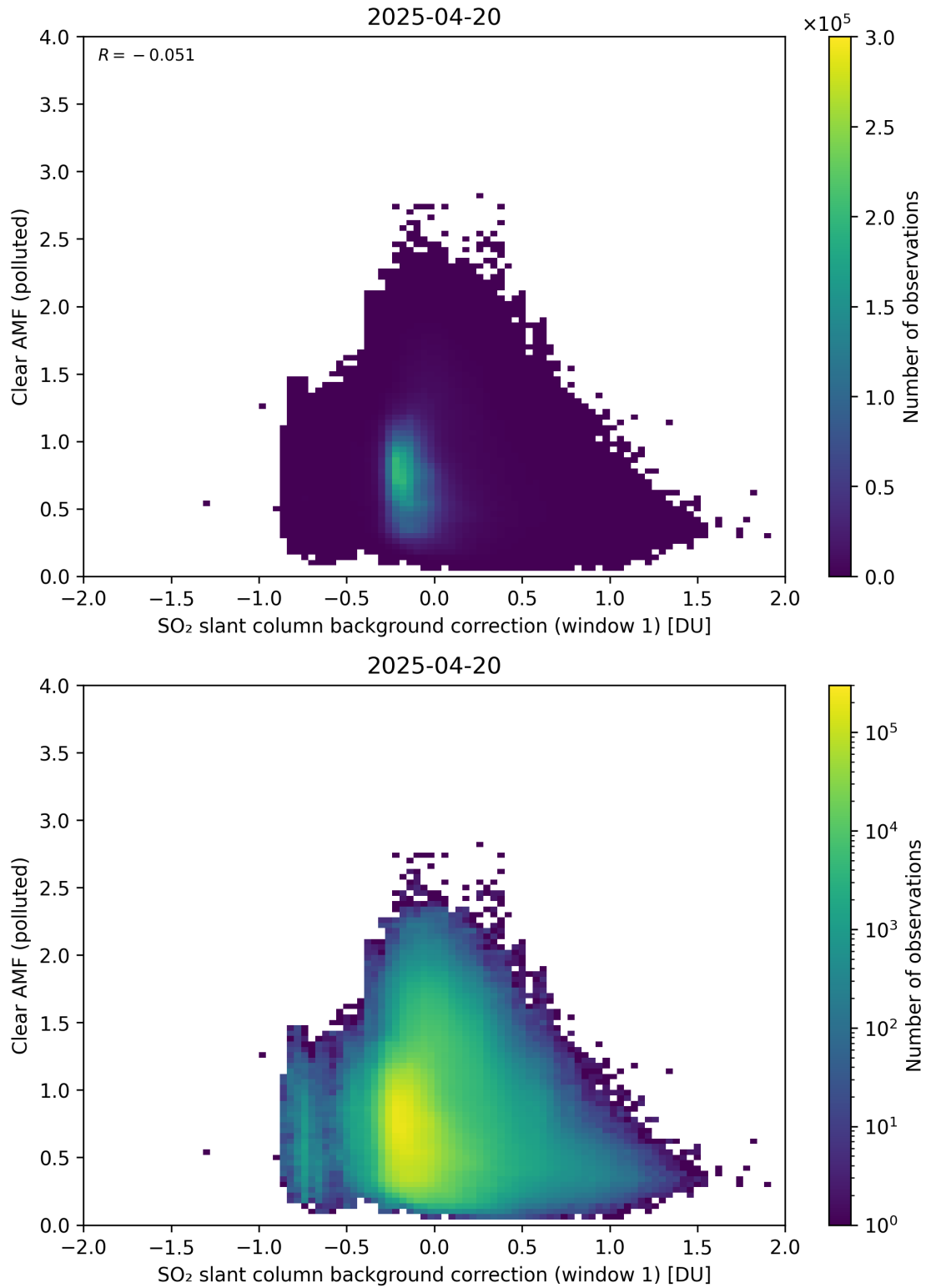
Figure 114: Scatter density plot of “SO 2 slant column background correction (window 1)” against “Clear AMF (polluted)” for 2025-04-19 to 2025-04-21.
