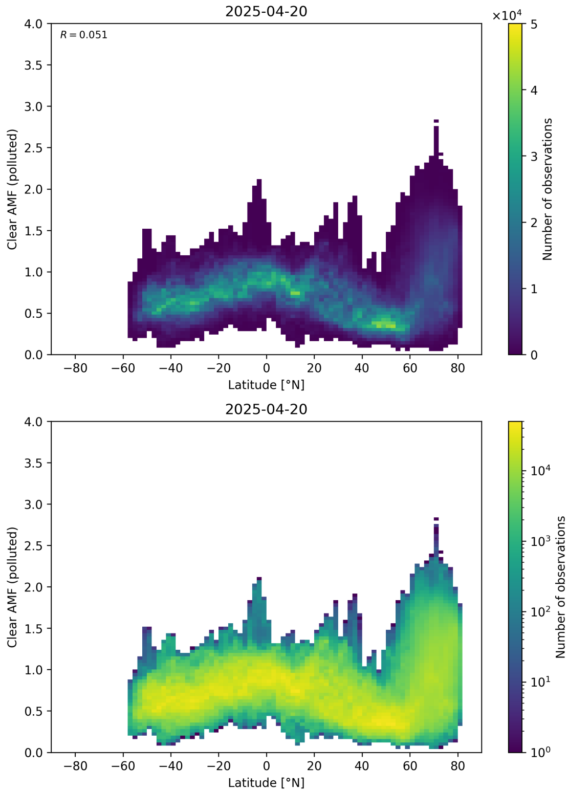
Figure 156: Scatter density plot of “Latitude” against “Clear AMF (polluted)” for 2025-04-19 to 2025-04-21.
