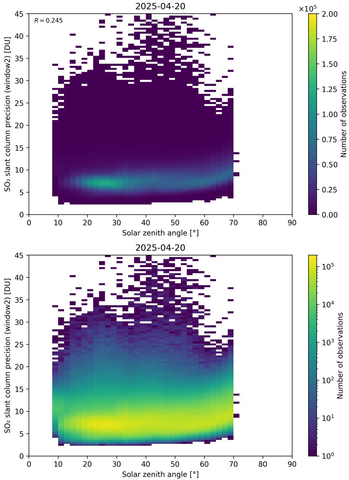
Figure 186: Scatter density plot of “Solar zenith angle” against “SO 2 slant column precision (window2)” for 2025-04-19 to 2025-04-21.
