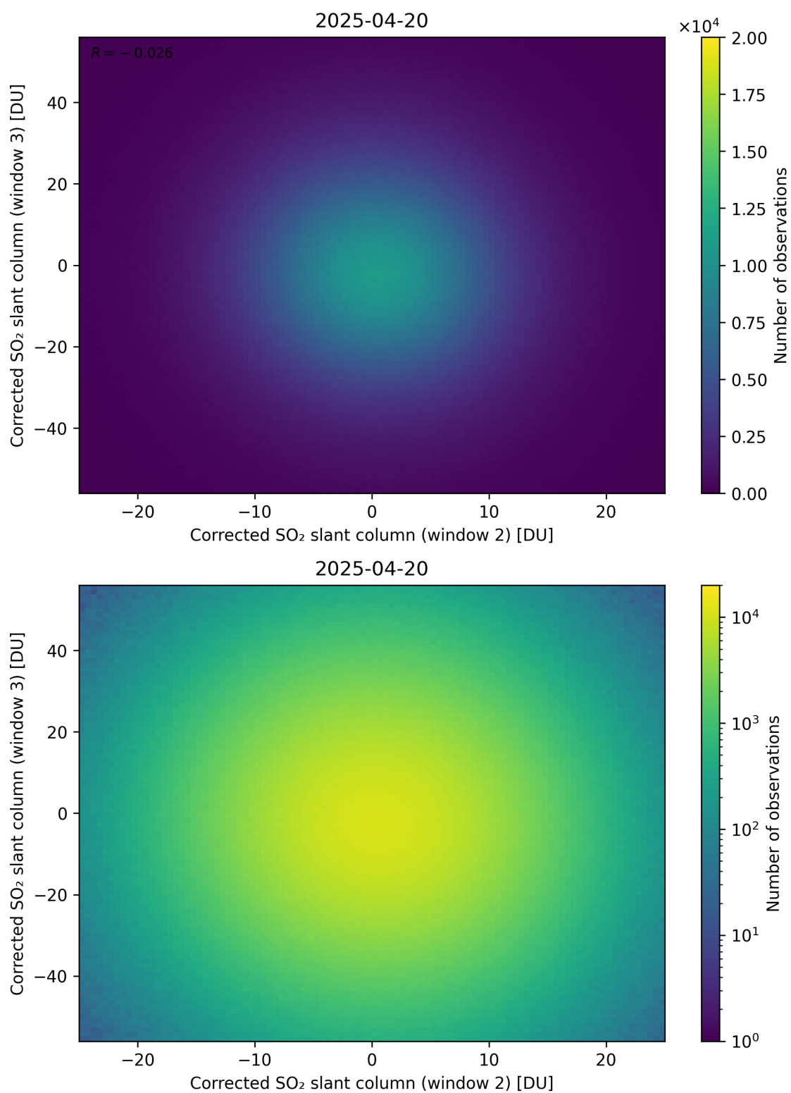
Figure 250: Scatter density plot of “Corrected SO 2 slant column (window 2)” against “Corrected SO 2 slant column (window 3)” for 2025-04-19 to 2025-04-21.
