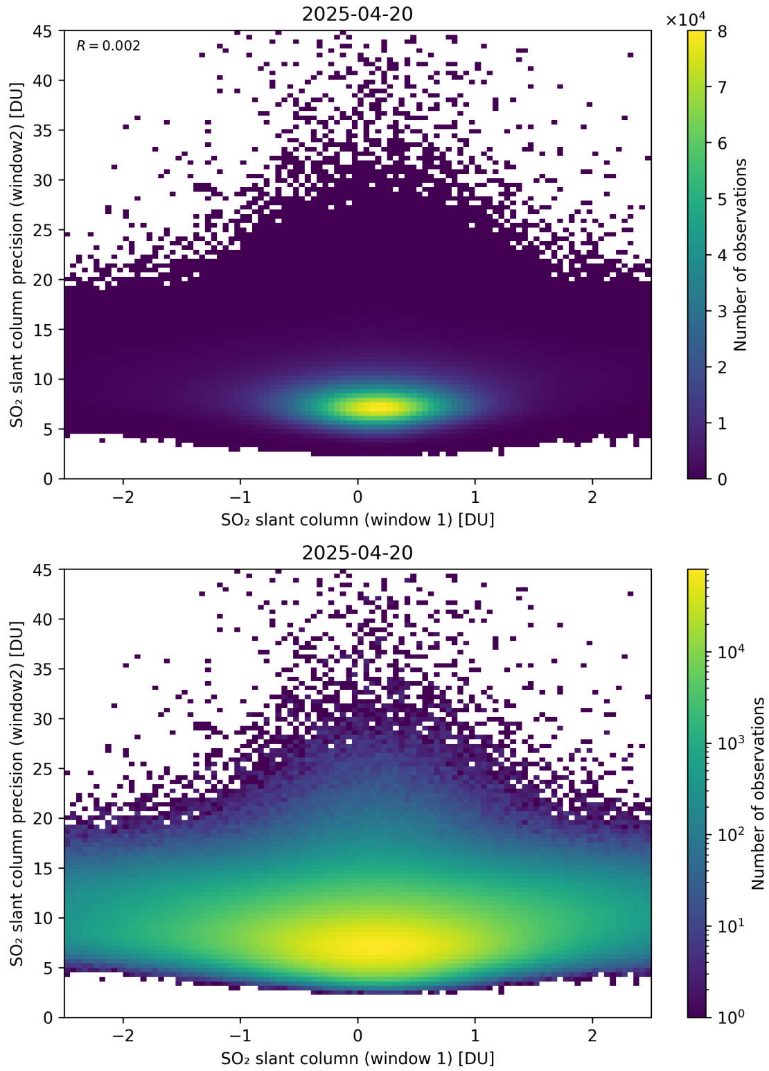
Figure 286: Scatter density plot of “SO 2 slant column (window 1)” against “SO 2 slant column precision (window2)” for 2025-04-19 to 2025-04-21.
