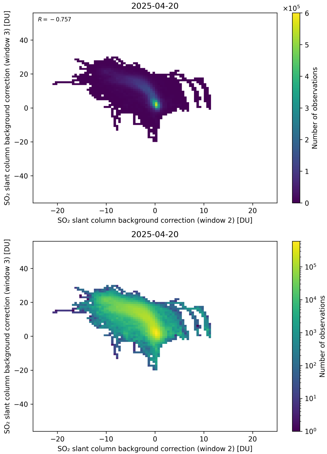
Figure 122: Scatter density plot of “SO 2 slant column background correction (window 2)” against “SO 2 slant column background correction (window 3)” for 2025-04-19 to 2025-04-21.
