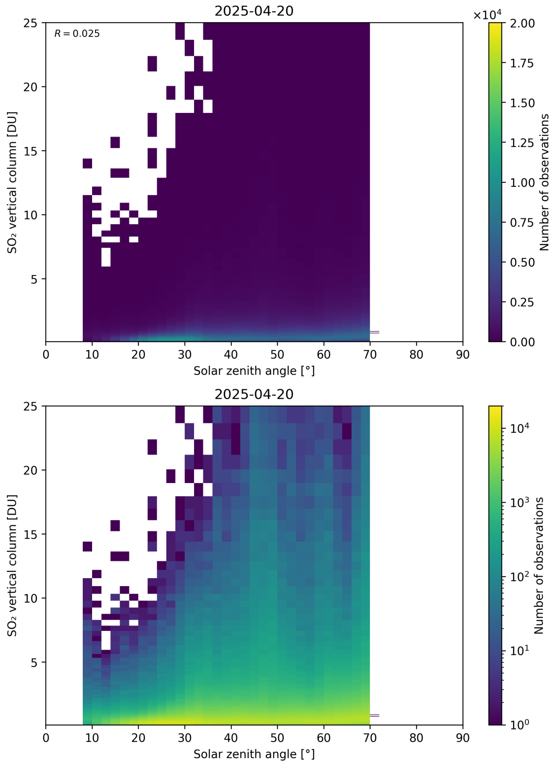
Figure 191: Scatter density plot of “Solar zenith angle” against “SO 2 vertical column” for 2025-04-19 to 2025-04-21.
