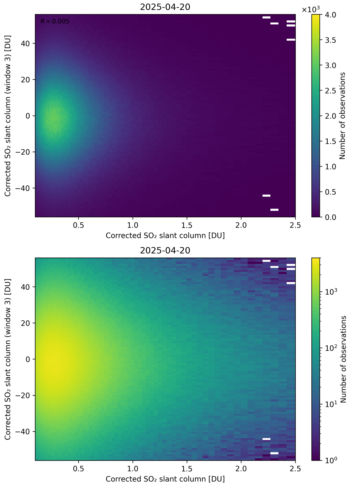
Figure 236: Scatter density plot of “Corrected SO 2 slant column” against “Corrected SO 2 slant column (window 3)” for 2025-04-19 to 2025-04-21.
