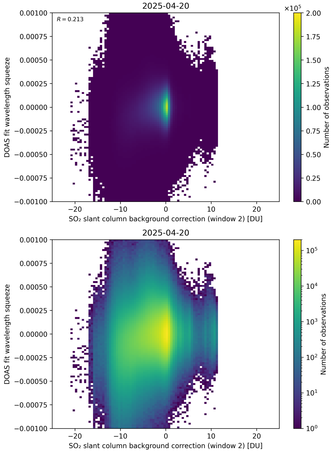
Figure 124: Scatter density plot of “SO 2 slant column background correction (window 2)” against “DOAS fit wavelength squeeze” for 2025-04-19 to 2025-04-21.
