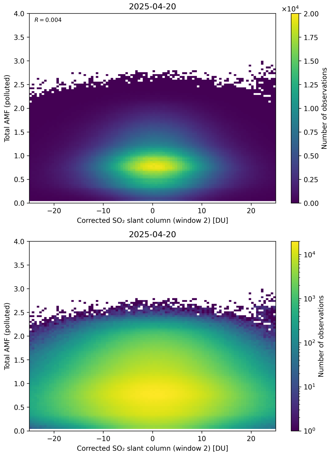
Figure 253: Scatter density plot of “Corrected SO 2 slant column (window 2)” against “Total AMF (polluted)” for 2025-04-19 to 2025-04-21.
