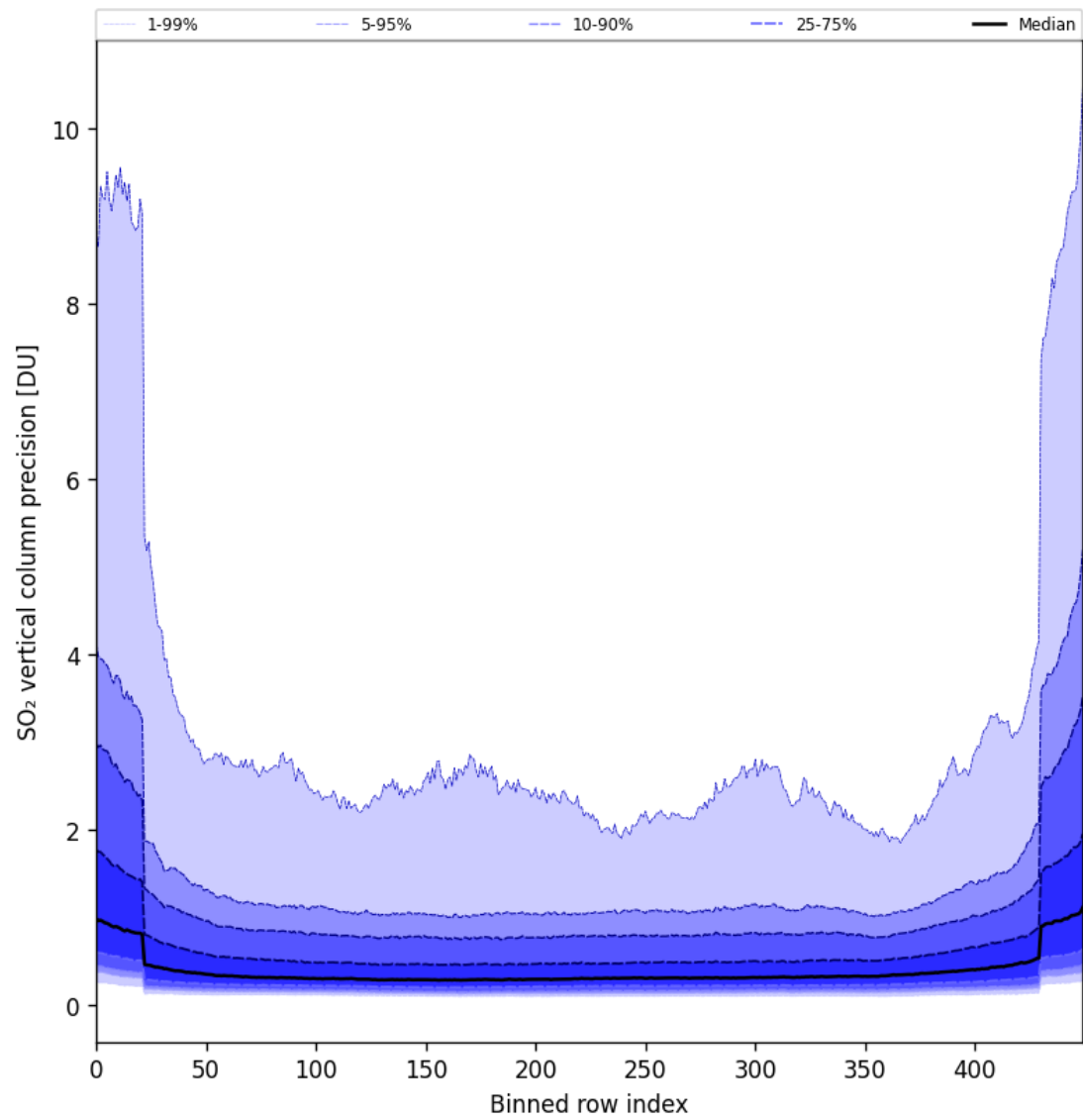
Figure 85: Along track statistics of “SO 2 vertical column precision” for 2025-04-19 to 2025-04-21
