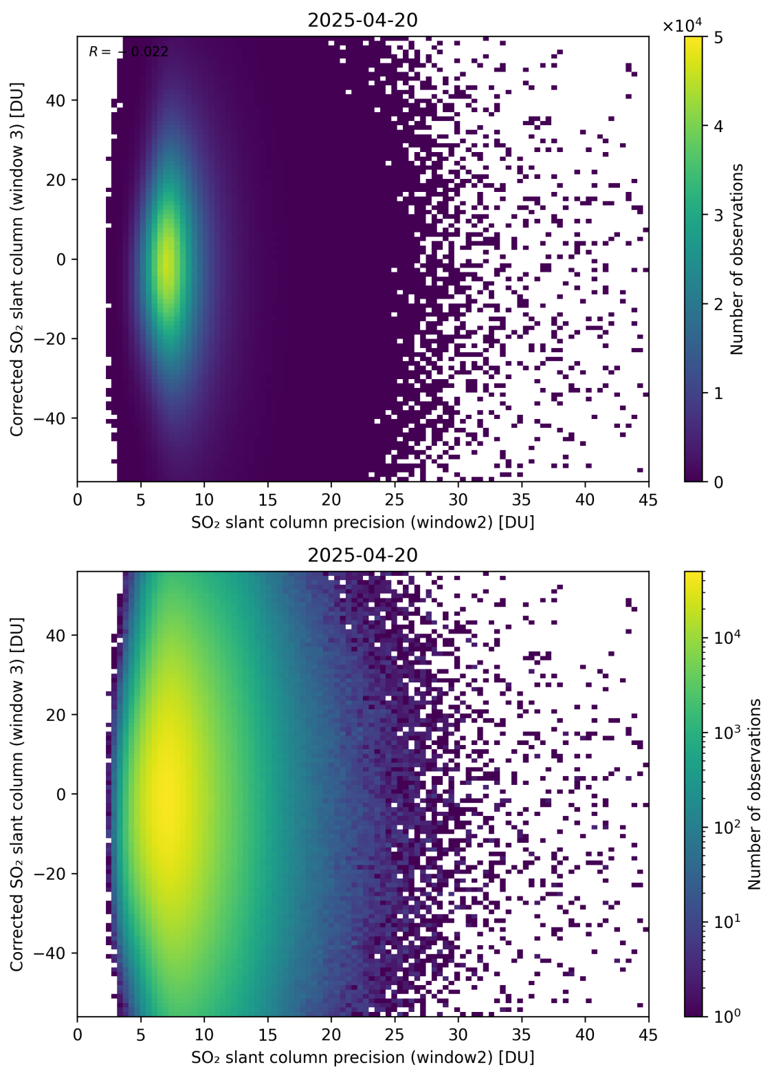
Figure 298: Scatter density plot of “SO 2 slant column precision (window2)” against “Corrected SO 2 slant column (window 3)” for 2025-04-19 to 2025-04-21.
