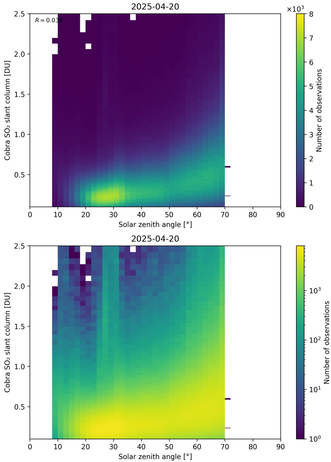
Figure 179: Scatter density plot of “Solar zenith angle” against “Cobra SO 2 slant column” for 2025-04-19 to 2025-04-21.
