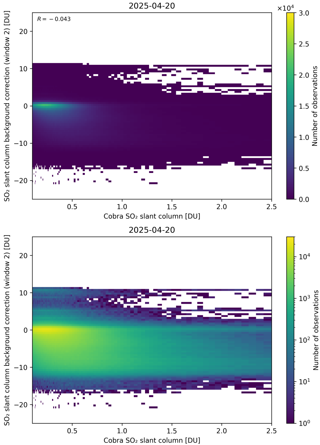
Figure 194: Scatter density plot of “Cobra SO 2 slant column” against “SO 2 slant column background correction (window 2)” for 2025-04-19 to 2025-04-21.
