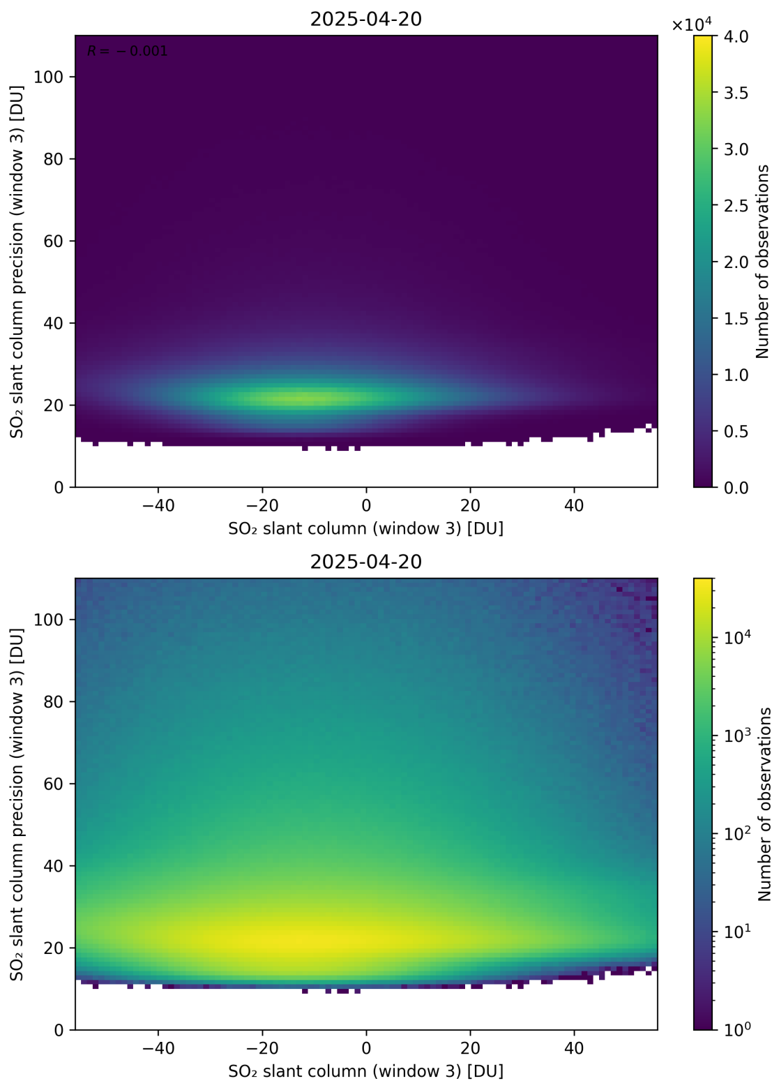
Figure 317: Scatter density plot of “SO 2 slant column (window 3)” against “SO 2 slant column precision (window 3)” for 2025-04-19 to 2025-04-21.
