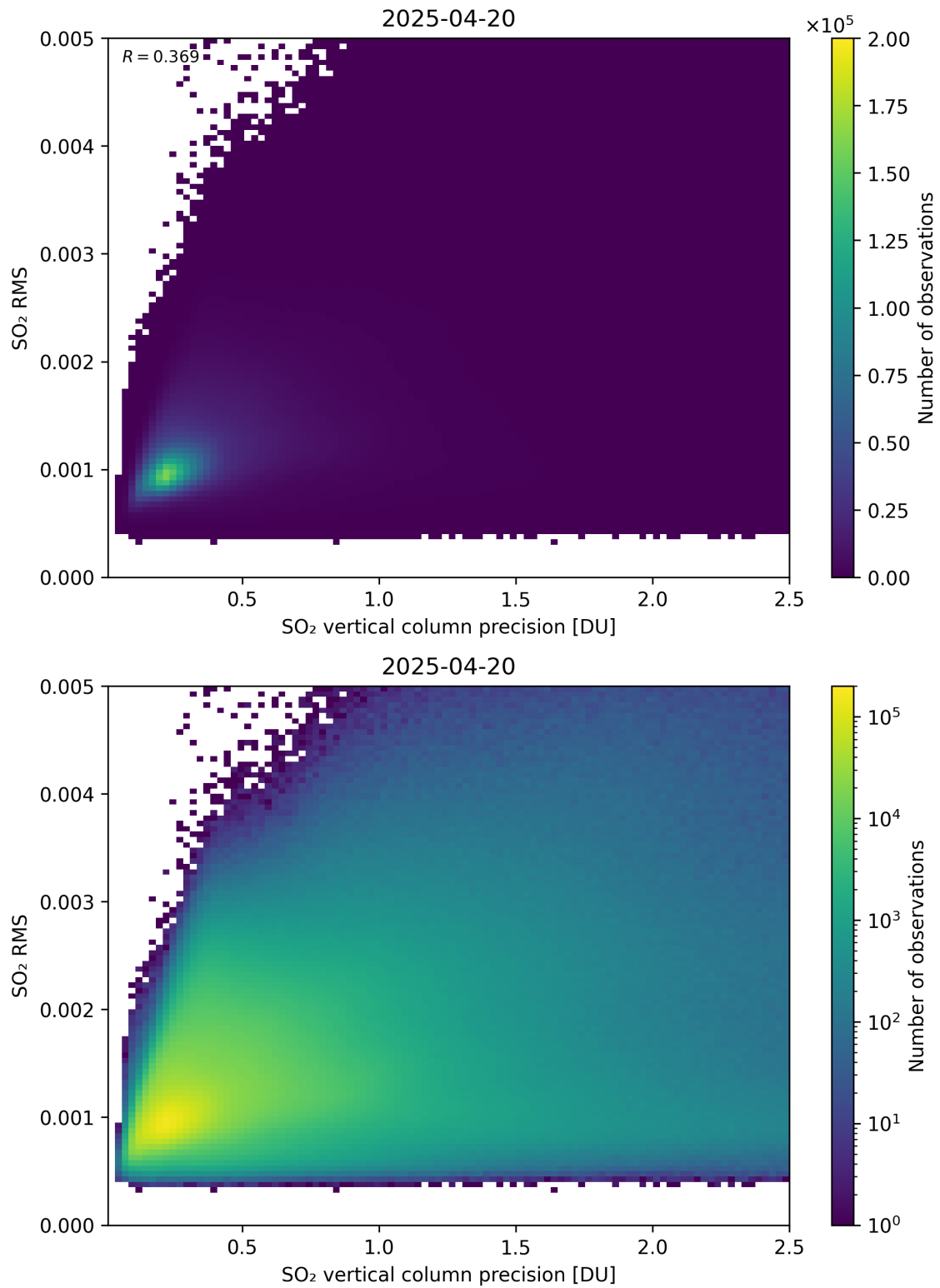
Figure 334: Scatter density plot of “SO 2 vertical column precision” against “SO 2 RMS” for 2025-04-19 to 2025-04-21.
