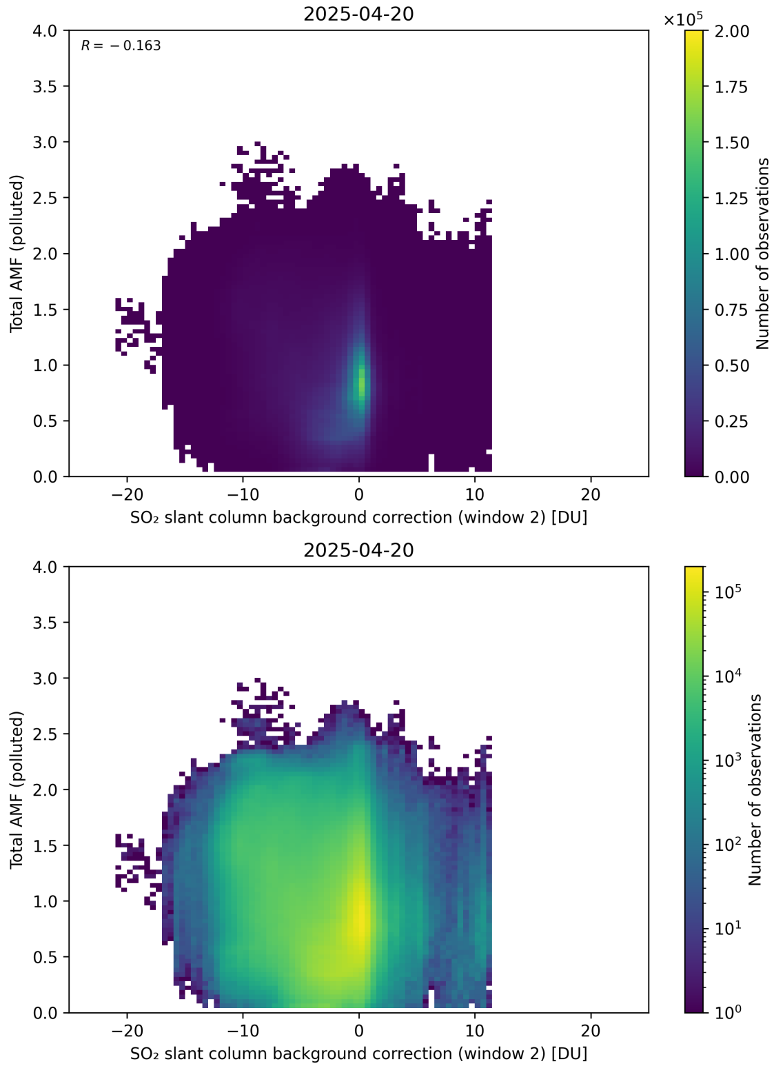
Figure 130: Scatter density plot of “SO 2 slant column background correction (window 2)” against “Total AMF (polluted)” for 2025-04-19 to 2025-04-21.
