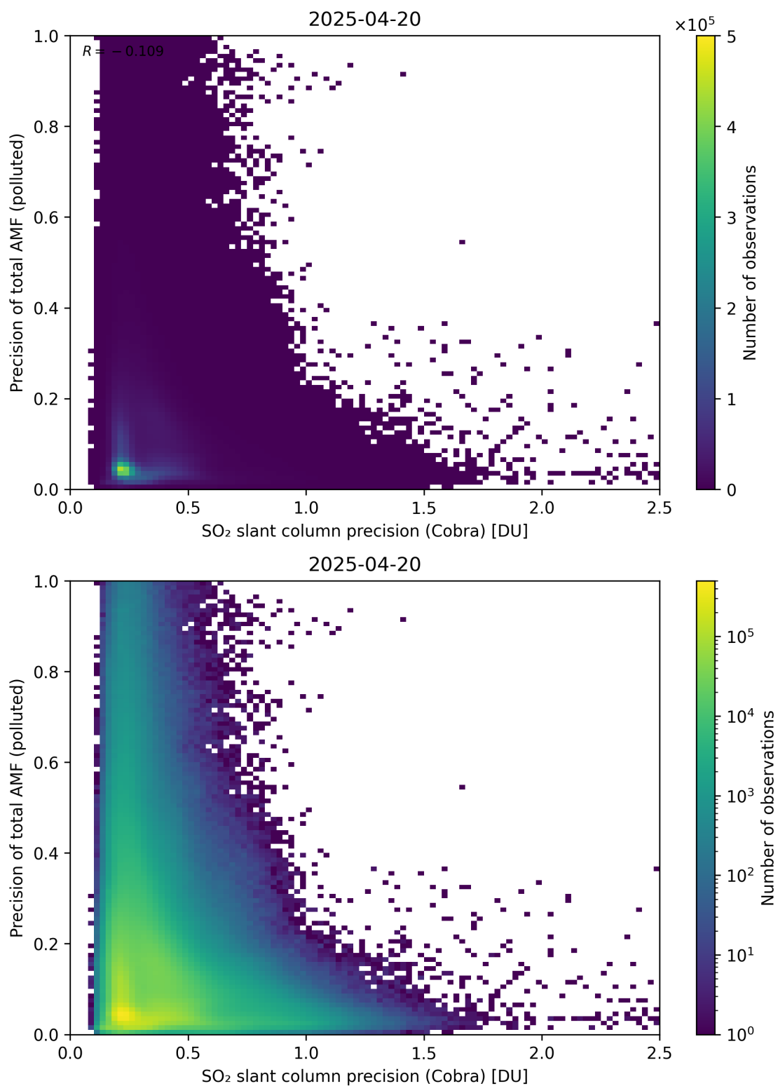
Figure 214: Scatter density plot of “SO 2 slant column precision (Cobra)” against “Precision of total AMF (polluted)” for 2025-04-19 to 2025-04-21.
