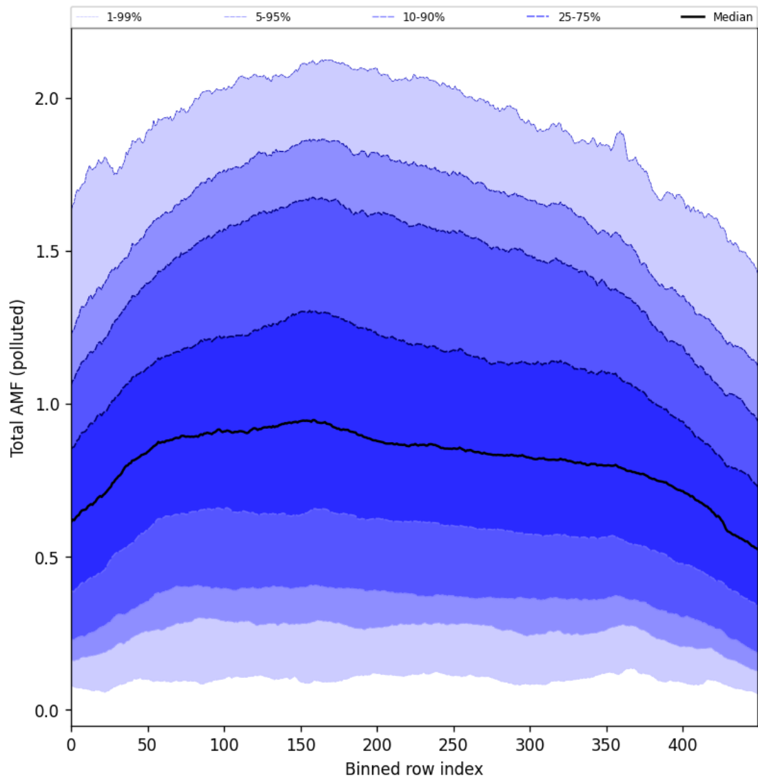
Figure 105: Along track statistics of “Total AMF (polluted)” for 2025-04-19 to 2025-04-21
