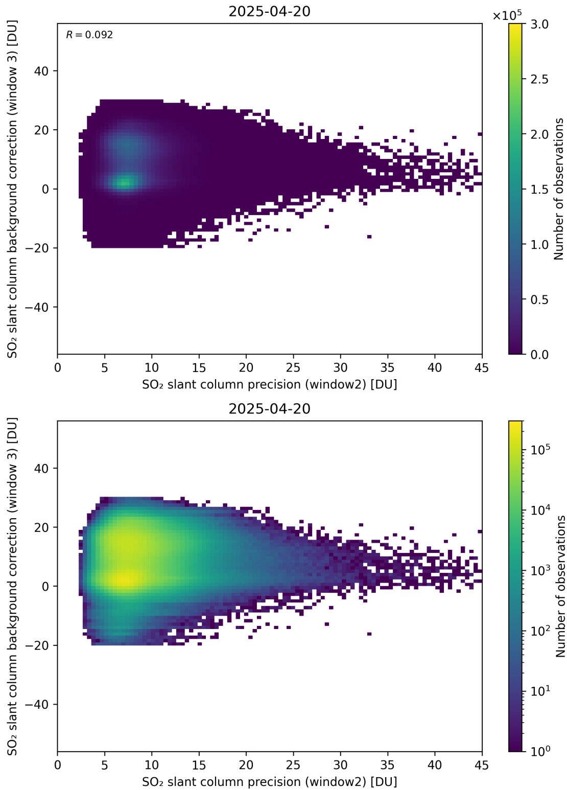
Figure 292: Scatter density plot of “SO 2 slant column precision (window2)” against “SO 2 slant column background correction (window 3)” for 2025-04-19 to 2025-04-21.
