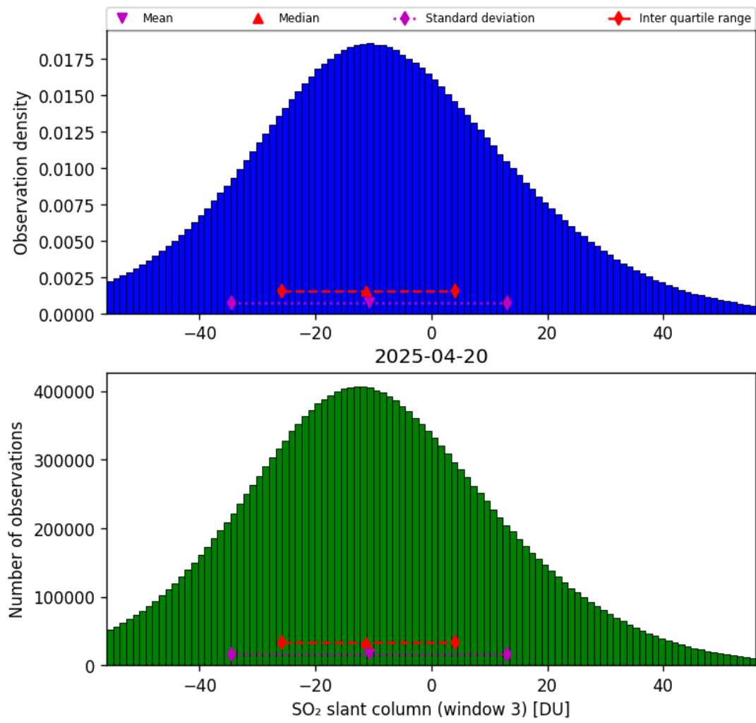
Figure 71: Histogram of “SO 2 slant column (window 3)” for 2025-04-19 to 2025-04-21
