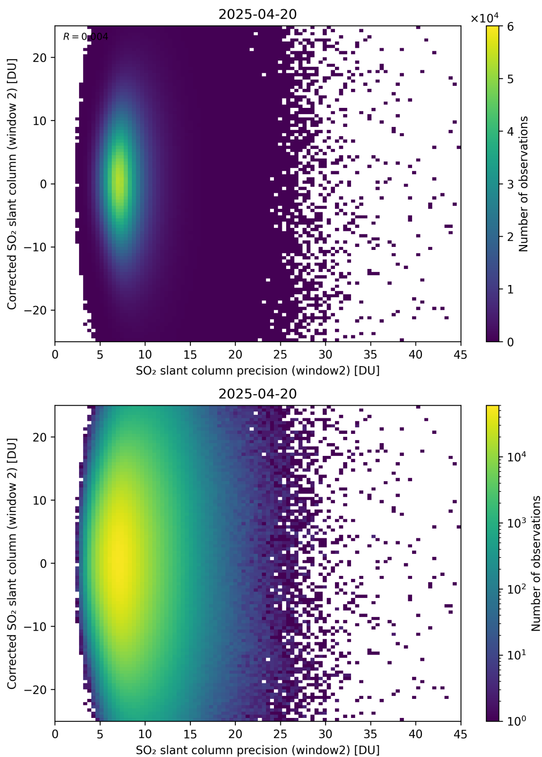
Figure 297: Scatter density plot of “SO 2 slant column precision (window2)” against “Corrected SO 2 slant column (window 2)” for 2025-04-19 to 2025-04-21.
