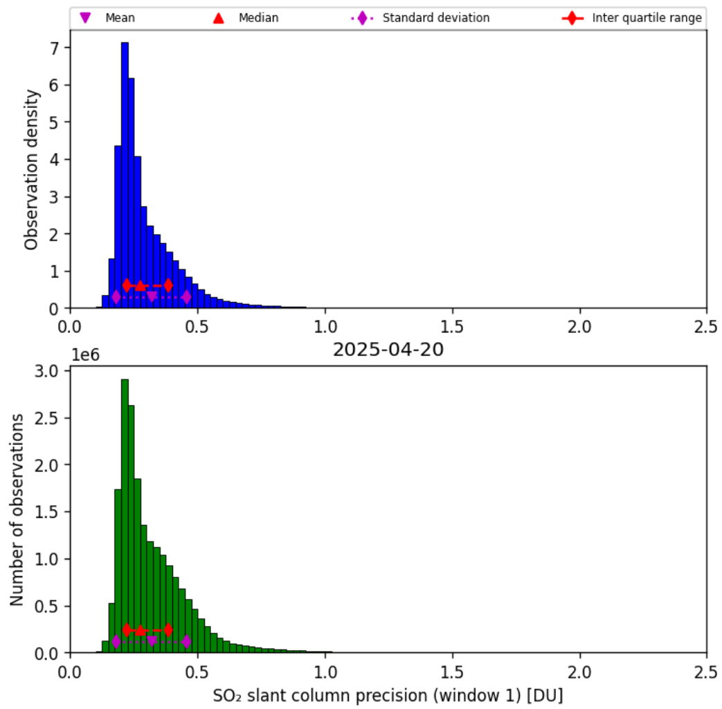
Figure 64: Histogram of “SO 2 slant column precision (window 1)” for 2025-04-19 to 2025-04-21
