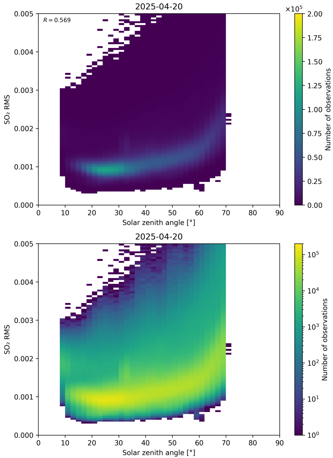
Figure 176: Scatter density plot of “Solar zenith angle” against “SO 2 RMS” for 2025-04-19 to 2025-04-21.
