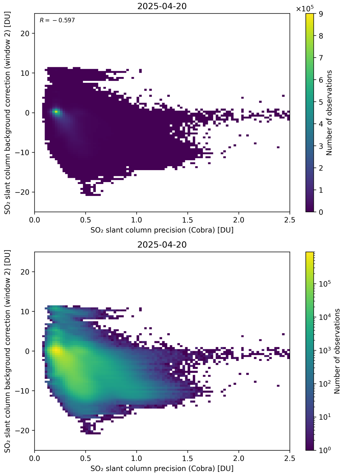
Figure 200: Scatter density plot of “SO 2 slant column precision (Cobra)” against “SO 2 slant column background correction (window 2)” for 2025-04-19 to 2025-04-21.
