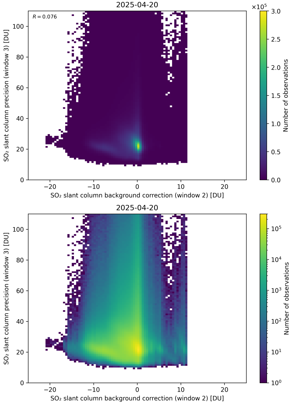
Figure 129: Scatter density plot of “SO 2 slant column background correction (window 2)” against “SO 2 slant column precision (window 3)” for 2025-04-19 to 2025-04-21.
