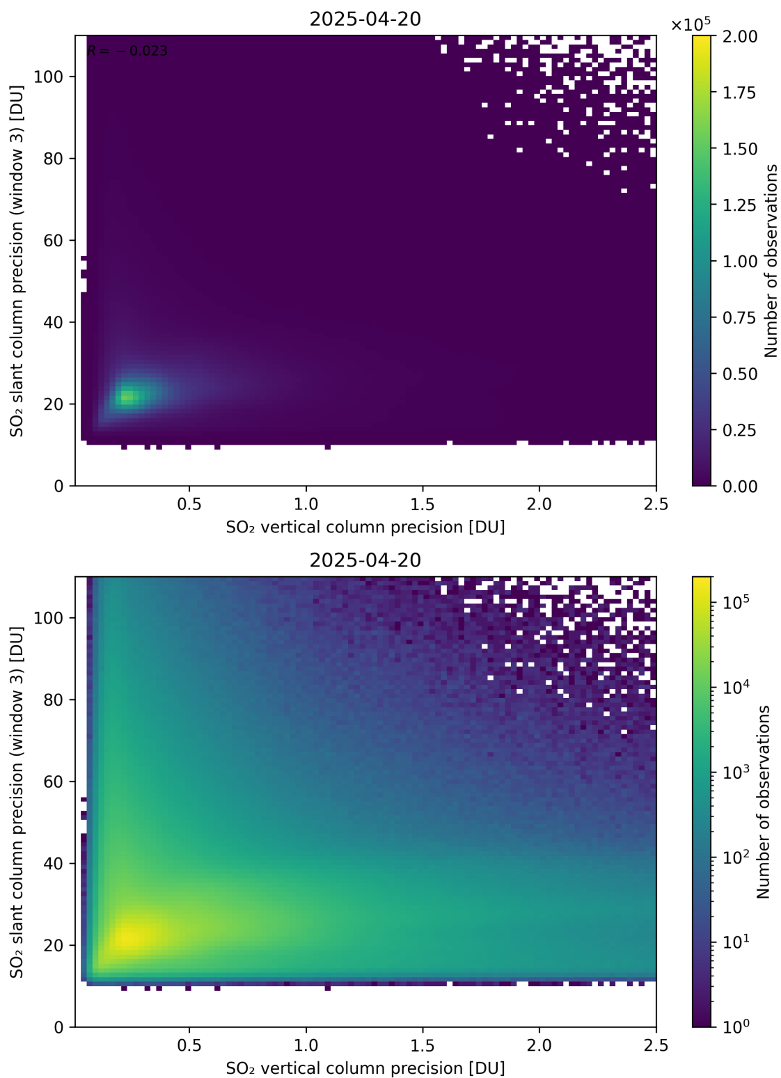
Figure 345: Scatter density plot of “SO 2 vertical column precision” against “SO 2 slant column precision (window 3)” for 2025-04-19 to 2025-04-21.
