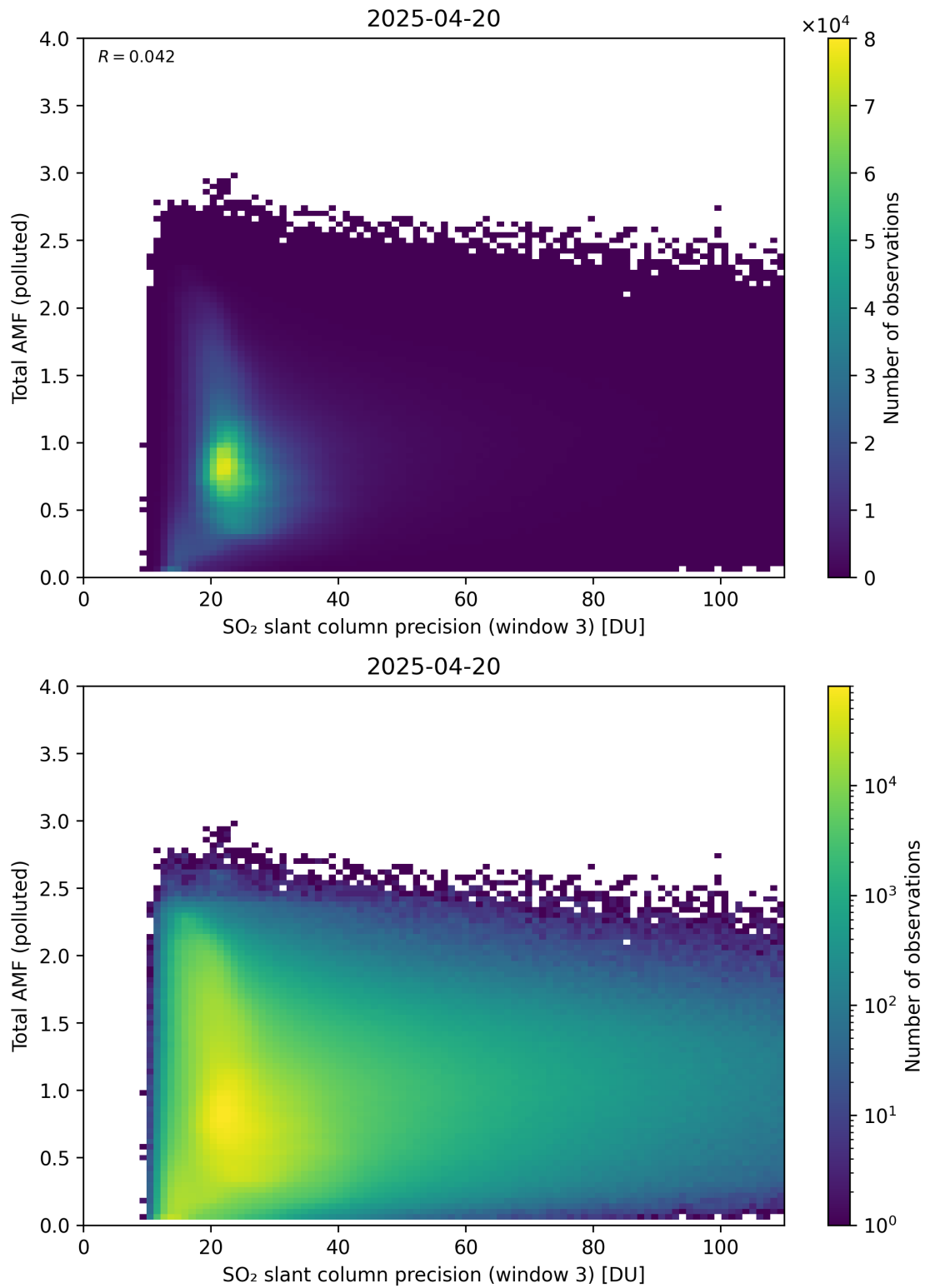
Figure 313: Scatter density plot of “SO 2 slant column precision (window 3)” against “Total AMF (polluted)” for 2025-04-19 to 2025-04-21.
