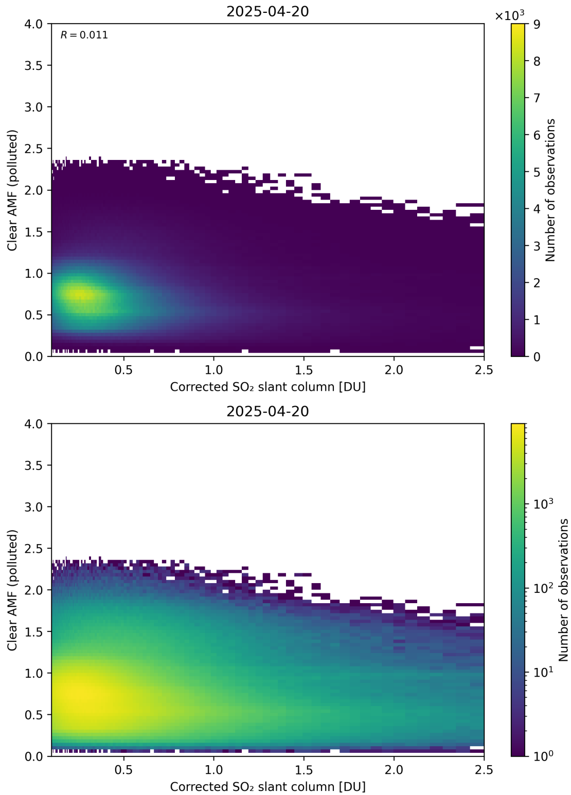
Figure 232: Scatter density plot of “Corrected SO 2 slant column” against “Clear AMF (polluted)” for 2025-04-19 to 2025-04-21.
