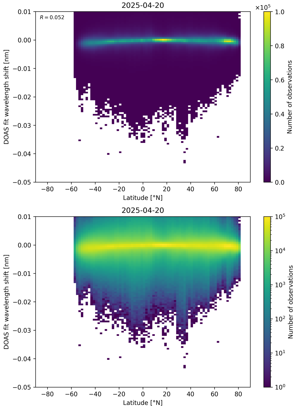
Figure 153: Scatter density plot of “Latitude” against “DOAS fit wavelength shift” for 2025-04-19 to 2025-04-21.
