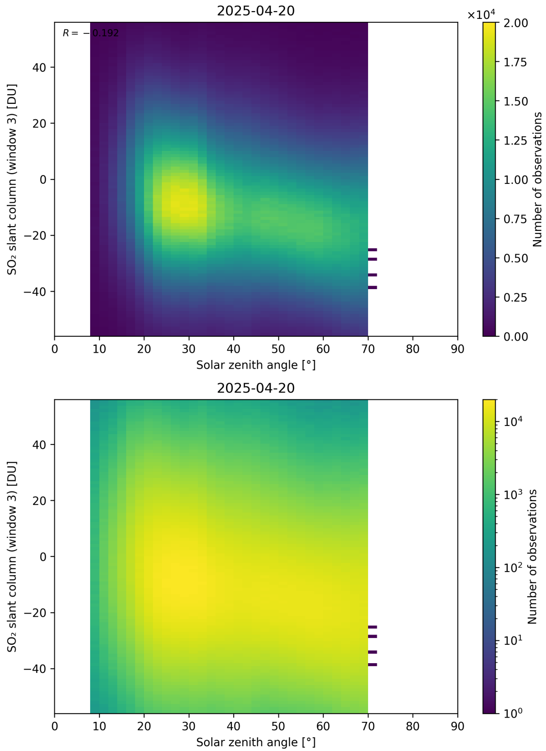
Figure 187: Scatter density plot of “Solar zenith angle” against “SO 2 slant column (window 3)” for 2025-04-19 to 2025-04-21.
