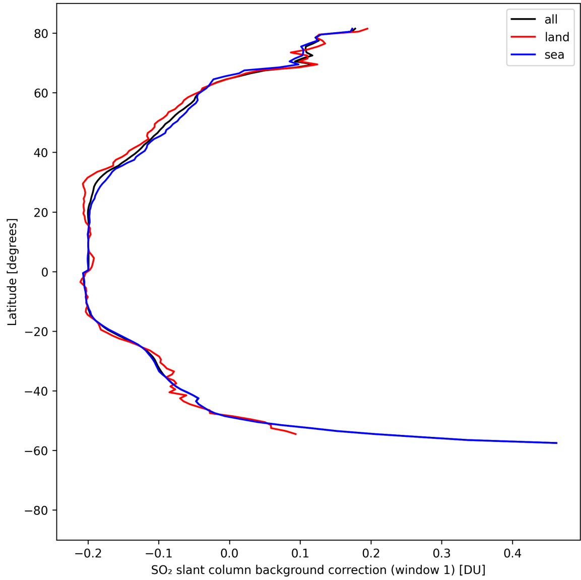
Figure 40: Zonal average of “SO 2 slant column background correction (window 1)” for 2025-04-19 to 2025-04-21.
