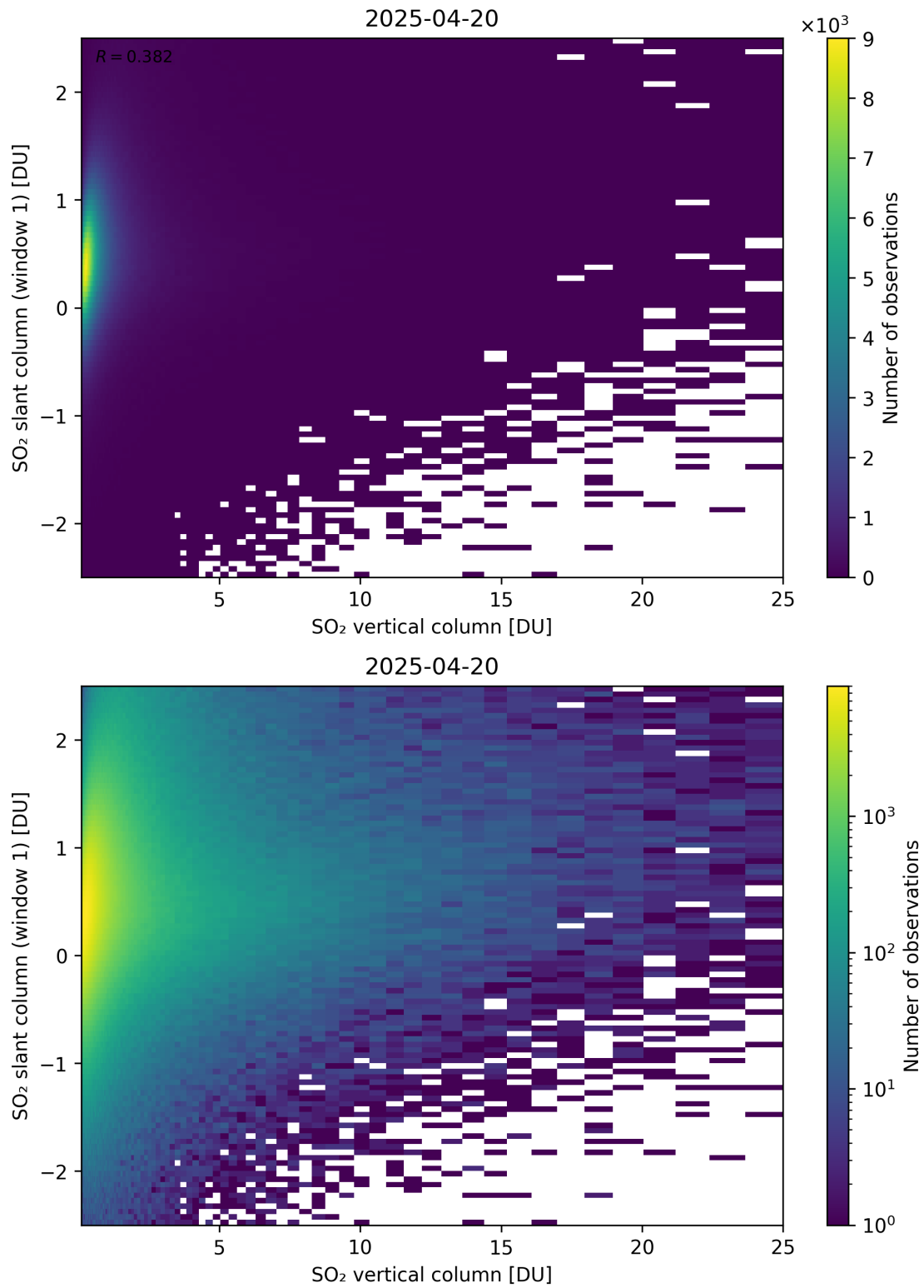
Figure 354: Scatter density plot of “SO 2 vertical column” against “SO 2 slant column (window 1)” for 2025-04-19 to 2025-04-21.
