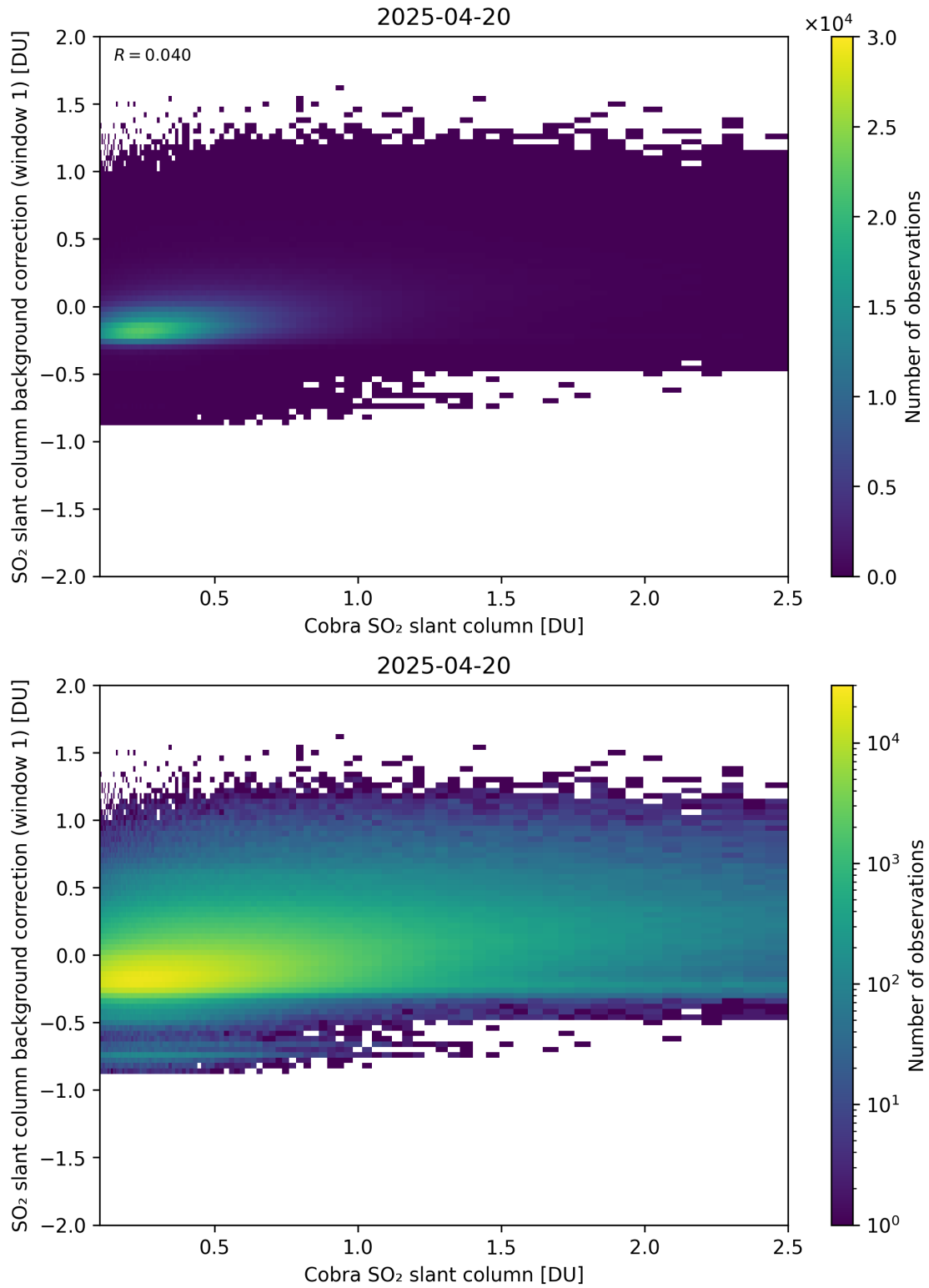
Figure 193: Scatter density plot of “Cobra SO 2 slant column” against “SO 2 slant column background correction (window 1)” for 2025-04-19 to 2025-04-21.
