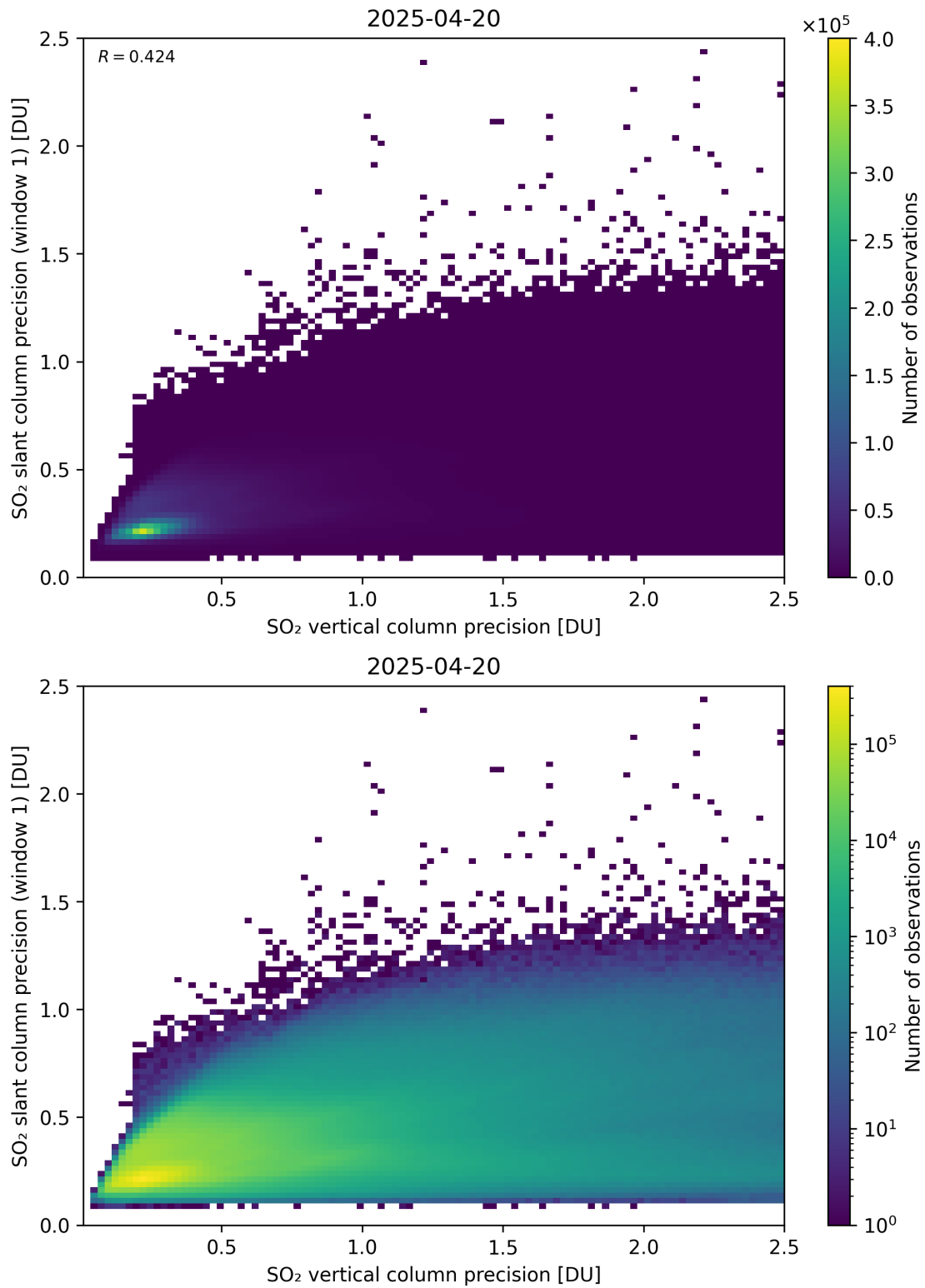
Figure 342: Scatter density plot of “SO 2 vertical column precision” against “SO 2 slant column precision (window 1)” for 2025-04-19 to 2025-04-21.
