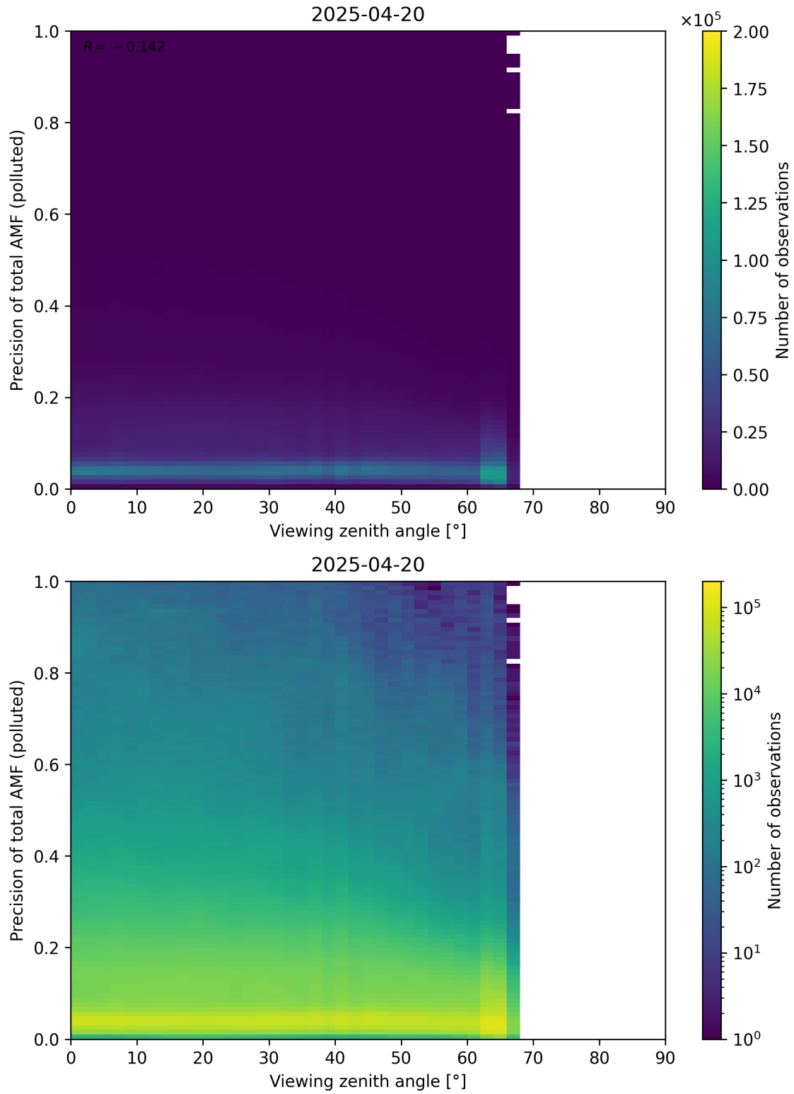
Figure 382: Scatter density plot of “Viewing zenith angle” against “Precision of total AMF (polluted)” for 2025-04-19 to 2025-04-21.
