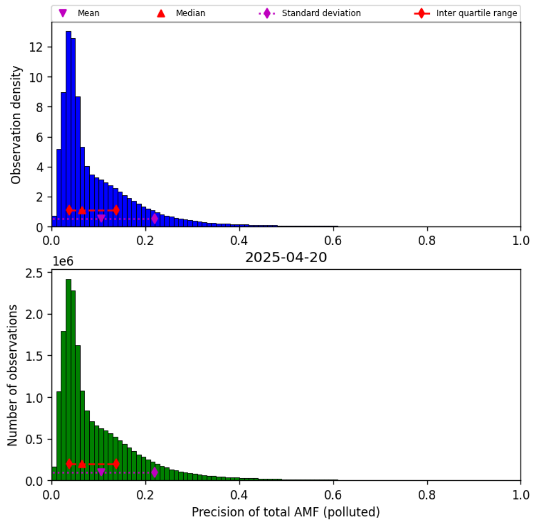
Figure 80: Histogram of “Precision of total AMF (polluted)” for 2025-04-19 to 2025-04-21
