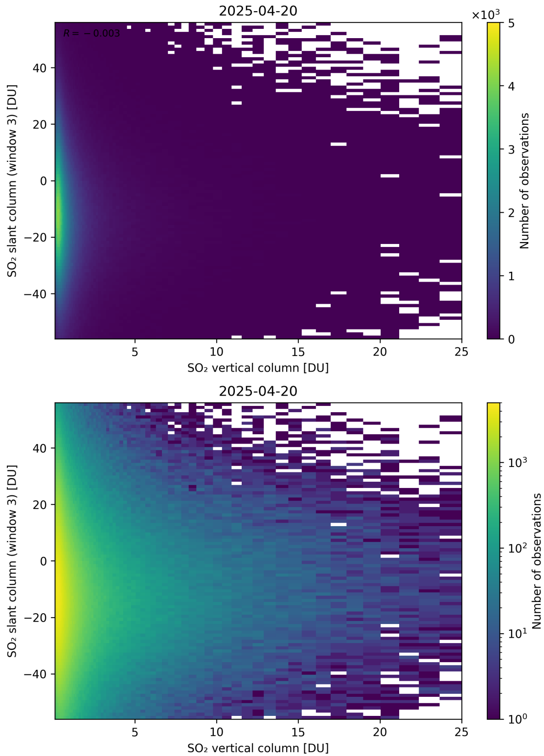
Figure 357: Scatter density plot of “SO 2 vertical column” against “SO 2 slant column (window 3)” for 2025-04-19 to 2025-04-21.
