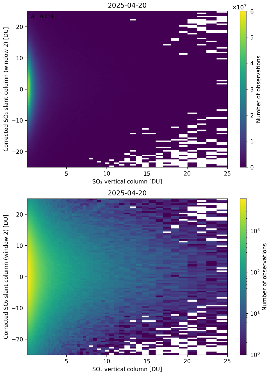
Figure 352: Scatter density plot of “SO 2 vertical column” against “Corrected SO 2 slant column (window 2)” for 2025-04-19 to 2025-04-21.
