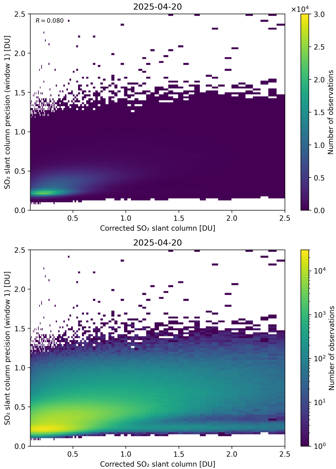
Figure 238: Scatter density plot of “Corrected SO 2 slant column” against “SO 2 slant column precision (window 1)” for 2025-04-19 to 2025-04-21.
