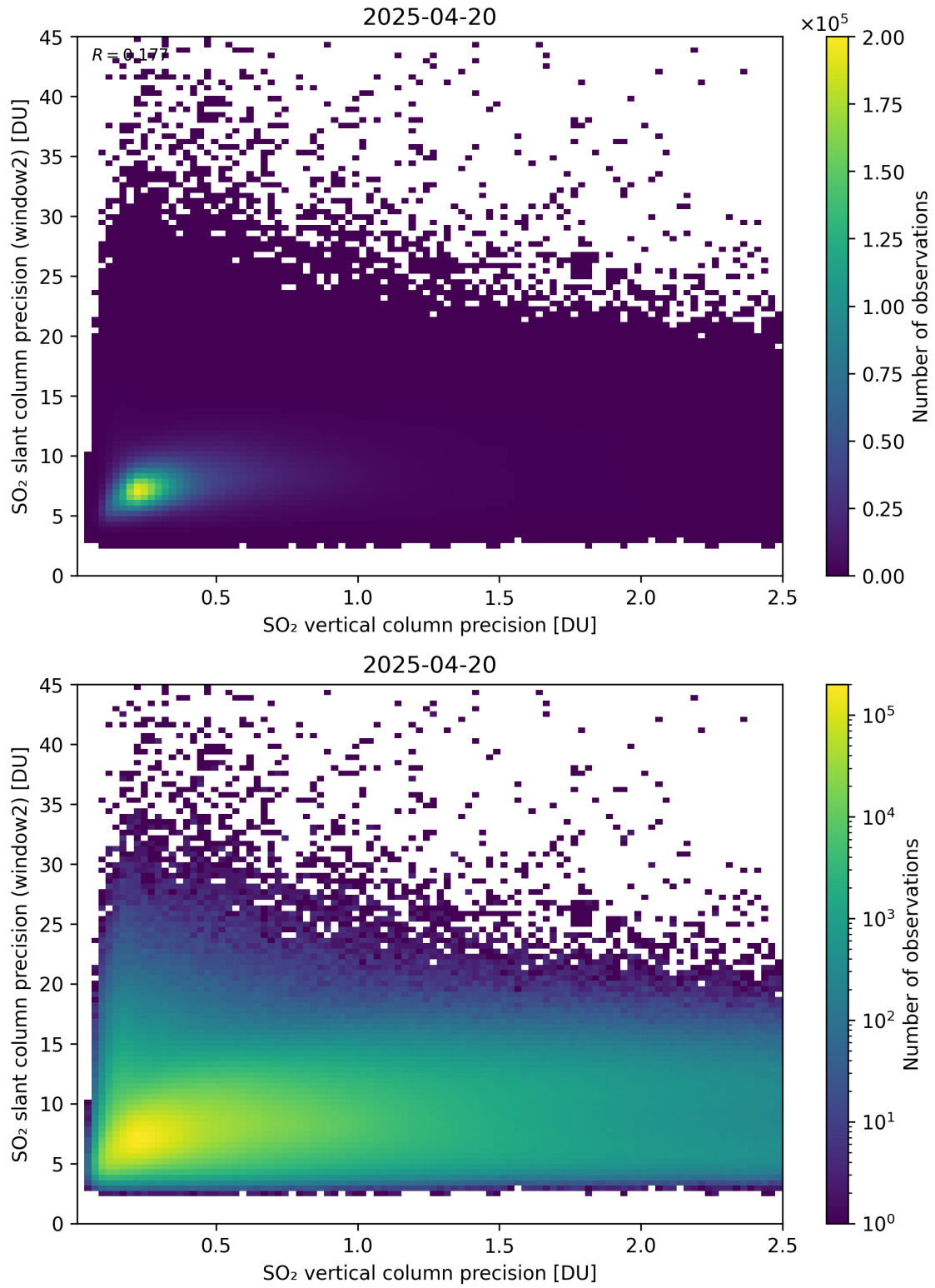
Figure 343: Scatter density plot of “SO 2 vertical column precision” against “SO 2 slant column precision (window2)” for 2025-04-19 to 2025-04-21.
