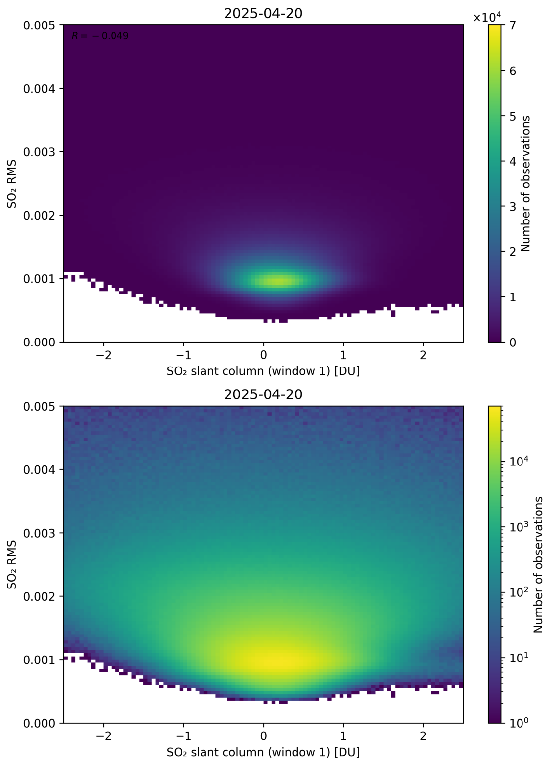
Figure 267: Scatter density plot of “SO 2 slant column (window 1)” against “SO 2 RMS” for 2025-04-19 to 2025-04-21.
