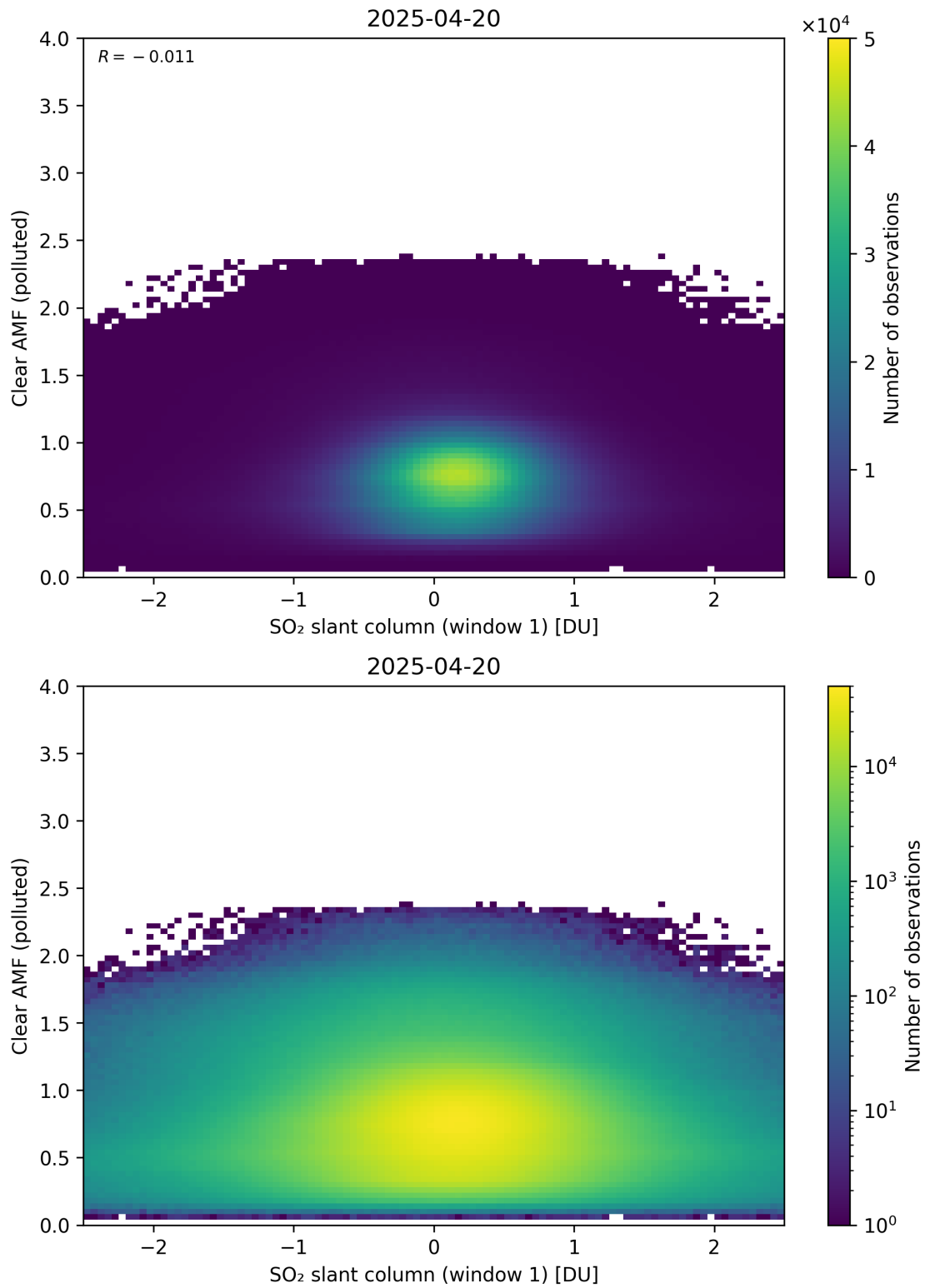
Figure 282: Scatter density plot of “SO 2 slant column (window 1)” against “Clear AMF (polluted)” for 2025-04-19 to 2025-04-21.
