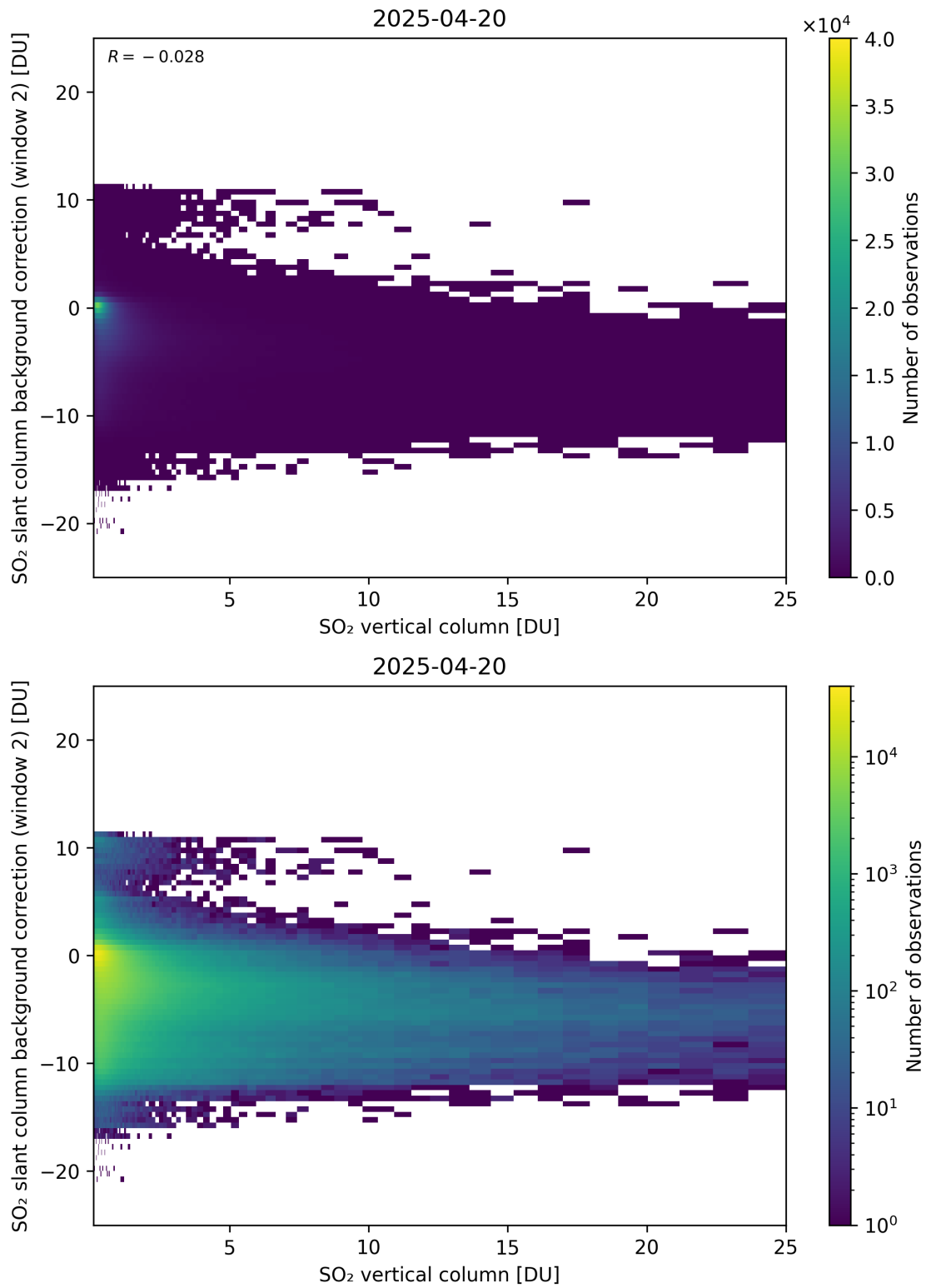
Figure 324: Scatter density plot of “SO 2 vertical column” against “SO 2 slant column background correction (window 2)” for 2025-04-19 to 2025-04-21.
