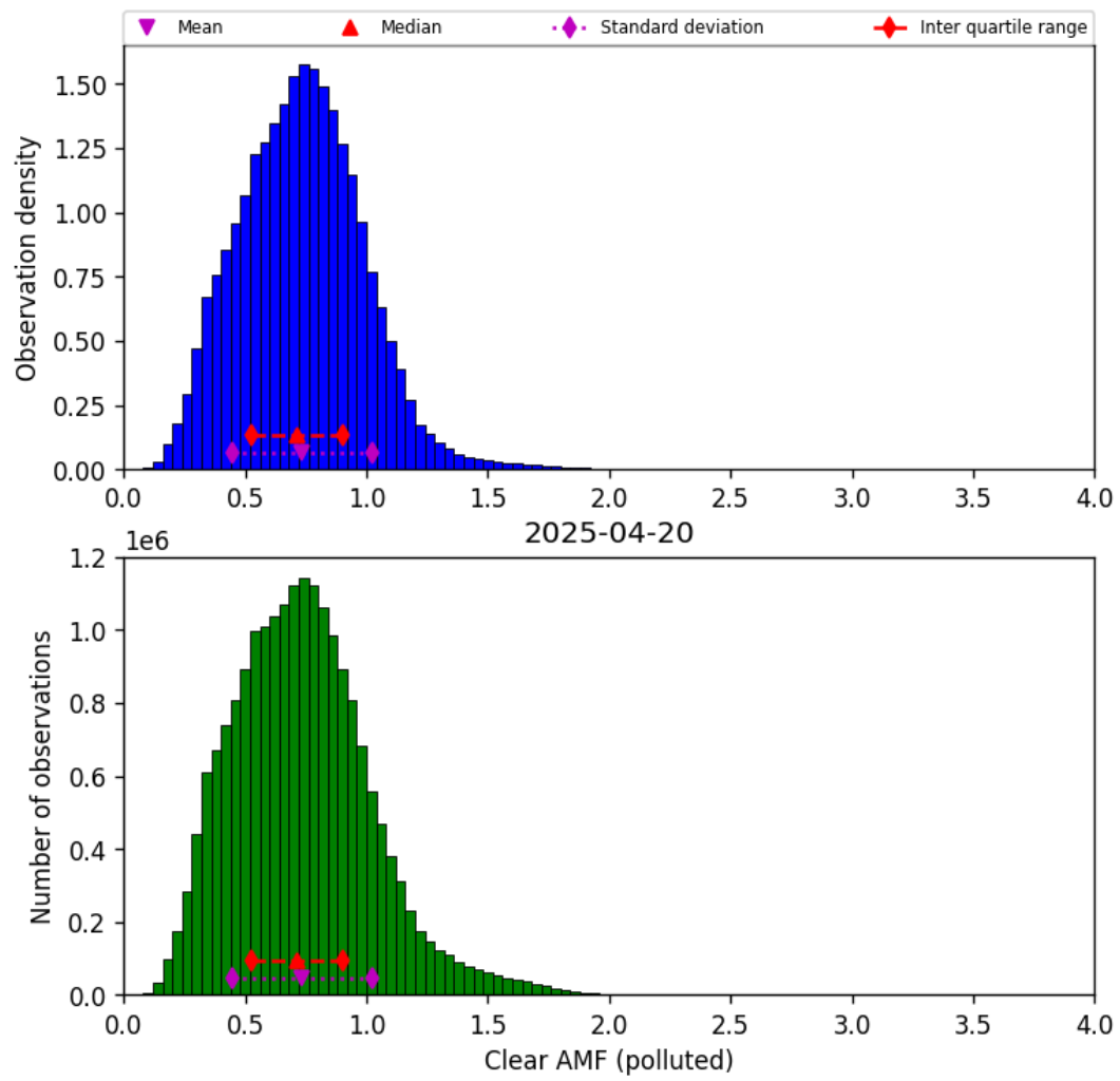
Figure 81: Histogram of “Clear AMF (polluted)” for 2025-04-19 to 2025-04-21
