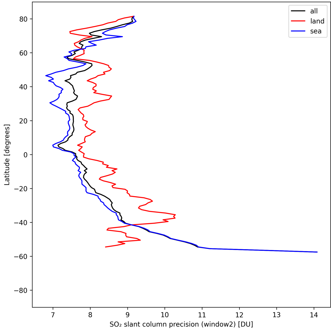
Figure 42: Zonal average of “SO 2 slant column precision (window2)” for 2025-04-19 to 2025-04-21.
