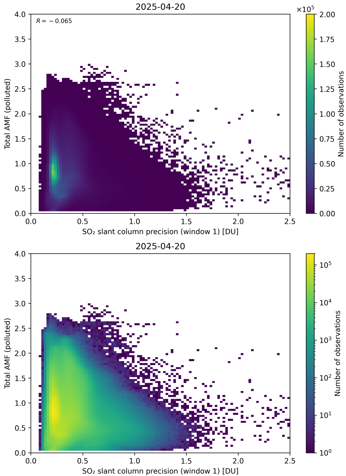
Figure 280: Scatter density plot of “SO 2 slant column precision (window 1)” against “Total AMF (polluted)” for 2025-04-19 to 2025-04-21.
