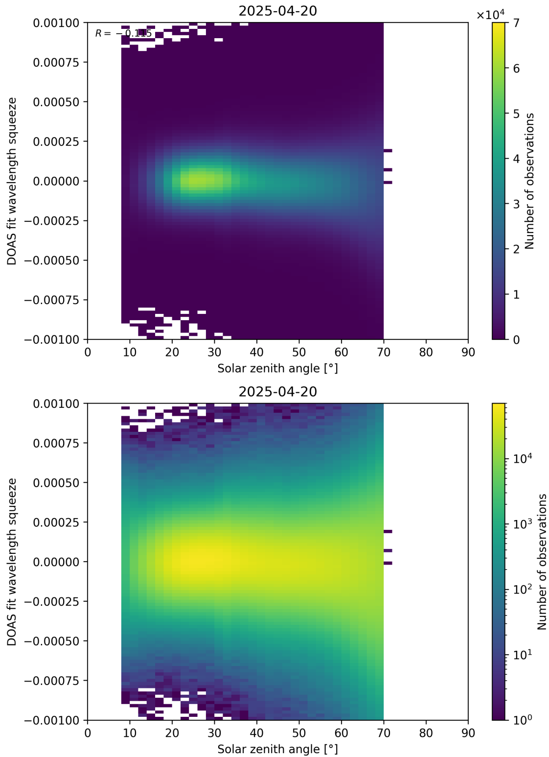
Figure 175: Scatter density plot of “Solar zenith angle” against “DOAS fit wavelength squeeze” for 2025-04-19 to 2025-04-21.
