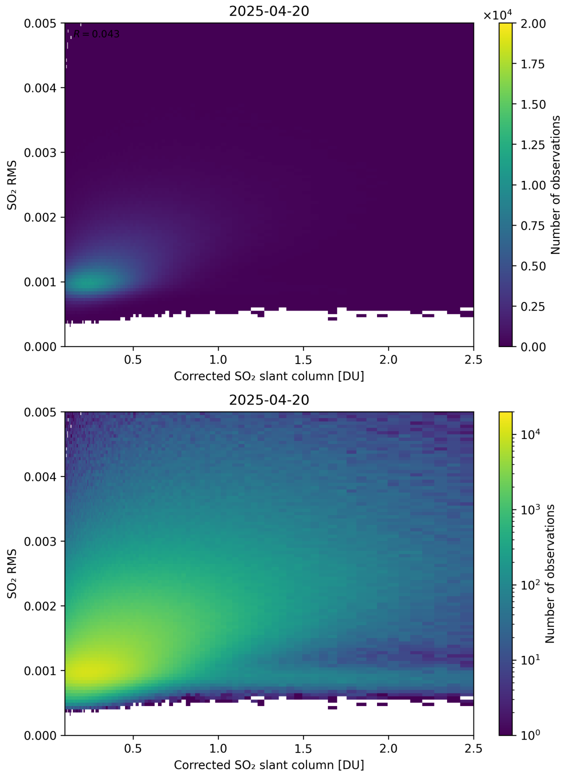
Figure 231: Scatter density plot of “Corrected SO 2 slant column” against “SO 2 RMS” for 2025-04-19 to 2025-04-21.
