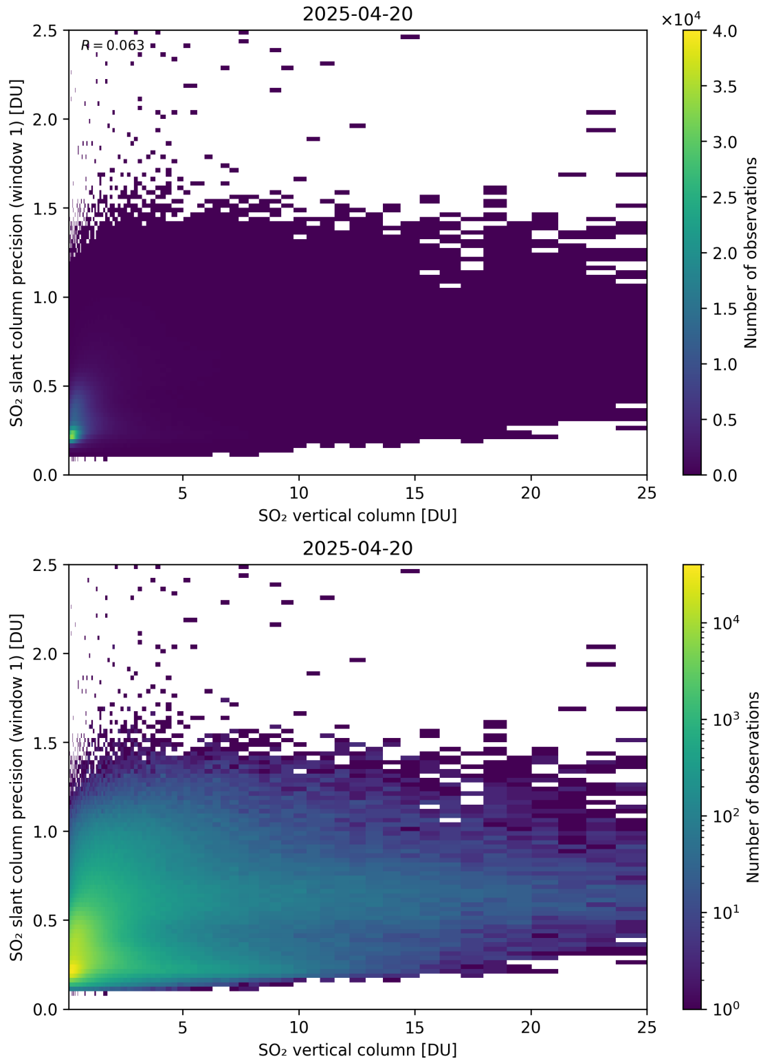
Figure 355: Scatter density plot of “SO 2 vertical column” against “SO 2 slant column precision (window 1)” for 2025-04-19 to 2025-04-21.
