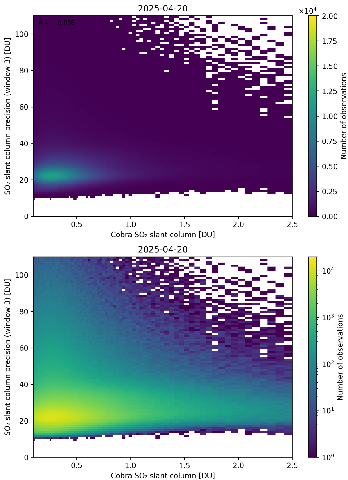
Figure 223: Scatter density plot of “Cobra SO 2 slant column” against “SO 2 slant column precision (window 3)” for 2025-04-19 to 2025-04-21.
