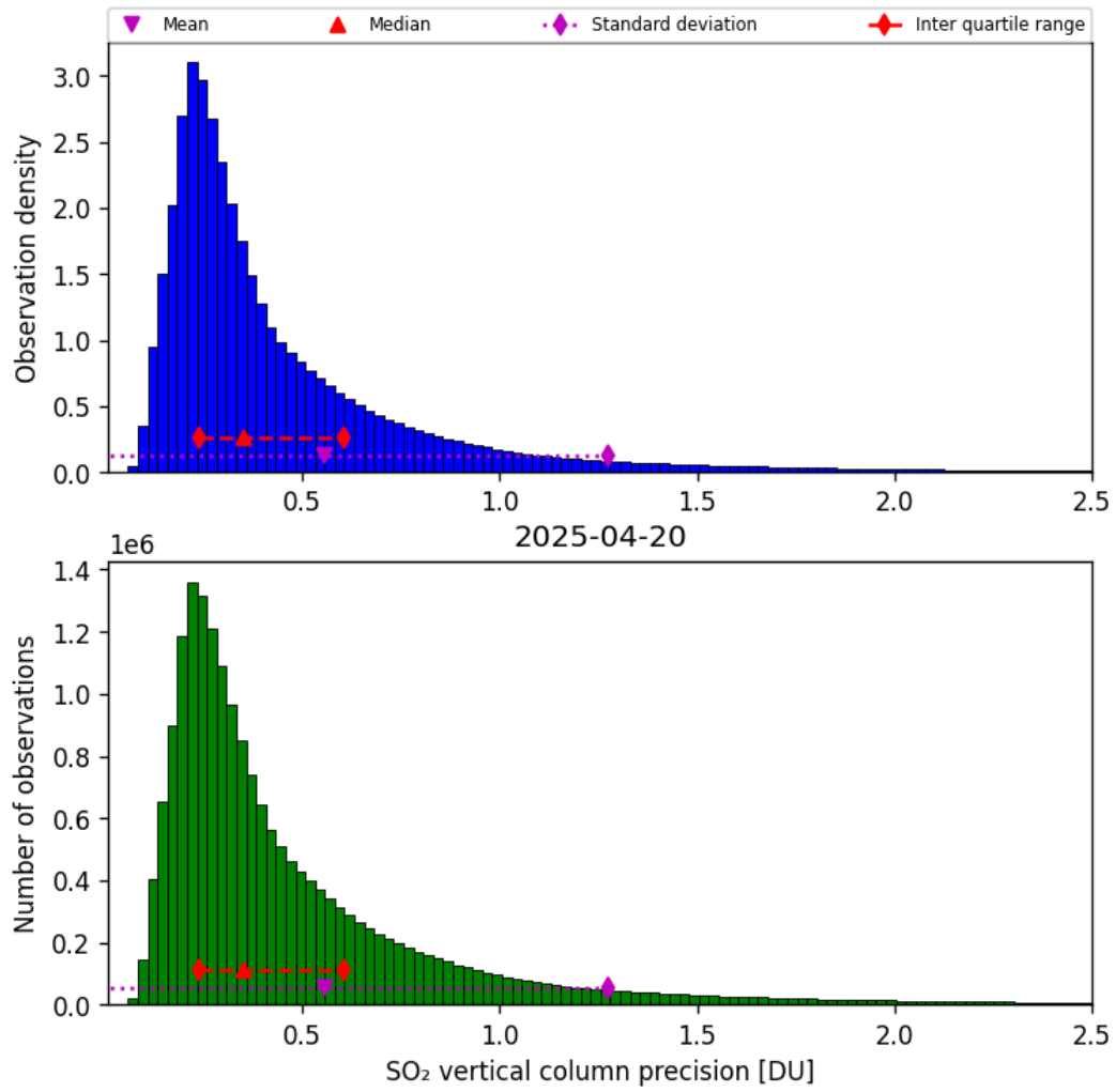
Figure 59: Histogram of “SO 2 vertical column precision” for 2025-04-19 to 2025-04-21
