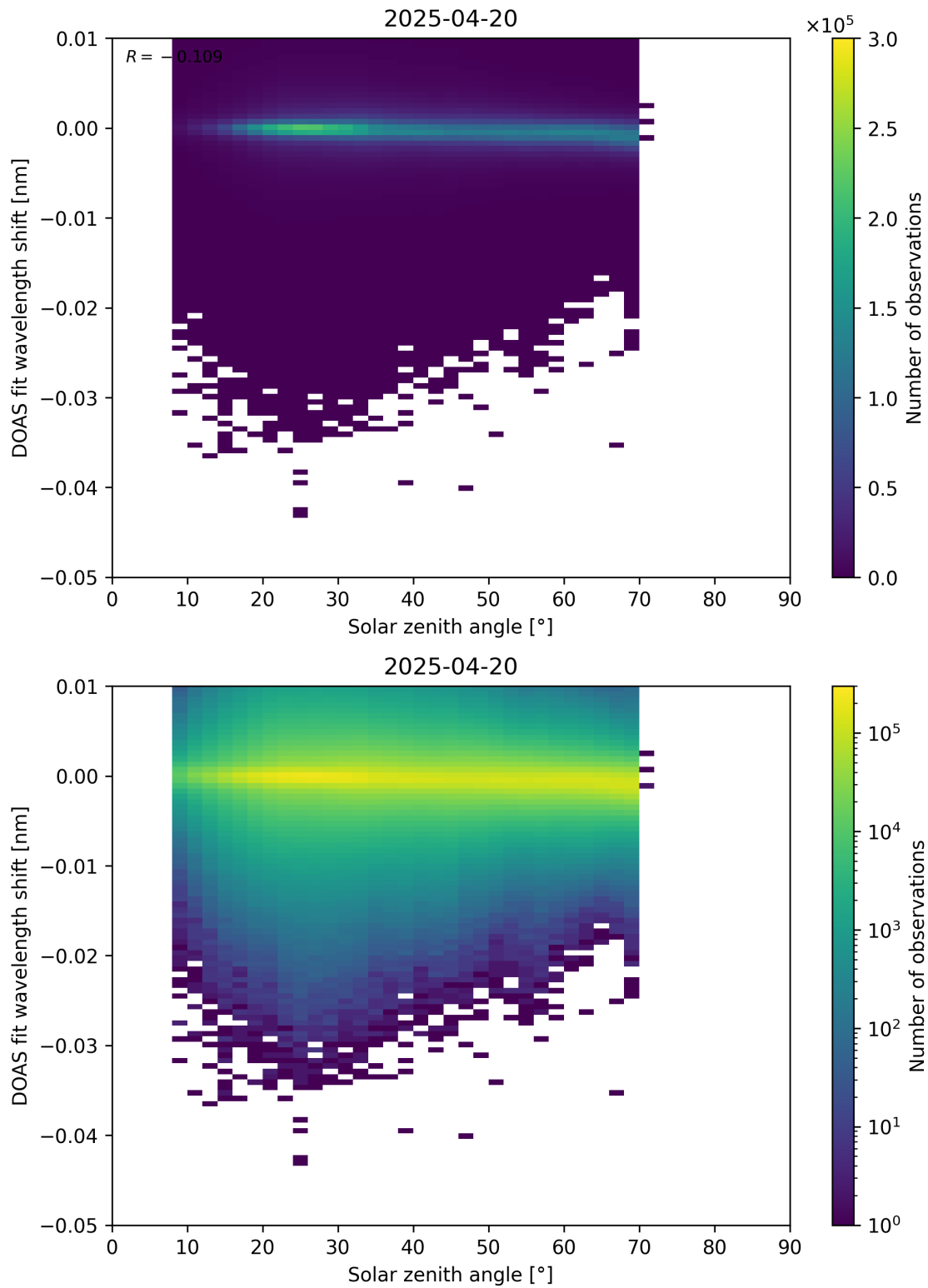
Figure 174: Scatter density plot of “Solar zenith angle” against “DOAS fit wavelength shift” for 2025-04-19 to 2025-04-21.
