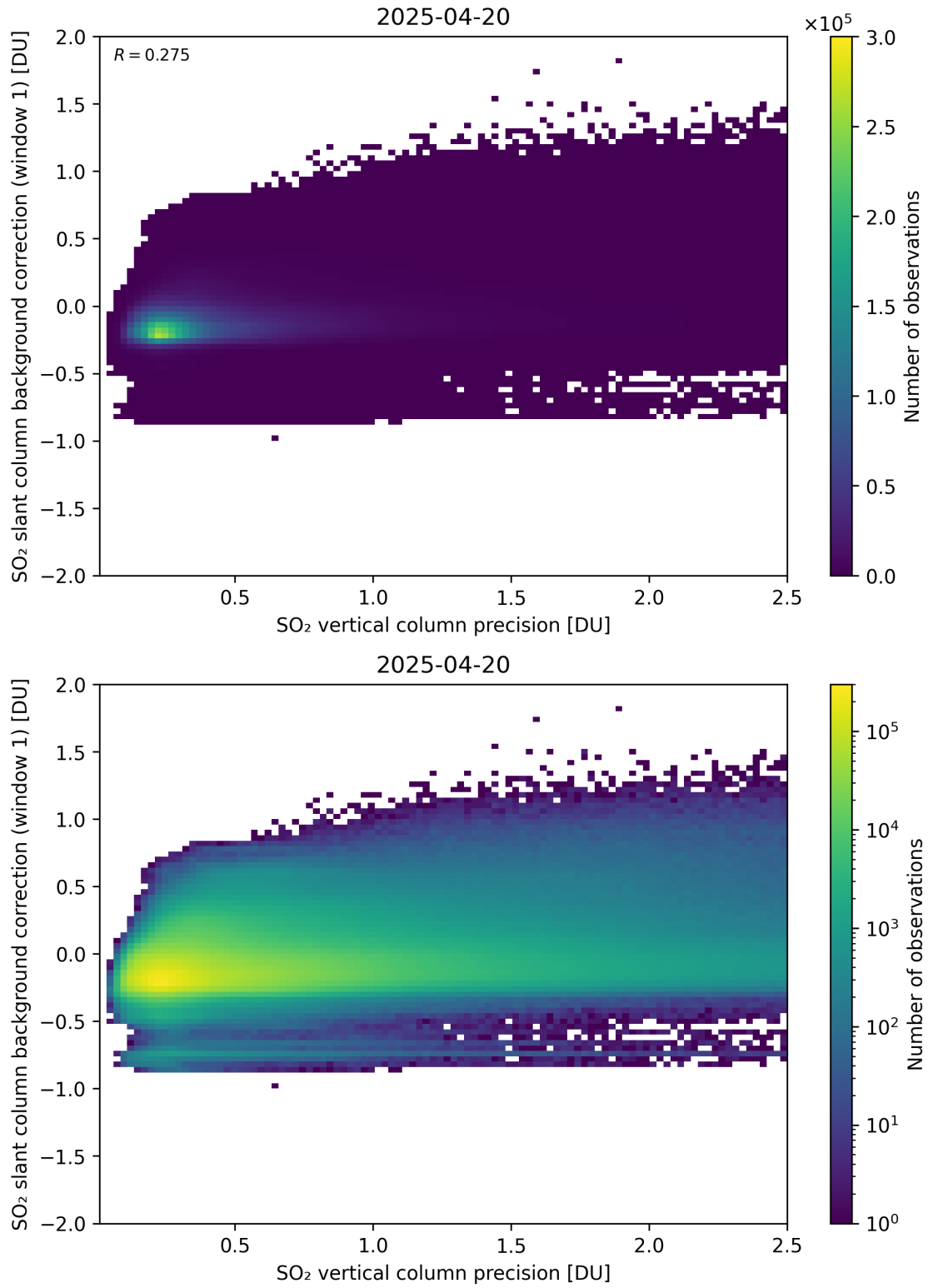
Figure 329: Scatter density plot of “SO 2 vertical column precision” against “SO 2 slant column background correction (window 1)” for 2025-04-19 to 2025-04-21.
