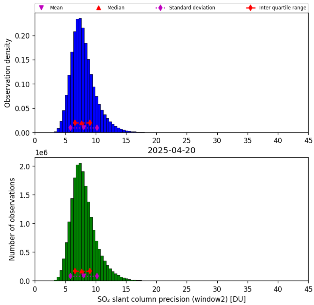
Figure 68: Histogram of “SO 2 slant column precision (window2)” for 2025-04-19 to 2025-04-21
