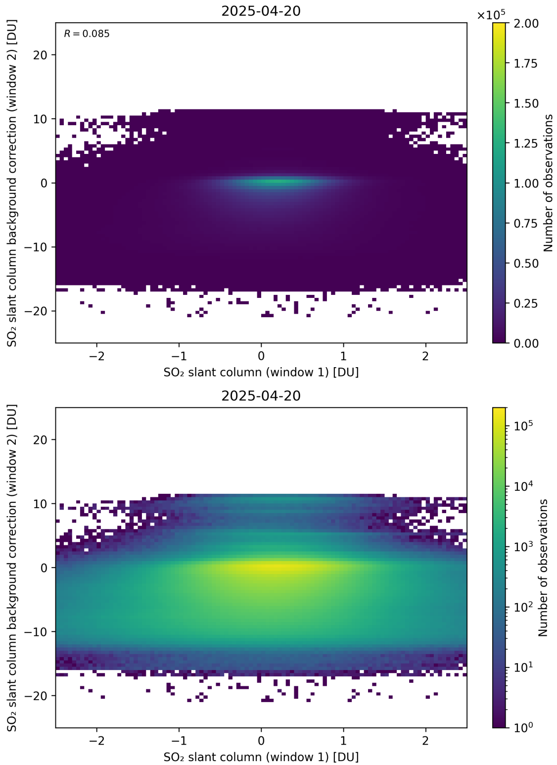
Figure 263: Scatter density plot of “SO 2 slant column (window 1)” against “SO 2 slant column background correction (window 2)” for 2025-04-19 to 2025-04-21.
