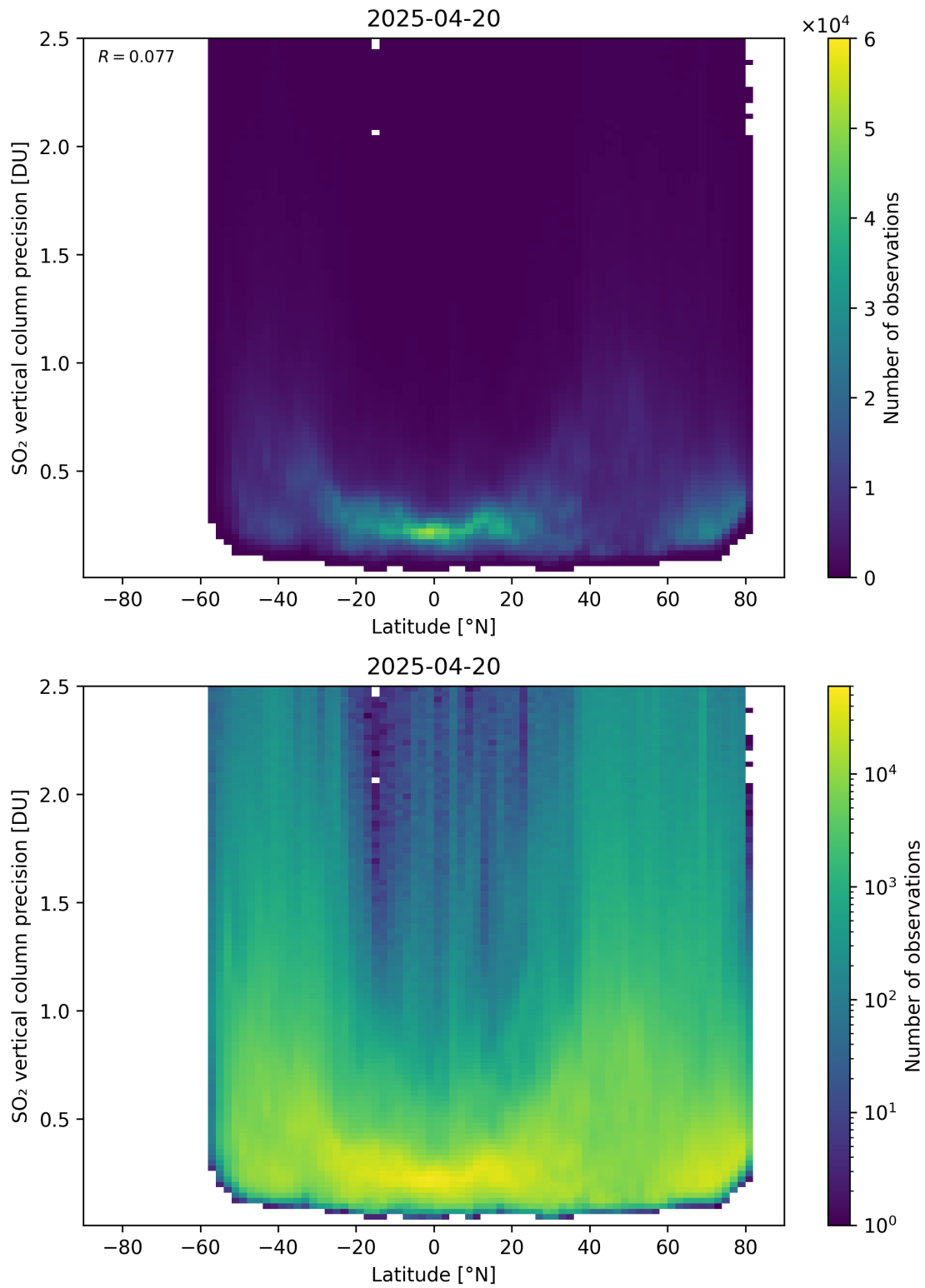
Figure 170: Scatter density plot of “Latitude” against “SO 2 vertical column precision” for 2025-04-19 to 2025-04-21.
