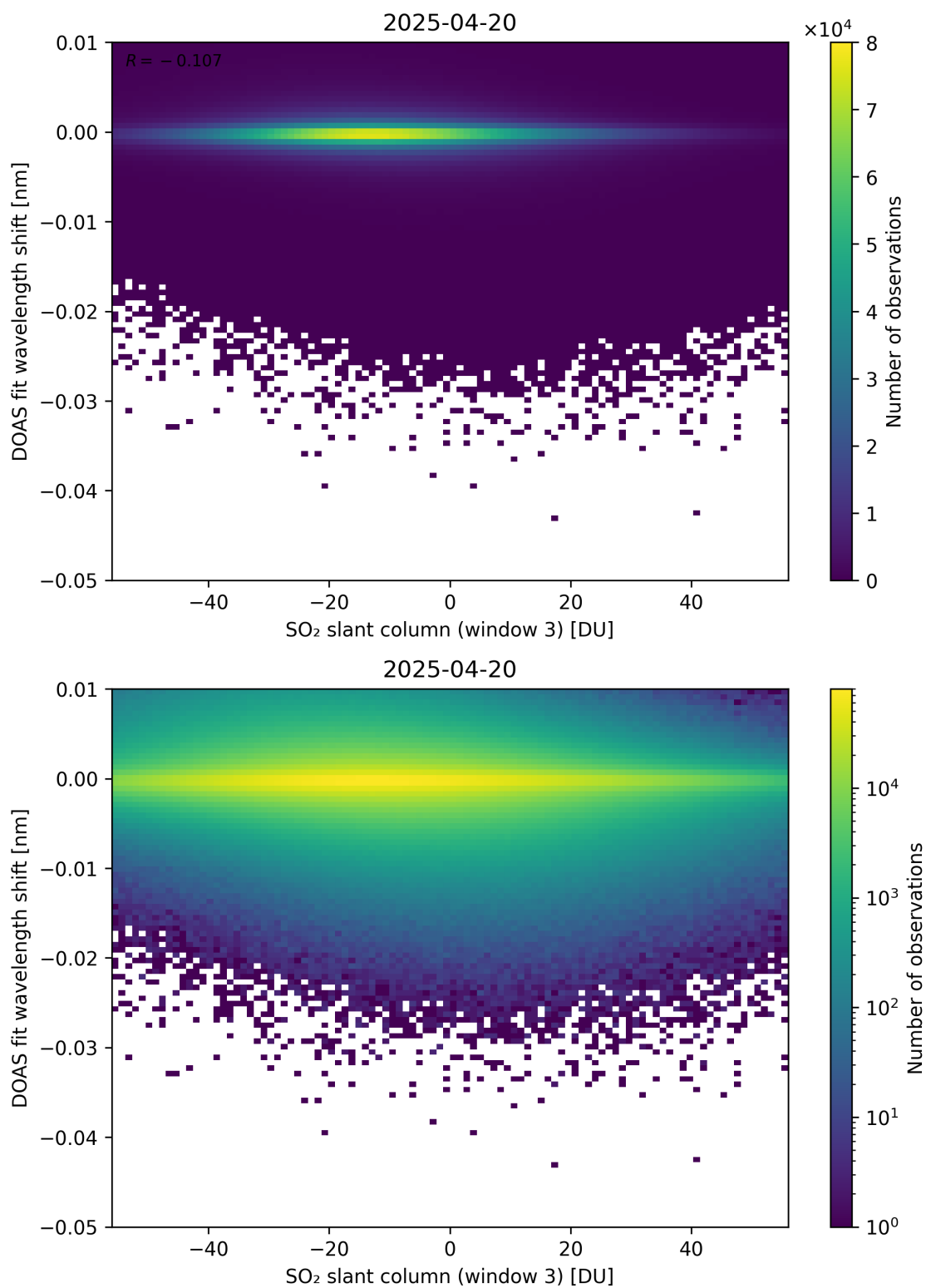
Figure 304: Scatter density plot of “SO 2 slant column (window 3)” against “DOAS fit wavelength shift” for 2025-04-19 to 2025-04-21.
