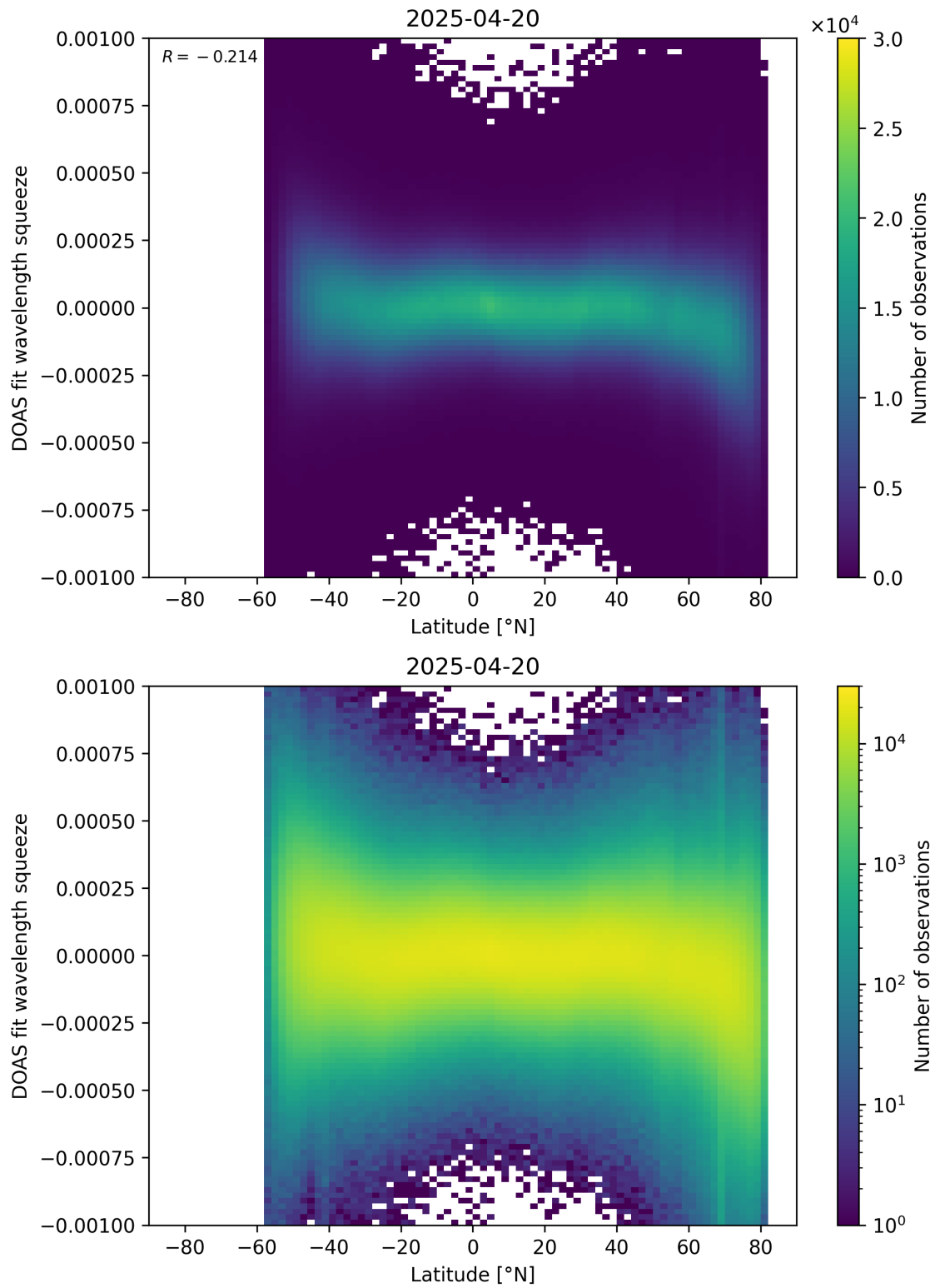
Figure 154: Scatter density plot of “Latitude” against “DOAS fit wavelength squeeze” for 2025-04-19 to 2025-04-21.
