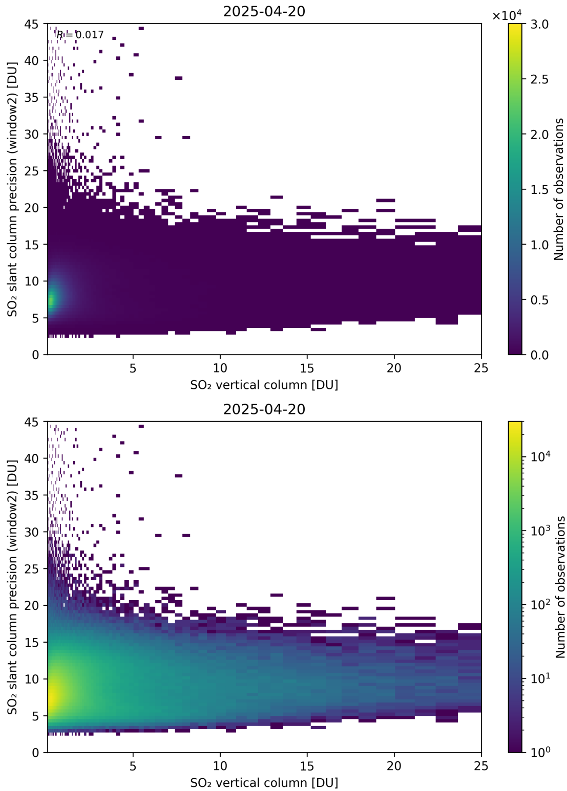
Figure 356: Scatter density plot of “SO 2 vertical column” against “SO 2 slant column precision (window2)” for 2025-04-19 to 2025-04-21.
