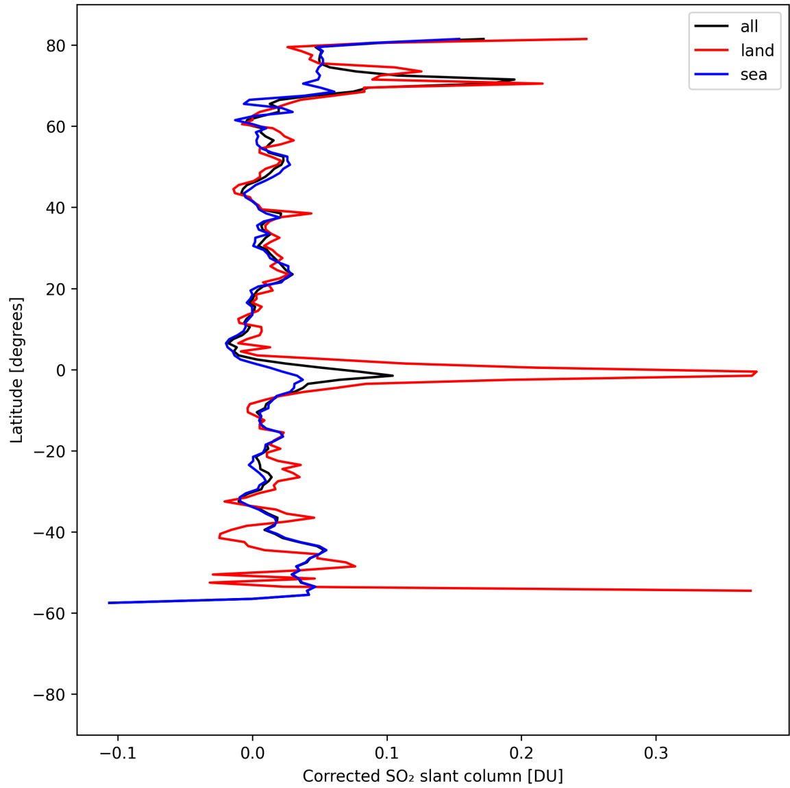
Figure 34: Zonal average of “Corrected SO 2 slant column” for 2025-04-19 to 2025-04-21.
