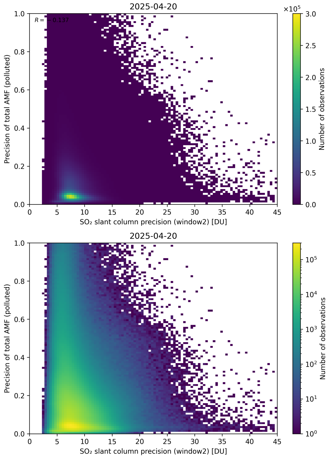
Figure 302: Scatter density plot of “SO 2 slant column precision (window2)” against “Precision of total AMF (polluted)” for 2025-04-19 to 2025-04-21.
