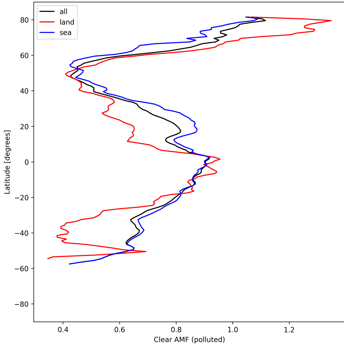
Figure 55: Zonal average of “Clear AMF (polluted)” for 2025-04-19 to 2025-04-21.
