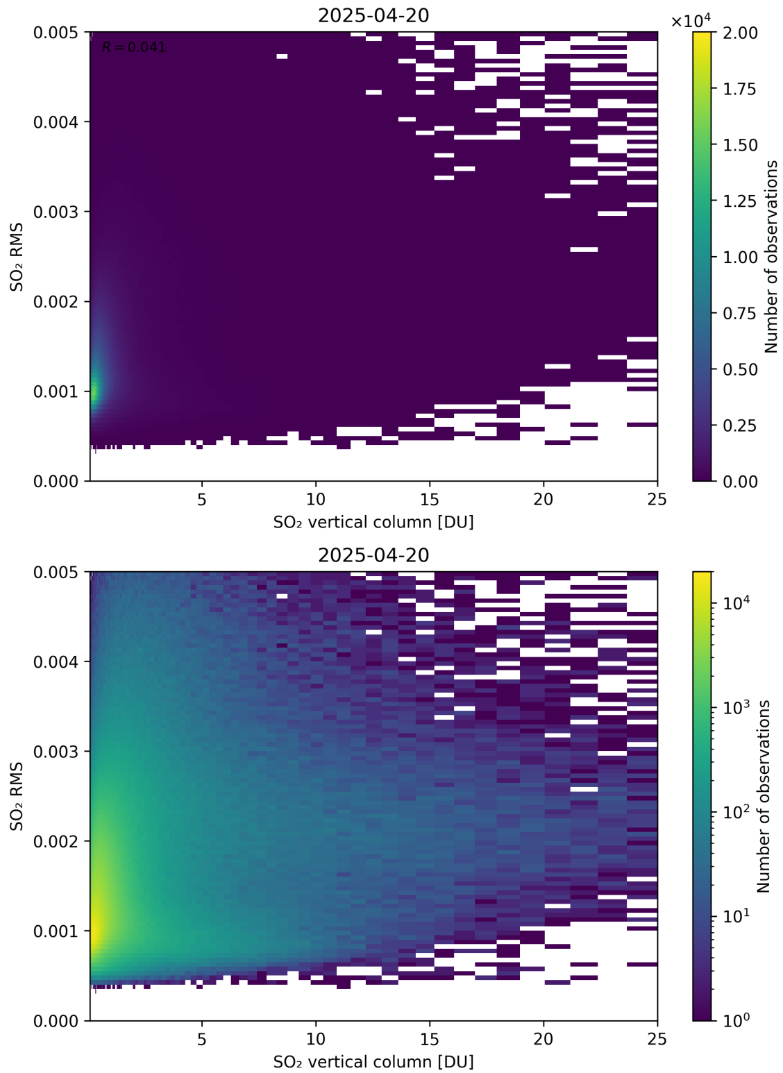
Figure 328: Scatter density plot of “SO 2 vertical column” against “SO 2 RMS” for 2025-04-19 to 2025-04-21.
