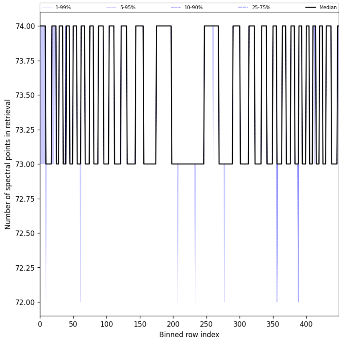
Figure 108: Along track statistics of “Number of spectral points in retrieval” for 2025-04-19 to 2025-04-21
