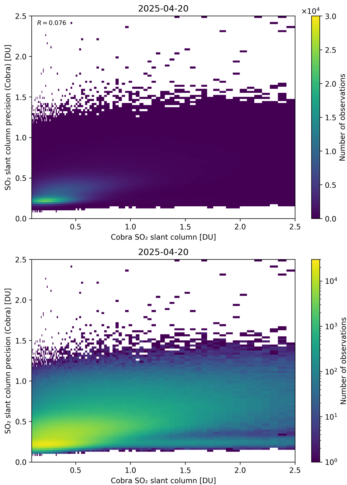
Figure 216: Scatter density plot of “Cobra SO 2 slant column” against “SO 2 slant column precision (Cobra)” for 2025-04-19 to 2025-04-21.
