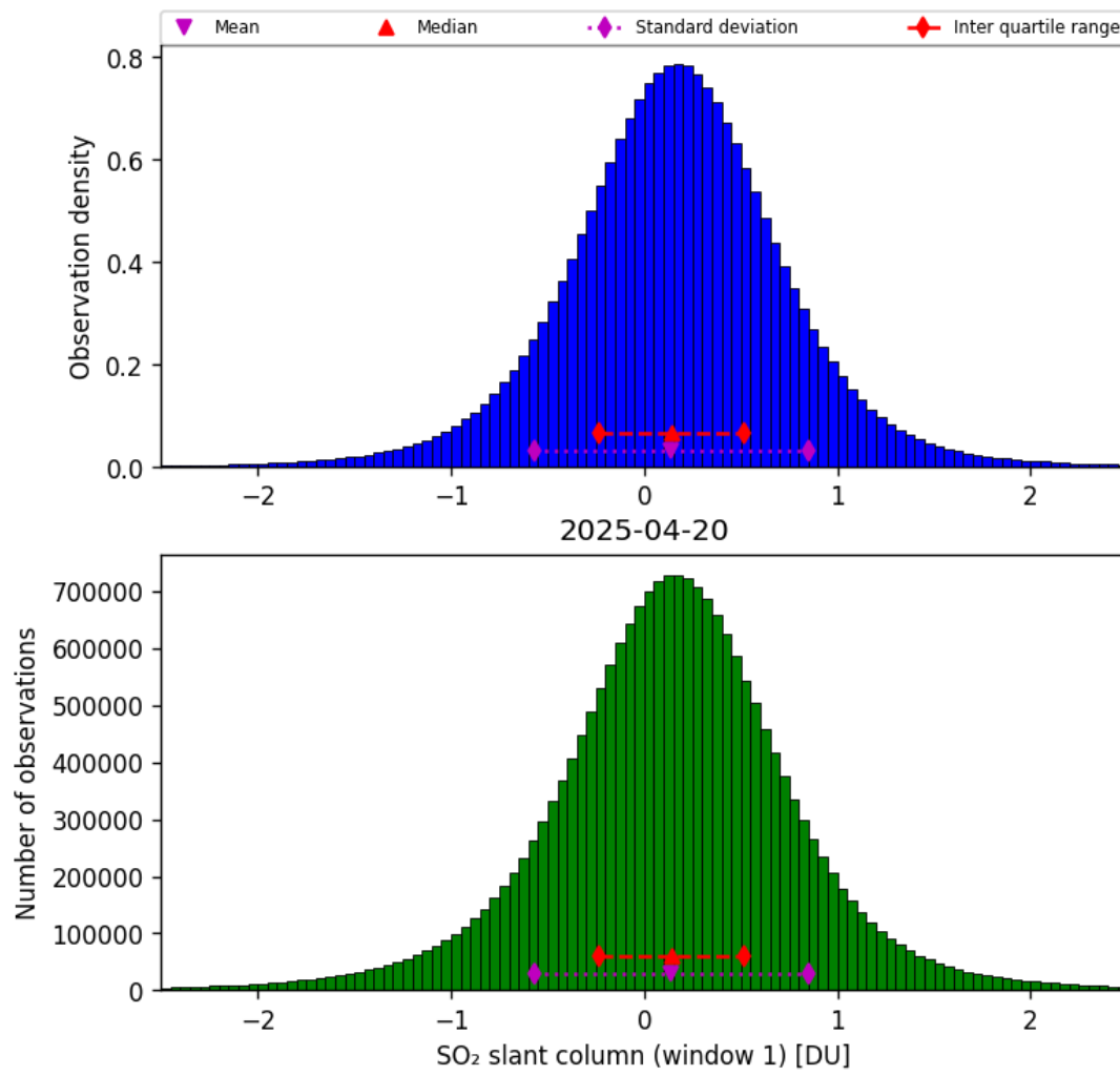
Figure 63: Histogram of “SO 2 slant column (window 1)” for 2025-04-19 to 2025-04-21
