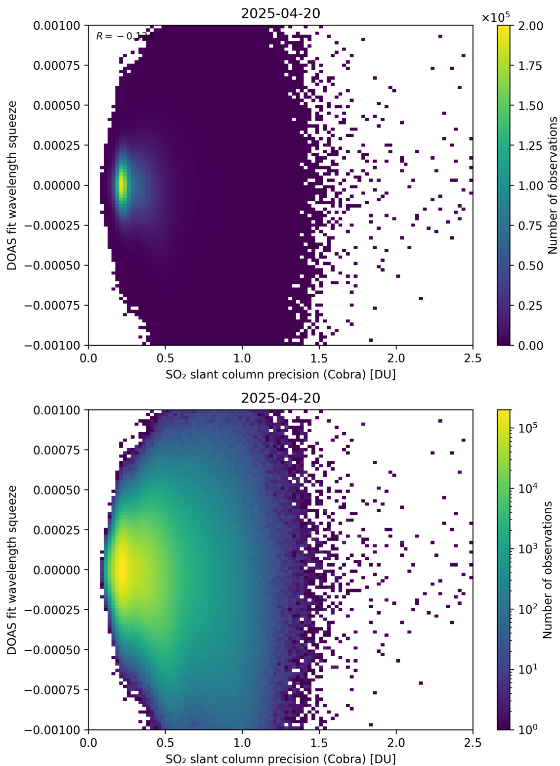
Figure 203: Scatter density plot of “SO 2 slant column precision (Cobra)” against “DOAS fit wavelength squeeze” for 2025-04-19 to 2025-04-21.
