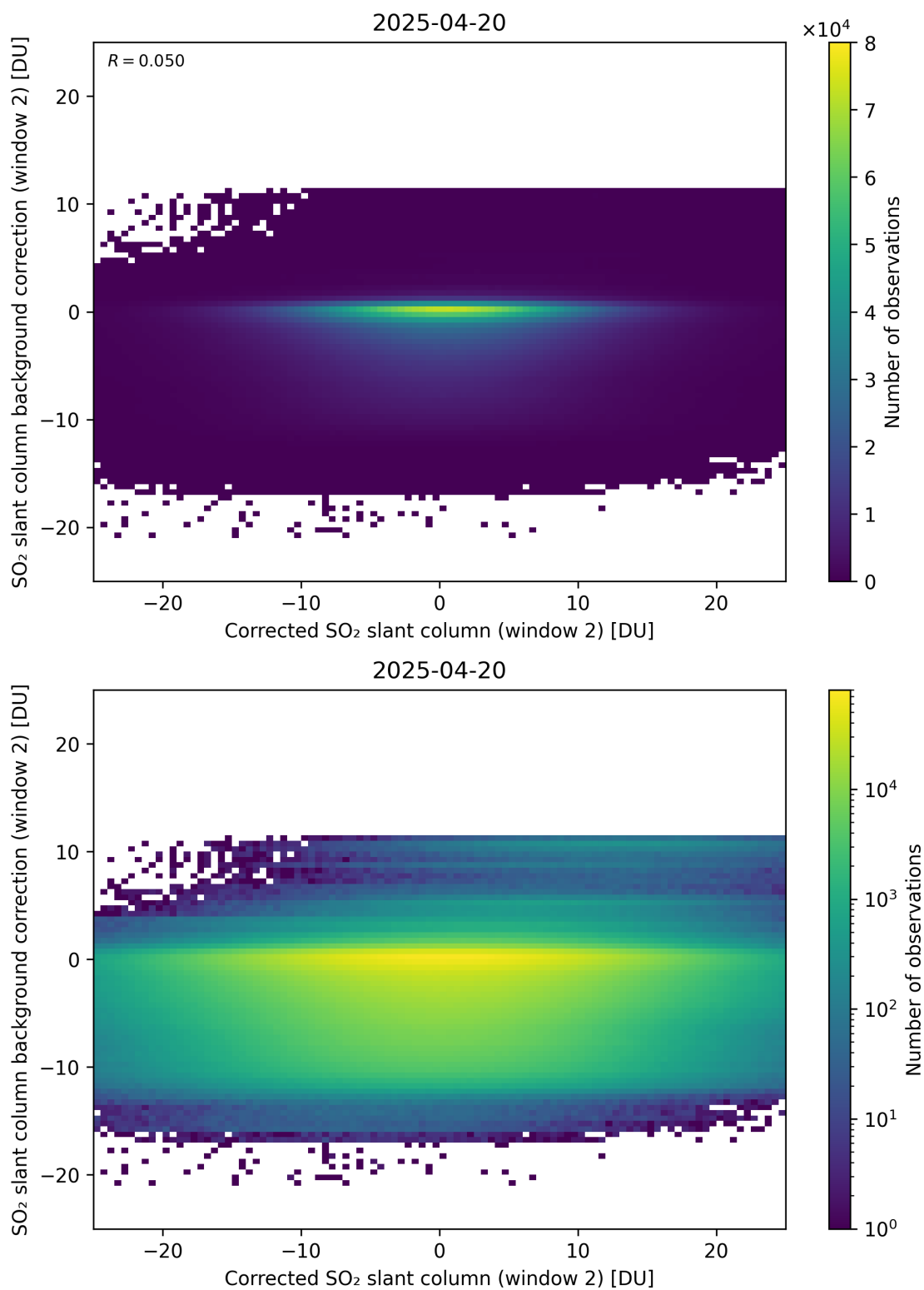
Figure 244: Scatter density plot of “Corrected SO 2 slant column (window 2)” against “SO 2 slant column background correction (window 2)” for 2025-04-19 to 2025-04-21.
