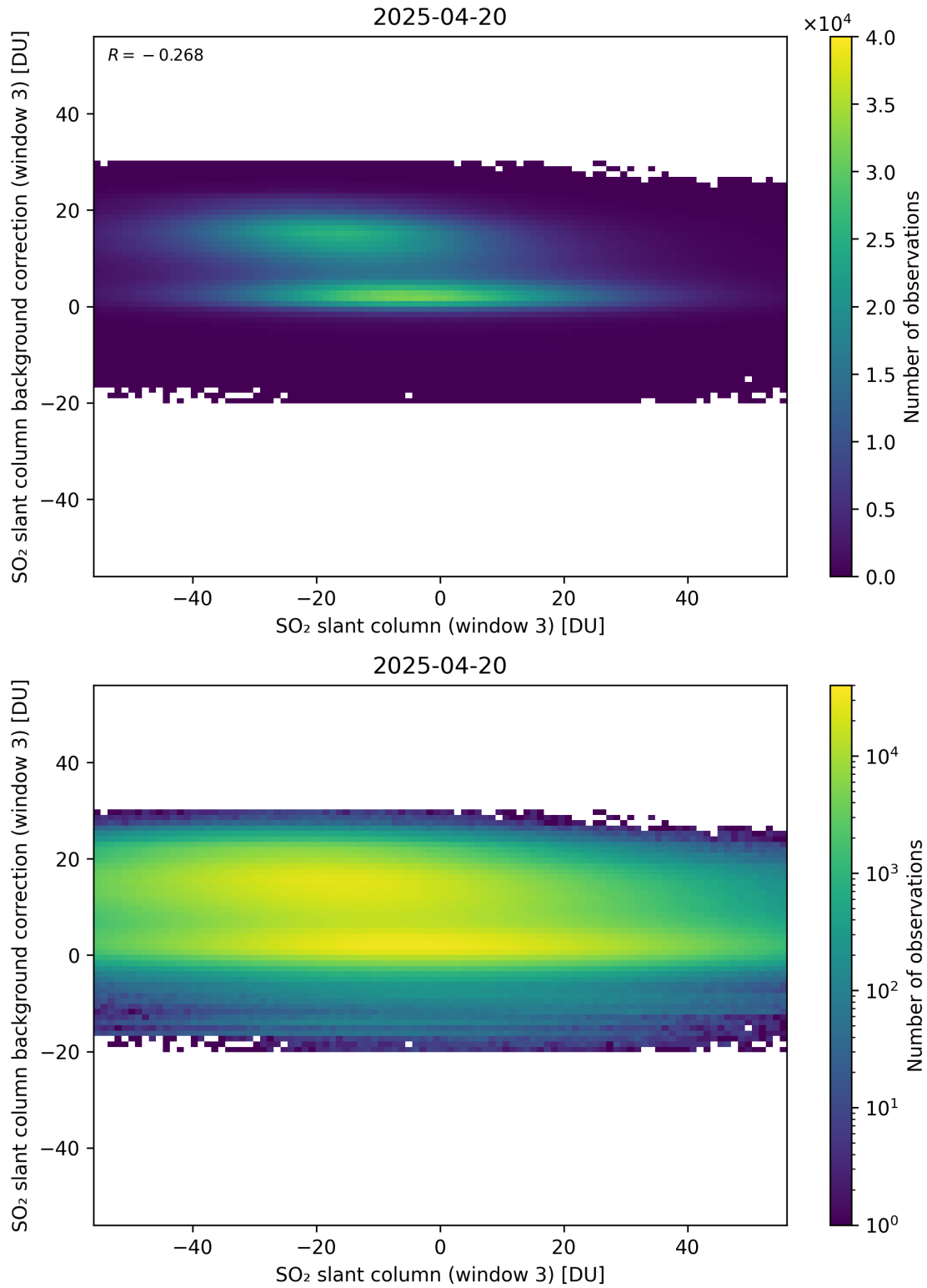
Figure 303: Scatter density plot of “SO 2 slant column (window 3)” against “SO 2 slant column background correction (window 3)” for 2025-04-19 to 2025-04-21.
