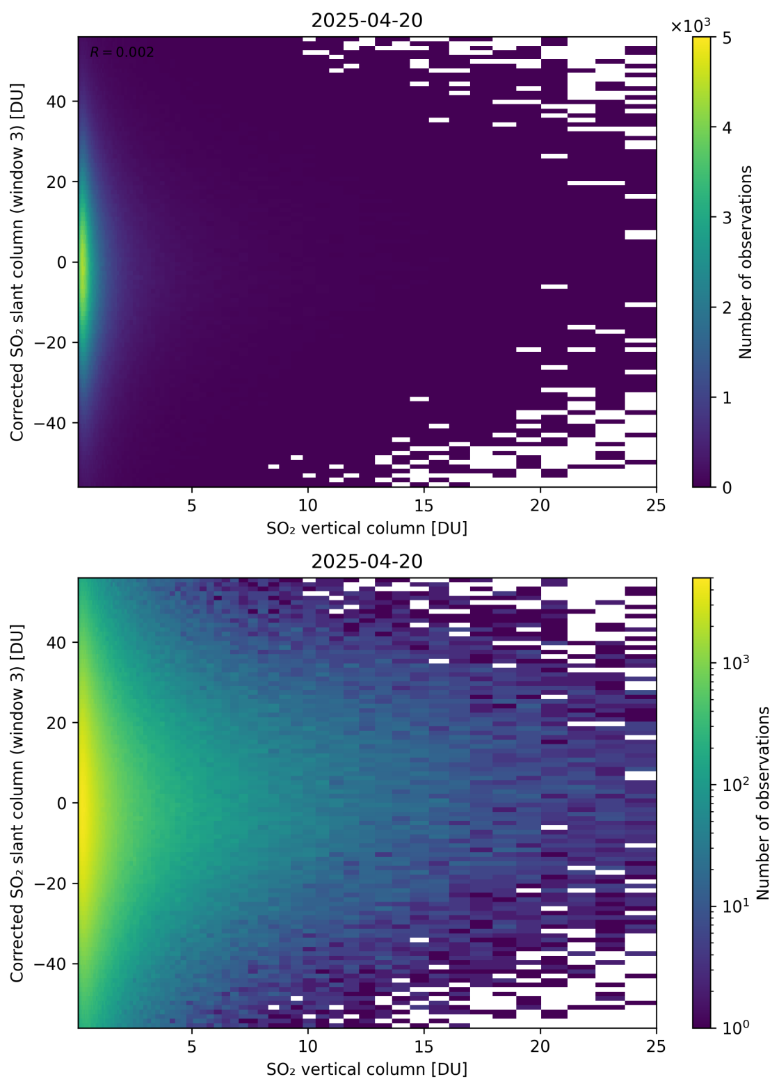
Figure 353: Scatter density plot of “SO 2 vertical column” against “Corrected SO 2 slant column (window 3)” for 2025-04-19 to 2025-04-21.
