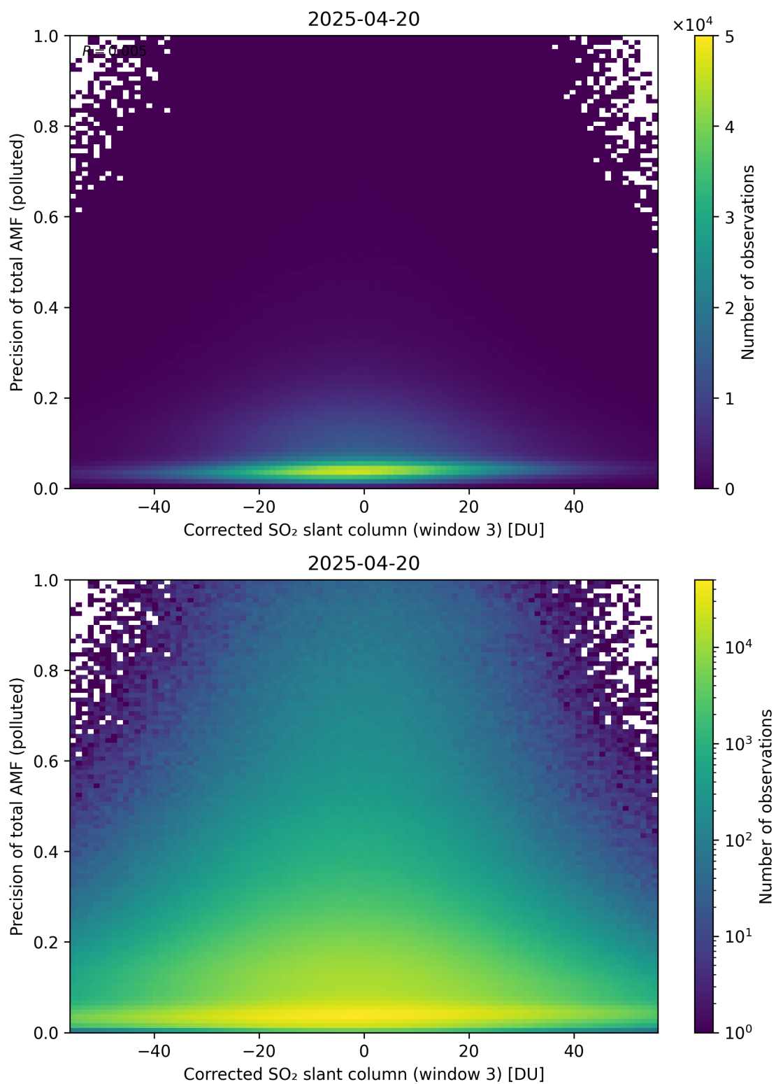
Figure 261: Scatter density plot of “Corrected SO 2 slant column (window 3)” against “Precision of total AMF (polluted)” for 2025-04-19 to 2025-04-21.
