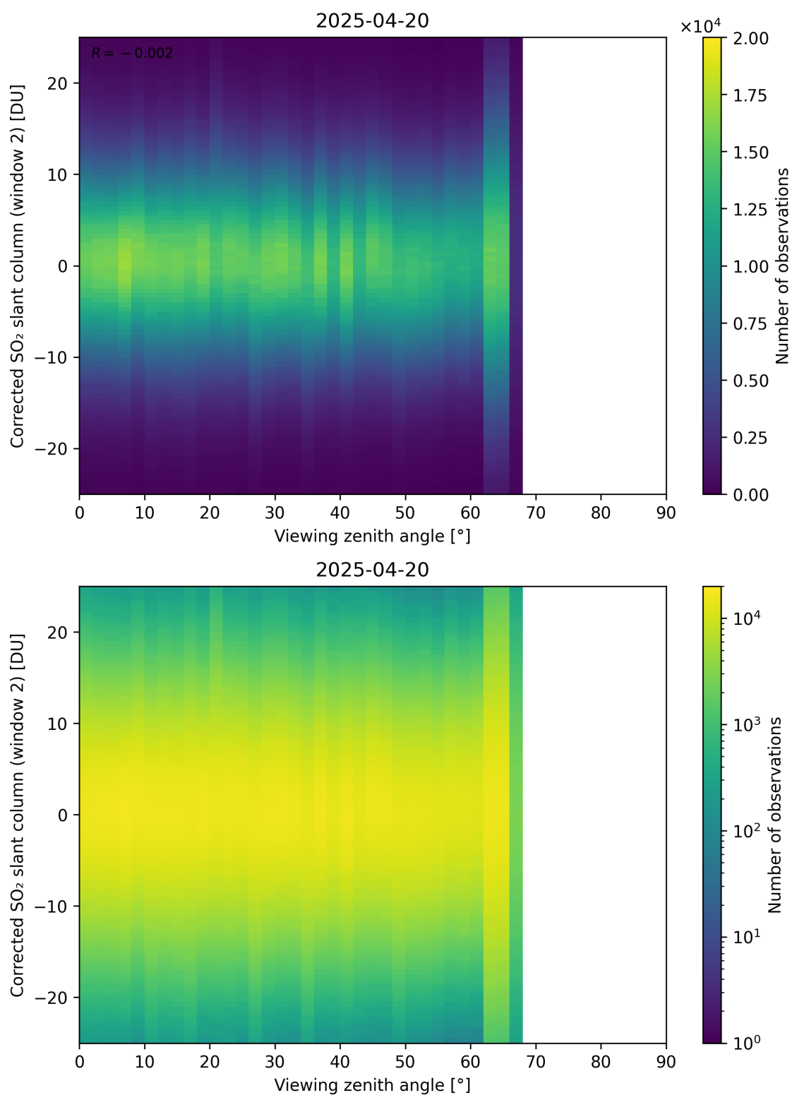
Figure 374: Scatter density plot of “Viewing zenith angle” against “Corrected SO 2 slant column (window 2)” for 2025-04-19 to 2025-04-21.
