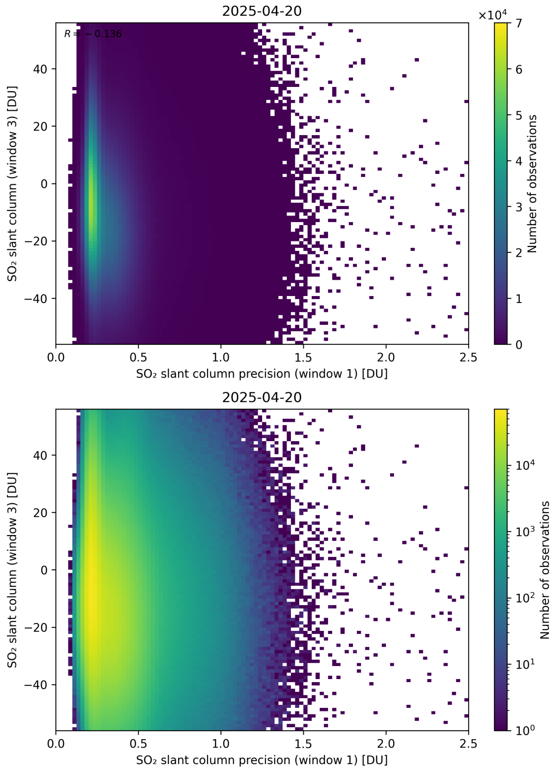
Figure 278: Scatter density plot of “SO 2 slant column precision (window 1)” against “SO 2 slant column (window 3)” for 2025-04-19 to 2025-04-21.
