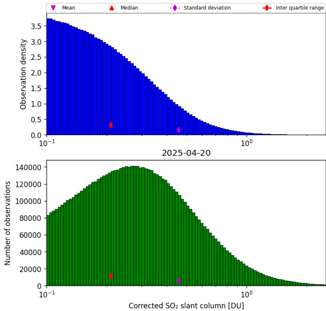
Figure 60: Histogram of "Corrected SO 2 slant column" for 2025-04-19 to 2025-04-21
