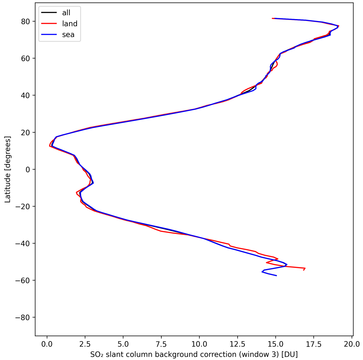
Figure 48: Zonal average of “SO 2 slant column background correction (window 3)” for 2025-04-19 to 2025-04-21.
