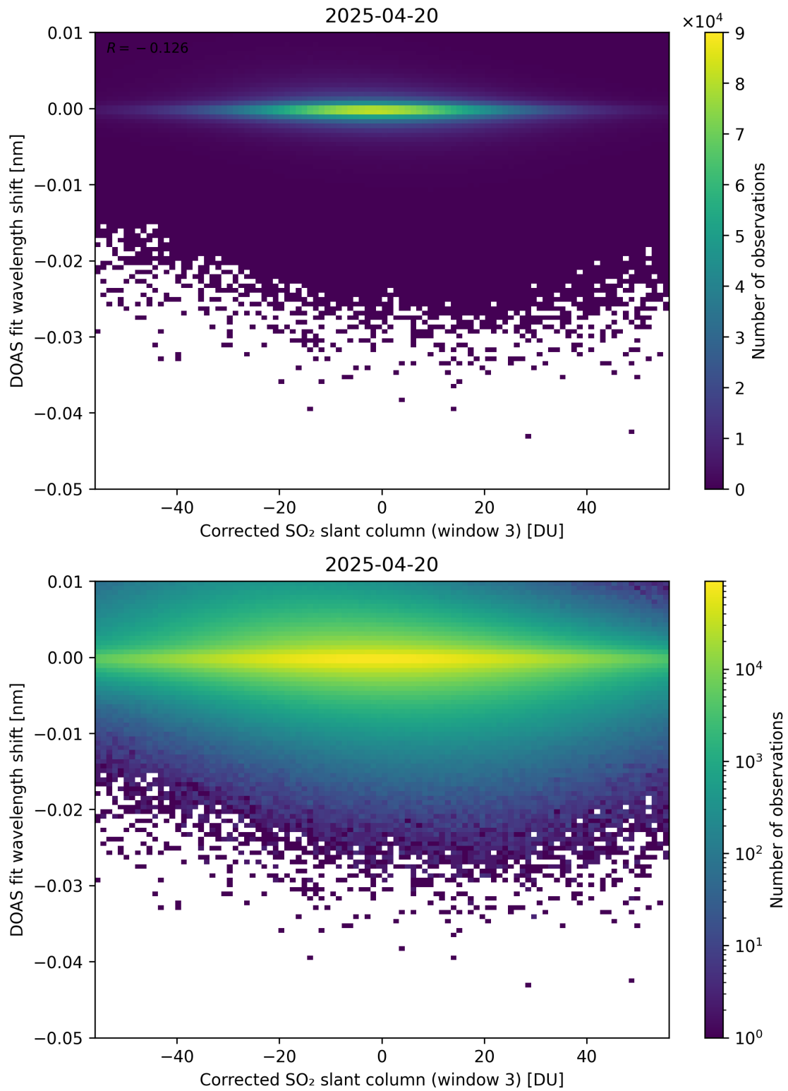
Figure 256: Scatter density plot of “Corrected SO 2 slant column (window 3)” against “DOAS fit wavelength shift” for 2025-04-19 to 2025-04-21.
