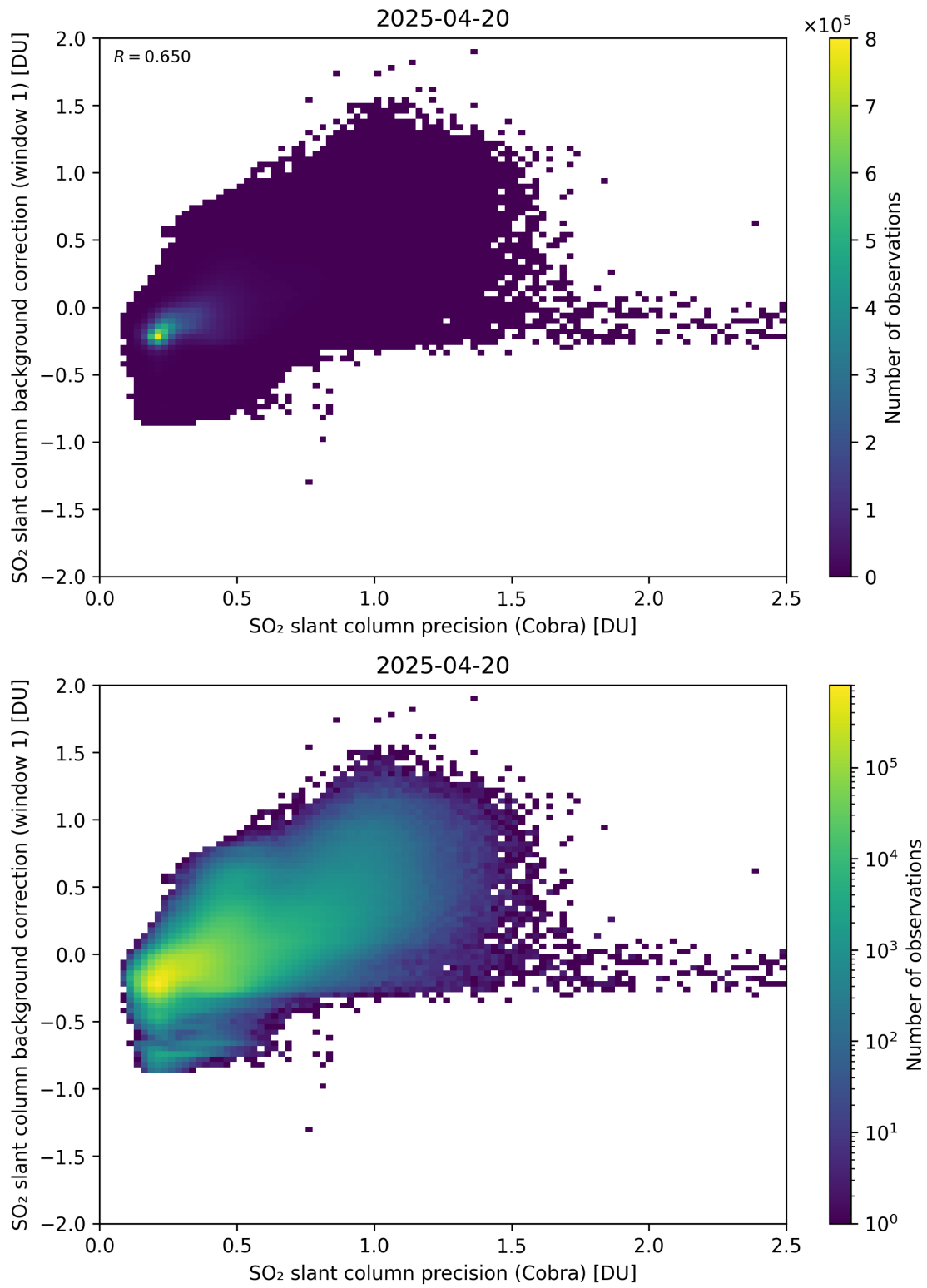
Figure 199: Scatter density plot of “SO 2 slant column precision (Cobra)” against “SO 2 slant column background correction (window 1)” for 2025-04-19 to 2025-04-21.
