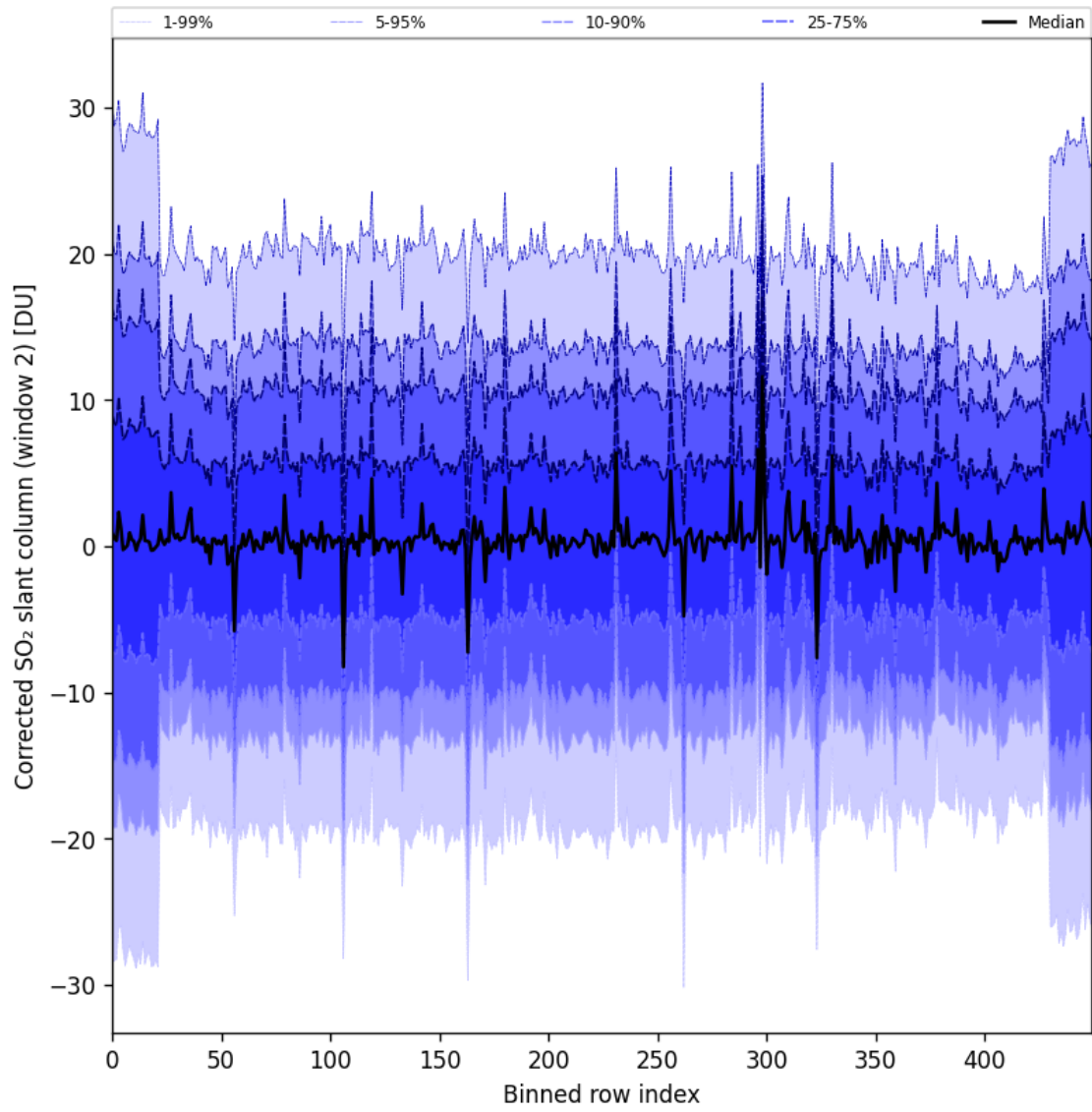
Figure 95: Along track statistics of “Corrected SO 2 slant column (window 2)” for 2025-04-19 to 2025-04-21
