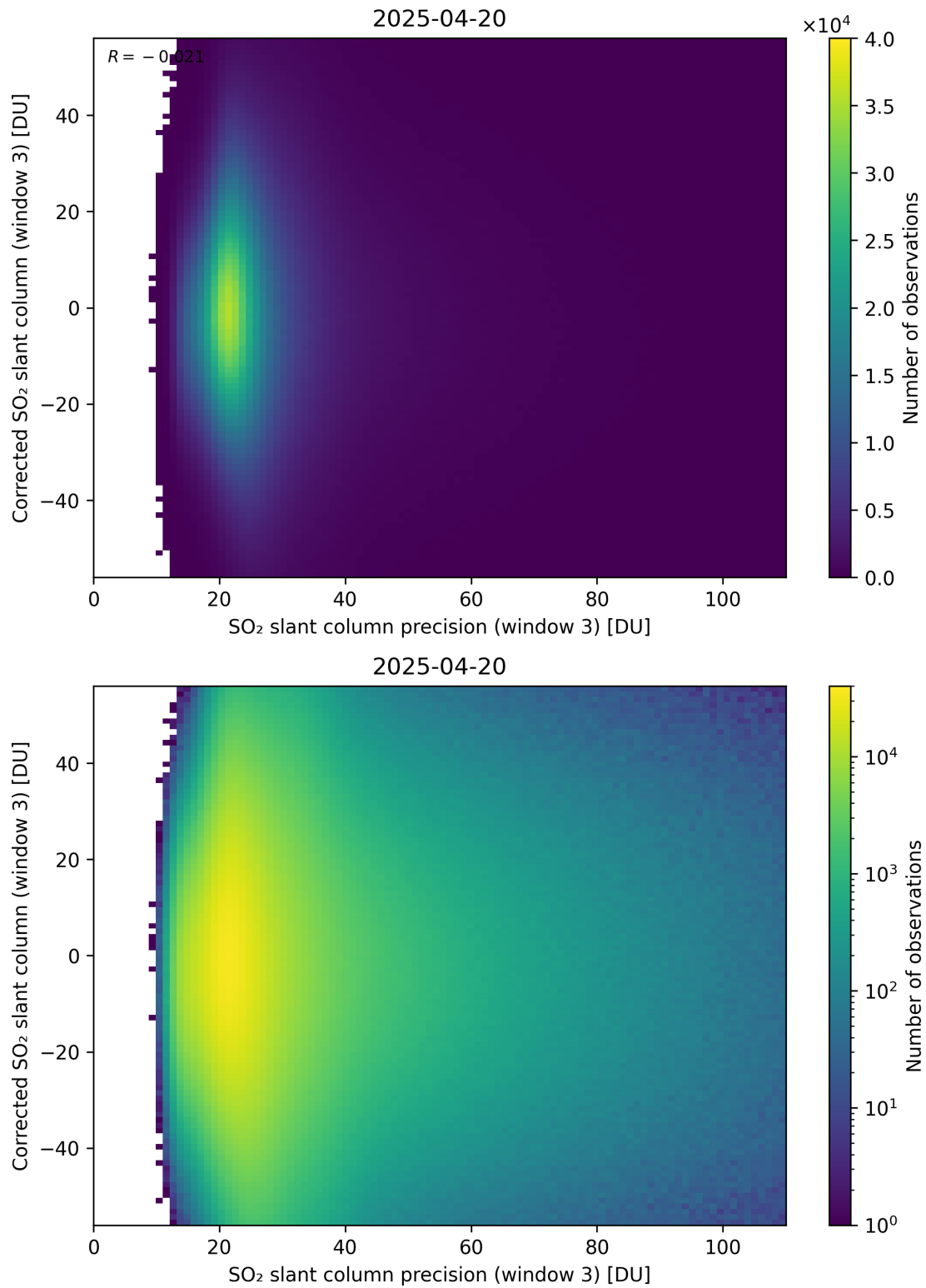
Figure 312: Scatter density plot of “SO 2 slant column precision (window 3)” against “Corrected SO 2 slant column (window 3)” for 2025-04-19 to 2025-04-21.
