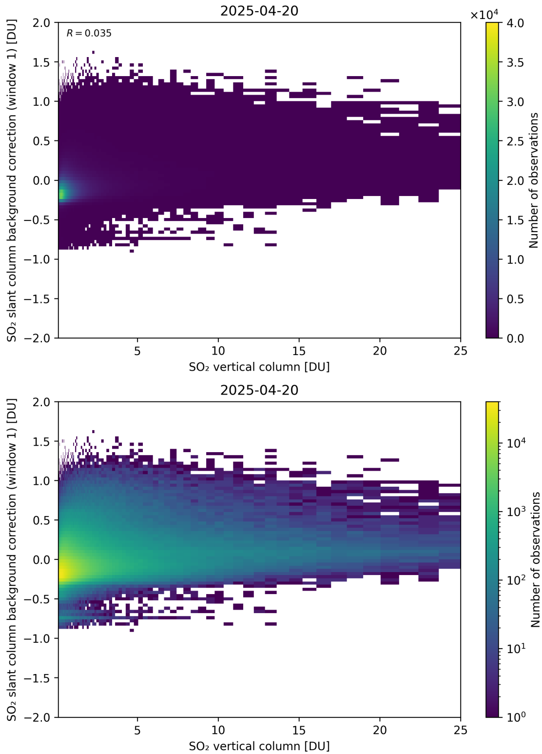
Figure 323: Scatter density plot of “SO 2 vertical column” against “SO 2 slant column background correction (window 1)” for 2025-04-19 to 2025-04-21.
