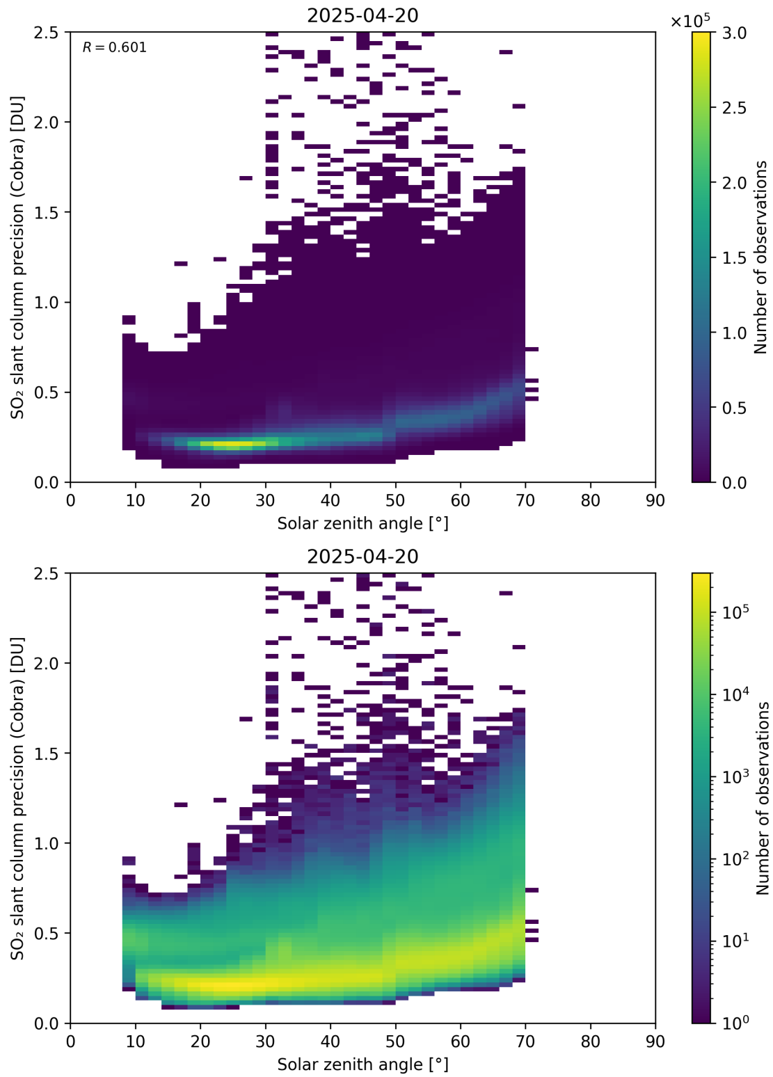
Figure 180: Scatter density plot of “Solar zenith angle” against “SO 2 slant column precision (Cobra)” for 2025-04-19 to 2025-04-21.
