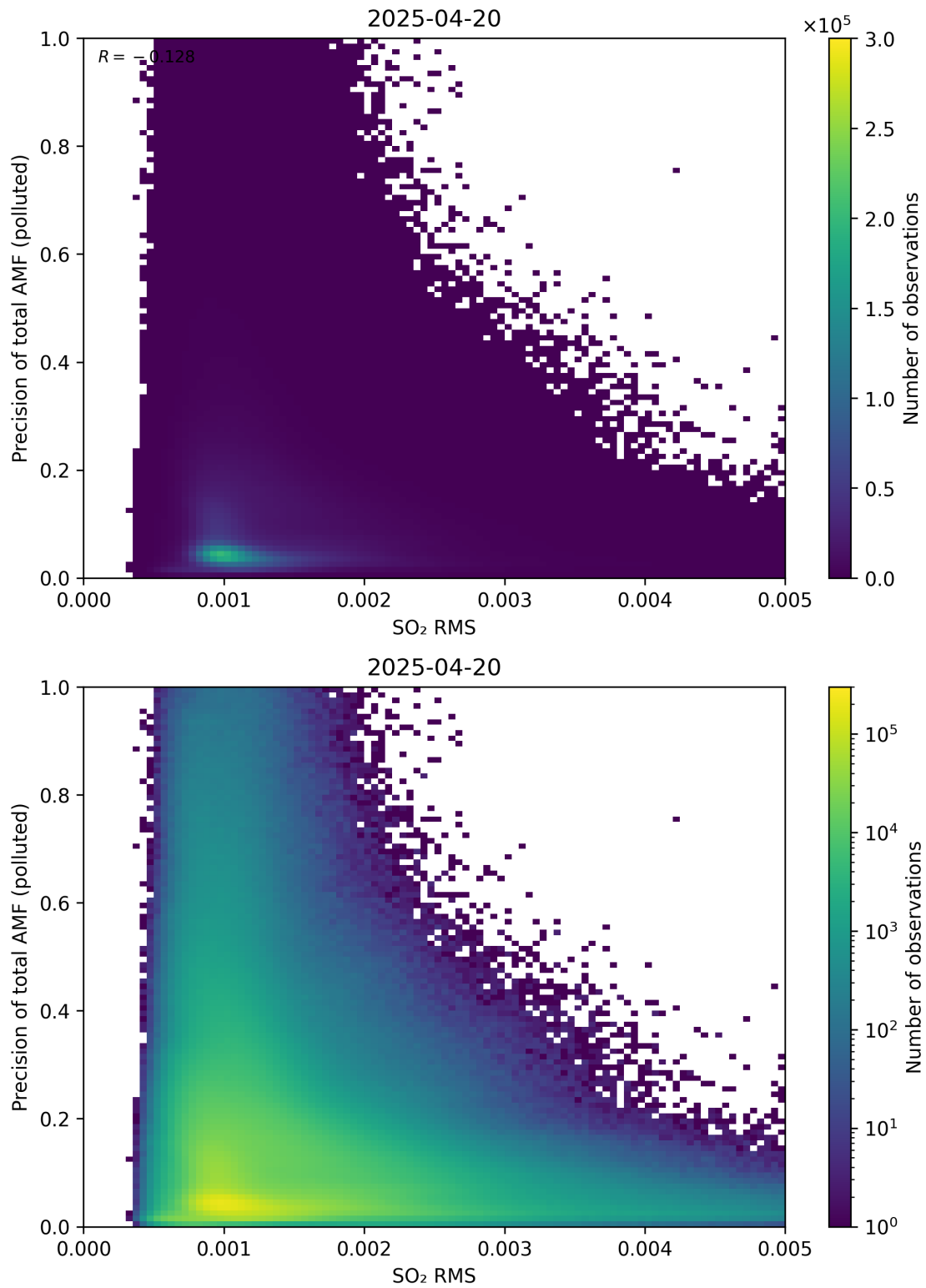
Figure 149: Scatter density plot of “SO 2 RMS” against “Precision of total AMF (polluted)” for 2025-04-19 to 2025-04-21.
