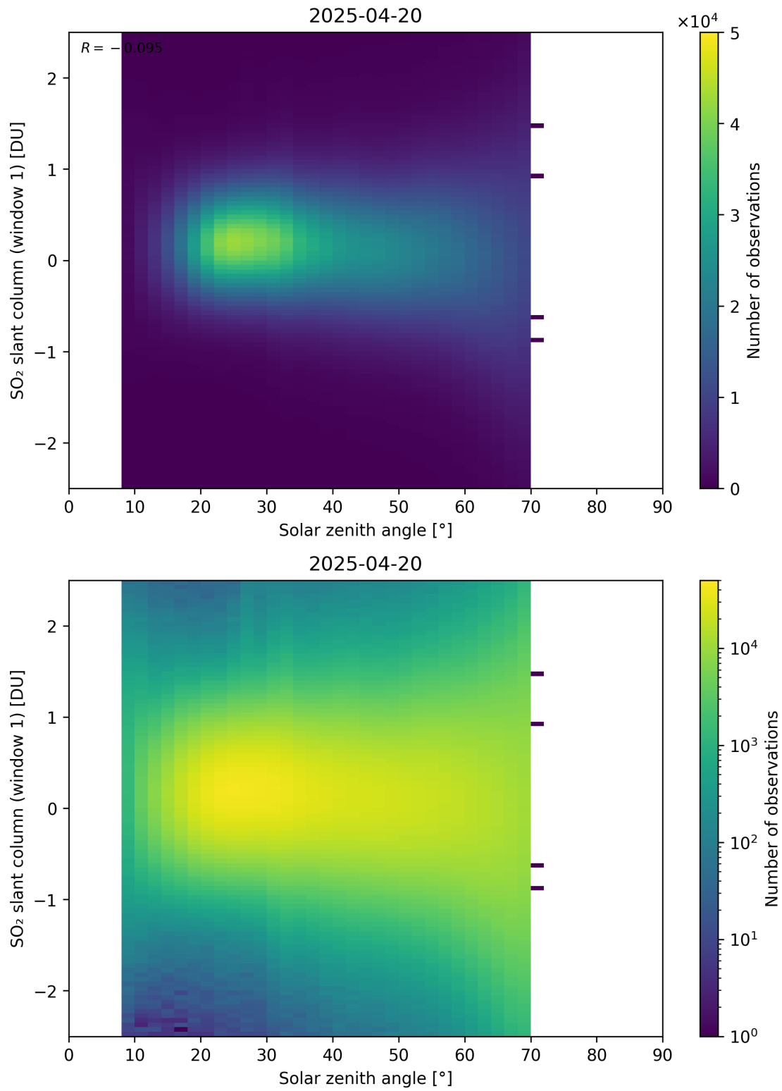
Figure 184: Scatter density plot of “Solar zenith angle” against “SO 2 slant column (window 1)” for 2025-04-19 to 2025-04-21.
