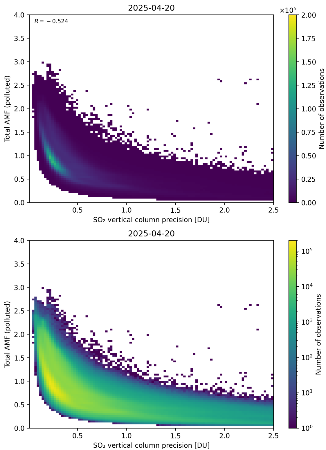
Figure 346: Scatter density plot of “SO 2 vertical column precision” against “Total AMF (polluted)” for 2025-04-19 to 2025-04-21.
