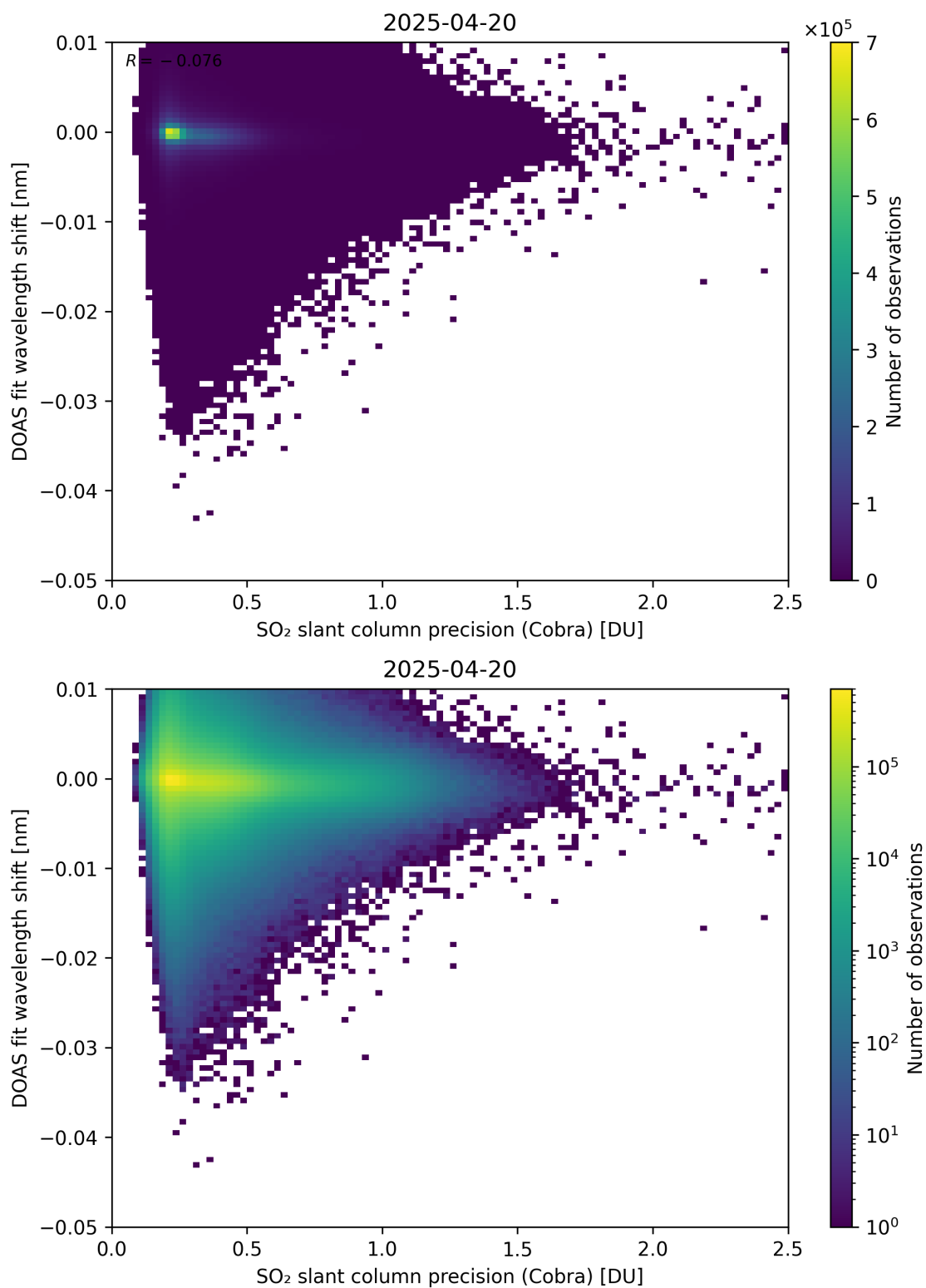
Figure 202: Scatter density plot of “SO 2 slant column precision (Cobra)” against “DOAS fit wavelength shift” for 2025-04-19 to 2025-04-21.
