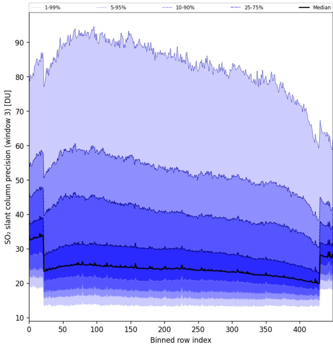
Figure 98: Along track statistics of “SO 2 slant column precision (window 3)” for 2025-04-19 to 2025-04-21
