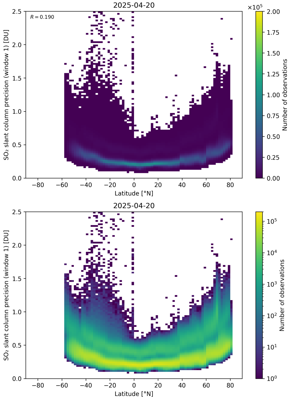
Figure 163: Scatter density plot of “Latitude” against “SO 2 slant column precision (window 1)” for 2025-04-19 to 2025-04-21.
