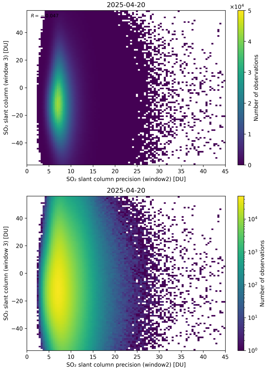
Figure 299: Scatter density plot of “SO 2 slant column precision (window2)” against “SO 2 slant column (window 3)” for 2025-04-19 to 2025-04-21.
