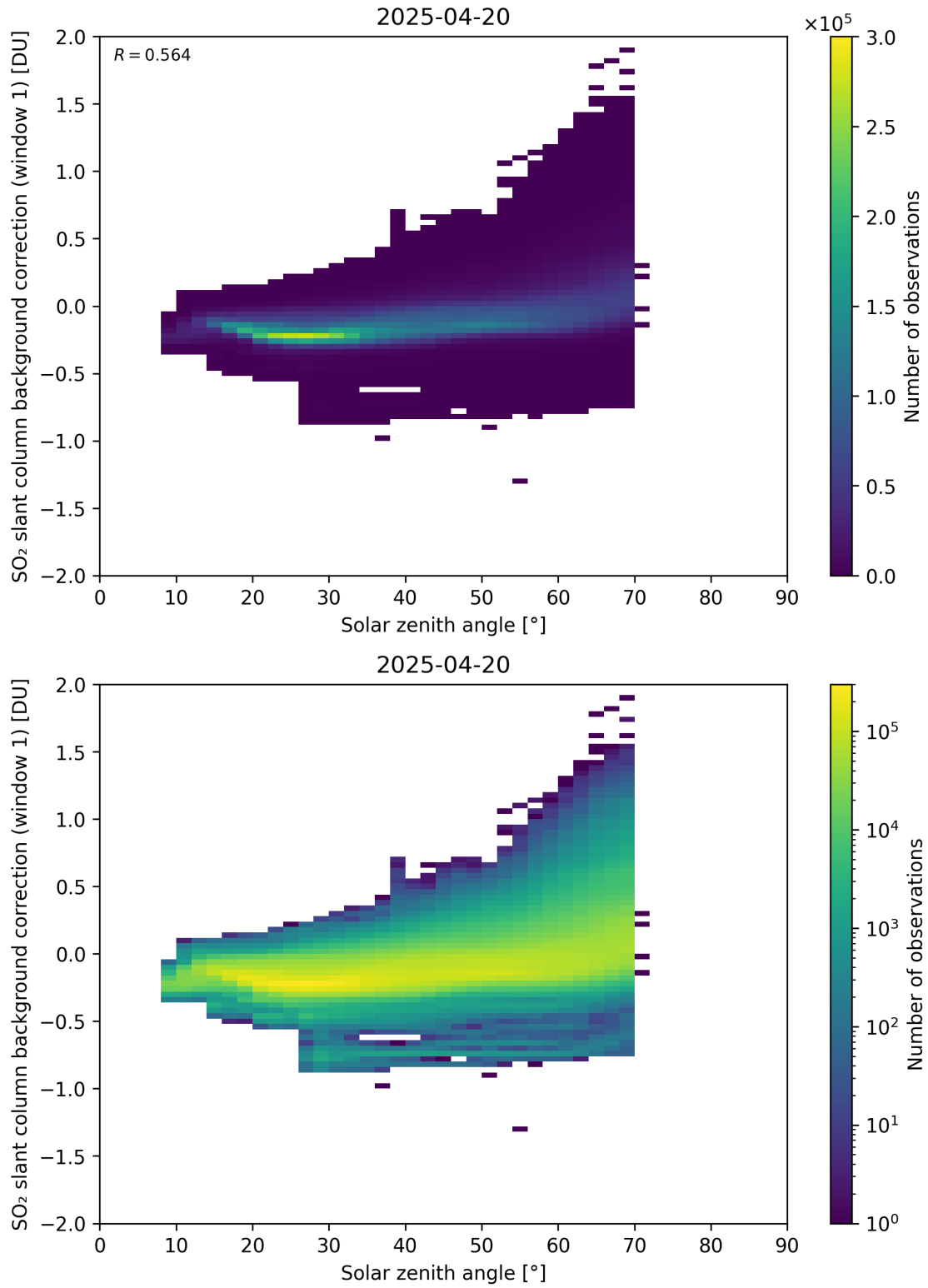
Figure 171: Scatter density plot of “Solar zenith angle” against “SO 2 slant column background correction (window 1)” for 2025-04-19 to 2025-04-21.
