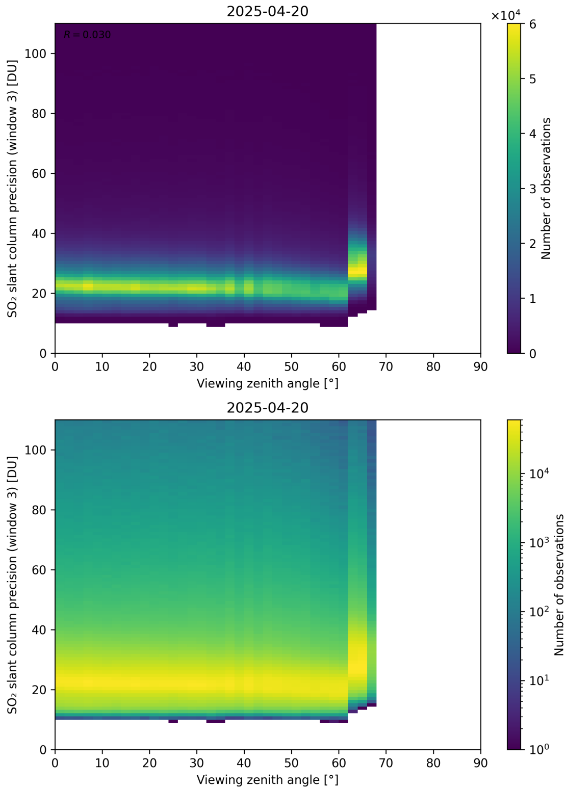
Figure 380: Scatter density plot of “Viewing zenith angle” against “SO 2 slant column precision (window 3)” for 2025-04-19 to 2025-04-21.
