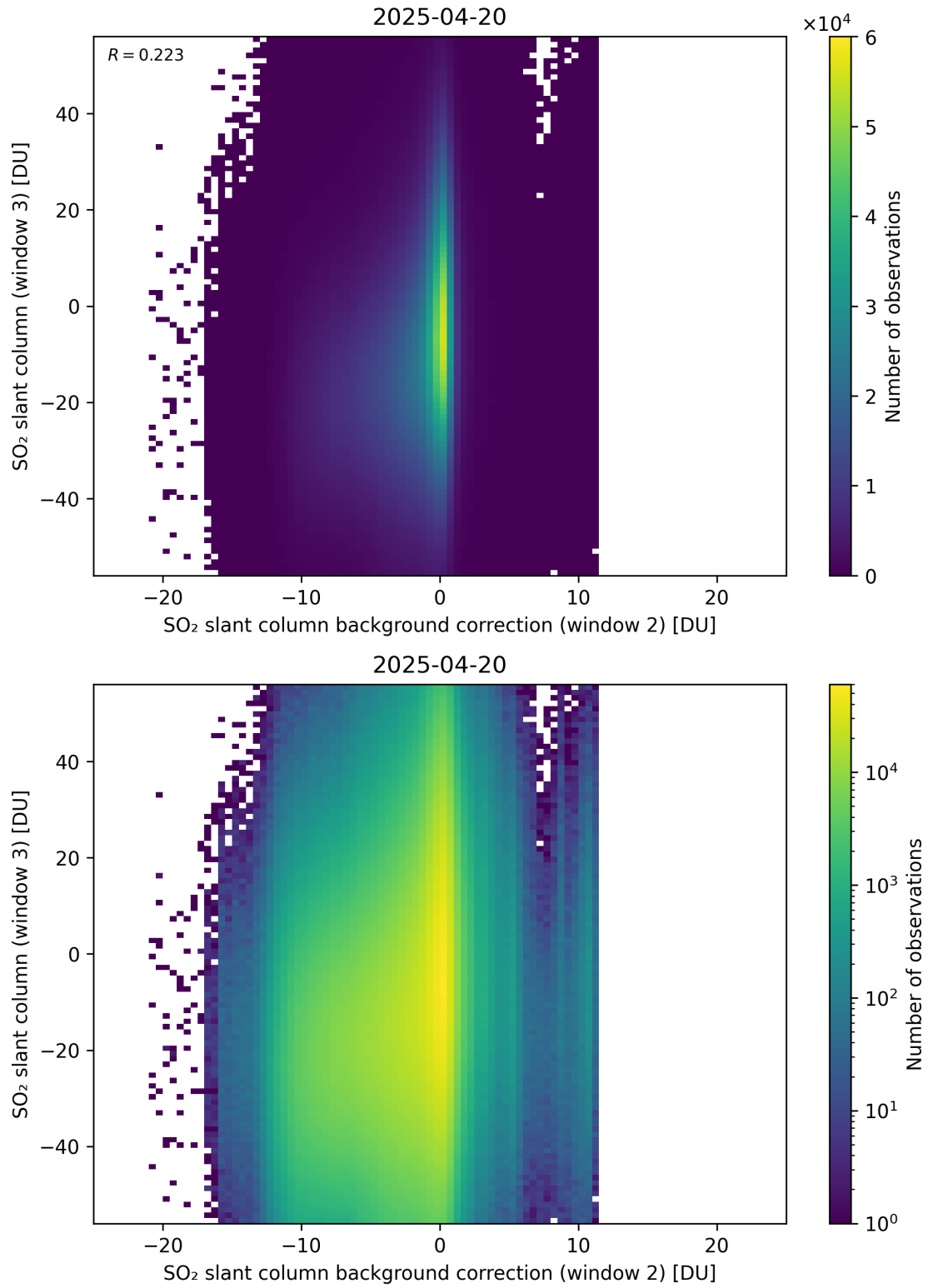
Figure 128: Scatter density plot of “SO 2 slant column background correction (window 2)” against “SO 2 slant column (window 3)” for 2025-04-19 to 2025-04-21.
