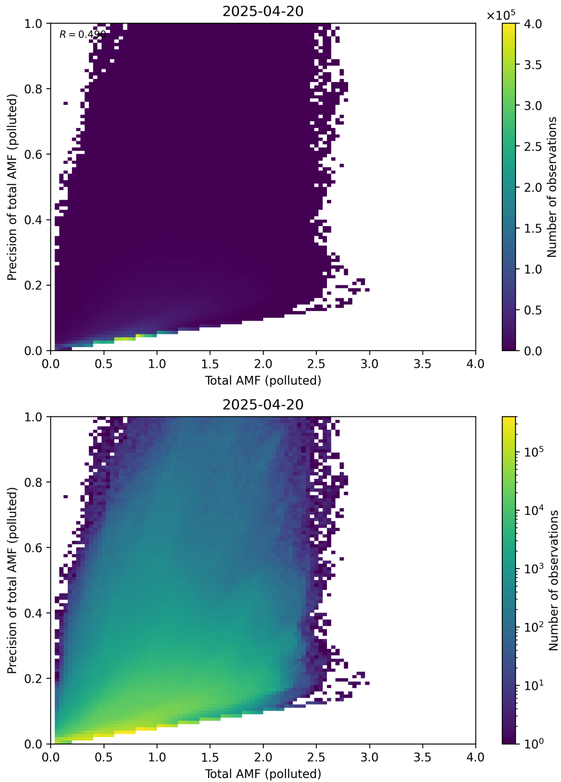
Figure 322: Scatter density plot of “Total AMF (polluted)” against “Precision of total AMF (polluted)” for 2025-04-19 to 2025-04-21.
