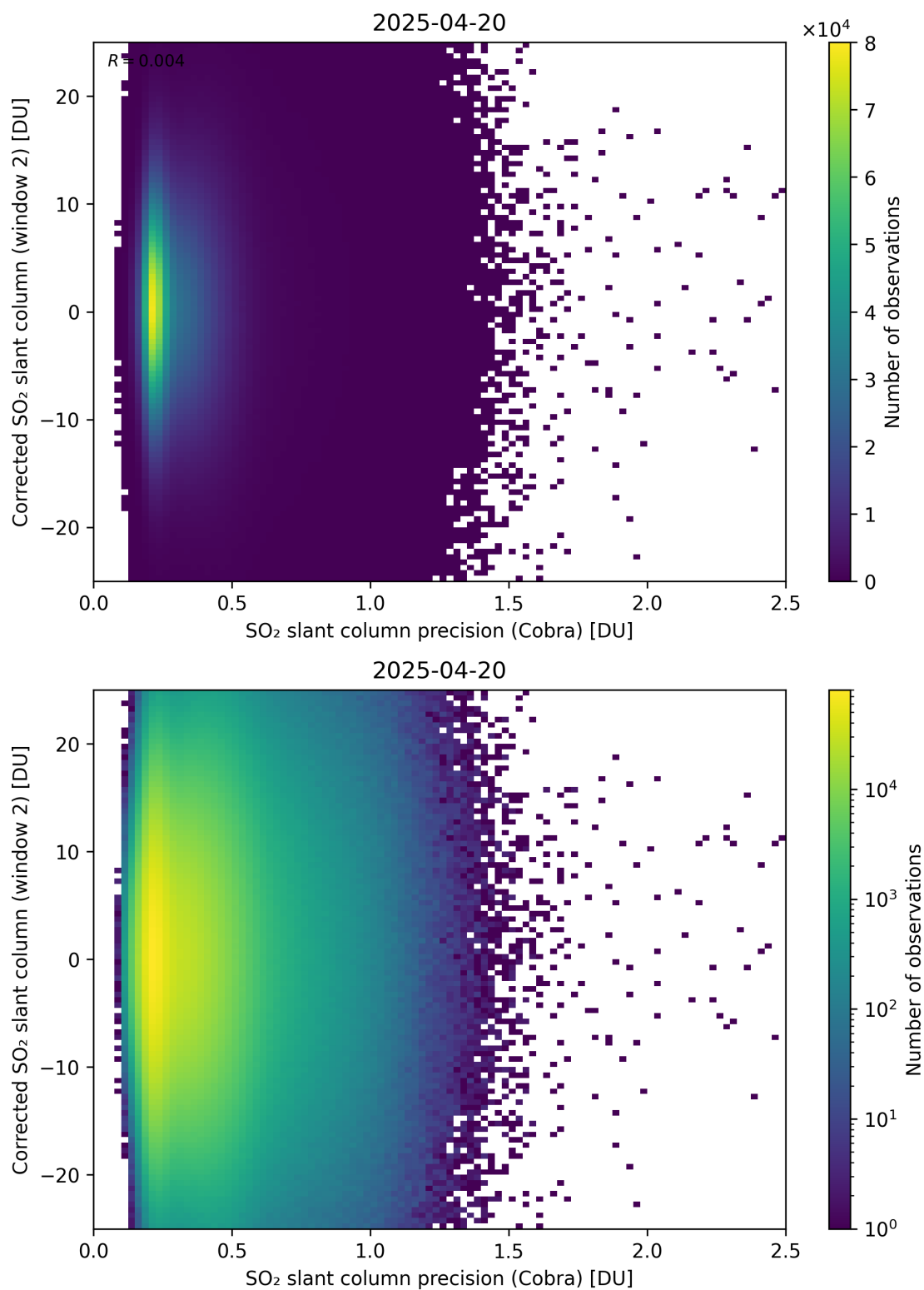
Figure 206: Scatter density plot of “SO 2 slant column precision (Cobra)” against “Corrected SO 2 slant column (window 2)” for 2025-04-19 to 2025-04-21.
