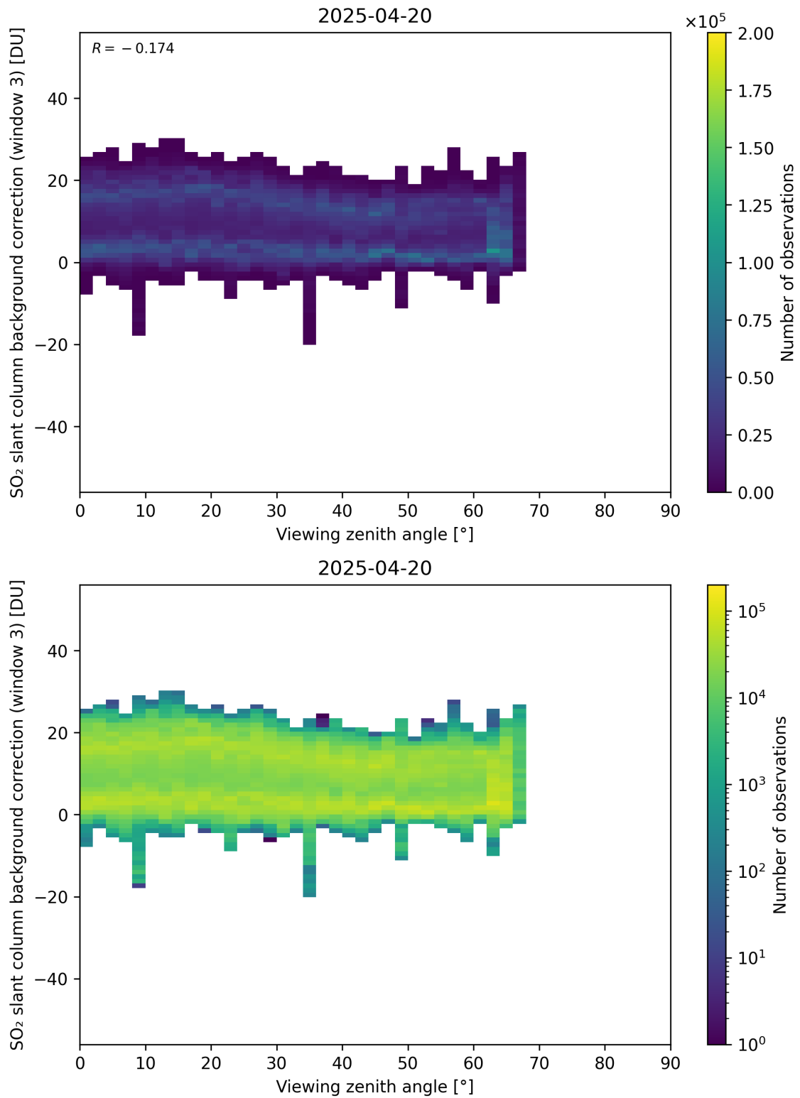
Figure 364: Scatter density plot of “Viewing zenith angle” against “SO 2 slant column background correction (window 3)” for 2025-04-19 to 2025-04-21.
