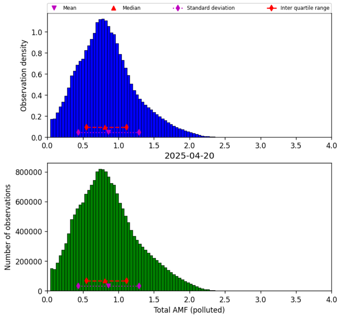
Figure 79: Histogram of “Total AMF (polluted)” for 2025-04-19 to 2025-04-21
