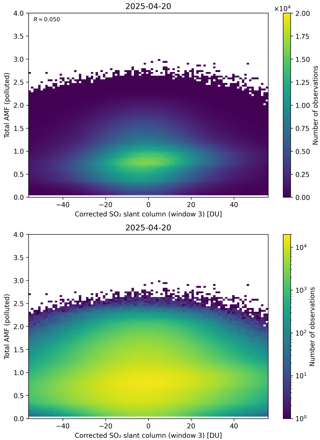
Figure 260: Scatter density plot of “Corrected SO 2 slant column (window 3)” against “Total AMF (polluted)” for 2025-04-19 to 2025-04-21.
