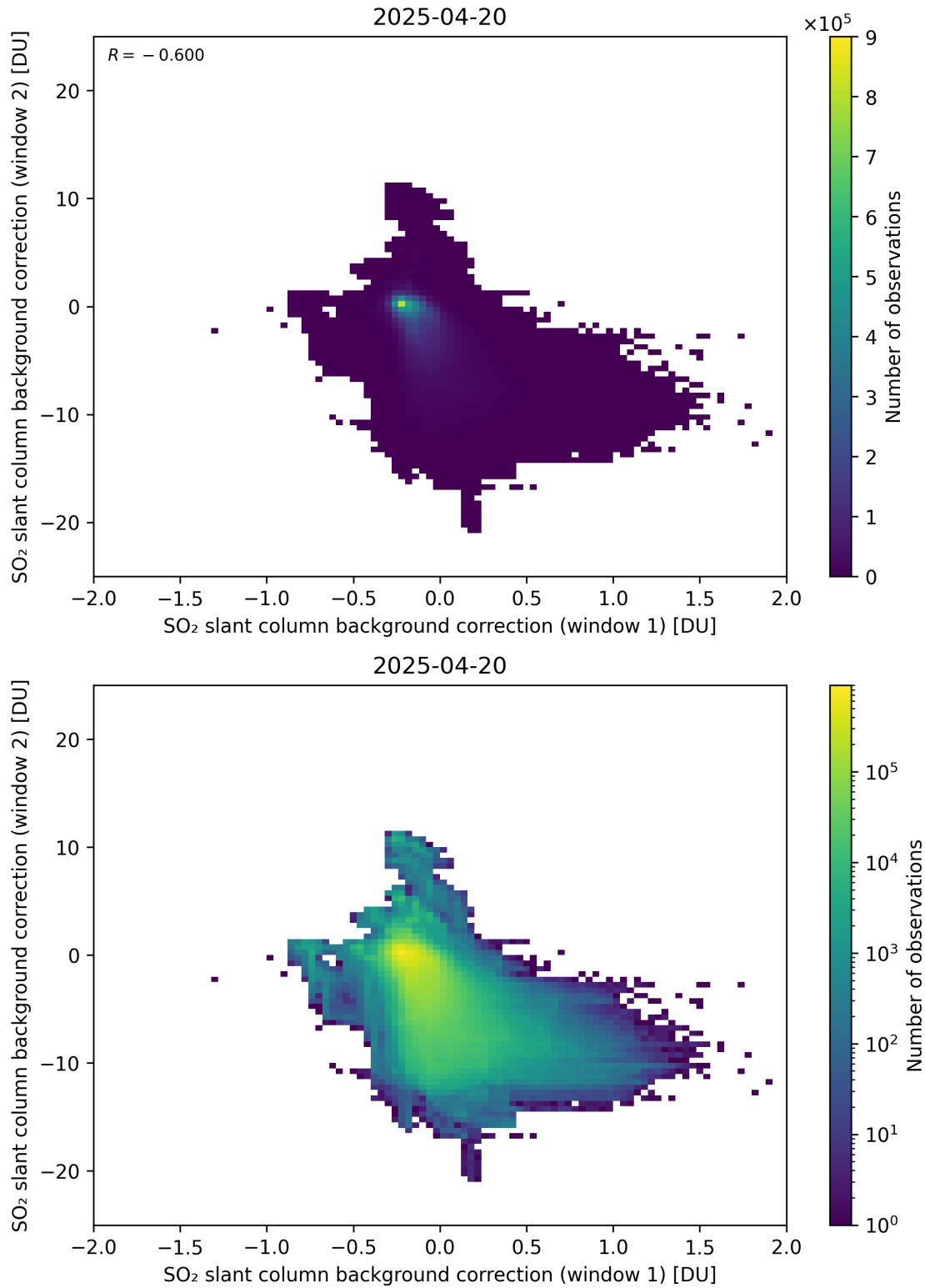
Figure 109: Scatter density plot of “SO 2 slant column background correction (window 1)” against “SO 2 slant column background correction (window 2)” for 2025-04-19 to 2025-04-21.
