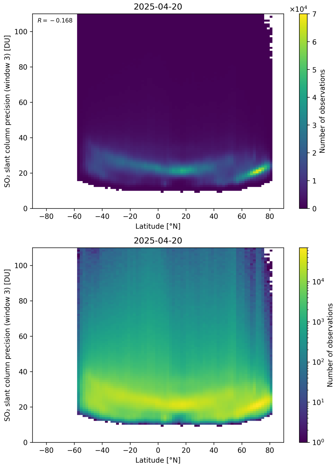
Figure 166: Scatter density plot of “Latitude” against “SO 2 slant column precision (window 3)” for 2025-04-19 to 2025-04-21.
