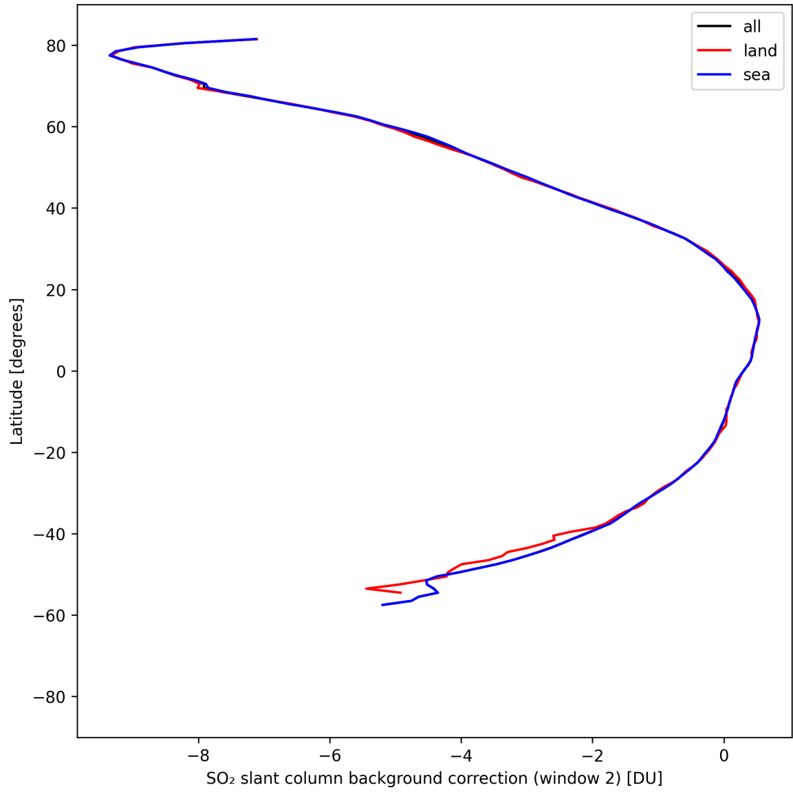
Figure 44: Zonal average of “SO 2 slant column background correction (window 2)” for 2025-04-19 to 2025-04-21.
