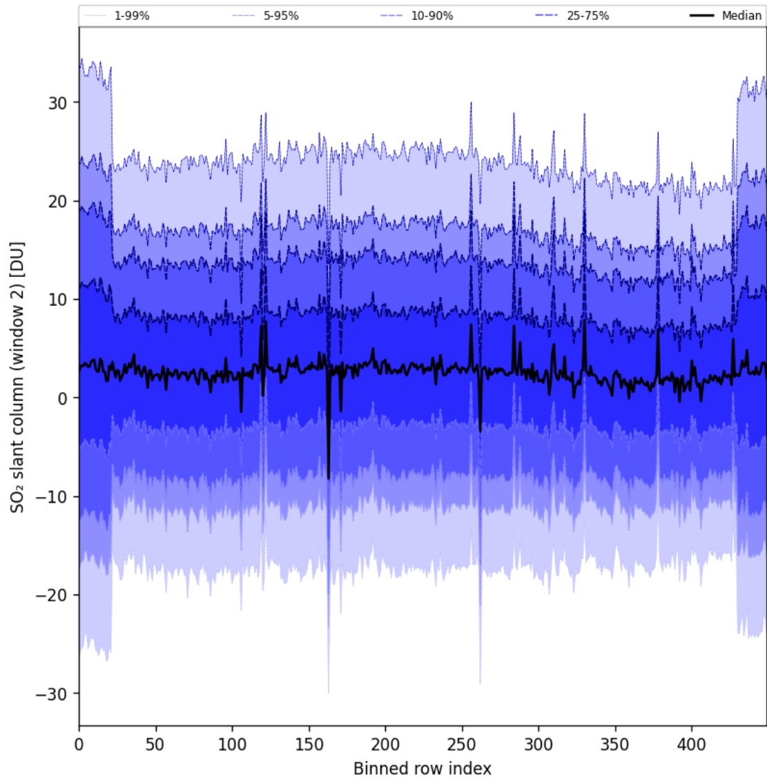
Figure 93: Along track statistics of “SO 2 slant column (window 2)” for 2025-04-19 to 2025-04-21
