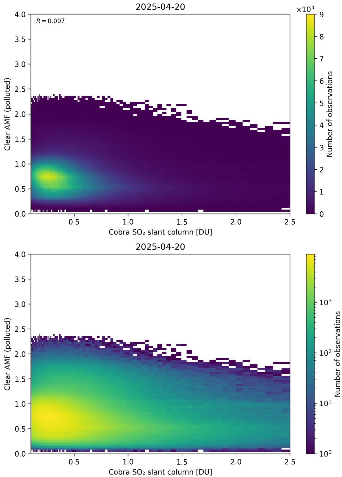
Figure 215: Scatter density plot of “Cobra SO 2 slant column” against “Clear AMF (polluted)” for 2025-04-19 to 2025-04-21.
