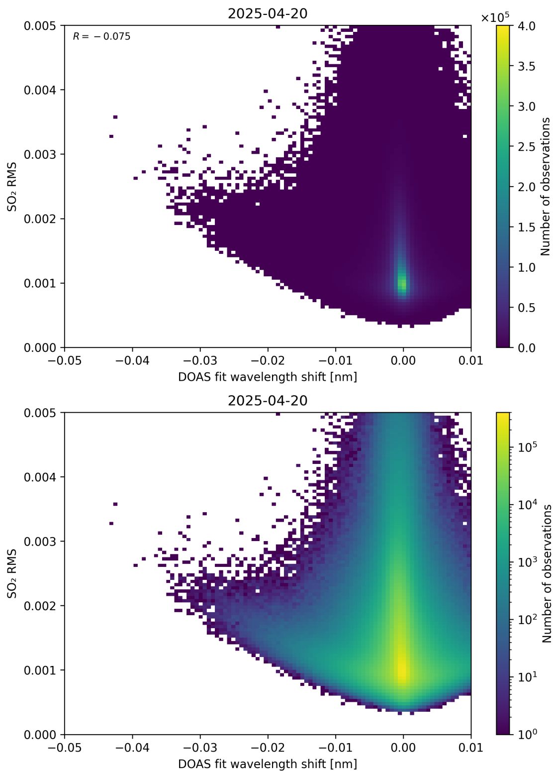
Figure 139: Scatter density plot of “DOAS fit wavelength shift” against “SO 2 RMS” for 2025-04-19 to 2025-04-21.
