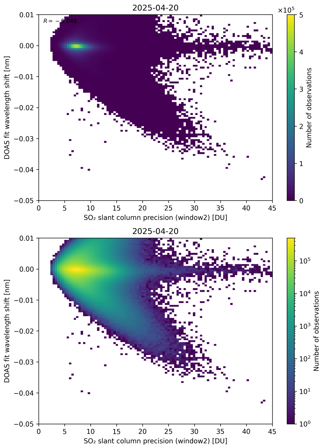
Figure 293: Scatter density plot of “SO 2 slant column precision (window2)” against “DOAS fit wavelength shift” for 2025-04-19 to 2025-04-21.
