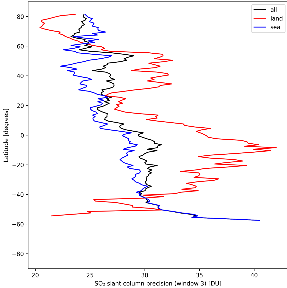
Figure 46: Zonal average of “SO 2 slant column precision (window 3)” for 2025-04-19 to 2025-04-21.
