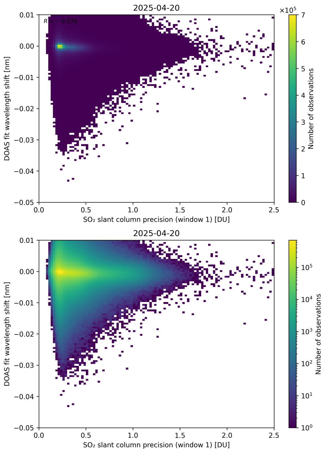
Figure 271: Scatter density plot of “SO 2 slant column precision (window 1)” against “DOAS fit wavelength shift” for 2025-04-19 to 2025-04-21.
