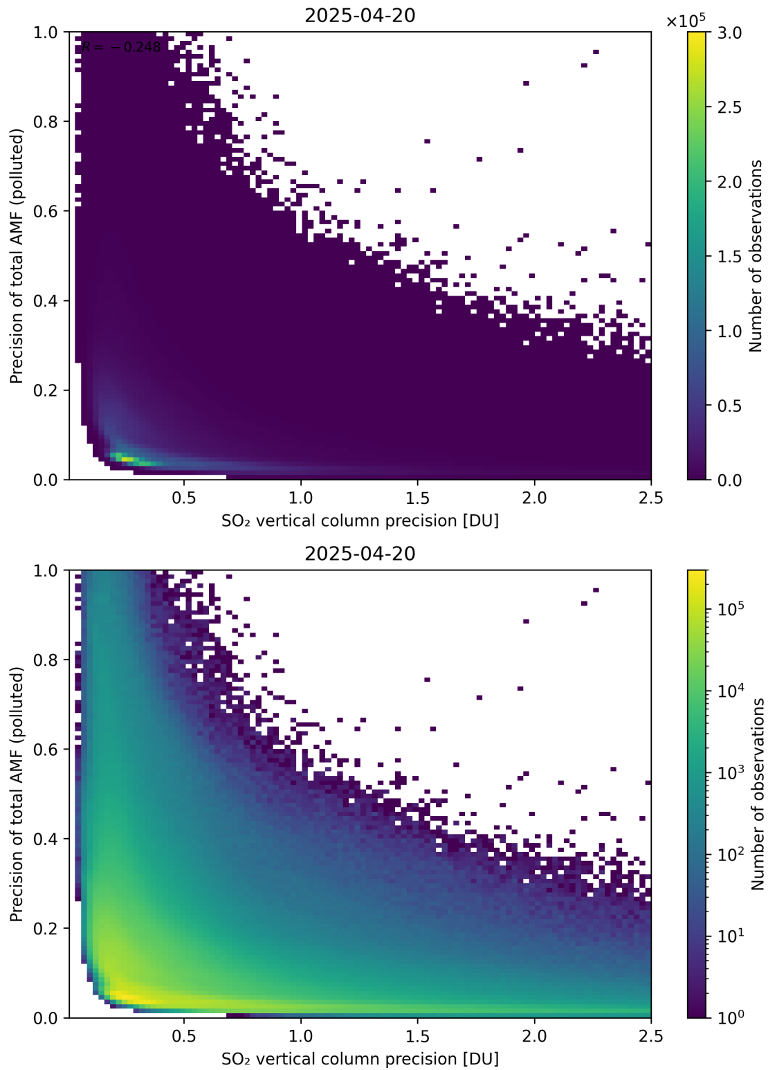
Figure 347: Scatter density plot of “SO 2 vertical column precision” against “Precision of total AMF (polluted)” for 2025-04-19 to 2025-04-21.
