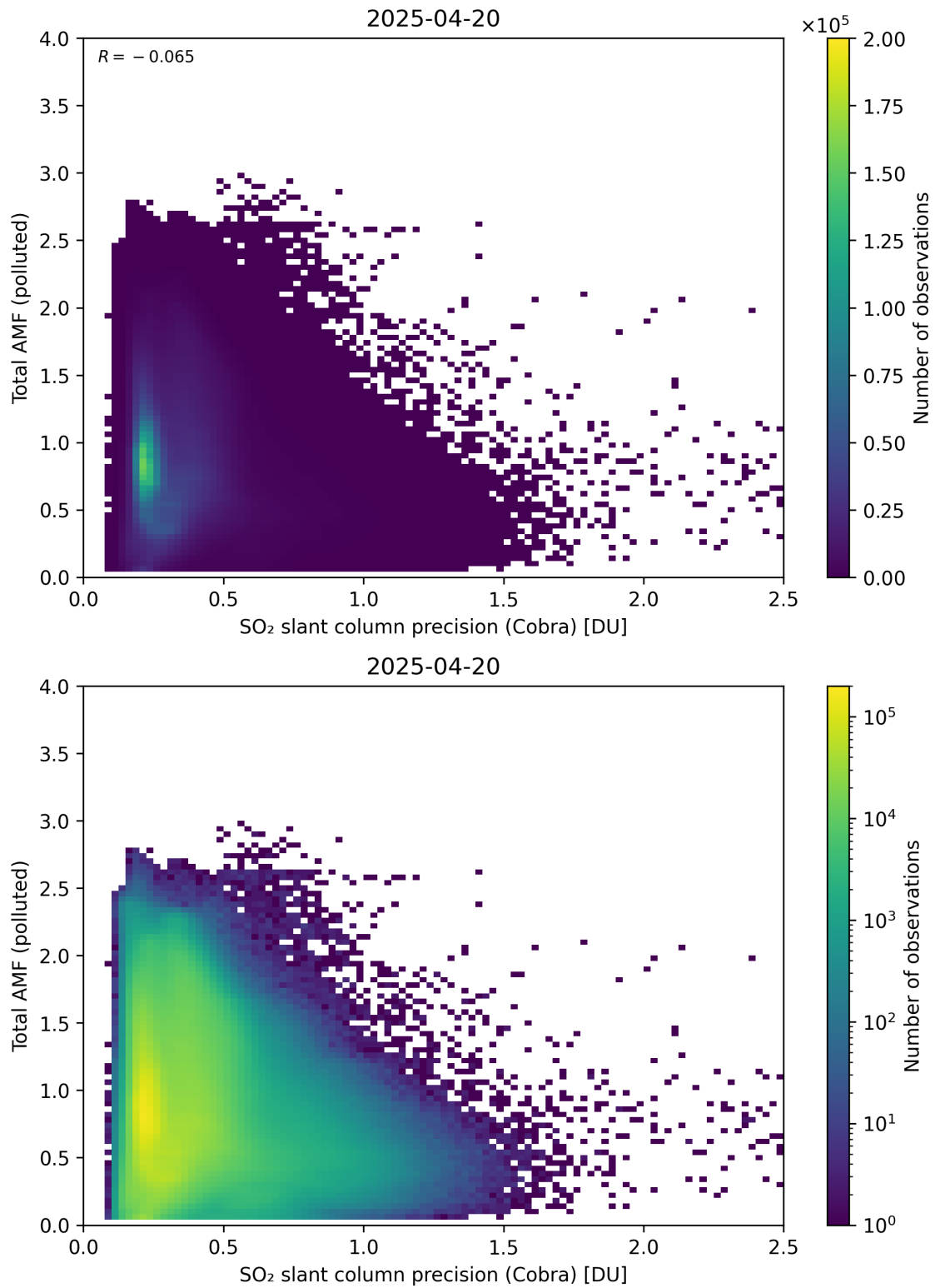
Figure 213: Scatter density plot of “SO 2 slant column precision (Cobra)” against “Total AMF (polluted)” for 2025-04-19 to 2025-04-21.
