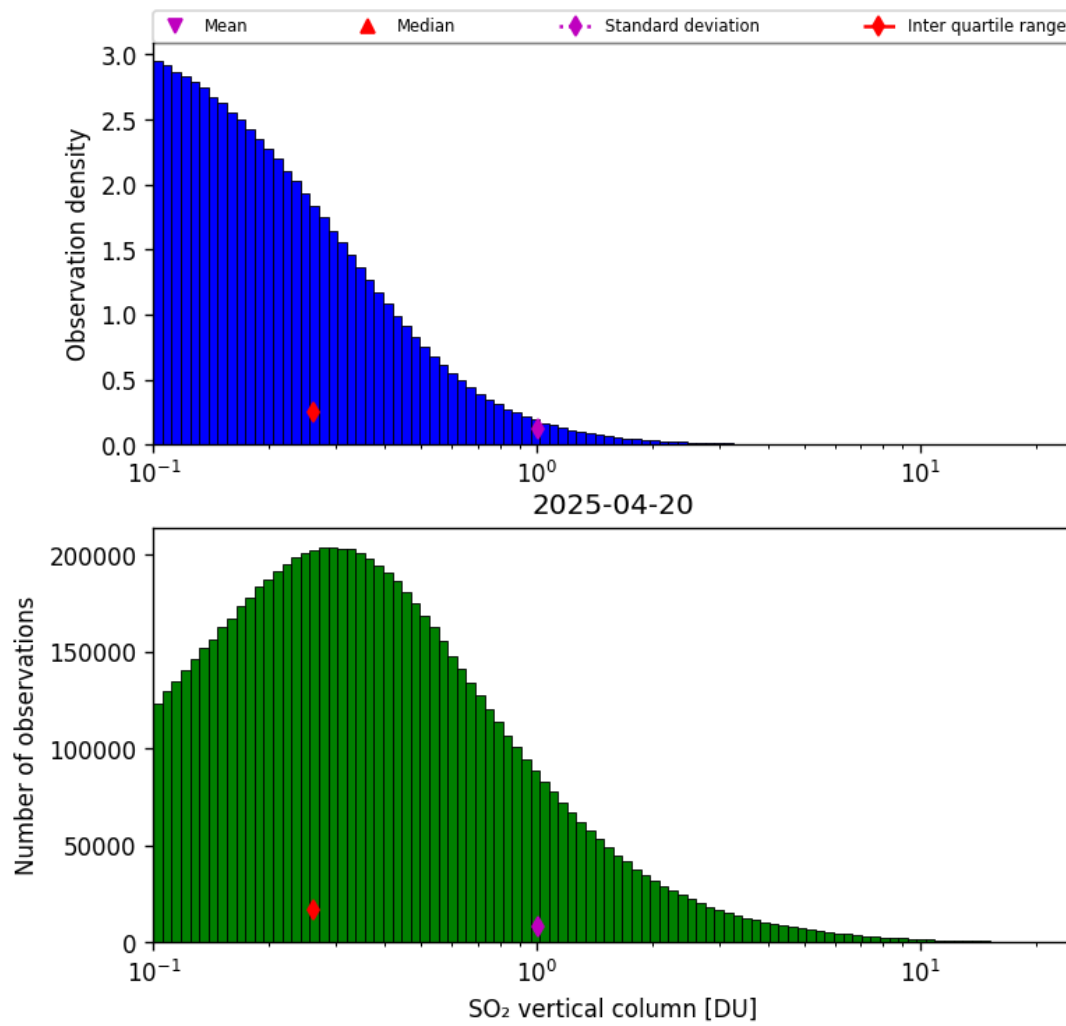
Figure 58: Histogram of “SO 2 vertical column” for 2025-04-19 to 2025-04-21
