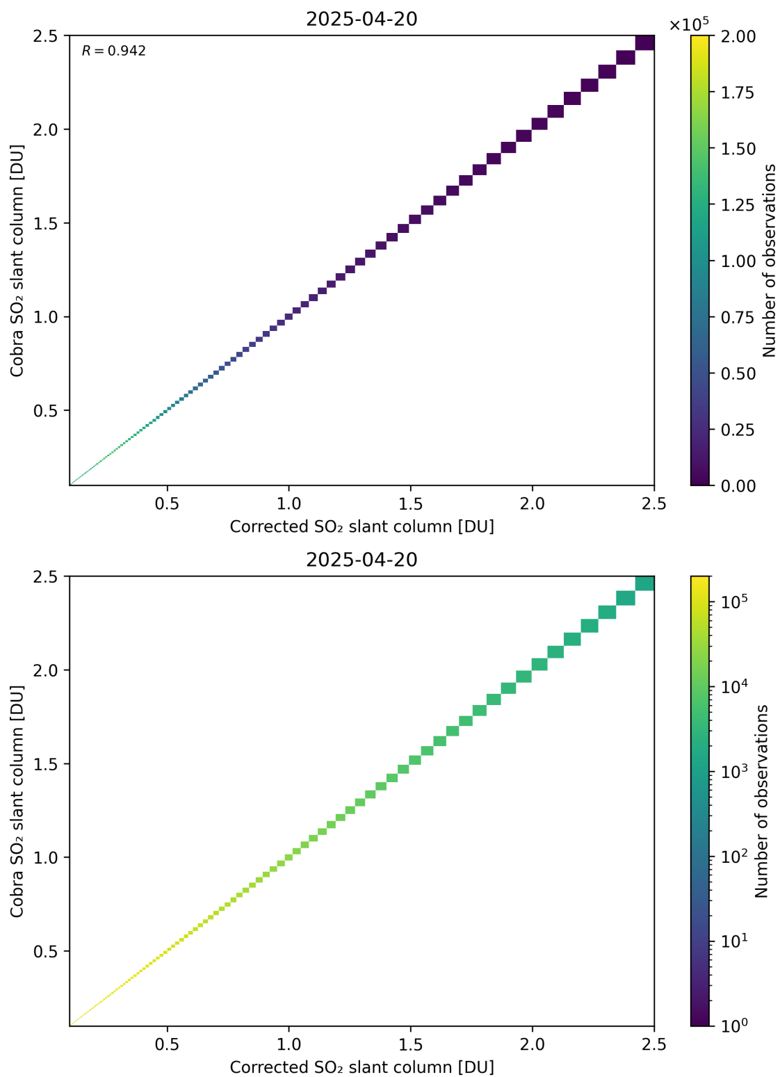
Figure 233: Scatter density plot of “Corrected SO 2 slant column” against “Cobra SO 2 slant column” for 2025-04-19 to 2025-04-21.
