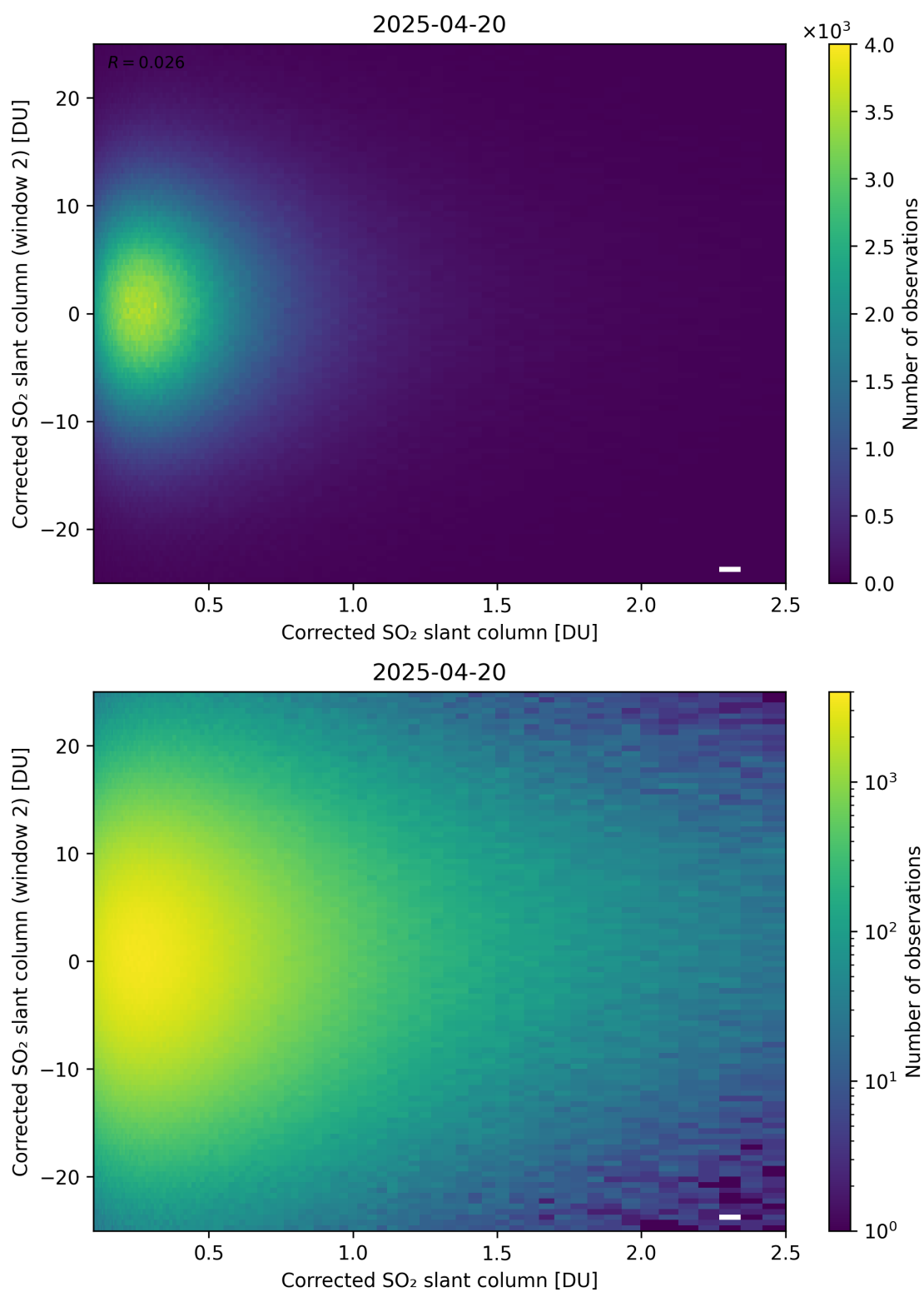
Figure 235: Scatter density plot of “Corrected SO 2 slant column” against “Corrected SO 2 slant column (window 2)” for 2025-04-19 to 2025-04-21.
