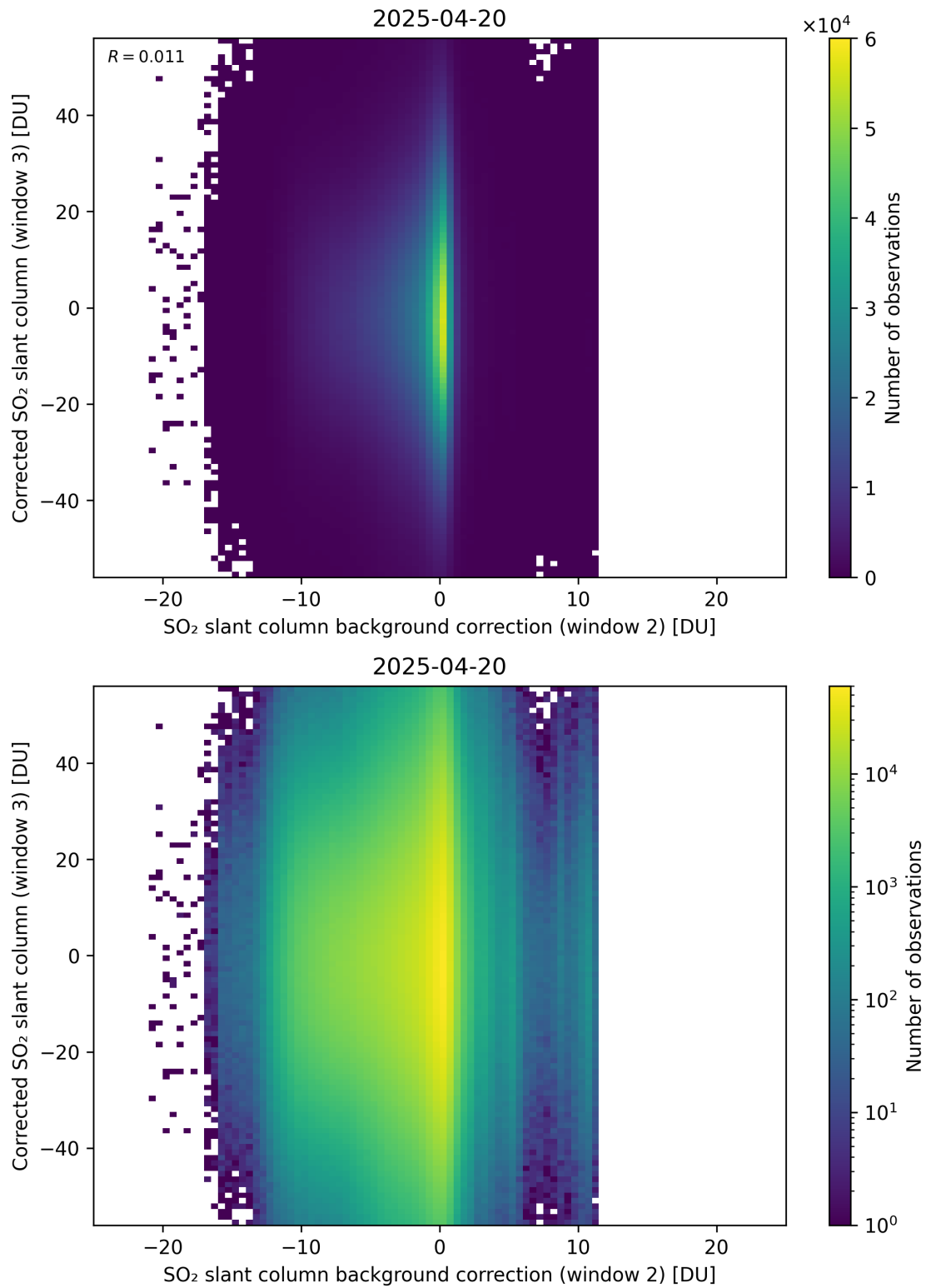
Figure 127: Scatter density plot of “SO 2 slant column background correction (window 2)” against “Corrected SO 2 slant column (window 3)” for 2025-04-19 to 2025-04-21.
