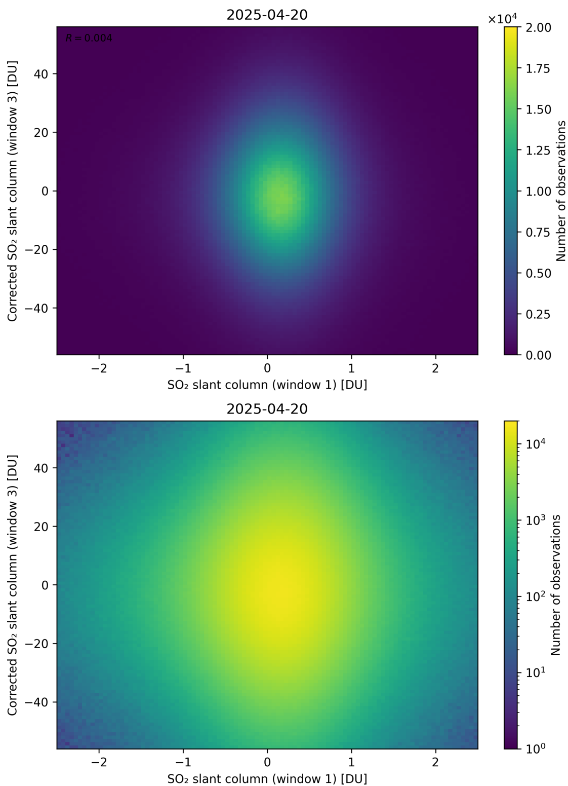
Figure 284: Scatter density plot of “SO 2 slant column (window 1)” against “Corrected SO 2 slant column (window 3)” for 2025-04-19 to 2025-04-21.
