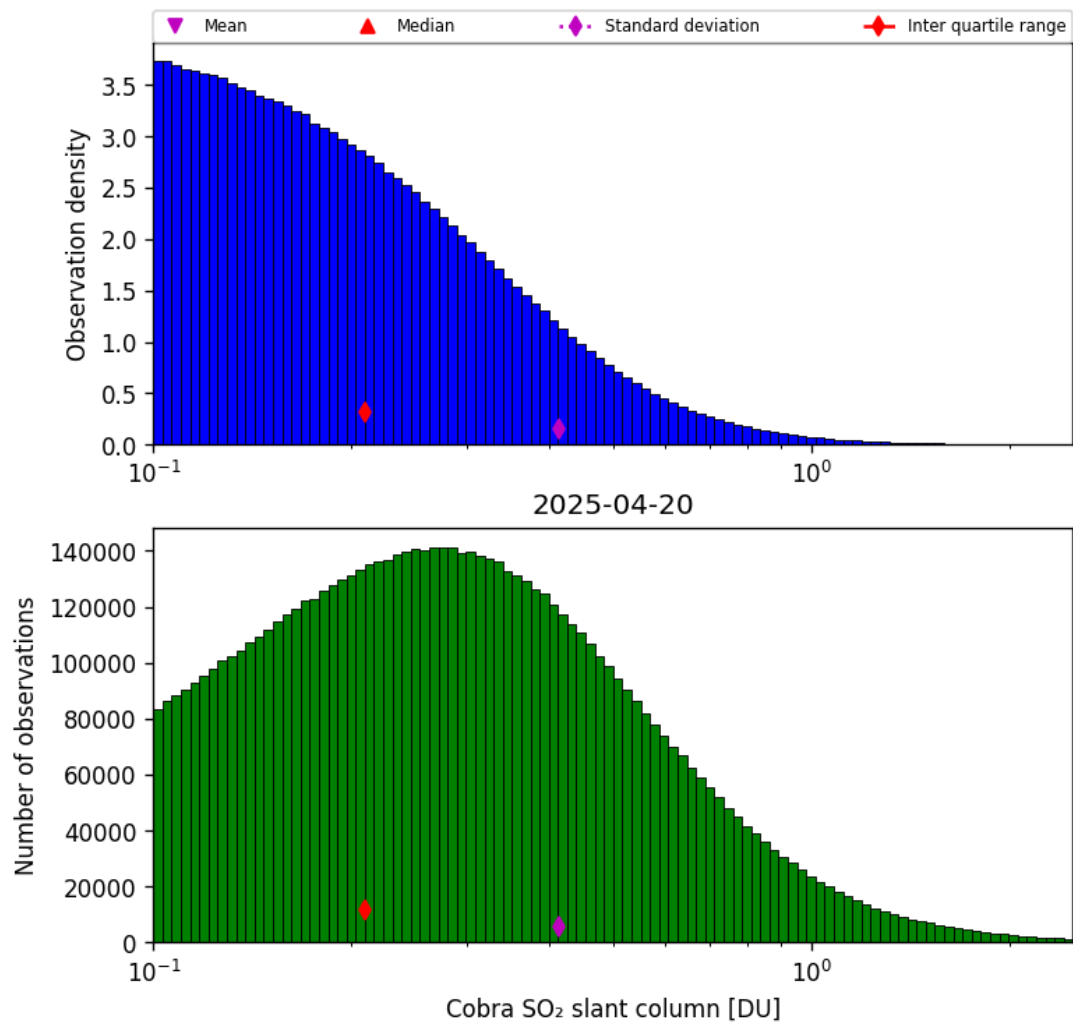
Figure 61: Histogram of “Cobra SO 2 slant column” for 2025-04-19 to 2025-04-21
