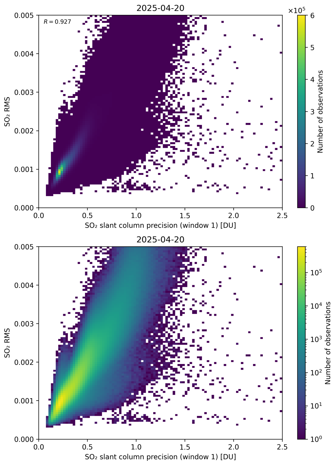
Figure 273: Scatter density plot of “SO 2 slant column precision (window 1)” against “SO 2 RMS” for 2025-04-19 to 2025-04-21.
