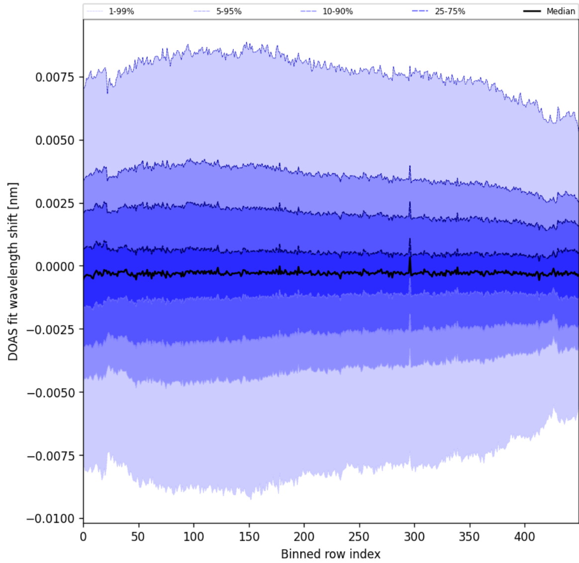
Figure 102: Along track statistics of “DOAS fit wavelength shift” for 2025-04-19 to 2025-04-21
