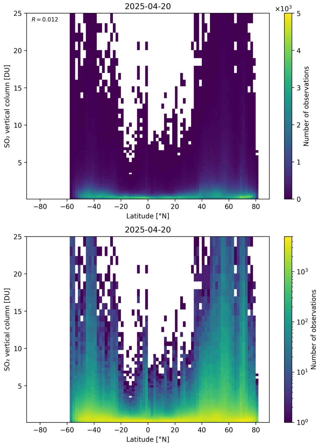
Figure 169: Scatter density plot of “Latitude” against “SO 2 vertical column” for 2025-04-19 to 2025-04-21.
