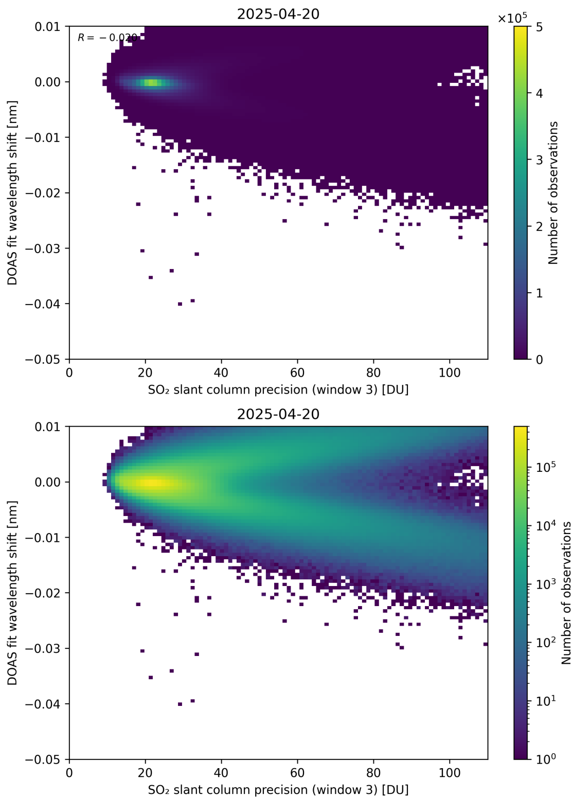
Figure 308: Scatter density plot of “SO 2 slant column precision (window 3)” against “DOAS fit wavelength shift” for 2025-04-19 to 2025-04-21.
