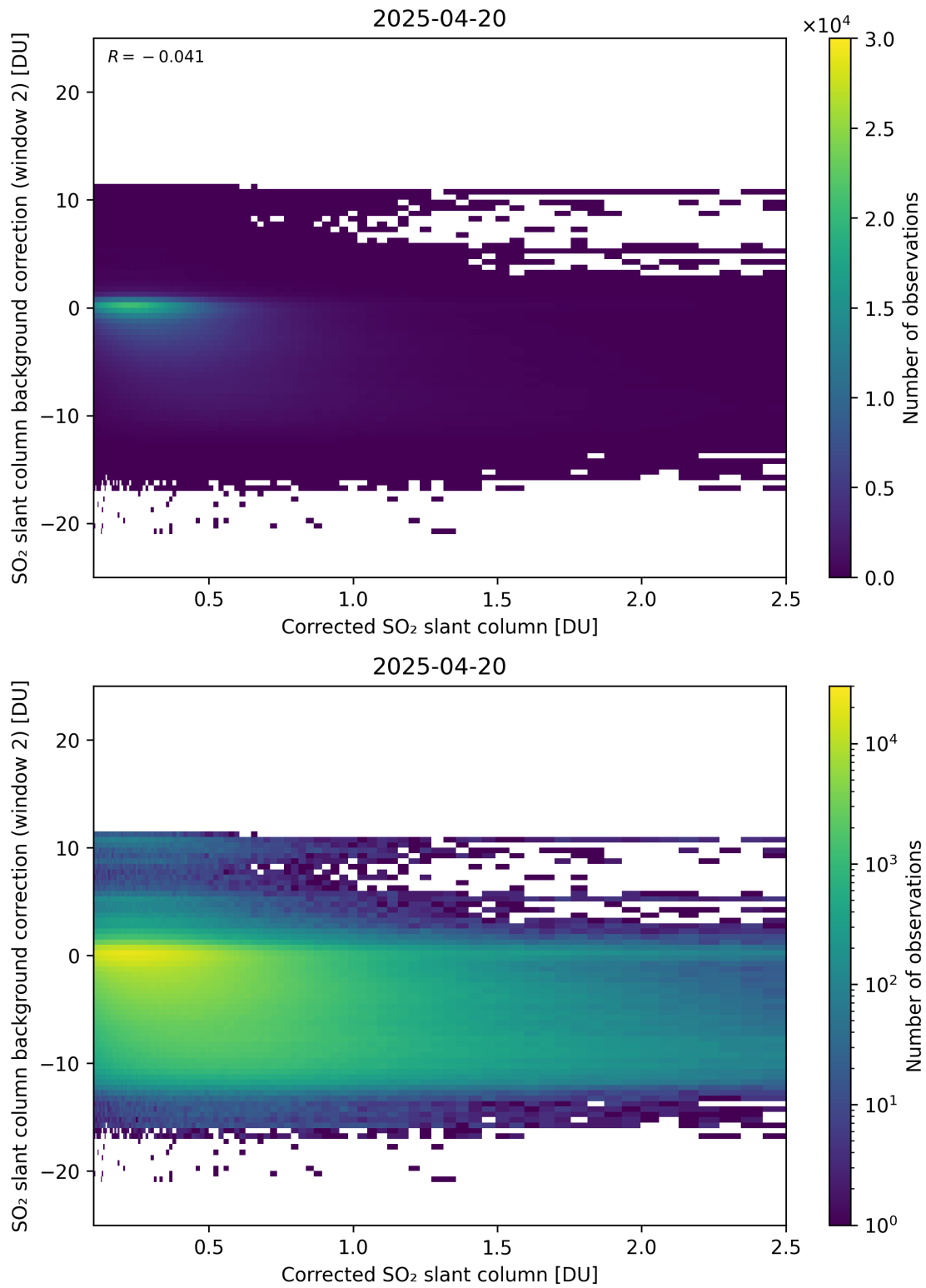
Figure 227: Scatter density plot of “Corrected SO 2 slant column” against “SO 2 slant column background correction (window 2)” for 2025-04-19 to 2025-04-21.
