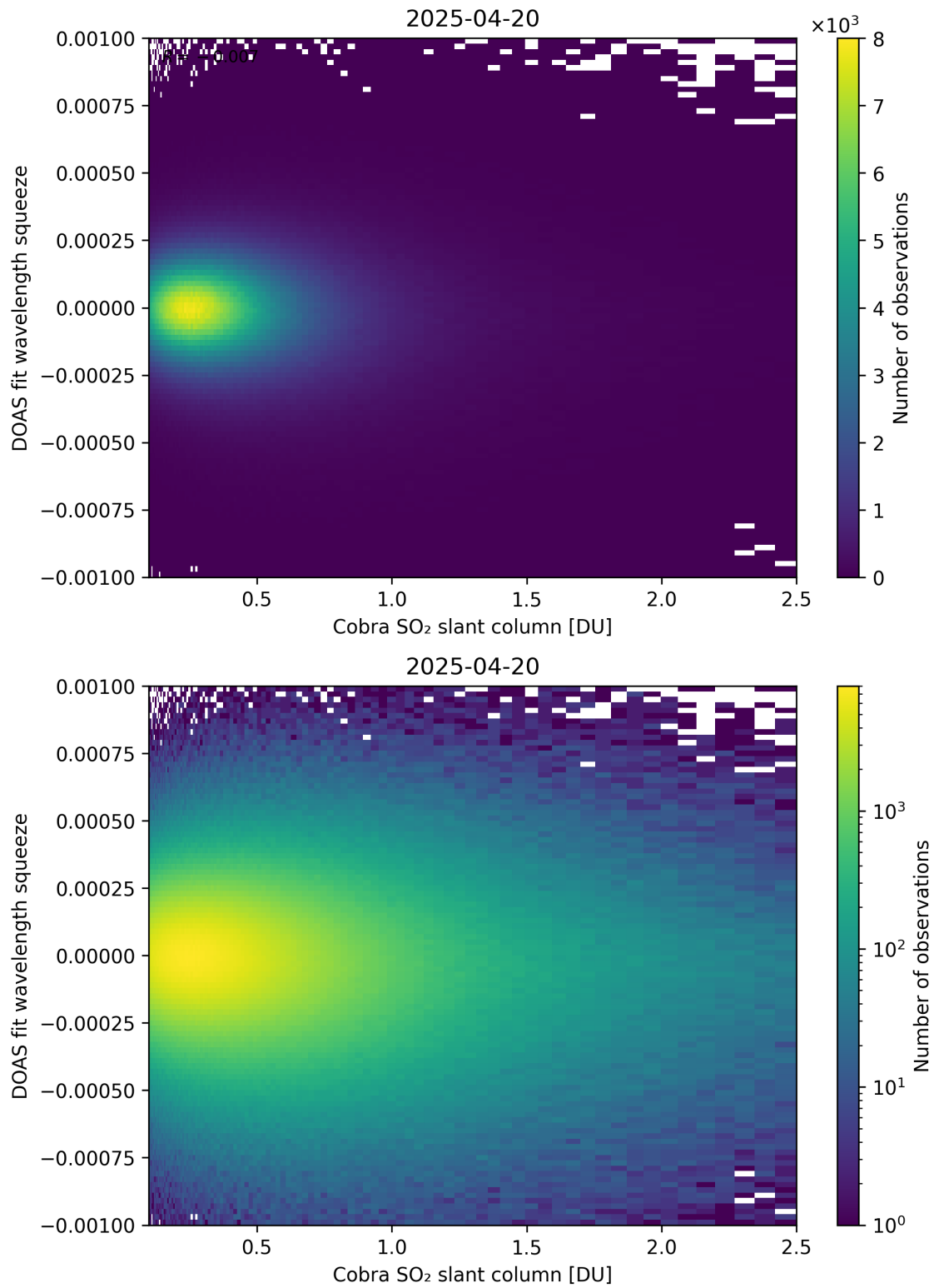
Figure 197: Scatter density plot of “Cobra SO 2 slant column” against “DOAS fit wavelength squeeze” for 2025-04-19 to 2025-04-21.
