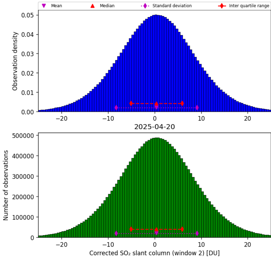
Figure 69: Histogram of “Corrected SO 2 slant column (window 2)” for 2025-04-19 to 2025-04-21
