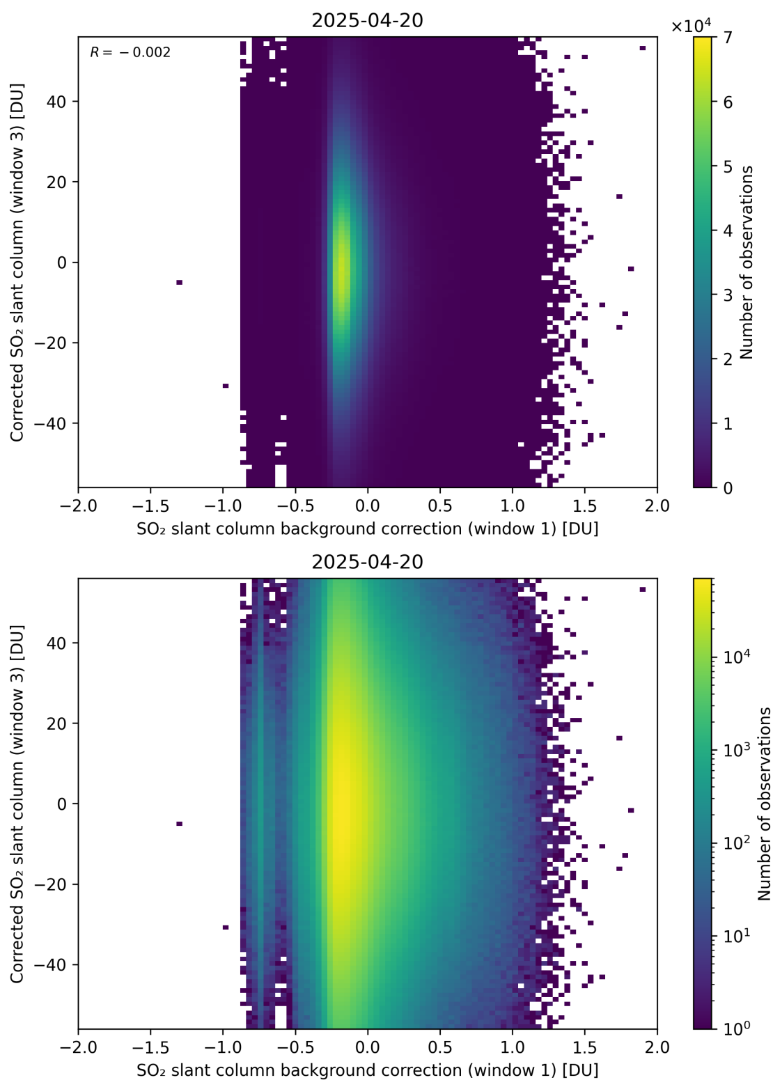
Figure 116: Scatter density plot of “SO 2 slant column background correction (window 1)” against “Corrected SO 2 slant column (window 3)” for 2025-04-19 to 2025-04-21.
