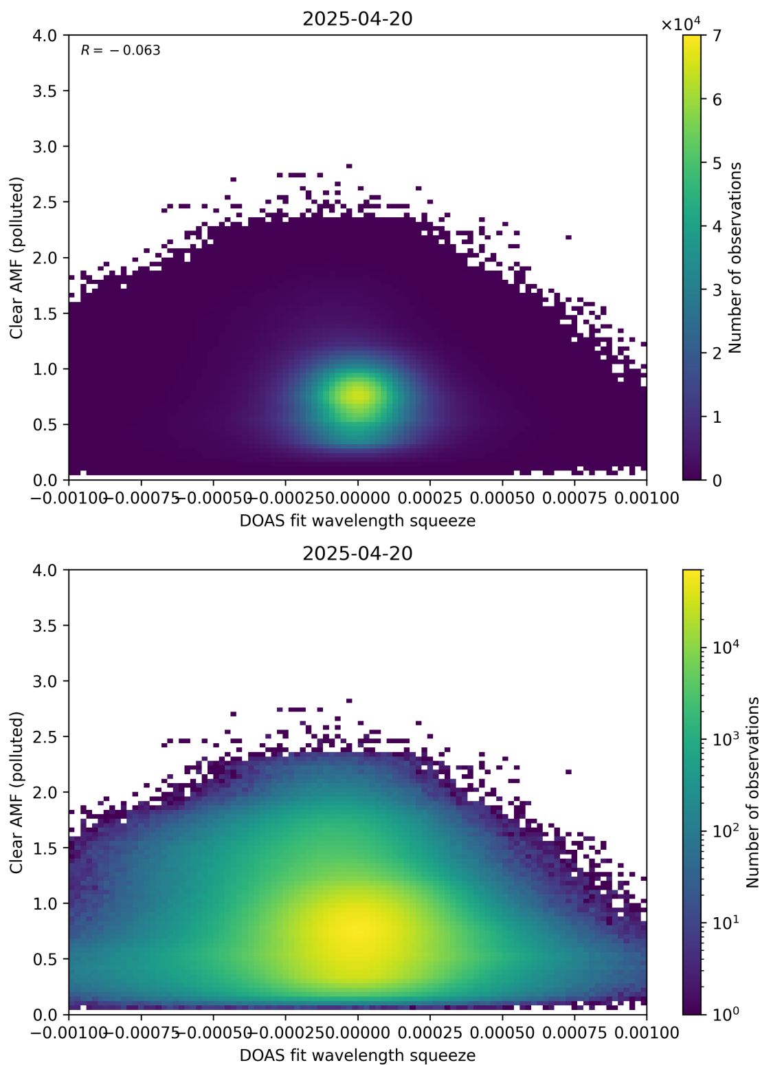
Figure 144: Scatter density plot of “DOAS fit wavelength squeeze” against “Clear AMF (polluted)” for 2025-04-19 to 2025-04-21.
