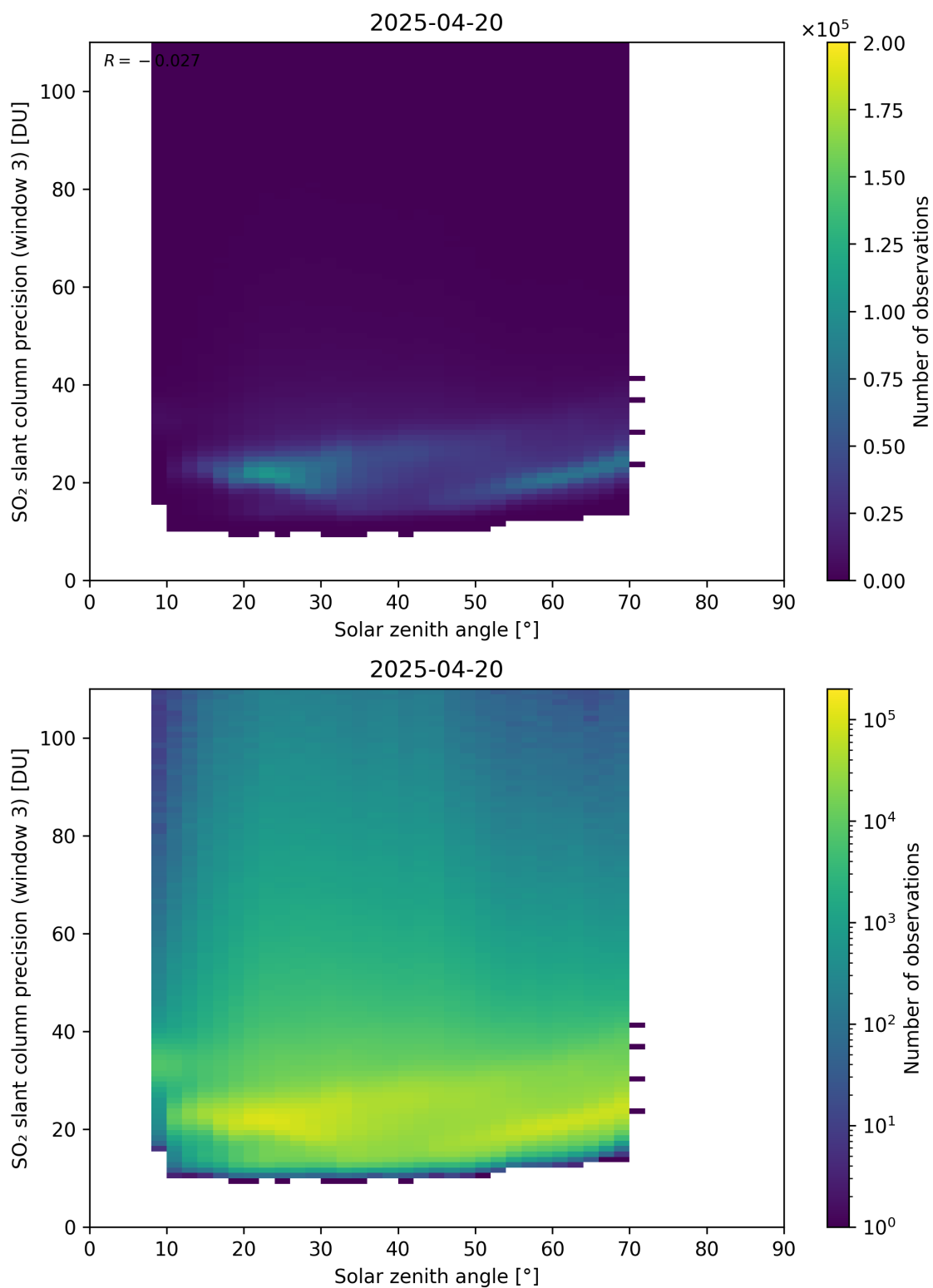
Figure 188: Scatter density plot of “Solar zenith angle” against “SO 2 slant column precision (window 3)” for 2025-04-19 to 2025-04-21.
