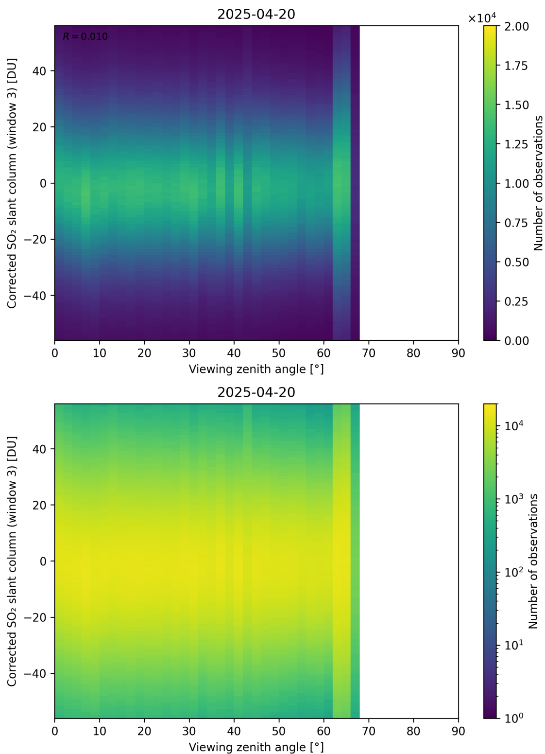
Figure 375: Scatter density plot of “Viewing zenith angle” against “Corrected SO 2 slant column (window 3)” for 2025-04-19 to 2025-04-21.
