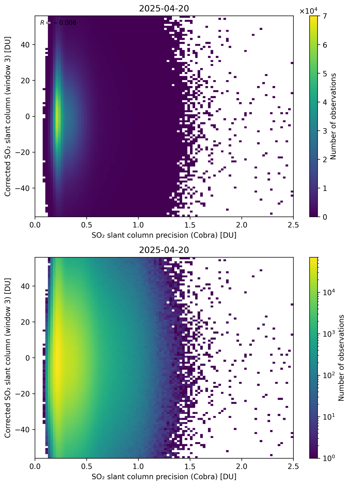
Figure 207: Scatter density plot of “SO 2 slant column precision (Cobra)” against “Corrected SO 2 slant column (window 3)” for 2025-04-19 to 2025-04-21.
