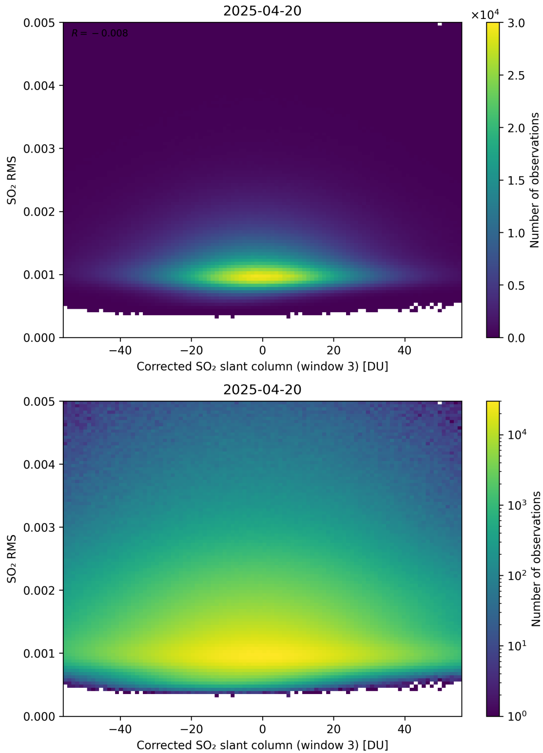
Figure 258: Scatter density plot of “Corrected SO 2 slant column (window 3)” against “SO 2 RMS” for 2025-04-19 to 2025-04-21.
