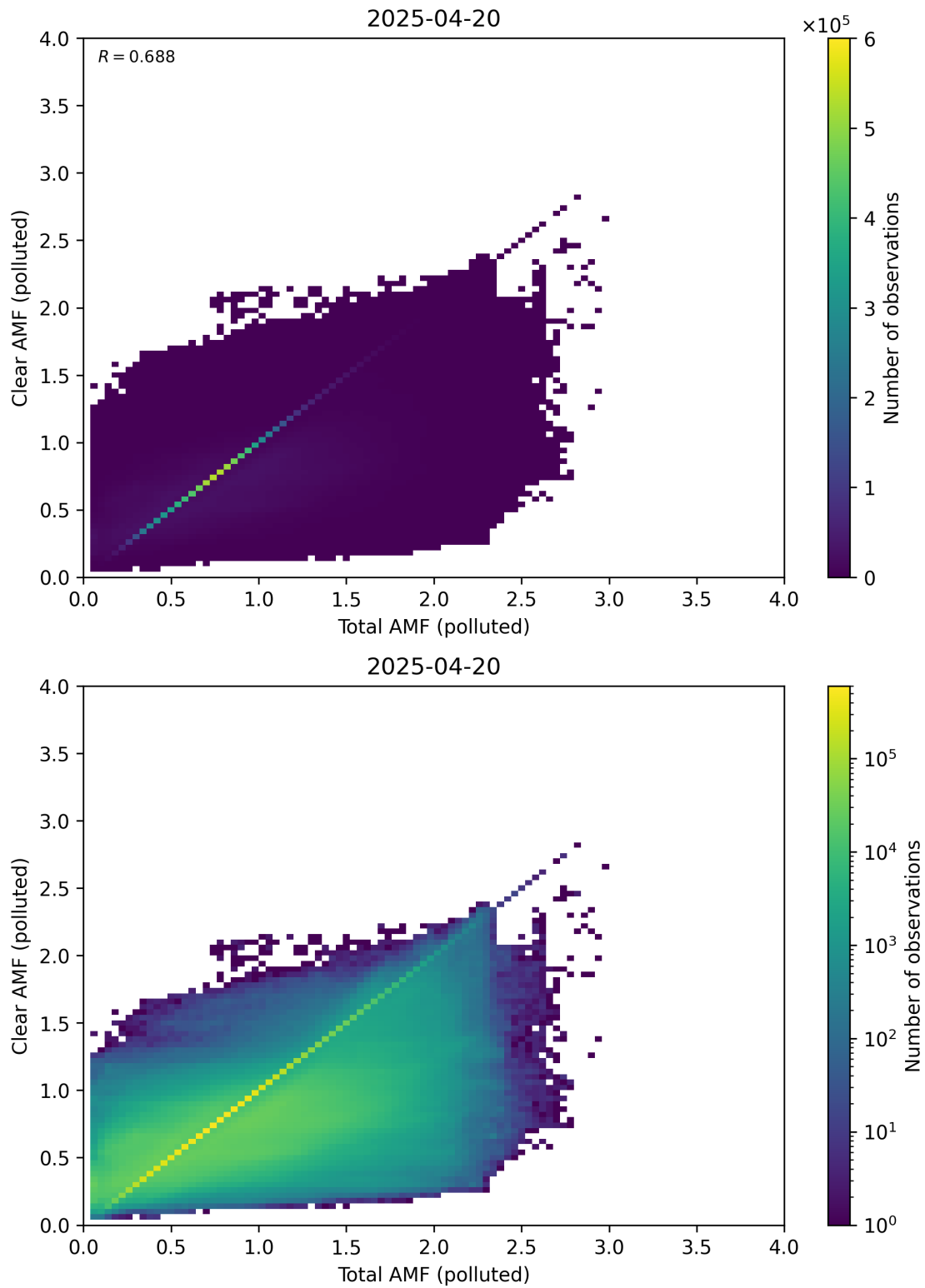
Figure 321: Scatter density plot of “Total AMF (polluted)” against “Clear AMF (polluted)” for 2025-04-19 to 2025-04-21.
