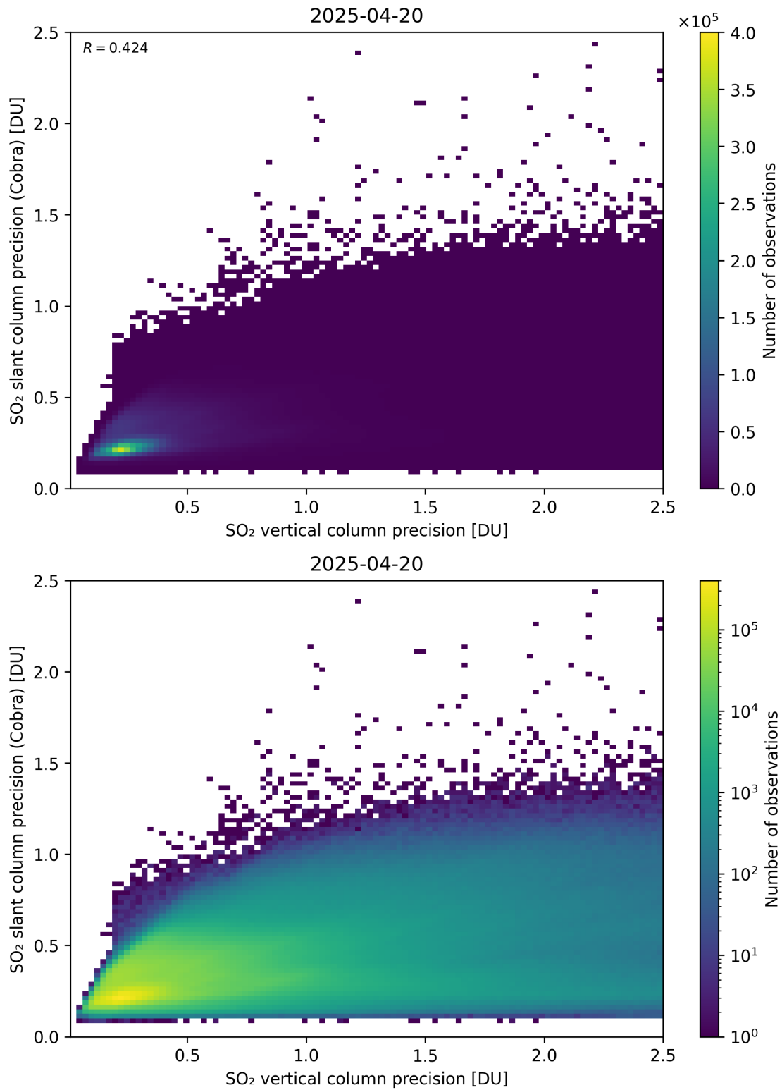
Figure 337: Scatter density plot of “SO 2 vertical column precision” against “SO 2 slant column precision (Cobra)” for 2025-04-19 to 2025-04-21.
