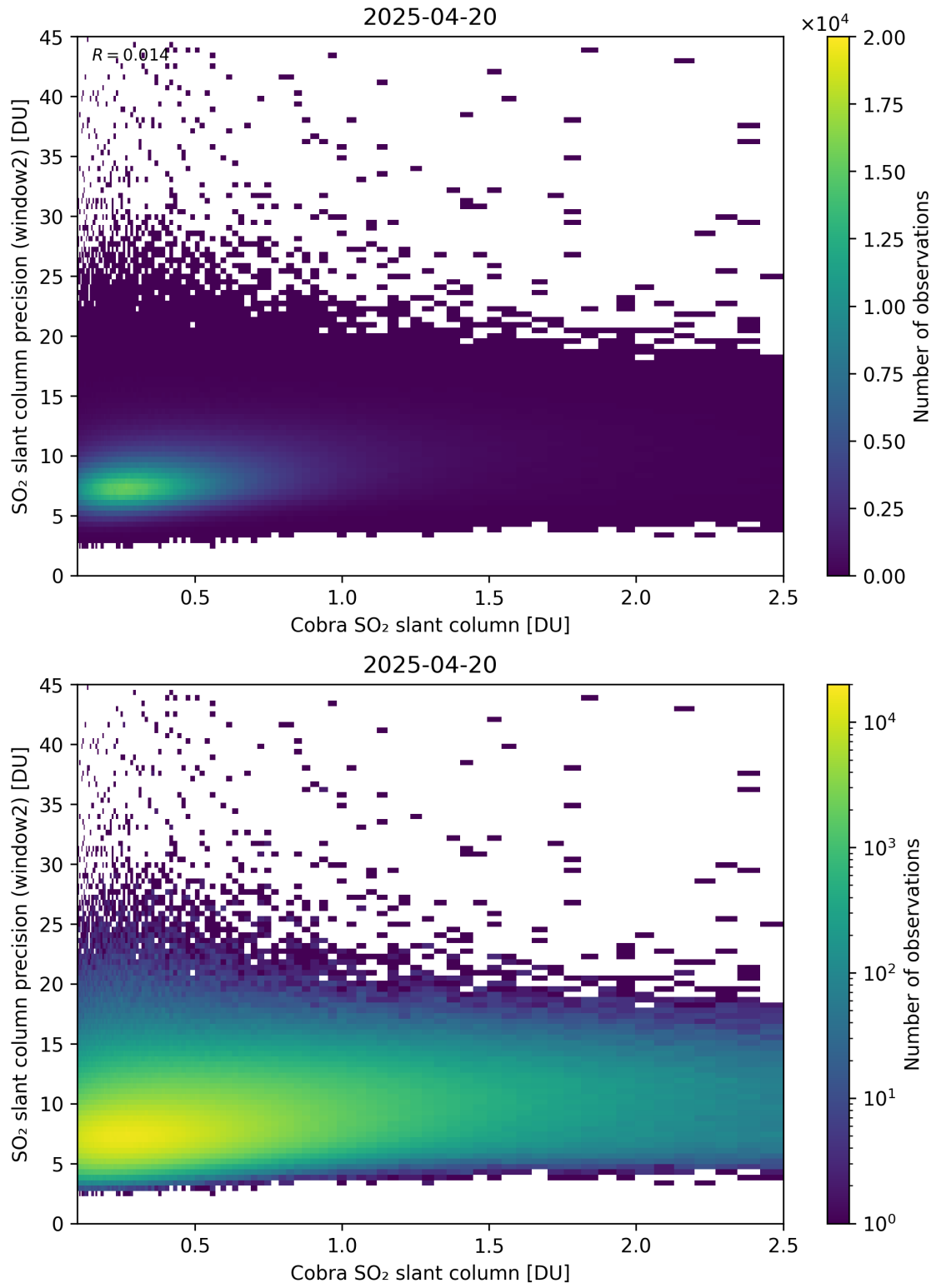
Figure 221: Scatter density plot of “Cobra SO 2 slant column” against “SO 2 slant column precision (window2)” for 2025-04-19 to 2025-04-21.
