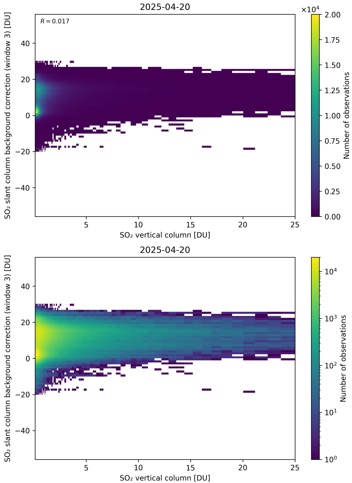
Figure 325: Scatter density plot of “SO 2 vertical column” against “SO 2 slant column background correction (window 3)” for 2025-04-19 to 2025-04-21.
