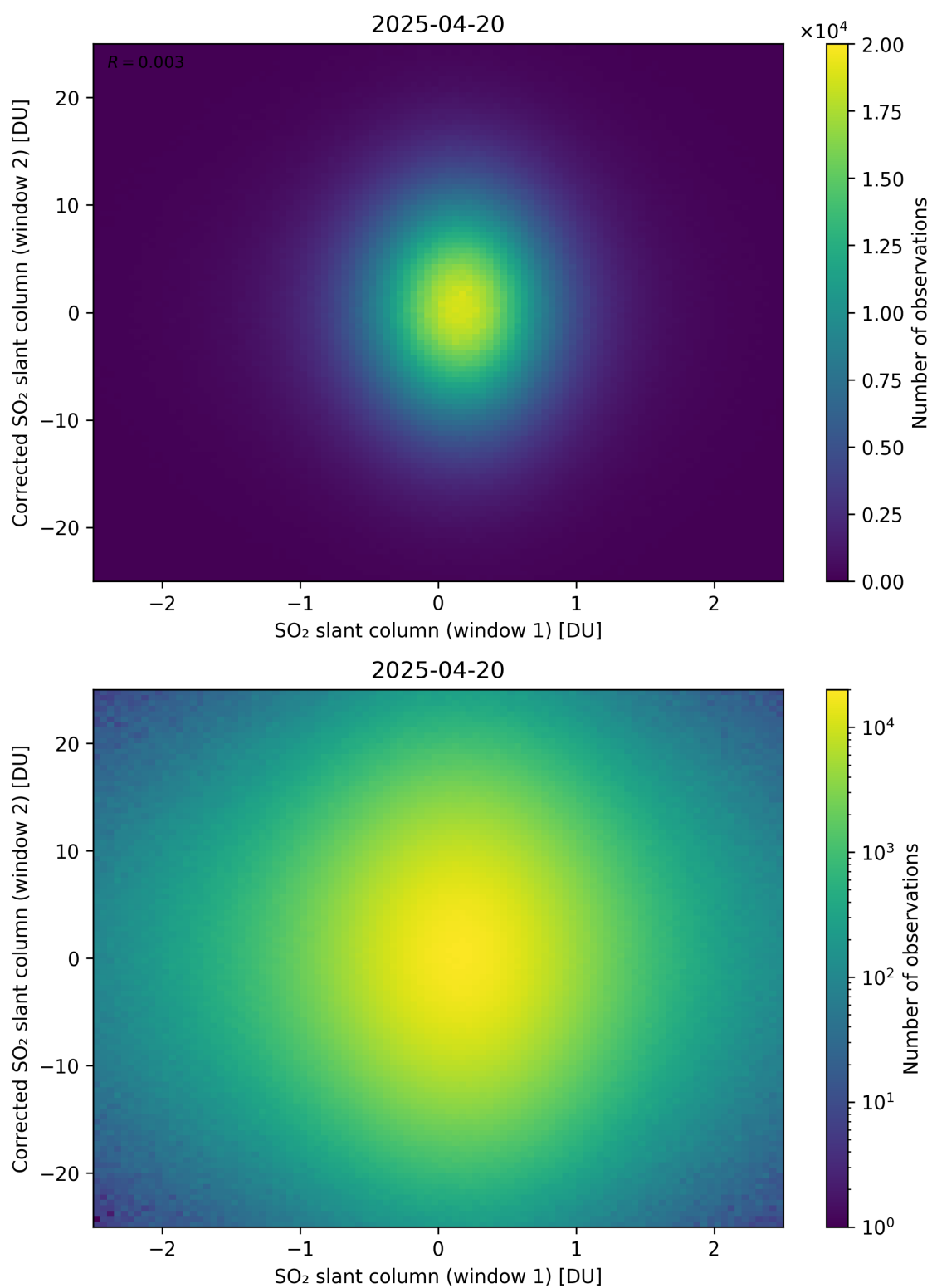
Figure 283: Scatter density plot of “SO 2 slant column (window 1)” against “Corrected SO 2 slant column (window 2)” for 2025-04-19 to 2025-04-21.
