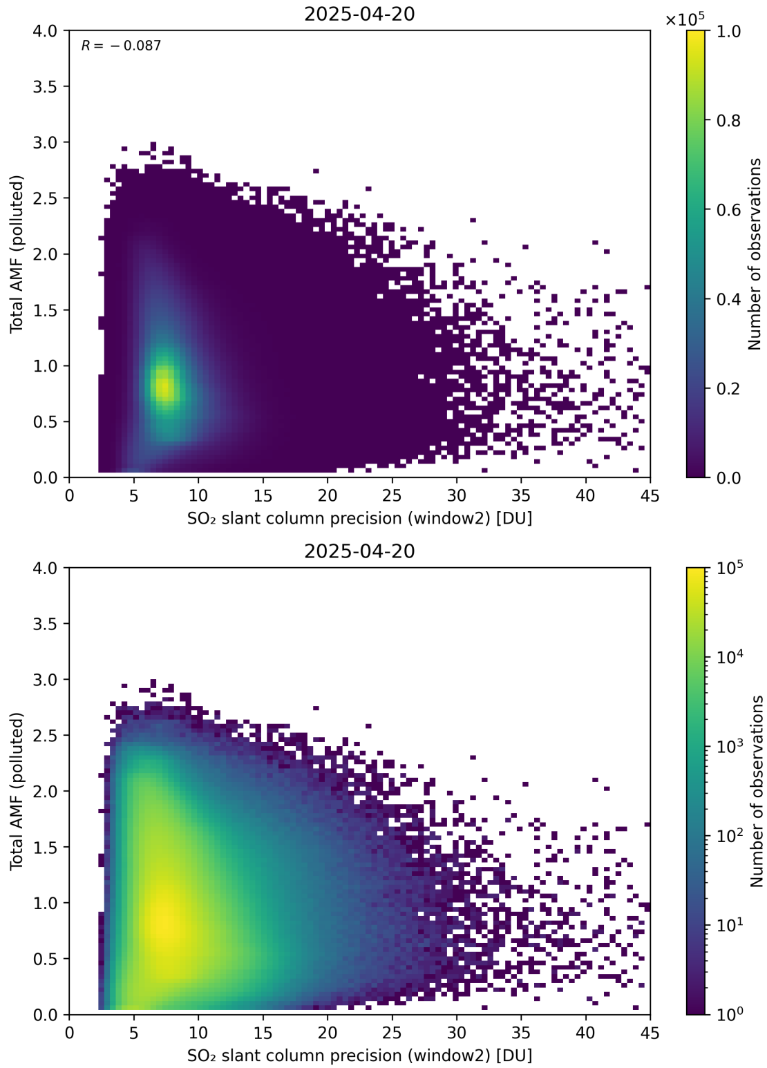
Figure 301: Scatter density plot of “SO 2 slant column precision (window2)” against “Total AMF (polluted)” for 2025-04-19 to 2025-04-21.
