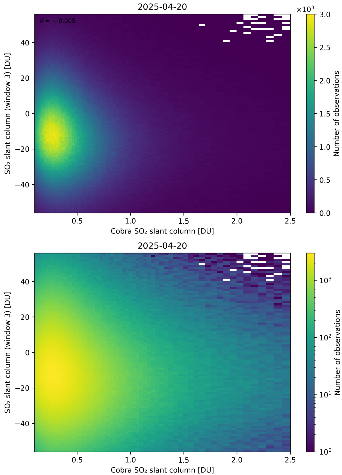
Figure 222: Scatter density plot of “Cobra SO 2 slant column” against “SO 2 slant column (window 3)” for 2025-04-19 to 2025-04-21.
