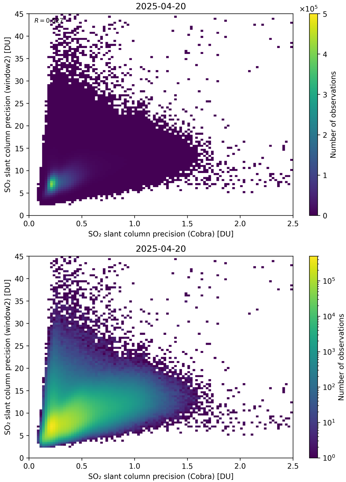
Figure 210: Scatter density plot of “SO 2 slant column precision (Cobra)” against “SO 2 slant column precision (window2)” for 2025-04-19 to 2025-04-21.
