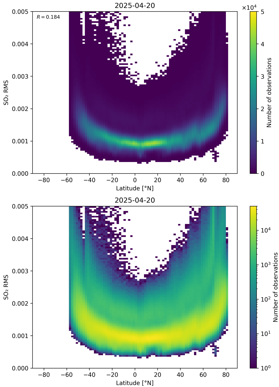
Figure 155: Scatter density plot of “Latitude” against “SO 2 RMS” for 2025-04-19 to 2025-04-21.
