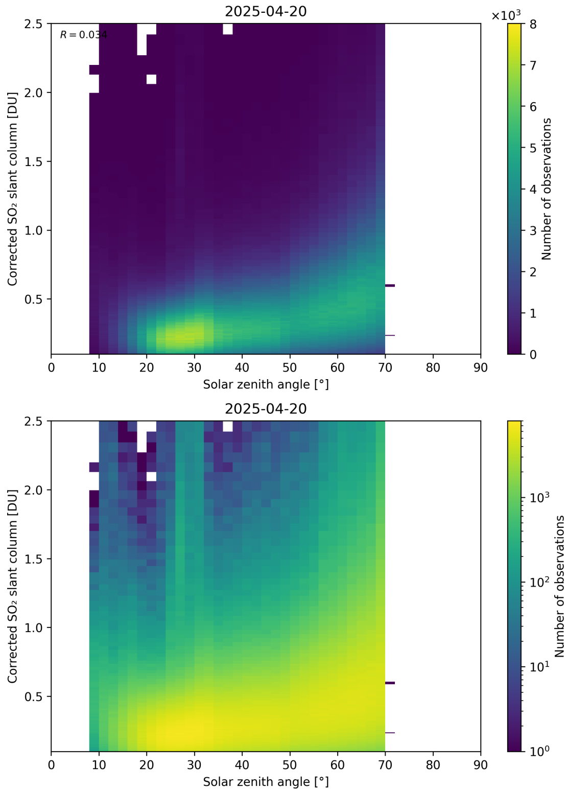
Figure 181: Scatter density plot of “Solar zenith angle” against “Corrected SO 2 slant column” for 2025-04-19 to 2025-04-21.
