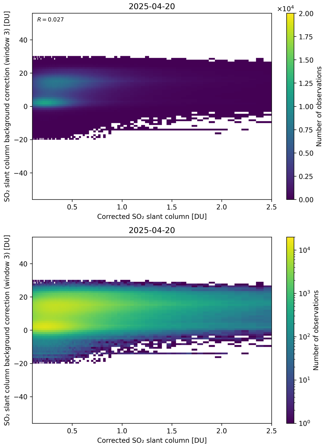
Figure 228: Scatter density plot of “Corrected SO 2 slant column” against “SO 2 slant column background correction (window 3)” for 2025-04-19 to 2025-04-21.
