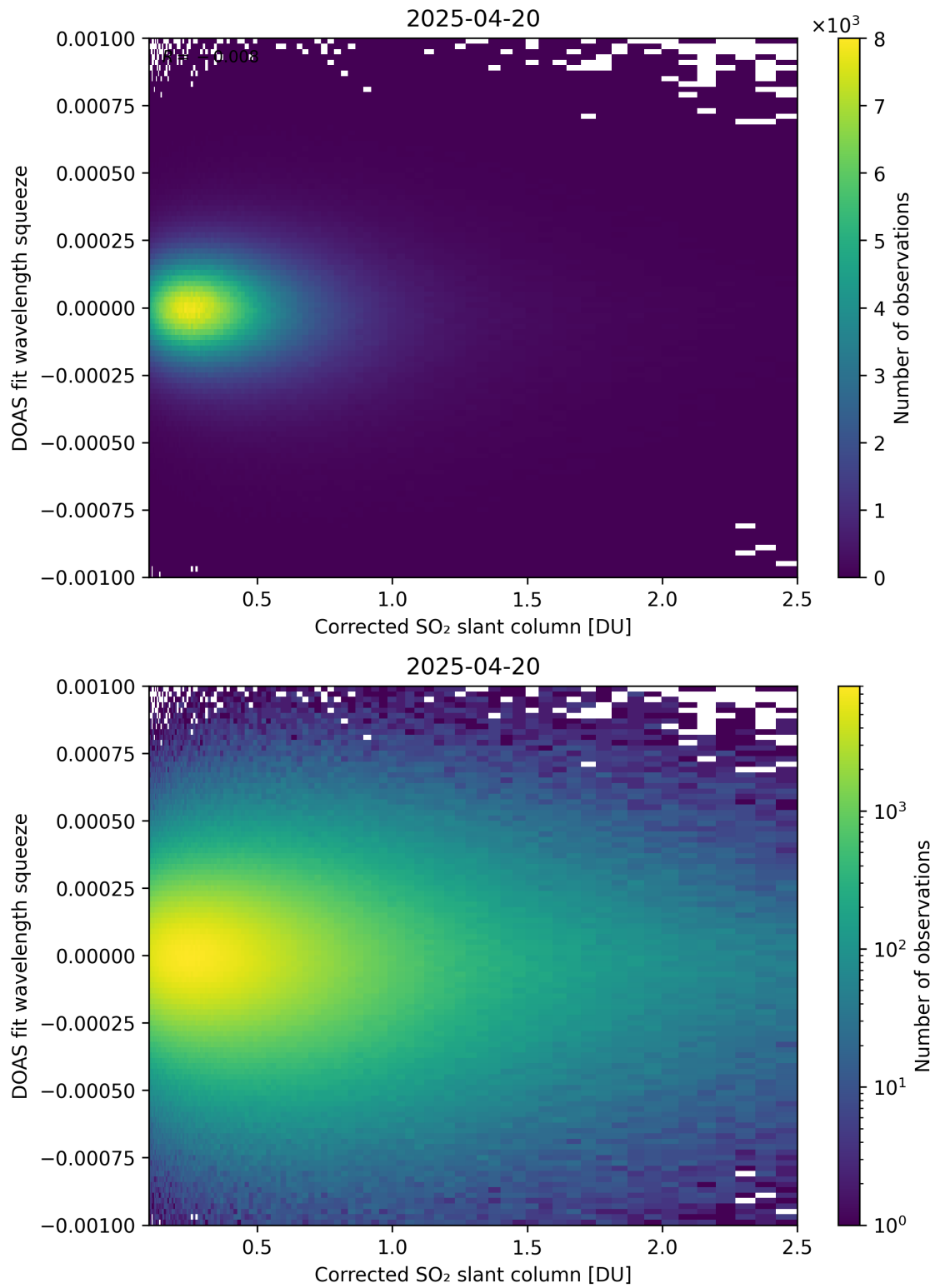
Figure 230: Scatter density plot of "Corrected SO 2 slant column" against "DOAS fit wavelength squeeze" for 2025-04-19 to 2025-04-21.
