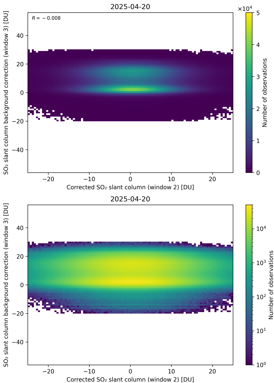
Figure 245: Scatter density plot of “Corrected SO 2 slant column (window 2)” against “SO 2 slant column background correction (window 3)” for 2025-04-19 to 2025-04-21.
