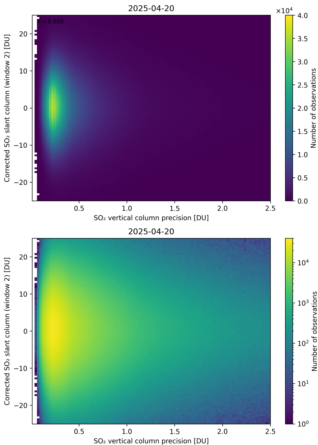
Figure 339: Scatter density plot of “SO 2 vertical column precision” against “Corrected SO 2 slant column (window 2)” for 2025-04-19 to 2025-04-21.
