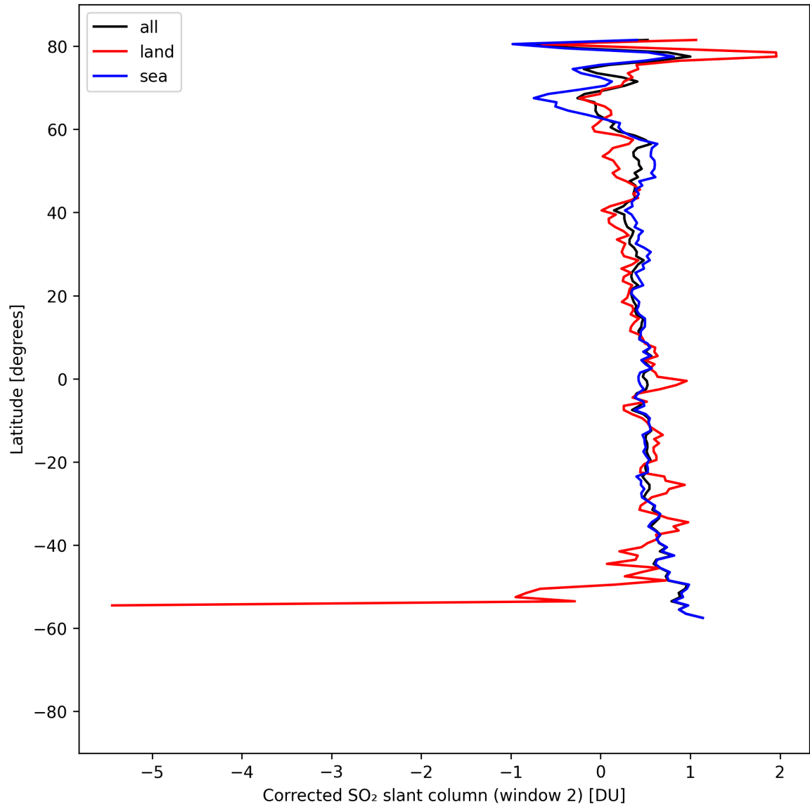
Figure 43: Zonal average of “Corrected SO 2 slant column (window 2)” for 2025-04-19 to 2025-04-21.
