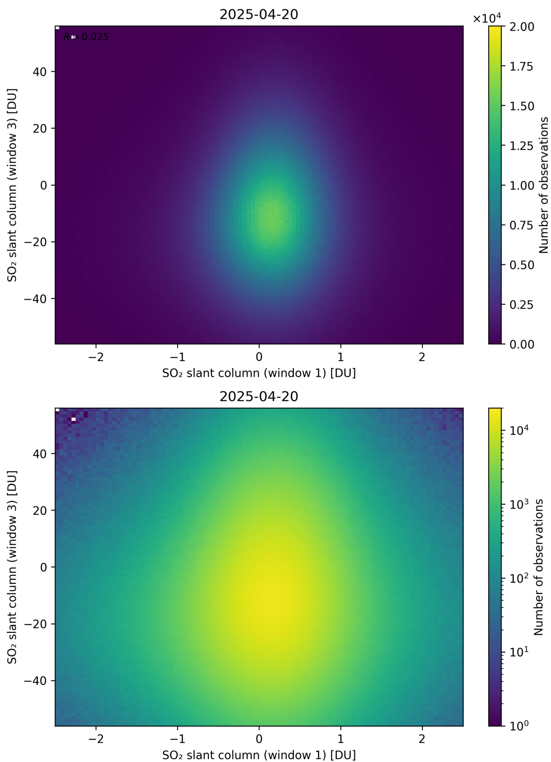
Figure 287: Scatter density plot of “SO 2 slant column (window 1)” against “SO 2 slant column (window 3)” for 2025-04-19 to 2025-04-21.
