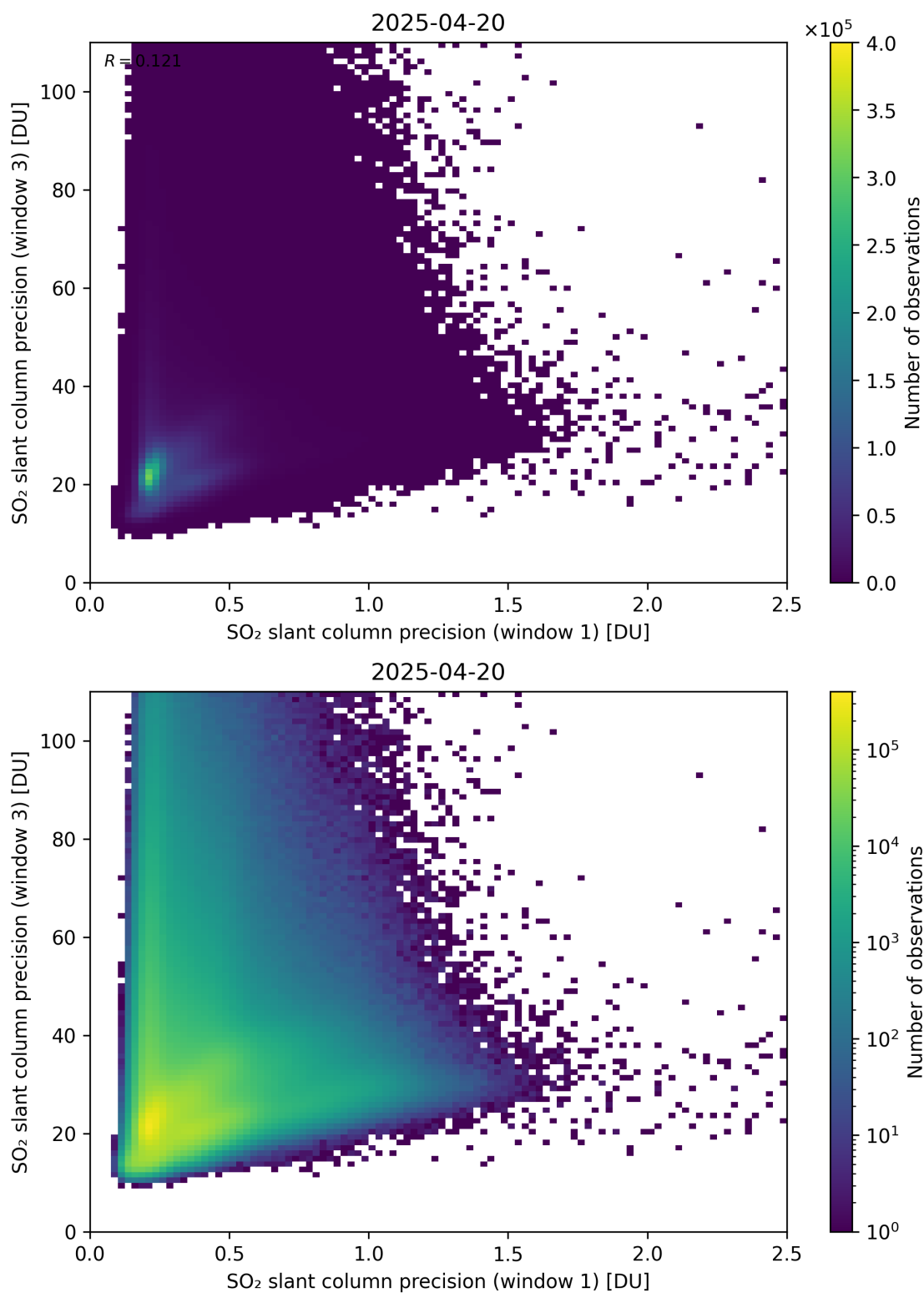
Figure 279: Scatter density plot of “SO 2 slant column precision (window 1)” against “SO 2 slant column precision (window 3)” for 2025-04-19 to 2025-04-21.
