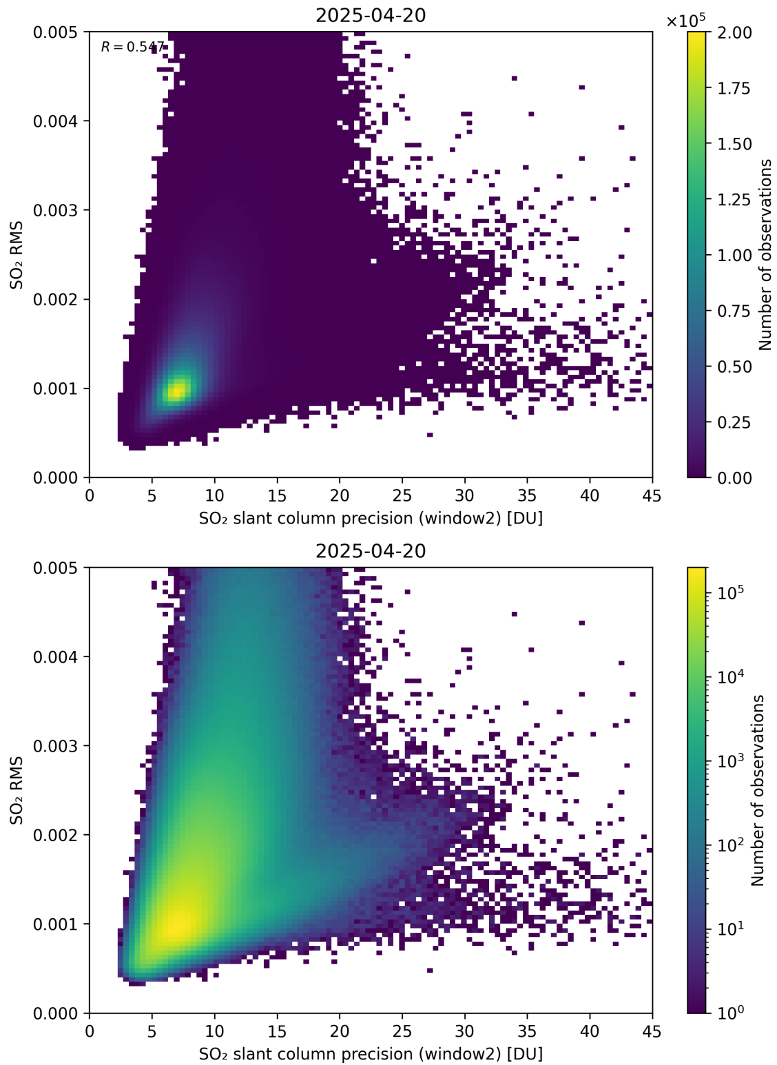
Figure 295: Scatter density plot of “SO 2 slant column precision (window2)” against “SO 2 RMS” for 2025-04-19 to 2025-04-21.
