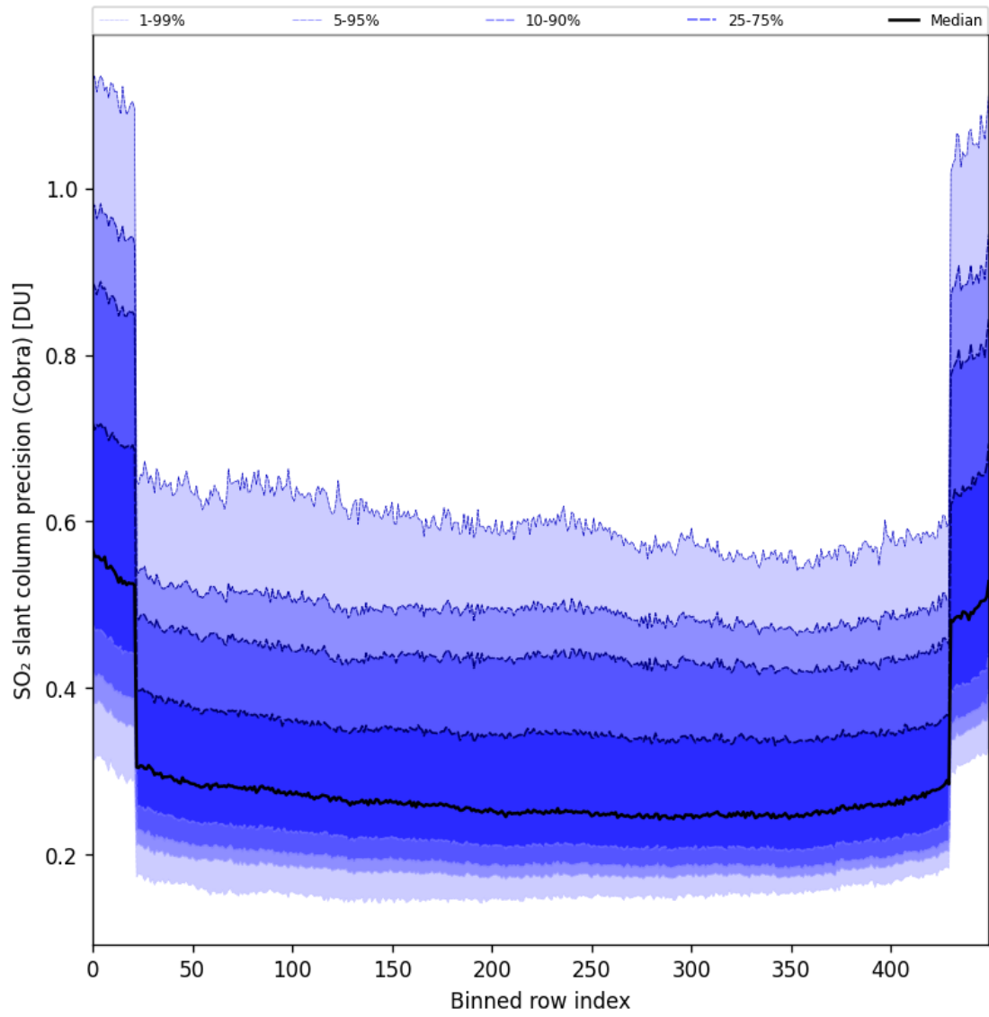
Figure 88: Along track statistics of “SO 2 slant column precision (Cobra)” for 2025-04-19 to 2025-04-21
