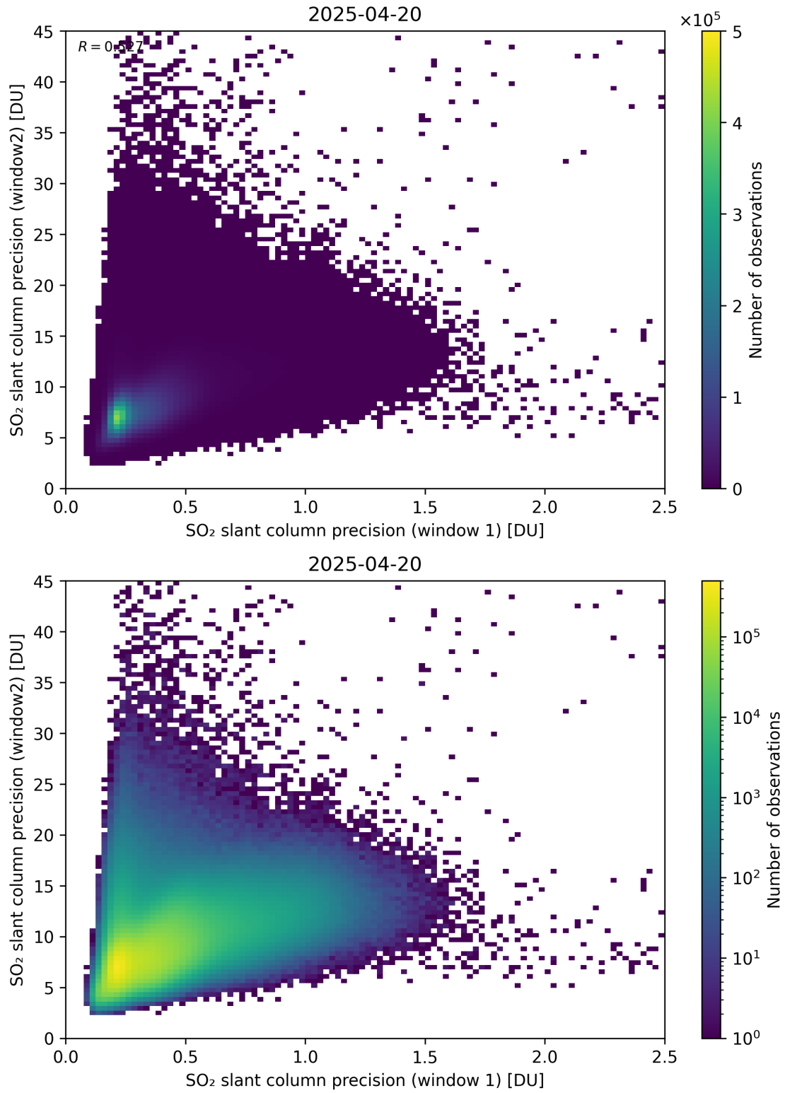
Figure 277: Scatter density plot of “SO 2 slant column precision (window 1)” against “SO 2 slant column precision (window 2)” for 2025-04-19 to 2025-04-21.
