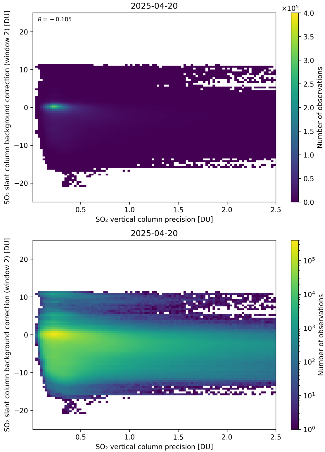
Figure 330: Scatter density plot of “SO 2 vertical column precision” against “SO 2 slant column background correction (window 2)” for 2025-04-19 to 2025-04-21.
