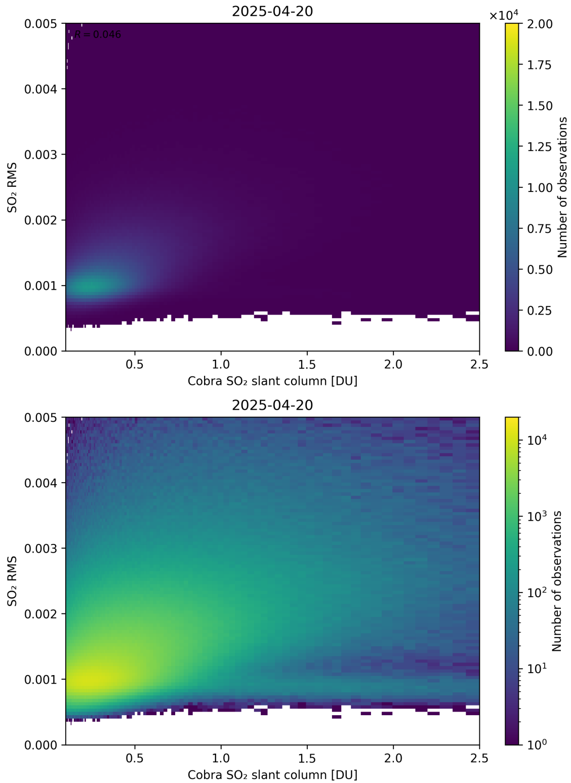
Figure 198: Scatter density plot of “Cobra SO 2 slant column” against “SO 2 RMS” for 2025-04-19 to 2025-04-21.
