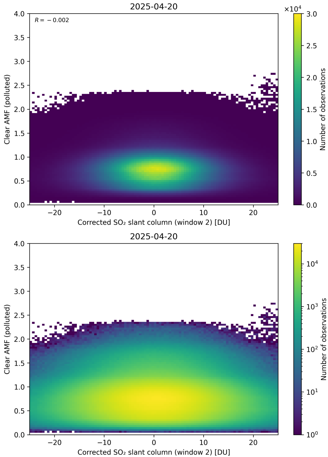
Figure 249: Scatter density plot of “Corrected SO 2 slant column (window 2)” against “Clear AMF (polluted)” for 2025-04-19 to 2025-04-21.
