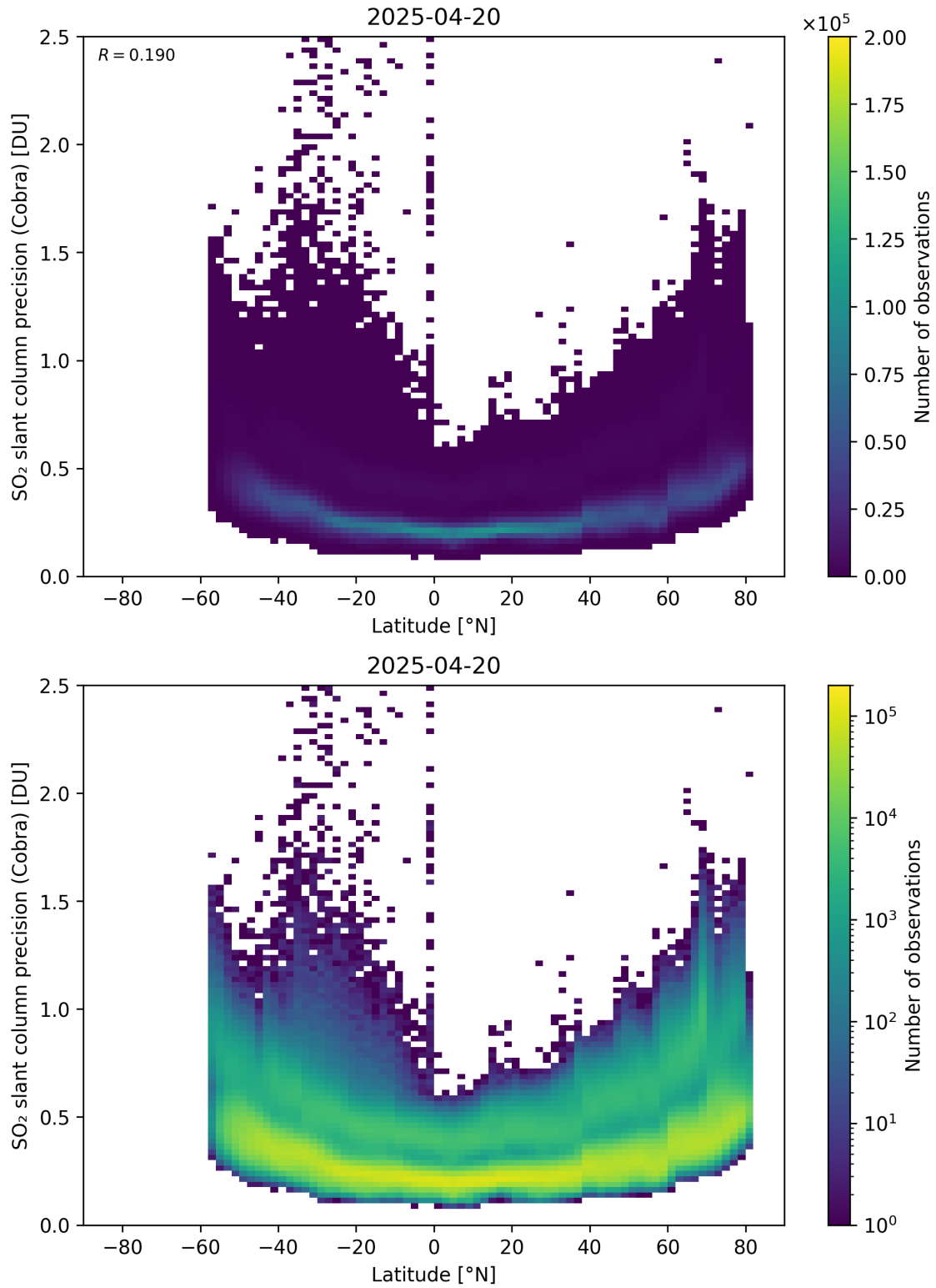
Figure 158: Scatter density plot of “Latitude” against “SO 2 slant column precision (Cobra)” for 2025-04-19 to 2025-04-21.
