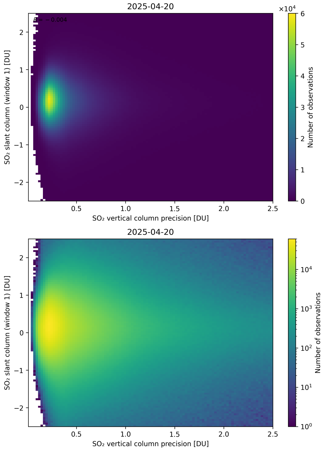
Figure 341: Scatter density plot of “SO 2 vertical column precision” against “SO 2 slant column (window 1)” for 2025-04-19 to 2025-04-21.
