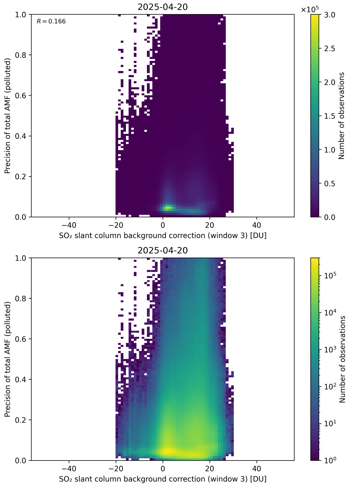
Figure 137: Scatter density plot of “SO 2 slant column background correction (window 3)” against “Precision of total AMF (polluted)” for 2025-04-19 to 2025-04-21.
