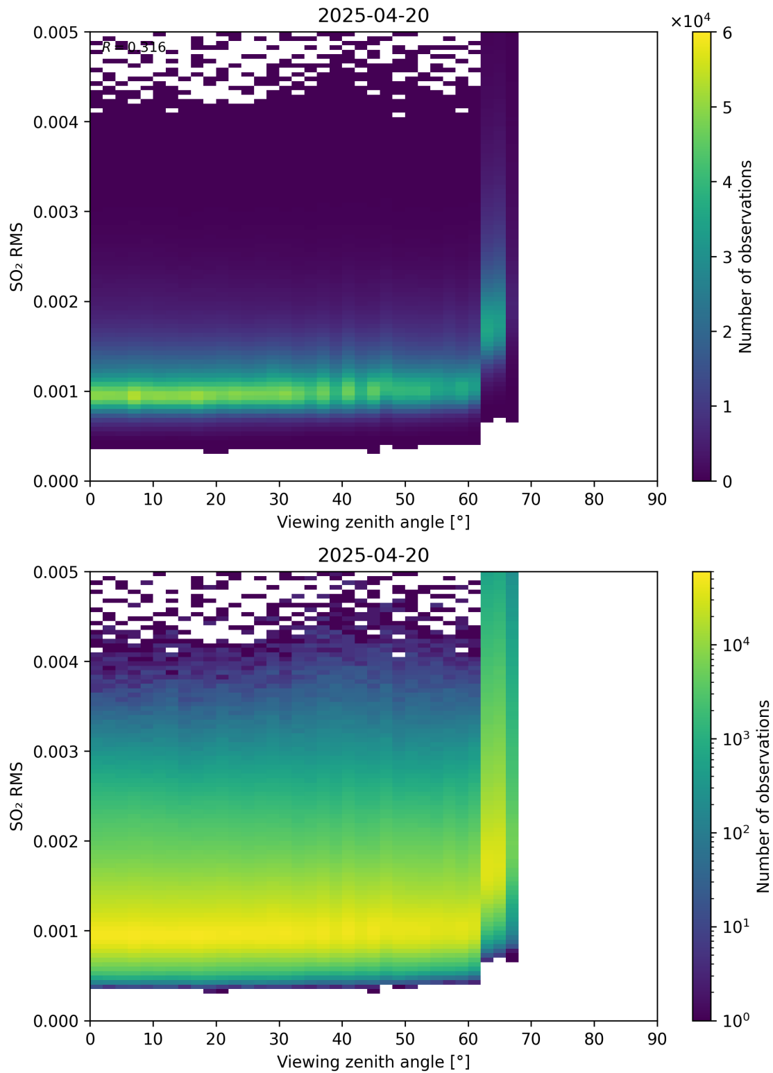
Figure 367: Scatter density plot of “Viewing zenith angle” against “SO 2 RMS” for 2025-04-19 to 2025-04-21.
