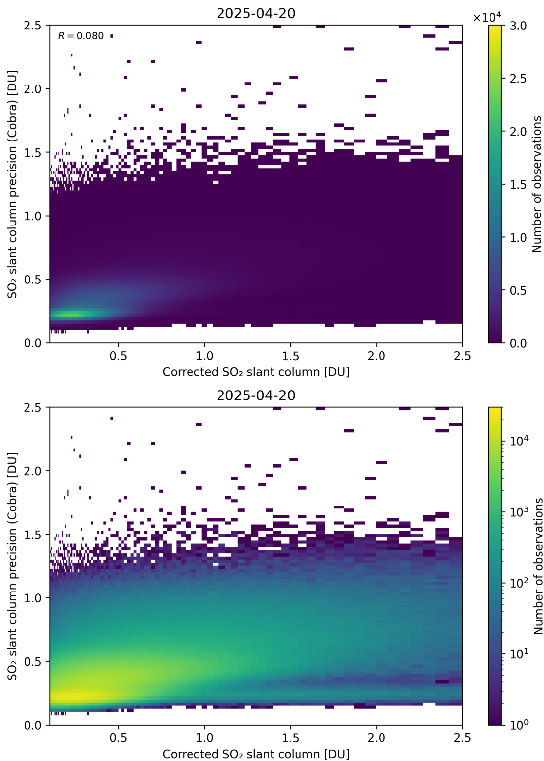
Figure 234: Scatter density plot of “Corrected SO 2 slant column” against “SO 2 slant column precision (Cobra)” for 2025-04-19 to 2025-04-21.
