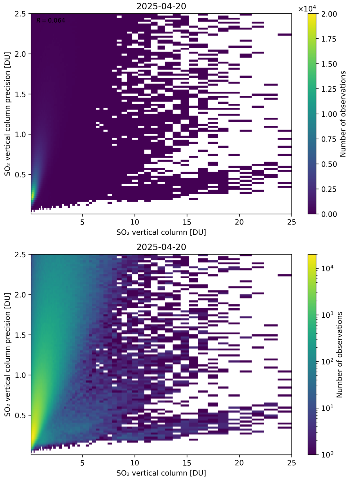
Figure 361: Scatter density plot of “SO 2 vertical column” against “SO 2 vertical column precision” for 2025-04-19 to 2025-04-21.
