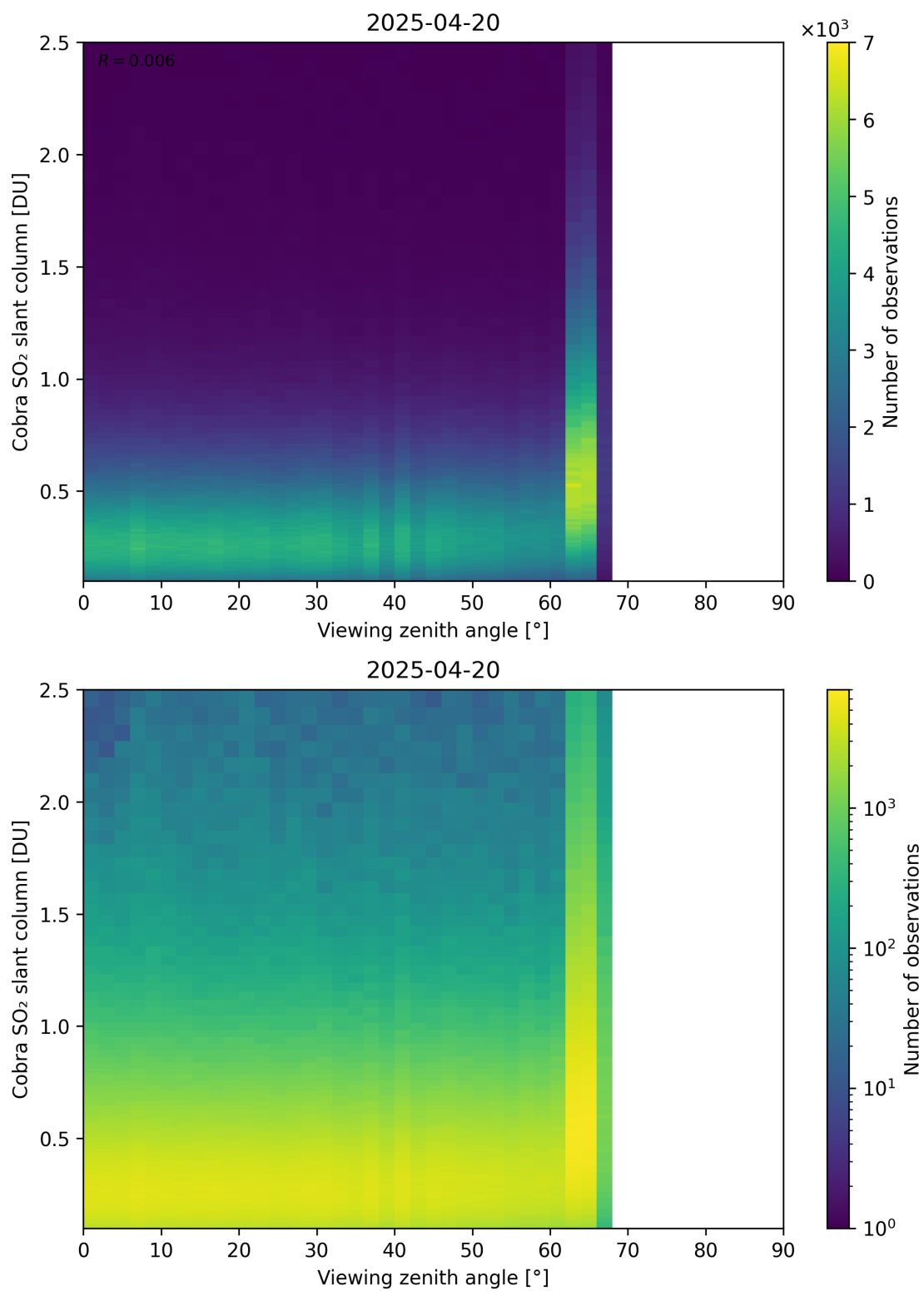
Figure 371: Scatter density plot of “Viewing zenith angle” against “Cobra SO 2 slant column” for 2025-04-19 to 2025-04-21.
