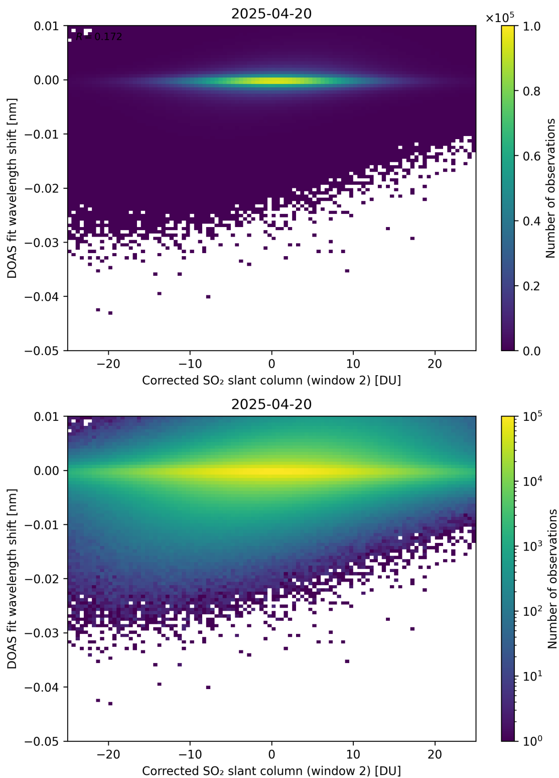
Figure 246: Scatter density plot of “Corrected SO 2 slant column (window 2)” against “DOAS fit wavelength shift” for 2025-04-19 to 2025-04-21.
