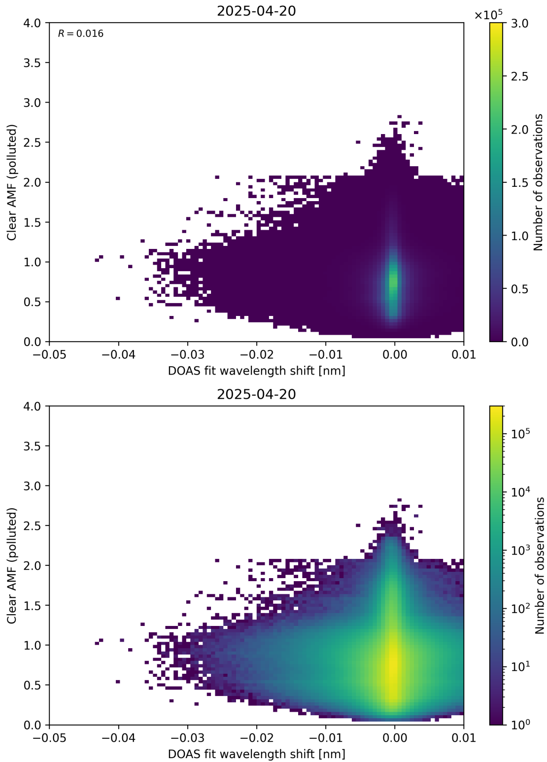
Figure 140: Scatter density plot of “DOAS fit wavelength shift” against “Clear AMF (polluted)” for 2025-04-19 to 2025-04-21.
