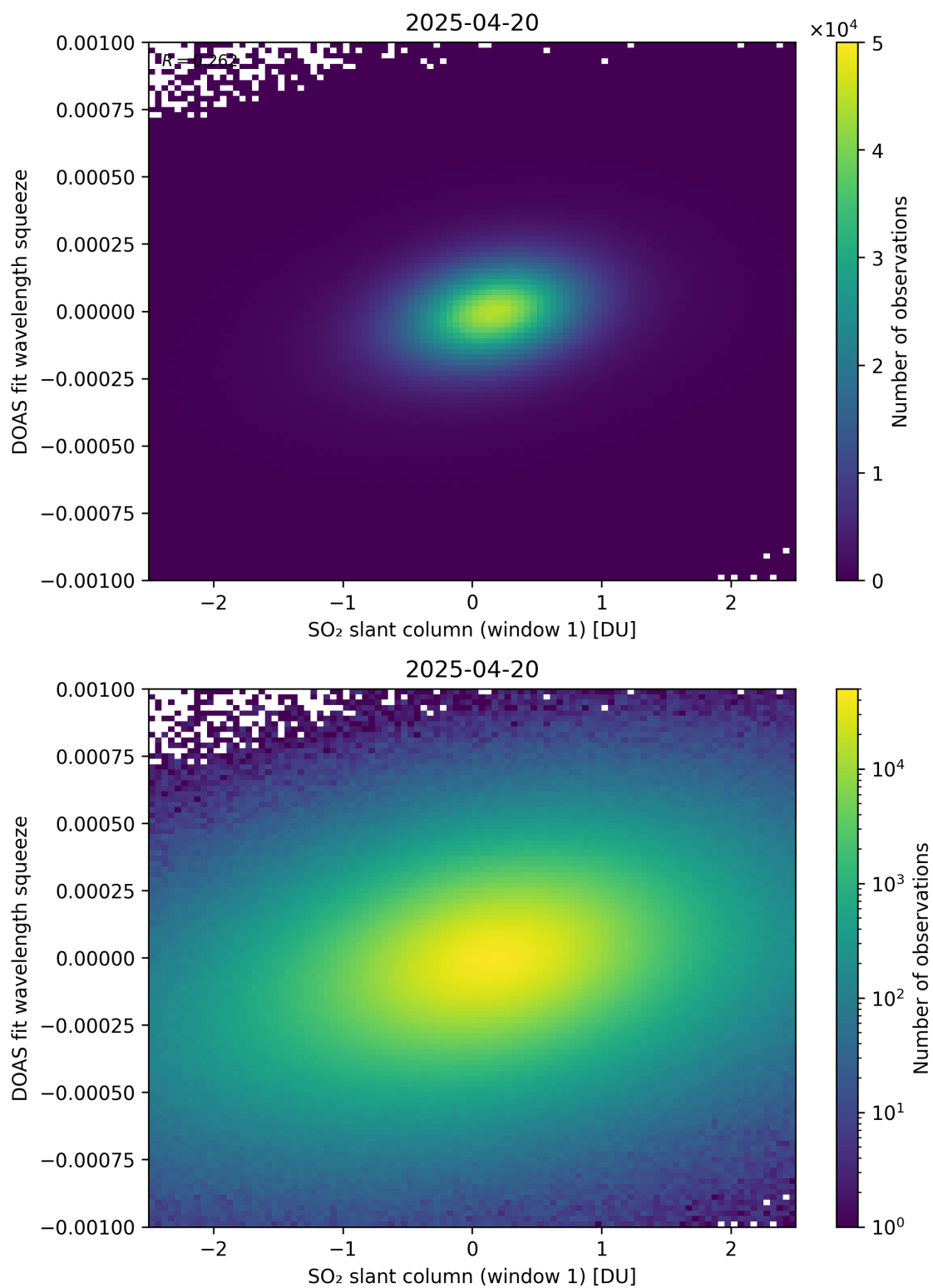
Figure 266: Scatter density plot of “SO 2 slant column (window 1)” against “DOAS fit wavelength squeeze” for 2025-04-19 to 2025-04-21.
