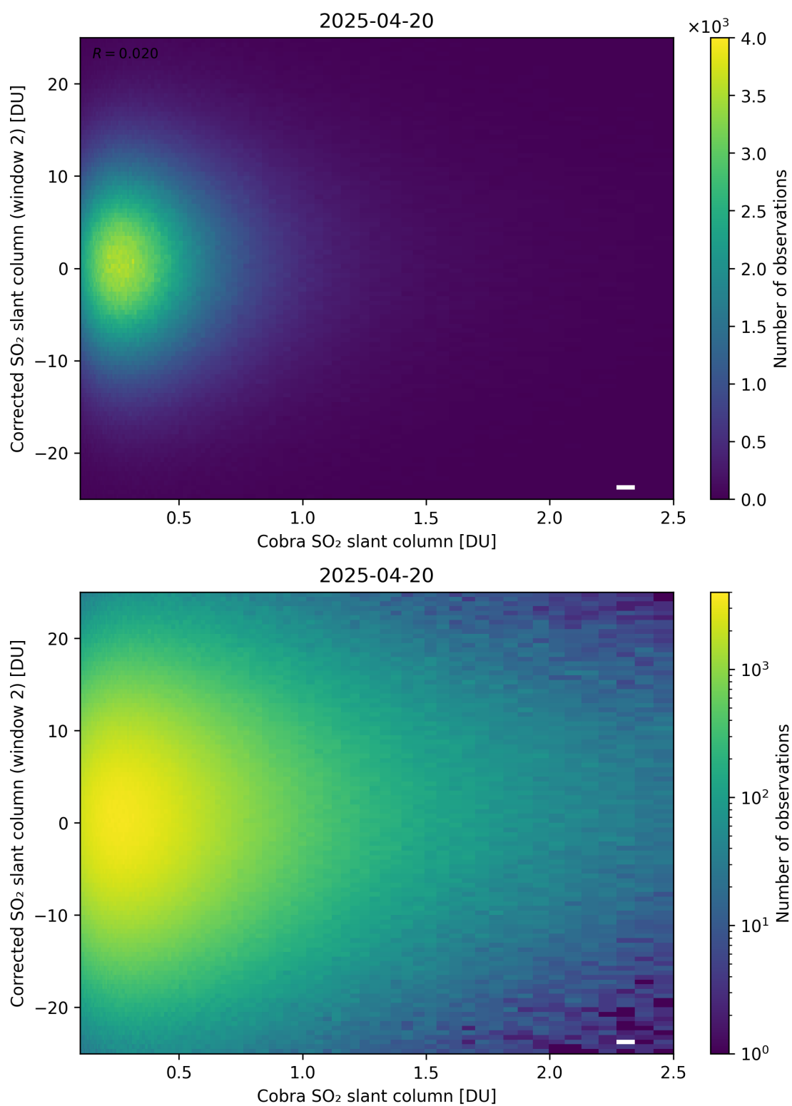
Figure 217: Scatter density plot of “Cobra SO 2 slant column” against “Corrected SO 2 slant column (window 2)” for 2025-04-19 to 2025-04-21.
