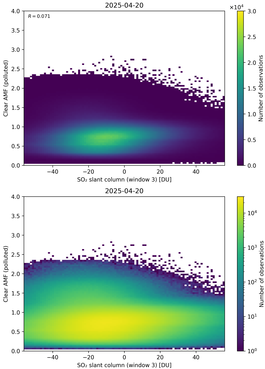
Figure 315: Scatter density plot of “SO 2 slant column (window 3)” against “Clear AMF (polluted)” for 2025-04-19 to 2025-04-21.
