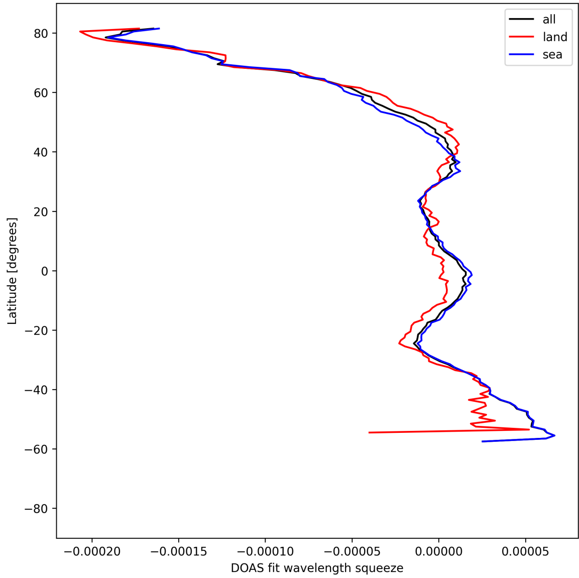
Figure 51: Zonal average of “DOAS fit wavelength squeeze” for 2025-04-19 to 2025-04-21.
