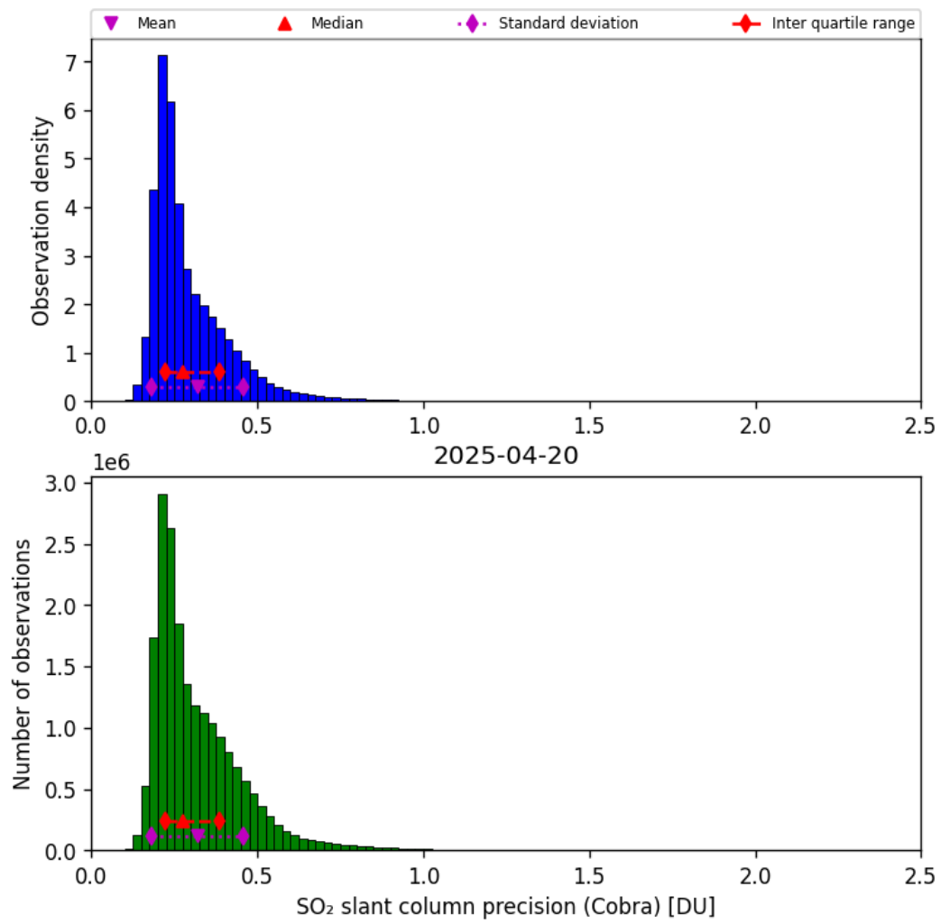
Figure 62: Histogram of “SO 2 slant column precision (Cobra)” for 2025-04-19 to 2025-04-21
