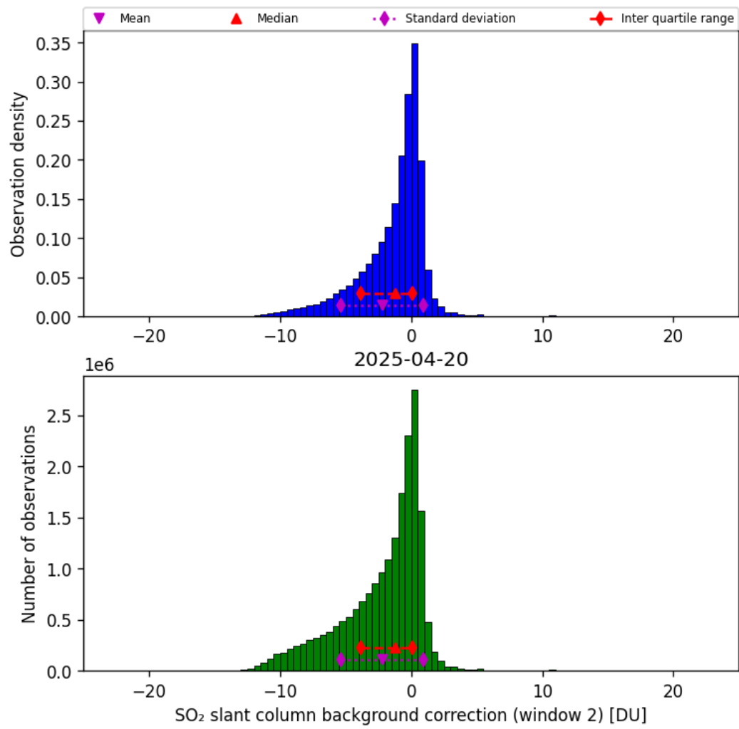
Figure 70: Histogram of “SO 2 slant column background correction (window 2)” for 2025-04-19 to 2025-04-21
