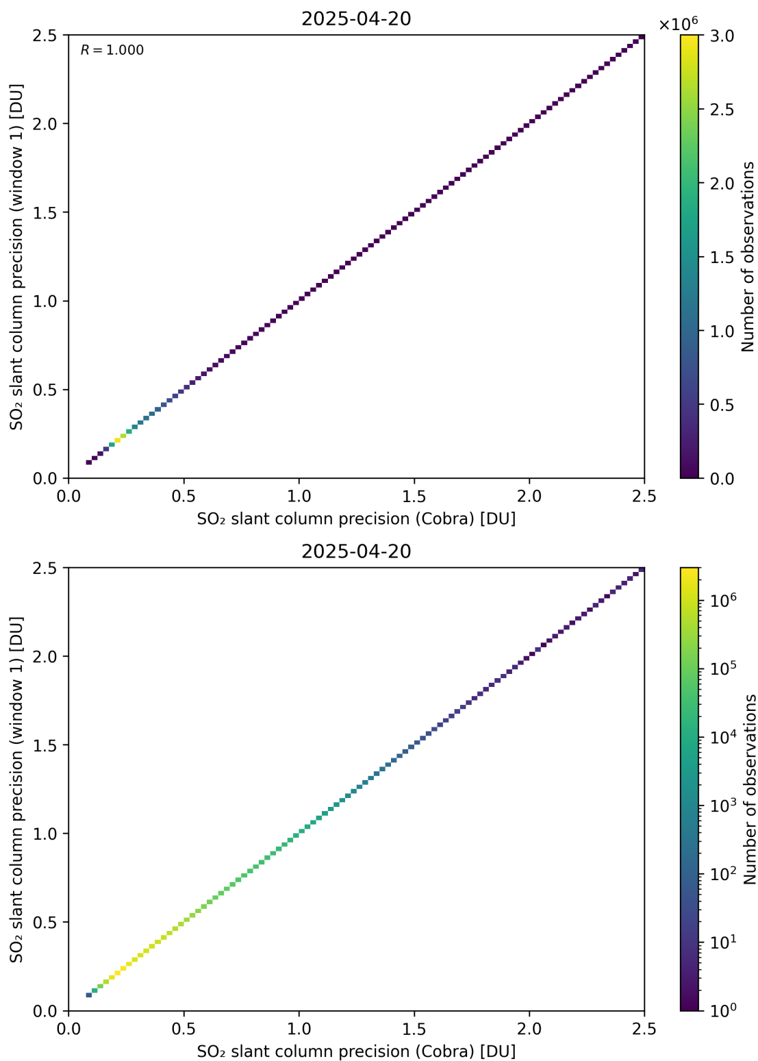
Figure 209: Scatter density plot of “SO 2 slant column precision (Cobra)” against “SO 2 slant column precision (window 1)” for 2025-04-19 to 2025-04-21.
