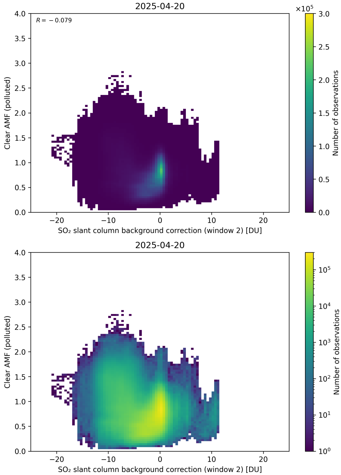
Figure 126: Scatter density plot of “SO 2 slant column background correction (window 2)” against “Clear AMF (polluted)” for 2025-04-19 to 2025-04-21.
