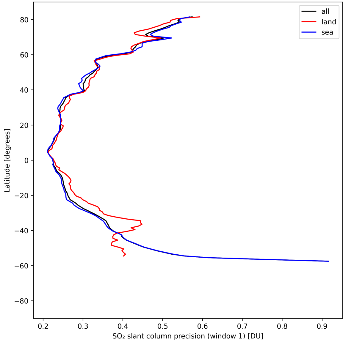
Figure 38: Zonal average of “SO 2 slant column precision (window 1)” for 2025-04-19 to 2025-04-21.
