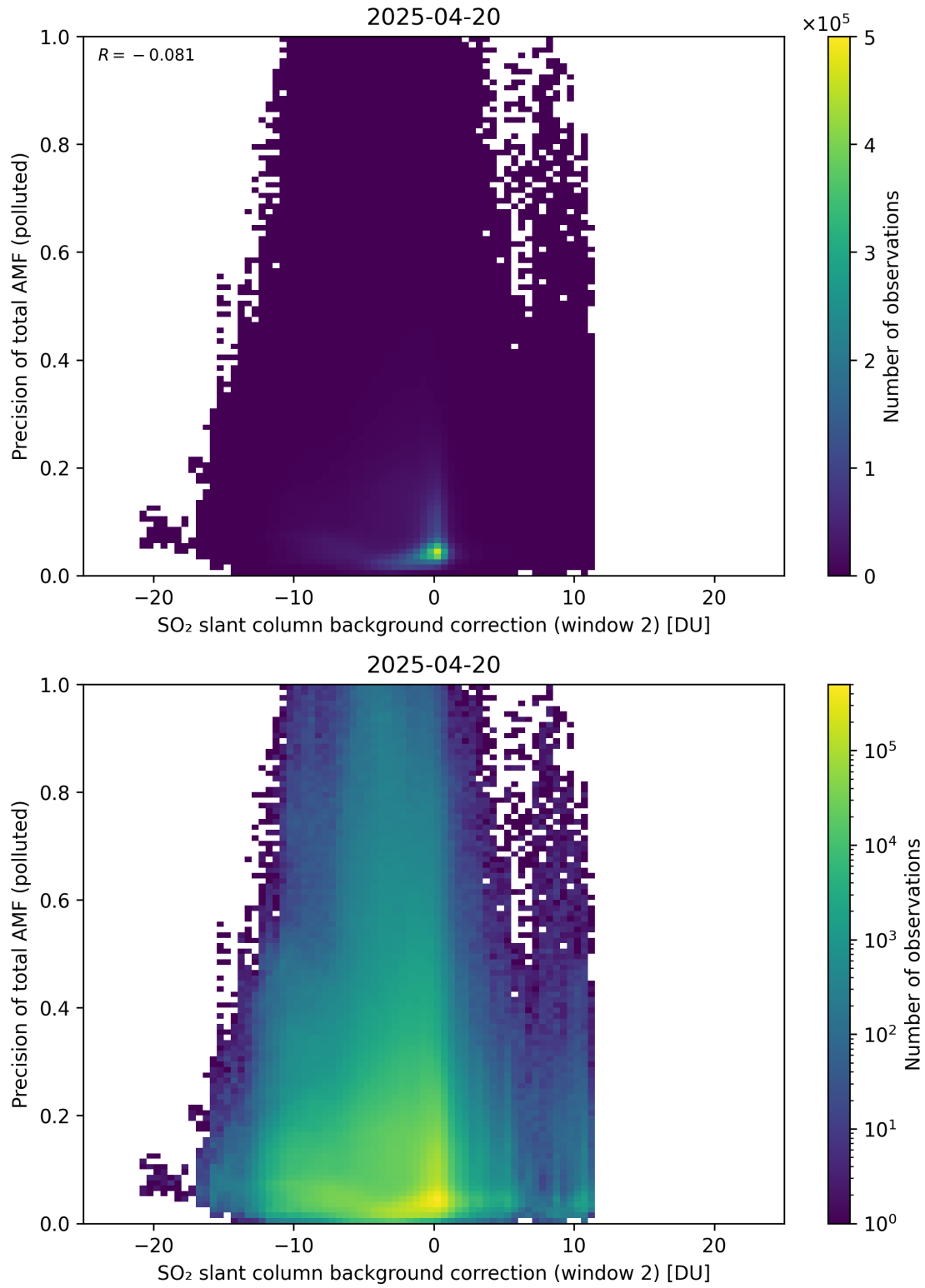
Figure 131: Scatter density plot of “SO 2 slant column background correction (window 2)” against “Precision of total AMF (polluted)” for 2025-04-19 to 2025-04-21.
