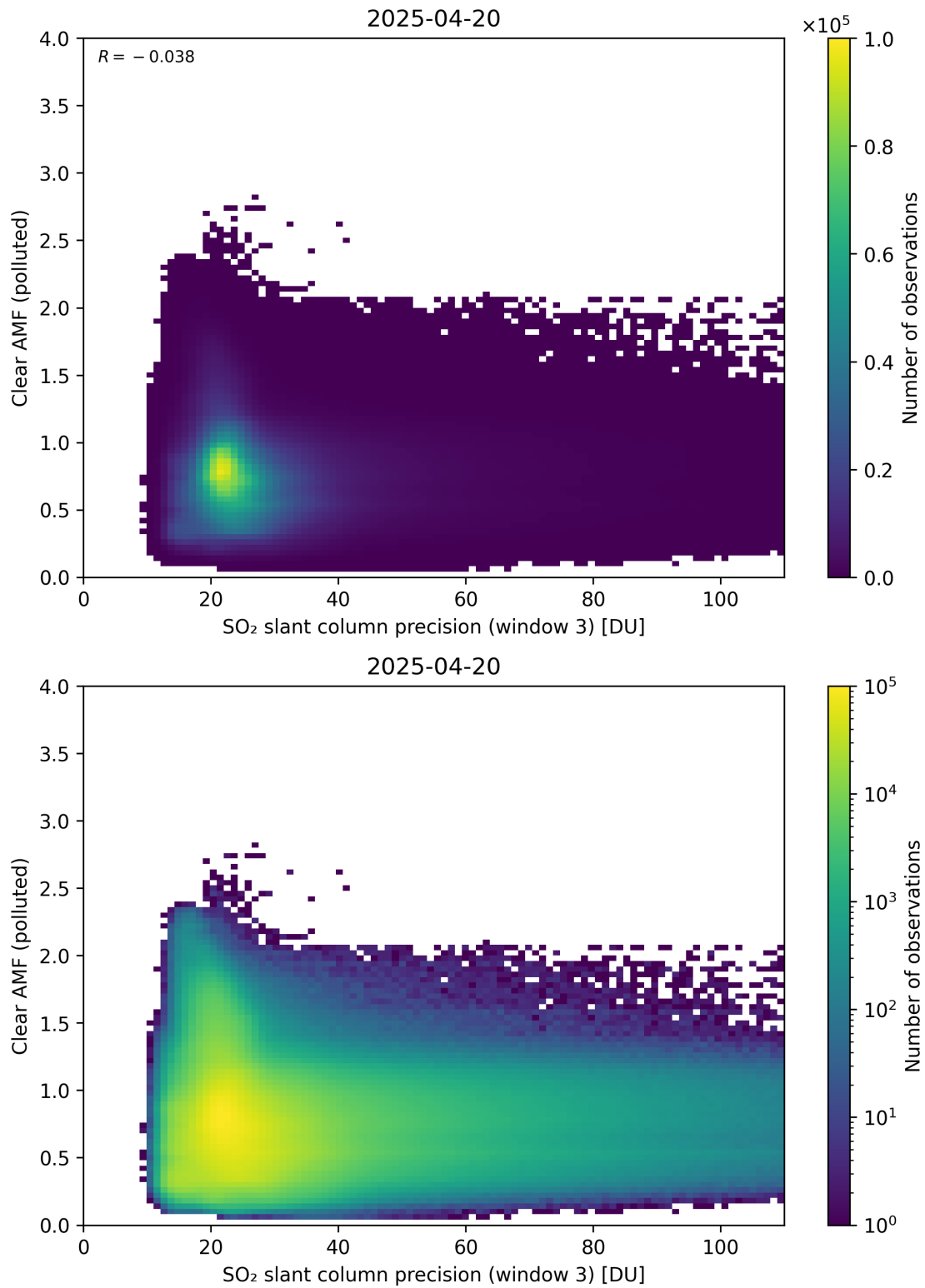
Figure 311: Scatter density plot of “SO 2 slant column precision (window 3)” against “Clear AMF (polluted)” for 2025-04-19 to 2025-04-21.
