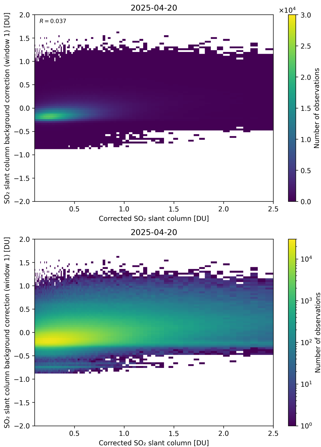
Figure 226: Scatter density plot of “Corrected SO 2 slant column” against “SO 2 slant column background correction (window 1)” for 2025-04-19 to 2025-04-21.
