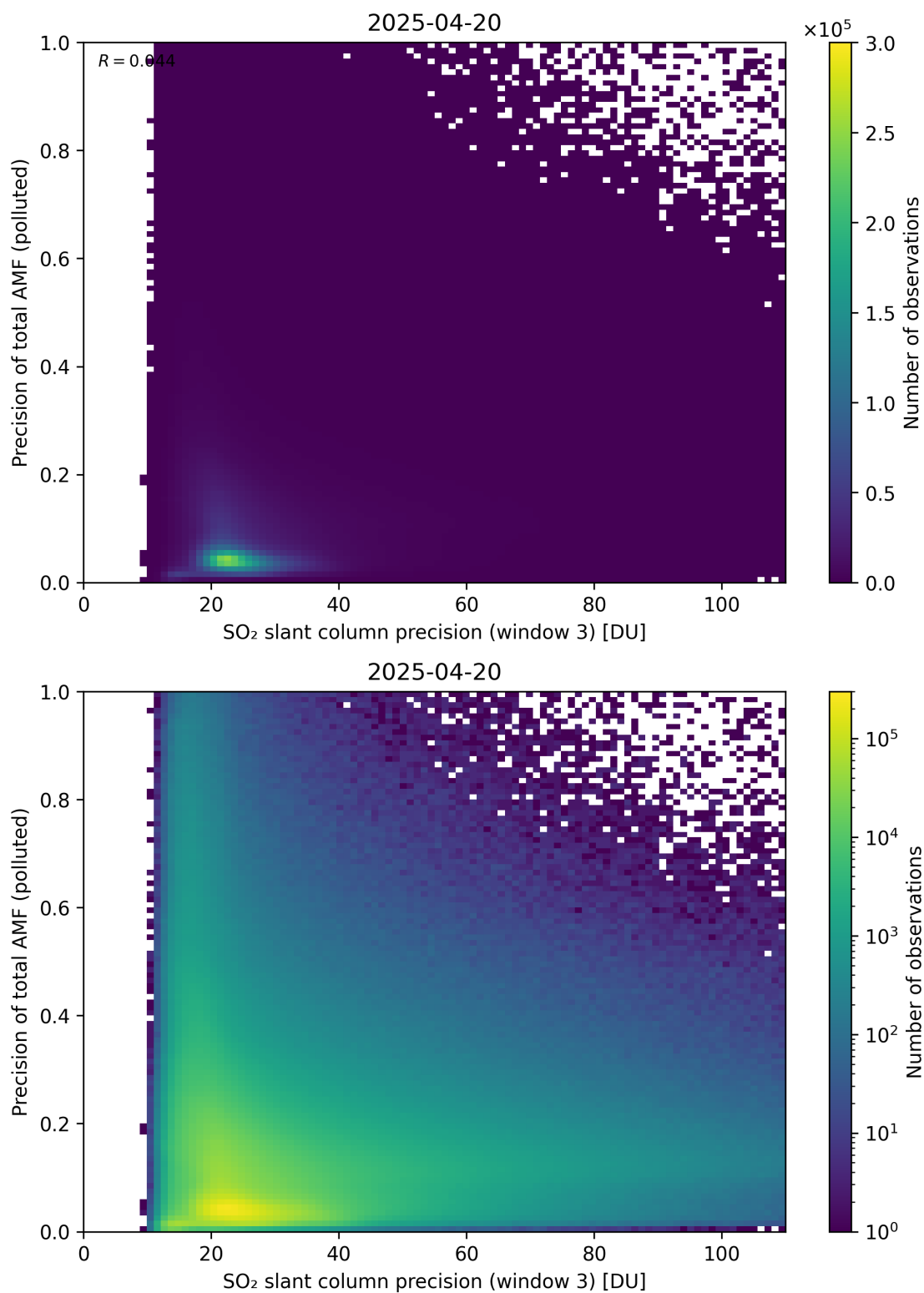
Figure 314: Scatter density plot of “SO 2 slant column precision (window 3)” against “Precision of total AMF (polluted)” for 2025-04-19 to 2025-04-21.
