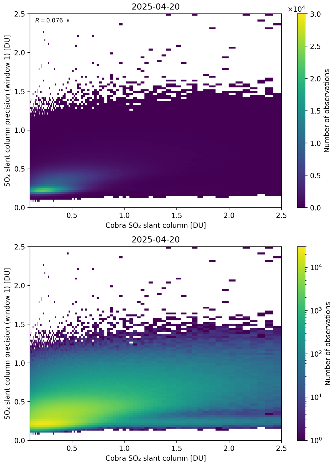
Figure 220: Scatter density plot of “Cobra SO 2 slant column” against “SO 2 slant column precision (window 1)” for 2025-04-19 to 2025-04-21.
