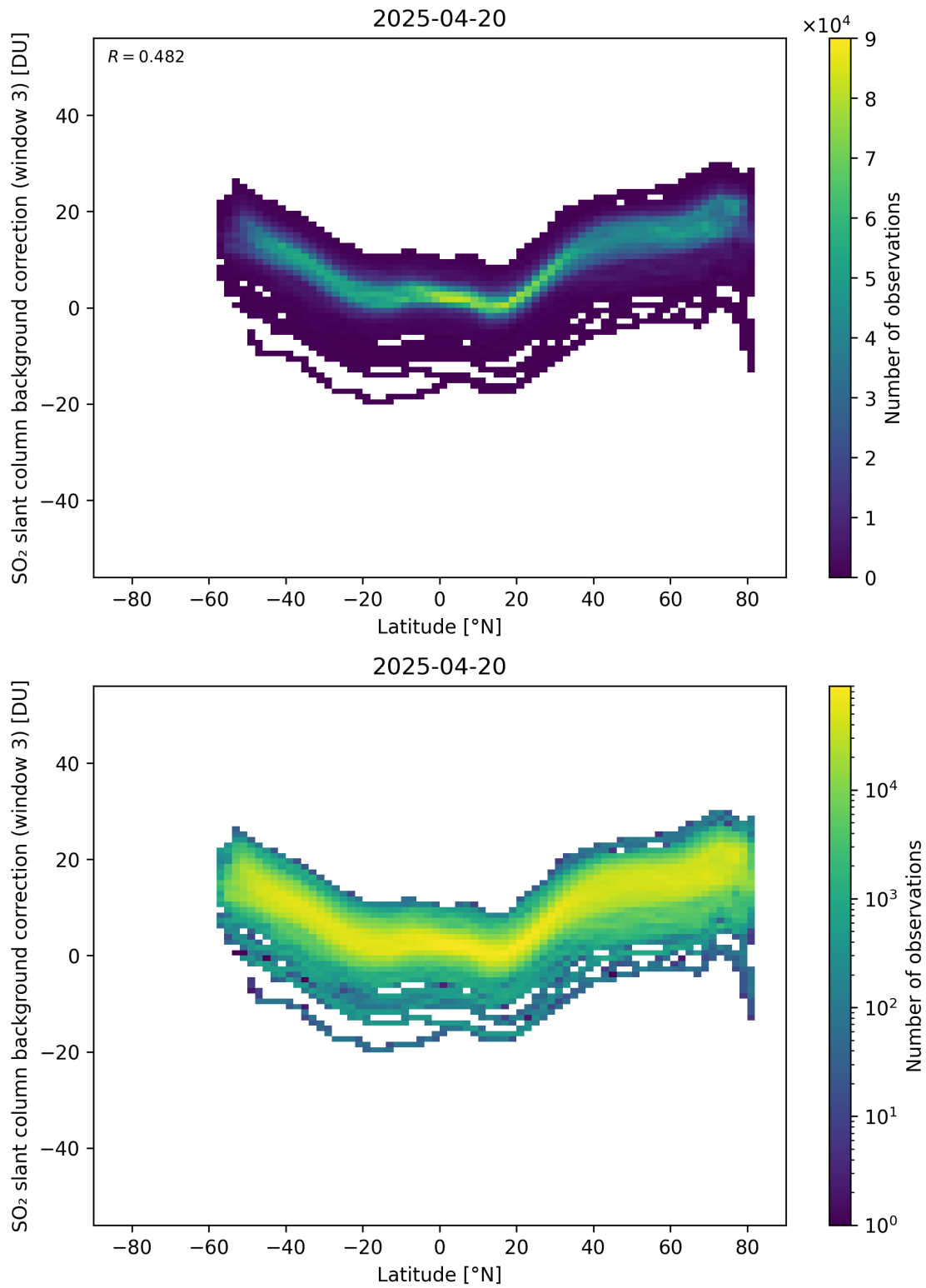
Figure 152: Scatter density plot of “Latitude” against “SO 2 slant column background correction (window 3)” for 2025-04-19 to 2025-04-21.
