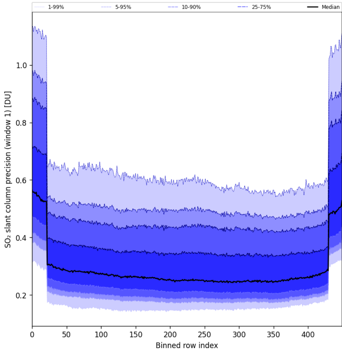
Figure 90: Along track statistics of “SO 2 slant column precision (window 1)” for 2025-04-19 to 2025-04-21
