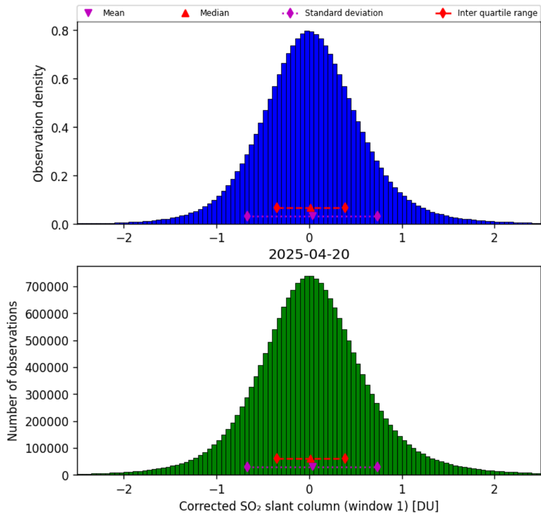
Figure 65: Histogram of “Corrected SO 2 slant column (window 1)” for 2025-04-19 to 2025-04-21
