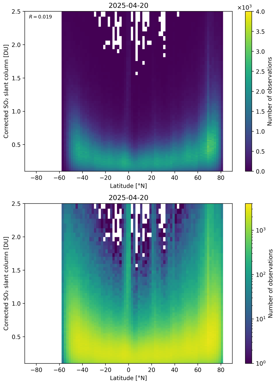
Figure 159: Scatter density plot of “Latitude” against “Corrected SO 2 slant column” for 2025-04-19 to 2025-04-21.
