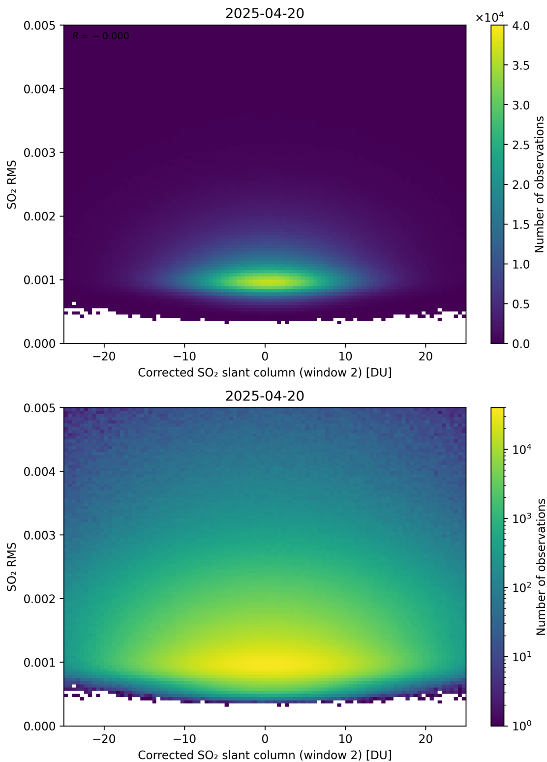
Figure 248: Scatter density plot of “Corrected SO 2 slant column (window 2)” against “SO 2 RMS” for 2025-04-19 to 2025-04-21.
