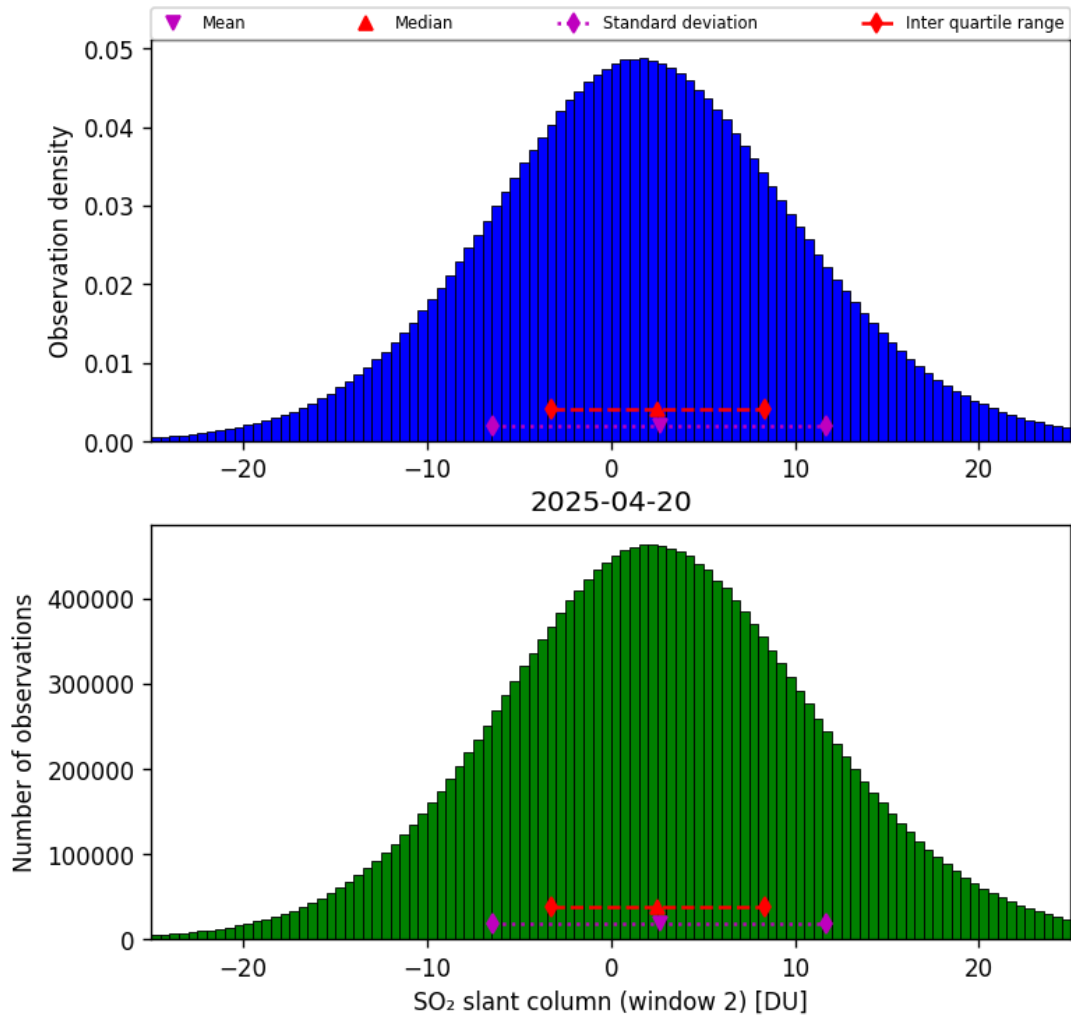
Figure 67: Histogram of “SO 2 slant column (window 2)” for 2025-04-19 to 2025-04-21
