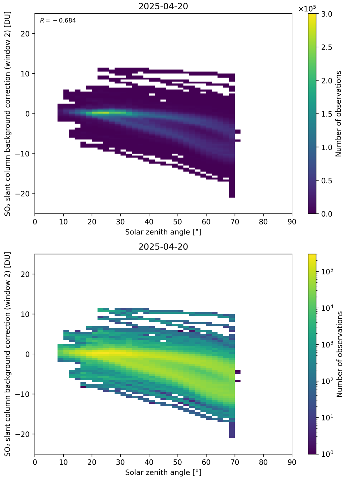
Figure 172: Scatter density plot of “Solar zenith angle” against “SO 2 slant column background correction (window 2)” for 2025-04-19 to 2025-04-21.
