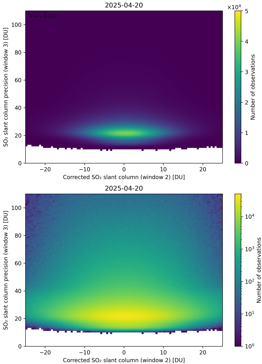
Figure 252: Scatter density plot of “Corrected SO 2 slant column (window 2)” against “SO 2 slant column precision (window 3)” for 2025-04-19 to 2025-04-21.
