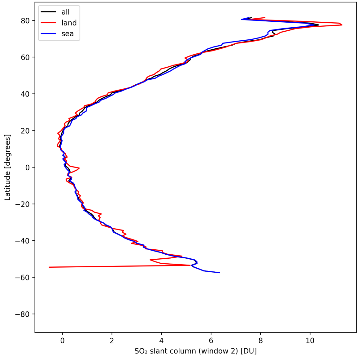
Figure 41: Zonal average of “SO 2 slant column (window 2)” for 2025-04-19 to 2025-04-21.
