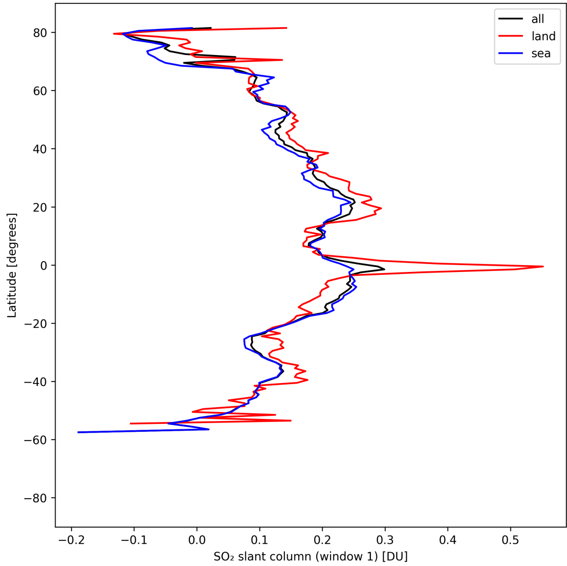
Figure 37: Zonal average of “SO 2 slant column (window 1)” for 2025-04-19 to 2025-04-21.
