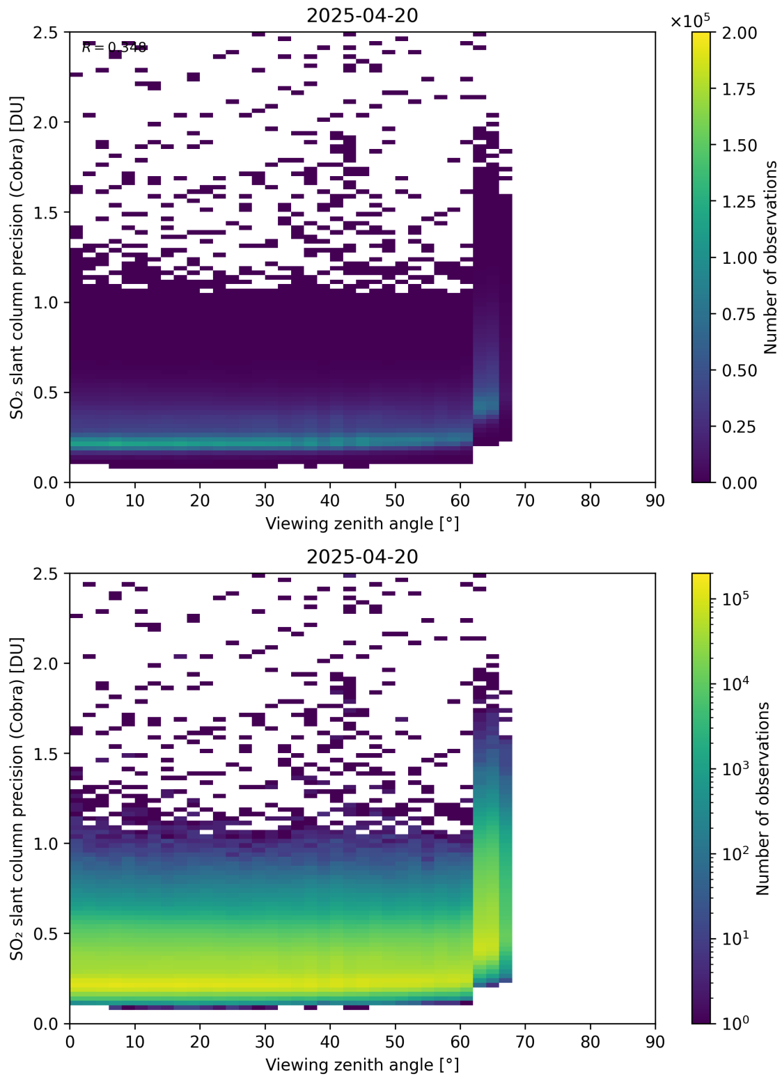
Figure 372: Scatter density plot of “Viewing zenith angle” against “SO 2 slant column precision (Cobra)” for 2025-04-19 to 2025-04-21.
