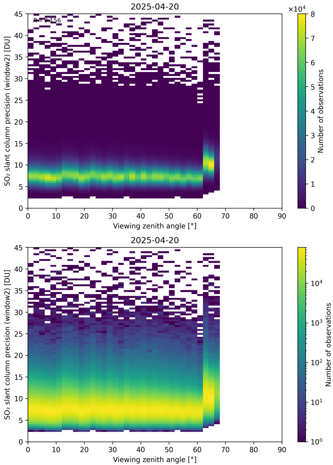
Figure 378: Scatter density plot of “Viewing zenith angle” against “SO 2 slant column precision (window2)” for 2025-04-19 to 2025-04-21.
