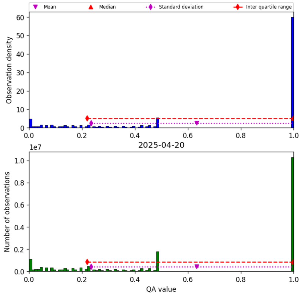
Figure 57: Histogram of “QA value” for 2025-04-19 to 2025-04-21
