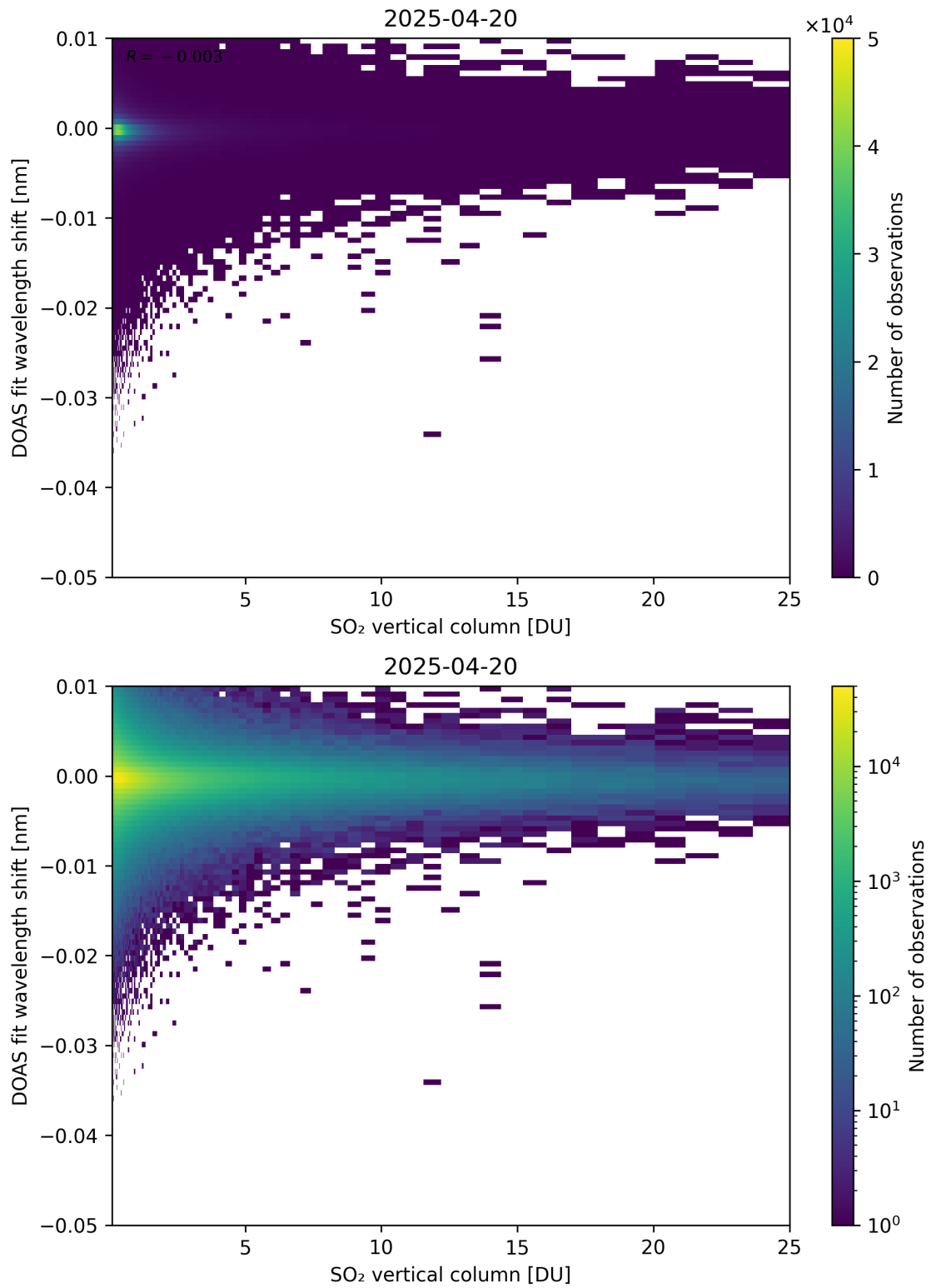
Figure 326: Scatter density plot of “SO 2 vertical column” against “DOAS fit wavelength shift” for 2025-04-19 to 2025-04-21.
