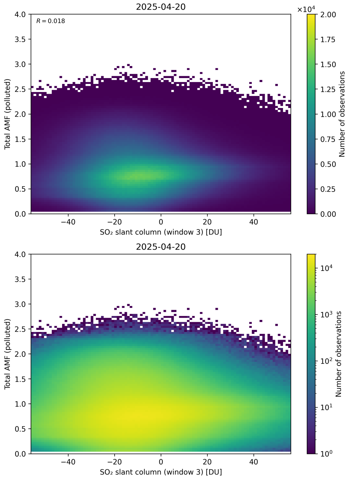
Figure 318: Scatter density plot of “SO 2 slant column (window 3)” against “Total AMF (polluted)” for 2025-04-19 to 2025-04-21.
