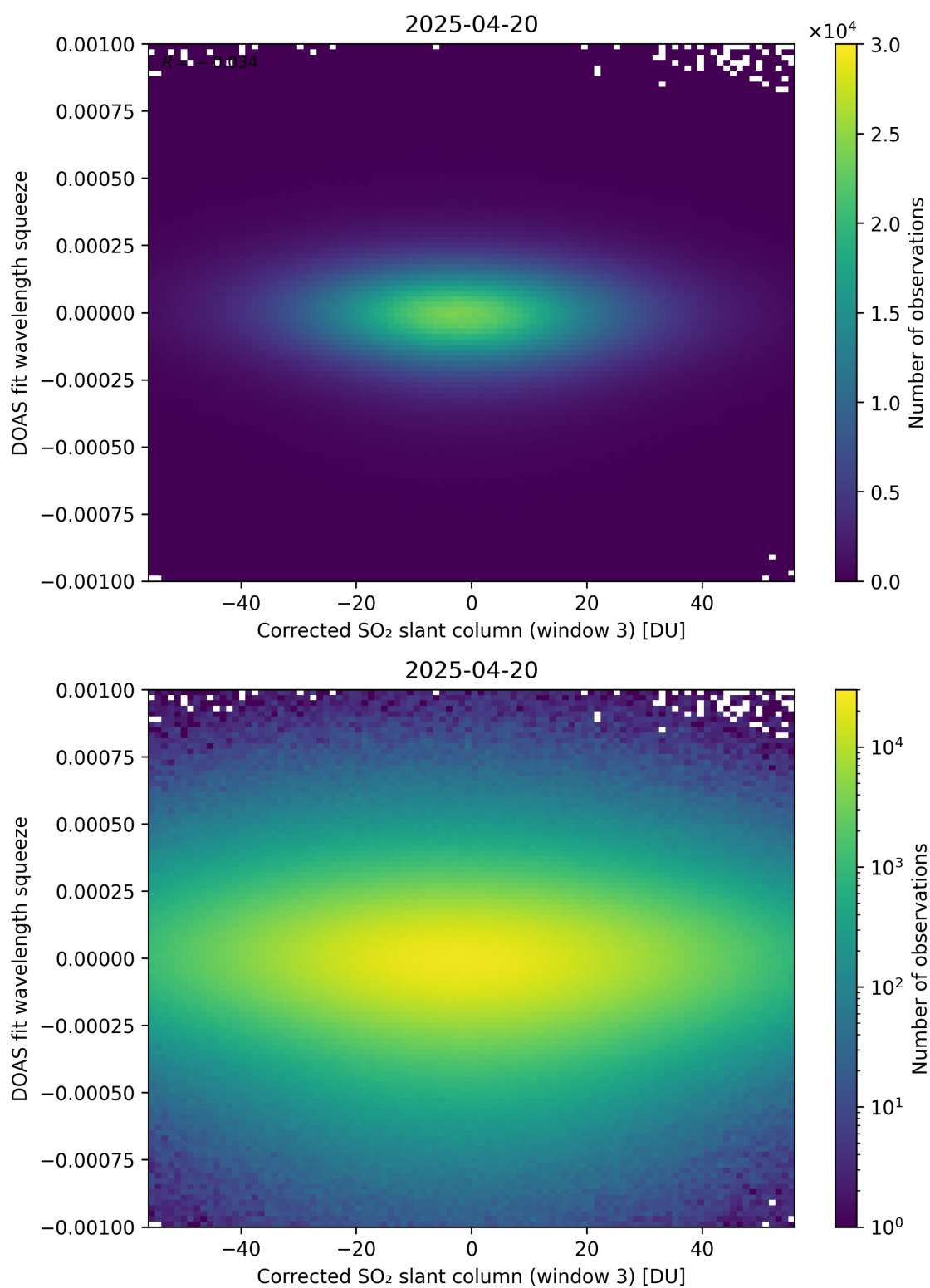
Figure 257: Scatter density plot of “Corrected SO 2 slant column (window 3)” against “DOAS fit wavelength squeeze” for 2025-04-19 to 2025-04-21.
