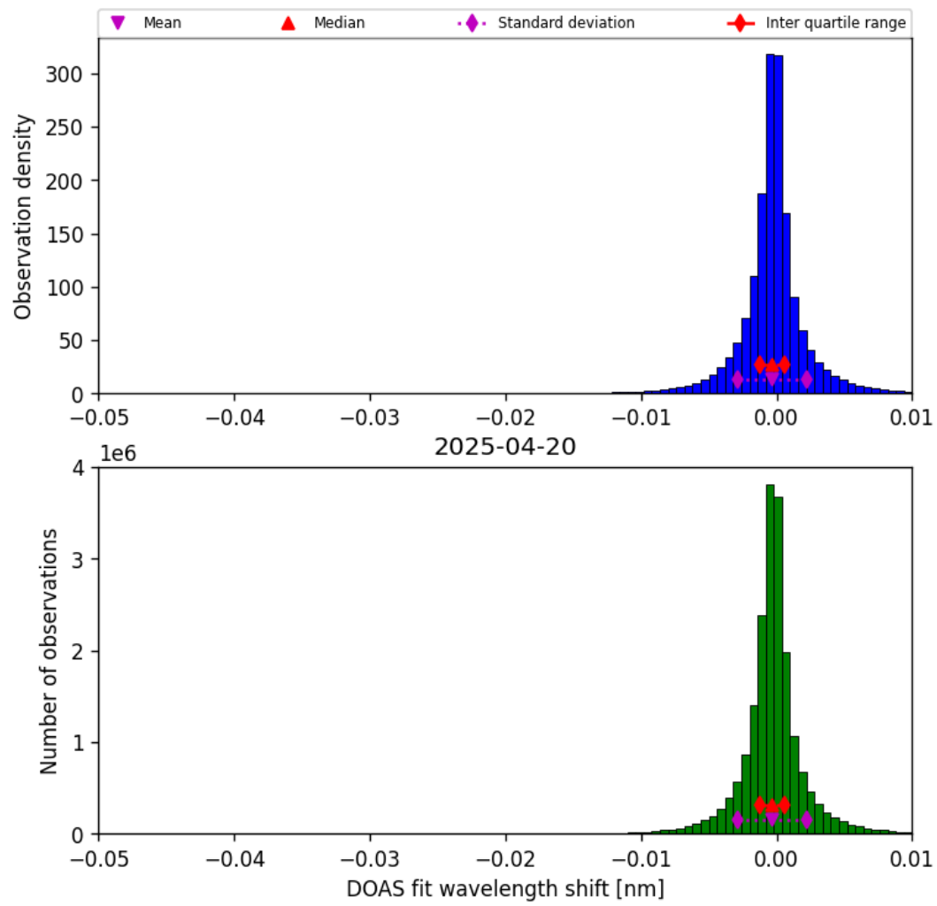
Figure 76: Histogram of “DOAS fit wavelength shift” for 2025-04-19 to 2025-04-21
