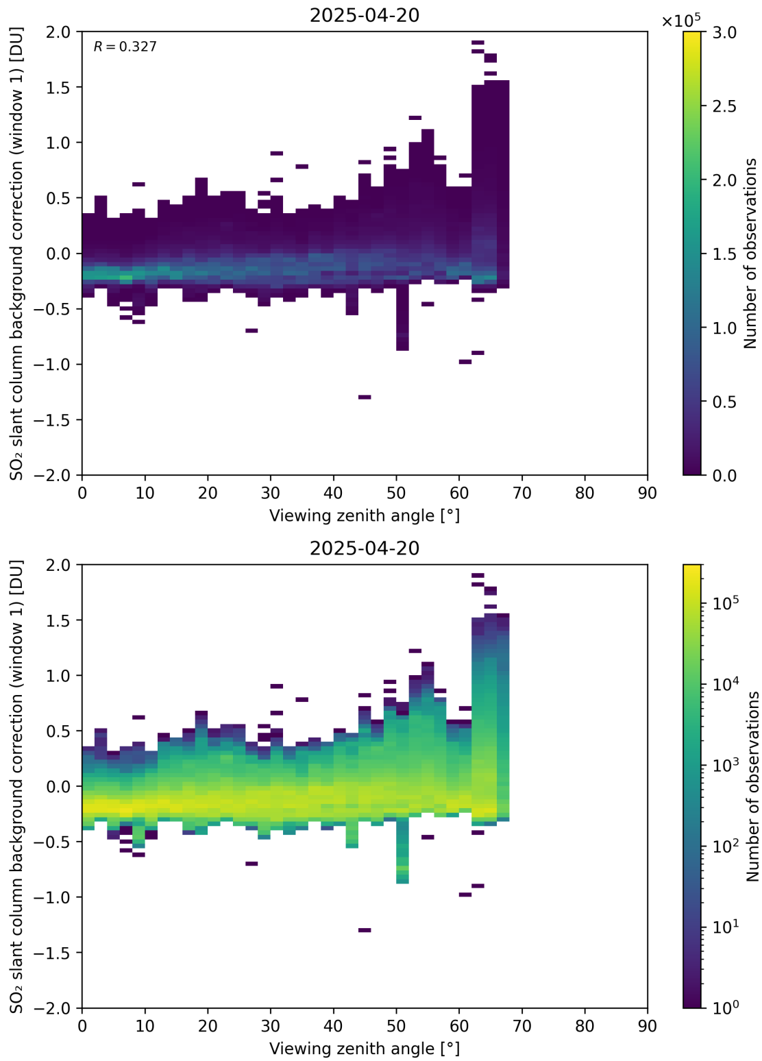
Figure 362: Scatter density plot of “Viewing zenith angle” against “SO 2 slant column background correction (window 1)” for 2025-04-19 to 2025-04-21.
