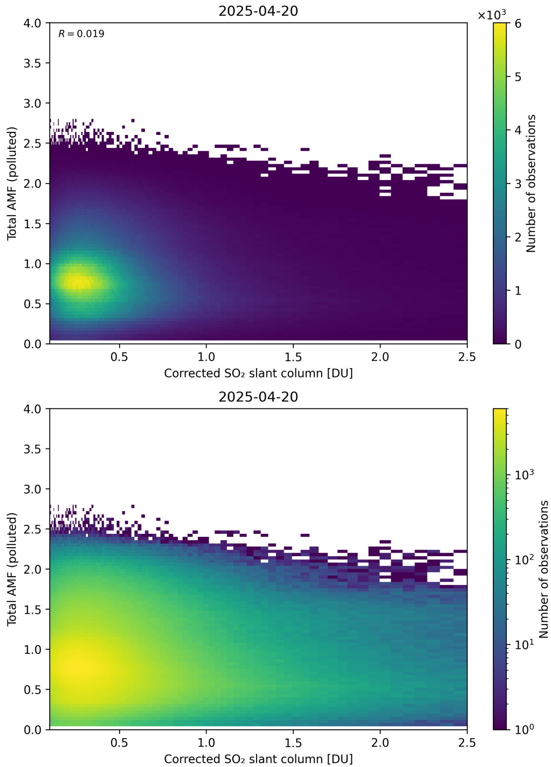
Figure 242: Scatter density plot of “Corrected SO 2 slant column” against “Total AMF (polluted)” for 2025-04-19 to 2025-04-21.
