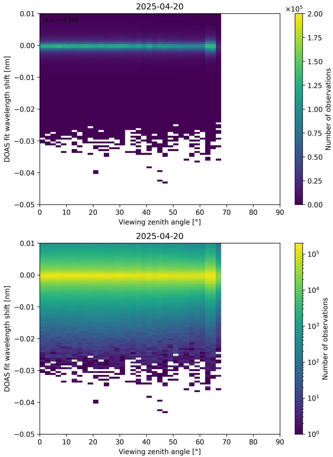
Figure 365: Scatter density plot of “Viewing zenith angle” against “DOAS fit wavelength shift” for 2025-04-19 to 2025-04-21.
