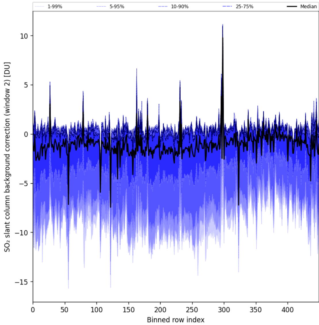
Figure 96: Along track statistics of “SO 2 slant column background correction (window 2)” for 2025-04-19 to 2025-04-21
