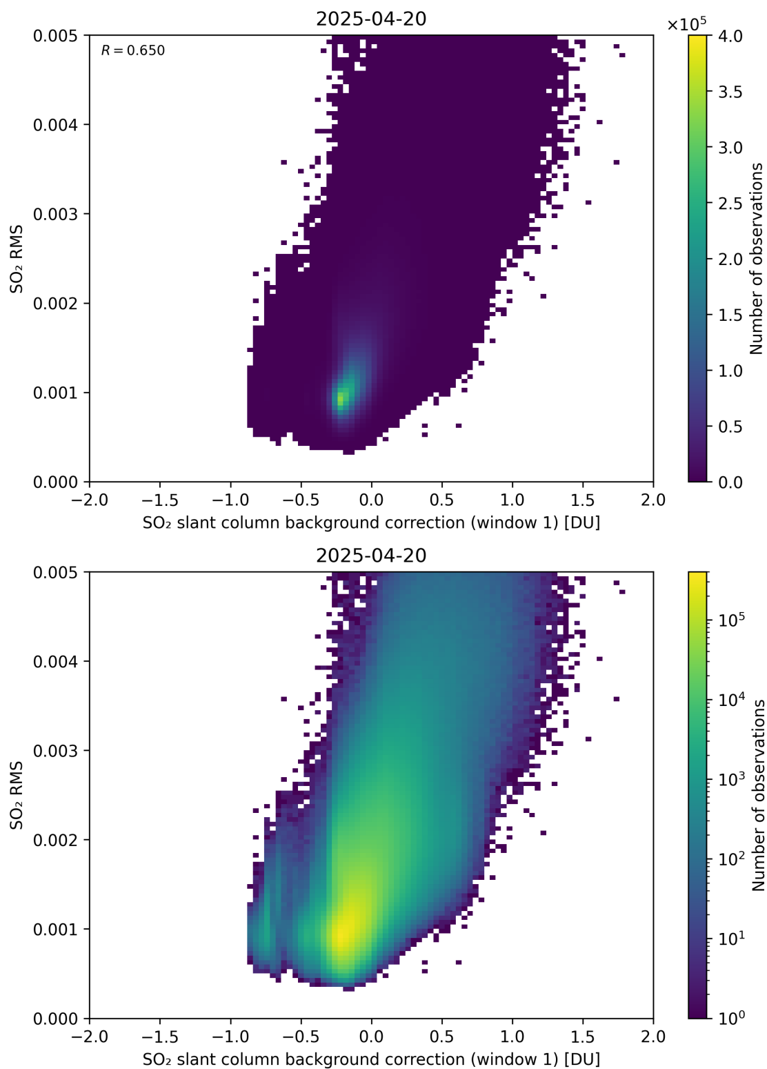
Figure 113: Scatter density plot of “SO 2 slant column background correction (window 1)” against “SO 2 RMS” for 2025-04-19 to 2025-04-21.
