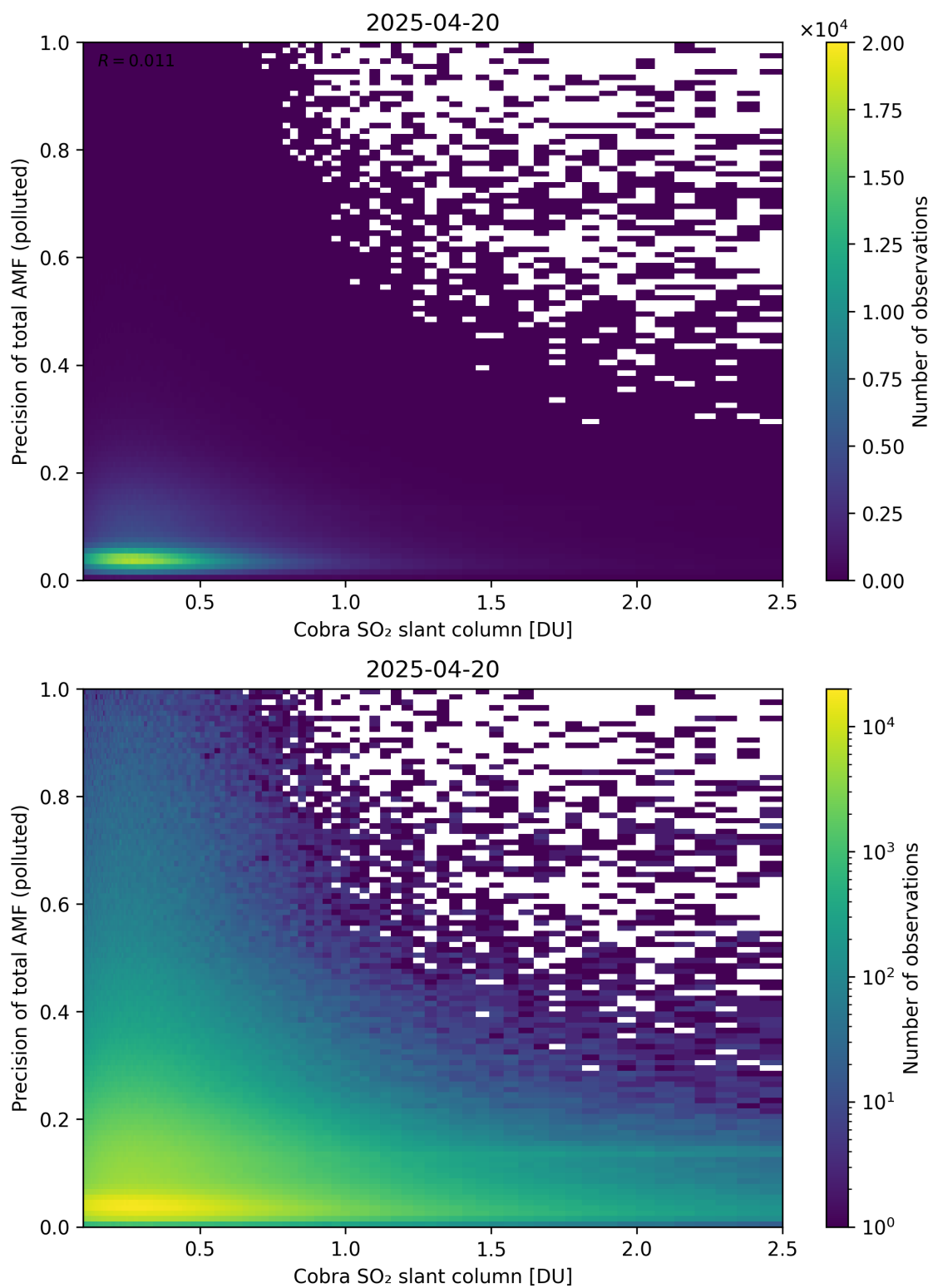
Figure 225: Scatter density plot of “Cobra SO 2 slant column” against “Precision of total AMF (polluted)” for 2025-04-19 to 2025-04-21.
