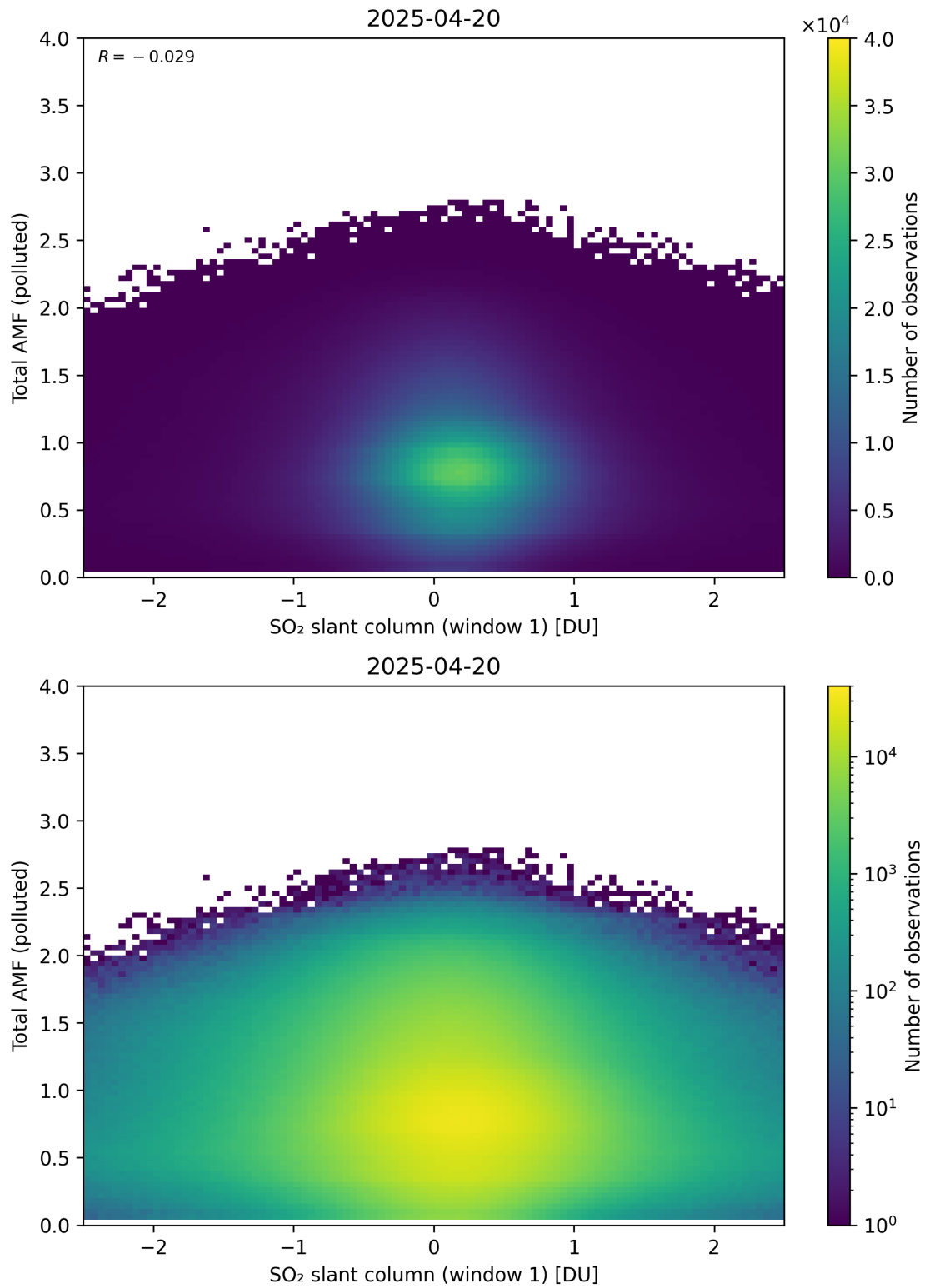
Figure 289: Scatter density plot of “SO 2 slant column (window 1)” against “Total AMF (polluted)” for 2025-04-19 to 2025-04-21.
