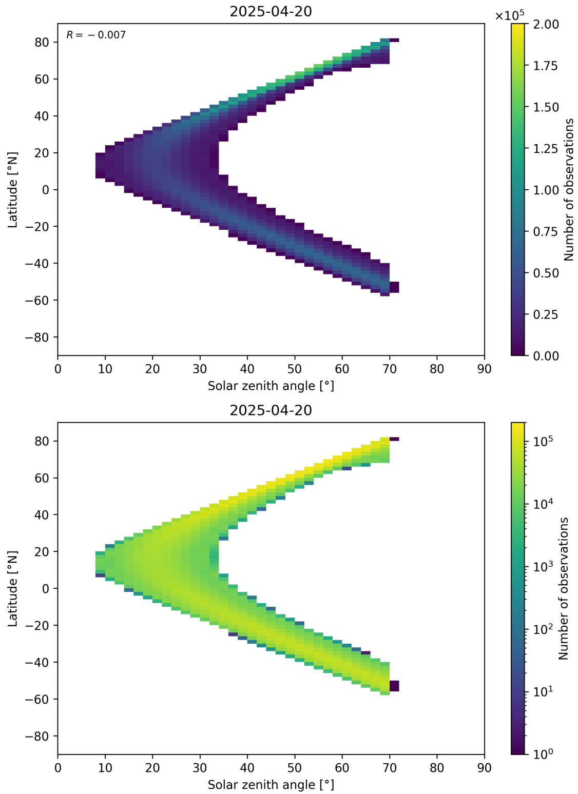
Figure 177: Scatter density plot of “Solar zenith angle” against “Latitude” for 2025-04-19 to 2025-04-21.
