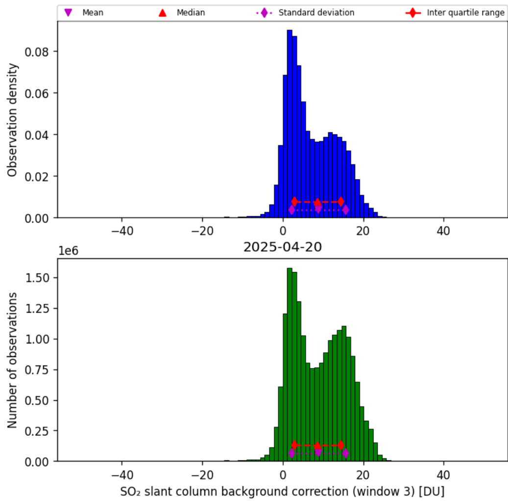
Figure 74: Histogram of “SO 2 slant column background correction (window 3)” for 2025-04-19 to 2025-04-21
