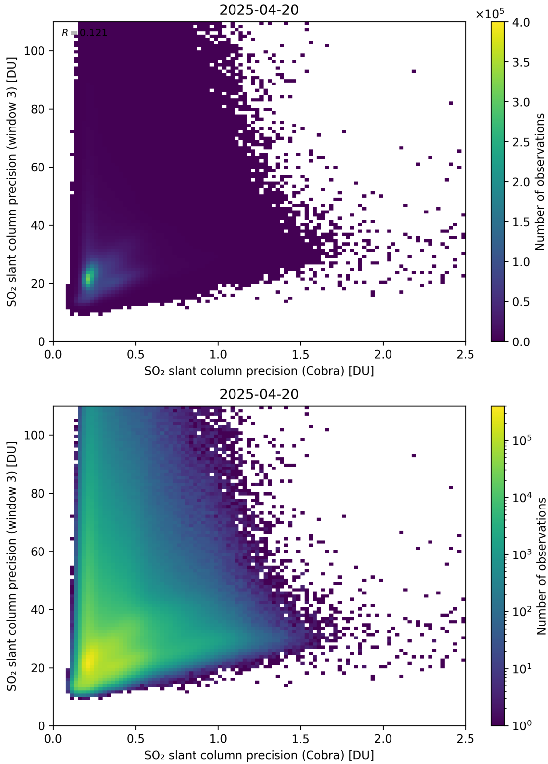
Figure 212: Scatter density plot of “SO 2 slant column precision (Cobra)” against “SO 2 slant column precision (window 3)” for 2025-04-19 to 2025-04-21.
