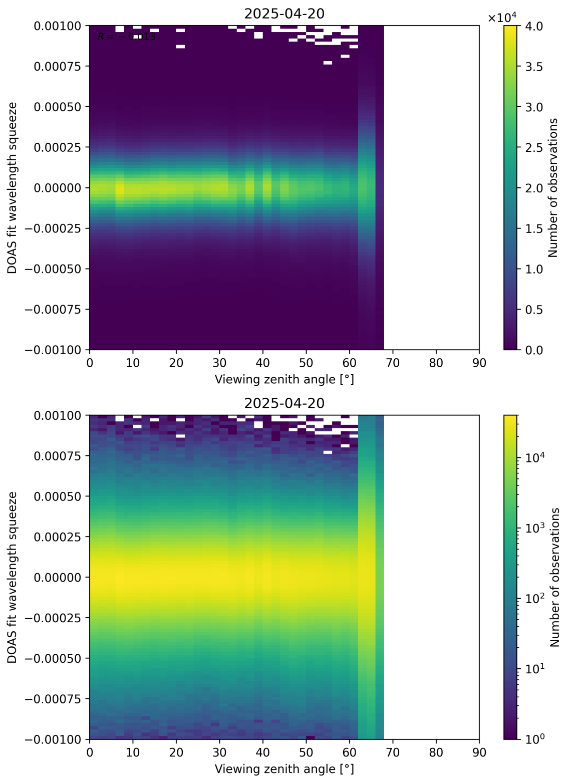
Figure 366: Scatter density plot of “Viewing zenith angle” against “DOAS fit wavelength squeeze” for 2025-04-19 to 2025-04-21.
