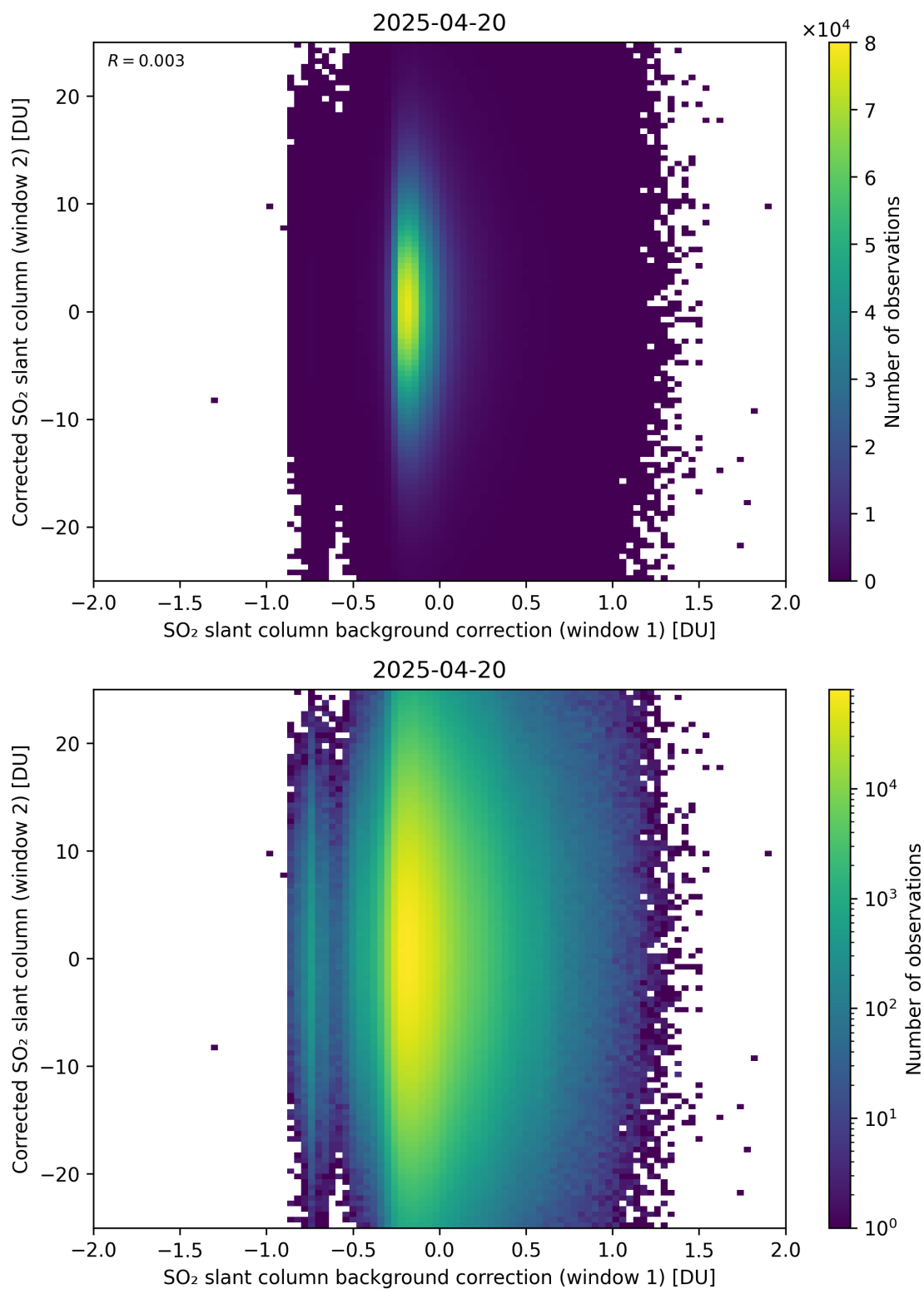
Figure 115: Scatter density plot of “SO 2 slant column background correction (window 1)” against “Corrected SO 2 slant column (window 2)” for 2025-04-19 to 2025-04-21.
