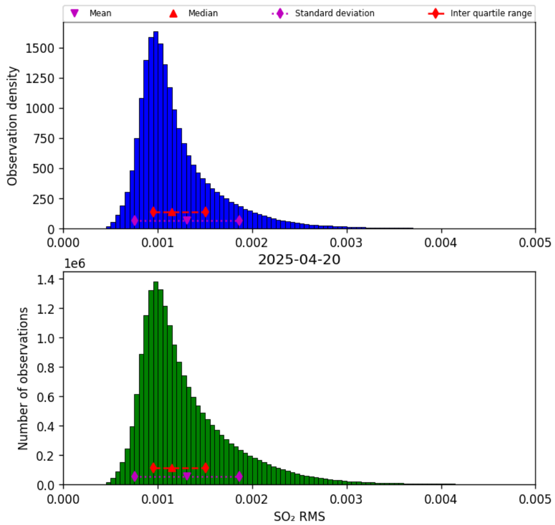
Figure 78: Histogram of “SO 2 RMS” for 2025-04-19 to 2025-04-21
