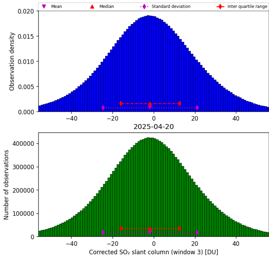
Figure 73: Histogram of “Corrected SO 2 slant column (window 3)” for 2025-04-19 to 2025-04-21
