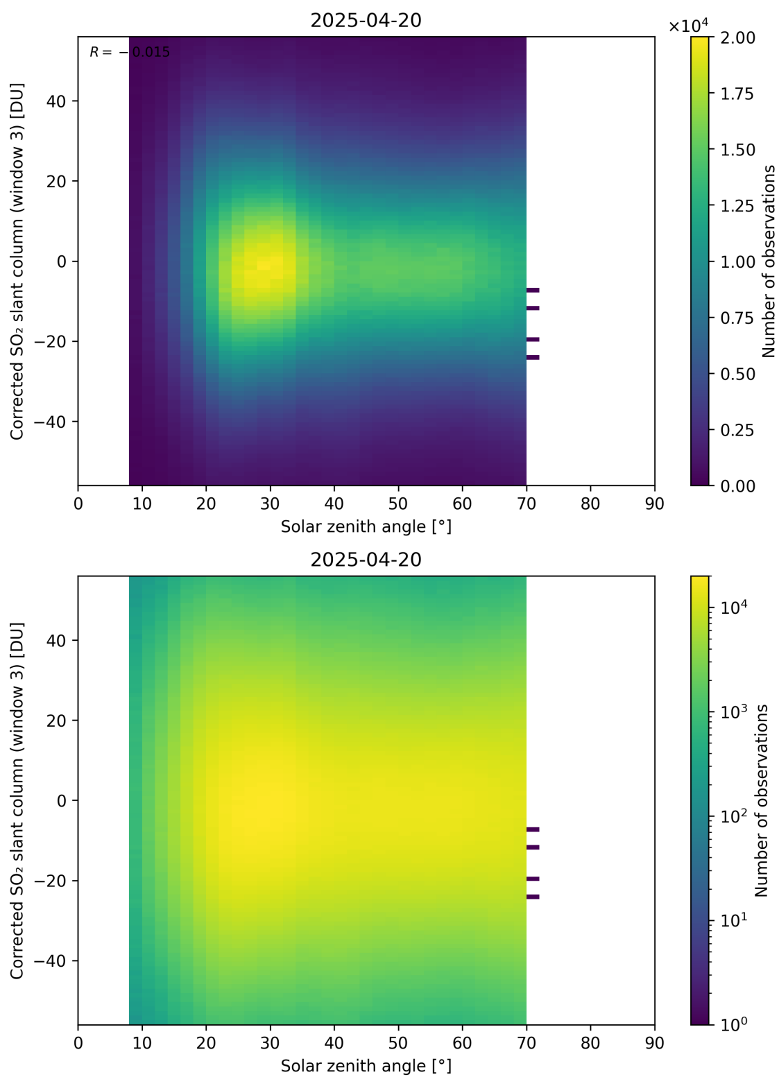
Figure 183: Scatter density plot of “Solar zenith angle” against “Corrected SO 2 slant column (window 3)” for 2025-04-19 to 2025-04-21.
