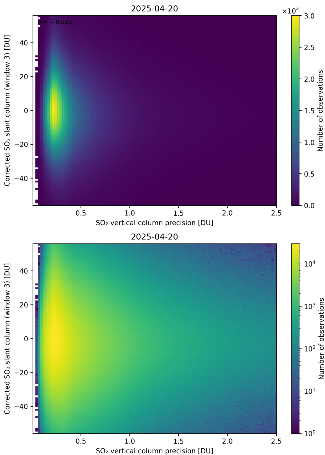
Figure 340: Scatter density plot of “SO 2 vertical column precision” against “Corrected SO 2 slant column (window 3)” for 2025-04-19 to 2025-04-21.
