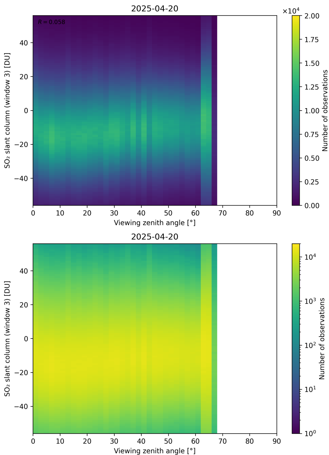
Figure 379: Scatter density plot of “Viewing zenith angle” against “SO 2 slant column (window 3)” for 2025-04-19 to 2025-04-21.
