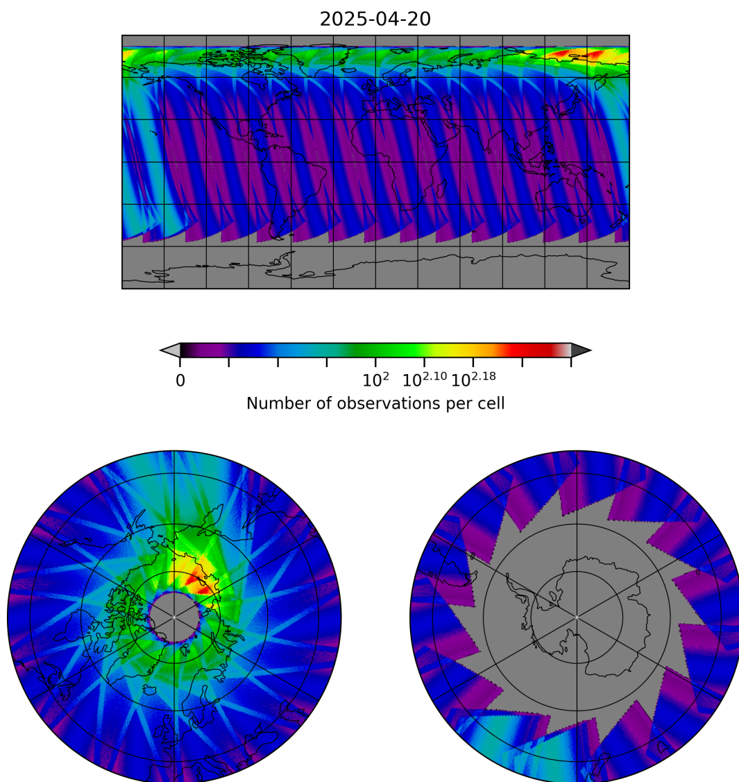
Figure 30: Map of the number of observations for 2025-04-19 to 2025-04-21
