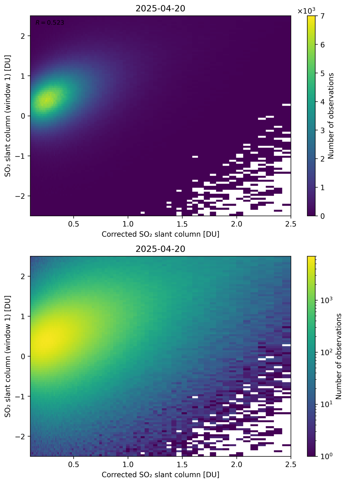
Figure 237: Scatter density plot of “Corrected SO 2 slant column” against “SO 2 slant column (window 1)” for 2025-04-19 to 2025-04-21.
