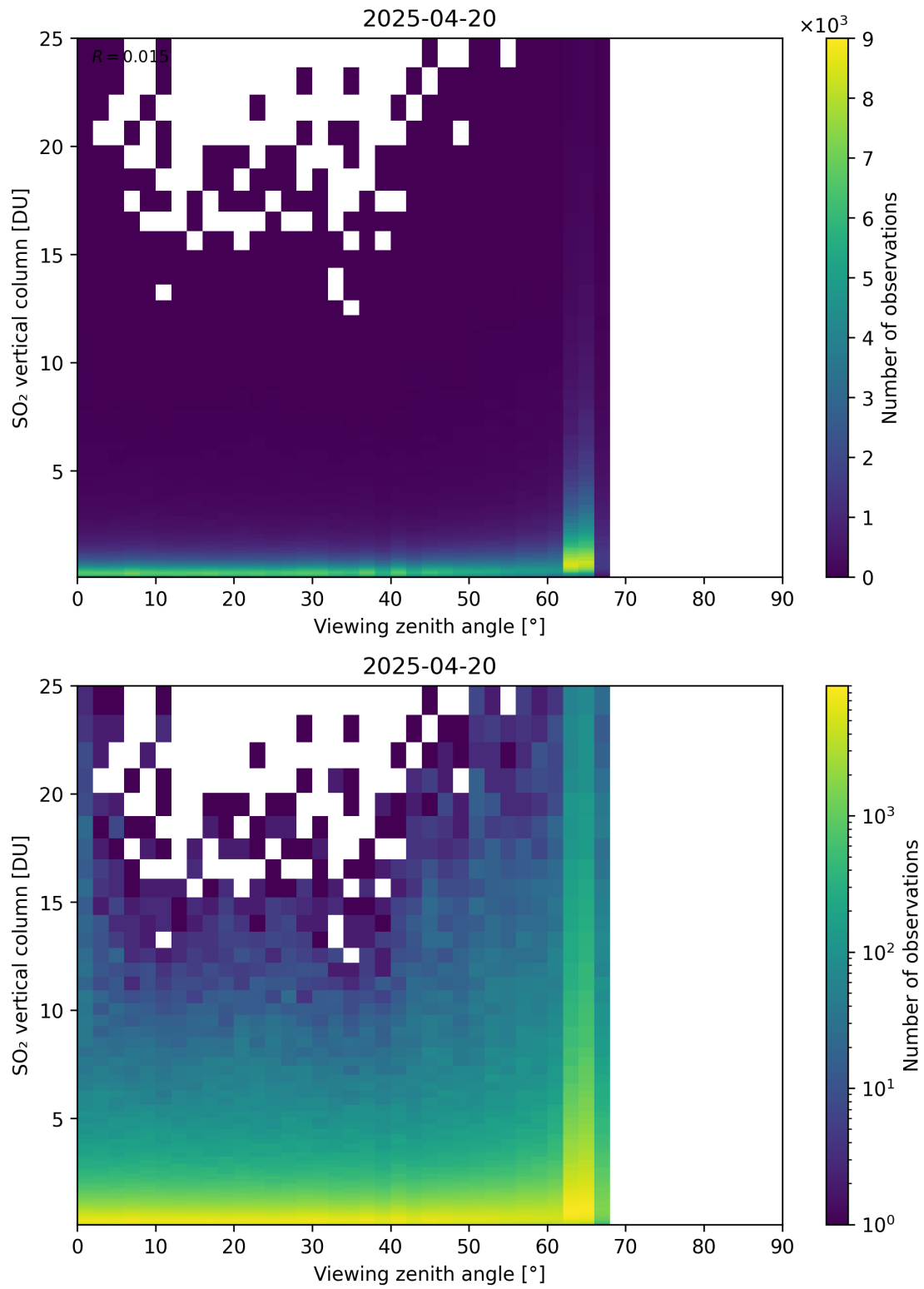
Figure 383: Scatter density plot of “Viewing zenith angle” against “SO 2 vertical column” for 2025-04-19 to 2025-04-21.
