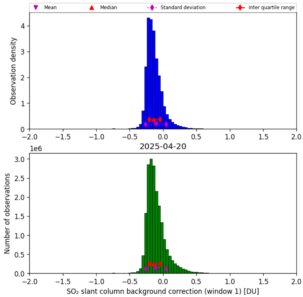
Figure 66: Histogram of “SO 2 slant column background correction (window 1)” for 2025-04-19 to 2025-04-21
