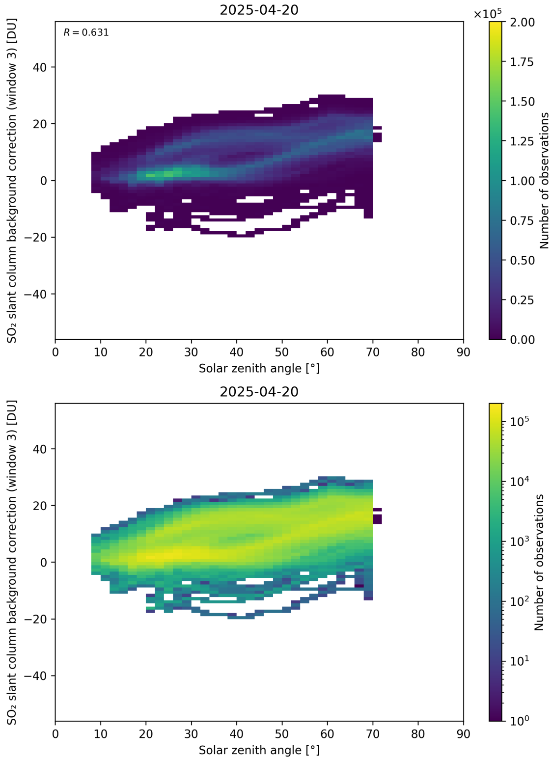
Figure 173: Scatter density plot of “Solar zenith angle” against “SO 2 slant column background correction (window 3)” for 2025-04-19 to 2025-04-21.
