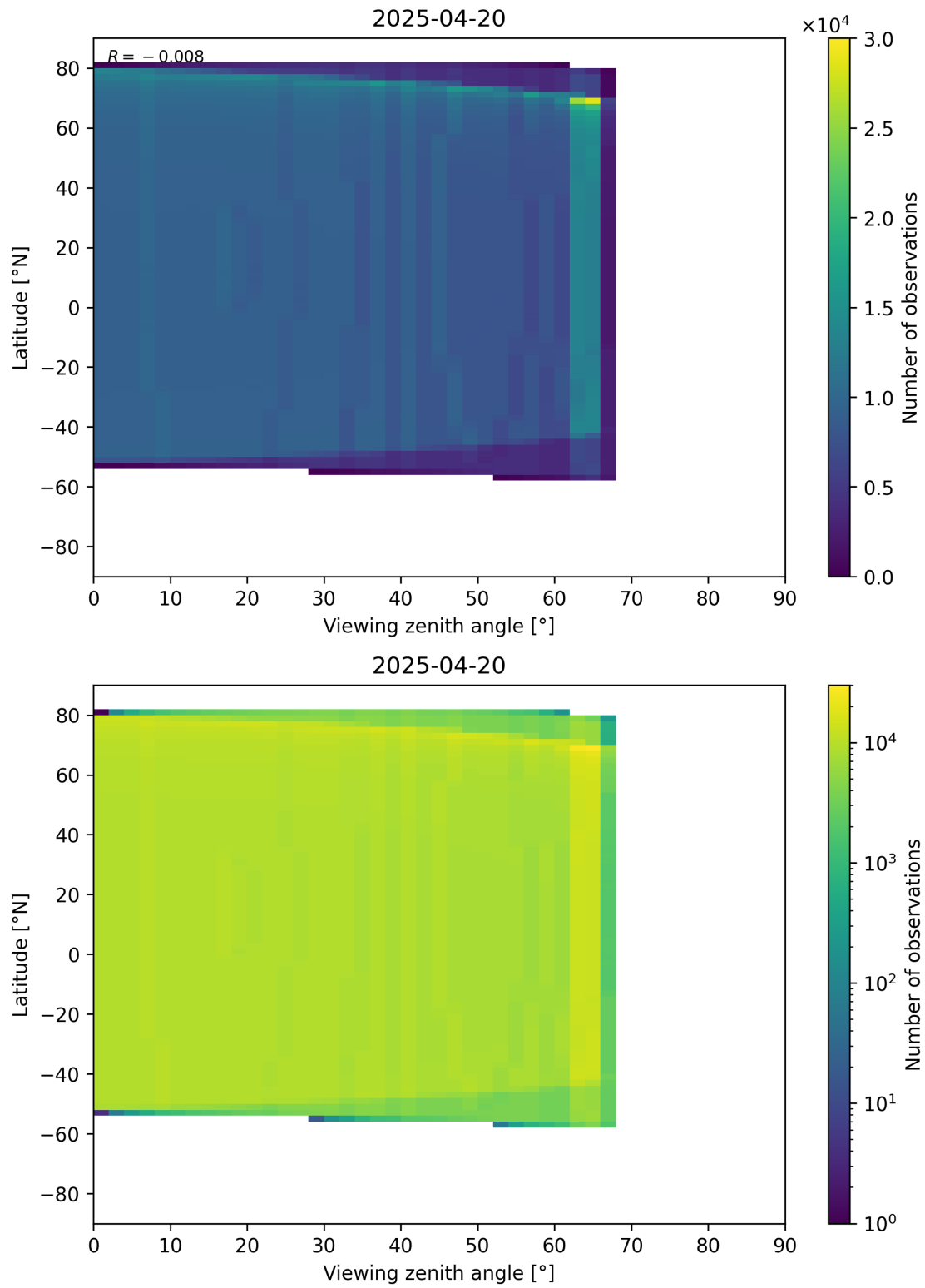
Figure 368: Scatter density plot of “Viewing zenith angle” against “Latitude” for 2025-04-19 to 2025-04-21.
