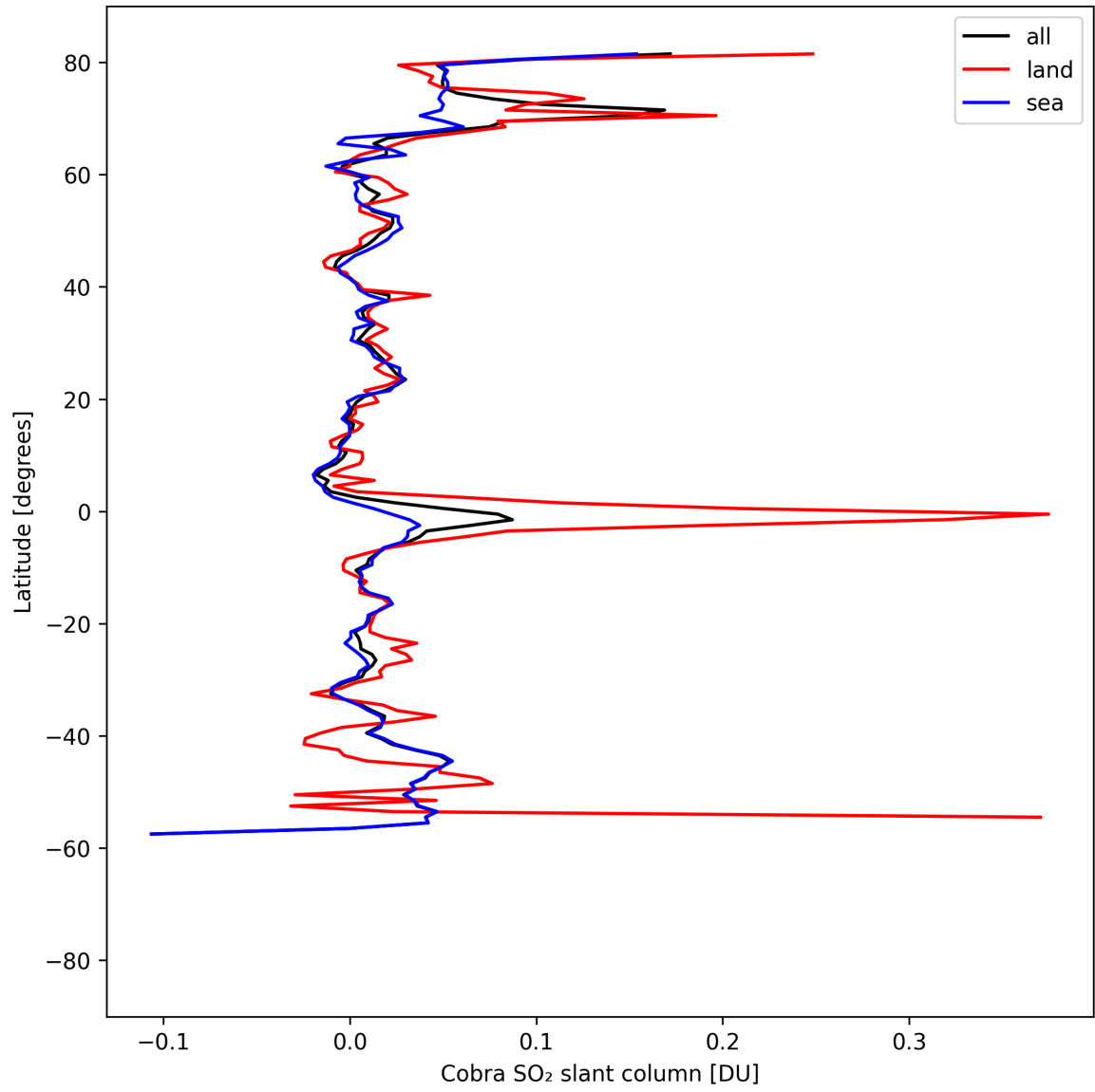
Figure 35: Zonal average of “Cobra SO 2 slant column” for 2025-04-19 to 2025-04-21.
