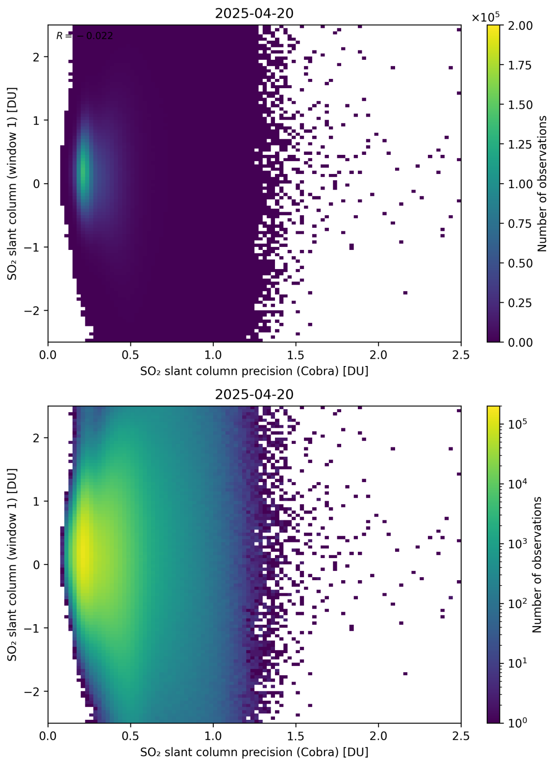
Figure 208: Scatter density plot of “SO 2 slant column precision (Cobra)” against “SO 2 slant column (window 1)” for 2025-04-19 to 2025-04-21.
