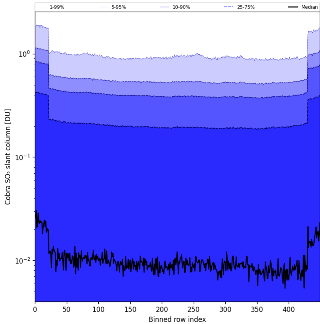
Figure 87: Along track statistics of “Cobra SO 2 slant column” for 2025-04-19 to 2025-04-21
