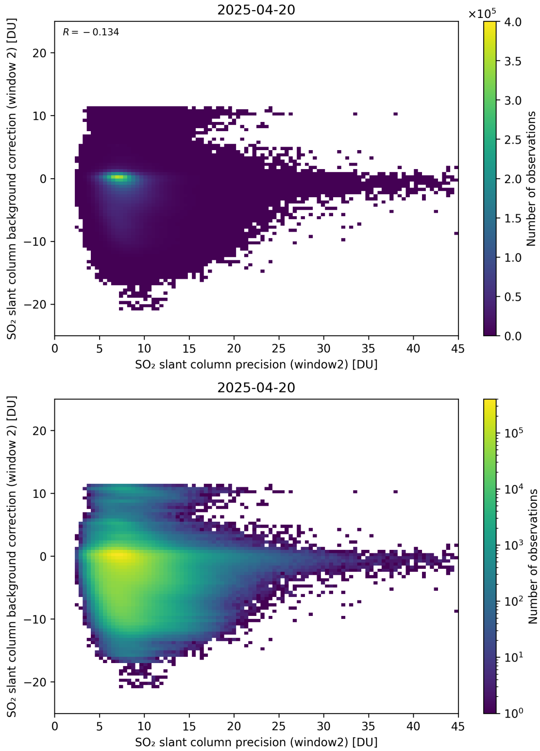
Figure 291: Scatter density plot of “SO 2 slant column precision (window2)” against “SO 2 slant column background correction (window 2)” for 2025-04-19 to 2025-04-21.
