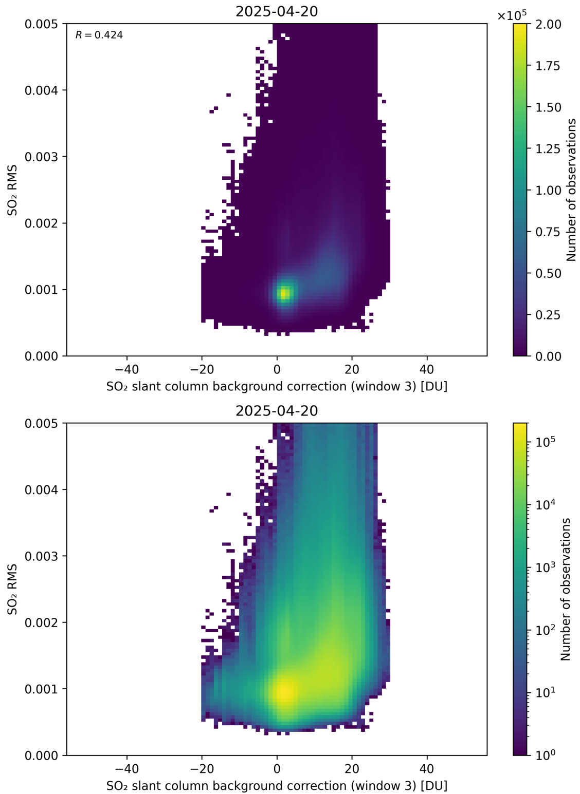
Figure 134: Scatter density plot of “SO 2 slant column background correction (window 3)” against “SO 2 RMS” for 2025-04-19 to 2025-04-21.
