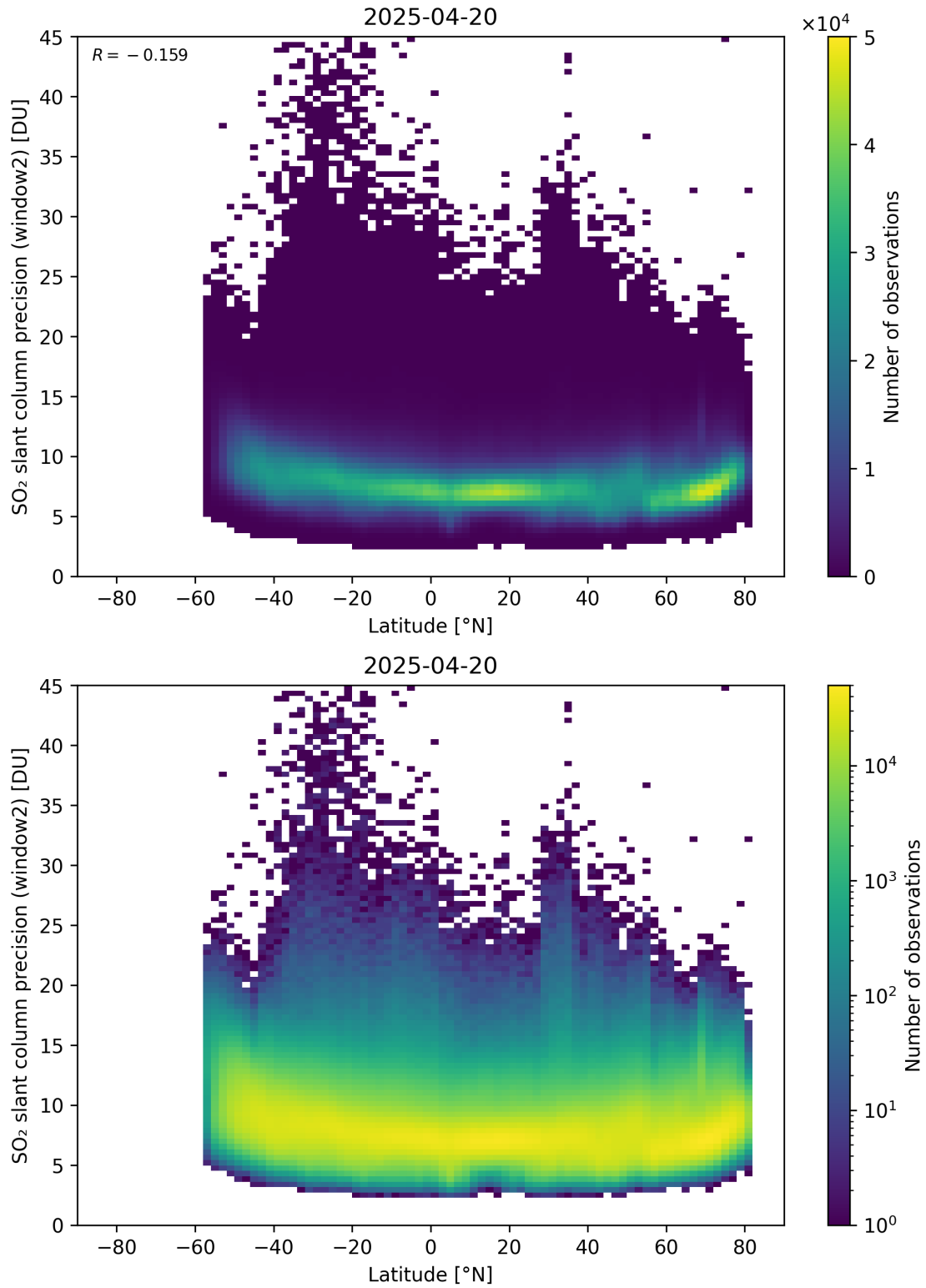
Figure 164: Scatter density plot of “Latitude” against “SO 2 slant column precision (window2)” for 2025-04-19 to 2025-04-21.
