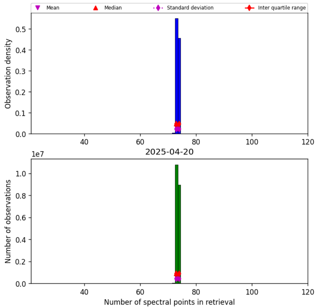
Figure 82: Histogram of “Number of spectral points in retrieval” for 2025-04-19 to 2025-04-21
