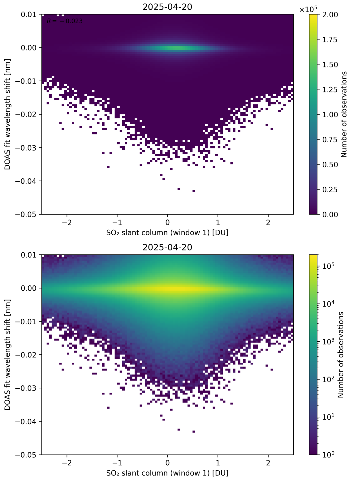
Figure 265: Scatter density plot of “SO 2 slant column (window 1)” against “DOAS fit wavelength shift” for 2025-04-19 to 2025-04-21.
