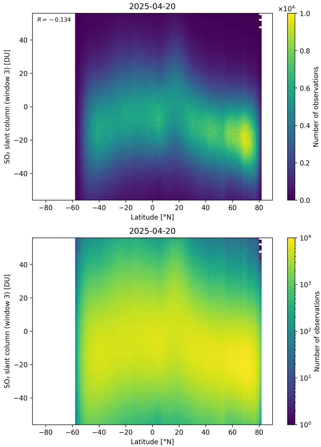
Figure 165: Scatter density plot of “Latitude” against “SO 2 slant column (window 3)” for 2025-04-19 to 2025-04-21.
