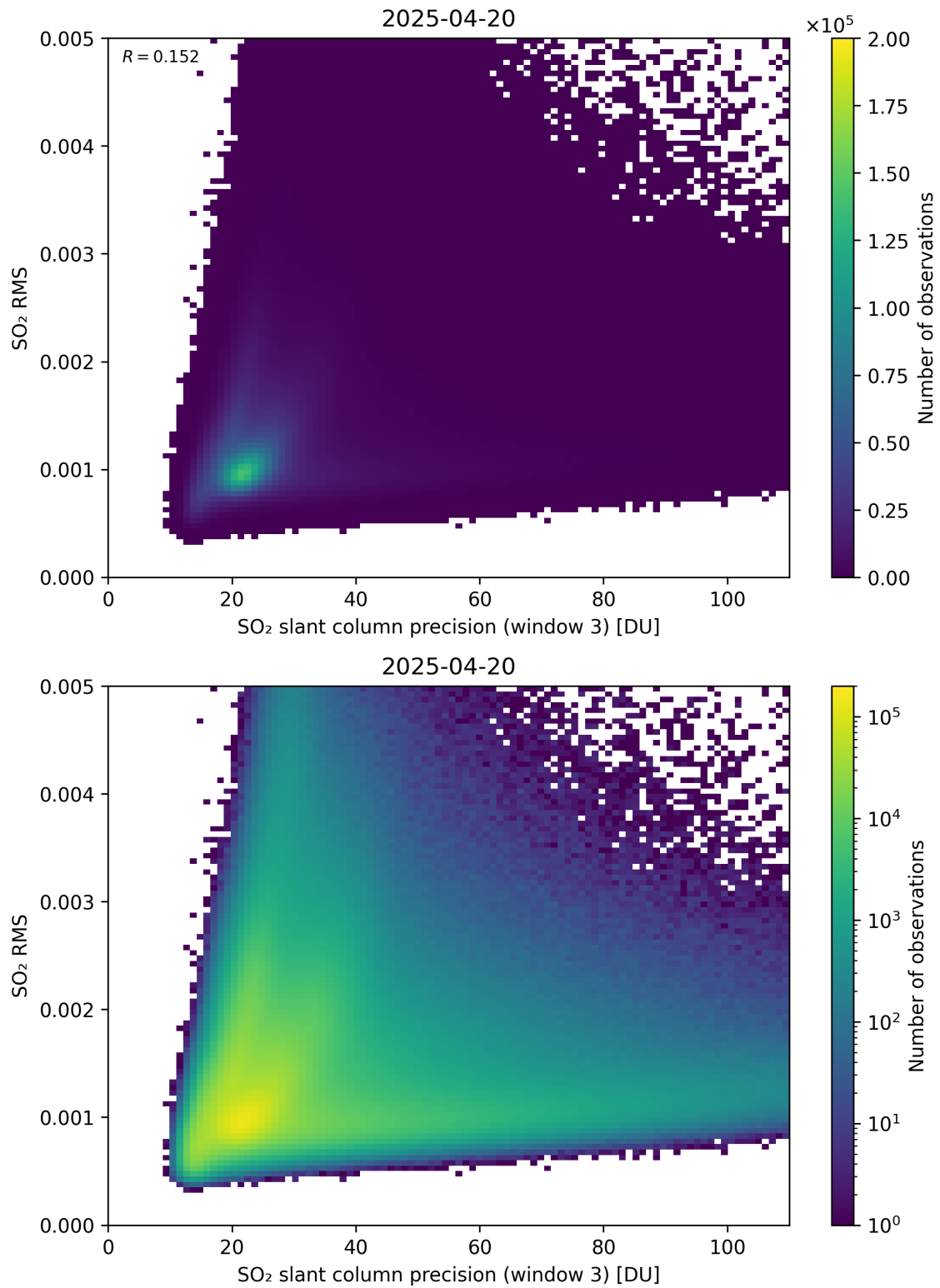
Figure 310: Scatter density plot of “SO 2 slant column precision (window 3)” against “SO 2 RMS” for 2025-04-19 to 2025-04-21.
