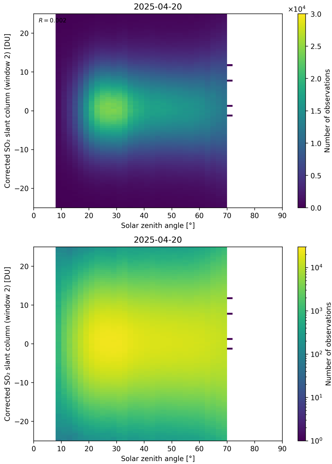
Figure 182: Scatter density plot of “Solar zenith angle” against “Corrected SO 2 slant column (window 2)” for 2025-04-19 to 2025-04-21.
