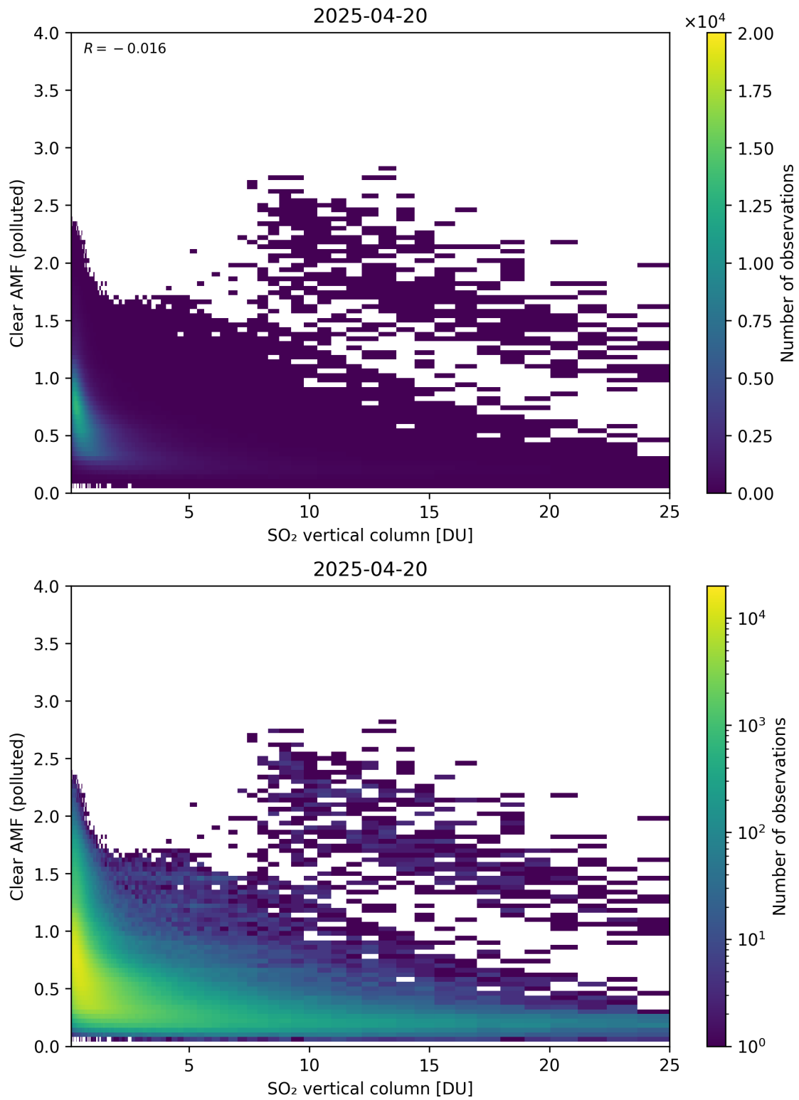
Figure 348: Scatter density plot of “SO 2 vertical column” against “Clear AMF (polluted)” for 2025-04-19 to 2025-04-21.
