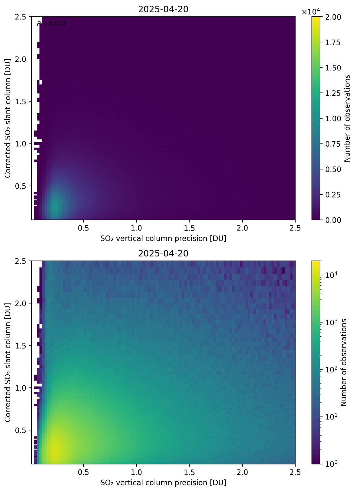
Figure 338: Scatter density plot of “SO 2 vertical column precision” against “Corrected SO 2 slant column” for 2025-04-19 to 2025-04-21.
