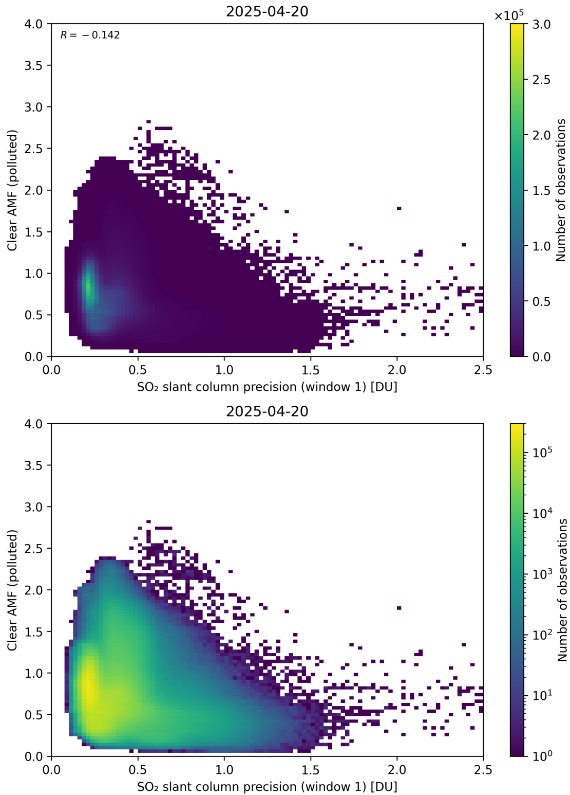
Figure 274: Scatter density plot of “SO 2 slant column precision (window 1)” against “Clear AMF (polluted)” for 2025-04-19 to 2025-04-21.
