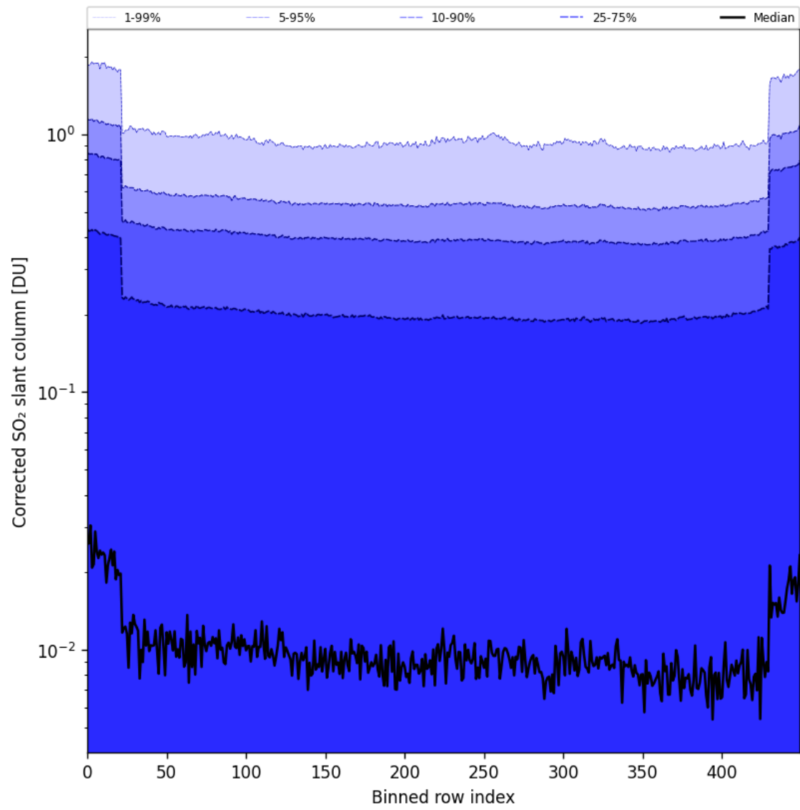
Figure 86: Along track statistics of "Corrected SO 2 slant column" for 2025-04-19 to 2025-04-21
