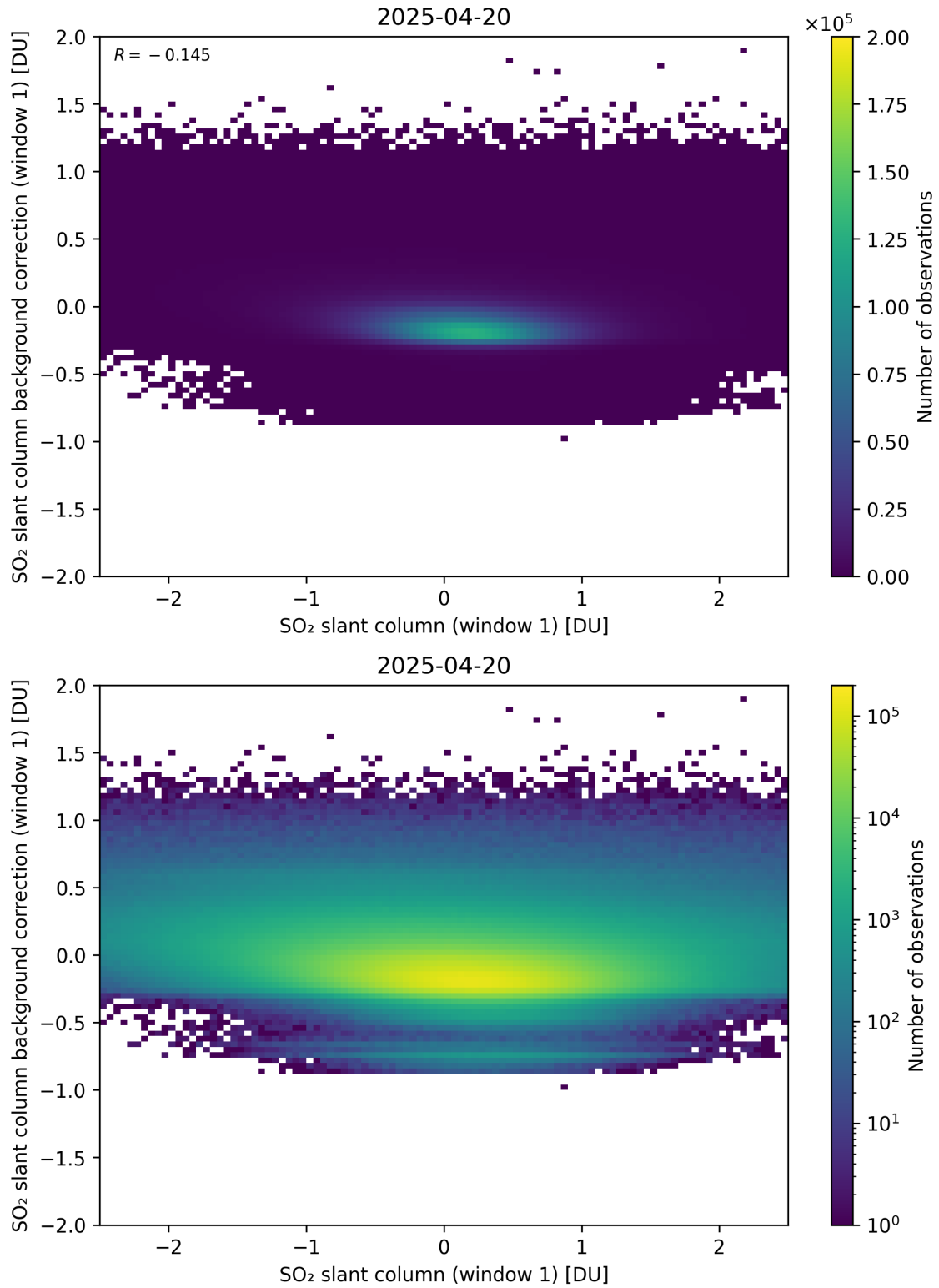
Figure 262: Scatter density plot of “SO 2 slant column (window 1)” against “SO 2 slant column background correction (window 1)” for 2025-04-19 to 2025-04-21.
