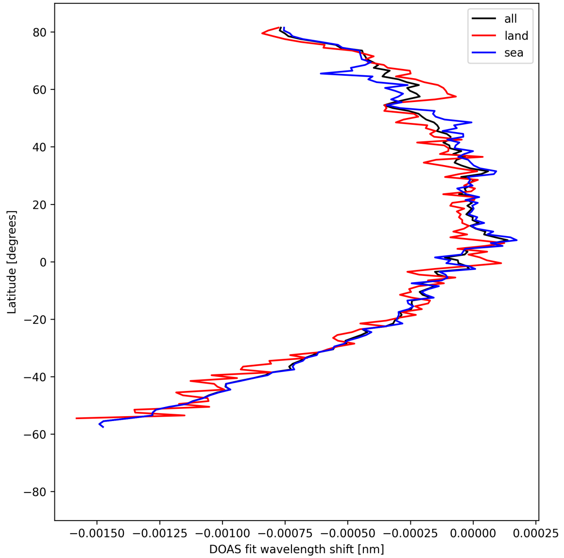
Figure 50: Zonal average of “DOAS fit wavelength shift” for 2025-04-19 to 2025-04-21.
