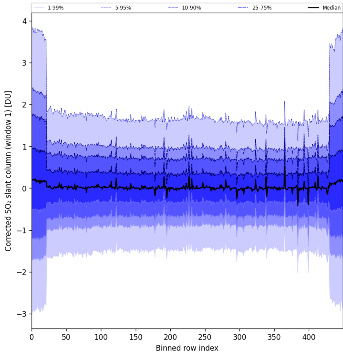
Figure 91: Along track statistics of “Corrected SO 2 slant column (window 1)” for 2025-04-19 to 2025-04-21
