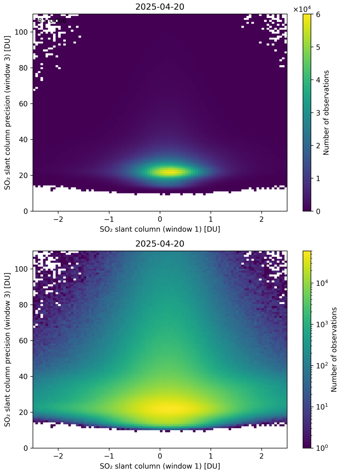
Figure 288: Scatter density plot of “SO 2 slant column (window 1)” against “SO 2 slant column precision (window 3)” for 2025-04-19 to 2025-04-21.
