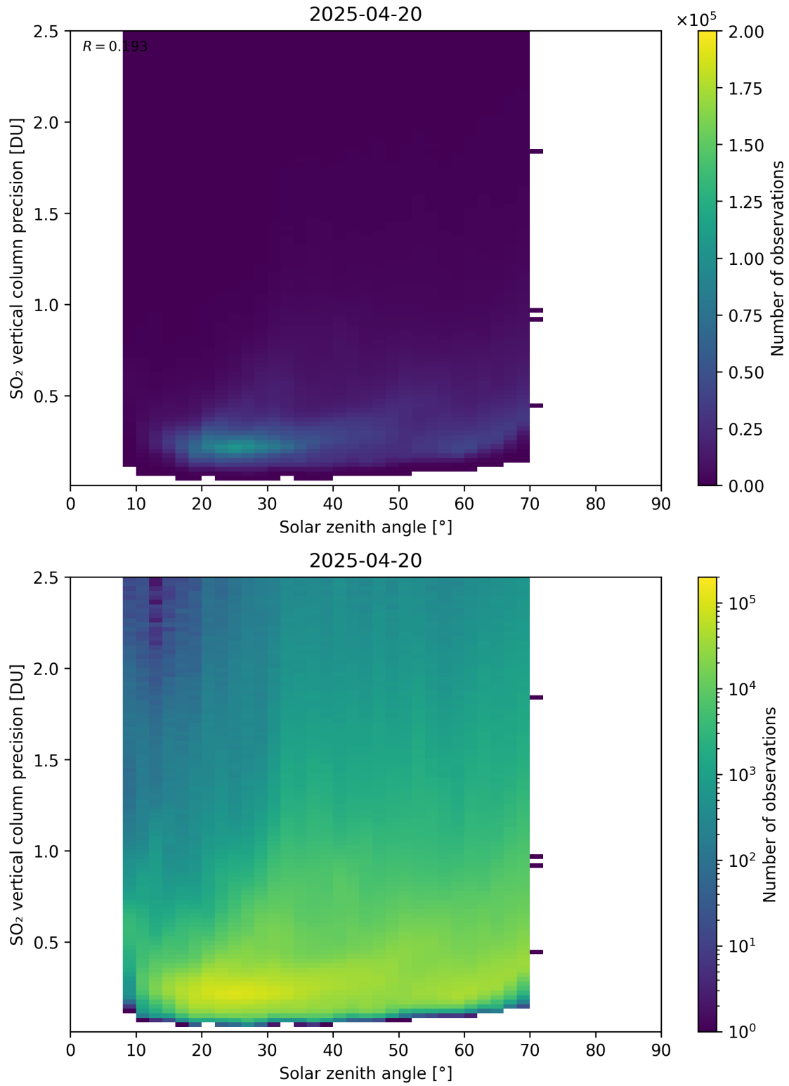
Figure 192: Scatter density plot of “Solar zenith angle” against “SO 2 vertical column precision” for 2025-04-19 to 2025-04-21.
