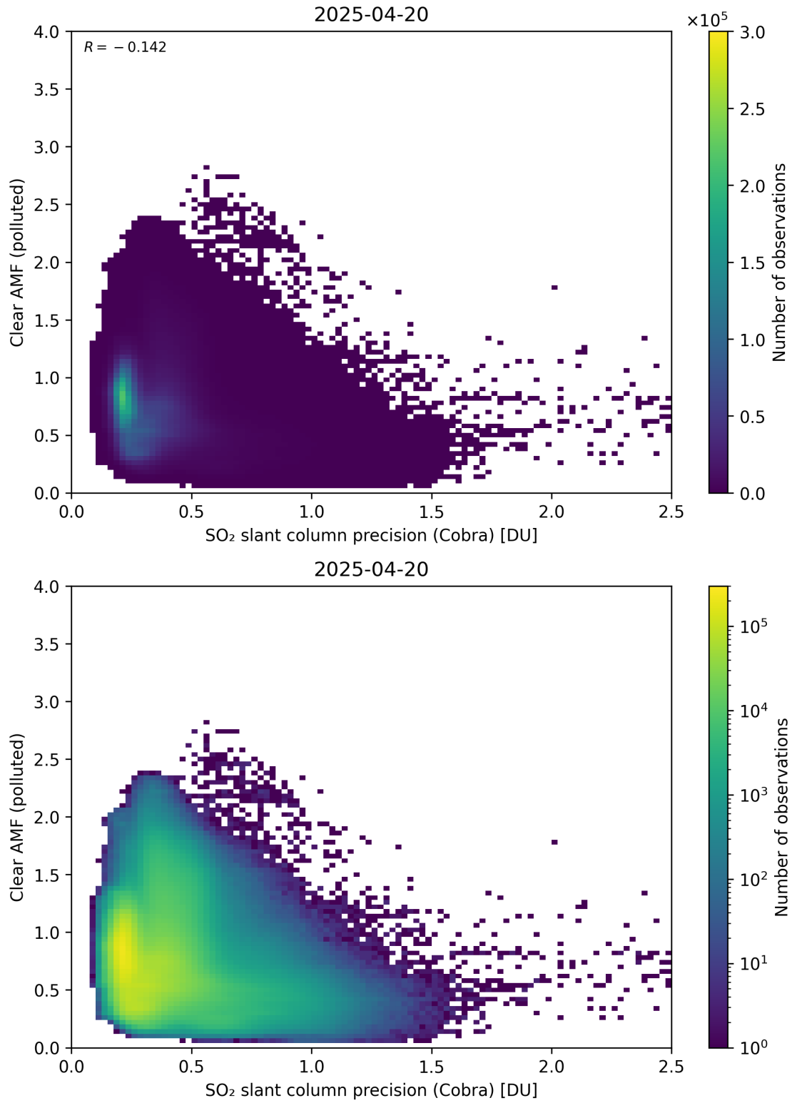
Figure 205: Scatter density plot of “SO 2 slant column precision (Cobra)” against “Clear AMF (polluted)” for 2025-04-19 to 2025-04-21.
