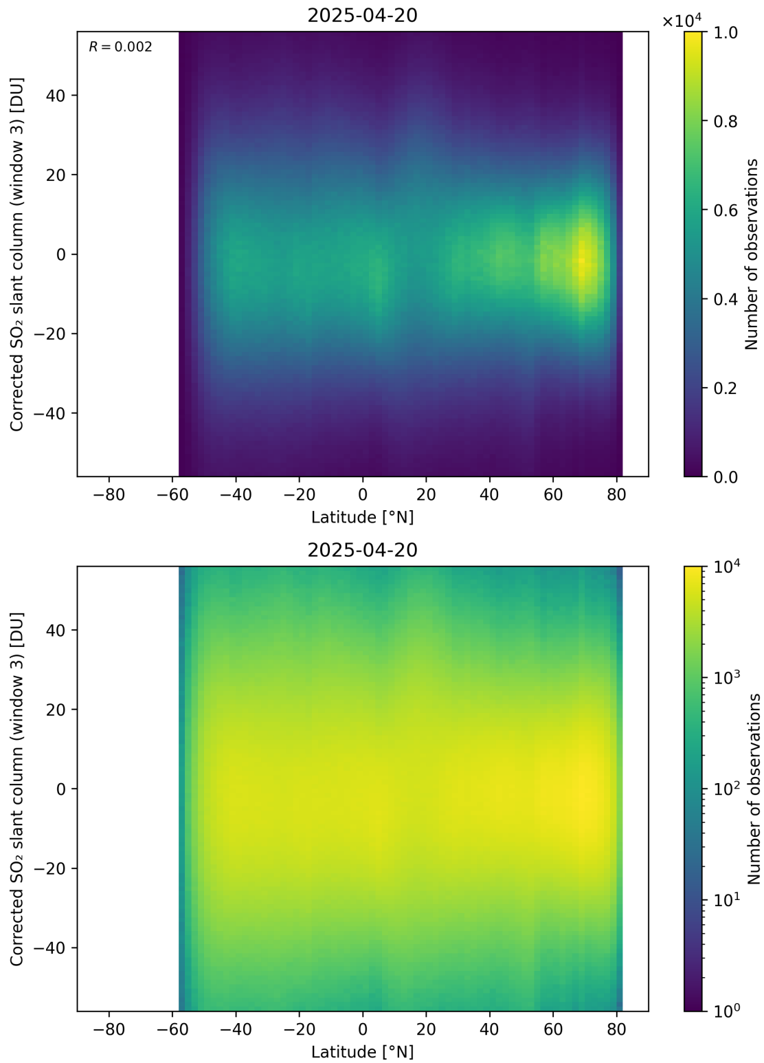
Figure 161: Scatter density plot of “Latitude” against “Corrected SO 2 slant column (window 3)” for 2025-04-19 to 2025-04-21.
