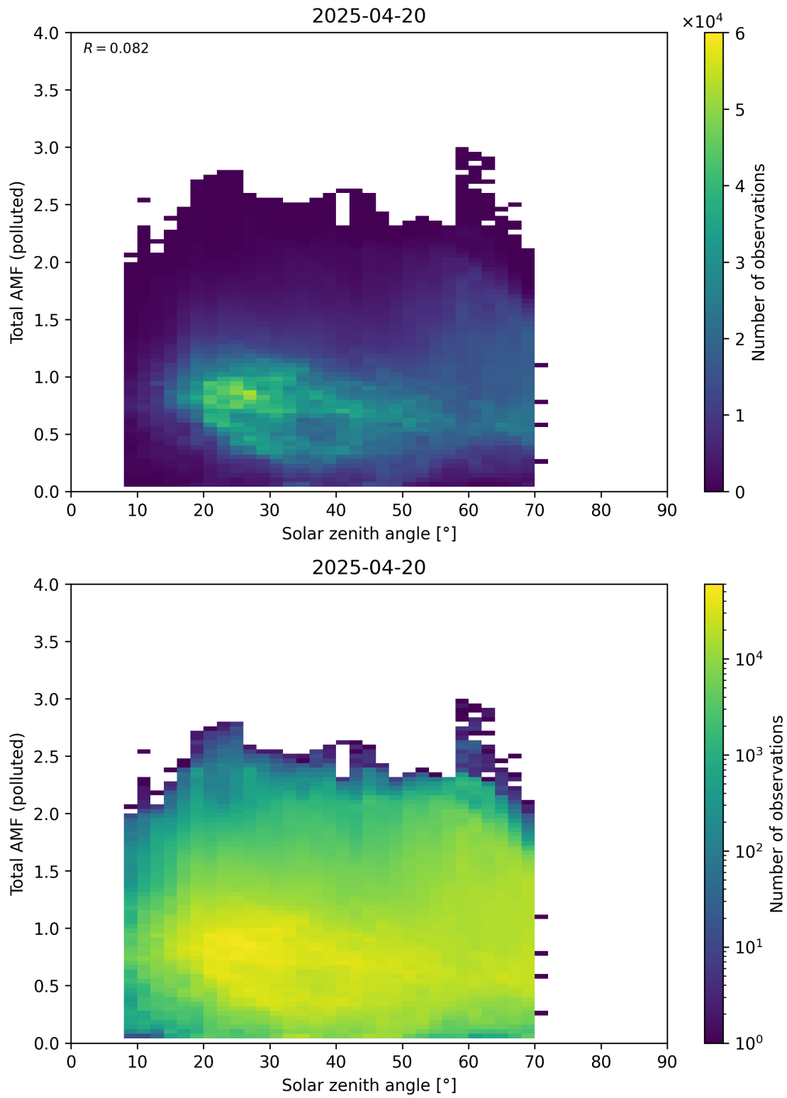
Figure 189: Scatter density plot of “Solar zenith angle” against “Total AMF (polluted)” for 2025-04-19 to 2025-04-21.
