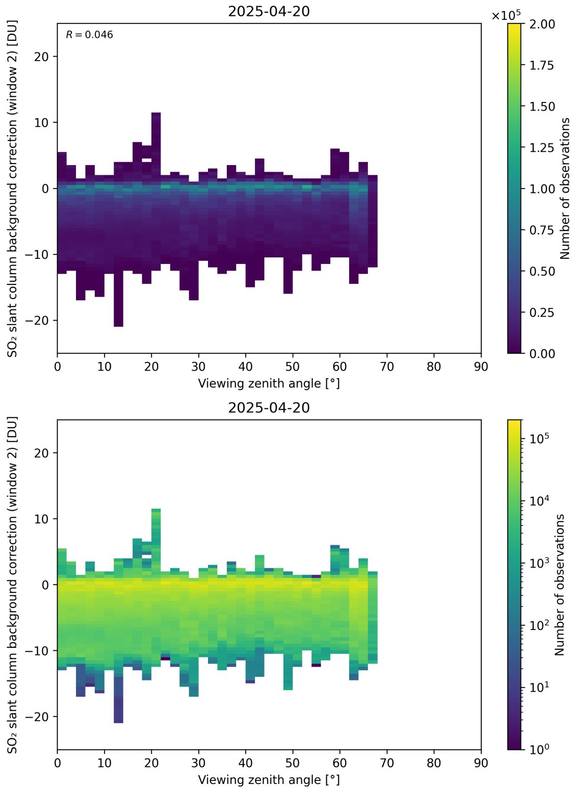
Figure 363: Scatter density plot of “Viewing zenith angle” against “SO 2 slant column background correction (window 2)” for 2025-04-19 to 2025-04-21.
