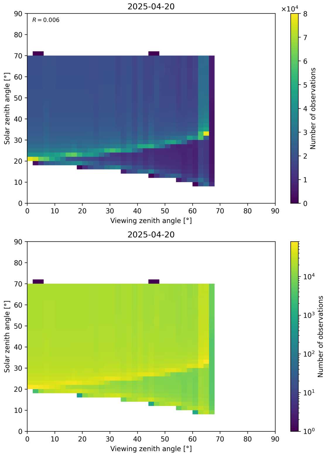
Figure 369: Scatter density plot of “Viewing zenith angle” against “Solar zenith angle” for 2025-04-19 to 2025-04-21.
