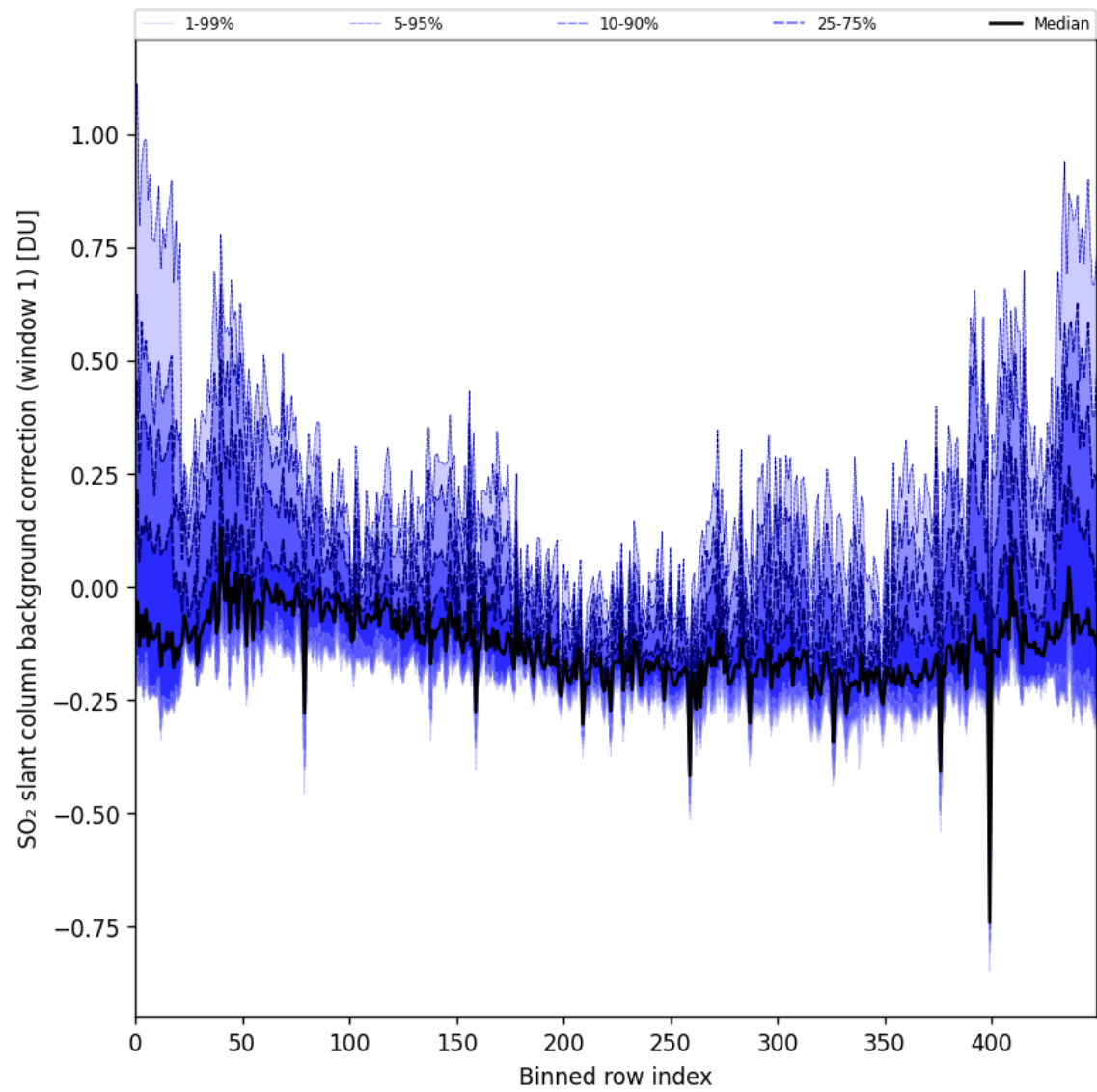
Figure 92: Along track statistics of “SO 2 slant column background correction (window 1)” for 2025-04-19 to 2025-04-21
