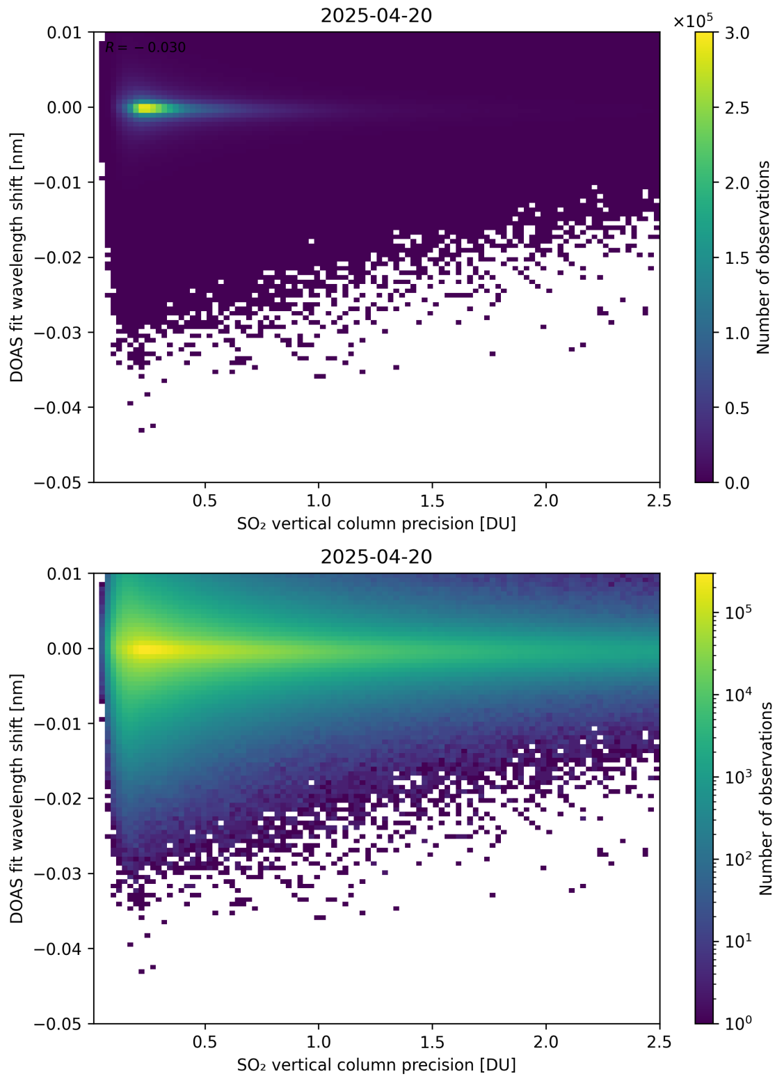
Figure 332: Scatter density plot of “SO 2 vertical column precision” against “DOAS fit wavelength shift” for 2025-04-19 to 2025-04-21.
