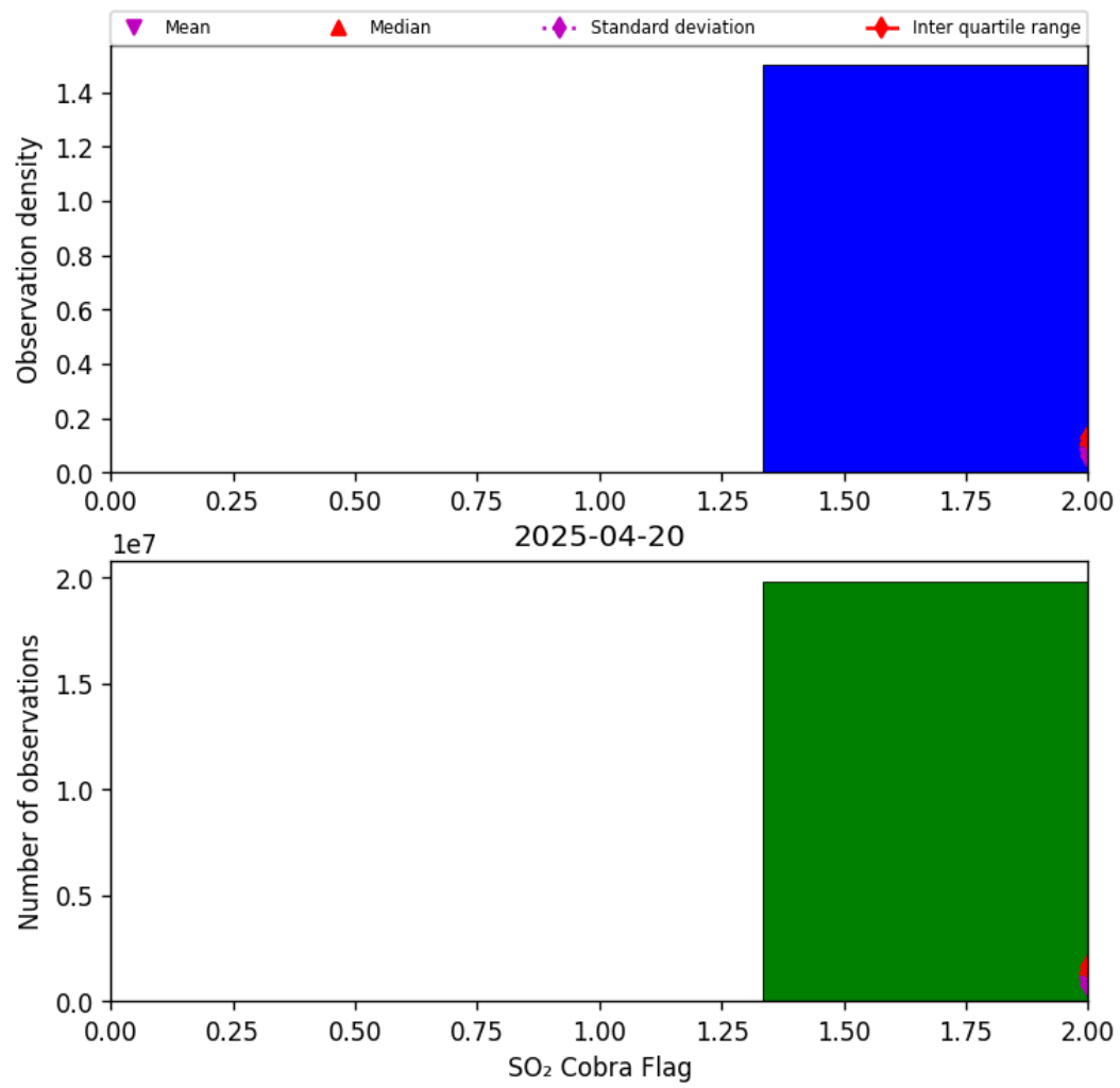
Figure 75: Histogram of “SO 2 Cobra Flag” for 2025-04-19 to 2025-04-21
