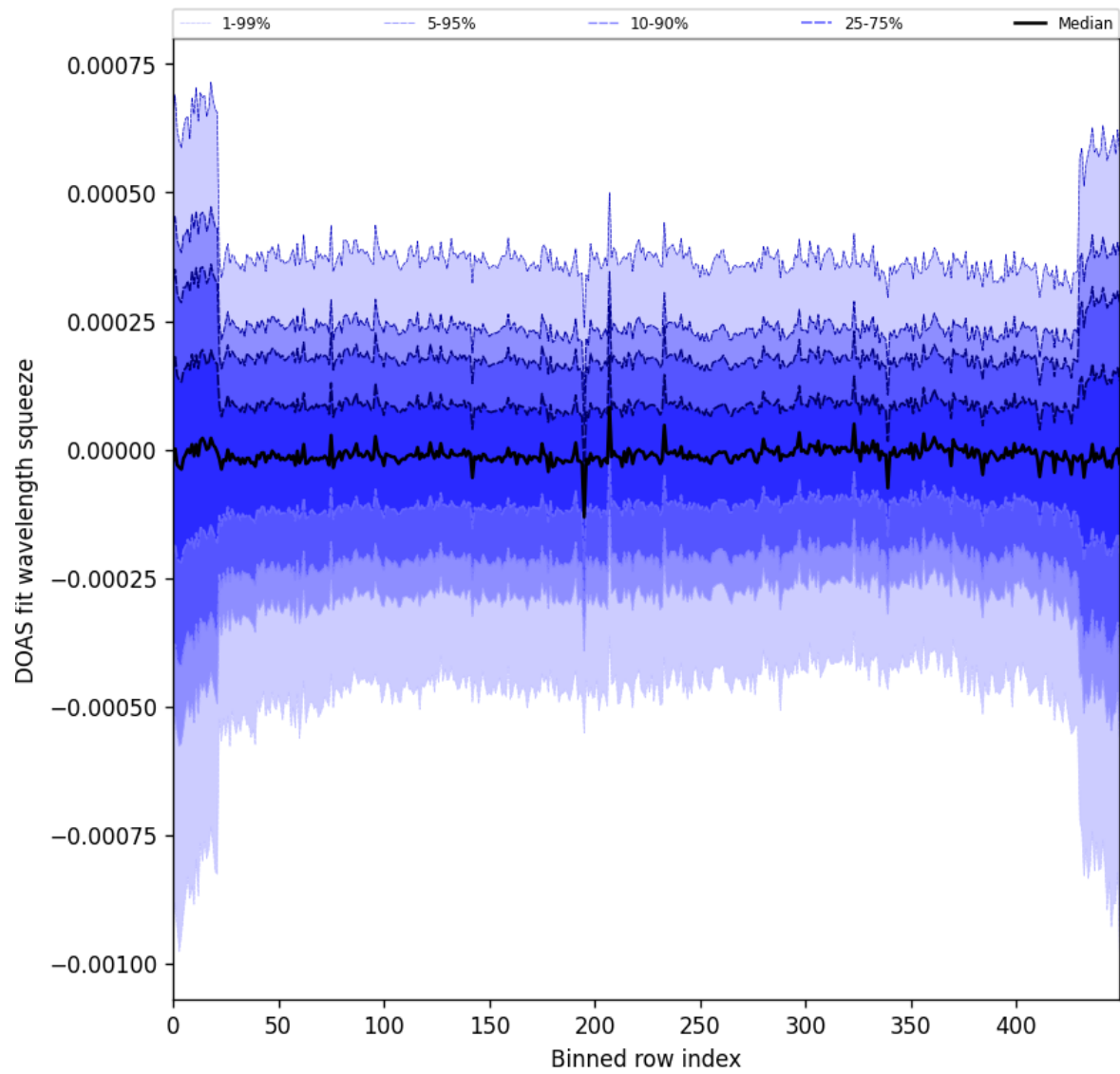
Figure 103: Along track statistics of “DOAS fit wavelength squeeze” for 2025-04-19 to 2025-04-21
