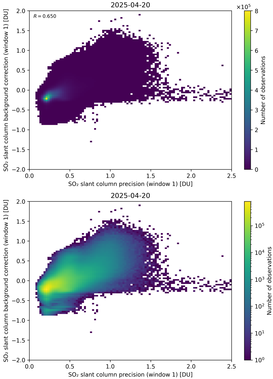
Figure 268: Scatter density plot of “SO 2 slant column precision (window 1)” against “SO 2 slant column background correction (window 1)” for 2025-04-19 to 2025-04-21.
