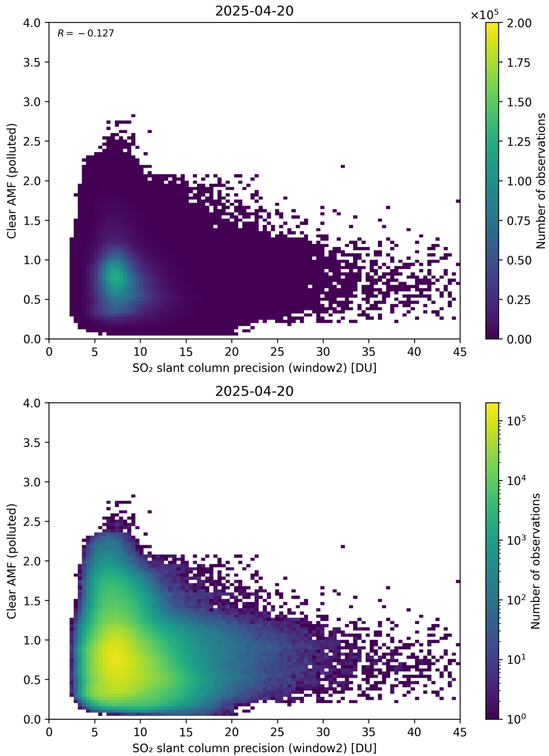
Figure 296: Scatter density plot of “SO 2 slant column precision (window2)” against “Clear AMF (polluted)” for 2025-04-19 to 2025-04-21.
