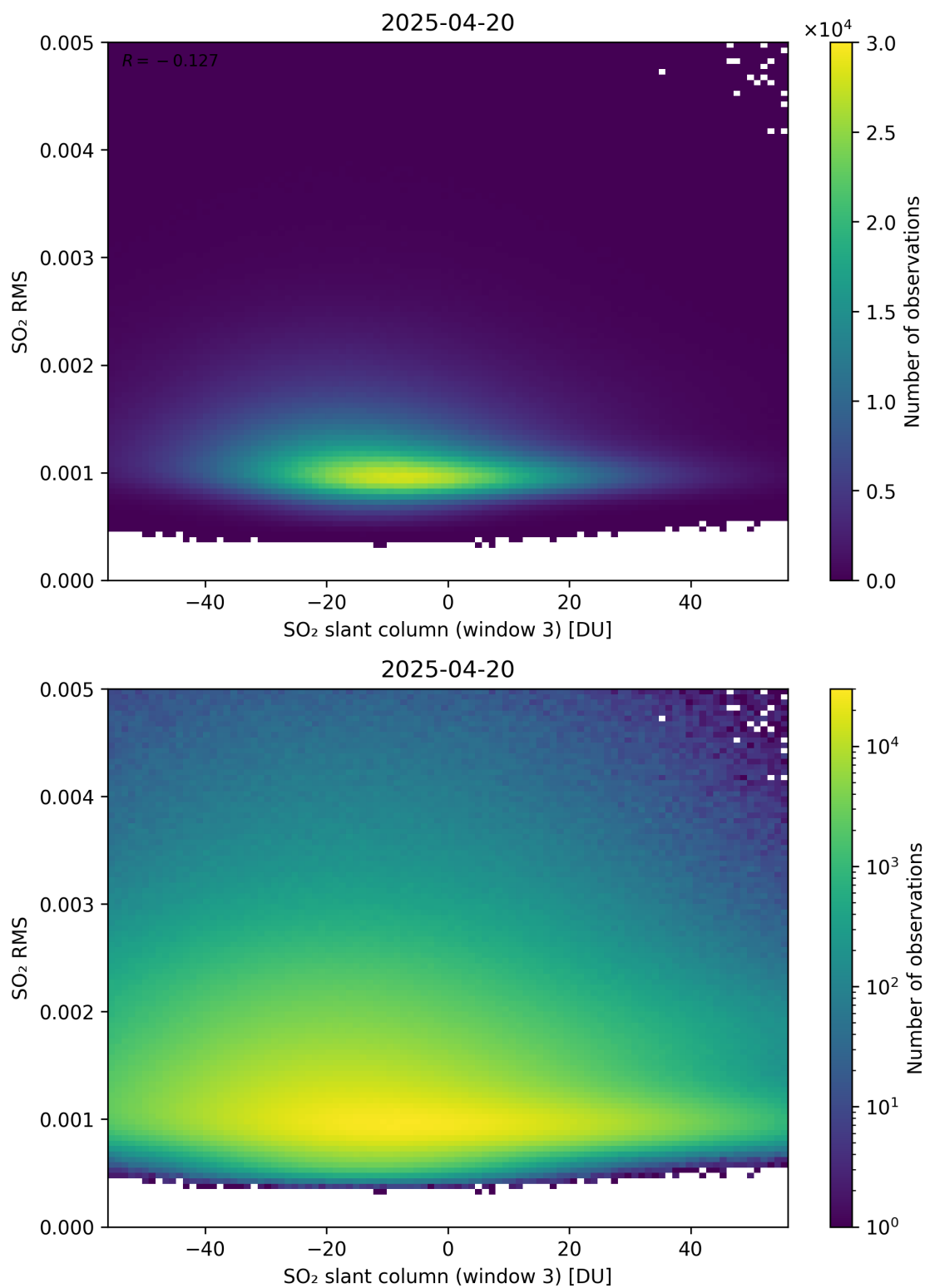
Figure 306: Scatter density plot of “SO 2 slant column (window 3)” against “SO 2 RMS” for 2025-04-19 to 2025-04-21.
