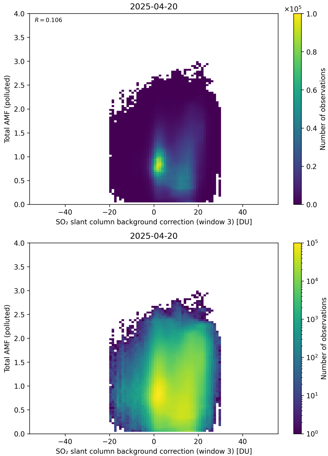
Figure 136: Scatter density plot of “SO 2 slant column background correction (window 3)” against “Total AMF (polluted)” for 2025-04-19 to 2025-04-21.
