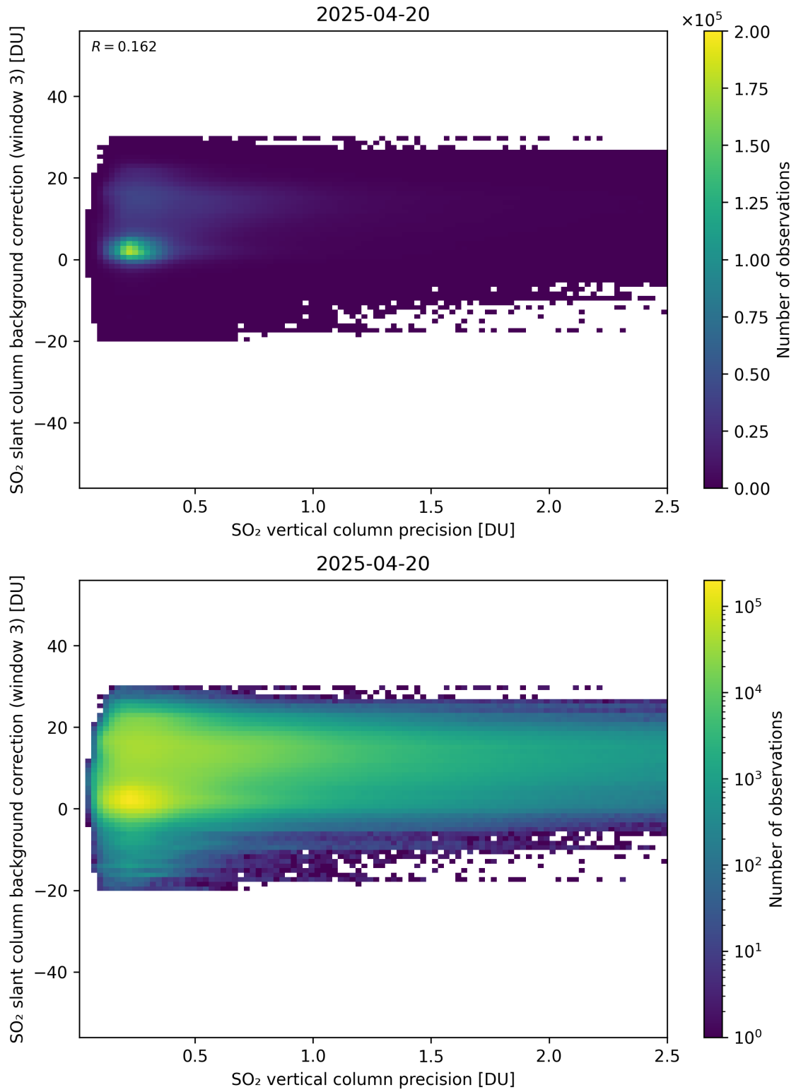
Figure 331: Scatter density plot of “SO 2 vertical column precision” against “SO 2 slant column background correction (window 3)” for 2025-04-19 to 2025-04-21.
