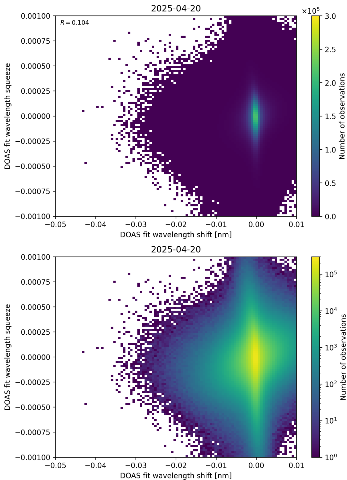
Figure 138: Scatter density plot of “DOAS fit wavelength shift” against “DOAS fit wavelength squeeze” for 2025-04-19 to 2025-04-21.
