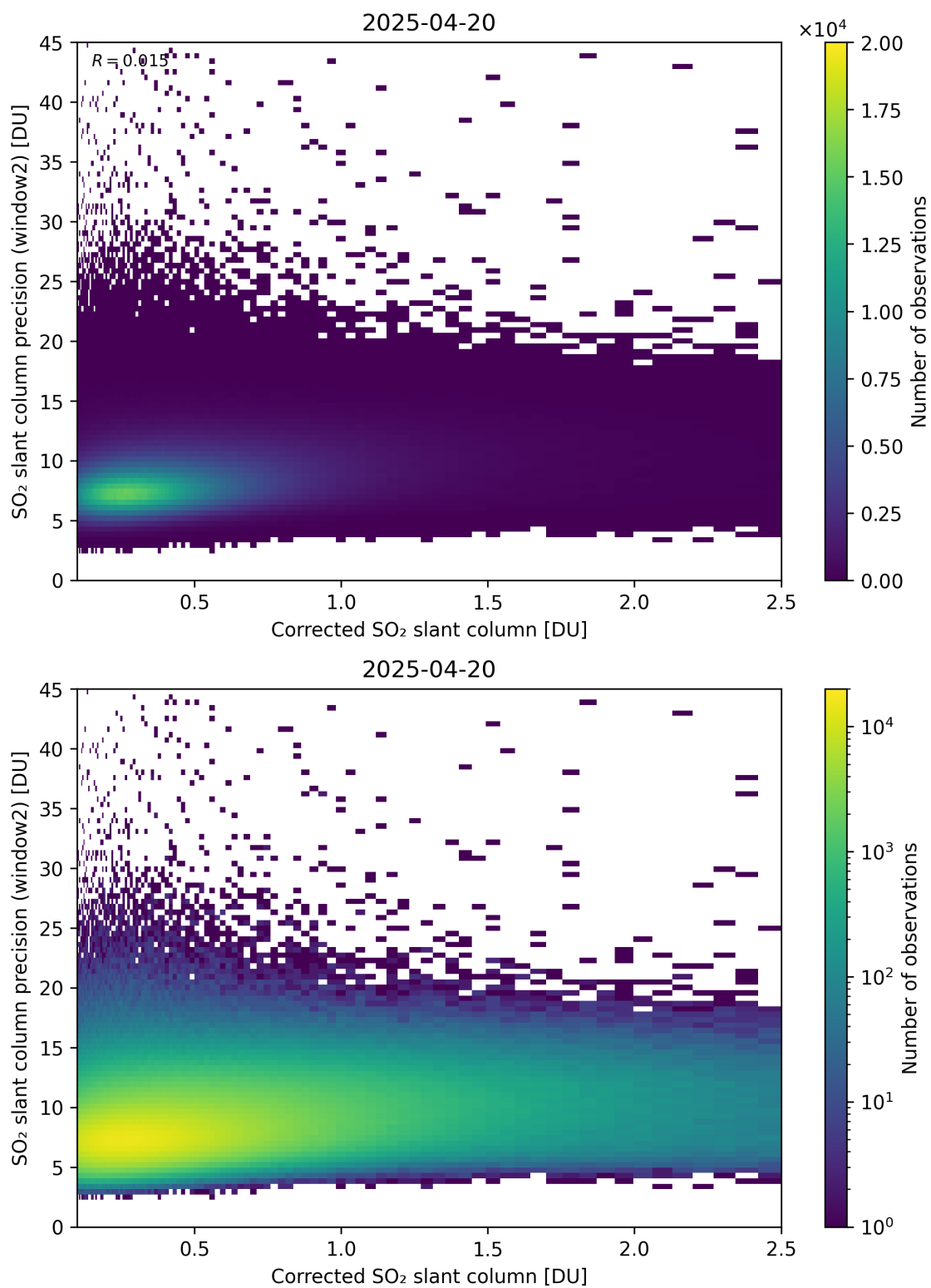
Figure 239: Scatter density plot of “Corrected SO 2 slant column” against “SO 2 slant column precision (window2)” for 2025-04-19 to 2025-04-21.
