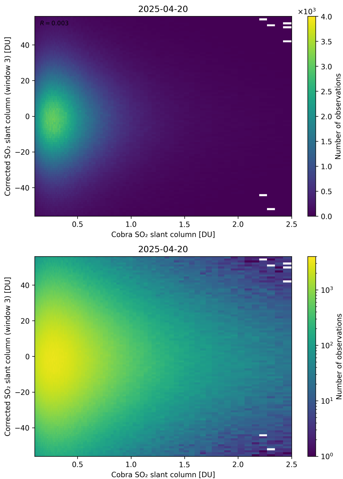
Figure 218: Scatter density plot of “Cobra SO 2 slant column” against “Corrected SO 2 slant column (window 3)” for 2025-04-19 to 2025-04-21.
