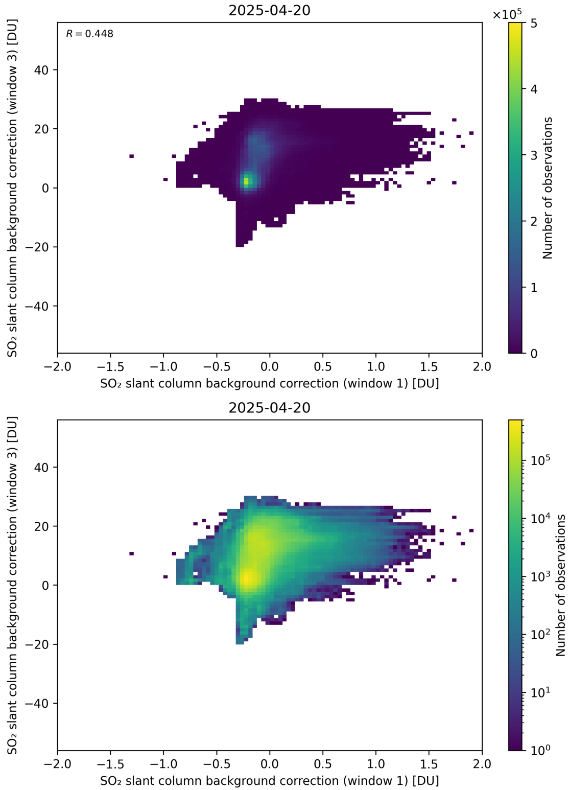
Figure 110: Scatter density plot of “SO 2 slant column background correction (window 1)” against “SO 2 slant column background correction (window 3)” for 2025-04-19 to 2025-04-21.
