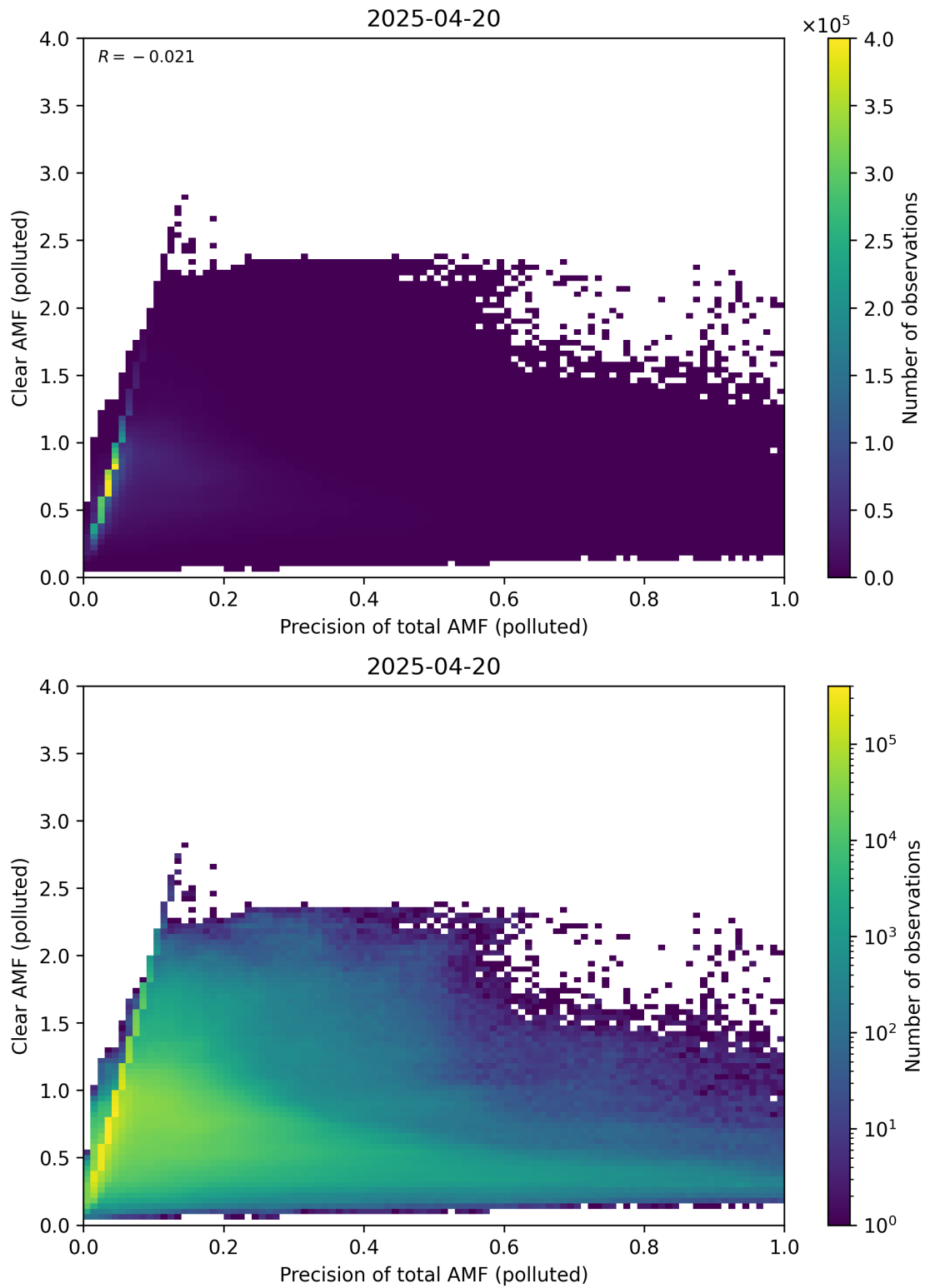
Figure 320: Scatter density plot of “Precision of total AMF (polluted)” against “Clear AMF (polluted)” for 2025-04-19 to 2025-04-21.
