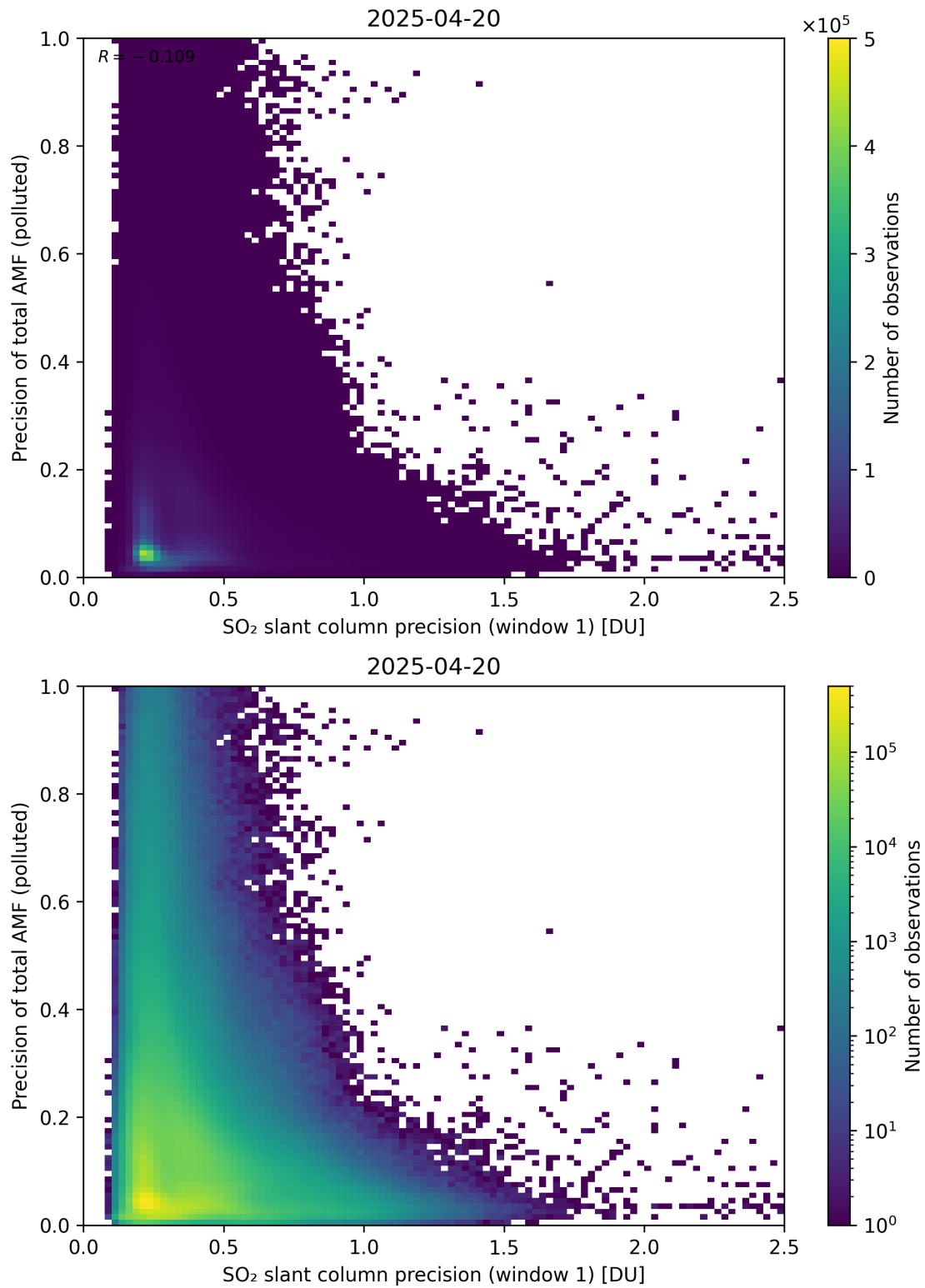
Figure 281: Scatter density plot of “SO 2 slant column precision (window 1)” against “Precision of total AMF (polluted)” for 2025-04-19 to 2025-04-21.
