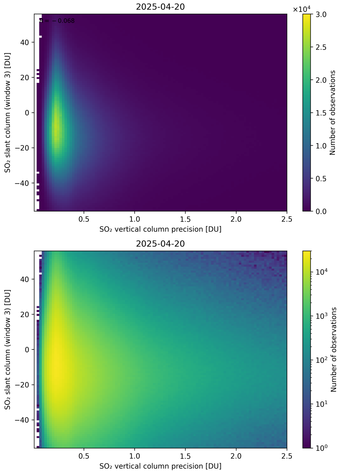
Figure 344: Scatter density plot of “SO 2 vertical column precision” against “SO 2 slant column (window 3)” for 2025-04-19 to 2025-04-21.
