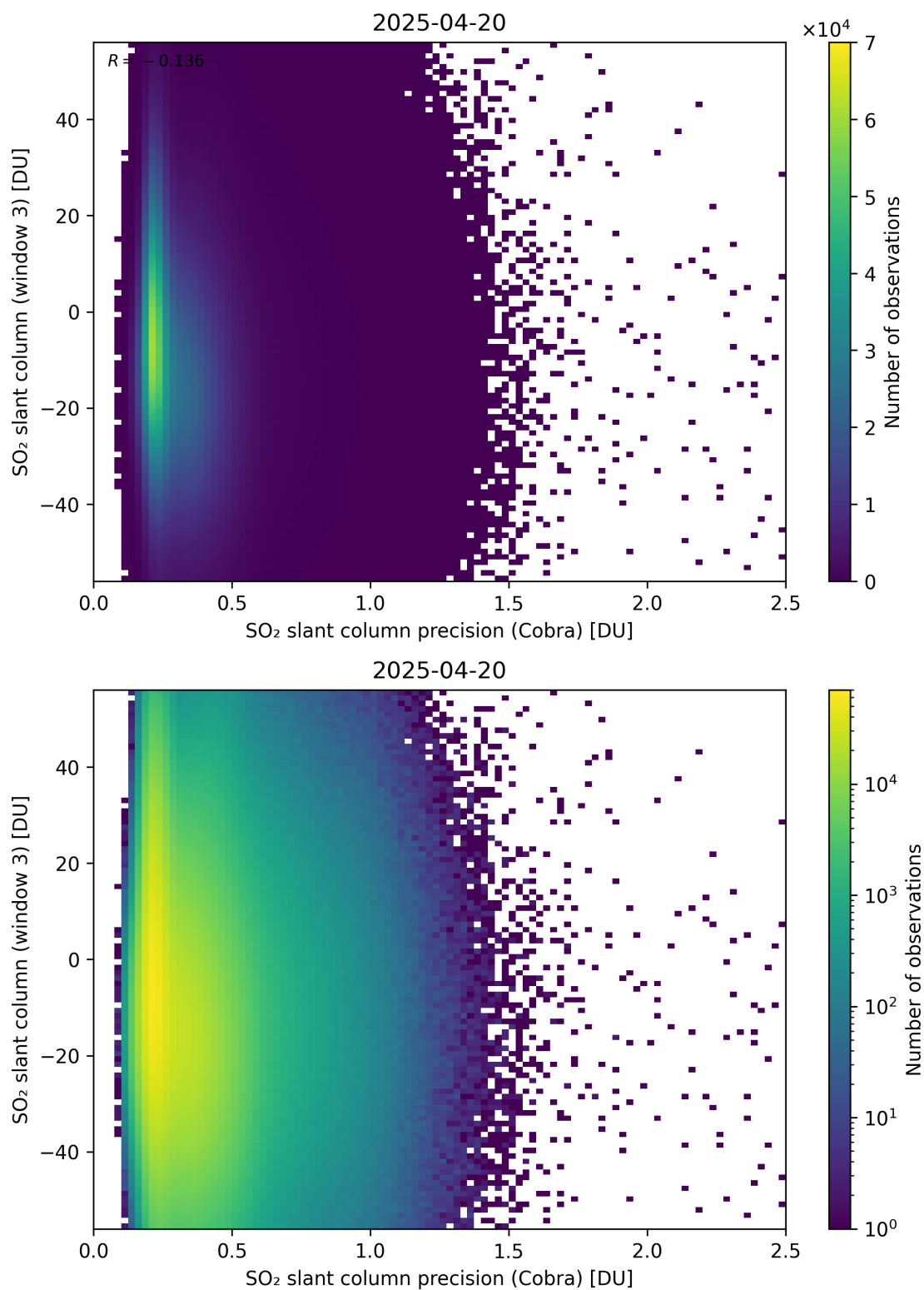
Figure 211: Scatter density plot of “SO 2 slant column precision (Cobra)” against “SO 2 slant column (window 3)” for 2025-04-19 to 2025-04-21.
