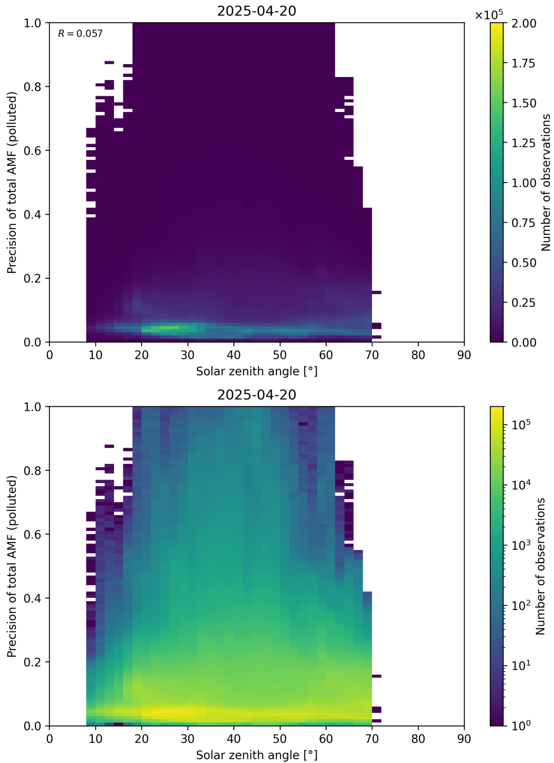
Figure 190: Scatter density plot of “Solar zenith angle” against “Precision of total AMF (polluted)” for 2025-04-19 to 2025-04-21.
