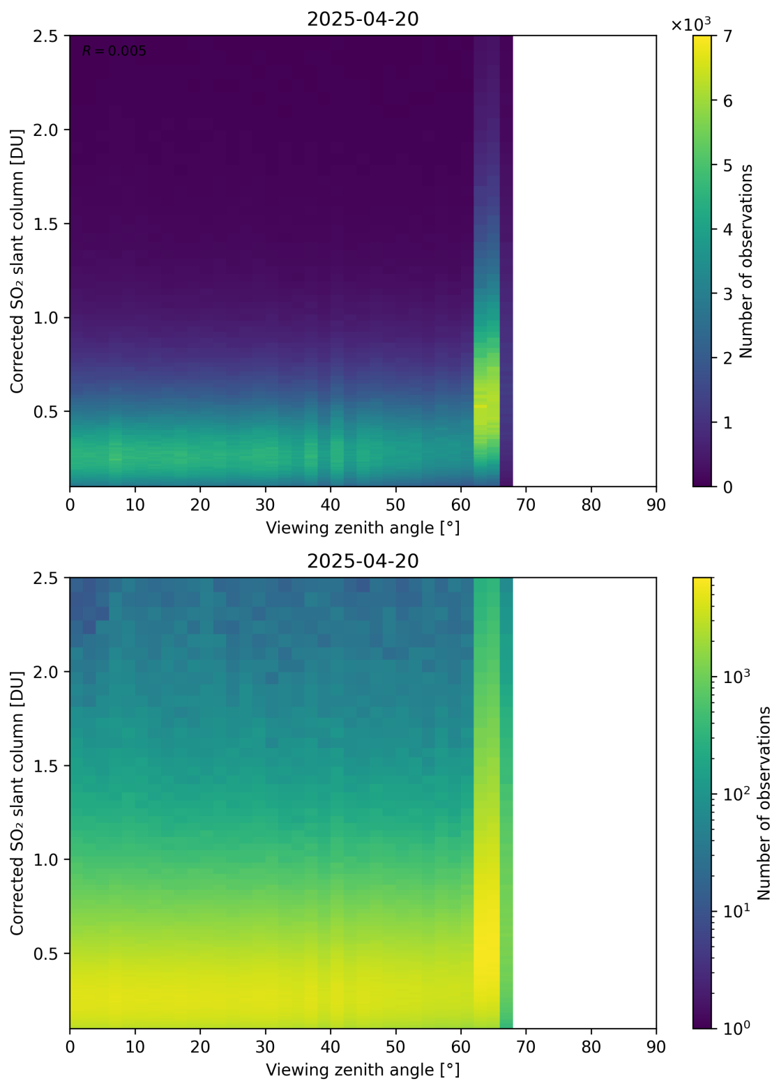
Figure 373: Scatter density plot of “Viewing zenith angle” against “Corrected SO 2 slant column” for 2025-04-19 to 2025-04-21.
