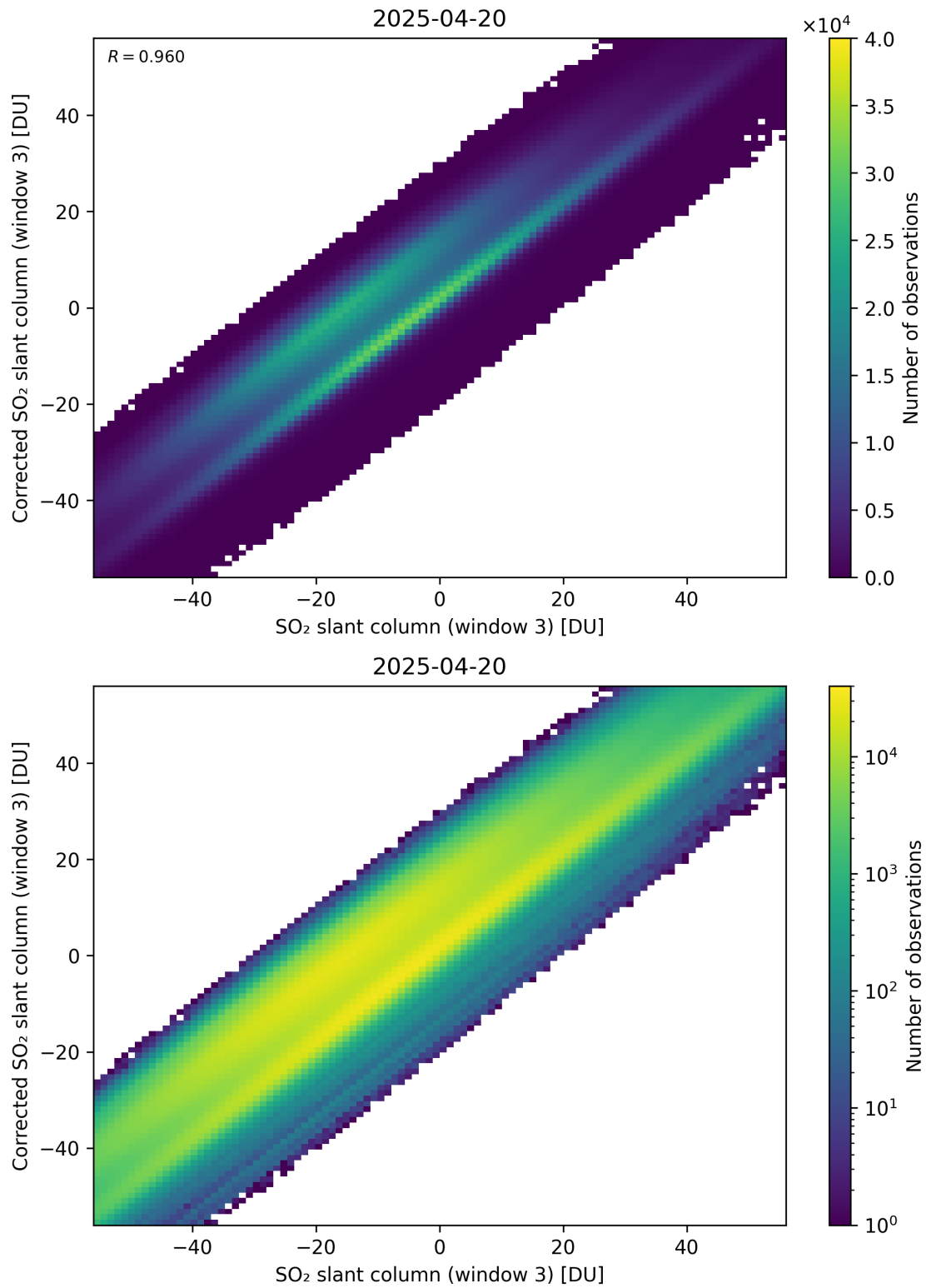
Figure 316: Scatter density plot of “SO 2 slant column (window 3)” against “Corrected SO 2 slant column (window 3)” for 2025-04-19 to 2025-04-21.
