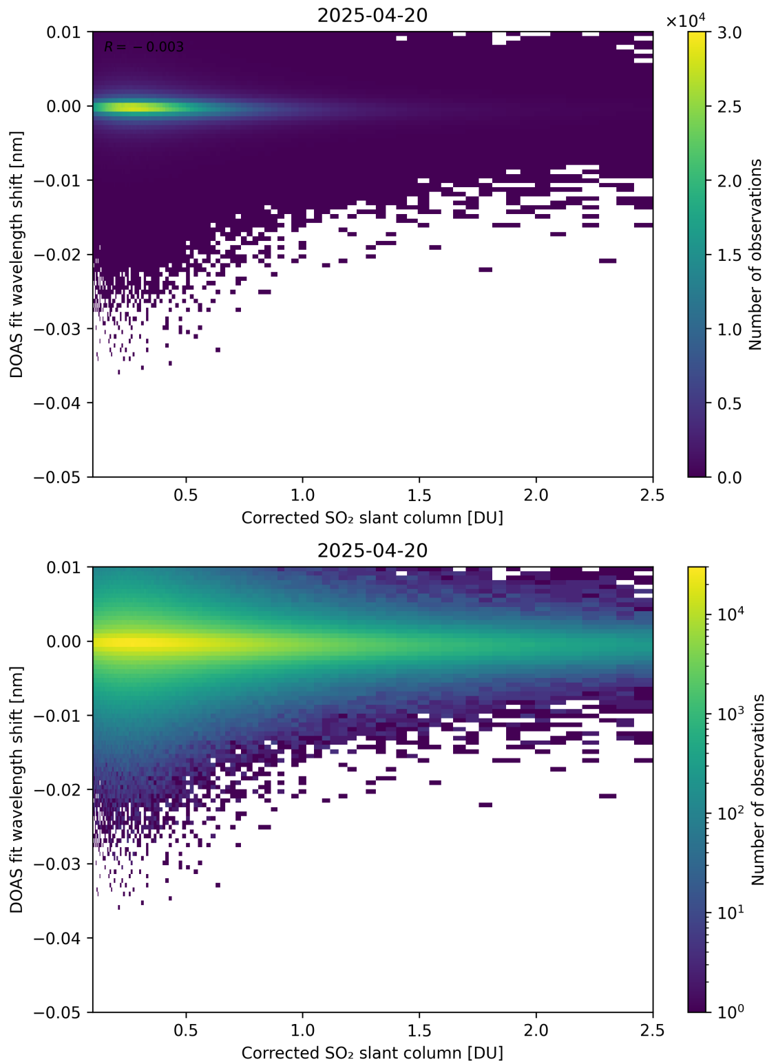
Figure 229: Scatter density plot of “Corrected SO 2 slant column” against “DOAS fit wavelength shift” for 2025-04-19 to 2025-04-21.
