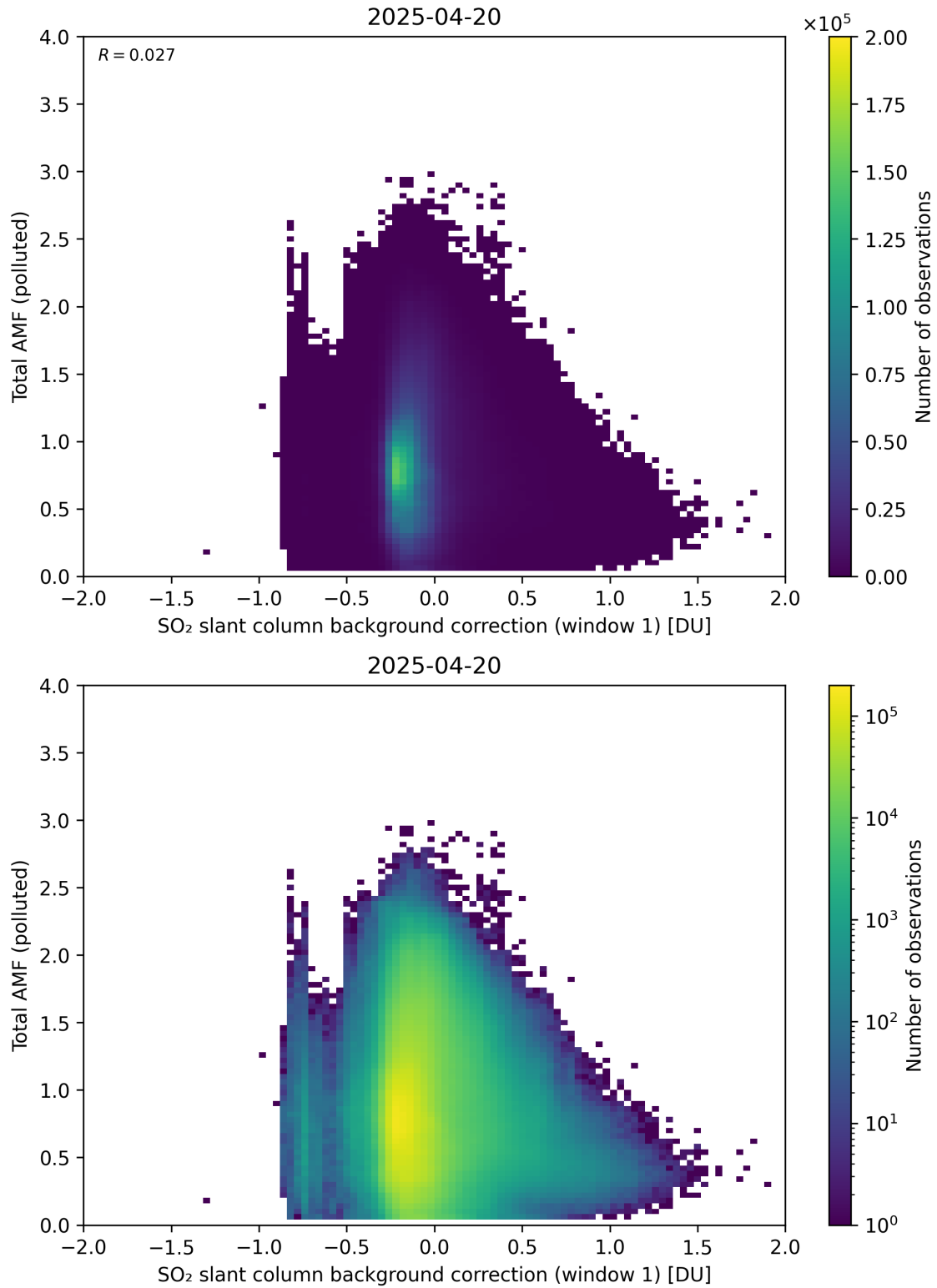
Figure 120: Scatter density plot of “SO 2 slant column background correction (window 1)” against “Total AMF (polluted)” for 2025-04-19 to 2025-04-21.
