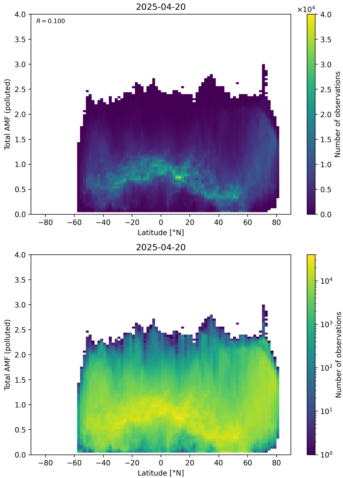
Figure 167: Scatter density plot of “Latitude” against “Total AMF (polluted)” for 2025-04-19 to 2025-04-21.
