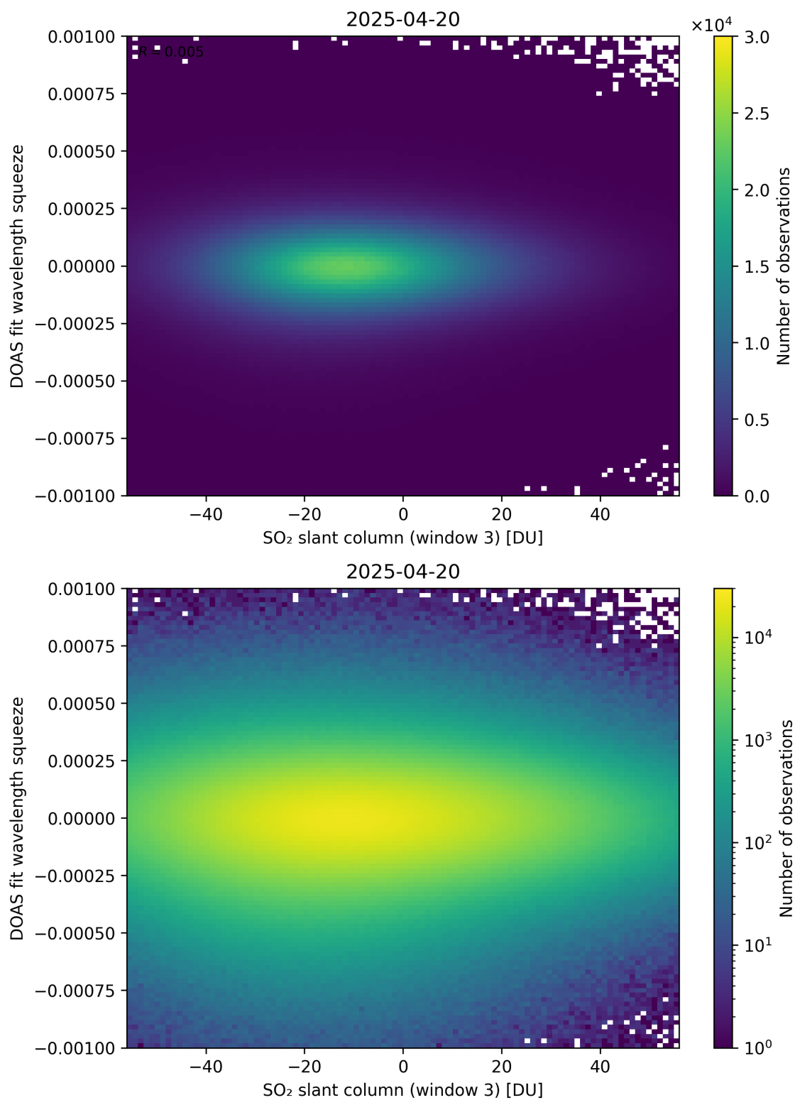
Figure 305: Scatter density plot of “SO 2 slant column (window 3)” against “DOAS fit wavelength squeeze” for 2025-04-19 to 2025-04-21.
