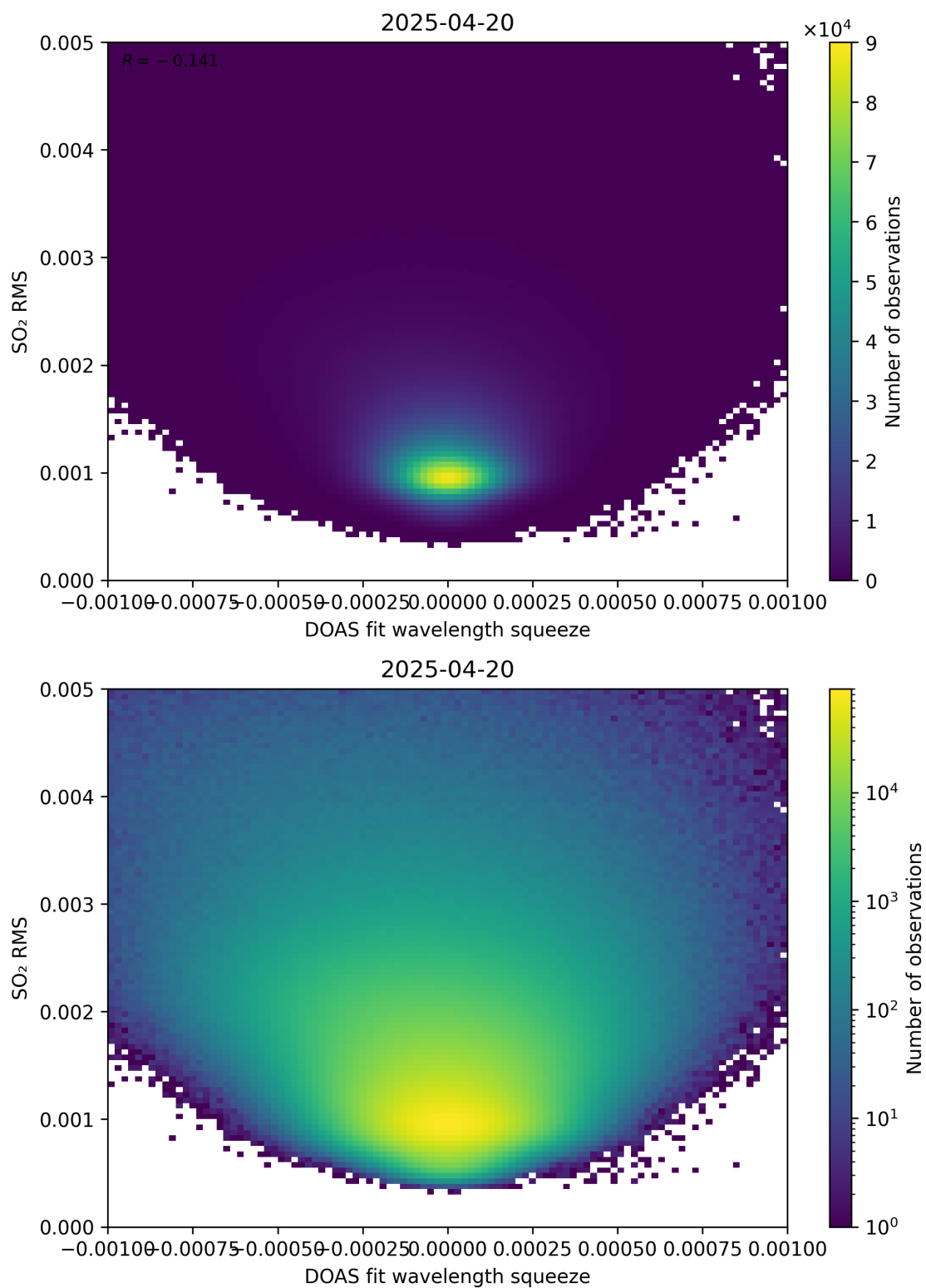
Figure 143: Scatter density plot of “DOAS fit wavelength squeeze” against “SO 2 RMS” for 2025-04-19 to 2025-04-21.
