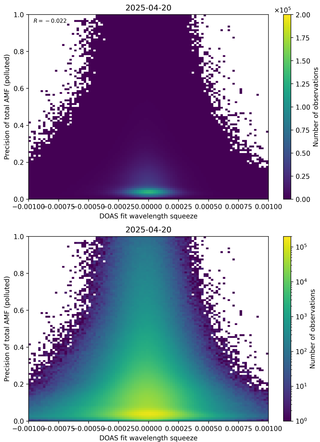
Figure 146: Scatter density plot of “DOAS fit wavelength squeeze” against “Precision of total AMF (polluted)” for 2025-04-19 to 2025-04-21.
