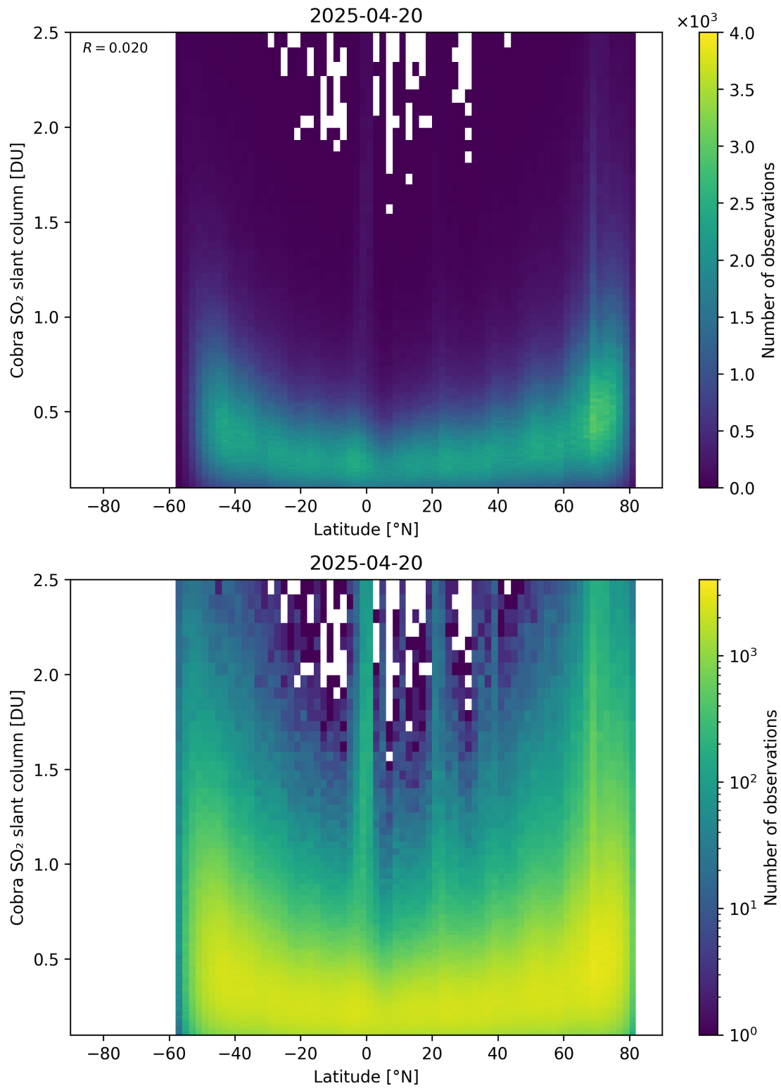
Figure 157: Scatter density plot of “Latitude” against “Cobra SO 2 slant column” for 2025-04-19 to 2025-04-21.
