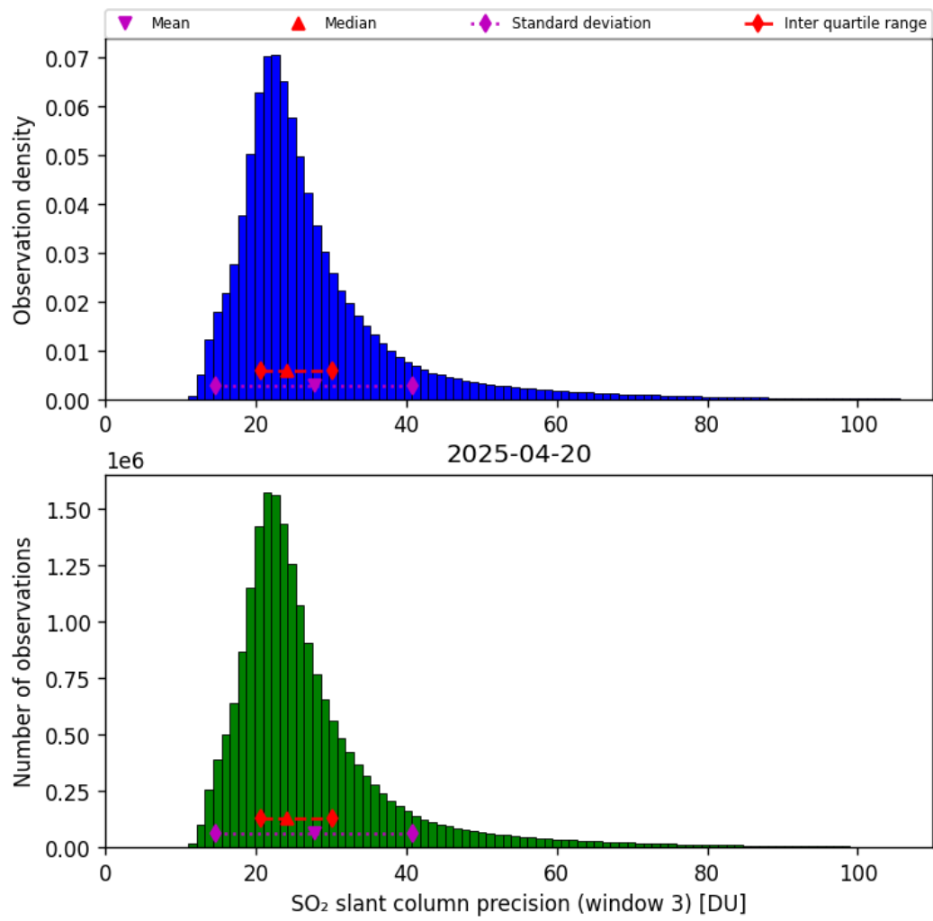
Figure 72: Histogram of “SO 2 slant column precision (window 3)” for 2025-04-19 to 2025-04-21
