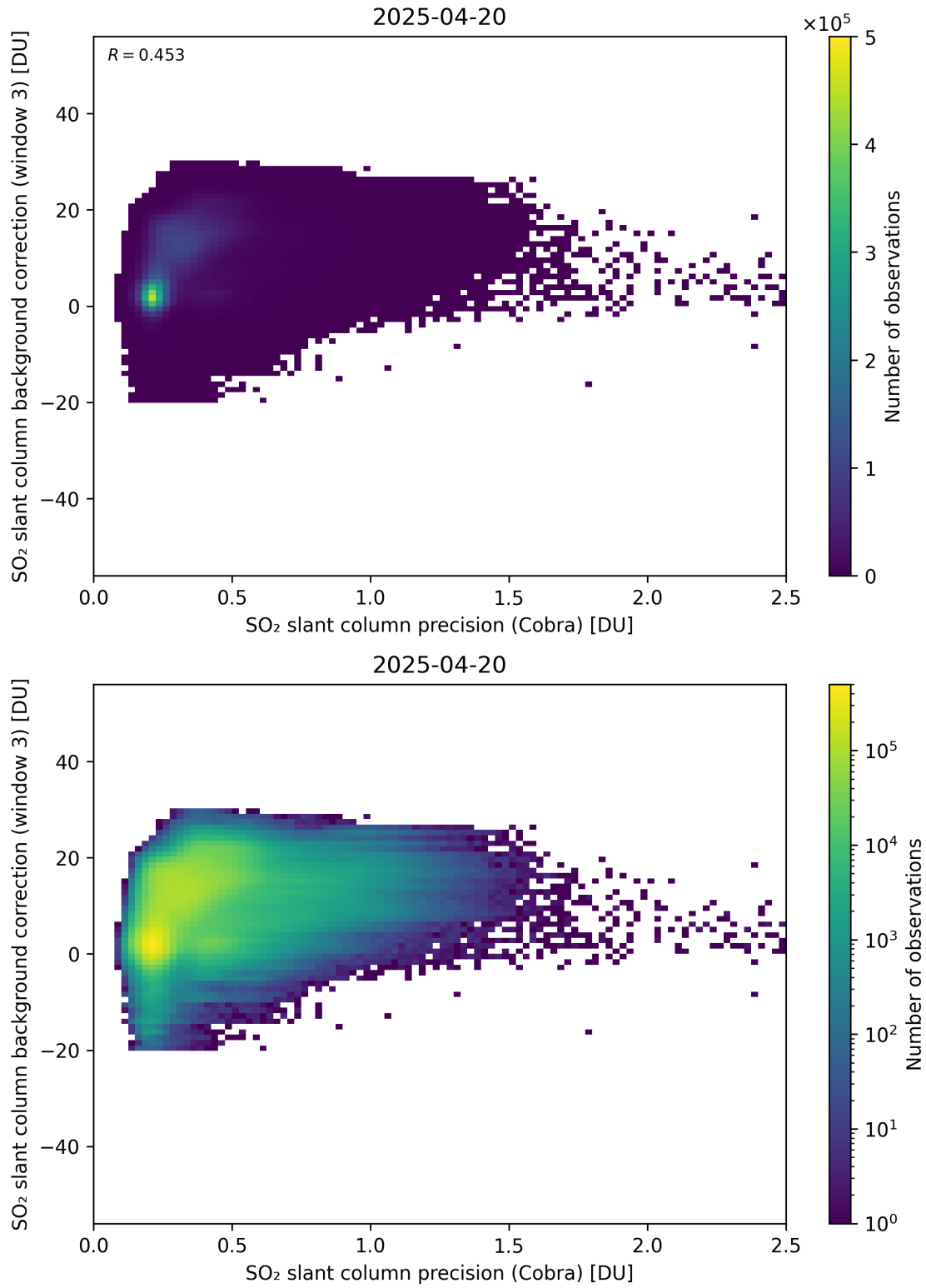
Figure 201: Scatter density plot of “SO 2 slant column precision (Cobra)” against “SO 2 slant column background correction (window 3)” for 2025-04-19 to 2025-04-21.
