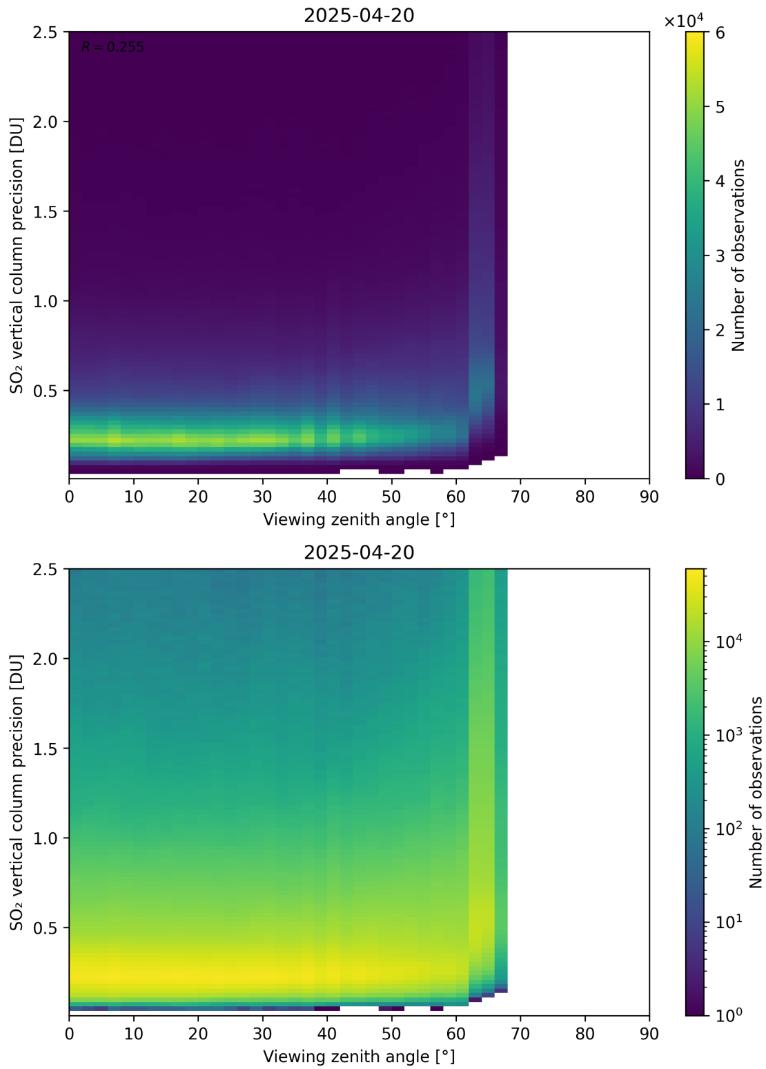
Figure 384: Scatter density plot of “Viewing zenith angle” against “SO 2 vertical column precision” for 2025-04-19 to 2025-04-21.
