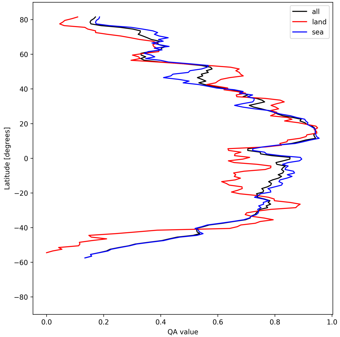
Figure 31: Zonal average of “QA value” for 2025-04-19 to 2025-04-21.
