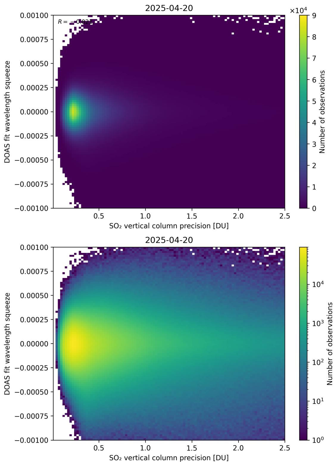
Figure 333: Scatter density plot of “SO 2 vertical column precision” against “DOAS fit wavelength squeeze” for 2025-04-19 to 2025-04-21.
