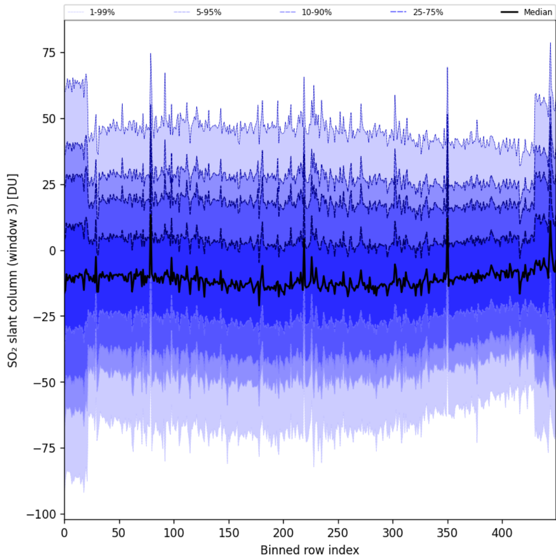
Figure 97: Along track statistics of “SO 2 slant column (window 3)” for 2025-04-19 to 2025-04-21
