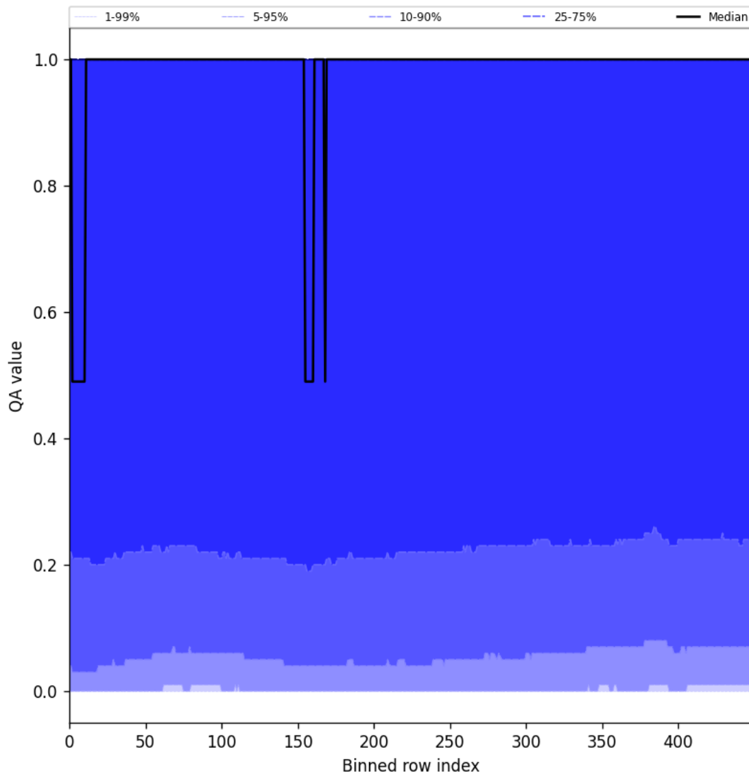
Figure 83: Along track statistics of “QA value” for 2025-04-19 to 2025-04-21
