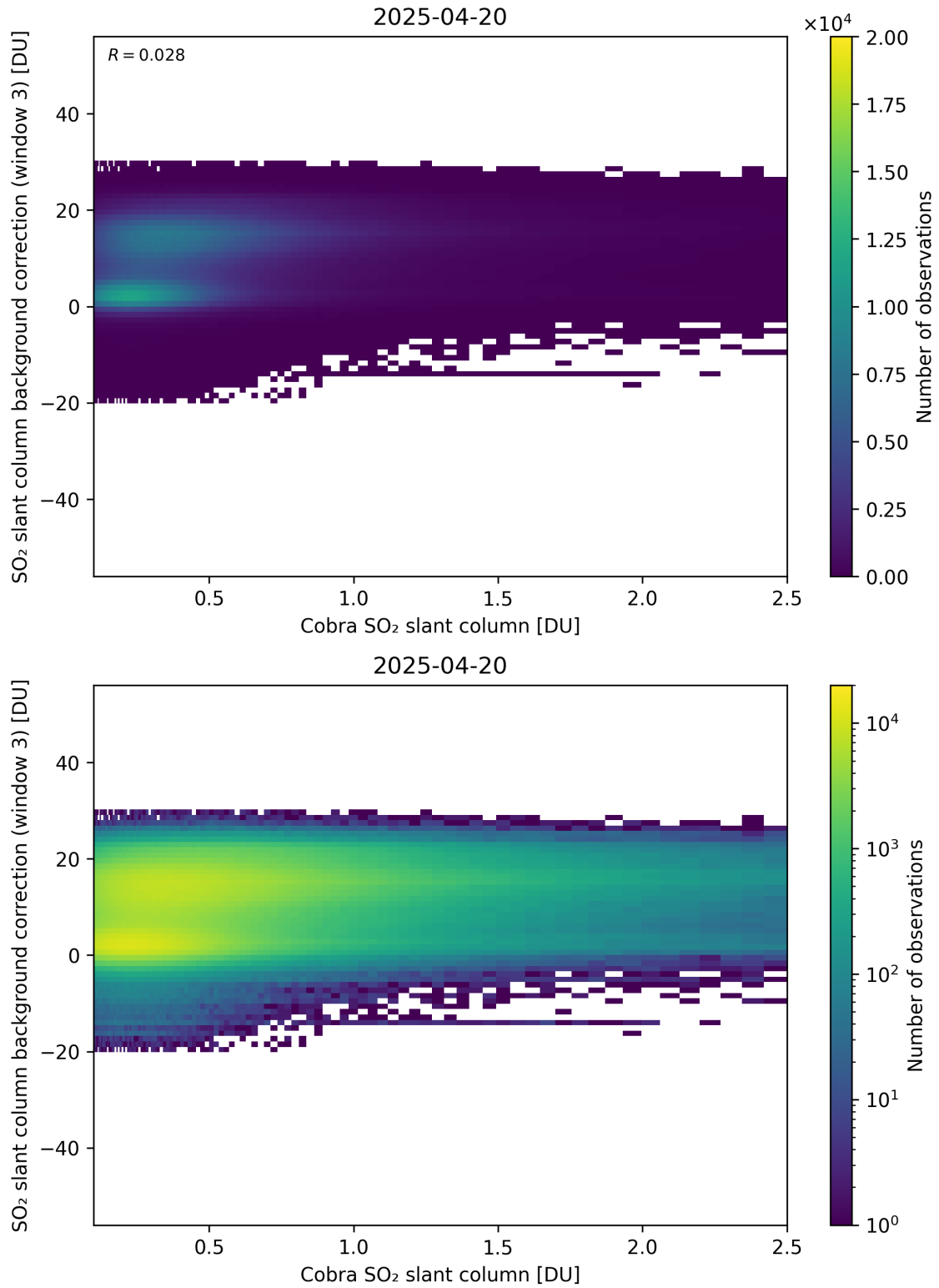
Figure 195: Scatter density plot of “Cobra SO 2 slant column” against “SO 2 slant column background correction (window 3)” for 2025-04-19 to 2025-04-21.
