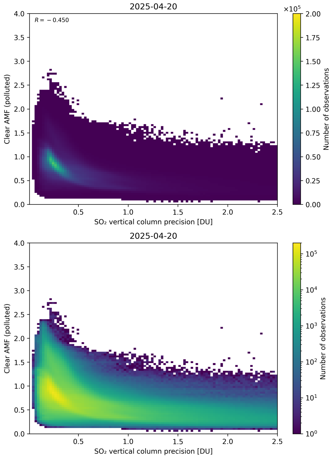
Figure 335: Scatter density plot of “SO 2 vertical column precision” against “Clear AMF (polluted)” for 2025-04-19 to 2025-04-21.
