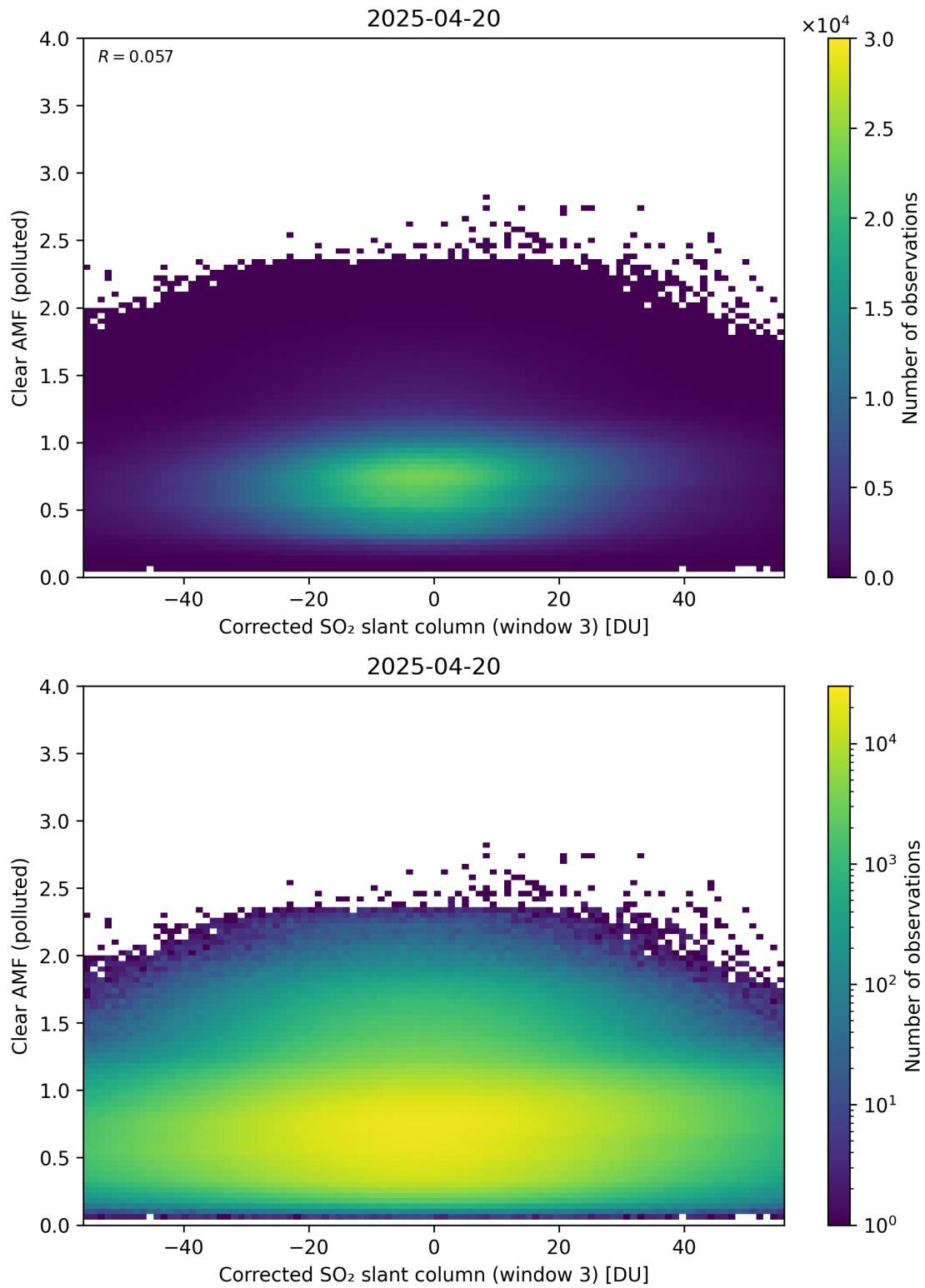
Figure 259: Scatter density plot of “Corrected SO 2 slant column (window 3)” against “Clear AMF (polluted)” for 2025-04-19 to 2025-04-21.
