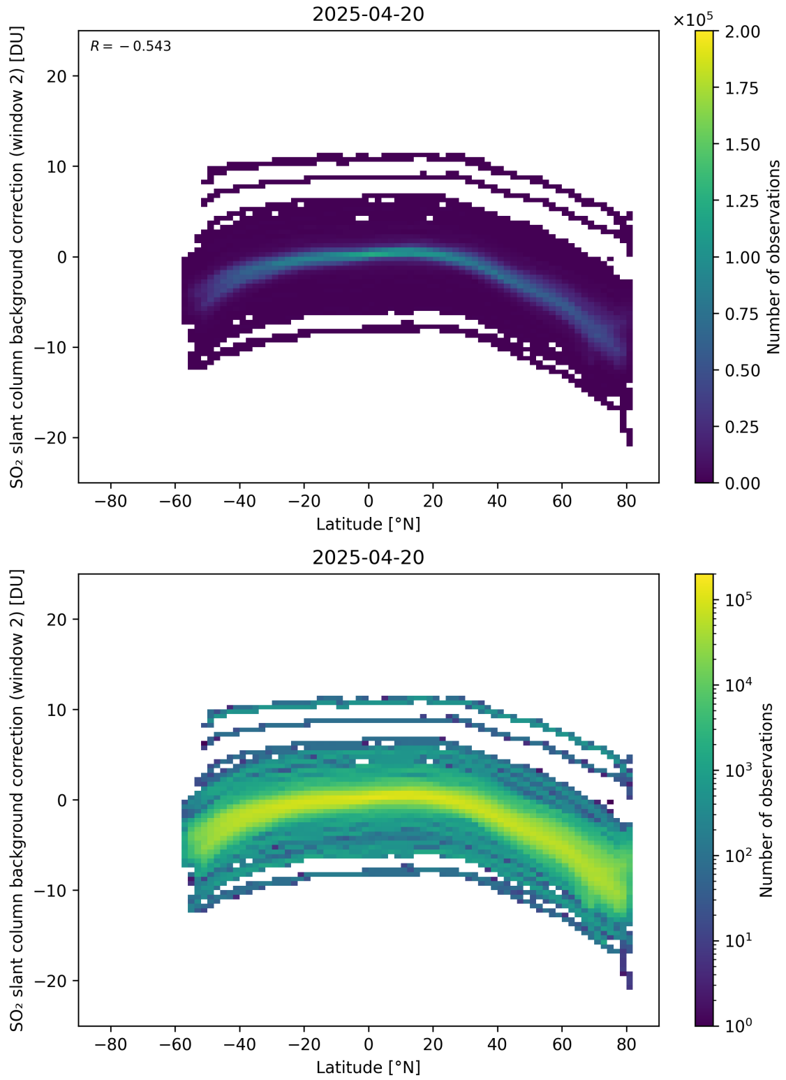
Figure 151: Scatter density plot of “Latitude” against “SO 2 slant column background correction (window 2)” for 2025-04-19 to 2025-04-21.
