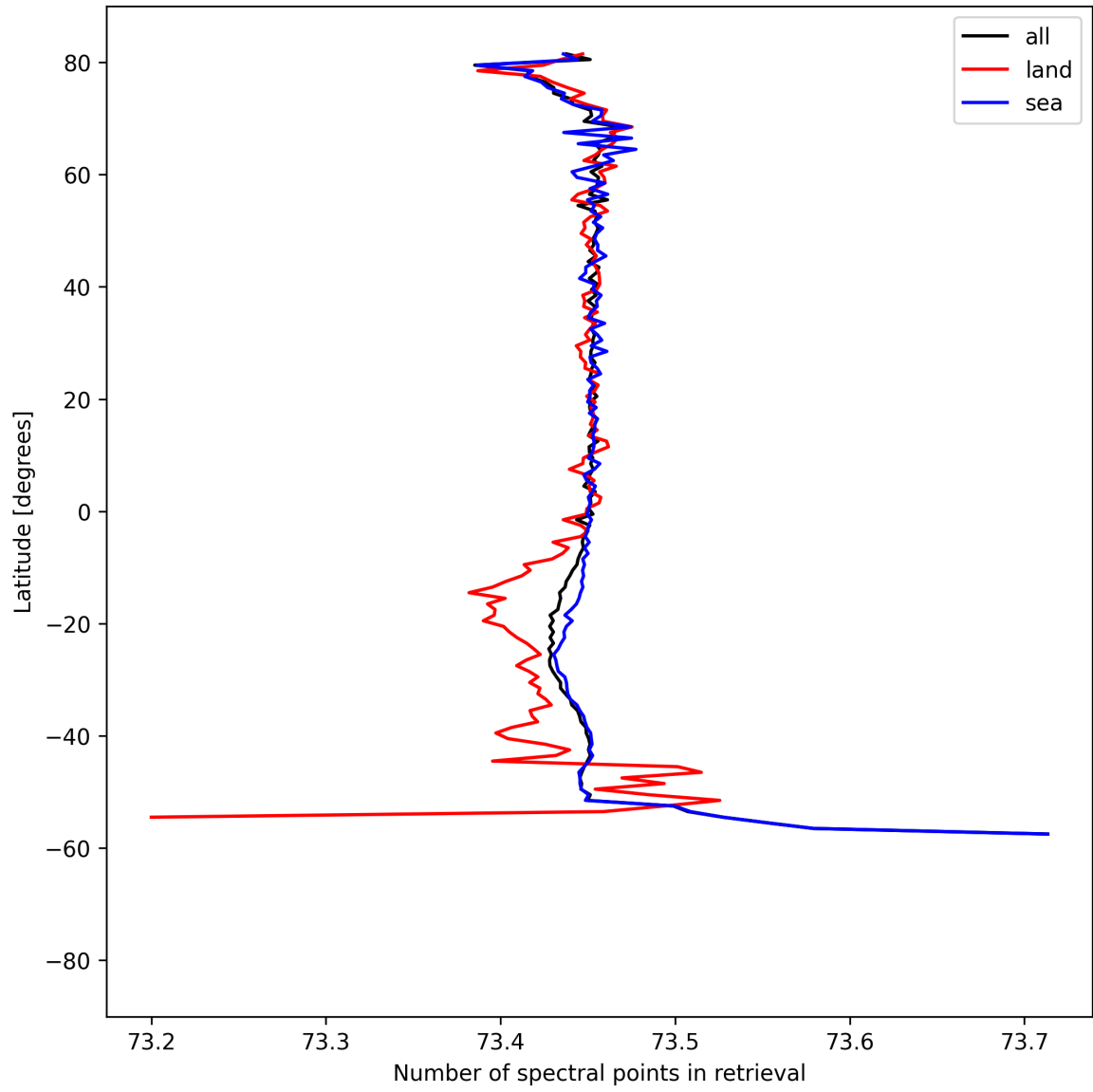
Figure 56: Zonal average of “Number of spectral points in retrieval” for 2025-04-19 to 2025-04-21.
