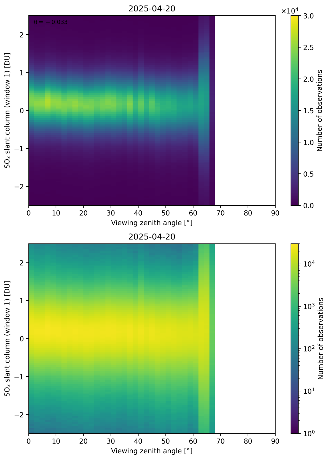
Figure 376: Scatter density plot of “Viewing zenith angle” against “SO 2 slant column (window 1)” for 2025-04-19 to 2025-04-21.
