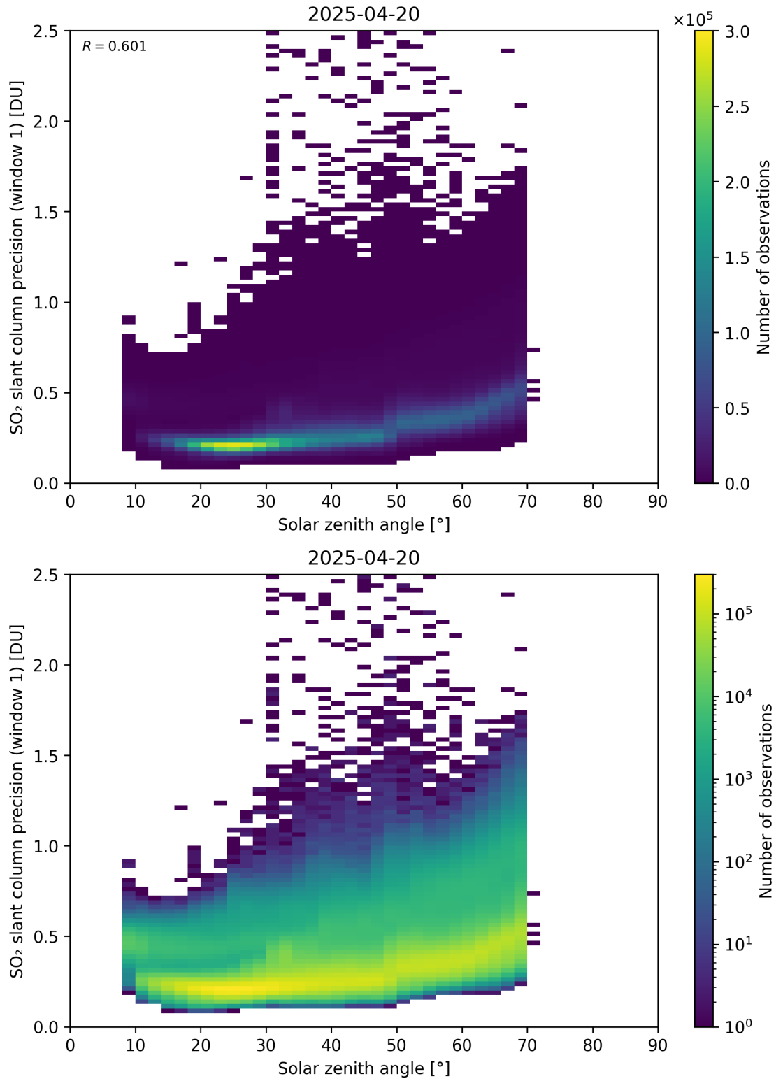
Figure 185: Scatter density plot of “Solar zenith angle” against “SO 2 slant column precision (window 1)” for 2025-04-19 to 2025-04-21.
