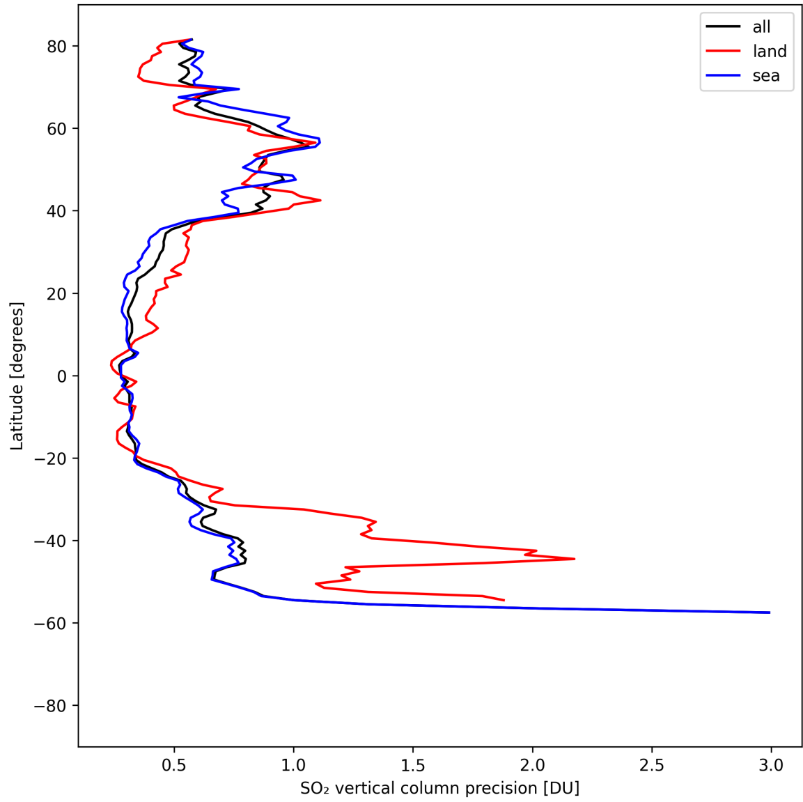
Figure 33: Zonal average of “SO 2 vertical column precision” for 2025-04-19 to 2025-04-21.
