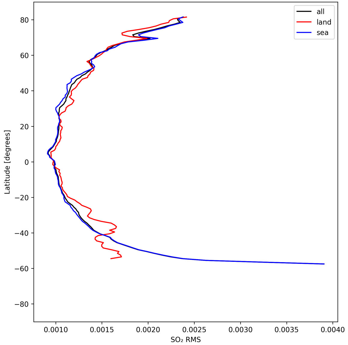
Figure 52: Zonal average of “SO 2 RMS” for 2025-04-19 to 2025-04-21.
