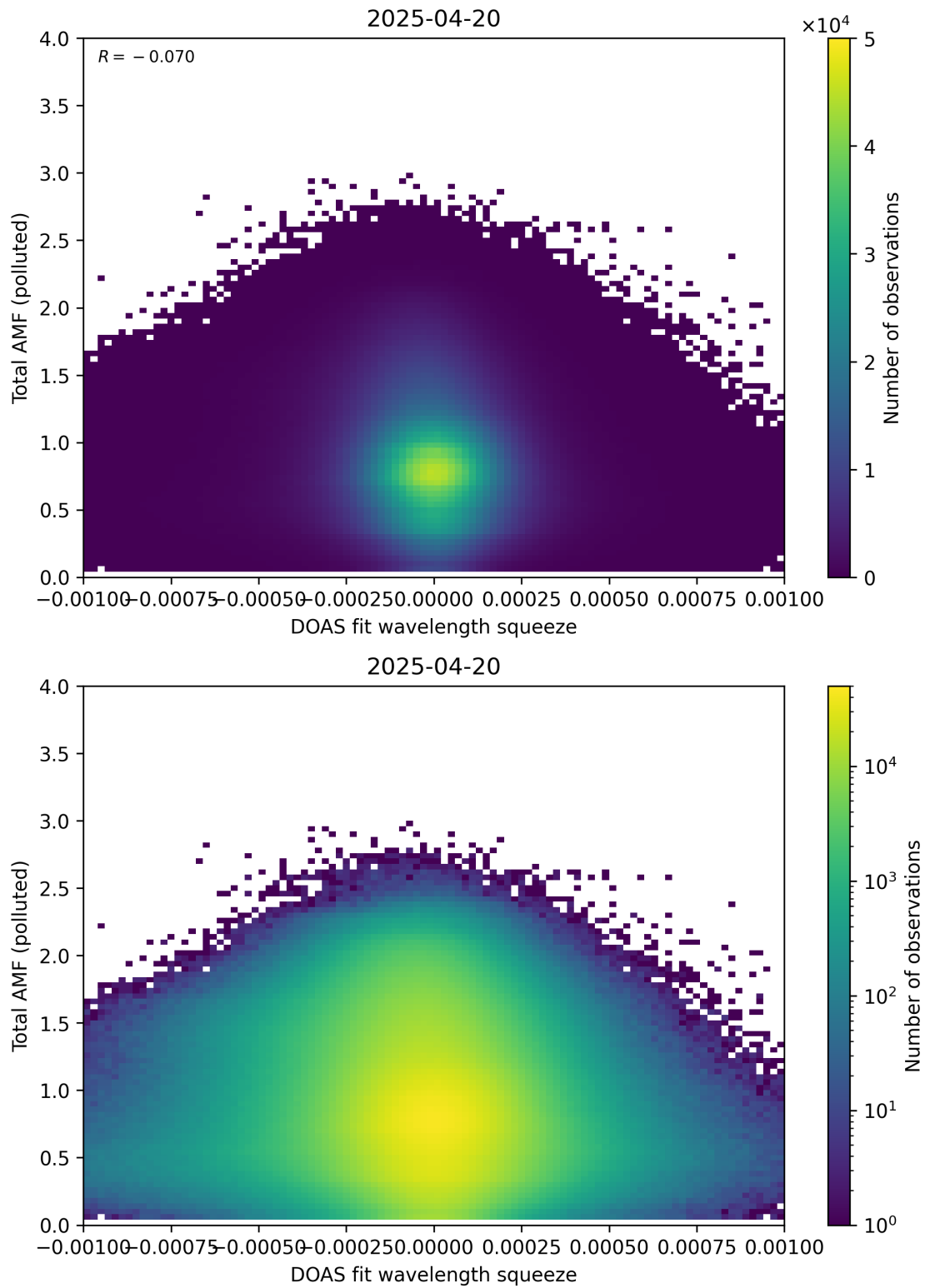
Figure 145: Scatter density plot of “DOAS fit wavelength squeeze” against “Total AMF (polluted)” for 2025-04-19 to 2025-04-21.
