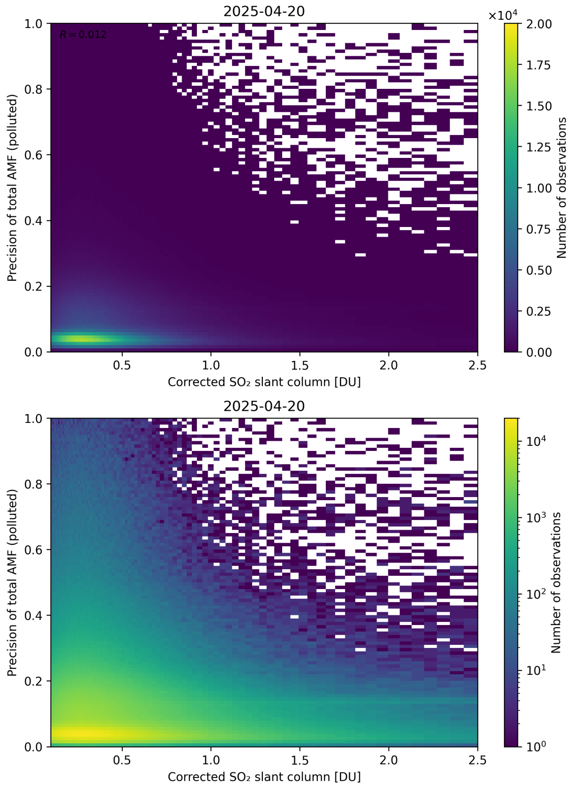
Figure 243: Scatter density plot of “Corrected SO 2 slant column” against “Precision of total AMF (polluted)” for 2025-04-19 to 2025-04-21.
