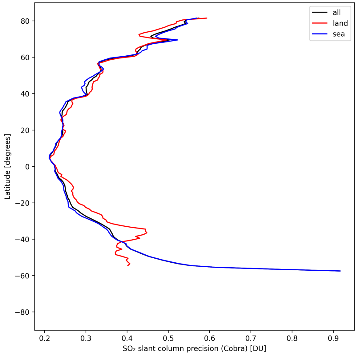
Figure 36: Zonal average of “SO 2 slant column precision (Cobra)” for 2025-04-19 to 2025-04-21.
