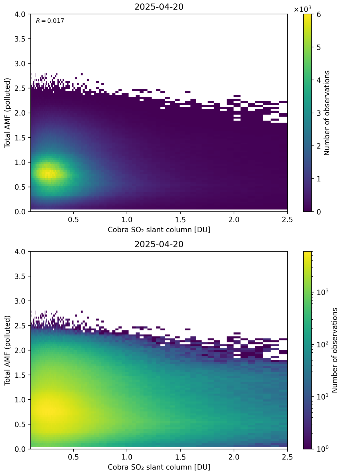
Figure 224: Scatter density plot of “Cobra SO 2 slant column” against “Total AMF (polluted)” for 2025-04-19 to 2025-04-21.
