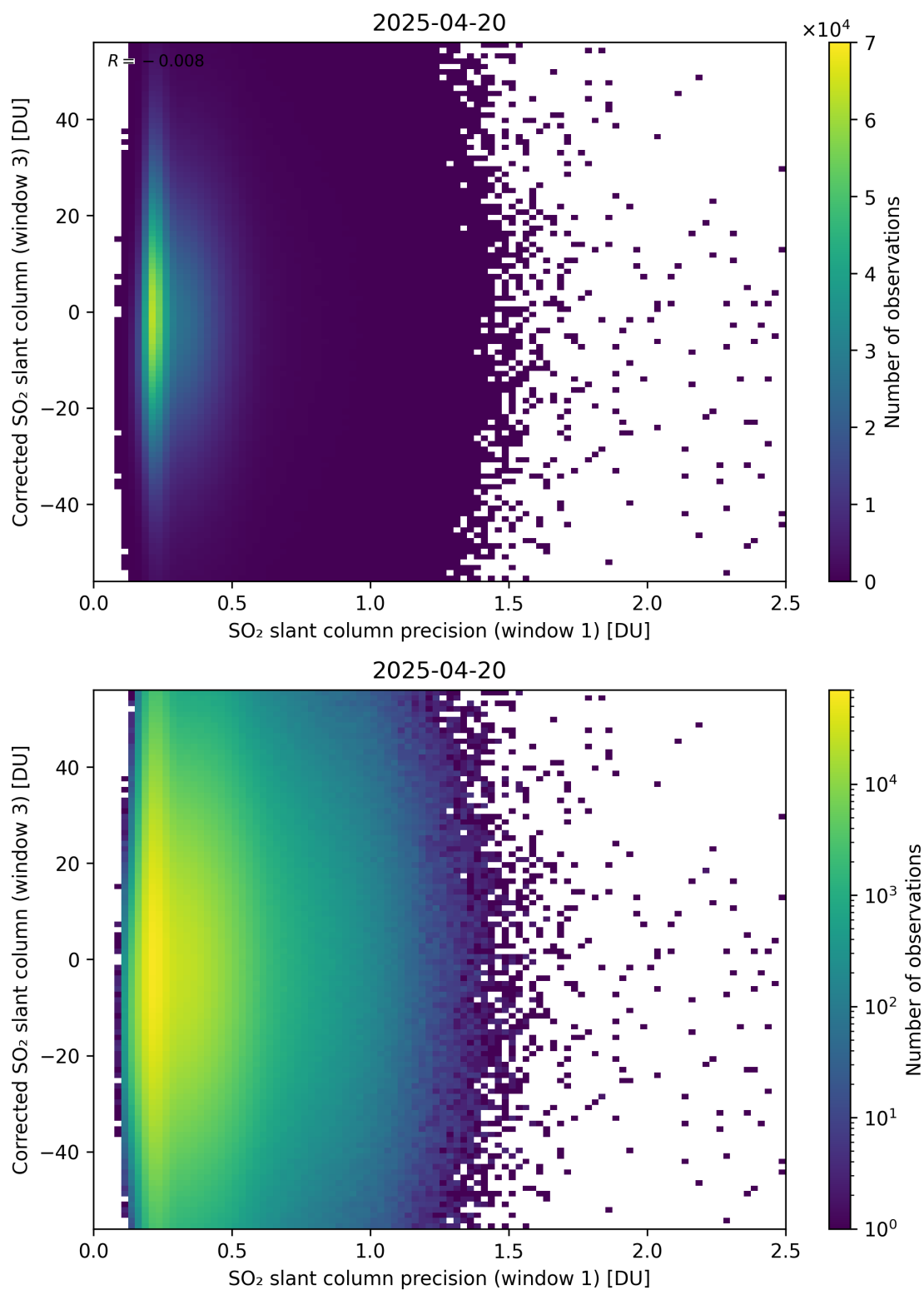
Figure 276: Scatter density plot of “SO 2 slant column precision (window 1)” against “Corrected SO 2 slant column (window 3)” for 2025-04-19 to 2025-04-21.
