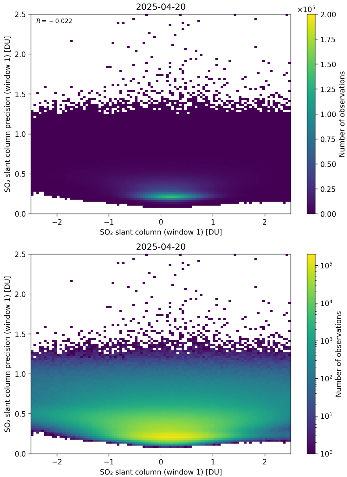
Figure 285: Scatter density plot of “SO 2 slant column (window 1)” against “SO 2 slant column precision (window 1)” for 2025-04-19 to 2025-04-21.
