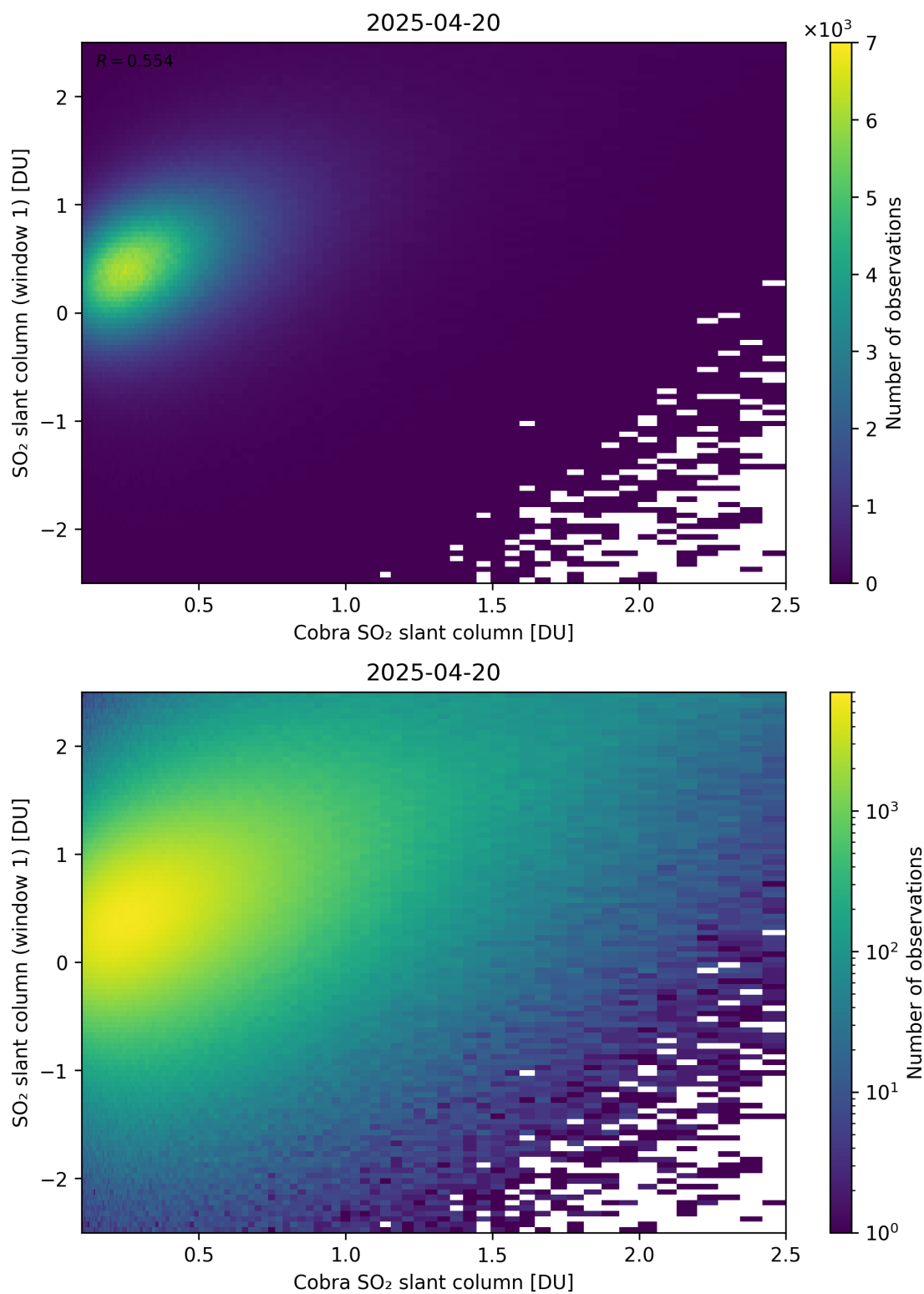
Figure 219: Scatter density plot of “Cobra SO 2 slant column” against “SO 2 slant column (window 1)” for 2025-04-19 to 2025-04-21.
