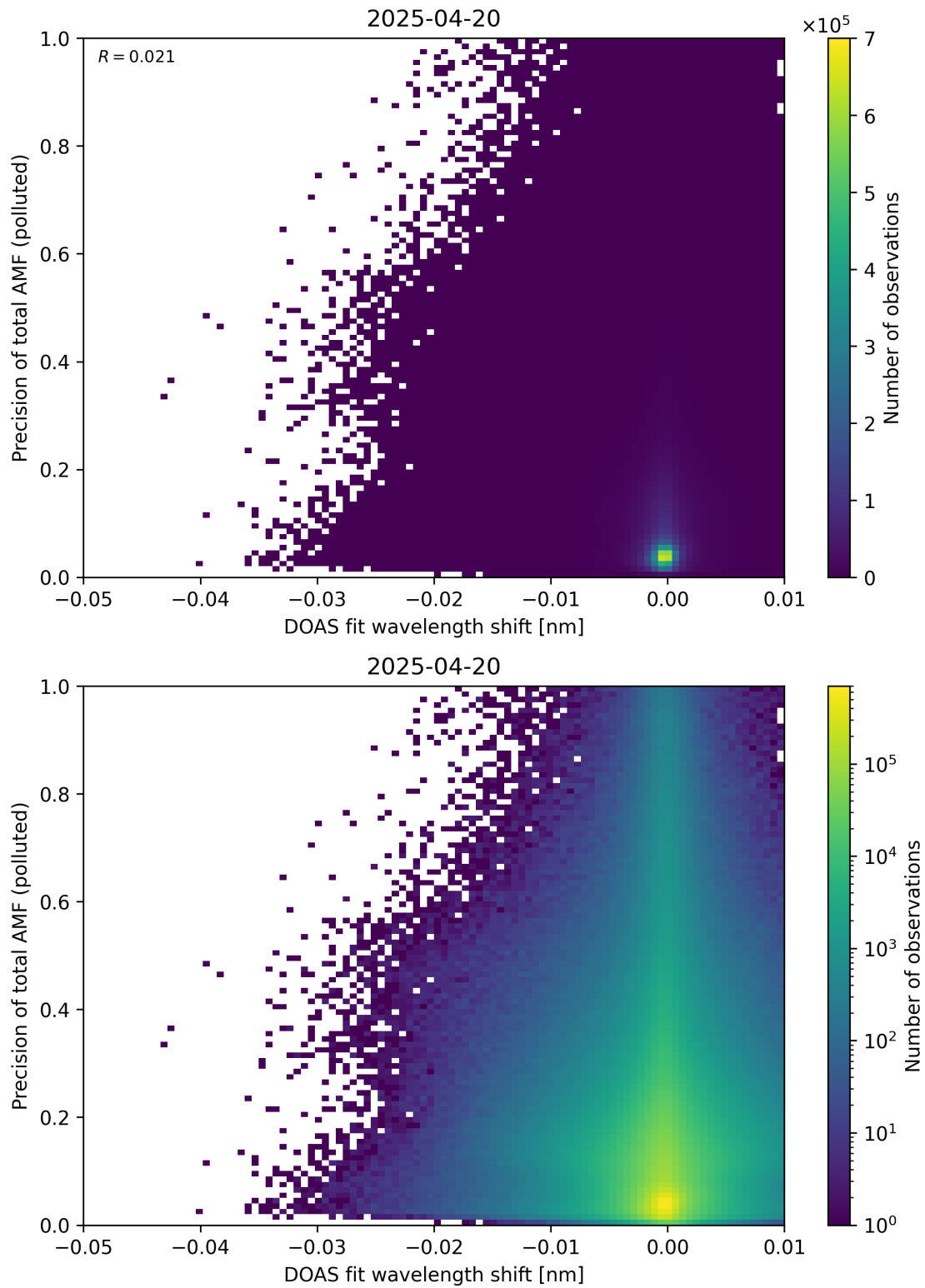
Figure 142: Scatter density plot of “DOAS fit wavelength shift” against “Precision of total AMF (polluted)” for 2025-04-19 to 2025-04-21.
