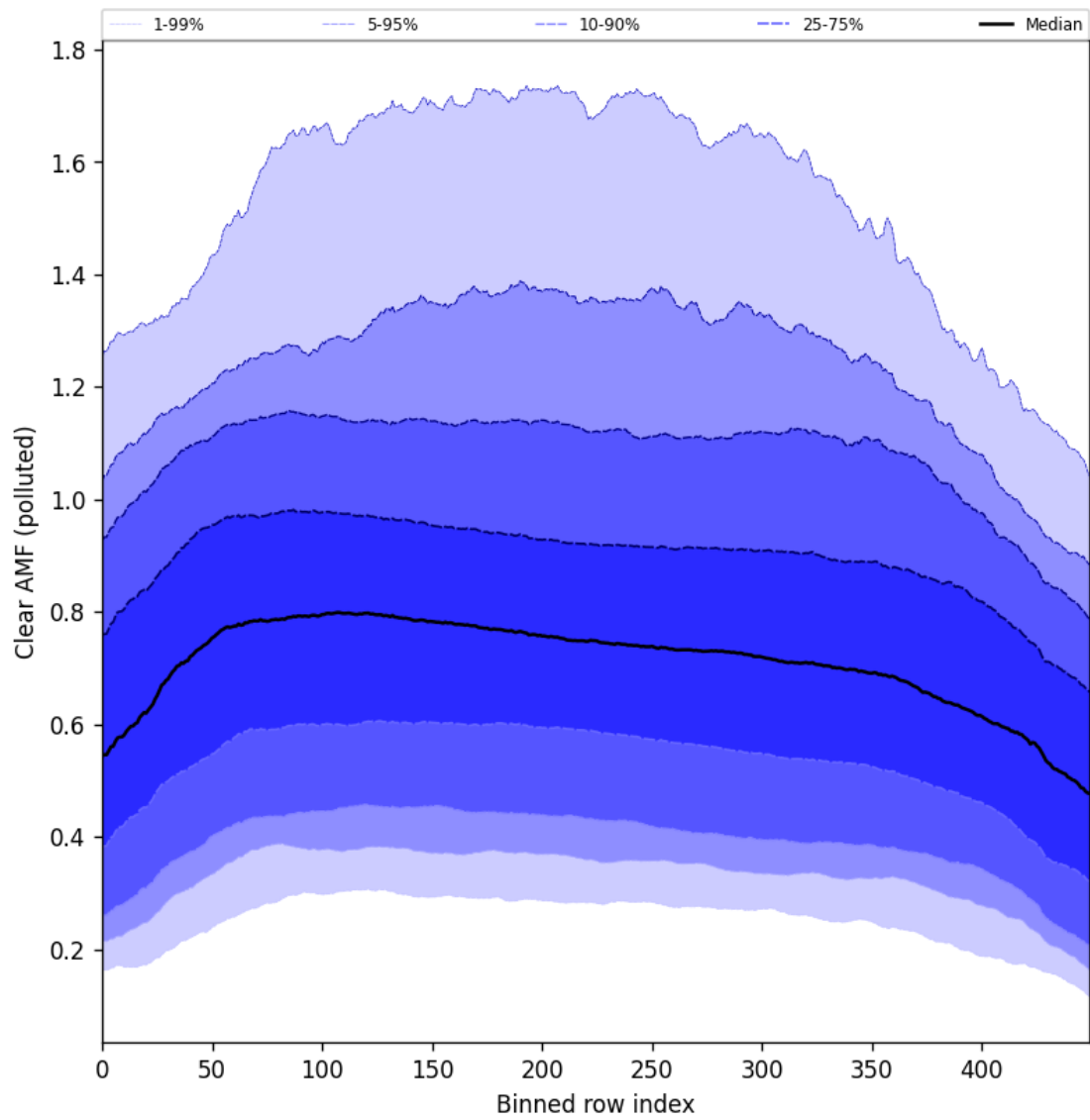
Figure 107: Along track statistics of “Clear AMF (polluted)” for 2025-04-19 to 2025-04-21
