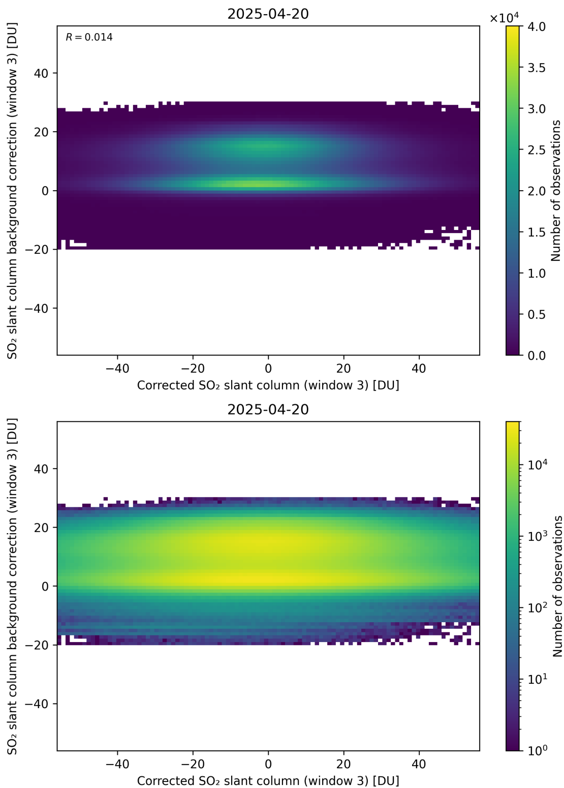
Figure 255: Scatter density plot of “Corrected SO 2 slant column (window 3)” against “SO 2 slant column background correction (window 3)” for 2025-04-19 to 2025-04-21.
