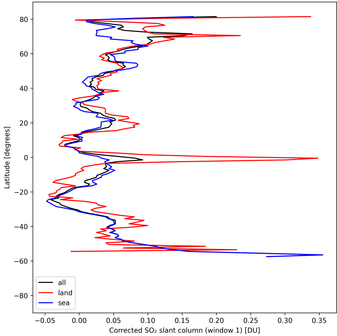
Figure 39: Zonal average of “Corrected SO 2 slant column (window 1)” for 2025-04-19 to 2025-04-21.
