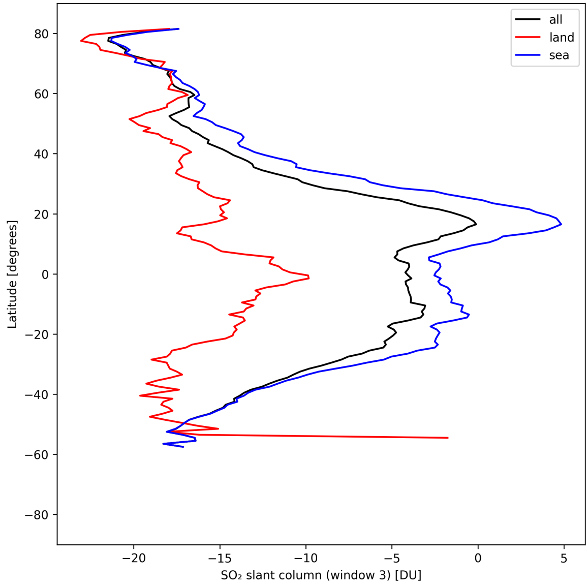
Figure 45: Zonal average of “SO 2 slant column (window 3)” for 2025-04-19 to 2025-04-21.
