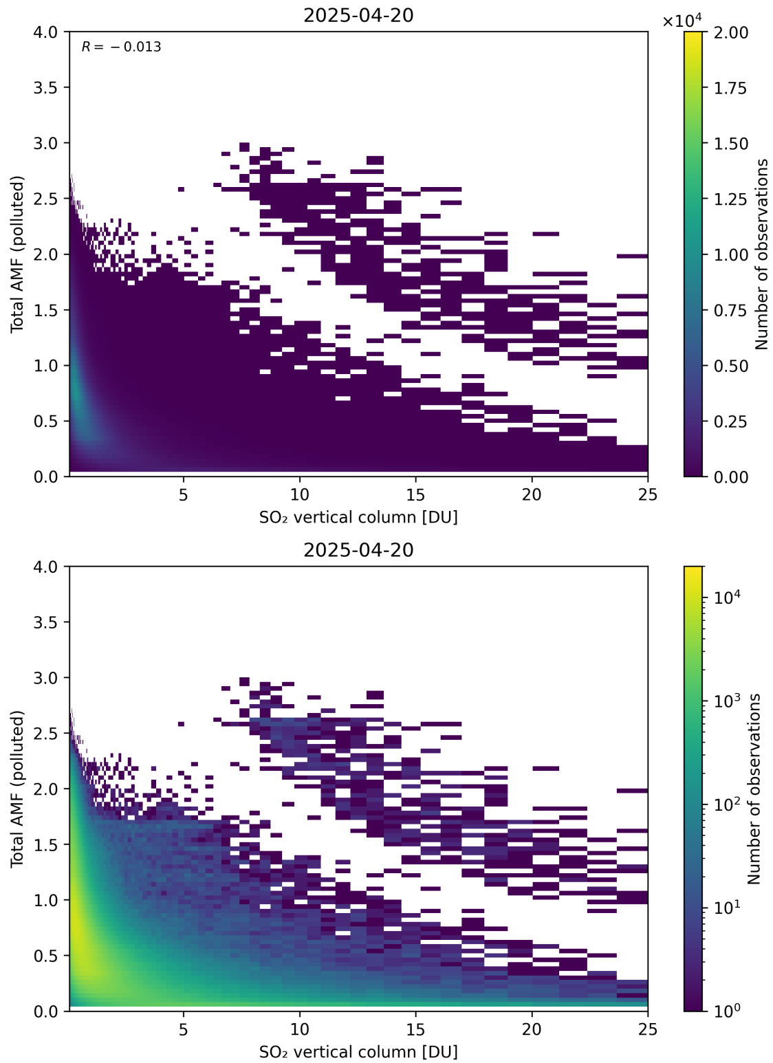
Figure 359: Scatter density plot of “SO 2 vertical column” against “Total AMF (polluted)” for 2025-04-19 to 2025-04-21.
