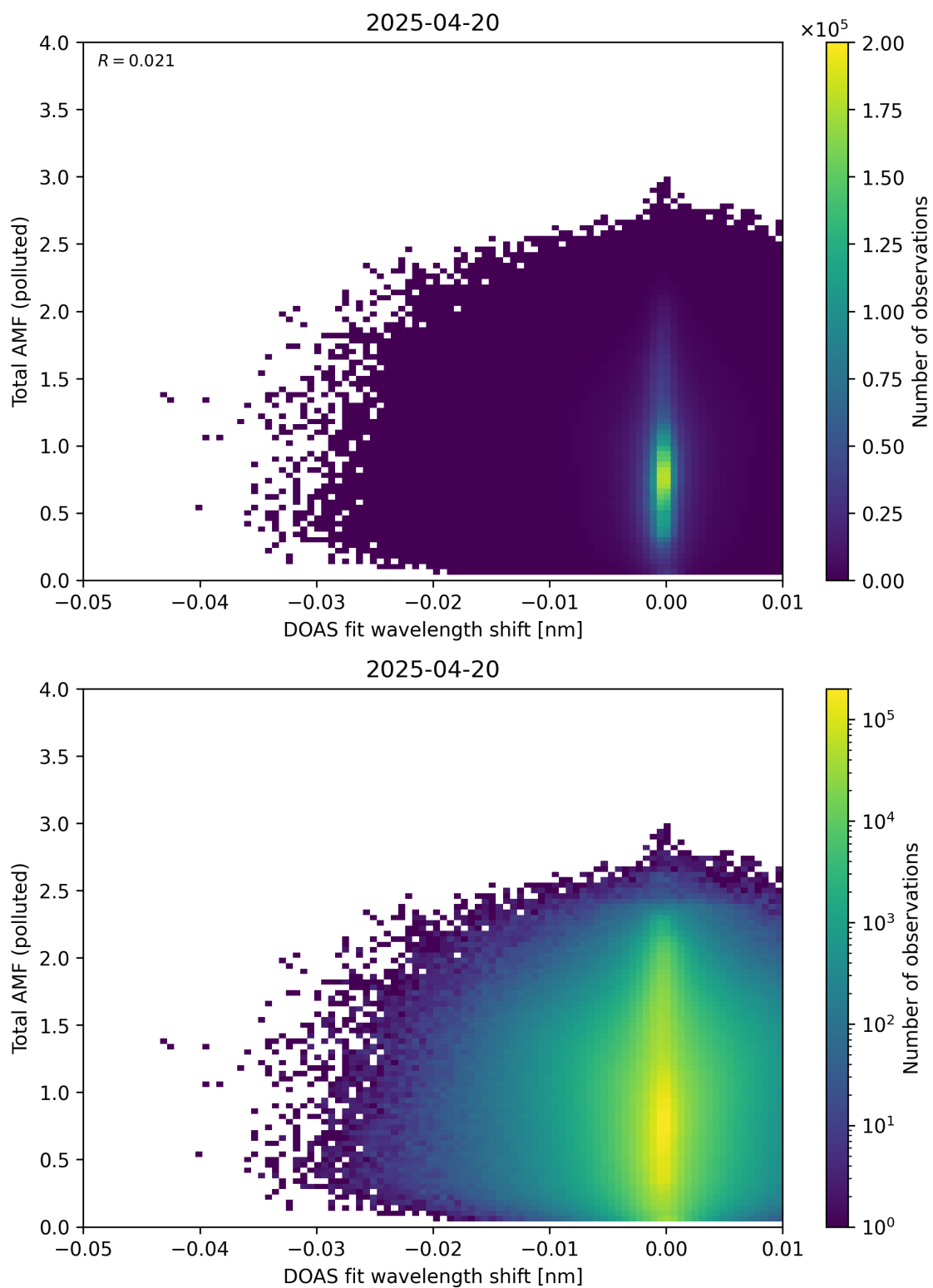
Figure 141: Scatter density plot of “DOAS fit wavelength shift” against “Total AMF (polluted)” for 2025-04-19 to 2025-04-21.
