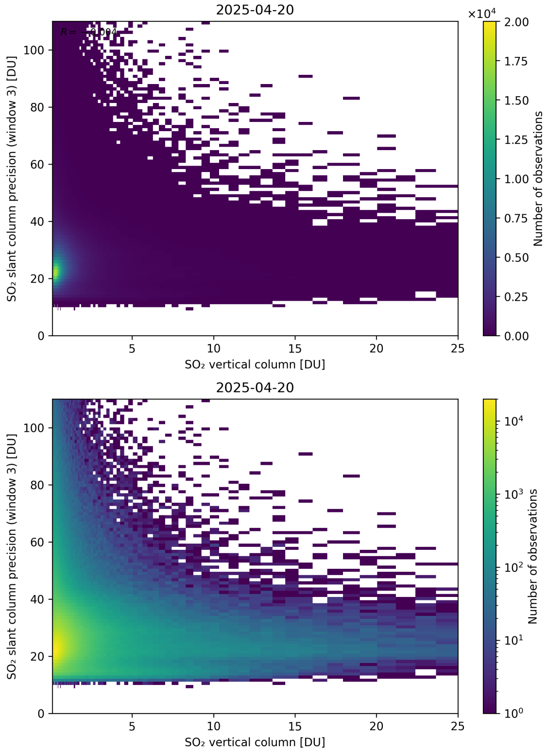
Figure 358: Scatter density plot of “SO 2 vertical column” against “SO 2 slant column precision (window 3)” for 2025-04-19 to 2025-04-21.
