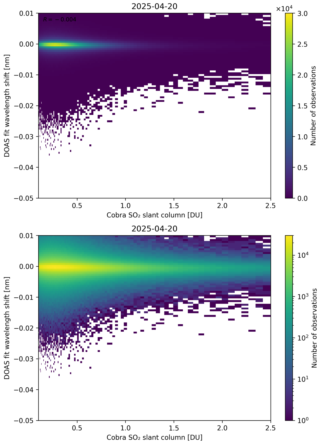
Figure 196: Scatter density plot of “Cobra SO 2 slant column” against “DOAS fit wavelength shift” for 2025-04-19 to 2025-04-21.
