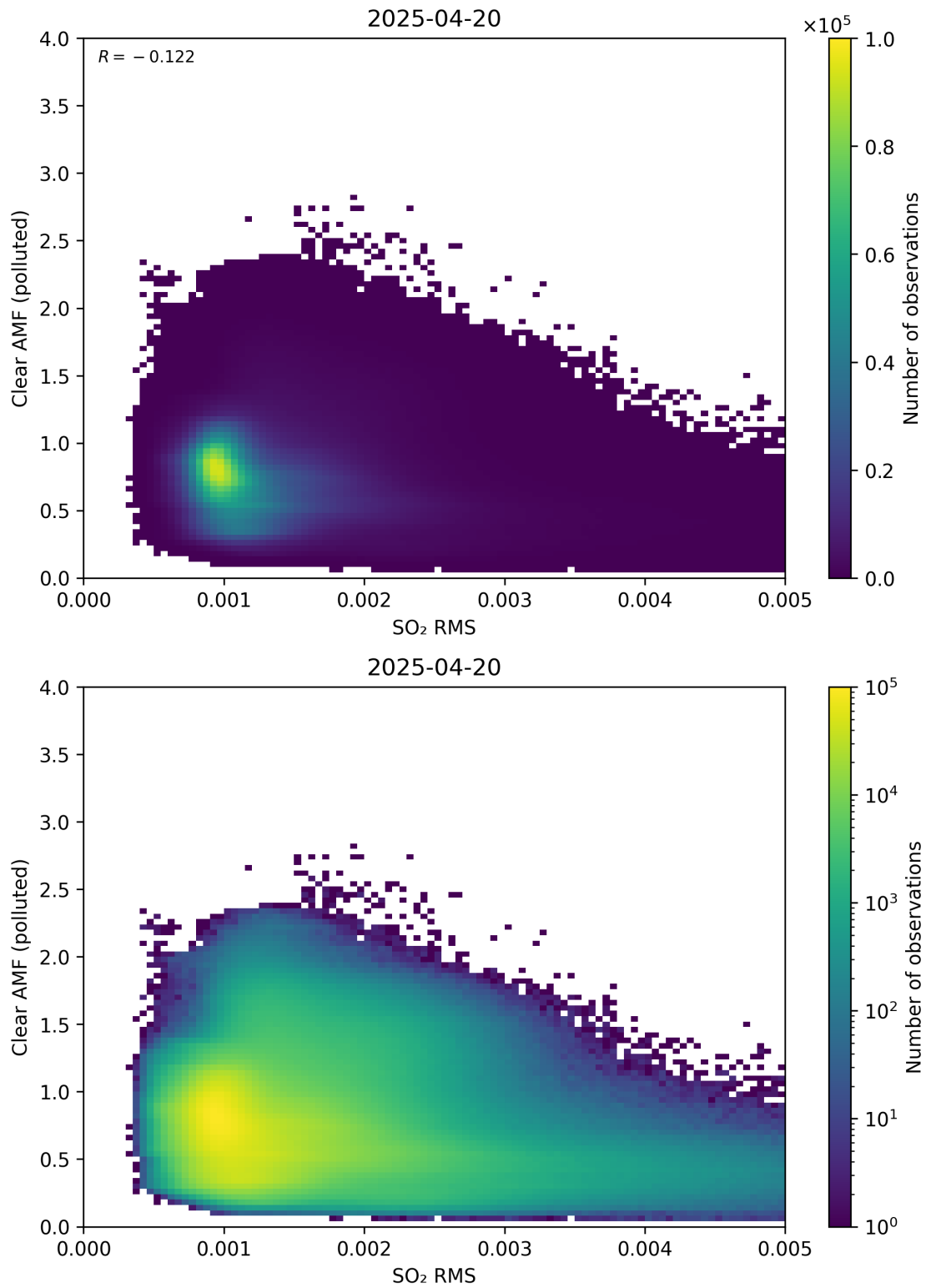
Figure 147: Scatter density plot of “SO 2 RMS” against “Clear AMF (polluted)” for 2025-04-19 to 2025-04-21.
