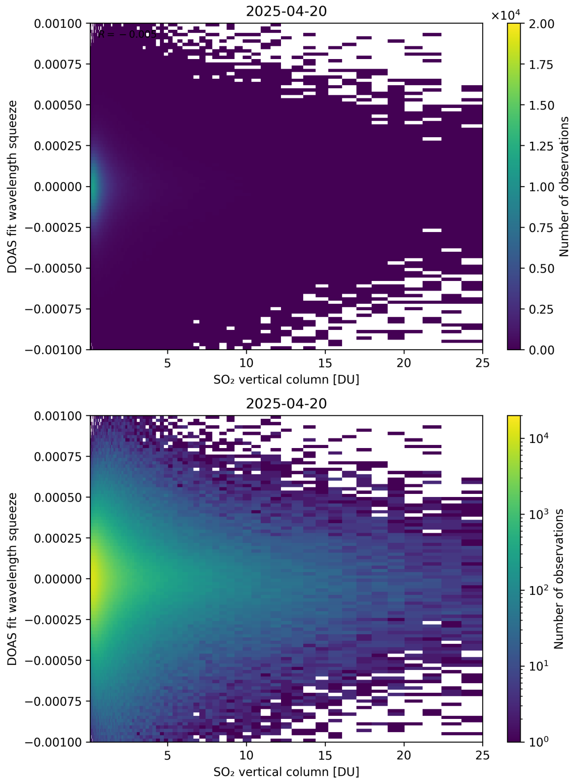
Figure 327: Scatter density plot of “SO 2 vertical column” against “DOAS fit wavelength squeeze” for 2025-04-19 to 2025-04-21.
