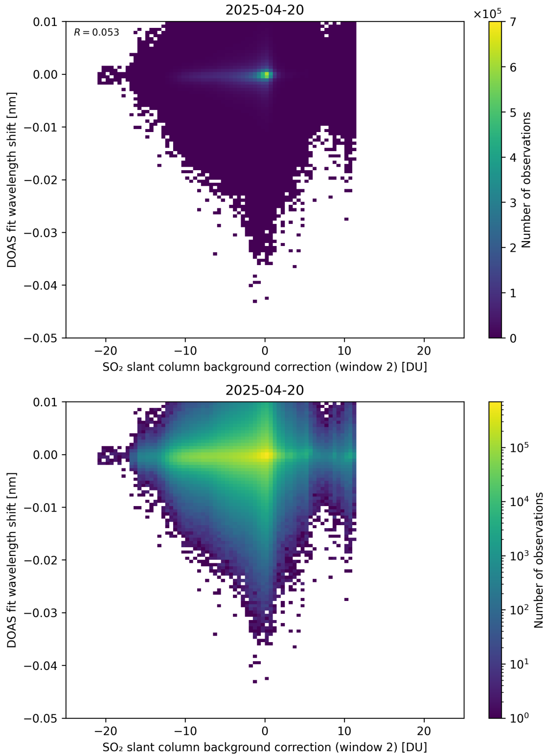
Figure 123: Scatter density plot of “SO 2 slant column background correction (window 2)” against “DOAS fit wavelength shift” for 2025-04-19 to 2025-04-21.
