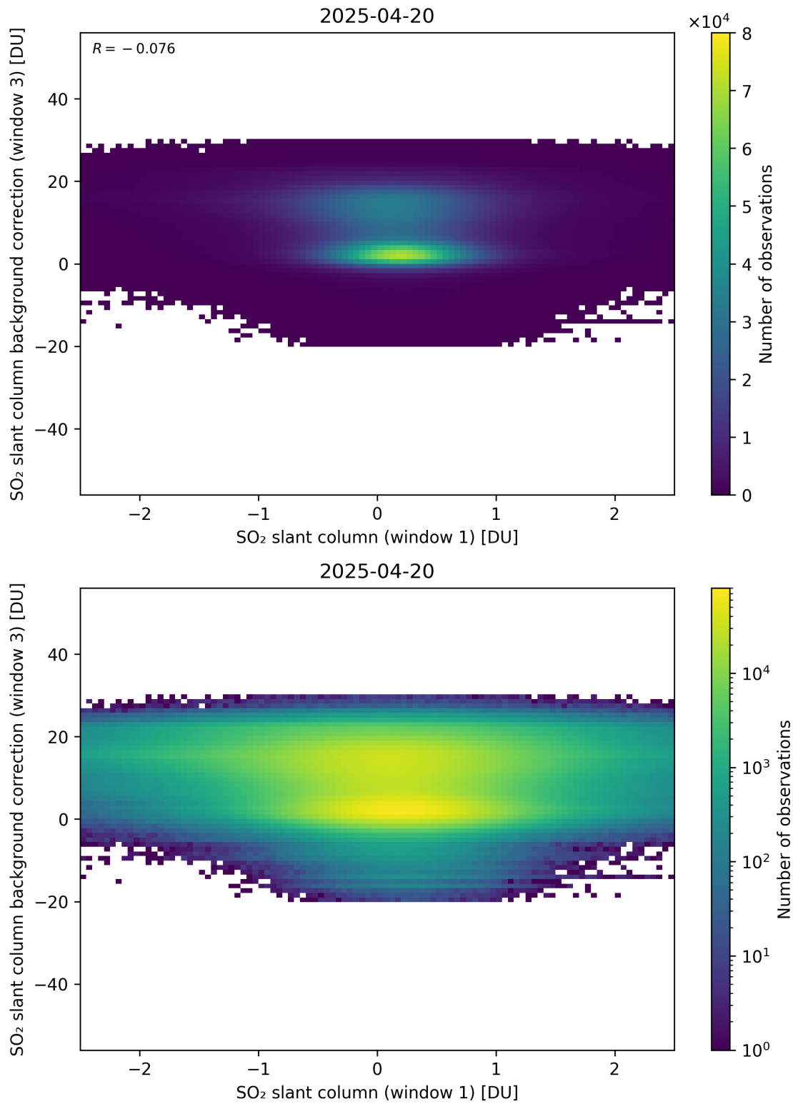
Figure 264: Scatter density plot of “SO 2 slant column (window 1)” against “SO 2 slant column background correction (window 3)” for 2025-04-19 to 2025-04-21.
