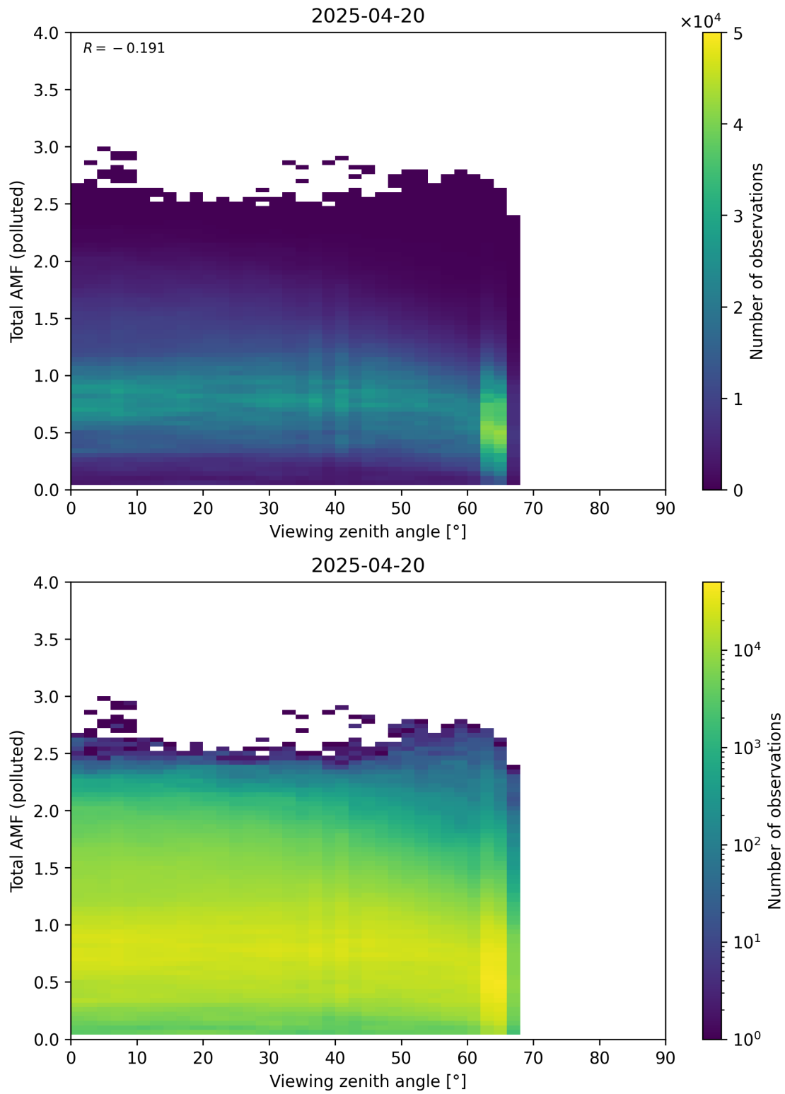
Figure 381: Scatter density plot of “Viewing zenith angle” against “Total AMF (polluted)” for 2025-04-19 to 2025-04-21.
