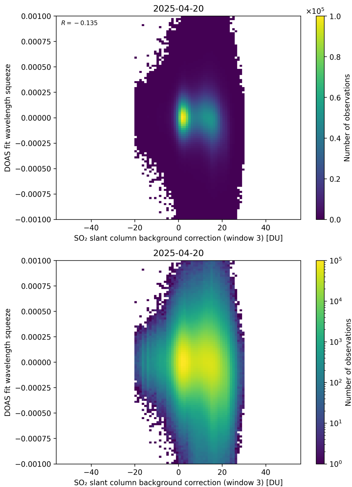
Figure 133: Scatter density plot of “SO 2 slant column background correction (window 3)” against “DOAS fit wavelength squeeze” for 2025-04-19 to 2025-04-21.
