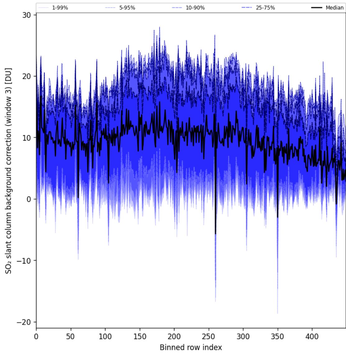
Figure 100: Along track statistics of “SO 2 slant column background correction (window 3)” for 2025-04-19 to 2025-04-21
