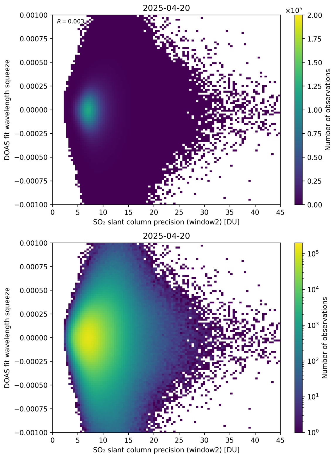
Figure 294: Scatter density plot of “SO 2 slant column precision (window2)” against “DOAS fit wavelength squeeze” for 2025-04-19 to 2025-04-21.
