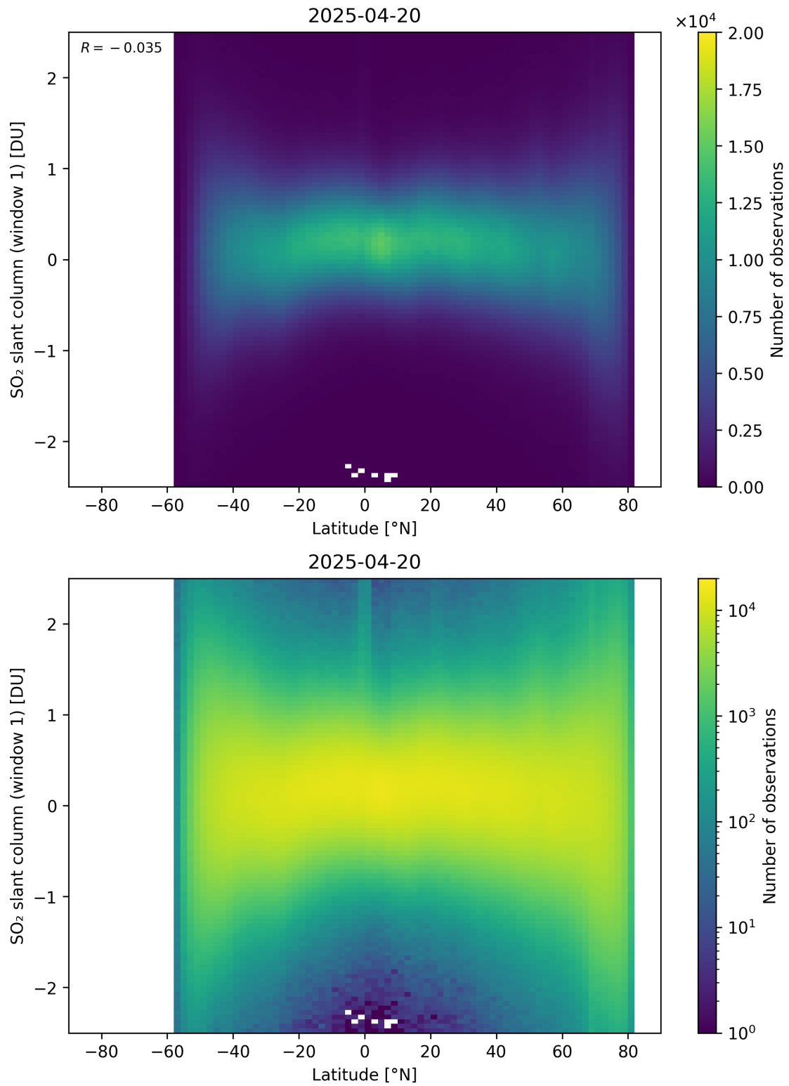
Figure 162: Scatter density plot of “Latitude” against “SO 2 slant column (window 1)” for 2025-04-19 to 2025-04-21.
