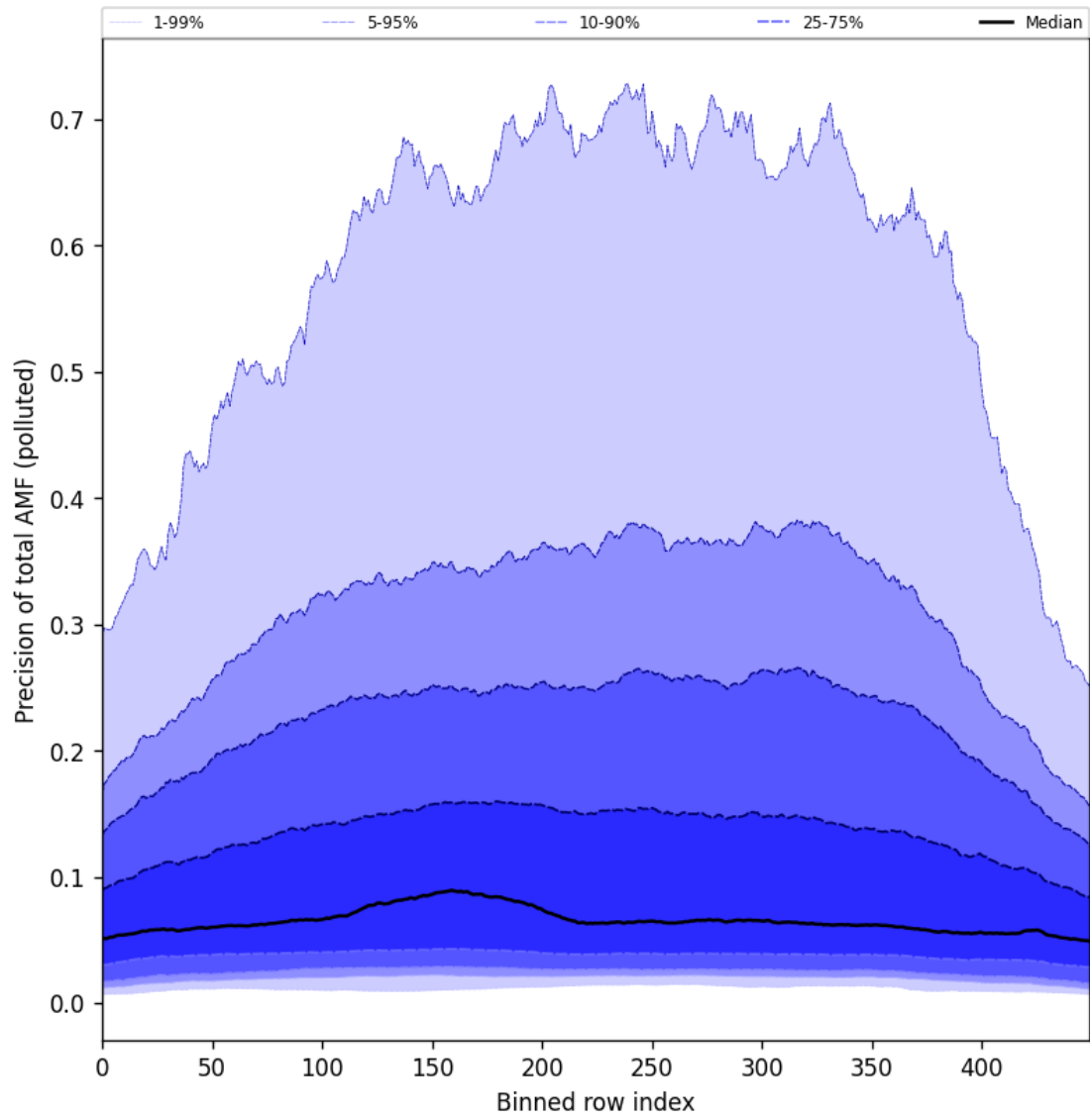
Figure 106: Along track statistics of “Precision of total AMF (polluted)” for 2025-04-20 to 2025-04-22
