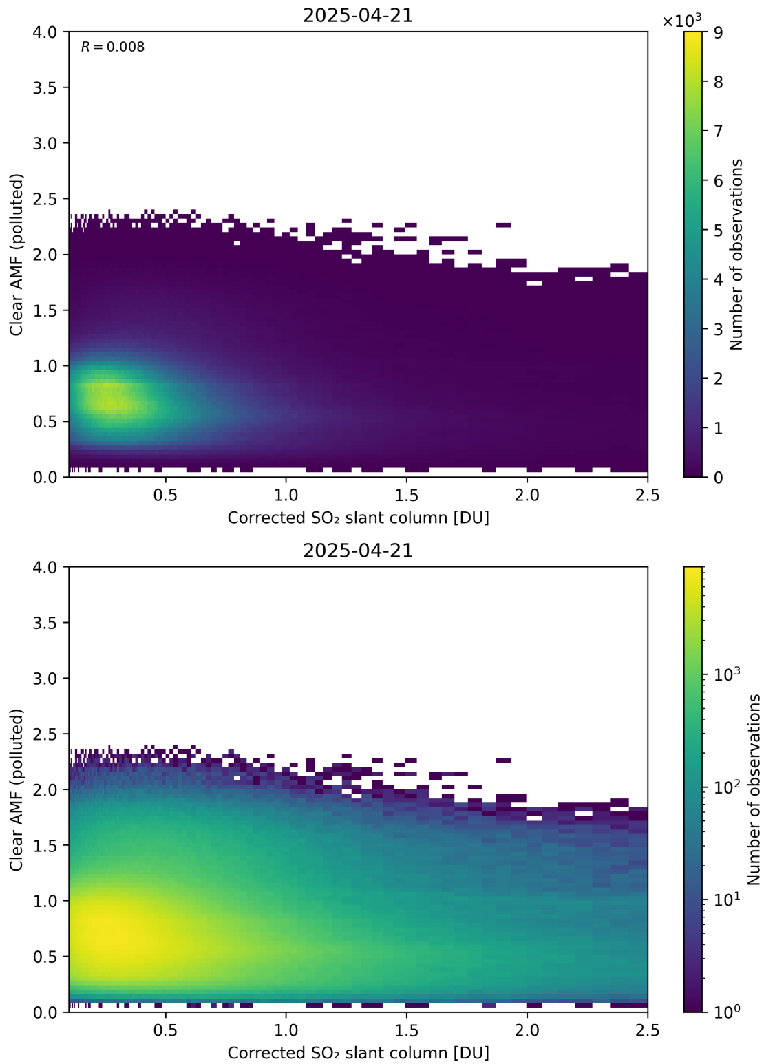
Figure 232: Scatter density plot of “Corrected SO 2 slant column” against “Clear AMF (polluted)” for 2025-04-20 to 2025-04-22.
