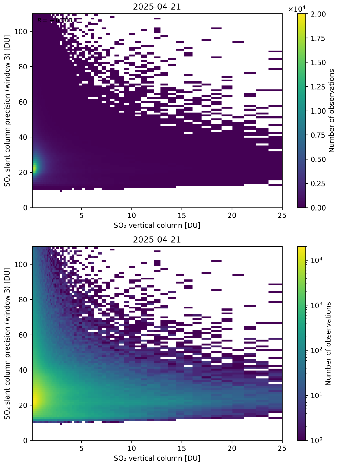
Figure 358: Scatter density plot of “SO 2 vertical column” against “SO 2 slant column precision (window 3)” for 2025-04-20 to 2025-04-22.
