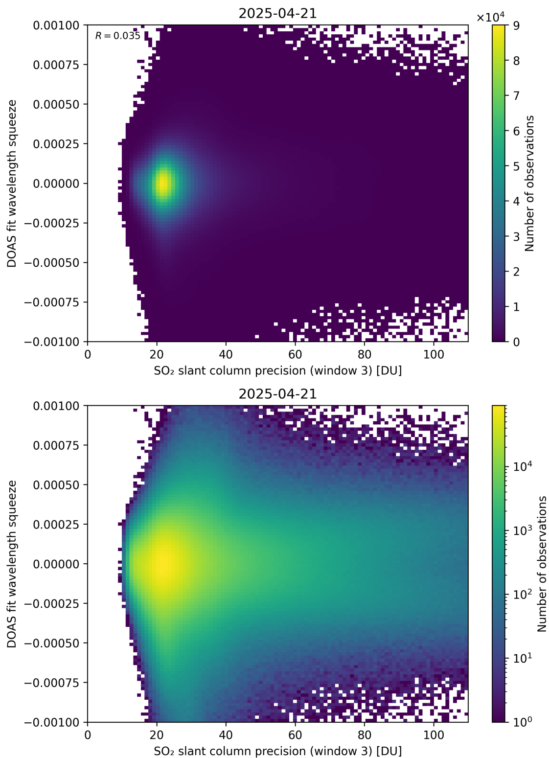
Figure 309: Scatter density plot of “SO 2 slant column precision (window 3)” against “DOAS fit wavelength squeeze” for 2025-04-20 to 2025-04-22.
