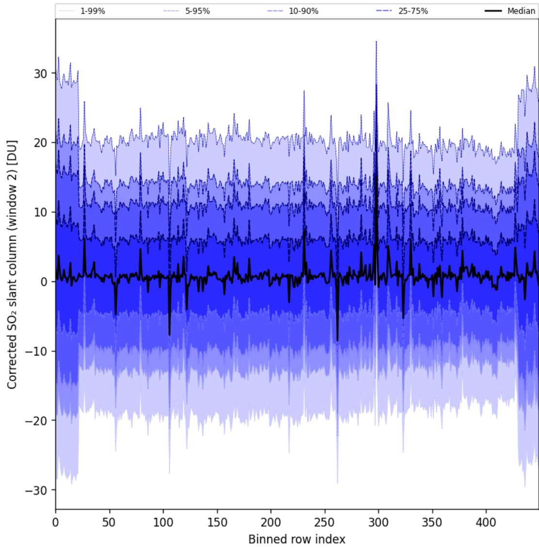
Figure 95: Along track statistics of “Corrected SO 2 slant column (window 2)” for 2025-04-20 to 2025-04-22
