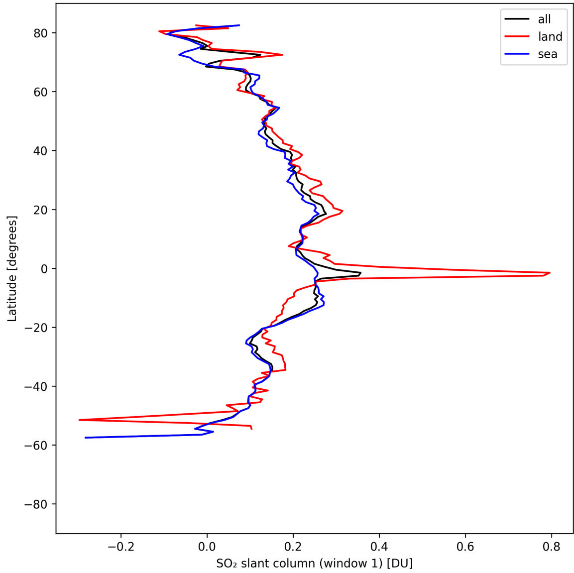
Figure 37: Zonal average of “SO 2 slant column (window 1)” for 2025-04-20 to 2025-04-22.
