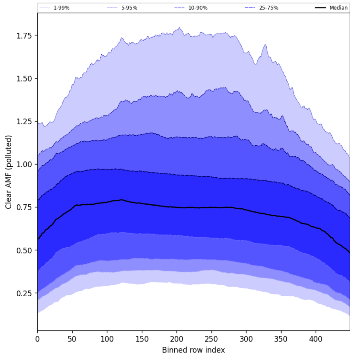
Figure 107: Along track statistics of “Clear AMF (polluted)” for 2025-04-20 to 2025-04-22
