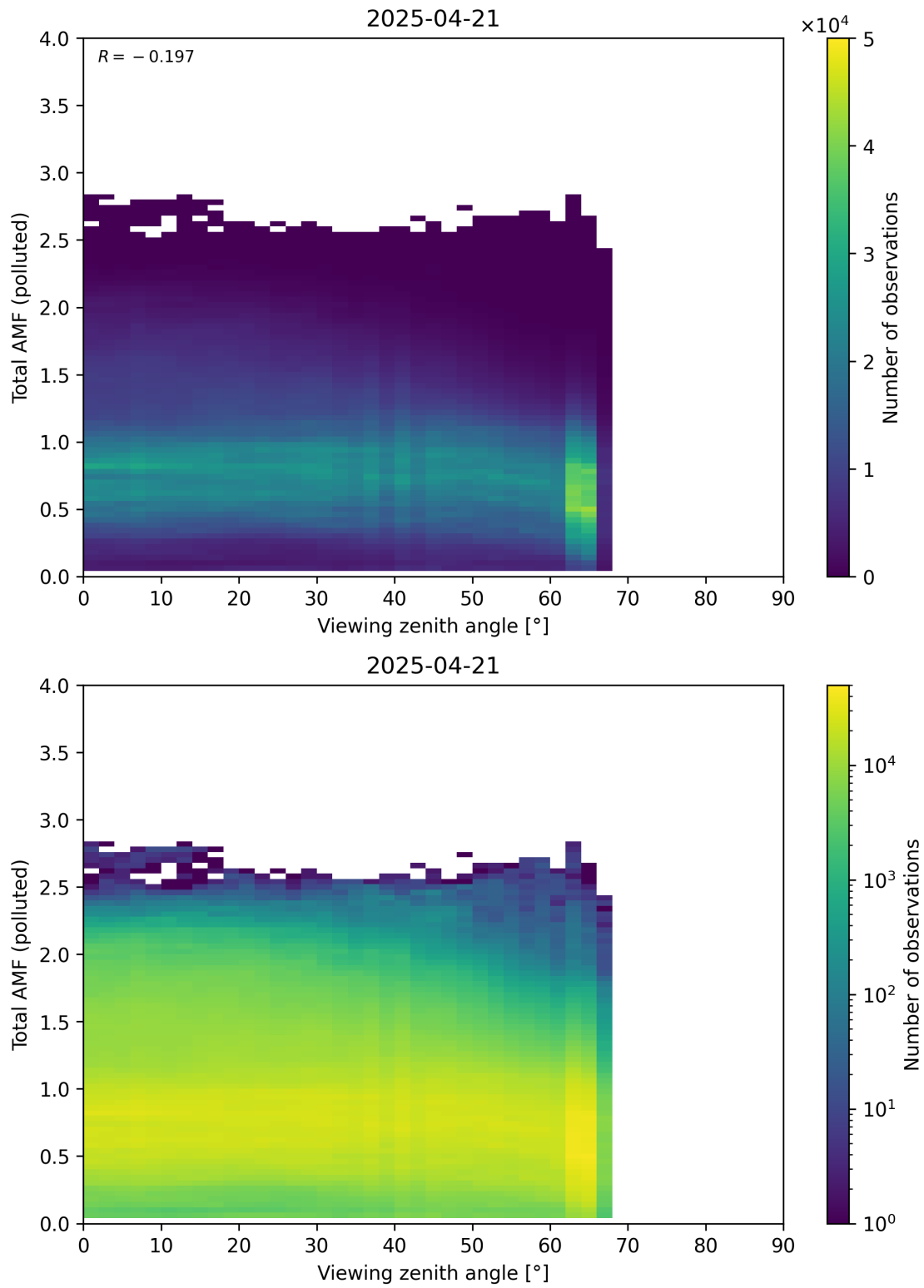
Figure 381: Scatter density plot of “Viewing zenith angle” against “Total AMF (polluted)” for 2025-04-20 to 2025-04-22.
