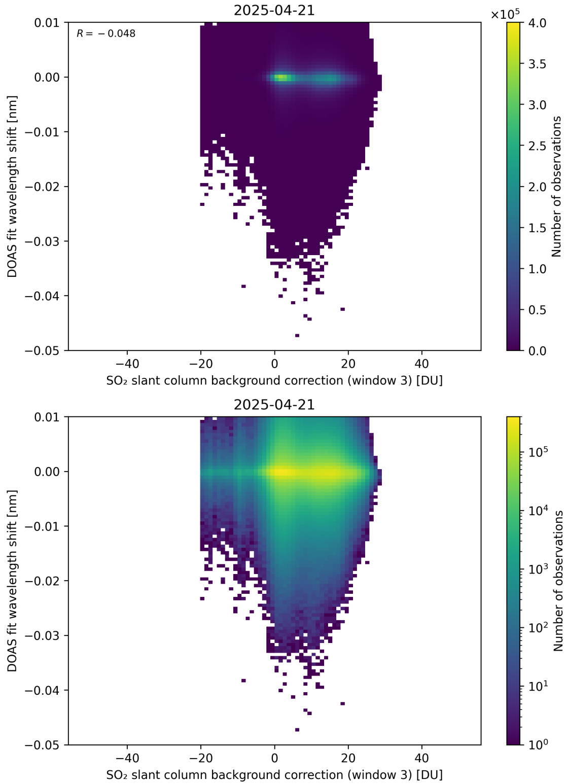
Figure 132: Scatter density plot of “SO 2 slant column background correction (window 3)” against “DOAS fit wavelength shift” for 2025-04-20 to 2025-04-22.
