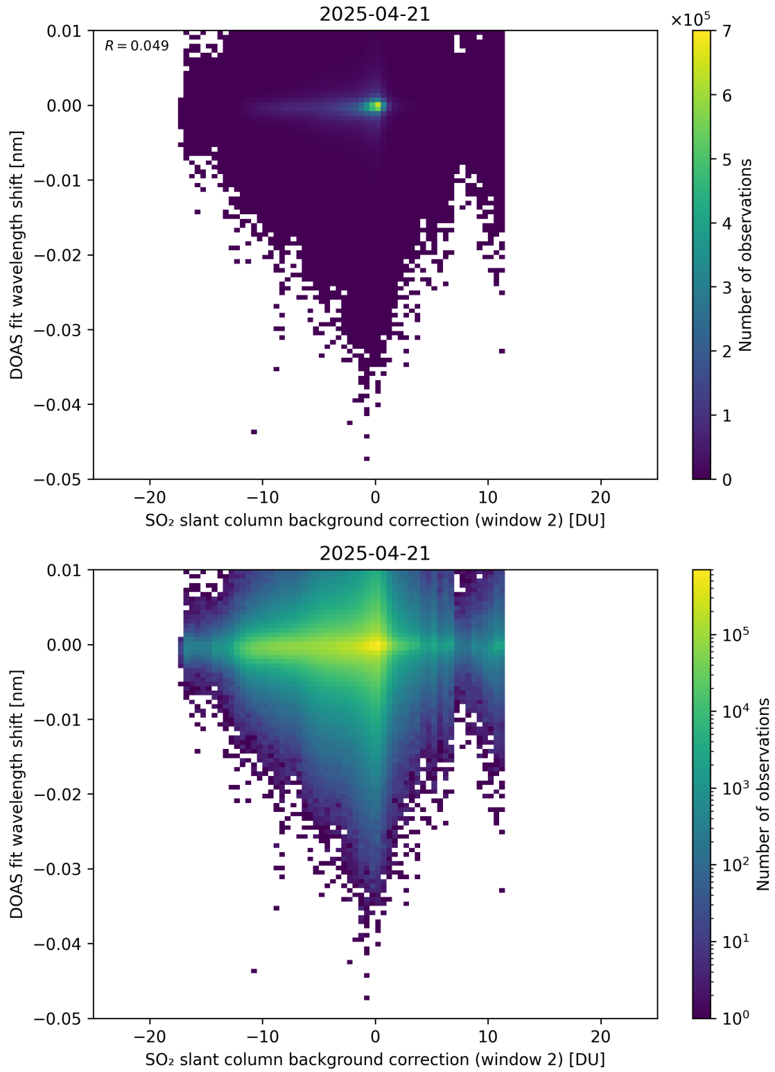
Figure 123: Scatter density plot of “SO 2 slant column background correction (window 2)” against “DOAS fit wavelength shift” for 2025-04-20 to 2025-04-22.
