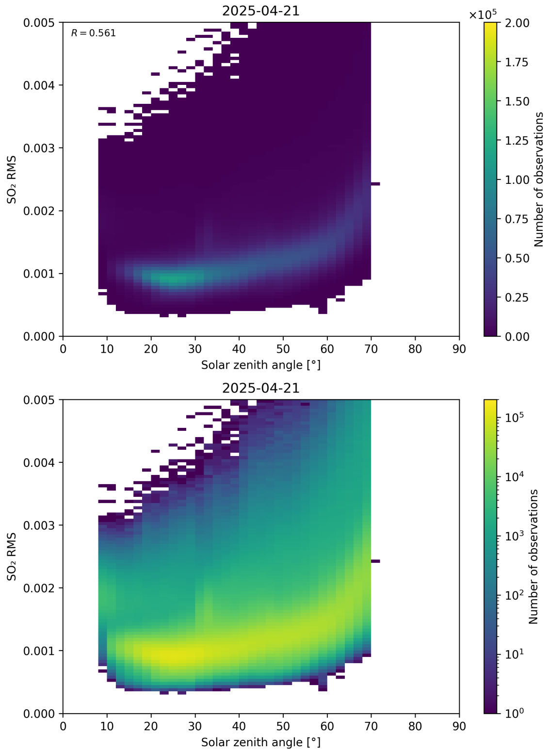
Figure 176: Scatter density plot of “Solar zenith angle” against “SO 2 RMS” for 2025-04-20 to 2025-04-22.
