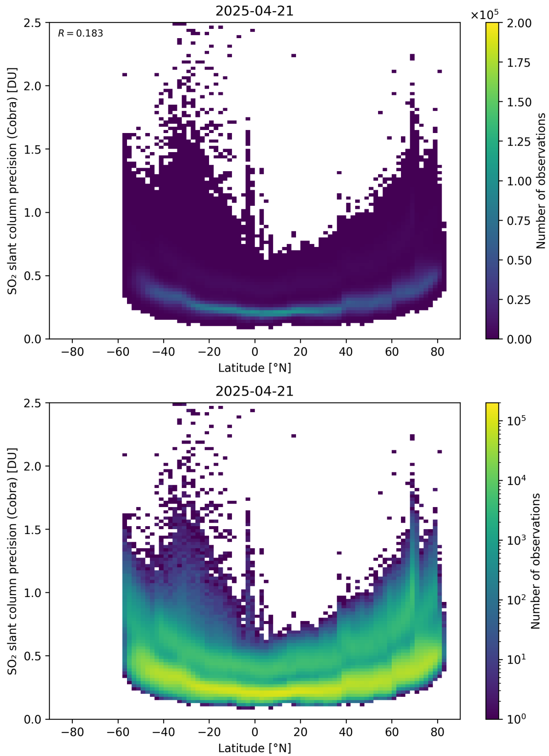
Figure 158: Scatter density plot of “Latitude” against “SO 2 slant column precision (Cobra)” for 2025-04-20 to 2025-04-22.
