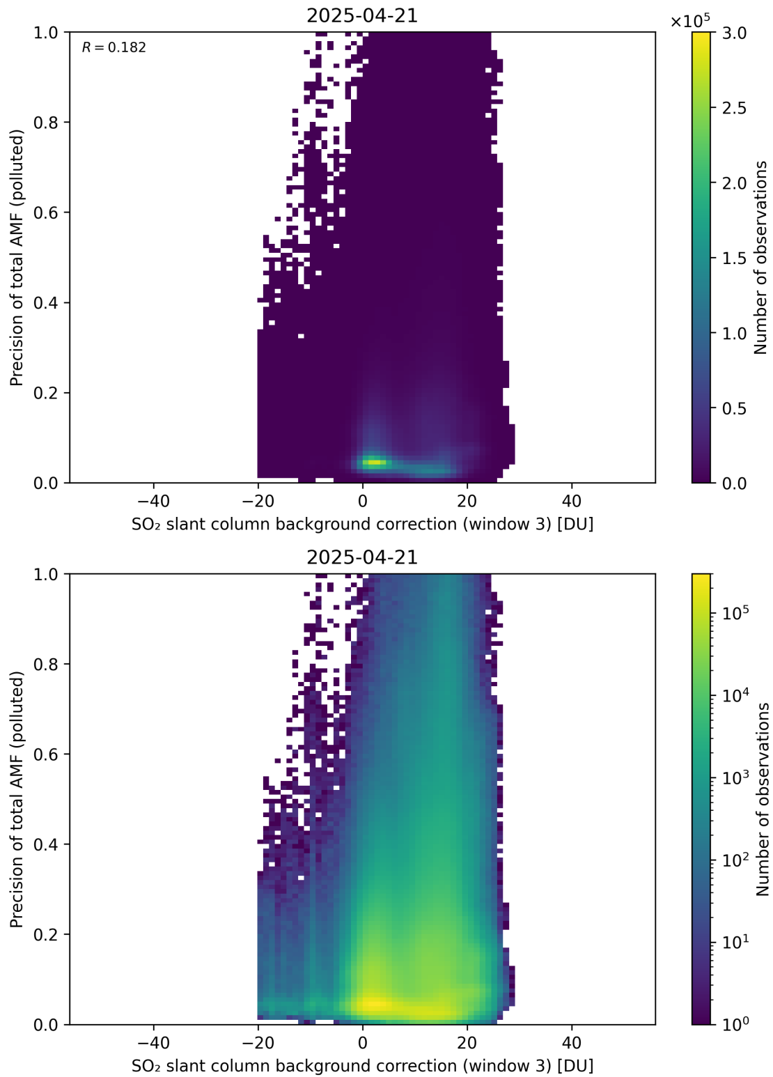
Figure 137: Scatter density plot of “SO 2 slant column background correction (window 3)” against “Precision of total AMF (polluted)” for 2025-04-20 to 2025-04-22.
