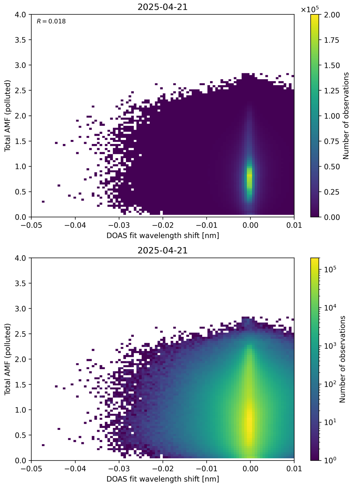
Figure 141: Scatter density plot of “DOAS fit wavelength shift” against “Total AMF (polluted)” for 2025-04-20 to 2025-04-22.
