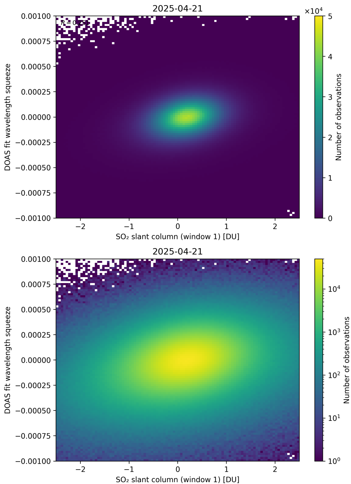
Figure 266: Scatter density plot of “SO 2 slant column (window 1)” against “DOAS fit wavelength squeeze” for 2025-04-20 to 2025-04-22.
