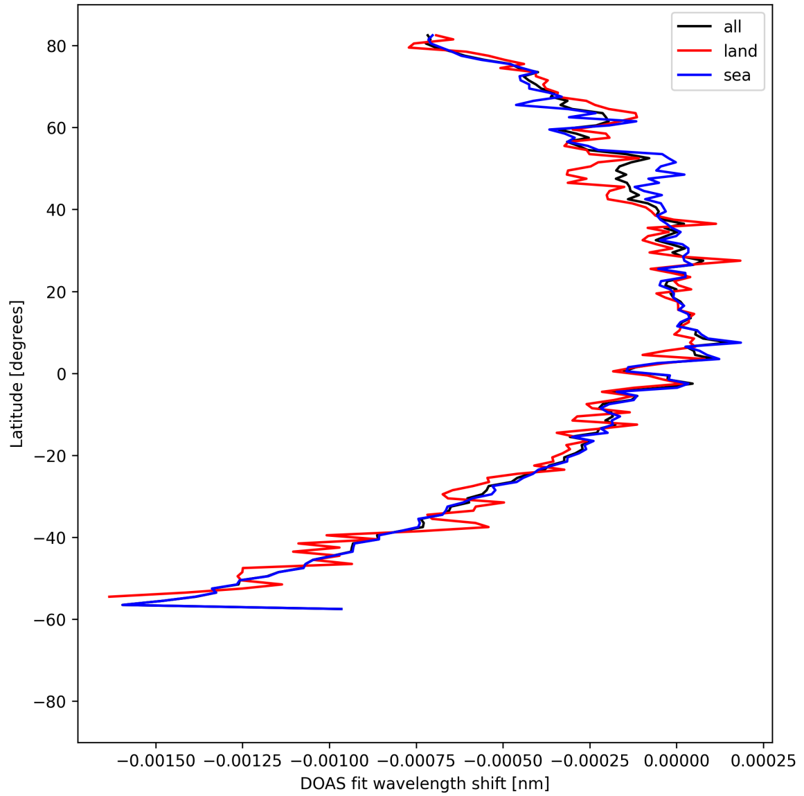
Figure 50: Zonal average of “DOAS fit wavelength shift” for 2025-04-20 to 2025-04-22.
