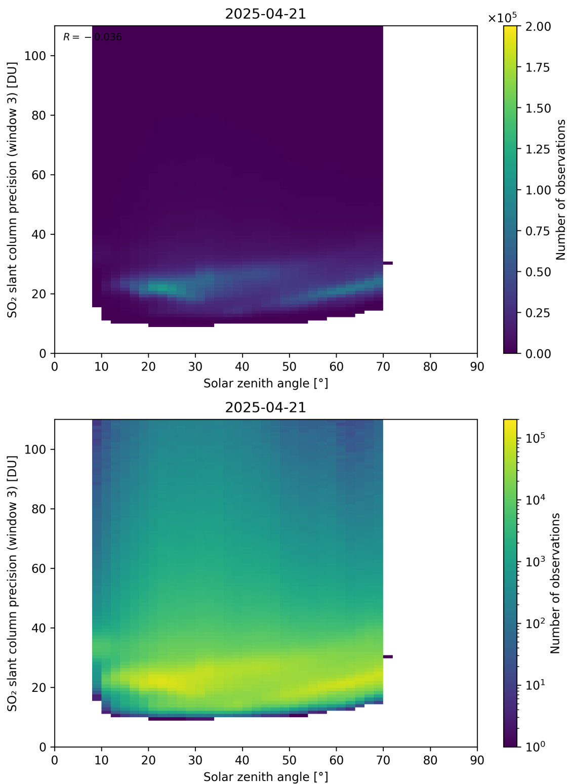
Figure 188: Scatter density plot of “Solar zenith angle” against “SO 2 slant column precision (window 3)” for 2025-04-20 to 2025-04-22.
