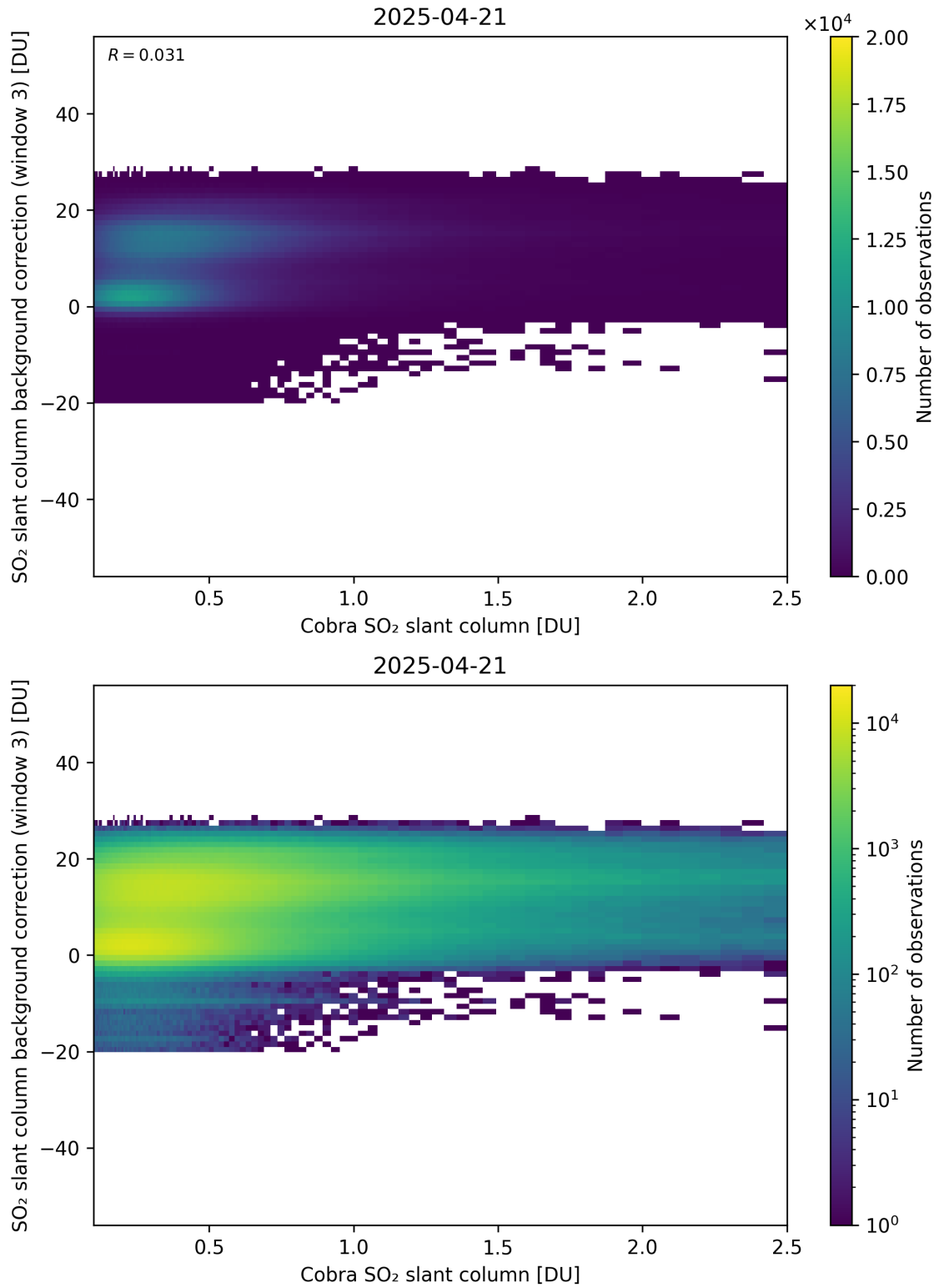
Figure 195: Scatter density plot of “Cobra SO 2 slant column” against “SO 2 slant column background correction (window 3)” for 2025-04-20 to 2025-04-22.
