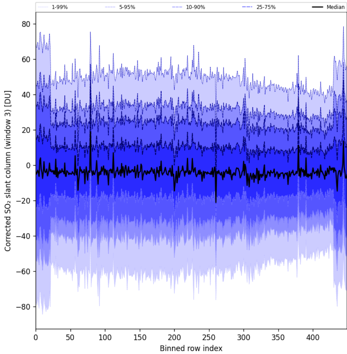
Figure 99: Along track statistics of “Corrected SO 2 slant column (window 3)” for 2025-04-20 to 2025-04-22
