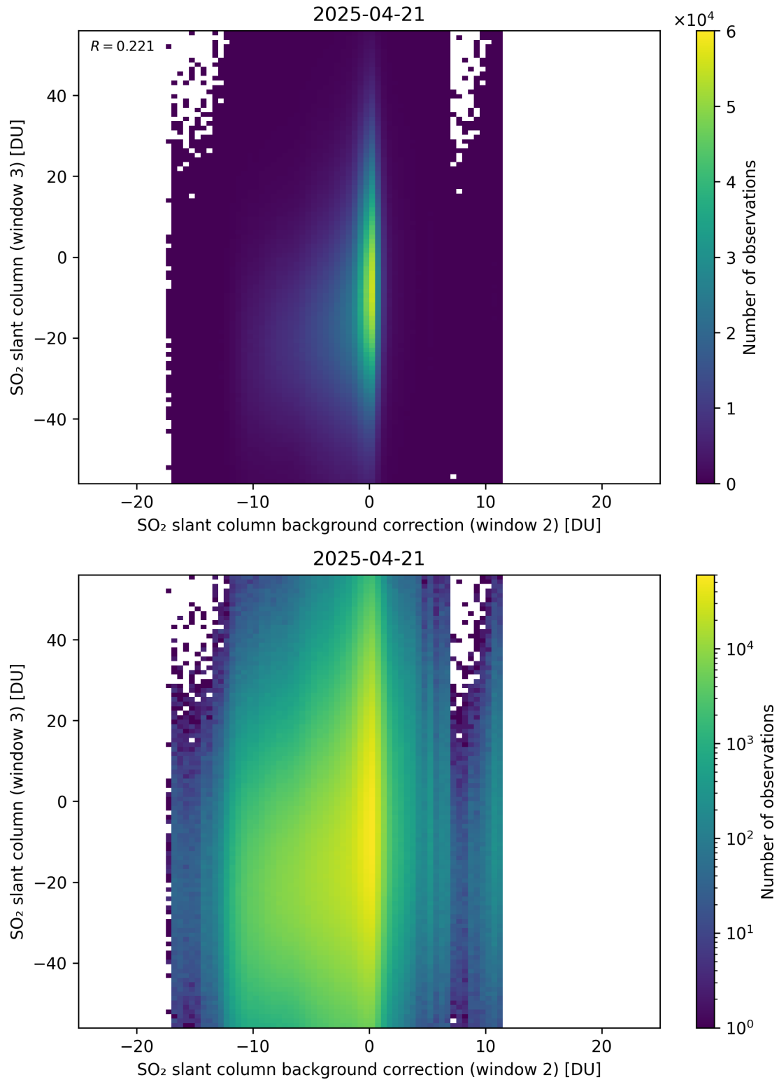
Figure 128: Scatter density plot of “SO 2 slant column background correction (window 2)” against “SO 2 slant column (window 3)” for 2025-04-20 to 2025-04-22.
