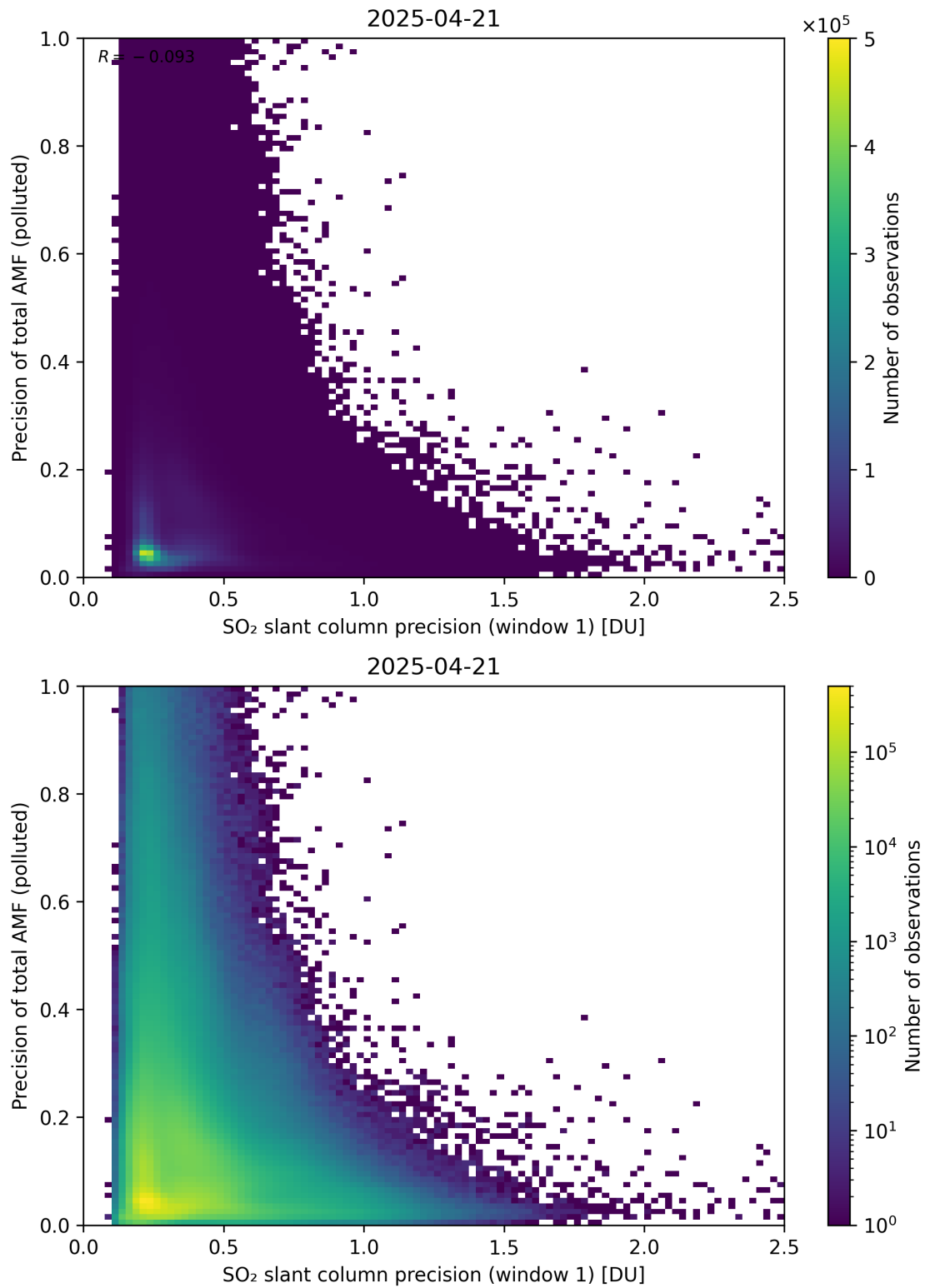
Figure 281: Scatter density plot of “SO 2 slant column precision (window 1)” against “Precision of total AMF (polluted)” for 2025-04-20 to 2025-04-22.
