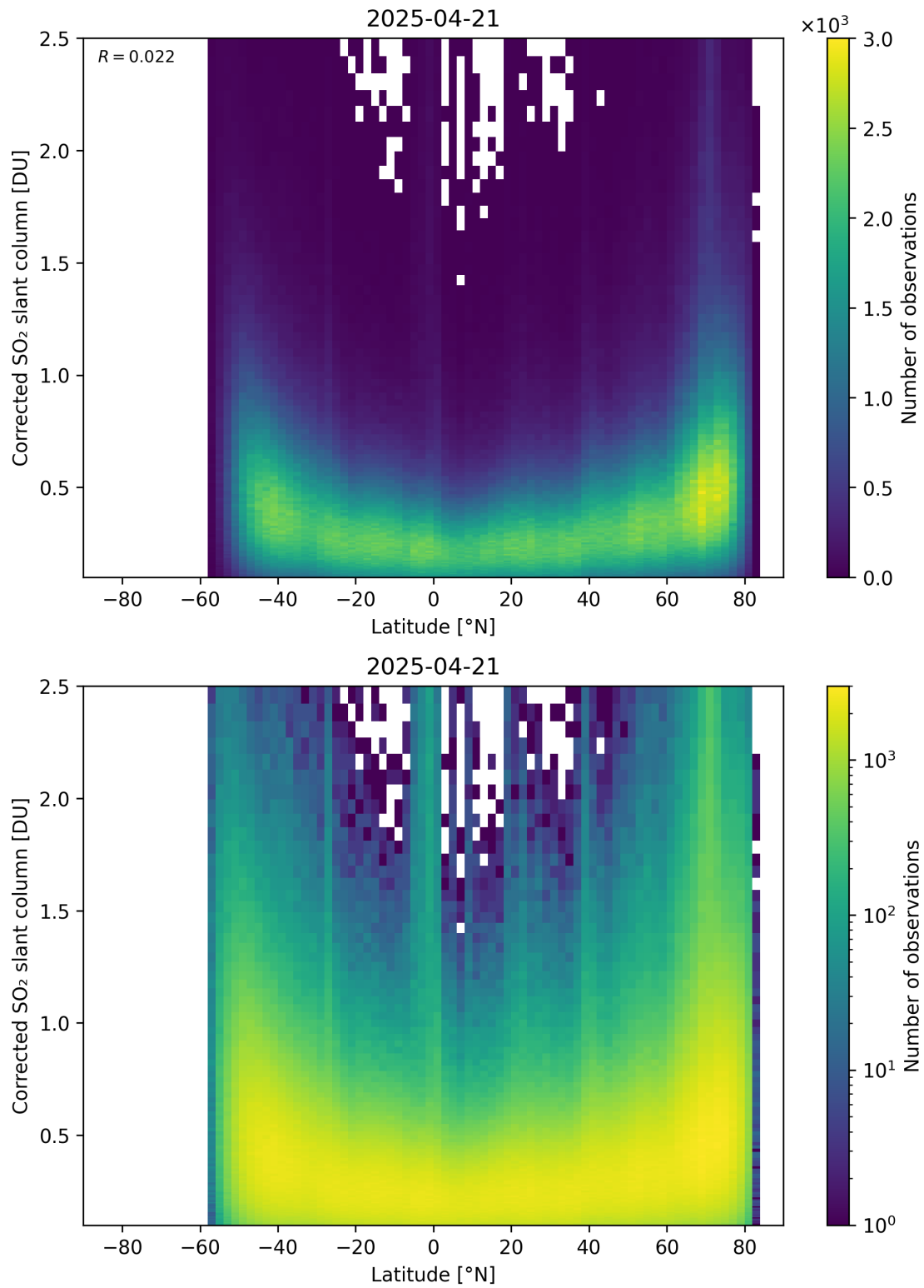
Figure 159: Scatter density plot of “Latitude” against “Corrected SO 2 slant column” for 2025-04-20 to 2025-04-22.
