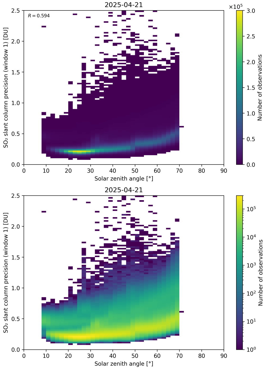
Figure 185: Scatter density plot of “Solar zenith angle” against “SO 2 slant column precision (window 1)” for 2025-04-20 to 2025-04-22.
