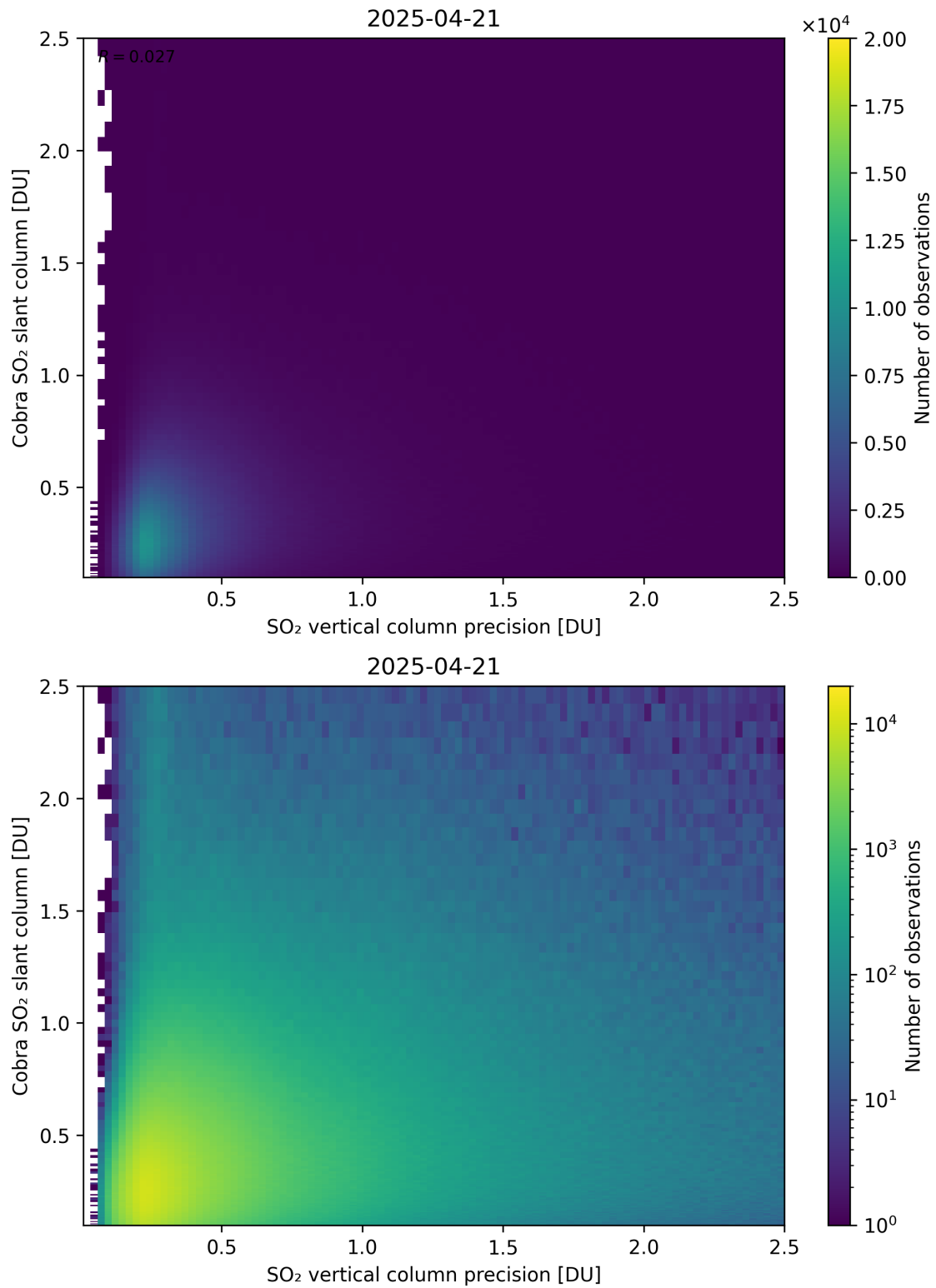
Figure 336: Scatter density plot of “SO 2 vertical column precision” against “Cobra SO 2 slant column” for 2025-04-20 to 2025-04-22.
