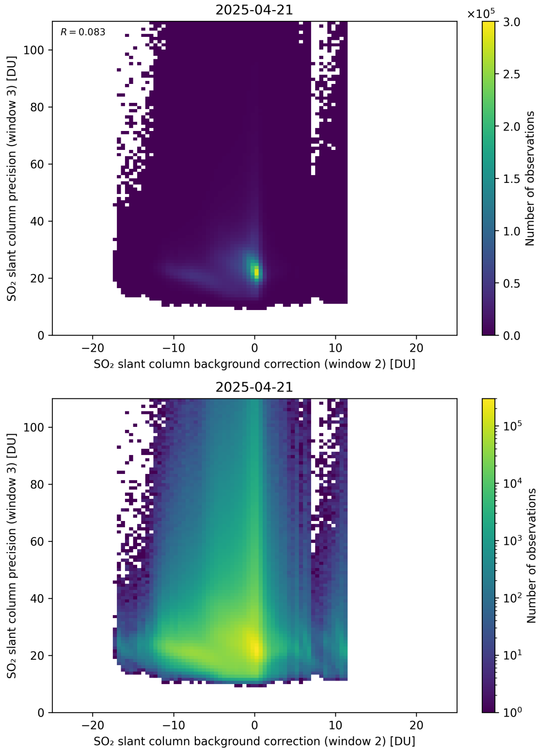
Figure 129: Scatter density plot of “SO 2 slant column background correction (window 2)” against “SO 2 slant column precision (window 3)” for 2025-04-20 to 2025-04-22.
