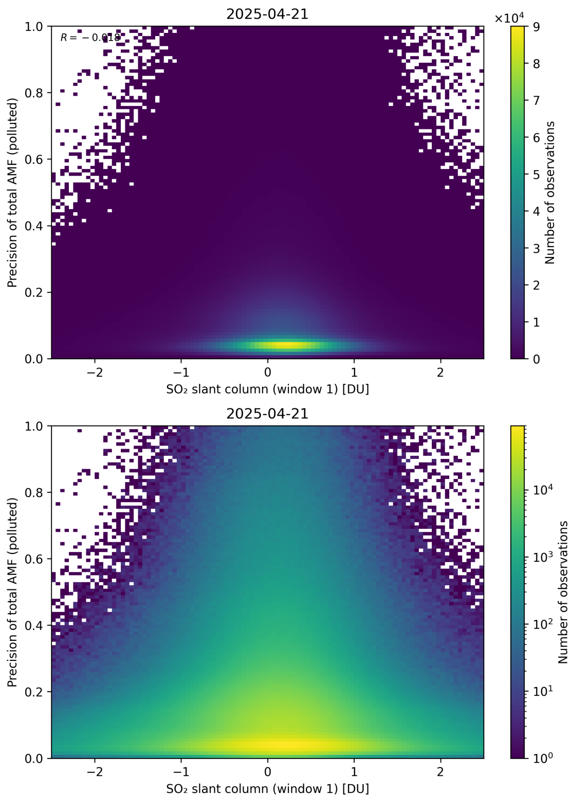
Figure 290: Scatter density plot of “SO 2 slant column (window 1)” against “Precision of total AMF (polluted)” for 2025-04-20 to 2025-04-22.
