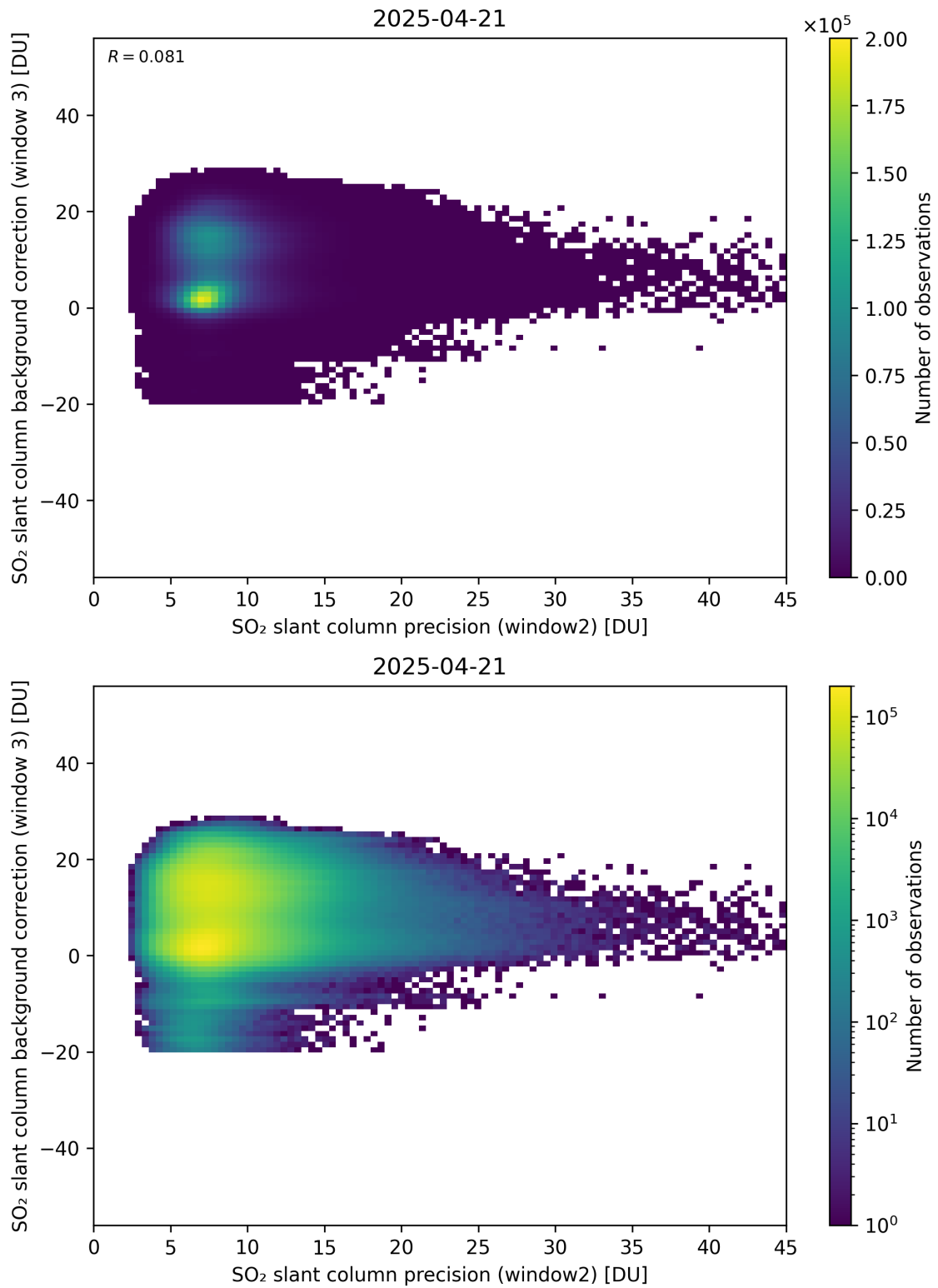
Figure 292: Scatter density plot of “SO 2 slant column precision (window2)” against “SO 2 slant column background correction (window 3)” for 2025-04-20 to 2025-04-22.
