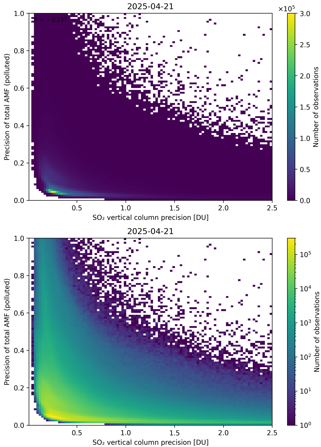
Figure 347: Scatter density plot of “SO 2 vertical column precision” against “Precision of total AMF (polluted)” for 2025-04-20 to 2025-04-22.
