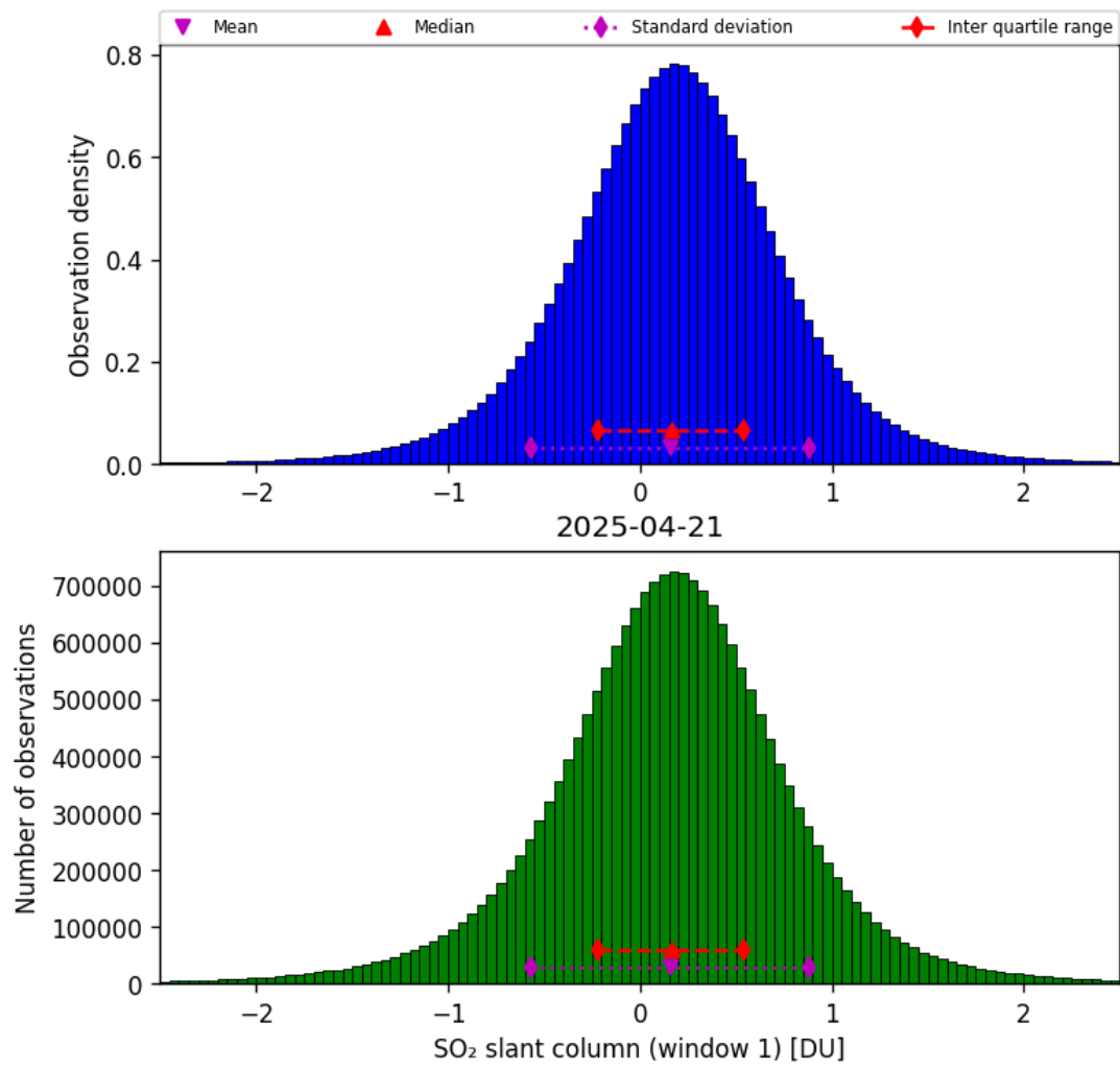
Figure 63: Histogram of “SO 2 slant column (window 1)” for 2025-04-20 to 2025-04-22
