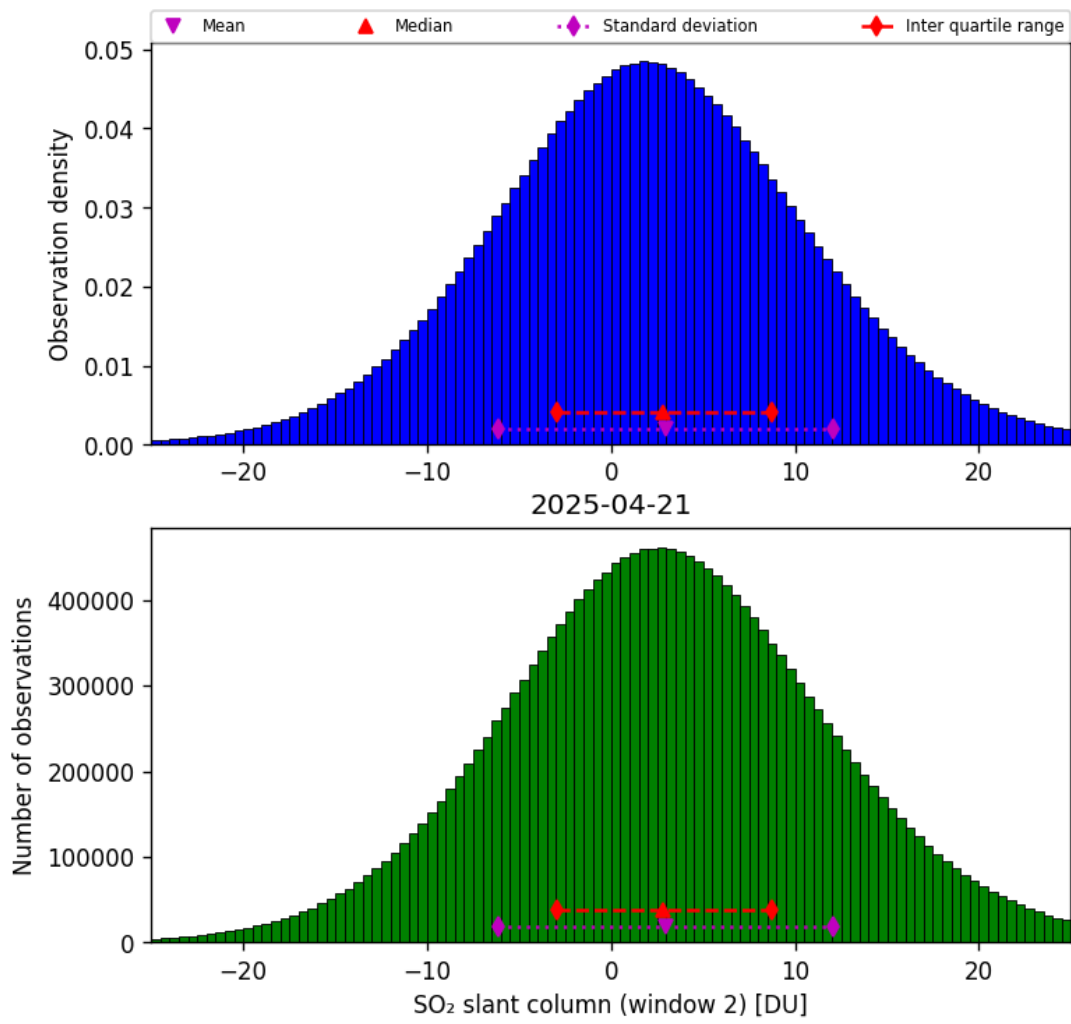
Figure 67: Histogram of “SO 2 slant column (window 2)” for 2025-04-20 to 2025-04-22
