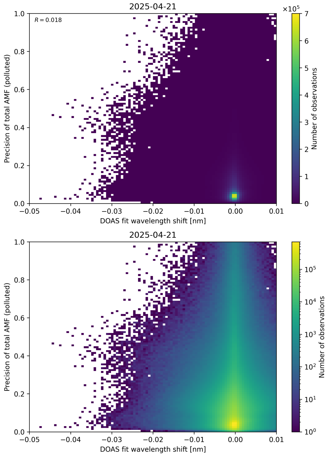
Figure 142: Scatter density plot of “DOAS fit wavelength shift” against “Precision of total AMF (polluted)” for 2025-04-20 to 2025-04-22.
