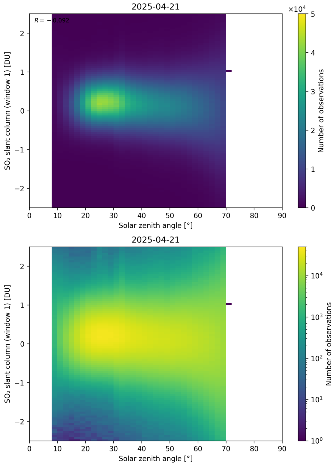
Figure 184: Scatter density plot of “Solar zenith angle” against “SO 2 slant column (window 1)” for 2025-04-20 to 2025-04-22.
