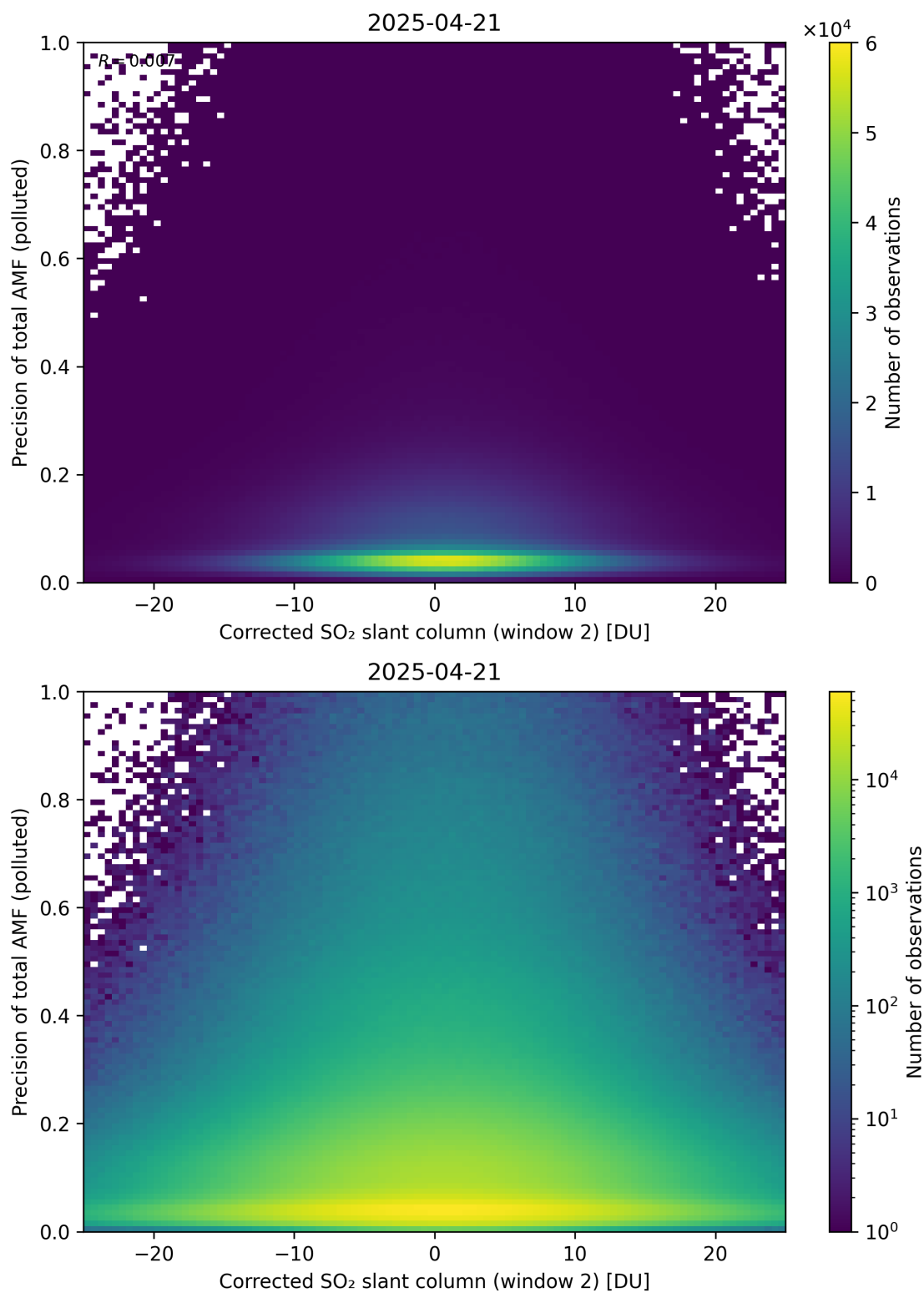
Figure 254: Scatter density plot of “Corrected SO 2 slant column (window 2)” against “Precision of total AMF (polluted)” for 2025-04-20 to 2025-04-22.
