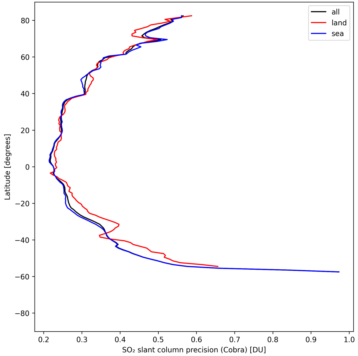
Figure 36: Zonal average of “SO 2 slant column precision (Cobra)” for 2025-04-20 to 2025-04-22.
