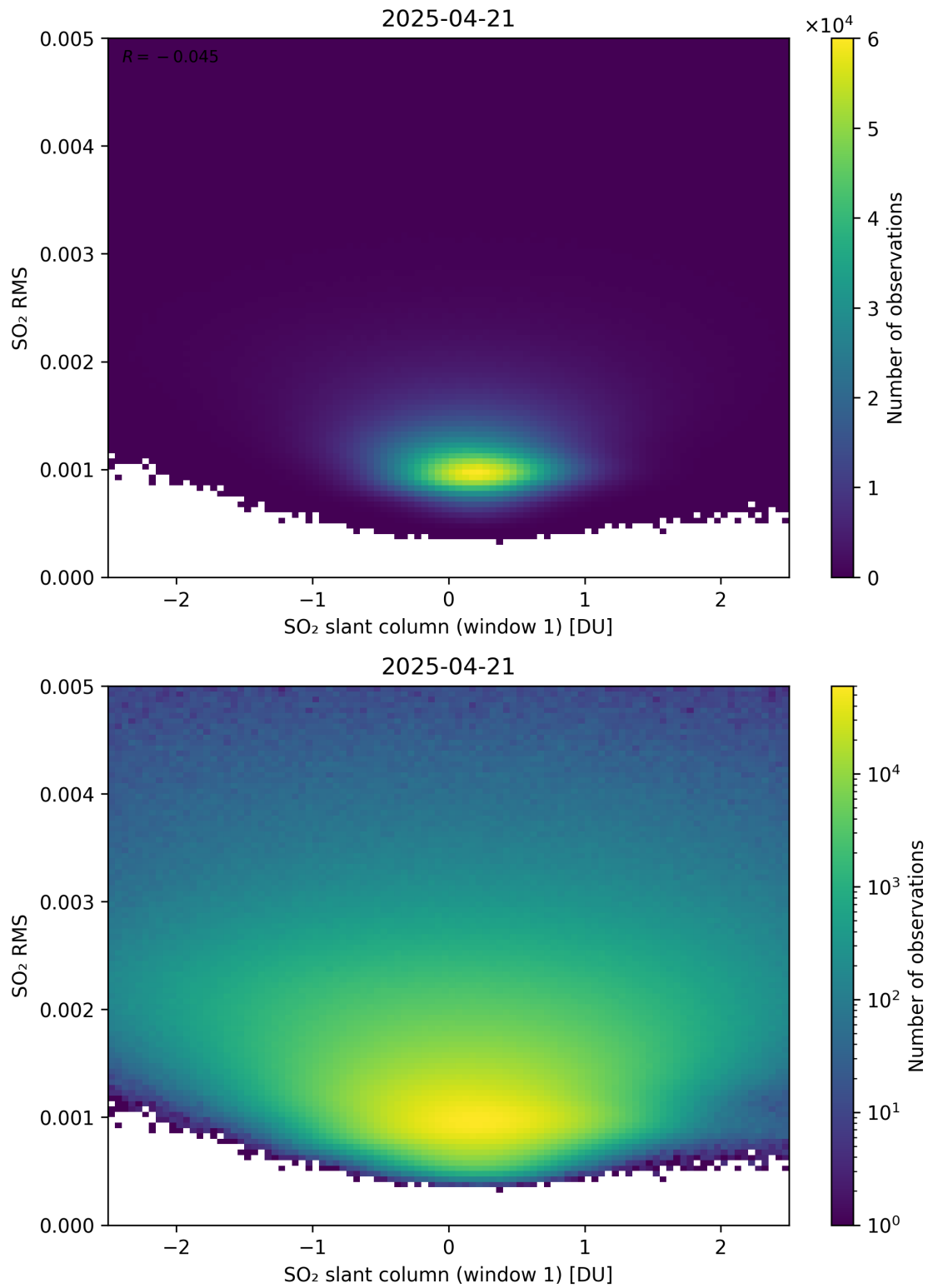
Figure 267: Scatter density plot of “SO 2 slant column (window 1)” against “SO 2 RMS” for 2025-04-20 to 2025-04-22.
