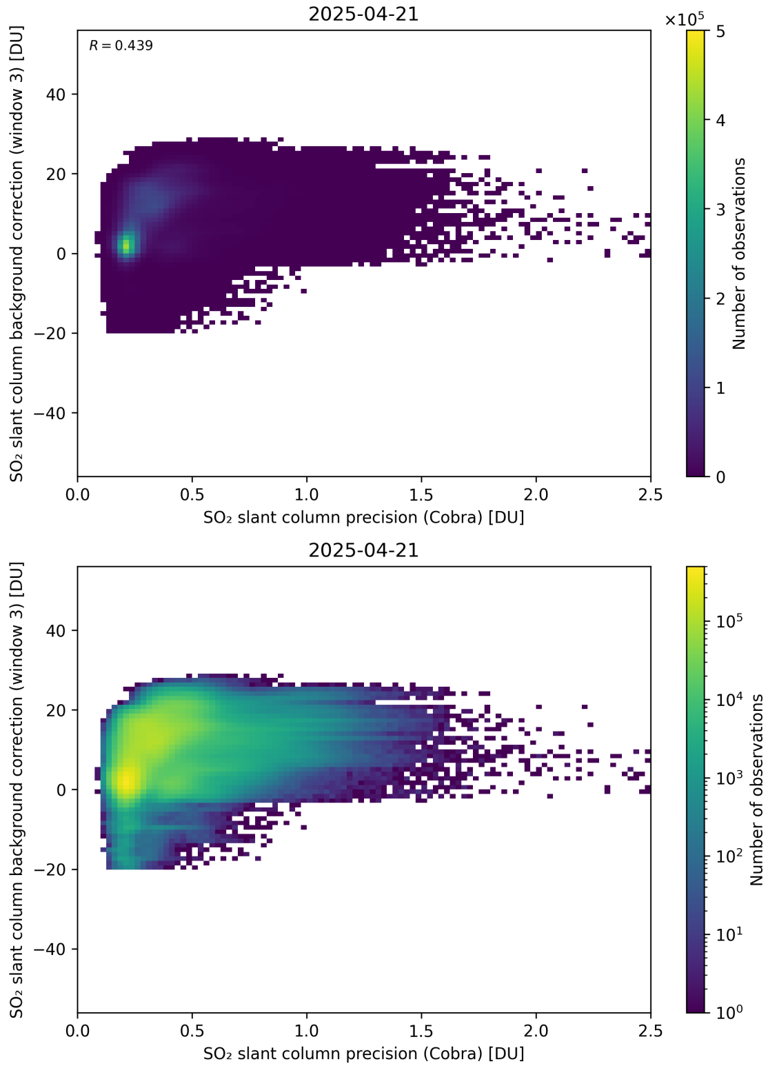
Figure 201: Scatter density plot of “SO 2 slant column precision (Cobra)” against “SO 2 slant column background correction (window 3)” for 2025-04-20 to 2025-04-22.
