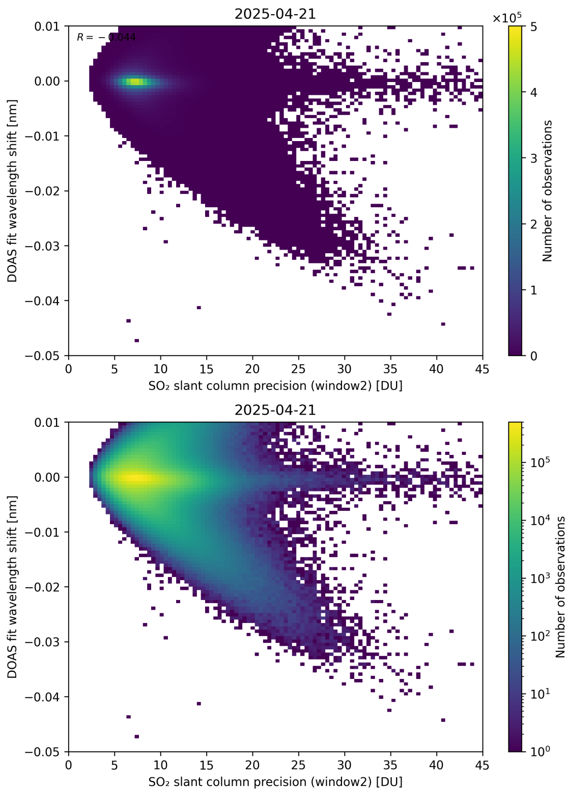
Figure 293: Scatter density plot of “SO 2 slant column precision (window2)” against “DOAS fit wavelength shift” for 2025-04-20 to 2025-04-22.
