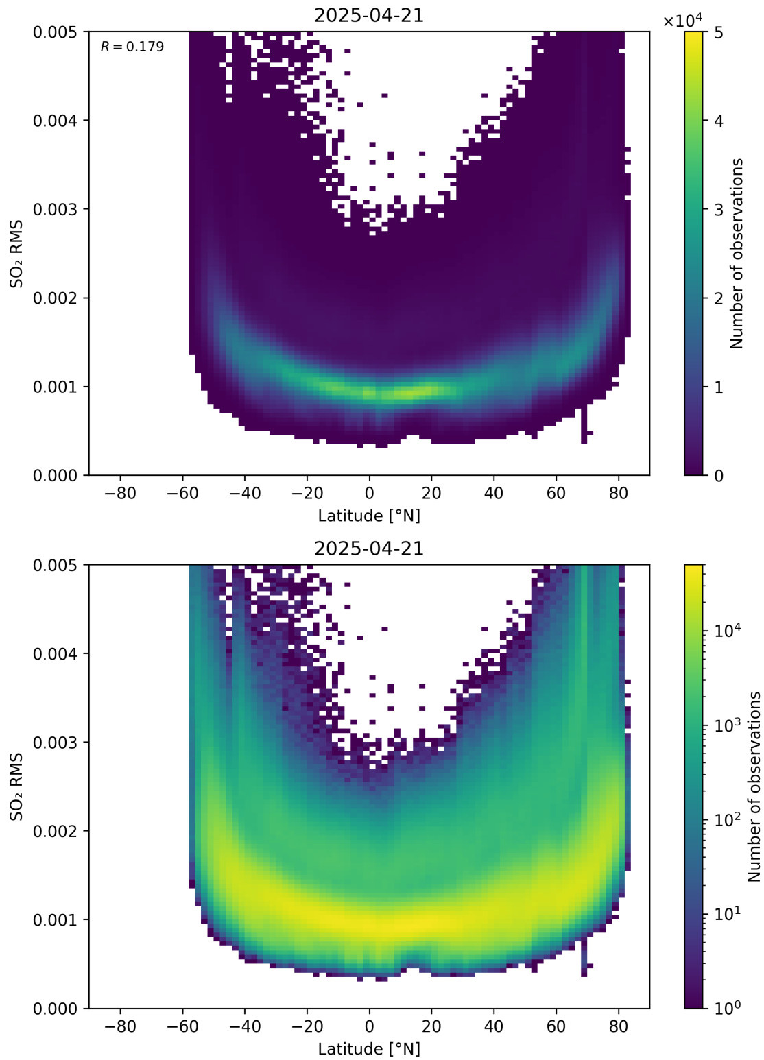
Figure 155: Scatter density plot of “Latitude” against “SO 2 RMS” for 2025-04-20 to 2025-04-22.
