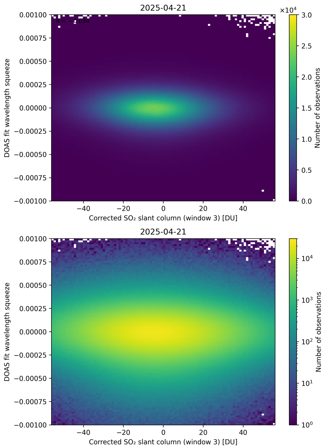
Figure 257: Scatter density plot of “Corrected SO 2 slant column (window 3)” against “DOAS fit wavelength squeeze” for 2025-04-20 to 2025-04-22.
