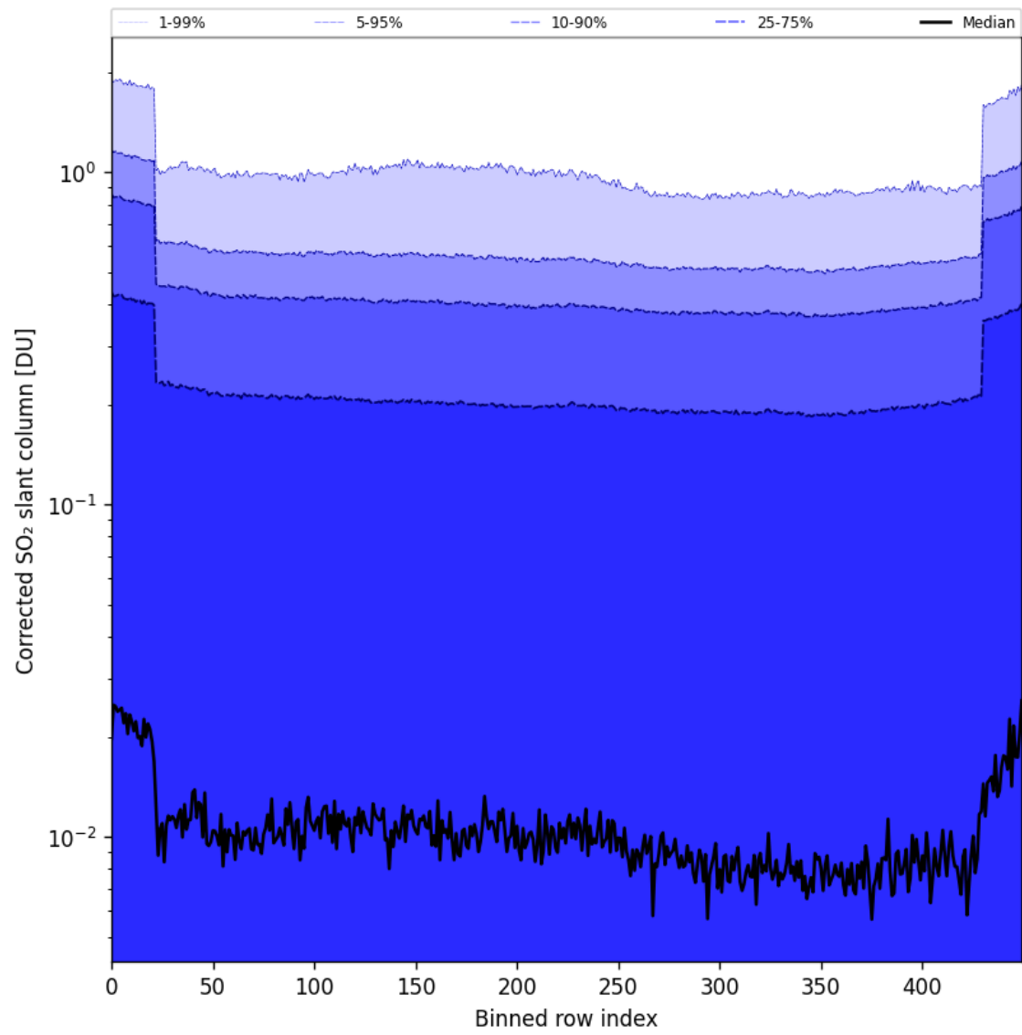
Figure 86: Along track statistics of “Corrected SO 2 slant column” for 2025-04-20 to 2025-04-22
