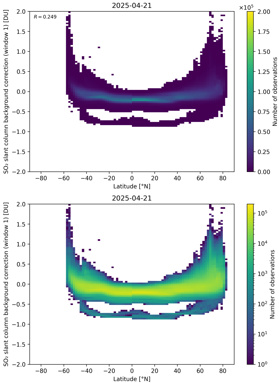
Figure 150: Scatter density plot of “Latitude” against “SO 2 slant column background correction (window 1)” for 2025-04-20 to 2025-04-22.
