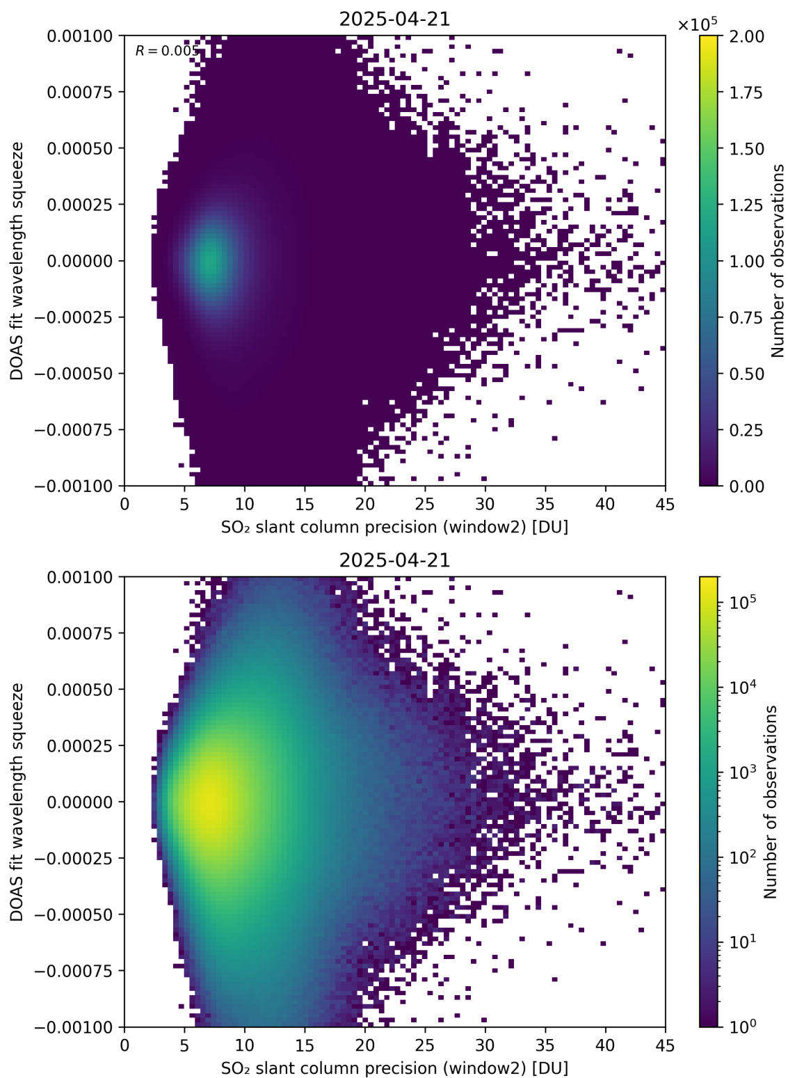
Figure 294: Scatter density plot of “SO 2 slant column precision (window2)” against “DOAS fit wavelength squeeze” for 2025-04-20 to 2025-04-22.
