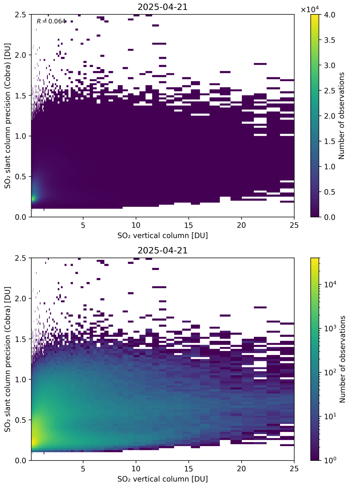
Figure 350: Scatter density plot of “SO 2 vertical column” against “SO 2 slant column precision (Cobra)” for 2025-04-20 to 2025-04-22.
