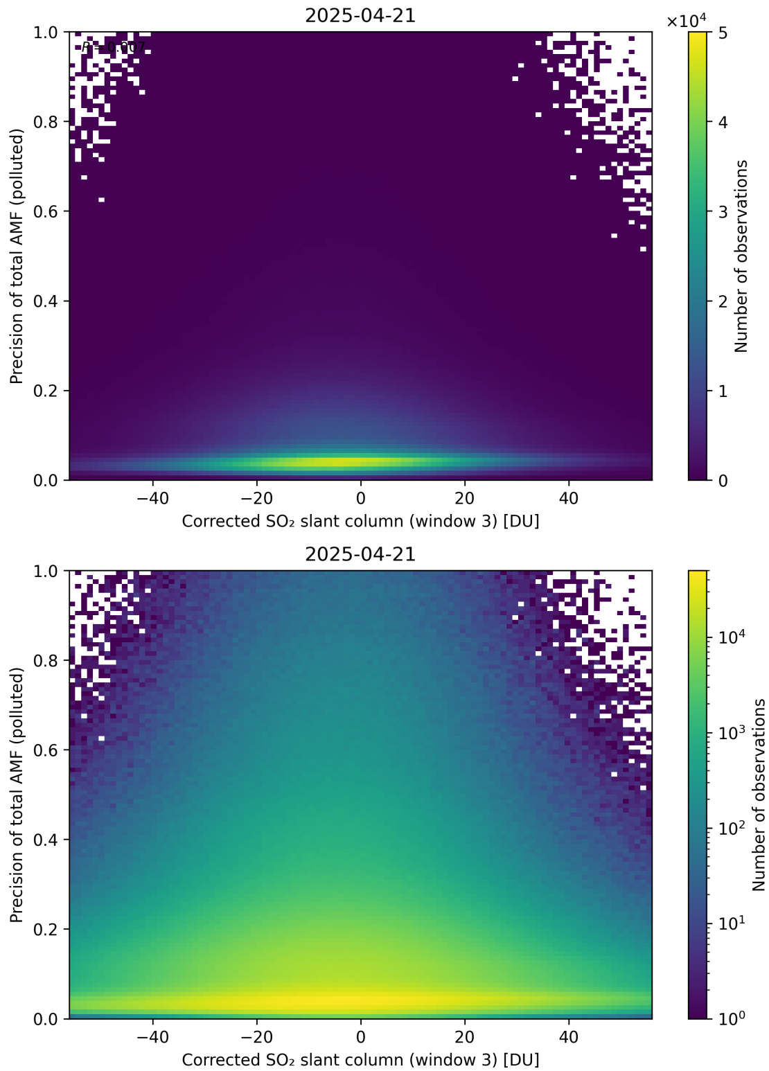
Figure 261: Scatter density plot of “Corrected SO 2 slant column (window 3)” against “Precision of total AMF (polluted)” for 2025-04-20 to 2025-04-22.
