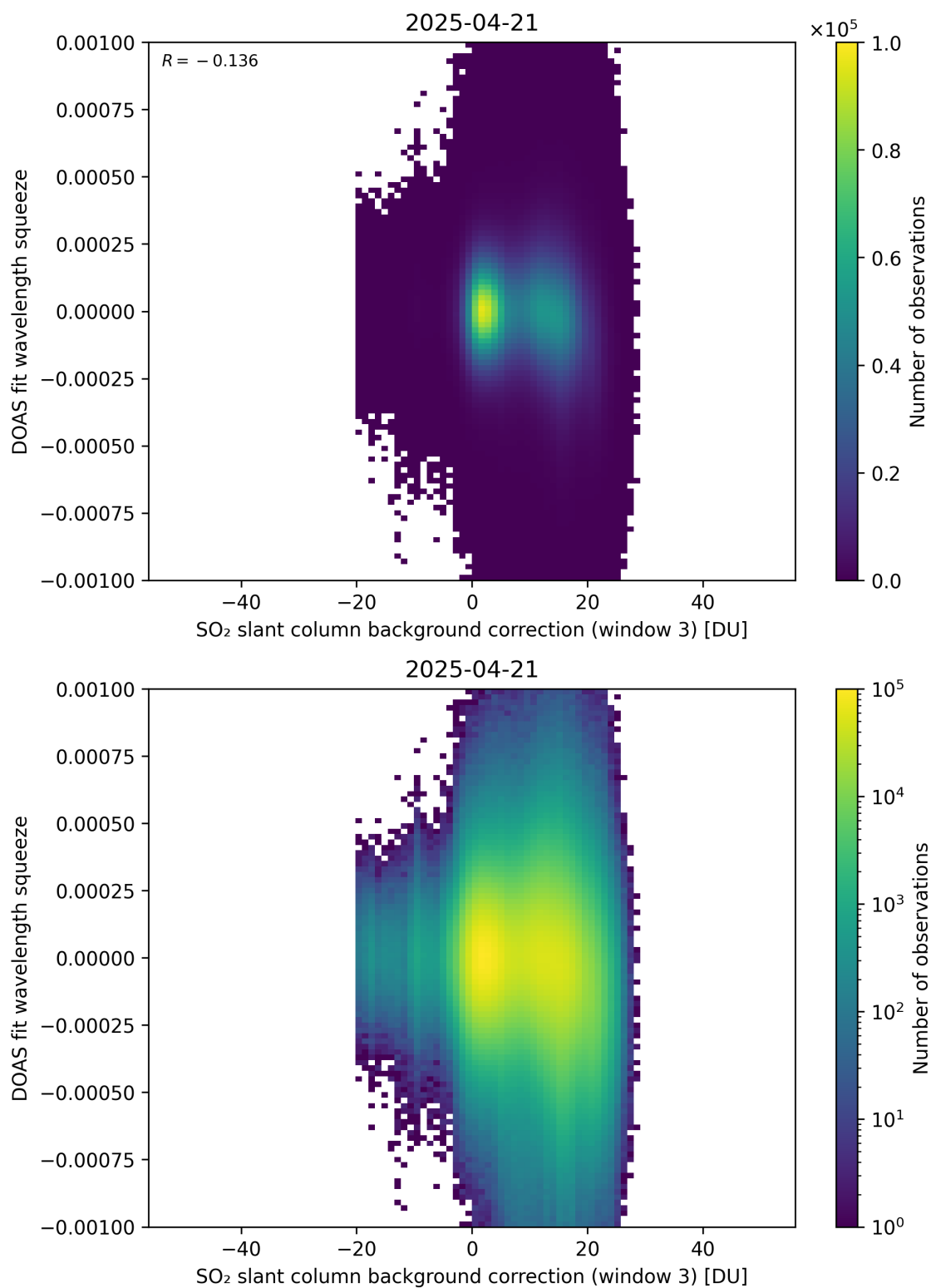
Figure 133: Scatter density plot of “SO 2 slant column background correction (window 3)” against “DOAS fit wavelength squeeze” for 2025-04-20 to 2025-04-22.
