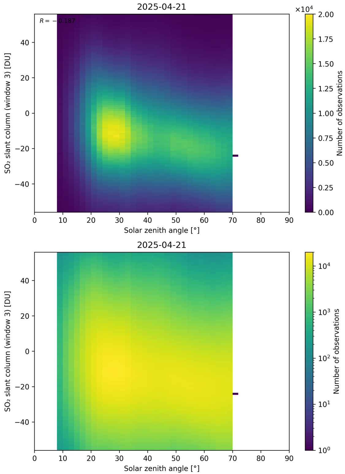
Figure 187: Scatter density plot of “Solar zenith angle” against “SO 2 slant column (window 3)” for 2025-04-20 to 2025-04-22.
