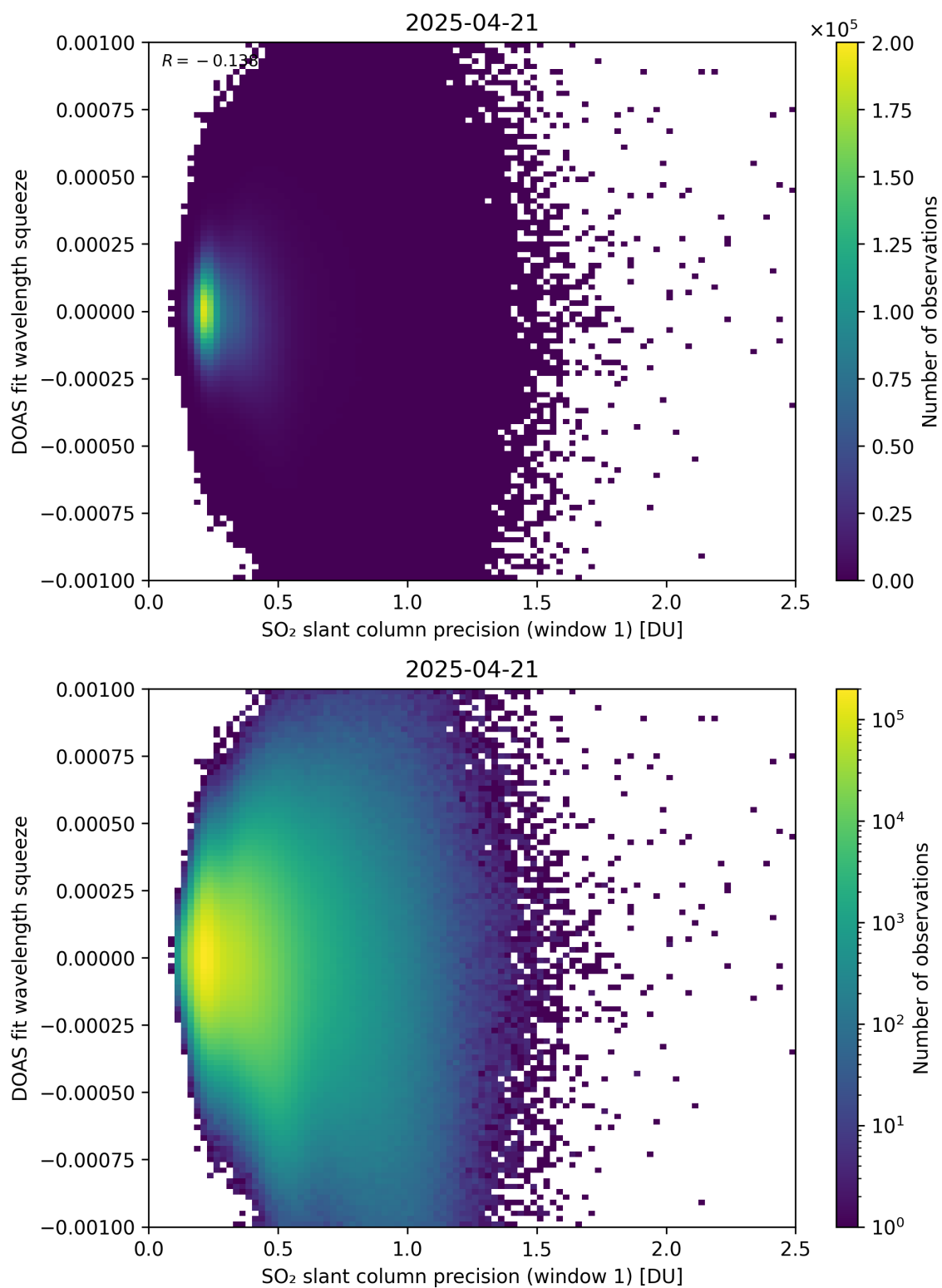
Figure 272: Scatter density plot of “SO 2 slant column precision (window 1)” against “DOAS fit wavelength squeeze” for 2025-04-20 to 2025-04-22.
