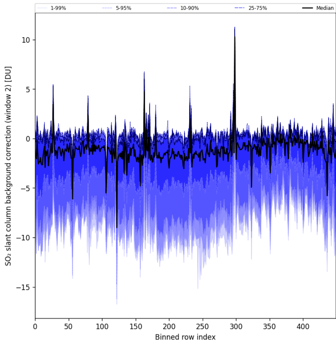
Figure 96: Along track statistics of “SO 2 slant column background correction (window 2)” for 2025-04-20 to 2025-04-22
