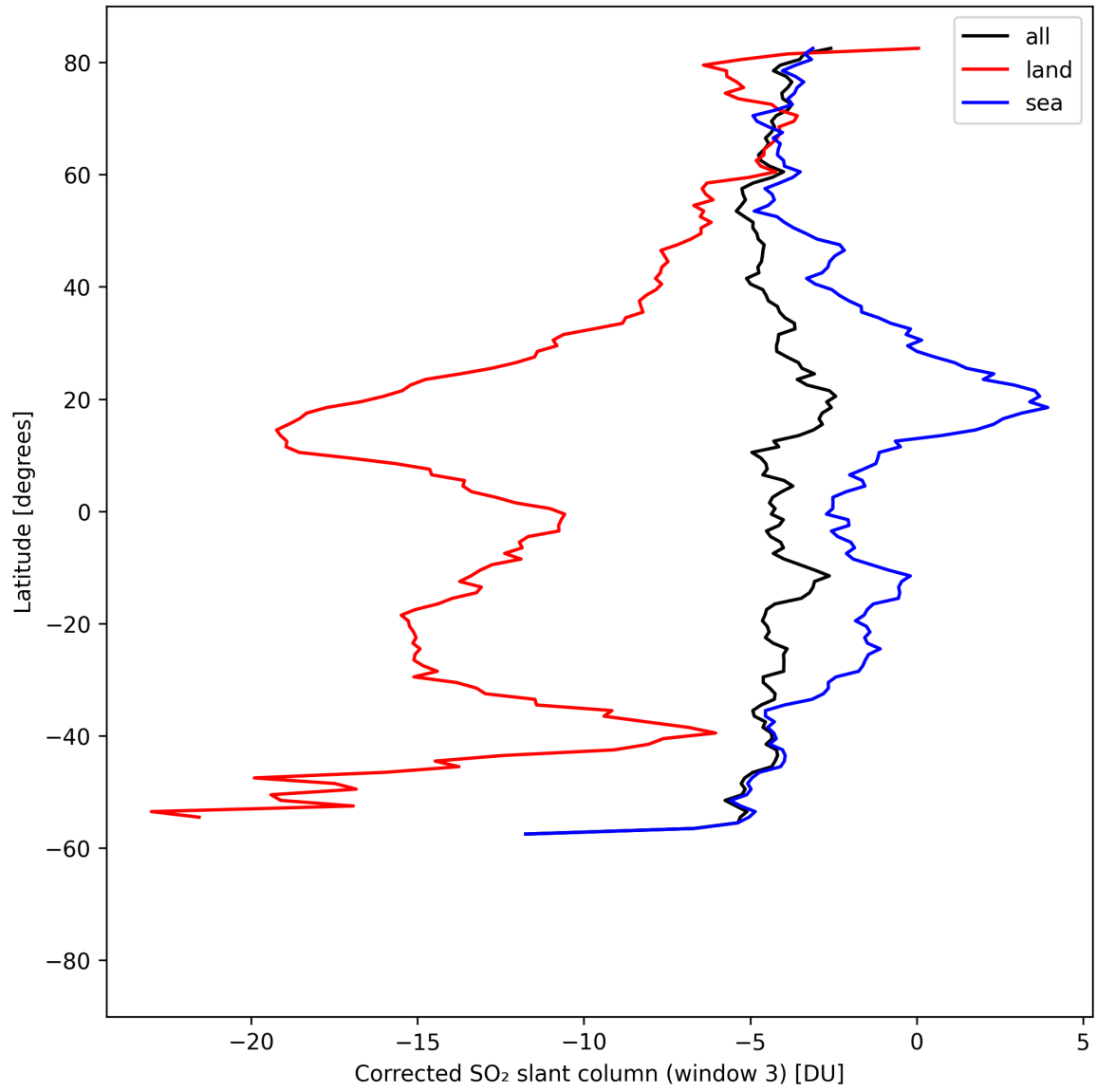
Figure 47: Zonal average of “Corrected SO 2 slant column (window 3)” for 2025-04-20 to 2025-04-22.
