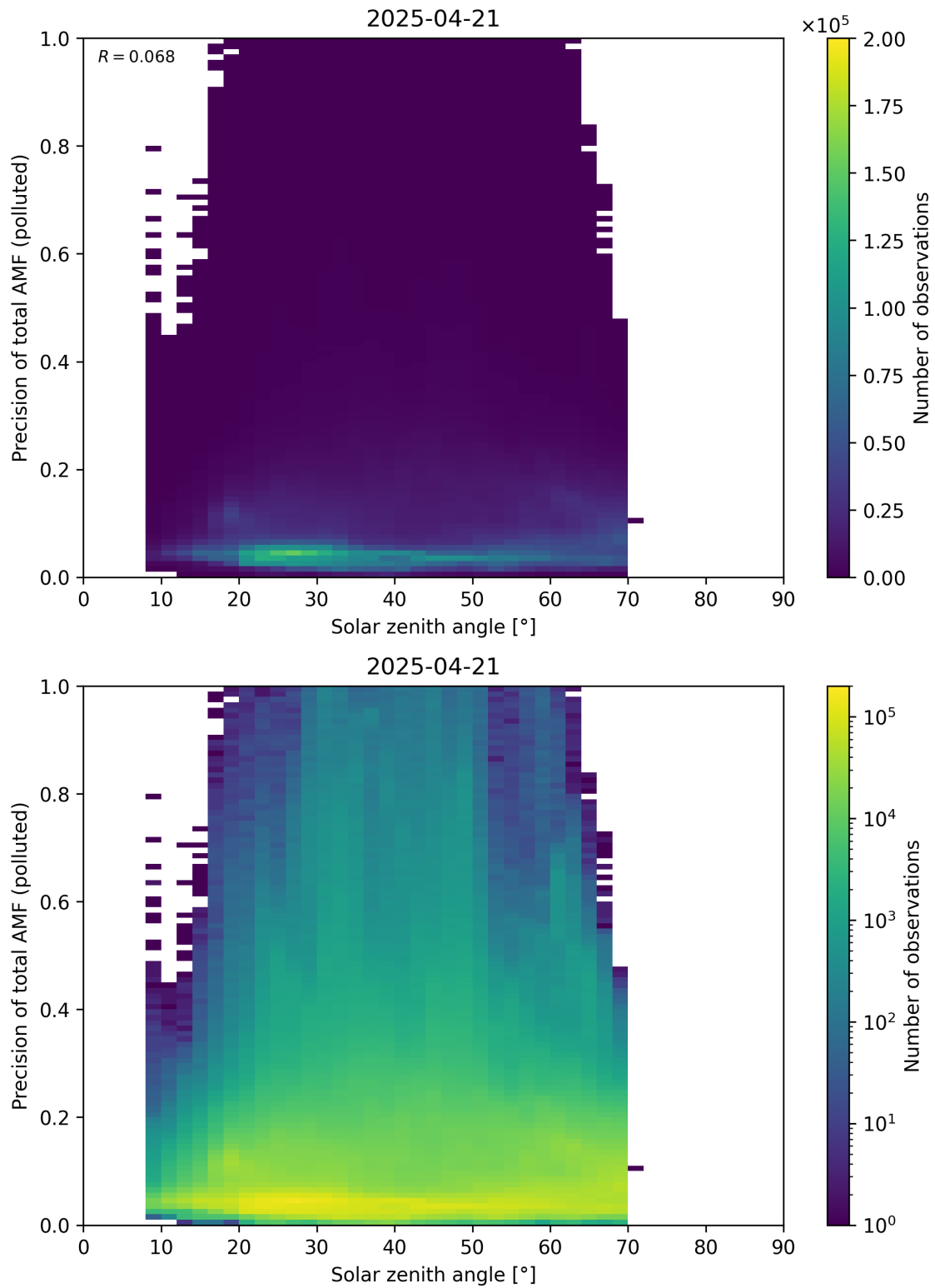
Figure 190: Scatter density plot of “Solar zenith angle” against “Precision of total AMF (polluted)” for 2025-04-20 to 2025-04-22.
