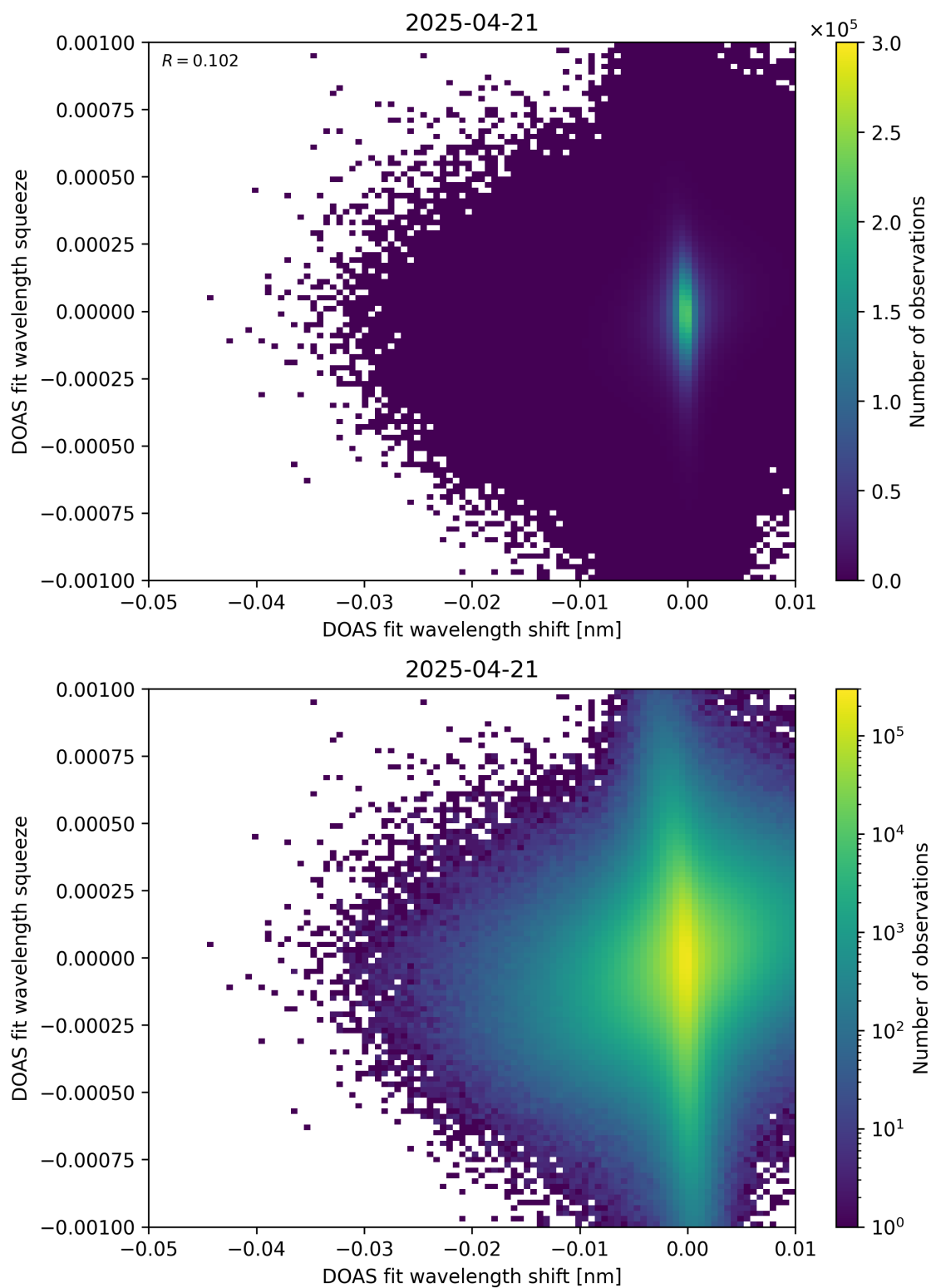
Figure 138: Scatter density plot of “DOAS fit wavelength shift” against “DOAS fit wavelength squeeze” for 2025-04-20 to 2025-04-22.
