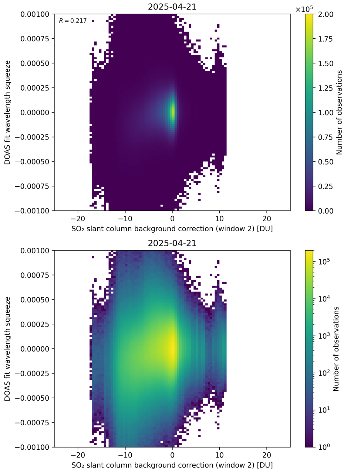
Figure 124: Scatter density plot of “SO 2 slant column background correction (window 2)” against “DOAS fit wavelength squeeze” for 2025-04-20 to 2025-04-22.
