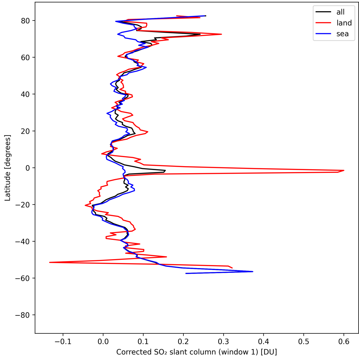
Figure 39: Zonal average of "Corrected SO 2 slant column (window 1)" for 2025-04-20 to 2025-04-22.
