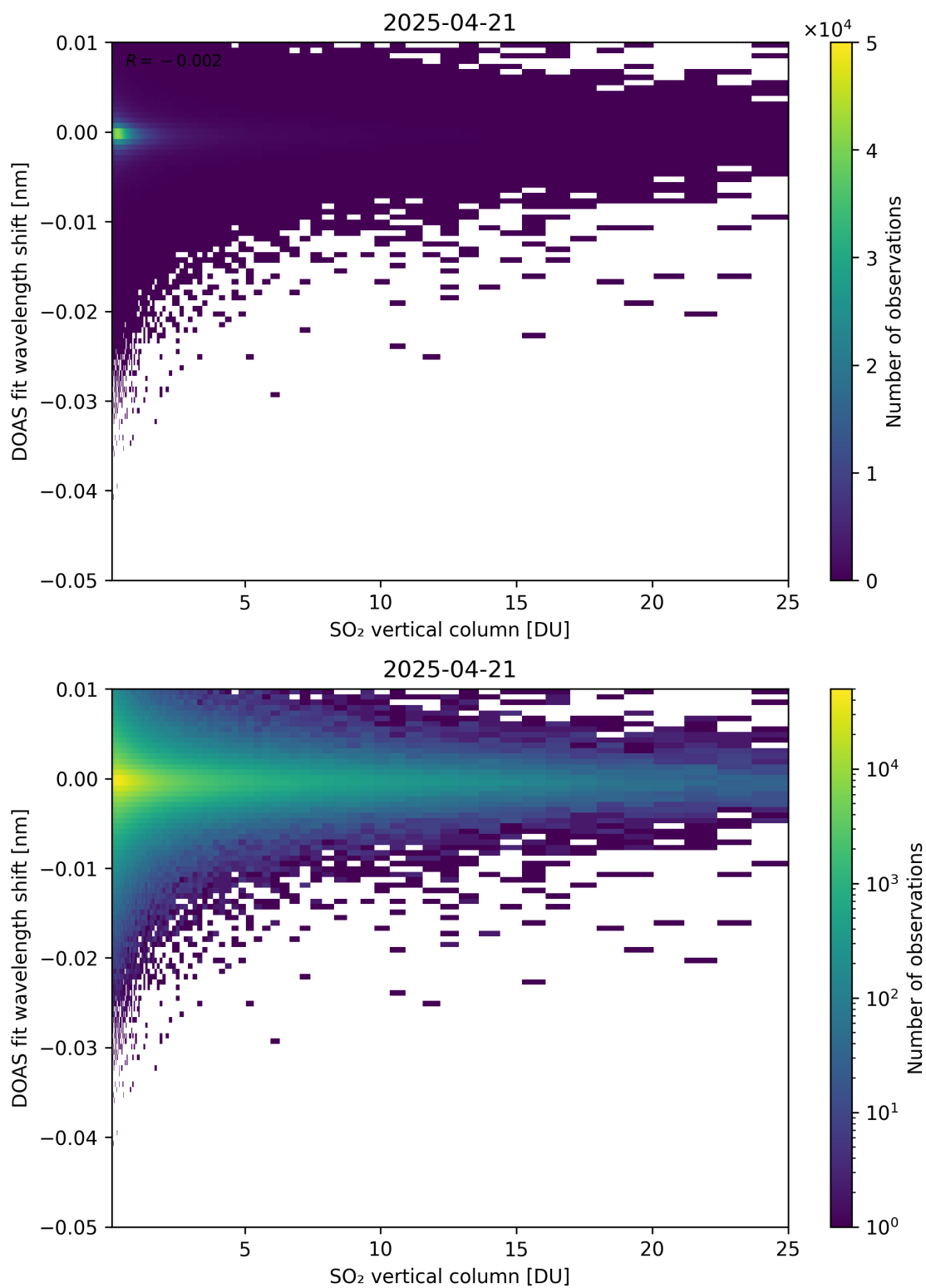
Figure 326: Scatter density plot of “SO 2 vertical column” against “DOAS fit wavelength shift” for 2025-04-20 to 2025-04-22.
