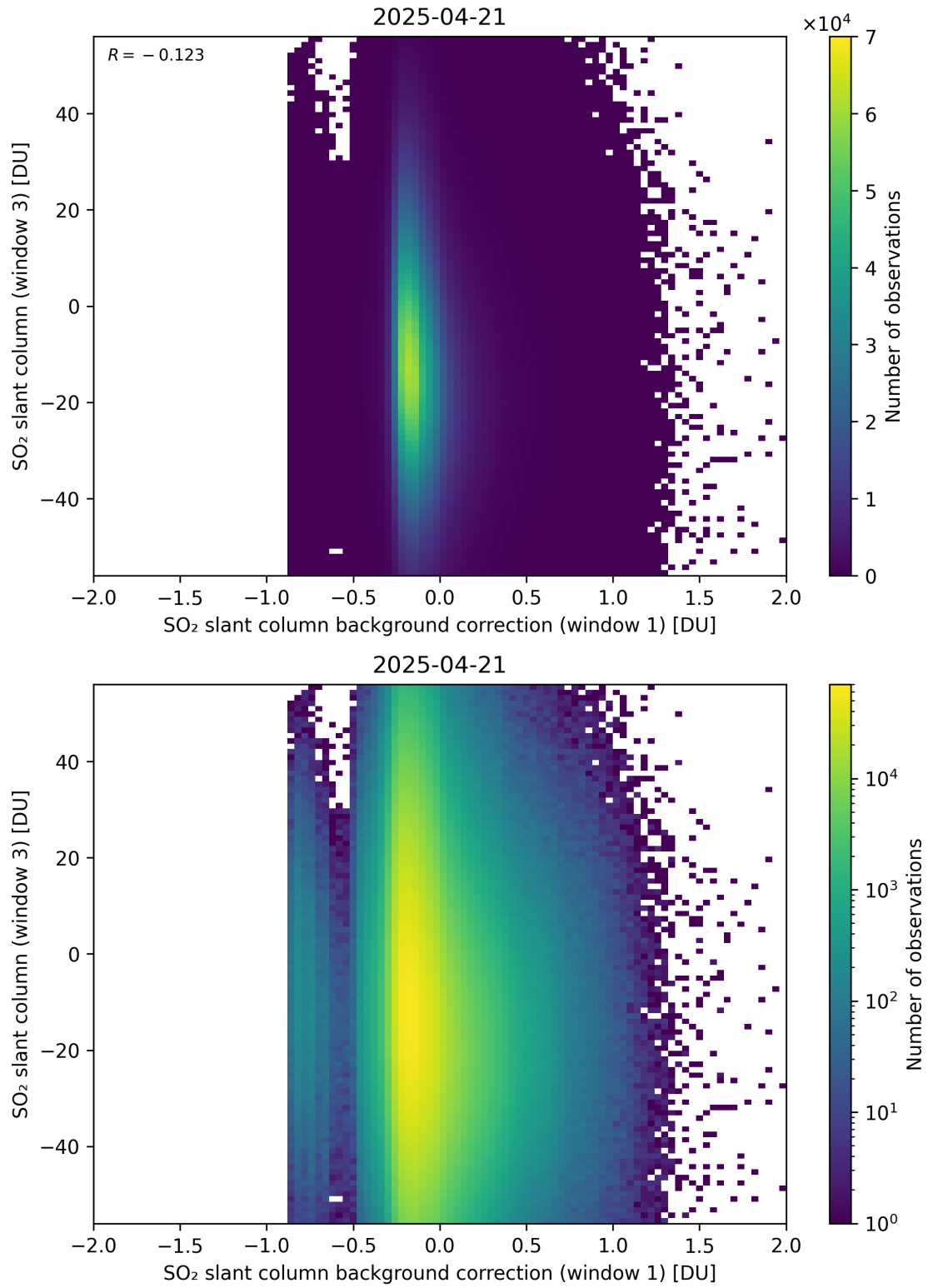
Figure 118: Scatter density plot of “SO 2 slant column background correction (window 1)” against “SO 2 slant column (window 3)” for 2025-04-20 to 2025-04-22.
