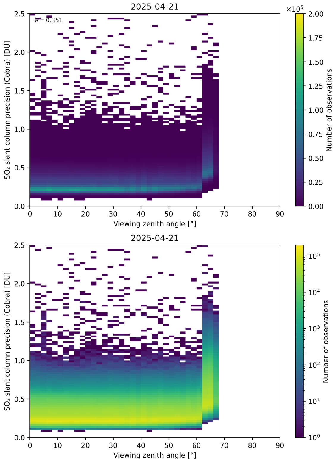
Figure 372: Scatter density plot of “Viewing zenith angle” against “SO 2 slant column precision (Cobra)” for 2025-04-20 to 2025-04-22.
