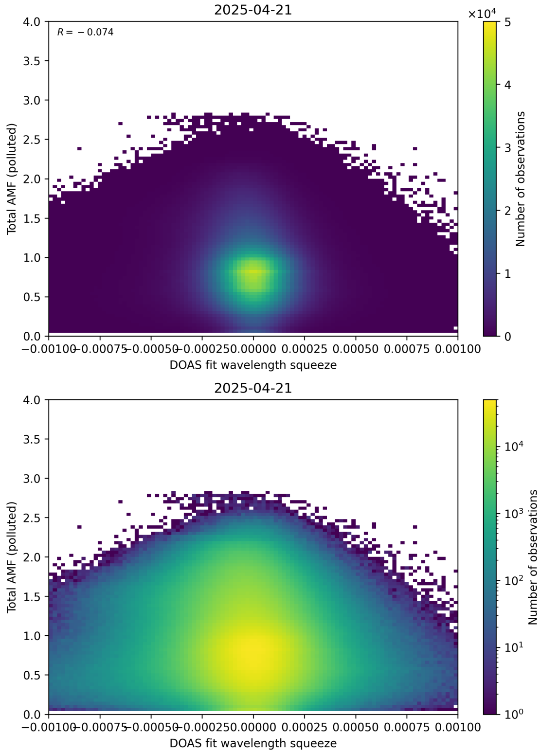
Figure 145: Scatter density plot of “DOAS fit wavelength squeeze” against “Total AMF (polluted)” for 2025-04-20 to 2025-04-22.
