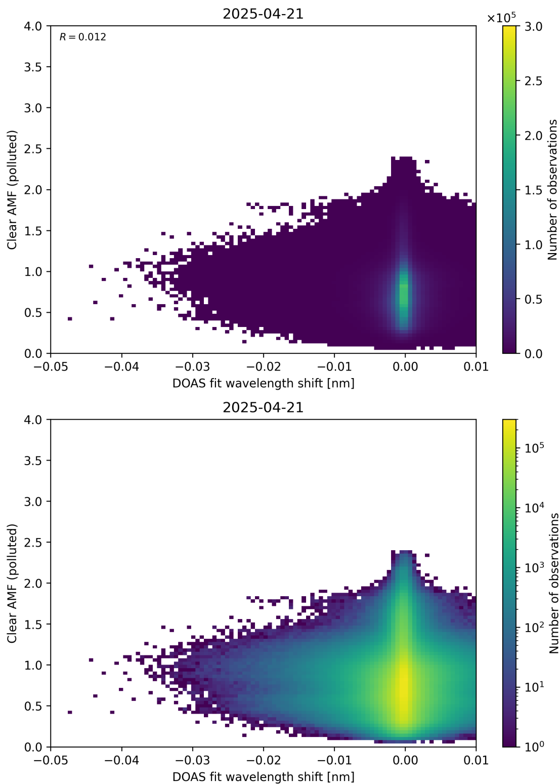
Figure 140: Scatter density plot of “DOAS fit wavelength shift” against “Clear AMF (polluted)” for 2025-04-20 to 2025-04-22.
