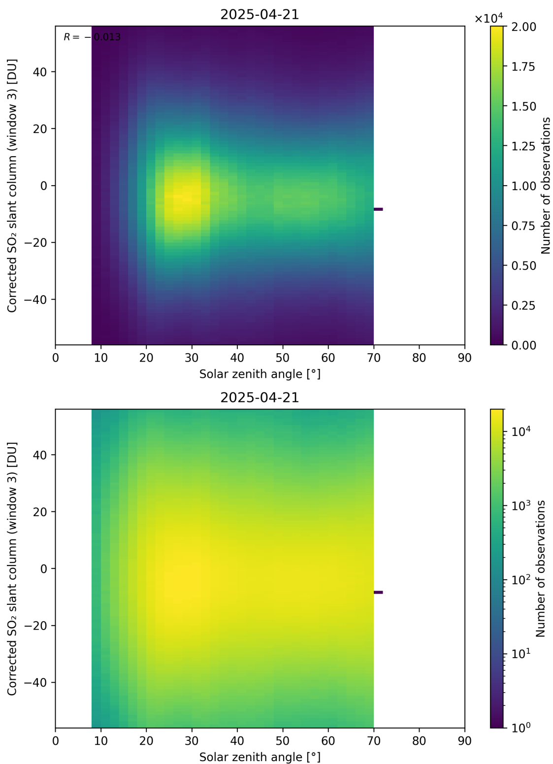
Figure 183: Scatter density plot of “Solar zenith angle” against “Corrected SO 2 slant column (window 3)” for 2025-04-20 to 2025-04-22.
