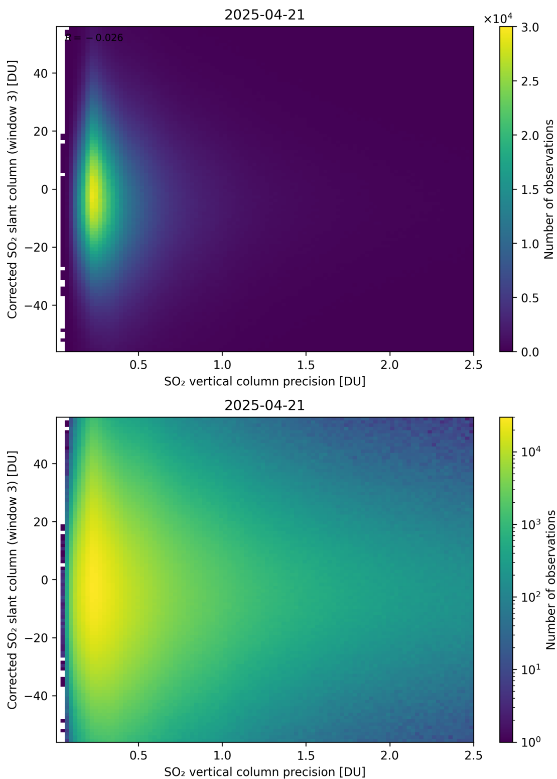
Figure 340: Scatter density plot of “SO 2 vertical column precision” against “Corrected SO 2 slant column (window 3)” for 2025-04-20 to 2025-04-22.
