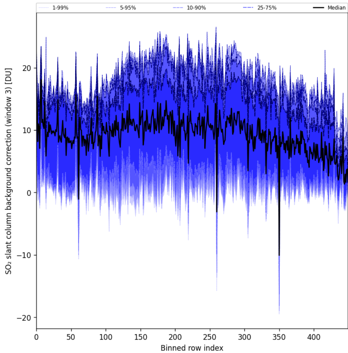
Figure 100: Along track statistics of “SO 2 slant column background correction (window 3)” for 2025-04-20 to 2025-04-22
