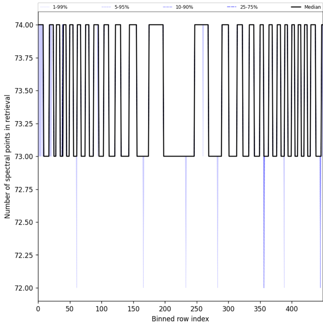
Figure 108: Along track statistics of “Number of spectral points in retrieval” for 2025-04-20 to 2025-04-22
