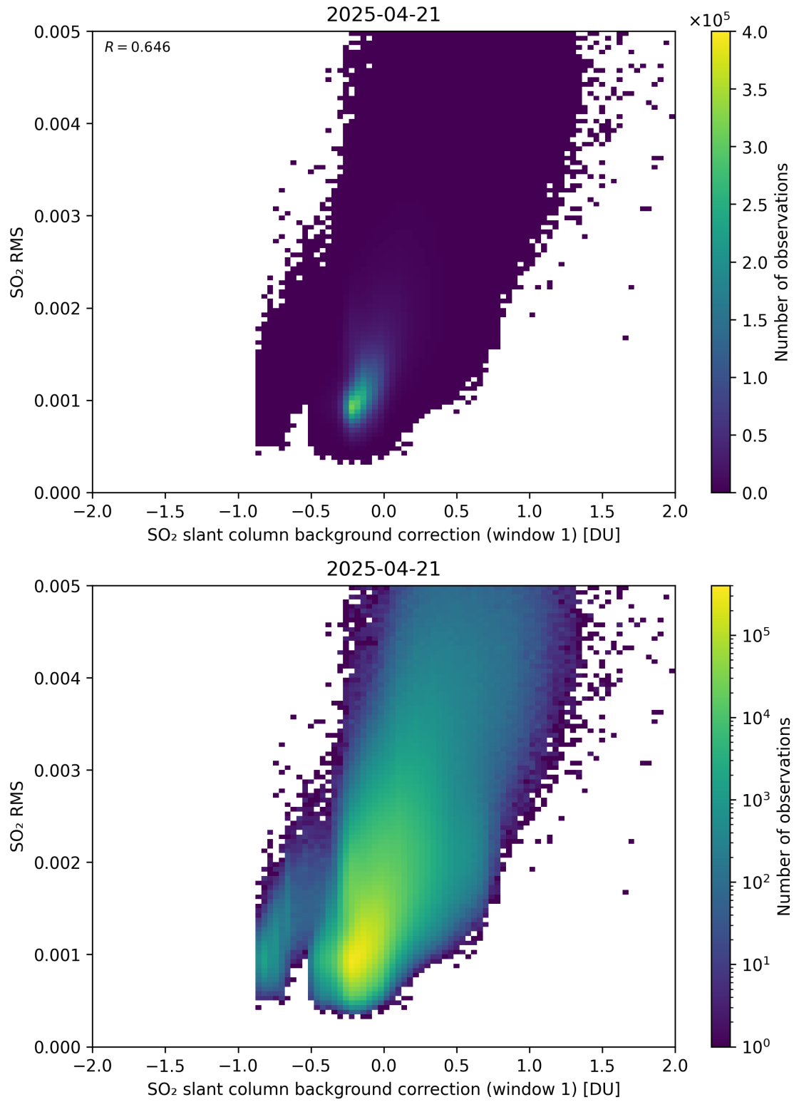
Figure 113: Scatter density plot of “SO 2 slant column background correction (window 1)” against “SO 2 RMS” for 2025-04-20 to 2025-04-22.
