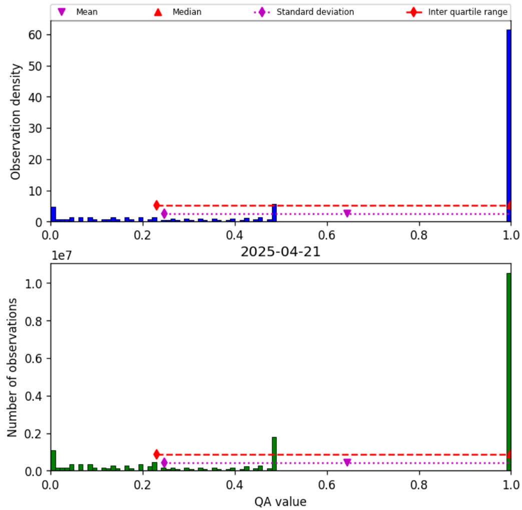
Figure 57: Histogram of “QA value” for 2025-04-20 to 2025-04-22
