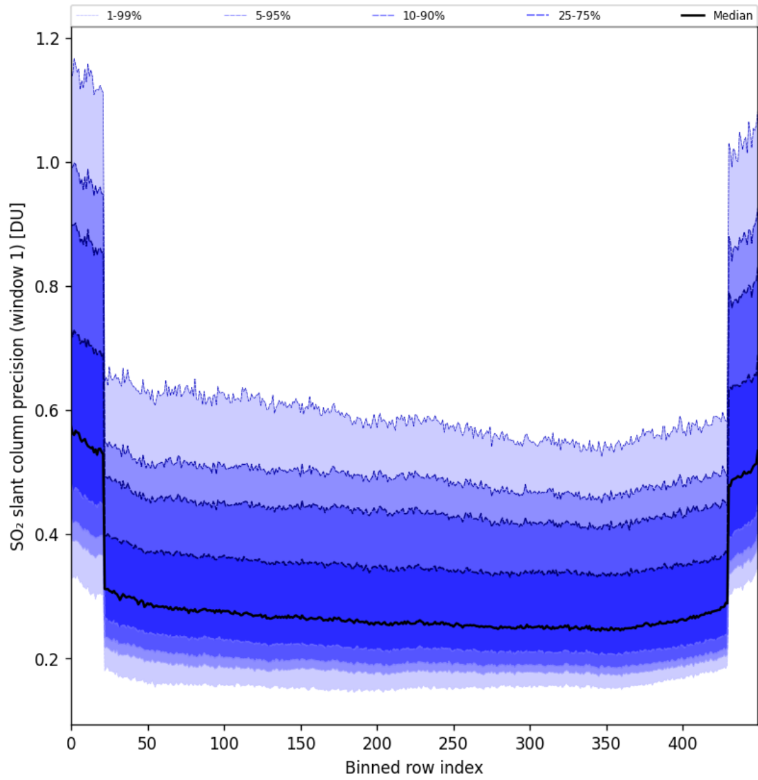
Figure 90: Along track statistics of “SO 2 slant column precision (window 1)” for 2025-04-20 to 2025-04-22
