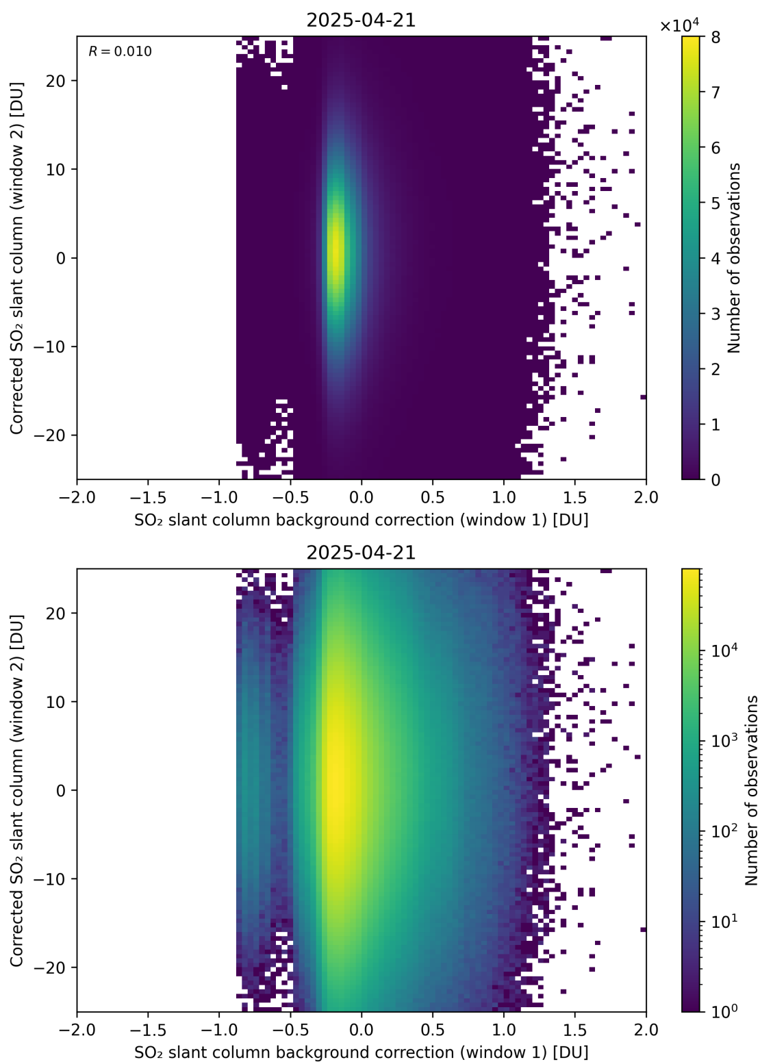
Figure 115: Scatter density plot of “SO 2 slant column background correction (window 1)” against “Corrected SO 2 slant column (window 2)” for 2025-04-20 to 2025-04-22.
