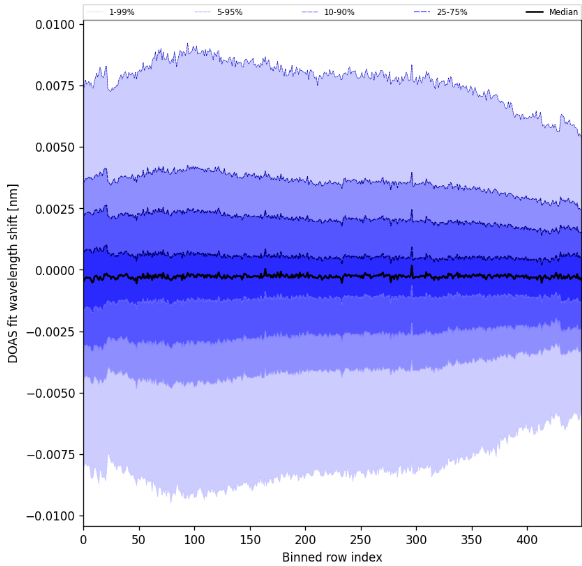
Figure 102: Along track statistics of “DOAS fit wavelength shift” for 2025-04-20 to 2025-04-22
