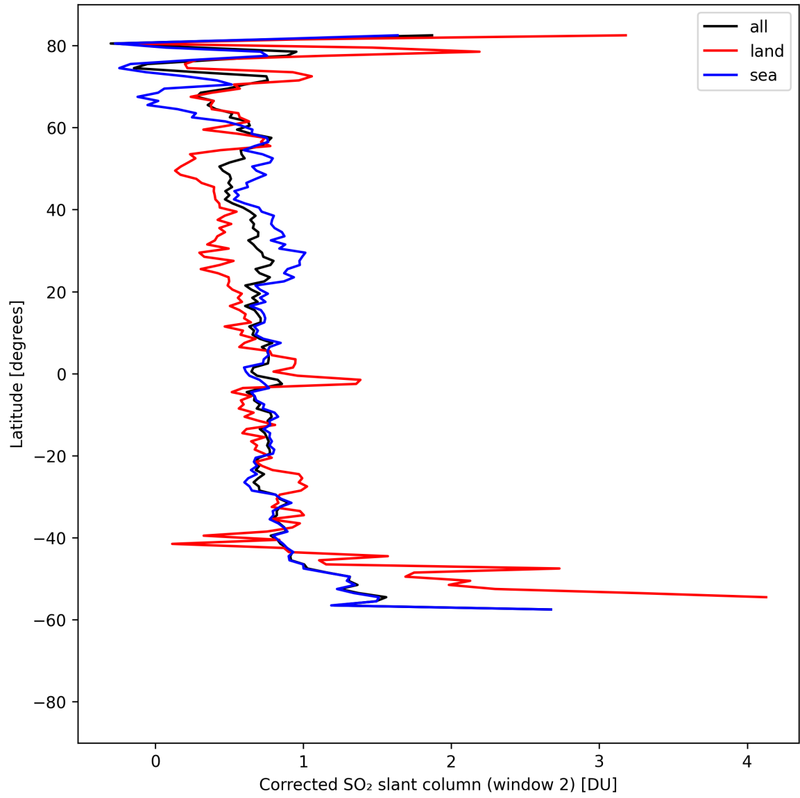
Figure 43: Zonal average of “Corrected SO 2 slant column (window 2)” for 2025-04-20 to 2025-04-22.
