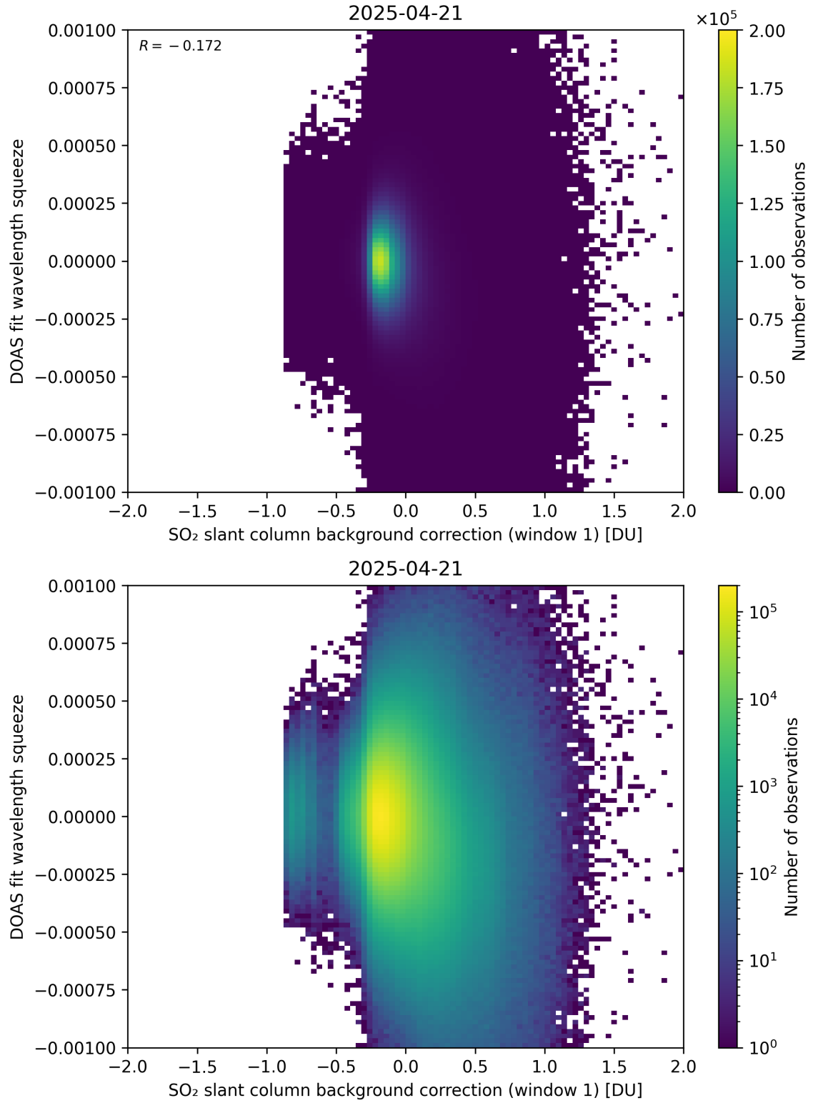
Figure 112: Scatter density plot of “SO 2 slant column background correction (window 1)” against “DOAS fit wavelength squeeze” for 2025-04-20 to 2025-04-22.
