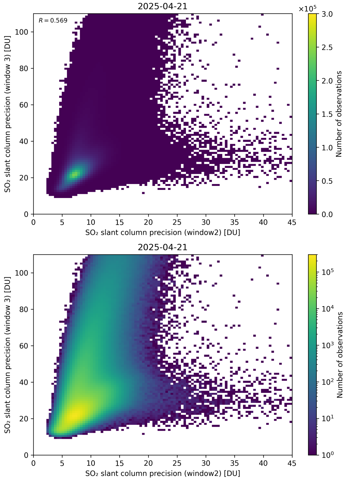
Figure 300: Scatter density plot of “SO 2 slant column precision (window2)” against “SO 2 slant column precision (window 3)” for 2025-04-20 to 2025-04-22.
