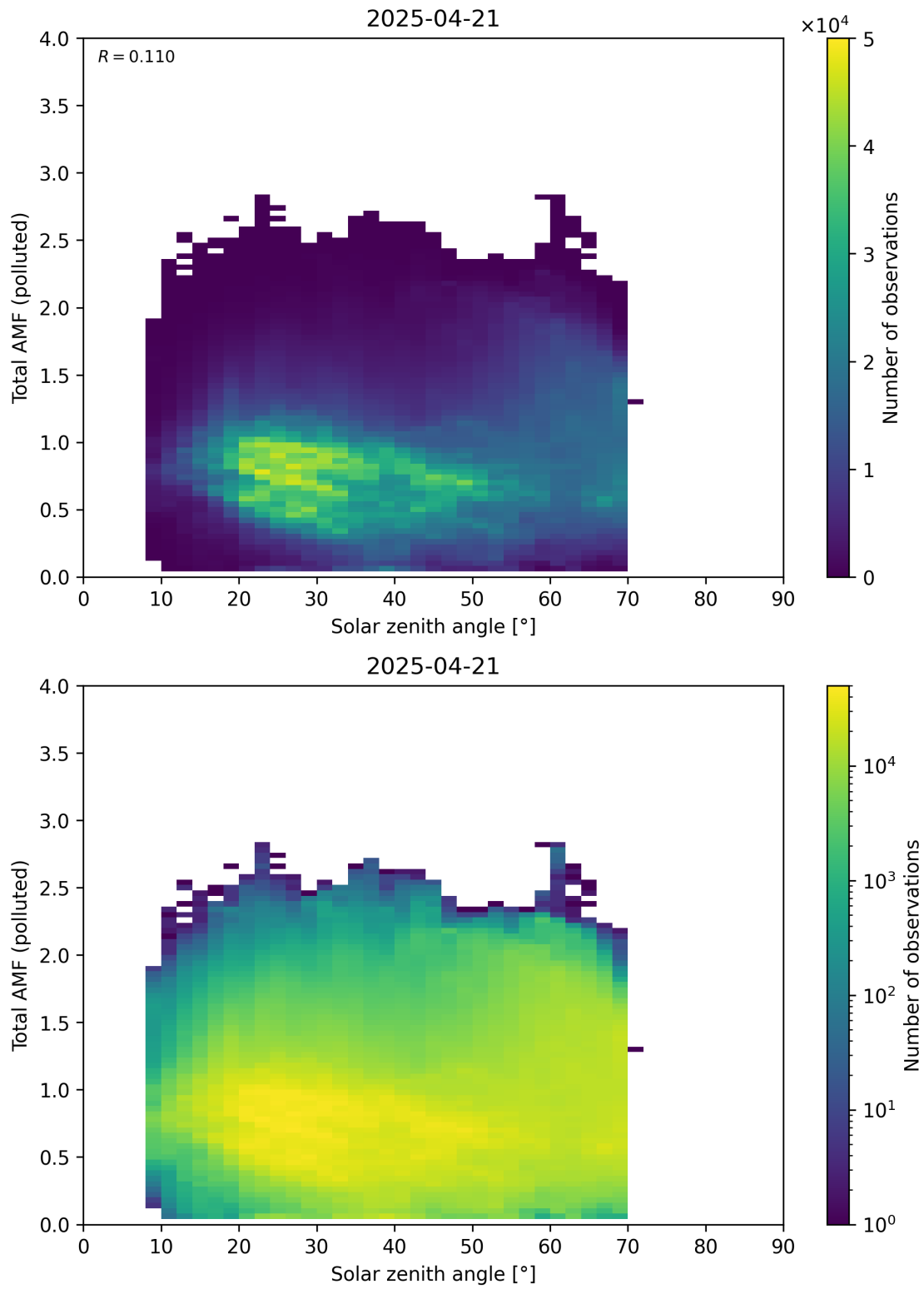
Figure 189: Scatter density plot of “Solar zenith angle” against “Total AMF (polluted)” for 2025-04-20 to 2025-04-22.
