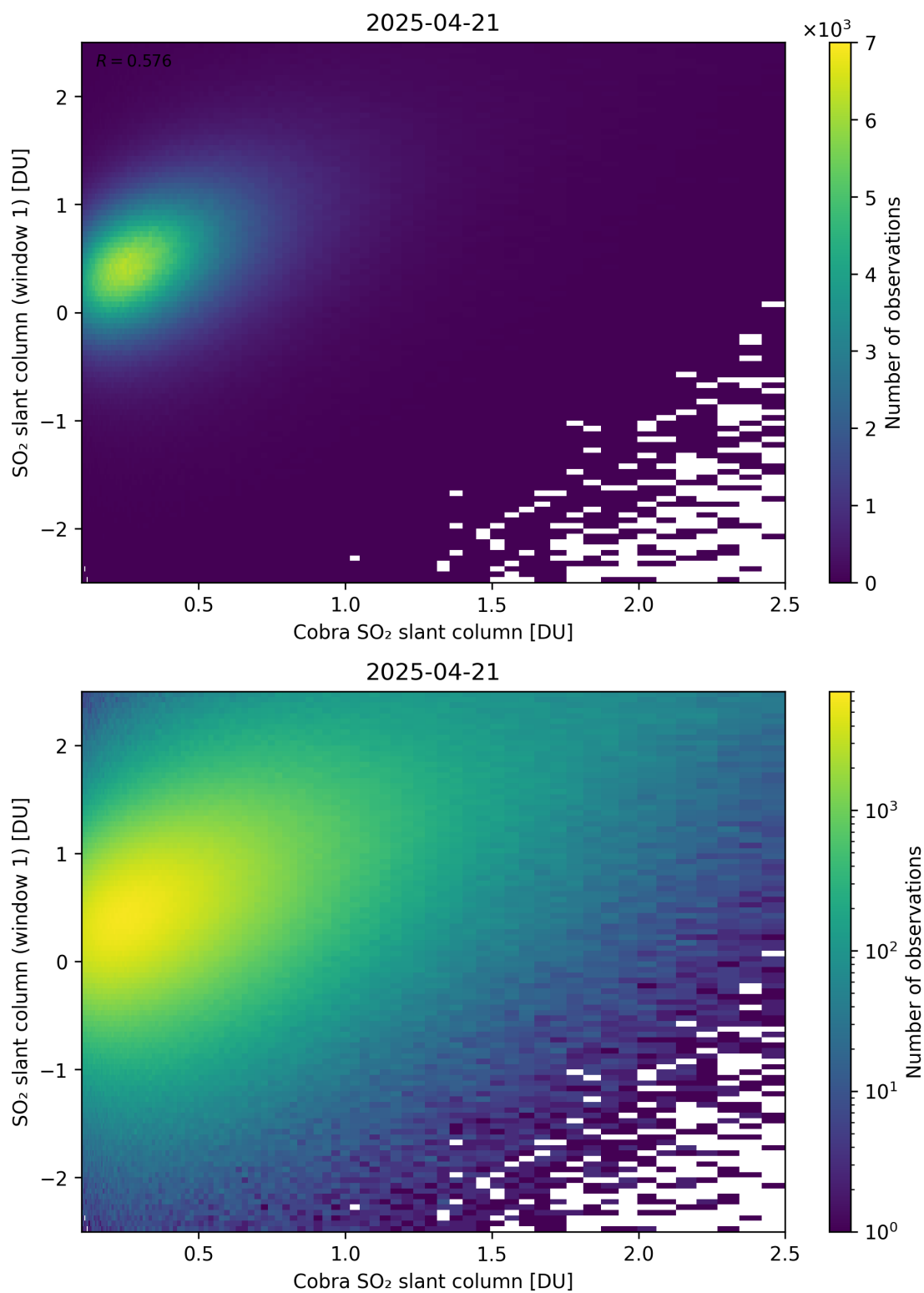
Figure 219: Scatter density plot of “Cobra SO 2 slant column” against “SO 2 slant column (window 1)” for 2025-04-20 to 2025-04-22.
