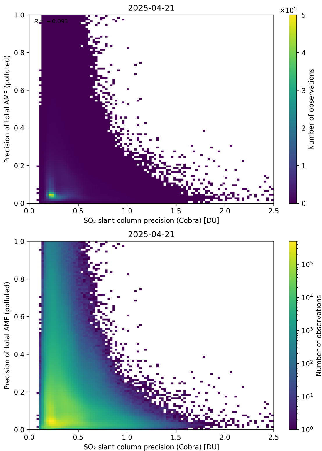
Figure 214: Scatter density plot of “SO 2 slant column precision (Cobra)” against “Precision of total AMF (polluted)” for 2025-04-20 to 2025-04-22.
