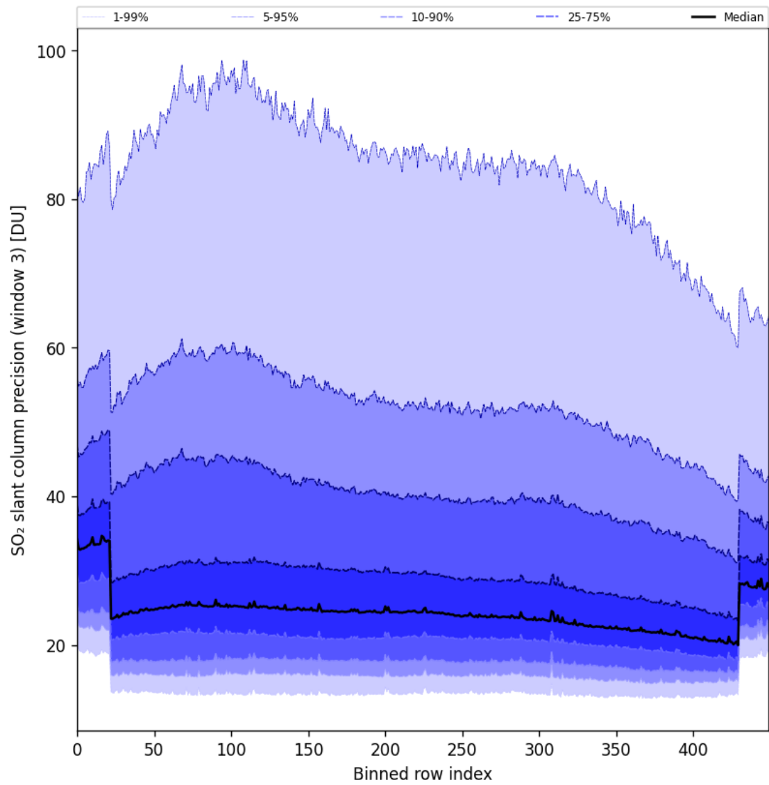
Figure 98: Along track statistics of “SO 2 slant column precision (window 3)” for 2025-04-20 to 2025-04-22
