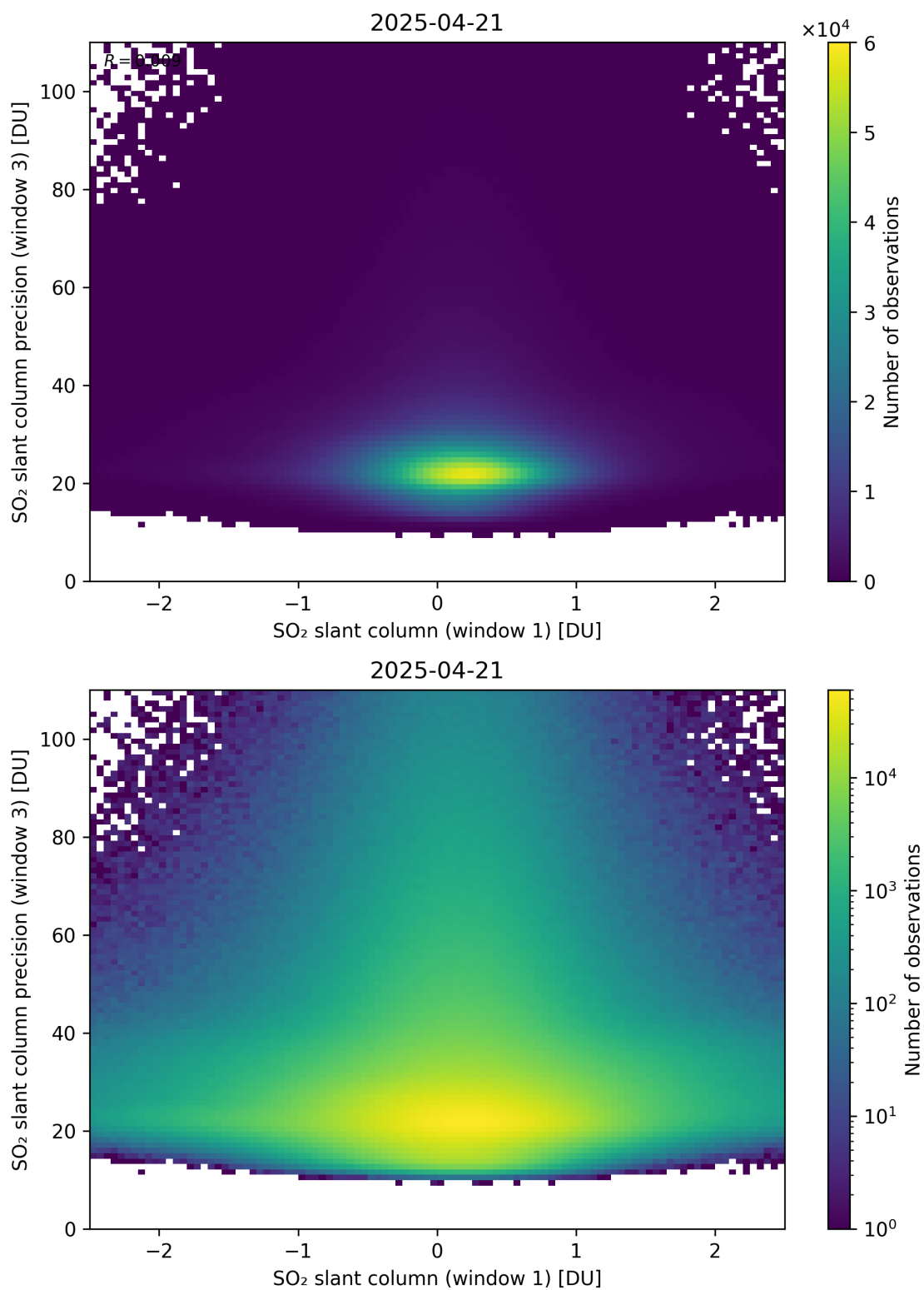
Figure 288: Scatter density plot of “SO 2 slant column (window 1)” against “SO 2 slant column precision (window 3)” for 2025-04-20 to 2025-04-22.
