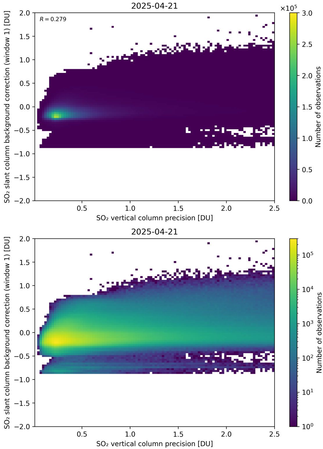
Figure 329: Scatter density plot of “SO 2 vertical column precision” against “SO 2 slant column background correction (window 1)” for 2025-04-20 to 2025-04-22.
