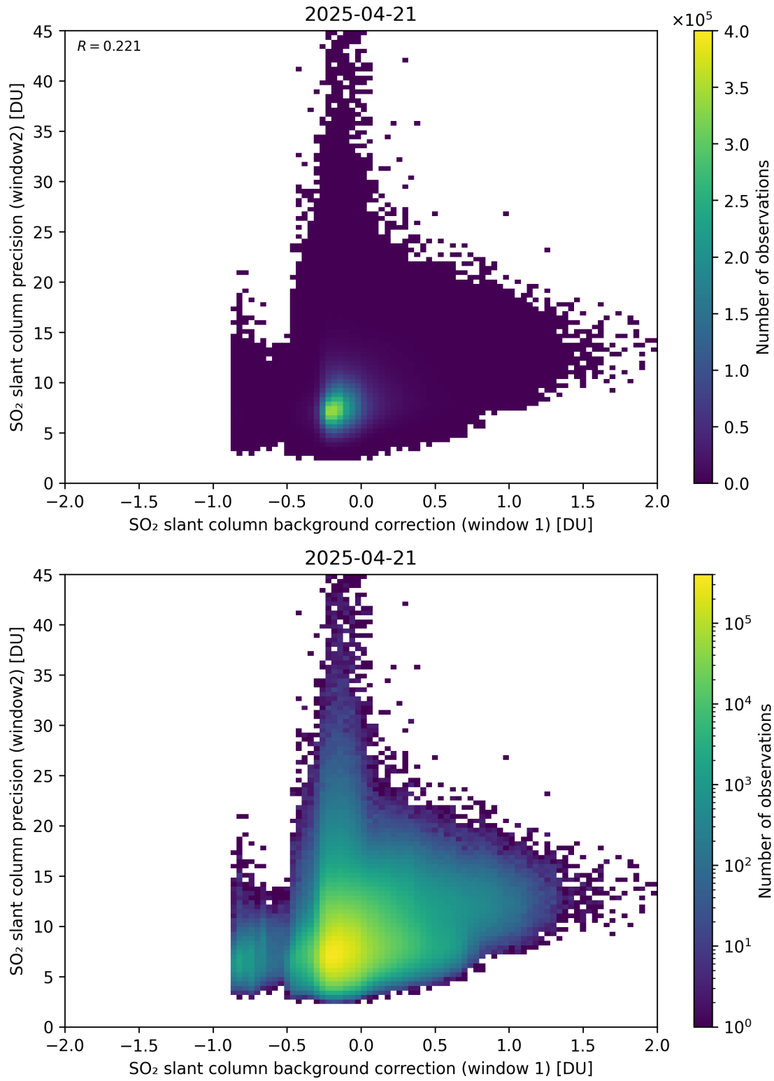
Figure 117: Scatter density plot of “SO 2 slant column background correction (window 1)” against “SO 2 slant column precision (window2)” for 2025-04-20 to 2025-04-22.
