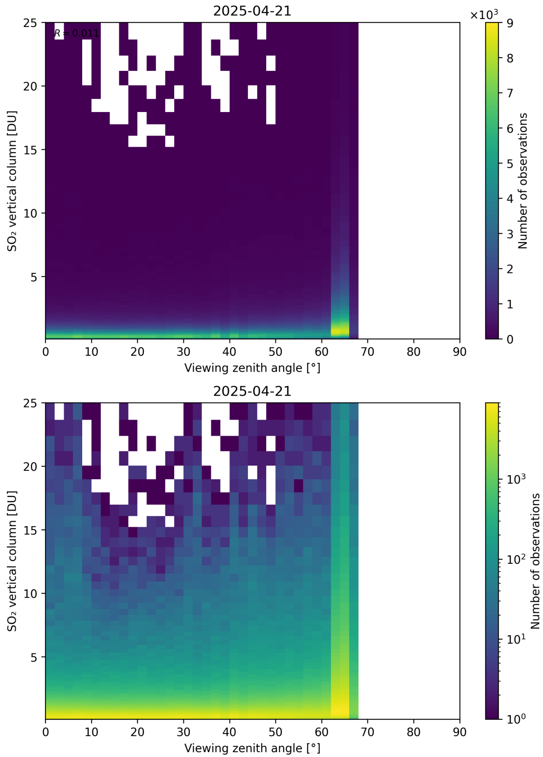
Figure 383: Scatter density plot of “Viewing zenith angle” against “SO 2 vertical column” for 2025-04-20 to 2025-04-22.
