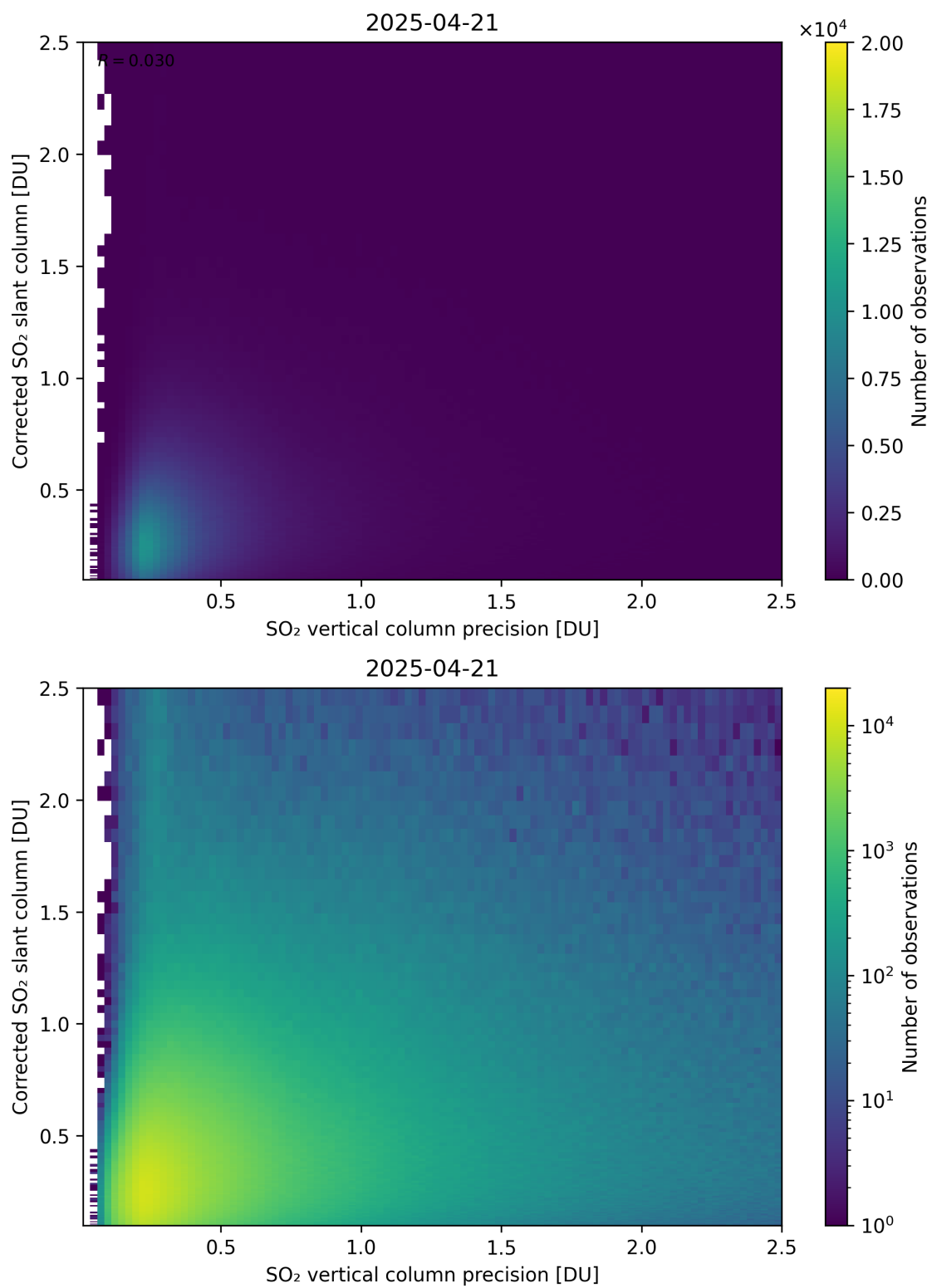
Figure 338: Scatter density plot of “SO 2 vertical column precision” against “Corrected SO 2 slant column” for 2025-04-20 to 2025-04-22.
