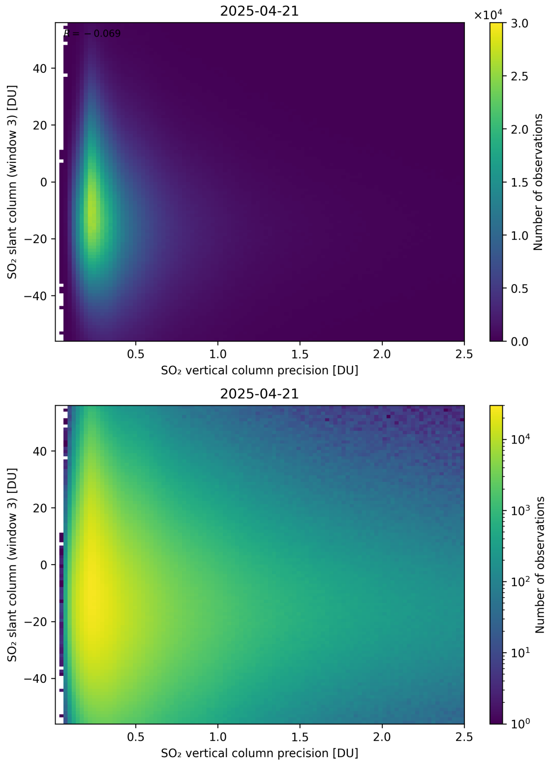
Figure 344: Scatter density plot of “SO 2 vertical column precision” against “SO 2 slant column (window 3)” for 2025-04-20 to 2025-04-22.
