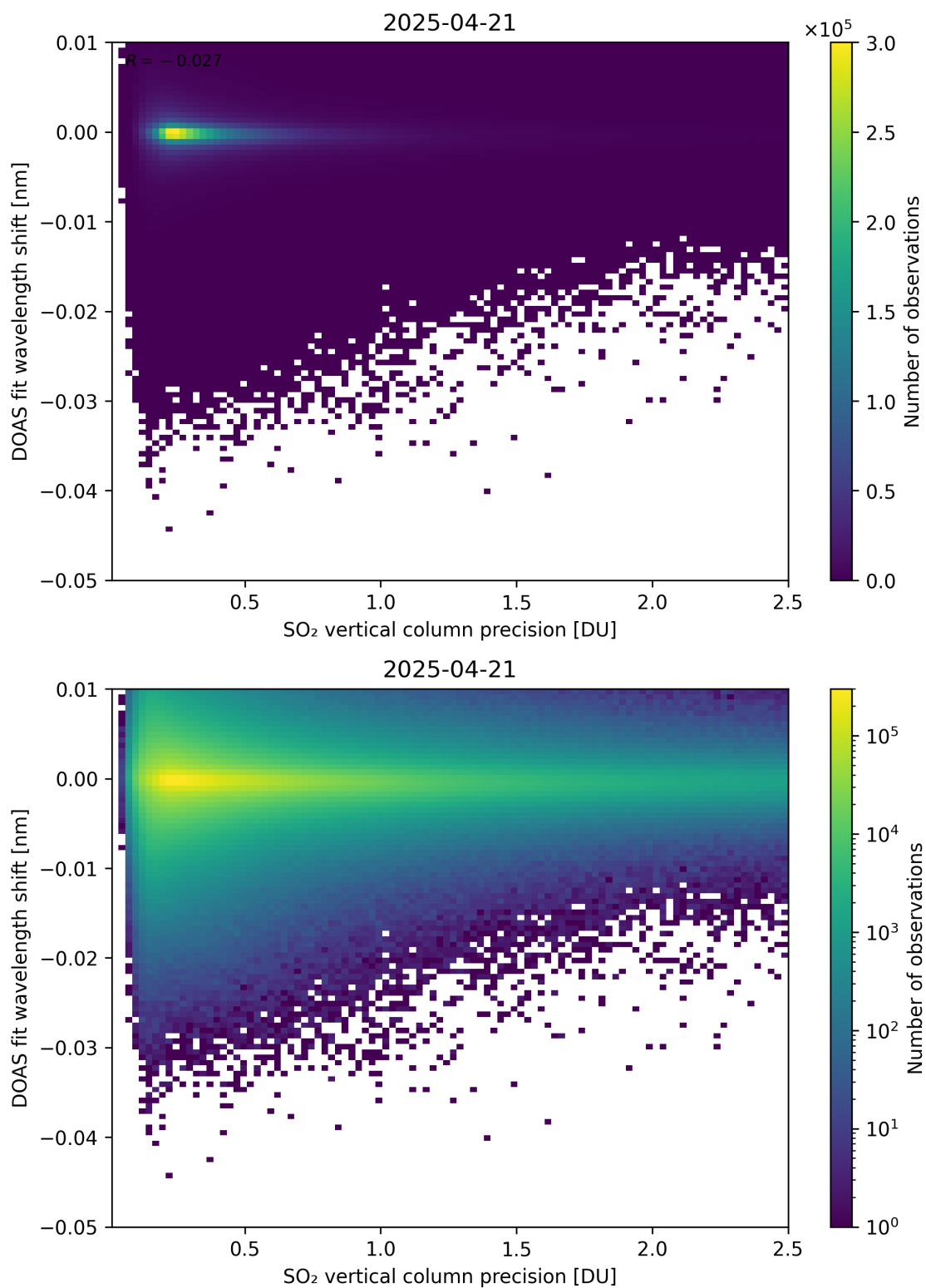
Figure 332: Scatter density plot of “SO 2 vertical column precision” against “DOAS fit wavelength shift” for 2025-04-20 to 2025-04-22.
