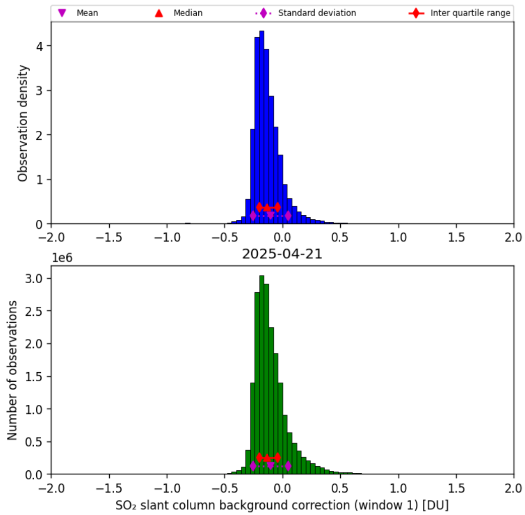
Figure 66: Histogram of “SO 2 slant column background correction (window 1)” for 2025-04-20 to 2025-04-22
