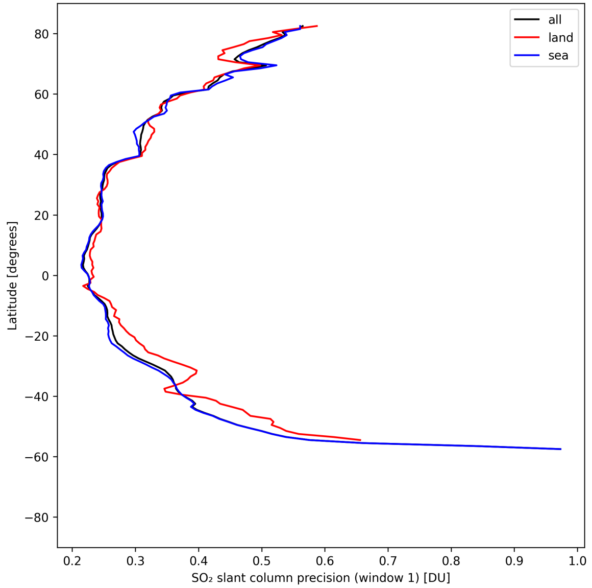
Figure 38: Zonal average of “SO 2 slant column precision (window 1)” for 2025-04-20 to 2025-04-22.
