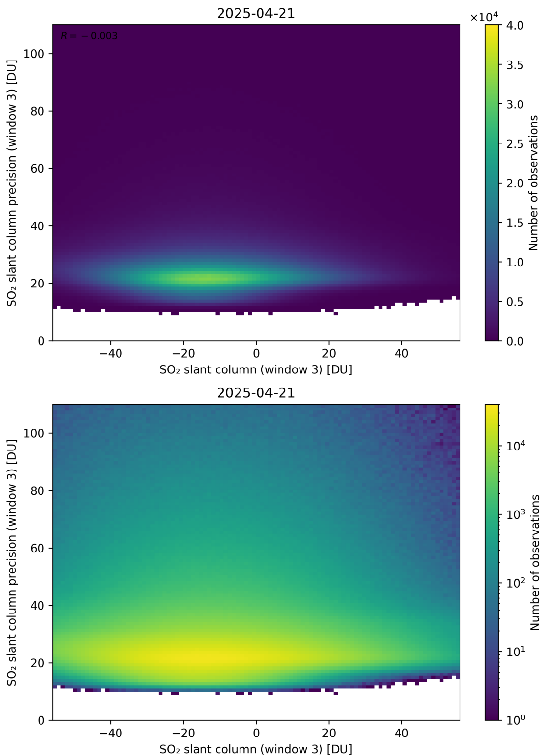
Figure 317: Scatter density plot of “SO 2 slant column (window 3)” against “SO 2 slant column precision (window 3)” for 2025-04-20 to 2025-04-22.
