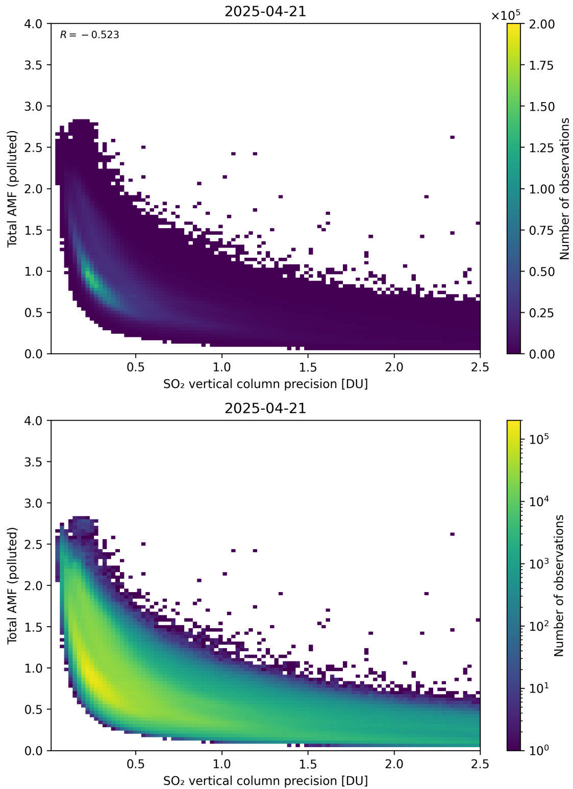
Figure 346: Scatter density plot of “SO 2 vertical column precision” against “Total AMF (polluted)” for 2025-04-20 to 2025-04-22.
