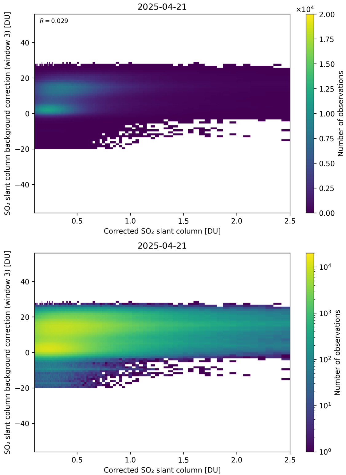
Figure 228: Scatter density plot of “Corrected SO 2 slant column” against “SO 2 slant column background correction (window 3)” for 2025-04-20 to 2025-04-22.
