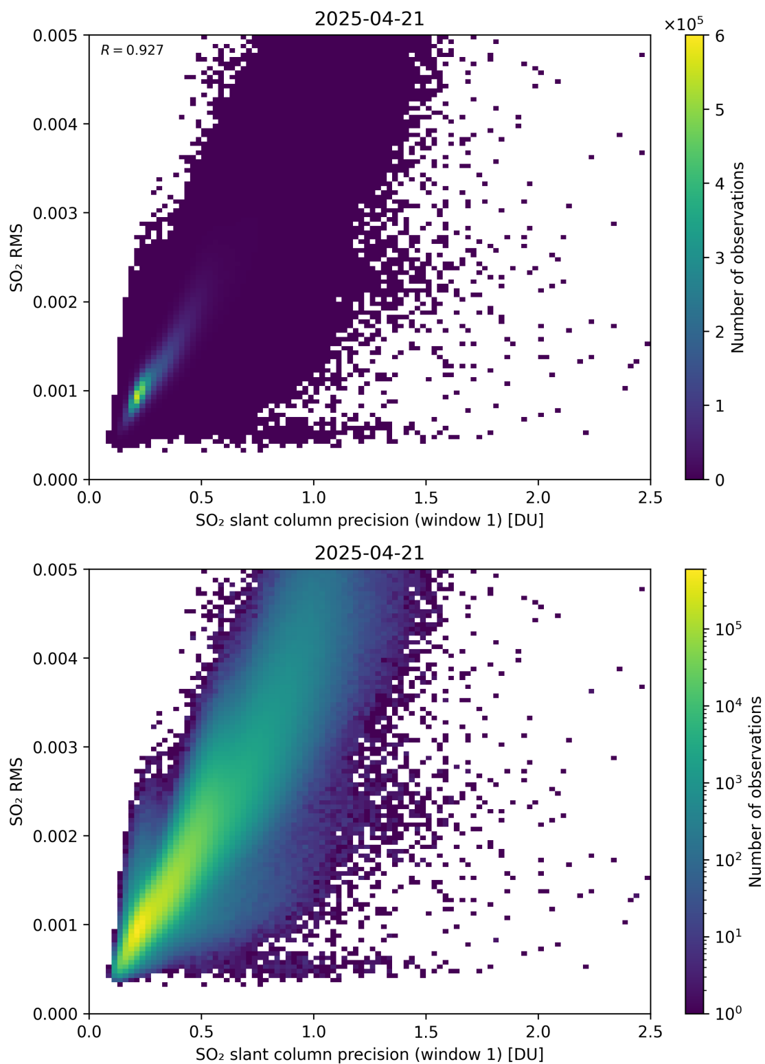
Figure 273: Scatter density plot of “SO 2 slant column precision (window 1)” against “SO 2 RMS” for 2025-04-20 to 2025-04-22.
