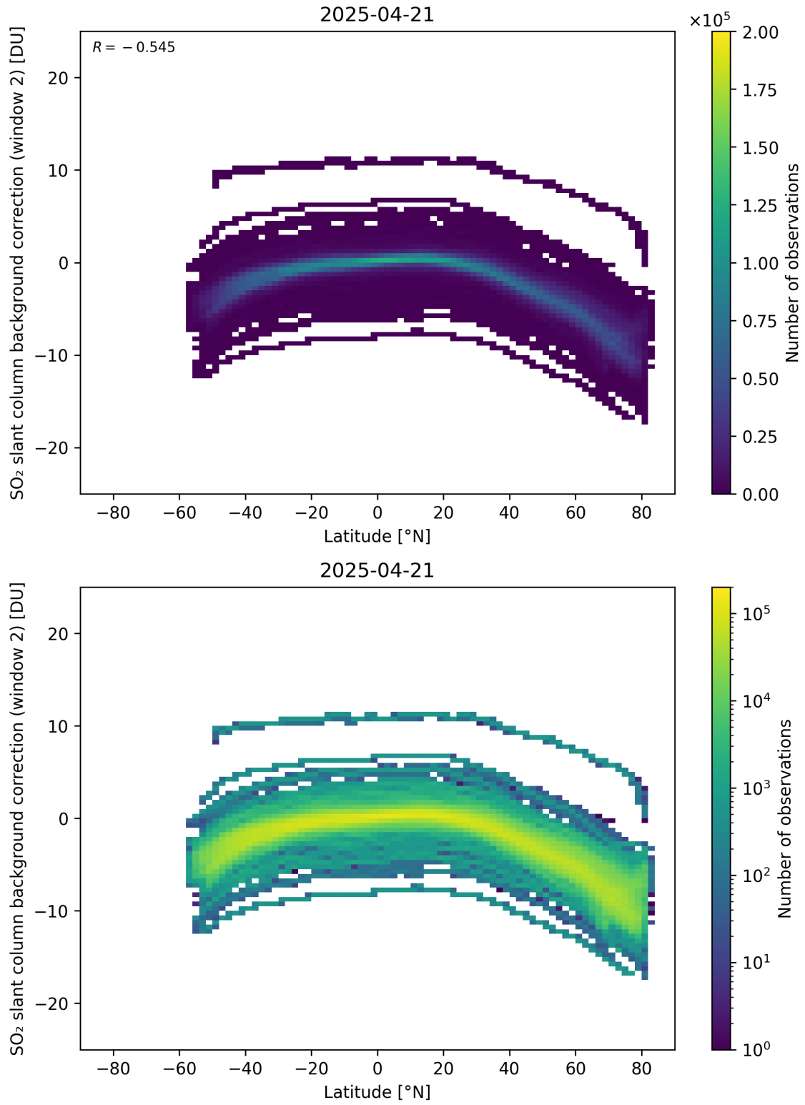
Figure 151: Scatter density plot of “Latitude” against “SO 2 slant column background correction (window 2)” for 2025-04-20 to 2025-04-22.
