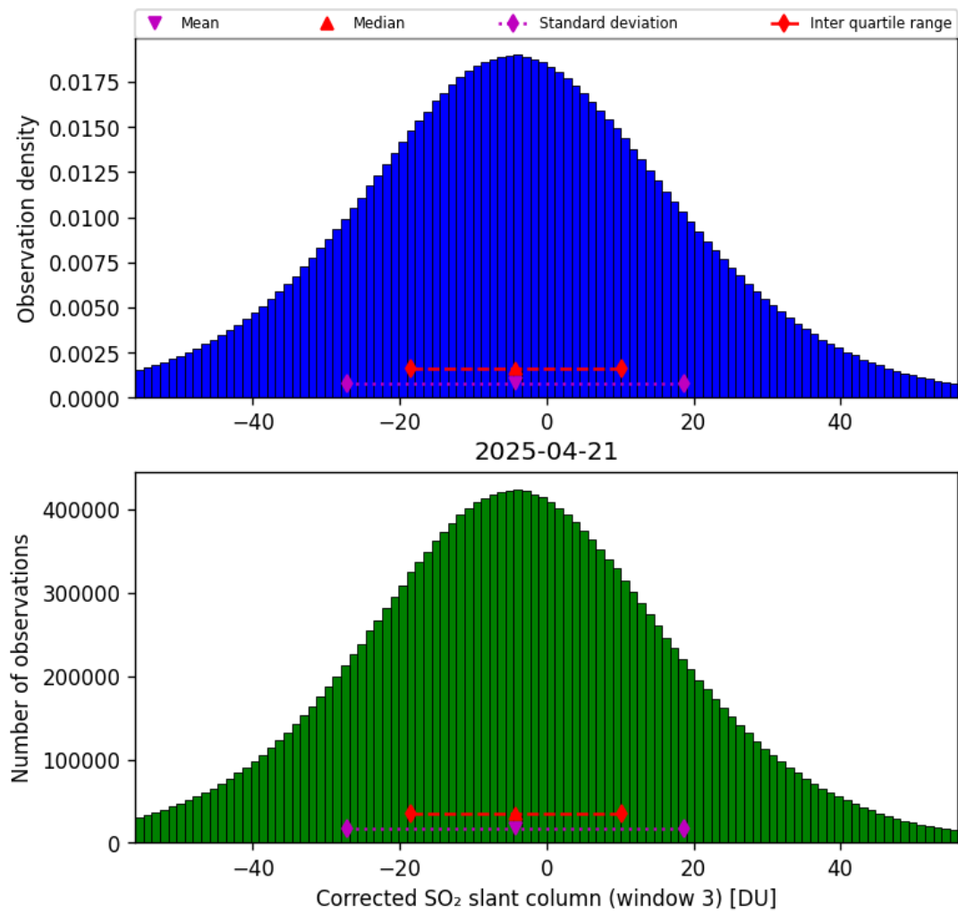
Figure 73: Histogram of “Corrected SO 2 slant column (window 3)” for 2025-04-20 to 2025-04-22
