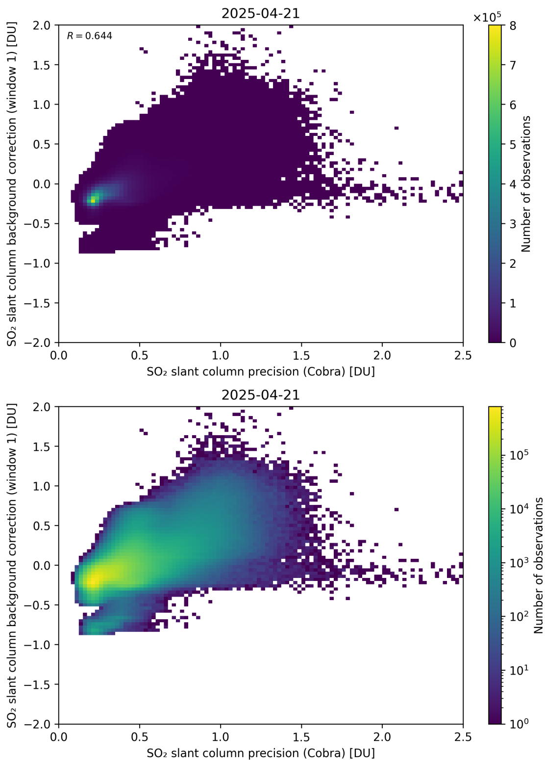
Figure 199: Scatter density plot of “SO 2 slant column precision (Cobra)” against “SO 2 slant column background correction (window 1)” for 2025-04-20 to 2025-04-22.
