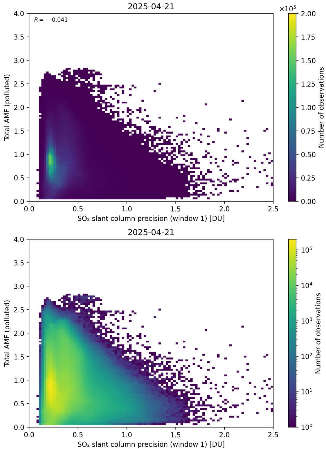
Figure 280: Scatter density plot of “SO 2 slant column precision (window 1)” against “Total AMF (polluted)” for 2025-04-20 to 2025-04-22.
