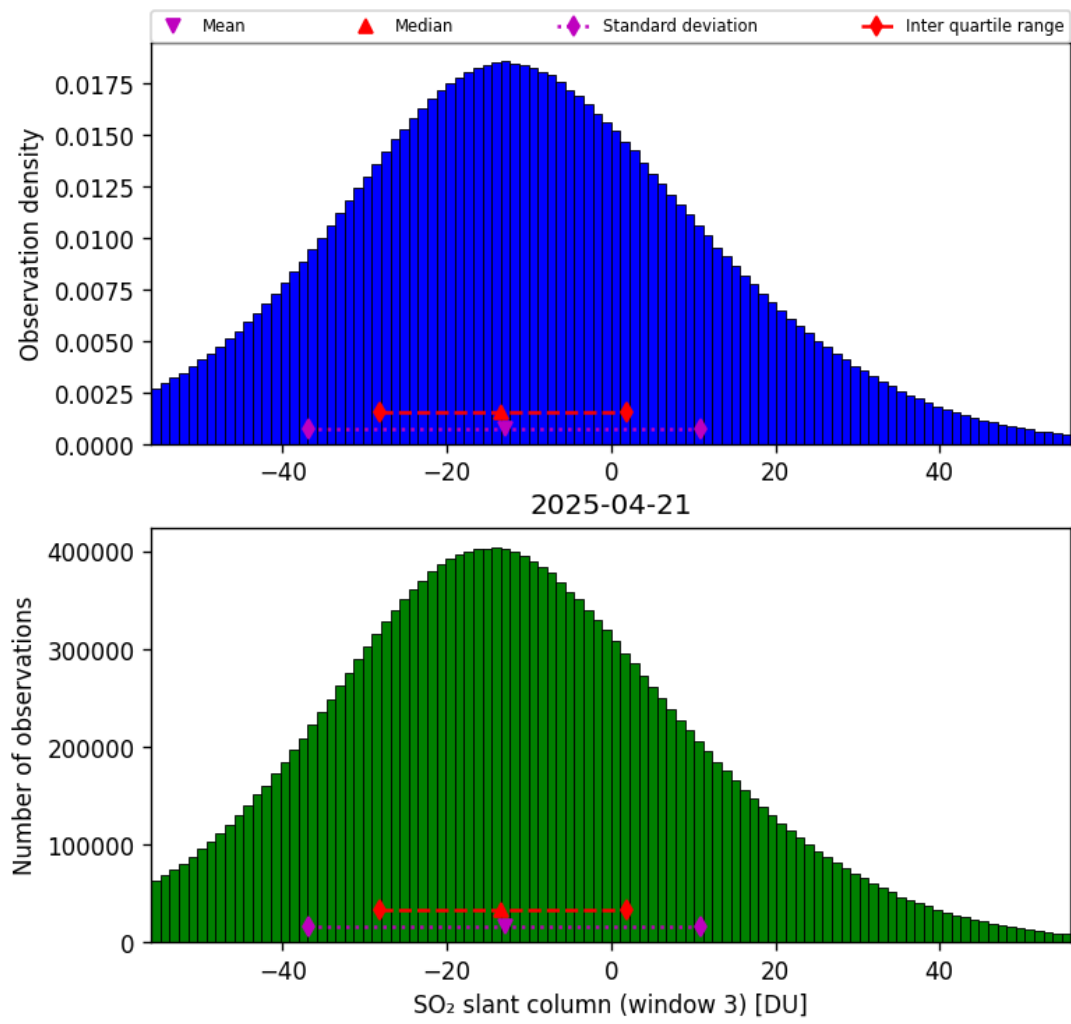
Figure 71: Histogram of “SO 2 slant column (window 3)” for 2025-04-20 to 2025-04-22
