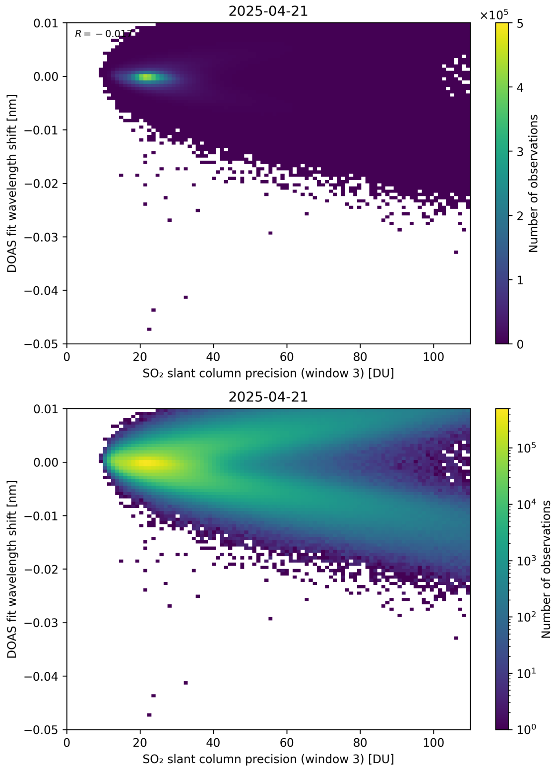
Figure 308: Scatter density plot of “SO 2 slant column precision (window 3)” against “DOAS fit wavelength shift” for 2025-04-20 to 2025-04-22.
