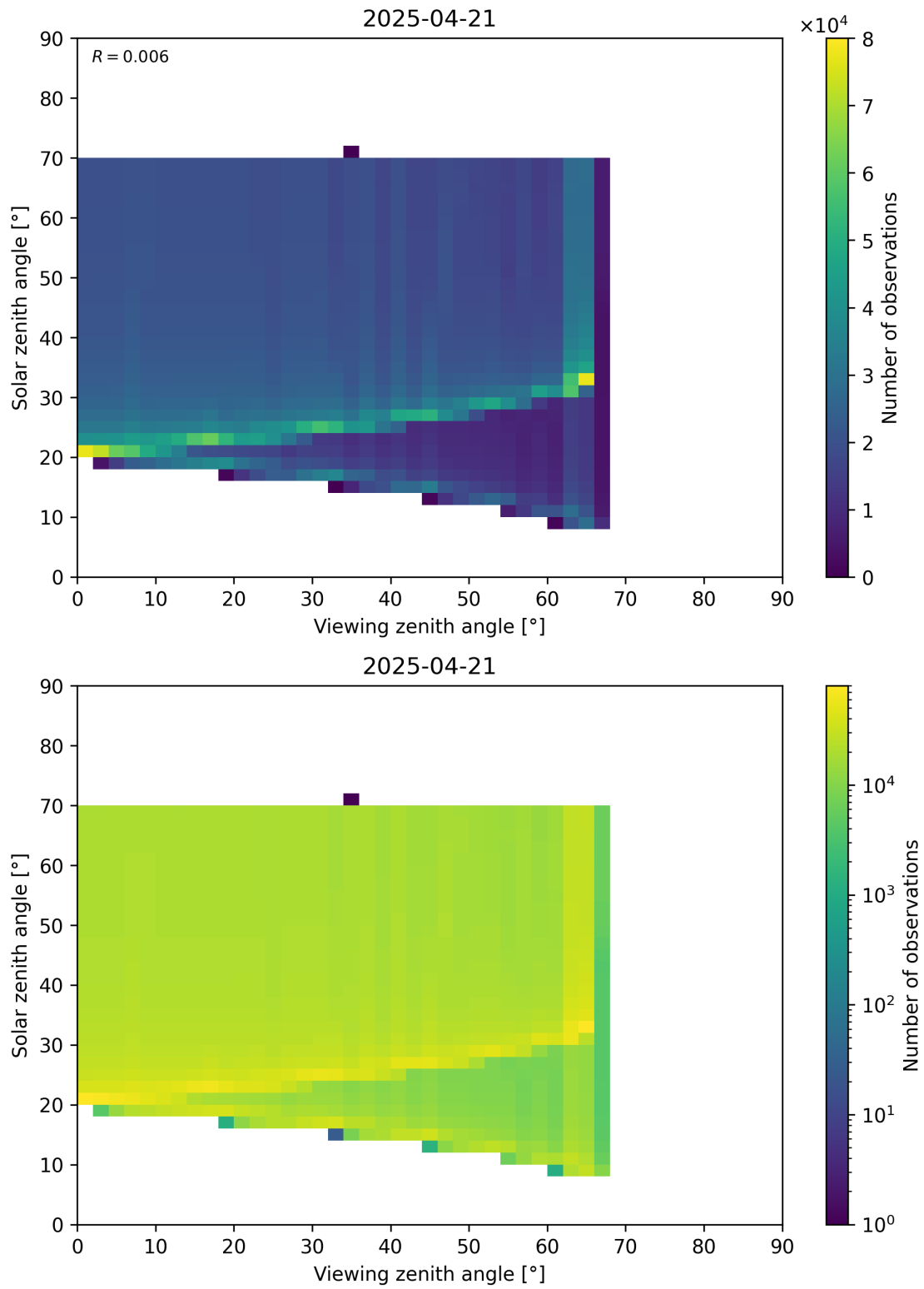
Figure 369: Scatter density plot of “Viewing zenith angle” against “Solar zenith angle” for 2025-04-20 to 2025-04-22.
