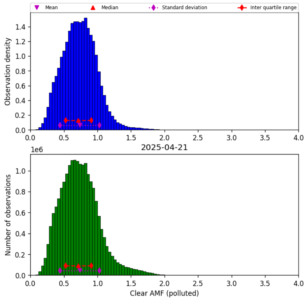
Figure 81: Histogram of “Clear AMF (polluted)” for 2025-04-20 to 2025-04-22
