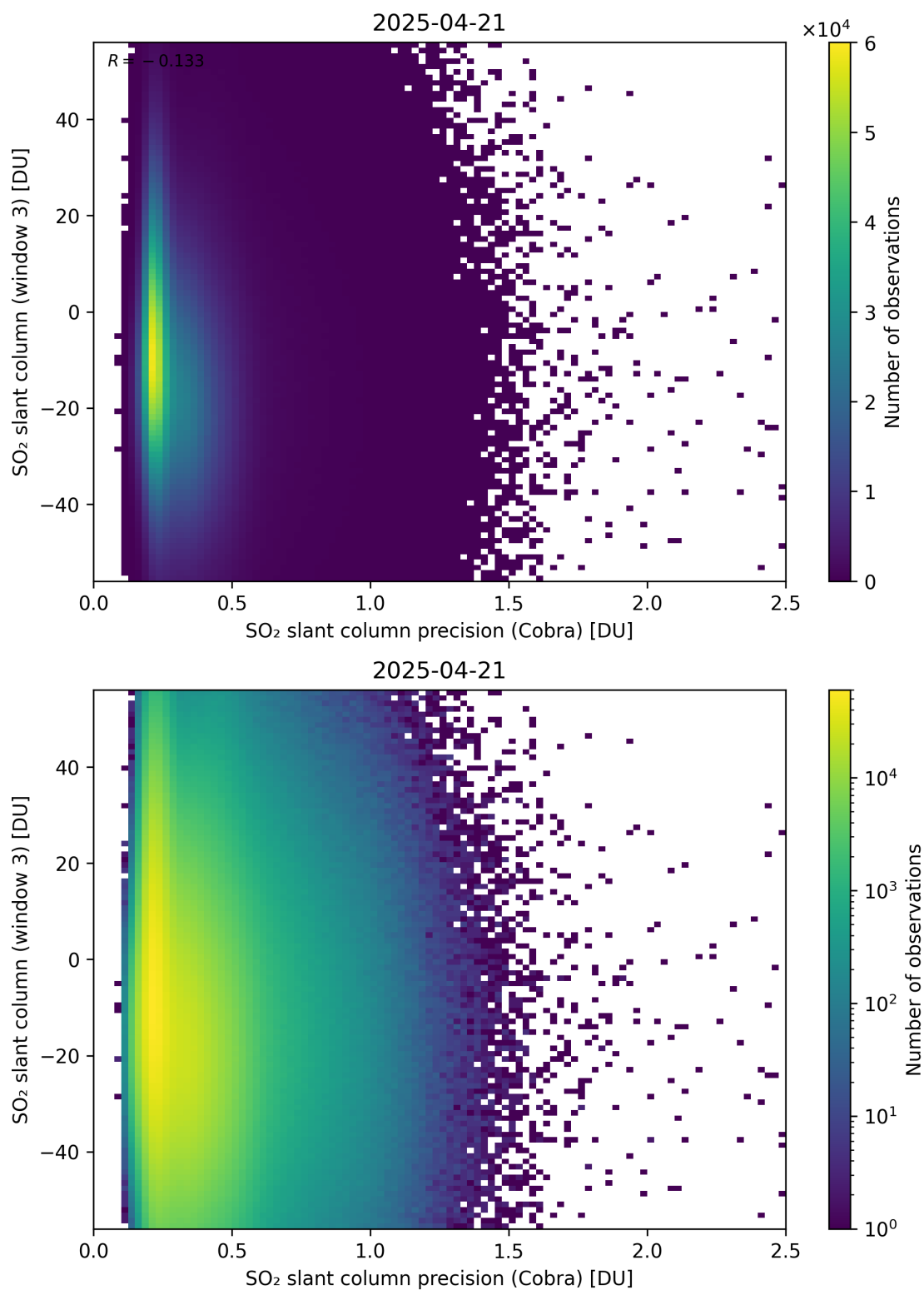
Figure 211: Scatter density plot of “SO 2 slant column precision (Cobra)” against “SO 2 slant column (window 3)” for 2025-04-20 to 2025-04-22.
