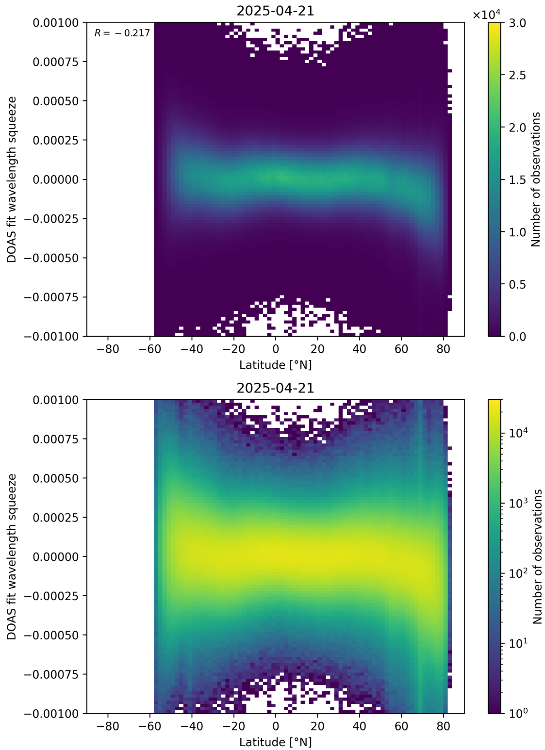
Figure 154: Scatter density plot of “Latitude” against “DOAS fit wavelength squeeze” for 2025-04-20 to 2025-04-22.
