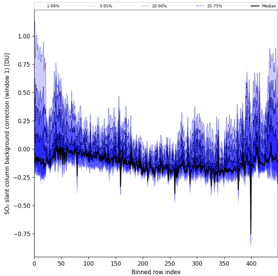
Figure 92: Along track statistics of “SO 2 slant column background correction (window 1)” for 2025-04-20 to 2025-04-22
