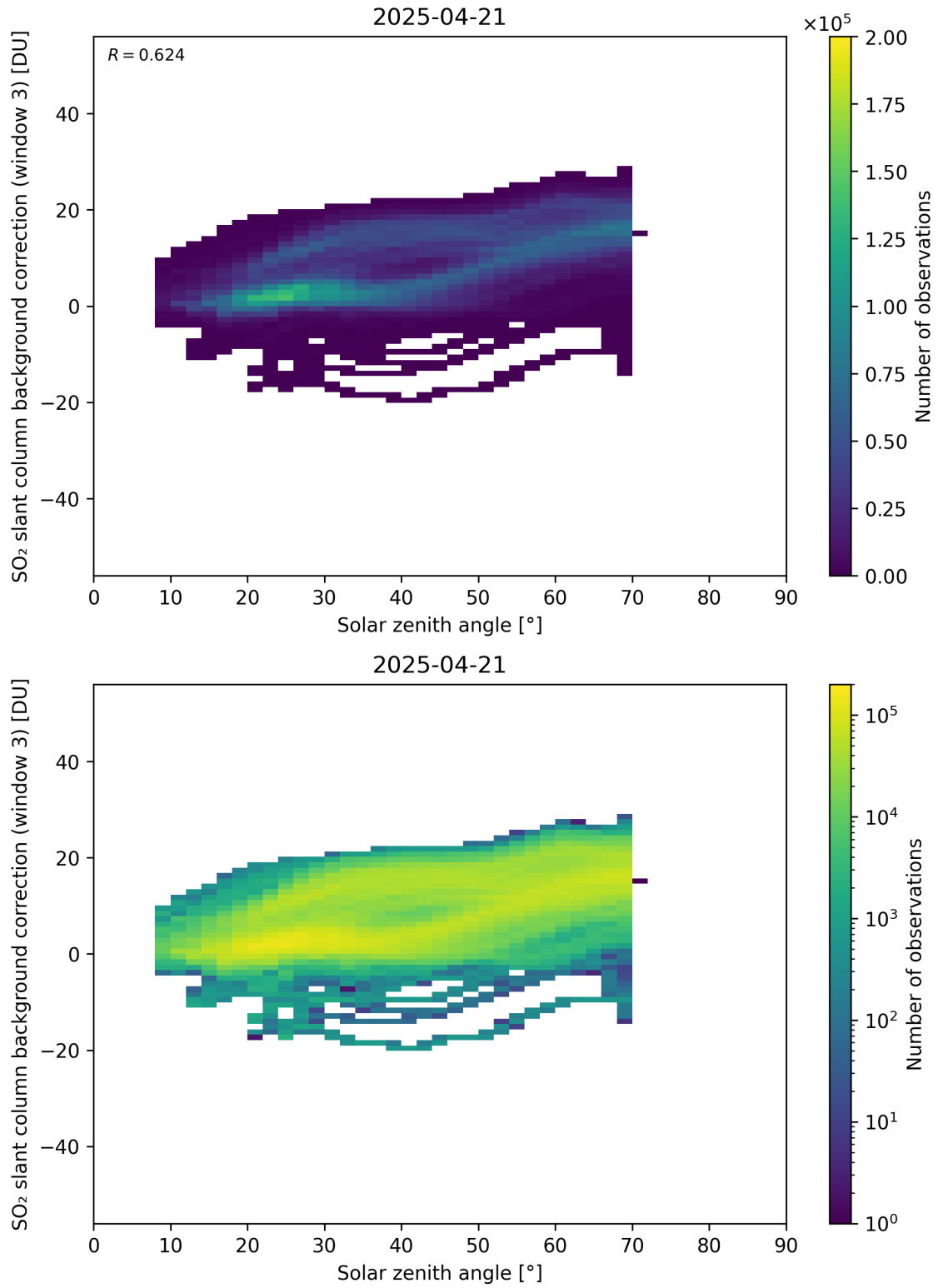
Figure 173: Scatter density plot of “Solar zenith angle” against “SO 2 slant column background correction (window 3)” for 2025-04-20 to 2025-04-22.
