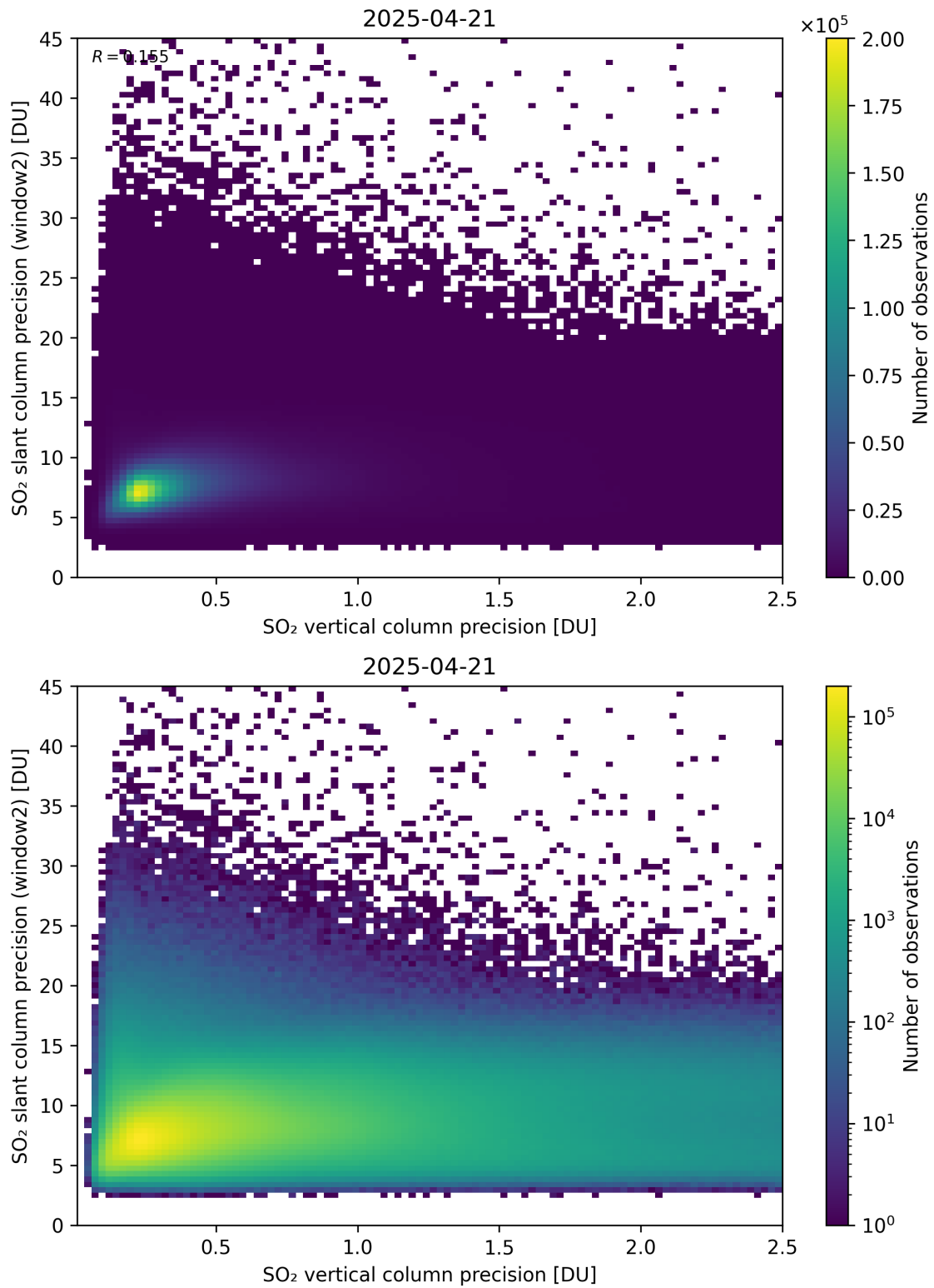
Figure 343: Scatter density plot of “SO 2 vertical column precision” against “SO 2 slant column precision (window2)” for 2025-04-20 to 2025-04-22.
