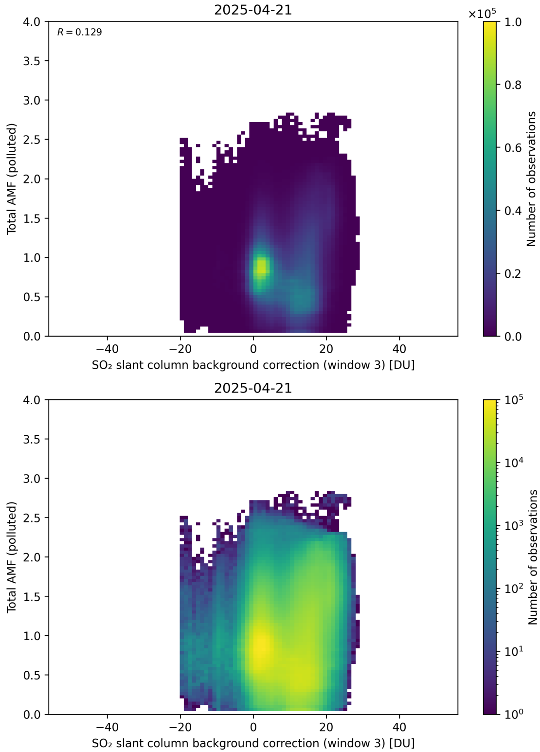
Figure 136: Scatter density plot of “SO 2 slant column background correction (window 3)” against “Total AMF (polluted)” for 2025-04-20 to 2025-04-22.
