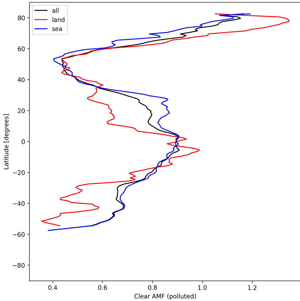
Figure 55: Zonal average of “Clear AMF (polluted)” for 2025-04-20 to 2025-04-22.
