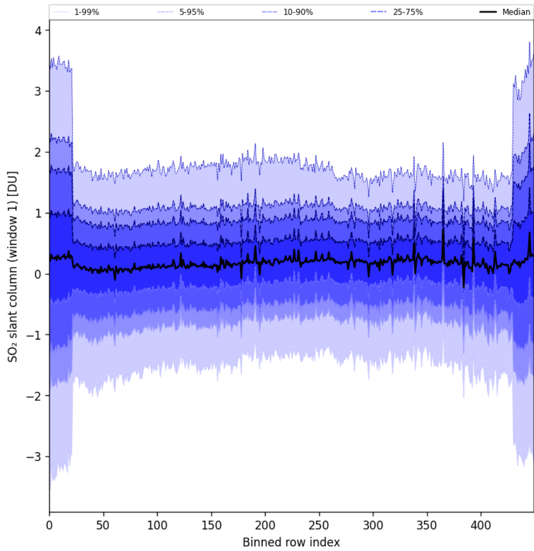
Figure 89: Along track statistics of “SO 2 slant column (window 1)” for 2025-04-20 to 2025-04-22
