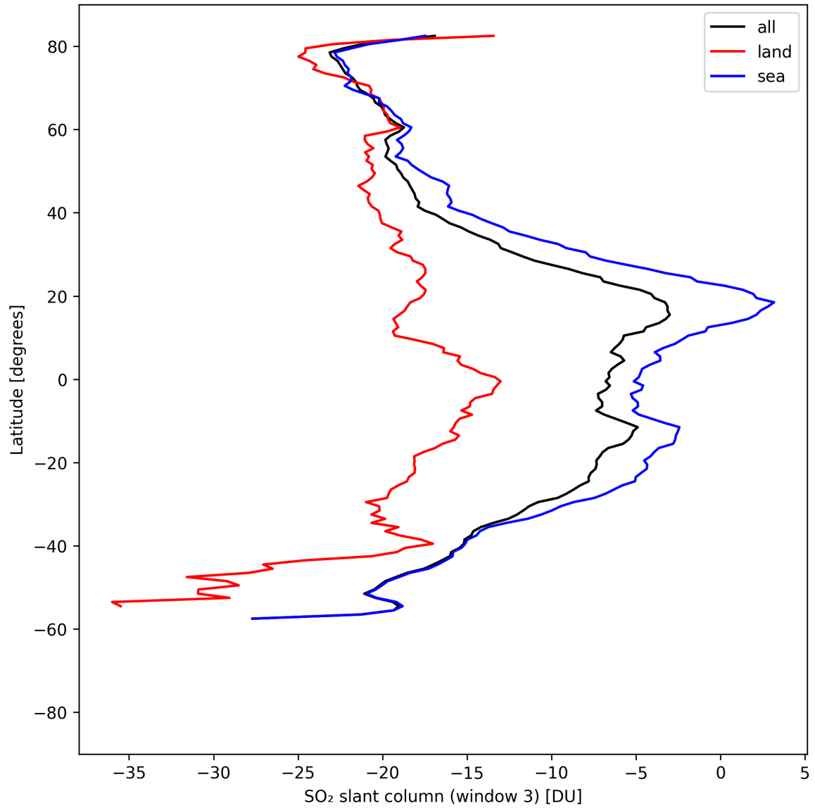
Figure 45: Zonal average of “SO 2 slant column (window 3)” for 2025-04-20 to 2025-04-22.
