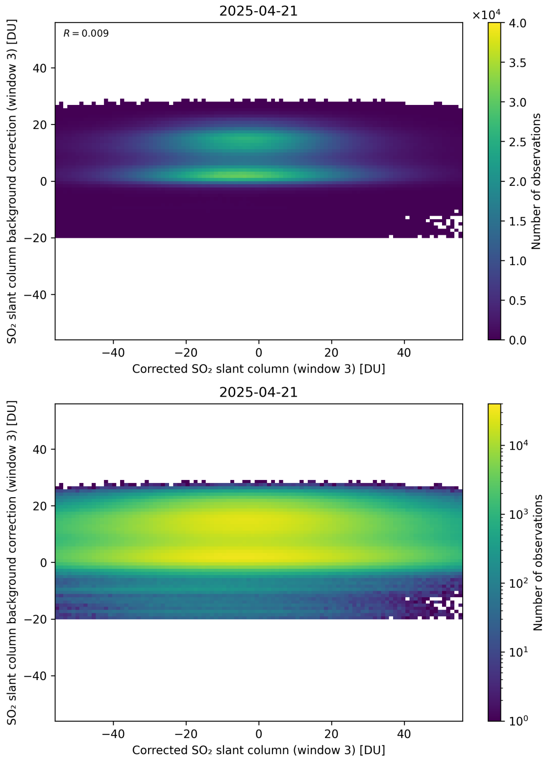
Figure 255: Scatter density plot of “Corrected SO 2 slant column (window 3)” against “SO 2 slant column background correction (window 3)” for 2025-04-20 to 2025-04-22.
