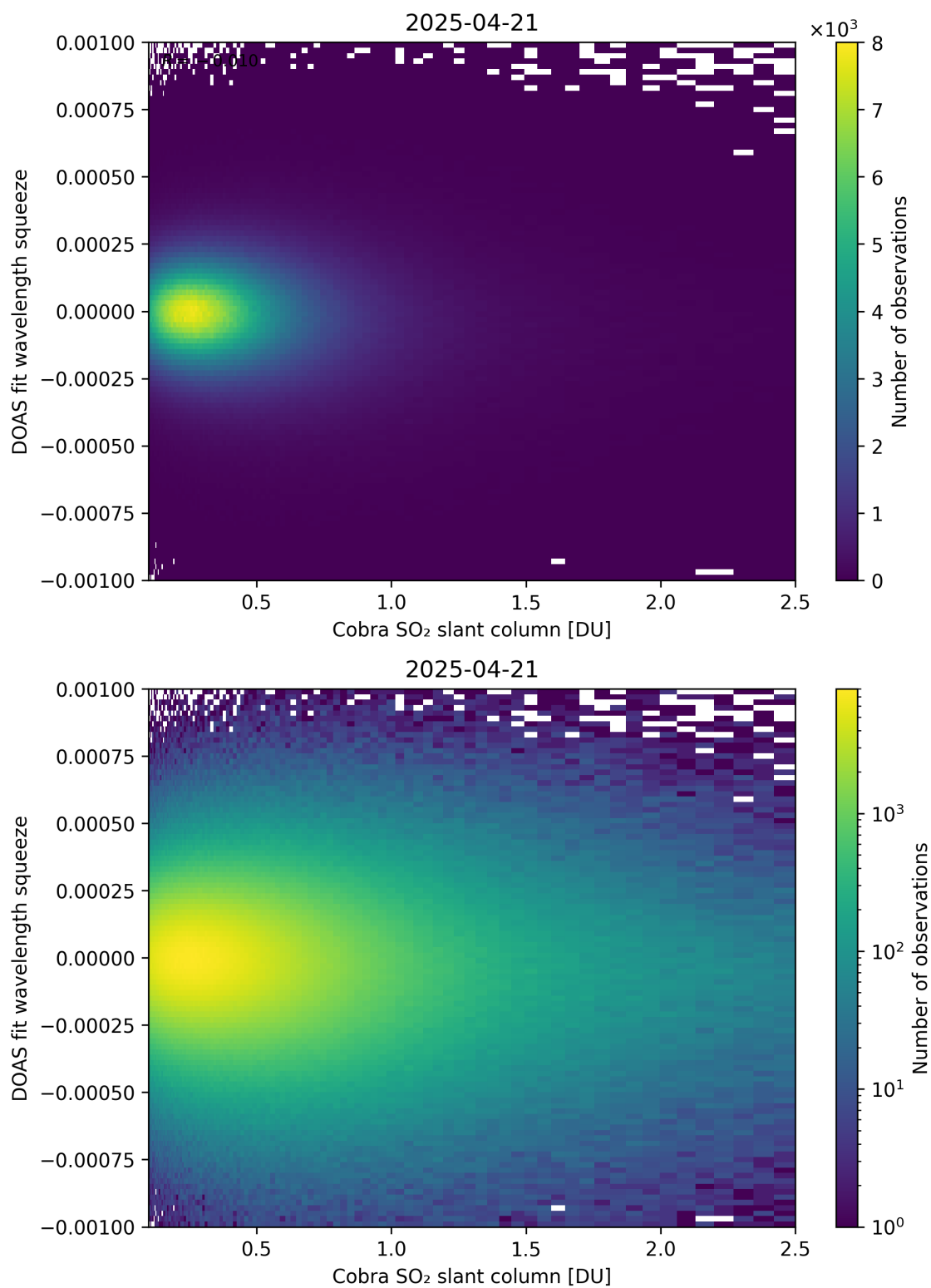
Figure 197: Scatter density plot of “Cobra SO 2 slant column” against “DOAS fit wavelength squeeze” for 2025-04-20 to 2025-04-22.
