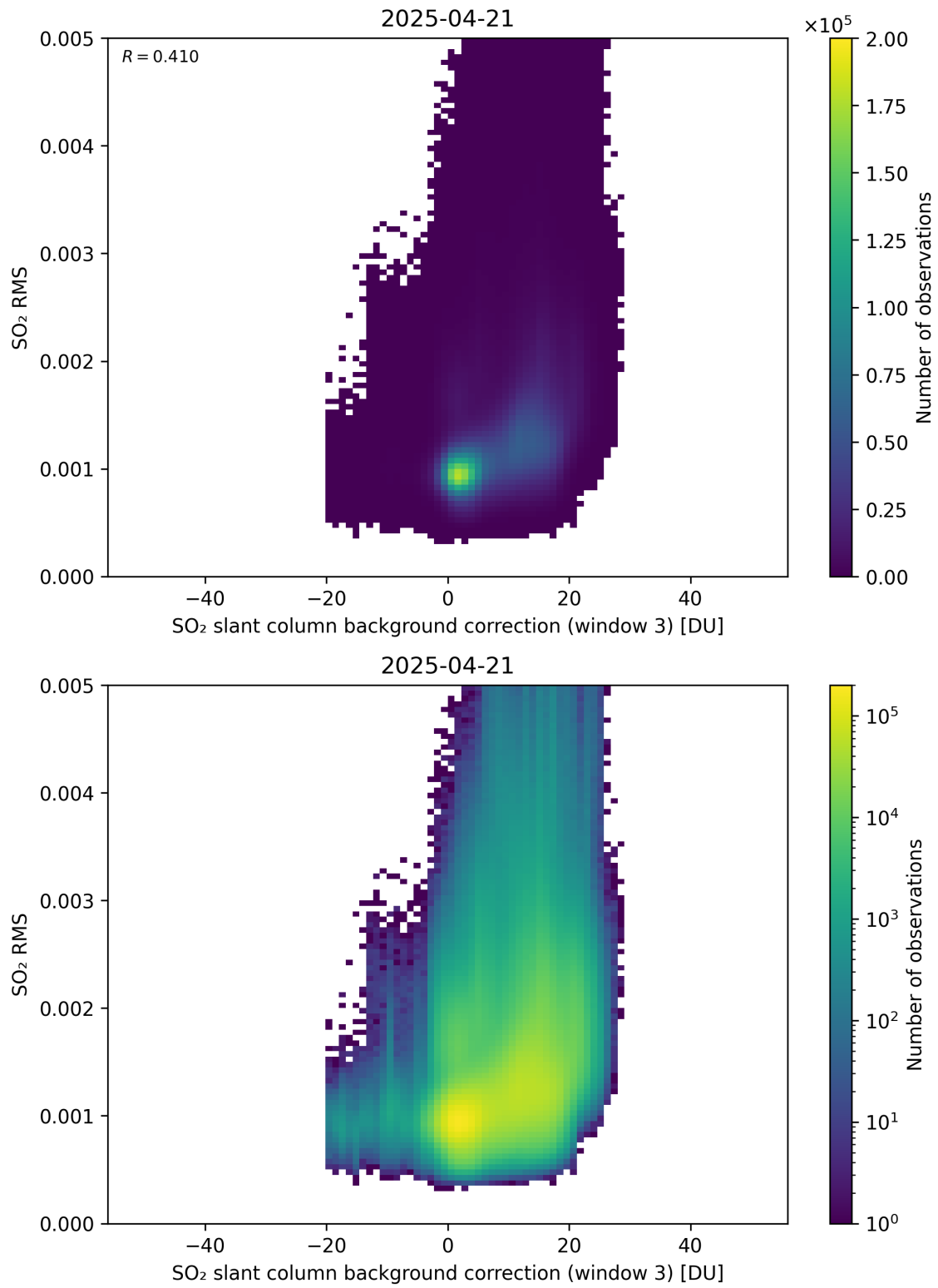
Figure 134: Scatter density plot of “SO 2 slant column background correction (window 3)” against “SO 2 RMS” for 2025-04-20 to 2025-04-22.
