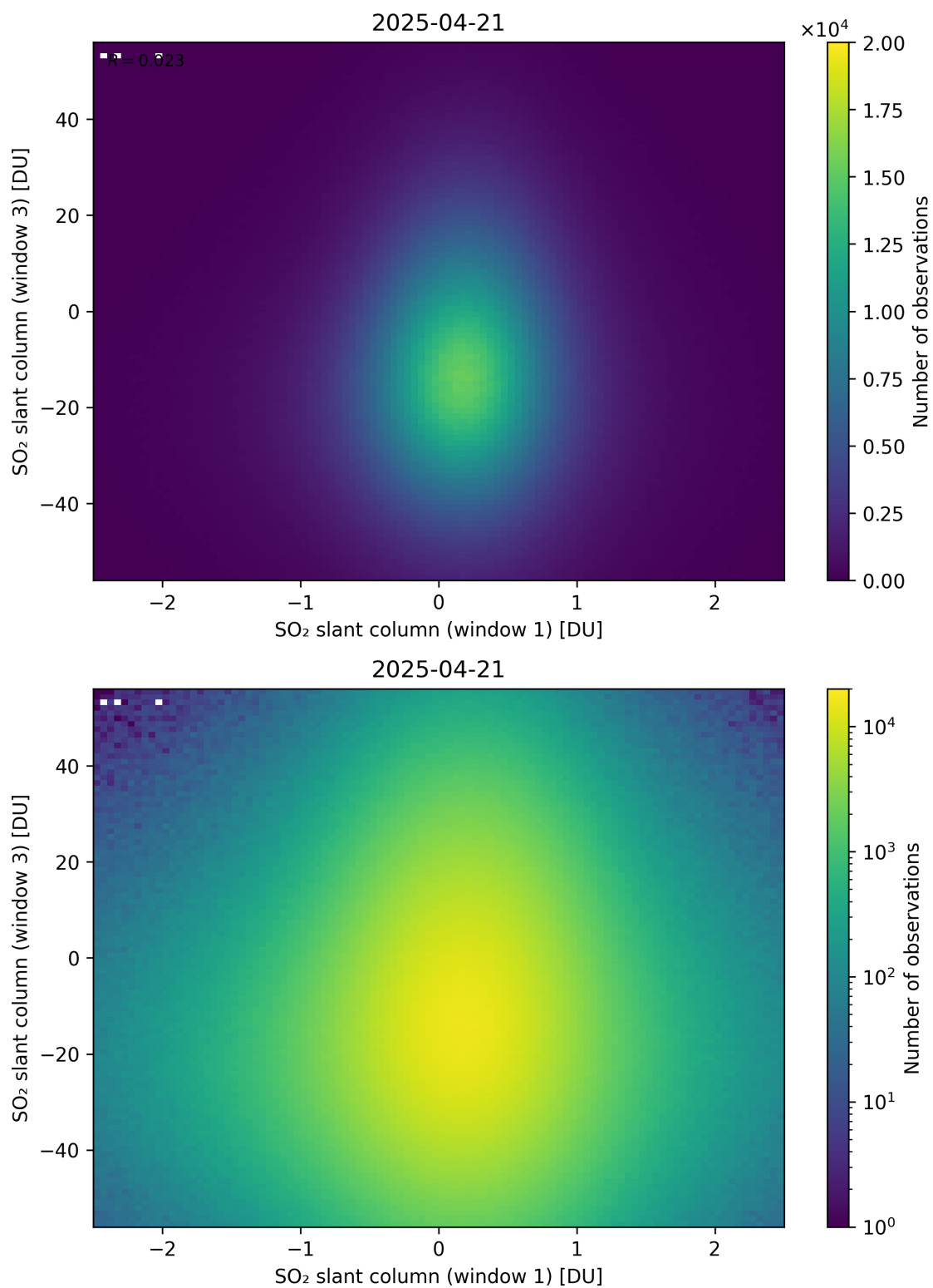
Figure 287: Scatter density plot of “SO 2 slant column (window 1)” against “SO 2 slant column (window 3)” for 2025-04-20 to 2025-04-22.
