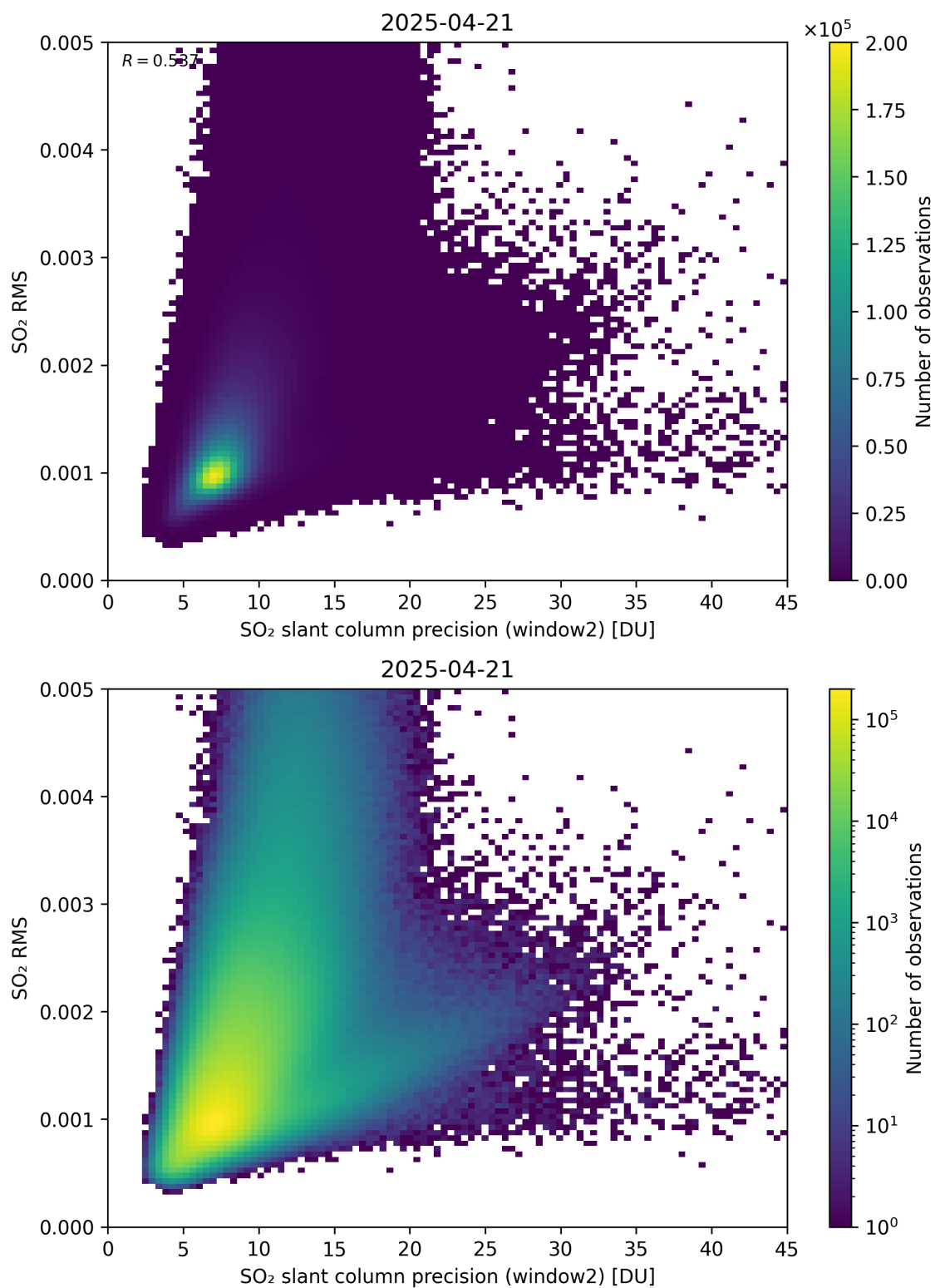
Figure 295: Scatter density plot of “SO 2 slant column precision (window2)” against “SO 2 RMS” for 2025-04-20 to 2025-04-22.
