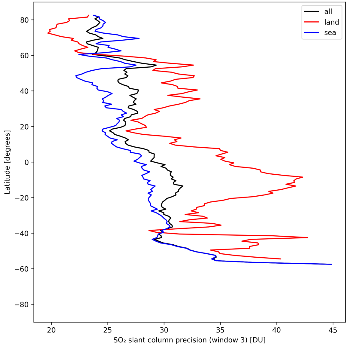
Figure 46: Zonal average of “SO 2 slant column precision (window 3)” for 2025-04-20 to 2025-04-22.
