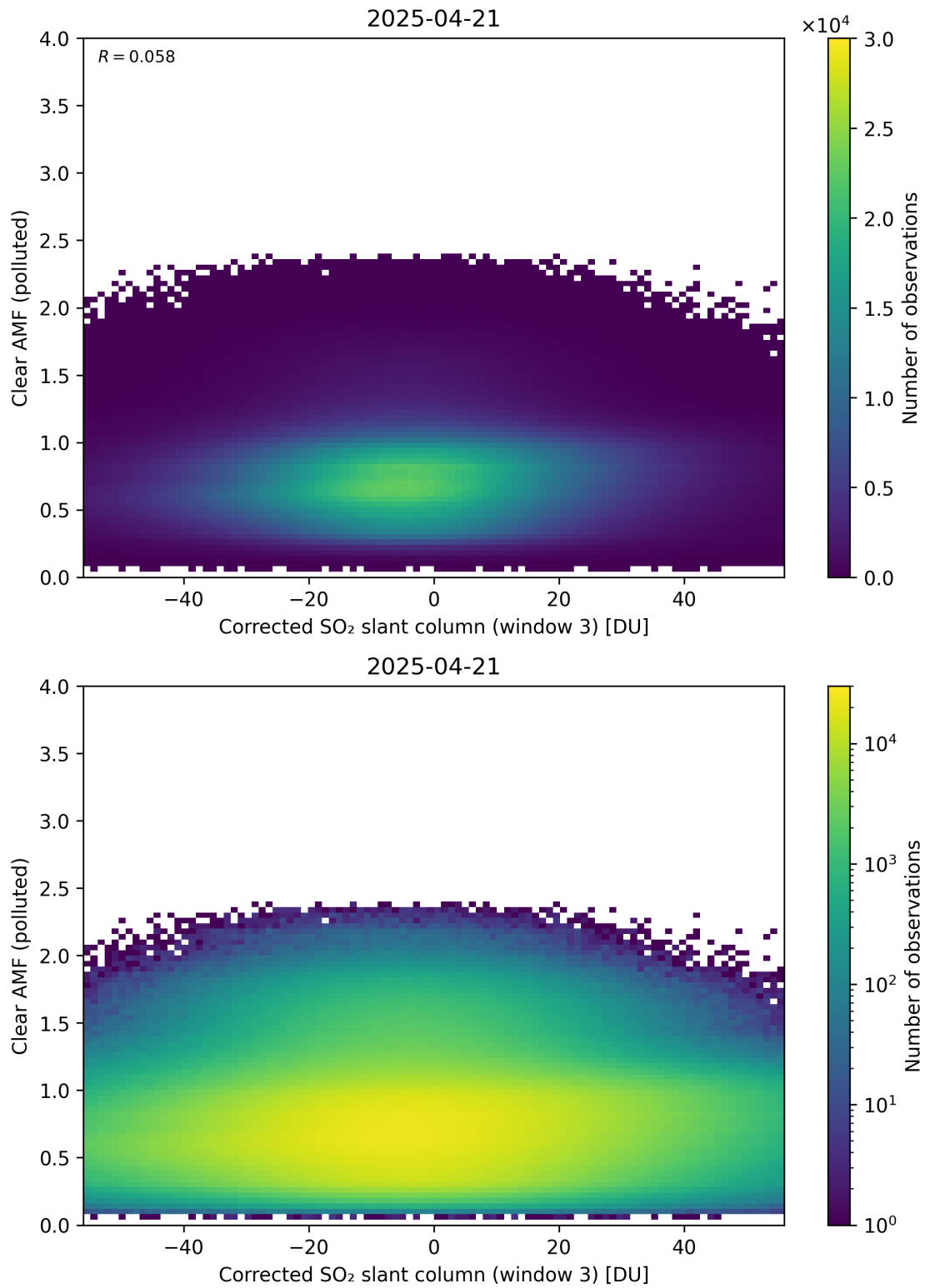
Figure 259: Scatter density plot of “Corrected SO 2 slant column (window 3)” against “Clear AMF (polluted)” for 2025-04-20 to 2025-04-22.
