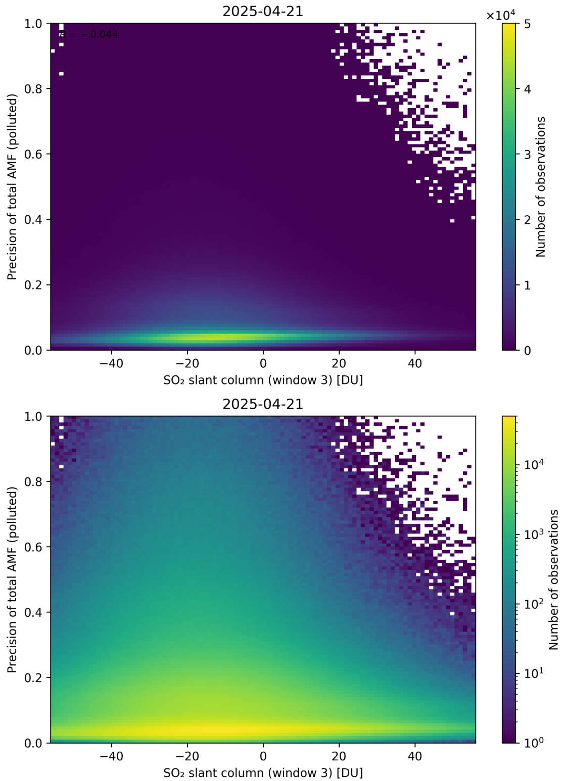
Figure 319: Scatter density plot of “SO 2 slant column (window 3)” against “Precision of total AMF (polluted)” for 2025-04-20 to 2025-04-22.
