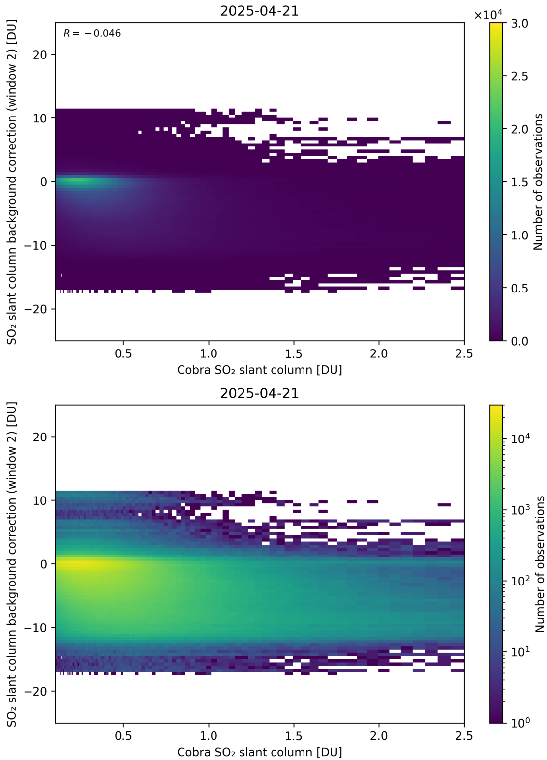
Figure 194: Scatter density plot of “Cobra SO 2 slant column” against “SO 2 slant column background correction (window 2)” for 2025-04-20 to 2025-04-22.
