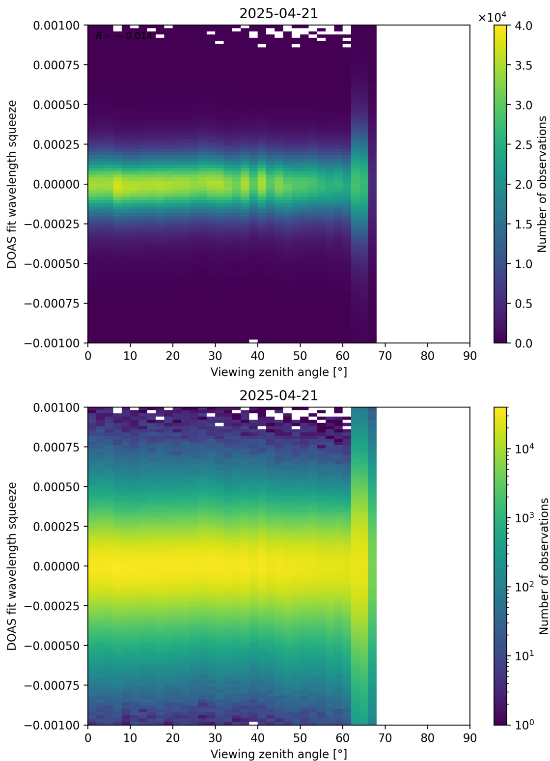
Figure 366: Scatter density plot of “Viewing zenith angle” against “DOAS fit wavelength squeeze” for 2025-04-20 to 2025-04-22.
