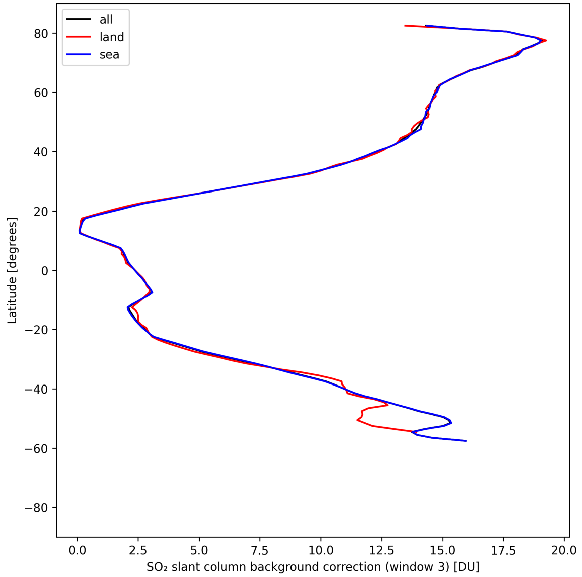
Figure 48: Zonal average of “SO 2 slant column background correction (window 3)” for 2025-04-20 to 2025-04-22.
