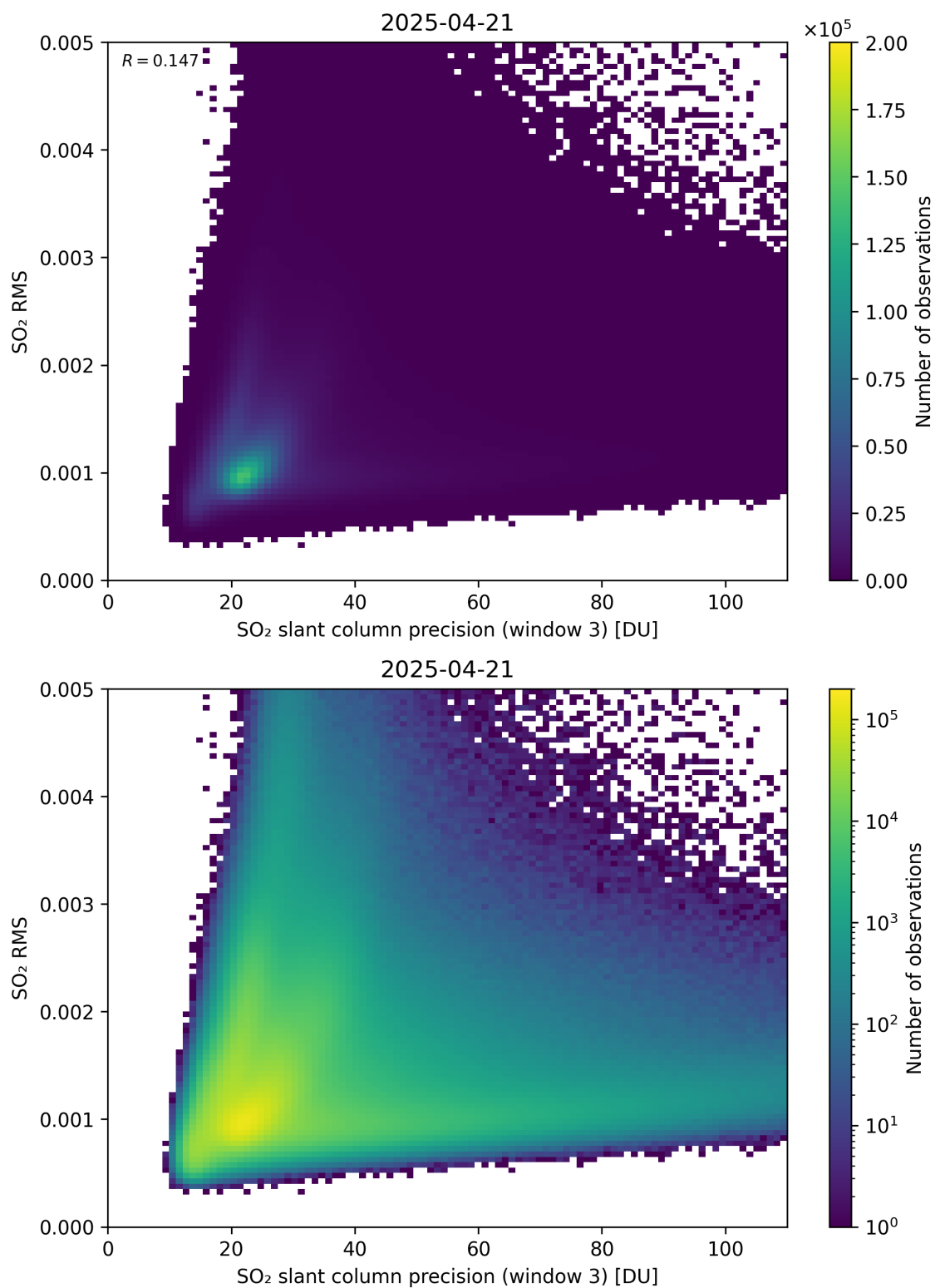
Figure 310: Scatter density plot of “SO 2 slant column precision (window 3)” against “SO 2 RMS” for 2025-04-20 to 2025-04-22.
