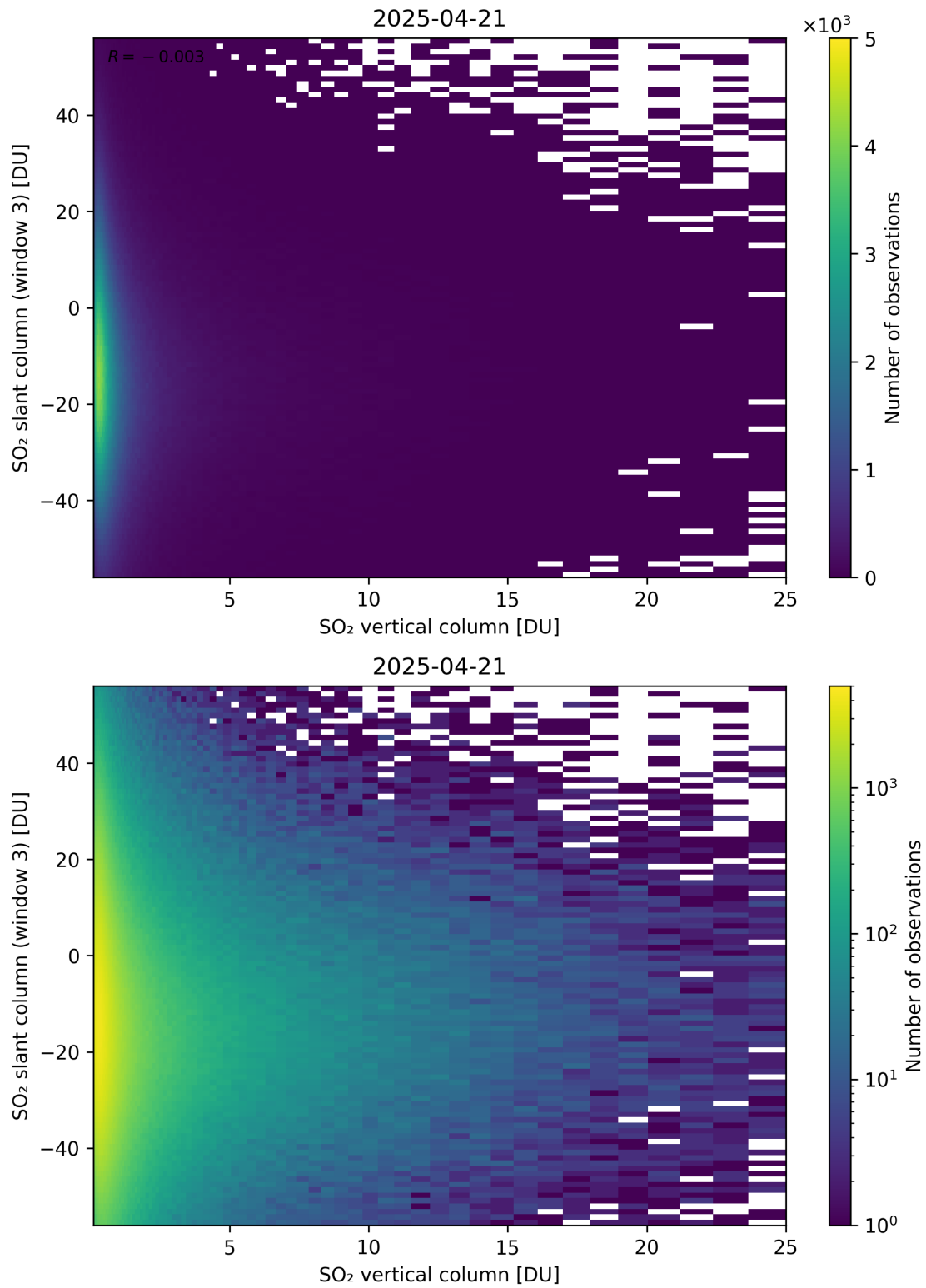
Figure 357: Scatter density plot of “SO 2 vertical column” against “SO 2 slant column (window 3)” for 2025-04-20 to 2025-04-22.
