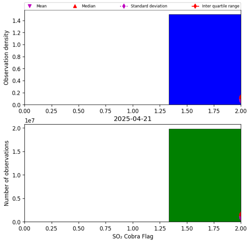
Figure 75: Histogram of “SO 2 Cobra Flag” for 2025-04-20 to 2025-04-22
