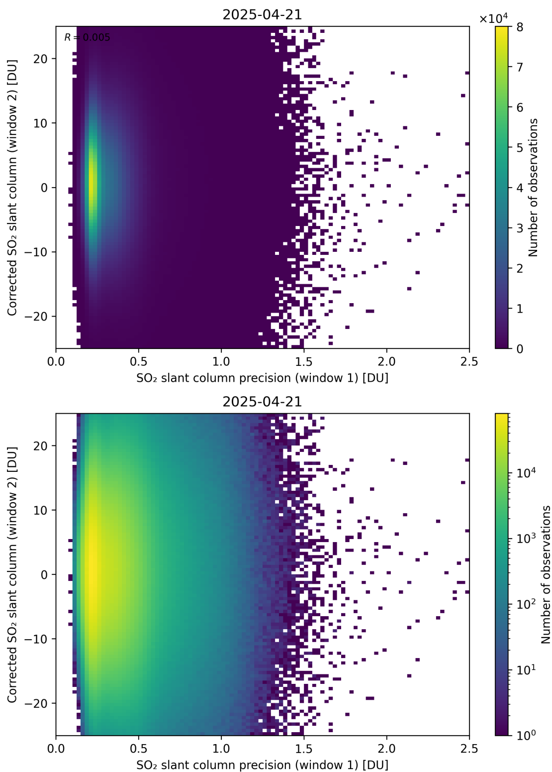
Figure 275: Scatter density plot of “SO 2 slant column precision (window 1)” against “Corrected SO 2 slant column (window 2)” for 2025-04-20 to 2025-04-22.
