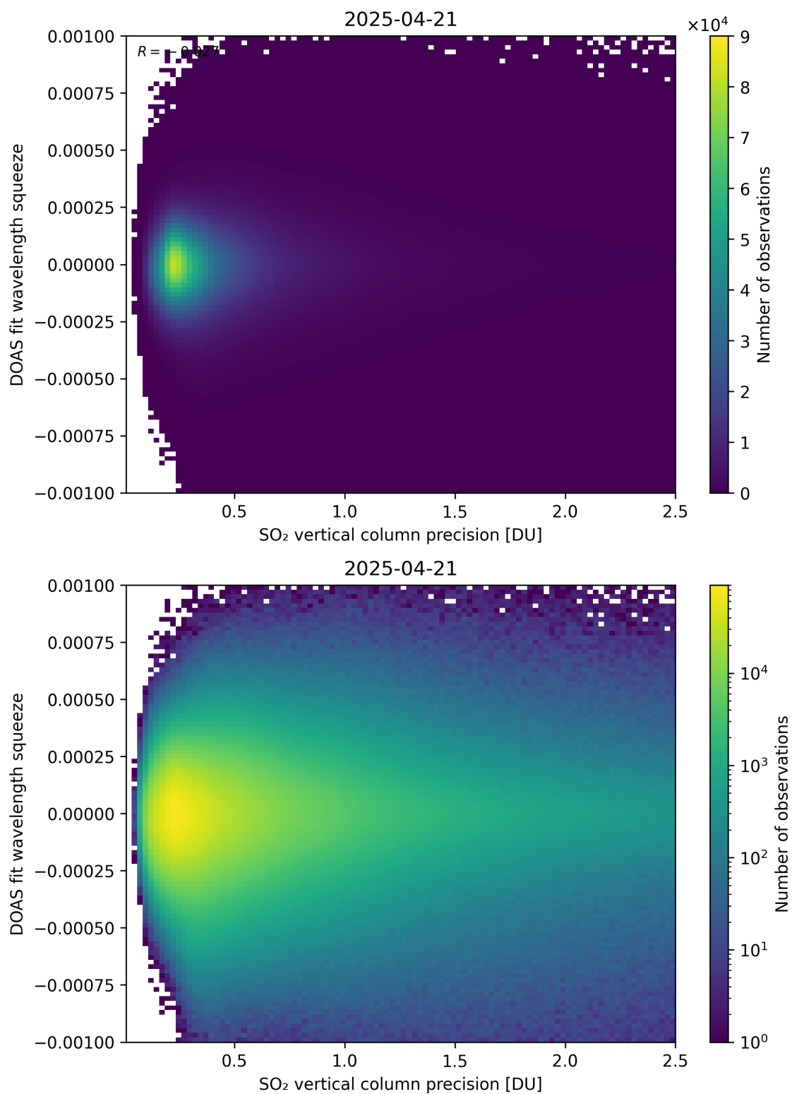
Figure 333: Scatter density plot of “SO 2 vertical column precision” against “DOAS fit wavelength squeeze” for 2025-04-20 to 2025-04-22.
