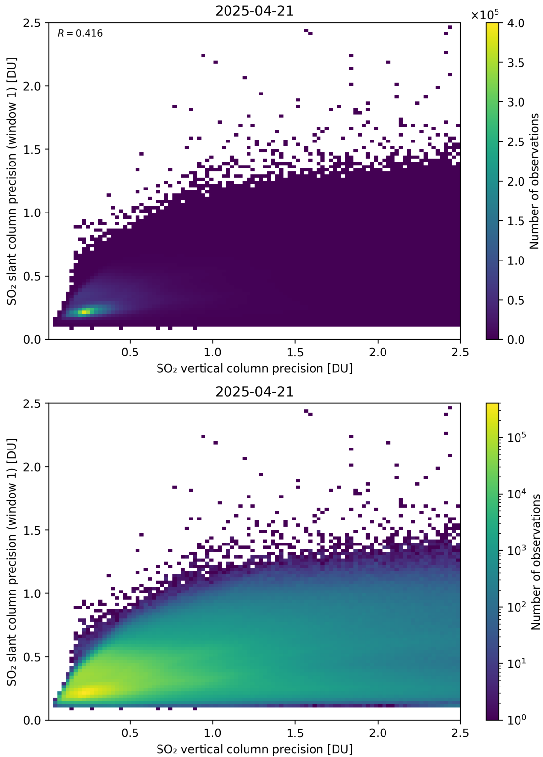
Figure 342: Scatter density plot of “SO 2 vertical column precision” against “SO 2 slant column precision (window 1)” for 2025-04-20 to 2025-04-22.
