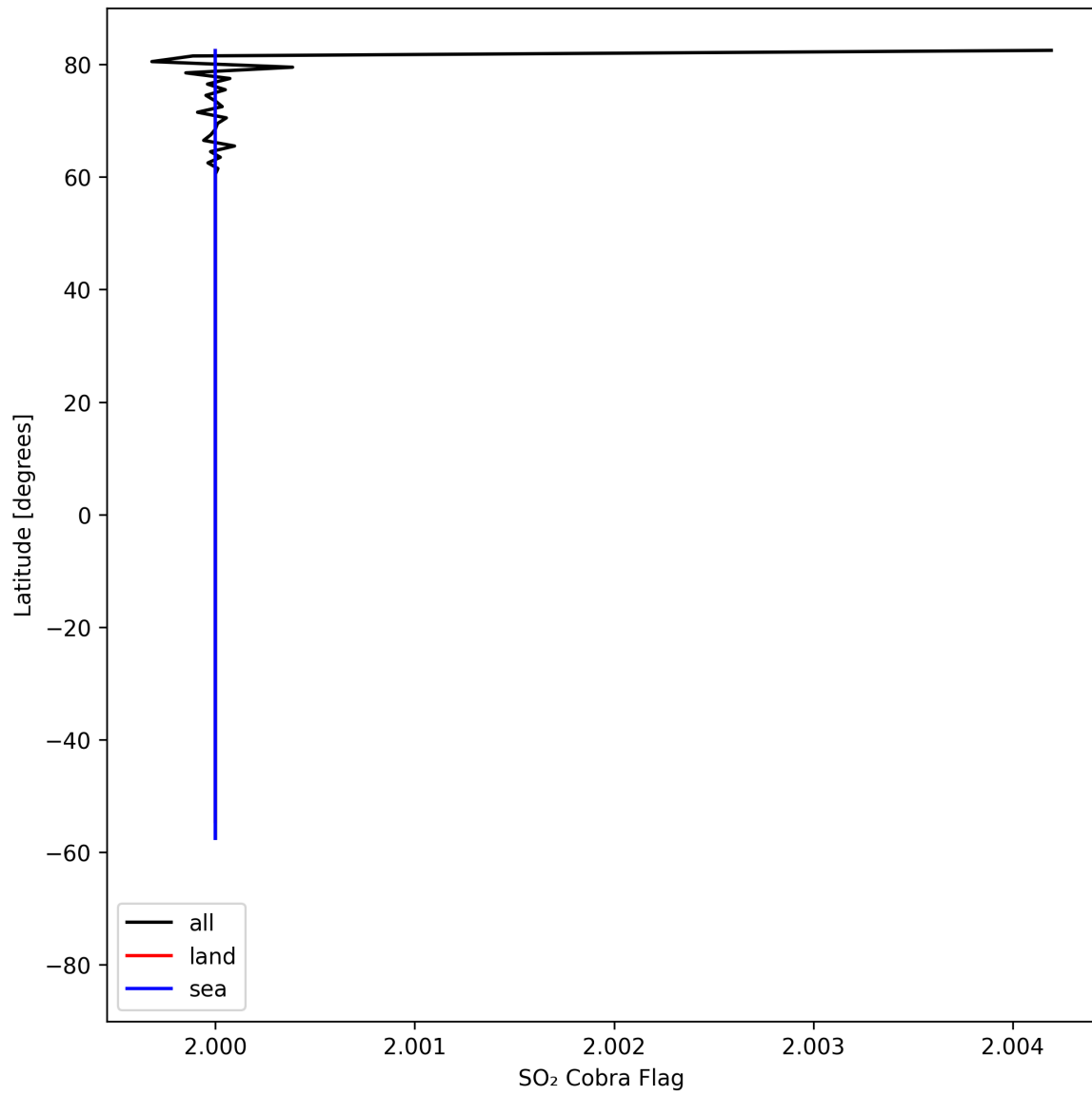
Figure 49: Zonal average of “SO 2 Cobra Flag” for 2025-04-20 to 2025-04-22.
