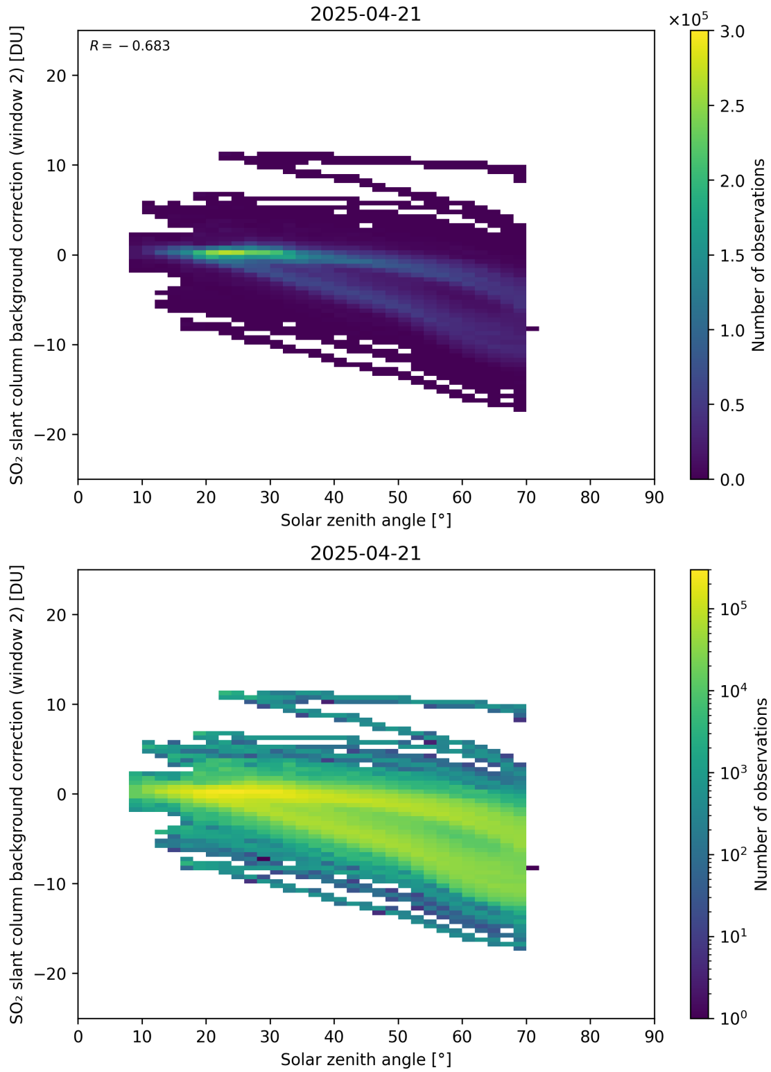
Figure 172: Scatter density plot of “Solar zenith angle” against “SO 2 slant column background correction (window 2)” for 2025-04-20 to 2025-04-22.
