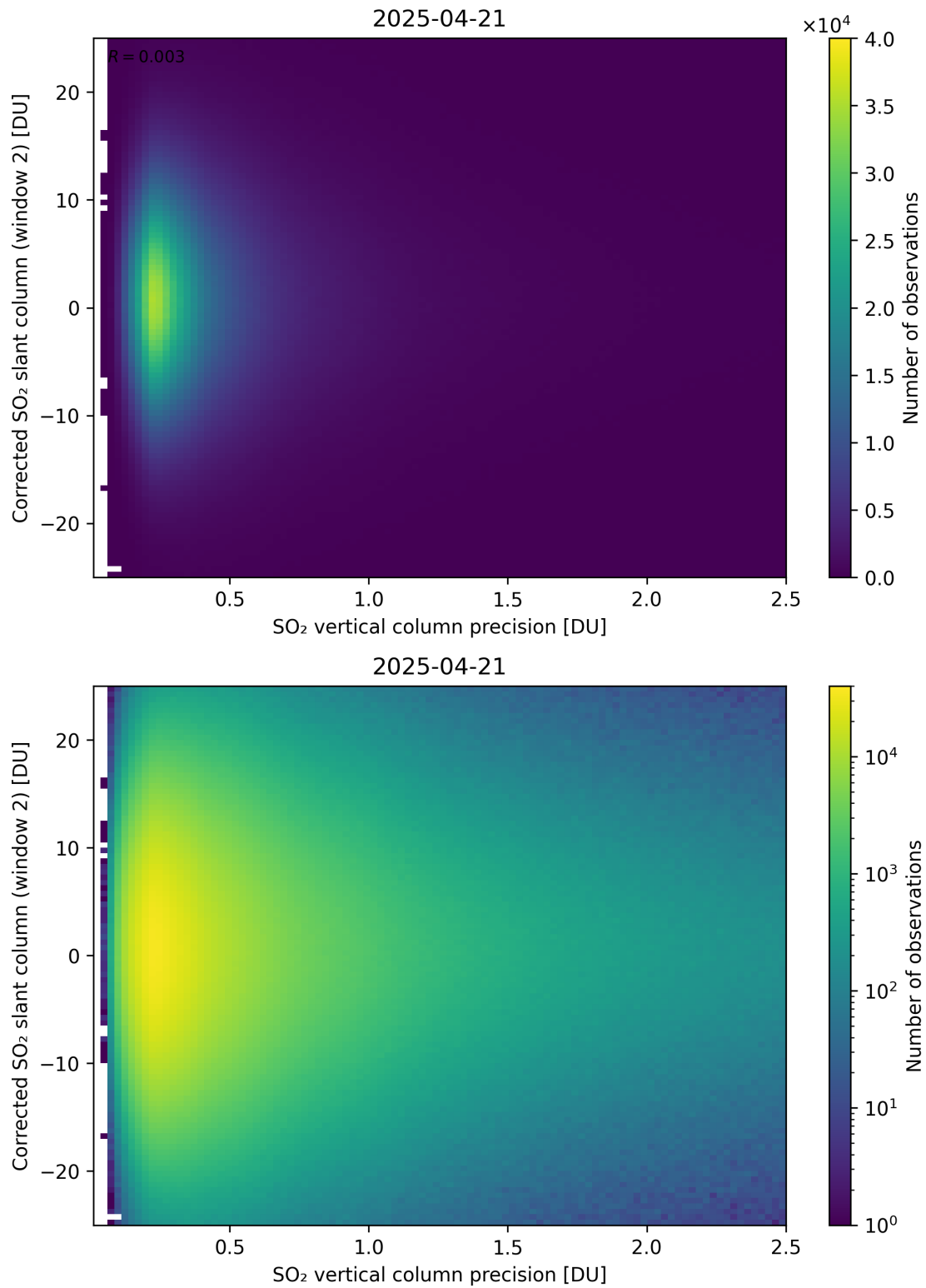
Figure 339: Scatter density plot of “SO 2 vertical column precision” against “Corrected SO 2 slant column (window 2)” for 2025-04-20 to 2025-04-22.
