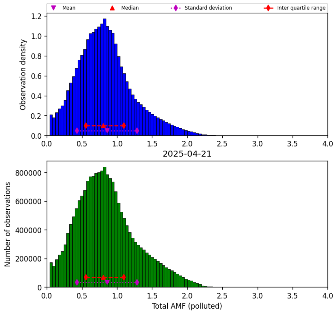
Figure 79: Histogram of “Total AMF (polluted)” for 2025-04-20 to 2025-04-22
