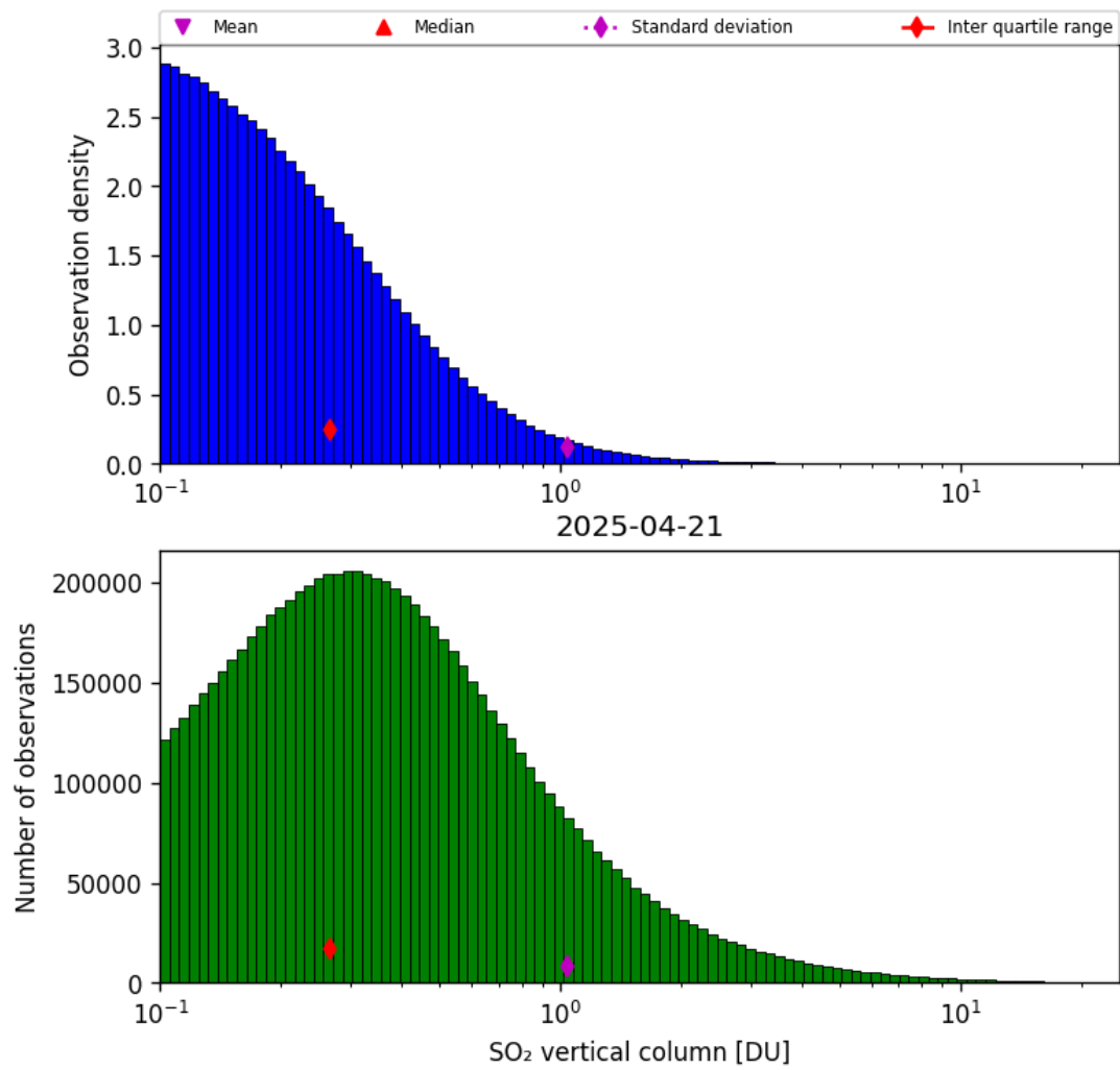
Figure 58: Histogram of “SO 2 vertical column” for 2025-04-20 to 2025-04-22
