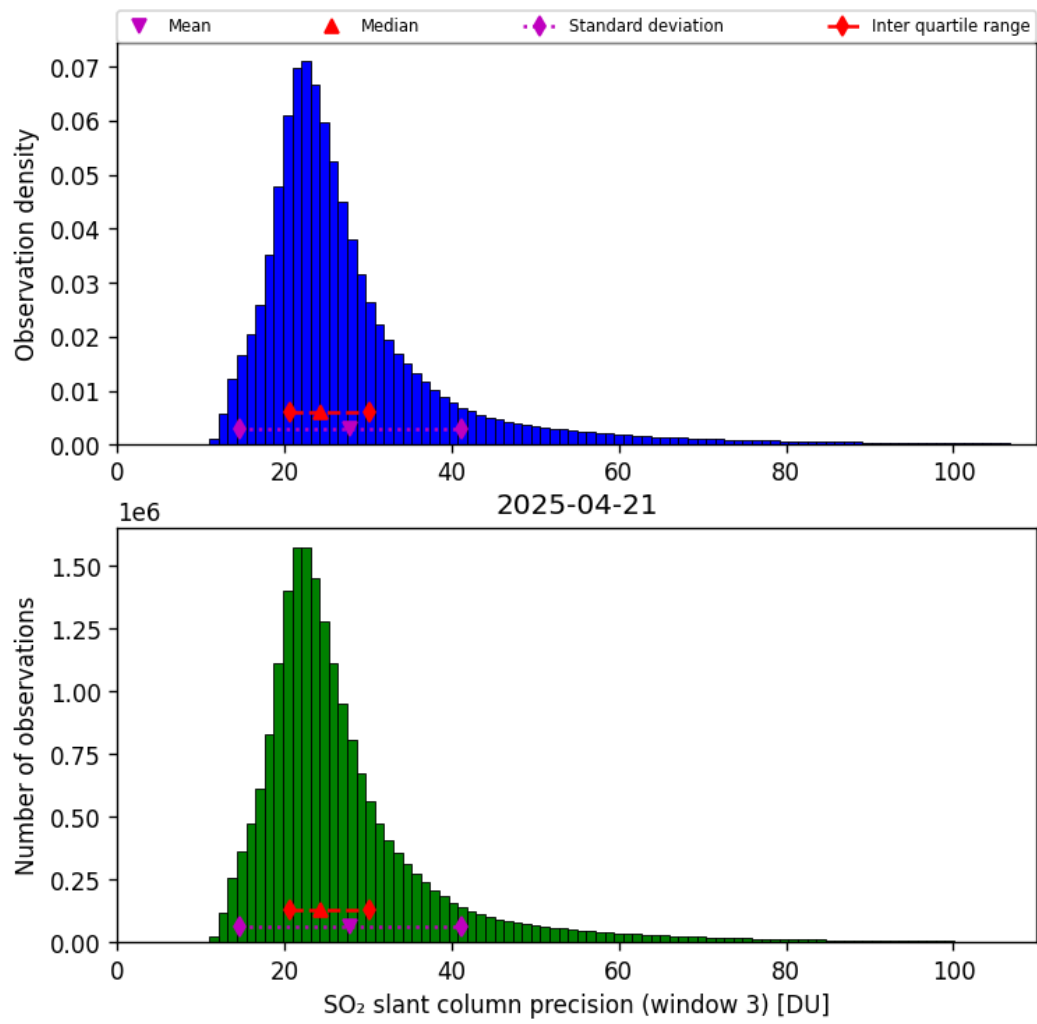
Figure 72: Histogram of “SO 2 slant column precision (window 3)” for 2025-04-20 to 2025-04-22
