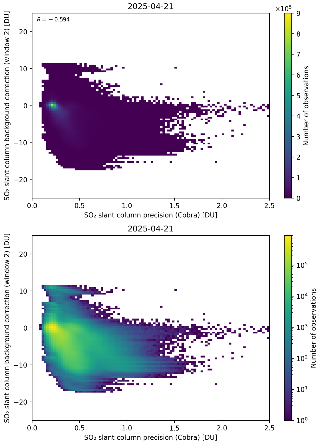
Figure 200: Scatter density plot of “SO 2 slant column precision (Cobra)” against “SO 2 slant column background correction (window 2)” for 2025-04-20 to 2025-04-22.
