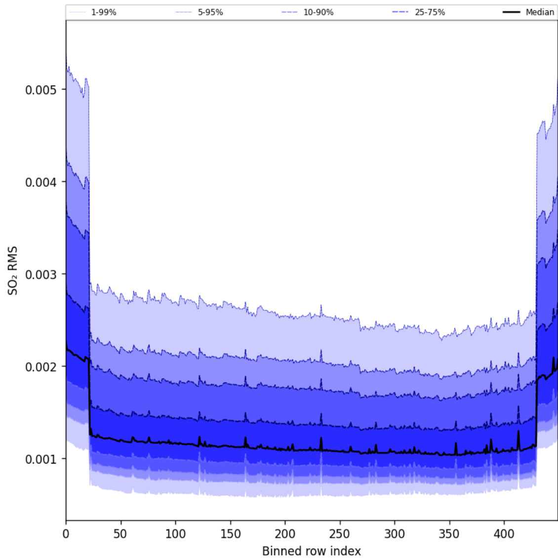
Figure 104: Along track statistics of “SO 2 RMS” for 2025-04-20 to 2025-04-22
