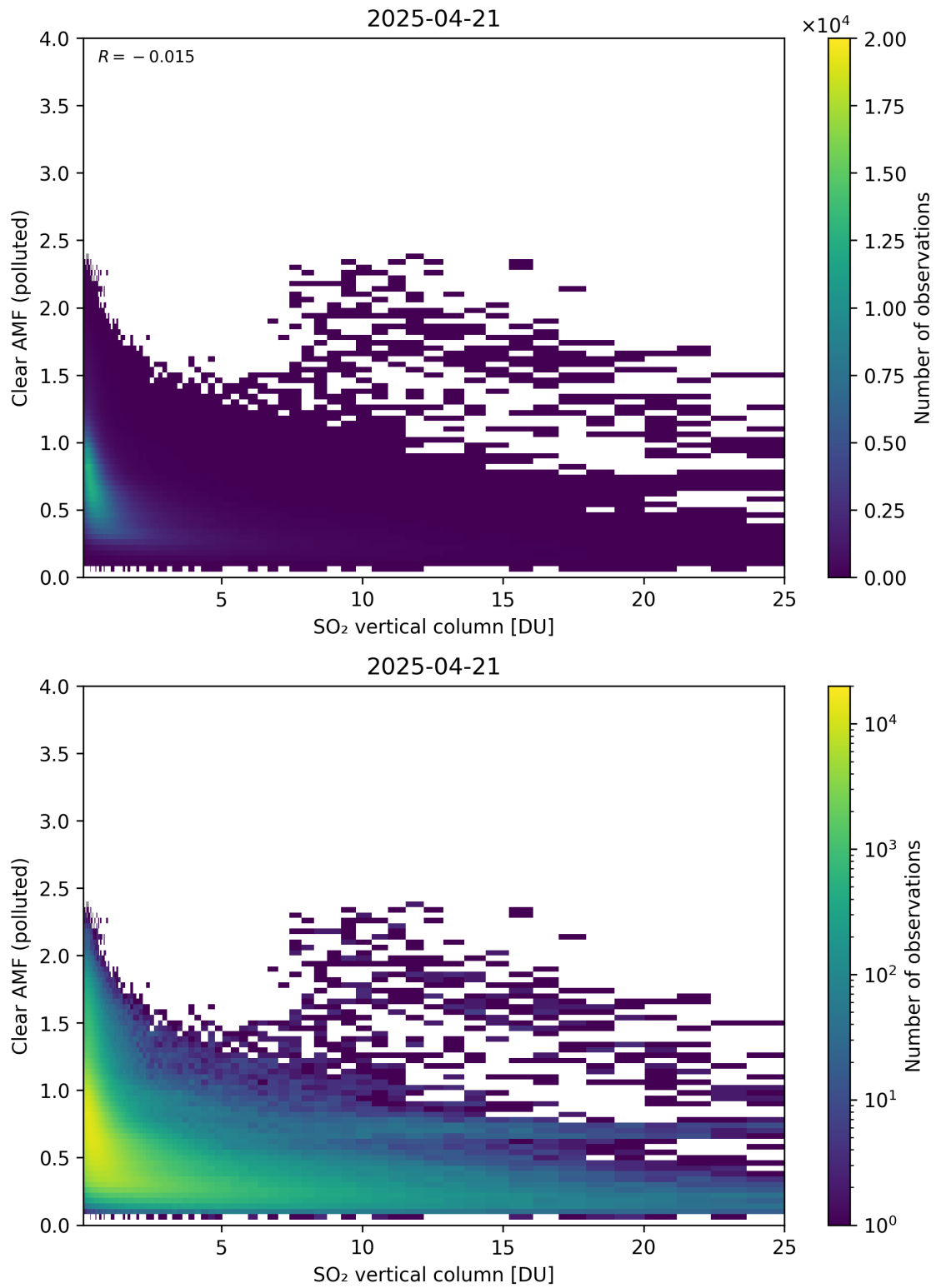
Figure 348: Scatter density plot of “SO 2 vertical column” against “Clear AMF (polluted)” for 2025-04-20 to 2025-04-22.
