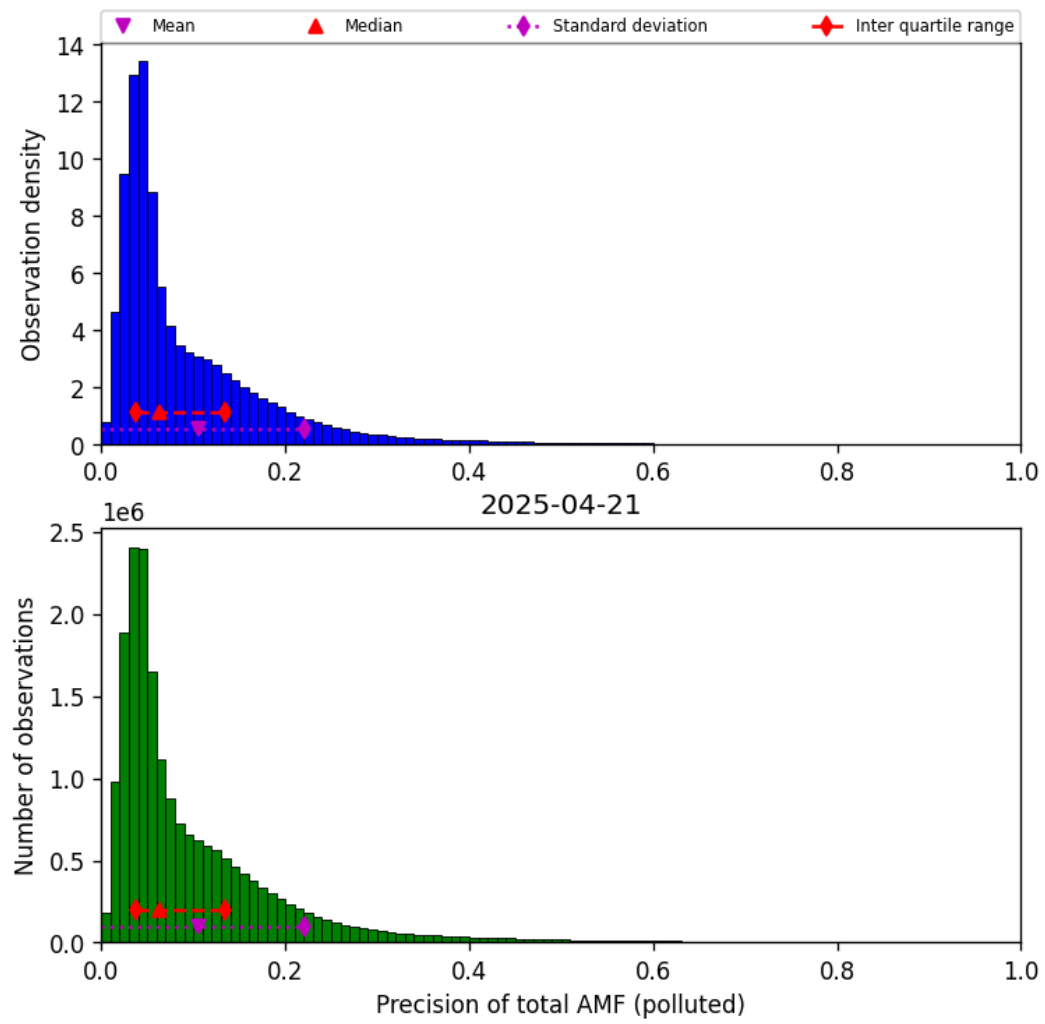
Figure 80: Histogram of “Precision of total AMF (polluted)” for 2025-04-20 to 2025-04-22
