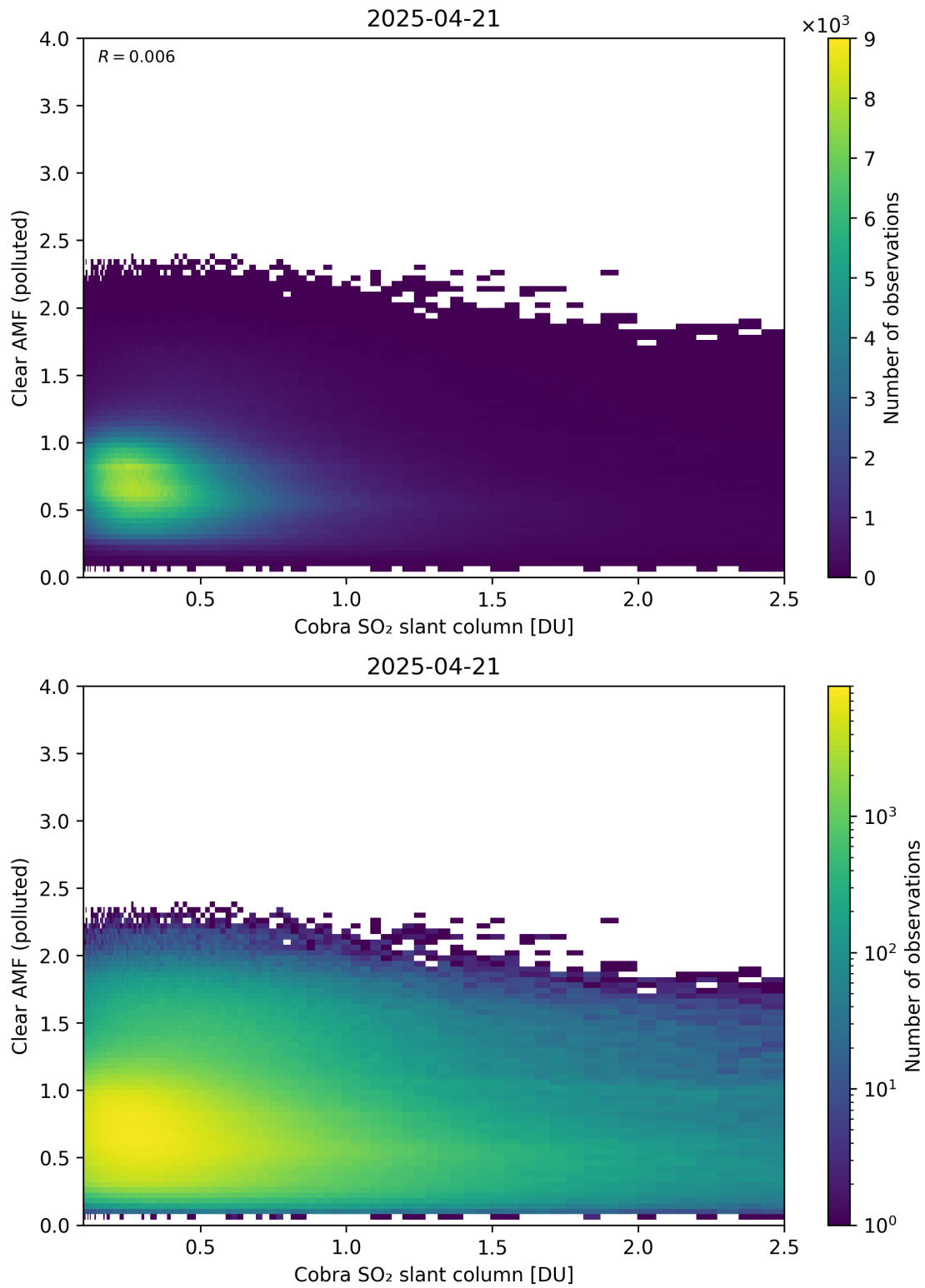
Figure 215: Scatter density plot of “Cobra SO 2 slant column” against “Clear AMF (polluted)” for 2025-04-20 to 2025-04-22.
