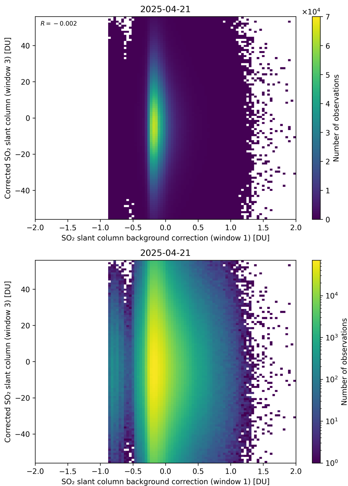
Figure 116: Scatter density plot of “SO 2 slant column background correction (window 1)” against “Corrected SO 2 slant column (window 3)” for 2025-04-20 to 2025-04-22.
