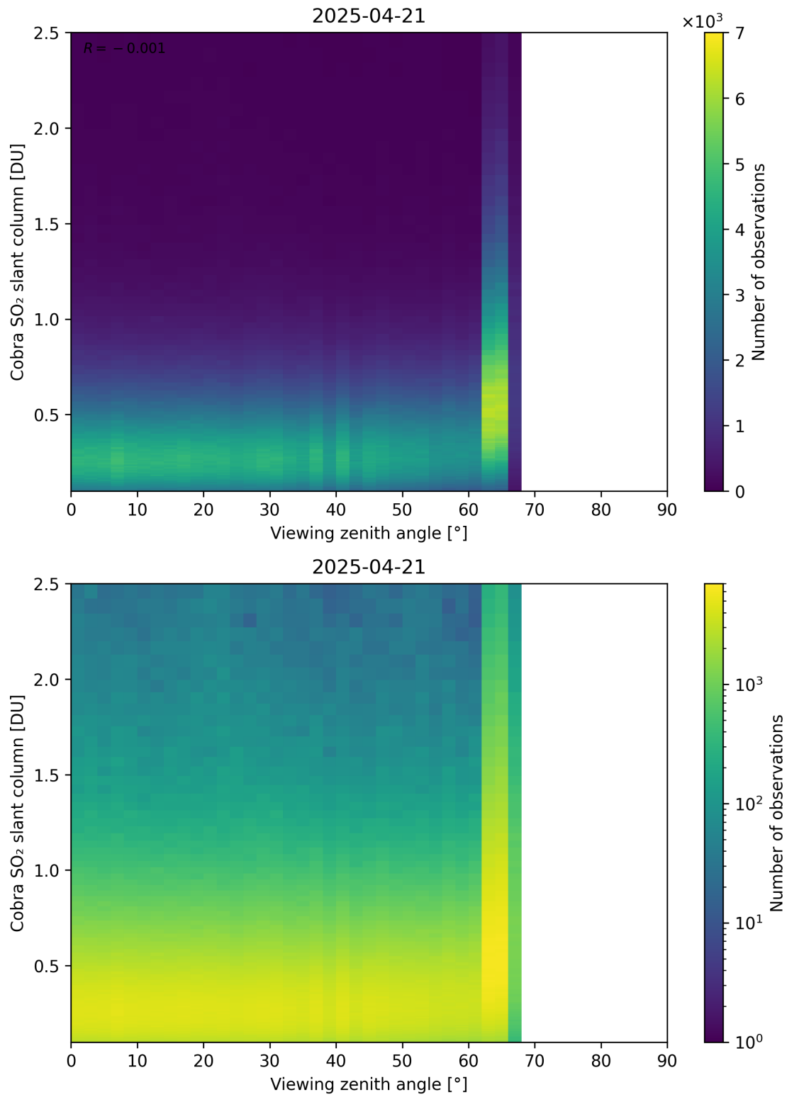
Figure 371: Scatter density plot of “Viewing zenith angle” against “Cobra SO 2 slant column” for 2025-04-20 to 2025-04-22.
