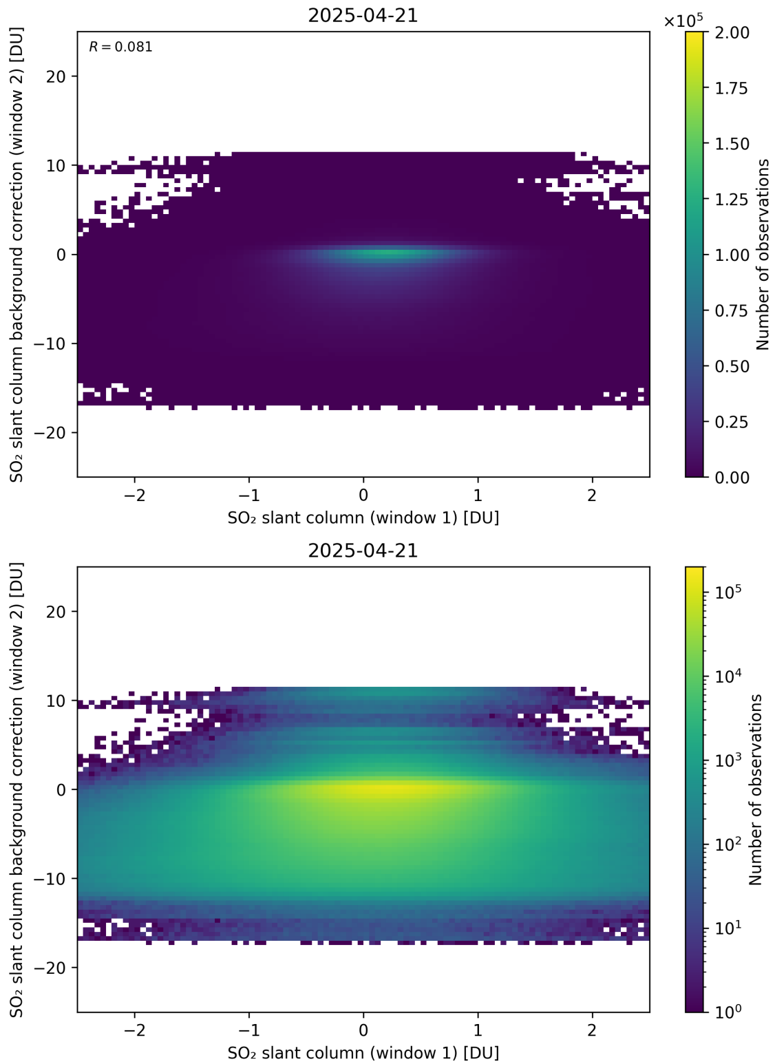
Figure 263: Scatter density plot of “SO 2 slant column (window 1)” against “SO 2 slant column background correction (window 2)” for 2025-04-20 to 2025-04-22.
