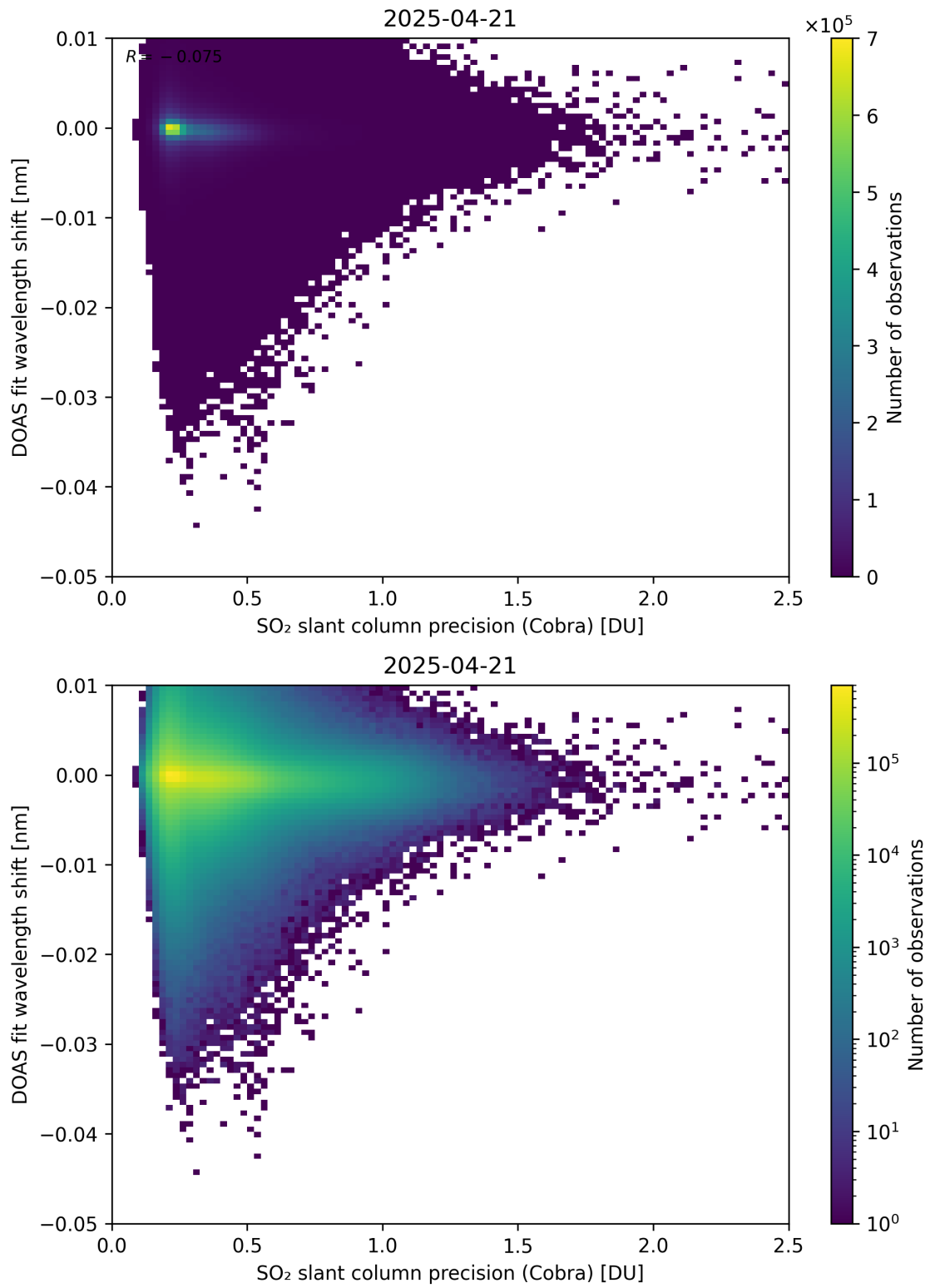
Figure 202: Scatter density plot of “SO 2 slant column precision (Cobra)” against “DOAS fit wavelength shift” for 2025-04-20 to 2025-04-22.
