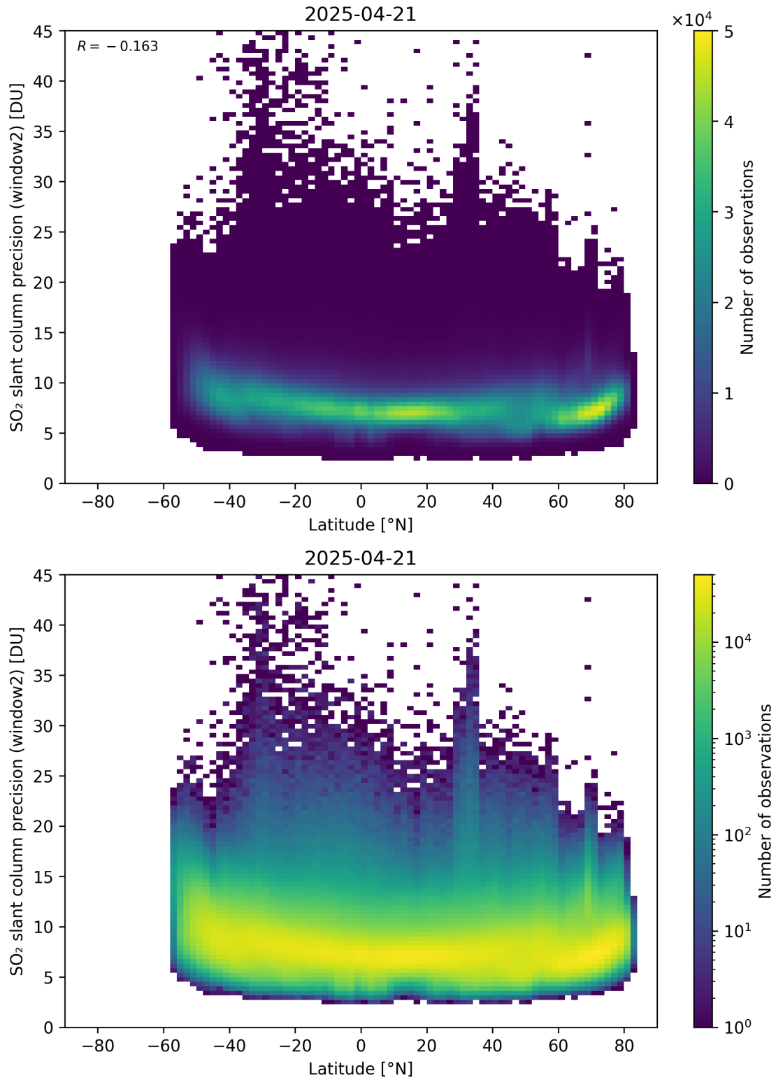
Figure 164: Scatter density plot of “Latitude” against “SO 2 slant column precision (window2)” for 2025-04-20 to 2025-04-22.
