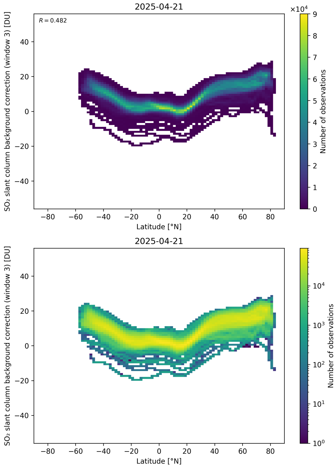
Figure 152: Scatter density plot of “Latitude” against “SO 2 slant column background correction (window 3)” for 2025-04-20 to 2025-04-22.
