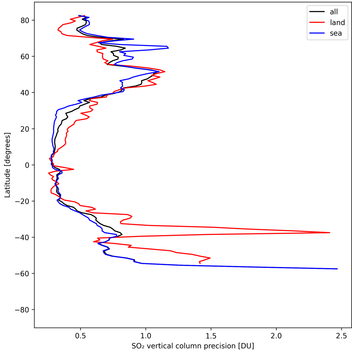
Figure 33: Zonal average of “SO 2 vertical column precision” for 2025-04-20 to 2025-04-22.
