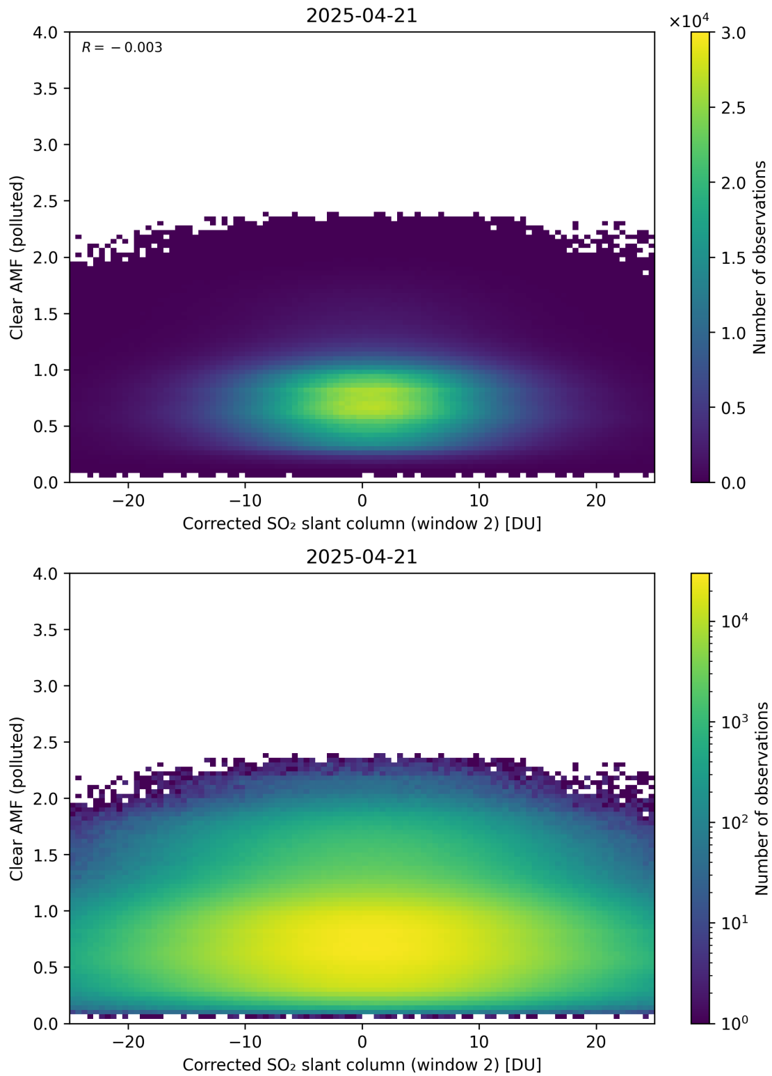
Figure 249: Scatter density plot of “Corrected SO 2 slant column (window 2)” against “Clear AMF (polluted)” for 2025-04-20 to 2025-04-22.
