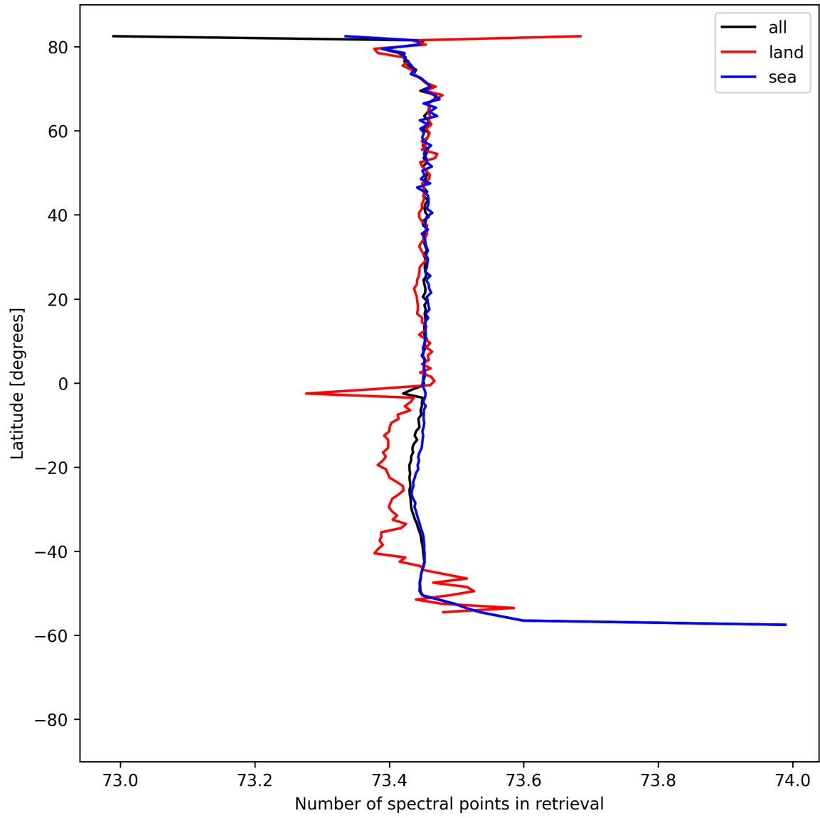
Figure 56: Zonal average of “Number of spectral points in retrieval” for 2025-04-20 to 2025-04-22.
