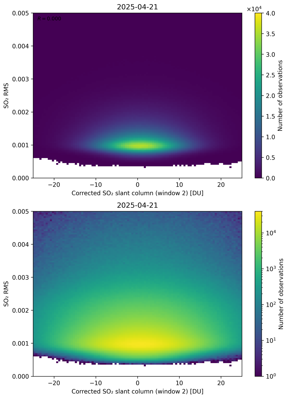
Figure 248: Scatter density plot of “Corrected SO 2 slant column (window 2)” against “SO 2 RMS” for 2025-04-20 to 2025-04-22.
