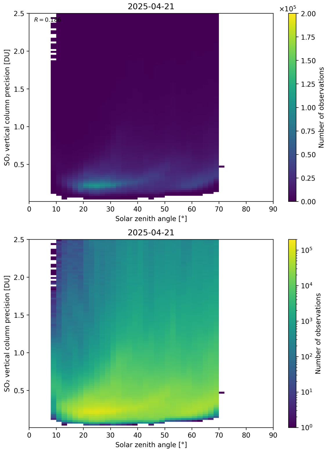
Figure 192: Scatter density plot of “Solar zenith angle” against “SO 2 vertical column precision” for 2025-04-20 to 2025-04-22.
