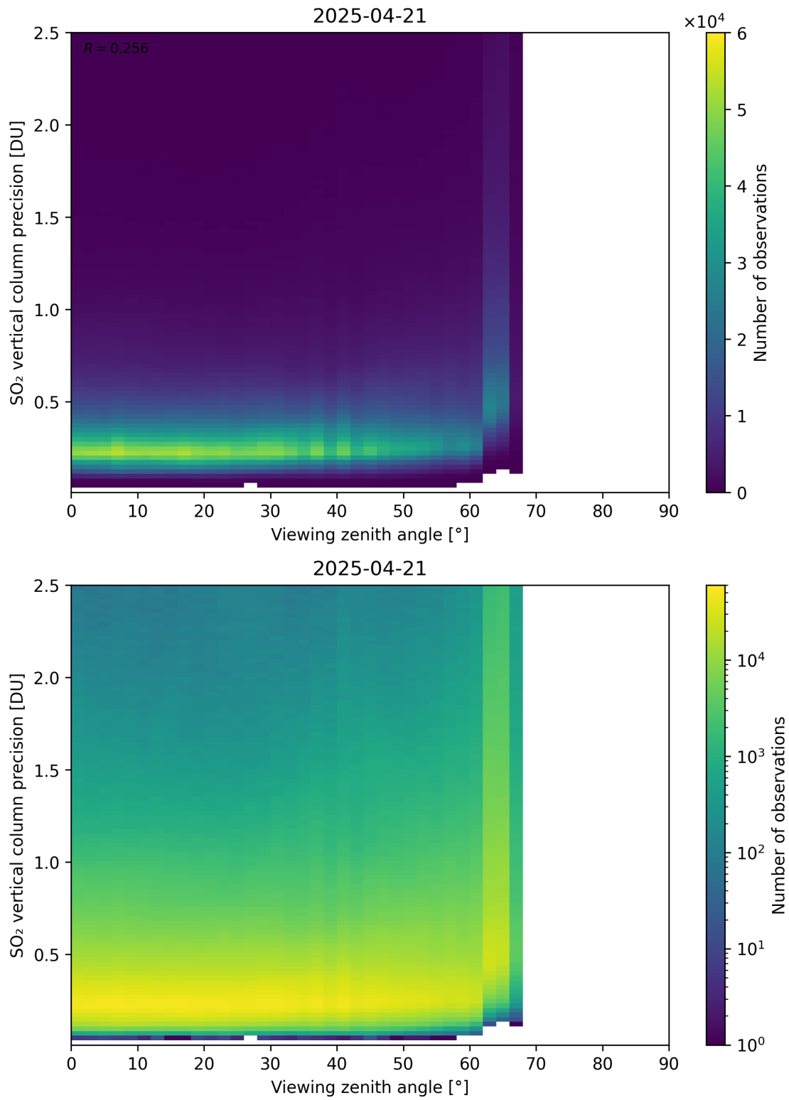
Figure 384: Scatter density plot of “Viewing zenith angle” against “SO 2 vertical column precision” for 2025-04-20 to 2025-04-22.
