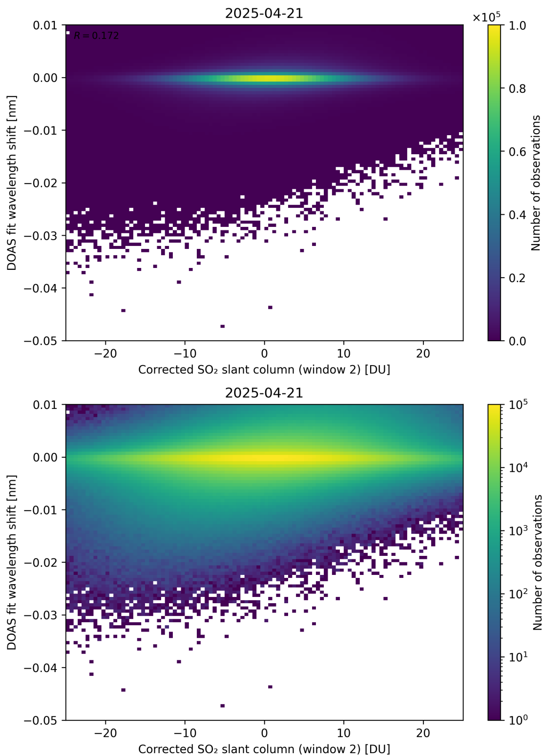
Figure 246: Scatter density plot of “Corrected SO 2 slant column (window 2)” against “DOAS fit wavelength shift” for 2025-04-20 to 2025-04-22.
