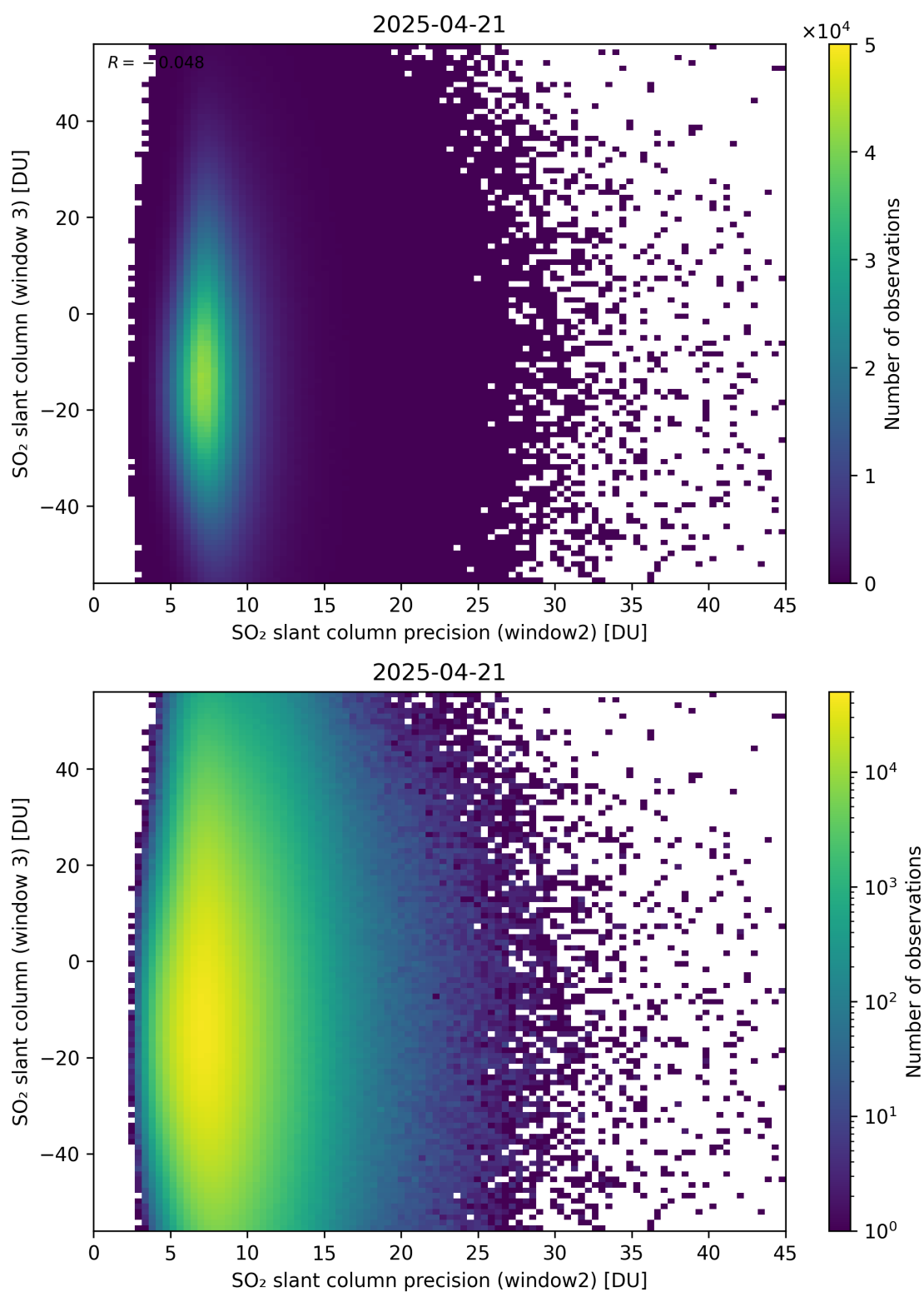
Figure 299: Scatter density plot of “SO 2 slant column precision (window2)” against “SO 2 slant column (window 3)” for 2025-04-20 to 2025-04-22.
