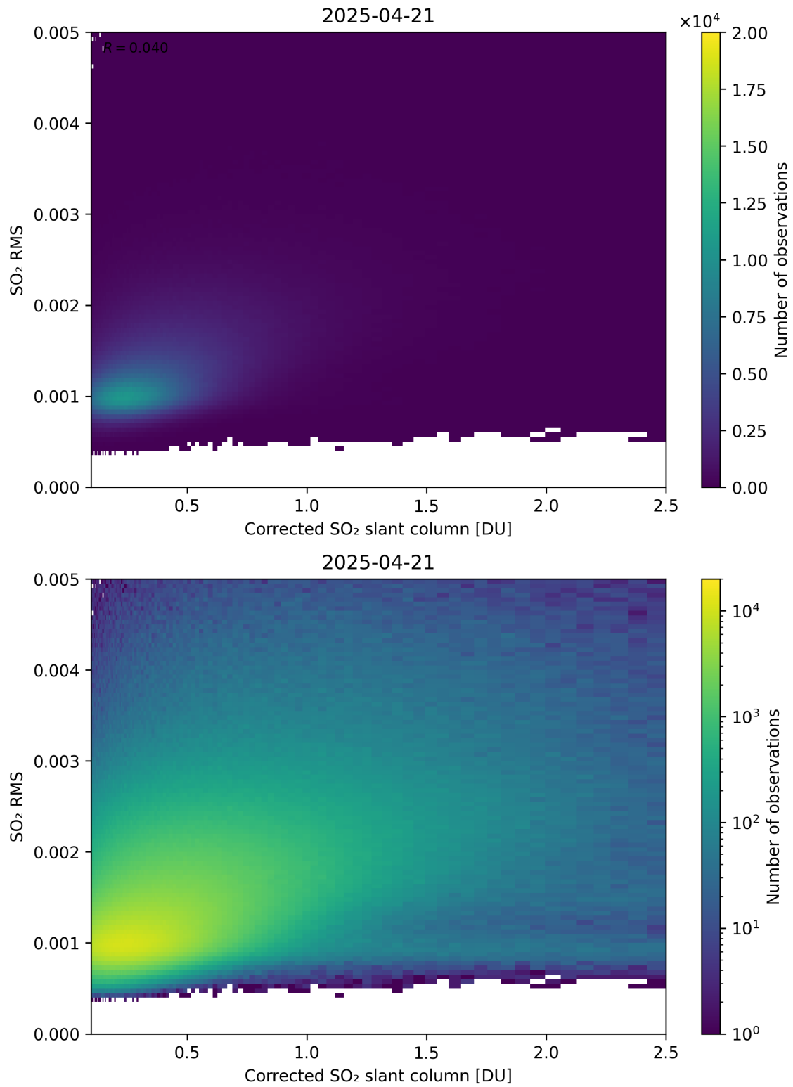
Figure 231: Scatter density plot of “Corrected SO 2 slant column” against “SO 2 RMS” for 2025-04-20 to 2025-04-22.
