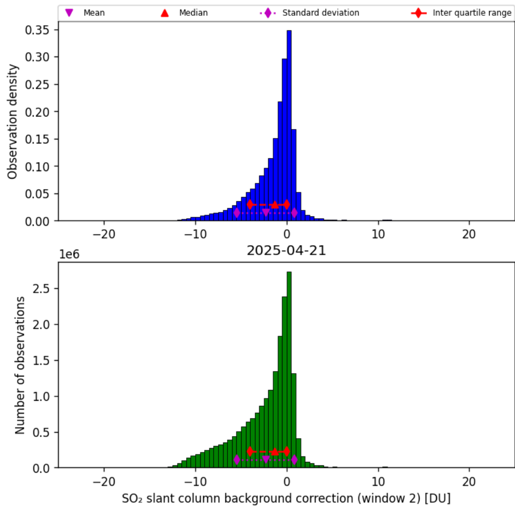
Figure 70: Histogram of “SO 2 slant column background correction (window 2)” for 2025-04-20 to 2025-04-22
