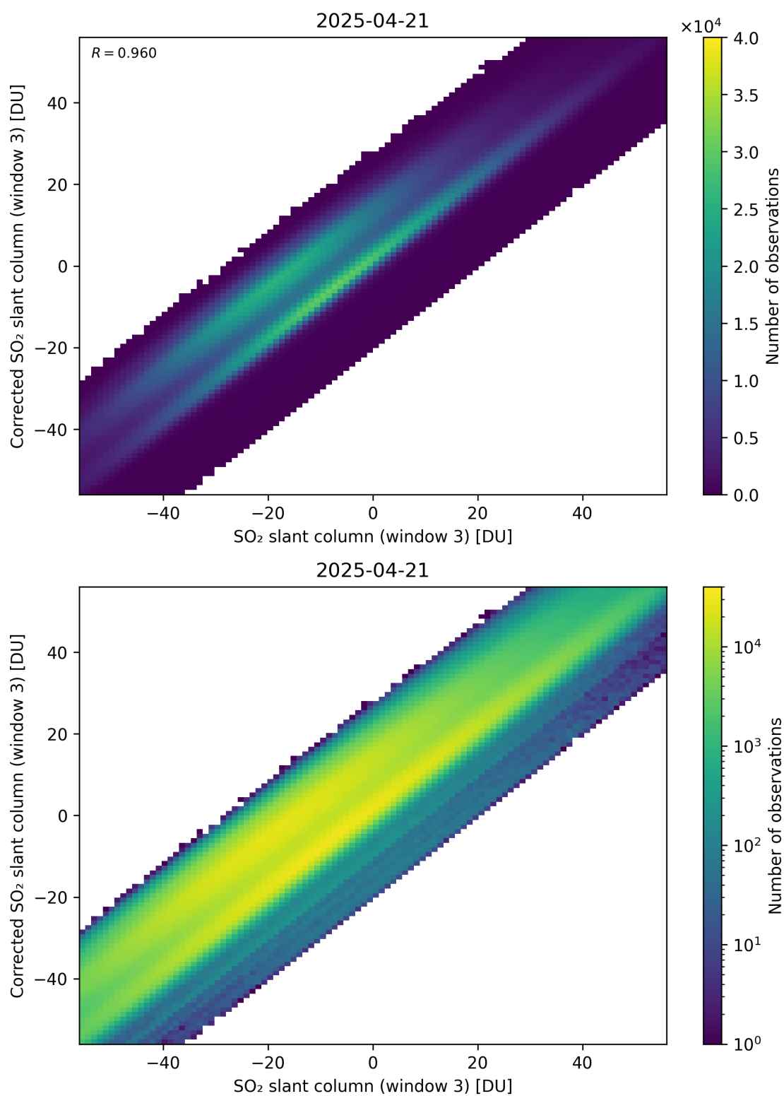
Figure 316: Scatter density plot of “SO 2 slant column (window 3)” against “Corrected SO 2 slant column (window 3)” for 2025-04-20 to 2025-04-22.
