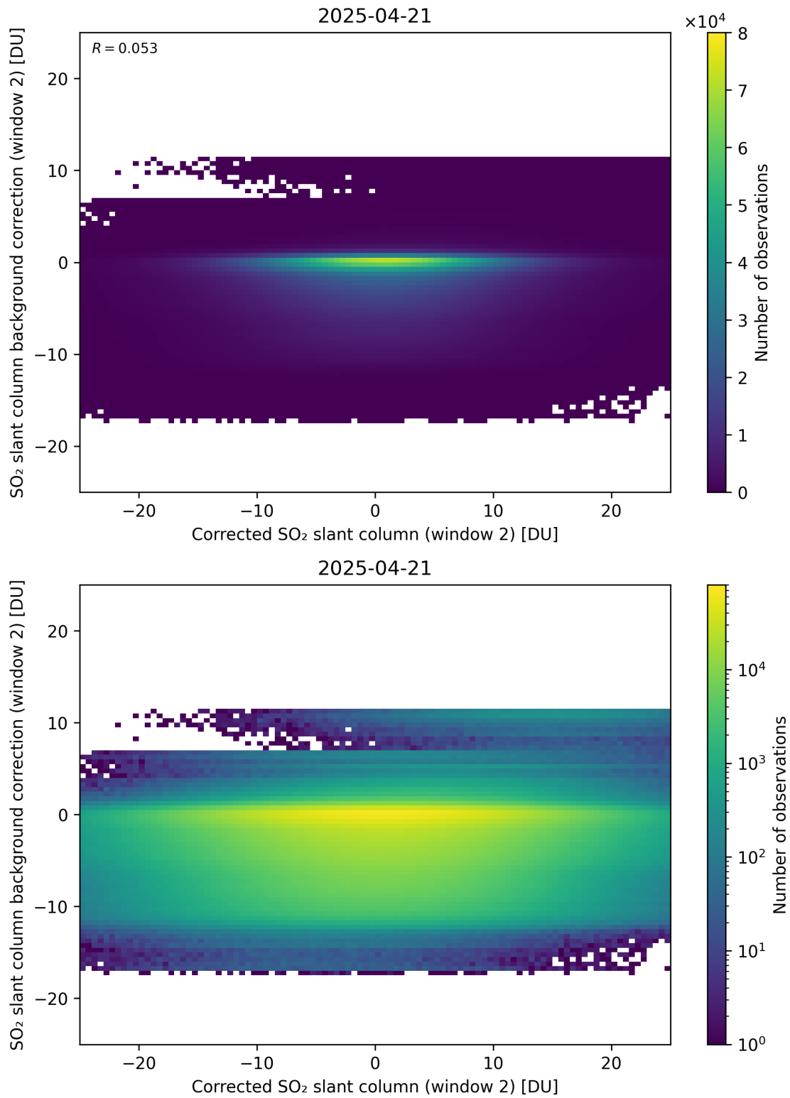
Figure 244: Scatter density plot of “Corrected SO 2 slant column (window 2)” against “SO 2 slant column background correction (window 2)” for 2025-04-20 to 2025-04-22.
