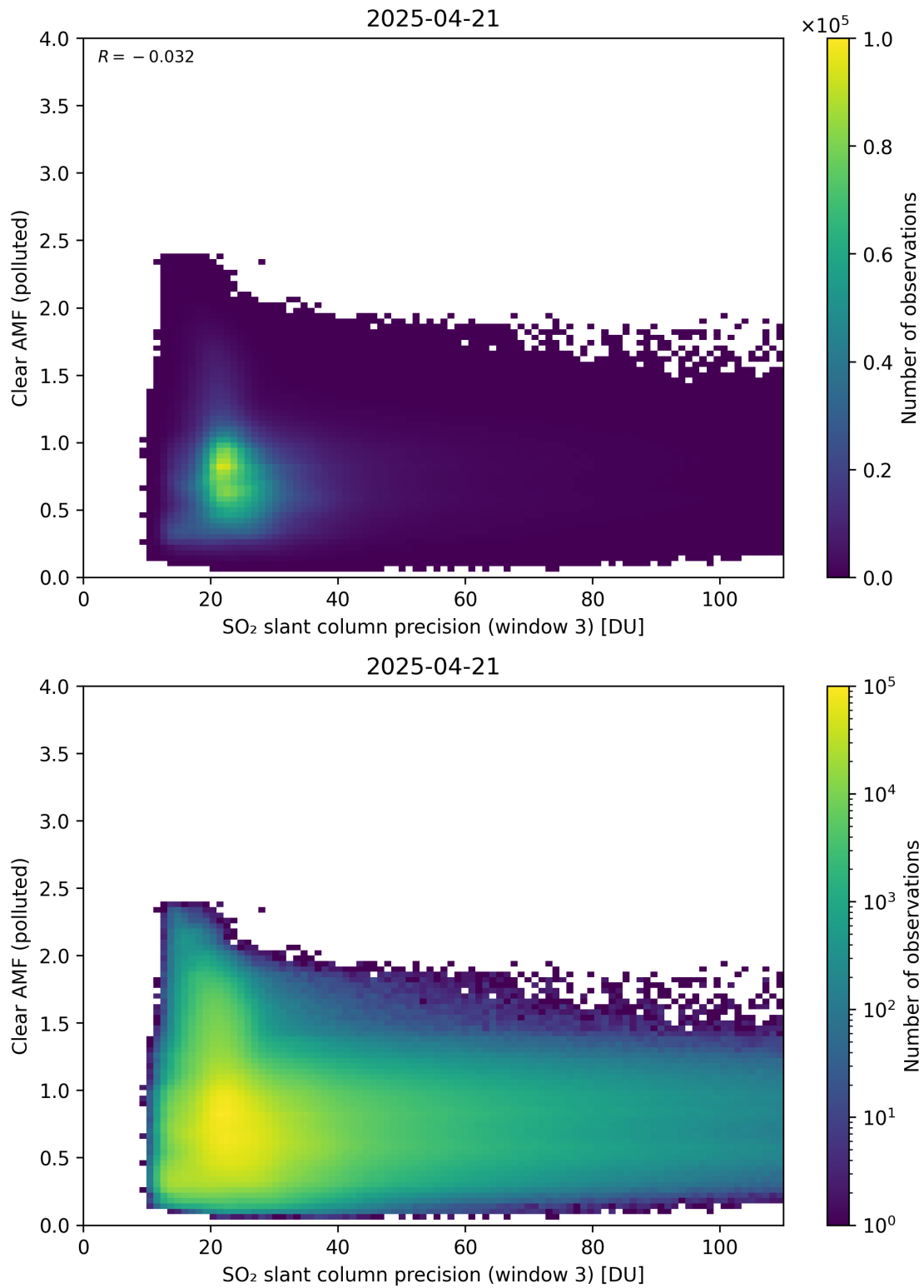
Figure 311: Scatter density plot of “SO 2 slant column precision (window 3)” against “Clear AMF (polluted)” for 2025-04-20 to 2025-04-22.
