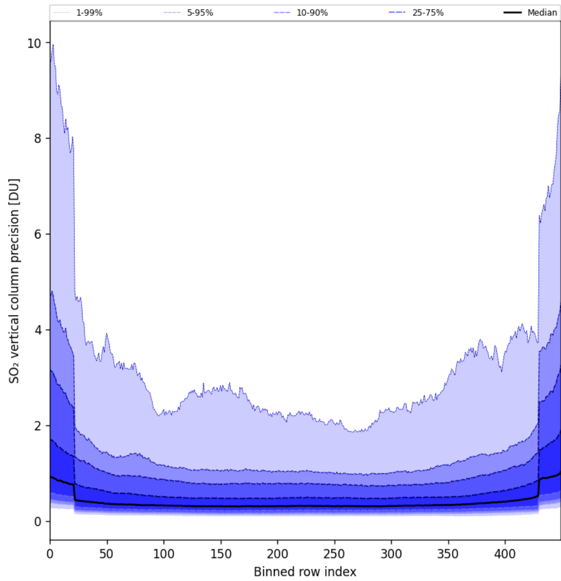
Figure 85: Along track statistics of “SO 2 vertical column precision” for 2025-04-20 to 2025-04-22
