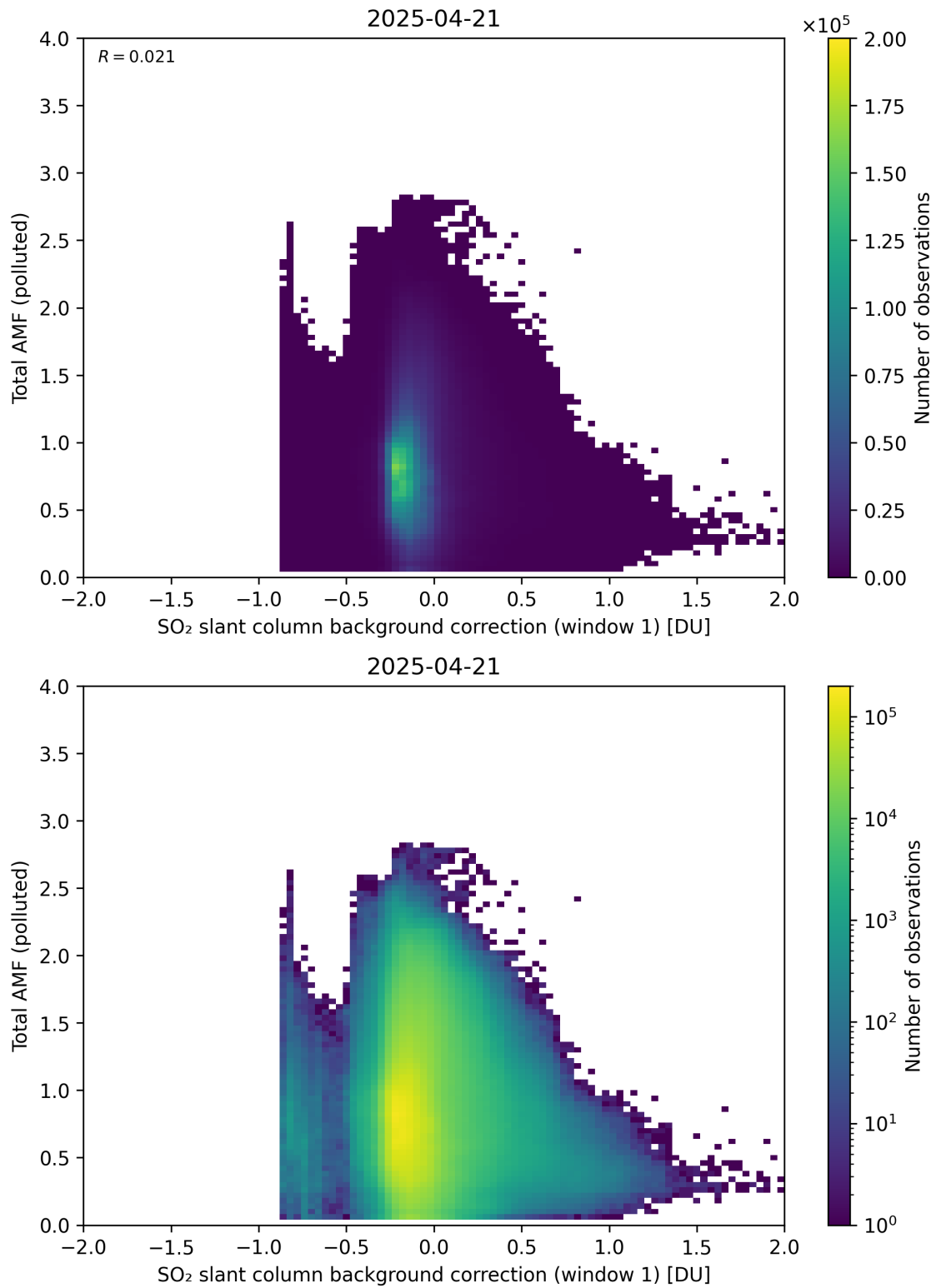
Figure 120: Scatter density plot of “SO 2 slant column background correction (window 1)” against “Total AMF (polluted)” for 2025-04-20 to 2025-04-22.
