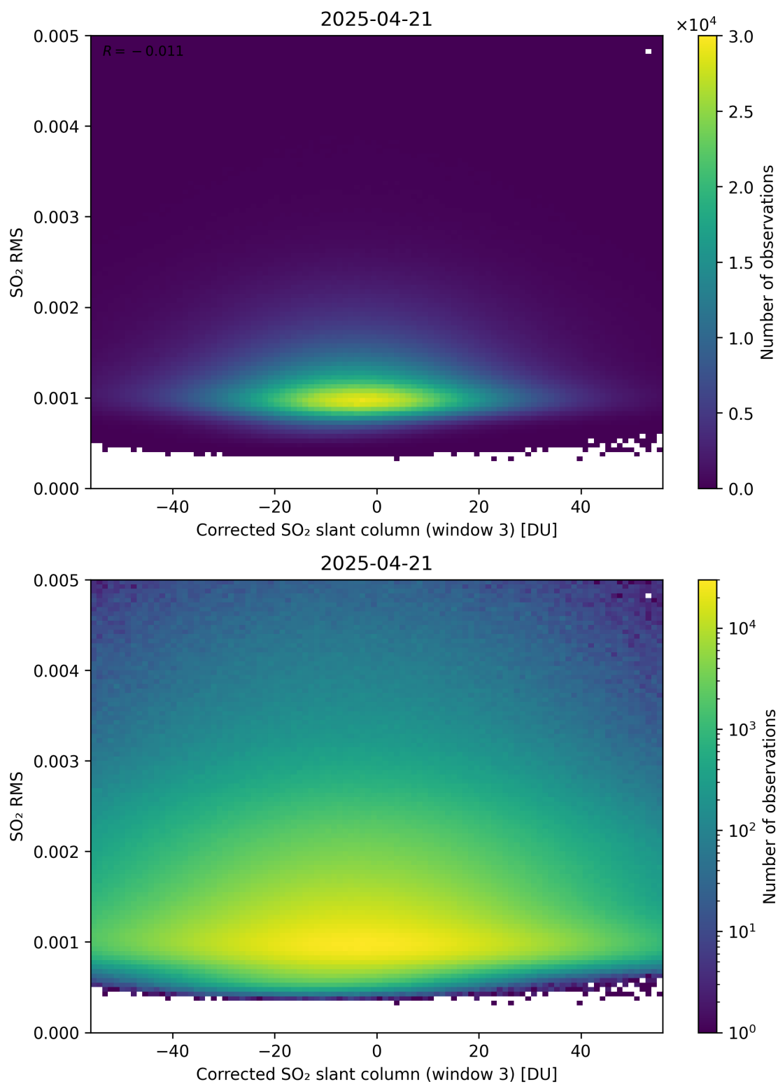
Figure 258: Scatter density plot of “Corrected SO 2 slant column (window 3)” against “SO 2 RMS” for 2025-04-20 to 2025-04-22.
