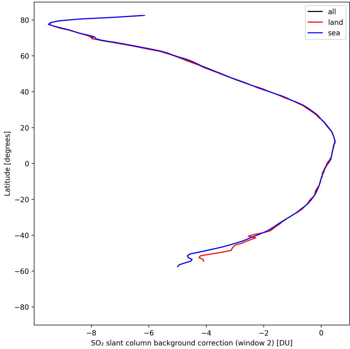
Figure 44: Zonal average of “SO 2 slant column background correction (window 2)” for 2025-04-20 to 2025-04-22.
