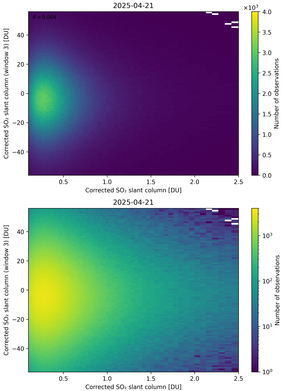
Figure 236: Scatter density plot of “Corrected SO 2 slant column” against “Corrected SO 2 slant column (window 3)” for 2025-04-20 to 2025-04-22.
