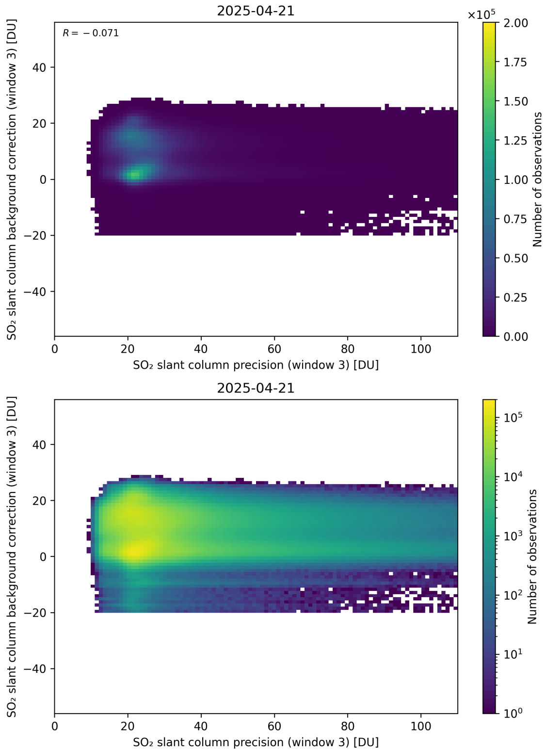
Figure 307: Scatter density plot of “SO 2 slant column precision (window 3)” against “SO 2 slant column background correction (window 3)” for 2025-04-20 to 2025-04-22.
