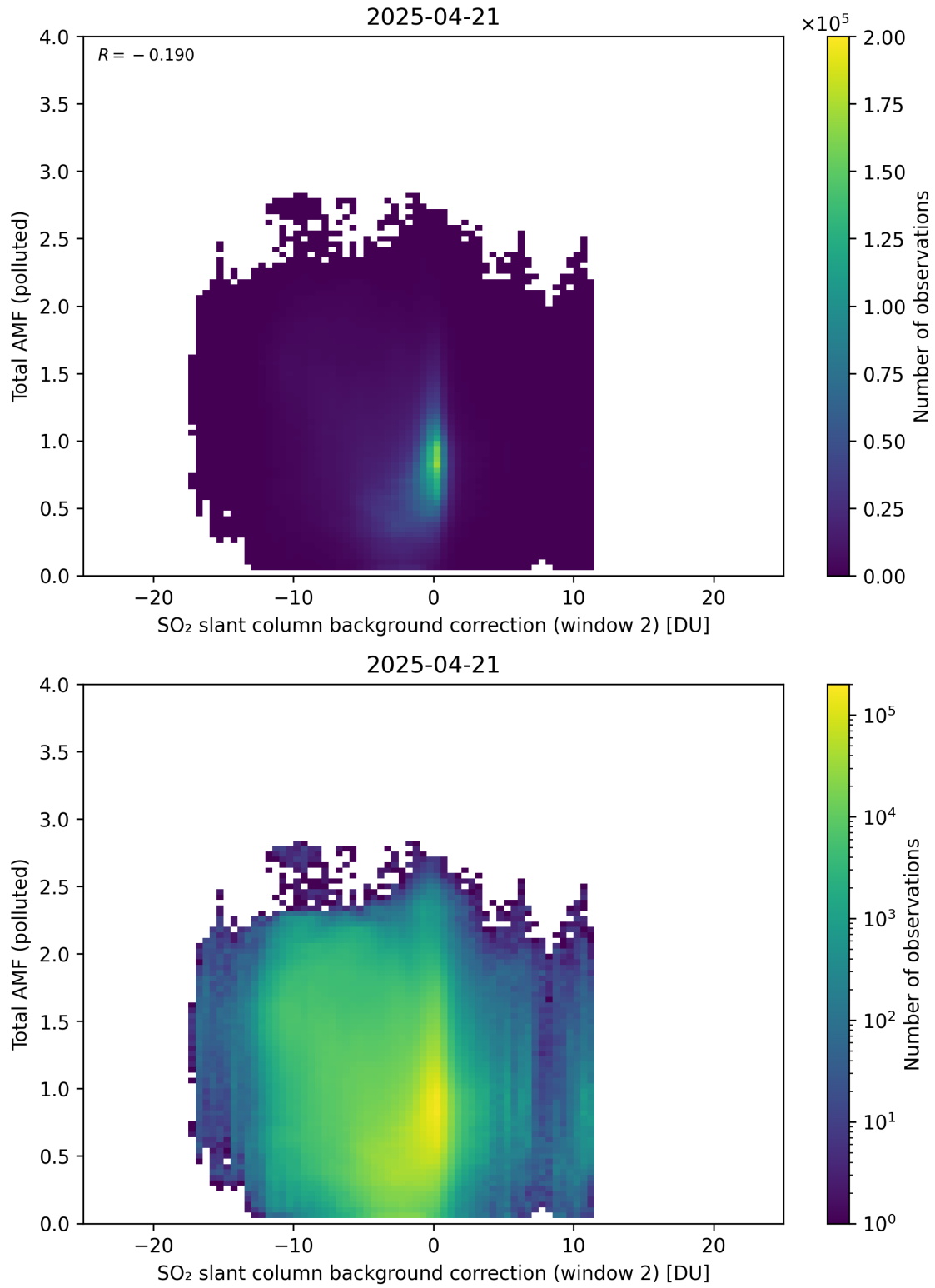
Figure 130: Scatter density plot of “SO 2 slant column background correction (window 2)” against “Total AMF (polluted)” for 2025-04-20 to 2025-04-22.
