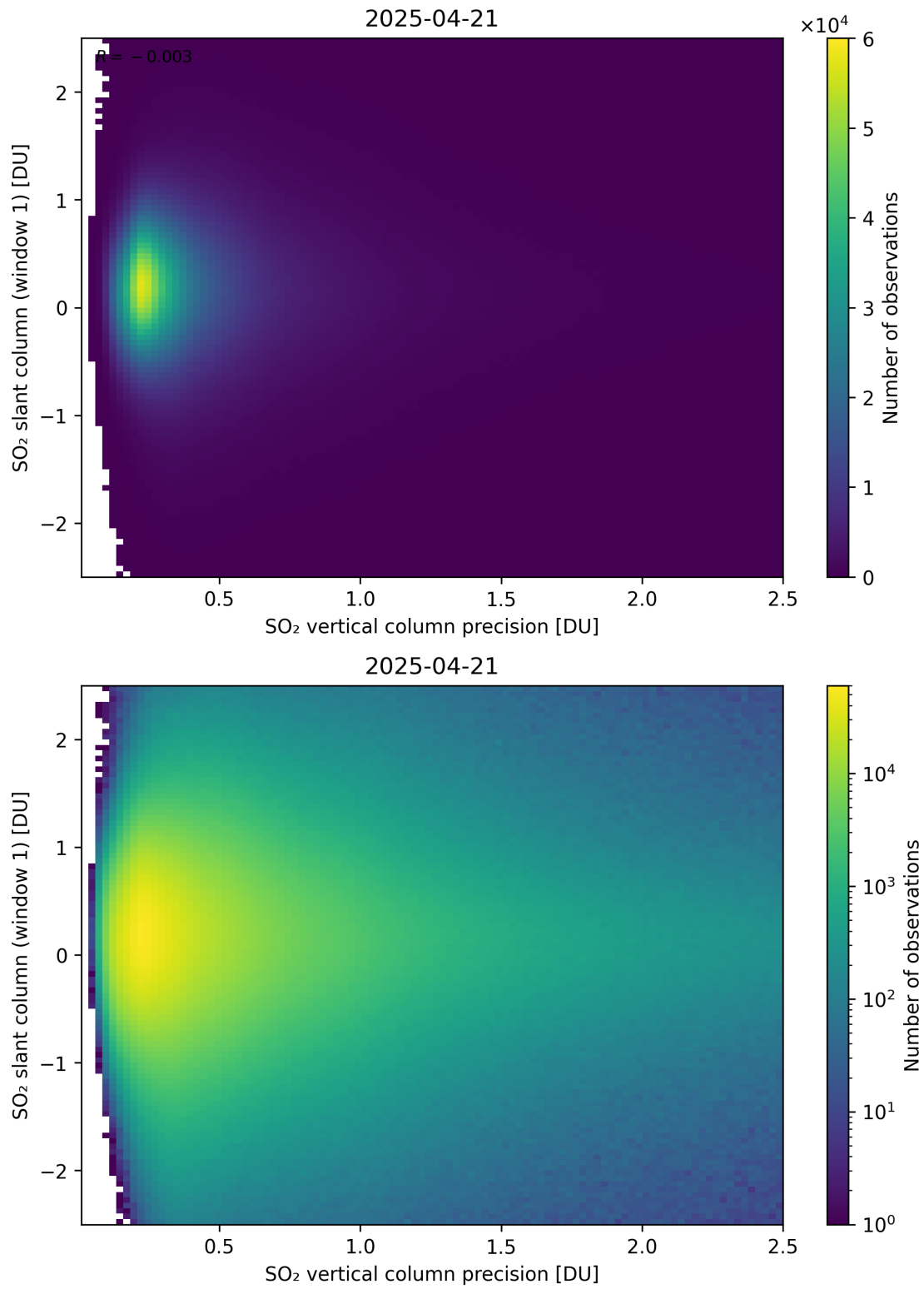
Figure 341: Scatter density plot of “SO 2 vertical column precision” against “SO 2 slant column (window 1)” for 2025-04-20 to 2025-04-22.
