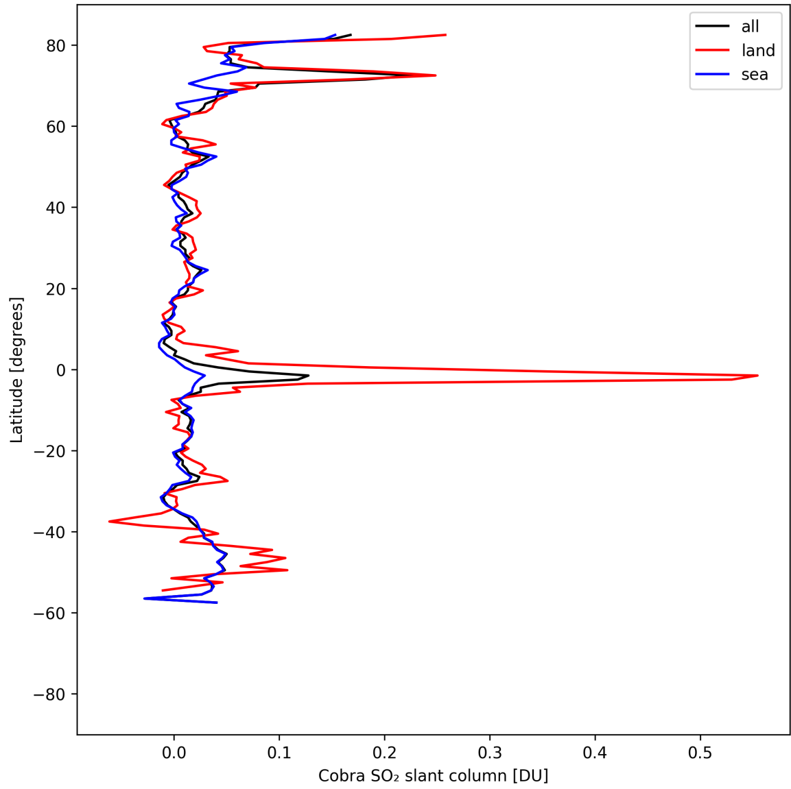
Figure 35: Zonal average of “Cobra SO 2 slant column” for 2025-04-20 to 2025-04-22.
