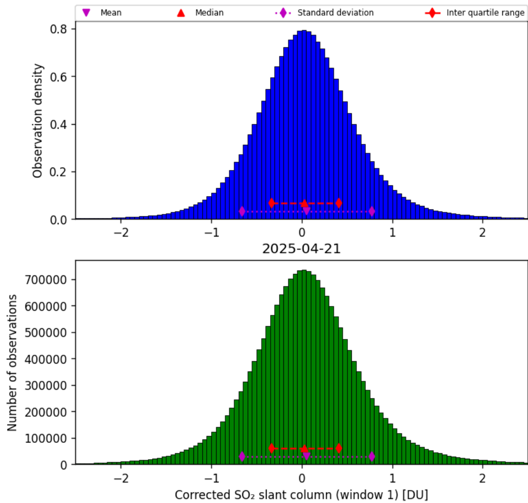
Figure 65: Histogram of “Corrected SO 2 slant column (window 1)” for 2025-04-20 to 2025-04-22
