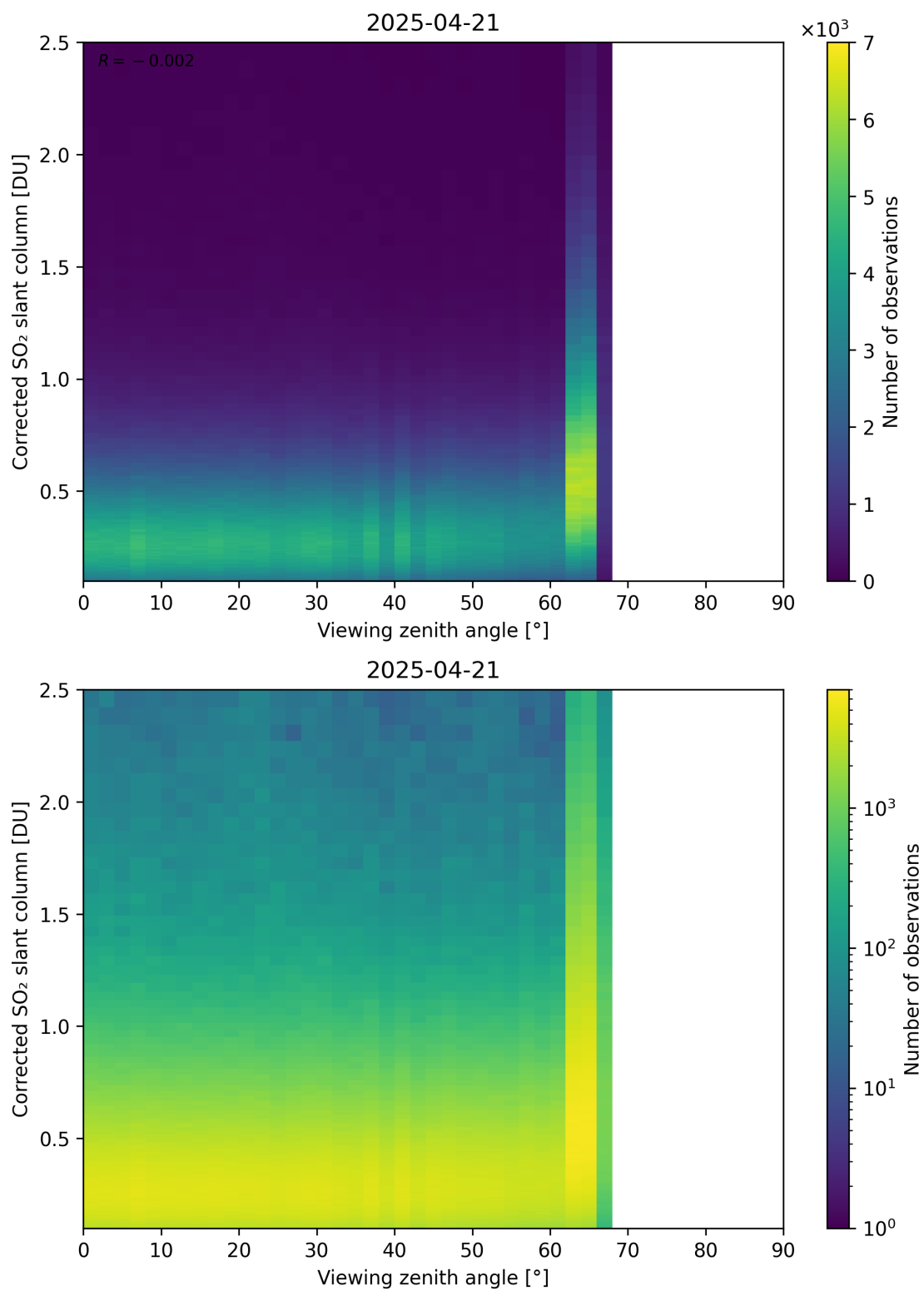
Figure 373: Scatter density plot of “Viewing zenith angle” against “Corrected SO 2 slant column” for 2025-04-20 to 2025-04-22.
