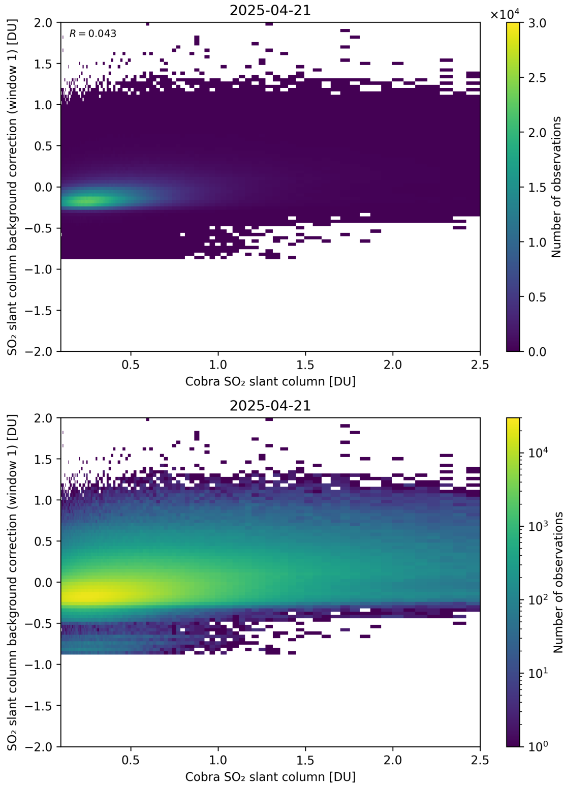
Figure 193: Scatter density plot of “Cobra SO 2 slant column” against “SO 2 slant column background correction (window 1)” for 2025-04-20 to 2025-04-22.
