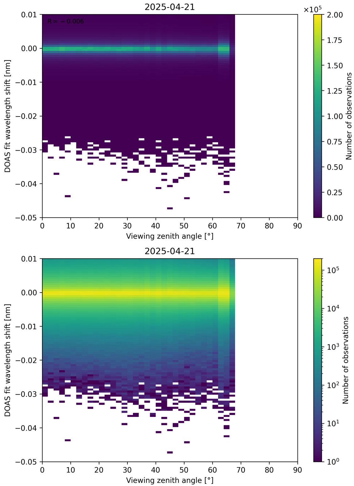
Figure 365: Scatter density plot of “Viewing zenith angle” against “DOAS fit wavelength shift” for 2025-04-20 to 2025-04-22.
