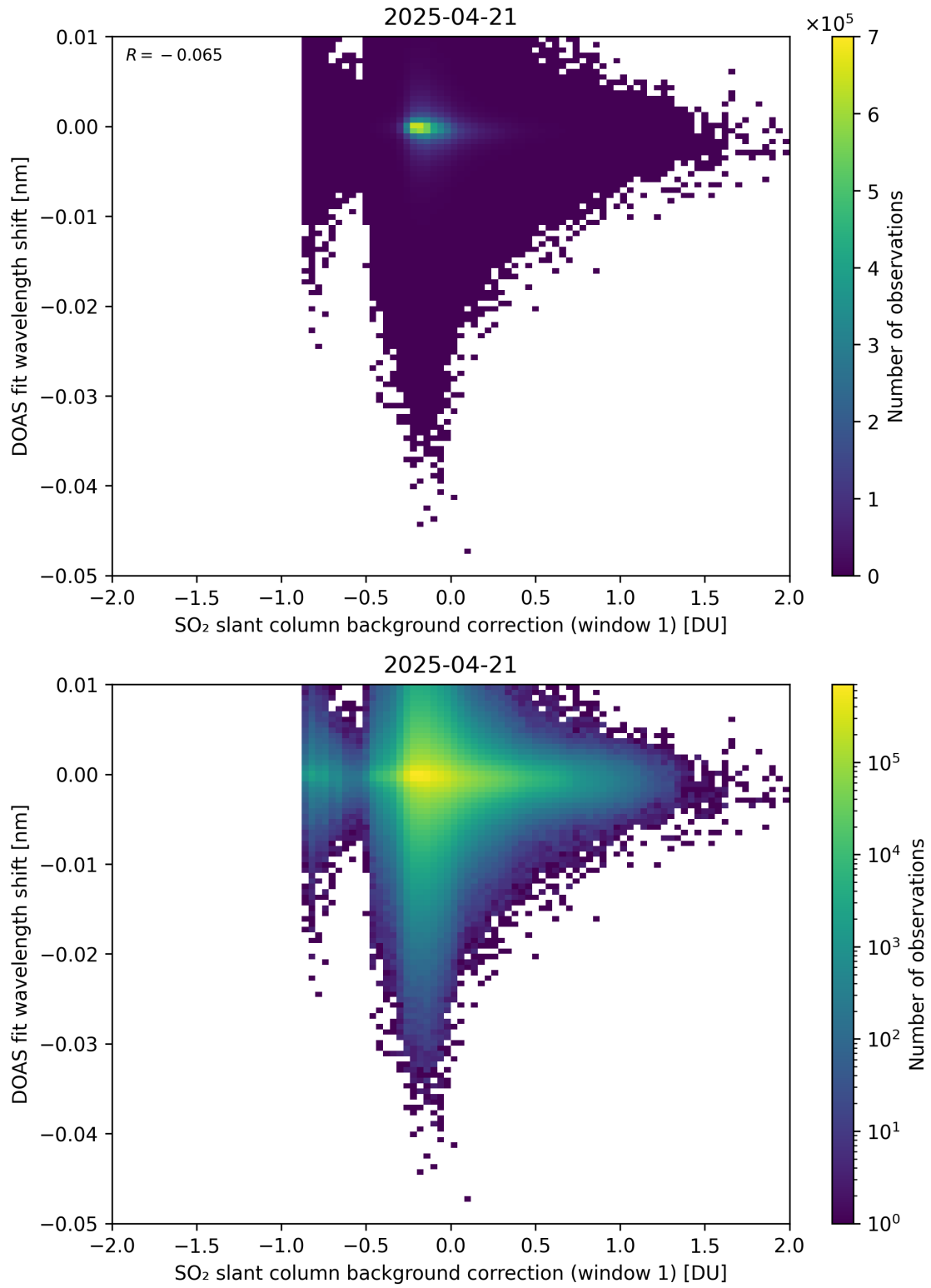
Figure 111: Scatter density plot of “SO 2 slant column background correction (window 1)” against “DOAS fit wavelength shift” for 2025-04-20 to 2025-04-22.
