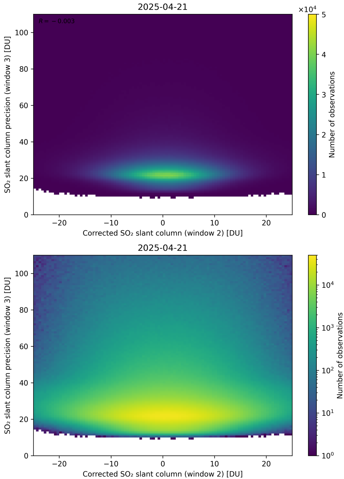
Figure 252: Scatter density plot of “Corrected SO 2 slant column (window 2)” against “SO 2 slant column precision (window 3)” for 2025-04-20 to 2025-04-22.
