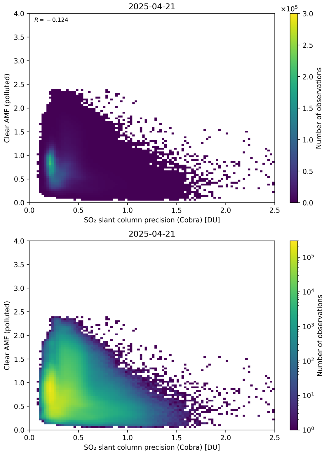
Figure 205: Scatter density plot of “SO 2 slant column precision (Cobra)” against “Clear AMF (polluted)” for 2025-04-20 to 2025-04-22.
