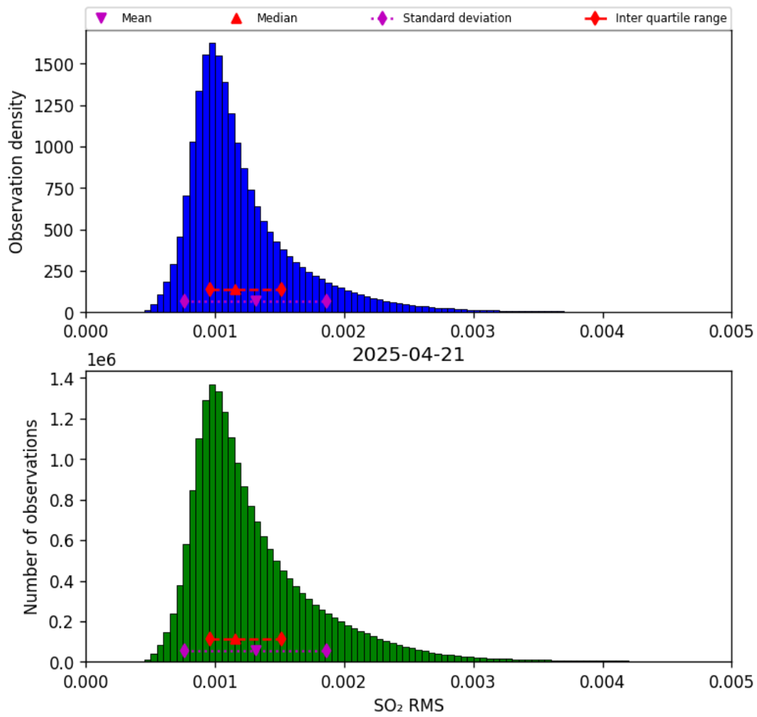
Figure 78: Histogram of “SO 2 RMS” for 2025-04-20 to 2025-04-22
