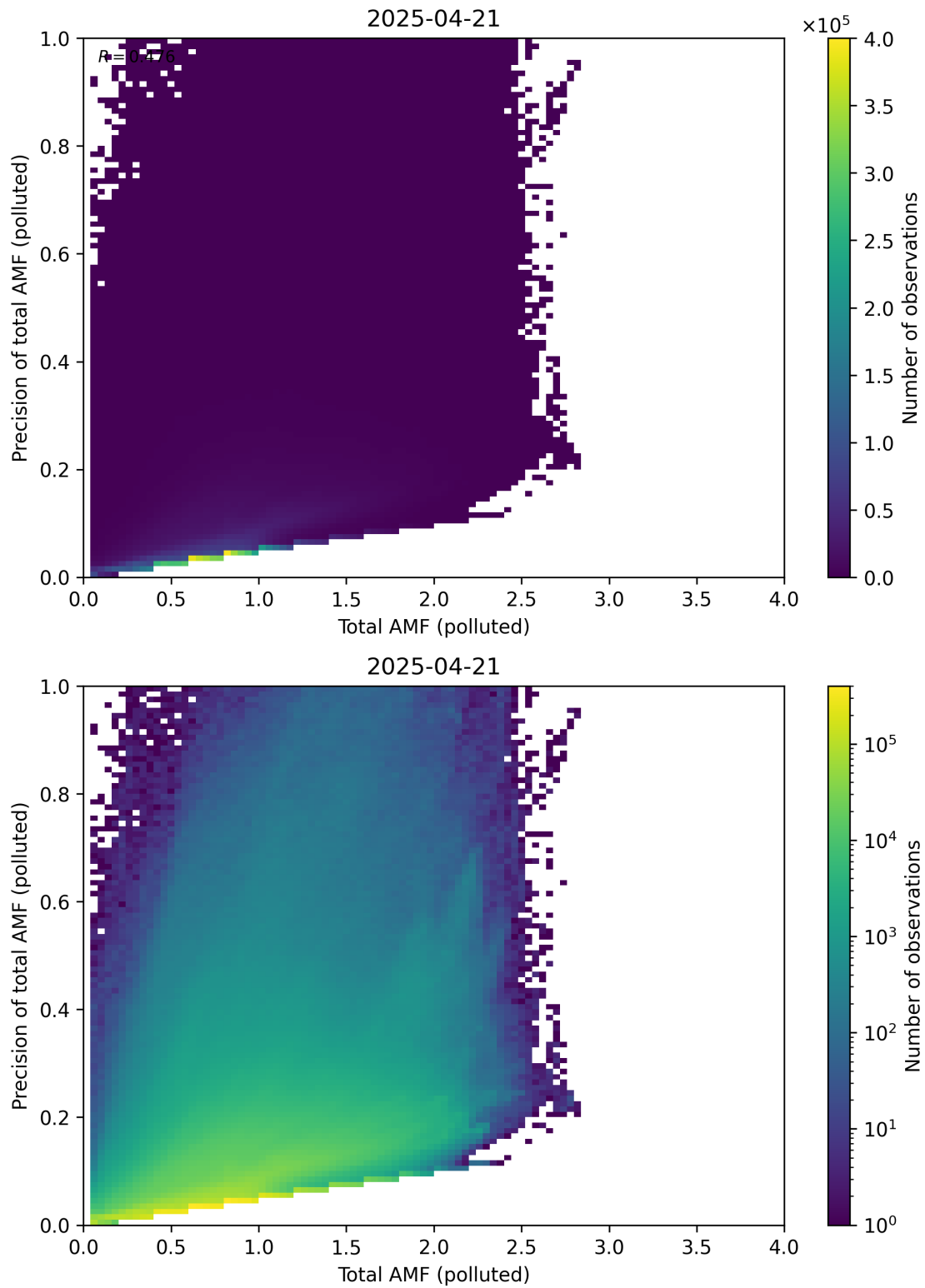
Figure 322: Scatter density plot of “Total AMF (polluted)” against “Precision of total AMF (polluted)” for 2025-04-20 to 2025-04-22.
