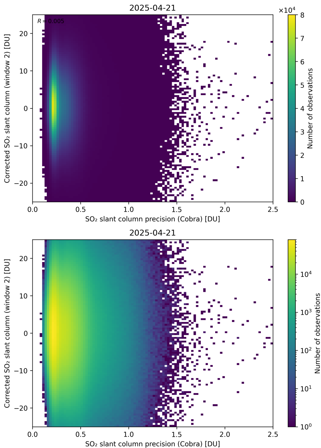
Figure 206: Scatter density plot of “SO 2 slant column precision (Cobra)” against “Corrected SO 2 slant column (window 2)” for 2025-04-20 to 2025-04-22.
