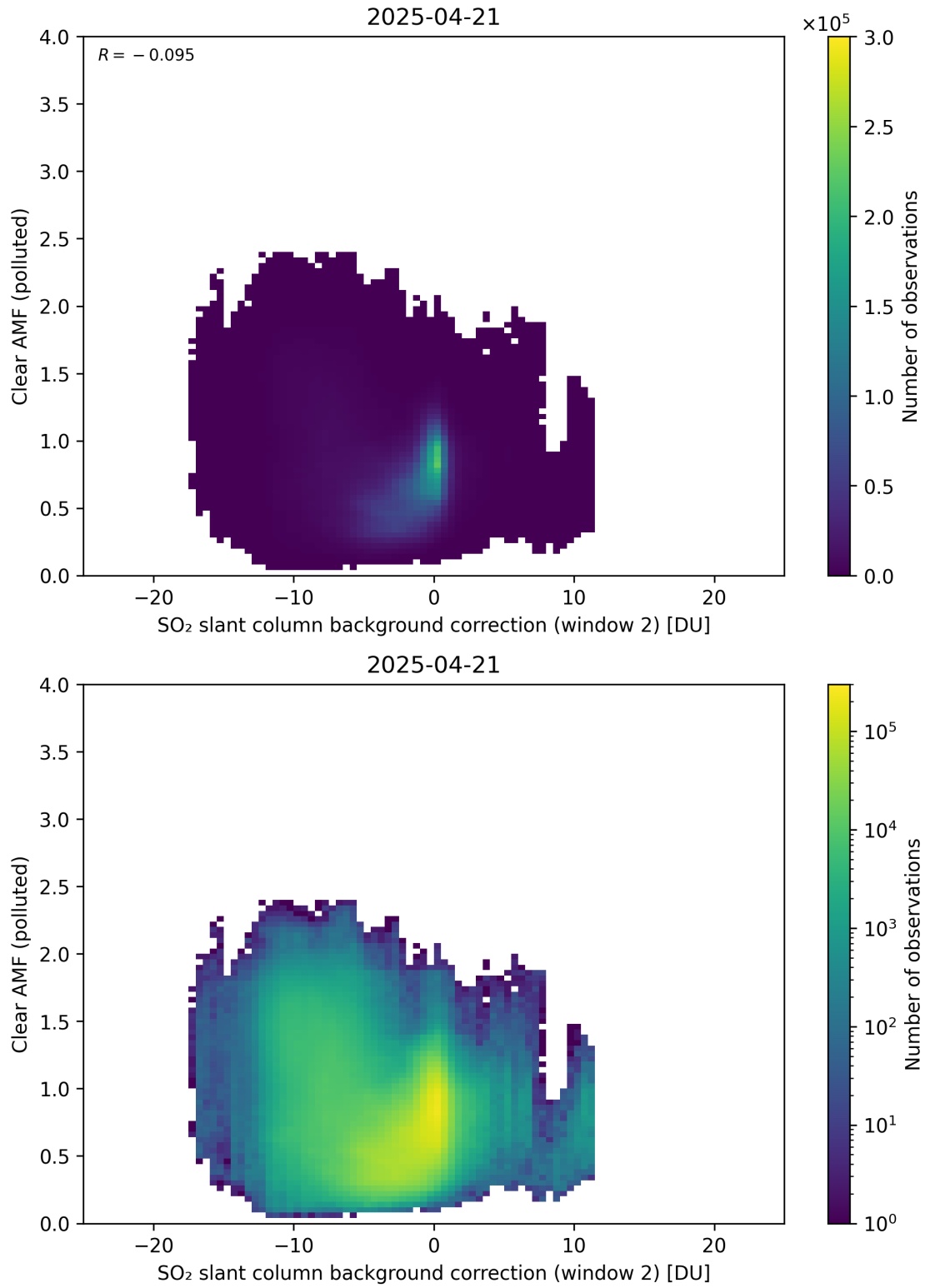
Figure 126: Scatter density plot of “SO 2 slant column background correction (window 2)” against “Clear AMF (polluted)” for 2025-04-20 to 2025-04-22.
