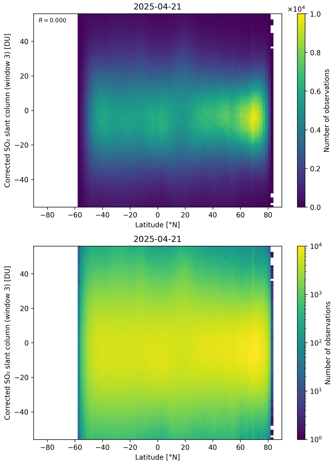
Figure 161: Scatter density plot of “Latitude” against “Corrected SO 2 slant column (window 3)” for 2025-04-20 to 2025-04-22.
