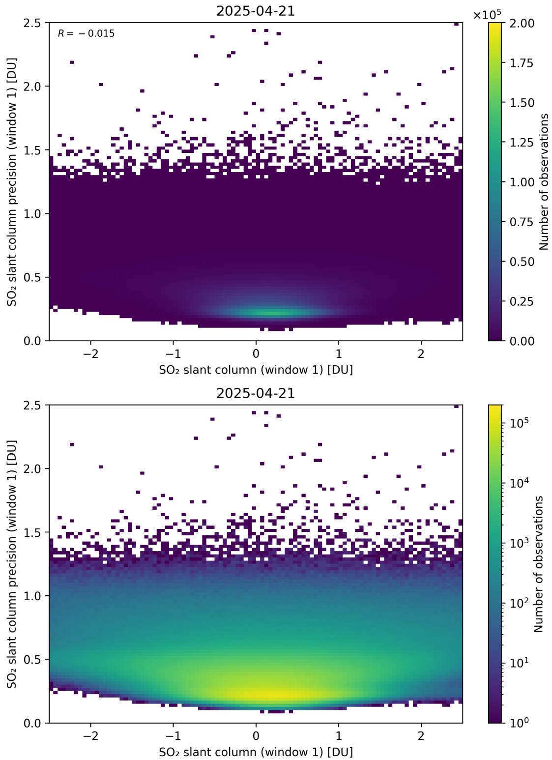
Figure 285: Scatter density plot of “SO 2 slant column (window 1)” against “SO 2 slant column precision (window 1)” for 2025-04-20 to 2025-04-22.
