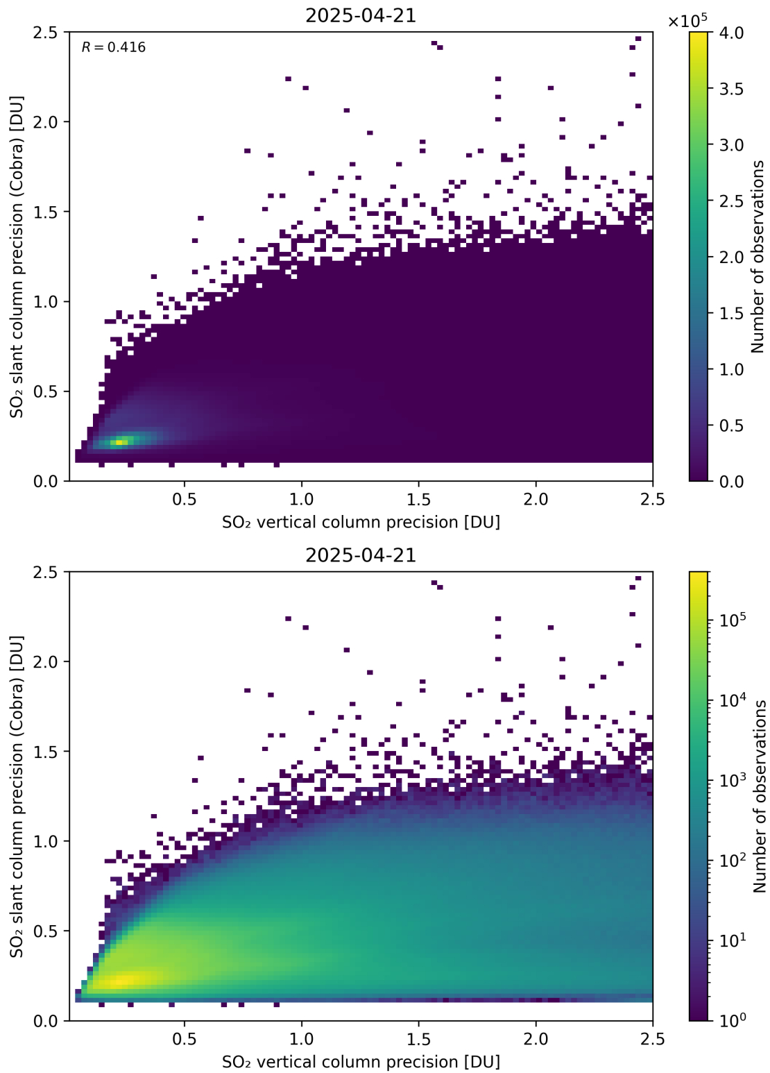
Figure 337: Scatter density plot of “SO 2 vertical column precision” against “SO 2 slant column precision (Cobra)” for 2025-04-20 to 2025-04-22.
