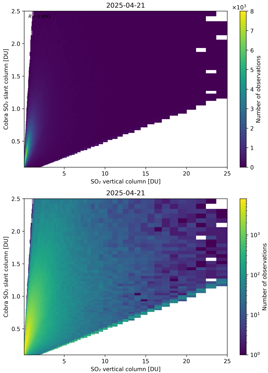
Figure 349: Scatter density plot of “SO 2 vertical column” against “Cobra SO 2 slant column” for 2025-04-20 to 2025-04-22.
