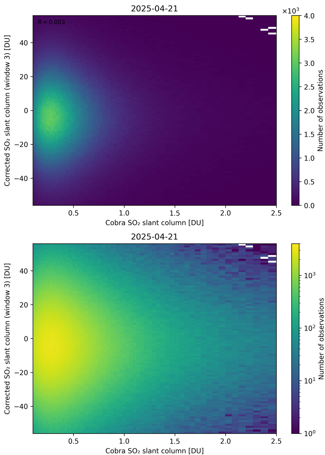
Figure 218: Scatter density plot of “Cobra SO 2 slant column” against “Corrected SO 2 slant column (window 3)” for 2025-04-20 to 2025-04-22.
