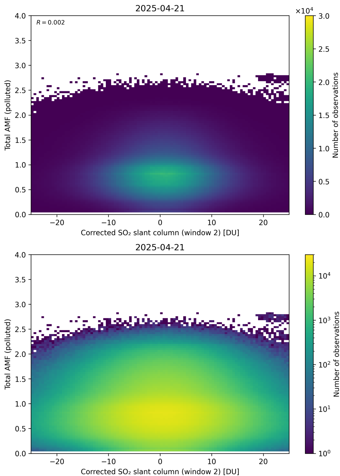
Figure 253: Scatter density plot of “Corrected SO 2 slant column (window 2)” against “Total AMF (polluted)” for 2025-04-20 to 2025-04-22.
