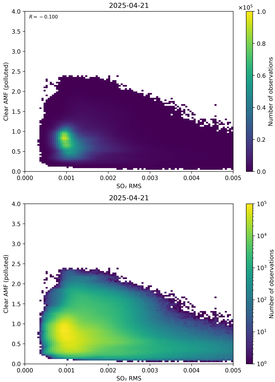
Figure 147: Scatter density plot of “SO 2 RMS” against “Clear AMF (polluted)” for 2025-04-20 to 2025-04-22.
