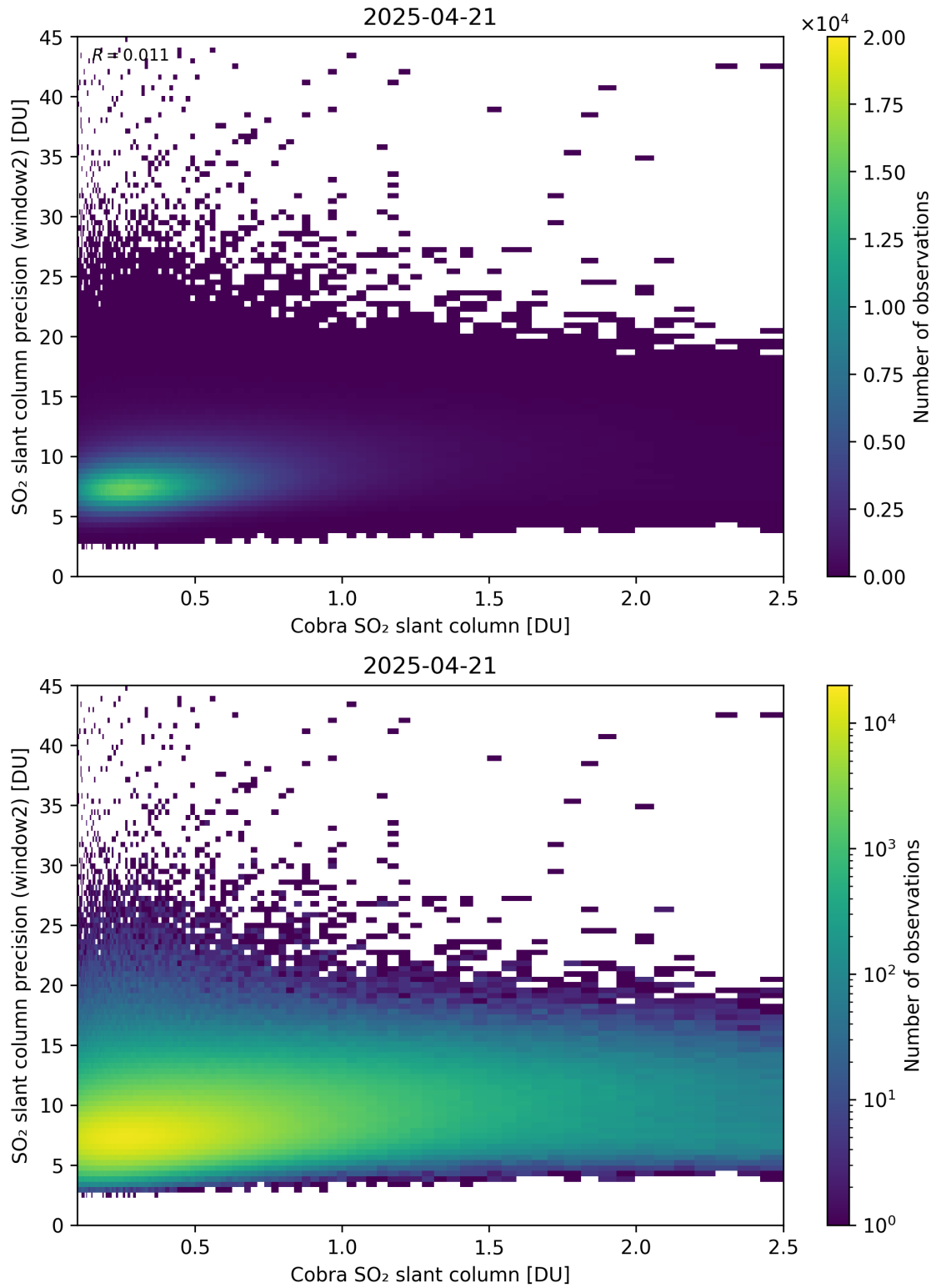
Figure 221: Scatter density plot of “Cobra SO 2 slant column” against “SO 2 slant column precision (window2)” for 2025-04-20 to 2025-04-22.
