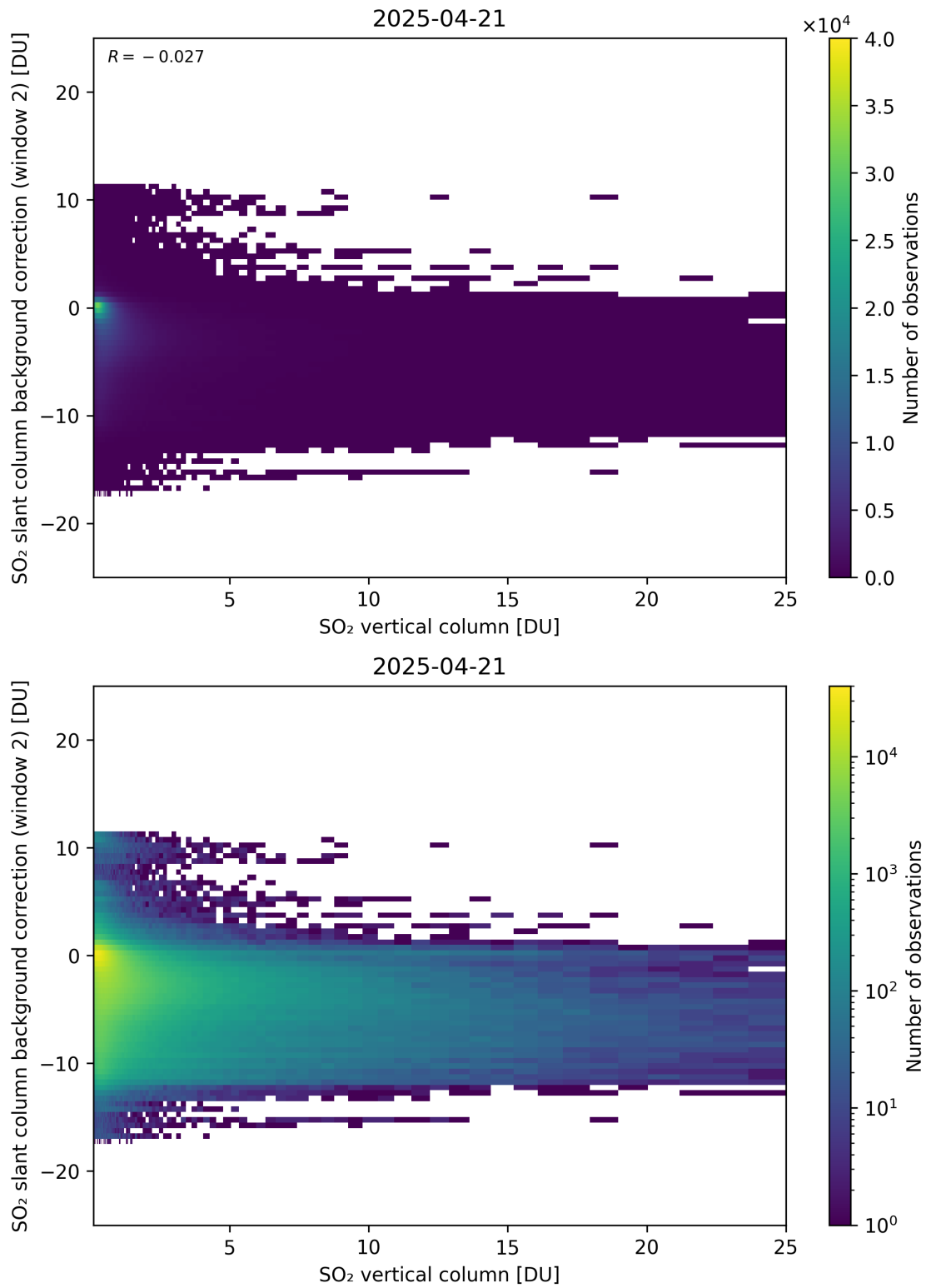
Figure 324: Scatter density plot of “SO 2 vertical column” against “SO 2 slant column background correction (window 2)” for 2025-04-20 to 2025-04-22.
