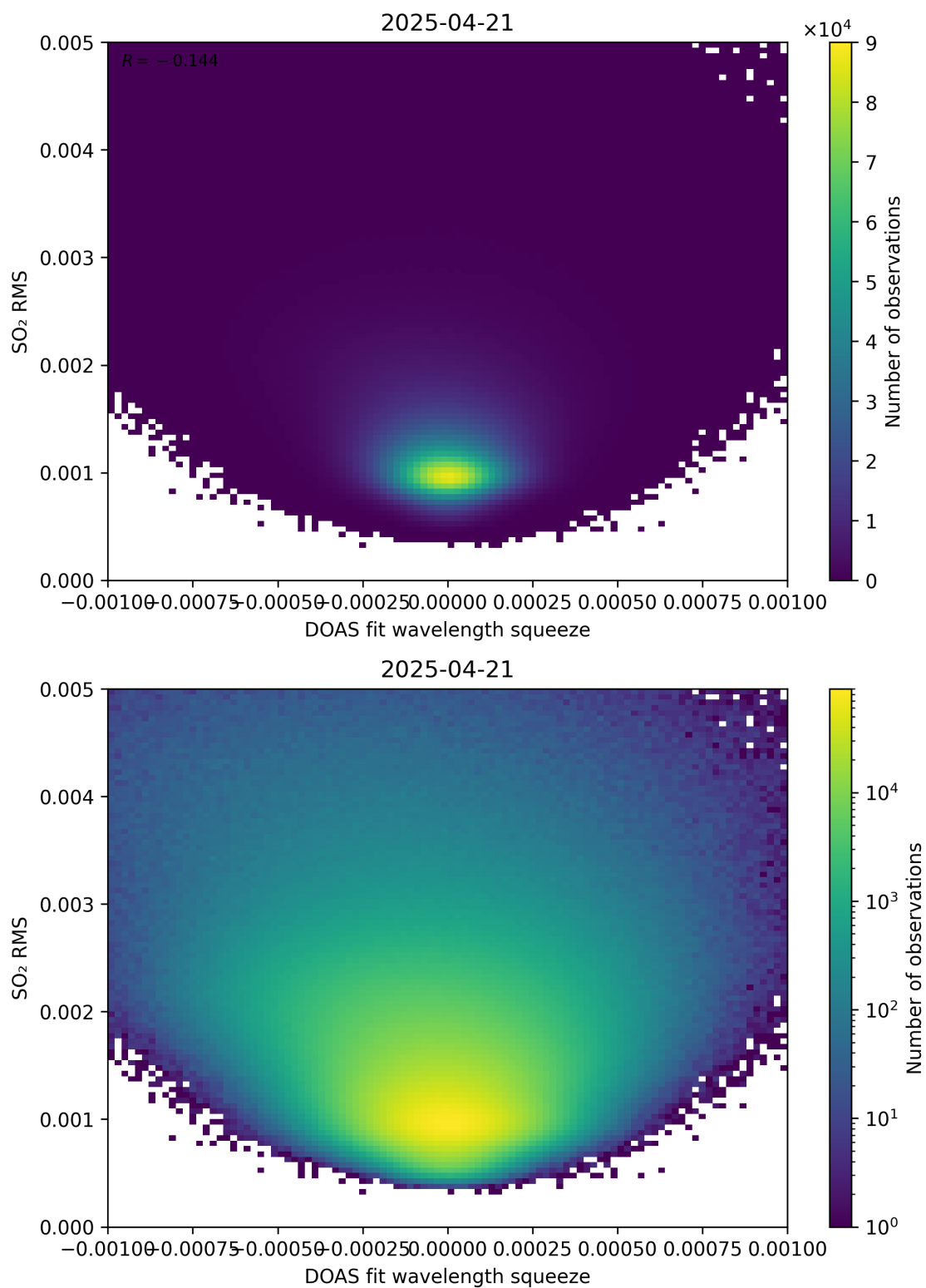
Figure 143: Scatter density plot of “DOAS fit wavelength squeeze” against “SO 2 RMS” for 2025-04-20 to 2025-04-22.
