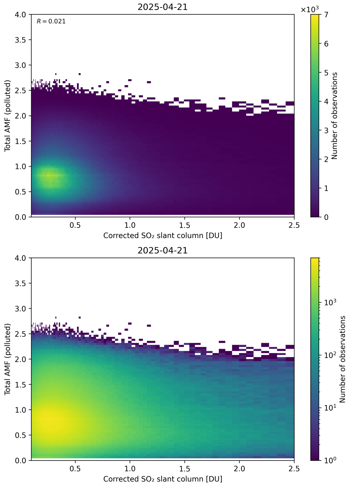
Figure 242: Scatter density plot of “Corrected SO 2 slant column” against “Total AMF (polluted)” for 2025-04-20 to 2025-04-22.
