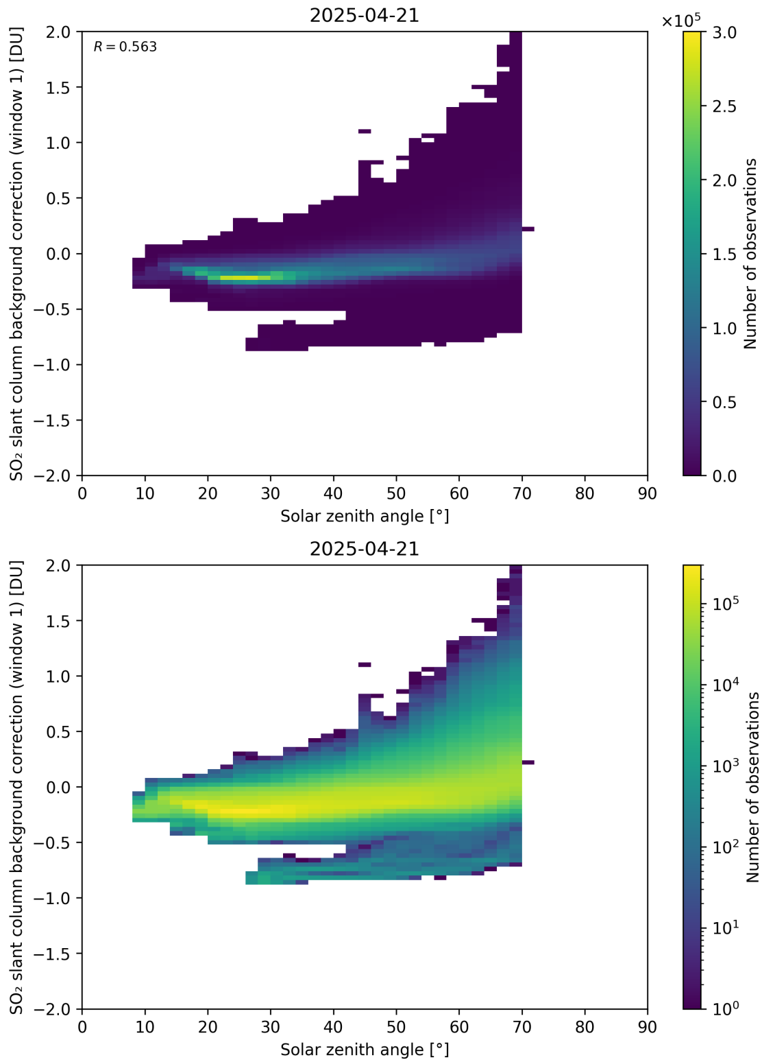
Figure 171: Scatter density plot of “Solar zenith angle” against “SO 2 slant column background correction (window 1)” for 2025-04-20 to 2025-04-22.
