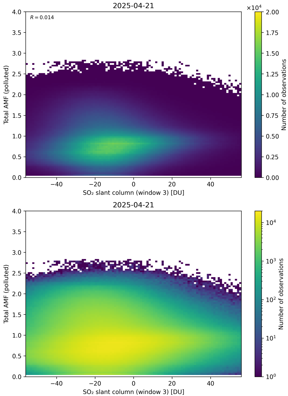
Figure 318: Scatter density plot of “SO 2 slant column (window 3)” against “Total AMF (polluted)” for 2025-04-20 to 2025-04-22.
