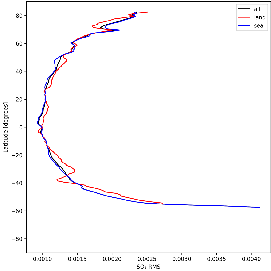
Figure 52: Zonal average of “SO 2 RMS” for 2025-04-20 to 2025-04-22.
