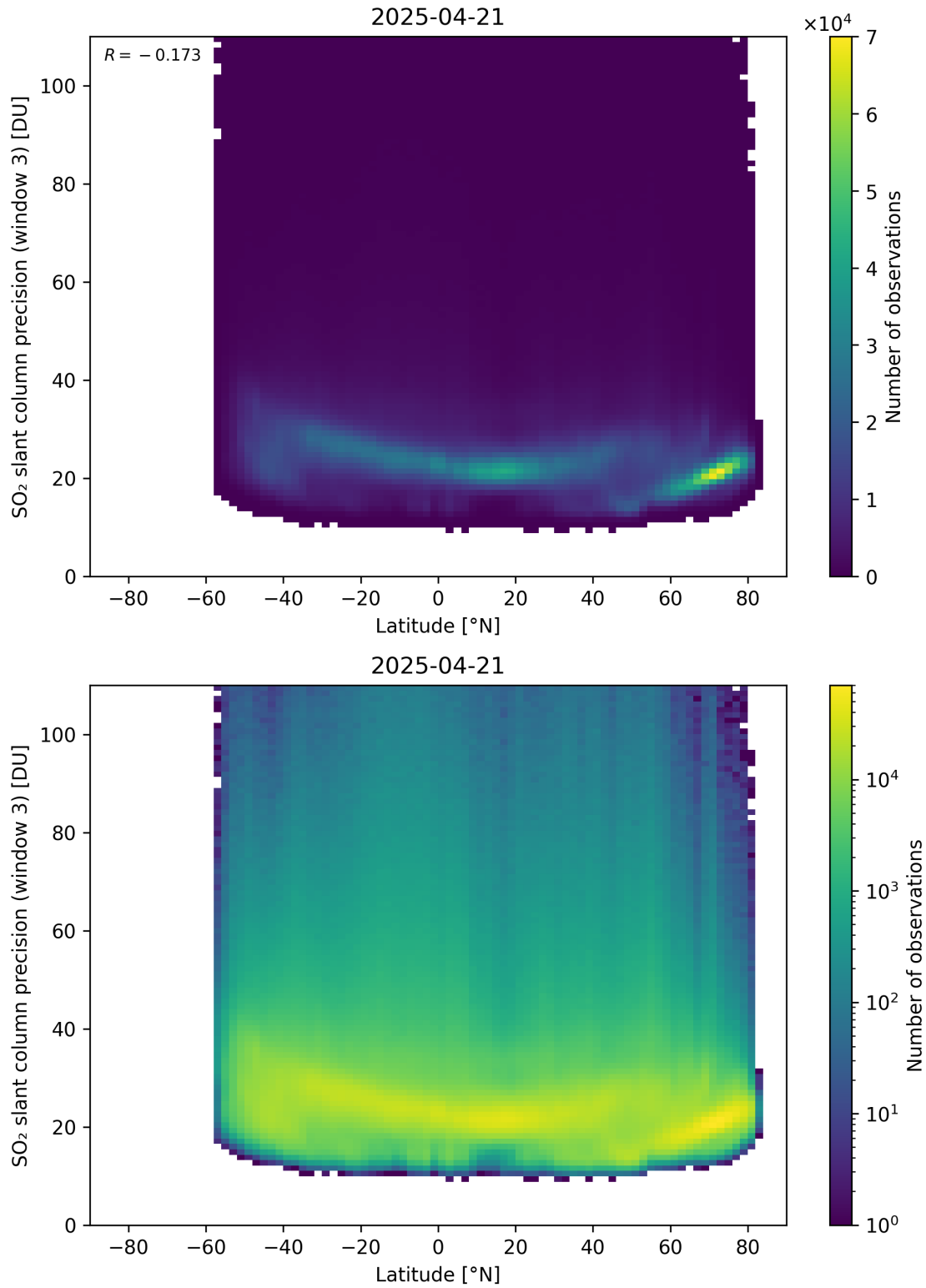
Figure 166: Scatter density plot of “Latitude” against “SO 2 slant column precision (window 3)” for 2025-04-20 to 2025-04-22.
