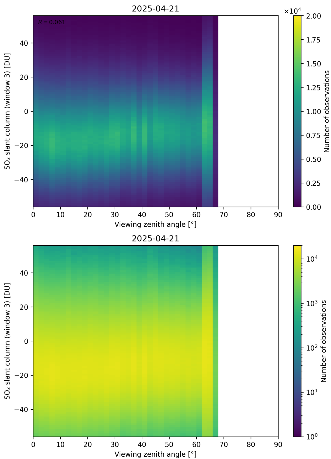
Figure 379: Scatter density plot of “Viewing zenith angle” against “SO 2 slant column (window 3)” for 2025-04-20 to 2025-04-22.
