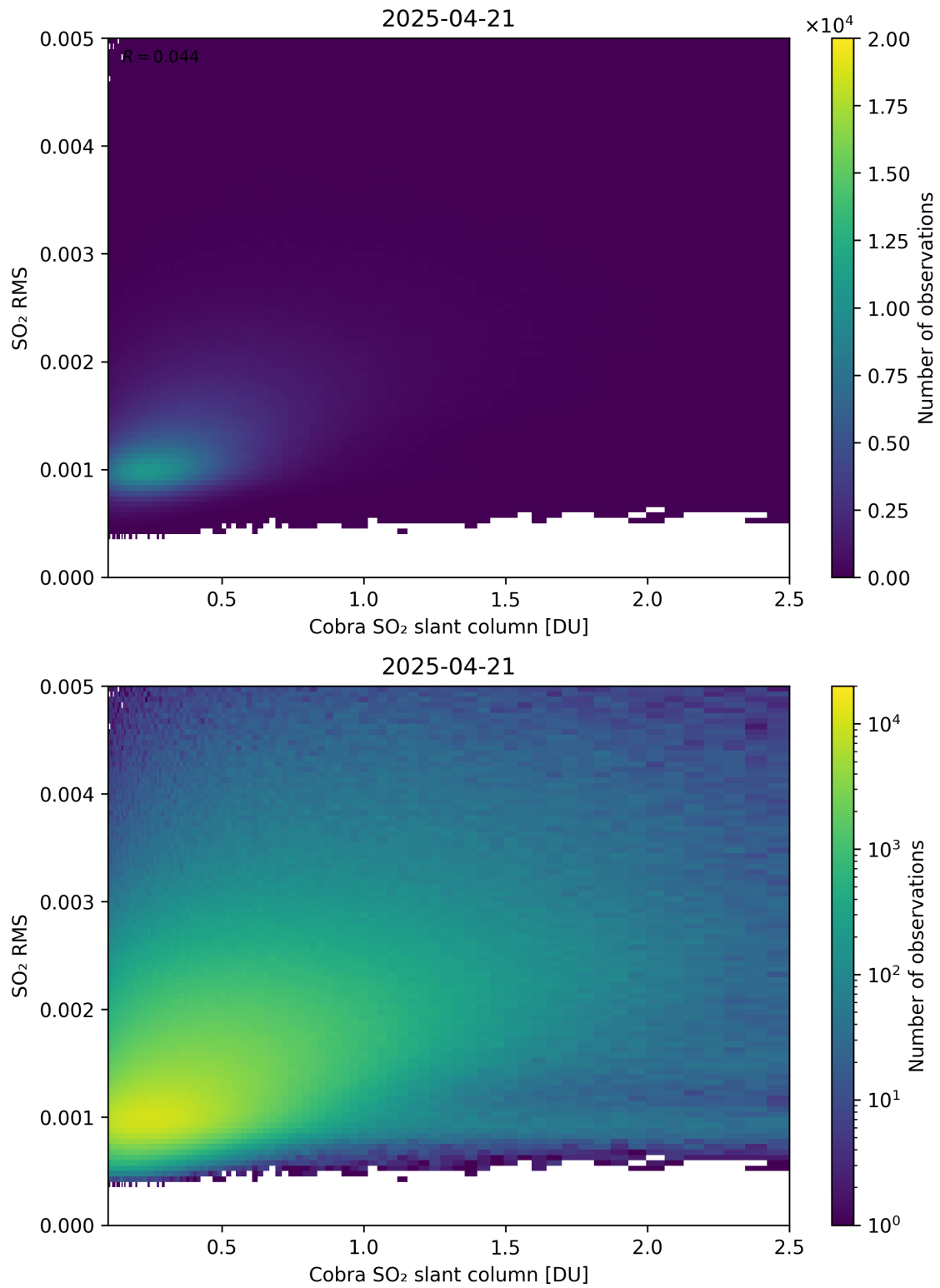
Figure 198: Scatter density plot of “Cobra SO 2 slant column” against “SO 2 RMS” for 2025-04-20 to 2025-04-22.
