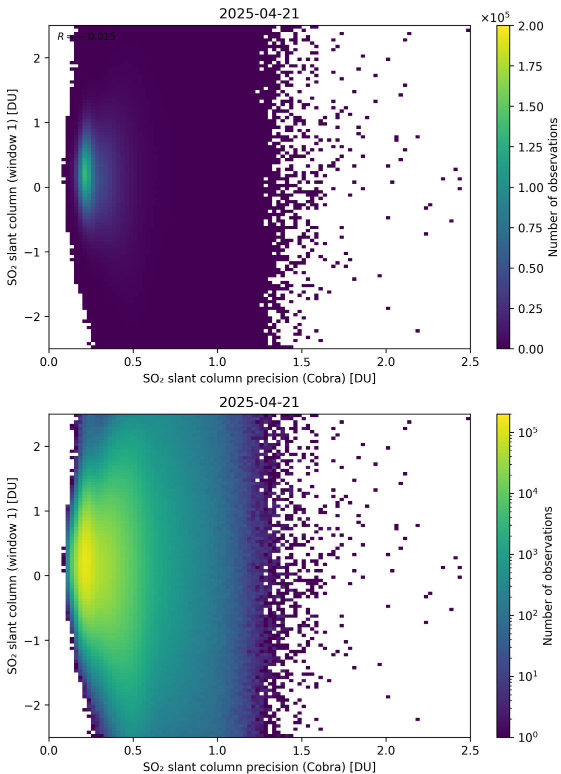
Figure 208: Scatter density plot of “SO 2 slant column precision (Cobra)” against “SO 2 slant column (window 1)” for 2025-04-20 to 2025-04-22.
