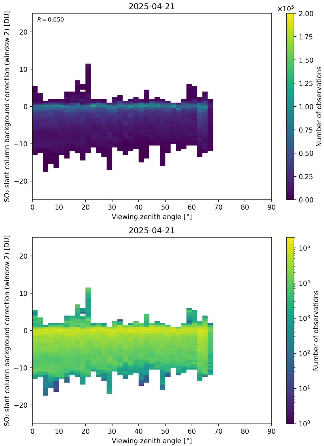
Figure 363: Scatter density plot of “Viewing zenith angle” against “SO 2 slant column background correction (window 2)” for 2025-04-20 to 2025-04-22.
