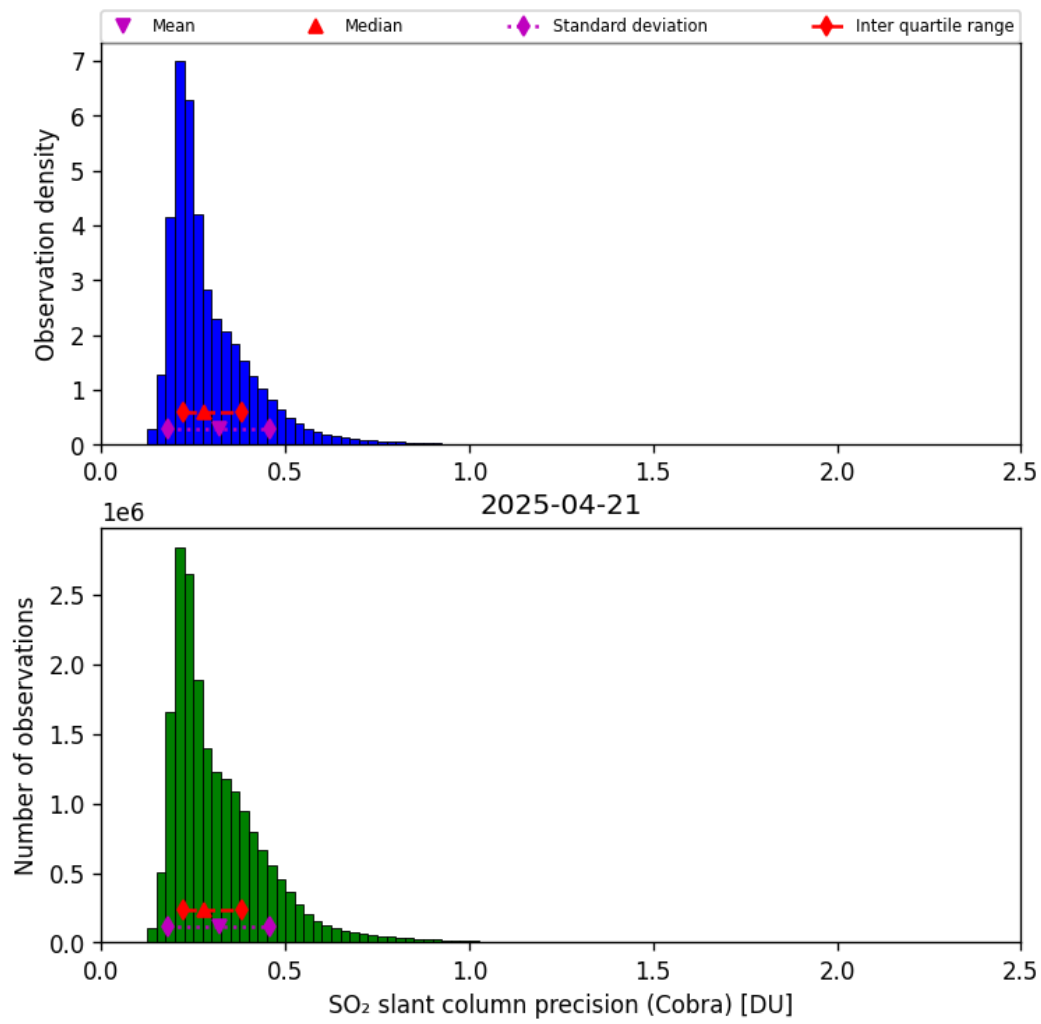
Figure 62: Histogram of “SO 2 slant column precision (Cobra)” for 2025-04-20 to 2025-04-22
