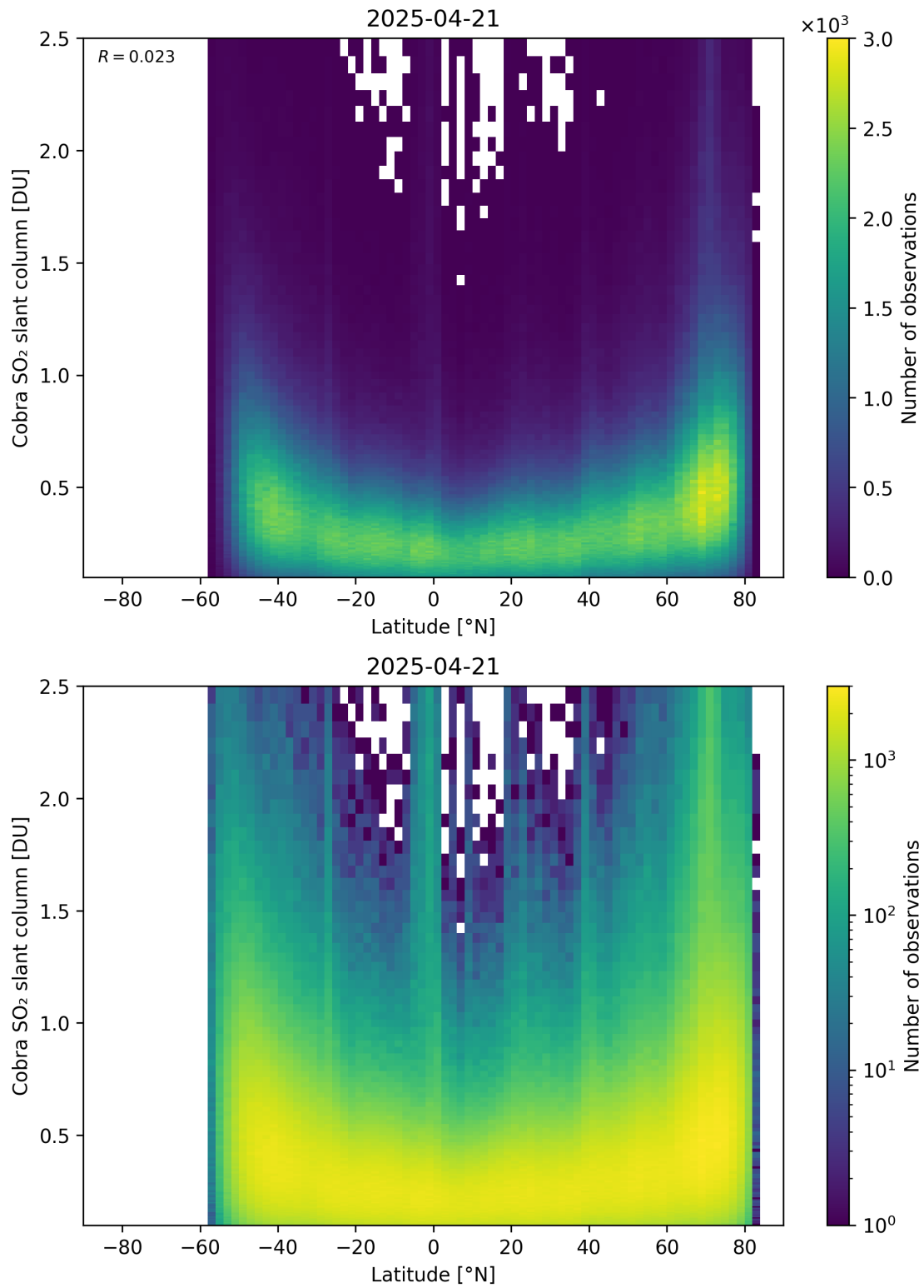
Figure 157: Scatter density plot of “Latitude” against “Cobra SO 2 slant column” for 2025-04-20 to 2025-04-22.
