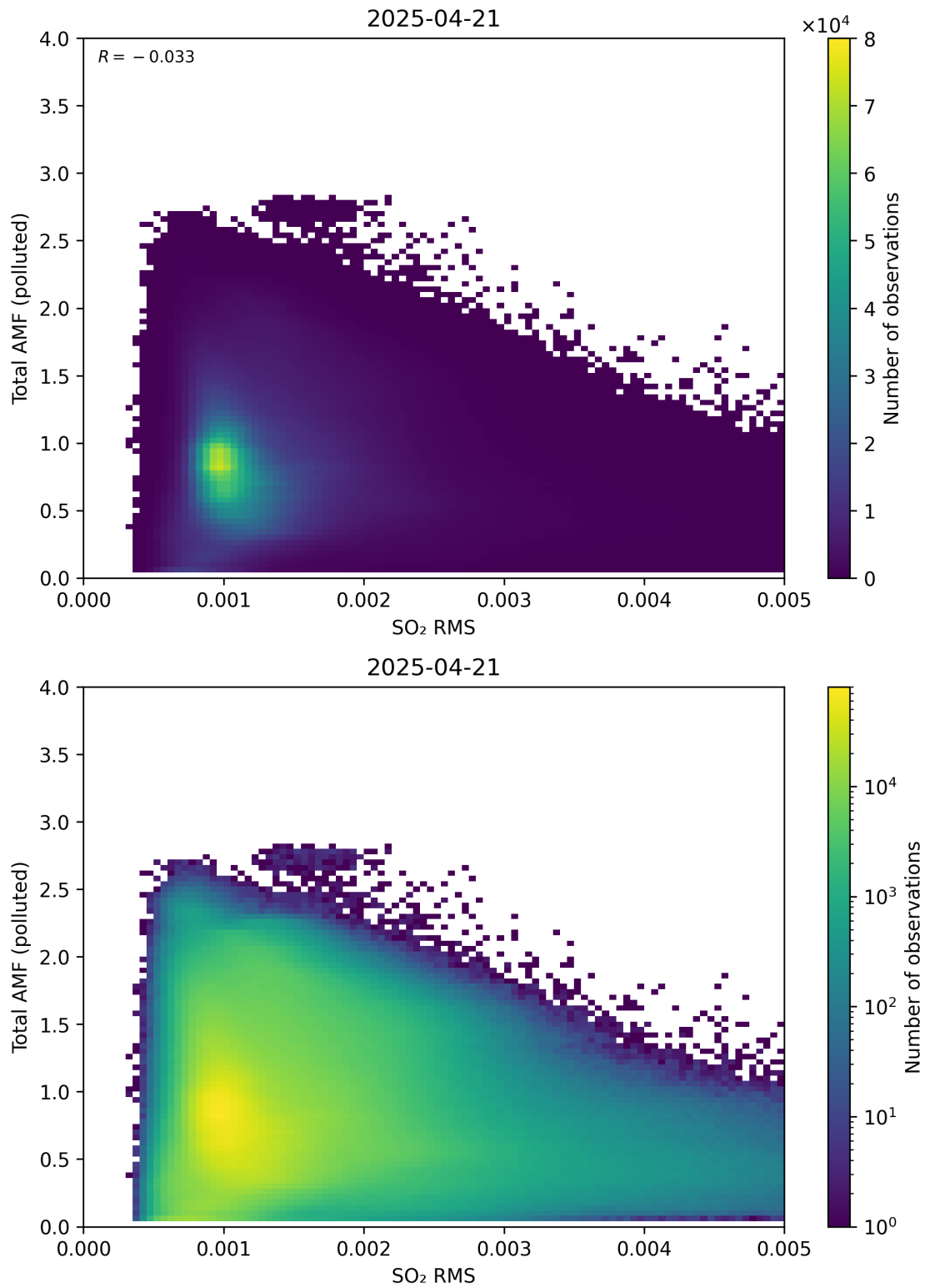
Figure 148: Scatter density plot of “SO 2 RMS” against “Total AMF (polluted)” for 2025-04-20 to 2025-04-22.
