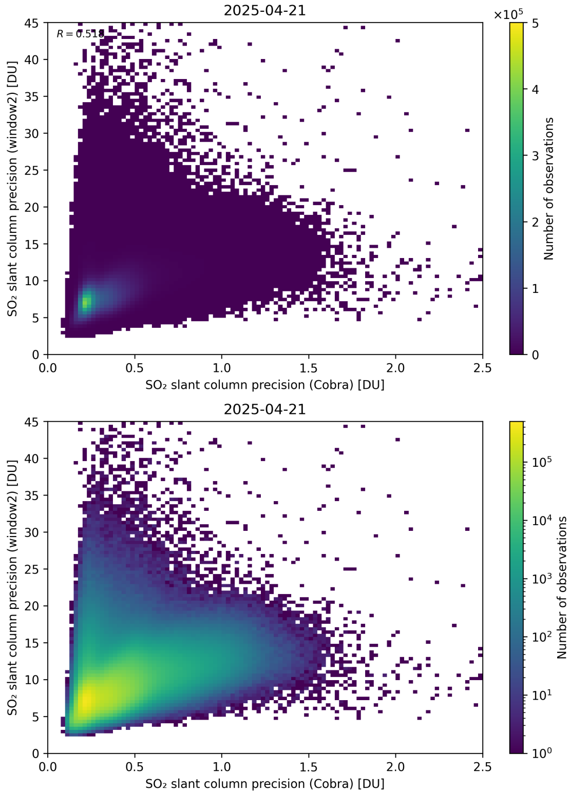
Figure 210: Scatter density plot of “SO 2 slant column precision (Cobra)” against “SO 2 slant column precision (window2)” for 2025-04-20 to 2025-04-22.
