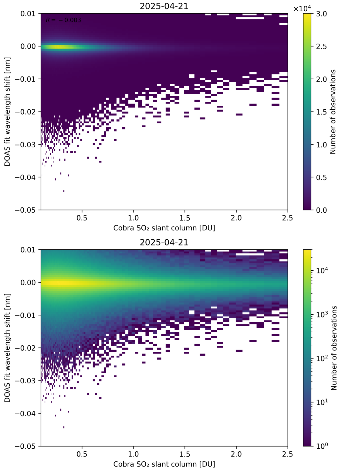
Figure 196: Scatter density plot of “Cobra SO 2 slant column” against “DOAS fit wavelength shift” for 2025-04-20 to 2025-04-22.
