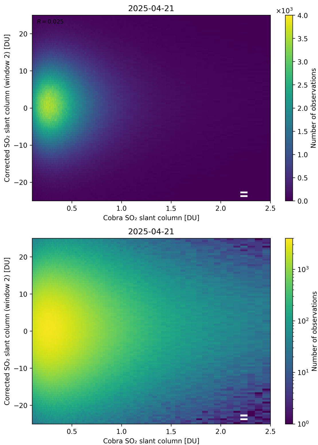
Figure 217: Scatter density plot of “Cobra SO 2 slant column” against “Corrected SO 2 slant column (window 2)” for 2025-04-20 to 2025-04-22.
