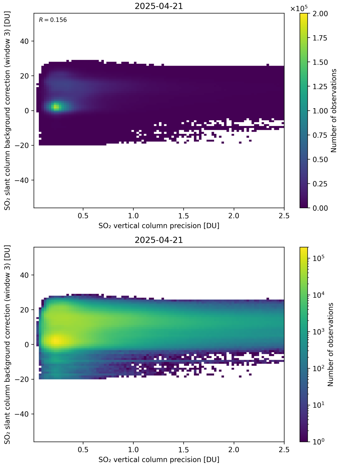
Figure 331: Scatter density plot of “SO 2 vertical column precision” against “SO 2 slant column background correction (window 3)” for 2025-04-20 to 2025-04-22.
