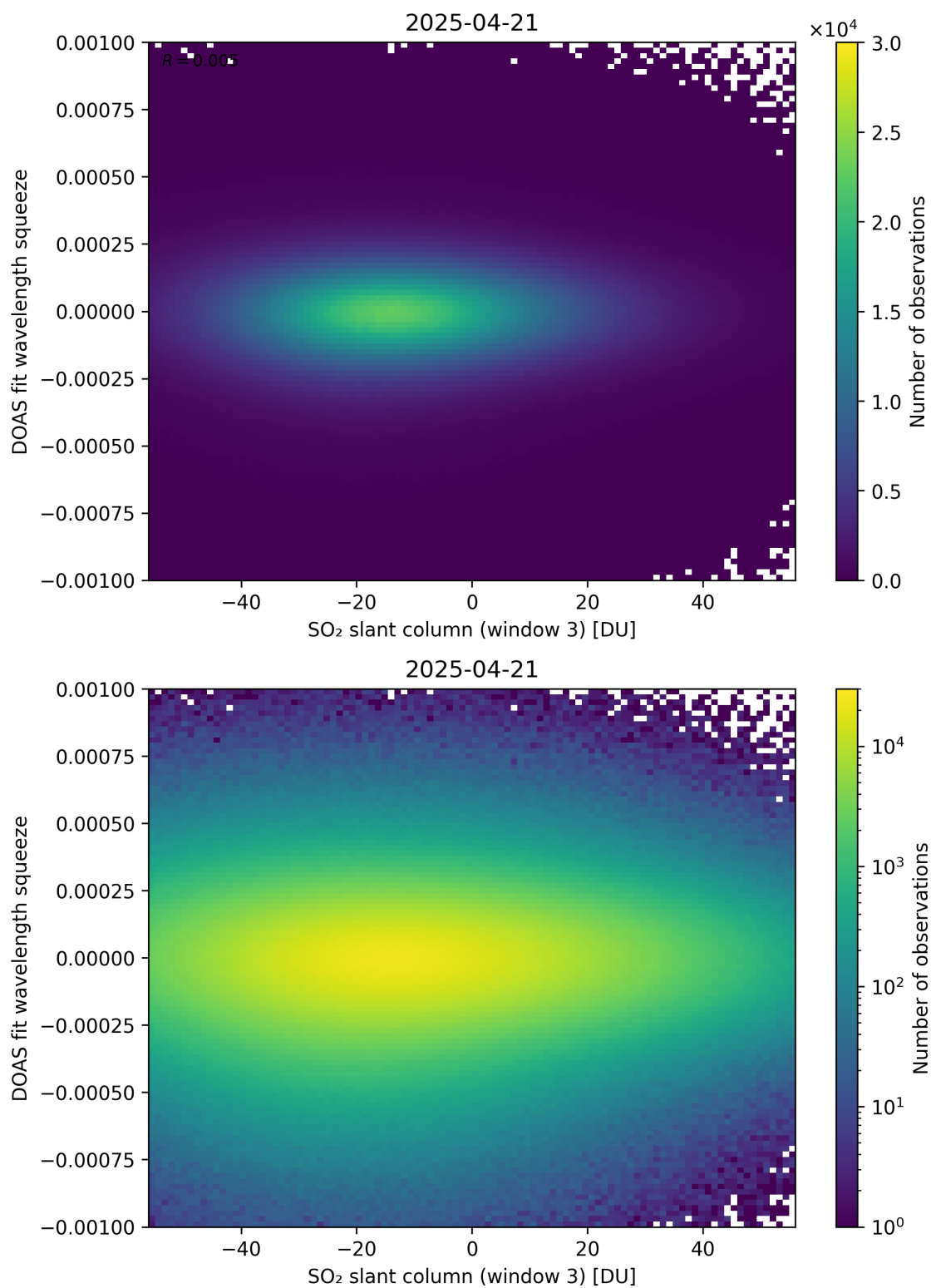
Figure 305: Scatter density plot of “SO 2 slant column (window 3)” against “DOAS fit wavelength squeeze” for 2025-04-20 to 2025-04-22.
