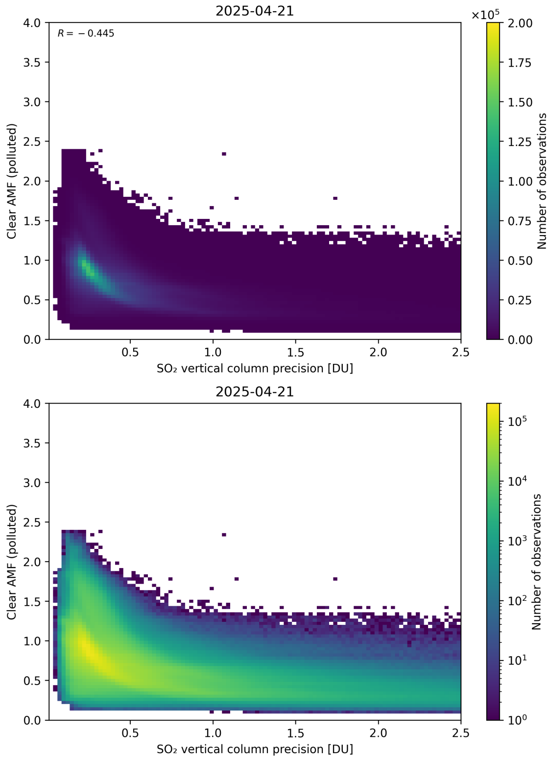
Figure 335: Scatter density plot of “SO 2 vertical column precision” against “Clear AMF (polluted)” for 2025-04-20 to 2025-04-22.
