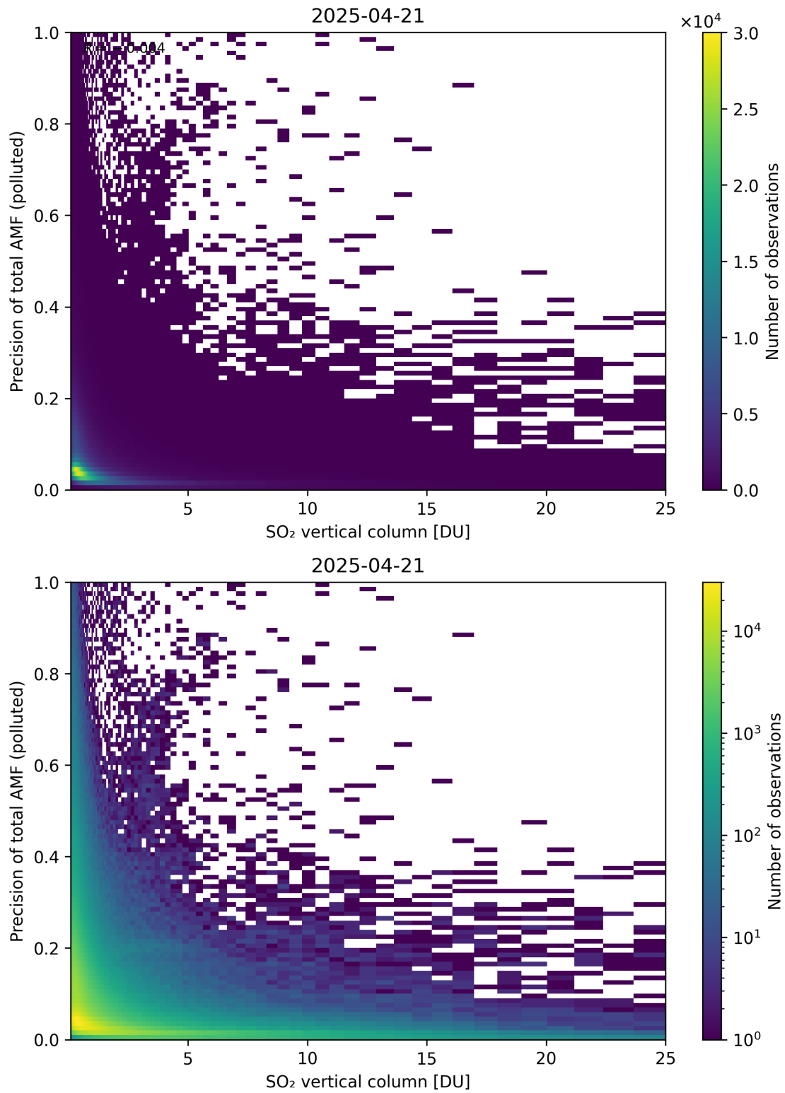
Figure 360: Scatter density plot of “SO 2 vertical column” against “Precision of total AMF (polluted)” for 2025-04-20 to 2025-04-22.
