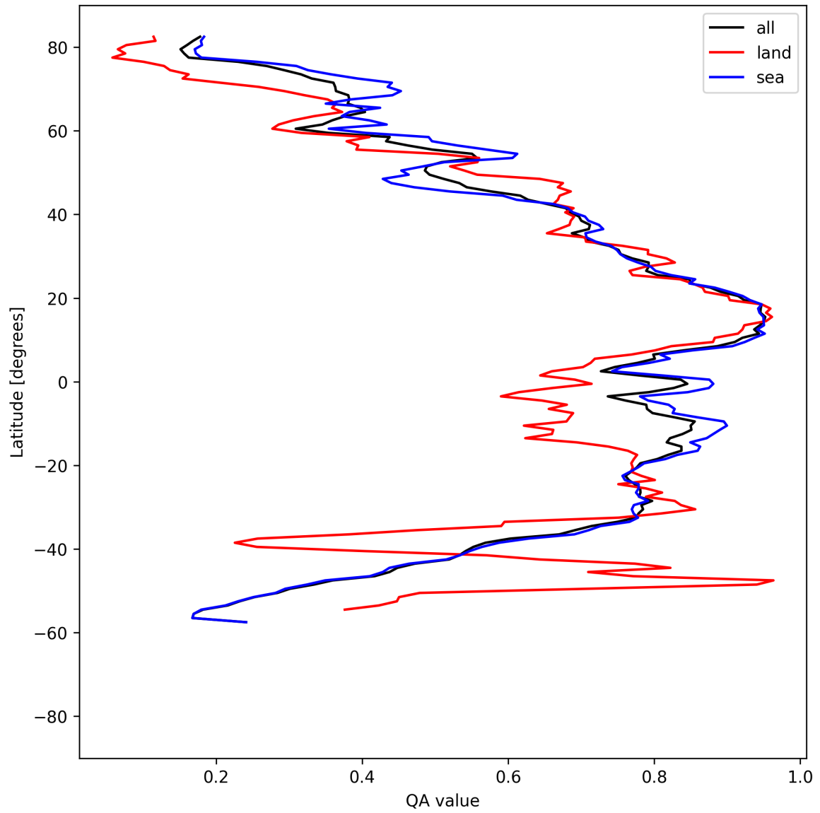
Figure 31: Zonal average of “QA value” for 2025-04-20 to 2025-04-22.
