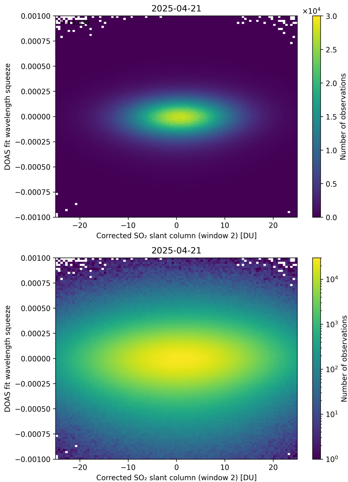
Figure 247: Scatter density plot of “Corrected SO 2 slant column (window 2)” against “DOAS fit wavelength squeeze” for 2025-04-20 to 2025-04-22.
