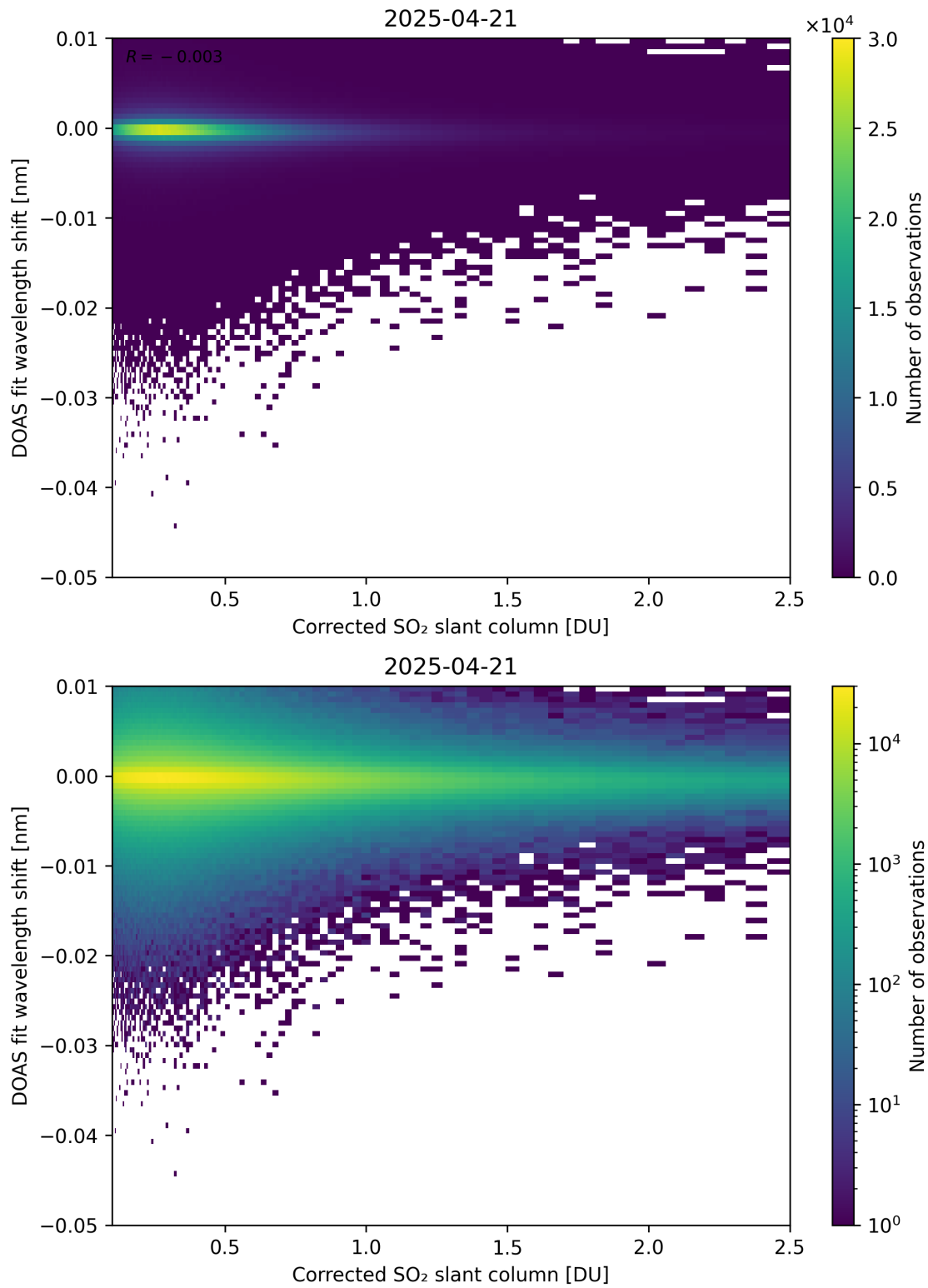
Figure 229: Scatter density plot of “Corrected SO 2 slant column” against “DOAS fit wavelength shift” for 2025-04-20 to 2025-04-22.
