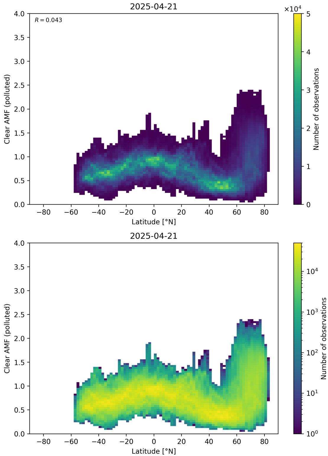
Figure 156: Scatter density plot of “Latitude” against “Clear AMF (polluted)” for 2025-04-20 to 2025-04-22.
