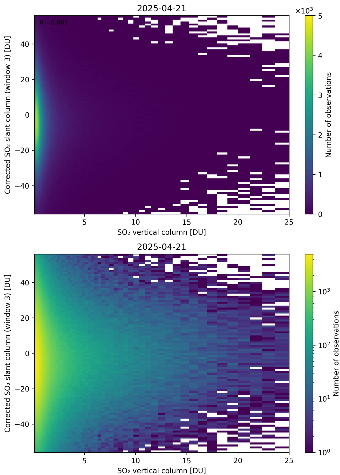
Figure 353: Scatter density plot of “SO 2 vertical column” against “Corrected SO 2 slant column (window 3)” for 2025-04-20 to 2025-04-22.
