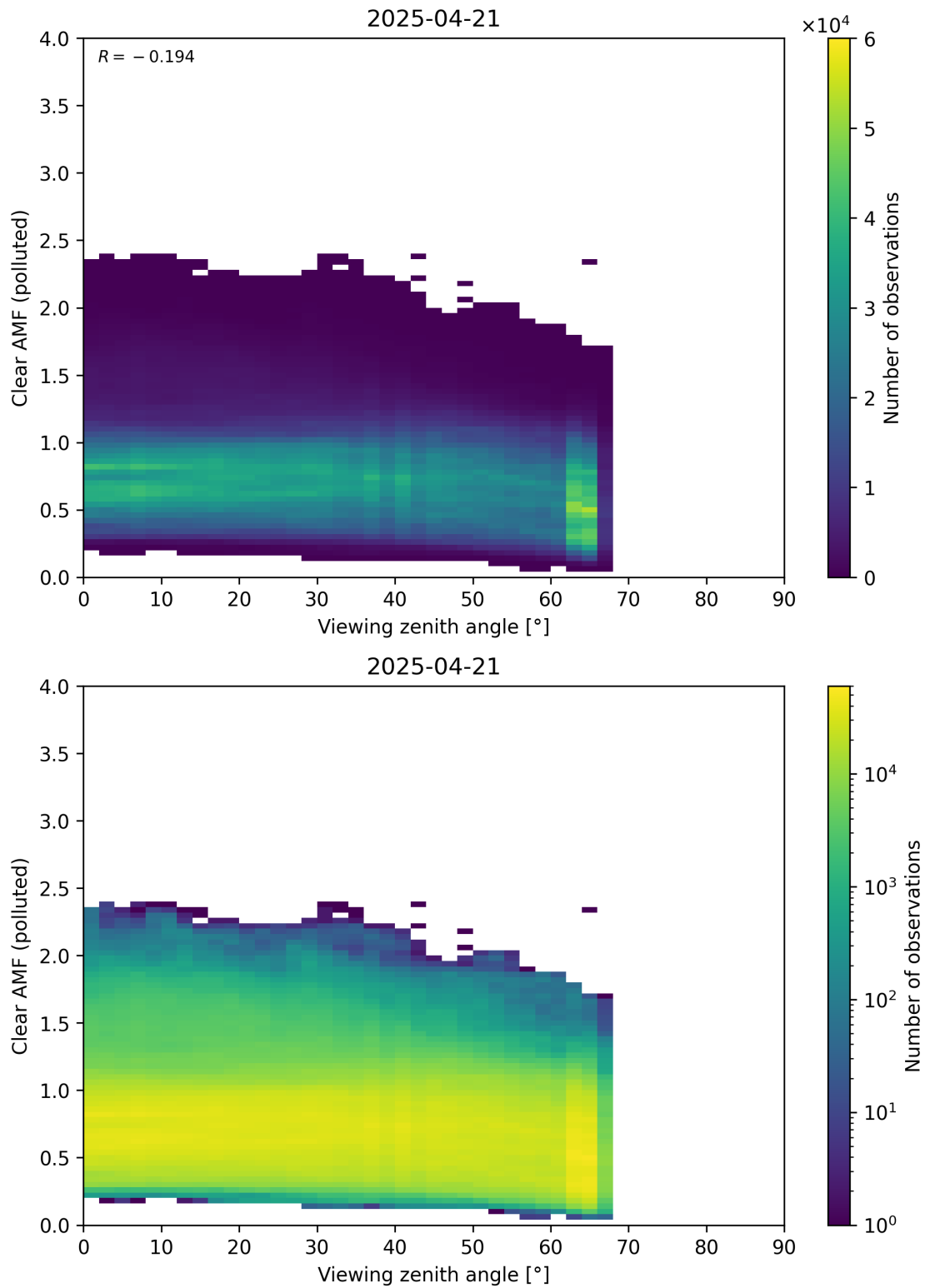
Figure 370: Scatter density plot of “Viewing zenith angle” against “Clear AMF (polluted)” for 2025-04-20 to 2025-04-22.
