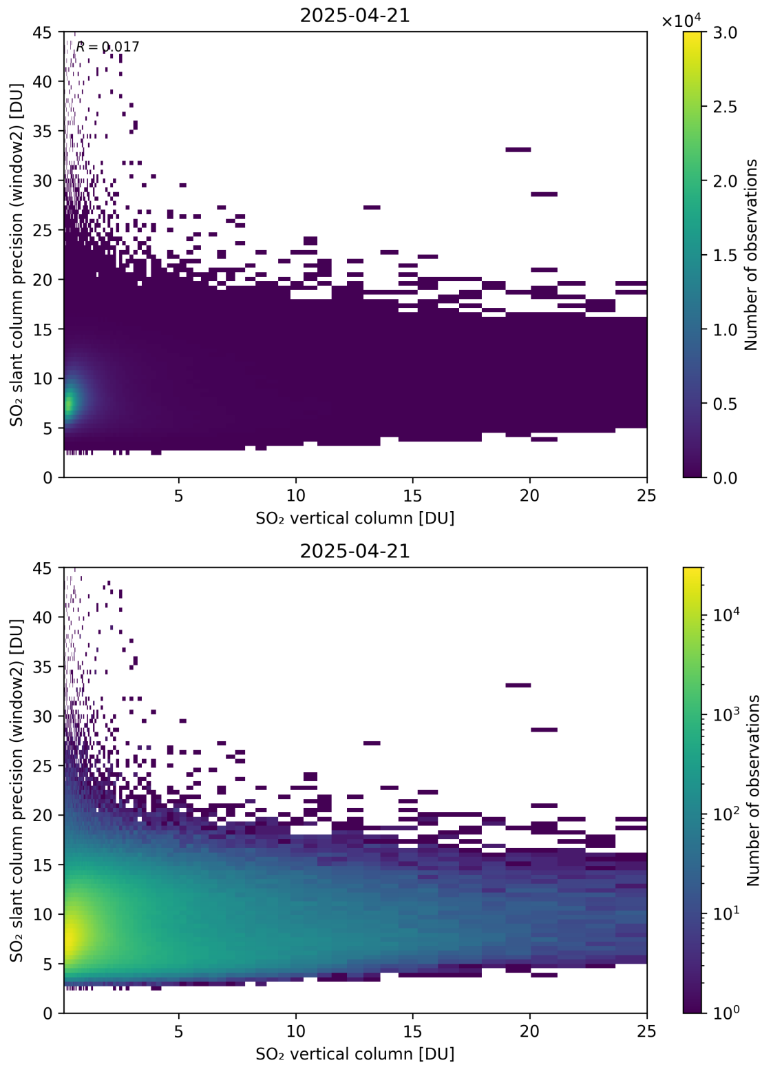
Figure 356: Scatter density plot of “SO 2 vertical column” against “SO 2 slant column precision (window2)” for 2025-04-20 to 2025-04-22.
