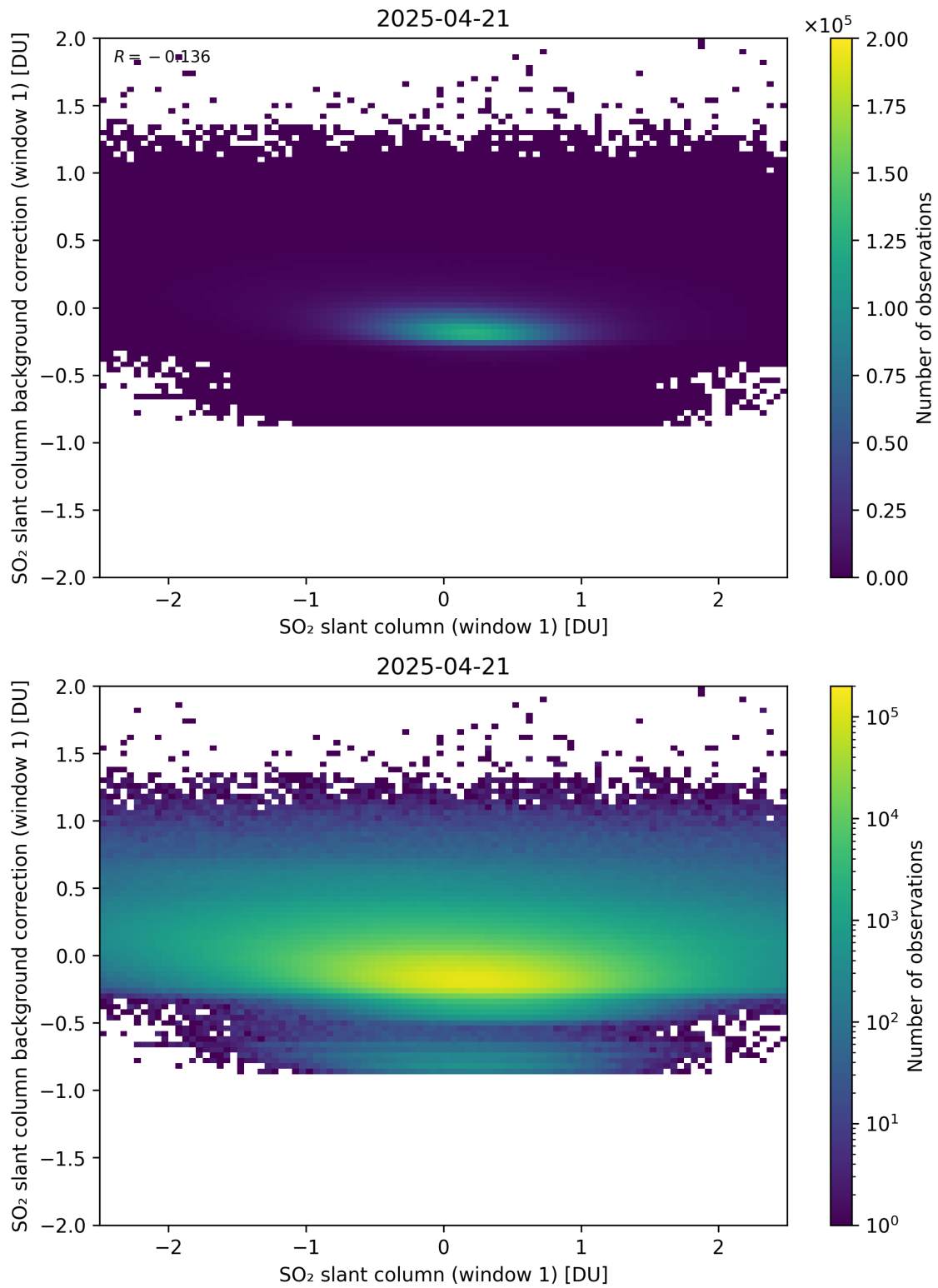
Figure 262: Scatter density plot of “SO 2 slant column (window 1)” against “SO 2 slant column background correction (window 1)” for 2025-04-20 to 2025-04-22.
