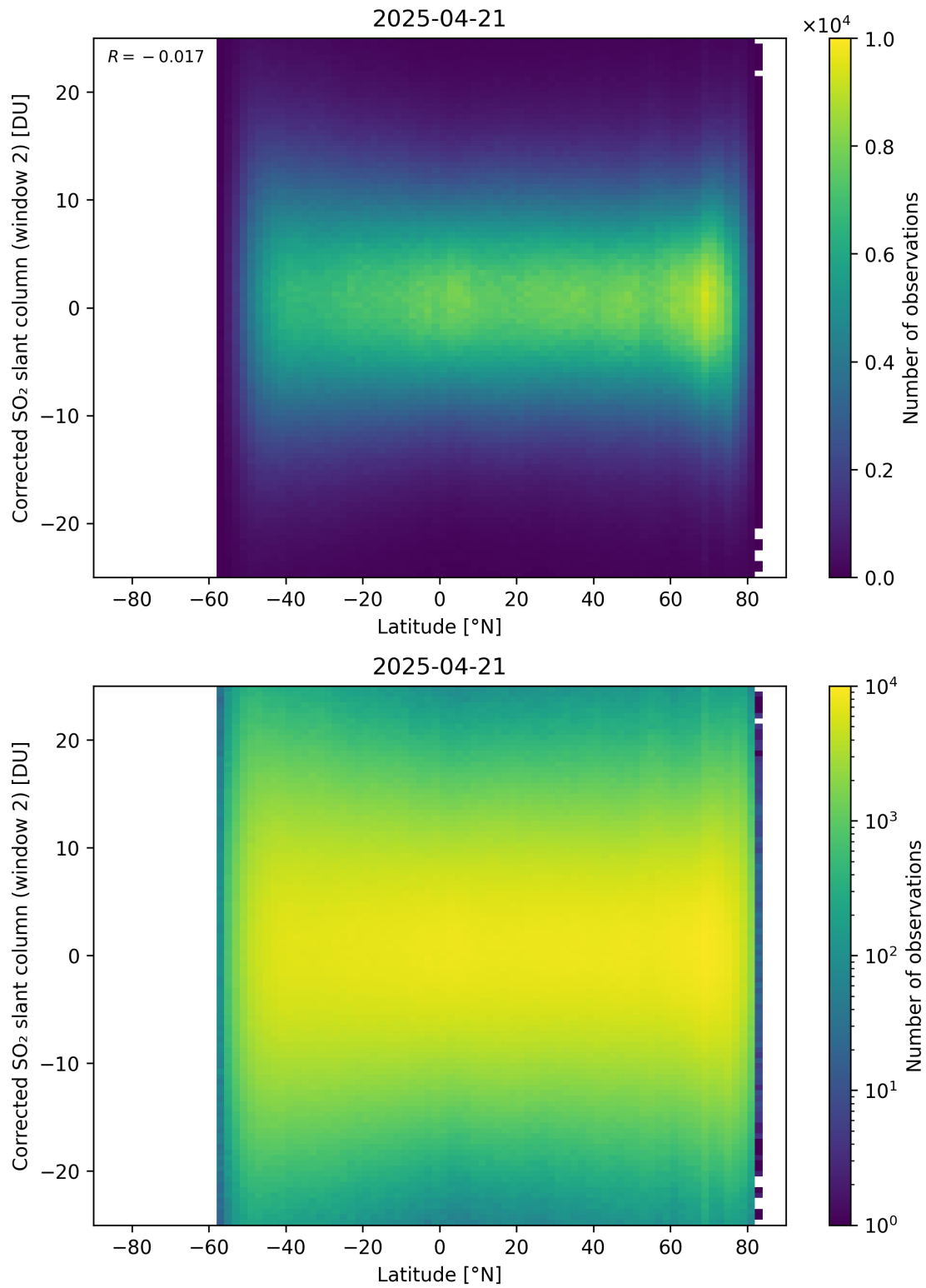
Figure 160: Scatter density plot of “Latitude” against “Corrected SO 2 slant column (window 2)” for 2025-04-20 to 2025-04-22.
