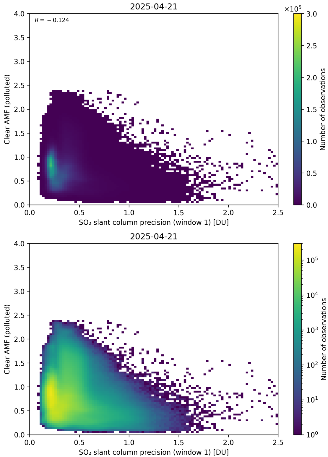
Figure 274: Scatter density plot of “SO 2 slant column precision (window 1)” against “Clear AMF (polluted)” for 2025-04-20 to 2025-04-22.
