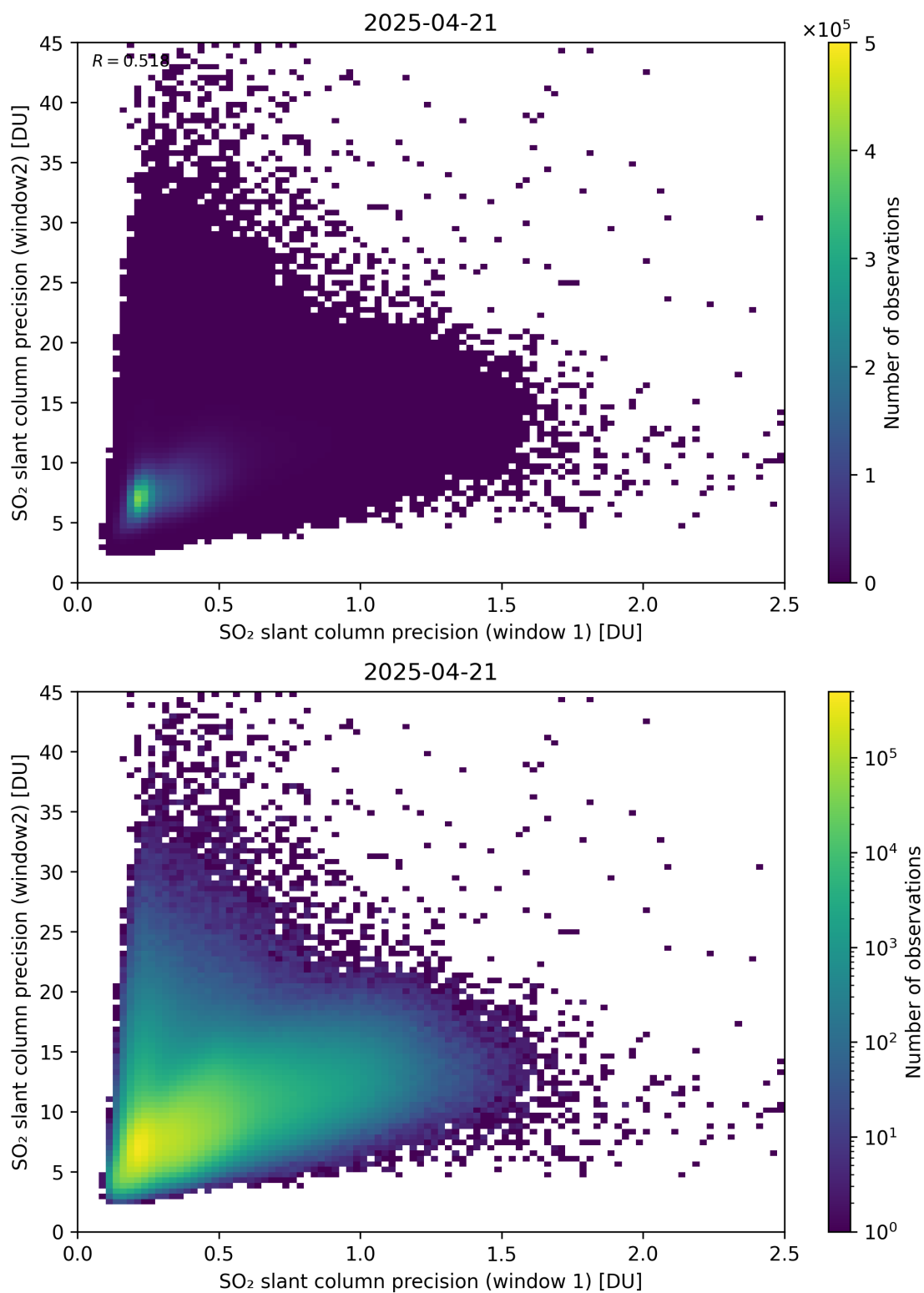
Figure 277: Scatter density plot of “SO 2 slant column precision (window 1)” against “SO 2 slant column precision (window2)” for 2025-04-20 to 2025-04-22.
