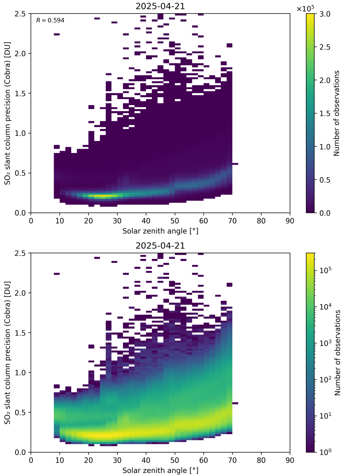
Figure 180: Scatter density plot of “Solar zenith angle” against “SO 2 slant column precision (Cobra)” for 2025-04-20 to 2025-04-22.
