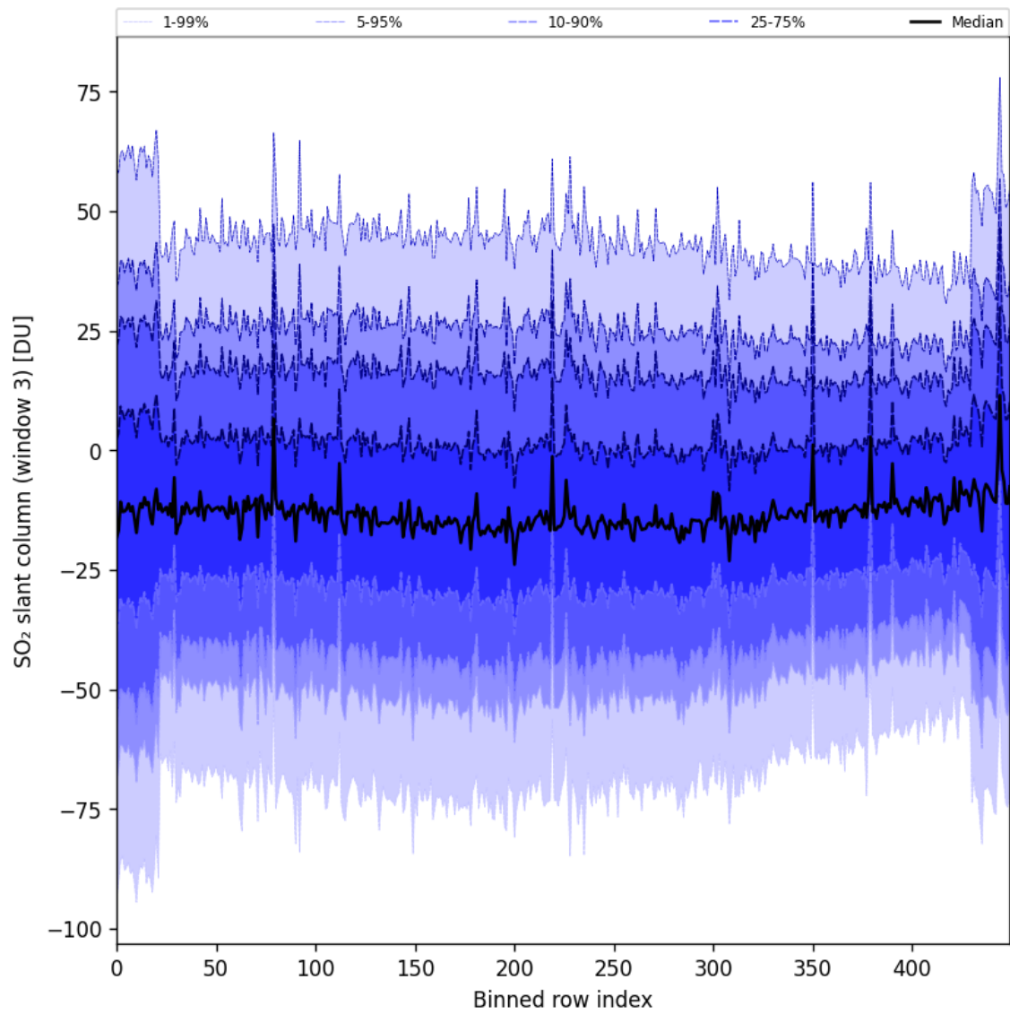
Figure 97: Along track statistics of “SO 2 slant column (window 3)” for 2025-04-20 to 2025-04-22
