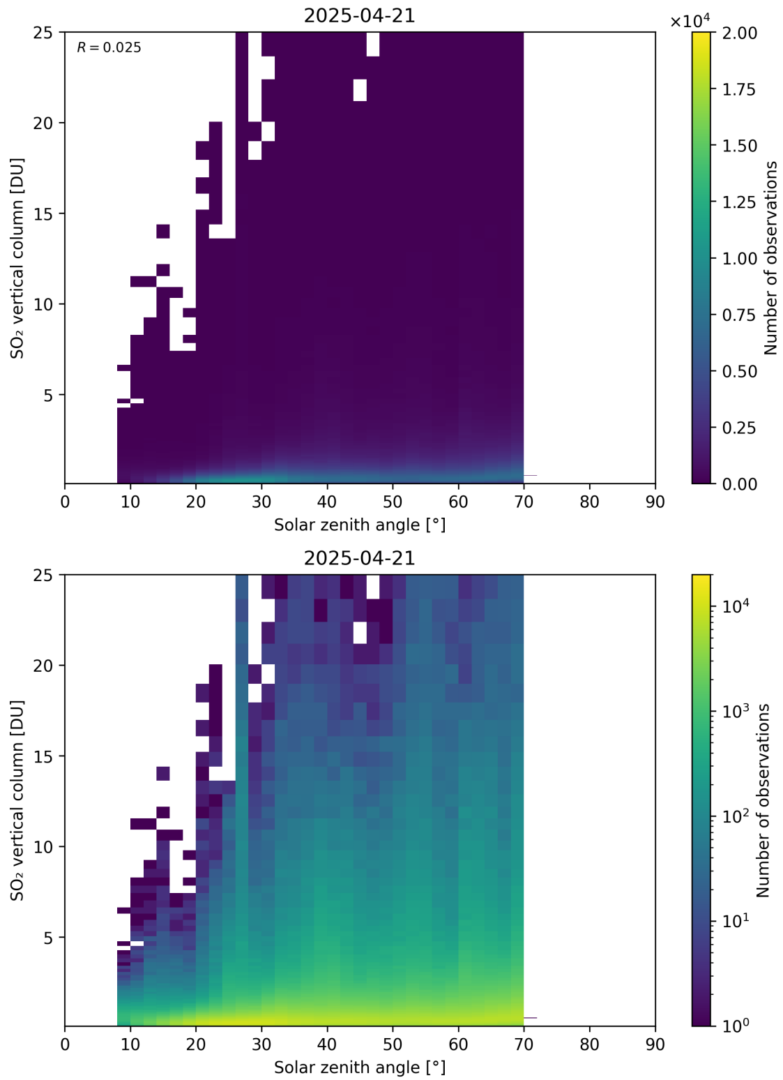
Figure 191: Scatter density plot of “Solar zenith angle” against “SO 2 vertical column” for 2025-04-20 to 2025-04-22.
