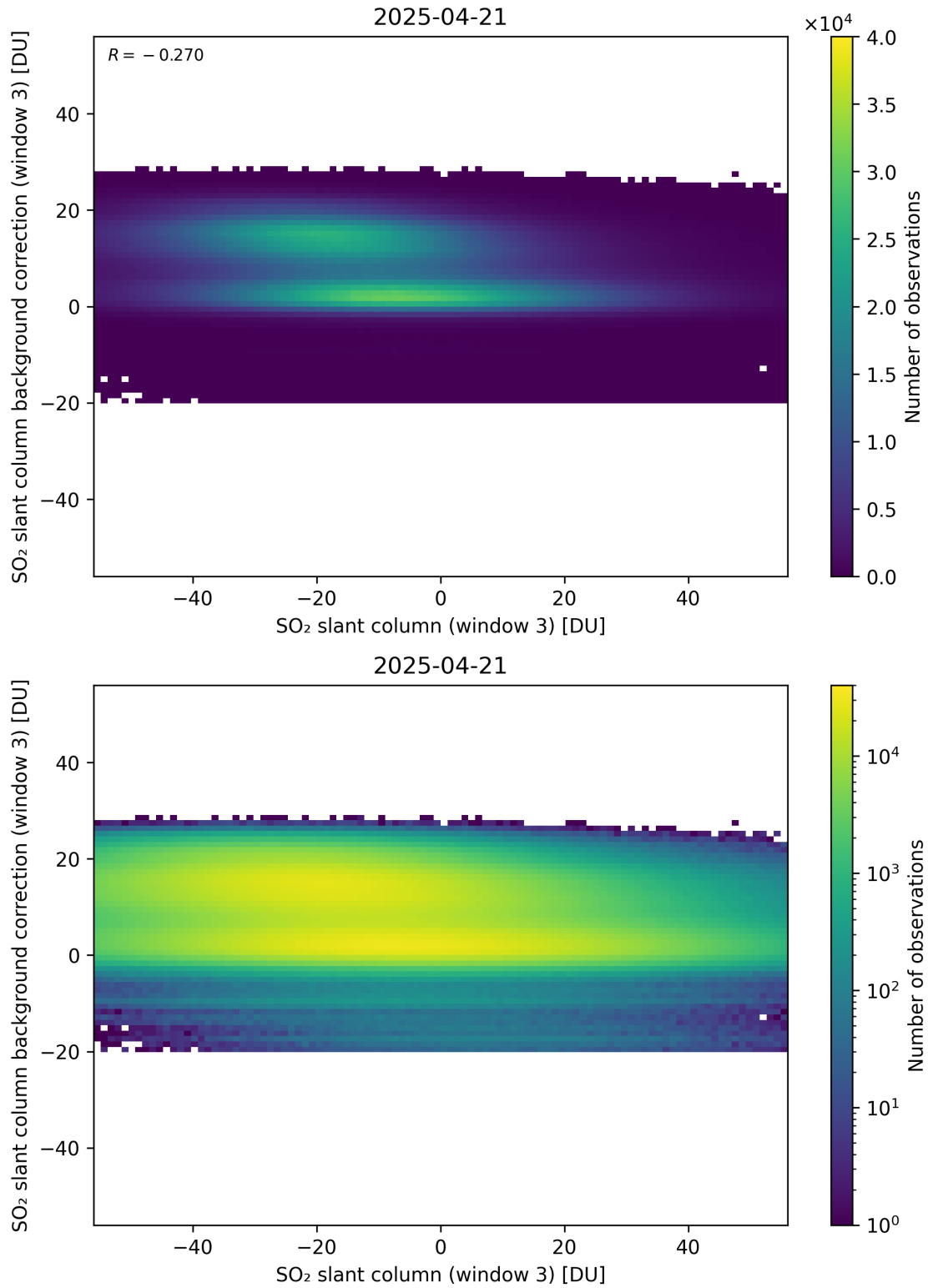
Figure 303: Scatter density plot of “SO 2 slant column (window 3)” against “SO 2 slant column background correction (window 3)” for 2025-04-20 to 2025-04-22.
