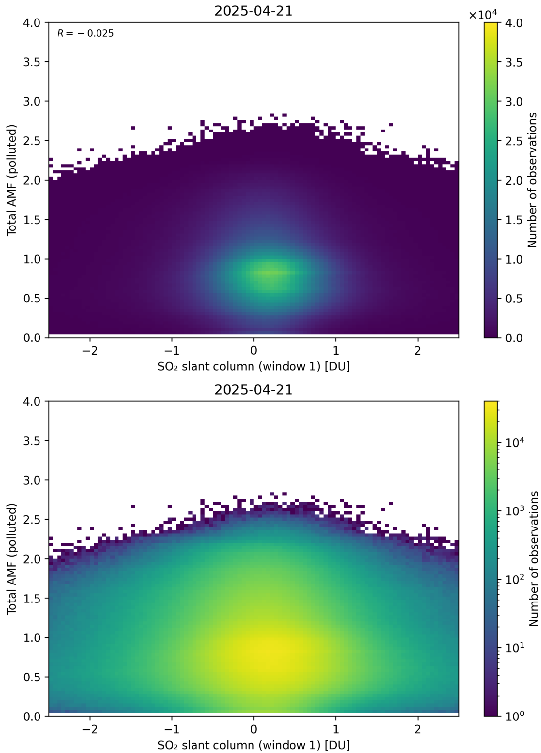
Figure 289: Scatter density plot of “SO 2 slant column (window 1)” against “Total AMF (polluted)” for 2025-04-20 to 2025-04-22.
