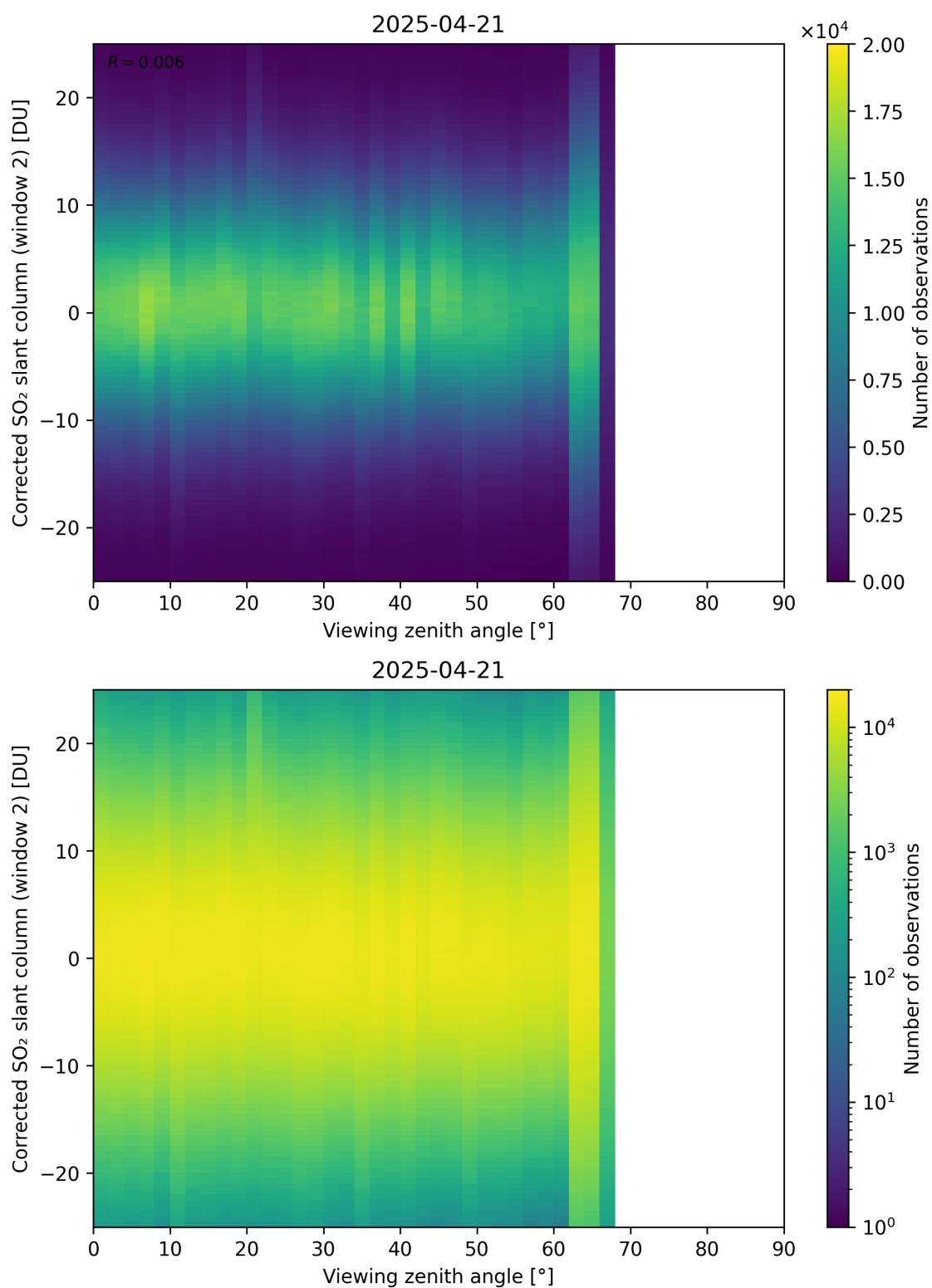
Figure 374: Scatter density plot of “Viewing zenith angle” against “Corrected SO 2 slant column (window 2)” for 2025-04-20 to 2025-04-22.
