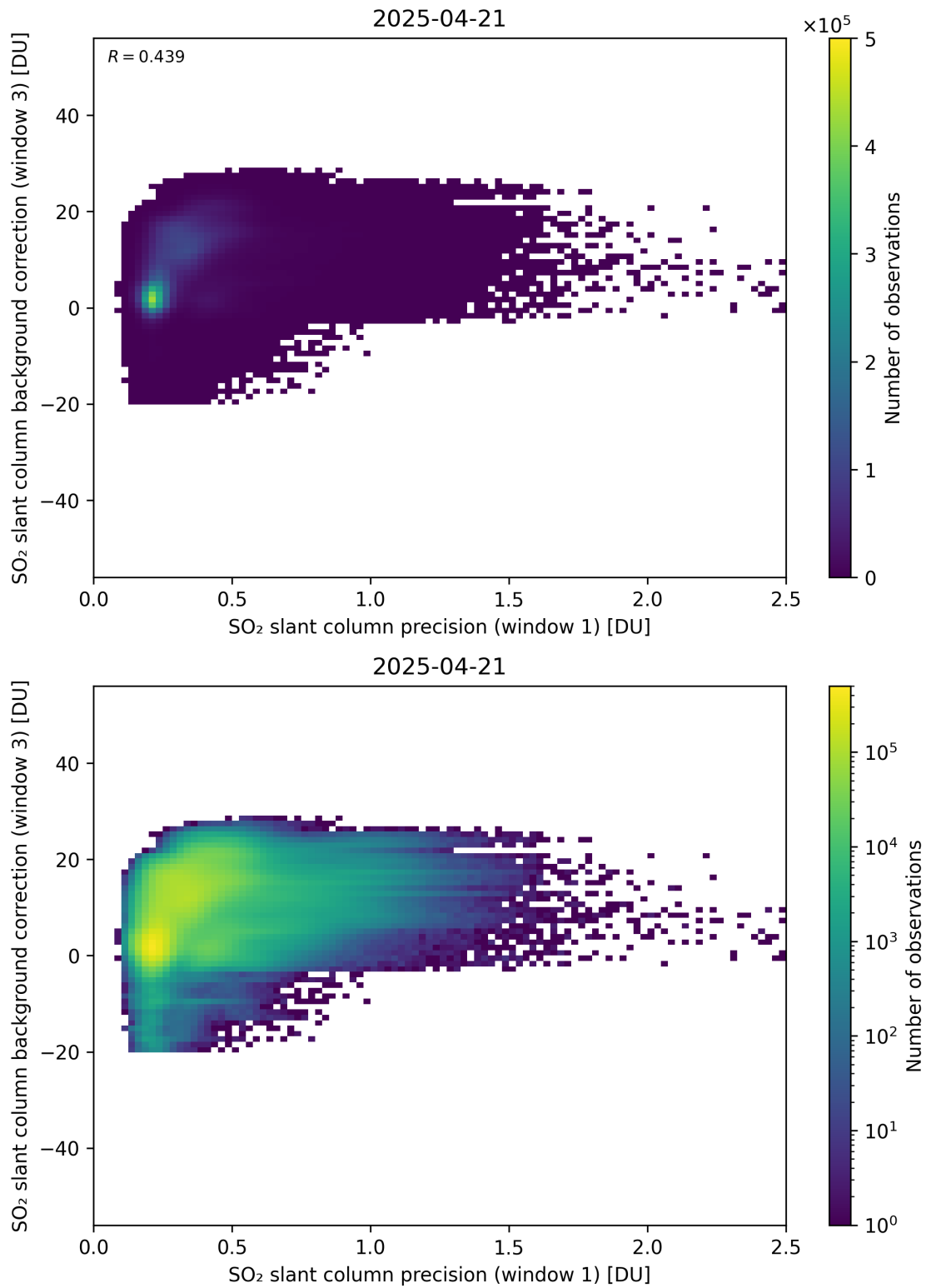
Figure 270: Scatter density plot of “SO 2 slant column precision (window 1)” against “SO 2 slant column background correction (window 3)” for 2025-04-20 to 2025-04-22.
