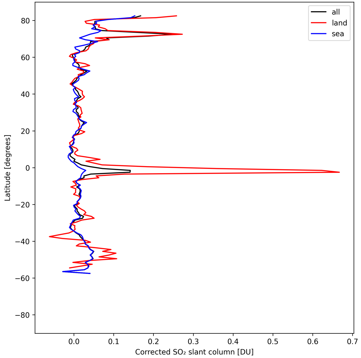
Figure 34: Zonal average of “Corrected SO 2 slant column” for 2025-04-20 to 2025-04-22.
