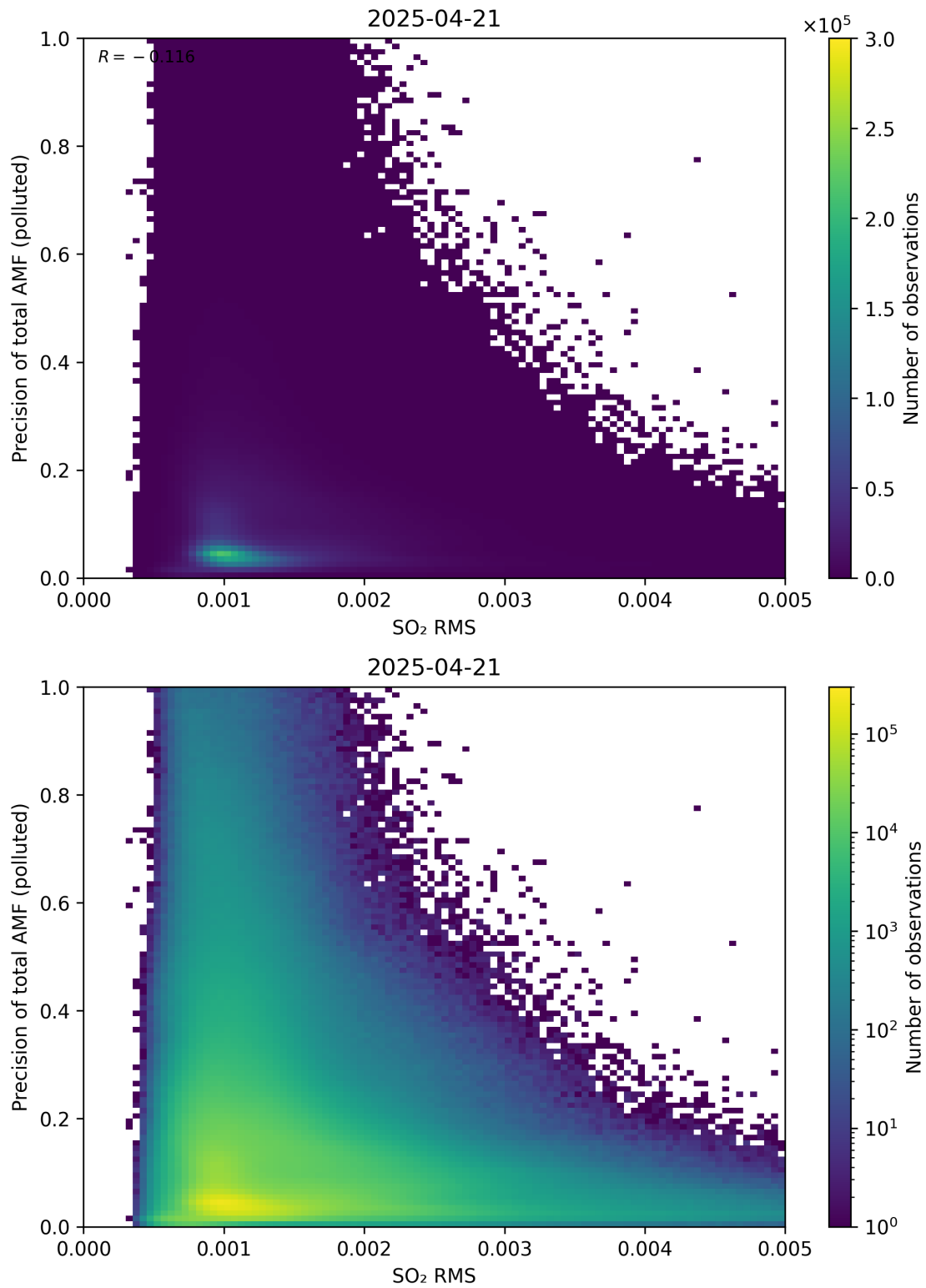
Figure 149: Scatter density plot of “SO 2 RMS” against “Precision of total AMF (polluted)” for 2025-04-20 to 2025-04-22.
