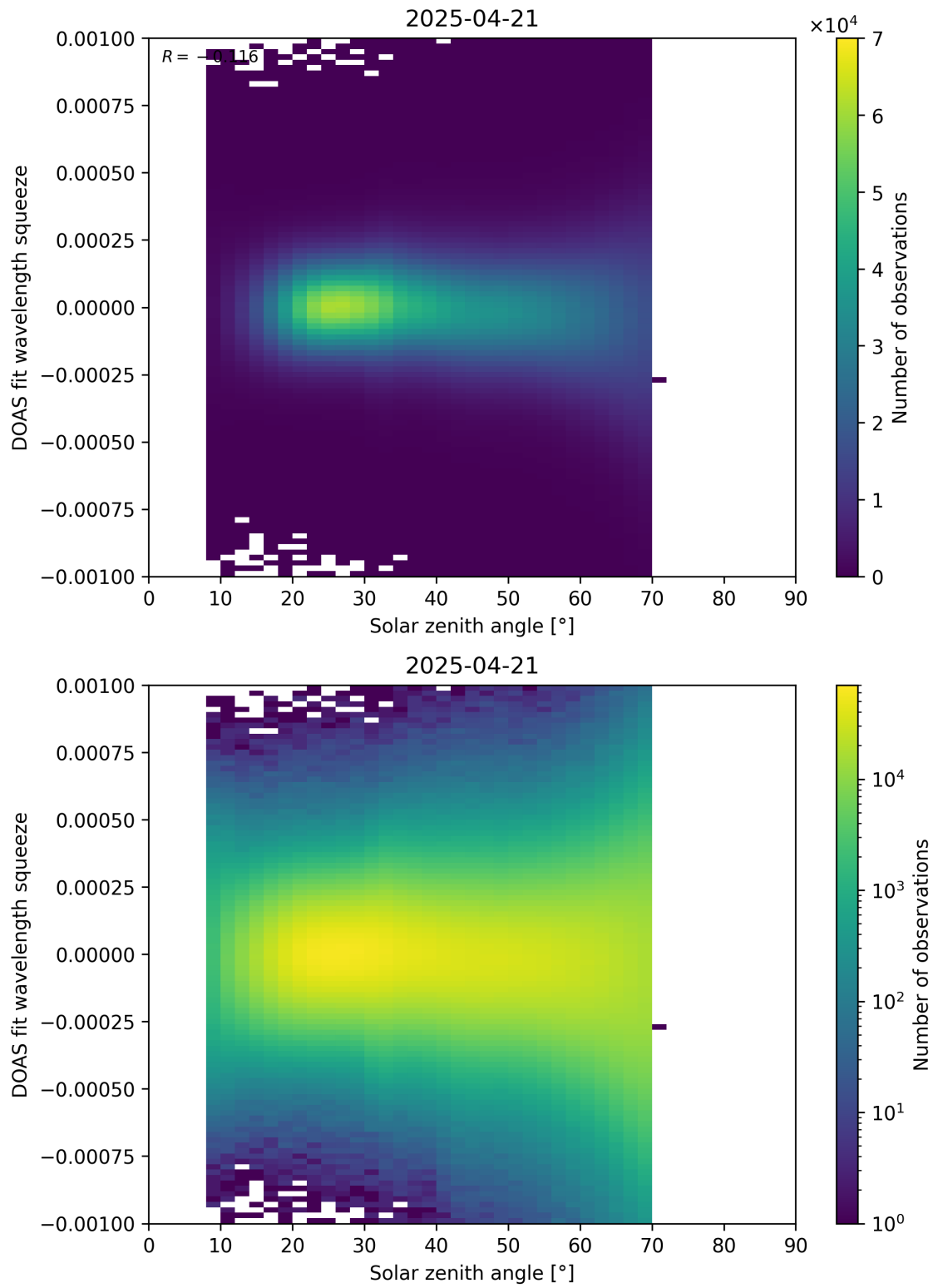
Figure 175: Scatter density plot of “Solar zenith angle” against “DOAS fit wavelength squeeze” for 2025-04-20 to 2025-04-22.
