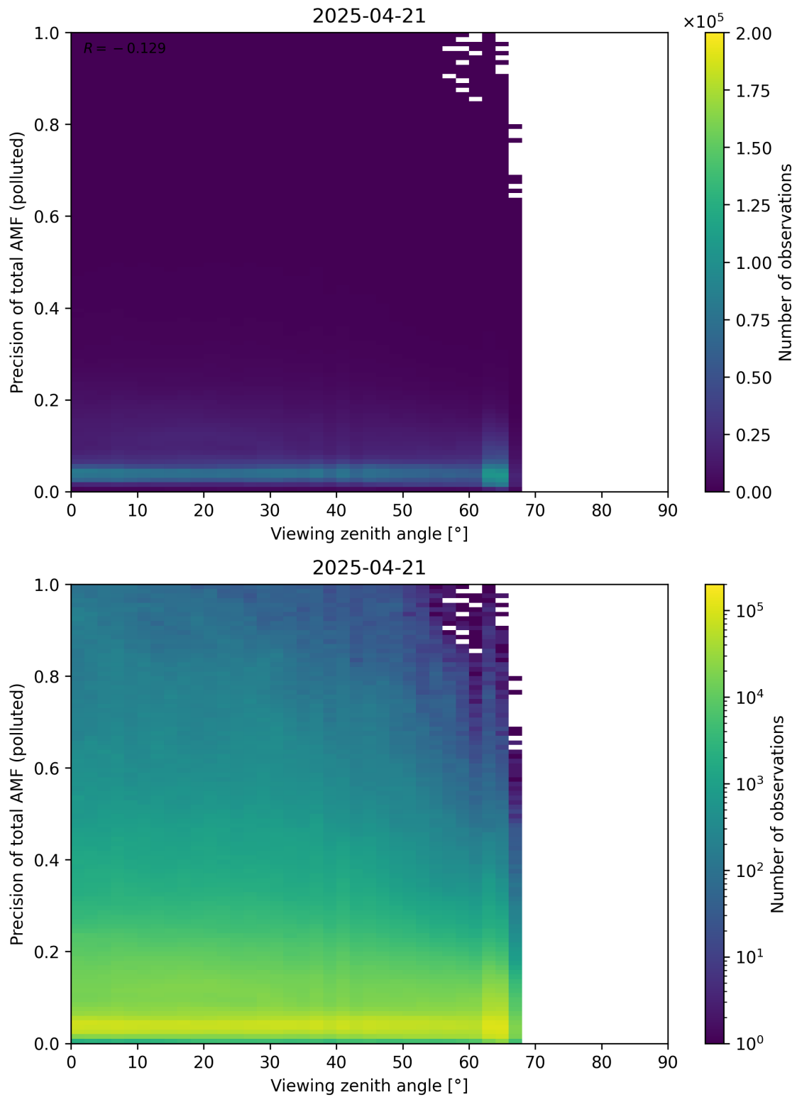
Figure 382: Scatter density plot of “Viewing zenith angle” against “Precision of total AMF (polluted)” for 2025-04-20 to 2025-04-22.
