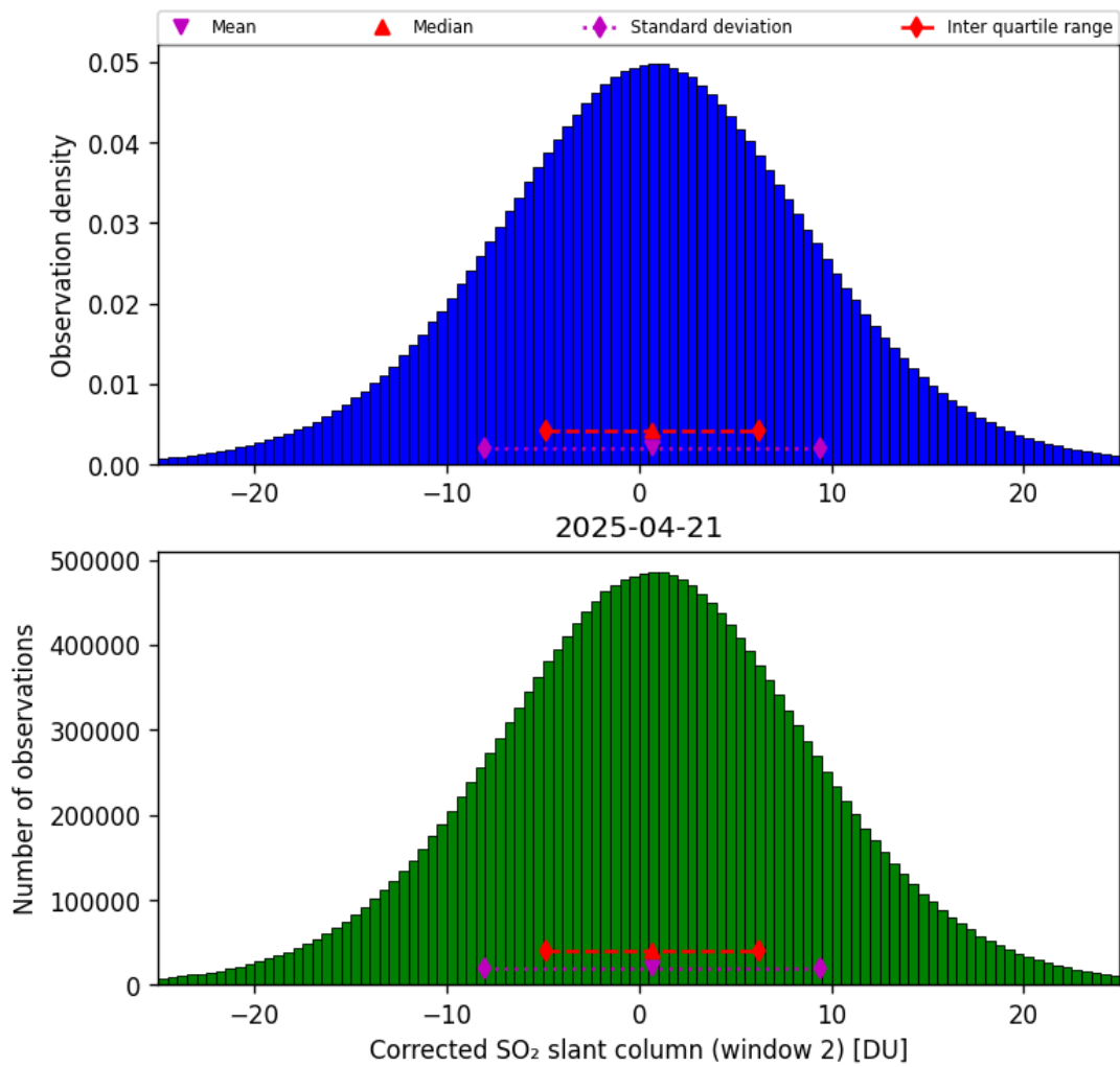
Figure 69: Histogram of “Corrected SO 2 slant column (window 2)” for 2025-04-20 to 2025-04-22
