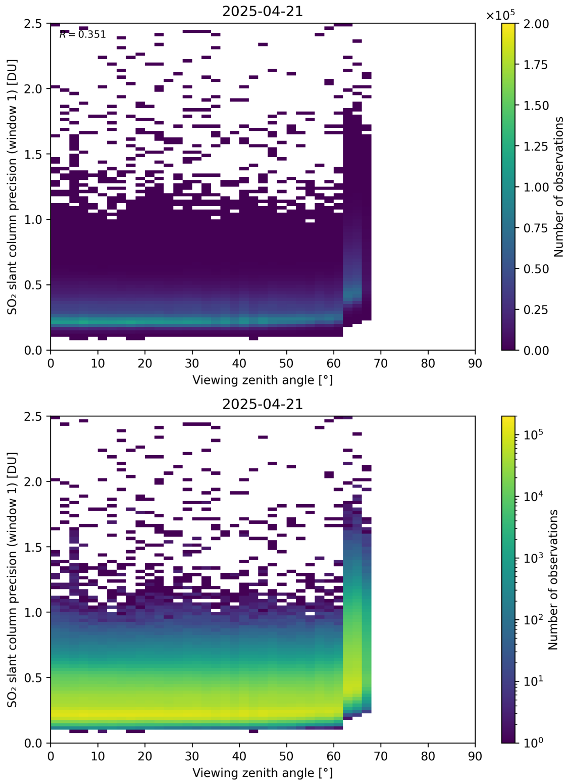
Figure 377: Scatter density plot of “Viewing zenith angle” against “SO 2 slant column precision (window 1)” for 2025-04-20 to 2025-04-22.
