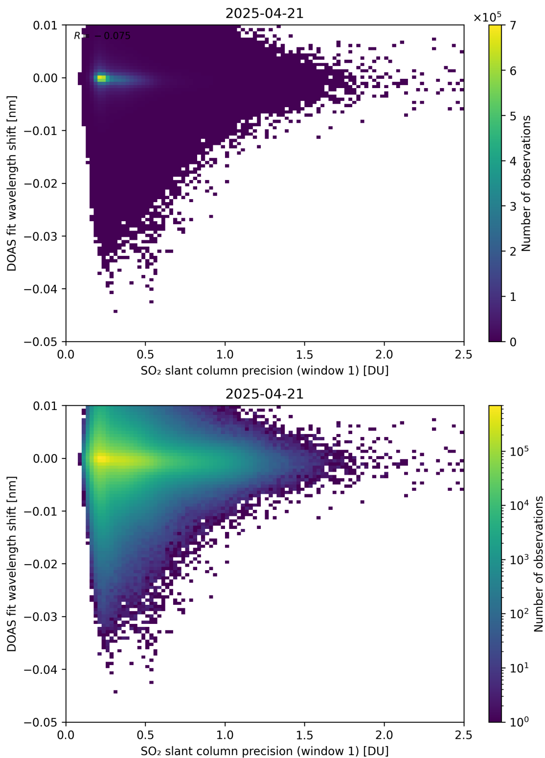
Figure 271: Scatter density plot of “SO 2 slant column precision (window 1)” against “DOAS fit wavelength shift” for 2025-04-20 to 2025-04-22.
