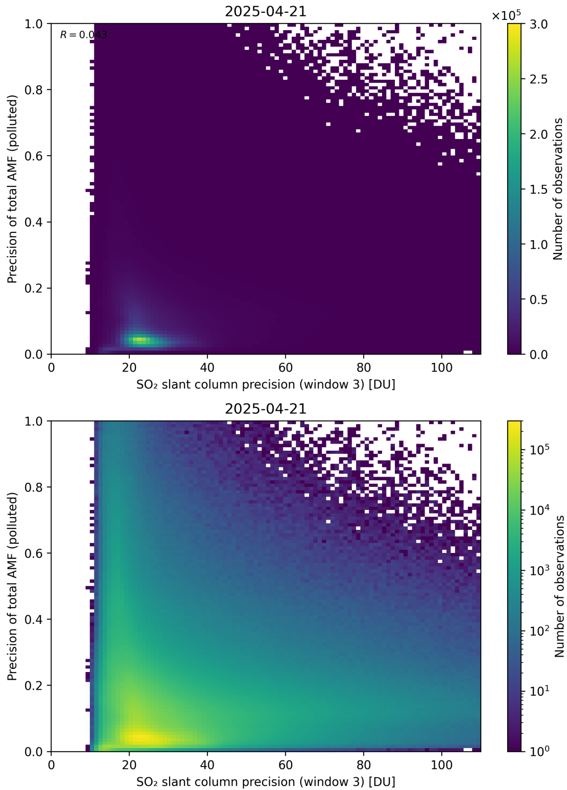
Figure 314: Scatter density plot of “SO 2 slant column precision (window 3)” against “Precision of total AMF (polluted)” for 2025-04-20 to 2025-04-22.
