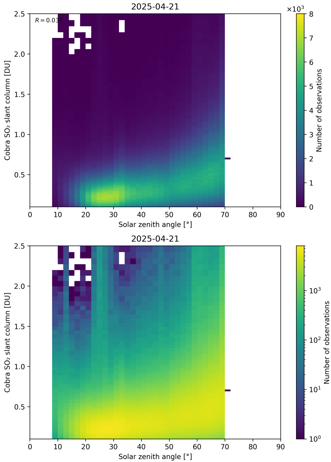
Figure 179: Scatter density plot of “Solar zenith angle” against “Cobra SO 2 slant column” for 2025-04-20 to 2025-04-22.
