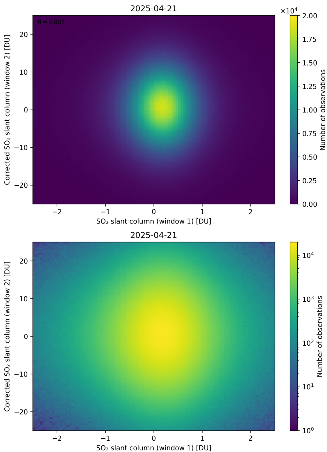
Figure 283: Scatter density plot of “SO 2 slant column (window 1)” against “Corrected SO 2 slant column (window 2)” for 2025-04-20 to 2025-04-22.
