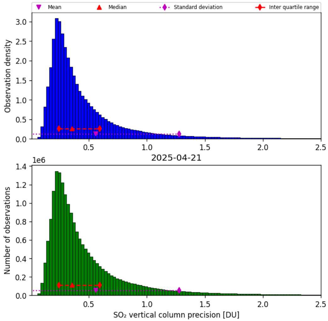
Figure 59: Histogram of “SO 2 vertical column precision” for 2025-04-20 to 2025-04-22
