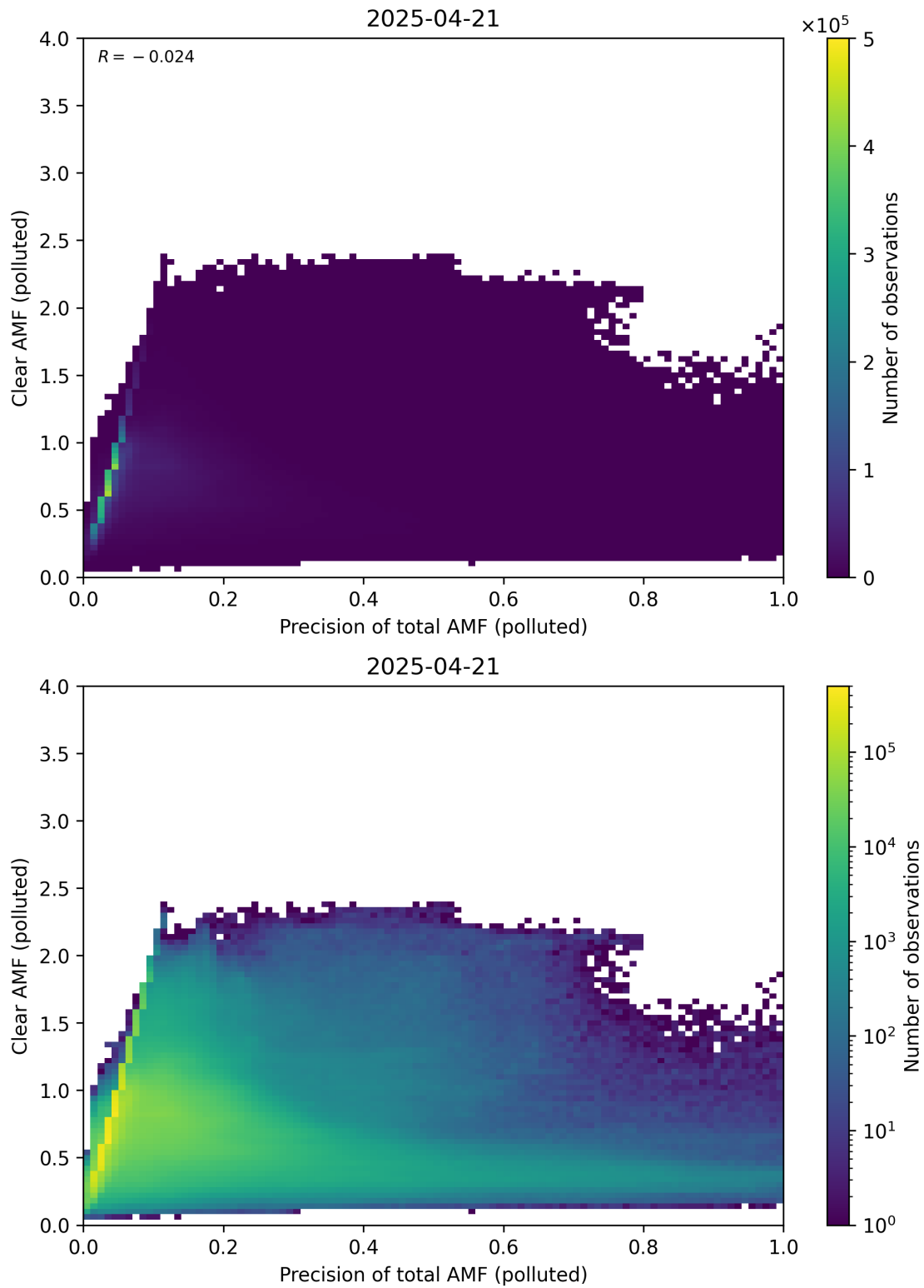
Figure 320: Scatter density plot of “Precision of total AMF (polluted)” against “Clear AMF (polluted)” for 2025-04-20 to 2025-04-22.
