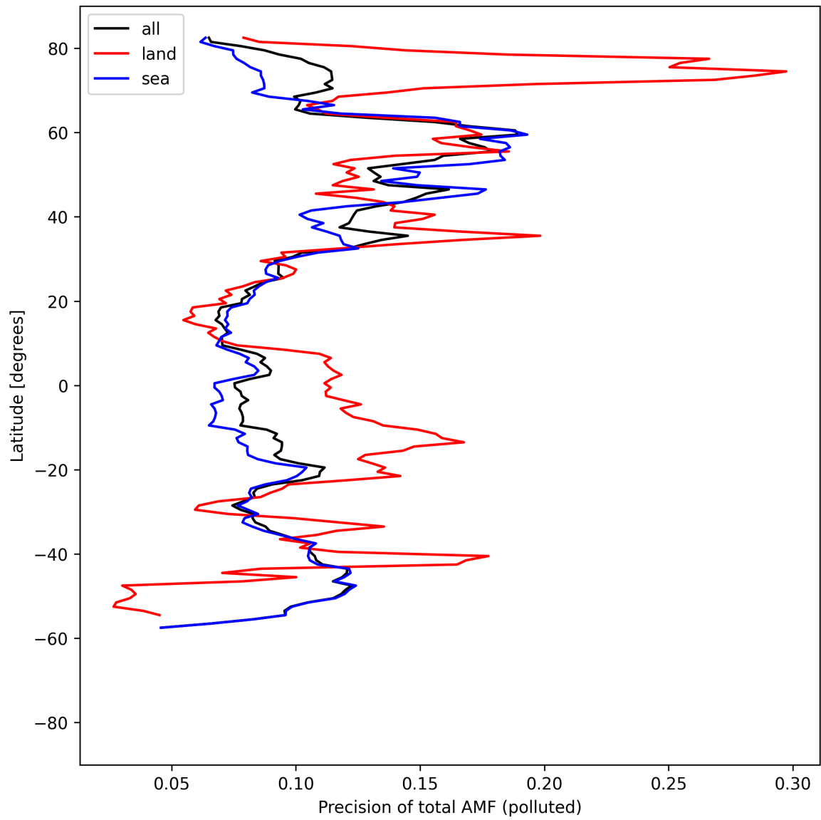
Figure 54: Zonal average of “Precision of total AMF (polluted)” for 2025-04-20 to 2025-04-22.
