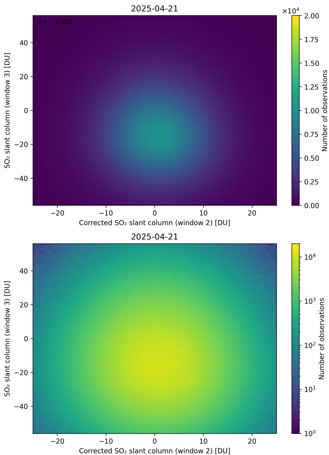
Figure 251: Scatter density plot of “Corrected SO 2 slant column (window 2)” against “SO 2 slant column (window 3)” for 2025-04-20 to 2025-04-22.
