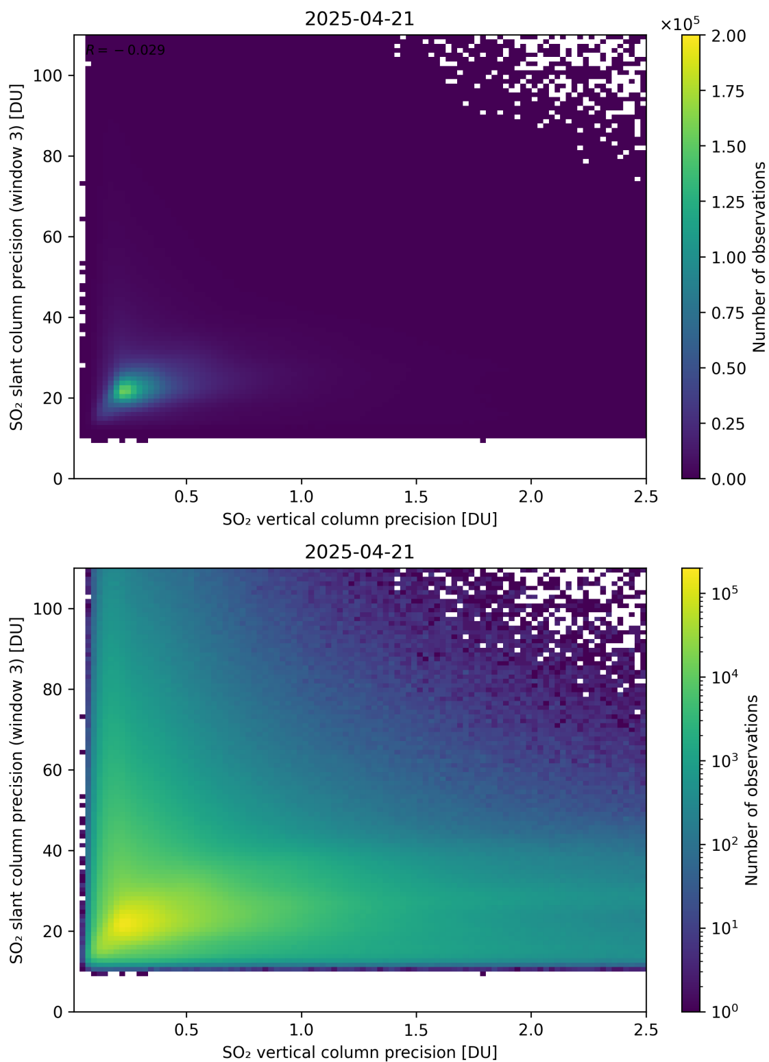
Figure 345: Scatter density plot of “SO 2 vertical column precision” against “SO 2 slant column precision (window 3)” for 2025-04-20 to 2025-04-22.
