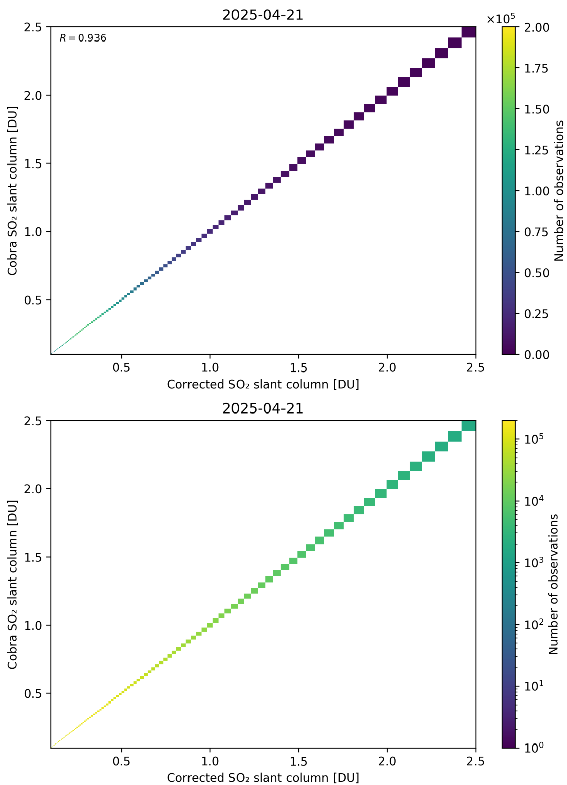
Figure 233: Scatter density plot of “Corrected SO 2 slant column” against “Cobra SO 2 slant column” for 2025-04-20 to 2025-04-22.
