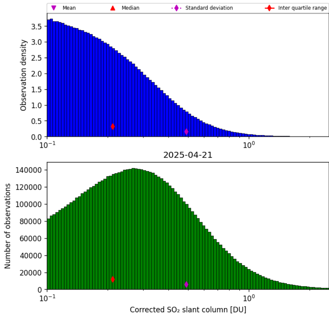
Figure 60: Histogram of “Corrected SO 2 slant column” for 2025-04-20 to 2025-04-22
