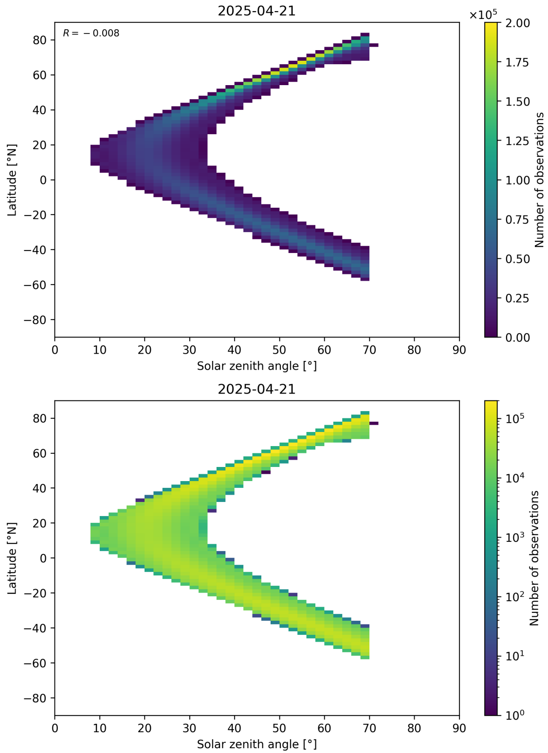
Figure 177: Scatter density plot of “Solar zenith angle” against “Latitude” for 2025-04-20 to 2025-04-22.
