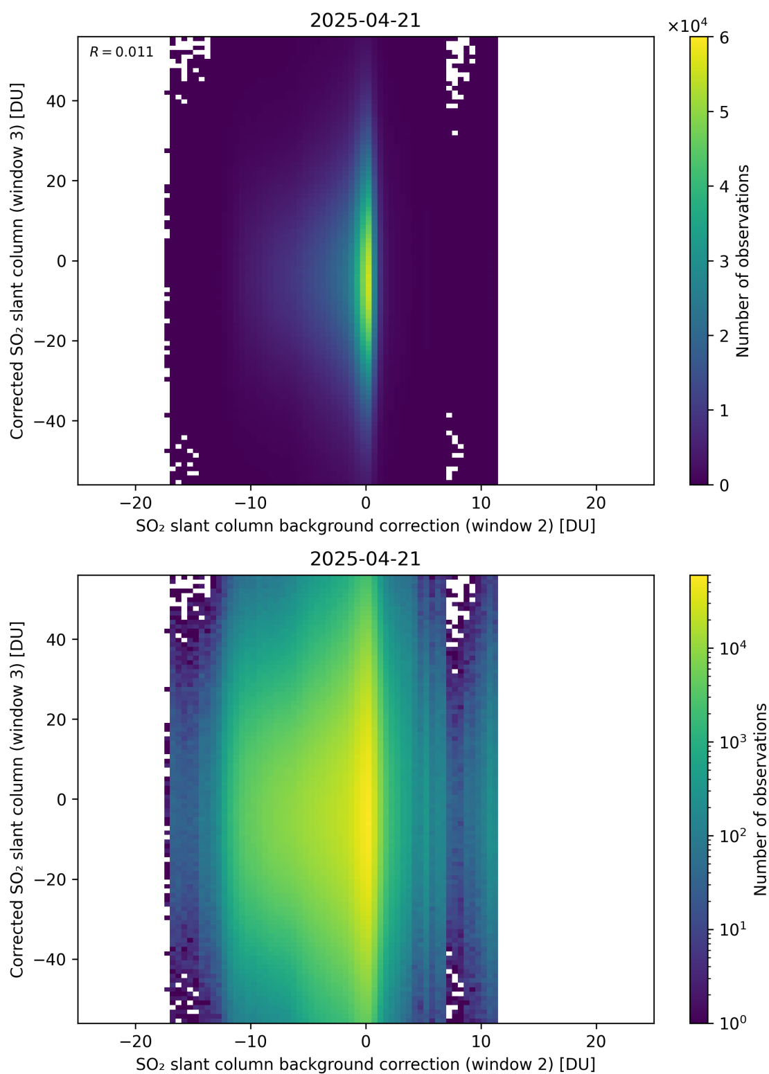
Figure 127: Scatter density plot of “SO 2 slant column background correction (window 2)” against “Corrected SO 2 slant column (window 3)” for 2025-04-20 to 2025-04-22.
