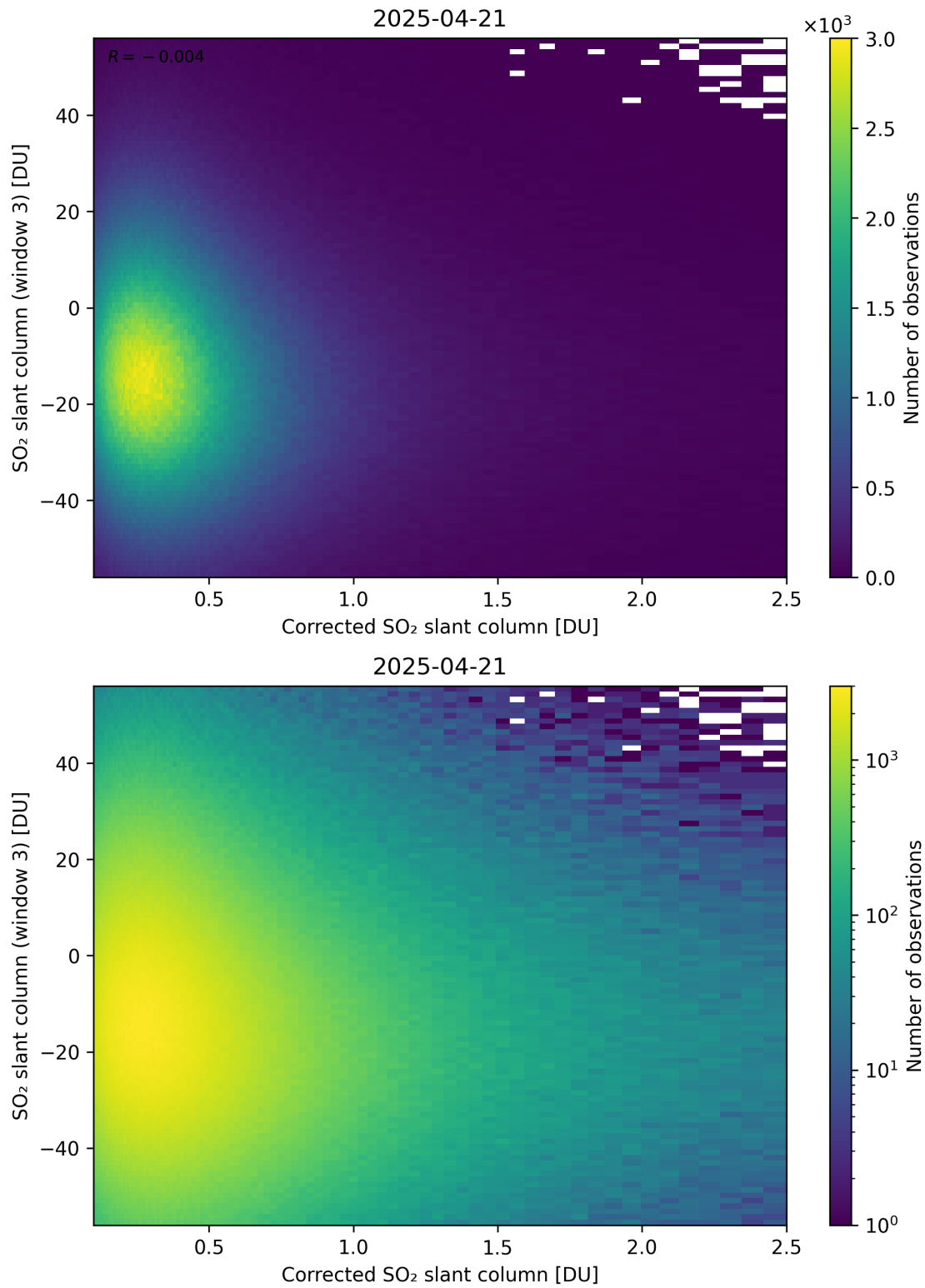
Figure 240: Scatter density plot of “Corrected SO 2 slant column” against “SO 2 slant column (window 3)” for 2025-04-20 to 2025-04-22.
