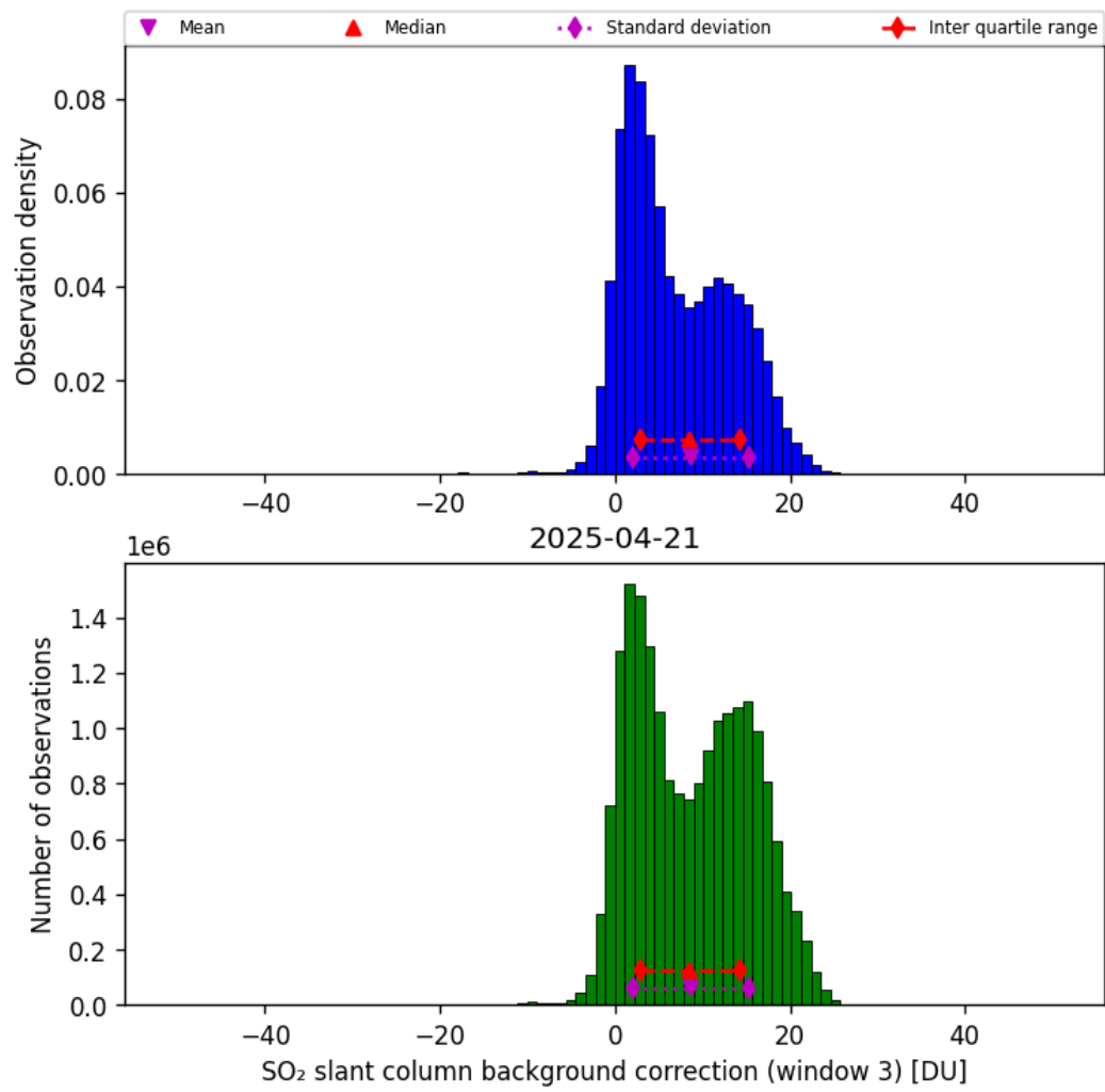
Figure 74: Histogram of “SO 2 slant column background correction (window 3)” for 2025-04-20 to 2025-04-22
