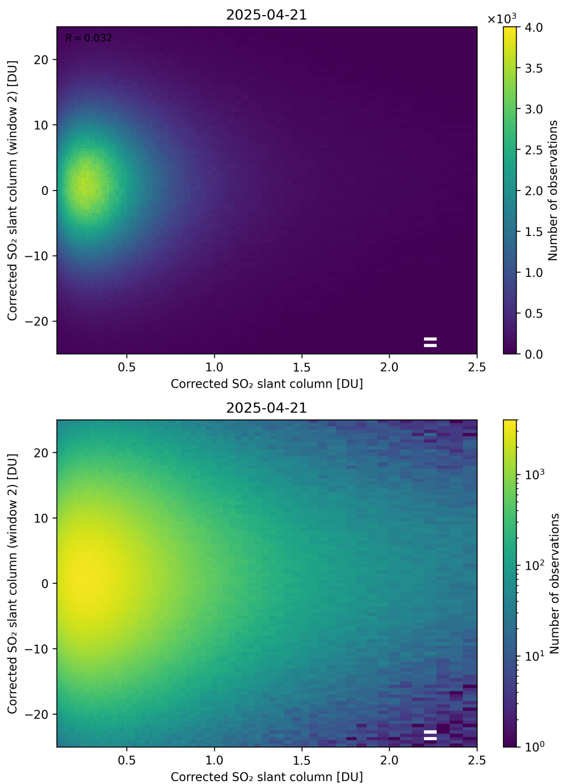
Figure 235: Scatter density plot of “Corrected SO 2 slant column” against “Corrected SO 2 slant column (window 2)” for 2025-04-20 to 2025-04-22.
