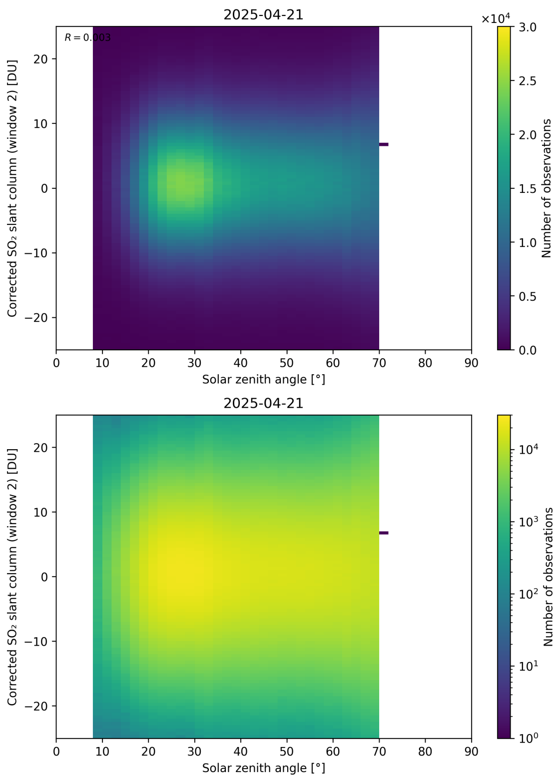
Figure 182: Scatter density plot of “Solar zenith angle” against “Corrected SO 2 slant column (window 2)” for 2025-04-20 to 2025-04-22.
