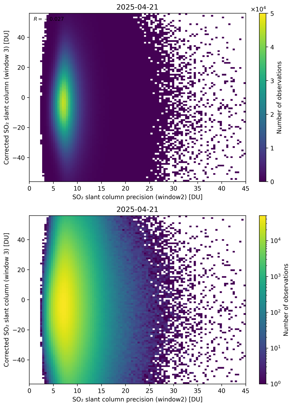
Figure 298: Scatter density plot of “SO 2 slant column precision (window2)” against “Corrected SO 2 slant column (window 3)” for 2025-04-20 to 2025-04-22.
