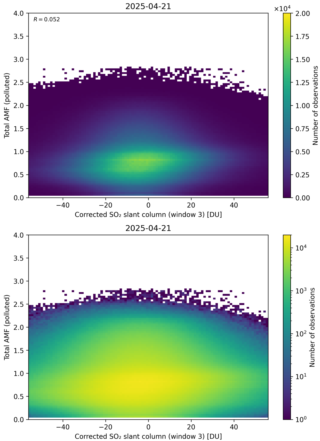
Figure 260: Scatter density plot of “Corrected SO 2 slant column (window 3)” against “Total AMF (polluted)” for 2025-04-20 to 2025-04-22.
