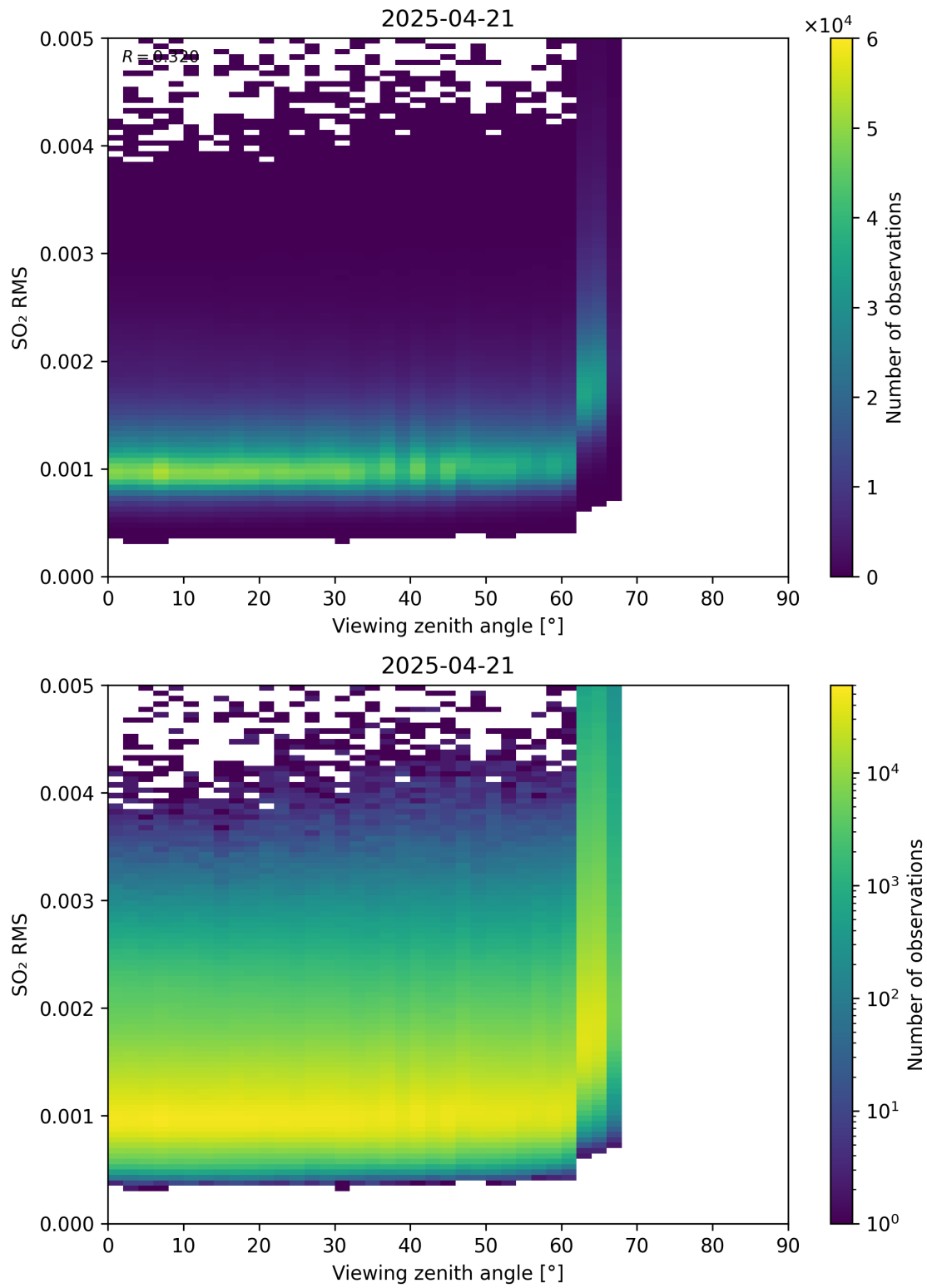
Figure 367: Scatter density plot of “Viewing zenith angle” against “SO 2 RMS” for 2025-04-20 to 2025-04-22.
