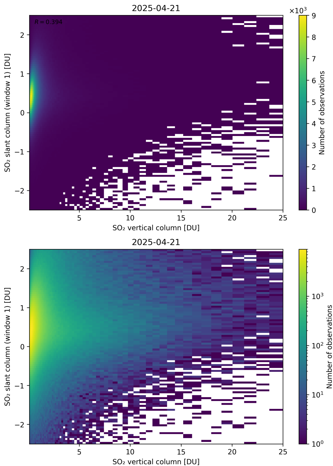
Figure 354: Scatter density plot of “SO 2 vertical column” against “SO 2 slant column (window 1)” for 2025-04-20 to 2025-04-22.
