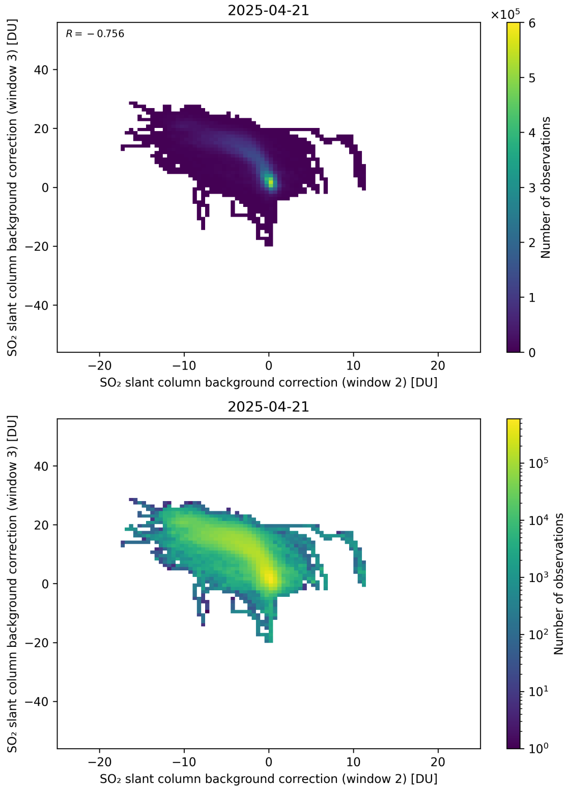
Figure 122: Scatter density plot of “SO 2 slant column background correction (window 2)” against “SO 2 slant column background correction (window 3)” for 2025-04-20 to 2025-04-22.
