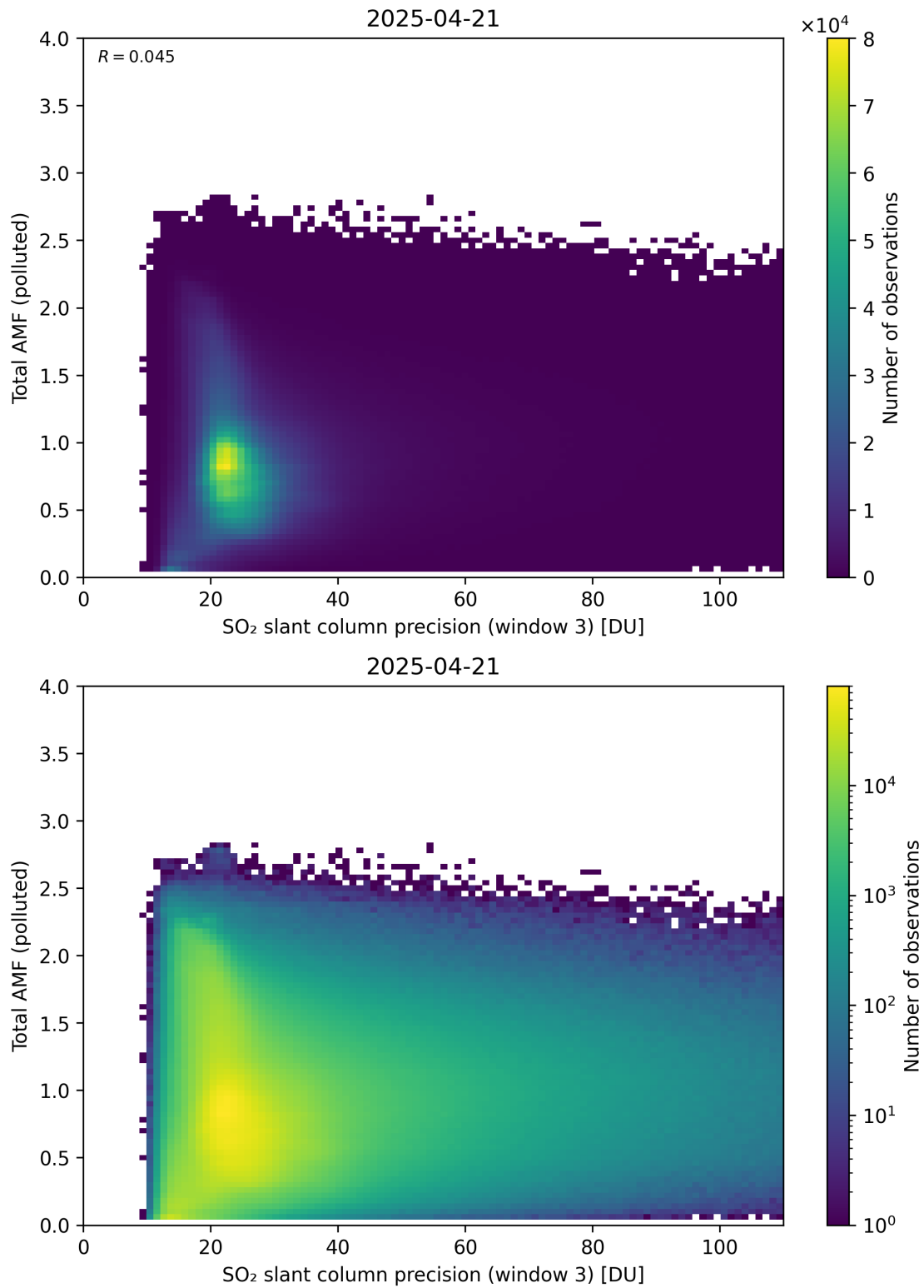
Figure 313: Scatter density plot of “SO 2 slant column precision (window 3)” against “Total AMF (polluted)” for 2025-04-20 to 2025-04-22.
