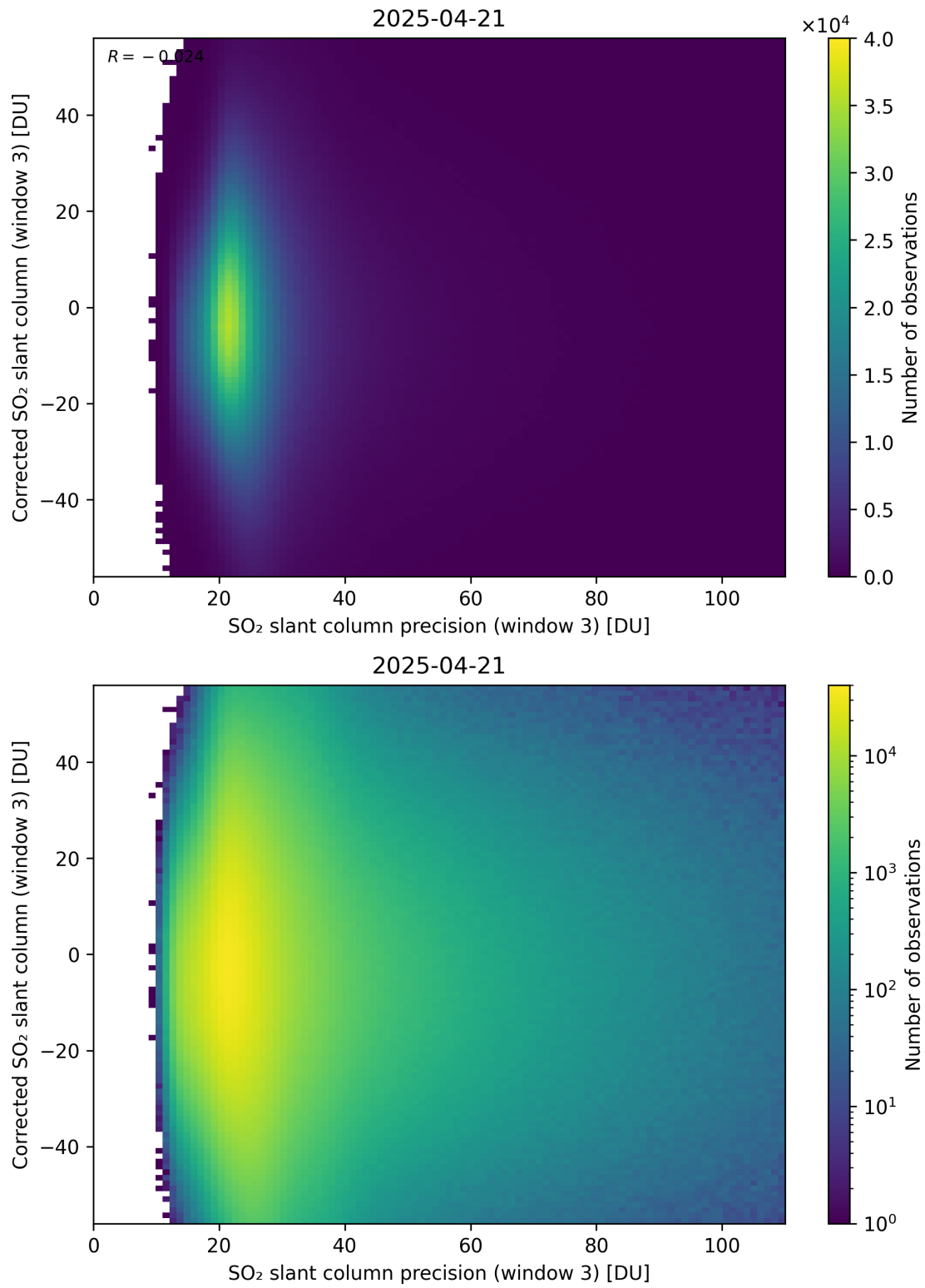
Figure 312: Scatter density plot of “SO 2 slant column precision (window 3)” against “Corrected SO 2 slant column (window 3)” for 2025-04-20 to 2025-04-22.
