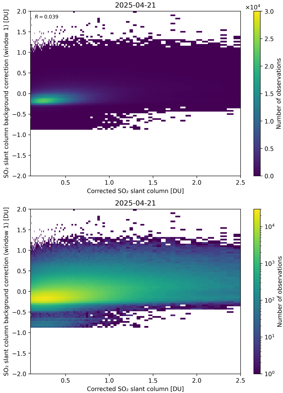
Figure 226: Scatter density plot of “Corrected SO 2 slant column” against “SO 2 slant column background correction (window 1)” for 2025-04-20 to 2025-04-22.
