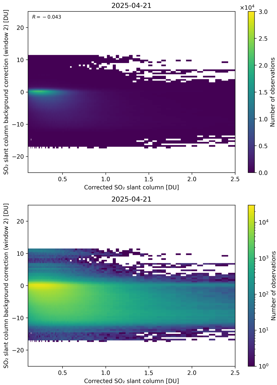
Figure 227: Scatter density plot of “Corrected SO 2 slant column” against “SO 2 slant column background correction (window 2)” for 2025-04-20 to 2025-04-22.
