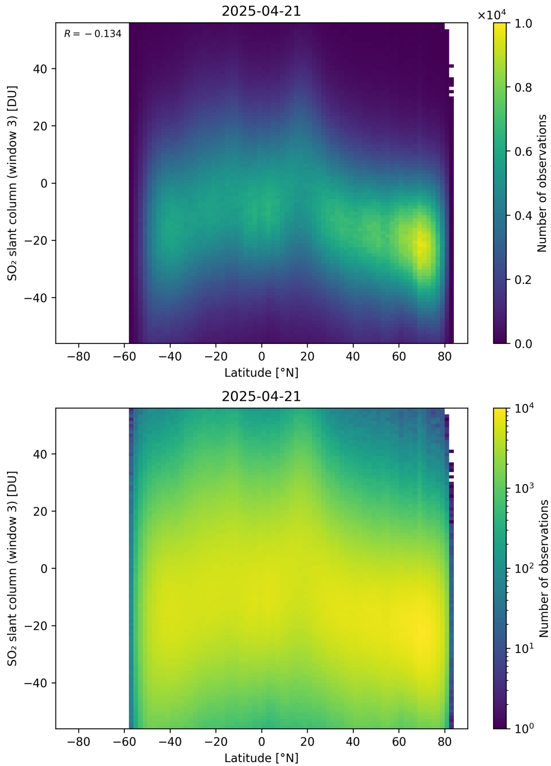
Figure 165: Scatter density plot of “Latitude” against “SO 2 slant column (window 3)” for 2025-04-20 to 2025-04-22.
