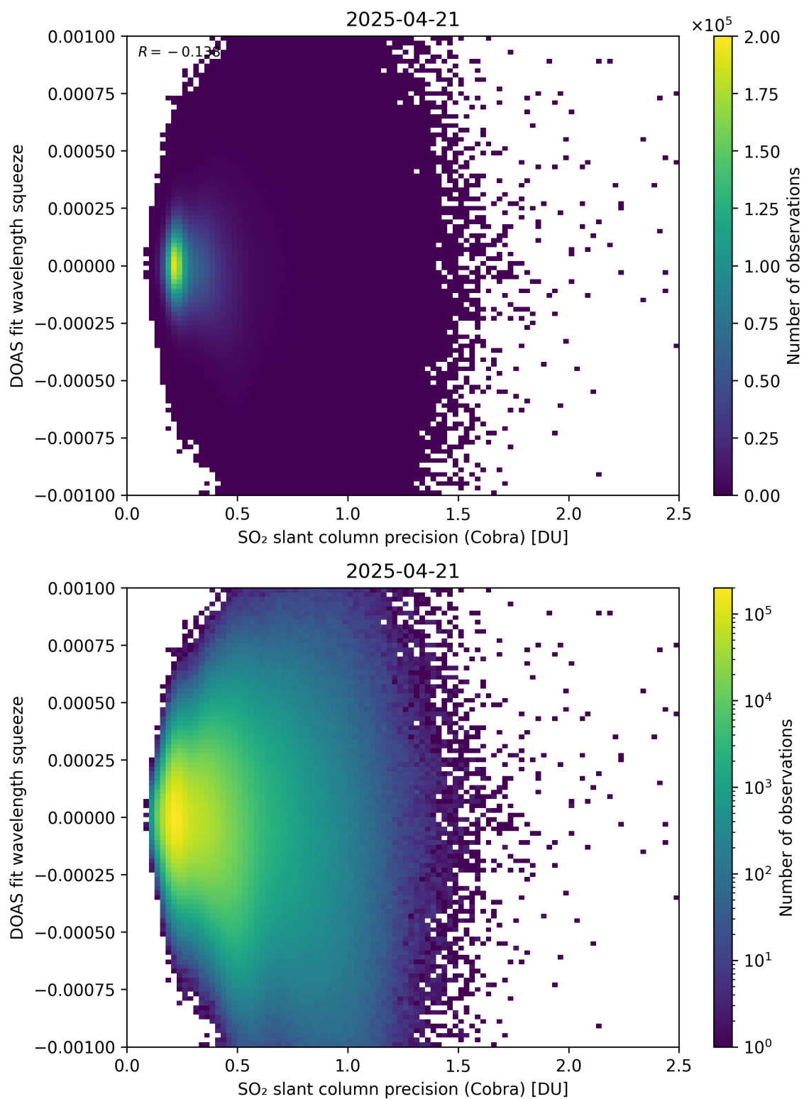
Figure 203: Scatter density plot of “SO 2 slant column precision (Cobra)” against “DOAS fit wavelength squeeze” for 2025-04-20 to 2025-04-22.
