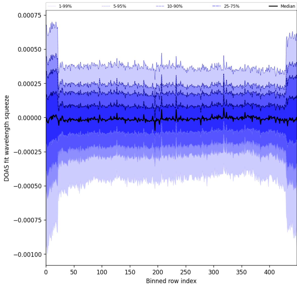
Figure 103: Along track statistics of “DOAS fit wavelength squeeze” for 2025-04-20 to 2025-04-22
