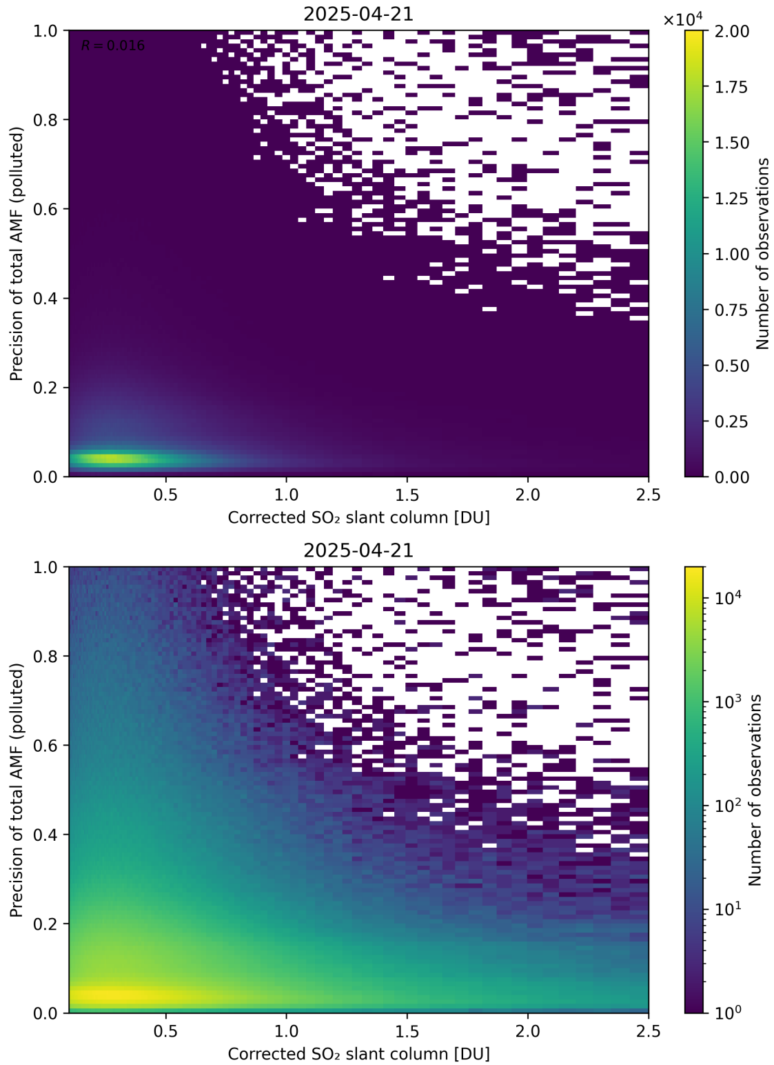
Figure 243: Scatter density plot of “Corrected SO 2 slant column” against “Precision of total AMF (polluted)” for 2025-04-20 to 2025-04-22.
