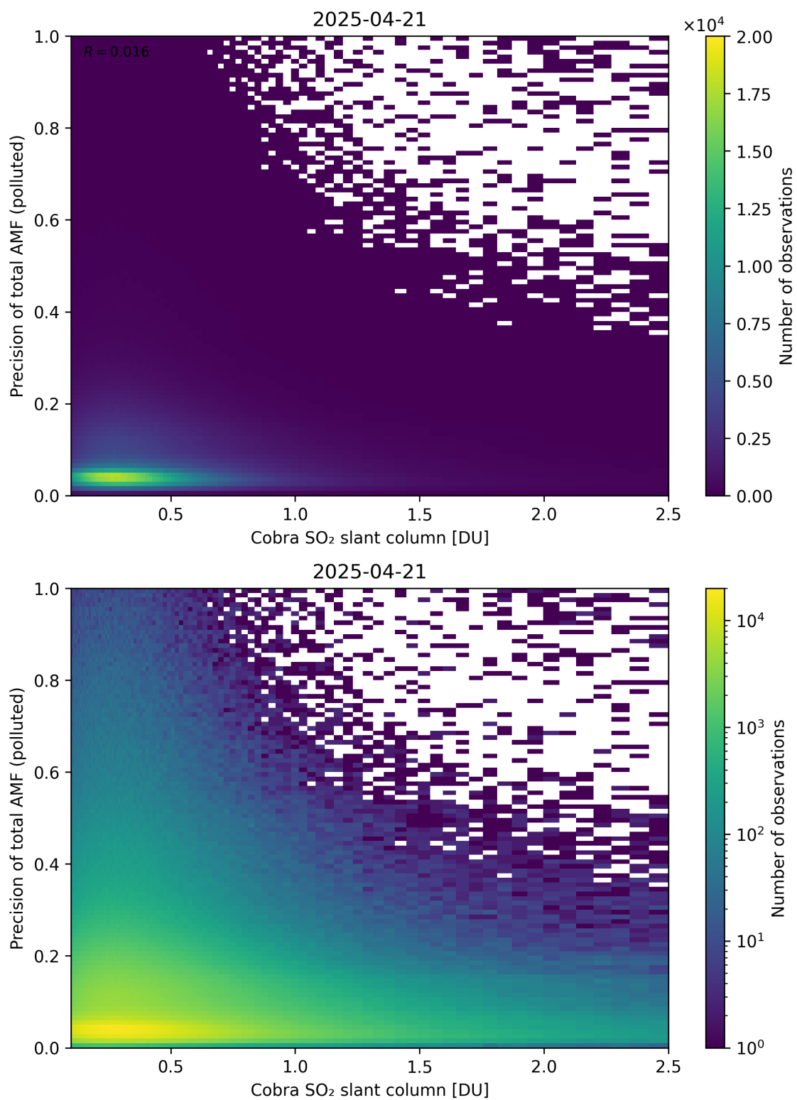
Figure 225: Scatter density plot of “Cobra SO 2 slant column” against “Precision of total AMF (polluted)” for 2025-04-20 to 2025-04-22.
