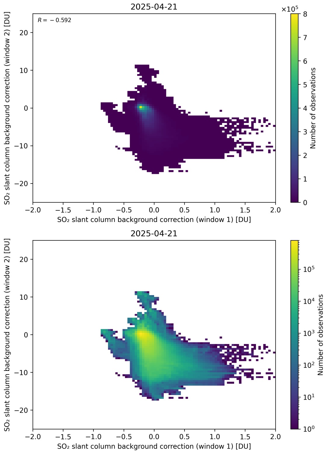
Figure 109: Scatter density plot of “SO 2 slant column background correction (window 1)” against “SO 2 slant column background correction (window 2)” for 2025-04-20 to 2025-04-22.
