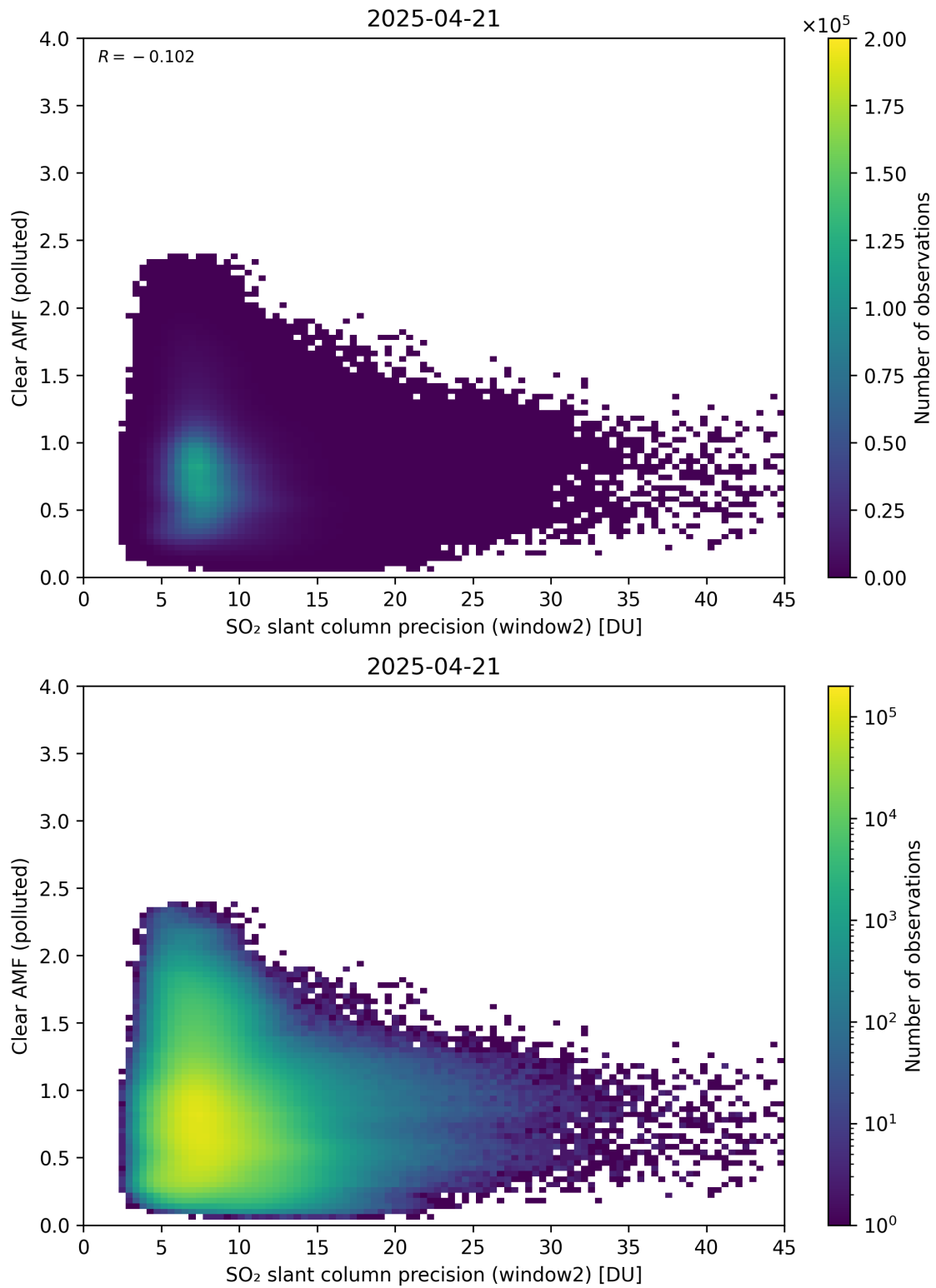
Figure 296: Scatter density plot of “SO 2 slant column precision (window2)” against “Clear AMF (polluted)” for 2025-04-20 to 2025-04-22.
