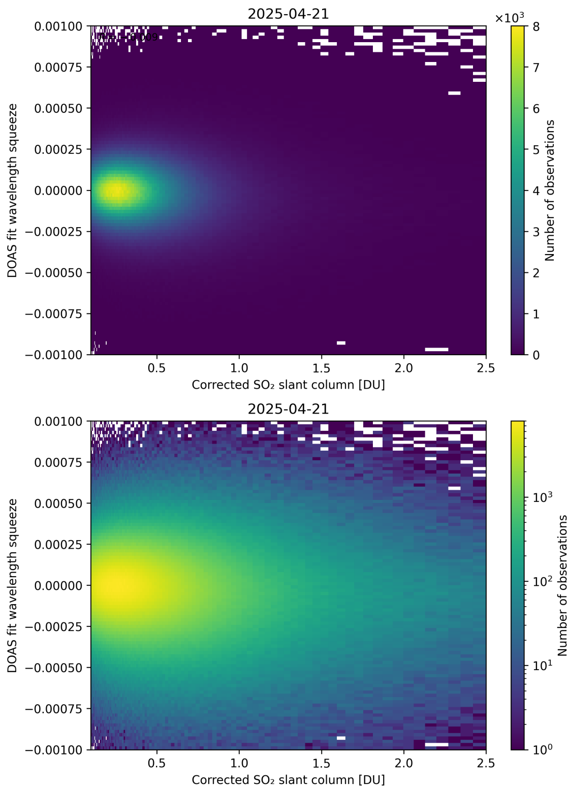
Figure 230: Scatter density plot of “Corrected SO 2 slant column” against “DOAS fit wavelength squeeze” for 2025-04-20 to 2025-04-22.
