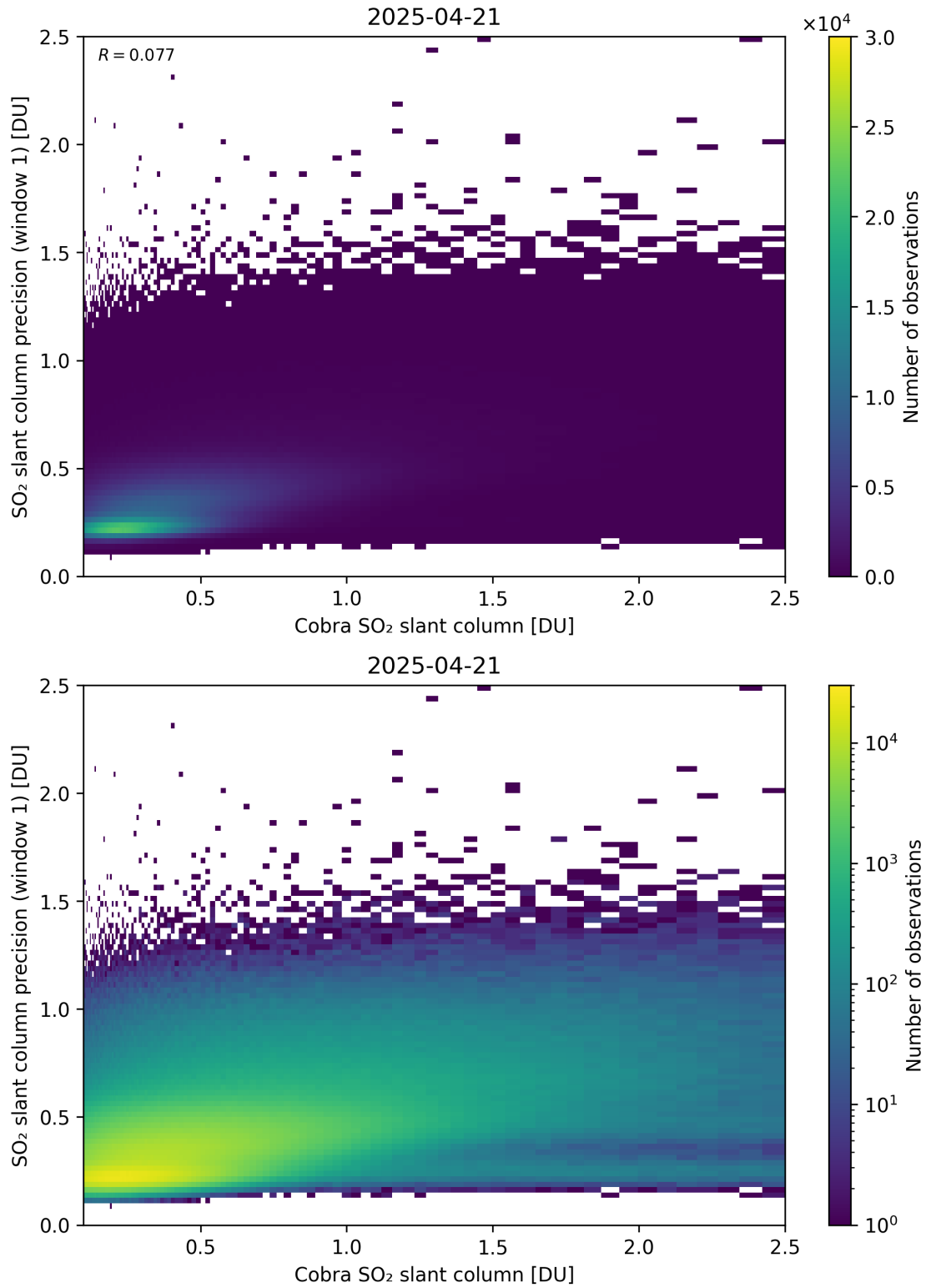
Figure 220: Scatter density plot of “Cobra SO 2 slant column” against “SO 2 slant column precision (window 1)” for 2025-04-20 to 2025-04-22.
