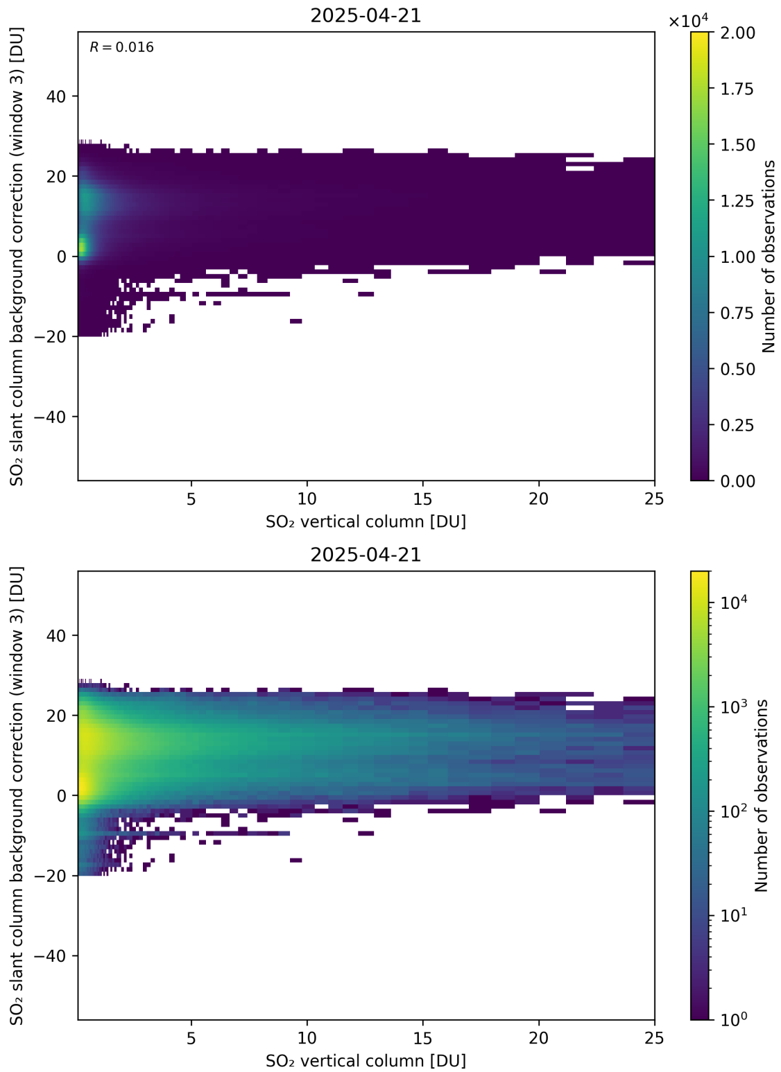
Figure 325: Scatter density plot of “SO 2 vertical column” against “SO 2 slant column background correction (window 3)” for 2025-04-20 to 2025-04-22.
