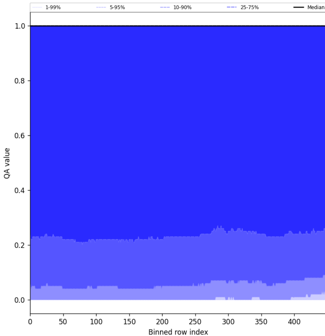
Figure 83: Along track statistics of “QA value” for 2025-04-20 to 2025-04-22
