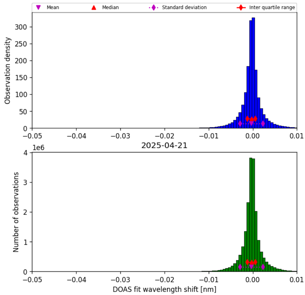
Figure 76: Histogram of “DOAS fit wavelength shift” for 2025-04-20 to 2025-04-22
