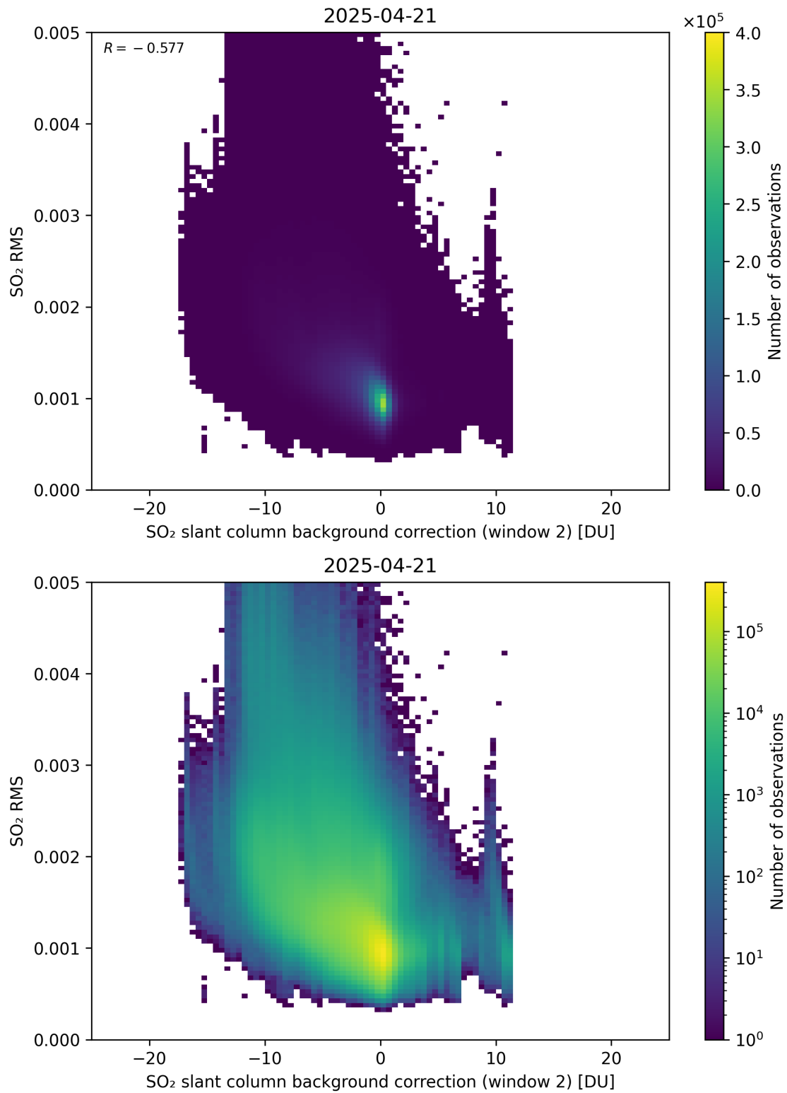
Figure 125: Scatter density plot of “SO 2 slant column background correction (window 2)” against “SO 2 RMS” for 2025-04-20 to 2025-04-22.
