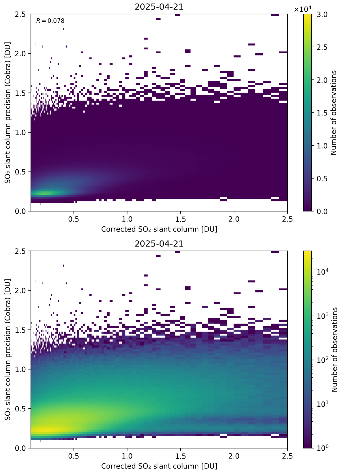
Figure 234: Scatter density plot of “Corrected SO 2 slant column” against “SO 2 slant column precision (Cobra)” for 2025-04-20 to 2025-04-22.
