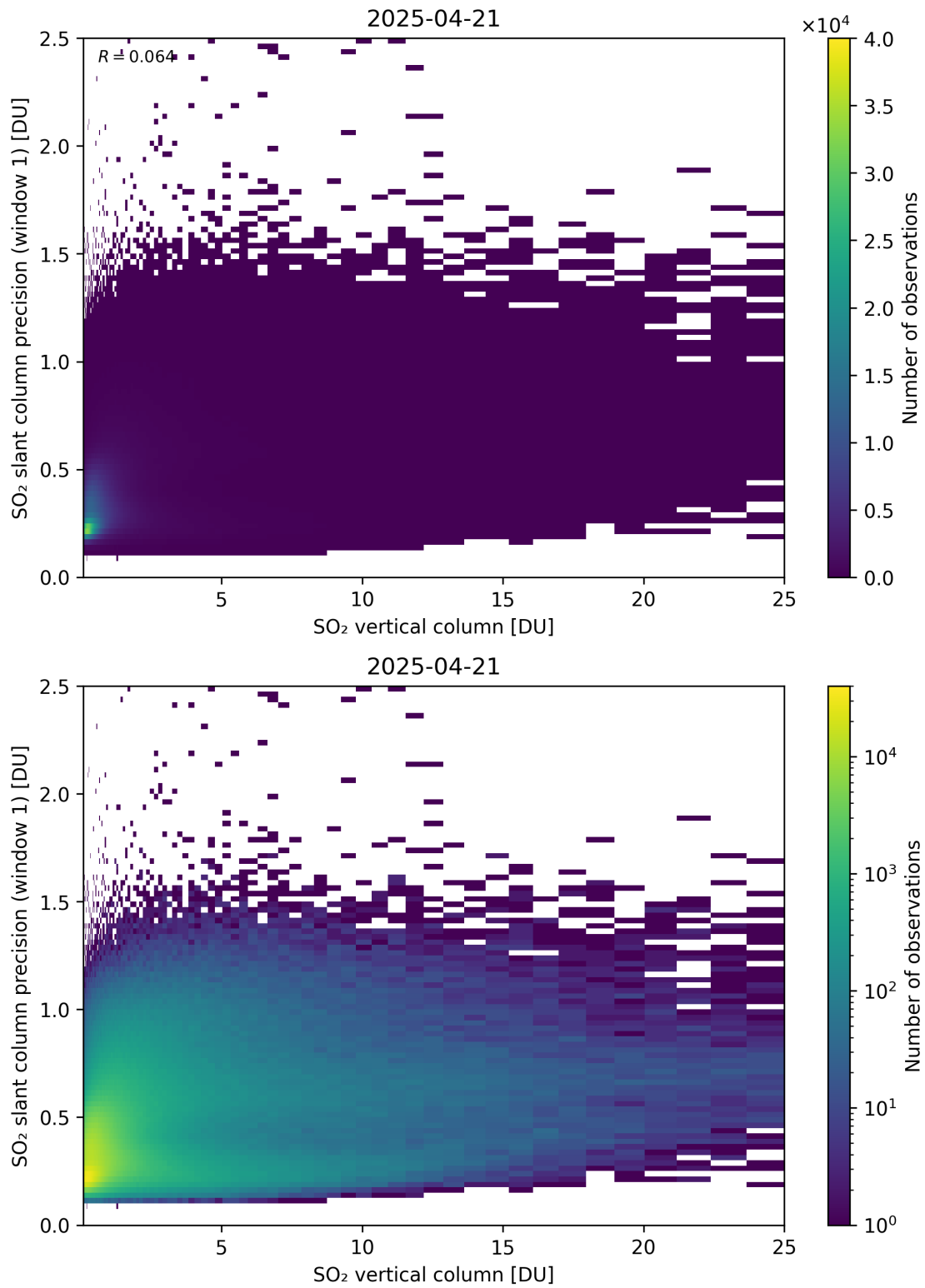
Figure 355: Scatter density plot of “SO 2 vertical column” against “SO 2 slant column precision (window 1)” for 2025-04-20 to 2025-04-22.
