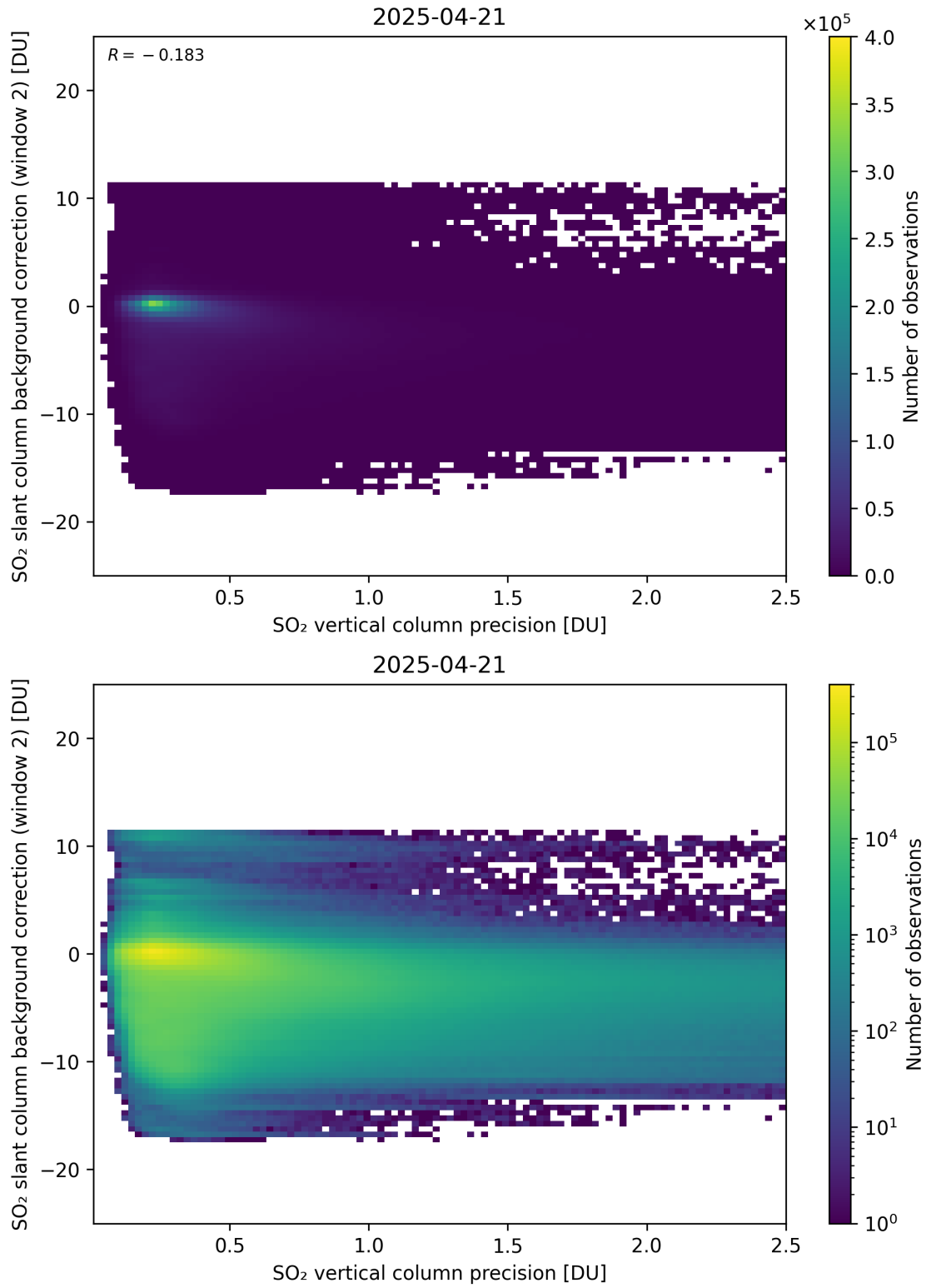
Figure 330: Scatter density plot of “SO 2 vertical column precision” against “SO 2 slant column background correction (window 2)” for 2025-04-20 to 2025-04-22.
