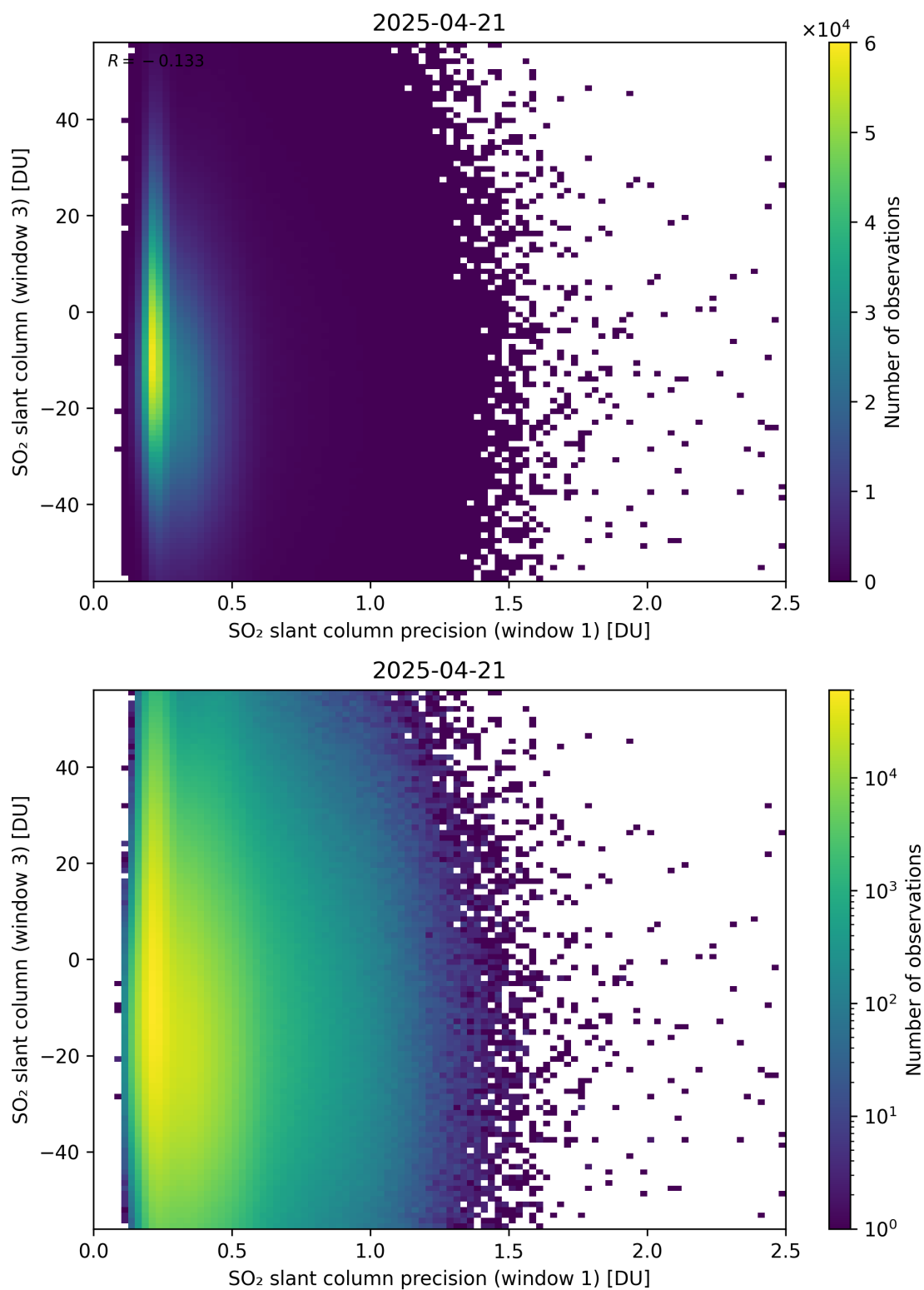
Figure 278: Scatter density plot of “SO 2 slant column precision (window 1)” against “SO 2 slant column (window 3)” for 2025-04-20 to 2025-04-22.
