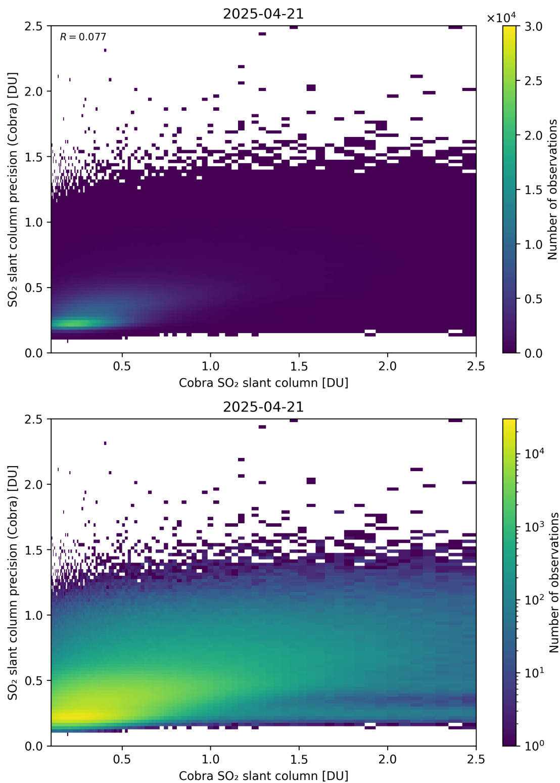
Figure 216: Scatter density plot of “Cobra SO 2 slant column” against “SO 2 slant column precision (Cobra)” for 2025-04-20 to 2025-04-22.
