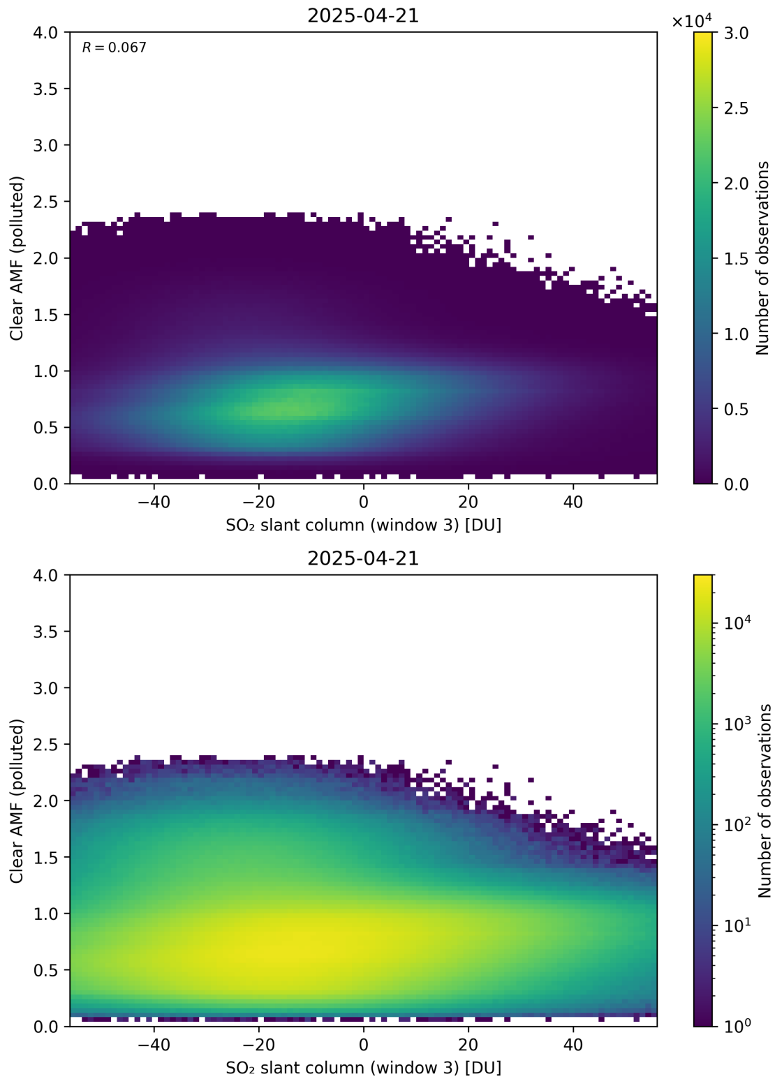
Figure 315: Scatter density plot of “SO 2 slant column (window 3)” against “Clear AMF (polluted)” for 2025-04-20 to 2025-04-22.
