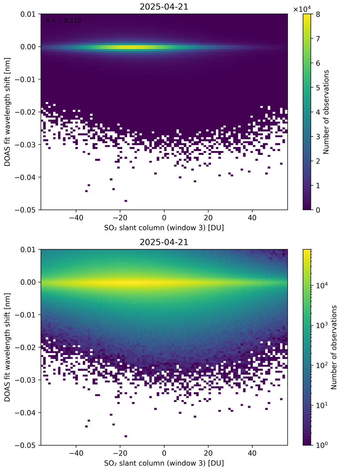
Figure 304: Scatter density plot of “SO 2 slant column (window 3)” against “DOAS fit wavelength shift” for 2025-04-20 to 2025-04-22.
