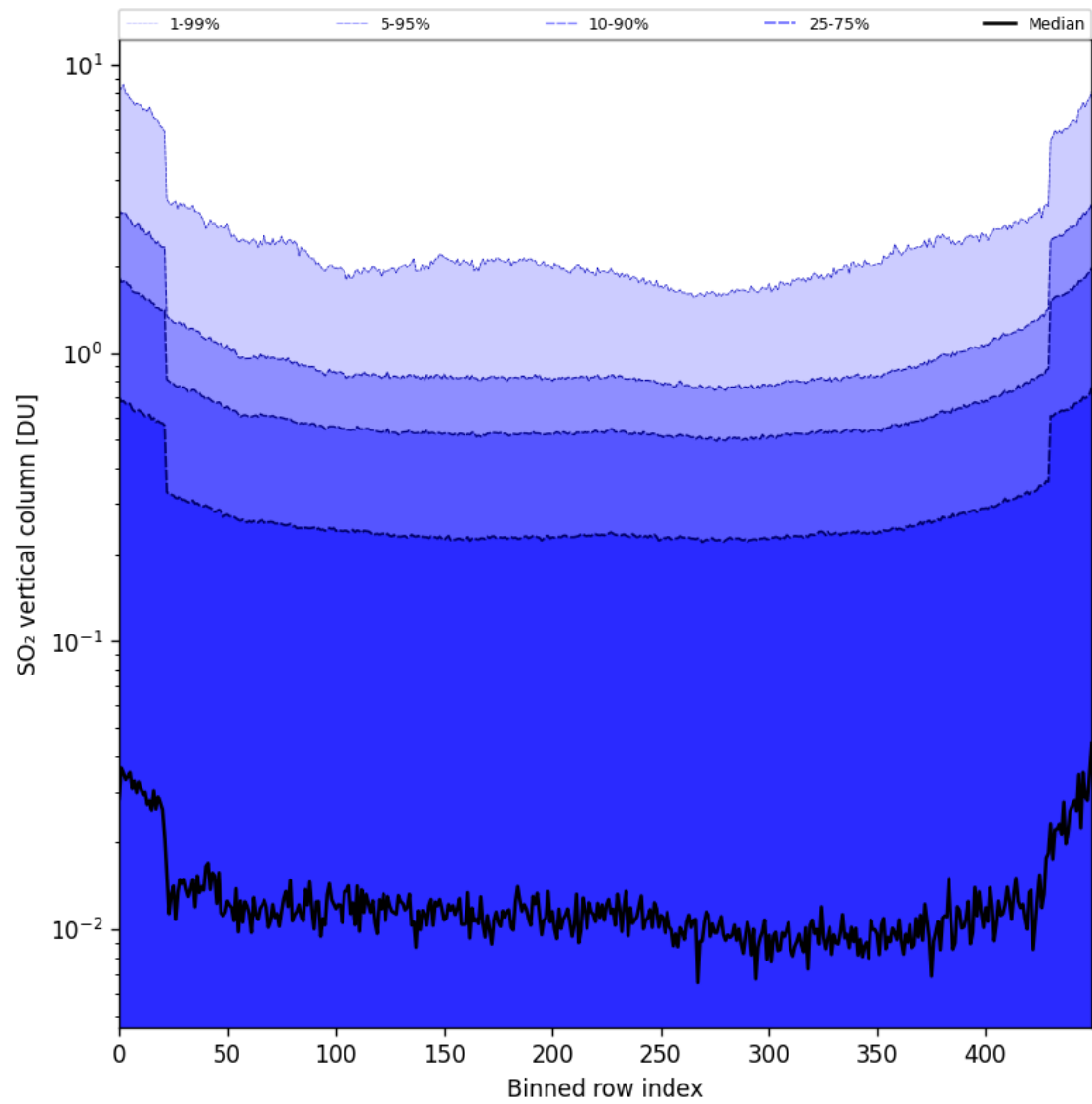
Figure 84: Along track statistics of “SO 2 vertical column” for 2025-04-20 to 2025-04-22
