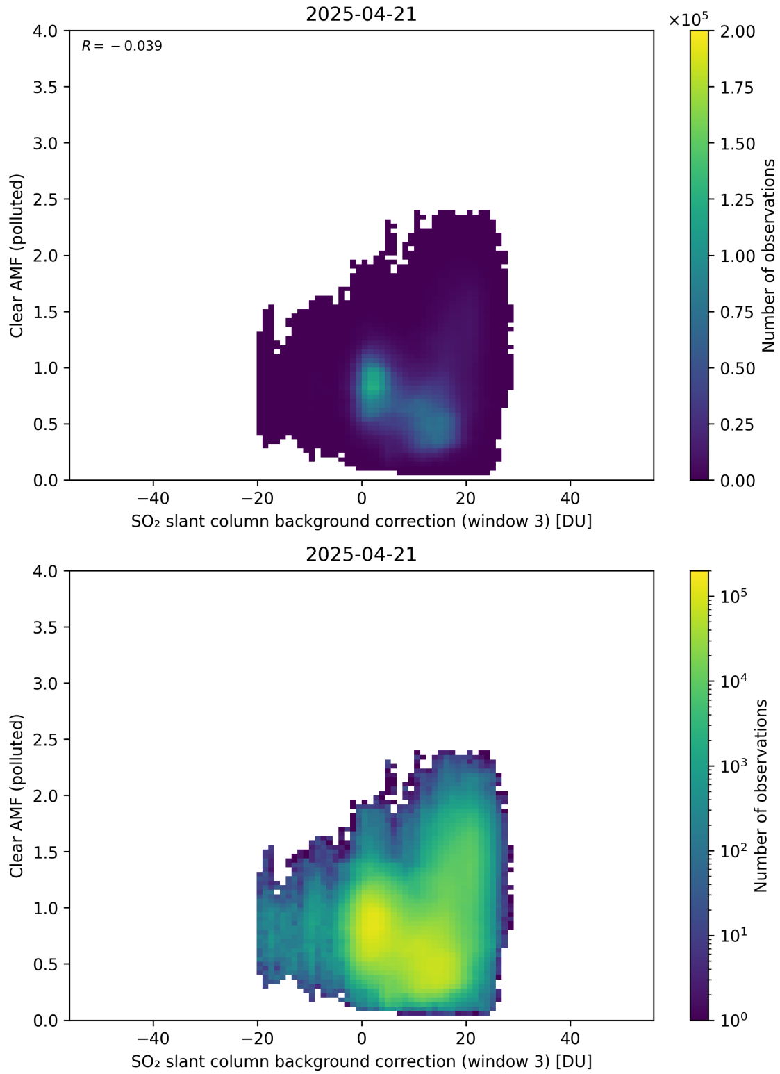
Figure 135: Scatter density plot of “SO 2 slant column background correction (window 3)” against “Clear AMF (polluted)” for 2025-04-20 to 2025-04-22.
