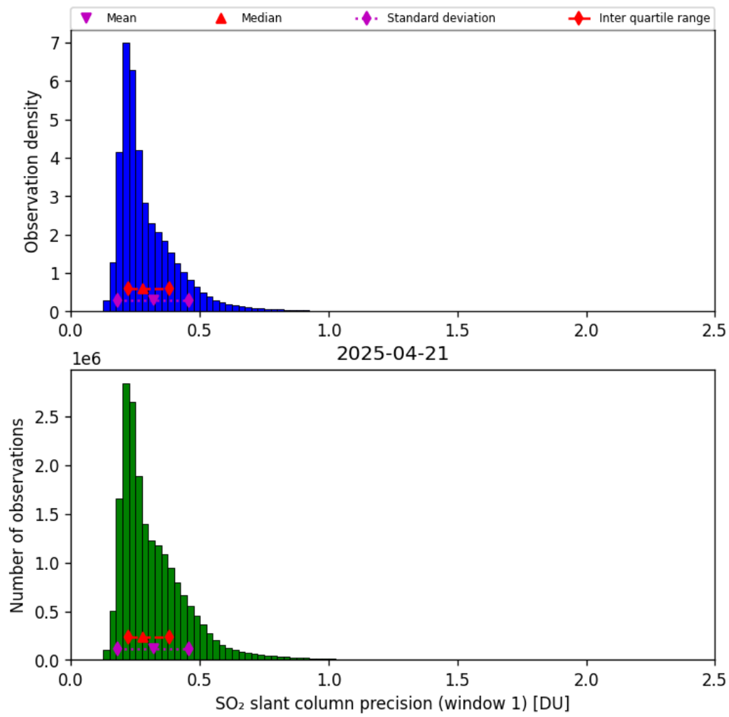
Figure 64: Histogram of “SO 2 slant column precision (window 1)” for 2025-04-20 to 2025-04-22
