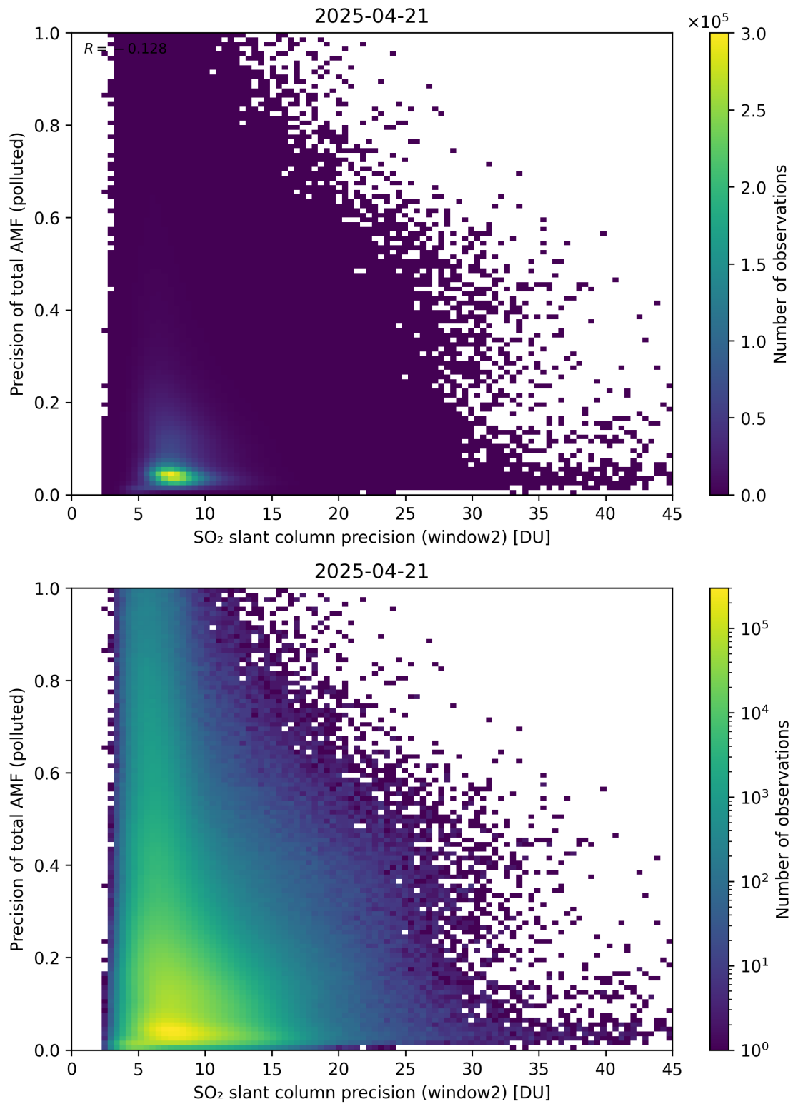
Figure 302: Scatter density plot of “SO 2 slant column precision (window2)” against “Precision of total AMF (polluted)” for 2025-04-20 to 2025-04-22.
