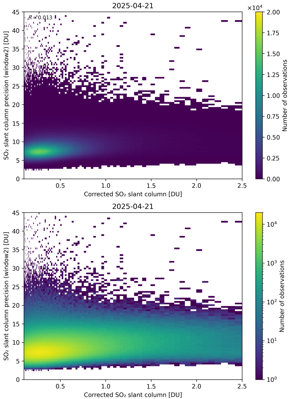
Figure 239: Scatter density plot of “Corrected SO 2 slant column” against “SO 2 slant column precision (window2)” for 2025-04-20 to 2025-04-22.
