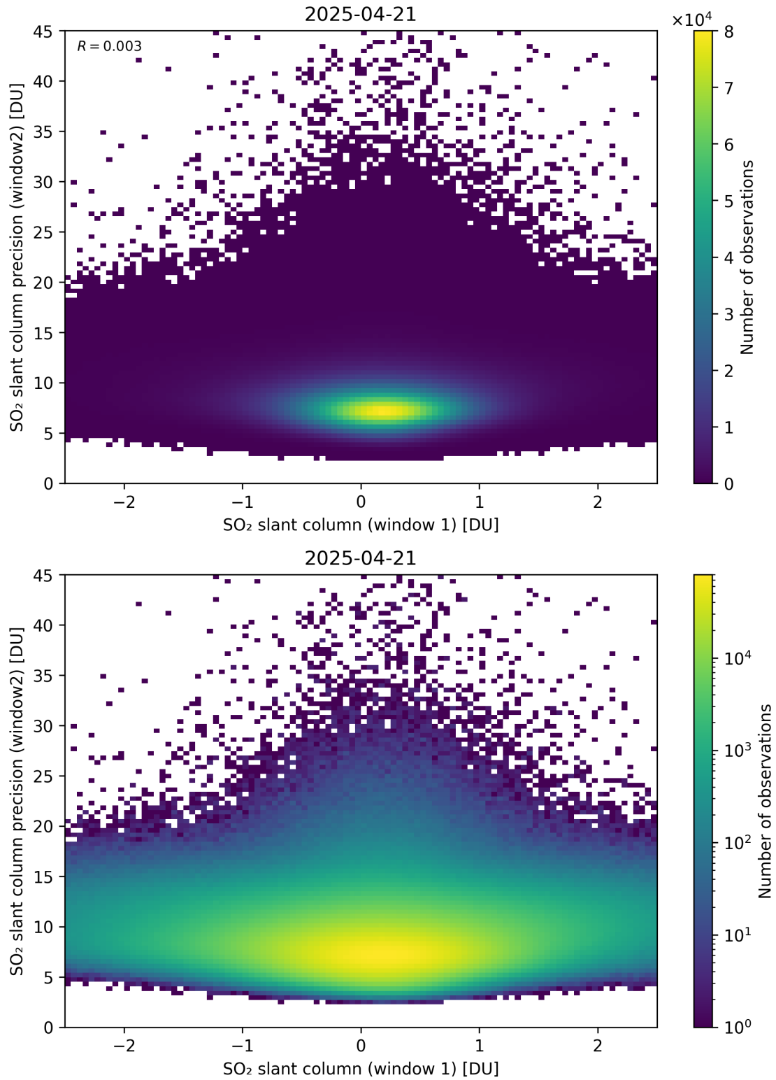
Figure 286: Scatter density plot of “SO 2 slant column (window 1)” against “SO 2 slant column precision (window2)” for 2025-04-20 to 2025-04-22.
