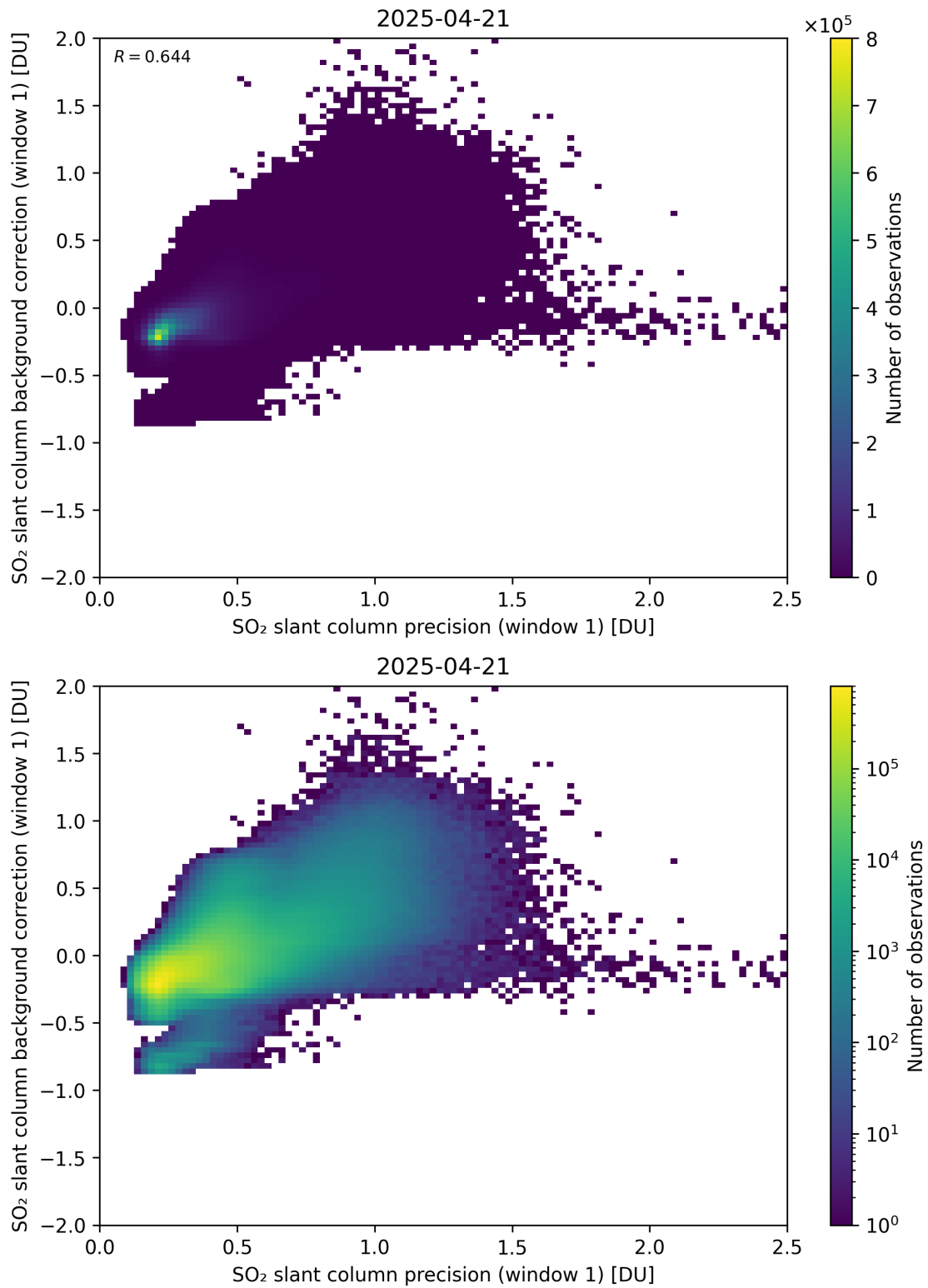
Figure 268: Scatter density plot of “SO 2 slant column precision (window 1)” against “SO 2 slant column background correction (window 1)” for 2025-04-20 to 2025-04-22.
