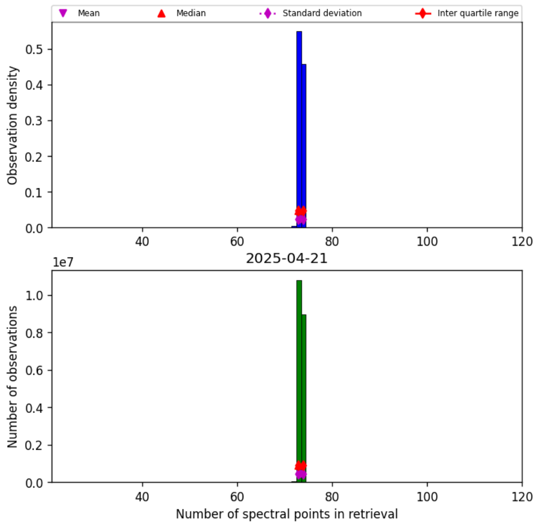
Figure 82: Histogram of “Number of spectral points in retrieval” for 2025-04-20 to 2025-04-22
