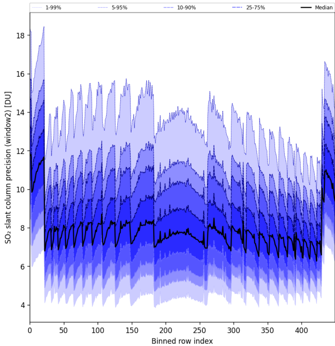
Figure 94: Along track statistics of “SO 2 slant column precision (window2)” for 2025-04-20 to 2025-04-22
