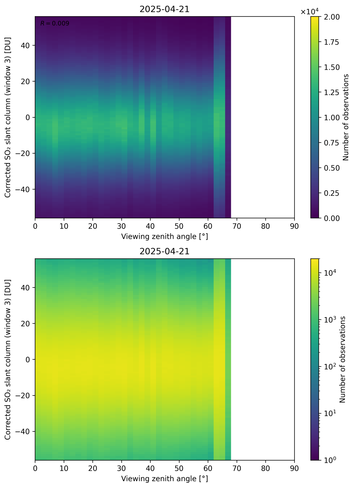
Figure 375: Scatter density plot of “Viewing zenith angle” against “Corrected SO 2 slant column (window 3)” for 2025-04-20 to 2025-04-22.
