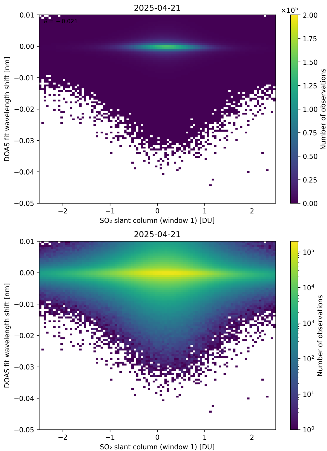
Figure 265: Scatter density plot of “SO 2 slant column (window 1)” against “DOAS fit wavelength shift” for 2025-04-20 to 2025-04-22.
