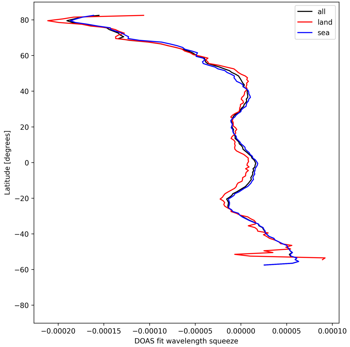
Figure 51: Zonal average of “DOAS fit wavelength squeeze” for 2025-04-20 to 2025-04-22.
