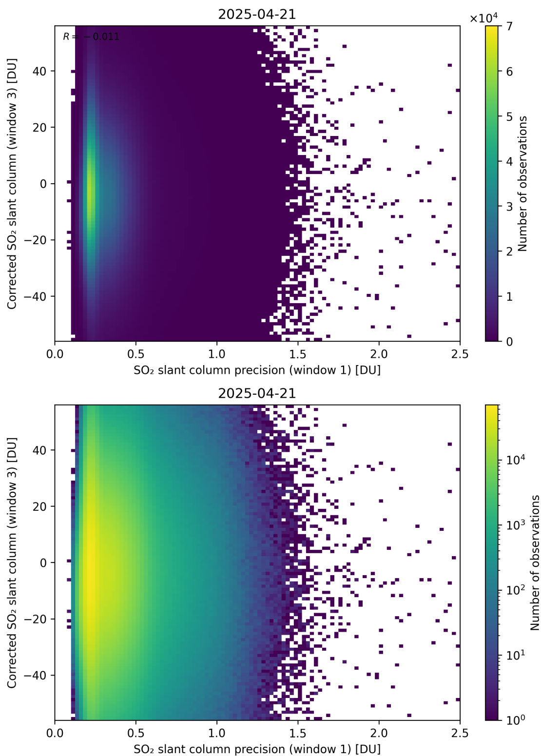
Figure 276: Scatter density plot of “SO 2 slant column precision (window 1)” against “Corrected SO 2 slant column (window 3)” for 2025-04-20 to 2025-04-22.
