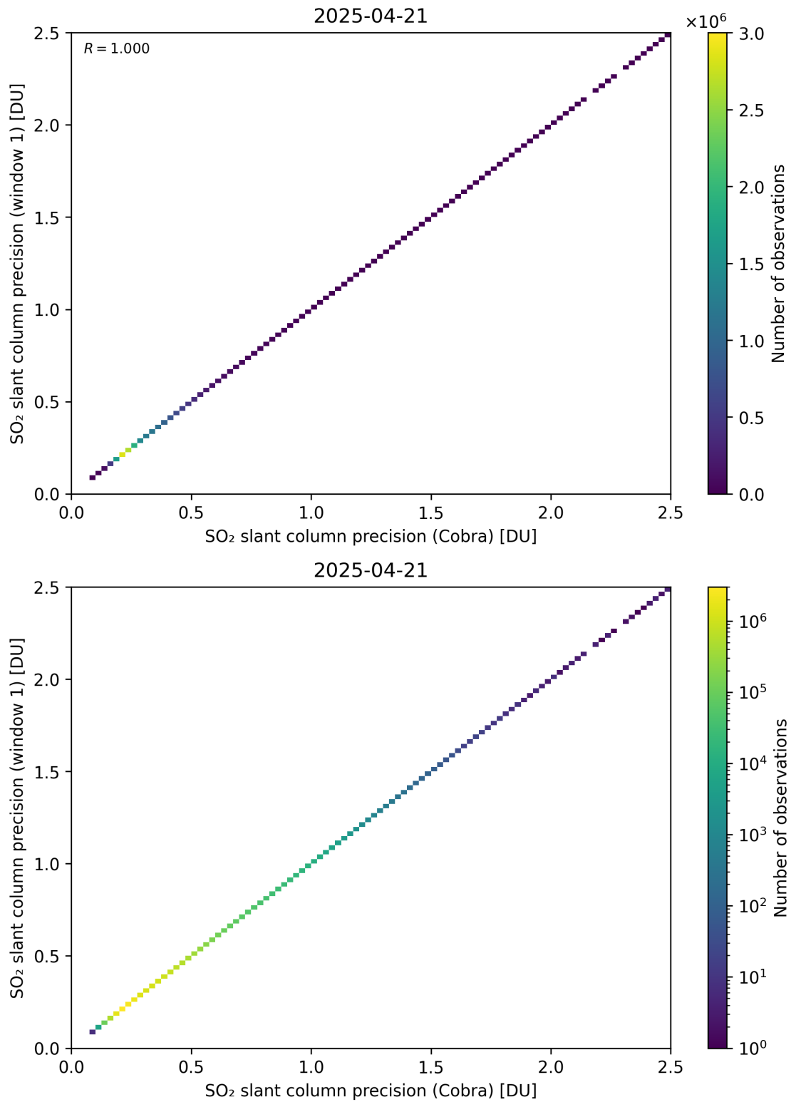
Figure 209: Scatter density plot of “SO 2 slant column precision (Cobra)” against “SO 2 slant column precision (window 1)” for 2025-04-20 to 2025-04-22.
