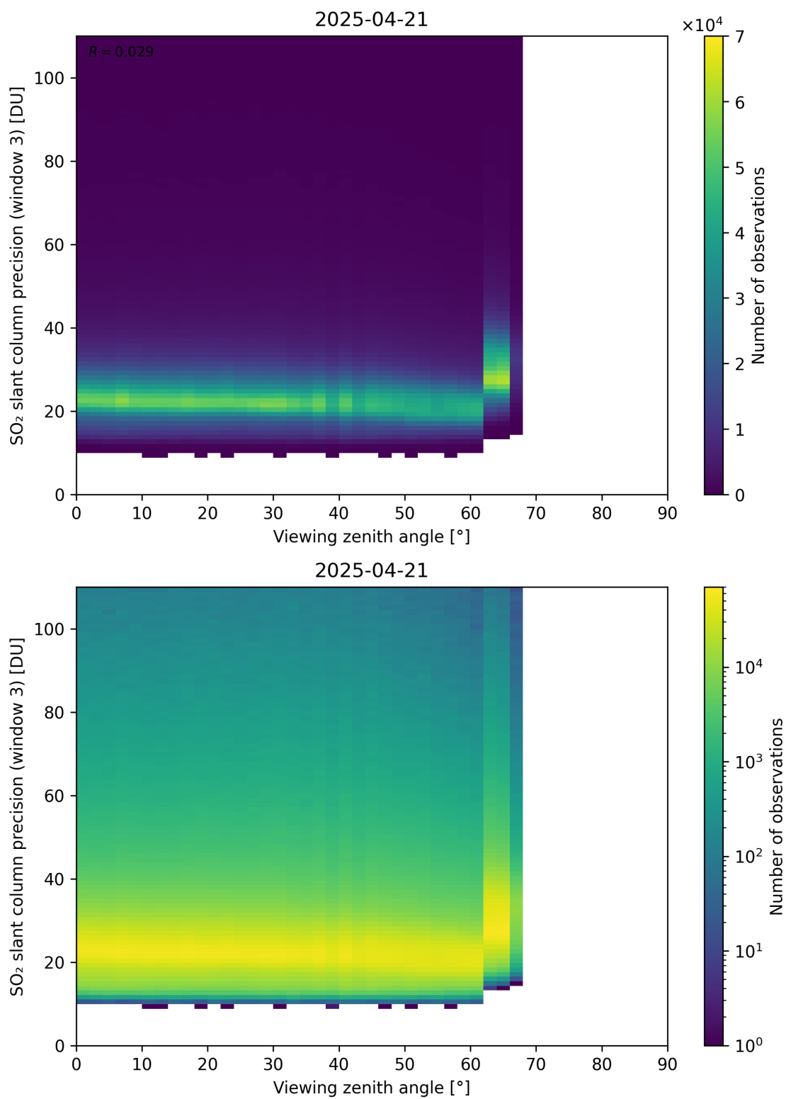
Figure 380: Scatter density plot of “Viewing zenith angle” against “SO 2 slant column precision (window 3)” for 2025-04-20 to 2025-04-22.
