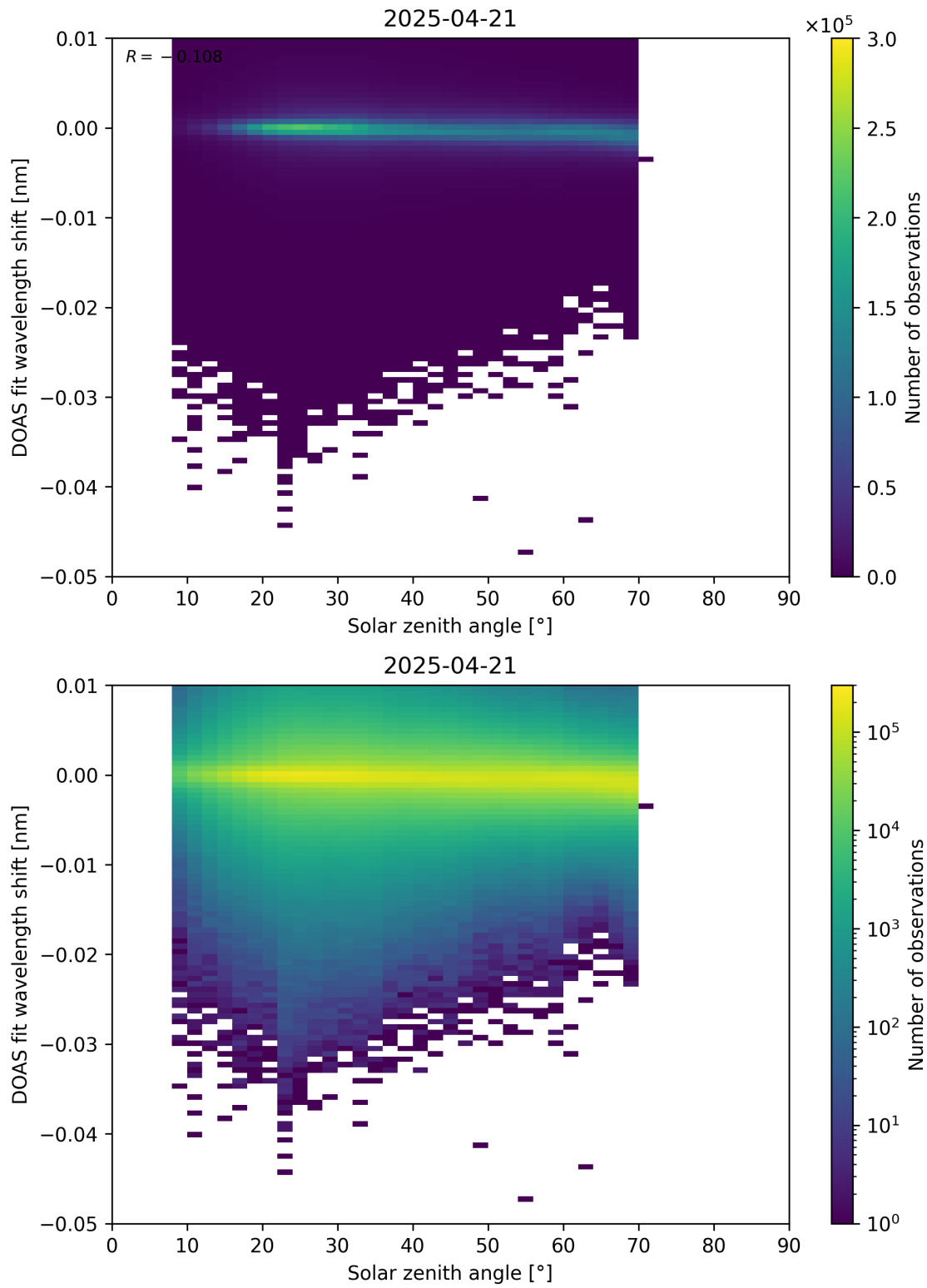
Figure 174: Scatter density plot of “Solar zenith angle” against “DOAS fit wavelength shift” for 2025-04-20 to 2025-04-22.
