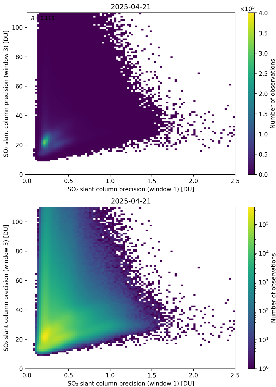
Figure 279: Scatter density plot of “SO 2 slant column precision (window 1)” against “SO 2 slant column precision (window 3)” for 2025-04-20 to 2025-04-22.
