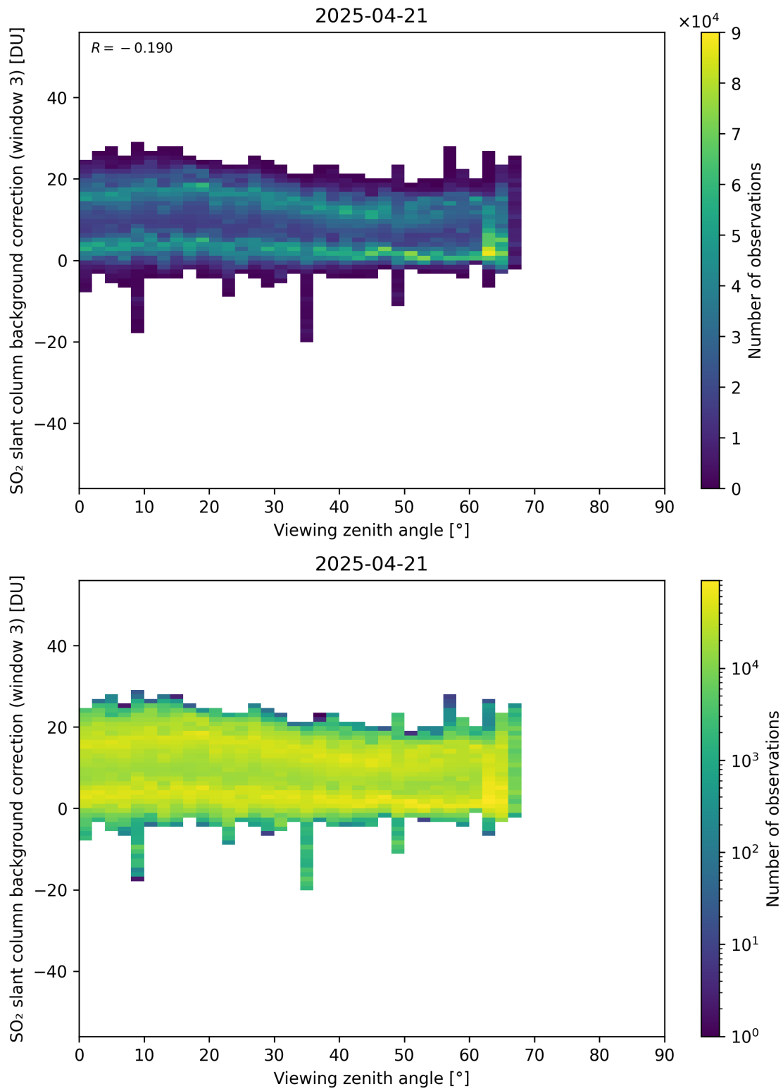
Figure 364: Scatter density plot of “Viewing zenith angle” against “SO 2 slant column background correction (window 3)” for 2025-04-20 to 2025-04-22.
