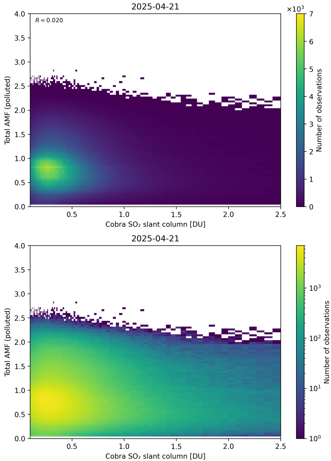
Figure 224: Scatter density plot of “Cobra SO 2 slant column” against “Total AMF (polluted)” for 2025-04-20 to 2025-04-22.
