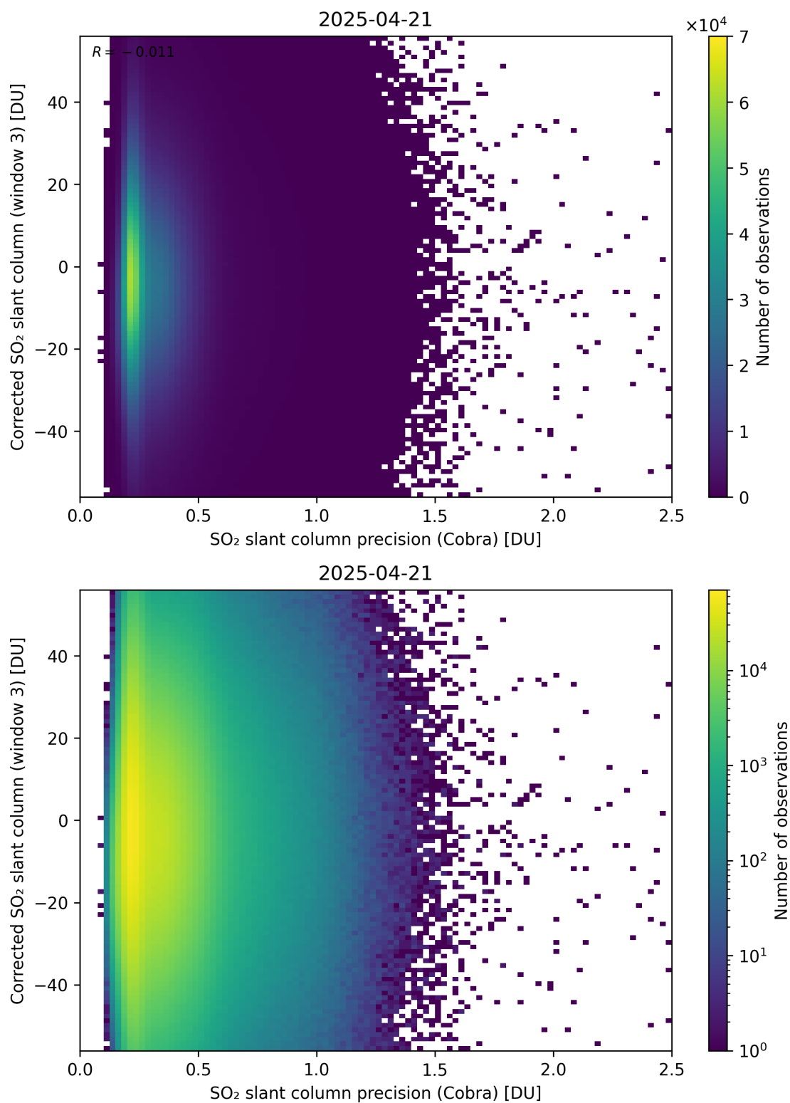
Figure 207: Scatter density plot of “SO 2 slant column precision (Cobra)” against “Corrected SO 2 slant column (window 3)” for 2025-04-20 to 2025-04-22.
