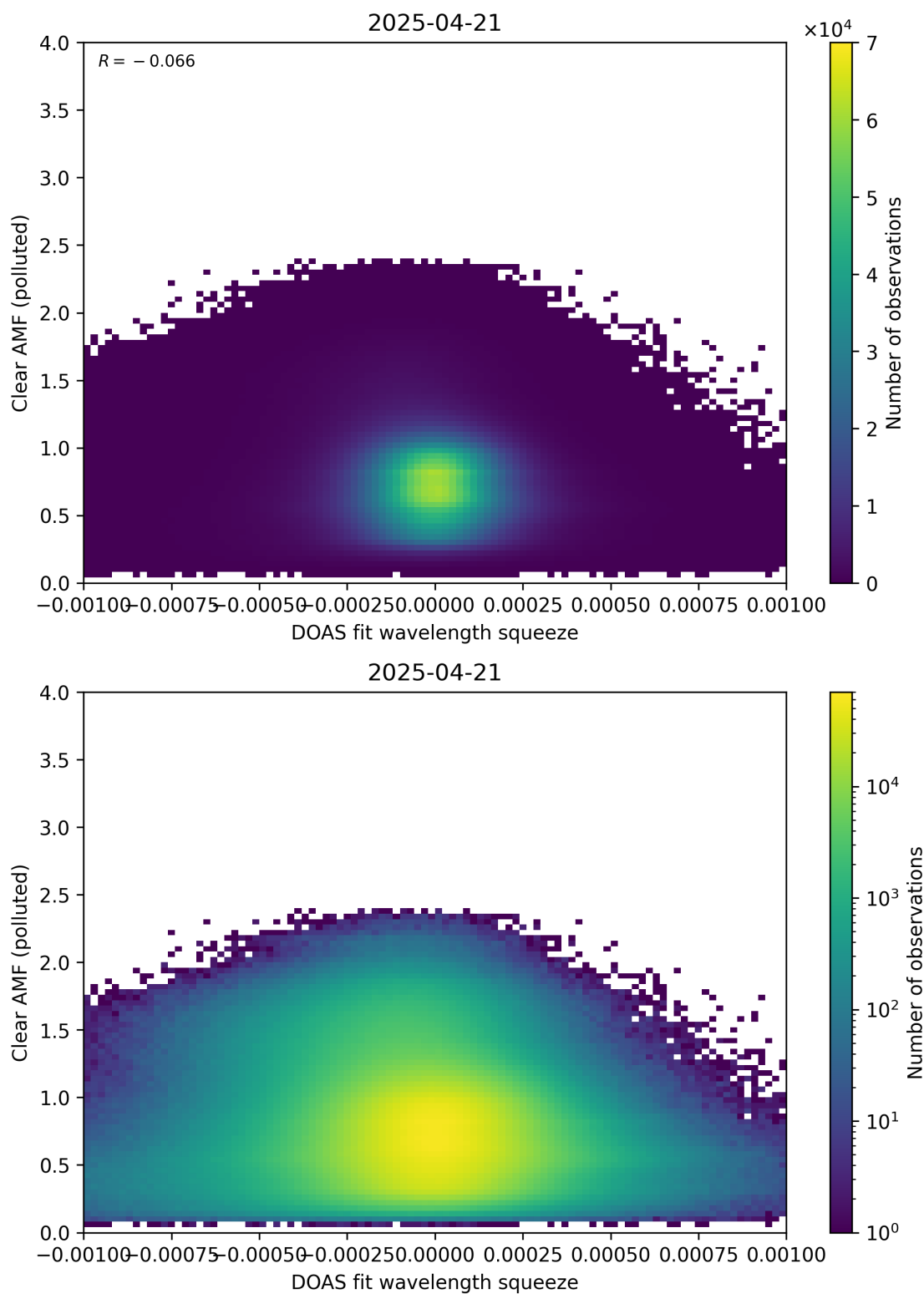
Figure 144: Scatter density plot of “DOAS fit wavelength squeeze” against “Clear AMF (polluted)” for 2025-04-20 to 2025-04-22.
