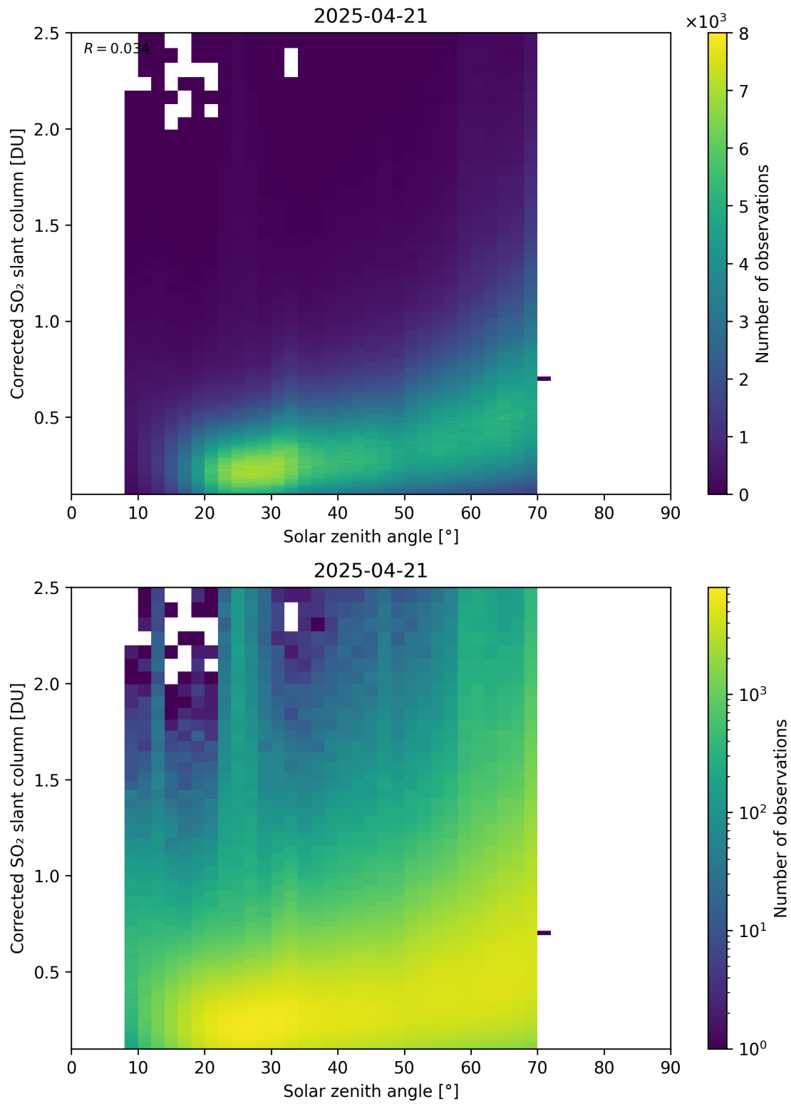
Figure 181: Scatter density plot of “Solar zenith angle” against “Corrected SO 2 slant column” for 2025-04-20 to 2025-04-22.
