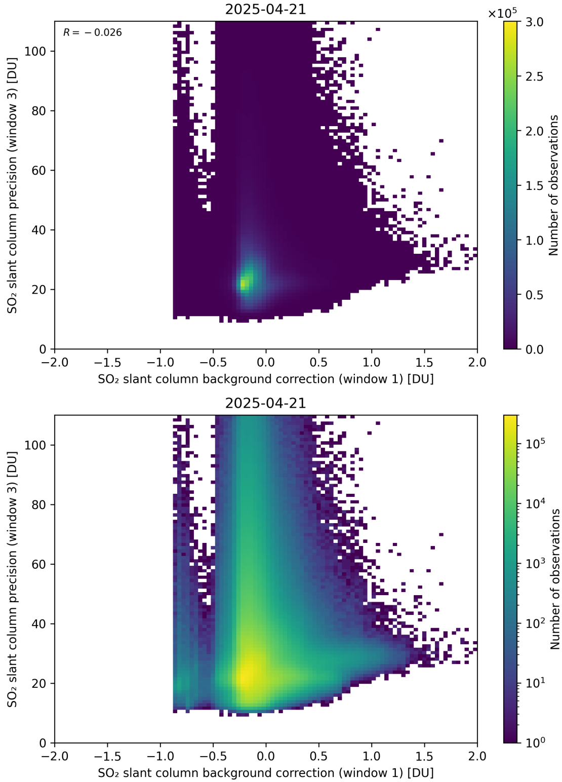
Figure 119: Scatter density plot of “SO 2 slant column background correction (window 1)” against “SO 2 slant column precision (window 3)” for 2025-04-20 to 2025-04-22.
