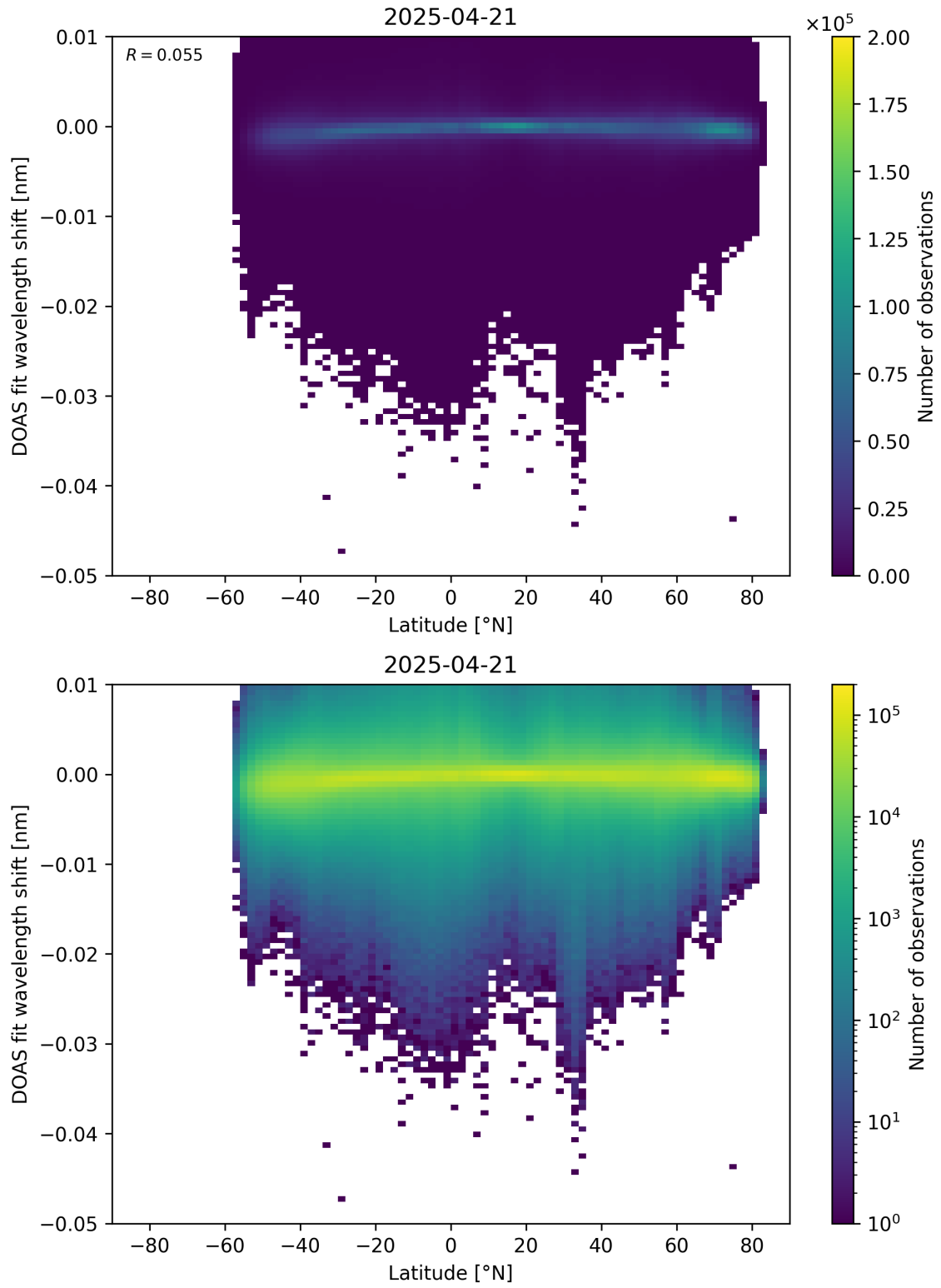
Figure 153: Scatter density plot of “Latitude” against “DOAS fit wavelength shift” for 2025-04-20 to 2025-04-22.
