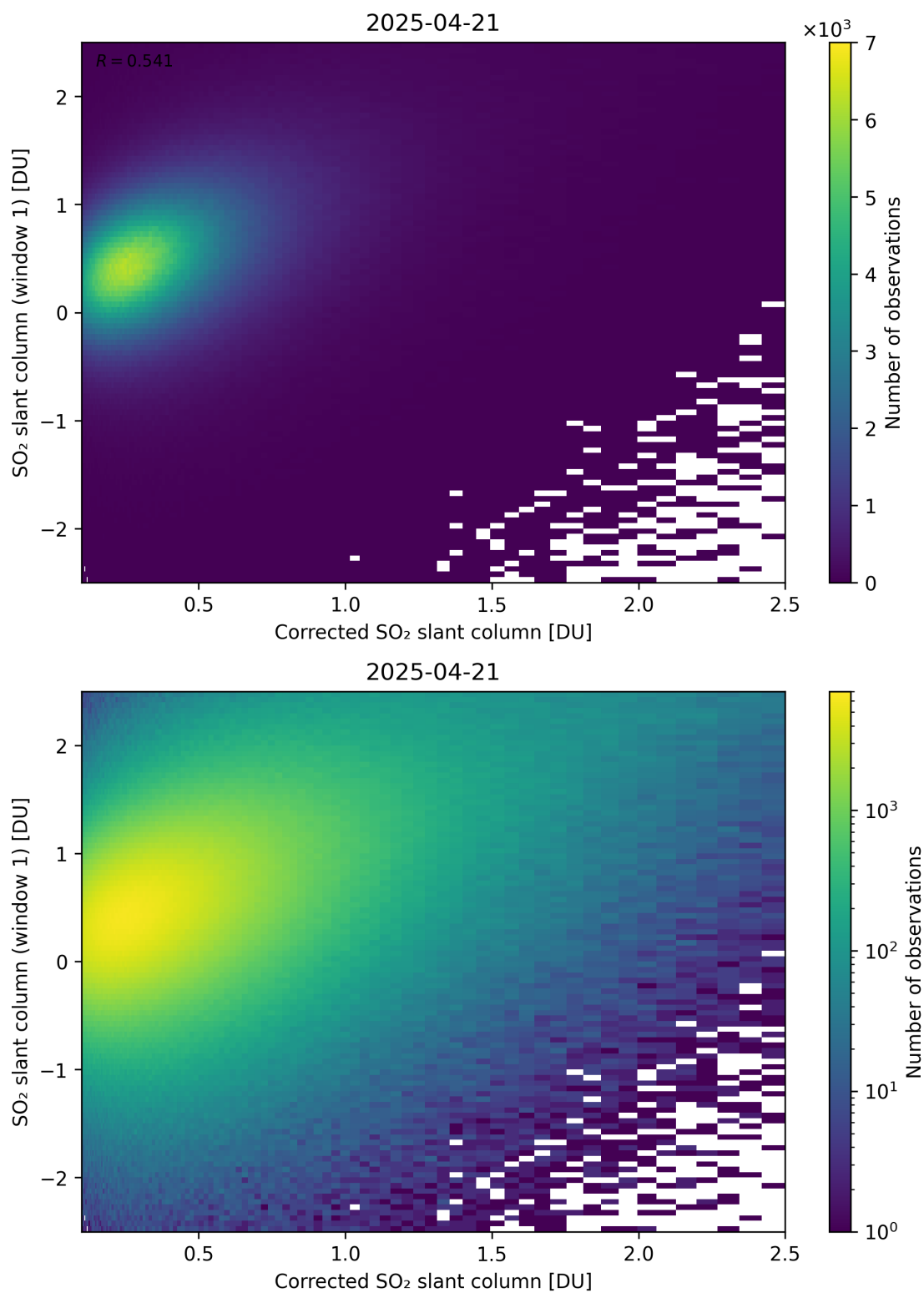
Figure 237: Scatter density plot of “Corrected SO 2 slant column” against “SO 2 slant column (window 1)” for 2025-04-20 to 2025-04-22.
