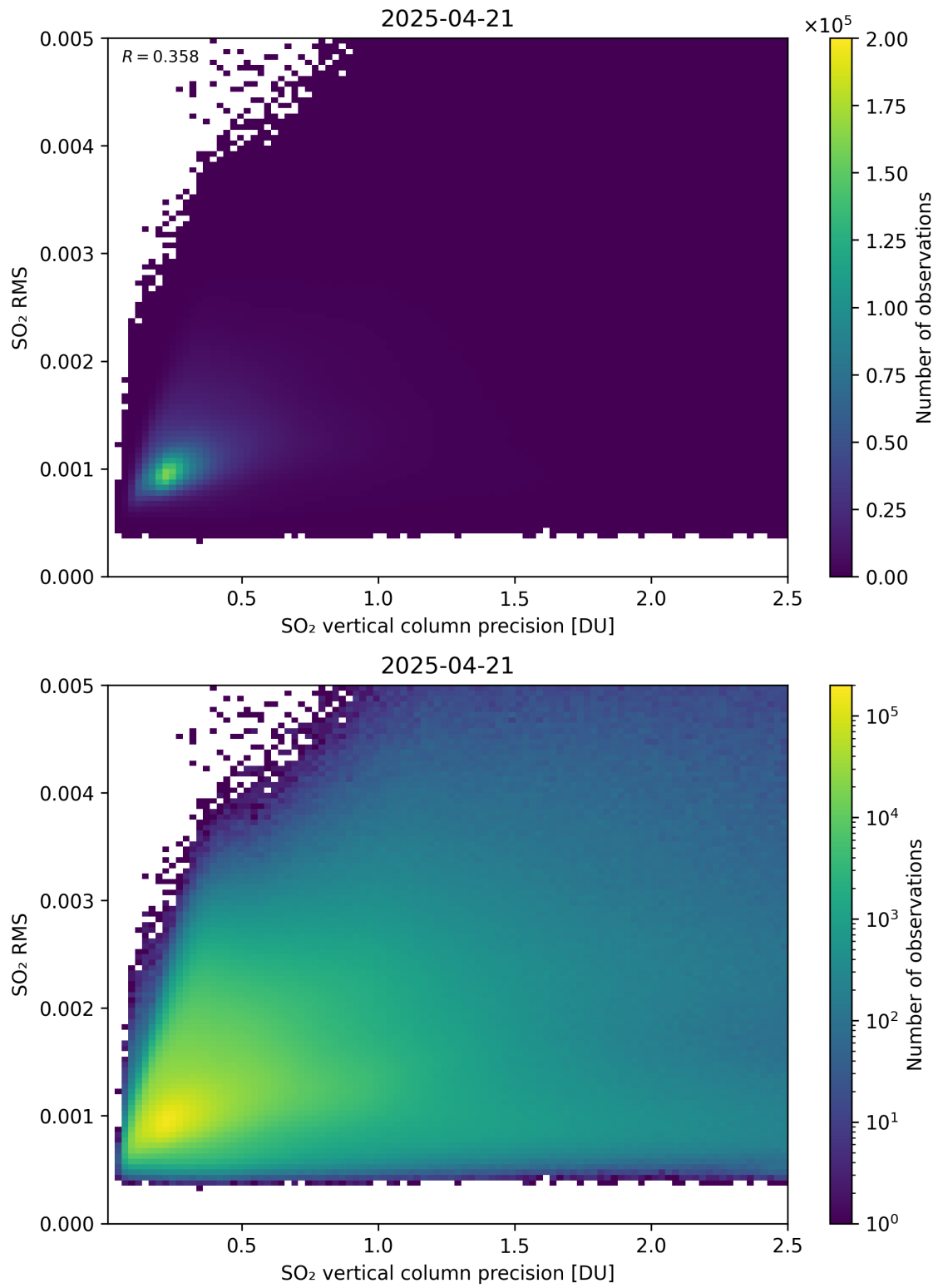
Figure 334: Scatter density plot of “SO 2 vertical column precision” against “SO 2 RMS” for 2025-04-20 to 2025-04-22.
