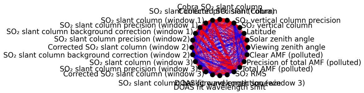
Figure 1: Map of correlation graph for 2025-04-20 to 2025-04-22.
