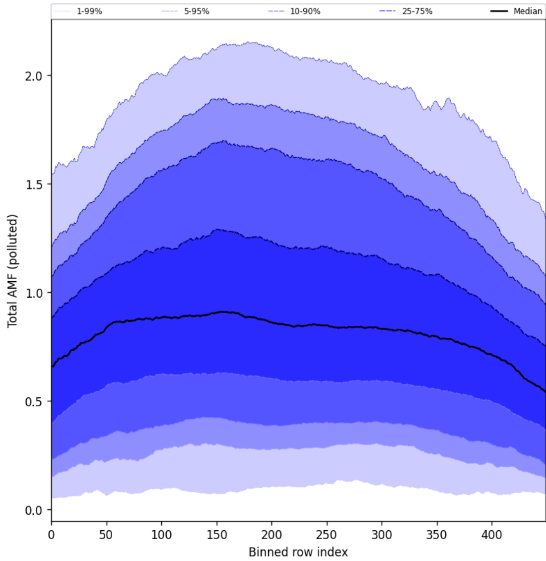
Figure 105: Along track statistics of “Total AMF (polluted)” for 2025-04-20 to 2025-04-22
