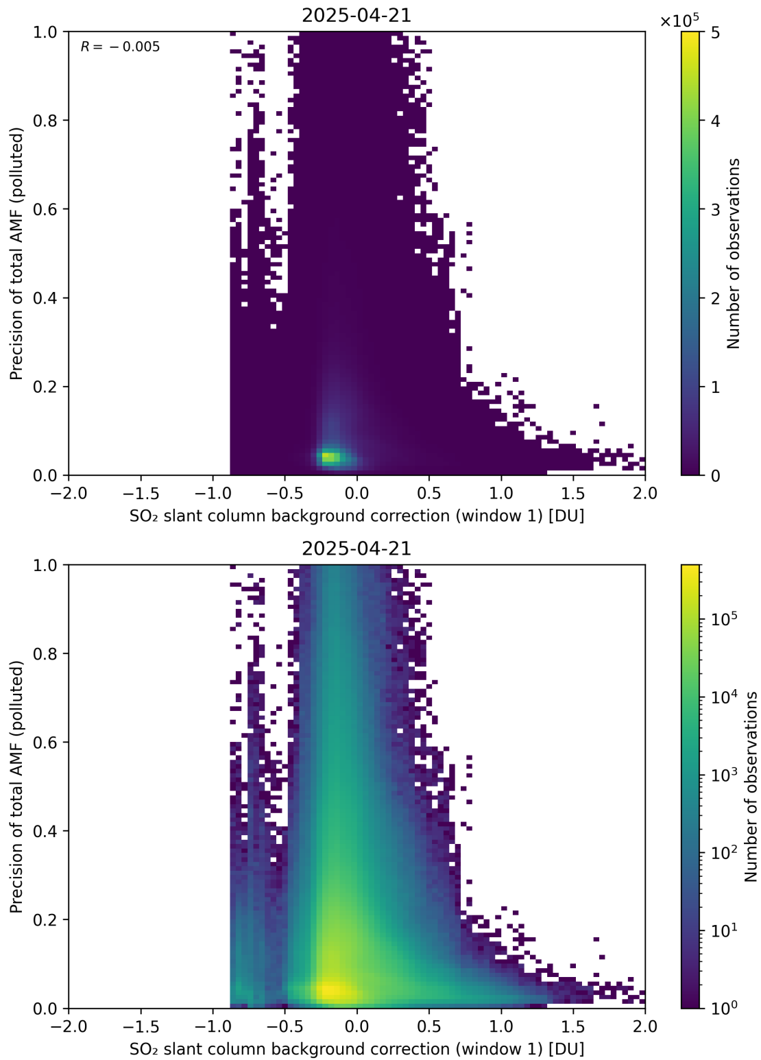
Figure 121: Scatter density plot of “SO 2 slant column background correction (window 1)” against “Precision of total AMF (polluted)” for 2025-04-20 to 2025-04-22.
