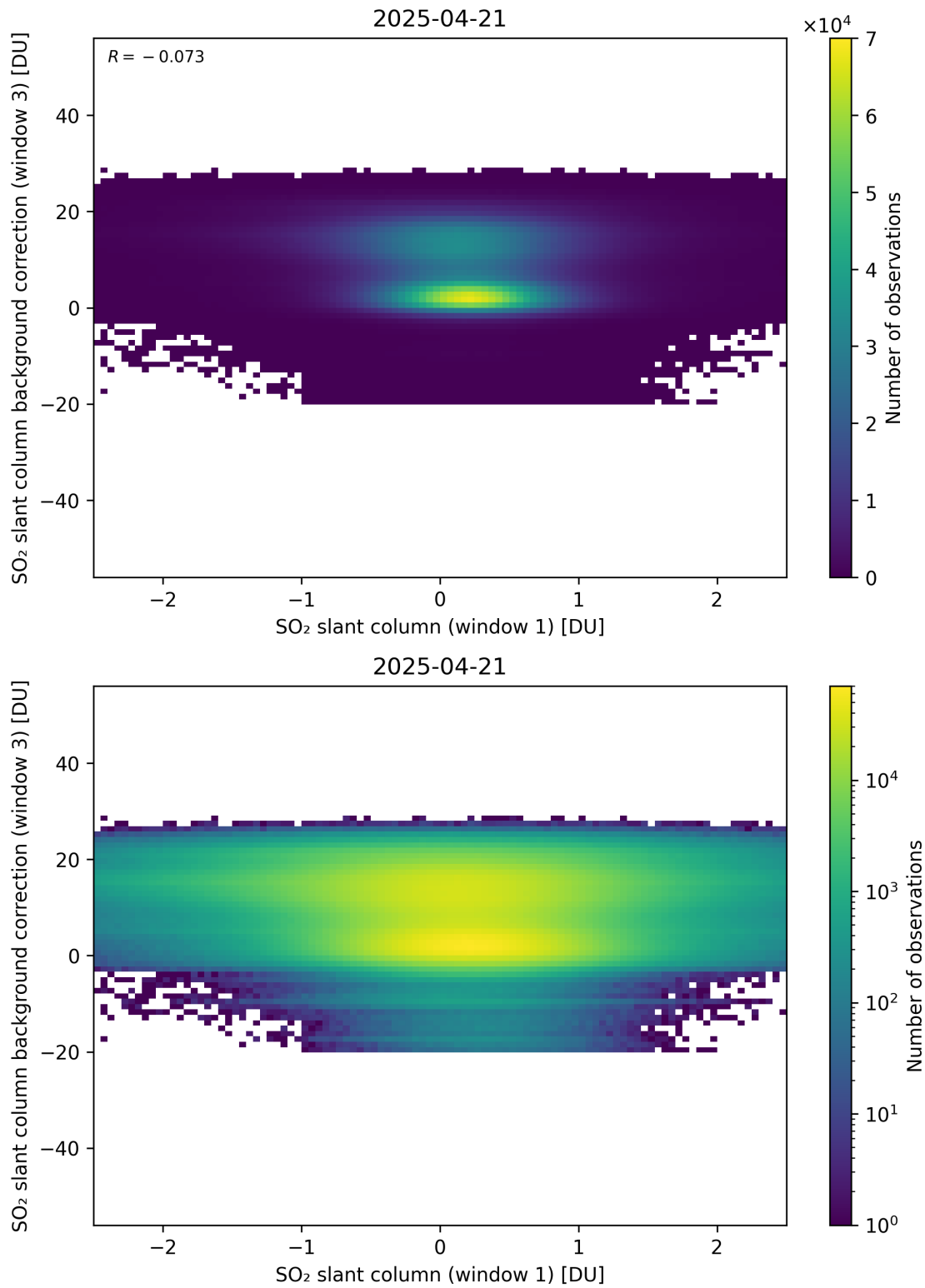
Figure 264: Scatter density plot of “SO 2 slant column (window 1)” against “SO 2 slant column background correction (window 3)” for 2025-04-20 to 2025-04-22.
