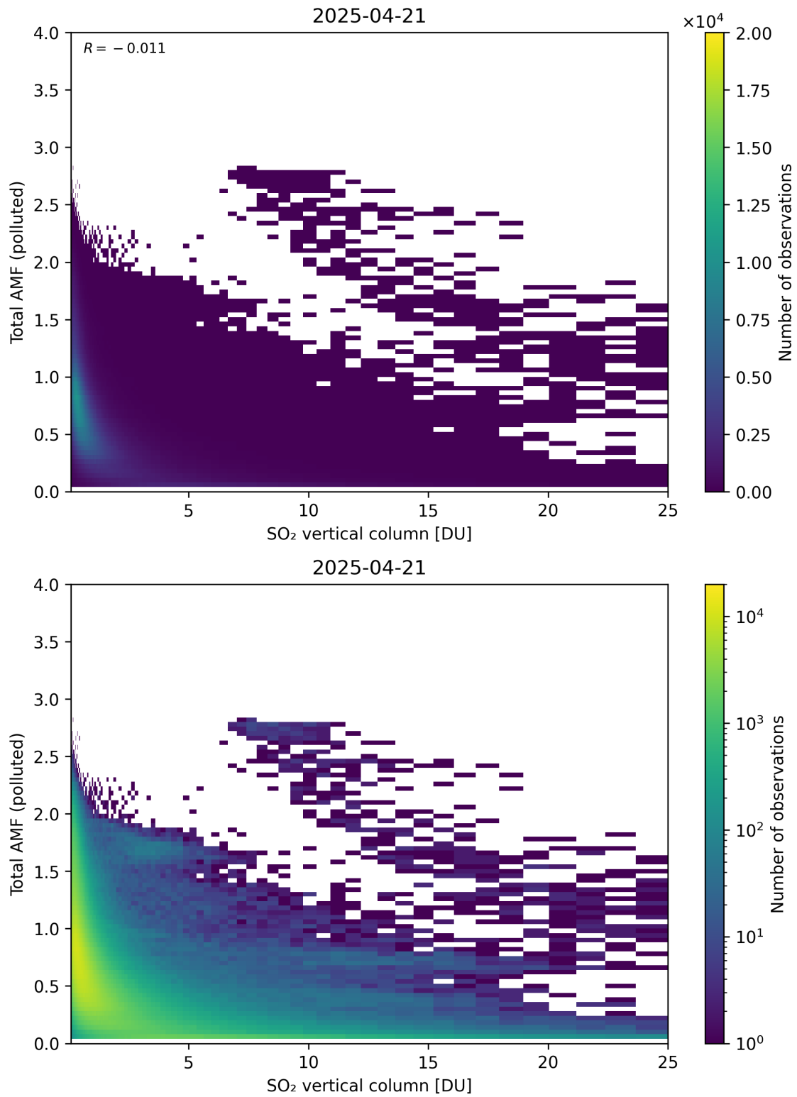
Figure 359: Scatter density plot of “SO 2 vertical column” against “Total AMF (polluted)” for 2025-04-20 to 2025-04-22.
