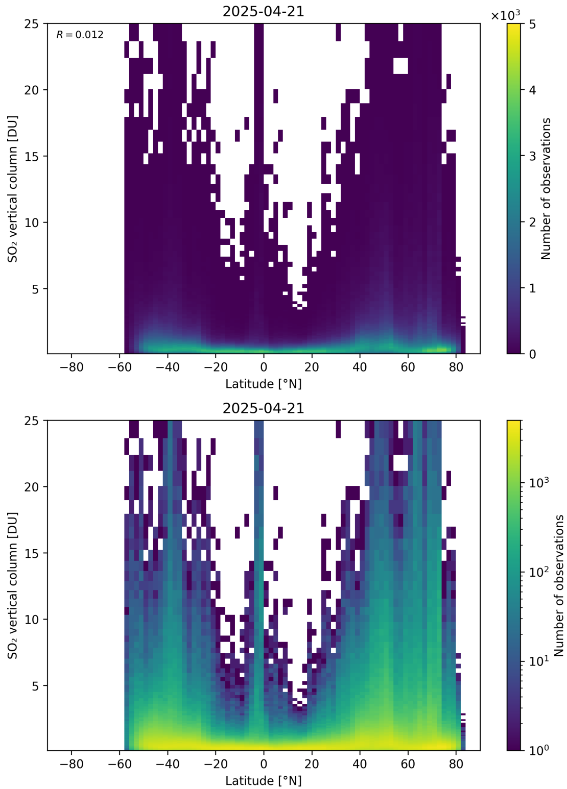
Figure 169: Scatter density plot of “Latitude” against “SO 2 vertical column” for 2025-04-20 to 2025-04-22.
