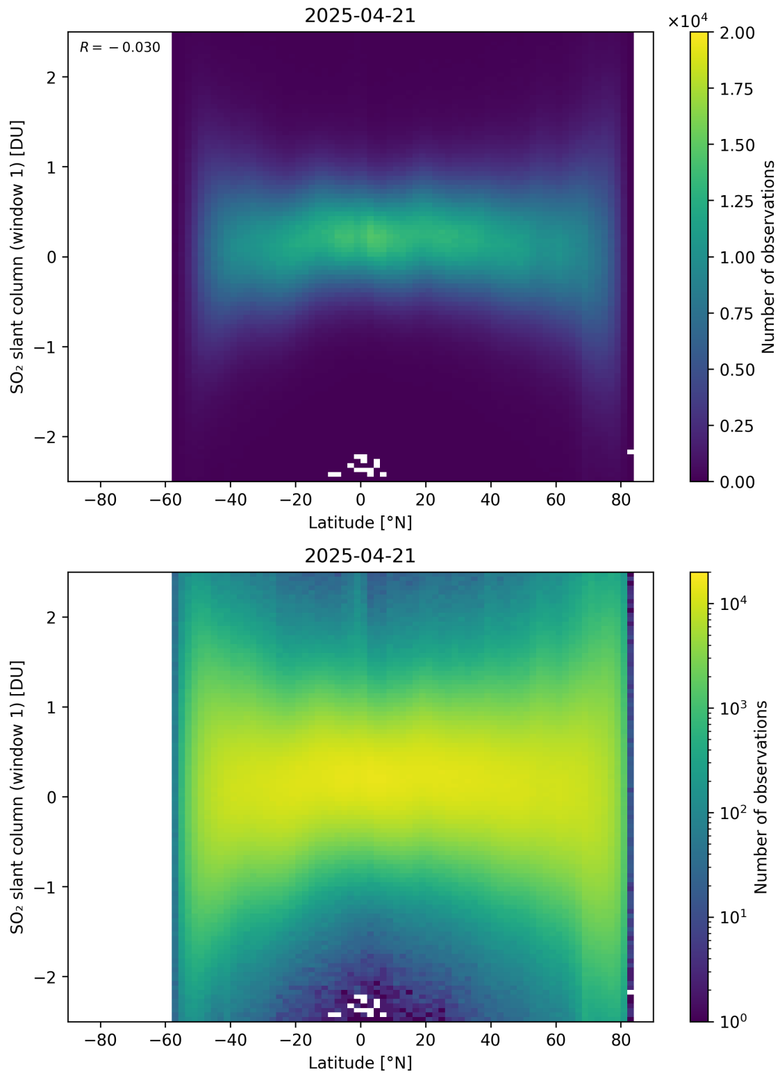
Figure 162: Scatter density plot of “Latitude” against “SO 2 slant column (window 1)” for 2025-04-20 to 2025-04-22.
