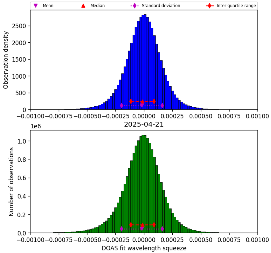
Figure 77: Histogram of “DOAS fit wavelength squeeze” for 2025-04-20 to 2025-04-22
