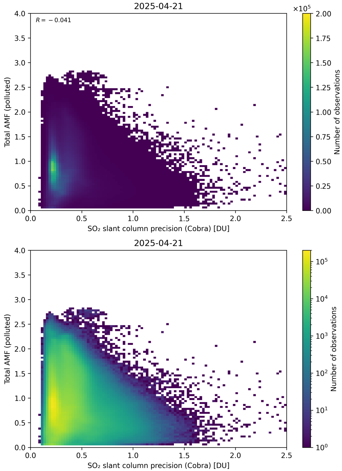
Figure 213: Scatter density plot of “SO 2 slant column precision (Cobra)” against “Total AMF (polluted)” for 2025-04-20 to 2025-04-22.
