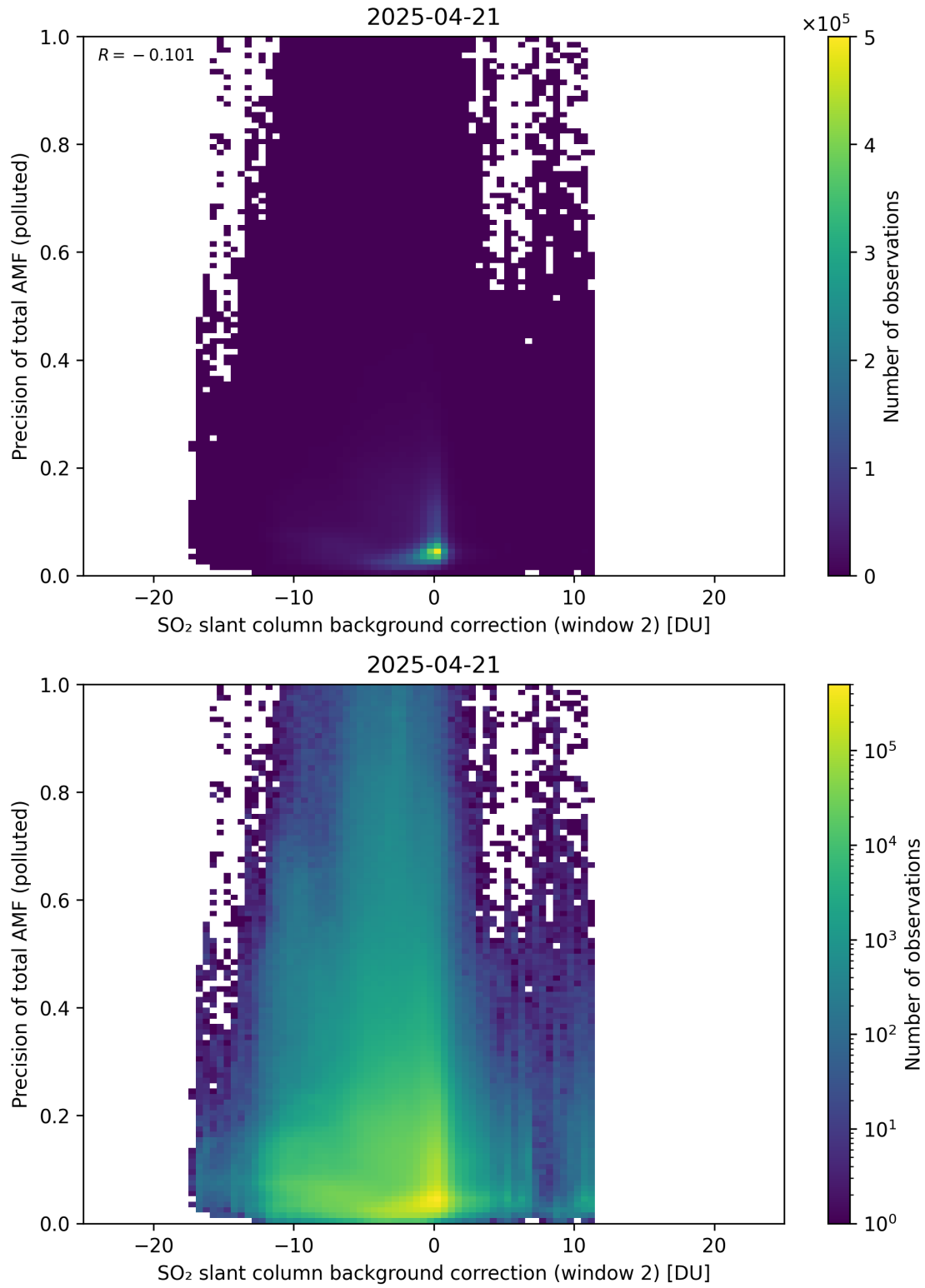
Figure 131: Scatter density plot of “SO 2 slant column background correction (window 2)” against “Precision of total AMF (polluted)” for 2025-04-20 to 2025-04-22.
