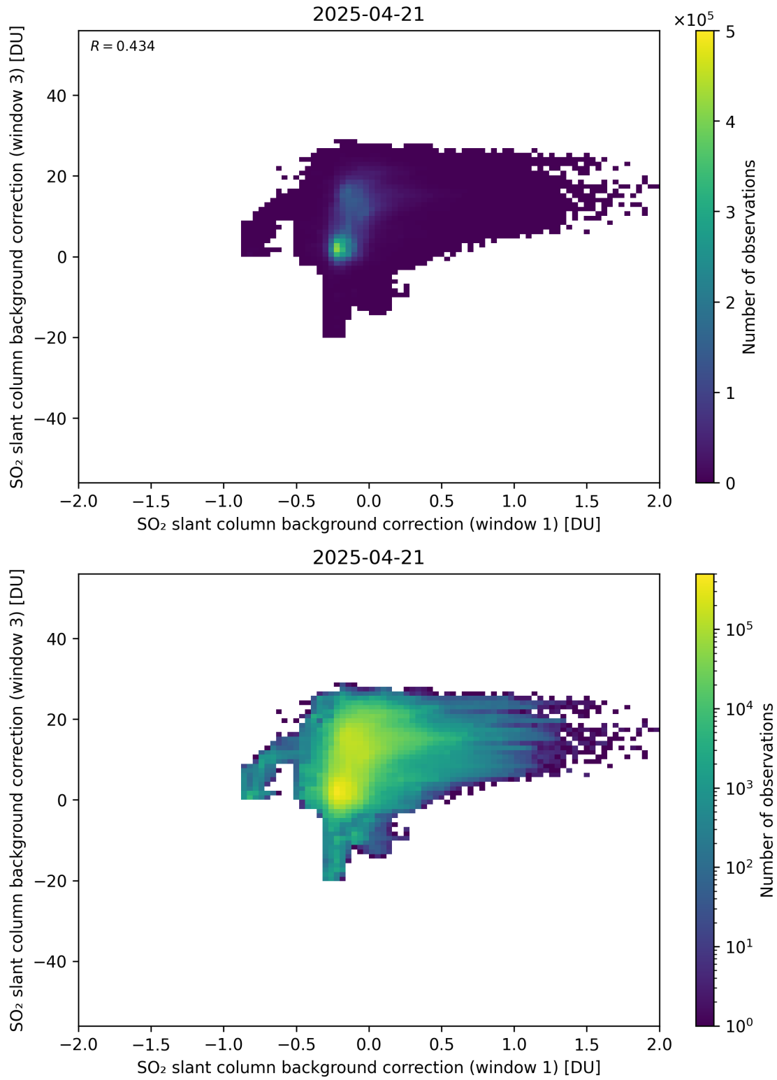
Figure 110: Scatter density plot of “SO 2 slant column background correction (window 1)” against “SO 2 slant column background correction (window 3)” for 2025-04-20 to 2025-04-22.
