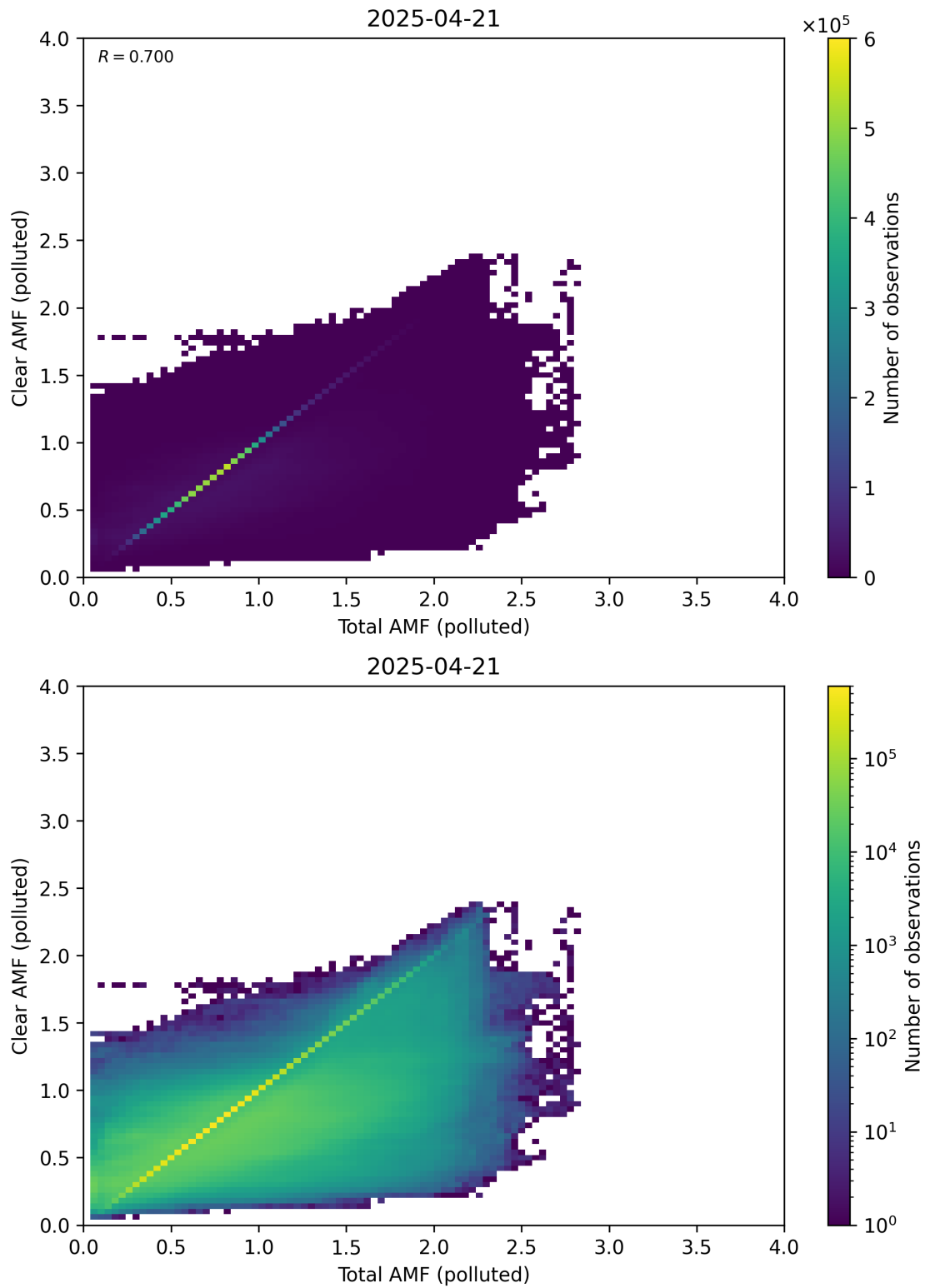
Figure 321: Scatter density plot of “Total AMF (polluted)” against “Clear AMF (polluted)” for 2025-04-20 to 2025-04-22.
