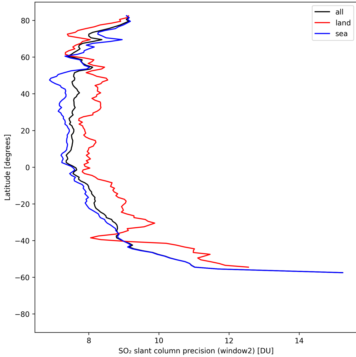
Figure 42: Zonal average of “SO 2 slant column precision (window2)” for 2025-04-20 to 2025-04-22.
