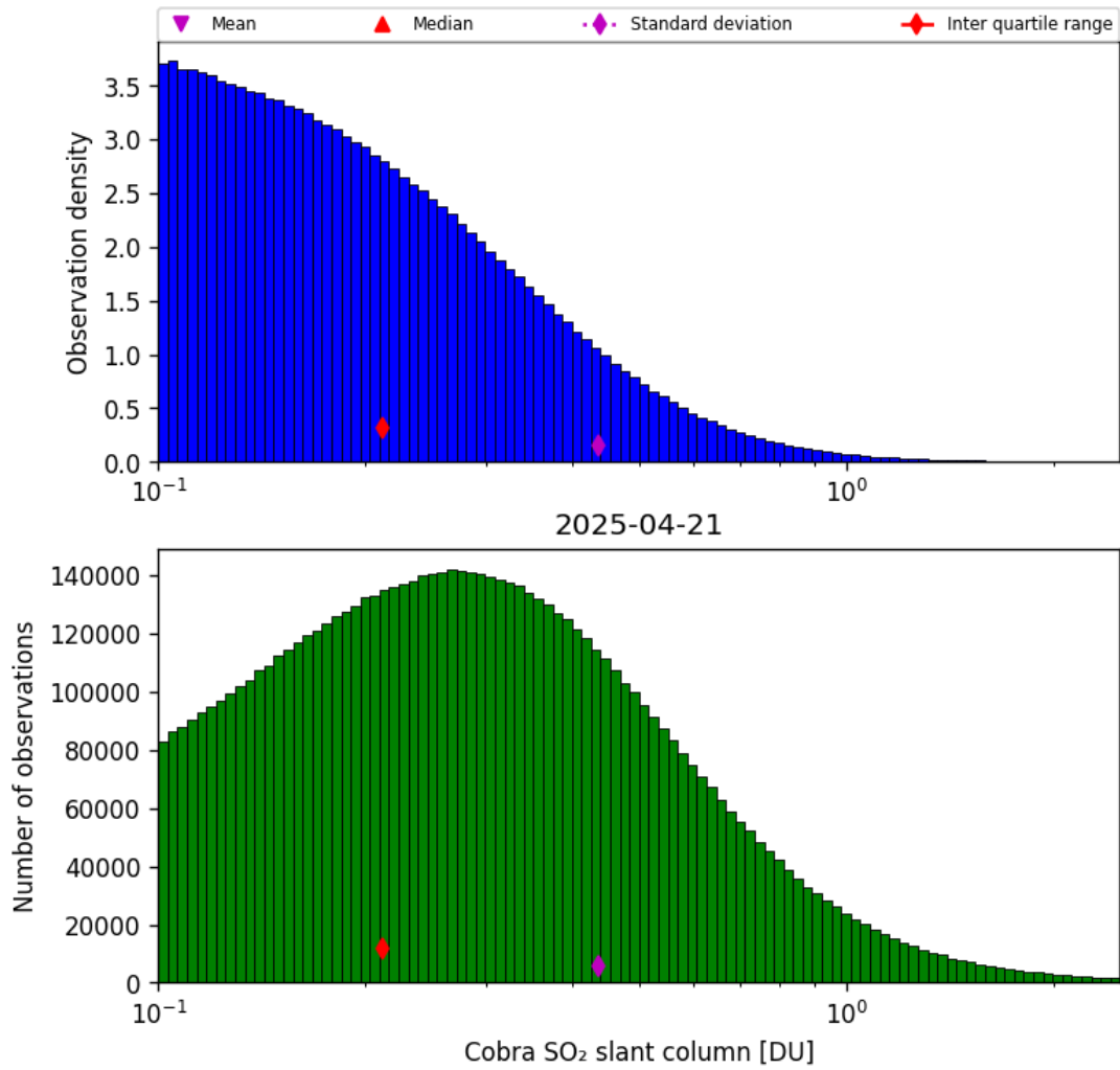
Figure 61: Histogram of “Cobra SO 2 slant column” for 2025-04-20 to 2025-04-22
