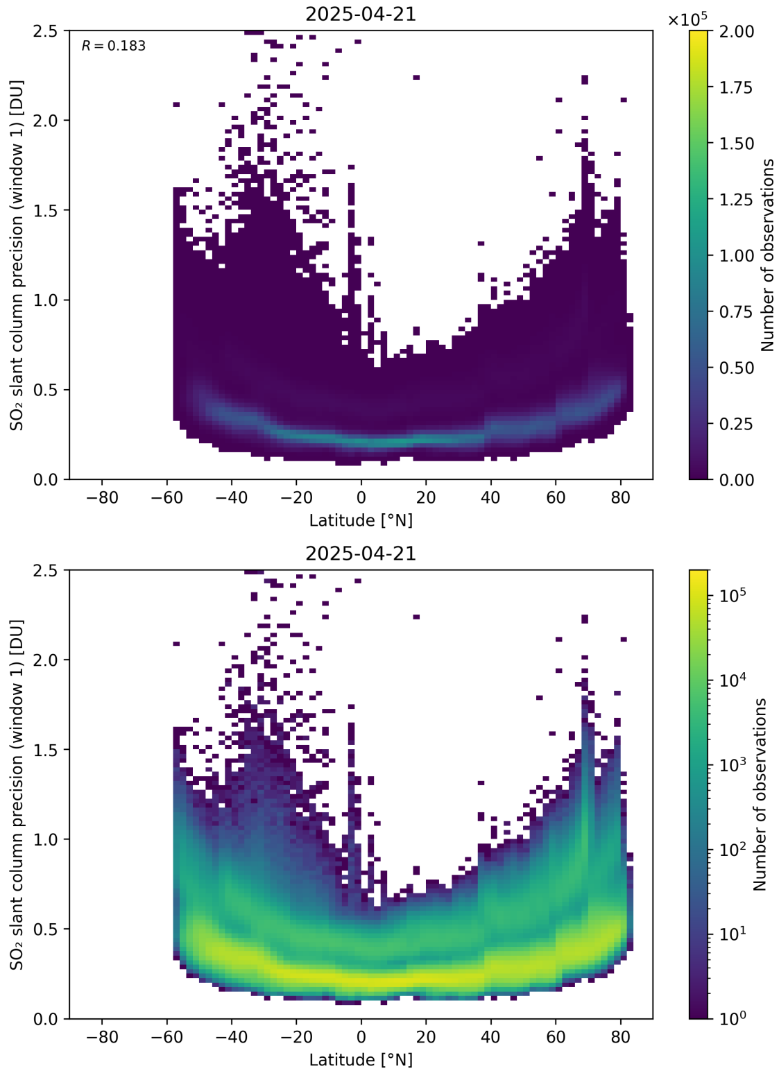
Figure 163: Scatter density plot of “Latitude” against “SO 2 slant column precision (window 1)” for 2025-04-20 to 2025-04-22.
