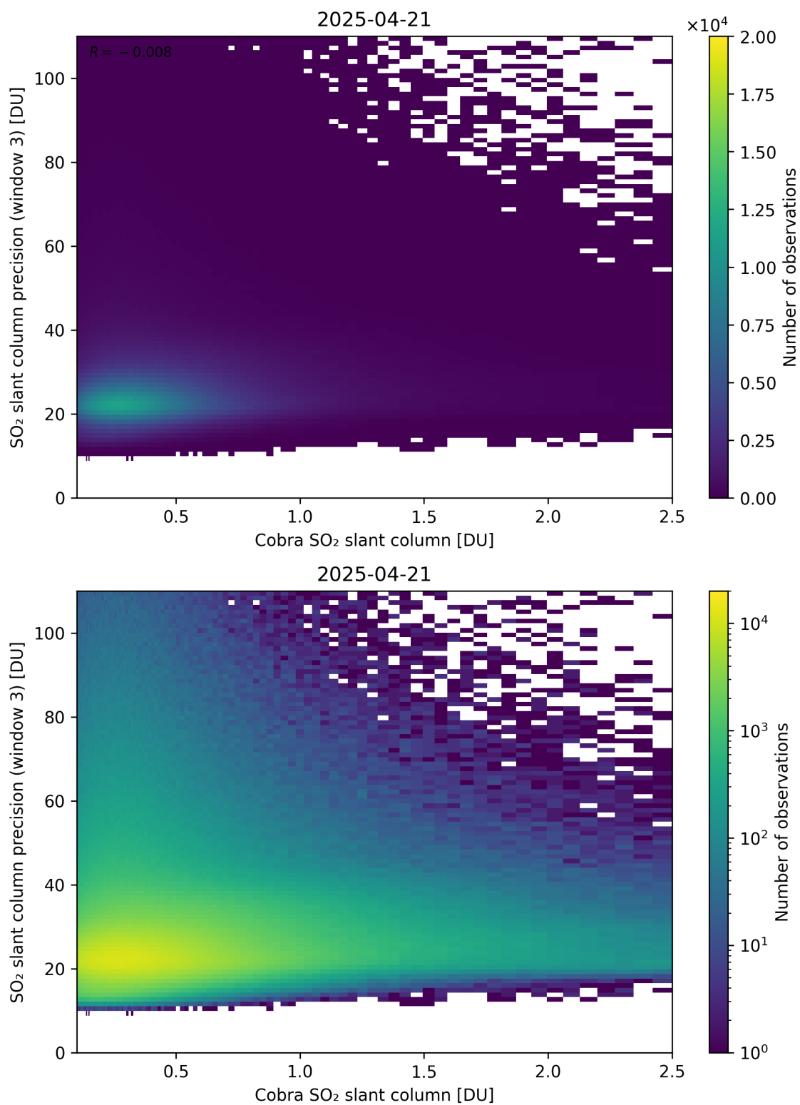
Figure 223: Scatter density plot of “Cobra SO 2 slant column” against “SO 2 slant column precision (window 3)” for 2025-04-20 to 2025-04-22.
