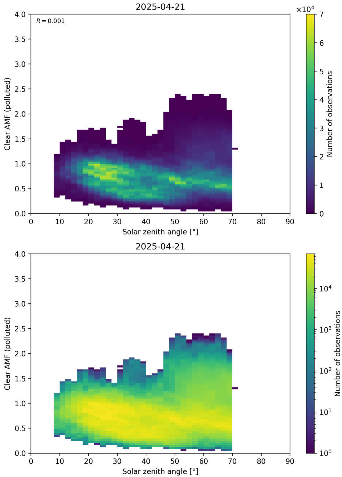
Figure 178: Scatter density plot of “Solar zenith angle” against “Clear AMF (polluted)” for 2025-04-20 to 2025-04-22.
