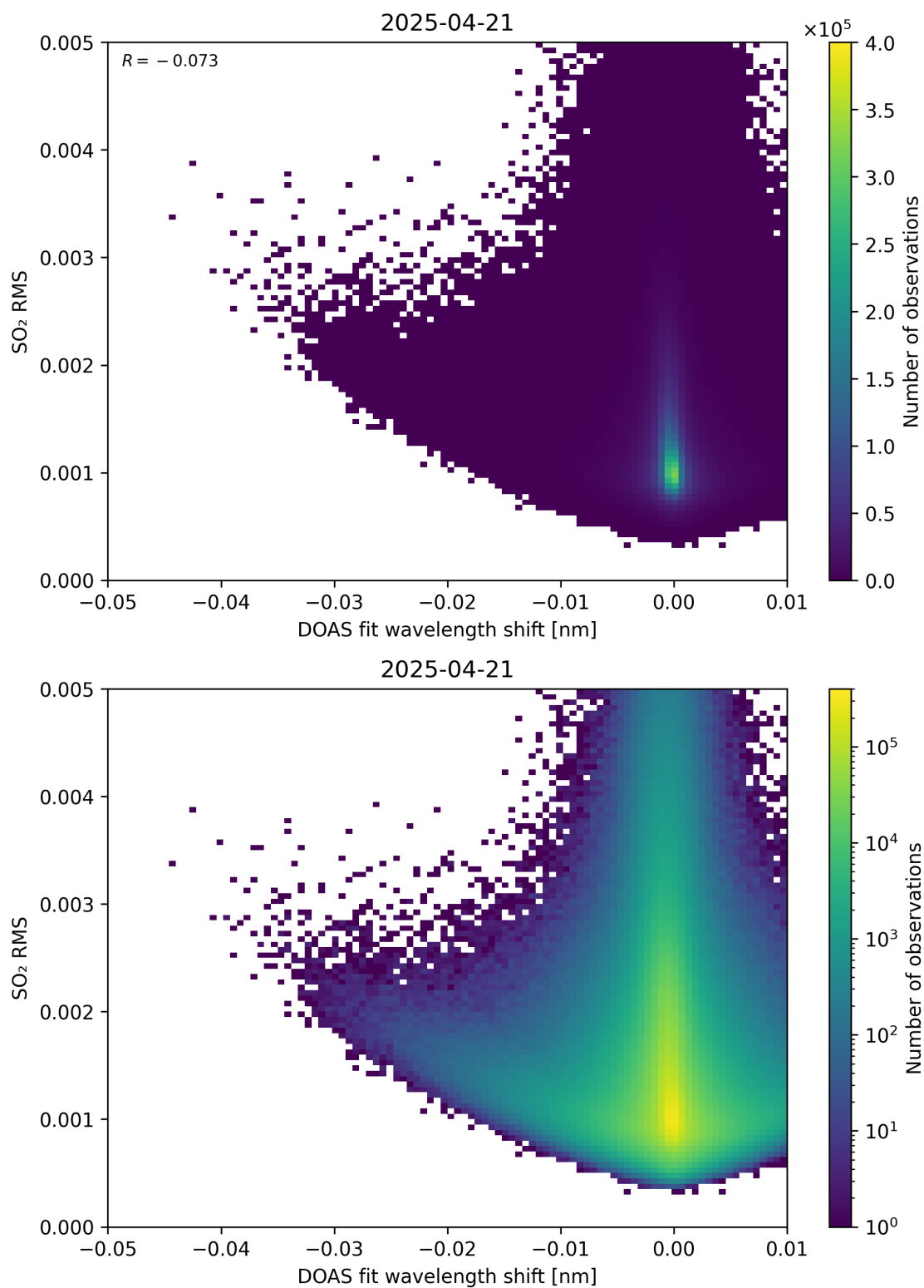
Figure 139: Scatter density plot of “DOAS fit wavelength shift” against “SO 2 RMS” for 2025-04-20 to 2025-04-22.
