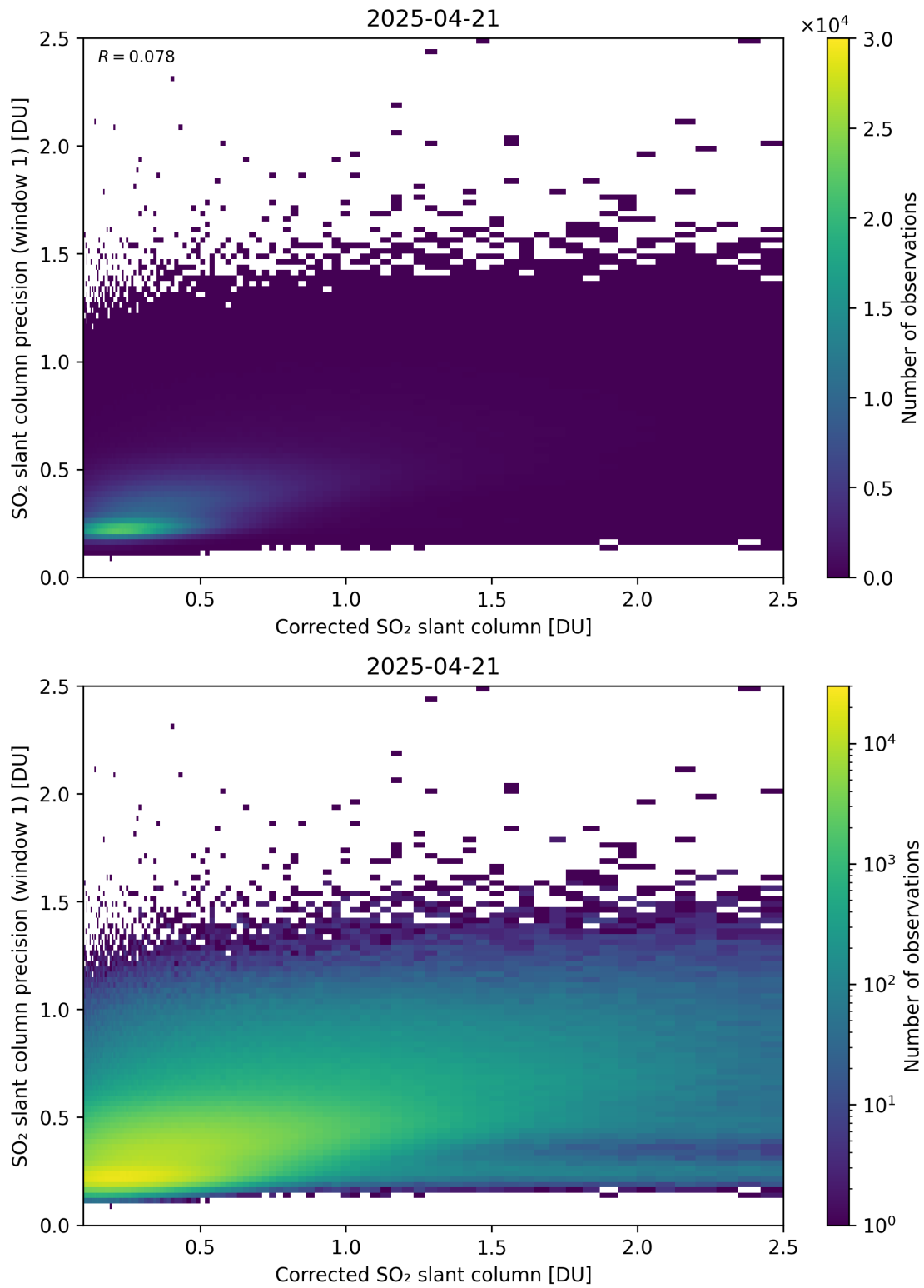
Figure 238: Scatter density plot of “Corrected SO 2 slant column” against “SO 2 slant column precision (window 1)” for 2025-04-20 to 2025-04-22.
