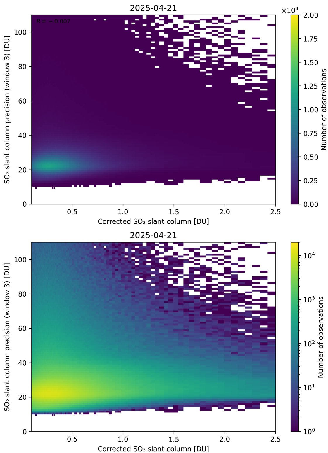
Figure 241: Scatter density plot of “Corrected SO 2 slant column” against “SO 2 slant column precision (window 3)” for 2025-04-20 to 2025-04-22.
