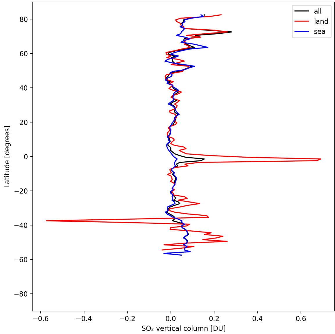
Figure 32: Zonal average of “SO 2 vertical column” for 2025-04-20 to 2025-04-22.
