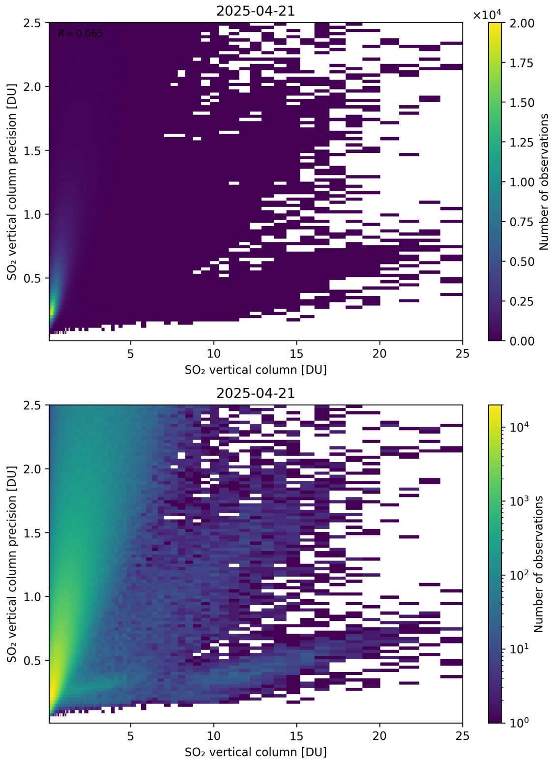
Figure 361: Scatter density plot of “SO 2 vertical column” against “SO 2 vertical column precision” for 2025-04-20 to 2025-04-22.
