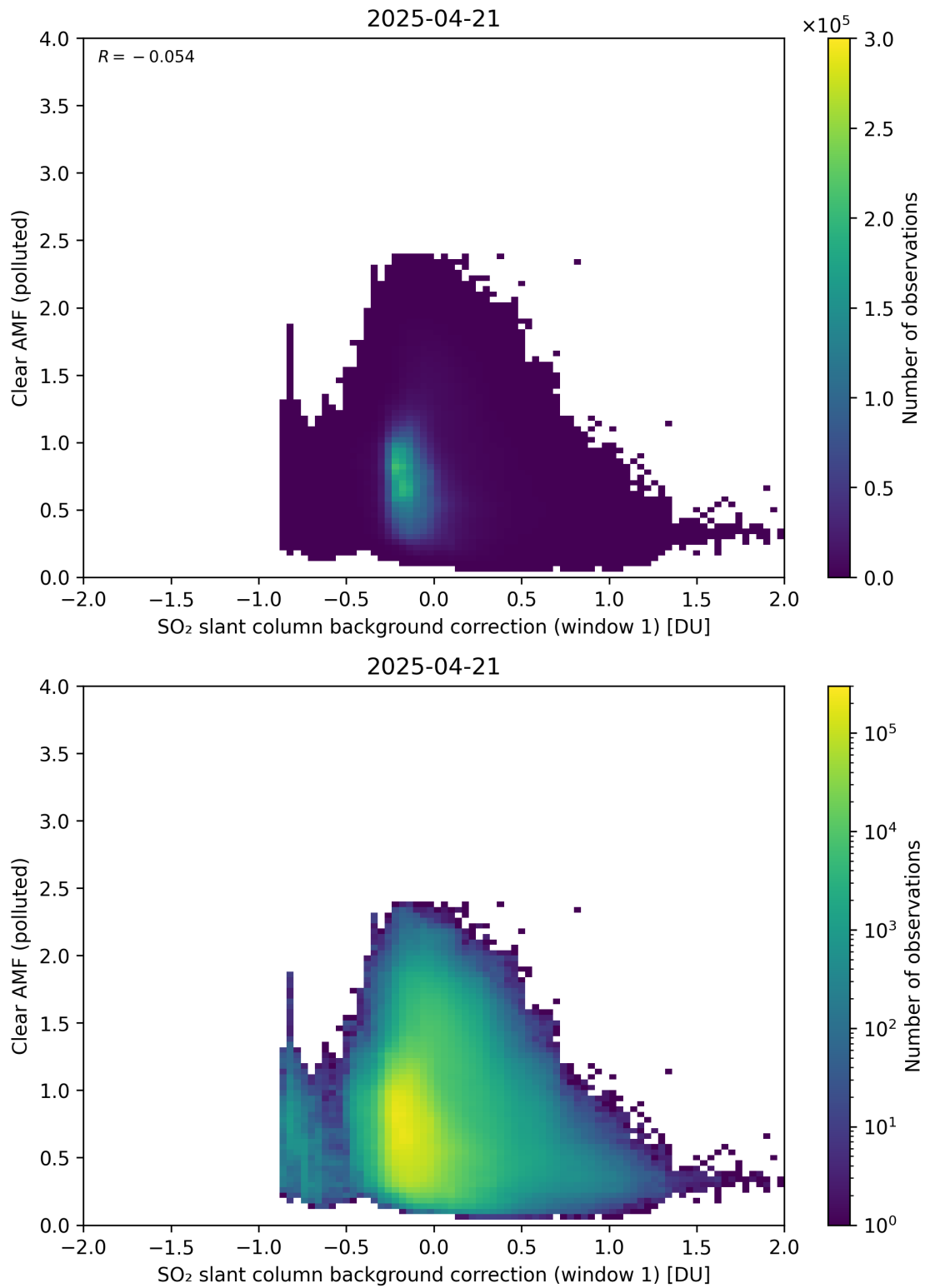
Figure 114: Scatter density plot of “SO 2 slant column background correction (window 1)” against “Clear AMF (polluted)” for 2025-04-20 to 2025-04-22.
