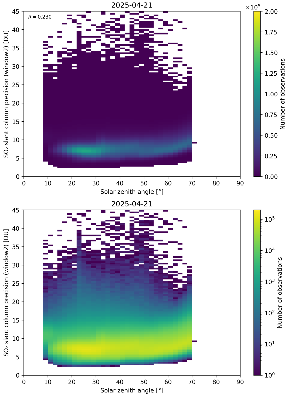
Figure 186: Scatter density plot of “Solar zenith angle” against “SO 2 slant column precision (window2)” for 2025-04-20 to 2025-04-22.
