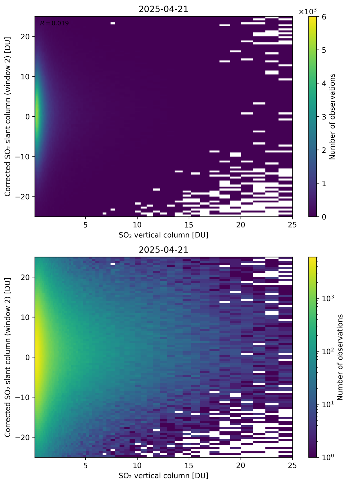
Figure 352: Scatter density plot of “SO 2 vertical column” against “Corrected SO 2 slant column (window 2)” for 2025-04-20 to 2025-04-22.
