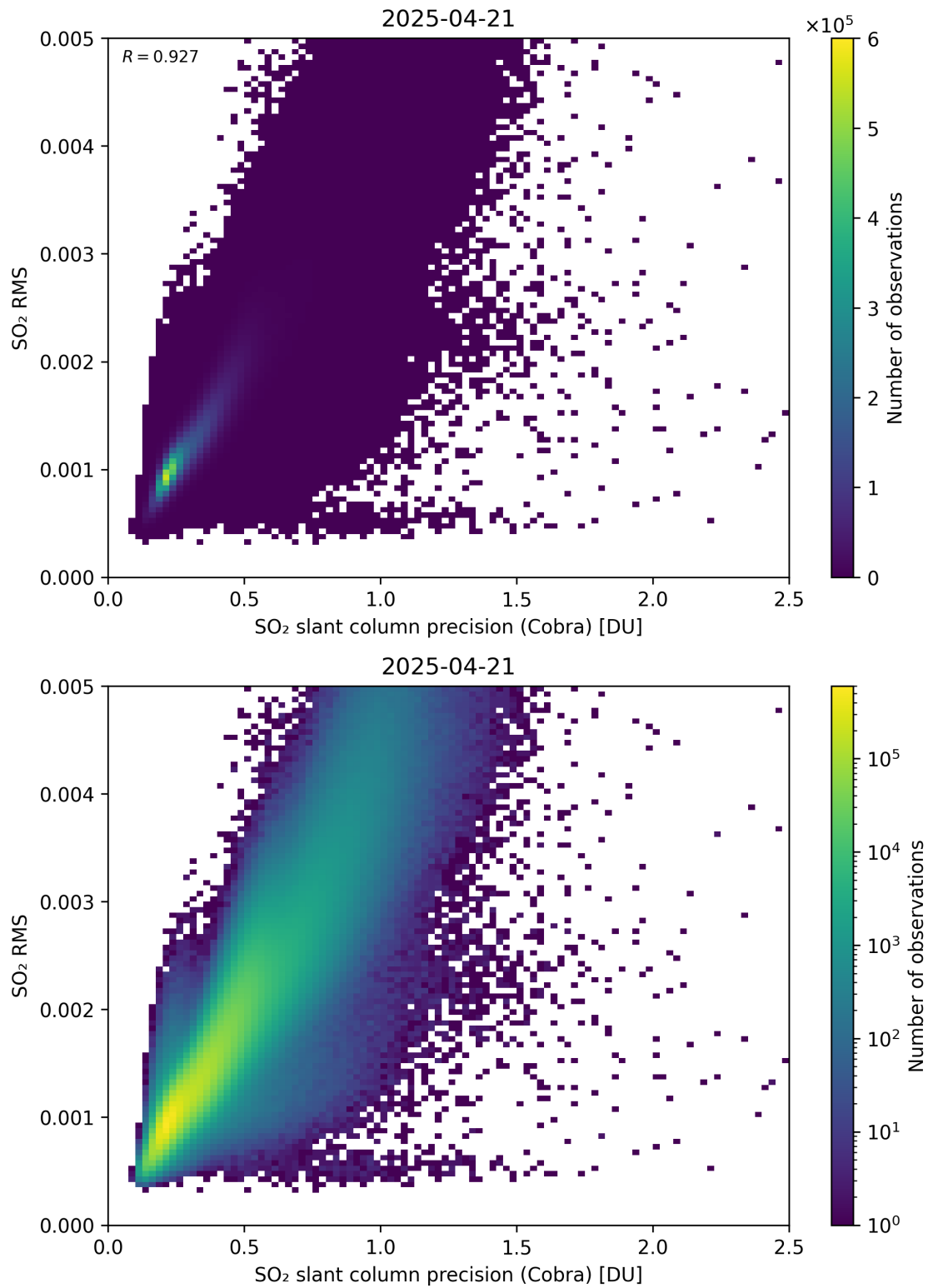
Figure 204: Scatter density plot of “SO 2 slant column precision (Cobra)” against “SO 2 RMS” for 2025-04-20 to 2025-04-22.
