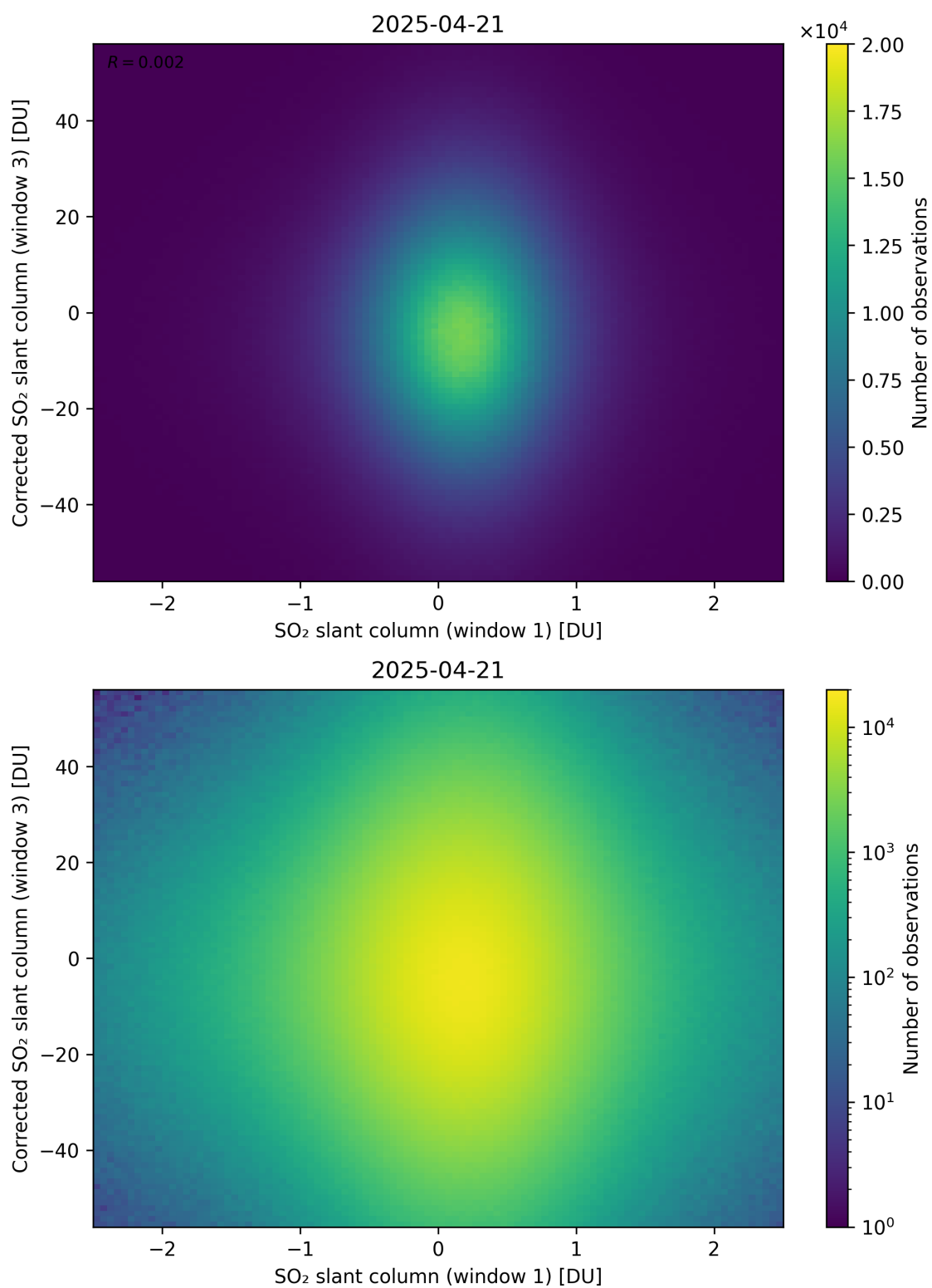
Figure 284: Scatter density plot of “SO 2 slant column (window 1)” against “Corrected SO 2 slant column (window 3)” for 2025-04-20 to 2025-04-22.
