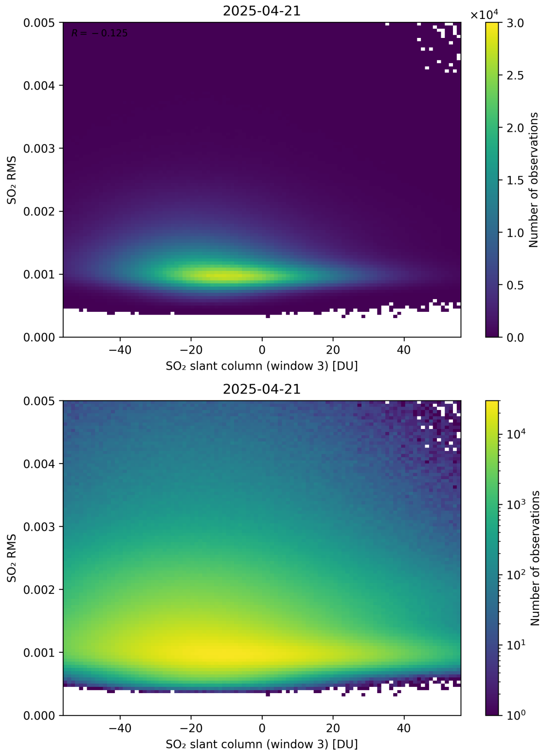
Figure 306: Scatter density plot of “SO 2 slant column (window 3)” against “SO 2 RMS” for 2025-04-20 to 2025-04-22.
