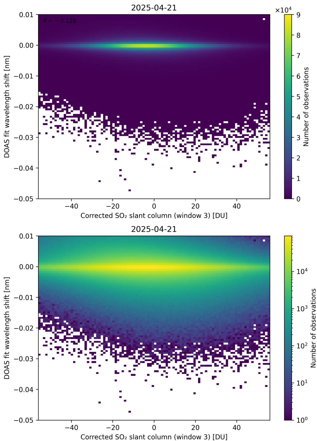
Figure 256: Scatter density plot of “Corrected SO 2 slant column (window 3)” against “DOAS fit wavelength shift” for 2025-04-20 to 2025-04-22.
