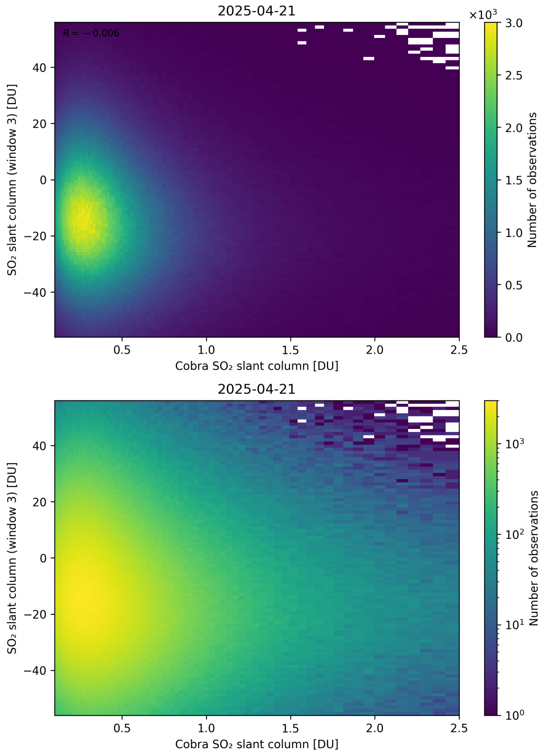
Figure 222: Scatter density plot of “Cobra SO 2 slant column” against “SO 2 slant column (window 3)” for 2025-04-20 to 2025-04-22.
