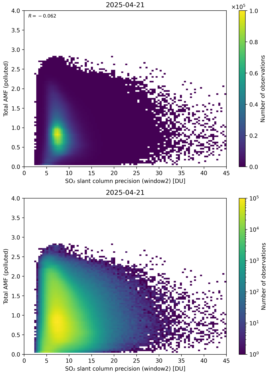
Figure 301: Scatter density plot of “SO 2 slant column precision (window2)” against “Total AMF (polluted)” for 2025-04-20 to 2025-04-22.
