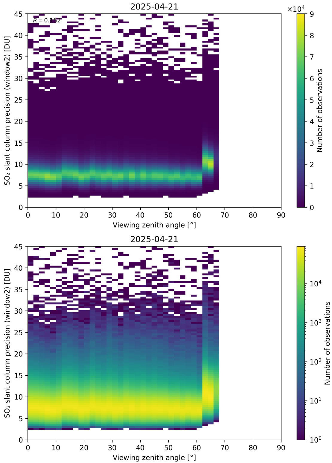
Figure 378: Scatter density plot of “Viewing zenith angle” against “SO 2 slant column precision (window2)” for 2025-04-20 to 2025-04-22.
