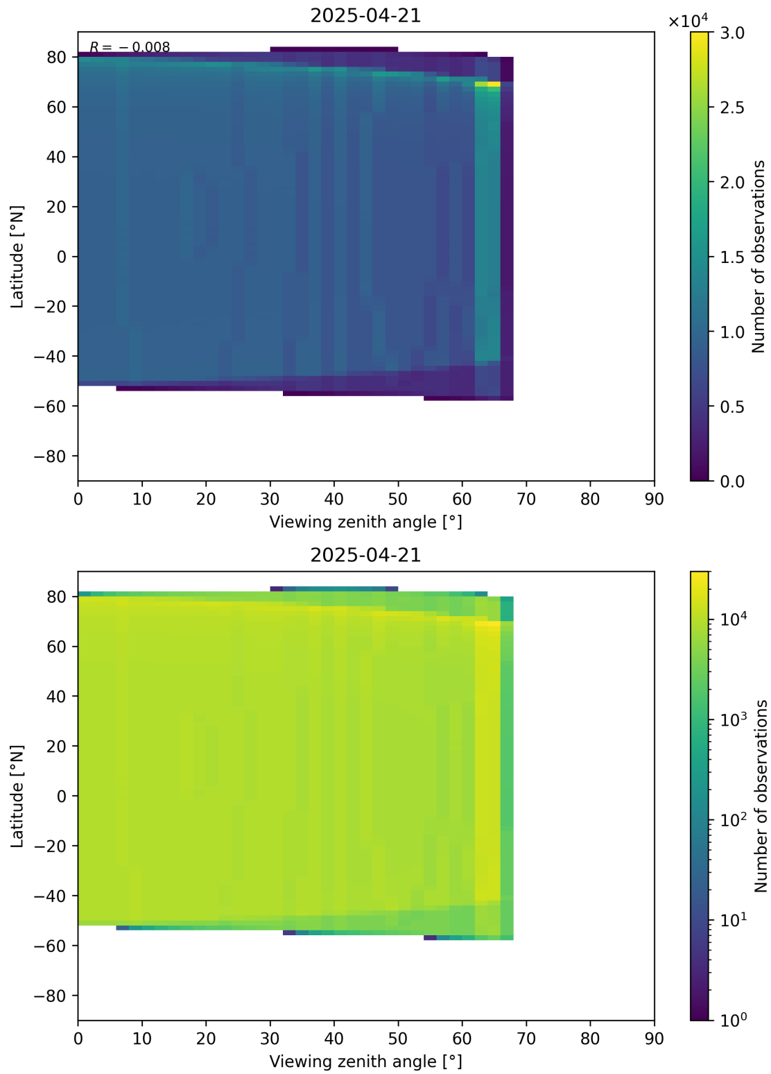
Figure 368: Scatter density plot of “Viewing zenith angle” against “Latitude” for 2025-04-20 to 2025-04-22.
