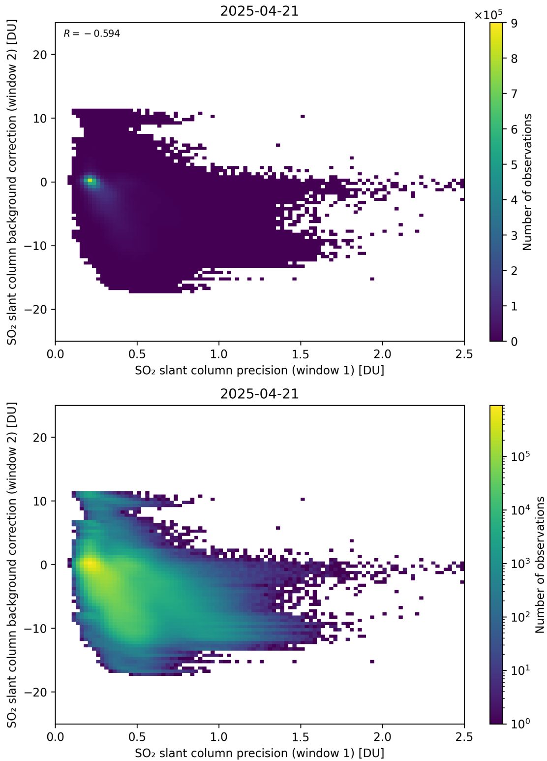
Figure 269: Scatter density plot of “SO 2 slant column precision (window 1)” against “SO 2 slant column background correction (window 2)” for 2025-04-20 to 2025-04-22.
