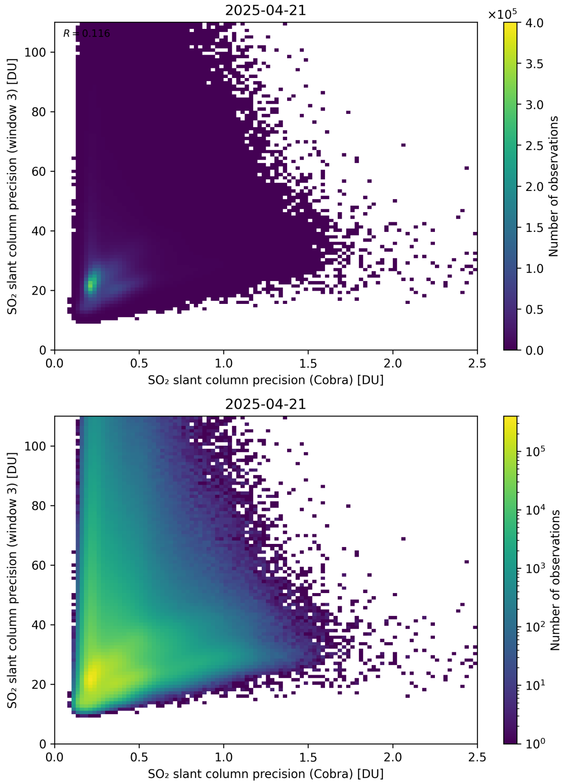
Figure 212: Scatter density plot of “SO 2 slant column precision (Cobra)” against “SO 2 slant column precision (window 3)” for 2025-04-20 to 2025-04-22.
