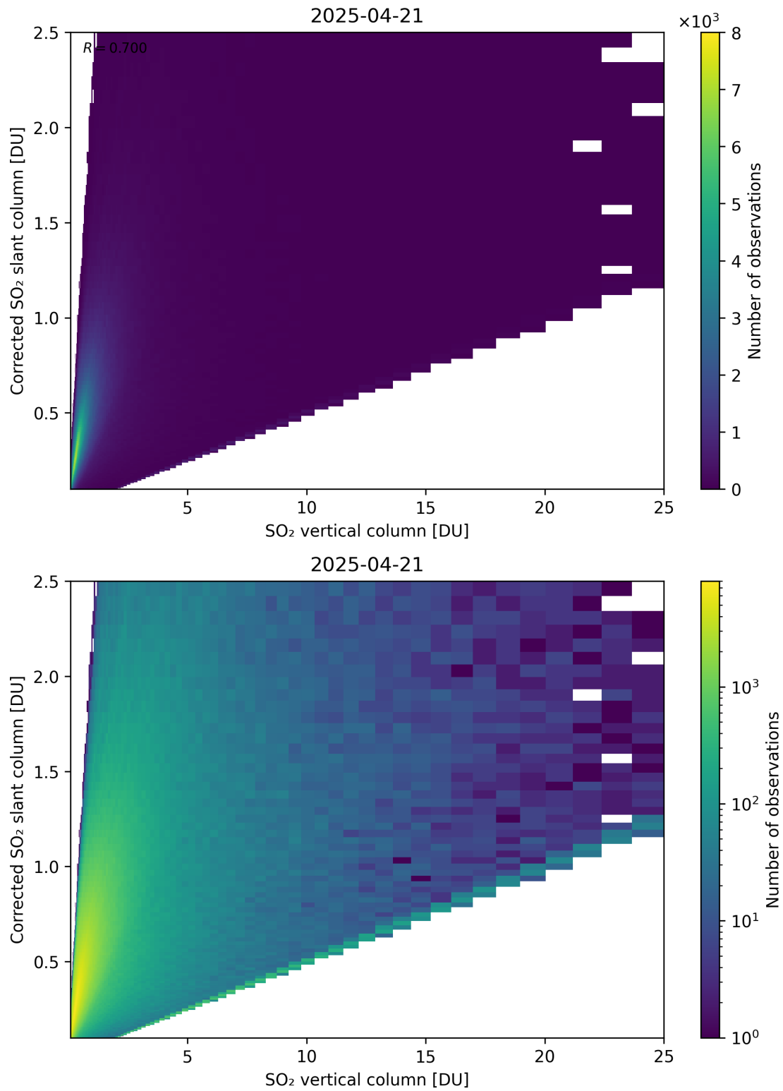
Figure 351: Scatter density plot of “SO 2 vertical column” against “Corrected SO 2 slant column” for 2025-04-20 to 2025-04-22.
