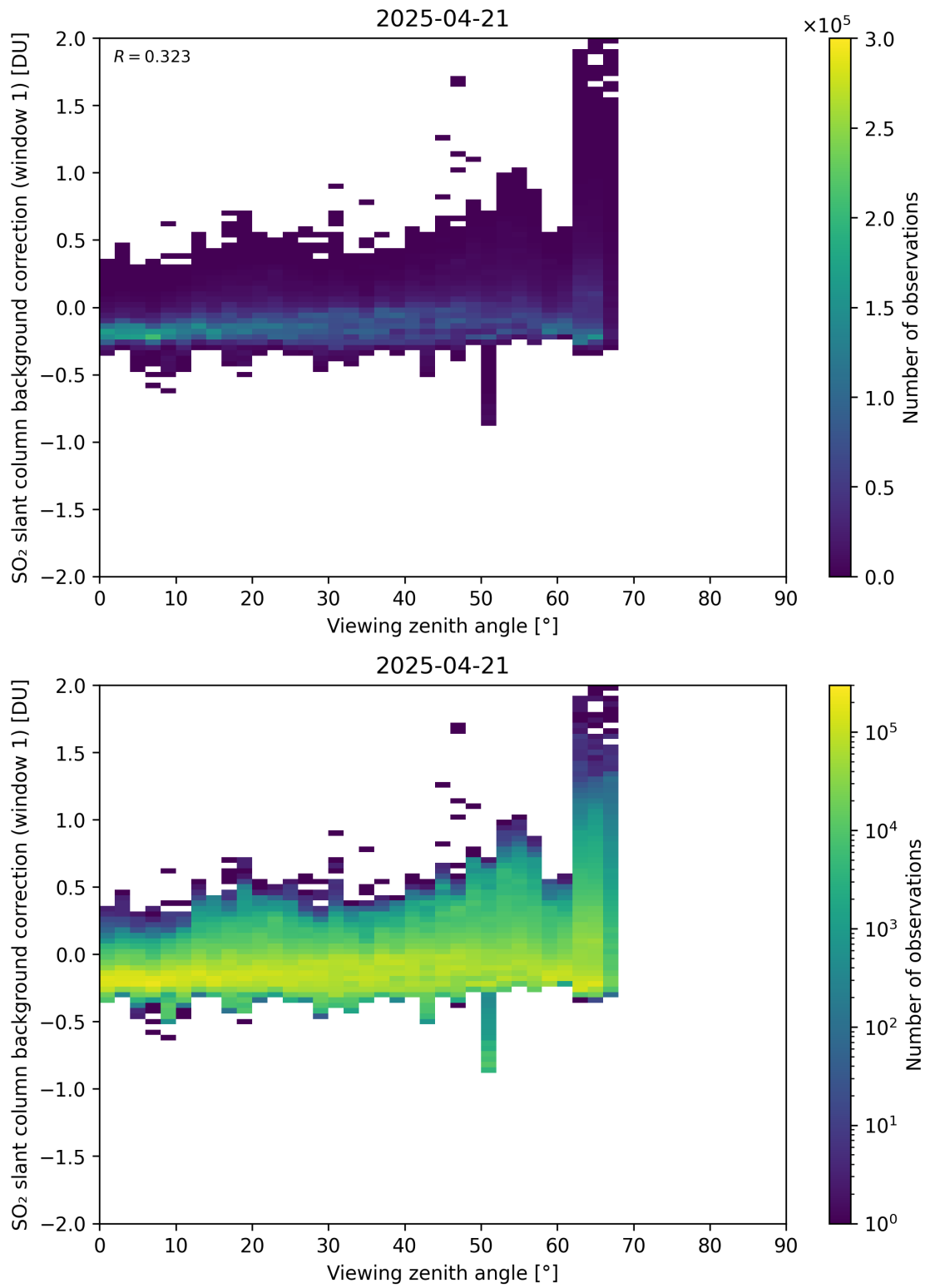
Figure 362: Scatter density plot of “Viewing zenith angle” against “SO 2 slant column background correction (window 1)” for 2025-04-20 to 2025-04-22.
