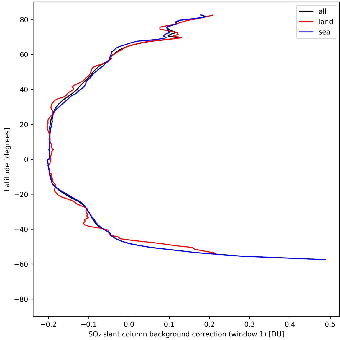
Figure 40: Zonal average of “SO 2 slant column background correction (window 1)” for 2025-04-20 to 2025-04-22.
