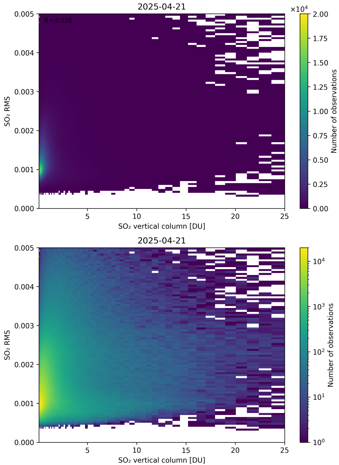
Figure 328: Scatter density plot of “SO 2 vertical column” against “SO 2 RMS” for 2025-04-20 to 2025-04-22.
