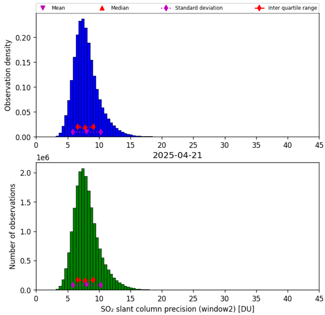
Figure 68: Histogram of “SO 2 slant column precision (window2)” for 2025-04-20 to 2025-04-22
