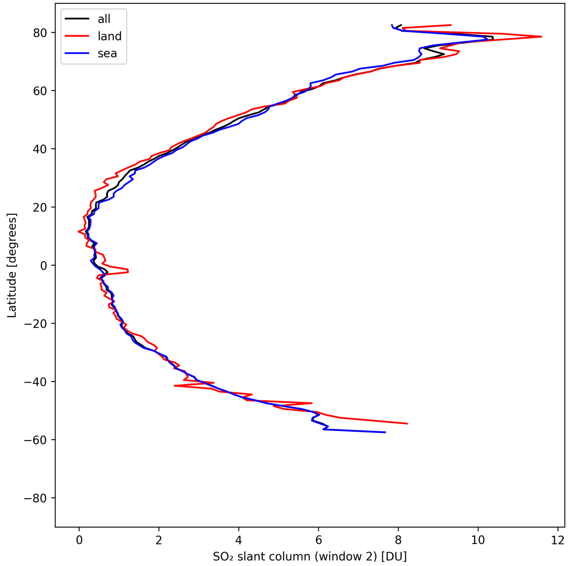
Figure 41: Zonal average of “SO 2 slant column (window 2)” for 2025-04-20 to 2025-04-22.
