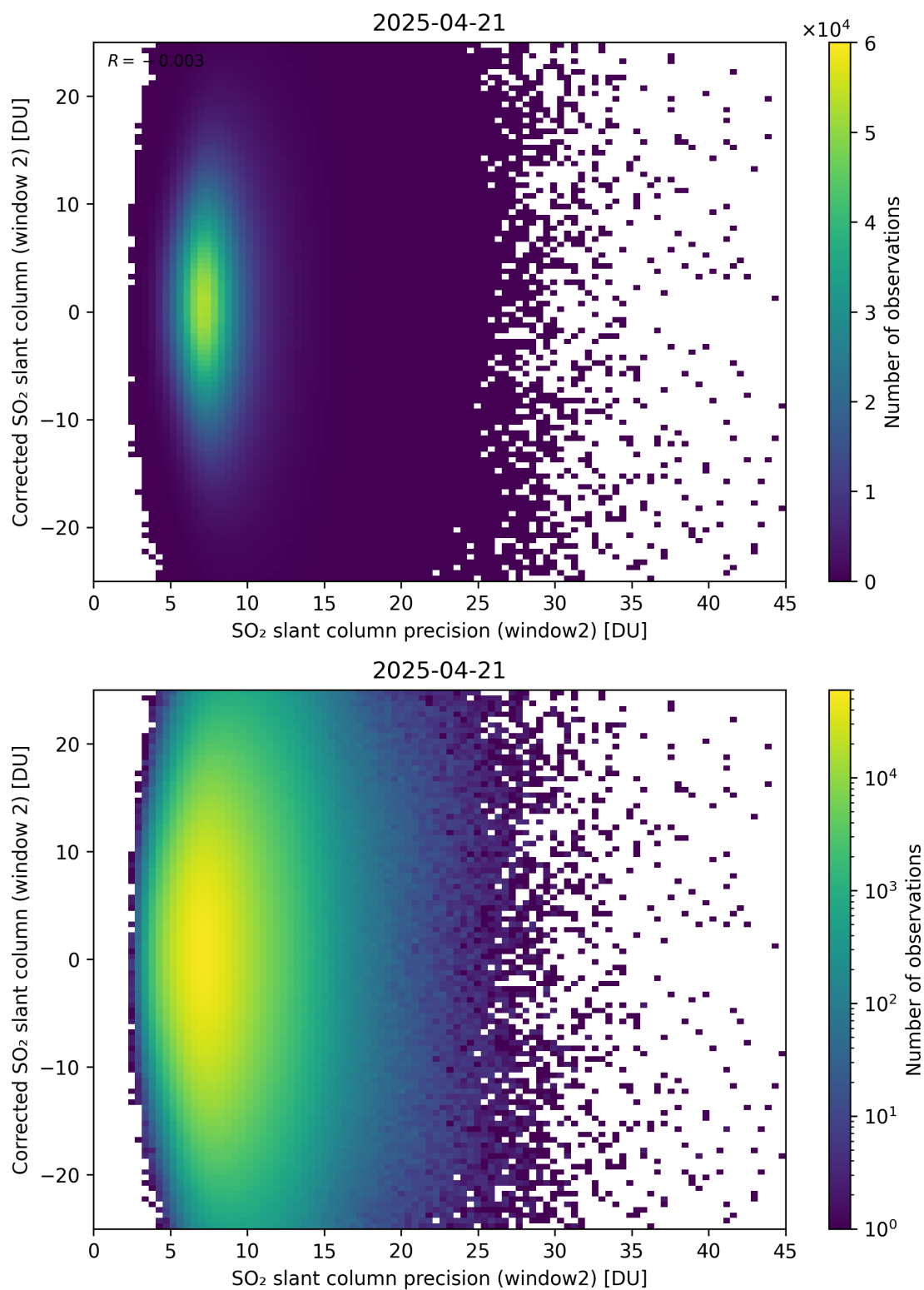
Figure 297: Scatter density plot of “SO 2 slant column precision (window2)” against “Corrected SO 2 slant column (window 2)” for 2025-04-20 to 2025-04-22.
