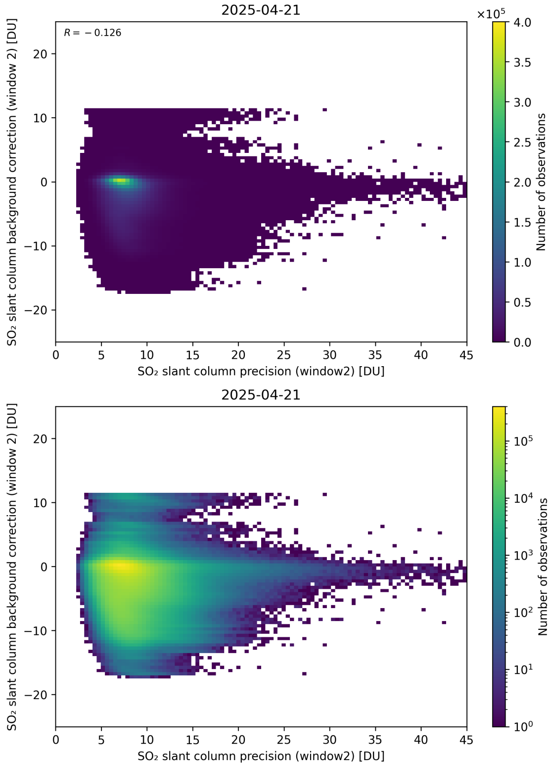
Figure 291: Scatter density plot of “SO 2 slant column precision (window2)” against “SO 2 slant column background correction (window 2)” for 2025-04-20 to 2025-04-22.
