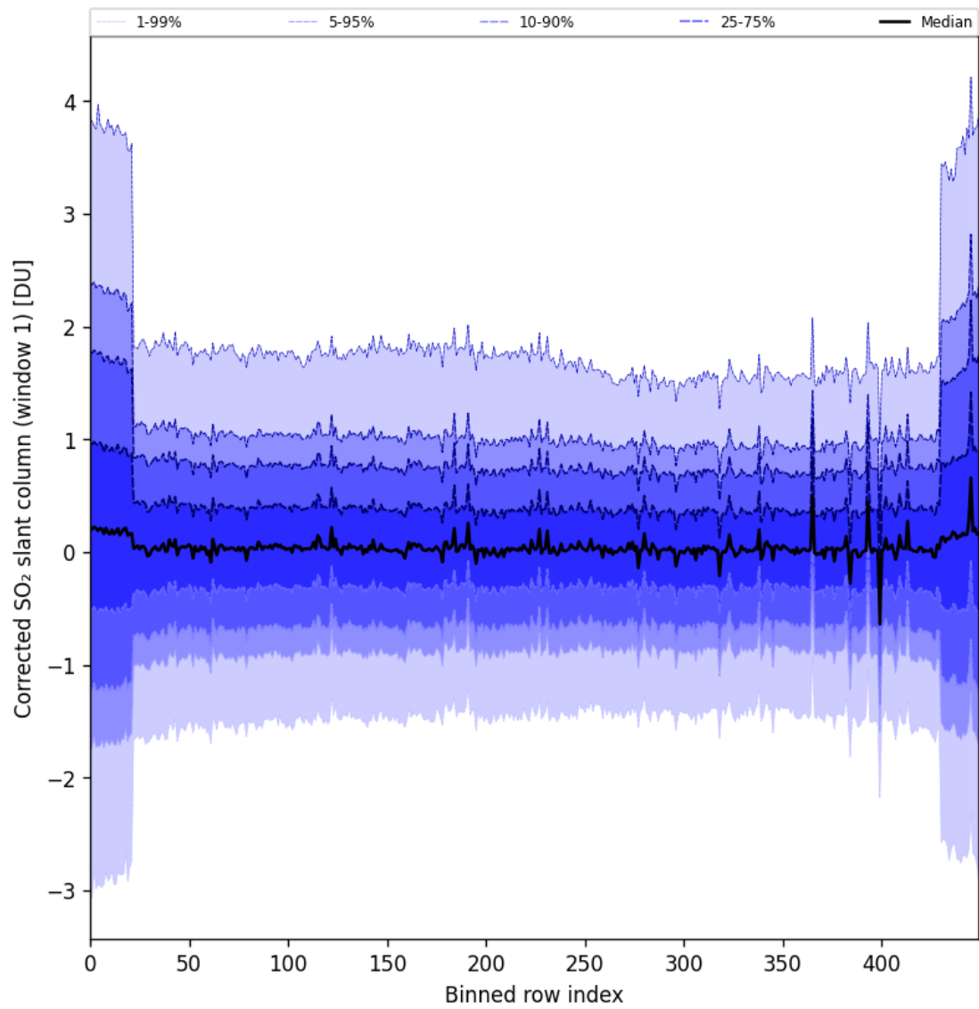
Figure 91: Along track statistics of “Corrected SO 2 slant column (window 1)” for 2025-04-20 to 2025-04-22
