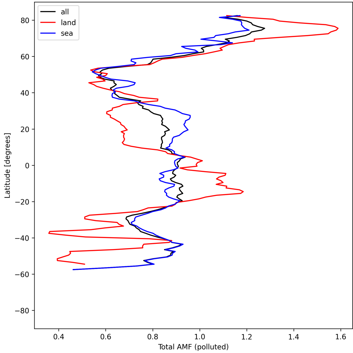
Figure 53: Zonal average of “Total AMF (polluted)” for 2025-04-20 to 2025-04-22.
