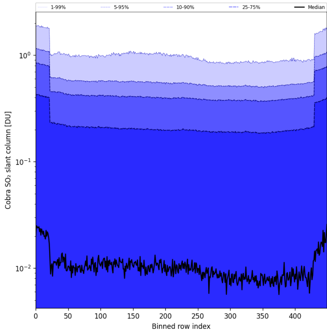
Figure 87: Along track statistics of “Cobra SO 2 slant column” for 2025-04-20 to 2025-04-22
