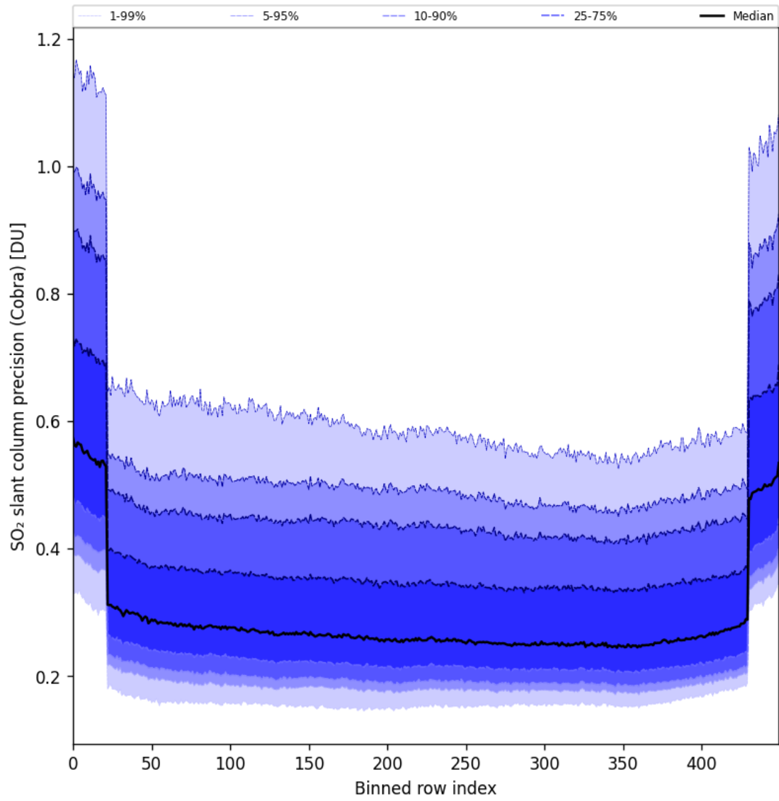
Figure 88: Along track statistics of “SO 2 slant column precision (Cobra)” for 2025-04-20 to 2025-04-22
