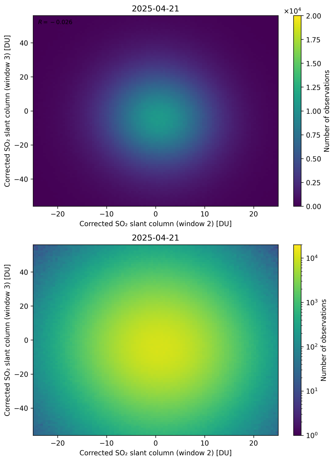
Figure 250: Scatter density plot of “Corrected SO 2 slant column (window 2)” against “Corrected SO 2 slant column (window 3)” for 2025-04-20 to 2025-04-22.
