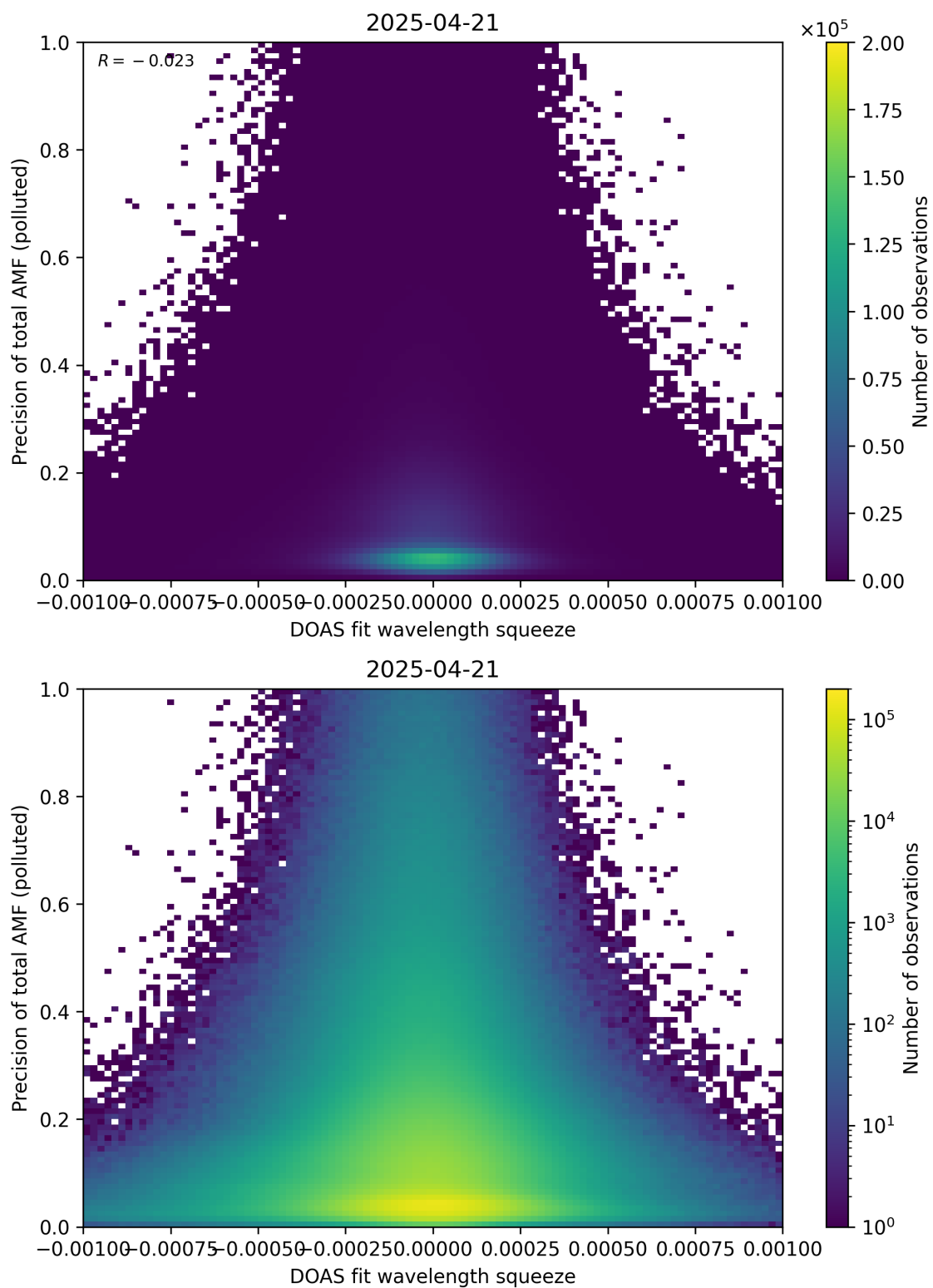
Figure 146: Scatter density plot of “DOAS fit wavelength squeeze” against “Precision of total AMF (polluted)” for 2025-04-20 to 2025-04-22.
