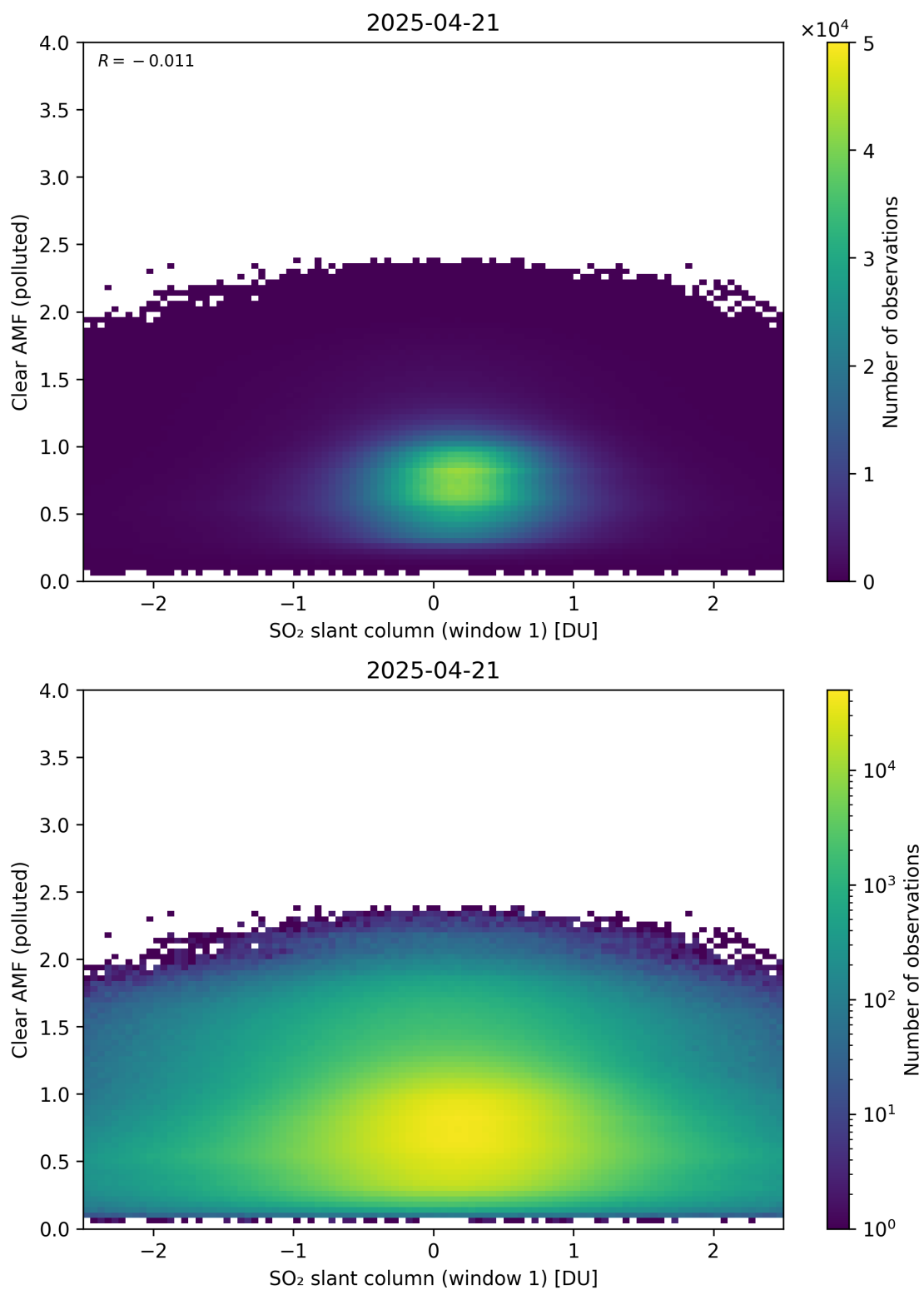
Figure 282: Scatter density plot of “SO 2 slant column (window 1)” against “Clear AMF (polluted)” for 2025-04-20 to 2025-04-22.
