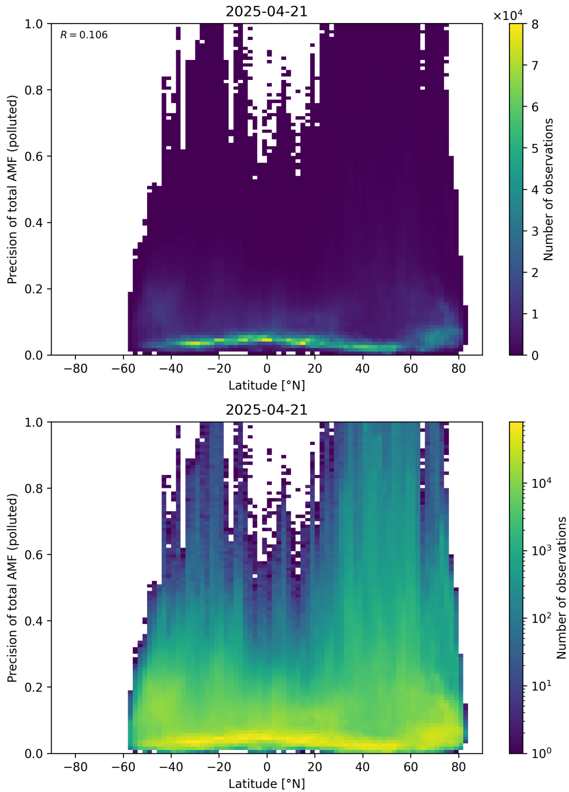
Figure 168: Scatter density plot of “Latitude” against “Precision of total AMF (polluted)” for 2025-04-20 to 2025-04-22.
