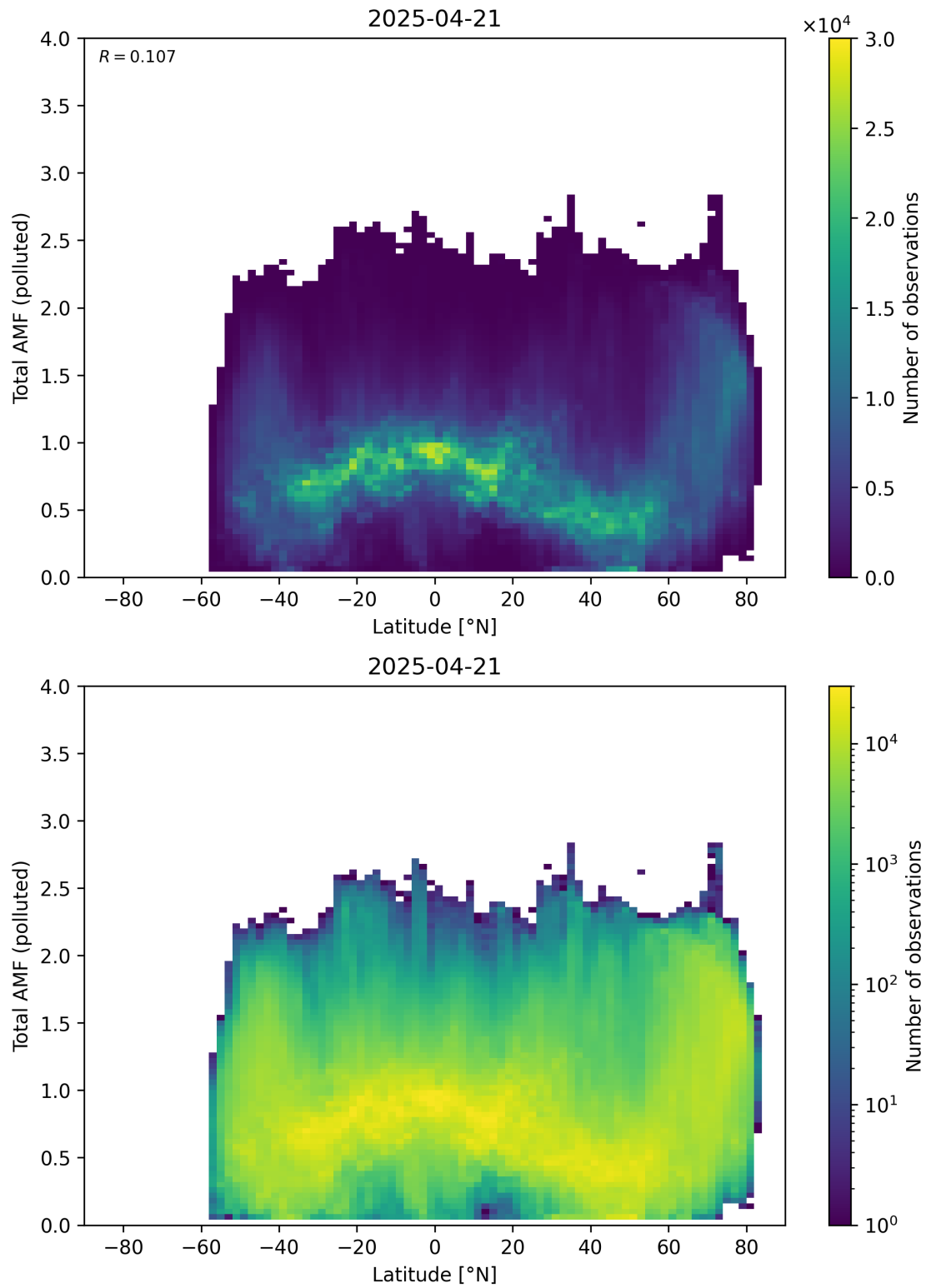
Figure 167: Scatter density plot of “Latitude” against “Total AMF (polluted)” for 2025-04-20 to 2025-04-22.
