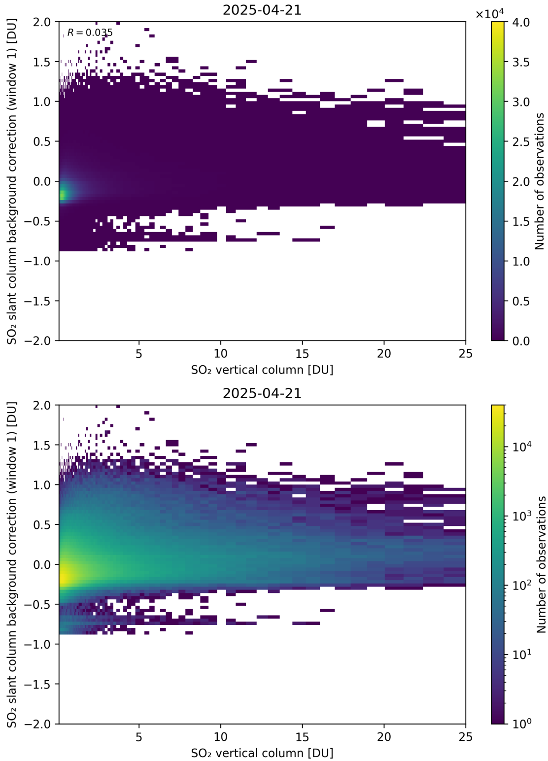
Figure 323: Scatter density plot of “SO 2 vertical column” against “SO 2 slant column background correction (window 1)” for 2025-04-20 to 2025-04-22.
