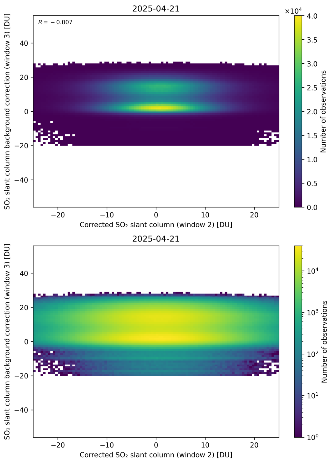
Figure 245: Scatter density plot of “Corrected SO 2 slant column (window 2)” against “SO 2 slant column background correction (window 3)” for 2025-04-20 to 2025-04-22.
