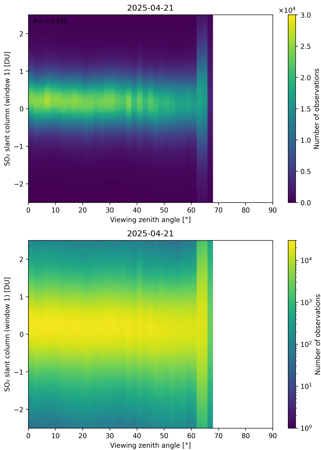
Figure 376: Scatter density plot of “Viewing zenith angle” against “SO 2 slant column (window 1)” for 2025-04-20 to 2025-04-22.
