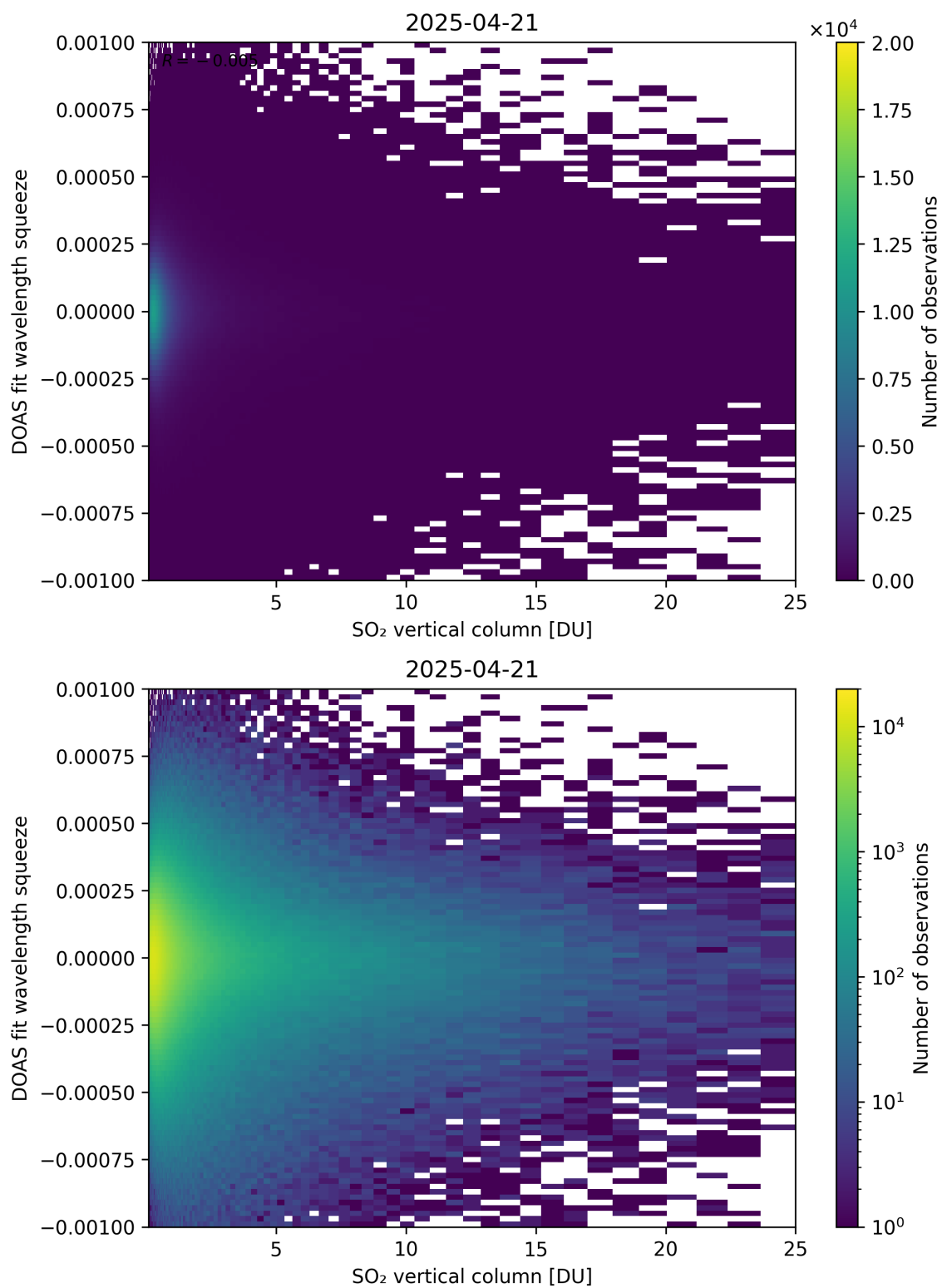
Figure 327: Scatter density plot of “SO 2 vertical column” against “DOAS fit wavelength squeeze” for 2025-04-20 to 2025-04-22.
