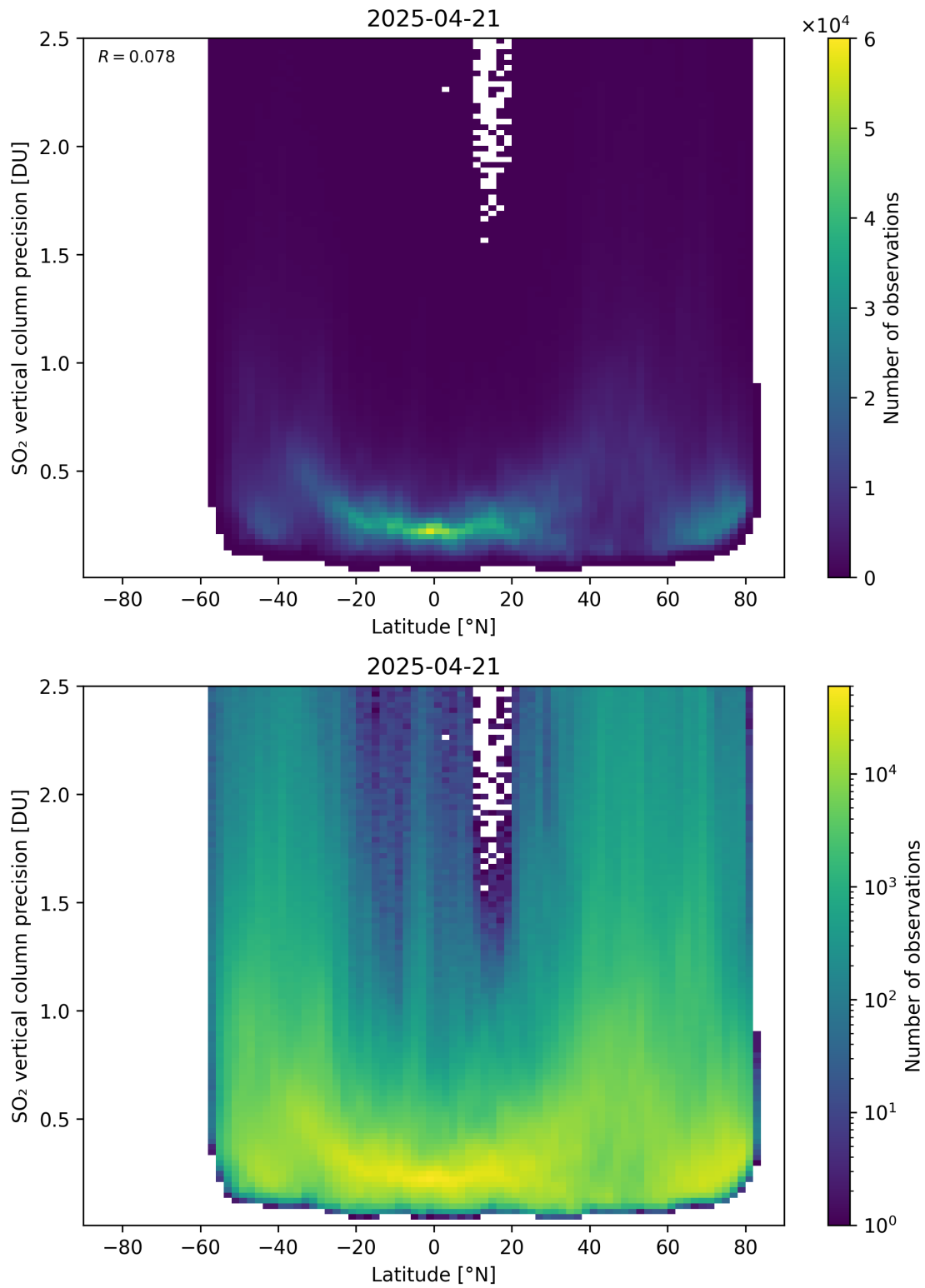
Figure 170: Scatter density plot of “Latitude” against “SO 2 vertical column precision” for 2025-04-20 to 2025-04-22.
