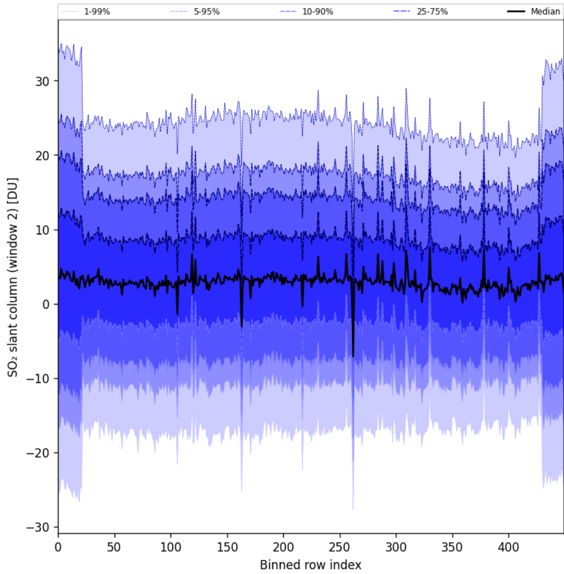
Figure 93: Along track statistics of “SO 2 slant column (window 2)” for 2025-04-20 to 2025-04-22
