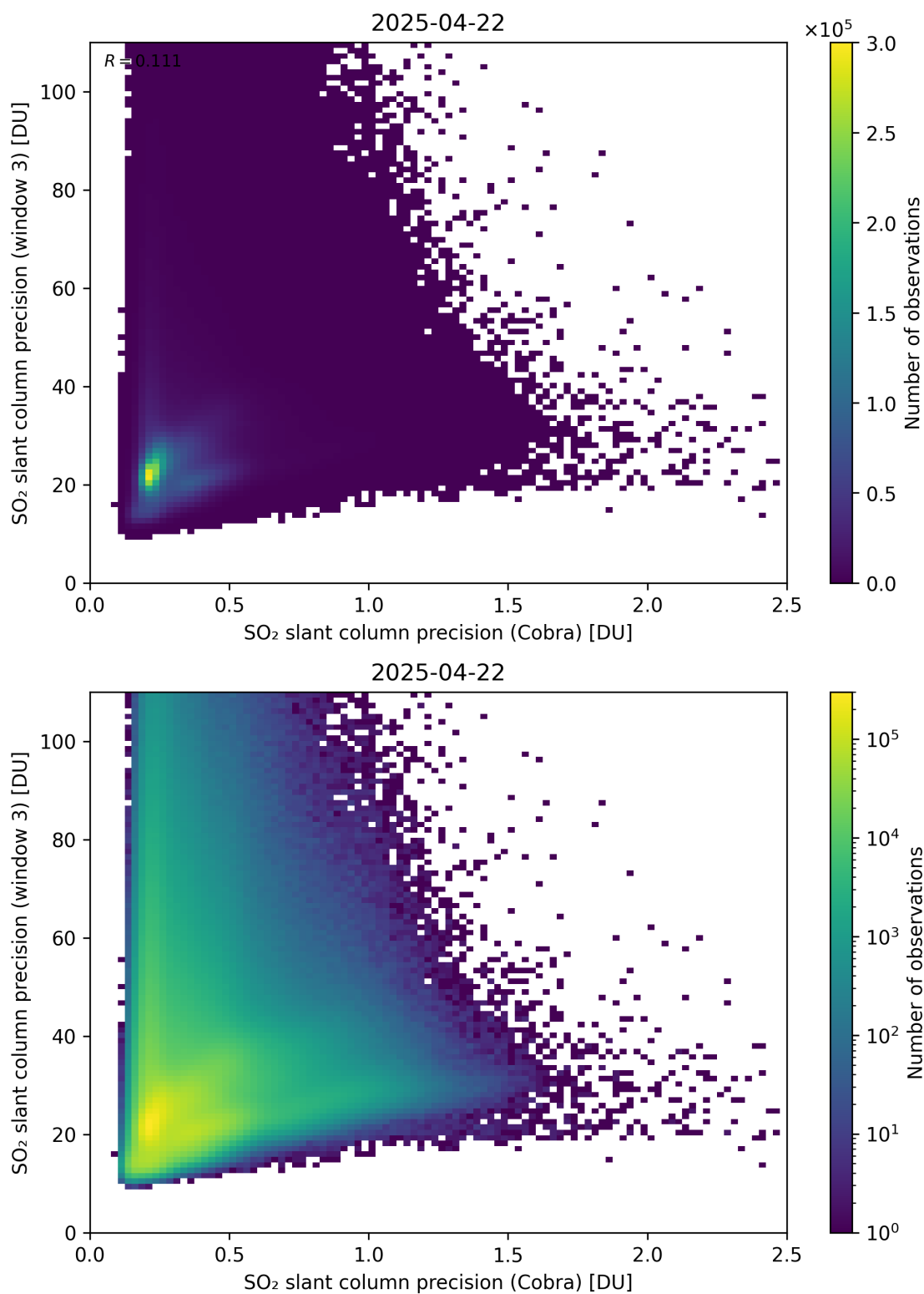
Figure 212: Scatter density plot of “SO 2 slant column precision (Cobra)” against “SO 2 slant column precision (window 3)” for 2025-04-21 to 2025-04-23.
