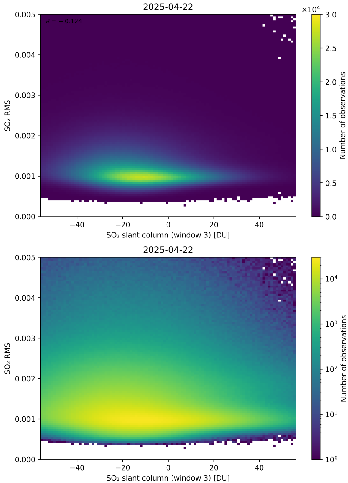
Figure 306: Scatter density plot of “SO 2 slant column (window 3)” against “SO 2 RMS” for 2025-04-21 to 2025-04-23.
