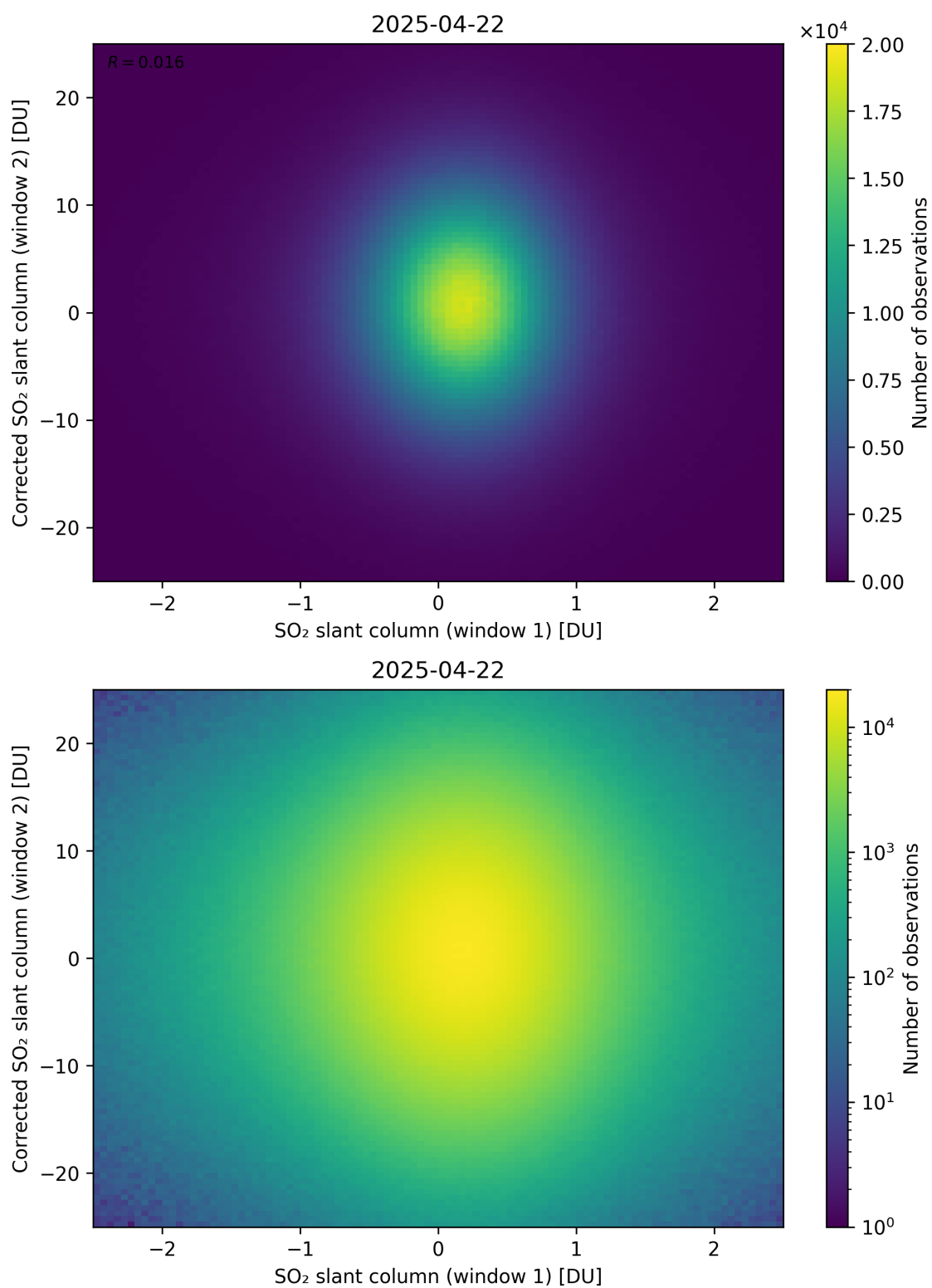
Figure 283: Scatter density plot of “SO 2 slant column (window 1)” against “Corrected SO 2 slant column (window 2)” for 2025-04-21 to 2025-04-23.
