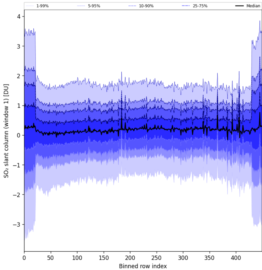
Figure 89: Along track statistics of "SO 2 slant column (window 1)" for 2025-04-21 to 2025-04-23
