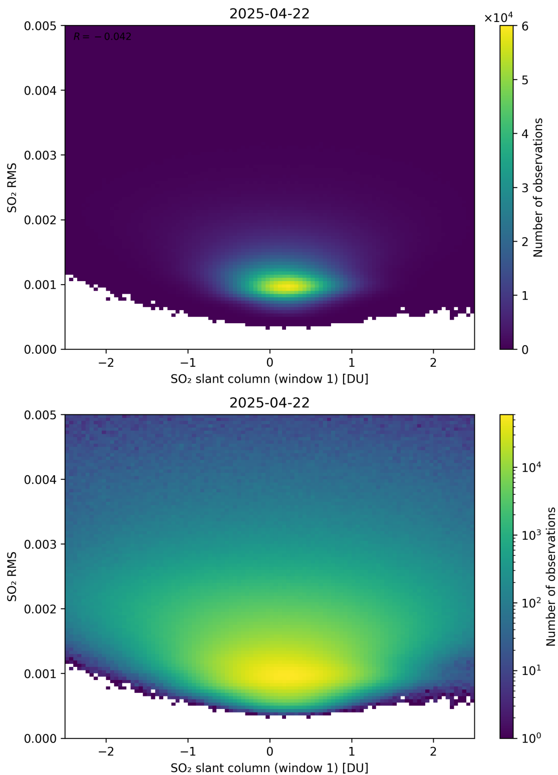
Figure 267: Scatter density plot of “SO 2 slant column (window 1)” against “SO 2 RMS” for 2025-04-21 to 2025-04-23.
