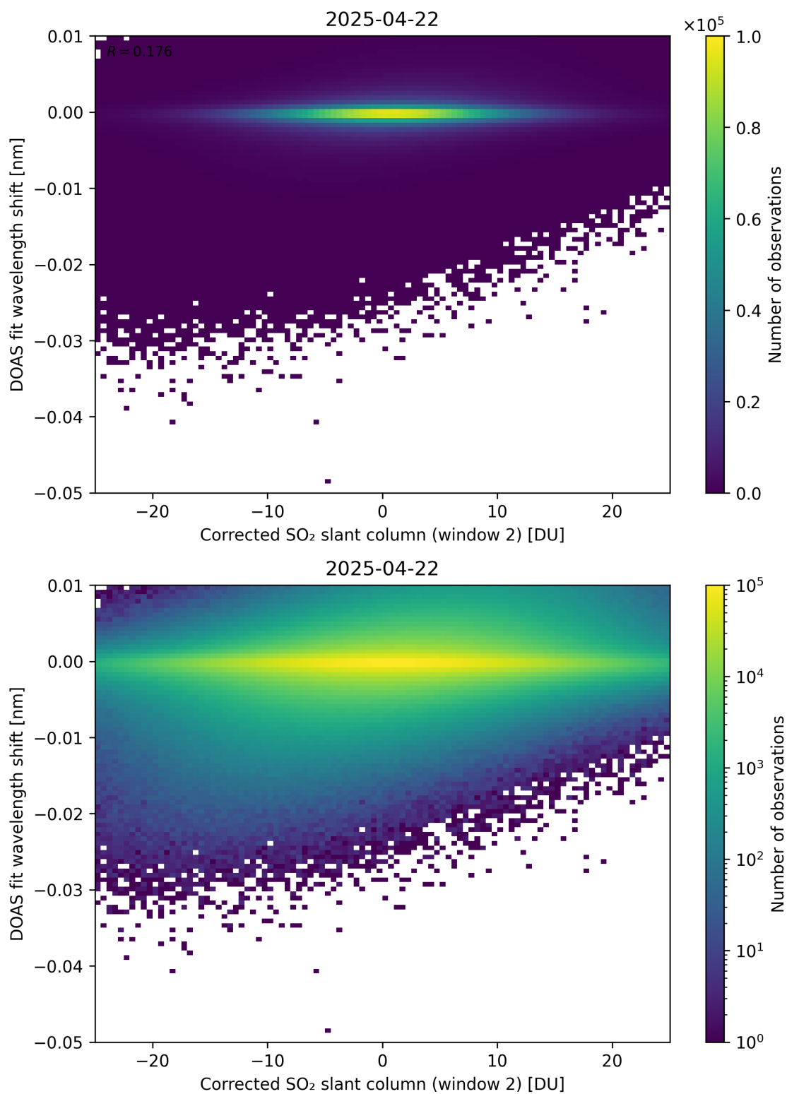
Figure 246: Scatter density plot of “Corrected SO 2 slant column (window 2)” against “DOAS fit wavelength shift” for 2025-04-21 to 2025-04-23.
