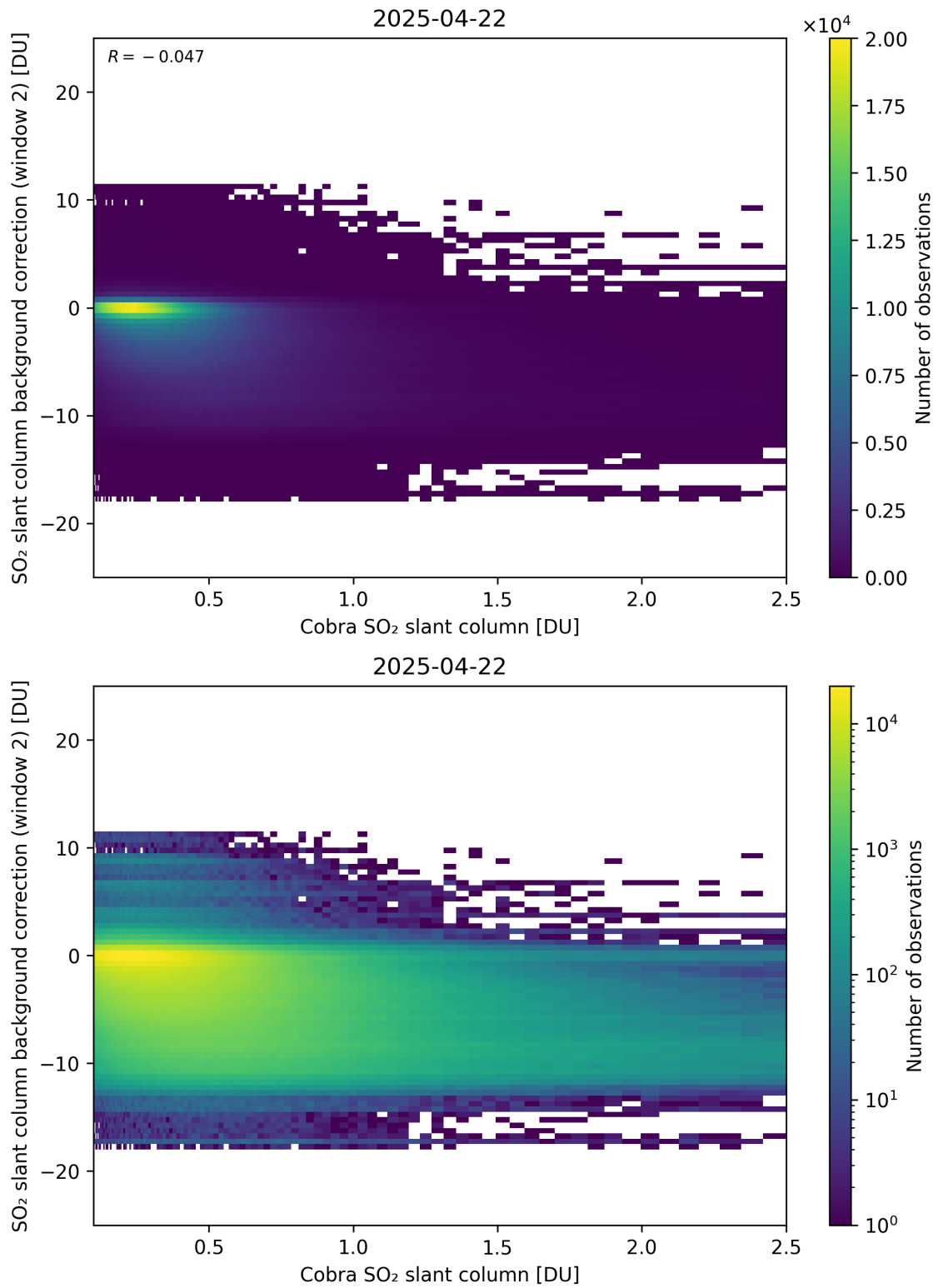
Figure 194: Scatter density plot of “Cobra SO 2 slant column” against “SO 2 slant column background correction (window 2)” for 2025-04-21 to 2025-04-23.
