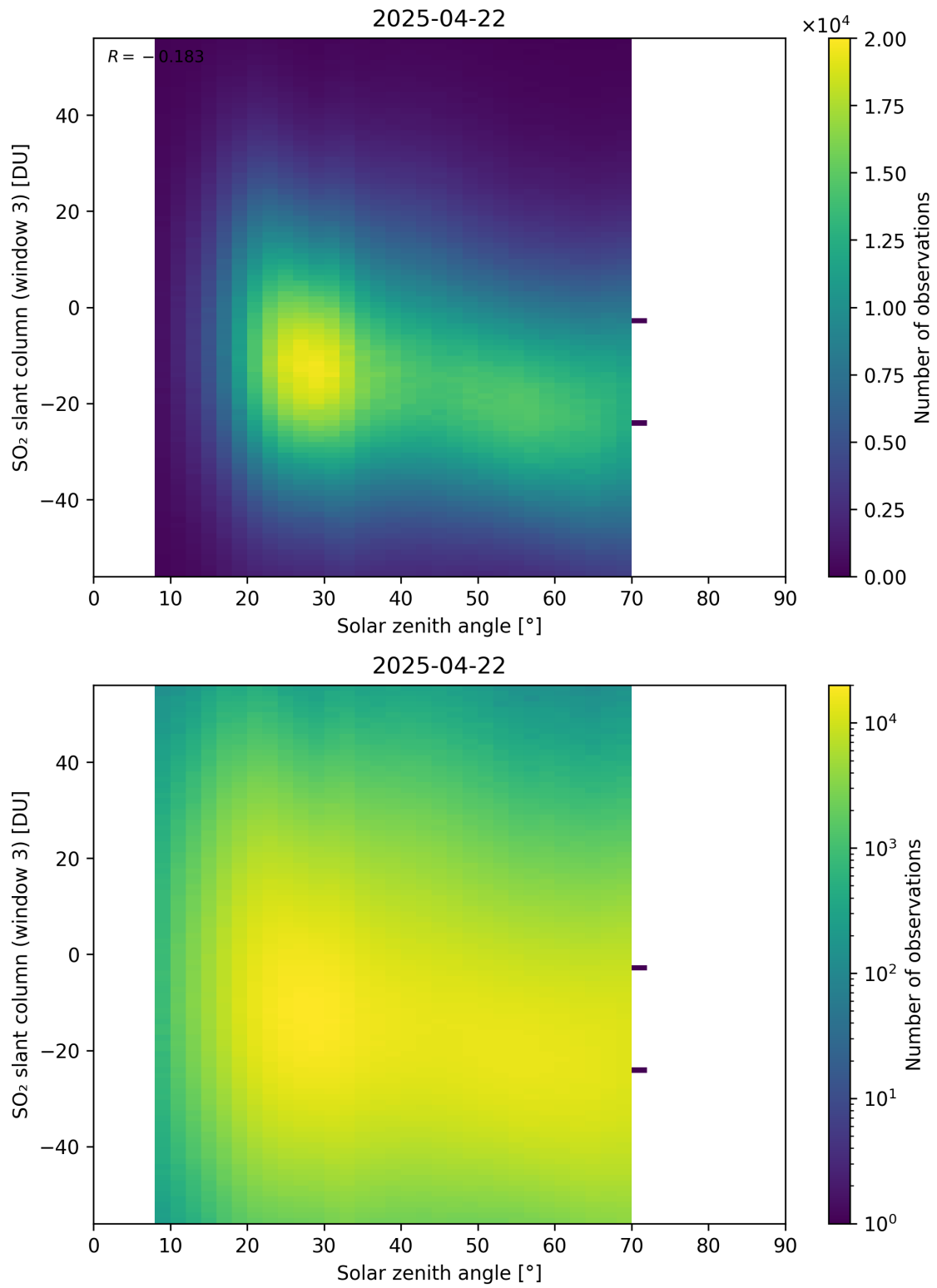
Figure 187: Scatter density plot of “Solar zenith angle” against “SO 2 slant column (window 3)” for 2025-04-21 to 2025-04-23.
