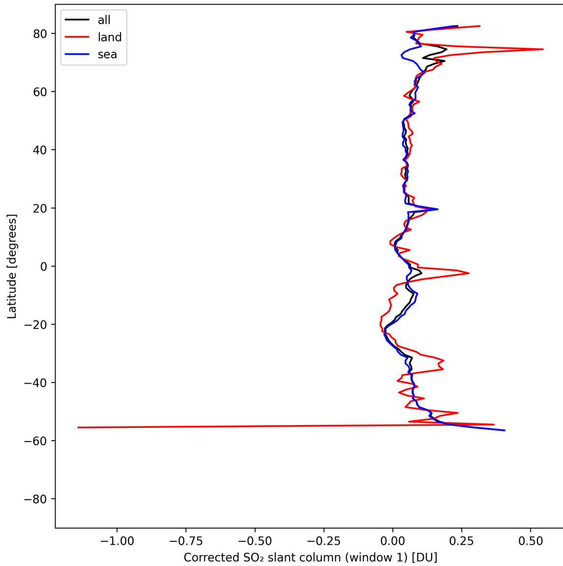
Figure 39: Zonal average of “Corrected SO 2 slant column (window 1)” for 2025-04-21 to 2025-04-23.
