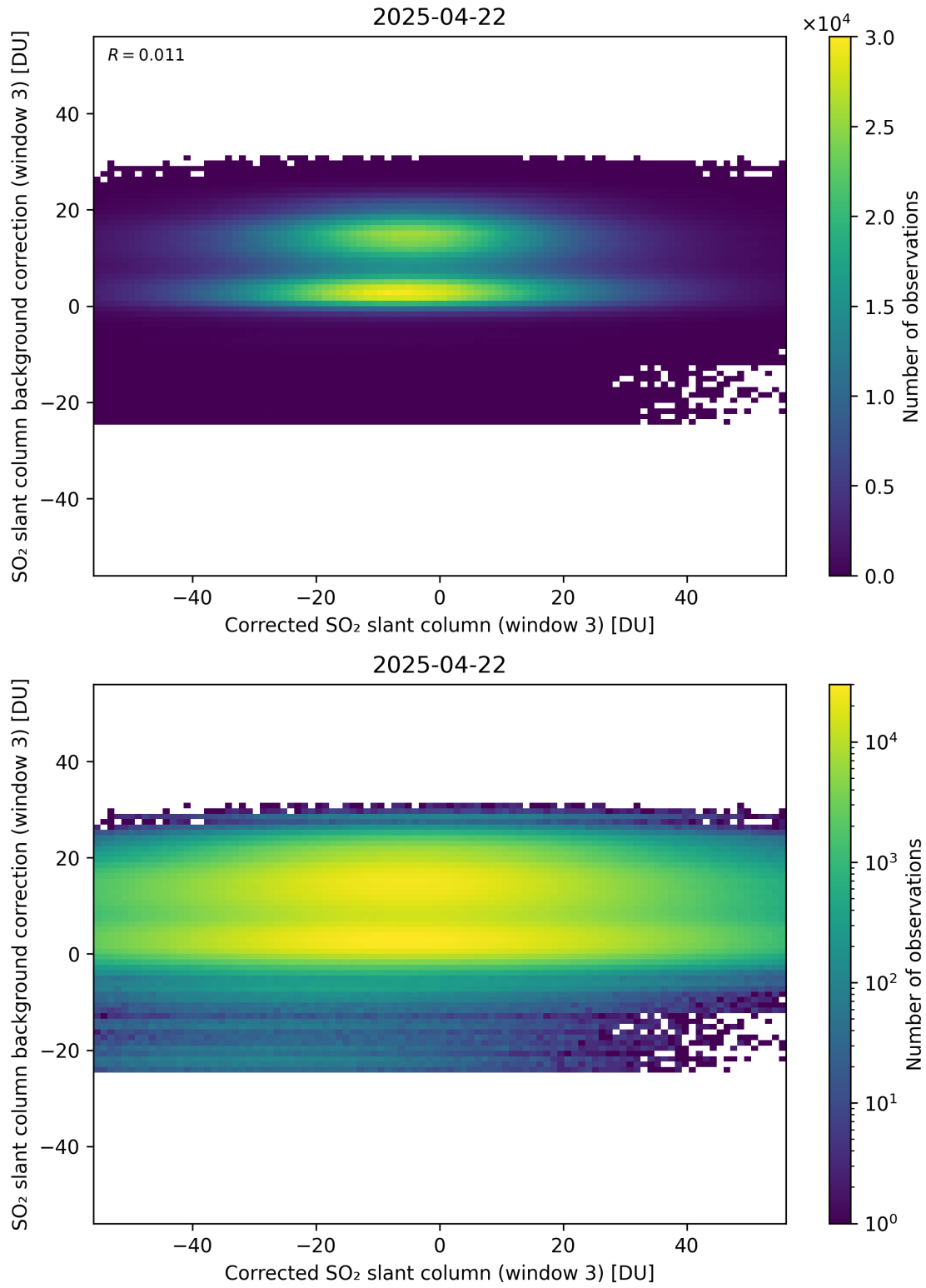
Figure 255: Scatter density plot of “Corrected SO 2 slant column (window 3)” against “SO 2 slant column background correction (window 3)” for 2025-04-21 to 2025-04-23.
