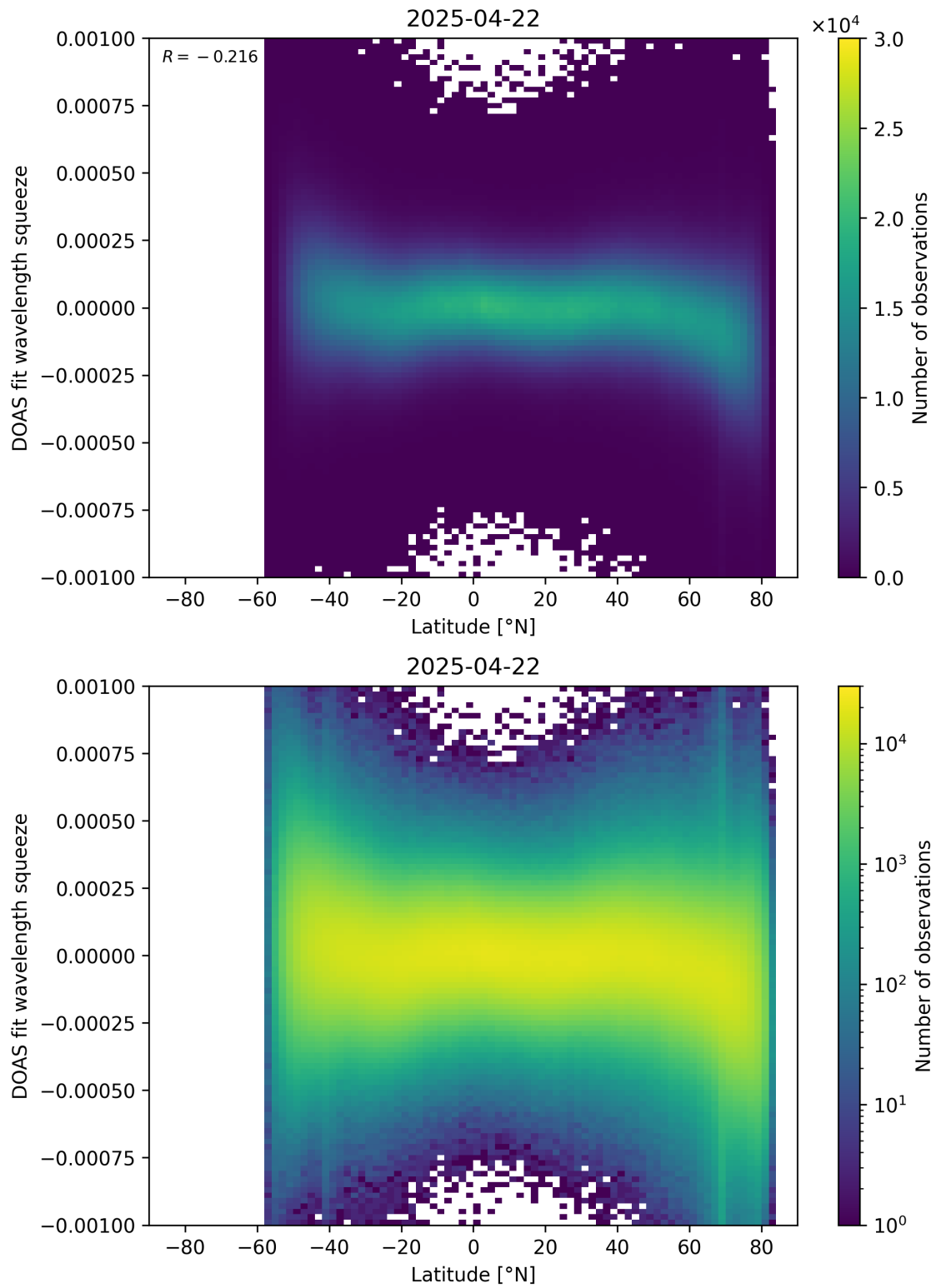
Figure 154: Scatter density plot of “Latitude” against “DOAS fit wavelength squeeze” for 2025-04-21 to 2025-04-23.
