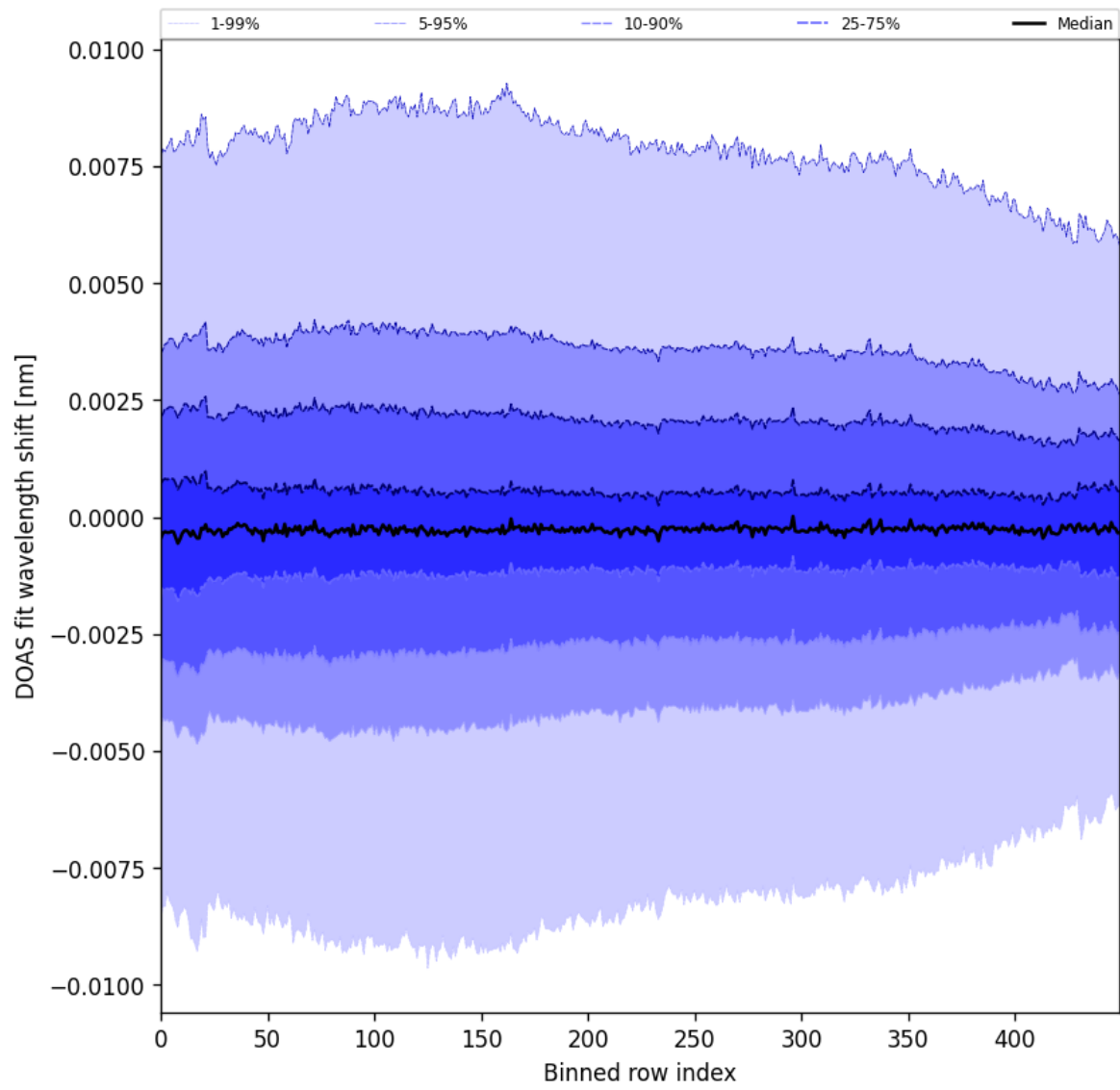
Figure 102: Along track statistics of “DOAS fit wavelength shift” for 2025-04-21 to 2025-04-23
