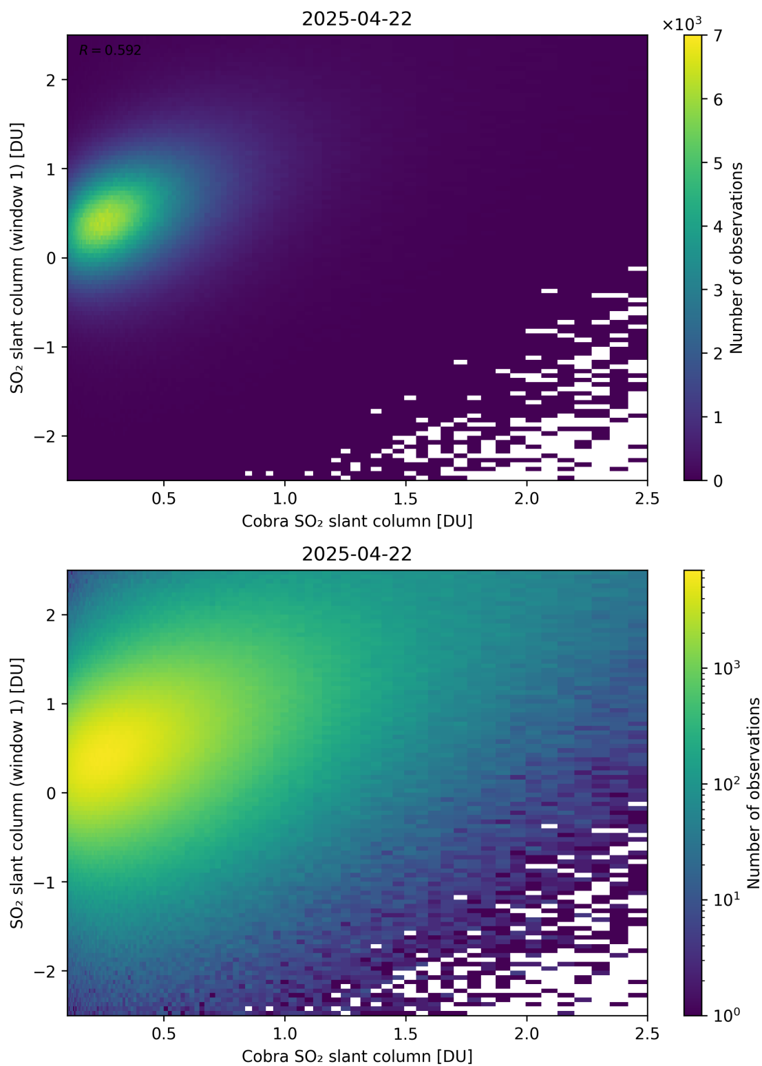
Figure 219: Scatter density plot of “Cobra SO 2 slant column” against “SO 2 slant column (window 1)” for 2025-04-21 to 2025-04-23.
