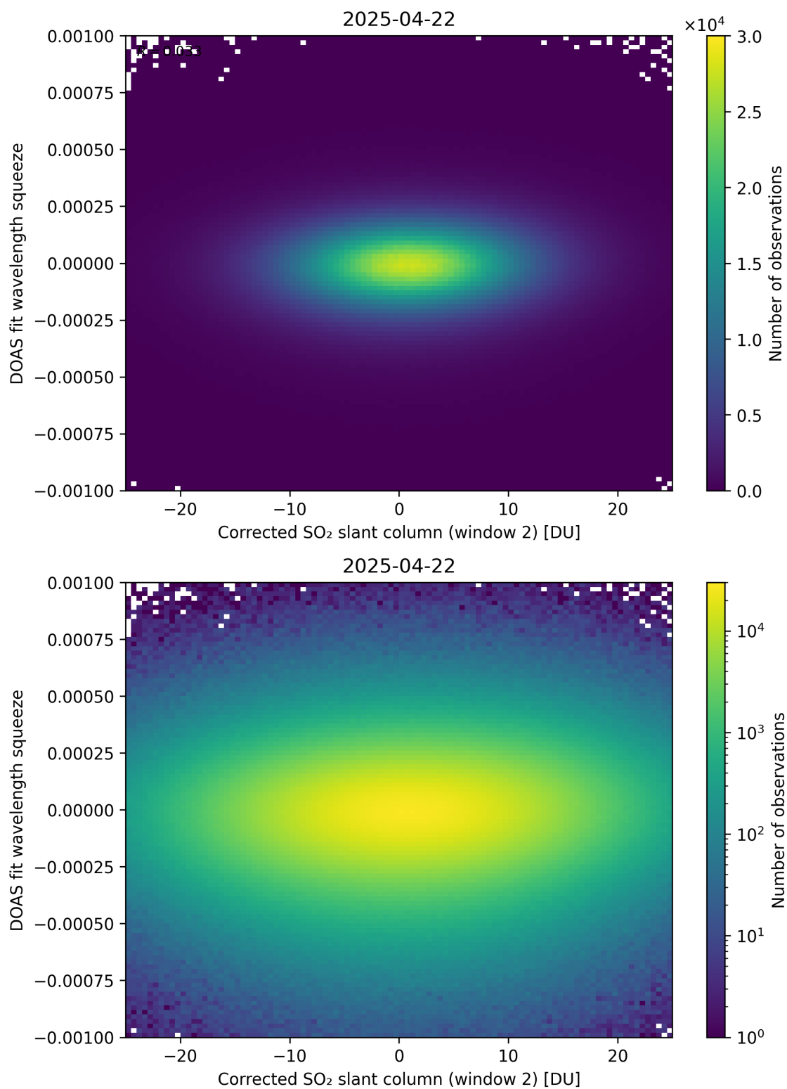
Figure 247: Scatter density plot of “Corrected SO 2 slant column (window 2)” against “DOAS fit wavelength squeeze” for 2025-04-21 to 2025-04-23.
