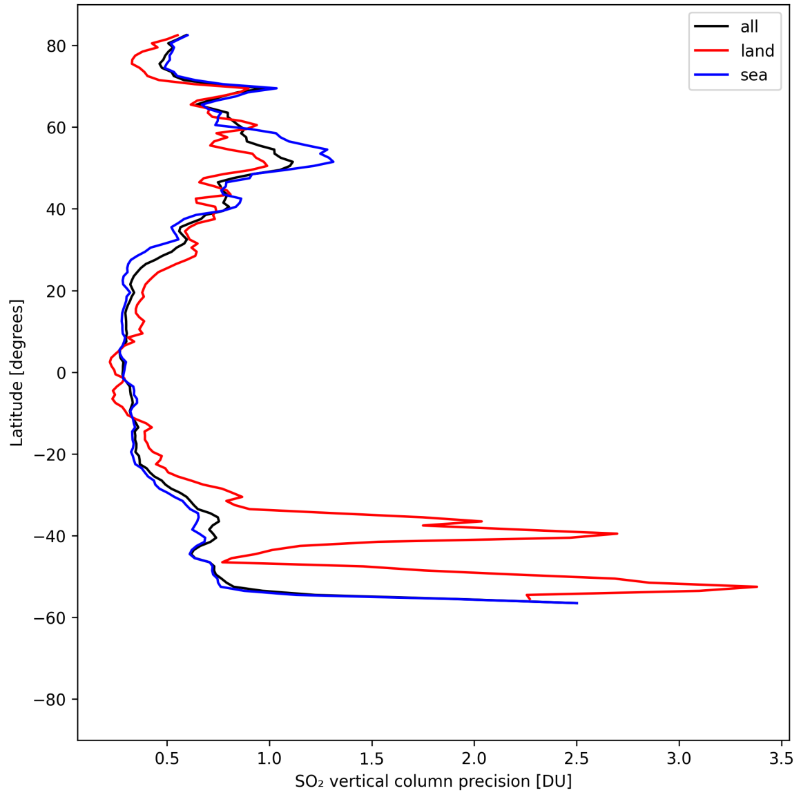
Figure 33: Zonal average of “SO 2 vertical column precision” for 2025-04-21 to 2025-04-23.
