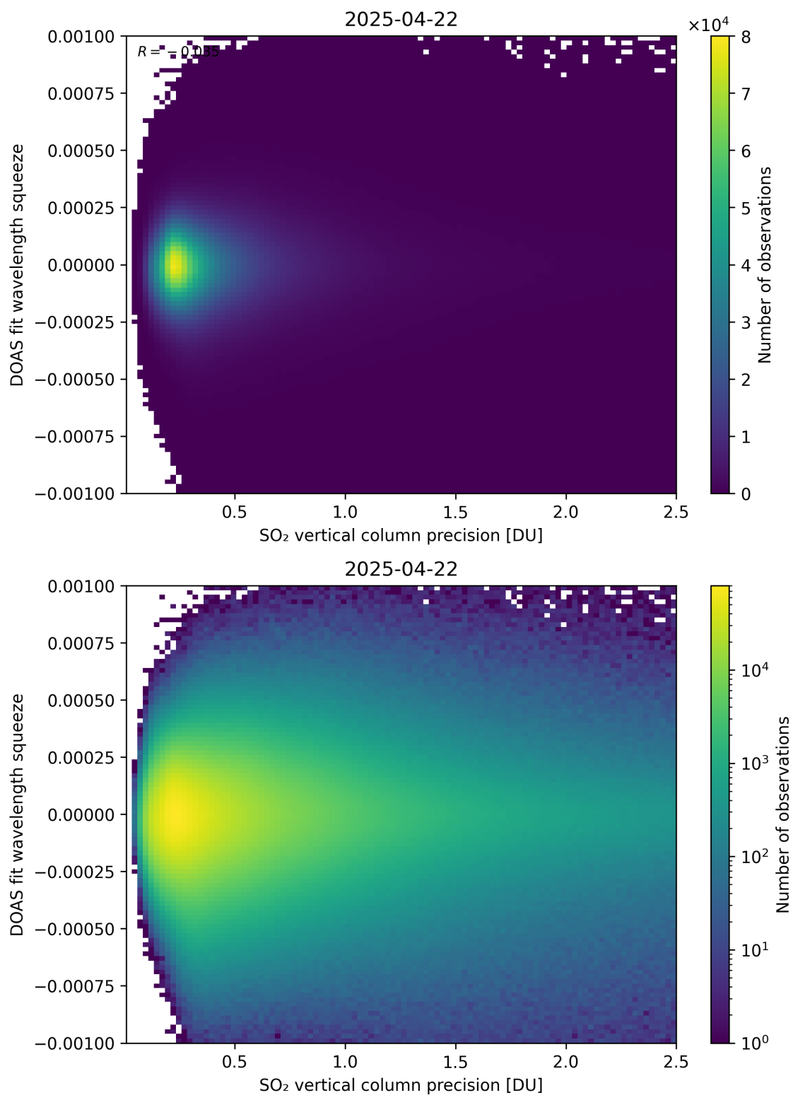
Figure 333: Scatter density plot of “SO 2 vertical column precision” against “DOAS fit wavelength squeeze” for 2025-04-21 to 2025-04-23.
