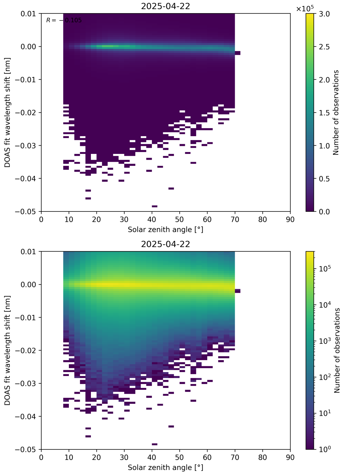
Figure 174: Scatter density plot of “Solar zenith angle” against “DOAS fit wavelength shift” for 2025-04-21 to 2025-04-23.
