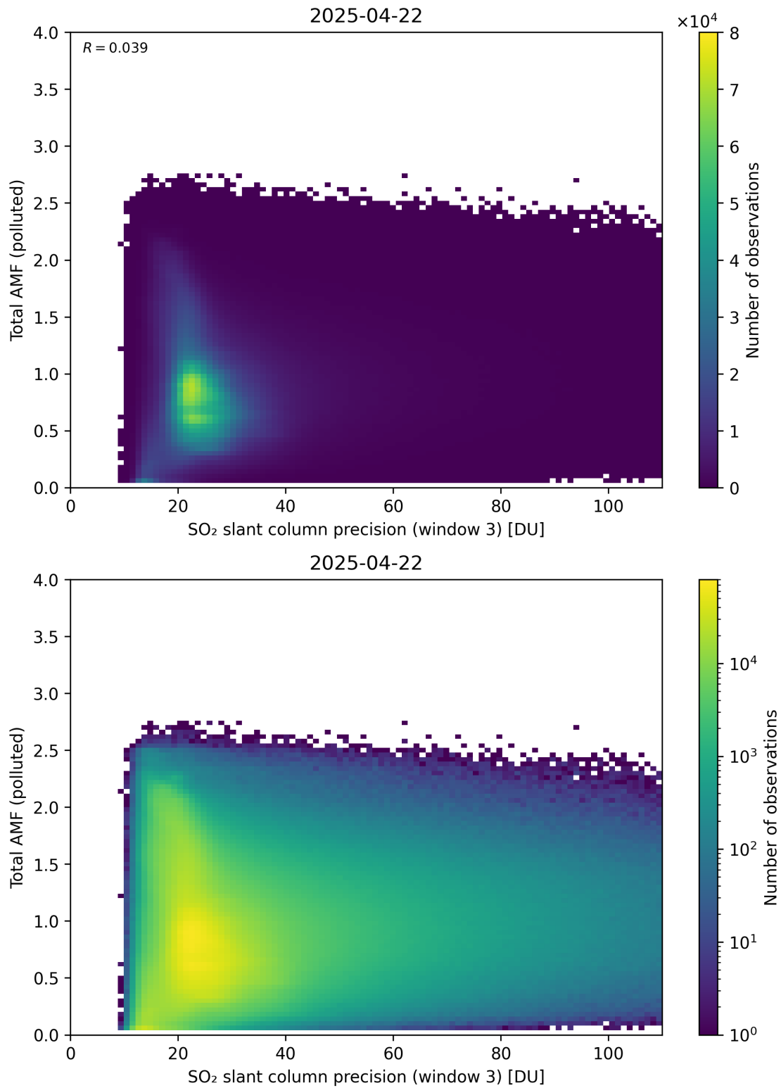
Figure 313: Scatter density plot of “SO 2 slant column precision (window 3)” against “Total AMF (polluted)” for 2025-04-21 to 2025-04-23.
