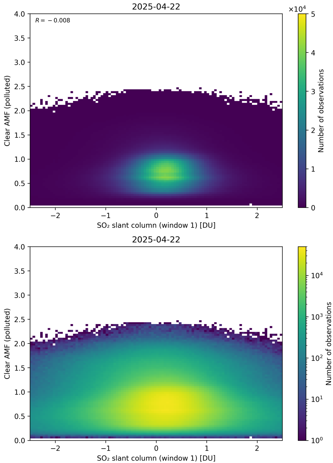
Figure 282: Scatter density plot of “SO 2 slant column (window 1)” against “Clear AMF (polluted)” for 2025-04-21 to 2025-04-23.
