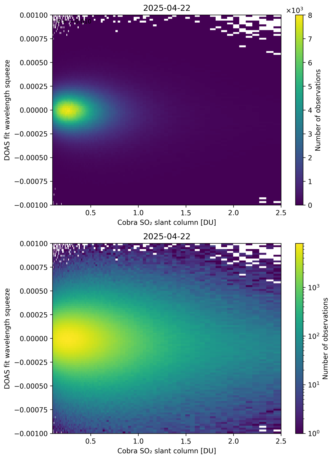
Figure 197: Scatter density plot of “Cobra SO 2 slant column” against “DOAS fit wavelength squeeze” for 2025-04-21 to 2025-04-23.
