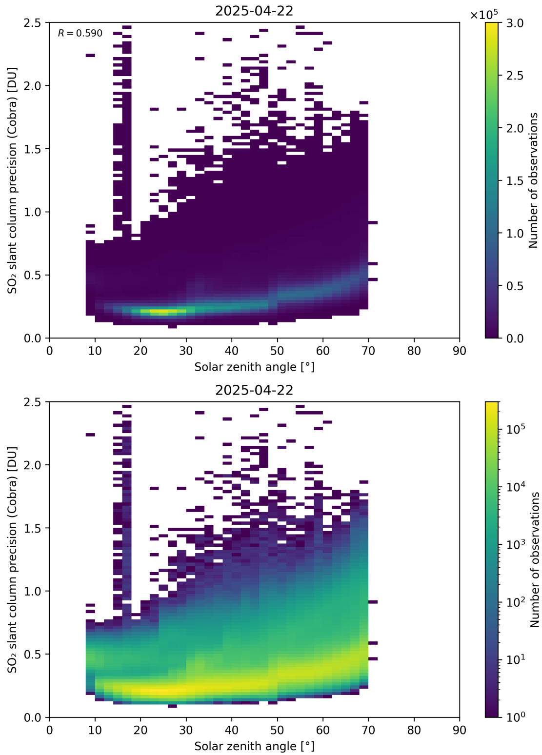
Figure 180: Scatter density plot of “Solar zenith angle” against “SO 2 slant column precision (Cobra)” for 2025-04-21 to 2025-04-23.
