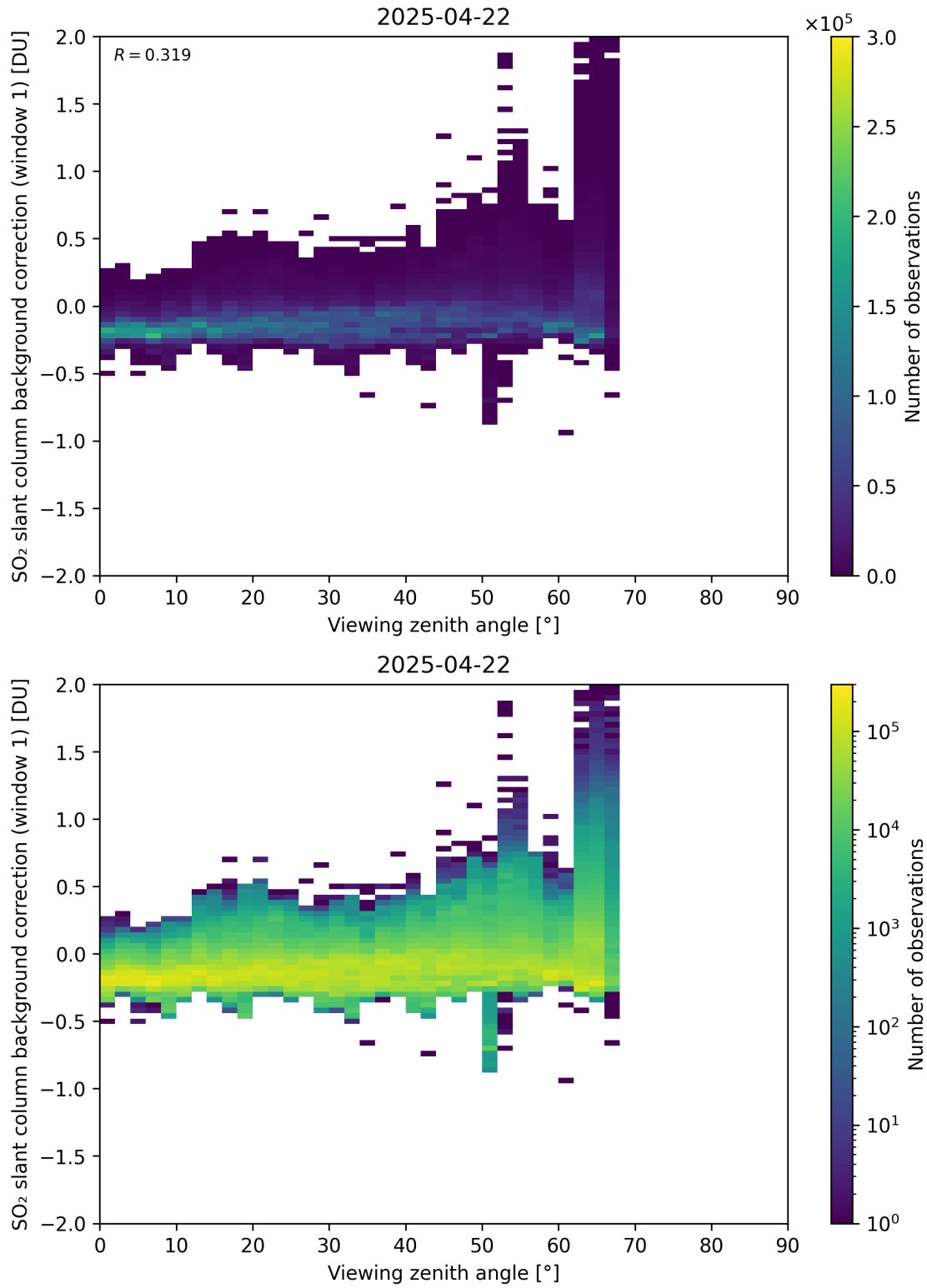
Figure 362: Scatter density plot of “Viewing zenith angle” against “SO 2 slant column background correction (window 1)” for 2025-04-21 to 2025-04-23.
