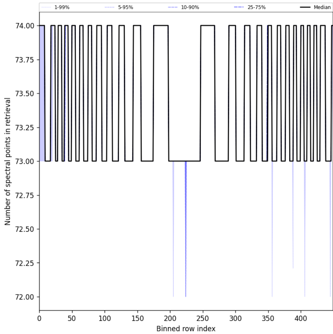
Figure 108: Along track statistics of “Number of spectral points in retrieval” for 2025-04-21 to 2025-04-23
