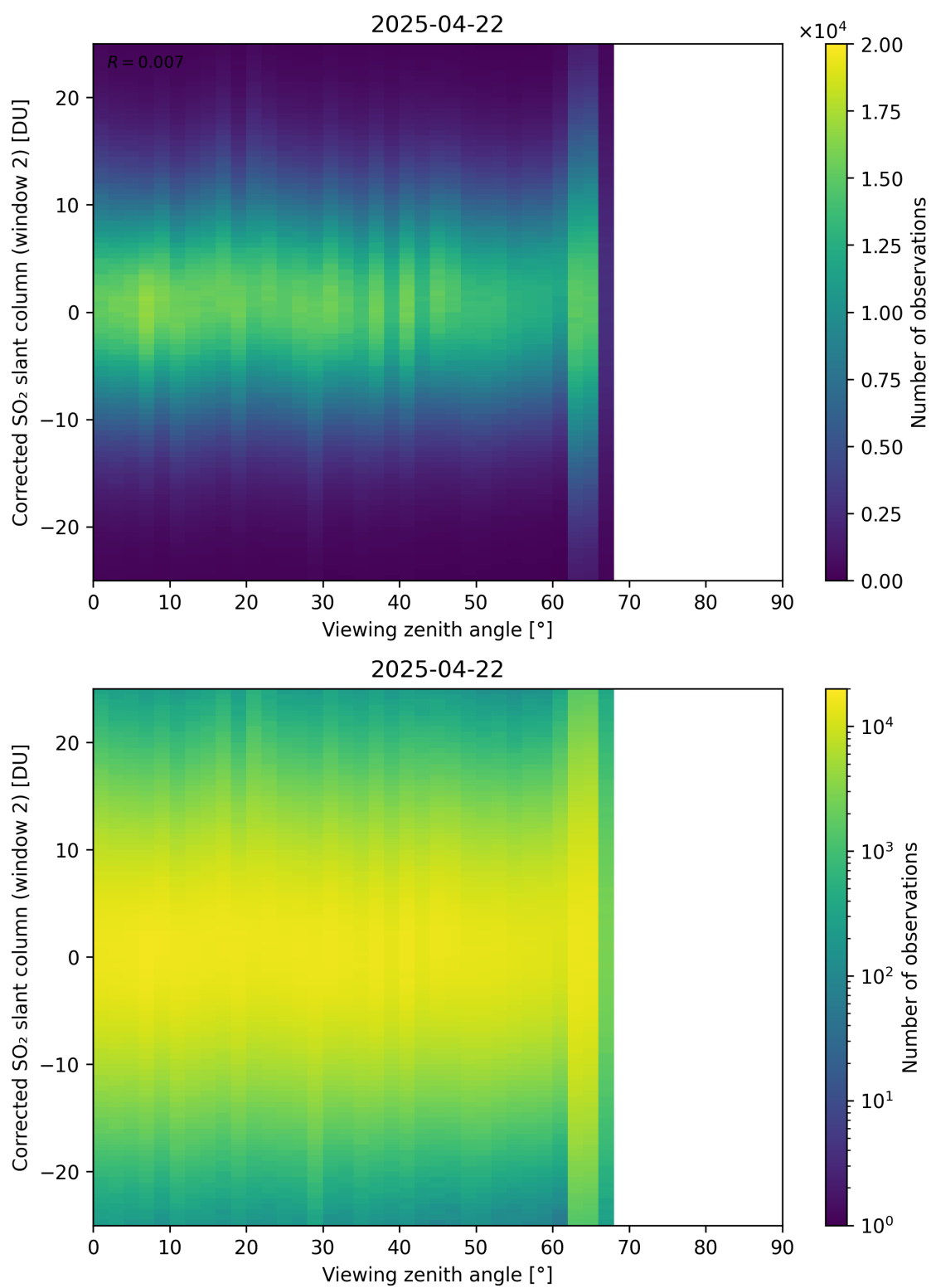
Figure 374: Scatter density plot of “Viewing zenith angle” against “Corrected SO 2 slant column (window 2)” for 2025-04-21 to 2025-04-23.
