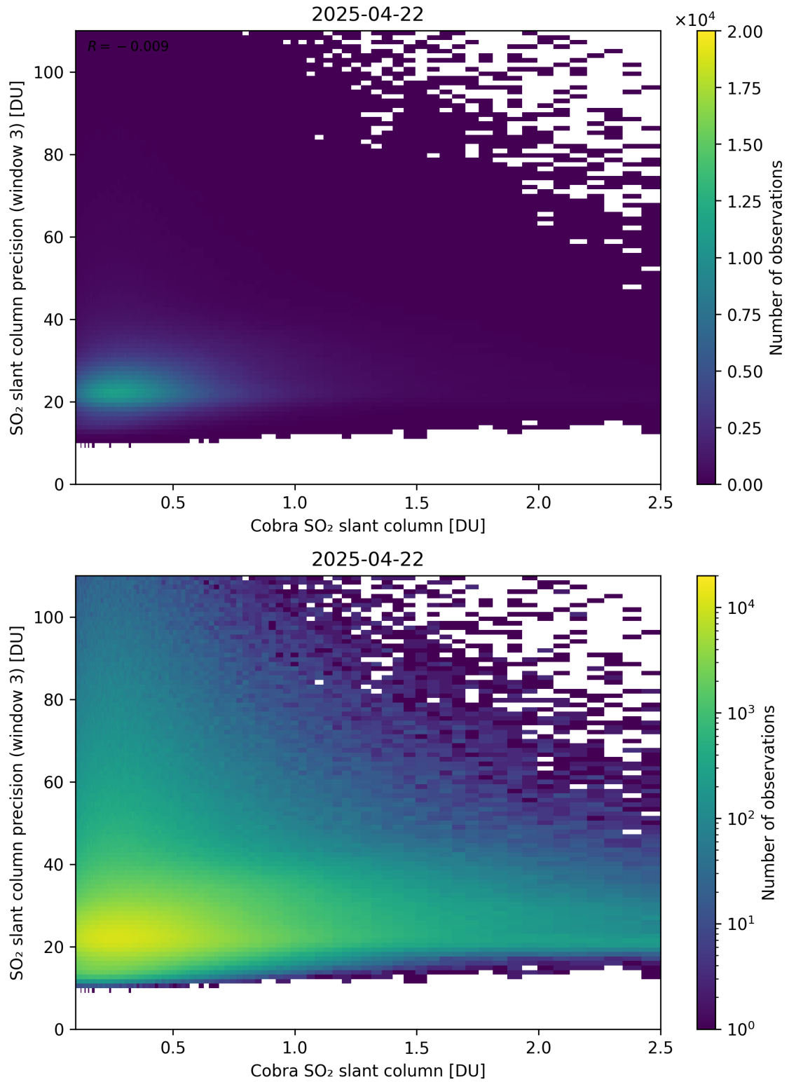
Figure 223: Scatter density plot of “Cobra SO 2 slant column” against “SO 2 slant column precision (window 3)” for 2025-04-21 to 2025-04-23.
