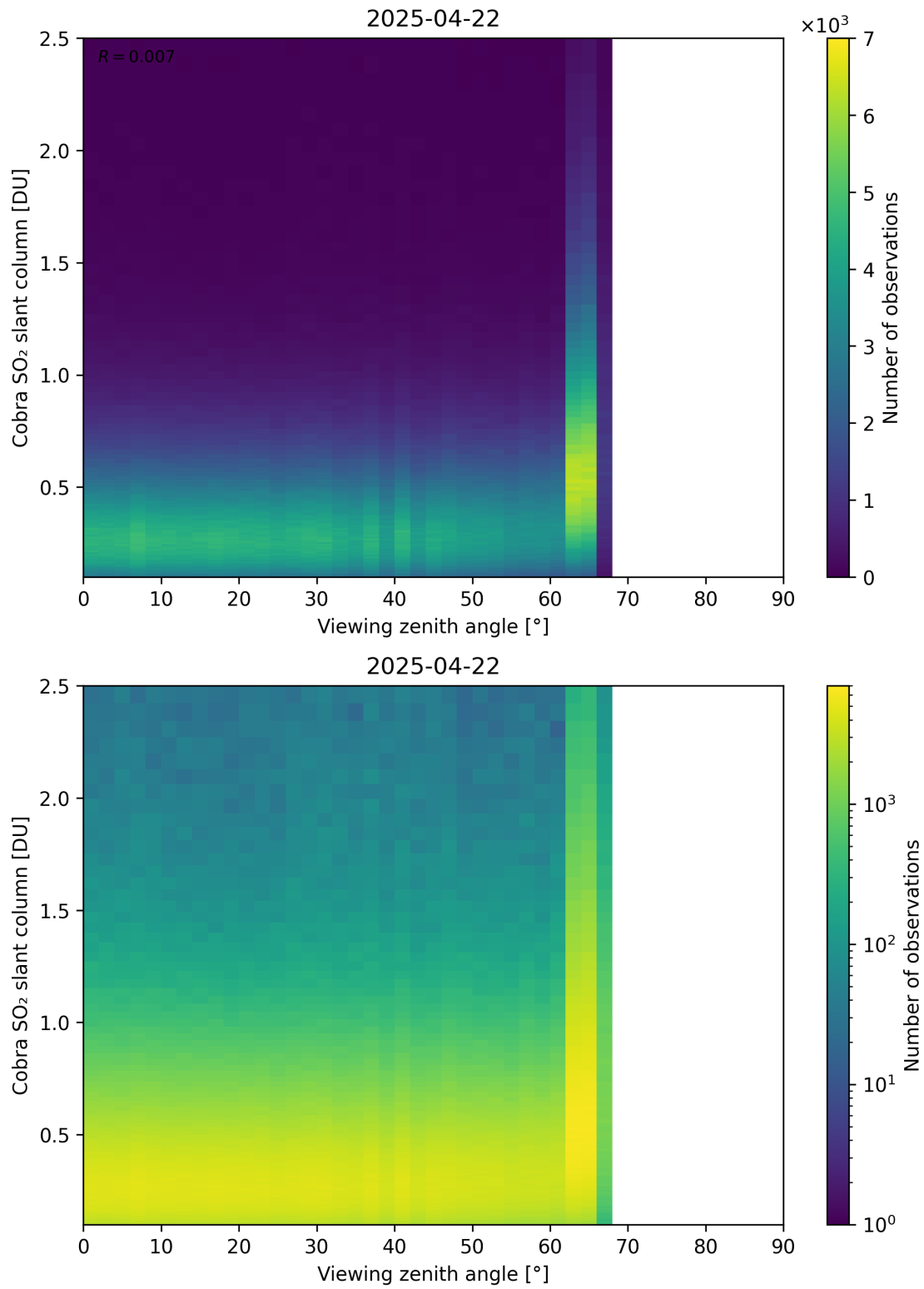
Figure 371: Scatter density plot of “Viewing zenith angle” against “Cobra SO 2 slant column” for 2025-04-21 to 2025-04-23.
