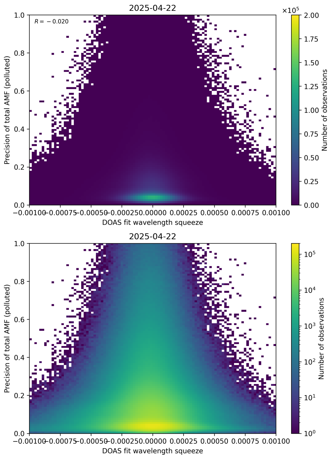
Figure 146: Scatter density plot of “DOAS fit wavelength squeeze” against “Precision of total AMF (polluted)” for 2025-04-21 to 2025-04-23.
