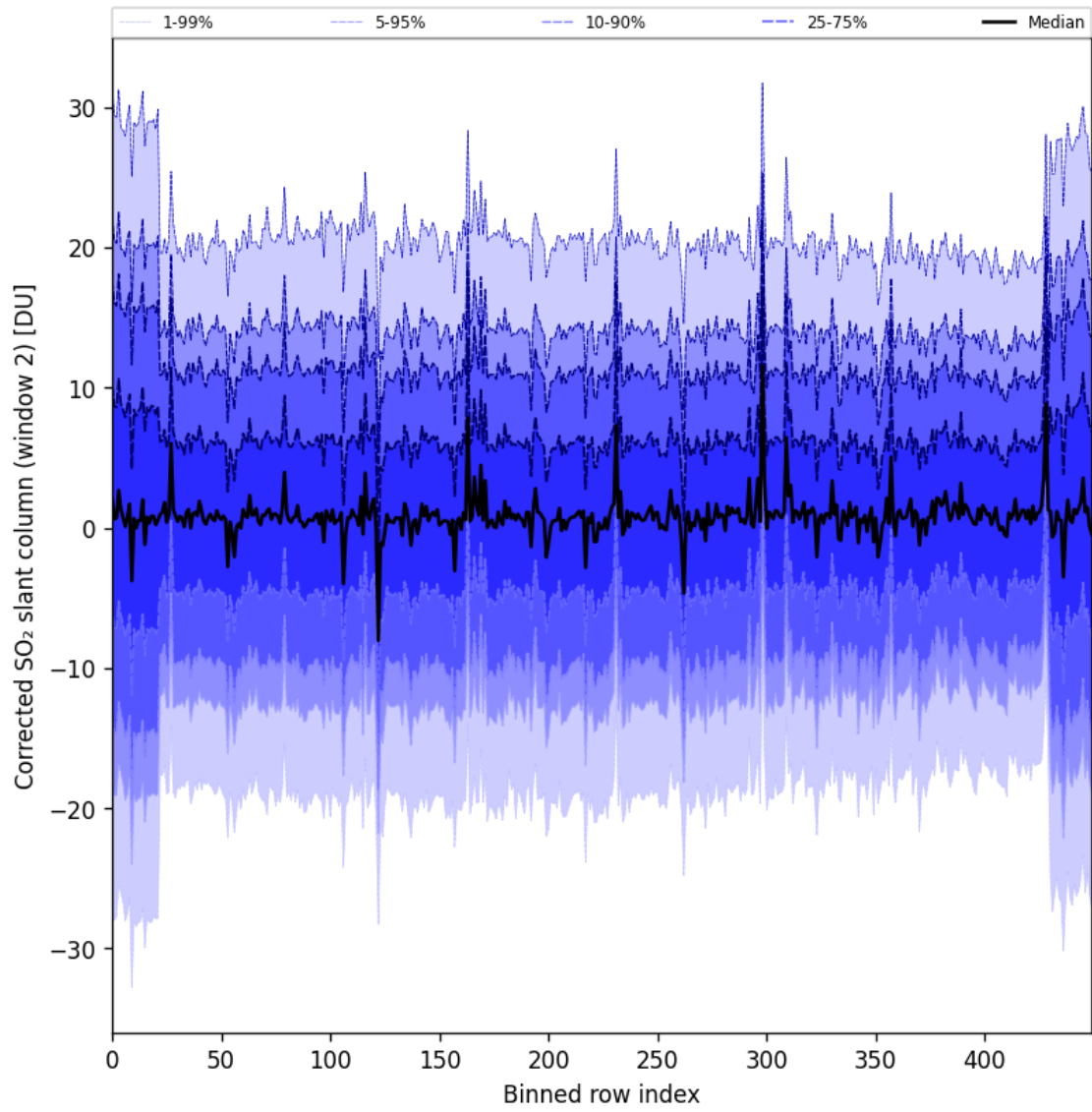
Figure 95: Along track statistics of “Corrected SO 2 slant column (window 2)” for 2025-04-21 to 2025-04-23
