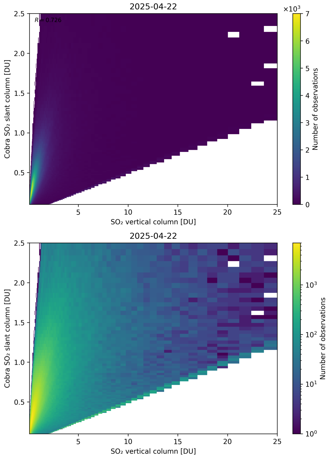
Figure 349: Scatter density plot of “SO 2 vertical column” against “Cobra SO 2 slant column” for 2025-04-21 to 2025-04-23.
