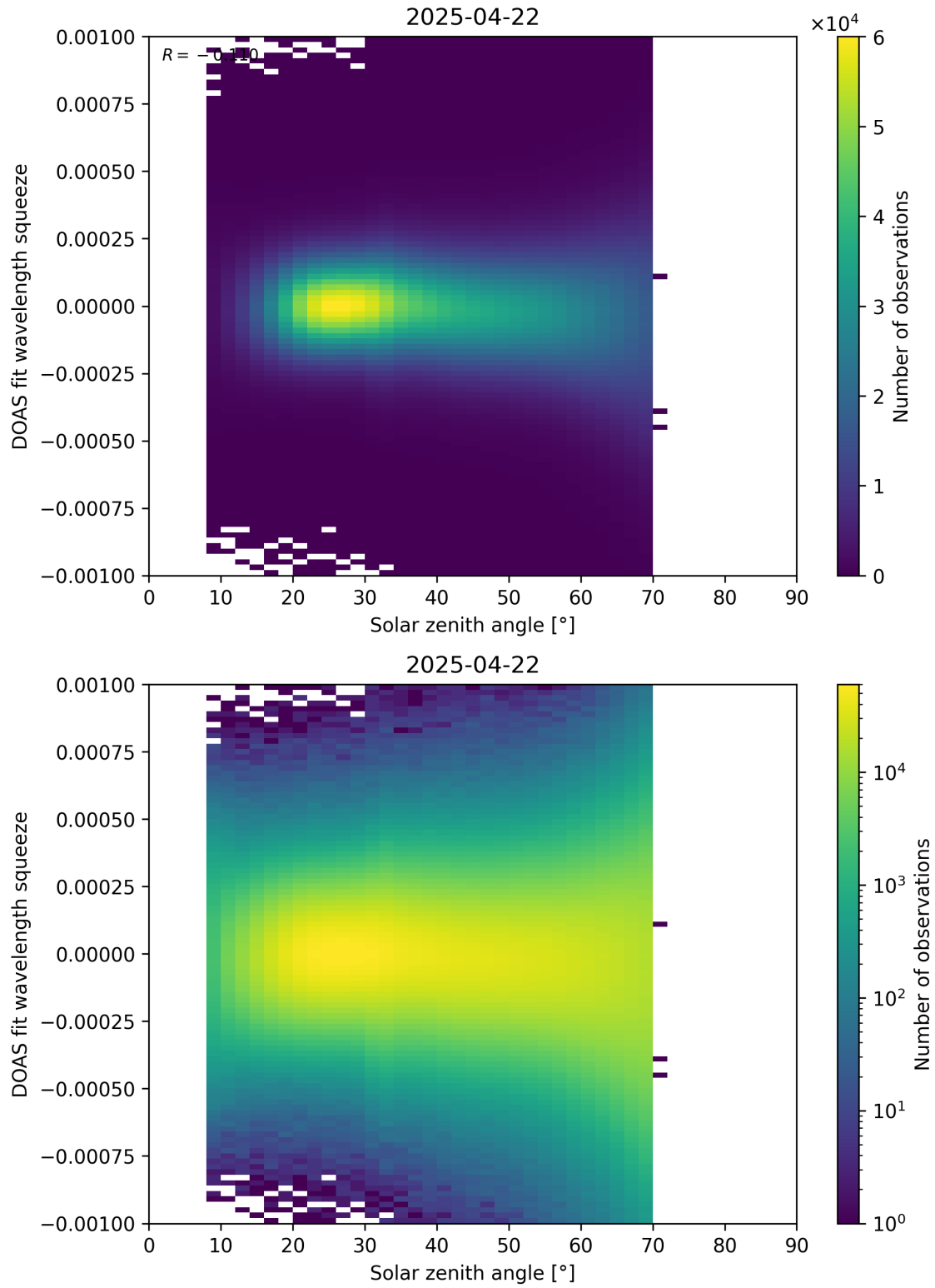
Figure 175: Scatter density plot of “Solar zenith angle” against “DOAS fit wavelength squeeze” for 2025-04-21 to 2025-04-23.
