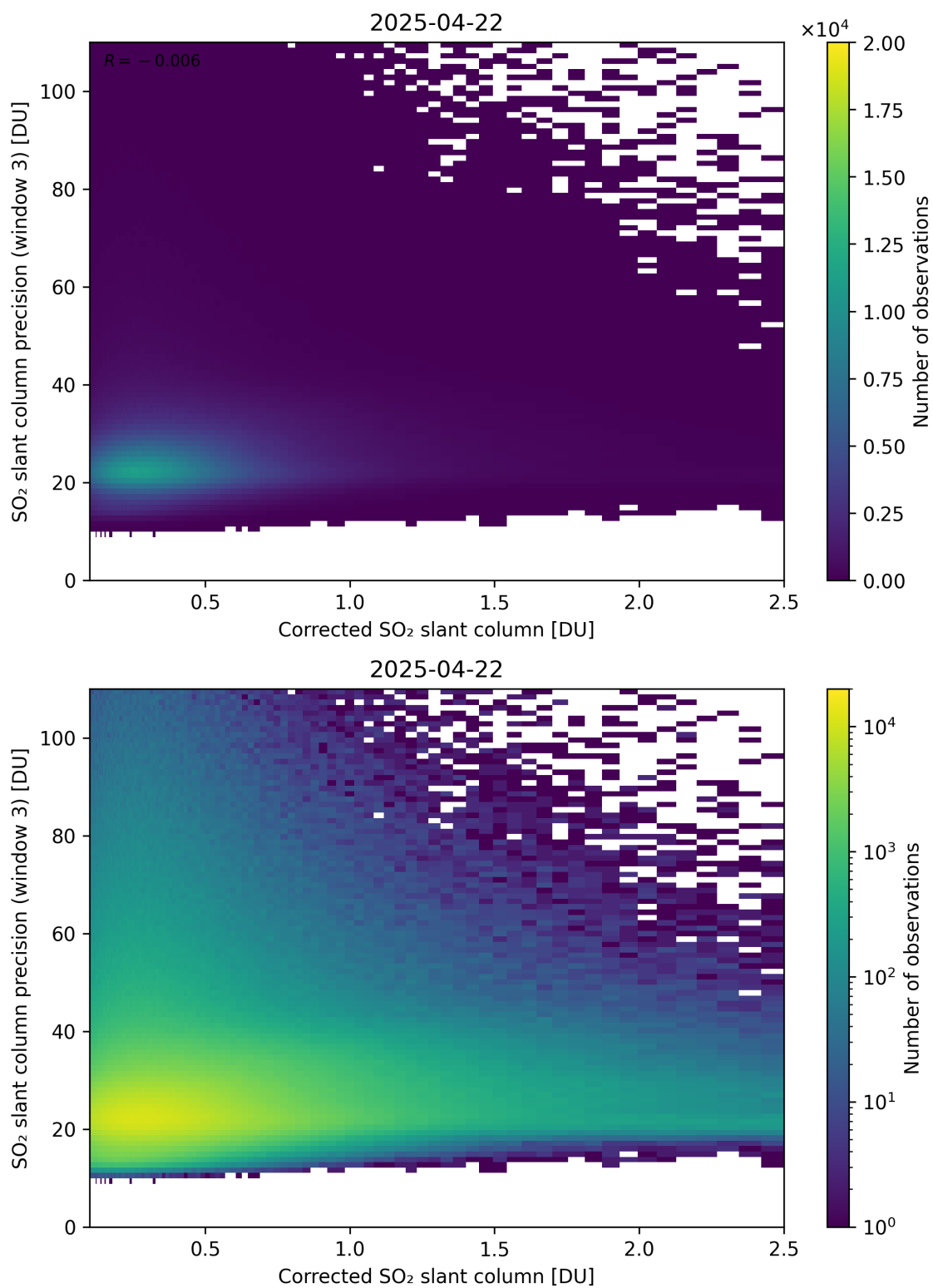
Figure 241: Scatter density plot of “Corrected SO 2 slant column” against “SO 2 slant column precision (window 3)” for 2025-04-21 to 2025-04-23.
