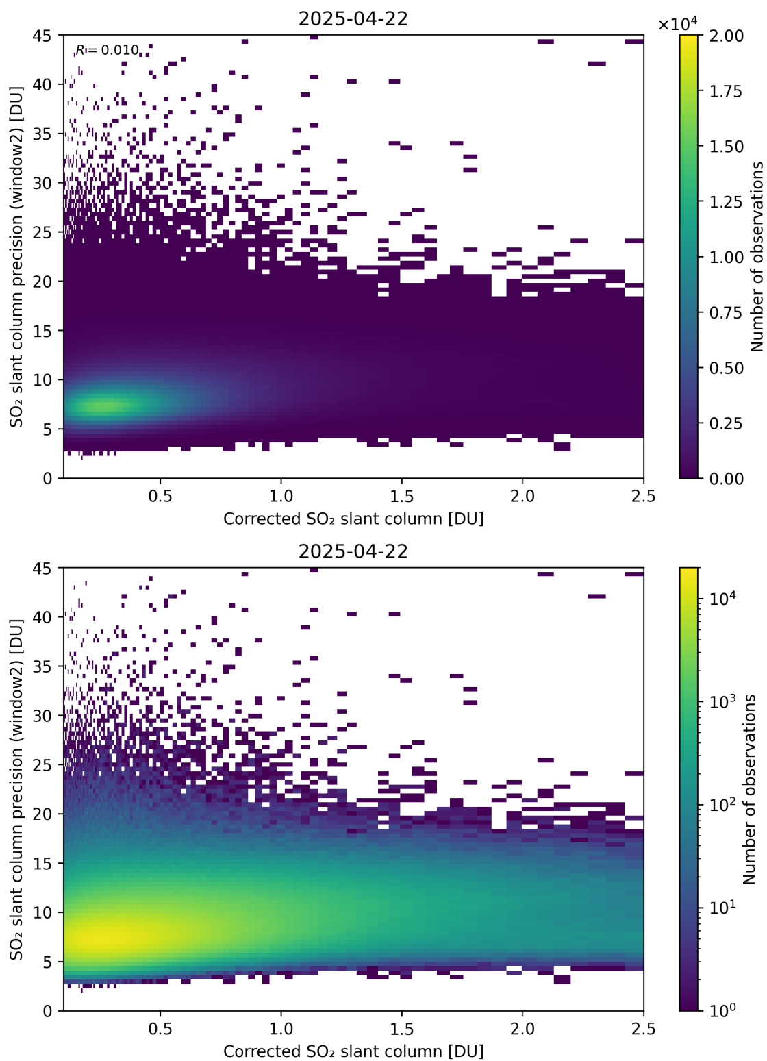
Figure 239: Scatter density plot of “Corrected SO 2 slant column” against “SO 2 slant column precision (window2)” for 2025-04-21 to 2025-04-23.
