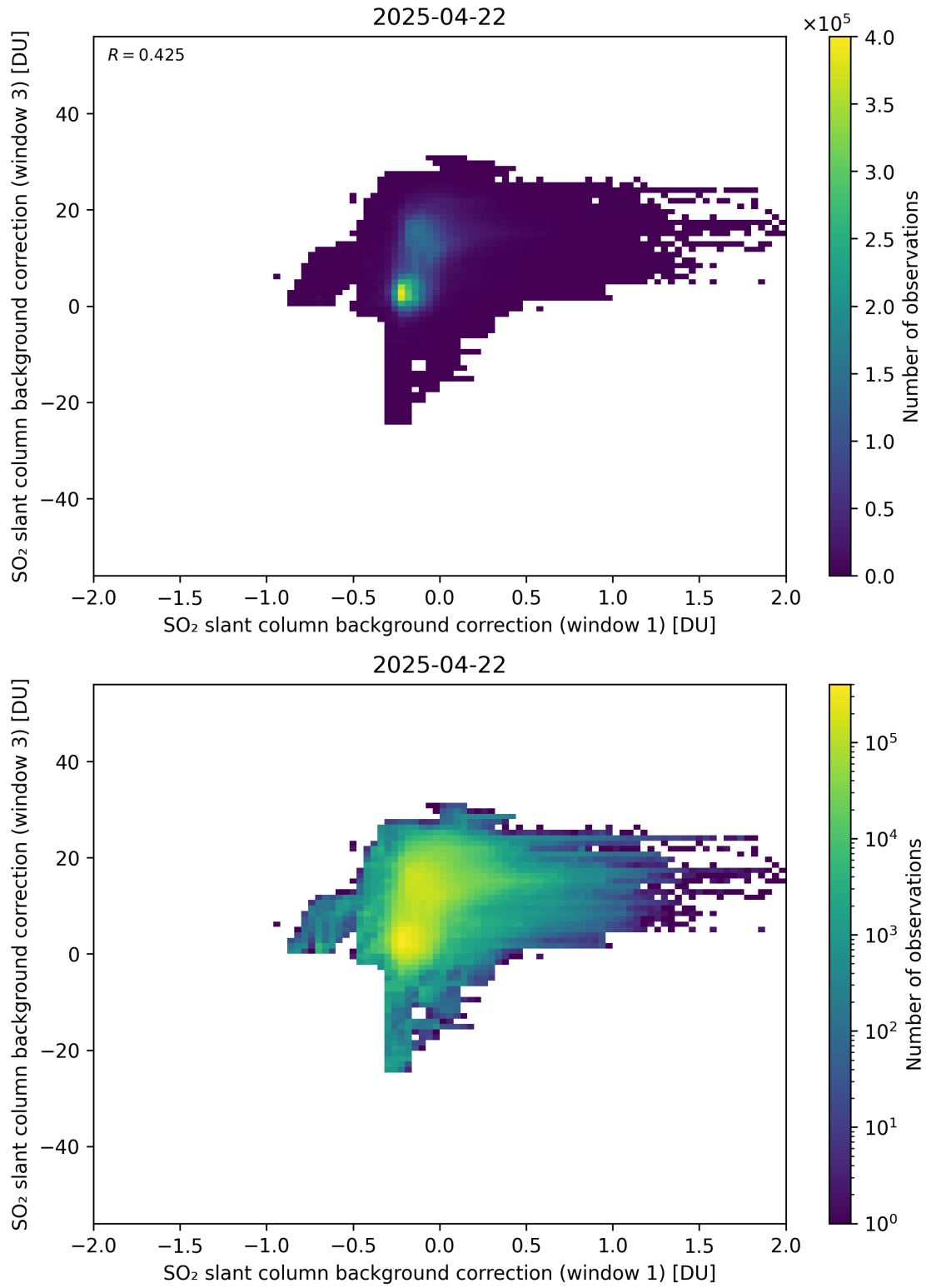
Figure 110: Scatter density plot of “SO 2 slant column background correction (window 1)” against “SO 2 slant column background correction (window 3)” for 2025-04-21 to 2025-04-23.
