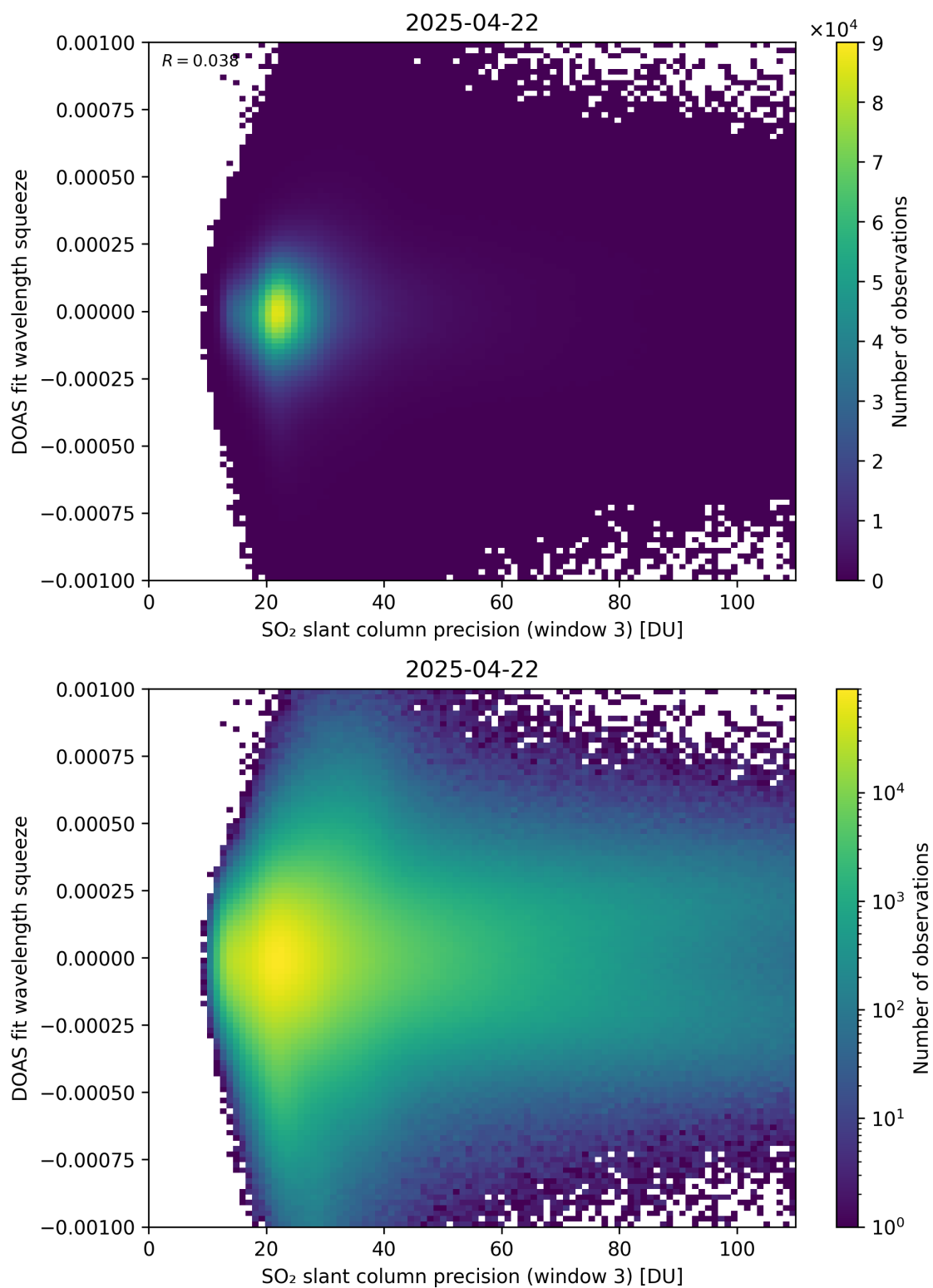
Figure 309: Scatter density plot of “SO 2 slant column precision (window 3)” against “DOAS fit wavelength squeeze” for 2025-04-21 to 2025-04-23.
