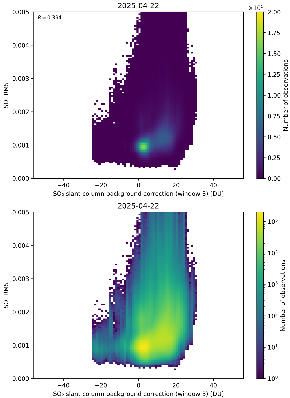
Figure 134: Scatter density plot of “SO 2 slant column background correction (window 3)” against “SO 2 RMS” for 2025-04-21 to 2025-04-23.
