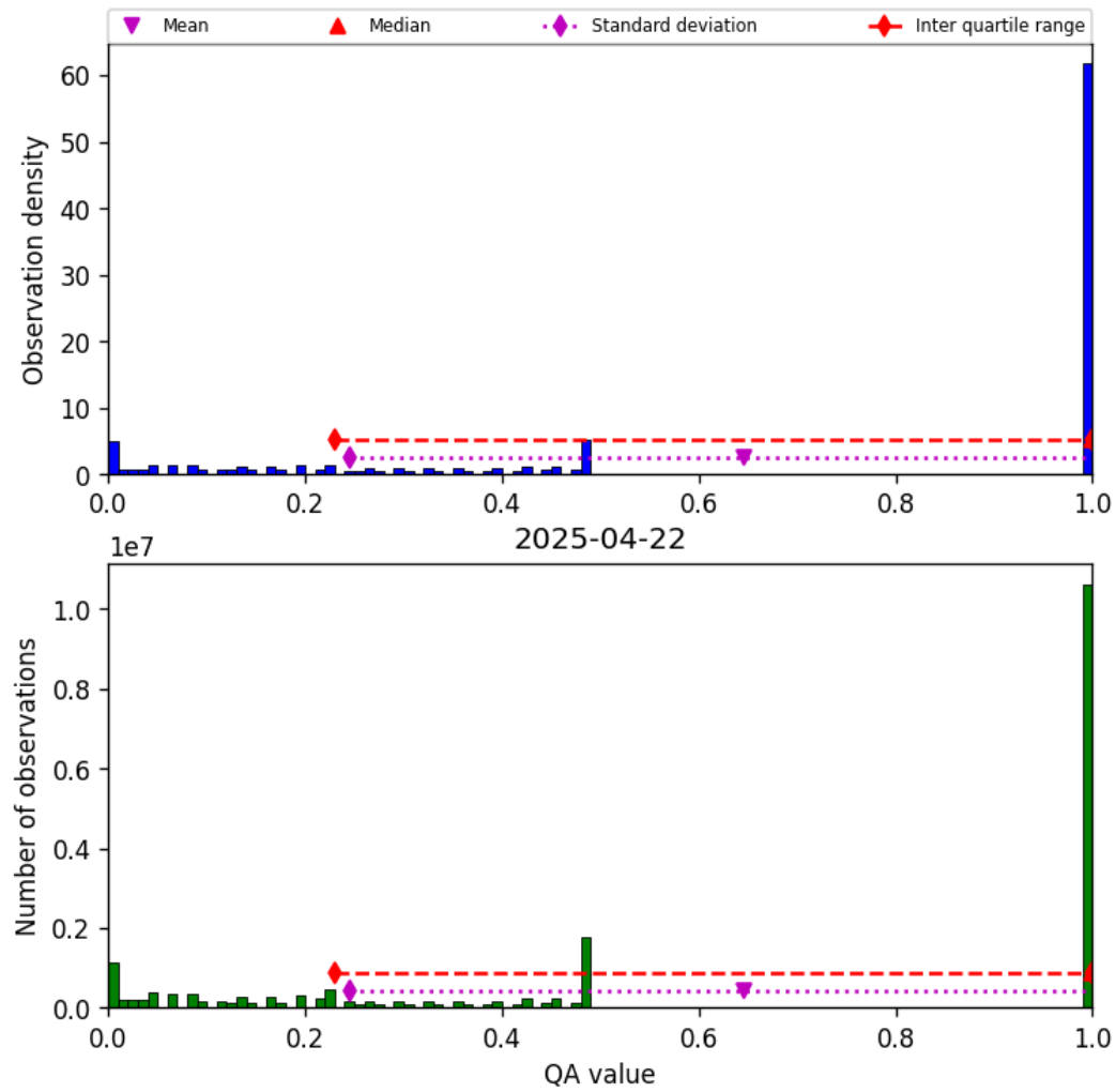
Figure 57: Histogram of “QA value” for 2025-04-21 to 2025-04-23
