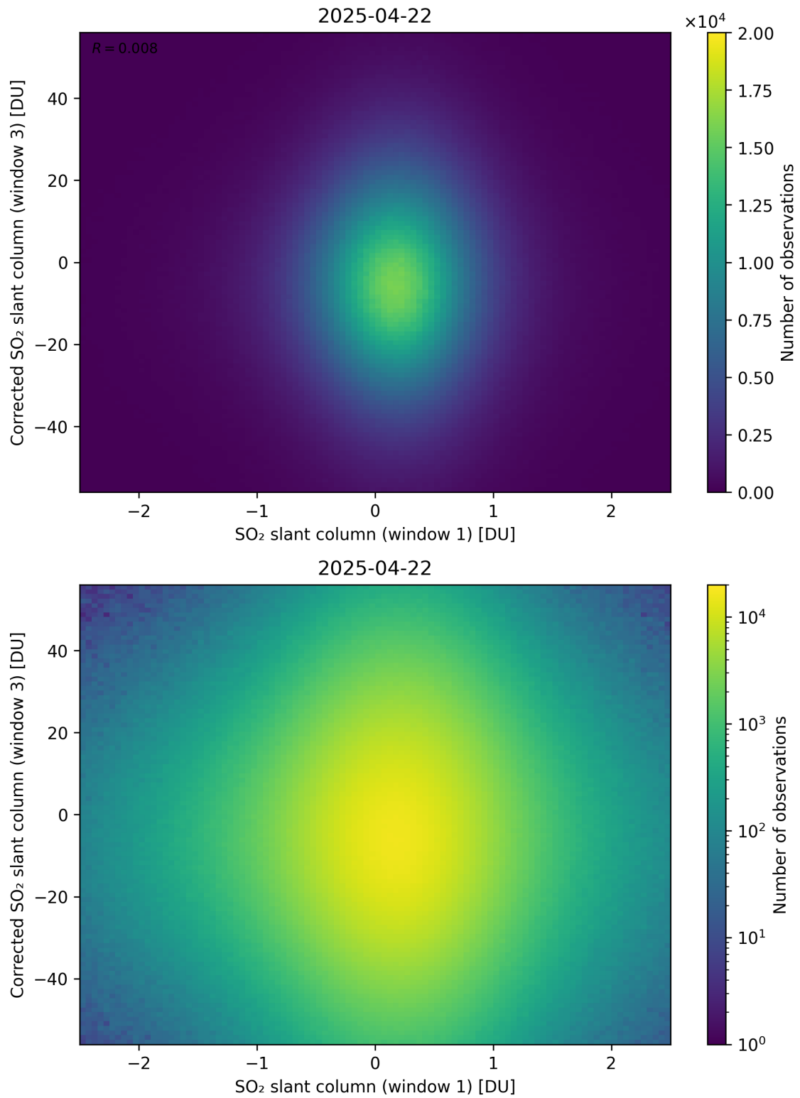
Figure 284: Scatter density plot of “SO 2 slant column (window 1)” against “Corrected SO 2 slant column (window 3)” for 2025-04-21 to 2025-04-23.
