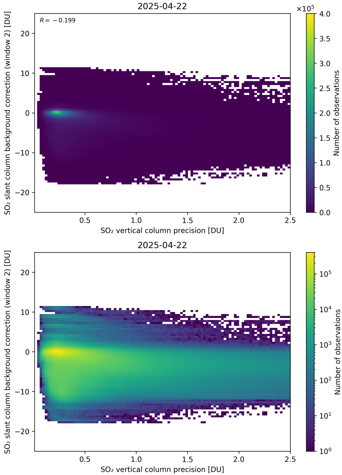
Figure 330: Scatter density plot of “SO 2 vertical column precision” against “SO 2 slant column background correction (window 2)” for 2025-04-21 to 2025-04-23.
