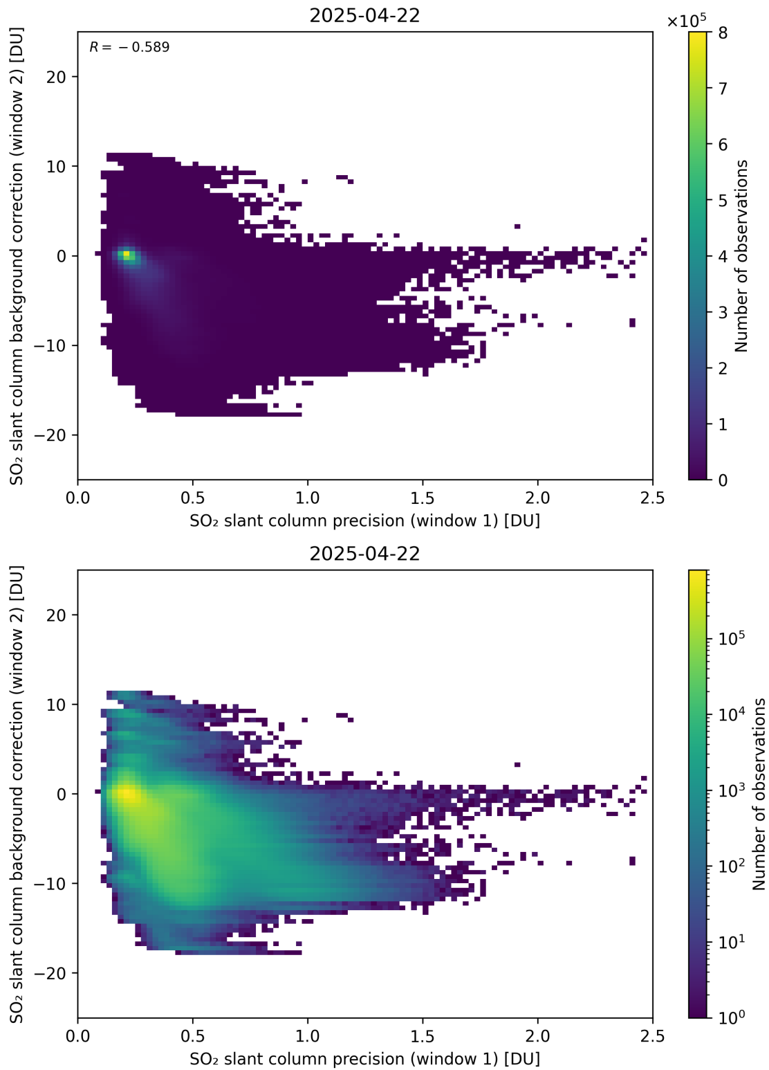
Figure 269: Scatter density plot of “SO 2 slant column precision (window 1)” against “SO 2 slant column background correction (window 2)” for 2025-04-21 to 2025-04-23.
