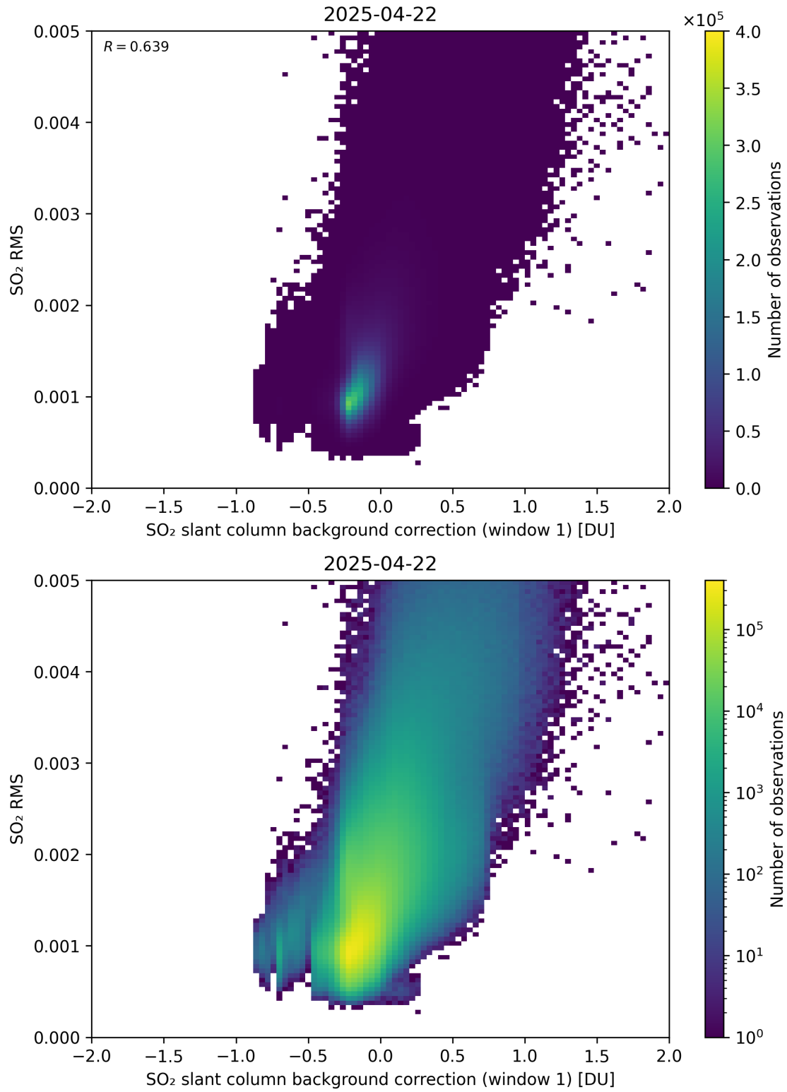
Figure 113: Scatter density plot of “SO 2 slant column background correction (window 1)” against “SO 2 RMS” for 2025-04-21 to 2025-04-23.
