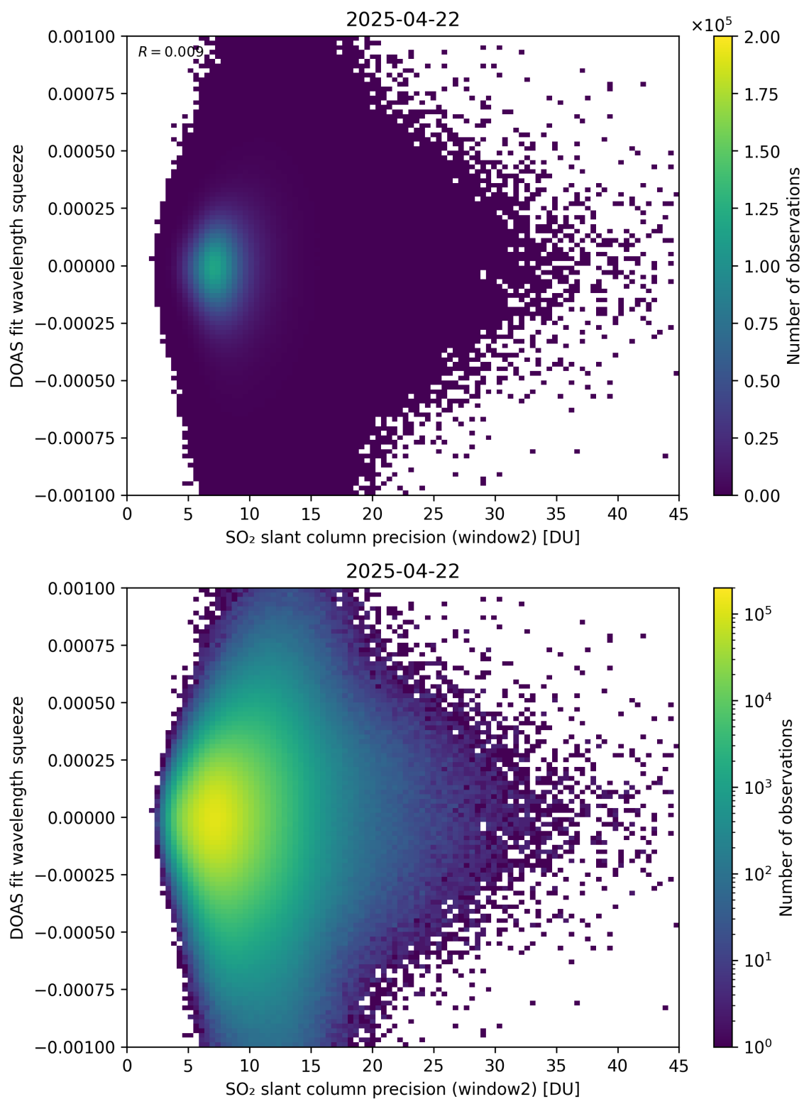
Figure 294: Scatter density plot of “SO 2 slant column precision (window2)” against “DOAS fit wavelength squeeze” for 2025-04-21 to 2025-04-23.
