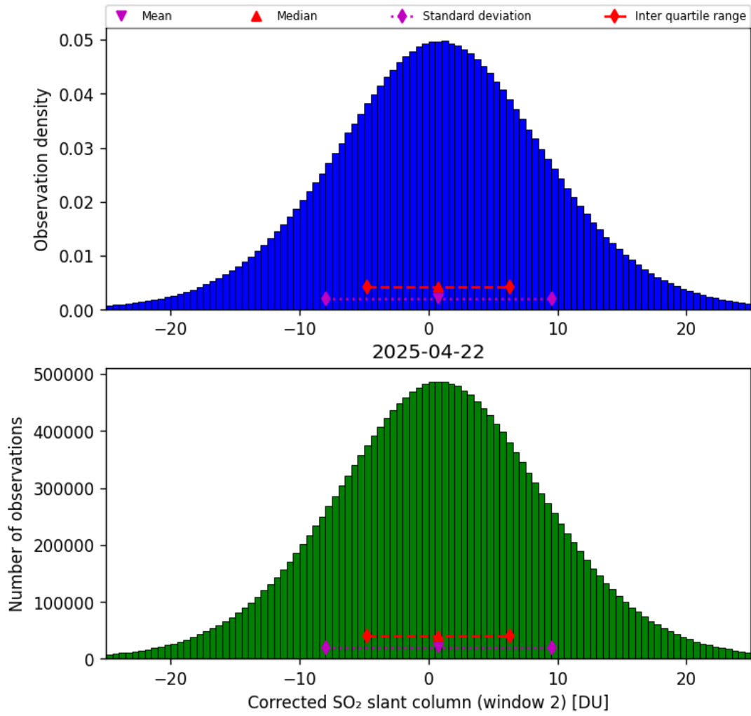
Figure 69: Histogram of “Corrected SO 2 slant column (window 2)” for 2025-04-21 to 2025-04-23
