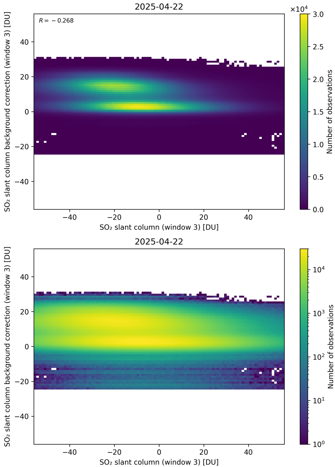
Figure 303: Scatter density plot of “SO 2 slant column (window 3)” against “SO 2 slant column background correction (window 3)” for 2025-04-21 to 2025-04-23.
