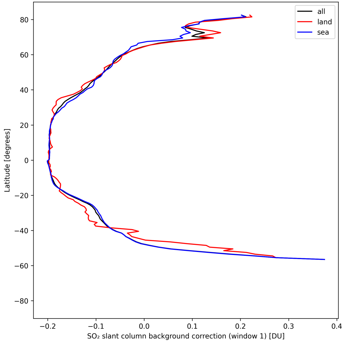
Figure 40: Zonal average of “SO 2 slant column background correction (window 1)” for 2025-04-21 to 2025-04-23.
