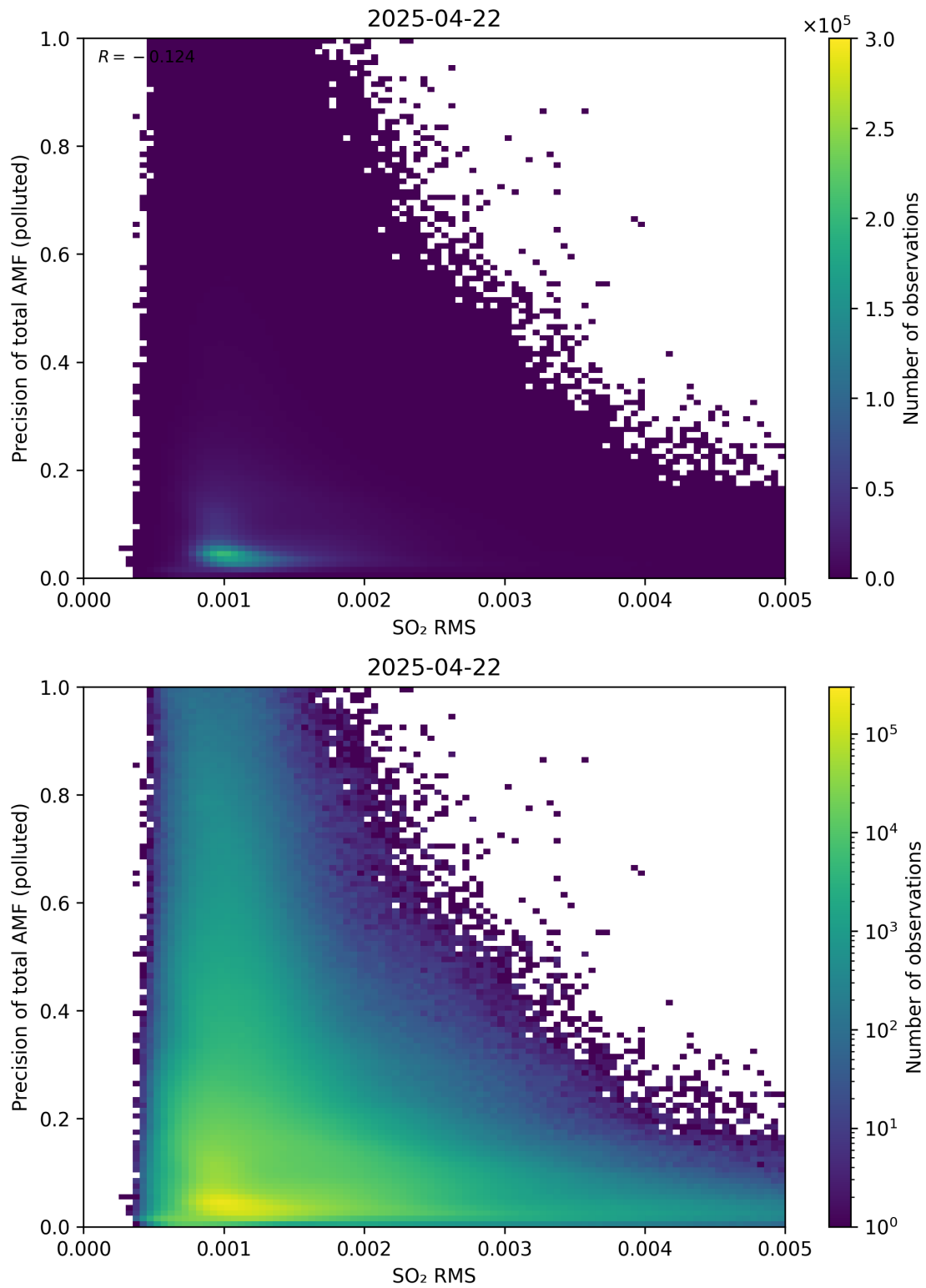
Figure 149: Scatter density plot of “SO 2 RMS” against “Precision of total AMF (polluted)” for 2025-04-21 to 2025-04-23.
