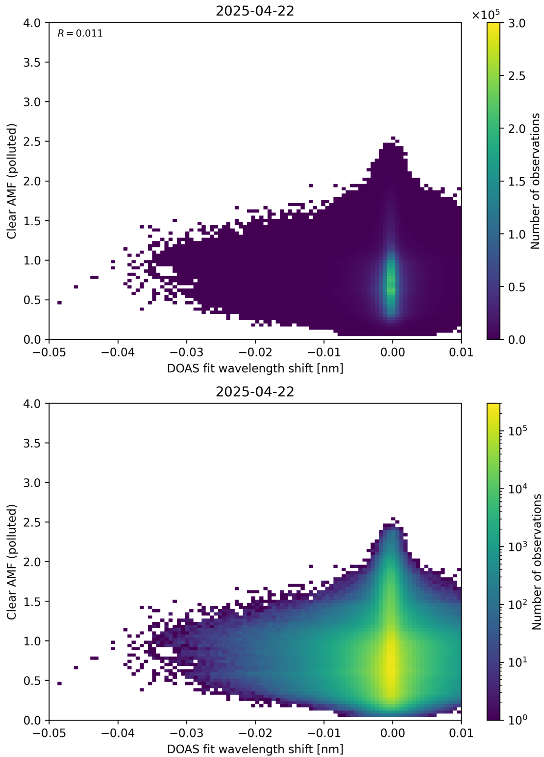
Figure 140: Scatter density plot of “DOAS fit wavelength shift” against “Clear AMF (polluted)” for 2025-04-21 to 2025-04-23.
