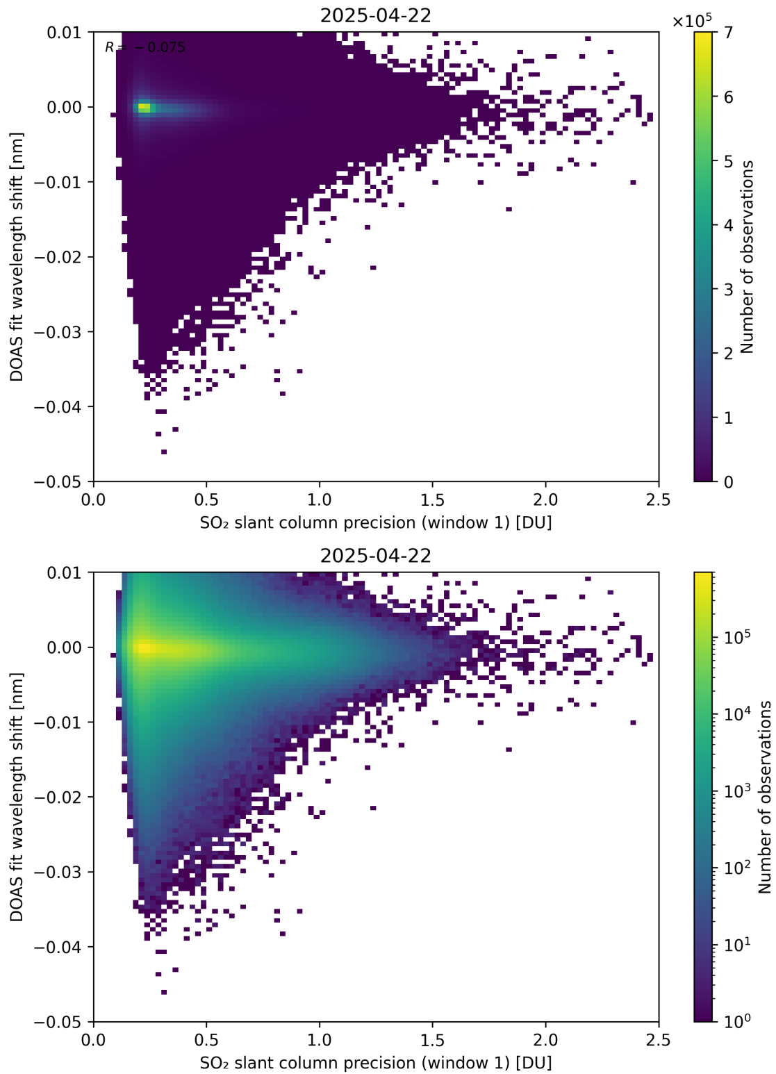
Figure 271: Scatter density plot of “SO 2 slant column precision (window 1)” against “DOAS fit wavelength shift” for 2025-04-21 to 2025-04-23.
