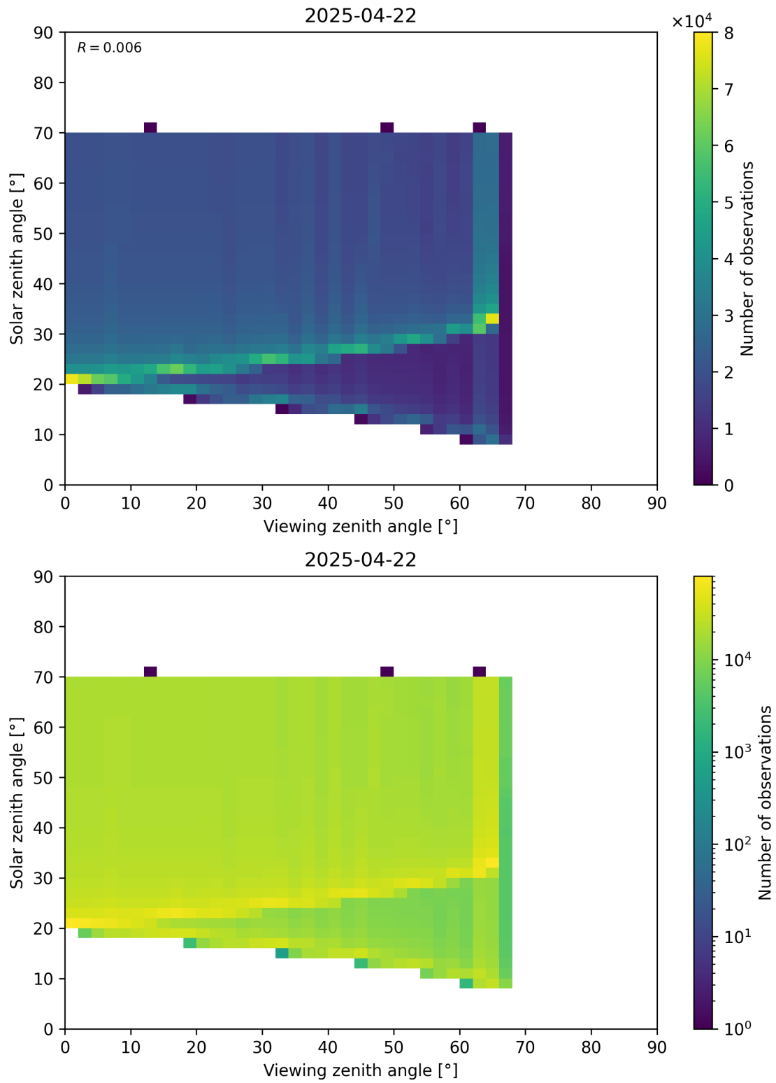
Figure 369: Scatter density plot of “Viewing zenith angle” against “Solar zenith angle” for 2025-04-21 to 2025-04-23.
