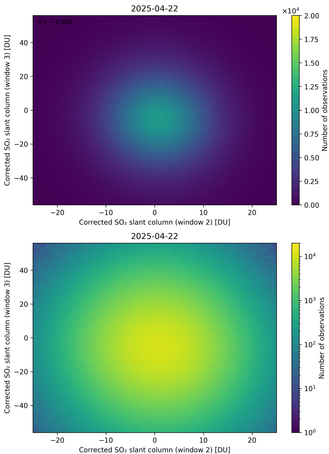
Figure 250: Scatter density plot of “Corrected SO 2 slant column (window 2)” against “Corrected SO 2 slant column (window 3)” for 2025-04-21 to 2025-04-23.
