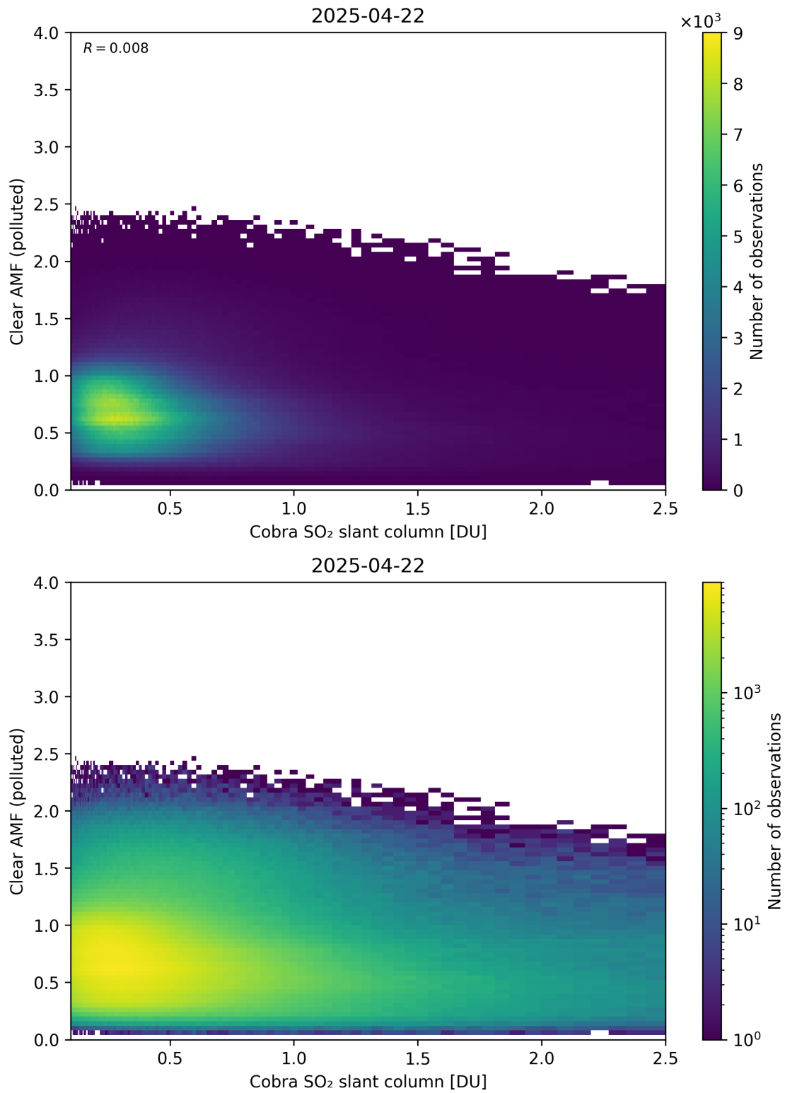
Figure 215: Scatter density plot of “Cobra SO 2 slant column” against “Clear AMF (polluted)” for 2025-04-21 to 2025-04-23.
