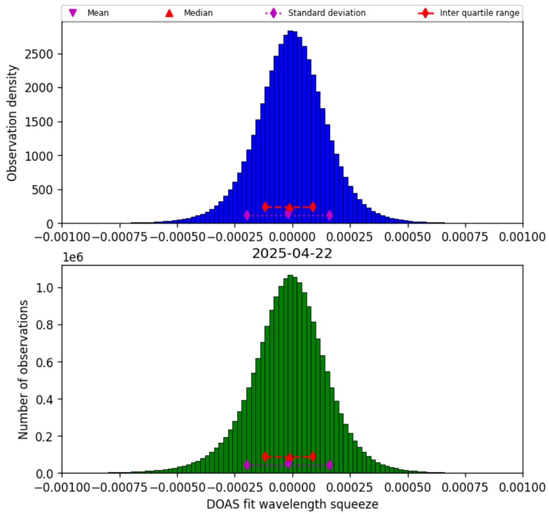
Figure 77: Histogram of “DOAS fit wavelength squeeze” for 2025-04-21 to 2025-04-23
