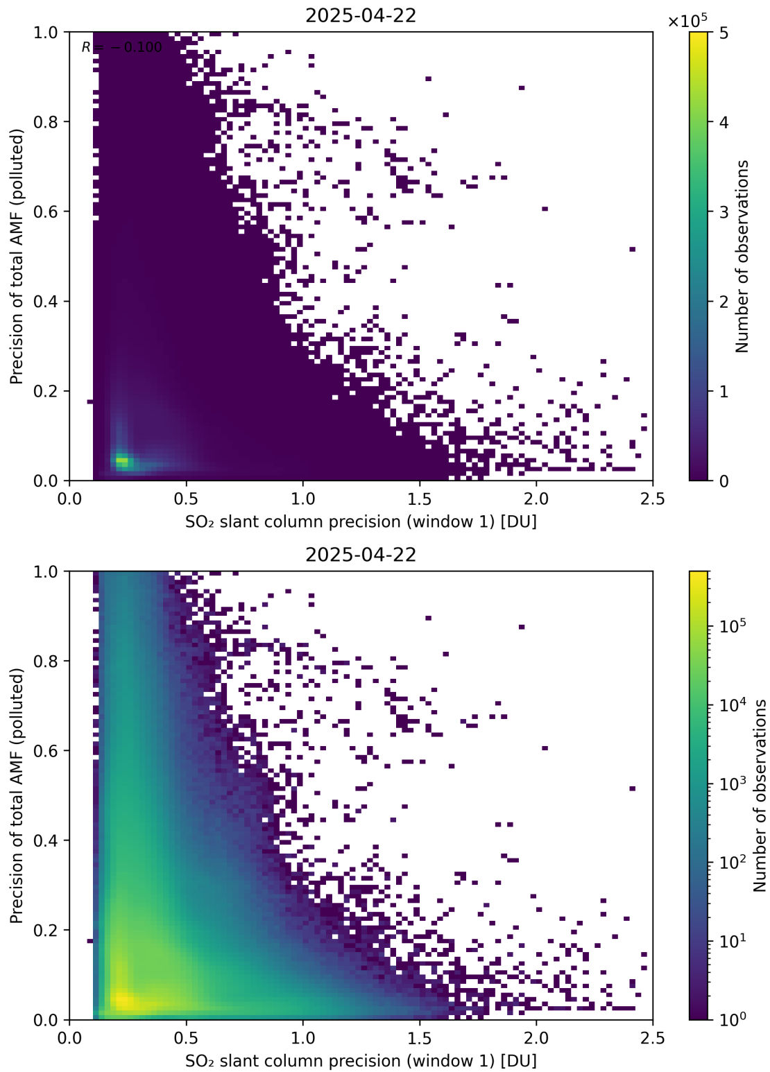
Figure 281: Scatter density plot of “SO 2 slant column precision (window 1)” against “Precision of total AMF (polluted)” for 2025-04-21 to 2025-04-23.
