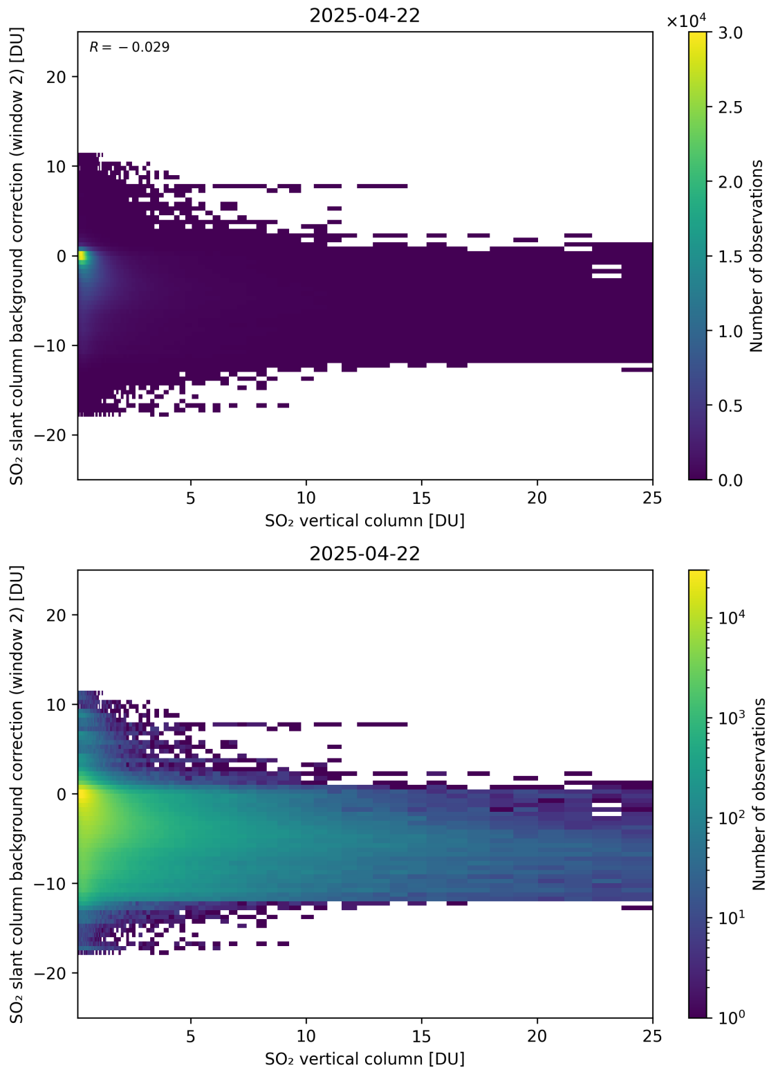
Figure 324: Scatter density plot of “SO 2 vertical column” against “SO 2 slant column background correction (window 2)” for 2025-04-21 to 2025-04-23.
