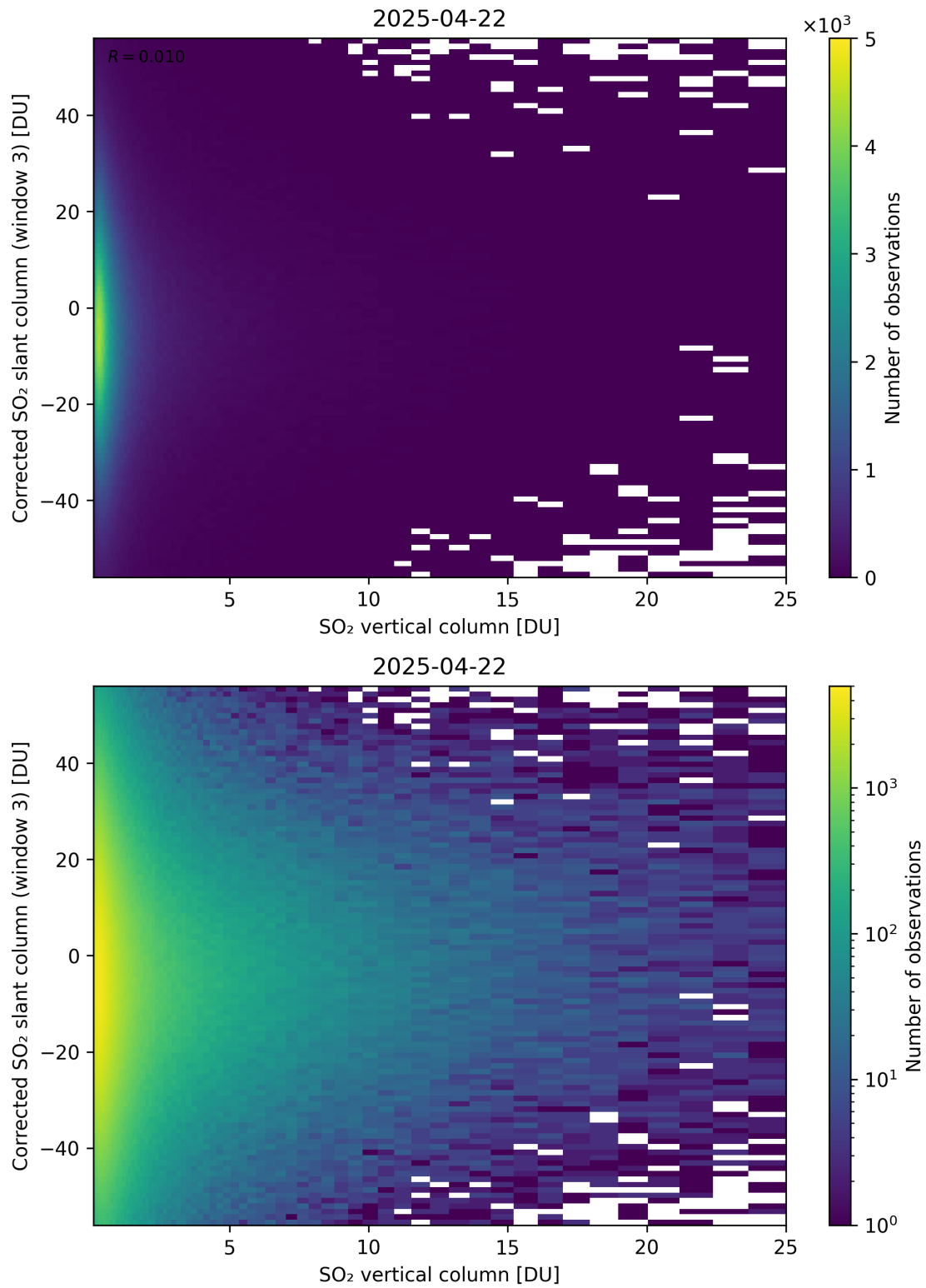
Figure 353: Scatter density plot of “SO 2 vertical column” against “Corrected SO 2 slant column (window 3)” for 2025-04-21 to 2025-04-23.
