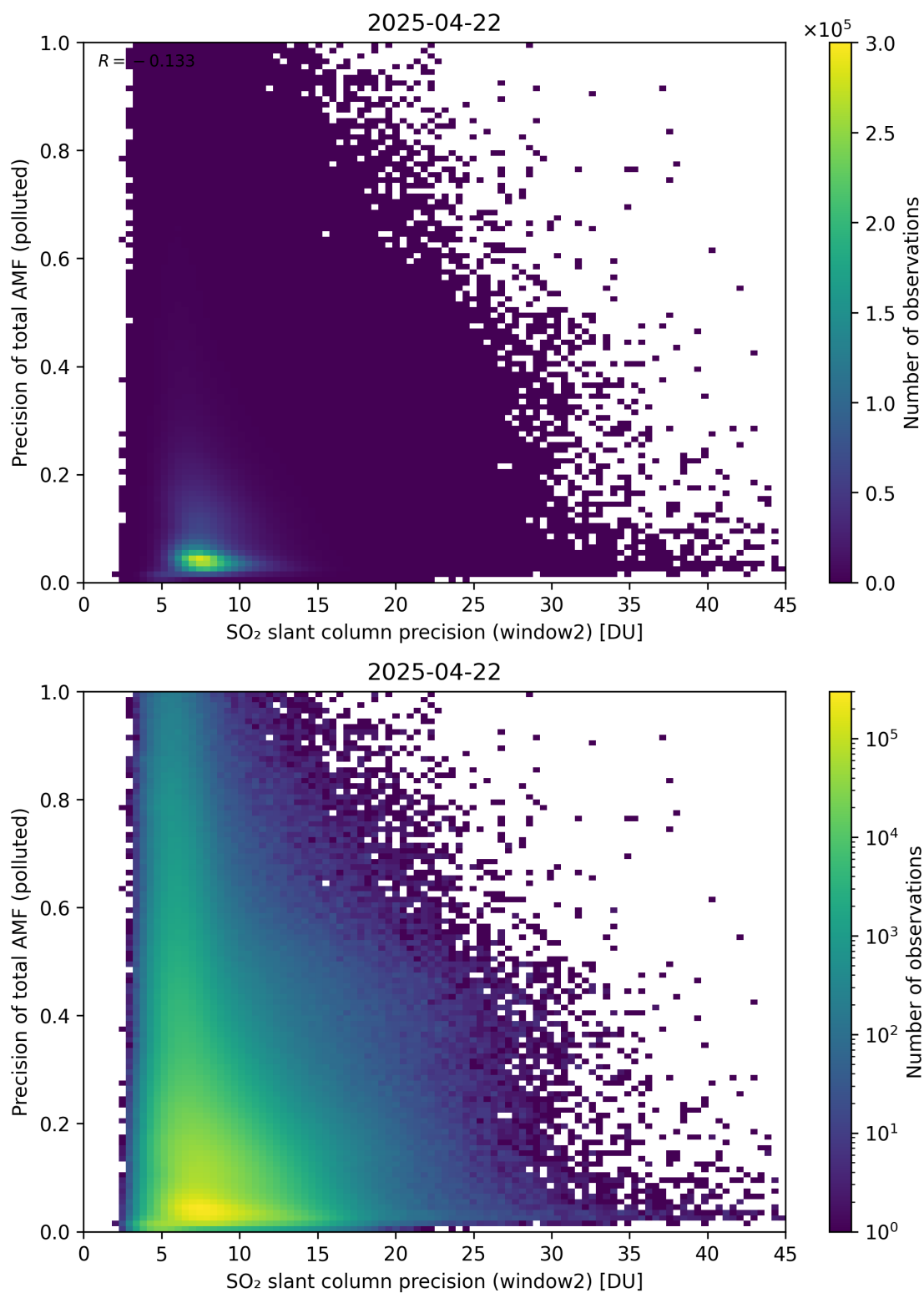
Figure 302: Scatter density plot of “SO 2 slant column precision (window2)” against “Precision of total AMF (polluted)” for 2025-04-21 to 2025-04-23.
