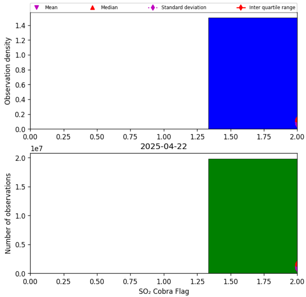
Figure 75: Histogram of “SO 2 Cobra Flag” for 2025-04-21 to 2025-04-23
