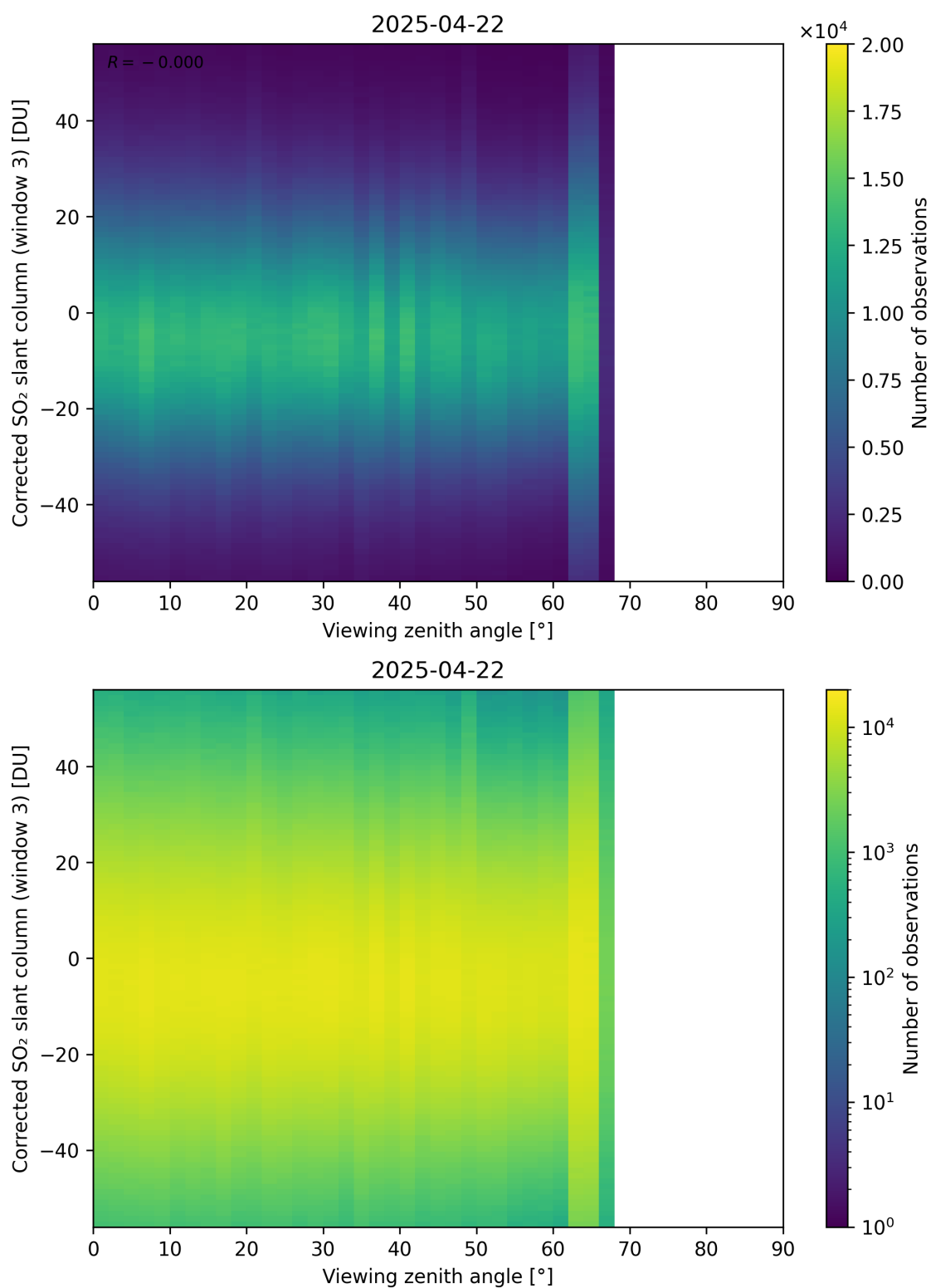
Figure 375: Scatter density plot of “Viewing zenith angle” against “Corrected SO 2 slant column (window 3)” for 2025-04-21 to 2025-04-23.
