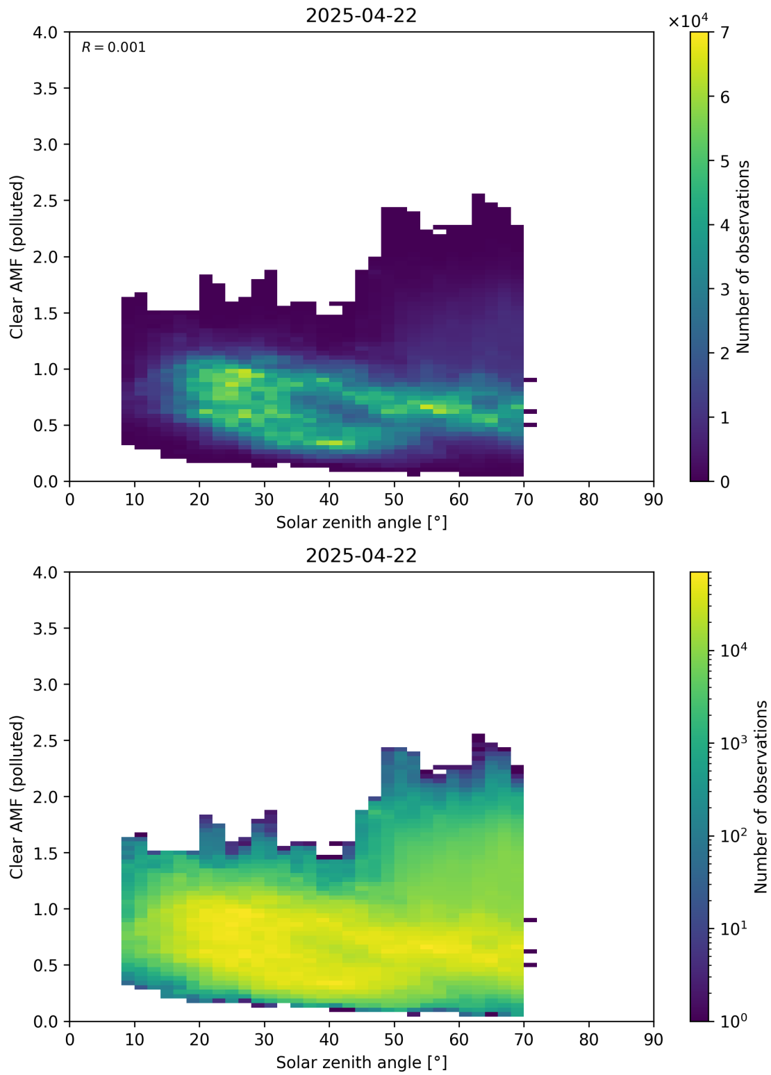
Figure 178: Scatter density plot of “Solar zenith angle” against “Clear AMF (polluted)” for 2025-04-21 to 2025-04-23.
