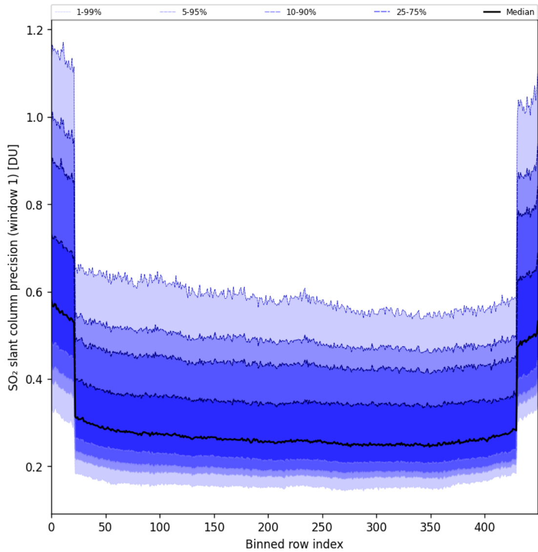
Figure 90: Along track statistics of “SO 2 slant column precision (window 1)” for 2025-04-21 to 2025-04-23
