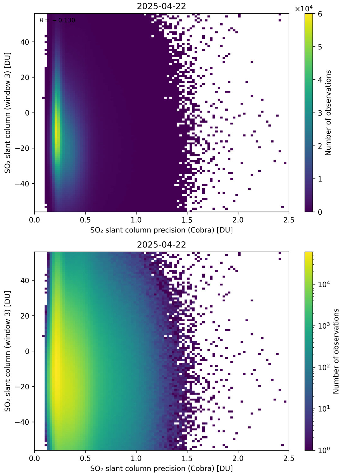
Figure 211: Scatter density plot of “SO 2 slant column precision (Cobra)” against “SO 2 slant column (window 3)” for 2025-04-21 to 2025-04-23.
