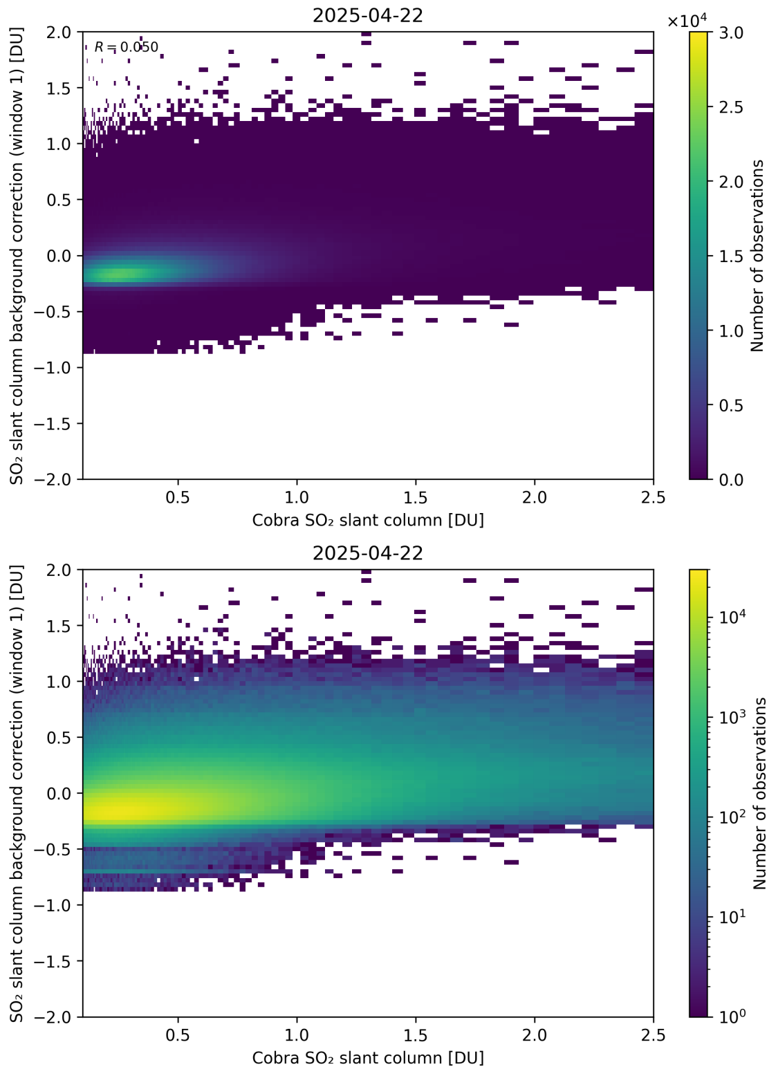
Figure 193: Scatter density plot of “Cobra SO 2 slant column” against “SO 2 slant column background correction (window 1)” for 2025-04-21 to 2025-04-23.
