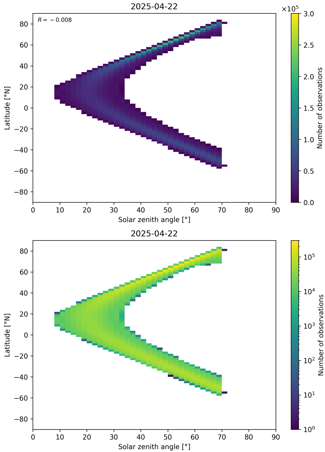
Figure 177: Scatter density plot of “Solar zenith angle” against “Latitude” for 2025-04-21 to 2025-04-23.
