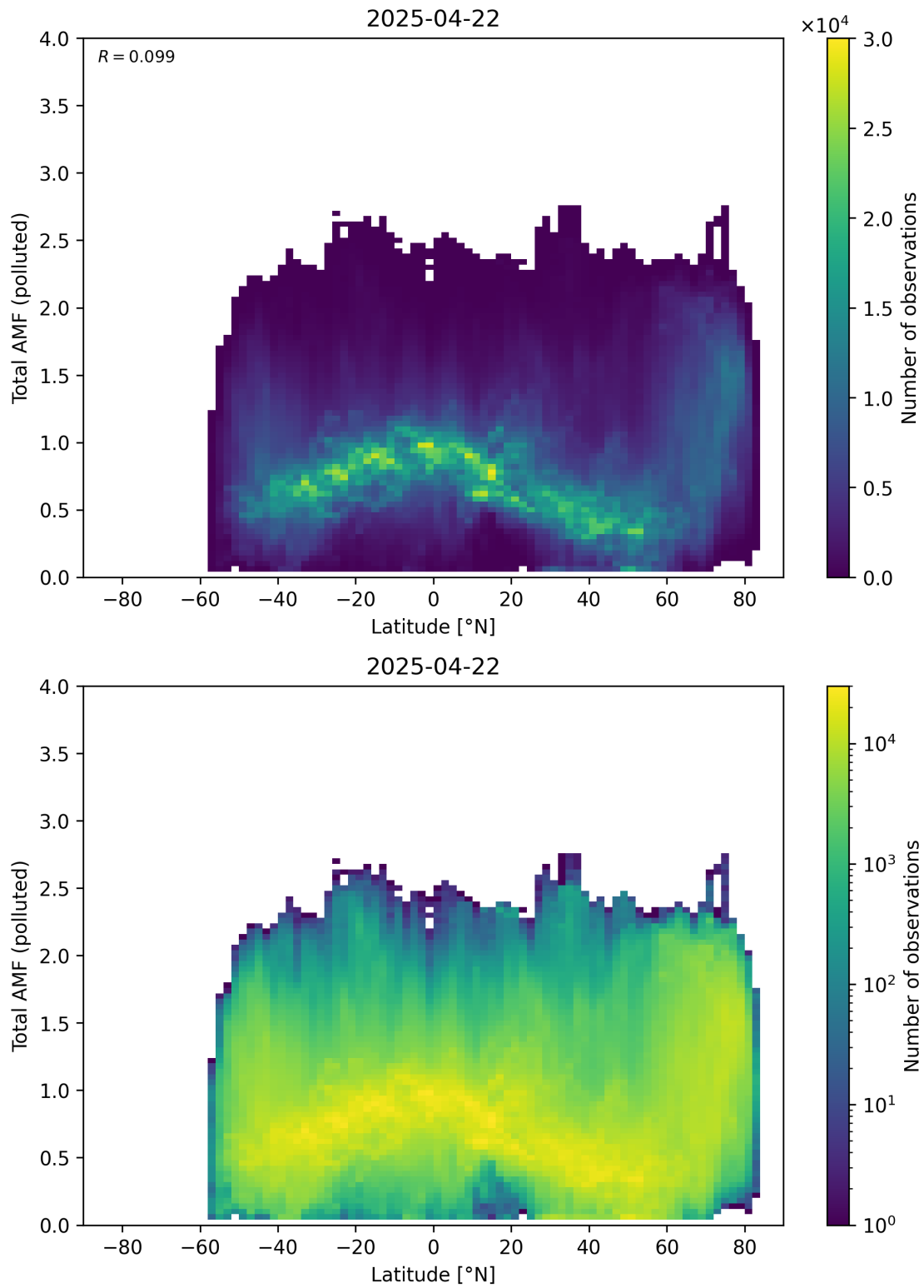
Figure 167: Scatter density plot of “Latitude” against “Total AMF (polluted)” for 2025-04-21 to 2025-04-23.
