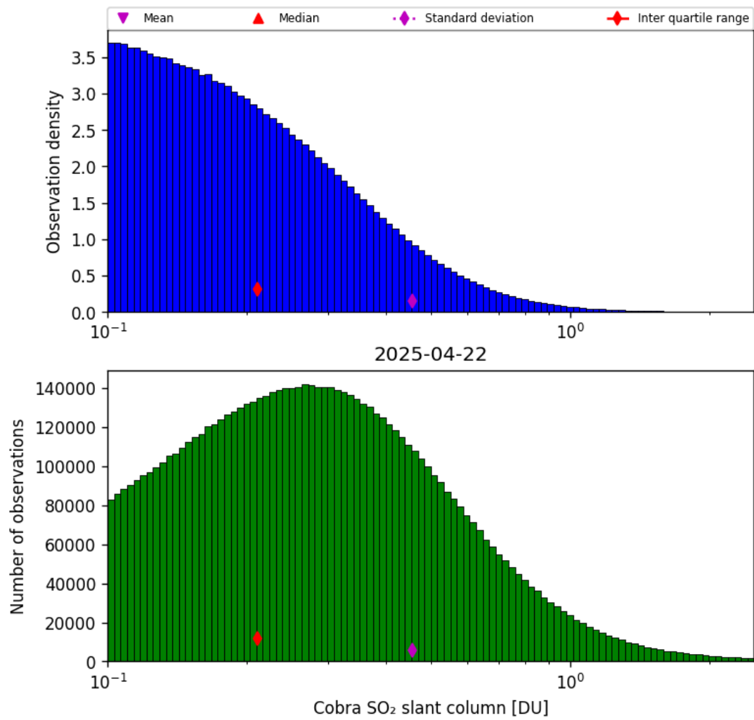
Figure 61: Histogram of “Cobra SO 2 slant column” for 2025-04-21 to 2025-04-23
