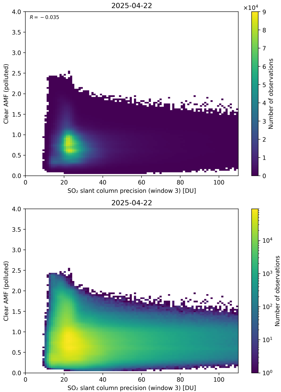
Figure 311: Scatter density plot of “SO 2 slant column precision (window 3)” against “Clear AMF (polluted)” for 2025-04-21 to 2025-04-23.
