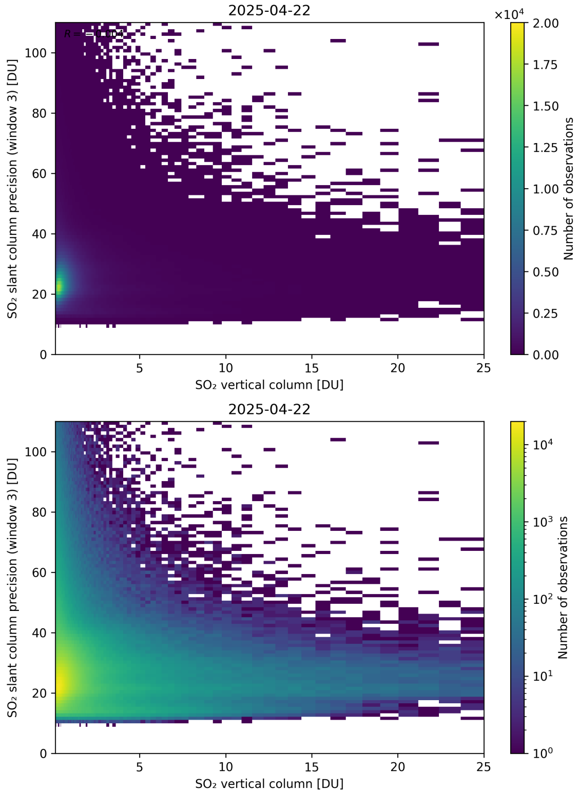
Figure 358: Scatter density plot of “SO 2 vertical column” against “SO 2 slant column precision (window 3)” for 2025-04-21 to 2025-04-23.
