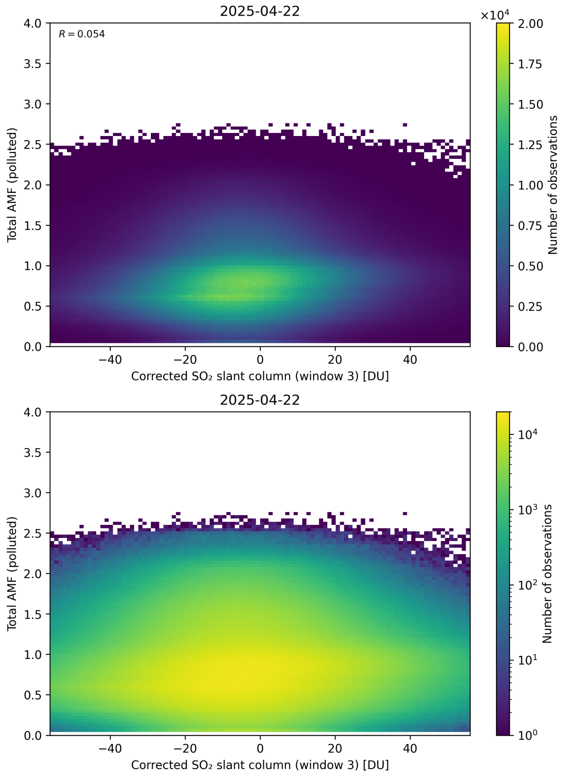
Figure 260: Scatter density plot of “Corrected SO 2 slant column (window 3)” against “Total AMF (polluted)” for 2025-04-21 to 2025-04-23.
