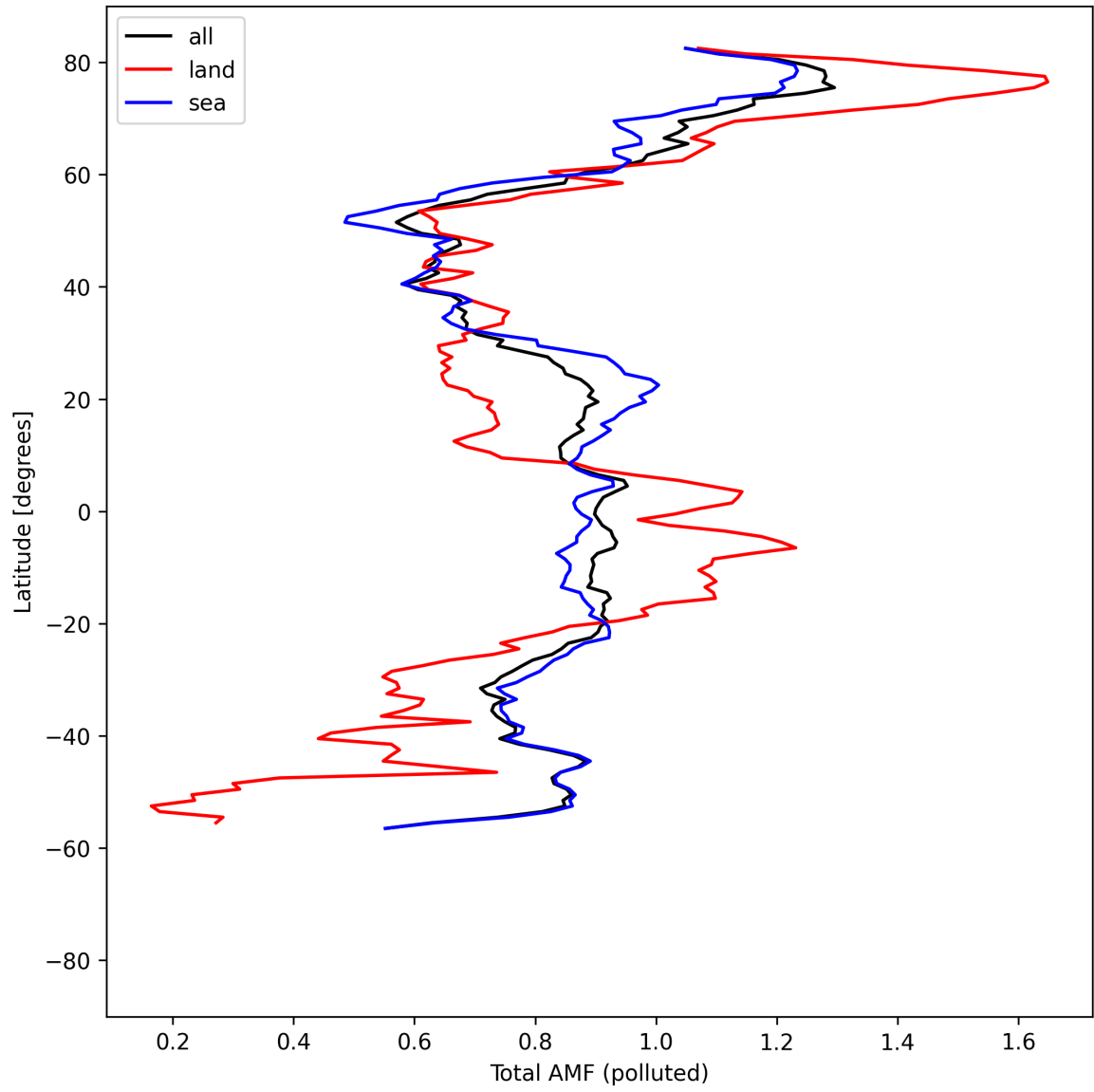
Figure 53: Zonal average of “Total AMF (polluted)” for 2025-04-21 to 2025-04-23.
