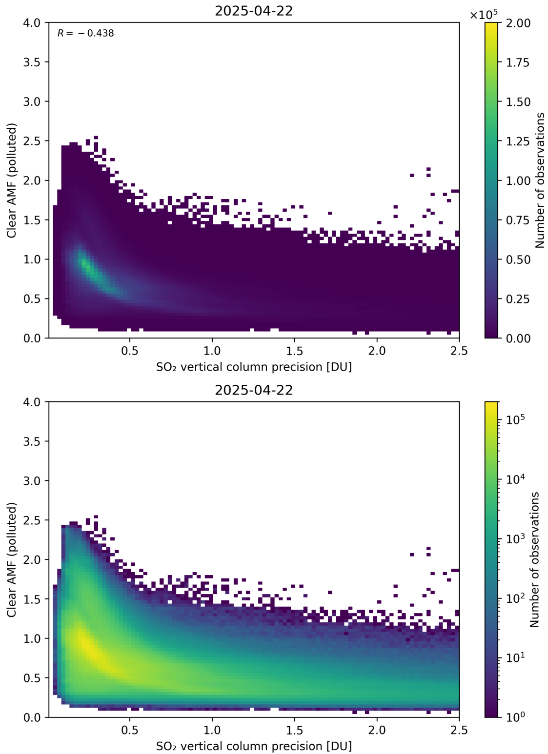
Figure 335: Scatter density plot of “SO 2 vertical column precision” against “Clear AMF (polluted)” for 2025-04-21 to 2025-04-23.
