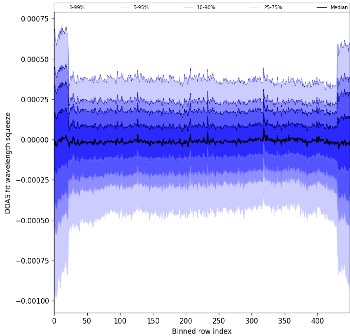
Figure 103: Along track statistics of “DOAS fit wavelength squeeze” for 2025-04-21 to 2025-04-23
