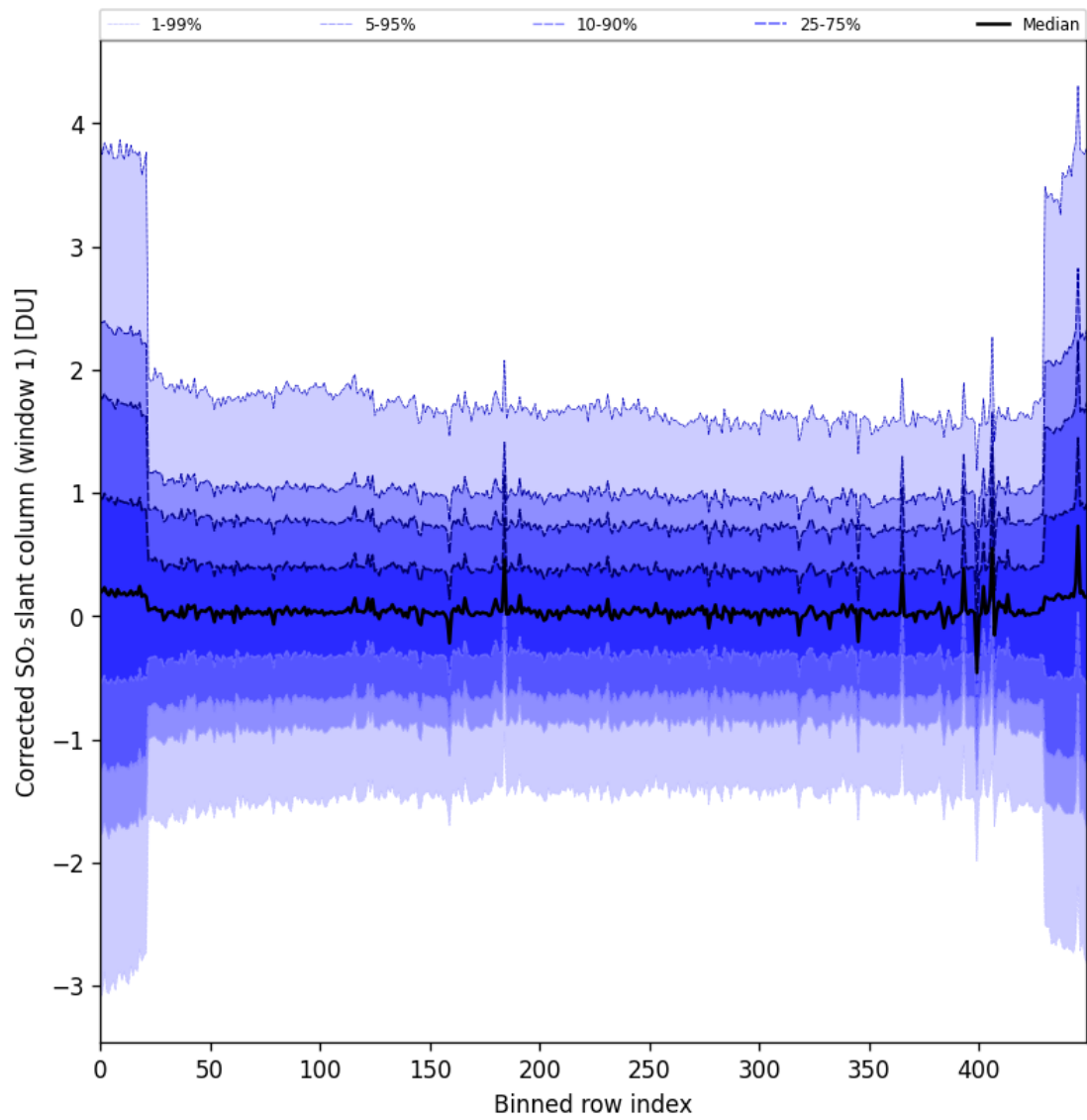
Figure 91: Along track statistics of “Corrected SO 2 slant column (window 1)” for 2025-04-21 to 2025-04-23
