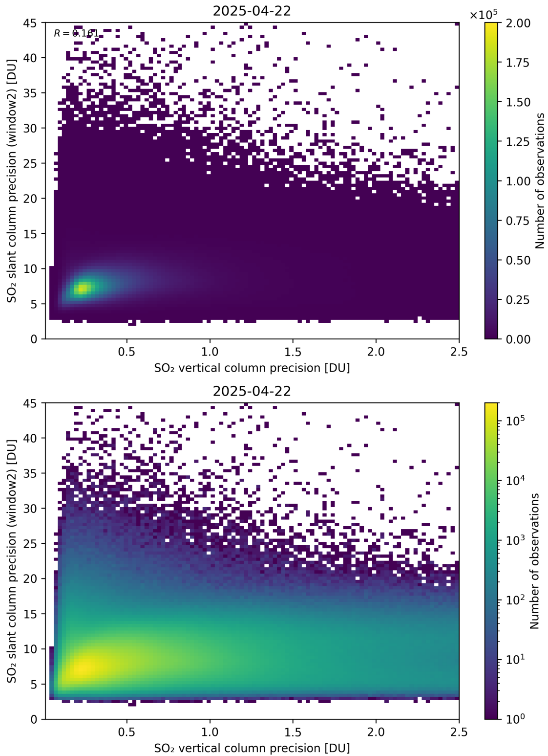
Figure 343: Scatter density plot of “SO 2 vertical column precision” against “SO 2 slant column precision (window2)” for 2025-04-21 to 2025-04-23.
