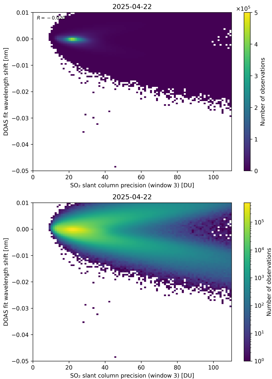
Figure 308: Scatter density plot of “SO 2 slant column precision (window 3)” against “DOAS fit wavelength shift” for 2025-04-21 to 2025-04-23.
