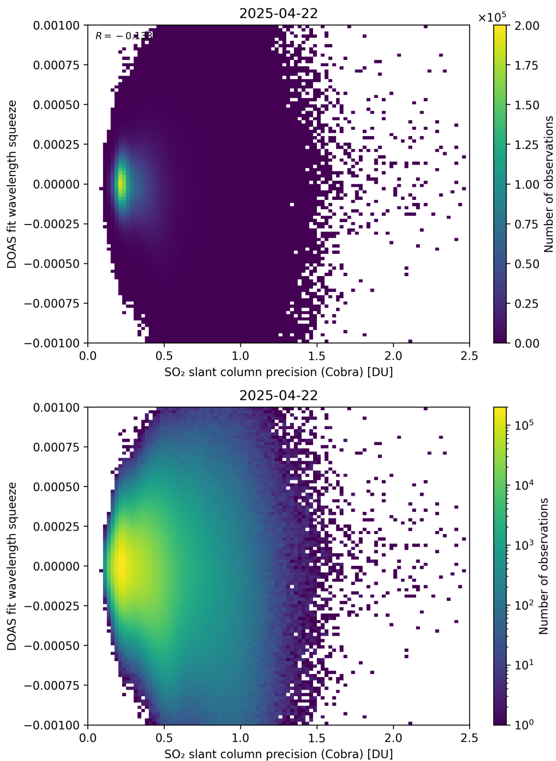
Figure 203: Scatter density plot of “SO 2 slant column precision (Cobra)” against “DOAS fit wavelength squeeze” for 2025-04-21 to 2025-04-23.
