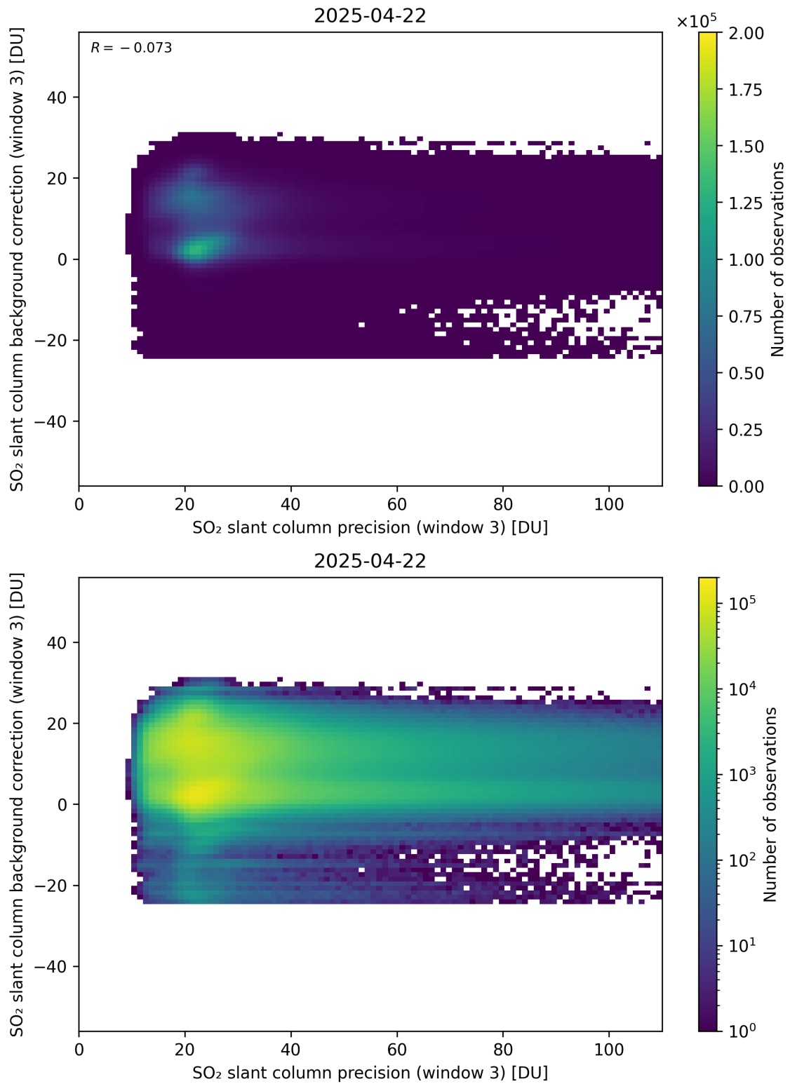
Figure 307: Scatter density plot of “SO 2 slant column precision (window 3)” against “SO 2 slant column background correction (window 3)” for 2025-04-21 to 2025-04-23.
