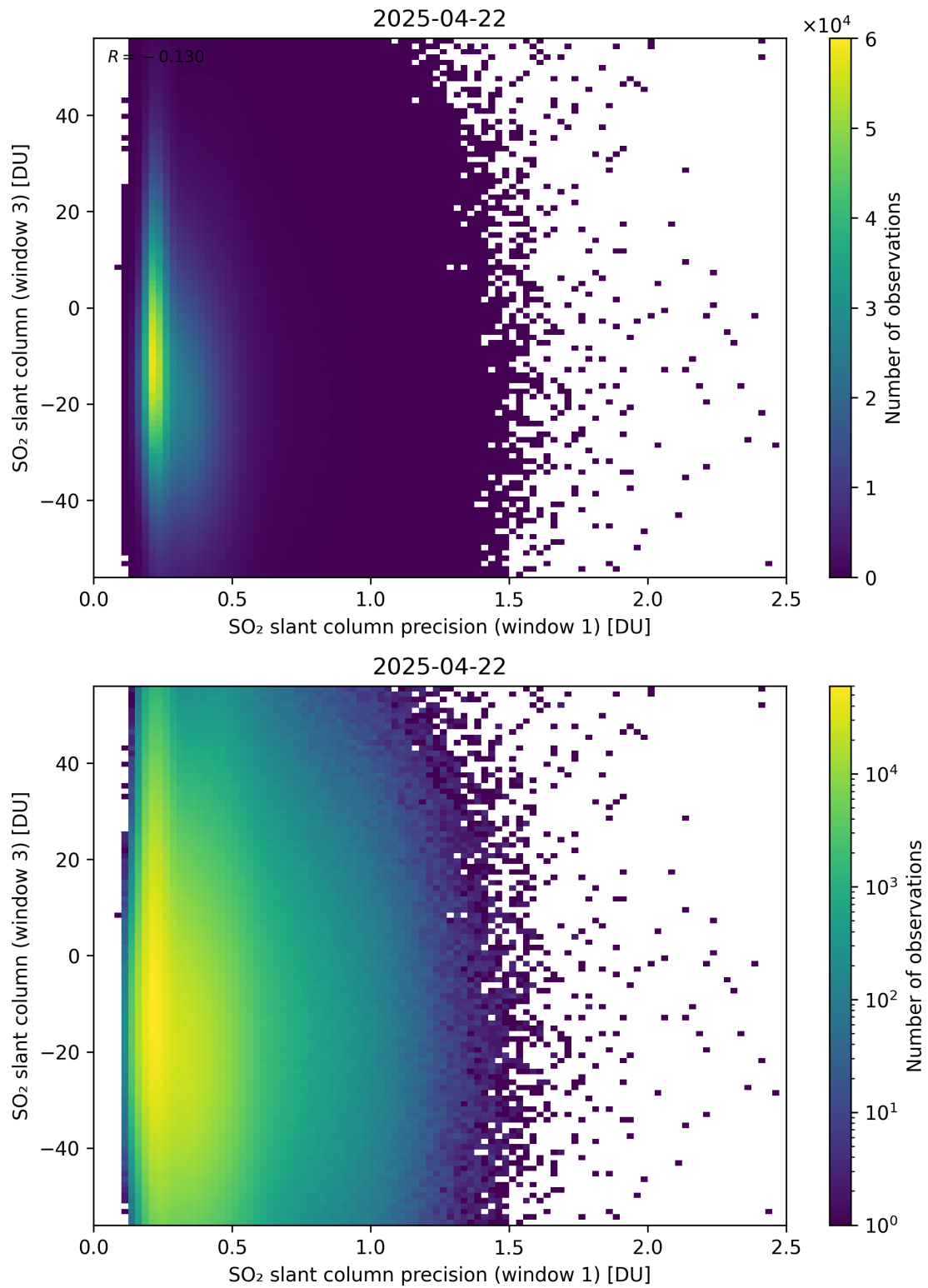
Figure 278: Scatter density plot of “SO 2 slant column precision (window 1)” against “SO 2 slant column (window 3)” for 2025-04-21 to 2025-04-23.
