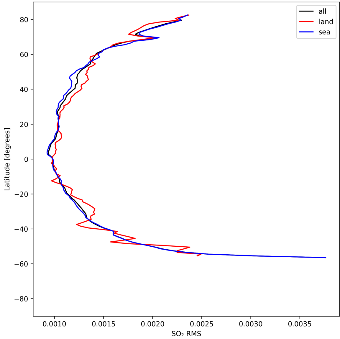
Figure 52: Zonal average of “SO 2 RMS” for 2025-04-21 to 2025-04-23.
