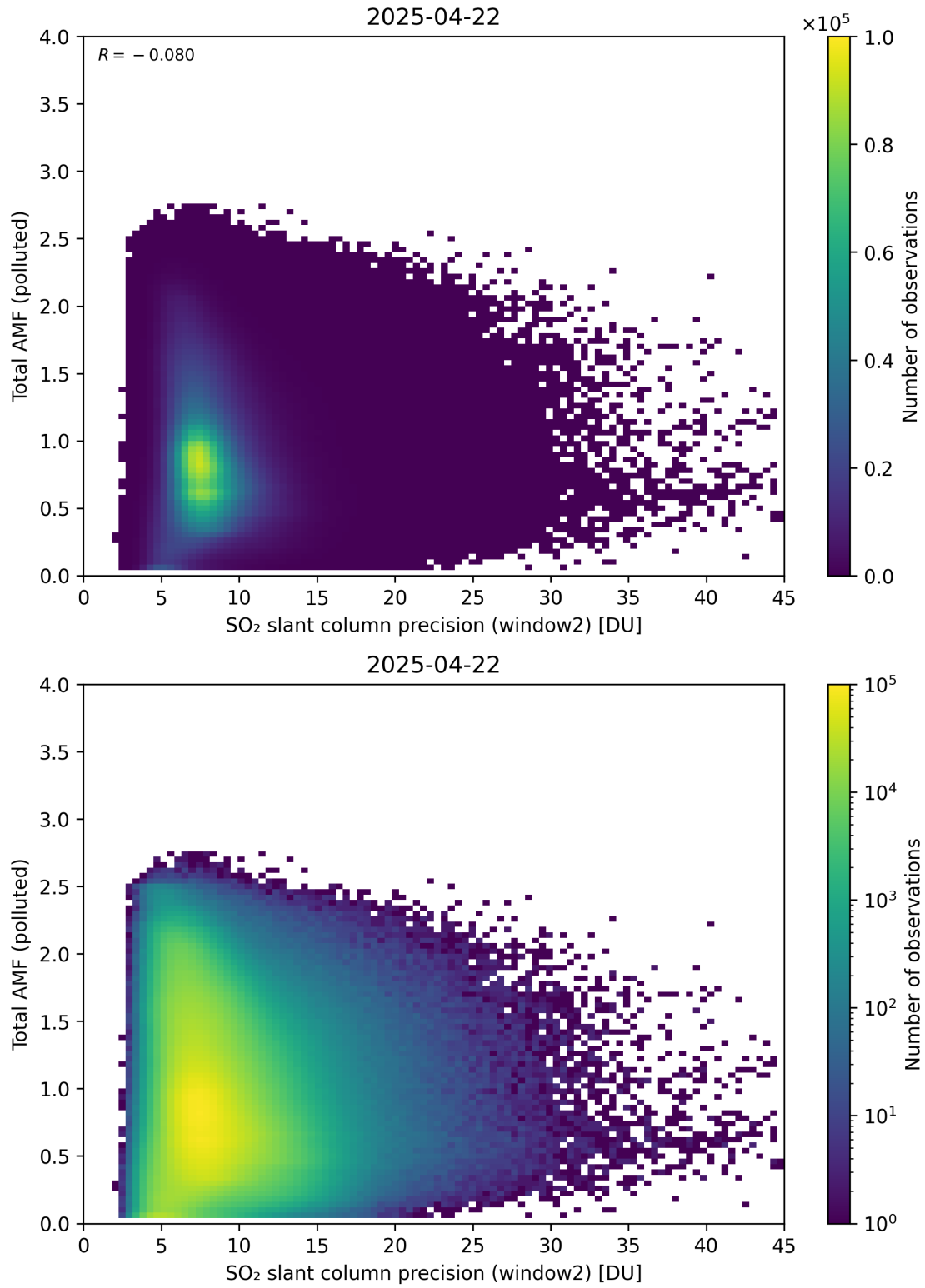
Figure 301: Scatter density plot of “SO 2 slant column precision (window2)” against “Total AMF (polluted)” for 2025-04-21 to 2025-04-23.
