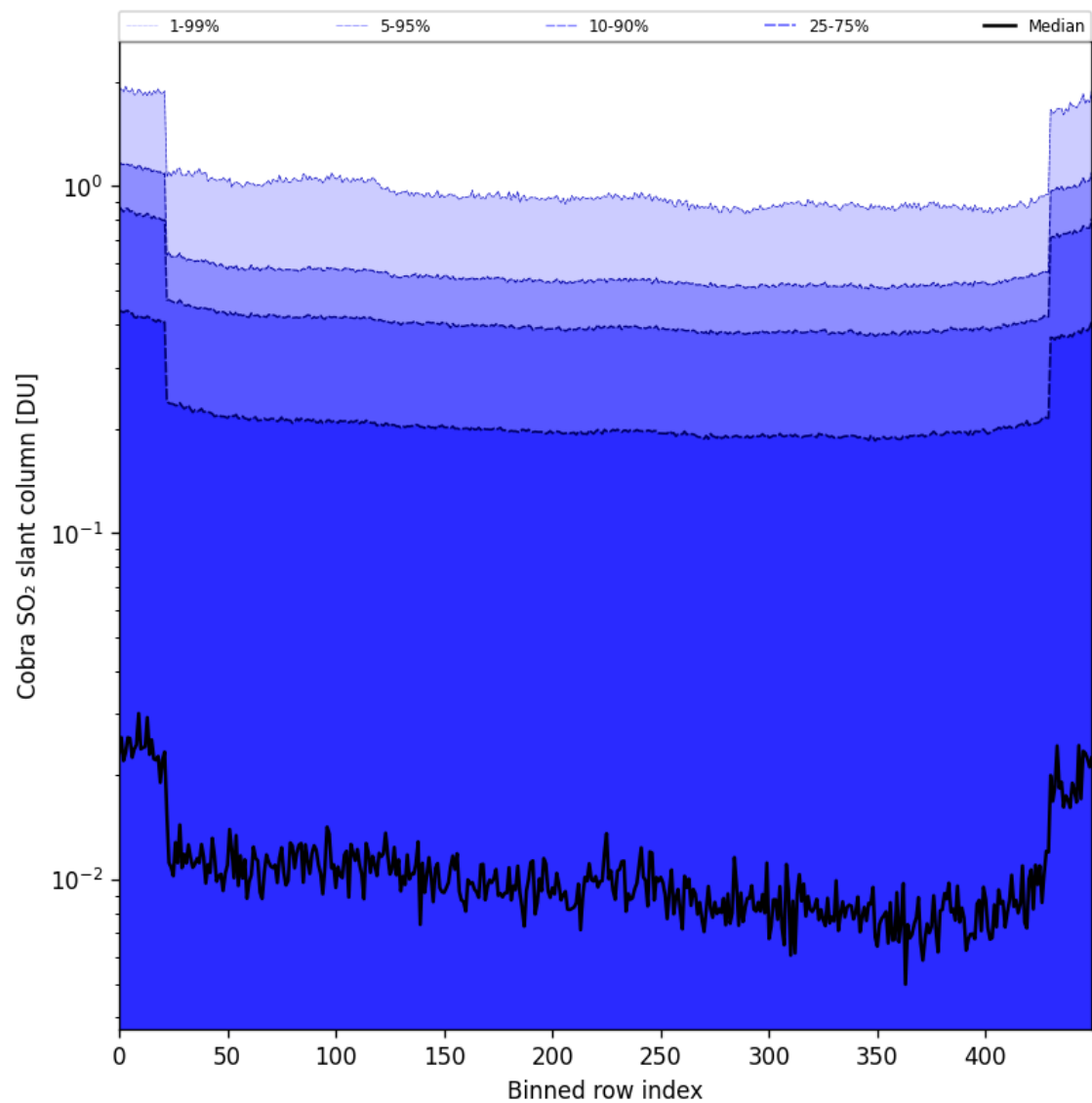
Figure 87: Along track statistics of “Cobra SO 2 slant column” for 2025-04-21 to 2025-04-23
