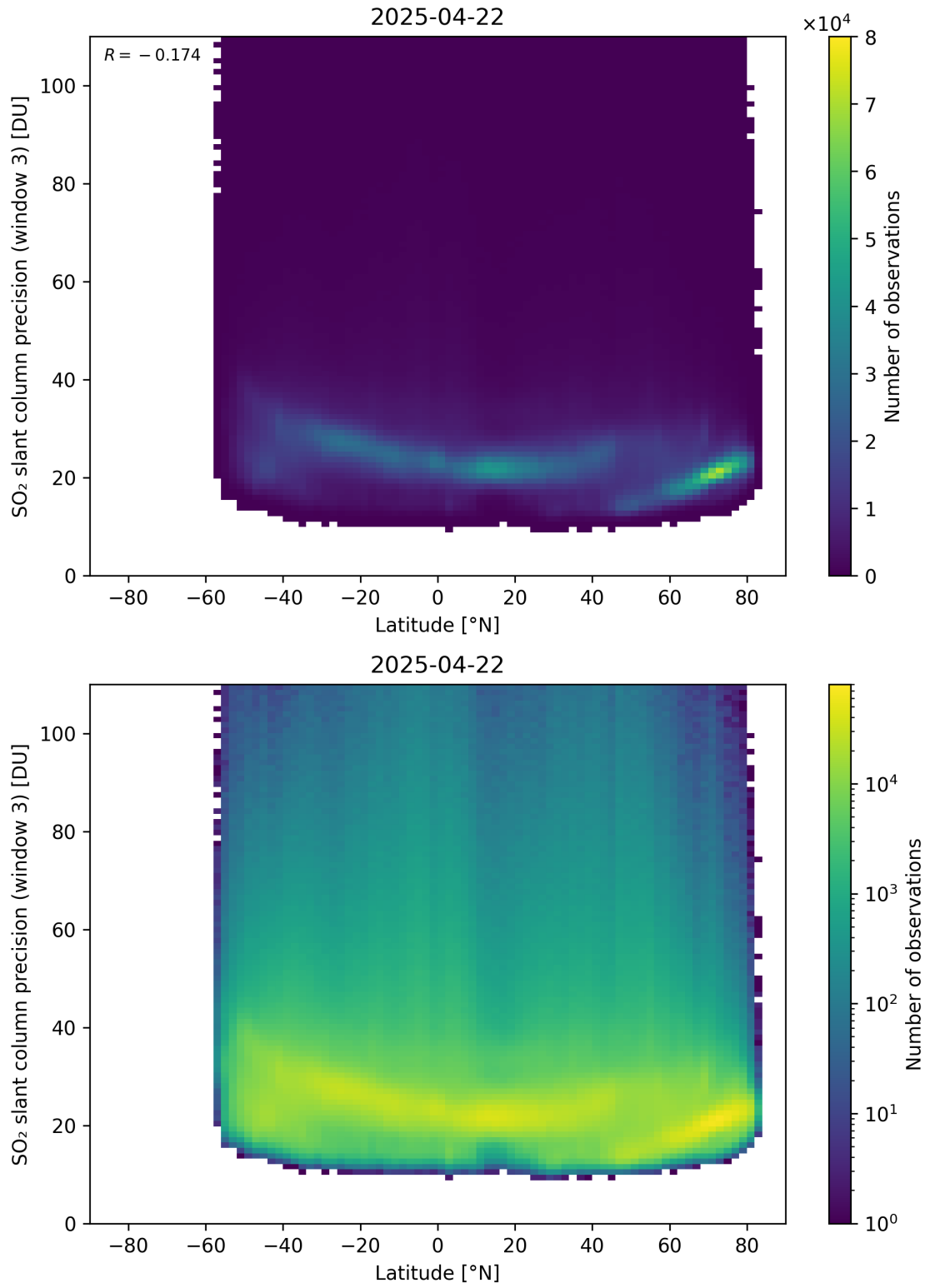
Figure 166: Scatter density plot of “Latitude” against “SO 2 slant column precision (window 3)” for 2025-04-21 to 2025-04-23.
