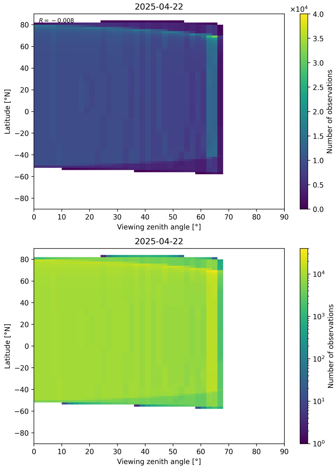
Figure 368: Scatter density plot of “Viewing zenith angle” against “Latitude” for 2025-04-21 to 2025-04-23.
