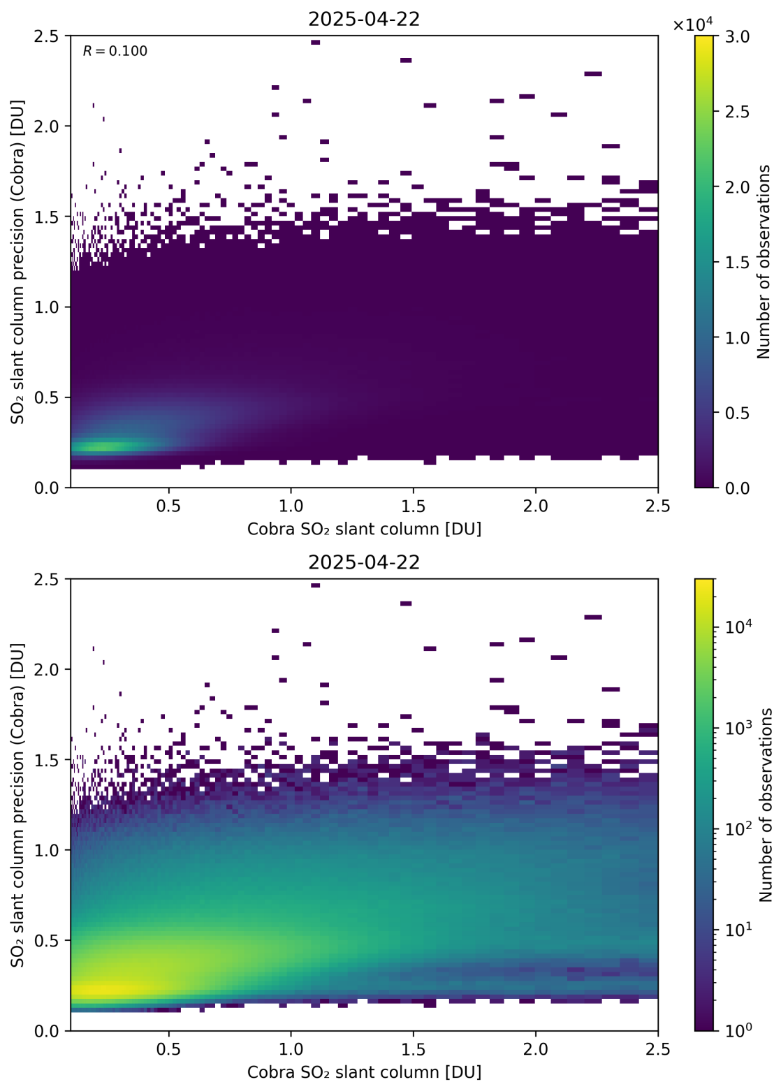
Figure 216: Scatter density plot of “Cobra SO 2 slant column” against “SO 2 slant column precision (Cobra)” for 2025-04-21 to 2025-04-23.
