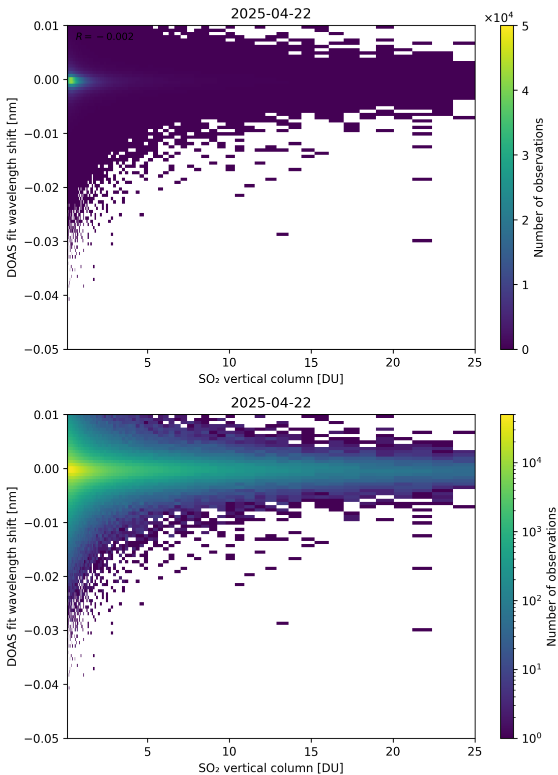
Figure 326: Scatter density plot of “SO 2 vertical column” against “DOAS fit wavelength shift” for 2025-04-21 to 2025-04-23.
