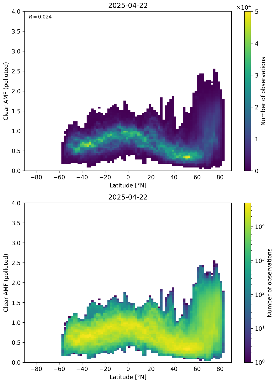
Figure 156: Scatter density plot of “Latitude” against “Clear AMF (polluted)” for 2025-04-21 to 2025-04-23.
