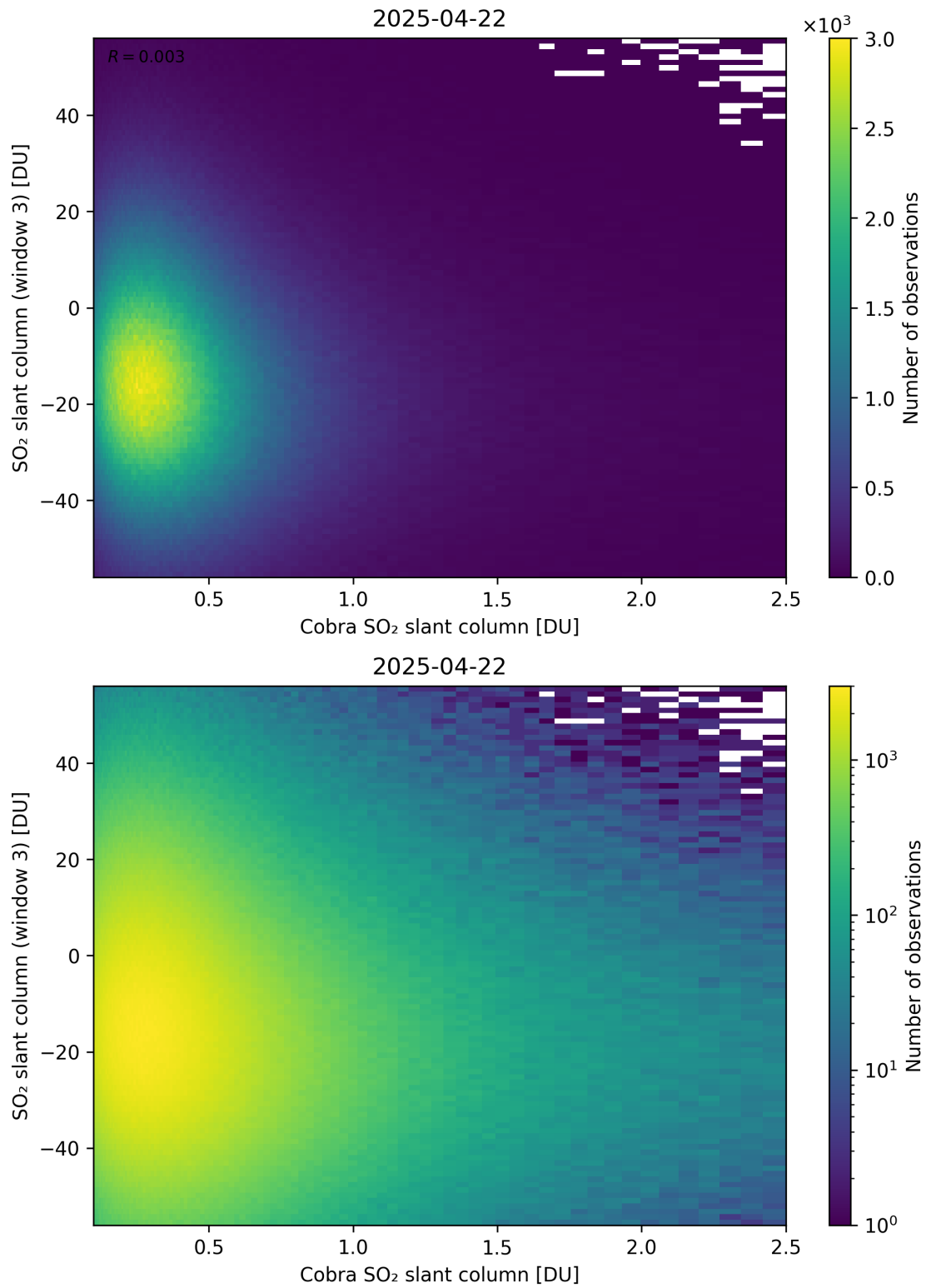
Figure 222: Scatter density plot of “Cobra SO 2 slant column” against “SO 2 slant column (window 3)” for 2025-04-21 to 2025-04-23.
