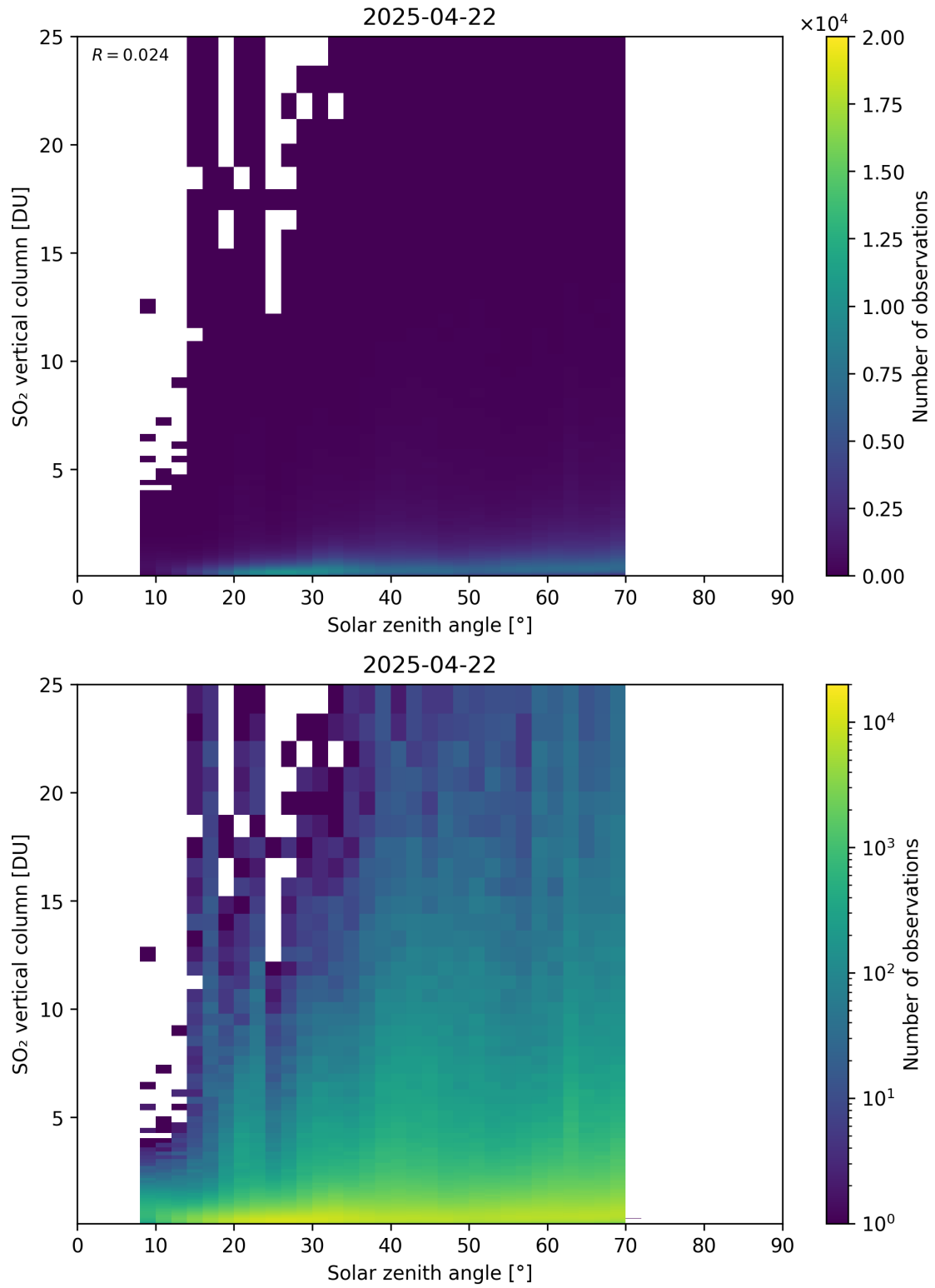
Figure 191: Scatter density plot of “Solar zenith angle” against “SO 2 vertical column” for 2025-04-21 to 2025-04-23.
