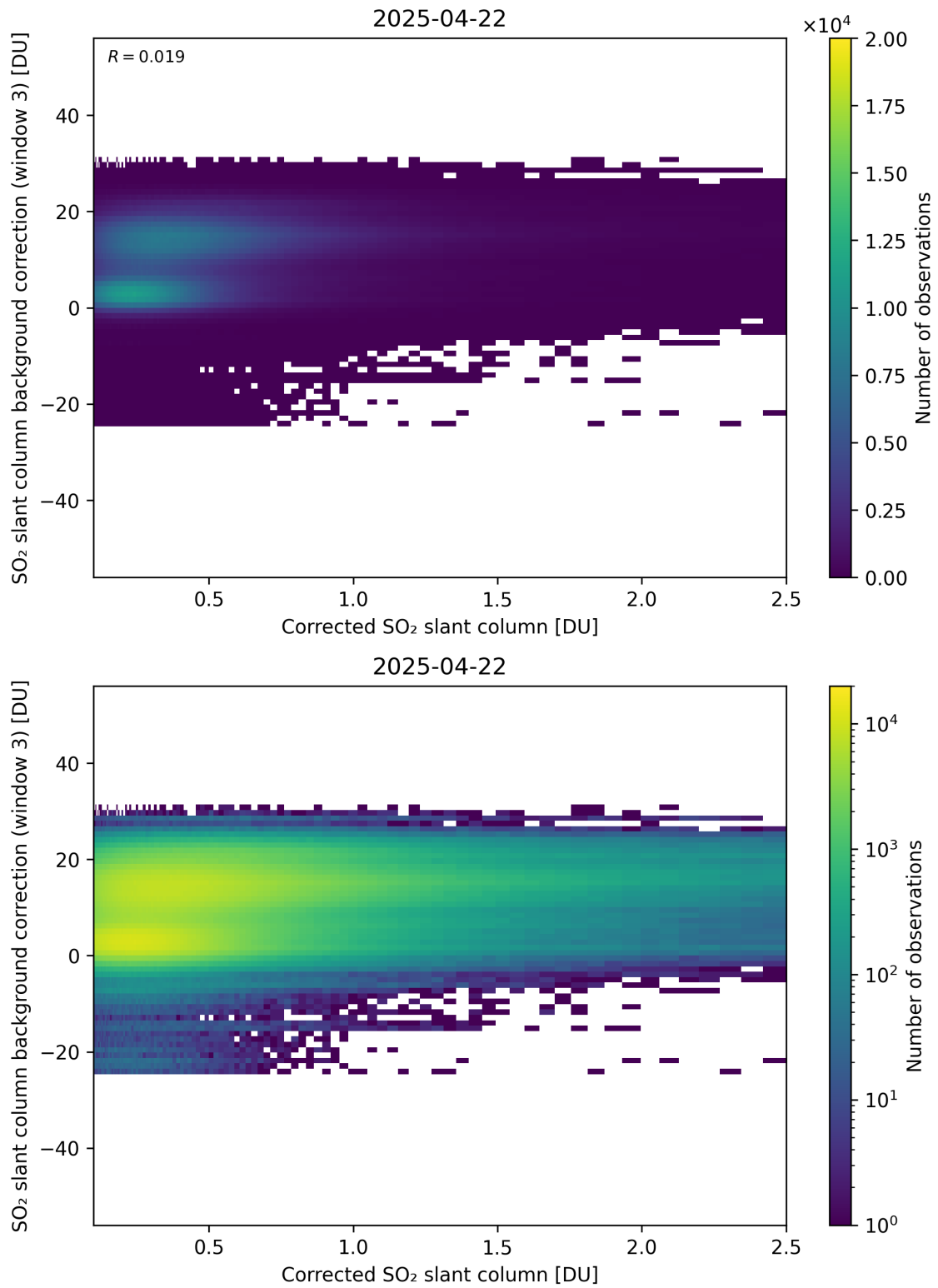
Figure 228: Scatter density plot of “Corrected SO 2 slant column” against “SO 2 slant column background correction (window 3)” for 2025-04-21 to 2025-04-23.
