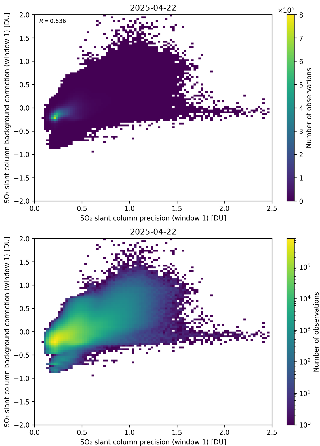
Figure 268: Scatter density plot of “SO 2 slant column precision (window 1)” against “SO 2 slant column background correction (window 1)” for 2025-04-21 to 2025-04-23.
