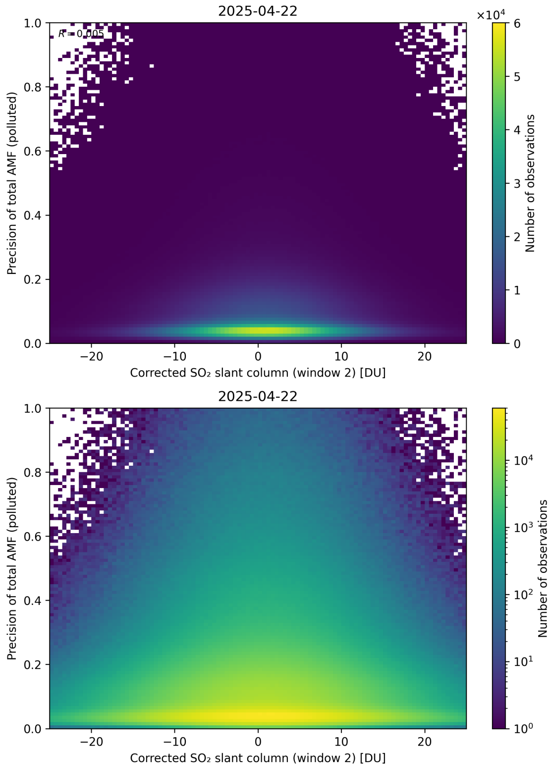
Figure 254: Scatter density plot of “Corrected SO 2 slant column (window 2)” against “Precision of total AMF (polluted)” for 2025-04-21 to 2025-04-23.
