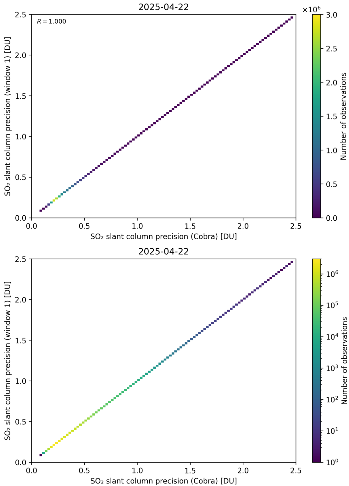
Figure 209: Scatter density plot of “SO 2 slant column precision (Cobra)” against “SO 2 slant column precision (window 1)” for 2025-04-21 to 2025-04-23.
