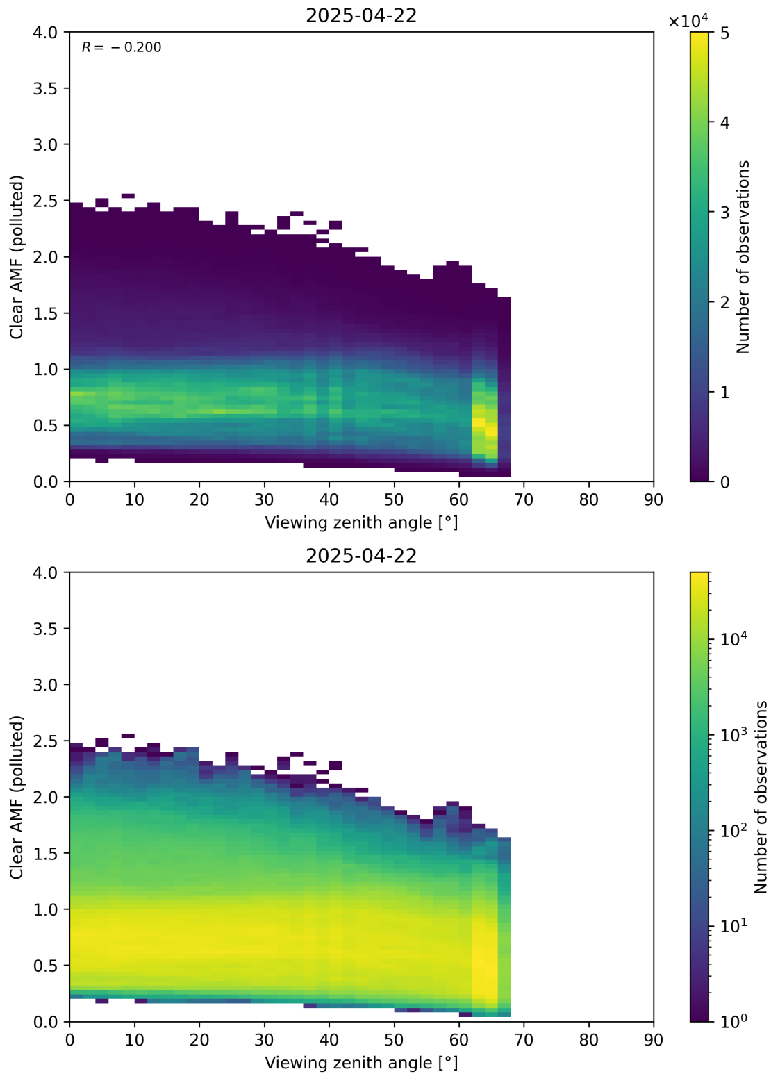
Figure 370: Scatter density plot of “Viewing zenith angle” against “Clear AMF (polluted)” for 2025-04-21 to 2025-04-23.
