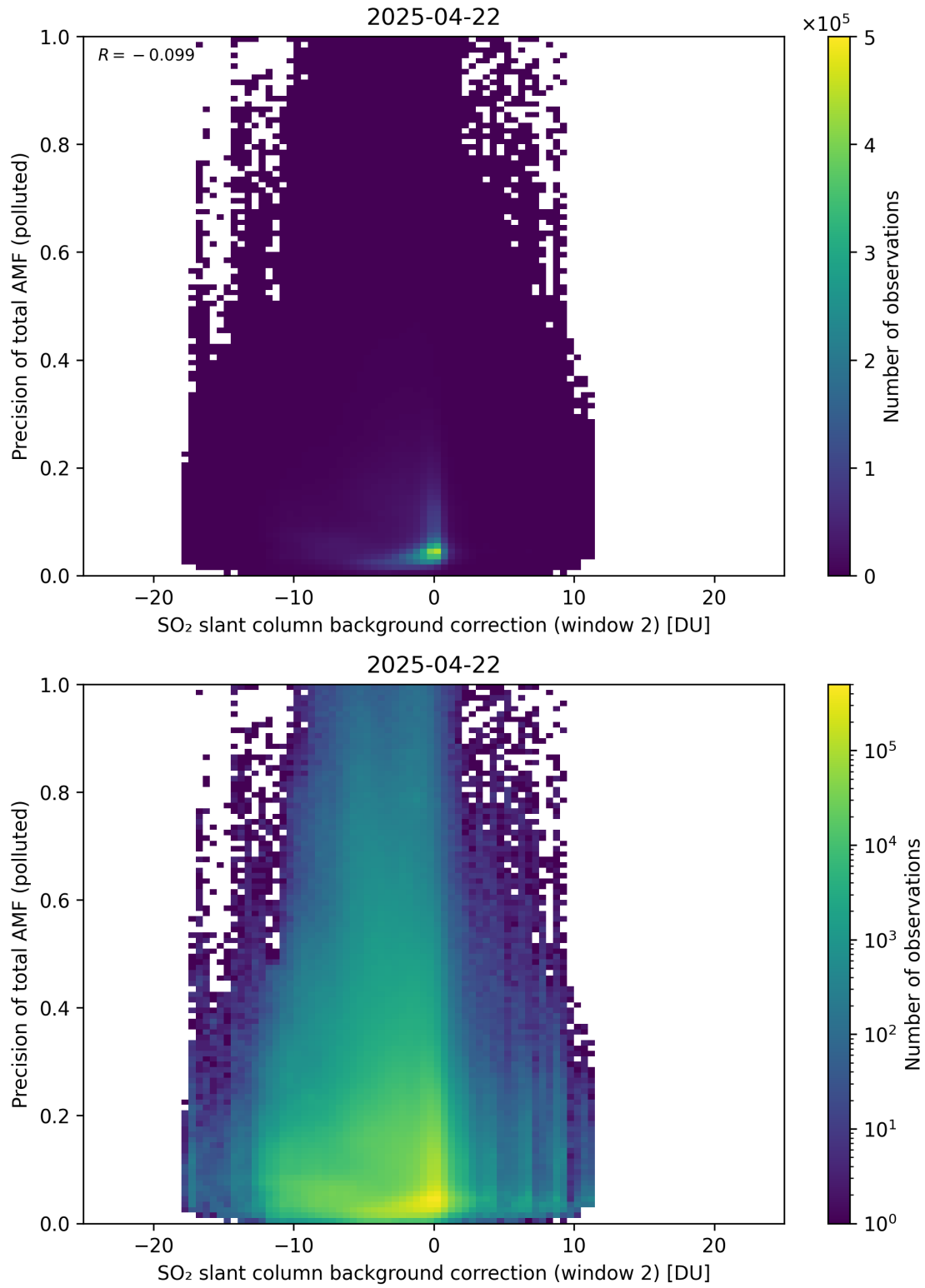
Figure 131: Scatter density plot of “SO 2 slant column background correction (window 2)” against “Precision of total AMF (polluted)” for 2025-04-21 to 2025-04-23.
