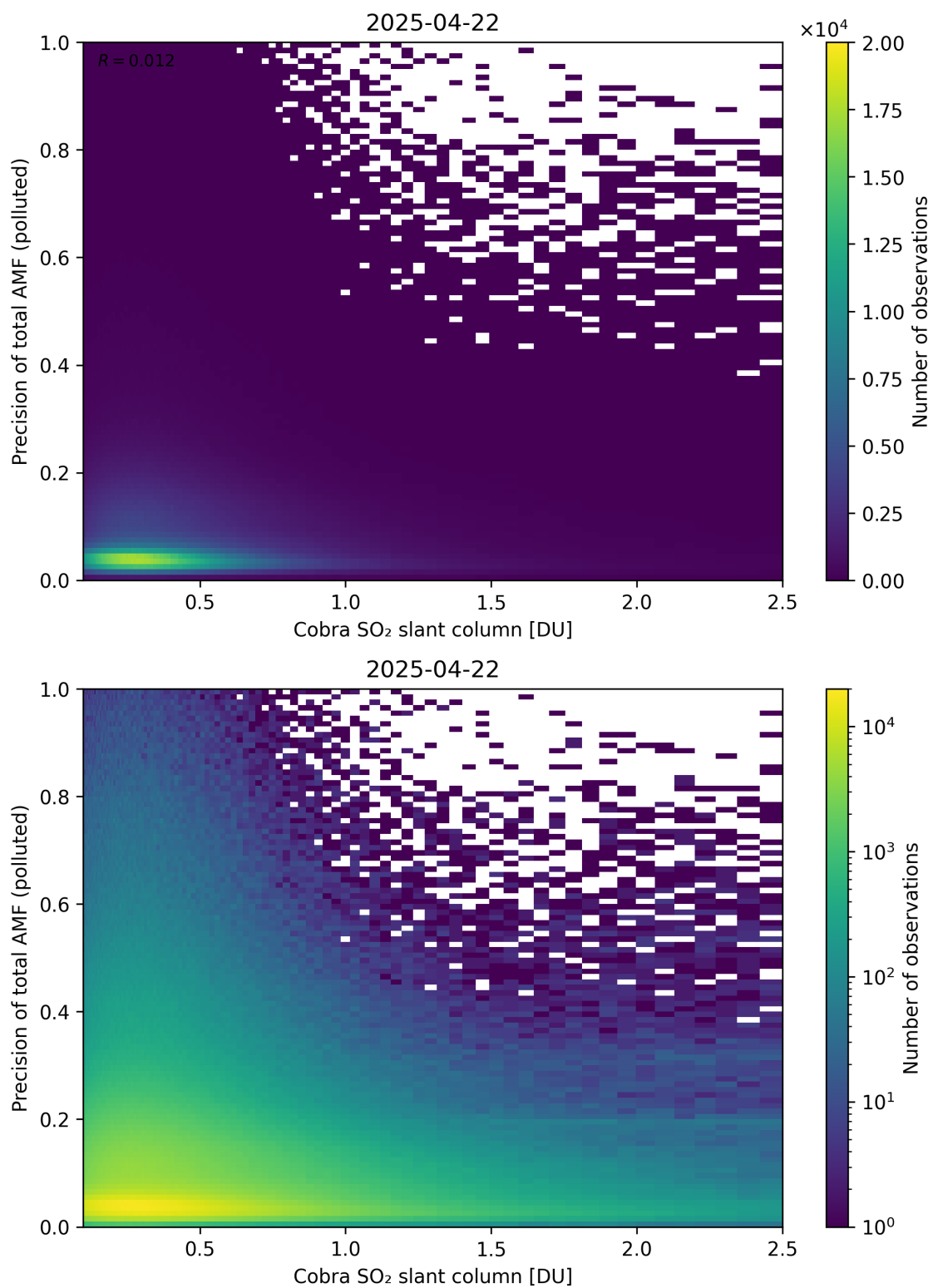
Figure 225: Scatter density plot of “Cobra SO 2 slant column” against “Precision of total AMF (polluted)” for 2025-04-21 to 2025-04-23.
