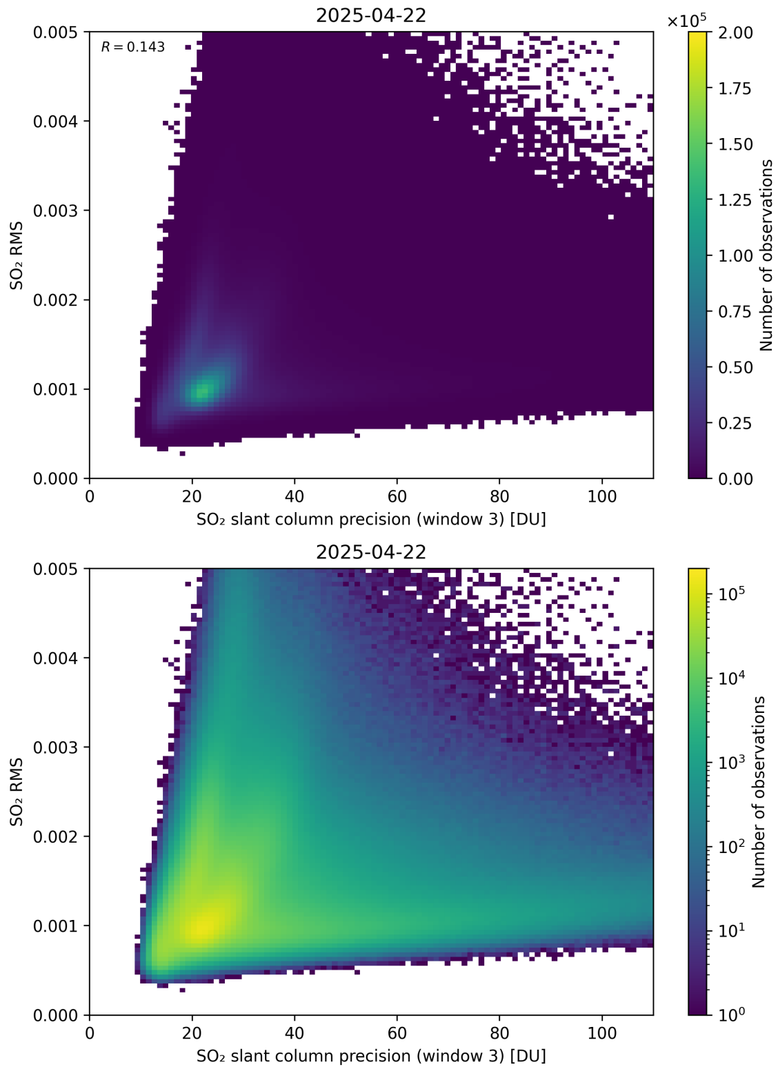
Figure 310: Scatter density plot of “SO 2 slant column precision (window 3)” against “SO 2 RMS” for 2025-04-21 to 2025-04-23.
