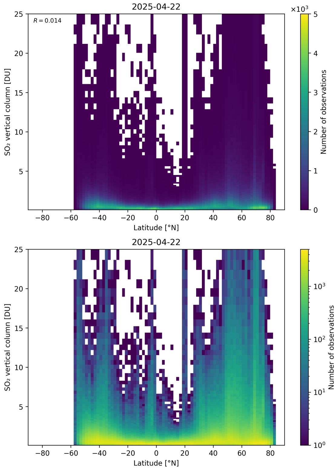
Figure 169: Scatter density plot of “Latitude” against “SO 2 vertical column” for 2025-04-21 to 2025-04-23.
