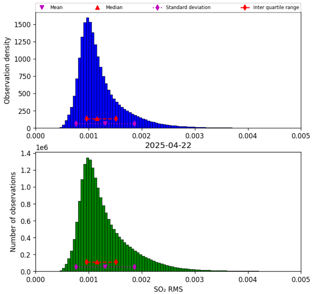
Figure 78: Histogram of “SO 2 RMS” for 2025-04-21 to 2025-04-23
