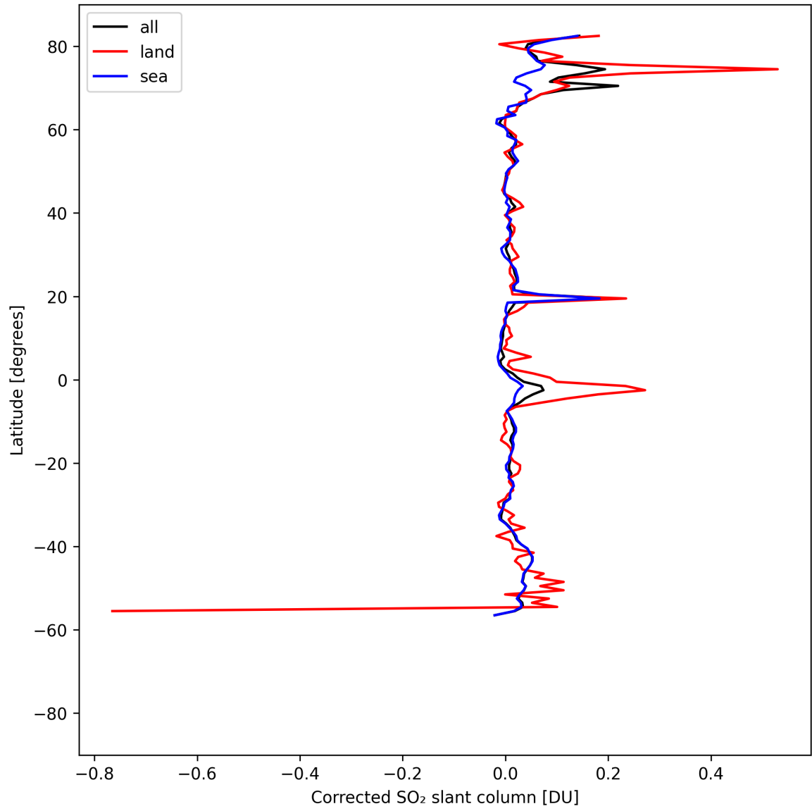
Figure 34: Zonal average of “Corrected SO 2 slant column” for 2025-04-21 to 2025-04-23.
