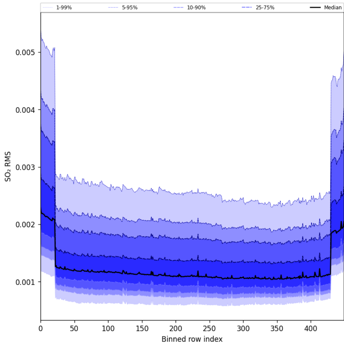
Figure 104: Along track statistics of “SO 2 RMS” for 2025-04-21 to 2025-04-23
