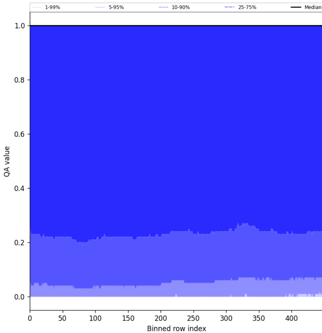
Figure 83: Along track statistics of “QA value” for 2025-04-21 to 2025-04-23
