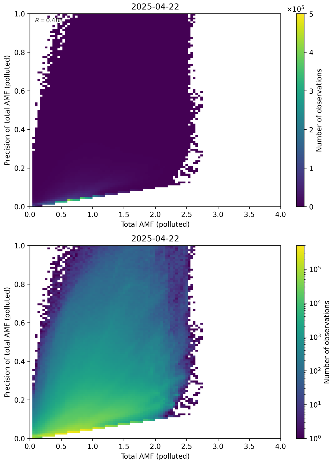
Figure 322: Scatter density plot of “Total AMF (polluted)” against “Precision of total AMF (polluted)” for 2025-04-21 to 2025-04-23.
