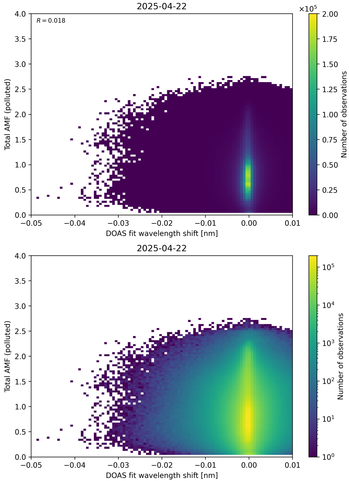
Figure 141: Scatter density plot of “DOAS fit wavelength shift” against “Total AMF (polluted)” for 2025-04-21 to 2025-04-23.
