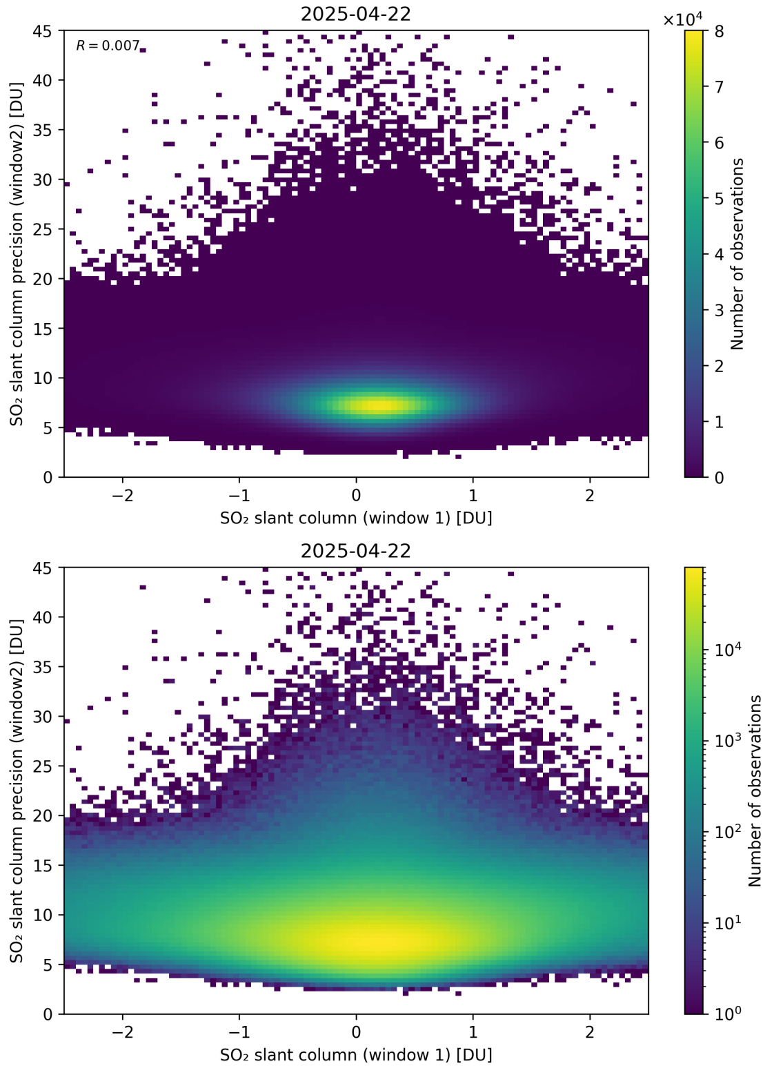
Figure 286: Scatter density plot of “SO 2 slant column (window 1)” against “SO 2 slant column precision (window2)” for 2025-04-21 to 2025-04-23.
