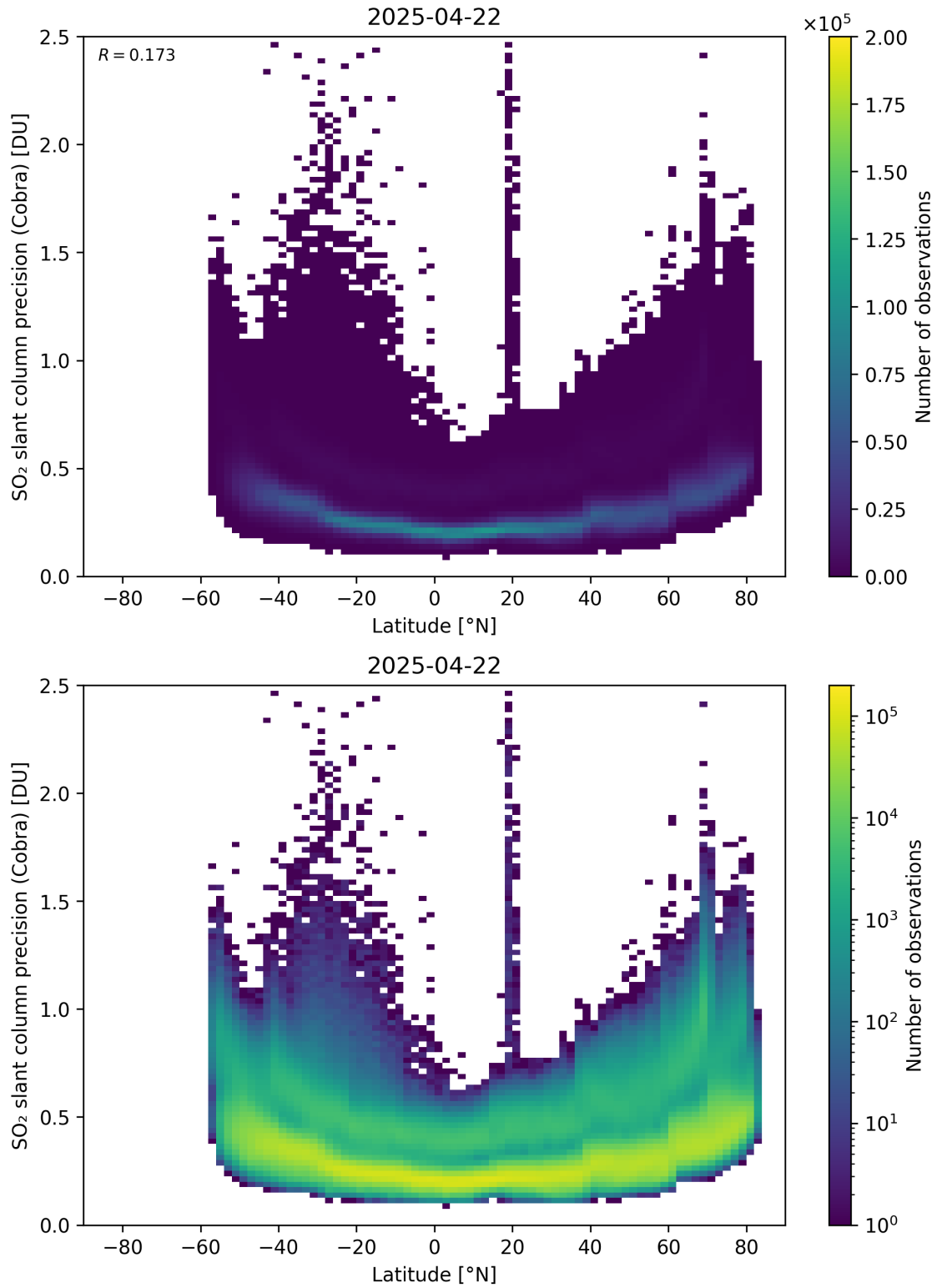
Figure 158: Scatter density plot of “Latitude” against “SO 2 slant column precision (Cobra)” for 2025-04-21 to 2025-04-23.
