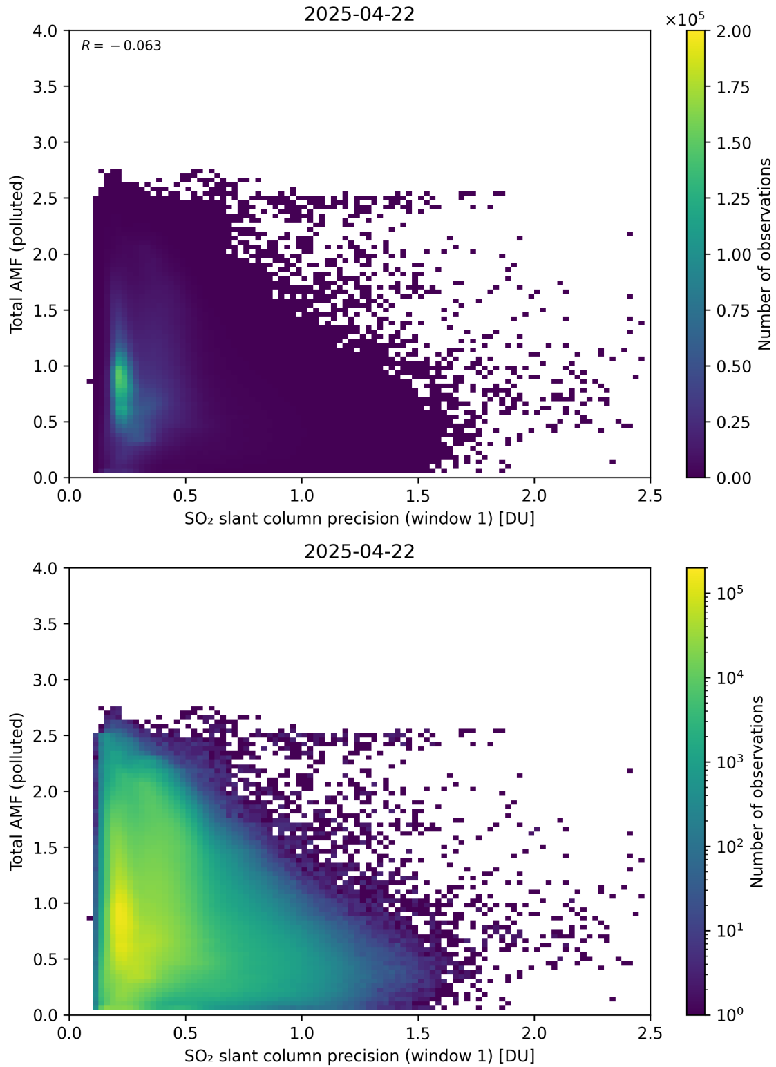
Figure 280: Scatter density plot of “SO 2 slant column precision (window 1)” against “Total AMF (polluted)” for 2025-04-21 to 2025-04-23.
