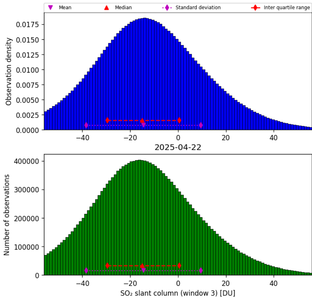
Figure 71: Histogram of “SO 2 slant column (window 3)” for 2025-04-21 to 2025-04-23
