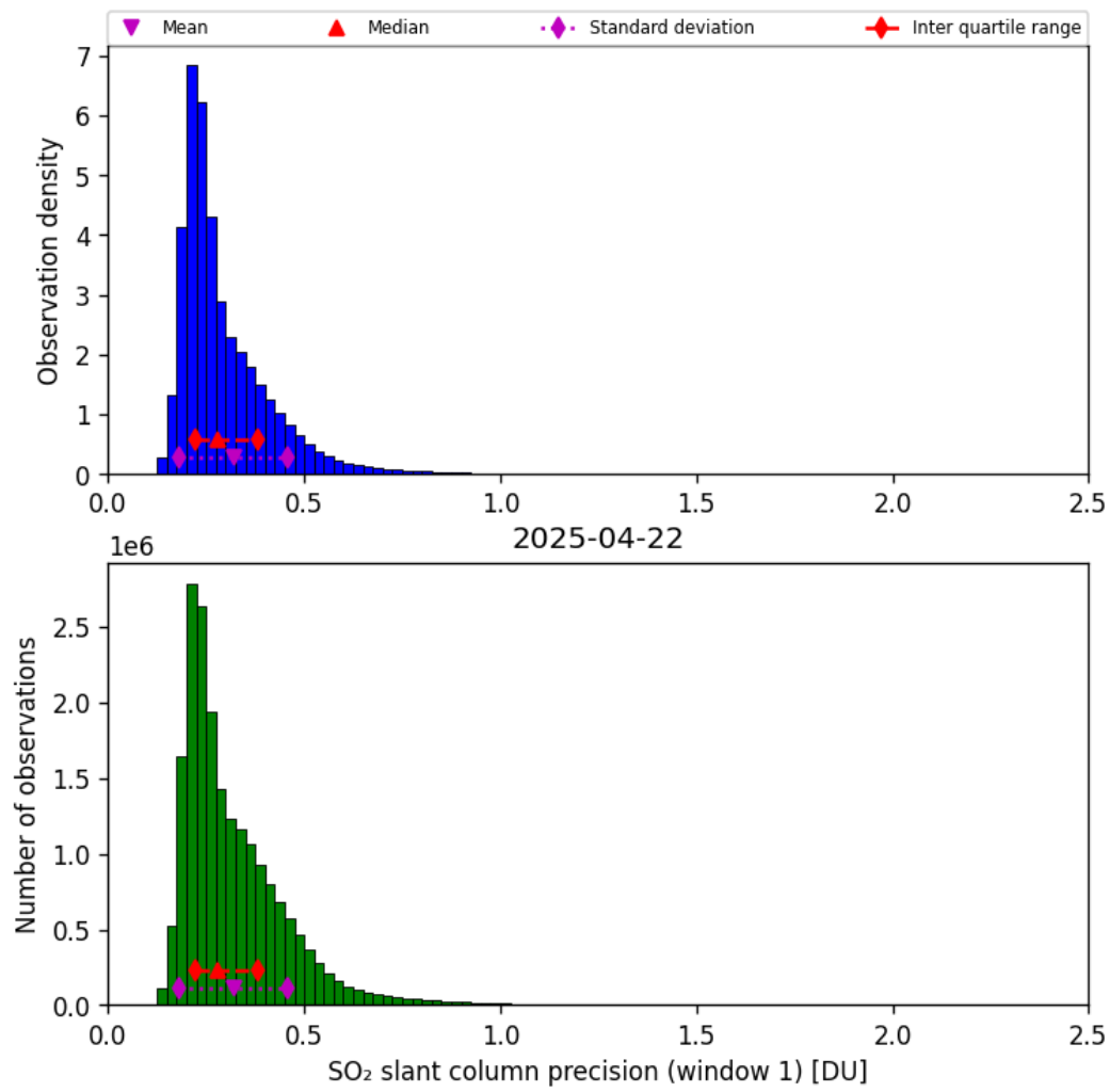
Figure 64: Histogram of “SO 2 slant column precision (window 1)” for 2025-04-21 to 2025-04-23
