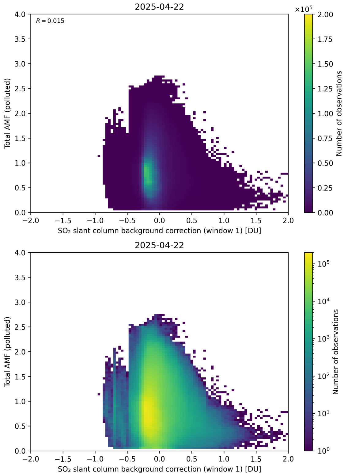
Figure 120: Scatter density plot of “SO 2 slant column background correction (window 1)” against “Total AMF (polluted)” for 2025-04-21 to 2025-04-23.
