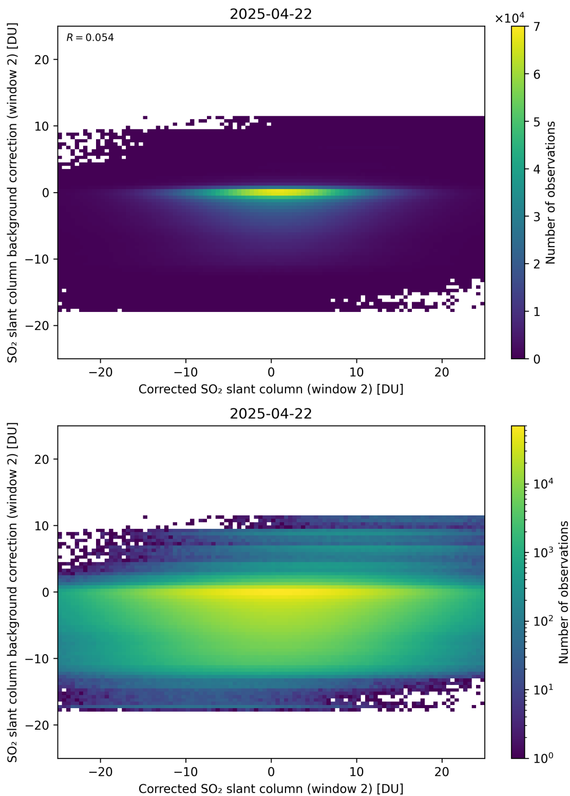
Figure 244: Scatter density plot of “Corrected SO 2 slant column (window 2)” against “SO 2 slant column background correction (window 2)” for 2025-04-21 to 2025-04-23.
