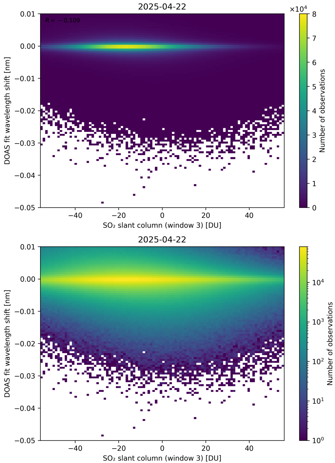
Figure 304: Scatter density plot of “SO 2 slant column (window 3)” against “DOAS fit wavelength shift” for 2025-04-21 to 2025-04-23.
