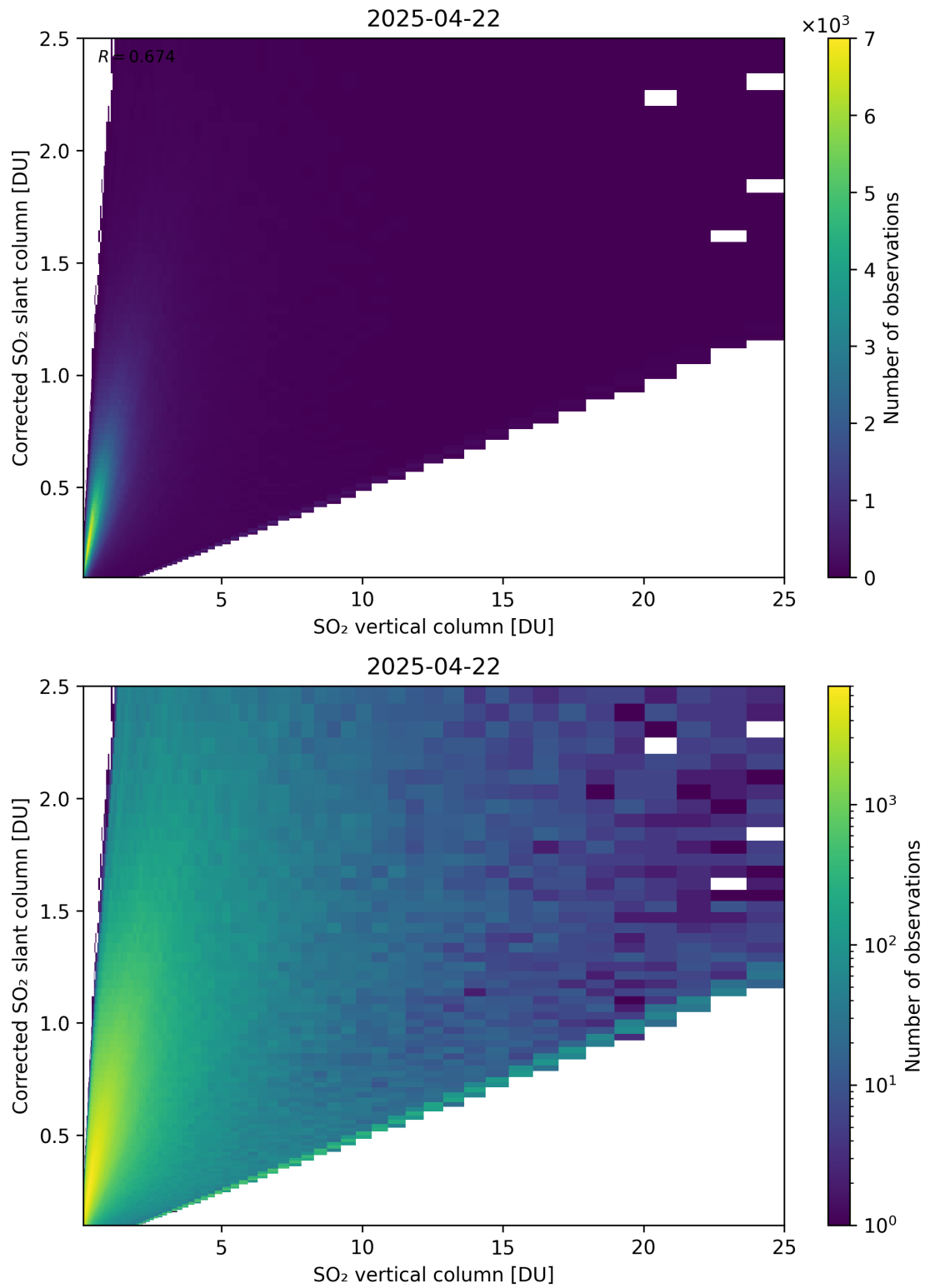
Figure 351: Scatter density plot of “SO 2 vertical column” against “Corrected SO 2 slant column” for 2025-04-21 to 2025-04-23.
