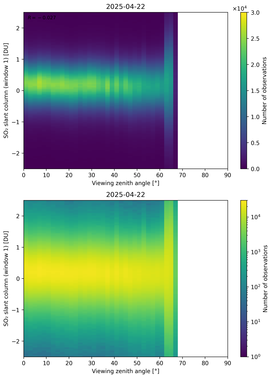
Figure 376: Scatter density plot of “Viewing zenith angle” against “SO 2 slant column (window 1)” for 2025-04-21 to 2025-04-23.
