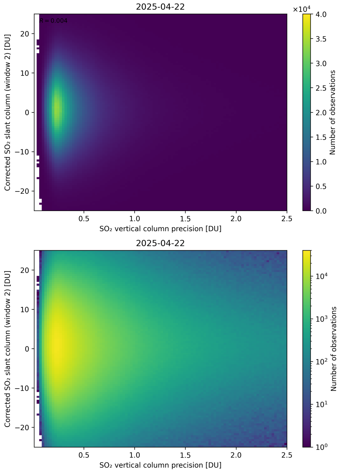
Figure 339: Scatter density plot of “SO 2 vertical column precision” against “Corrected SO 2 slant column (window 2)” for 2025-04-21 to 2025-04-23.
