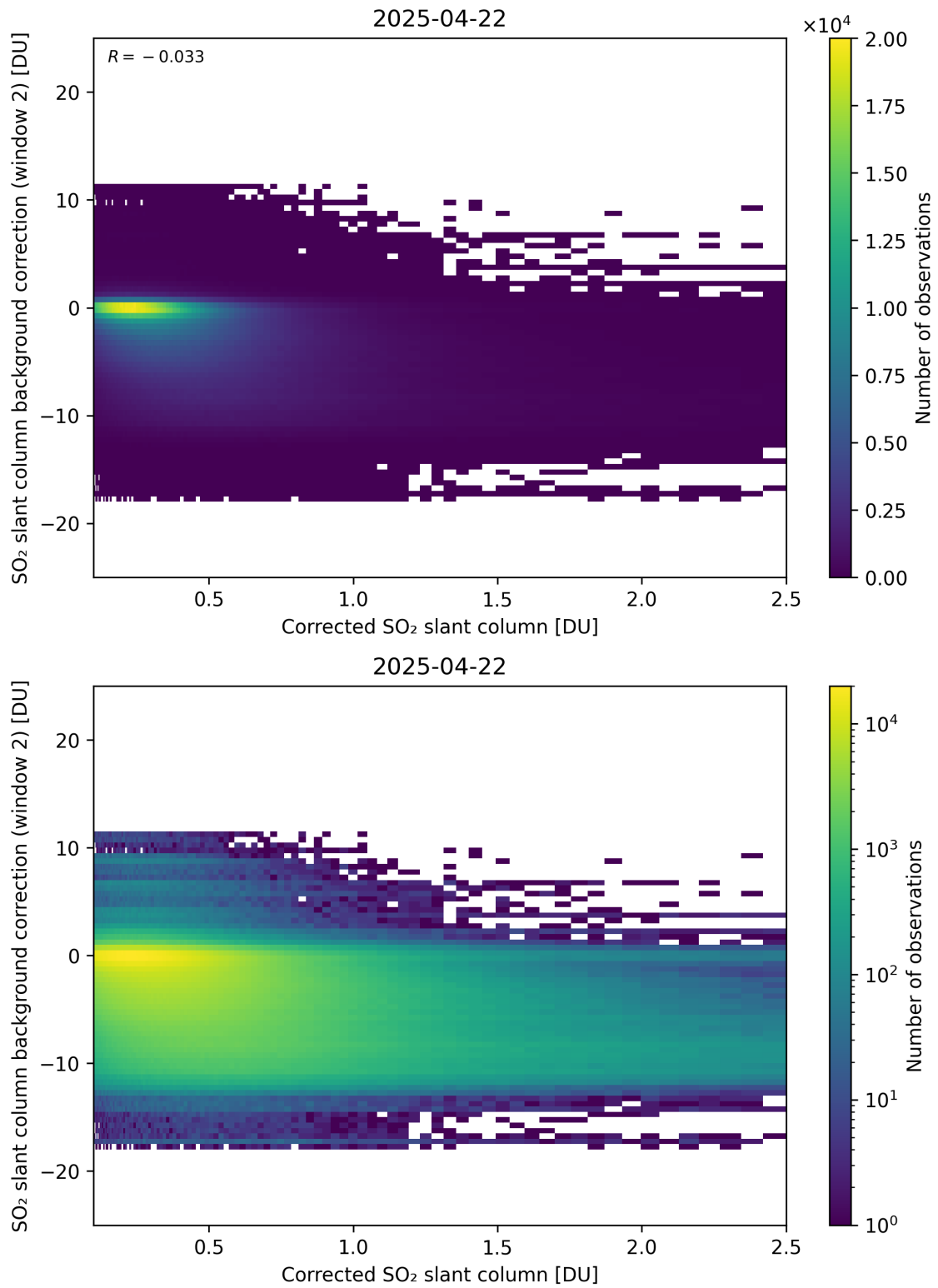
Figure 227: Scatter density plot of “Corrected SO 2 slant column” against “SO 2 slant column background correction (window 2)” for 2025-04-21 to 2025-04-23.
