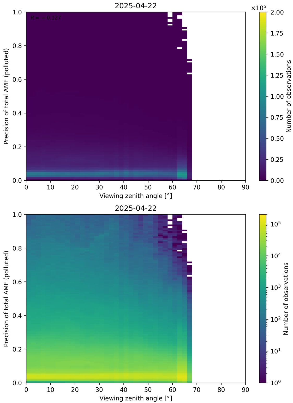
Figure 382: Scatter density plot of “Viewing zenith angle” against “Precision of total AMF (polluted)” for 2025-04-21 to 2025-04-23.
