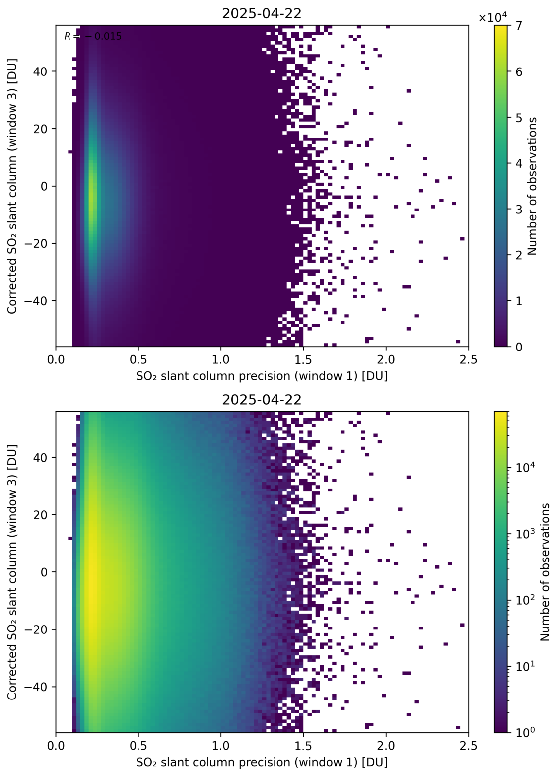
Figure 276: Scatter density plot of “SO 2 slant column precision (window 1)” against “Corrected SO 2 slant column (window 3)” for 2025-04-21 to 2025-04-23.
