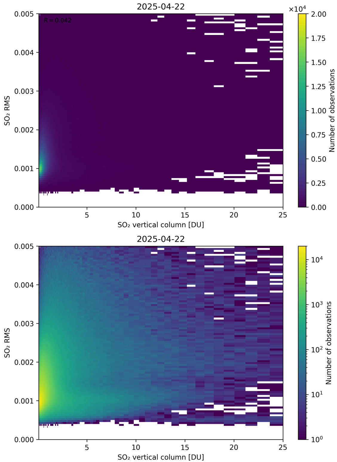
Figure 328: Scatter density plot of “SO 2 vertical column” against “SO 2 RMS” for 2025-04-21 to 2025-04-23.
