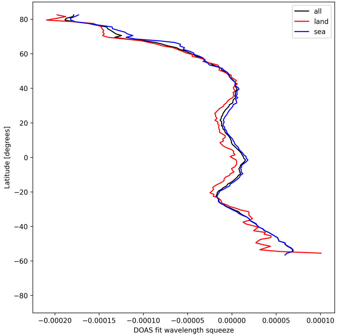
Figure 51: Zonal average of “DOAS fit wavelength squeeze” for 2025-04-21 to 2025-04-23.
