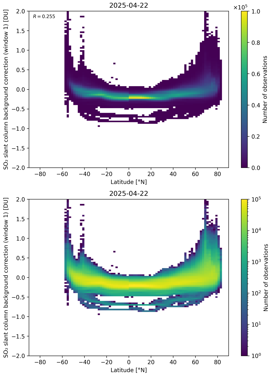
Figure 150: Scatter density plot of “Latitude” against “SO 2 slant column background correction (window 1)” for 2025-04-21 to 2025-04-23.
