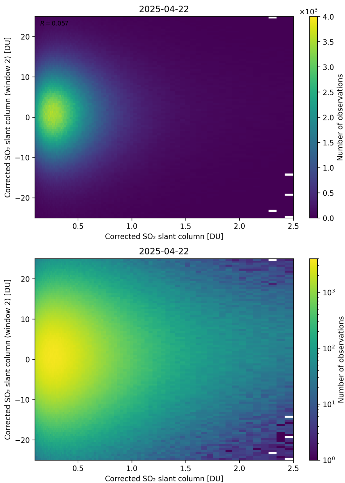
Figure 235: Scatter density plot of “Corrected SO 2 slant column” against “Corrected SO 2 slant column (window 2)” for 2025-04-21 to 2025-04-23.
