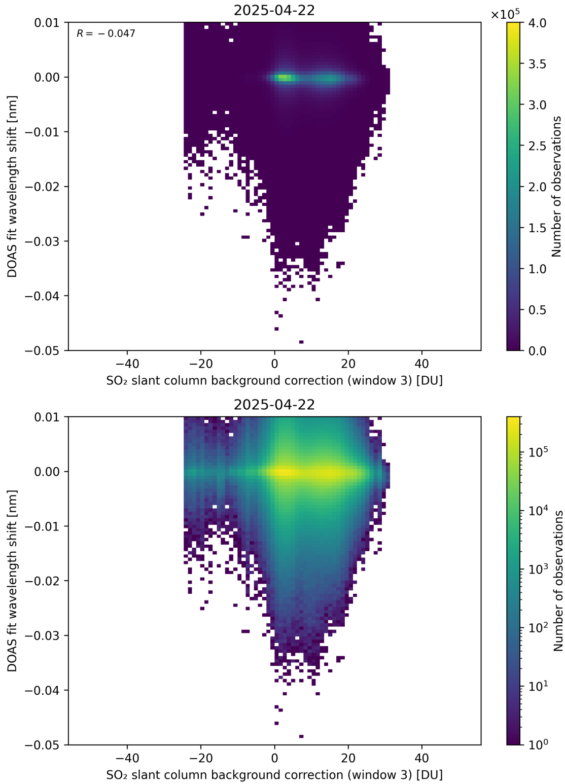
Figure 132: Scatter density plot of “SO 2 slant column background correction (window 3)” against “DOAS fit wavelength shift” for 2025-04-21 to 2025-04-23.
