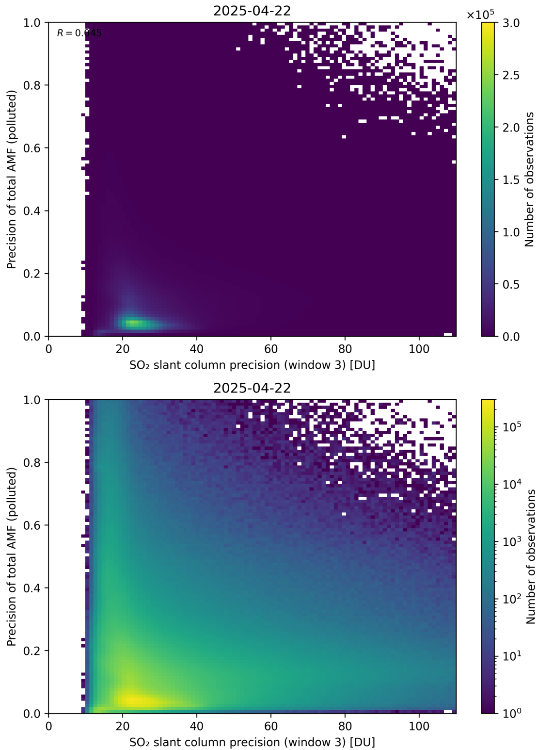
Figure 314: Scatter density plot of “SO 2 slant column precision (window 3)” against “Precision of total AMF (polluted)” for 2025-04-21 to 2025-04-23.
