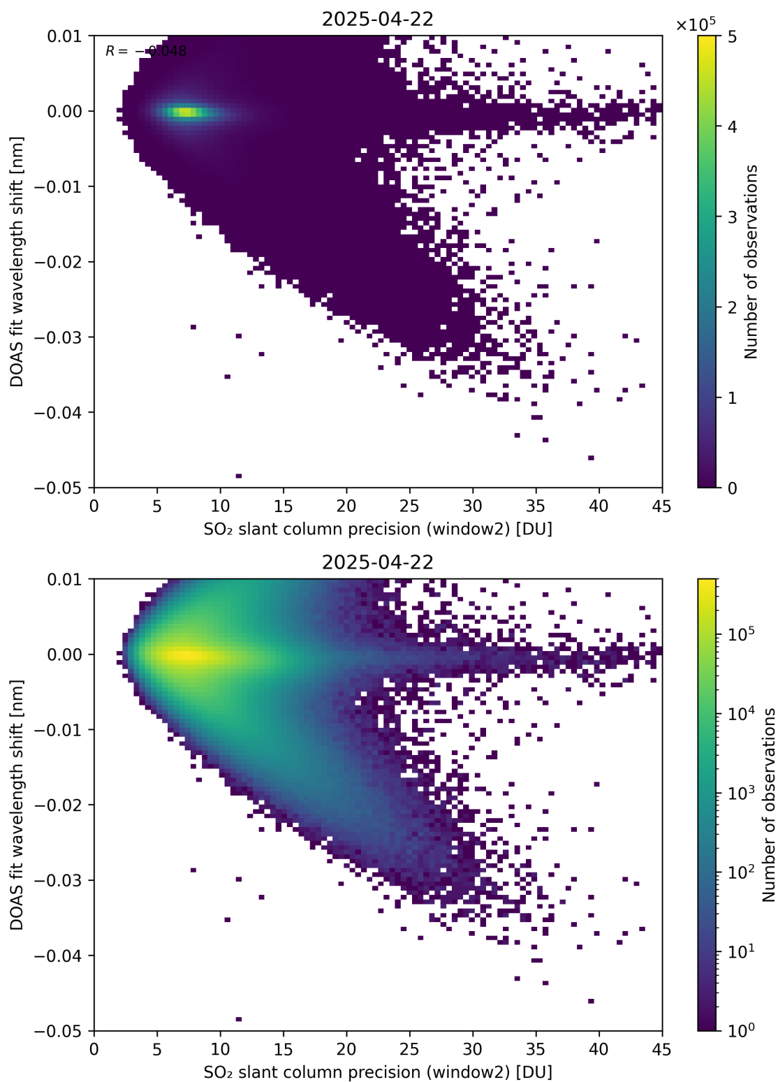
Figure 293: Scatter density plot of “SO 2 slant column precision (window2)” against “DOAS fit wavelength shift” for 2025-04-21 to 2025-04-23.
