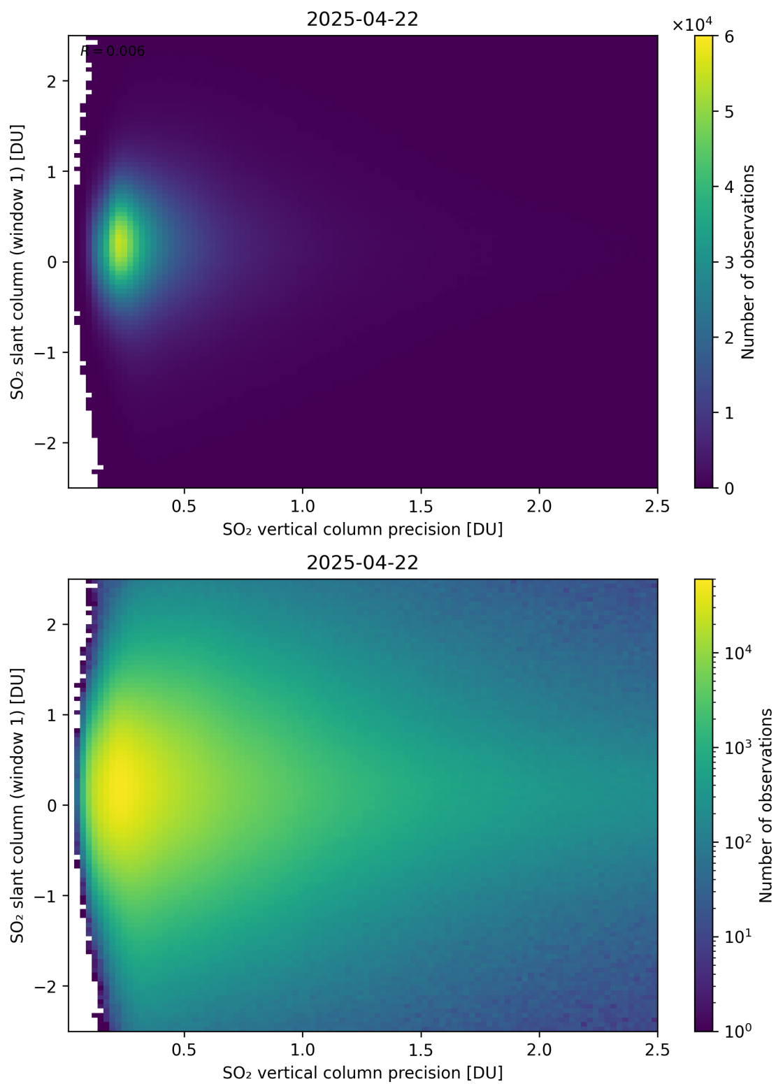
Figure 341: Scatter density plot of “SO 2 vertical column precision” against “SO 2 slant column (window 1)” for 2025-04-21 to 2025-04-23.
