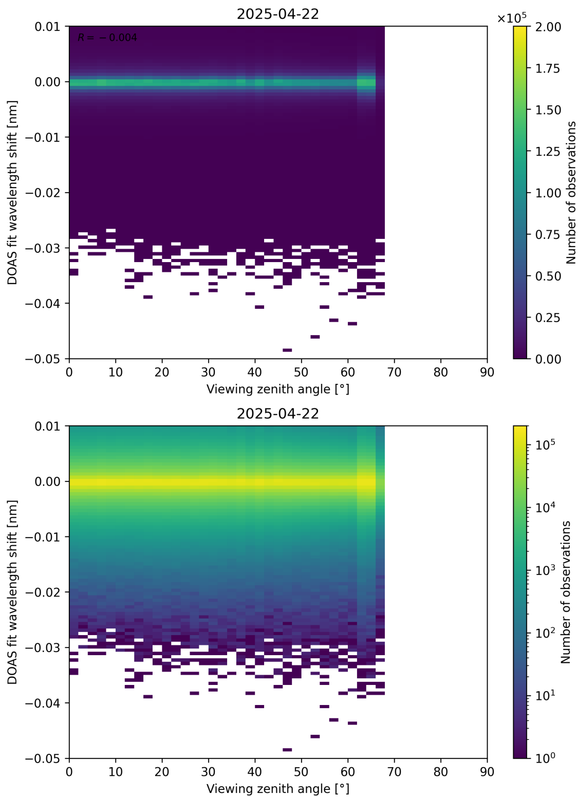
Figure 365: Scatter density plot of “Viewing zenith angle” against “DOAS fit wavelength shift” for 2025-04-21 to 2025-04-23.
