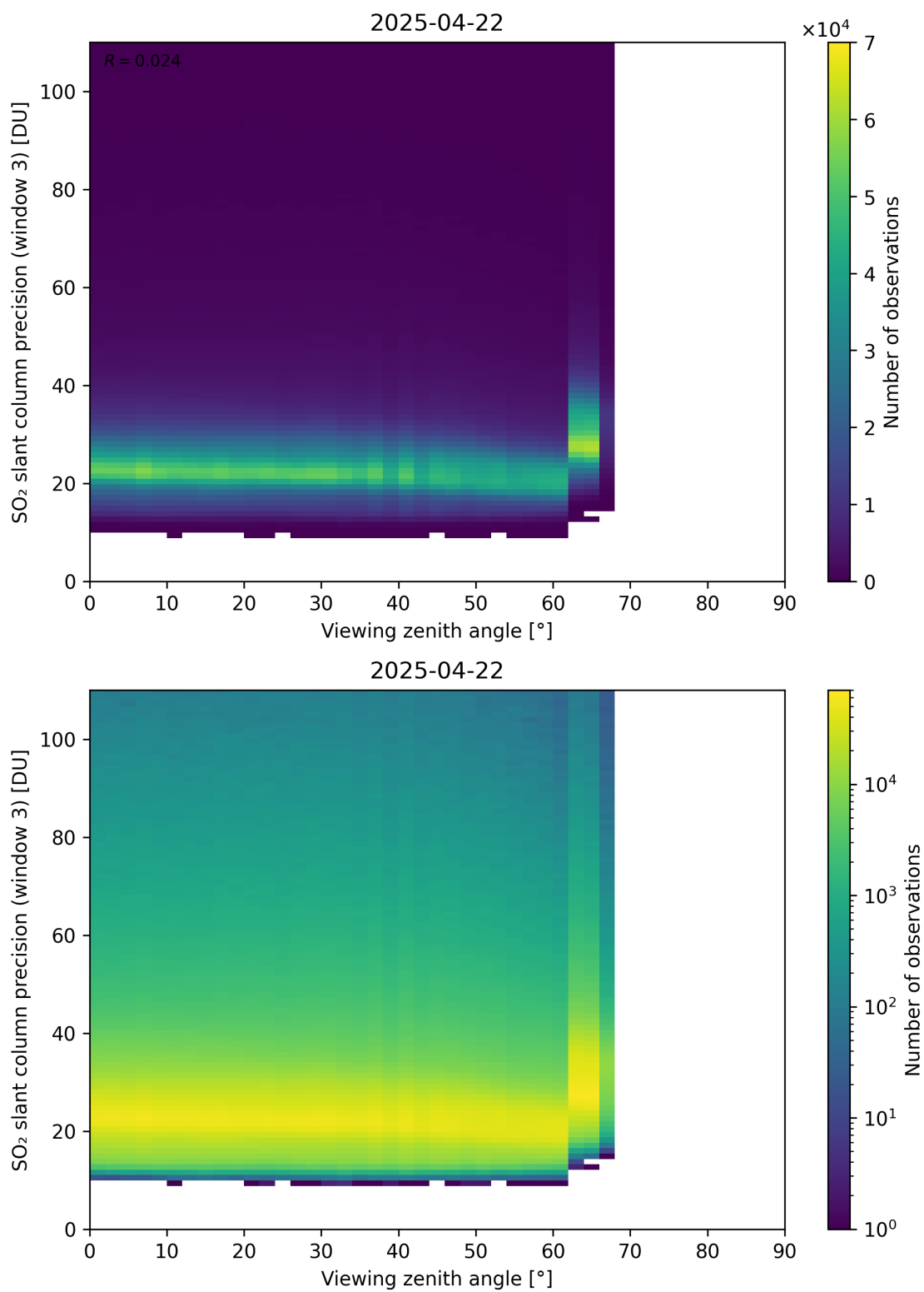
Figure 380: Scatter density plot of “Viewing zenith angle” against “SO 2 slant column precision (window 3)” for 2025-04-21 to 2025-04-23.
