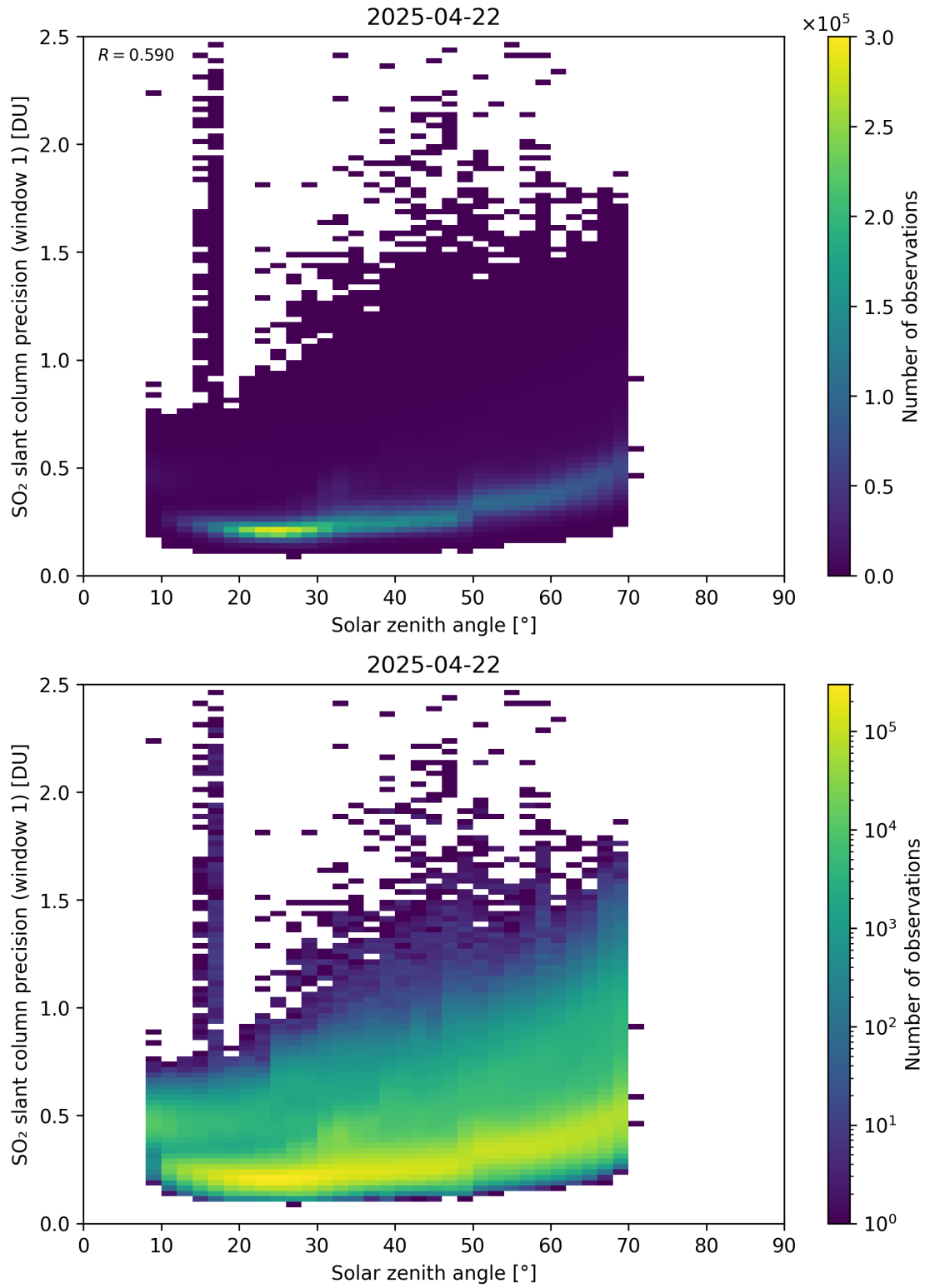
Figure 185: Scatter density plot of “Solar zenith angle” against “SO 2 slant column precision (window 1)” for 2025-04-21 to 2025-04-23.
