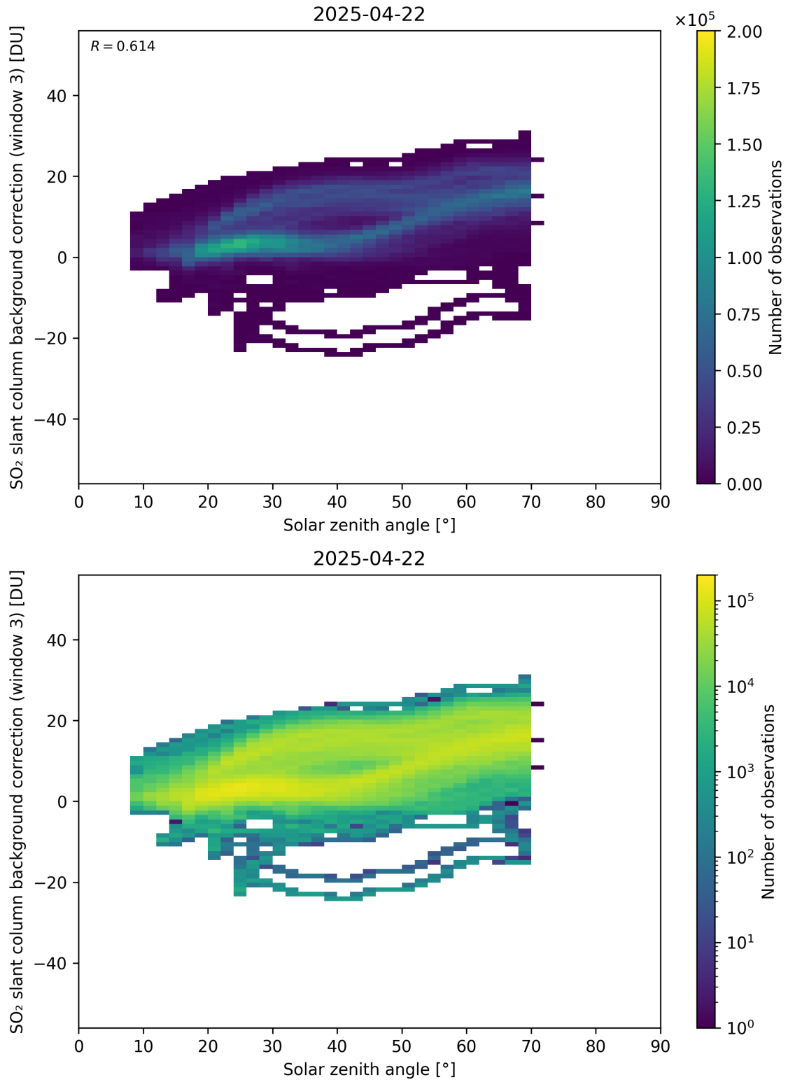
Figure 173: Scatter density plot of “Solar zenith angle” against “SO 2 slant column background correction (window 3)” for 2025-04-21 to 2025-04-23.
