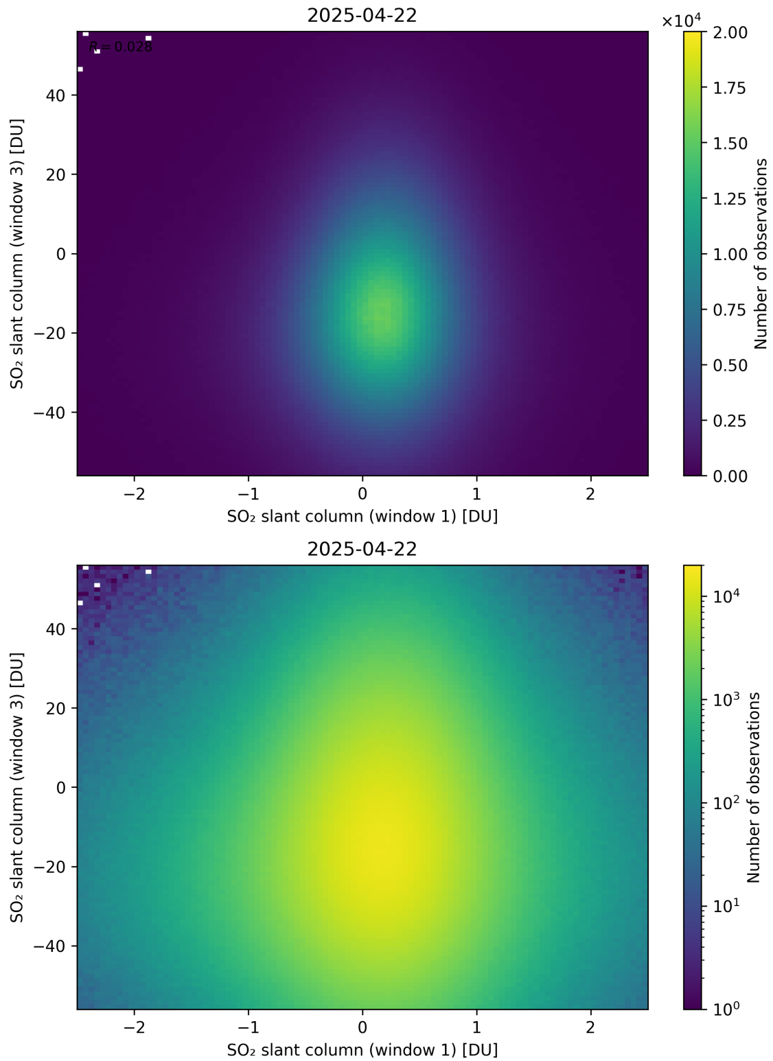
Figure 287: Scatter density plot of “SO 2 slant column (window 1)” against “SO 2 slant column (window 3)” for 2025-04-21 to 2025-04-23.
