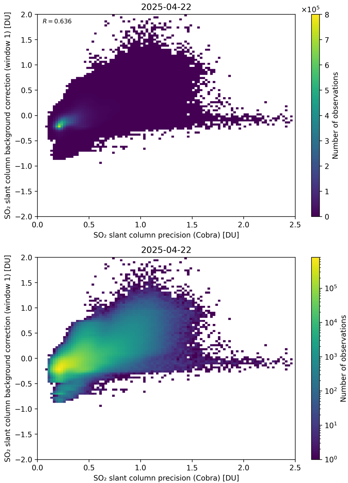
Figure 199: Scatter density plot of “SO 2 slant column precision (Cobra)” against “SO 2 slant column background correction (window 1)” for 2025-04-21 to 2025-04-23.
