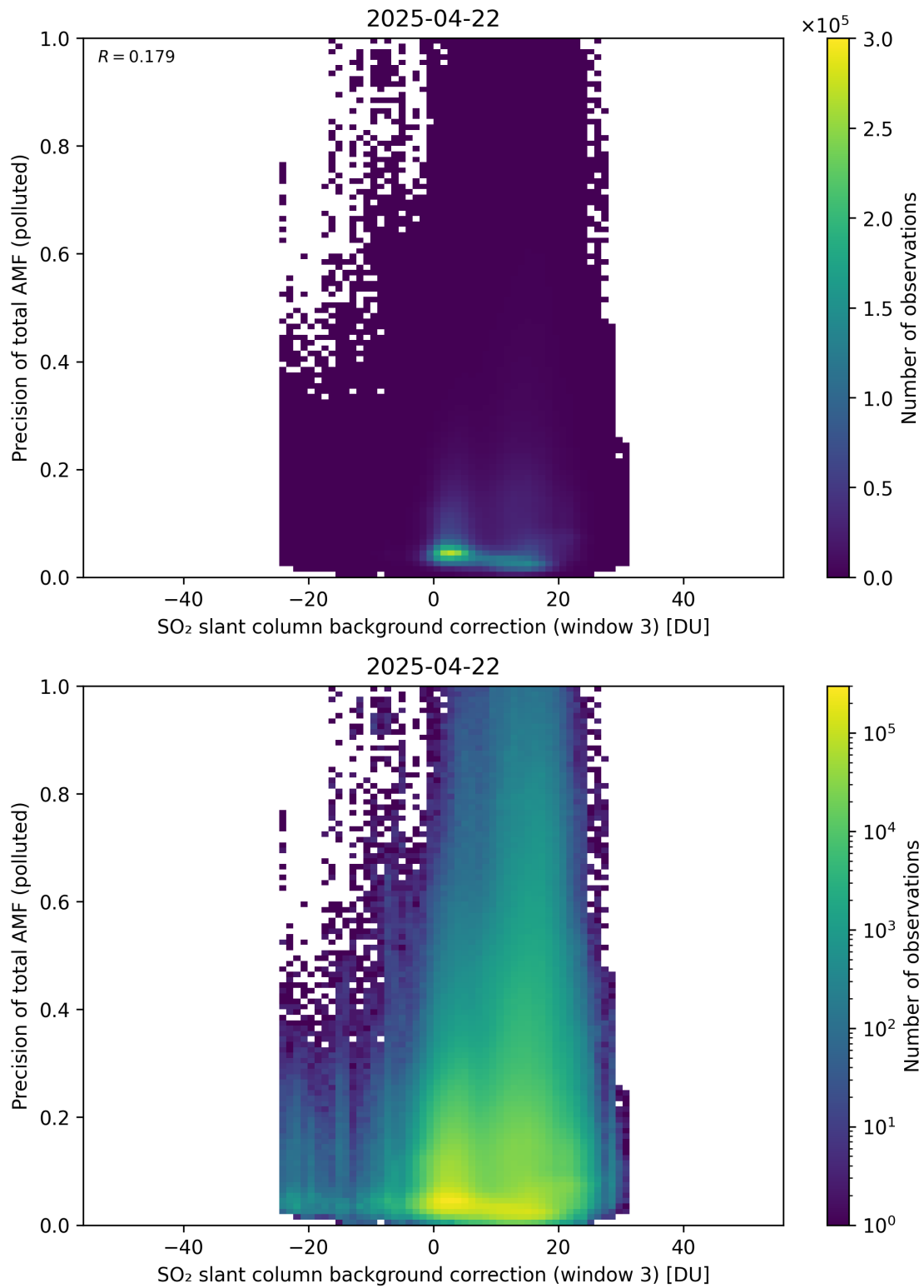
Figure 137: Scatter density plot of “SO 2 slant column background correction (window 3)” against “Precision of total AMF (polluted)” for 2025-04-21 to 2025-04-23.
