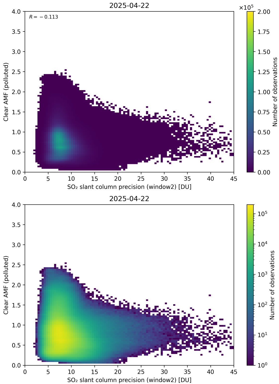
Figure 296: Scatter density plot of “SO 2 slant column precision (window2)” against “Clear AMF (polluted)” for 2025-04-21 to 2025-04-23.
