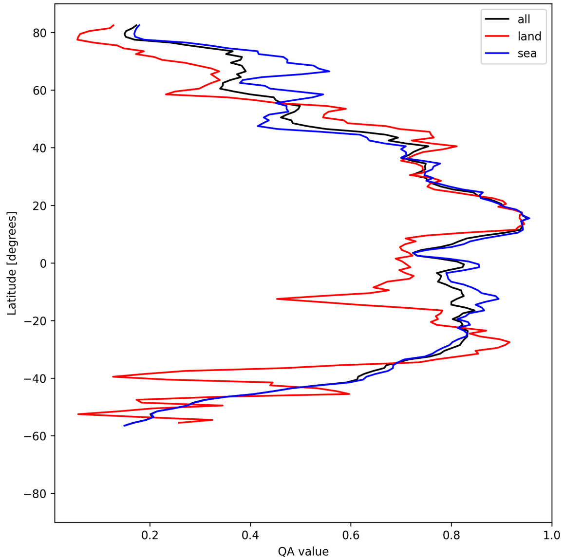
Figure 31: Zonal average of “QA value” for 2025-04-21 to 2025-04-23.
