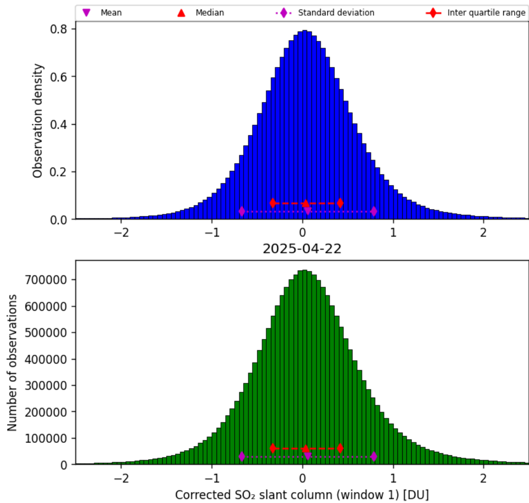
Figure 65: Histogram of “Corrected SO 2 slant column (window 1)” for 2025-04-21 to 2025-04-23
