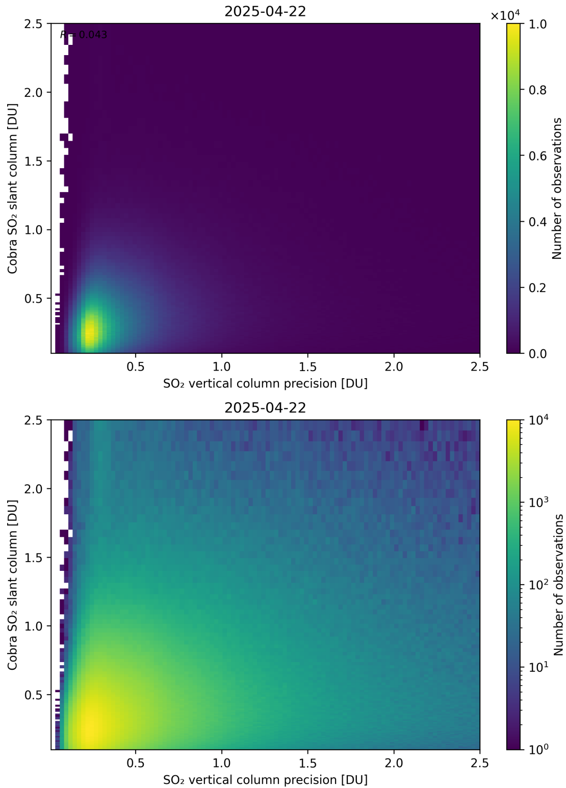
Figure 336: Scatter density plot of “SO 2 vertical column precision” against “Cobra SO 2 slant column” for 2025-04-21 to 2025-04-23.
