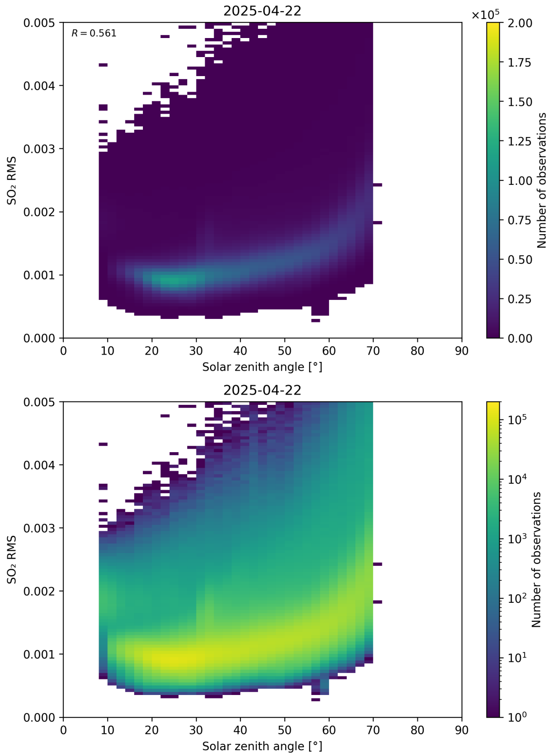
Figure 176: Scatter density plot of “Solar zenith angle” against “SO 2 RMS” for 2025-04-21 to 2025-04-23.
