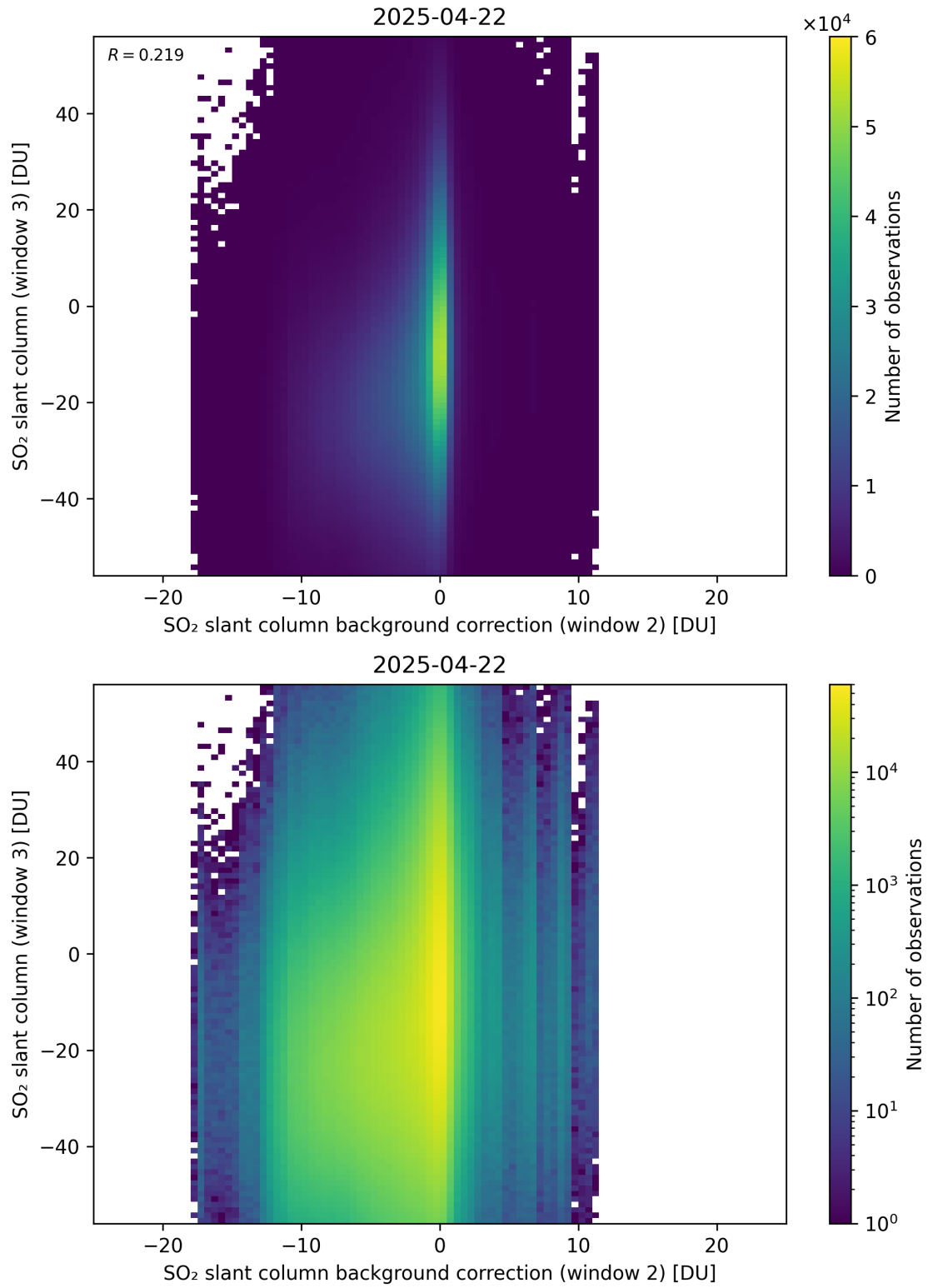
Figure 128: Scatter density plot of “SO 2 slant column background correction (window 2)” against “SO 2 slant column (window 3)” for 2025-04-21 to 2025-04-23.
