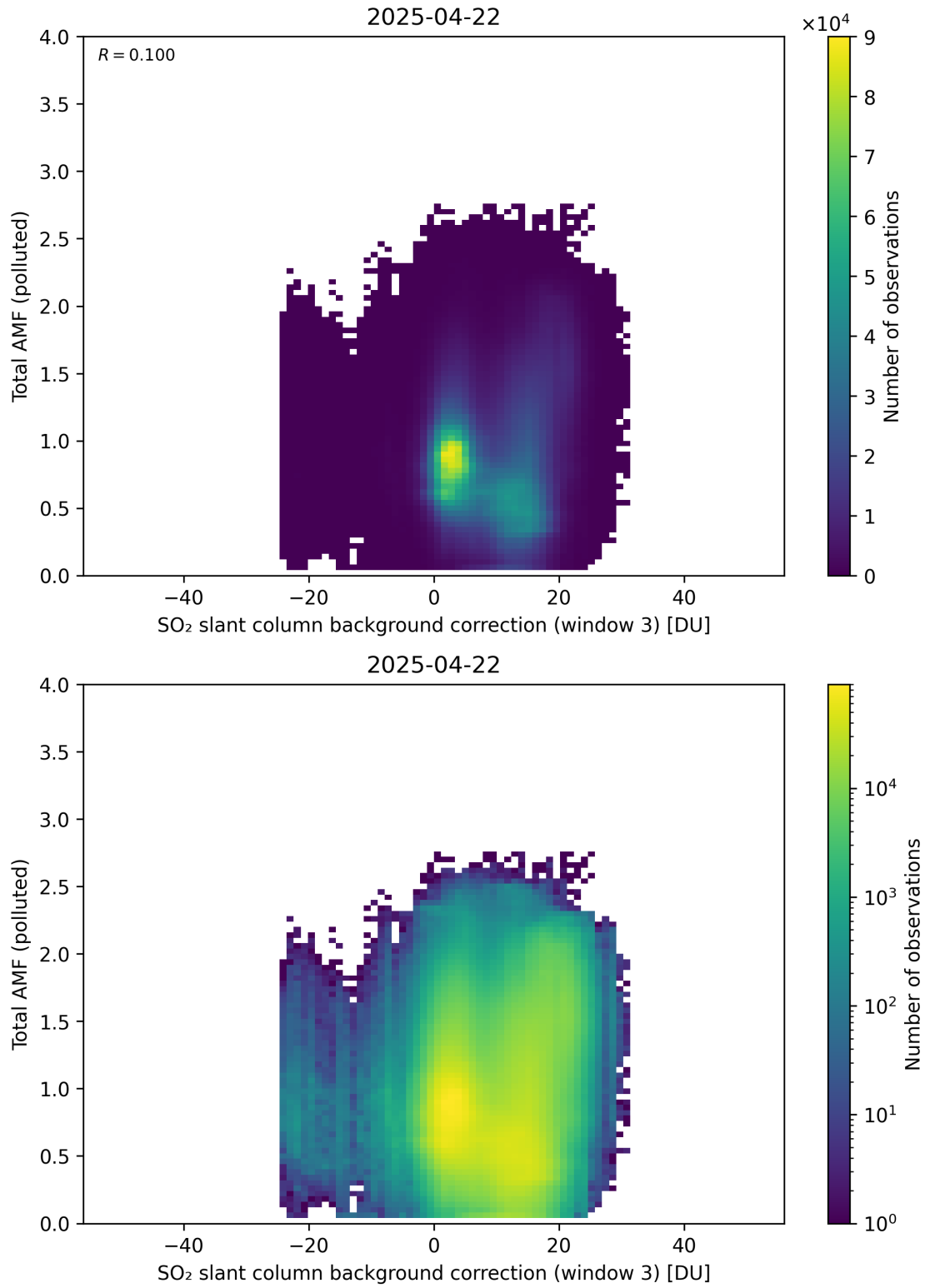
Figure 136: Scatter density plot of “SO 2 slant column background correction (window 3)” against “Total AMF (polluted)” for 2025-04-21 to 2025-04-23.
