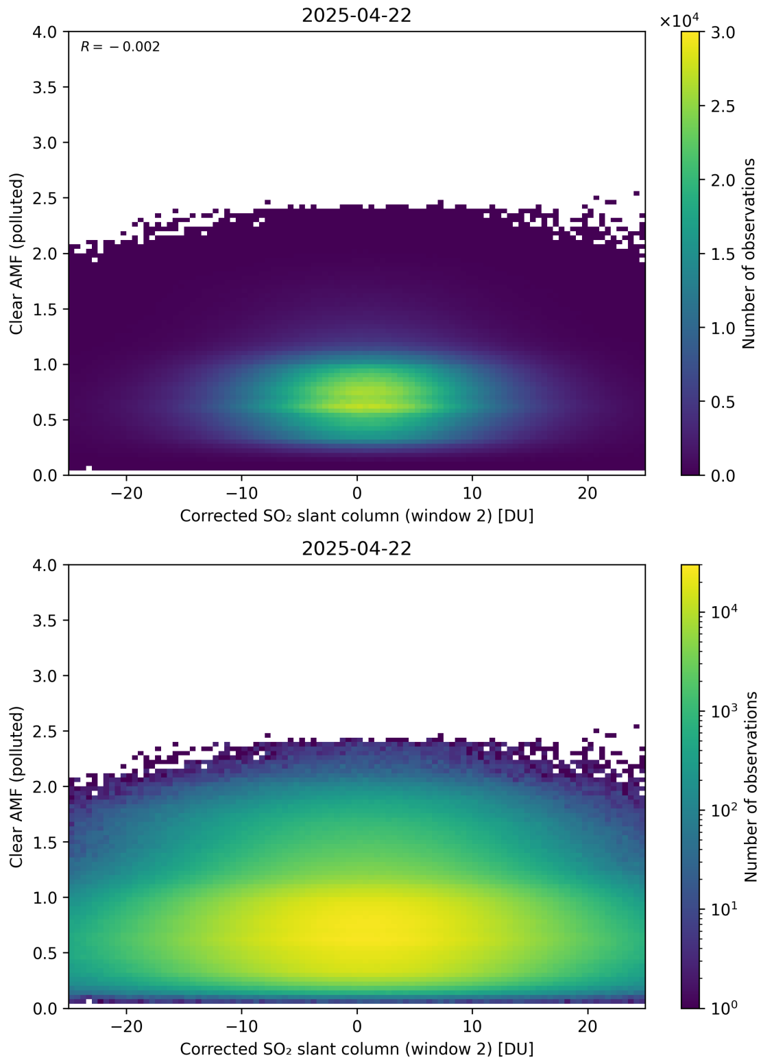
Figure 249: Scatter density plot of “Corrected SO 2 slant column (window 2)” against “Clear AMF (polluted)” for 2025-04-21 to 2025-04-23.
