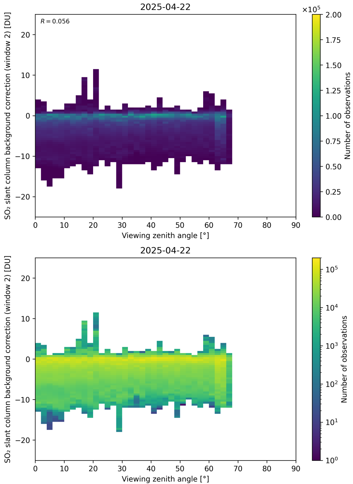
Figure 363: Scatter density plot of “Viewing zenith angle” against “SO 2 slant column background correction (window 2)” for 2025-04-21 to 2025-04-23.
