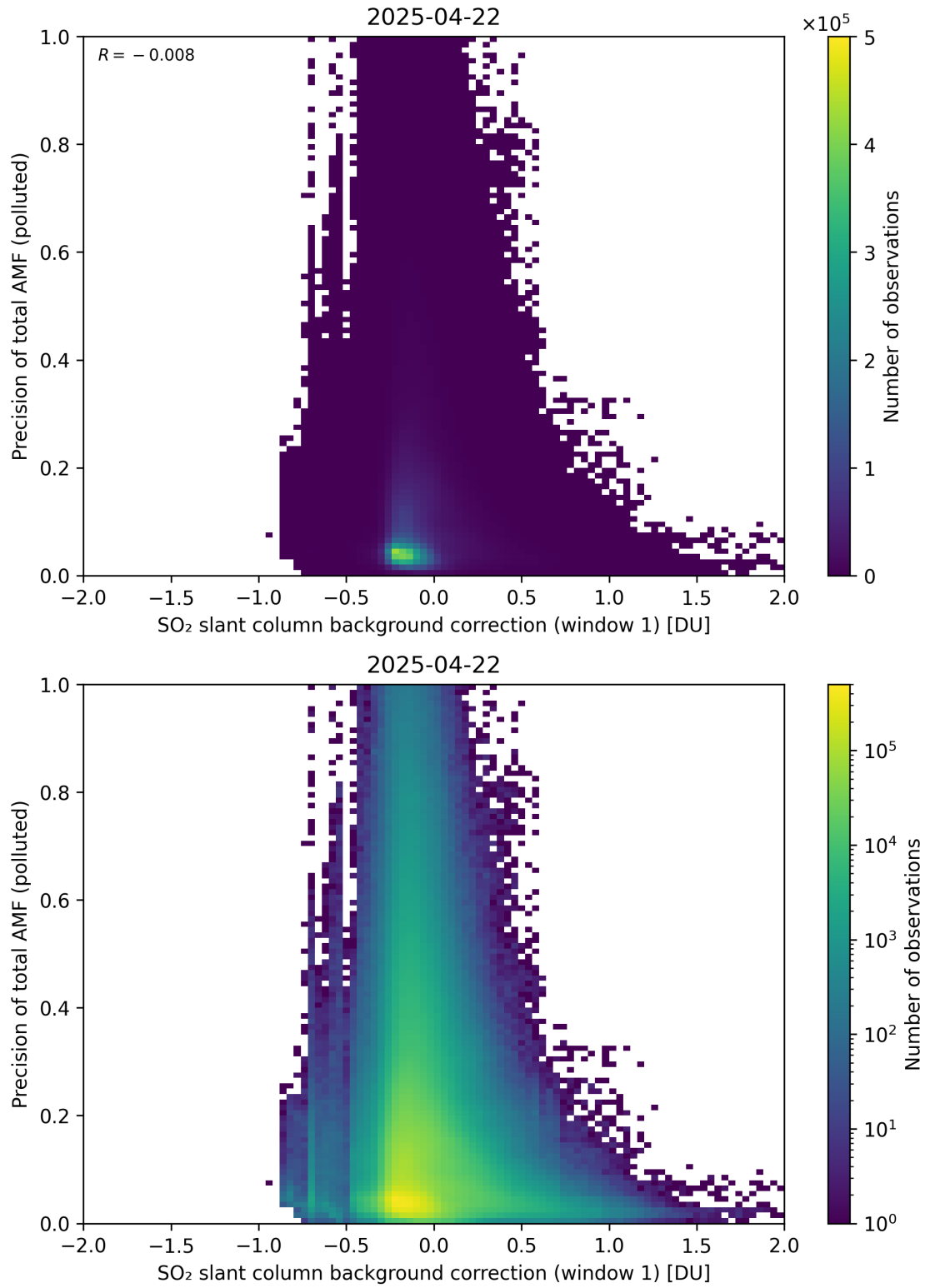
Figure 121: Scatter density plot of “SO 2 slant column background correction (window 1)” against “Precision of total AMF (polluted)” for 2025-04-21 to 2025-04-23.
