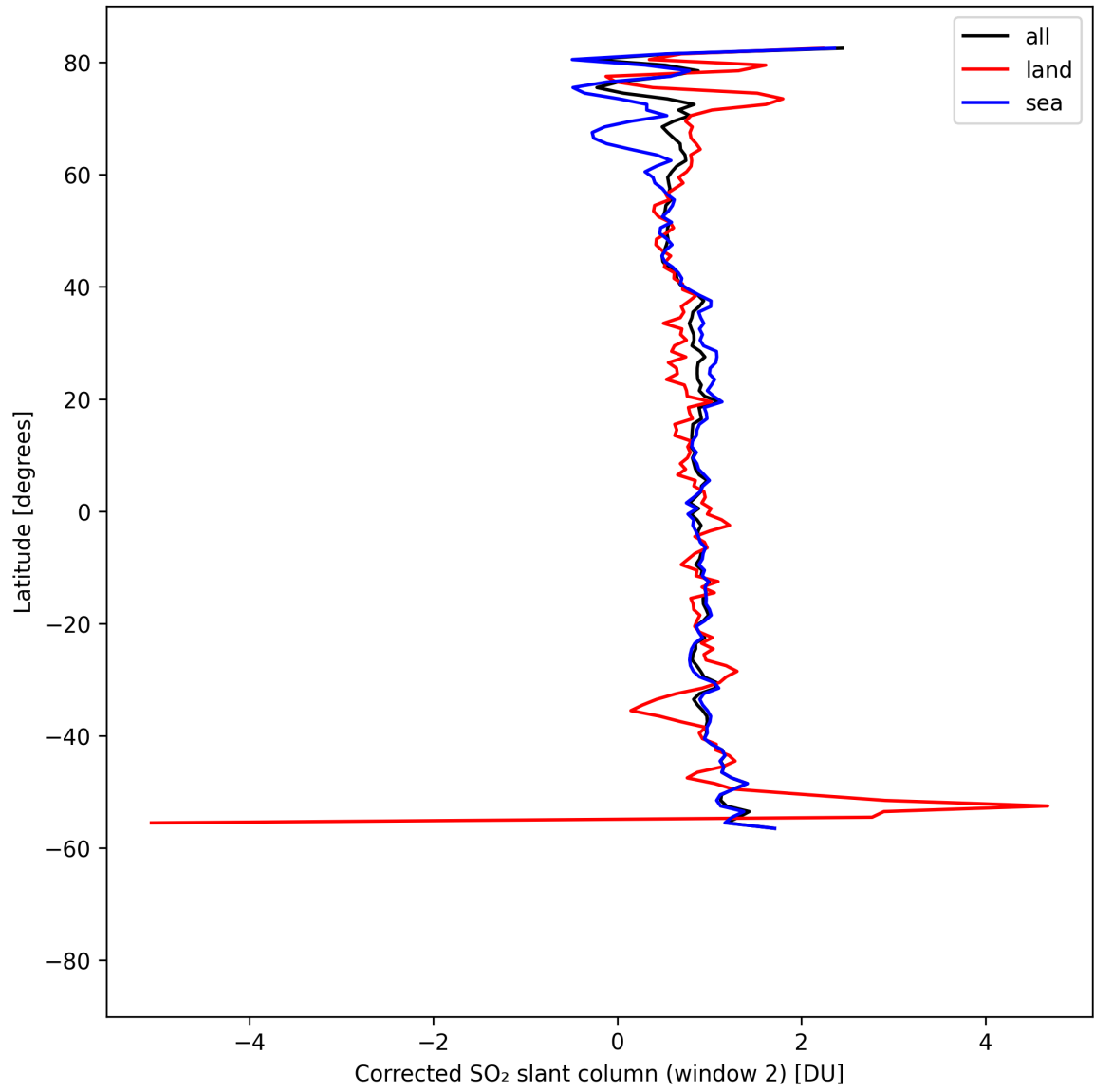
Figure 43: Zonal average of “Corrected SO 2 slant column (window 2)” for 2025-04-21 to 2025-04-23.
