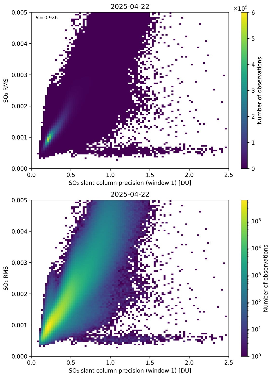
Figure 273: Scatter density plot of “SO 2 slant column precision (window 1)” against “SO 2 RMS” for 2025-04-21 to 2025-04-23.
