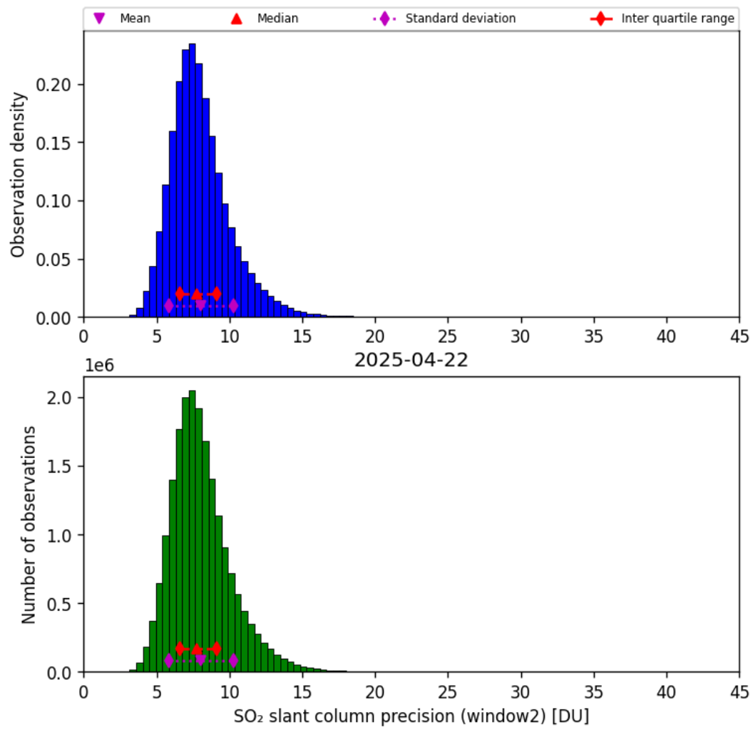
Figure 68: Histogram of “SO 2 slant column precision (window2)” for 2025-04-21 to 2025-04-23
