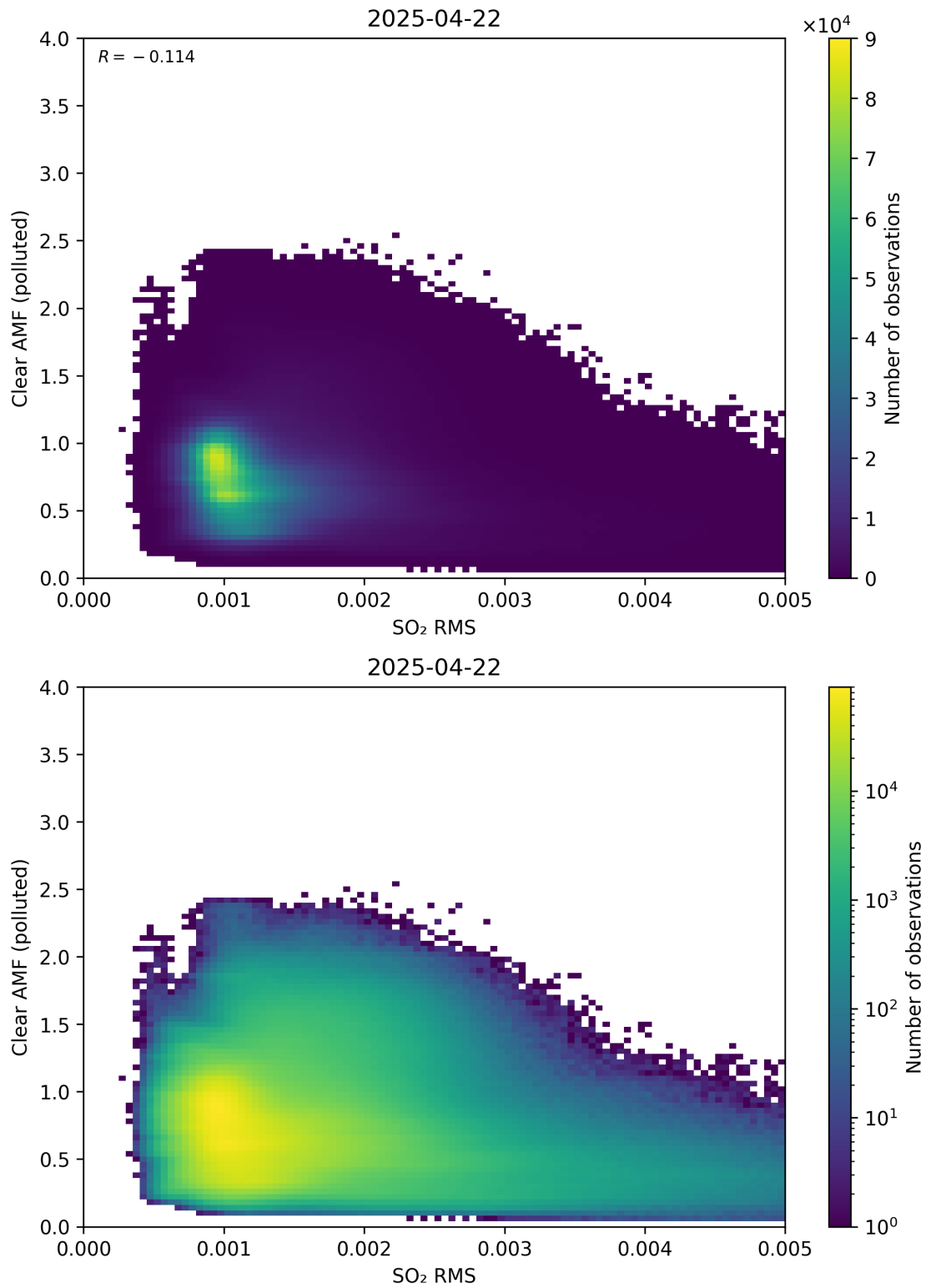
Figure 147: Scatter density plot of “SO 2 RMS” against “Clear AMF (polluted)” for 2025-04-21 to 2025-04-23.
