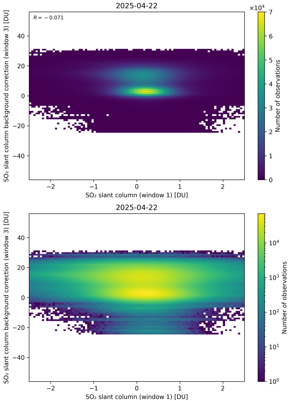
Figure 264: Scatter density plot of “SO 2 slant column (window 1)” against “SO 2 slant column background correction (window 3)” for 2025-04-21 to 2025-04-23.
