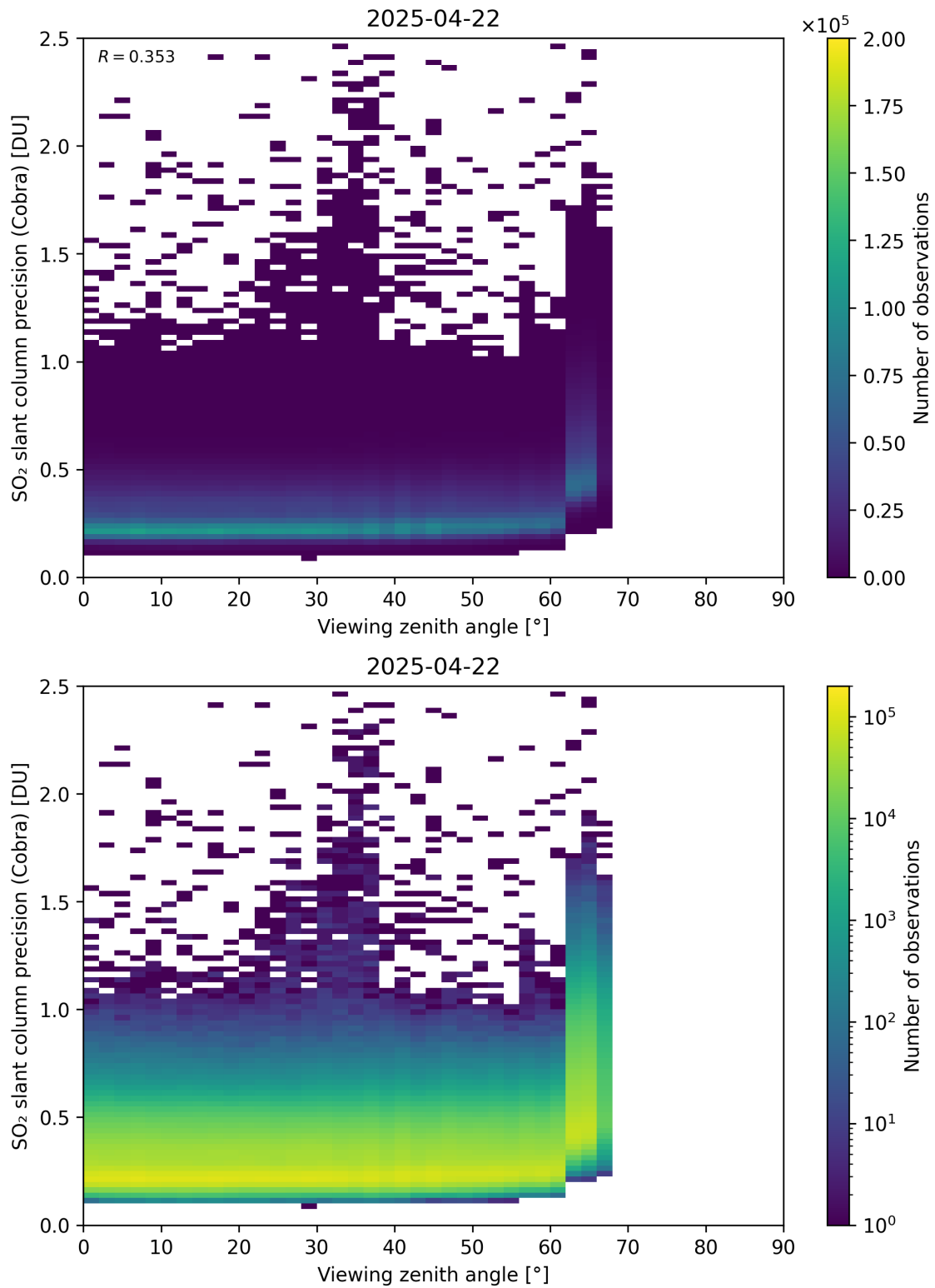
Figure 372: Scatter density plot of “Viewing zenith angle” against “SO 2 slant column precision (Cobra)” for 2025-04-21 to 2025-04-23.
