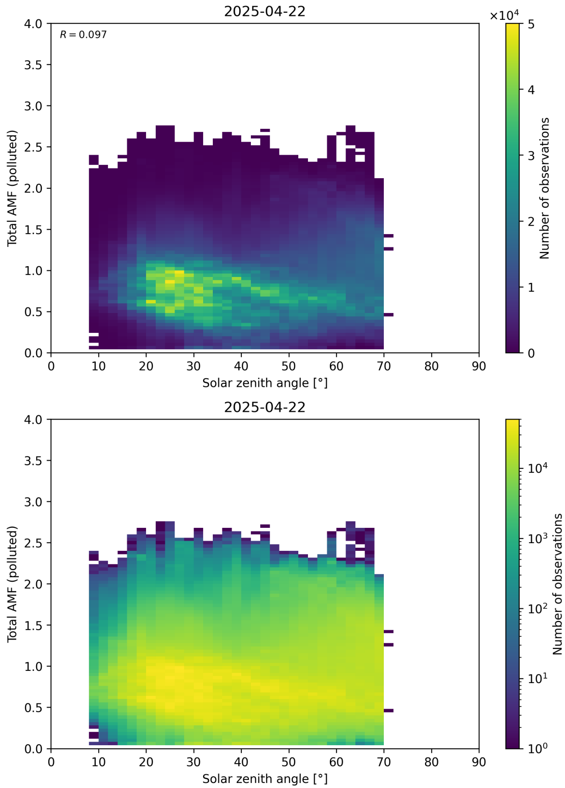
Figure 189: Scatter density plot of “Solar zenith angle” against “Total AMF (polluted)” for 2025-04-21 to 2025-04-23.
