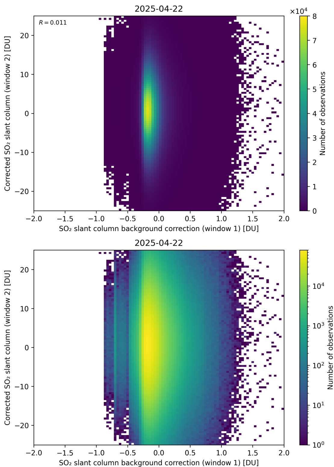
Figure 115: Scatter density plot of “SO 2 slant column background correction (window 1)” against “Corrected SO 2 slant column (window 2)” for 2025-04-21 to 2025-04-23.
