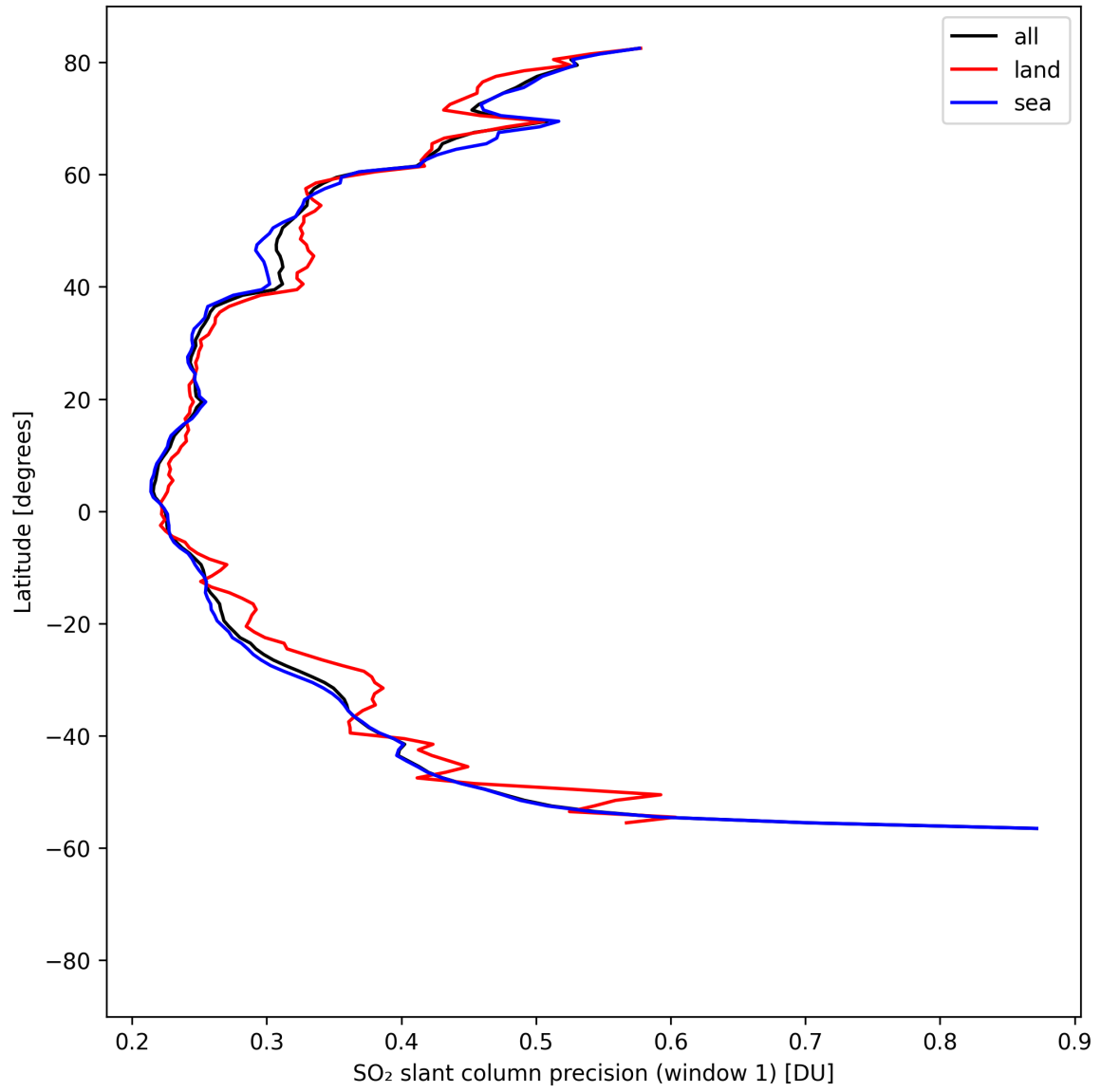
Figure 38: Zonal average of “SO 2 slant column precision (window 1)” for 2025-04-21 to 2025-04-23.
