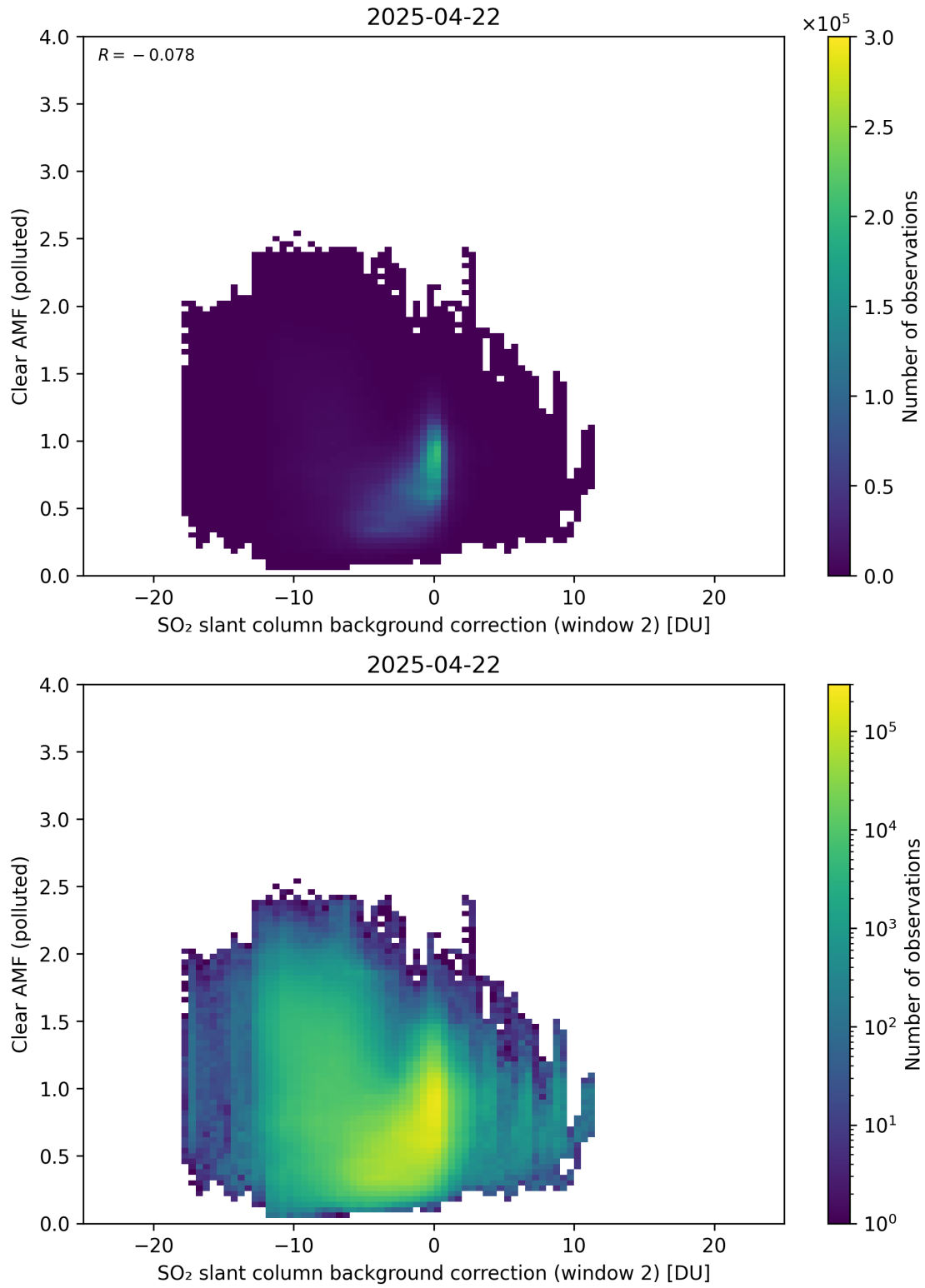
Figure 126: Scatter density plot of “SO 2 slant column background correction (window 2)” against “Clear AMF (polluted)” for 2025-04-21 to 2025-04-23.
