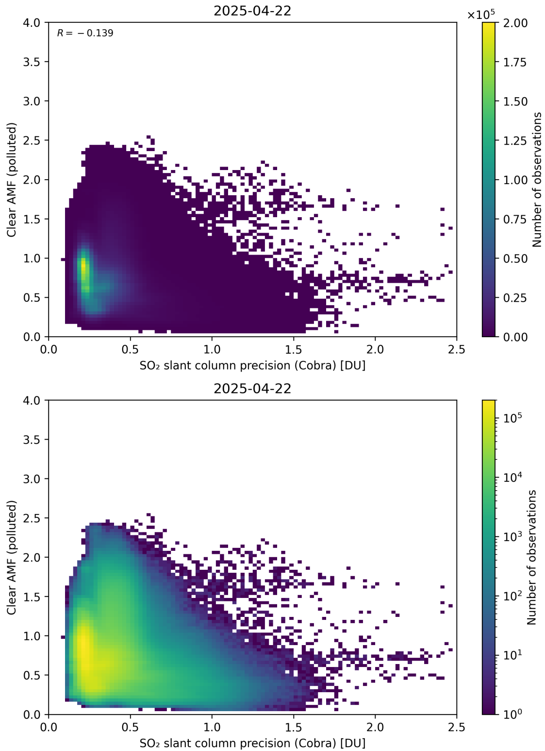
Figure 205: Scatter density plot of “SO 2 slant column precision (Cobra)” against “Clear AMF (polluted)” for 2025-04-21 to 2025-04-23.
