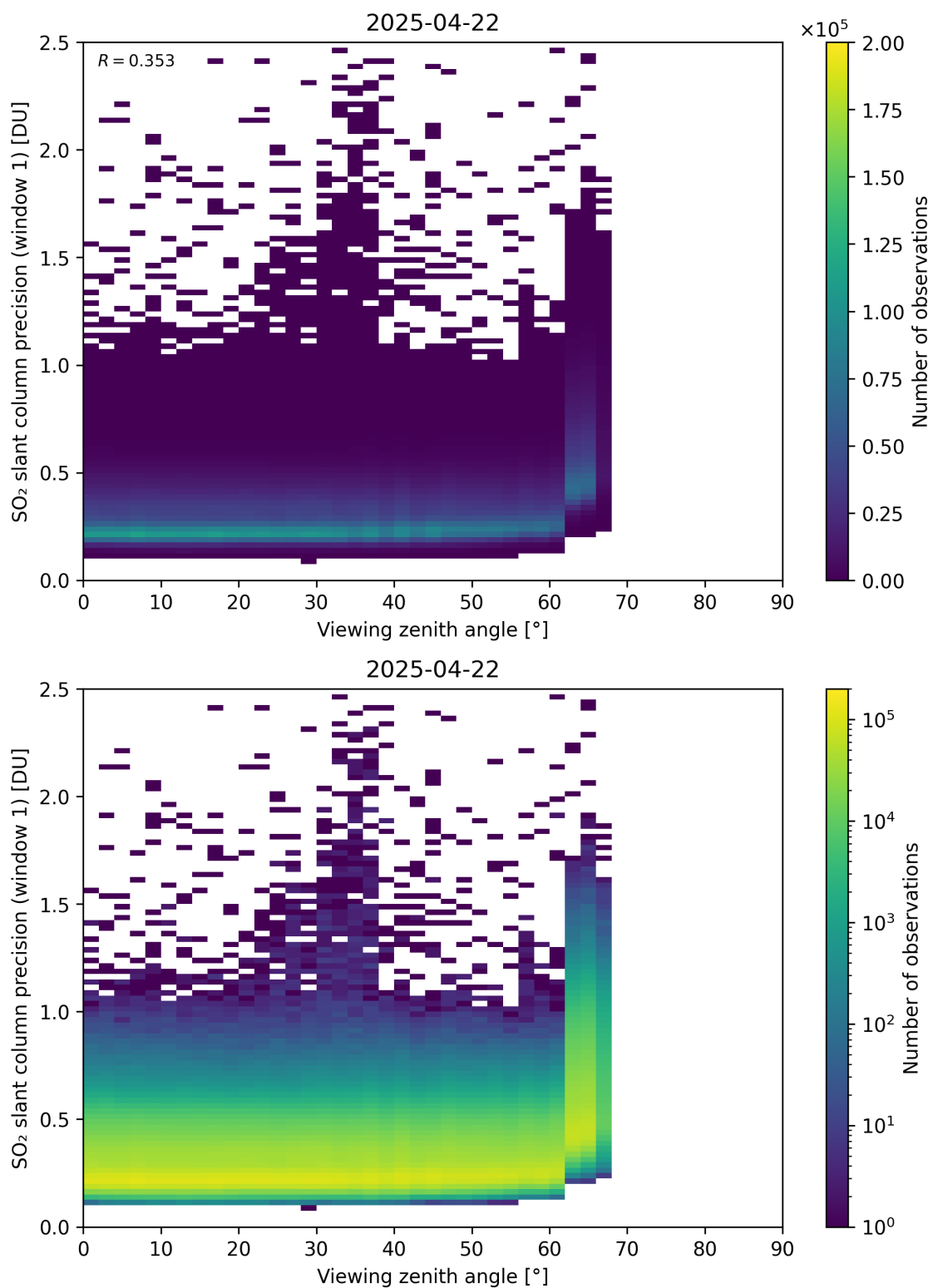
Figure 377: Scatter density plot of “Viewing zenith angle” against “SO 2 slant column precision (window 1)” for 2025-04-21 to 2025-04-23.
