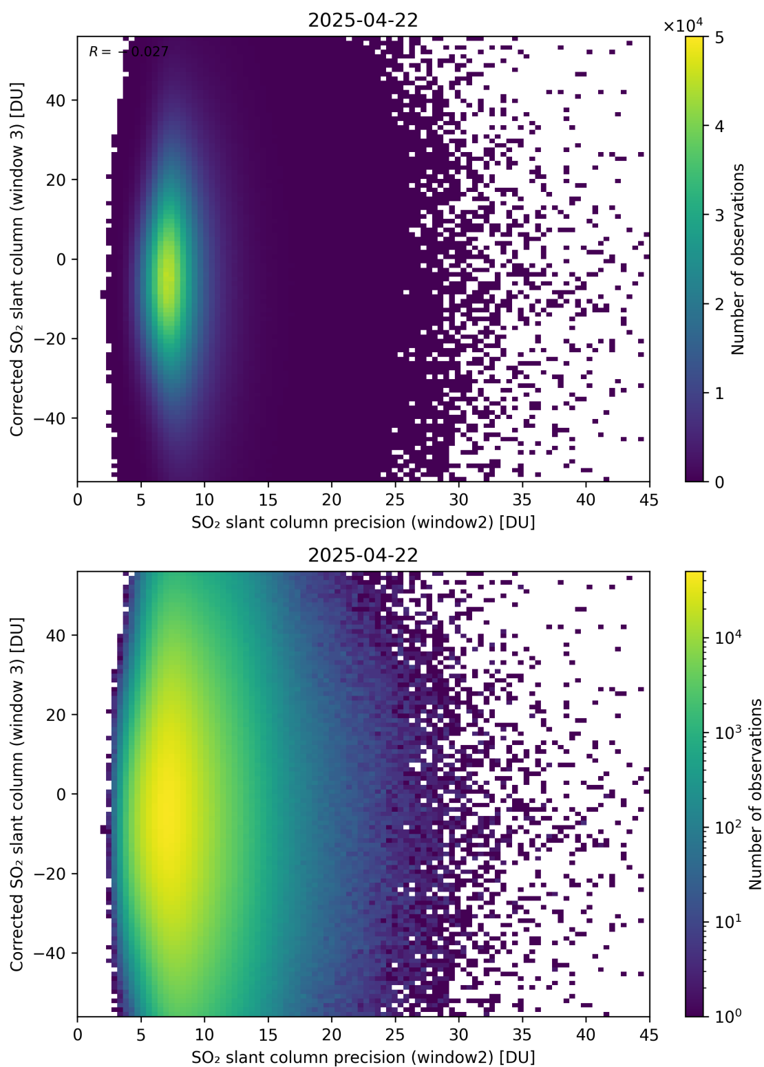
Figure 298: Scatter density plot of “SO 2 slant column precision (window2)” against “Corrected SO 2 slant column (window 3)” for 2025-04-21 to 2025-04-23.
