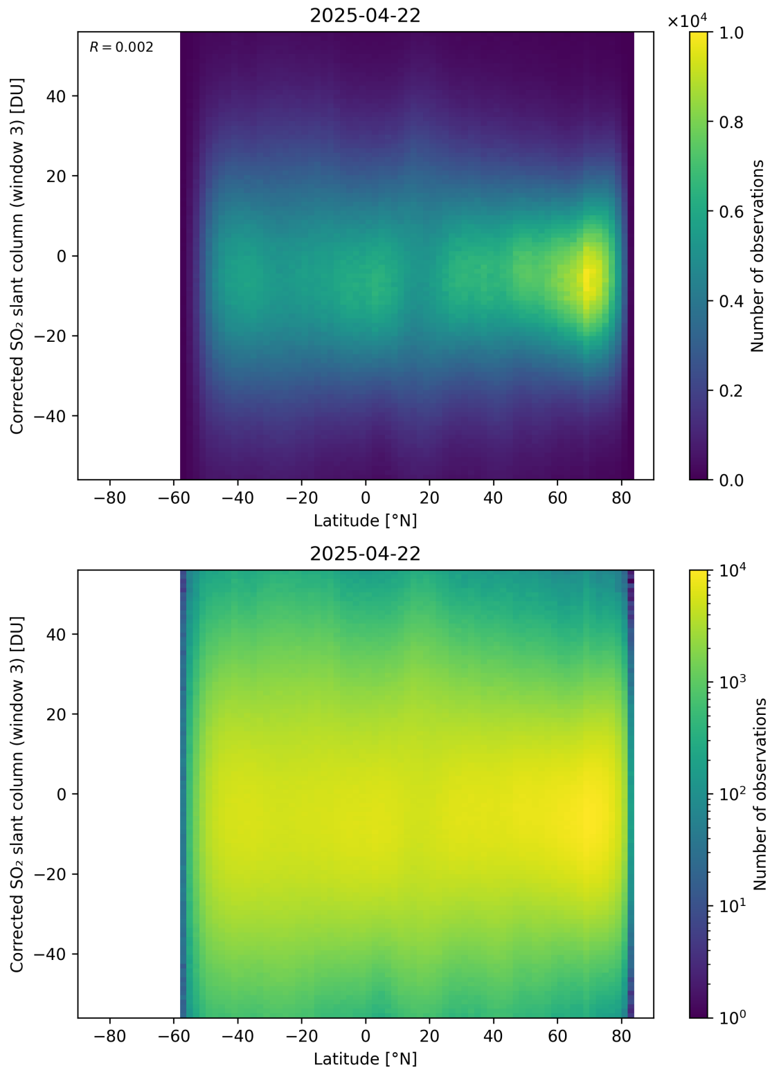
Figure 161: Scatter density plot of “Latitude” against “Corrected SO 2 slant column (window 3)” for 2025-04-21 to 2025-04-23.
