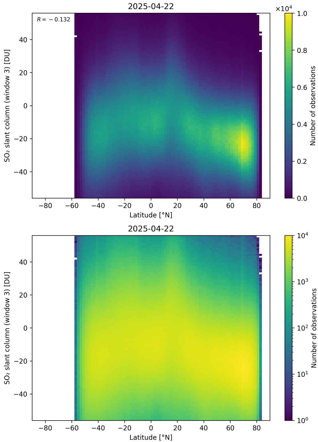
Figure 165: Scatter density plot of “Latitude” against “SO 2 slant column (window 3)” for 2025-04-21 to 2025-04-23.
