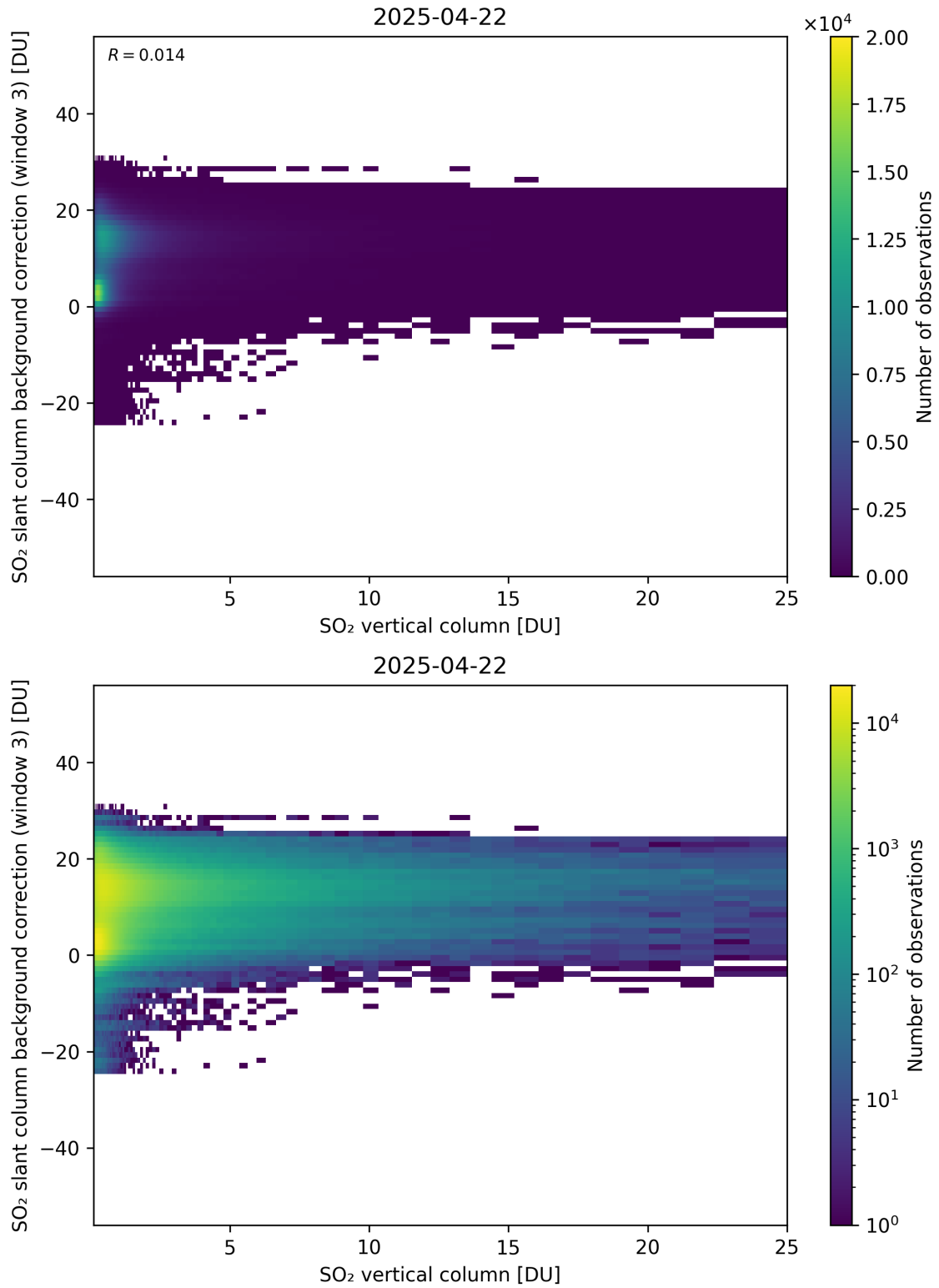
Figure 325: Scatter density plot of “SO 2 vertical column” against “SO 2 slant column background correction (window 3)” for 2025-04-21 to 2025-04-23.
