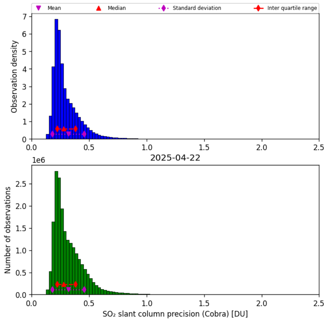
Figure 62: Histogram of “SO 2 slant column precision (Cobra)” for 2025-04-21 to 2025-04-23
