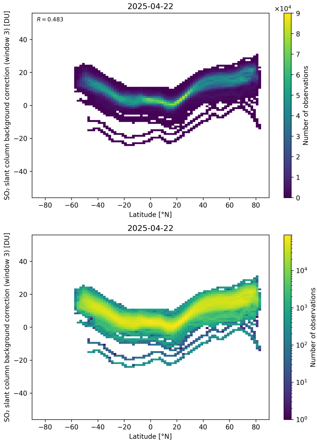
Figure 152: Scatter density plot of “Latitude” against “SO 2 slant column background correction (window 3)” for 2025-04-21 to 2025-04-23.
