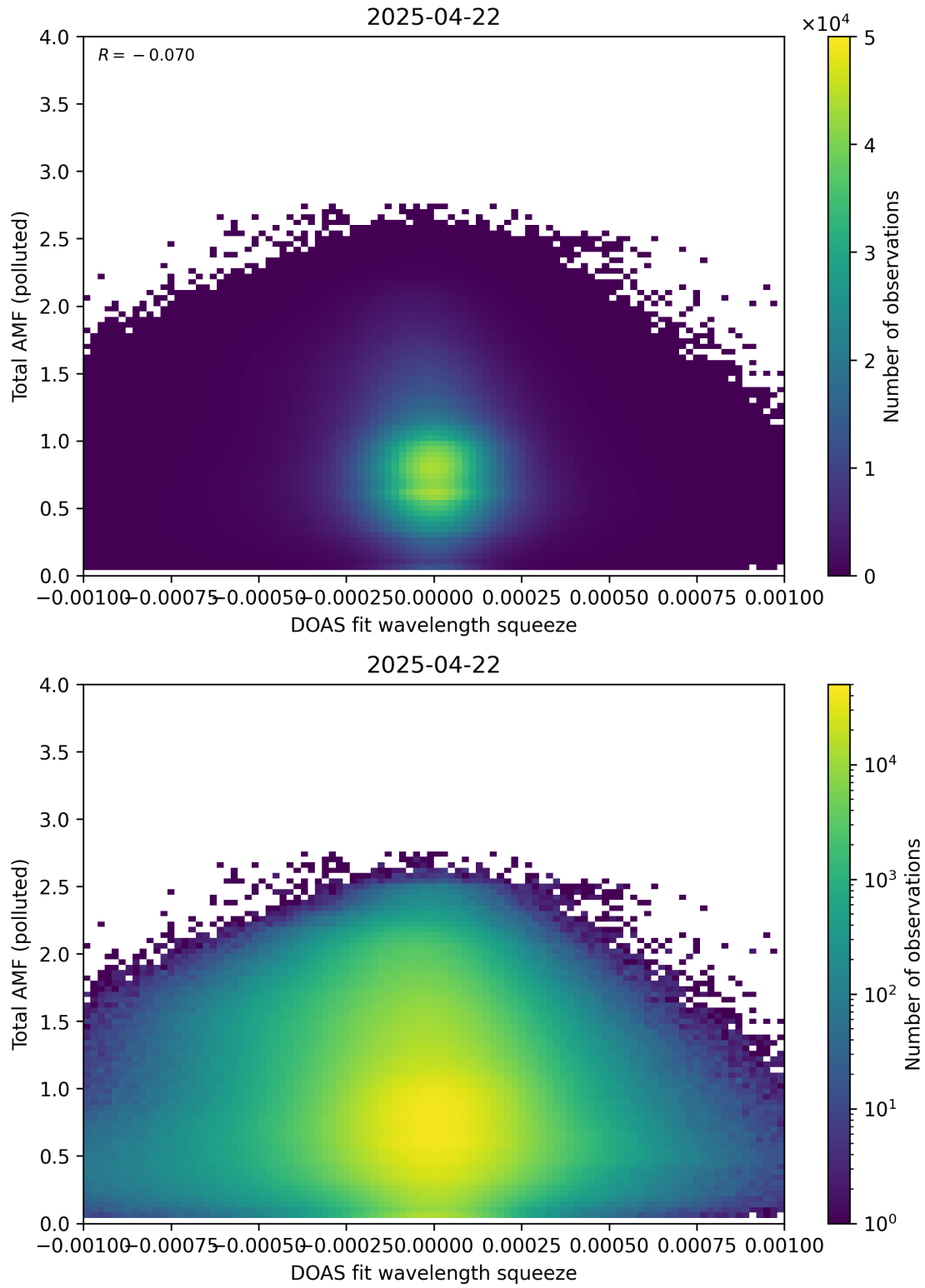
Figure 145: Scatter density plot of “DOAS fit wavelength squeeze” against “Total AMF (polluted)” for 2025-04-21 to 2025-04-23.
