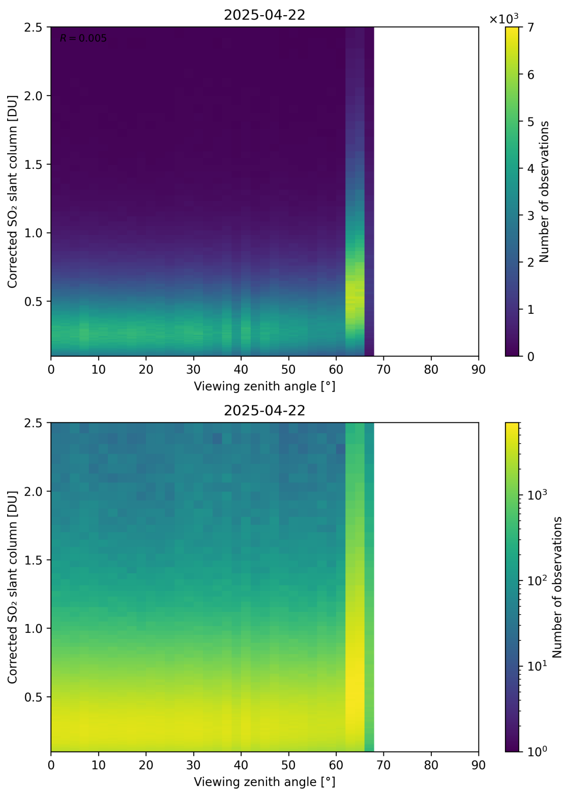
Figure 373: Scatter density plot of “Viewing zenith angle” against “Corrected SO 2 slant column” for 2025-04-21 to 2025-04-23.
