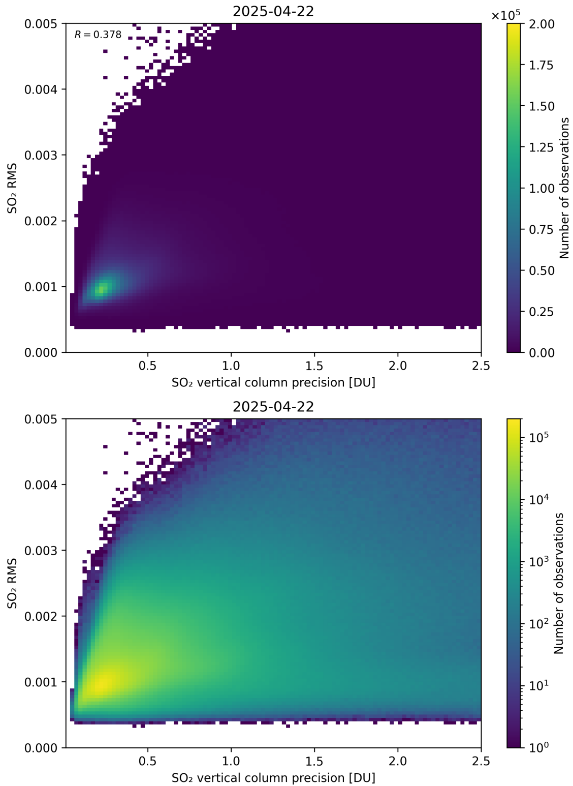
Figure 334: Scatter density plot of “SO 2 vertical column precision” against “SO 2 RMS” for 2025-04-21 to 2025-04-23.
