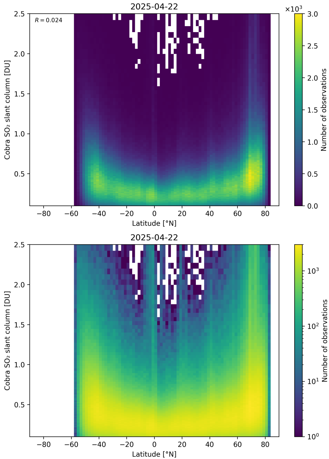
Figure 157: Scatter density plot of “Latitude” against “Cobra SO 2 slant column” for 2025-04-21 to 2025-04-23.
