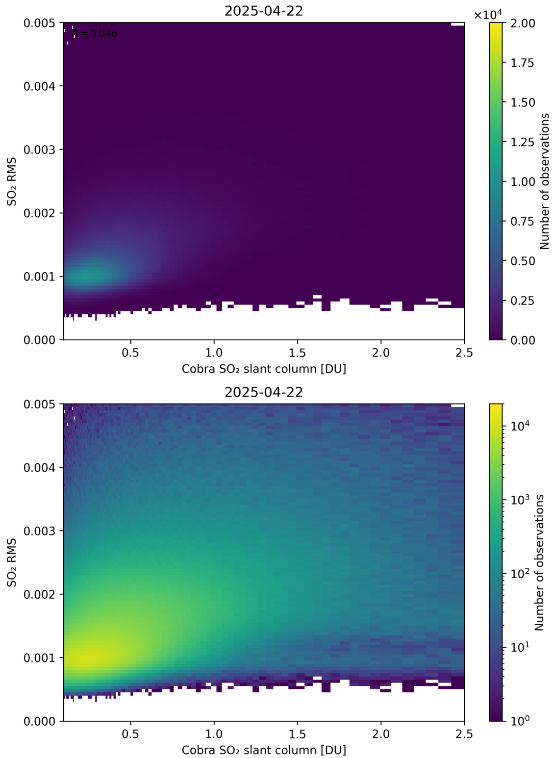
Figure 198: Scatter density plot of “Cobra SO 2 slant column” against “SO 2 RMS” for 2025-04-21 to 2025-04-23.
