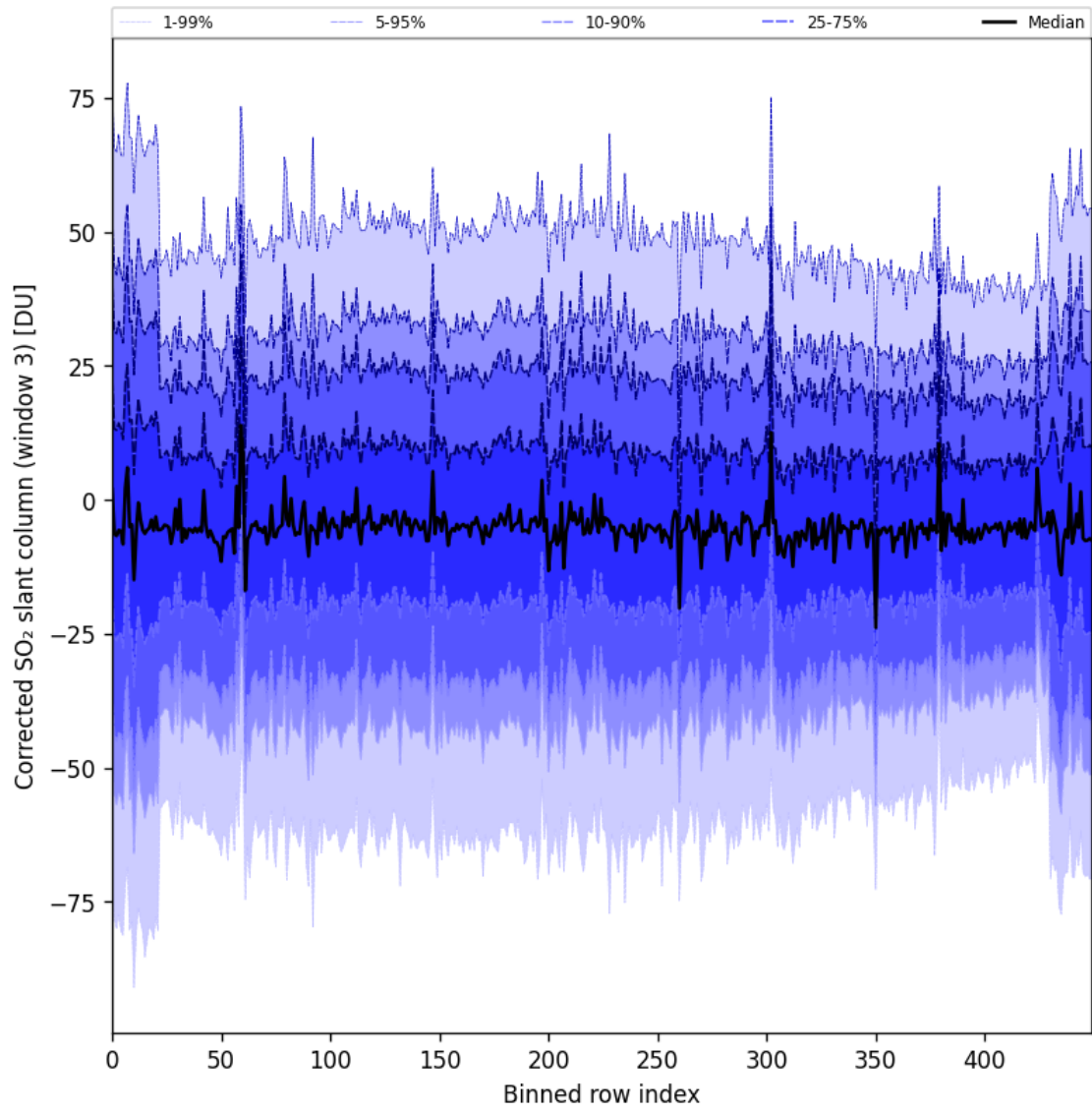
Figure 99: Along track statistics of “Corrected SO 2 slant column (window 3)” for 2025-04-21 to 2025-04-23
