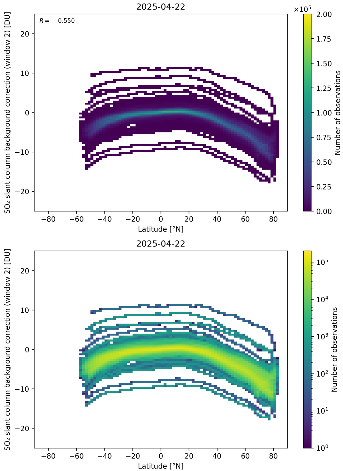
Figure 151: Scatter density plot of “Latitude” against “SO 2 slant column background correction (window 2)” for 2025-04-21 to 2025-04-23.
