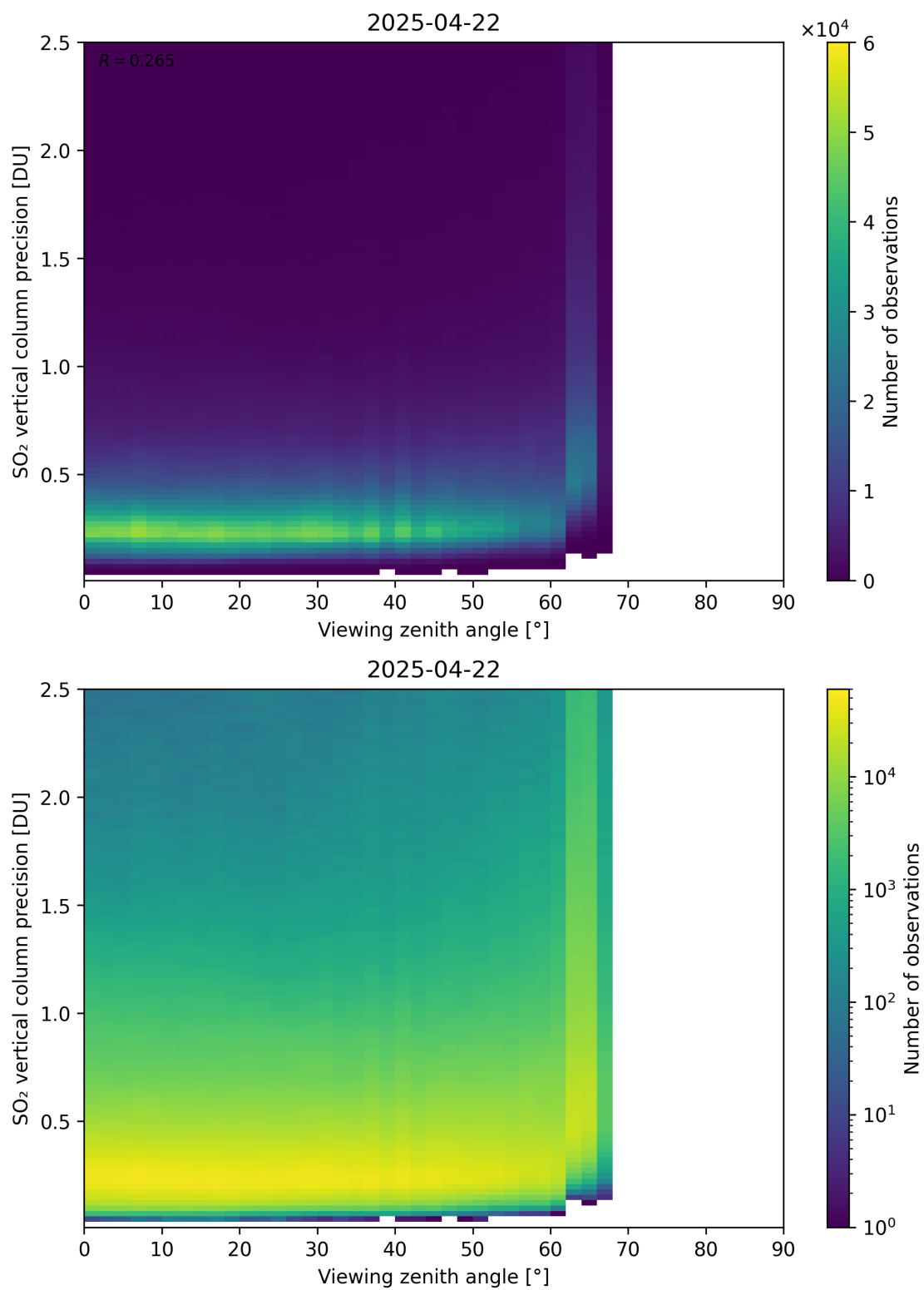
Figure 384: Scatter density plot of “Viewing zenith angle” against “SO 2 vertical column precision” for 2025-04-21 to 2025-04-23.
