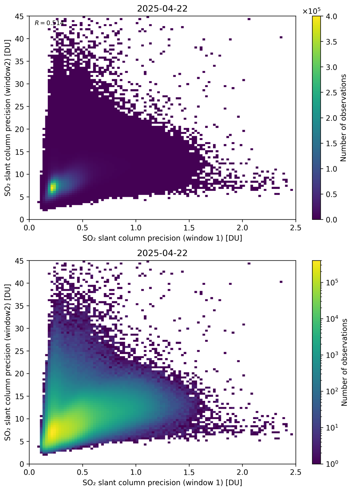
Figure 277: Scatter density plot of “SO 2 slant column precision (window 1)” against “SO 2 slant column precision (window2)” for 2025-04-21 to 2025-04-23.
