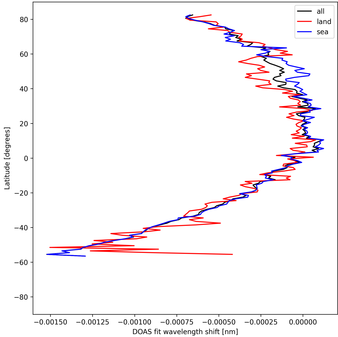
Figure 50: Zonal average of “DOAS fit wavelength shift” for 2025-04-21 to 2025-04-23.
