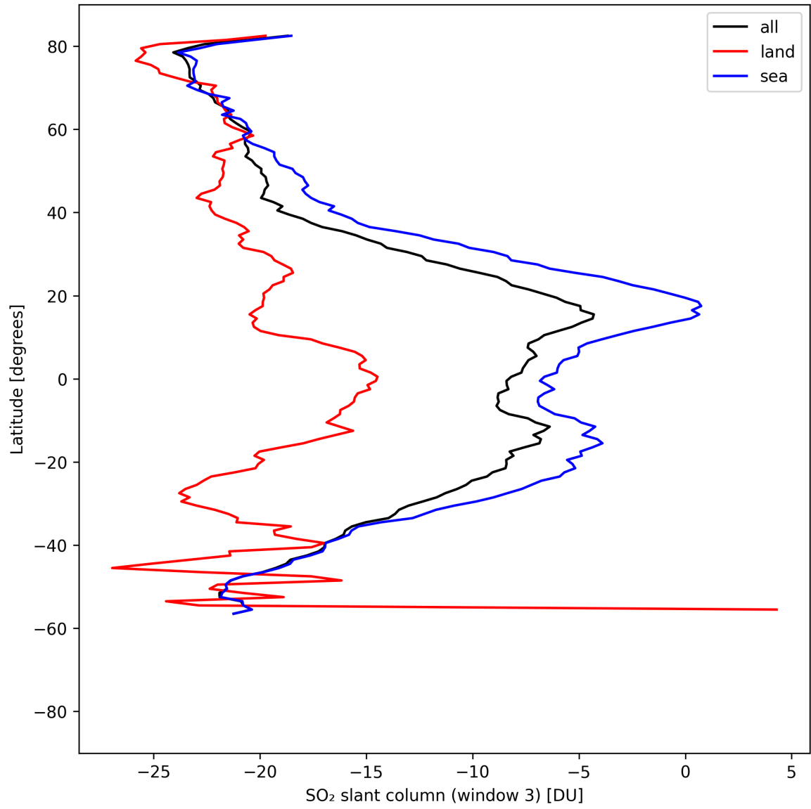
Figure 45: Zonal average of “SO 2 slant column (window 3)” for 2025-04-21 to 2025-04-23.
