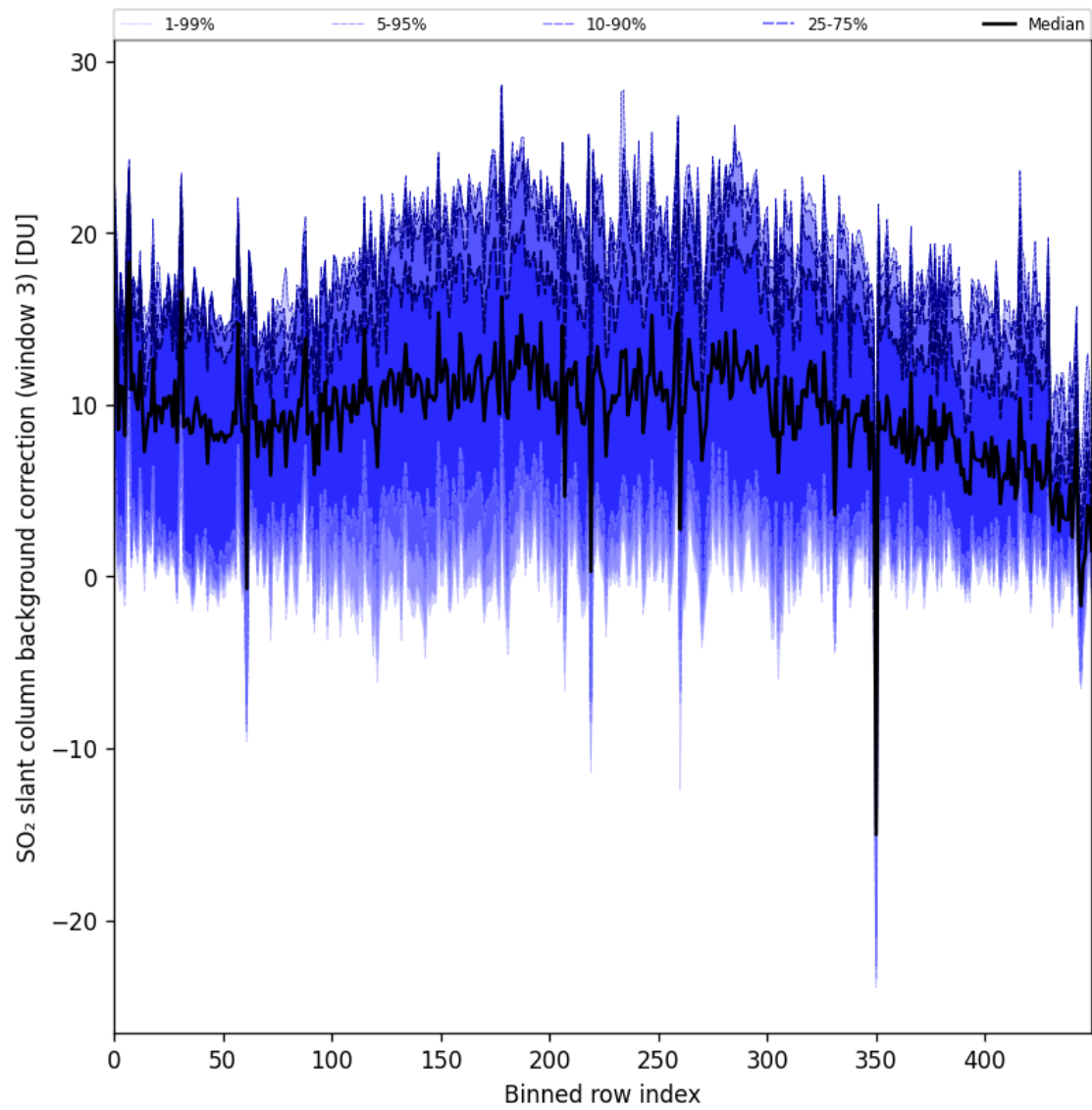
Figure 100: Along track statistics of “SO 2 slant column background correction (window 3)” for 2025-04-21 to 2025-04-23
