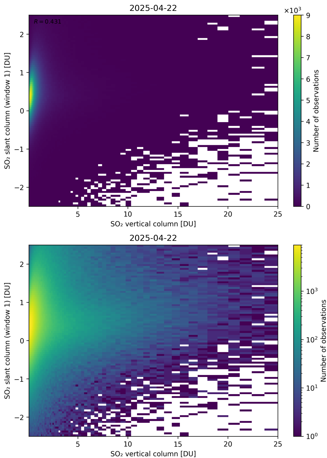
Figure 354: Scatter density plot of “SO 2 vertical column” against “SO 2 slant column (window 1)” for 2025-04-21 to 2025-04-23.
