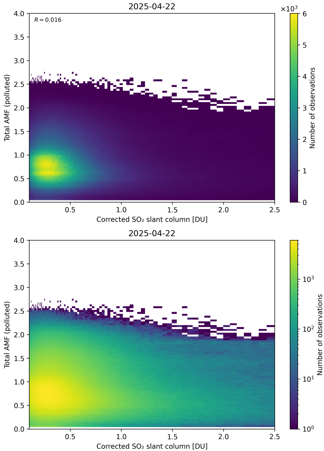
Figure 242: Scatter density plot of “Corrected SO 2 slant column” against “Total AMF (polluted)” for 2025-04-21 to 2025-04-23.
