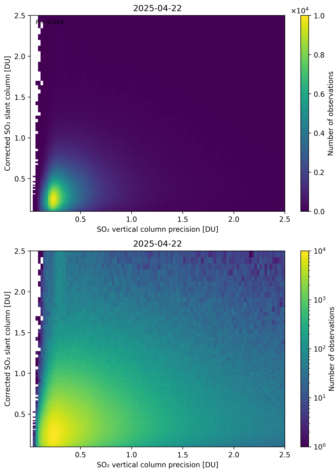
Figure 338: Scatter density plot of “SO 2 vertical column precision” against “Corrected SO 2 slant column” for 2025-04-21 to 2025-04-23.
