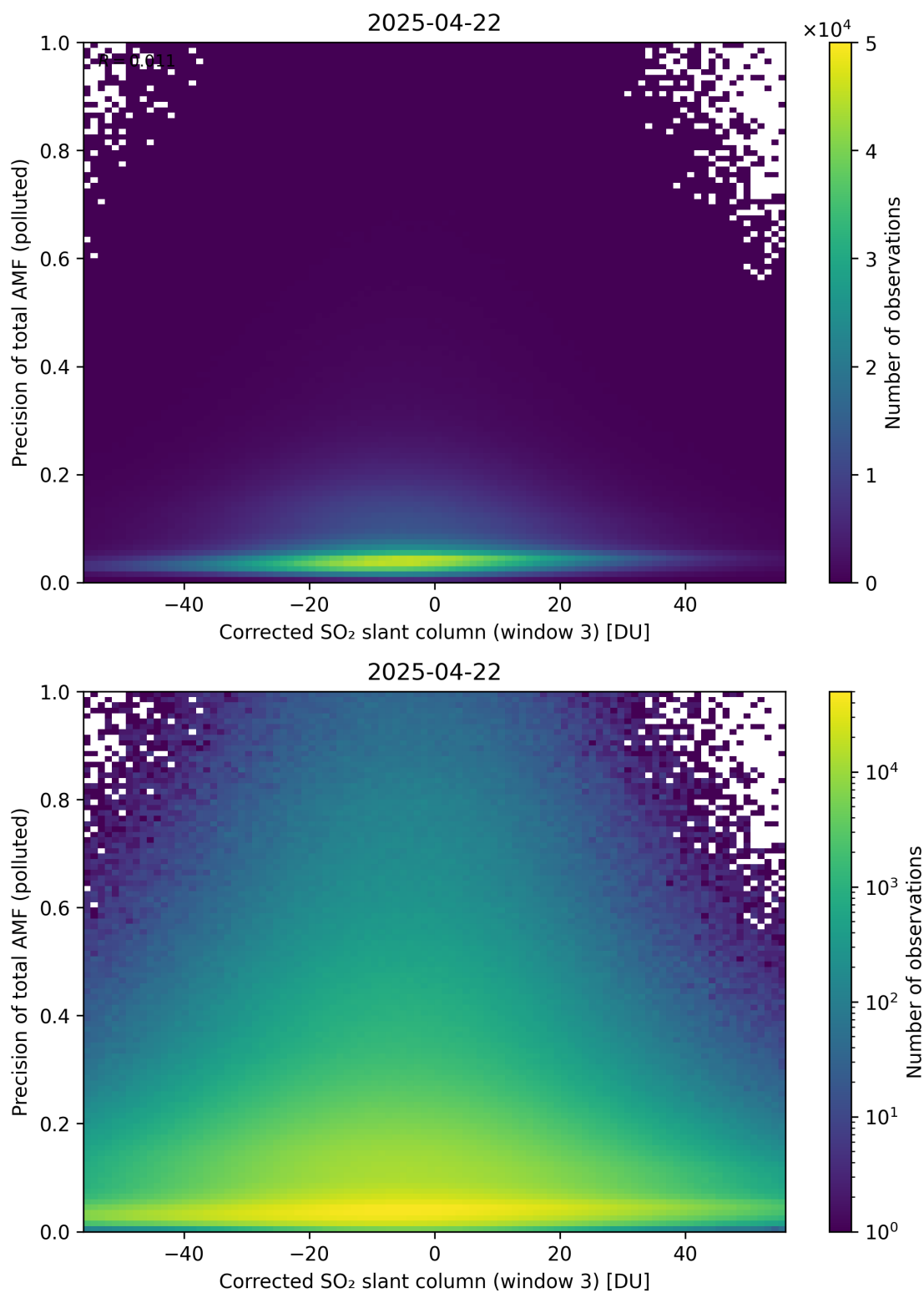
Figure 261: Scatter density plot of “Corrected SO 2 slant column (window 3)” against “Precision of total AMF (polluted)” for 2025-04-21 to 2025-04-23.
