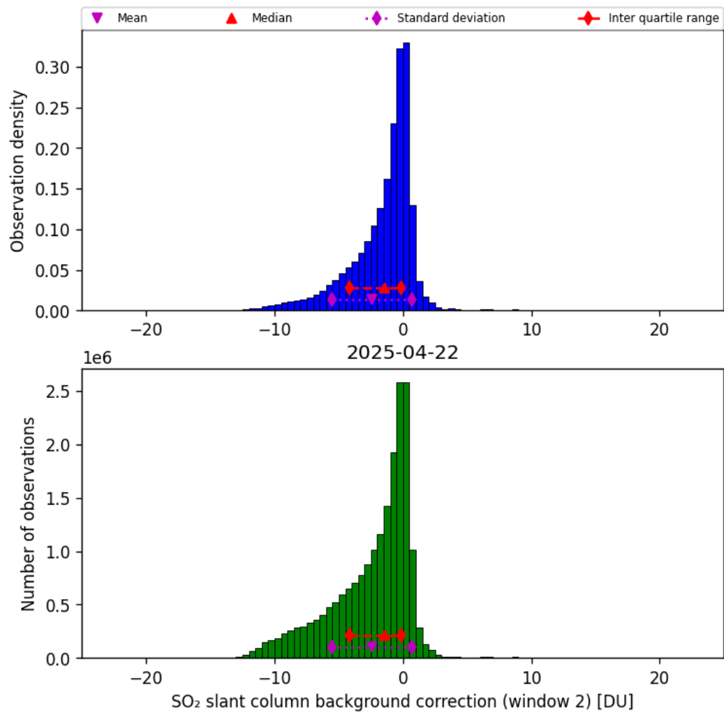
Figure 70: Histogram of “SO 2 slant column background correction (window 2)” for 2025-04-21 to 2025-04-23
