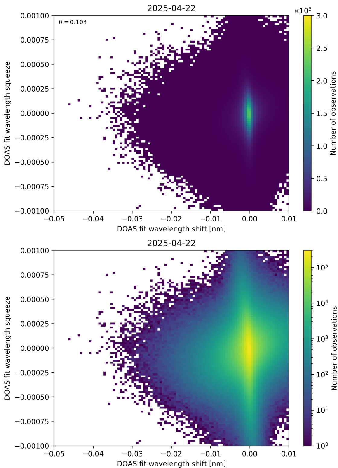
Figure 138: Scatter density plot of “DOAS fit wavelength shift” against “DOAS fit wavelength squeeze” for 2025-04-21 to 2025-04-23.
