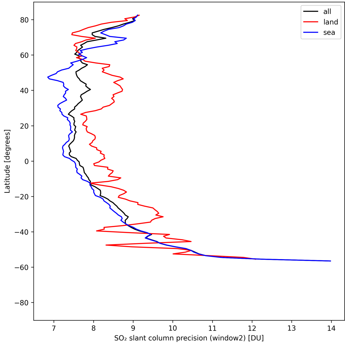
Figure 42: Zonal average of “SO 2 slant column precision (window2)” for 2025-04-21 to 2025-04-23.
