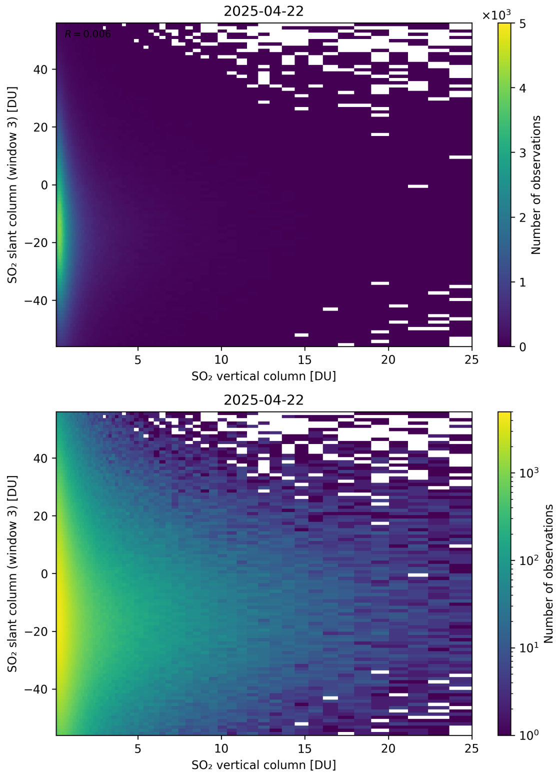
Figure 357: Scatter density plot of “SO 2 vertical column” against “SO 2 slant column (window 3)” for 2025-04-21 to 2025-04-23.
