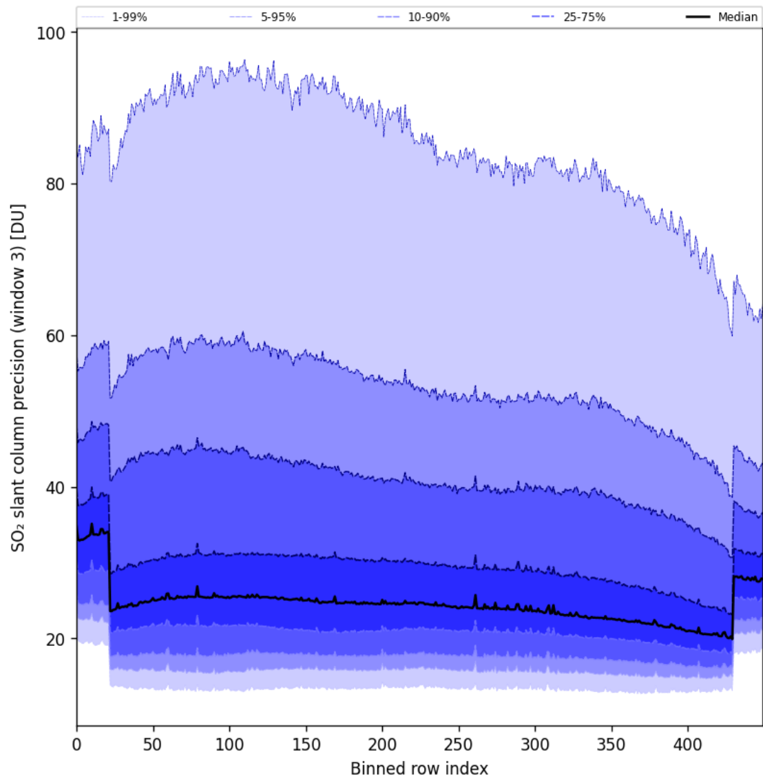
Figure 98: Along track statistics of “SO 2 slant column precision (window 3)” for 2025-04-21 to 2025-04-23
