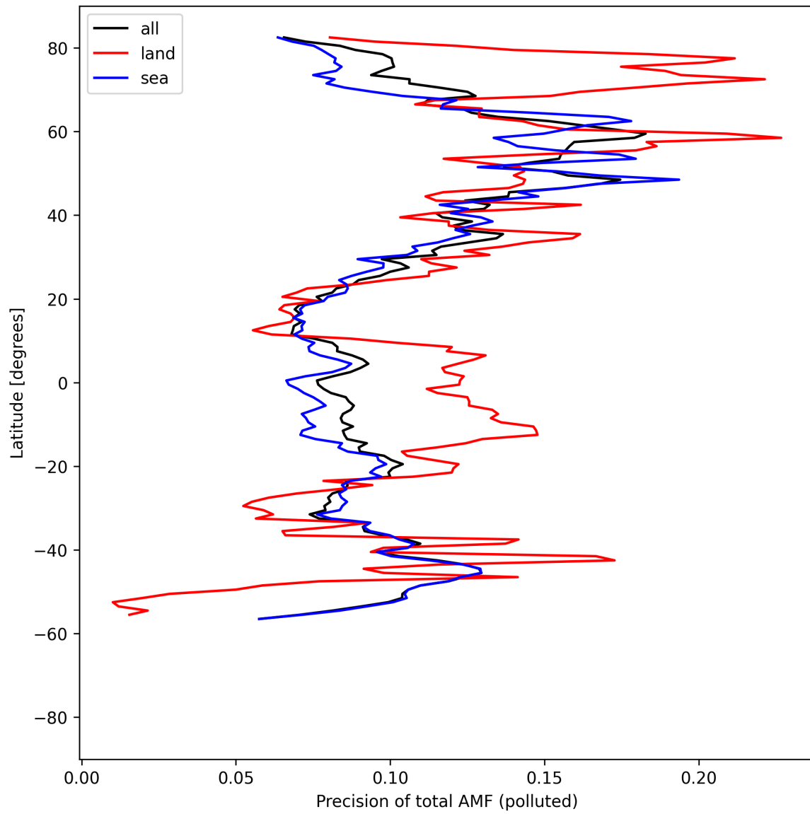
Figure 54: Zonal average of “Precision of total AMF (polluted)” for 2025-04-21 to 2025-04-23.
