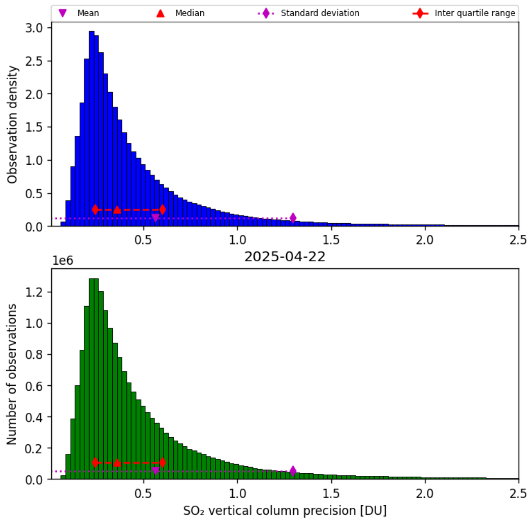
Figure 59: Histogram of “SO 2 vertical column precision” for 2025-04-21 to 2025-04-23
