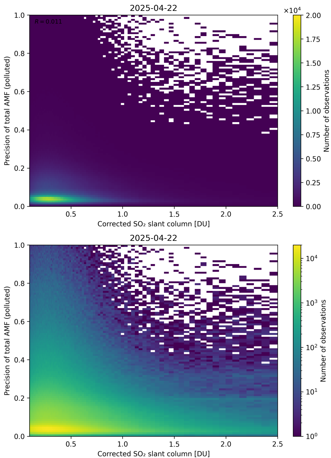
Figure 243: Scatter density plot of “Corrected SO 2 slant column” against “Precision of total AMF (polluted)” for 2025-04-21 to 2025-04-23.
