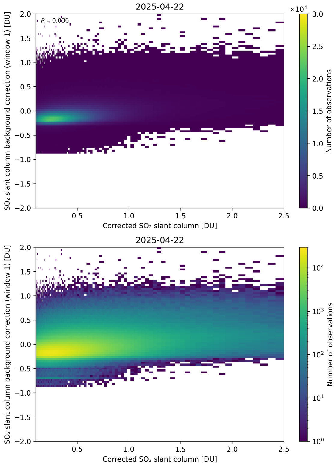
Figure 226: Scatter density plot of “Corrected SO 2 slant column” against “SO 2 slant column background correction (window 1)” for 2025-04-21 to 2025-04-23.
