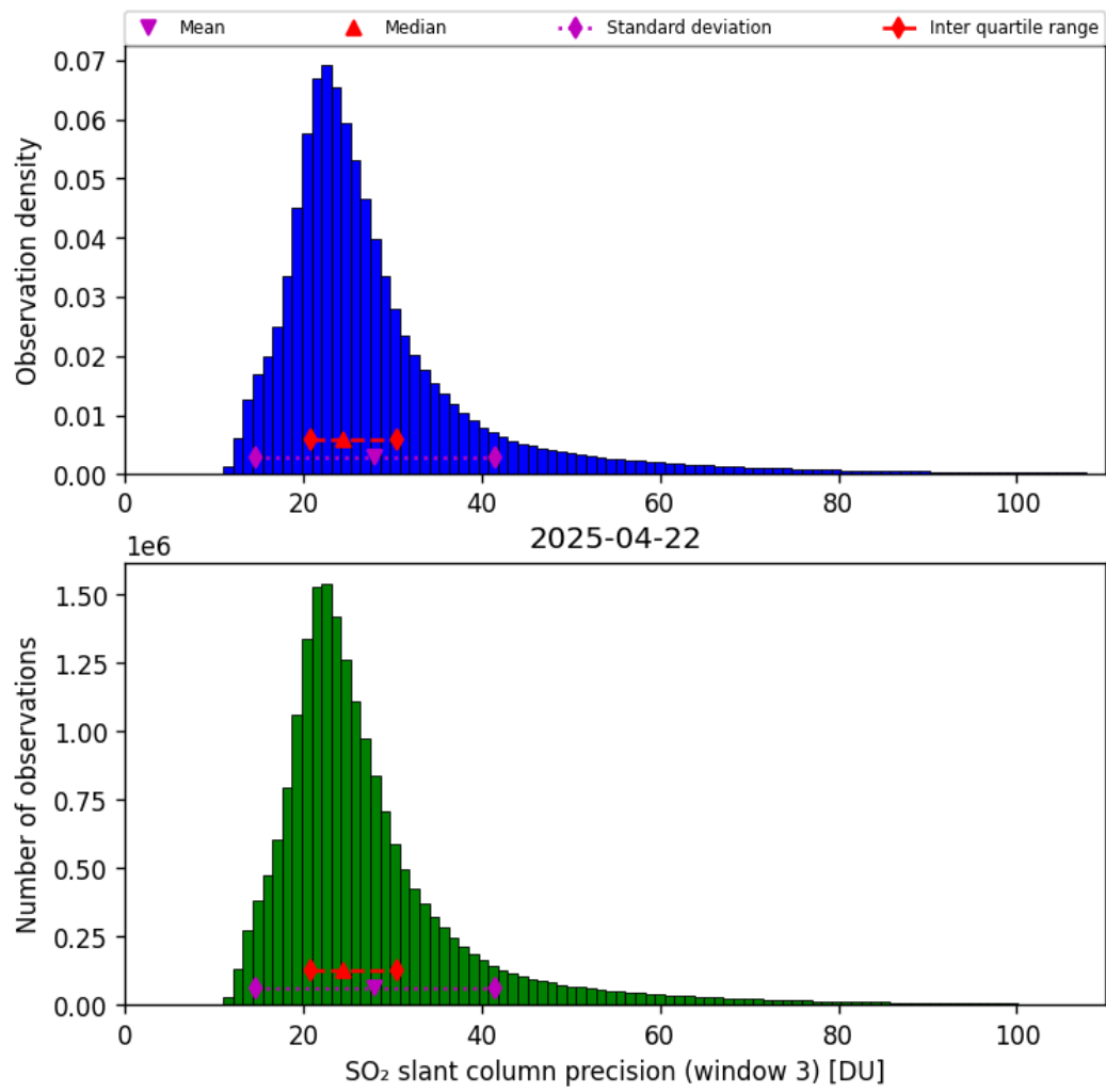
Figure 72: Histogram of “SO 2 slant column precision (window 3)” for 2025-04-21 to 2025-04-23
