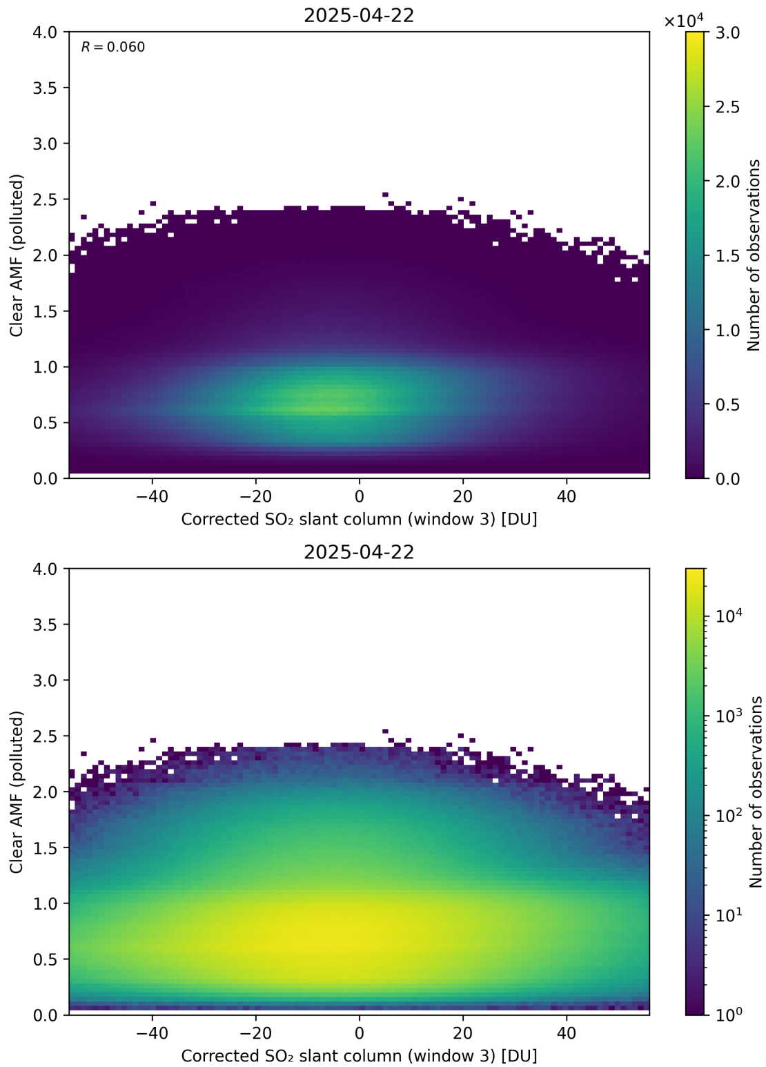
Figure 259: Scatter density plot of “Corrected SO 2 slant column (window 3)” against “Clear AMF (polluted)” for 2025-04-21 to 2025-04-23.
