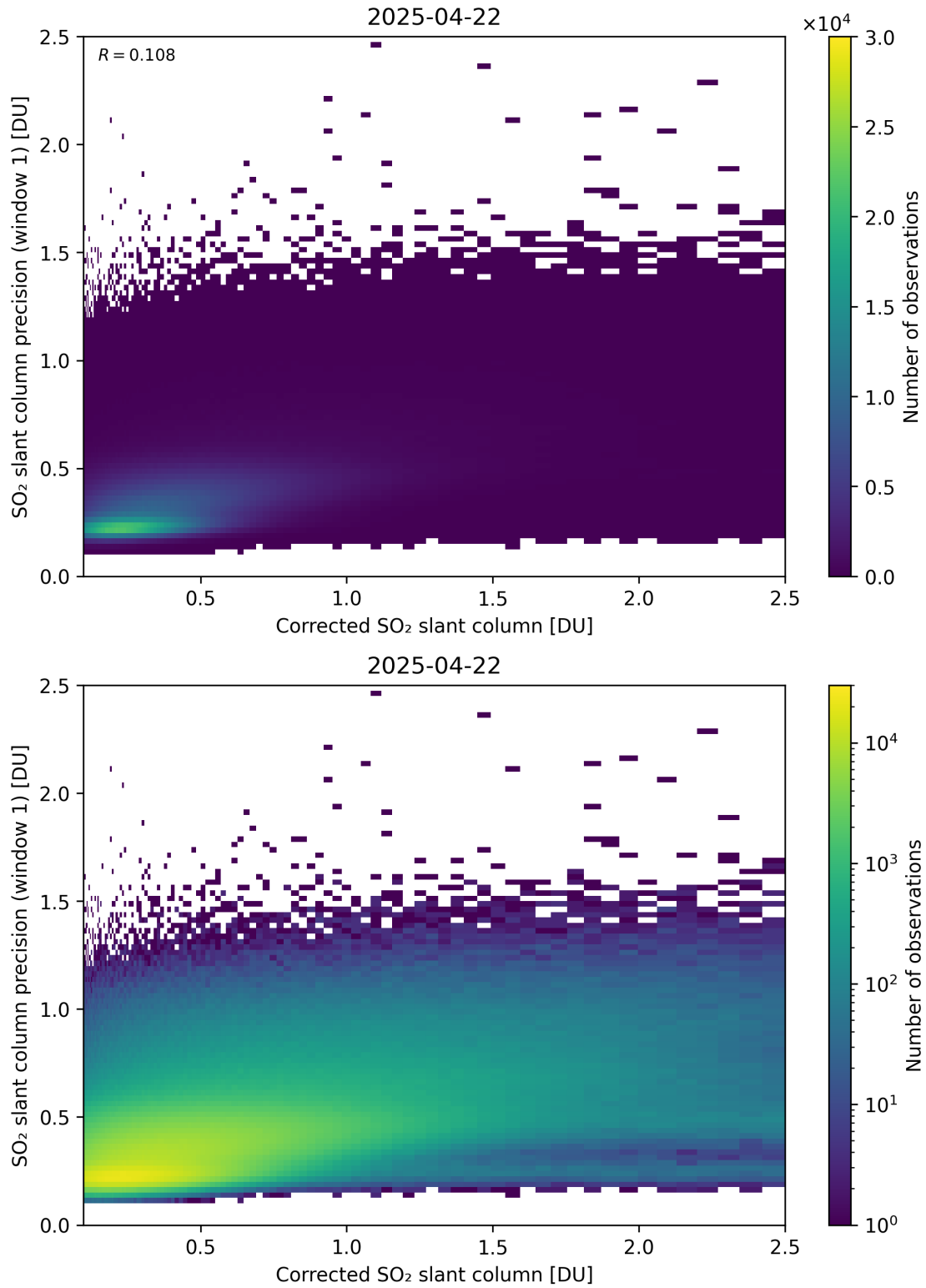
Figure 238: Scatter density plot of “Corrected SO 2 slant column” against “SO 2 slant column precision (window 1)” for 2025-04-21 to 2025-04-23.
