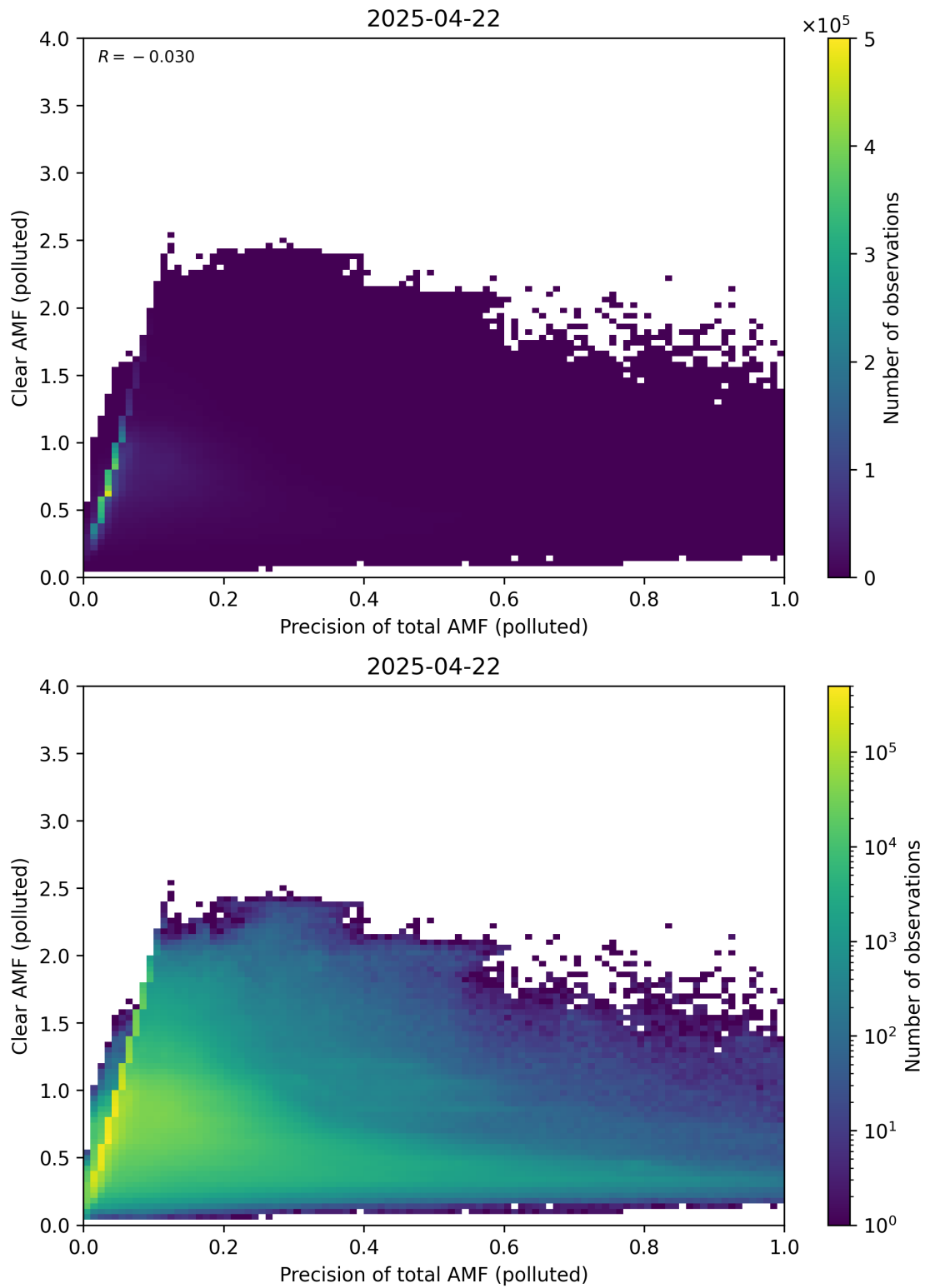
Figure 320: Scatter density plot of “Precision of total AMF (polluted)” against “Clear AMF (polluted)” for 2025-04-21 to 2025-04-23.
