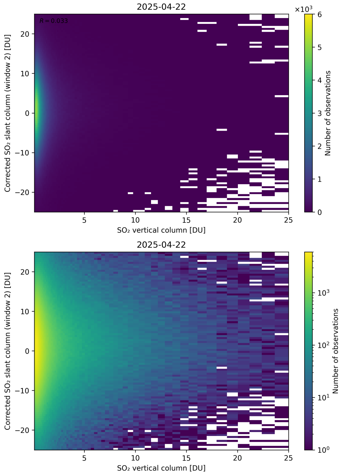
Figure 352: Scatter density plot of “SO 2 vertical column” against “Corrected SO 2 slant column (window 2)” for 2025-04-21 to 2025-04-23.
