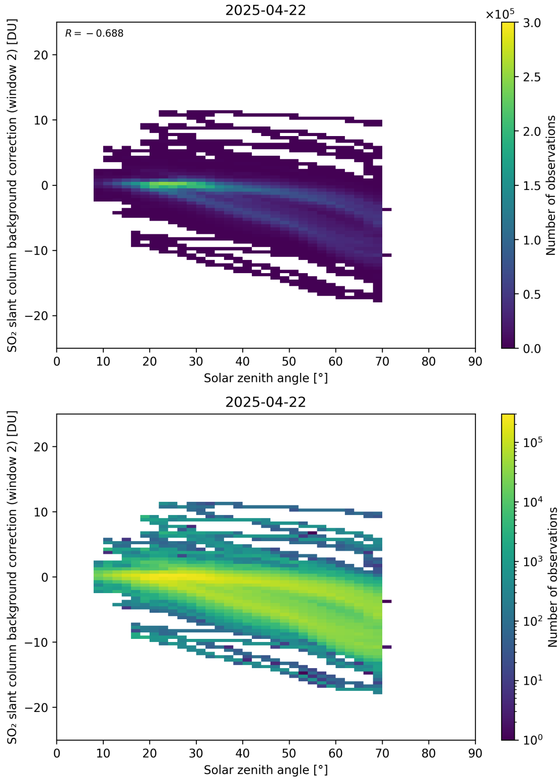
Figure 172: Scatter density plot of “Solar zenith angle” against “SO 2 slant column background correction (window 2)” for 2025-04-21 to 2025-04-23.
