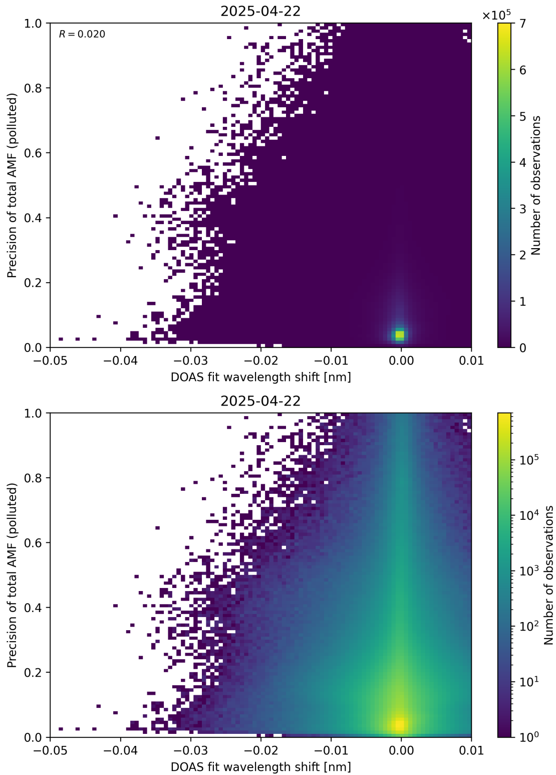
Figure 142: Scatter density plot of “DOAS fit wavelength shift” against “Precision of total AMF (polluted)” for 2025-04-21 to 2025-04-23.
