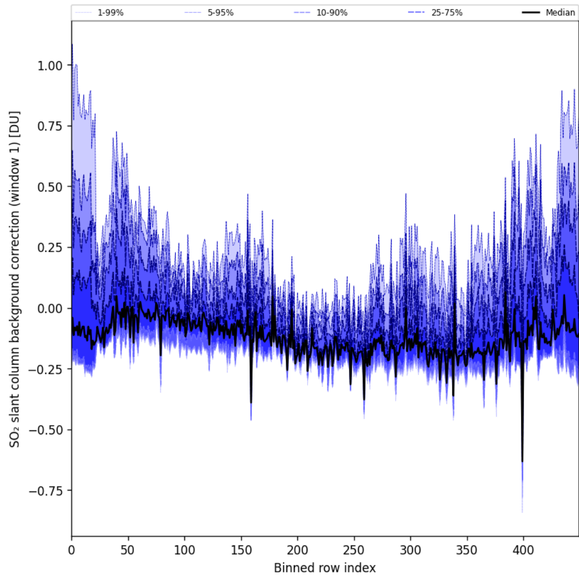
Figure 92: Along track statistics of “SO 2 slant column background correction (window 1)” for 2025-04-21 to 2025-04-23
