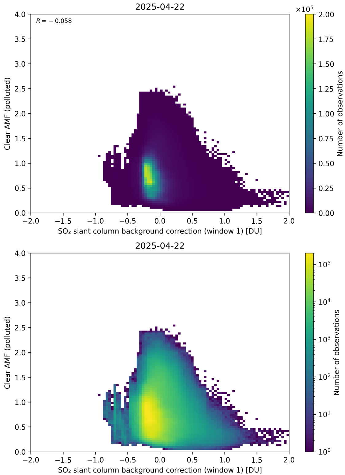
Figure 114: Scatter density plot of “SO 2 slant column background correction (window 1)” against “Clear AMF (polluted)” for 2025-04-21 to 2025-04-23.
