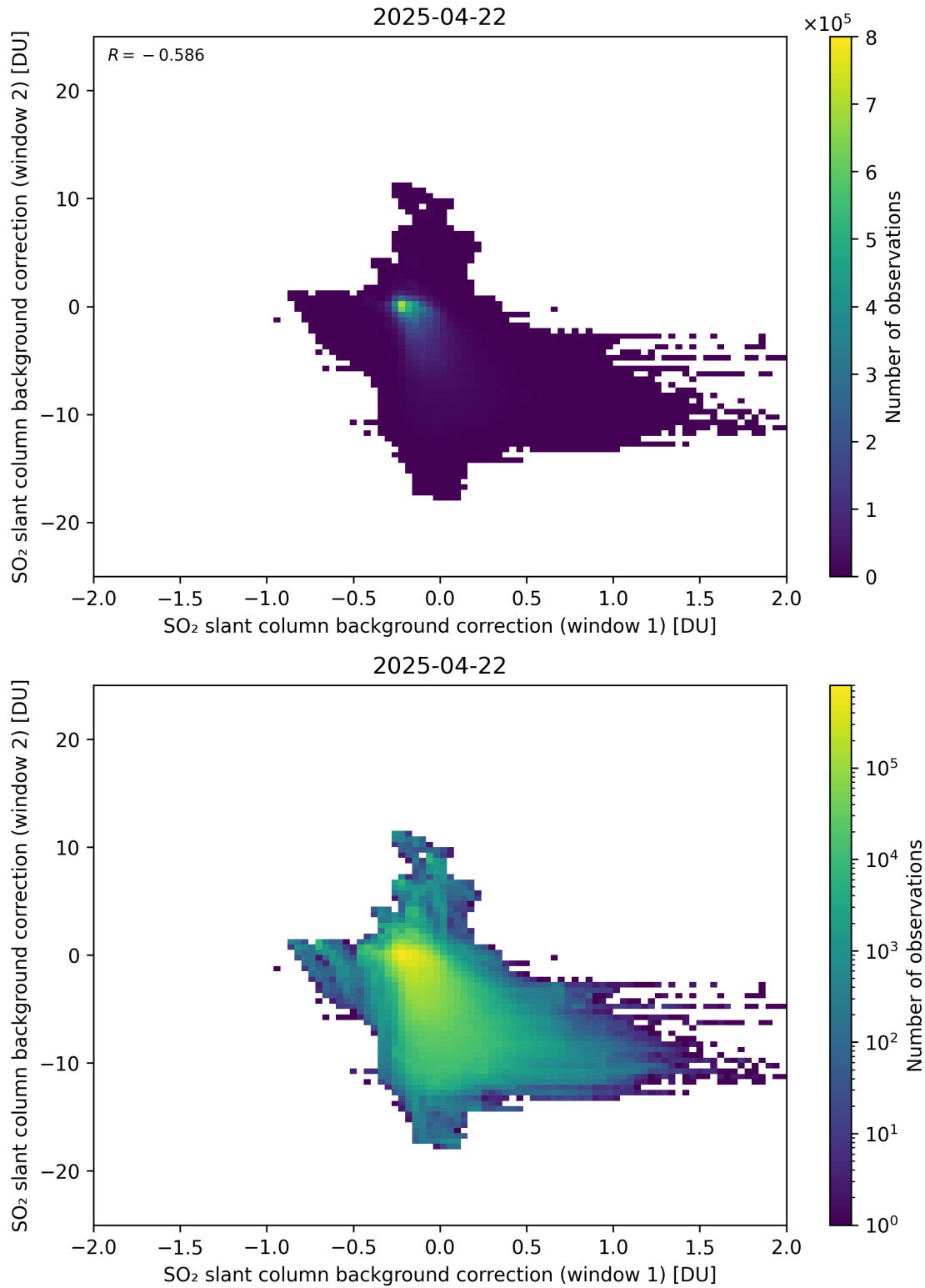
Figure 109: Scatter density plot of “SO 2 slant column background correction (window 1)” against “SO 2 slant column background correction (window 2)” for 2025-04-21 to 2025-04-23.
