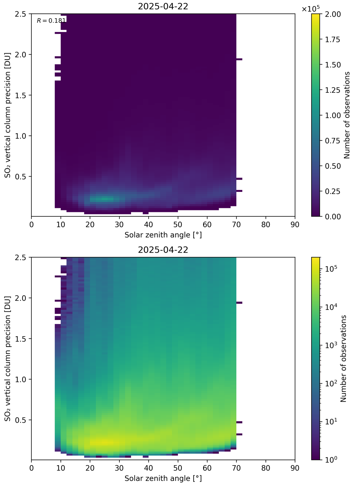
Figure 192: Scatter density plot of “Solar zenith angle” against “SO 2 vertical column precision” for 2025-04-21 to 2025-04-23.
