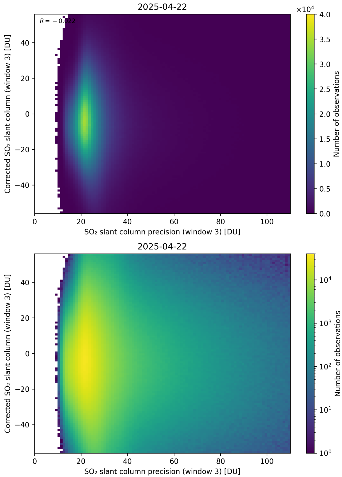
Figure 312: Scatter density plot of “SO 2 slant column precision (window 3)” against “Corrected SO 2 slant column (window 3)” for 2025-04-21 to 2025-04-23.
