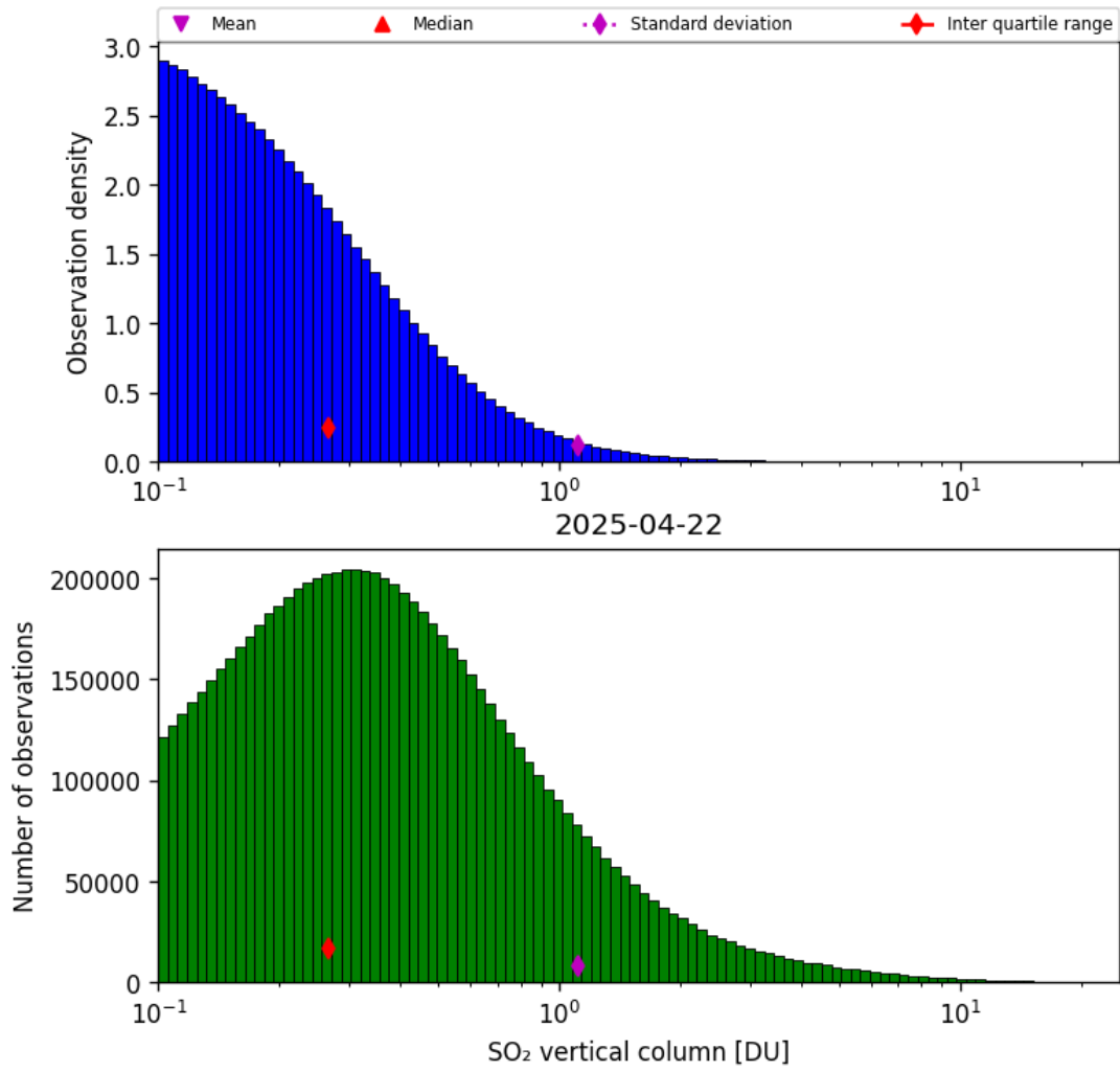
Figure 58: Histogram of “SO 2 vertical column” for 2025-04-21 to 2025-04-23
