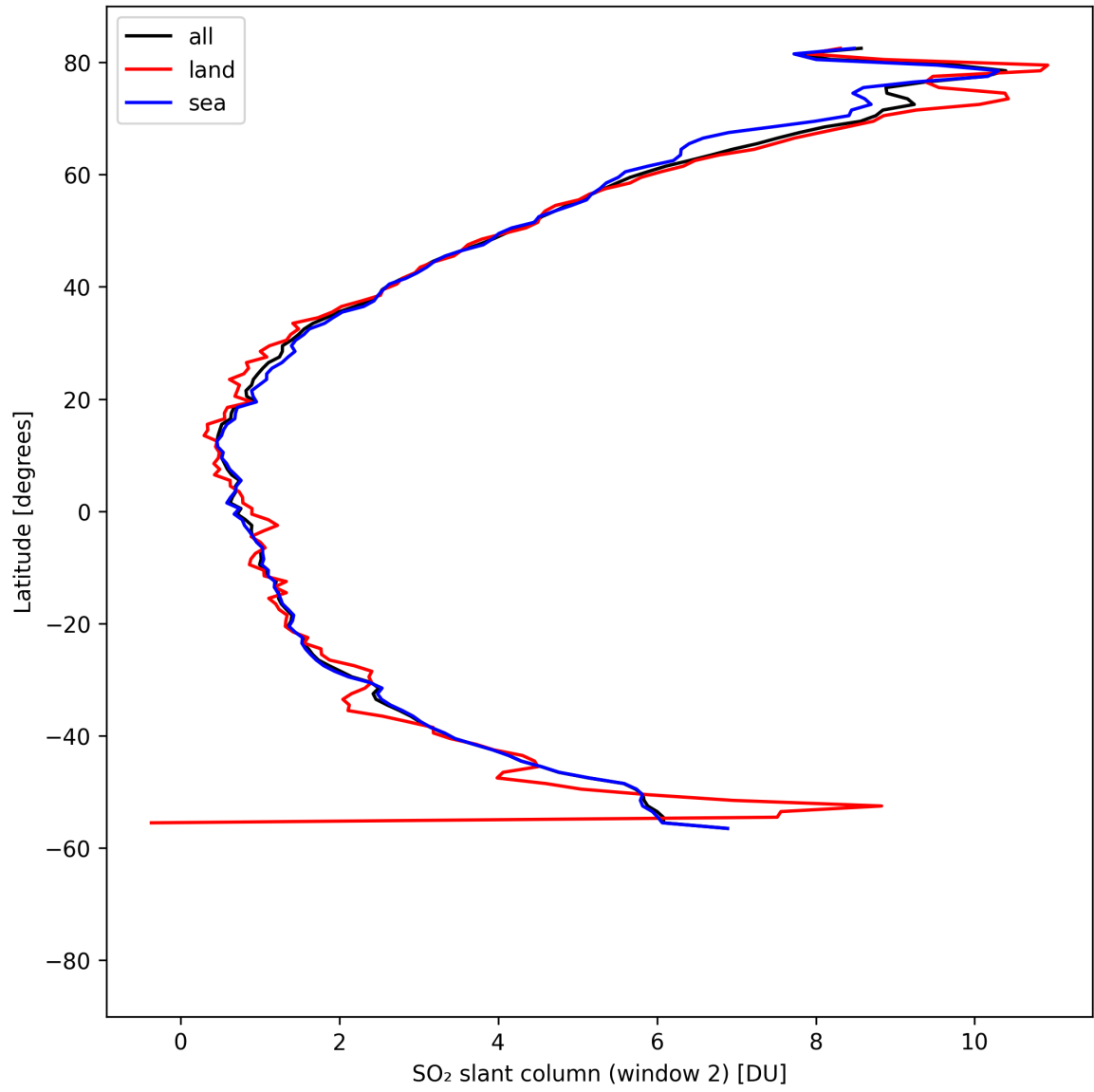
Figure 41: Zonal average of “SO 2 slant column (window 2)” for 2025-04-21 to 2025-04-23.
