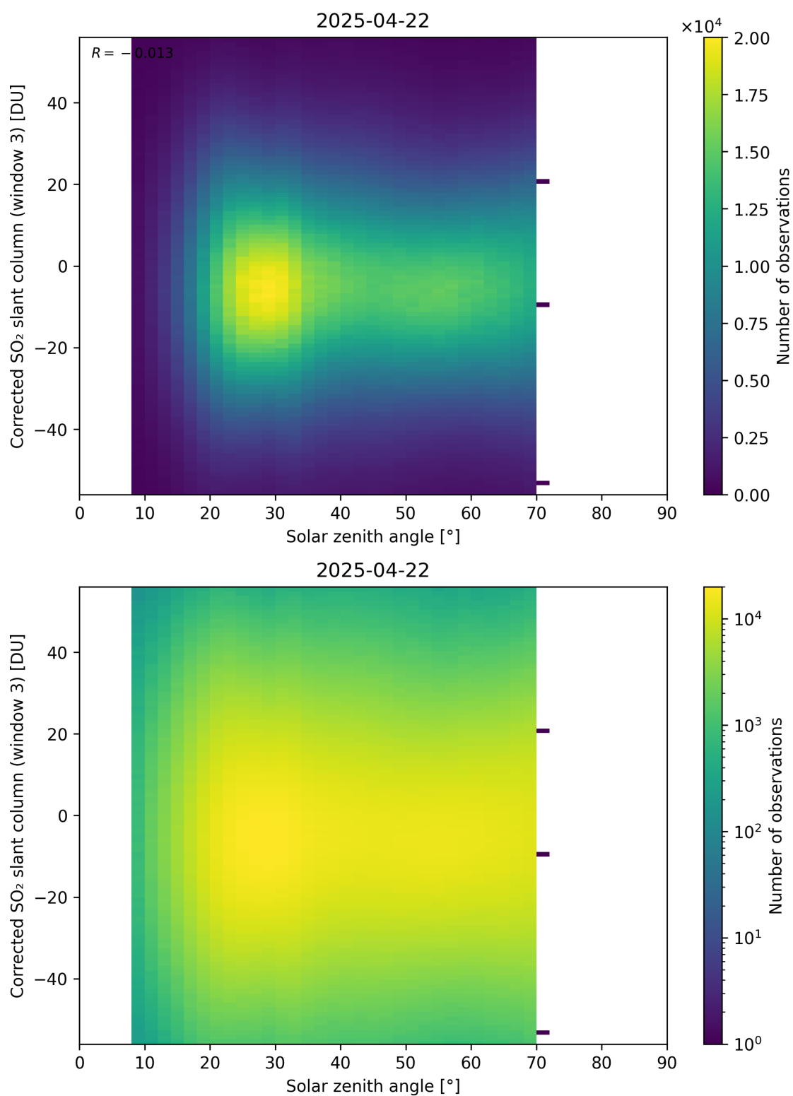
Figure 183: Scatter density plot of “Solar zenith angle” against “Corrected SO 2 slant column (window 3)” for 2025-04-21 to 2025-04-23.
