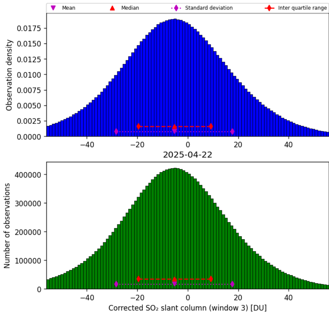
Figure 73: Histogram of “Corrected SO 2 slant column (window 3)” for 2025-04-21 to 2025-04-23
