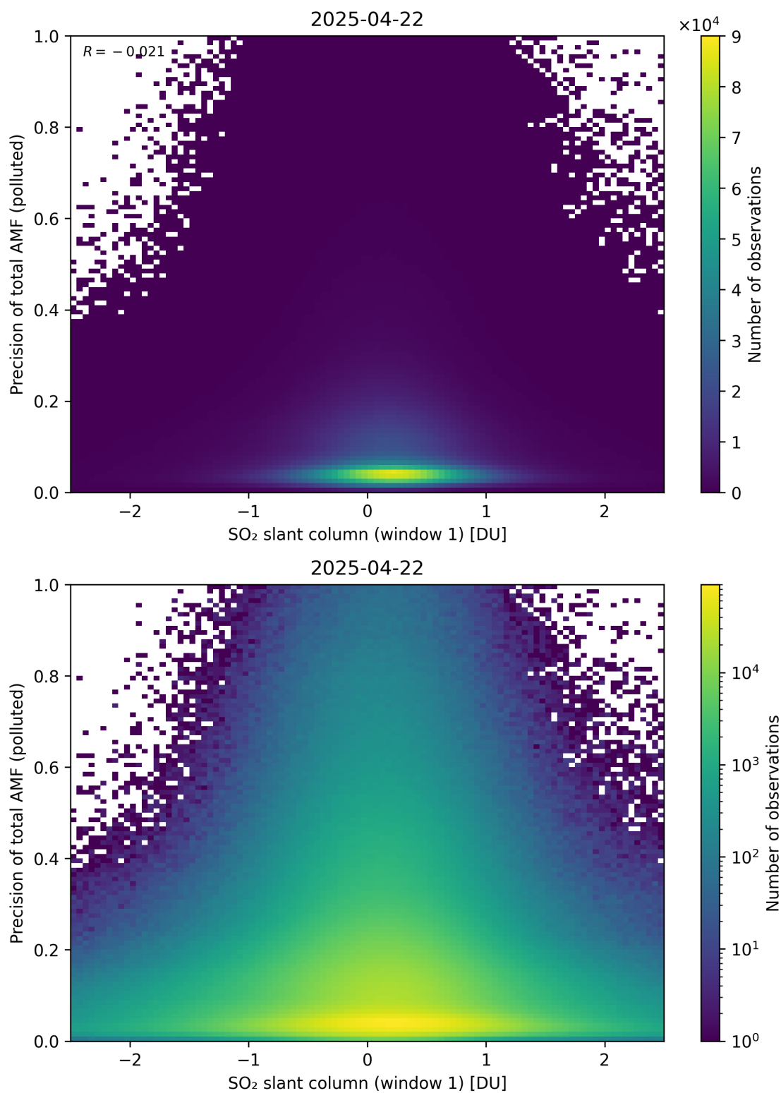
Figure 290: Scatter density plot of “SO 2 slant column (window 1)” against “Precision of total AMF (polluted)” for 2025-04-21 to 2025-04-23.
