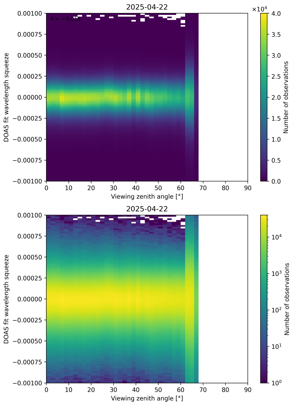
Figure 366: Scatter density plot of “Viewing zenith angle” against “DOAS fit wavelength squeeze” for 2025-04-21 to 2025-04-23.
