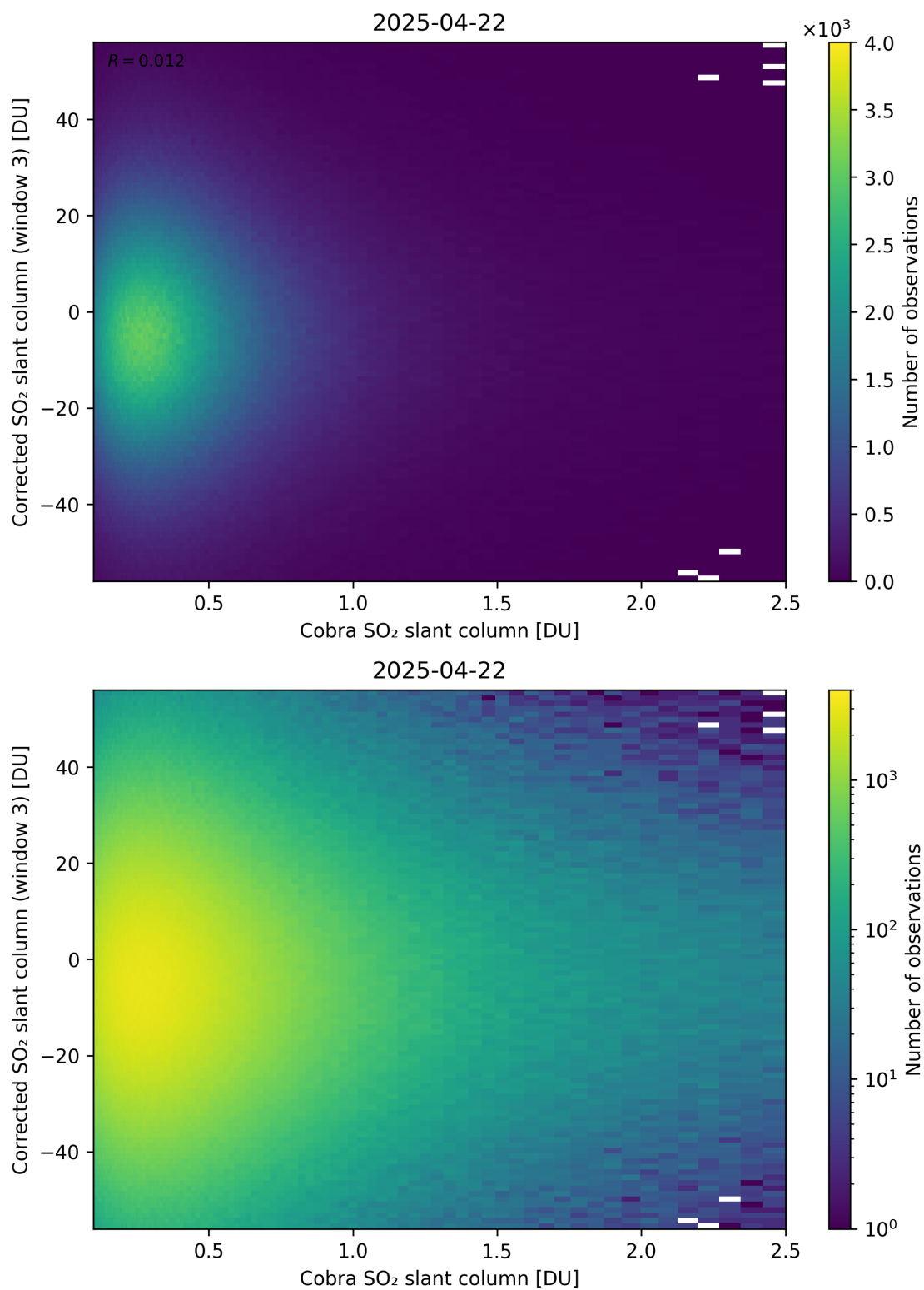
Figure 218: Scatter density plot of “Cobra SO 2 slant column” against “Corrected SO 2 slant column (window 3)” for 2025-04-21 to 2025-04-23.
