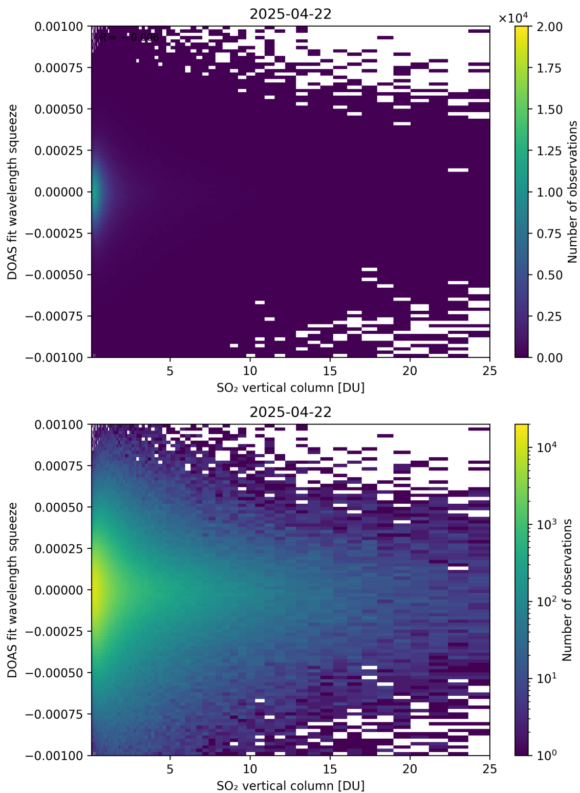
Figure 327: Scatter density plot of “SO 2 vertical column” against “DOAS fit wavelength squeeze” for 2025-04-21 to 2025-04-23.
