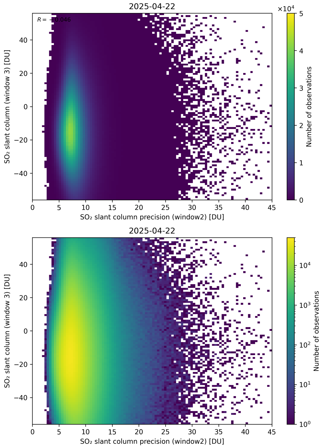
Figure 299: Scatter density plot of “SO 2 slant column precision (window2)” against “SO 2 slant column (window 3)” for 2025-04-21 to 2025-04-23.
