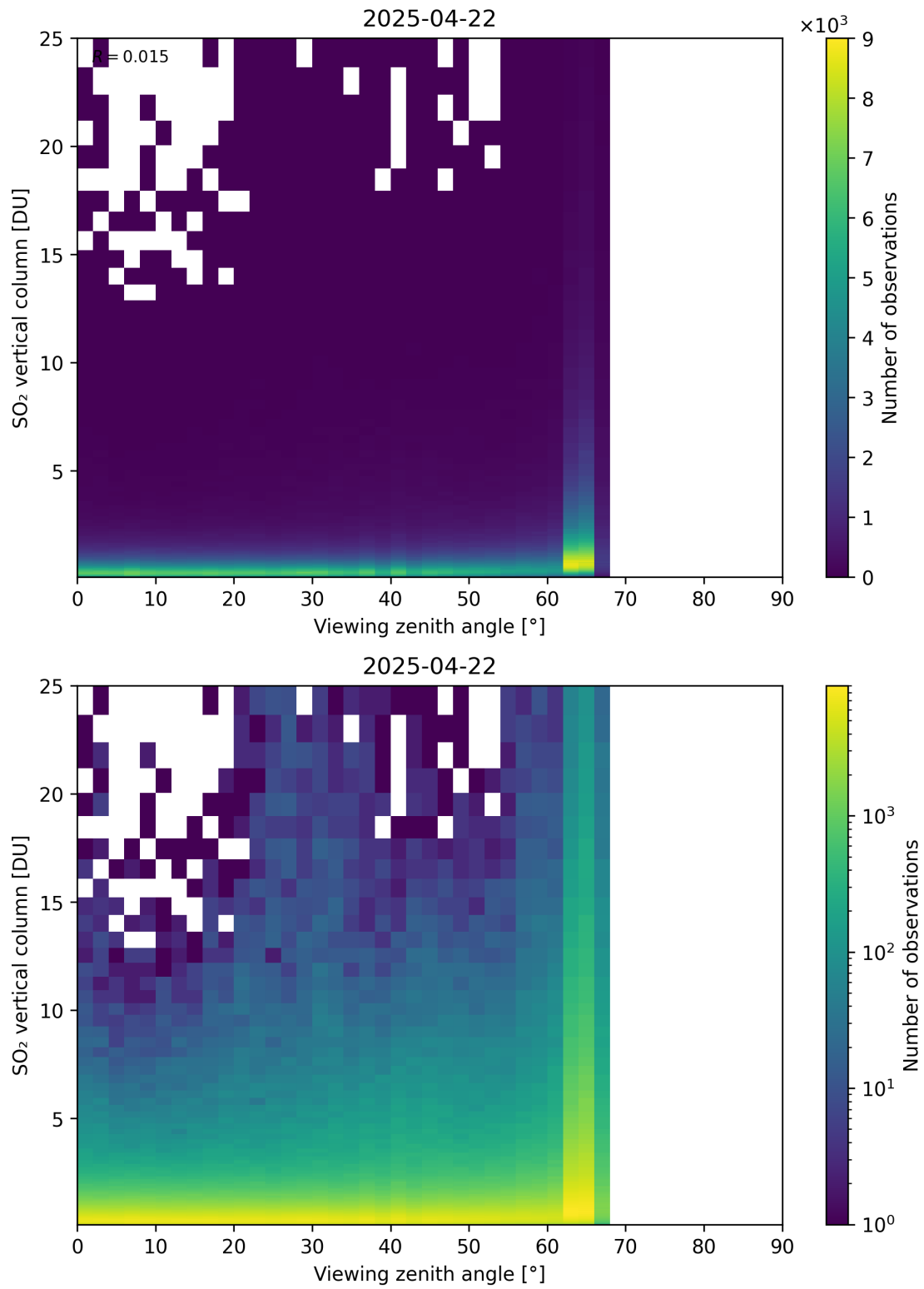
Figure 383: Scatter density plot of “Viewing zenith angle” against “SO 2 vertical column” for 2025-04-21 to 2025-04-23.
