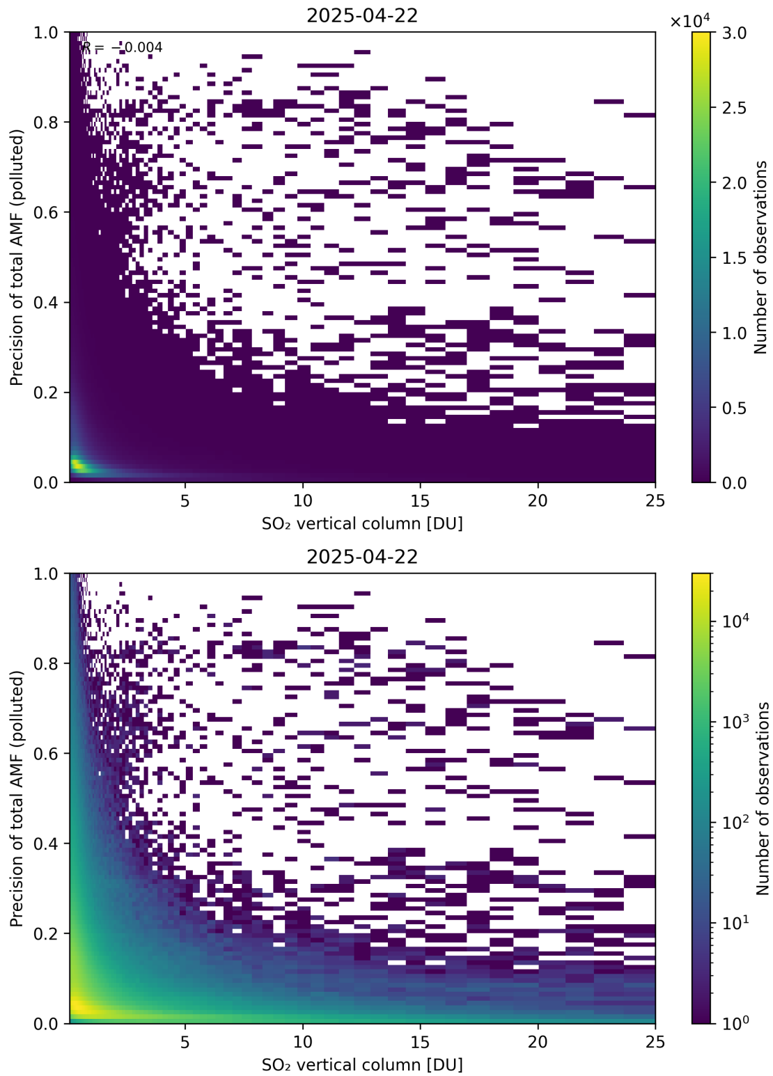
Figure 360: Scatter density plot of “SO 2 vertical column” against “Precision of total AMF (polluted)” for 2025-04-21 to 2025-04-23.
