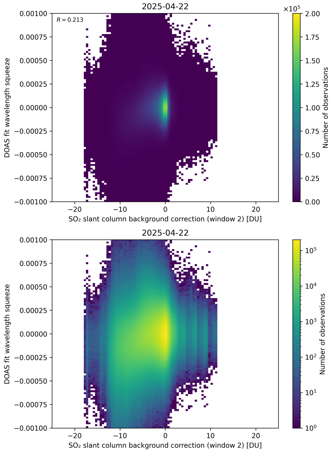
Figure 124: Scatter density plot of “SO 2 slant column background correction (window 2)” against “DOAS fit wavelength squeeze” for 2025-04-21 to 2025-04-23.
