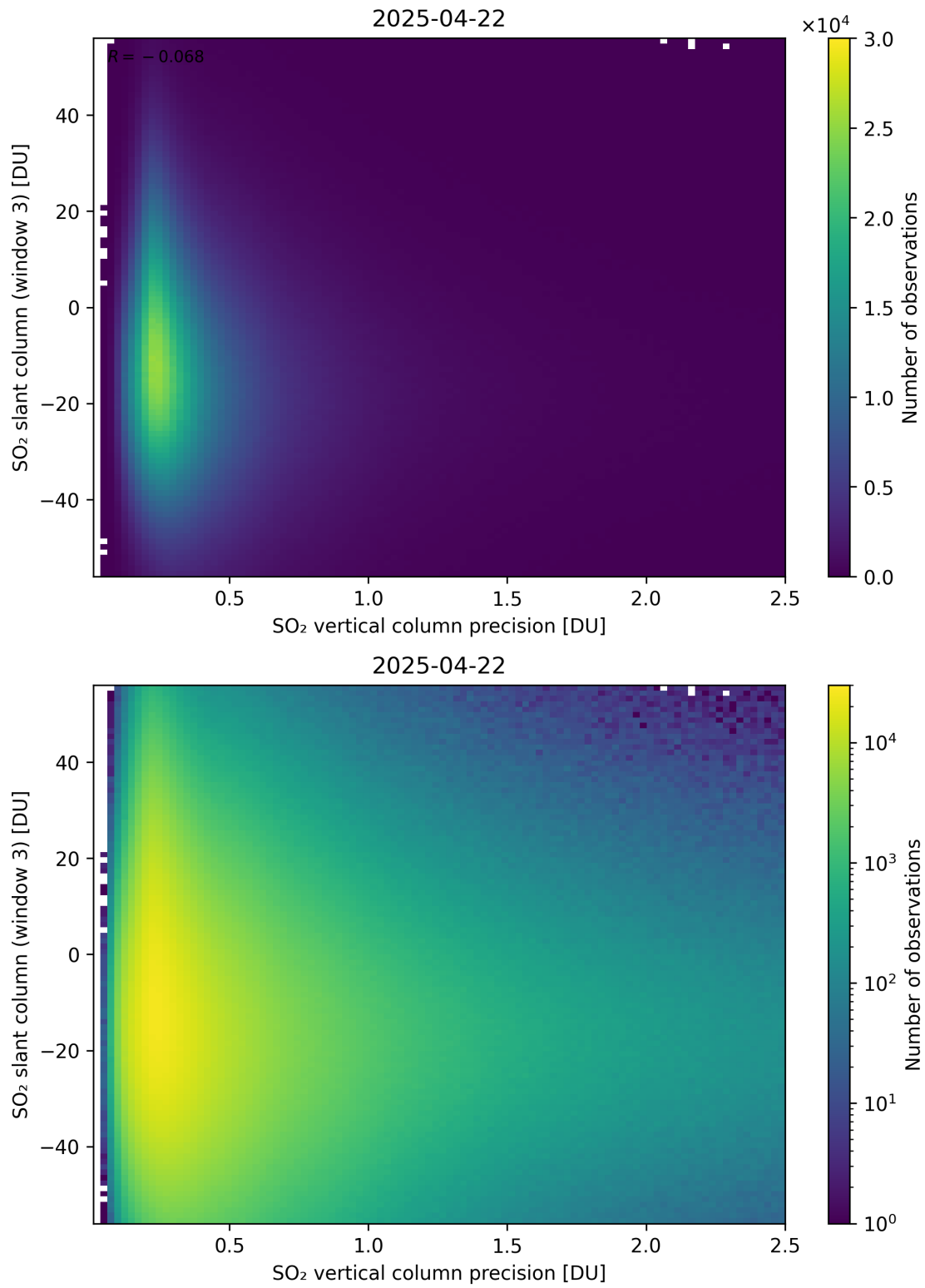
Figure 344: Scatter density plot of “SO 2 vertical column precision” against “SO 2 slant column (window 3)” for 2025-04-21 to 2025-04-23.
