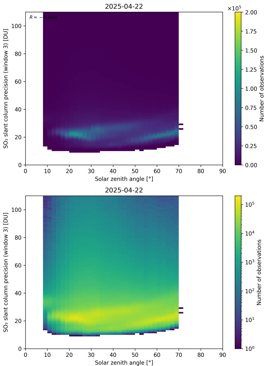
Figure 188: Scatter density plot of “Solar zenith angle” against “SO 2 slant column precision (window 3)” for 2025-04-21 to 2025-04-23.
