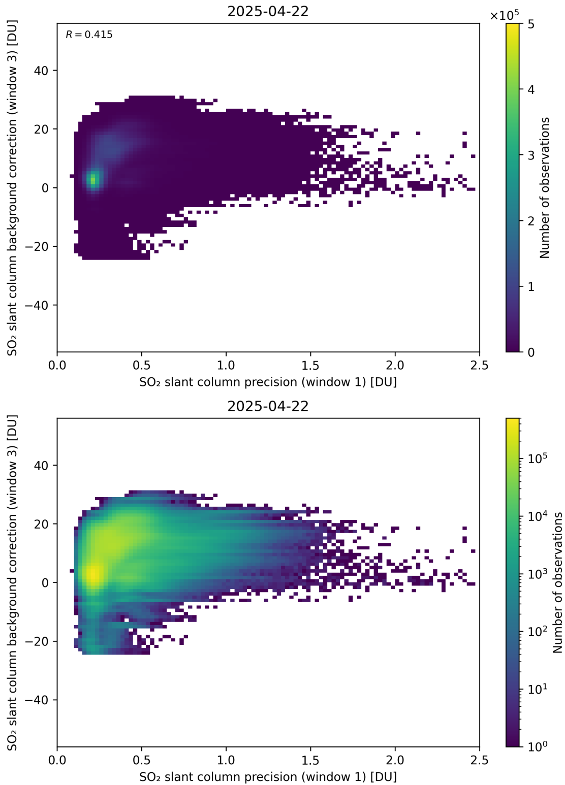
Figure 270: Scatter density plot of “SO 2 slant column precision (window 1)” against “SO 2 slant column background correction (window 3)” for 2025-04-21 to 2025-04-23.
