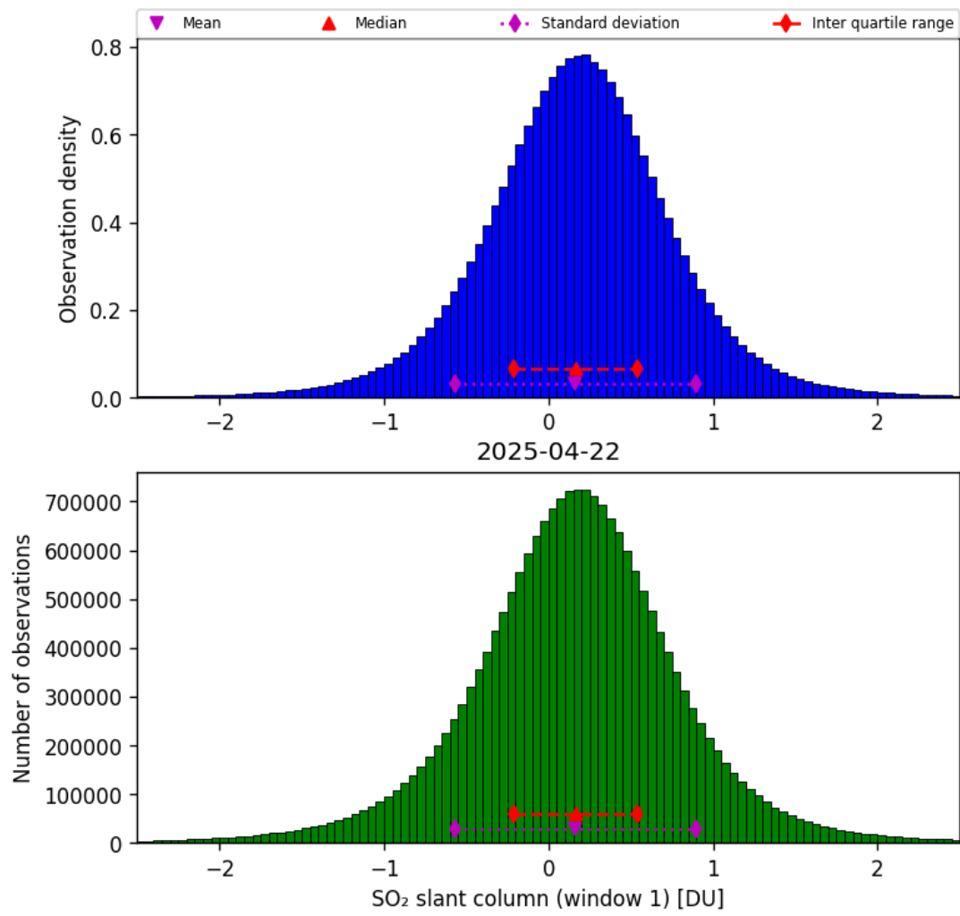
Figure 63: Histogram of “SO 2 slant column (window 1)” for 2025-04-21 to 2025-04-23
