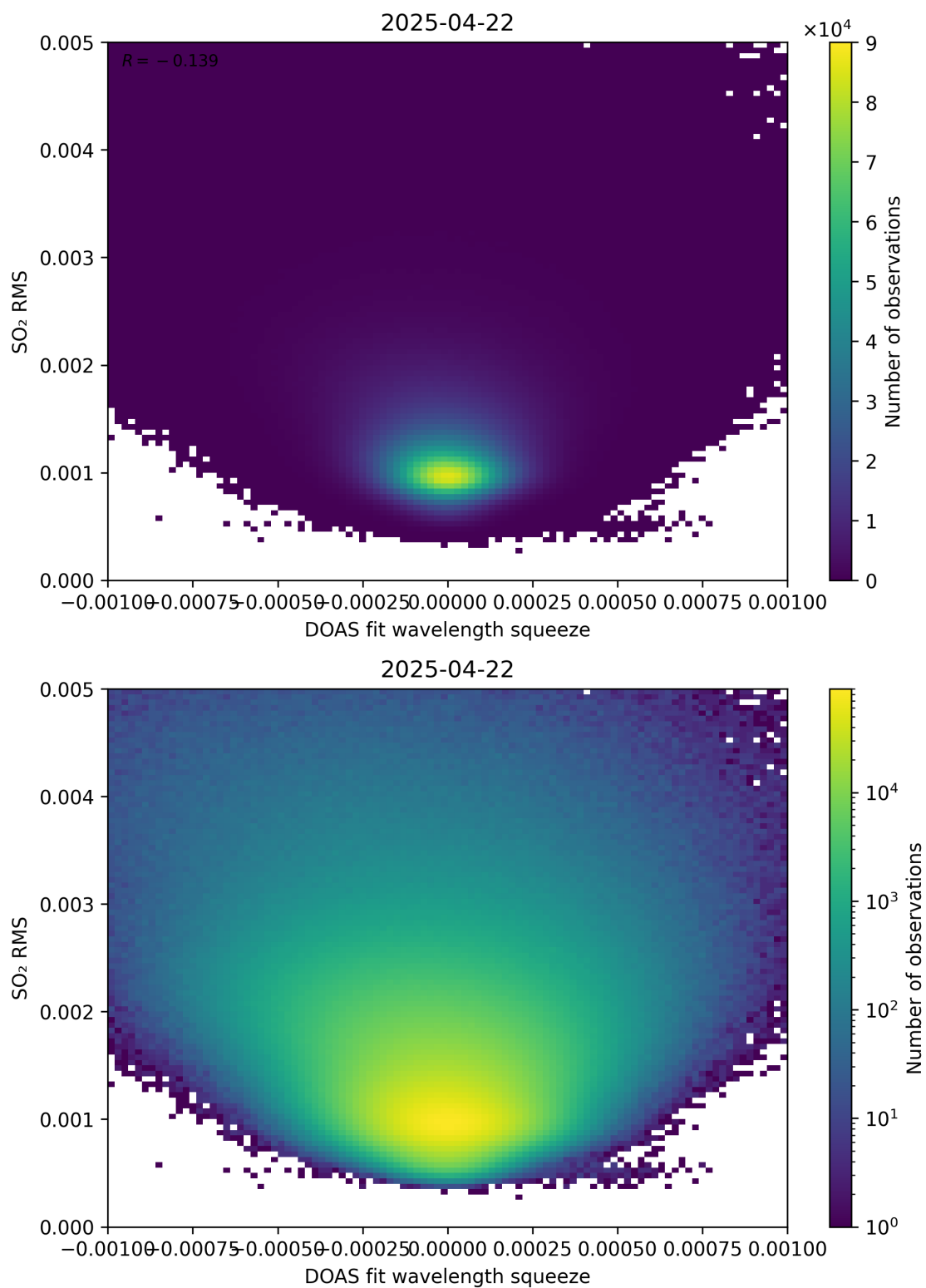
Figure 143: Scatter density plot of “DOAS fit wavelength squeeze” against “SO 2 RMS” for 2025-04-21 to 2025-04-23.
