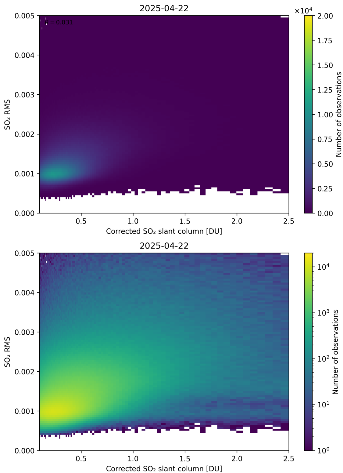
Figure 231: Scatter density plot of “Corrected SO 2 slant column” against “SO 2 RMS” for 2025-04-21 to 2025-04-23.
