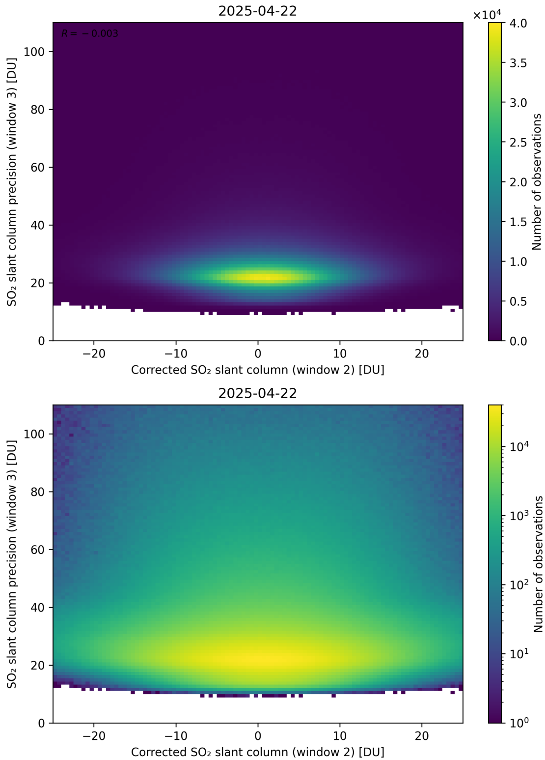
Figure 252: Scatter density plot of “Corrected SO 2 slant column (window 2)” against “SO 2 slant column precision (window 3)” for 2025-04-21 to 2025-04-23.
