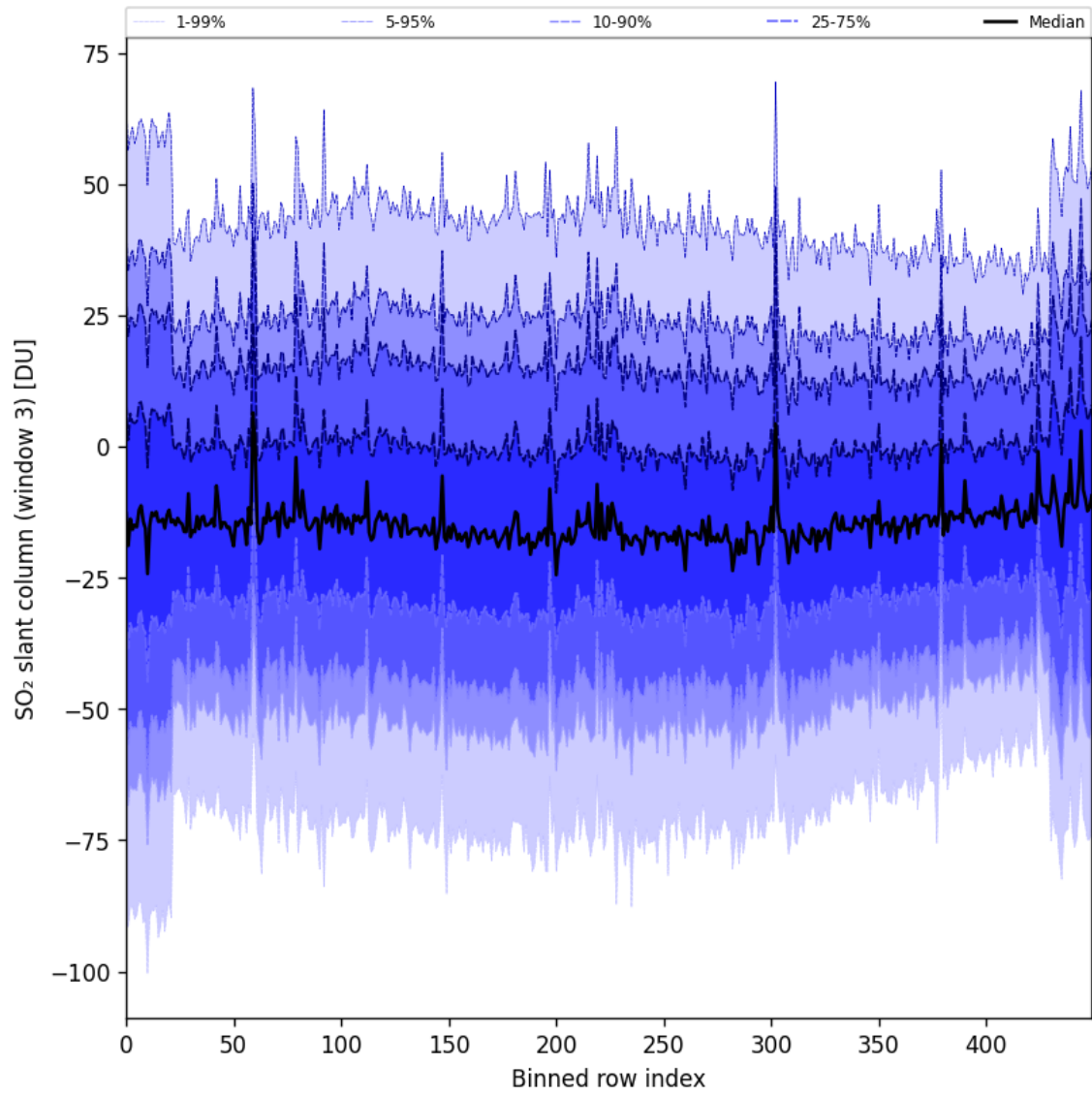
Figure 97: Along track statistics of “SO 2 slant column (window 3)” for 2025-04-21 to 2025-04-23
