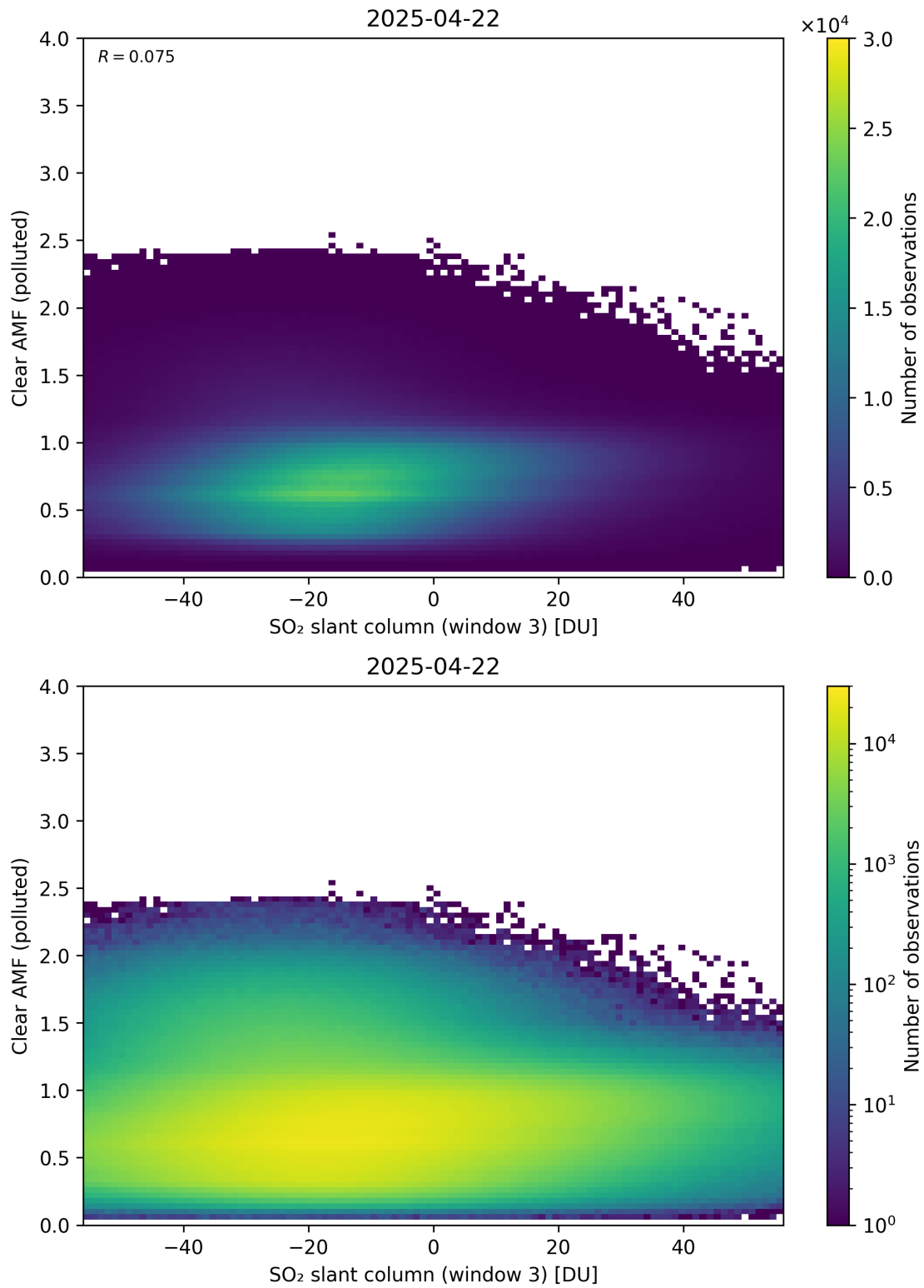
Figure 315: Scatter density plot of “SO 2 slant column (window 3)” against “Clear AMF (polluted)” for 2025-04-21 to 2025-04-23.
