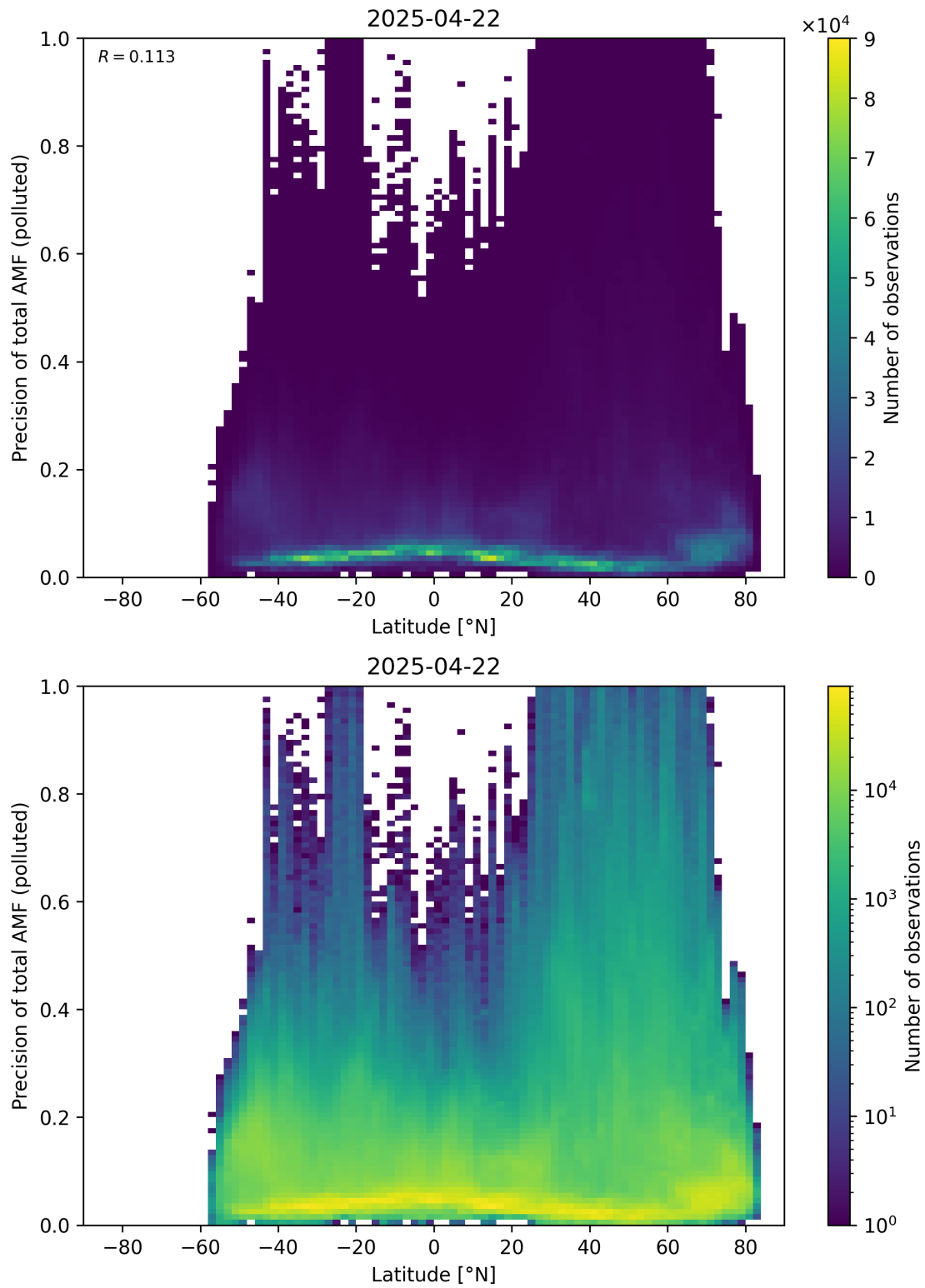
Figure 168: Scatter density plot of “Latitude” against “Precision of total AMF (polluted)” for 2025-04-21 to 2025-04-23.
