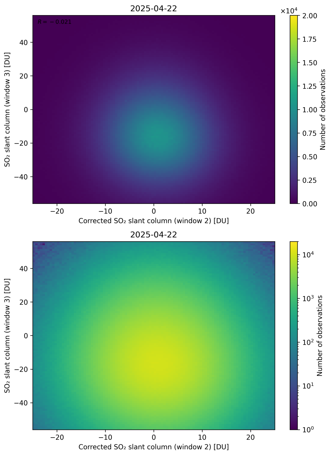
Figure 251: Scatter density plot of “Corrected SO 2 slant column (window 2)” against “SO 2 slant column (window 3)” for 2025-04-21 to 2025-04-23.
