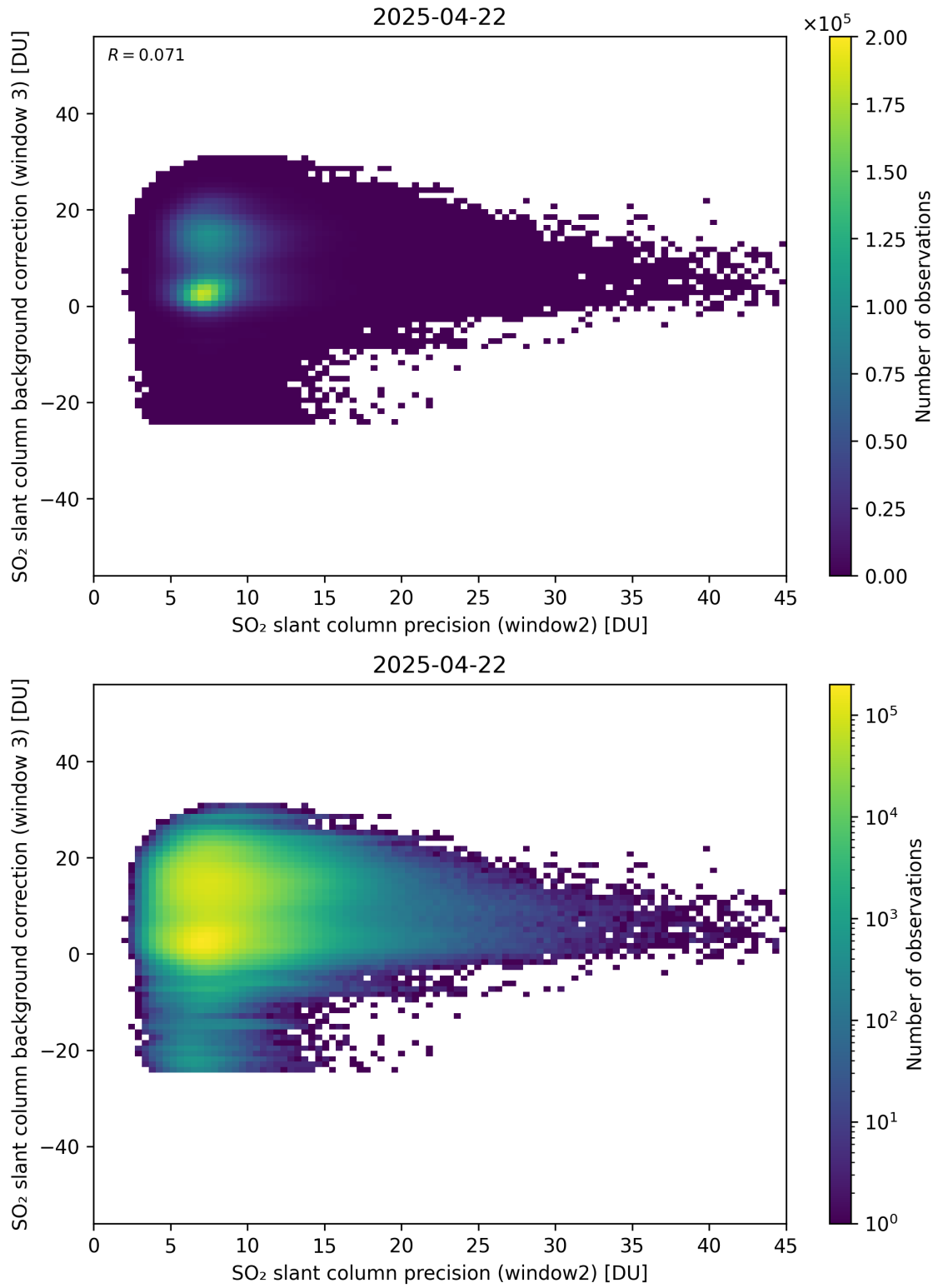
Figure 292: Scatter density plot of “SO 2 slant column precision (window2)” against “SO 2 slant column background correction (window 3)” for 2025-04-21 to 2025-04-23.
