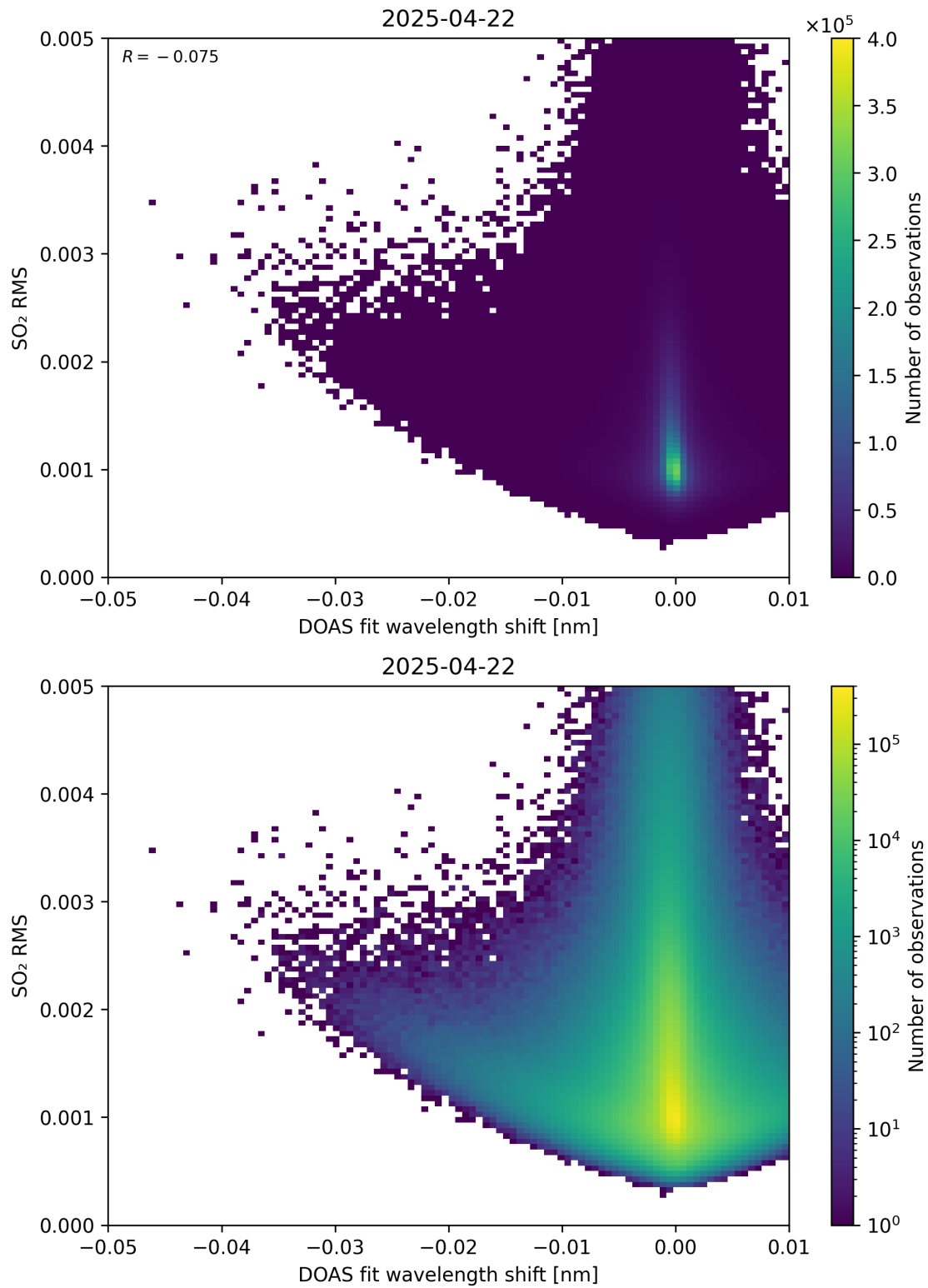
Figure 139: Scatter density plot of “DOAS fit wavelength shift” against “SO 2 RMS” for 2025-04-21 to 2025-04-23.
