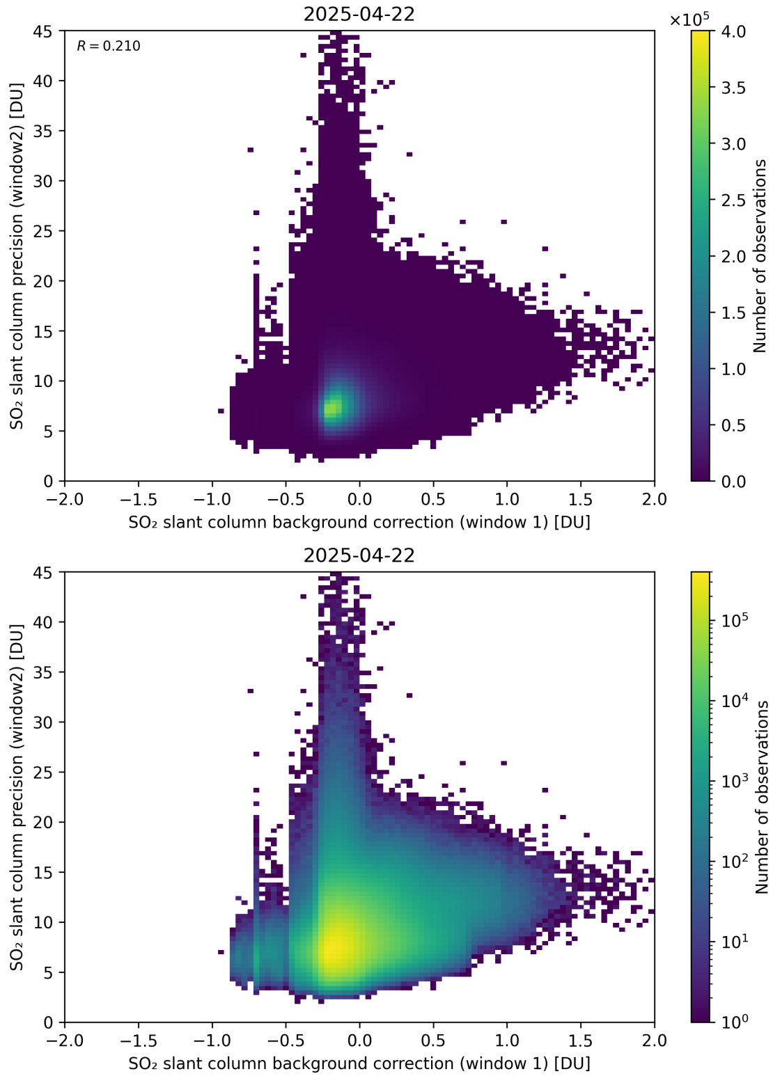
Figure 117: Scatter density plot of “SO 2 slant column background correction (window 1)” against “SO 2 slant column precision (window2)” for 2025-04-21 to 2025-04-23.
