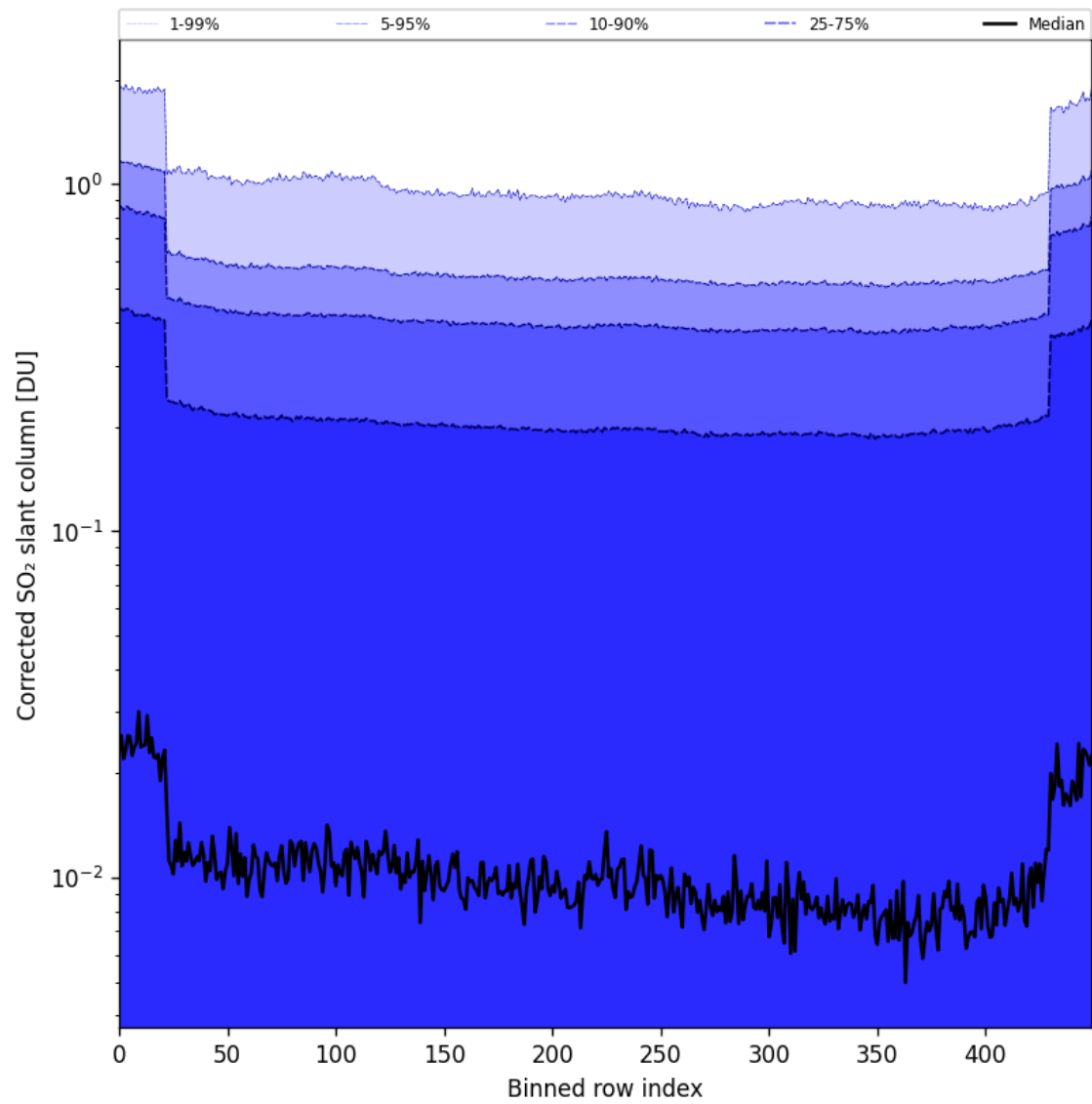
Figure 86: Along track statistics of “Corrected SO 2 slant column” for 2025-04-21 to 2025-04-23
