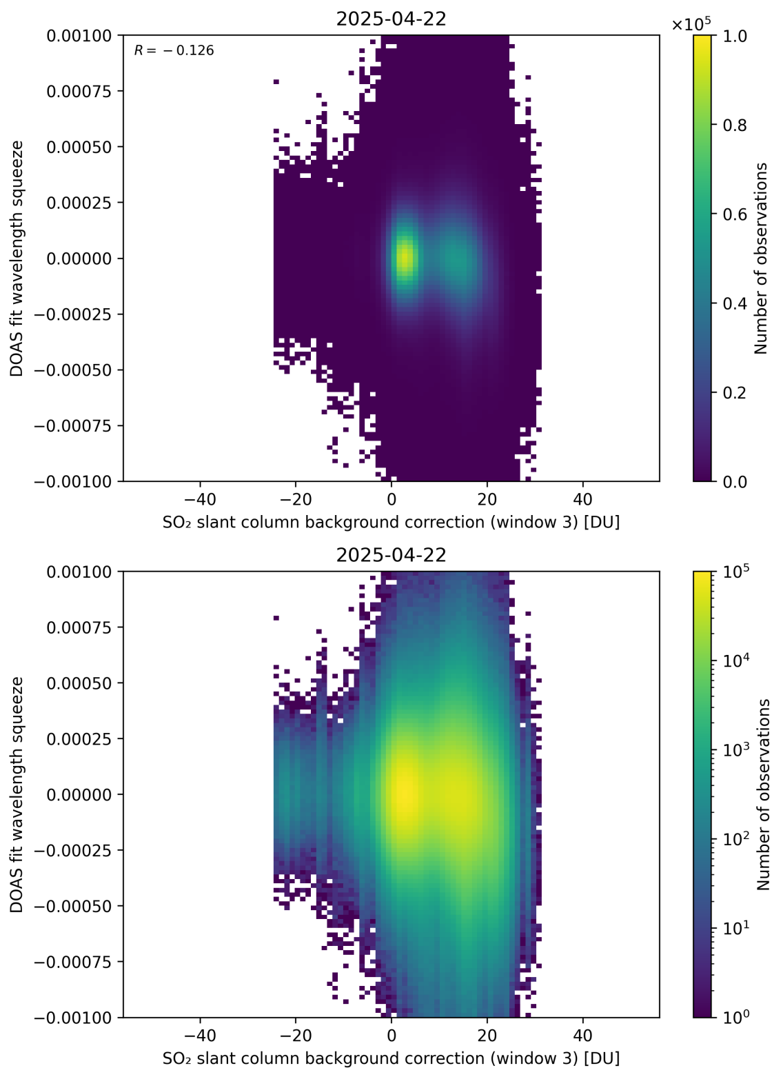
Figure 133: Scatter density plot of “SO 2 slant column background correction (window 3)” against “DOAS fit wavelength squeeze” for 2025-04-21 to 2025-04-23.
