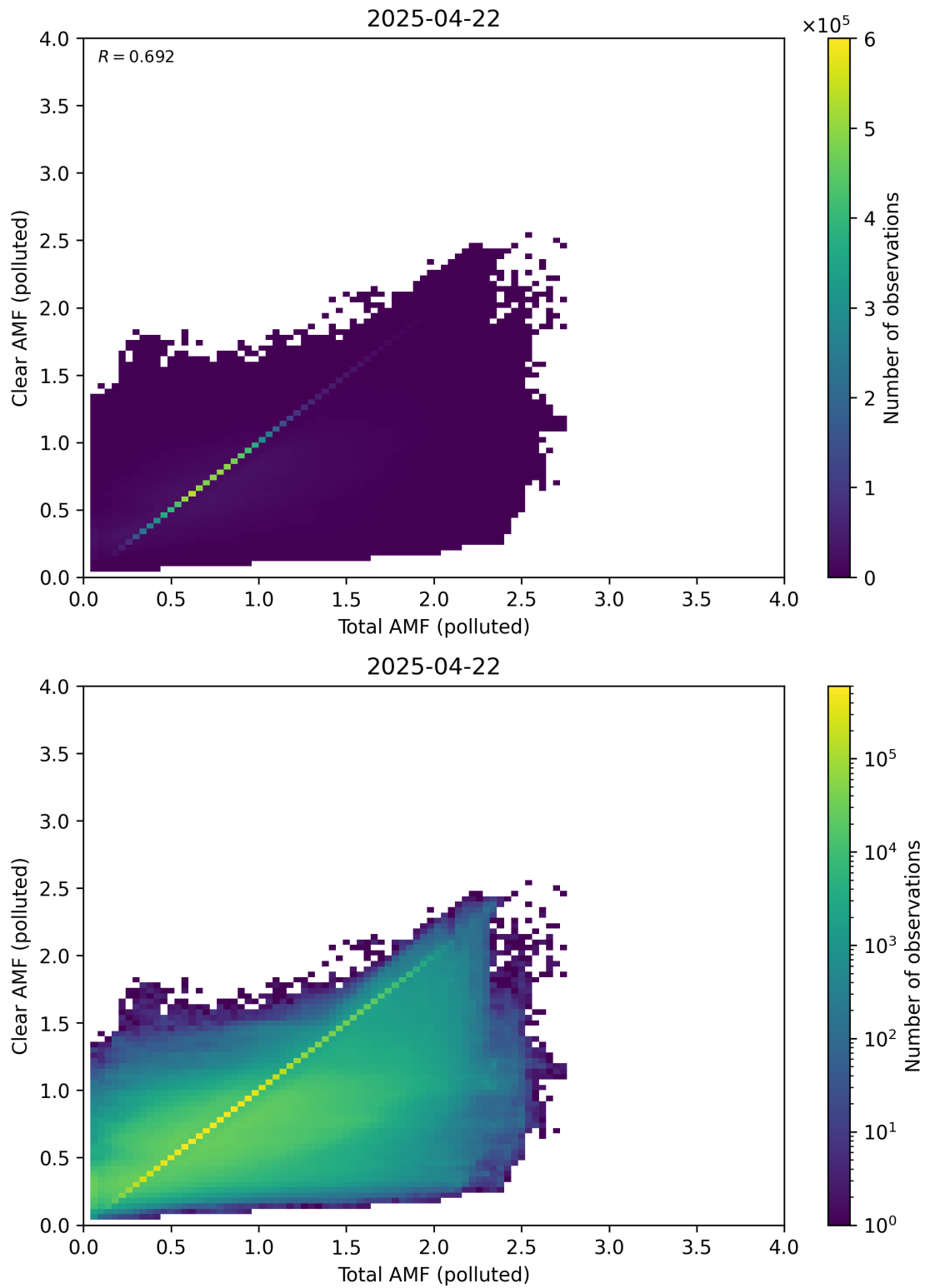
Figure 321: Scatter density plot of “Total AMF (polluted)” against “Clear AMF (polluted)” for 2025-04-21 to 2025-04-23.
