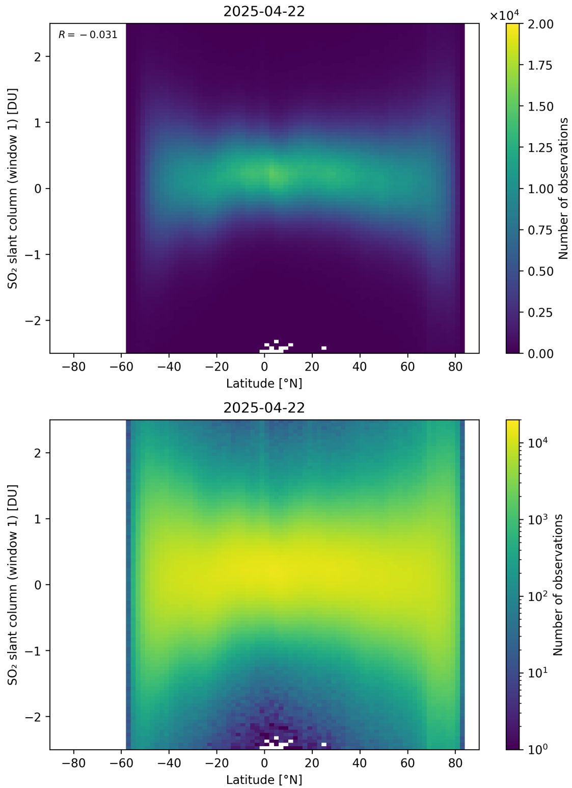
Figure 162: Scatter density plot of “Latitude” against “SO 2 slant column (window 1)” for 2025-04-21 to 2025-04-23.
