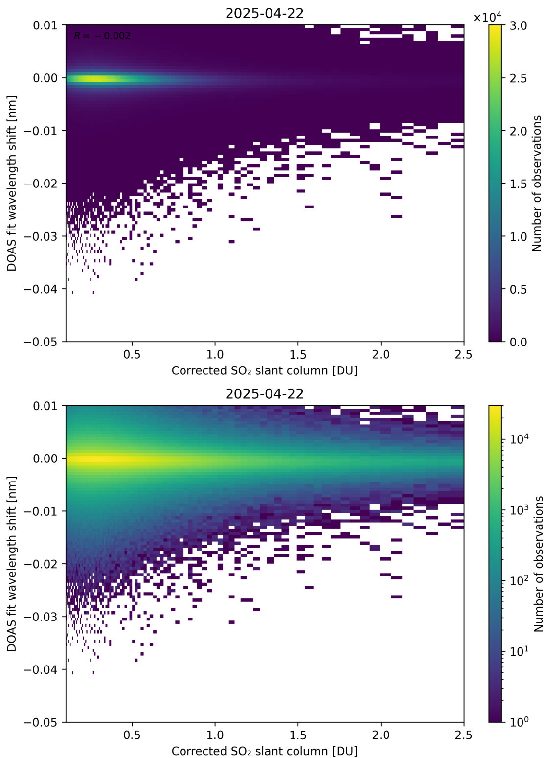
Figure 229: Scatter density plot of “Corrected SO 2 slant column” against “DOAS fit wavelength shift” for 2025-04-21 to 2025-04-23.
