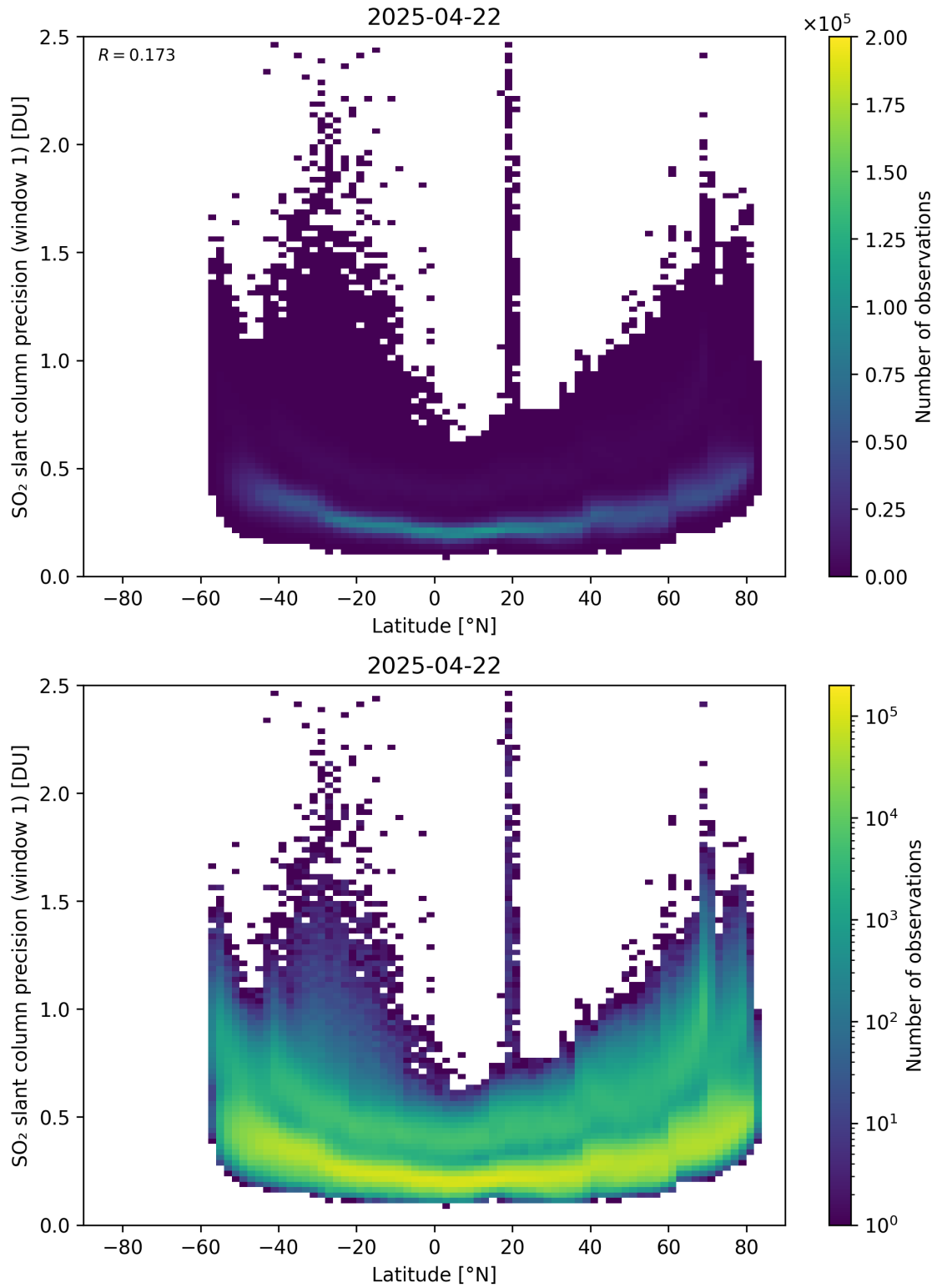
Figure 163: Scatter density plot of “Latitude” against “SO 2 slant column precision (window 1)” for 2025-04-21 to 2025-04-23.
