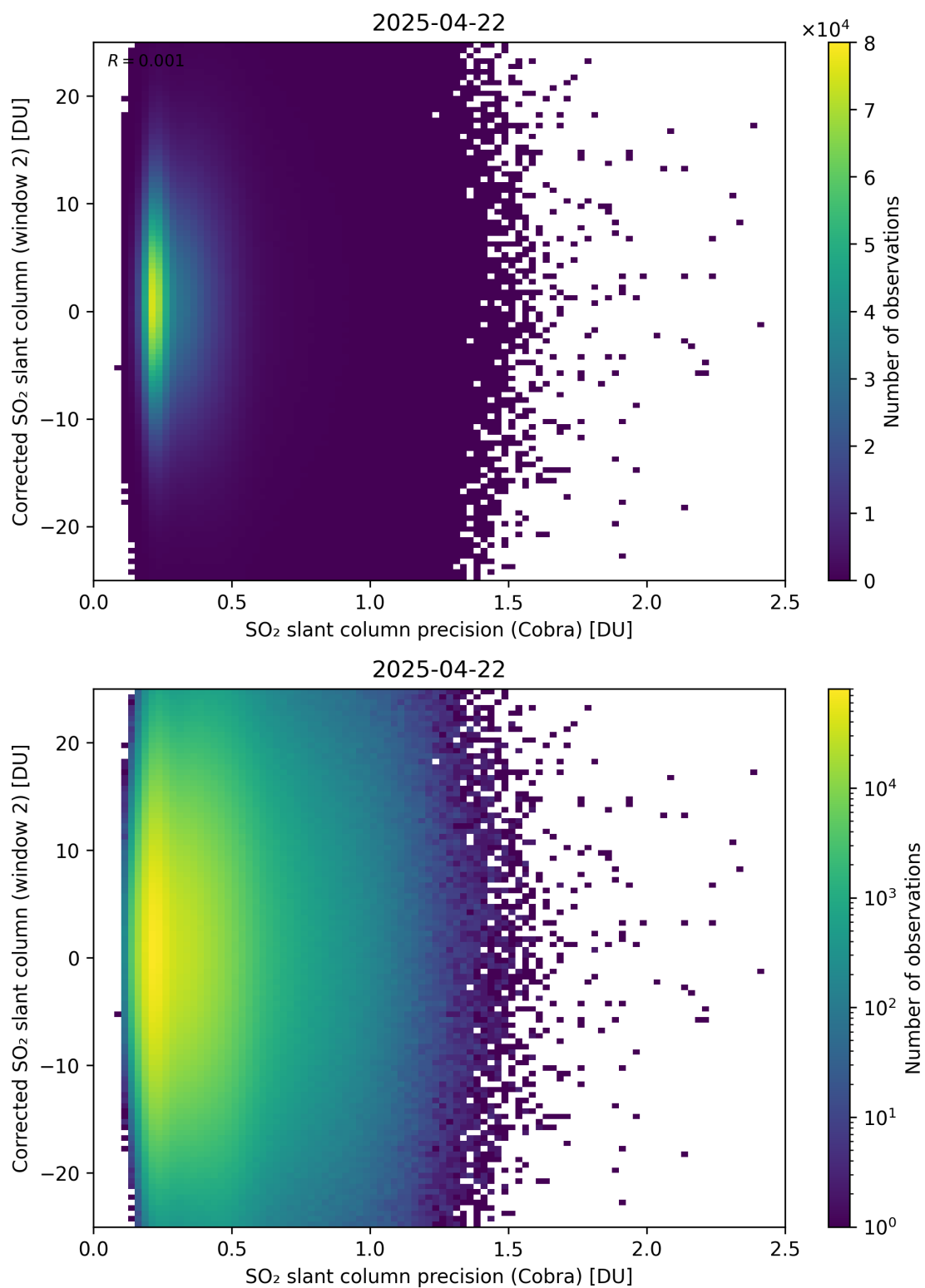
Figure 206: Scatter density plot of “SO 2 slant column precision (Cobra)” against “Corrected SO 2 slant column (window 2)” for 2025-04-21 to 2025-04-23.
