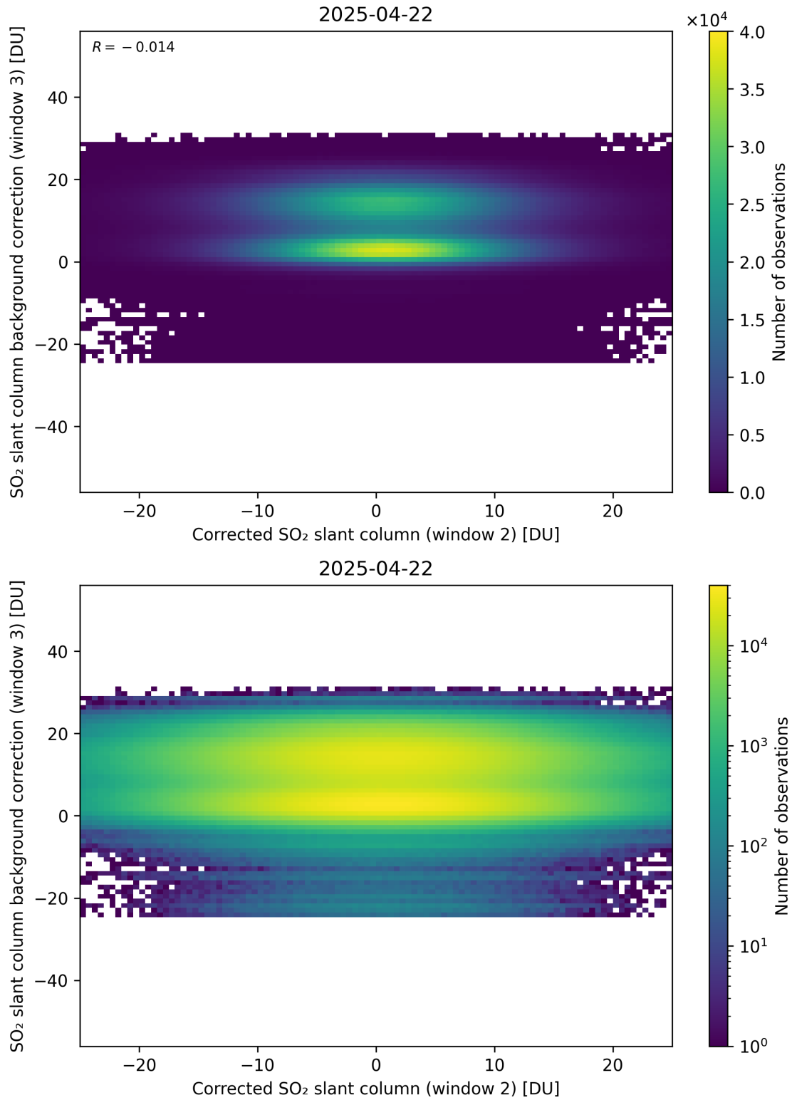
Figure 245: Scatter density plot of “Corrected SO 2 slant column (window 2)” against “SO 2 slant column background correction (window 3)” for 2025-04-21 to 2025-04-23.
