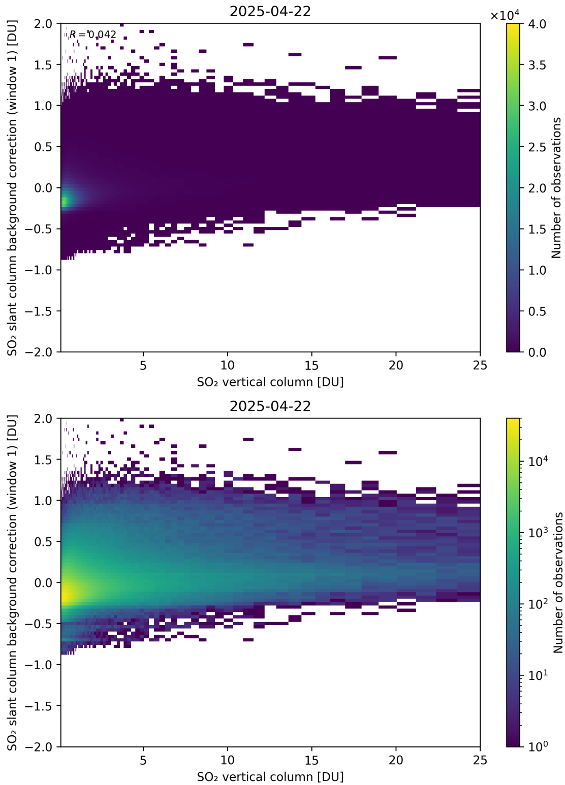
Figure 323: Scatter density plot of “SO 2 vertical column” against “SO 2 slant column background correction (window 1)” for 2025-04-21 to 2025-04-23.
