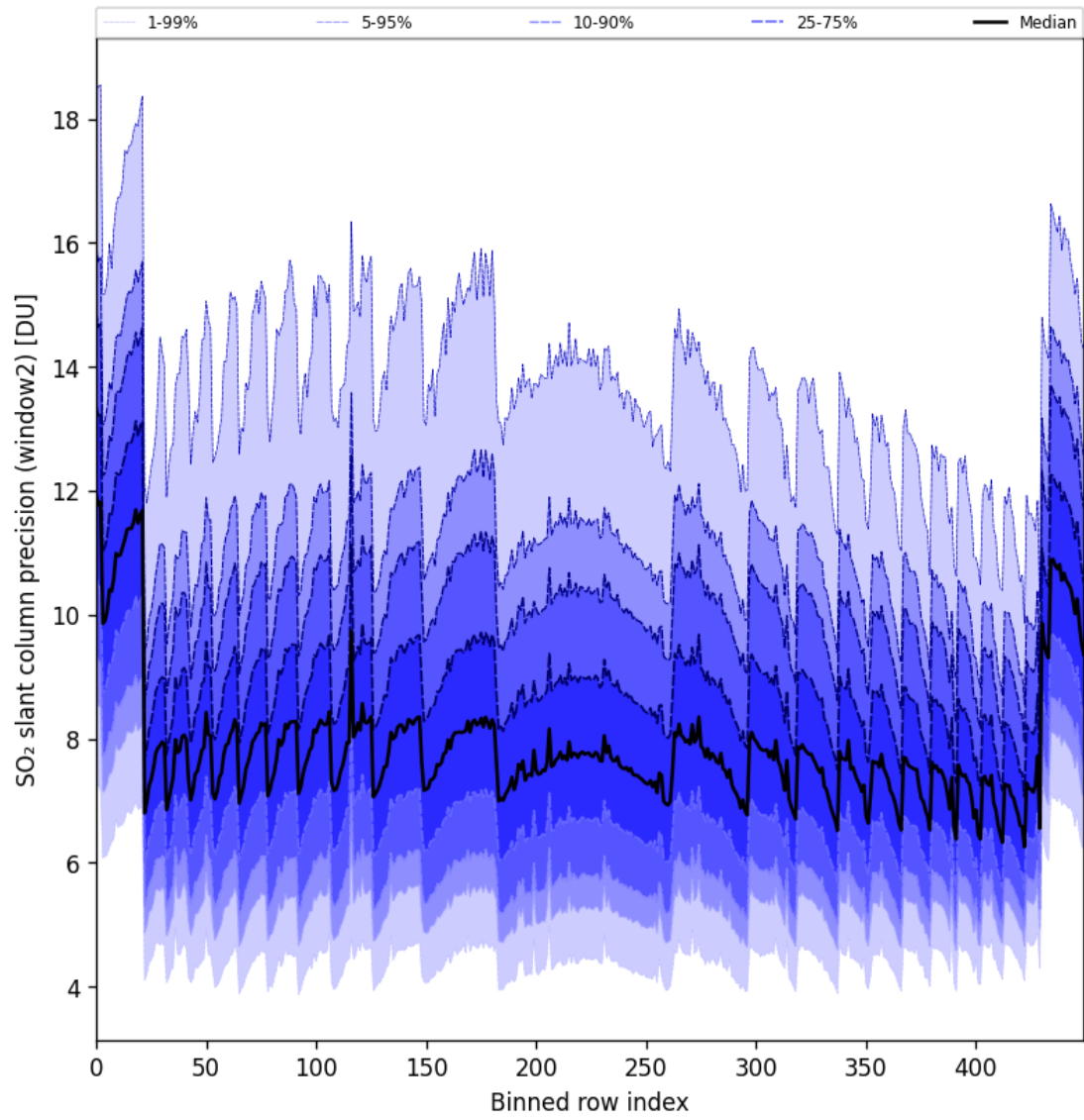
Figure 94: Along track statistics of “SO 2 slant column precision (window2)” for 2025-04-21 to 2025-04-23
