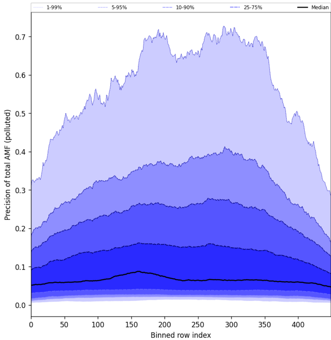
Figure 106: Along track statistics of “Precision of total AMF (polluted)” for 2025-04-21 to 2025-04-23
