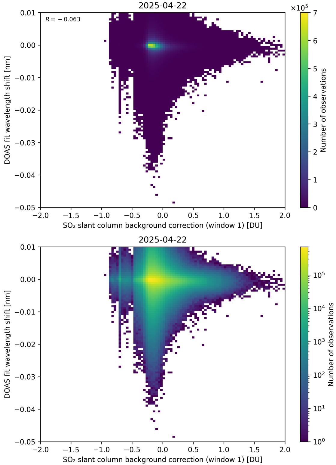
Figure 111: Scatter density plot of “SO 2 slant column background correction (window 1)” against “DOAS fit wavelength shift” for 2025-04-21 to 2025-04-23.
