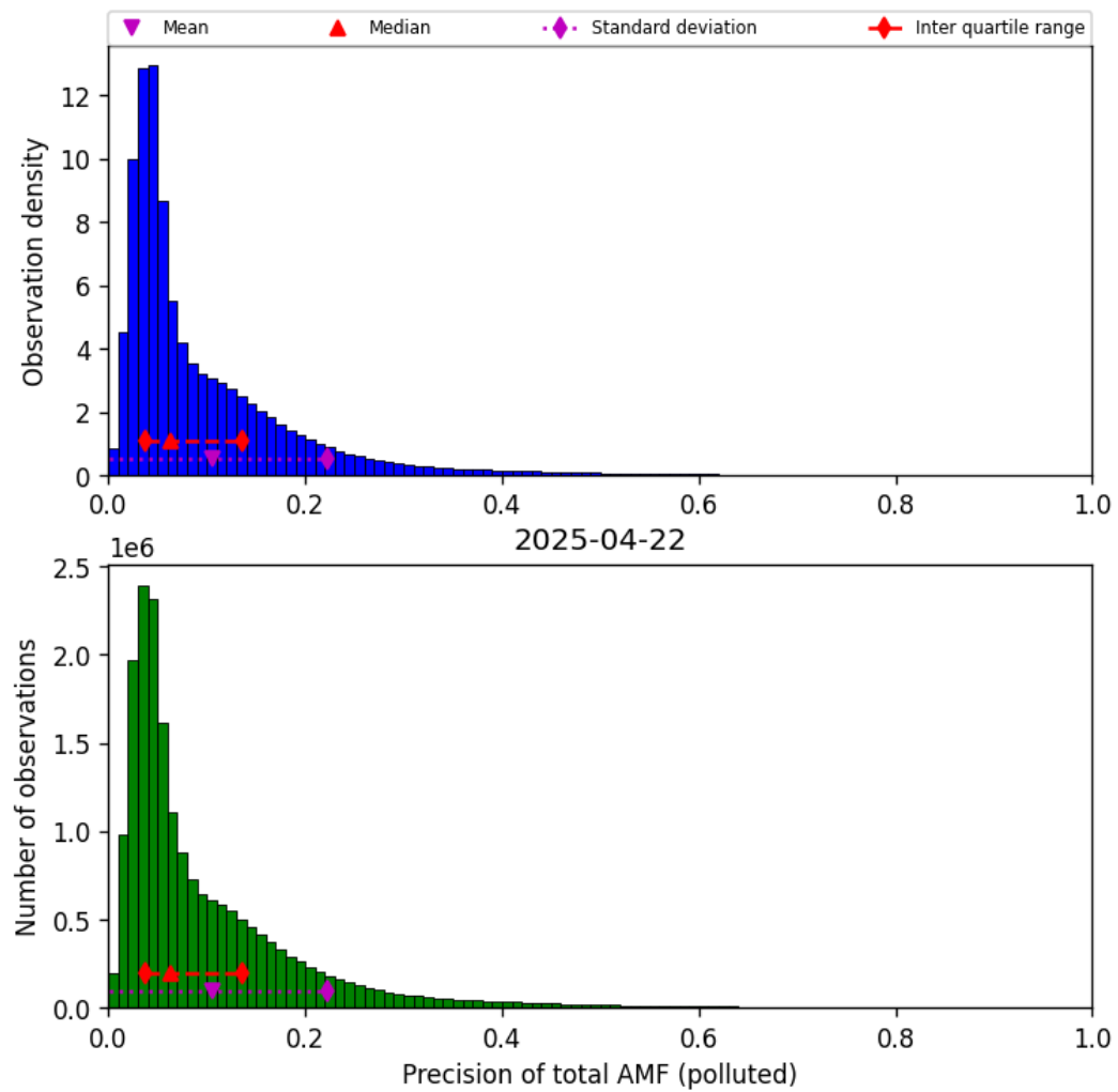
Figure 80: Histogram of “Precision of total AMF (polluted)” for 2025-04-21 to 2025-04-23
