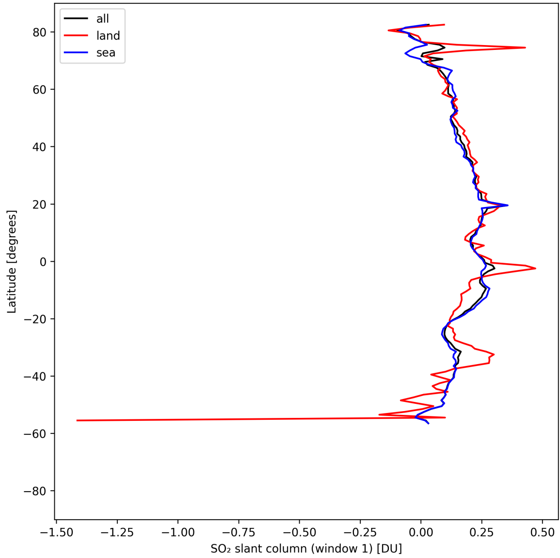
Figure 37: Zonal average of “SO 2 slant column (window 1)” for 2025-04-21 to 2025-04-23.
