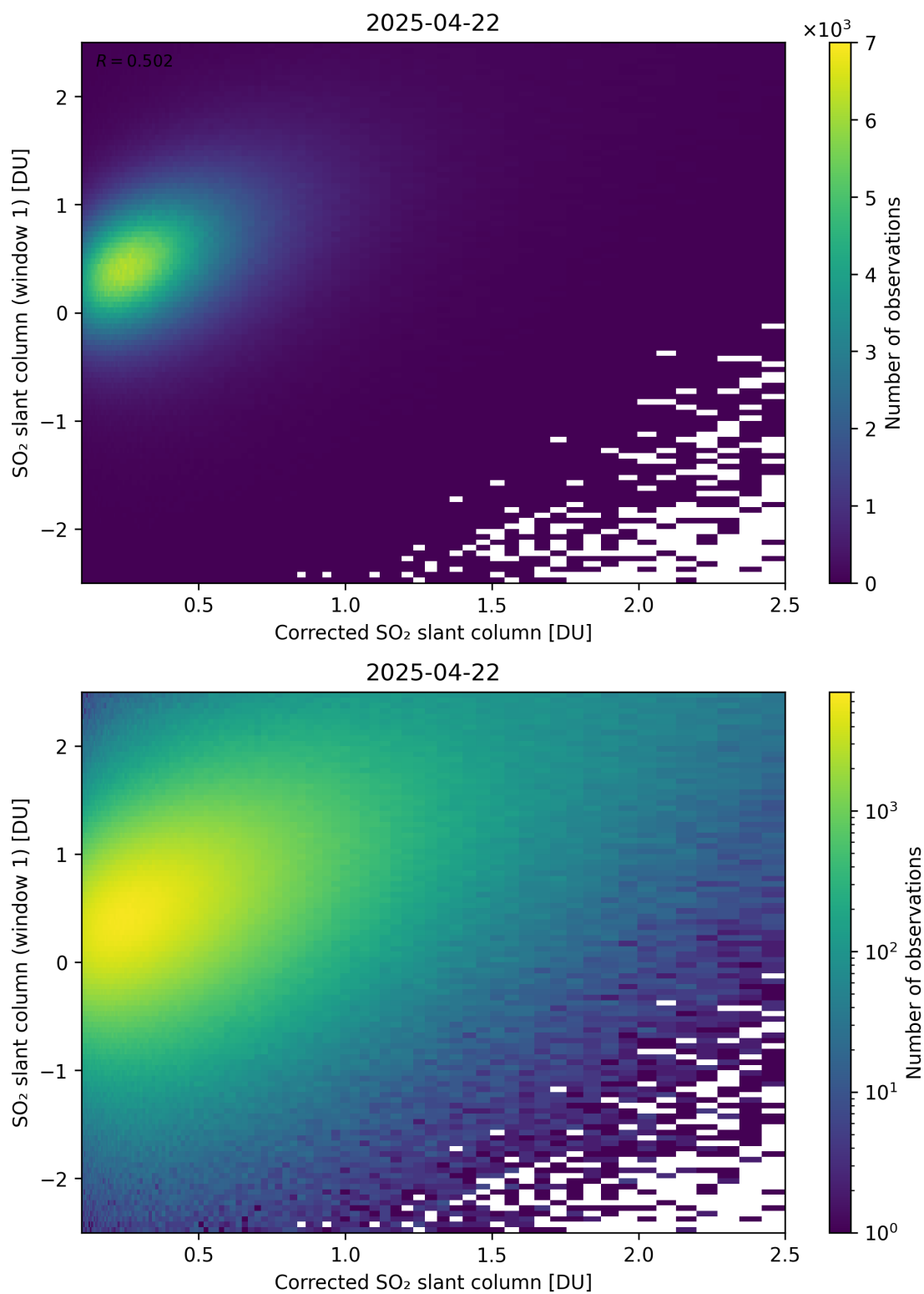
Figure 237: Scatter density plot of “Corrected SO 2 slant column” against “SO 2 slant column (window 1)” for 2025-04-21 to 2025-04-23.
