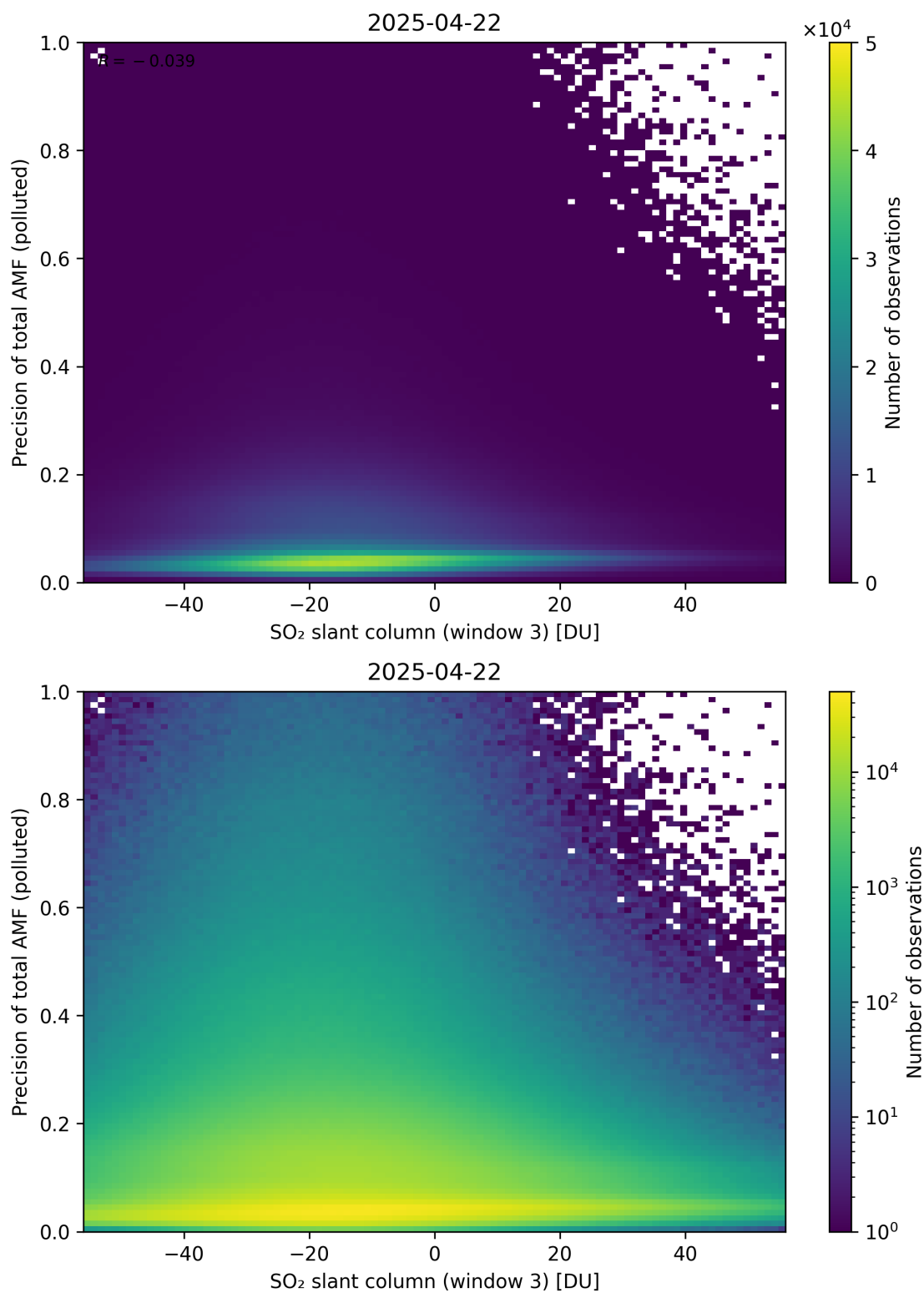
Figure 319: Scatter density plot of “SO 2 slant column (window 3)” against “Precision of total AMF (polluted)” for 2025-04-21 to 2025-04-23.
