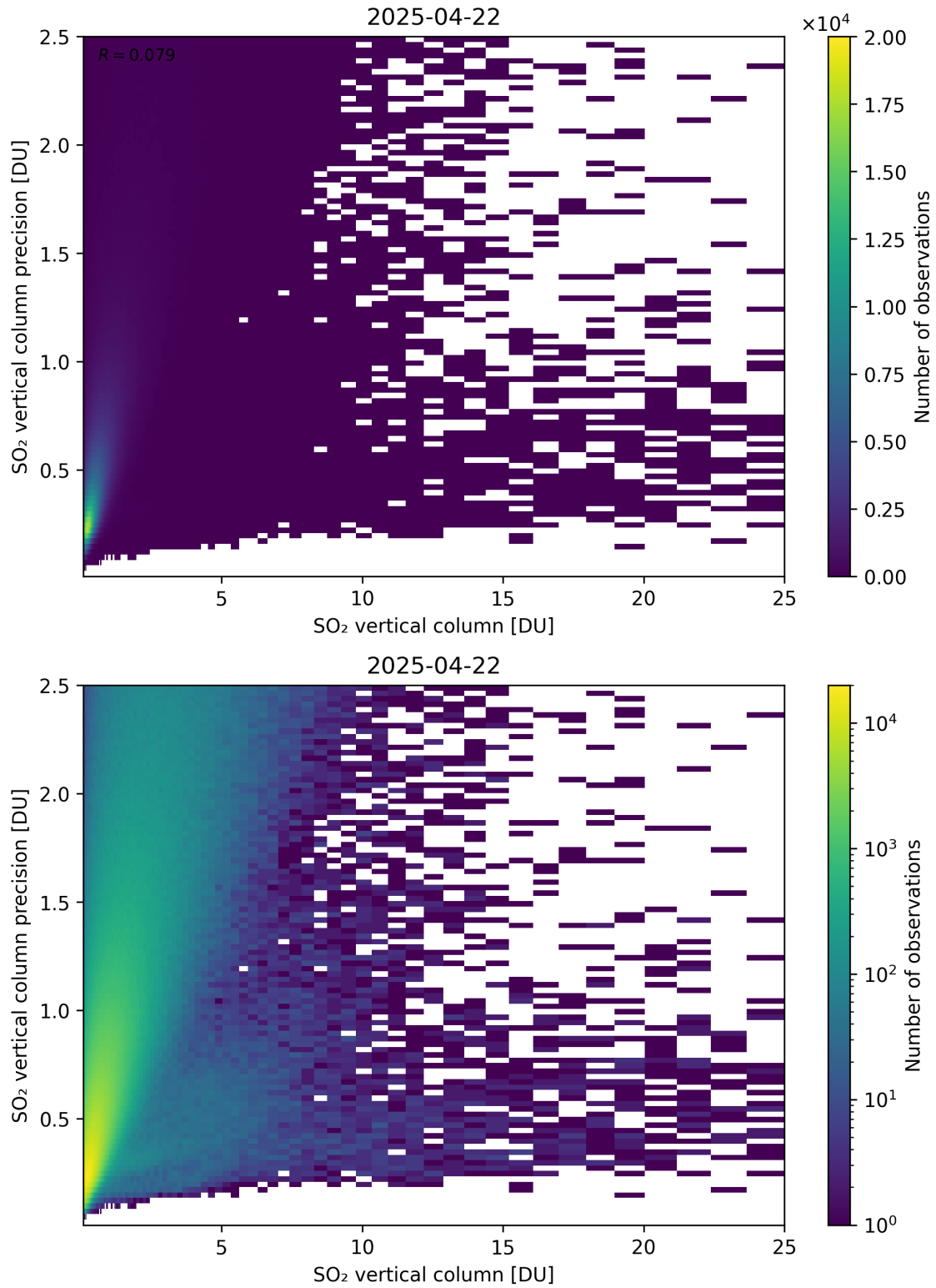
Figure 361: Scatter density plot of “SO 2 vertical column” against “SO 2 vertical column precision” for 2025-04-21 to 2025-04-23.
