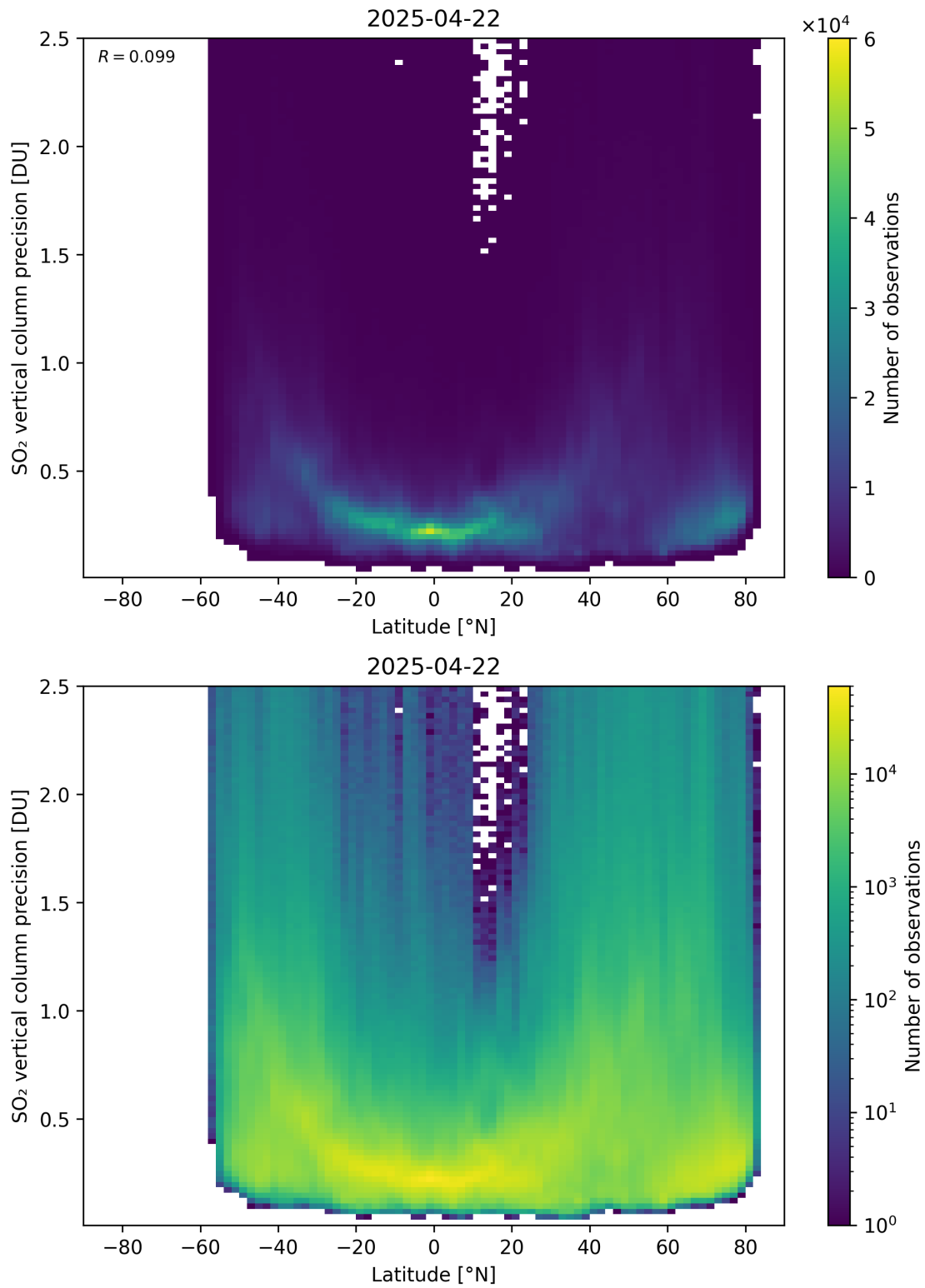
Figure 170: Scatter density plot of “Latitude” against “SO 2 vertical column precision” for 2025-04-21 to 2025-04-23.
