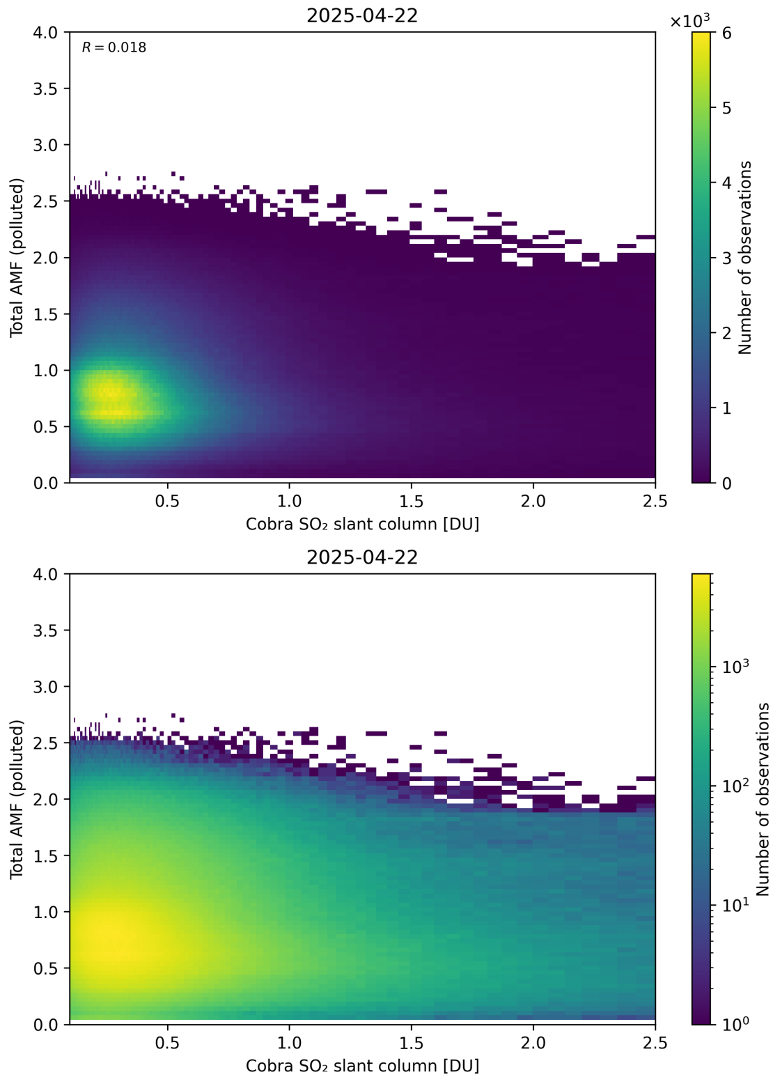
Figure 224: Scatter density plot of “Cobra SO 2 slant column” against “Total AMF (polluted)” for 2025-04-21 to 2025-04-23.
