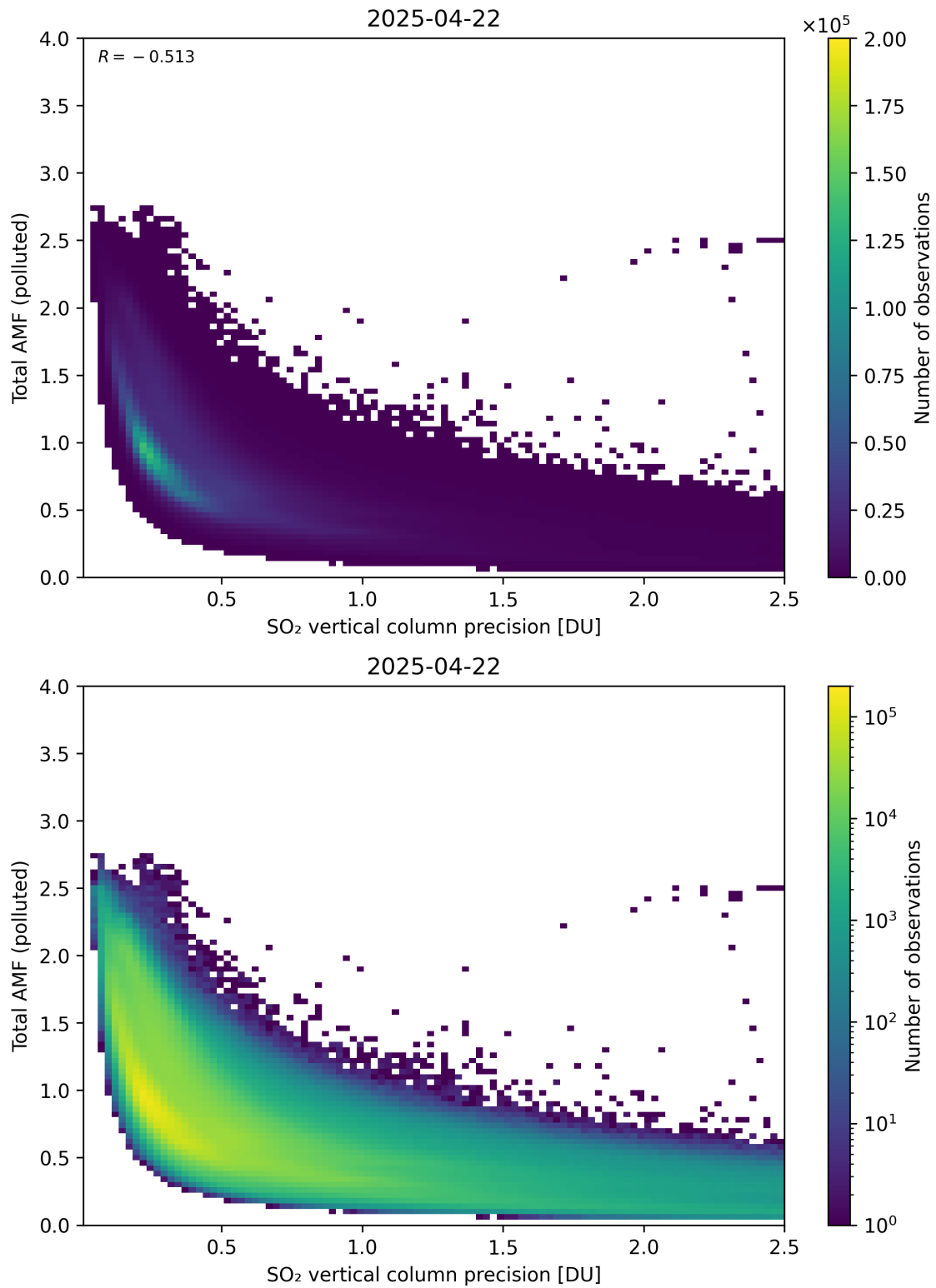
Figure 346: Scatter density plot of “SO 2 vertical column precision” against “Total AMF (polluted)” for 2025-04-21 to 2025-04-23.
