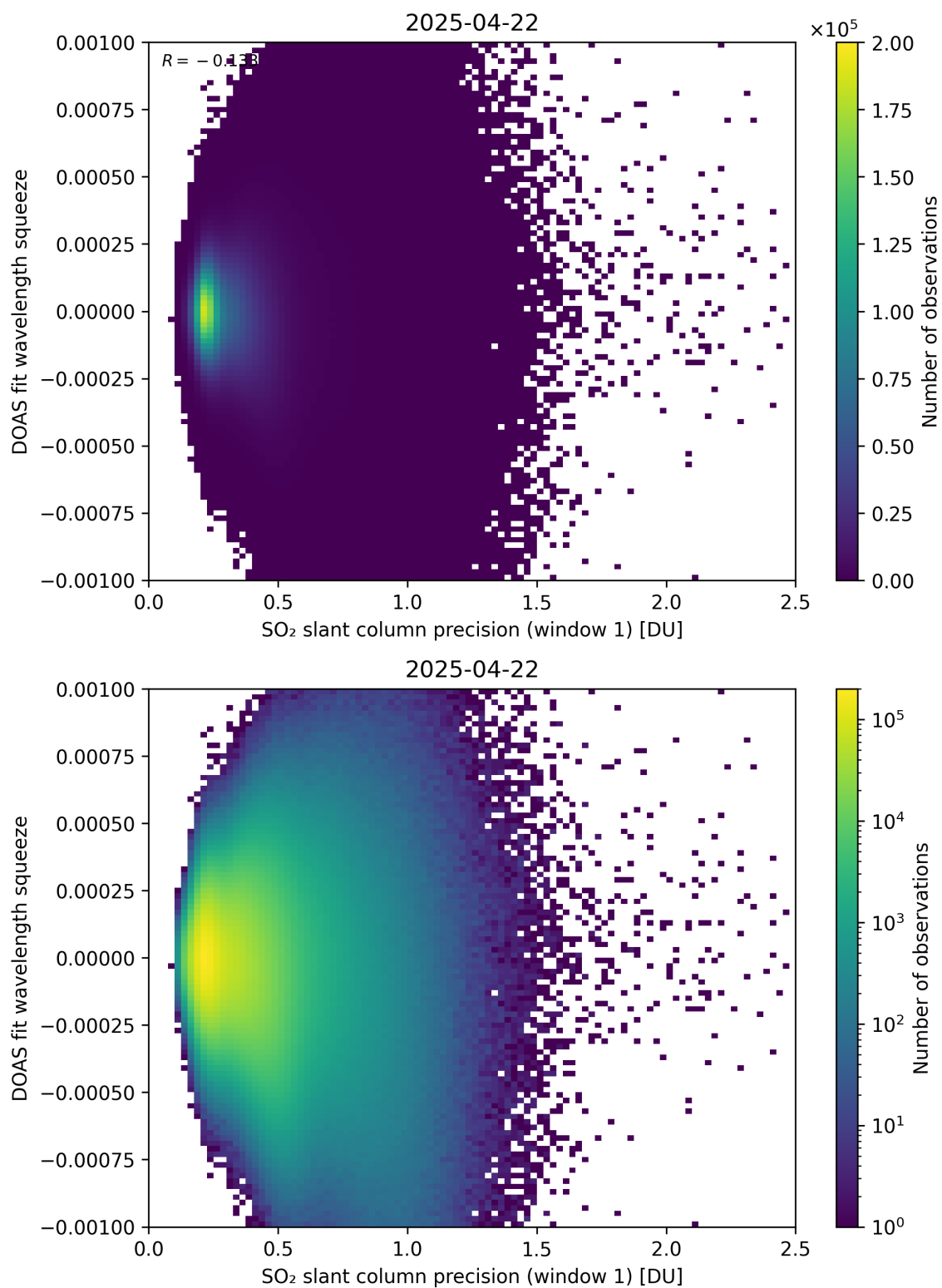
Figure 272: Scatter density plot of “SO 2 slant column precision (window 1)” against “DOAS fit wavelength squeeze” for 2025-04-21 to 2025-04-23.
