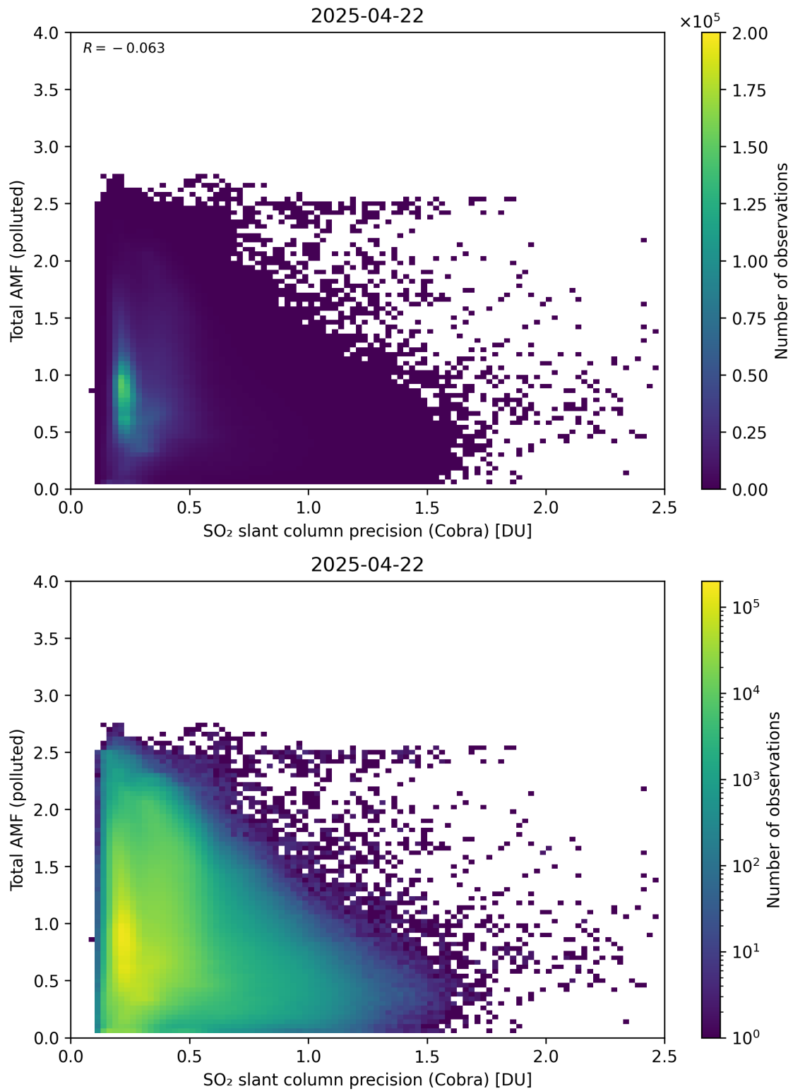
Figure 213: Scatter density plot of “SO 2 slant column precision (Cobra)” against “Total AMF (polluted)” for 2025-04-21 to 2025-04-23.
