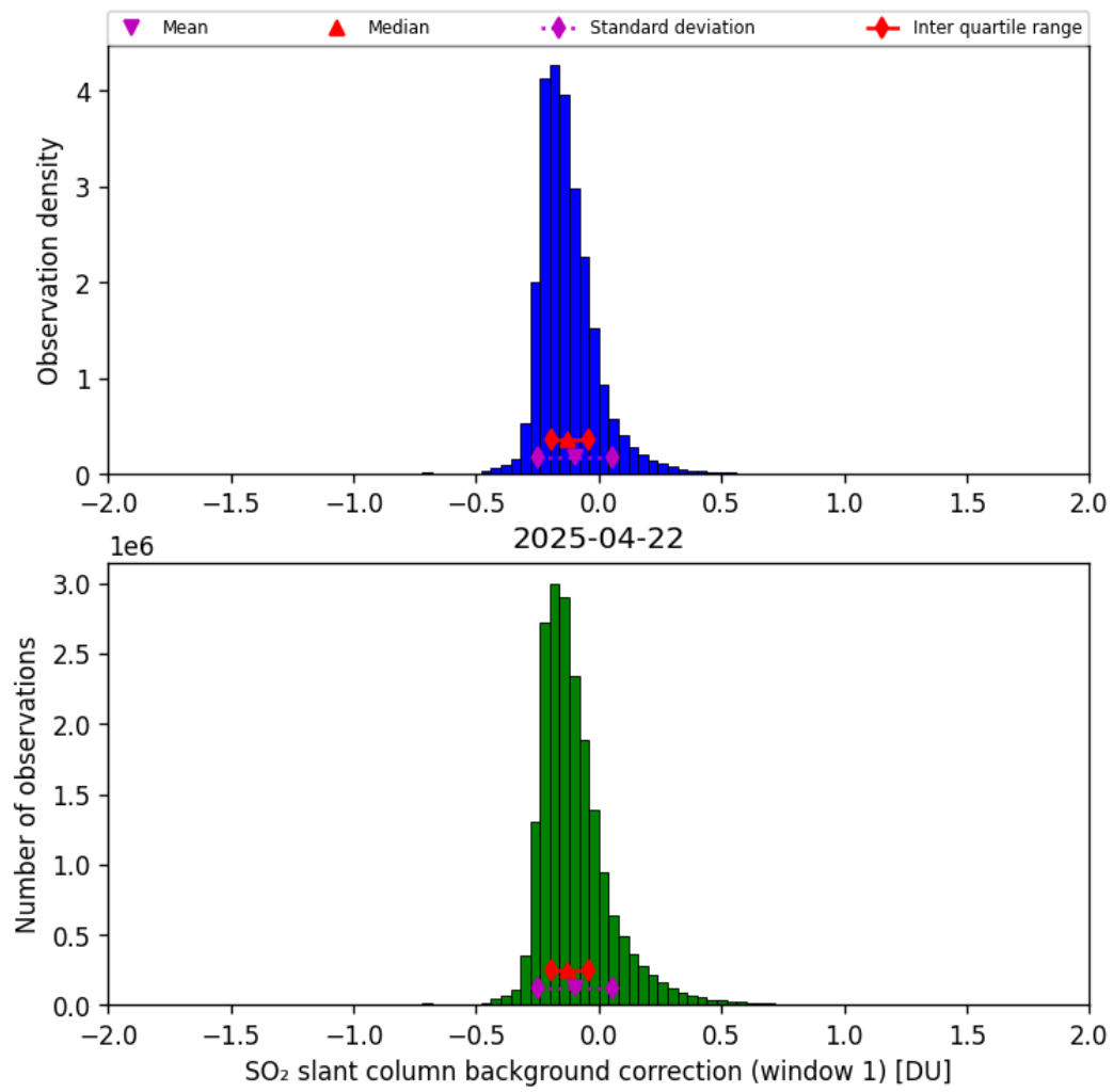
Figure 66: Histogram of “SO 2 slant column background correction (window 1)” for 2025-04-21 to 2025-04-23
