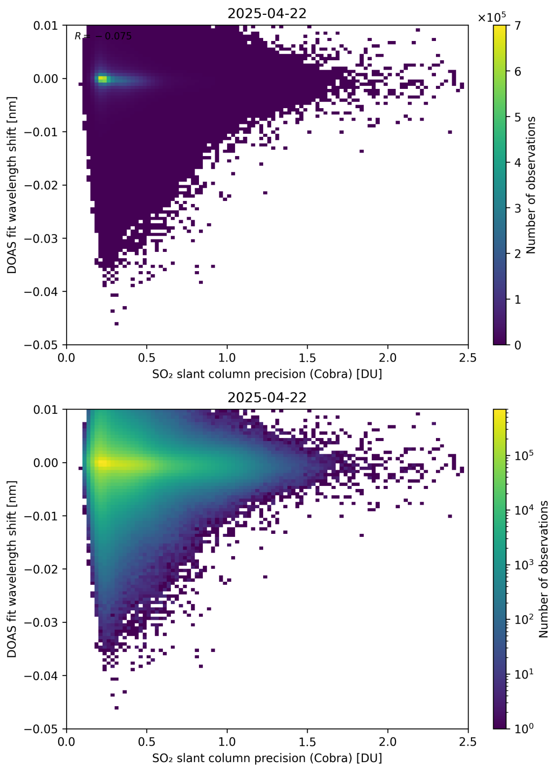
Figure 202: Scatter density plot of “SO 2 slant column precision (Cobra)” against “DOAS fit wavelength shift” for 2025-04-21 to 2025-04-23.
