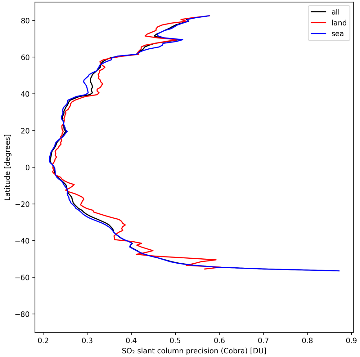
Figure 36: Zonal average of “SO 2 slant column precision (Cobra)” for 2025-04-21 to 2025-04-23.
