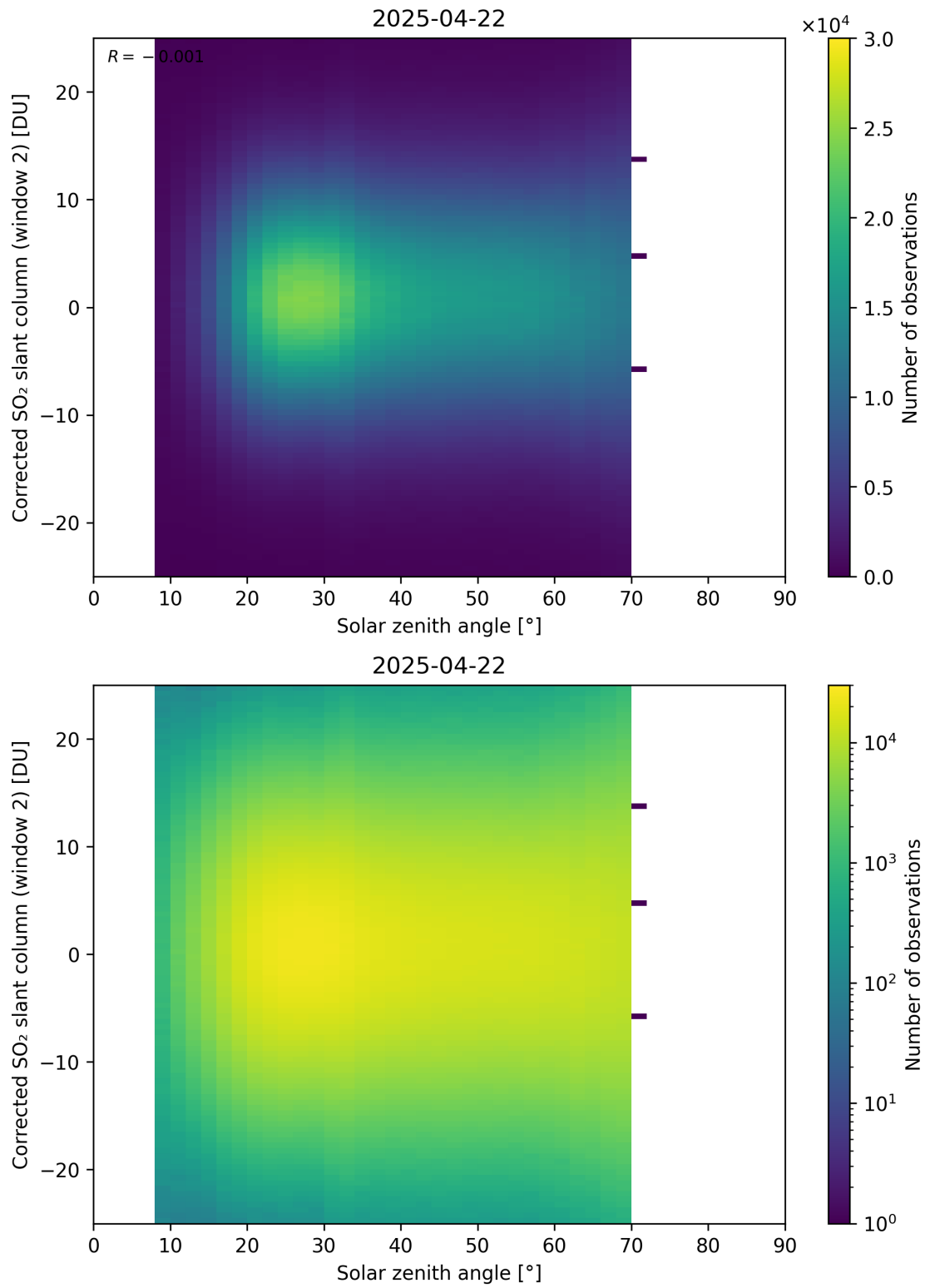
Figure 182: Scatter density plot of “Solar zenith angle” against “Corrected SO 2 slant column (window 2)” for 2025-04-21 to 2025-04-23.
