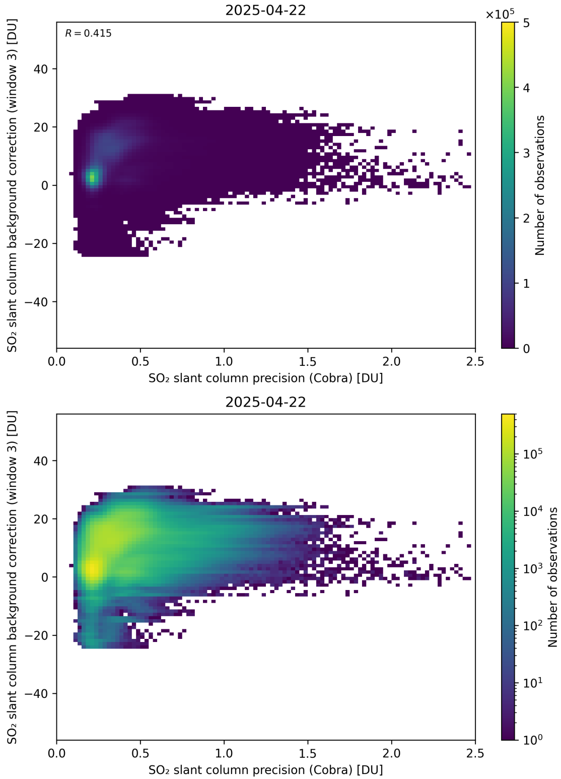
Figure 201: Scatter density plot of “SO 2 slant column precision (Cobra)” against “SO 2 slant column background correction (window 3)” for 2025-04-21 to 2025-04-23.
