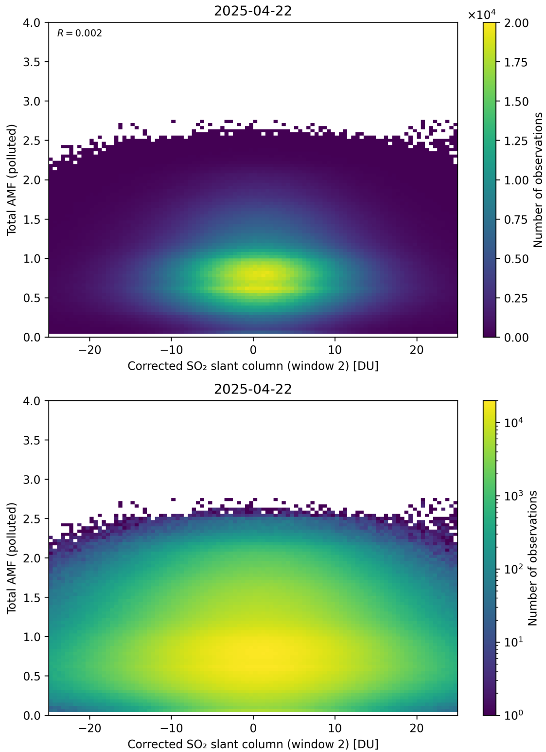
Figure 253: Scatter density plot of “Corrected SO 2 slant column (window 2)” against “Total AMF (polluted)” for 2025-04-21 to 2025-04-23.
