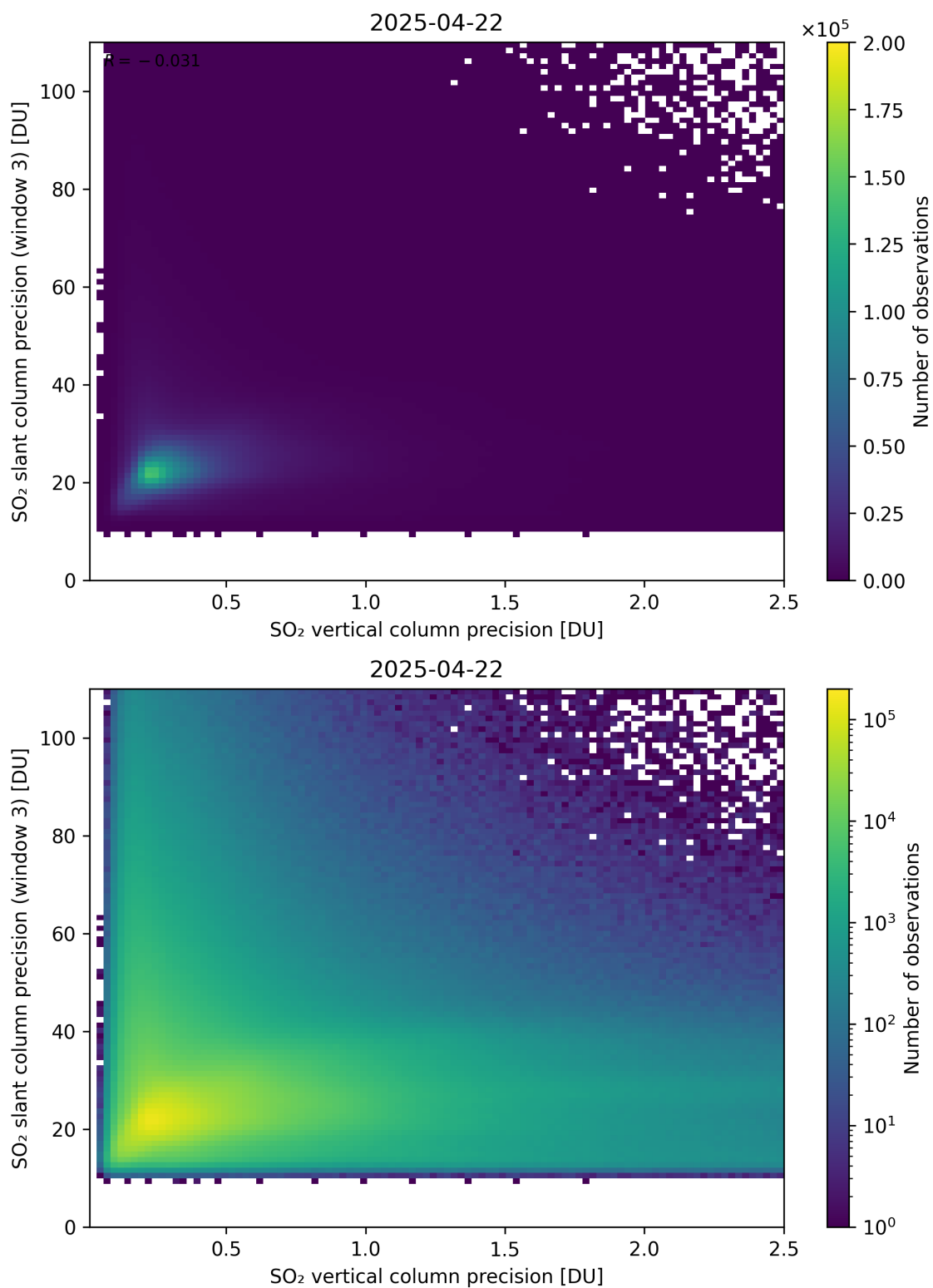
Figure 345: Scatter density plot of “SO 2 vertical column precision” against “SO 2 slant column precision (window 3)” for 2025-04-21 to 2025-04-23.
