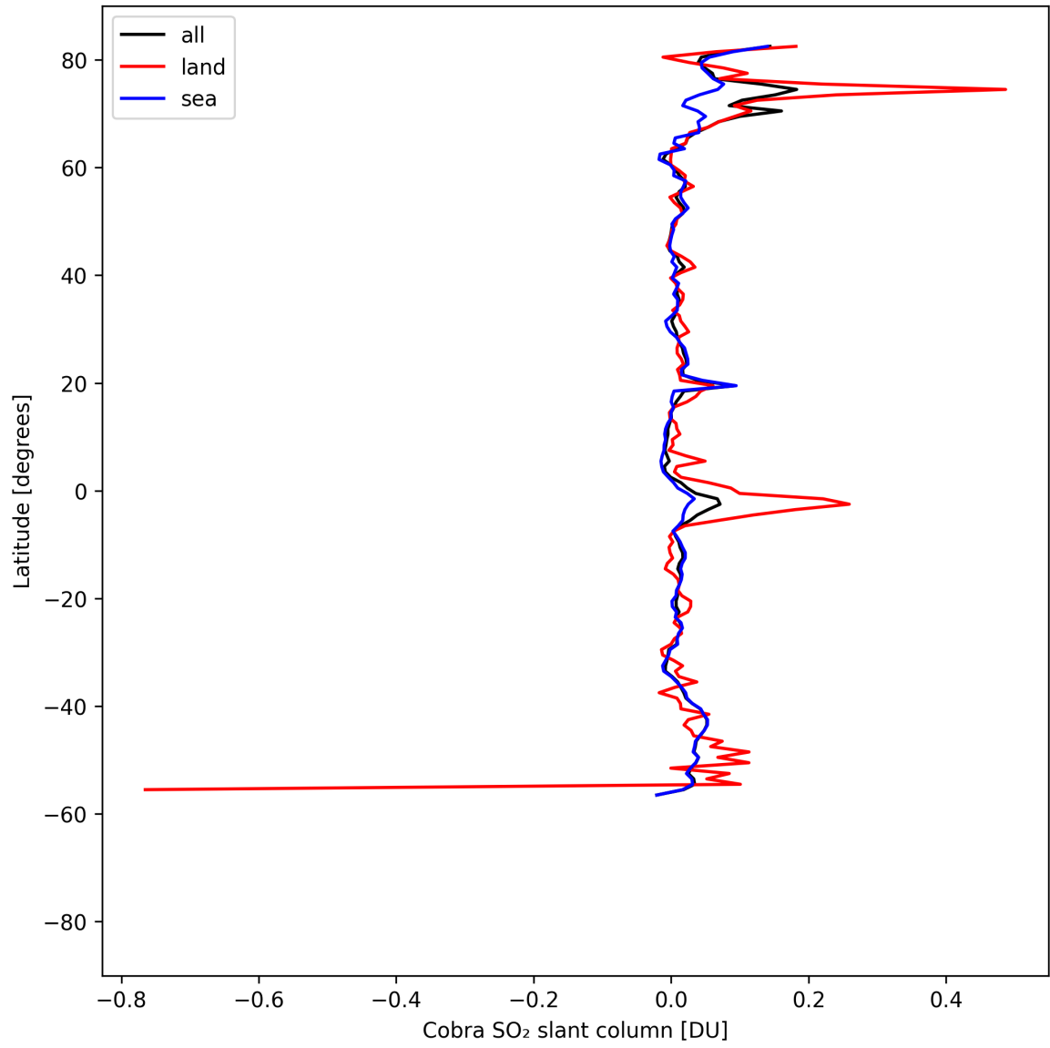
Figure 35: Zonal average of “Cobra SO 2 slant column” for 2025-04-21 to 2025-04-23.
