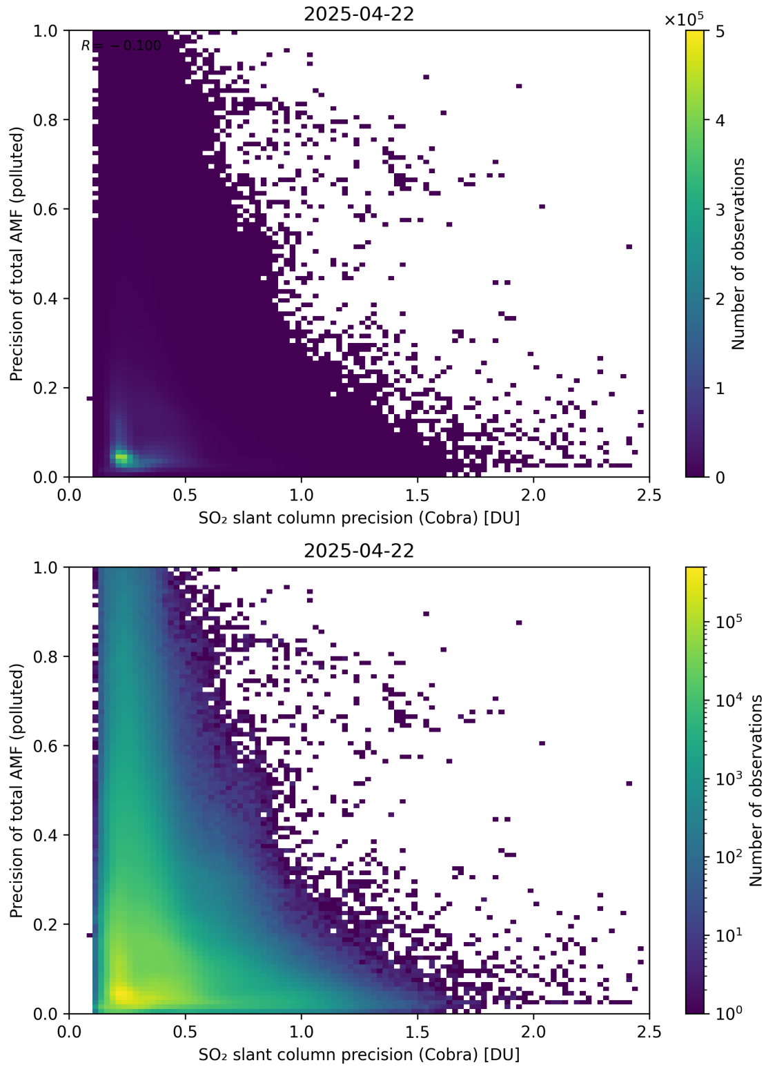
Figure 214: Scatter density plot of “SO 2 slant column precision (Cobra)” against “Precision of total AMF (polluted)” for 2025-04-21 to 2025-04-23.
