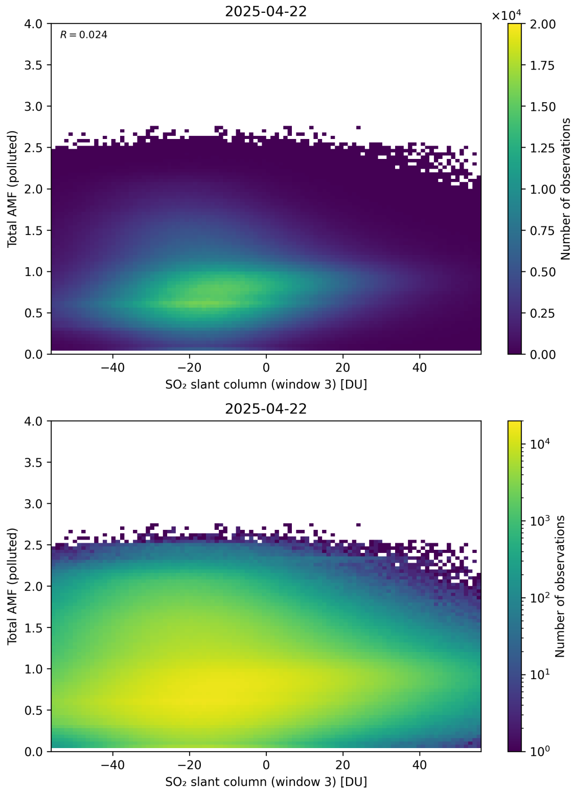
Figure 318: Scatter density plot of “SO 2 slant column (window 3)” against “Total AMF (polluted)” for 2025-04-21 to 2025-04-23.
