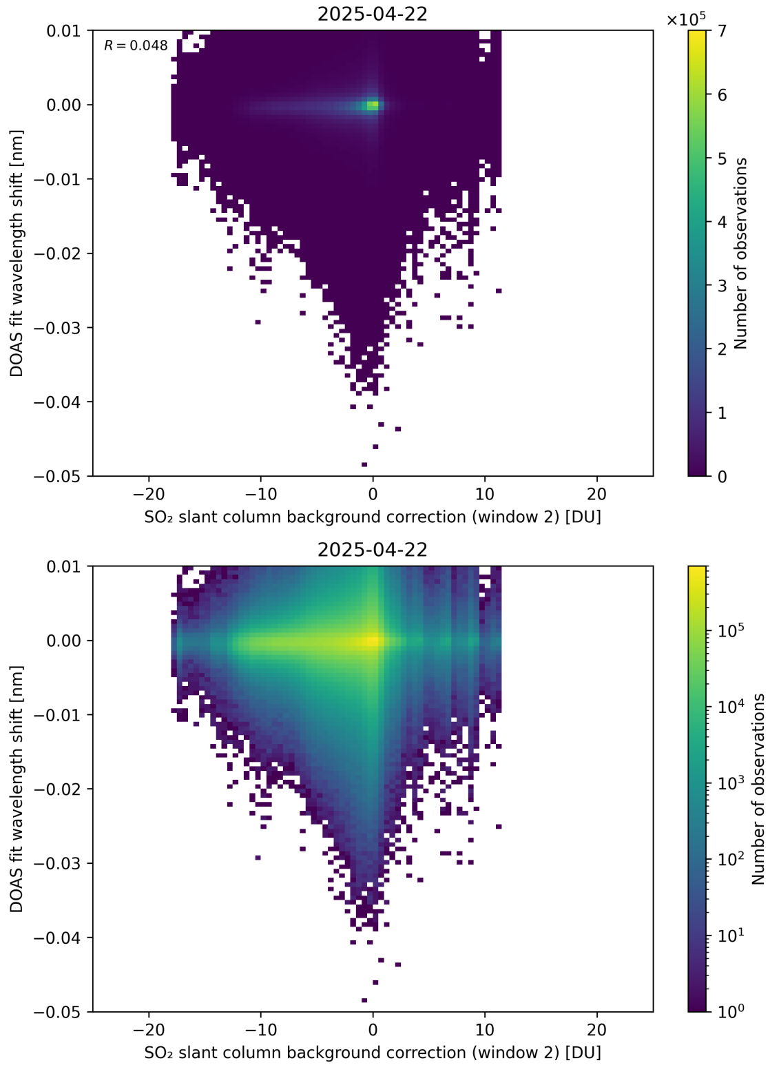
Figure 123: Scatter density plot of “SO 2 slant column background correction (window 2)” against “DOAS fit wavelength shift” for 2025-04-21 to 2025-04-23.
