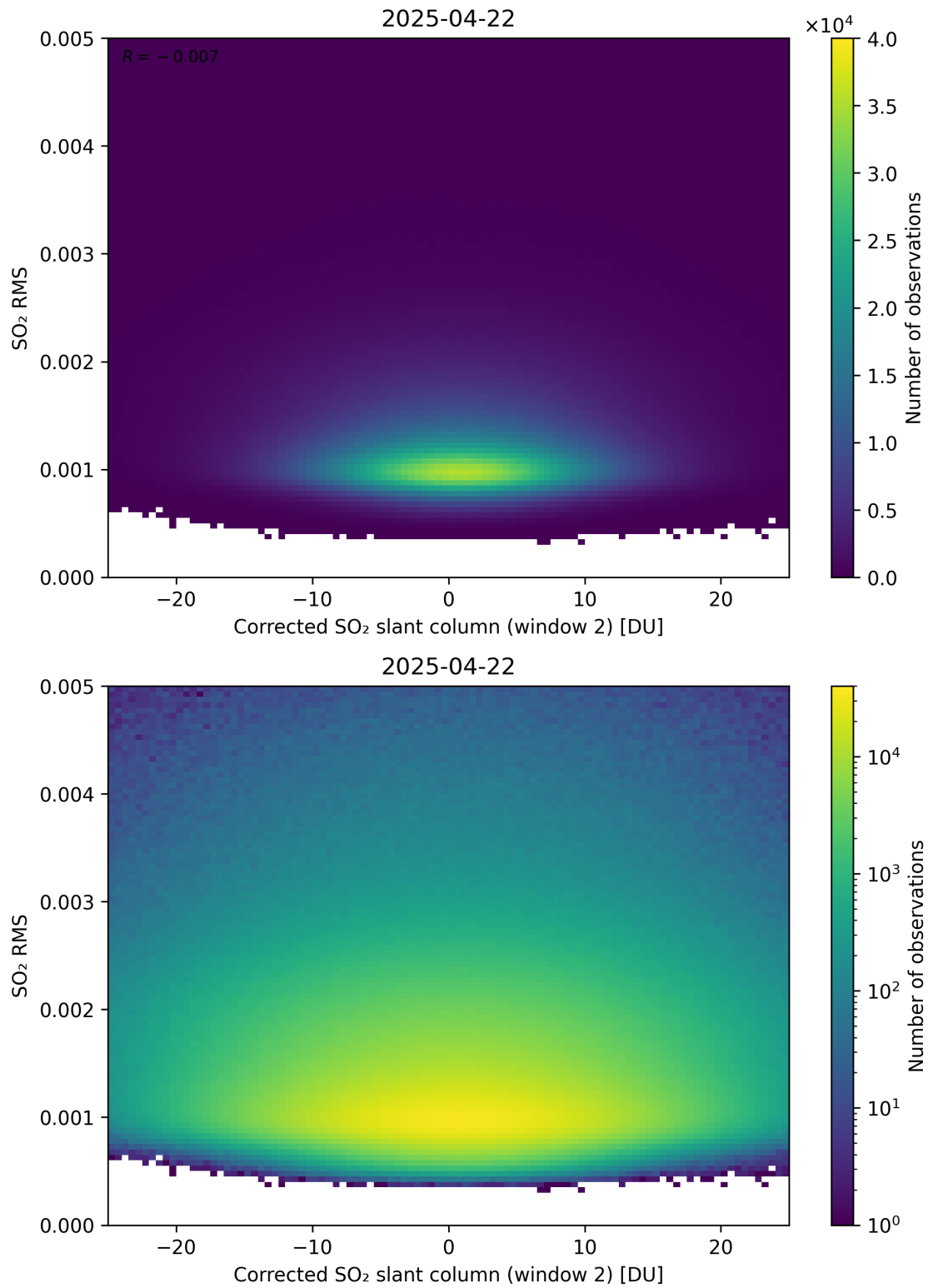
Figure 248: Scatter density plot of “Corrected SO 2 slant column (window 2)” against “SO 2 RMS” for 2025-04-21 to 2025-04-23.
