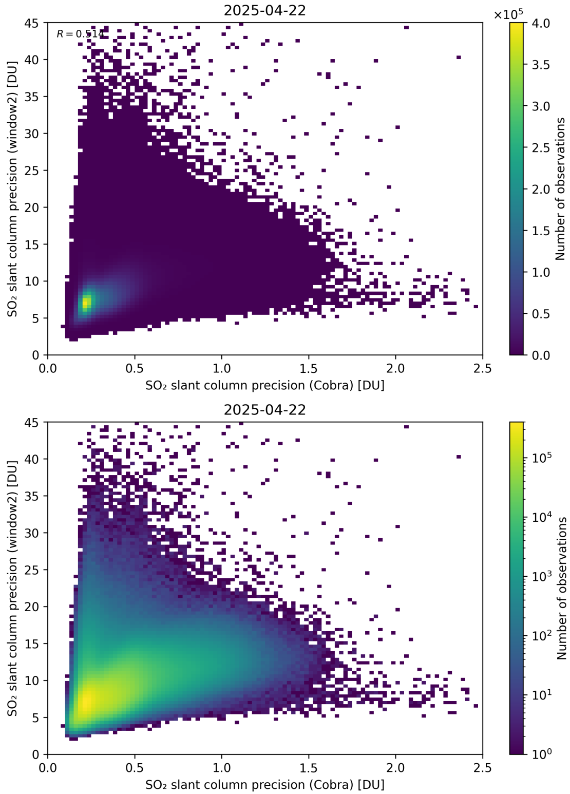
Figure 210: Scatter density plot of “SO 2 slant column precision (Cobra)” against “SO 2 slant column precision (window2)” for 2025-04-21 to 2025-04-23.
