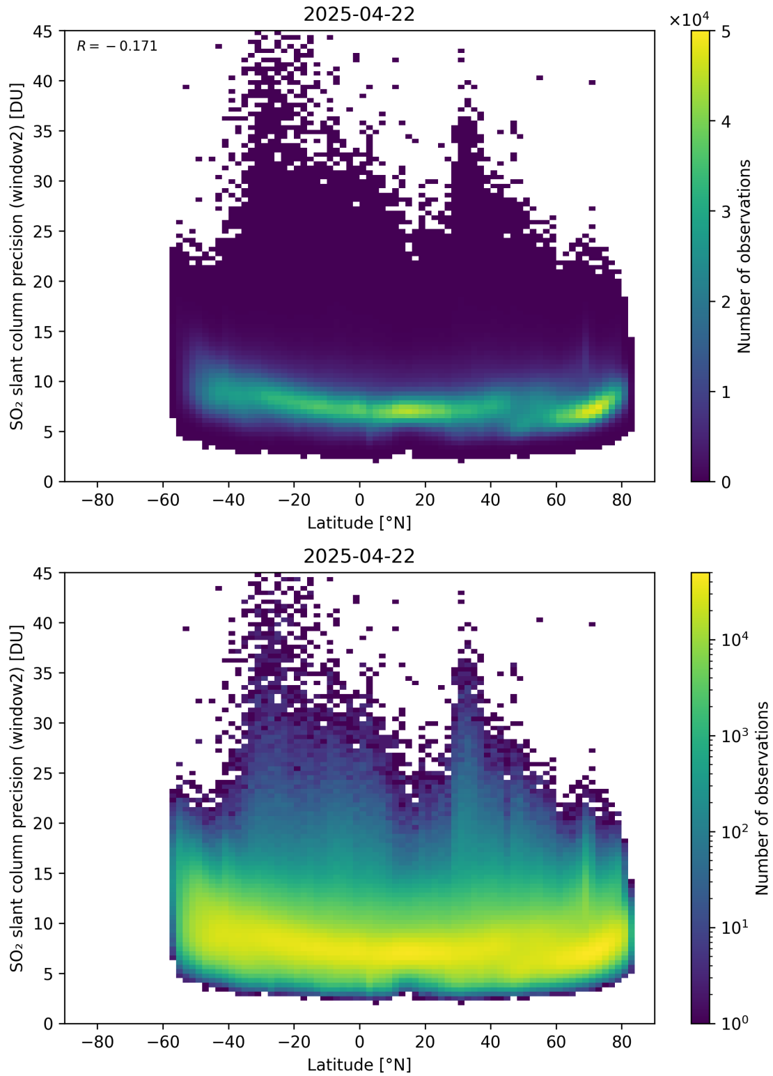
Figure 164: Scatter density plot of “Latitude” against “SO 2 slant column precision (window2)” for 2025-04-21 to 2025-04-23.
