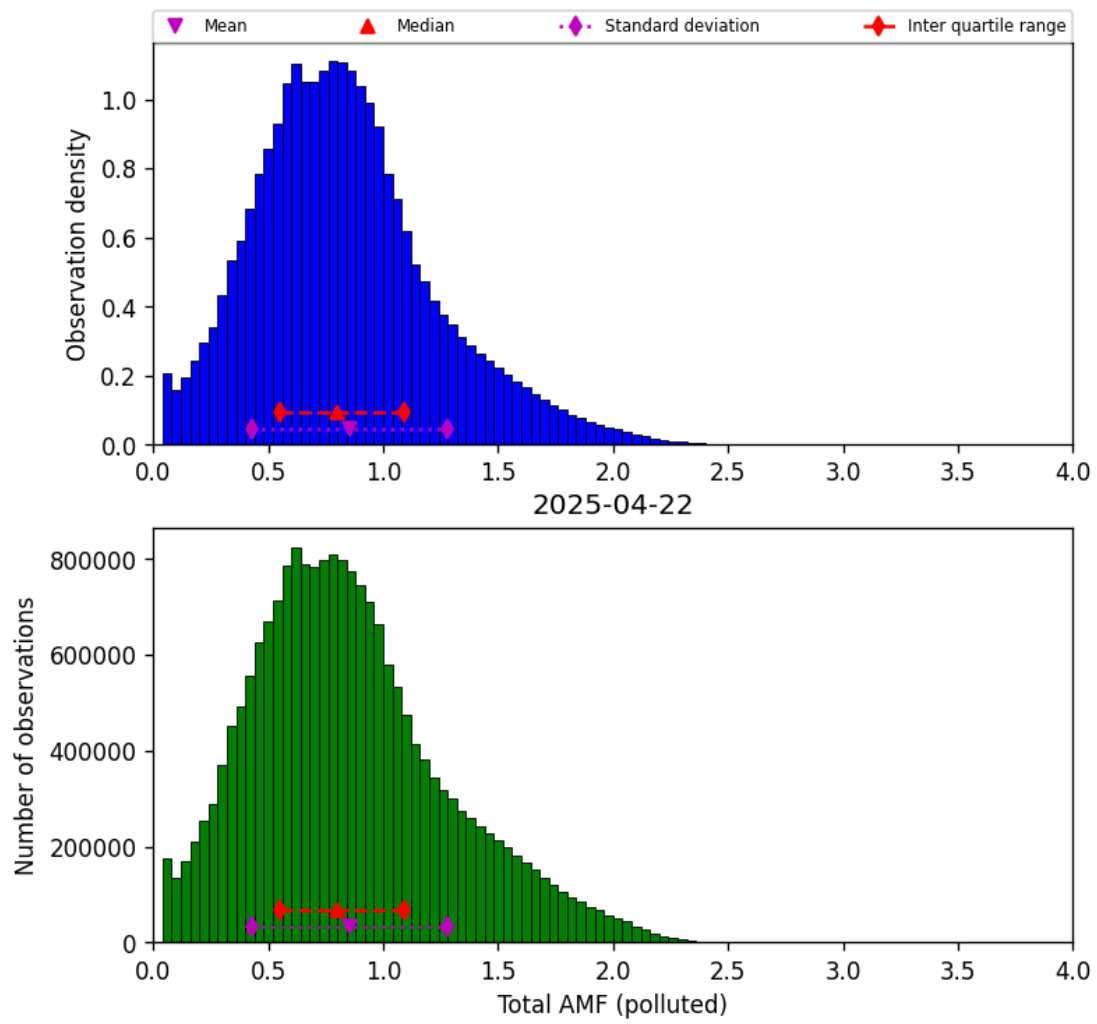
Figure 79: Histogram of “Total AMF (polluted)” for 2025-04-21 to 2025-04-23
