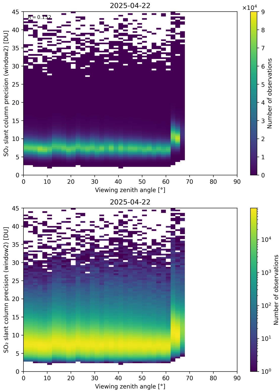
Figure 378: Scatter density plot of “Viewing zenith angle” against “SO 2 slant column precision (window2)” for 2025-04-21 to 2025-04-23.
