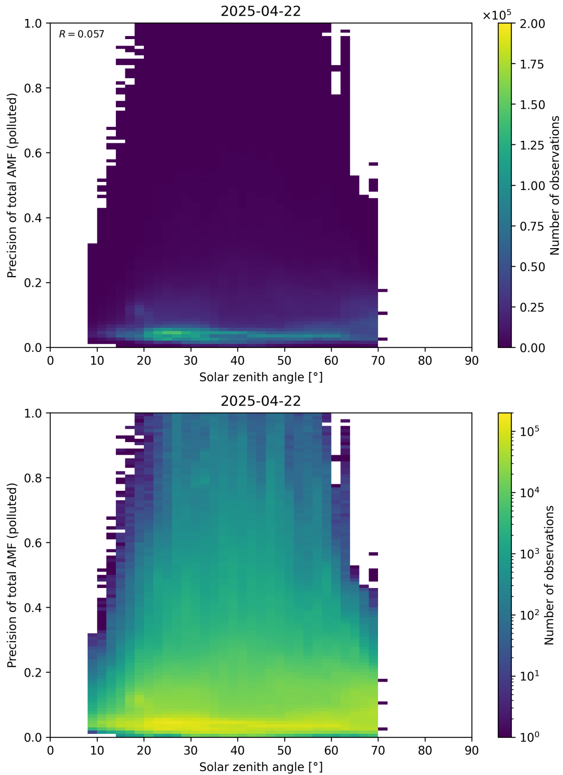
Figure 190: Scatter density plot of “Solar zenith angle” against “Precision of total AMF (polluted)” for 2025-04-21 to 2025-04-23.
