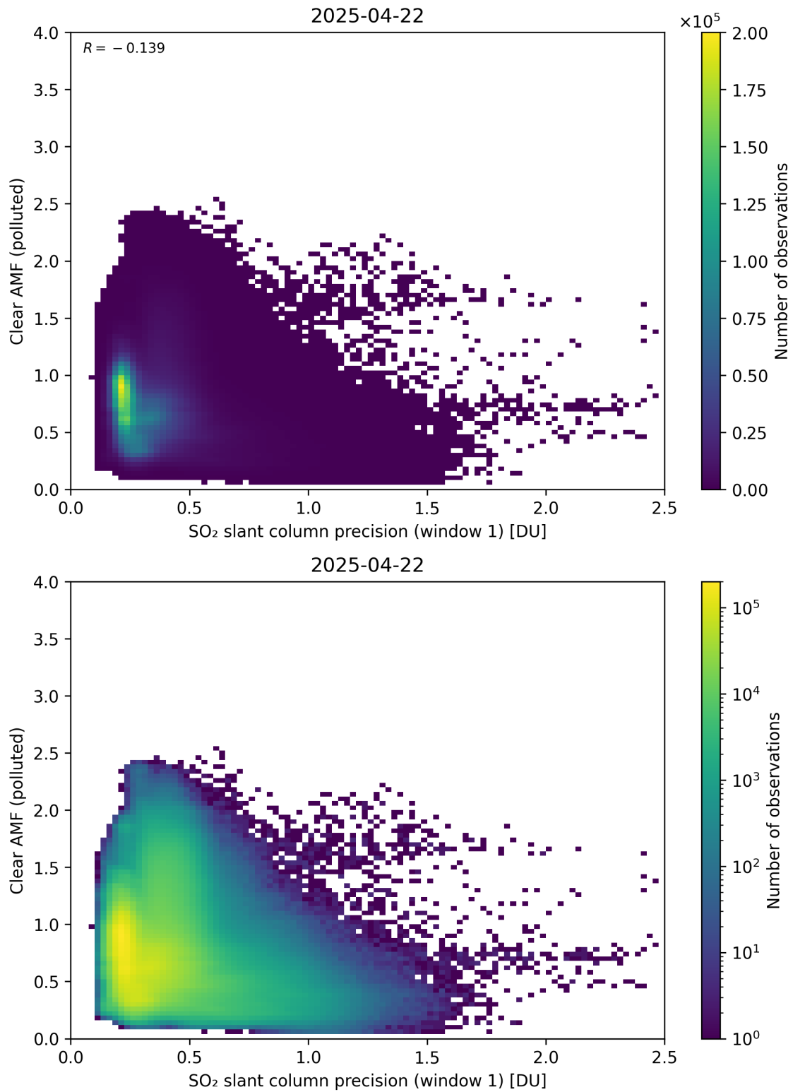
Figure 274: Scatter density plot of “SO 2 slant column precision (window 1)” against “Clear AMF (polluted)” for 2025-04-21 to 2025-04-23.
