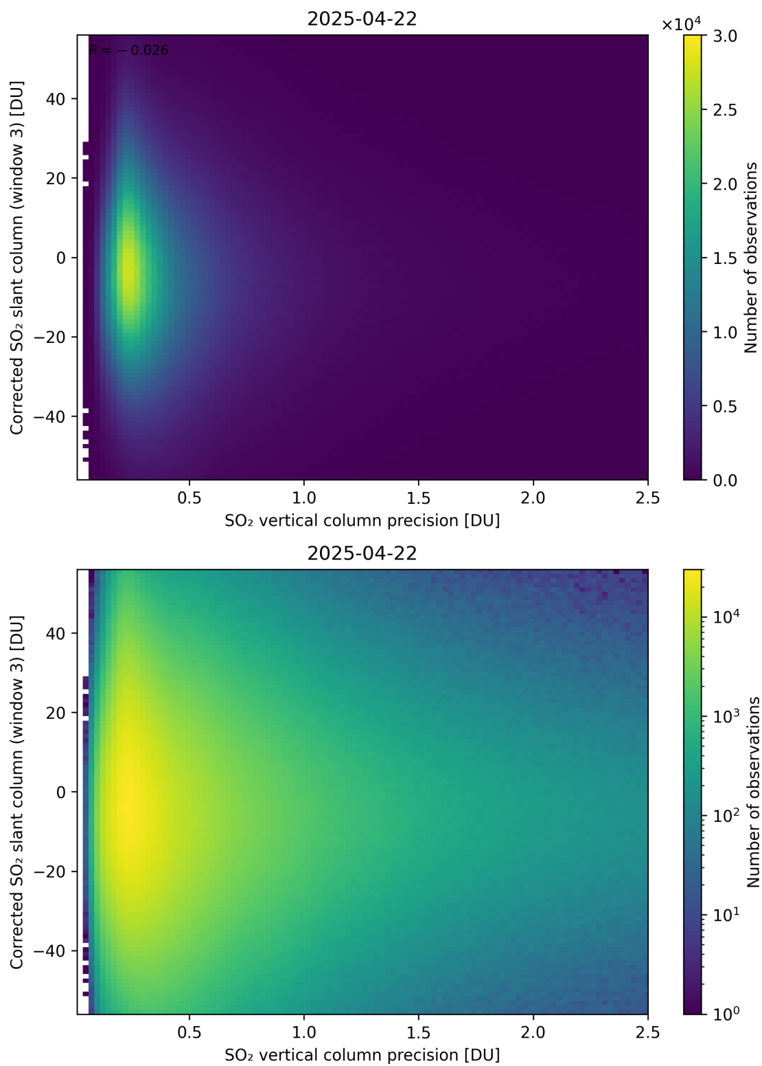
Figure 340: Scatter density plot of “SO 2 vertical column precision” against “Corrected SO 2 slant column (window 3)” for 2025-04-21 to 2025-04-23.
