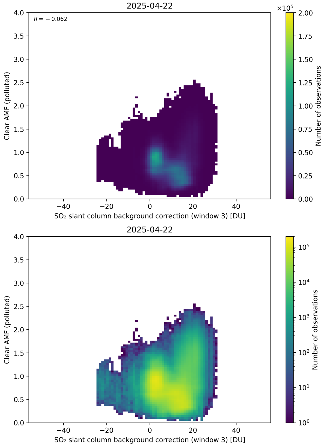
Figure 135: Scatter density plot of “SO 2 slant column background correction (window 3)” against “Clear AMF (polluted)” for 2025-04-21 to 2025-04-23.
