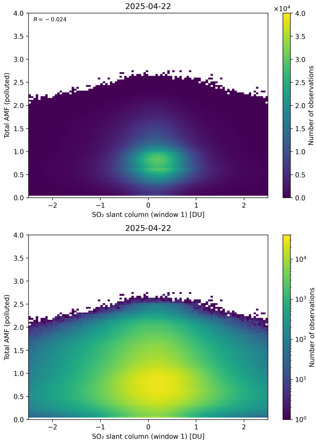
Figure 289: Scatter density plot of “SO 2 slant column (window 1)” against “Total AMF (polluted)” for 2025-04-21 to 2025-04-23.
