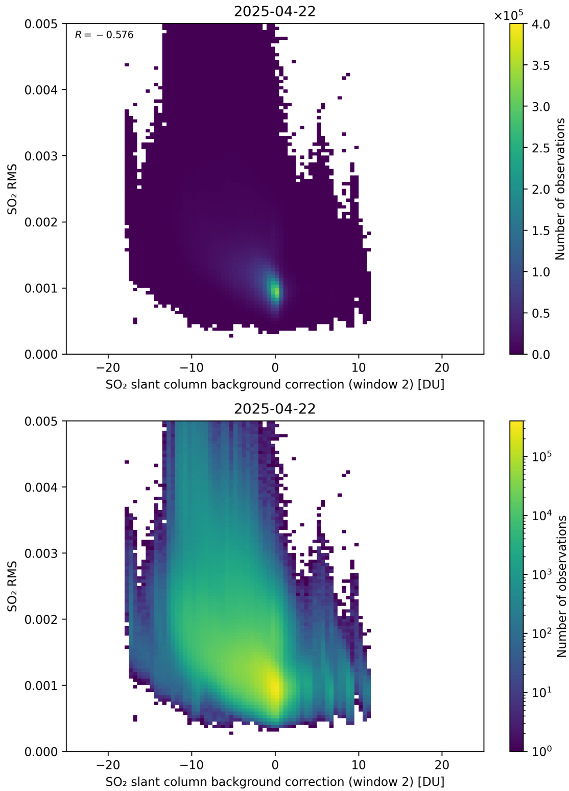
Figure 125: Scatter density plot of “SO 2 slant column background correction (window 2)” against “SO 2 RMS” for 2025-04-21 to 2025-04-23.
