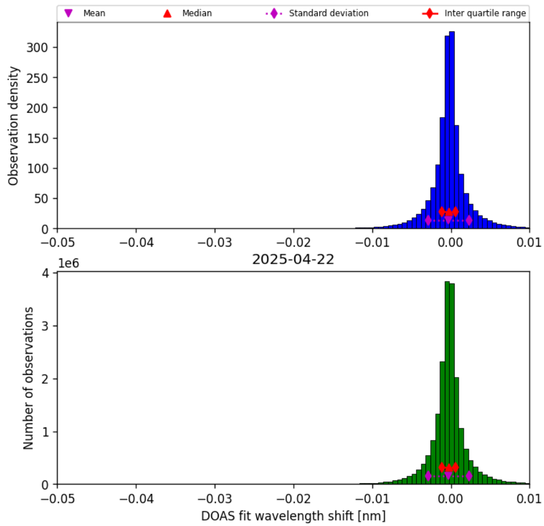
Figure 76: Histogram of “DOAS fit wavelength shift” for 2025-04-21 to 2025-04-23
