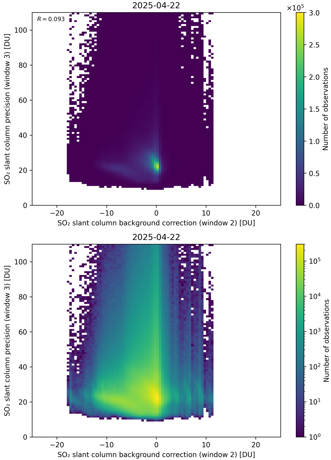
Figure 129: Scatter density plot of “SO 2 slant column background correction (window 2)” against “SO 2 slant column precision (window 3)” for 2025-04-21 to 2025-04-23.
