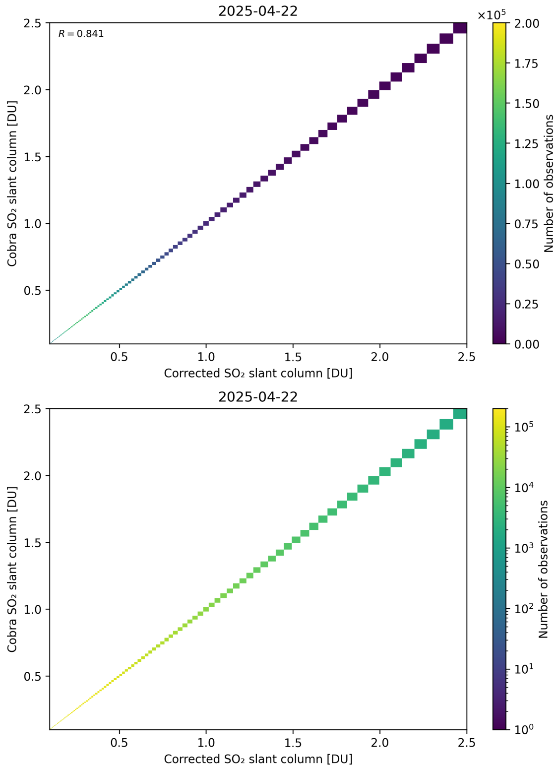
Figure 233: Scatter density plot of “Corrected SO 2 slant column” against “Cobra SO 2 slant column” for 2025-04-21 to 2025-04-23.
