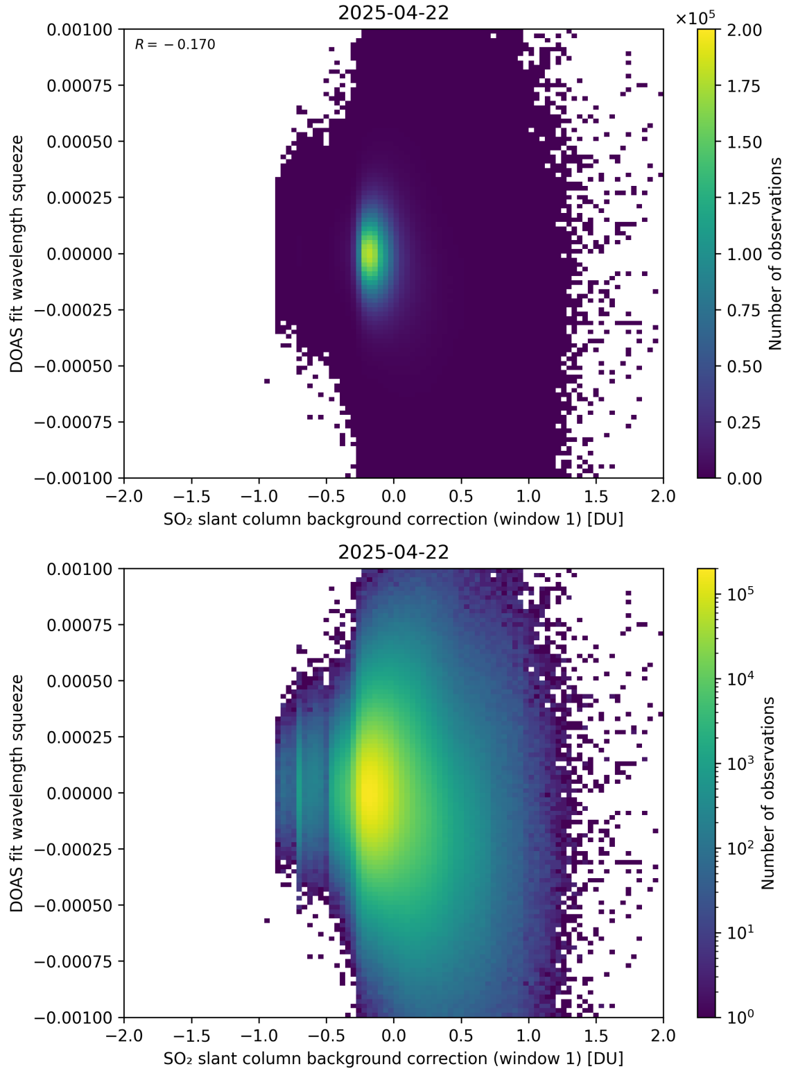
Figure 112: Scatter density plot of “SO 2 slant column background correction (window 1)” against “DOAS fit wavelength squeeze” for 2025-04-21 to 2025-04-23.
