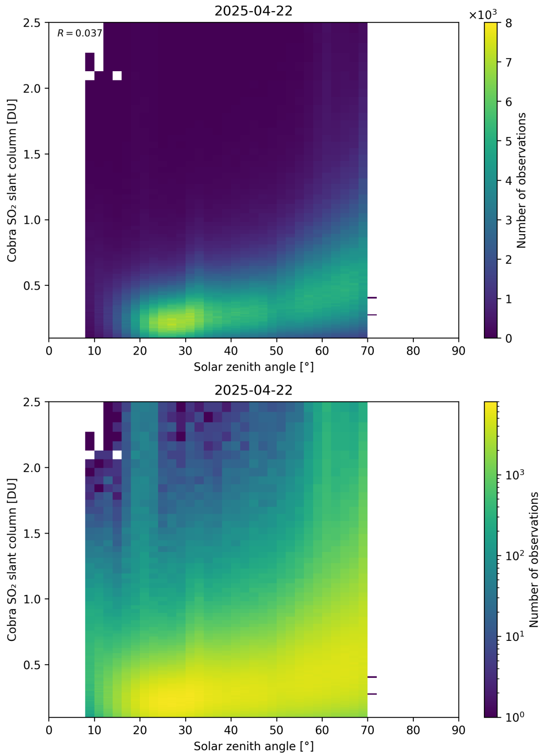
Figure 179: Scatter density plot of “Solar zenith angle” against “Cobra SO 2 slant column” for 2025-04-21 to 2025-04-23.
