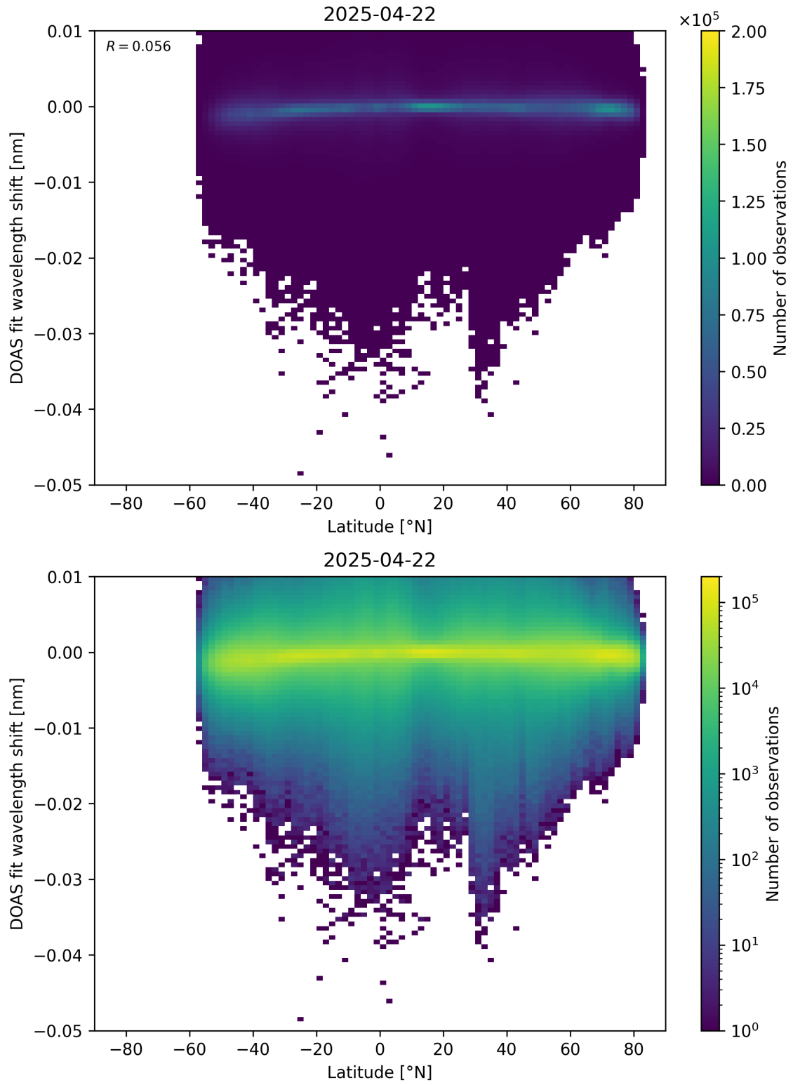
Figure 153: Scatter density plot of “Latitude” against “DOAS fit wavelength shift” for 2025-04-21 to 2025-04-23.
