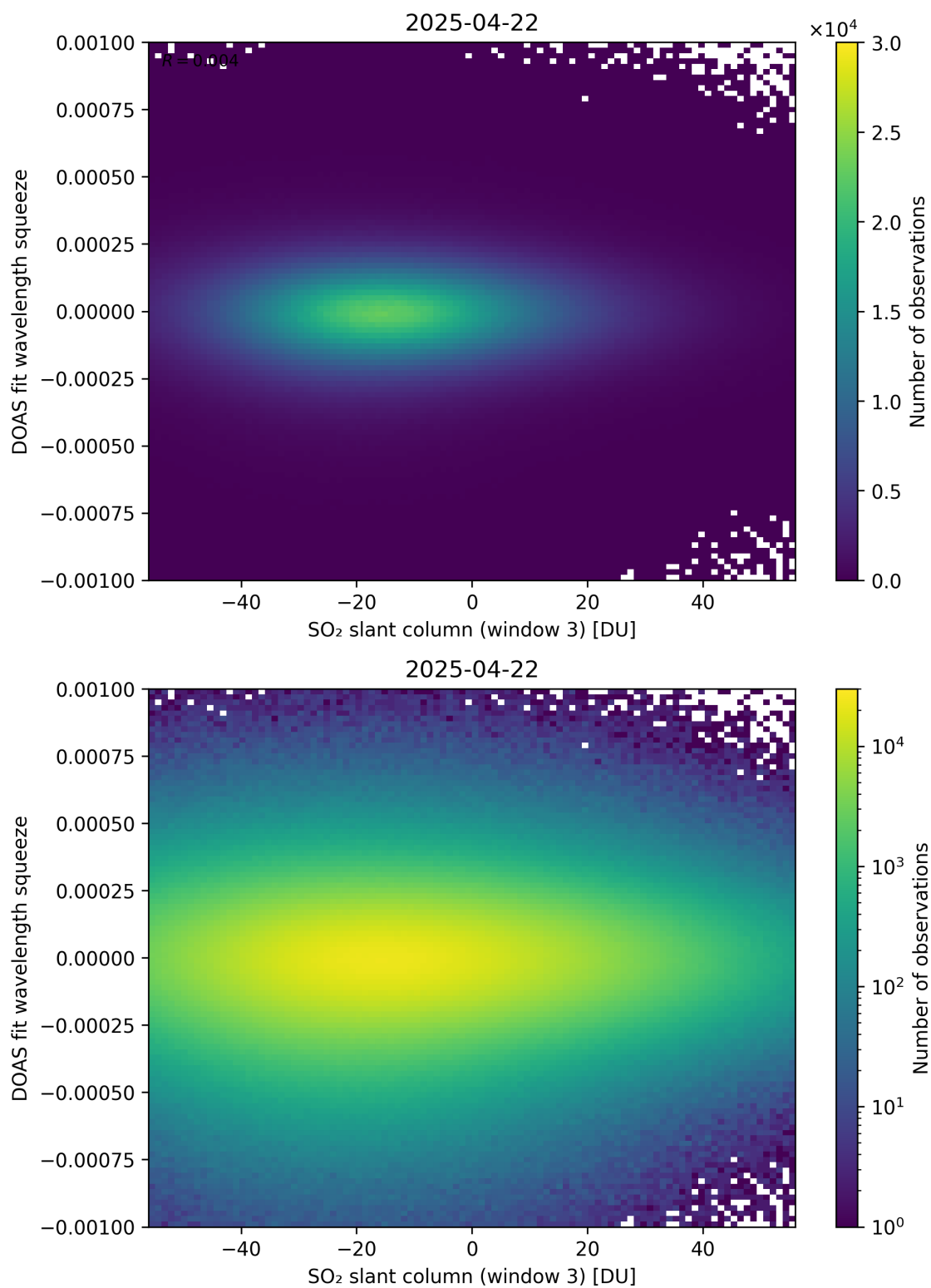
Figure 305: Scatter density plot of “SO 2 slant column (window 3)” against “DOAS fit wavelength squeeze” for 2025-04-21 to 2025-04-23.
