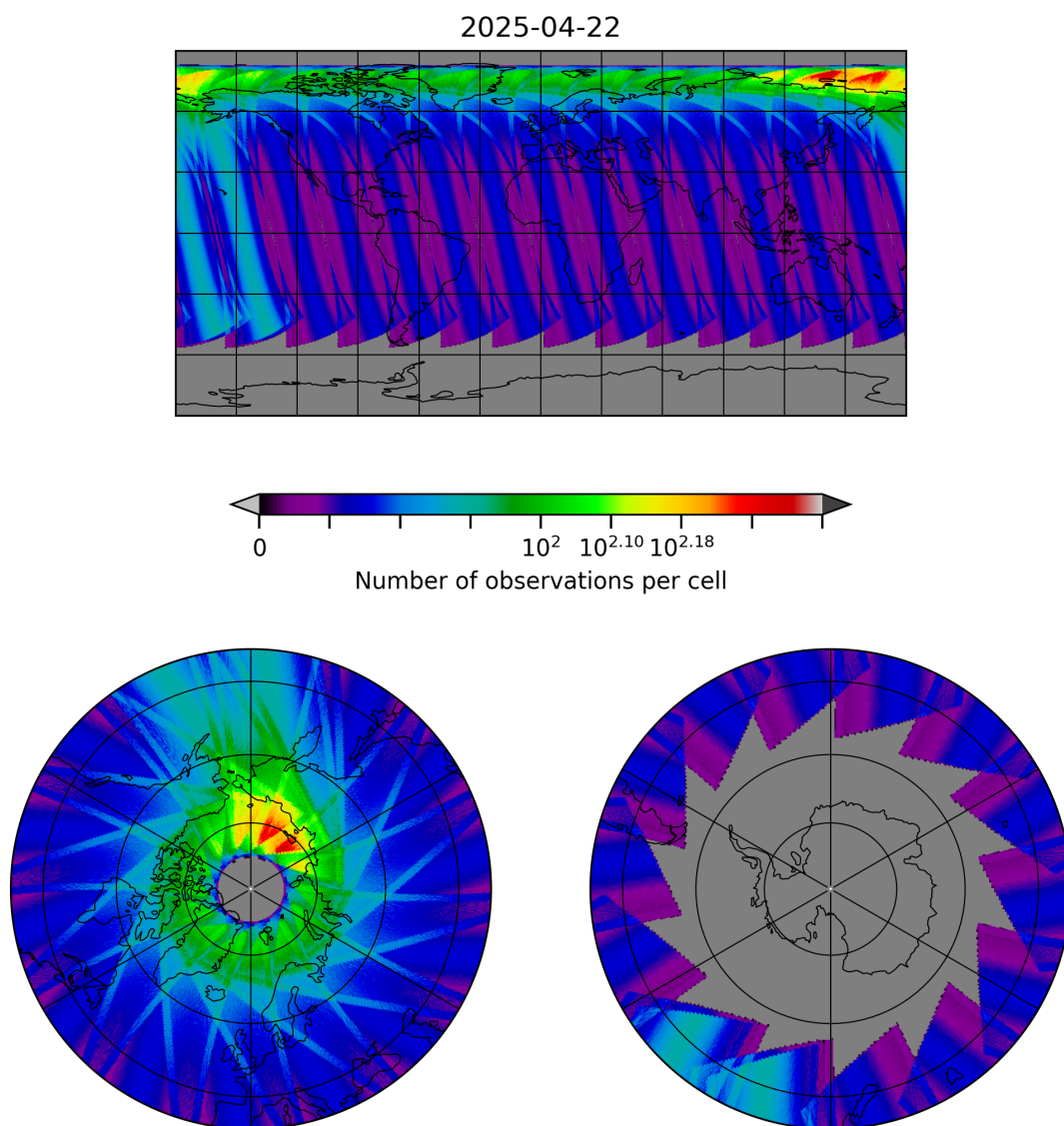
Figure 30: Map of the number of observations for 2025-04-21 to 2025-04-23
