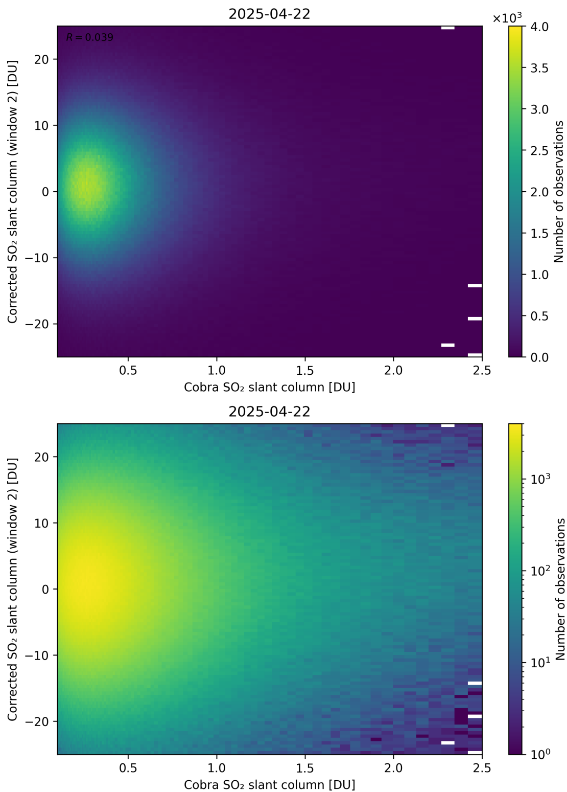
Figure 217: Scatter density plot of “Cobra SO 2 slant column” against “Corrected SO 2 slant column (window 2)” for 2025-04-21 to 2025-04-23.
