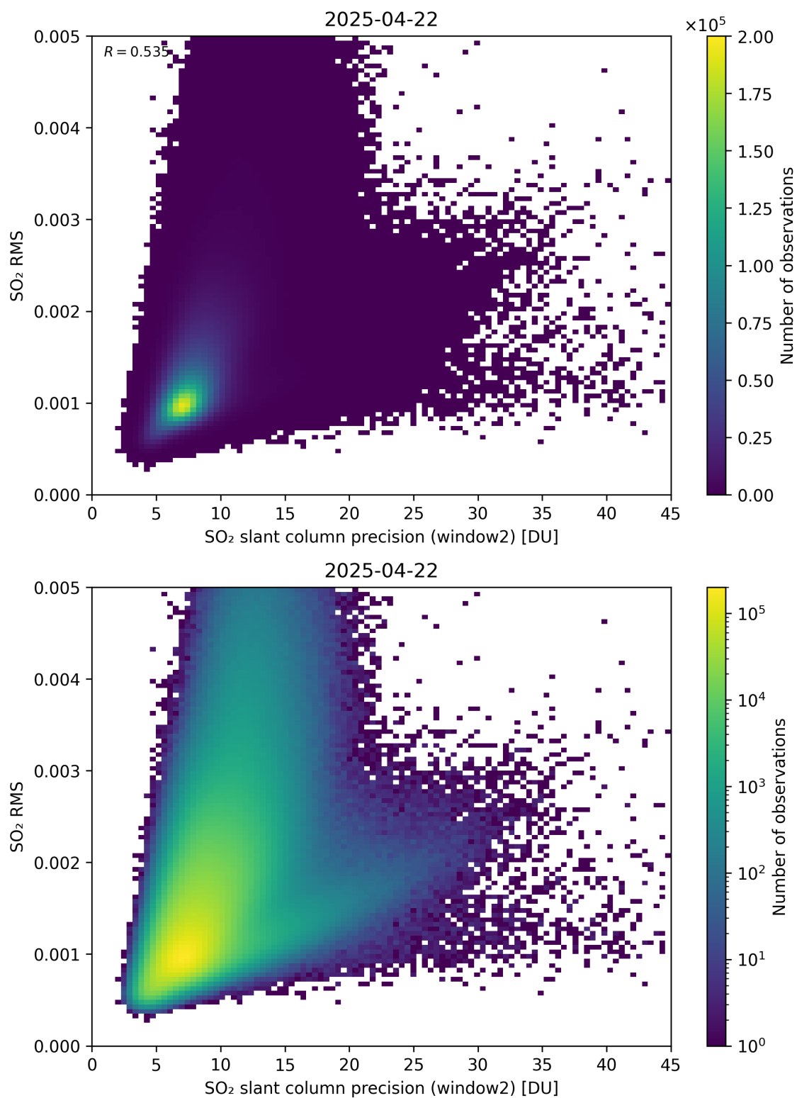
Figure 295: Scatter density plot of “SO 2 slant column precision (window2)” against “SO 2 RMS” for 2025-04-21 to 2025-04-23.
