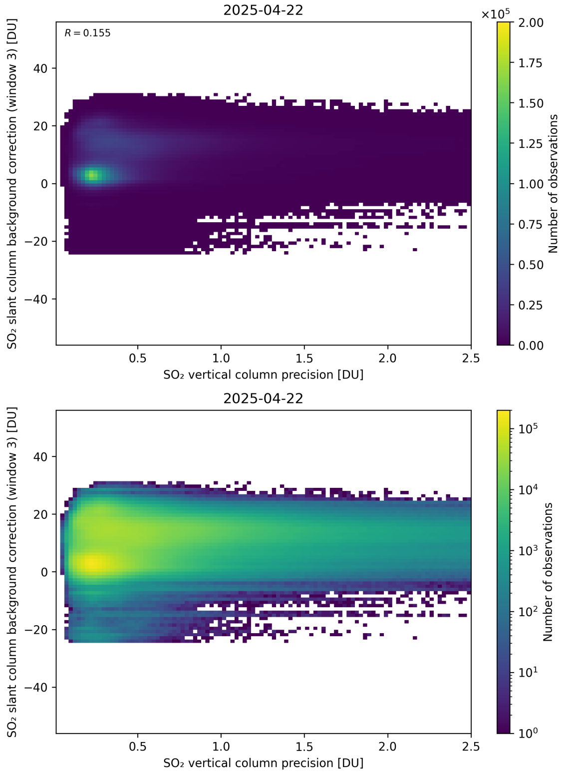
Figure 331: Scatter density plot of “SO 2 vertical column precision” against “SO 2 slant column background correction (window 3)” for 2025-04-21 to 2025-04-23.
