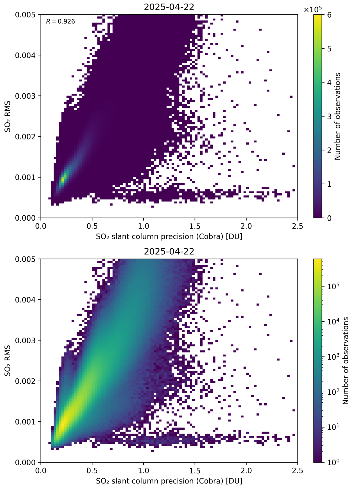
Figure 204: Scatter density plot of “SO 2 slant column precision (Cobra)” against “SO 2 RMS” for 2025-04-21 to 2025-04-23.
