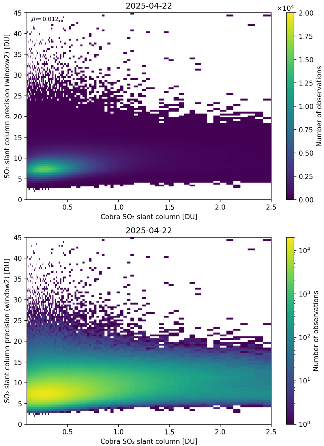
Figure 221: Scatter density plot of “Cobra SO 2 slant column” against “SO 2 slant column precision (window2)” for 2025-04-21 to 2025-04-23.
