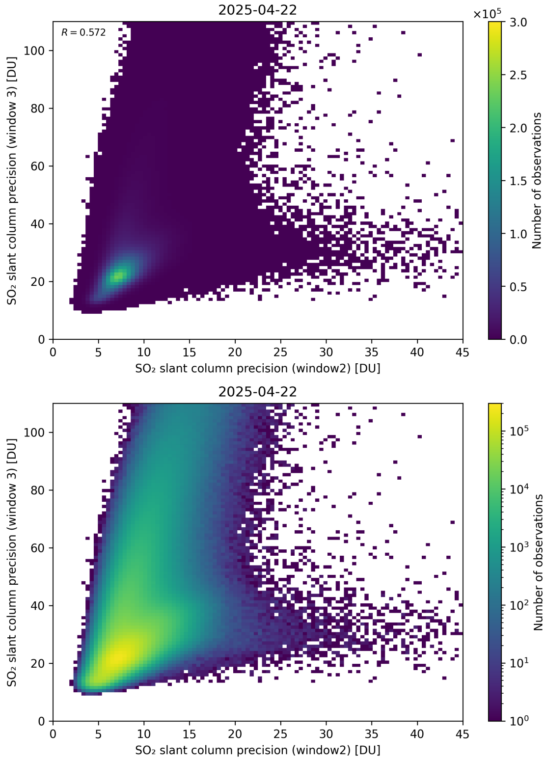
Figure 300: Scatter density plot of “SO 2 slant column precision (window2)” against “SO 2 slant column precision (window 3)” for 2025-04-21 to 2025-04-23.
