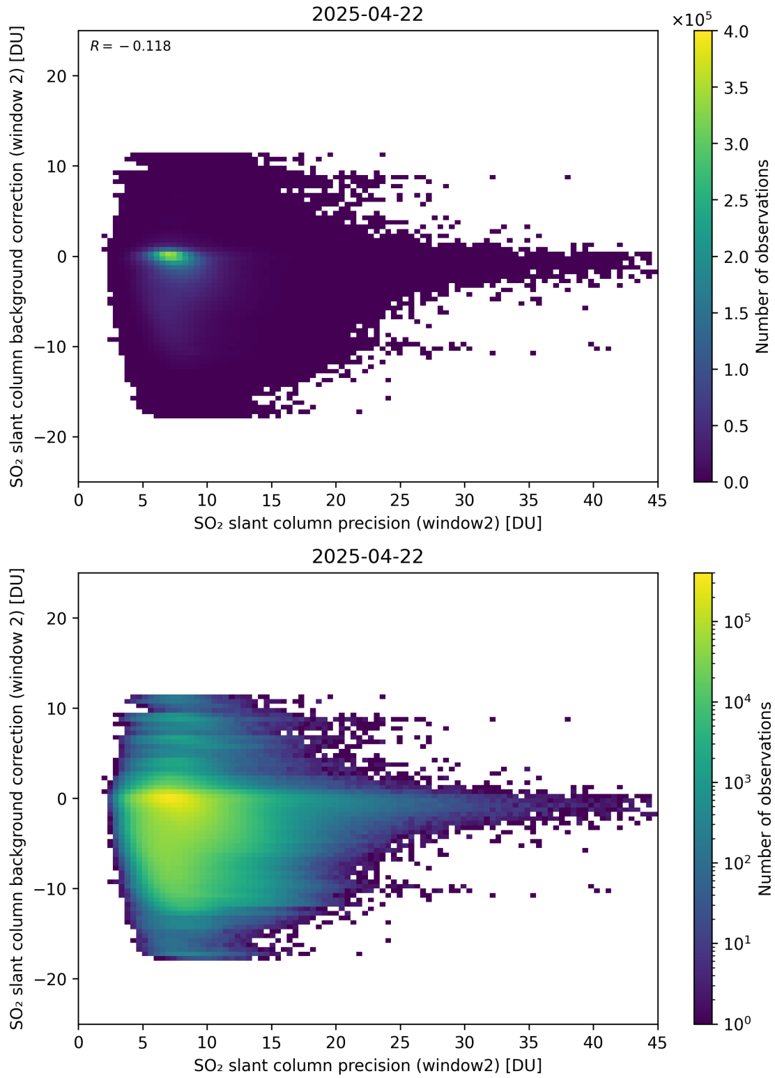
Figure 291: Scatter density plot of “SO 2 slant column precision (window2)” against “SO 2 slant column background correction (window 2)” for 2025-04-21 to 2025-04-23.
