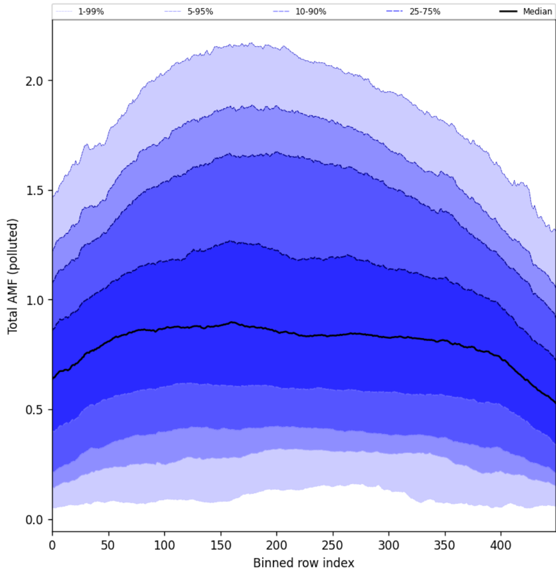
Figure 105: Along track statistics of “Total AMF (polluted)” for 2025-04-21 to 2025-04-23
