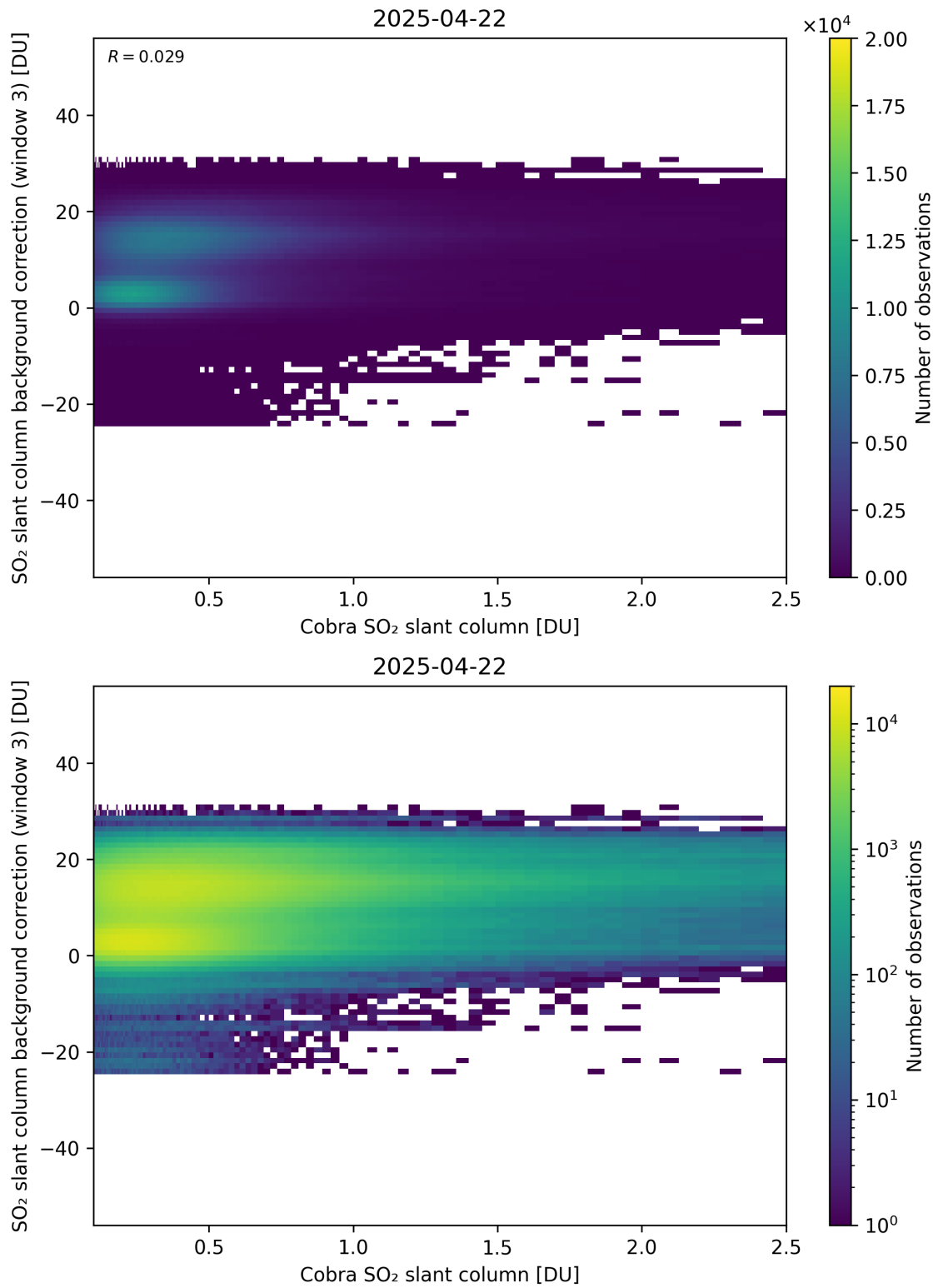
Figure 195: Scatter density plot of “Cobra SO 2 slant column” against “SO 2 slant column background correction (window 3)” for 2025-04-21 to 2025-04-23.
