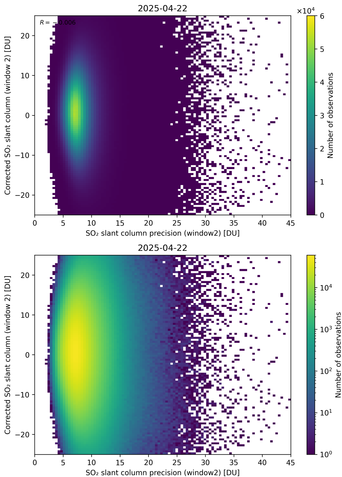
Figure 297: Scatter density plot of “SO 2 slant column precision (window2)” against “Corrected SO 2 slant column (window 2)” for 2025-04-21 to 2025-04-23.
