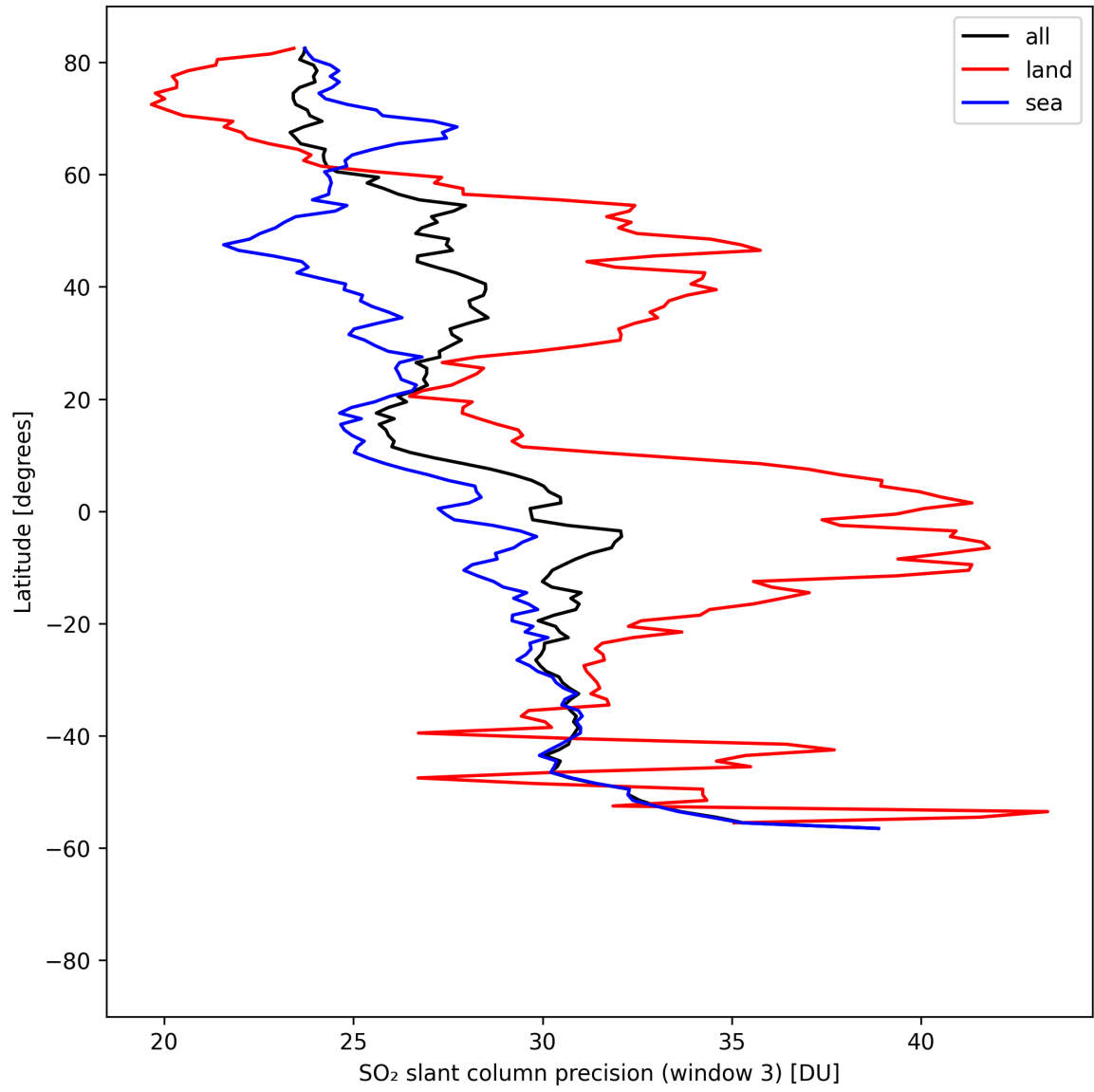
Figure 46: Zonal average of “SO 2 slant column precision (window 3)” for 2025-04-21 to 2025-04-23.
