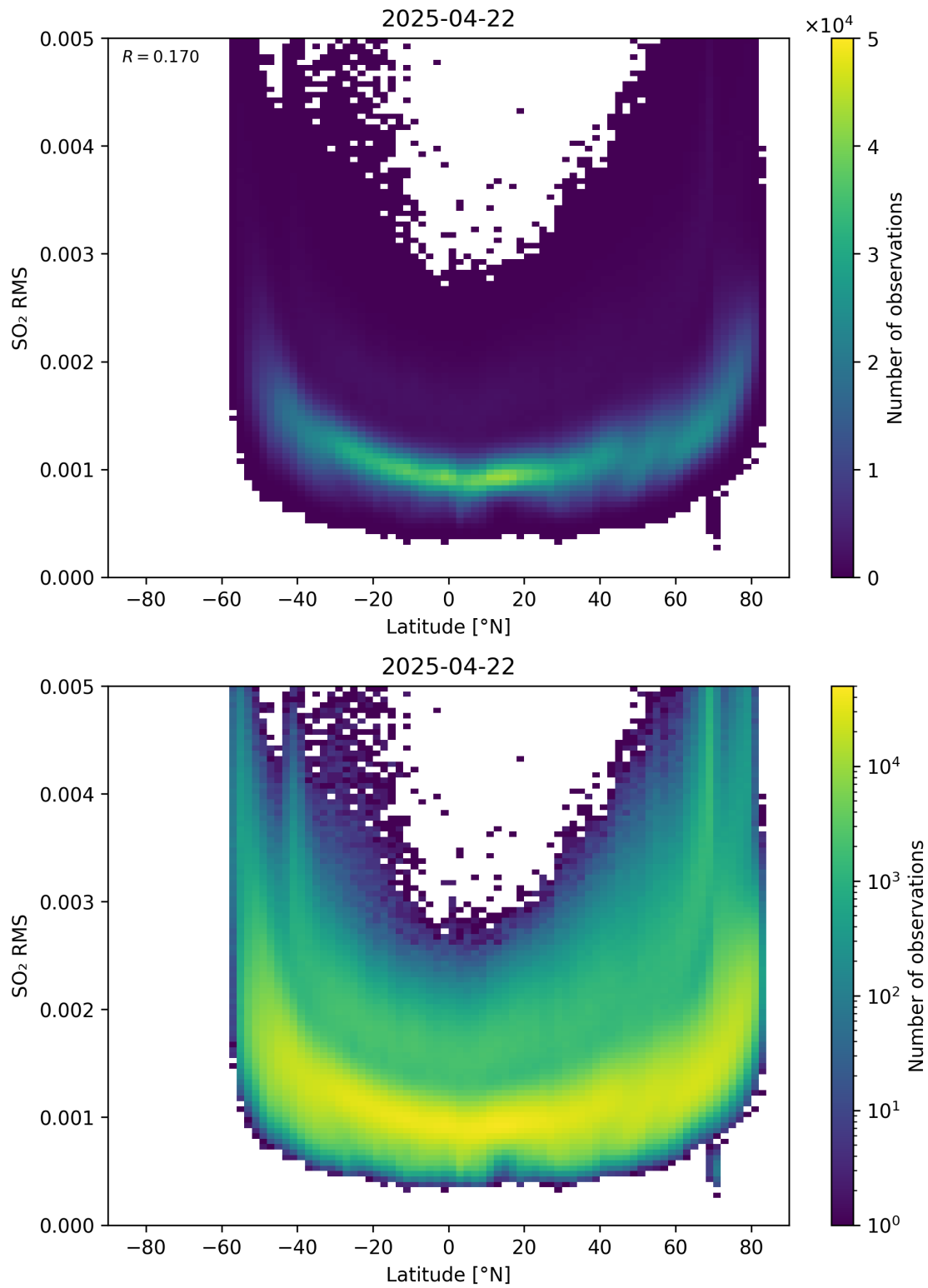
Figure 155: Scatter density plot of “Latitude” against “SO 2 RMS” for 2025-04-21 to 2025-04-23.
