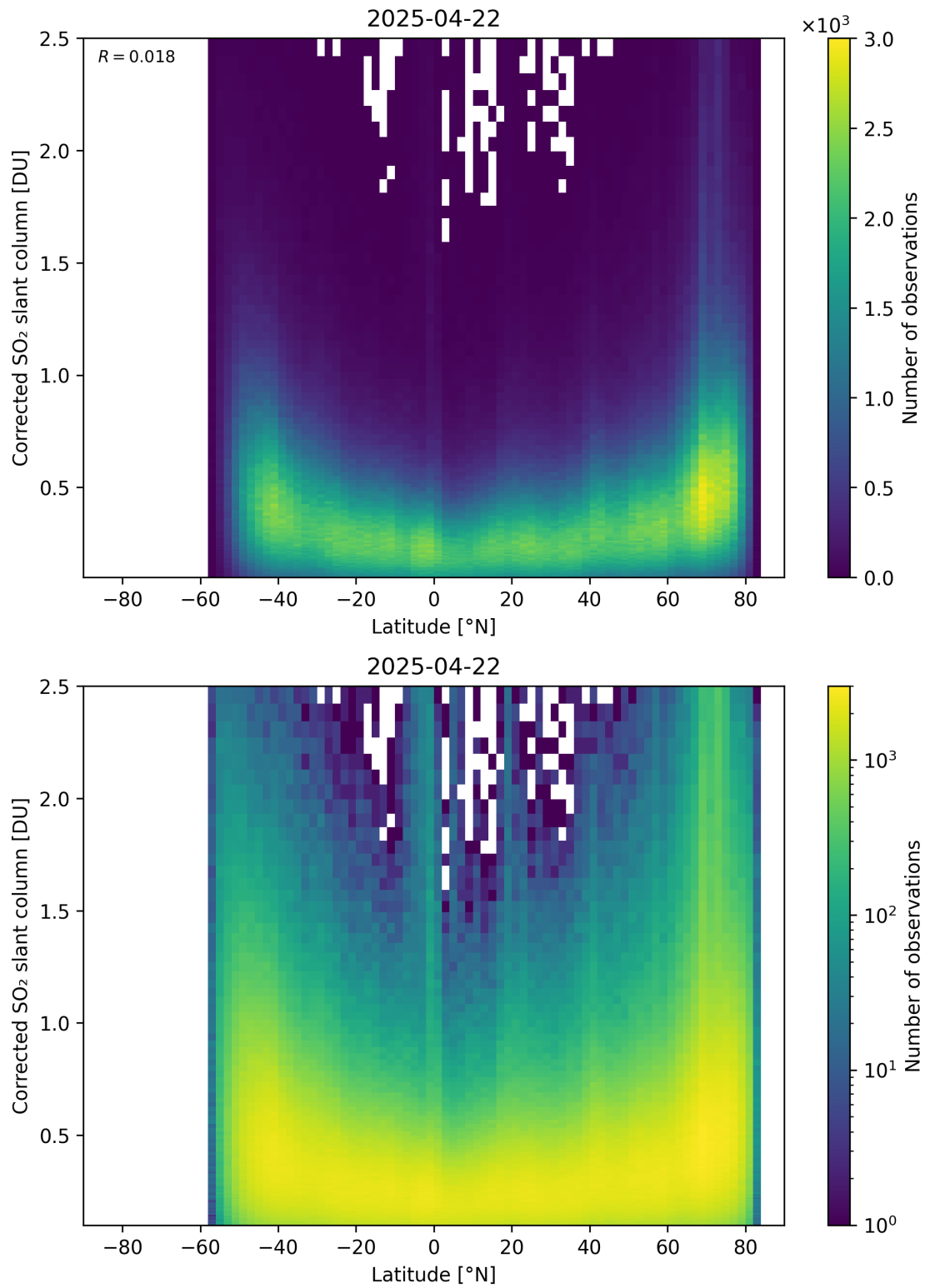
Figure 159: Scatter density plot of “Latitude” against “Corrected SO 2 slant column” for 2025-04-21 to 2025-04-23.
