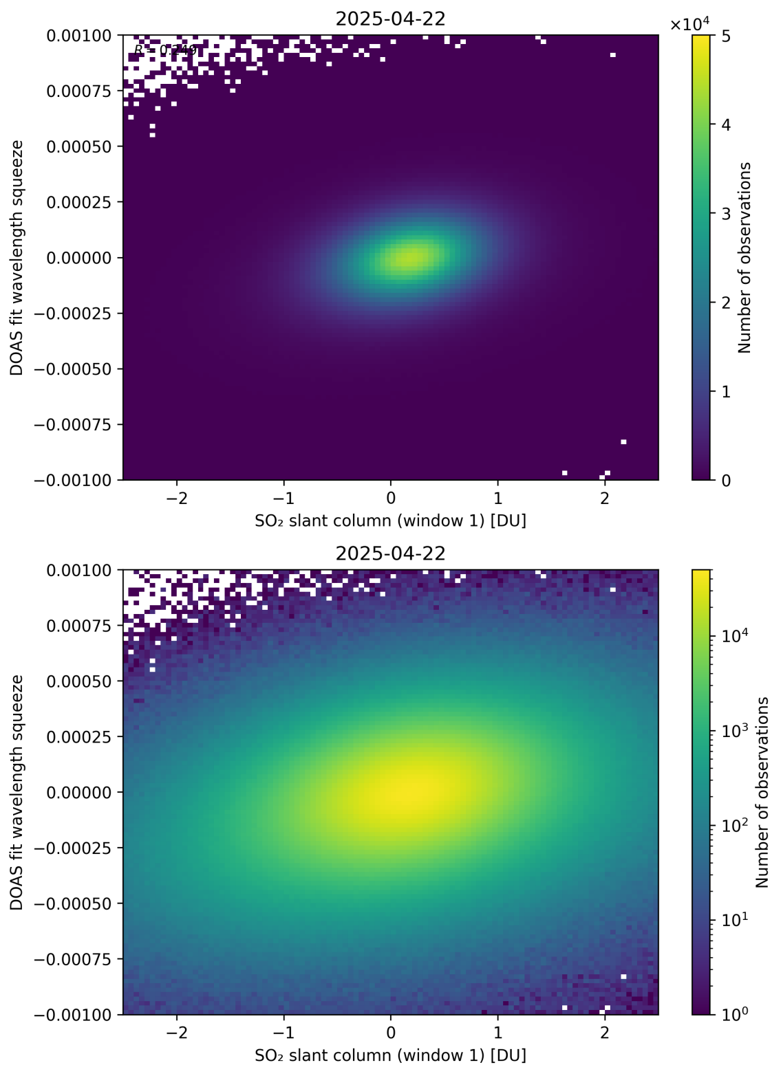
Figure 266: Scatter density plot of “SO 2 slant column (window 1)” against “DOAS fit wavelength squeeze” for 2025-04-21 to 2025-04-23.
