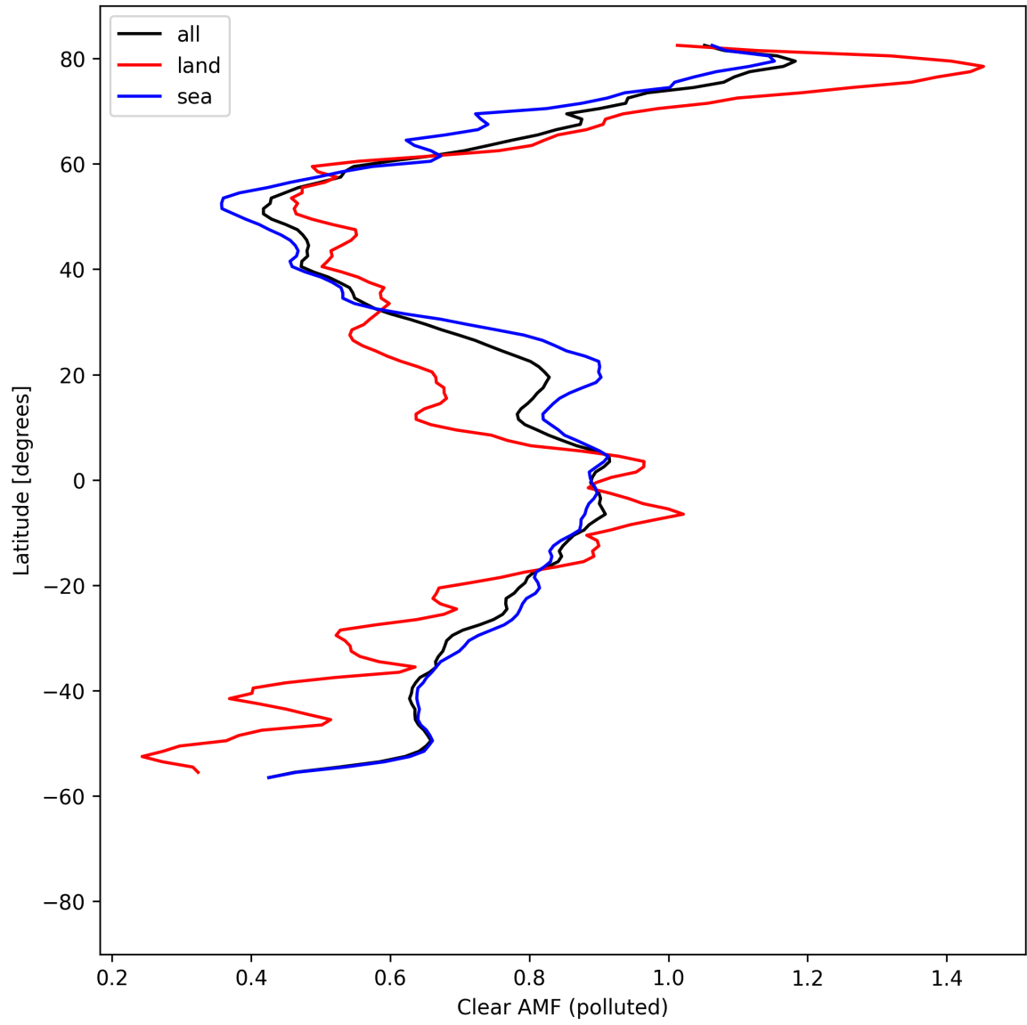
Figure 55: Zonal average of “Clear AMF (polluted)” for 2025-04-21 to 2025-04-23.
