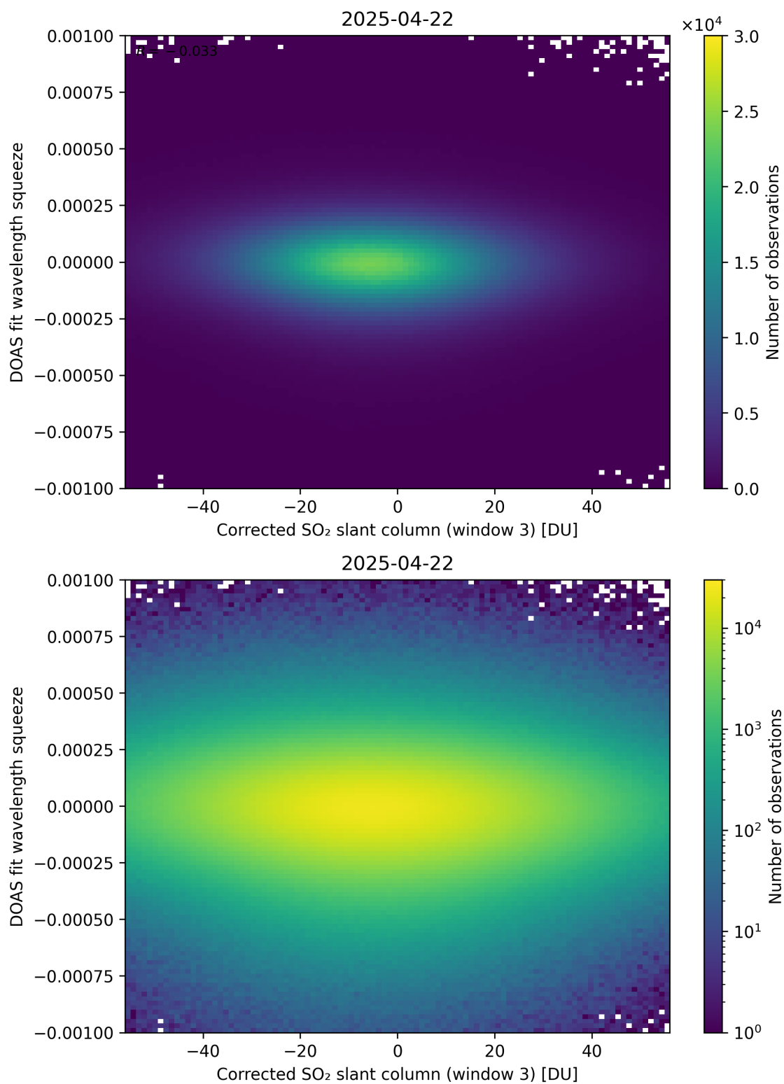
Figure 257: Scatter density plot of “Corrected SO 2 slant column (window 3)” against “DOAS fit wavelength squeeze” for 2025-04-21 to 2025-04-23.
