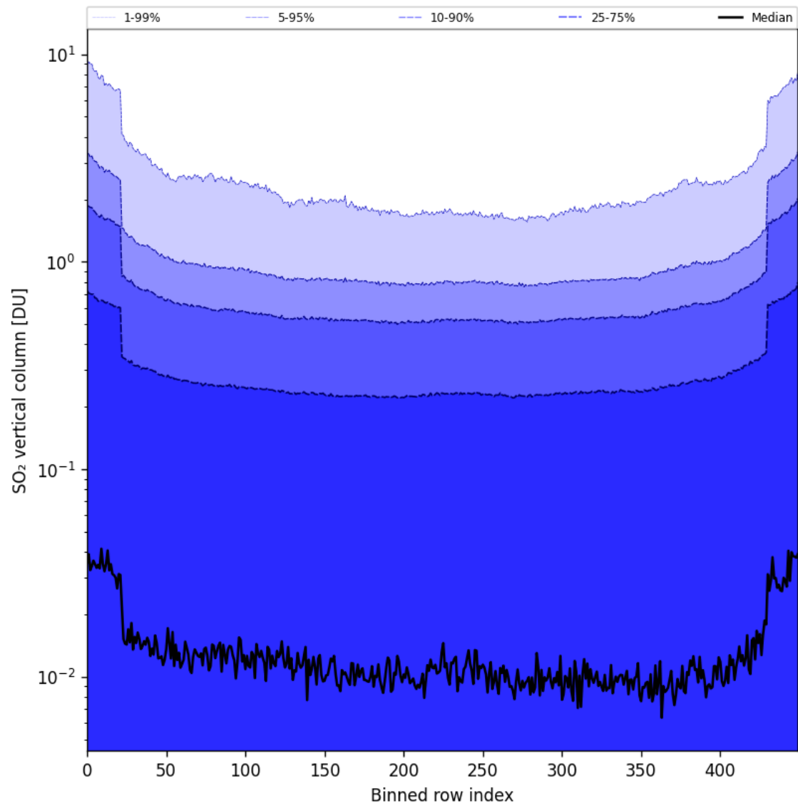
Figure 84: Along track statistics of “SO 2 vertical column” for 2025-04-21 to 2025-04-23
