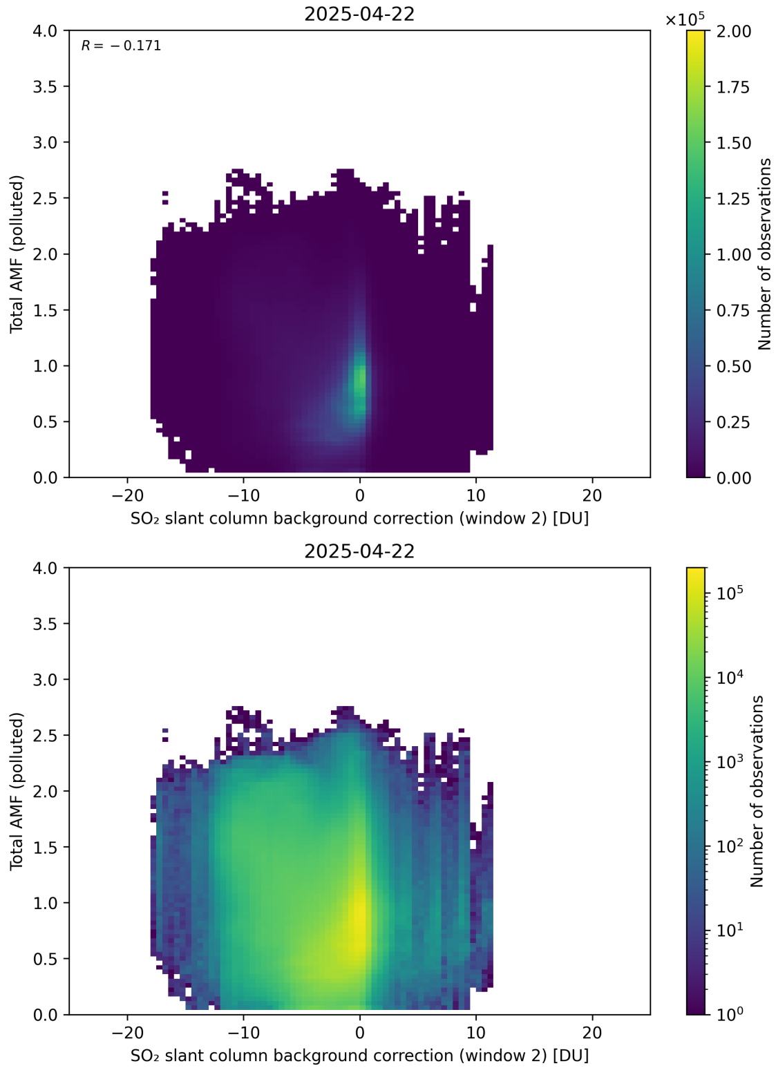
Figure 130: Scatter density plot of “SO 2 slant column background correction (window 2)” against “Total AMF (polluted)” for 2025-04-21 to 2025-04-23.
