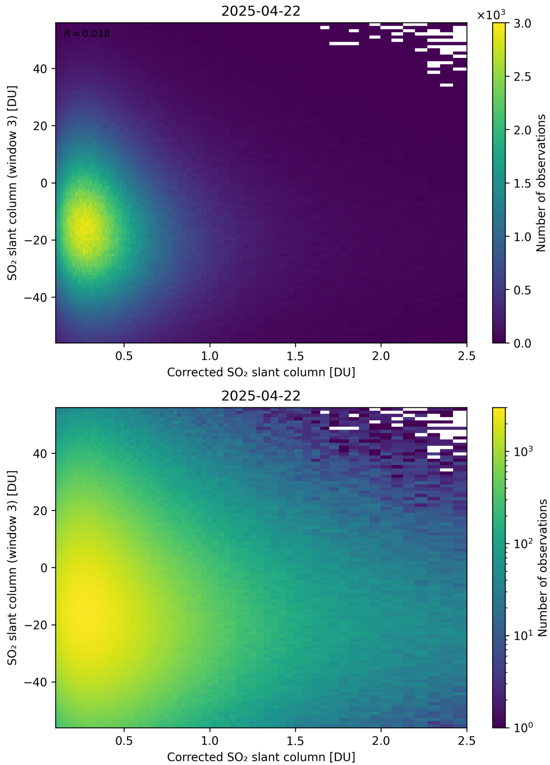
Figure 240: Scatter density plot of “Corrected SO 2 slant column” against “SO 2 slant column (window 3)” for 2025-04-21 to 2025-04-23.
