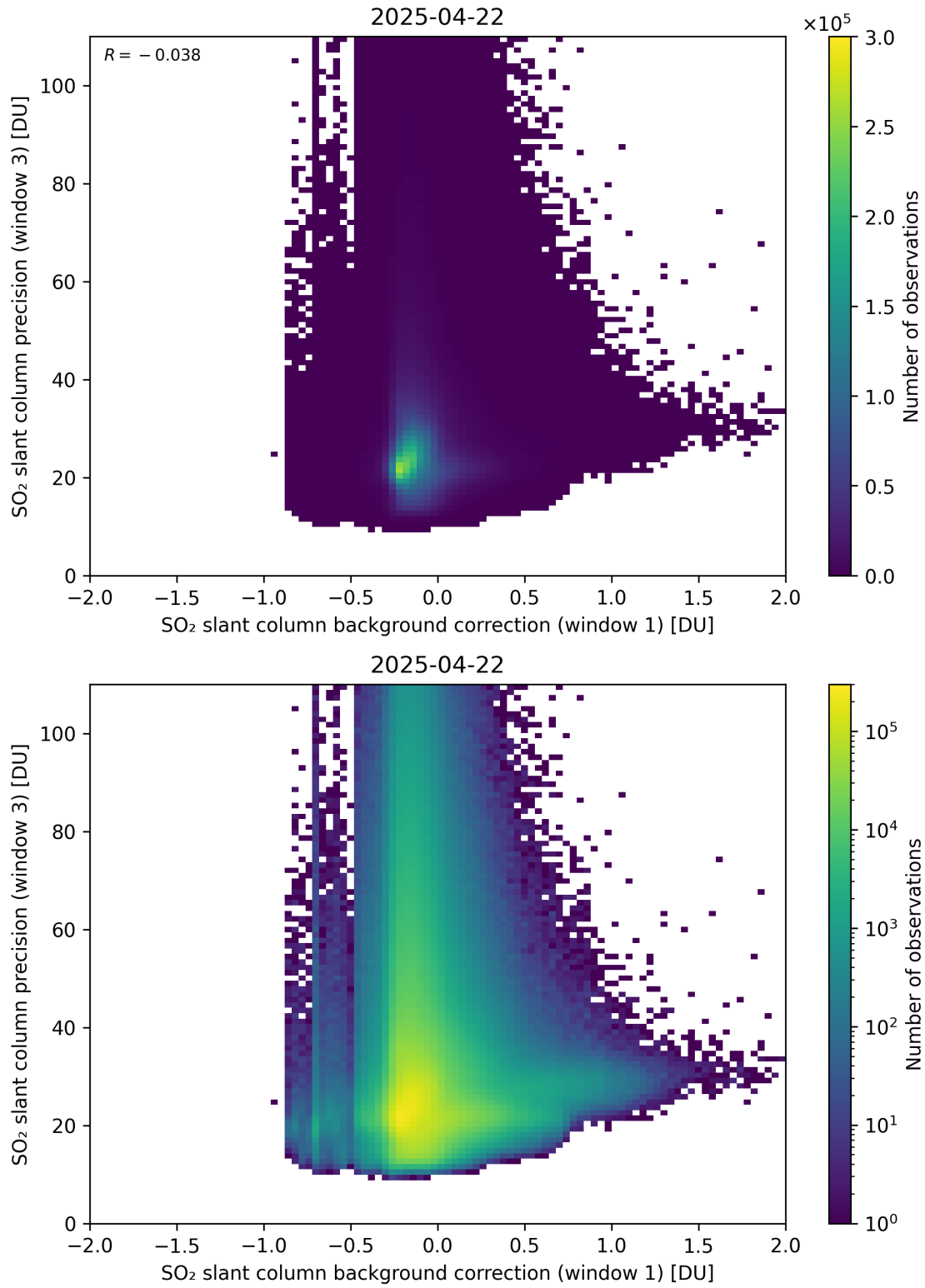
Figure 119: Scatter density plot of “SO 2 slant column background correction (window 1)” against “SO 2 slant column precision (window 3)” for 2025-04-21 to 2025-04-23.
