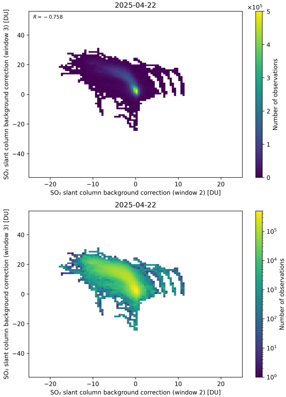
Figure 122: Scatter density plot of “SO 2 slant column background correction (window 2)” against “SO 2 slant column background correction (window 3)” for 2025-04-21 to 2025-04-23.
