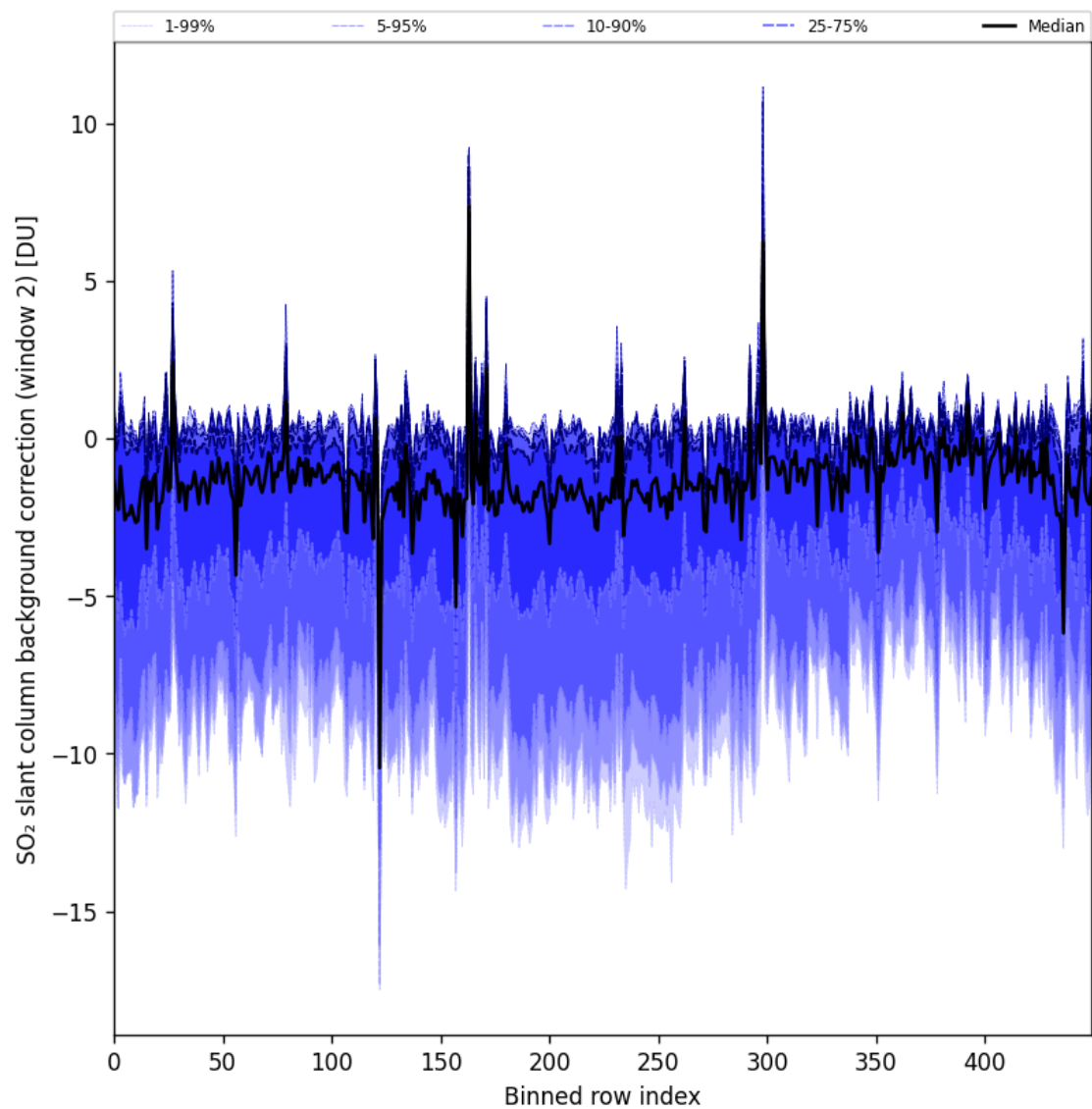
Figure 96: Along track statistics of “SO 2 slant column background correction (window 2)” for 2025-04-21 to 2025-04-23
