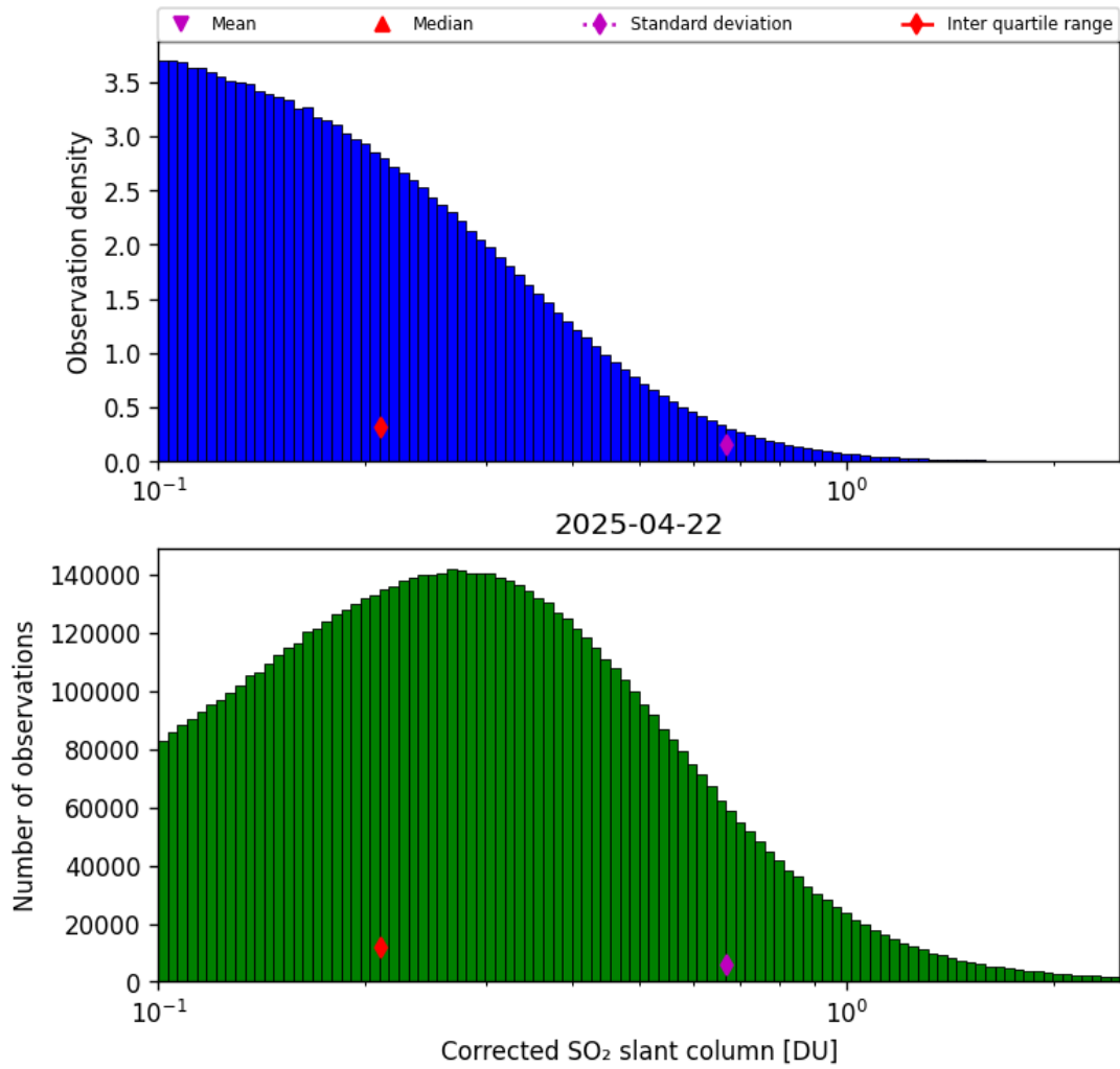
Figure 60: Histogram of "Corrected SO 2 slant column" for 2025-04-21 to 2025-04-23
