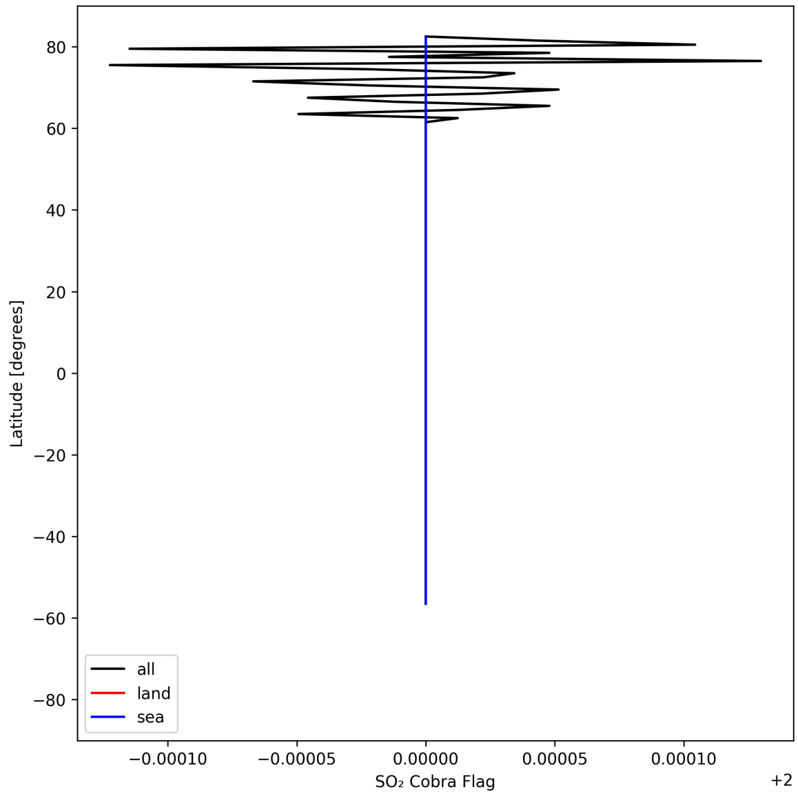
Figure 49: Zonal average of “SO 2 Cobra Flag” for 2025-04-21 to 2025-04-23.
