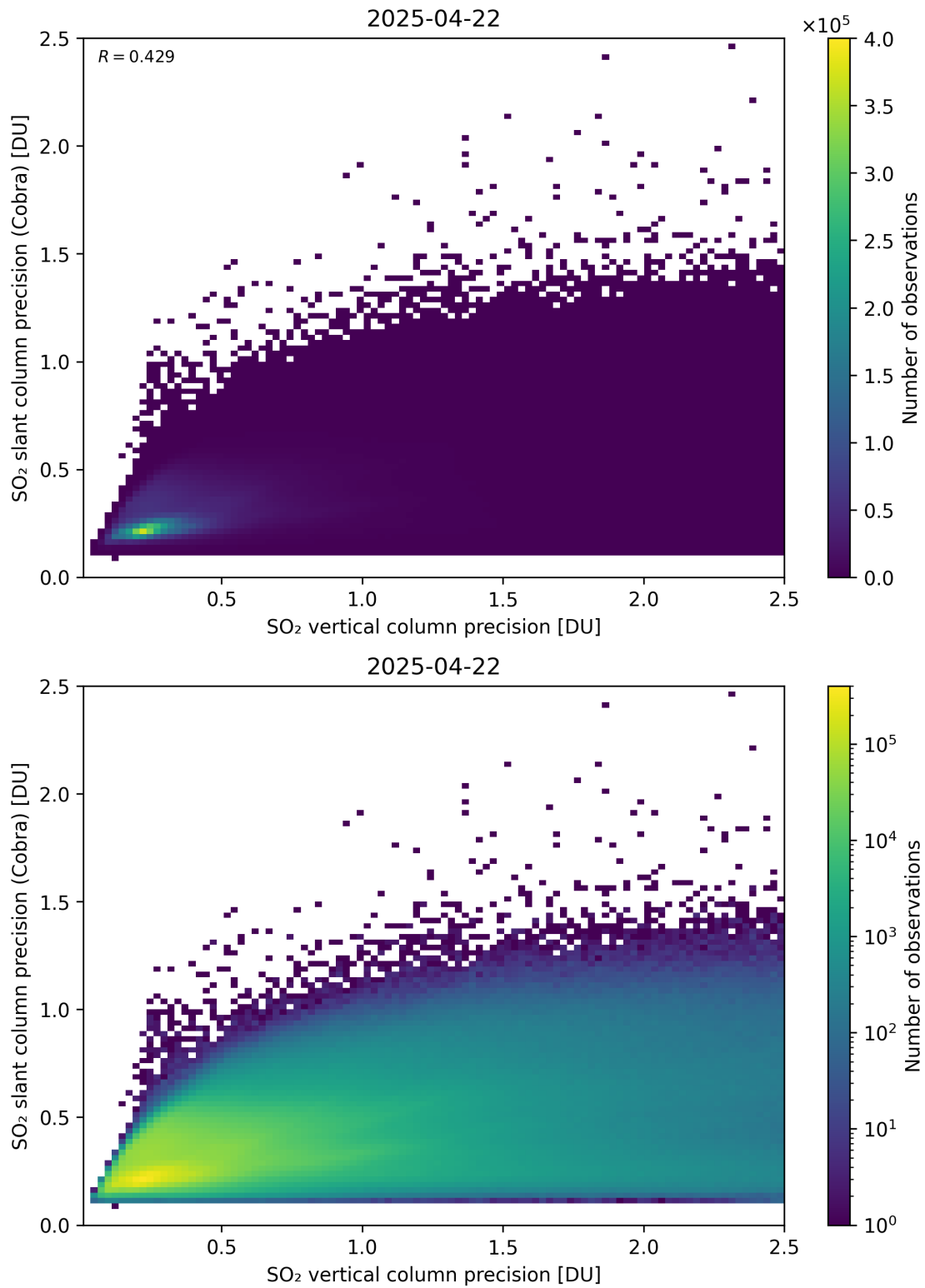
Figure 337: Scatter density plot of “SO 2 vertical column precision” against “SO 2 slant column precision (Cobra)” for 2025-04-21 to 2025-04-23.
