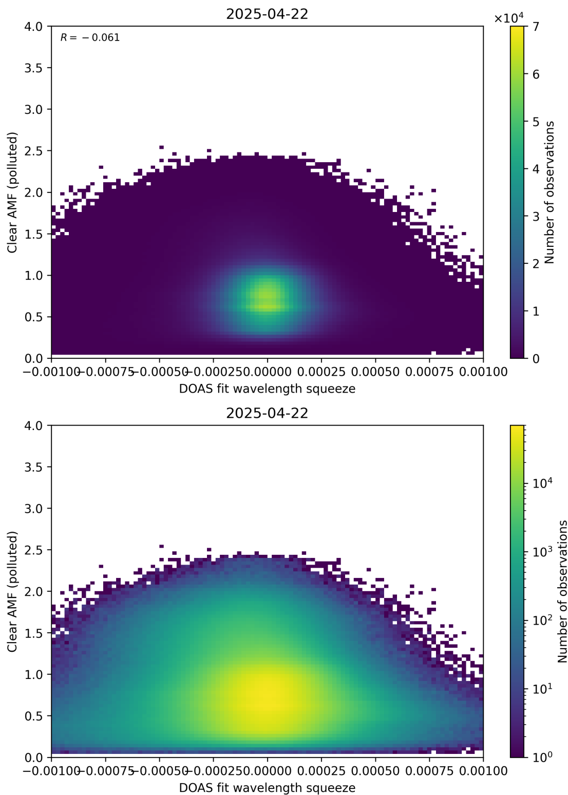
Figure 144: Scatter density plot of “DOAS fit wavelength squeeze” against “Clear AMF (polluted)” for 2025-04-21 to 2025-04-23.
