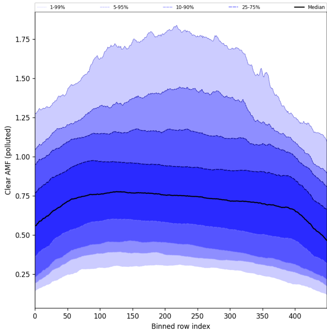
Figure 107: Along track statistics of “Clear AMF (polluted)” for 2025-04-21 to 2025-04-23
