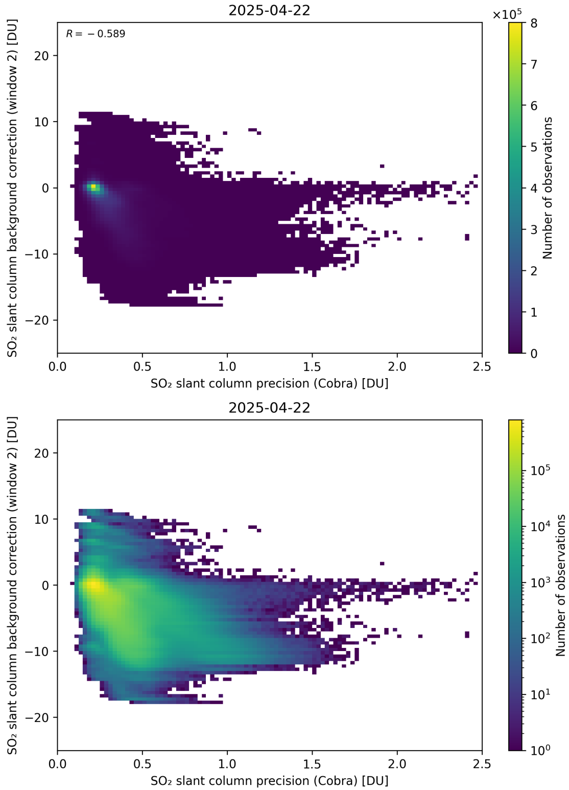
Figure 200: Scatter density plot of “SO 2 slant column precision (Cobra)” against “SO 2 slant column background correction (window 2)” for 2025-04-21 to 2025-04-23.
