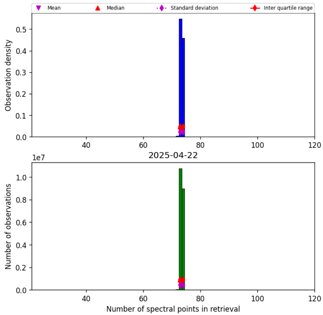
Figure 82: Histogram of “Number of spectral points in retrieval” for 2025-04-21 to 2025-04-23
