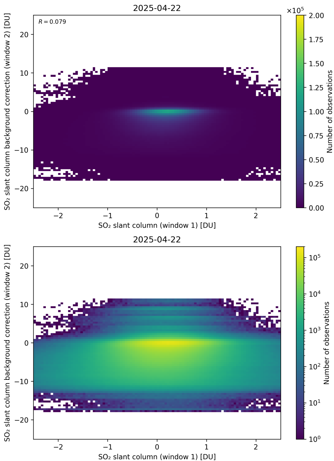
Figure 263: Scatter density plot of “SO 2 slant column (window 1)” against “SO 2 slant column background correction (window 2)” for 2025-04-21 to 2025-04-23.
