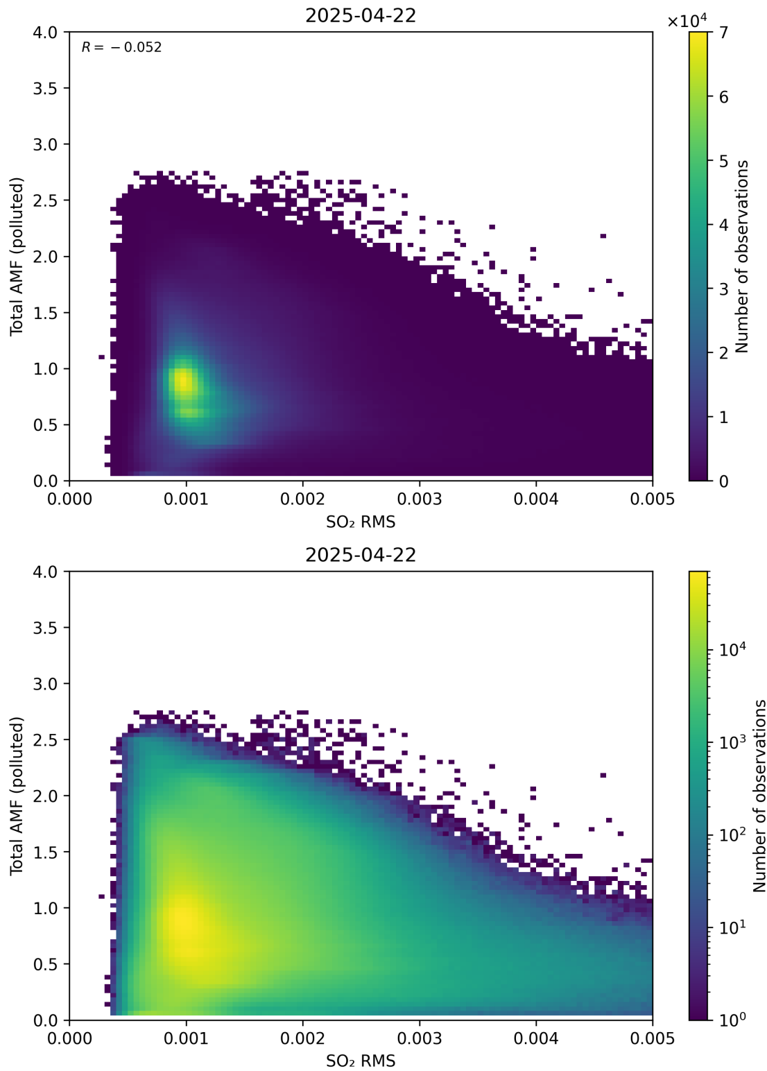
Figure 148: Scatter density plot of “SO 2 RMS” against “Total AMF (polluted)” for 2025-04-21 to 2025-04-23.
