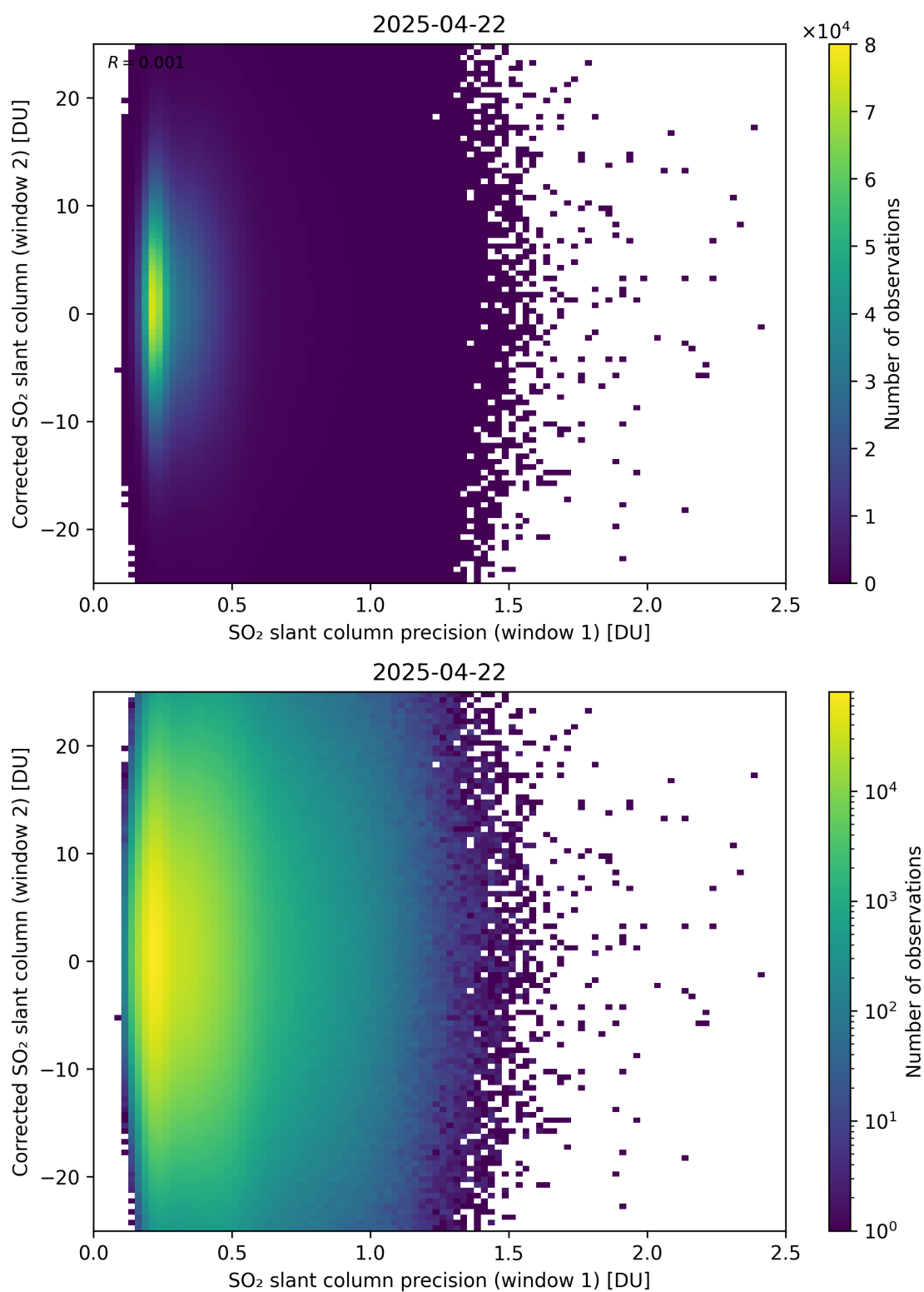
Figure 275: Scatter density plot of “SO 2 slant column precision (window 1)” against “Corrected SO 2 slant column (window 2)” for 2025-04-21 to 2025-04-23.
