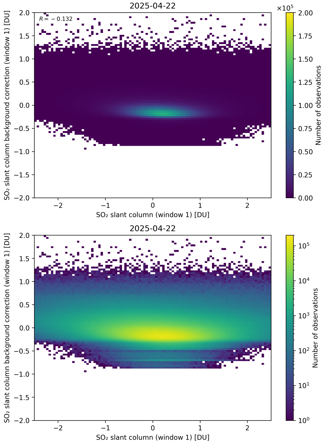
Figure 262: Scatter density plot of “SO 2 slant column (window 1)” against “SO 2 slant column background correction (window 1)” for 2025-04-21 to 2025-04-23.
