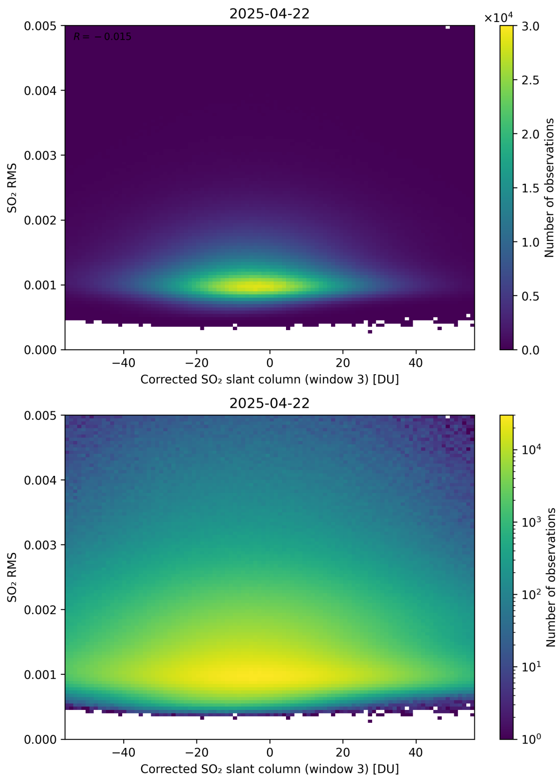
Figure 258: Scatter density plot of “Corrected SO 2 slant column (window 3)” against “SO 2 RMS” for 2025-04-21 to 2025-04-23.
