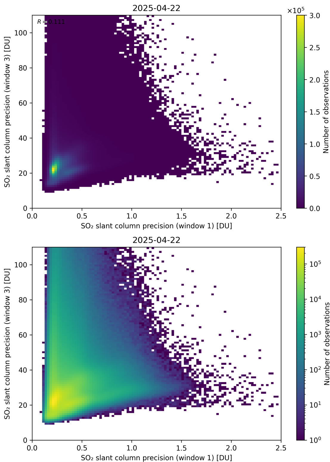
Figure 279: Scatter density plot of “SO 2 slant column precision (window 1)” against “SO 2 slant column precision (window 3)” for 2025-04-21 to 2025-04-23.
