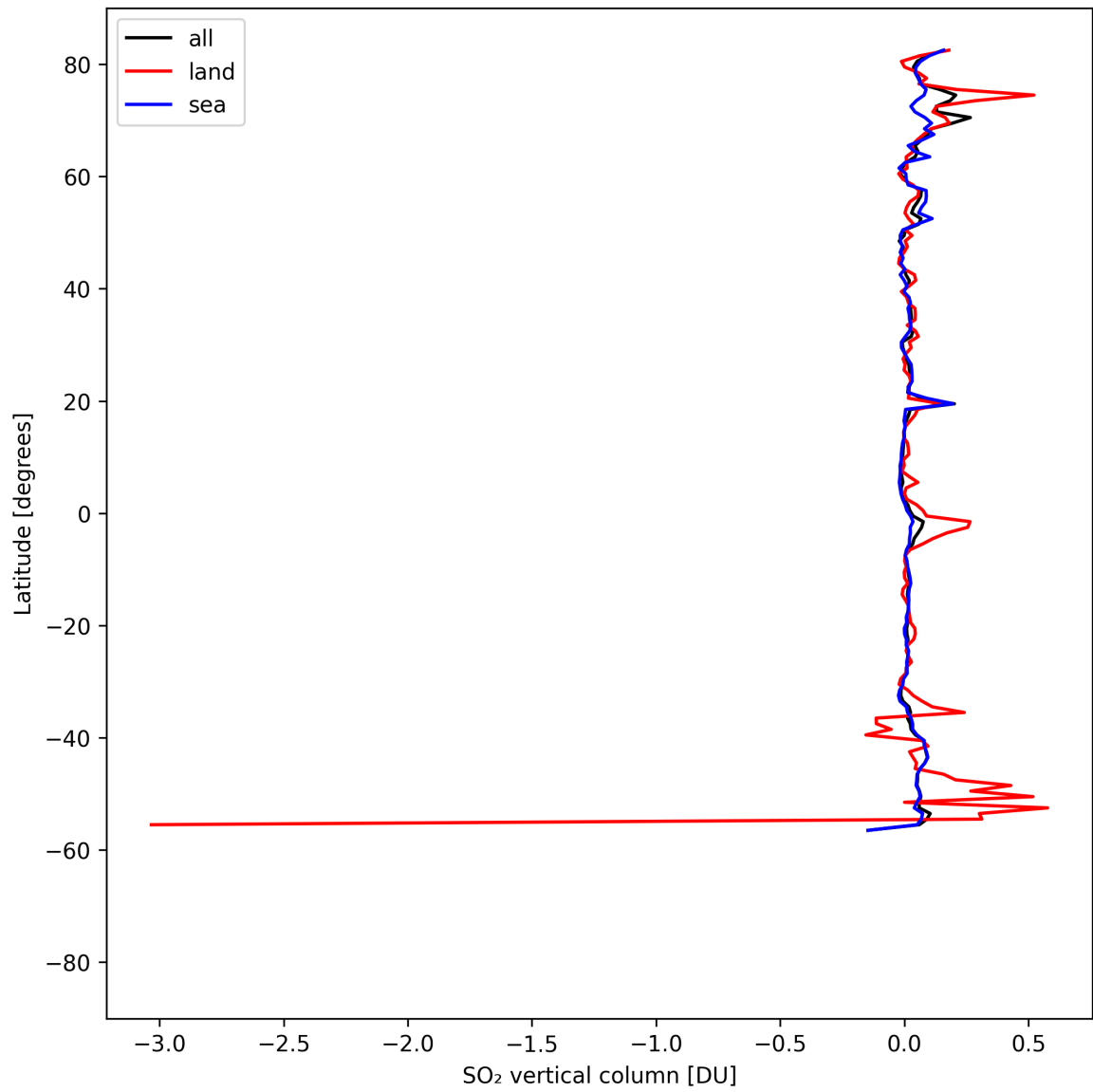
Figure 32: Zonal average of “SO 2 vertical column” for 2025-04-21 to 2025-04-23.
