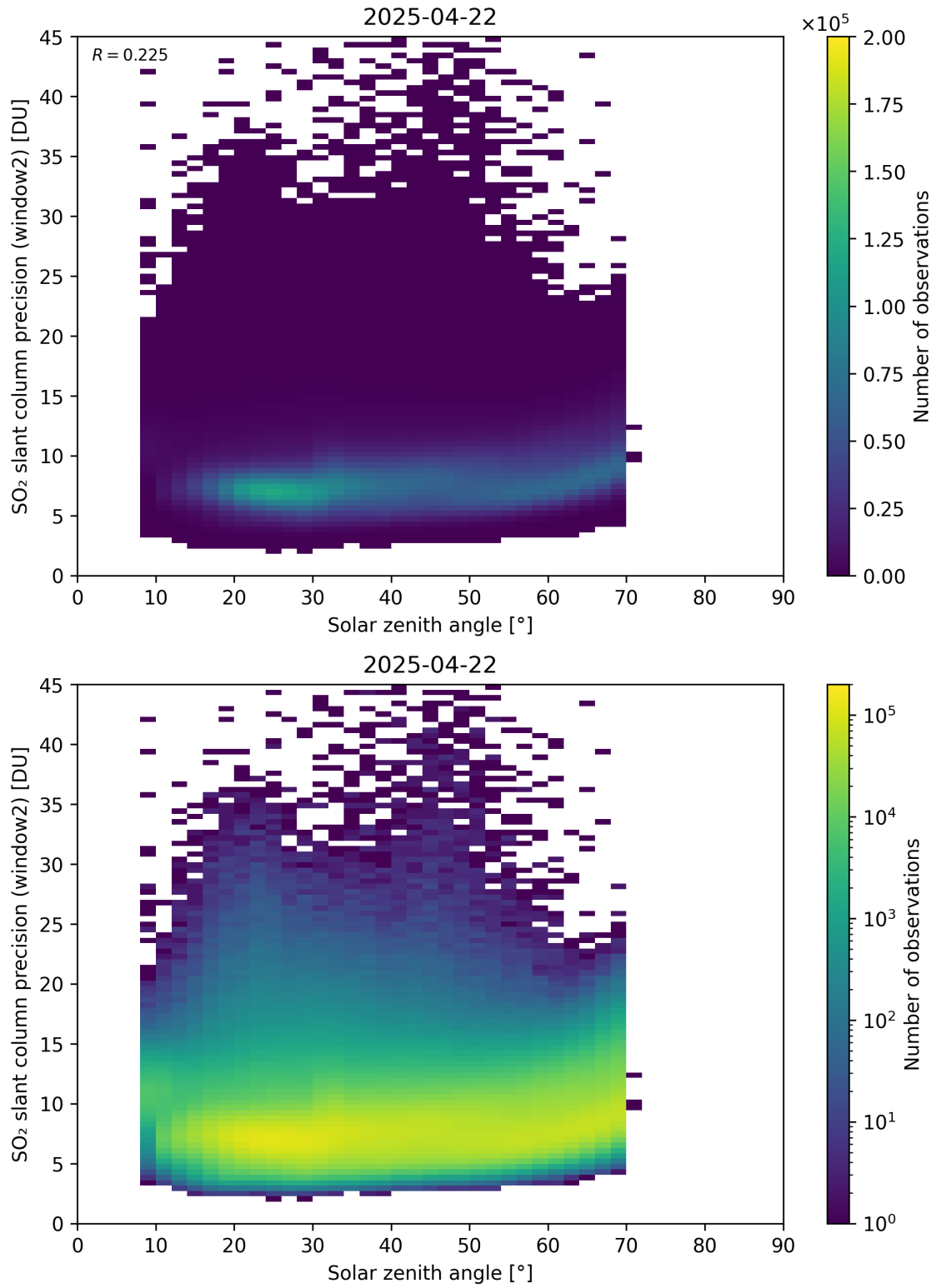
Figure 186: Scatter density plot of “Solar zenith angle” against “SO 2 slant column precision (window2)” for 2025-04-21 to 2025-04-23.
