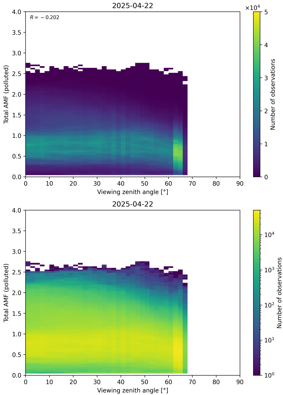
Figure 381: Scatter density plot of “Viewing zenith angle” against “Total AMF (polluted)” for 2025-04-21 to 2025-04-23.
