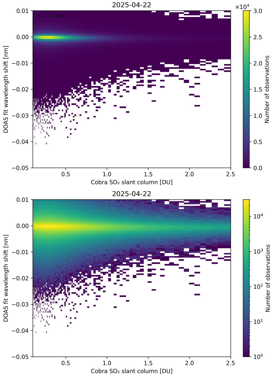
Figure 196: Scatter density plot of “Cobra SO 2 slant column” against “DOAS fit wavelength shift” for 2025-04-21 to 2025-04-23.
