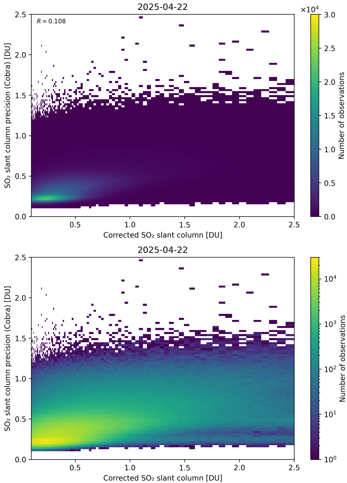
Figure 234: Scatter density plot of “Corrected SO 2 slant column” against “SO 2 slant column precision (Cobra)” for 2025-04-21 to 2025-04-23.
