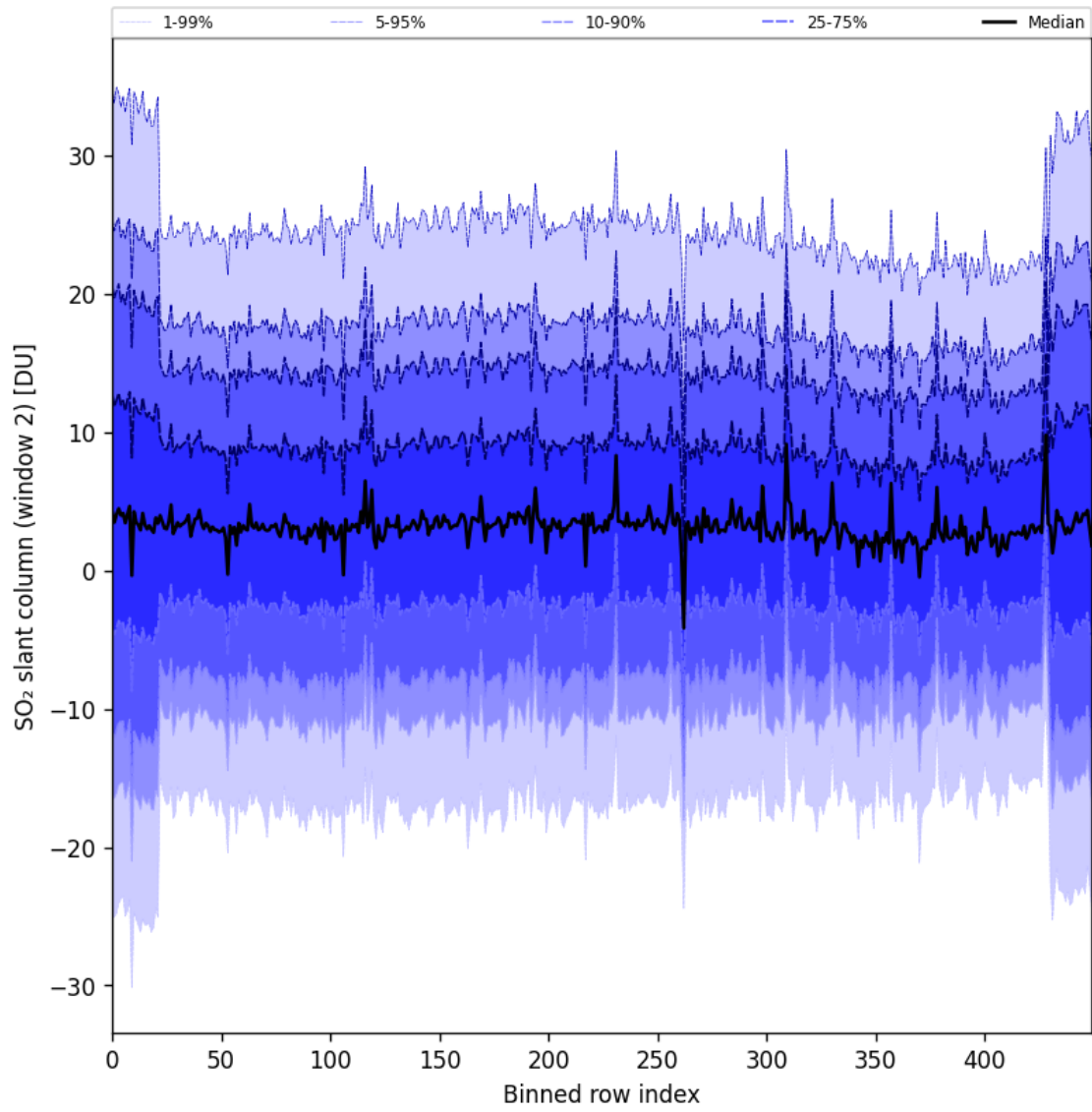
Figure 93: Along track statistics of “SO 2 slant column (window 2)” for 2025-04-21 to 2025-04-23
