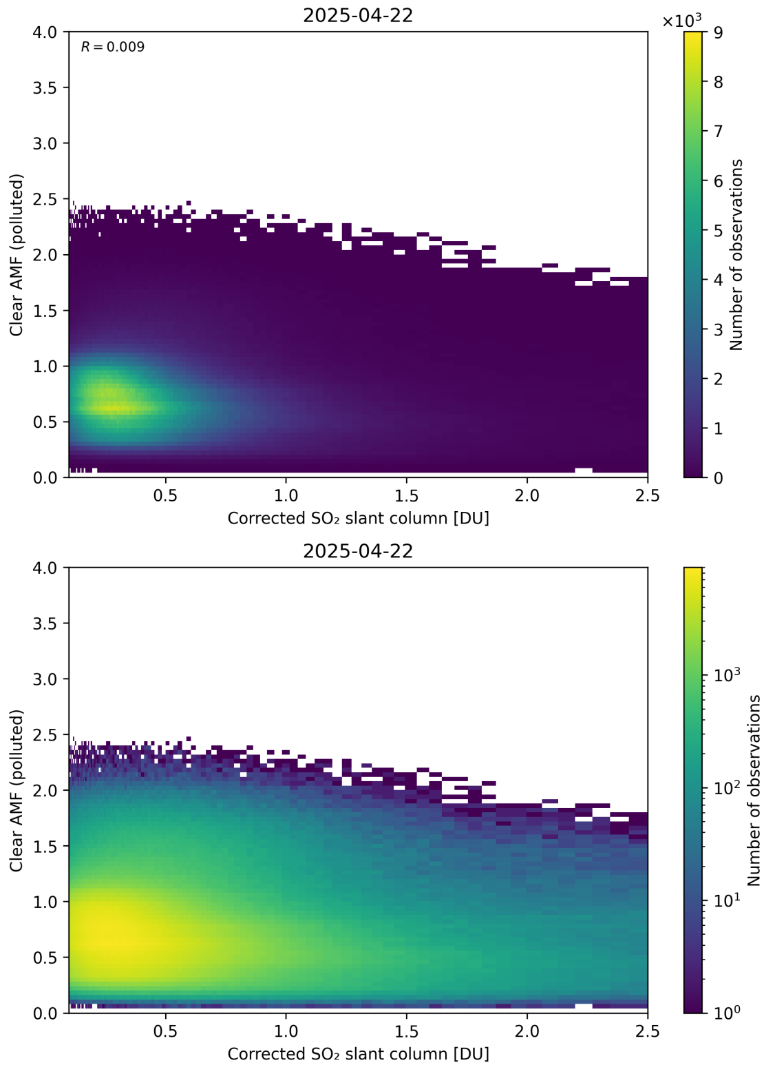
Figure 232: Scatter density plot of “Corrected SO 2 slant column” against “Clear AMF (polluted)” for 2025-04-21 to 2025-04-23.
