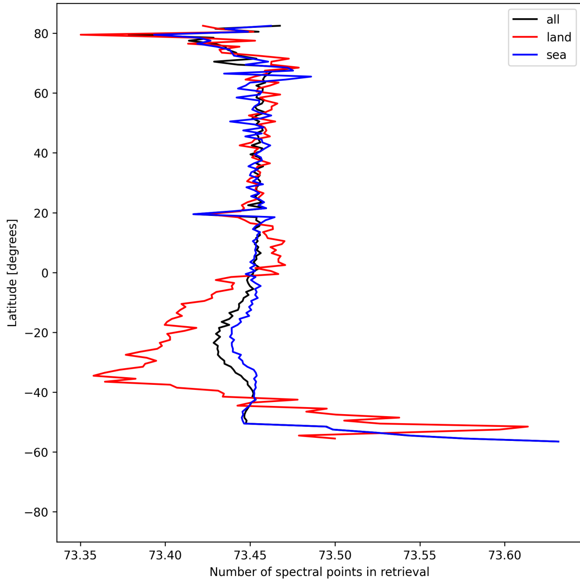
Figure 56: Zonal average of “Number of spectral points in retrieval” for 2025-04-21 to 2025-04-23.
