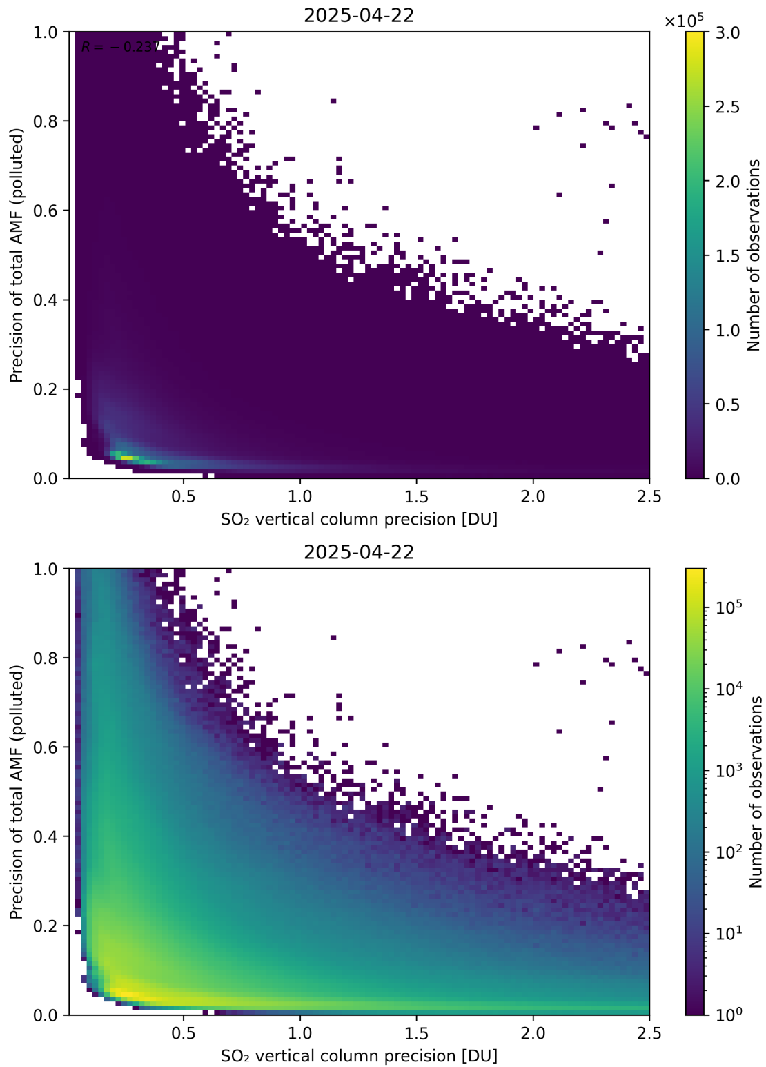
Figure 347: Scatter density plot of “SO 2 vertical column precision” against “Precision of total AMF (polluted)” for 2025-04-21 to 2025-04-23.
