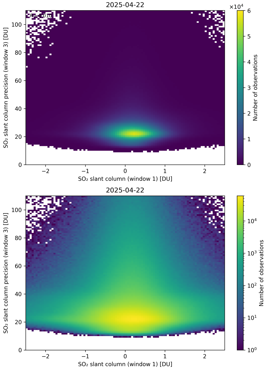
Figure 288: Scatter density plot of “SO 2 slant column (window 1)” against “SO 2 slant column precision (window 3)” for 2025-04-21 to 2025-04-23.
