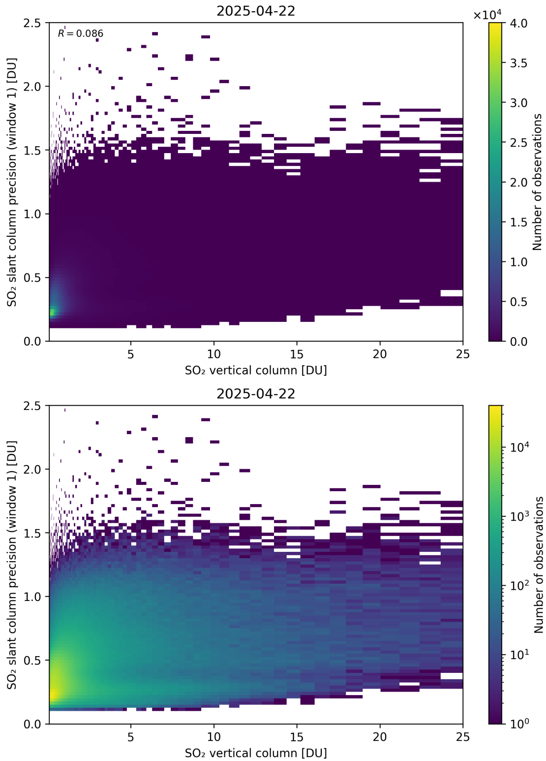
Figure 355: Scatter density plot of “SO 2 vertical column” against “SO 2 slant column precision (window 1)” for 2025-04-21 to 2025-04-23.
