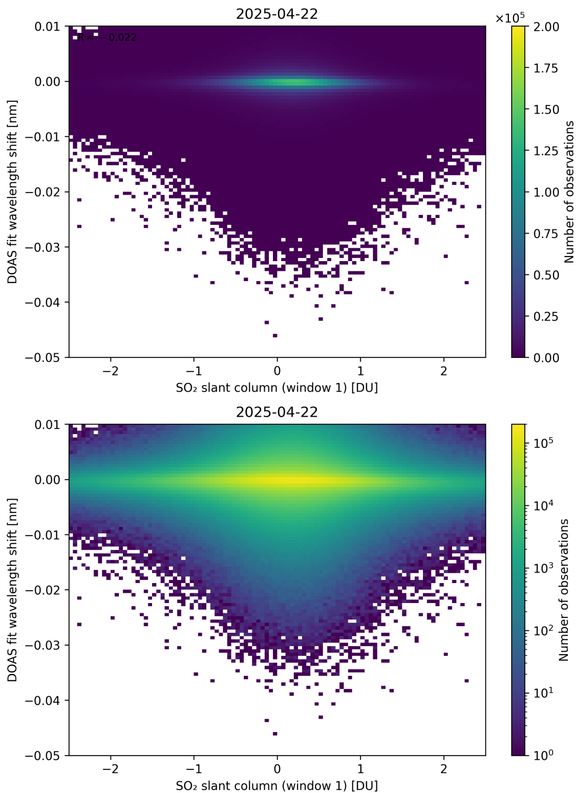
Figure 265: Scatter density plot of “SO 2 slant column (window 1)” against “DOAS fit wavelength shift” for 2025-04-21 to 2025-04-23.
