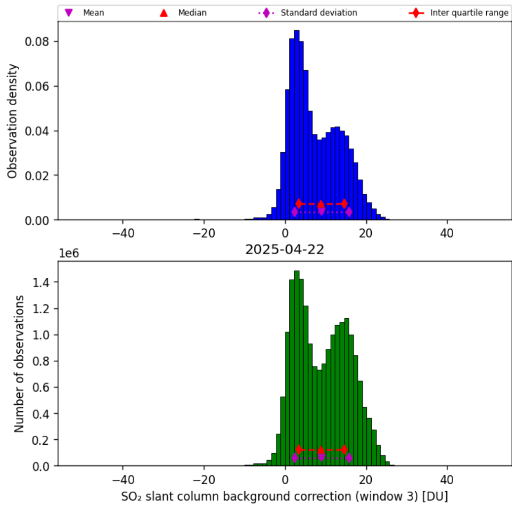
Figure 74: Histogram of "SO 2 slant column background correction (window 3)" for 2025-04-21 to 2025-04-23
