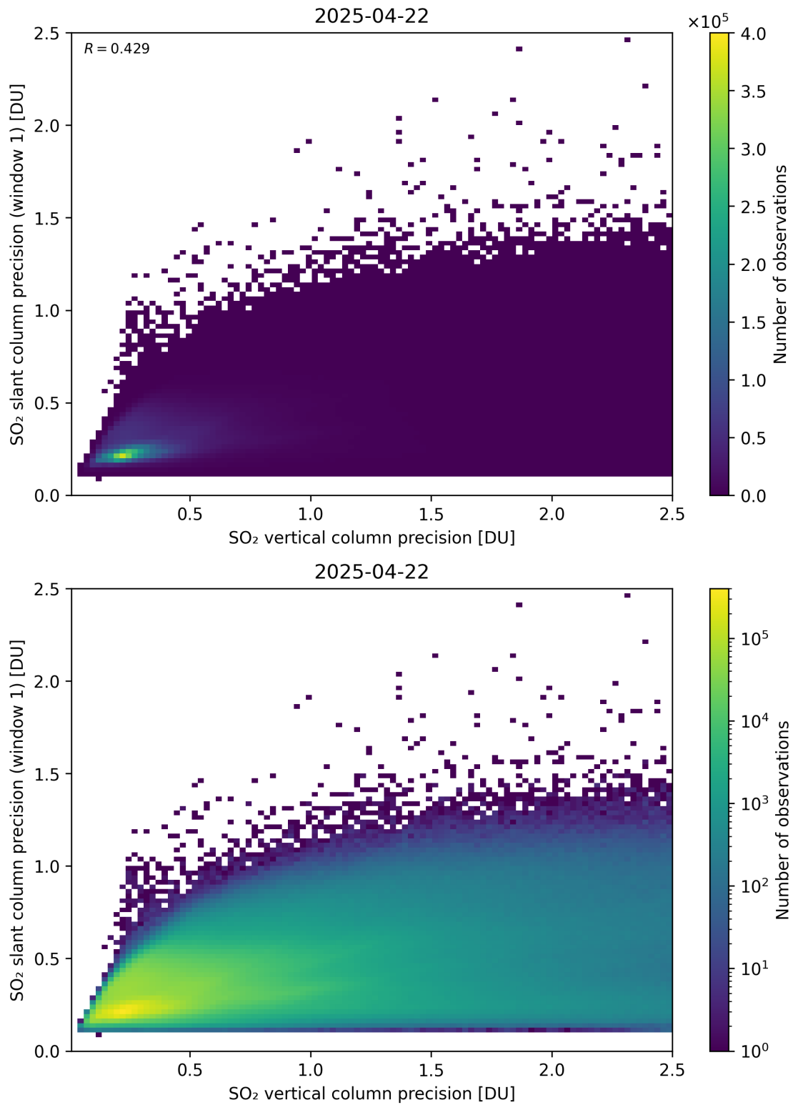
Figure 342: Scatter density plot of “SO 2 vertical column precision” against “SO 2 slant column precision (window 1)” for 2025-04-21 to 2025-04-23.
