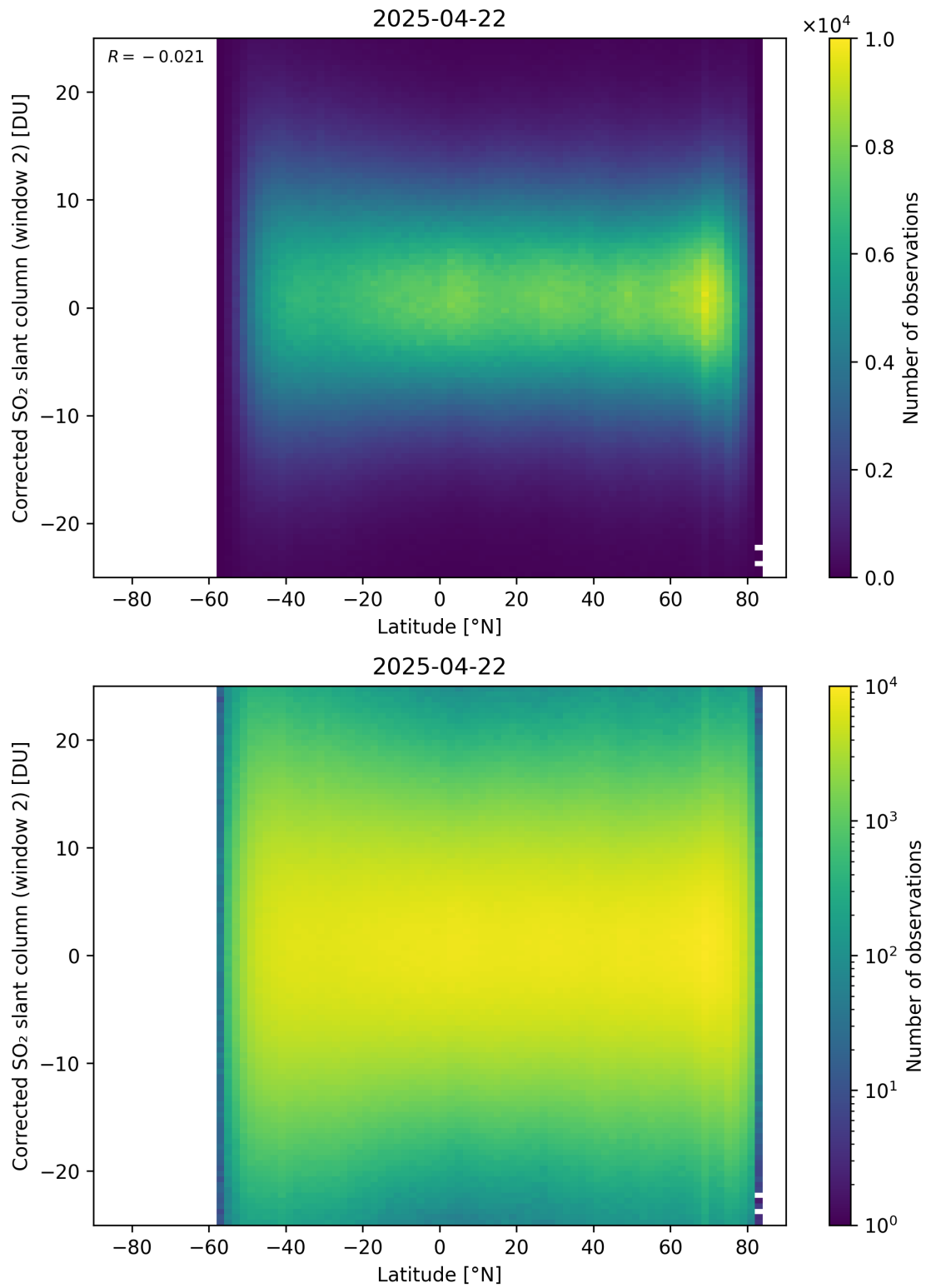
Figure 160: Scatter density plot of “Latitude” against “Corrected SO 2 slant column (window 2)” for 2025-04-21 to 2025-04-23.
