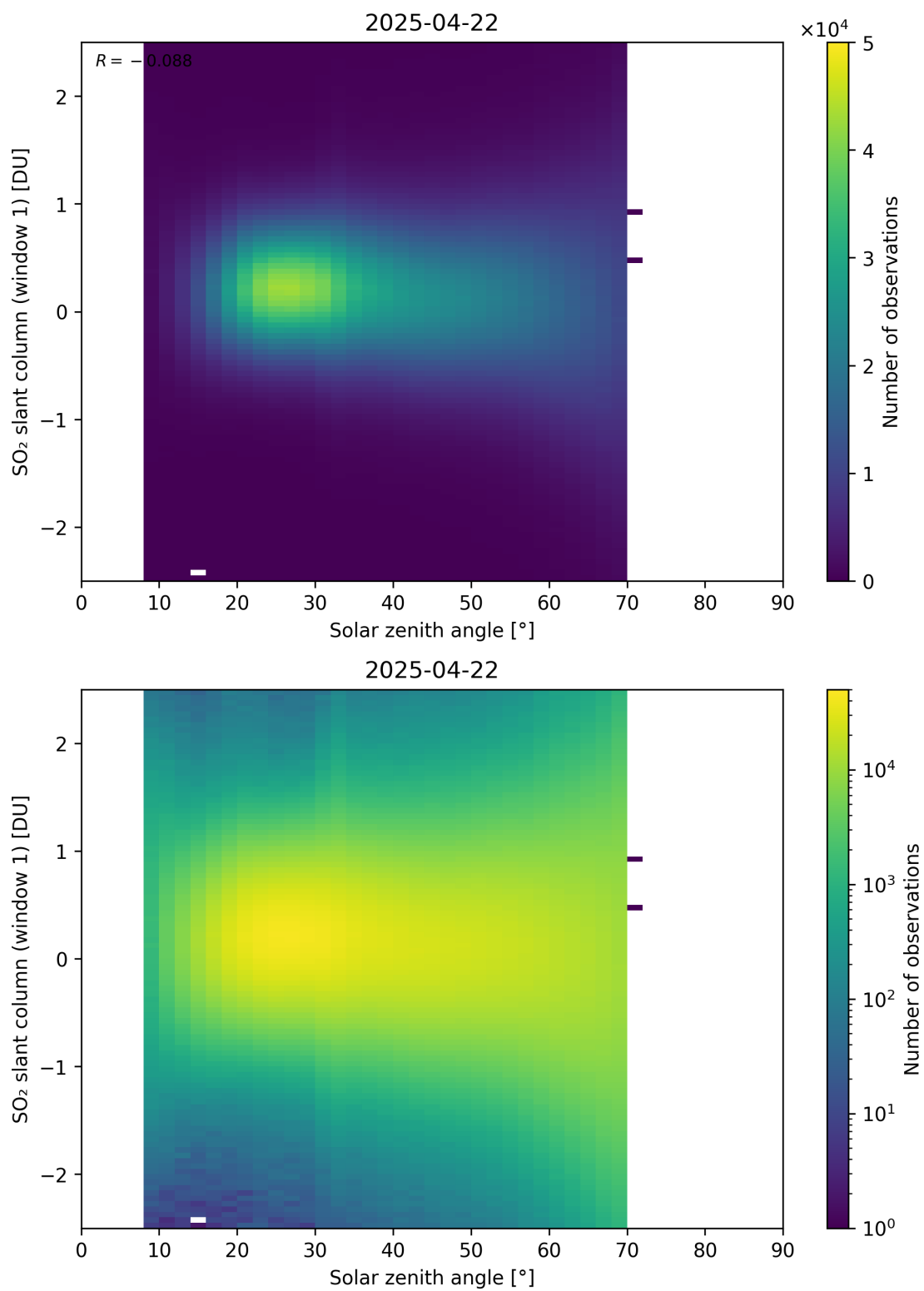
Figure 184: Scatter density plot of “Solar zenith angle” against “SO 2 slant column (window 1)” for 2025-04-21 to 2025-04-23.
