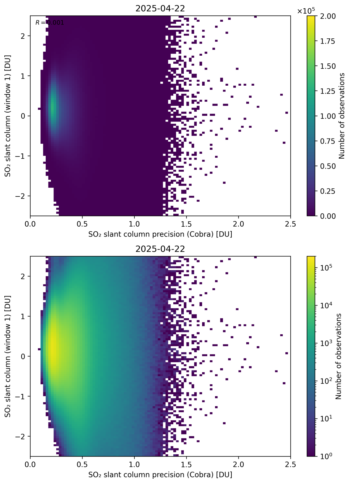
Figure 208: Scatter density plot of “SO 2 slant column precision (Cobra)” against “SO 2 slant column (window 1)” for 2025-04-21 to 2025-04-23.
