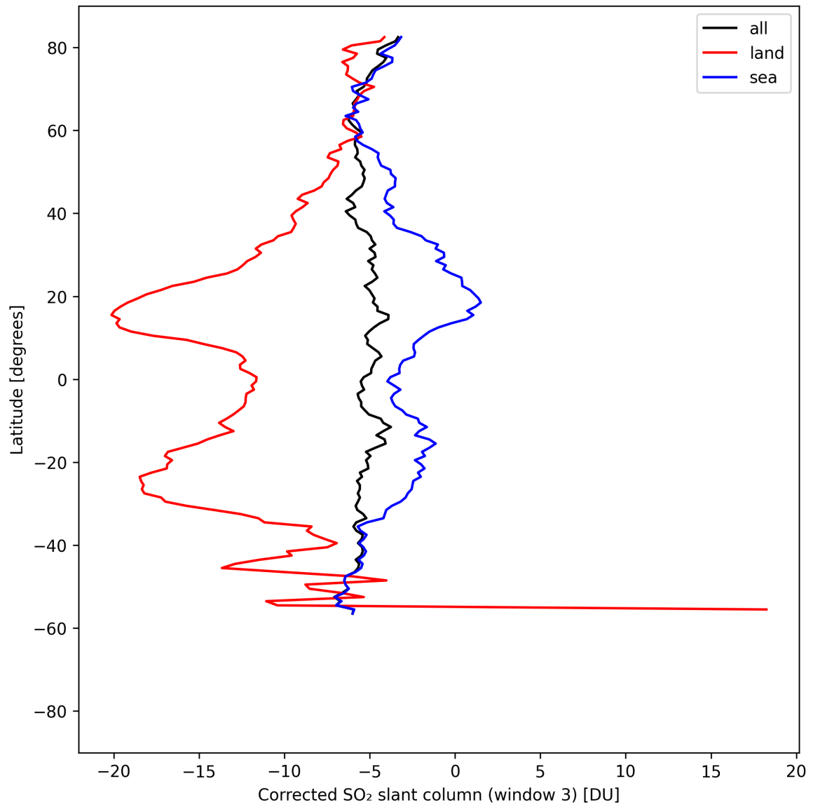
Figure 47: Zonal average of “Corrected SO 2 slant column (window 3)” for 2025-04-21 to 2025-04-23.
