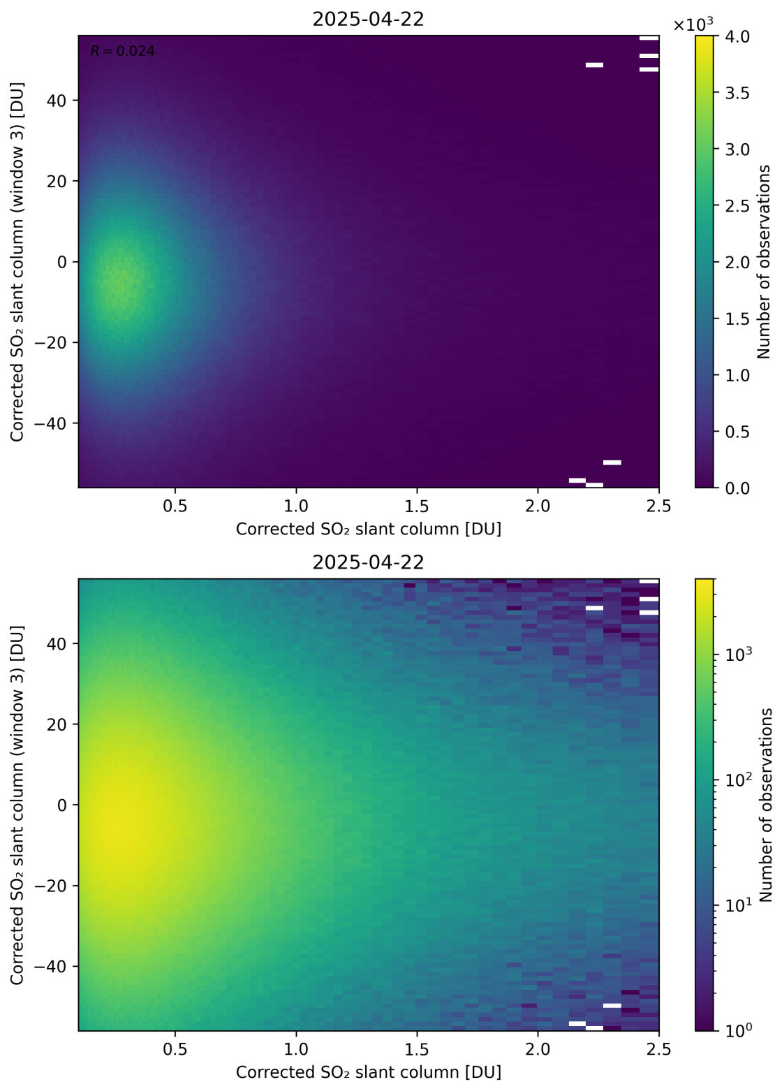
Figure 236: Scatter density plot of “Corrected SO 2 slant column” against “Corrected SO 2 slant column (window 3)” for 2025-04-21 to 2025-04-23.
