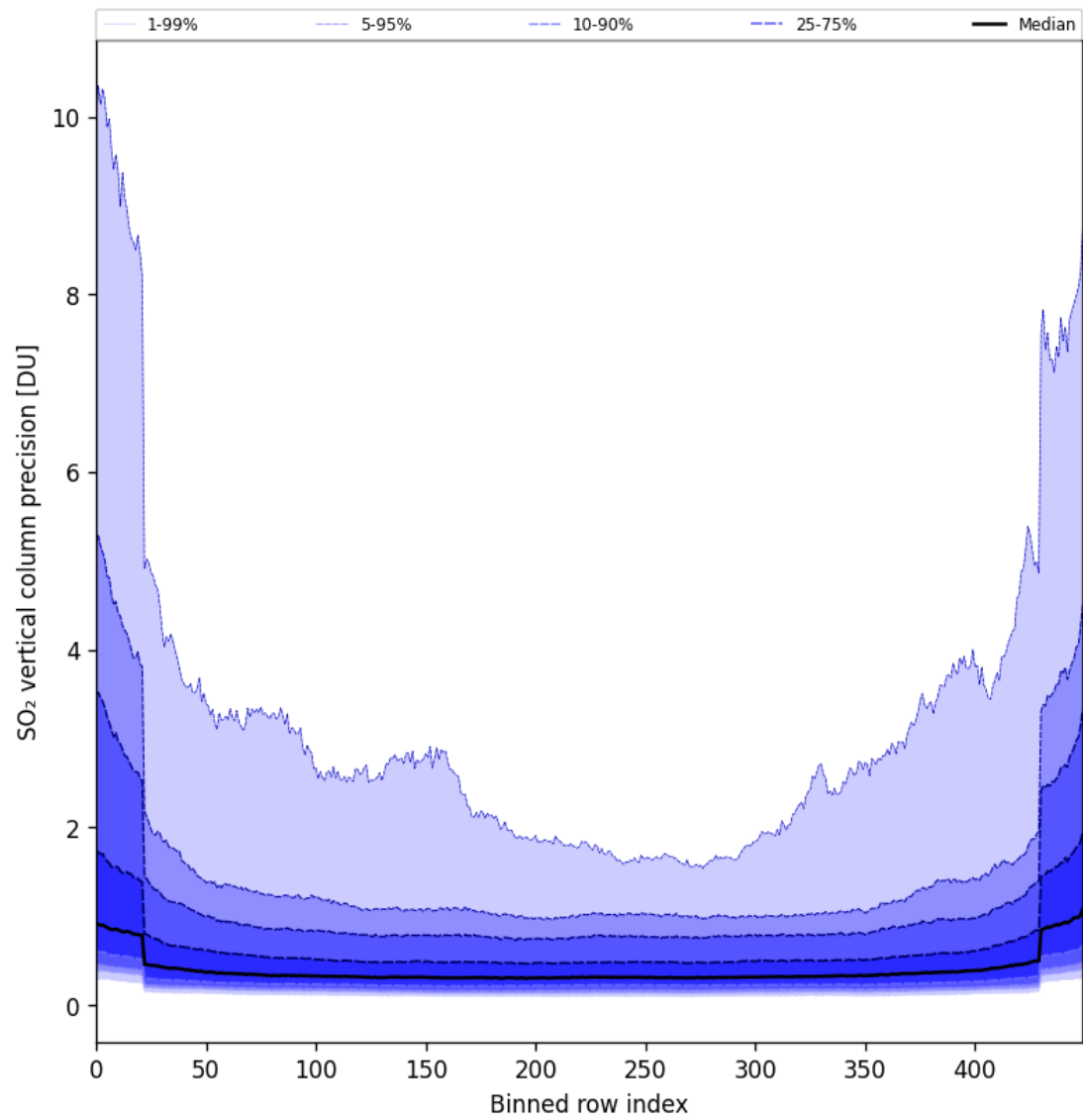
Figure 85: Along track statistics of “SO 2 vertical column precision” for 2025-04-21 to 2025-04-23
