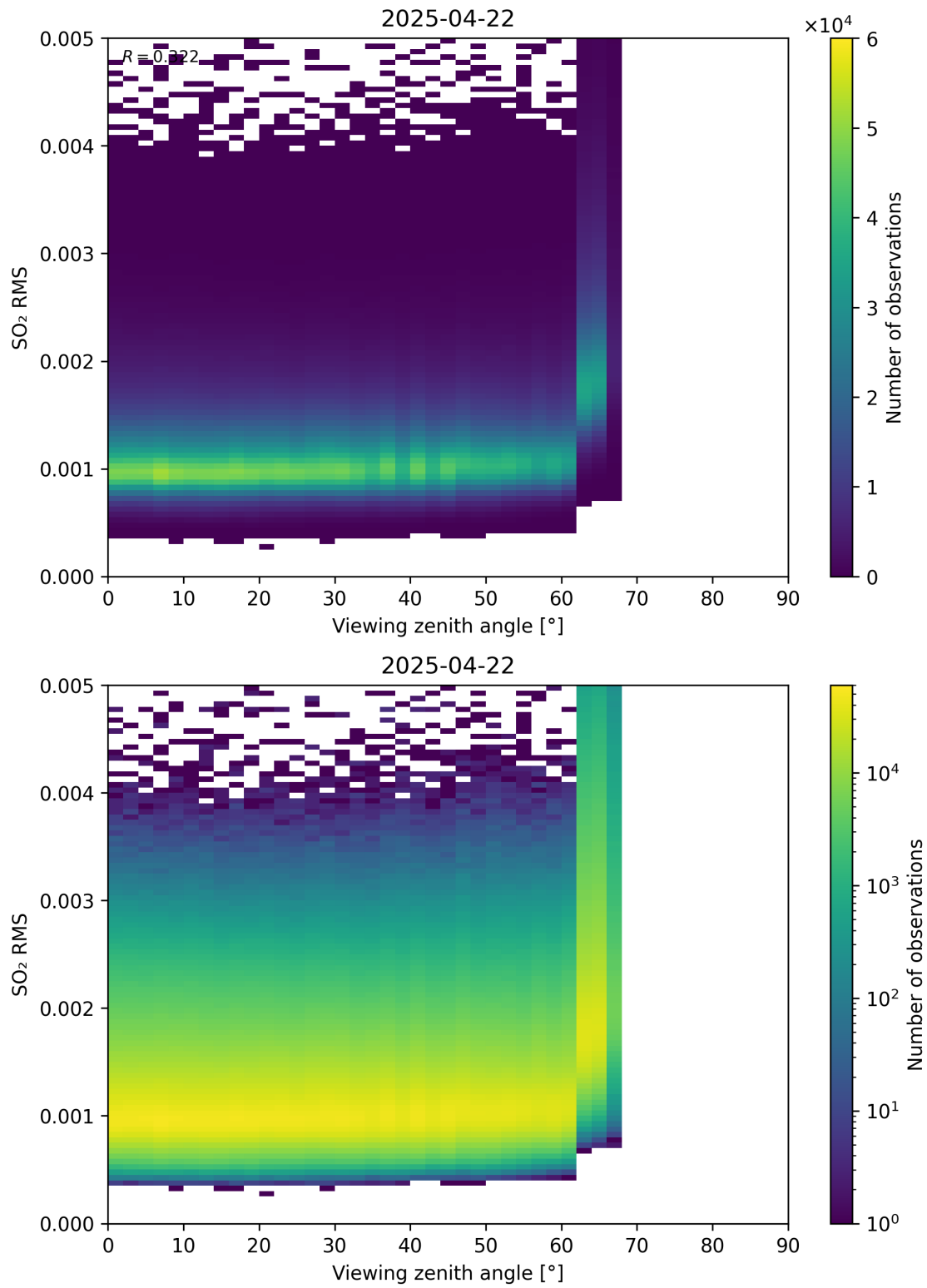
Figure 367: Scatter density plot of “Viewing zenith angle” against “SO 2 RMS” for 2025-04-21 to 2025-04-23.
