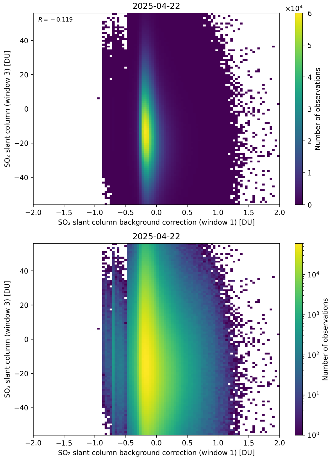
Figure 118: Scatter density plot of “SO 2 slant column background correction (window 1)” against “SO 2 slant column (window 3)” for 2025-04-21 to 2025-04-23.
