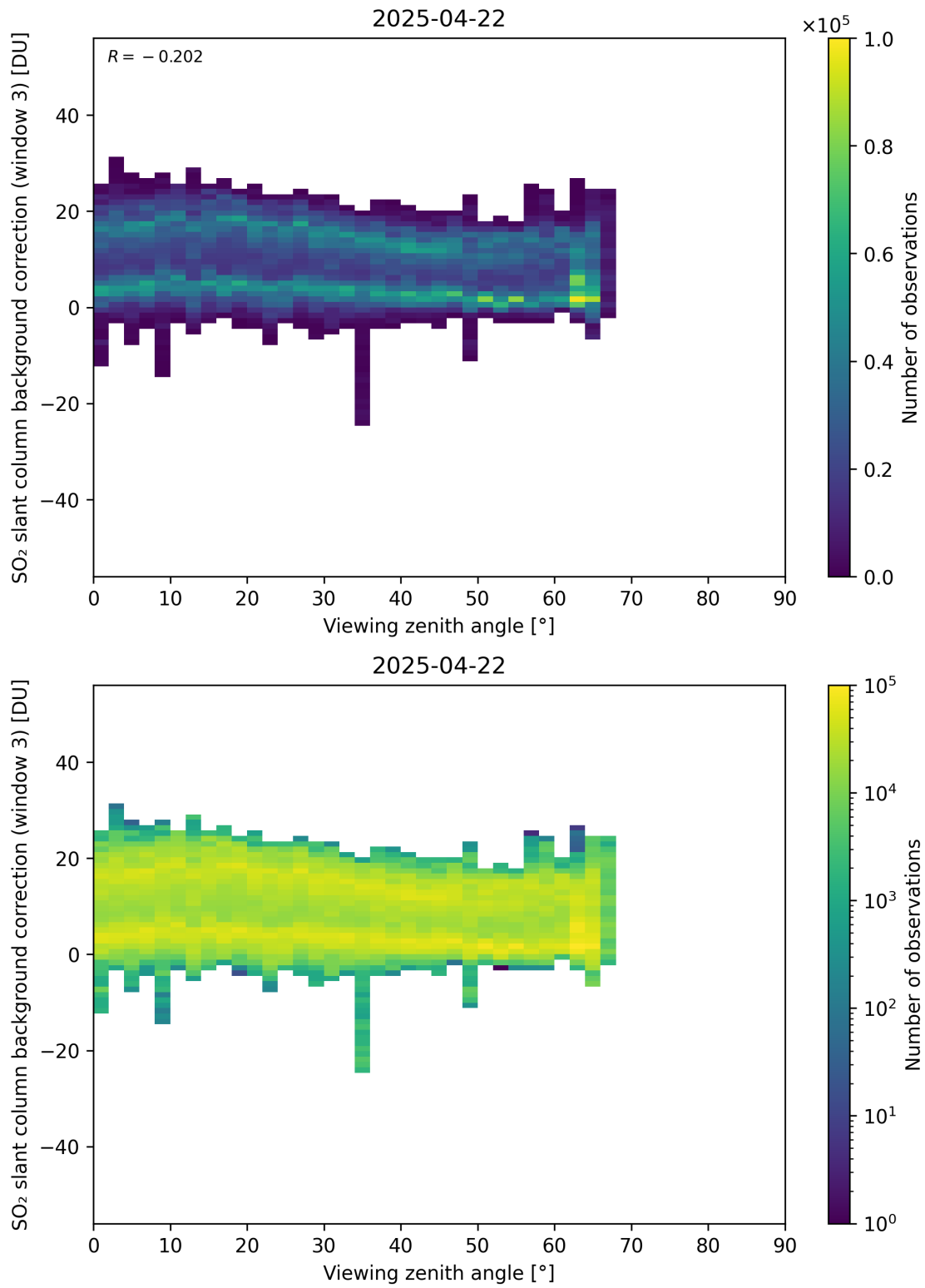
Figure 364: Scatter density plot of “Viewing zenith angle” against “SO 2 slant column background correction (window 3)” for 2025-04-21 to 2025-04-23.
