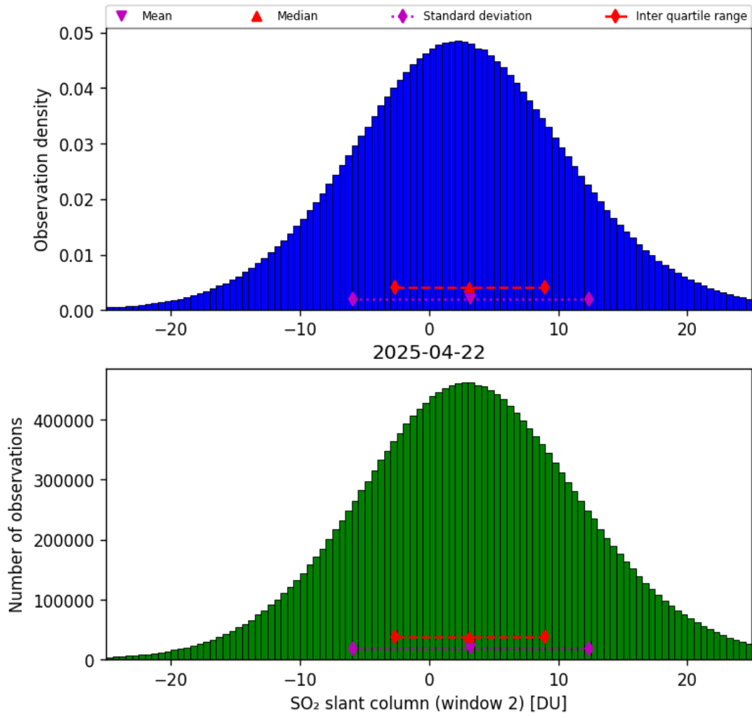
Figure 67: Histogram of “SO 2 slant column (window 2)” for 2025-04-21 to 2025-04-23
