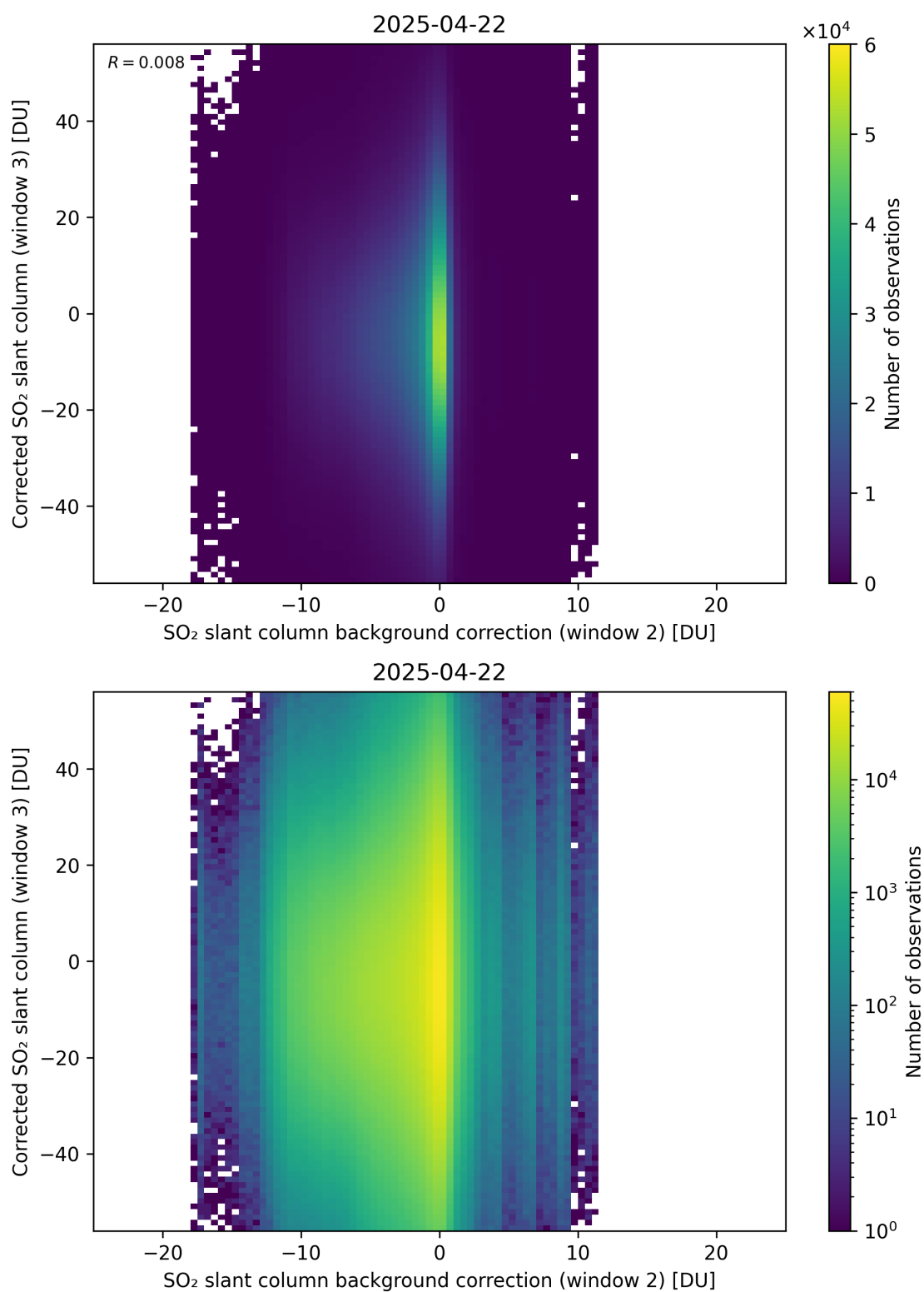
Figure 127: Scatter density plot of “SO 2 slant column background correction (window 2)” against “Corrected SO 2 slant column (window 3)” for 2025-04-21 to 2025-04-23.
