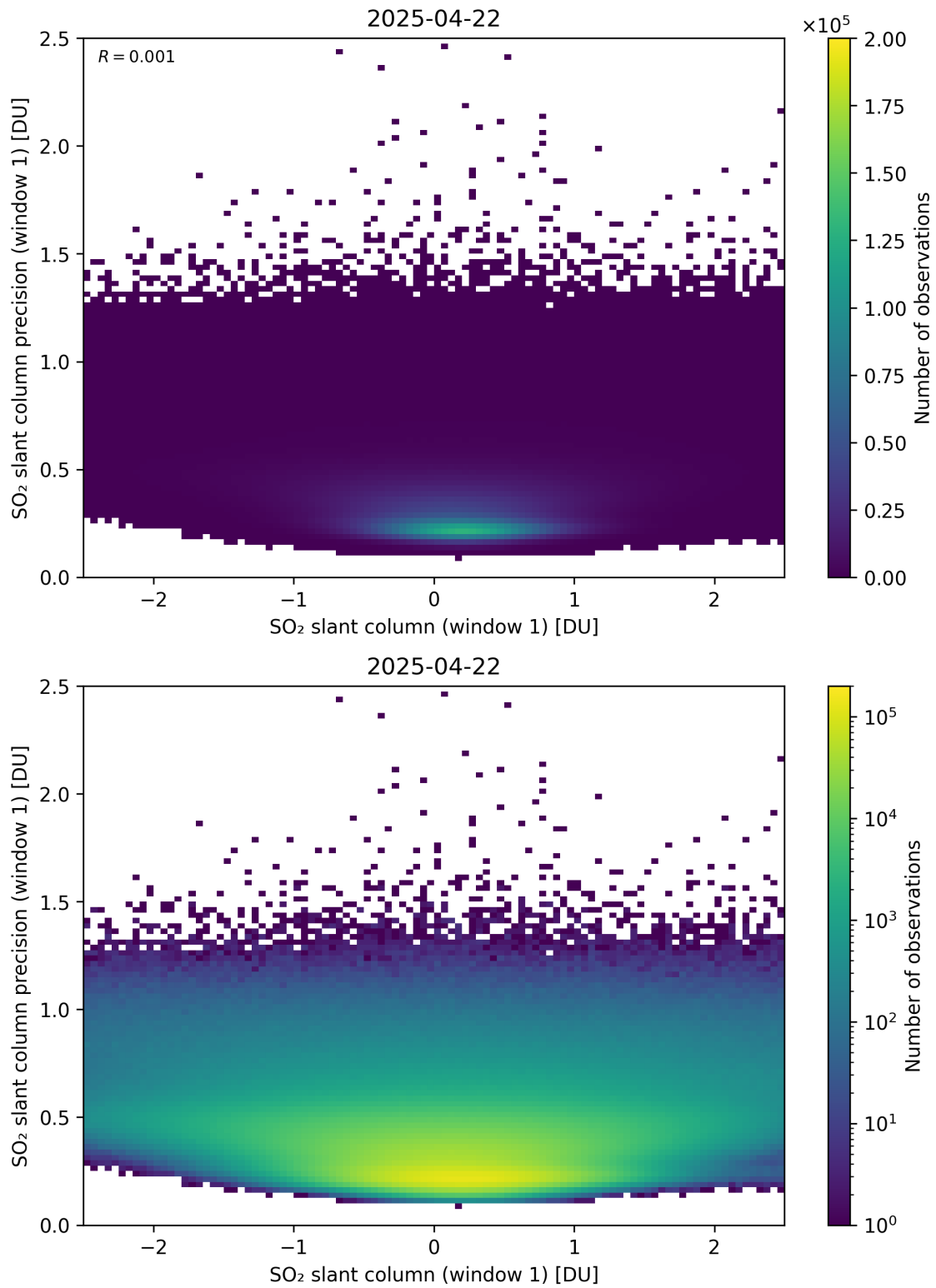
Figure 285: Scatter density plot of “SO 2 slant column (window 1)” against “SO 2 slant column precision (window 1)” for 2025-04-21 to 2025-04-23.
