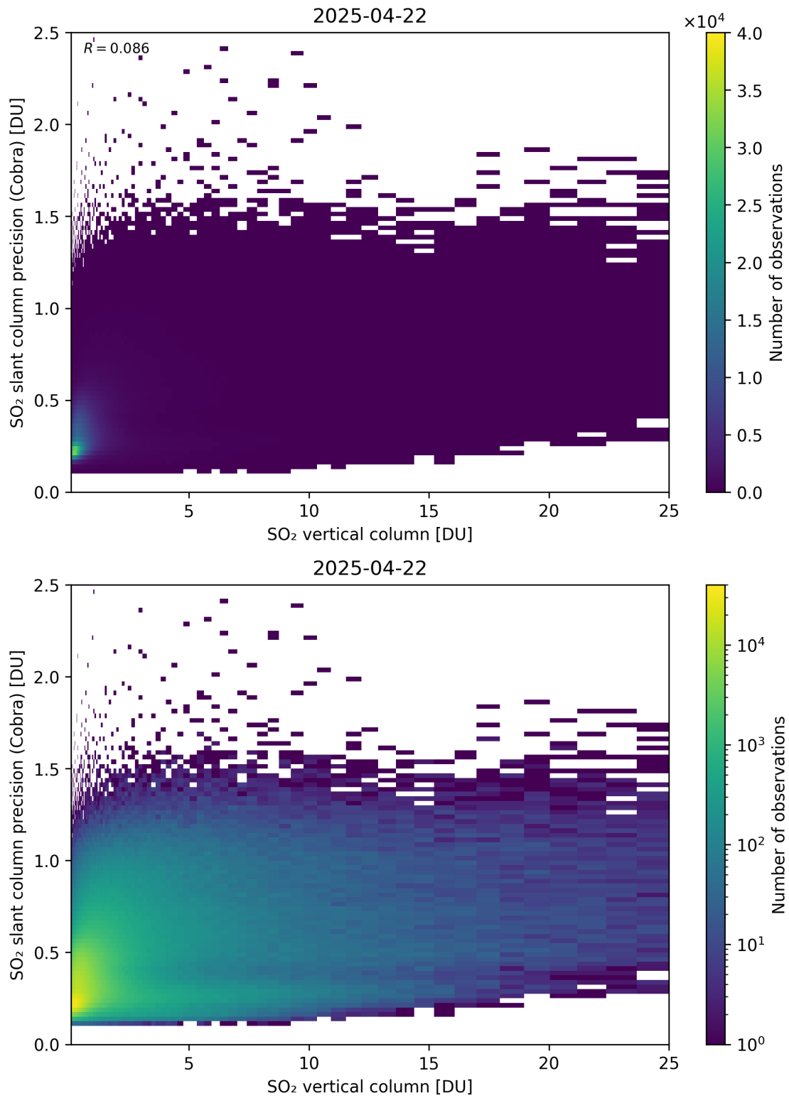
Figure 350: Scatter density plot of “SO 2 vertical column” against “SO 2 slant column precision (Cobra)” for 2025-04-21 to 2025-04-23.
