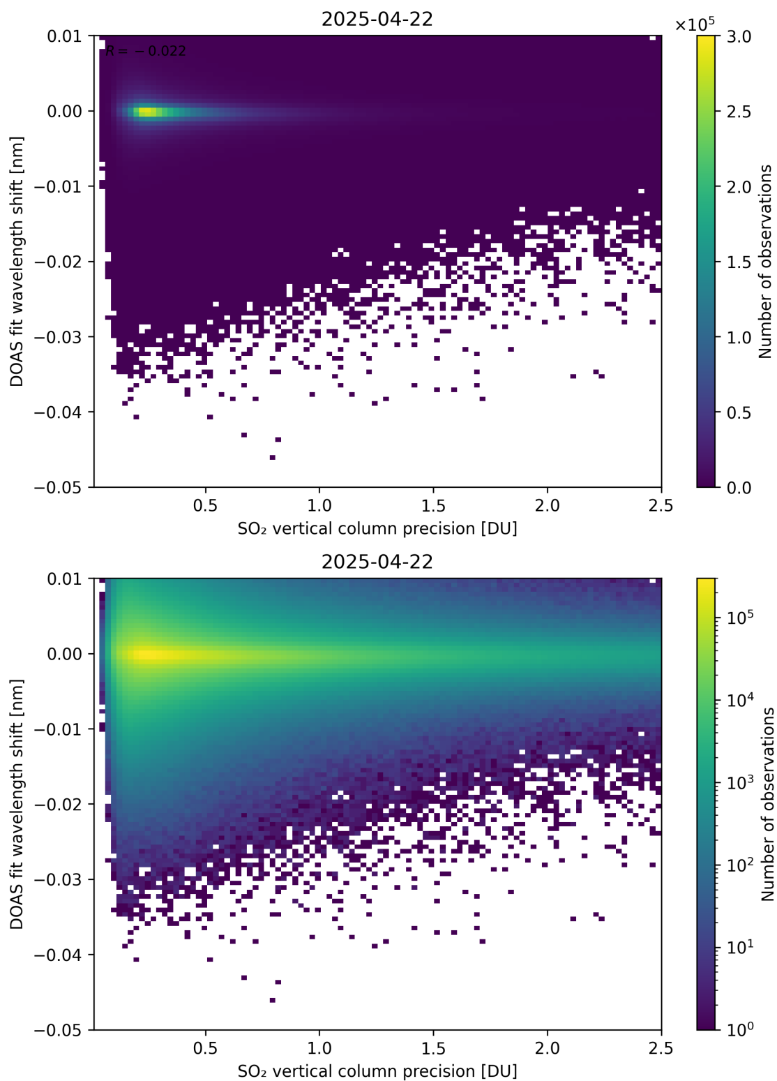
Figure 332: Scatter density plot of “SO 2 vertical column precision” against “DOAS fit wavelength shift” for 2025-04-21 to 2025-04-23.
