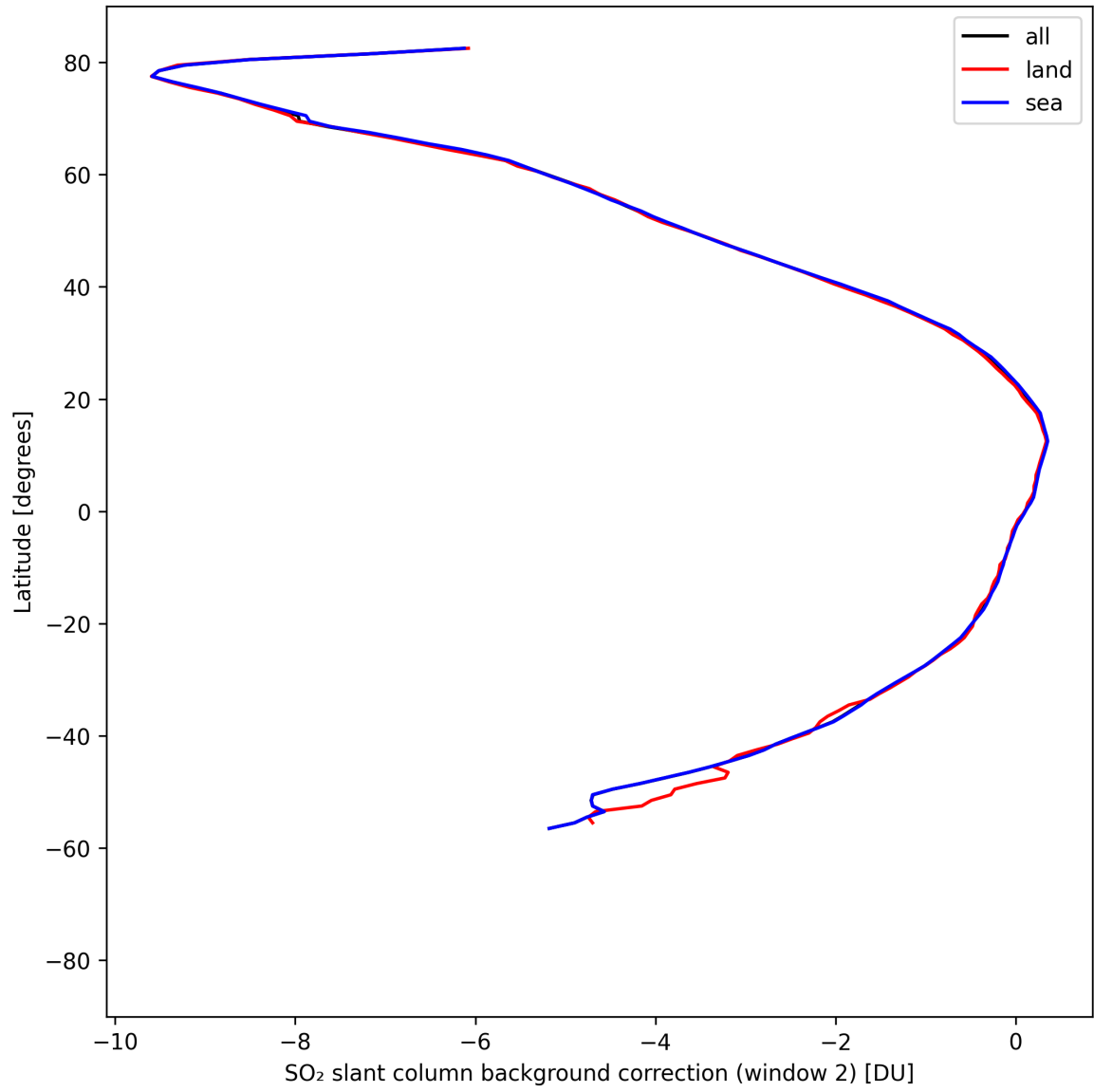
Figure 44: Zonal average of “SO 2 slant column background correction (window 2)” for 2025-04-21 to 2025-04-23.
