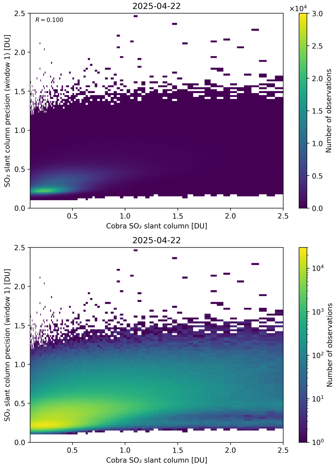
Figure 220: Scatter density plot of “Cobra SO 2 slant column” against “SO 2 slant column precision (window 1)” for 2025-04-21 to 2025-04-23.
