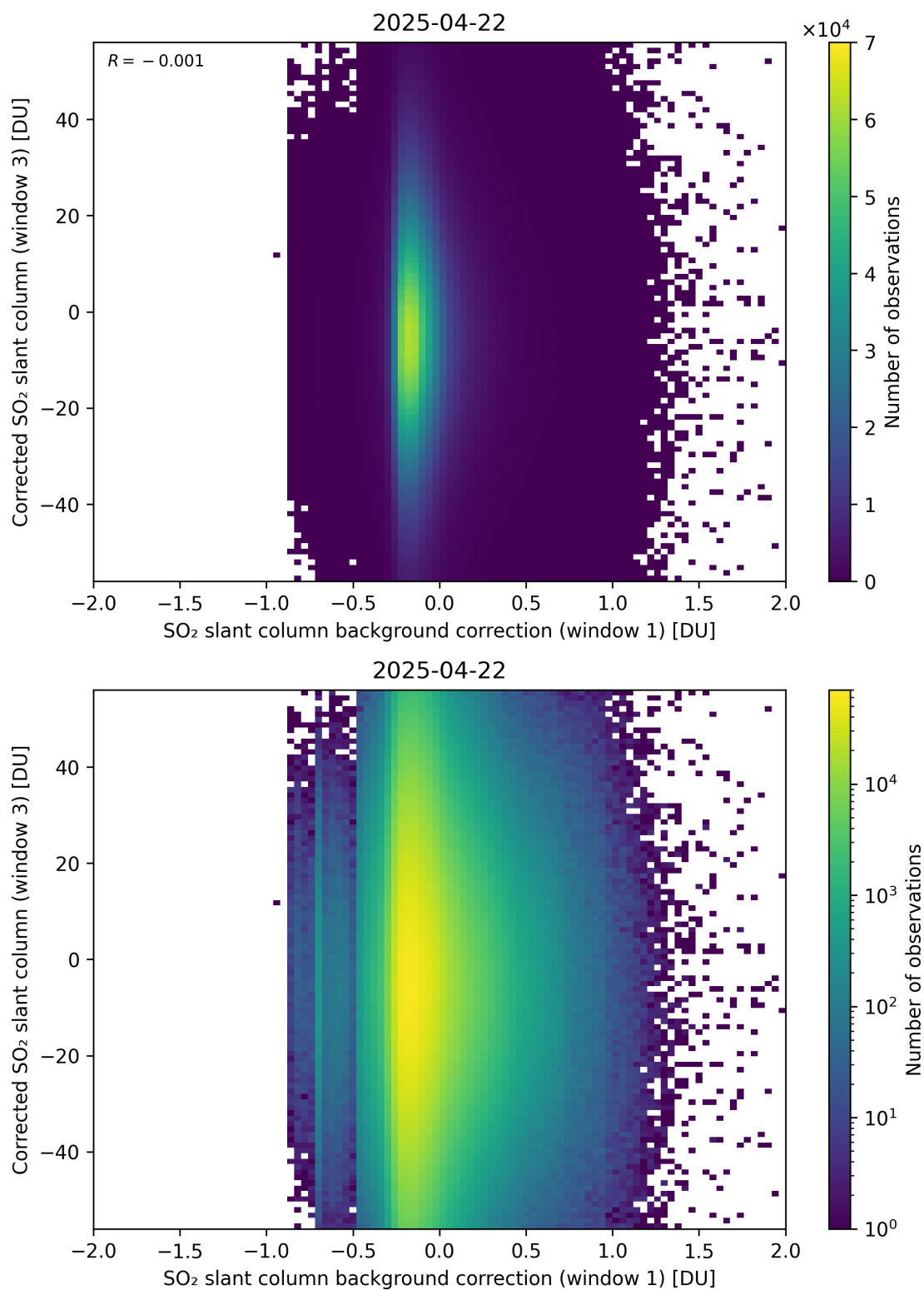
Figure 116: Scatter density plot of “SO 2 slant column background correction (window 1)” against “Corrected SO 2 slant column (window 3)” for 2025-04-21 to 2025-04-23.
