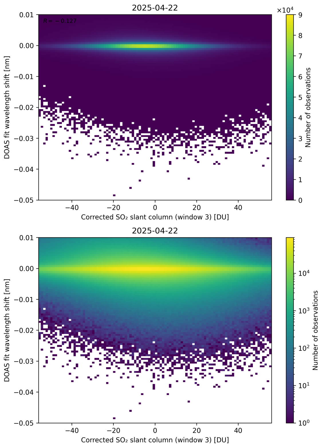
Figure 256: Scatter density plot of “Corrected SO 2 slant column (window 3)” against “DOAS fit wavelength shift” for 2025-04-21 to 2025-04-23.
