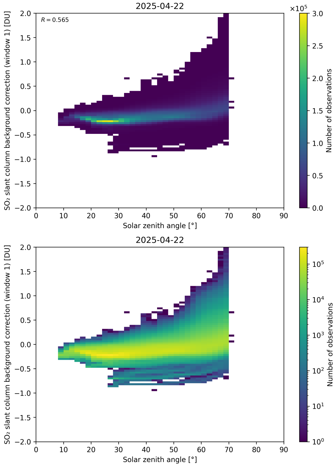
Figure 171: Scatter density plot of “Solar zenith angle” against “SO 2 slant column background correction (window 1)” for 2025-04-21 to 2025-04-23.
