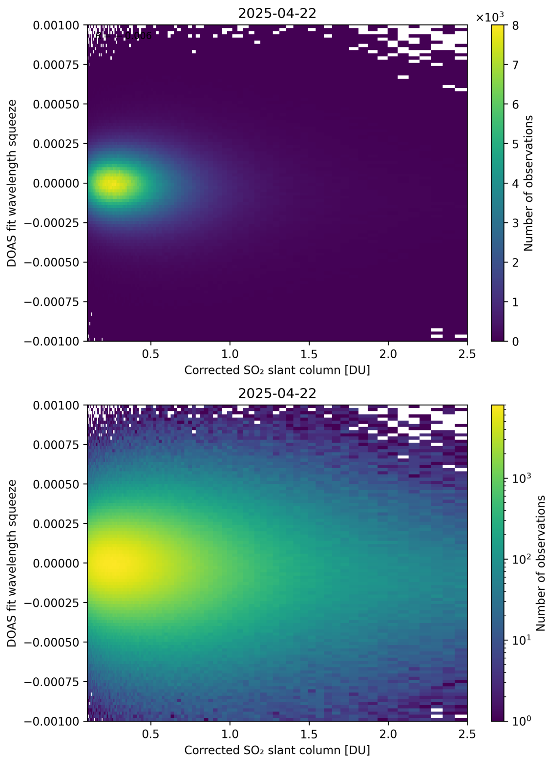
Figure 230: Scatter density plot of “Corrected SO 2 slant column” against “DOAS fit wavelength squeeze” for 2025-04-21 to 2025-04-23.
