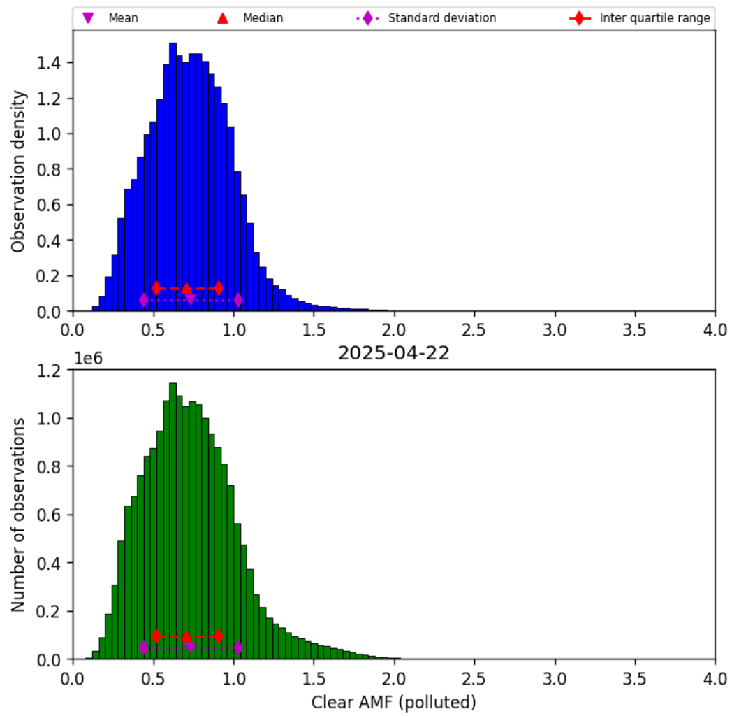
Figure 81: Histogram of “Clear AMF (polluted)” for 2025-04-21 to 2025-04-23
