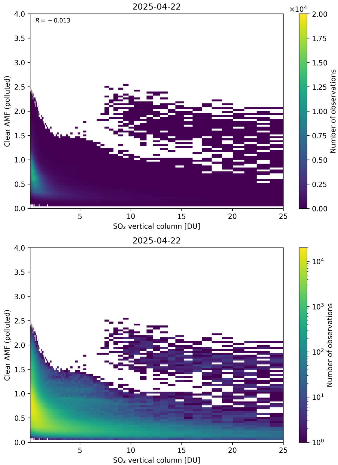
Figure 348: Scatter density plot of “SO 2 vertical column” against “Clear AMF (polluted)” for 2025-04-21 to 2025-04-23.
