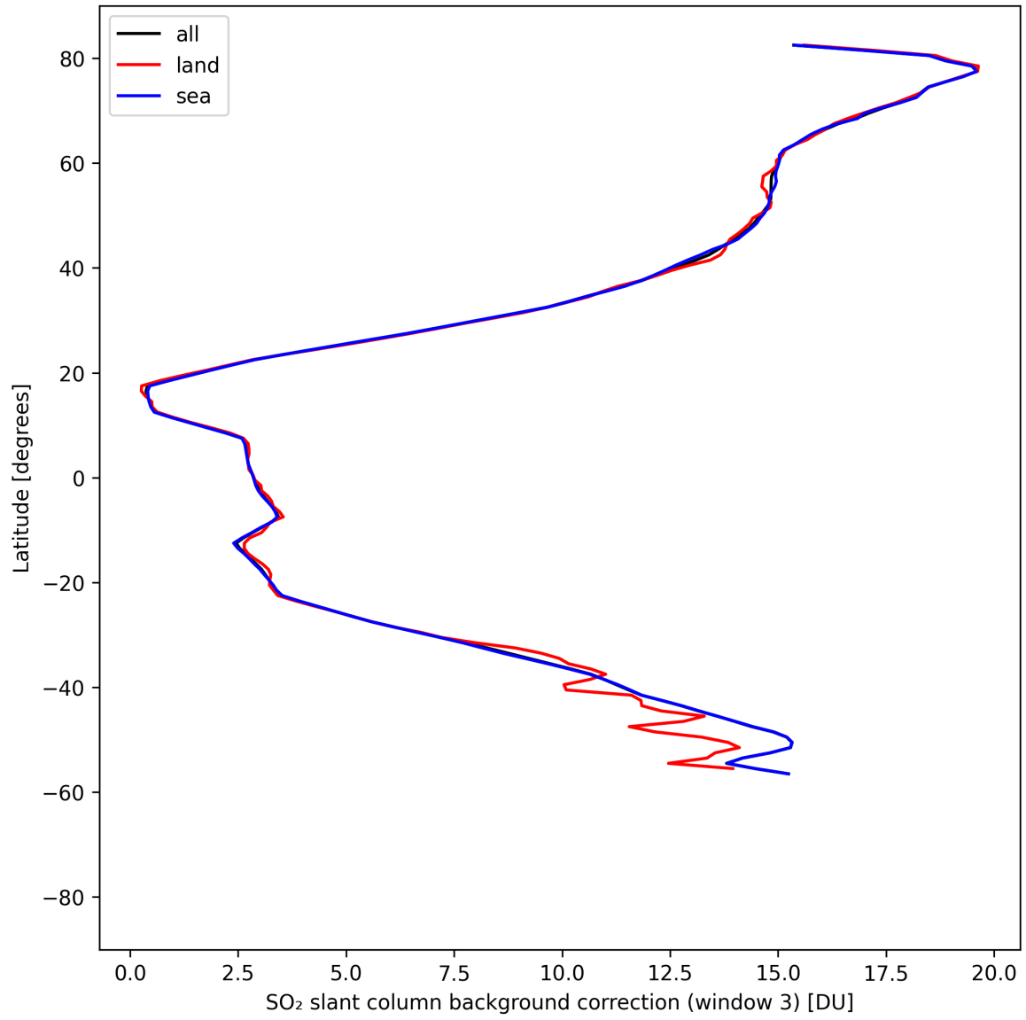
Figure 48: Zonal average of "SO 2 slant column background correction (window 3)" for 2025-04-21 to 2025-04-23.
