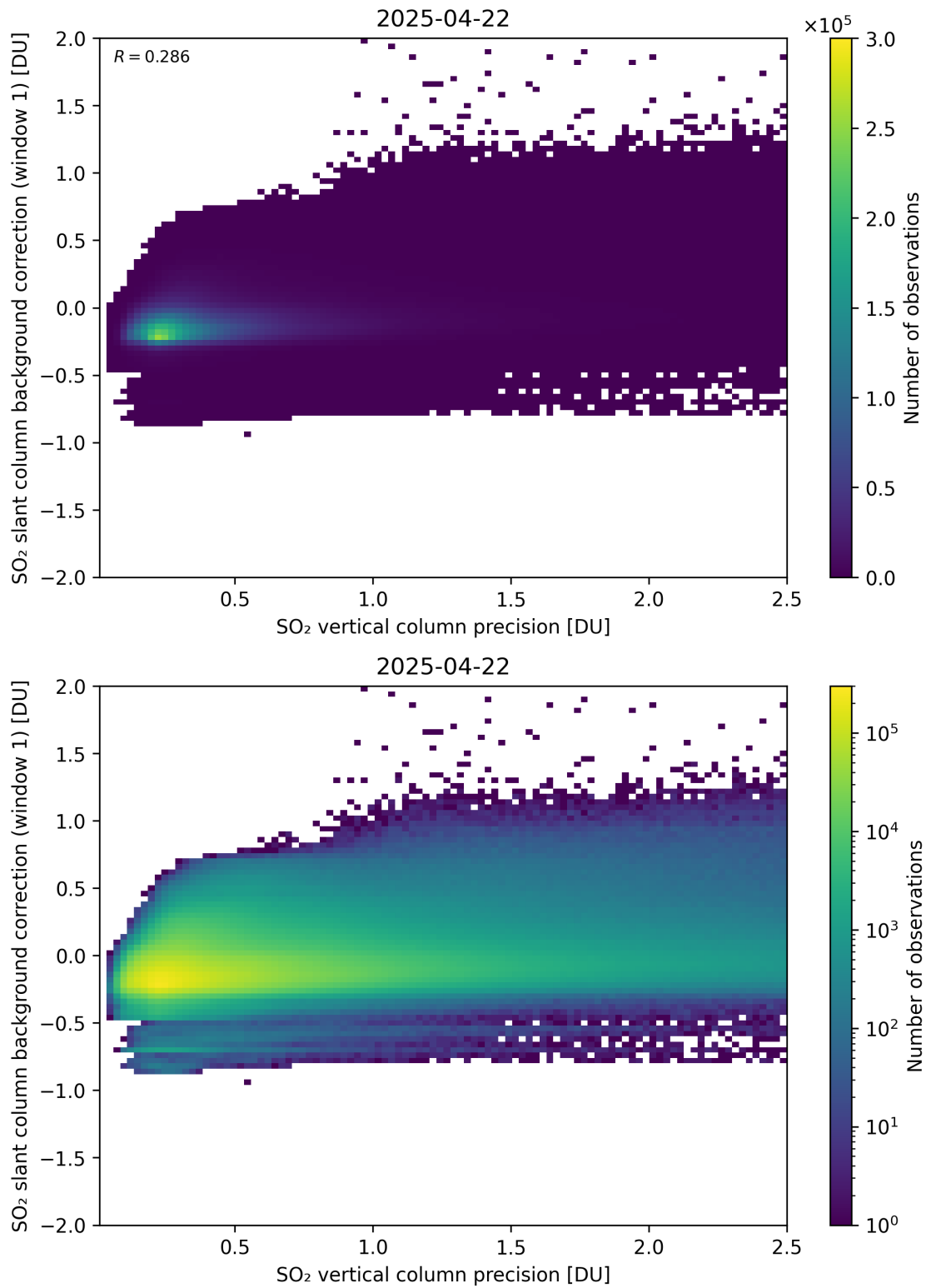
Figure 329: Scatter density plot of “SO 2 vertical column precision” against “SO 2 slant column background correction (window 1)” for 2025-04-21 to 2025-04-23.
