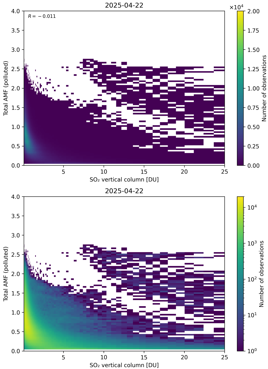
Figure 359: Scatter density plot of “SO 2 vertical column” against “Total AMF (polluted)” for 2025-04-21 to 2025-04-23.
