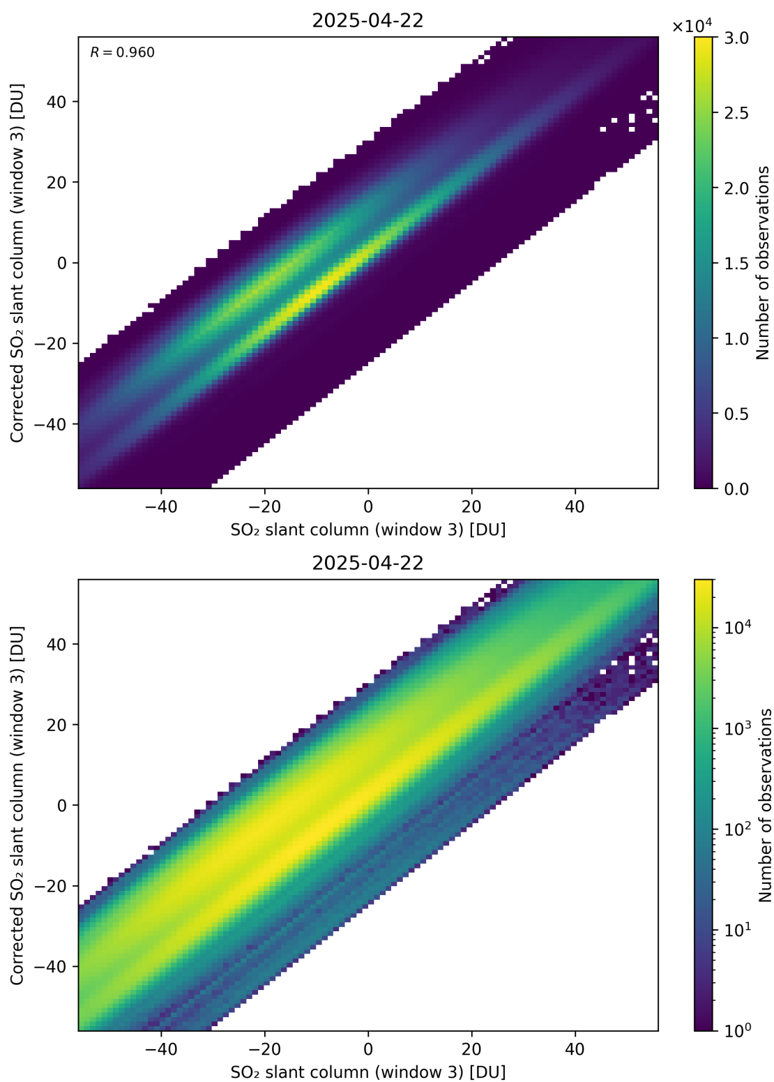
Figure 316: Scatter density plot of “SO 2 slant column (window 3)” against “Corrected SO 2 slant column (window 3)” for 2025-04-21 to 2025-04-23.
