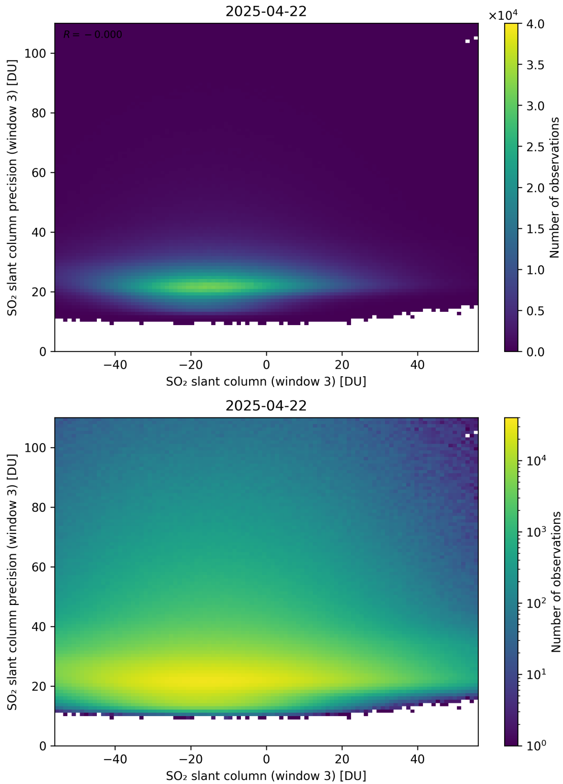
Figure 317: Scatter density plot of “SO 2 slant column (window 3)” against “SO 2 slant column precision (window 3)” for 2025-04-21 to 2025-04-23.
