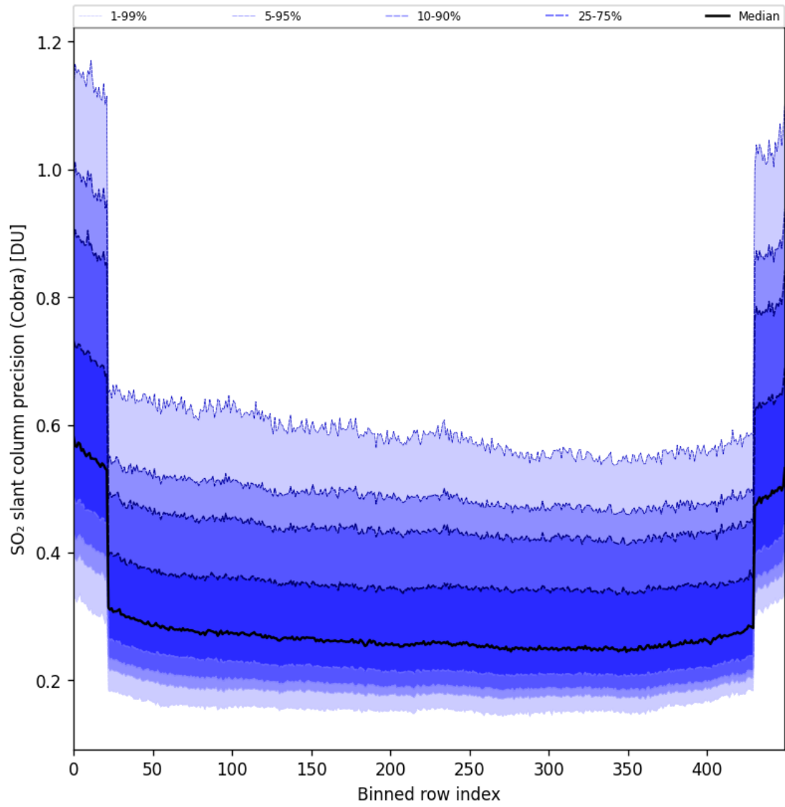
Figure 88: Along track statistics of “SO 2 slant column precision (Cobra)” for 2025-04-21 to 2025-04-23
