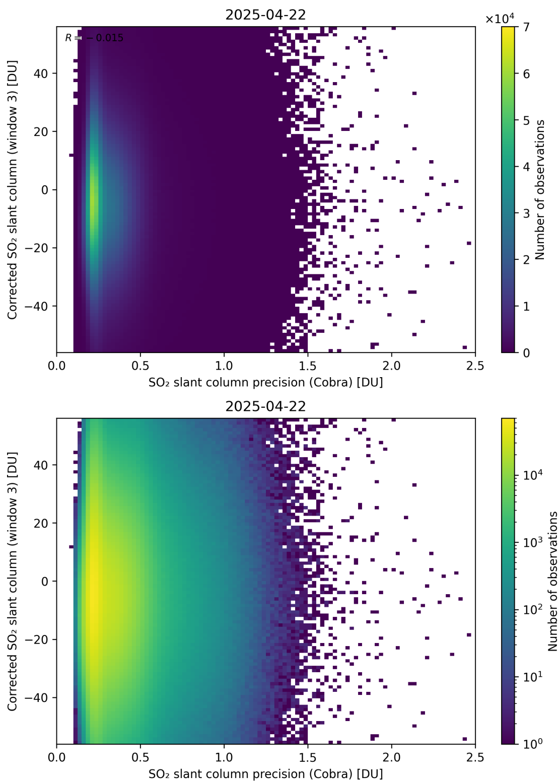
Figure 207: Scatter density plot of “SO 2 slant column precision (Cobra)” against “Corrected SO 2 slant column (window 3)” for 2025-04-21 to 2025-04-23.
