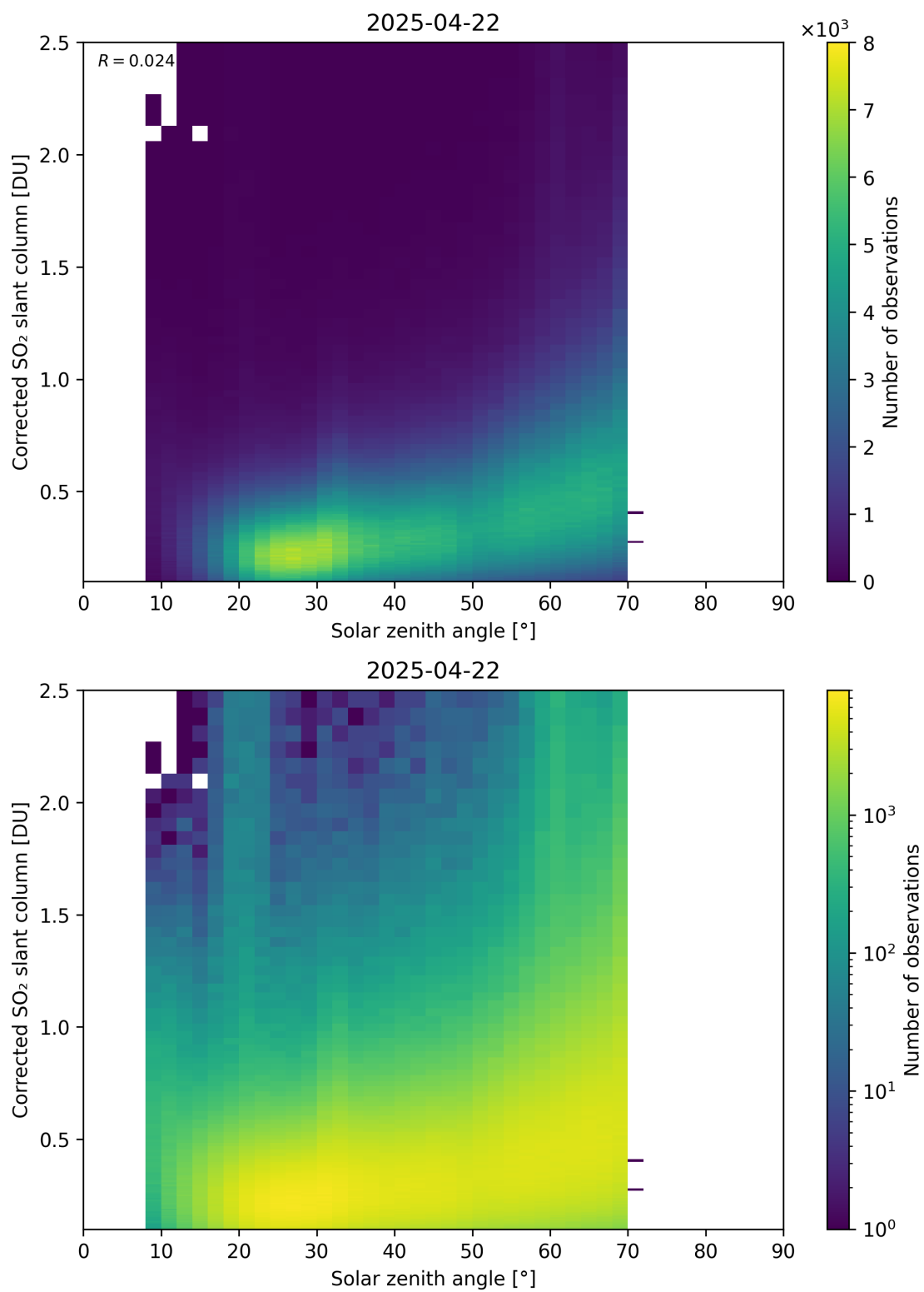
Figure 181: Scatter density plot of “Solar zenith angle” against “Corrected SO 2 slant column” for 2025-04-21 to 2025-04-23.
