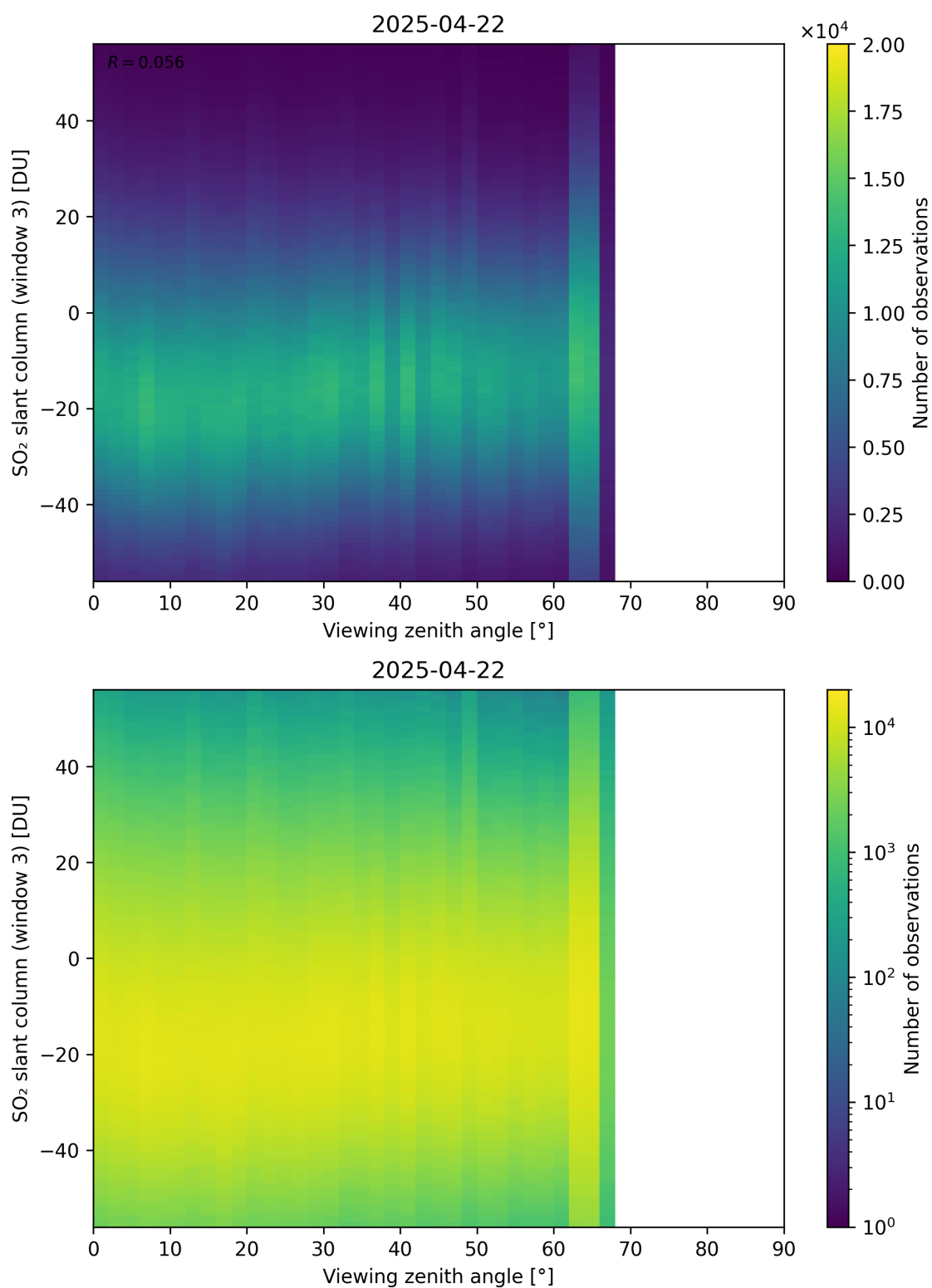
Figure 379: Scatter density plot of “Viewing zenith angle” against “SO 2 slant column (window 3)” for 2025-04-21 to 2025-04-23.
