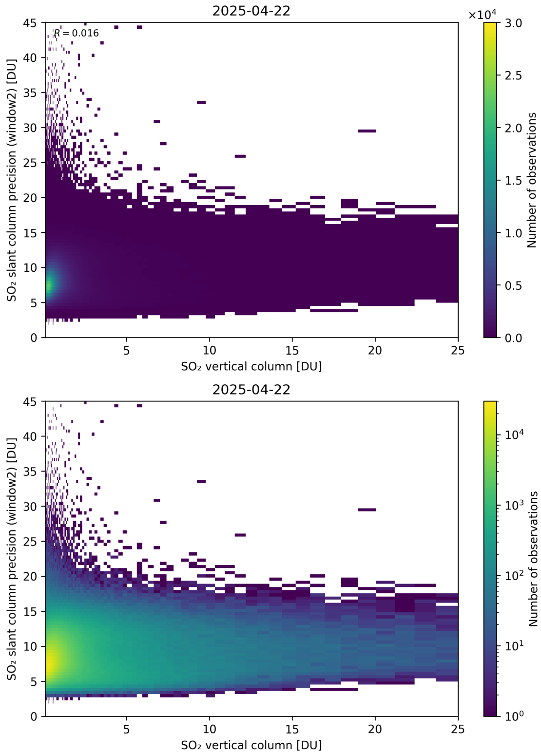
Figure 356: Scatter density plot of “SO 2 vertical column” against “SO 2 slant column precision (window2)” for 2025-04-21 to 2025-04-23.
