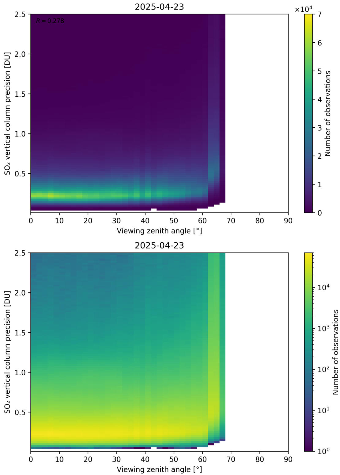
Figure 384: Scatter density plot of “Viewing zenith angle” against “SO 2 vertical column precision” for 2025-04-22 to 2025-04-24.
