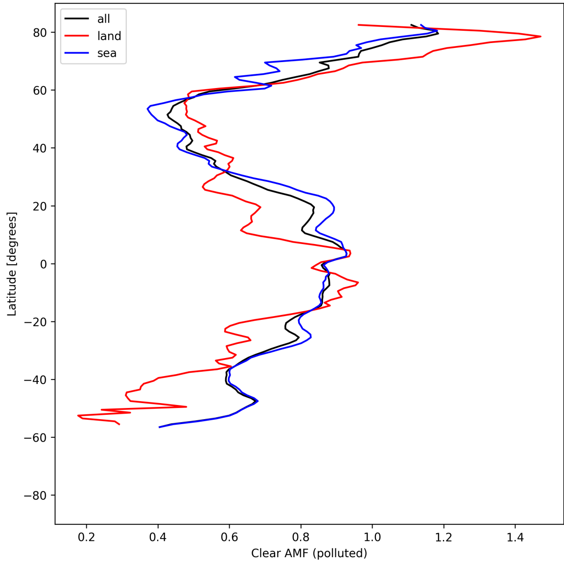
Figure 55: Zonal average of “Clear AMF (polluted)” for 2025-04-22 to 2025-04-24.
