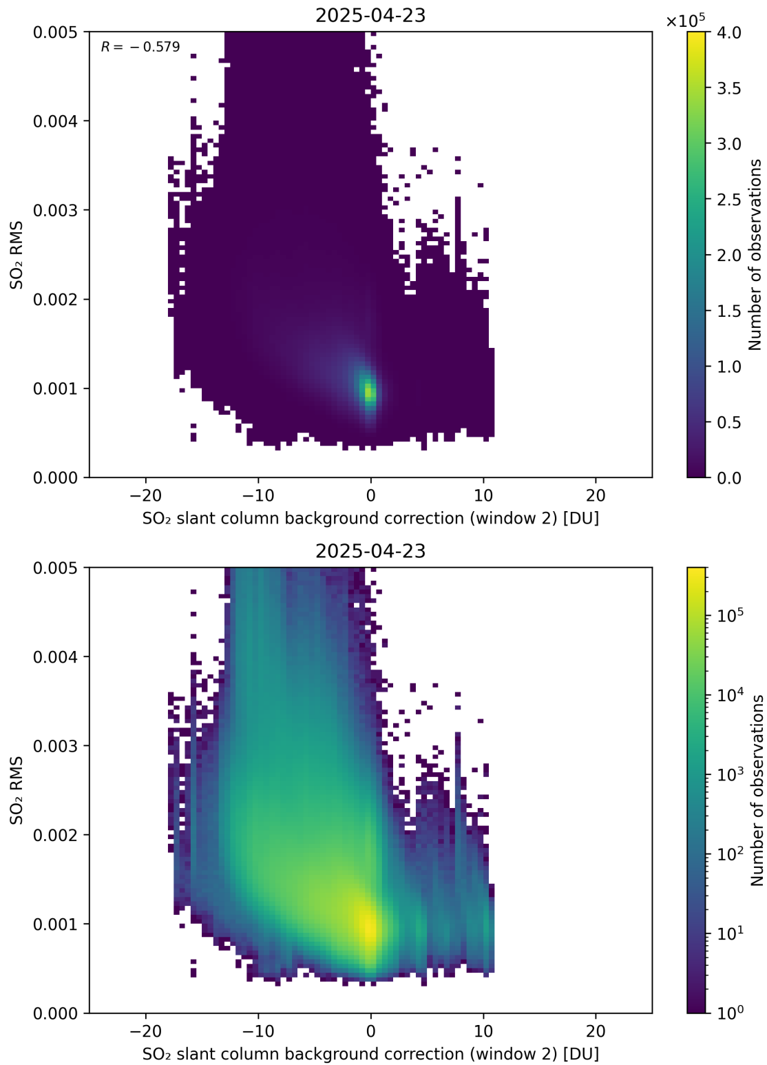
Figure 125: Scatter density plot of “SO 2 slant column background correction (window 2)” against “SO 2 RMS” for 2025-04-22 to 2025-04-24.
