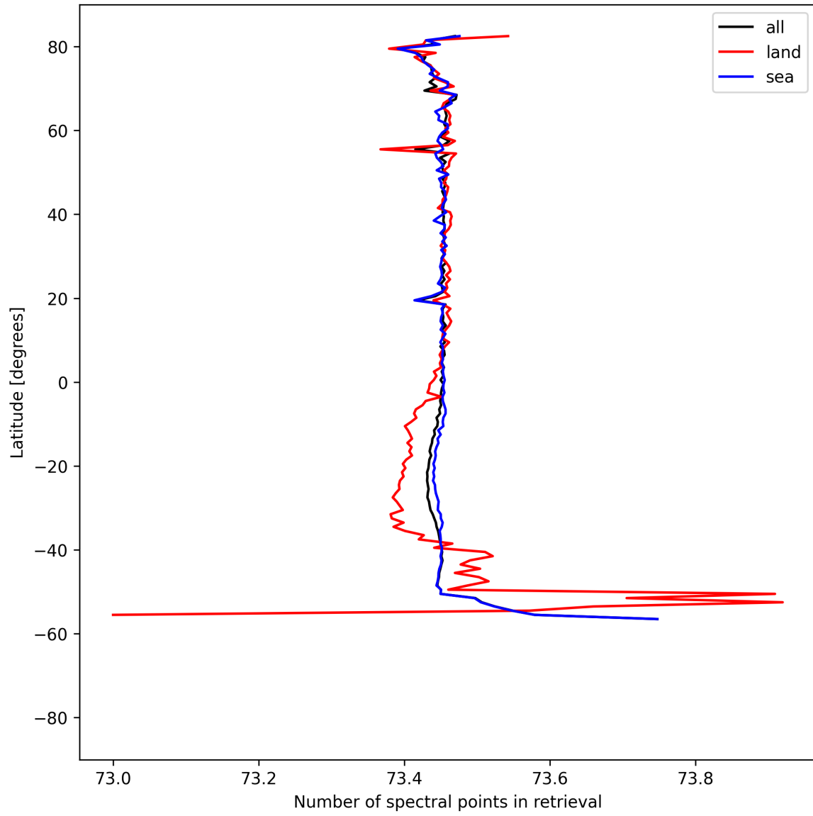
Figure 56: Zonal average of “Number of spectral points in retrieval” for 2025-04-22 to 2025-04-24.
