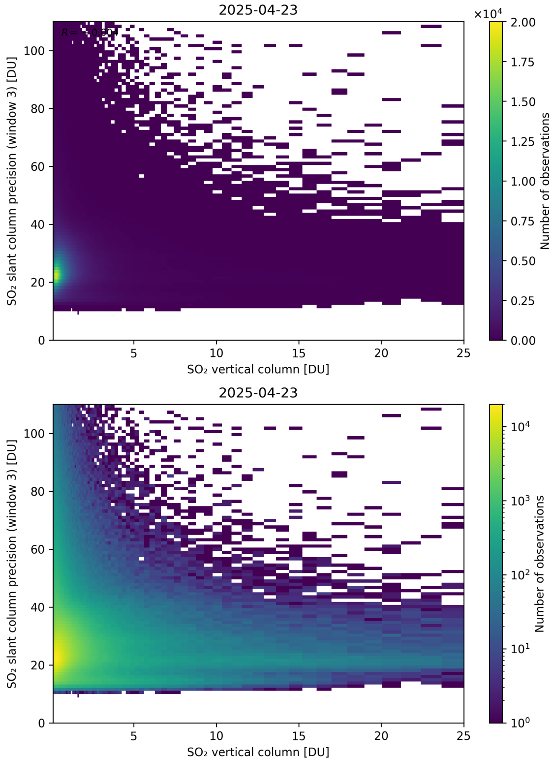
Figure 358: Scatter density plot of “SO 2 vertical column” against “SO 2 slant column precision (window 3)” for 2025-04-22 to 2025-04-24.
