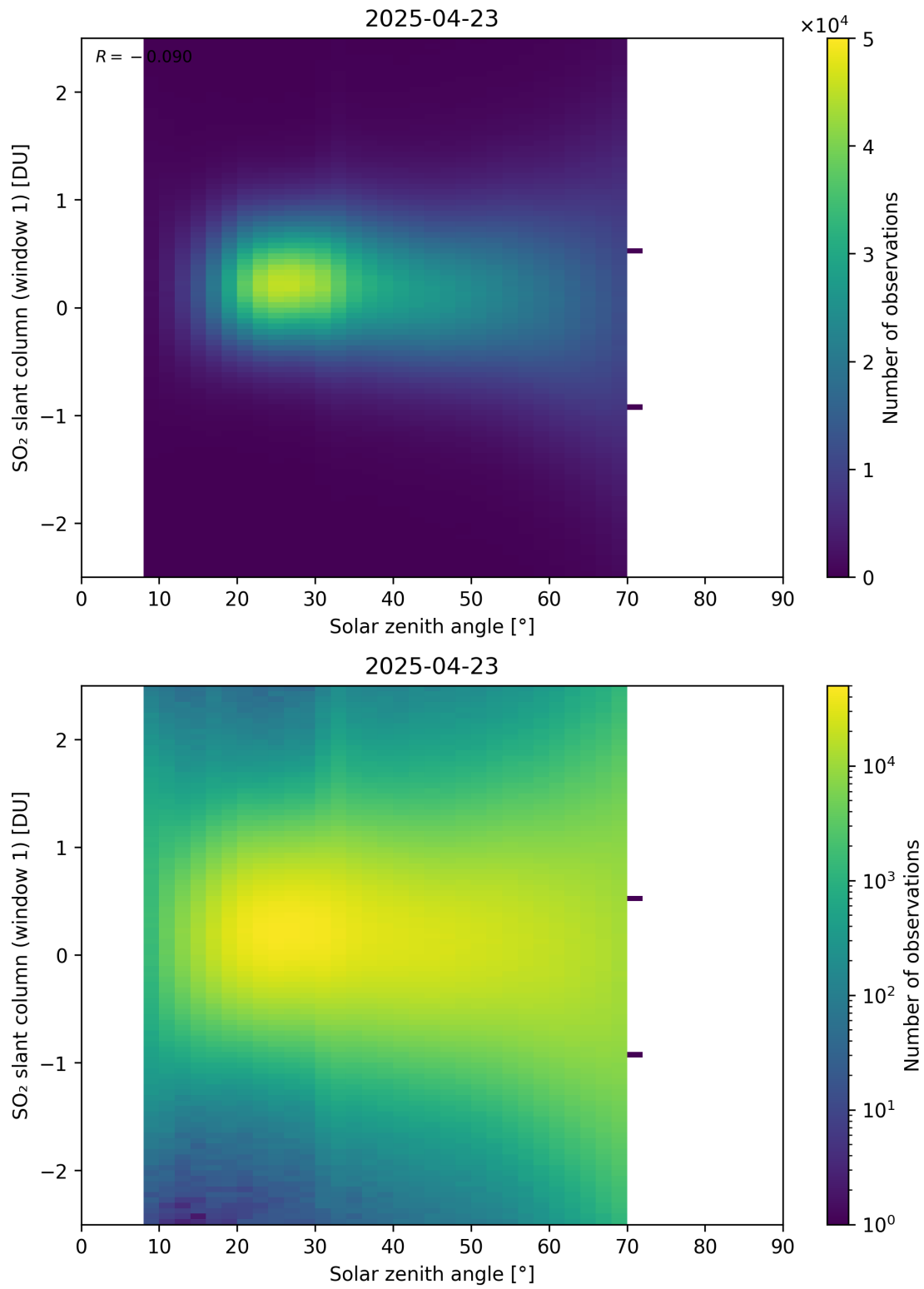
Figure 184: Scatter density plot of “Solar zenith angle” against “SO 2 slant column (window 1)” for 2025-04-22 to 2025-04-24.
