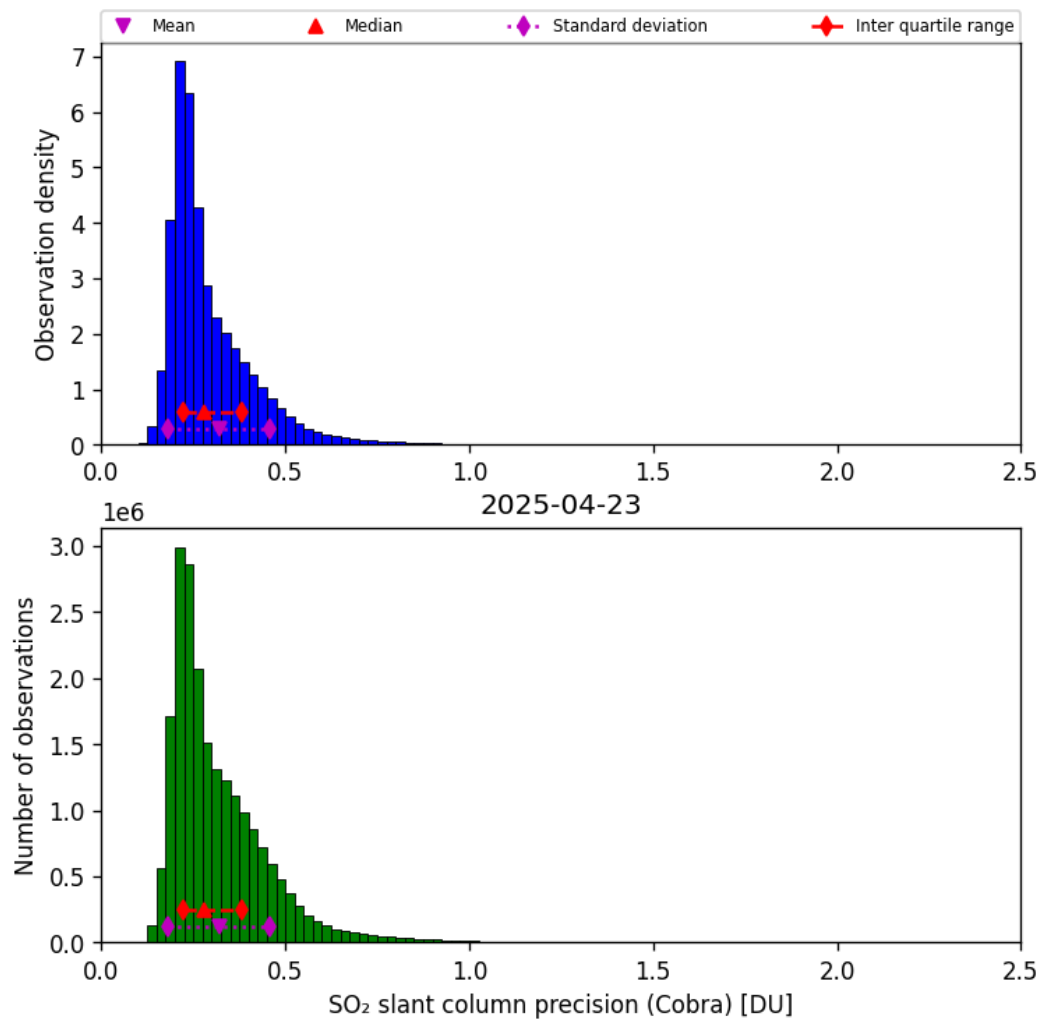
Figure 62: Histogram of “SO 2 slant column precision (Cobra)” for 2025-04-22 to 2025-04-24
