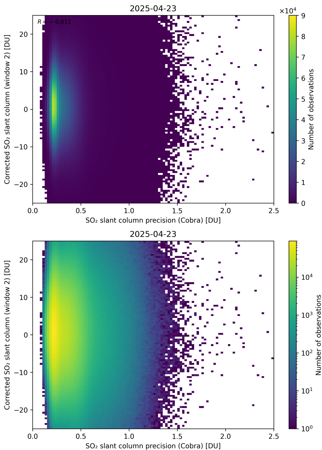
Figure 206: Scatter density plot of “SO 2 slant column precision (Cobra)” against “Corrected SO 2 slant column (window 2)” for 2025-04-22 to 2025-04-24.
