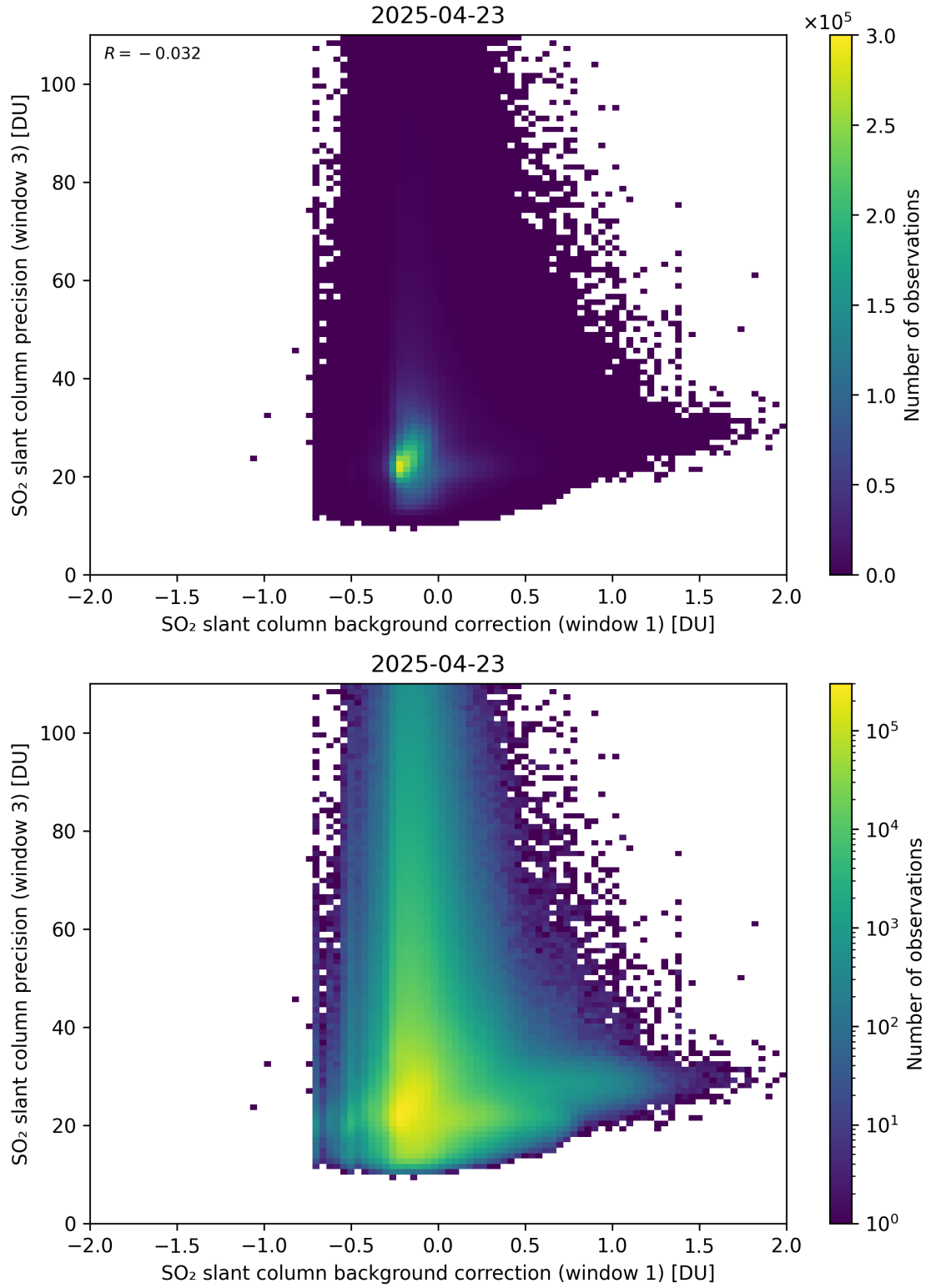
Figure 119: Scatter density plot of “SO 2 slant column background correction (window 1)” against “SO 2 slant column precision (window 3)” for 2025-04-22 to 2025-04-24.
