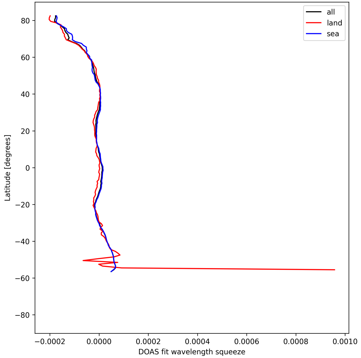
Figure 51: Zonal average of “DOAS fit wavelength squeeze” for 2025-04-22 to 2025-04-24.
