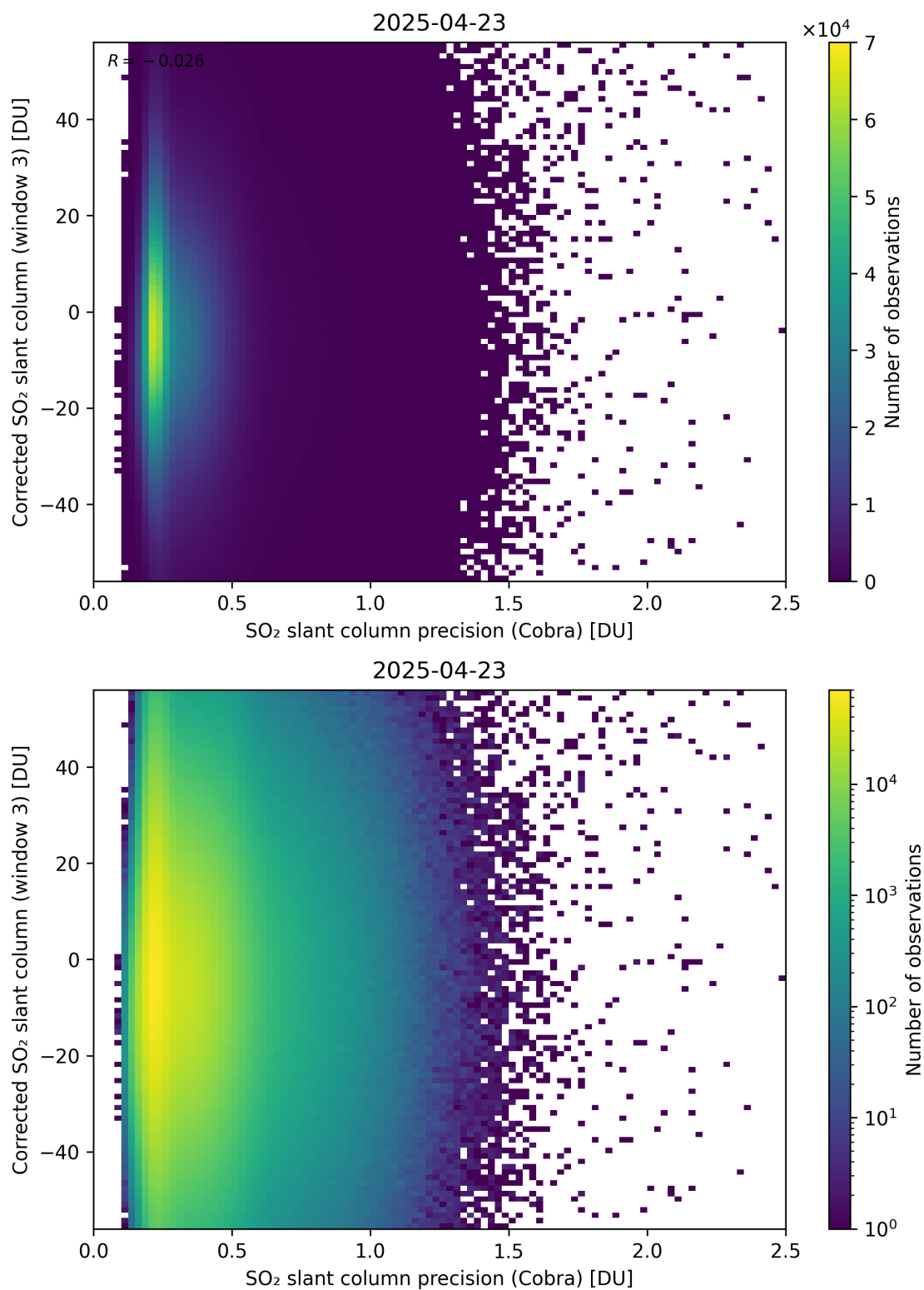
Figure 207: Scatter density plot of “SO 2 slant column precision (Cobra)” against “Corrected SO 2 slant column (window 3)” for 2025-04-22 to 2025-04-24.
