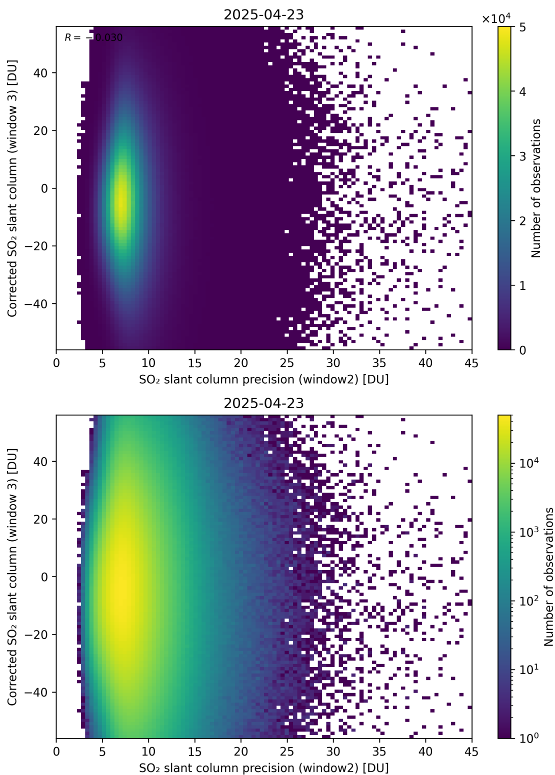
Figure 298: Scatter density plot of “SO 2 slant column precision (window2)” against “Corrected SO 2 slant column (window 3)” for 2025-04-22 to 2025-04-24.
