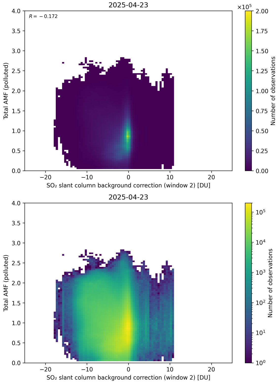
Figure 130: Scatter density plot of “SO 2 slant column background correction (window 2)” against “Total AMF (polluted)” for 2025-04-22 to 2025-04-24.
