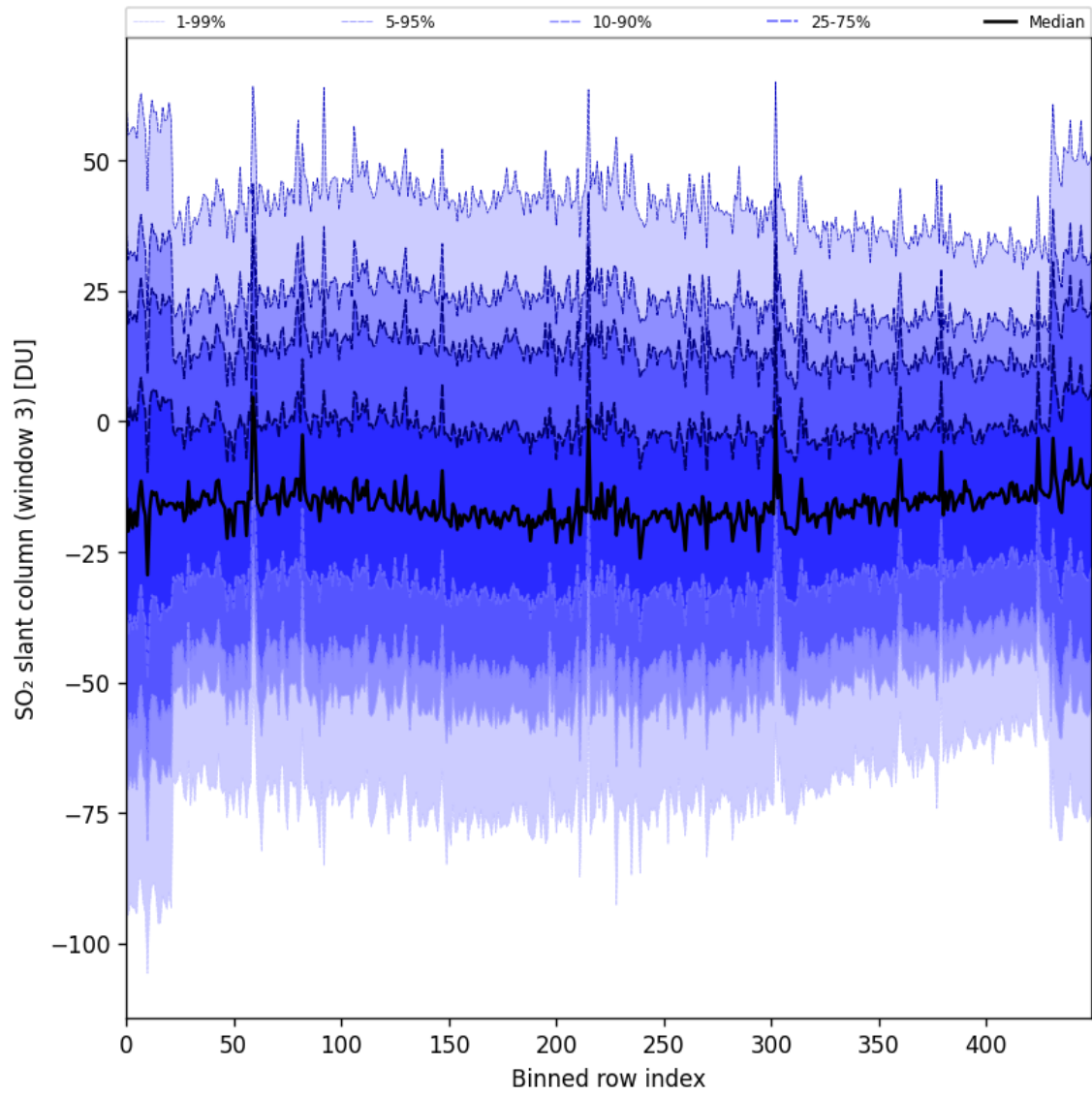
Figure 97: Along track statistics of “SO 2 slant column (window 3)” for 2025-04-22 to 2025-04-24
