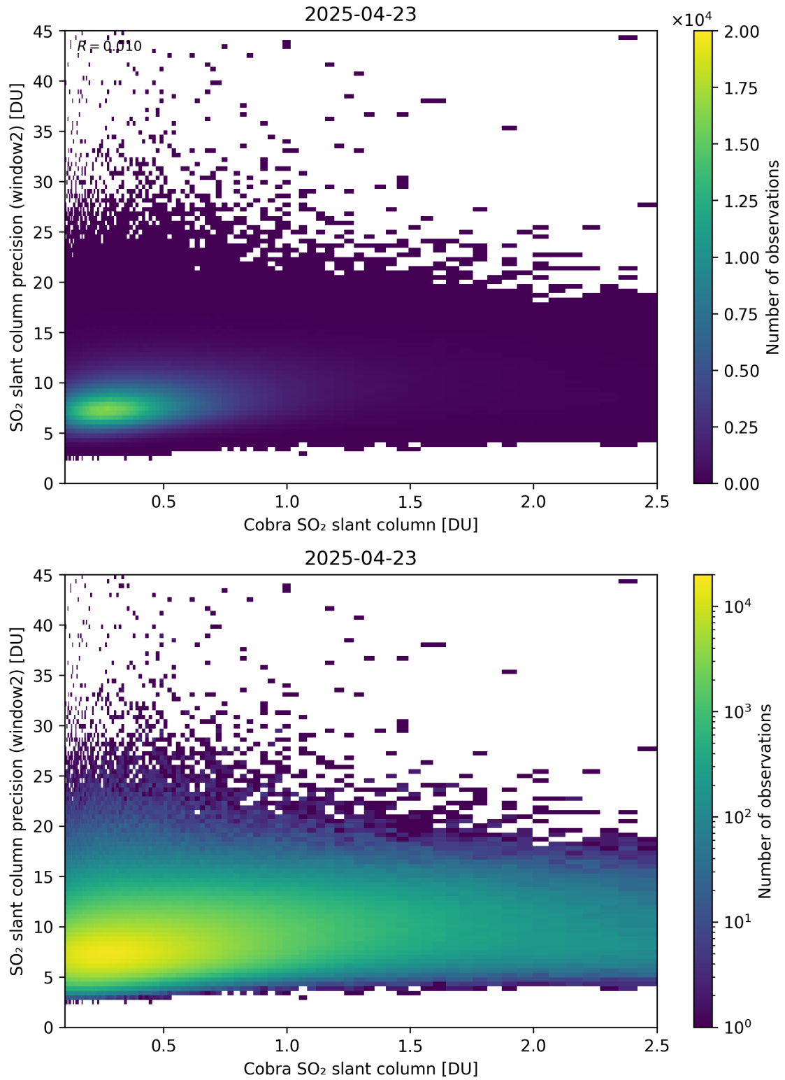
Figure 221: Scatter density plot of “Cobra SO 2 slant column” against “SO 2 slant column precision (window2)” for 2025-04-22 to 2025-04-24.
