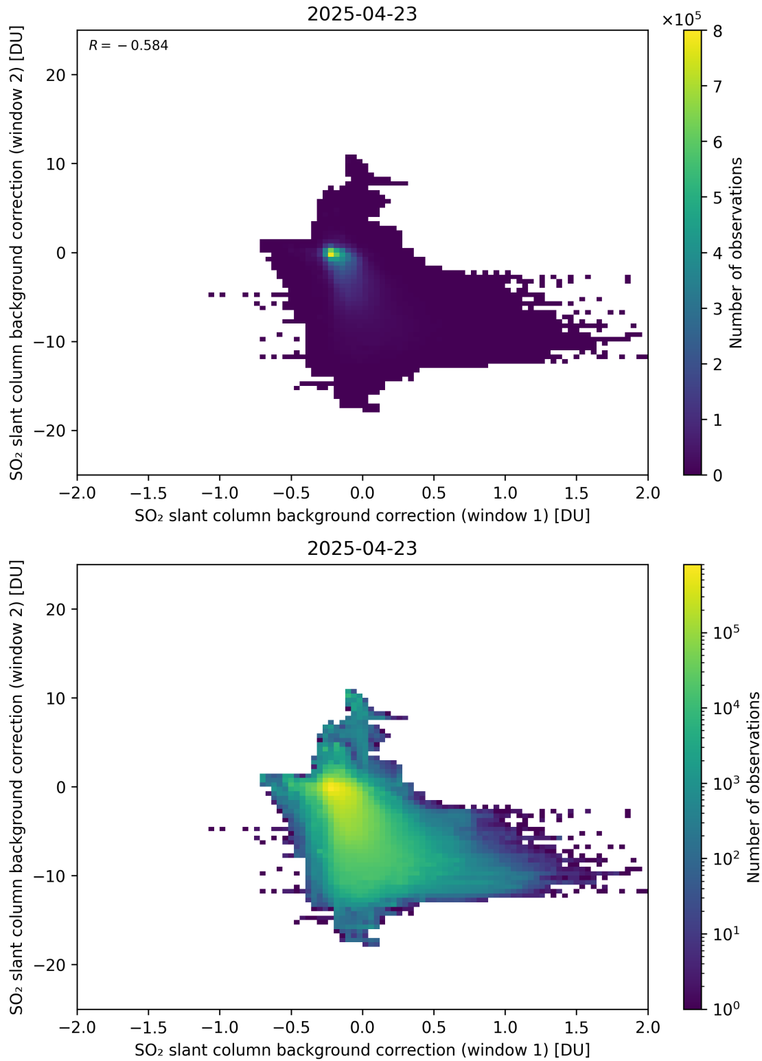
Figure 109: Scatter density plot of “SO 2 slant column background correction (window 1)” against “SO 2 slant column background correction (window 2)” for 2025-04-22 to 2025-04-24.
