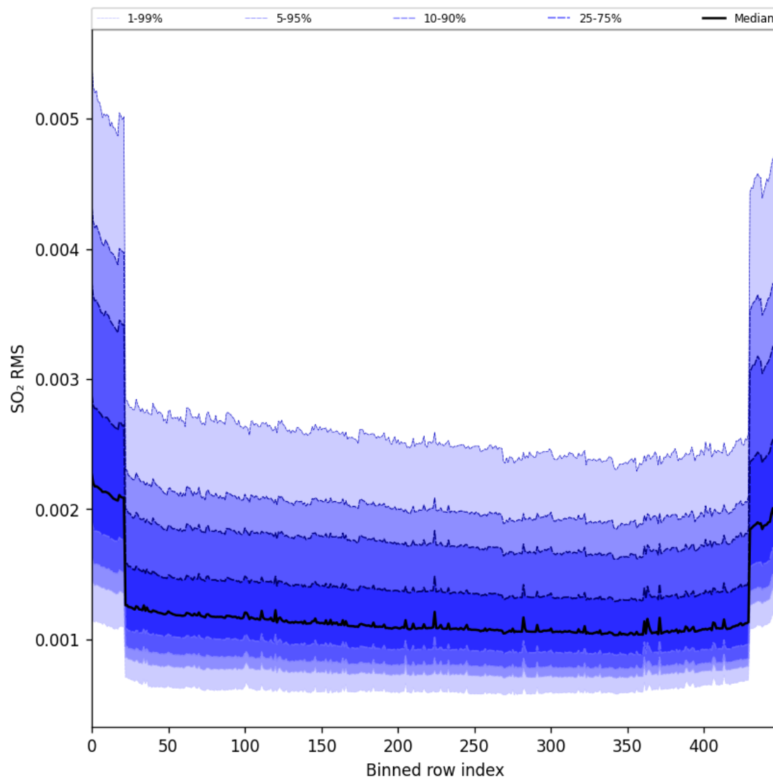
Figure 104: Along track statistics of “SO 2 RMS” for 2025-04-22 to 2025-04-24
