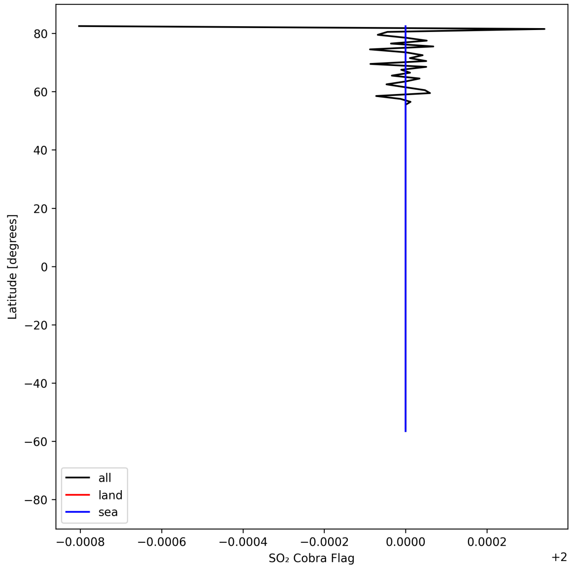
Figure 49: Zonal average of “SO 2 Cobra Flag” for 2025-04-22 to 2025-04-24.
