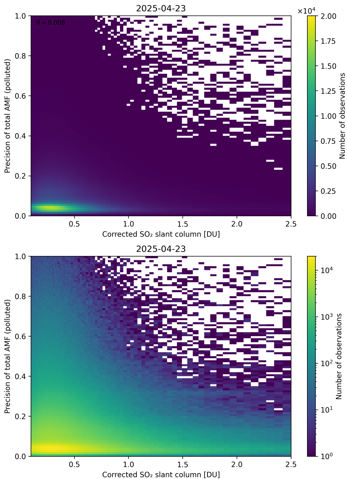
Figure 243: Scatter density plot of “Corrected SO 2 slant column” against “Precision of total AMF (polluted)” for 2025-04-22 to 2025-04-24.
