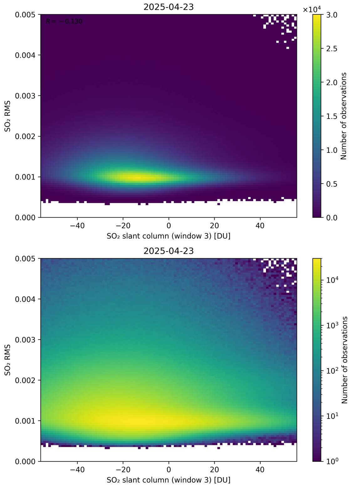
Figure 306: Scatter density plot of “SO 2 slant column (window 3)” against “SO 2 RMS” for 2025-04-22 to 2025-04-24.
