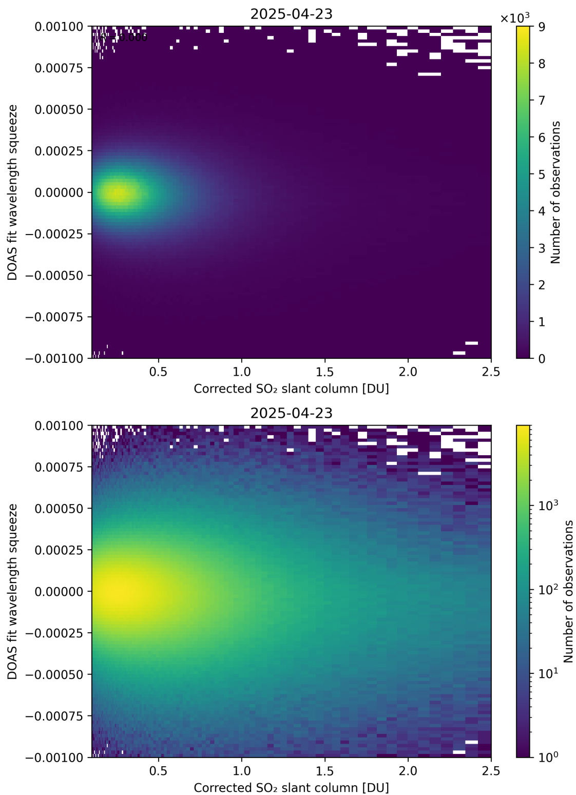
Figure 230: Scatter density plot of "Corrected SO 2 slant column" against "DOAS fit wavelength squeeze" for 2025-04-22 to 2025-04-24.
