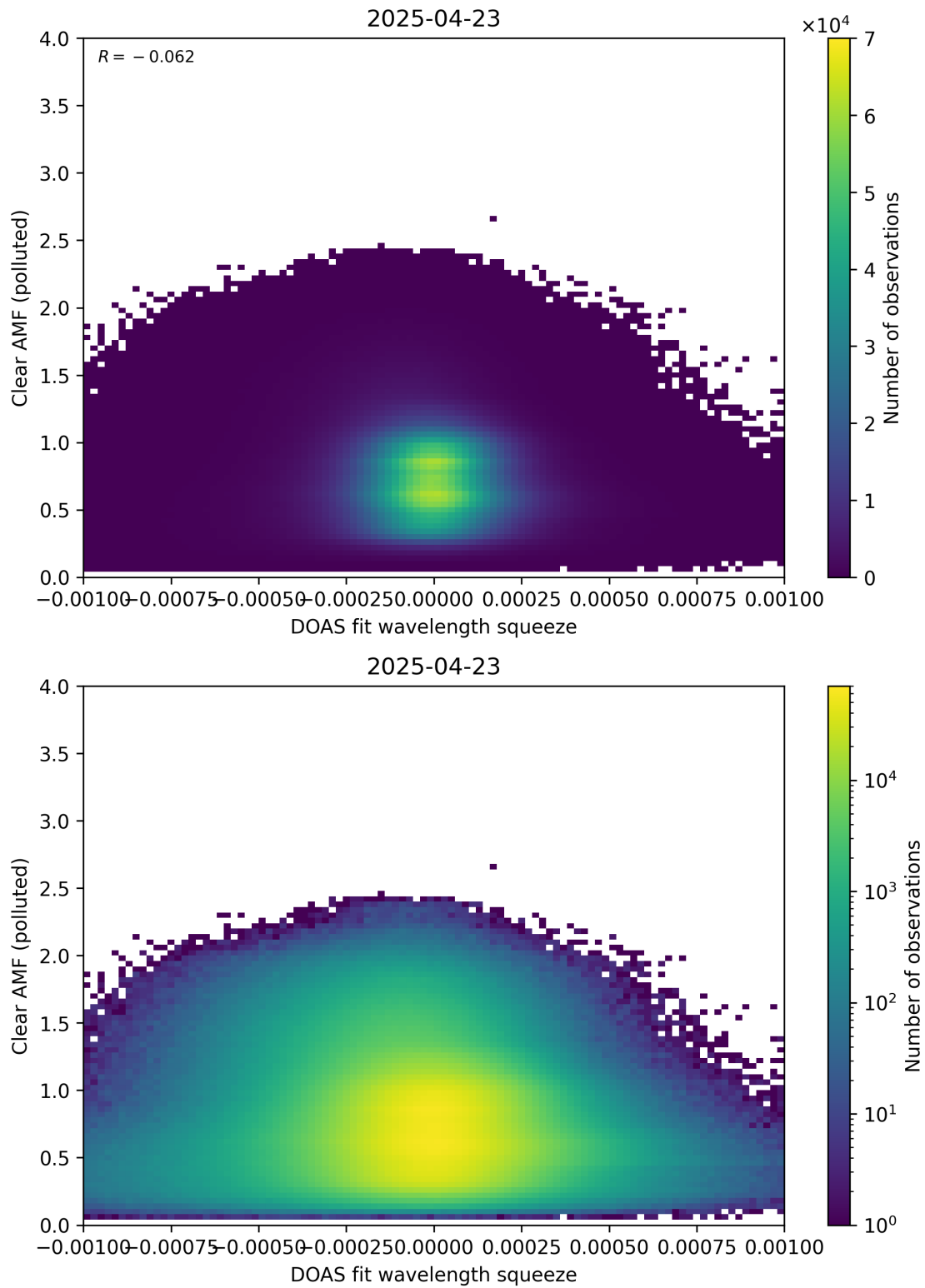
Figure 144: Scatter density plot of “DOAS fit wavelength squeeze” against “Clear AMF (polluted)” for 2025-04-22 to 2025-04-24.
