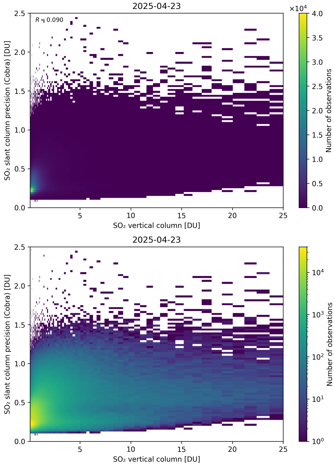
Figure 350: Scatter density plot of “SO 2 vertical column” against “SO 2 slant column precision (Cobra)” for 2025-04-22 to 2025-04-24.
