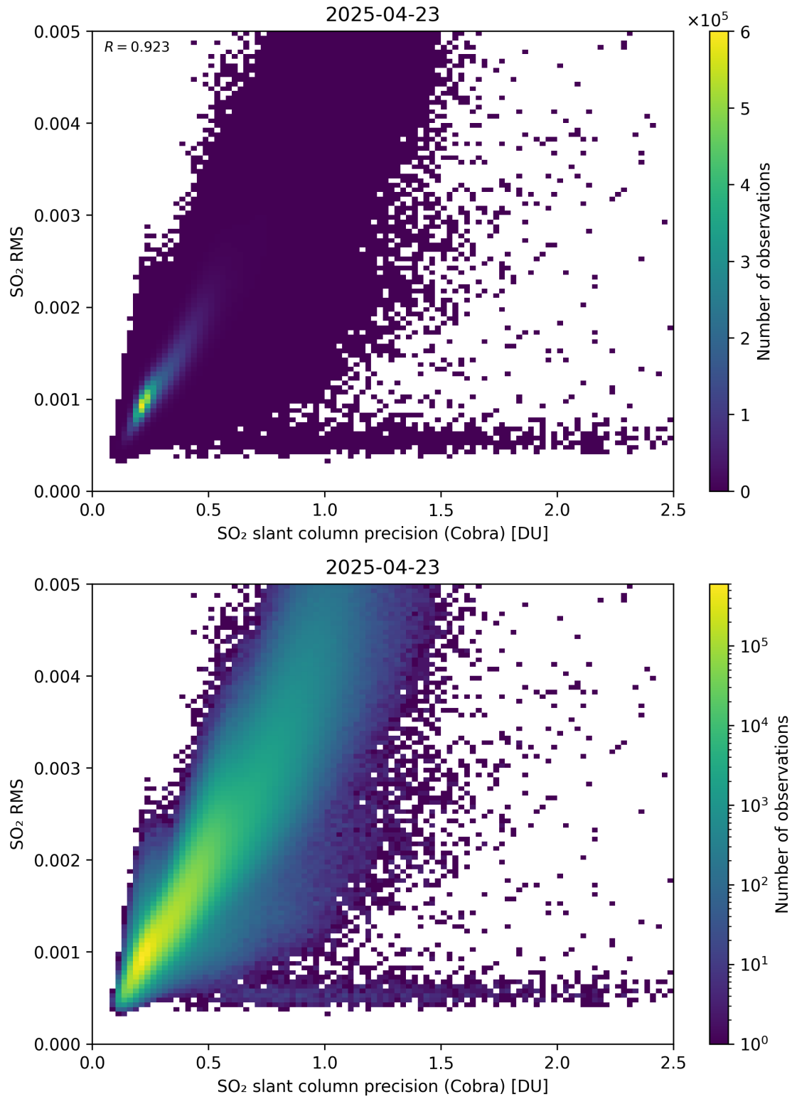
Figure 204: Scatter density plot of “SO 2 slant column precision (Cobra)” against “SO 2 RMS” for 2025-04-22 to 2025-04-24.
