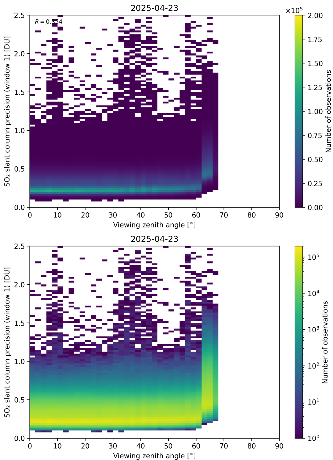
Figure 377: Scatter density plot of “Viewing zenith angle” against “SO 2 slant column precision (window 1)” for 2025-04-22 to 2025-04-24.
