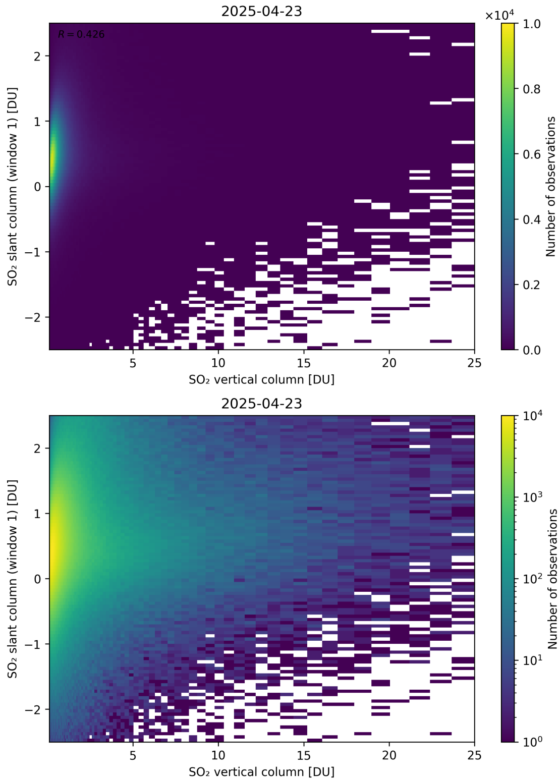
Figure 354: Scatter density plot of “SO 2 vertical column” against “SO 2 slant column (window 1)” for 2025-04-22 to 2025-04-24.
