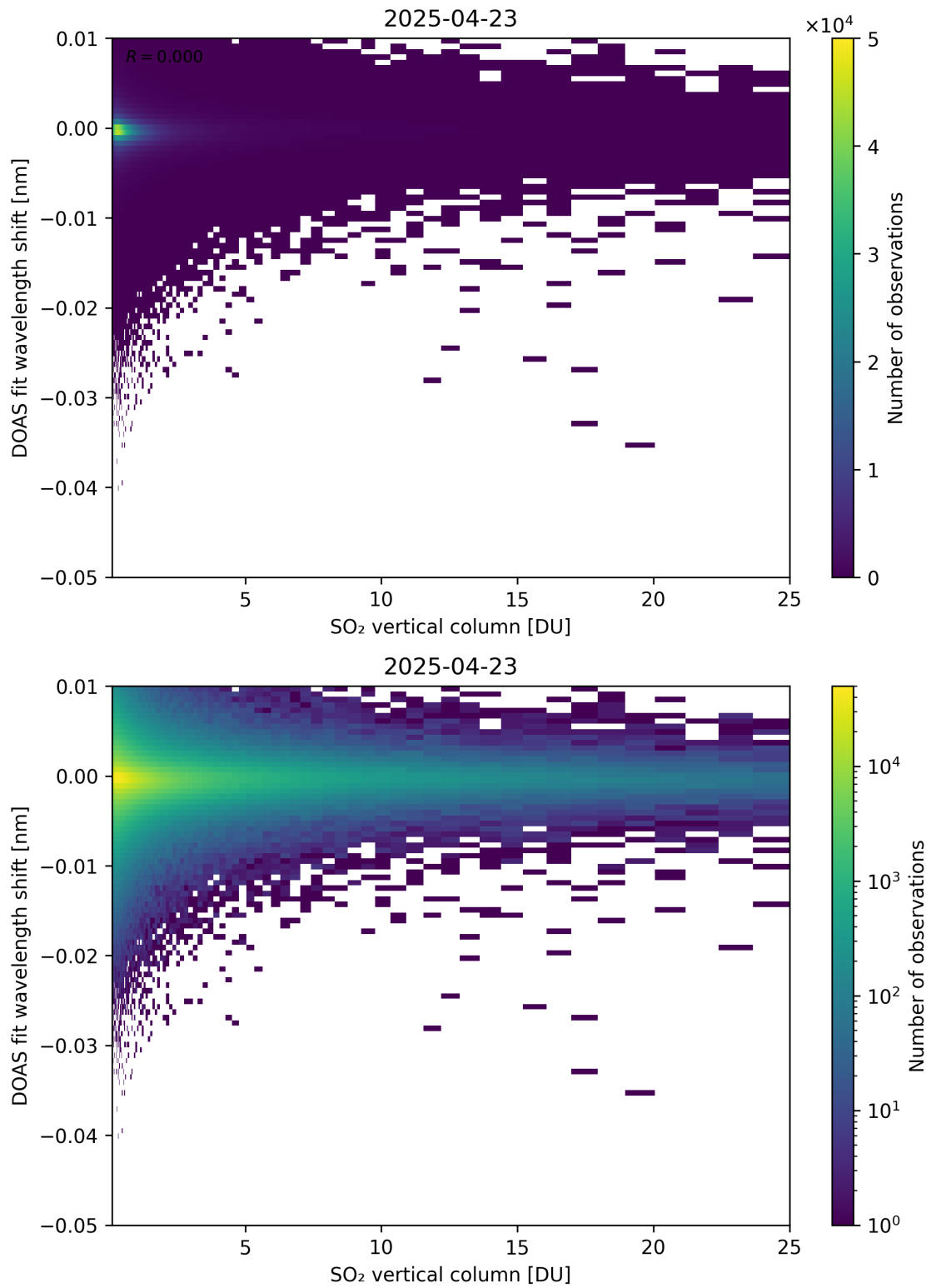
Figure 326: Scatter density plot of “SO 2 vertical column” against “DOAS fit wavelength shift” for 2025-04-22 to 2025-04-24.
