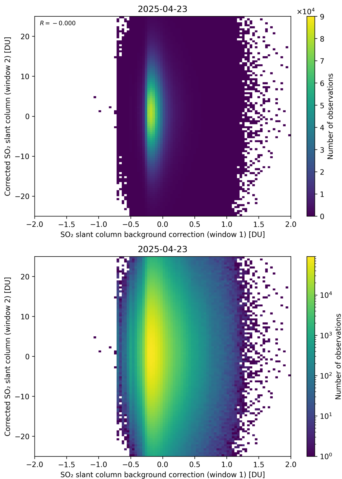
Figure 115: Scatter density plot of “SO 2 slant column background correction (window 1)” against “Corrected SO 2 slant column (window 2)” for 2025-04-22 to 2025-04-24.
