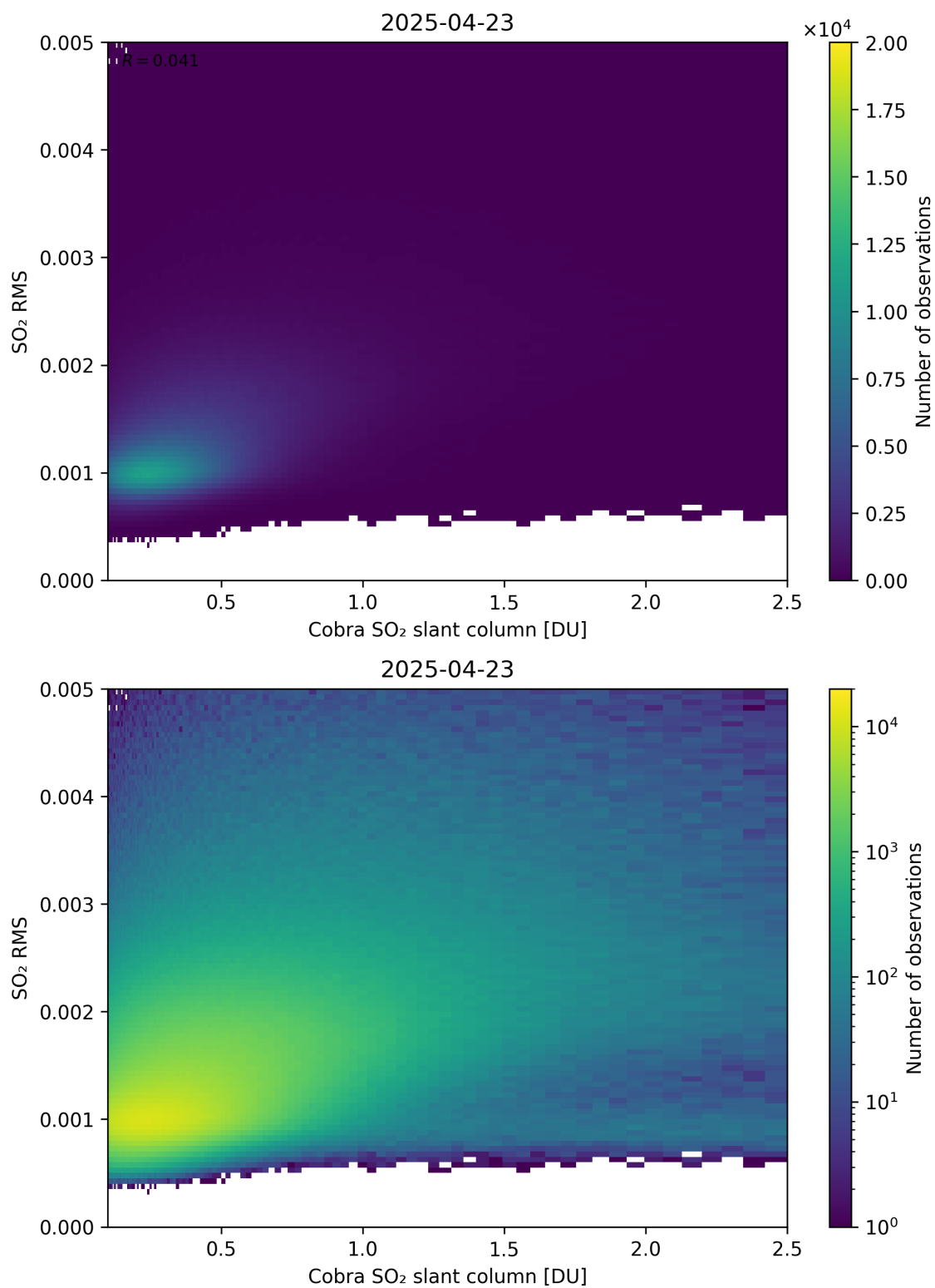
Figure 198: Scatter density plot of “Cobra SO 2 slant column” against “SO 2 RMS” for 2025-04-22 to 2025-04-24.
