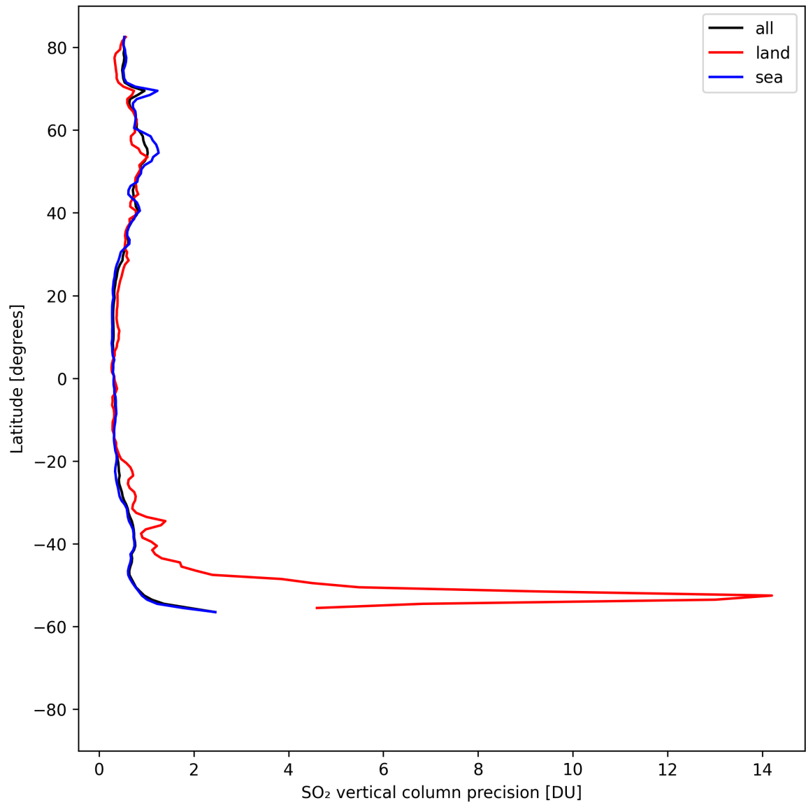
Figure 33: Zonal average of “SO 2 vertical column precision” for 2025-04-22 to 2025-04-24.
