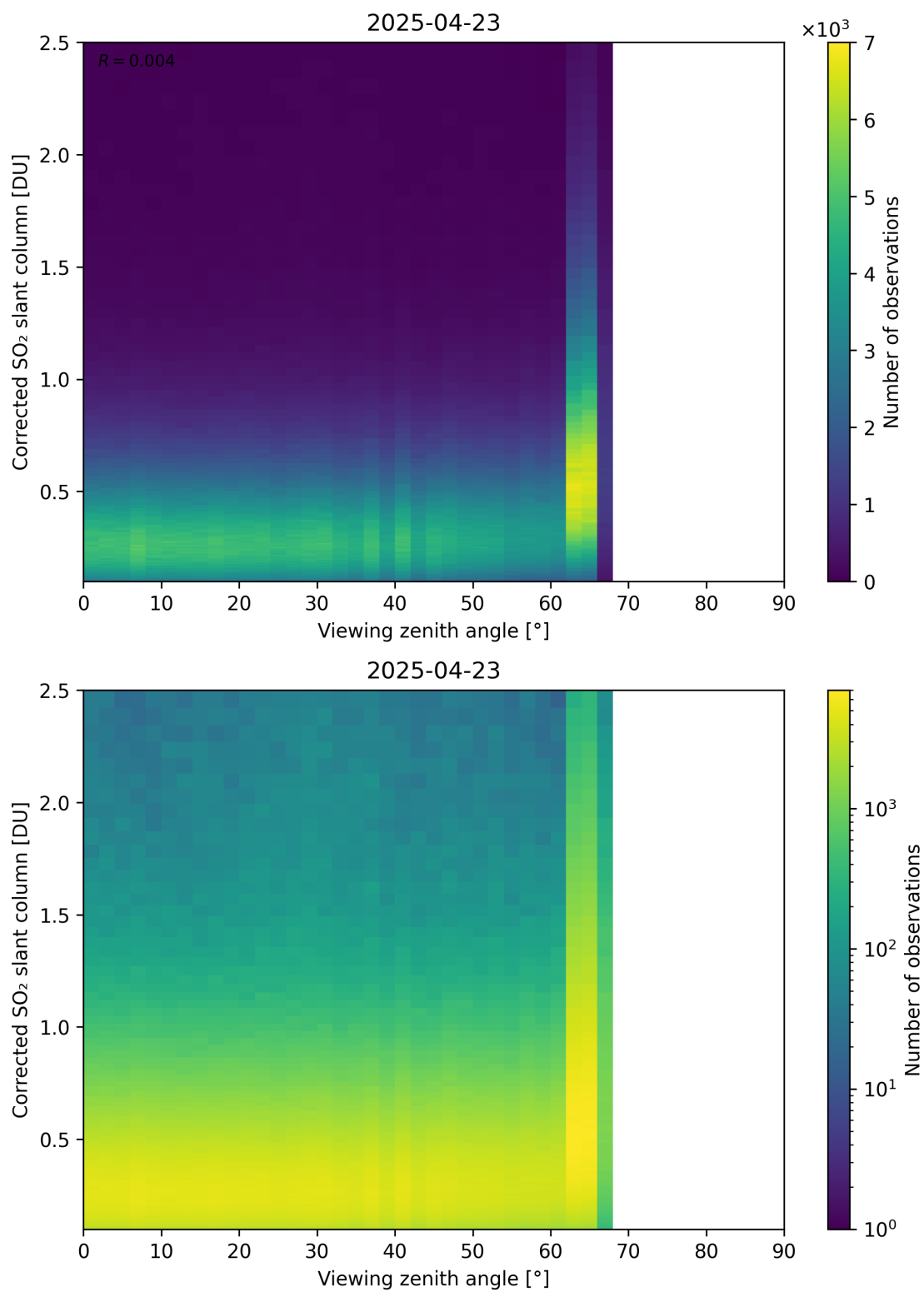
Figure 373: Scatter density plot of “Viewing zenith angle” against “Corrected SO 2 slant column” for 2025-04-22 to 2025-04-24.
