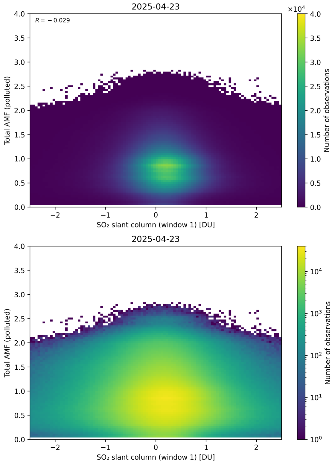
Figure 289: Scatter density plot of “SO 2 slant column (window 1)” against “Total AMF (polluted)” for 2025-04-22 to 2025-04-24.
