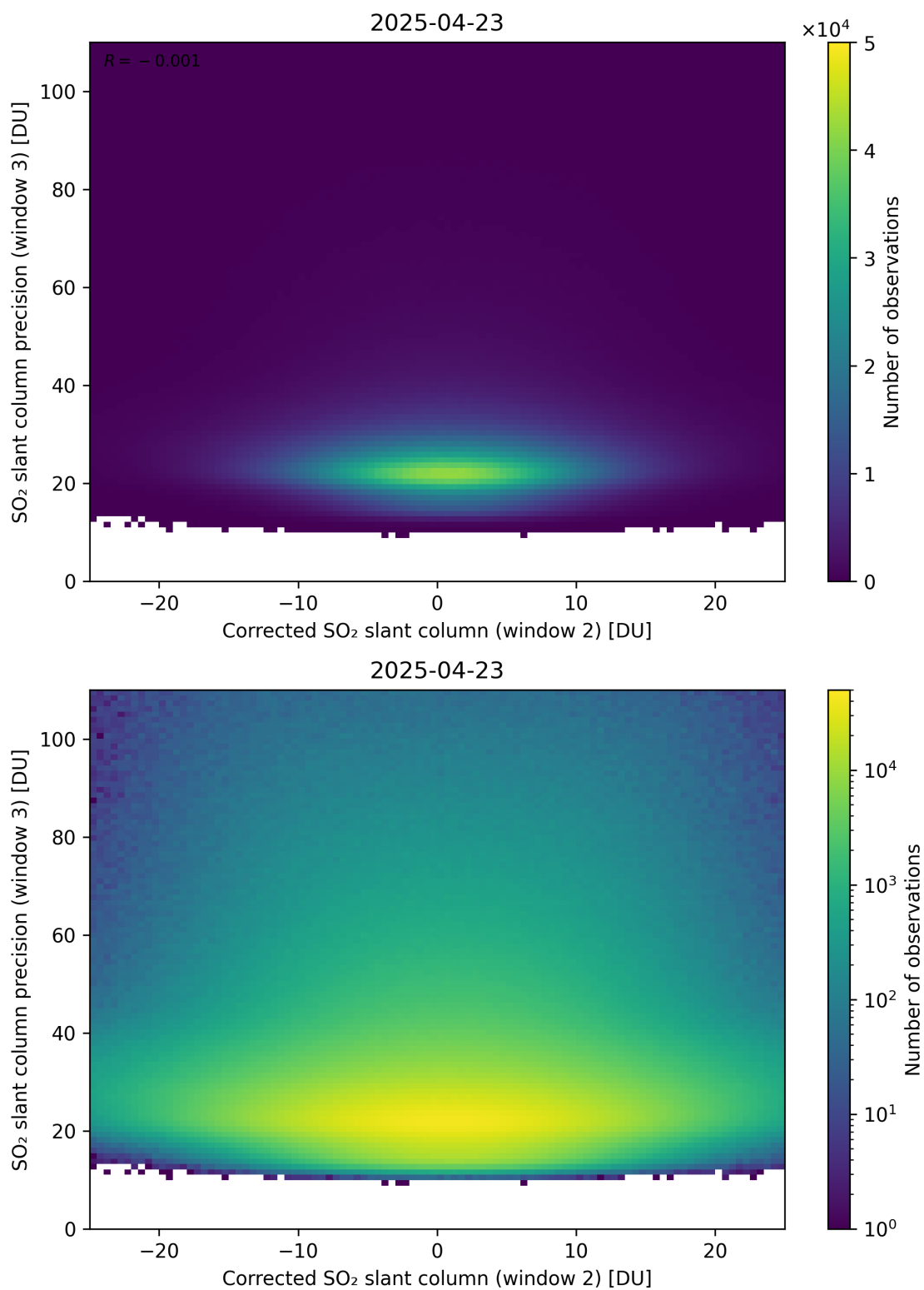
Figure 252: Scatter density plot of “Corrected SO 2 slant column (window 2)” against “SO 2 slant column precision (window 3)” for 2025-04-22 to 2025-04-24.
