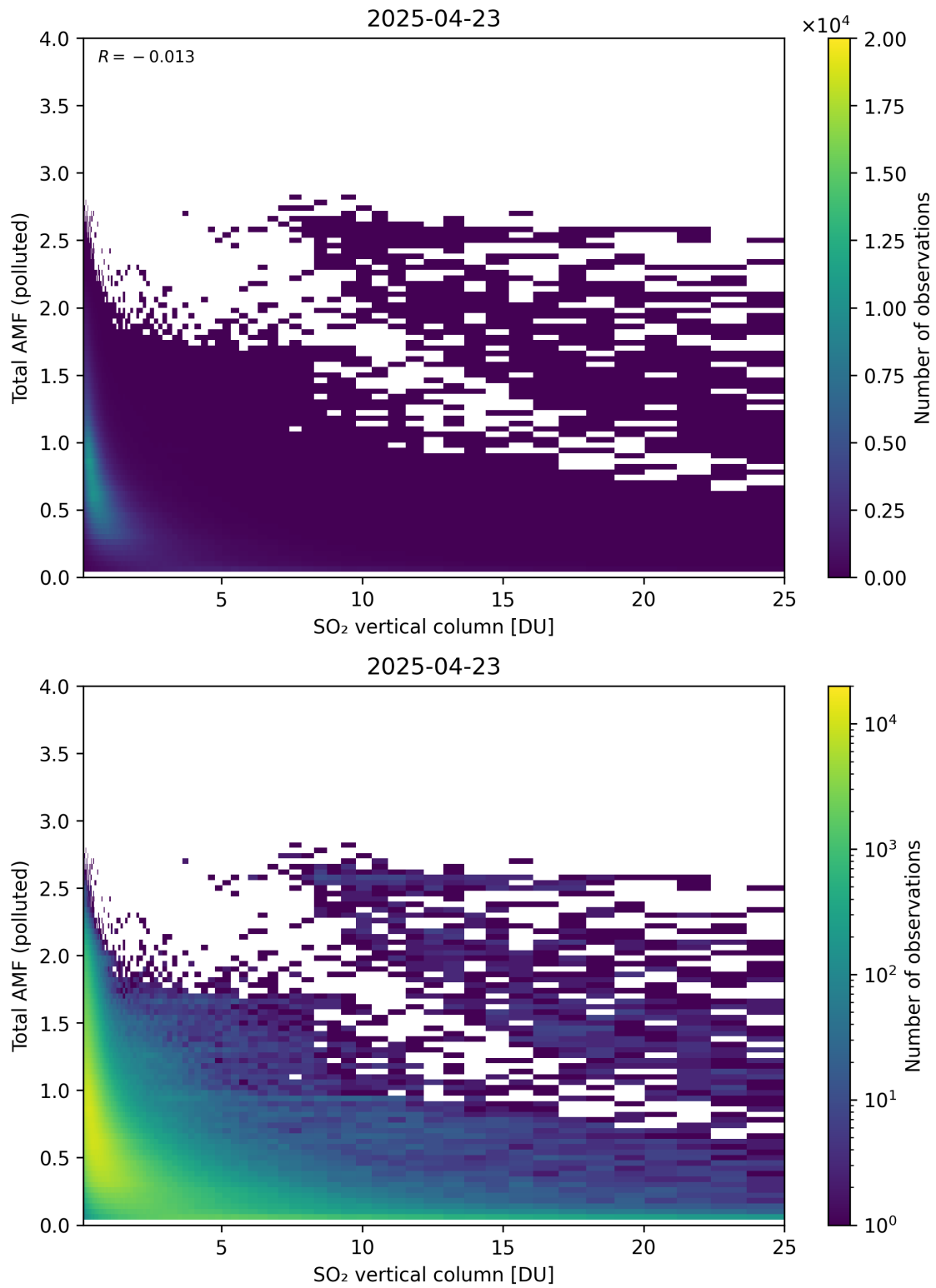
Figure 359: Scatter density plot of “SO 2 vertical column” against “Total AMF (polluted)” for 2025-04-22 to 2025-04-24.
