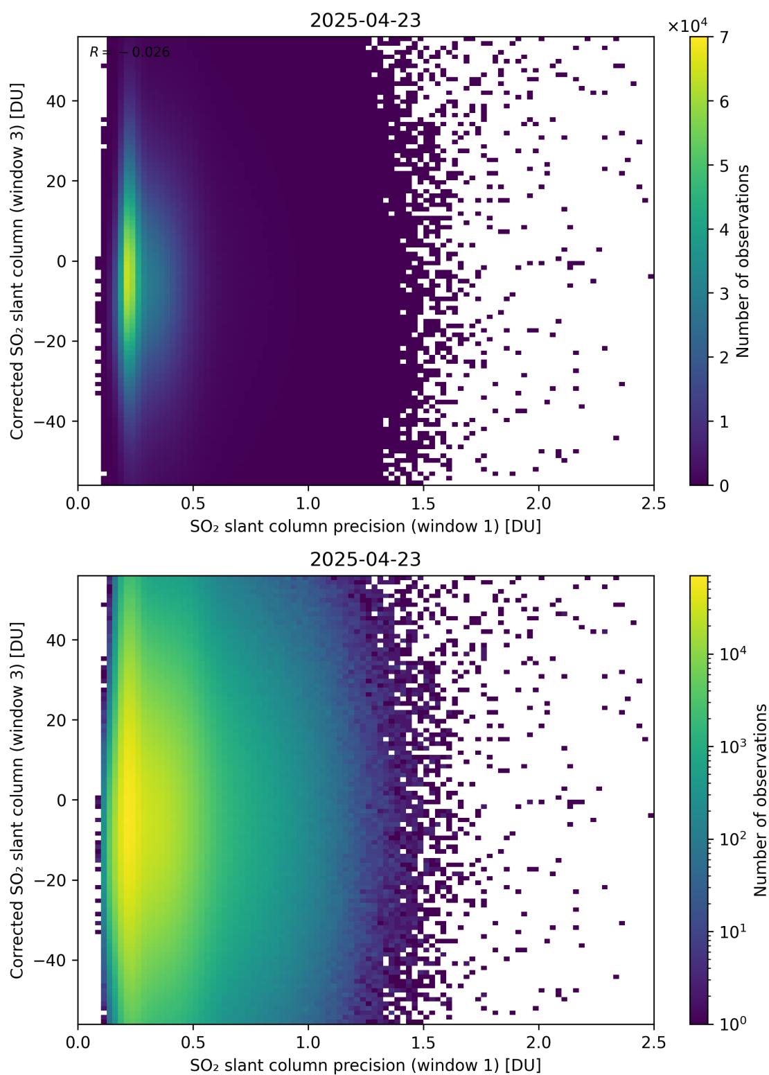
Figure 276: Scatter density plot of “SO 2 slant column precision (window 1)” against “Corrected SO 2 slant column (window 3)” for 2025-04-22 to 2025-04-24.
