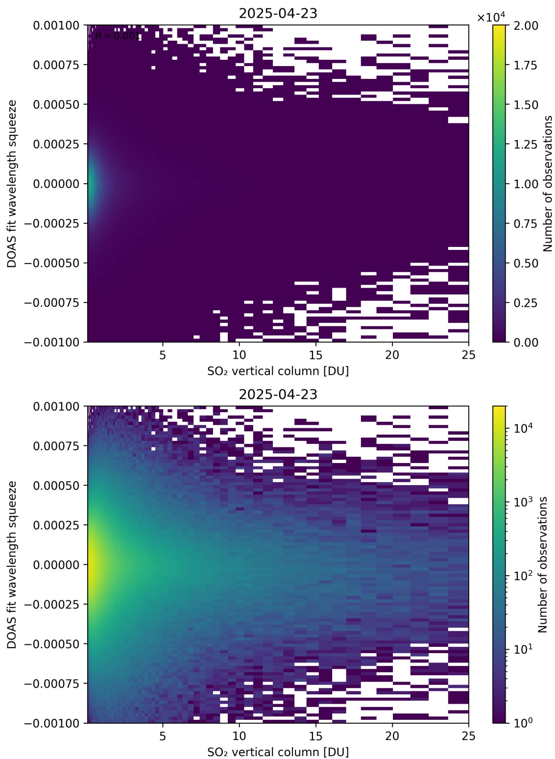
Figure 327: Scatter density plot of “SO 2 vertical column” against “DOAS fit wavelength squeeze” for 2025-04-22 to 2025-04-24.
