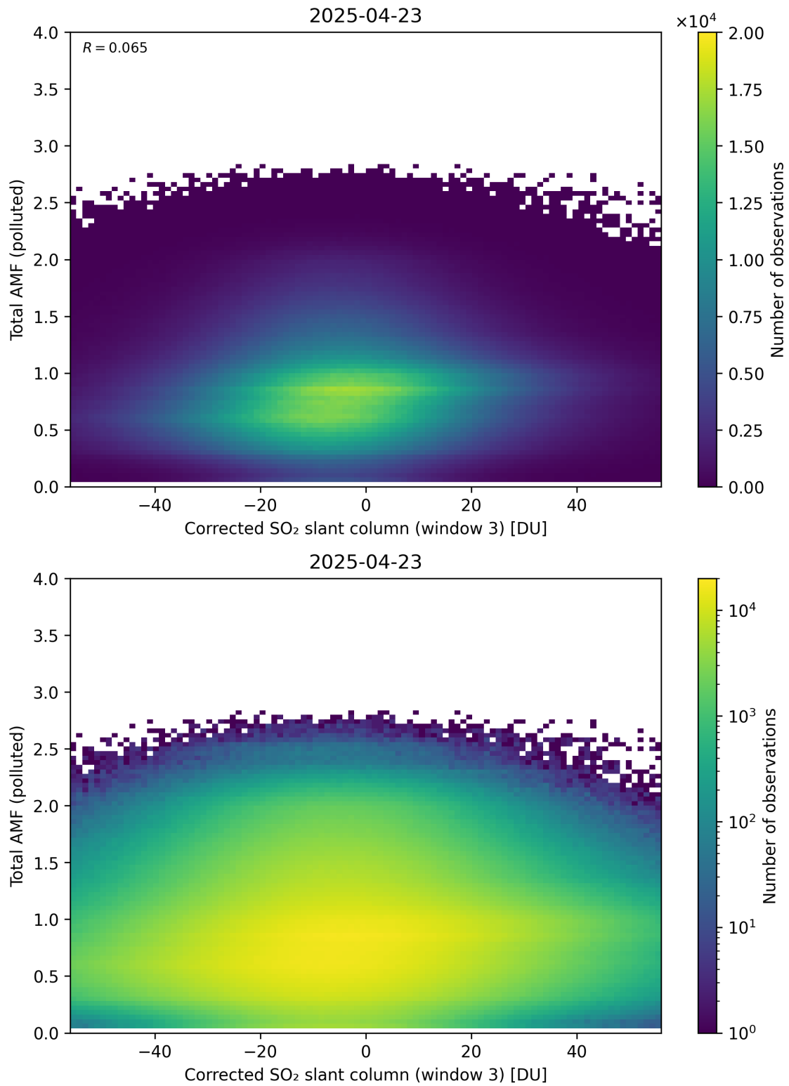
Figure 260: Scatter density plot of “Corrected SO 2 slant column (window 3)” against “Total AMF (polluted)” for 2025-04-22 to 2025-04-24.
