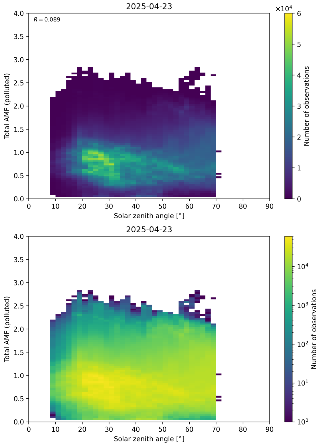
Figure 189: Scatter density plot of “Solar zenith angle” against “Total AMF (polluted)” for 2025-04-22 to 2025-04-24.
