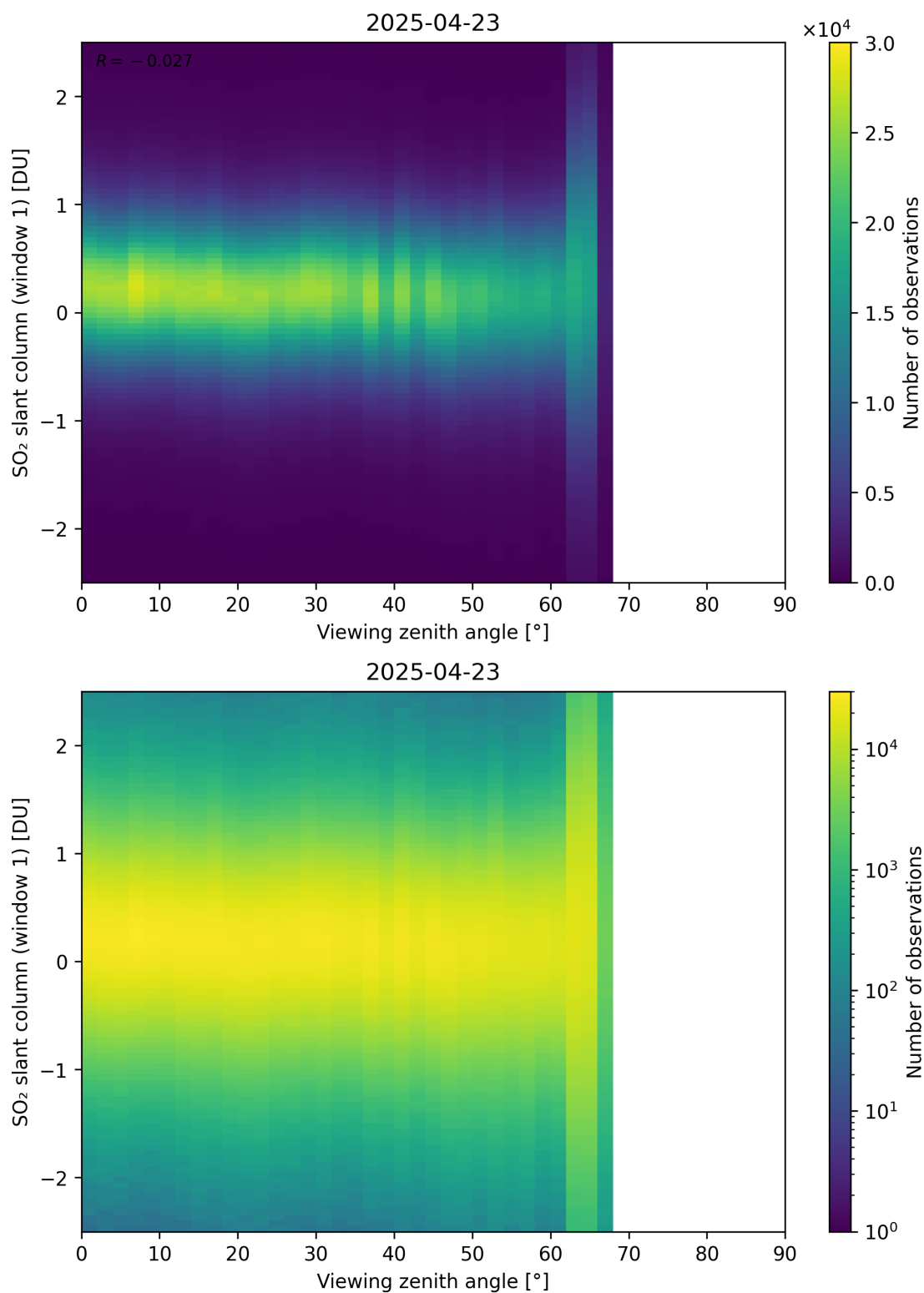
Figure 376: Scatter density plot of “Viewing zenith angle” against “SO 2 slant column (window 1)” for 2025-04-22 to 2025-04-24.
