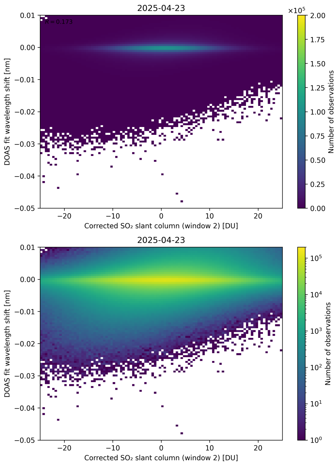
Figure 246: Scatter density plot of “Corrected SO 2 slant column (window 2)” against “DOAS fit wavelength shift” for 2025-04-22 to 2025-04-24.
