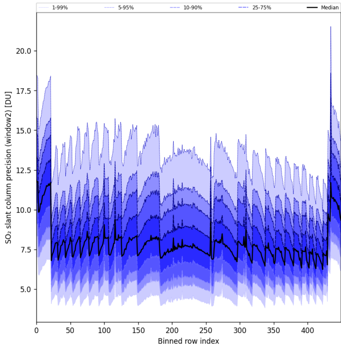
Figure 94: Along track statistics of “SO 2 slant column precision (window2)” for 2025-04-22 to 2025-04-24
