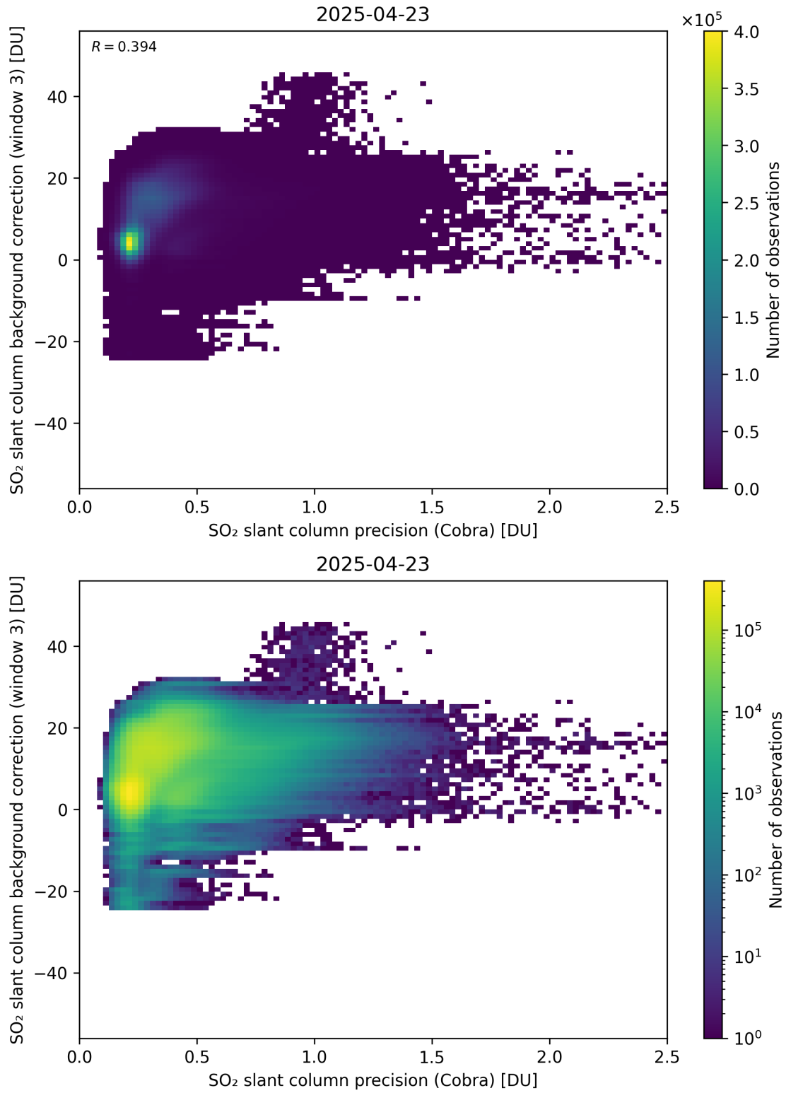
Figure 201: Scatter density plot of “SO 2 slant column precision (Cobra)” against “SO 2 slant column background correction (window 3)” for 2025-04-22 to 2025-04-24.
