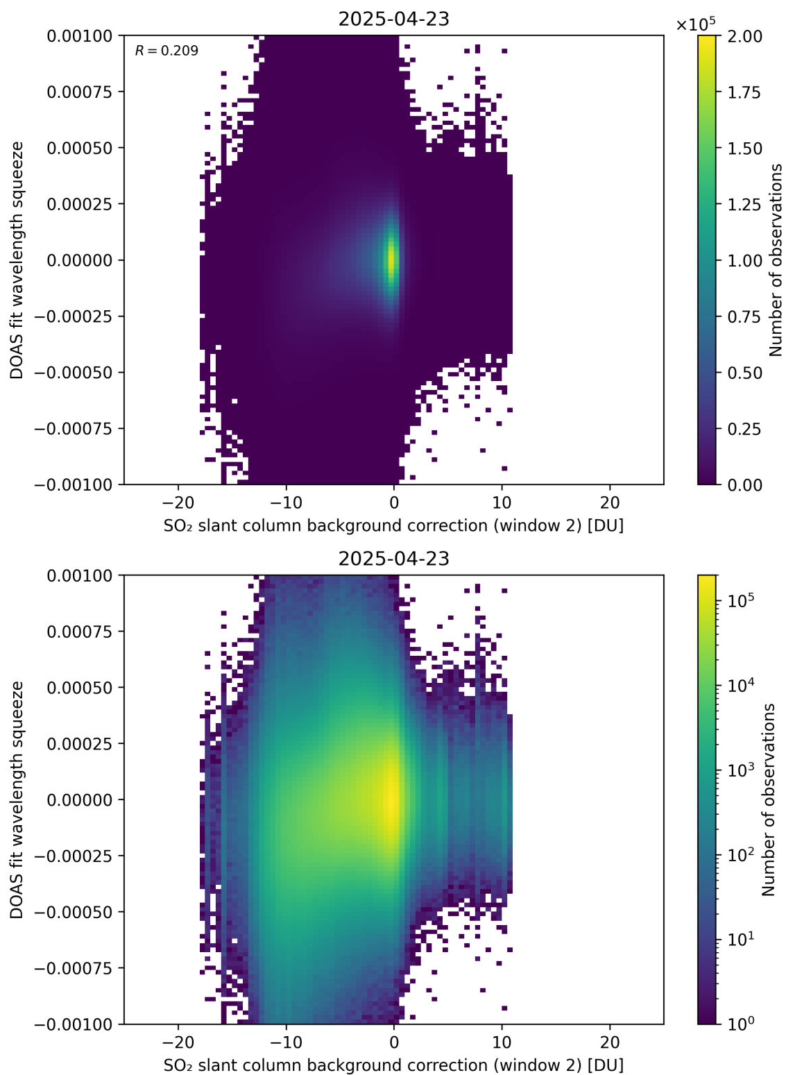
Figure 124: Scatter density plot of “SO 2 slant column background correction (window 2)” against “DOAS fit wavelength squeeze” for 2025-04-22 to 2025-04-24.
