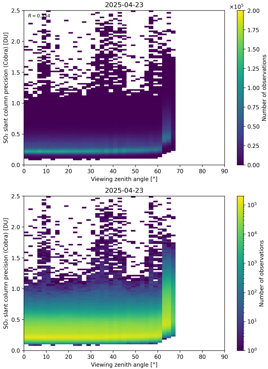
Figure 372: Scatter density plot of “Viewing zenith angle” against “SO 2 slant column precision (Cobra)” for 2025-04-22 to 2025-04-24.
