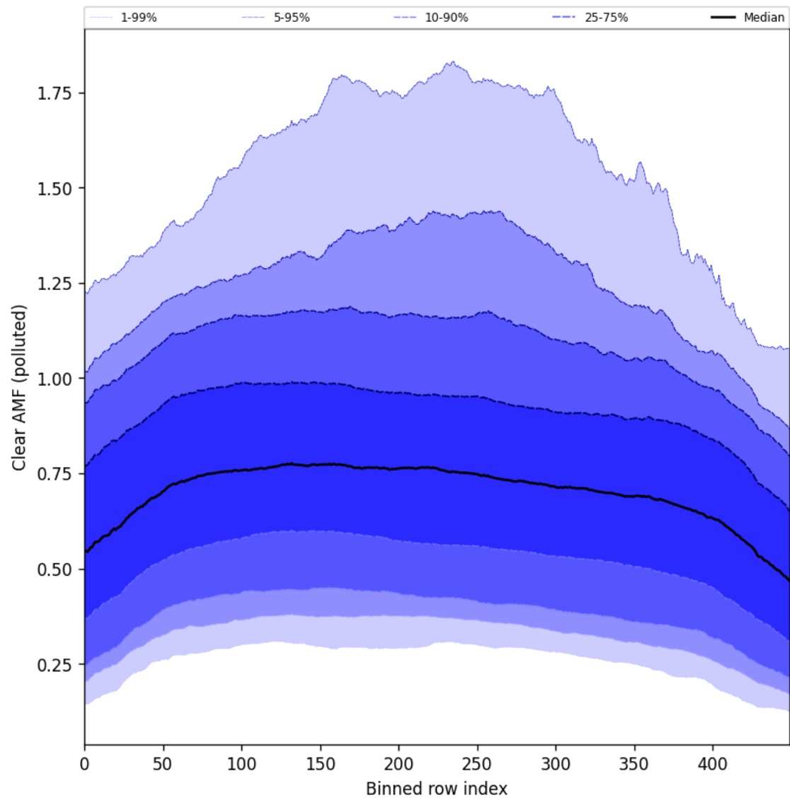
Figure 107: Along track statistics of “Clear AMF (polluted)” for 2025-04-22 to 2025-04-24
