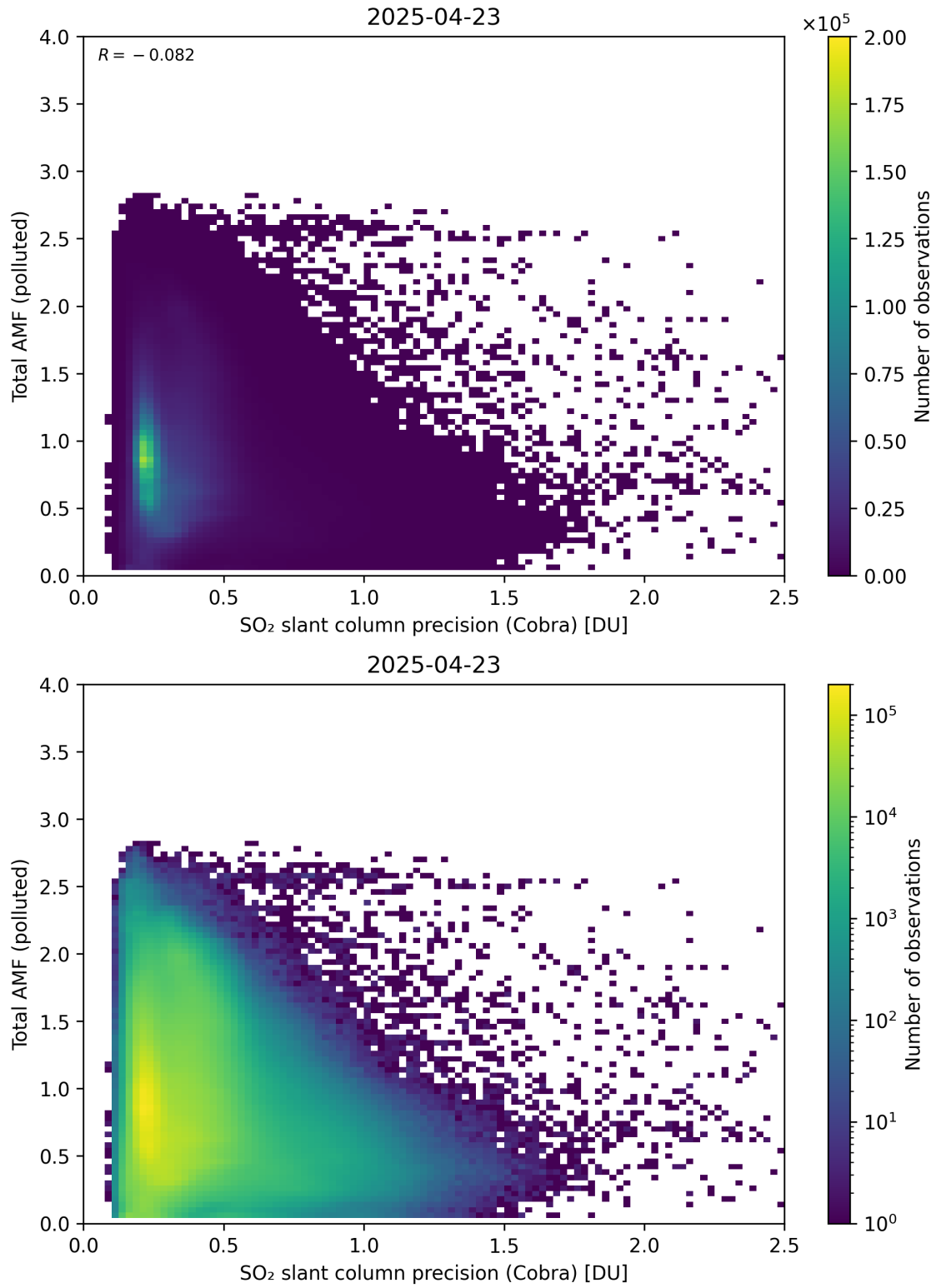
Figure 213: Scatter density plot of “SO 2 slant column precision (Cobra)” against “Total AMF (polluted)” for 2025-04-22 to 2025-04-24.
