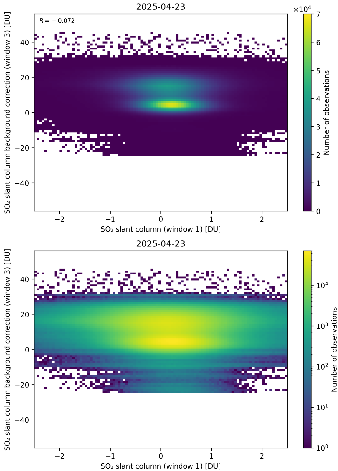
Figure 264: Scatter density plot of “SO 2 slant column (window 1)” against “SO 2 slant column background correction (window 3)” for 2025-04-22 to 2025-04-24.
