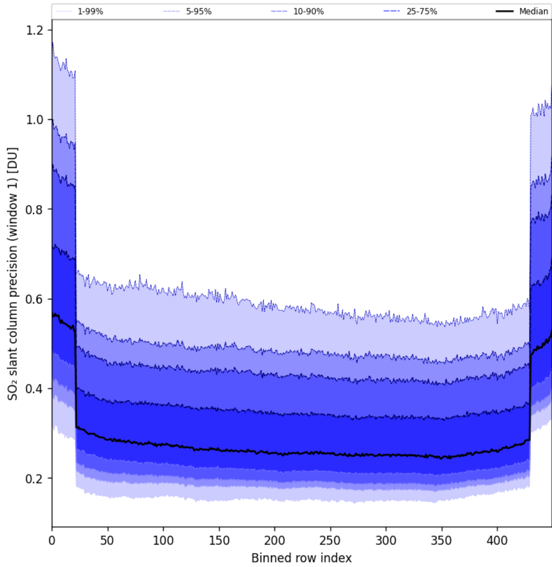
Figure 90: Along track statistics of “SO 2 slant column precision (window 1)” for 2025-04-22 to 2025-04-24
