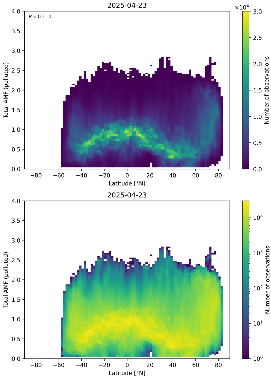
Figure 167: Scatter density plot of “Latitude” against “Total AMF (polluted)” for 2025-04-22 to 2025-04-24.
