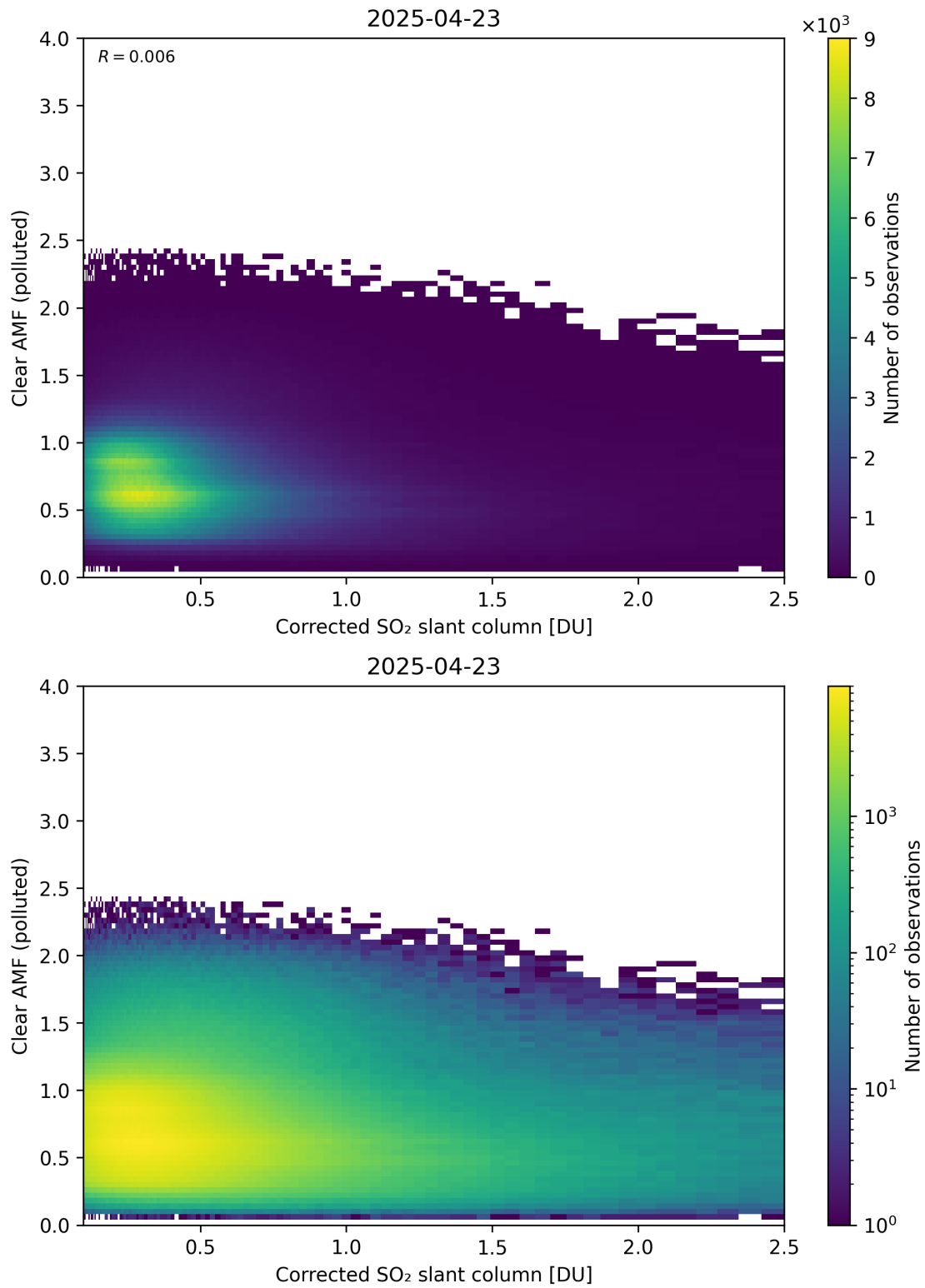
Figure 232: Scatter density plot of “Corrected SO 2 slant column” against “Clear AMF (polluted)” for 2025-04-22 to 2025-04-24.
