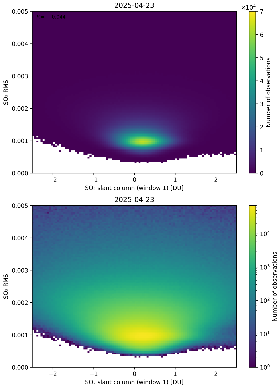
Figure 267: Scatter density plot of “SO 2 slant column (window 1)” against “SO 2 RMS” for 2025-04-22 to 2025-04-24.
