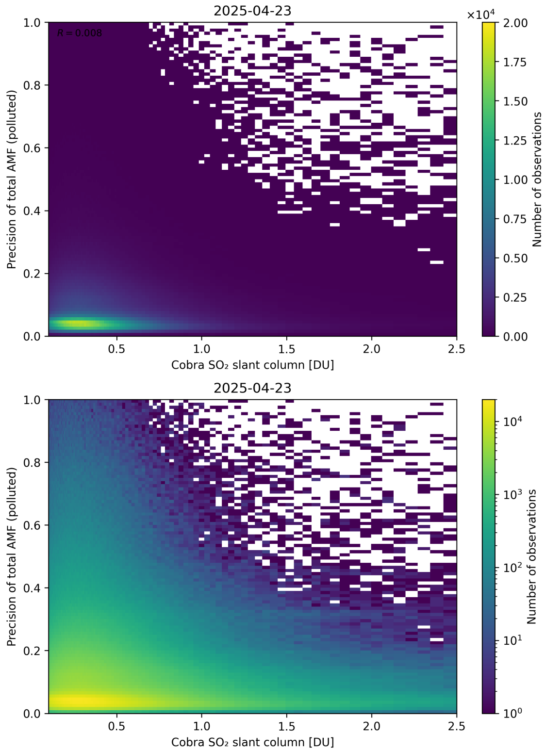
Figure 225: Scatter density plot of “Cobra SO 2 slant column” against “Precision of total AMF (polluted)” for 2025-04-22 to 2025-04-24.
