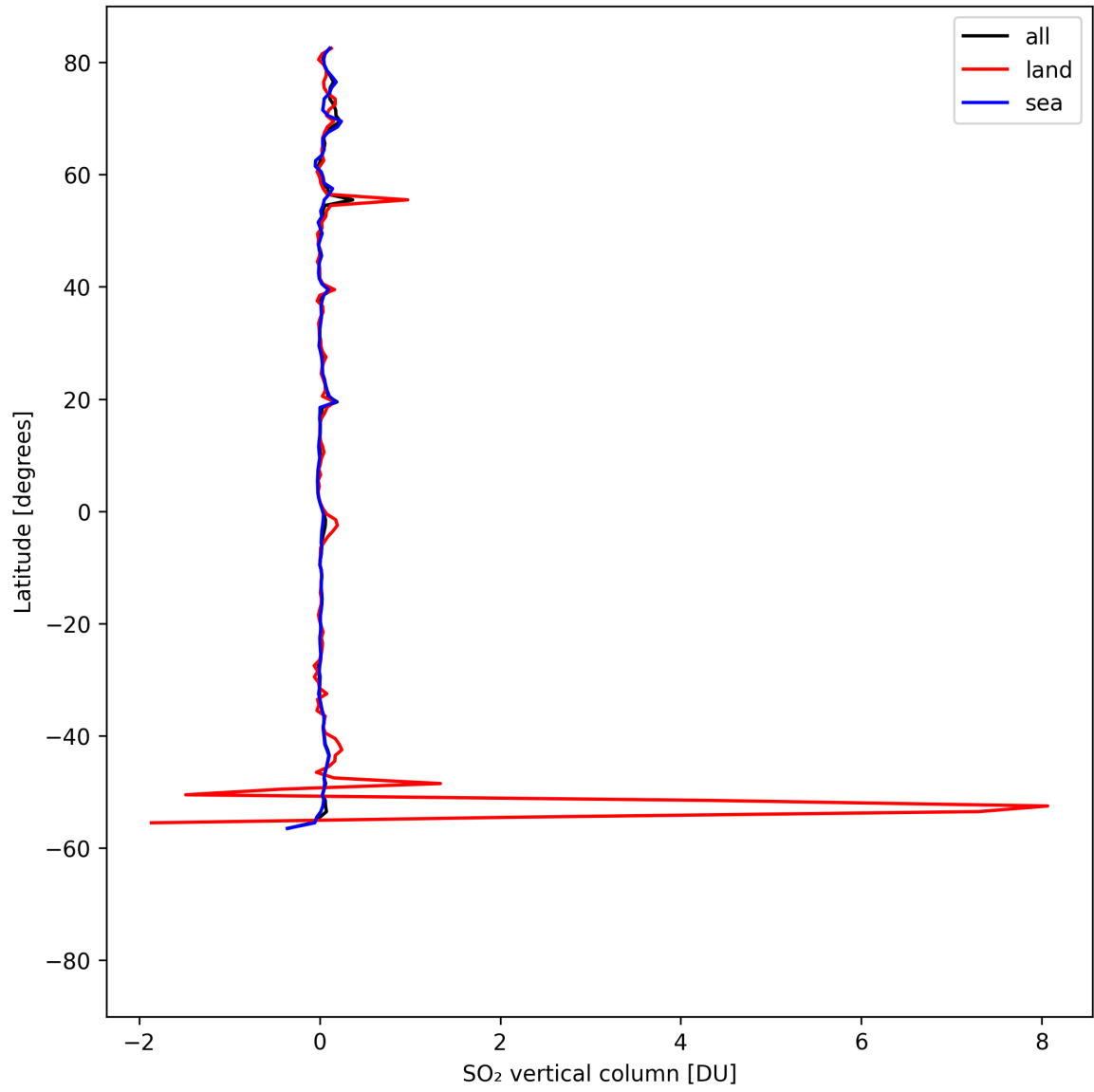
Figure 32: Zonal average of “SO 2 vertical column” for 2025-04-22 to 2025-04-24.
