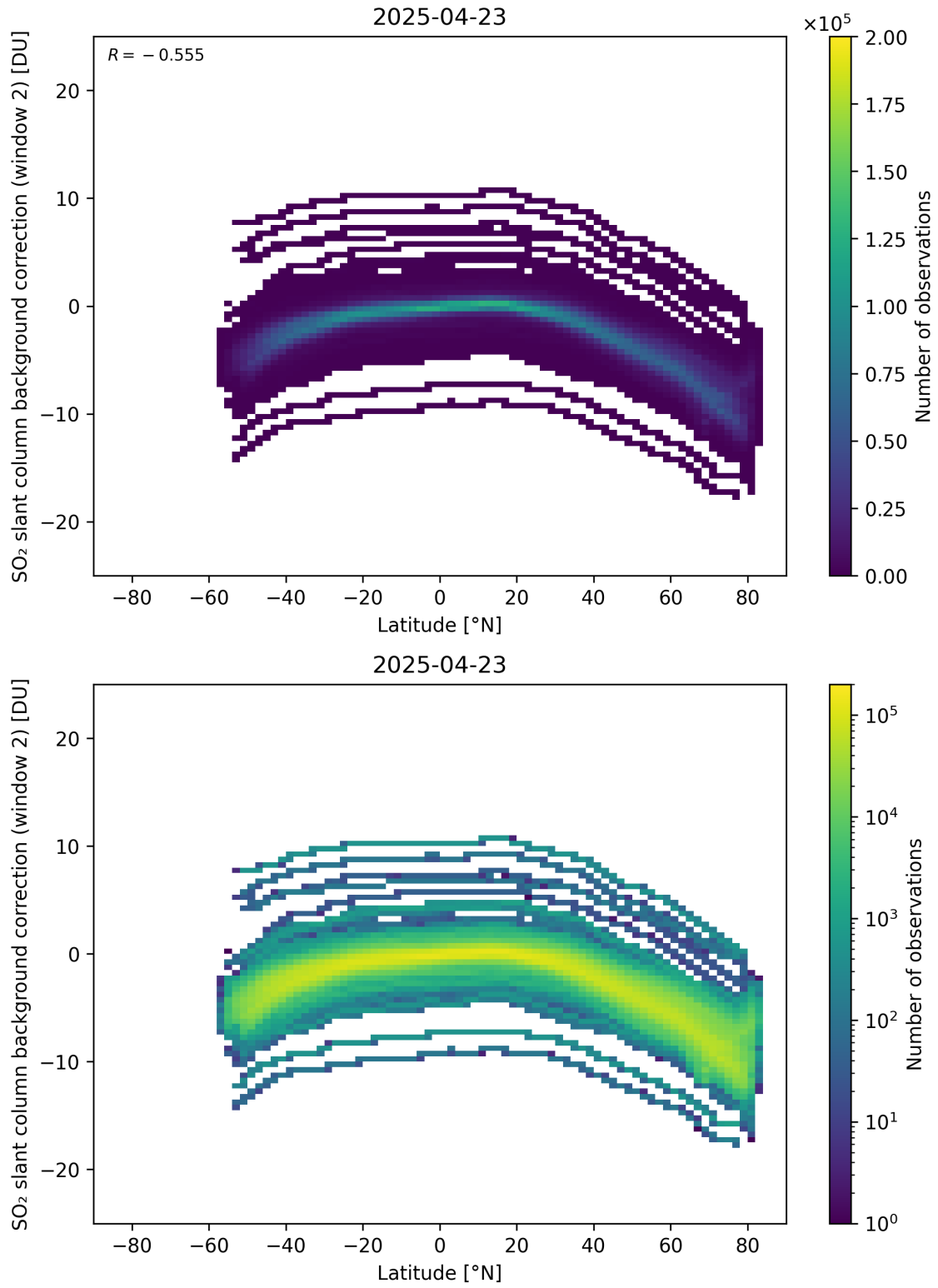
Figure 151: Scatter density plot of “Latitude” against “SO 2 slant column background correction (window 2)” for 2025-04-22 to 2025-04-24.
