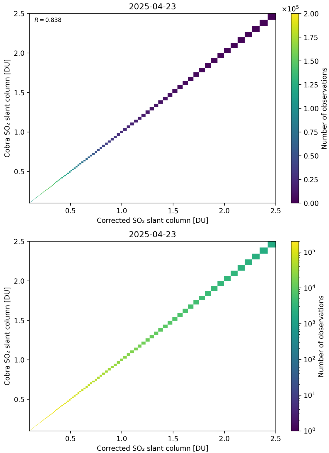
Figure 233: Scatter density plot of “Corrected SO 2 slant column” against “Cobra SO 2 slant column” for 2025-04-22 to 2025-04-24.
