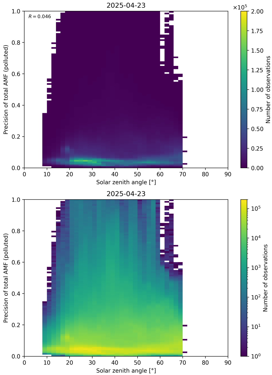
Figure 190: Scatter density plot of “Solar zenith angle” against “Precision of total AMF (polluted)” for 2025-04-22 to 2025-04-24.
