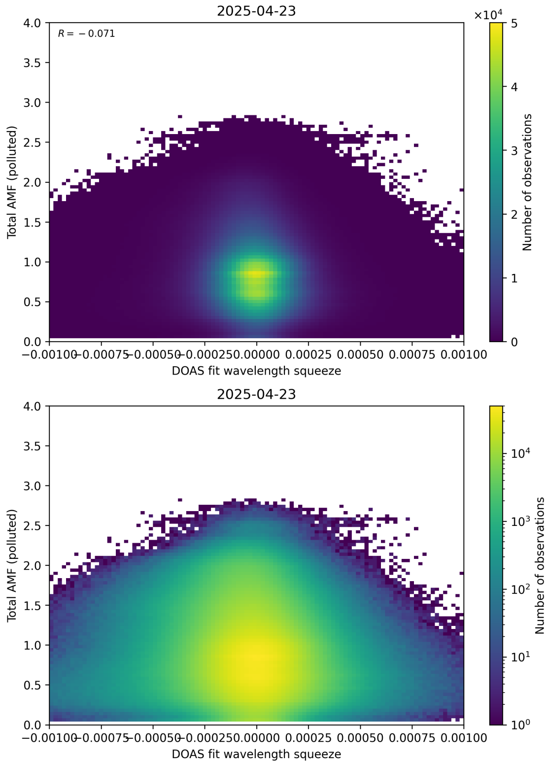
Figure 145: Scatter density plot of “DOAS fit wavelength squeeze” against “Total AMF (polluted)” for 2025-04-22 to 2025-04-24.
