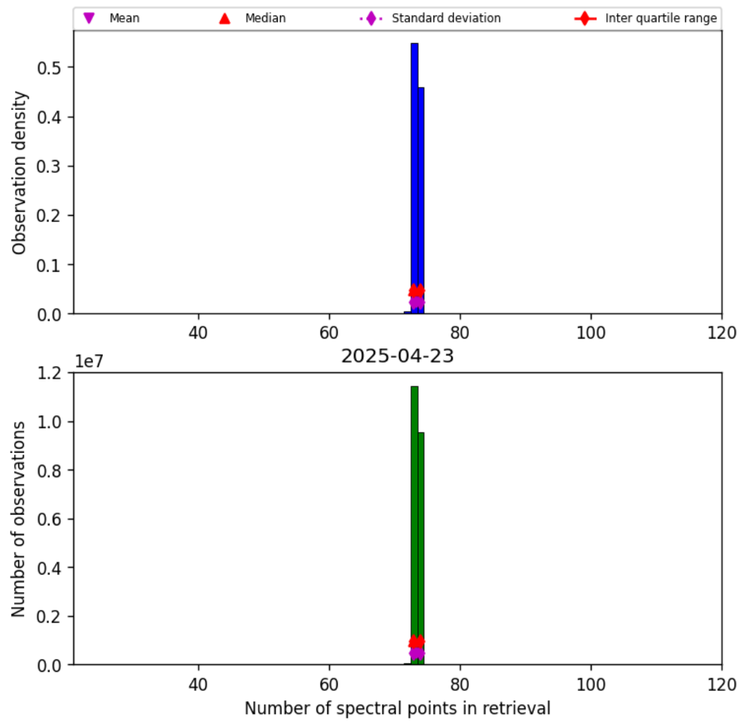
Figure 82: Histogram of “Number of spectral points in retrieval” for 2025-04-22 to 2025-04-24
