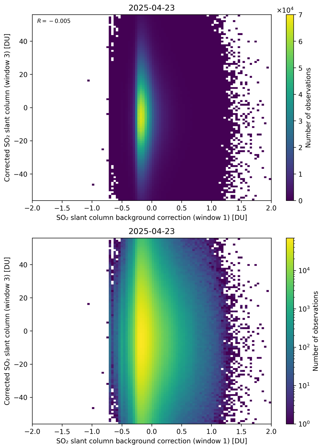
Figure 116: Scatter density plot of “SO 2 slant column background correction (window 1)” against “Corrected SO 2 slant column (window 3)” for 2025-04-22 to 2025-04-24.
