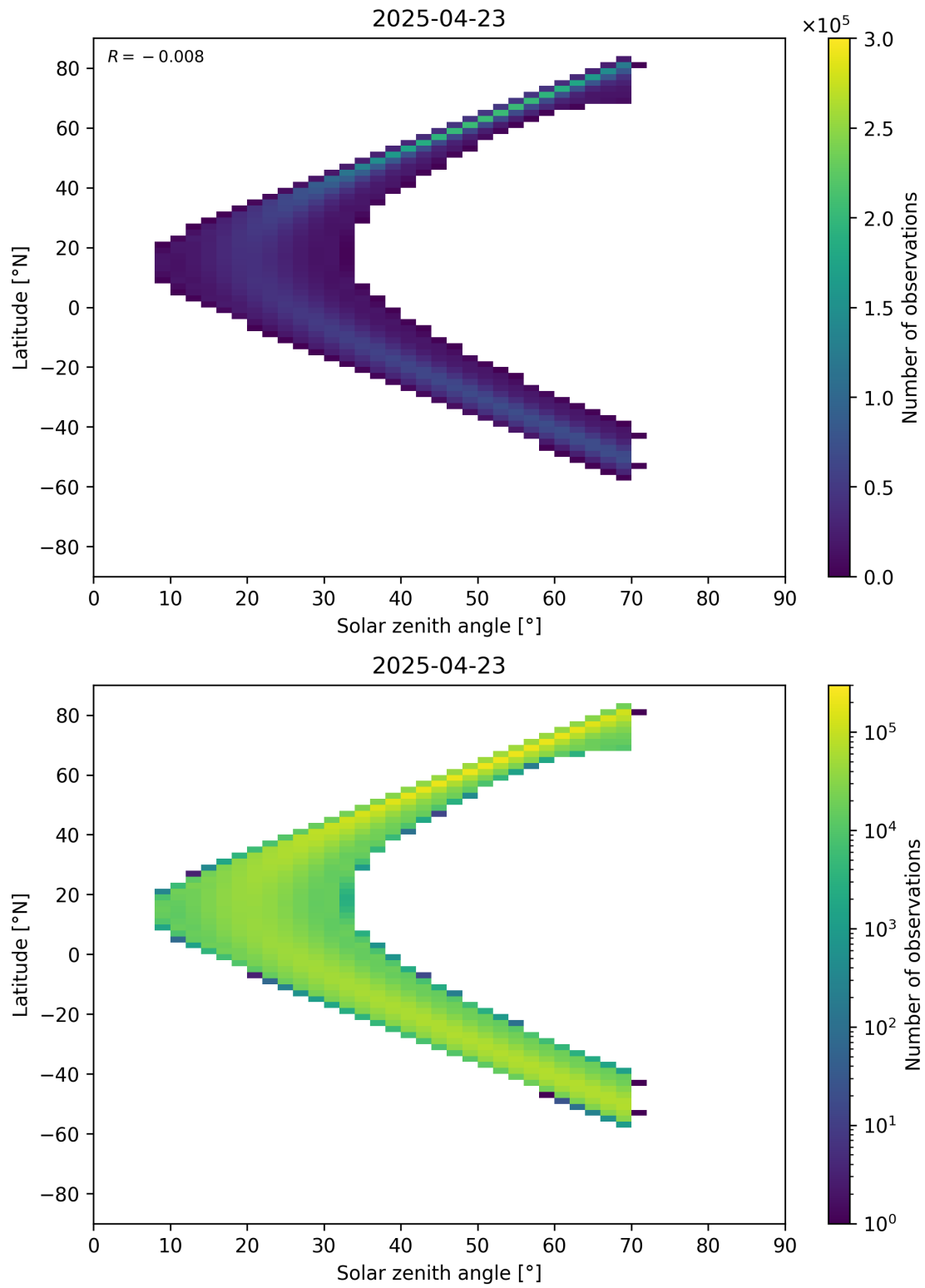
Figure 177: Scatter density plot of “Solar zenith angle” against “Latitude” for 2025-04-22 to 2025-04-24.
