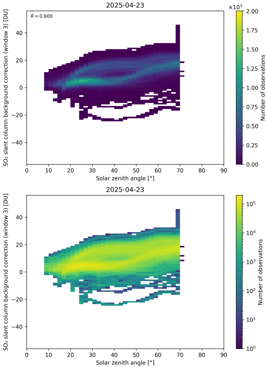
Figure 173: Scatter density plot of “Solar zenith angle” against “SO 2 slant column background correction (window 3)” for 2025-04-22 to 2025-04-24.
