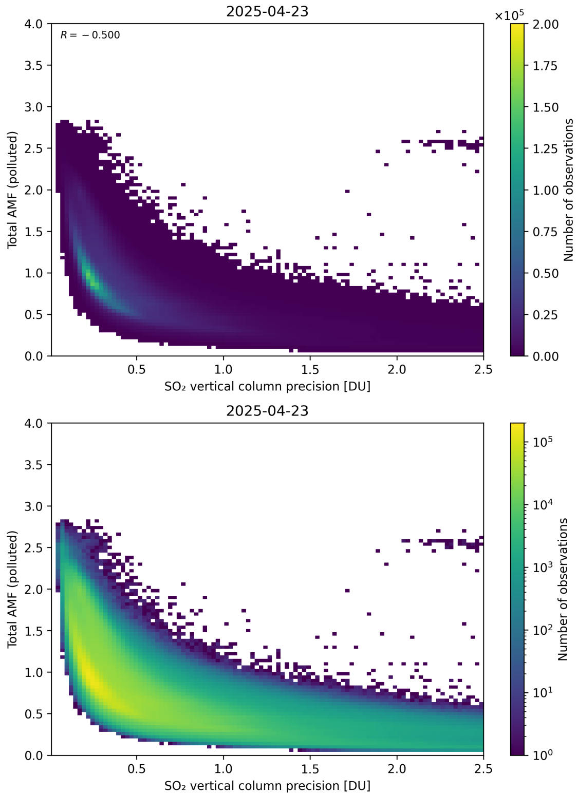
Figure 346: Scatter density plot of “SO 2 vertical column precision” against “Total AMF (polluted)” for 2025-04-22 to 2025-04-24.
