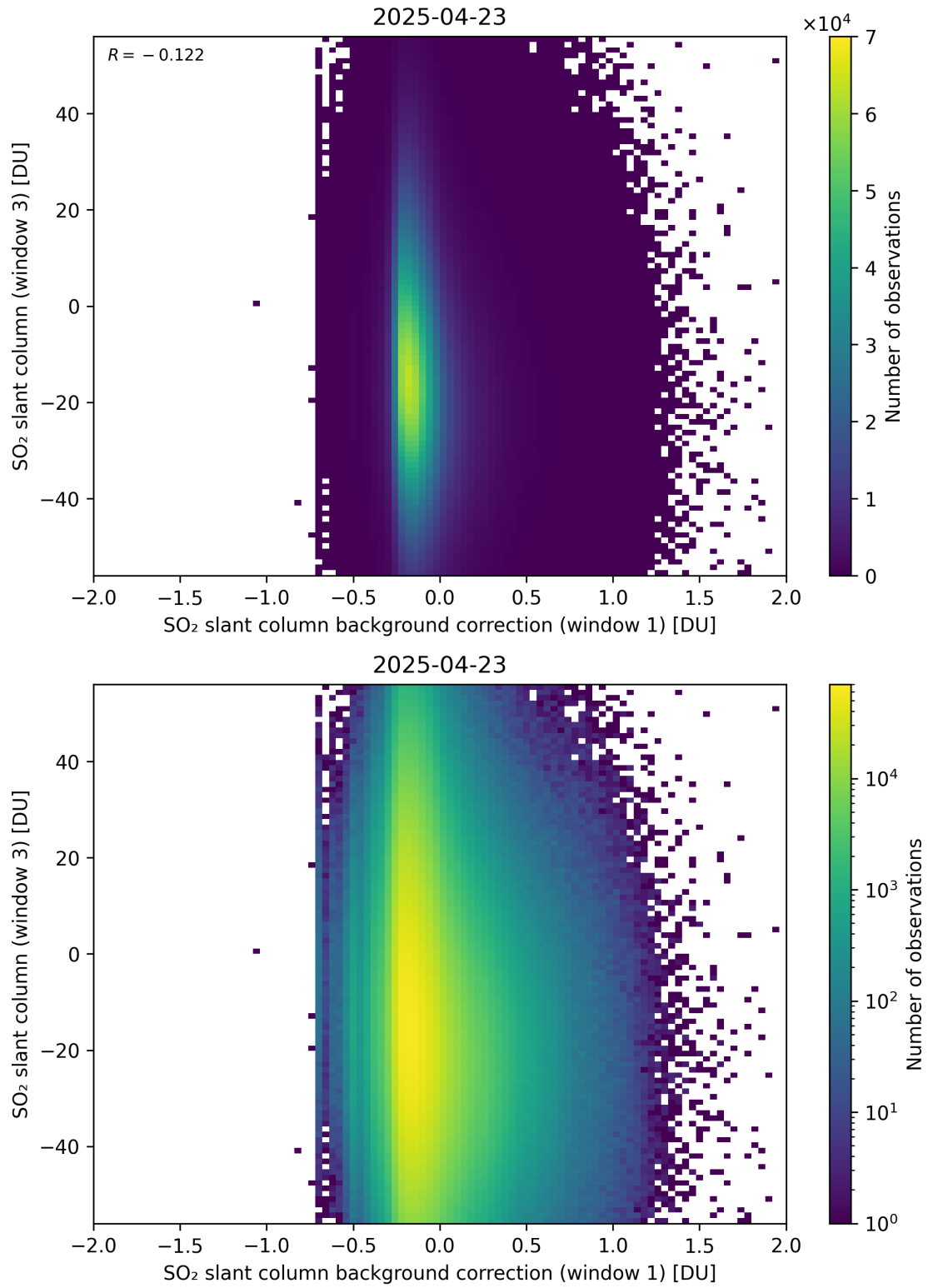
Figure 118: Scatter density plot of “SO 2 slant column background correction (window 1)” against “SO 2 slant column (window 3)” for 2025-04-22 to 2025-04-24.
