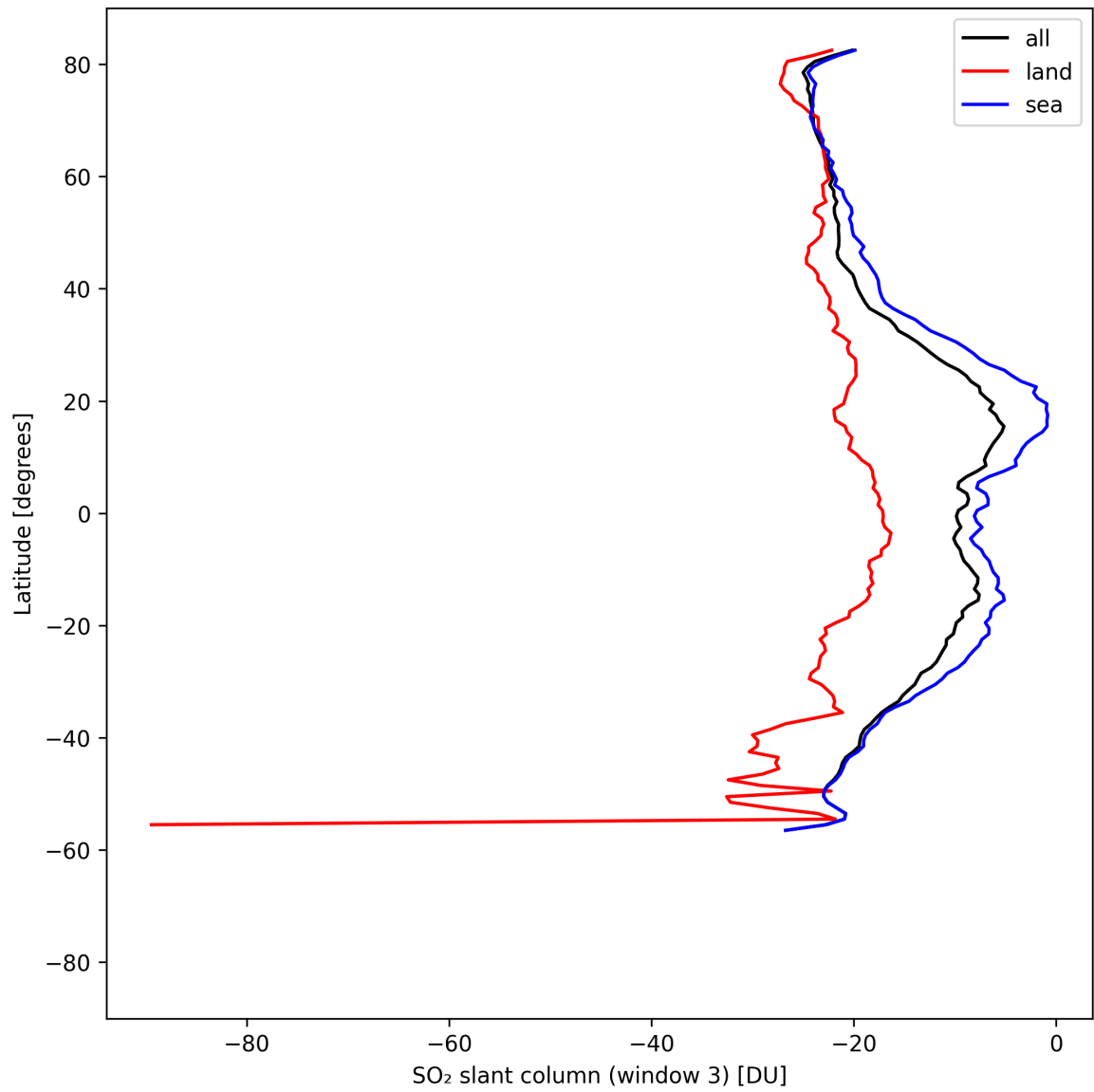
Figure 45: Zonal average of “SO 2 slant column (window 3)” for 2025-04-22 to 2025-04-24.
