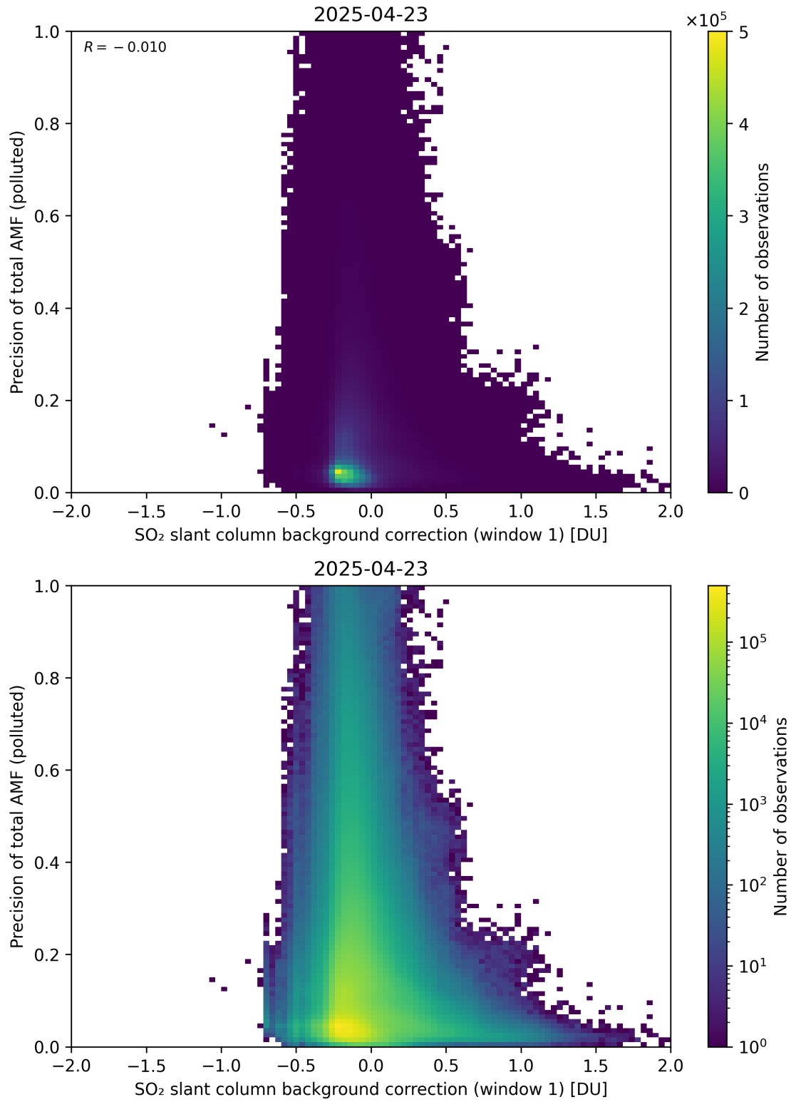
Figure 121: Scatter density plot of “SO 2 slant column background correction (window 1)” against “Precision of total AMF (polluted)” for 2025-04-22 to 2025-04-24.
