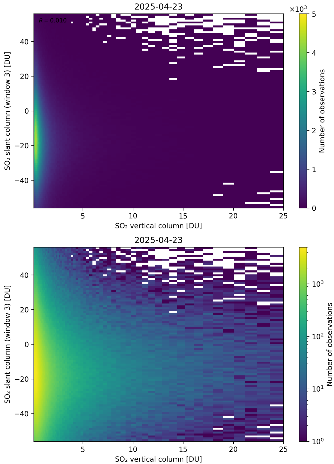
Figure 357: Scatter density plot of “SO 2 vertical column” against “SO 2 slant column (window 3)” for 2025-04-22 to 2025-04-24.
