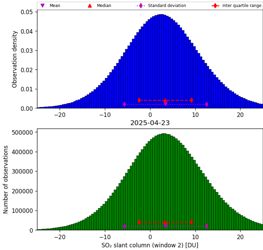
Figure 67: Histogram of “SO 2 slant column (window 2)” for 2025-04-22 to 2025-04-24
