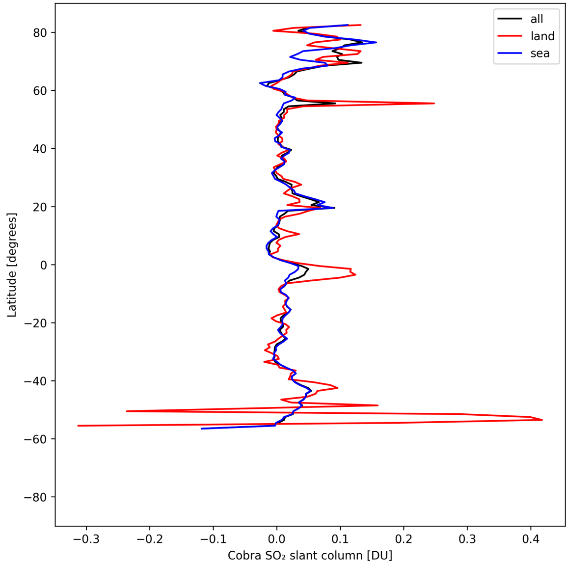
Figure 35: Zonal average of “Cobra SO 2 slant column” for 2025-04-22 to 2025-04-24.
