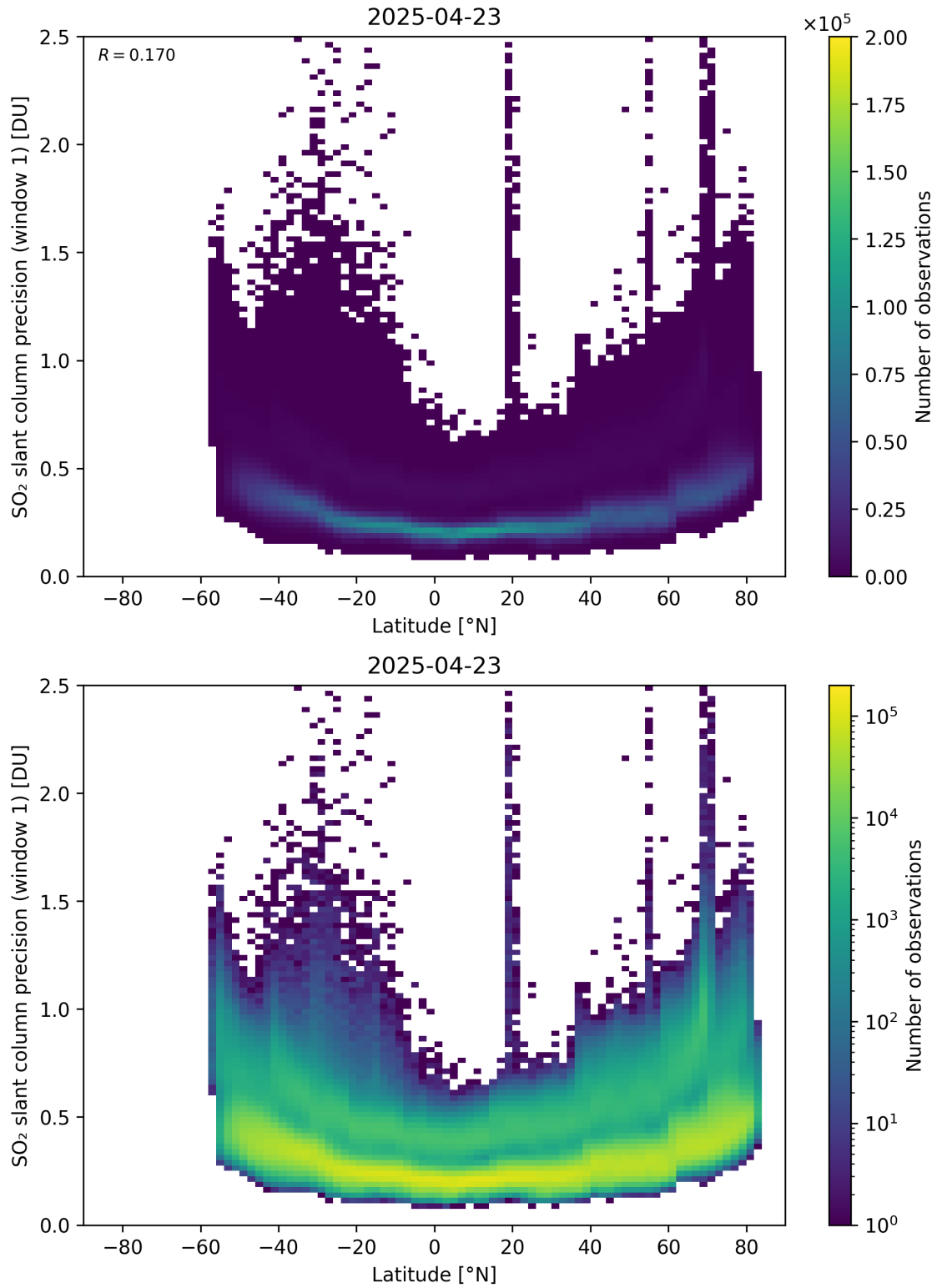
Figure 163: Scatter density plot of “Latitude” against “SO 2 slant column precision (window 1)” for 2025-04-22 to 2025-04-24.
