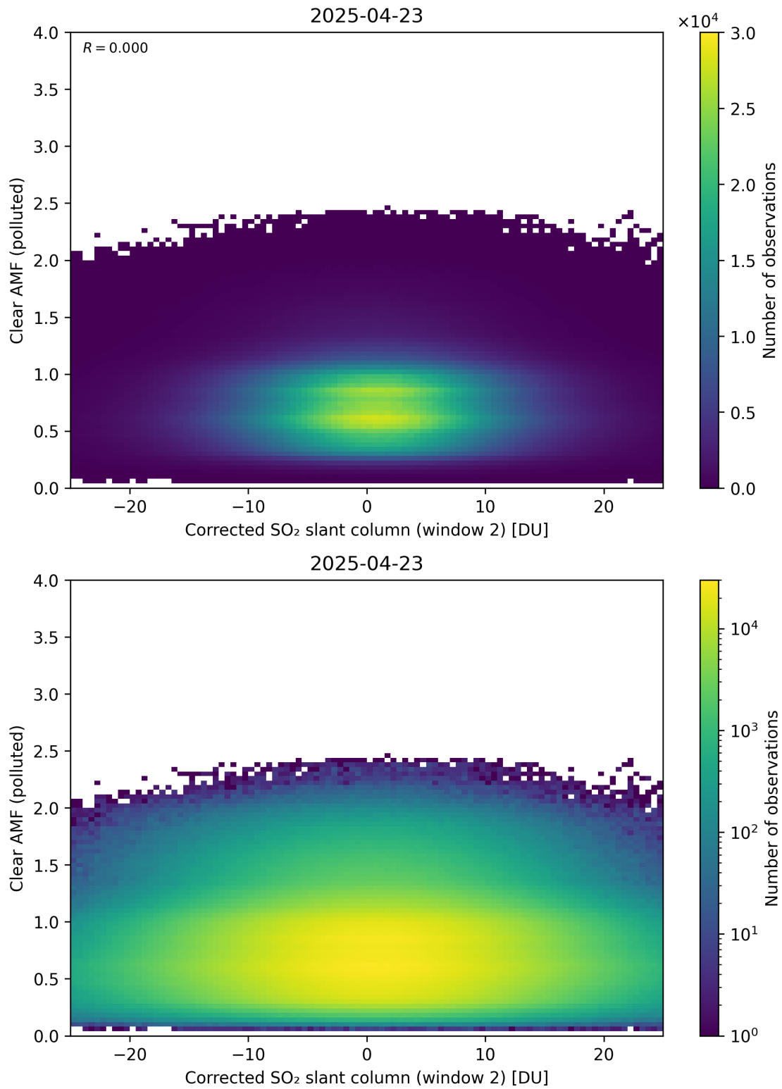
Figure 249: Scatter density plot of “Corrected SO 2 slant column (window 2)” against “Clear AMF (polluted)” for 2025-04-22 to 2025-04-24.
