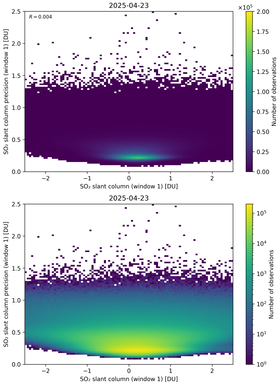
Figure 285: Scatter density plot of “SO 2 slant column (window 1)” against “SO 2 slant column precision (window 1)” for 2025-04-22 to 2025-04-24.
