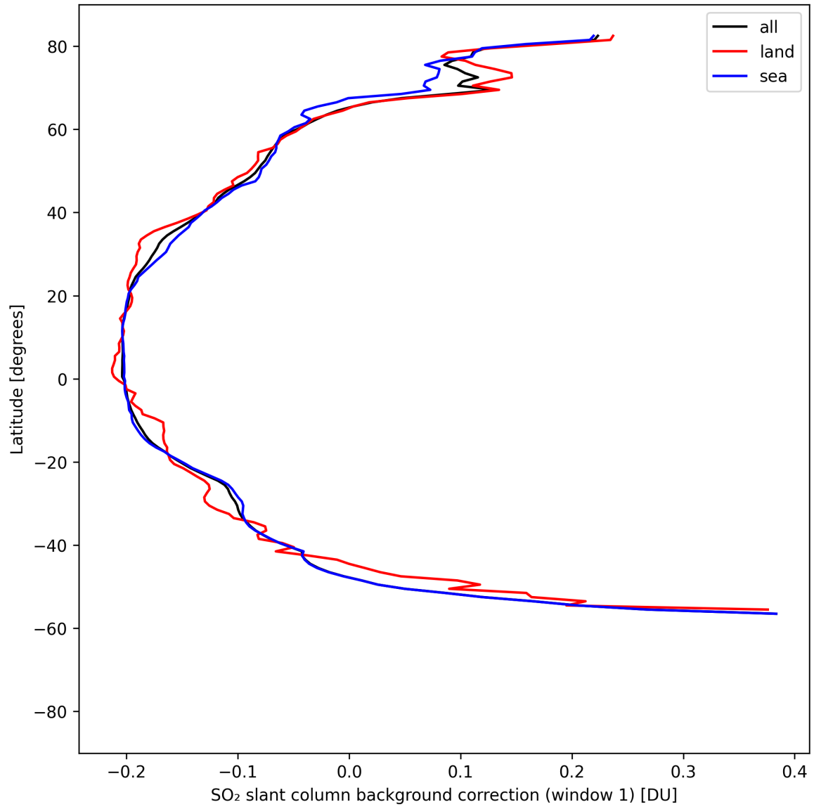
Figure 40: Zonal average of “SO 2 slant column background correction (window 1)” for 2025-04-22 to 2025-04-24.
