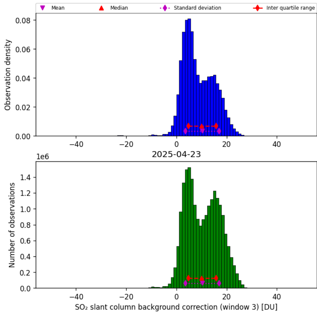
Figure 74: Histogram of “SO 2 slant column background correction (window 3)” for 2025-04-22 to 2025-04-24
