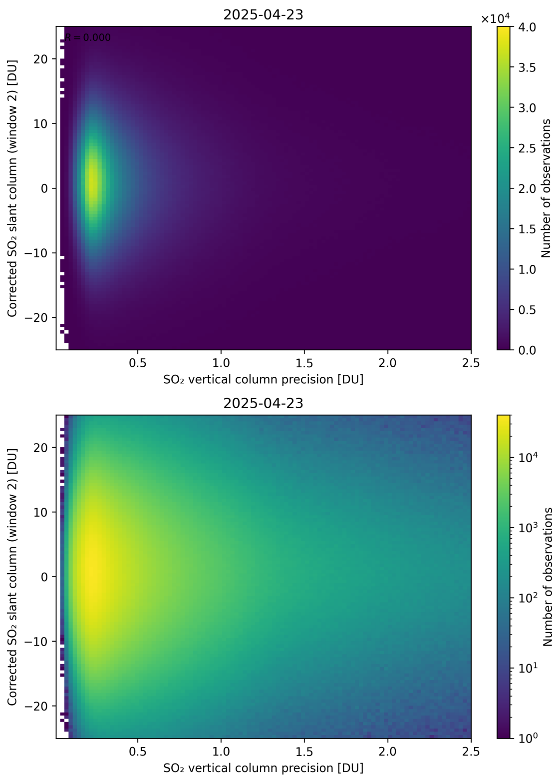
Figure 339: Scatter density plot of “SO 2 vertical column precision” against “Corrected SO 2 slant column (window 2)” for 2025-04-22 to 2025-04-24.
