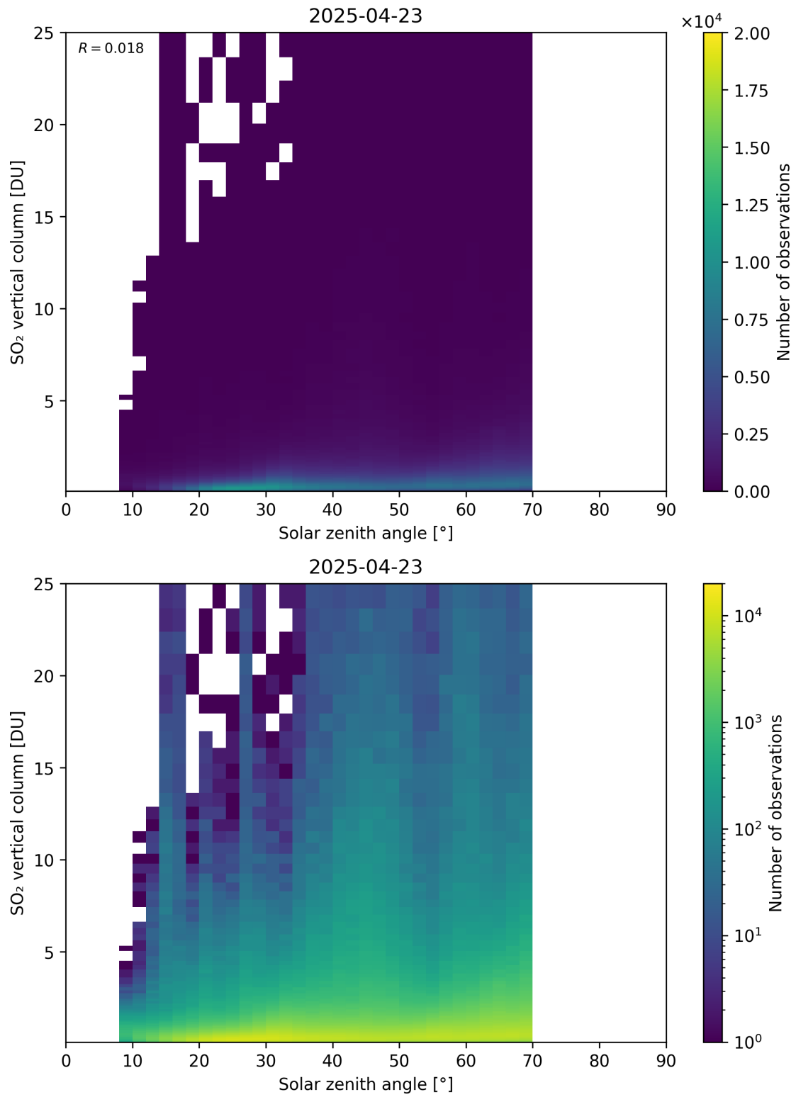
Figure 191: Scatter density plot of “Solar zenith angle” against “SO 2 vertical column” for 2025-04-22 to 2025-04-24.
