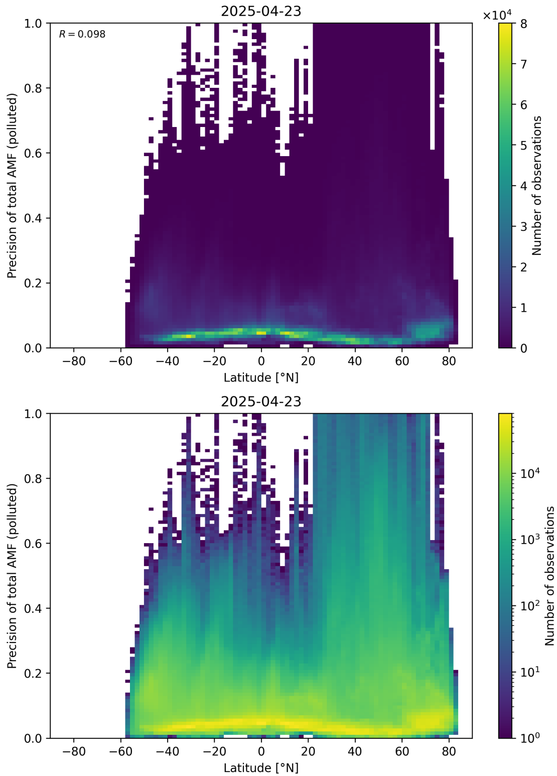
Figure 168: Scatter density plot of “Latitude” against “Precision of total AMF (polluted)” for 2025-04-22 to 2025-04-24.
