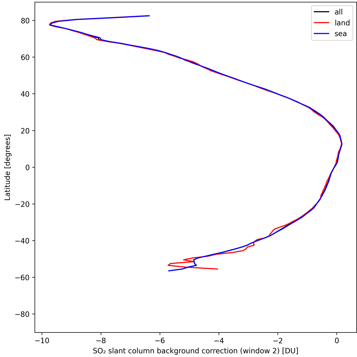
Figure 44: Zonal average of “SO 2 slant column background correction (window 2)” for 2025-04-22 to 2025-04-24.
