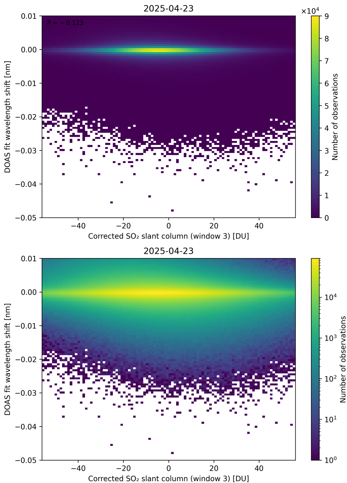
Figure 256: Scatter density plot of “Corrected SO 2 slant column (window 3)” against “DOAS fit wavelength shift” for 2025-04-22 to 2025-04-24.
