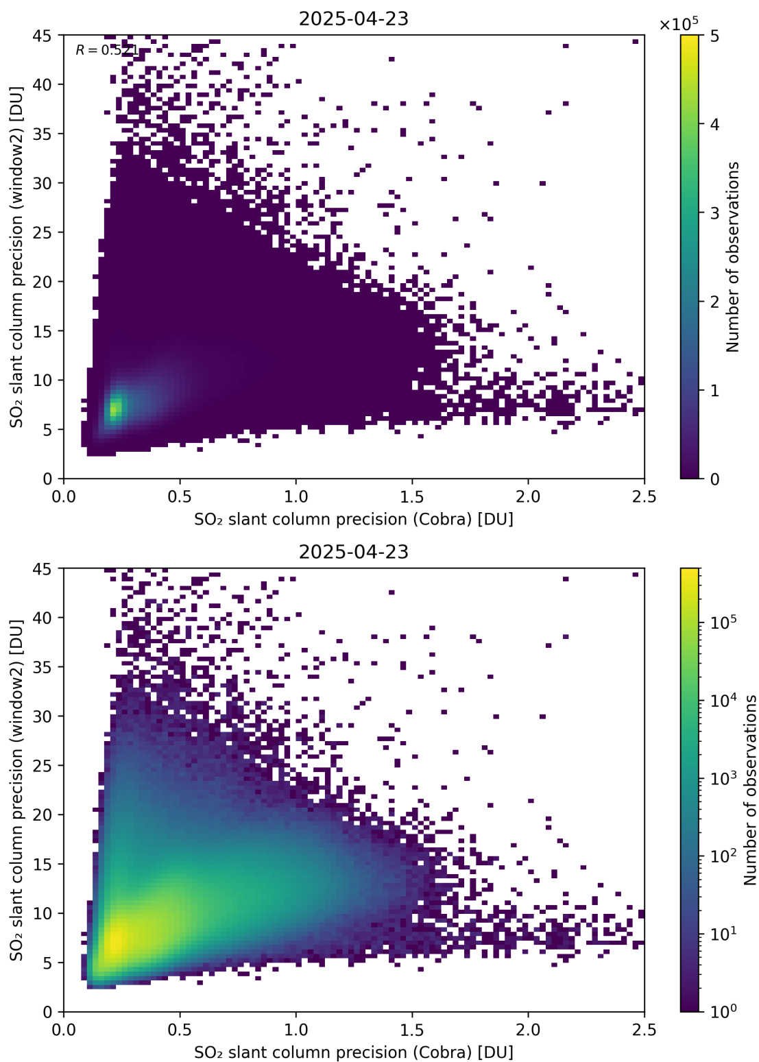
Figure 210: Scatter density plot of “SO 2 slant column precision (Cobra)” against “SO 2 slant column precision (window2)” for 2025-04-22 to 2025-04-24.
