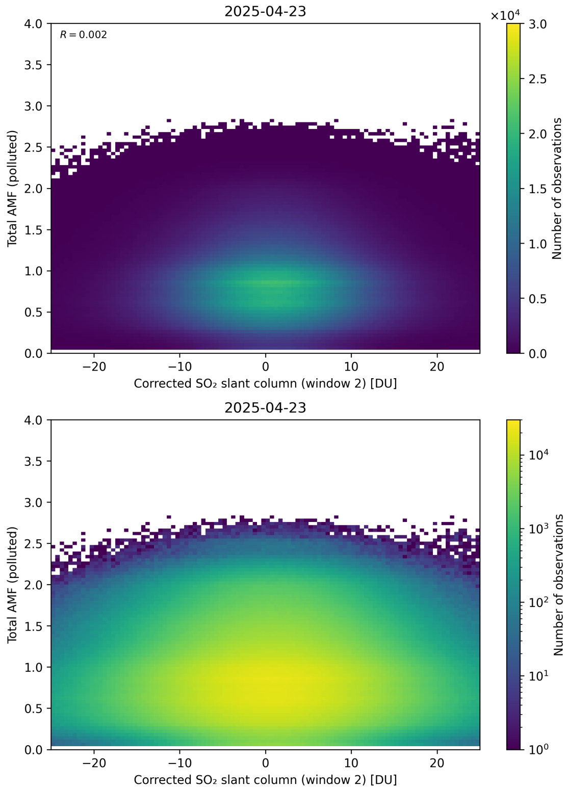
Figure 253: Scatter density plot of “Corrected SO 2 slant column (window 2)” against “Total AMF (polluted)” for 2025-04-22 to 2025-04-24.
