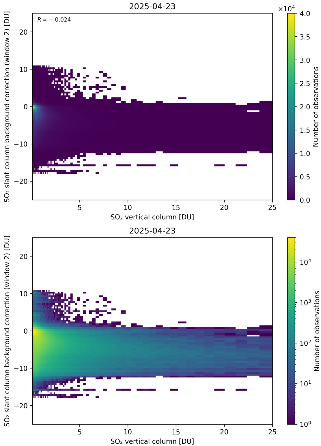
Figure 324: Scatter density plot of “SO 2 vertical column” against “SO 2 slant column background correction (window 2)” for 2025-04-22 to 2025-04-24.
