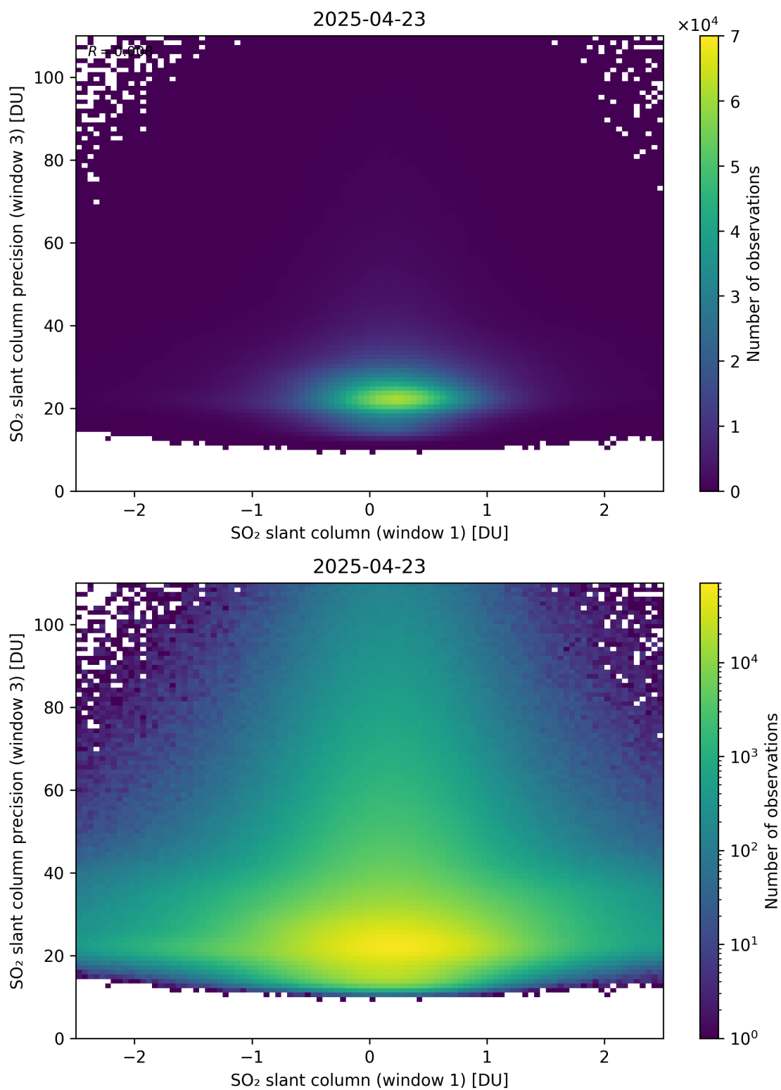
Figure 288: Scatter density plot of “SO 2 slant column (window 1)” against “SO 2 slant column precision (window 3)” for 2025-04-22 to 2025-04-24.
