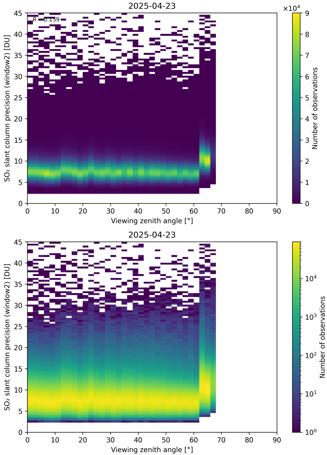
Figure 378: Scatter density plot of “Viewing zenith angle” against “SO 2 slant column precision (window2)” for 2025-04-22 to 2025-04-24.
