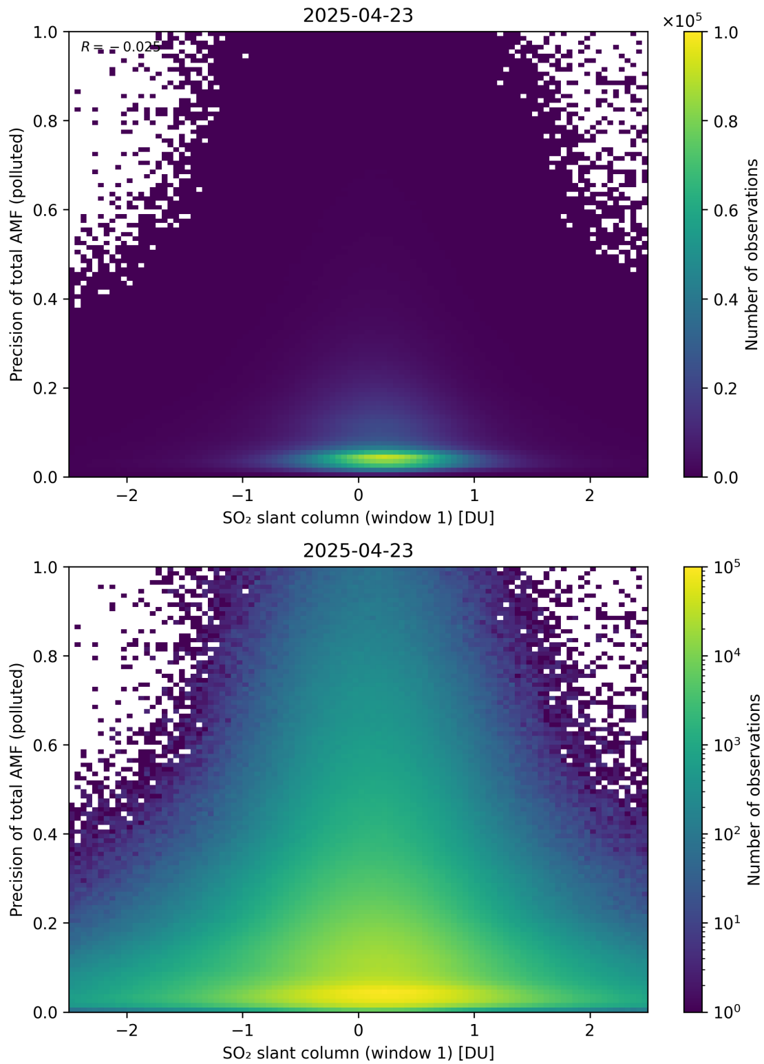
Figure 290: Scatter density plot of “SO 2 slant column (window 1)” against “Precision of total AMF (polluted)” for 2025-04-22 to 2025-04-24.
