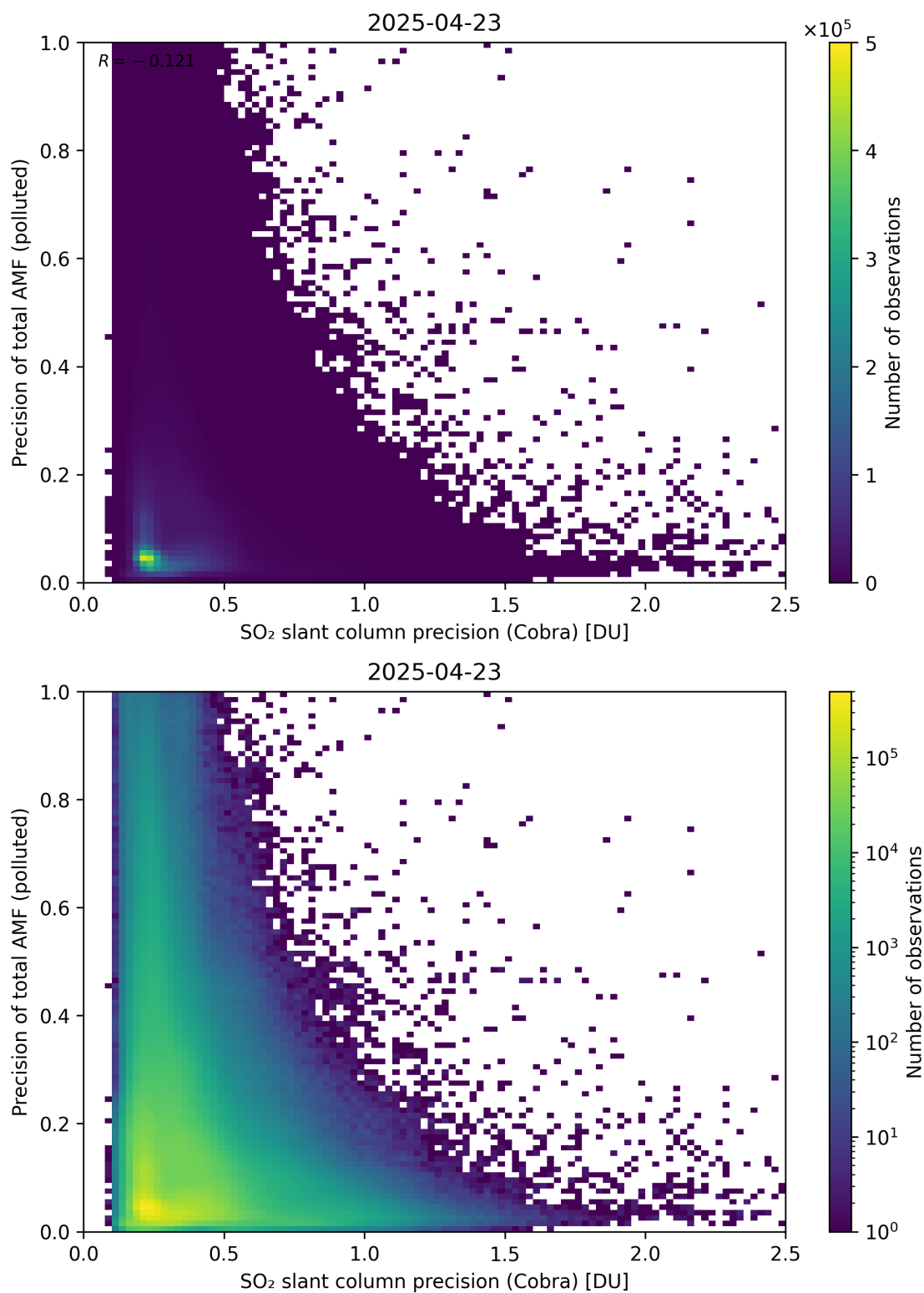
Figure 214: Scatter density plot of “SO 2 slant column precision (Cobra)” against “Precision of total AMF (polluted)” for 2025-04-22 to 2025-04-24.
