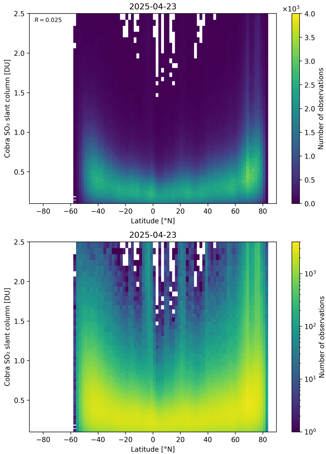
Figure 157: Scatter density plot of “Latitude” against “Cobra SO 2 slant column” for 2025-04-22 to 2025-04-24.
