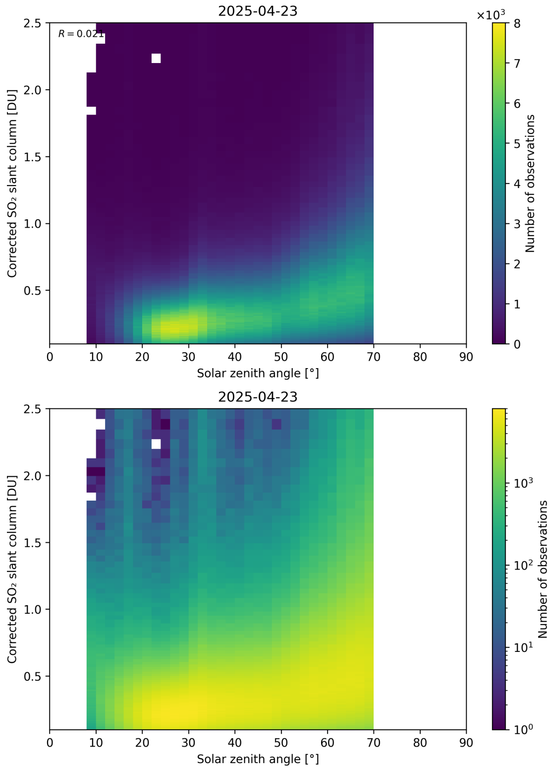
Figure 181: Scatter density plot of “Solar zenith angle” against “Corrected SO 2 slant column” for 2025-04-22 to 2025-04-24.
