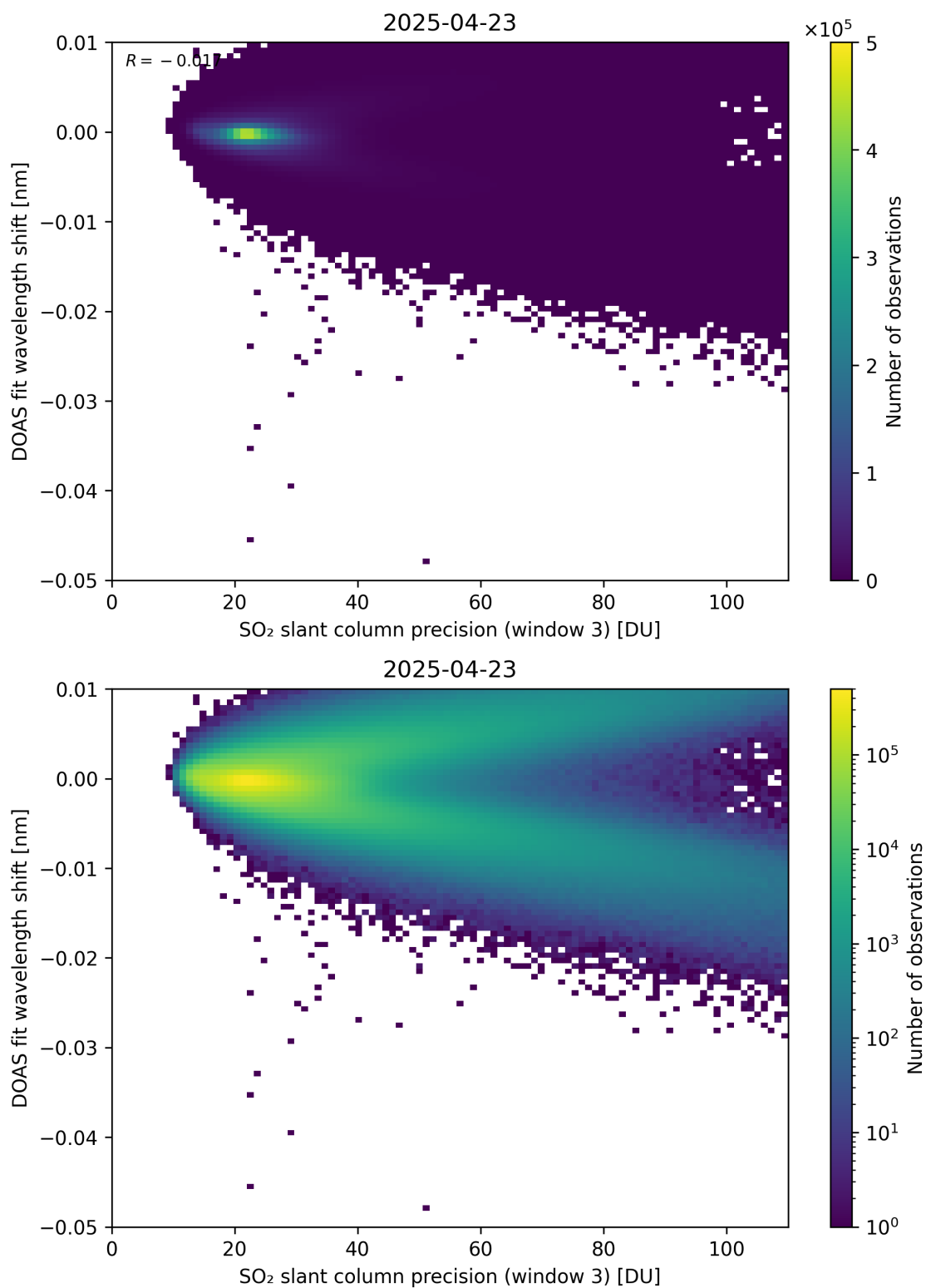
Figure 308: Scatter density plot of “SO 2 slant column precision (window 3)” against “DOAS fit wavelength shift” for 2025-04-22 to 2025-04-24.
