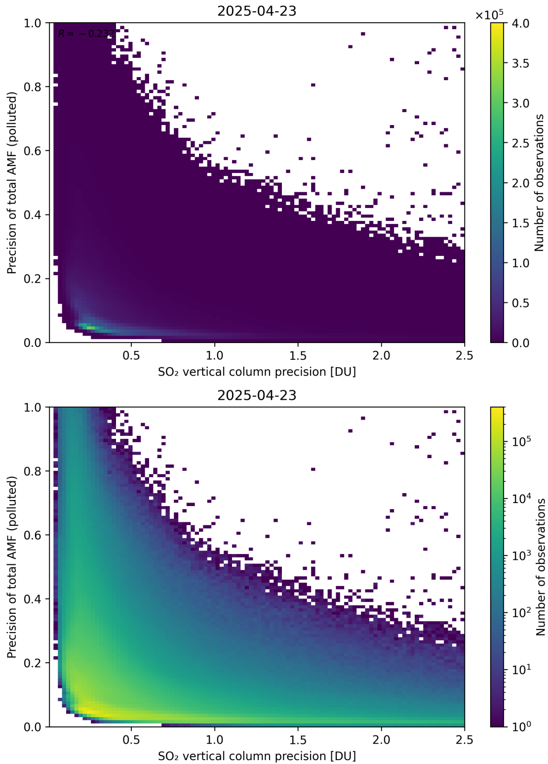
Figure 347: Scatter density plot of “SO 2 vertical column precision” against “Precision of total AMF (polluted)” for 2025-04-22 to 2025-04-24.
