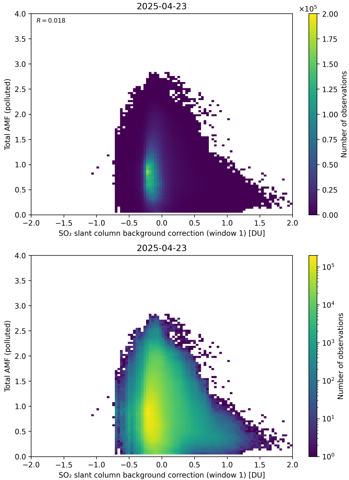
Figure 120: Scatter density plot of “SO 2 slant column background correction (window 1)” against “Total AMF (polluted)” for 2025-04-22 to 2025-04-24.
