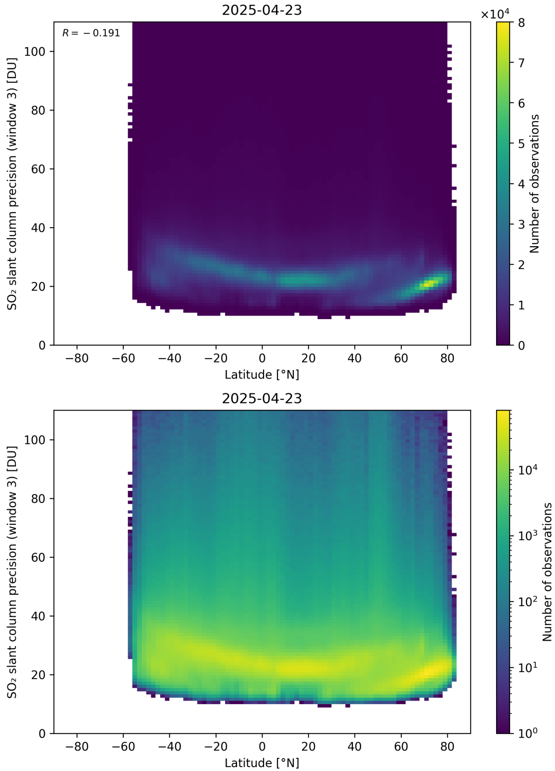
Figure 166: Scatter density plot of “Latitude” against “SO 2 slant column precision (window 3)” for 2025-04-22 to 2025-04-24.
