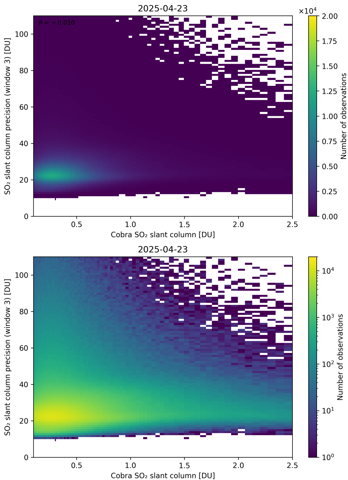
Figure 223: Scatter density plot of “Cobra SO 2 slant column” against “SO 2 slant column precision (window 3)” for 2025-04-22 to 2025-04-24.
