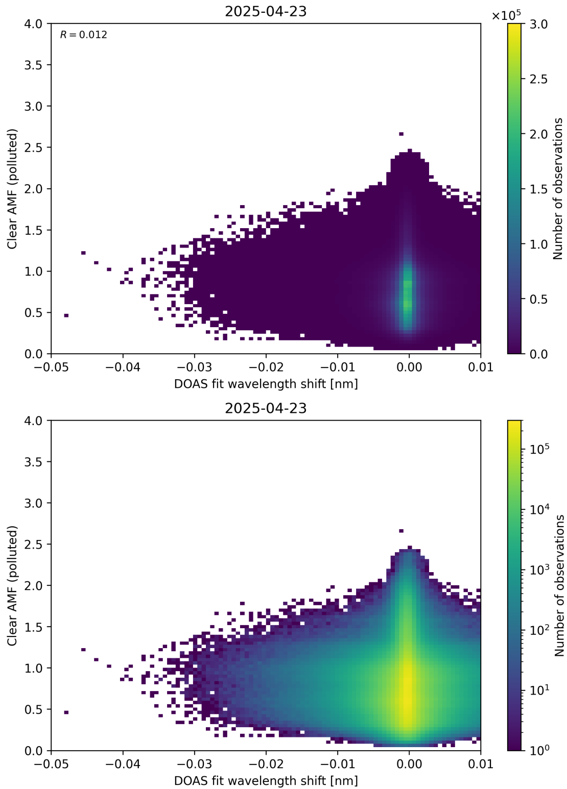
Figure 140: Scatter density plot of “DOAS fit wavelength shift” against “Clear AMF (polluted)” for 2025-04-22 to 2025-04-24.
