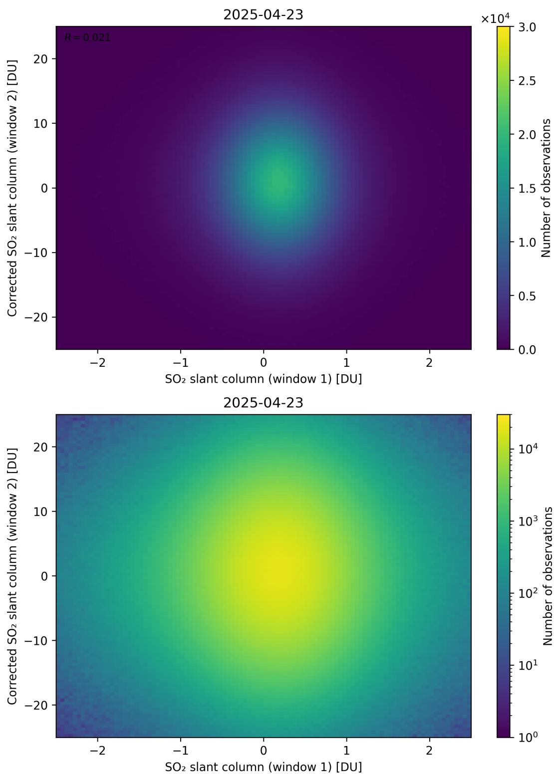
Figure 283: Scatter density plot of “SO 2 slant column (window 1)” against “Corrected SO 2 slant column (window 2)” for 2025-04-22 to 2025-04-24.
