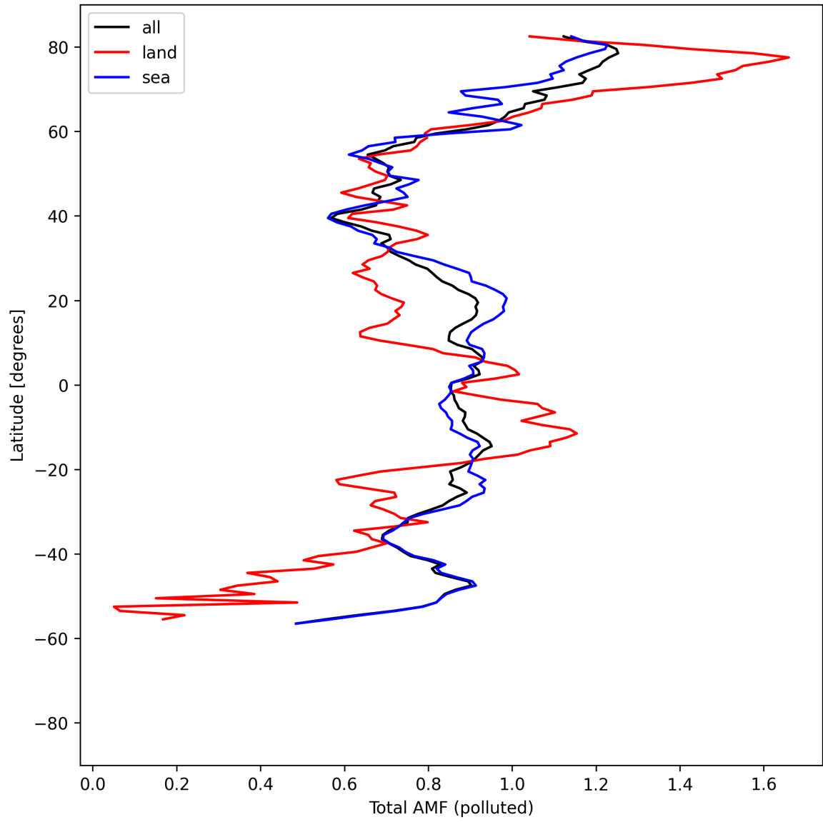
Figure 53: Zonal average of “Total AMF (polluted)” for 2025-04-22 to 2025-04-24.
