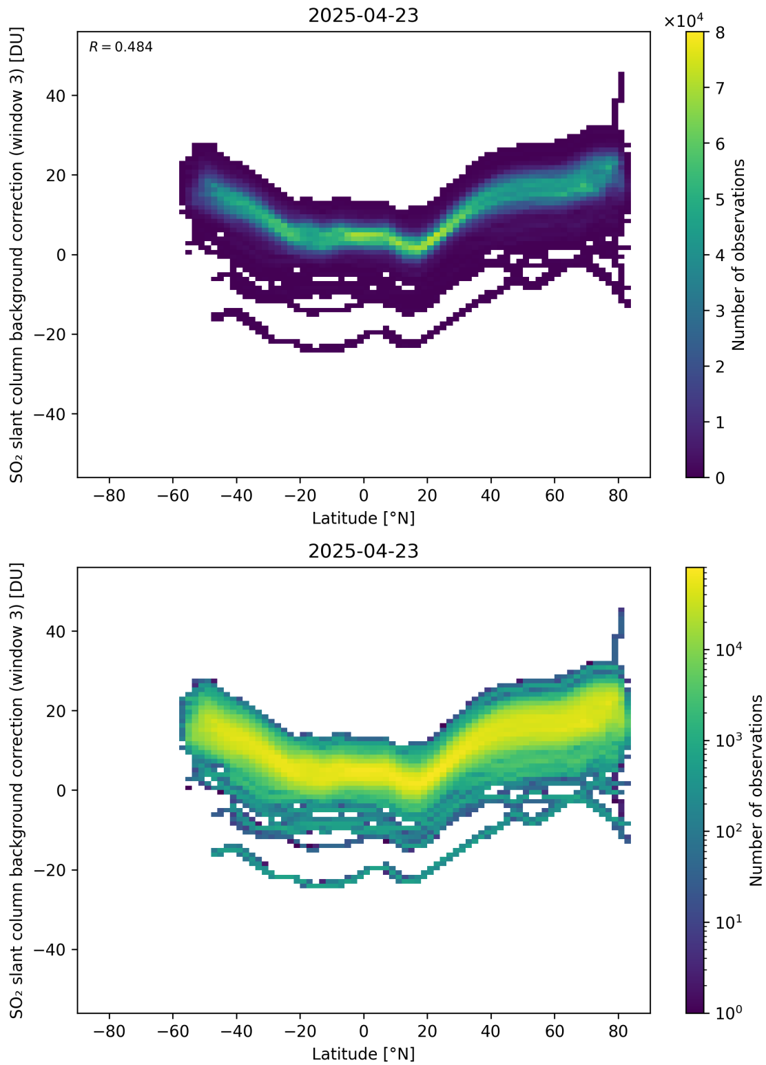
Figure 152: Scatter density plot of “Latitude” against “SO 2 slant column background correction (window 3)” for 2025-04-22 to 2025-04-24.
