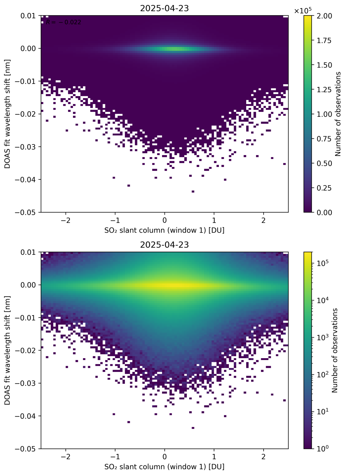
Figure 265: Scatter density plot of “SO 2 slant column (window 1)” against “DOAS fit wavelength shift” for 2025-04-22 to 2025-04-24.
