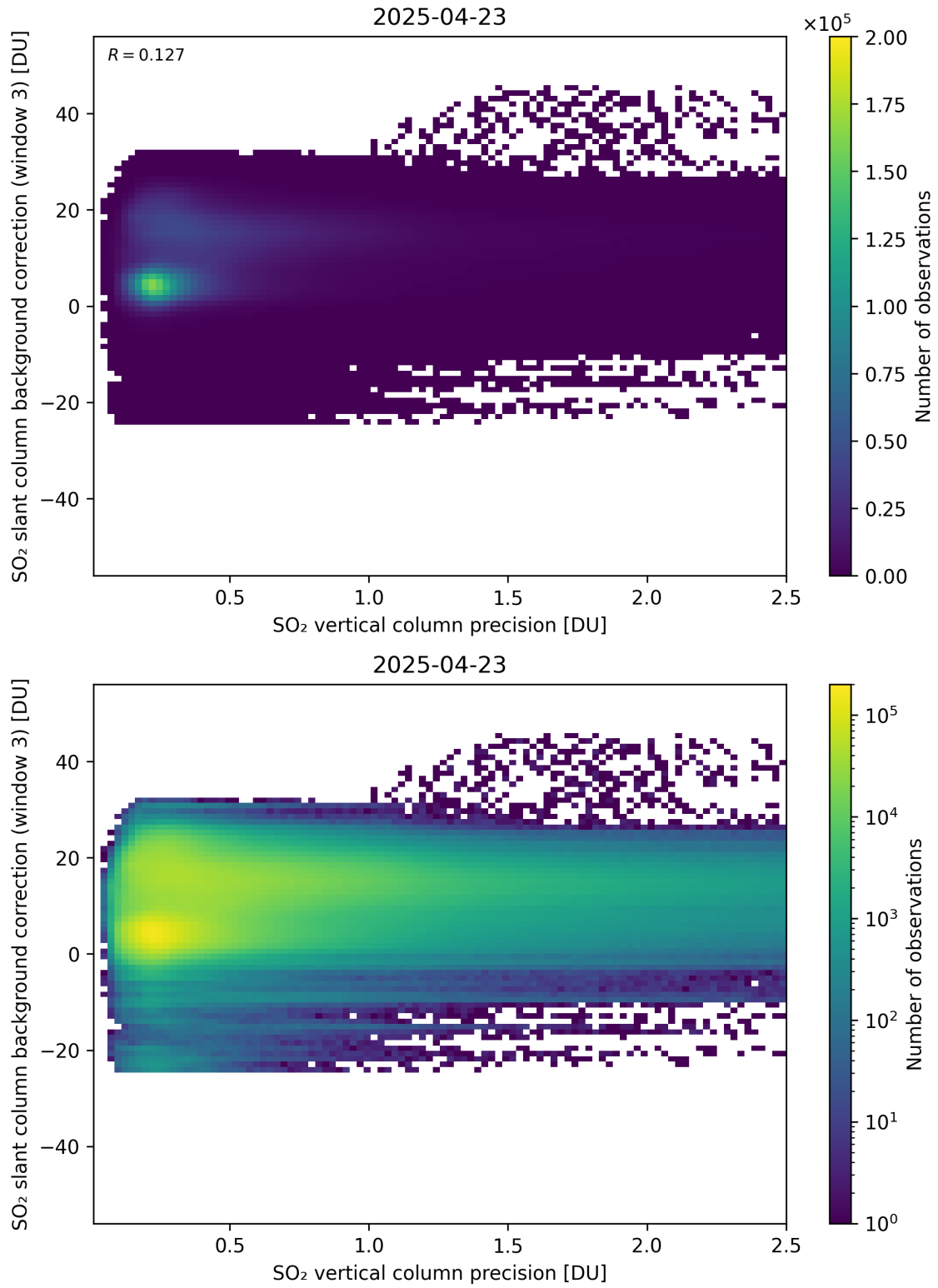
Figure 331: Scatter density plot of “SO 2 vertical column precision” against “SO 2 slant column background correction (window 3)” for 2025-04-22 to 2025-04-24.
