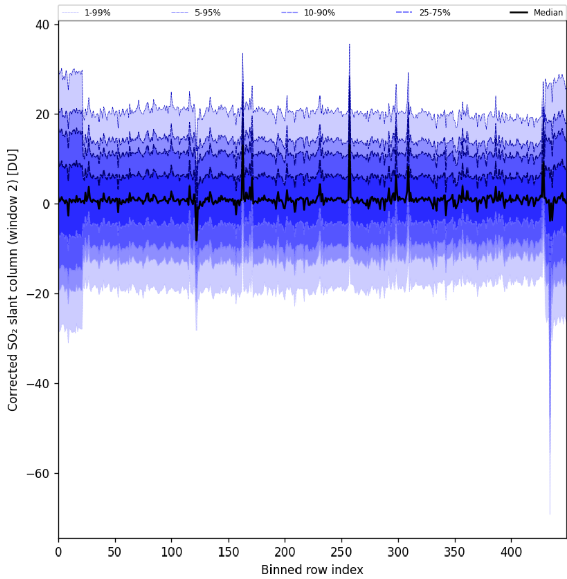
Figure 95: Along track statistics of “Corrected SO 2 slant column (window 2)” for 2025-04-22 to 2025-04-24
