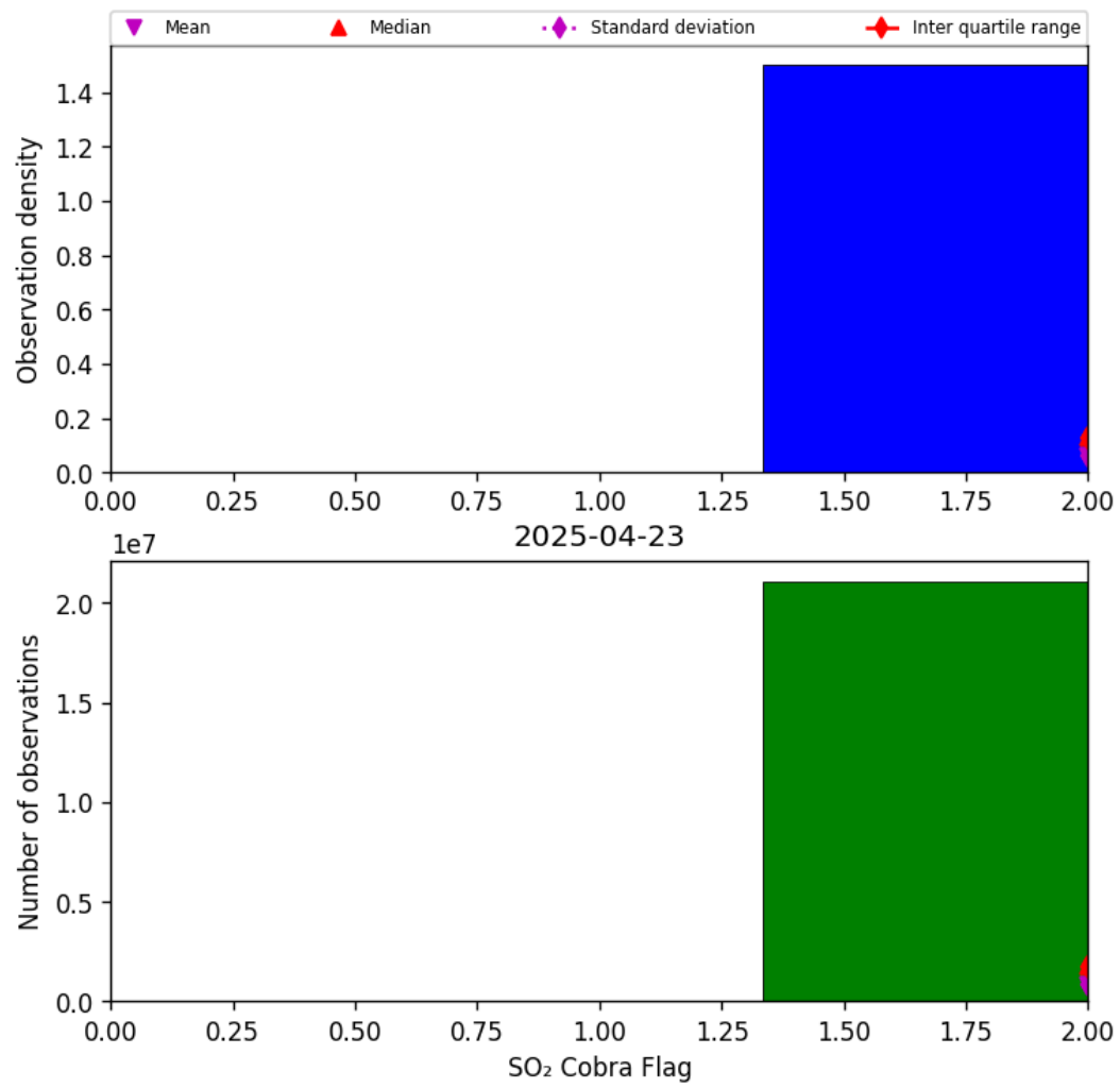
Figure 75: Histogram of “SO 2 Cobra Flag” for 2025-04-22 to 2025-04-24
