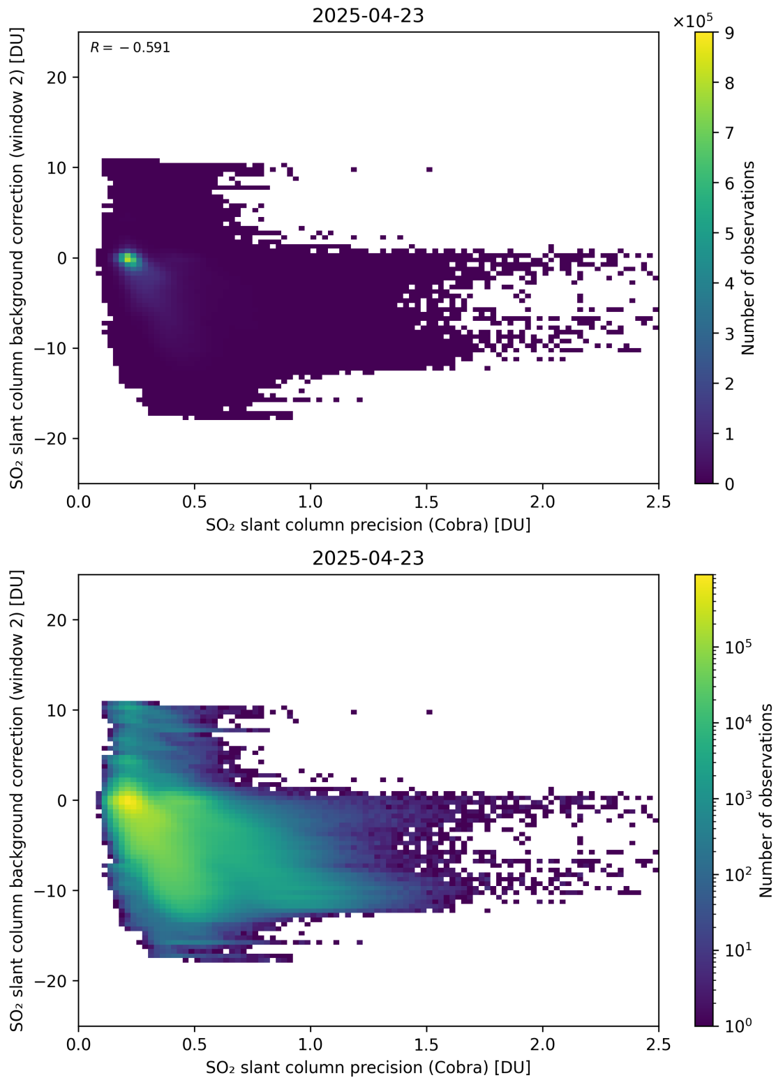
Figure 200: Scatter density plot of “SO 2 slant column precision (Cobra)” against “SO 2 slant column background correction (window 2)” for 2025-04-22 to 2025-04-24.
