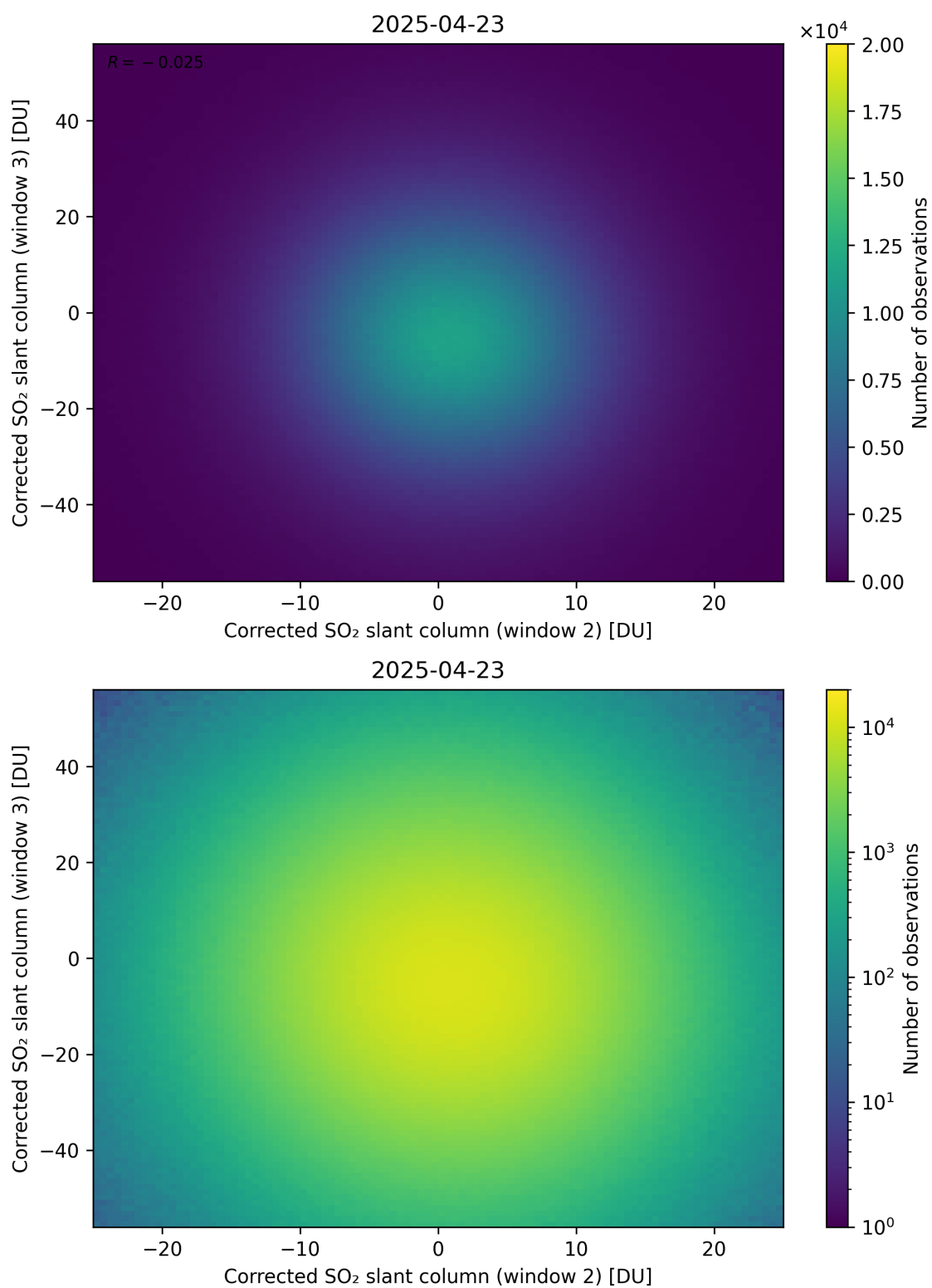
Figure 250: Scatter density plot of “Corrected SO 2 slant column (window 2)” against “Corrected SO 2 slant column (window 3)” for 2025-04-22 to 2025-04-24.
