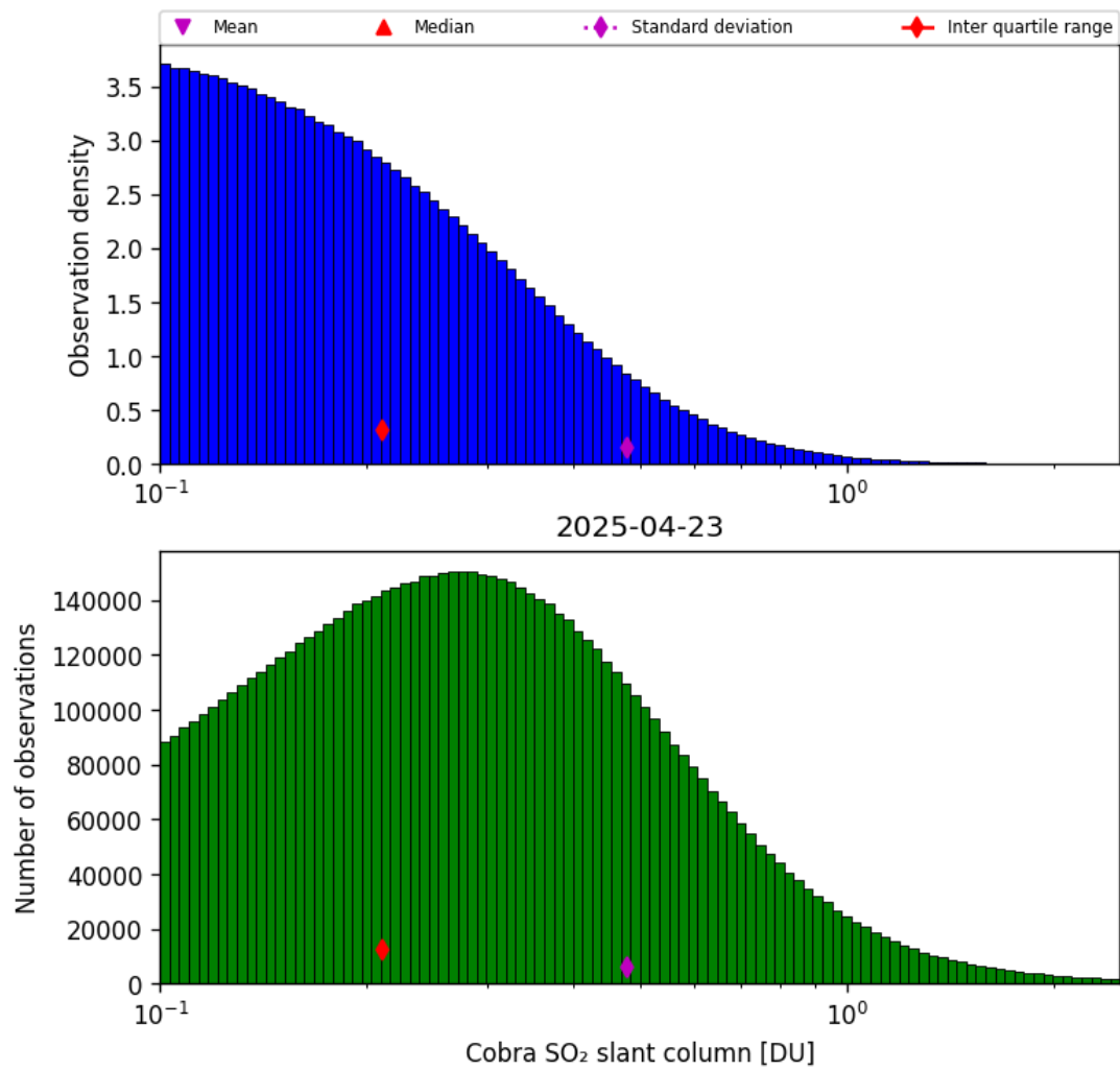
Figure 61: Histogram of “Cobra SO 2 slant column” for 2025-04-22 to 2025-04-24
