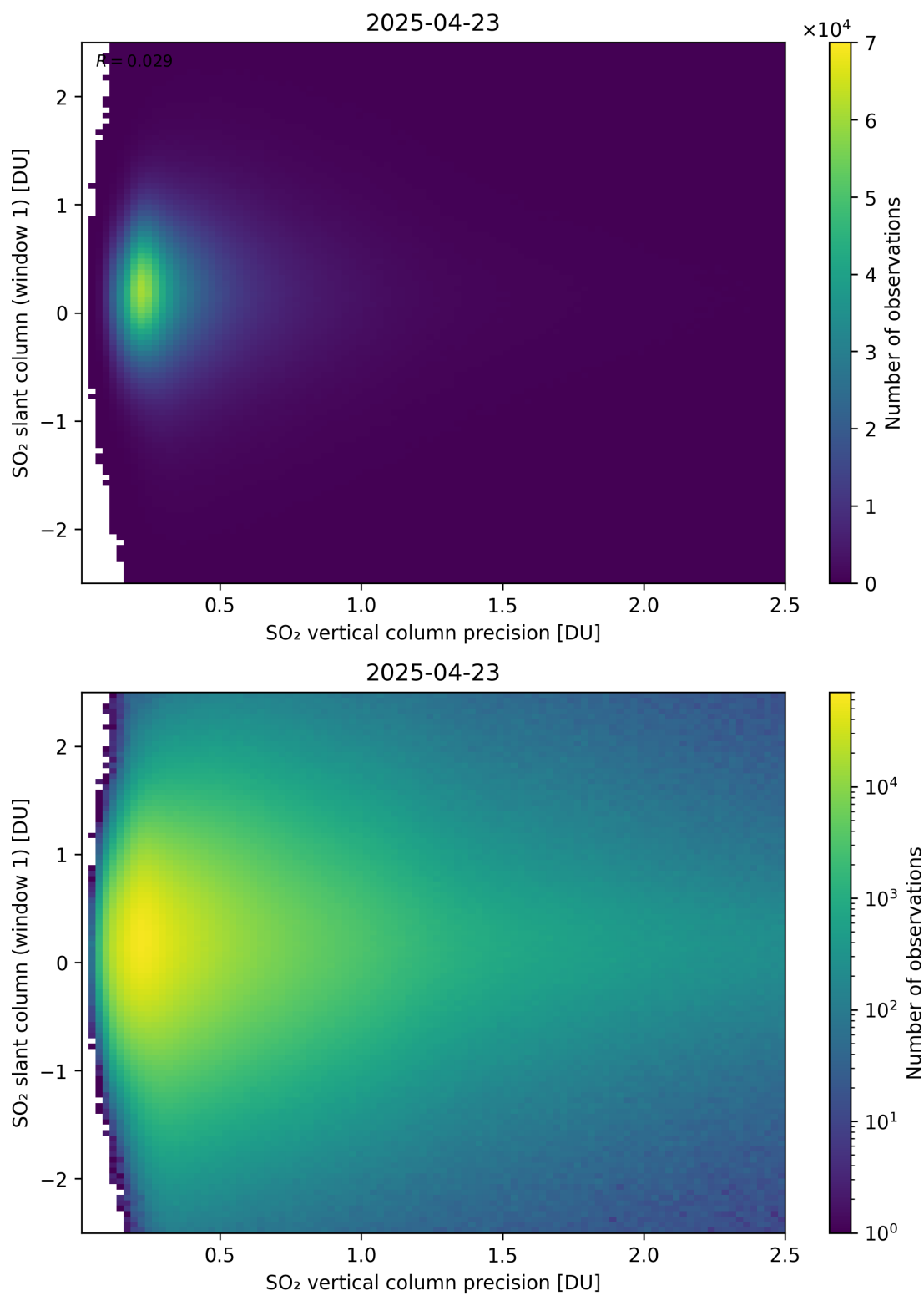
Figure 341: Scatter density plot of “SO 2 vertical column precision” against “SO 2 slant column (window 1)” for 2025-04-22 to 2025-04-24.
