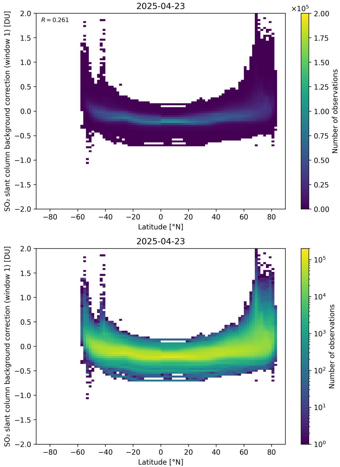
Figure 150: Scatter density plot of “Latitude” against “SO 2 slant column background correction (window 1)” for 2025-04-22 to 2025-04-24.
