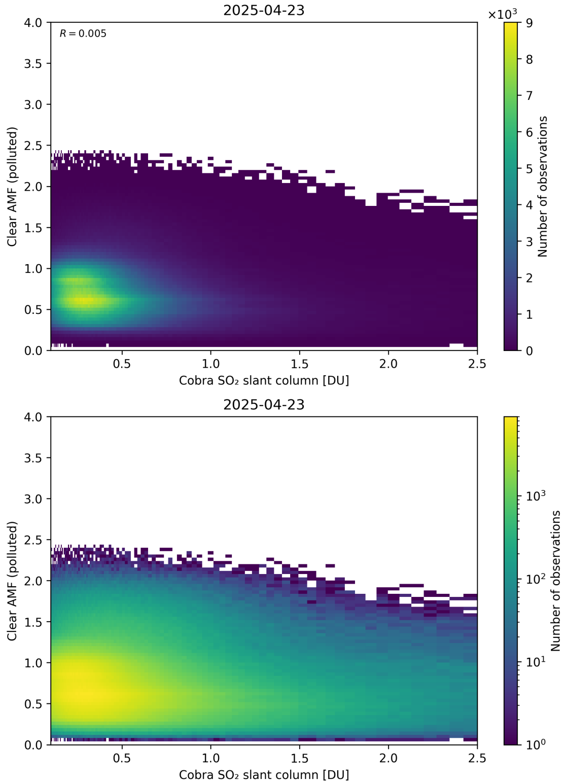
Figure 215: Scatter density plot of “Cobra SO 2 slant column” against “Clear AMF (polluted)” for 2025-04-22 to 2025-04-24.
