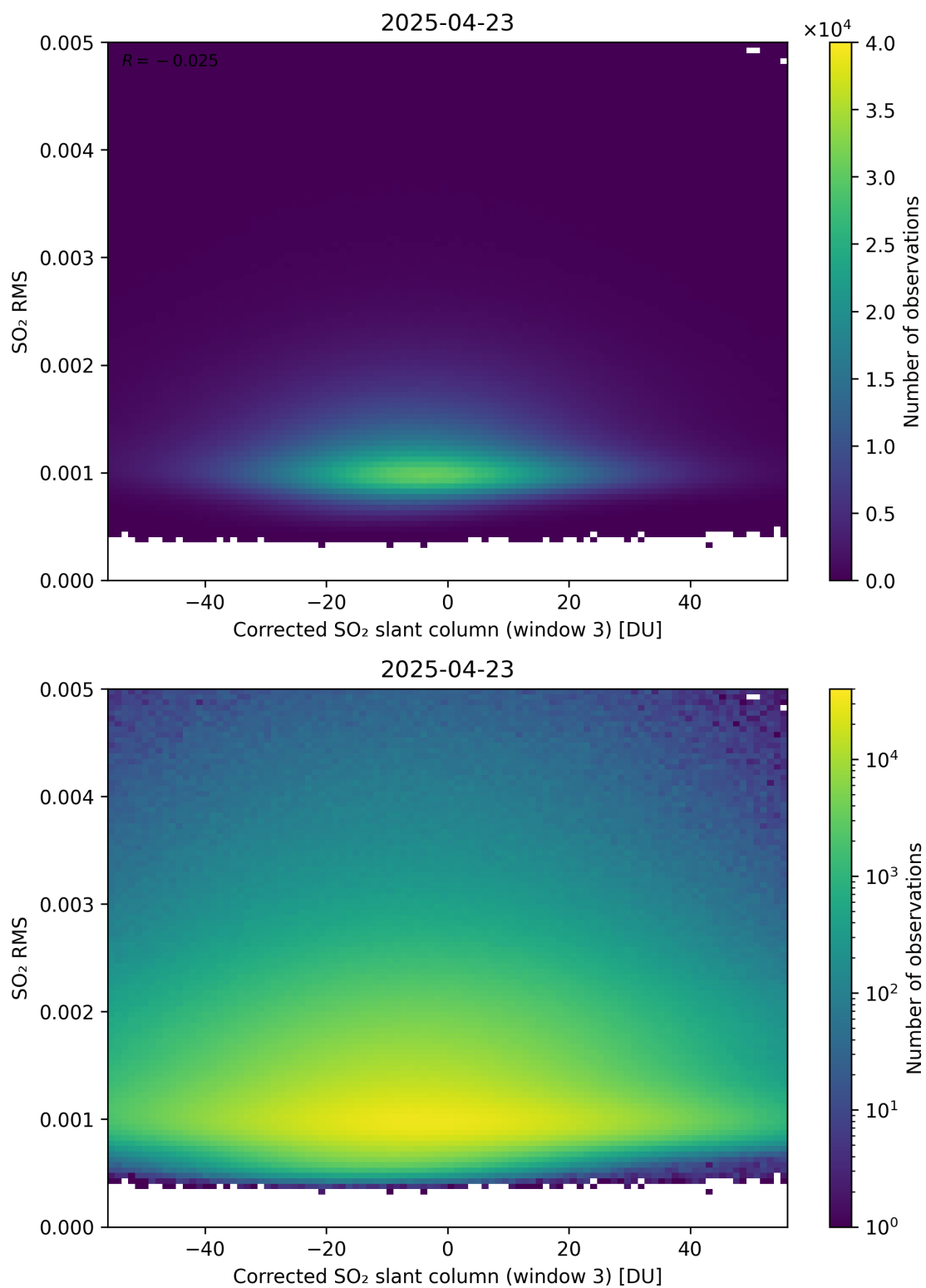
Figure 258: Scatter density plot of “Corrected SO 2 slant column (window 3)” against “SO 2 RMS” for 2025-04-22 to 2025-04-24.
