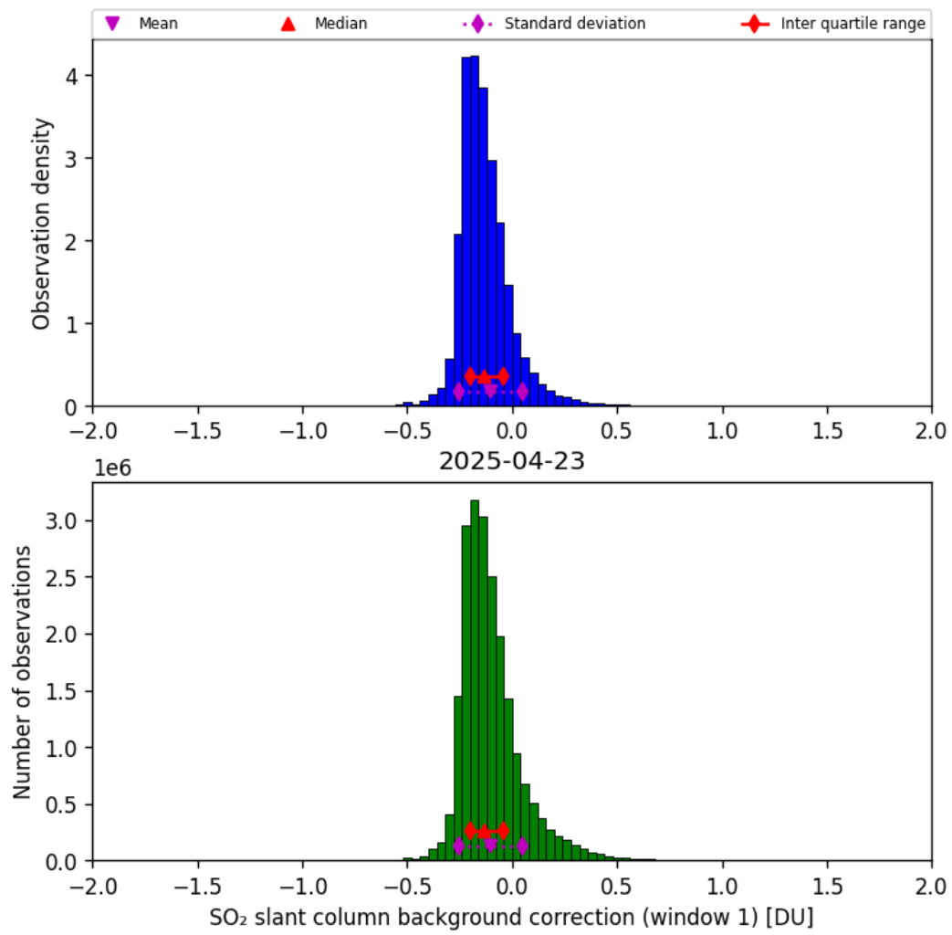
Figure 66: Histogram of “SO 2 slant column background correction (window 1)” for 2025-04-22 to 2025-04-24
