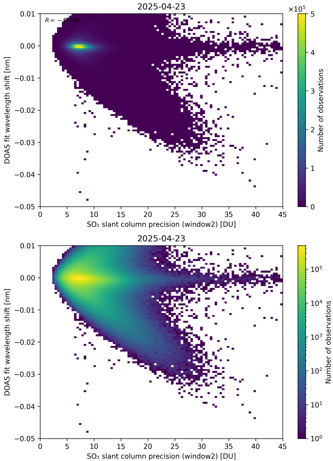
Figure 293: Scatter density plot of “SO 2 slant column precision (window2)” against “DOAS fit wavelength shift” for 2025-04-22 to 2025-04-24.
