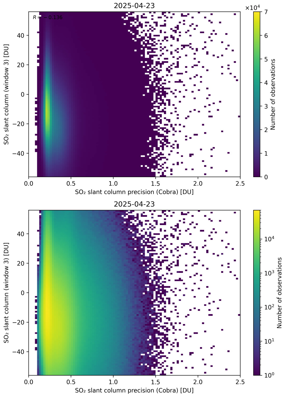
Figure 211: Scatter density plot of “SO 2 slant column precision (Cobra)” against “SO 2 slant column (window 3)” for 2025-04-22 to 2025-04-24.
