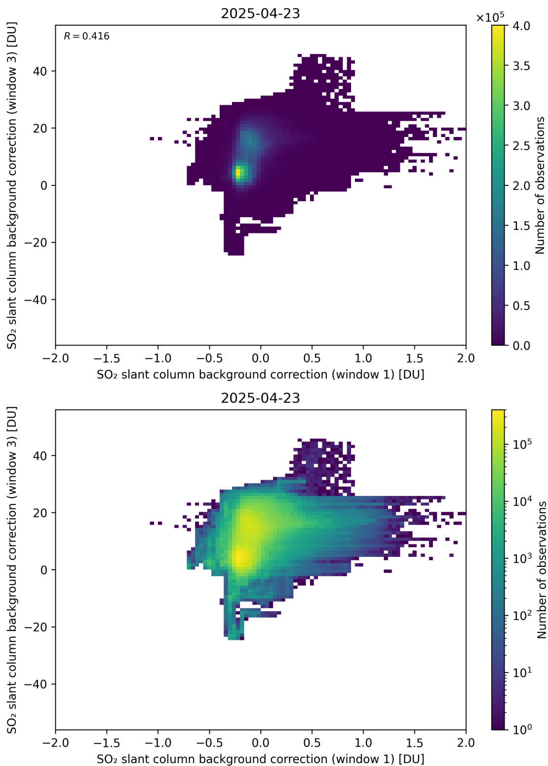
Figure 110: Scatter density plot of “SO 2 slant column background correction (window 1)” against “SO 2 slant column background correction (window 3)” for 2025-04-22 to 2025-04-24.
