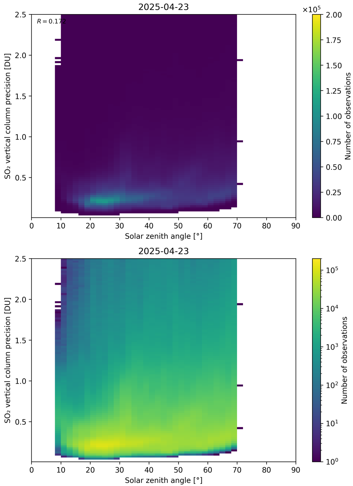
Figure 192: Scatter density plot of “Solar zenith angle” against “SO 2 vertical column precision” for 2025-04-22 to 2025-04-24.
