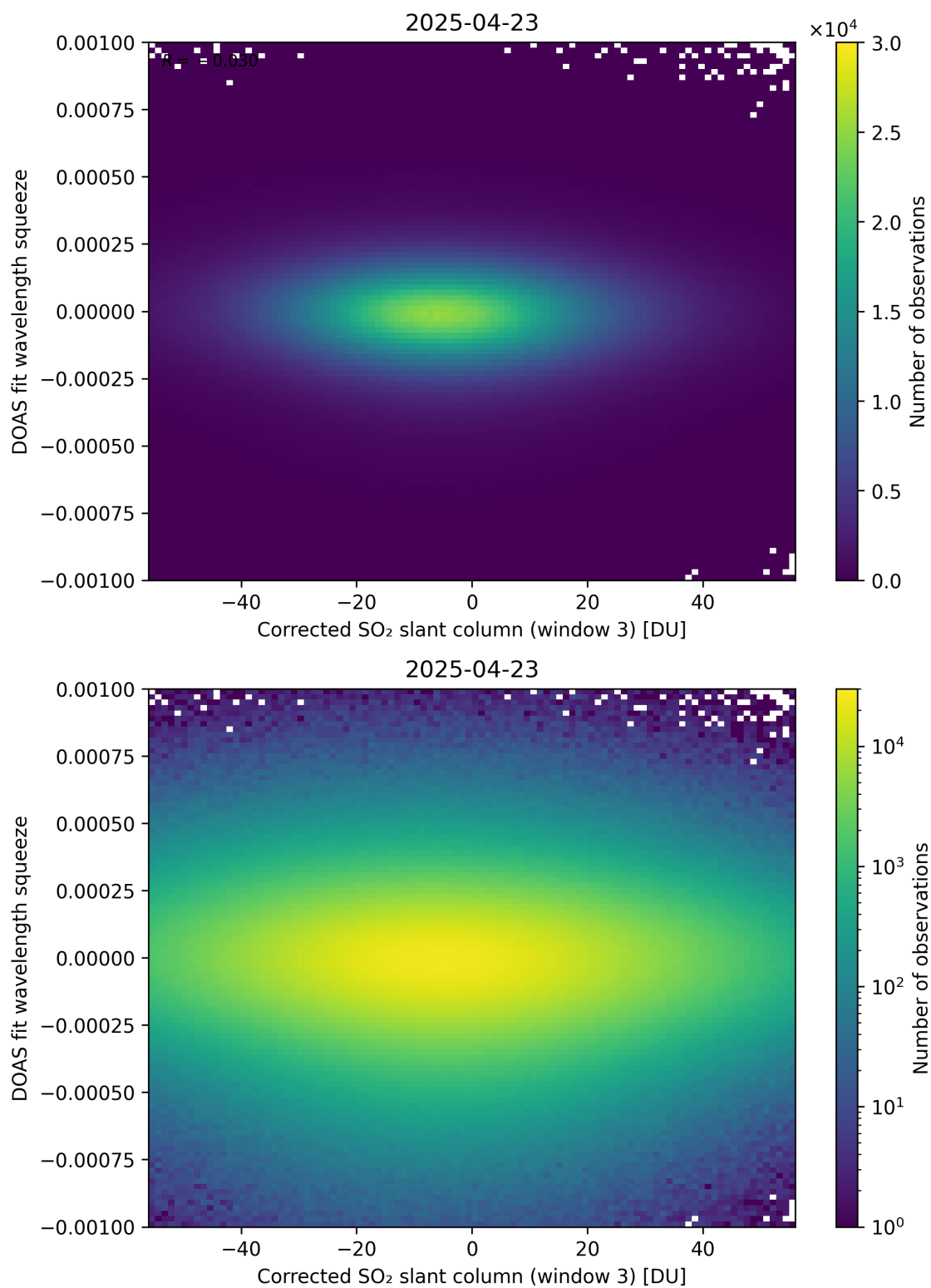
Figure 257: Scatter density plot of “Corrected SO 2 slant column (window 3)” against “DOAS fit wavelength squeeze” for 2025-04-22 to 2025-04-24.
