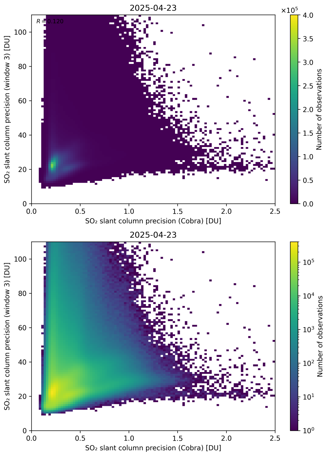
Figure 212: Scatter density plot of “SO 2 slant column precision (Cobra)” against “SO 2 slant column precision (window 3)” for 2025-04-22 to 2025-04-24.
