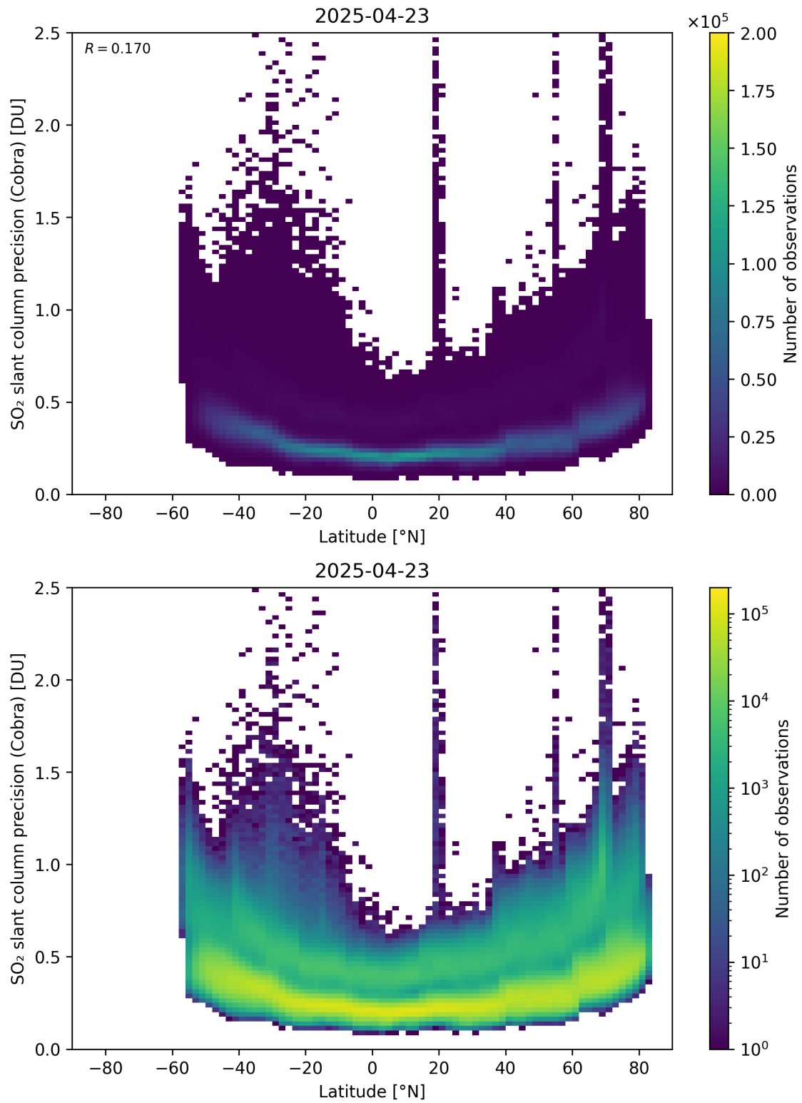
Figure 158: Scatter density plot of “Latitude” against “SO 2 slant column precision (Cobra)” for 2025-04-22 to 2025-04-24.
