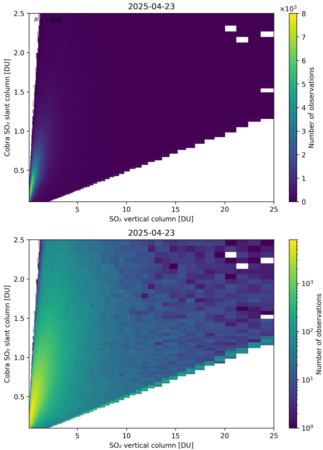
Figure 349: Scatter density plot of “SO 2 vertical column” against “Cobra SO 2 slant column” for 2025-04-22 to 2025-04-24.
