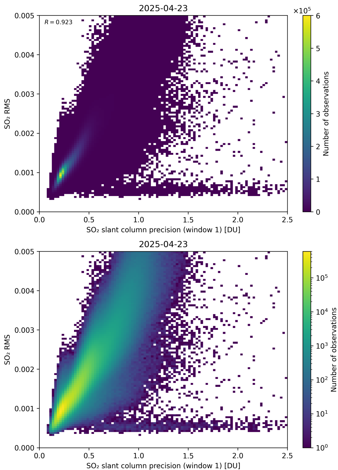
Figure 273: Scatter density plot of “SO 2 slant column precision (window 1)” against “SO 2 RMS” for 2025-04-22 to 2025-04-24.
