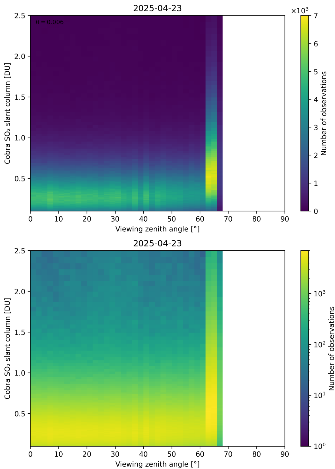
Figure 371: Scatter density plot of “Viewing zenith angle” against “Cobra SO 2 slant column” for 2025-04-22 to 2025-04-24.
