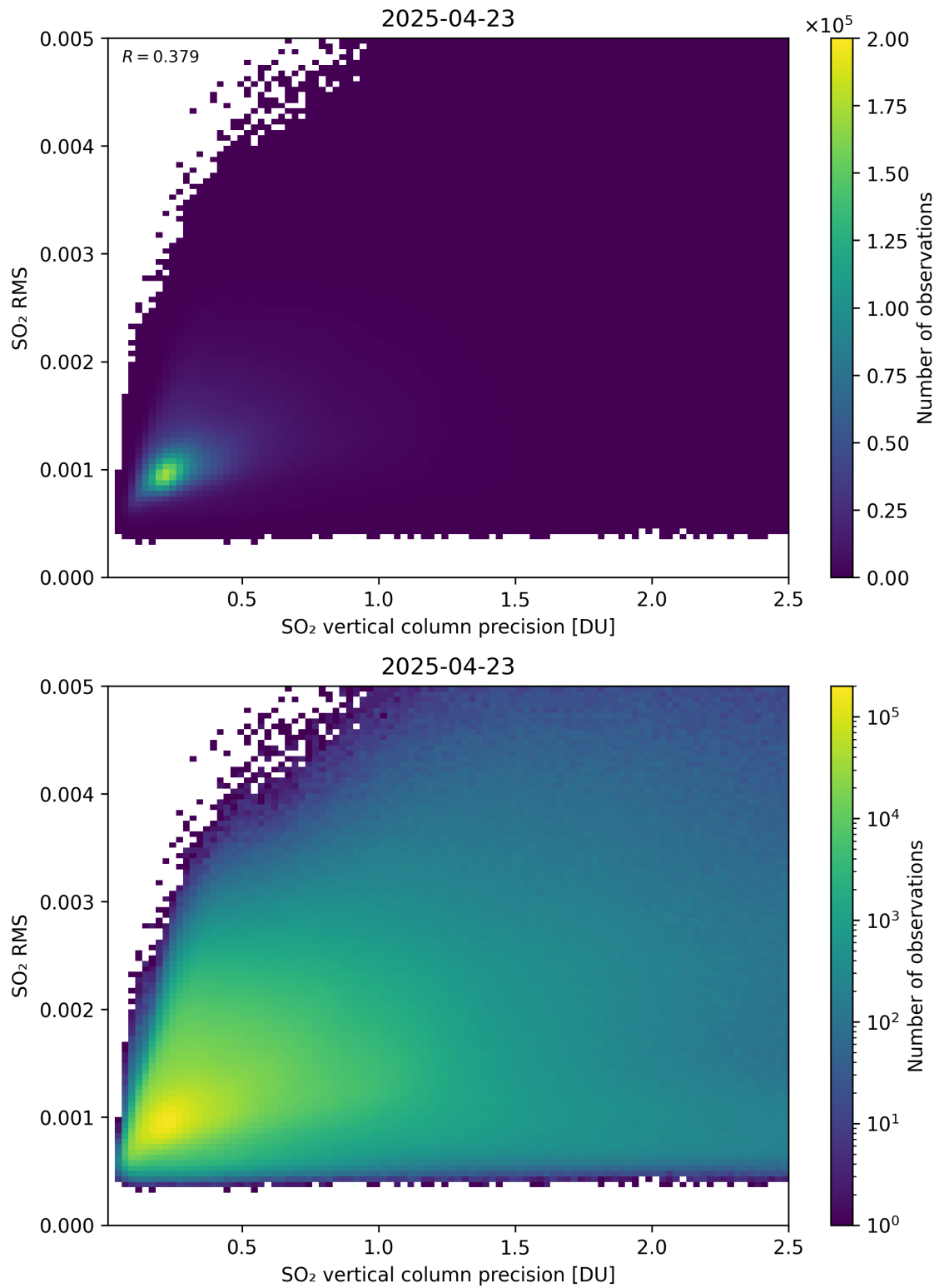
Figure 334: Scatter density plot of “SO 2 vertical column precision” against “SO 2 RMS” for 2025-04-22 to 2025-04-24.
