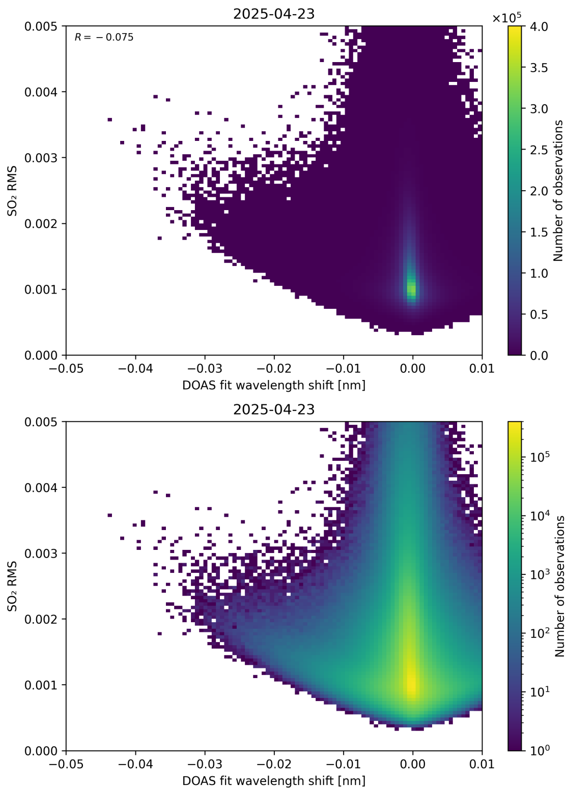
Figure 139: Scatter density plot of “DOAS fit wavelength shift” against “SO 2 RMS” for 2025-04-22 to 2025-04-24.
