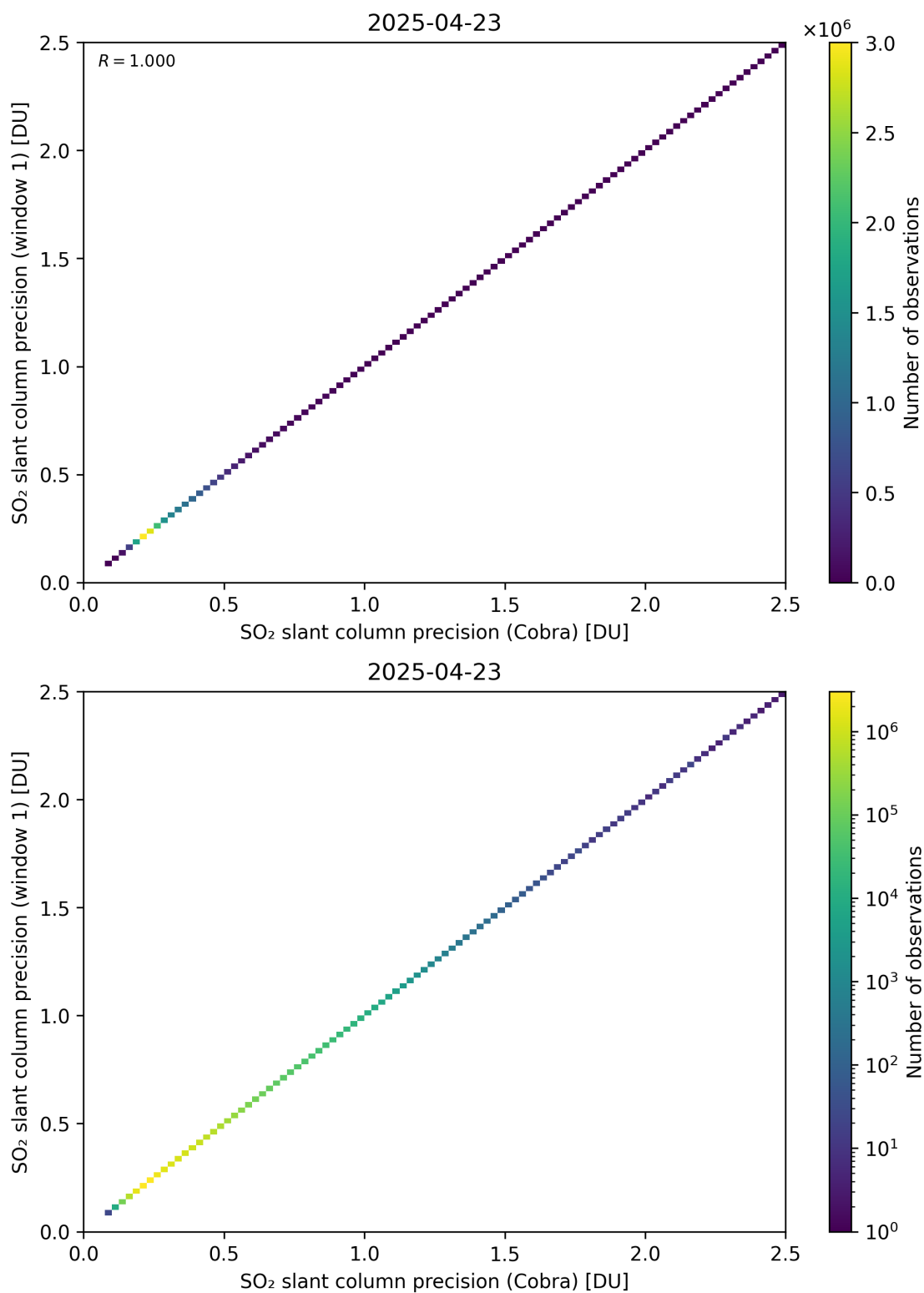
Figure 209: Scatter density plot of “SO 2 slant column precision (Cobra)” against “SO 2 slant column precision (window 1)” for 2025-04-22 to 2025-04-24.
