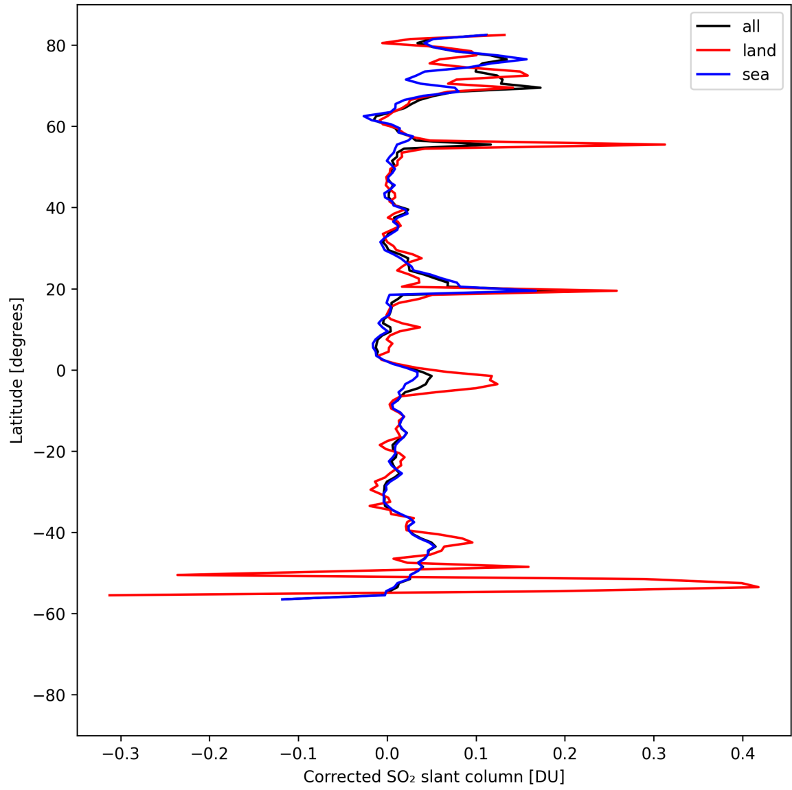
Figure 34: Zonal average of “Corrected SO 2 slant column” for 2025-04-22 to 2025-04-24.
