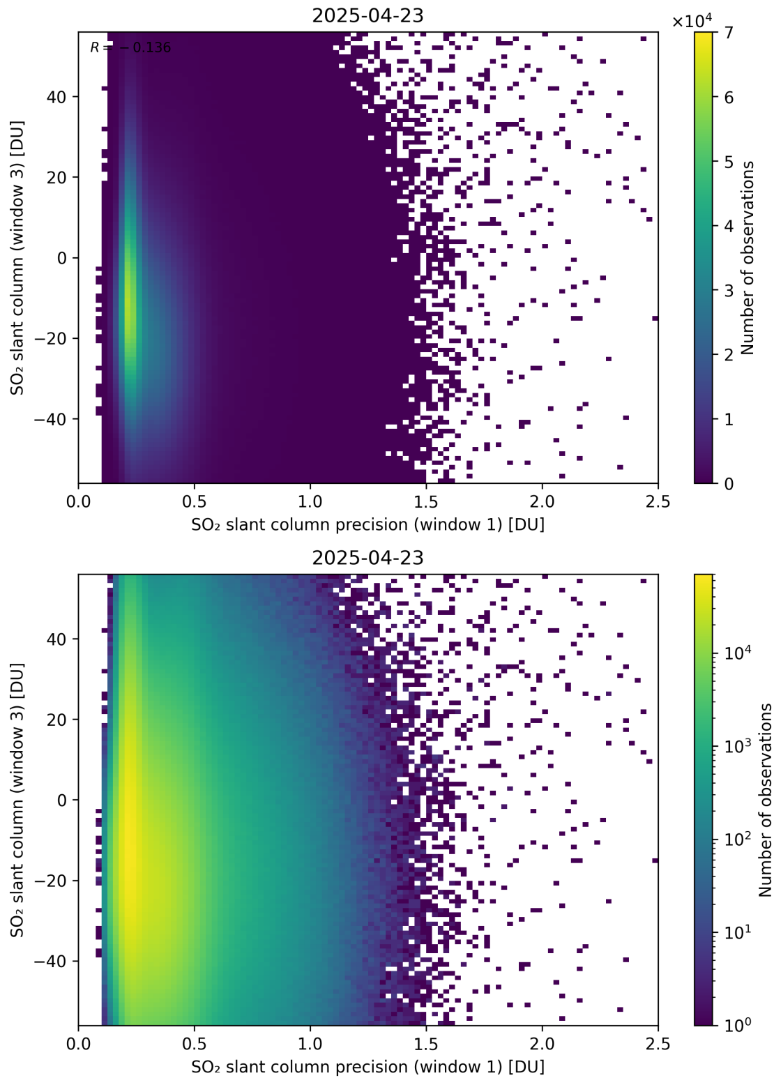
Figure 278: Scatter density plot of “SO 2 slant column precision (window 1)” against “SO 2 slant column (window 3)” for 2025-04-22 to 2025-04-24.
