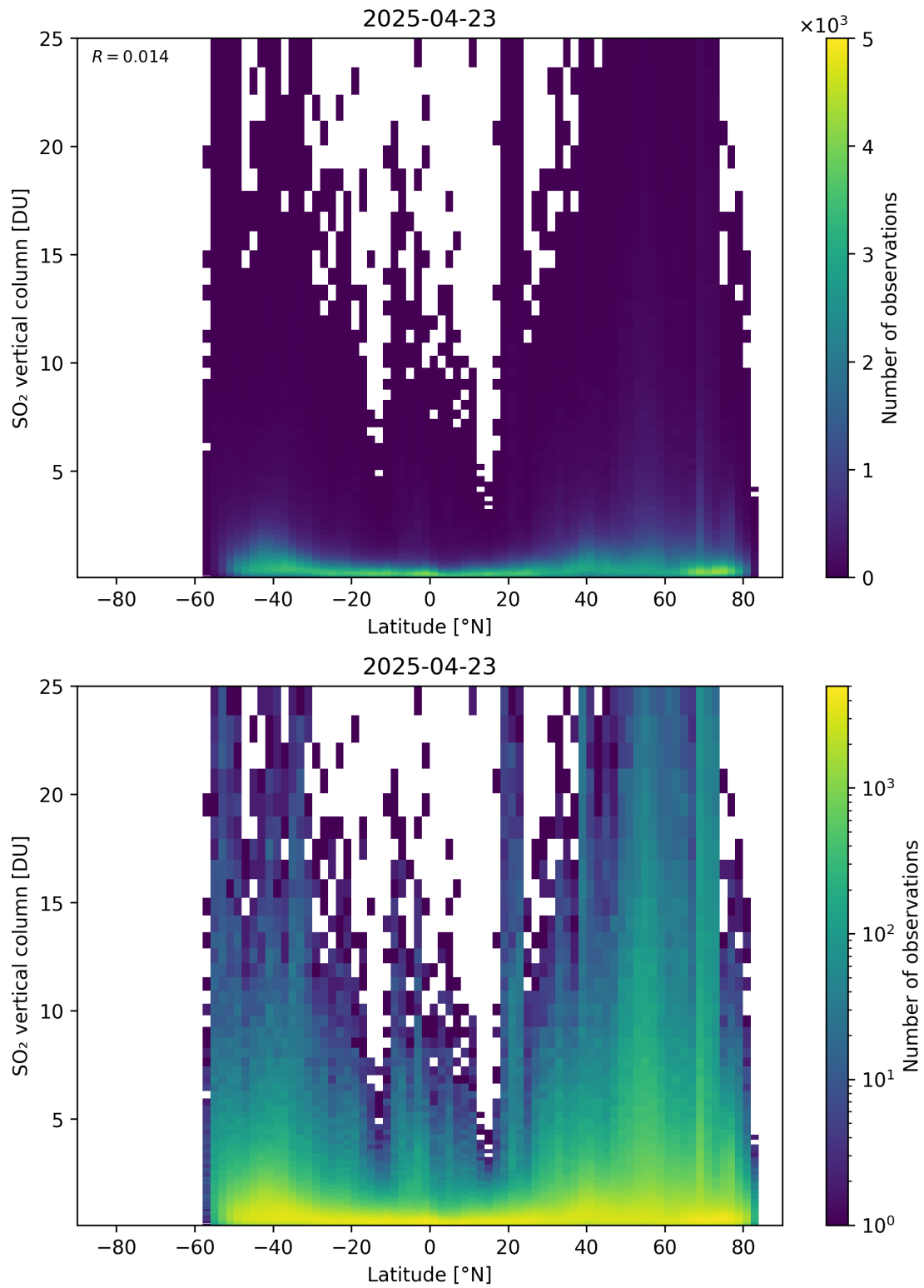
Figure 169: Scatter density plot of “Latitude” against “SO 2 vertical column” for 2025-04-22 to 2025-04-24.
