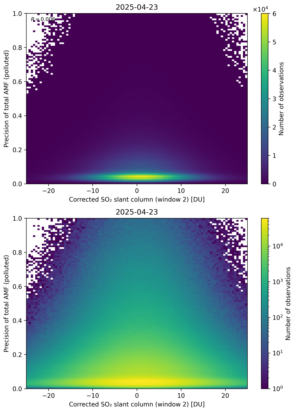
Figure 254: Scatter density plot of “Corrected SO 2 slant column (window 2)” against “Precision of total AMF (polluted)” for 2025-04-22 to 2025-04-24.
