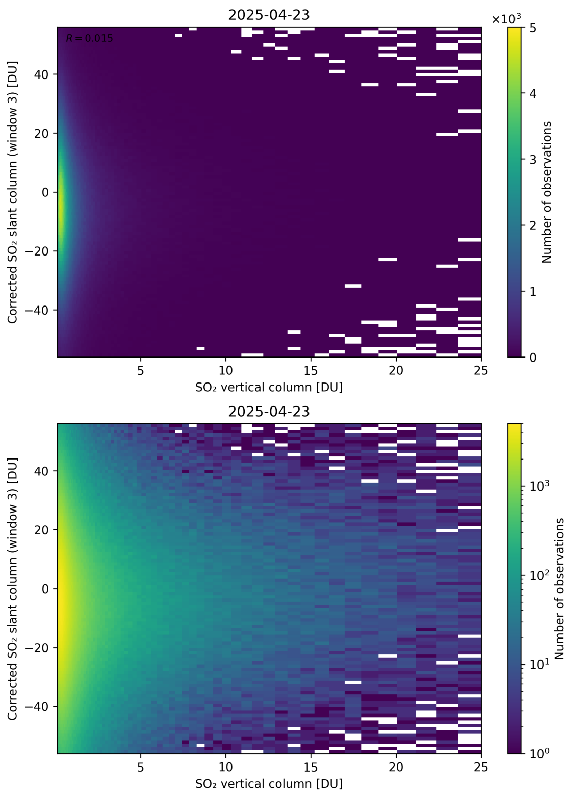
Figure 353: Scatter density plot of “SO 2 vertical column” against “Corrected SO 2 slant column (window 3)” for 2025-04-22 to 2025-04-24.
