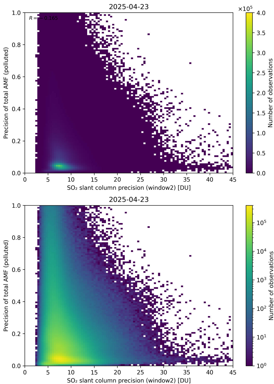
Figure 302: Scatter density plot of “SO 2 slant column precision (window2)” against “Precision of total AMF (polluted)” for 2025-04-22 to 2025-04-24.
