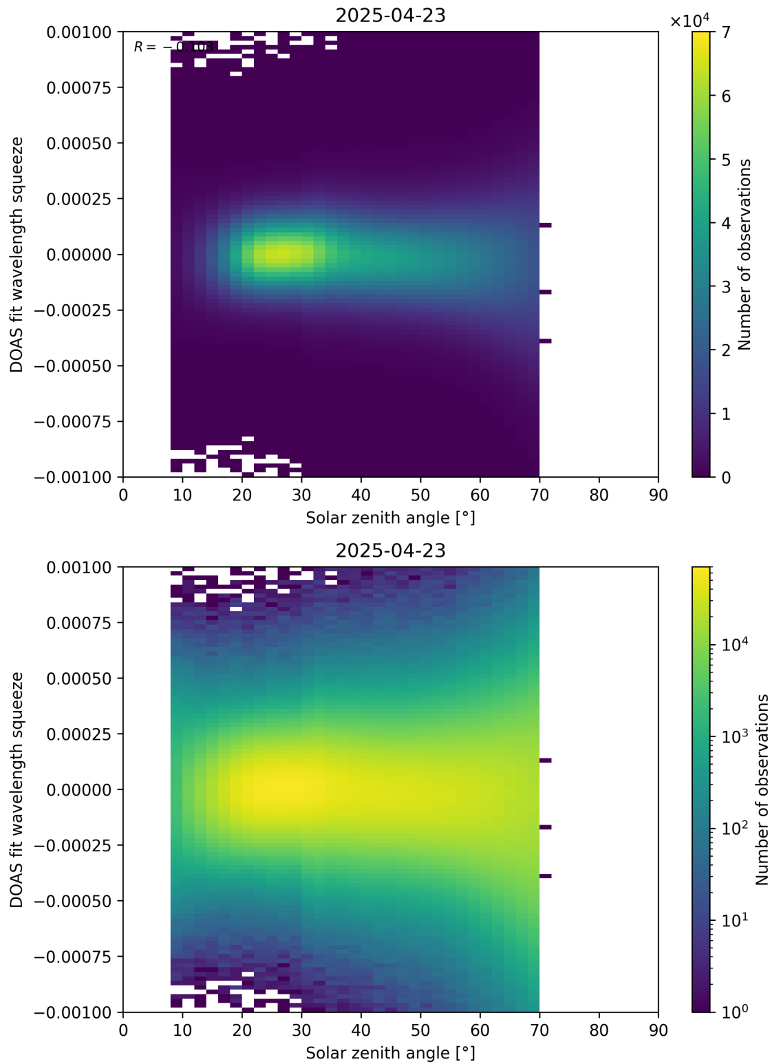
Figure 175: Scatter density plot of “Solar zenith angle” against “DOAS fit wavelength squeeze” for 2025-04-22 to 2025-04-24.
