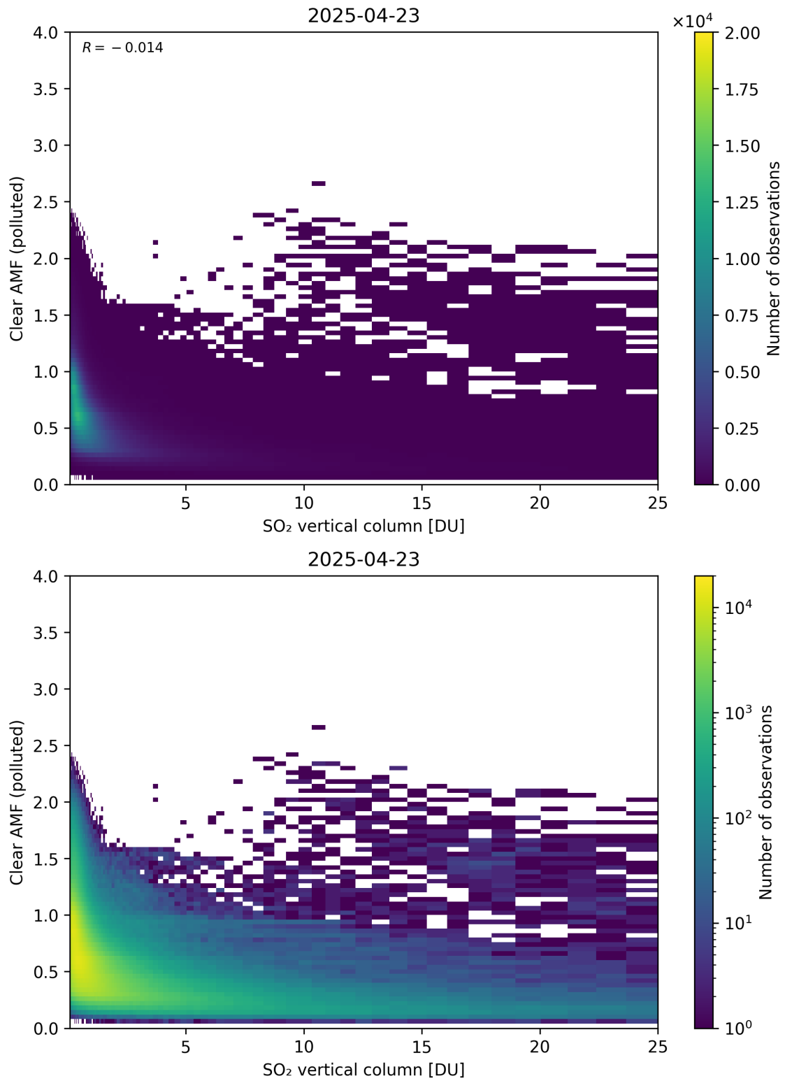
Figure 348: Scatter density plot of “SO 2 vertical column” against “Clear AMF (polluted)” for 2025-04-22 to 2025-04-24.
