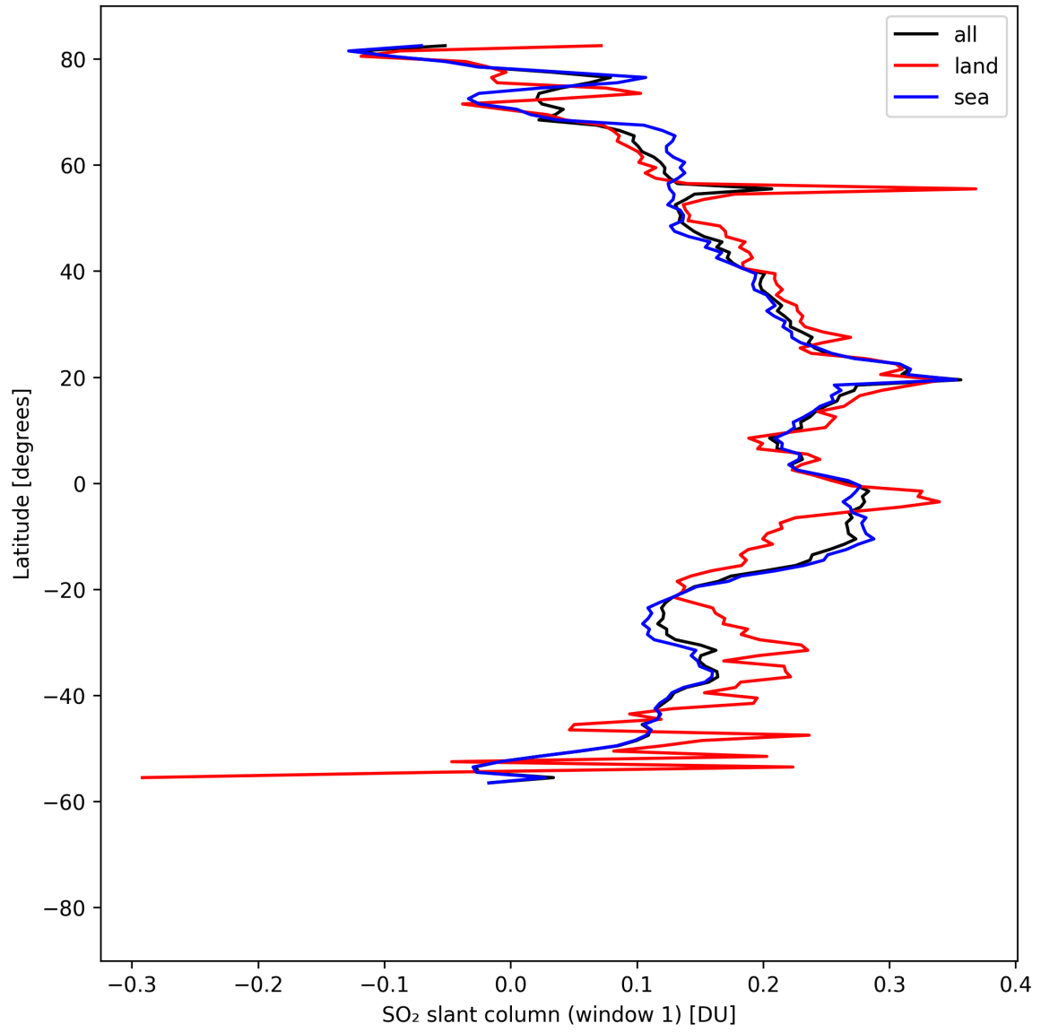
Figure 37: Zonal average of “SO 2 slant column (window 1)” for 2025-04-22 to 2025-04-24.
