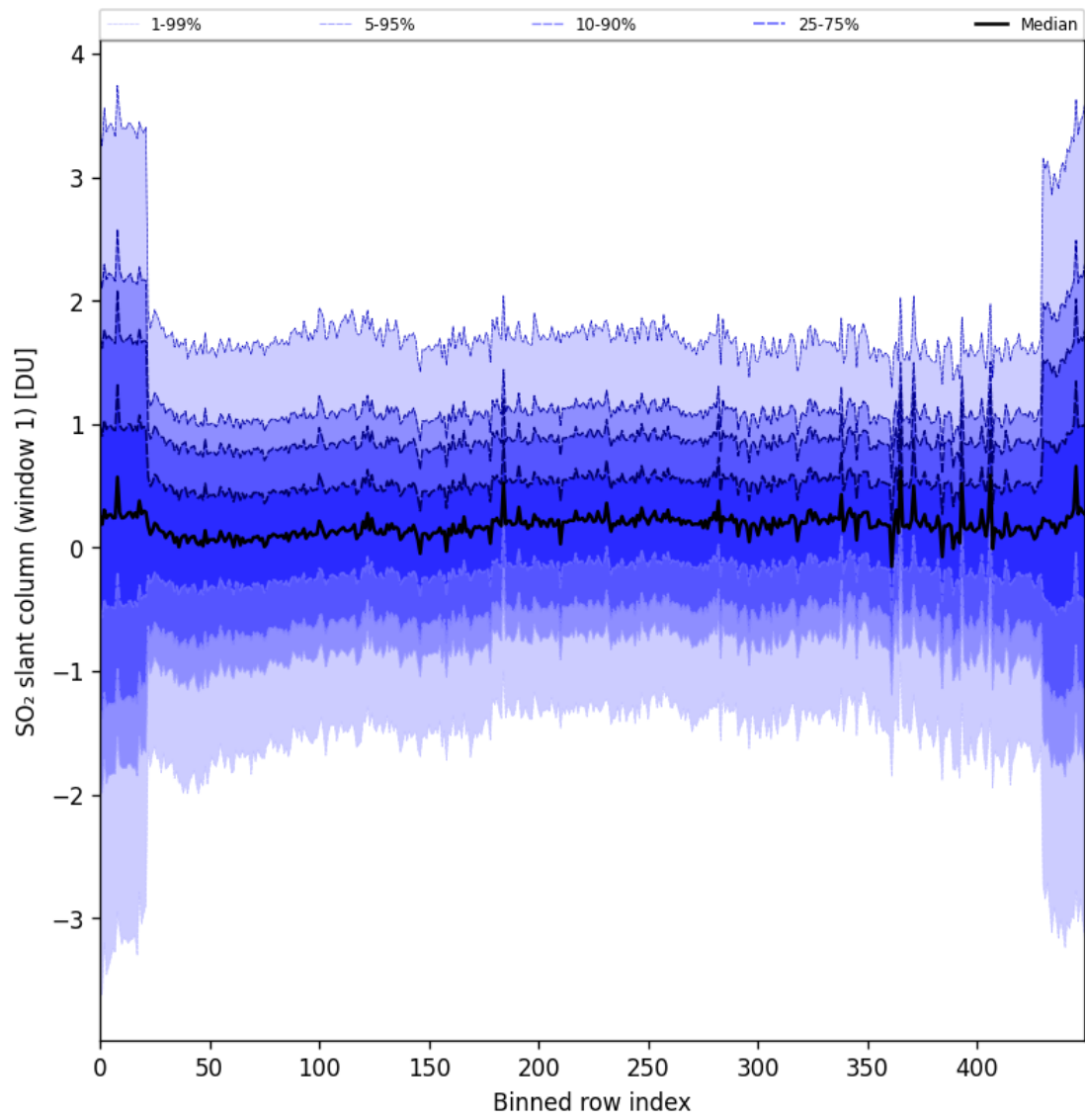
Figure 89: Along track statistics of “SO 2 slant column (window 1)” for 2025-04-22 to 2025-04-24
