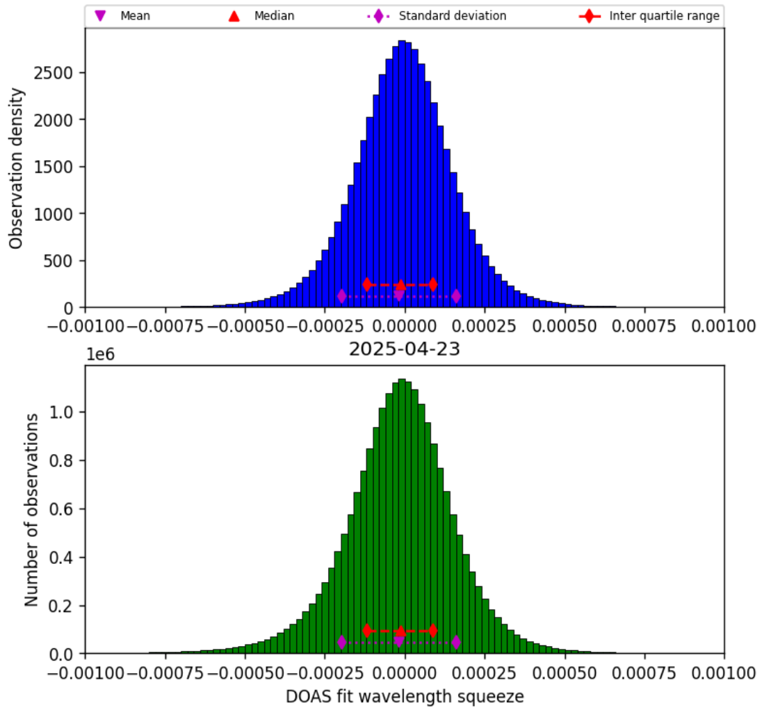
Figure 77: Histogram of “DOAS fit wavelength squeeze” for 2025-04-22 to 2025-04-24
