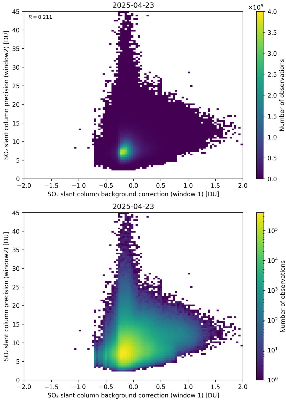
Figure 117: Scatter density plot of “SO 2 slant column background correction (window 1)” against “SO 2 slant column precision (window2)” for 2025-04-22 to 2025-04-24.
