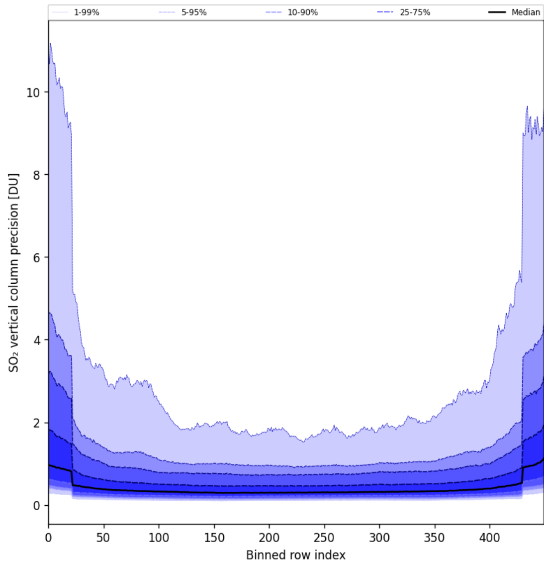
Figure 85: Along track statistics of “SO 2 vertical column precision” for 2025-04-22 to 2025-04-24
