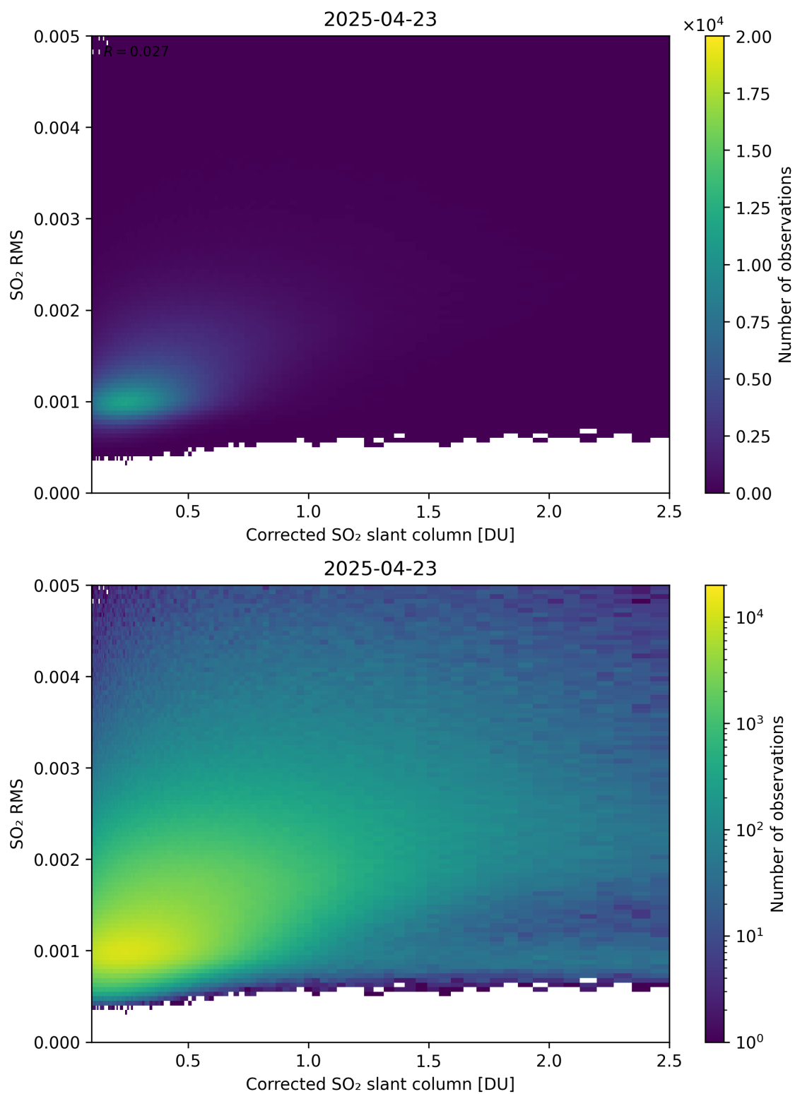
Figure 231: Scatter density plot of “Corrected SO 2 slant column” against “SO 2 RMS” for 2025-04-22 to 2025-04-24.
