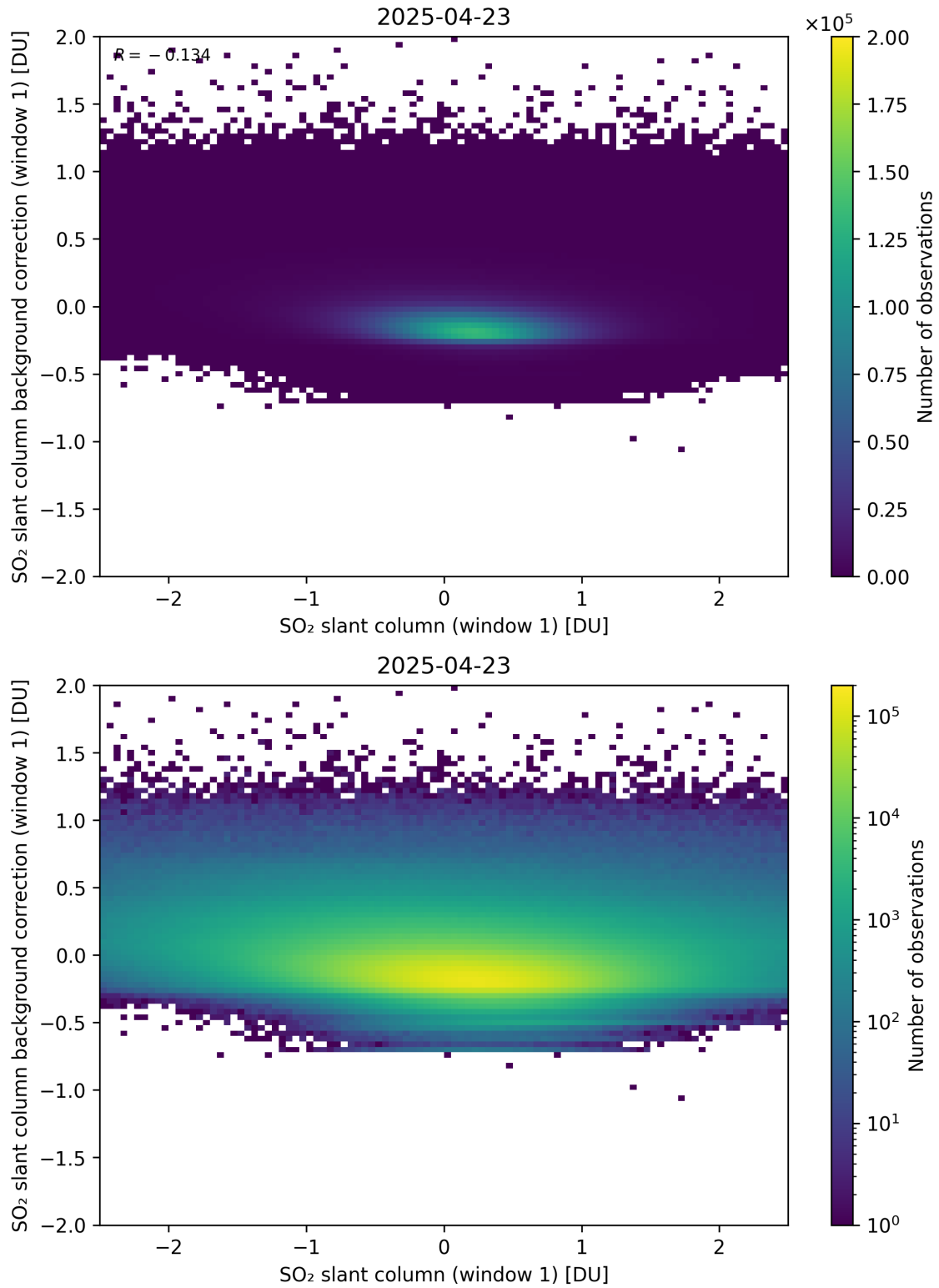
Figure 262: Scatter density plot of “SO 2 slant column (window 1)” against “SO 2 slant column background correction (window 1)” for 2025-04-22 to 2025-04-24.
