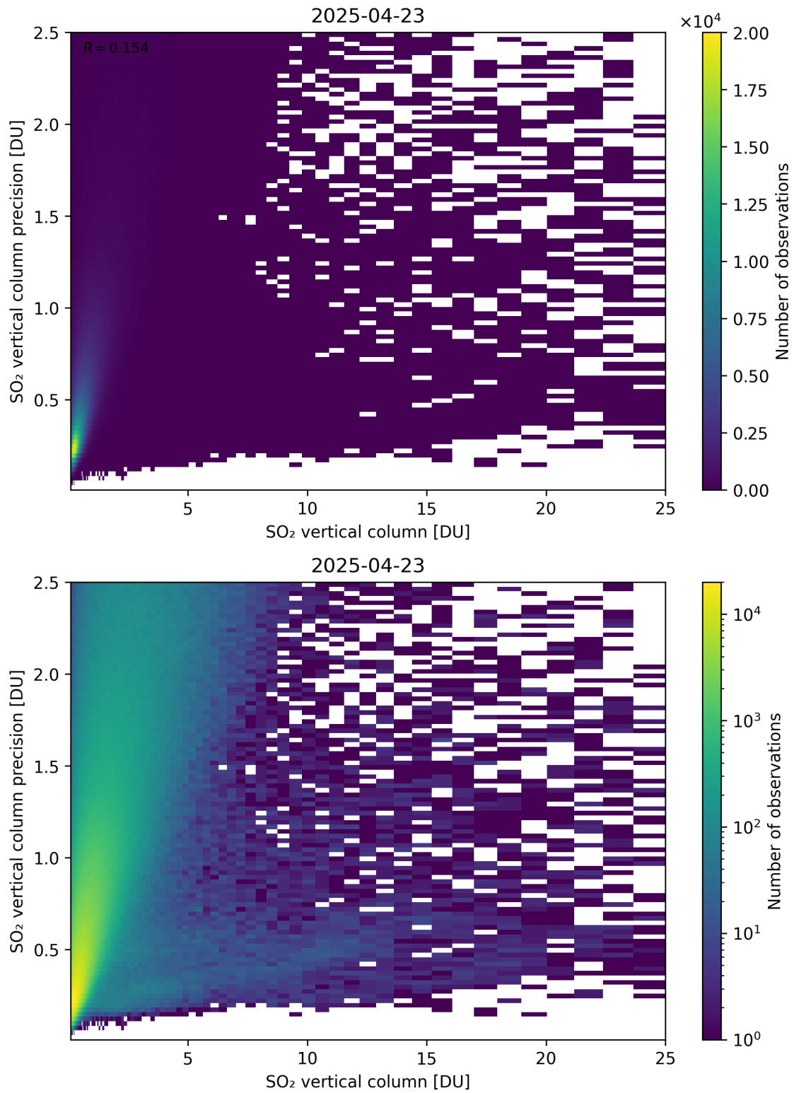
Figure 361: Scatter density plot of “SO 2 vertical column” against “SO 2 vertical column precision” for 2025-04-22 to 2025-04-24.
