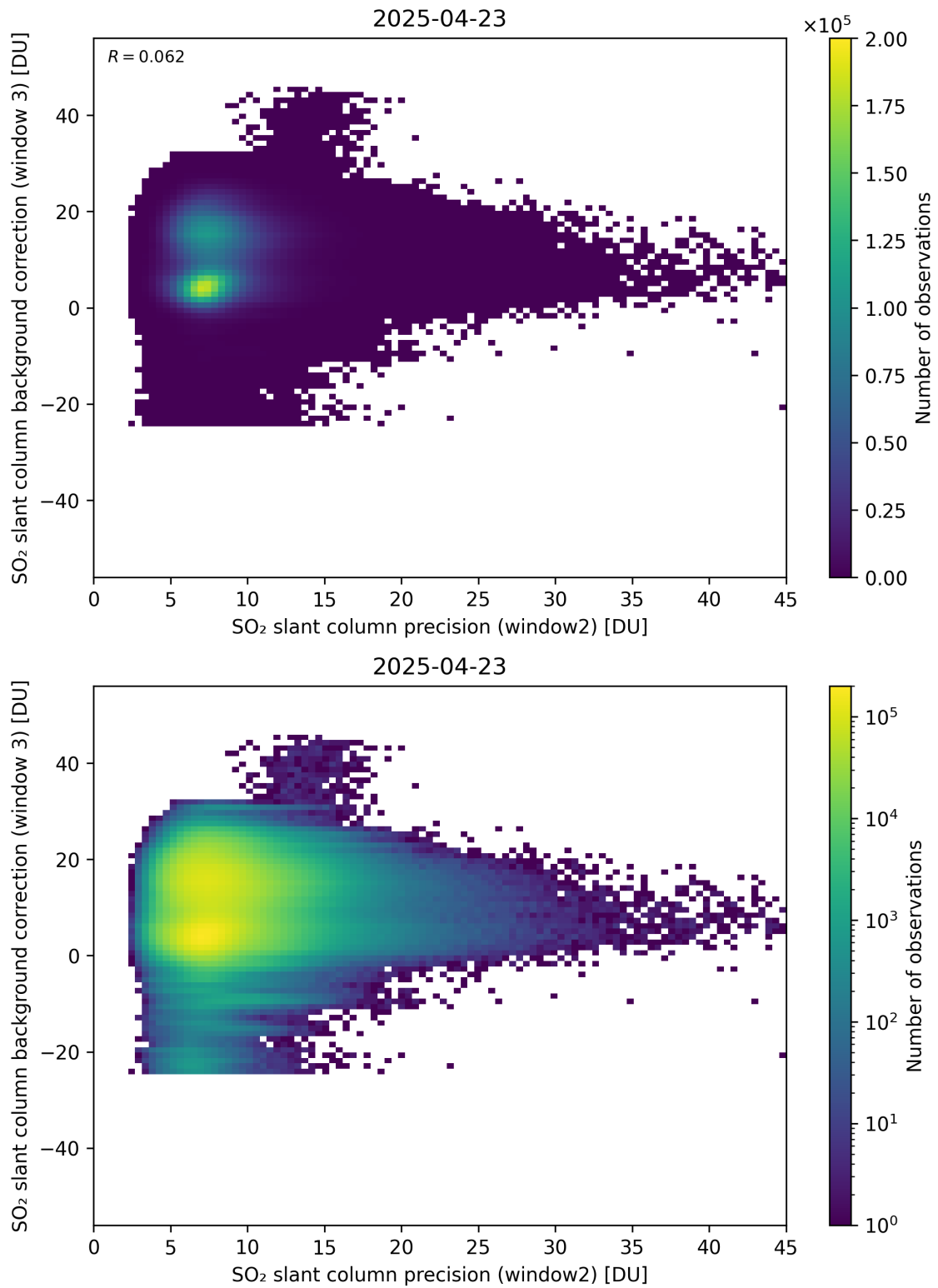
Figure 292: Scatter density plot of “SO 2 slant column precision (window2)” against “SO 2 slant column background correction (window 3)” for 2025-04-22 to 2025-04-24.
