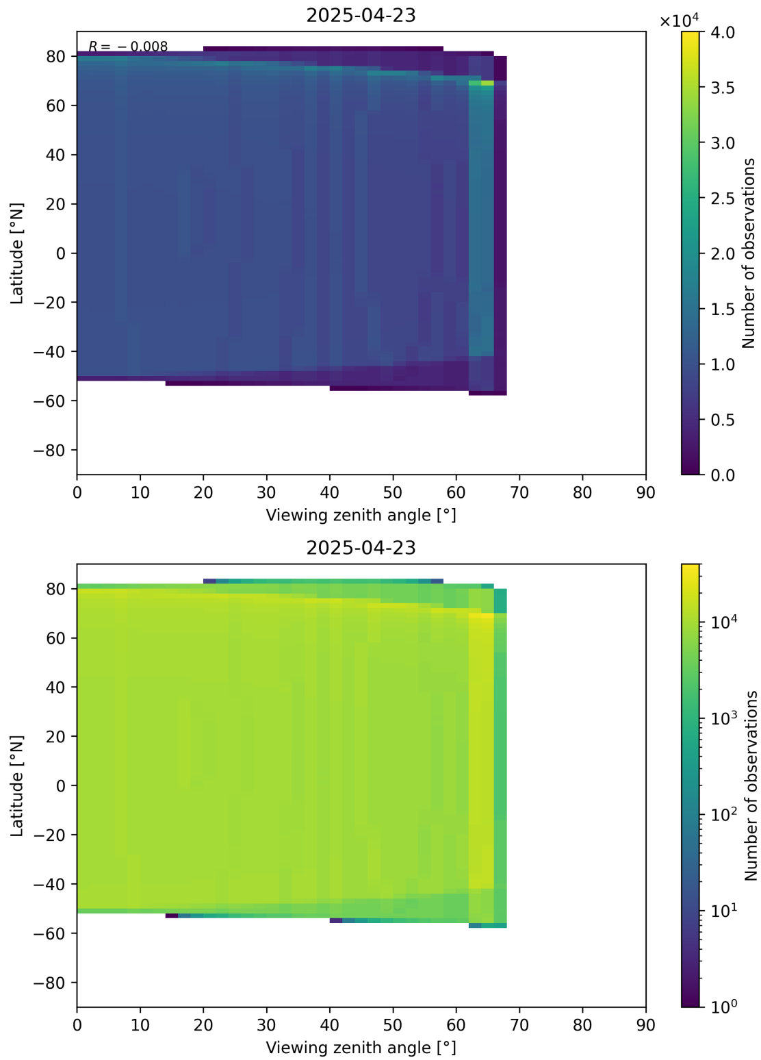
Figure 368: Scatter density plot of “Viewing zenith angle” against “Latitude” for 2025-04-22 to 2025-04-24.
