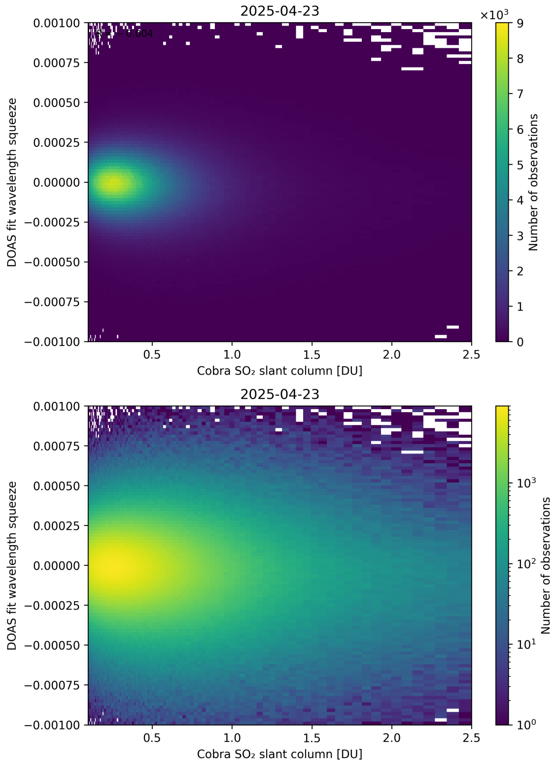
Figure 197: Scatter density plot of “Cobra SO 2 slant column” against “DOAS fit wavelength squeeze” for 2025-04-22 to 2025-04-24.
