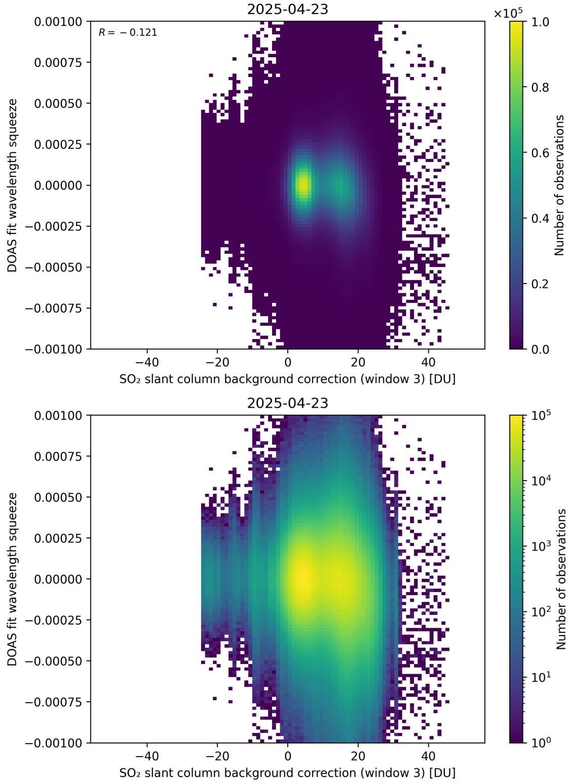
Figure 133: Scatter density plot of “SO 2 slant column background correction (window 3)” against “DOAS fit wavelength squeeze” for 2025-04-22 to 2025-04-24.
