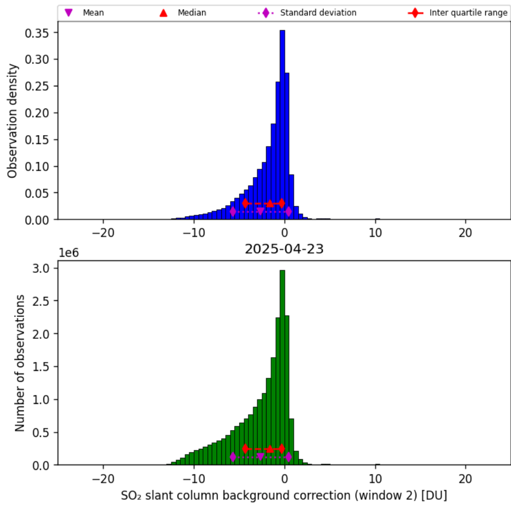
Figure 70: Histogram of “SO 2 slant column background correction (window 2)” for 2025-04-22 to 2025-04-24
