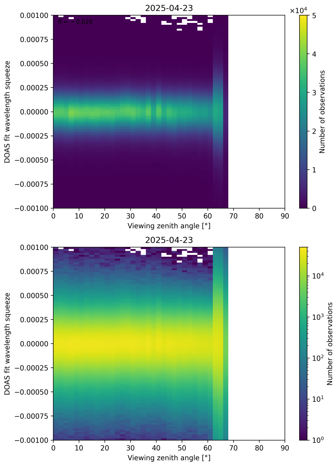
Figure 366: Scatter density plot of “Viewing zenith angle” against “DOAS fit wavelength squeeze” for 2025-04-22 to 2025-04-24.
