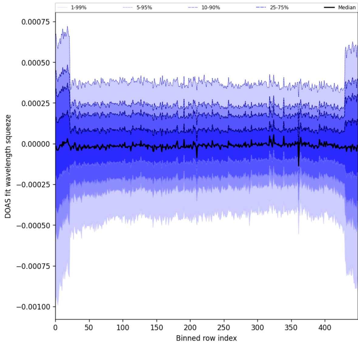
Figure 103: Along track statistics of “DOAS fit wavelength squeeze” for 2025-04-22 to 2025-04-24
