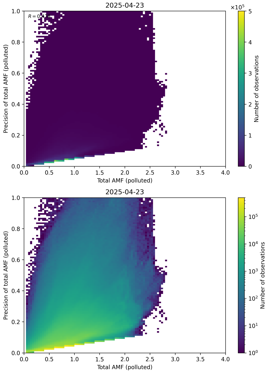
Figure 322: Scatter density plot of “Total AMF (polluted)” against “Precision of total AMF (polluted)” for 2025-04-22 to 2025-04-24.
