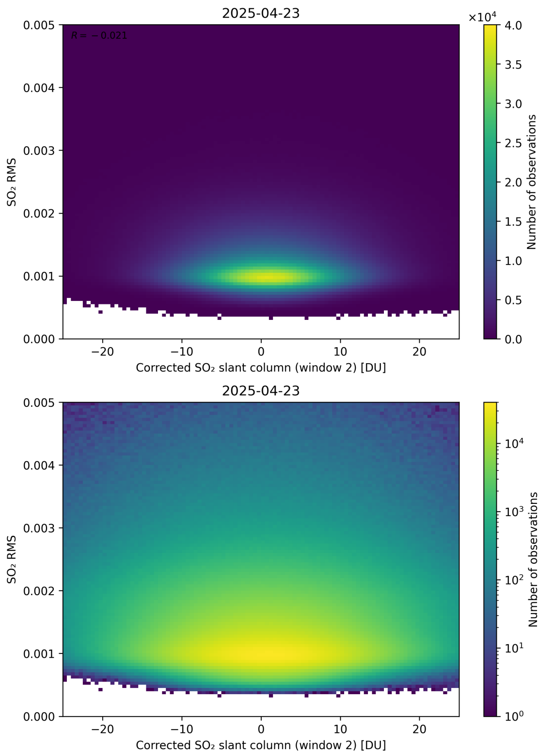
Figure 248: Scatter density plot of “Corrected SO 2 slant column (window 2)” against “SO 2 RMS” for 2025-04-22 to 2025-04-24.
