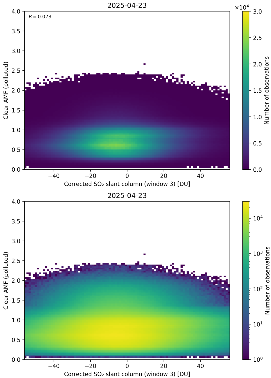
Figure 259: Scatter density plot of “Corrected SO 2 slant column (window 3)” against “Clear AMF (polluted)” for 2025-04-22 to 2025-04-24.
