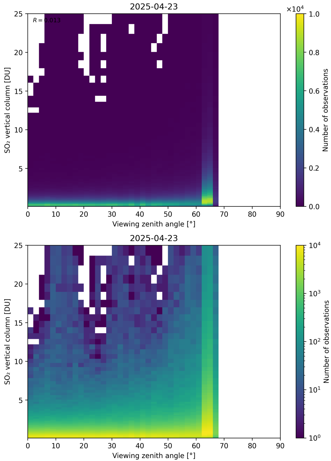
Figure 383: Scatter density plot of “Viewing zenith angle” against “SO 2 vertical column” for 2025-04-22 to 2025-04-24.
