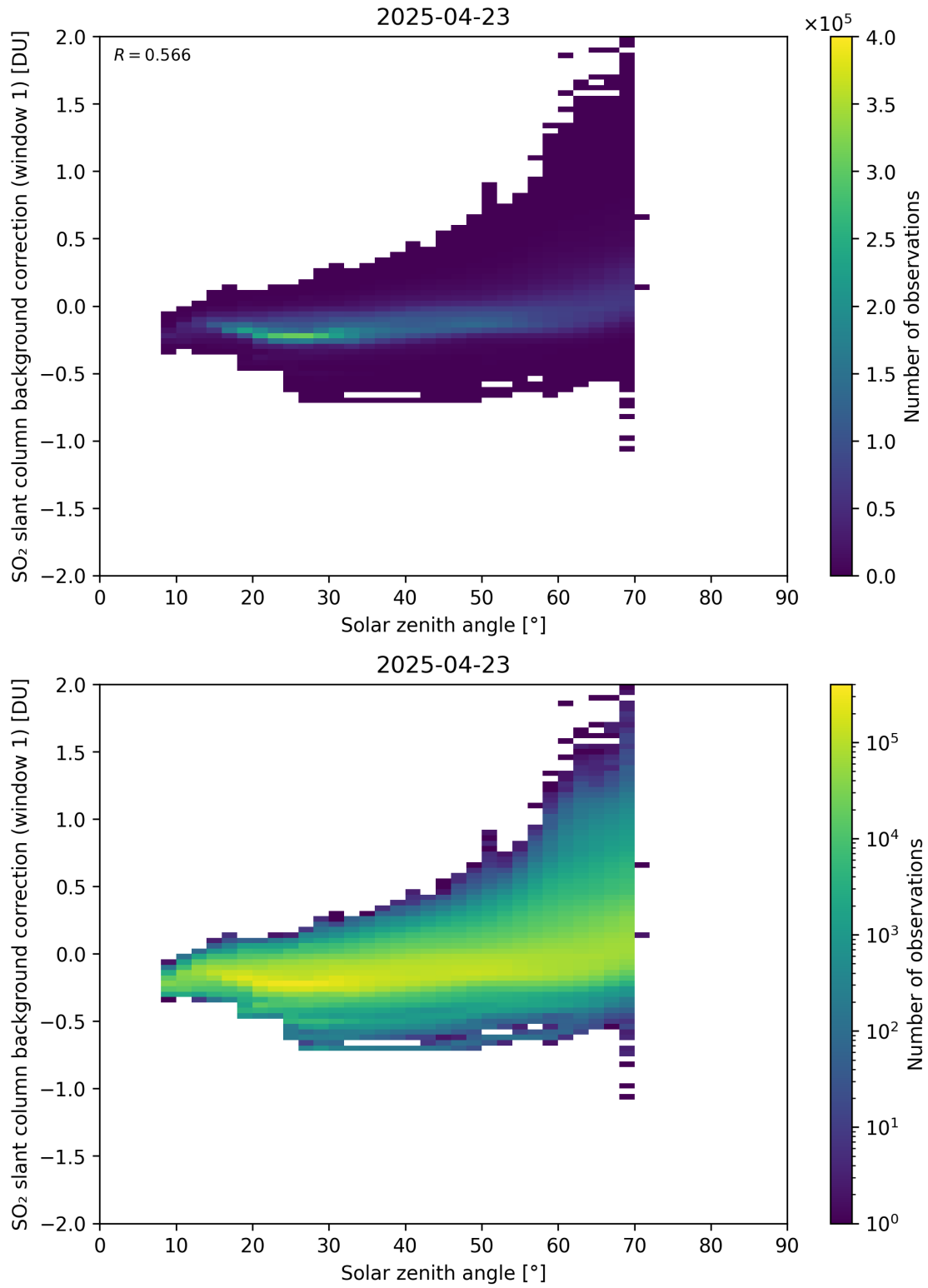
Figure 171: Scatter density plot of “Solar zenith angle” against “SO 2 slant column background correction (window 1)” for 2025-04-22 to 2025-04-24.
