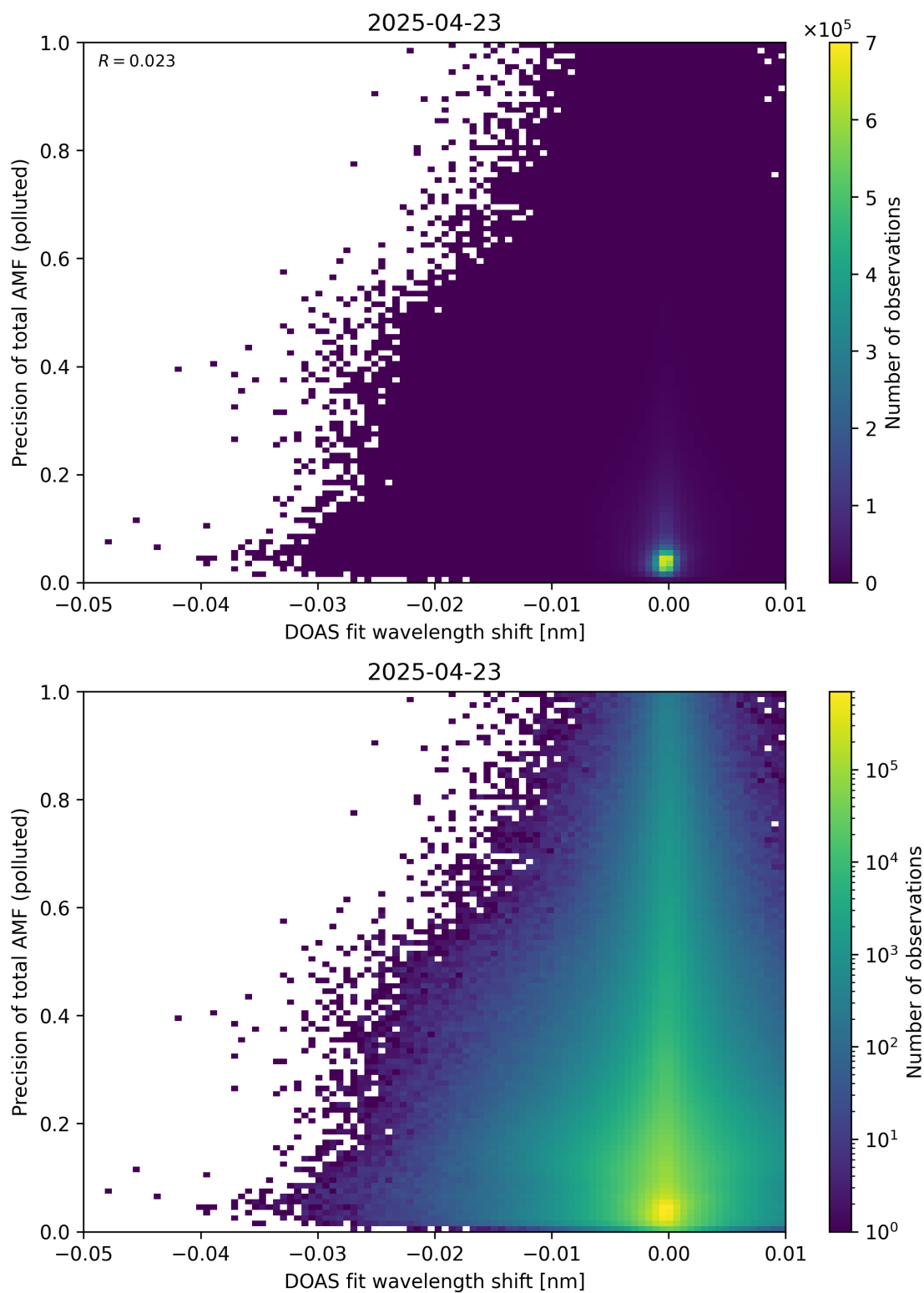
Figure 142: Scatter density plot of “DOAS fit wavelength shift” against “Precision of total AMF (polluted)” for 2025-04-22 to 2025-04-24.
