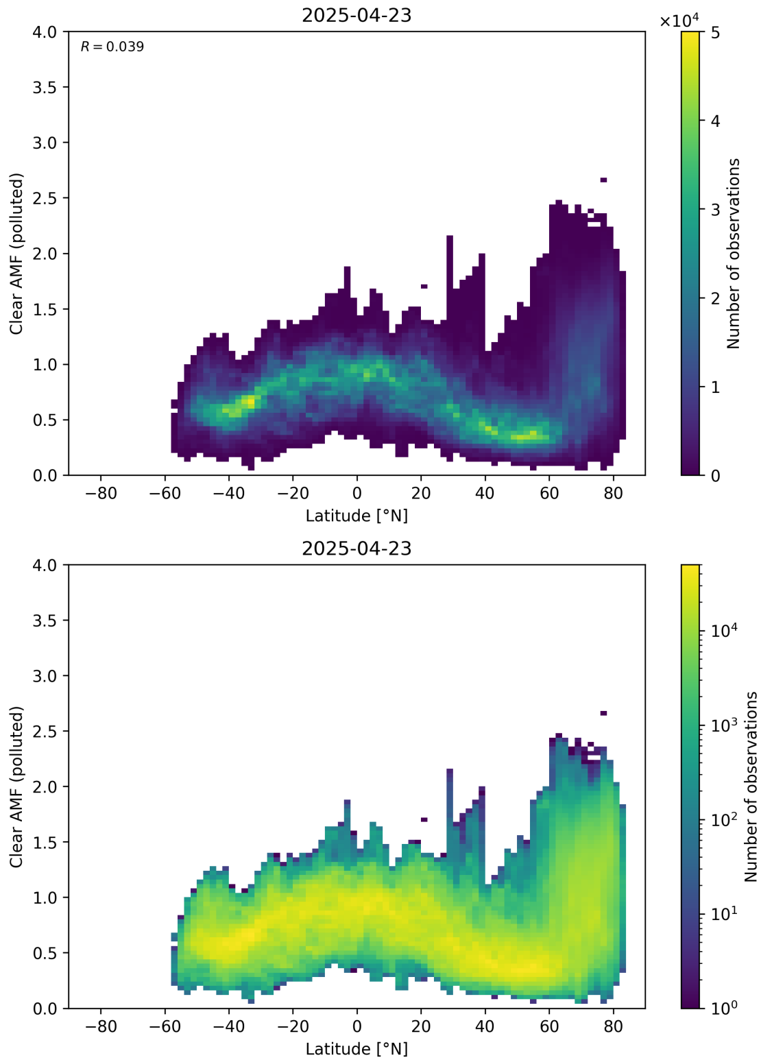
Figure 156: Scatter density plot of “Latitude” against “Clear AMF (polluted)” for 2025-04-22 to 2025-04-24.
