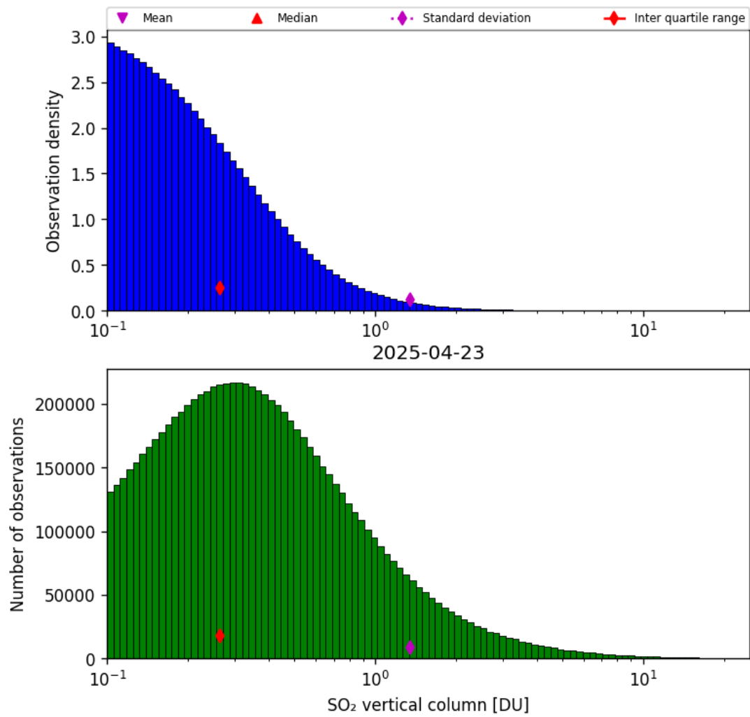
Figure 58: Histogram of “SO 2 vertical column” for 2025-04-22 to 2025-04-24
