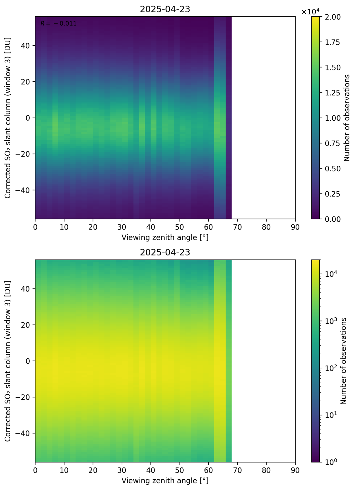
Figure 375: Scatter density plot of “Viewing zenith angle” against “Corrected SO 2 slant column (window 3)” for 2025-04-22 to 2025-04-24.
