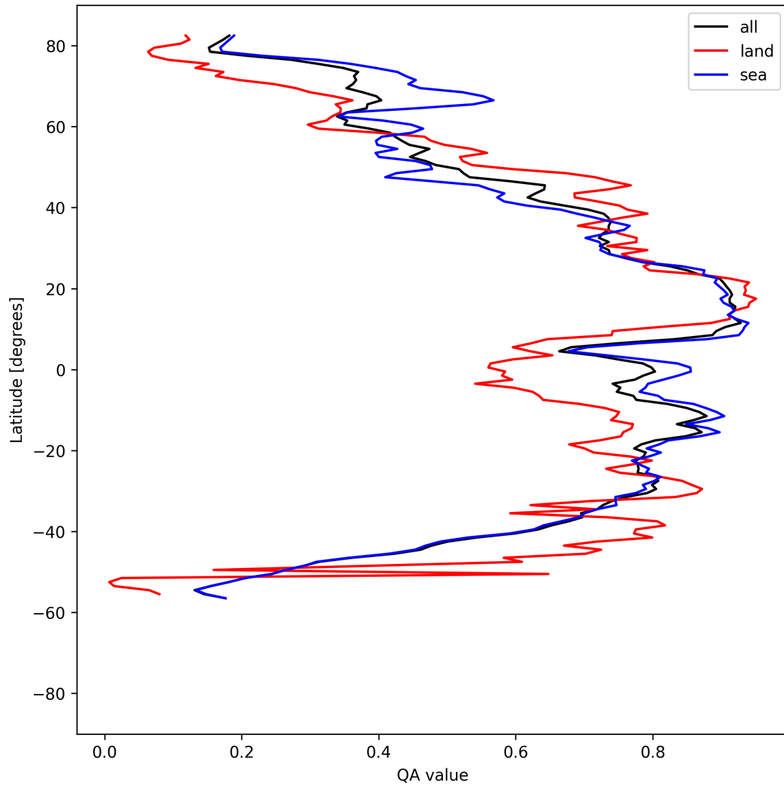
Figure 31: Zonal average of “QA value” for 2025-04-22 to 2025-04-24.
