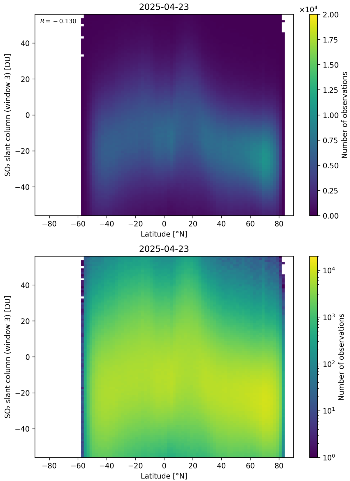
Figure 165: Scatter density plot of “Latitude” against “SO 2 slant column (window 3)” for 2025-04-22 to 2025-04-24.
