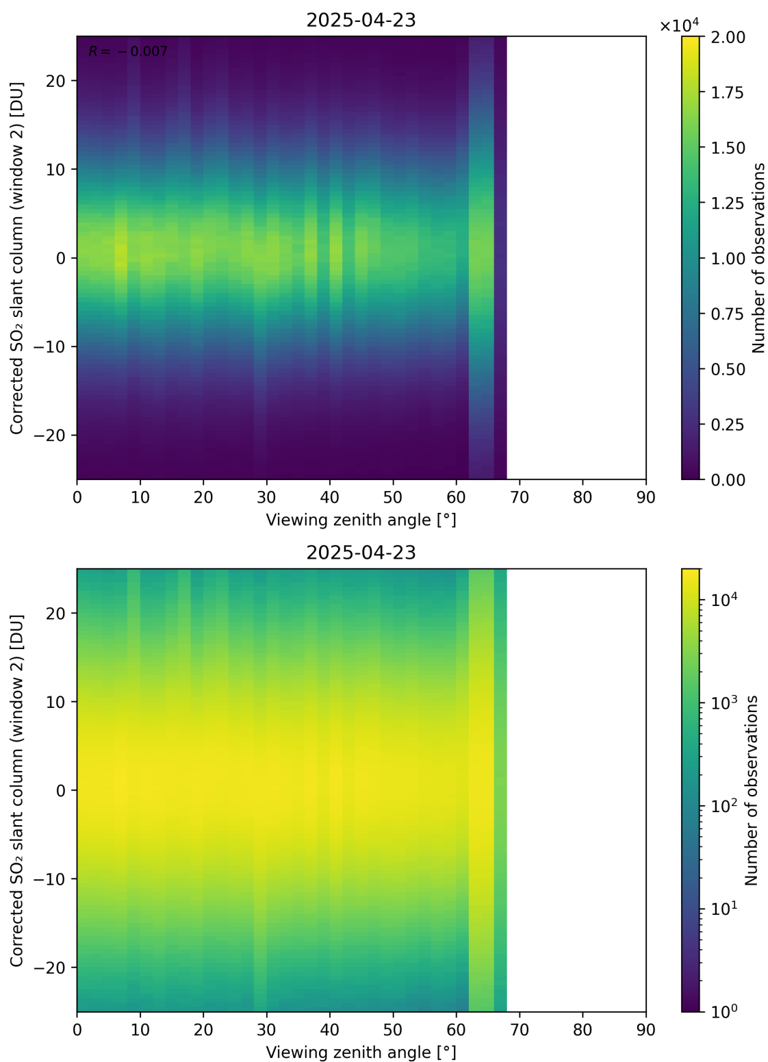
Figure 374: Scatter density plot of “Viewing zenith angle” against “Corrected SO 2 slant column (window 2)” for 2025-04-22 to 2025-04-24.
