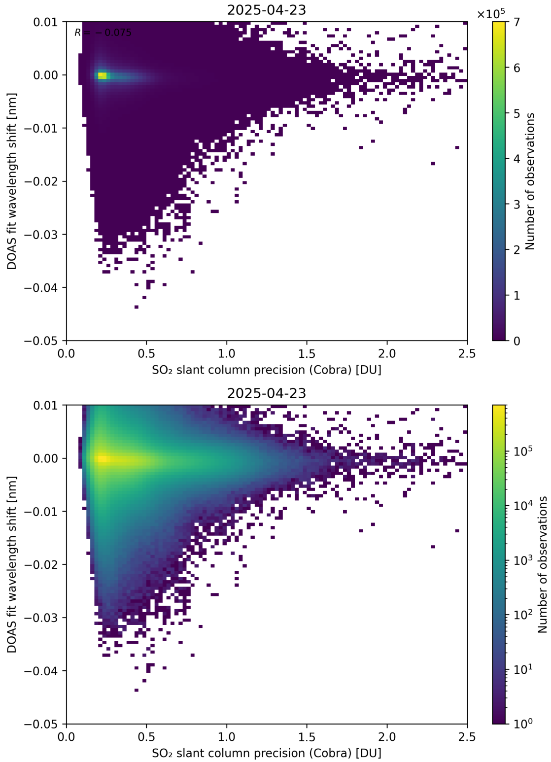
Figure 202: Scatter density plot of “SO 2 slant column precision (Cobra)” against “DOAS fit wavelength shift” for 2025-04-22 to 2025-04-24.
