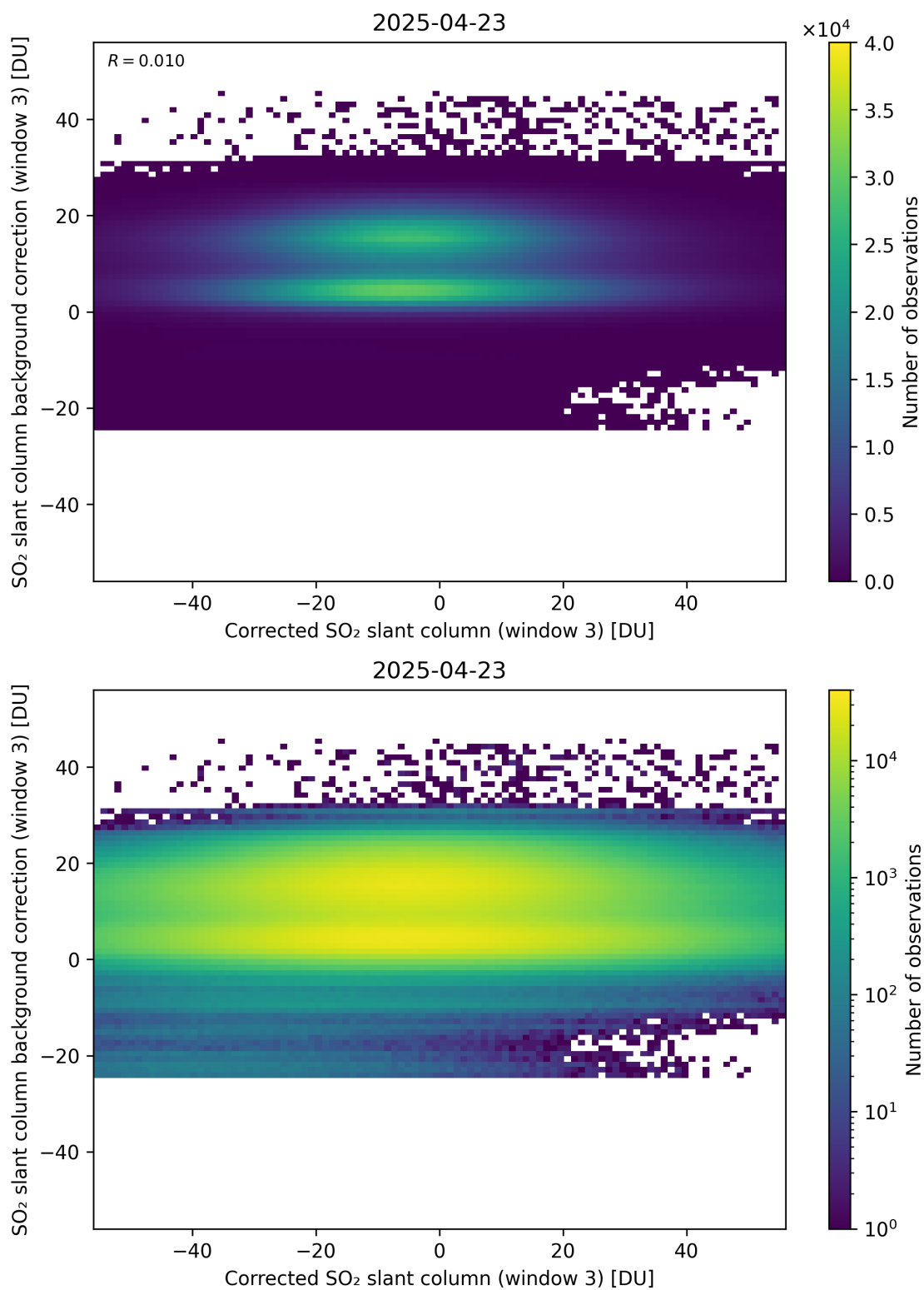
Figure 255: Scatter density plot of “Corrected SO 2 slant column (window 3)” against “SO 2 slant column background correction (window 3)” for 2025-04-22 to 2025-04-24.
