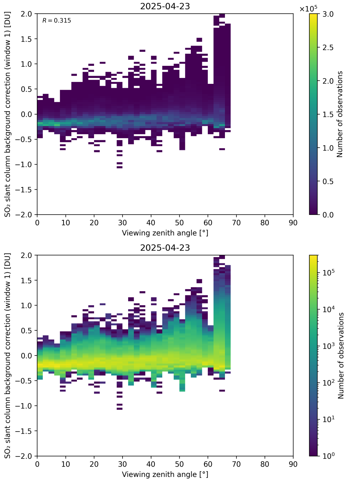
Figure 362: Scatter density plot of “Viewing zenith angle” against “SO 2 slant column background correction (window 1)” for 2025-04-22 to 2025-04-24.
