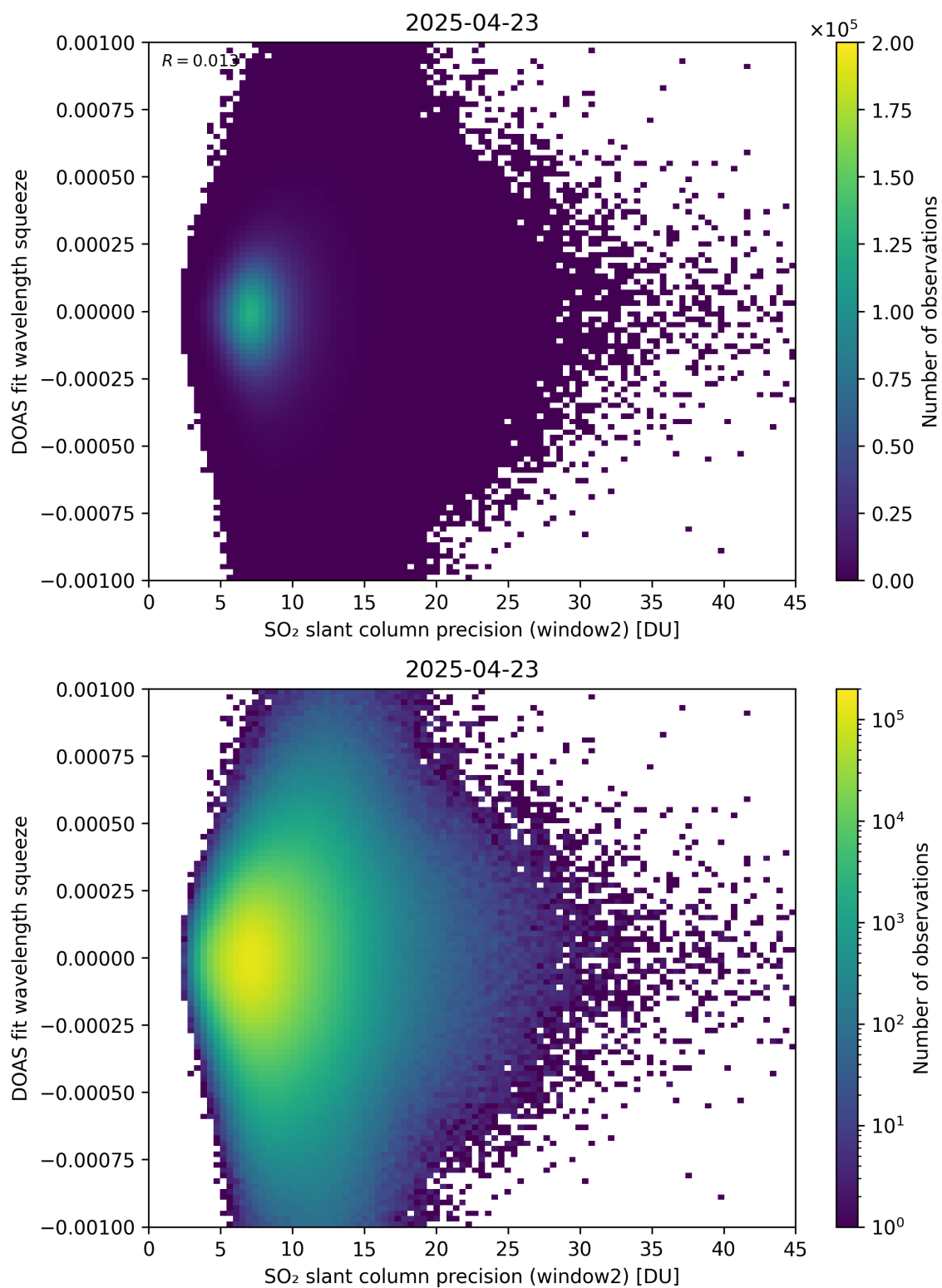
Figure 294: Scatter density plot of “SO 2 slant column precision (window2)” against “DOAS fit wavelength squeeze” for 2025-04-22 to 2025-04-24.
