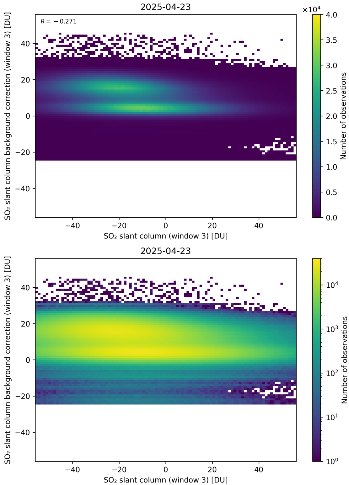
Figure 303: Scatter density plot of “SO 2 slant column (window 3)” against “SO 2 slant column background correction (window 3)” for 2025-04-22 to 2025-04-24.
