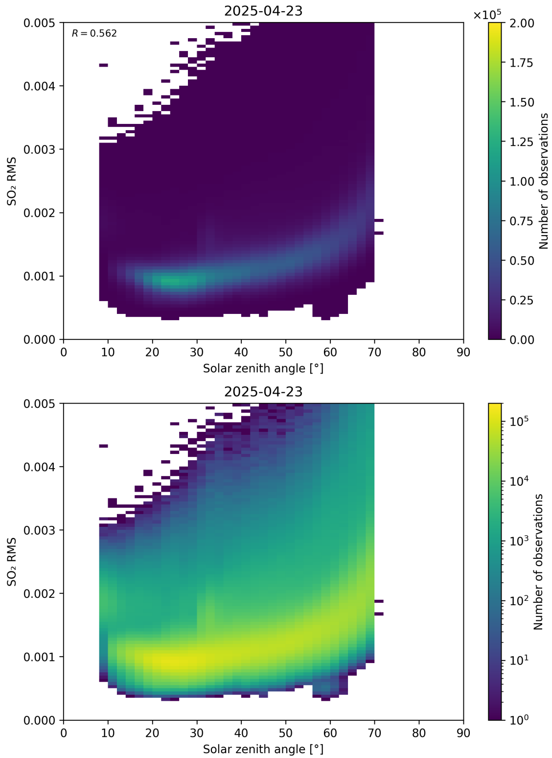
Figure 176: Scatter density plot of “Solar zenith angle” against “SO 2 RMS” for 2025-04-22 to 2025-04-24.
