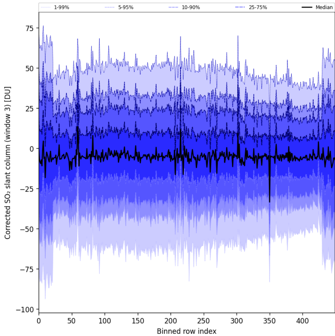
Figure 99: Along track statistics of “Corrected SO 2 slant column (window 3)” for 2025-04-22 to 2025-04-24
