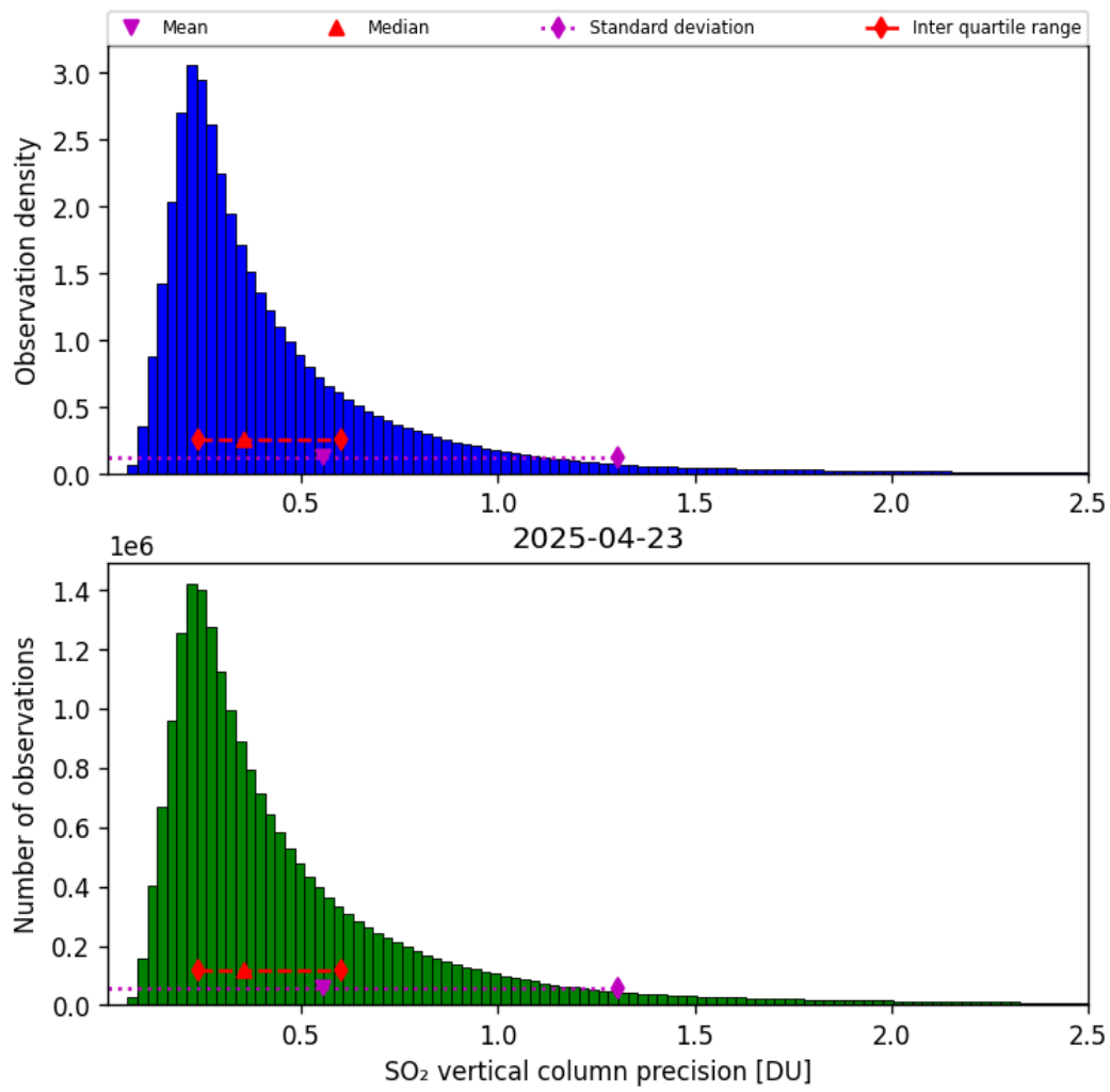
Figure 59: Histogram of “SO 2 vertical column precision” for 2025-04-22 to 2025-04-24
