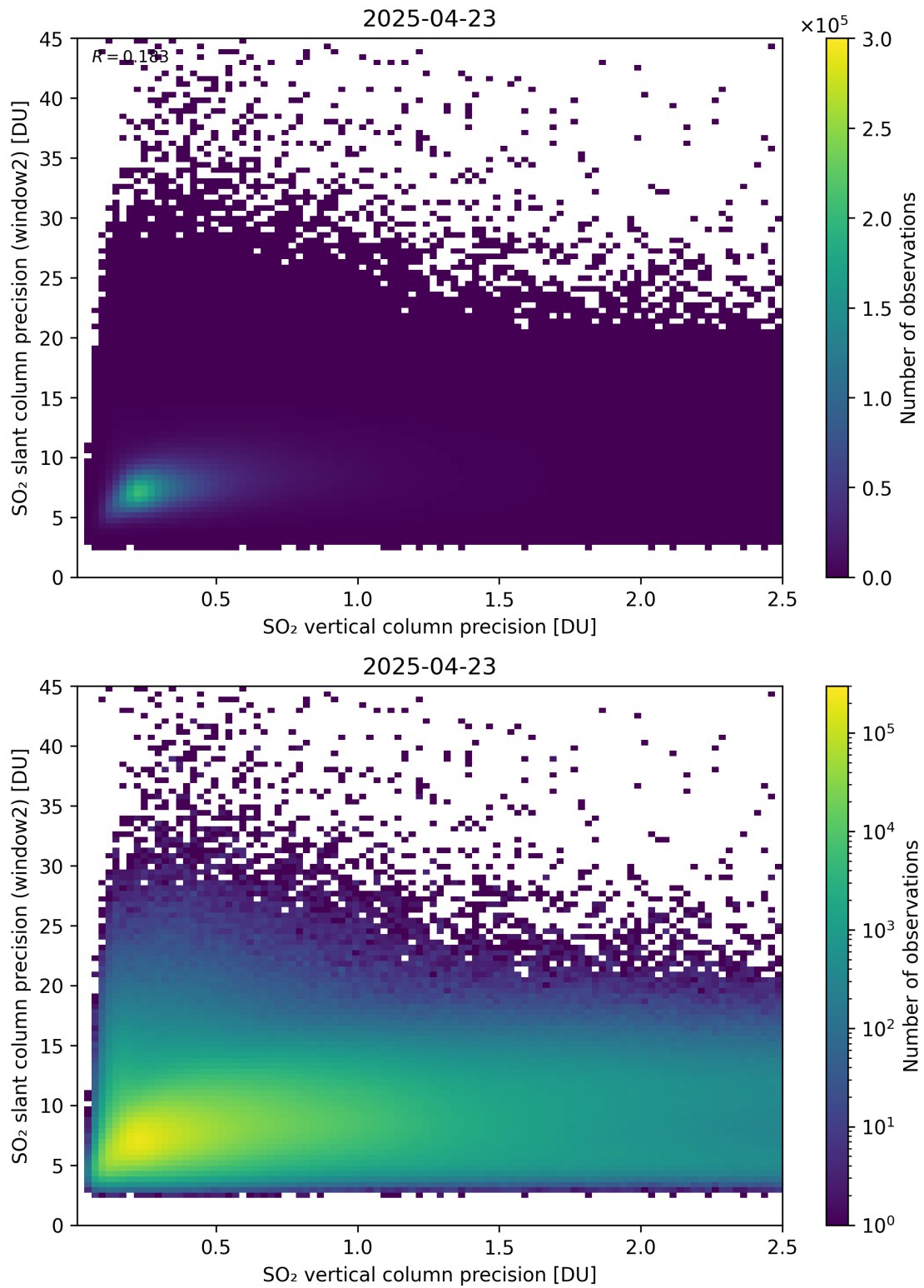
Figure 343: Scatter density plot of “SO 2 vertical column precision” against “SO 2 slant column precision (window2)” for 2025-04-22 to 2025-04-24.
