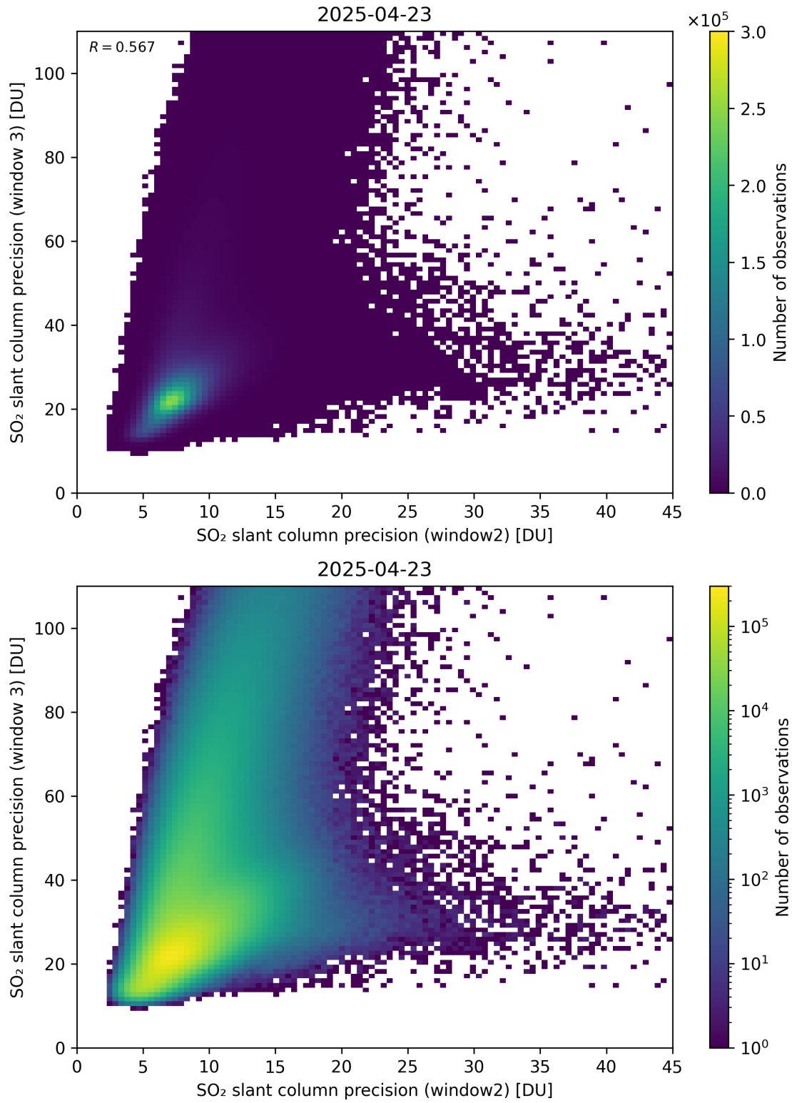
Figure 300: Scatter density plot of “SO 2 slant column precision (window2)” against “SO 2 slant column precision (window 3)” for 2025-04-22 to 2025-04-24.
