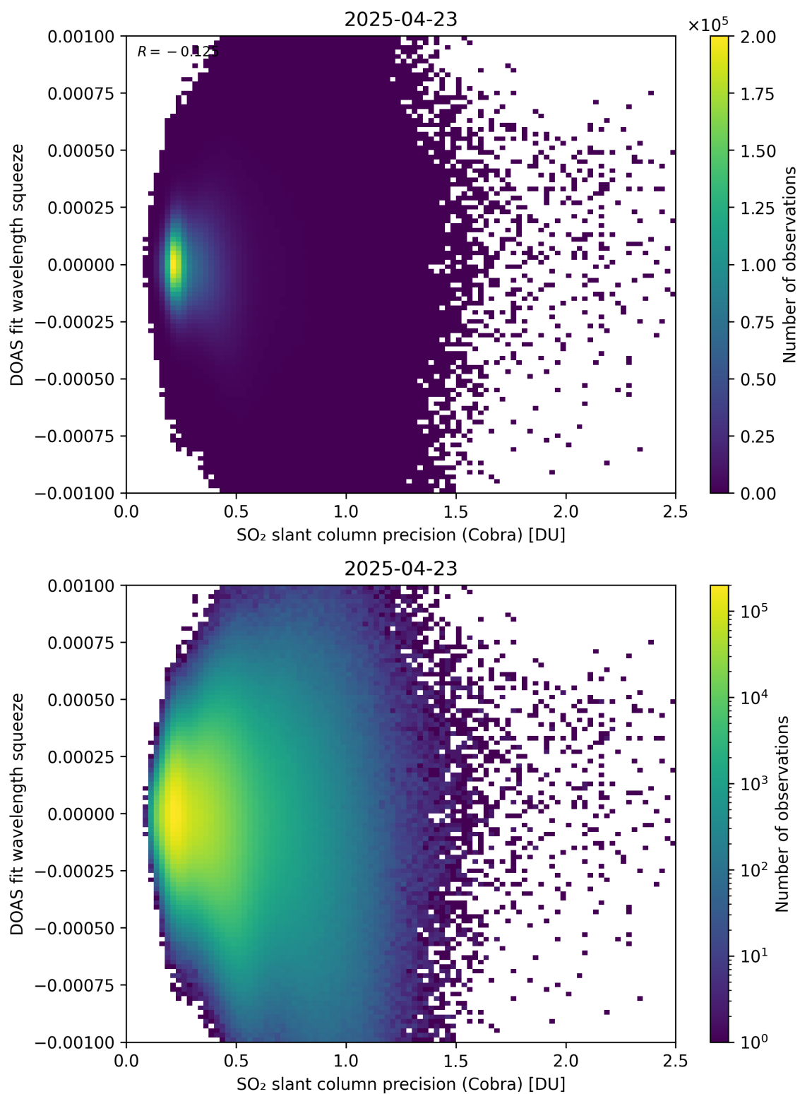
Figure 203: Scatter density plot of “SO 2 slant column precision (Cobra)” against “DOAS fit wavelength squeeze” for 2025-04-22 to 2025-04-24.
