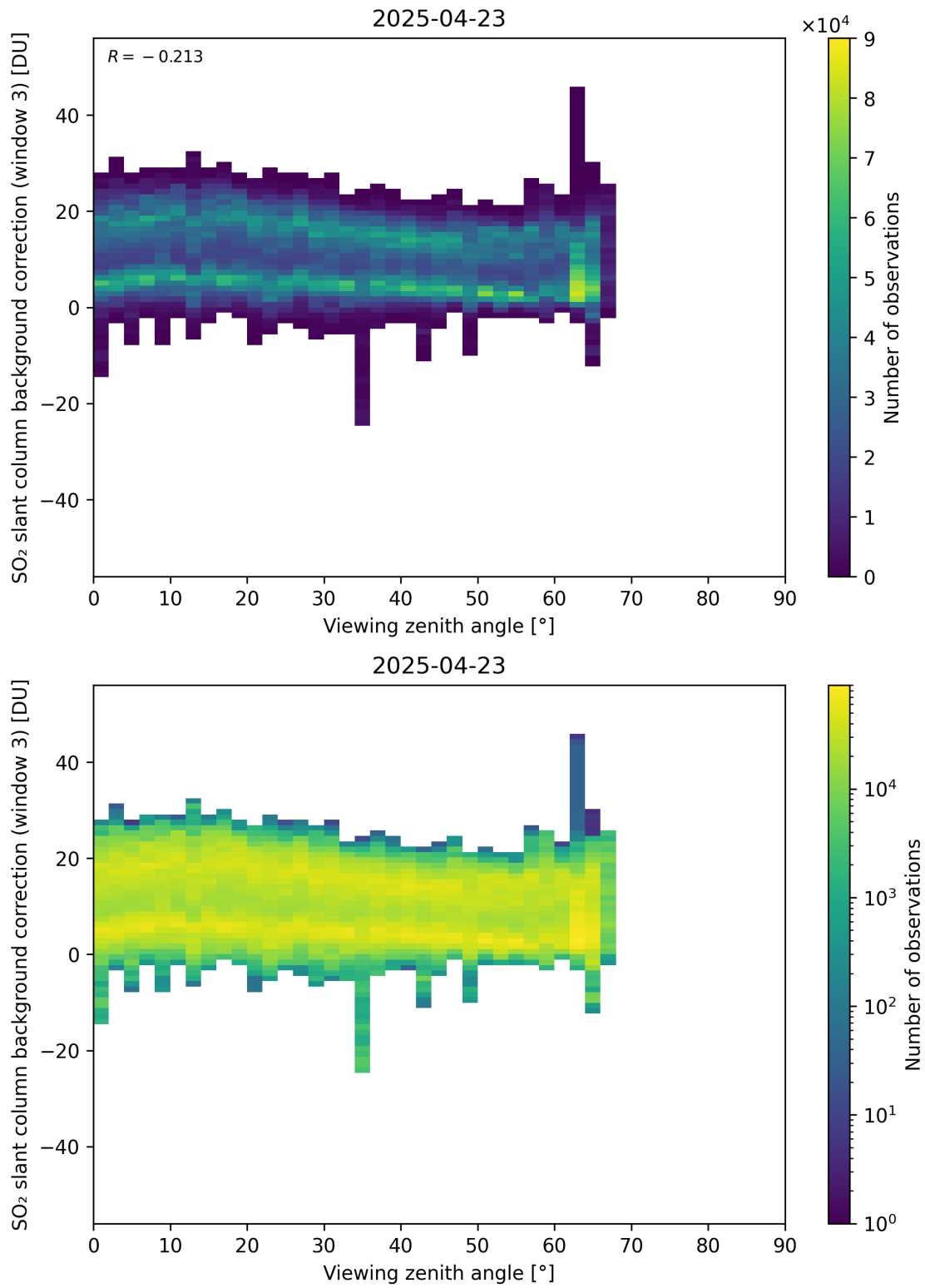
Figure 364: Scatter density plot of “Viewing zenith angle” against “SO 2 slant column background correction (window 3)” for 2025-04-22 to 2025-04-24.
