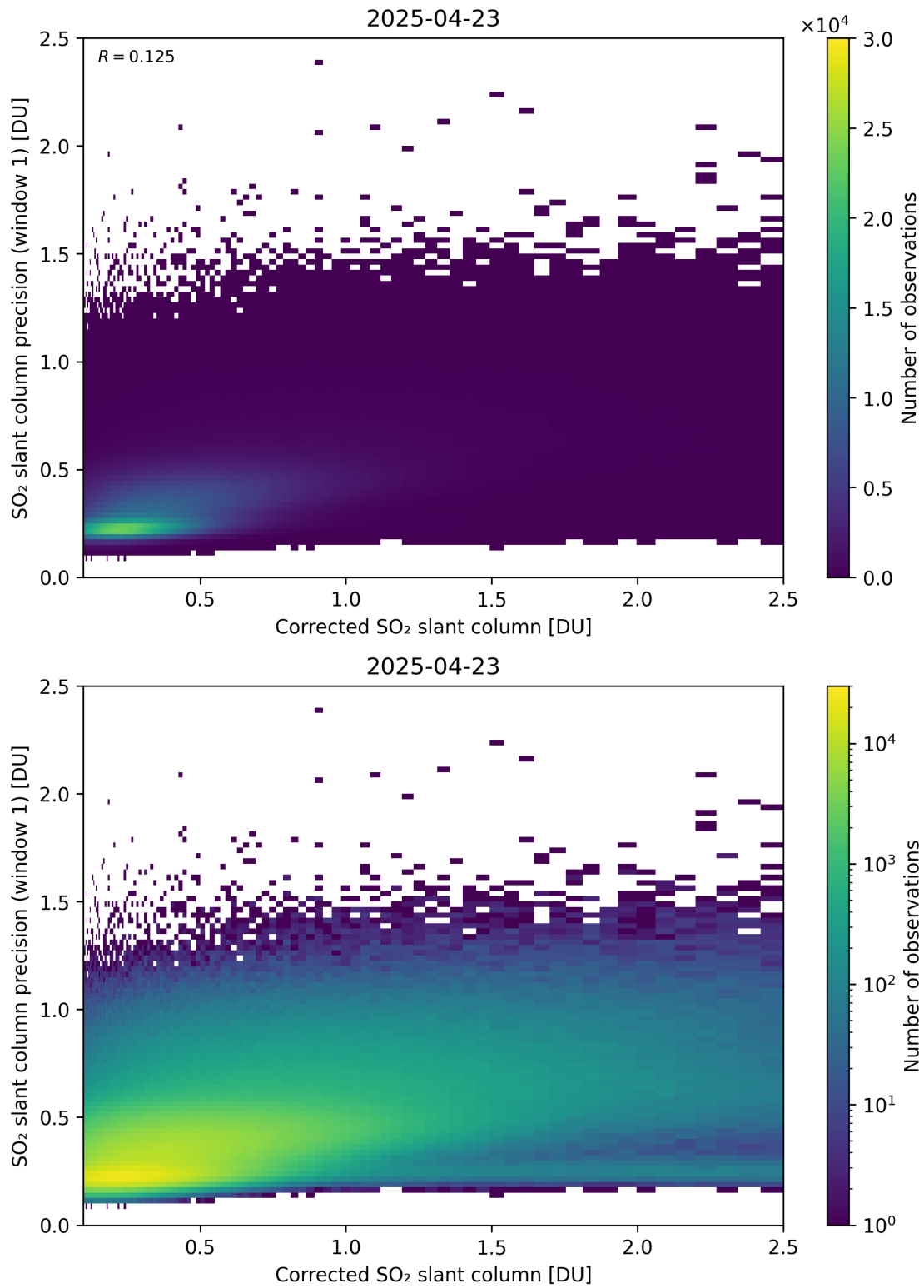
Figure 238: Scatter density plot of “Corrected SO 2 slant column” against “SO 2 slant column precision (window 1)” for 2025-04-22 to 2025-04-24.
