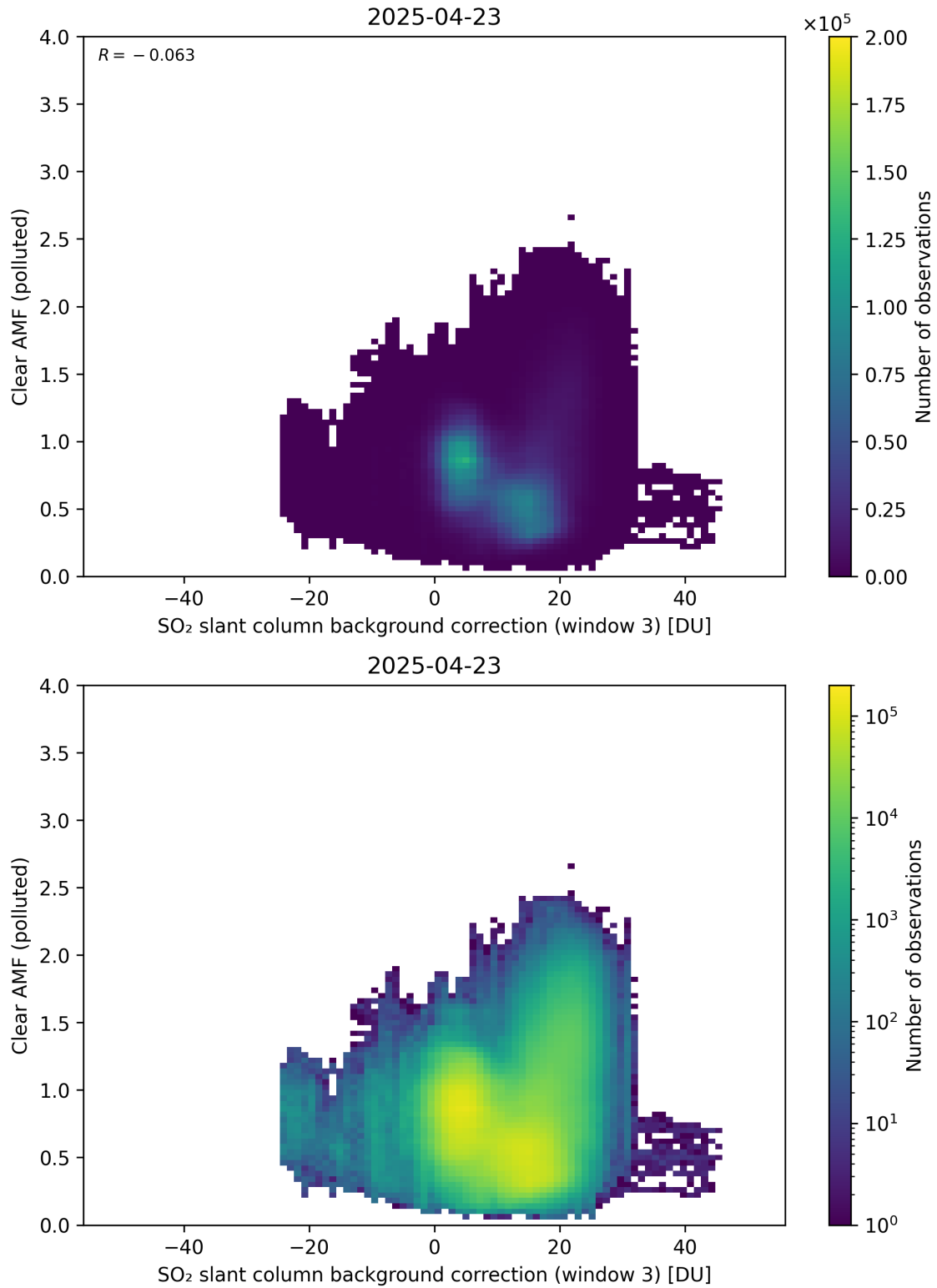
Figure 135: Scatter density plot of “SO 2 slant column background correction (window 3)” against “Clear AMF (polluted)” for 2025-04-22 to 2025-04-24.
