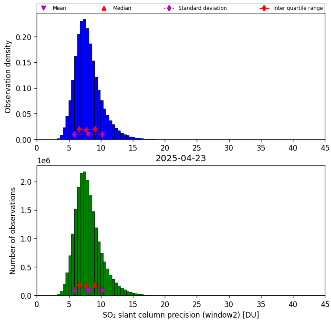
Figure 68: Histogram of “SO 2 slant column precision (window2)” for 2025-04-22 to 2025-04-24
