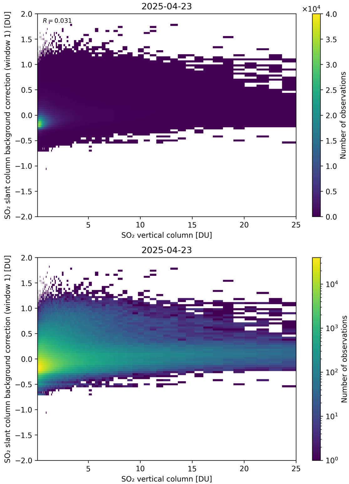
Figure 323: Scatter density plot of “SO 2 vertical column” against “SO 2 slant column background correction (window 1)” for 2025-04-22 to 2025-04-24.
