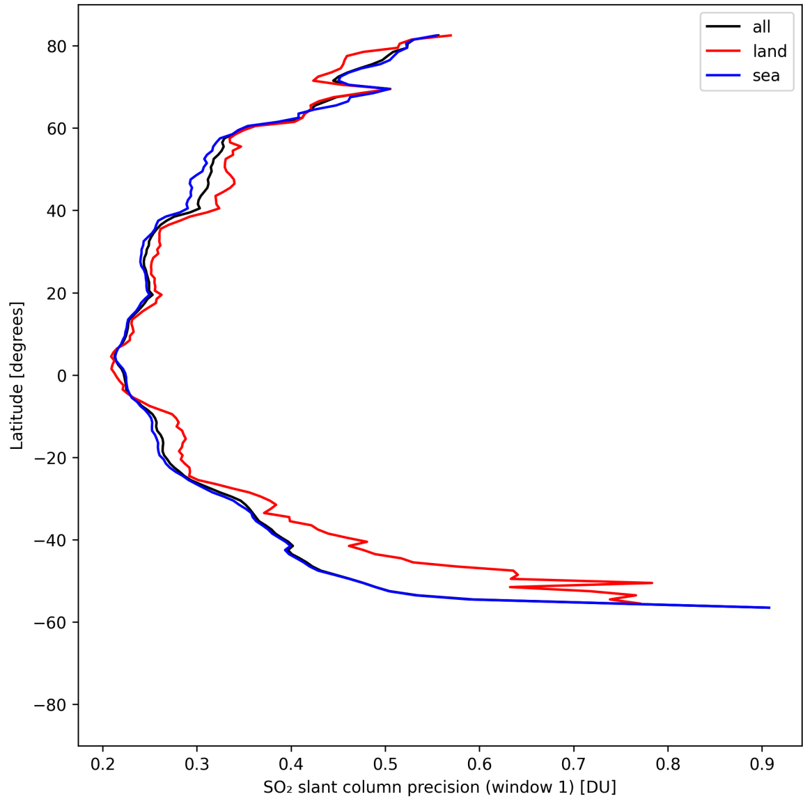
Figure 38: Zonal average of “SO 2 slant column precision (window 1)” for 2025-04-22 to 2025-04-24.
