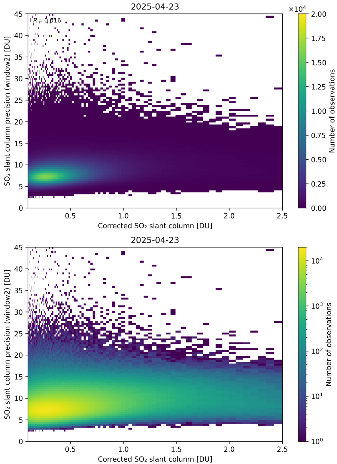
Figure 239: Scatter density plot of “Corrected SO 2 slant column” against “SO 2 slant column precision (window2)” for 2025-04-22 to 2025-04-24.
