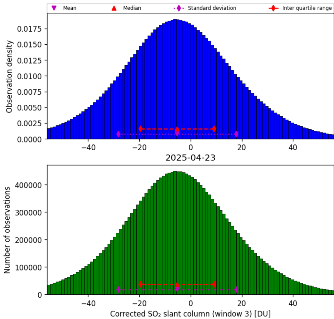
Figure 73: Histogram of “Corrected SO 2 slant column (window 3)” for 2025-04-22 to 2025-04-24
