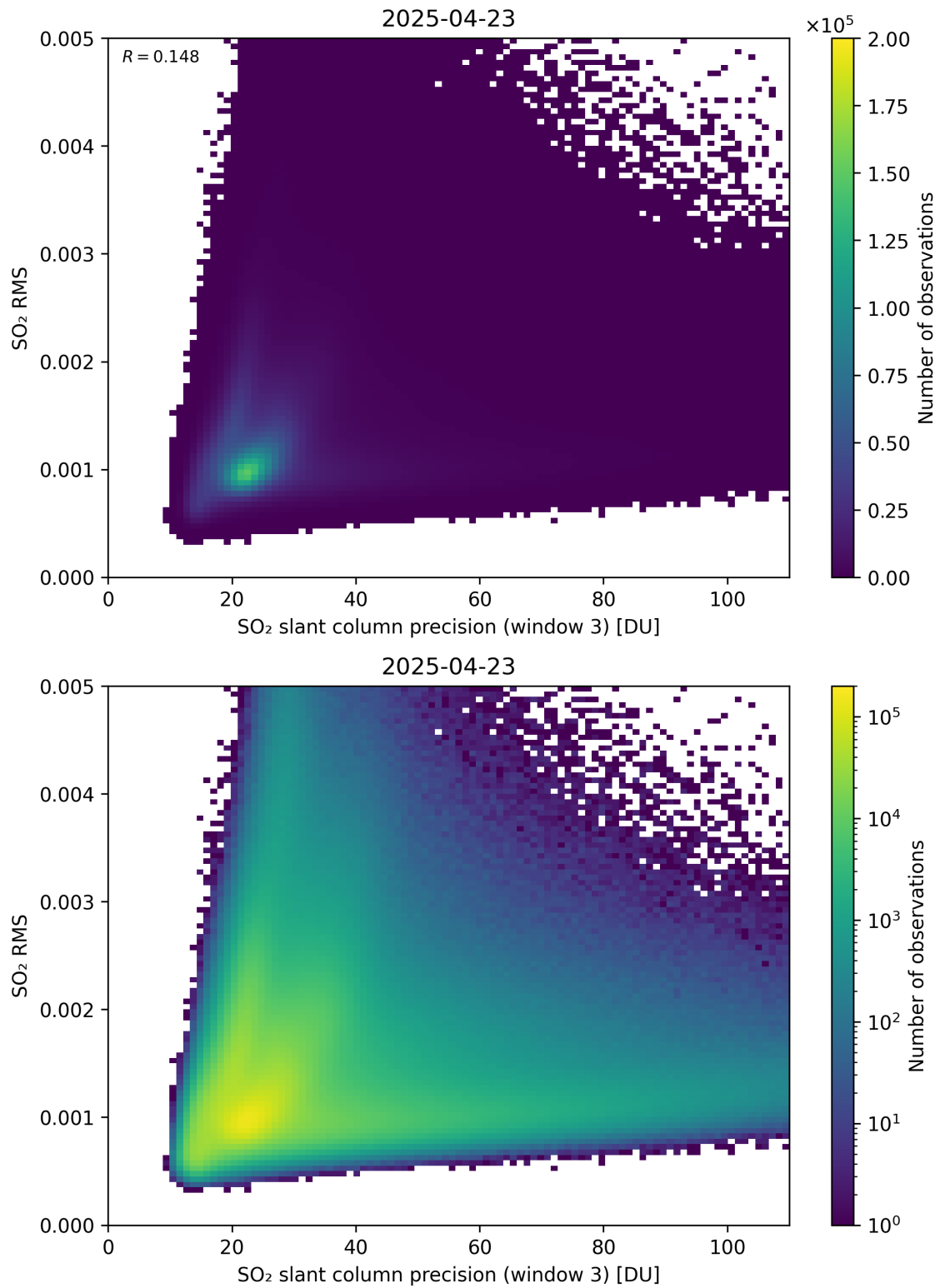
Figure 310: Scatter density plot of “SO 2 slant column precision (window 3)” against “SO 2 RMS” for 2025-04-22 to 2025-04-24.
