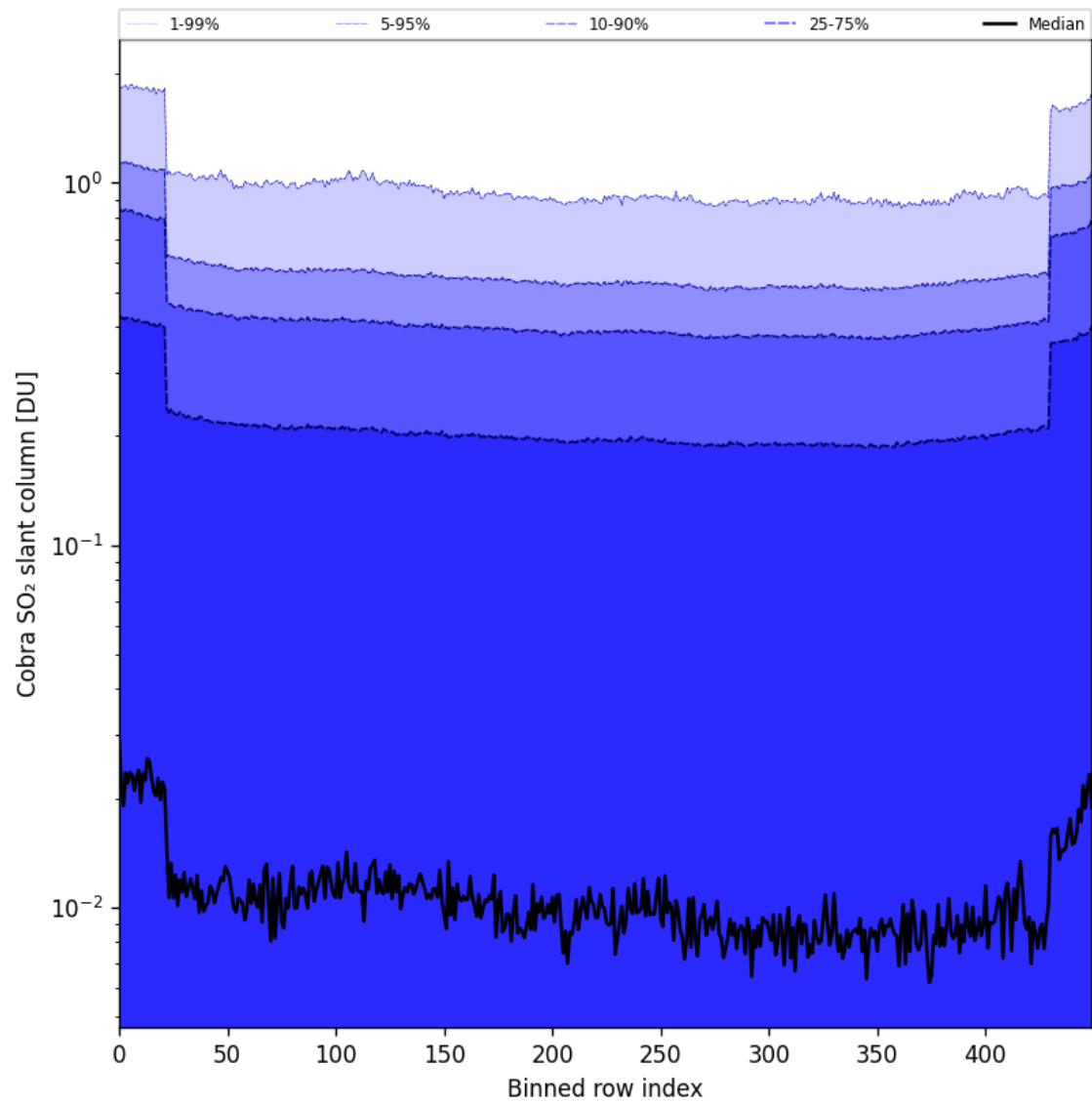
Figure 87: Along track statistics of “Cobra SO 2 slant column” for 2025-04-22 to 2025-04-24
