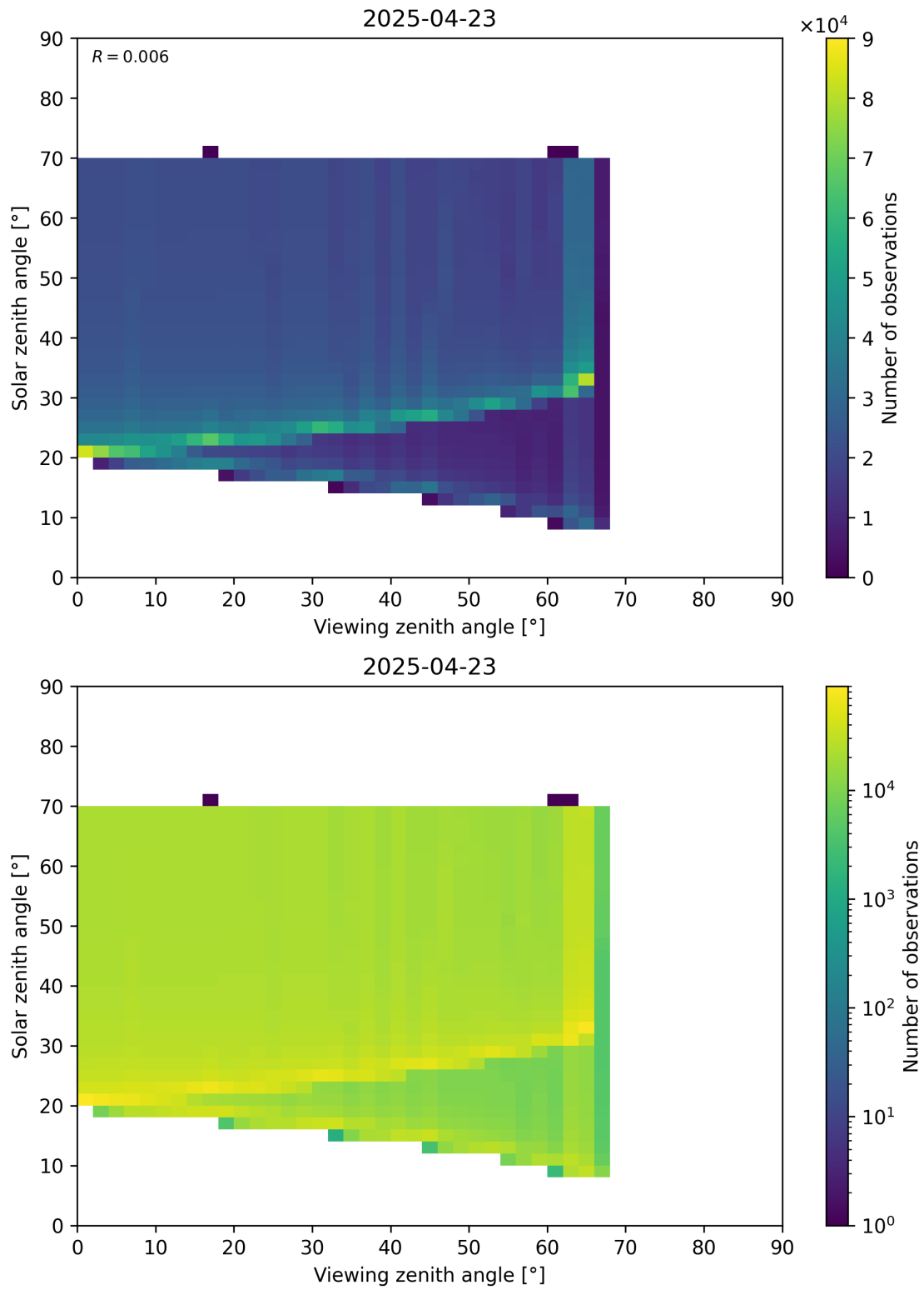
Figure 369: Scatter density plot of “Viewing zenith angle” against “Solar zenith angle” for 2025-04-22 to 2025-04-24.
