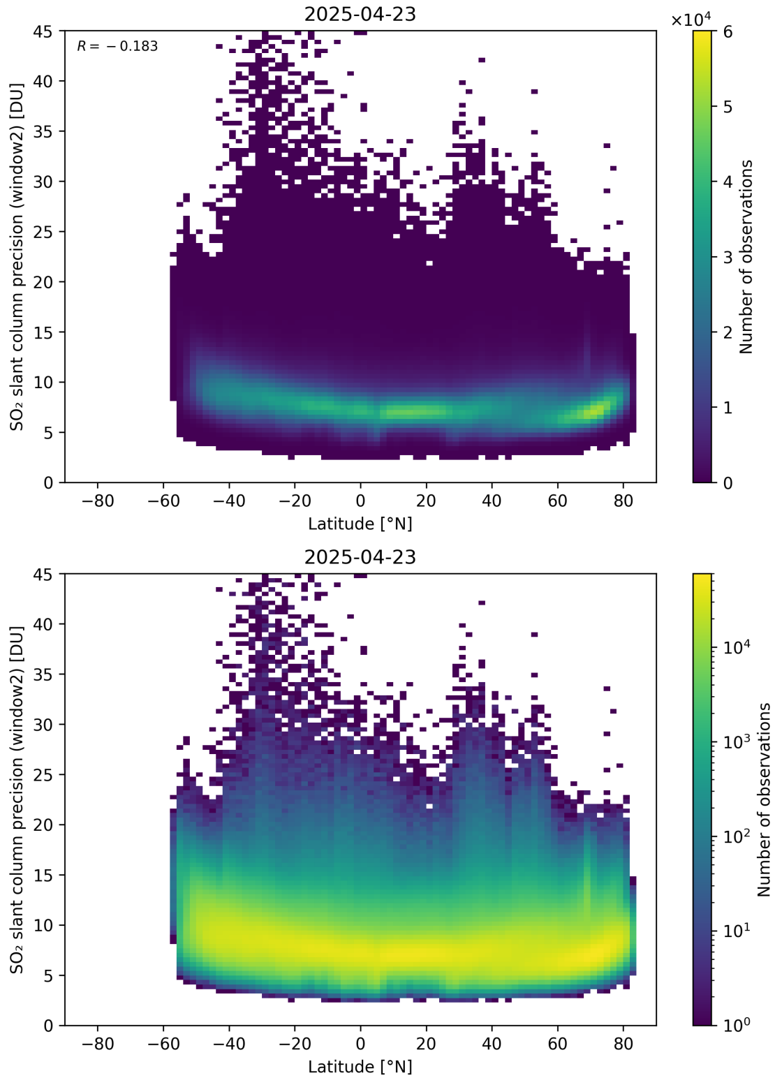
Figure 164: Scatter density plot of “Latitude” against “SO 2 slant column precision (window2)” for 2025-04-22 to 2025-04-24.
