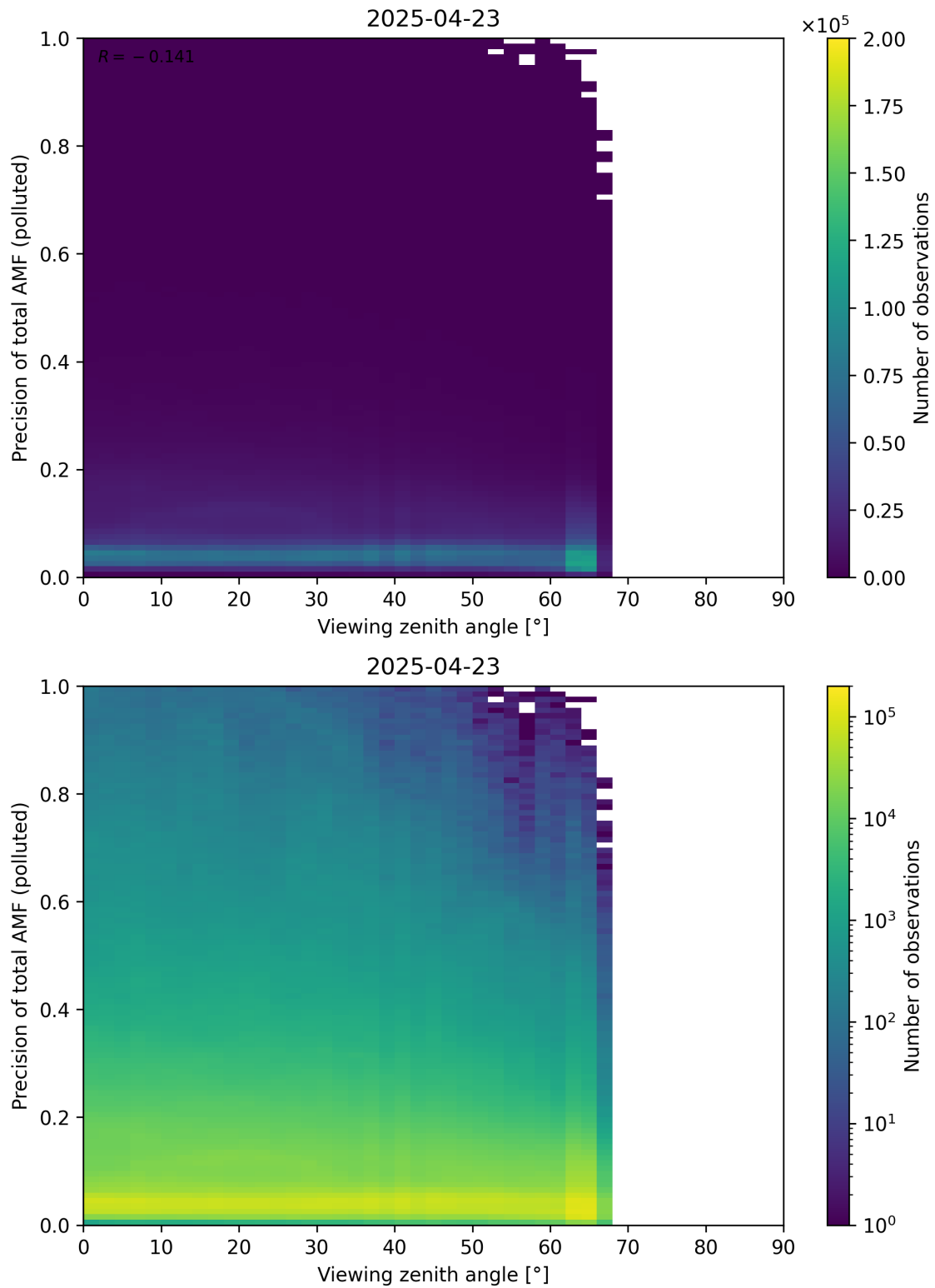
Figure 382: Scatter density plot of “Viewing zenith angle” against “Precision of total AMF (polluted)” for 2025-04-22 to 2025-04-24.
