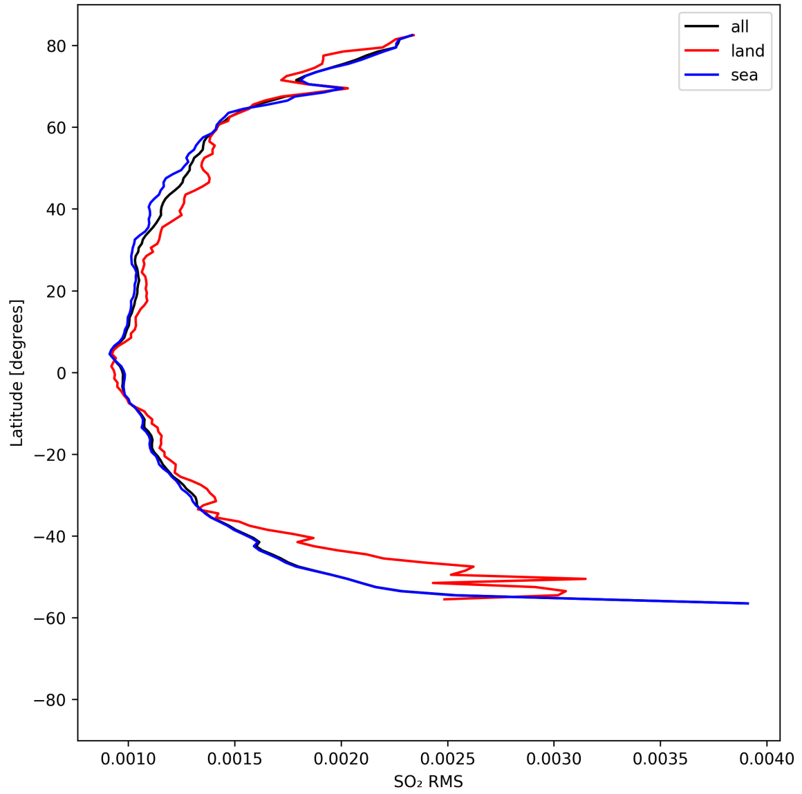
Figure 52: Zonal average of “SO 2 RMS” for 2025-04-22 to 2025-04-24.
