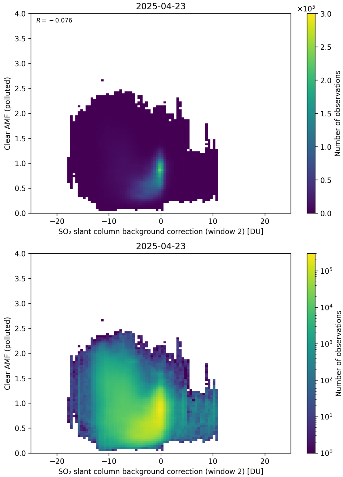
Figure 126: Scatter density plot of “SO 2 slant column background correction (window 2)” against “Clear AMF (polluted)” for 2025-04-22 to 2025-04-24.
