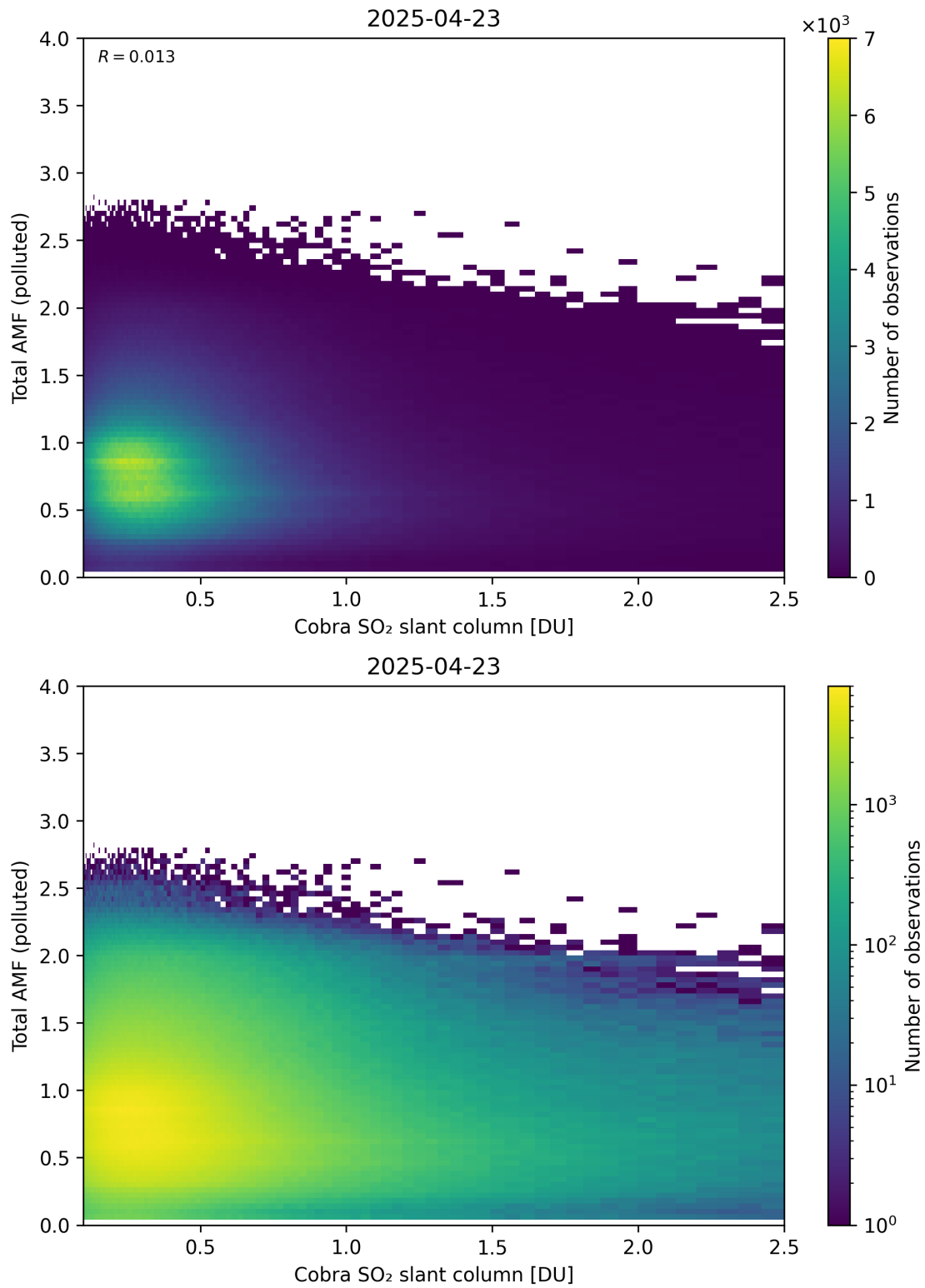
Figure 224: Scatter density plot of “Cobra SO 2 slant column” against “Total AMF (polluted)” for 2025-04-22 to 2025-04-24.
