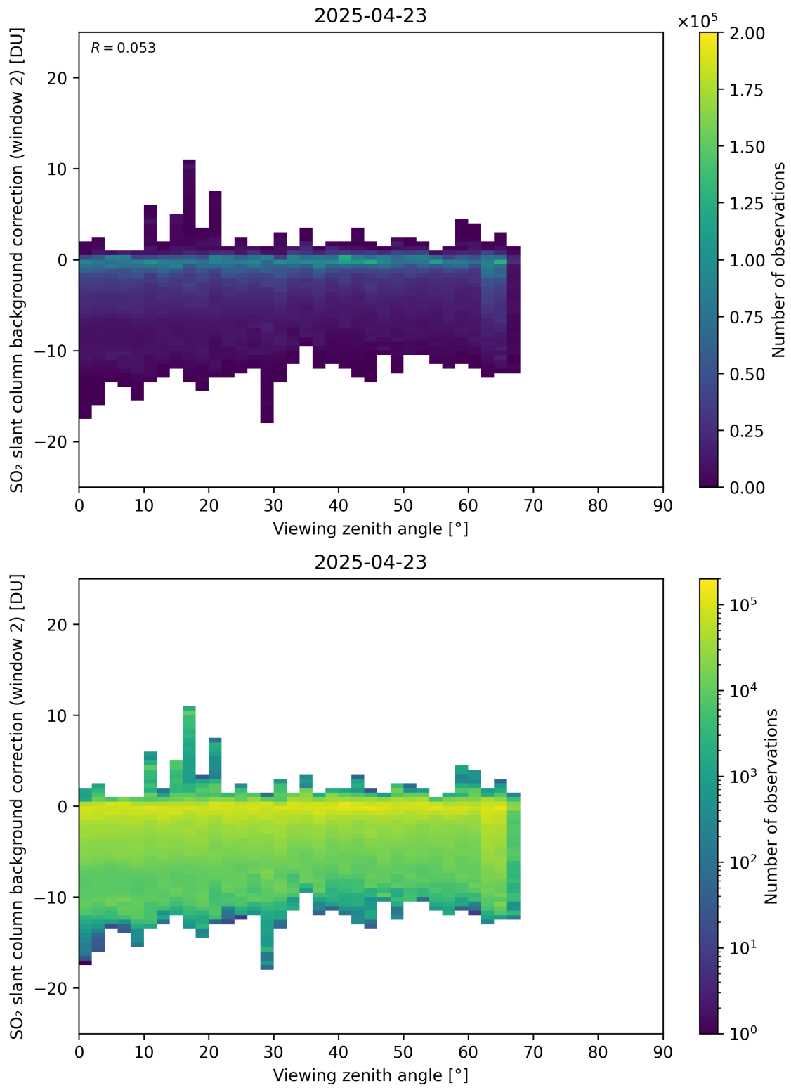
Figure 363: Scatter density plot of “Viewing zenith angle” against “SO 2 slant column background correction (window 2)” for 2025-04-22 to 2025-04-24.
