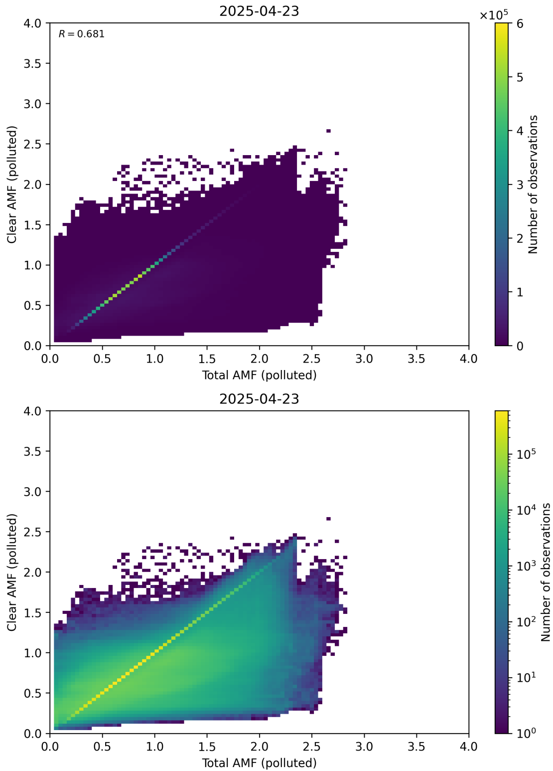
Figure 321: Scatter density plot of “Total AMF (polluted)” against “Clear AMF (polluted)” for 2025-04-22 to 2025-04-24.
