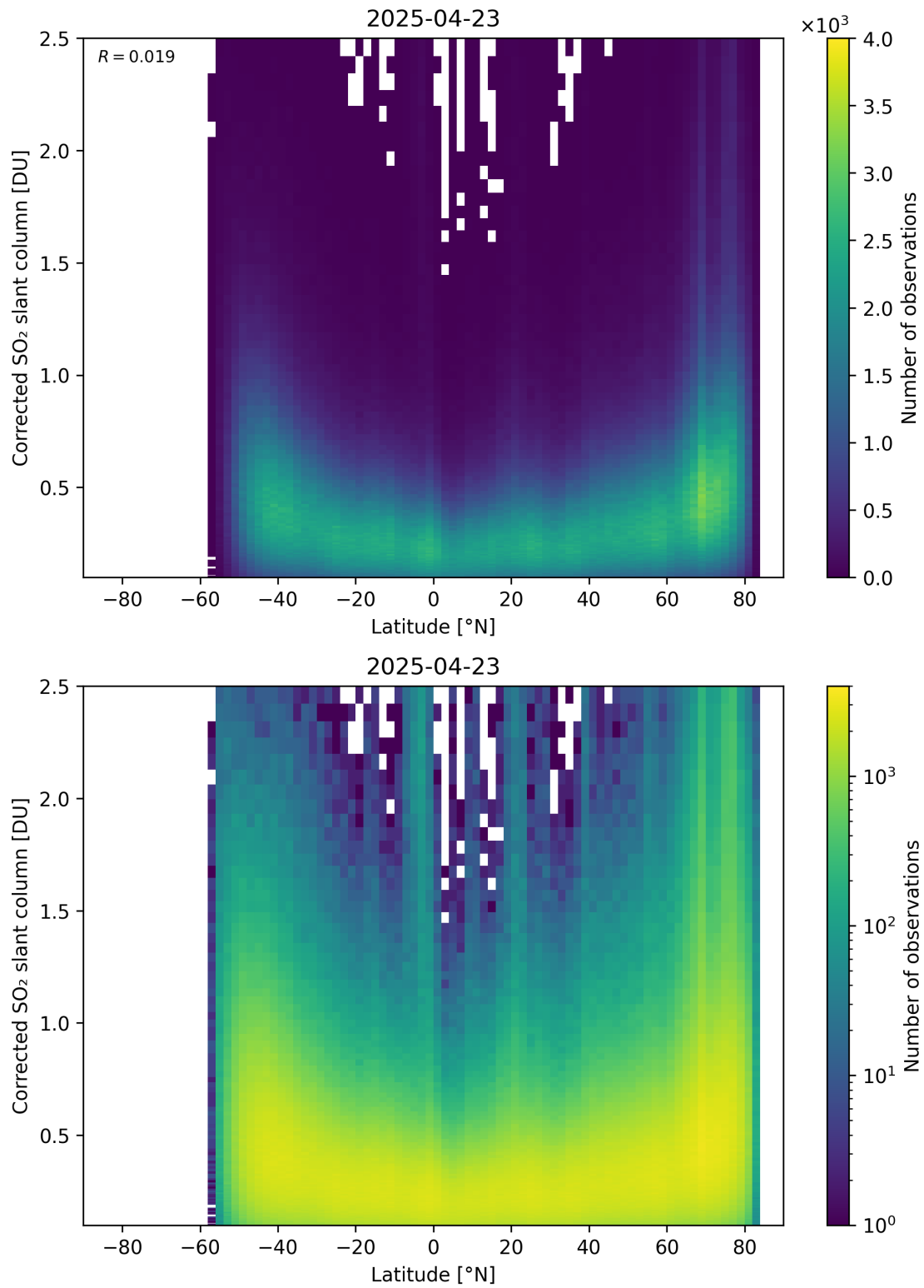
Figure 159: Scatter density plot of “Latitude” against “Corrected SO 2 slant column” for 2025-04-22 to 2025-04-24.
