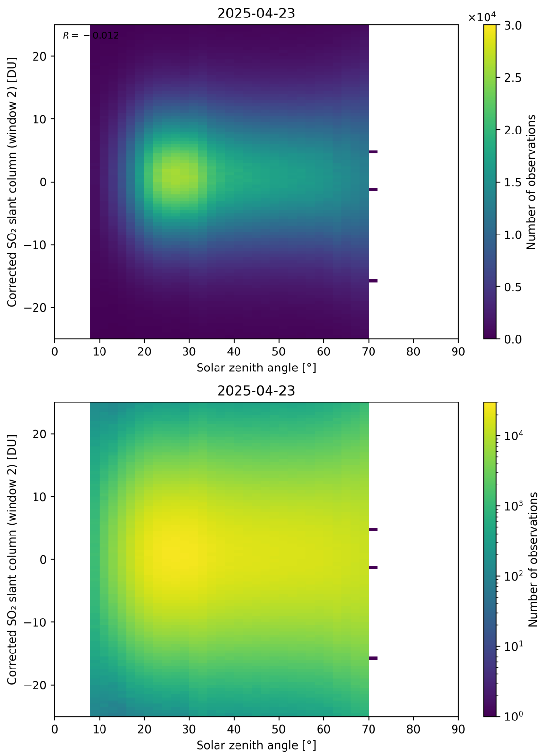
Figure 182: Scatter density plot of “Solar zenith angle” against “Corrected SO 2 slant column (window 2)” for 2025-04-22 to 2025-04-24.
