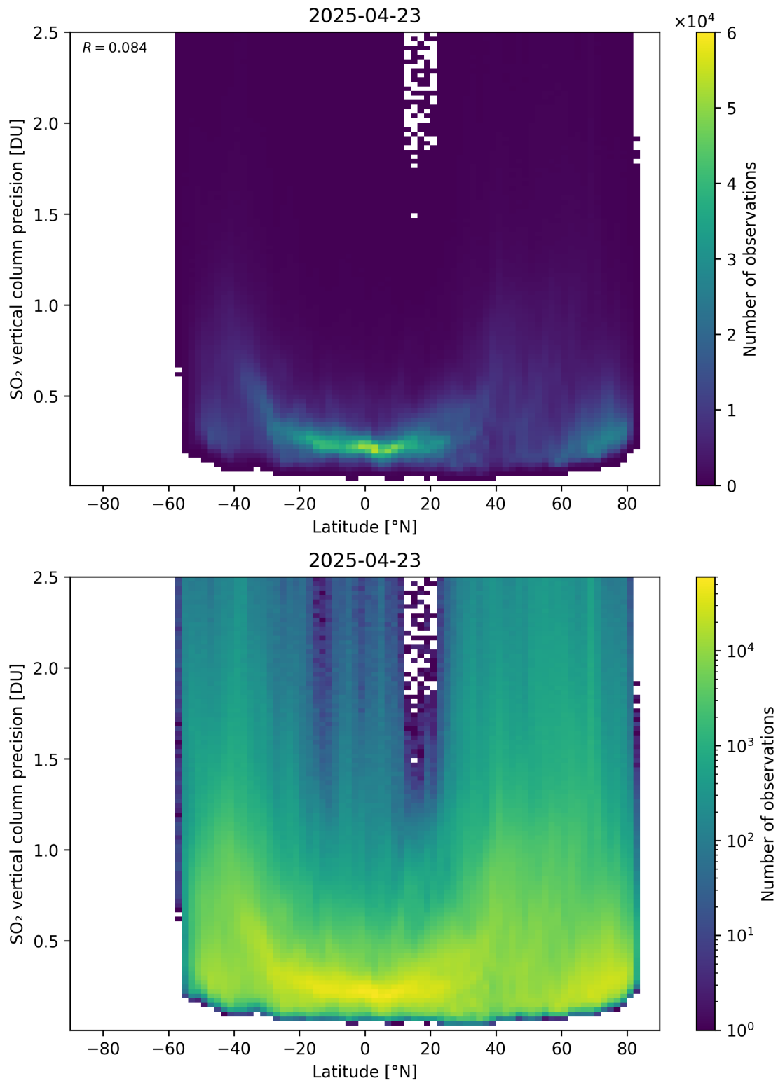
Figure 170: Scatter density plot of “Latitude” against “SO 2 vertical column precision” for 2025-04-22 to 2025-04-24.
