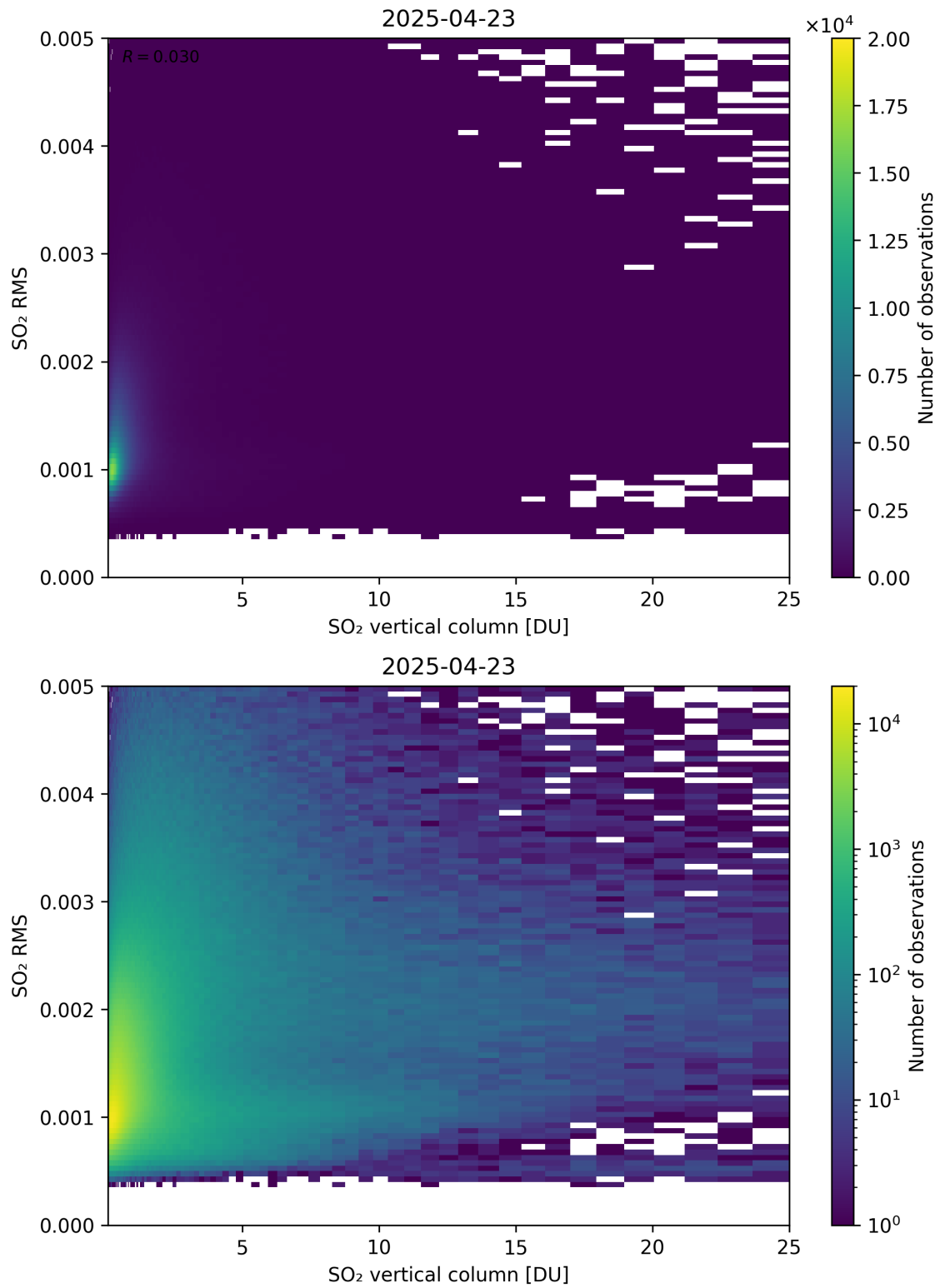
Figure 328: Scatter density plot of “SO 2 vertical column” against “SO 2 RMS” for 2025-04-22 to 2025-04-24.
