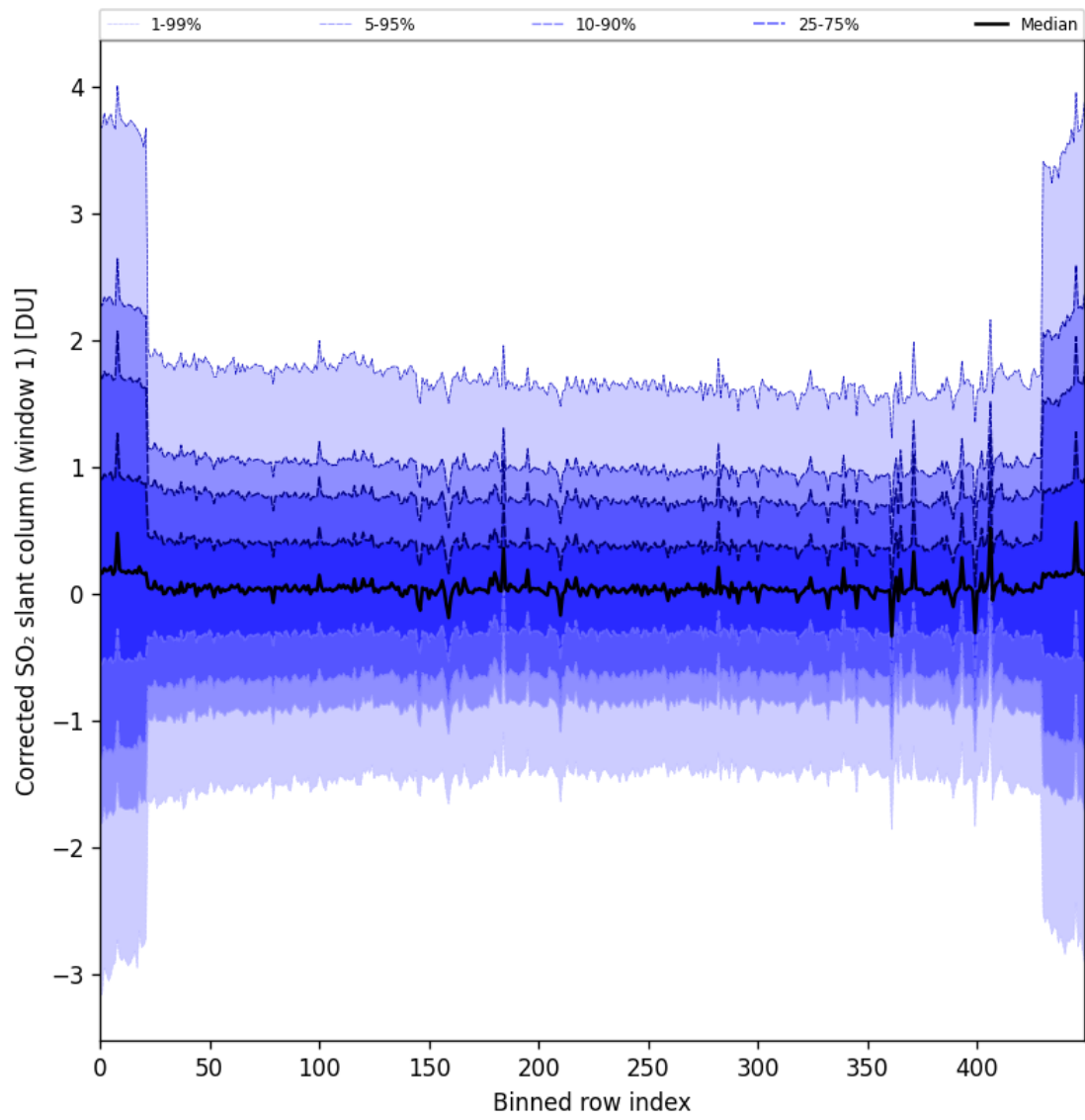
Figure 91: Along track statistics of “Corrected SO 2 slant column (window 1)” for 2025-04-22 to 2025-04-24
