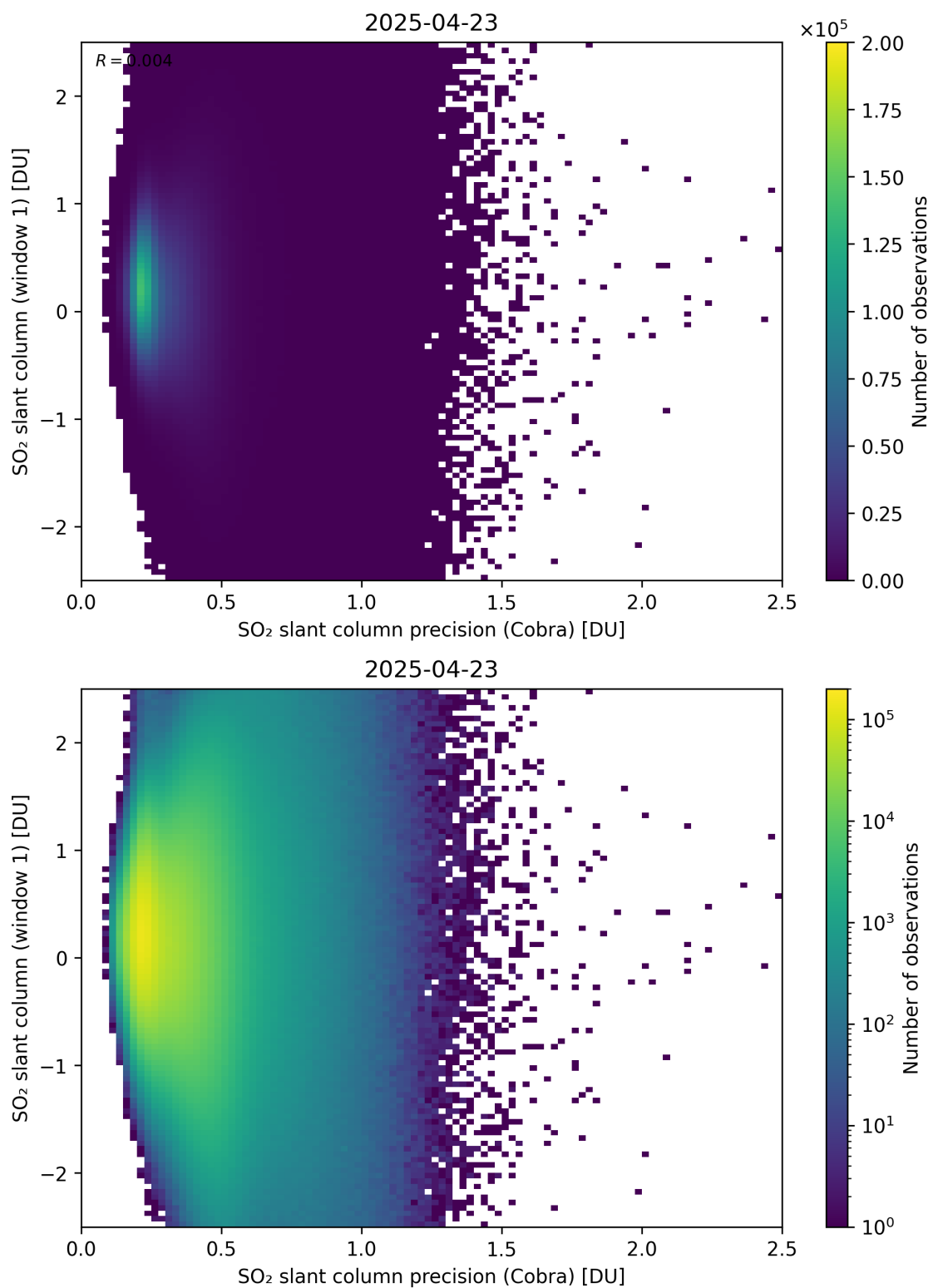
Figure 208: Scatter density plot of “SO 2 slant column precision (Cobra)” against “SO 2 slant column (window 1)” for 2025-04-22 to 2025-04-24.
