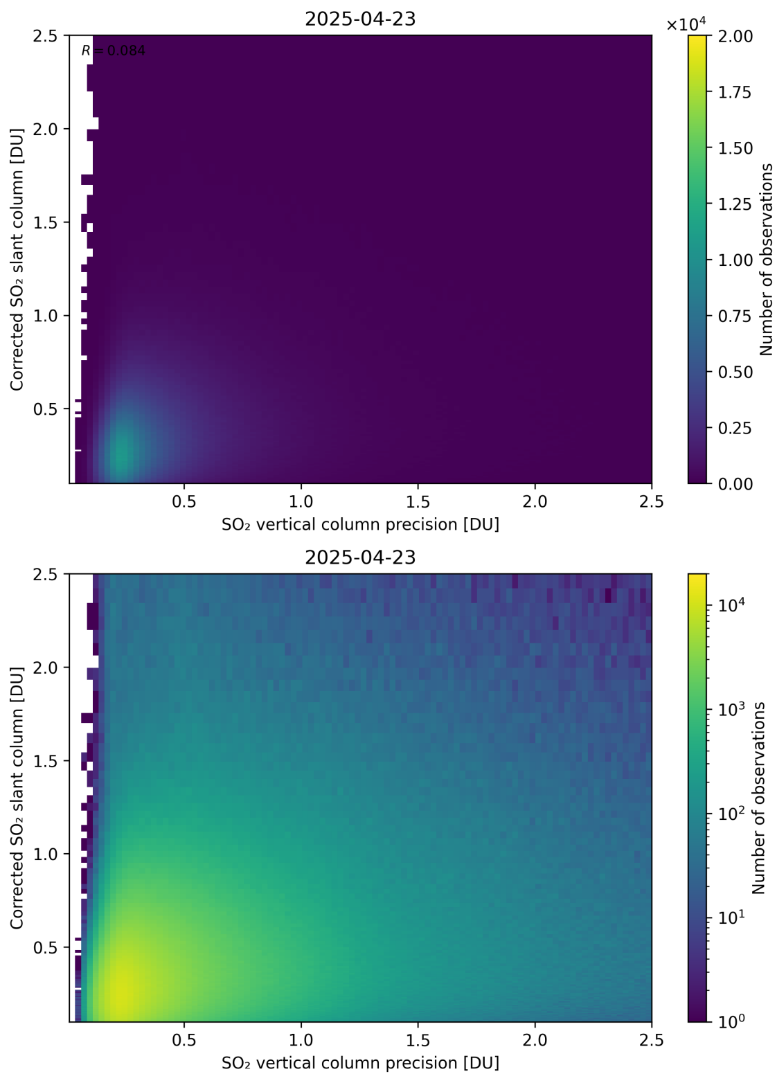
Figure 338: Scatter density plot of “SO 2 vertical column precision” against “Corrected SO 2 slant column” for 2025-04-22 to 2025-04-24.
