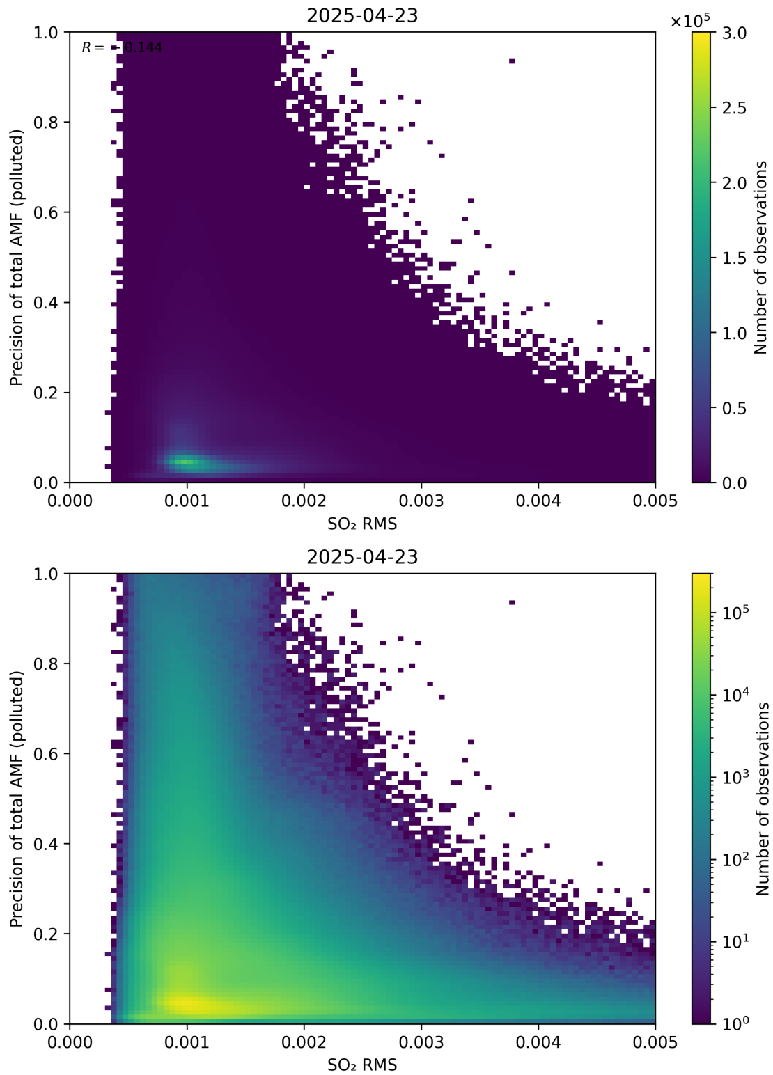
Figure 149: Scatter density plot of “SO 2 RMS” against “Precision of total AMF (polluted)” for 2025-04-22 to 2025-04-24.
