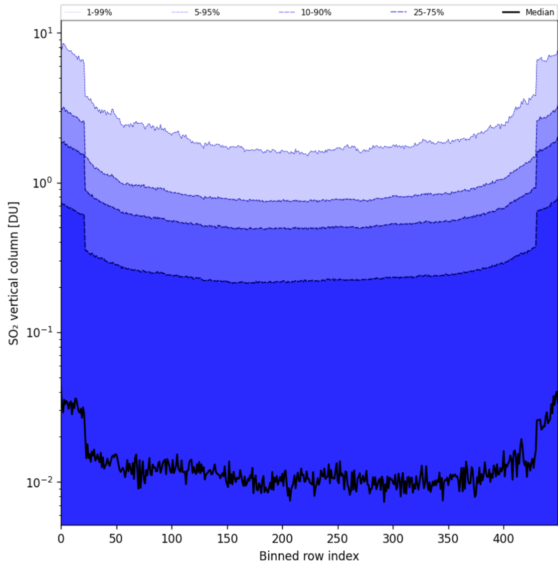
Figure 84: Along track statistics of “SO 2 vertical column” for 2025-04-22 to 2025-04-24
