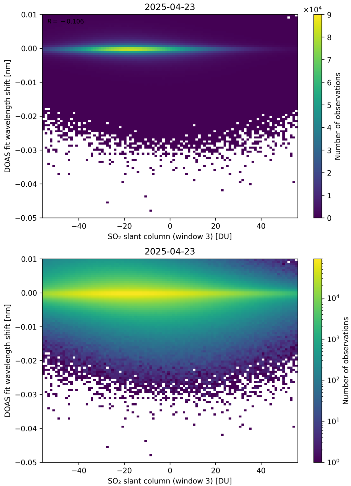
Figure 304: Scatter density plot of “SO 2 slant column (window 3)” against “DOAS fit wavelength shift” for 2025-04-22 to 2025-04-24.
