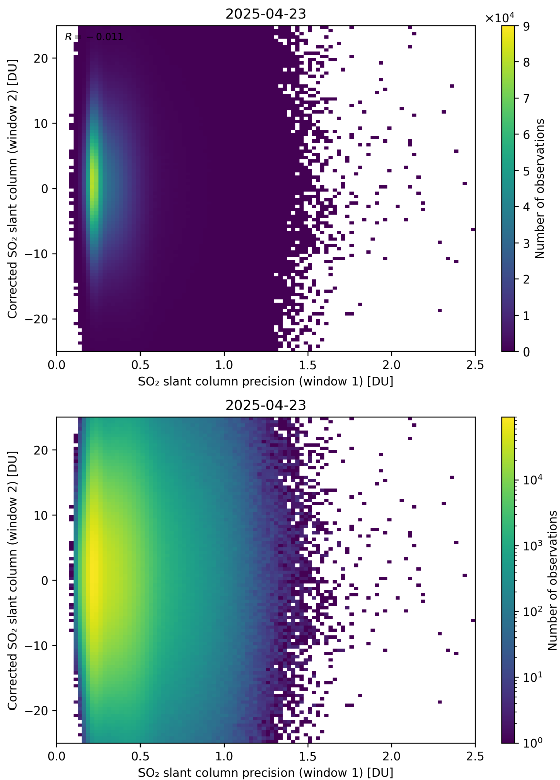
Figure 275: Scatter density plot of “SO 2 slant column precision (window 1)” against “Corrected SO 2 slant column (window 2)” for 2025-04-22 to 2025-04-24.
