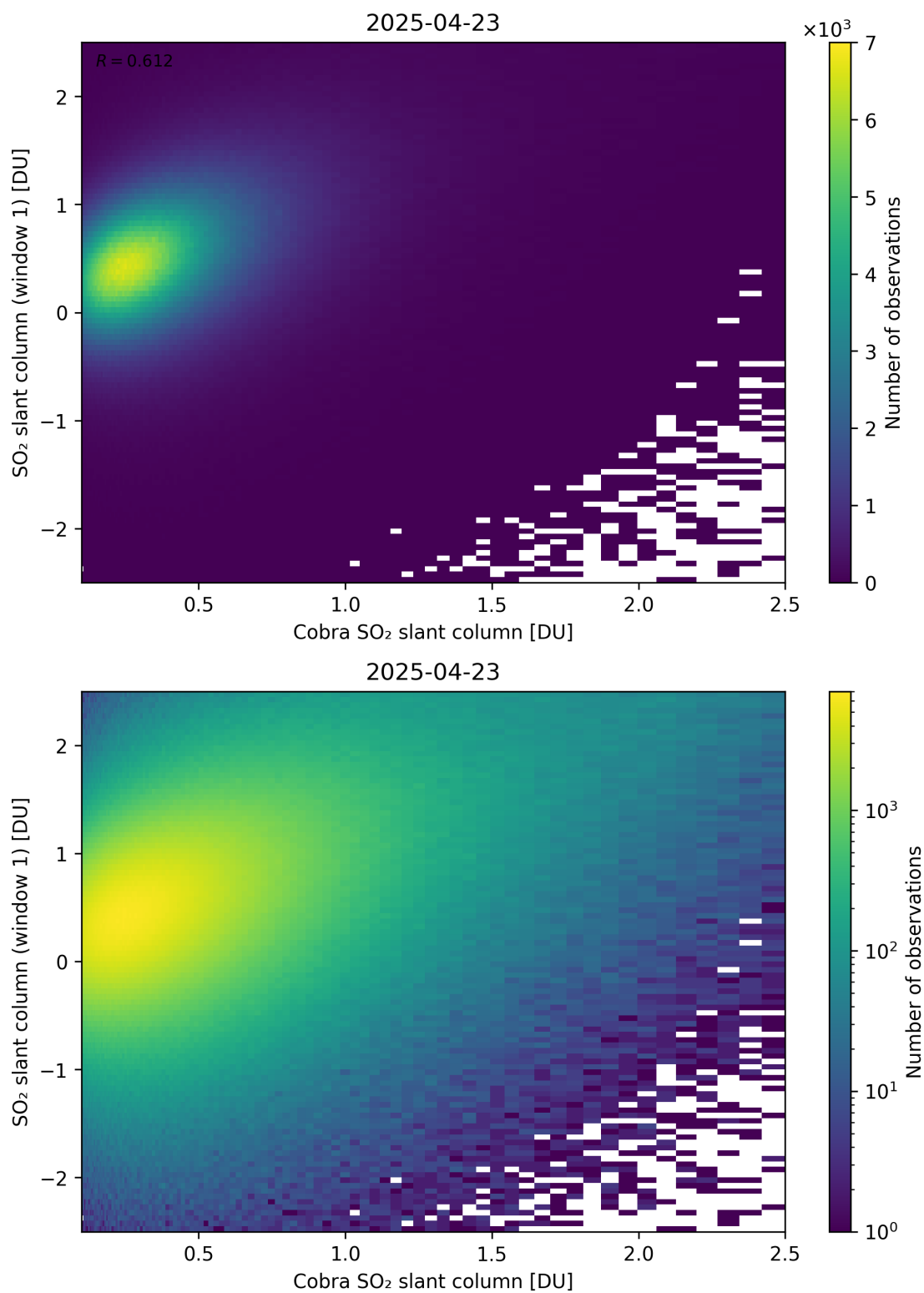
Figure 219: Scatter density plot of “Cobra SO 2 slant column” against “SO 2 slant column (window 1)” for 2025-04-22 to 2025-04-24.
