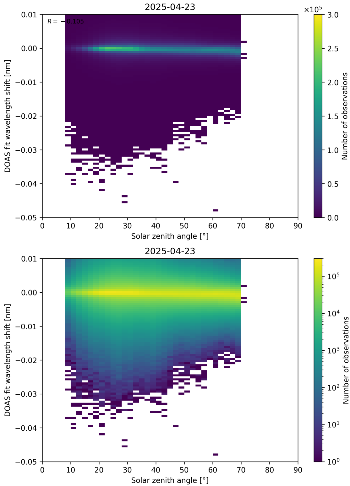
Figure 174: Scatter density plot of “Solar zenith angle” against “DOAS fit wavelength shift” for 2025-04-22 to 2025-04-24.
