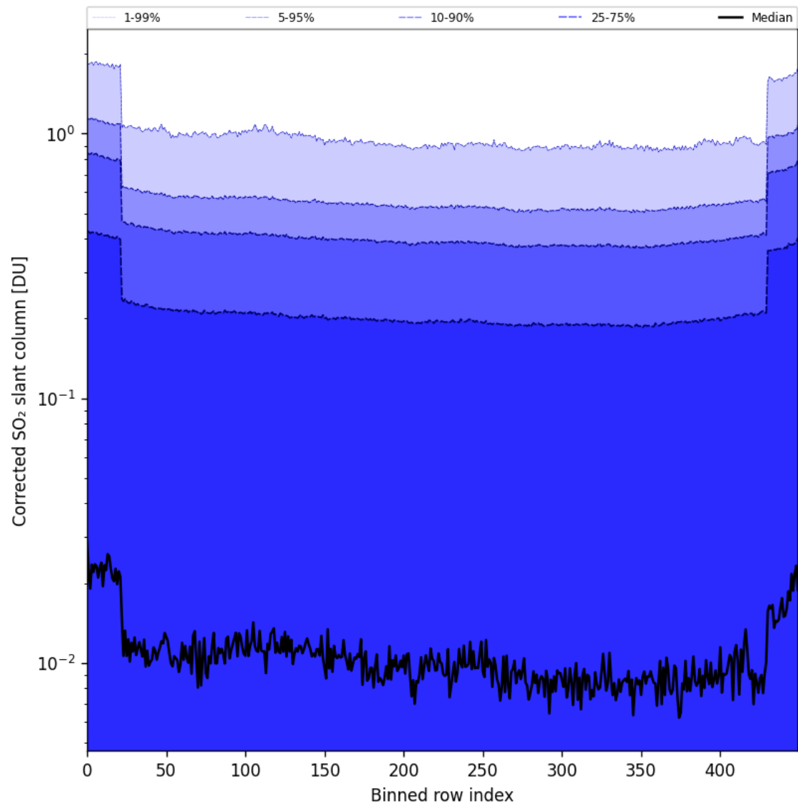
Figure 86: Along track statistics of “Corrected SO 2 slant column” for 2025-04-22 to 2025-04-24
