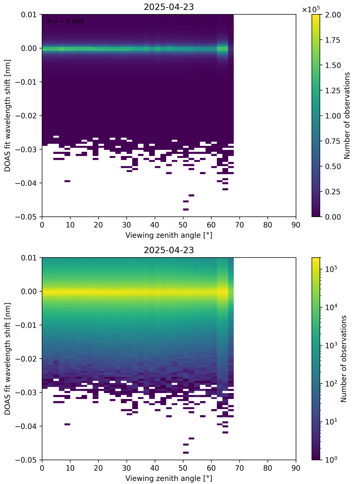
Figure 365: Scatter density plot of “Viewing zenith angle” against “DOAS fit wavelength shift” for 2025-04-22 to 2025-04-24.
