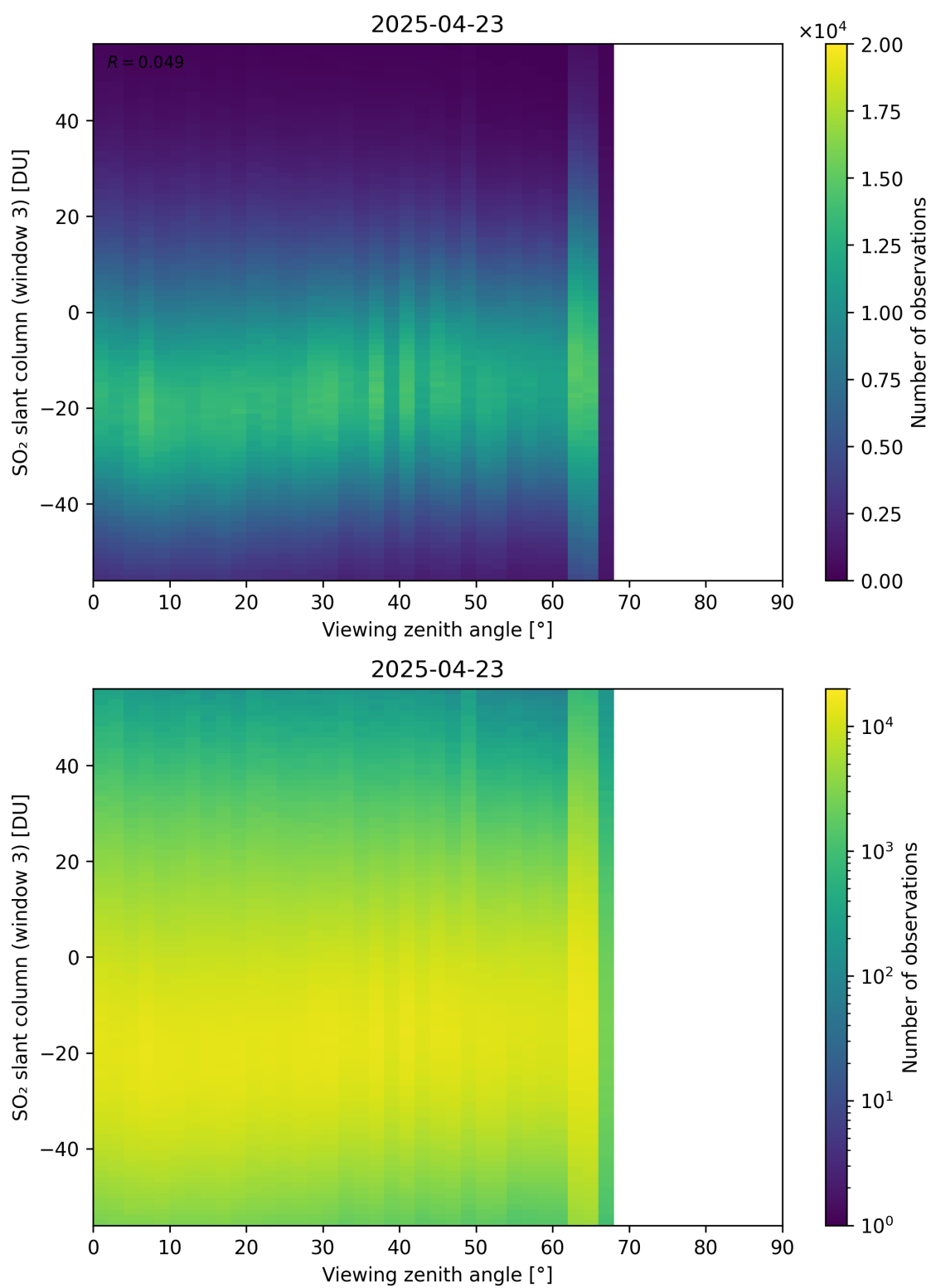
Figure 379: Scatter density plot of “Viewing zenith angle” against “SO 2 slant column (window 3)” for 2025-04-22 to 2025-04-24.
