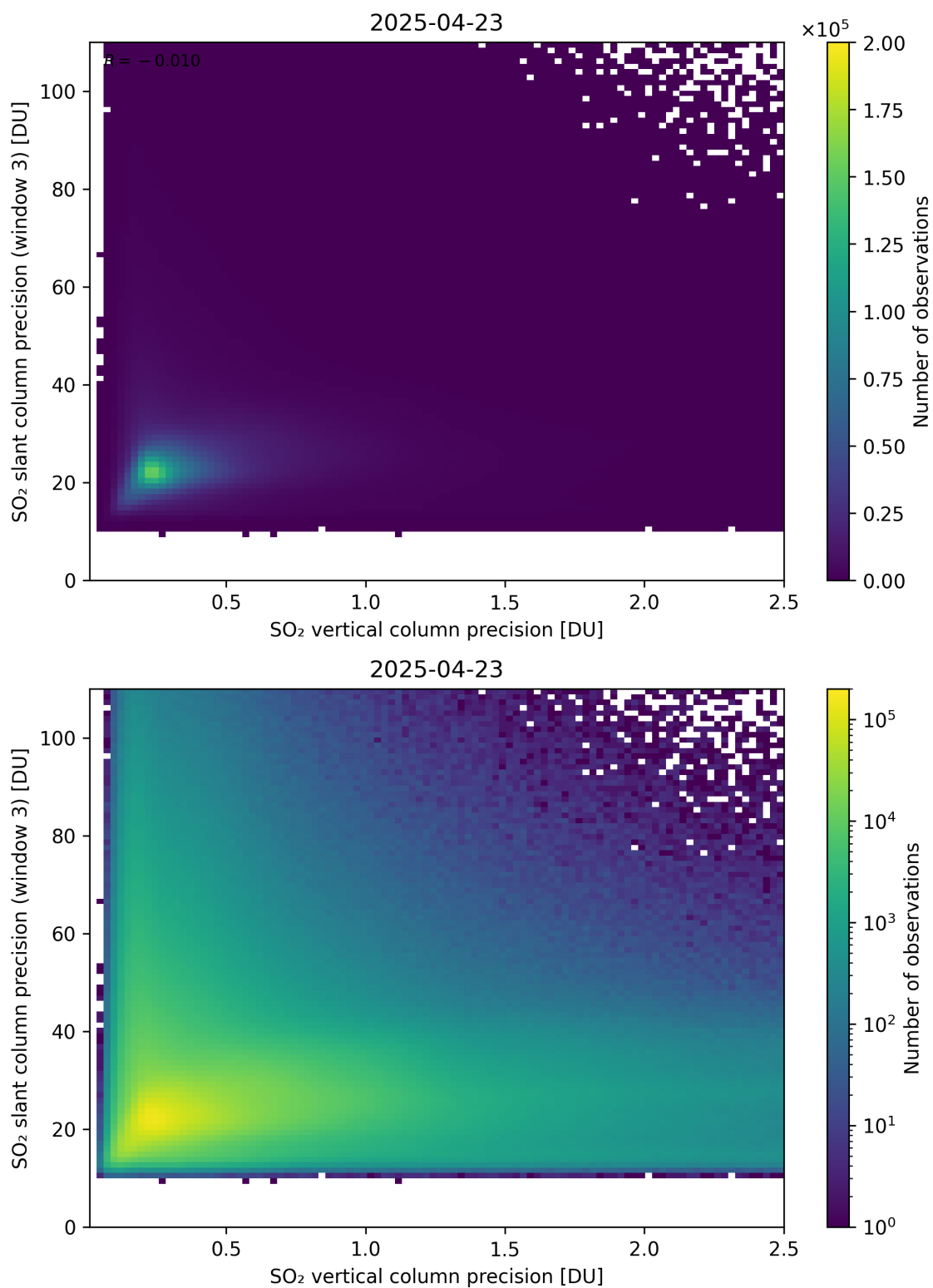
Figure 345: Scatter density plot of “SO 2 vertical column precision” against “SO 2 slant column precision (window 3)” for 2025-04-22 to 2025-04-24.
