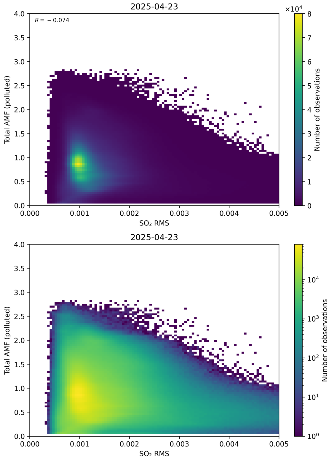
Figure 148: Scatter density plot of “SO 2 RMS” against “Total AMF (polluted)” for 2025-04-22 to 2025-04-24.
