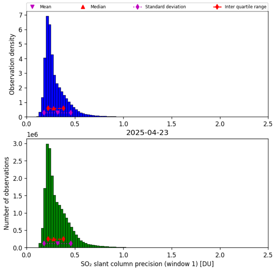
Figure 64: Histogram of “SO 2 slant column precision (window 1)” for 2025-04-22 to 2025-04-24
