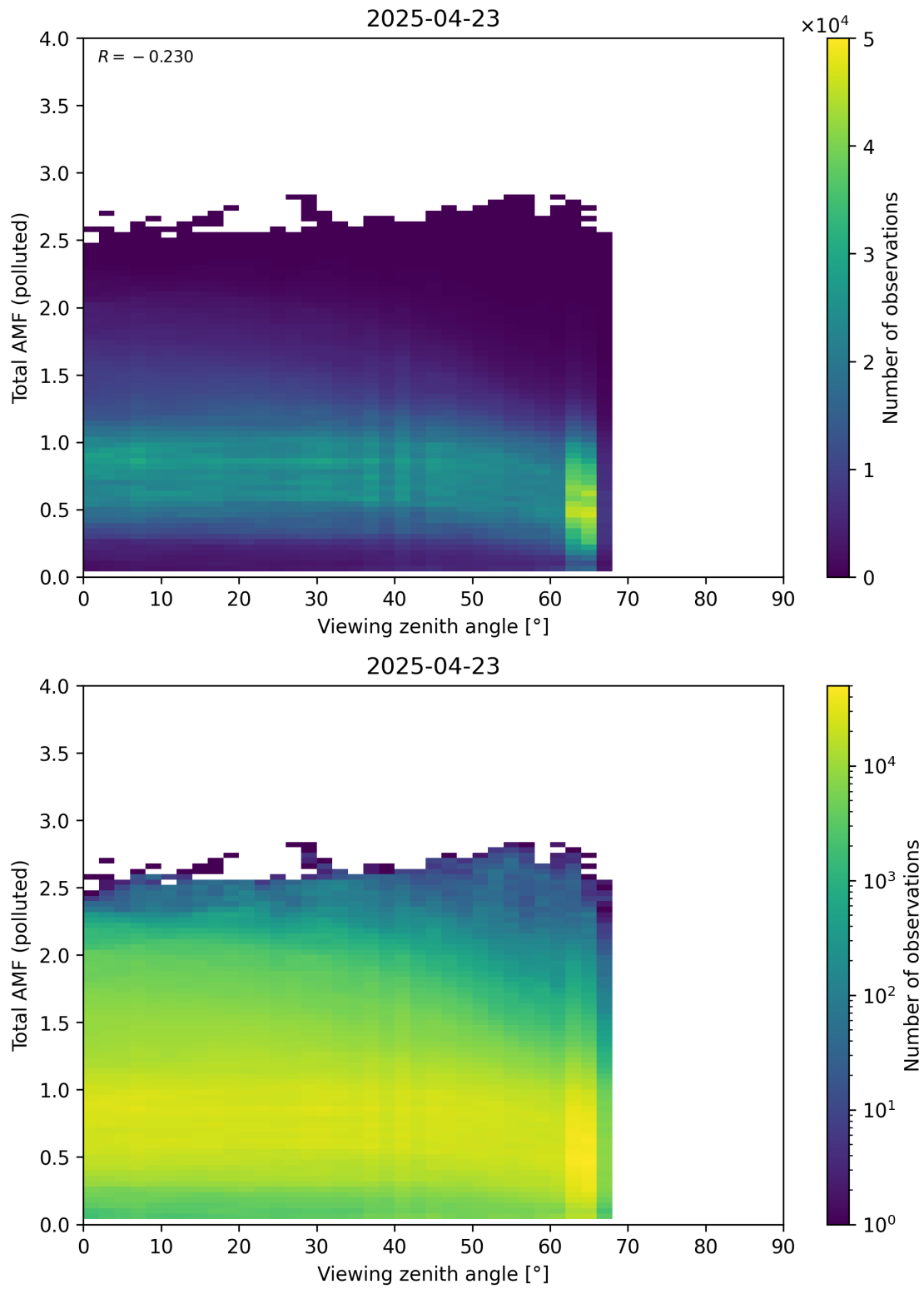
Figure 381: Scatter density plot of “Viewing zenith angle” against “Total AMF (polluted)” for 2025-04-22 to 2025-04-24.
