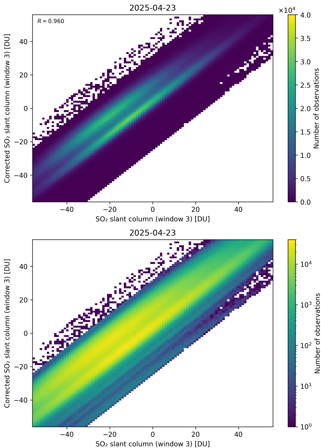
Figure 316: Scatter density plot of “SO 2 slant column (window 3)” against “Corrected SO 2 slant column (window 3)” for 2025-04-22 to 2025-04-24.
