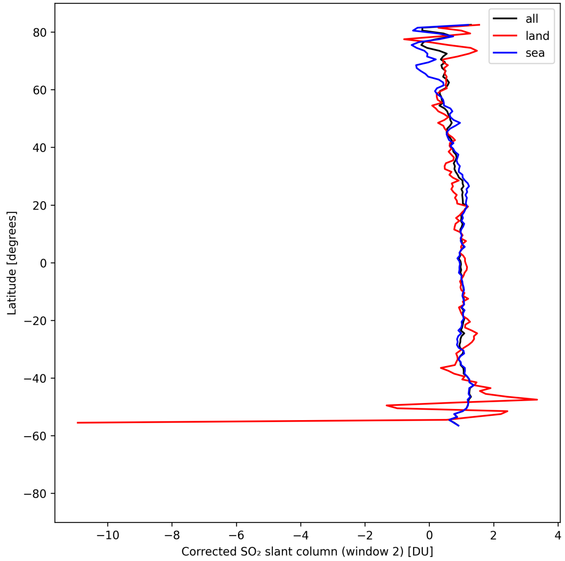
Figure 43: Zonal average of “Corrected SO 2 slant column (window 2)” for 2025-04-22 to 2025-04-24.
