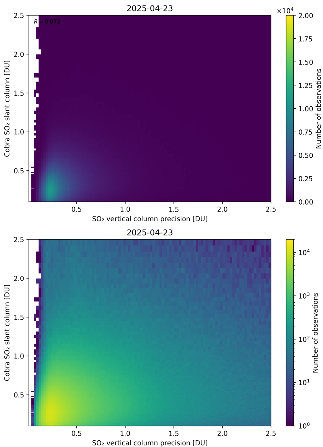
Figure 336: Scatter density plot of “SO 2 vertical column precision” against “Cobra SO 2 slant column” for 2025-04-22 to 2025-04-24.
