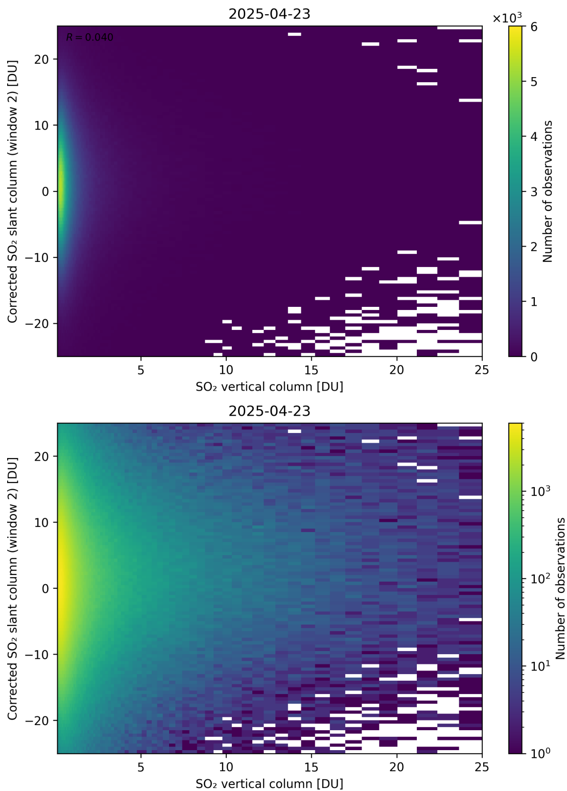
Figure 352: Scatter density plot of “SO 2 vertical column” against “Corrected SO 2 slant column (window 2)” for 2025-04-22 to 2025-04-24.
