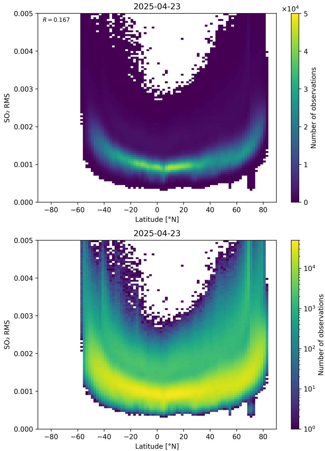
Figure 155: Scatter density plot of “Latitude” against “SO 2 RMS” for 2025-04-22 to 2025-04-24.
