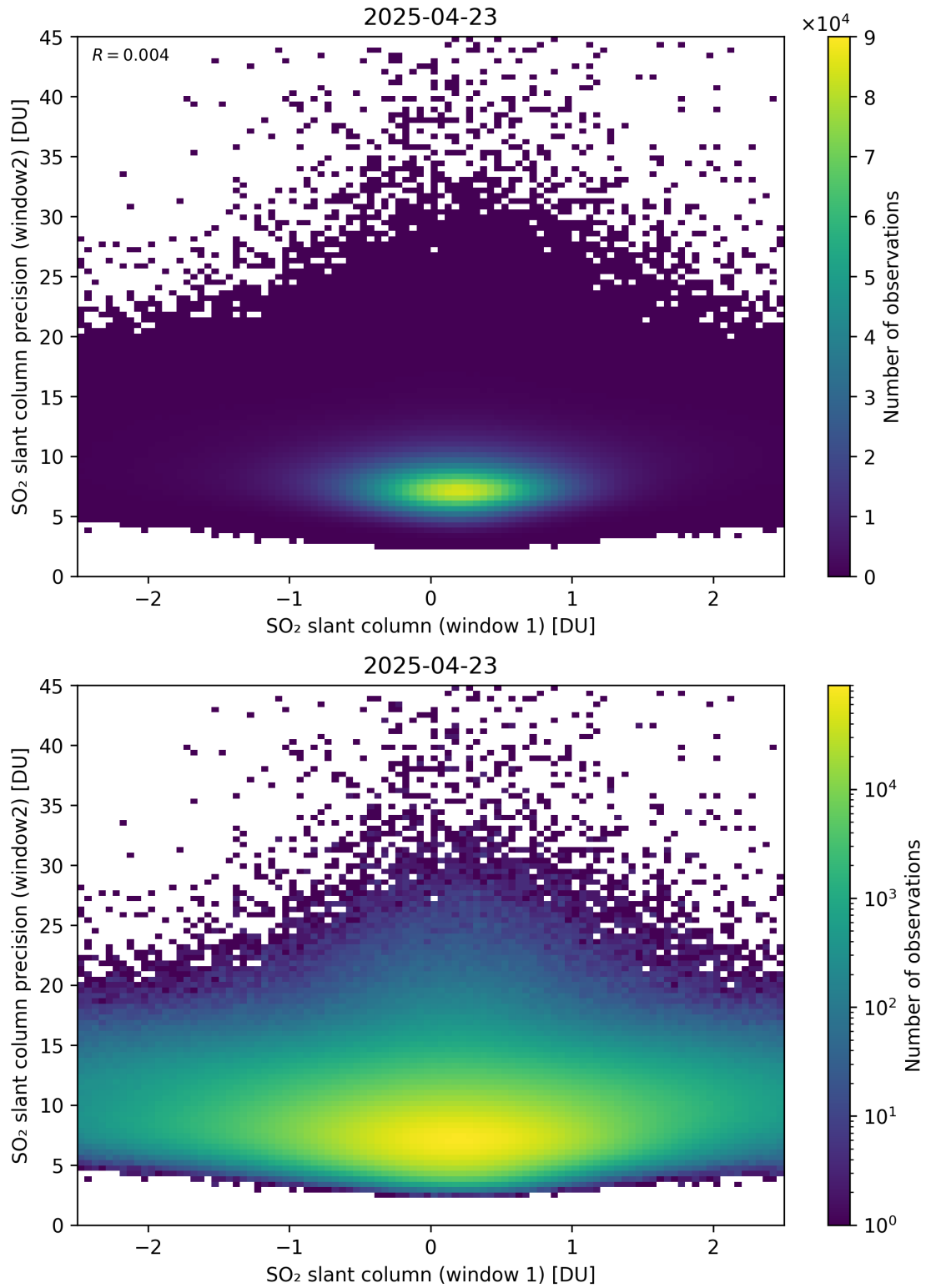
Figure 286: Scatter density plot of “SO 2 slant column (window 1)” against “SO 2 slant column precision (window2)” for 2025-04-22 to 2025-04-24.
