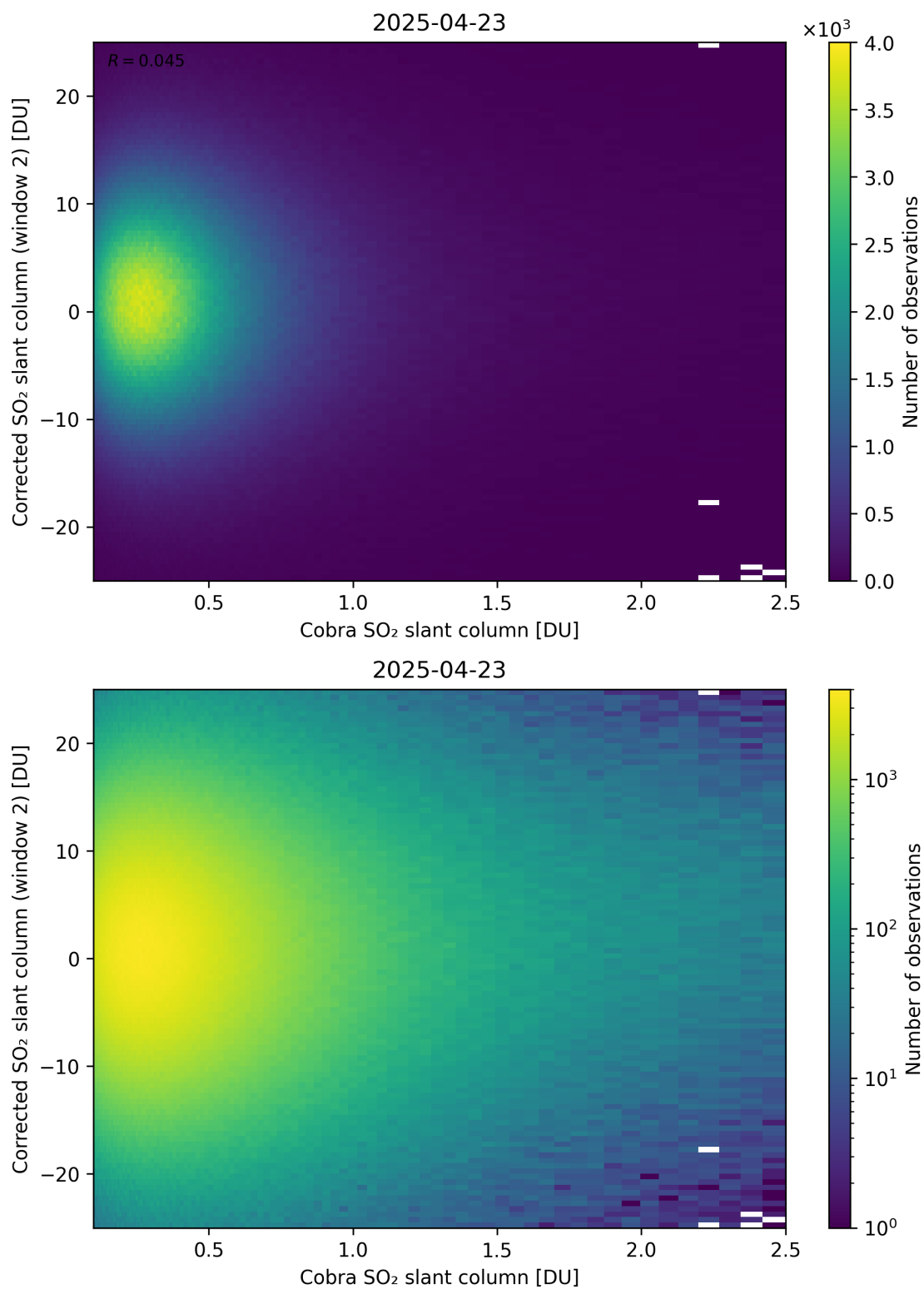
Figure 217: Scatter density plot of “Cobra SO 2 slant column” against “Corrected SO 2 slant column (window 2)” for 2025-04-22 to 2025-04-24.
