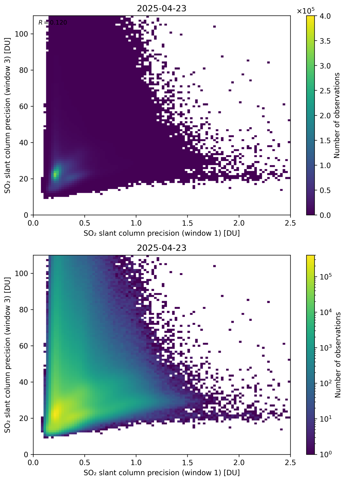
Figure 279: Scatter density plot of “SO 2 slant column precision (window 1)” against “SO 2 slant column precision (window 3)” for 2025-04-22 to 2025-04-24.
