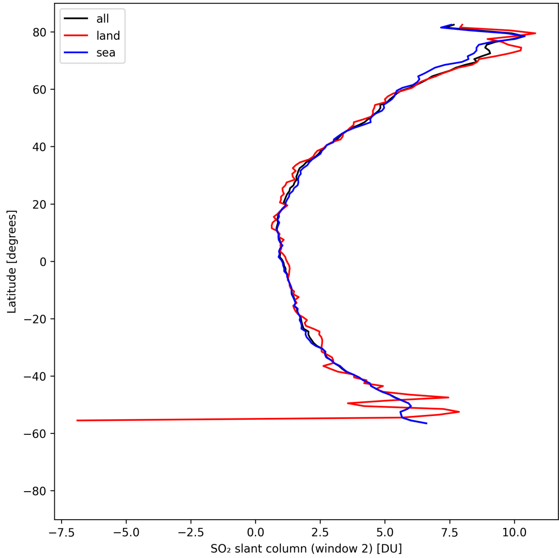
Figure 41: Zonal average of “SO 2 slant column (window 2)” for 2025-04-22 to 2025-04-24.
