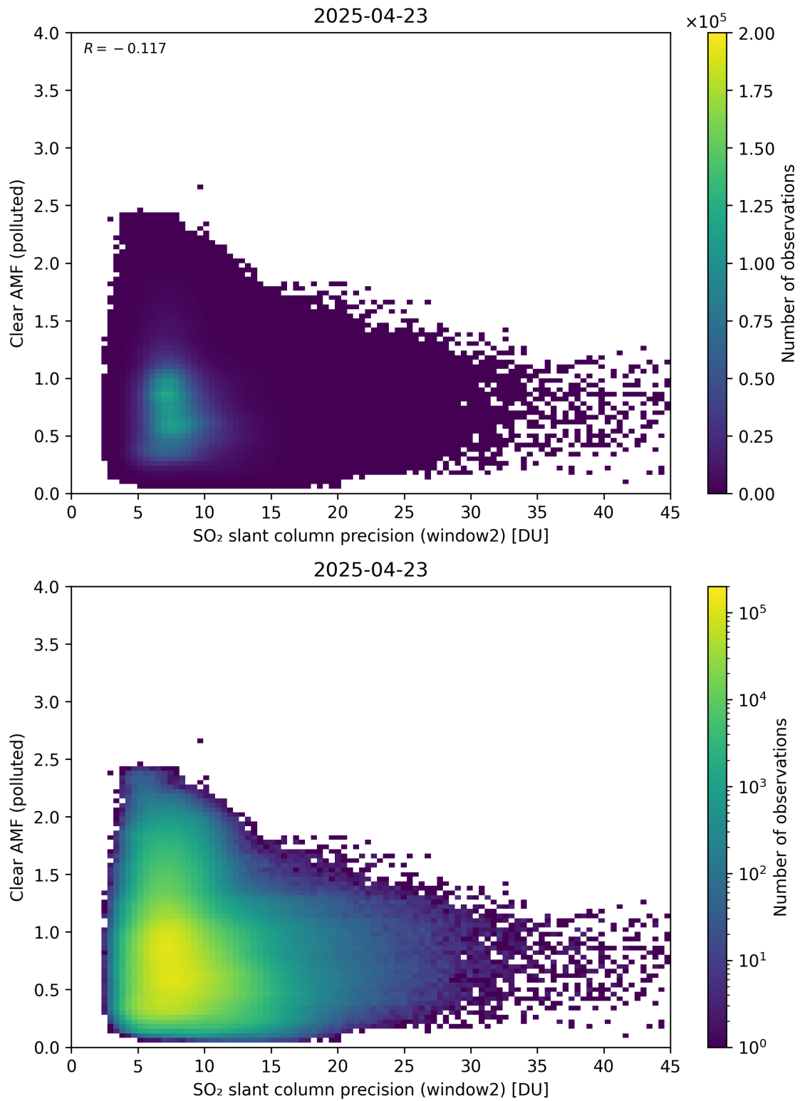
Figure 296: Scatter density plot of “SO 2 slant column precision (window2)” against “Clear AMF (polluted)” for 2025-04-22 to 2025-04-24.
