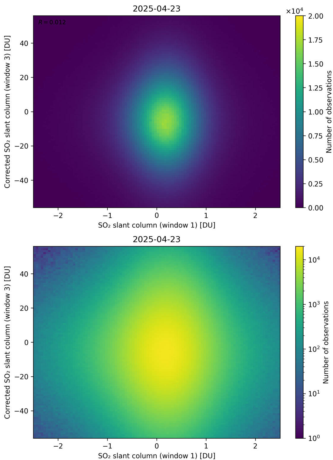
Figure 284: Scatter density plot of “SO 2 slant column (window 1)” against “Corrected SO 2 slant column (window 3)” for 2025-04-22 to 2025-04-24.
