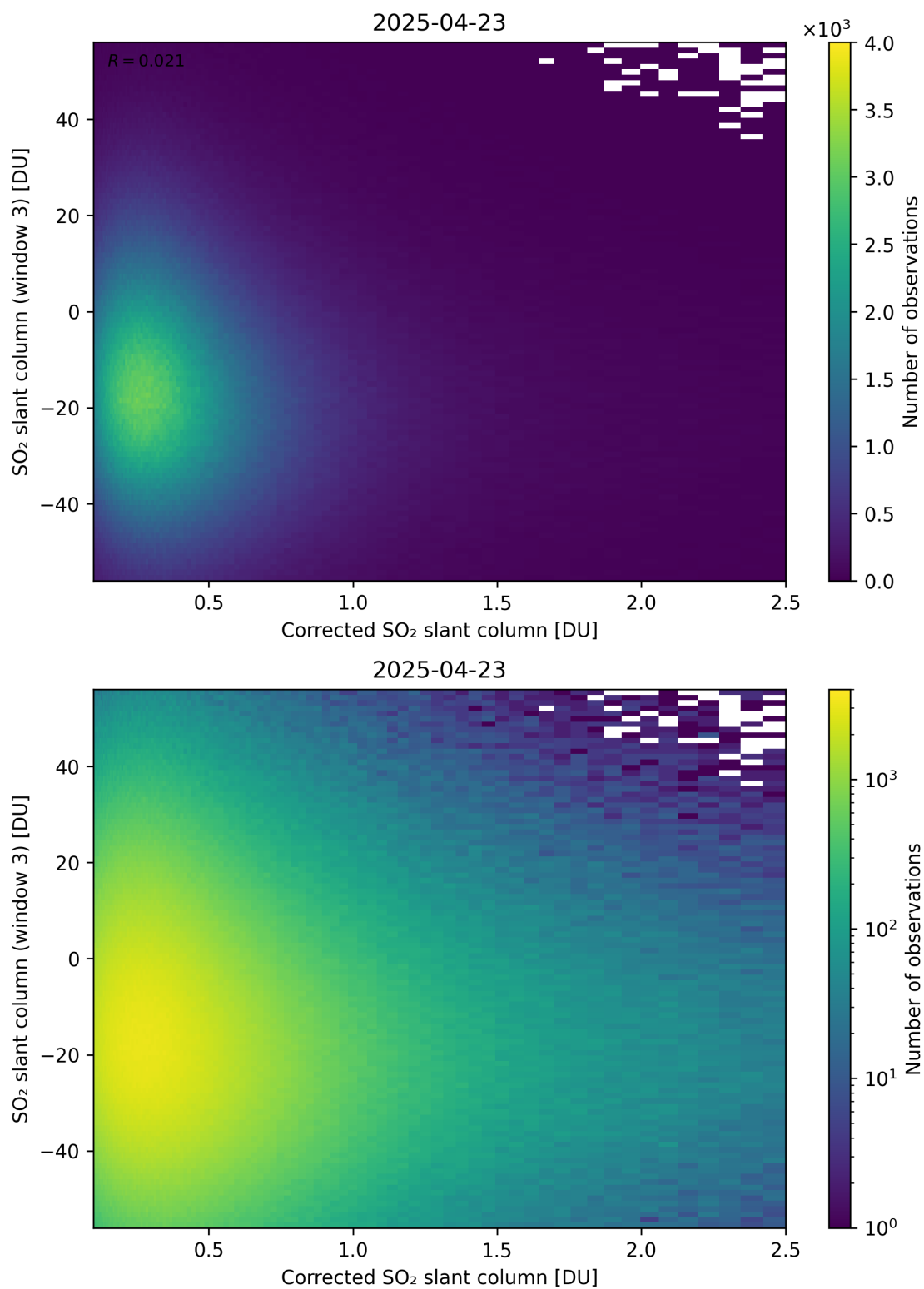
Figure 240: Scatter density plot of “Corrected SO 2 slant column” against “SO 2 slant column (window 3)” for 2025-04-22 to 2025-04-24.
