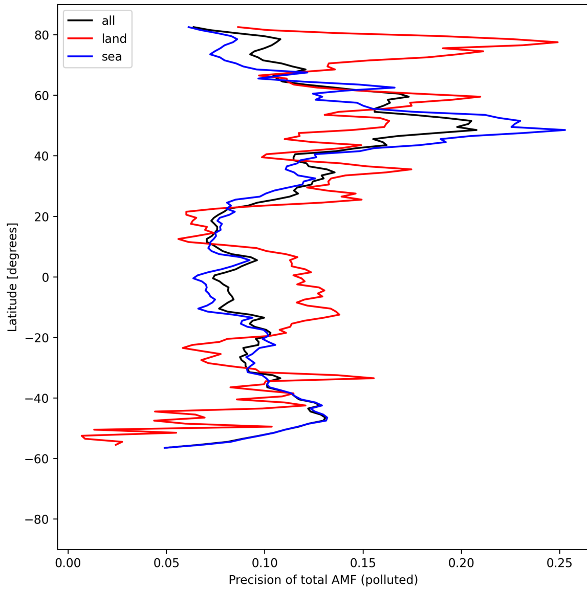
Figure 54: Zonal average of “Precision of total AMF (polluted)” for 2025-04-22 to 2025-04-24.
