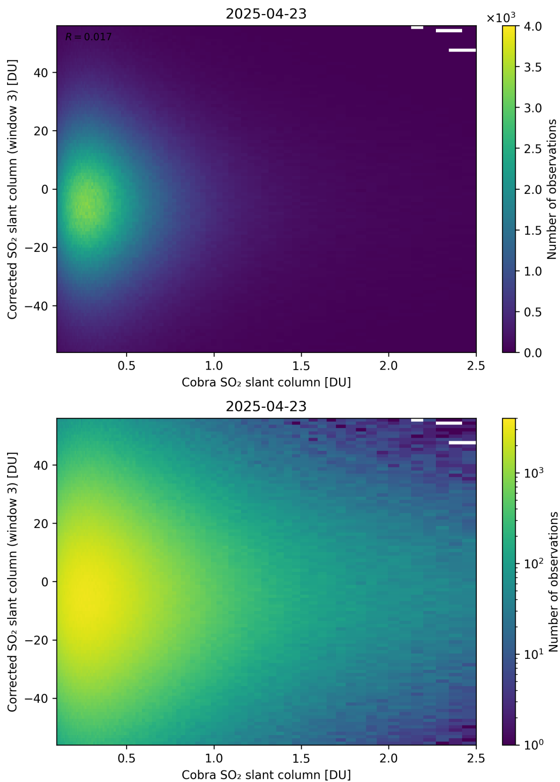
Figure 218: Scatter density plot of “Cobra SO 2 slant column” against “Corrected SO 2 slant column (window 3)” for 2025-04-22 to 2025-04-24.
