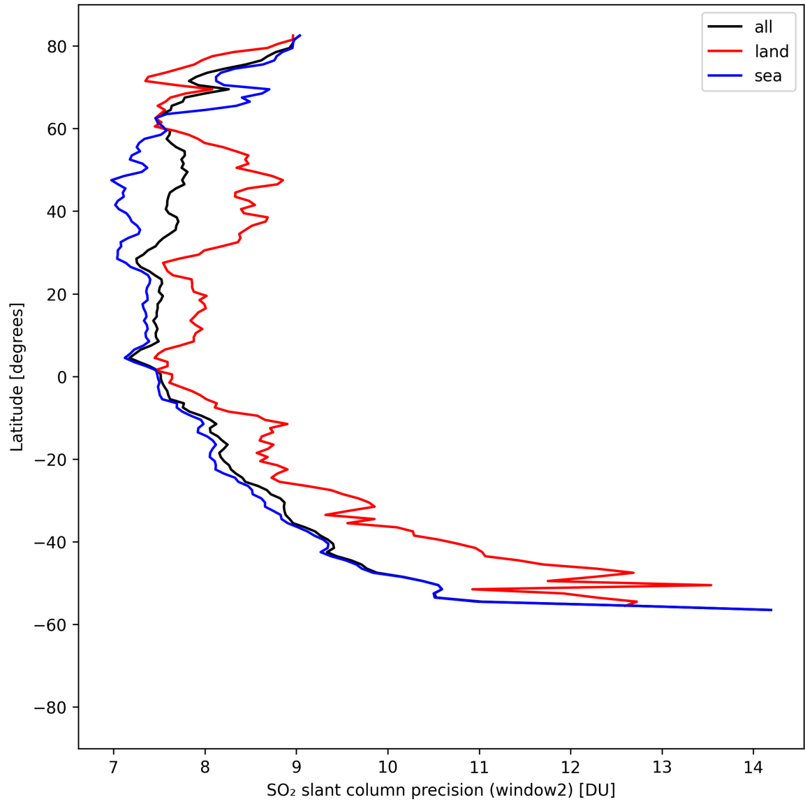
Figure 42: Zonal average of “SO 2 slant column precision (window2)” for 2025-04-22 to 2025-04-24.
