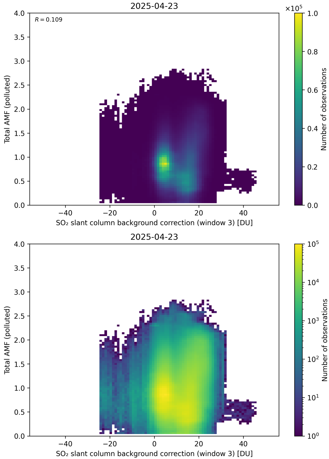
Figure 136: Scatter density plot of “SO 2 slant column background correction (window 3)” against “Total AMF (polluted)” for 2025-04-22 to 2025-04-24.
