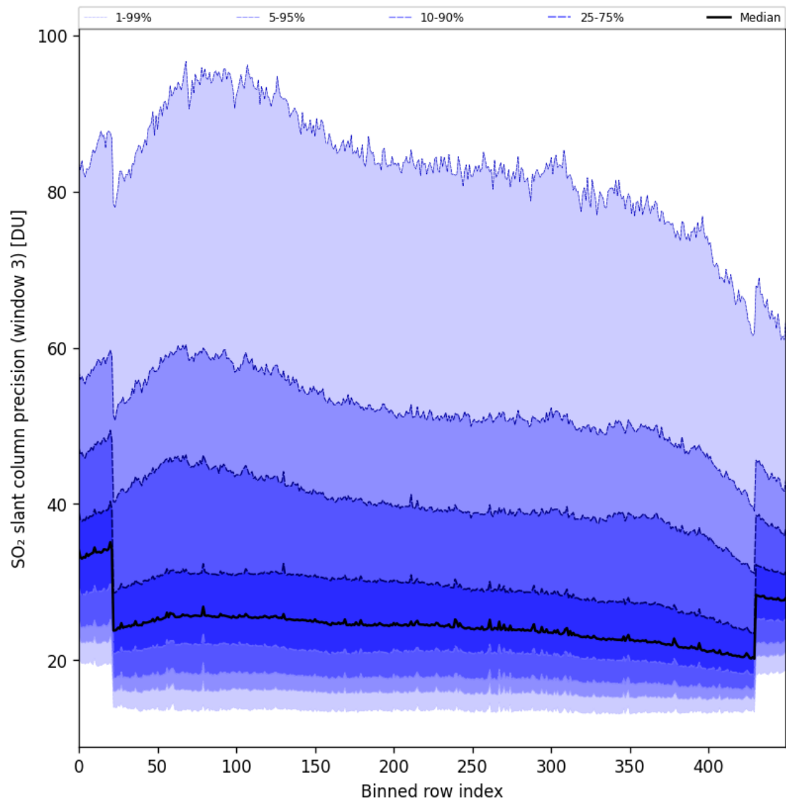
Figure 98: Along track statistics of “SO 2 slant column precision (window 3)” for 2025-04-22 to 2025-04-24
