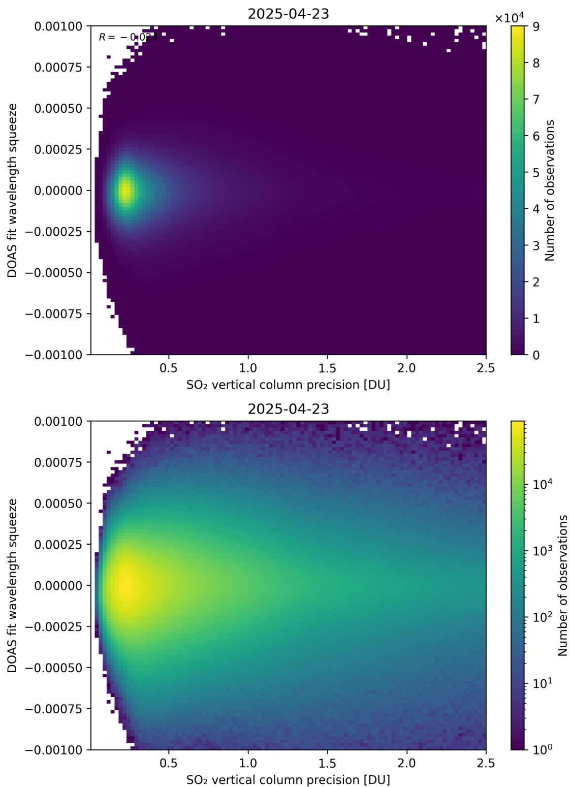
Figure 333: Scatter density plot of “SO 2 vertical column precision” against “DOAS fit wavelength squeeze” for 2025-04-22 to 2025-04-24.
