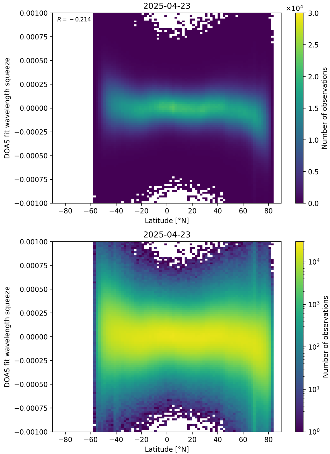
Figure 154: Scatter density plot of “Latitude” against “DOAS fit wavelength squeeze” for 2025-04-22 to 2025-04-24.
