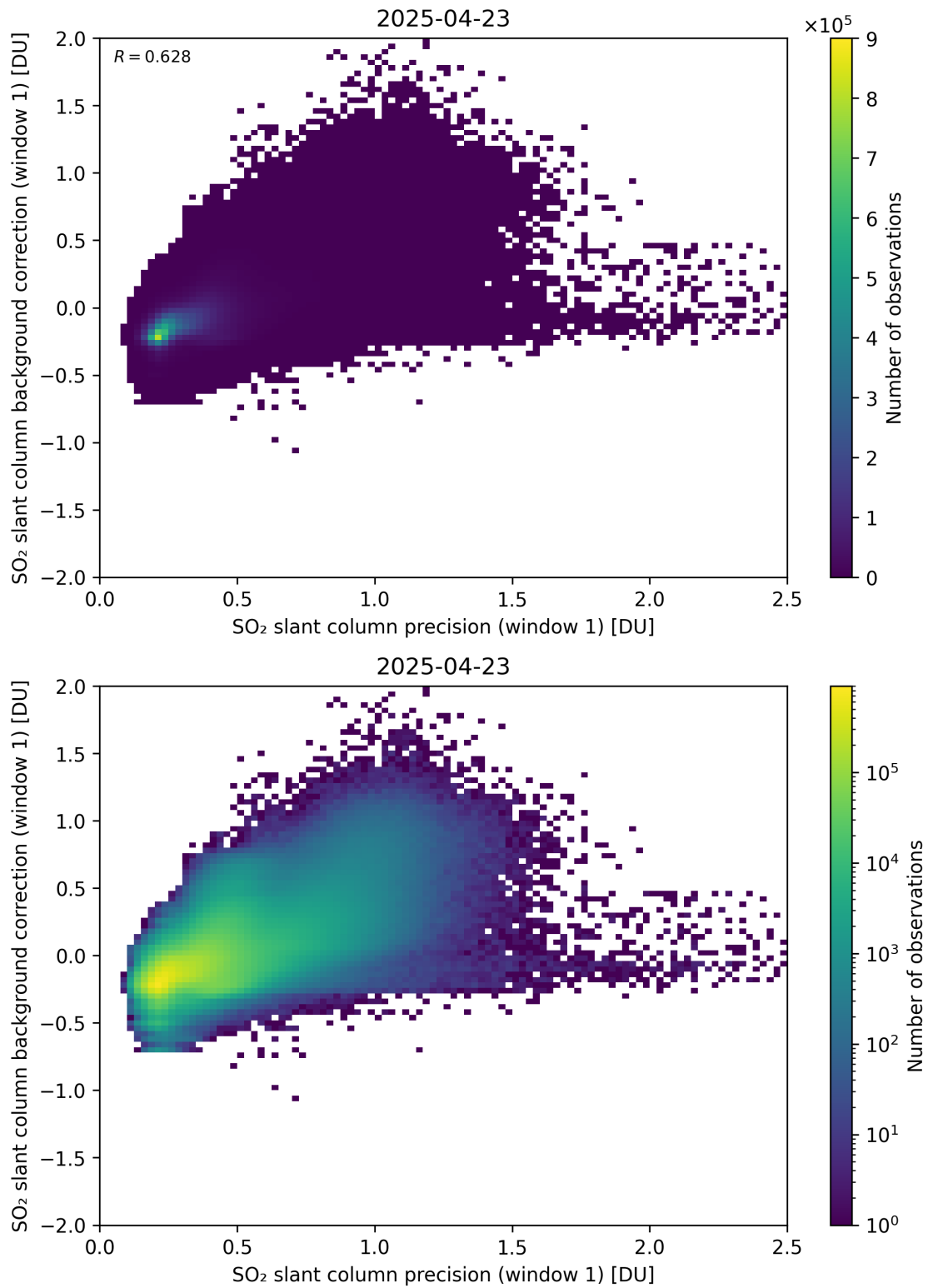
Figure 268: Scatter density plot of “SO 2 slant column precision (window 1)” against “SO 2 slant column background correction (window 1)” for 2025-04-22 to 2025-04-24.
