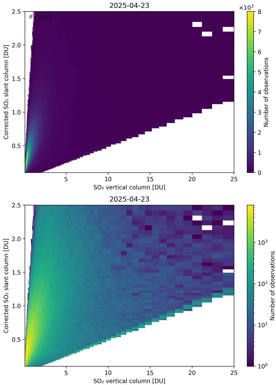
Figure 351: Scatter density plot of “SO 2 vertical column” against “Corrected SO 2 slant column” for 2025-04-22 to 2025-04-24.
