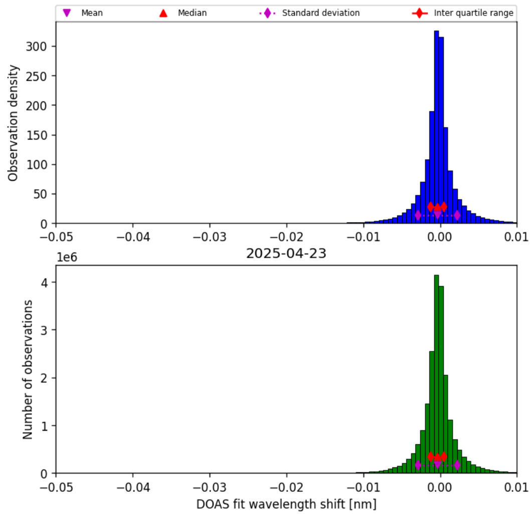
Figure 76: Histogram of “DOAS fit wavelength shift” for 2025-04-22 to 2025-04-24
