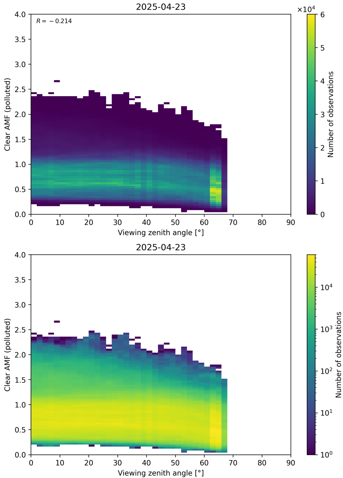
Figure 370: Scatter density plot of “Viewing zenith angle” against “Clear AMF (polluted)” for 2025-04-22 to 2025-04-24.
