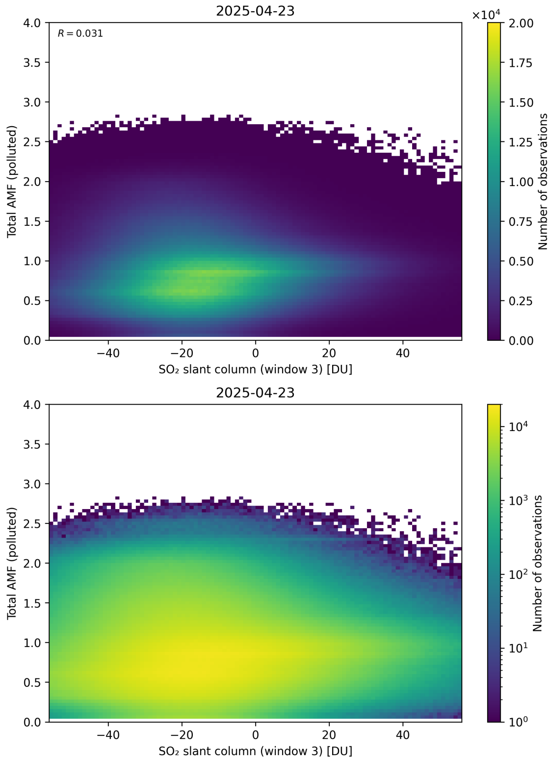
Figure 318: Scatter density plot of “SO 2 slant column (window 3)” against “Total AMF (polluted)” for 2025-04-22 to 2025-04-24.
