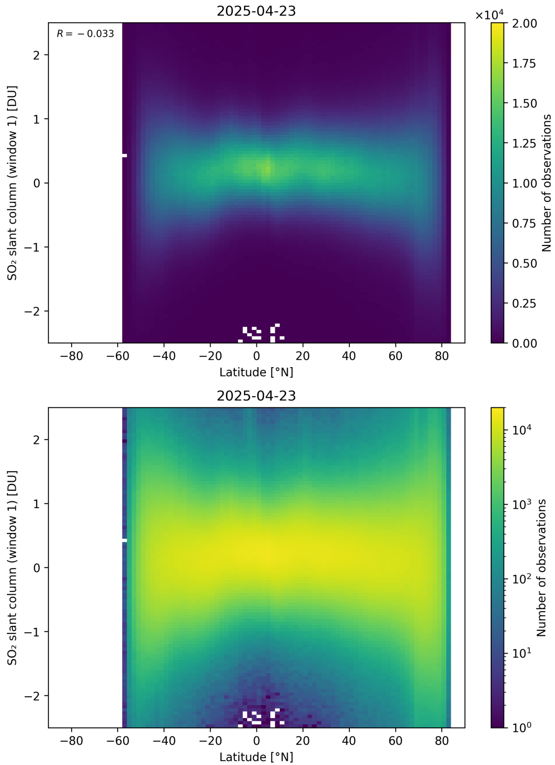
Figure 162: Scatter density plot of “Latitude” against “SO 2 slant column (window 1)” for 2025-04-22 to 2025-04-24.
