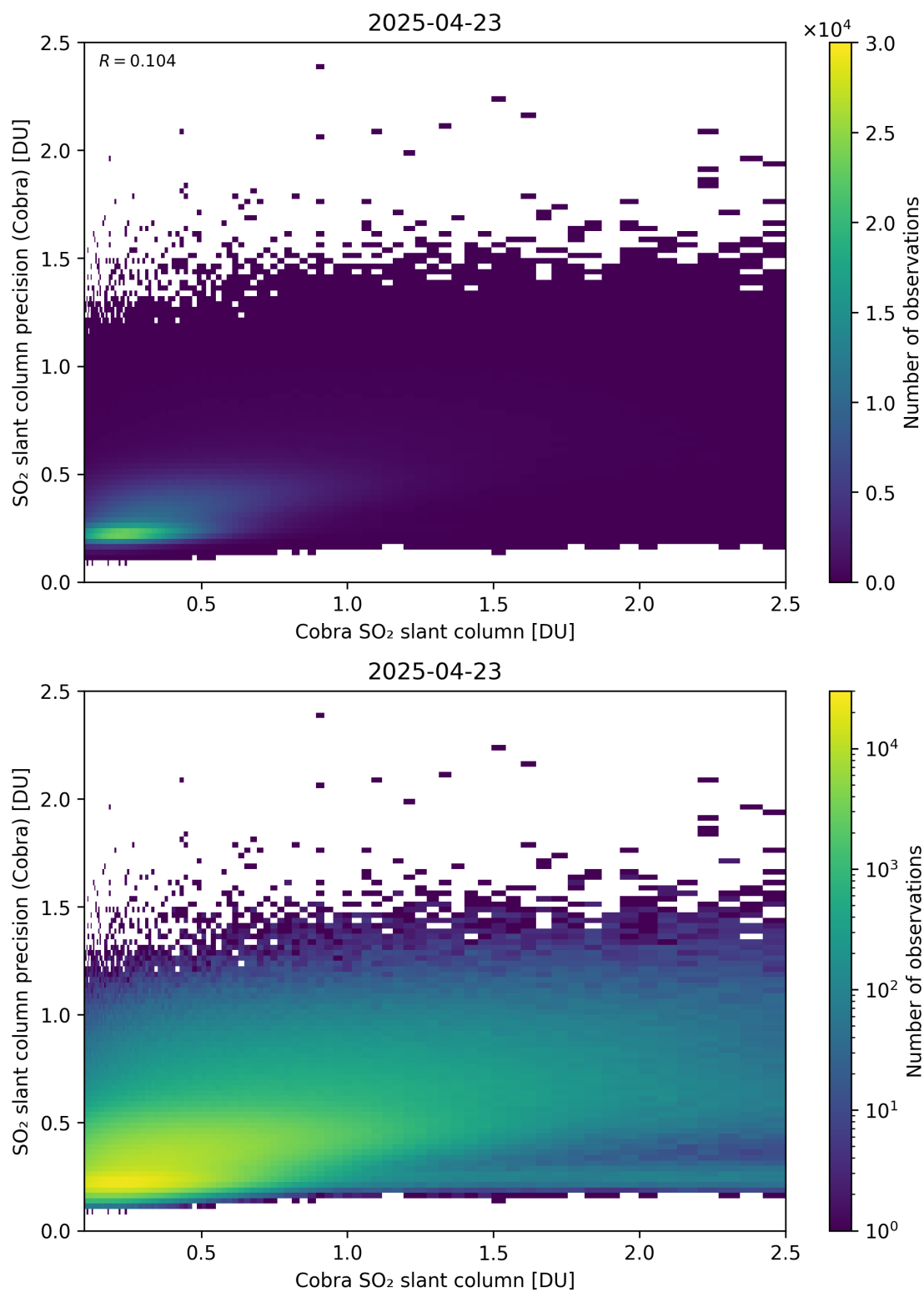
Figure 216: Scatter density plot of “Cobra SO 2 slant column” against “SO 2 slant column precision (Cobra)” for 2025-04-22 to 2025-04-24.
