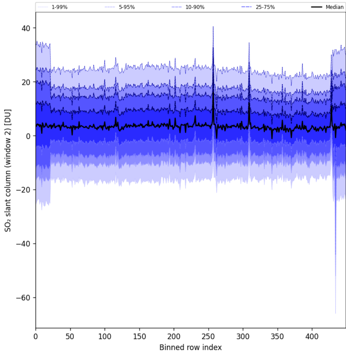
Figure 93: Along track statistics of “SO 2 slant column (window 2)” for 2025-04-22 to 2025-04-24
