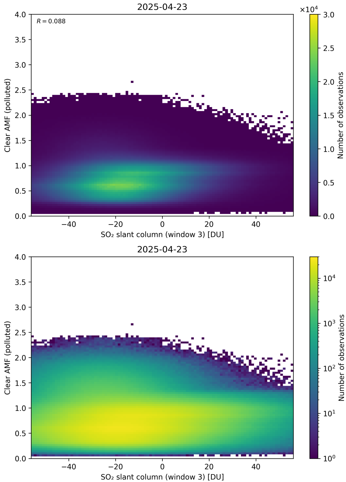
Figure 315: Scatter density plot of “SO 2 slant column (window 3)” against “Clear AMF (polluted)” for 2025-04-22 to 2025-04-24.
