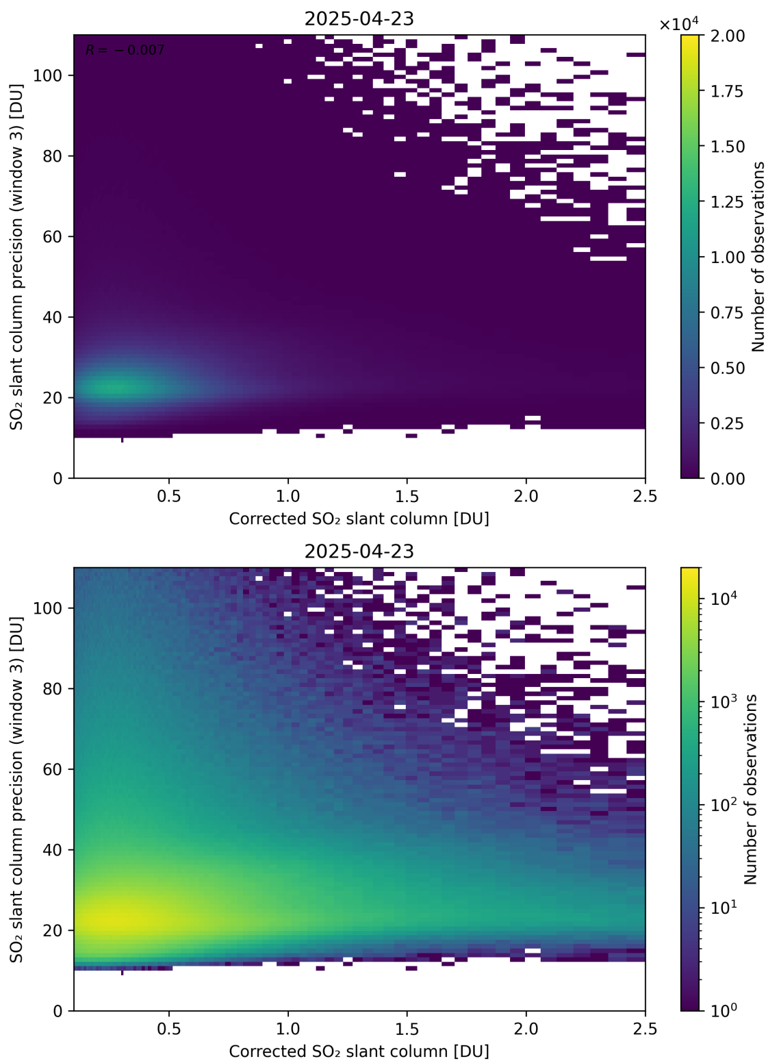
Figure 241: Scatter density plot of “Corrected SO 2 slant column” against “SO 2 slant column precision (window 3)” for 2025-04-22 to 2025-04-24.
