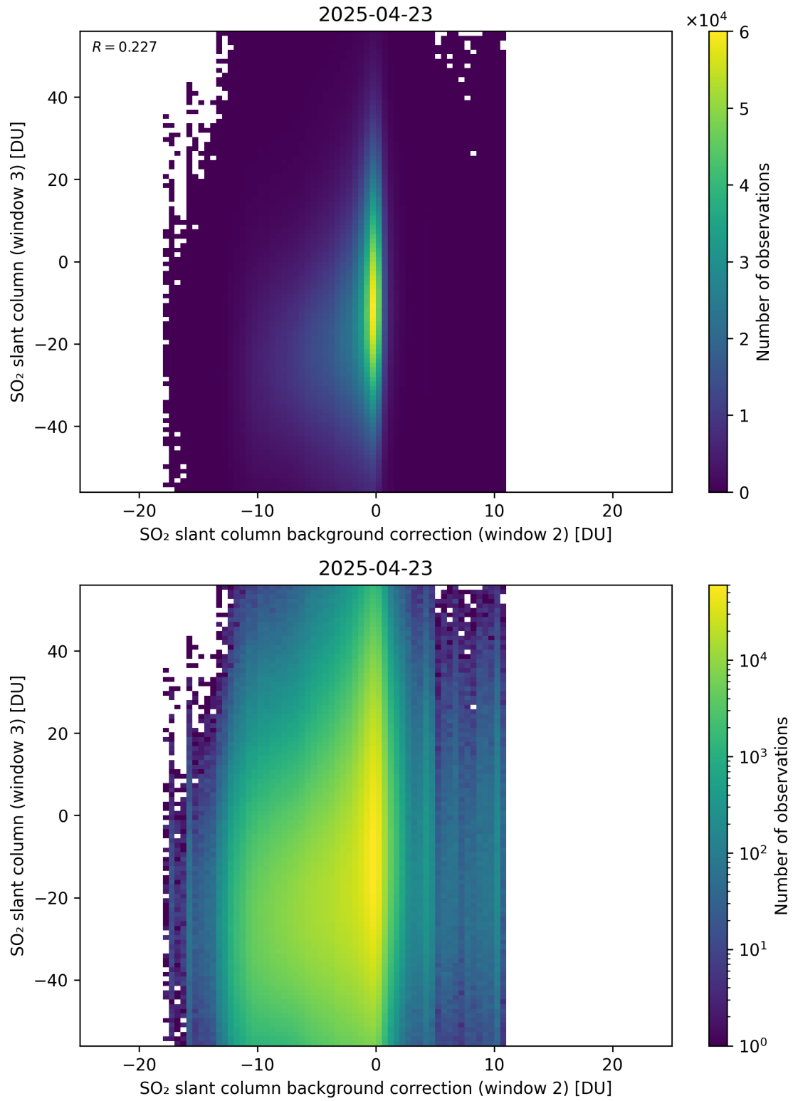
Figure 128: Scatter density plot of “SO 2 slant column background correction (window 2)” against “SO 2 slant column (window 3)” for 2025-04-22 to 2025-04-24.
