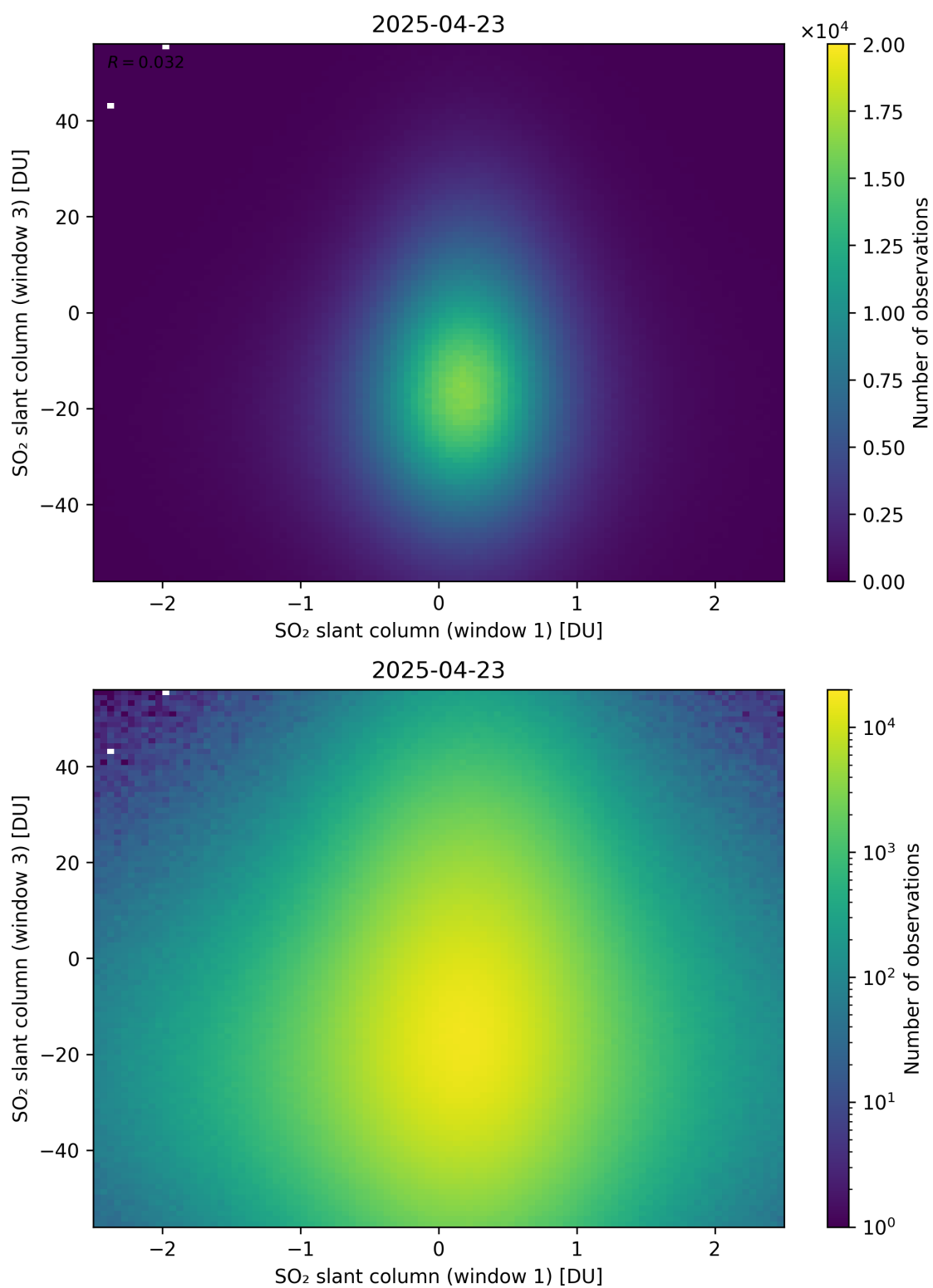
Figure 287: Scatter density plot of “SO 2 slant column (window 1)” against “SO 2 slant column (window 3)” for 2025-04-22 to 2025-04-24.
