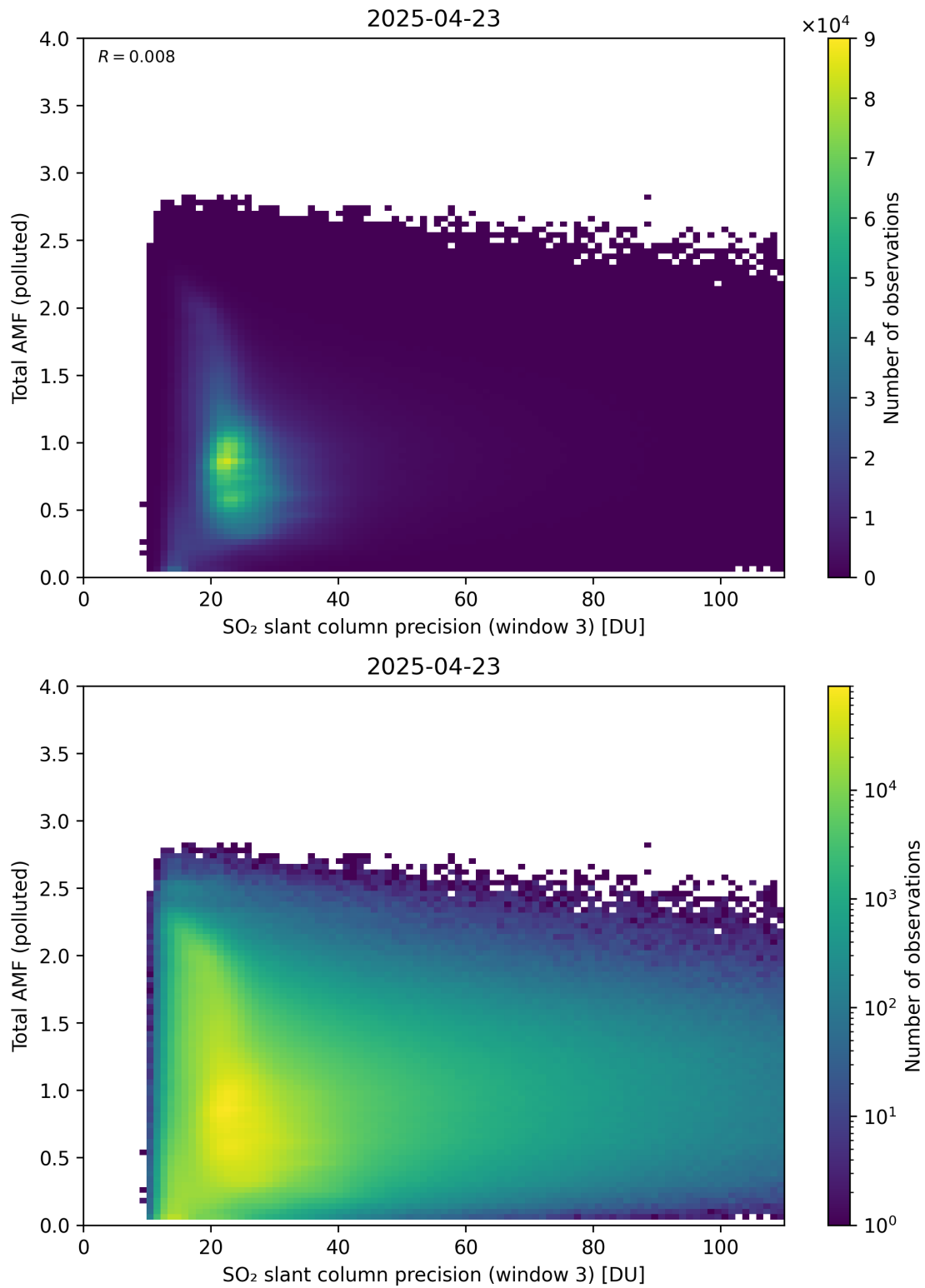
Figure 313: Scatter density plot of “SO 2 slant column precision (window 3)” against “Total AMF (polluted)” for 2025-04-22 to 2025-04-24.
