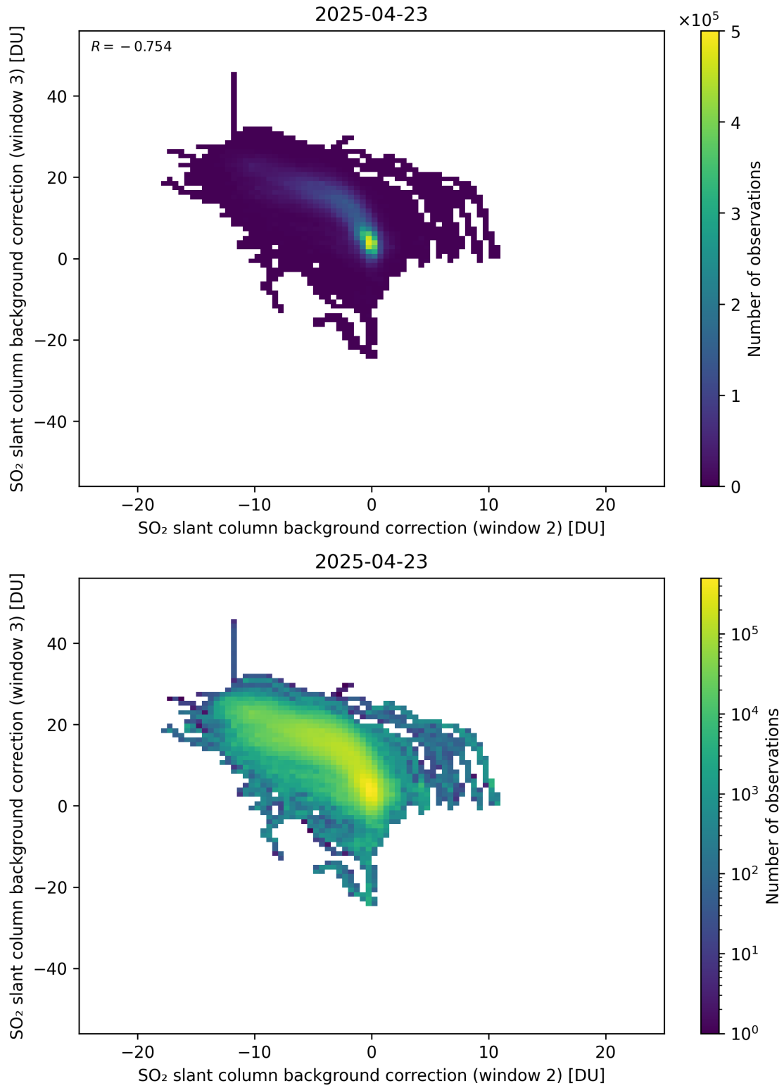
Figure 122: Scatter density plot of “SO 2 slant column background correction (window 2)” against “SO 2 slant column background correction (window 3)” for 2025-04-22 to 2025-04-24.
