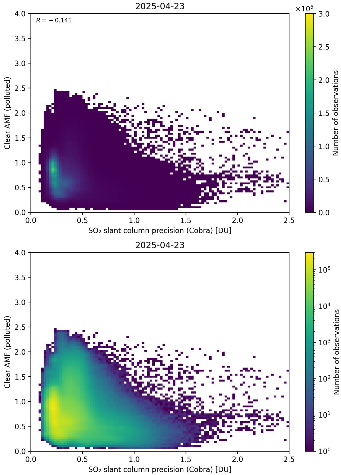
Figure 205: Scatter density plot of “SO 2 slant column precision (Cobra)” against “Clear AMF (polluted)” for 2025-04-22 to 2025-04-24.
