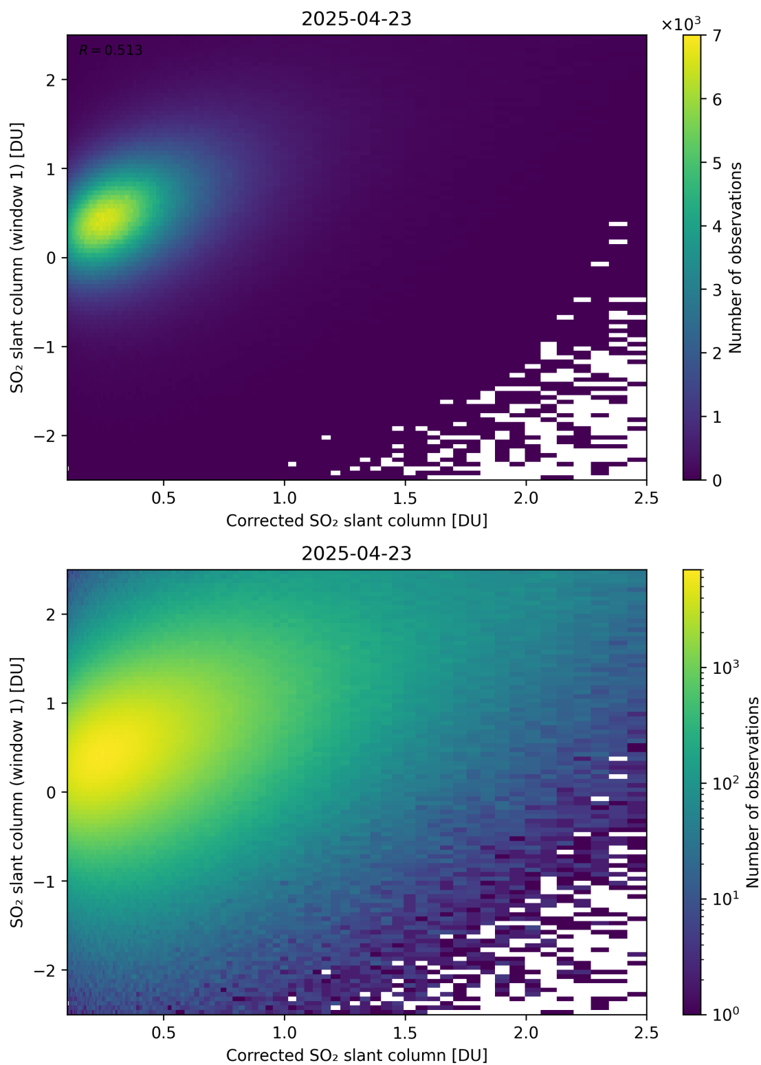
Figure 237: Scatter density plot of “Corrected SO 2 slant column” against “SO 2 slant column (window 1)” for 2025-04-22 to 2025-04-24.
