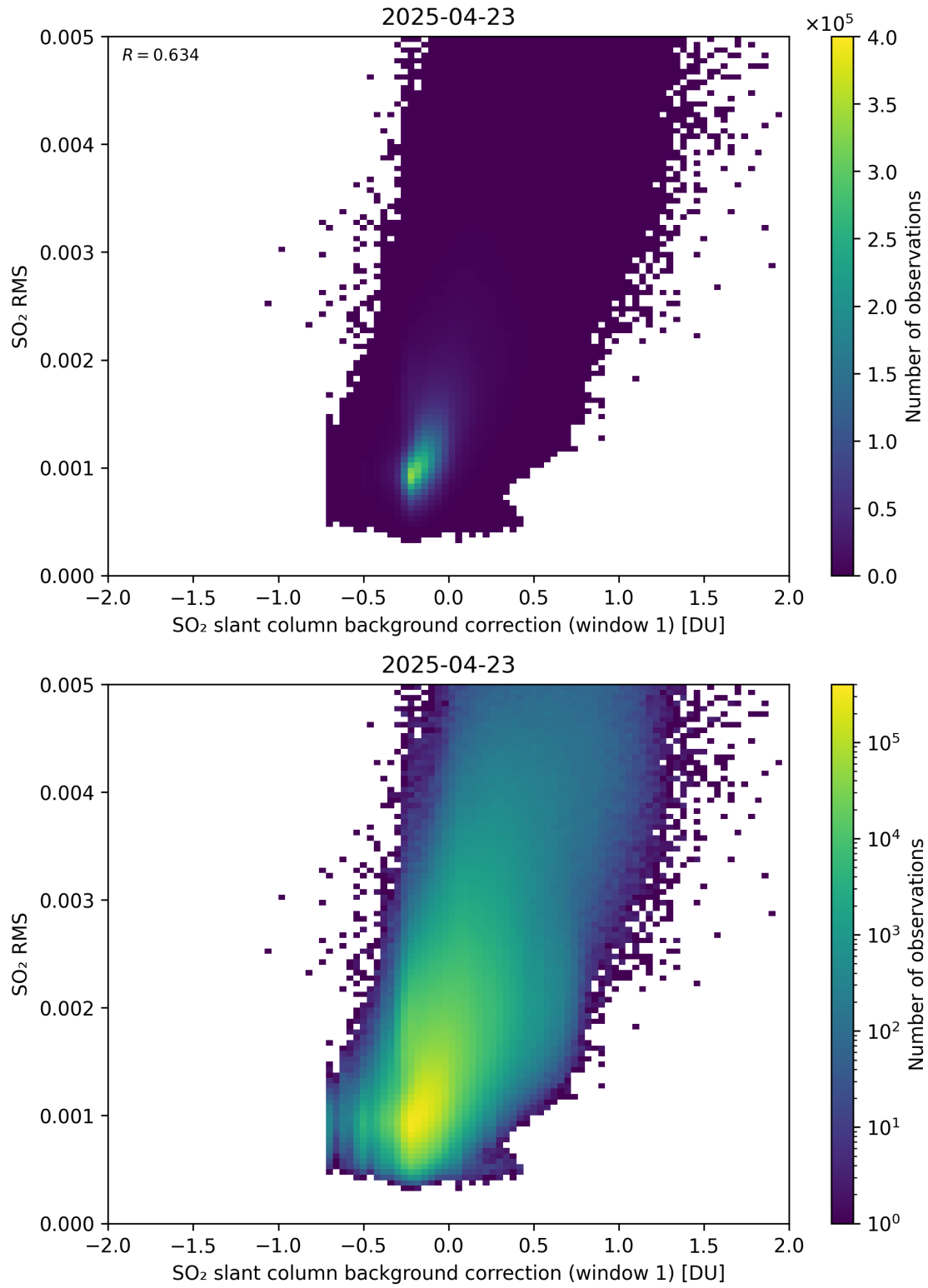
Figure 113: Scatter density plot of “SO 2 slant column background correction (window 1)” against “SO 2 RMS” for 2025-04-22 to 2025-04-24.
