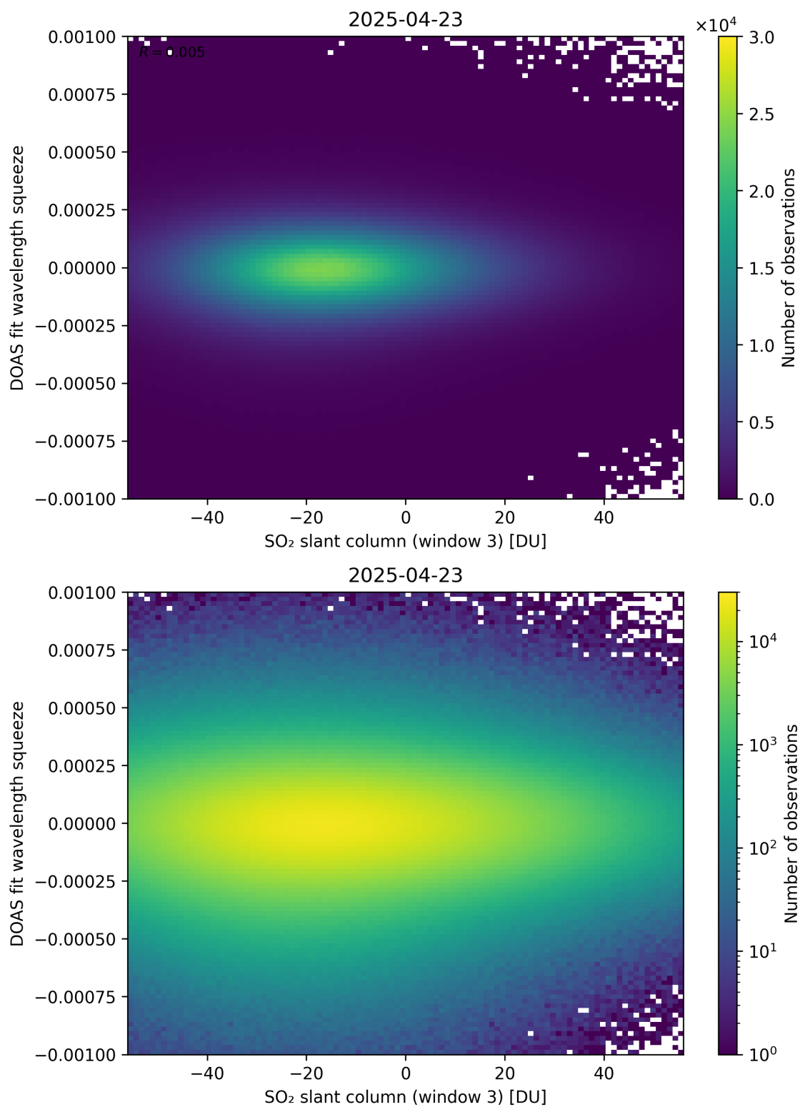
Figure 305: Scatter density plot of “SO 2 slant column (window 3)” against “DOAS fit wavelength squeeze” for 2025-04-22 to 2025-04-24.
