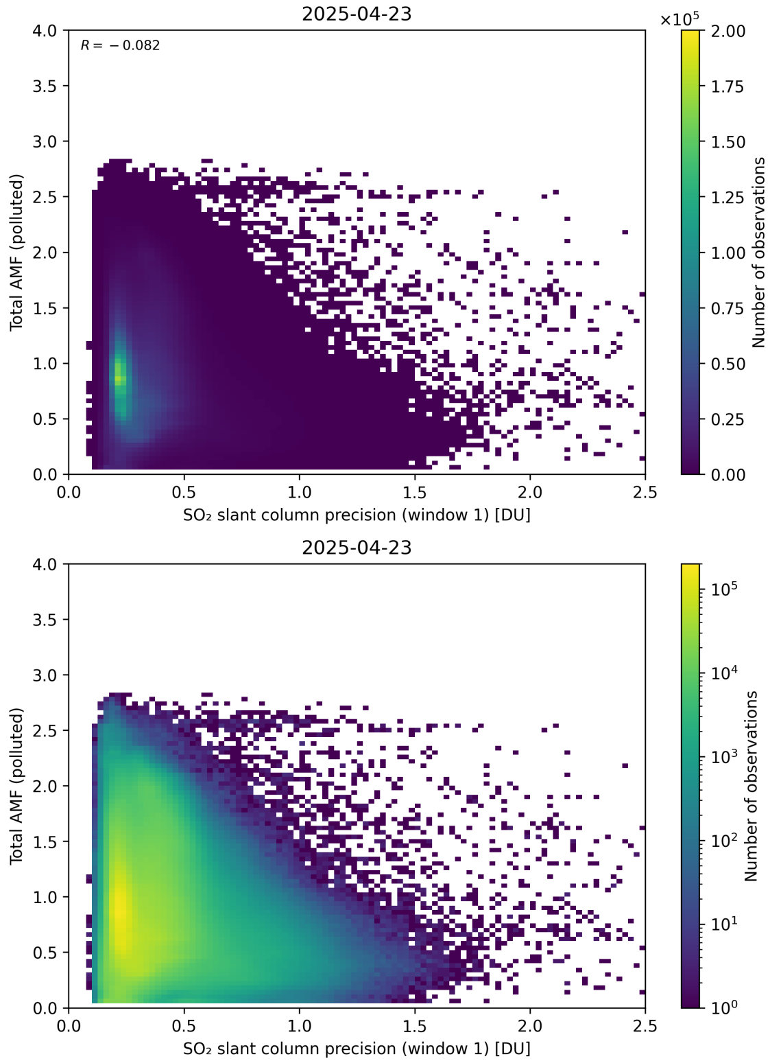
Figure 280: Scatter density plot of “SO 2 slant column precision (window 1)” against “Total AMF (polluted)” for 2025-04-22 to 2025-04-24.
