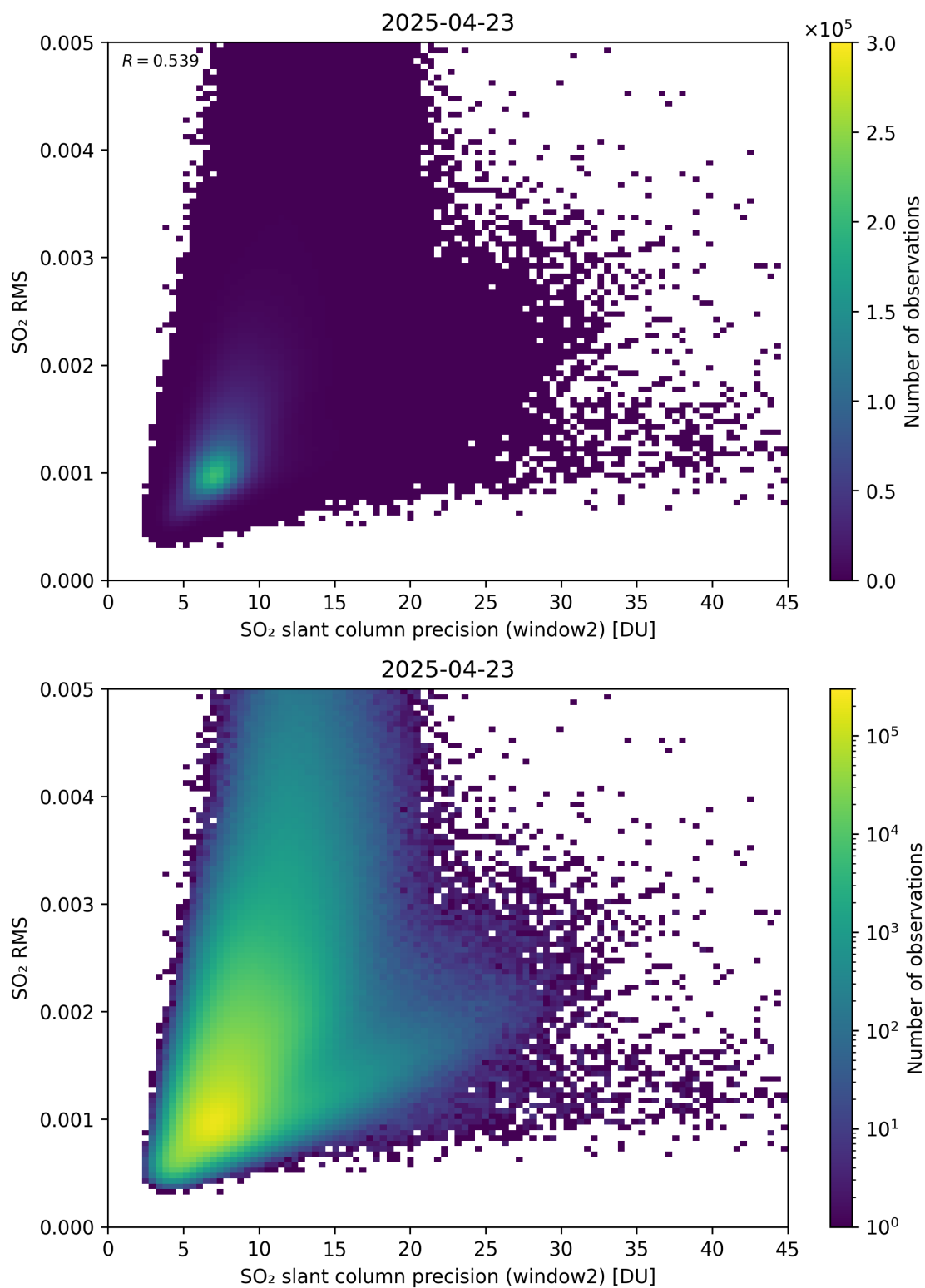
Figure 295: Scatter density plot of “SO 2 slant column precision (window2)” against “SO 2 RMS” for 2025-04-22 to 2025-04-24.
