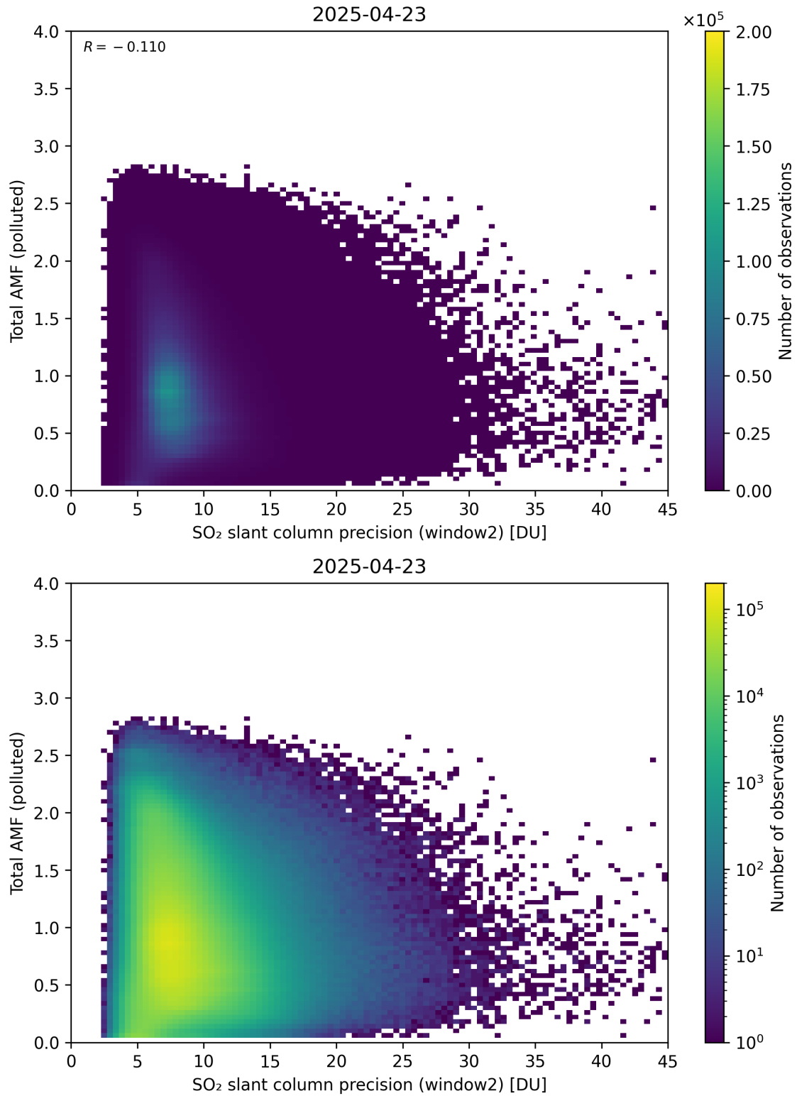
Figure 301: Scatter density plot of “SO 2 slant column precision (window2)” against “Total AMF (polluted)” for 2025-04-22 to 2025-04-24.
