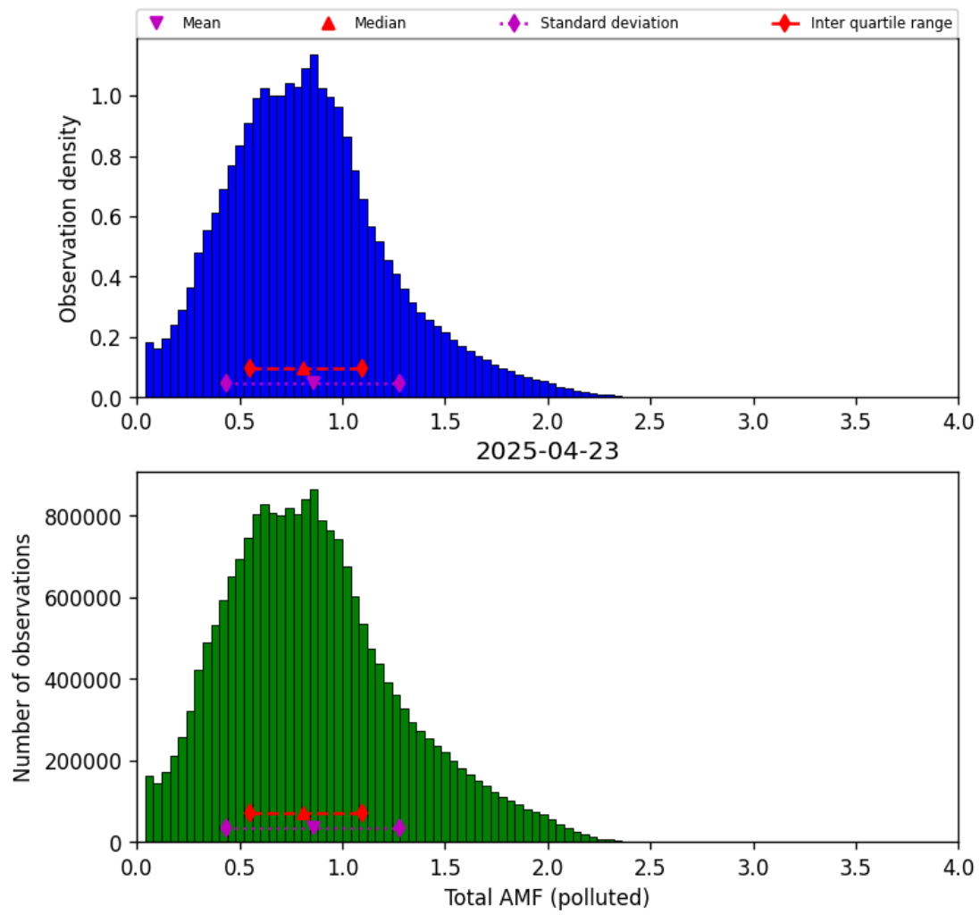
Figure 79: Histogram of “Total AMF (polluted)” for 2025-04-22 to 2025-04-24
