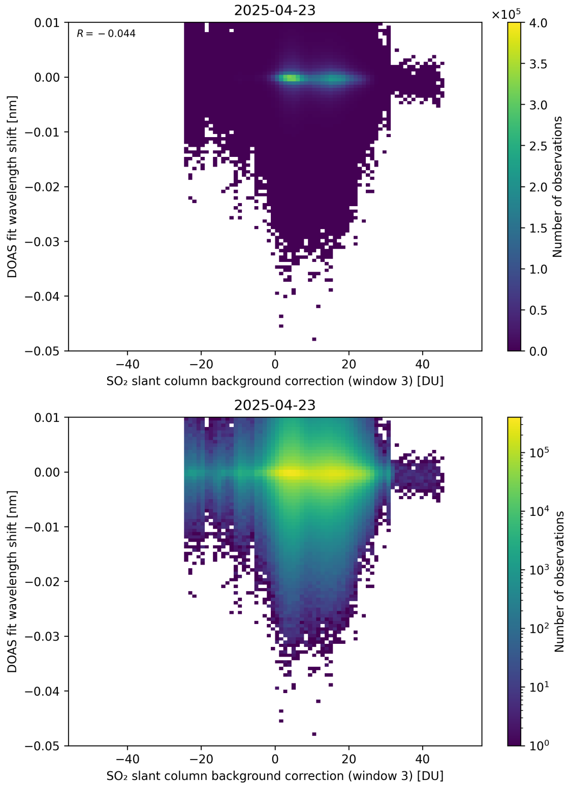
Figure 132: Scatter density plot of “SO 2 slant column background correction (window 3)” against “DOAS fit wavelength shift” for 2025-04-22 to 2025-04-24.
