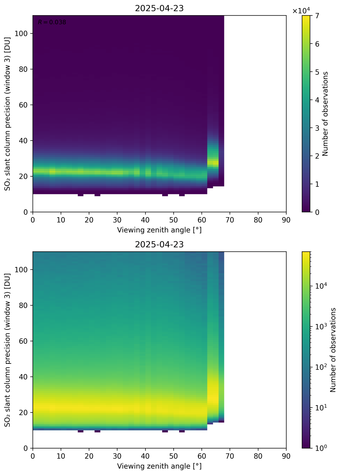
Figure 380: Scatter density plot of “Viewing zenith angle” against “SO 2 slant column precision (window 3)” for 2025-04-22 to 2025-04-24.
