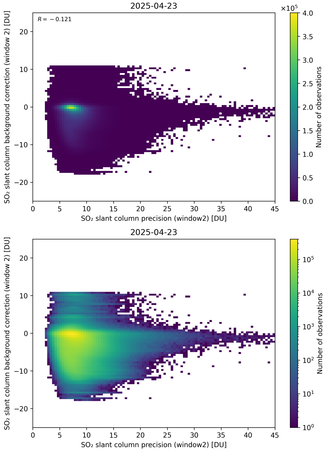
Figure 291: Scatter density plot of “SO 2 slant column precision (window2)” against “SO 2 slant column background correction (window 2)” for 2025-04-22 to 2025-04-24.
