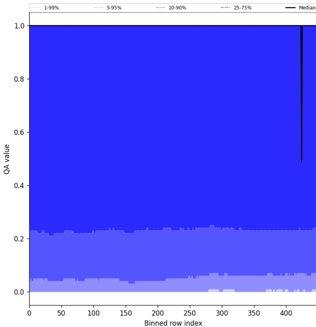
Figure 83: Along track statistics of “QA value” for 2025-04-22 to 2025-04-24
