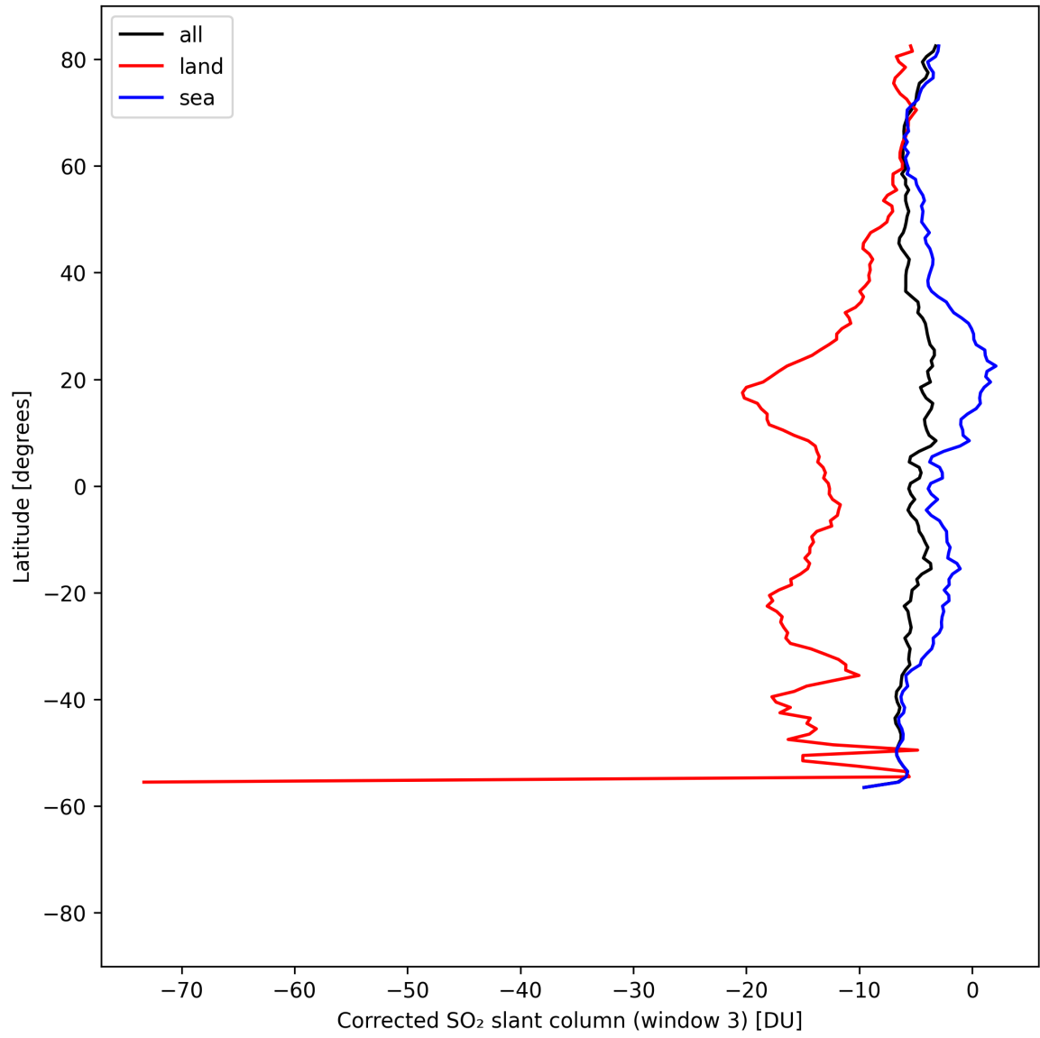
Figure 47: Zonal average of “Corrected SO 2 slant column (window 3)” for 2025-04-22 to 2025-04-24.
