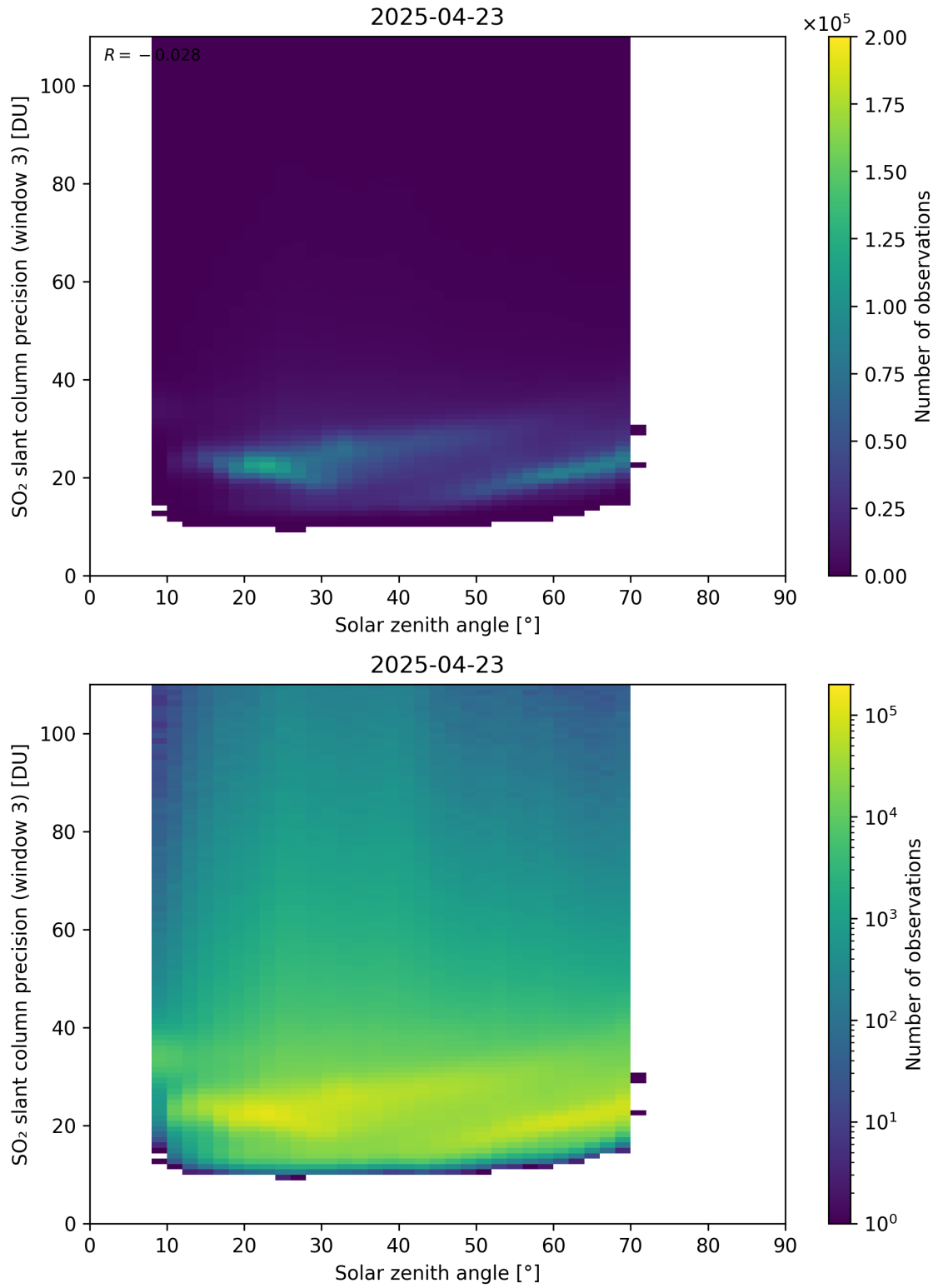
Figure 188: Scatter density plot of “Solar zenith angle” against “SO 2 slant column precision (window 3)” for 2025-04-22 to 2025-04-24.
