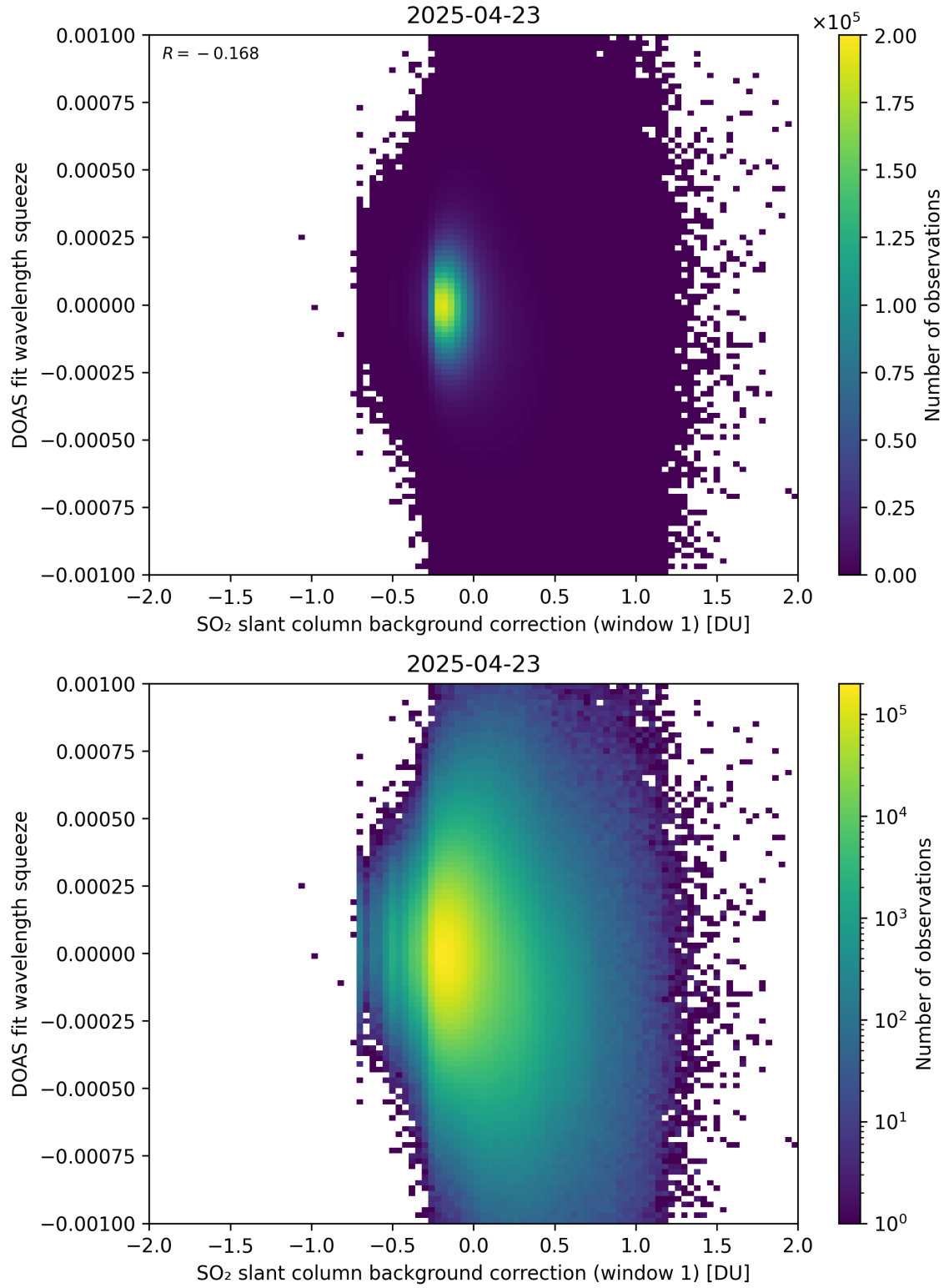
Figure 112: Scatter density plot of “SO 2 slant column background correction (window 1)” against “DOAS fit wavelength squeeze” for 2025-04-22 to 2025-04-24.
