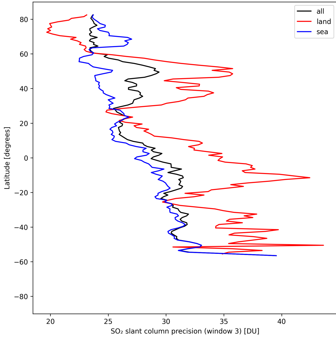
Figure 46: Zonal average of “SO 2 slant column precision (window 3)” for 2025-04-22 to 2025-04-24.
