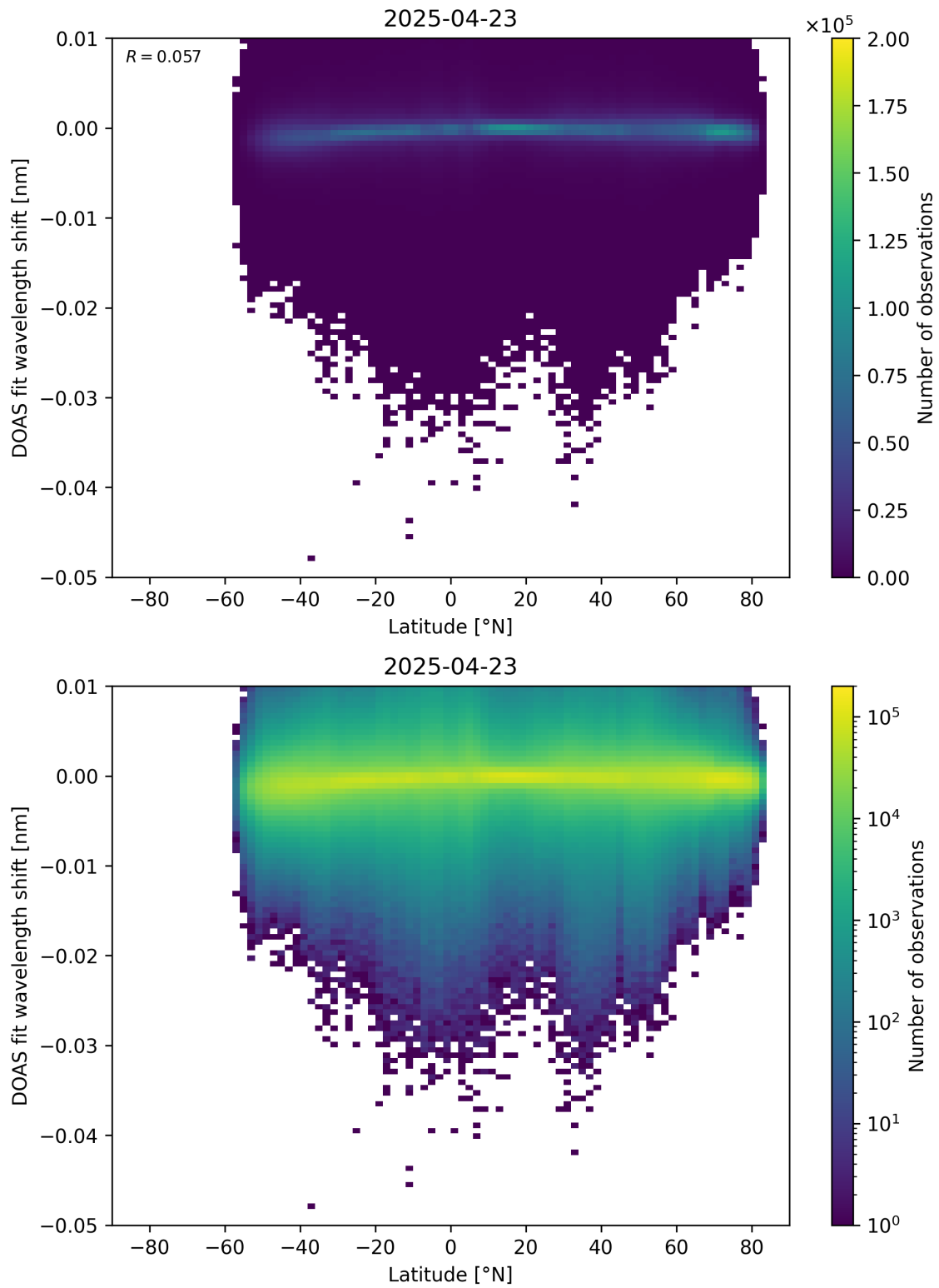
Figure 153: Scatter density plot of “Latitude” against “DOAS fit wavelength shift” for 2025-04-22 to 2025-04-24.
