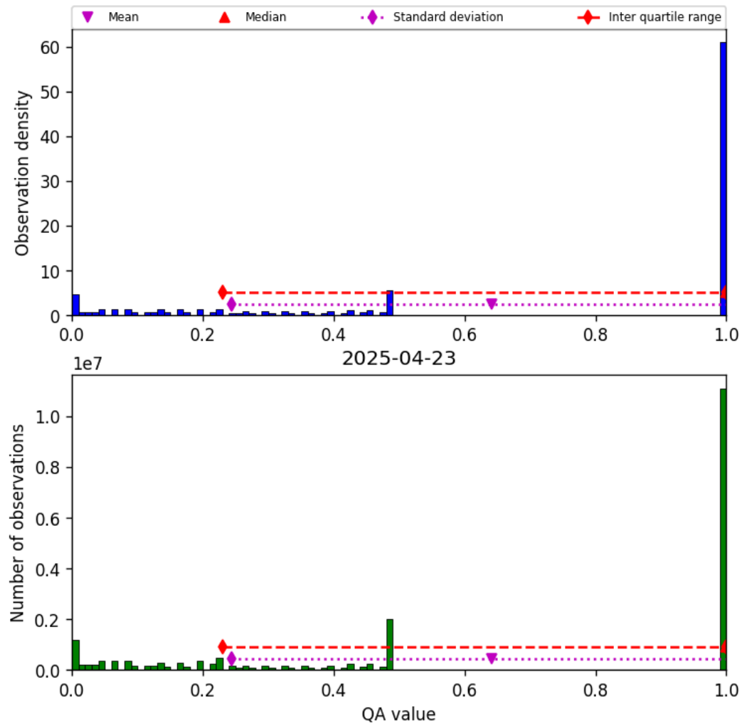
Figure 57: Histogram of “QA value” for 2025-04-22 to 2025-04-24
