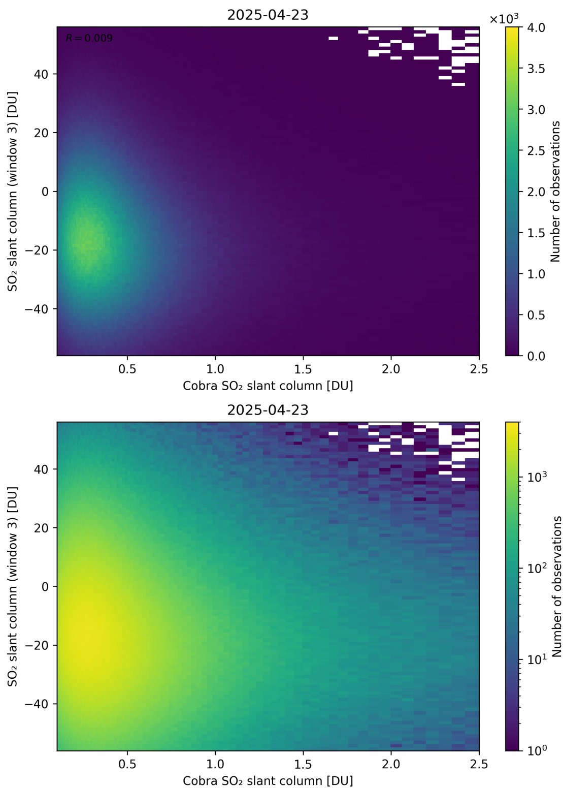
Figure 222: Scatter density plot of “Cobra SO 2 slant column” against “SO 2 slant column (window 3)” for 2025-04-22 to 2025-04-24.
