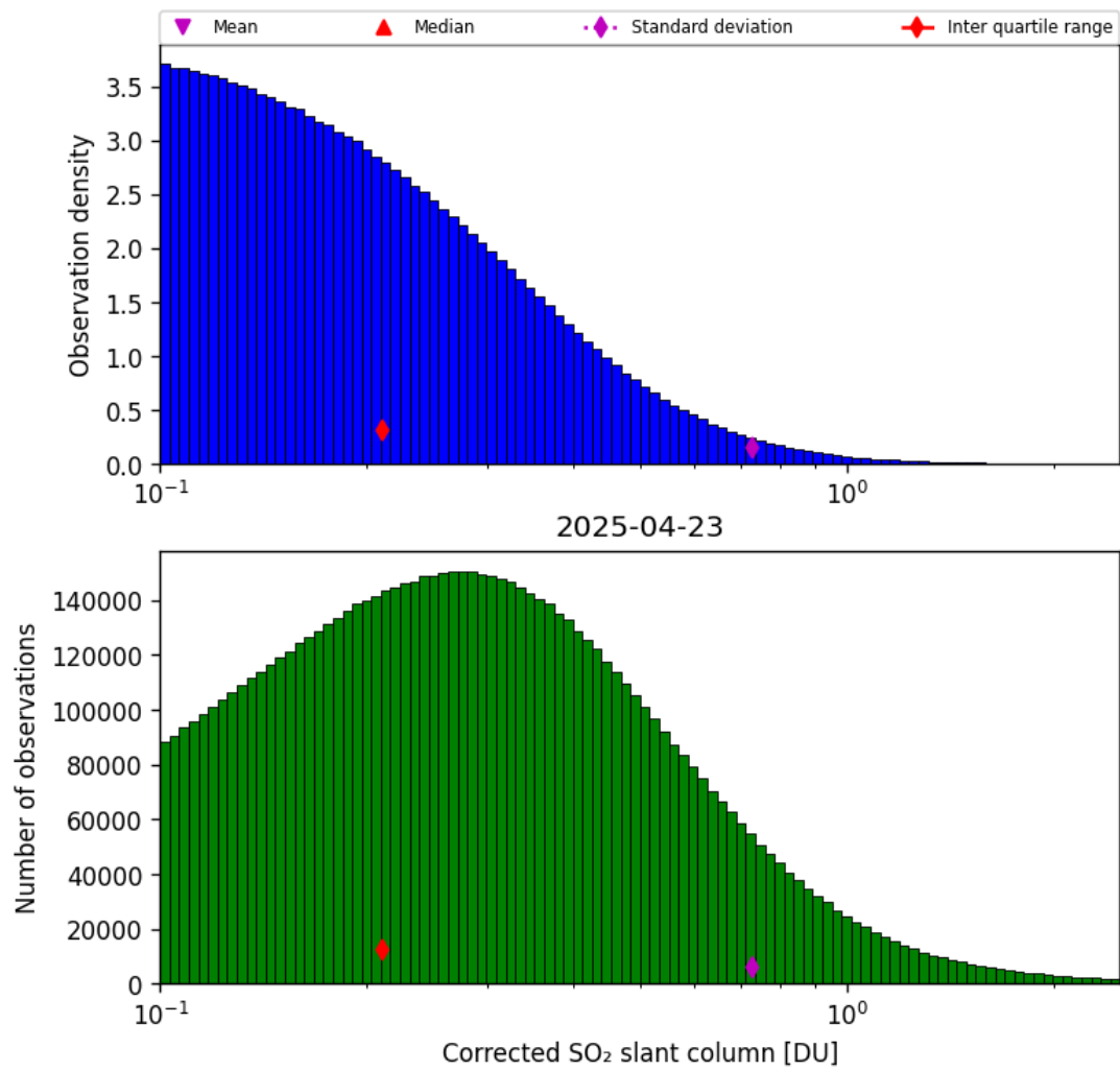
Figure 60: Histogram of “Corrected SO 2 slant column” for 2025-04-22 to 2025-04-24
