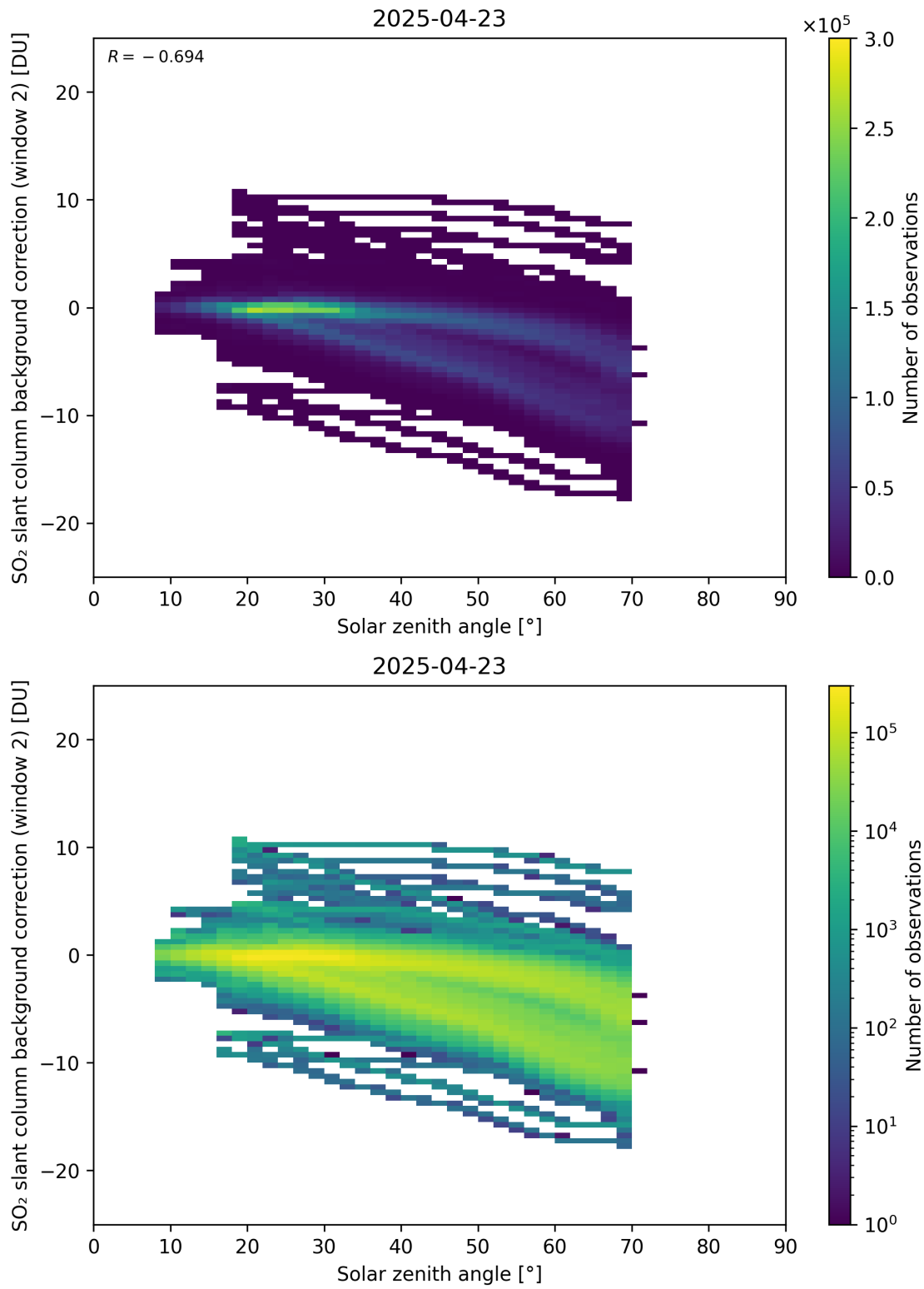
Figure 172: Scatter density plot of “Solar zenith angle” against “SO 2 slant column background correction (window 2)” for 2025-04-22 to 2025-04-24.
