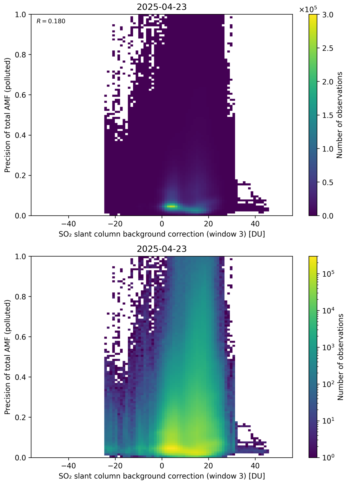
Figure 137: Scatter density plot of “SO 2 slant column background correction (window 3)” against “Precision of total AMF (polluted)” for 2025-04-22 to 2025-04-24.
