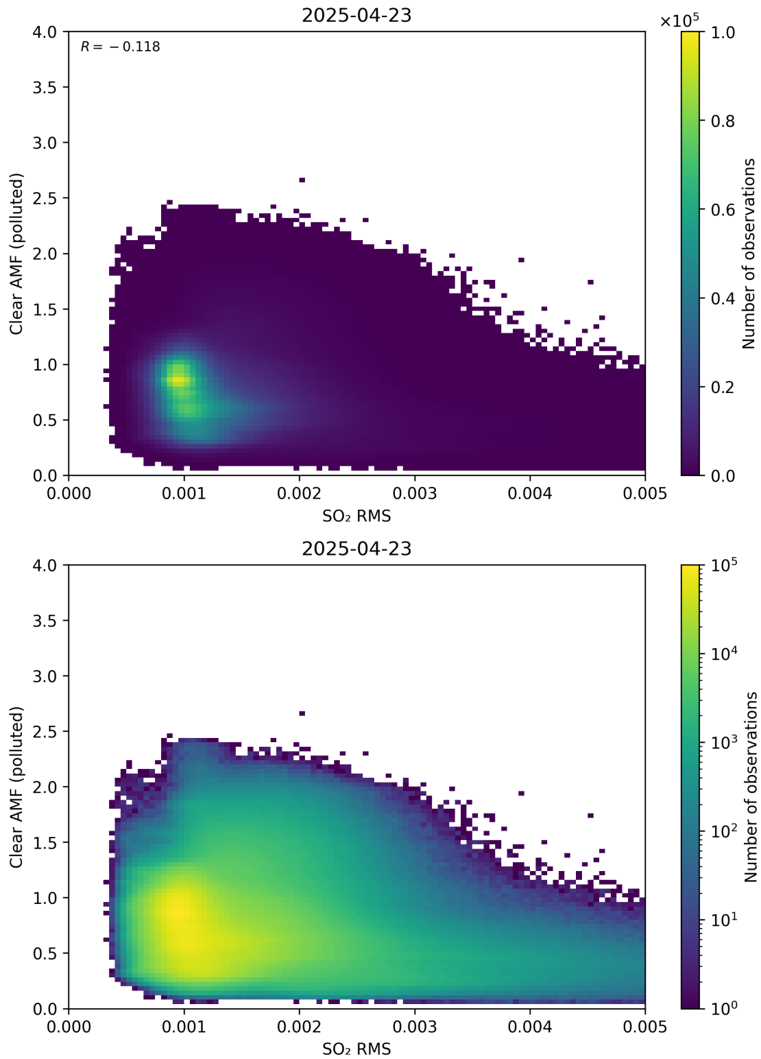
Figure 147: Scatter density plot of “SO 2 RMS” against “Clear AMF (polluted)” for 2025-04-22 to 2025-04-24.
