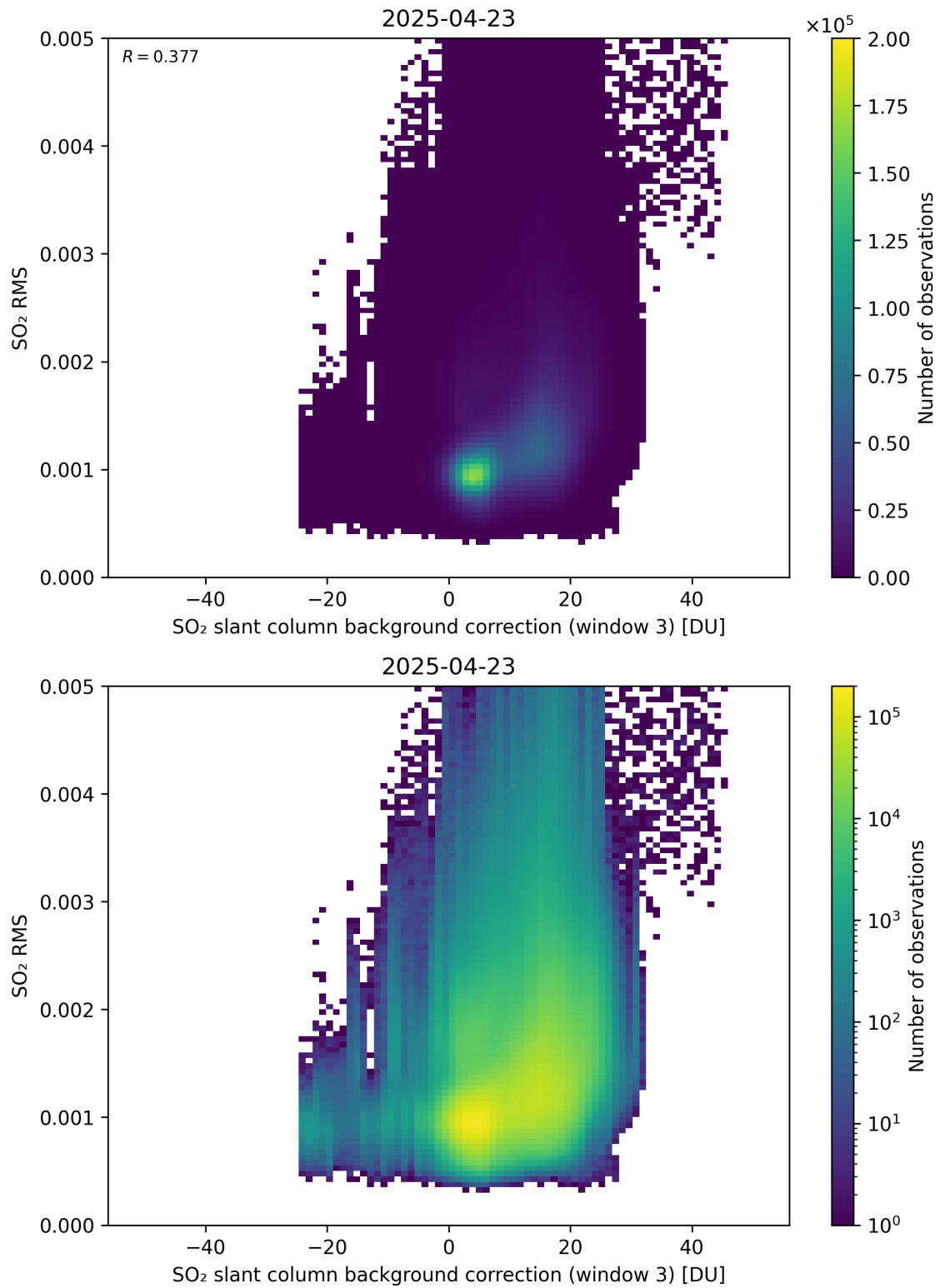
Figure 134: Scatter density plot of “SO 2 slant column background correction (window 3)” against “SO 2 RMS” for 2025-04-22 to 2025-04-24.
