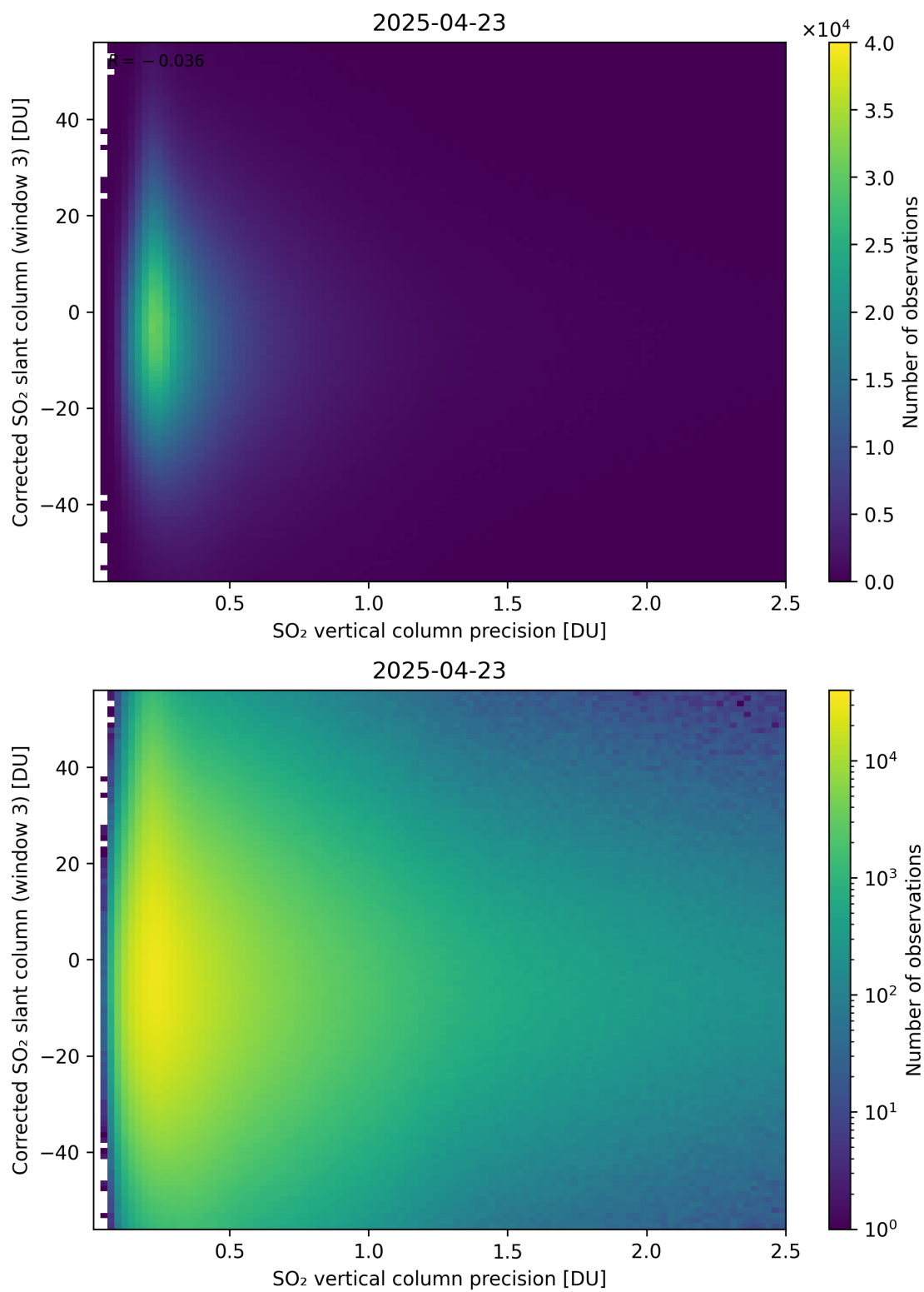
Figure 340: Scatter density plot of “SO 2 vertical column precision” against “Corrected SO 2 slant column (window 3)” for 2025-04-22 to 2025-04-24.
