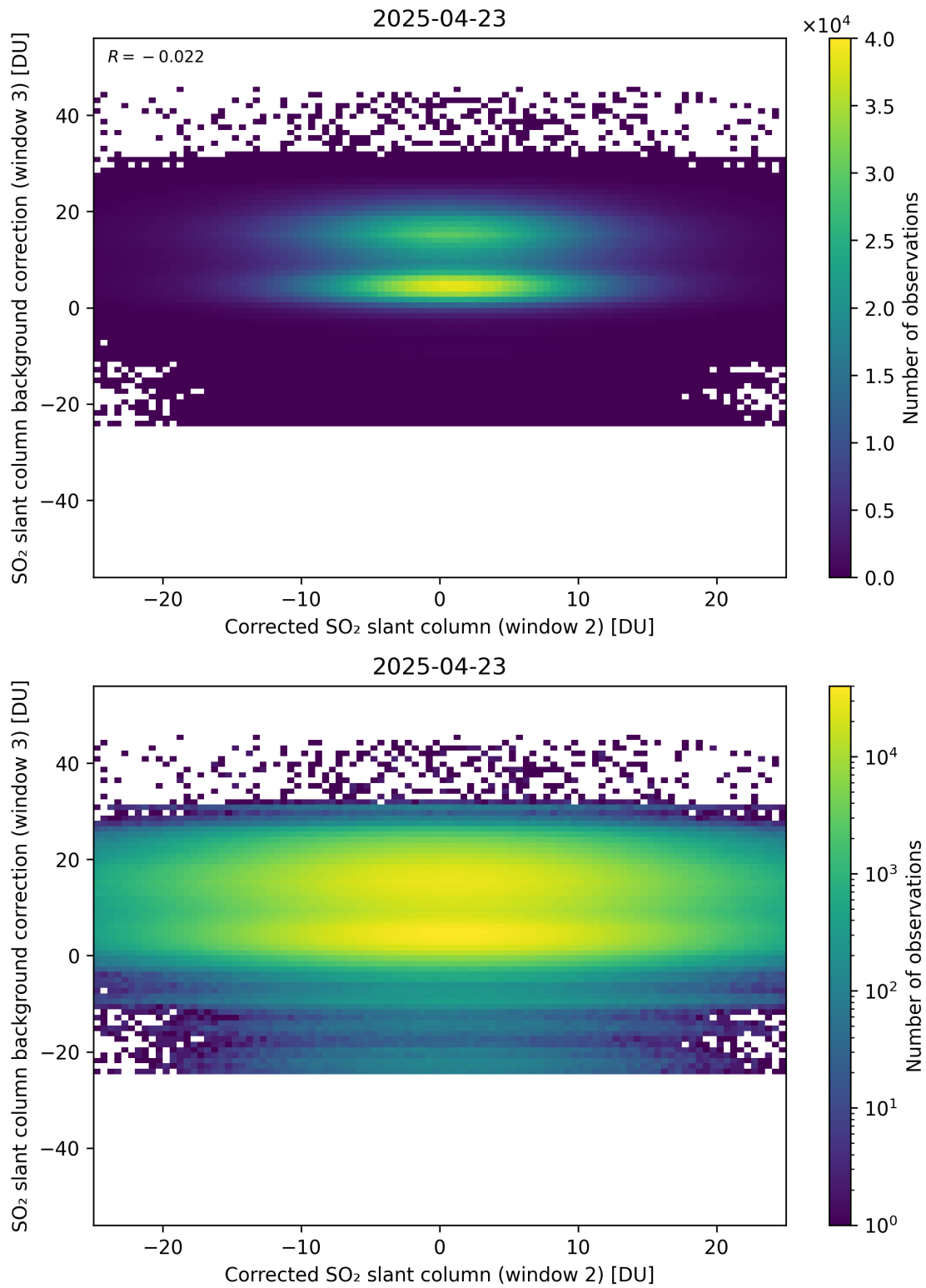
Figure 245: Scatter density plot of “Corrected SO 2 slant column (window 2)” against “SO 2 slant column background correction (window 3)” for 2025-04-22 to 2025-04-24.
