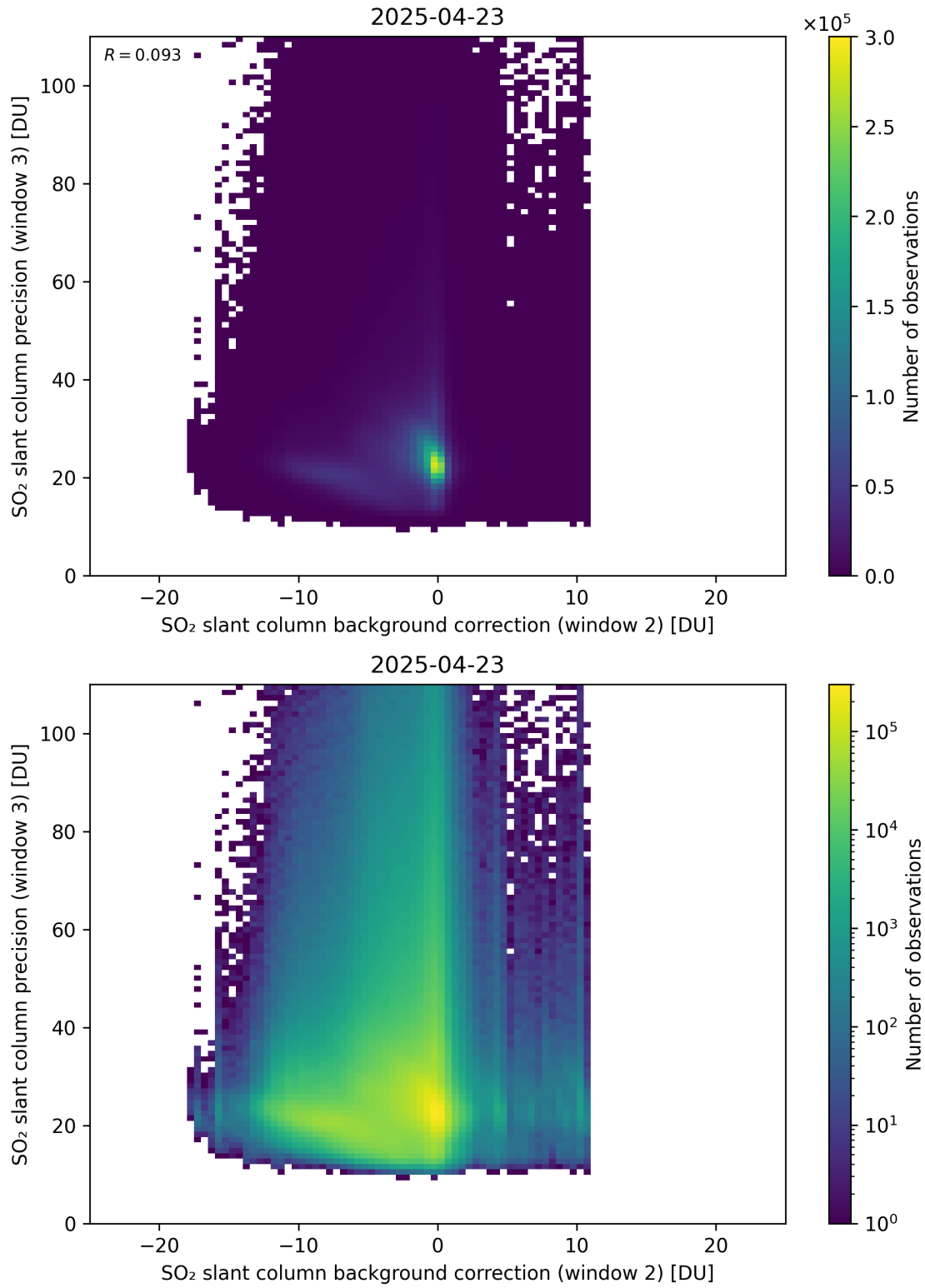
Figure 129: Scatter density plot of “SO 2 slant column background correction (window 2)” against “SO 2 slant column precision (window 3)” for 2025-04-22 to 2025-04-24.
