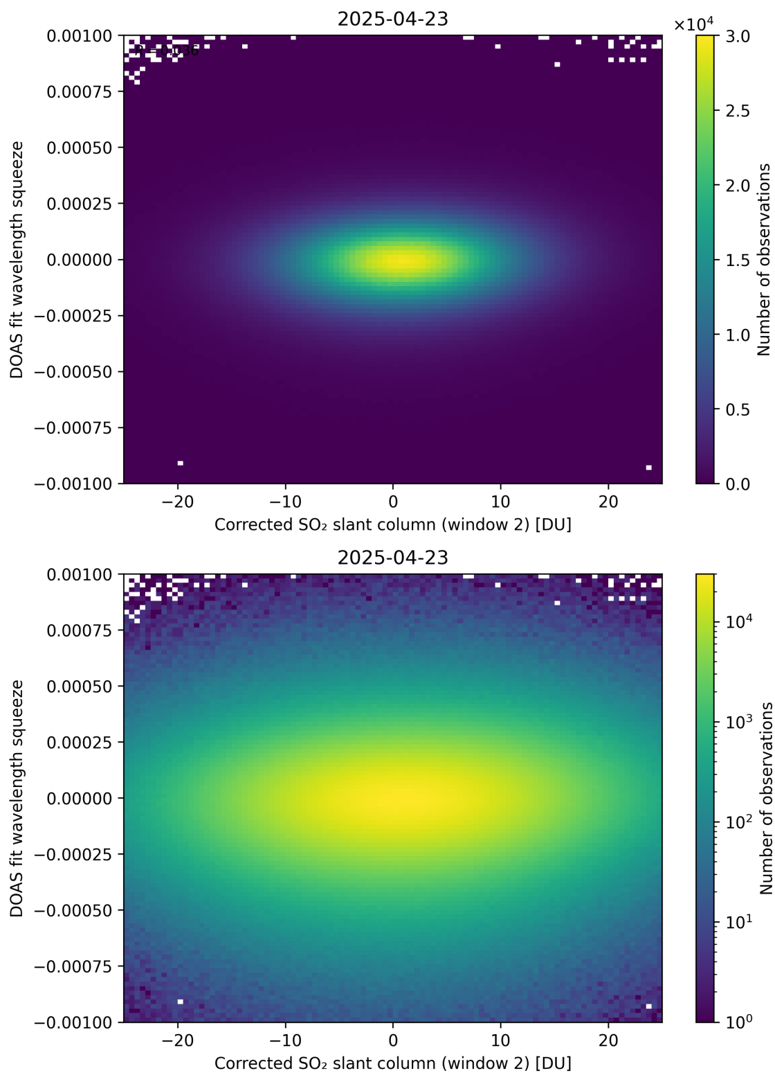
Figure 247: Scatter density plot of “Corrected SO 2 slant column (window 2)” against “DOAS fit wavelength squeeze” for 2025-04-22 to 2025-04-24.
