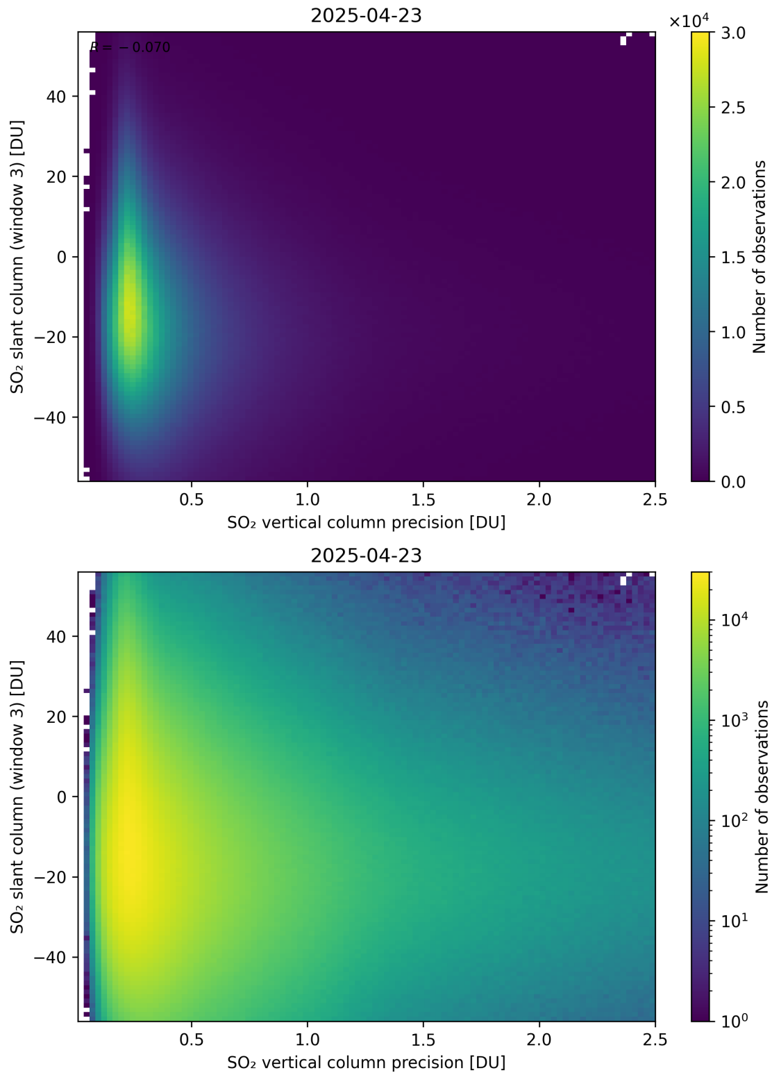
Figure 344: Scatter density plot of “SO 2 vertical column precision” against “SO 2 slant column (window 3)” for 2025-04-22 to 2025-04-24.
