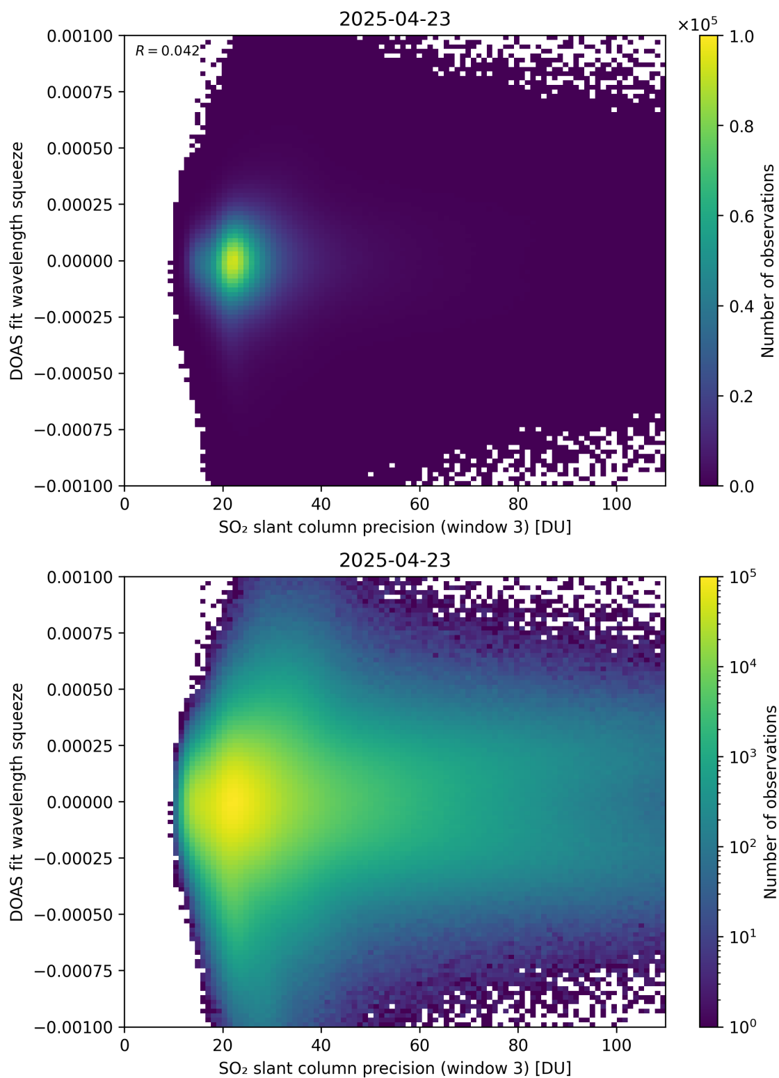
Figure 309: Scatter density plot of “SO 2 slant column precision (window 3)” against “DOAS fit wavelength squeeze” for 2025-04-22 to 2025-04-24.
