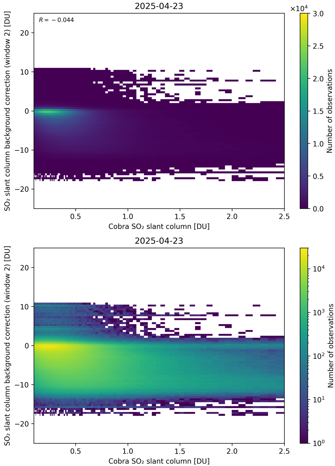
Figure 194: Scatter density plot of “Cobra SO 2 slant column” against “SO 2 slant column background correction (window 2)” for 2025-04-22 to 2025-04-24.
