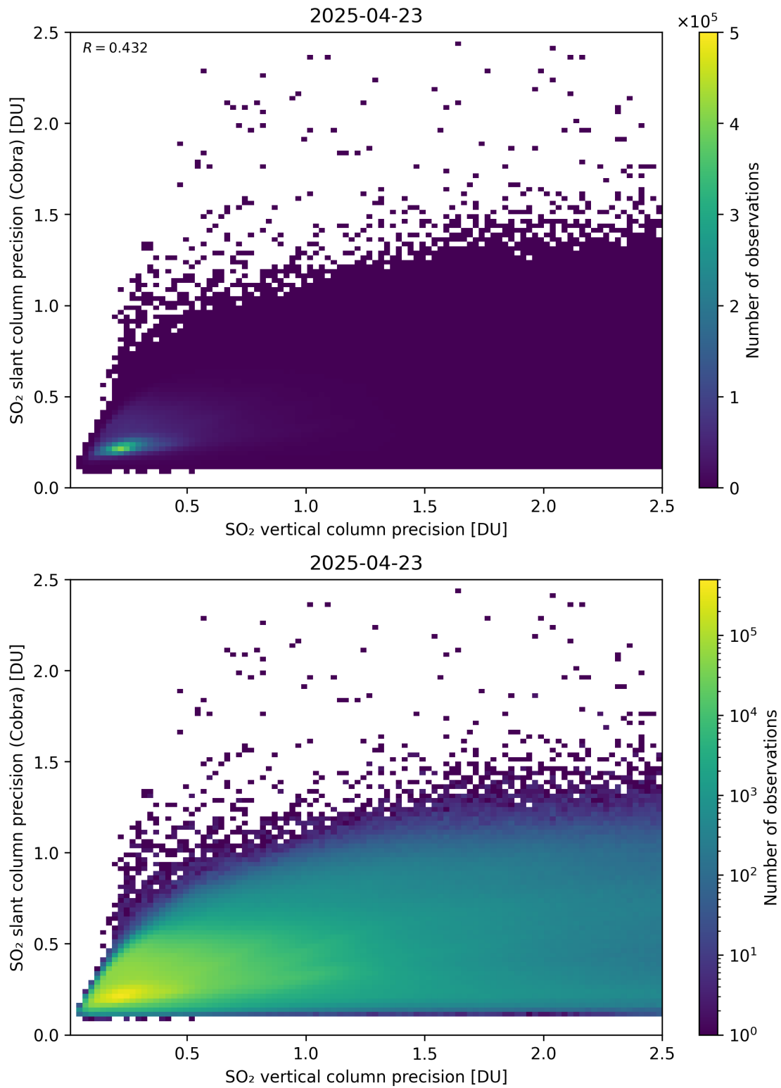
Figure 337: Scatter density plot of “SO 2 vertical column precision” against “SO 2 slant column precision (Cobra)” for 2025-04-22 to 2025-04-24.
