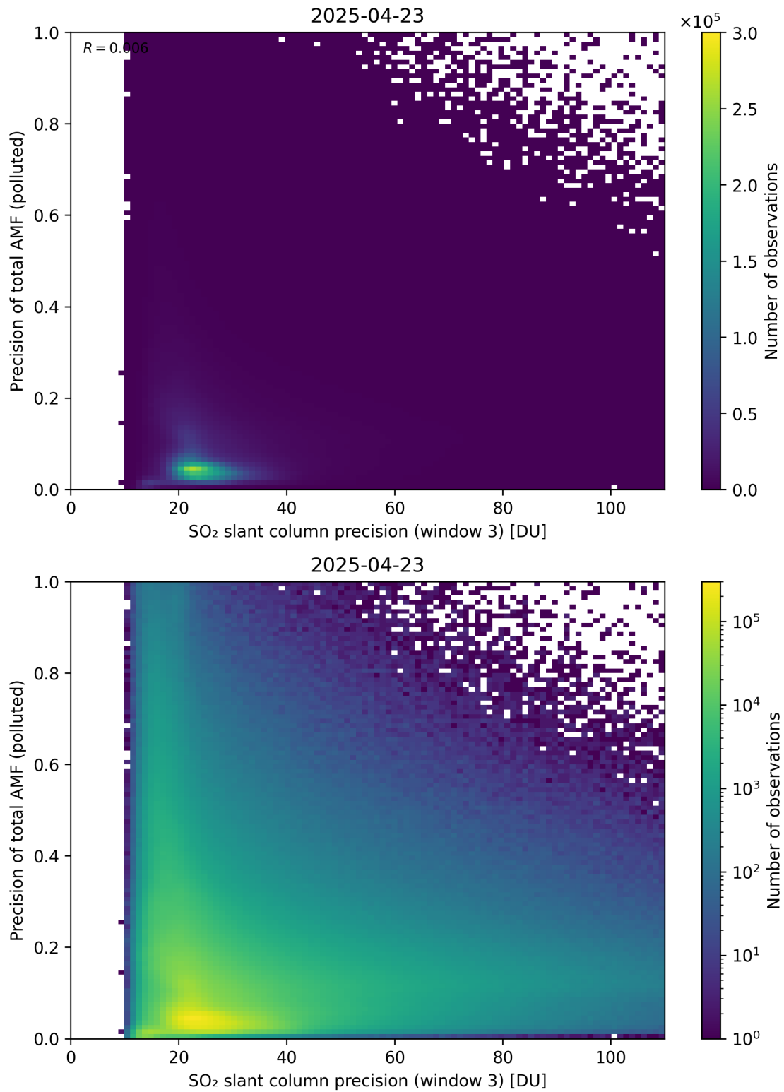
Figure 314: Scatter density plot of “SO 2 slant column precision (window 3)” against “Precision of total AMF (polluted)” for 2025-04-22 to 2025-04-24.
