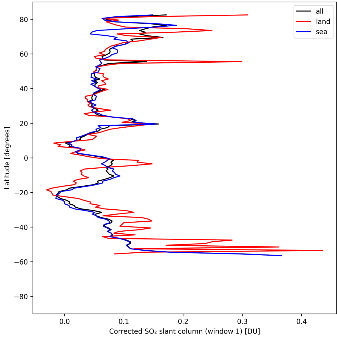
Figure 39: Zonal average of “Corrected SO 2 slant column (window 1)” for 2025-04-22 to 2025-04-24.
