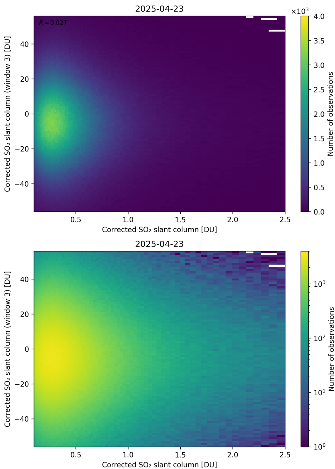
Figure 236: Scatter density plot of “Corrected SO 2 slant column” against “Corrected SO 2 slant column (window 3)” for 2025-04-22 to 2025-04-24.
