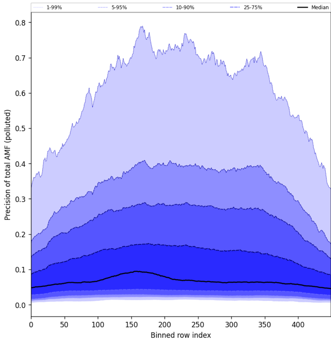
Figure 106: Along track statistics of “Precision of total AMF (polluted)” for 2025-04-22 to 2025-04-24
