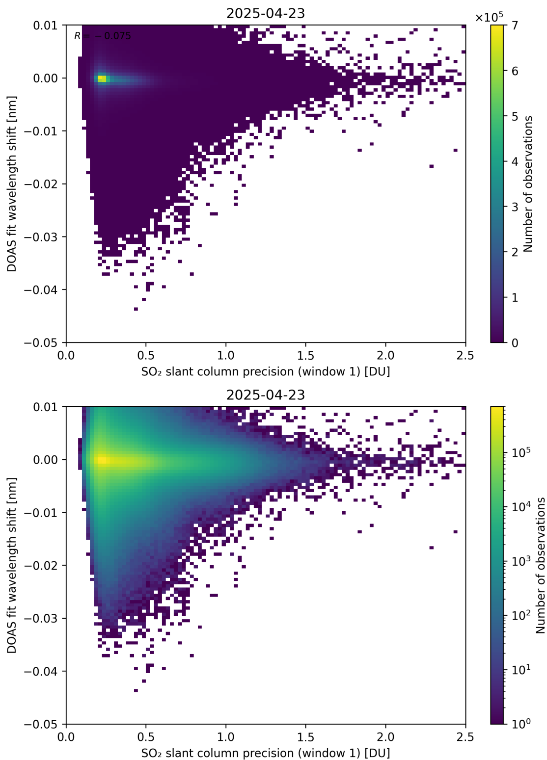
Figure 271: Scatter density plot of “SO 2 slant column precision (window 1)” against “DOAS fit wavelength shift” for 2025-04-22 to 2025-04-24.
