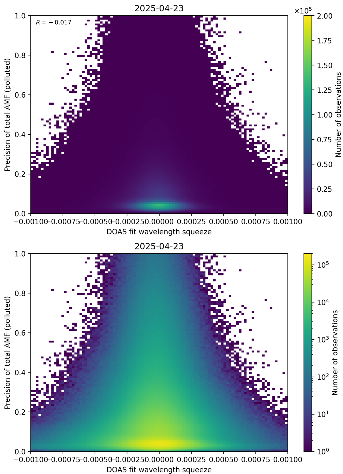
Figure 146: Scatter density plot of “DOAS fit wavelength squeeze” against “Precision of total AMF (polluted)” for 2025-04-22 to 2025-04-24.
