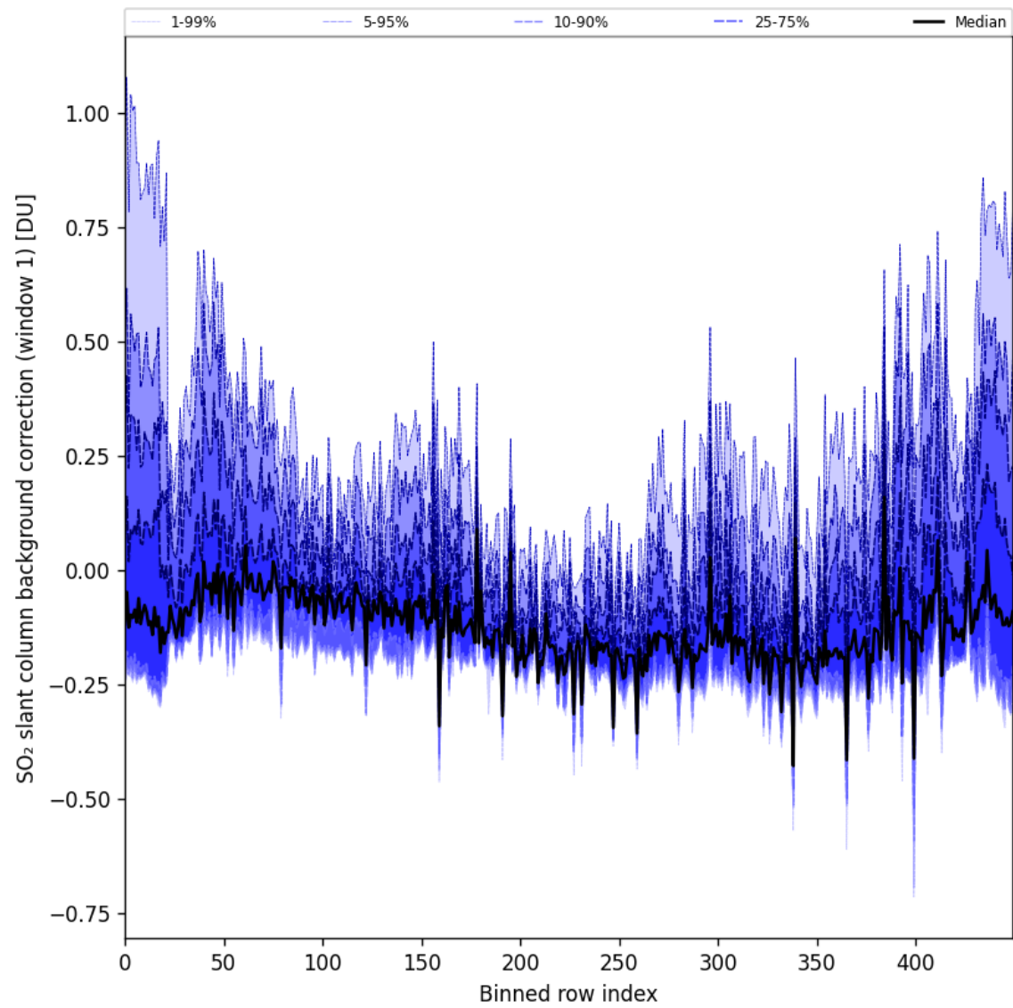
Figure 92: Along track statistics of “SO 2 slant column background correction (window 1)” for 2025-04-22 to 2025-04-24
