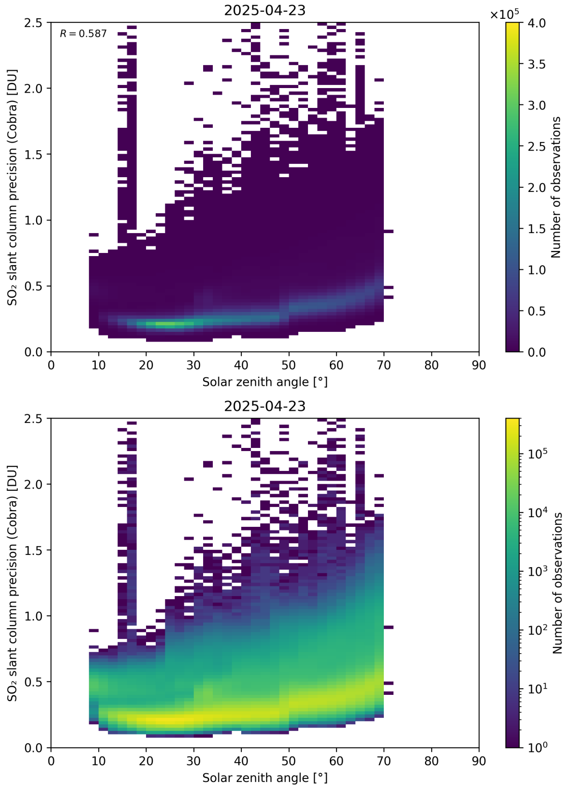
Figure 180: Scatter density plot of “Solar zenith angle” against “SO 2 slant column precision (Cobra)” for 2025-04-22 to 2025-04-24.
