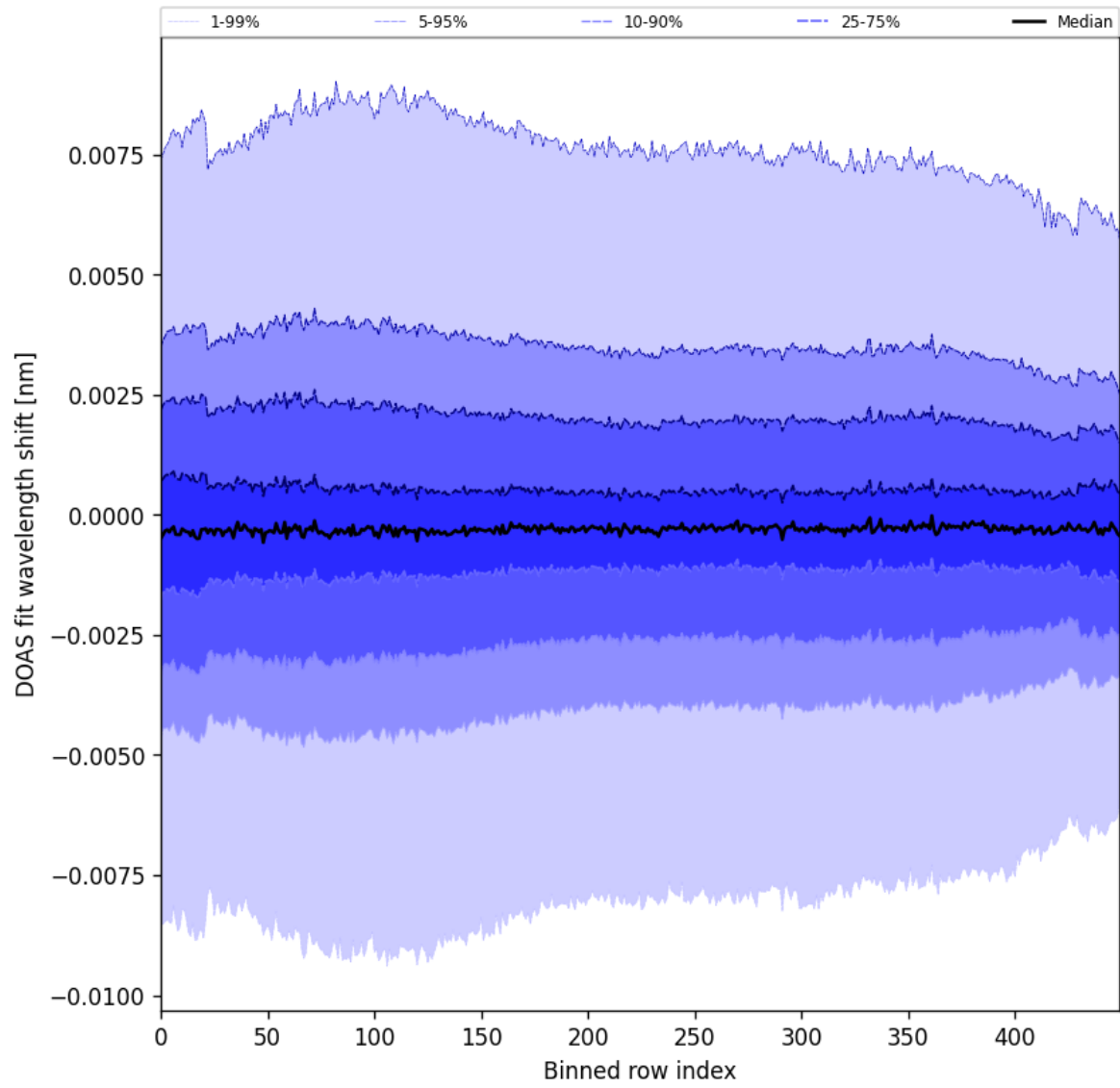
Figure 102: Along track statistics of “DOAS fit wavelength shift” for 2025-04-22 to 2025-04-24
