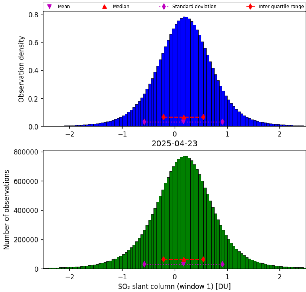
Figure 63: Histogram of “SO 2 slant column (window 1)” for 2025-04-22 to 2025-04-24
