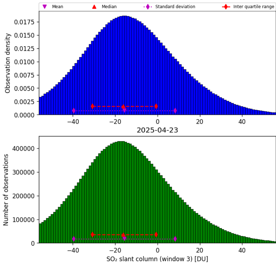
Figure 71: Histogram of “SO 2 slant column (window 3)” for 2025-04-22 to 2025-04-24
