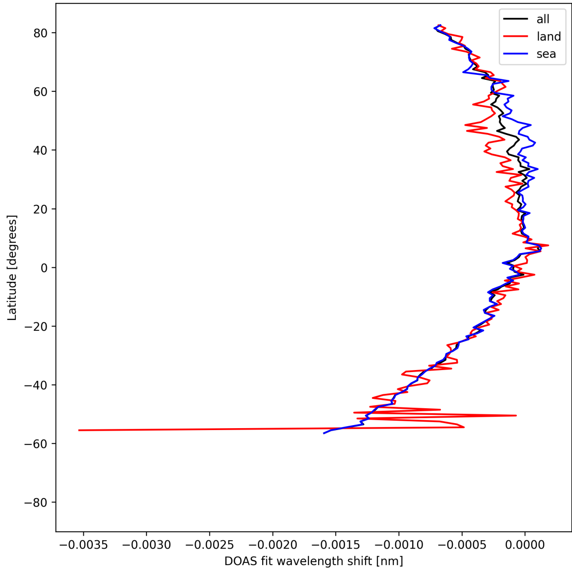
Figure 50: Zonal average of “DOAS fit wavelength shift” for 2025-04-22 to 2025-04-24.
