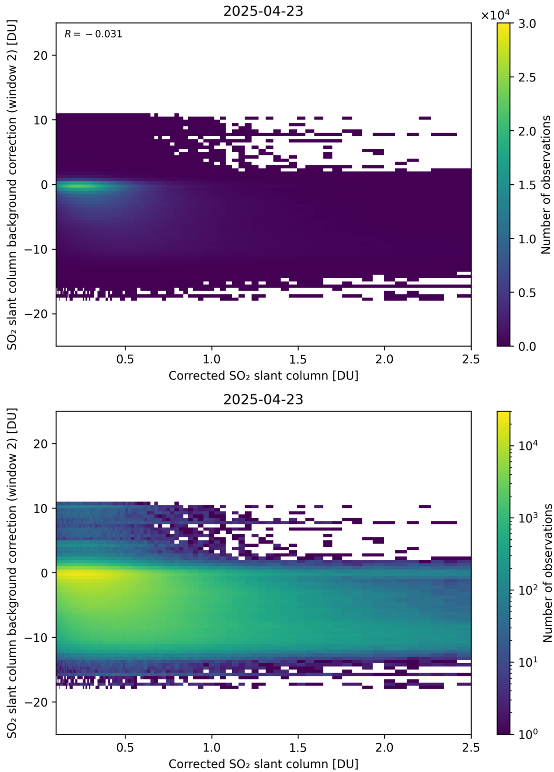
Figure 227: Scatter density plot of “Corrected SO 2 slant column” against “SO 2 slant column background correction (window 2)” for 2025-04-22 to 2025-04-24.
