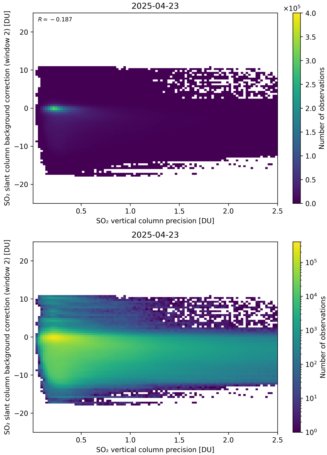
Figure 330: Scatter density plot of “SO 2 vertical column precision” against “SO 2 slant column background correction (window 2)” for 2025-04-22 to 2025-04-24.
