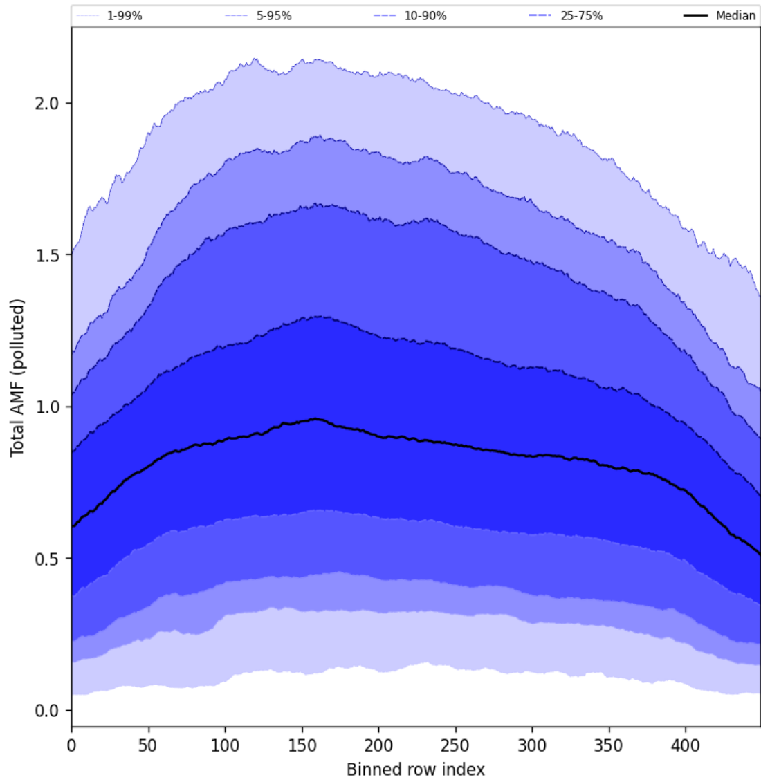
Figure 105: Along track statistics of “Total AMF (polluted)” for 2025-04-22 to 2025-04-24
