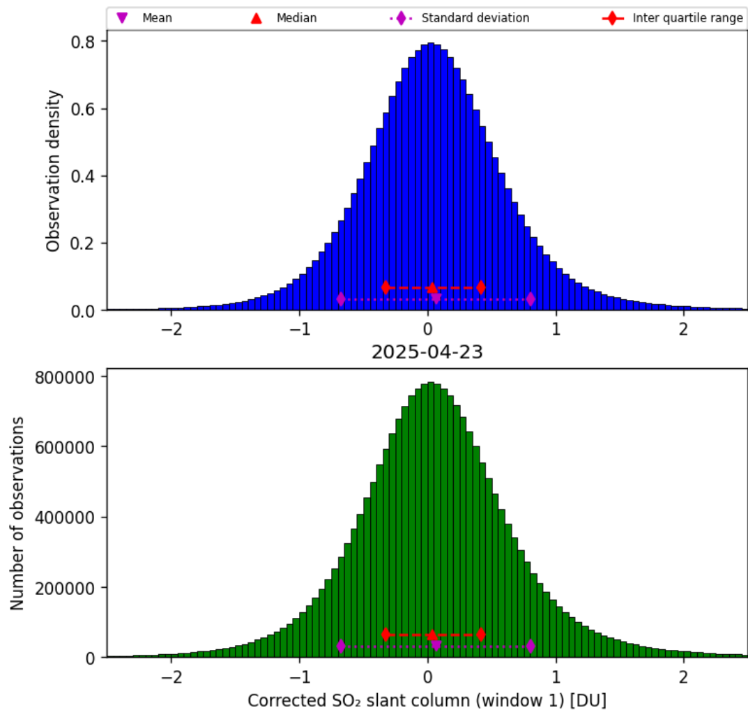
Figure 65: Histogram of “Corrected SO 2 slant column (window 1)” for 2025-04-22 to 2025-04-24
