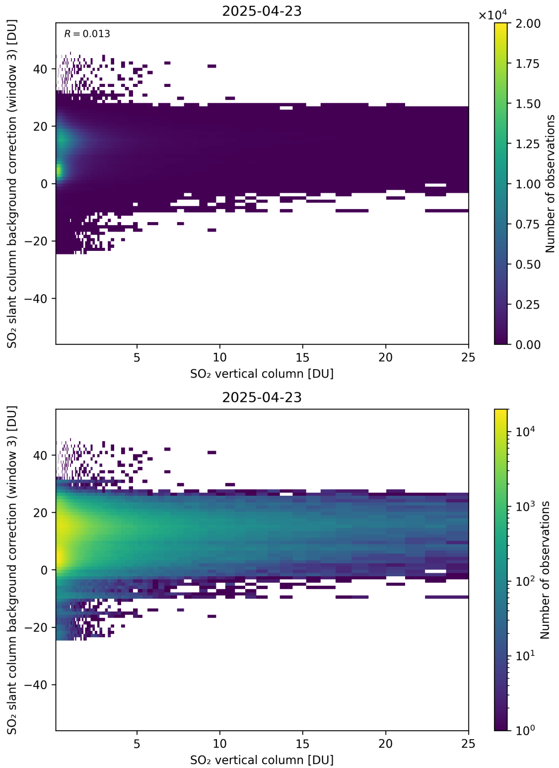
Figure 325: Scatter density plot of “SO 2 vertical column” against “SO 2 slant column background correction (window 3)” for 2025-04-22 to 2025-04-24.
