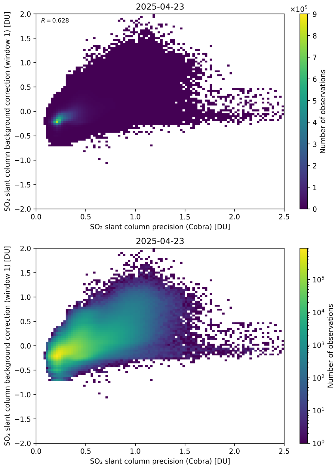
Figure 199: Scatter density plot of “SO 2 slant column precision (Cobra)” against “SO 2 slant column background correction (window 1)” for 2025-04-22 to 2025-04-24.
