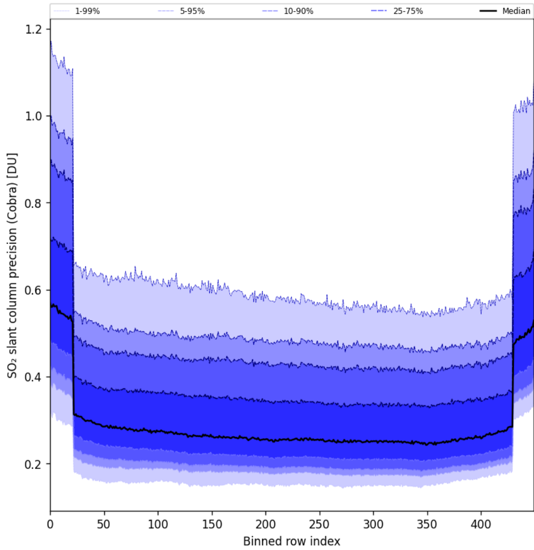
Figure 88: Along track statistics of “SO 2 slant column precision (Cobra)” for 2025-04-22 to 2025-04-24
