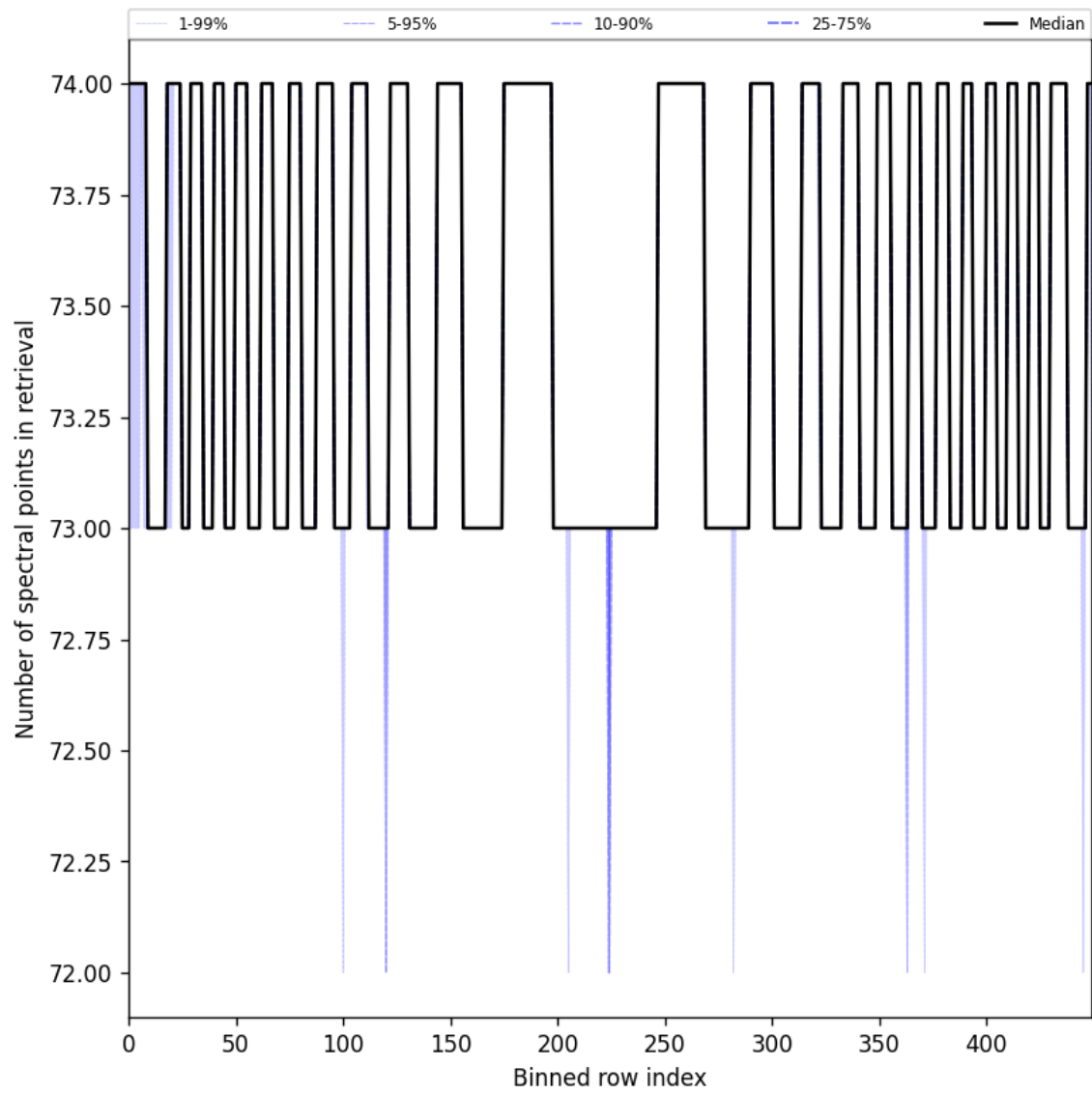
Figure 108: Along track statistics of “Number of spectral points in retrieval” for 2025-04-22 to 2025-04-24
