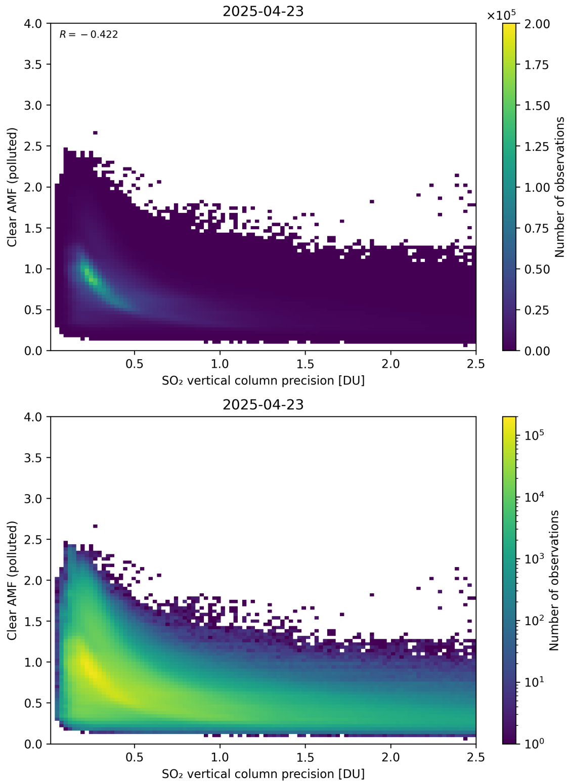
Figure 335: Scatter density plot of “SO 2 vertical column precision” against “Clear AMF (polluted)” for 2025-04-22 to 2025-04-24.
