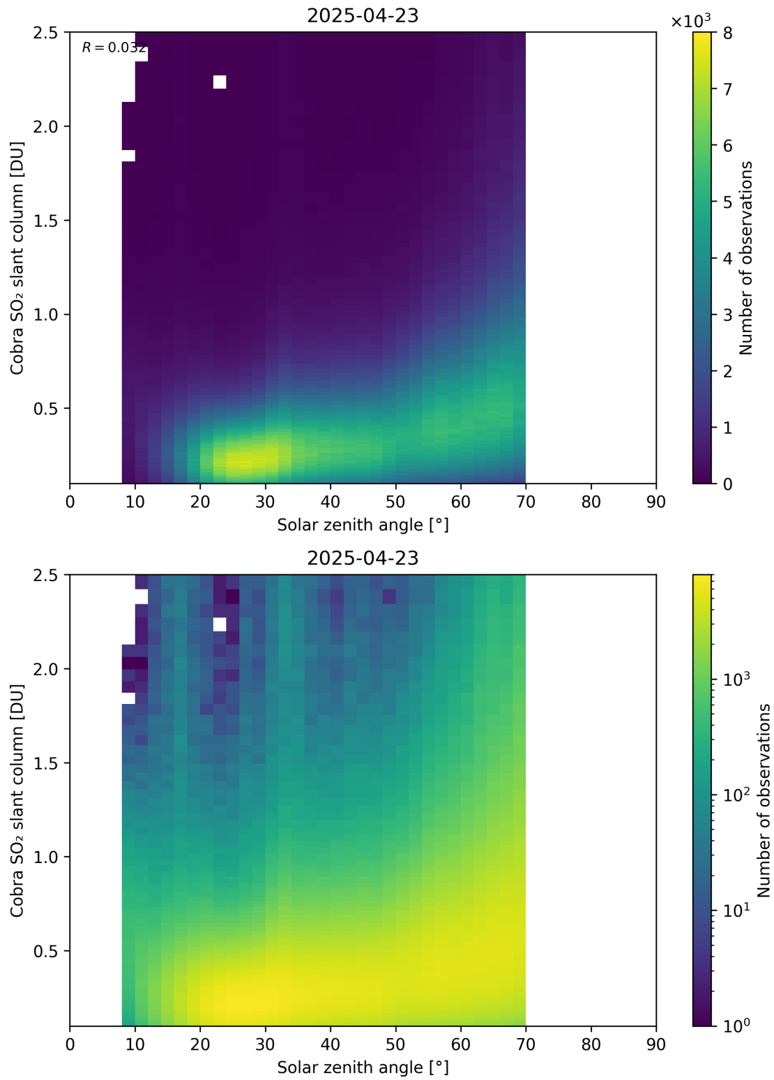
Figure 179: Scatter density plot of “Solar zenith angle” against “Cobra SO 2 slant column” for 2025-04-22 to 2025-04-24.
