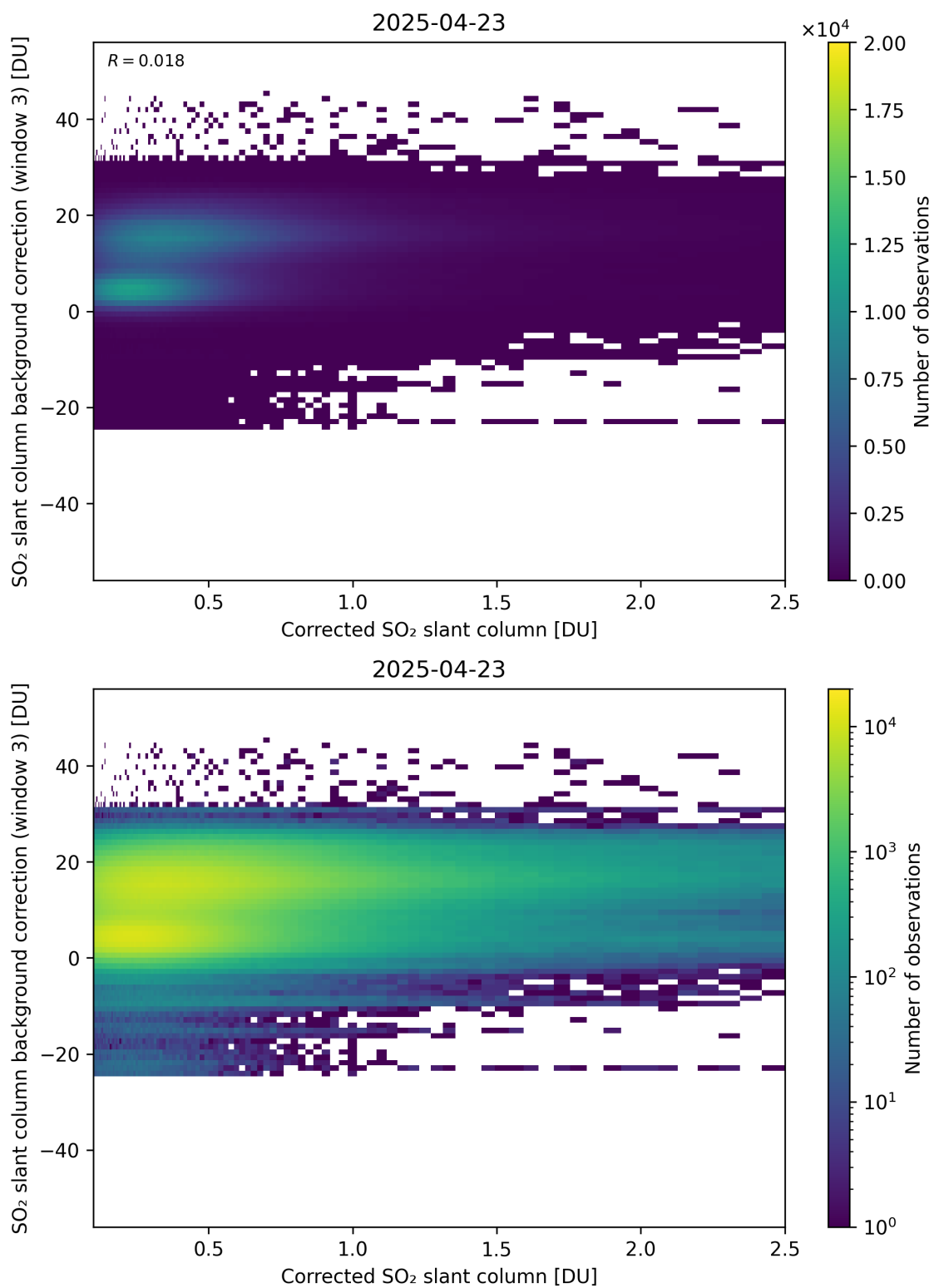
Figure 228: Scatter density plot of “Corrected SO 2 slant column” against “SO 2 slant column background correction (window 3)” for 2025-04-22 to 2025-04-24.
