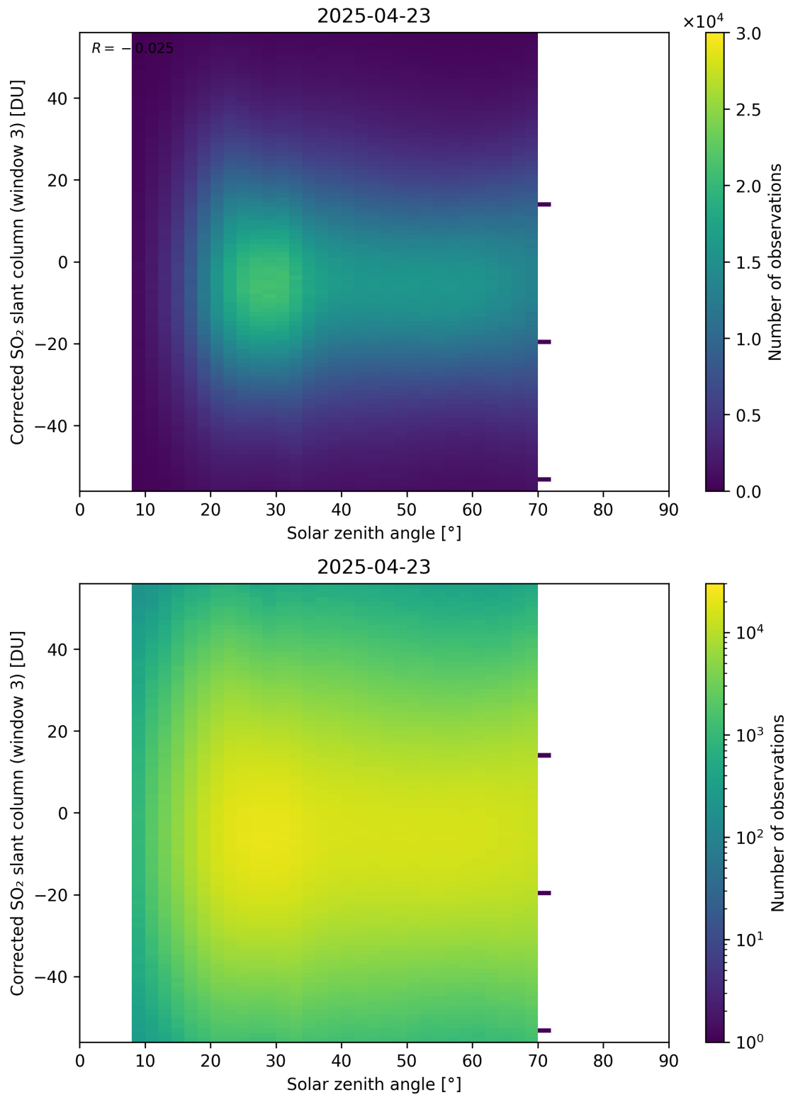
Figure 183: Scatter density plot of “Solar zenith angle” against “Corrected SO 2 slant column (window 3)” for 2025-04-22 to 2025-04-24.
