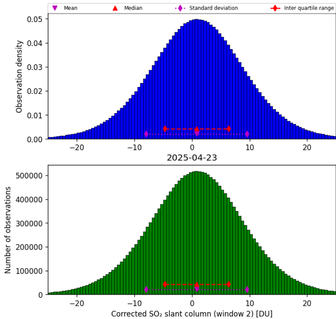
Figure 69: Histogram of “Corrected SO 2 slant column (window 2)” for 2025-04-22 to 2025-04-24
