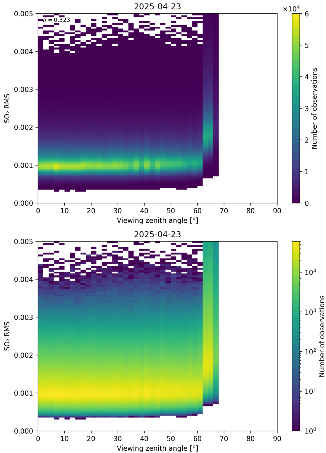
Figure 367: Scatter density plot of “Viewing zenith angle” against “SO 2 RMS” for 2025-04-22 to 2025-04-24.
