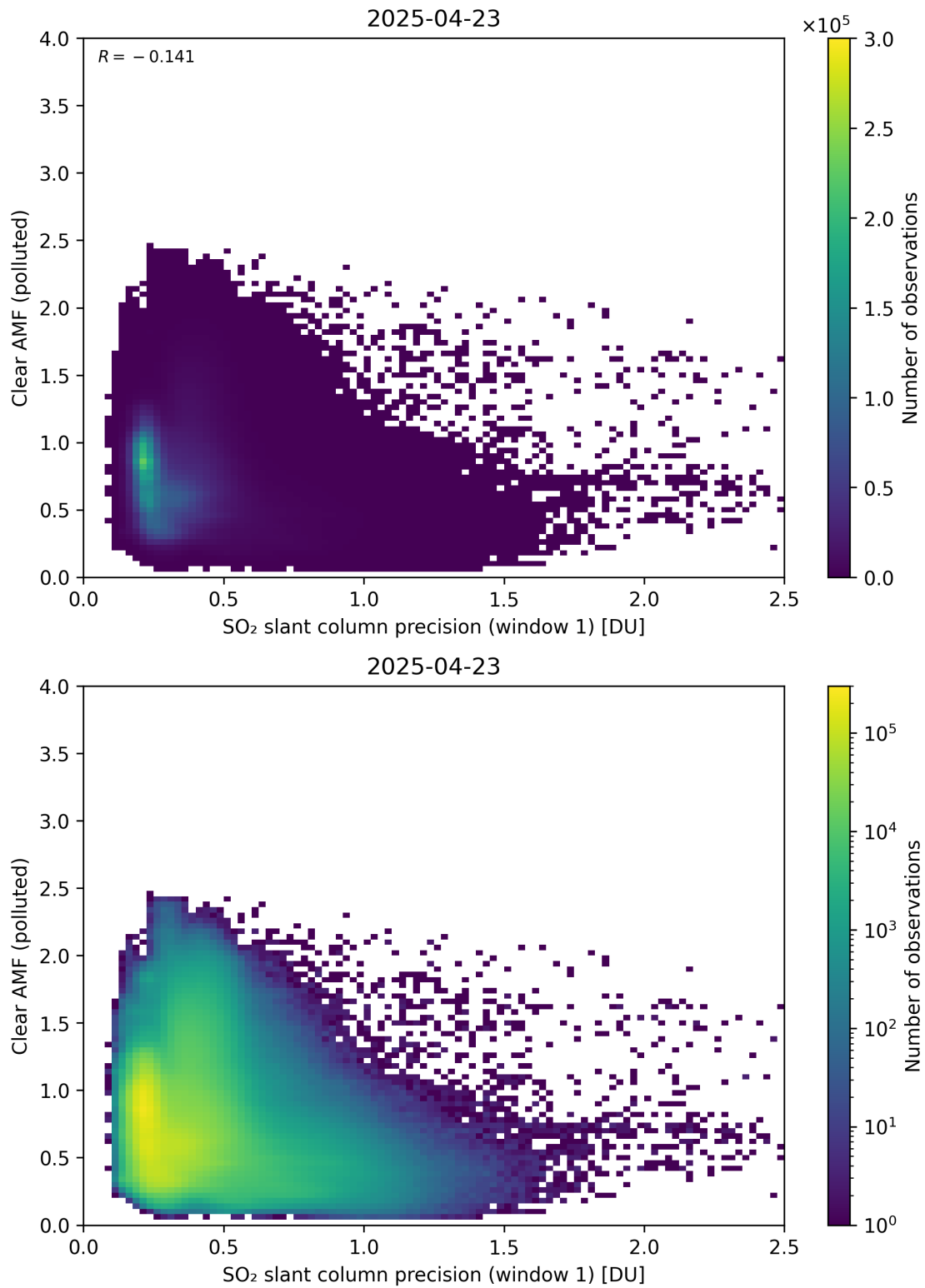
Figure 274: Scatter density plot of “SO 2 slant column precision (window 1)” against “Clear AMF (polluted)” for 2025-04-22 to 2025-04-24.
