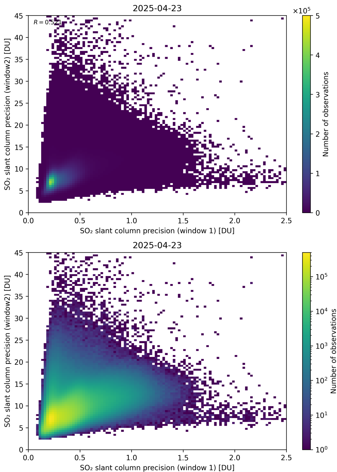
Figure 277: Scatter density plot of “SO 2 slant column precision (window 1)” against “SO 2 slant column precision (window2)” for 2025-04-22 to 2025-04-24.
