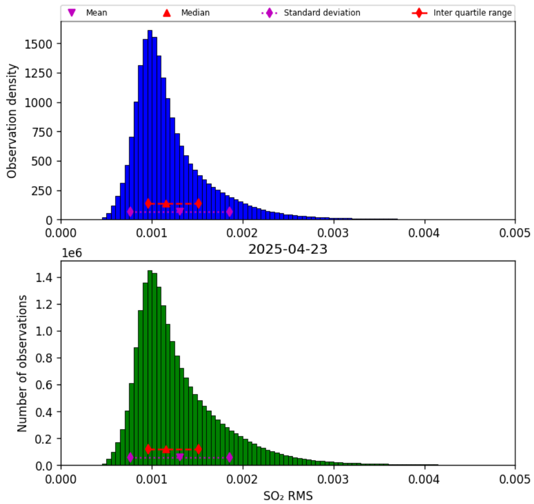
Figure 78: Histogram of “SO 2 RMS” for 2025-04-22 to 2025-04-24
