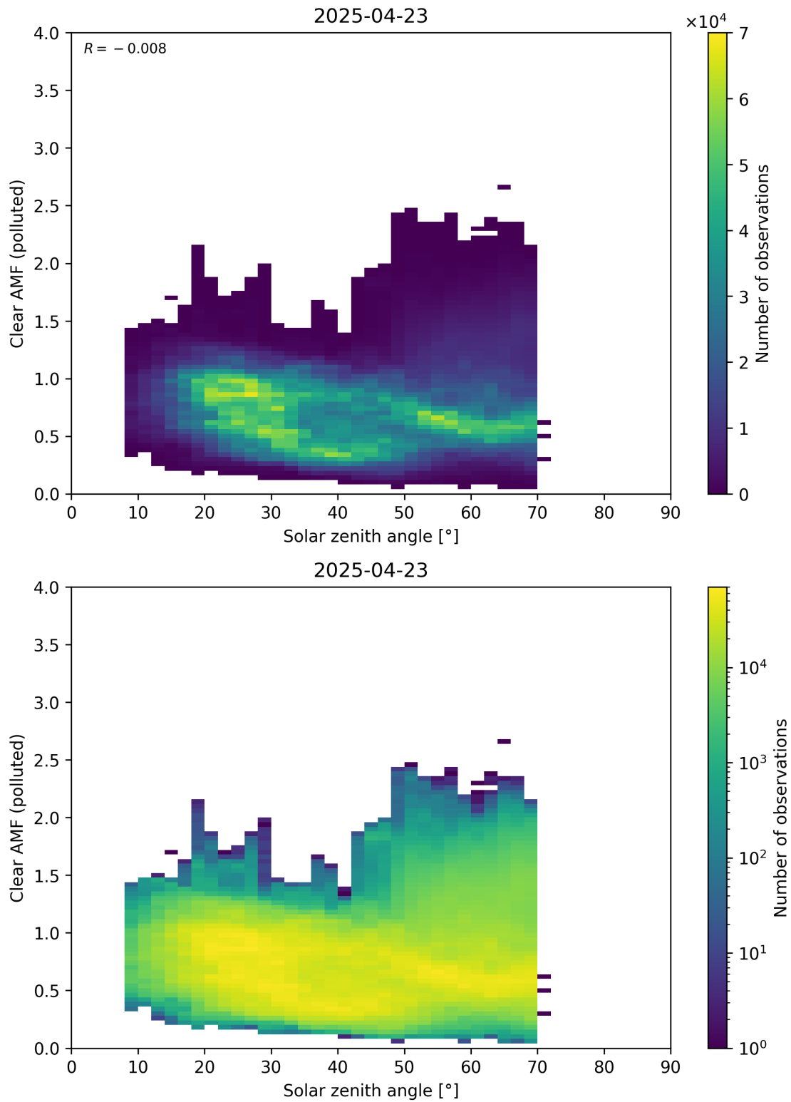
Figure 178: Scatter density plot of “Solar zenith angle” against “Clear AMF (polluted)” for 2025-04-22 to 2025-04-24.
