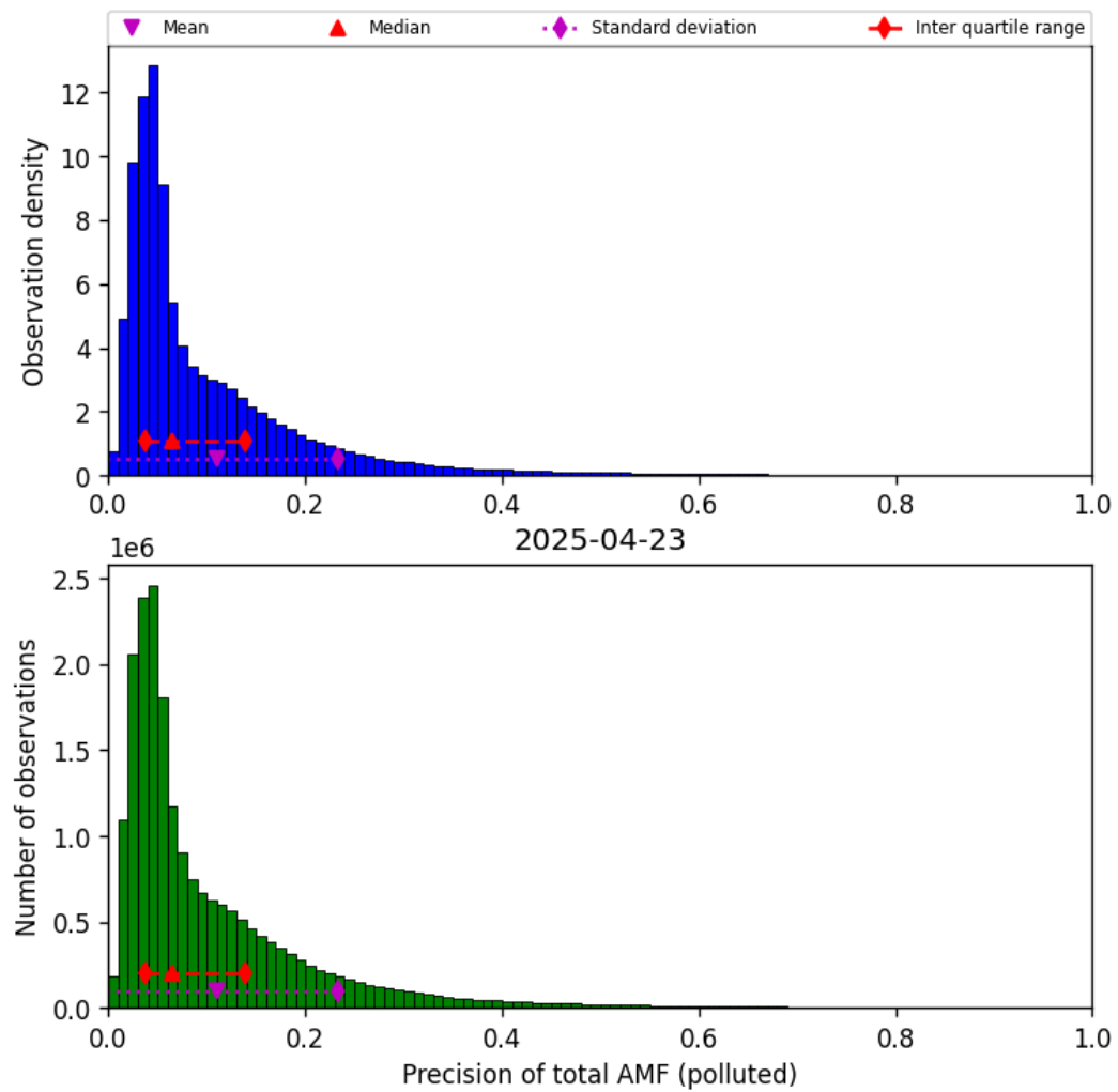
Figure 80: Histogram of “Precision of total AMF (polluted)” for 2025-04-22 to 2025-04-24
