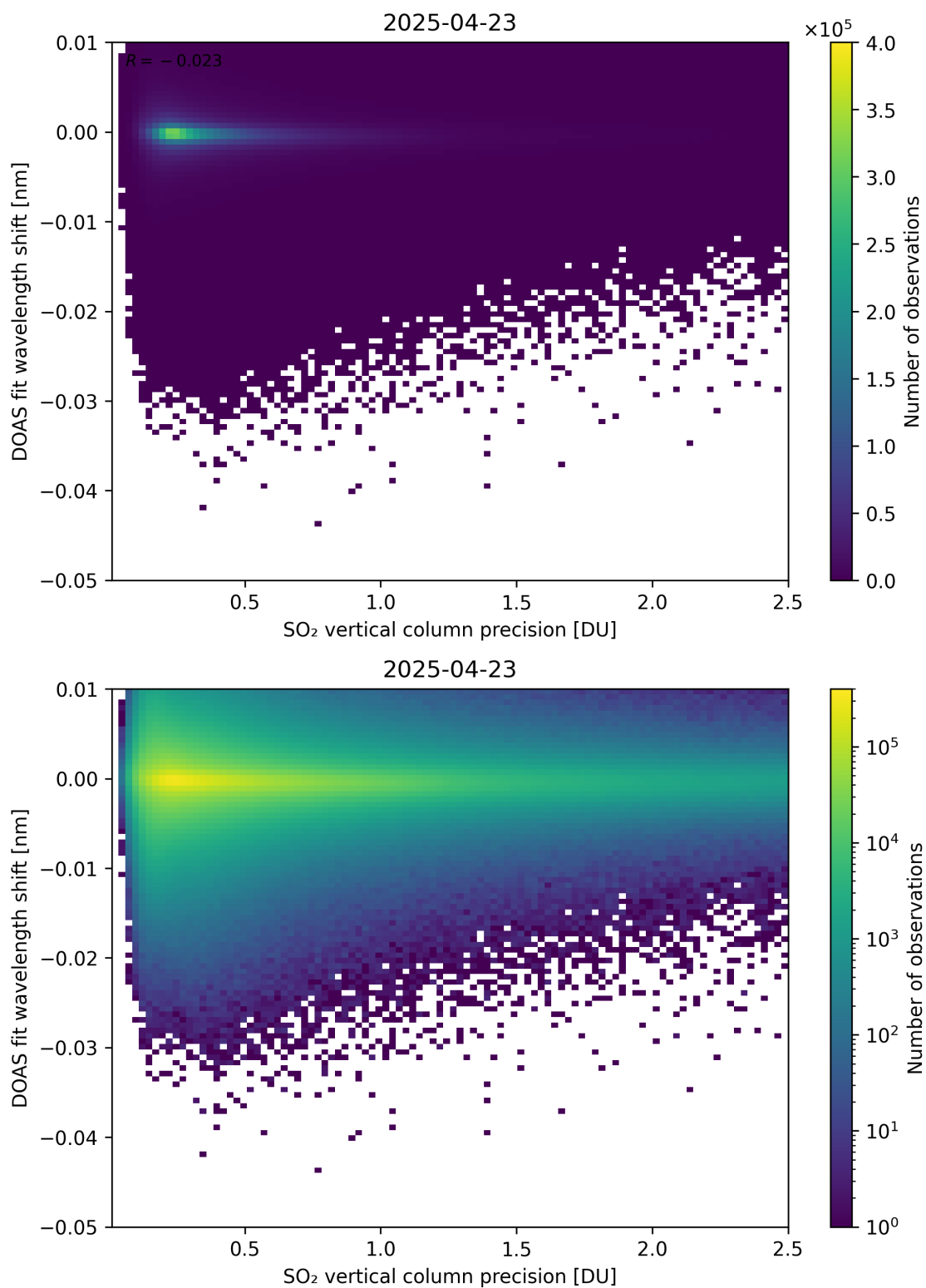
Figure 332: Scatter density plot of “SO 2 vertical column precision” against “DOAS fit wavelength shift” for 2025-04-22 to 2025-04-24.
