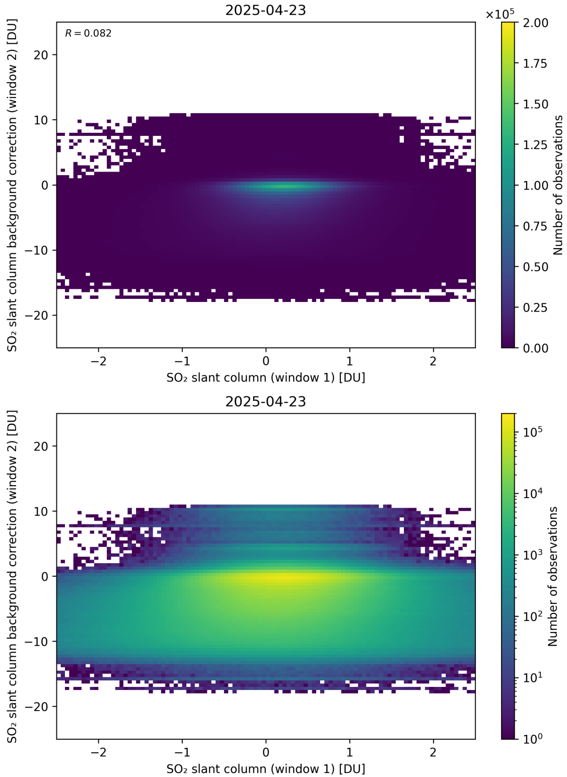
Figure 263: Scatter density plot of “SO 2 slant column (window 1)” against “SO 2 slant column background correction (window 2)” for 2025-04-22 to 2025-04-24.
