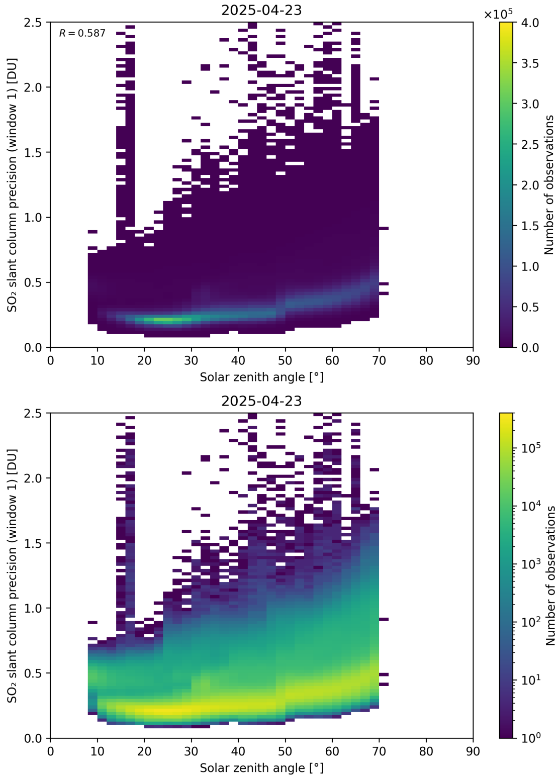
Figure 185: Scatter density plot of “Solar zenith angle” against “SO 2 slant column precision (window 1)” for 2025-04-22 to 2025-04-24.
