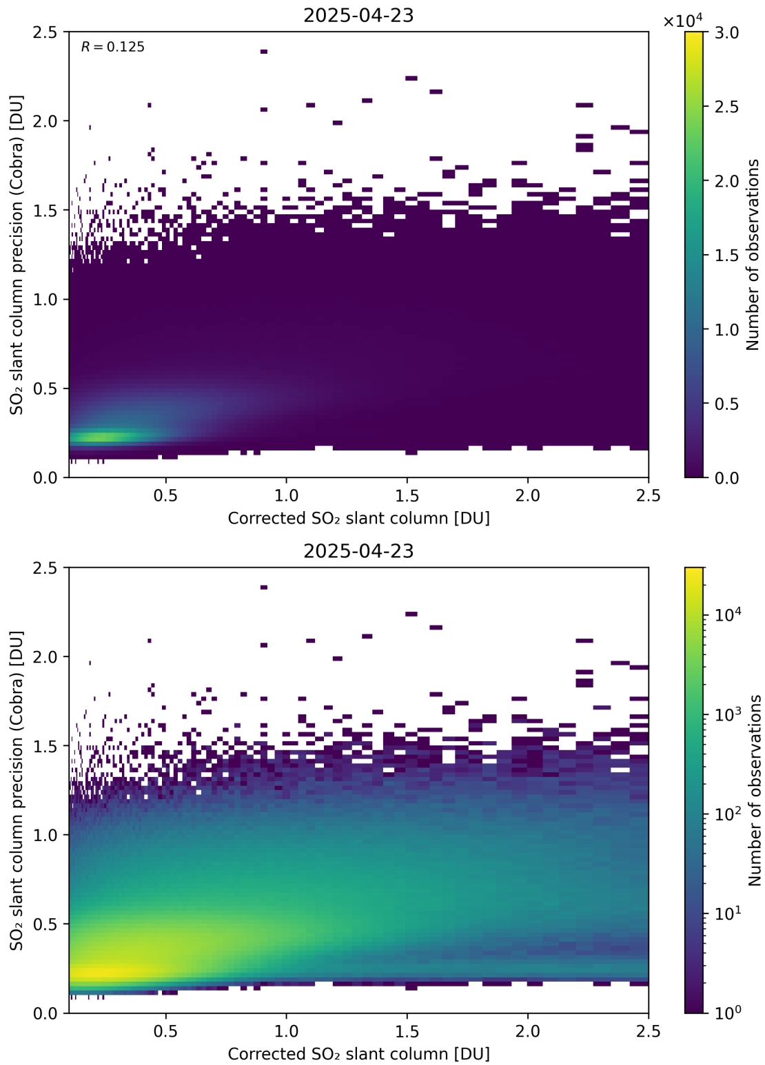
Figure 234: Scatter density plot of “Corrected SO 2 slant column” against “SO 2 slant column precision (Cobra)” for 2025-04-22 to 2025-04-24.
