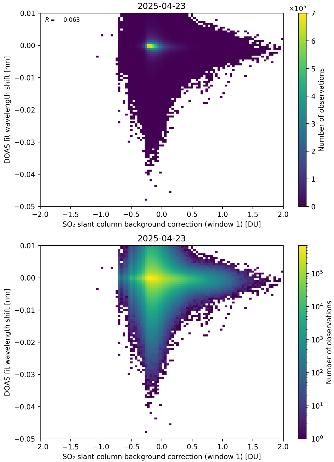
Figure 111: Scatter density plot of “SO 2 slant column background correction (window 1)” against “DOAS fit wavelength shift” for 2025-04-22 to 2025-04-24.
