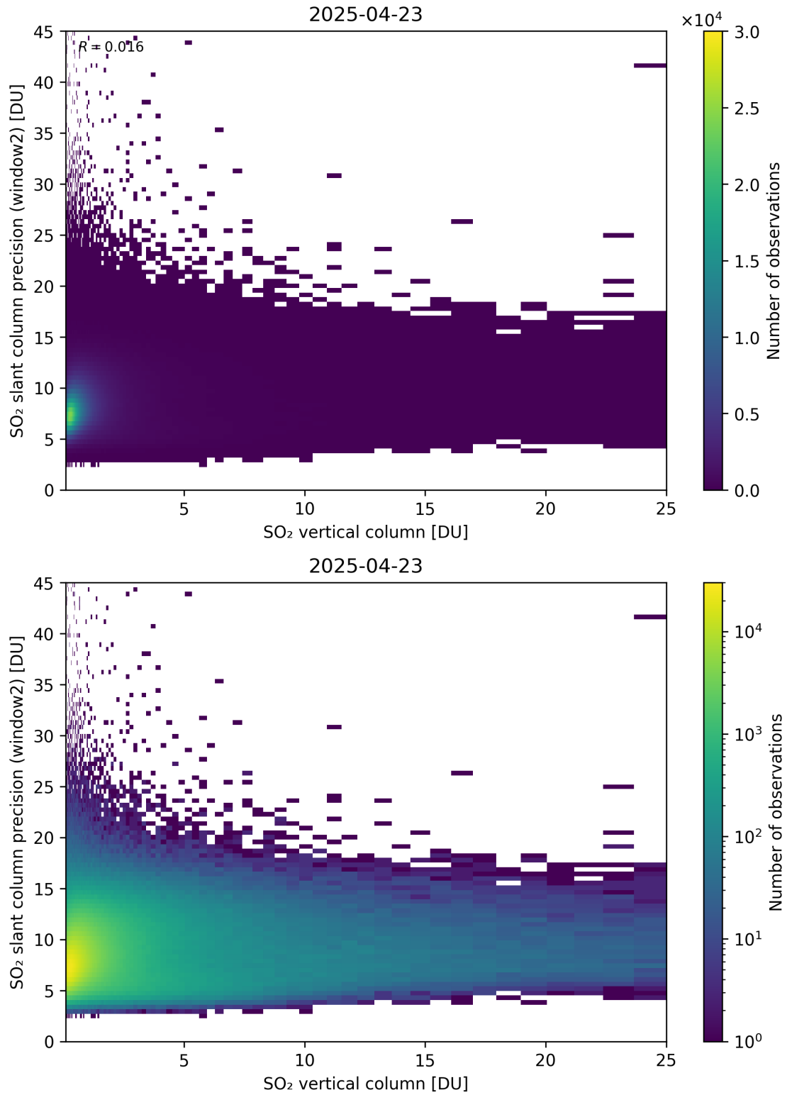
Figure 356: Scatter density plot of “SO 2 vertical column” against “SO 2 slant column precision (window2)” for 2025-04-22 to 2025-04-24.
