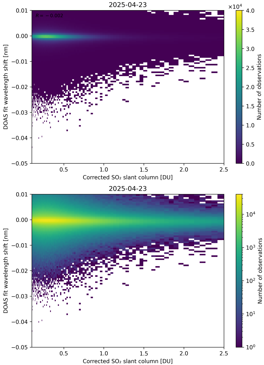
Figure 229: Scatter density plot of “Corrected SO 2 slant column” against “DOAS fit wavelength shift” for 2025-04-22 to 2025-04-24.
