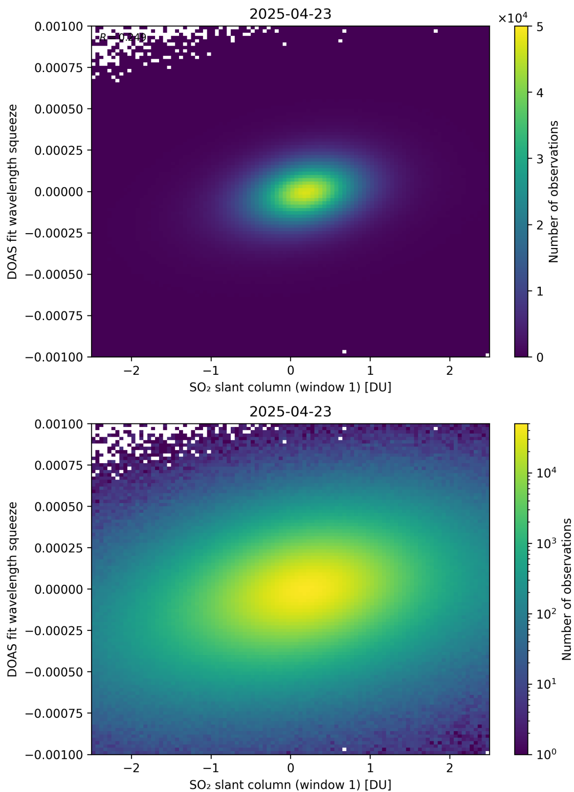
Figure 266: Scatter density plot of “SO 2 slant column (window 1)” against “DOAS fit wavelength squeeze” for 2025-04-22 to 2025-04-24.
