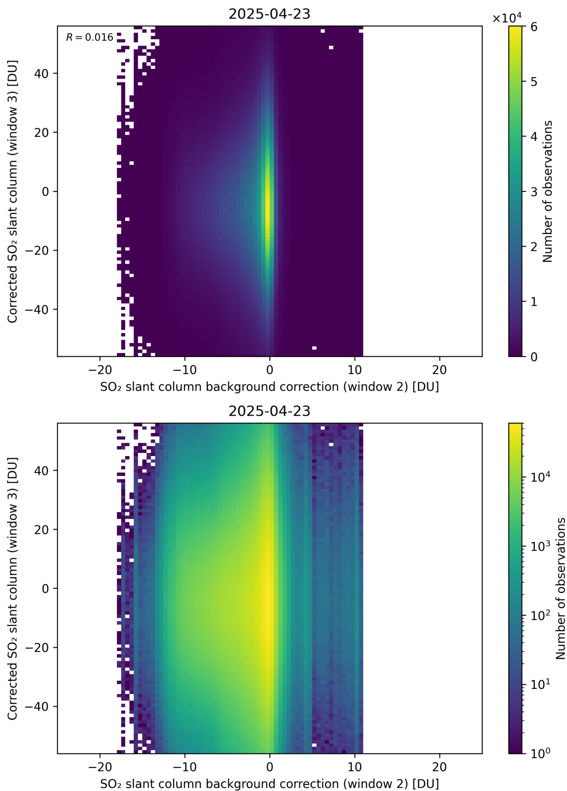
Figure 127: Scatter density plot of “SO 2 slant column background correction (window 2)” against “Corrected SO 2 slant column (window 3)” for 2025-04-22 to 2025-04-24.
