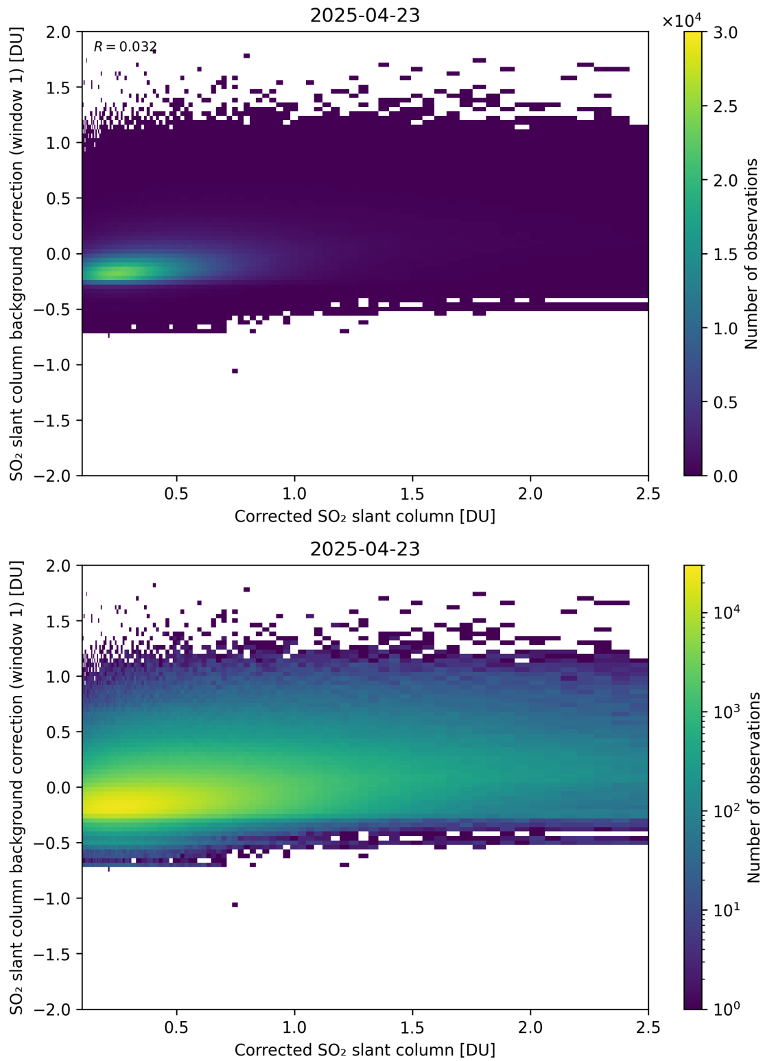
Figure 226: Scatter density plot of “Corrected SO 2 slant column” against “SO 2 slant column background correction (window 1)” for 2025-04-22 to 2025-04-24.
