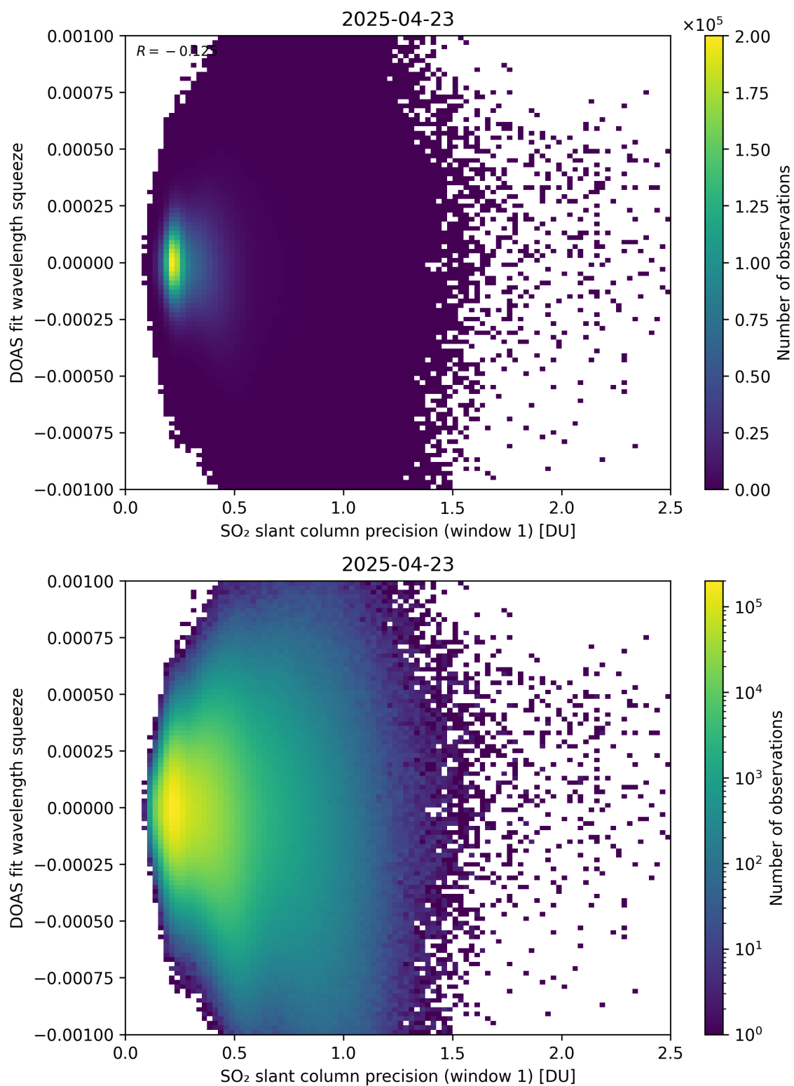
Figure 272: Scatter density plot of “SO 2 slant column precision (window 1)” against “DOAS fit wavelength squeeze” for 2025-04-22 to 2025-04-24.
