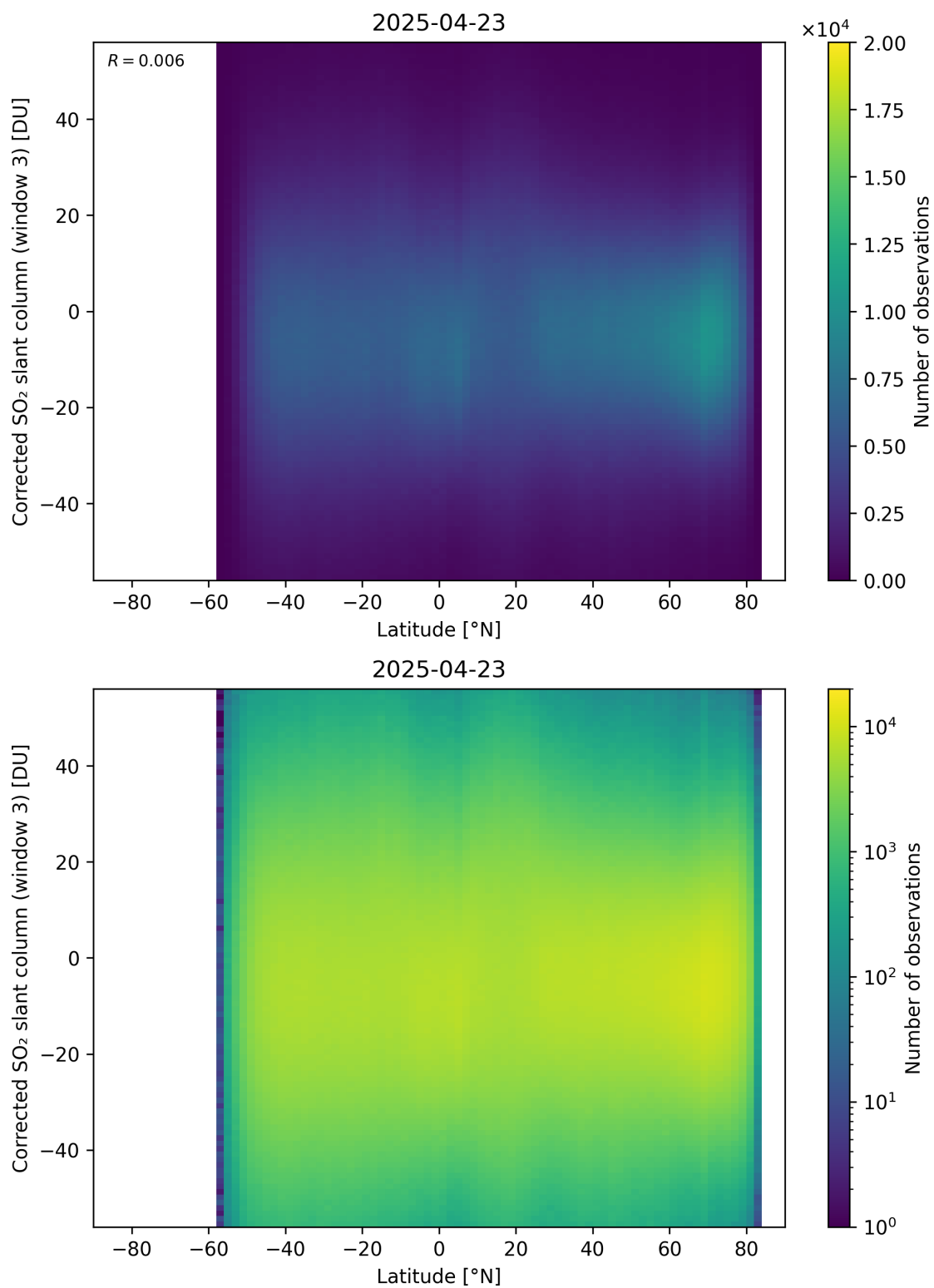
Figure 161: Scatter density plot of “Latitude” against “Corrected SO 2 slant column (window 3)” for 2025-04-22 to 2025-04-24.
