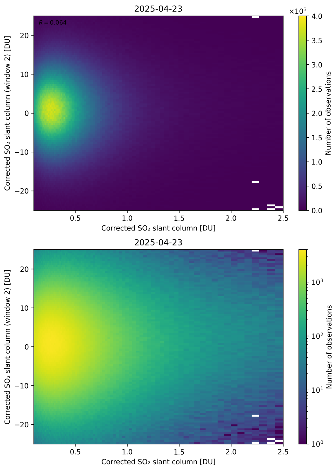
Figure 235: Scatter density plot of “Corrected SO 2 slant column” against “Corrected SO 2 slant column (window 2)” for 2025-04-22 to 2025-04-24.
