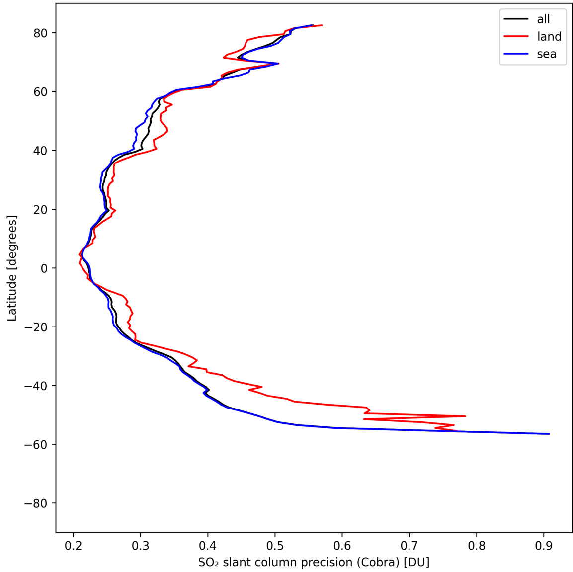
Figure 36: Zonal average of “SO 2 slant column precision (Cobra)” for 2025-04-22 to 2025-04-24.
