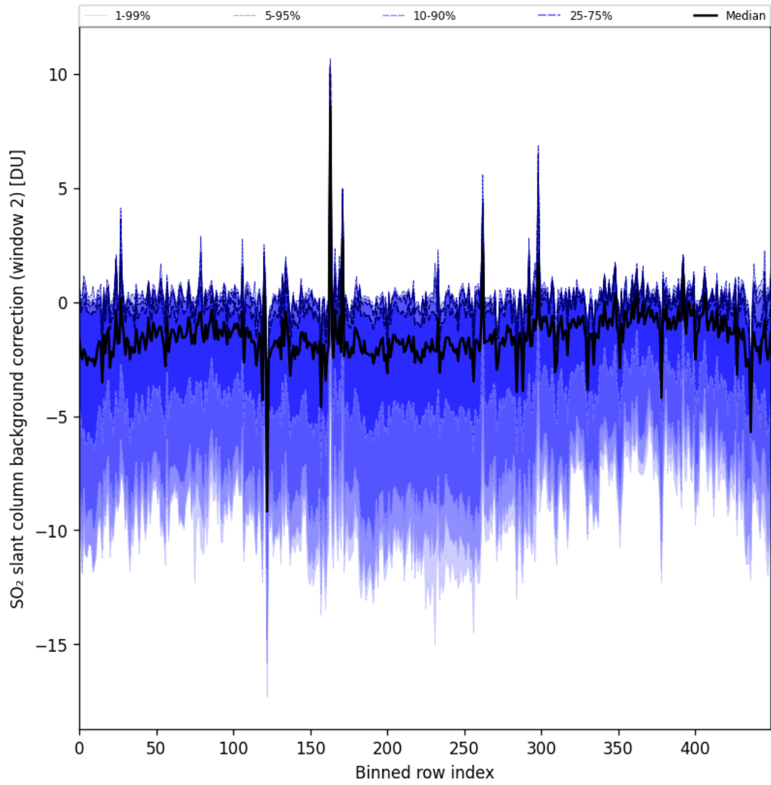
Figure 96: Along track statistics of “SO 2 slant column background correction (window 2)” for 2025-04-22 to 2025-04-24
