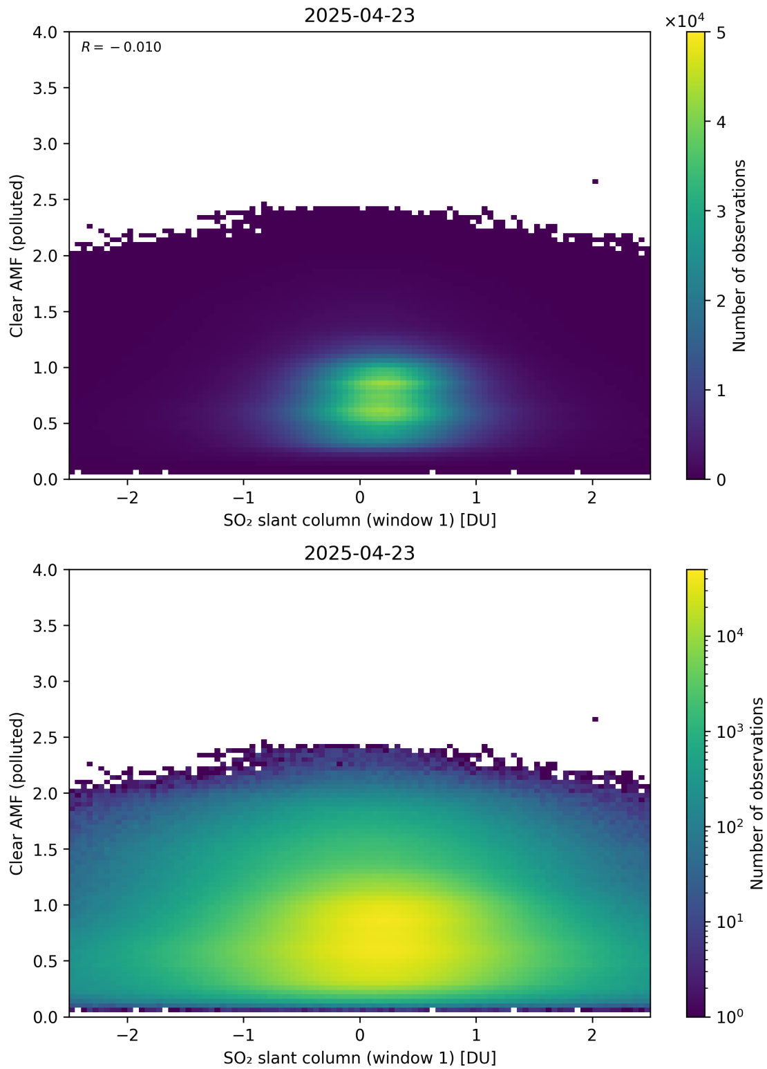
Figure 282: Scatter density plot of “SO 2 slant column (window 1)” against “Clear AMF (polluted)” for 2025-04-22 to 2025-04-24.
