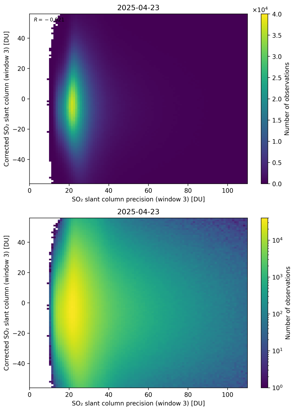
Figure 312: Scatter density plot of “SO 2 slant column precision (window 3)” against “Corrected SO 2 slant column (window 3)” for 2025-04-22 to 2025-04-24.
