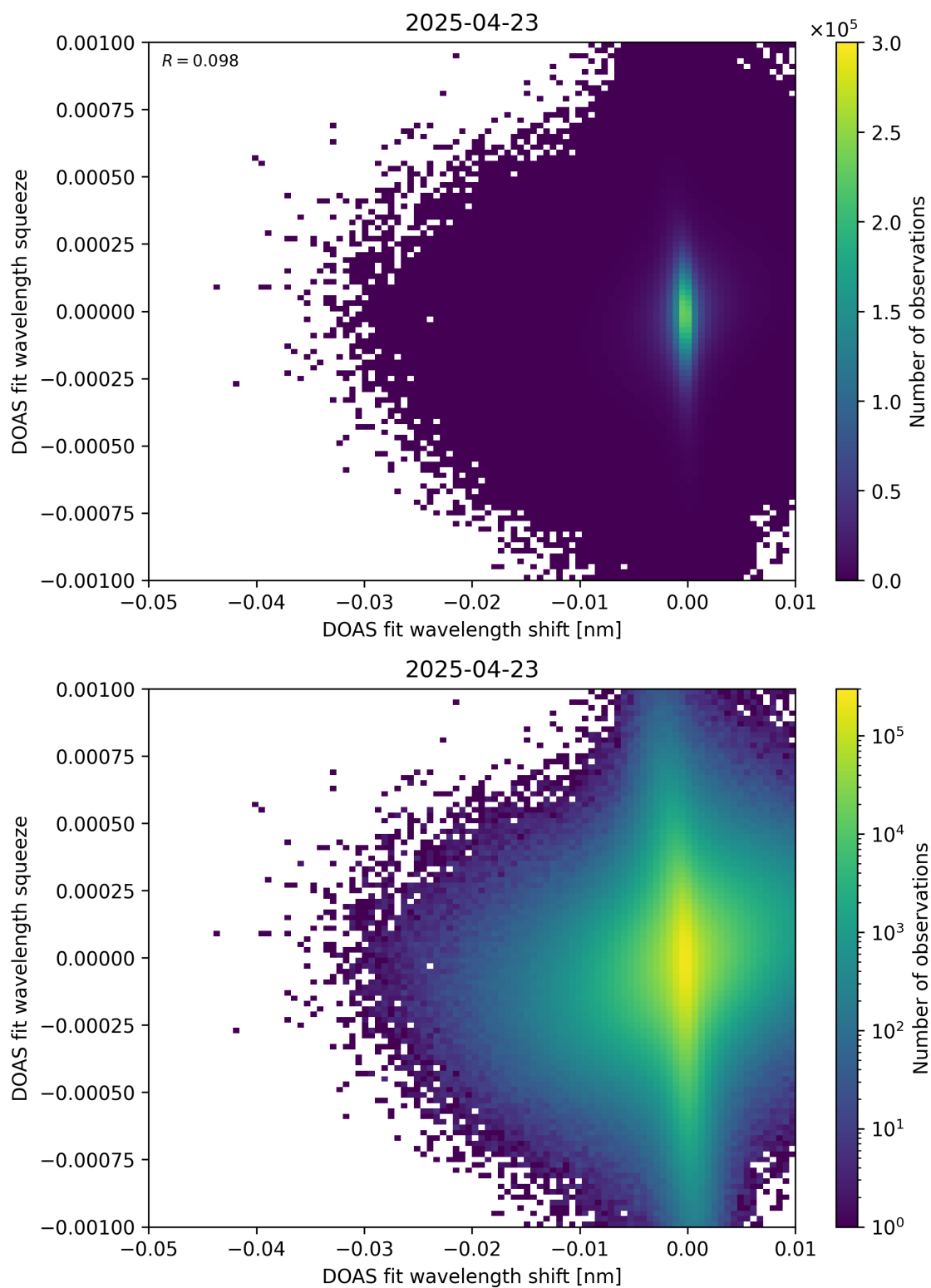
Figure 138: Scatter density plot of “DOAS fit wavelength shift” against “DOAS fit wavelength squeeze” for 2025-04-22 to 2025-04-24.
