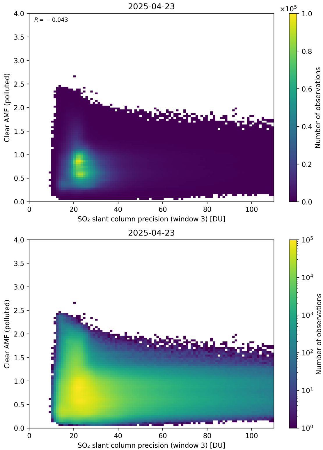
Figure 311: Scatter density plot of “SO 2 slant column precision (window 3)” against “Clear AMF (polluted)” for 2025-04-22 to 2025-04-24.
