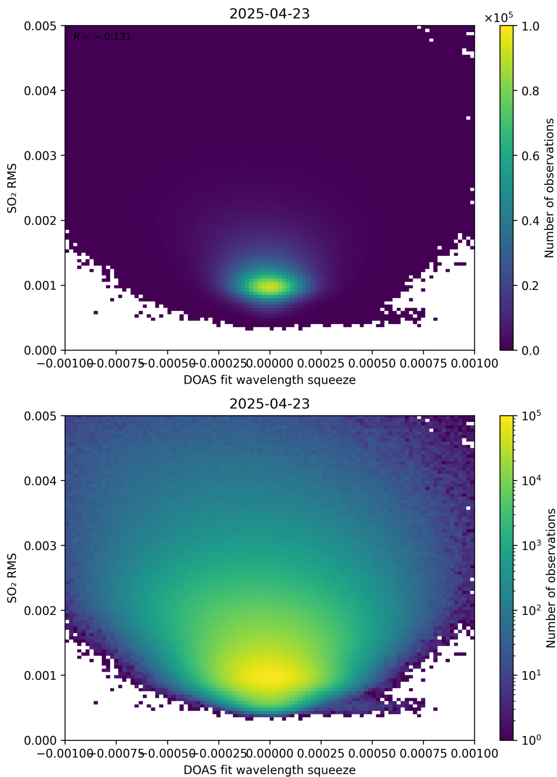
Figure 143: Scatter density plot of “DOAS fit wavelength squeeze” against “SO 2 RMS” for 2025-04-22 to 2025-04-24.
