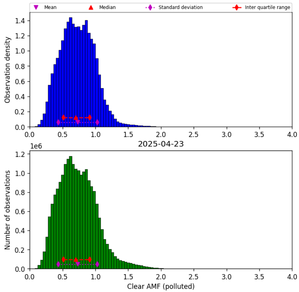
Figure 81: Histogram of “Clear AMF (polluted)” for 2025-04-22 to 2025-04-24
