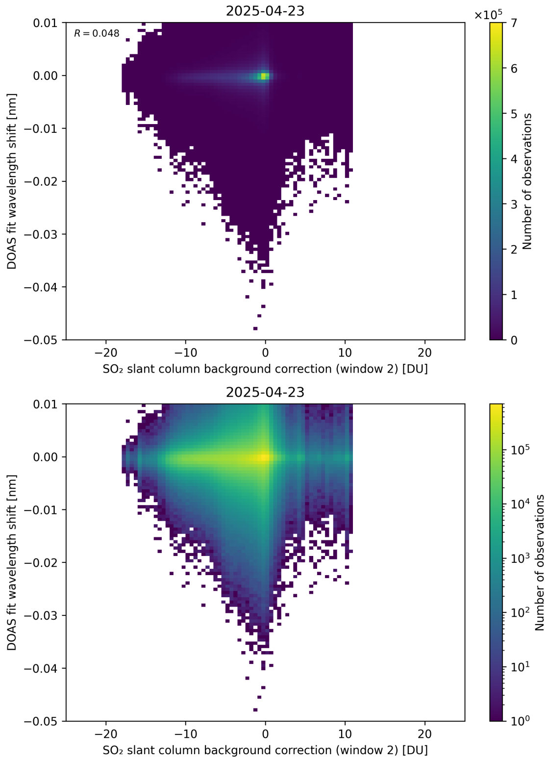
Figure 123: Scatter density plot of “SO 2 slant column background correction (window 2)” against “DOAS fit wavelength shift” for 2025-04-22 to 2025-04-24.
