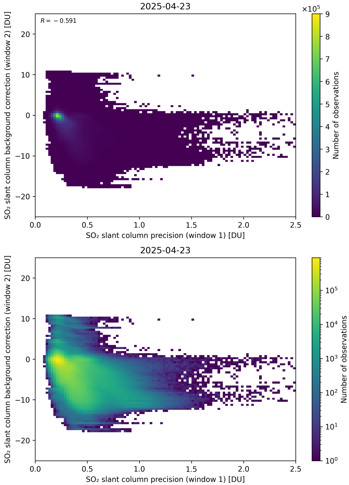
Figure 269: Scatter density plot of “SO 2 slant column precision (window 1)” against “SO 2 slant column background correction (window 2)” for 2025-04-22 to 2025-04-24.
