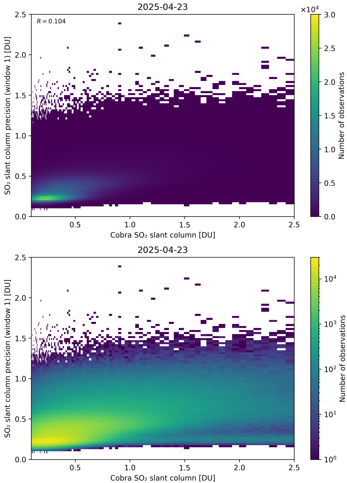
Figure 220: Scatter density plot of “Cobra SO 2 slant column” against “SO 2 slant column precision (window 1)” for 2025-04-22 to 2025-04-24.
