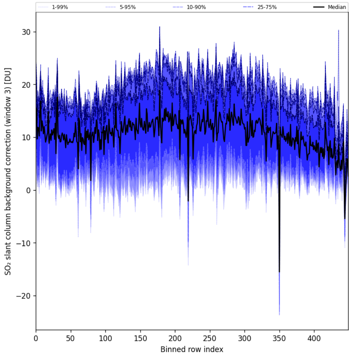
Figure 100: Along track statistics of “SO 2 slant column background correction (window 3)” for 2025-04-22 to 2025-04-24
