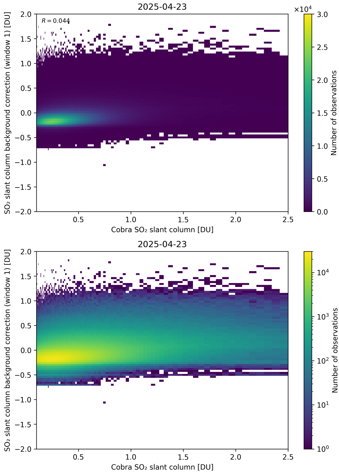
Figure 193: Scatter density plot of “Cobra SO 2 slant column” against “SO 2 slant column background correction (window 1)” for 2025-04-22 to 2025-04-24.
