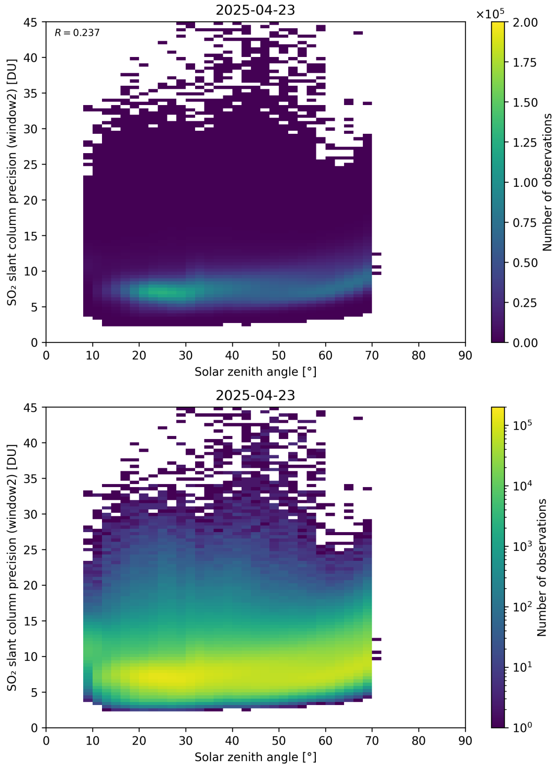
Figure 186: Scatter density plot of “Solar zenith angle” against “SO 2 slant column precision (window2)” for 2025-04-22 to 2025-04-24.
