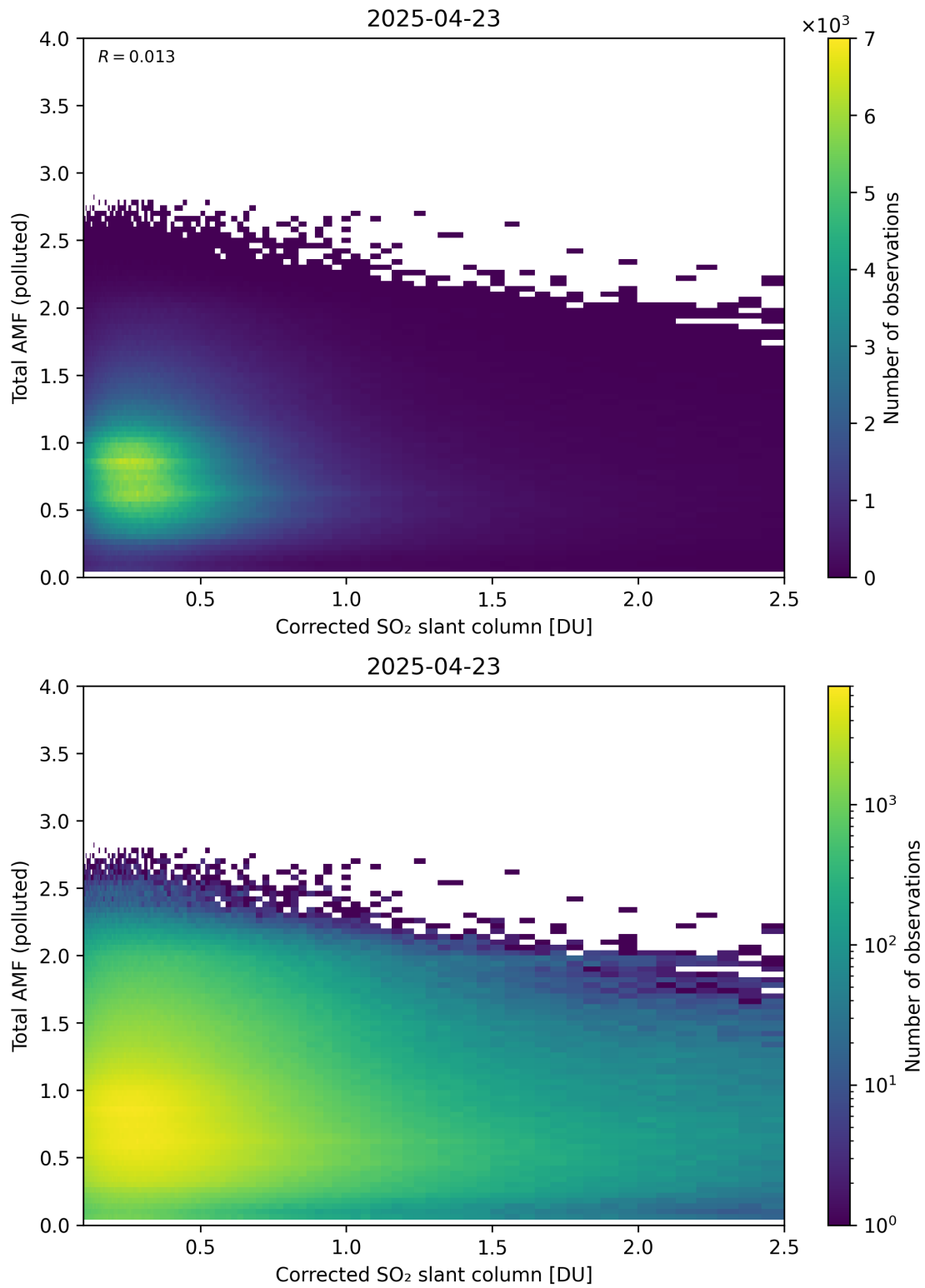
Figure 242: Scatter density plot of “Corrected SO 2 slant column” against “Total AMF (polluted)” for 2025-04-22 to 2025-04-24.
