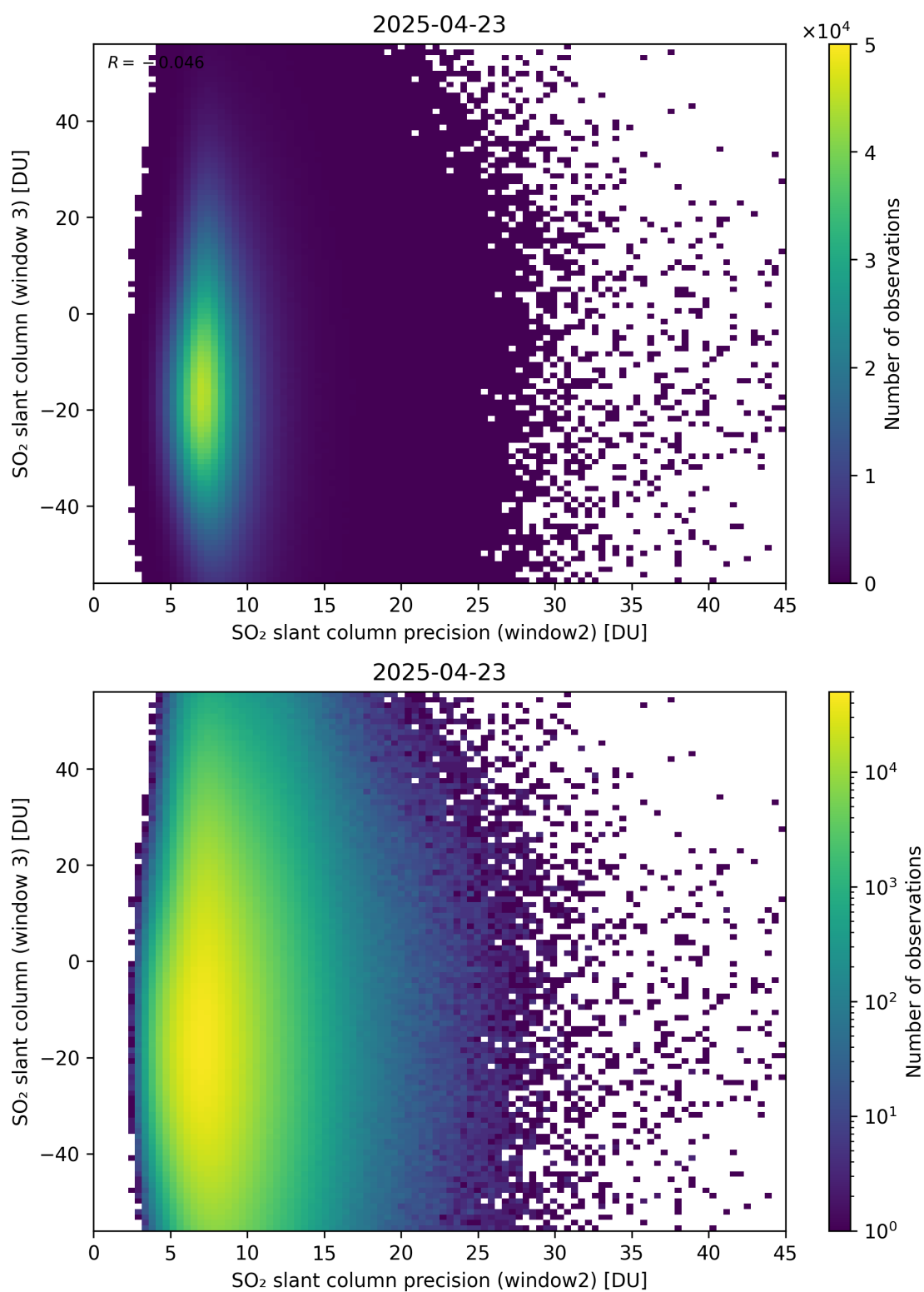
Figure 299: Scatter density plot of “SO 2 slant column precision (window2)” against “SO 2 slant column (window 3)” for 2025-04-22 to 2025-04-24.
