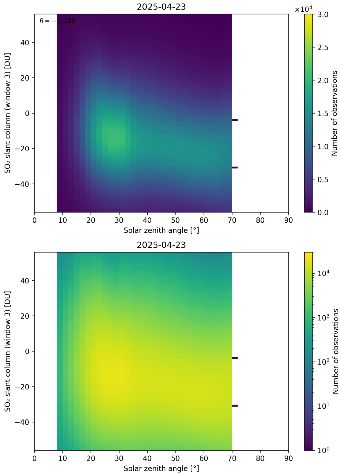
Figure 187: Scatter density plot of “Solar zenith angle” against “SO 2 slant column (window 3)” for 2025-04-22 to 2025-04-24.
