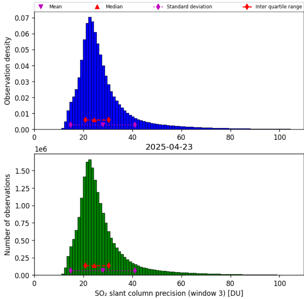
Figure 72: Histogram of “SO 2 slant column precision (window 3)” for 2025-04-22 to 2025-04-24
