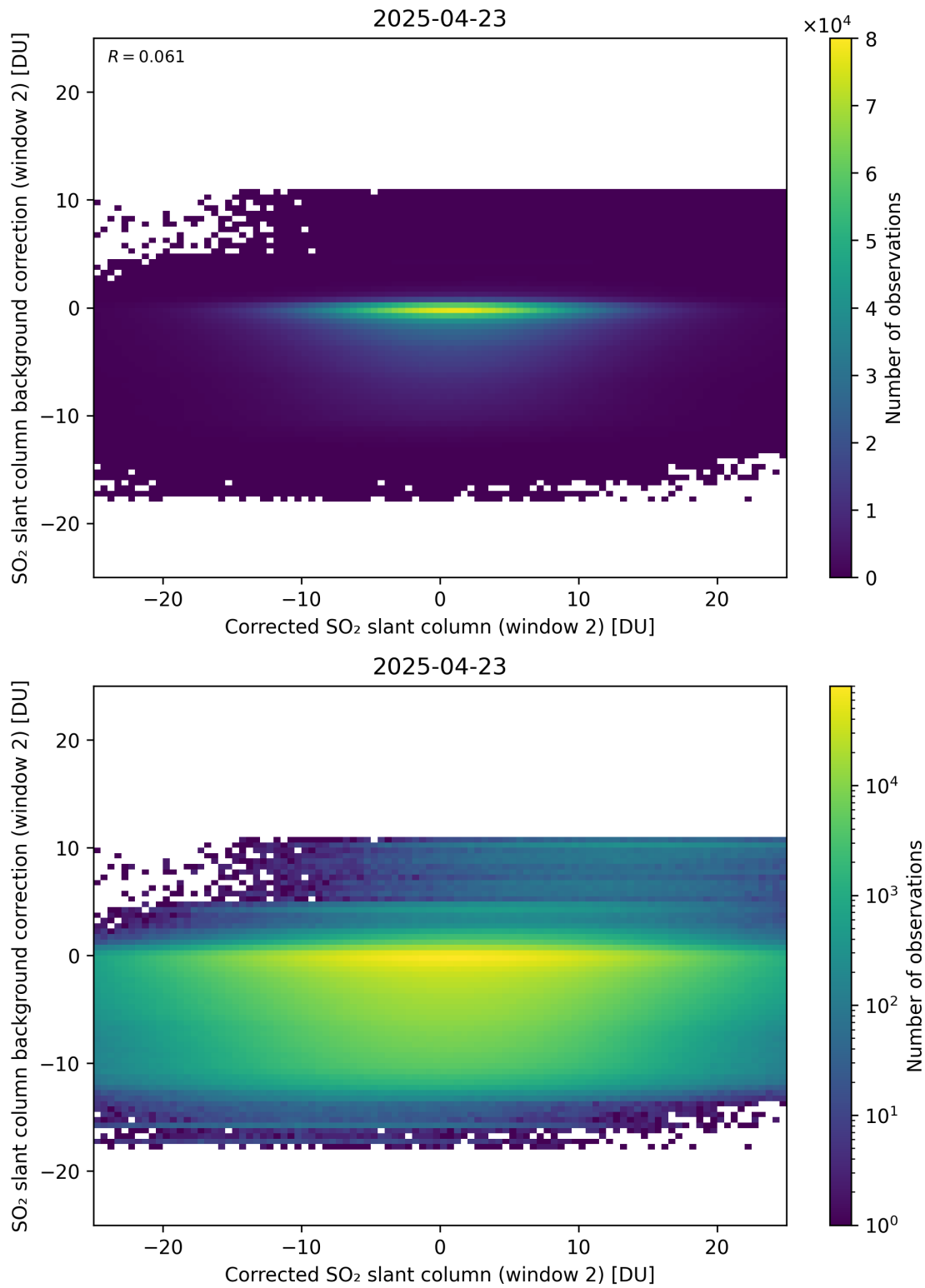
Figure 244: Scatter density plot of “Corrected SO 2 slant column (window 2)” against “SO 2 slant column background correction (window 2)” for 2025-04-22 to 2025-04-24.
