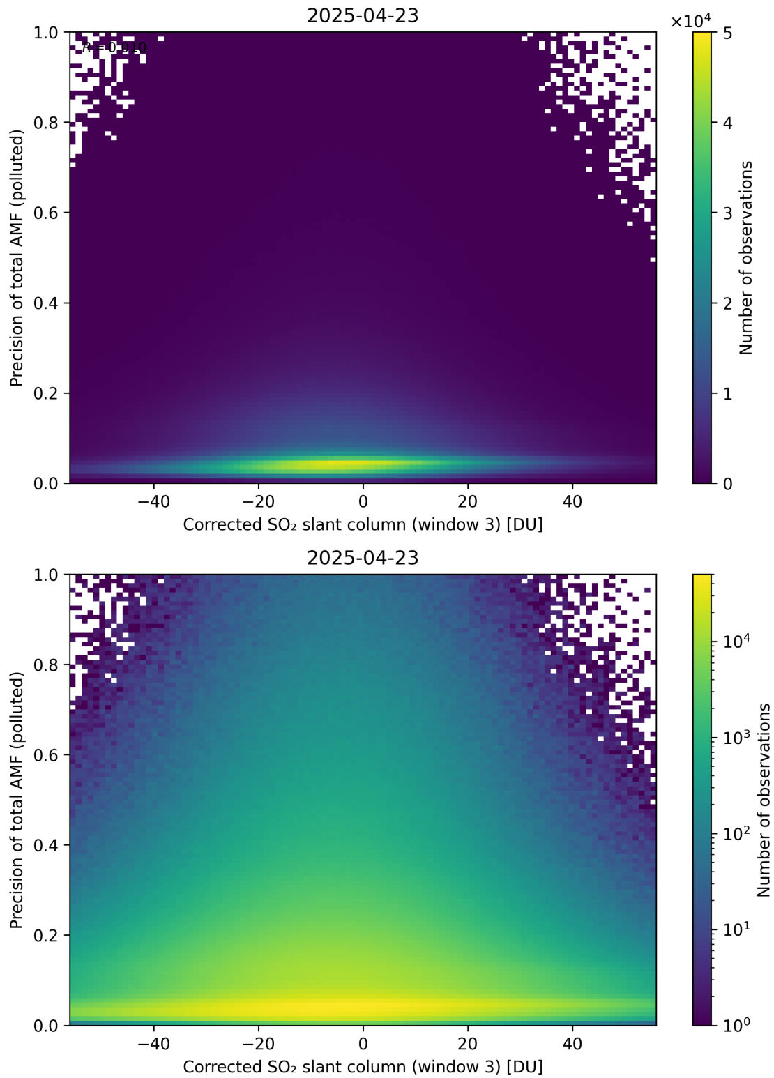
Figure 261: Scatter density plot of “Corrected SO 2 slant column (window 3)” against “Precision of total AMF (polluted)” for 2025-04-22 to 2025-04-24.
