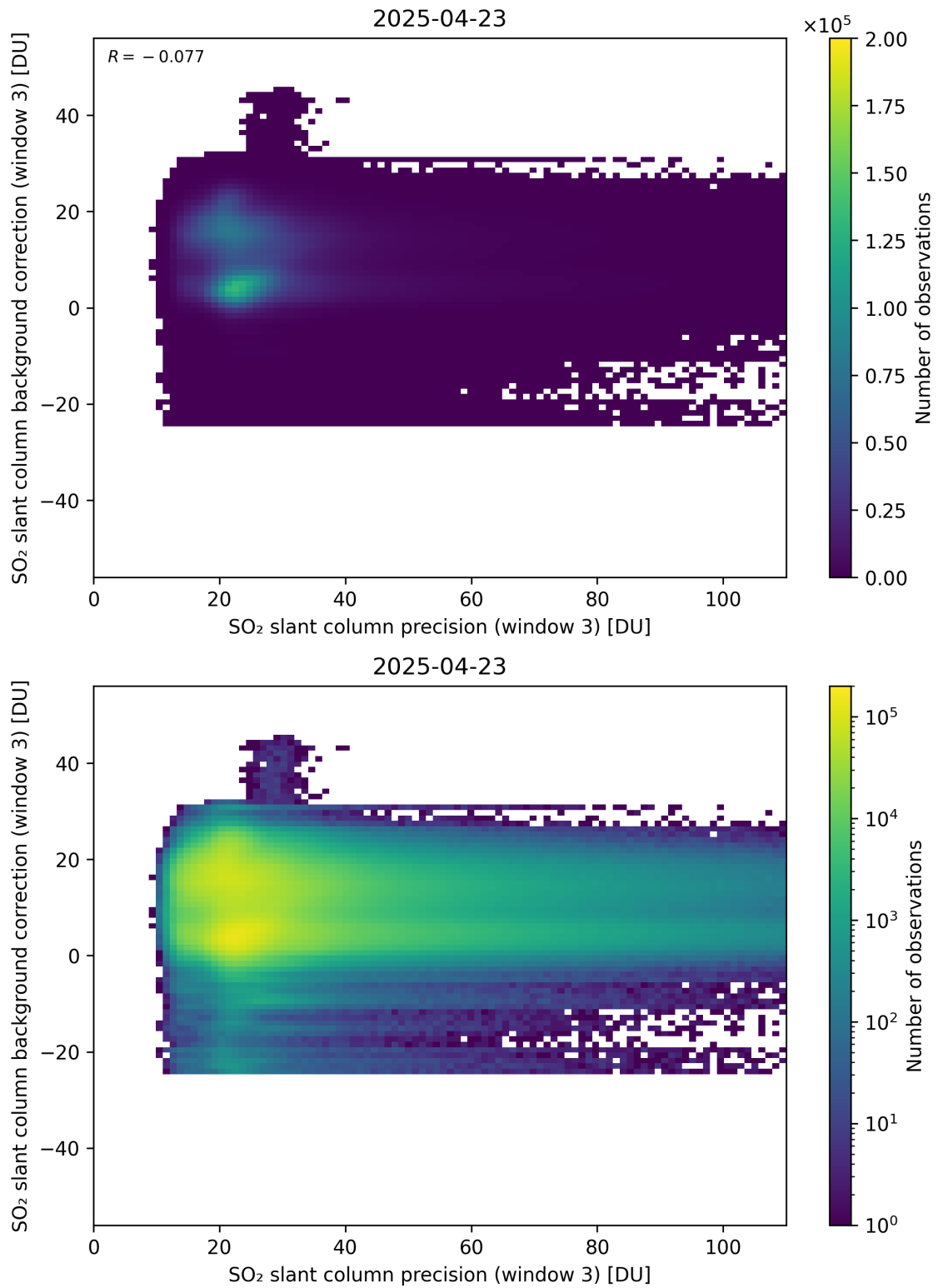
Figure 307: Scatter density plot of “SO 2 slant column precision (window 3)” against “SO 2 slant column background correction (window 3)” for 2025-04-22 to 2025-04-24.
