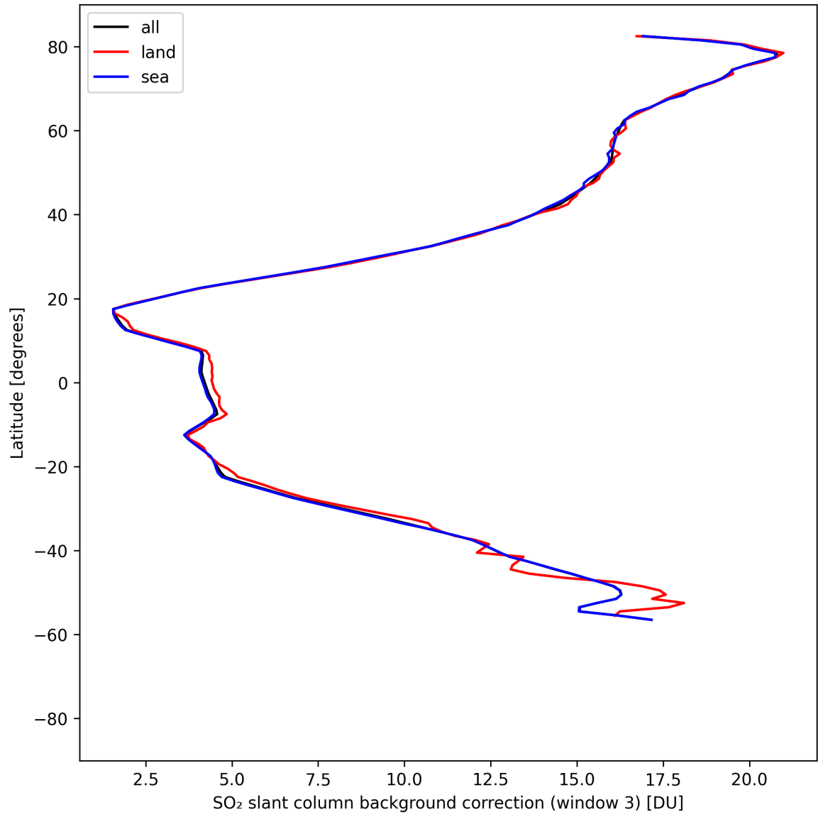
Figure 48: Zonal average of “SO 2 slant column background correction (window 3)” for 2025-04-22 to 2025-04-24.
