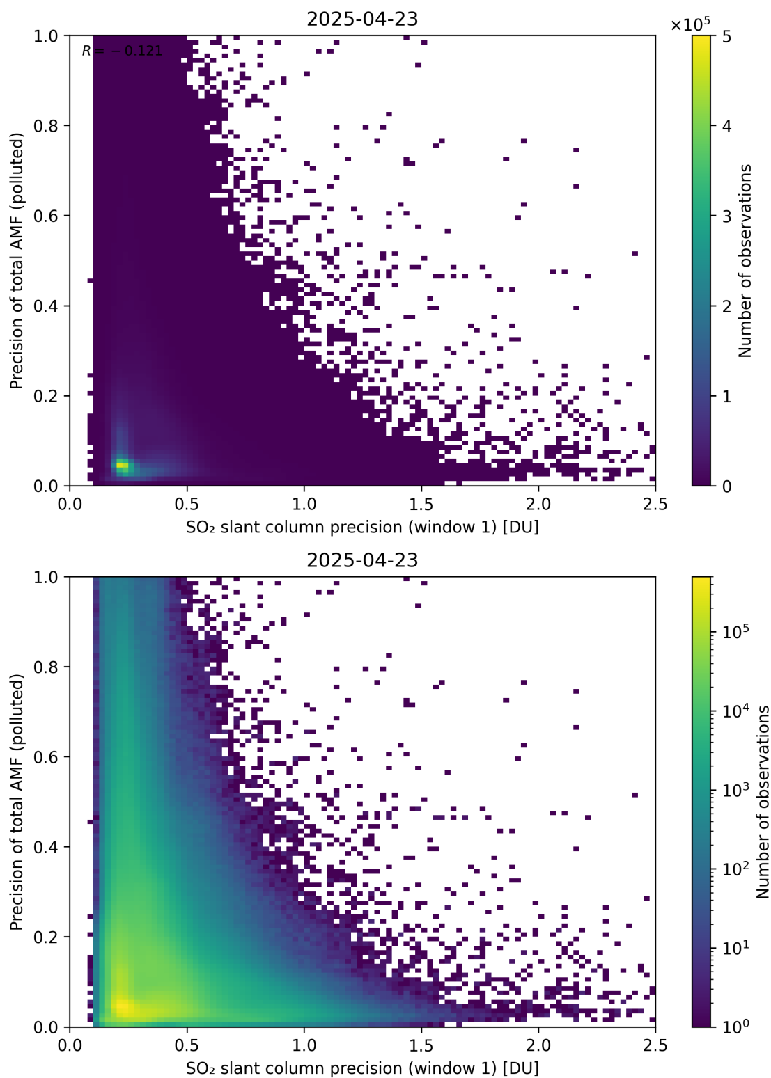
Figure 281: Scatter density plot of “SO 2 slant column precision (window 1)” against “Precision of total AMF (polluted)” for 2025-04-22 to 2025-04-24.
