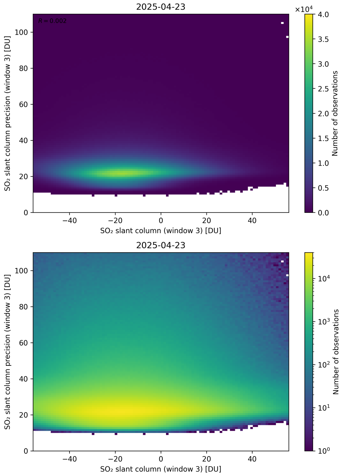
Figure 317: Scatter density plot of “SO 2 slant column (window 3)” against “SO 2 slant column precision (window 3)” for 2025-04-22 to 2025-04-24.
