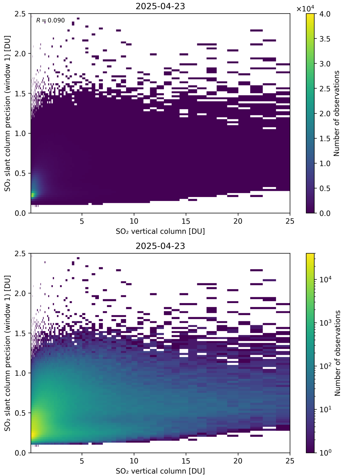
Figure 355: Scatter density plot of “SO 2 vertical column” against “SO 2 slant column precision (window 1)” for 2025-04-22 to 2025-04-24.
