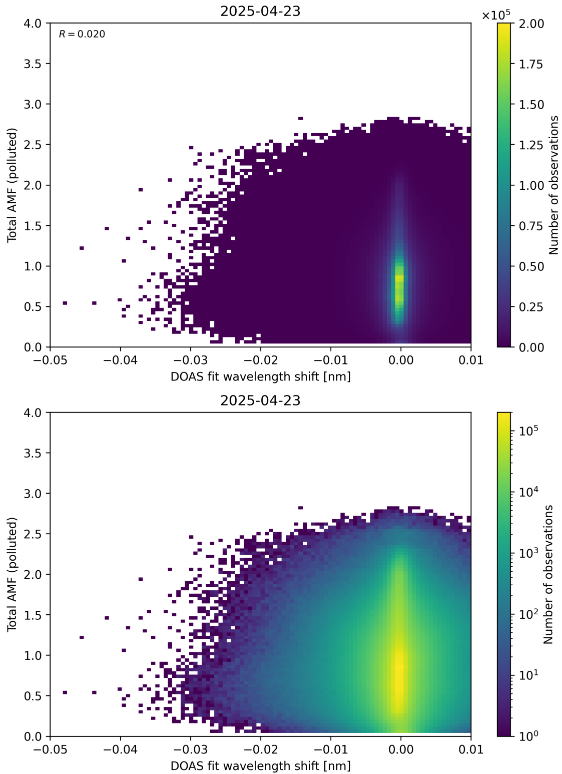
Figure 141: Scatter density plot of “DOAS fit wavelength shift” against “Total AMF (polluted)” for 2025-04-22 to 2025-04-24.
