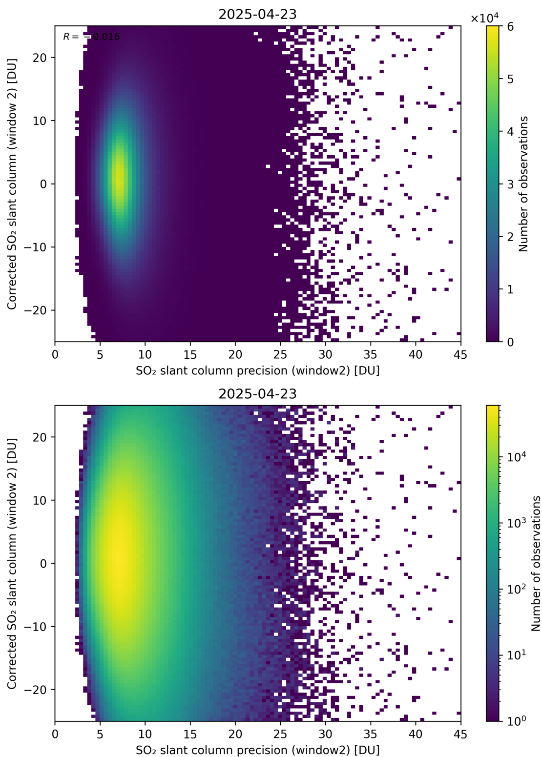
Figure 297: Scatter density plot of “SO 2 slant column precision (window2)” against “Corrected SO 2 slant column (window 2)” for 2025-04-22 to 2025-04-24.
