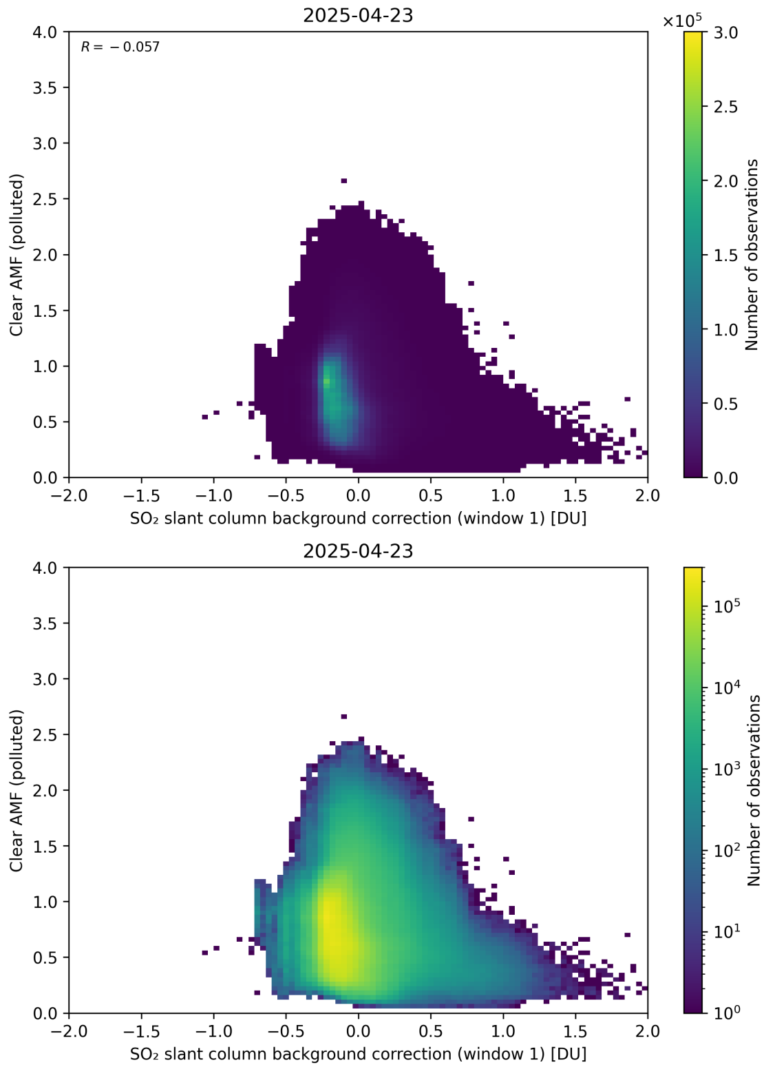
Figure 114: Scatter density plot of “SO 2 slant column background correction (window 1)” against “Clear AMF (polluted)” for 2025-04-22 to 2025-04-24.
