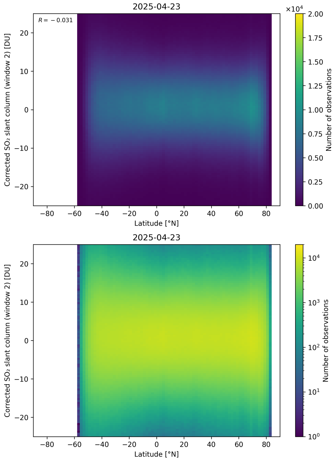
Figure 160: Scatter density plot of “Latitude” against “Corrected SO 2 slant column (window 2)” for 2025-04-22 to 2025-04-24.
