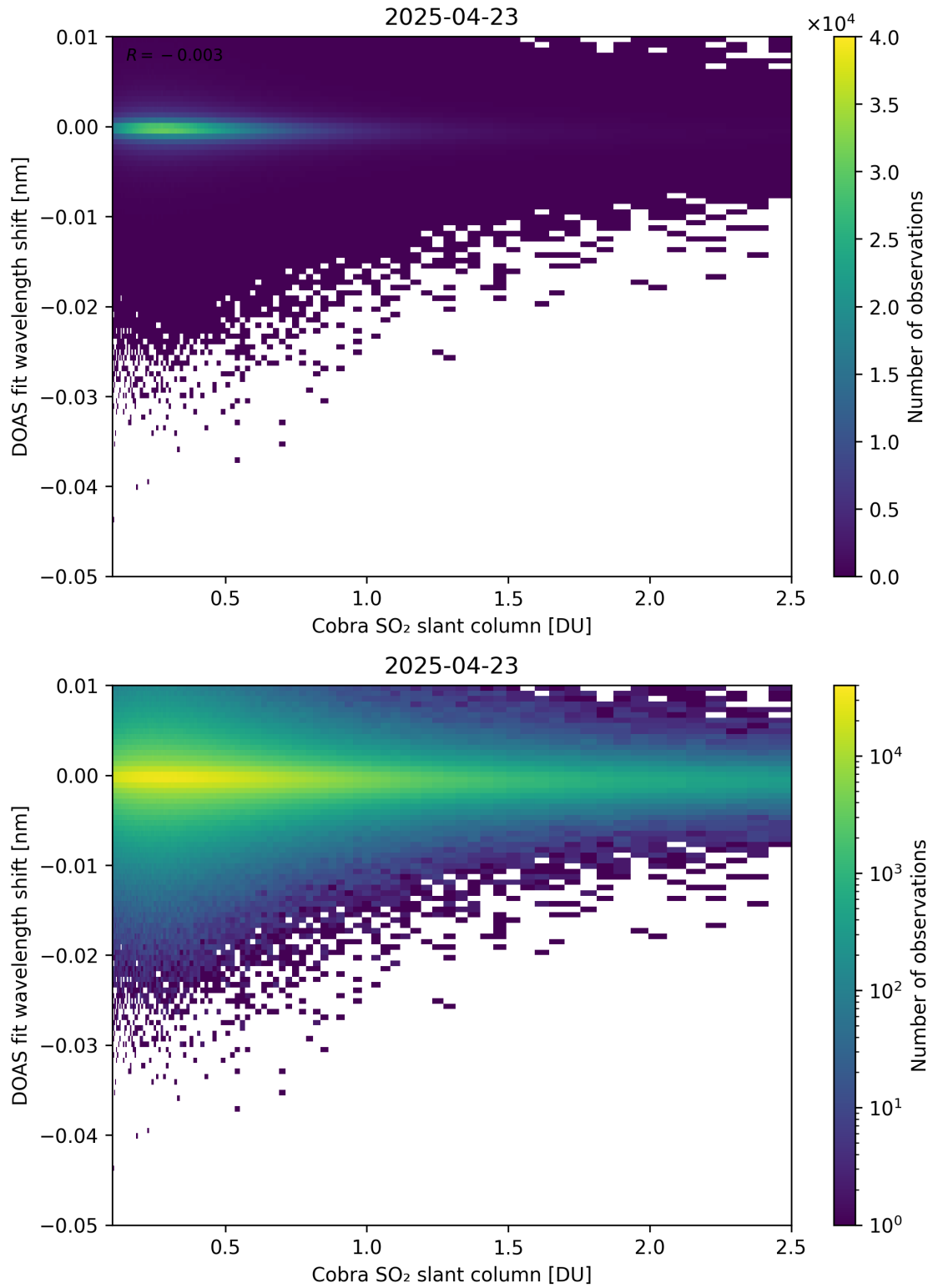
Figure 196: Scatter density plot of “Cobra SO 2 slant column” against “DOAS fit wavelength shift” for 2025-04-22 to 2025-04-24.
