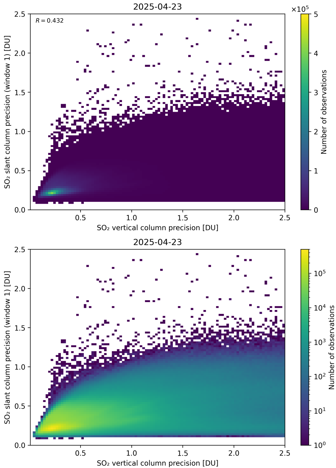
Figure 342: Scatter density plot of “SO 2 vertical column precision” against “SO 2 slant column precision (window 1)” for 2025-04-22 to 2025-04-24.
