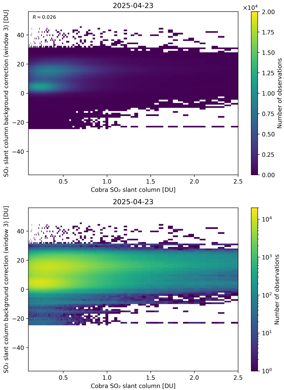
Figure 195: Scatter density plot of “Cobra SO 2 slant column” against “SO 2 slant column background correction (window 3)” for 2025-04-22 to 2025-04-24.
