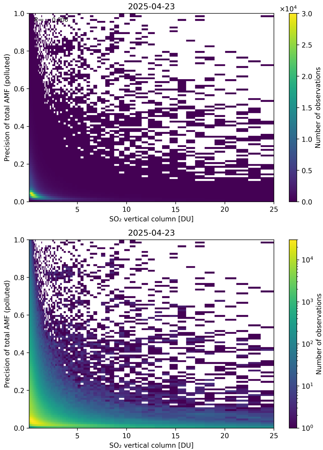
Figure 360: Scatter density plot of “SO 2 vertical column” against “Precision of total AMF (polluted)” for 2025-04-22 to 2025-04-24.
