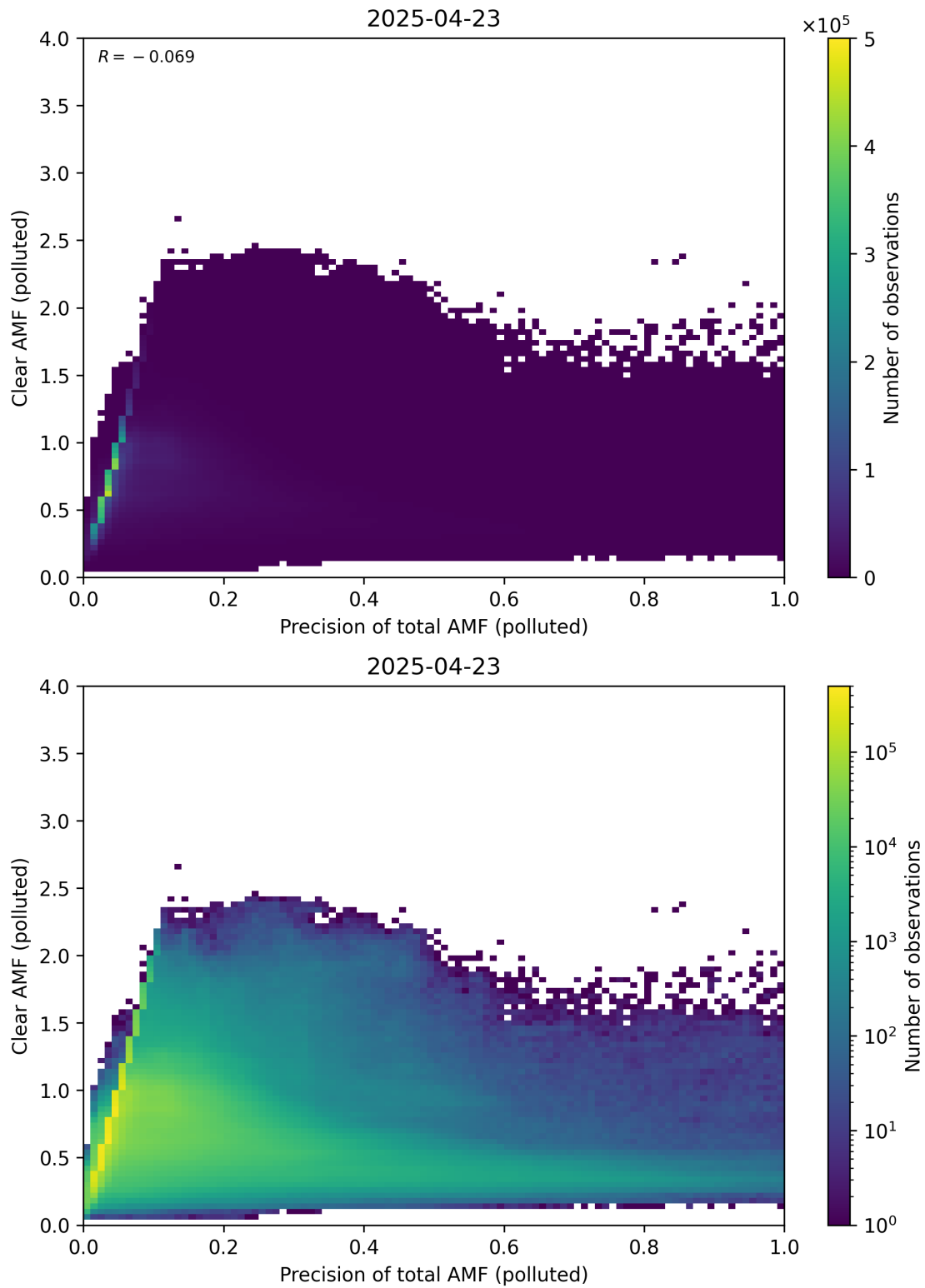
Figure 320: Scatter density plot of “Precision of total AMF (polluted)” against “Clear AMF (polluted)” for 2025-04-22 to 2025-04-24.
