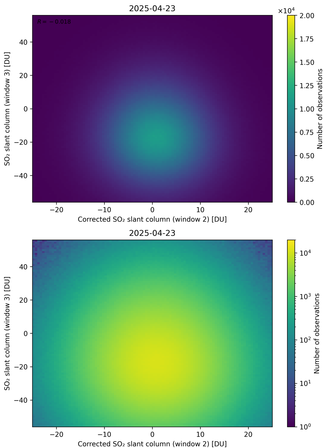
Figure 251: Scatter density plot of “Corrected SO 2 slant column (window 2)” against “SO 2 slant column (window 3)” for 2025-04-22 to 2025-04-24.
