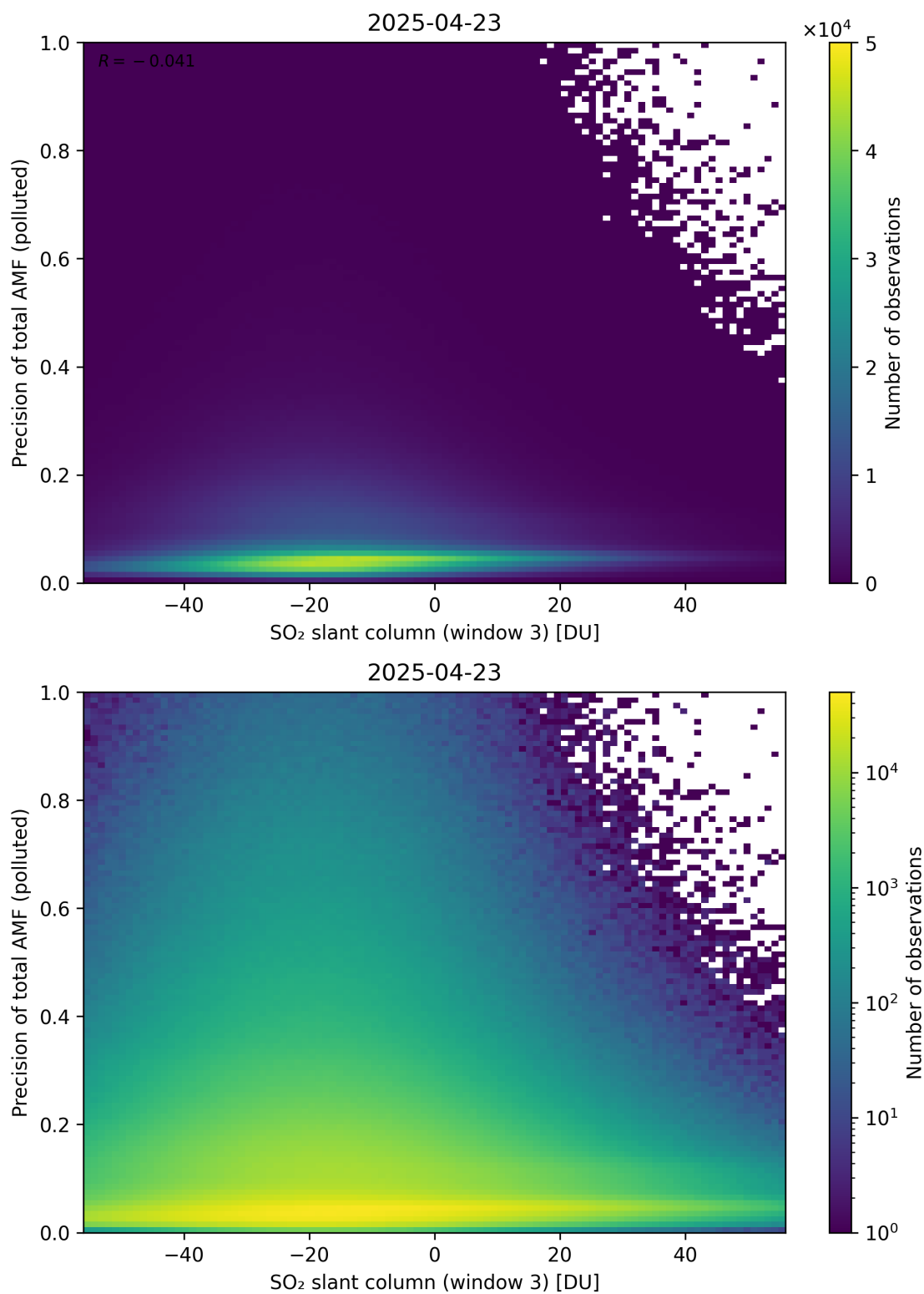
Figure 319: Scatter density plot of “SO 2 slant column (window 3)” against “Precision of total AMF (polluted)” for 2025-04-22 to 2025-04-24.
