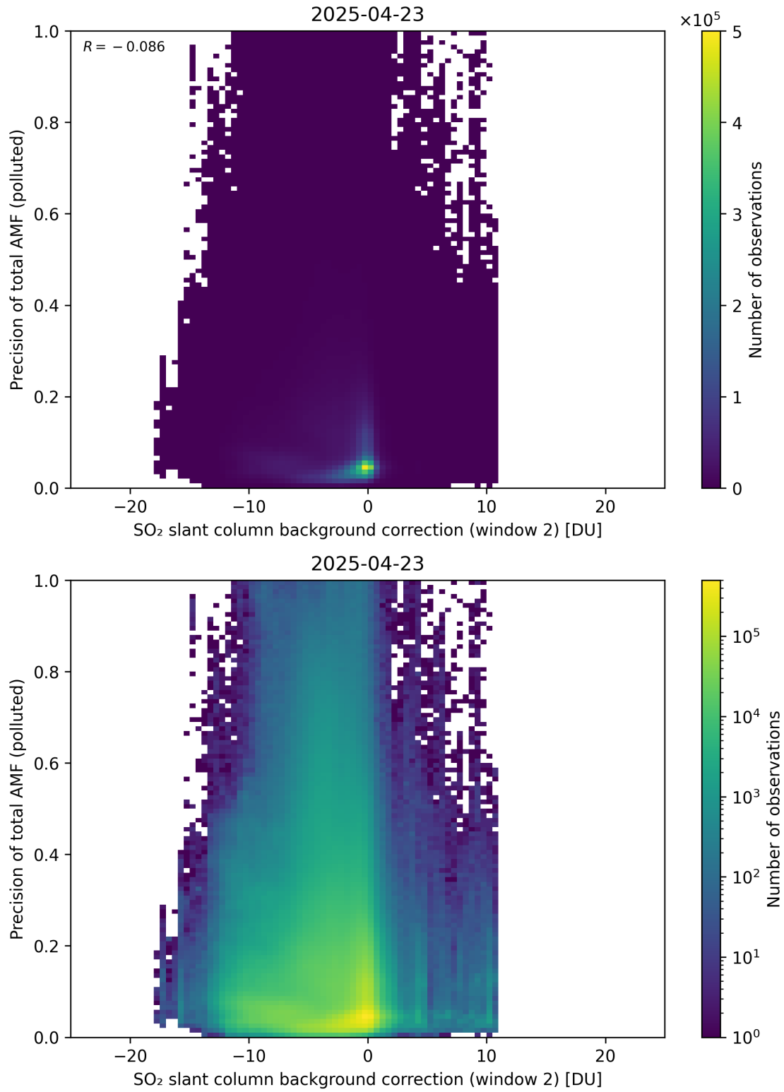
Figure 131: Scatter density plot of “SO 2 slant column background correction (window 2)” against “Precision of total AMF (polluted)” for 2025-04-22 to 2025-04-24.
