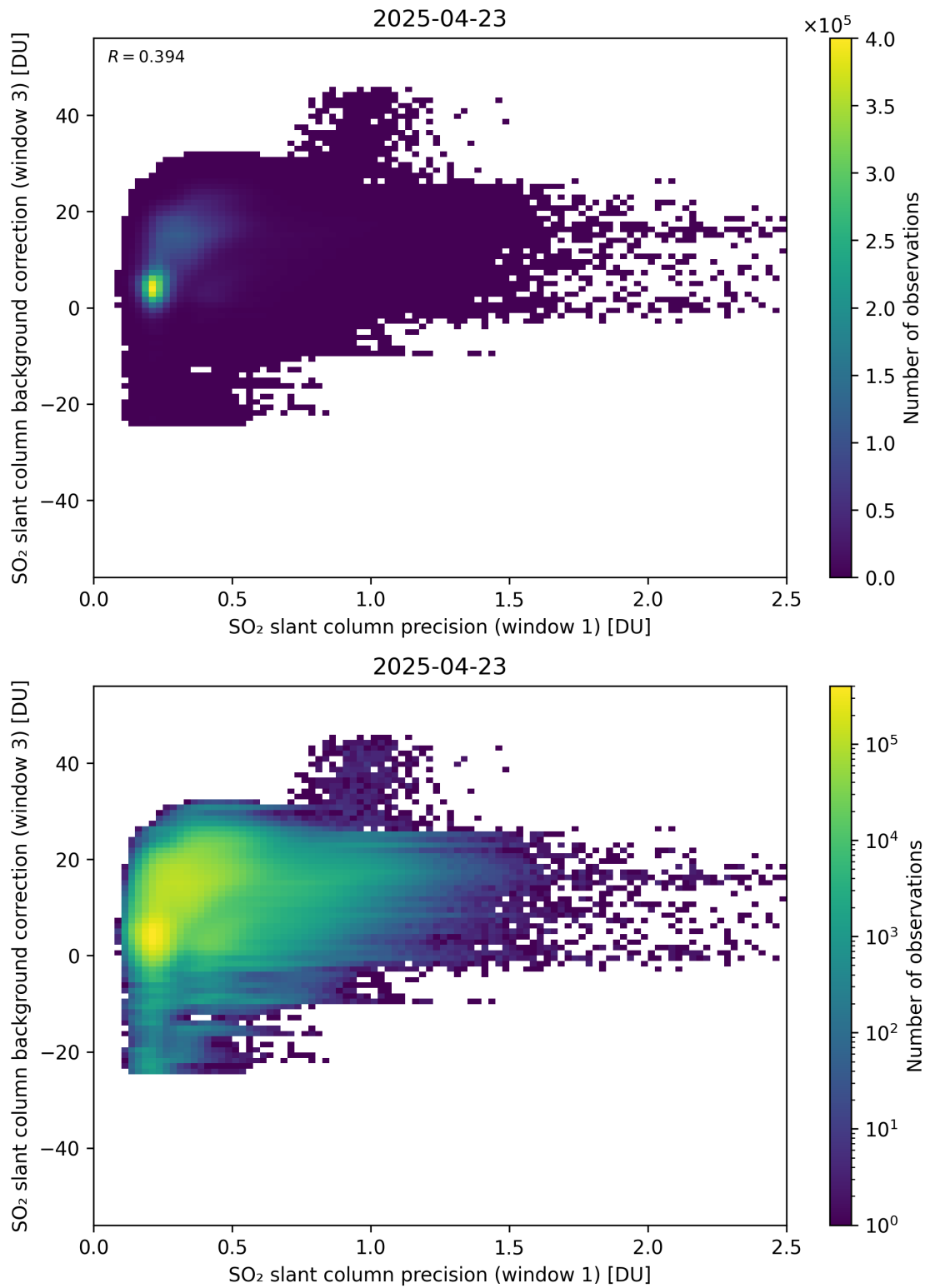
Figure 270: Scatter density plot of “SO 2 slant column precision (window 1)” against “SO 2 slant column background correction (window 3)” for 2025-04-22 to 2025-04-24.
