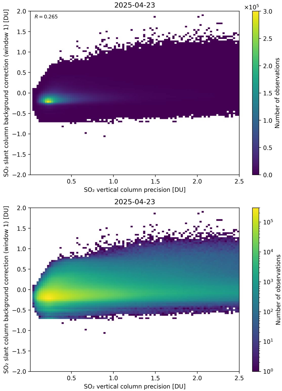
Figure 329: Scatter density plot of “SO 2 vertical column precision” against “SO 2 slant column background correction (window 1)” for 2025-04-22 to 2025-04-24.
