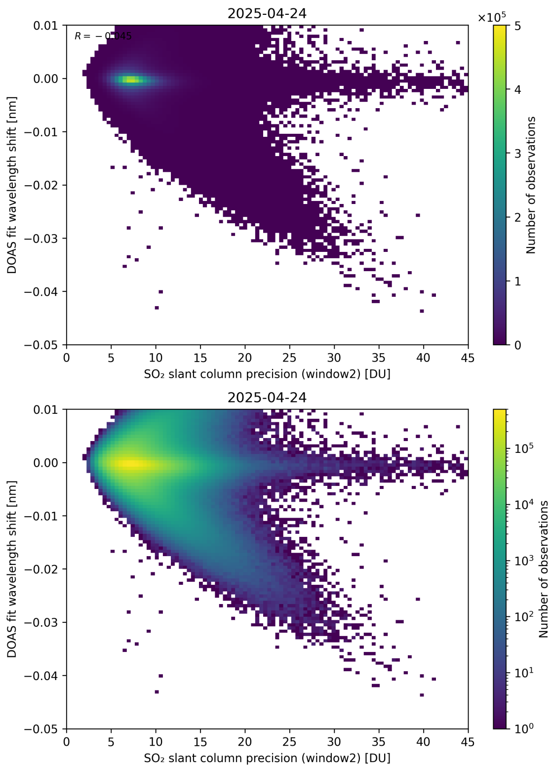
Figure 293: Scatter density plot of “SO 2 slant column precision (window2)” against “DOAS fit wavelength shift” for 2025-04-24 to 2025-04-25.
