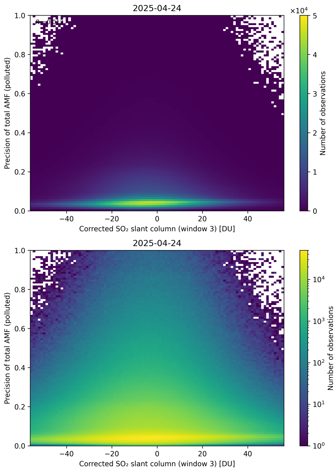
Figure 261: Scatter density plot of “Corrected SO 2 slant column (window 3)” against “Precision of total AMF (polluted)” for 2025-04-24 to 2025-04-25.
