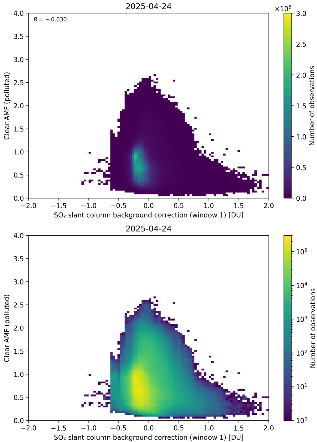
Figure 114: Scatter density plot of “SO 2 slant column background correction (window 1)” against “Clear AMF (polluted)” for 2025-04-24 to 2025-04-25.
