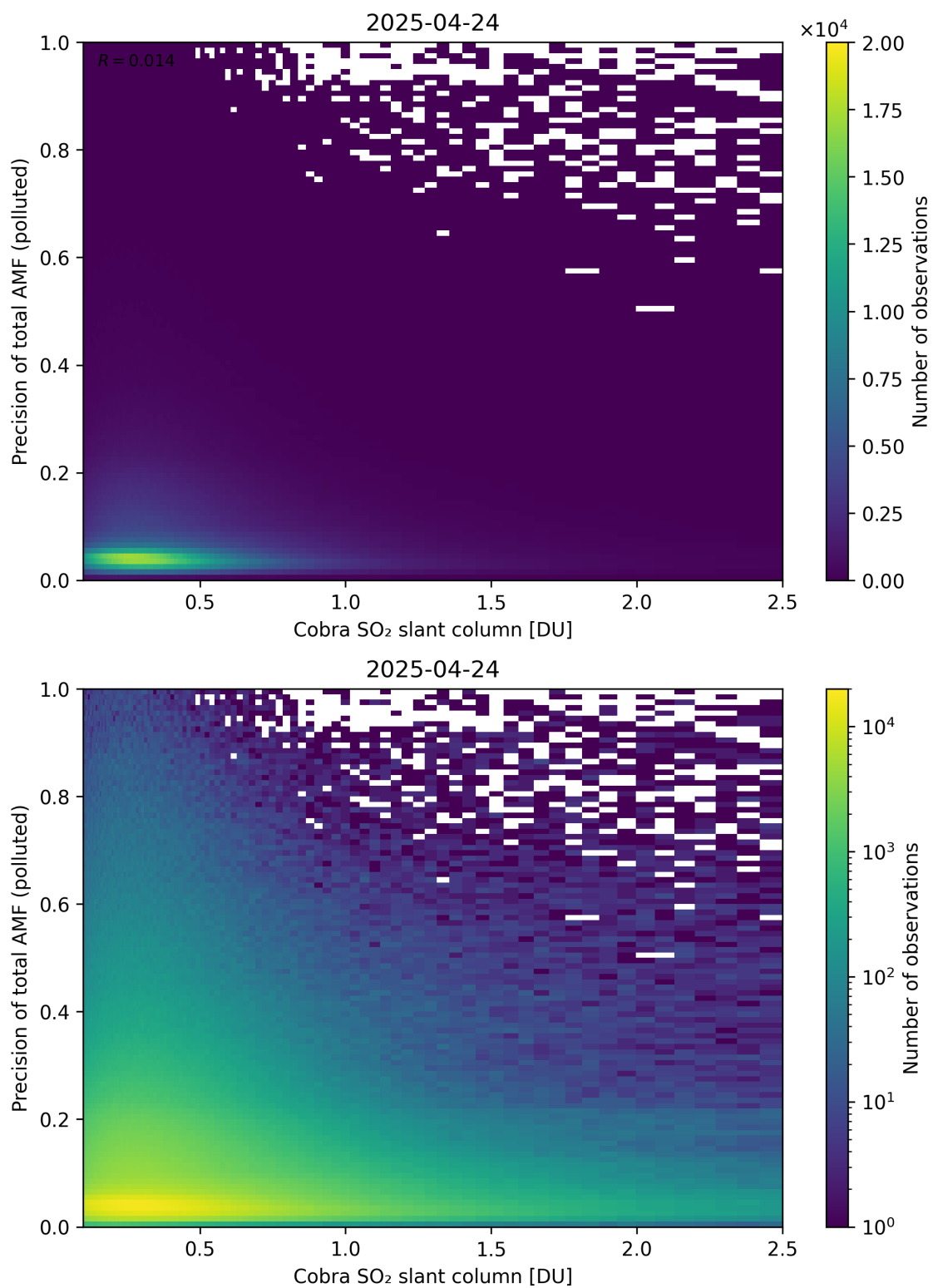
Figure 225: Scatter density plot of “Cobra SO 2 slant column” against “Precision of total AMF (polluted)” for 2025-04-24 to 2025-04-25.
