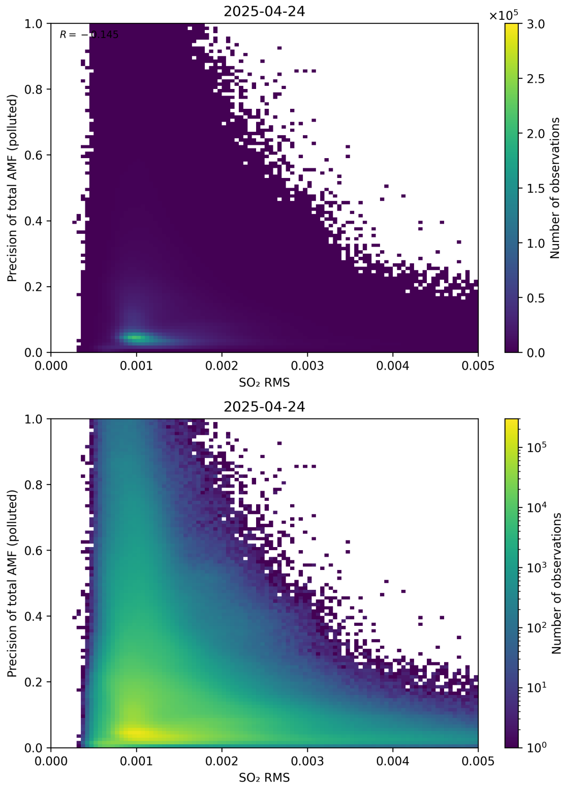
Figure 149: Scatter density plot of “SO 2 RMS” against “Precision of total AMF (polluted)” for 2025-04-24 to 2025-04-25.
