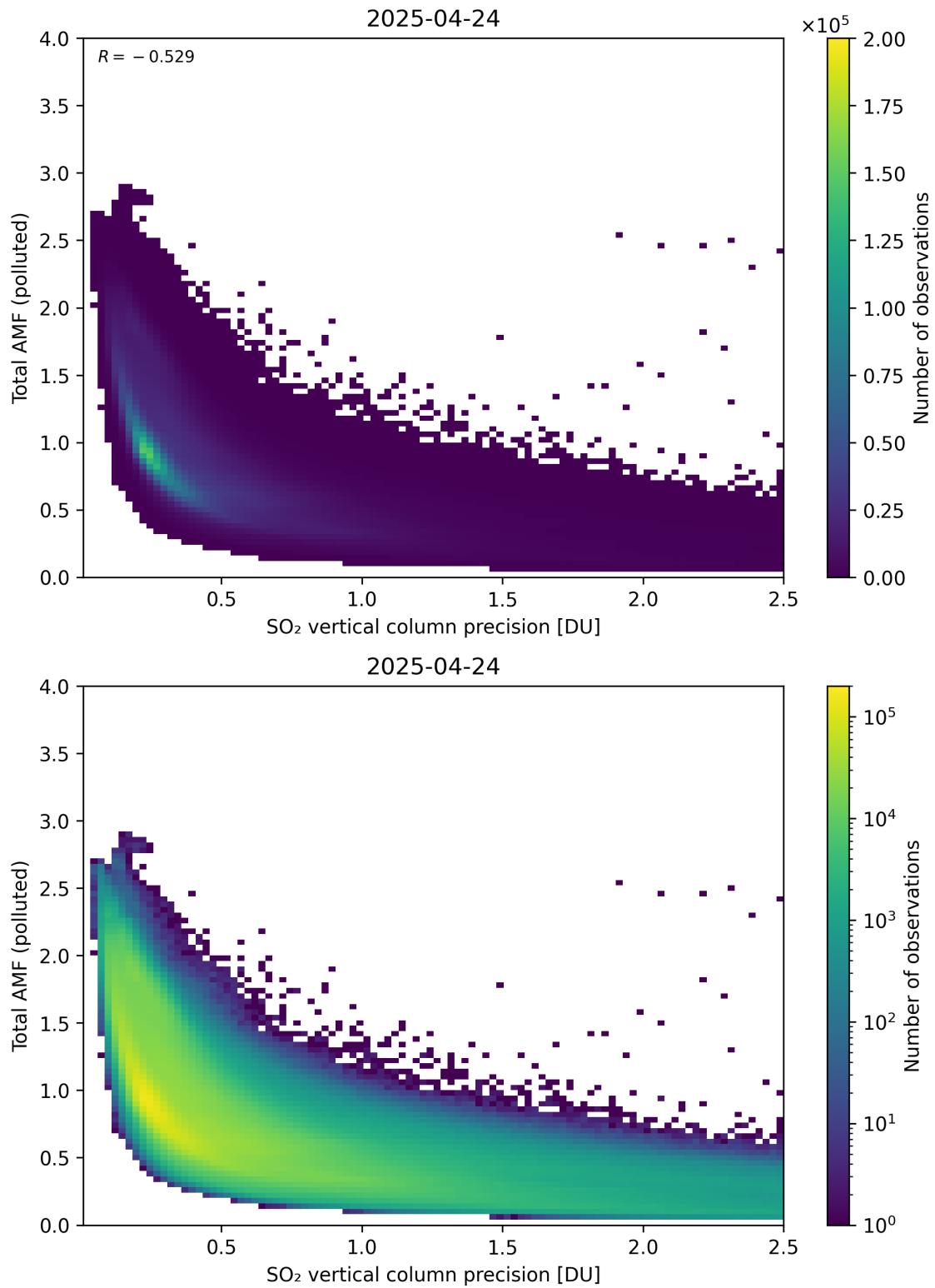
Figure 346: Scatter density plot of “SO 2 vertical column precision” against “Total AMF (polluted)” for 2025-04-24 to 2025-04-25.
