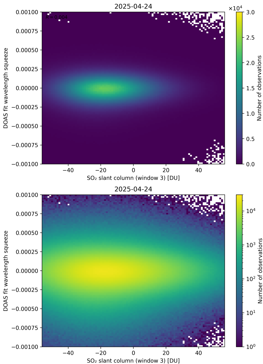
Figure 305: Scatter density plot of “SO 2 slant column (window 3)” against “DOAS fit wavelength squeeze” for 2025-04-24 to 2025-04-25.
