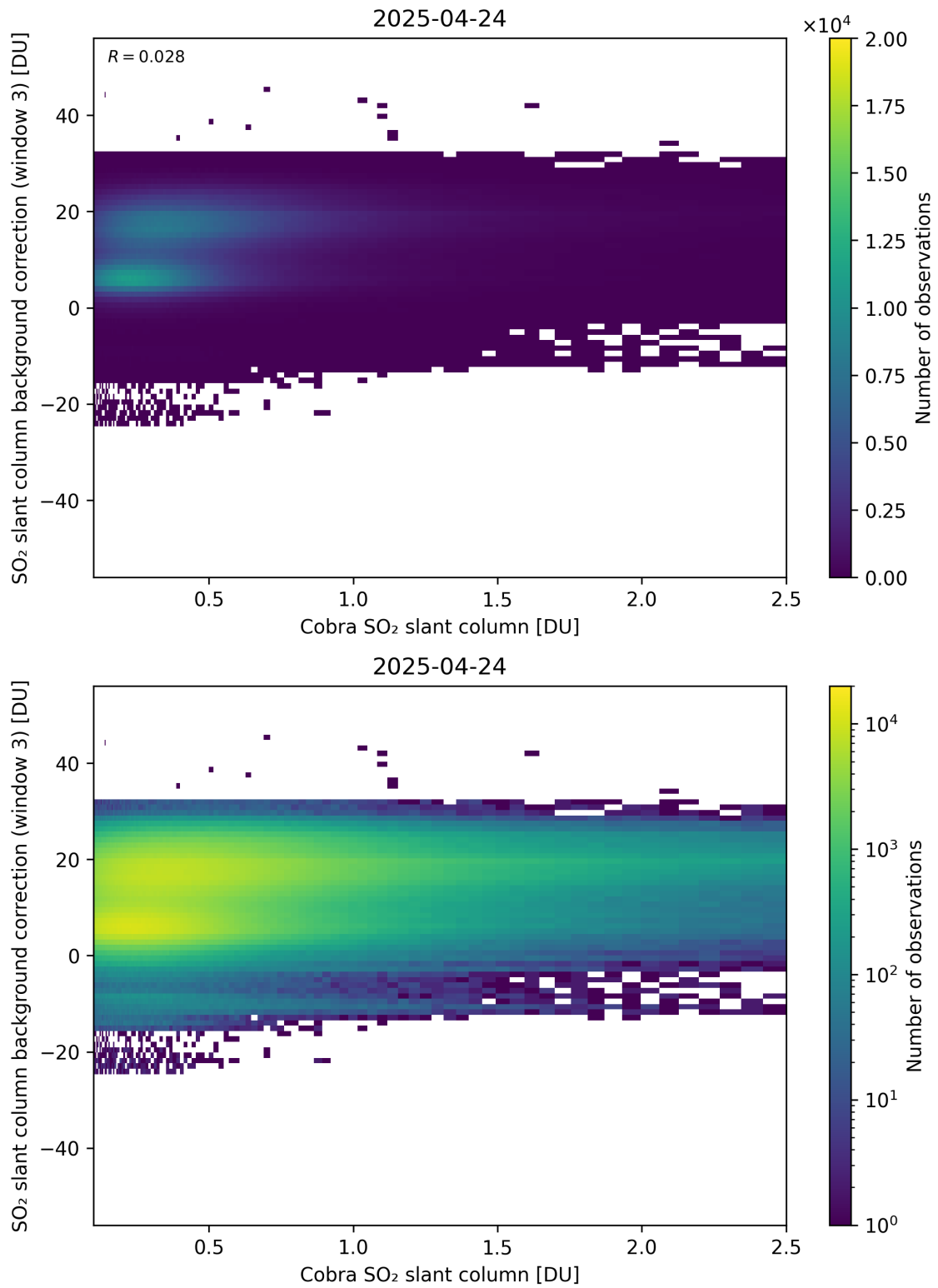
Figure 195: Scatter density plot of “Cobra SO 2 slant column” against “SO 2 slant column background correction (window 3)” for 2025-04-24 to 2025-04-25.
