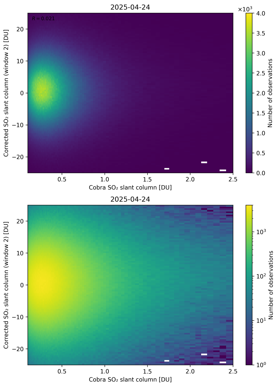
Figure 217: Scatter density plot of “Cobra SO 2 slant column” against “Corrected SO 2 slant column (window 2)” for 2025-04-24 to 2025-04-25.
