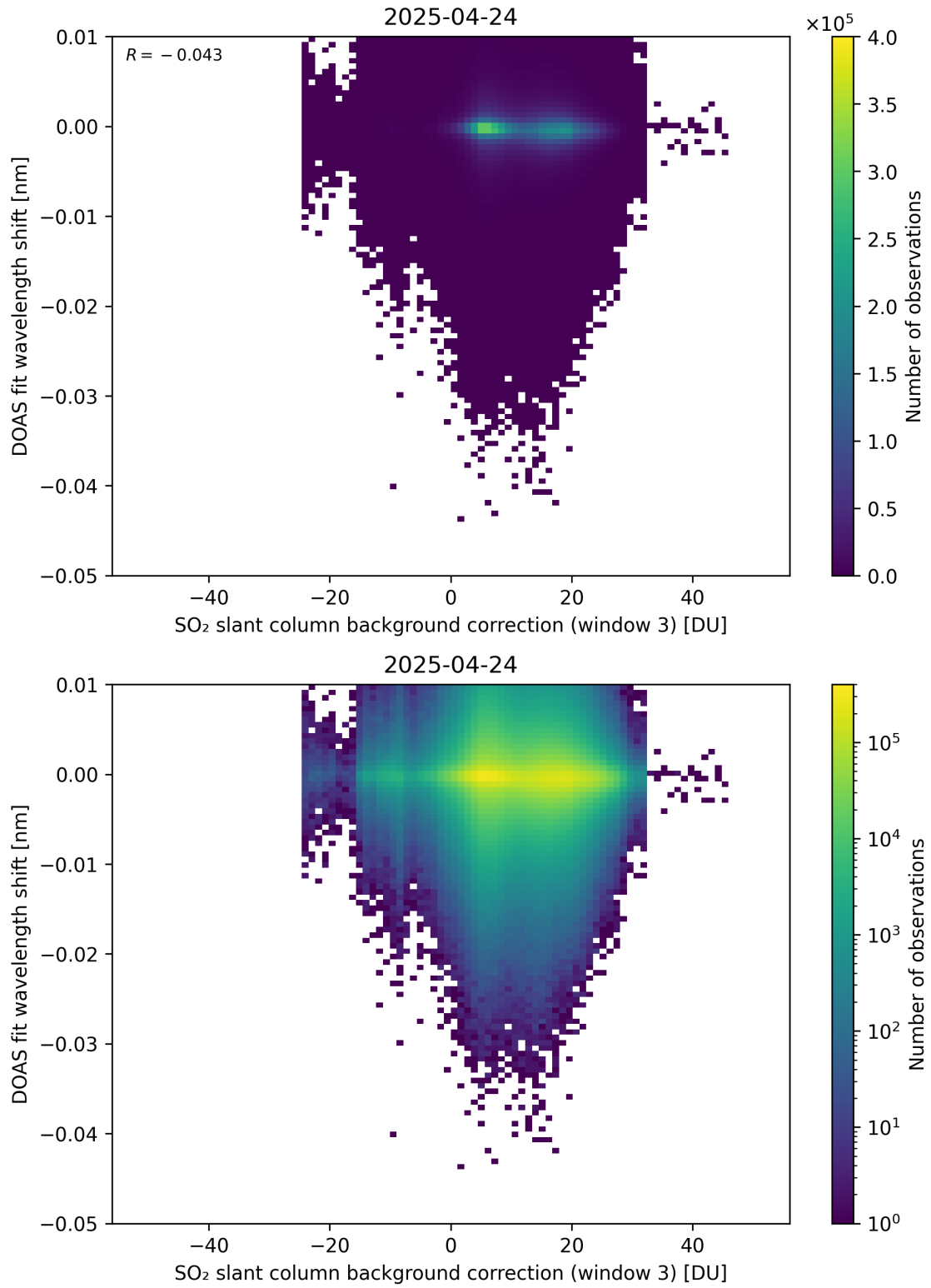
Figure 132: Scatter density plot of “SO 2 slant column background correction (window 3)” against “DOAS fit wavelength shift” for 2025-04-24 to 2025-04-25.
