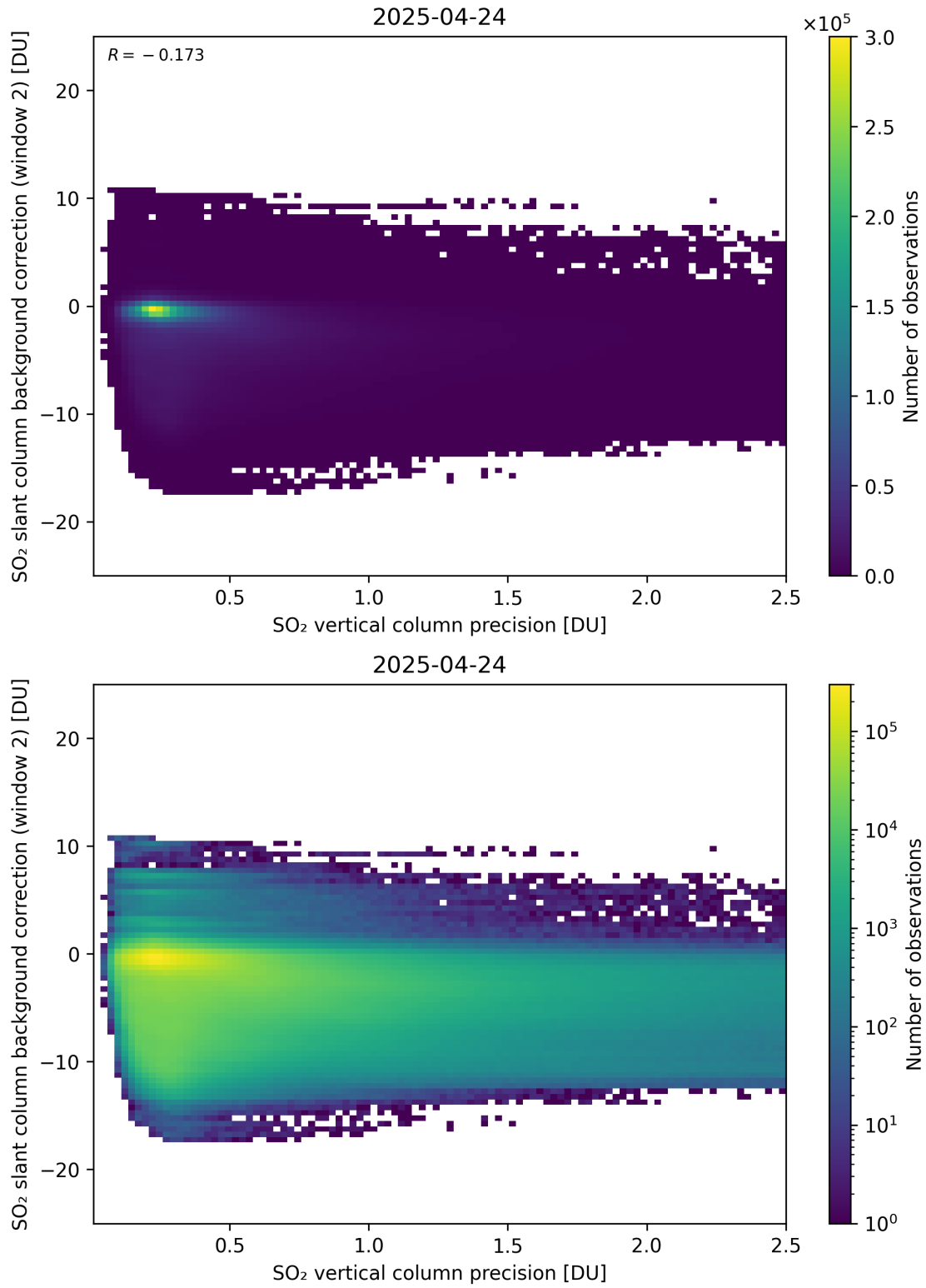
Figure 330: Scatter density plot of “SO 2 vertical column precision” against “SO 2 slant column background correction (window 2)” for 2025-04-24 to 2025-04-25.
