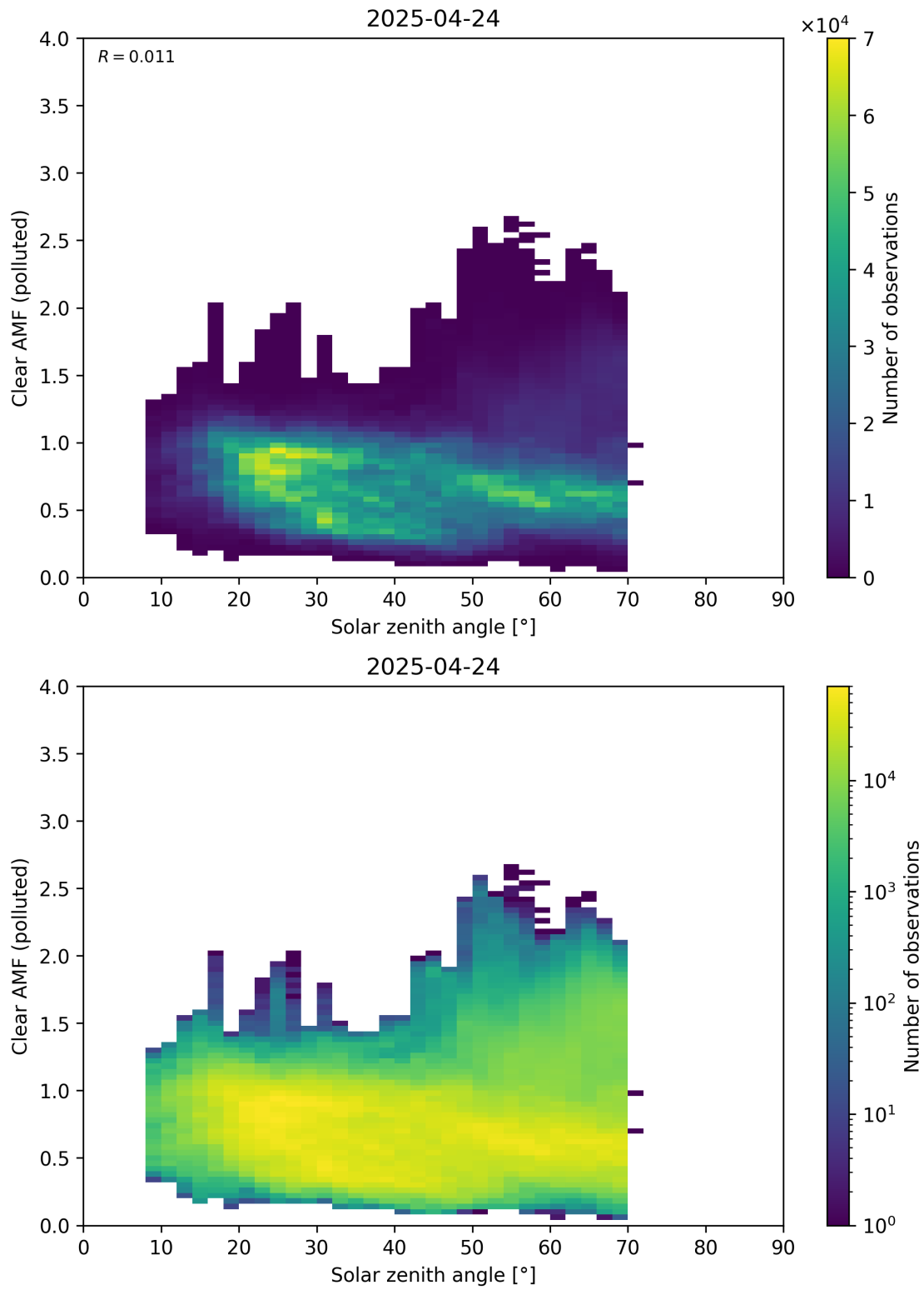
Figure 178: Scatter density plot of “Solar zenith angle” against “Clear AMF (polluted)” for 2025-04-24 to 2025-04-25.
