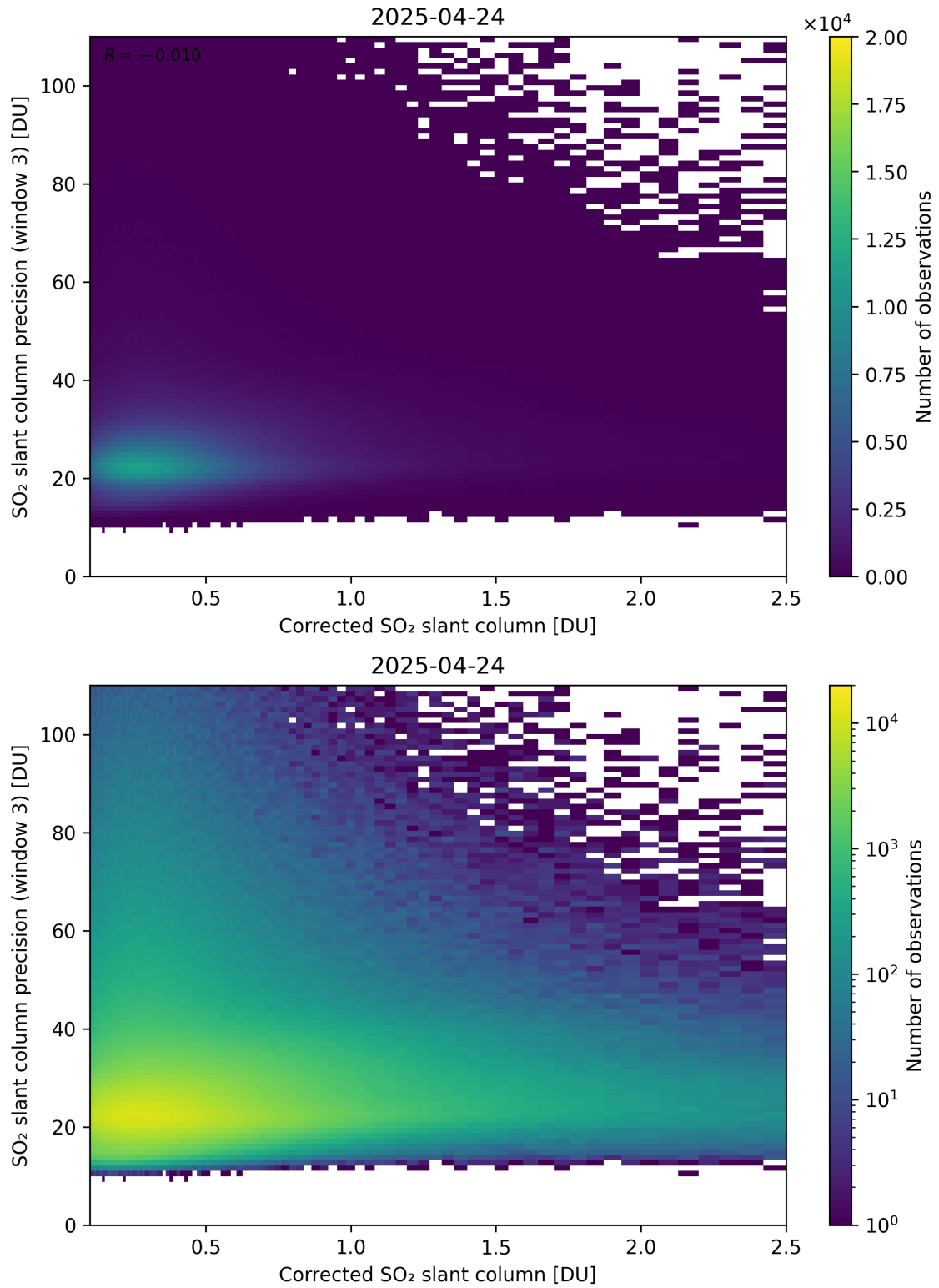
Figure 241: Scatter density plot of “Corrected SO 2 slant column” against “SO 2 slant column precision (window 3)” for 2025-04-24 to 2025-04-25.
