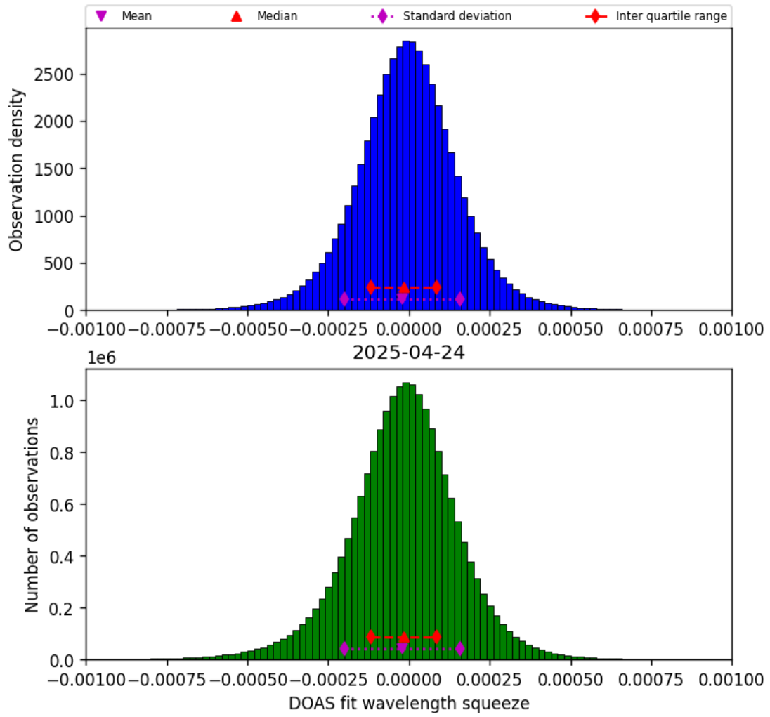
Figure 77: Histogram of “DOAS fit wavelength squeeze” for 2025-04-24 to 2025-04-25
