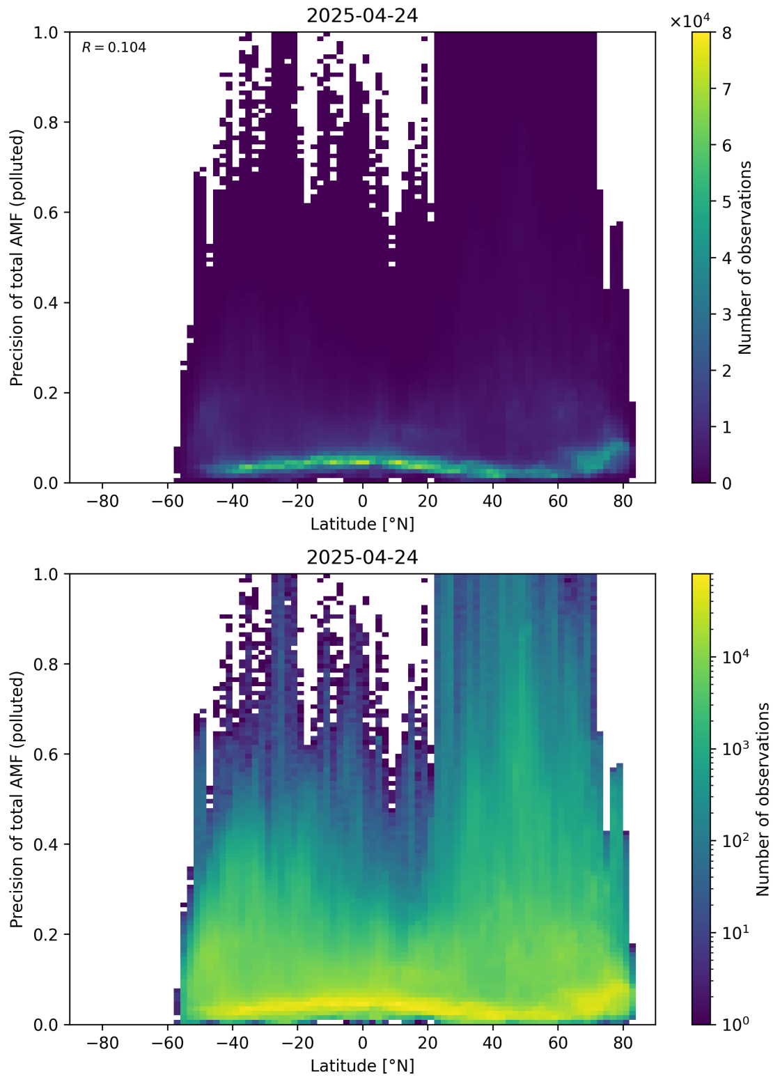
Figure 168: Scatter density plot of “Latitude” against “Precision of total AMF (polluted)” for 2025-04-24 to 2025-04-25.
