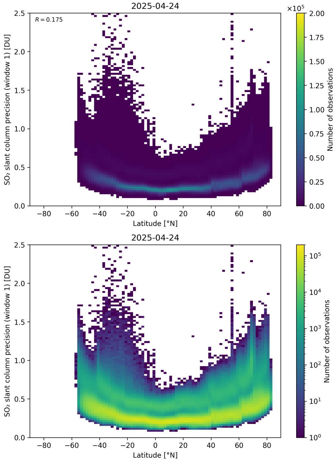
Figure 163: Scatter density plot of “Latitude” against “SO 2 slant column precision (window 1)” for 2025-04-24 to 2025-04-25.
