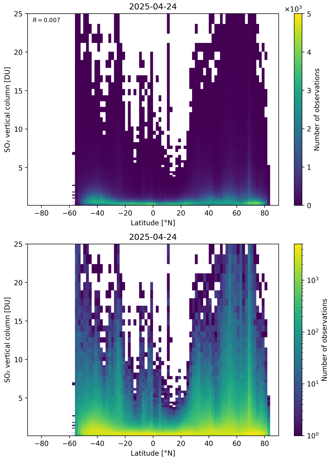
Figure 169: Scatter density plot of “Latitude” against “SO 2 vertical column” for 2025-04-24 to 2025-04-25.
