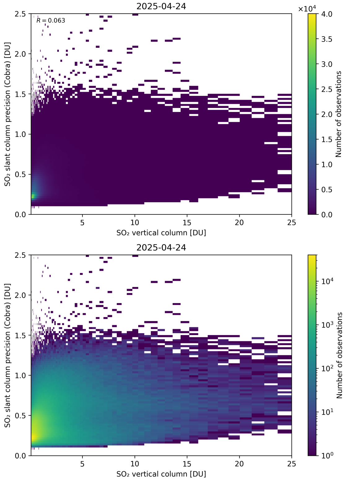
Figure 350: Scatter density plot of “SO 2 vertical column” against “SO 2 slant column precision (Cobra)” for 2025-04-24 to 2025-04-25.
