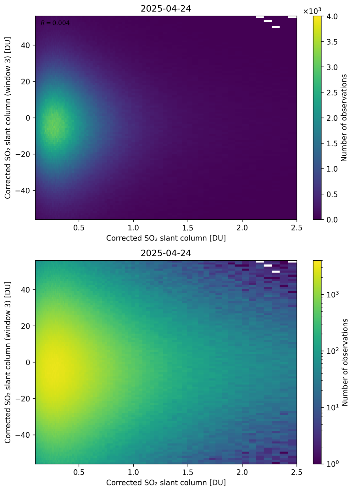
Figure 236: Scatter density plot of “Corrected SO 2 slant column” against “Corrected SO 2 slant column (window 3)” for 2025-04-24 to 2025-04-25.
