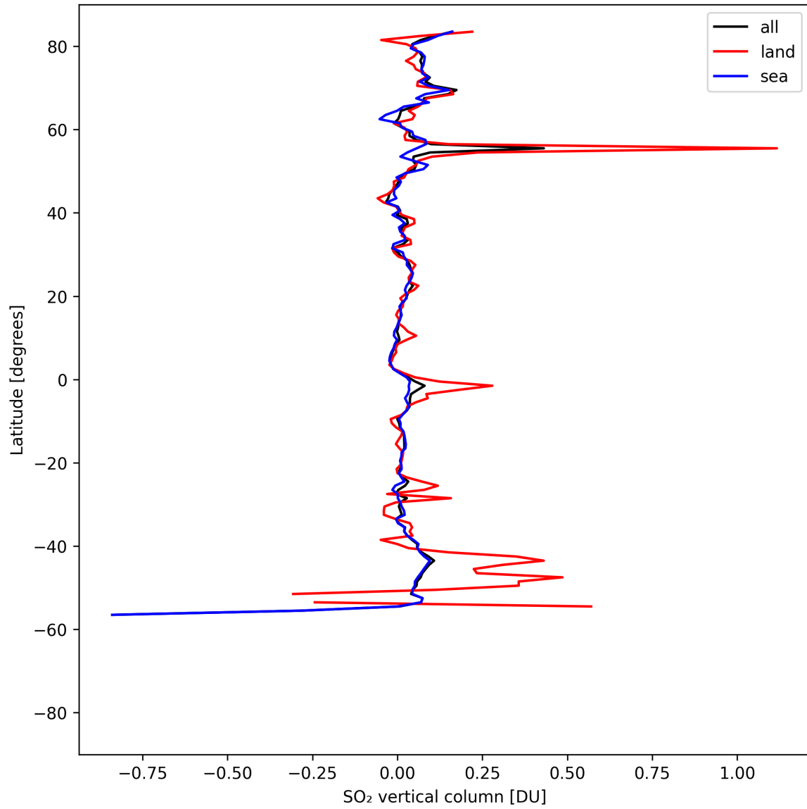
Figure 32: Zonal average of “SO 2 vertical column” for 2025-04-24 to 2025-04-25.
