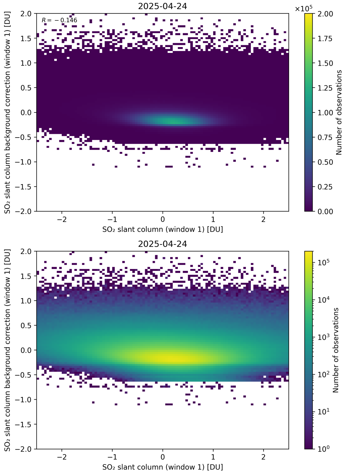
Figure 262: Scatter density plot of “SO 2 slant column (window 1)” against “SO 2 slant column background correction (window 1)” for 2025-04-24 to 2025-04-25.
