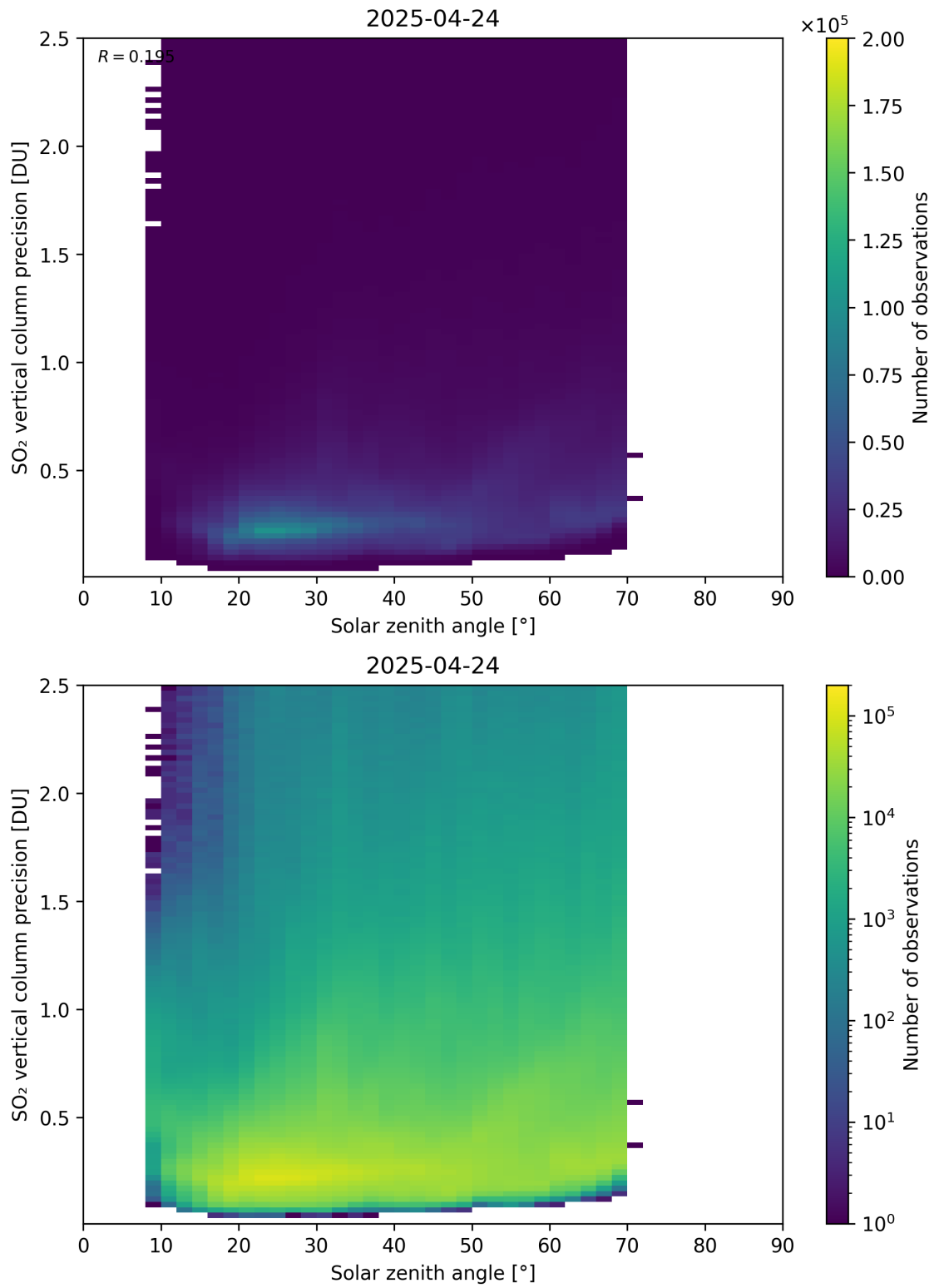
Figure 192: Scatter density plot of “Solar zenith angle” against “SO 2 vertical column precision” for 2025-04-24 to 2025-04-25.
