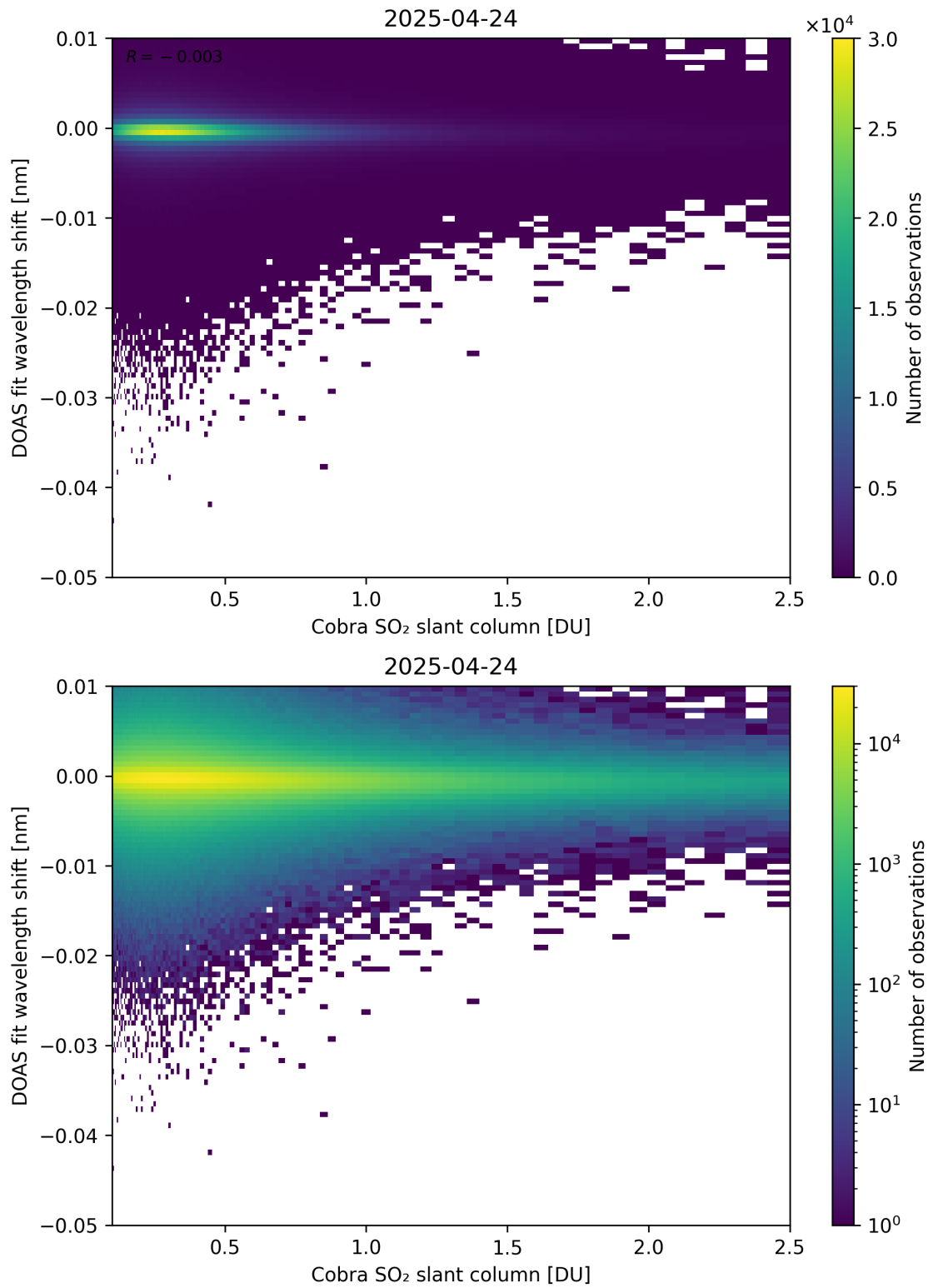
Figure 196: Scatter density plot of “Cobra SO 2 slant column” against “DOAS fit wavelength shift” for 2025-04-24 to 2025-04-25.
