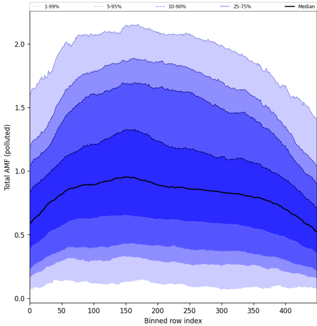
Figure 105: Along track statistics of “Total AMF (polluted)” for 2025-04-24 to 2025-04-25
