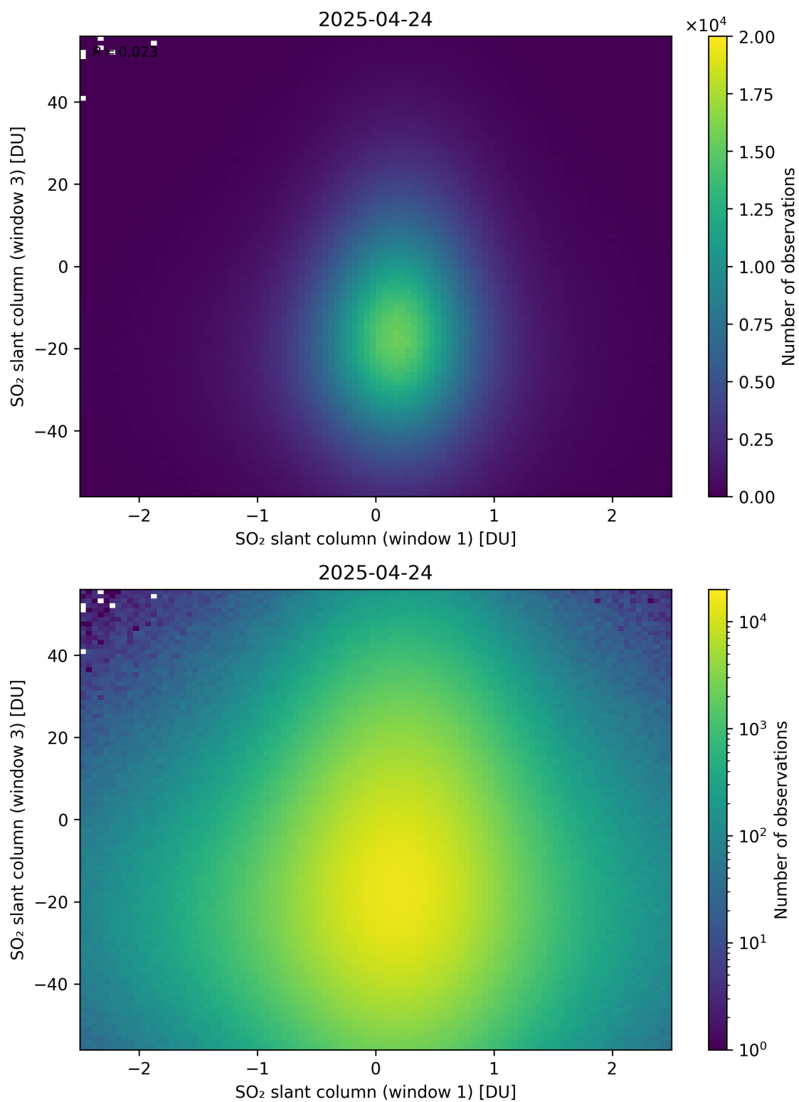
Figure 287: Scatter density plot of “SO 2 slant column (window 1)” against “SO 2 slant column (window 3)” for 2025-04-24 to 2025-04-25.
