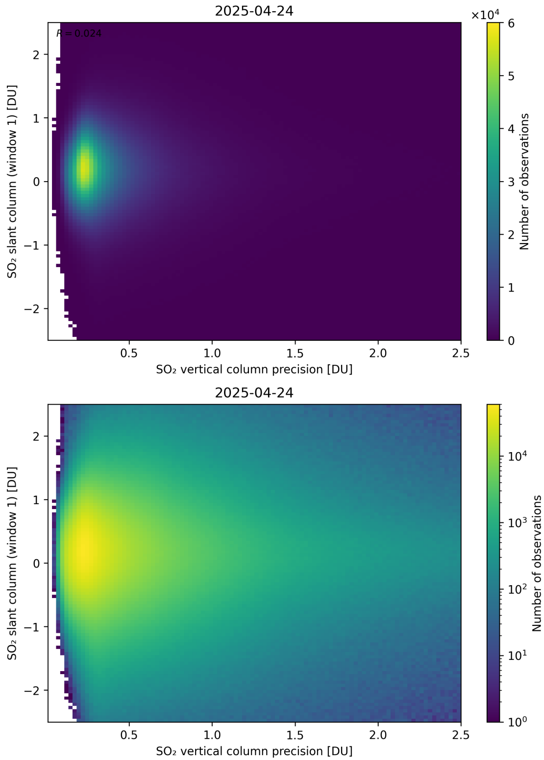
Figure 341: Scatter density plot of “SO 2 vertical column precision” against “SO 2 slant column (window 1)” for 2025-04-24 to 2025-04-25.
