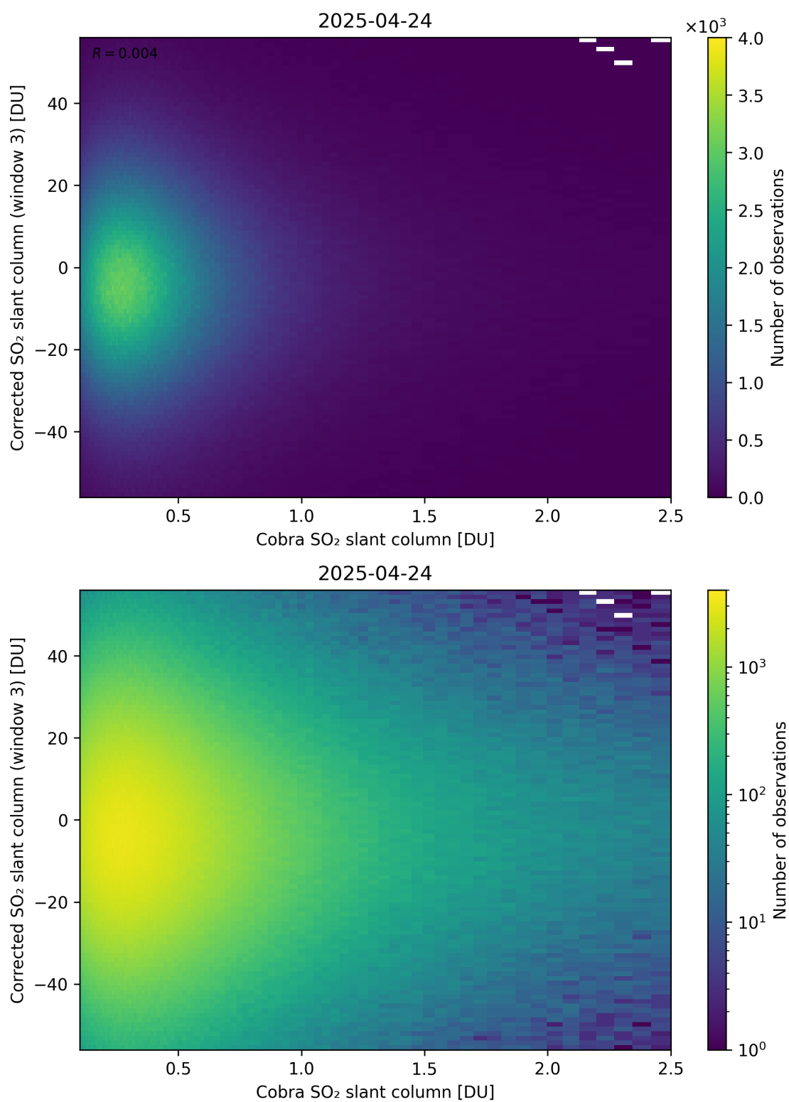
Figure 218: Scatter density plot of “Cobra SO 2 slant column” against “Corrected SO 2 slant column (window 3)” for 2025-04-24 to 2025-04-25.
