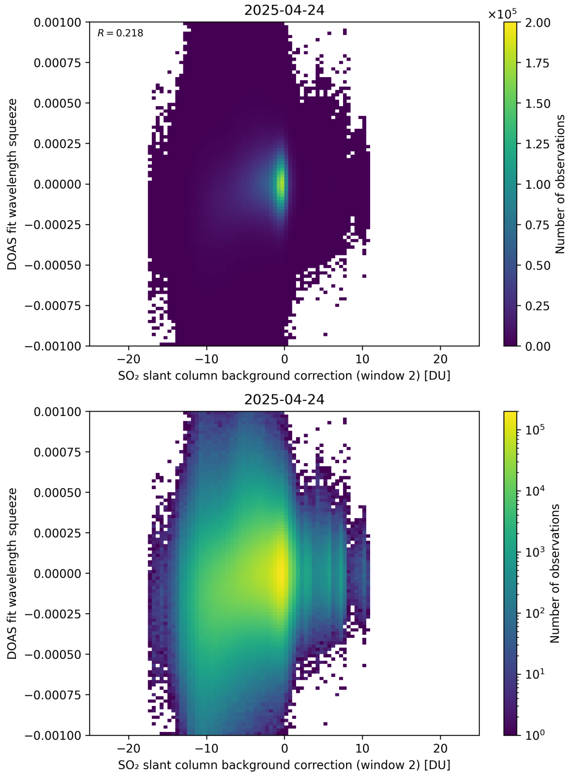
Figure 124: Scatter density plot of “SO 2 slant column background correction (window 2)” against “DOAS fit wavelength squeeze” for 2025-04-24 to 2025-04-25.
