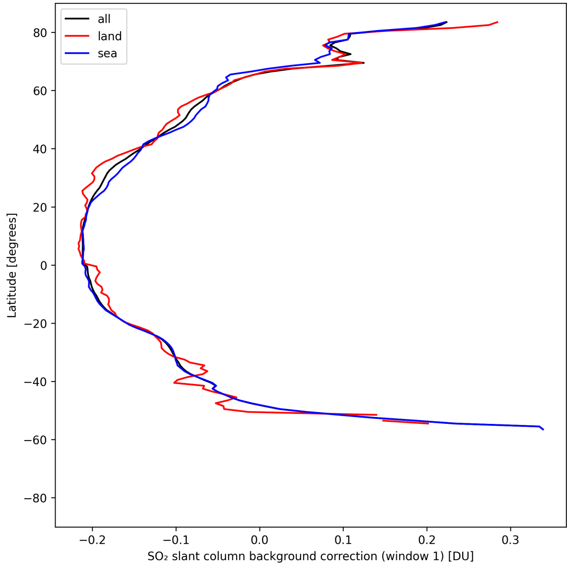
Figure 40: Zonal average of “SO 2 slant column background correction (window 1)” for 2025-04-24 to 2025-04-25.
