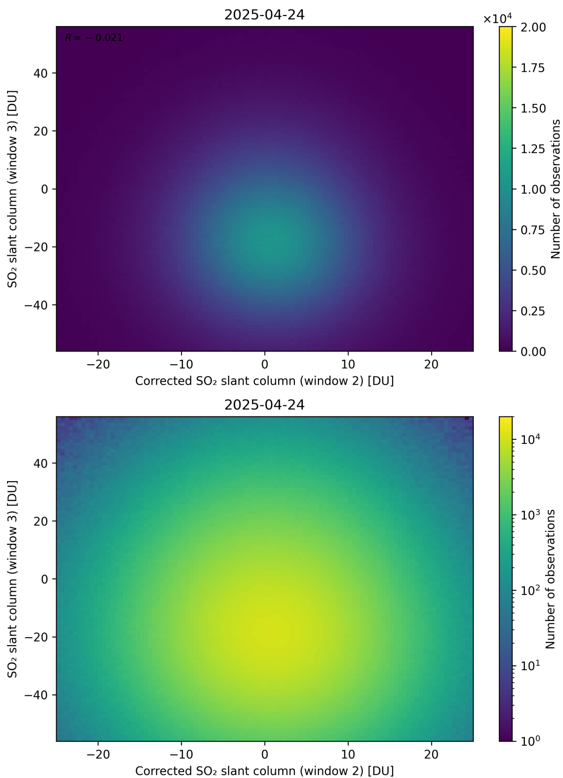
Figure 251: Scatter density plot of “Corrected SO 2 slant column (window 2)” against “SO 2 slant column (window 3)” for 2025-04-24 to 2025-04-25.
