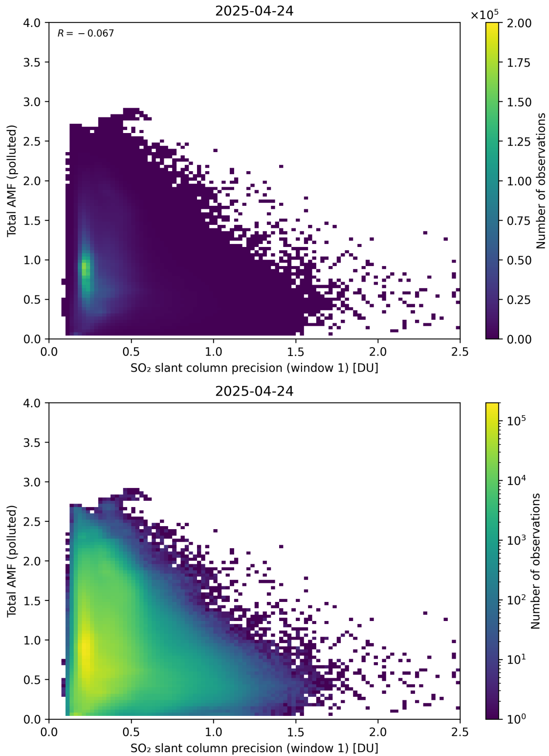
Figure 280: Scatter density plot of “SO 2 slant column precision (window 1)” against “Total AMF (polluted)” for 2025-04-24 to 2025-04-25.
