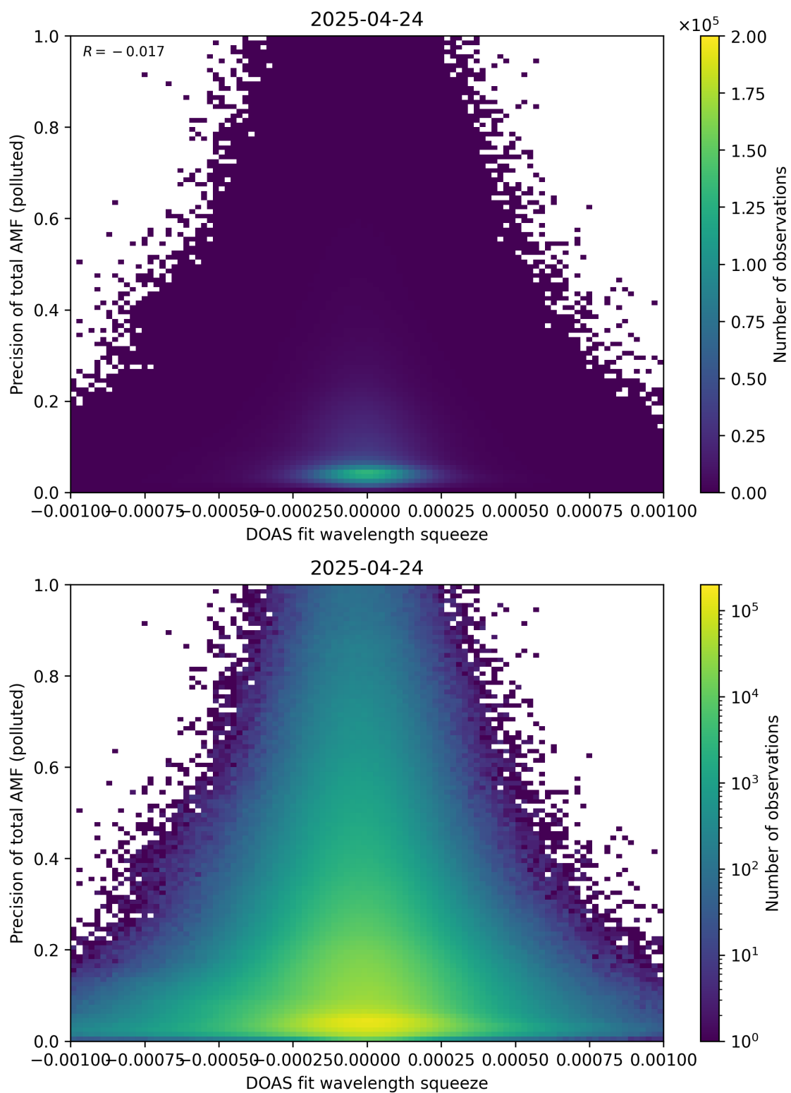
Figure 146: Scatter density plot of “DOAS fit wavelength squeeze” against “Precision of total AMF (polluted)” for 2025-04-24 to 2025-04-25.
