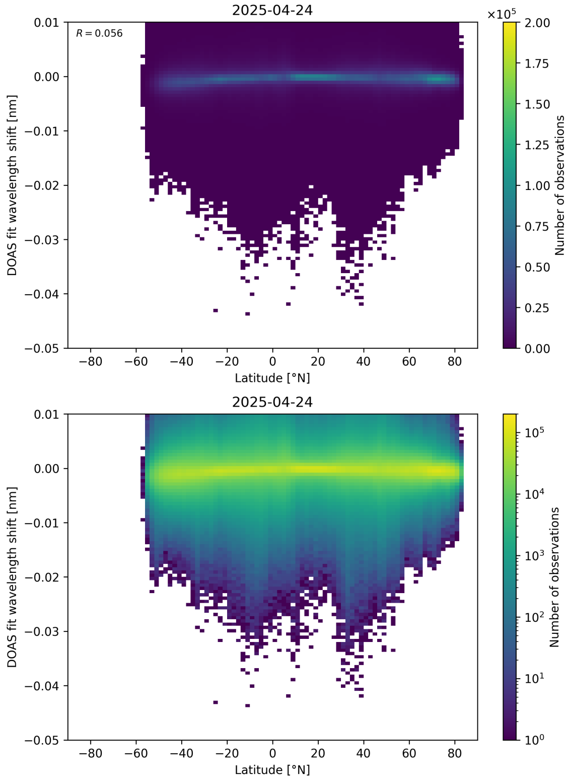
Figure 153: Scatter density plot of “Latitude” against “DOAS fit wavelength shift” for 2025-04-24 to 2025-04-25.
