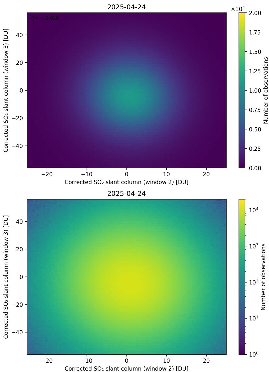
Figure 250: Scatter density plot of “Corrected SO 2 slant column (window 2)” against “Corrected SO 2 slant column (window 3)” for 2025-04-24 to 2025-04-25.
