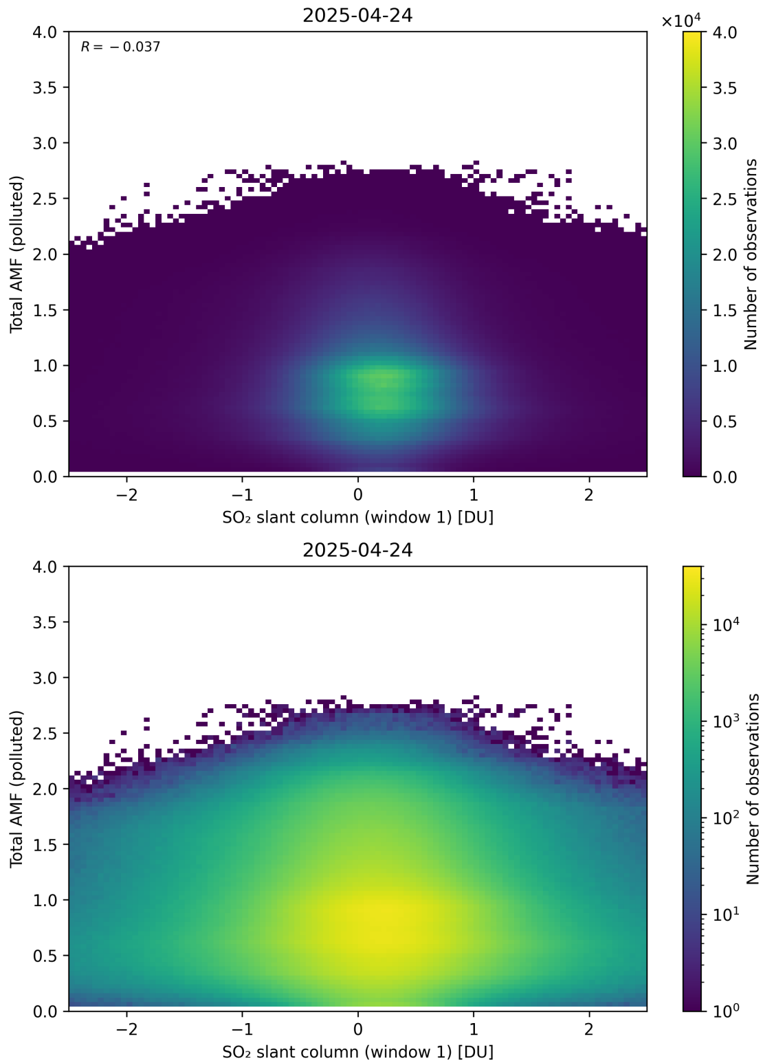
Figure 289: Scatter density plot of “SO 2 slant column (window 1)” against “Total AMF (polluted)” for 2025-04-24 to 2025-04-25.
