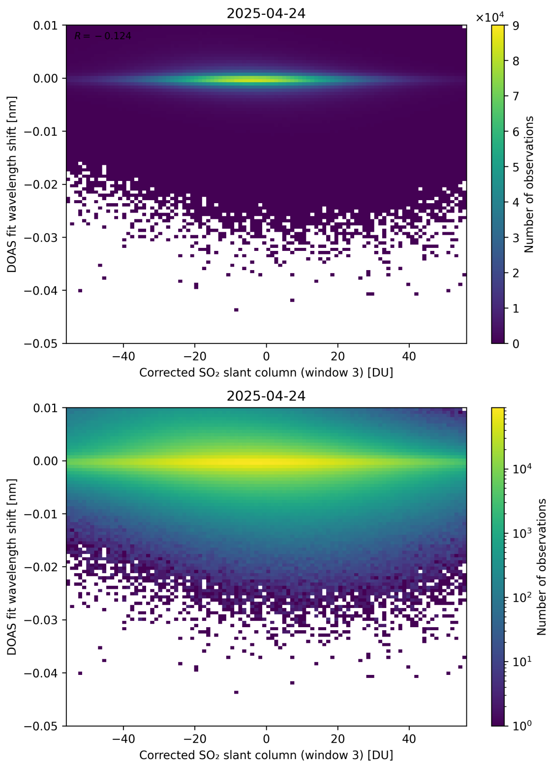
Figure 256: Scatter density plot of “Corrected SO 2 slant column (window 3)” against “DOAS fit wavelength shift” for 2025-04-24 to 2025-04-25.
