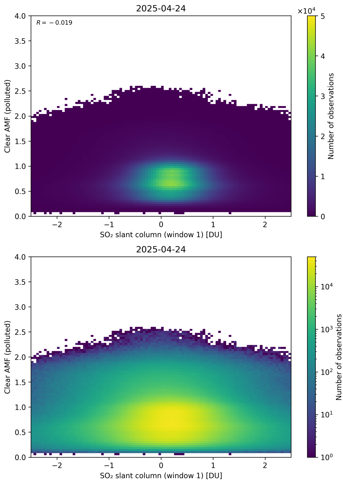
Figure 282: Scatter density plot of “SO 2 slant column (window 1)” against “Clear AMF (polluted)” for 2025-04-24 to 2025-04-25.
