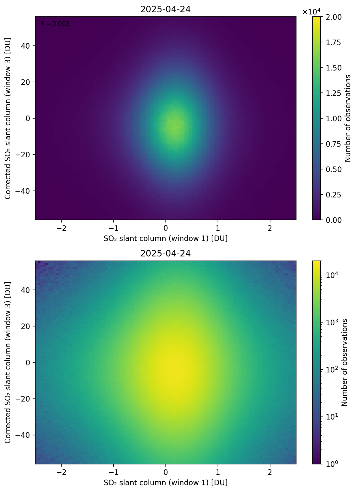
Figure 284: Scatter density plot of “SO 2 slant column (window 1)” against “Corrected SO 2 slant column (window 3)” for 2025-04-24 to 2025-04-25.
