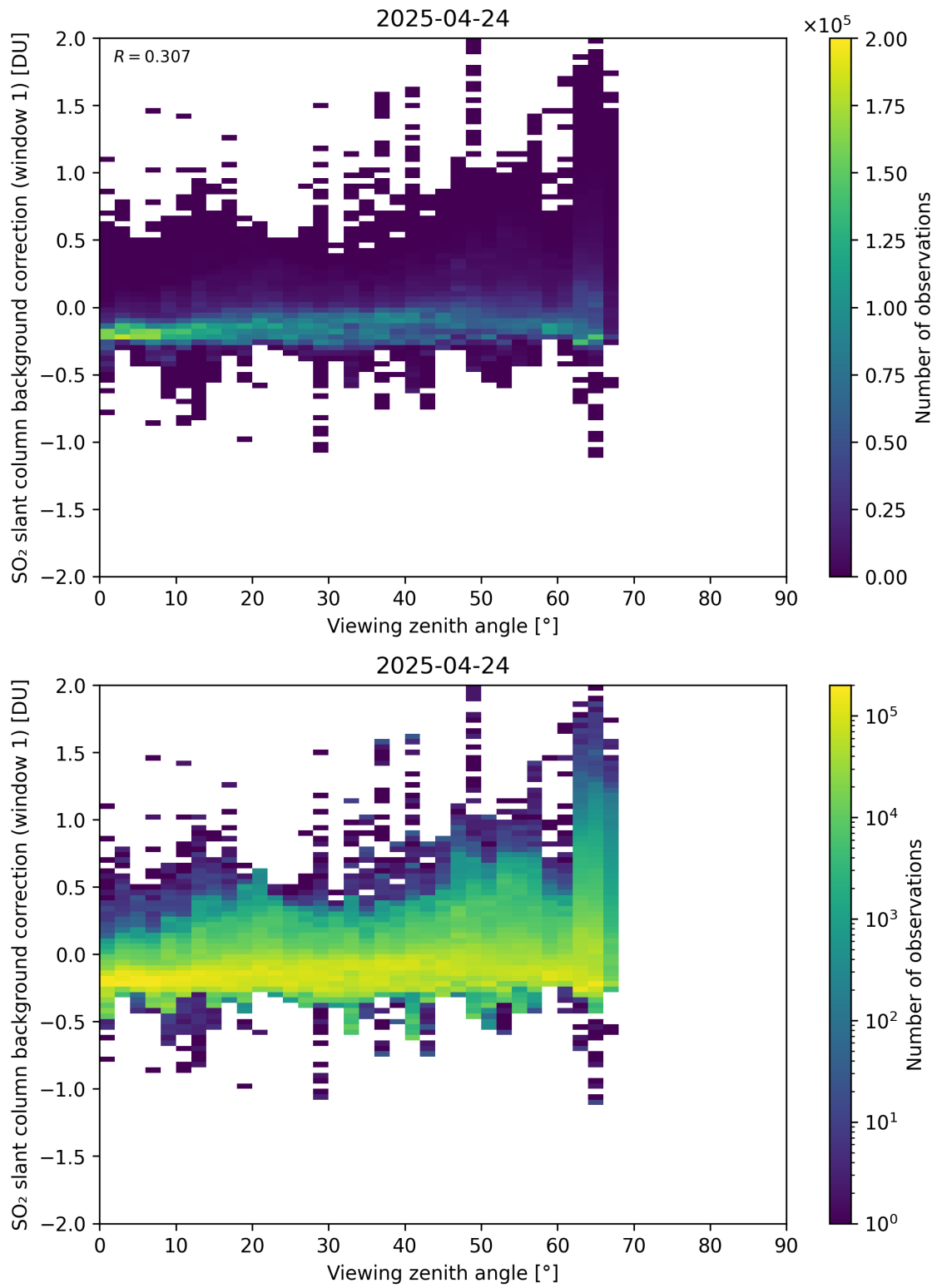
Figure 362: Scatter density plot of “Viewing zenith angle” against “SO 2 slant column background correction (window 1)” for 2025-04-24 to 2025-04-25.
