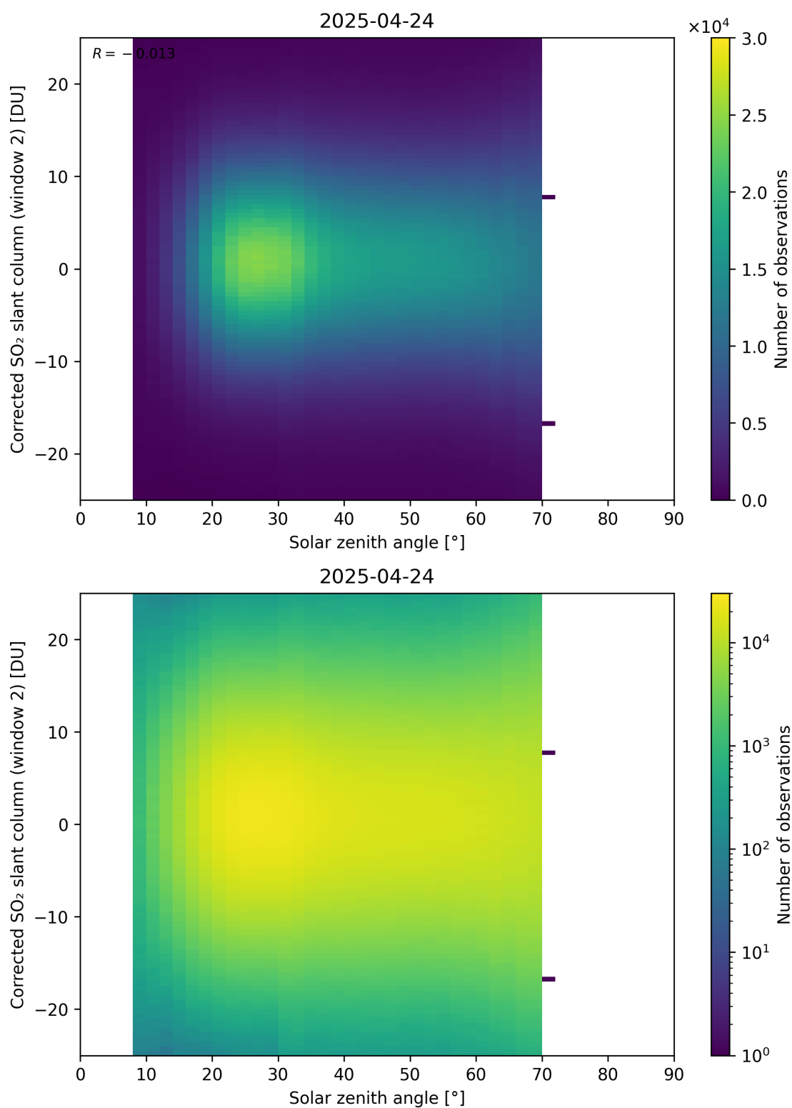
Figure 182: Scatter density plot of “Solar zenith angle” against “Corrected SO 2 slant column (window 2)” for 2025-04-24 to 2025-04-25.
