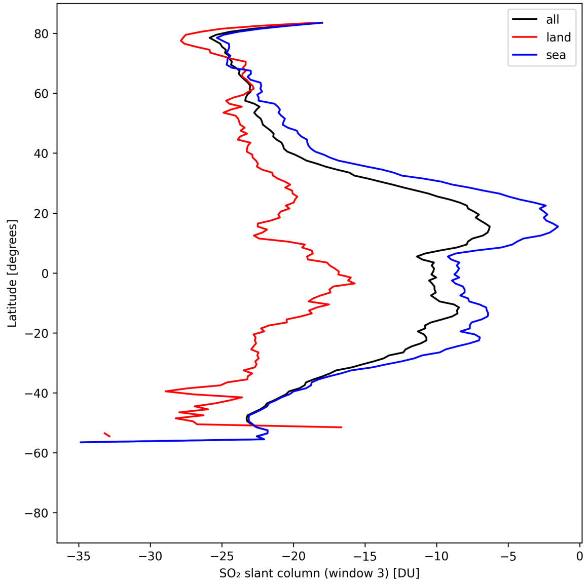
Figure 45: Zonal average of “SO 2 slant column (window 3)” for 2025-04-24 to 2025-04-25.
