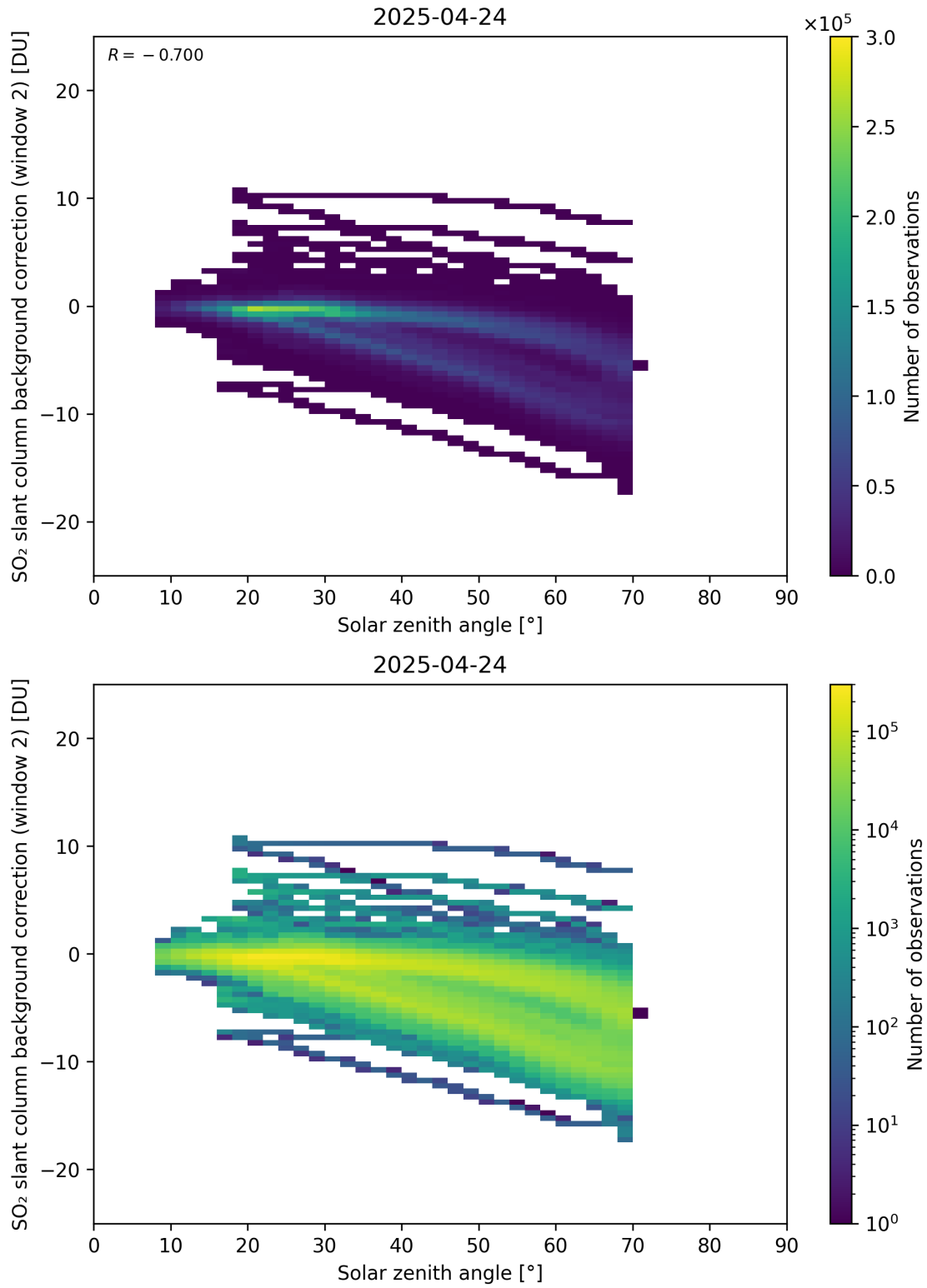
Figure 172: Scatter density plot of “Solar zenith angle” against “SO 2 slant column background correction (window 2)” for 2025-04-24 to 2025-04-25.
