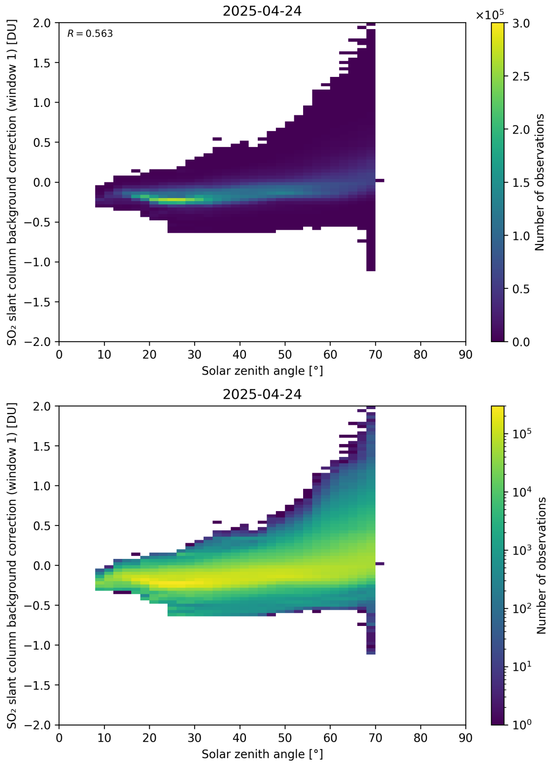
Figure 171: Scatter density plot of “Solar zenith angle” against “SO 2 slant column background correction (window 1)” for 2025-04-24 to 2025-04-25.
