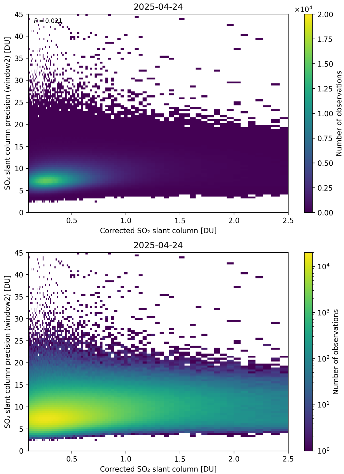
Figure 239: Scatter density plot of “Corrected SO 2 slant column” against “SO 2 slant column precision (window2)” for 2025-04-24 to 2025-04-25.
