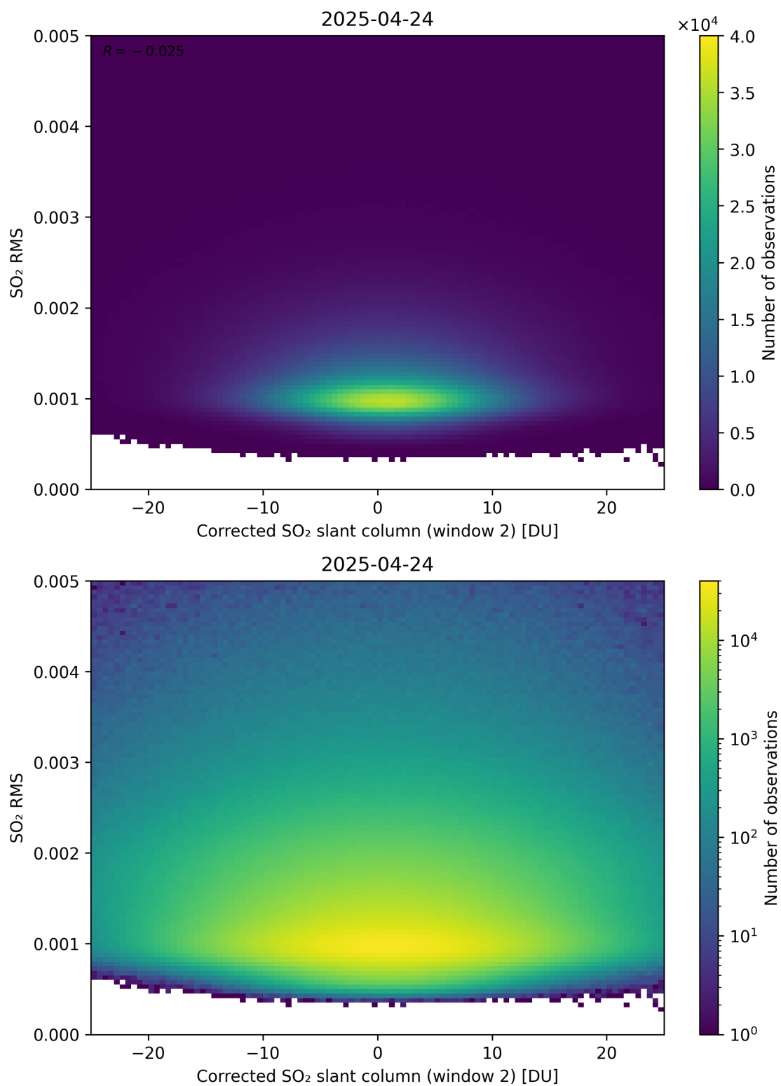
Figure 248: Scatter density plot of “Corrected SO 2 slant column (window 2)” against “SO 2 RMS” for 2025-04-24 to 2025-04-25.
