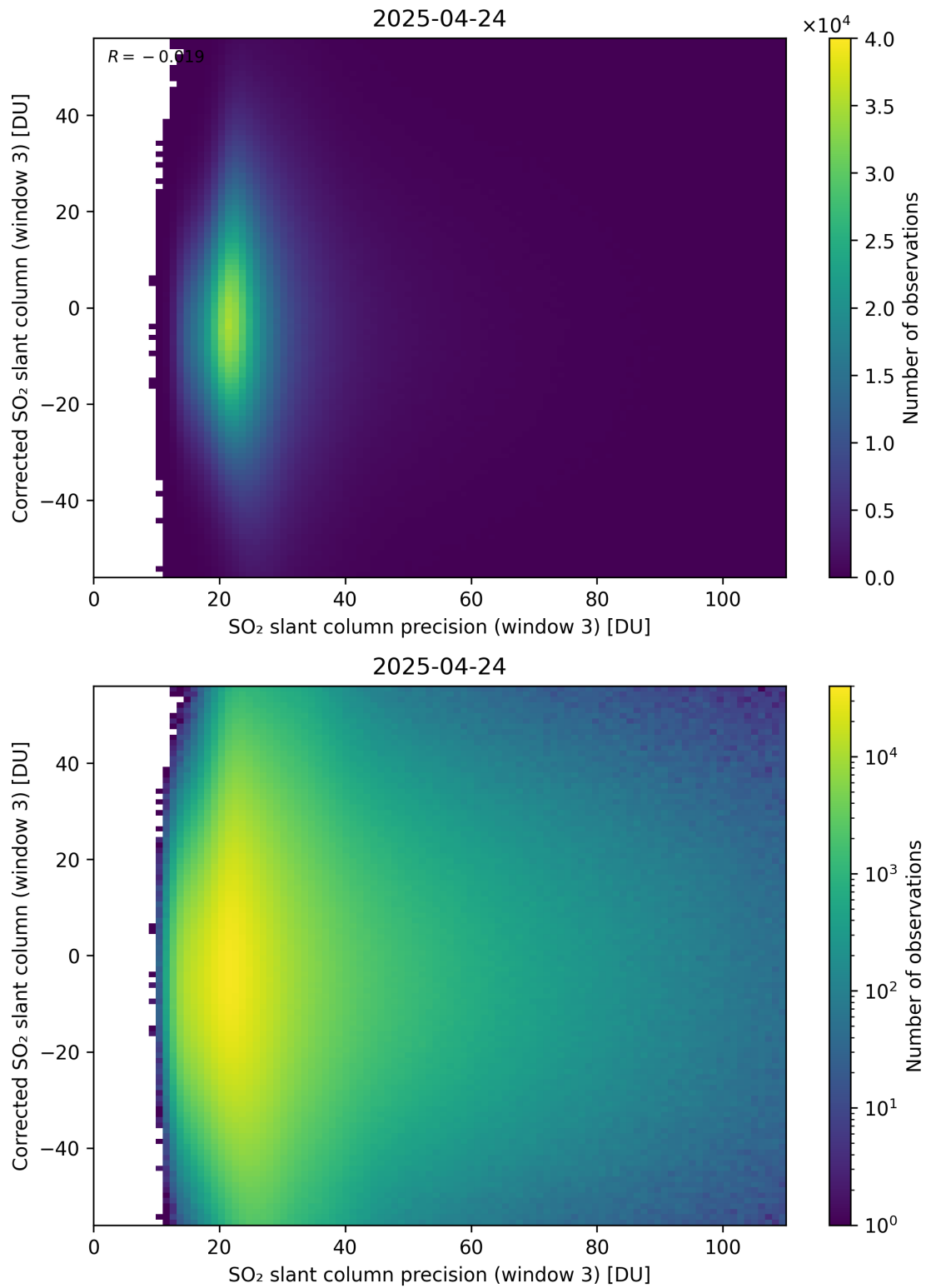
Figure 312: Scatter density plot of “SO 2 slant column precision (window 3)” against “Corrected SO 2 slant column (window 3)” for 2025-04-24 to 2025-04-25.
