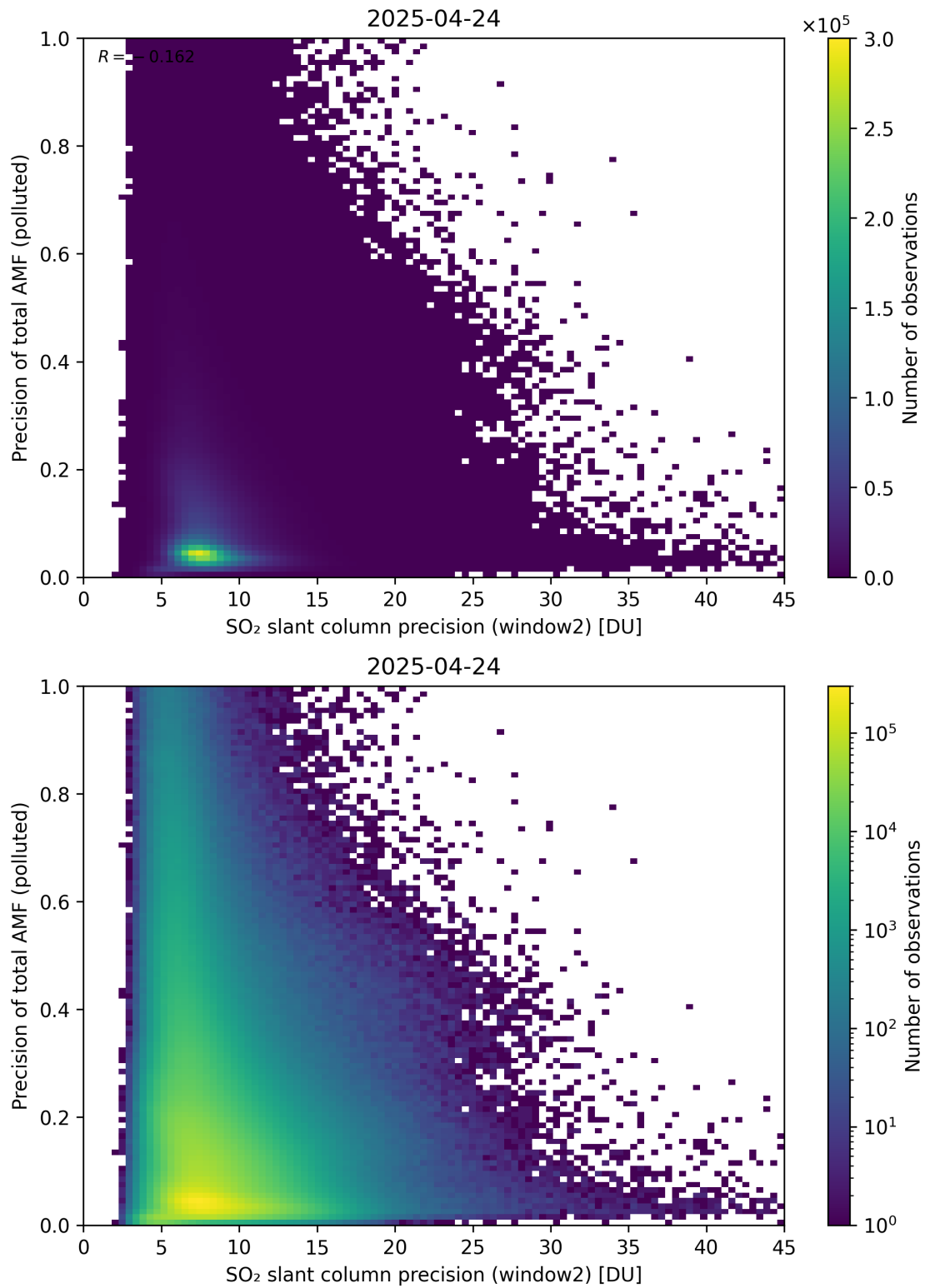
Figure 302: Scatter density plot of “SO 2 slant column precision (window2)” against “Precision of total AMF (polluted)” for 2025-04-24 to 2025-04-25.
