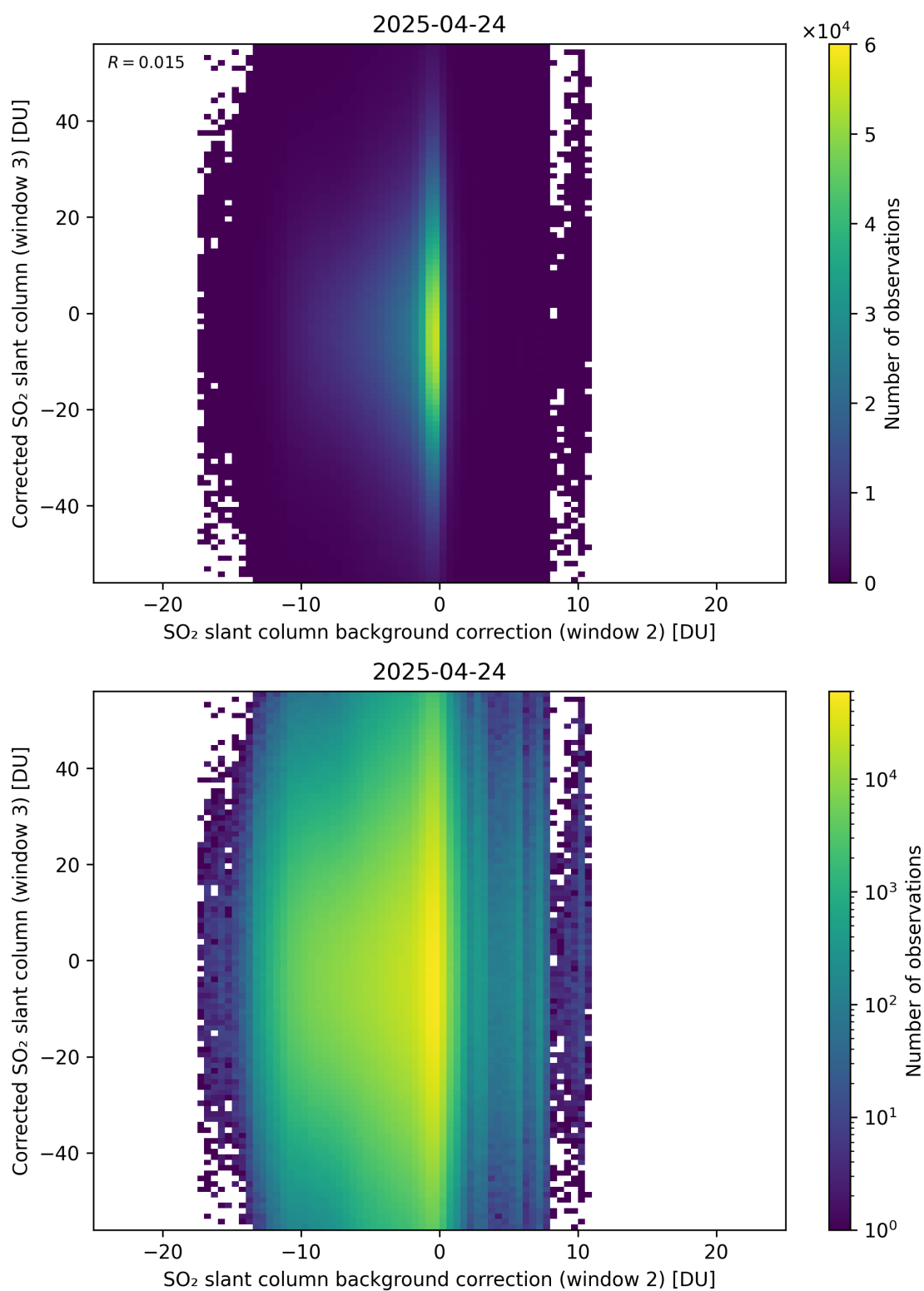
Figure 127: Scatter density plot of “SO 2 slant column background correction (window 2)” against “Corrected SO 2 slant column (window 3)” for 2025-04-24 to 2025-04-25.
