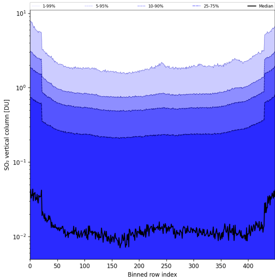
Figure 84: Along track statistics of “SO 2 vertical column” for 2025-04-24 to 2025-04-25
