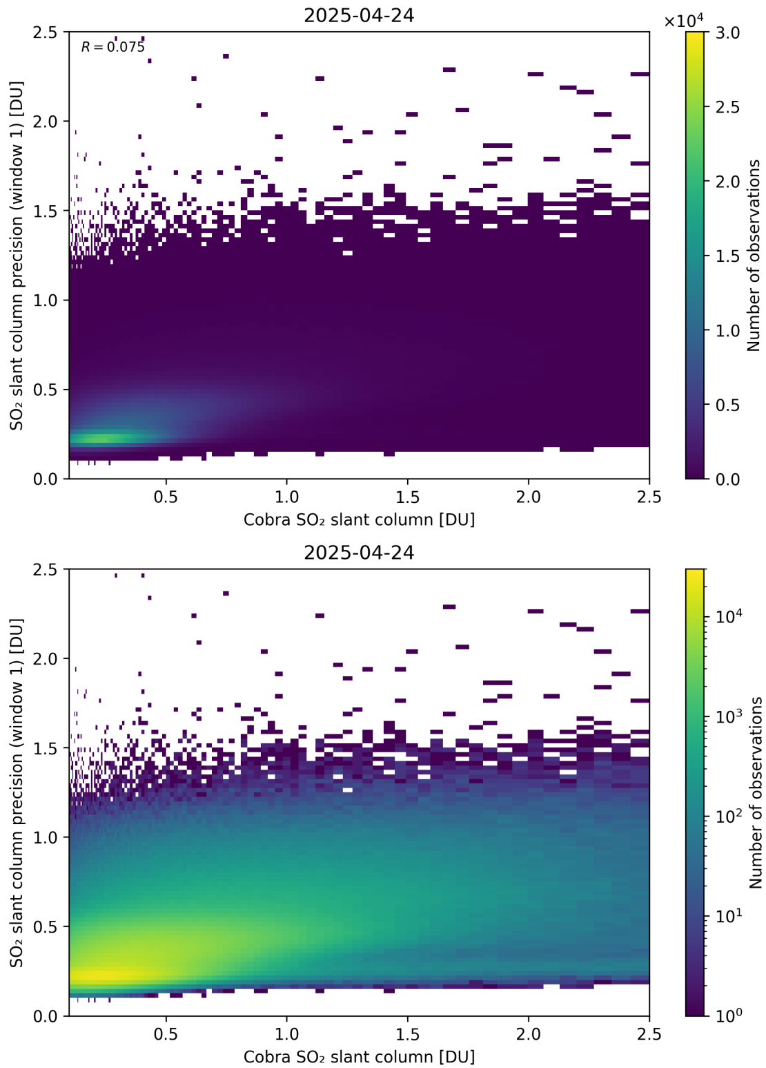
Figure 220: Scatter density plot of “Cobra SO 2 slant column” against “SO 2 slant column precision (window 1)” for 2025-04-24 to 2025-04-25.
