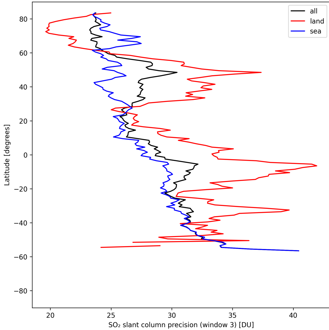
Figure 46: Zonal average of “SO 2 slant column precision (window 3)” for 2025-04-24 to 2025-04-25.
