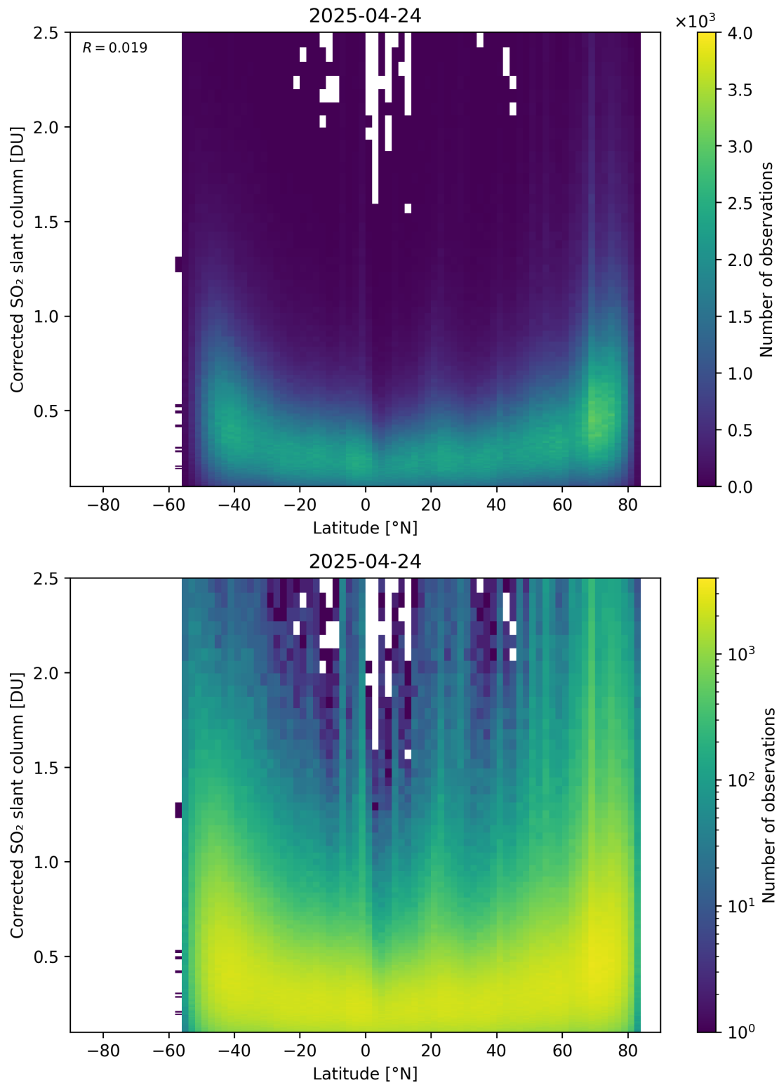
Figure 159: Scatter density plot of “Latitude” against “Corrected SO 2 slant column” for 2025-04-24 to 2025-04-25.
