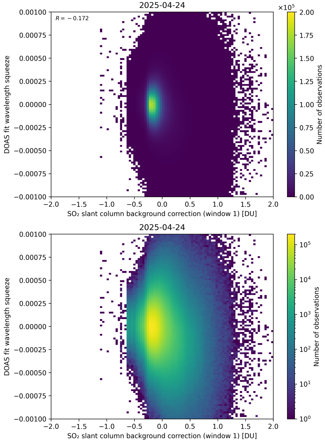
Figure 112: Scatter density plot of “SO 2 slant column background correction (window 1)” against “DOAS fit wavelength squeeze” for 2025-04-24 to 2025-04-25.
