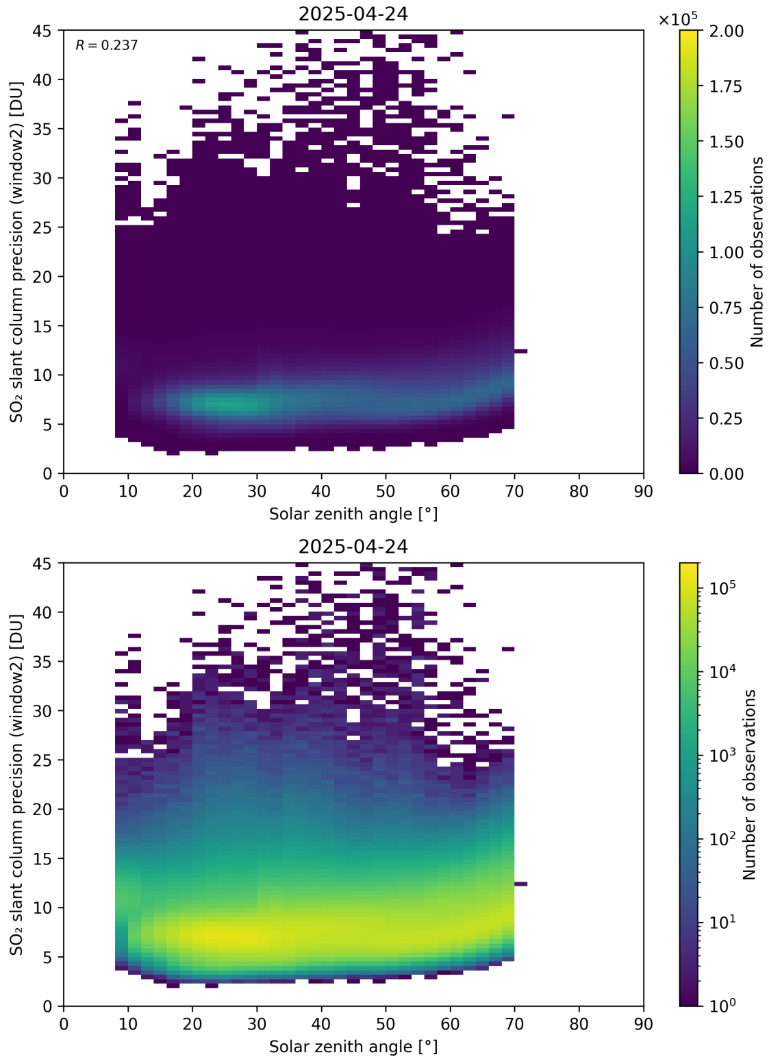
Figure 186: Scatter density plot of “Solar zenith angle” against “SO 2 slant column precision (window2)” for 2025-04-24 to 2025-04-25.
