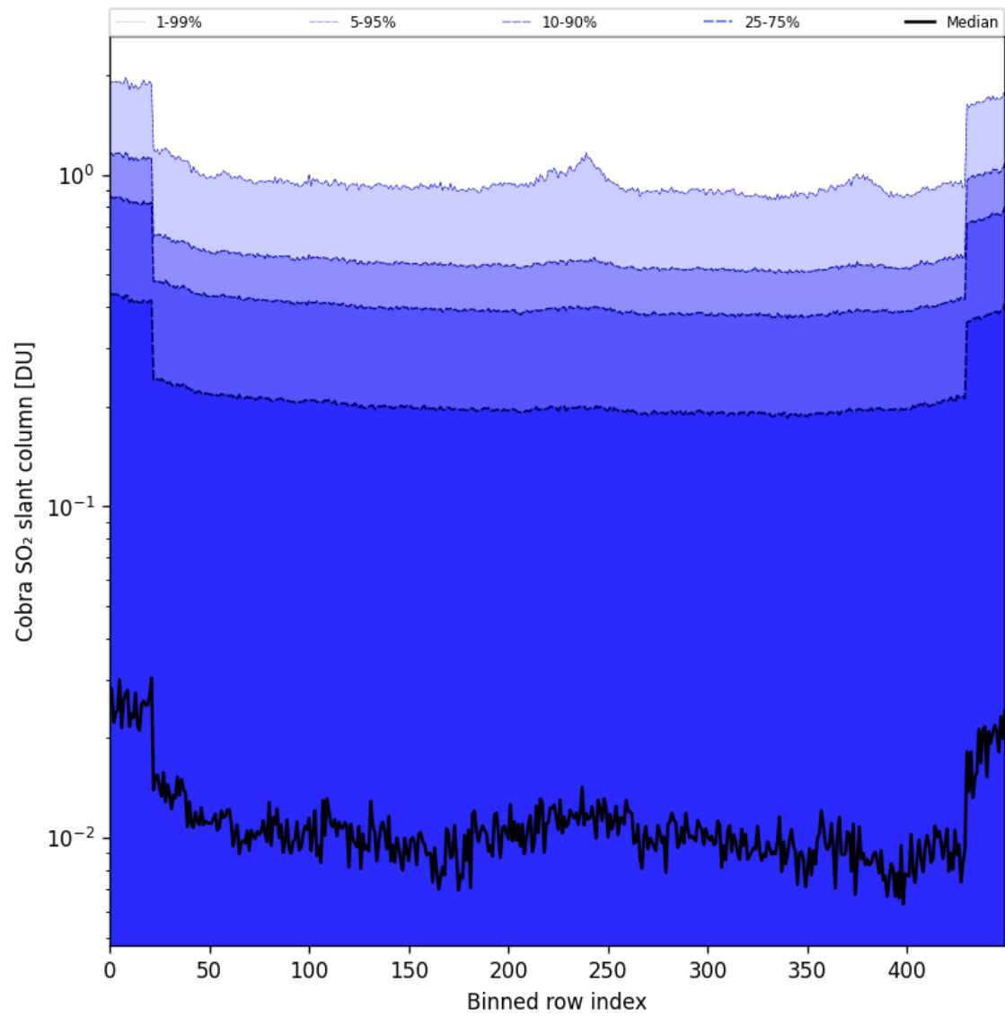
Figure 87: Along track statistics of “Cobra SO 2 slant column” for 2025-04-24 to 2025-04-25
