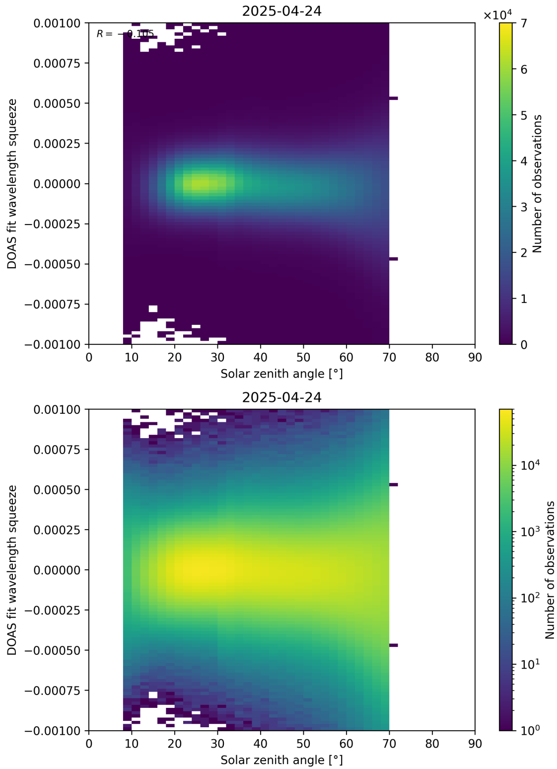
Figure 175: Scatter density plot of “Solar zenith angle” against “DOAS fit wavelength squeeze” for 2025-04-24 to 2025-04-25.
