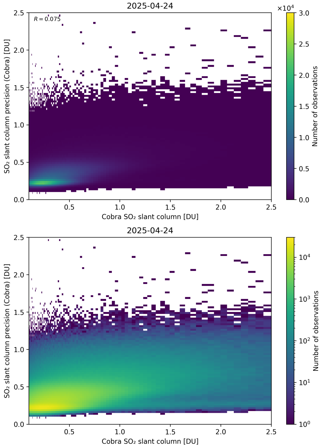
Figure 216: Scatter density plot of “Cobra SO 2 slant column” against “SO 2 slant column precision (Cobra)” for 2025-04-24 to 2025-04-25.
