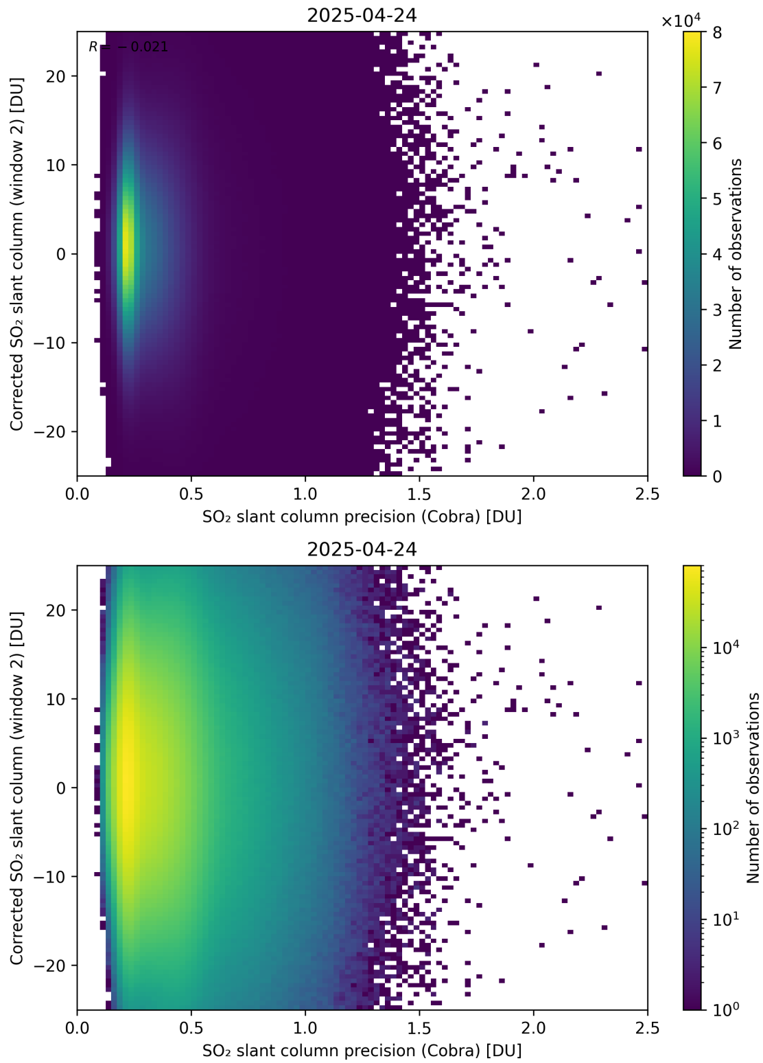
Figure 206: Scatter density plot of “SO 2 slant column precision (Cobra)” against “Corrected SO 2 slant column (window 2)” for 2025-04-24 to 2025-04-25.
