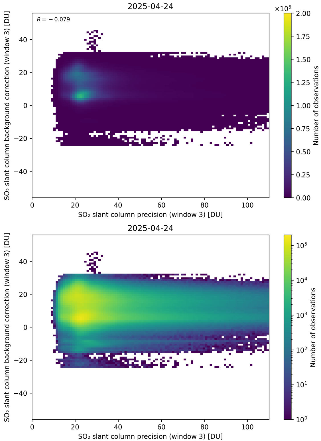
Figure 307: Scatter density plot of “SO 2 slant column precision (window 3)” against “SO 2 slant column background correction (window 3)” for 2025-04-24 to 2025-04-25.
