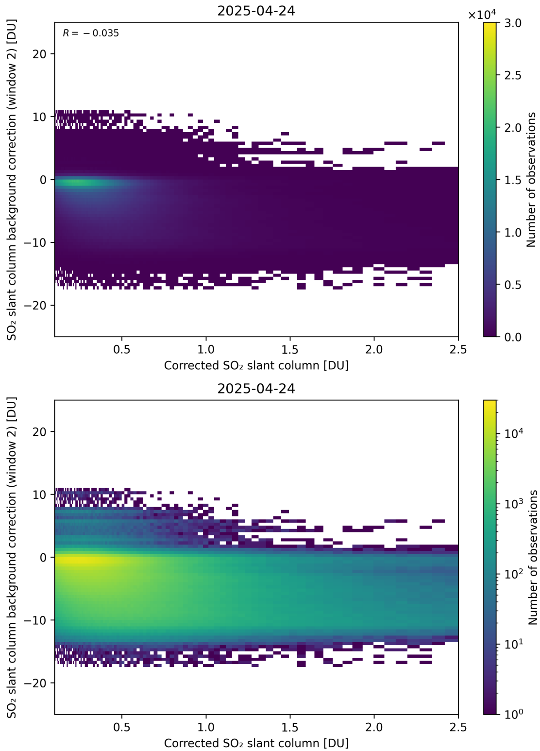
Figure 227: Scatter density plot of “Corrected SO 2 slant column” against “SO 2 slant column background correction (window 2)” for 2025-04-24 to 2025-04-25.
