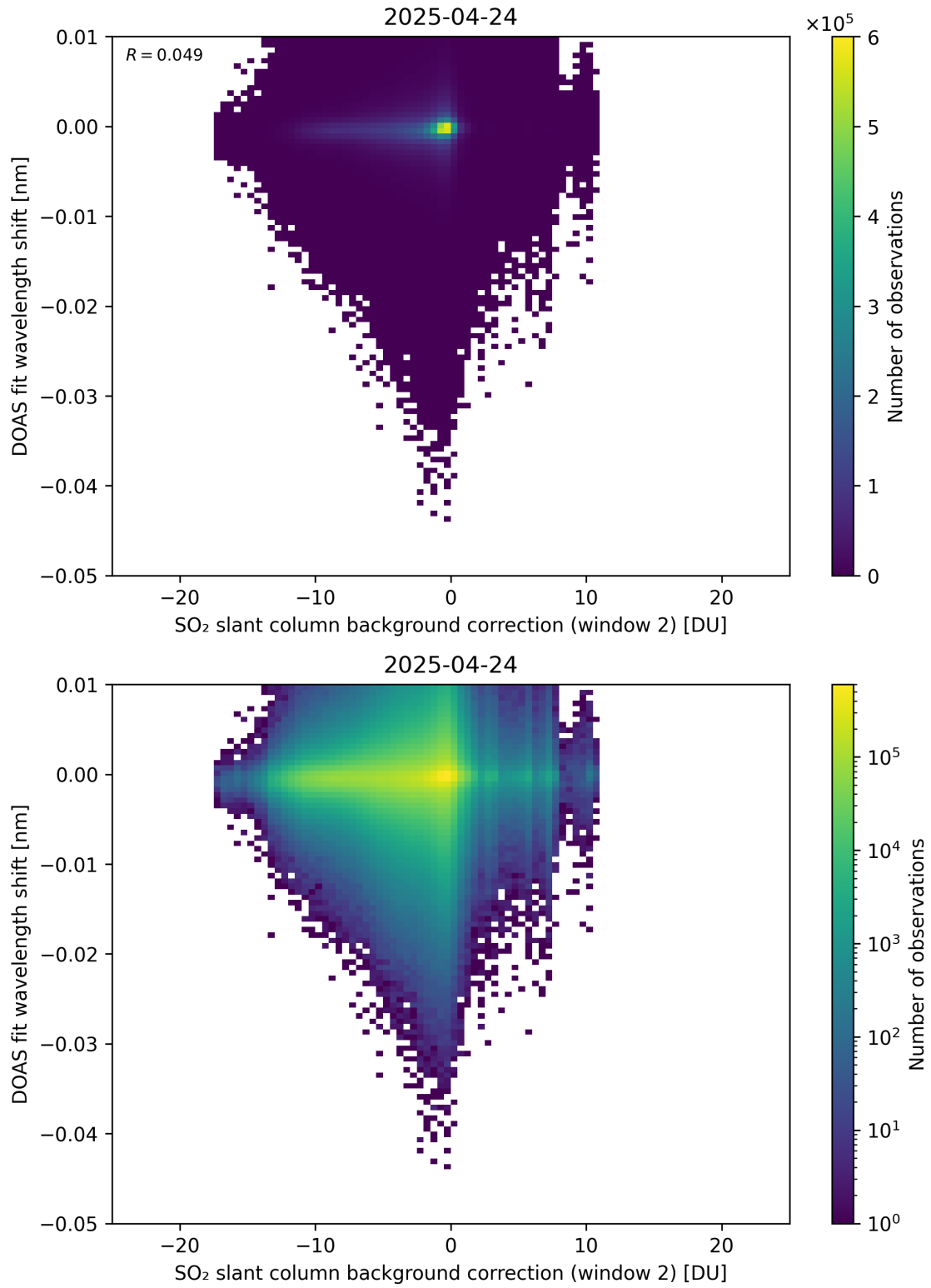
Figure 123: Scatter density plot of “SO 2 slant column background correction (window 2)” against “DOAS fit wavelength shift” for 2025-04-24 to 2025-04-25.
