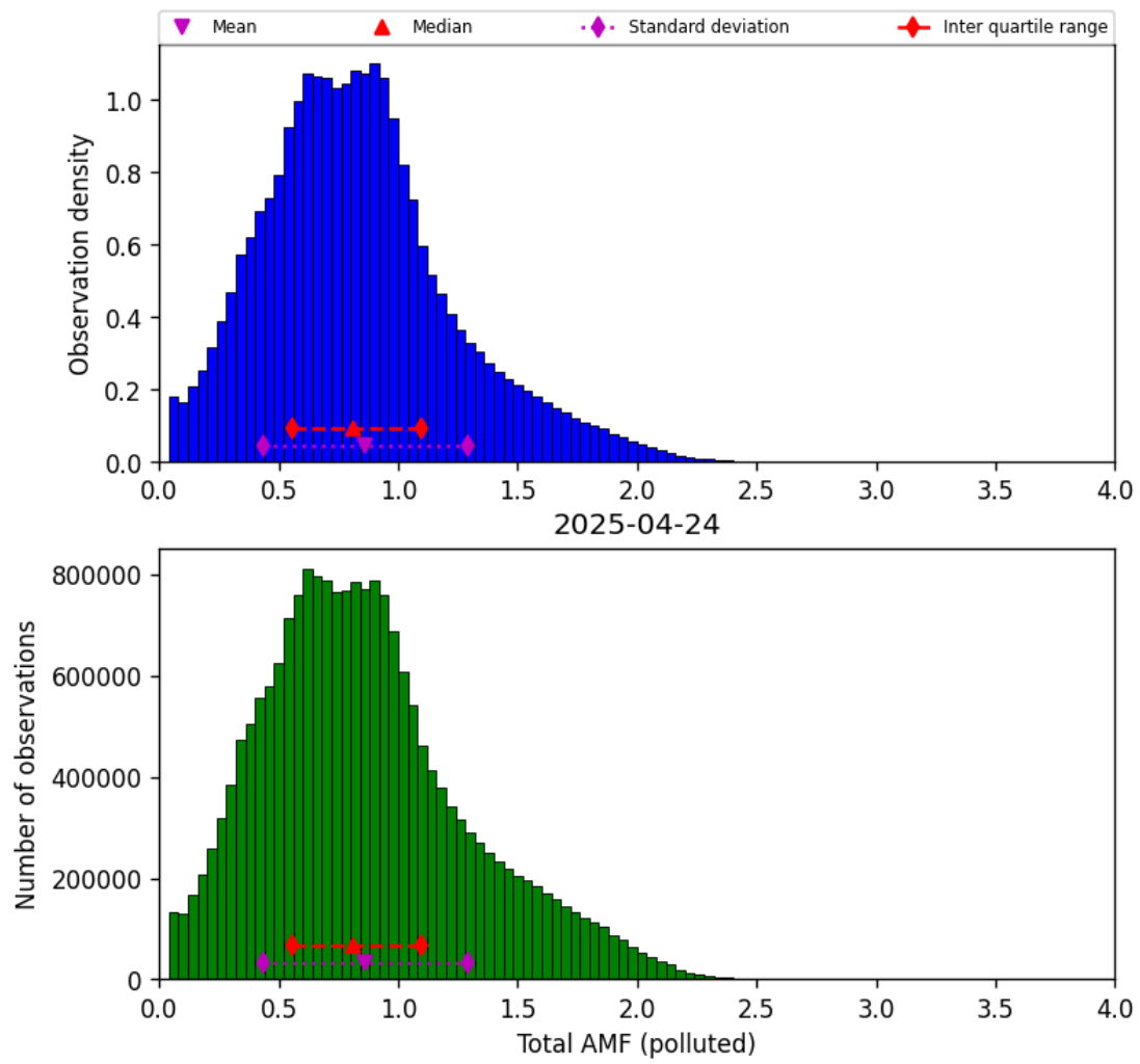
Figure 79: Histogram of “Total AMF (polluted)” for 2025-04-24 to 2025-04-25
