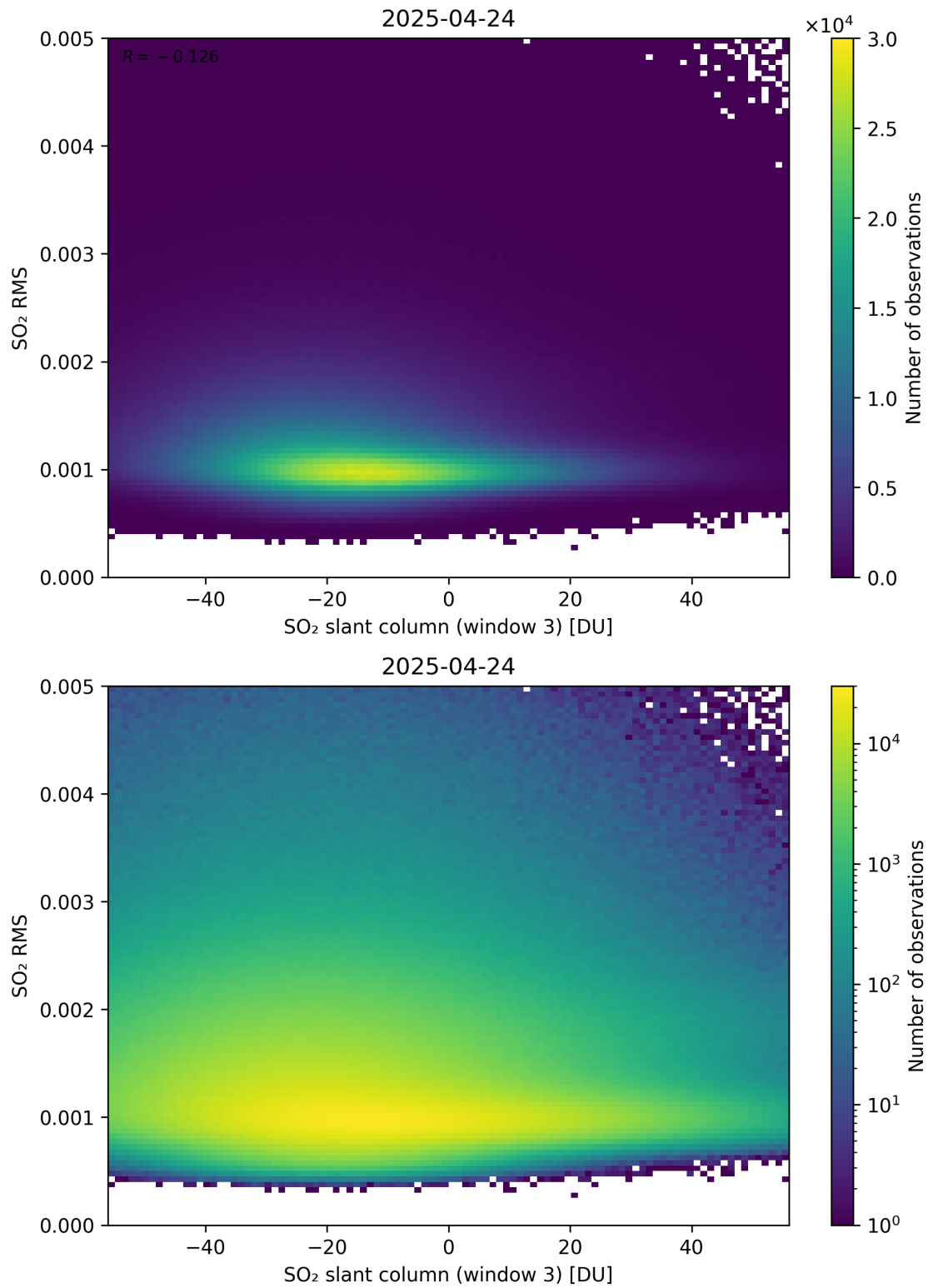
Figure 306: Scatter density plot of “SO 2 slant column (window 3)” against “SO 2 RMS” for 2025-04-24 to 2025-04-25.
