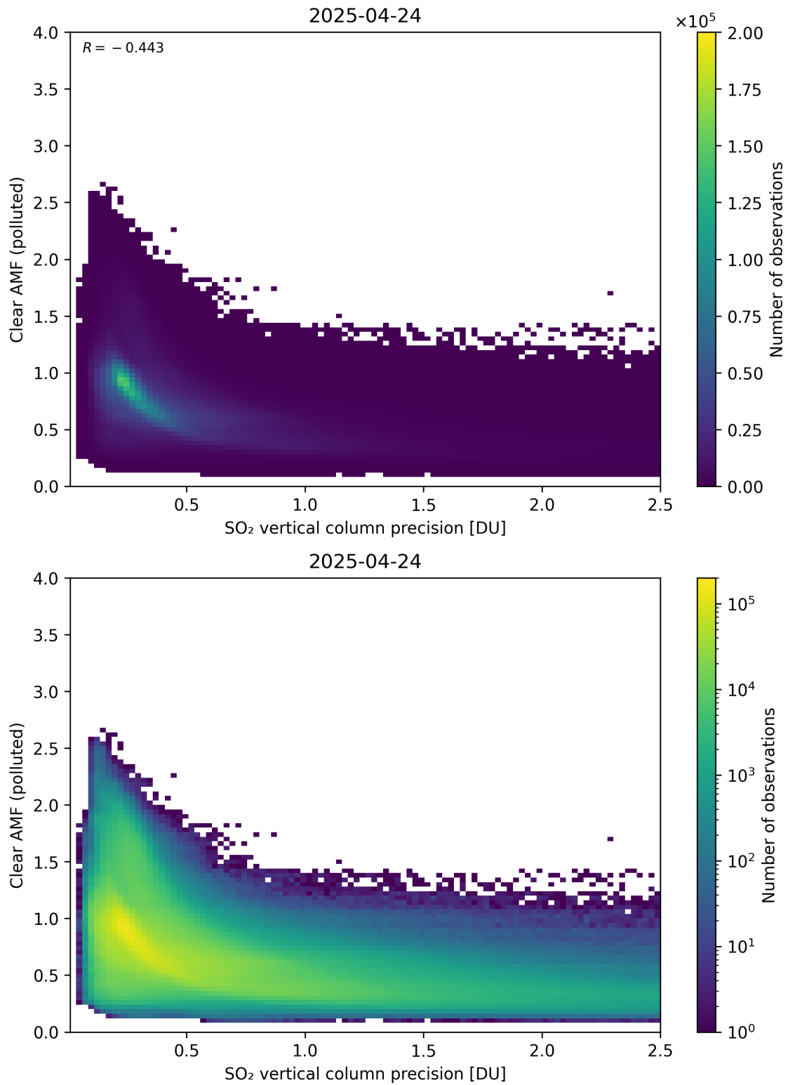
Figure 335: Scatter density plot of “SO 2 vertical column precision” against “Clear AMF (polluted)” for 2025-04-24 to 2025-04-25.
