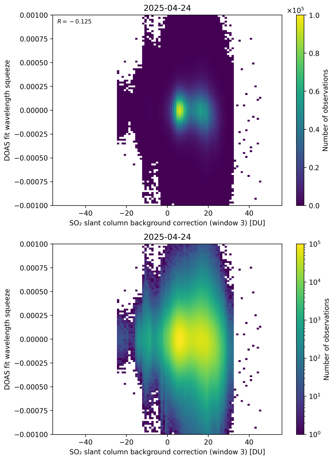
Figure 133: Scatter density plot of “SO 2 slant column background correction (window 3)” against “DOAS fit wavelength squeeze” for 2025-04-24 to 2025-04-25.
