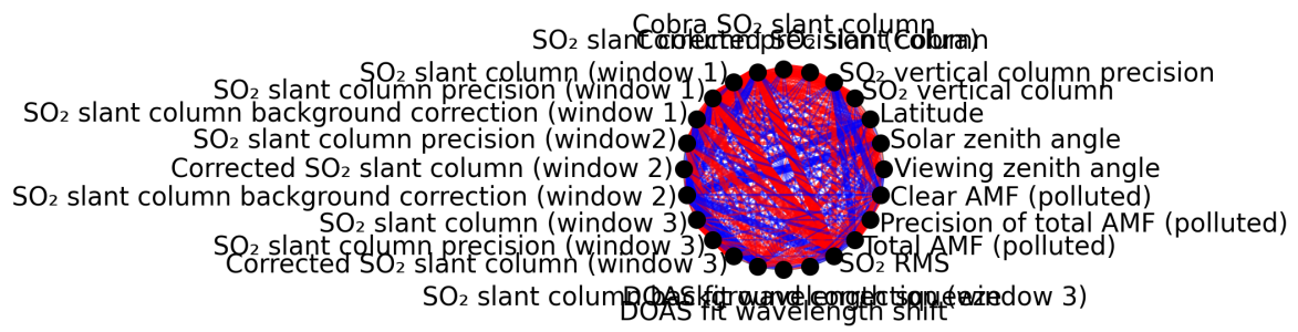
Figure 1: Map of correlation graph for 2025-04-24 to 2025-04-25.
