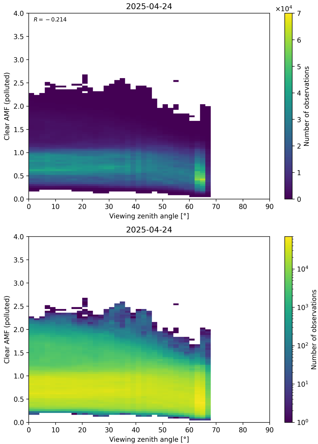
Figure 370: Scatter density plot of “Viewing zenith angle” against “Clear AMF (polluted)” for 2025-04-24 to 2025-04-25.
