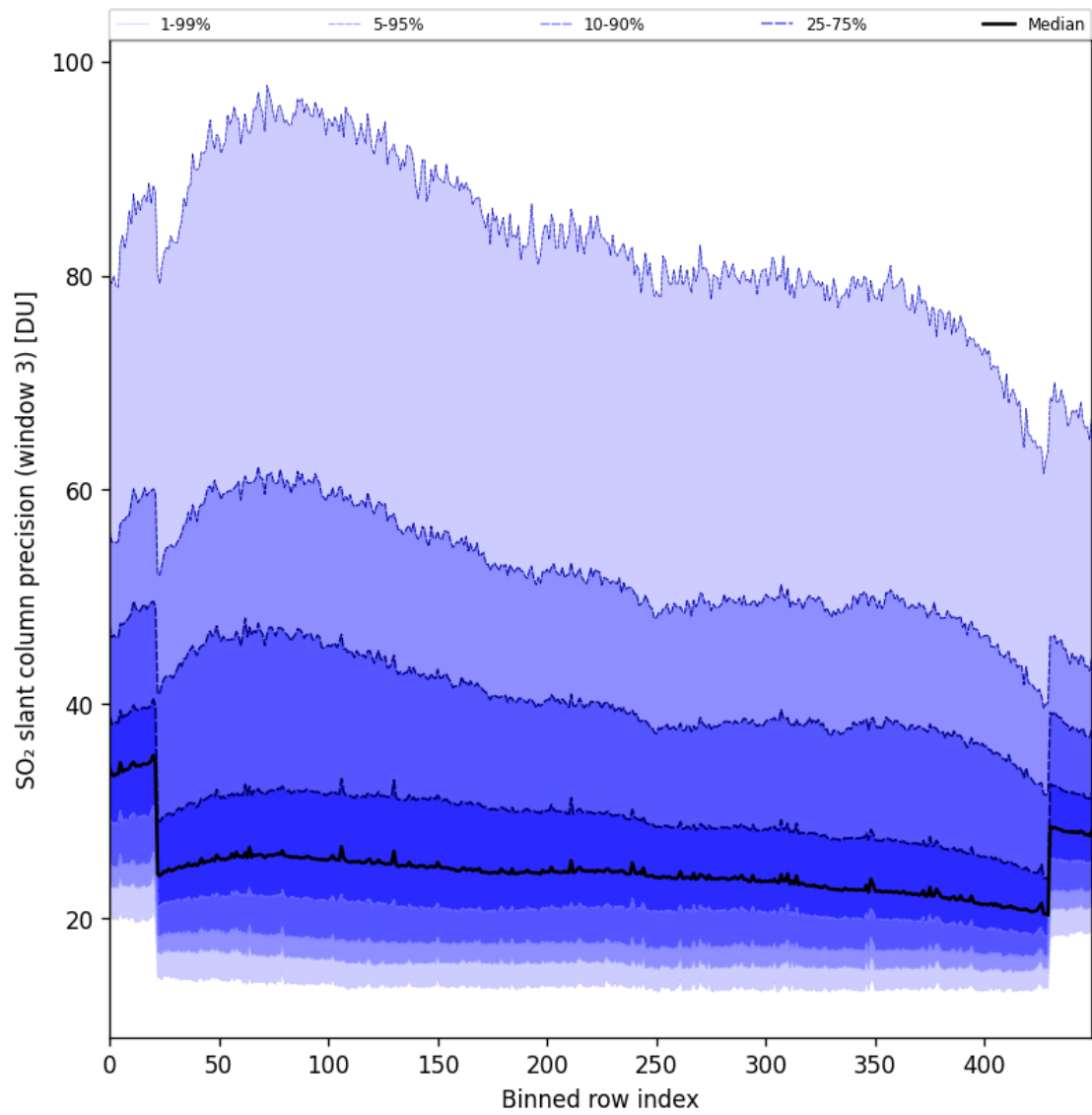
Figure 98: Along track statistics of “SO 2 slant column precision (window 3)” for 2025-04-24 to 2025-04-25
