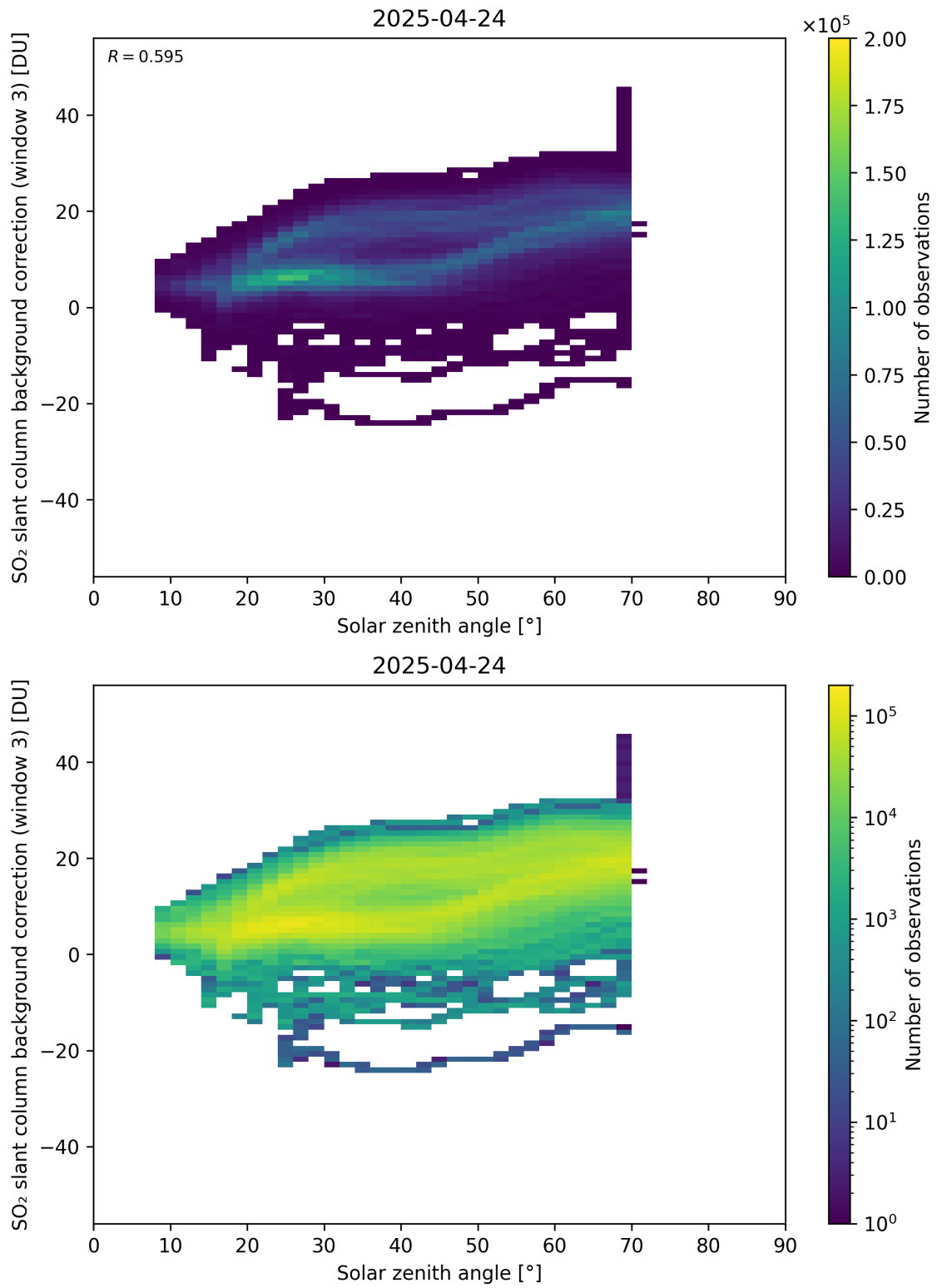
Figure 173: Scatter density plot of “Solar zenith angle” against “SO 2 slant column background correction (window 3)” for 2025-04-24 to 2025-04-25.
