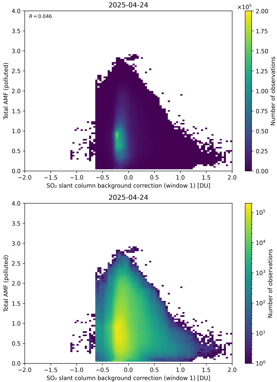
Figure 120: Scatter density plot of “SO 2 slant column background correction (window 1)” against “Total AMF (polluted)” for 2025-04-24 to 2025-04-25.
