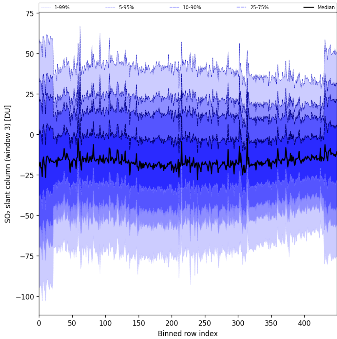
Figure 97: Along track statistics of “SO 2 slant column (window 3)” for 2025-04-24 to 2025-04-25
