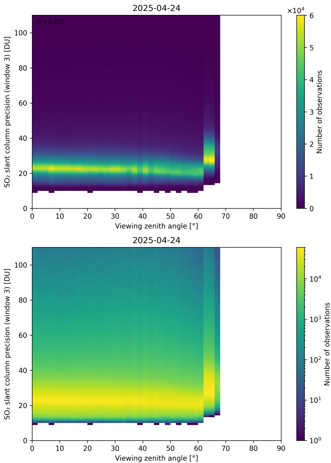
Figure 380: Scatter density plot of “Viewing zenith angle” against “SO 2 slant column precision (window 3)” for 2025-04-24 to 2025-04-25.
