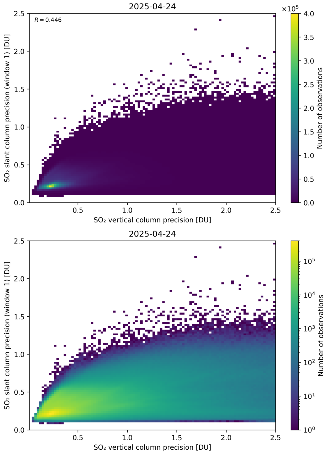
Figure 342: Scatter density plot of “SO 2 vertical column precision” against “SO 2 slant column precision (window 1)” for 2025-04-24 to 2025-04-25.
