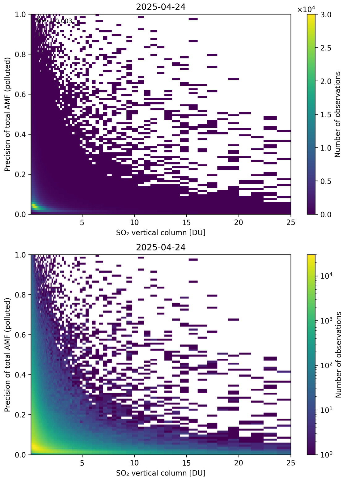
Figure 360: Scatter density plot of “SO 2 vertical column” against “Precision of total AMF (polluted)” for 2025-04-24 to 2025-04-25.
