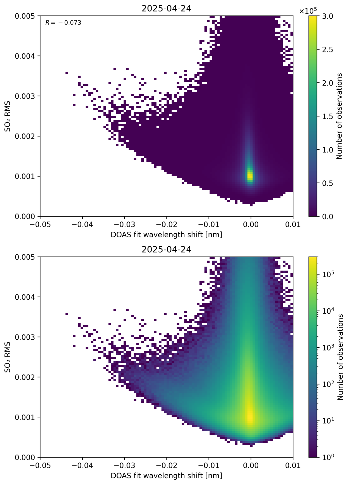
Figure 139: Scatter density plot of “DOAS fit wavelength shift” against “SO 2 RMS” for 2025-04-24 to 2025-04-25.
