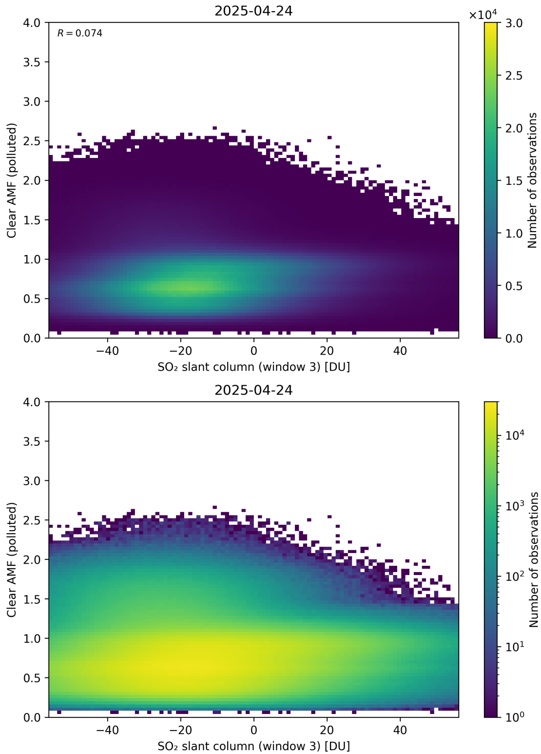
Figure 315: Scatter density plot of “SO 2 slant column (window 3)” against “Clear AMF (polluted)” for 2025-04-24 to 2025-04-25.
