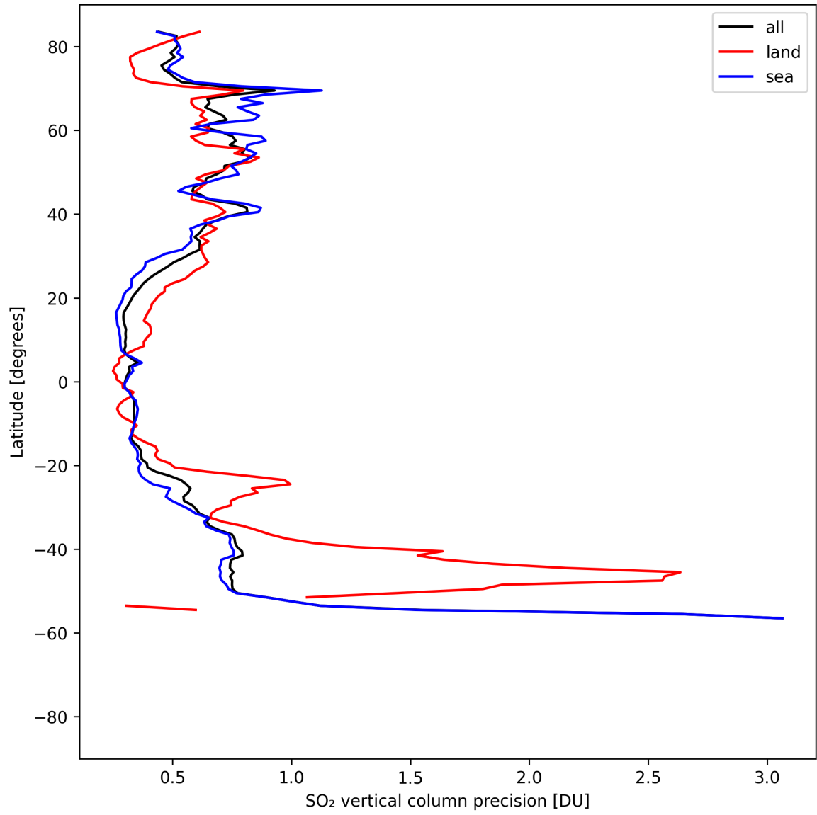
Figure 33: Zonal average of “SO 2 vertical column precision” for 2025-04-24 to 2025-04-25.
