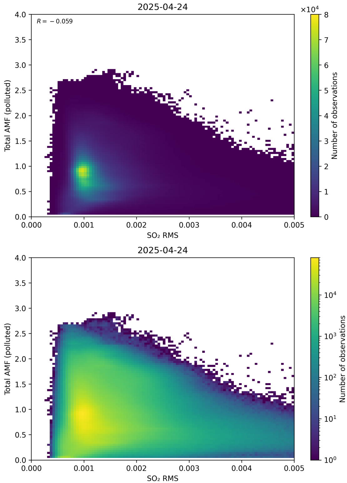
Figure 148: Scatter density plot of “SO 2 RMS” against “Total AMF (polluted)” for 2025-04-24 to 2025-04-25.
