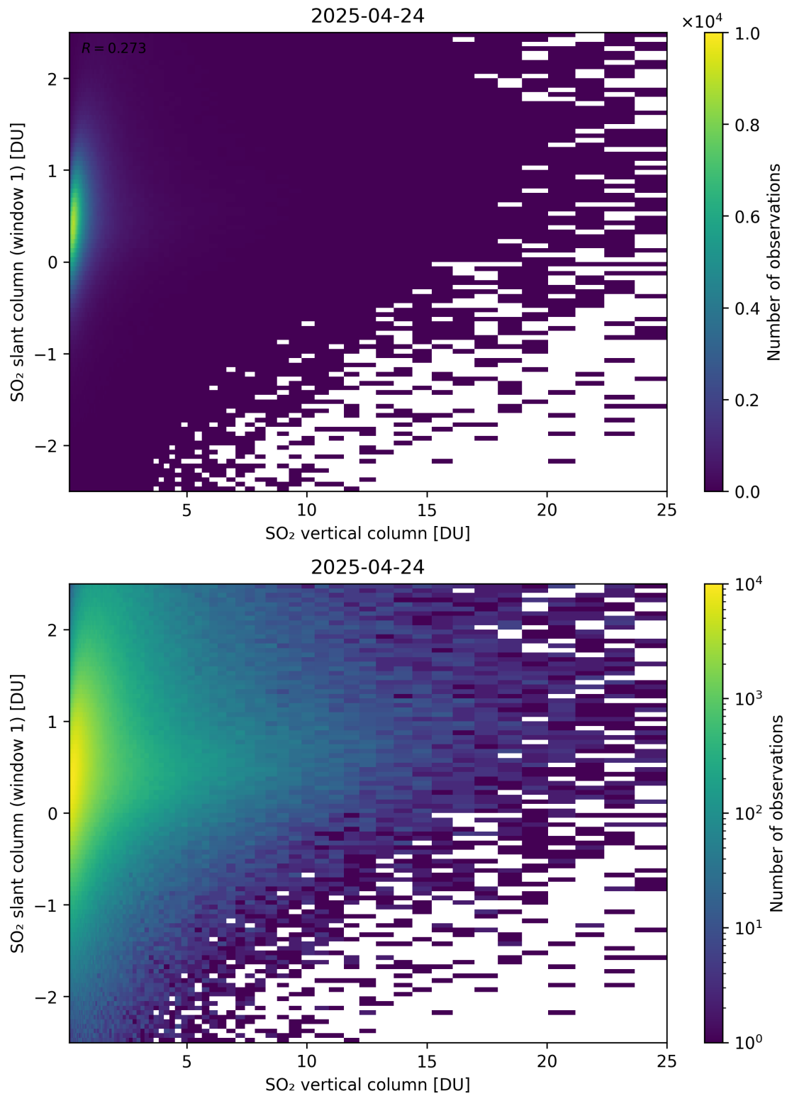
Figure 354: Scatter density plot of “SO 2 vertical column” against “SO 2 slant column (window 1)” for 2025-04-24 to 2025-04-25.
