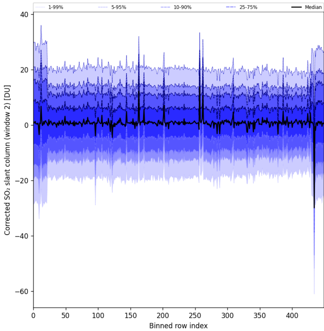
Figure 95: Along track statistics of “Corrected SO 2 slant column (window 2)” for 2025-04-24 to 2025-04-25
