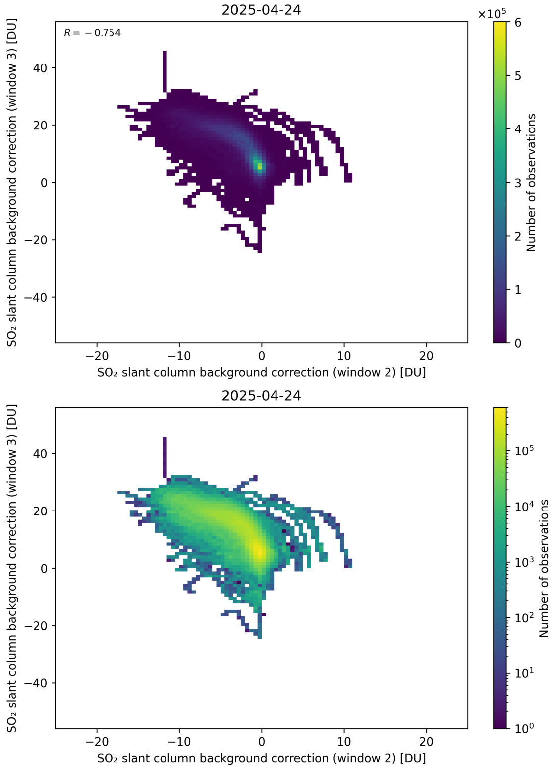
Figure 122: Scatter density plot of “SO 2 slant column background correction (window 2)” against “SO 2 slant column background correction (window 3)” for 2025-04-24 to 2025-04-25.
