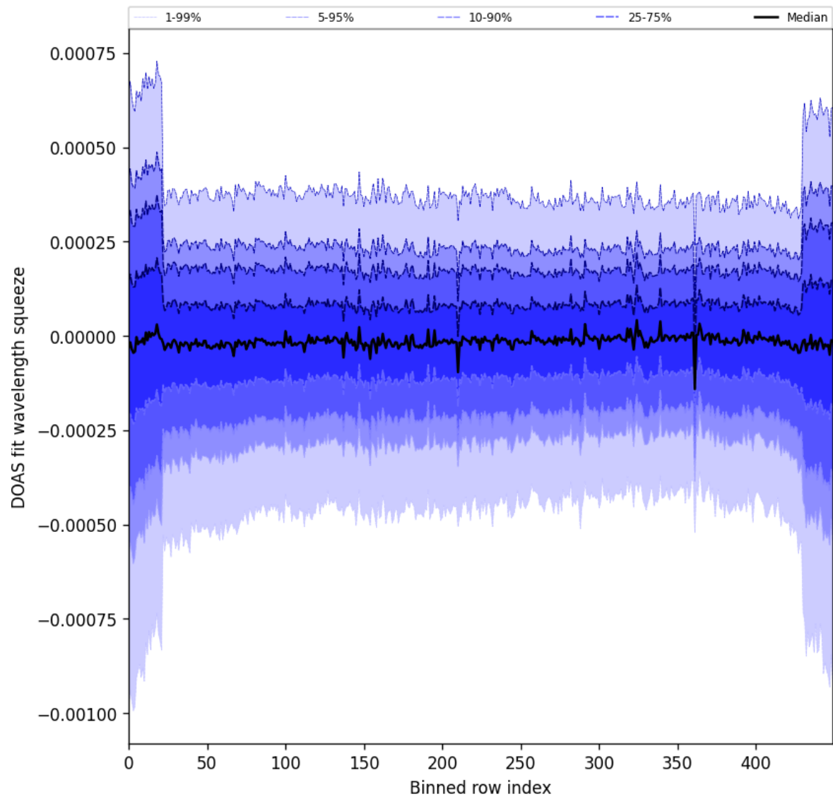
Figure 103: Along track statistics of “DOAS fit wavelength squeeze” for 2025-04-24 to 2025-04-25
