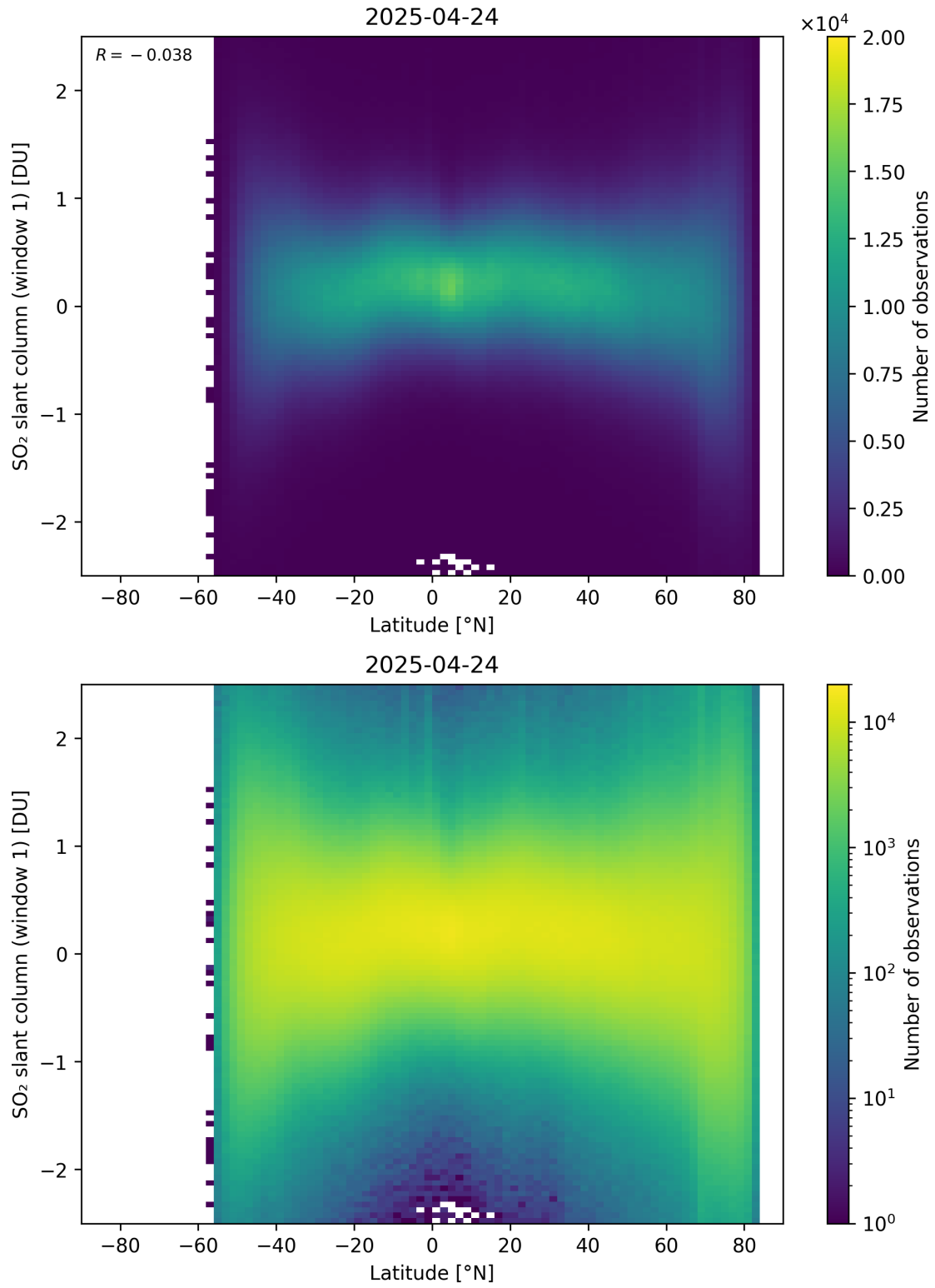
Figure 162: Scatter density plot of “Latitude” against “SO 2 slant column (window 1)” for 2025-04-24 to 2025-04-25.
