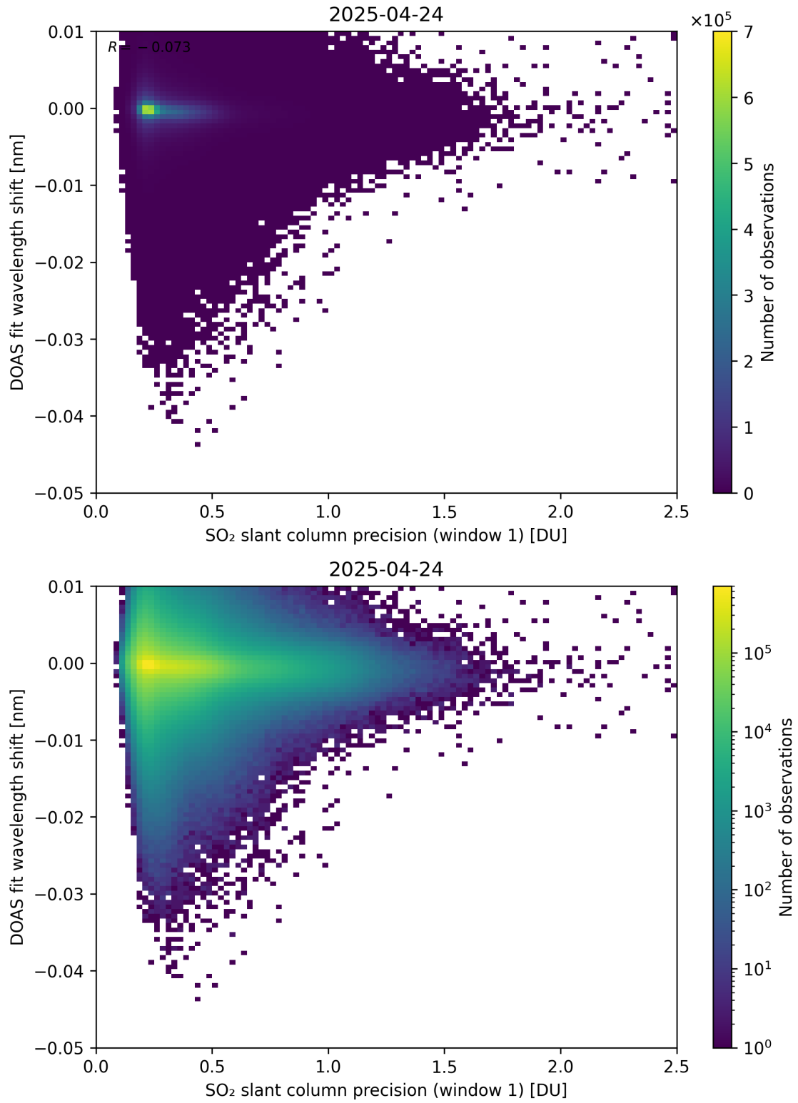
Figure 271: Scatter density plot of “SO 2 slant column precision (window 1)” against “DOAS fit wavelength shift” for 2025-04-24 to 2025-04-25.
