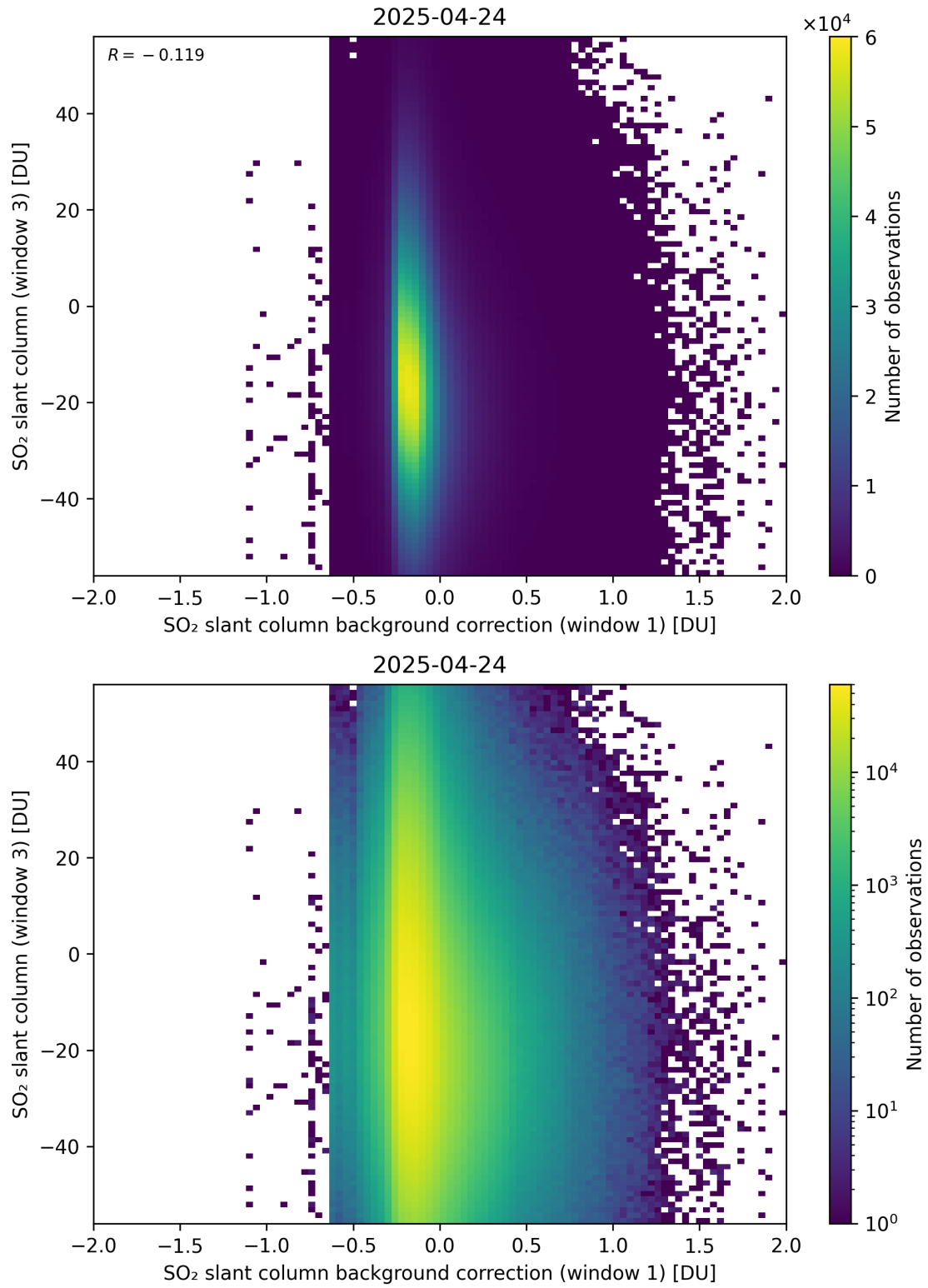
Figure 118: Scatter density plot of “SO 2 slant column background correction (window 1)” against “SO 2 slant column (window 3)” for 2025-04-24 to 2025-04-25.
