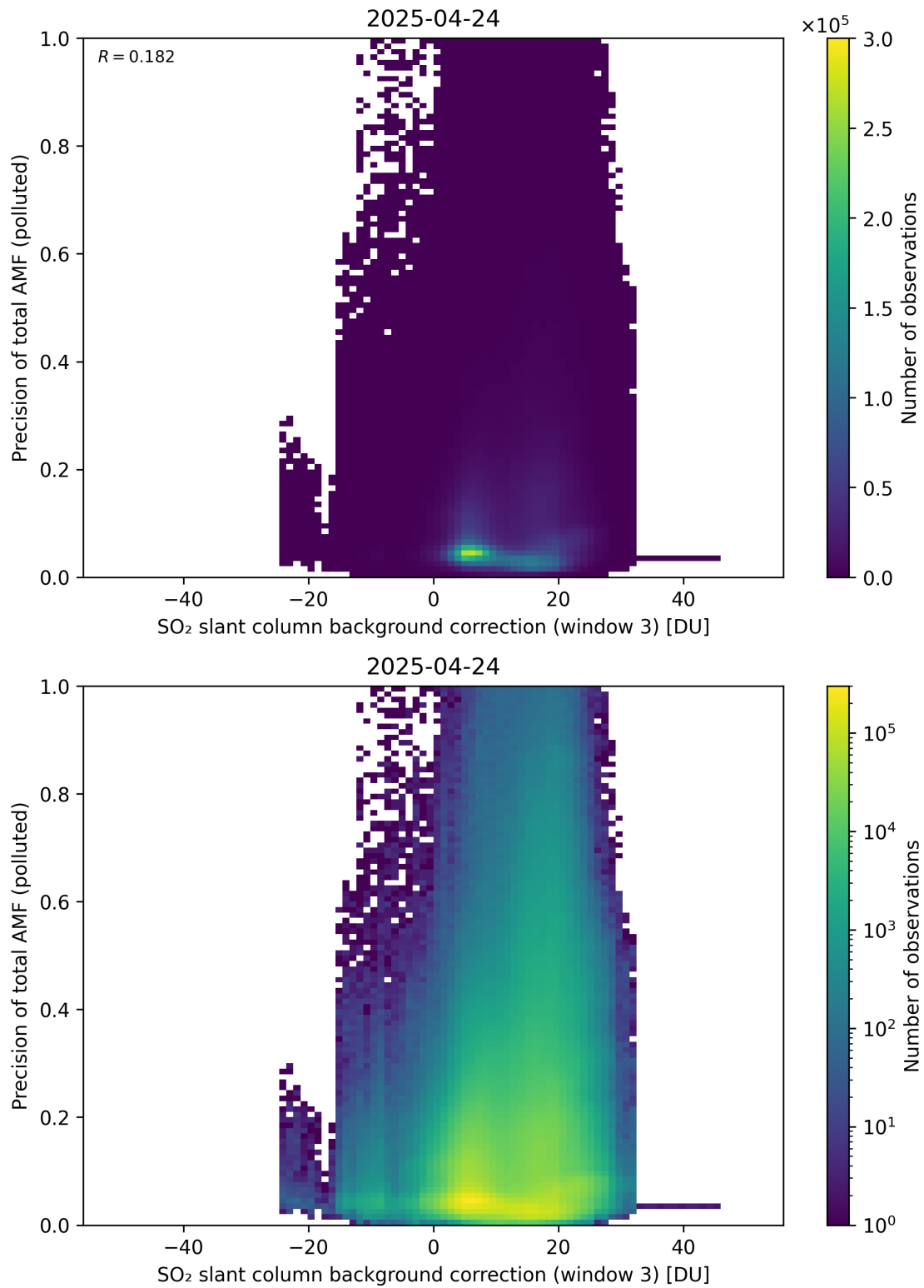
Figure 137: Scatter density plot of “SO 2 slant column background correction (window 3)” against “Precision of total AMF (polluted)” for 2025-04-24 to 2025-04-25.
