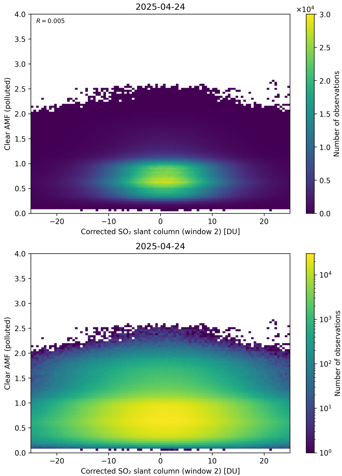
Figure 249: Scatter density plot of “Corrected SO 2 slant column (window 2)” against “Clear AMF (polluted)” for 2025-04-24 to 2025-04-25.
