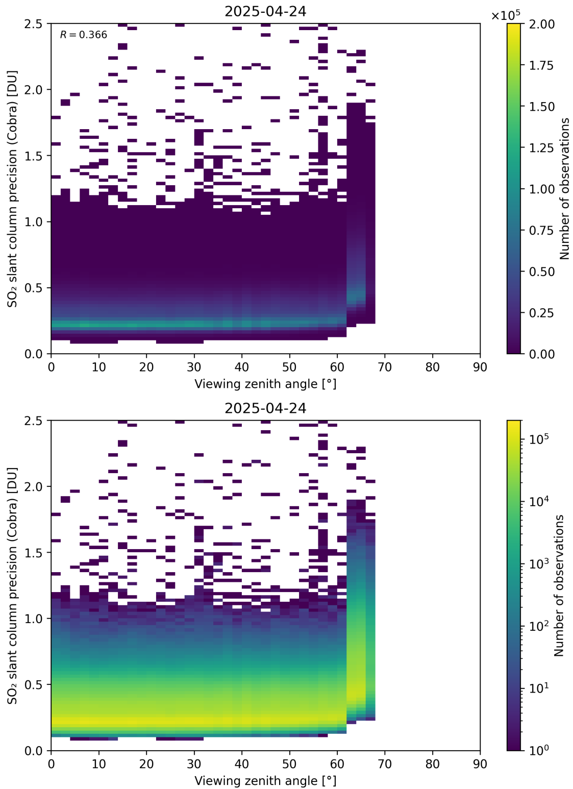
Figure 372: Scatter density plot of “Viewing zenith angle” against “SO 2 slant column precision (Cobra)” for 2025-04-24 to 2025-04-25.
