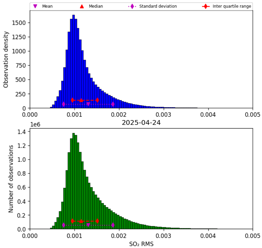
Figure 78: Histogram of "SO 2 RMS" for 2025-04-24 to 2025-04-25
