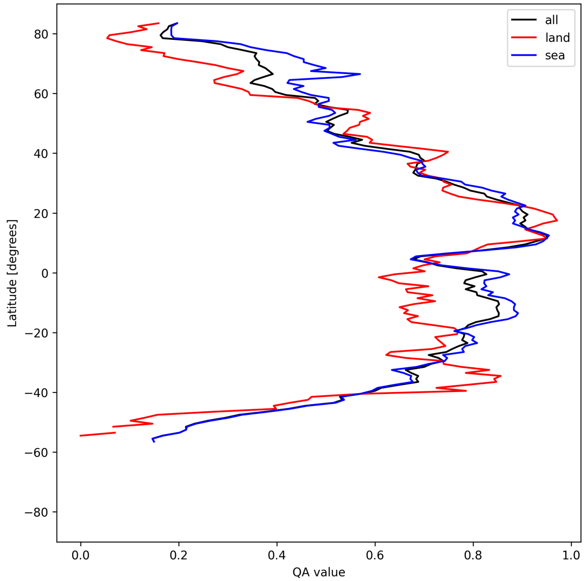
Figure 31: Zonal average of “QA value” for 2025-04-24 to 2025-04-25.
