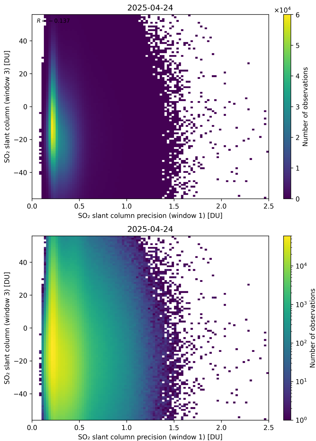
Figure 278: Scatter density plot of “SO 2 slant column precision (window 1)” against “SO 2 slant column (window 3)” for 2025-04-24 to 2025-04-25.
