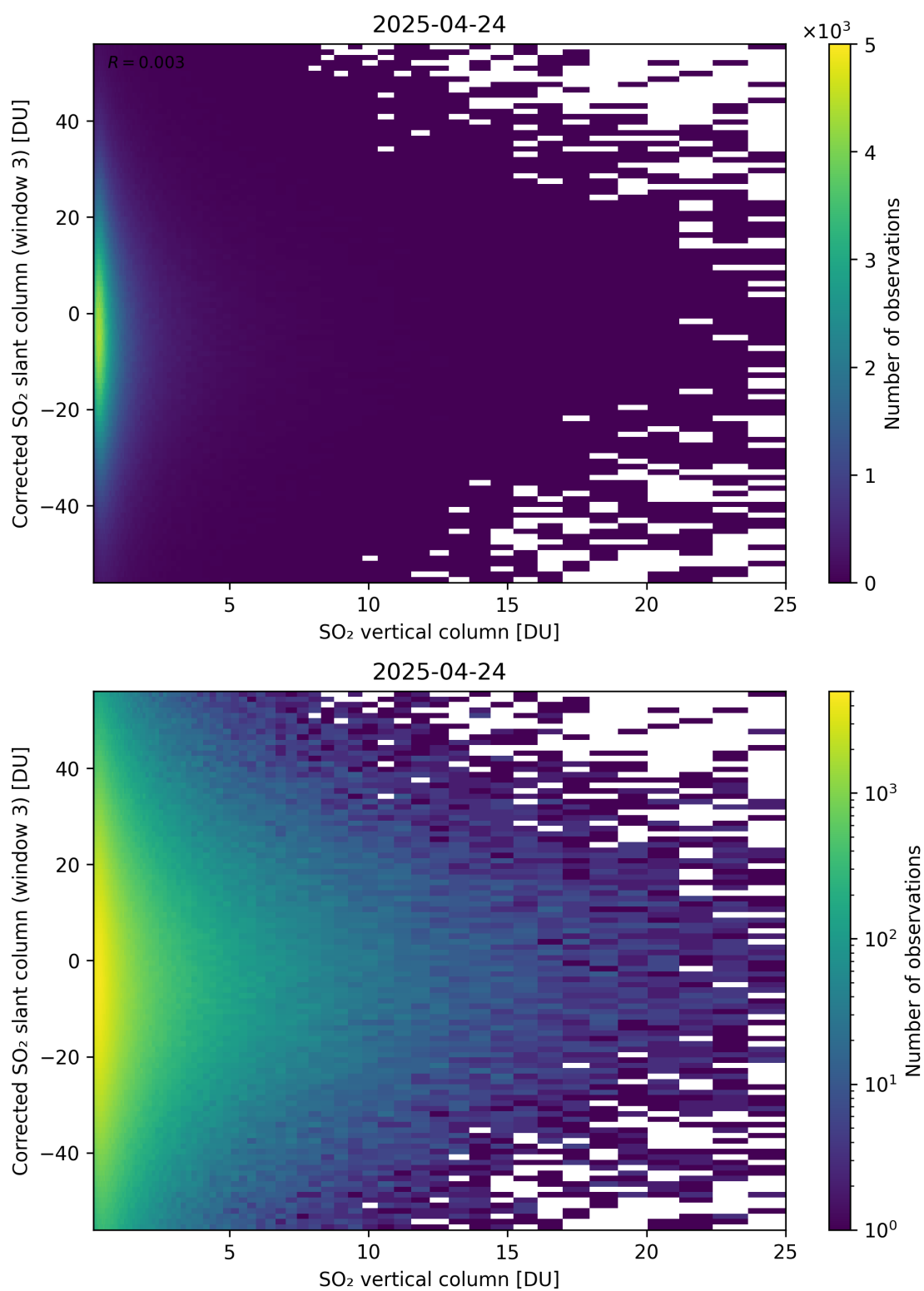
Figure 353: Scatter density plot of “SO 2 vertical column” against “Corrected SO 2 slant column (window 3)” for 2025-04-24 to 2025-04-25.
