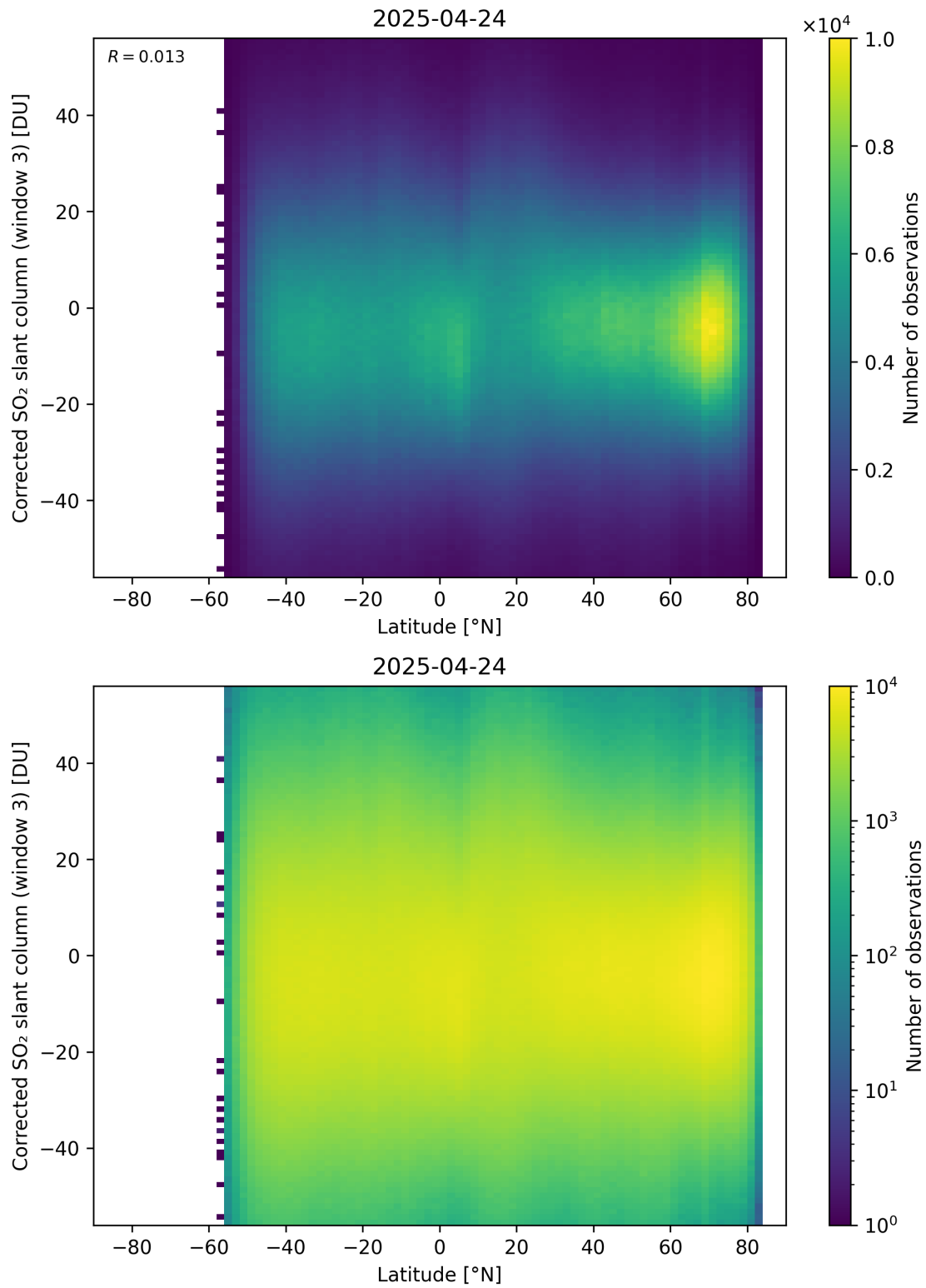
Figure 161: Scatter density plot of “Latitude” against “Corrected SO 2 slant column (window 3)” for 2025-04-24 to 2025-04-25.
