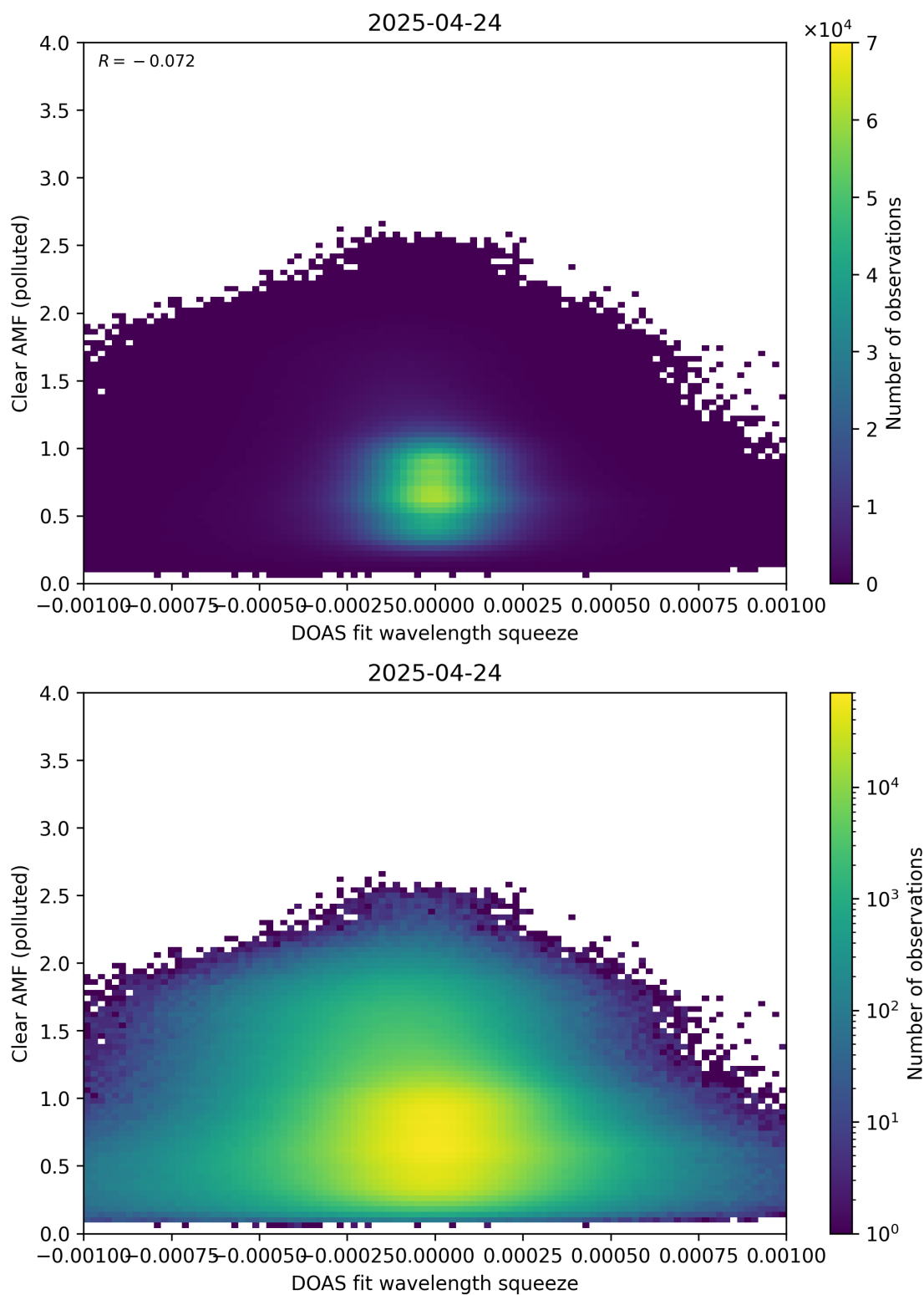
Figure 144: Scatter density plot of “DOAS fit wavelength squeeze” against “Clear AMF (polluted)” for 2025-04-24 to 2025-04-25.
