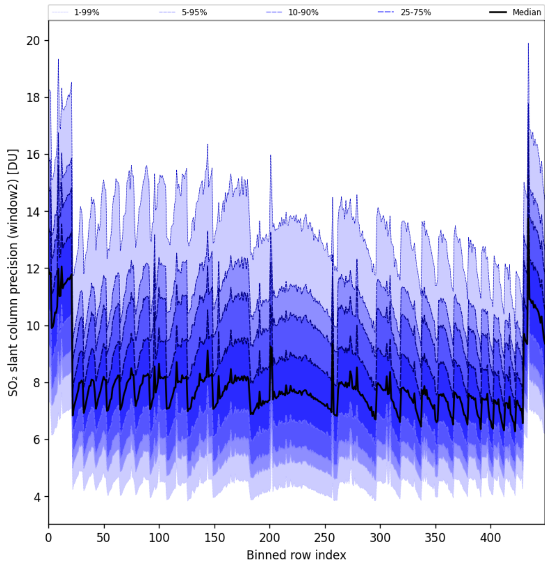
Figure 94: Along track statistics of “SO 2 slant column precision (window2)” for 2025-04-24 to 2025-04-25
