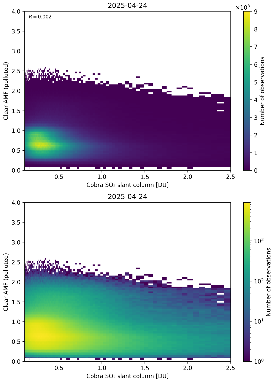
Figure 215: Scatter density plot of “Cobra SO 2 slant column” against “Clear AMF (polluted)” for 2025-04-24 to 2025-04-25.
