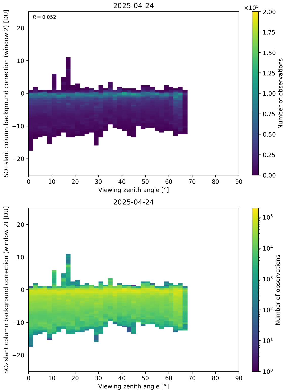
Figure 363: Scatter density plot of “Viewing zenith angle” against “SO 2 slant column background correction (window 2)” for 2025-04-24 to 2025-04-25.
