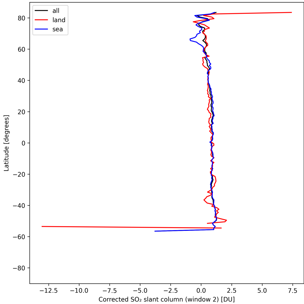
Figure 43: Zonal average of “Corrected SO 2 slant column (window 2)” for 2025-04-24 to 2025-04-25.
