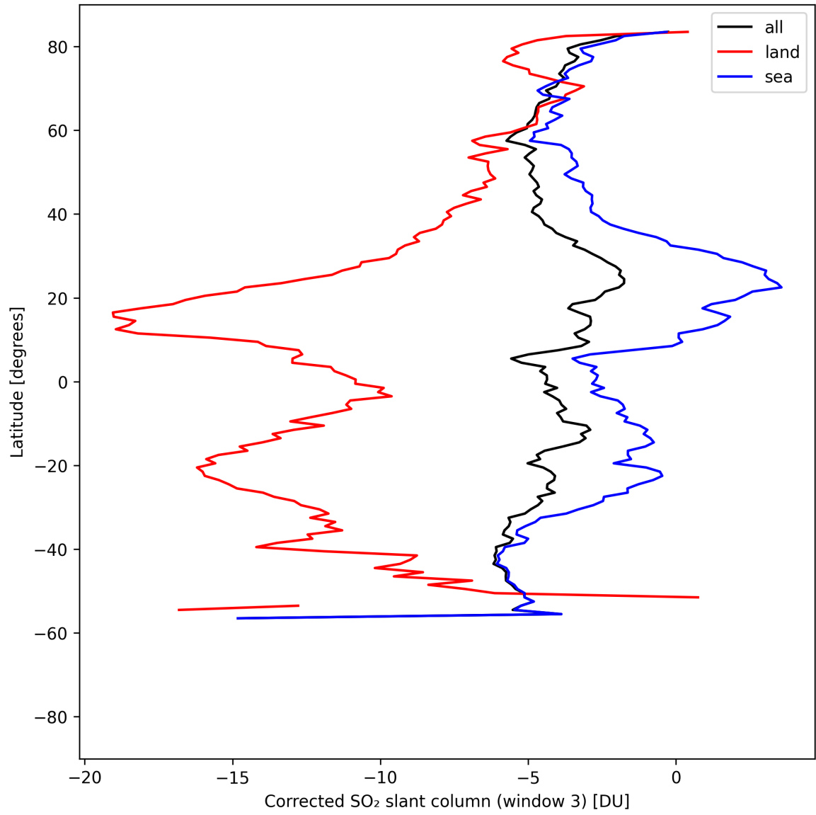
Figure 47: Zonal average of “Corrected SO 2 slant column (window 3)” for 2025-04-24 to 2025-04-25.
