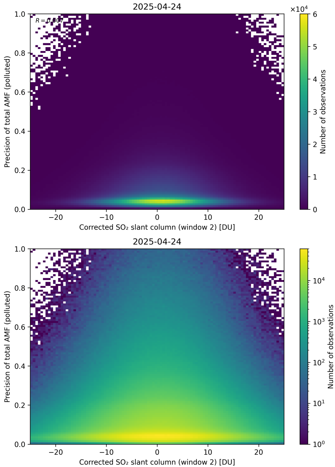
Figure 254: Scatter density plot of “Corrected SO 2 slant column (window 2)” against “Precision of total AMF (polluted)” for 2025-04-24 to 2025-04-25.
