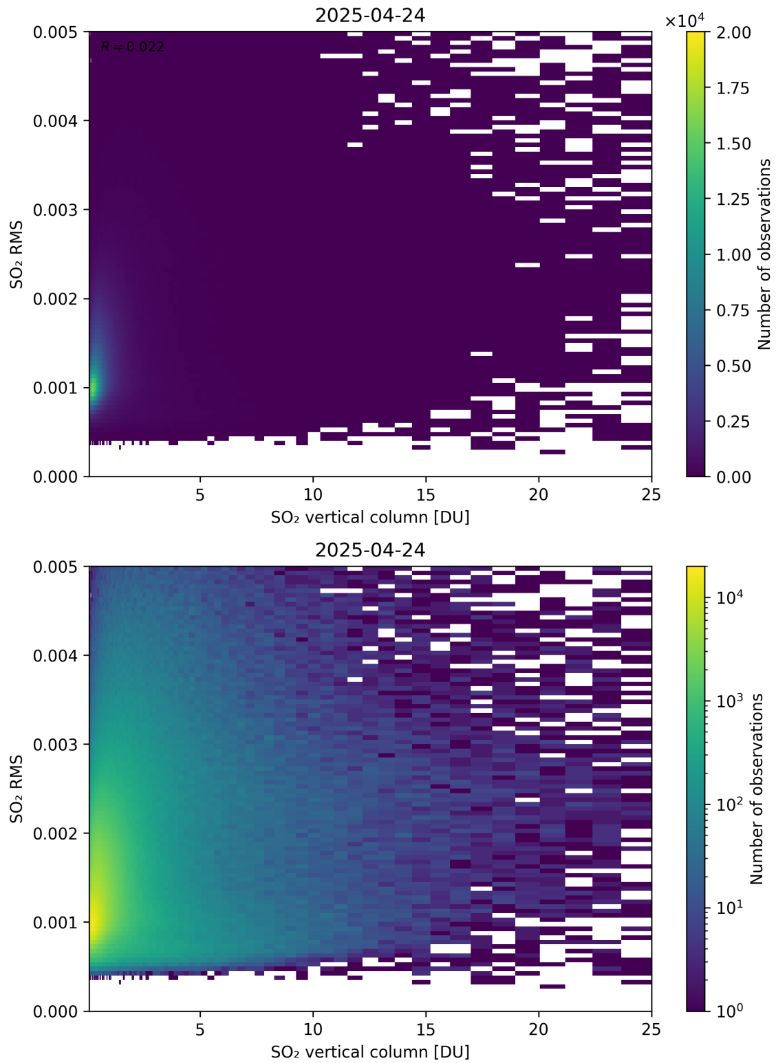
Figure 328: Scatter density plot of “SO 2 vertical column” against “SO 2 RMS” for 2025-04-24 to 2025-04-25.
