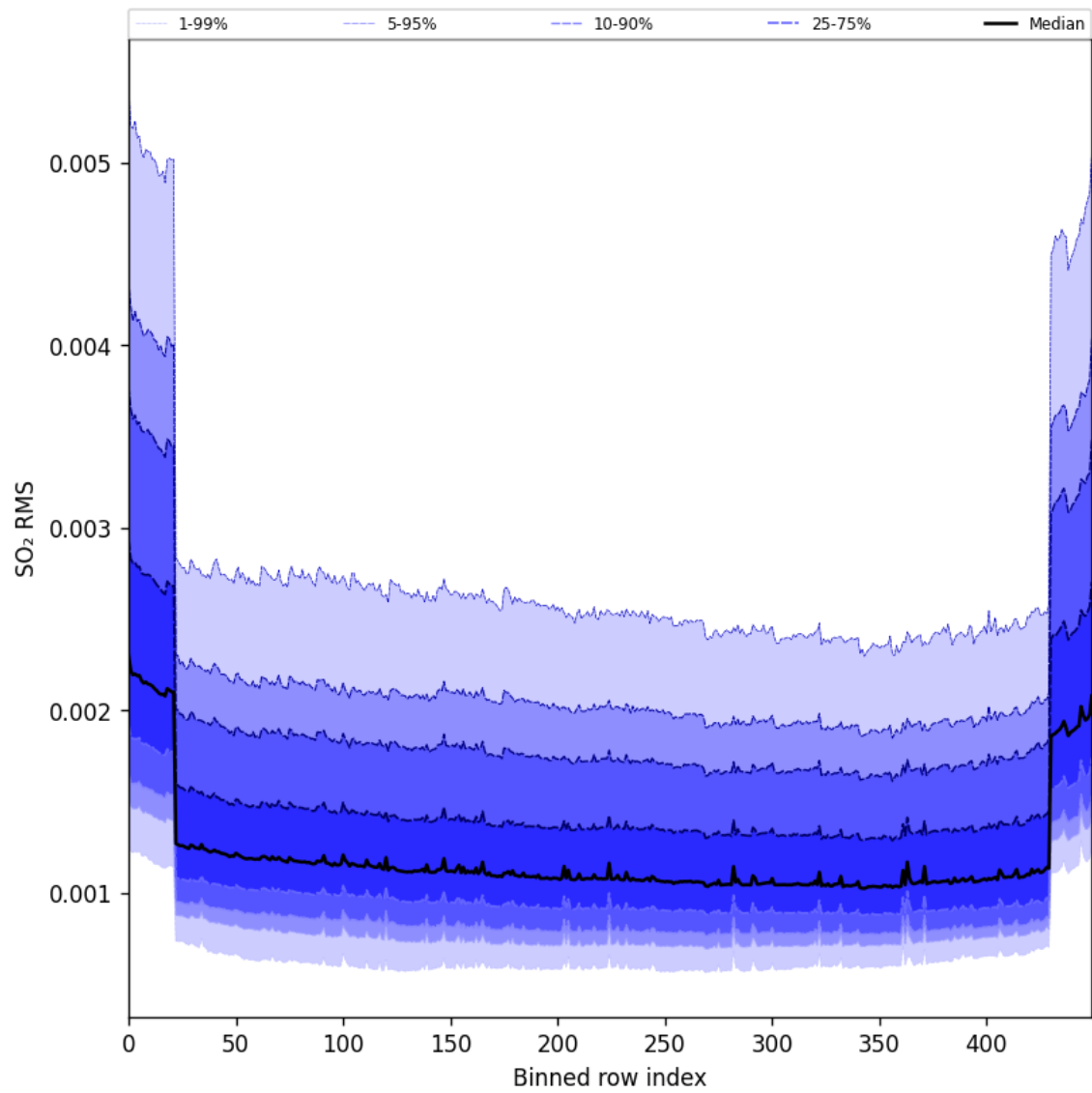
Figure 104: Along track statistics of “SO 2 RMS” for 2025-04-24 to 2025-04-25
