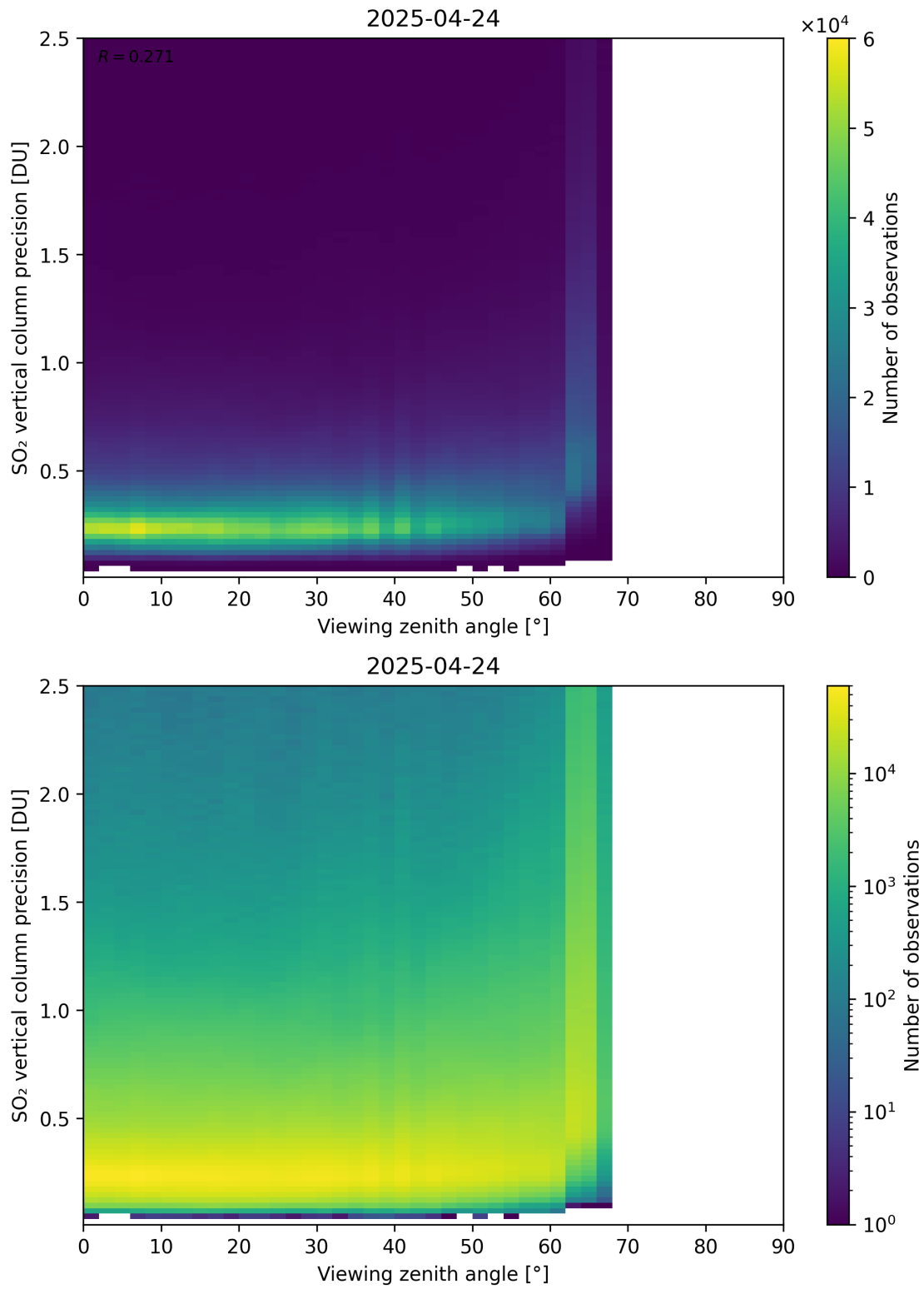
Figure 384: Scatter density plot of “Viewing zenith angle” against “SO 2 vertical column precision” for 2025-04-24 to 2025-04-25.
