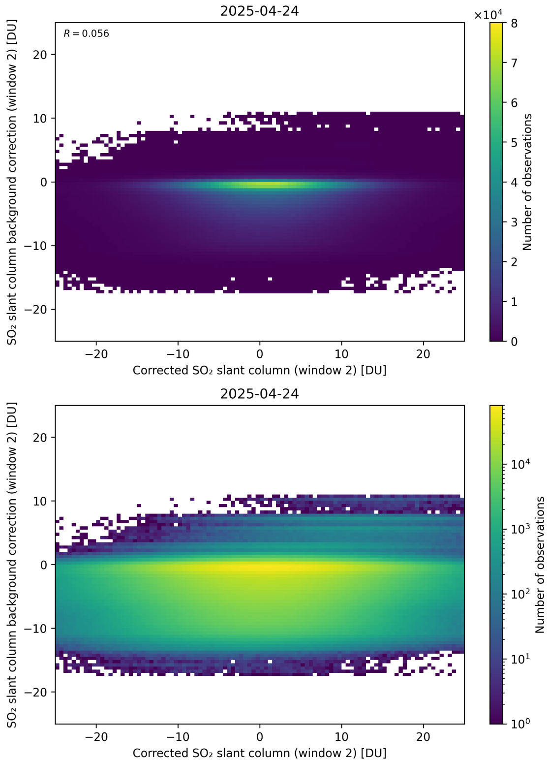
Figure 244: Scatter density plot of “Corrected SO 2 slant column (window 2)” against “SO 2 slant column background correction (window 2)” for 2025-04-24 to 2025-04-25.
