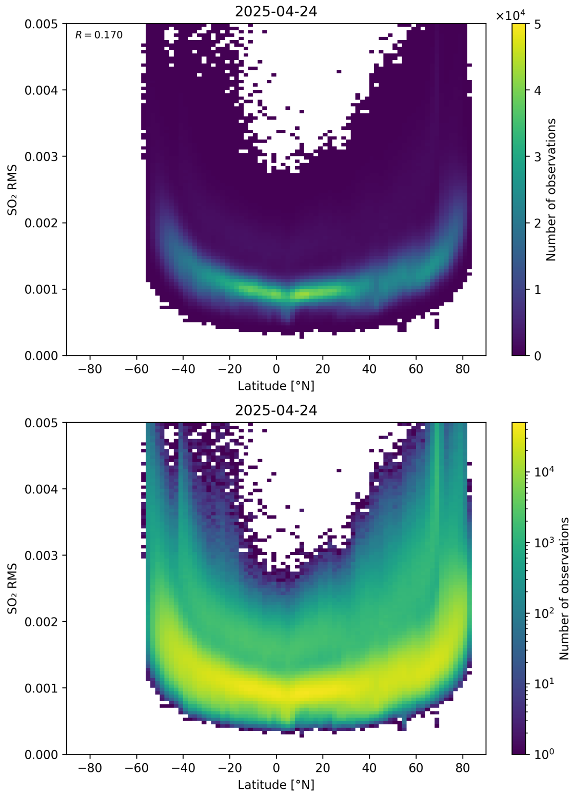
Figure 155: Scatter density plot of “Latitude” against “SO 2 RMS” for 2025-04-24 to 2025-04-25.
