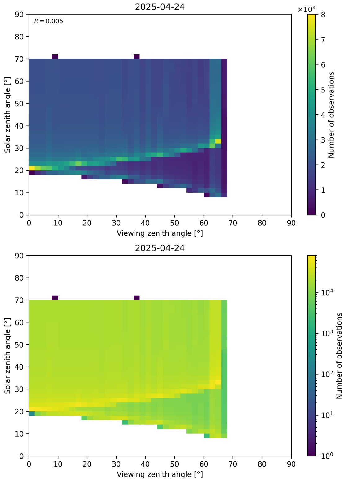
Figure 369: Scatter density plot of “Viewing zenith angle” against “Solar zenith angle” for 2025-04-24 to 2025-04-25.
