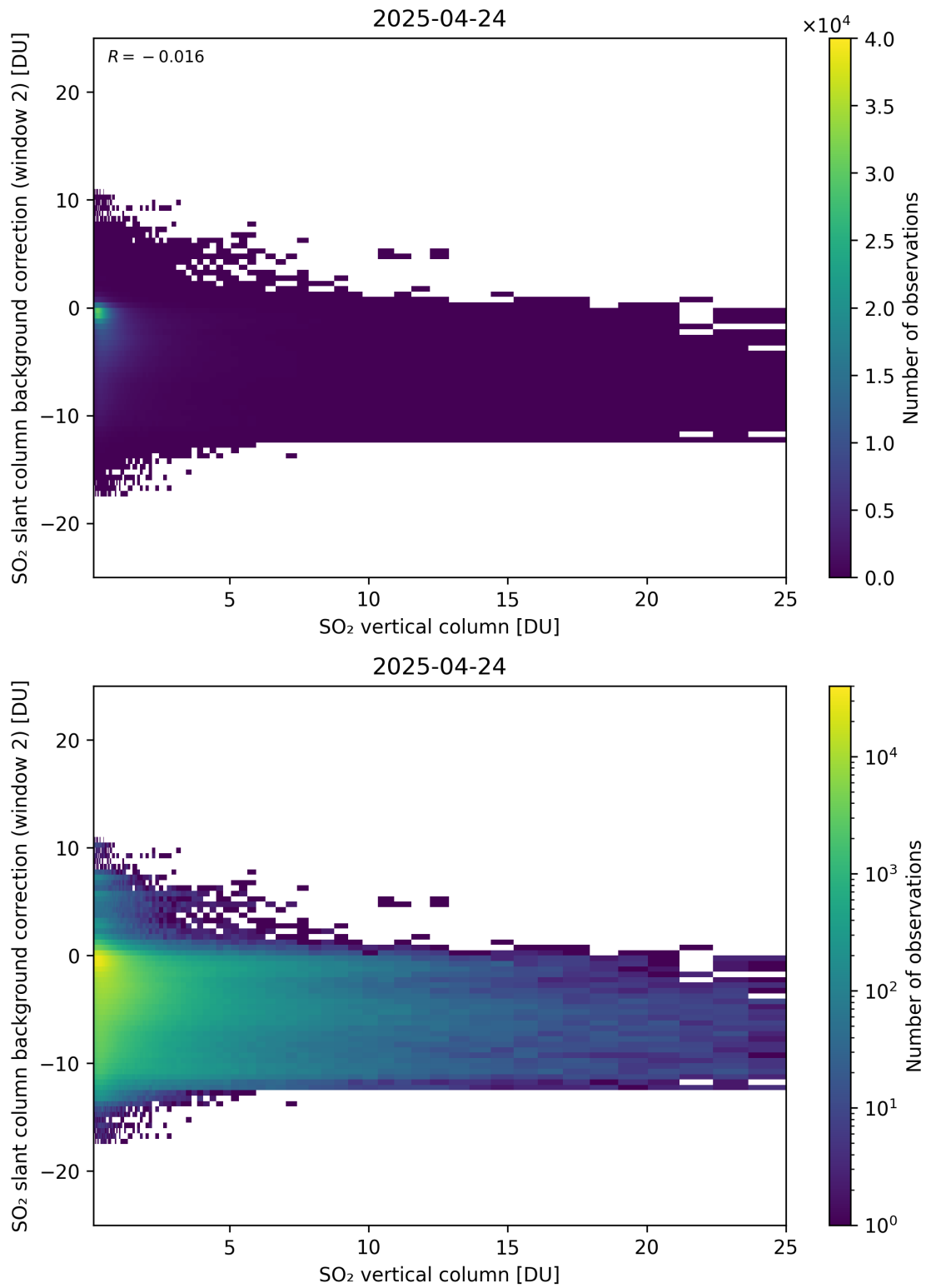
Figure 324: Scatter density plot of “SO 2 vertical column” against “SO 2 slant column background correction (window 2)” for 2025-04-24 to 2025-04-25.
