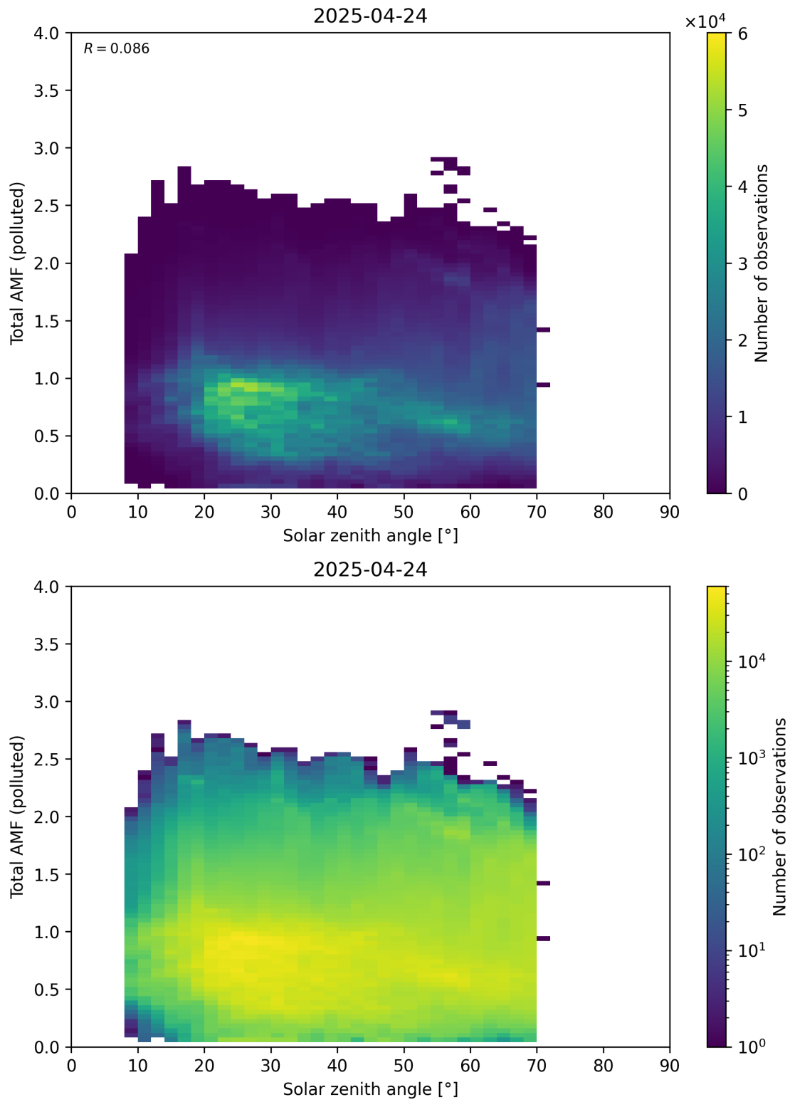
Figure 189: Scatter density plot of “Solar zenith angle” against “Total AMF (polluted)” for 2025-04-24 to 2025-04-25.
