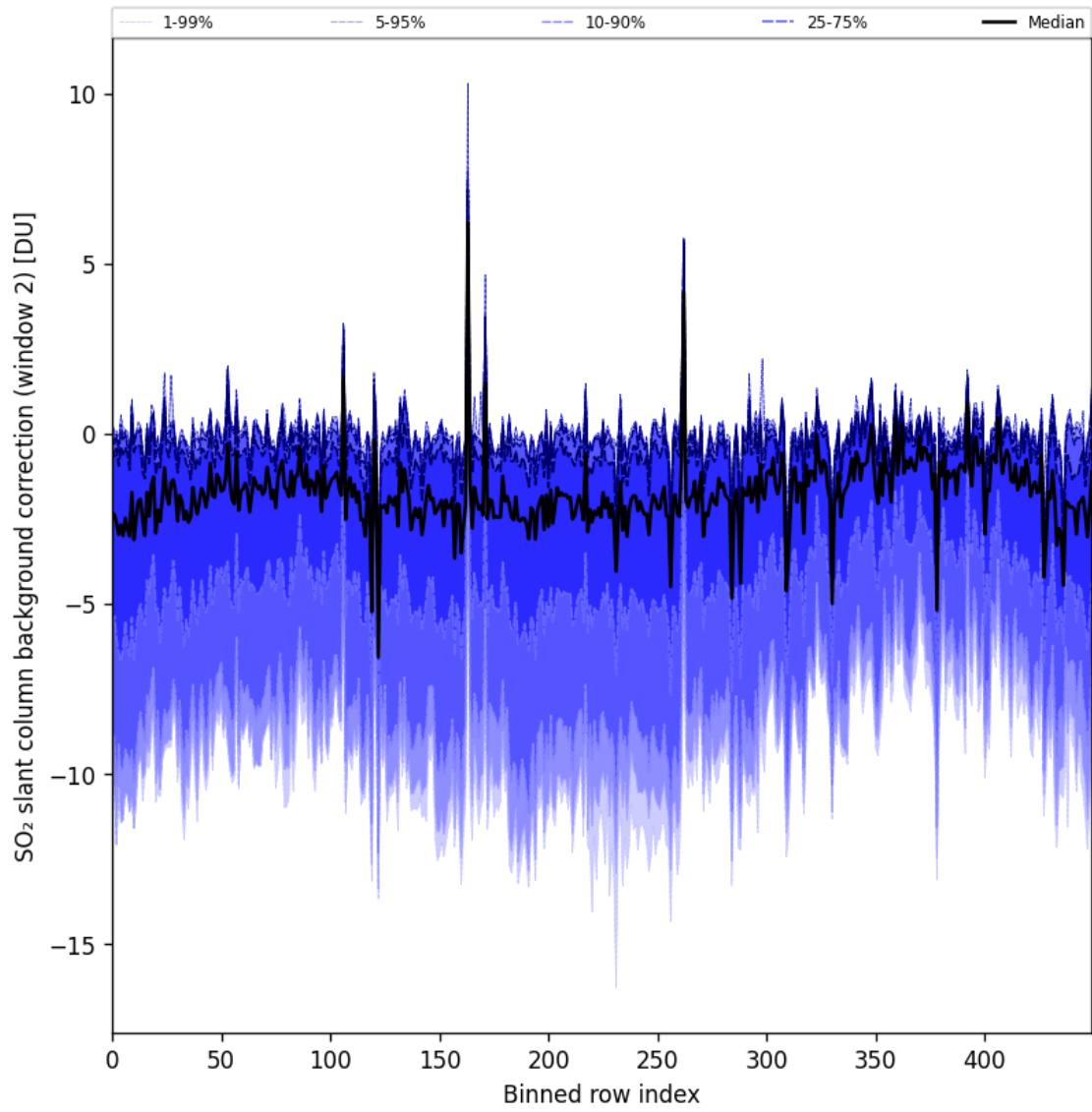
Figure 96: Along track statistics of “SO 2 slant column background correction (window 2)” for 2025-04-24 to 2025-04-25
