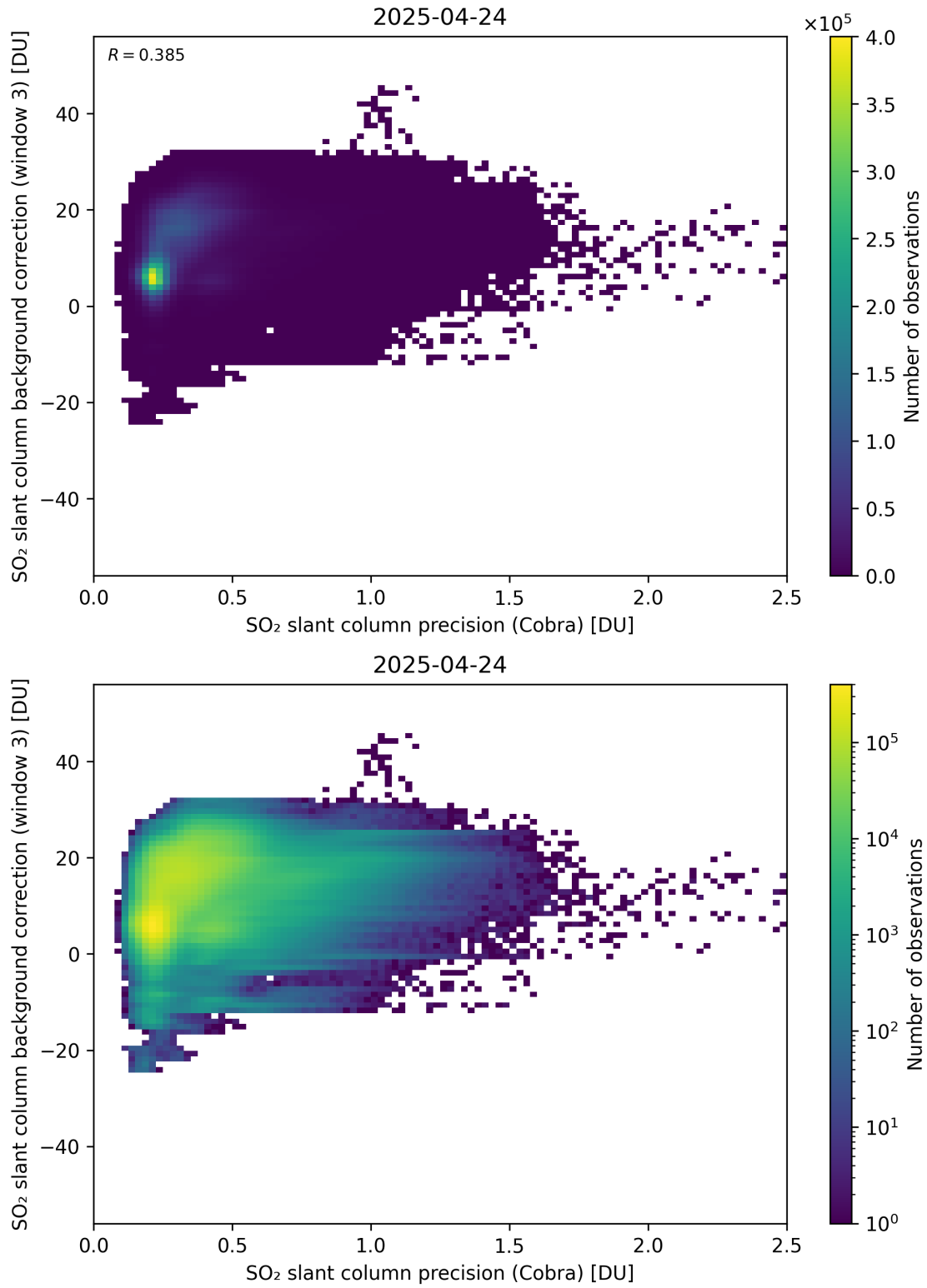
Figure 201: Scatter density plot of “SO 2 slant column precision (Cobra)” against “SO 2 slant column background correction (window 3)” for 2025-04-24 to 2025-04-25.
