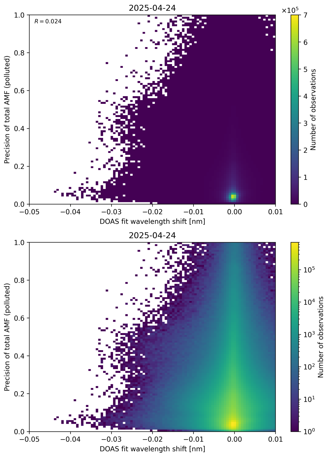
Figure 142: Scatter density plot of “DOAS fit wavelength shift” against “Precision of total AMF (polluted)” for 2025-04-24 to 2025-04-25.
