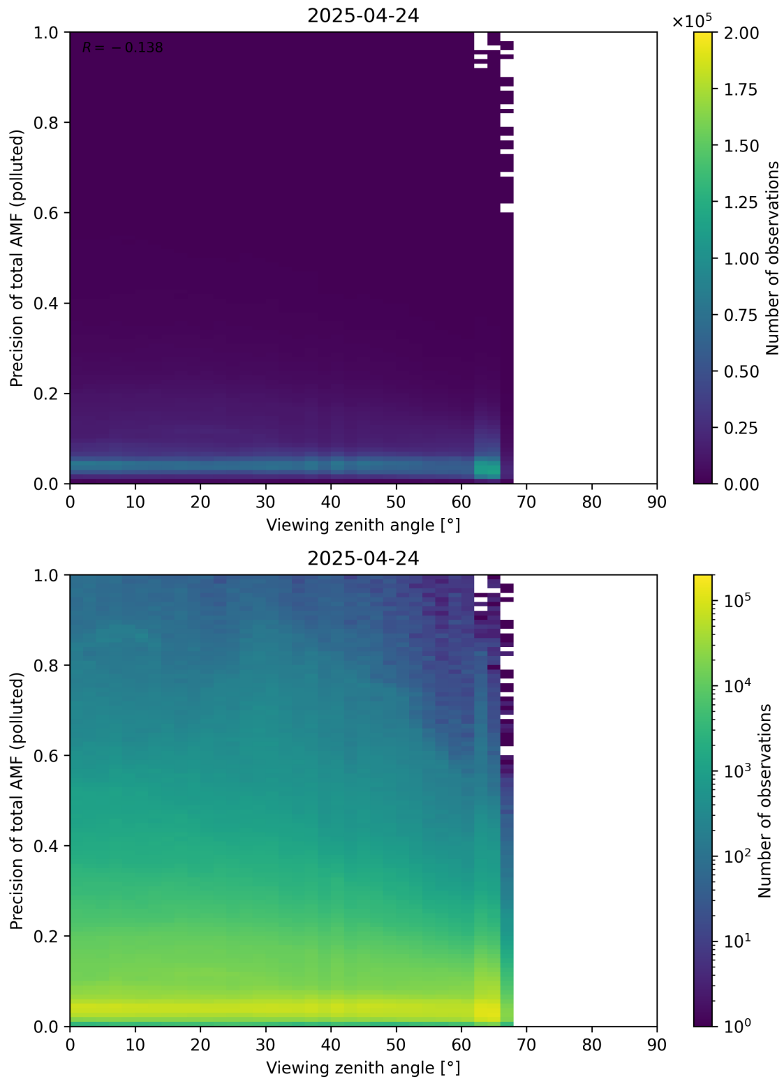
Figure 382: Scatter density plot of “Viewing zenith angle” against “Precision of total AMF (polluted)” for 2025-04-24 to 2025-04-25.
