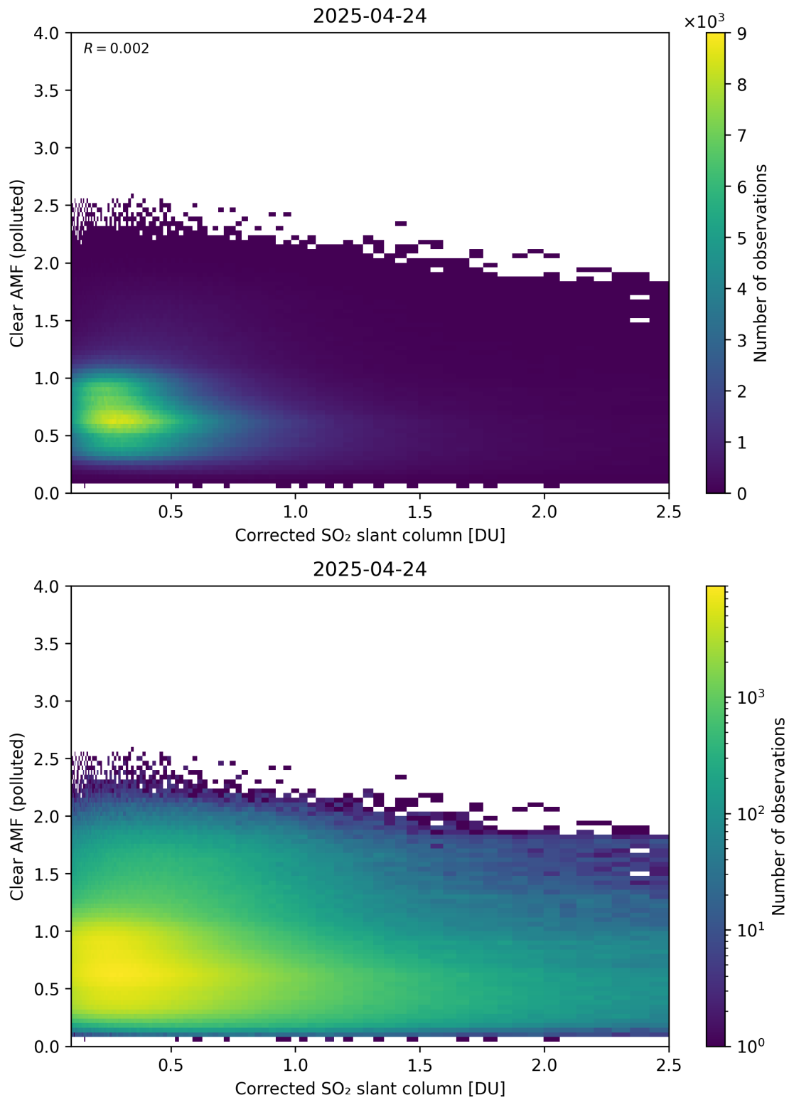
Figure 232: Scatter density plot of “Corrected SO 2 slant column” against “Clear AMF (polluted)” for 2025-04-24 to 2025-04-25.
