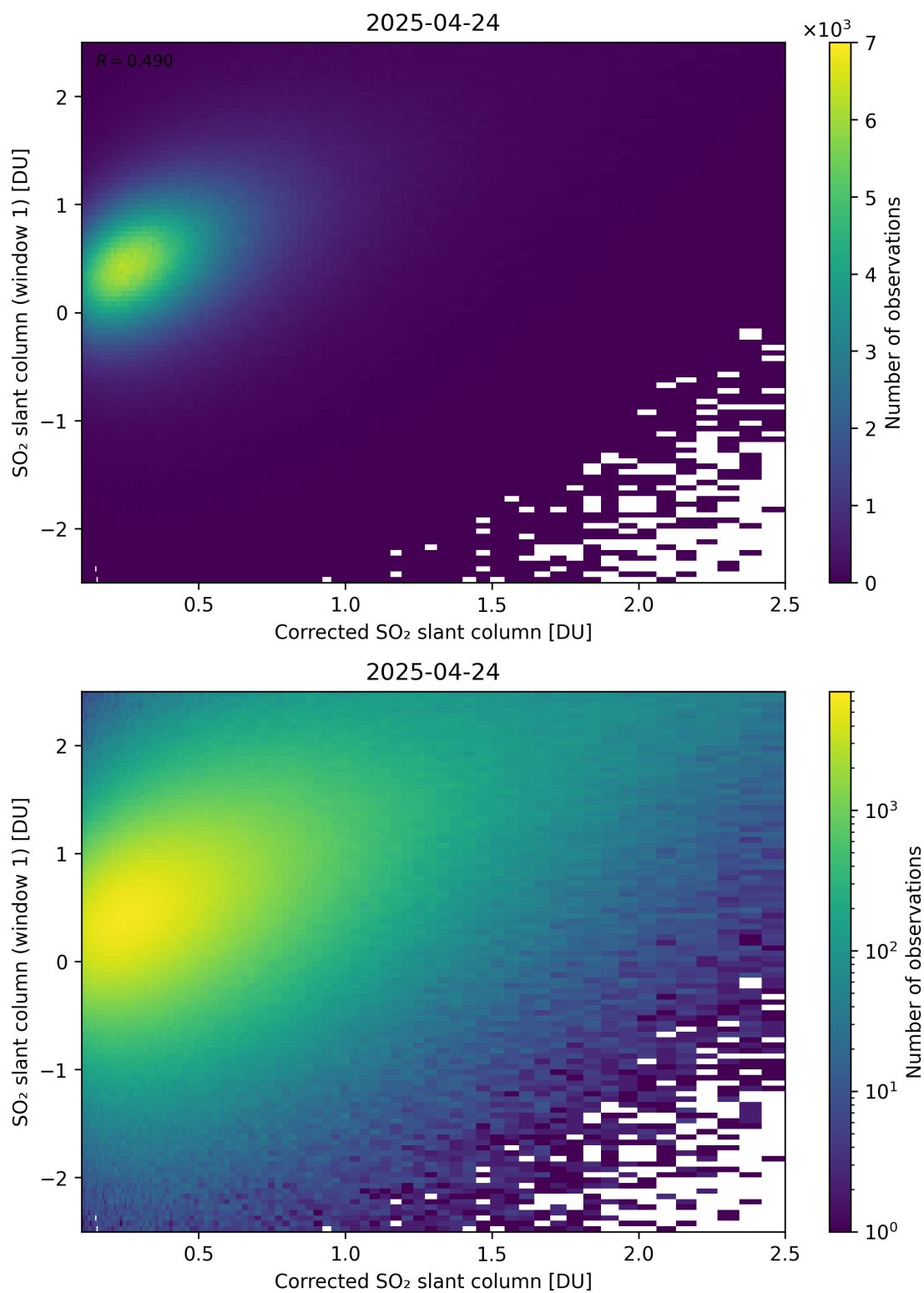
Figure 237: Scatter density plot of “Corrected SO 2 slant column” against “SO 2 slant column (window 1)” for 2025-04-24 to 2025-04-25.
