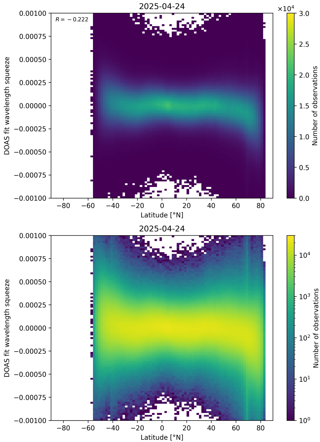
Figure 154: Scatter density plot of “Latitude” against “DOAS fit wavelength squeeze” for 2025-04-24 to 2025-04-25.
