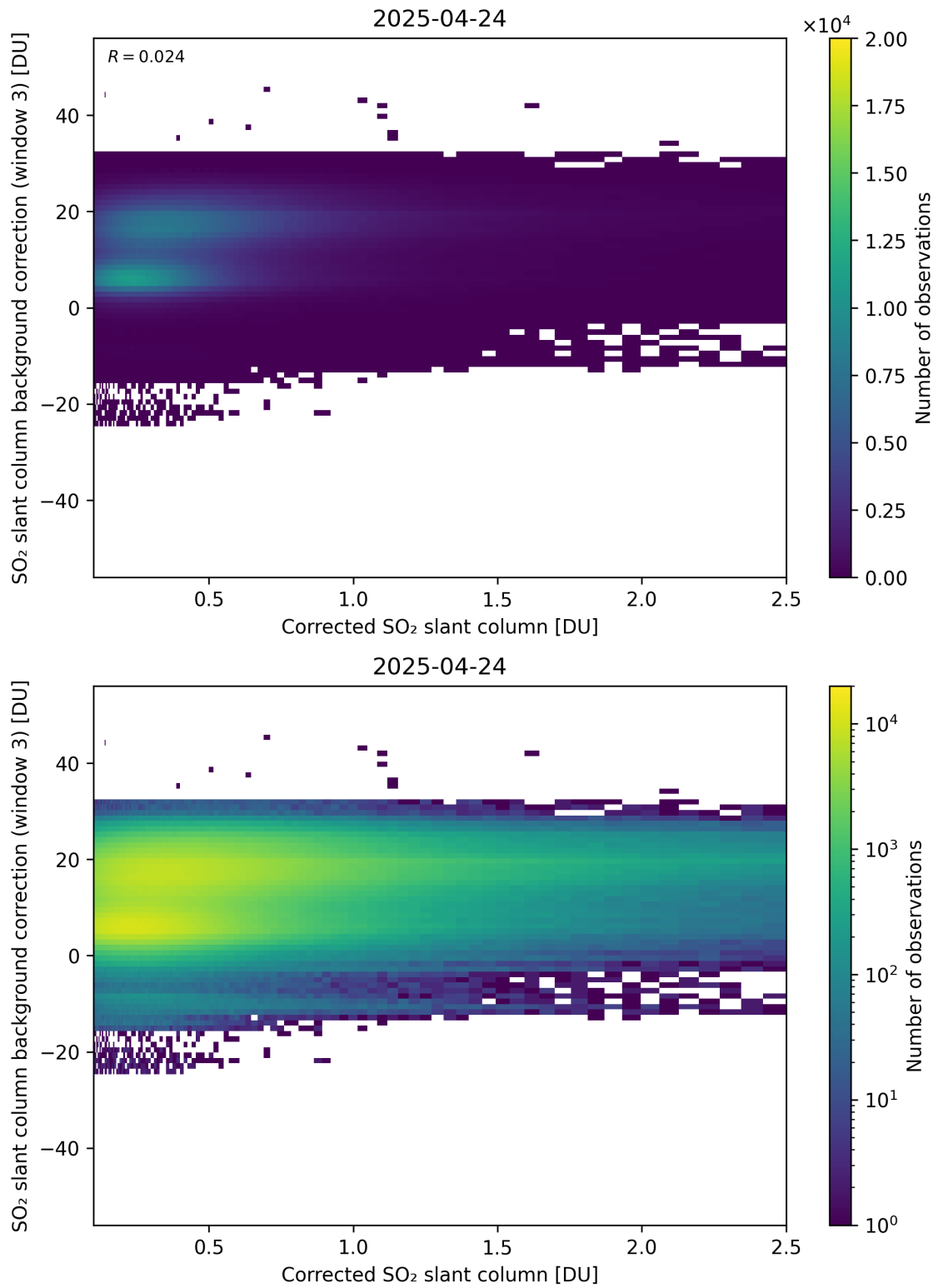
Figure 228: Scatter density plot of “Corrected SO 2 slant column” against “SO 2 slant column background correction (window 3)” for 2025-04-24 to 2025-04-25.
