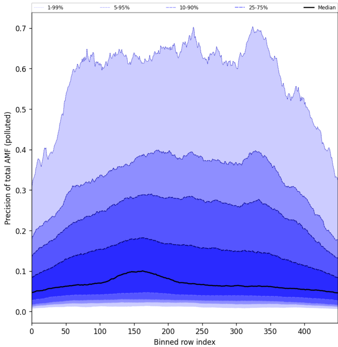
Figure 106: Along track statistics of “Precision of total AMF (polluted)” for 2025-04-24 to 2025-04-25
