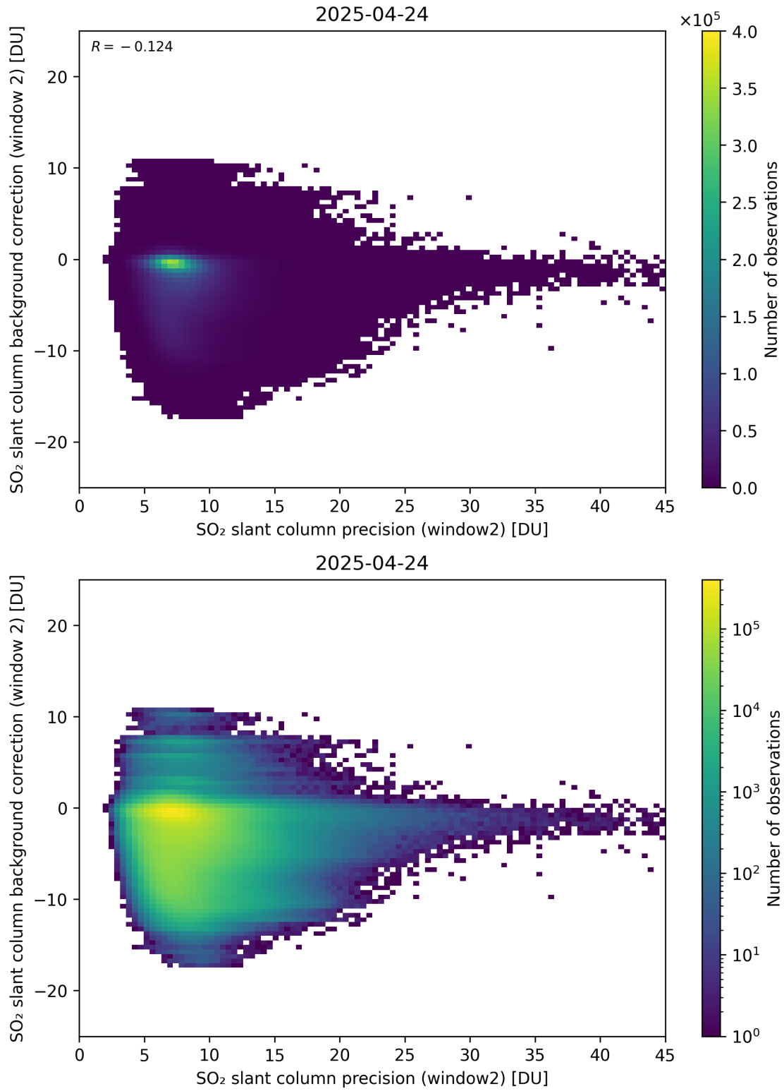
Figure 291: Scatter density plot of “SO 2 slant column precision (window2)” against “SO 2 slant column background correction (window 2)” for 2025-04-24 to 2025-04-25.
