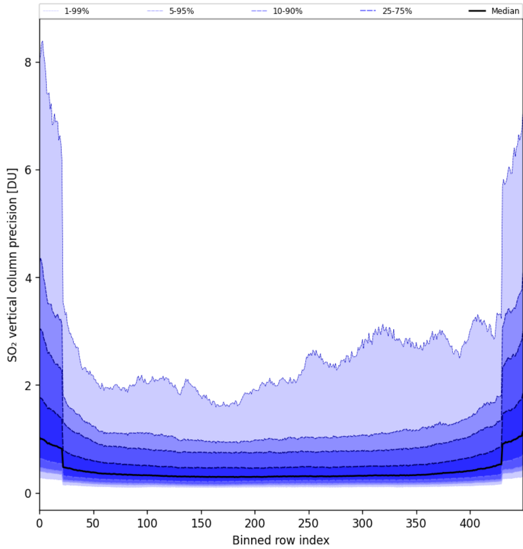
Figure 85: Along track statistics of “SO 2 vertical column precision” for 2025-04-24 to 2025-04-25
