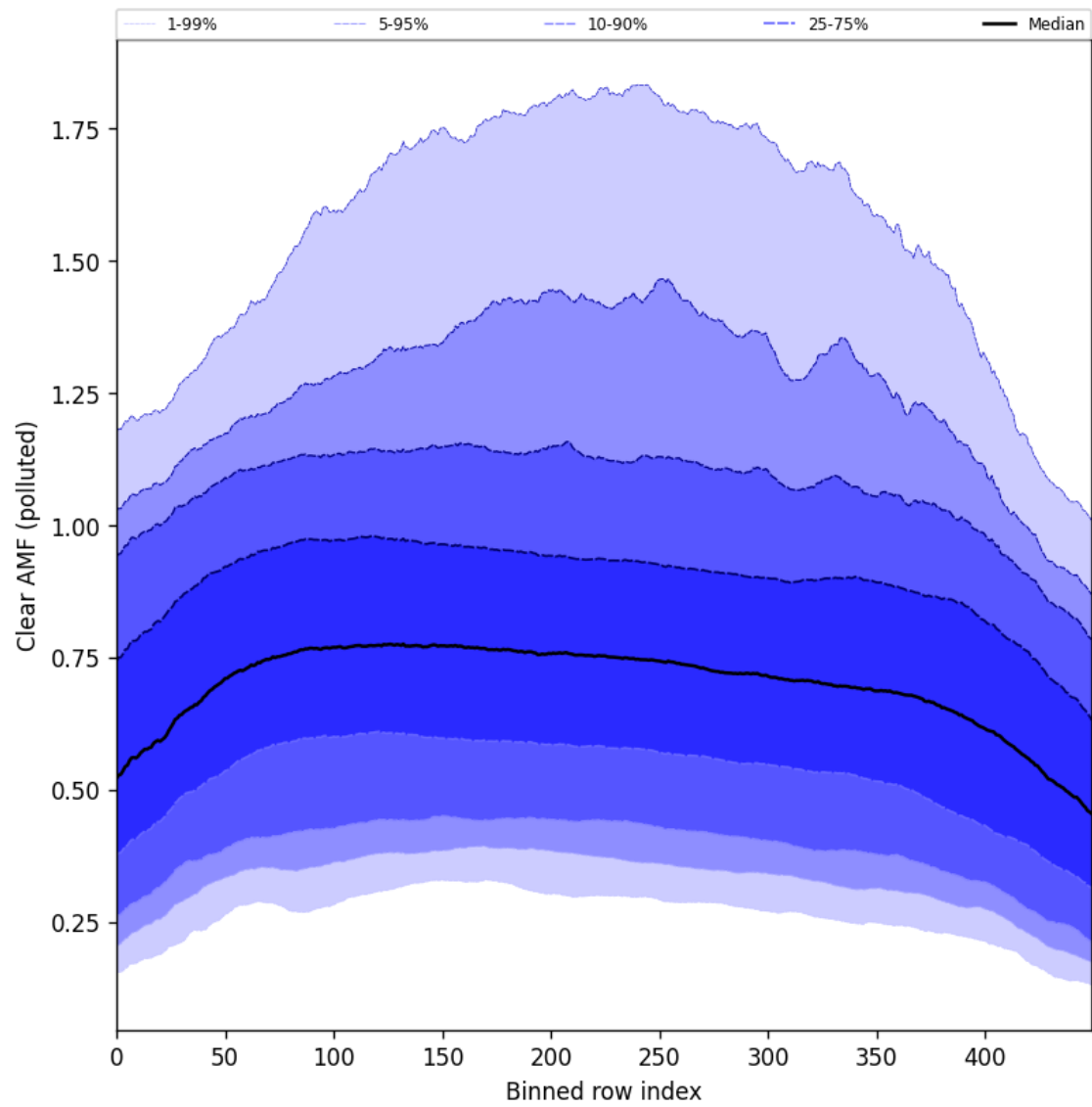
Figure 107: Along track statistics of “Clear AMF (polluted)” for 2025-04-24 to 2025-04-25
