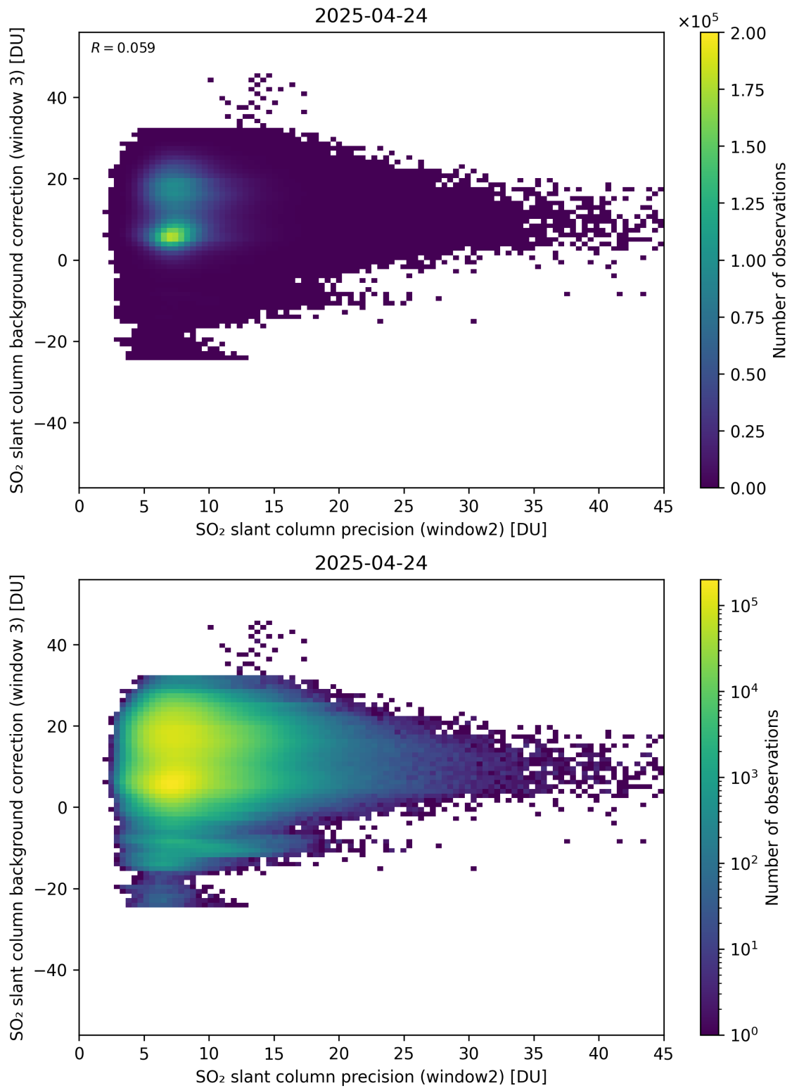
Figure 292: Scatter density plot of “SO 2 slant column precision (window2)” against “SO 2 slant column background correction (window 3)” for 2025-04-24 to 2025-04-25.
