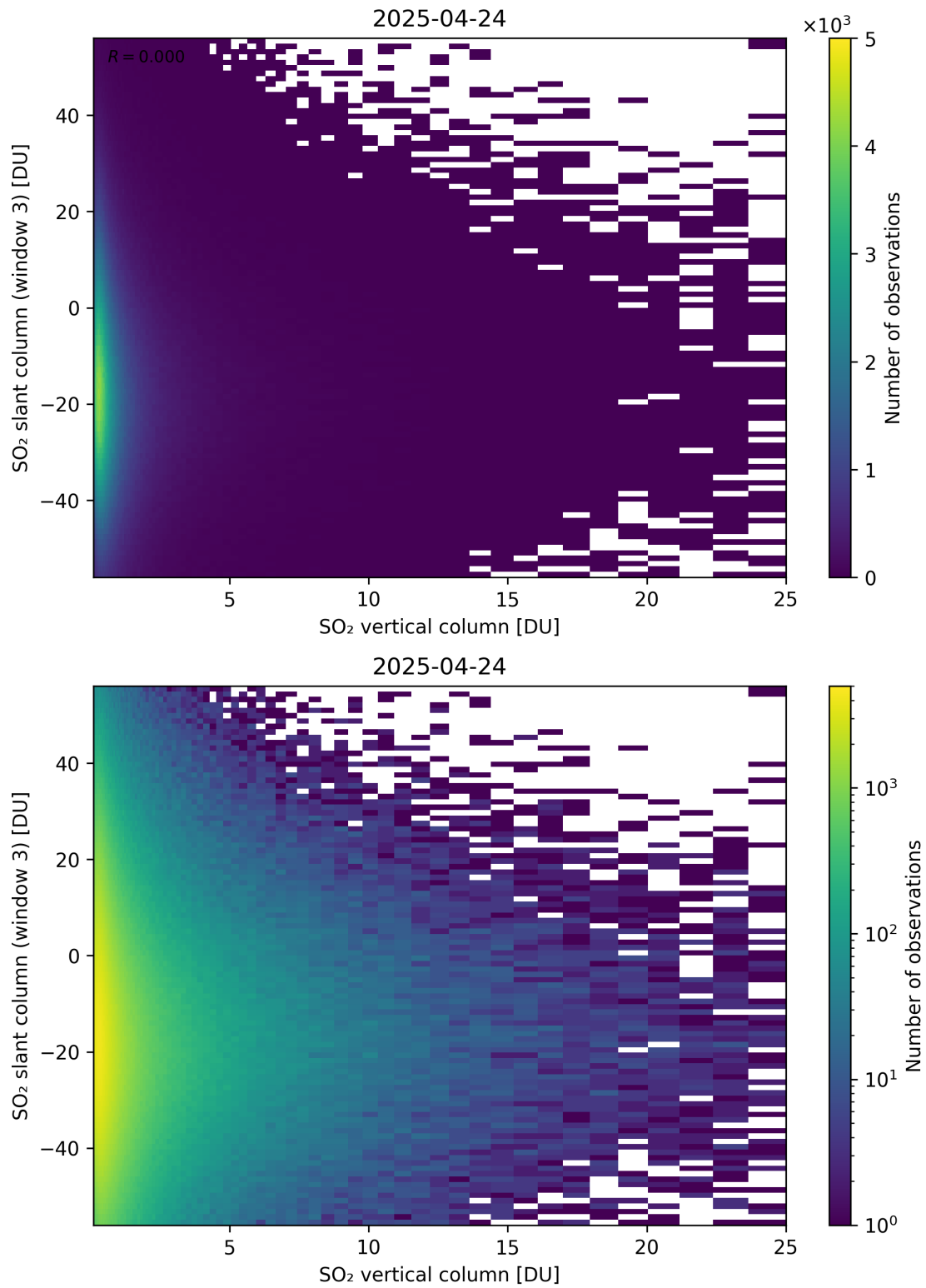
Figure 357: Scatter density plot of “SO 2 vertical column” against “SO 2 slant column (window 3)” for 2025-04-24 to 2025-04-25.
