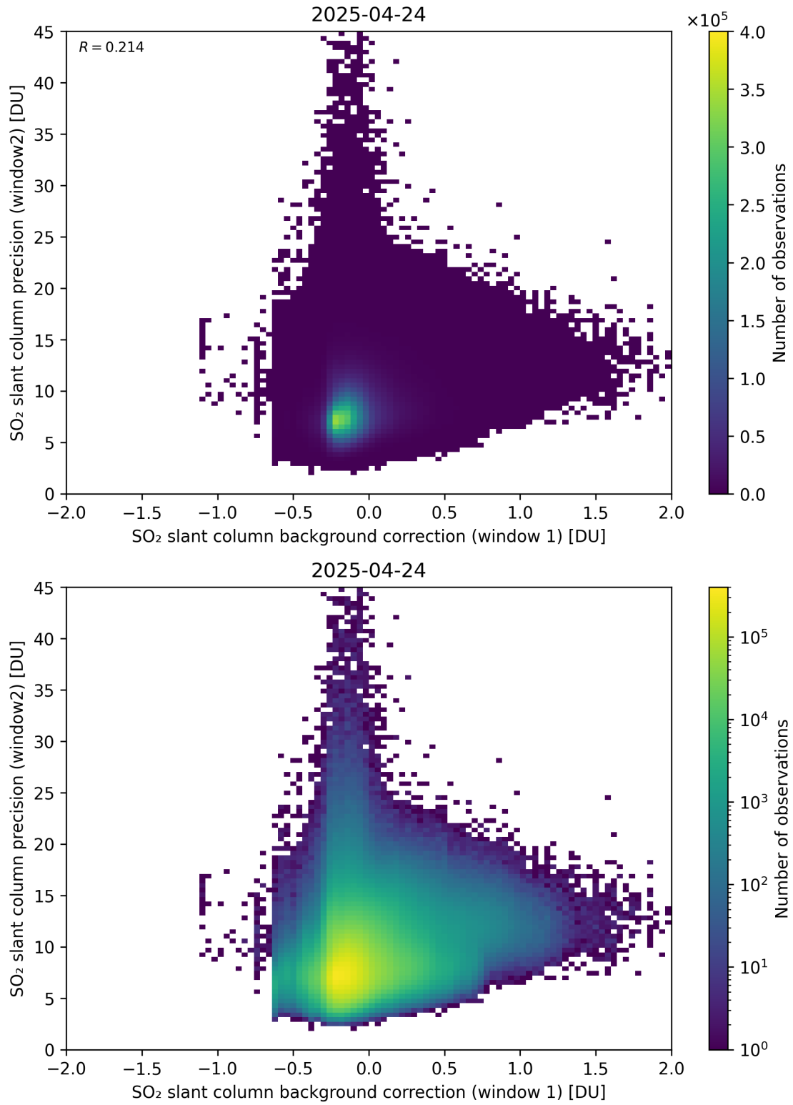
Figure 117: Scatter density plot of “SO 2 slant column background correction (window 1)” against “SO 2 slant column precision (window2)” for 2025-04-24 to 2025-04-25.
