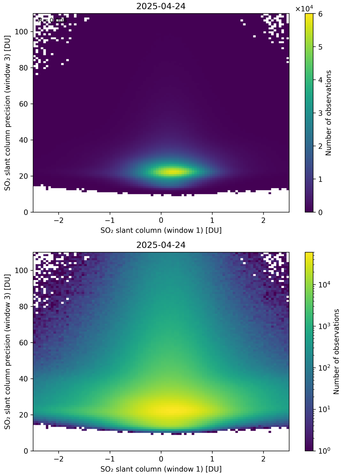
Figure 288: Scatter density plot of “SO 2 slant column (window 1)” against “SO 2 slant column precision (window 3)” for 2025-04-24 to 2025-04-25.
