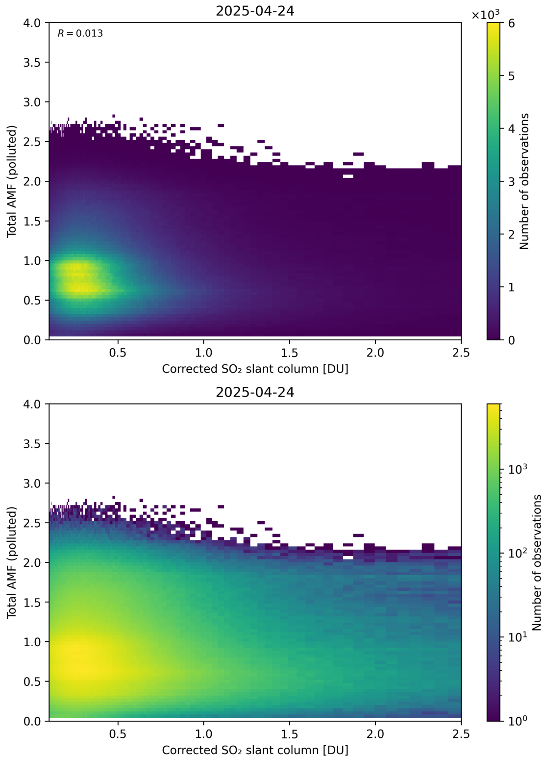
Figure 242: Scatter density plot of “Corrected SO 2 slant column” against “Total AMF (polluted)” for 2025-04-24 to 2025-04-25.
