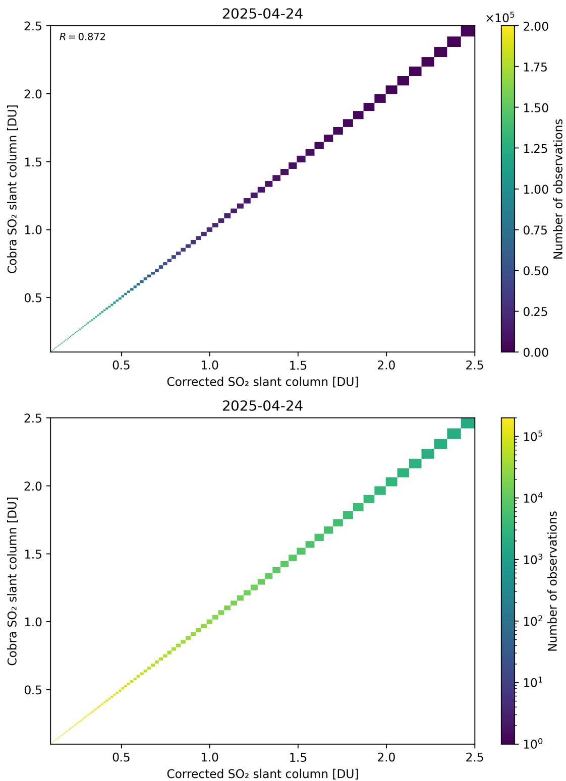
Figure 233: Scatter density plot of “Corrected SO 2 slant column” against “Cobra SO 2 slant column” for 2025-04-24 to 2025-04-25.
