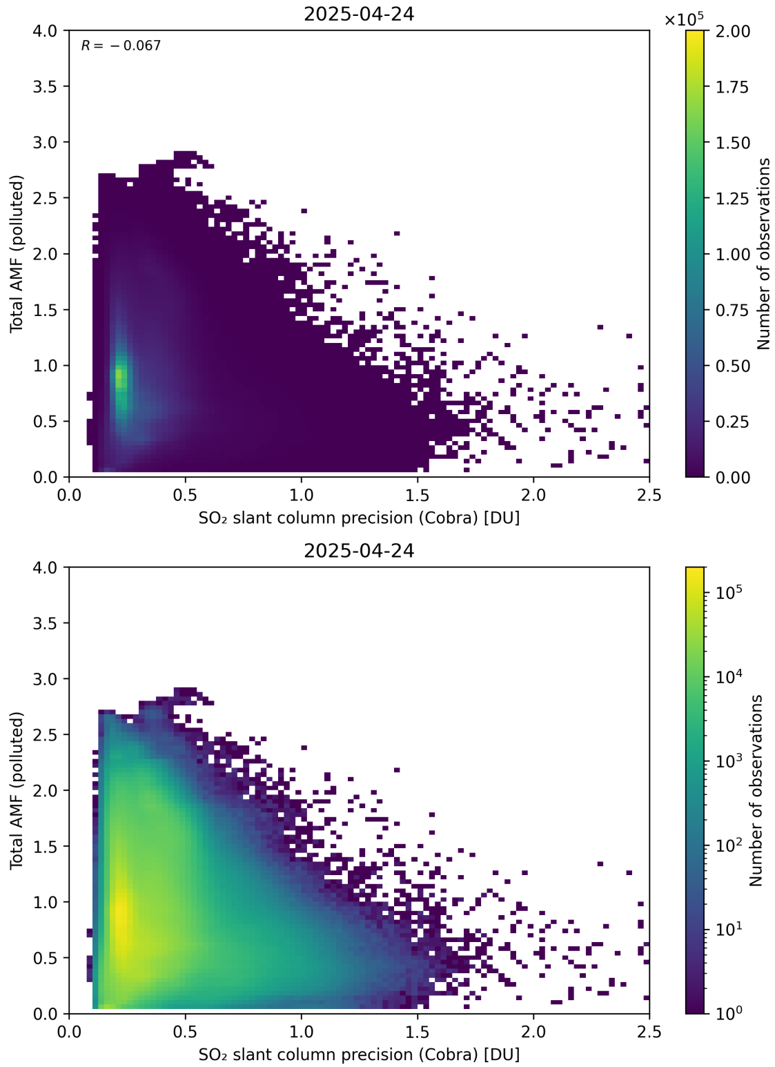
Figure 213: Scatter density plot of “SO 2 slant column precision (Cobra)” against “Total AMF (polluted)” for 2025-04-24 to 2025-04-25.
