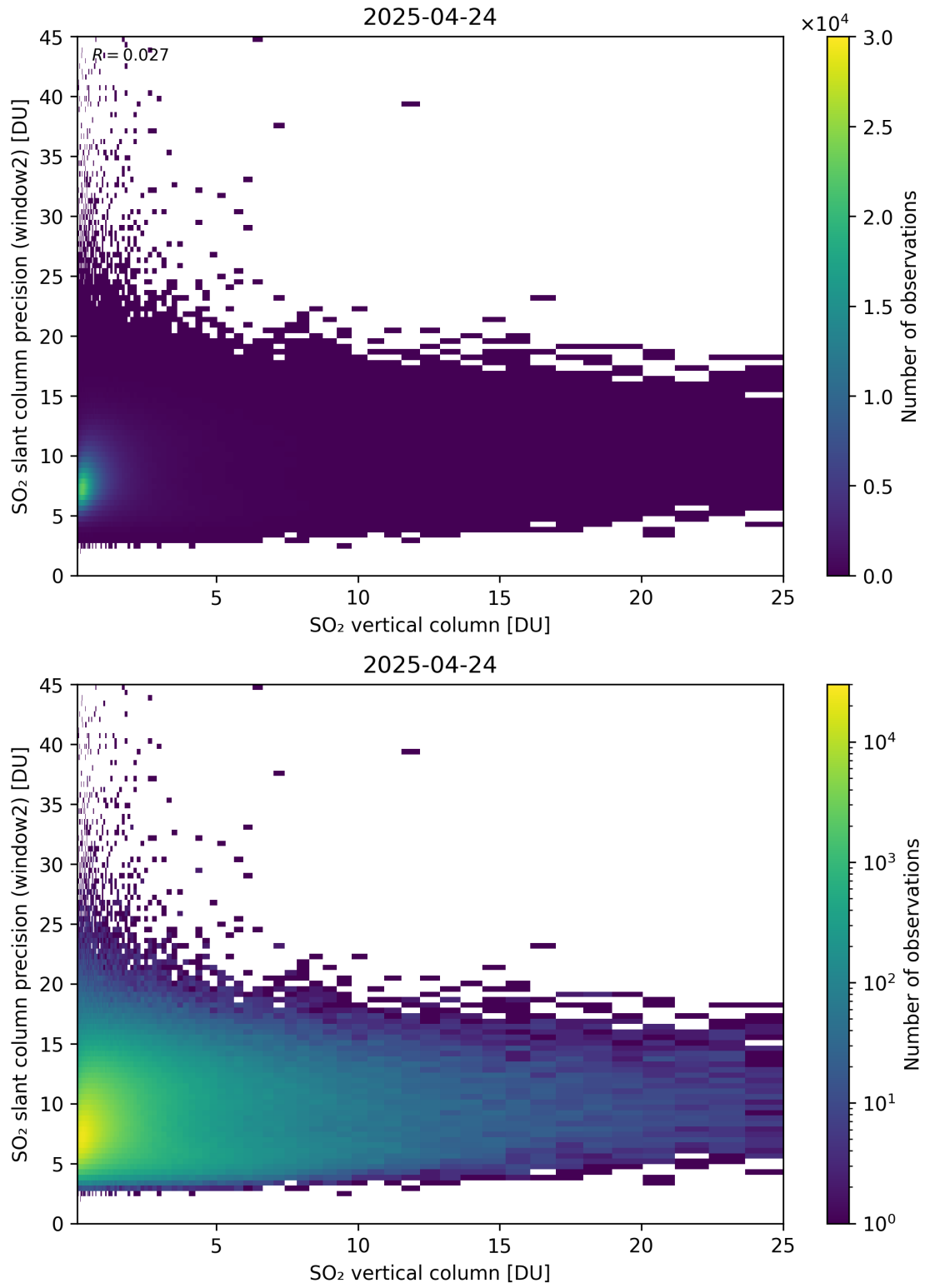
Figure 356: Scatter density plot of “SO 2 vertical column” against “SO 2 slant column precision (window2)” for 2025-04-24 to 2025-04-25.
