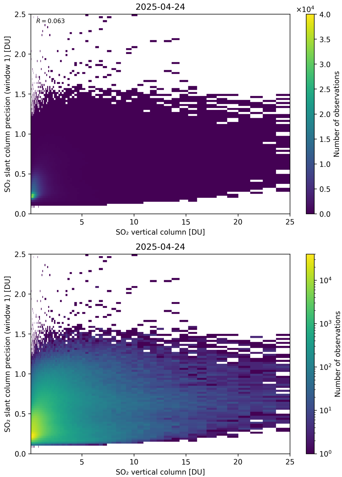
Figure 355: Scatter density plot of “SO 2 vertical column” against “SO 2 slant column precision (window 1)” for 2025-04-24 to 2025-04-25.
