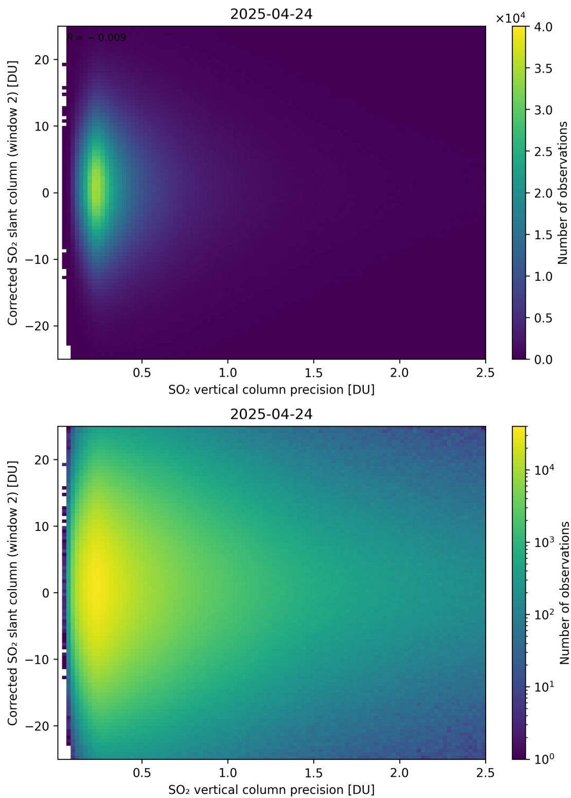
Figure 339: Scatter density plot of “SO 2 vertical column precision” against “Corrected SO 2 slant column (window 2)” for 2025-04-24 to 2025-04-25.
