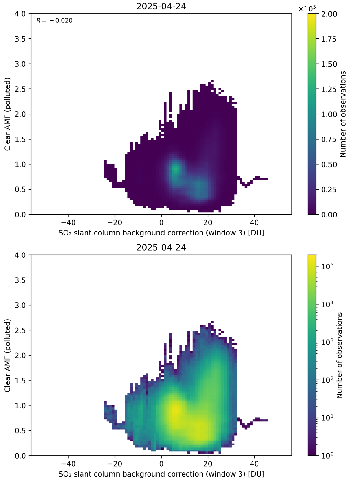
Figure 135: Scatter density plot of “SO 2 slant column background correction (window 3)” against “Clear AMF (polluted)” for 2025-04-24 to 2025-04-25.
