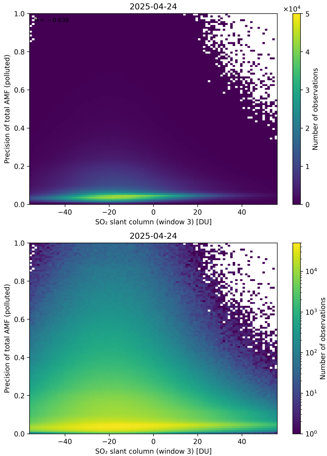
Figure 319: Scatter density plot of “SO 2 slant column (window 3)” against “Precision of total AMF (polluted)” for 2025-04-24 to 2025-04-25.
