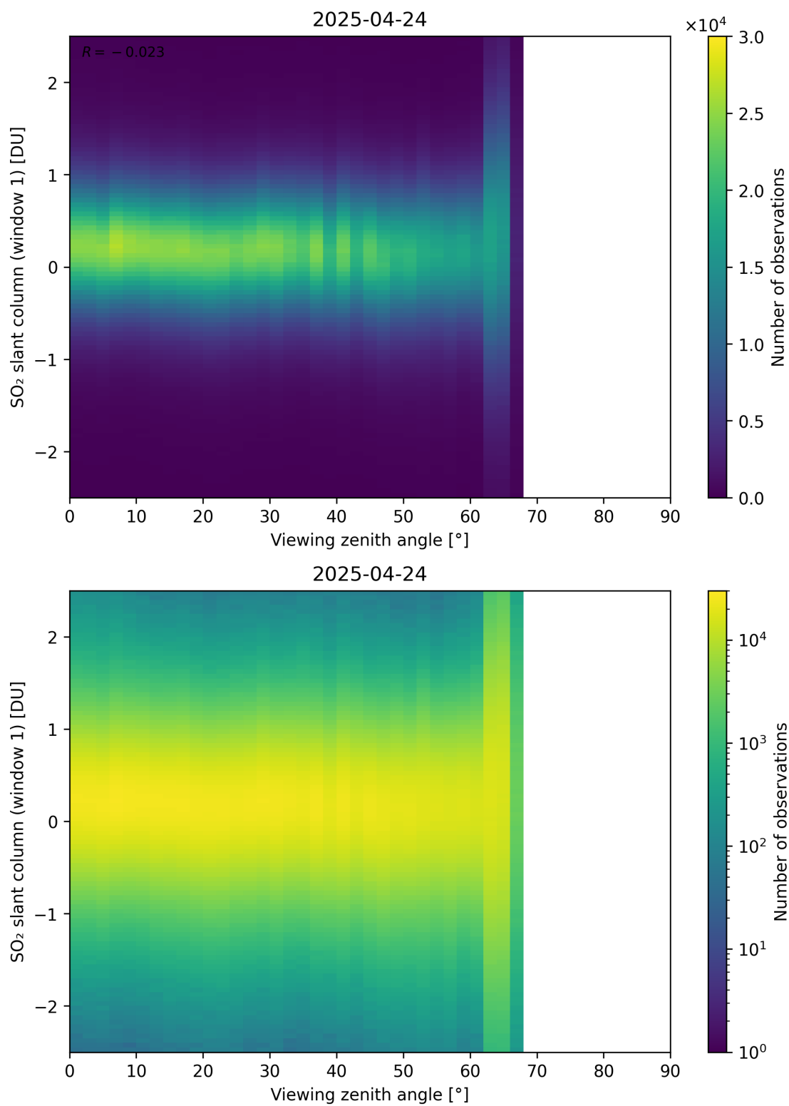
Figure 376: Scatter density plot of “Viewing zenith angle” against “SO 2 slant column (window 1)” for 2025-04-24 to 2025-04-25.
