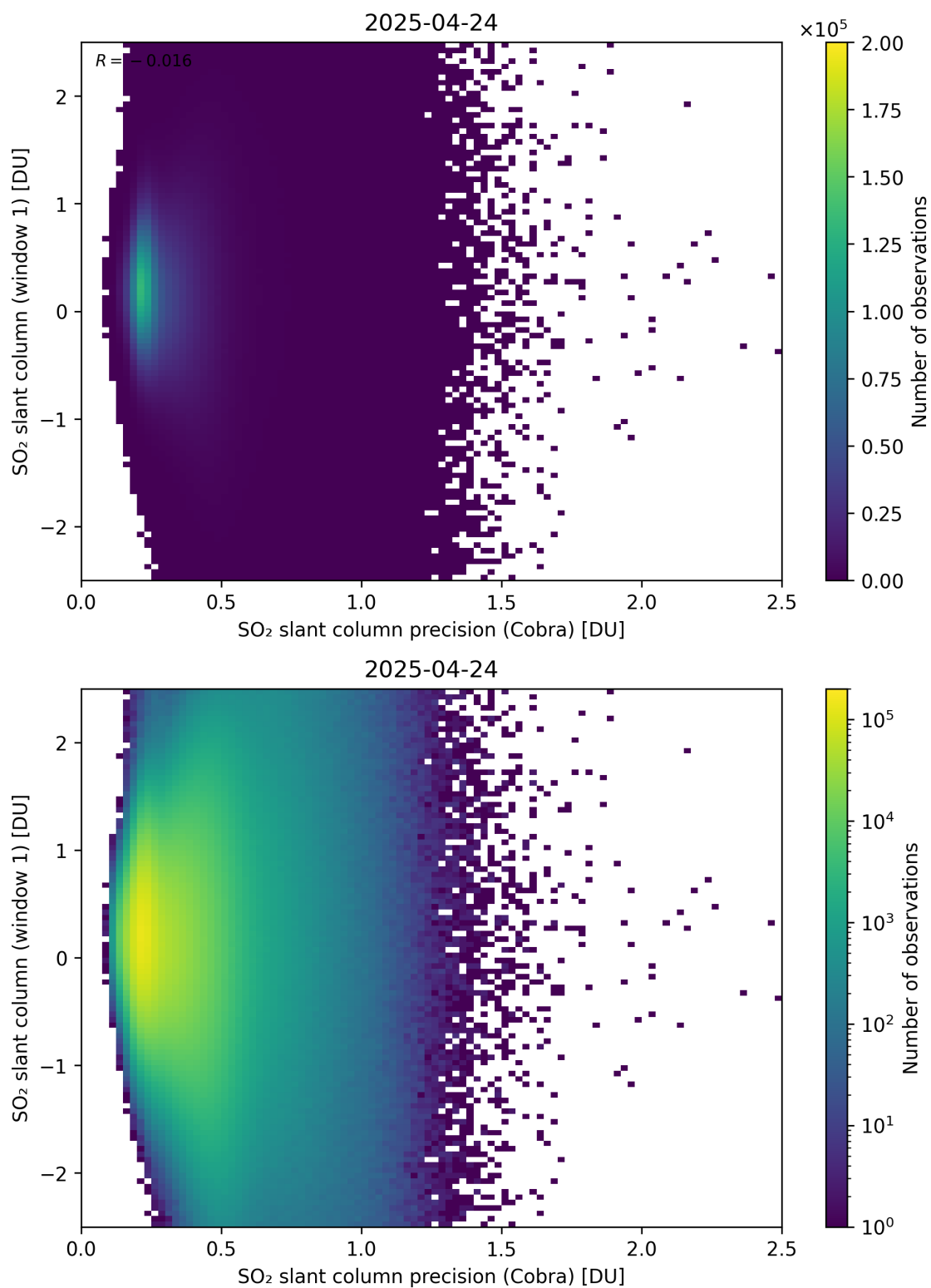
Figure 208: Scatter density plot of “SO 2 slant column precision (Cobra)” against “SO 2 slant column (window 1)” for 2025-04-24 to 2025-04-25.
