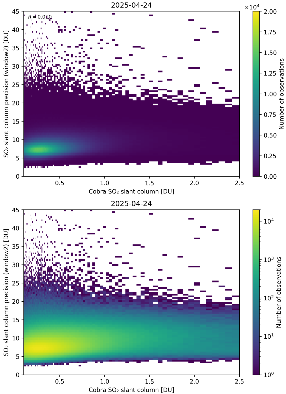
Figure 221: Scatter density plot of “Cobra SO 2 slant column” against “SO 2 slant column precision (window2)” for 2025-04-24 to 2025-04-25.
