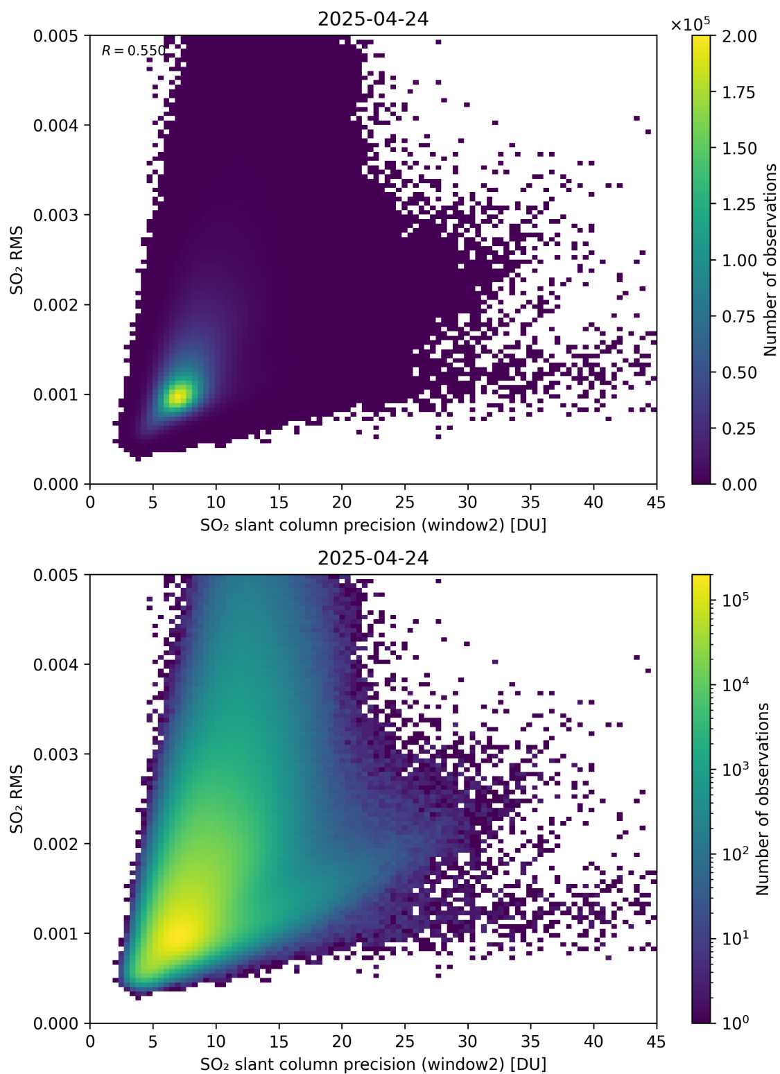
Figure 295: Scatter density plot of “SO 2 slant column precision (window2)” against “SO 2 RMS” for 2025-04-24 to 2025-04-25.
