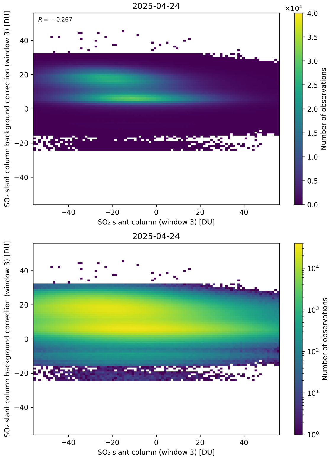
Figure 303: Scatter density plot of “SO 2 slant column (window 3)” against “SO 2 slant column background correction (window 3)” for 2025-04-24 to 2025-04-25.
