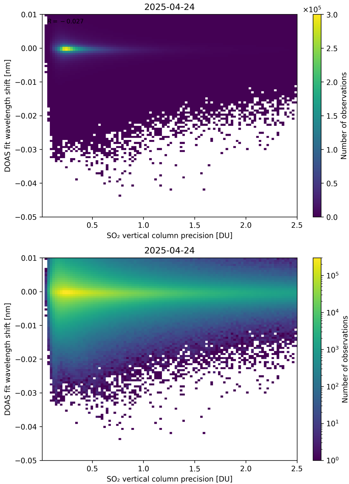
Figure 332: Scatter density plot of “SO 2 vertical column precision” against “DOAS fit wavelength shift” for 2025-04-24 to 2025-04-25.
