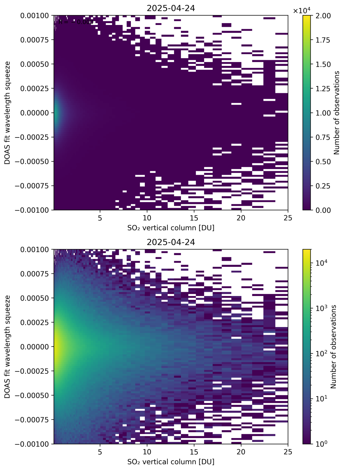
Figure 327: Scatter density plot of “SO 2 vertical column” against “DOAS fit wavelength squeeze” for 2025-04-24 to 2025-04-25.
