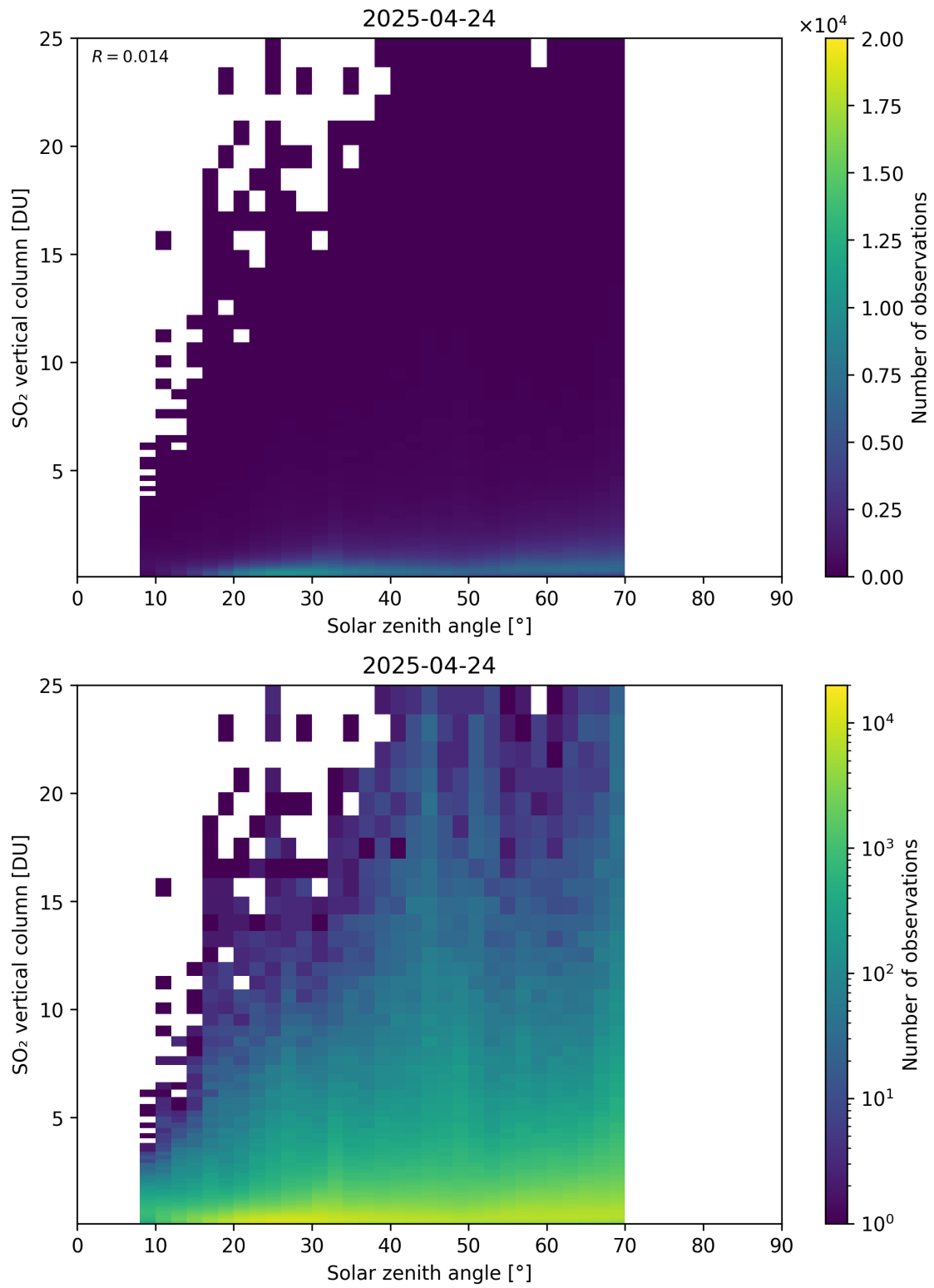
Figure 191: Scatter density plot of “Solar zenith angle” against “SO 2 vertical column” for 2025-04-24 to 2025-04-25.
