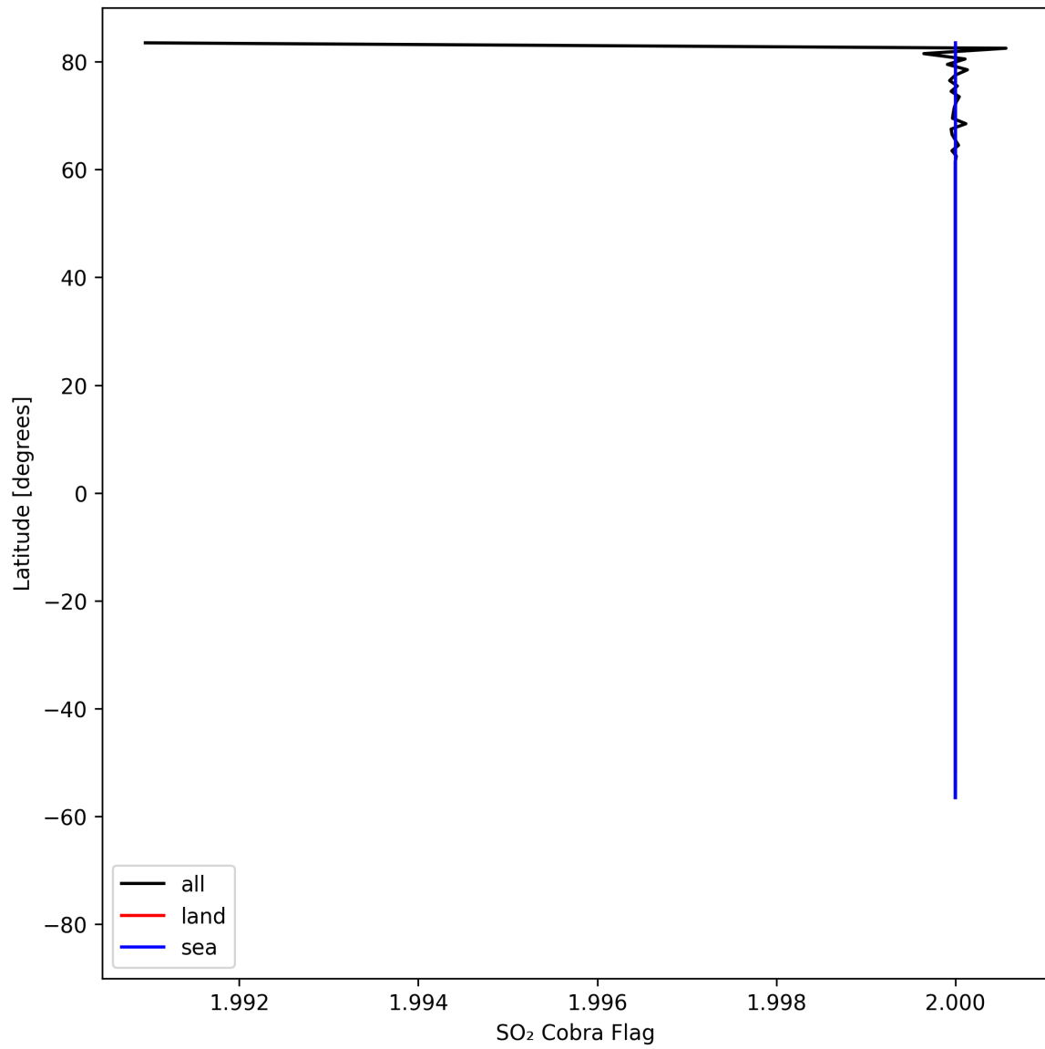
Figure 49: Zonal average of “SO 2 Cobra Flag” for 2025-04-24 to 2025-04-25.
