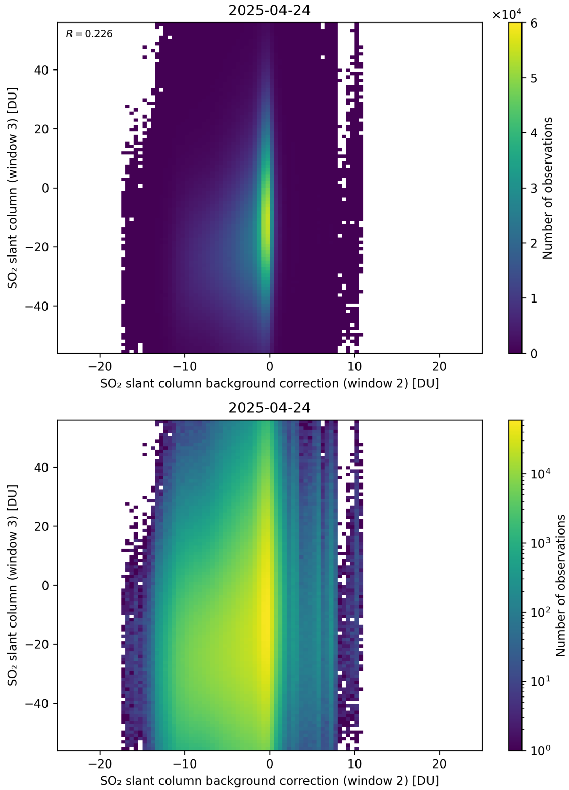
Figure 128: Scatter density plot of “SO 2 slant column background correction (window 2)” against “SO 2 slant column (window 3)” for 2025-04-24 to 2025-04-25.
