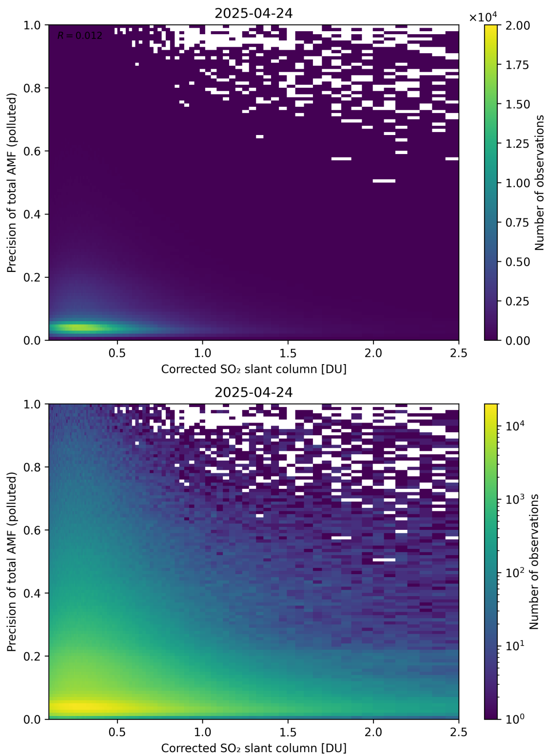
Figure 243: Scatter density plot of “Corrected SO 2 slant column” against “Precision of total AMF (polluted)” for 2025-04-24 to 2025-04-25.
