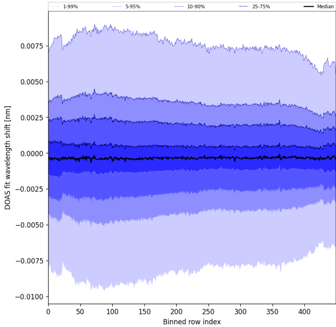
Figure 102: Along track statistics of “DOAS fit wavelength shift” for 2025-04-24 to 2025-04-25
