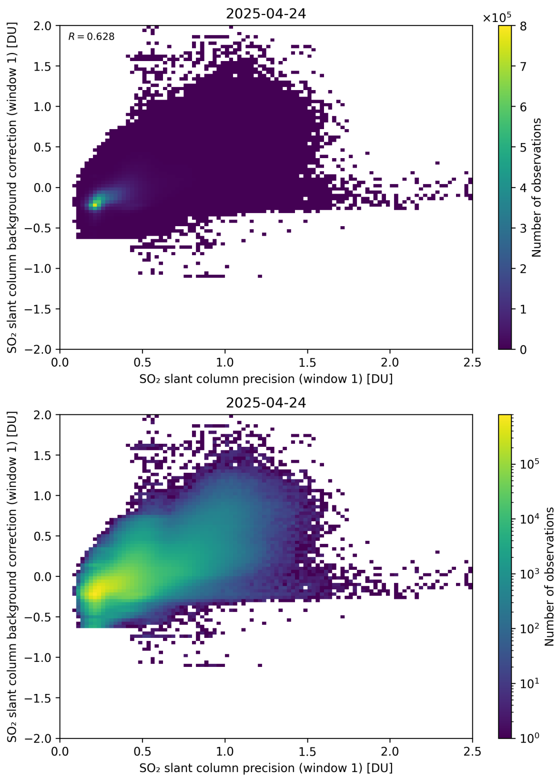
Figure 268: Scatter density plot of “SO 2 slant column precision (window 1)” against “SO 2 slant column background correction (window 1)” for 2025-04-24 to 2025-04-25.
