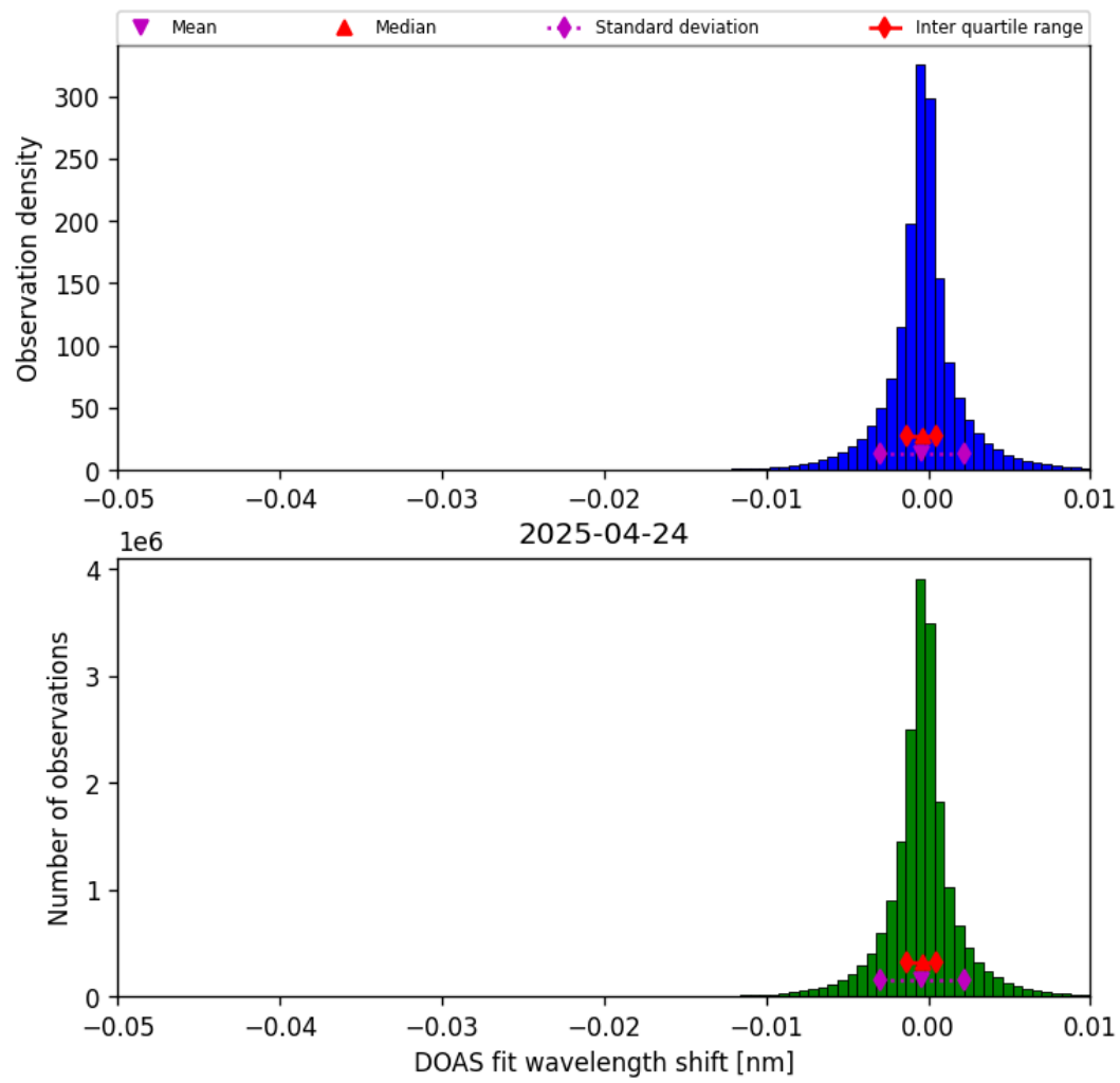
Figure 76: Histogram of “DOAS fit wavelength shift” for 2025-04-24 to 2025-04-25
