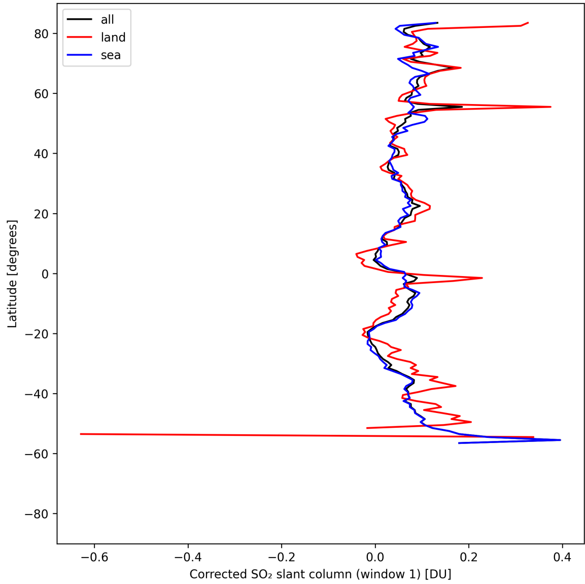
Figure 39: Zonal average of “Corrected SO 2 slant column (window 1)” for 2025-04-24 to 2025-04-25.
