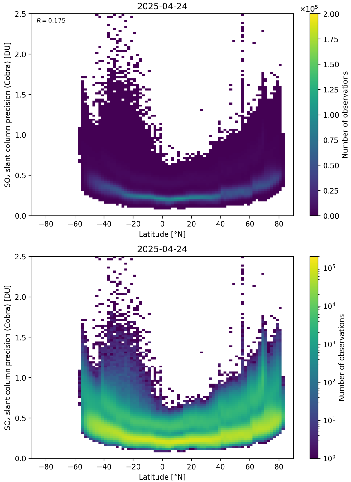
Figure 158: Scatter density plot of “Latitude” against “SO 2 slant column precision (Cobra)” for 2025-04-24 to 2025-04-25.
