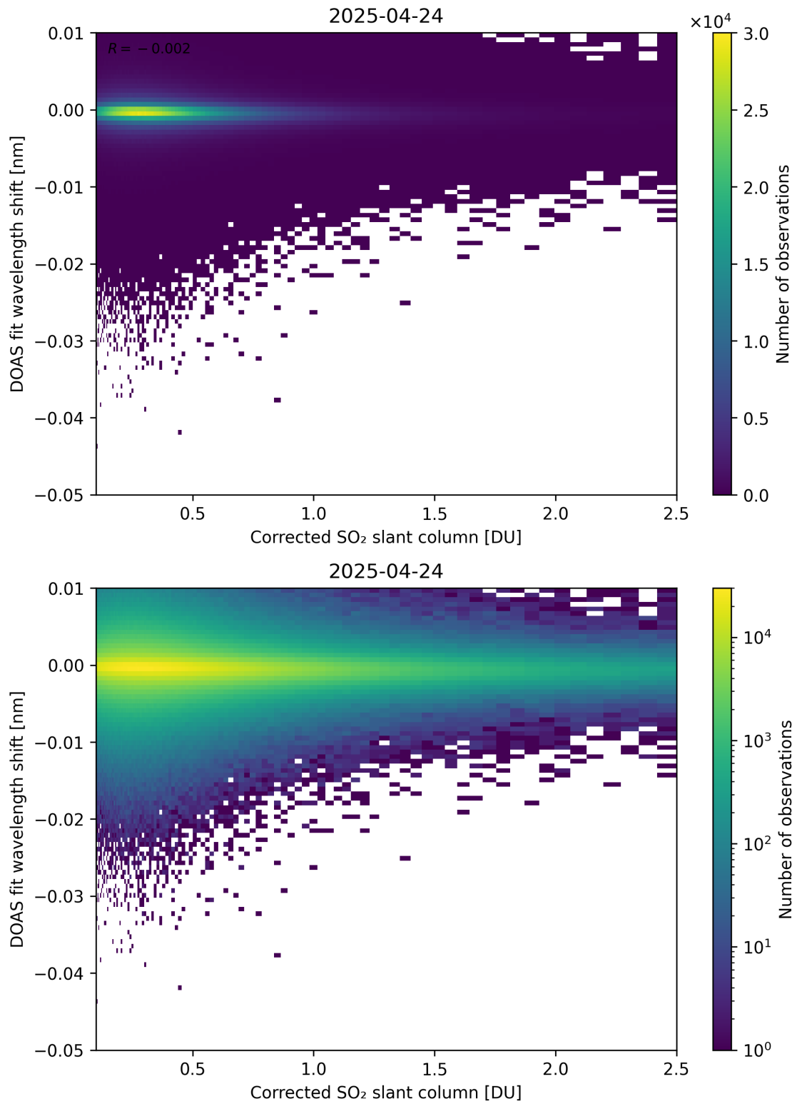
Figure 229: Scatter density plot of “Corrected SO 2 slant column” against “DOAS fit wavelength shift” for 2025-04-24 to 2025-04-25.
