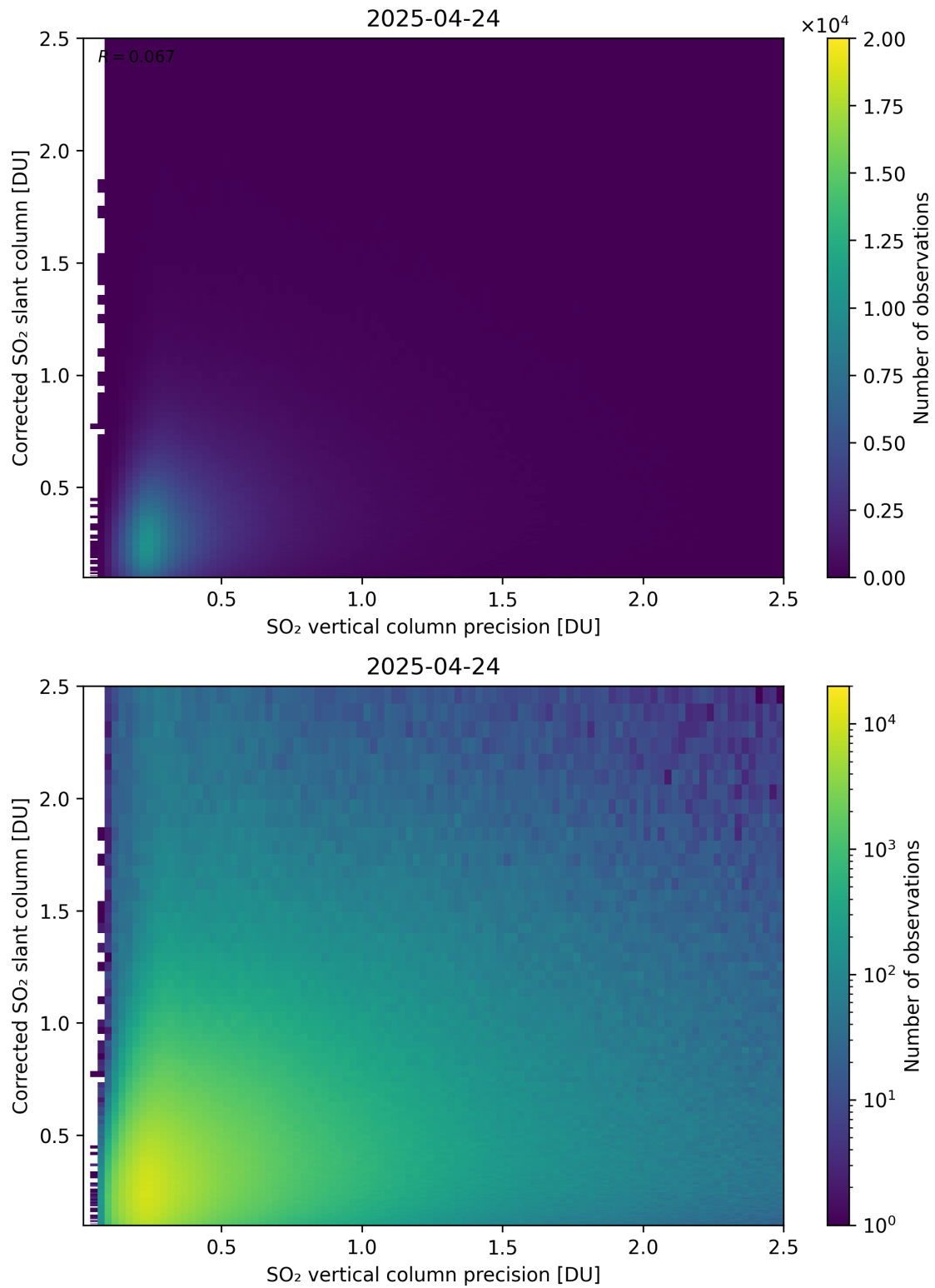
Figure 338: Scatter density plot of “SO 2 vertical column precision” against “Corrected SO 2 slant column” for 2025-04-24 to 2025-04-25.
