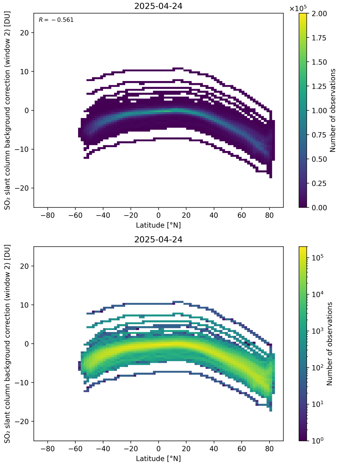
Figure 151: Scatter density plot of “Latitude” against “SO 2 slant column background correction (window 2)” for 2025-04-24 to 2025-04-25.
