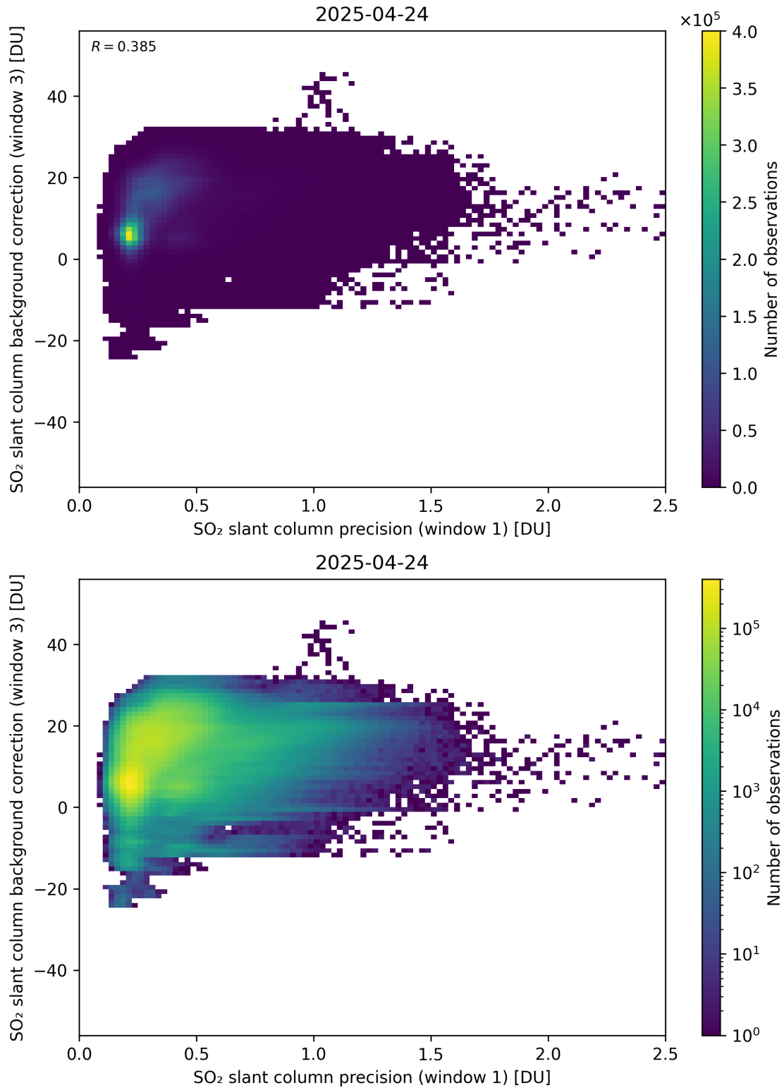
Figure 270: Scatter density plot of “SO 2 slant column precision (window 1)” against “SO 2 slant column background correction (window 3)” for 2025-04-24 to 2025-04-25.
