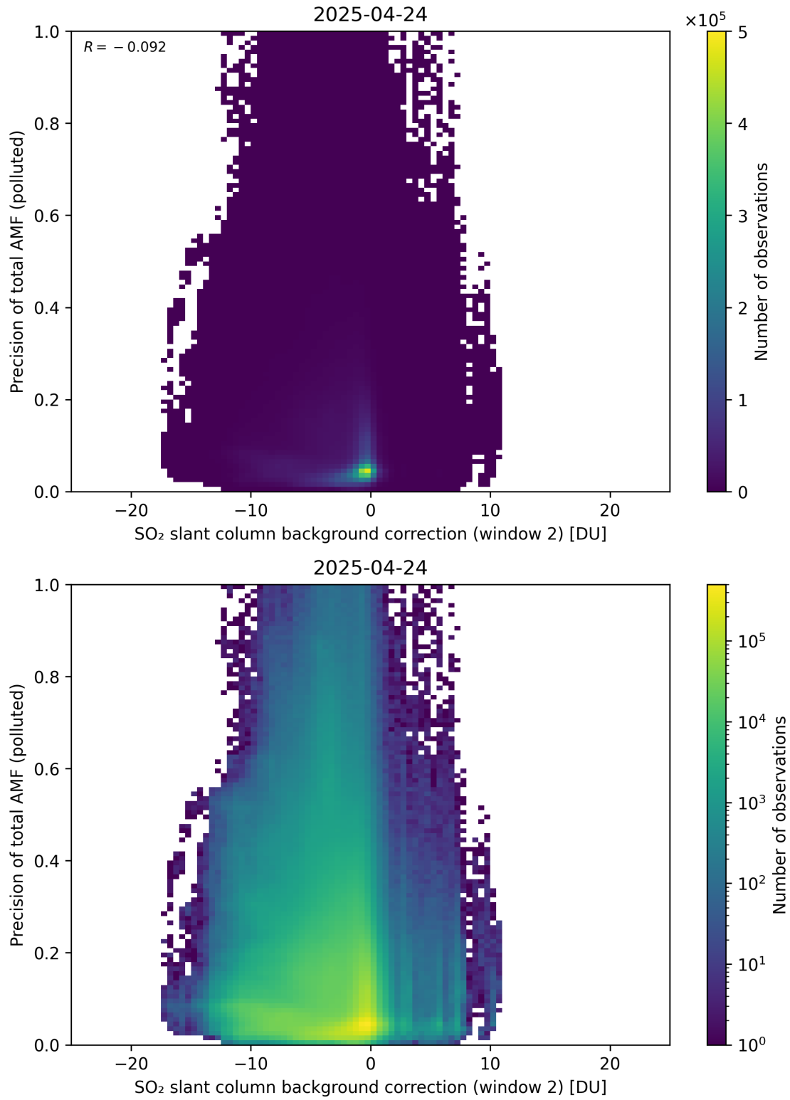
Figure 131: Scatter density plot of “SO 2 slant column background correction (window 2)” against “Precision of total AMF (polluted)” for 2025-04-24 to 2025-04-25.
