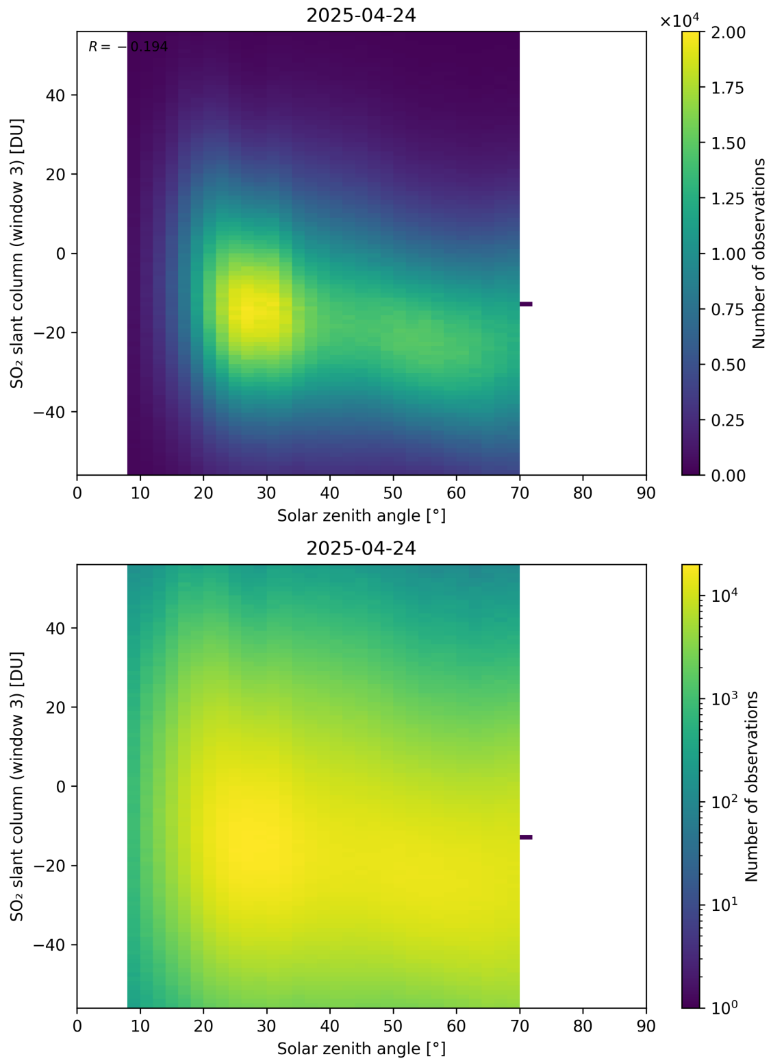
Figure 187: Scatter density plot of “Solar zenith angle” against “SO 2 slant column (window 3)” for 2025-04-24 to 2025-04-25.
