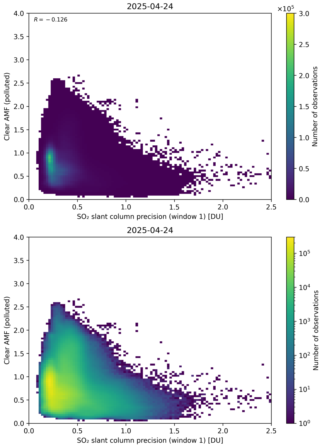
Figure 274: Scatter density plot of “SO 2 slant column precision (window 1)” against “Clear AMF (polluted)” for 2025-04-24 to 2025-04-25.
