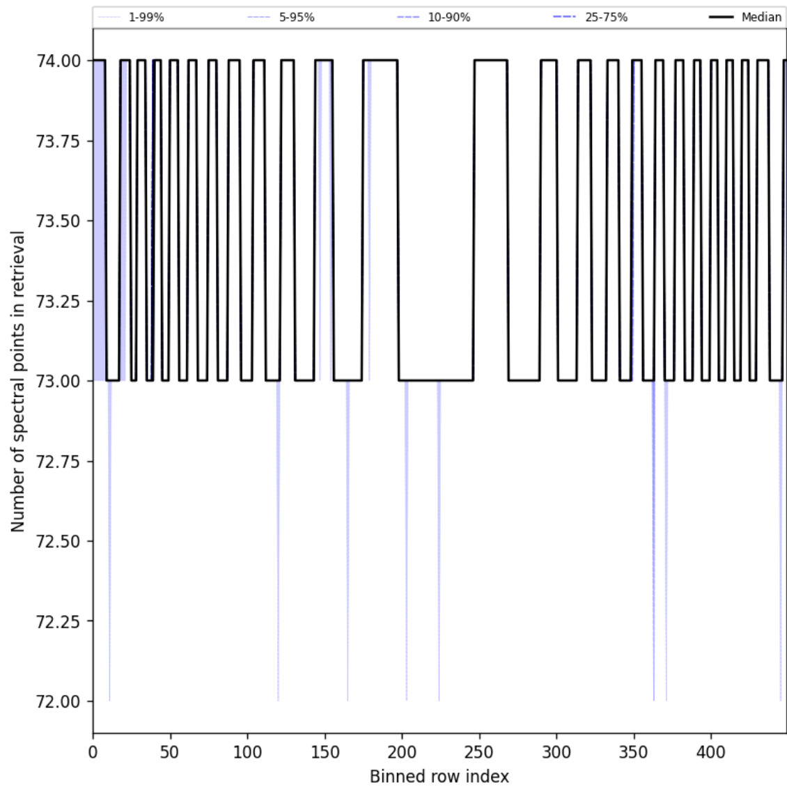
Figure 108: Along track statistics of “Number of spectral points in retrieval” for 2025-04-24 to 2025-04-25
