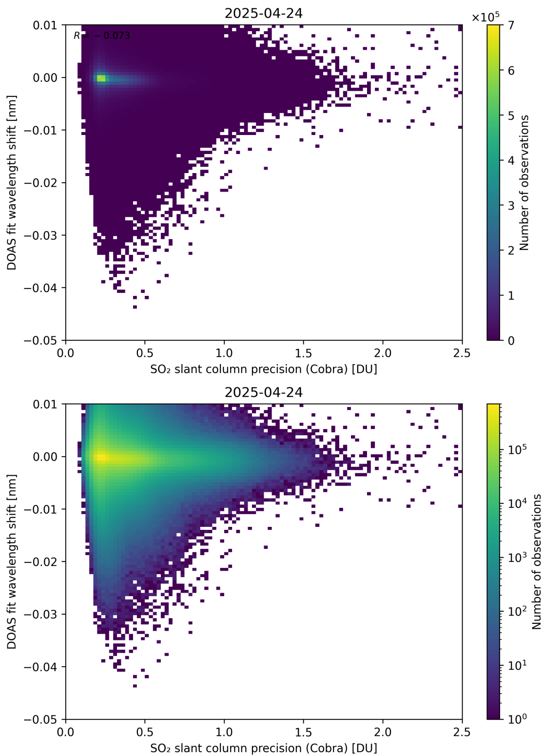
Figure 202: Scatter density plot of “SO 2 slant column precision (Cobra)” against “DOAS fit wavelength shift” for 2025-04-24 to 2025-04-25.
