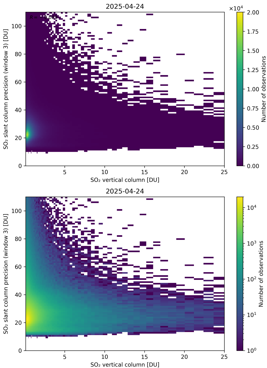
Figure 358: Scatter density plot of “SO 2 vertical column” against “SO 2 slant column precision (window 3)” for 2025-04-24 to 2025-04-25.
