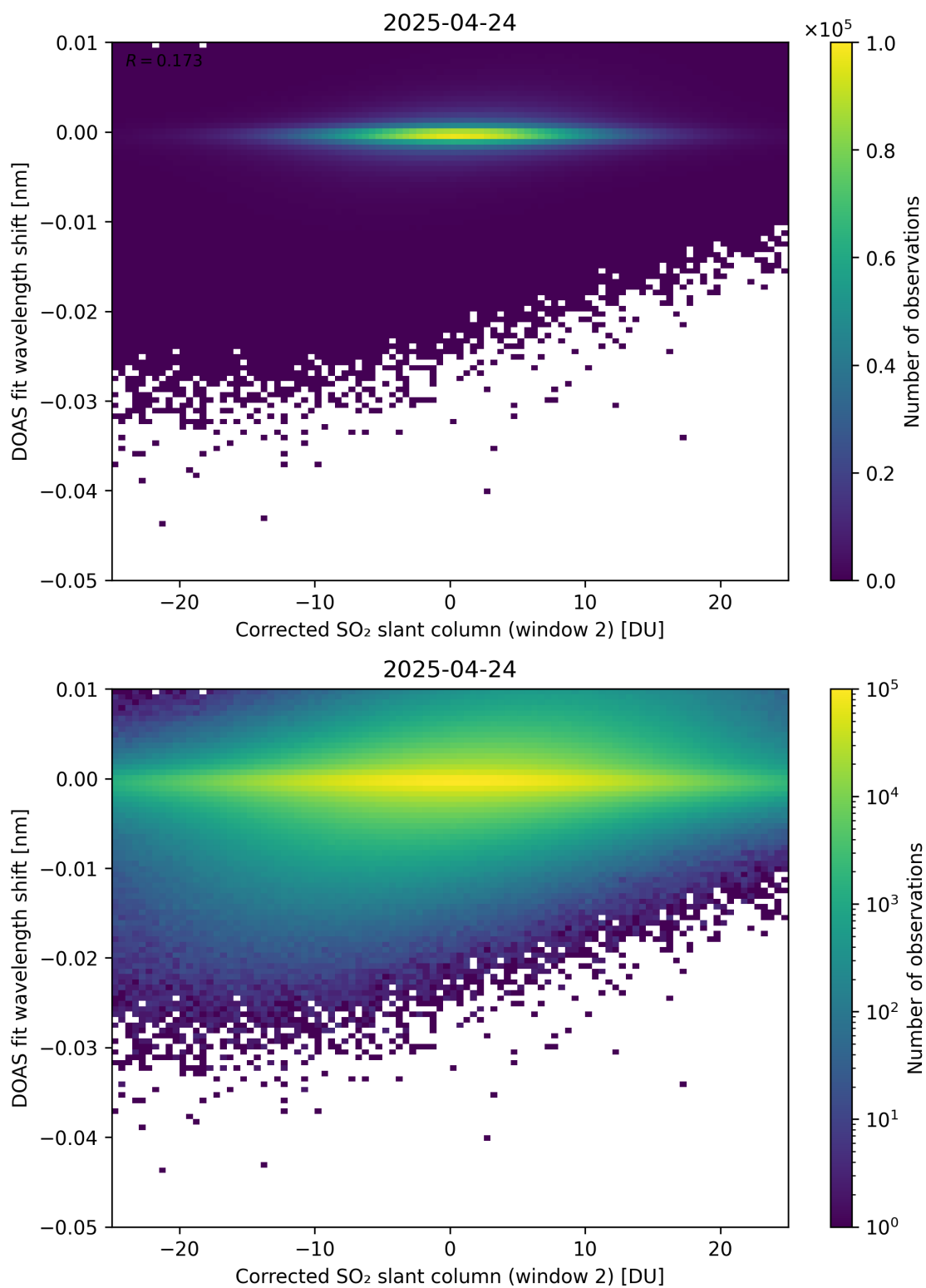
Figure 246: Scatter density plot of “Corrected SO 2 slant column (window 2)” against “DOAS fit wavelength shift” for 2025-04-24 to 2025-04-25.
