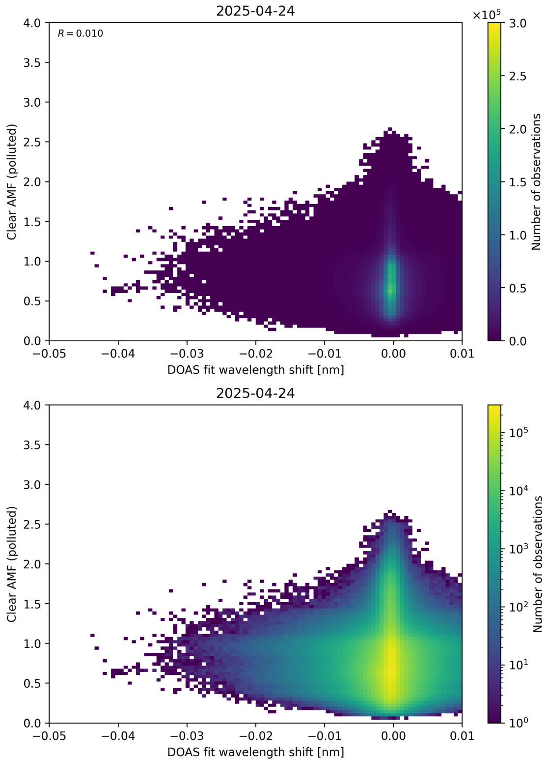
Figure 140: Scatter density plot of “DOAS fit wavelength shift” against “Clear AMF (polluted)” for 2025-04-24 to 2025-04-25.
