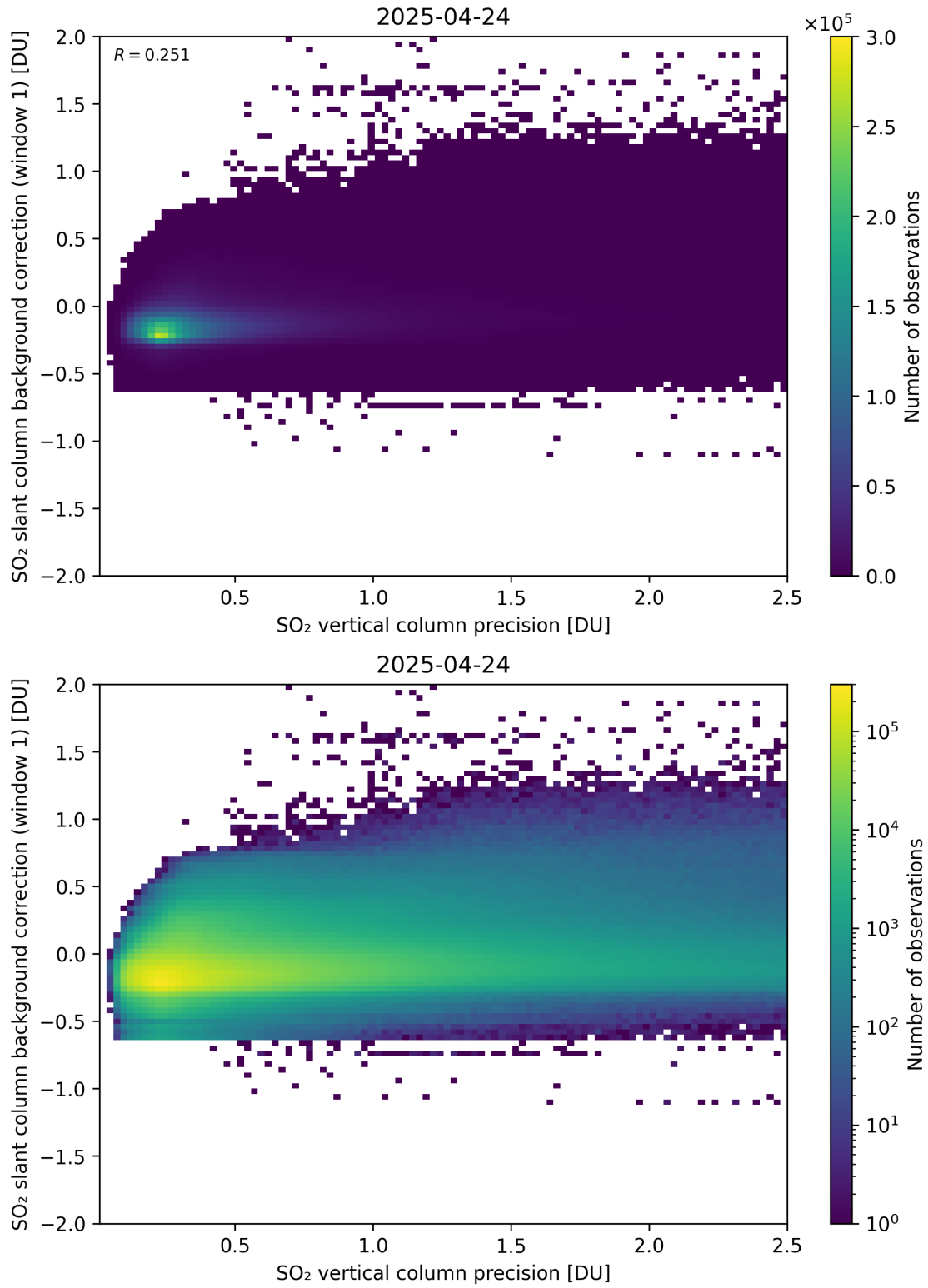
Figure 329: Scatter density plot of “SO 2 vertical column precision” against “SO 2 slant column background correction (window 1)” for 2025-04-24 to 2025-04-25.
