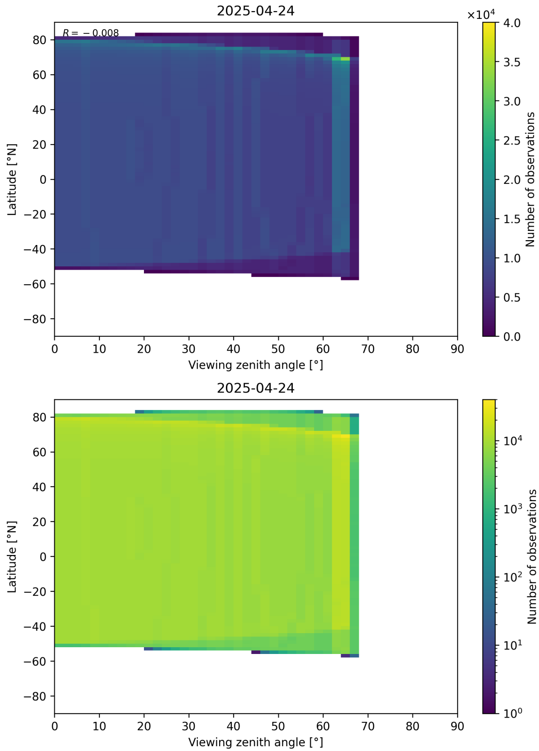
Figure 368: Scatter density plot of “Viewing zenith angle” against “Latitude” for 2025-04-24 to 2025-04-25.
