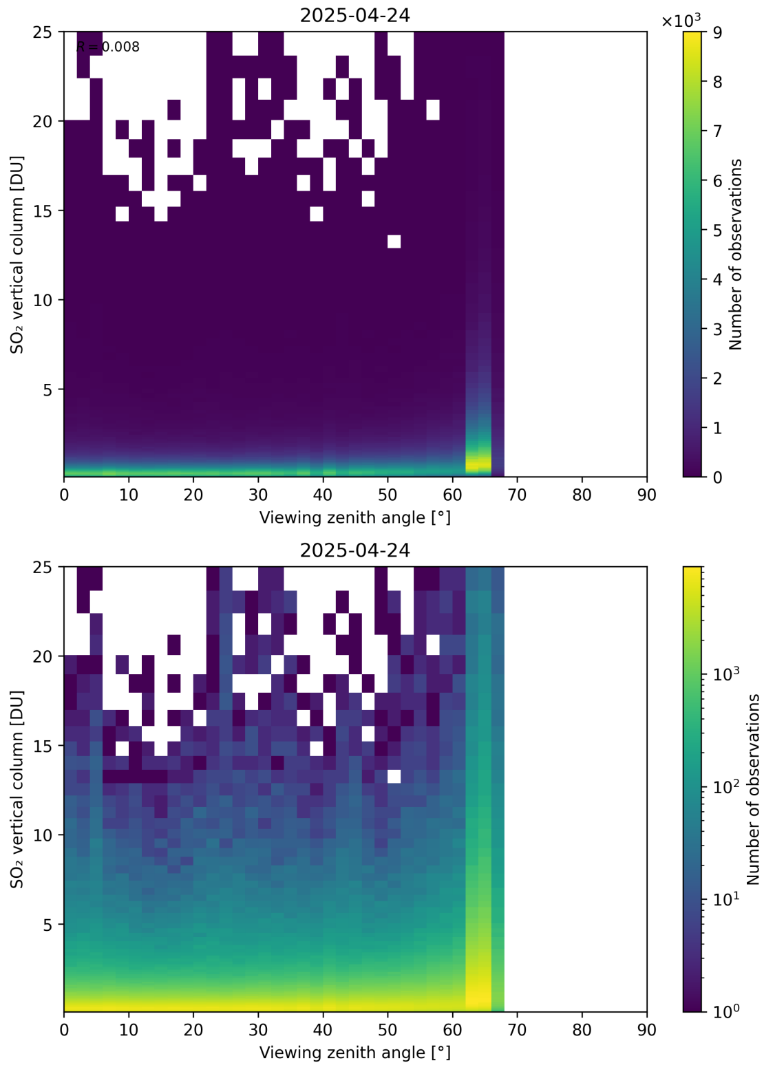
Figure 383: Scatter density plot of “Viewing zenith angle” against “SO 2 vertical column” for 2025-04-24 to 2025-04-25.
