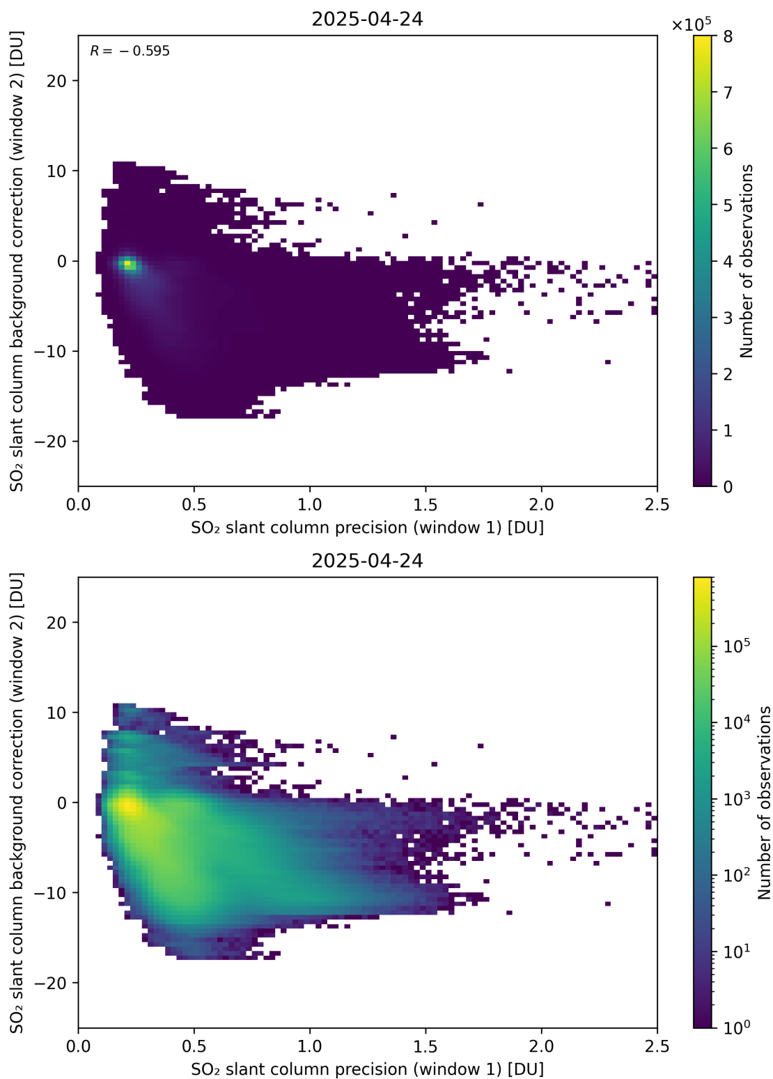
Figure 269: Scatter density plot of “SO 2 slant column precision (window 1)” against “SO 2 slant column background correction (window 2)” for 2025-04-24 to 2025-04-25.
