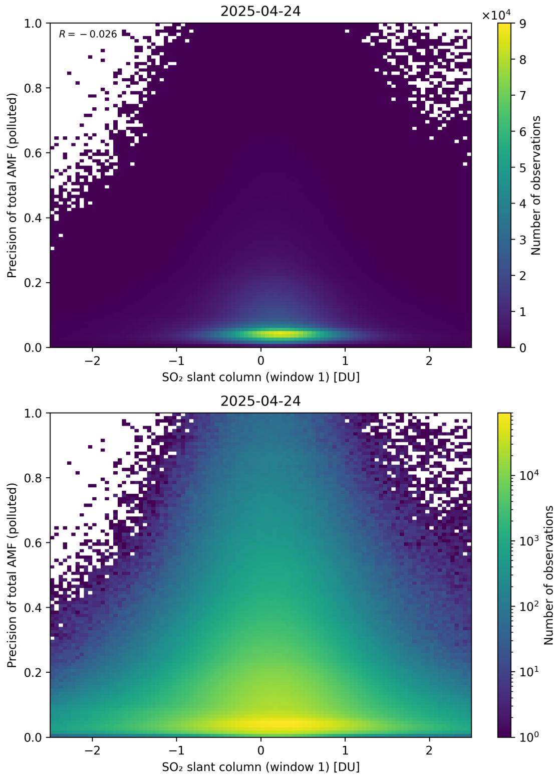
Figure 290: Scatter density plot of “SO 2 slant column (window 1)” against “Precision of total AMF (polluted)” for 2025-04-24 to 2025-04-25.
