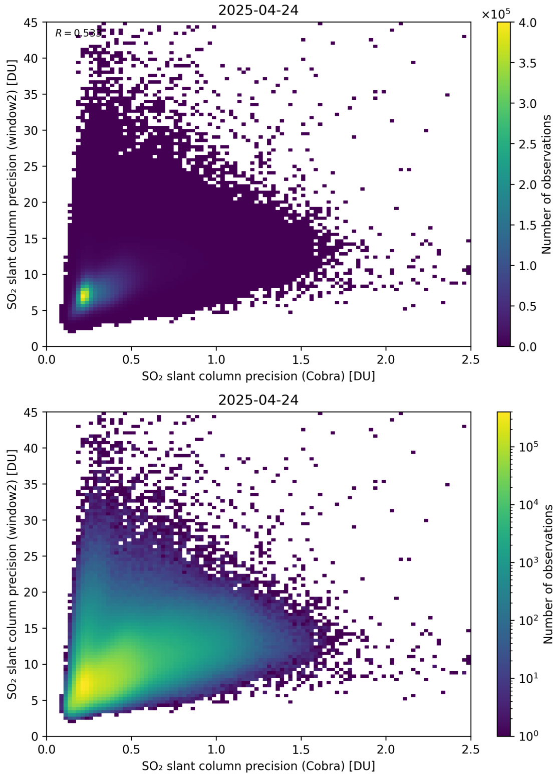
Figure 210: Scatter density plot of “SO 2 slant column precision (Cobra)” against “SO 2 slant column precision (window2)” for 2025-04-24 to 2025-04-25.
