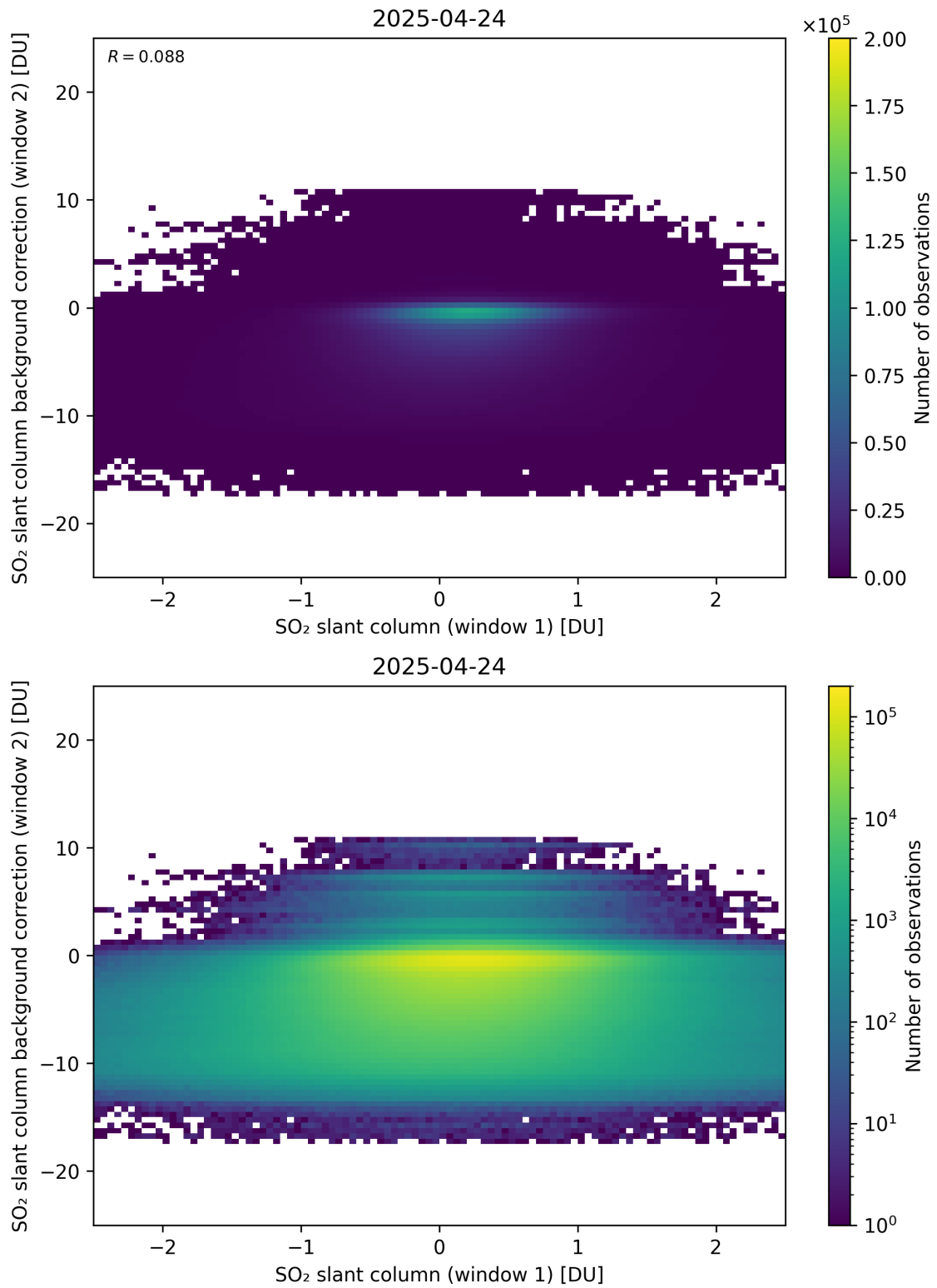
Figure 263: Scatter density plot of “SO 2 slant column (window 1)” against “SO 2 slant column background correction (window 2)” for 2025-04-24 to 2025-04-25.
