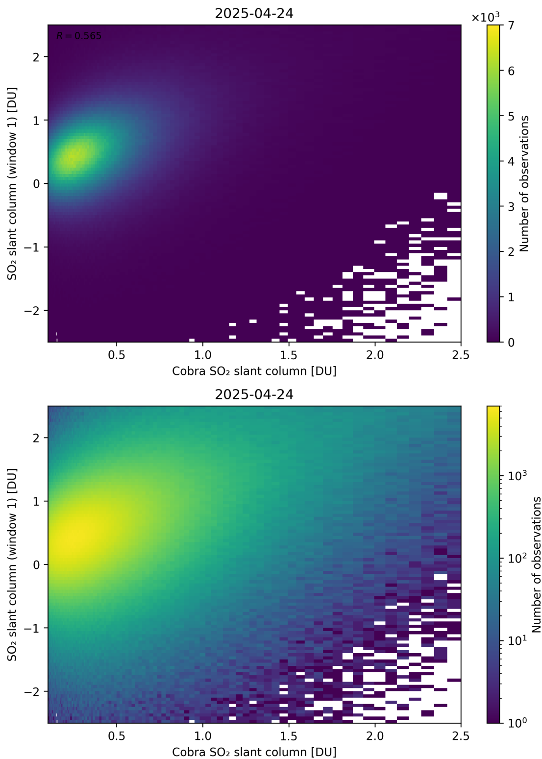
Figure 219: Scatter density plot of “Cobra SO 2 slant column” against “SO 2 slant column (window 1)” for 2025-04-24 to 2025-04-25.
