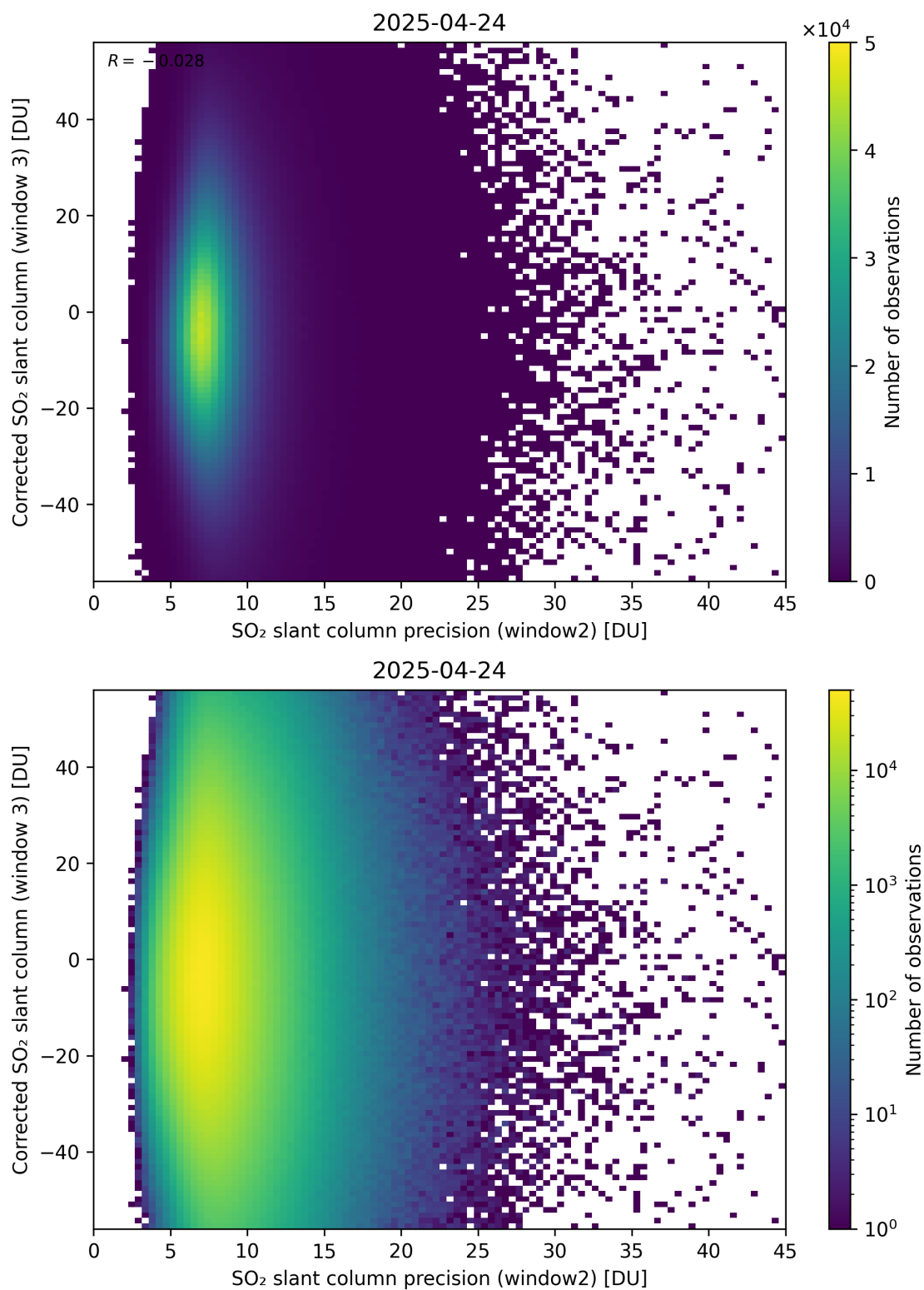
Figure 298: Scatter density plot of “SO 2 slant column precision (window2)” against “Corrected SO 2 slant column (window 3)” for 2025-04-24 to 2025-04-25.
