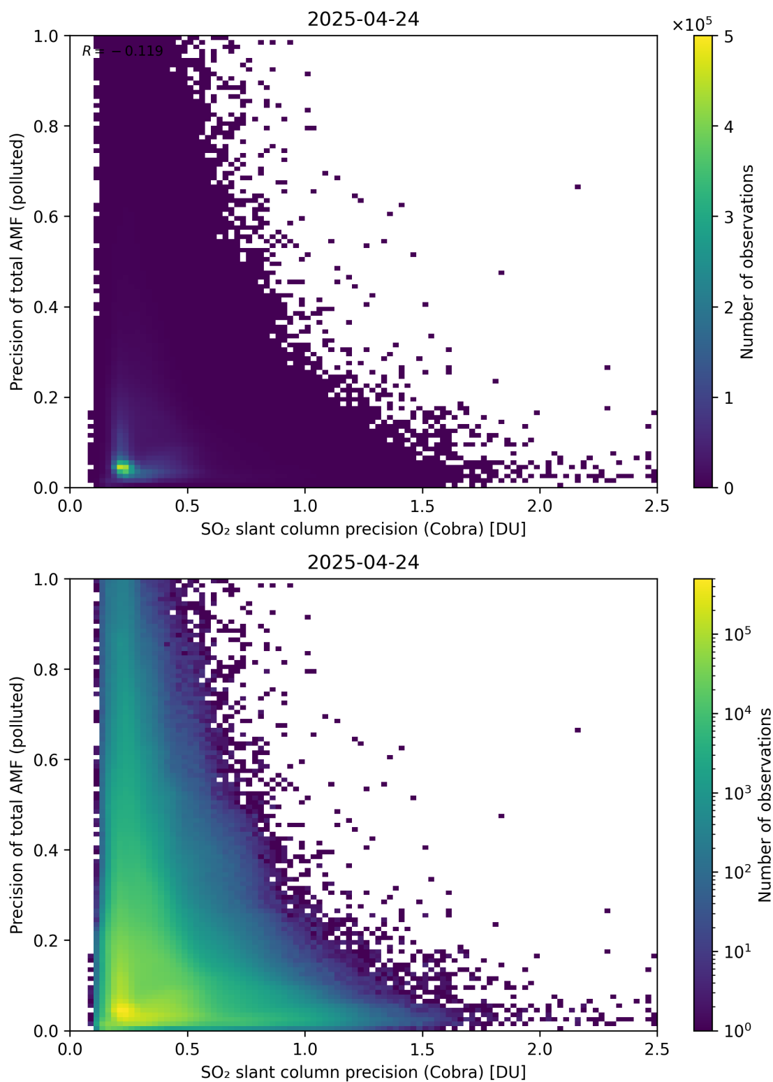
Figure 214: Scatter density plot of “SO 2 slant column precision (Cobra)” against “Precision of total AMF (polluted)” for 2025-04-24 to 2025-04-25.
