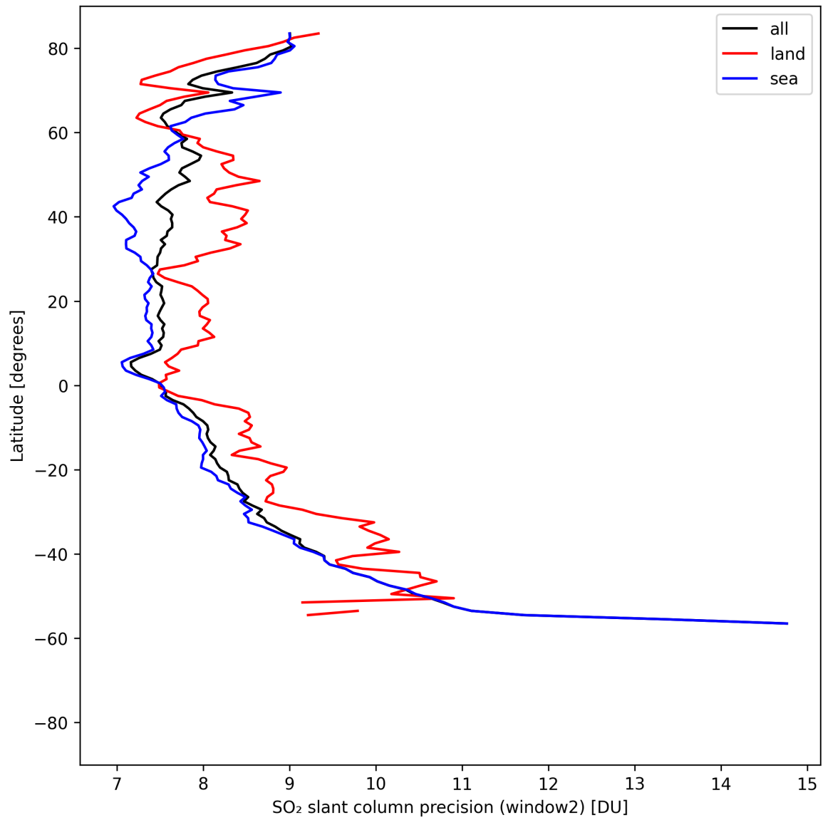
Figure 42: Zonal average of “SO 2 slant column precision (window2)” for 2025-04-24 to 2025-04-25.
