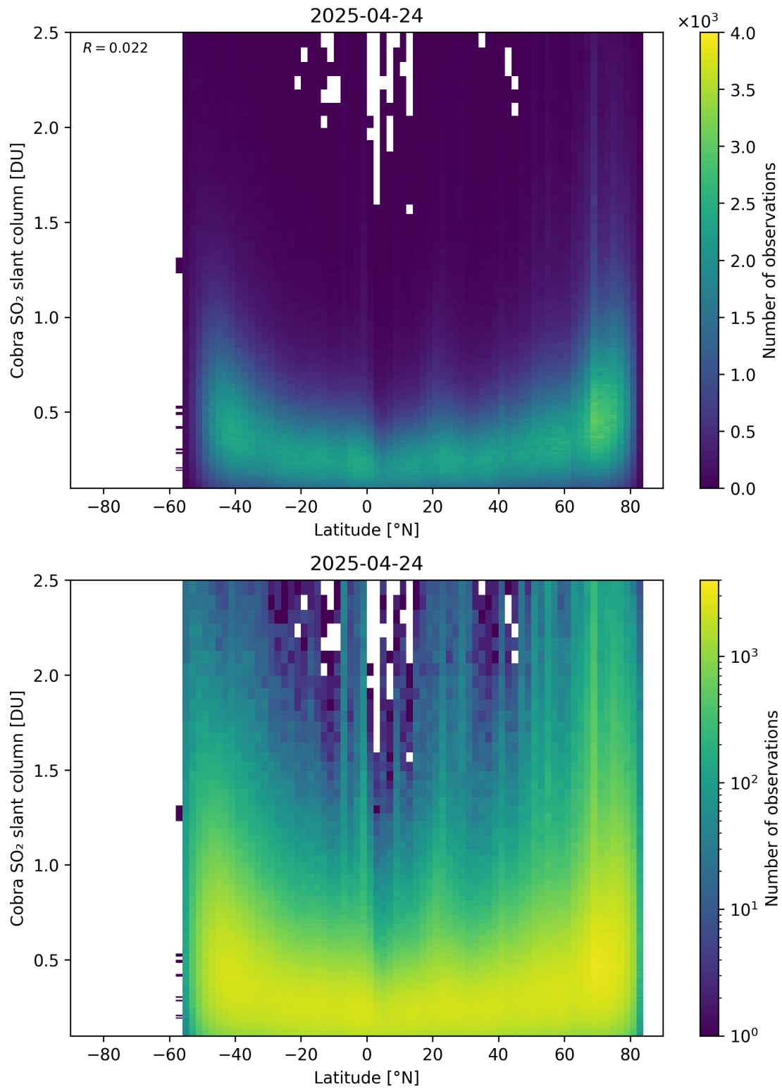
Figure 157: Scatter density plot of “Latitude” against “Cobra SO 2 slant column” for 2025-04-24 to 2025-04-25.
