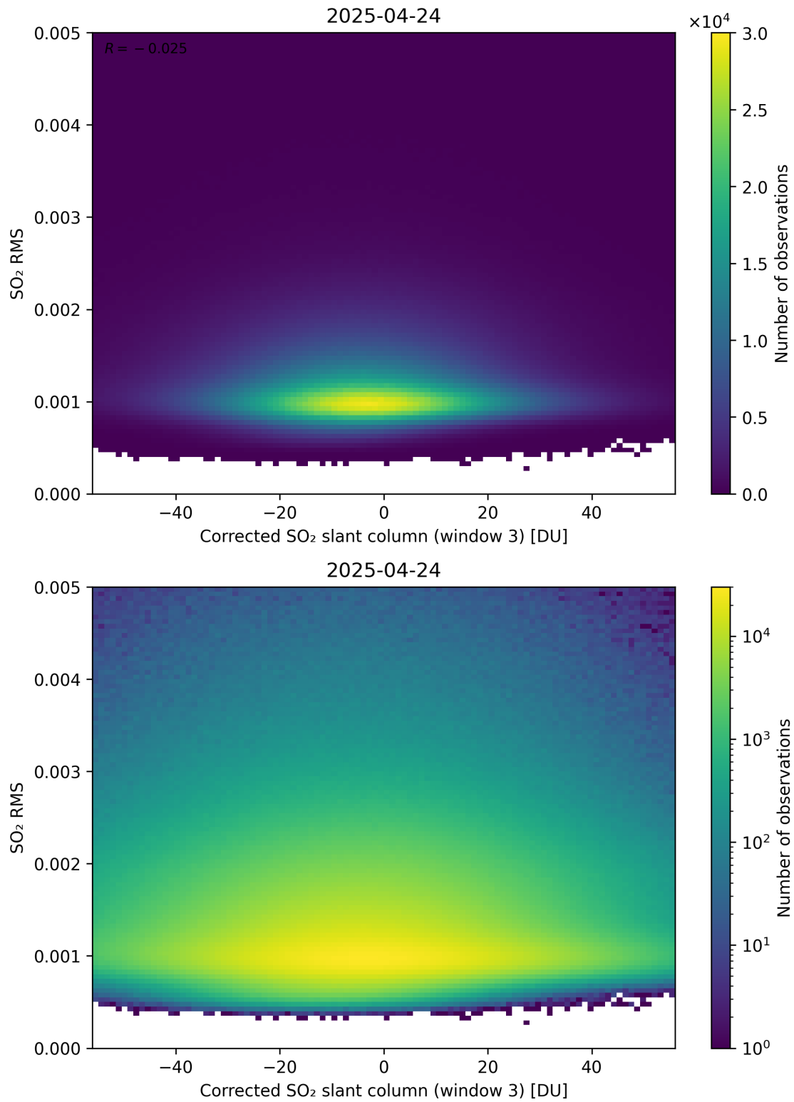
Figure 258: Scatter density plot of “Corrected SO 2 slant column (window 3)” against “SO 2 RMS” for 2025-04-24 to 2025-04-25.
