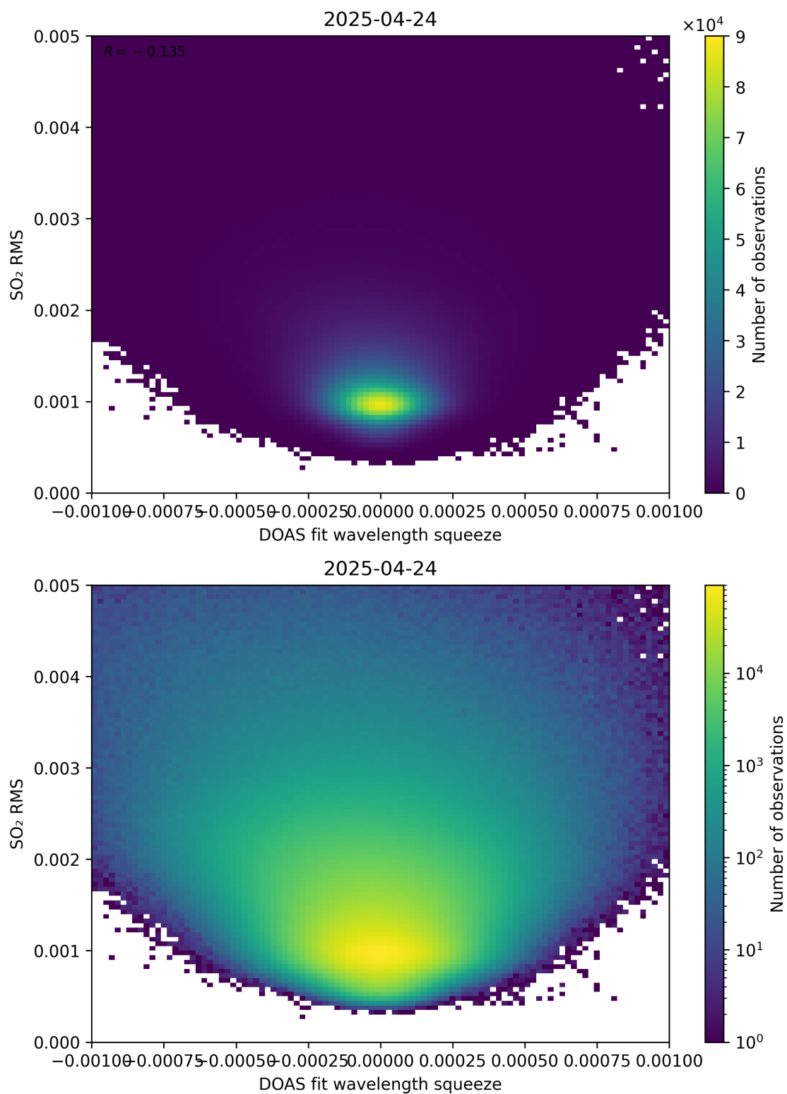
Figure 143: Scatter density plot of “DOAS fit wavelength squeeze” against “SO 2 RMS” for 2025-04-24 to 2025-04-25.
