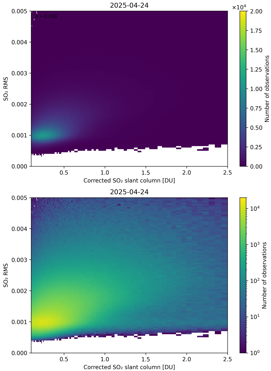
Figure 231: Scatter density plot of “Corrected SO 2 slant column” against “SO 2 RMS” for 2025-04-24 to 2025-04-25.
