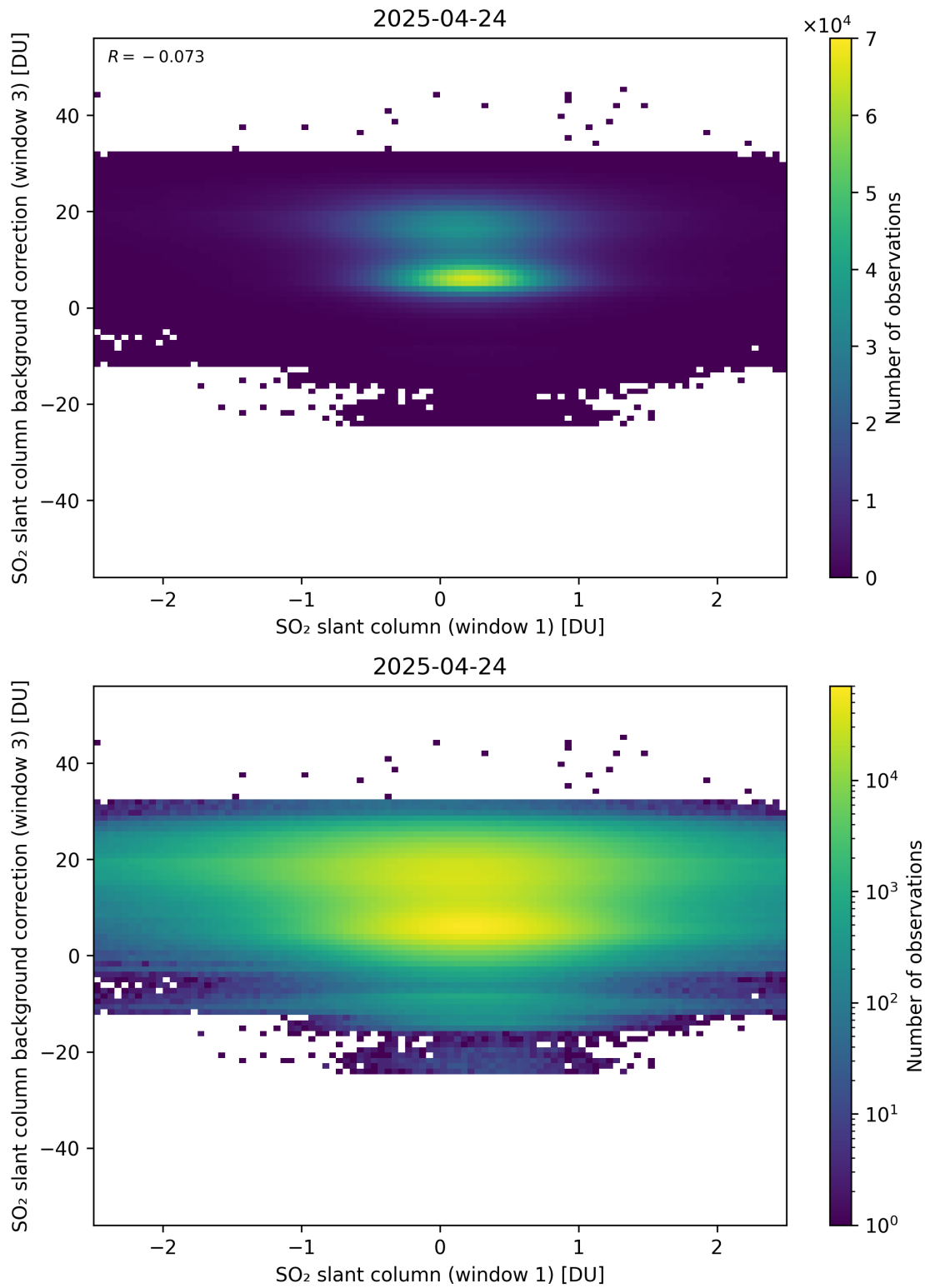
Figure 264: Scatter density plot of “SO 2 slant column (window 1)” against “SO 2 slant column background correction (window 3)” for 2025-04-24 to 2025-04-25.
