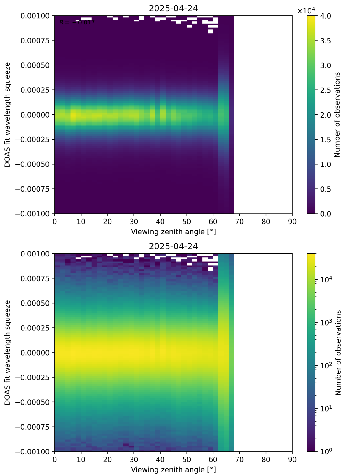
Figure 366: Scatter density plot of “Viewing zenith angle” against “DOAS fit wavelength squeeze” for 2025-04-24 to 2025-04-25.
