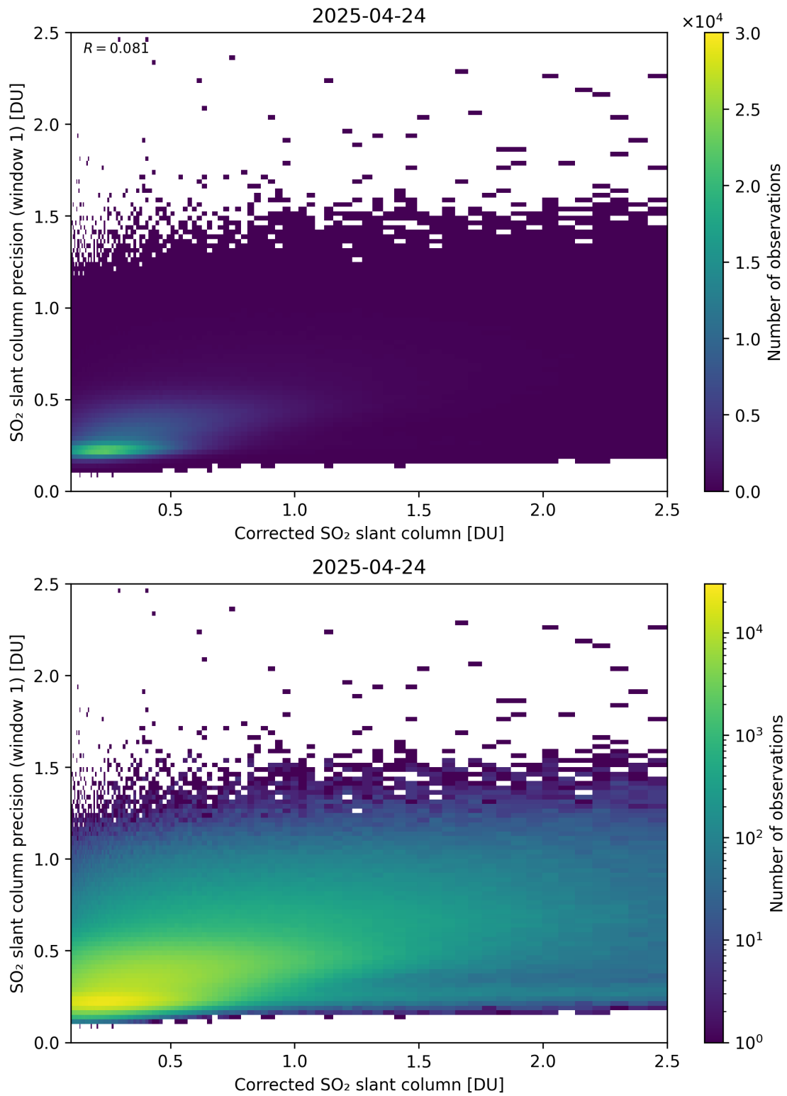
Figure 238: Scatter density plot of “Corrected SO 2 slant column” against “SO 2 slant column precision (window 1)” for 2025-04-24 to 2025-04-25.
