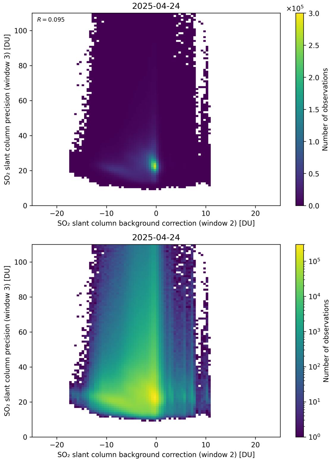
Figure 129: Scatter density plot of “SO 2 slant column background correction (window 2)” against “SO 2 slant column precision (window 3)” for 2025-04-24 to 2025-04-25.
