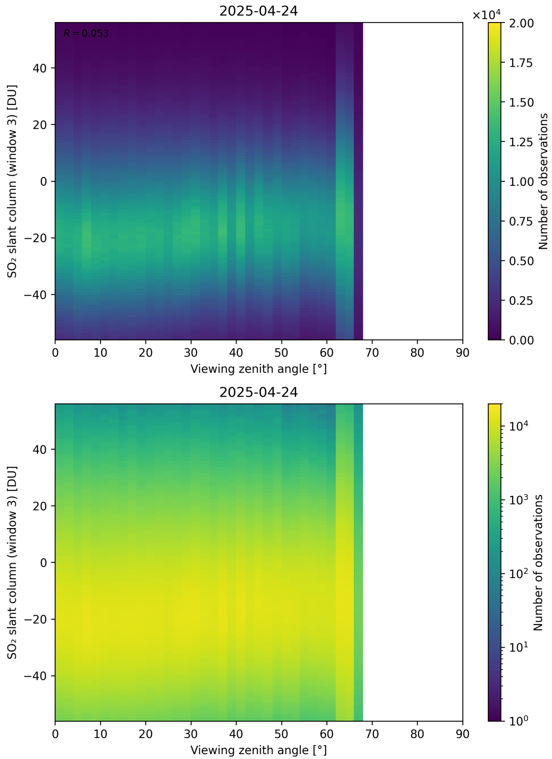
Figure 379: Scatter density plot of “Viewing zenith angle” against “SO 2 slant column (window 3)” for 2025-04-24 to 2025-04-25.
