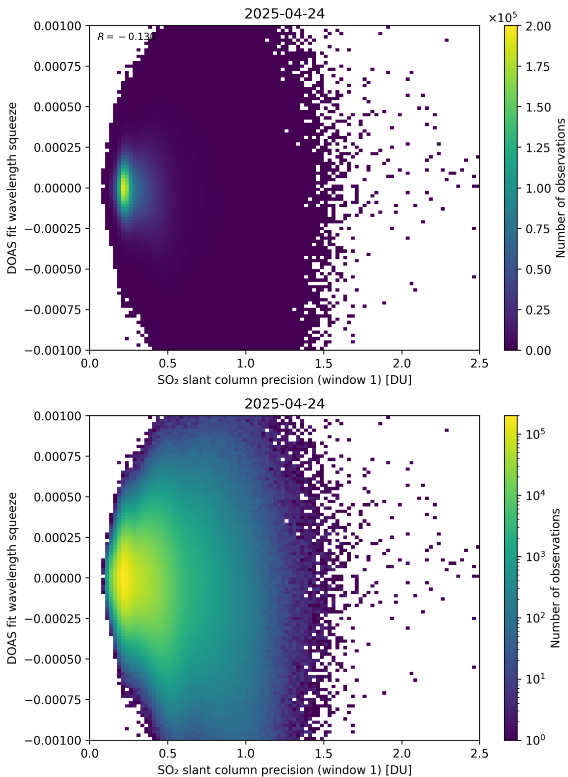
Figure 272: Scatter density plot of “SO 2 slant column precision (window 1)” against “DOAS fit wavelength squeeze” for 2025-04-24 to 2025-04-25.
