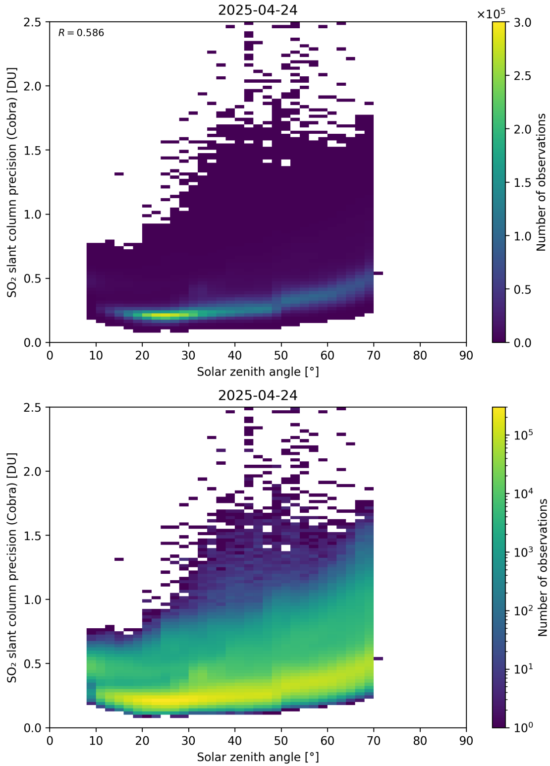
Figure 180: Scatter density plot of “Solar zenith angle” against “SO 2 slant column precision (Cobra)” for 2025-04-24 to 2025-04-25.
