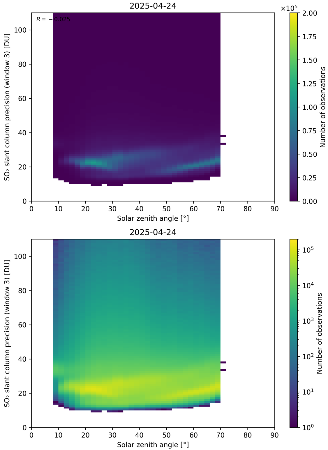
Figure 188: Scatter density plot of “Solar zenith angle” against “SO 2 slant column precision (window 3)” for 2025-04-24 to 2025-04-25.
