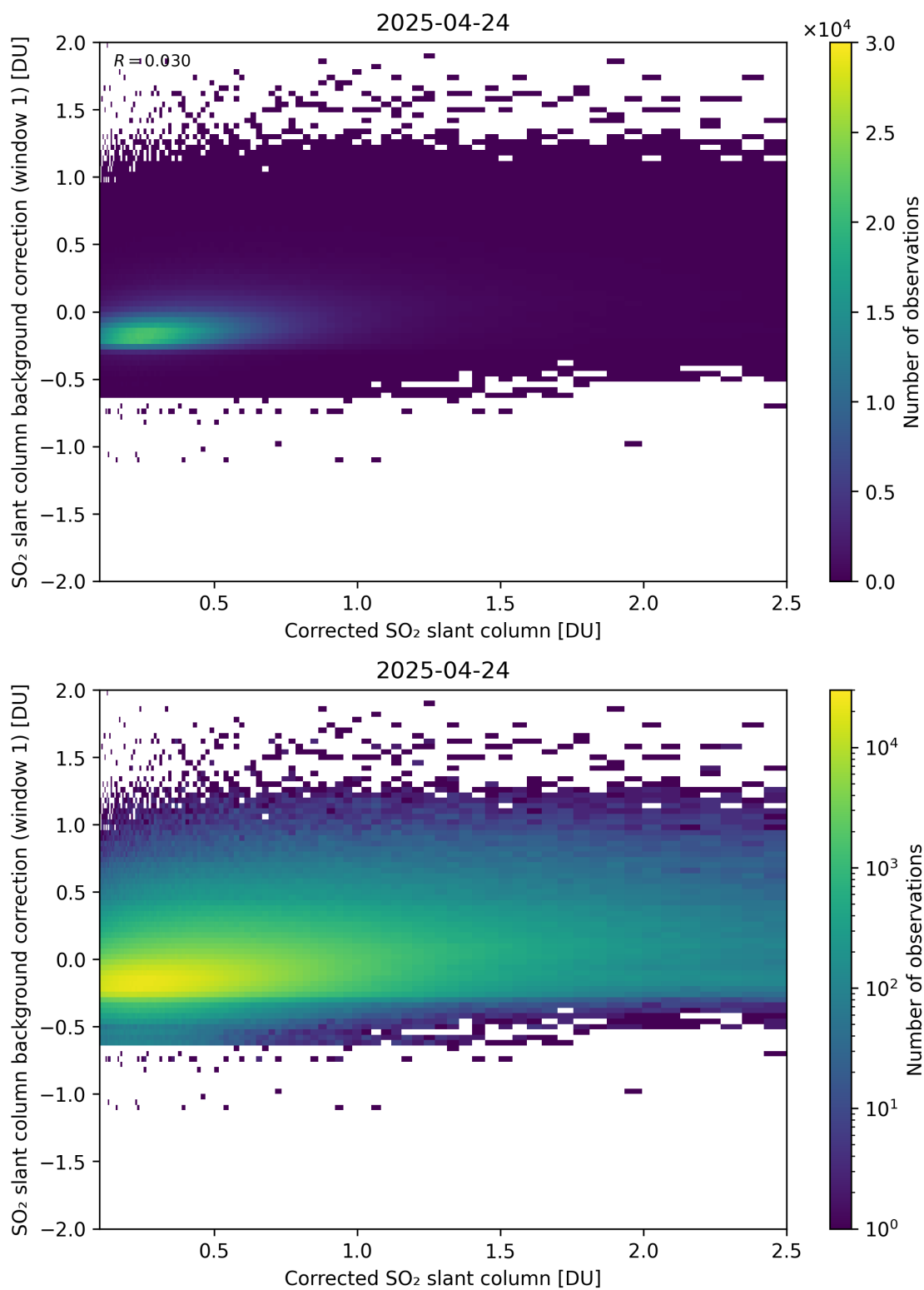
Figure 226: Scatter density plot of “Corrected SO 2 slant column” against “SO 2 slant column background correction (window 1)” for 2025-04-24 to 2025-04-25.
