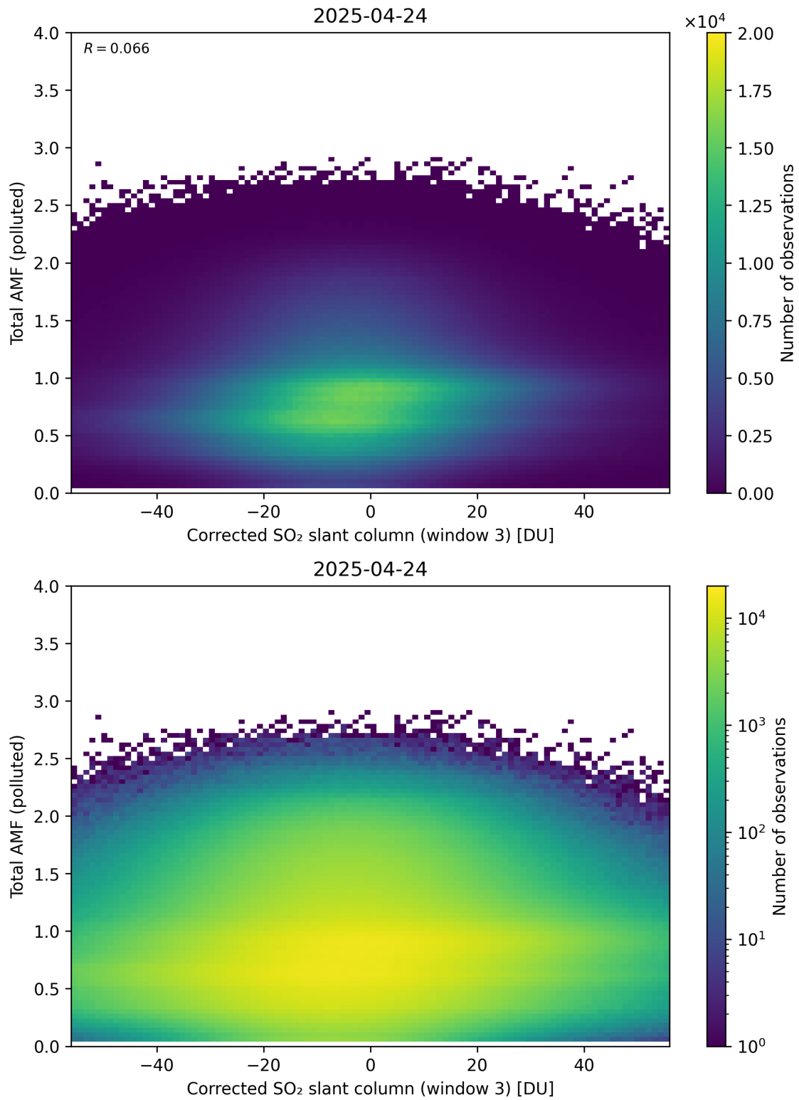
Figure 260: Scatter density plot of “Corrected SO 2 slant column (window 3)” against “Total AMF (polluted)” for 2025-04-24 to 2025-04-25.
