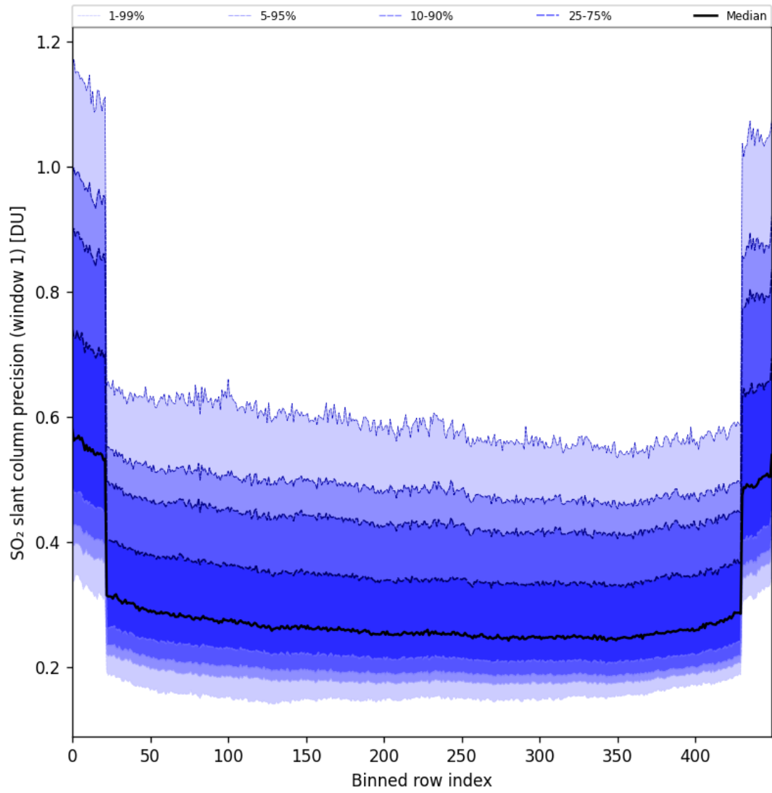
Figure 90: Along track statistics of “SO 2 slant column precision (window 1)” for 2025-04-24 to 2025-04-25
