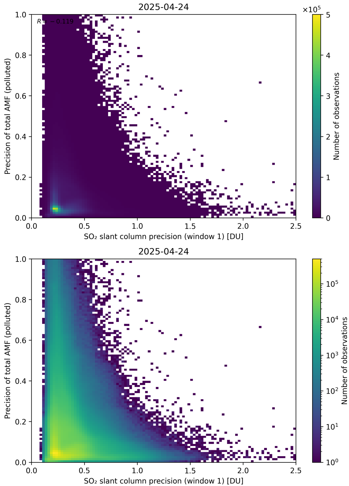
Figure 281: Scatter density plot of “SO 2 slant column precision (window 1)” against “Precision of total AMF (polluted)” for 2025-04-24 to 2025-04-25.
