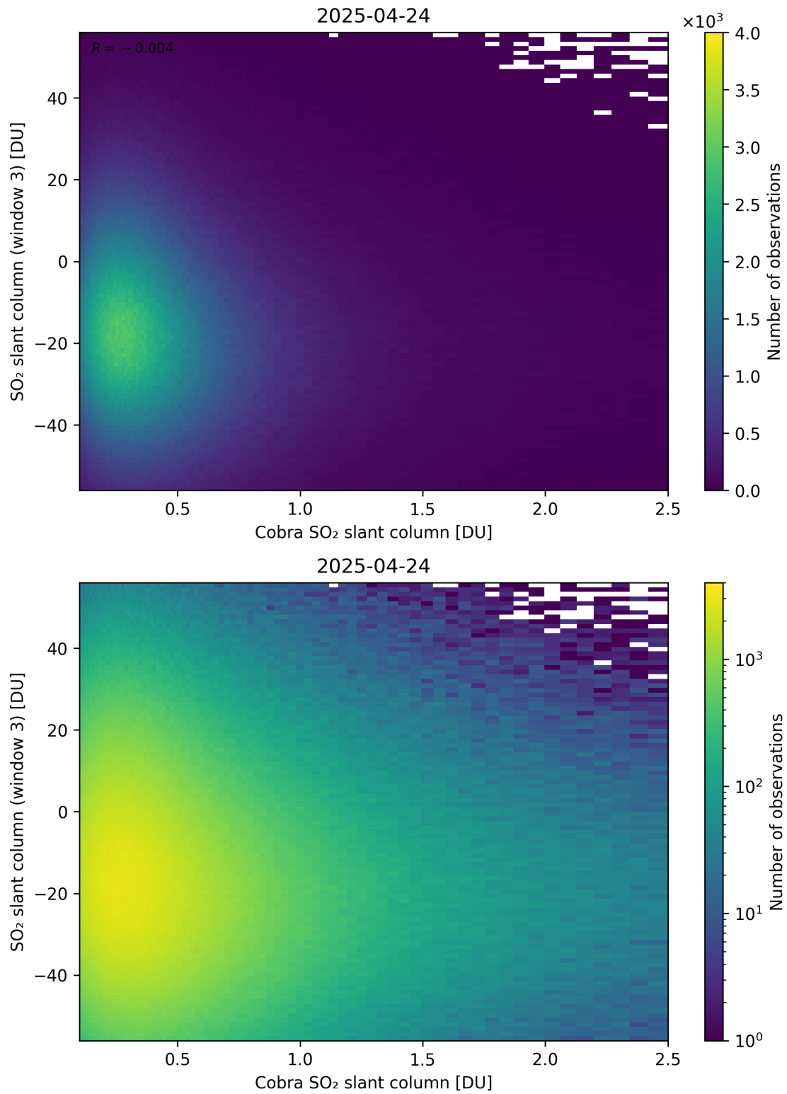
Figure 222: Scatter density plot of “Cobra SO 2 slant column” against “SO 2 slant column (window 3)” for 2025-04-24 to 2025-04-25.
