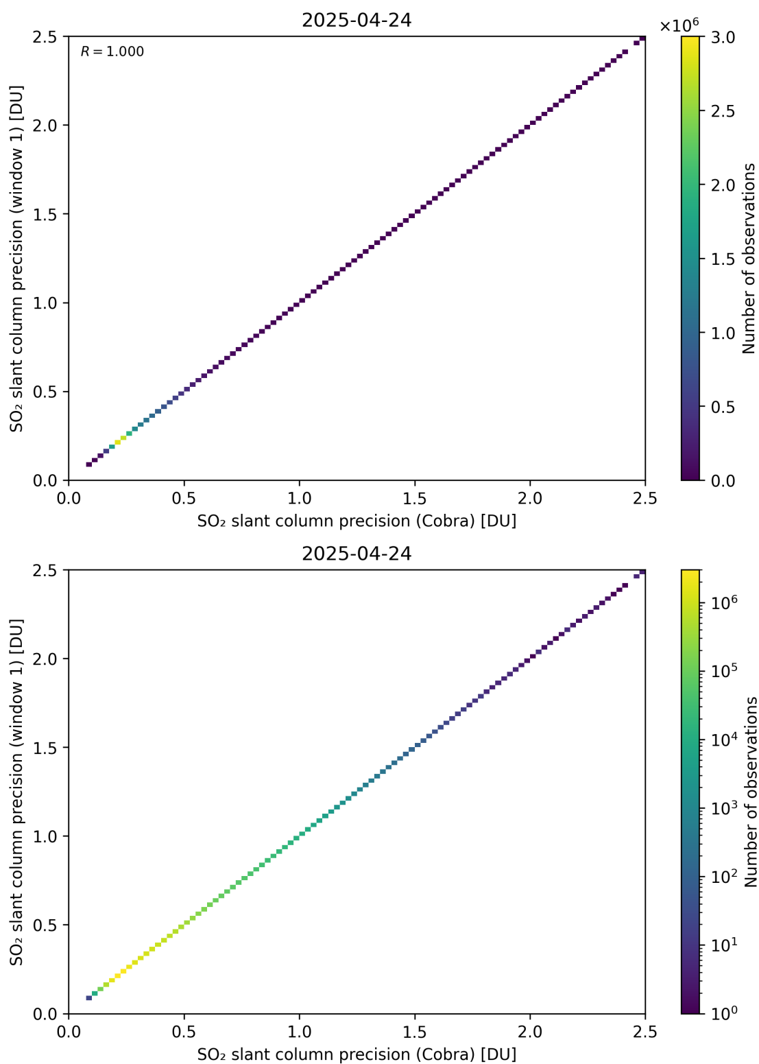
Figure 209: Scatter density plot of “SO 2 slant column precision (Cobra)” against “SO 2 slant column precision (window 1)” for 2025-04-24 to 2025-04-25.
