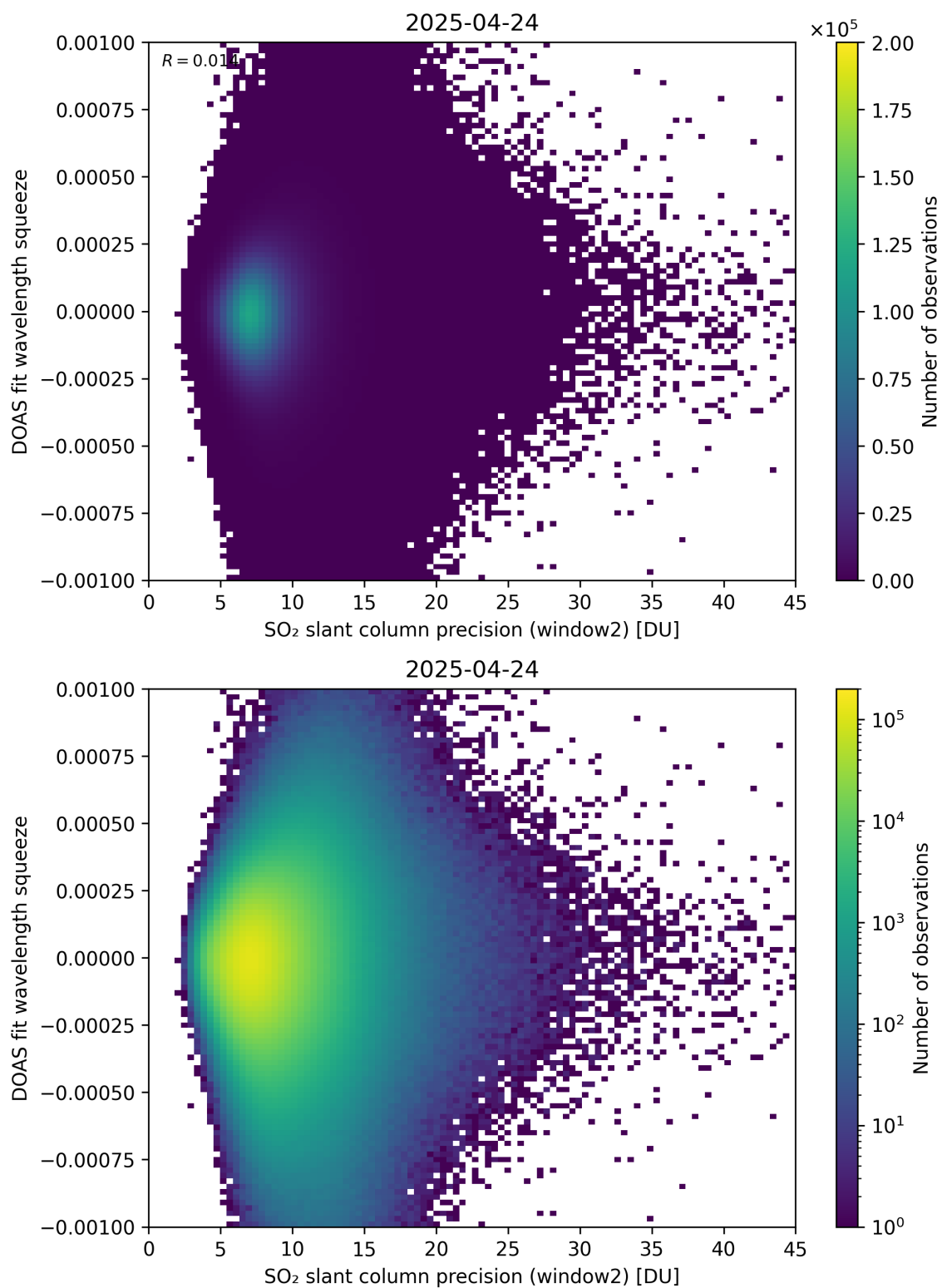
Figure 294: Scatter density plot of “SO 2 slant column precision (window2)” against “DOAS fit wavelength squeeze” for 2025-04-24 to 2025-04-25.
