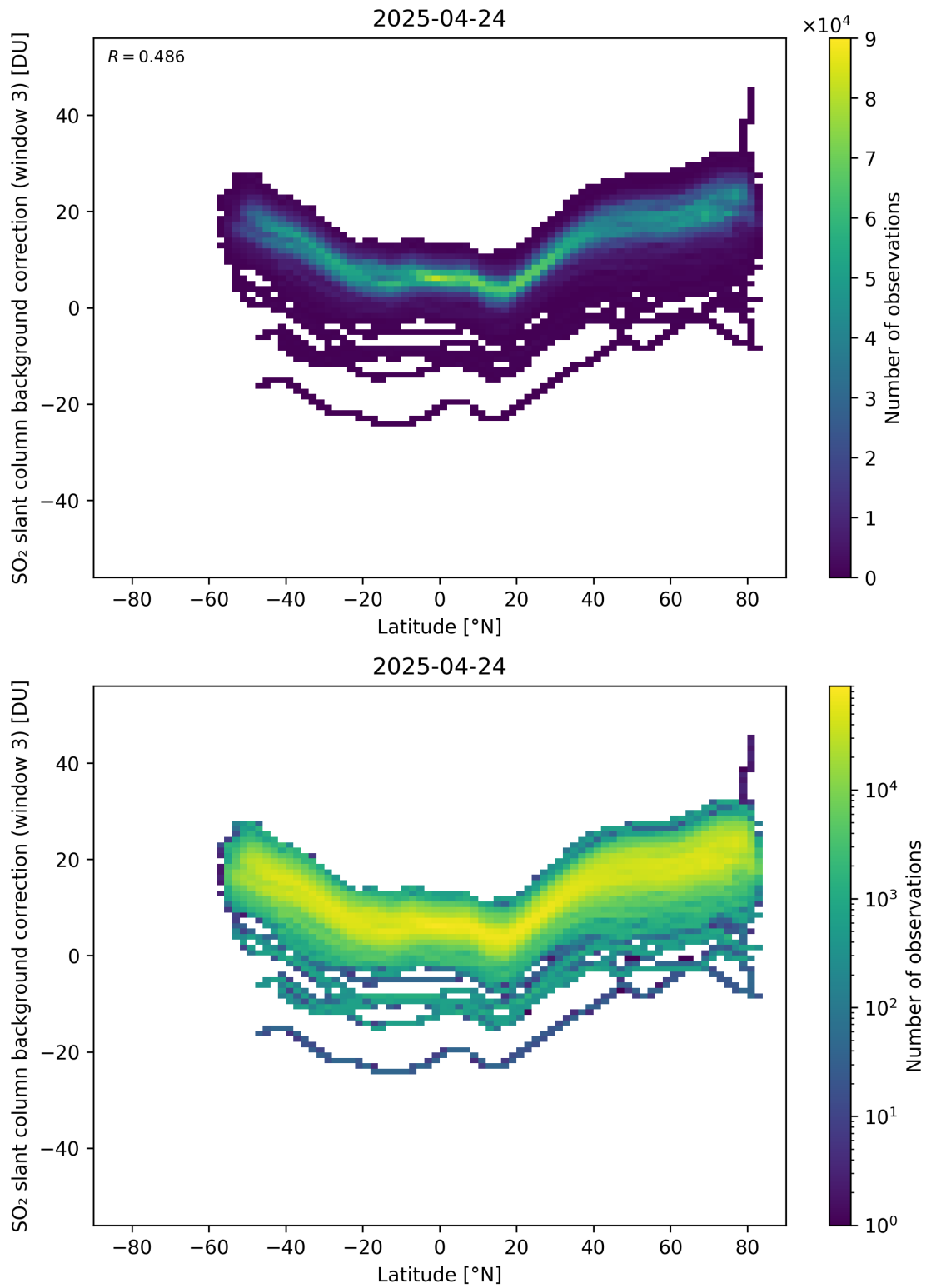
Figure 152: Scatter density plot of “Latitude” against “SO 2 slant column background correction (window 3)” for 2025-04-24 to 2025-04-25.
