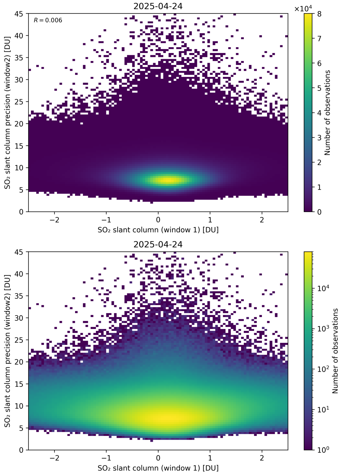
Figure 286: Scatter density plot of “SO 2 slant column (window 1)” against “SO 2 slant column precision (window2)” for 2025-04-24 to 2025-04-25.
