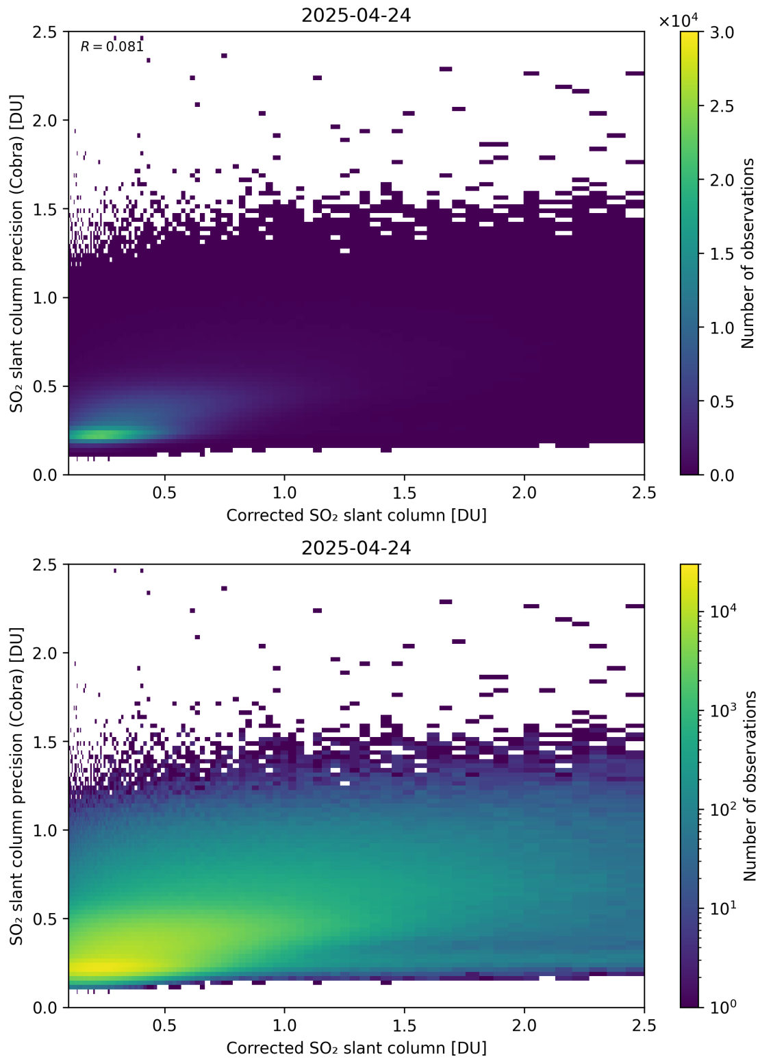
Figure 234: Scatter density plot of “Corrected SO 2 slant column” against “SO 2 slant column precision (Cobra)” for 2025-04-24 to 2025-04-25.
