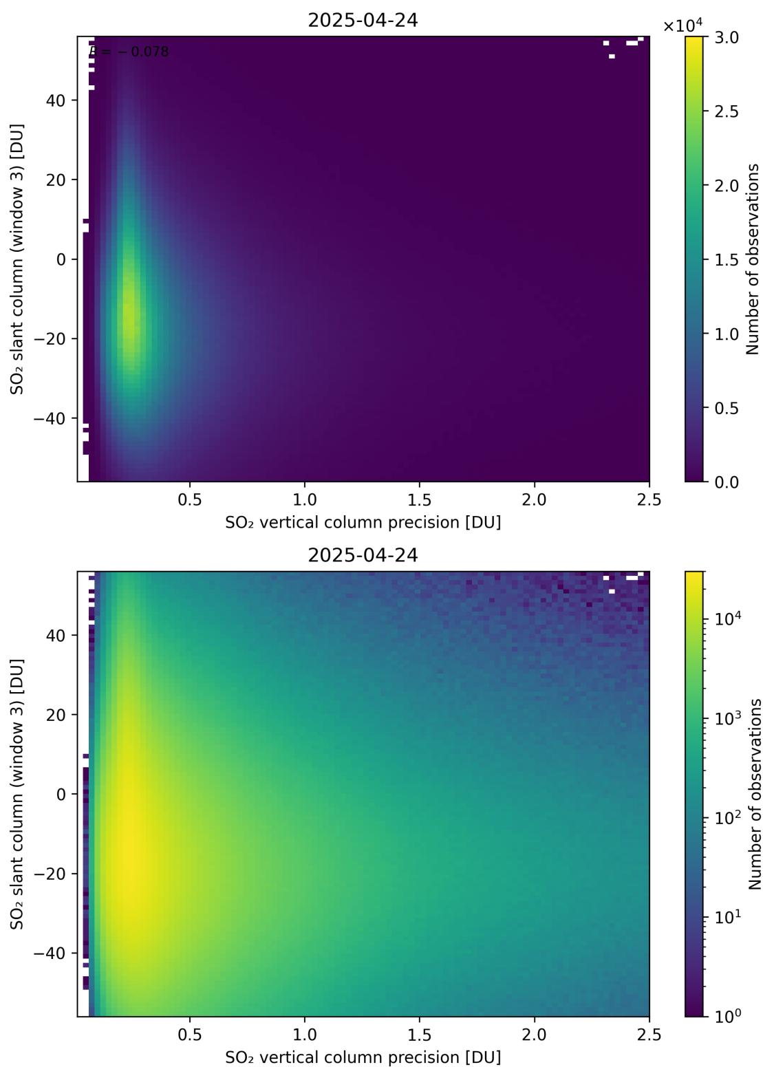
Figure 344: Scatter density plot of “SO 2 vertical column precision” against “SO 2 slant column (window 3)” for 2025-04-24 to 2025-04-25.
