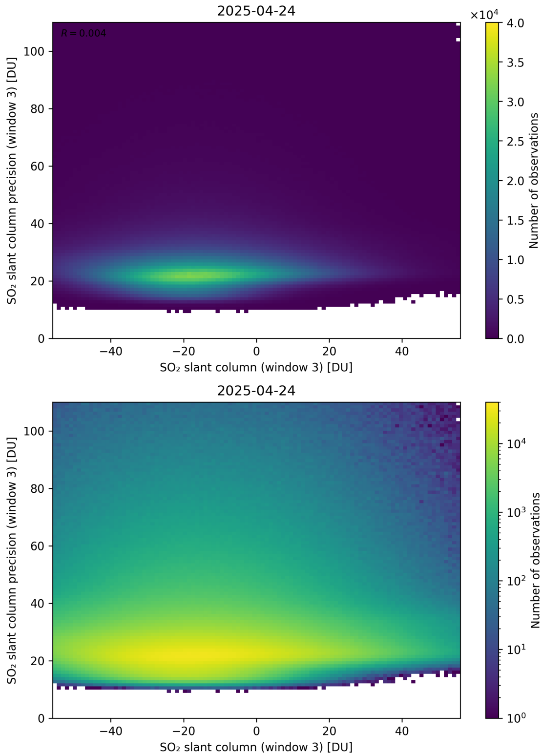
Figure 317: Scatter density plot of “SO 2 slant column (window 3)” against “SO 2 slant column precision (window 3)” for 2025-04-24 to 2025-04-25.
