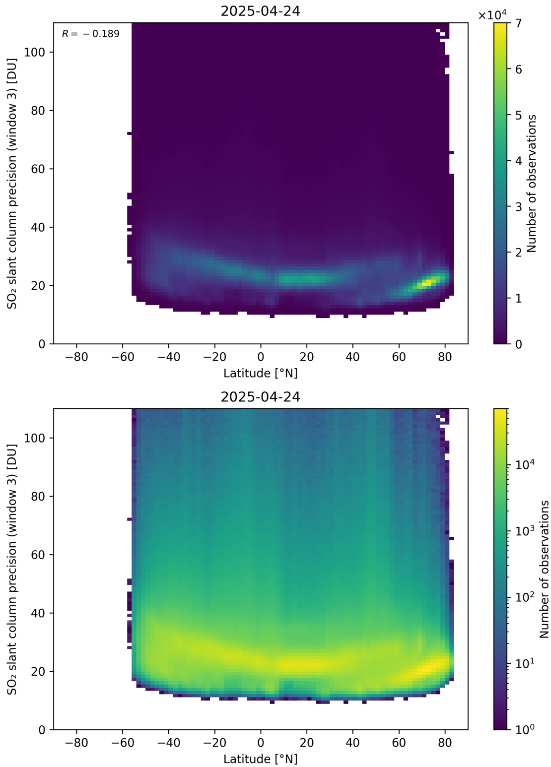
Figure 166: Scatter density plot of “Latitude” against “SO 2 slant column precision (window 3)” for 2025-04-24 to 2025-04-25.
