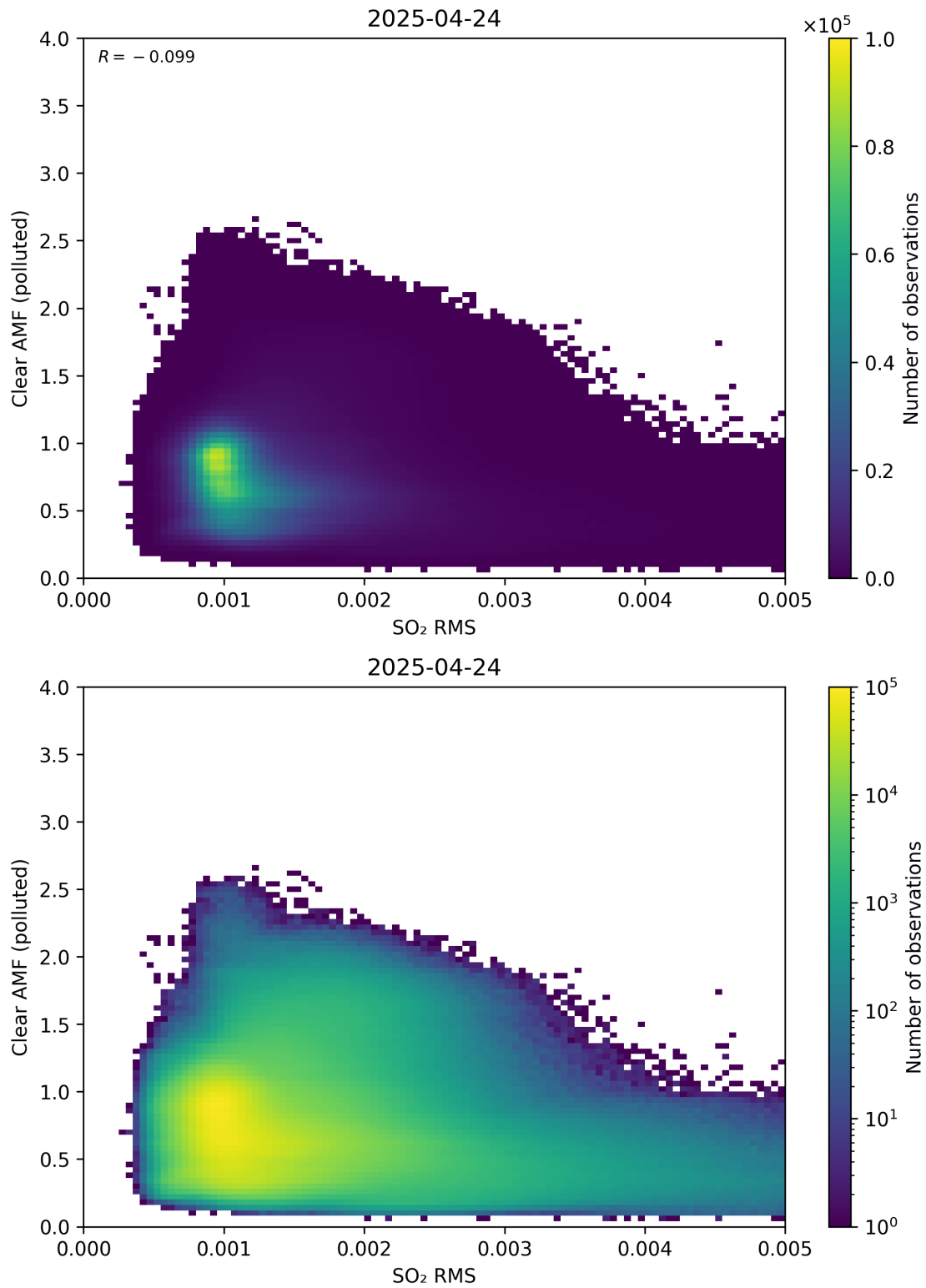
Figure 147: Scatter density plot of “SO 2 RMS” against “Clear AMF (polluted)” for 2025-04-24 to 2025-04-25.
