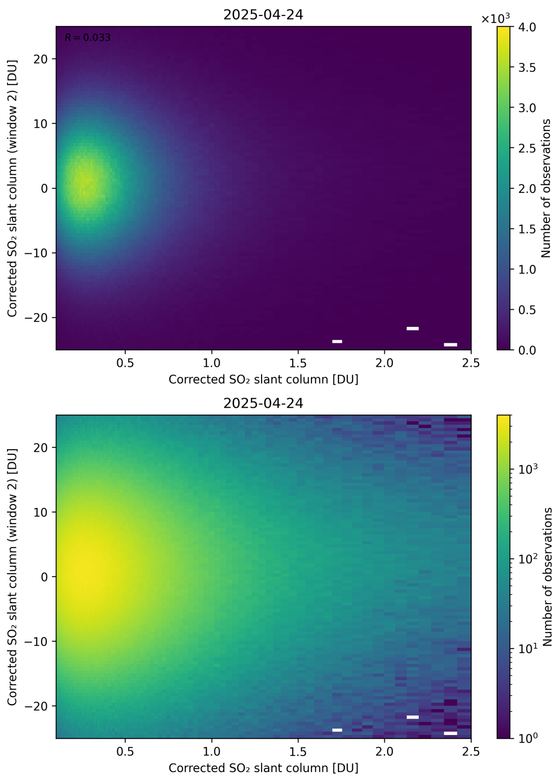
Figure 235: Scatter density plot of “Corrected SO 2 slant column” against “Corrected SO 2 slant column (window 2)” for 2025-04-24 to 2025-04-25.
