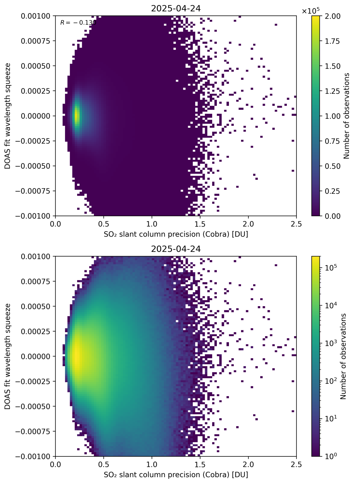
Figure 203: Scatter density plot of “SO 2 slant column precision (Cobra)” against “DOAS fit wavelength squeeze” for 2025-04-24 to 2025-04-25.
