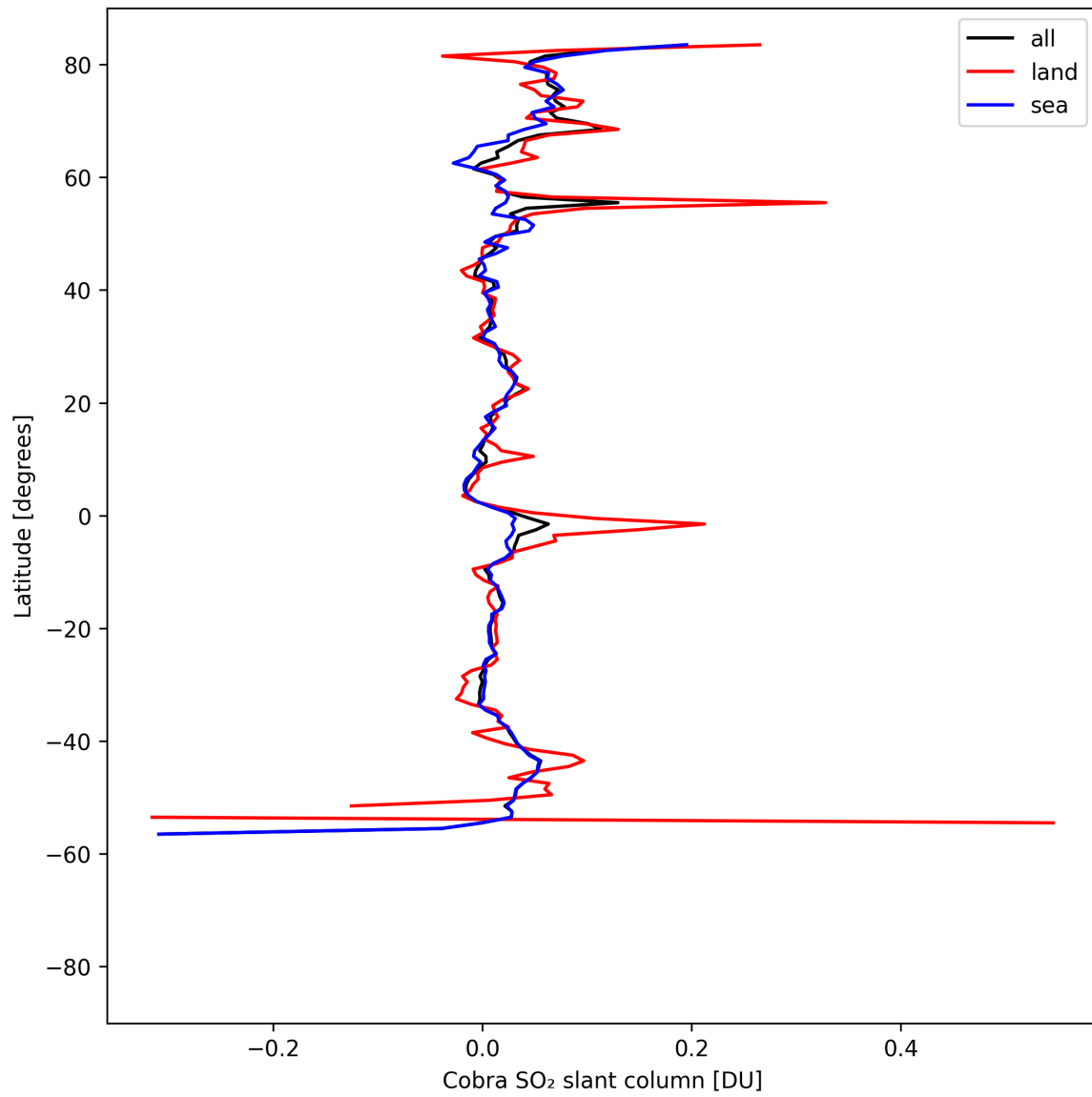
Figure 35: Zonal average of “Cobra SO 2 slant column” for 2025-04-24 to 2025-04-25.
