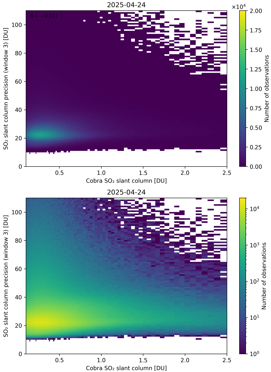
Figure 223: Scatter density plot of “Cobra SO 2 slant column” against “SO 2 slant column precision (window 3)” for 2025-04-24 to 2025-04-25.
