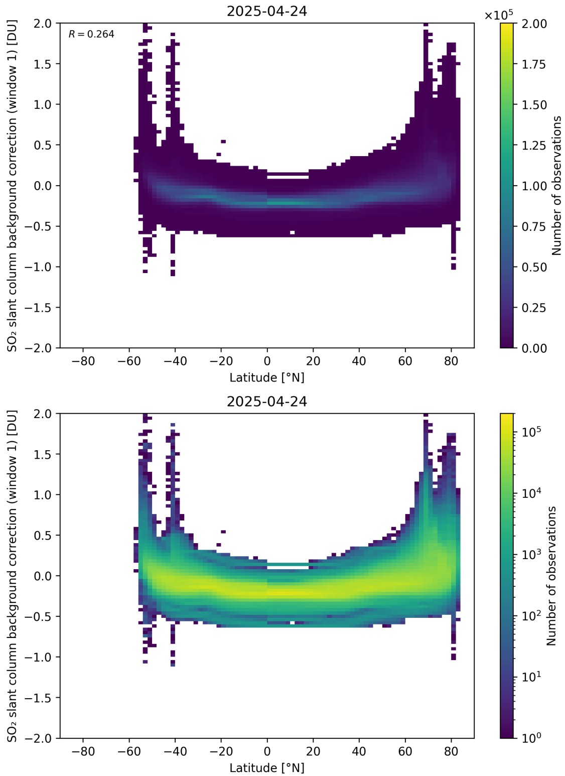
Figure 150: Scatter density plot of “Latitude” against “SO 2 slant column background correction (window 1)” for 2025-04-24 to 2025-04-25.
