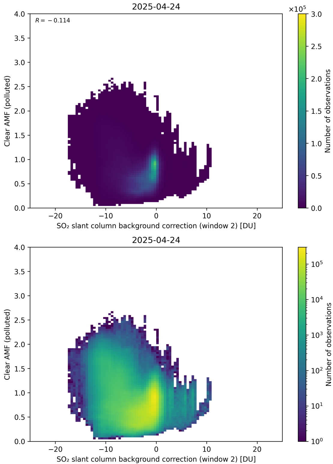
Figure 126: Scatter density plot of “SO 2 slant column background correction (window 2)” against “Clear AMF (polluted)” for 2025-04-24 to 2025-04-25.
