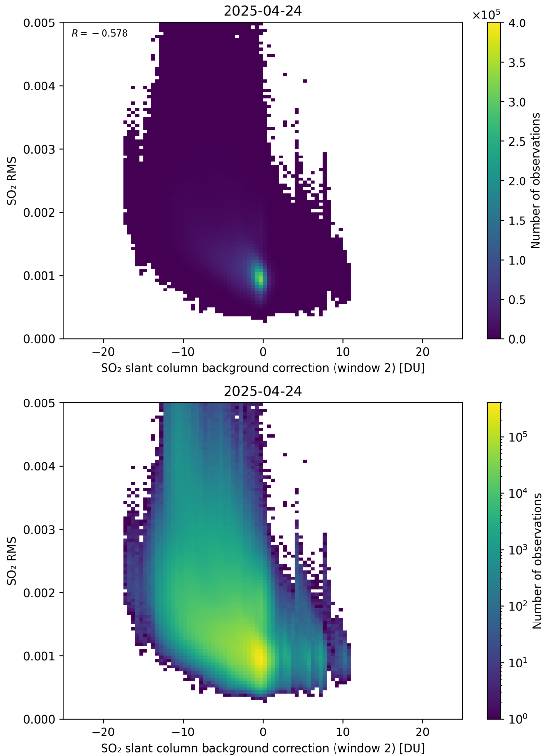
Figure 125: Scatter density plot of “SO 2 slant column background correction (window 2)” against “SO 2 RMS” for 2025-04-24 to 2025-04-25.
