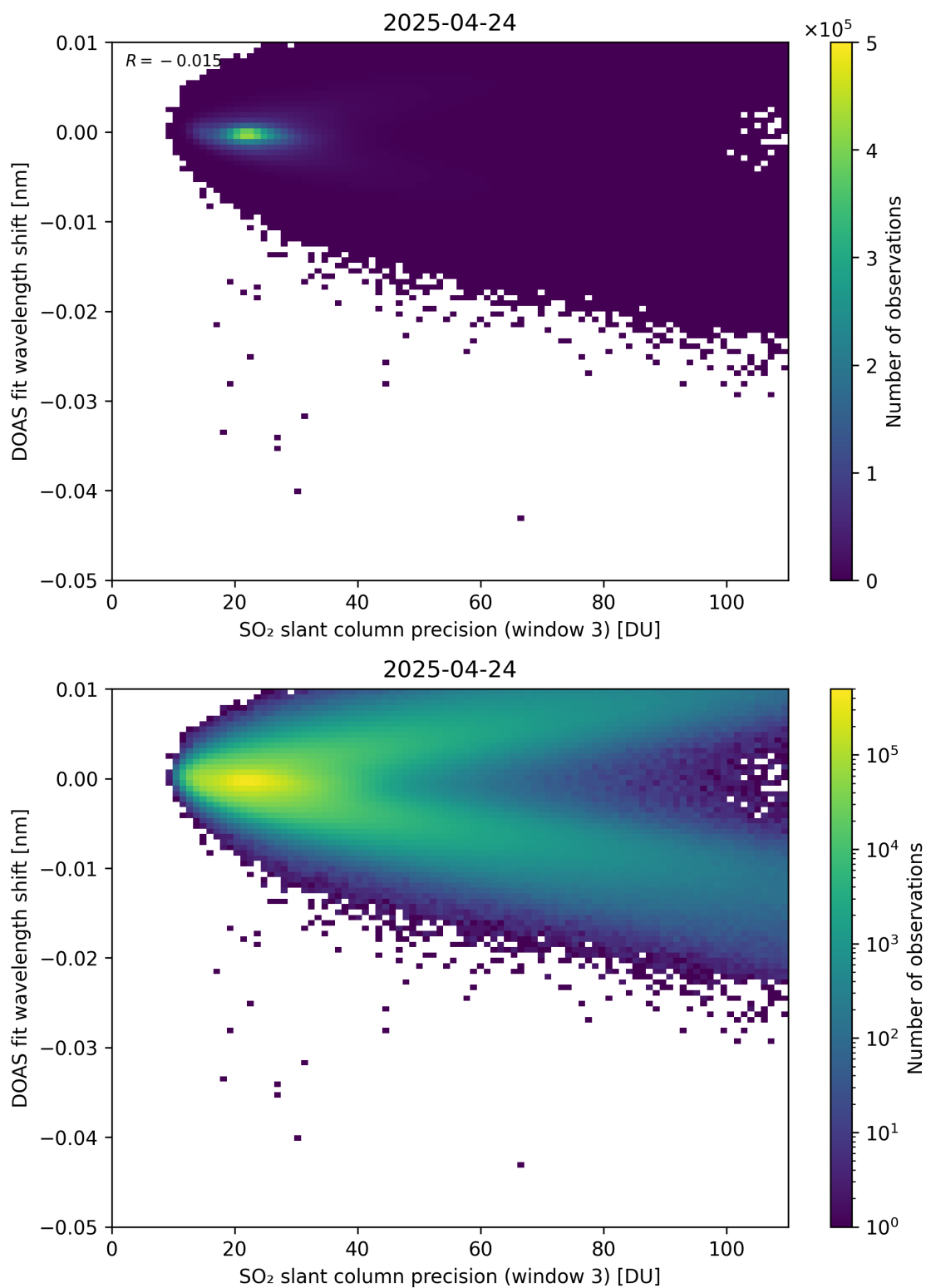
Figure 308: Scatter density plot of “SO 2 slant column precision (window 3)” against “DOAS fit wavelength shift” for 2025-04-24 to 2025-04-25.
