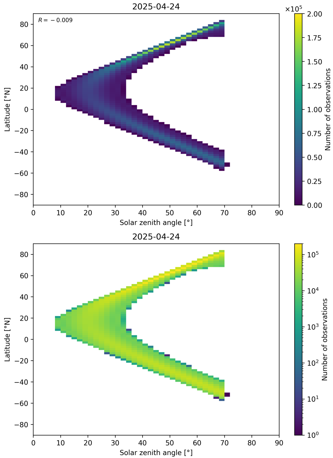
Figure 177: Scatter density plot of “Solar zenith angle” against “Latitude” for 2025-04-24 to 2025-04-25.
