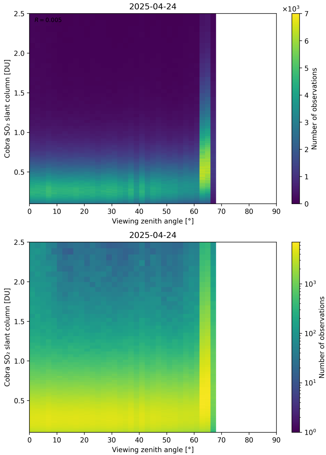
Figure 371: Scatter density plot of “Viewing zenith angle” against “Cobra SO 2 slant column” for 2025-04-24 to 2025-04-25.
