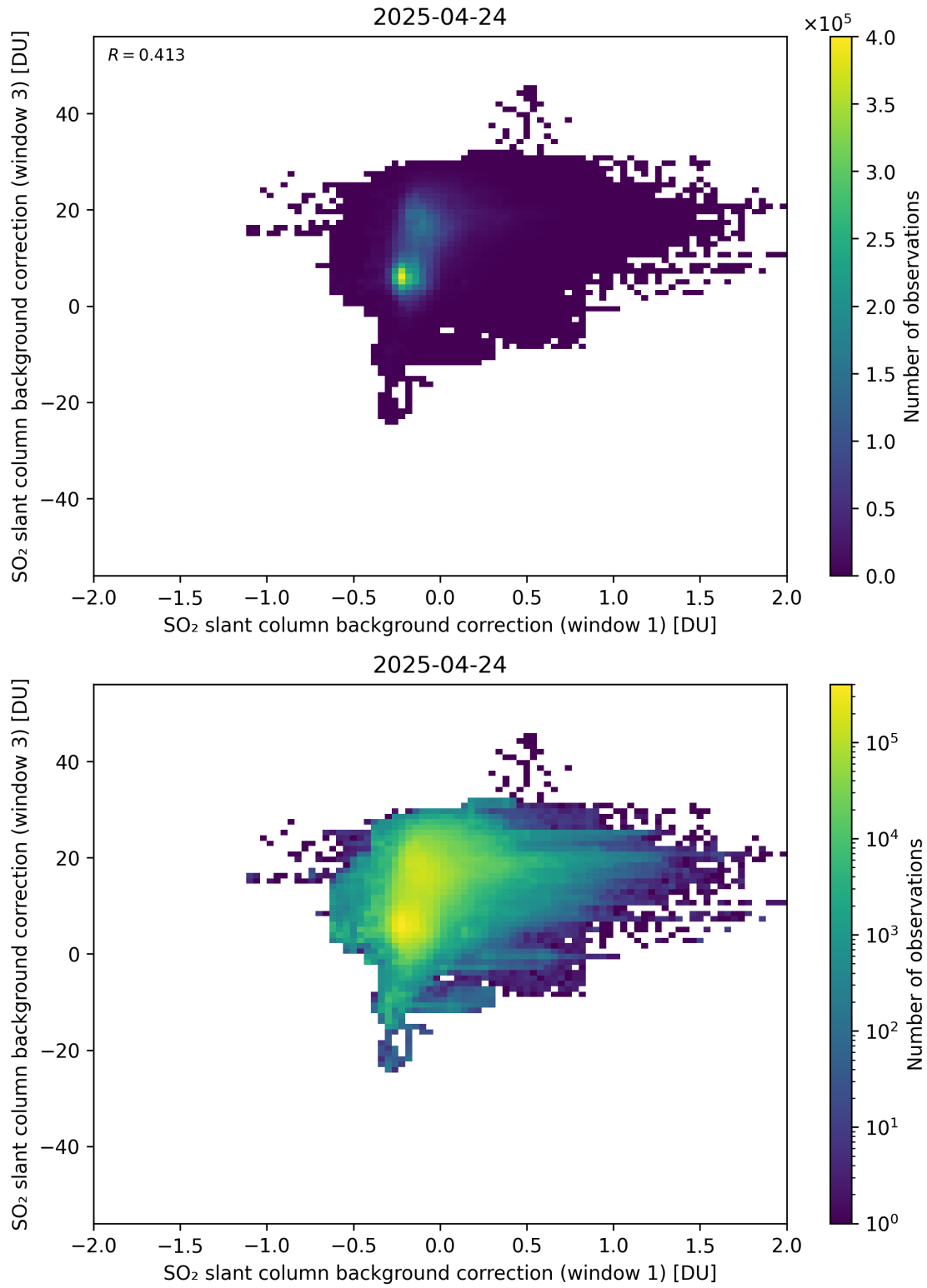
Figure 110: Scatter density plot of “SO 2 slant column background correction (window 1)” against “SO 2 slant column background correction (window 3)” for 2025-04-24 to 2025-04-25.
