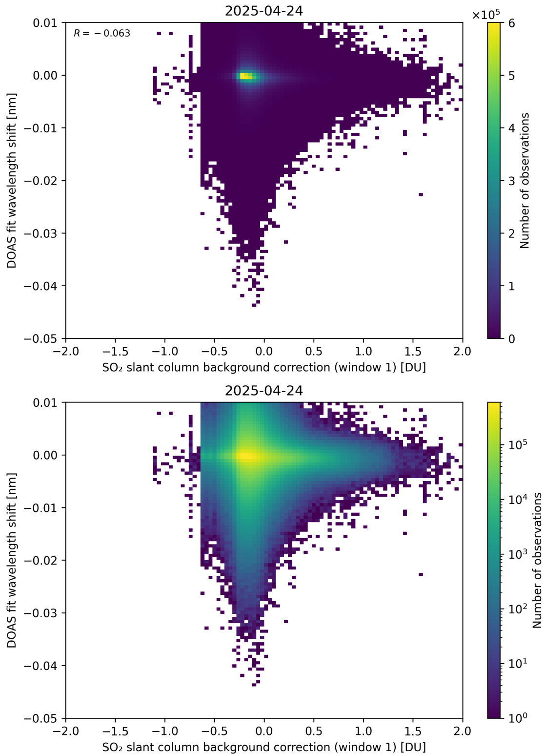
Figure 111: Scatter density plot of “SO 2 slant column background correction (window 1)” against “DOAS fit wavelength shift” for 2025-04-24 to 2025-04-25.
