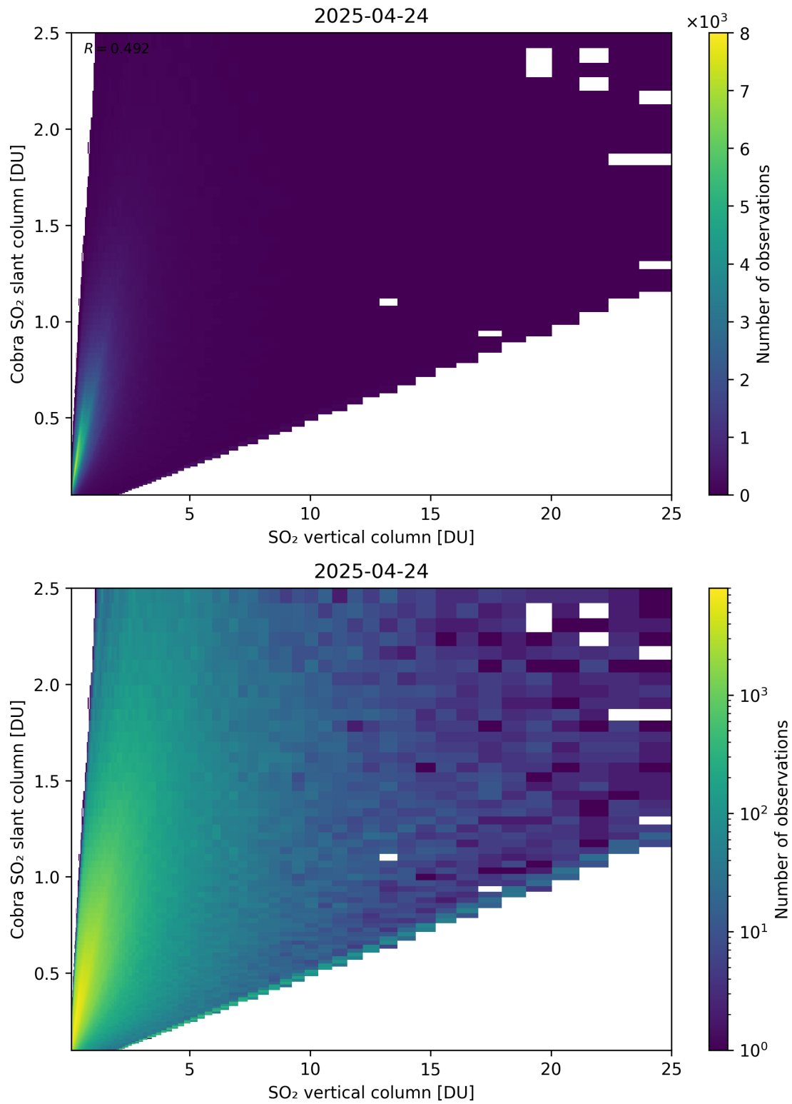
Figure 349: Scatter density plot of “SO 2 vertical column” against “Cobra SO 2 slant column” for 2025-04-24 to 2025-04-25.
