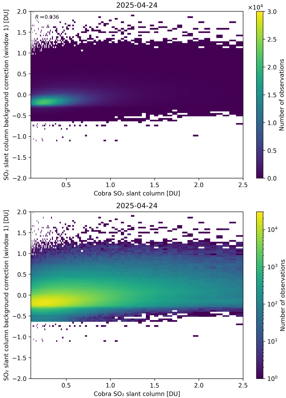
Figure 193: Scatter density plot of “Cobra SO 2 slant column” against “SO 2 slant column background correction (window 1)” for 2025-04-24 to 2025-04-25.
