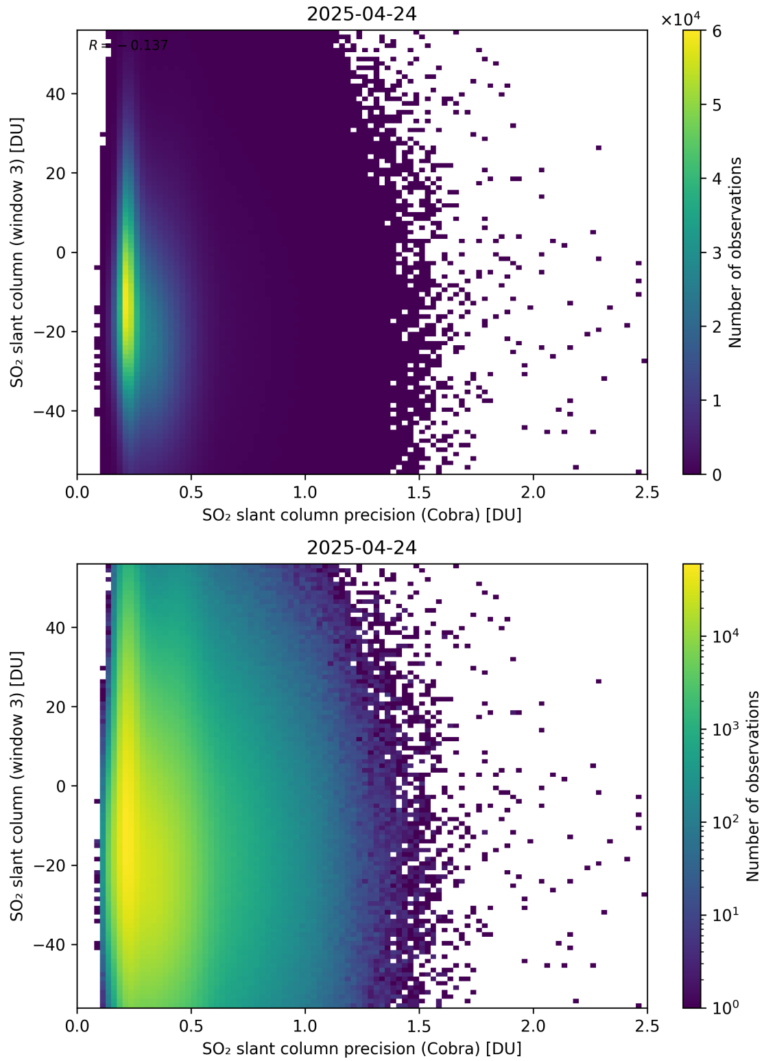
Figure 211: Scatter density plot of “SO 2 slant column precision (Cobra)” against “SO 2 slant column (window 3)” for 2025-04-24 to 2025-04-25.
