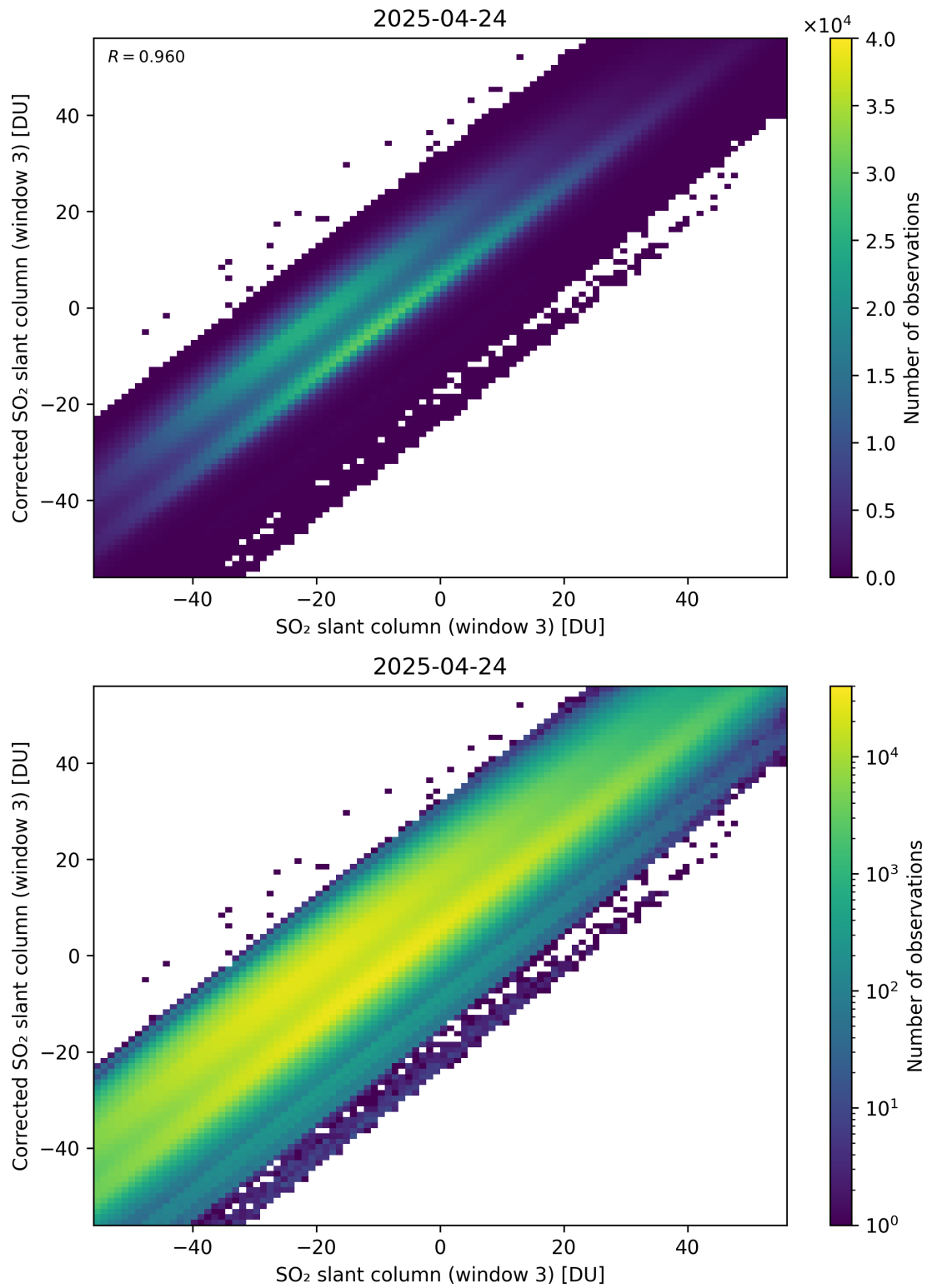
Figure 316: Scatter density plot of “SO 2 slant column (window 3)” against “Corrected SO 2 slant column (window 3)” for 2025-04-24 to 2025-04-25.
