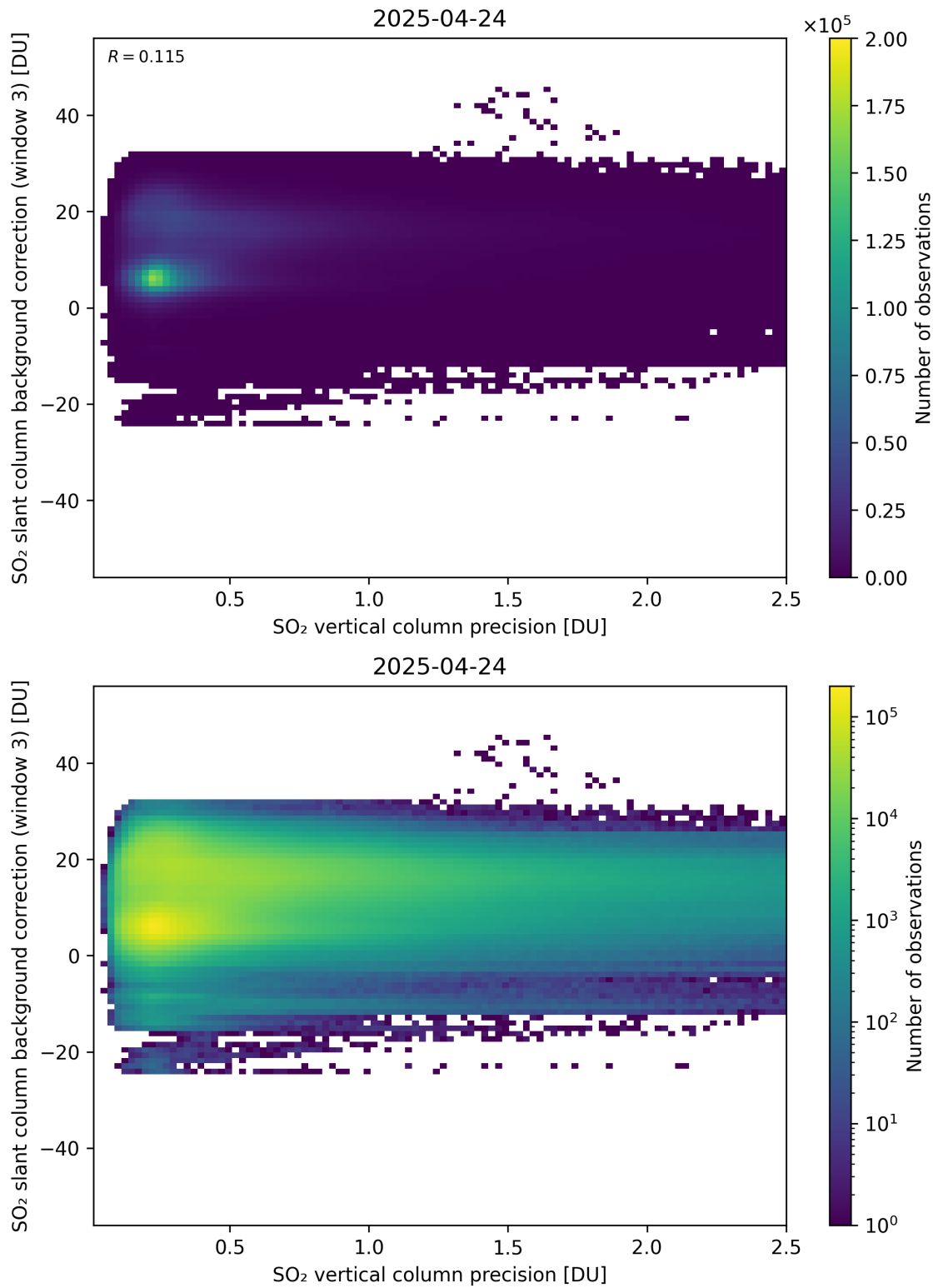
Figure 331: Scatter density plot of “SO 2 vertical column precision” against “SO 2 slant column background correction (window 3)” for 2025-04-24 to 2025-04-25.
