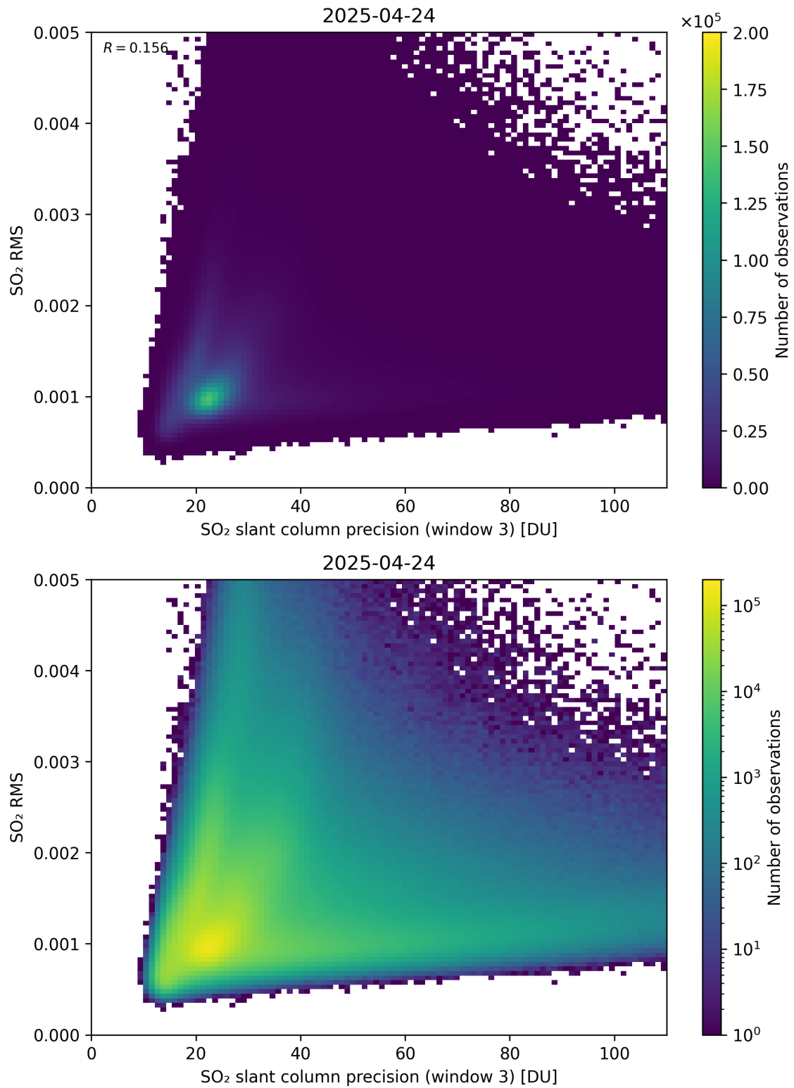
Figure 310: Scatter density plot of “SO 2 slant column precision (window 3)” against “SO 2 RMS” for 2025-04-24 to 2025-04-25.
