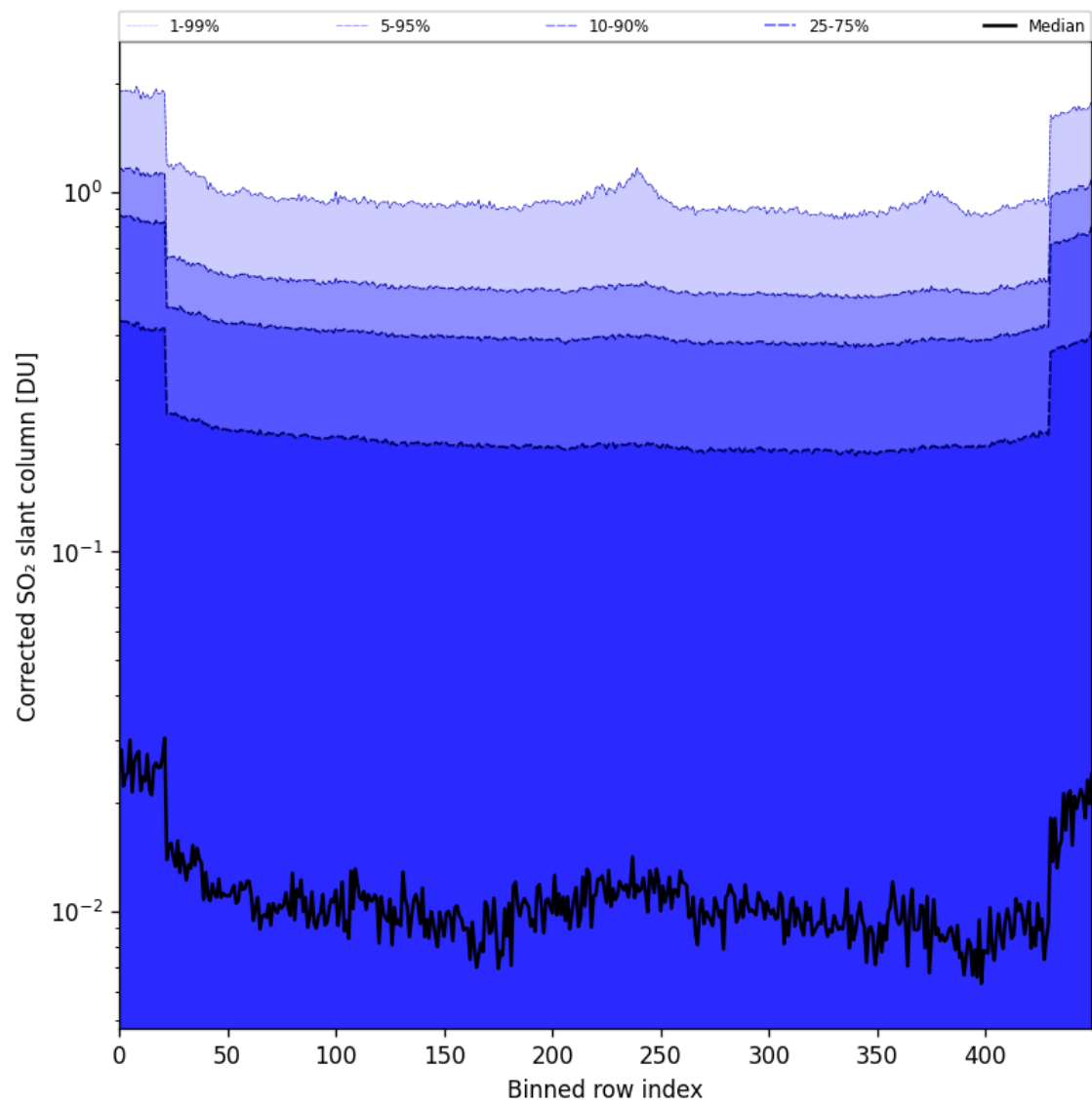
Figure 86: Along track statistics of “Corrected SO 2 slant column” for 2025-04-24 to 2025-04-25
