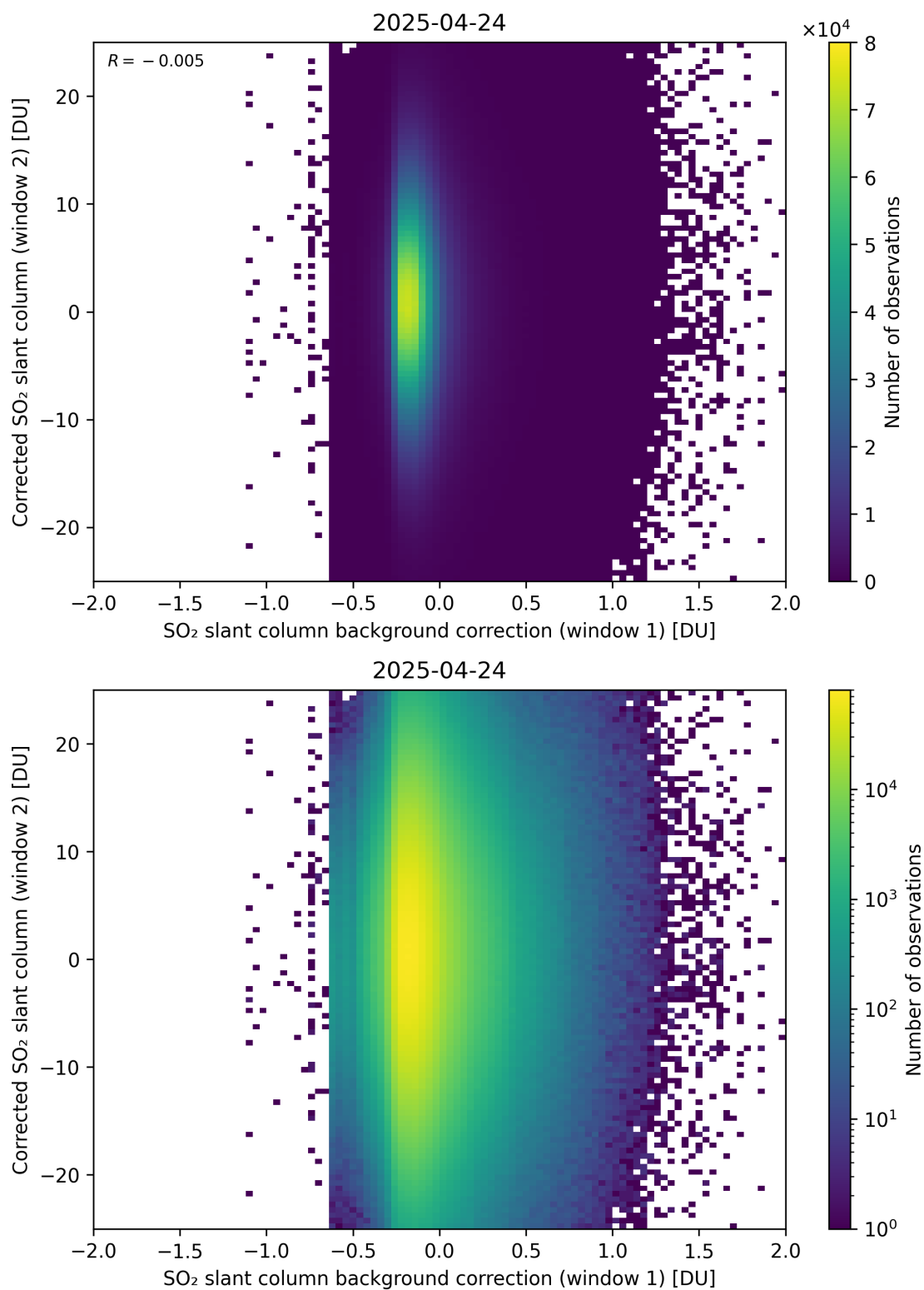
Figure 115: Scatter density plot of “SO 2 slant column background correction (window 1)” against “Corrected SO 2 slant column (window 2)” for 2025-04-24 to 2025-04-25.
