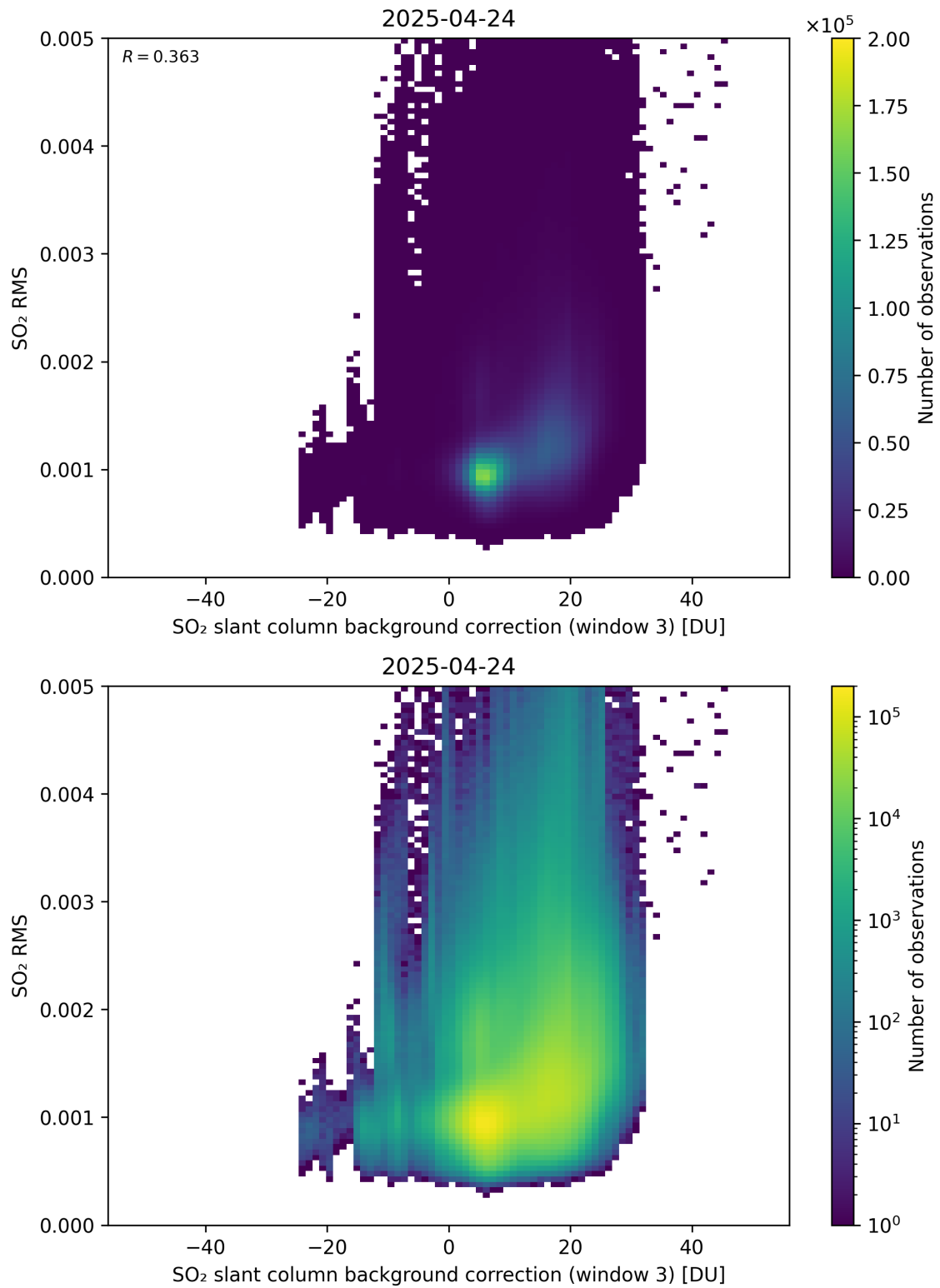
Figure 134: Scatter density plot of “SO 2 slant column background correction (window 3)” against “SO 2 RMS” for 2025-04-24 to 2025-04-25.
