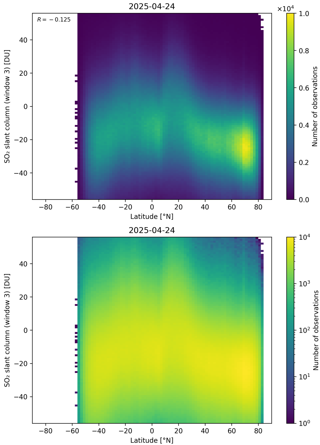
Figure 165: Scatter density plot of “Latitude” against “SO 2 slant column (window 3)” for 2025-04-24 to 2025-04-25.
