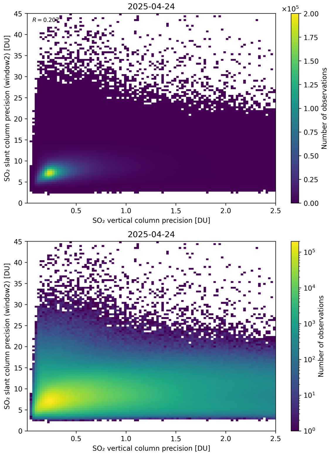
Figure 343: Scatter density plot of “SO 2 vertical column precision” against “SO 2 slant column precision (window2)” for 2025-04-24 to 2025-04-25.
