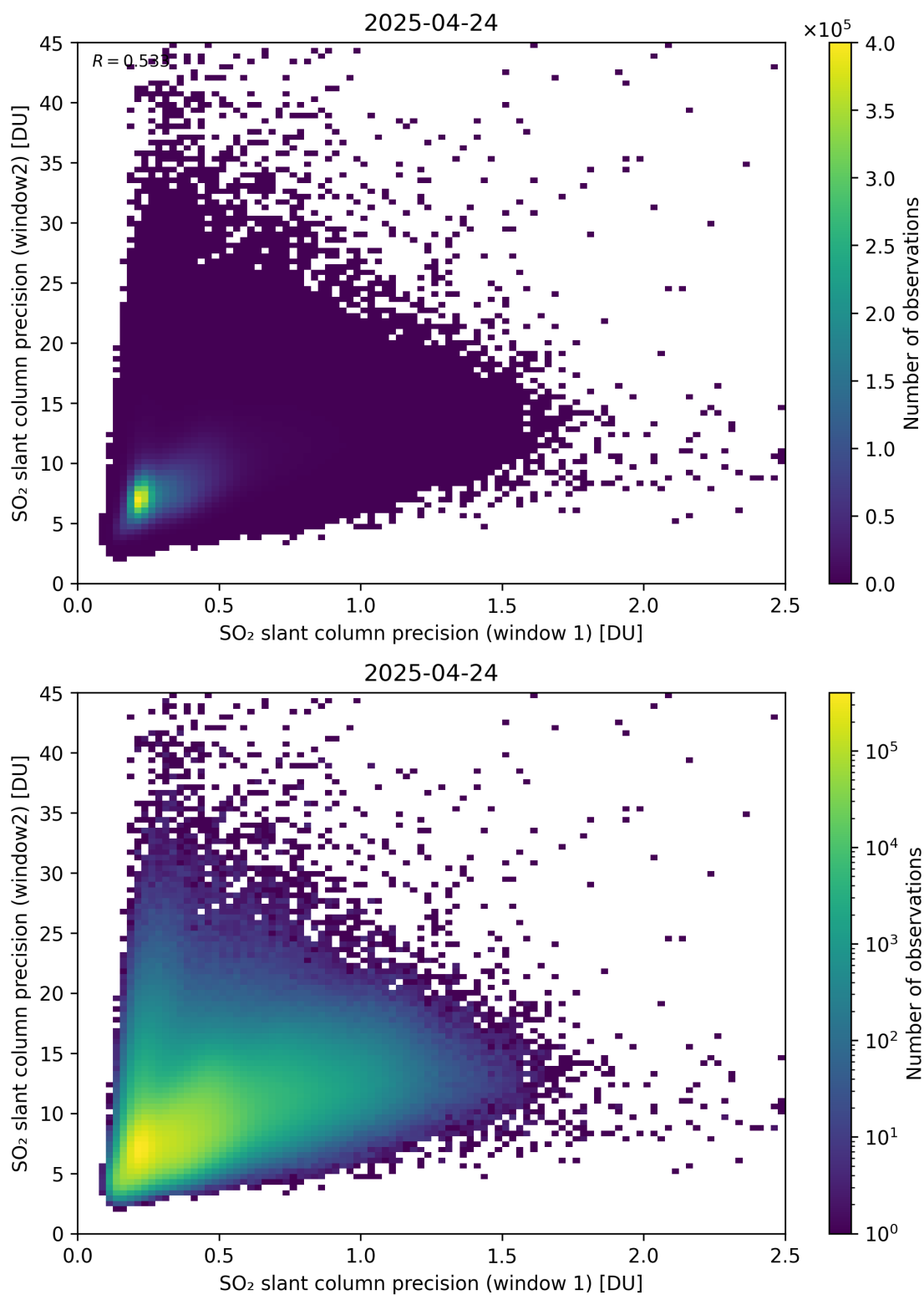
Figure 277: Scatter density plot of “SO 2 slant column precision (window 1)” against “SO 2 slant column precision (window2)” for 2025-04-24 to 2025-04-25.
