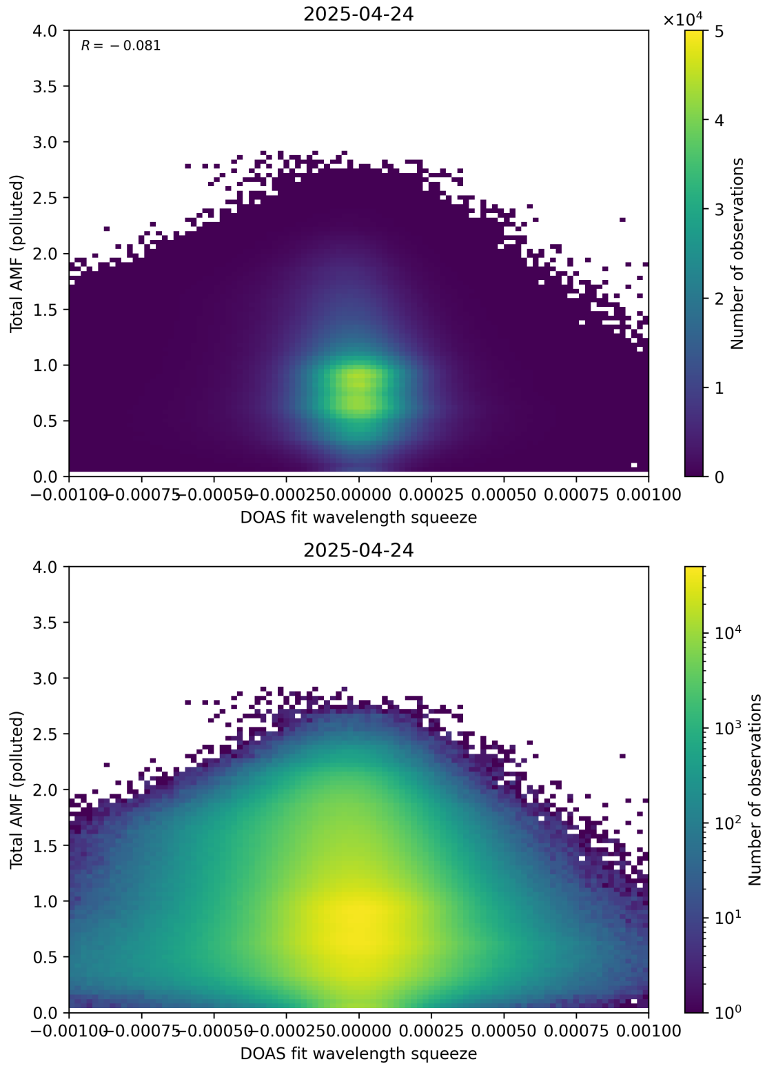
Figure 145: Scatter density plot of “DOAS fit wavelength squeeze” against “Total AMF (polluted)” for 2025-04-24 to 2025-04-25.
