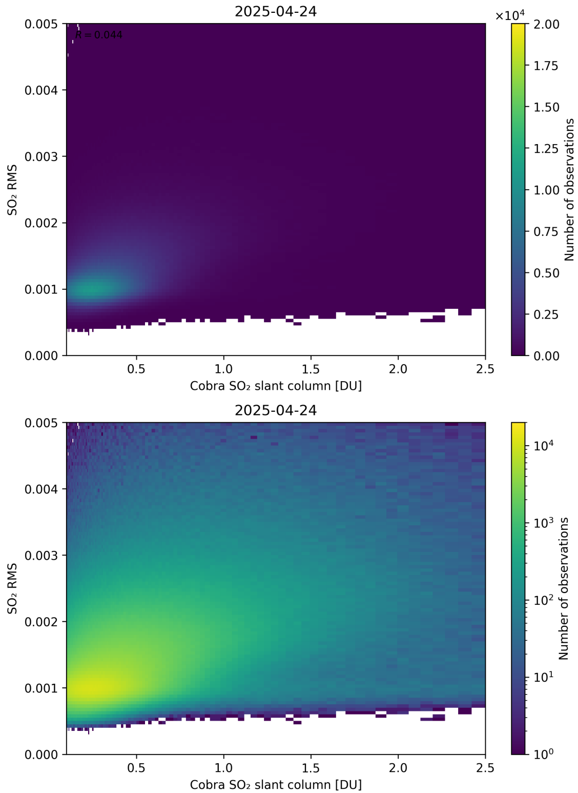
Figure 198: Scatter density plot of “Cobra SO 2 slant column” against “SO 2 RMS” for 2025-04-24 to 2025-04-25.
