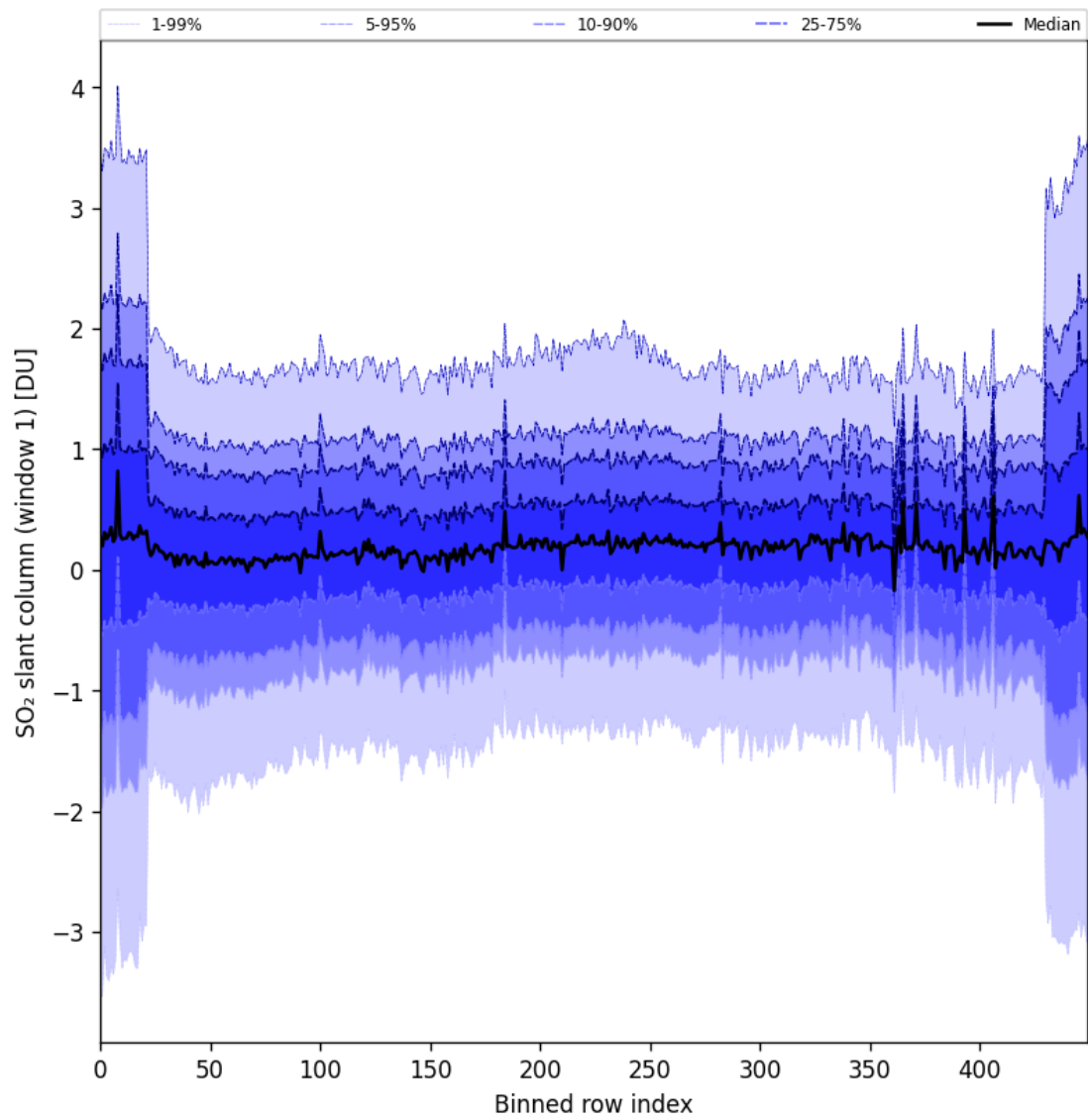
Figure 89: Along track statistics of “SO 2 slant column (window 1)” for 2025-04-24 to 2025-04-25
