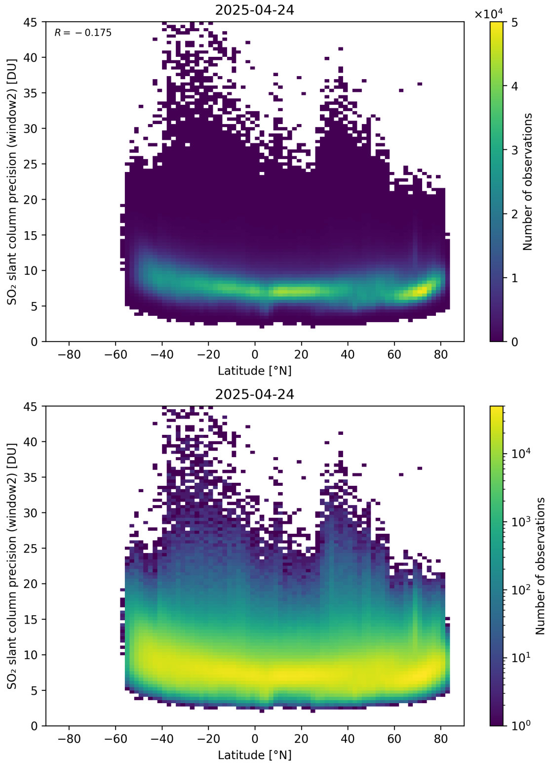
Figure 164: Scatter density plot of “Latitude” against “SO 2 slant column precision (window2)” for 2025-04-24 to 2025-04-25.
