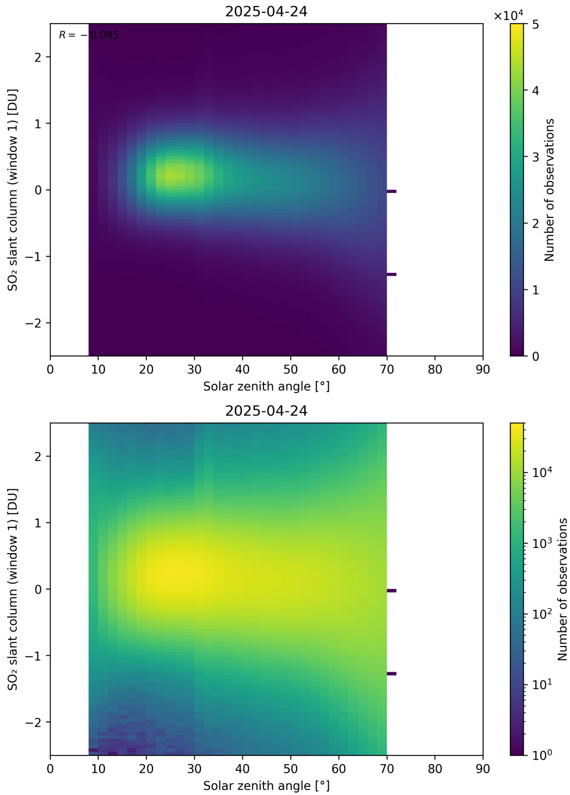
Figure 184: Scatter density plot of “Solar zenith angle” against “SO 2 slant column (window 1)” for 2025-04-24 to 2025-04-25.
