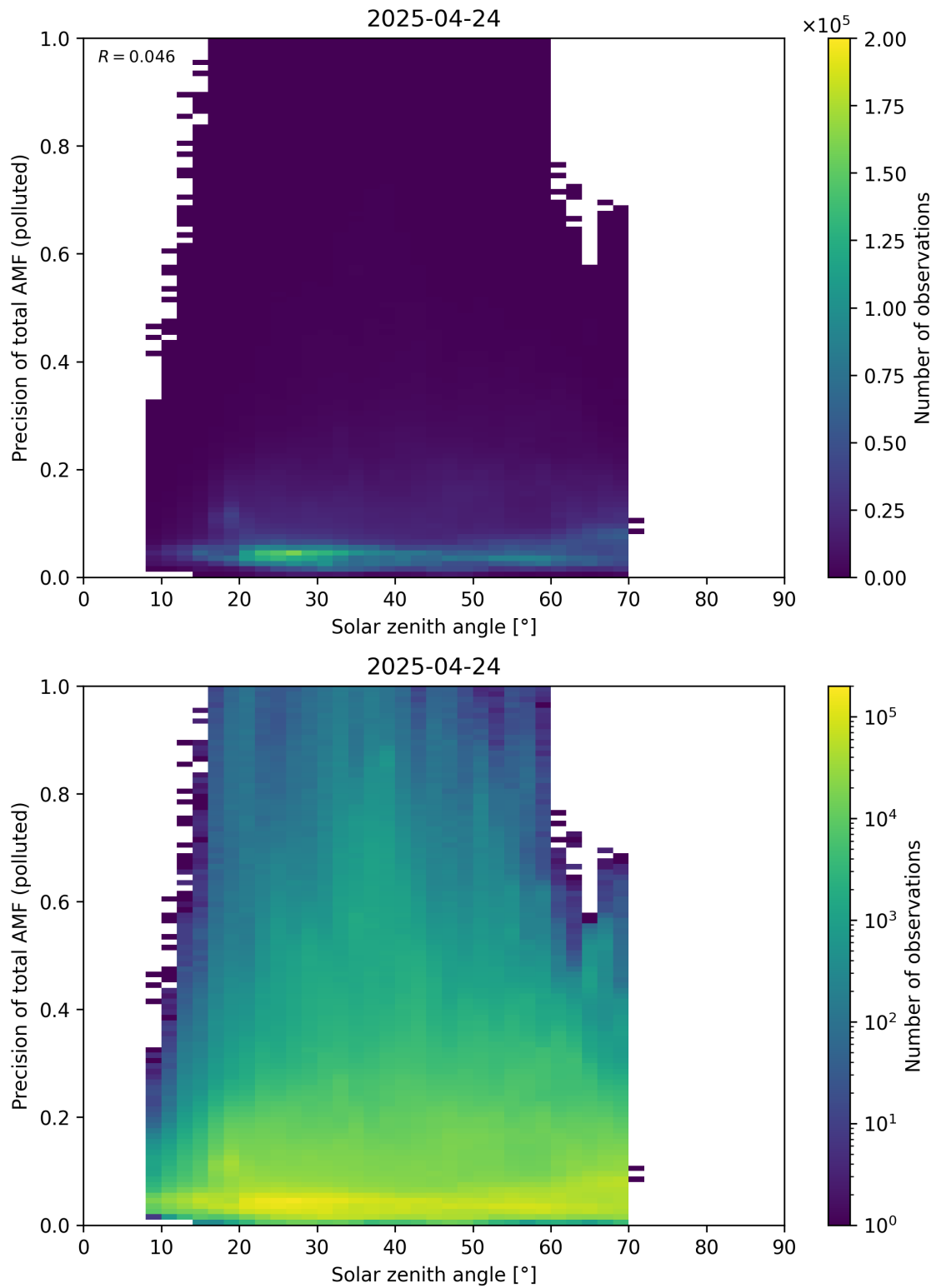
Figure 190: Scatter density plot of “Solar zenith angle” against “Precision of total AMF (polluted)” for 2025-04-24 to 2025-04-25.
