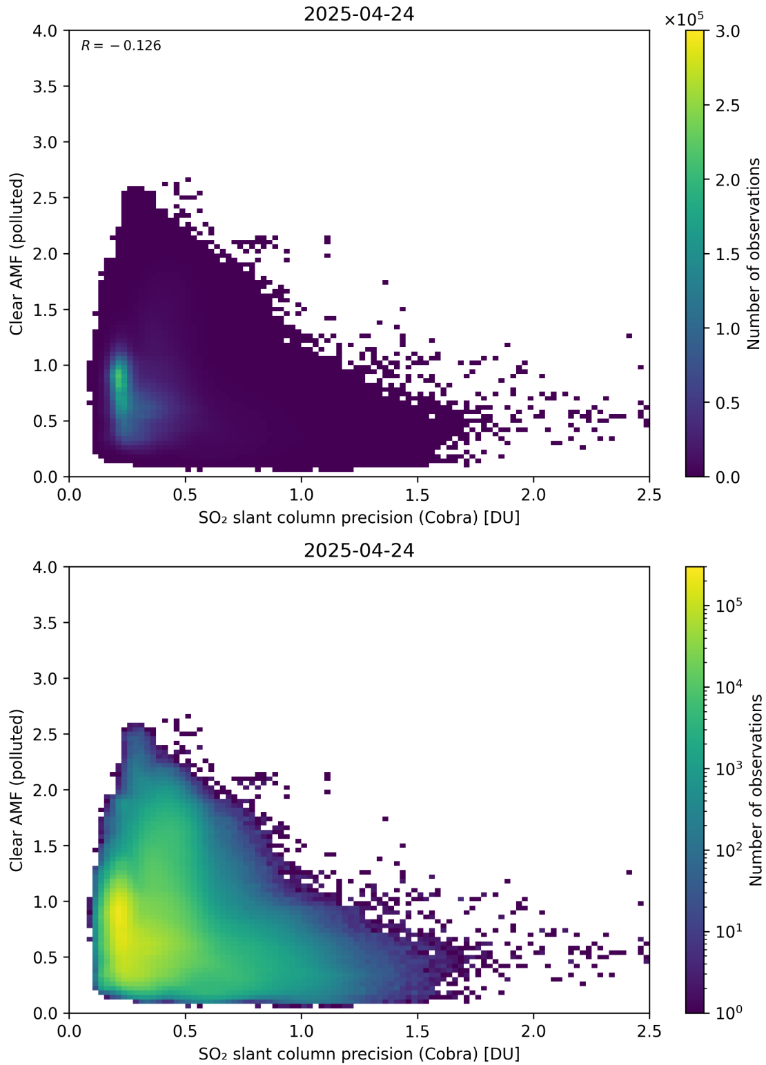
Figure 205: Scatter density plot of “SO 2 slant column precision (Cobra)” against “Clear AMF (polluted)” for 2025-04-24 to 2025-04-25.
