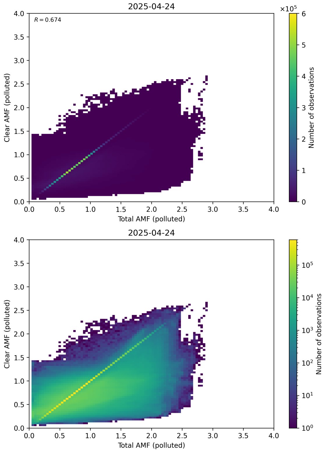
Figure 321: Scatter density plot of “Total AMF (polluted)” against “Clear AMF (polluted)” for 2025-04-24 to 2025-04-25.
