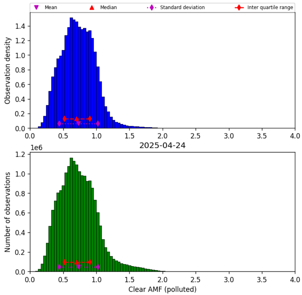
Figure 81: Histogram of "Clear AMF (polluted)" for 2025-04-24 to 2025-04-25
