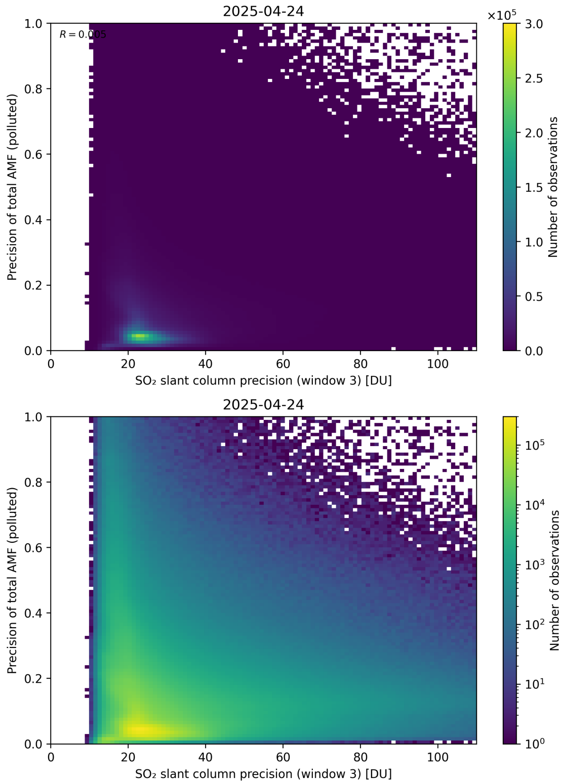
Figure 314: Scatter density plot of “SO 2 slant column precision (window 3)” against “Precision of total AMF (polluted)” for 2025-04-24 to 2025-04-25.
