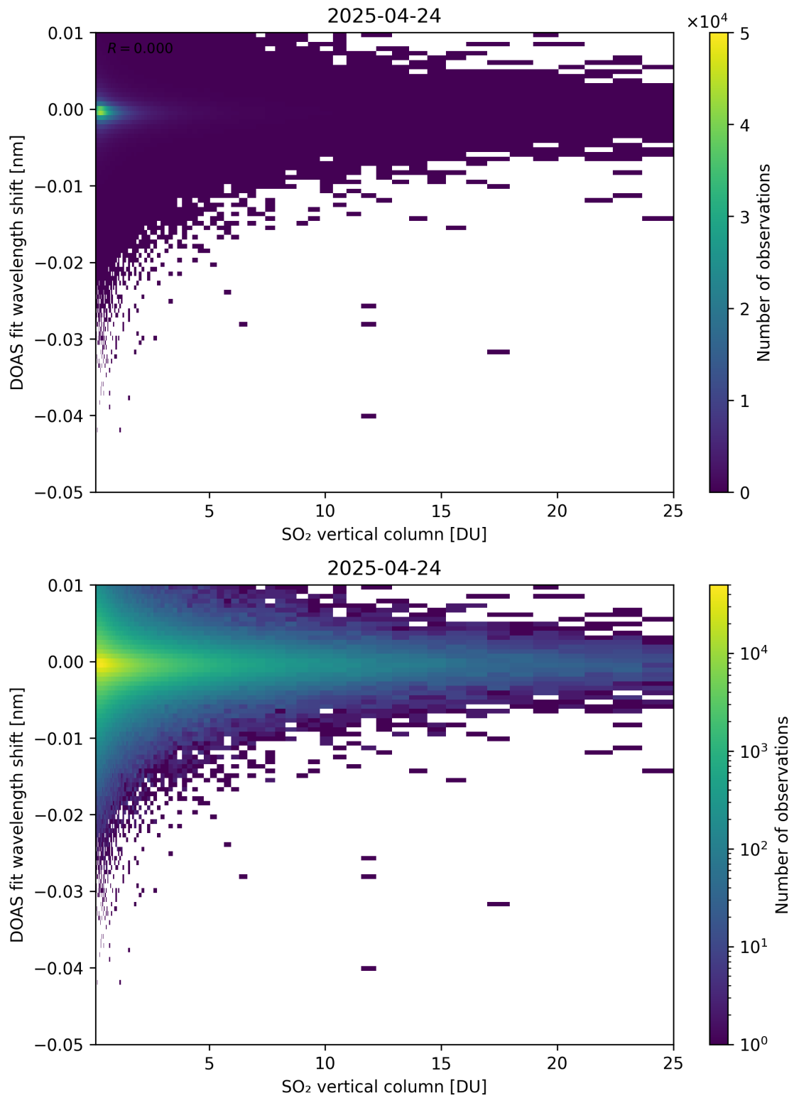
Figure 326: Scatter density plot of “SO 2 vertical column” against “DOAS fit wavelength shift” for 2025-04-24 to 2025-04-25.
