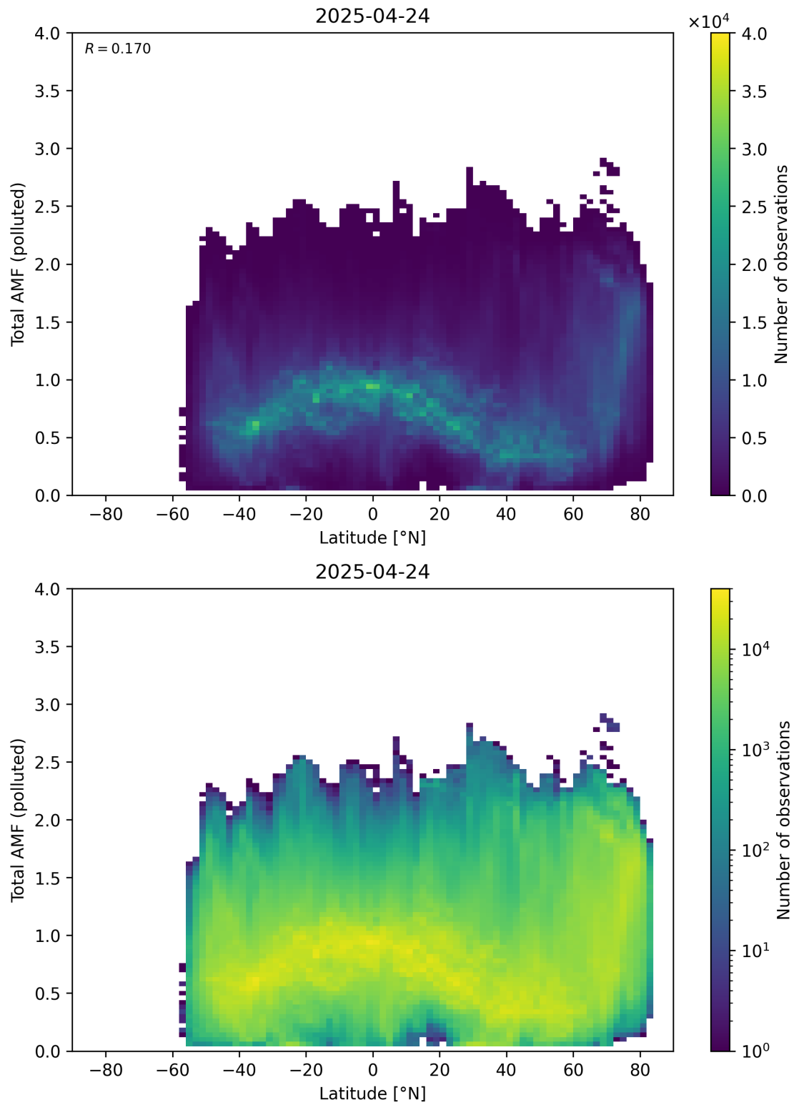
Figure 167: Scatter density plot of “Latitude” against “Total AMF (polluted)” for 2025-04-24 to 2025-04-25.
