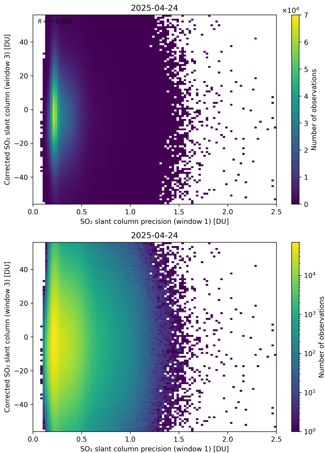
Figure 276: Scatter density plot of “SO 2 slant column precision (window 1)” against “Corrected SO 2 slant column (window 3)” for 2025-04-24 to 2025-04-25.
