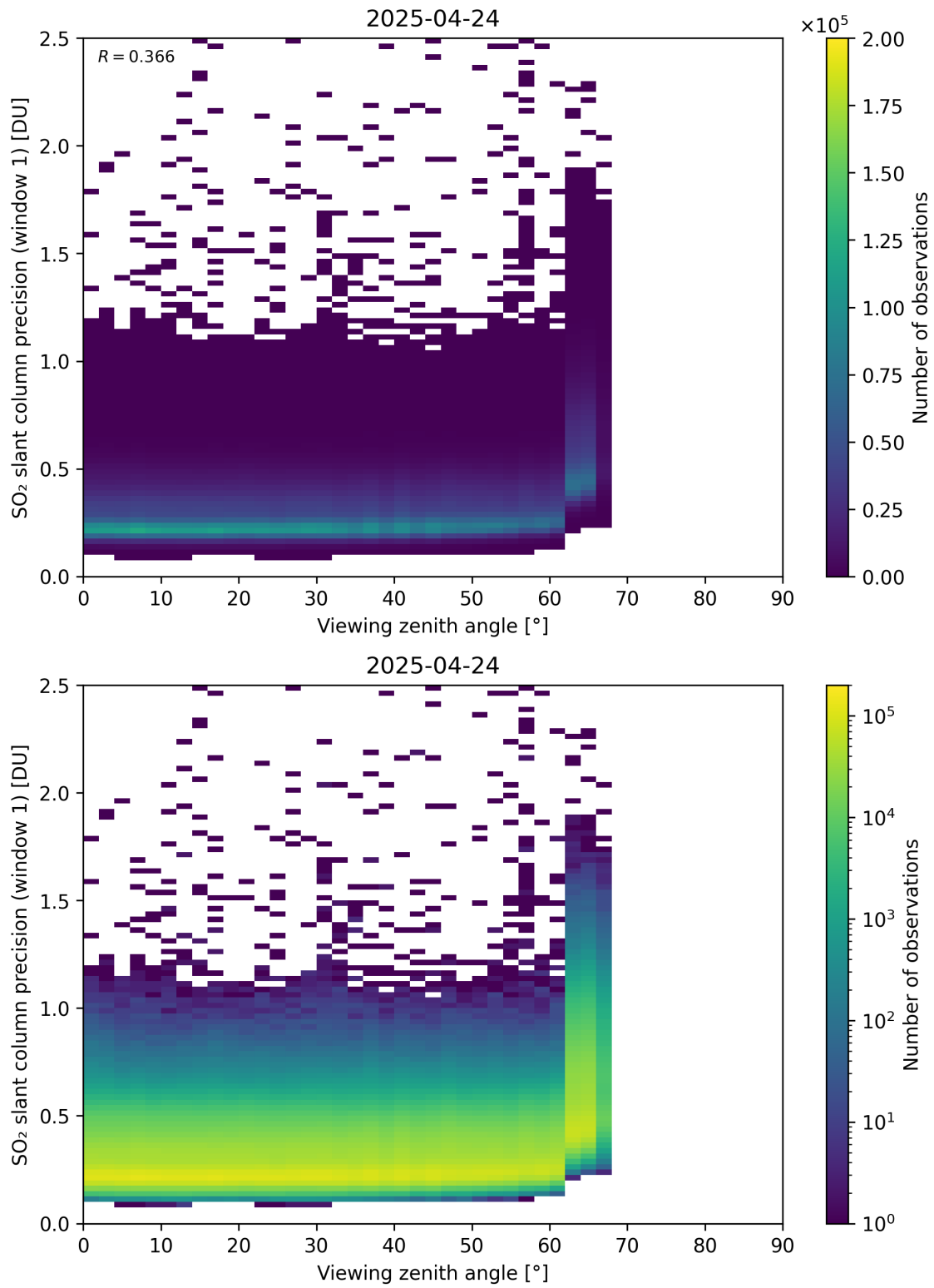
Figure 377: Scatter density plot of “Viewing zenith angle” against “SO 2 slant column precision (window 1)” for 2025-04-24 to 2025-04-25.
