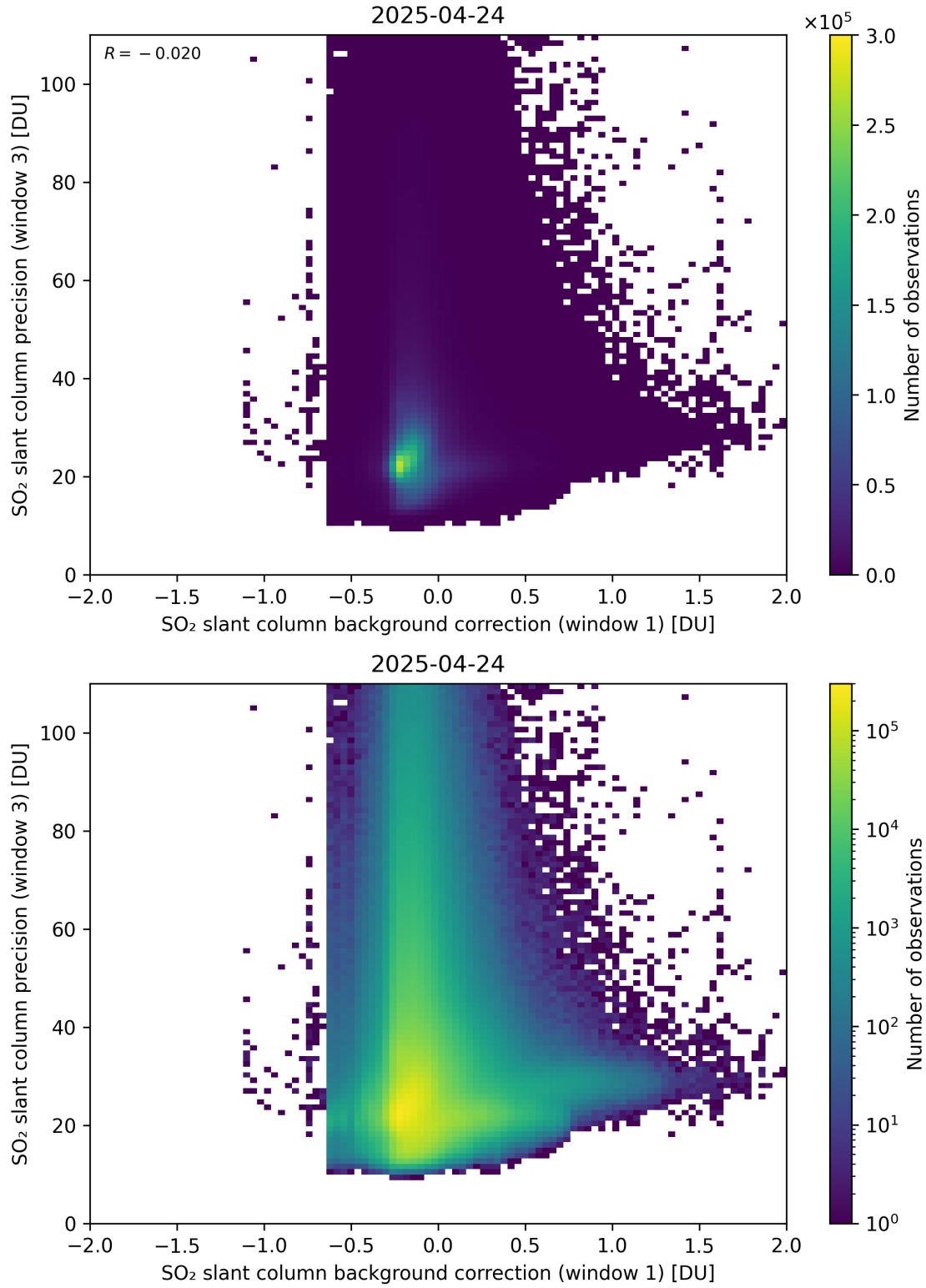
Figure 119: Scatter density plot of “SO 2 slant column background correction (window 1)” against “SO 2 slant column precision (window 3)” for 2025-04-24 to 2025-04-25.
