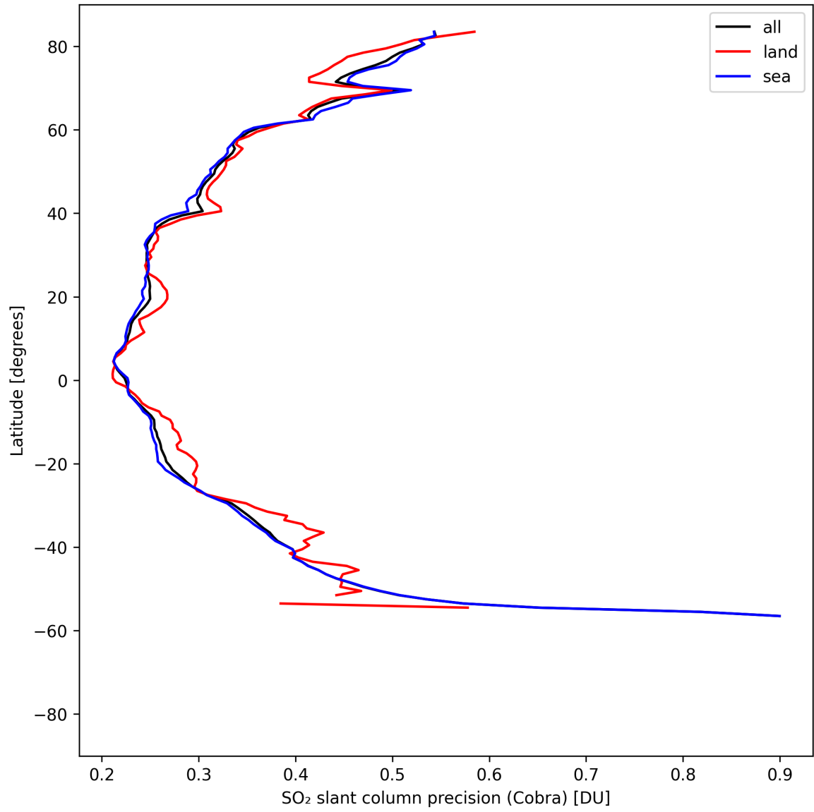
Figure 36: Zonal average of "SO 2 slant column precision (Cobra)" for 2025-04-24 to 2025-04-25.
