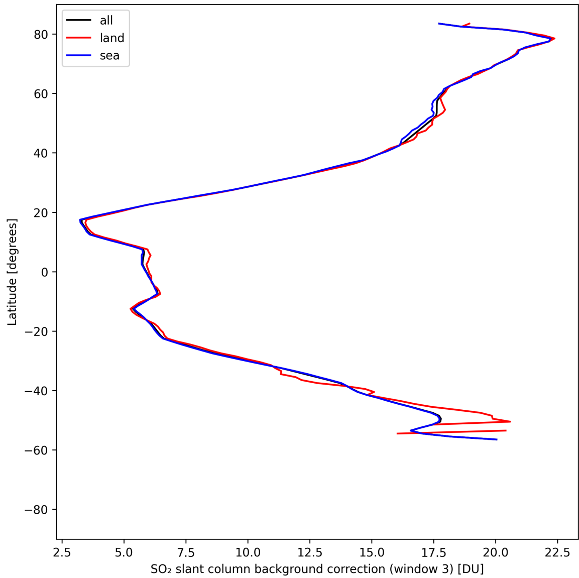
Figure 48: Zonal average of “SO 2 slant column background correction (window 3)” for 2025-04-24 to 2025-04-25.
