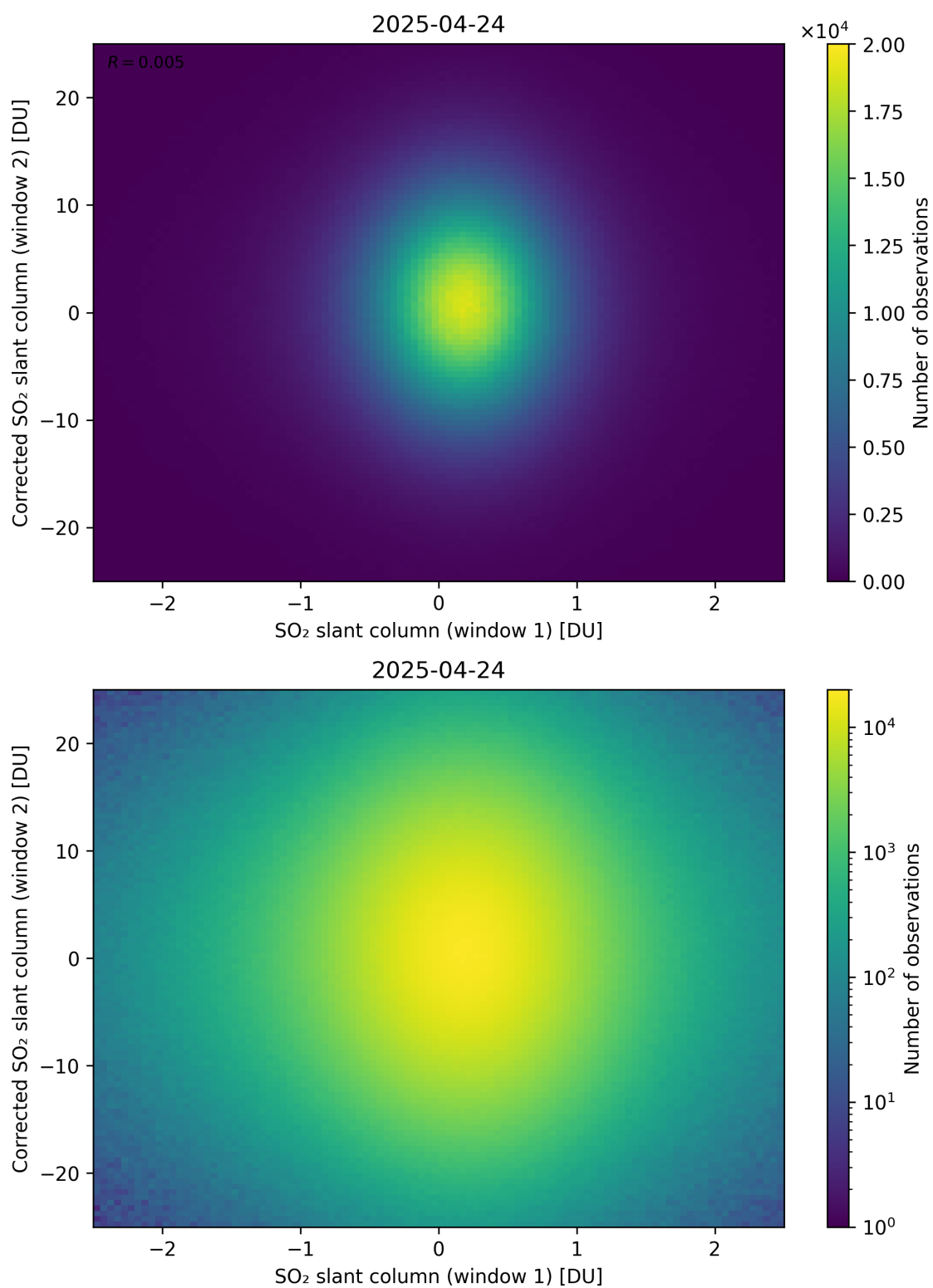
Figure 283: Scatter density plot of “SO 2 slant column (window 1)” against “Corrected SO 2 slant column (window 2)” for 2025-04-24 to 2025-04-25.
