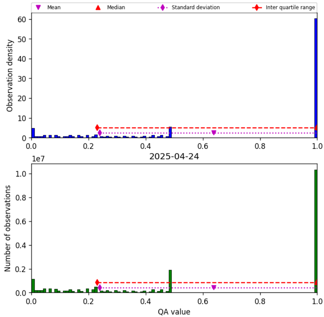
Figure 57: Histogram of “QA value” for 2025-04-24 to 2025-04-25
