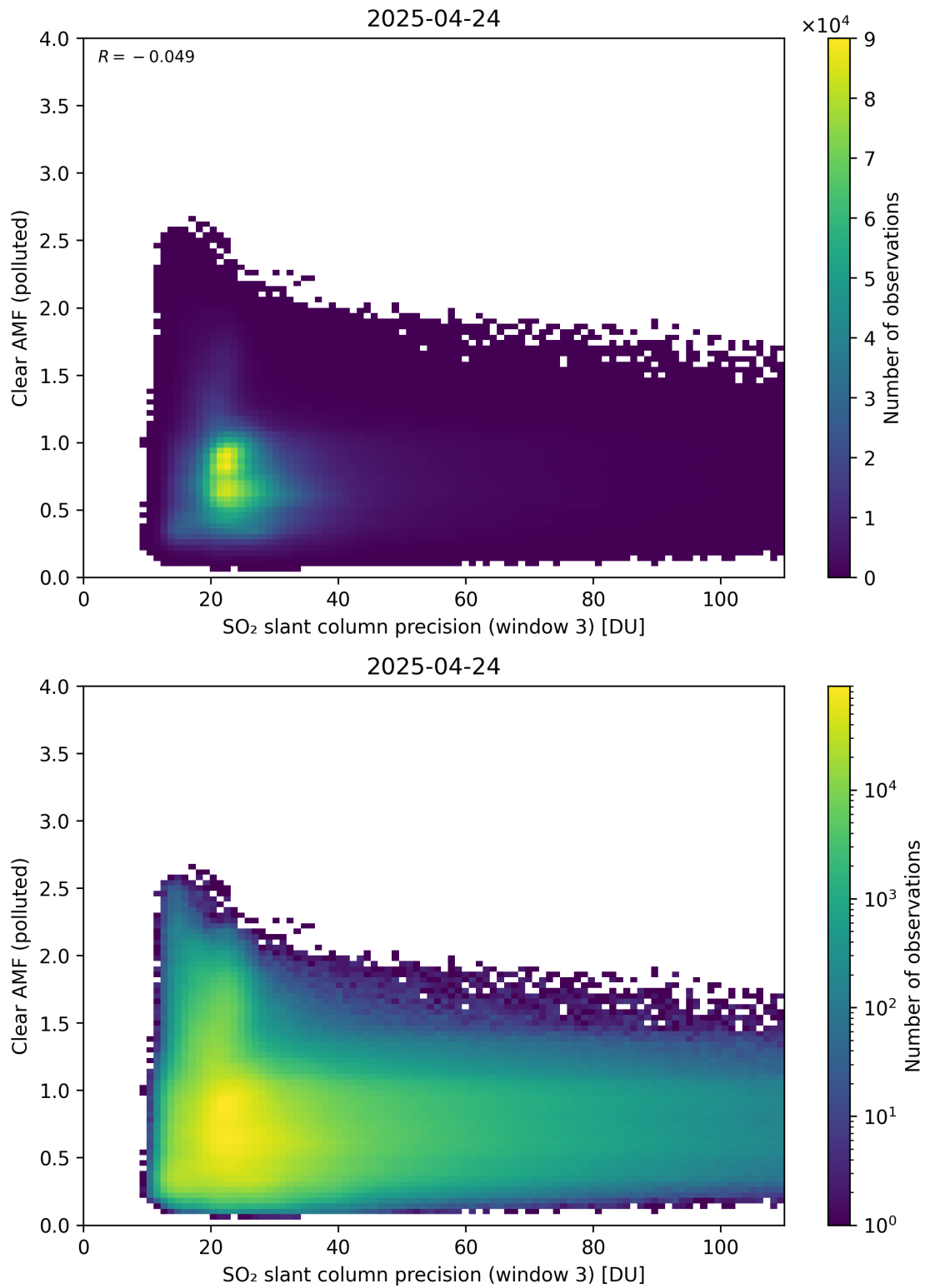
Figure 311: Scatter density plot of “SO 2 slant column precision (window 3)” against “Clear AMF (polluted)” for 2025-04-24 to 2025-04-25.
