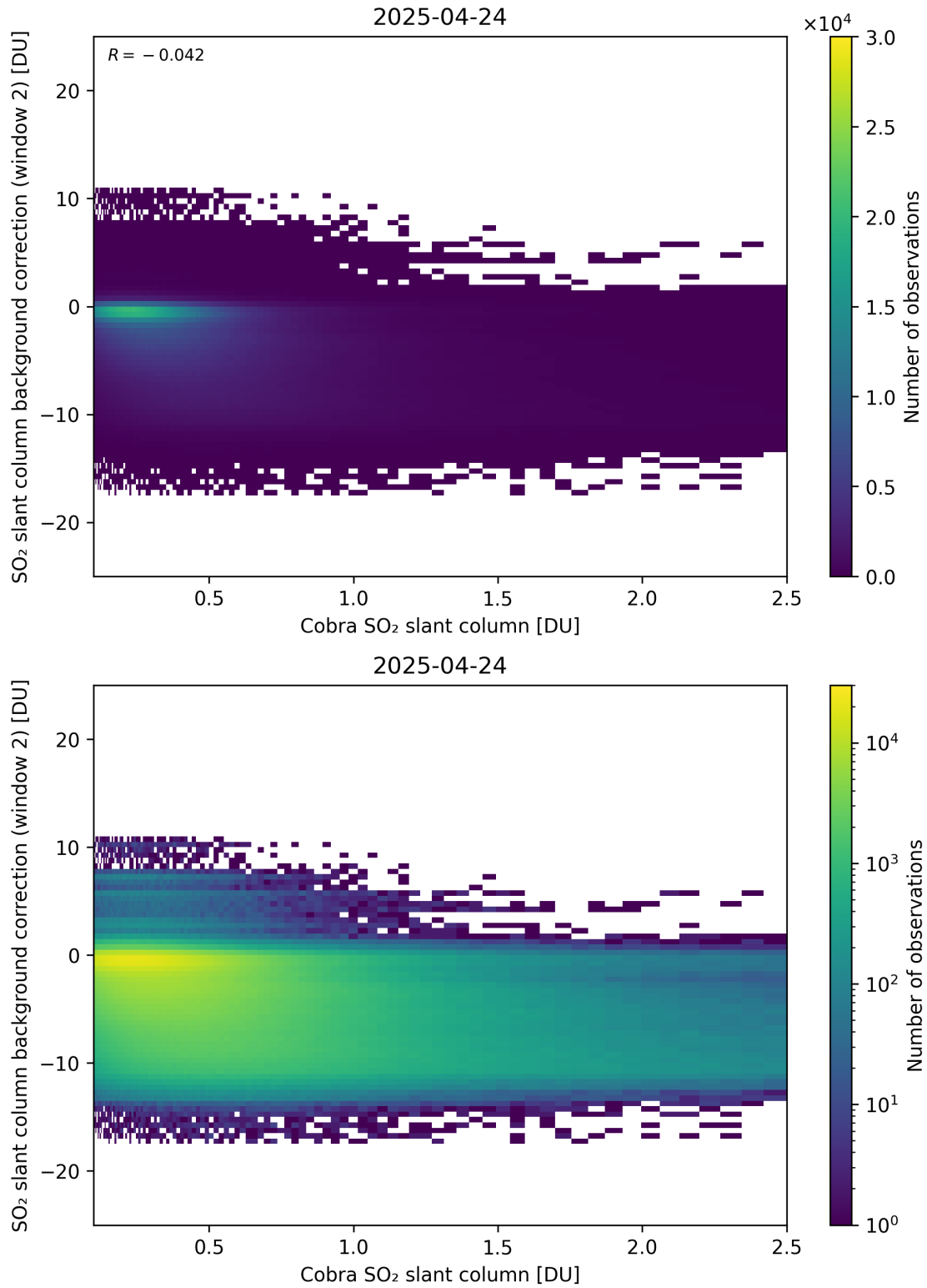
Figure 194: Scatter density plot of “Cobra SO 2 slant column” against “SO 2 slant column background correction (window 2)” for 2025-04-24 to 2025-04-25.
