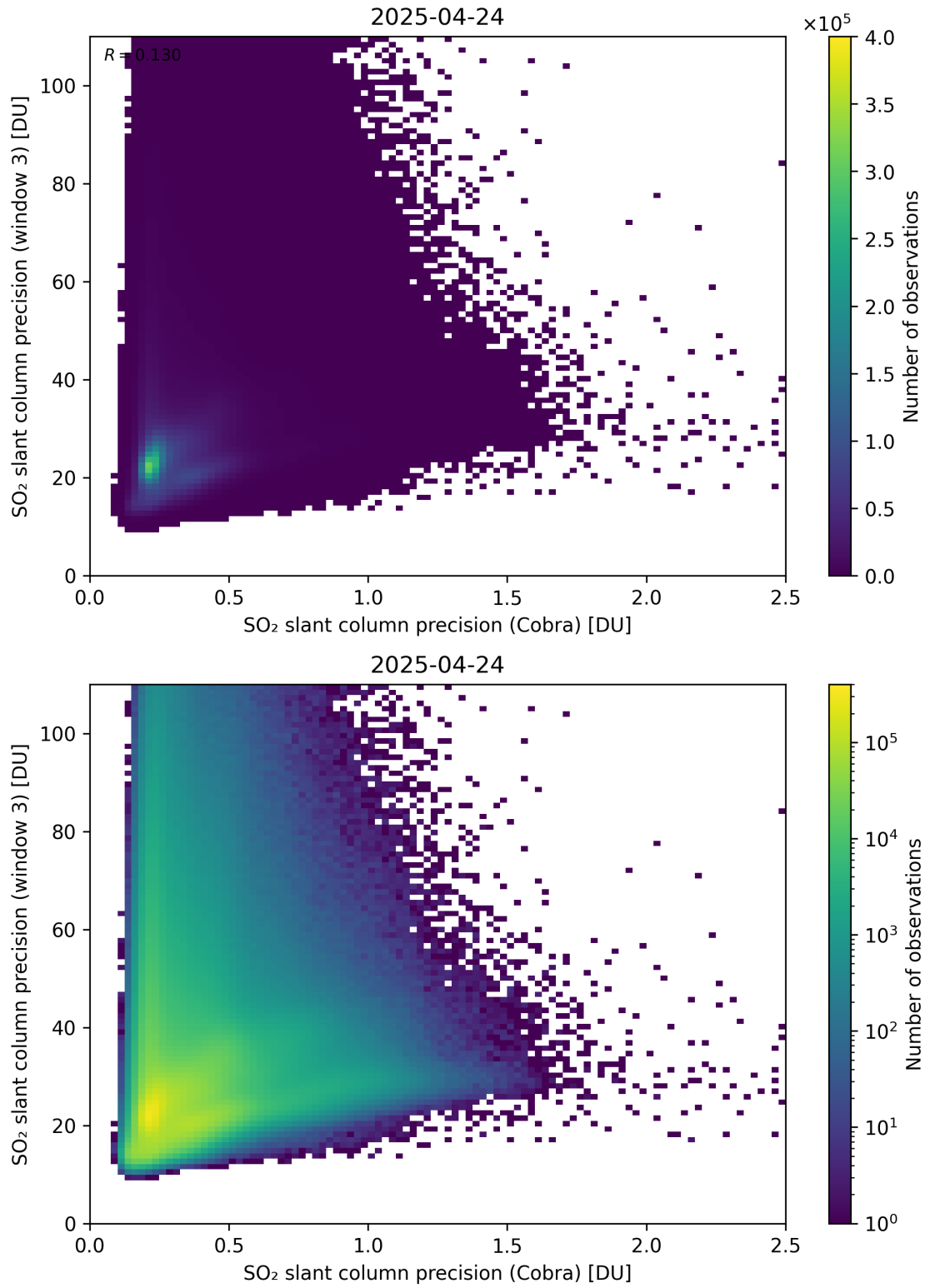
Figure 212: Scatter density plot of “SO 2 slant column precision (Cobra)” against “SO 2 slant column precision (window 3)” for 2025-04-24 to 2025-04-25.
