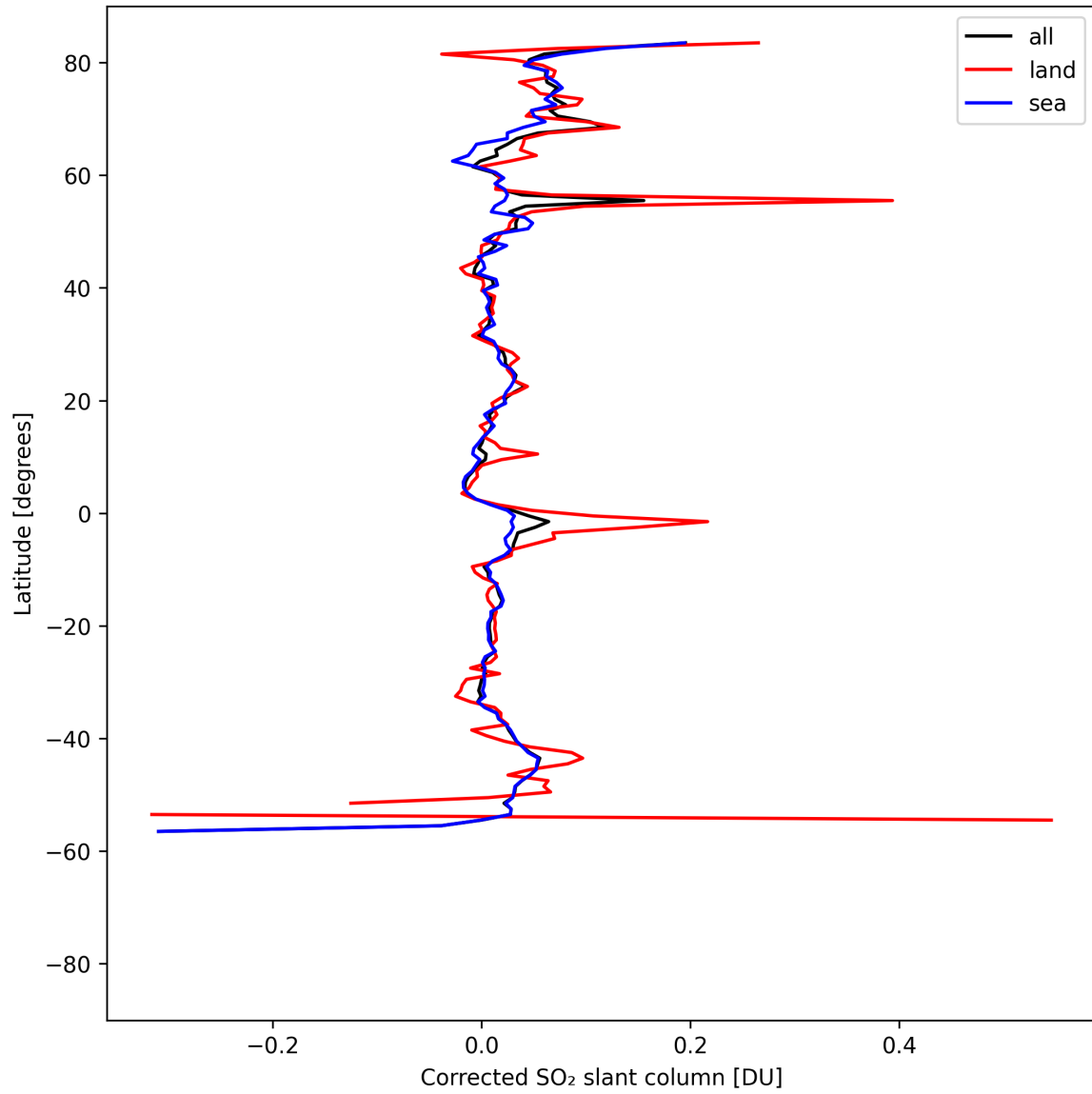
Figure 34: Zonal average of "Corrected SO 2 slant column" for 2025-04-24 to 2025-04-25.
