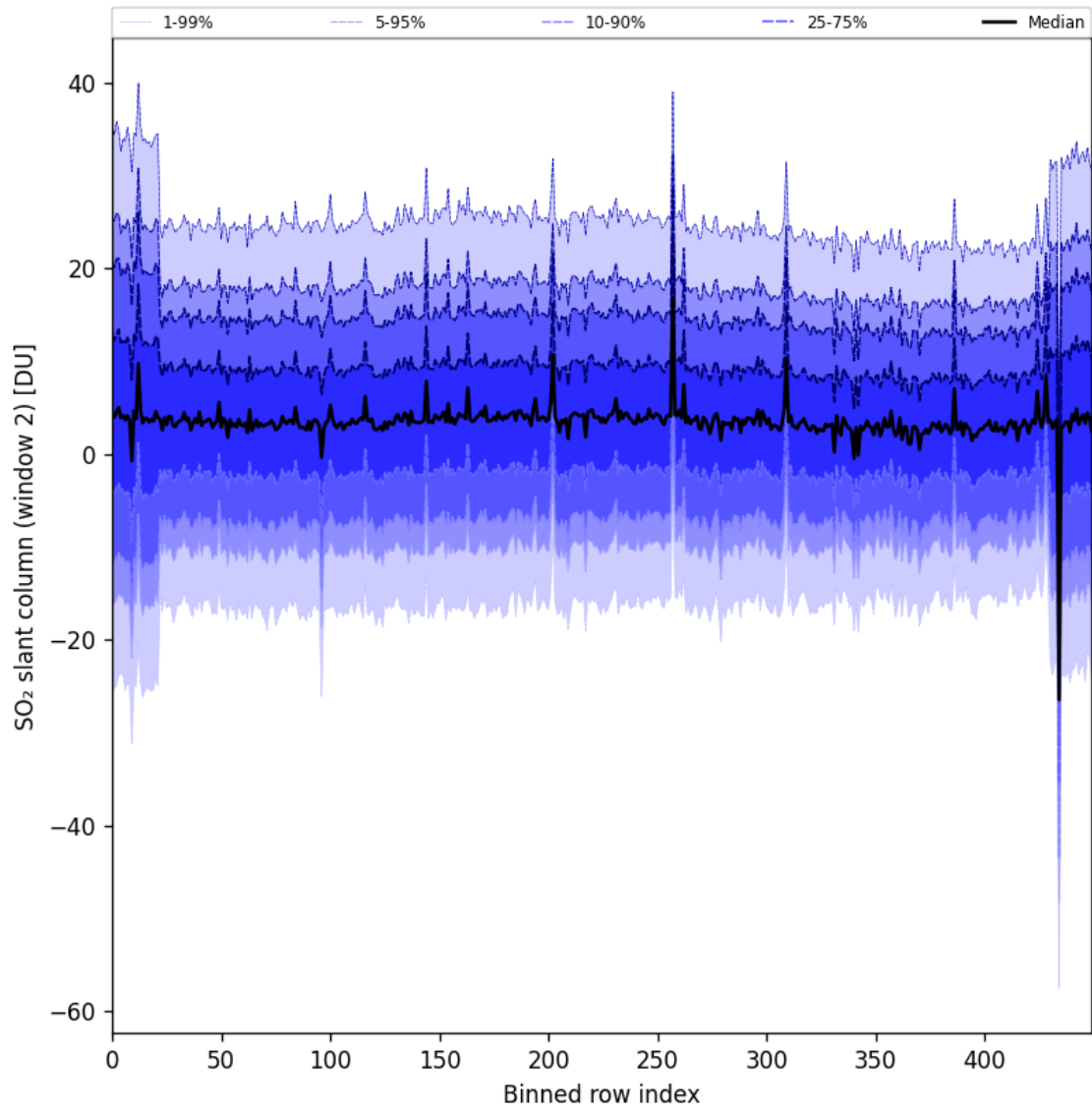
Figure 93: Along track statistics of “SO 2 slant column (window 2)” for 2025-04-24 to 2025-04-25
