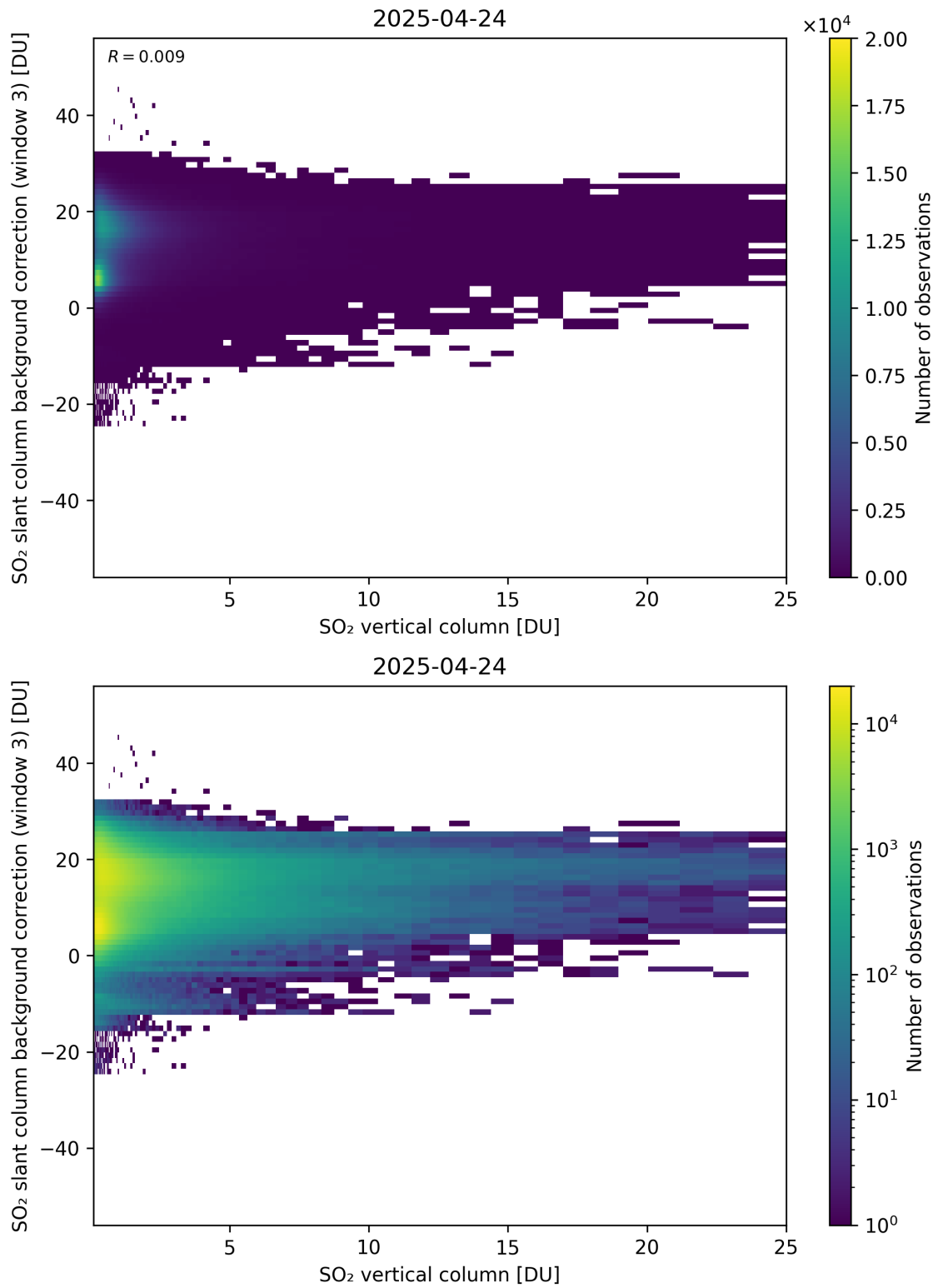
Figure 325: Scatter density plot of “SO 2 vertical column” against “SO 2 slant column background correction (window 3)” for 2025-04-24 to 2025-04-25.
