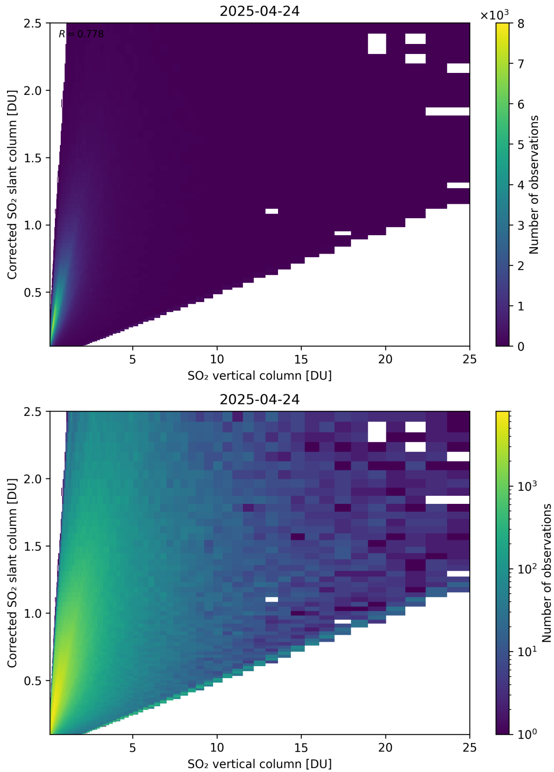
Figure 351: Scatter density plot of “SO 2 vertical column” against “Corrected SO 2 slant column” for 2025-04-24 to 2025-04-25.
