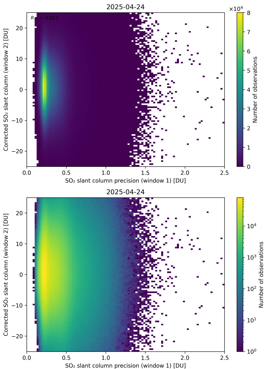
Figure 275: Scatter density plot of “SO 2 slant column precision (window 1)” against “Corrected SO 2 slant column (window 2)” for 2025-04-24 to 2025-04-25.
