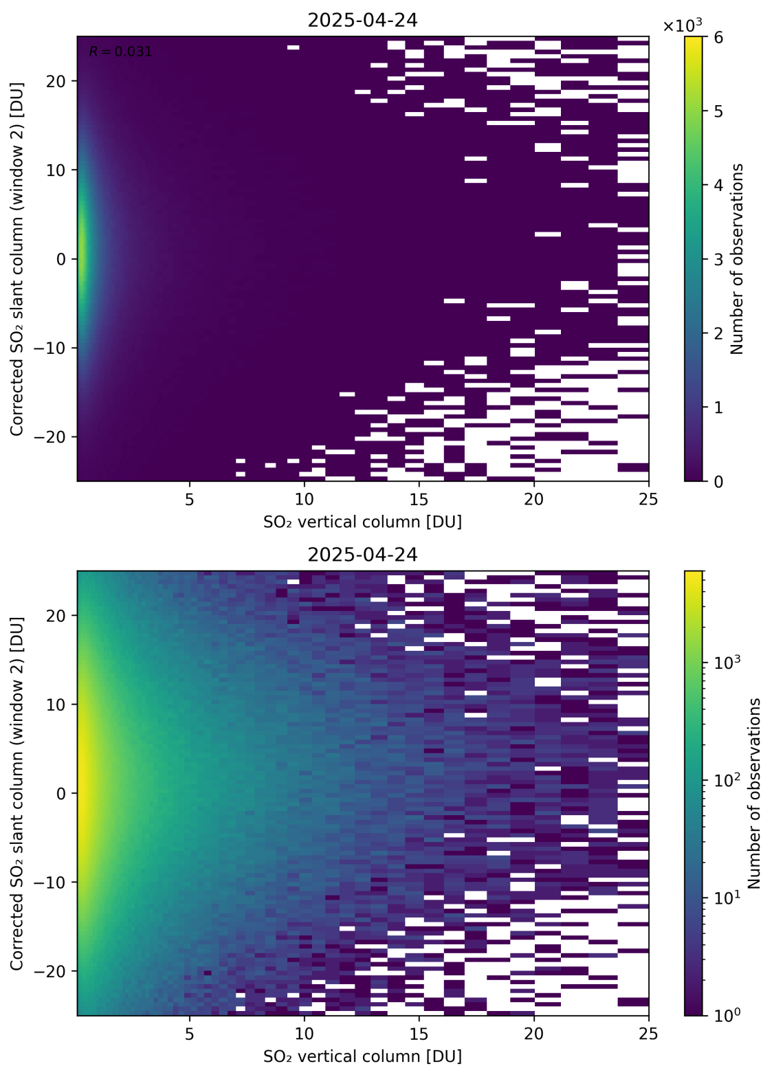
Figure 352: Scatter density plot of “SO 2 vertical column” against “Corrected SO 2 slant column (window 2)” for 2025-04-24 to 2025-04-25.
