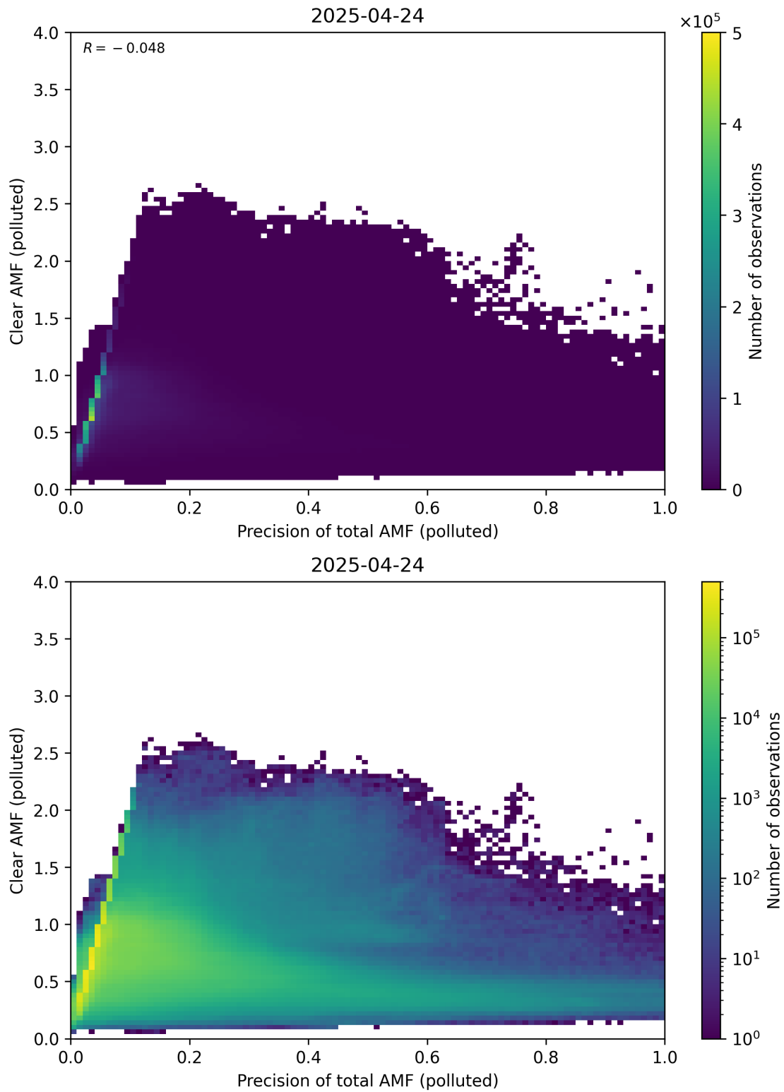
Figure 320: Scatter density plot of “Precision of total AMF (polluted)” against “Clear AMF (polluted)” for 2025-04-24 to 2025-04-25.
