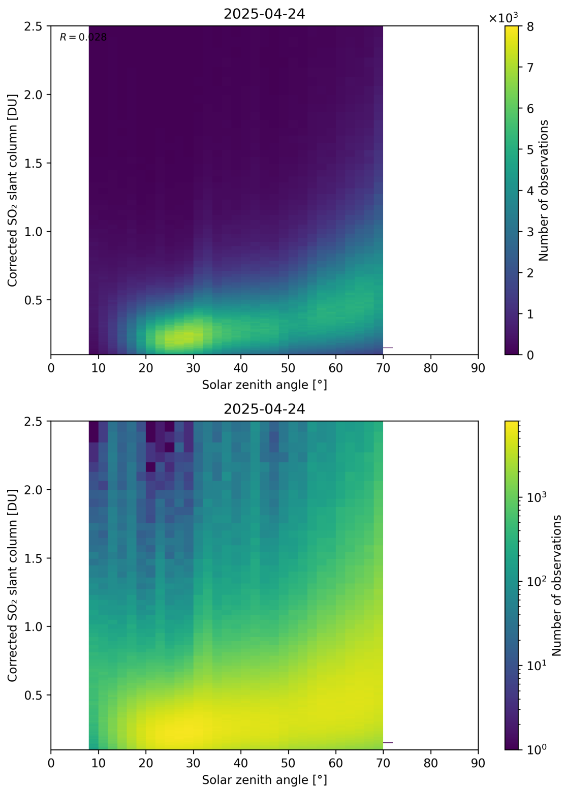
Figure 181: Scatter density plot of “Solar zenith angle” against “Corrected SO 2 slant column” for 2025-04-24 to 2025-04-25.
