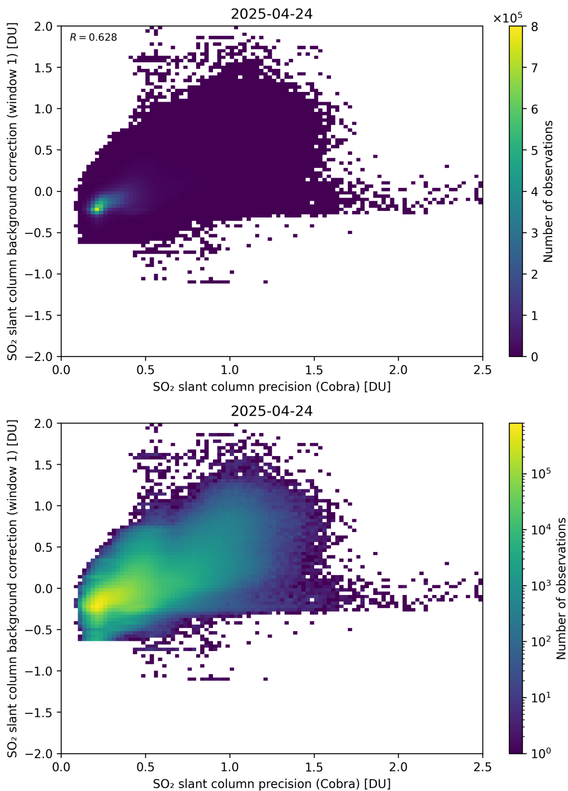
Figure 199: Scatter density plot of “SO 2 slant column precision (Cobra)” against “SO 2 slant column background correction (window 1)” for 2025-04-24 to 2025-04-25.
