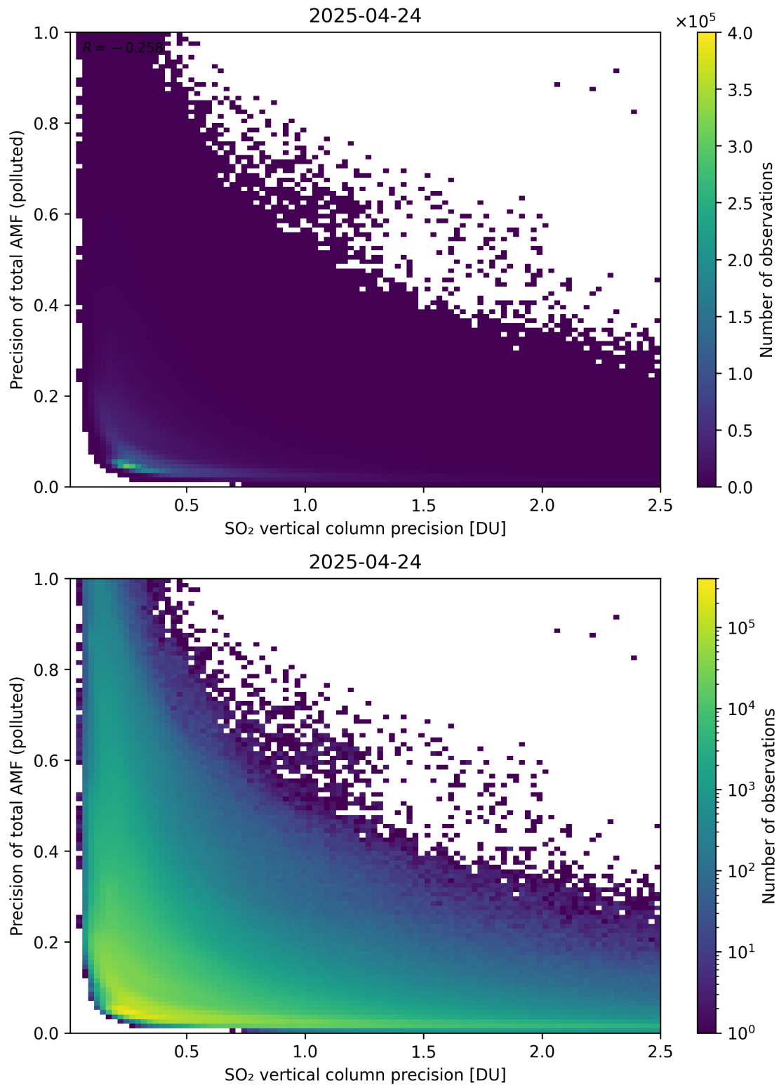
Figure 347: Scatter density plot of “SO 2 vertical column precision” against “Precision of total AMF (polluted)” for 2025-04-24 to 2025-04-25.
