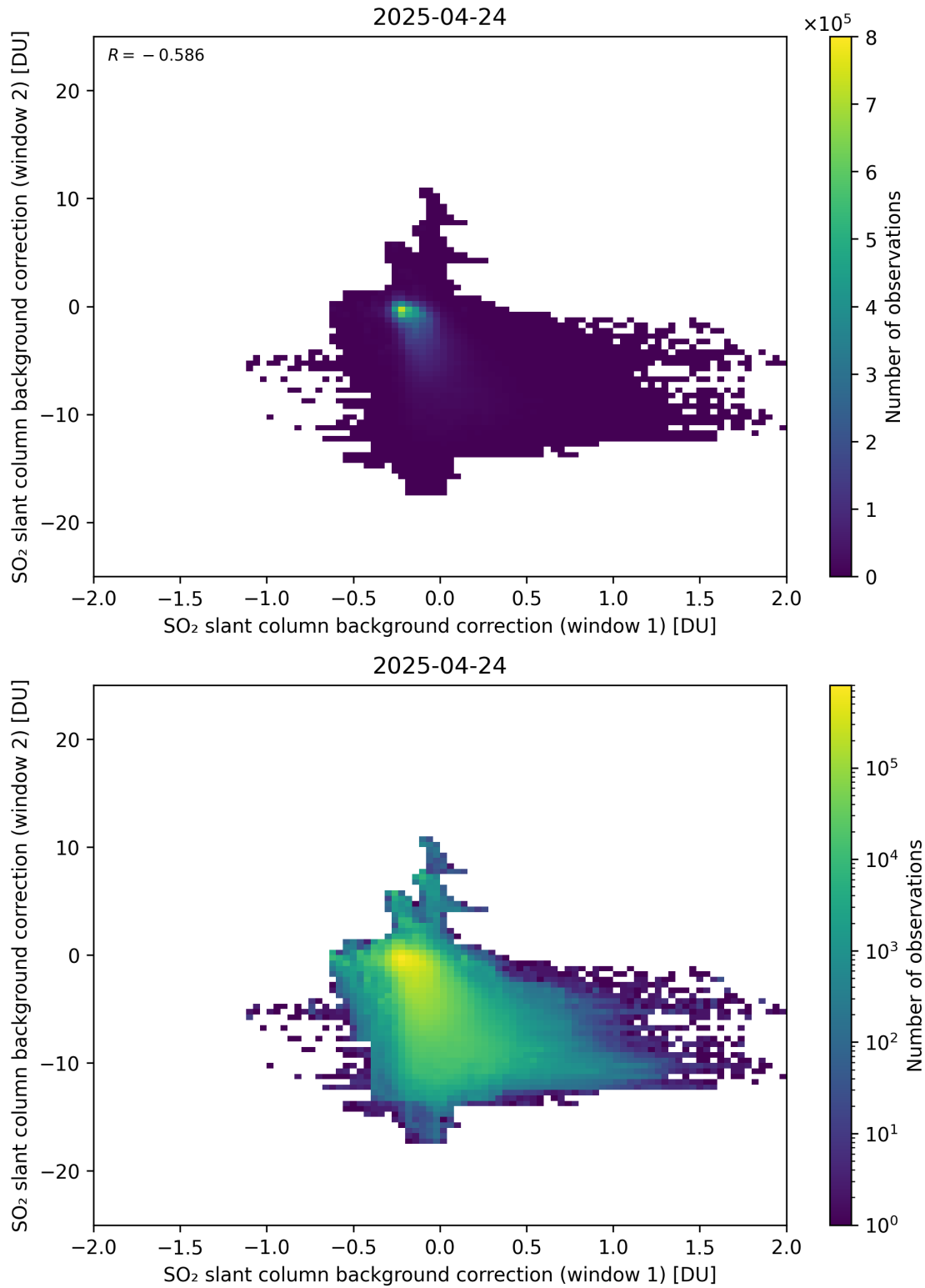
Figure 109: Scatter density plot of “SO 2 slant column background correction (window 1)” against “SO 2 slant column background correction (window 2)” for 2025-04-24 to 2025-04-25.
