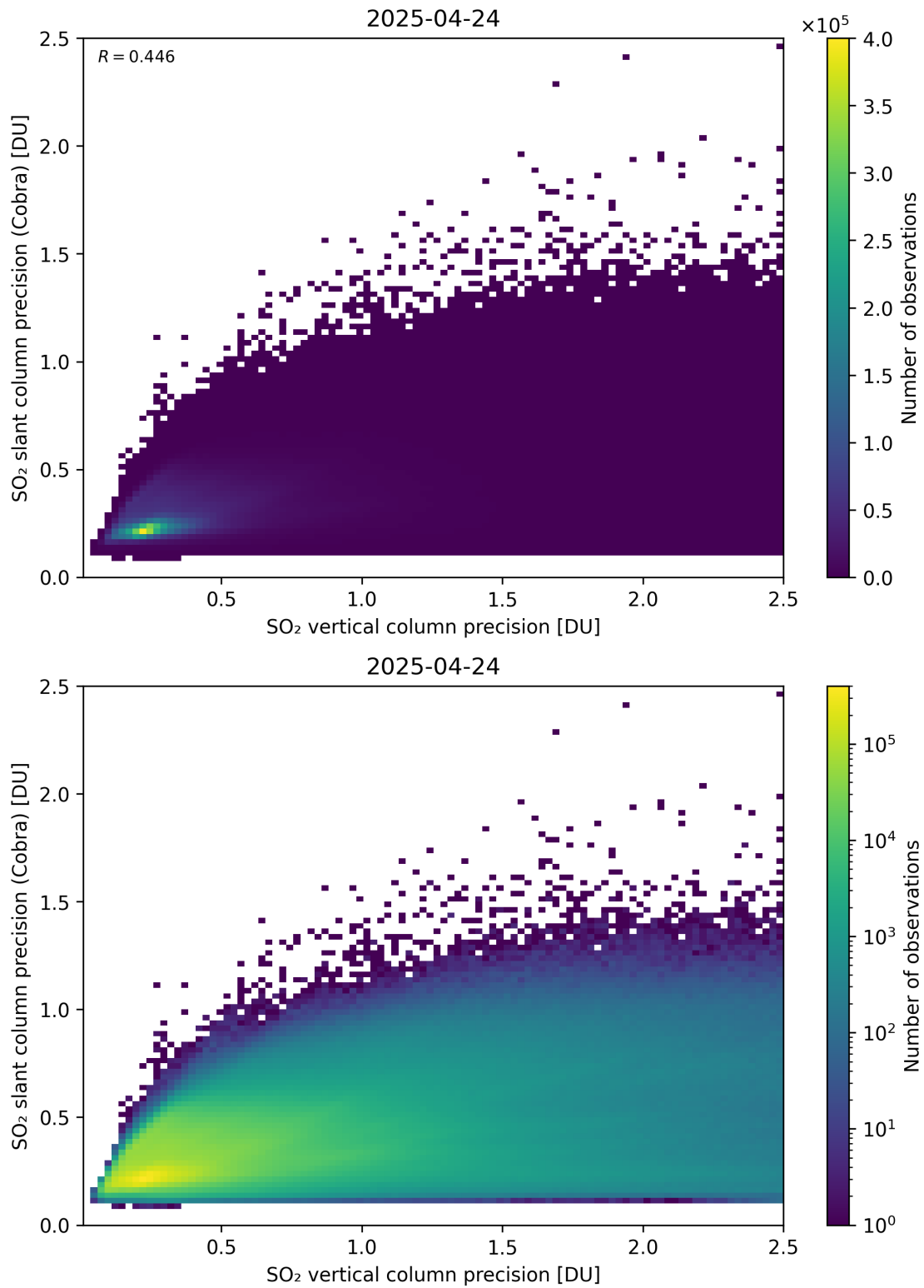
Figure 337: Scatter density plot of “SO 2 vertical column precision” against “SO 2 slant column precision (Cobra)” for 2025-04-24 to 2025-04-25.
