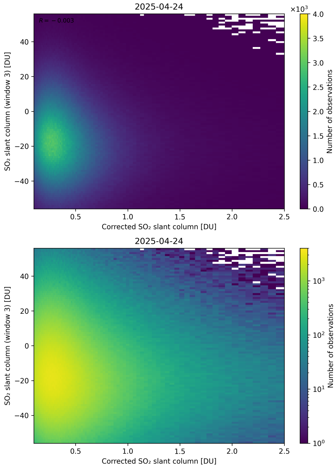
Figure 240: Scatter density plot of “Corrected SO 2 slant column” against “SO 2 slant column (window 3)” for 2025-04-24 to 2025-04-25.
