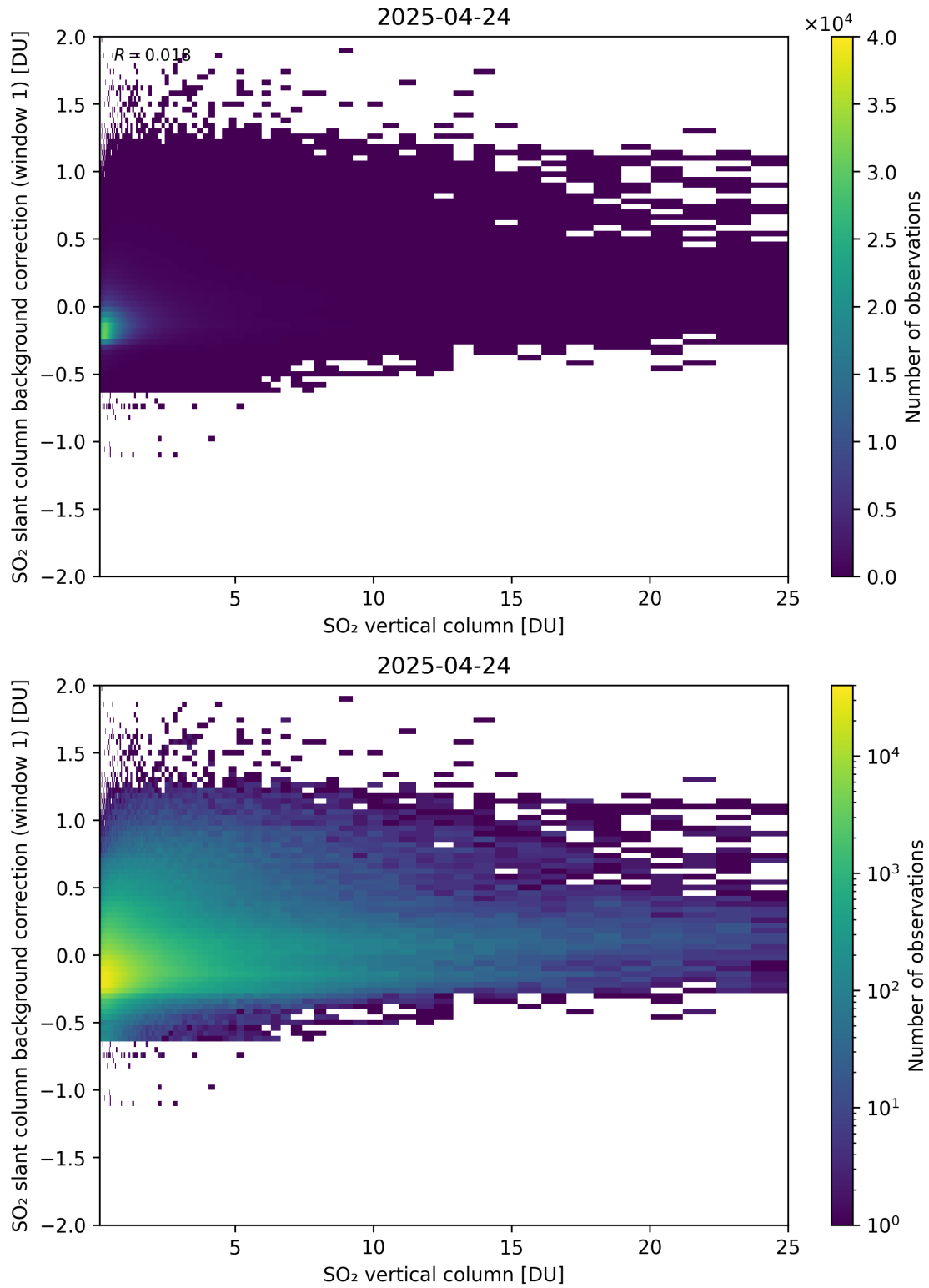
Figure 323: Scatter density plot of “SO 2 vertical column” against “SO 2 slant column background correction (window 1)” for 2025-04-24 to 2025-04-25.
