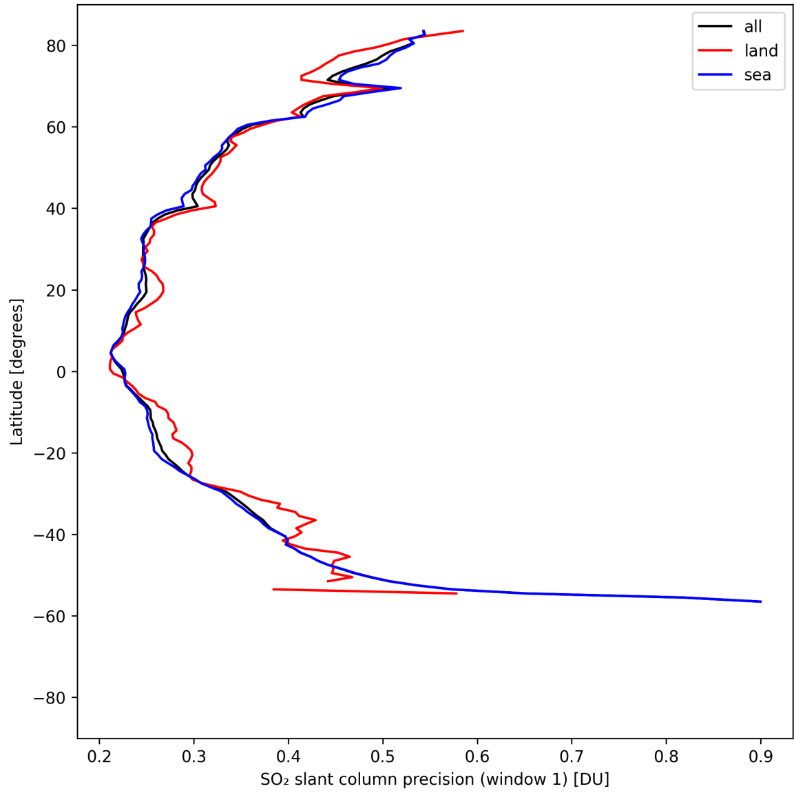
Figure 38: Zonal average of “SO 2 slant column precision (window 1)” for 2025-04-24 to 2025-04-25.
