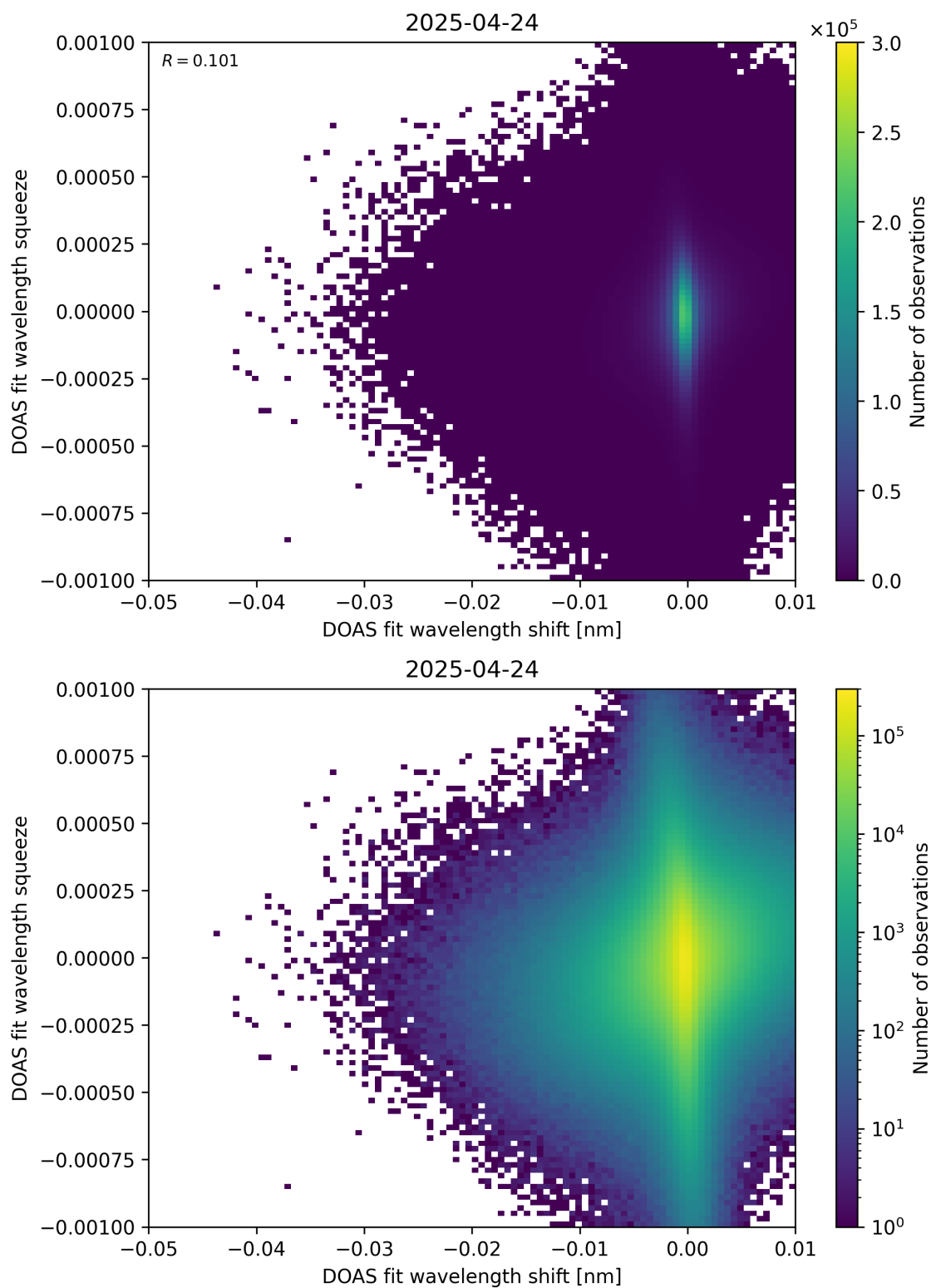
Figure 138: Scatter density plot of “DOAS fit wavelength shift” against “DOAS fit wavelength squeeze” for 2025-04-24 to 2025-04-25.
