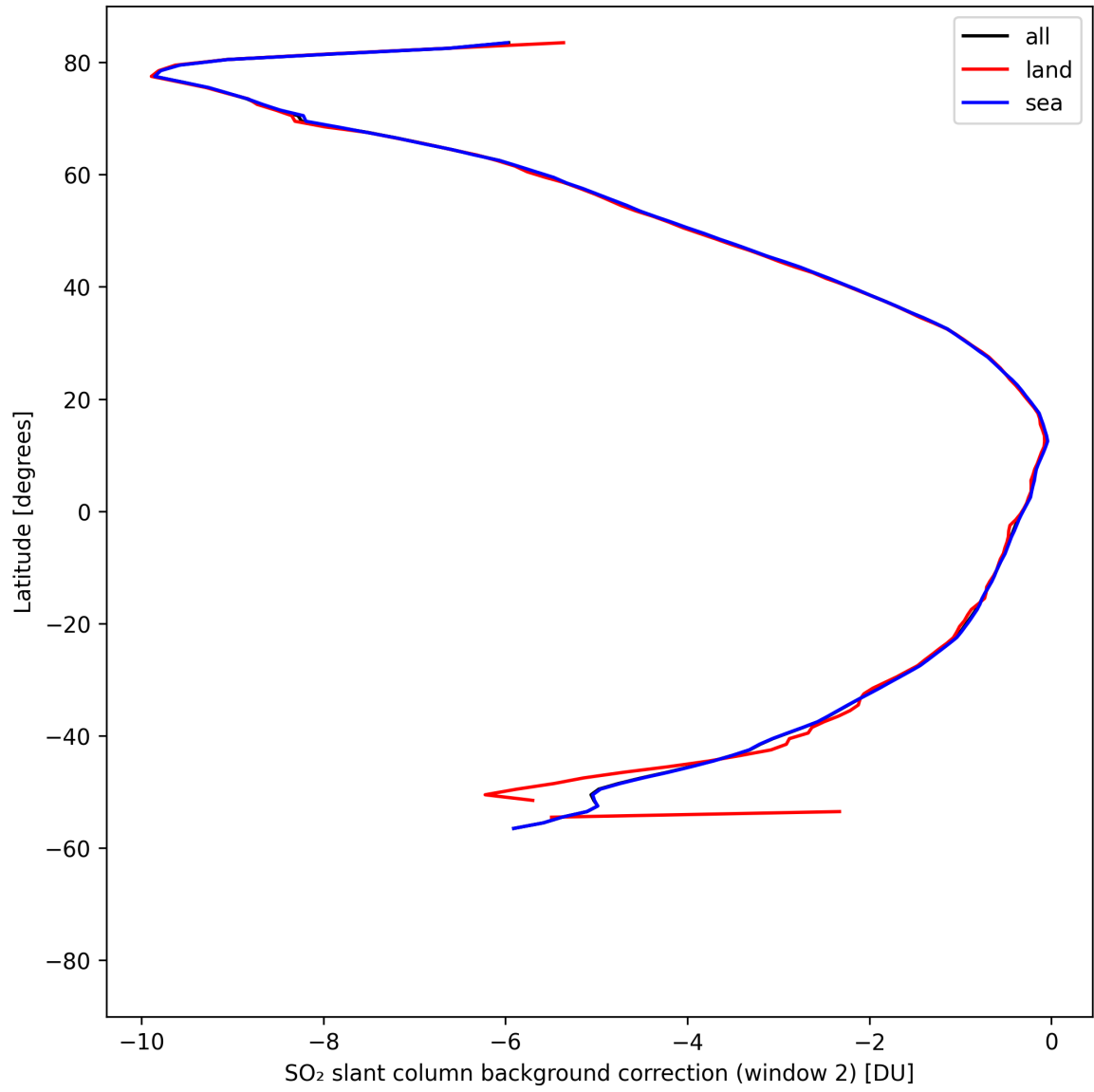
Figure 44: Zonal average of “SO 2 slant column background correction (window 2)” for 2025-04-24 to 2025-04-25.
