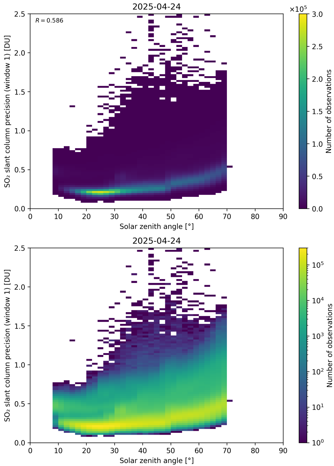
Figure 185: Scatter density plot of “Solar zenith angle” against “SO 2 slant column precision (window 1)” for 2025-04-24 to 2025-04-25.
