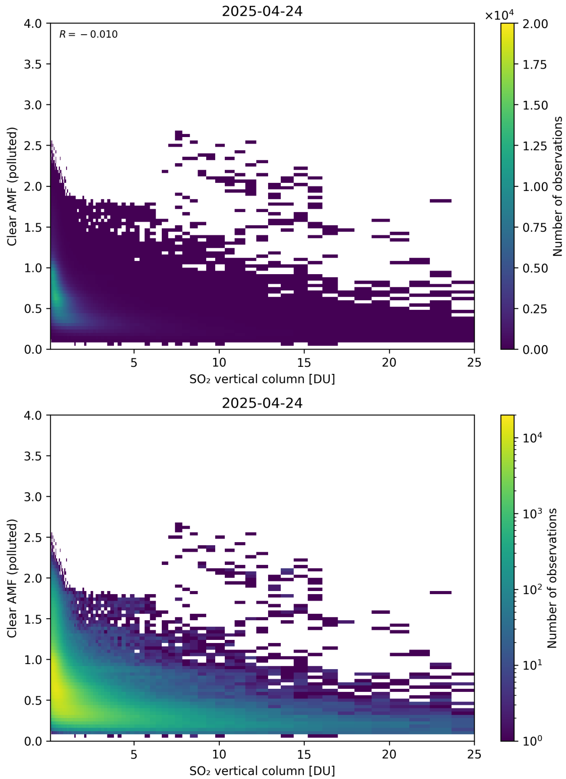
Figure 348: Scatter density plot of “SO 2 vertical column” against “Clear AMF (polluted)” for 2025-04-24 to 2025-04-25.
