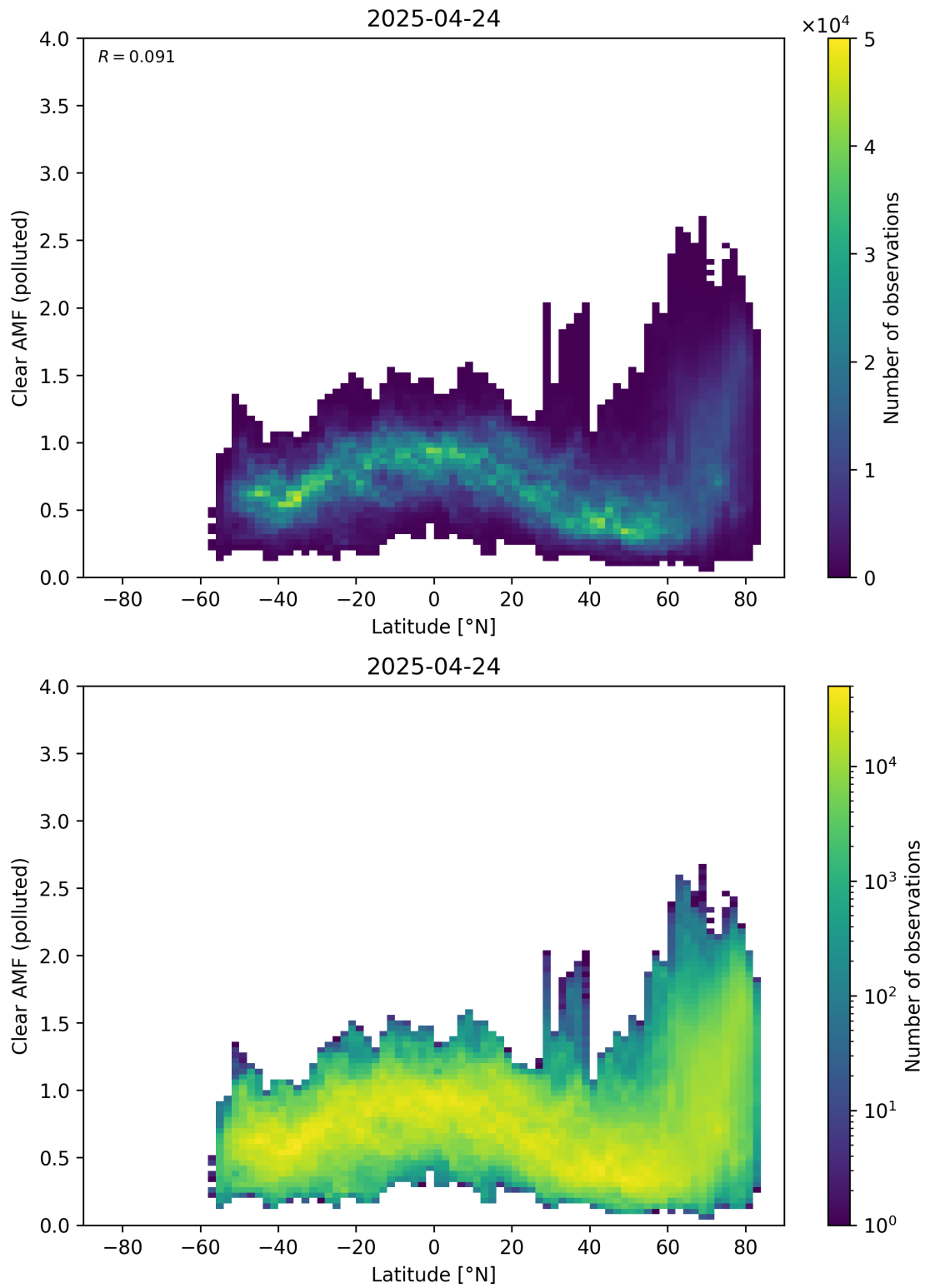
Figure 156: Scatter density plot of “Latitude” against “Clear AMF (polluted)” for 2025-04-24 to 2025-04-25.
