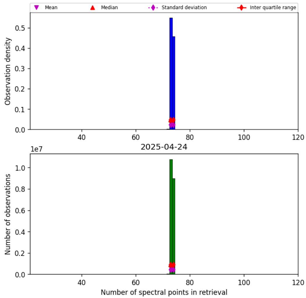
Figure 82: Histogram of “Number of spectral points in retrieval” for 2025-04-24 to 2025-04-25
