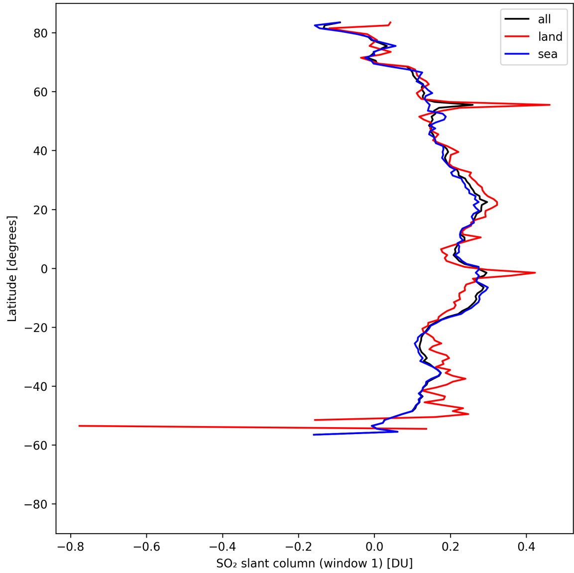
Figure 37: Zonal average of “SO 2 slant column (window 1)” for 2025-04-24 to 2025-04-25.
