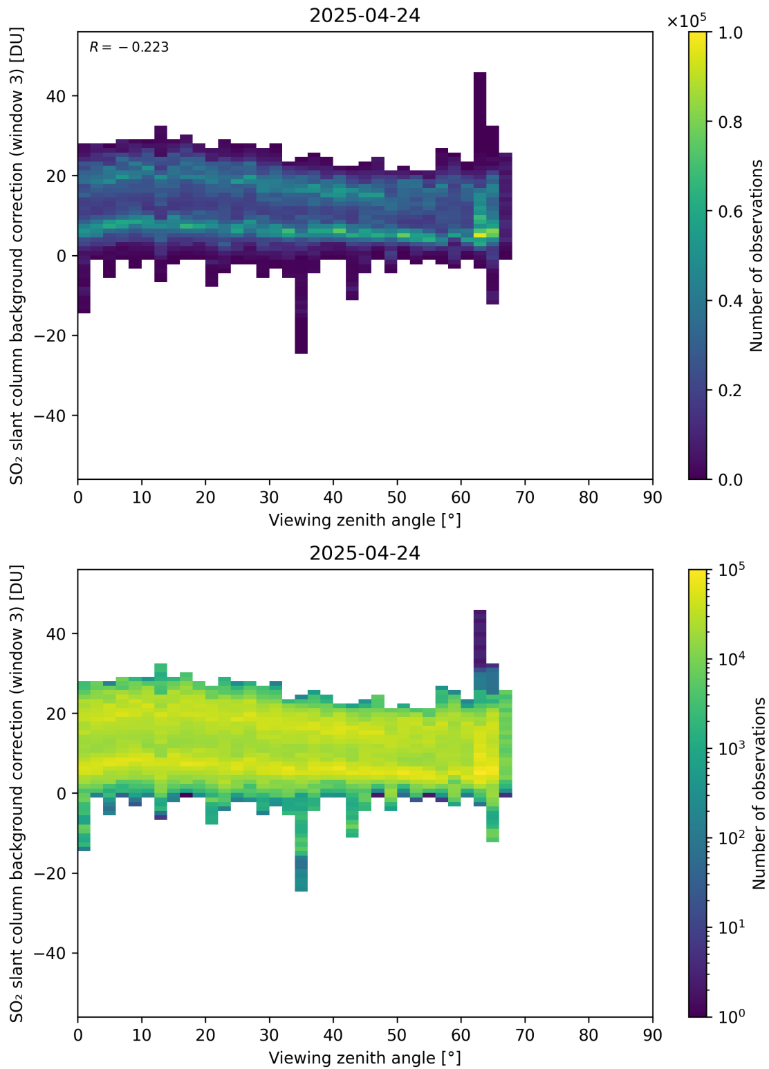
Figure 364: Scatter density plot of “Viewing zenith angle” against “SO 2 slant column background correction (window 3)” for 2025-04-24 to 2025-04-25.
