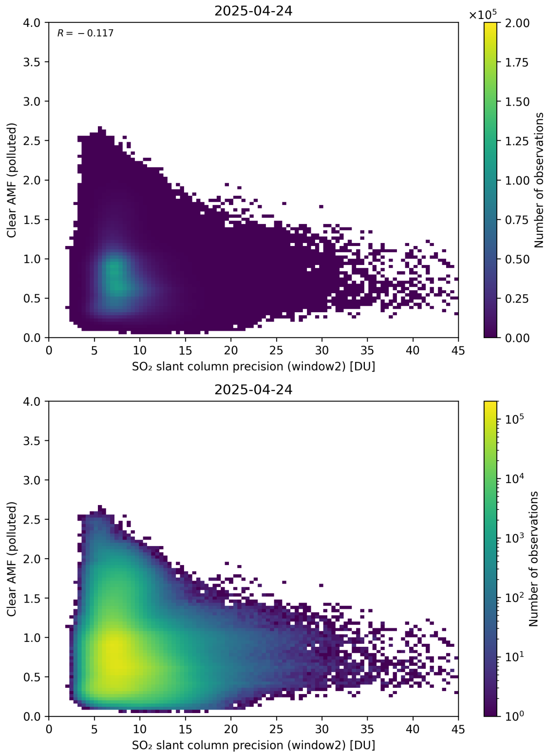
Figure 296: Scatter density plot of “SO 2 slant column precision (window2)” against “Clear AMF (polluted)” for 2025-04-24 to 2025-04-25.
