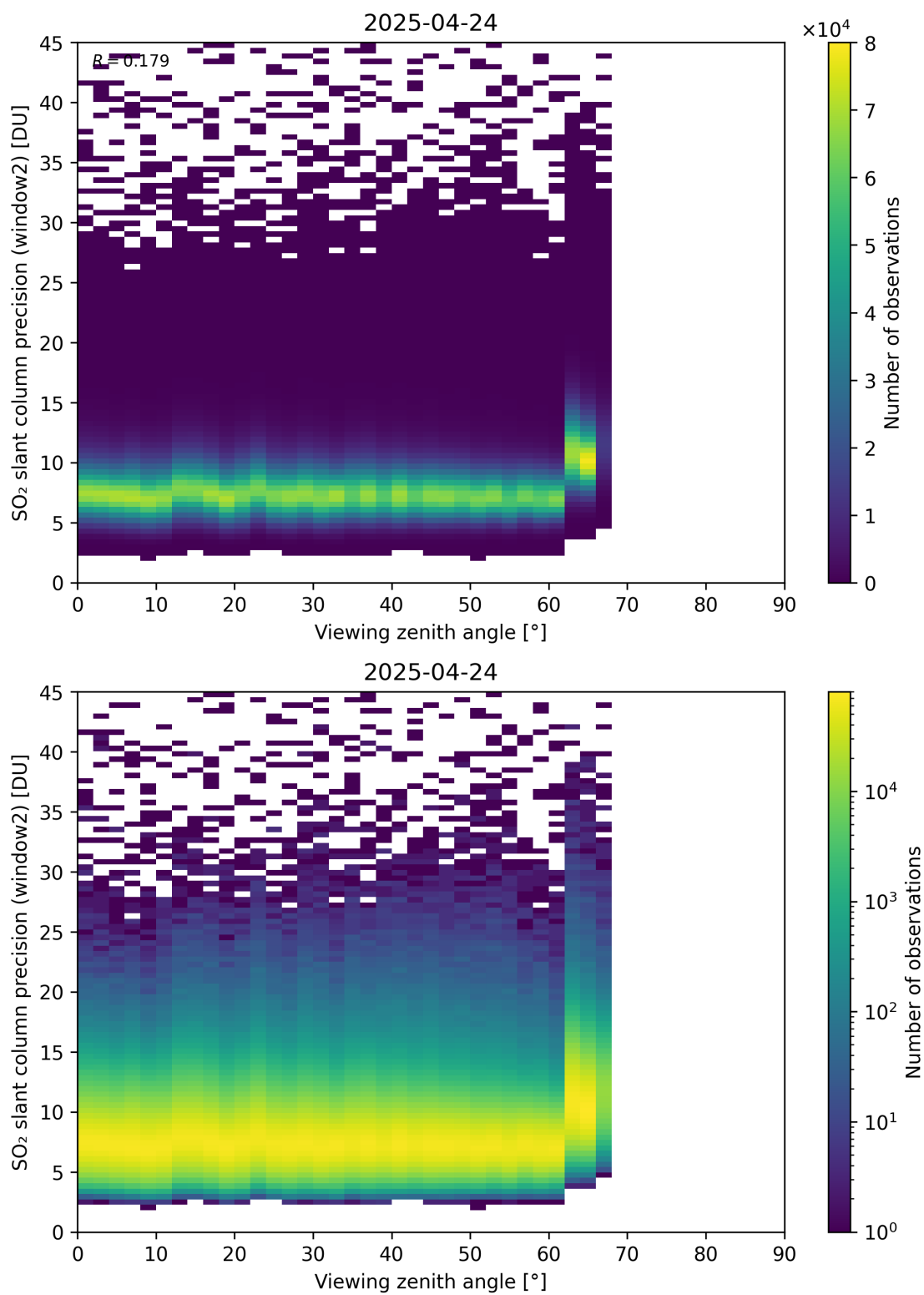
Figure 378: Scatter density plot of “Viewing zenith angle” against “SO 2 slant column precision (window2)” for 2025-04-24 to 2025-04-25.
