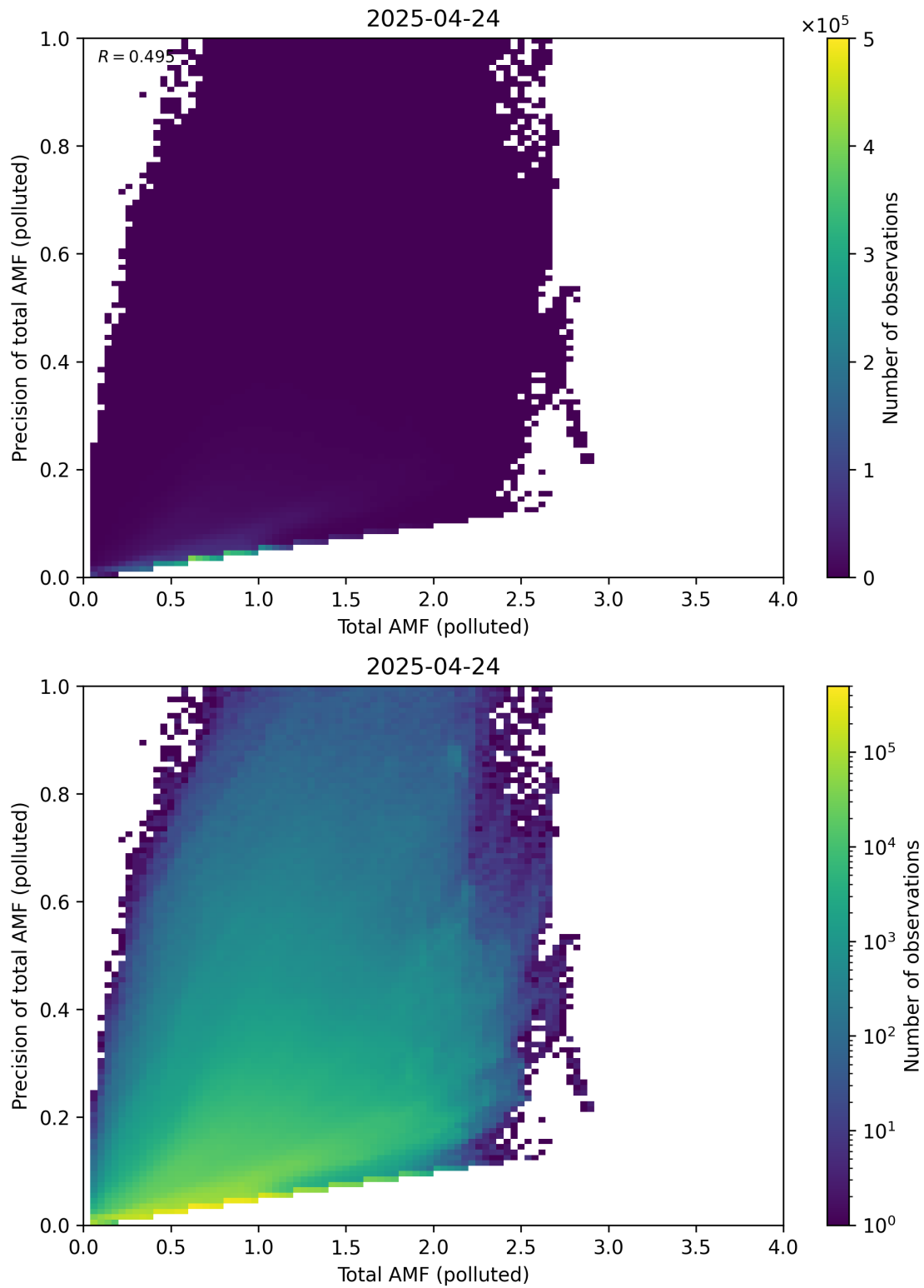
Figure 322: Scatter density plot of “Total AMF (polluted)” against “Precision of total AMF (polluted)” for 2025-04-24 to 2025-04-25.
