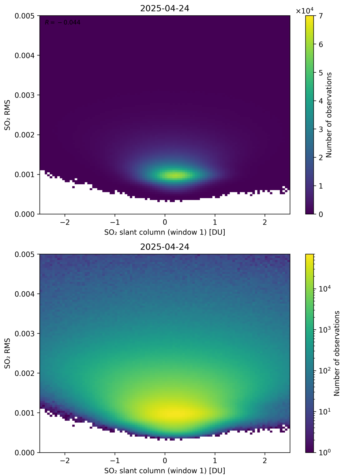
Figure 267: Scatter density plot of “SO 2 slant column (window 1)” against “SO 2 RMS” for 2025-04-24 to 2025-04-25.
