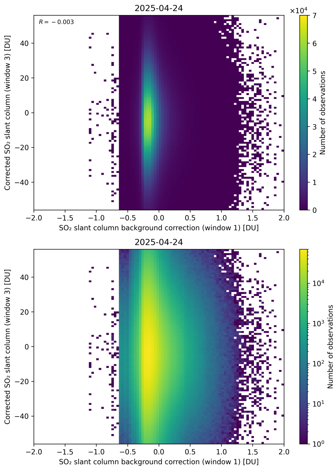
Figure 116: Scatter density plot of “SO 2 slant column background correction (window 1)” against “Corrected SO 2 slant column (window 3)” for 2025-04-24 to 2025-04-25.
