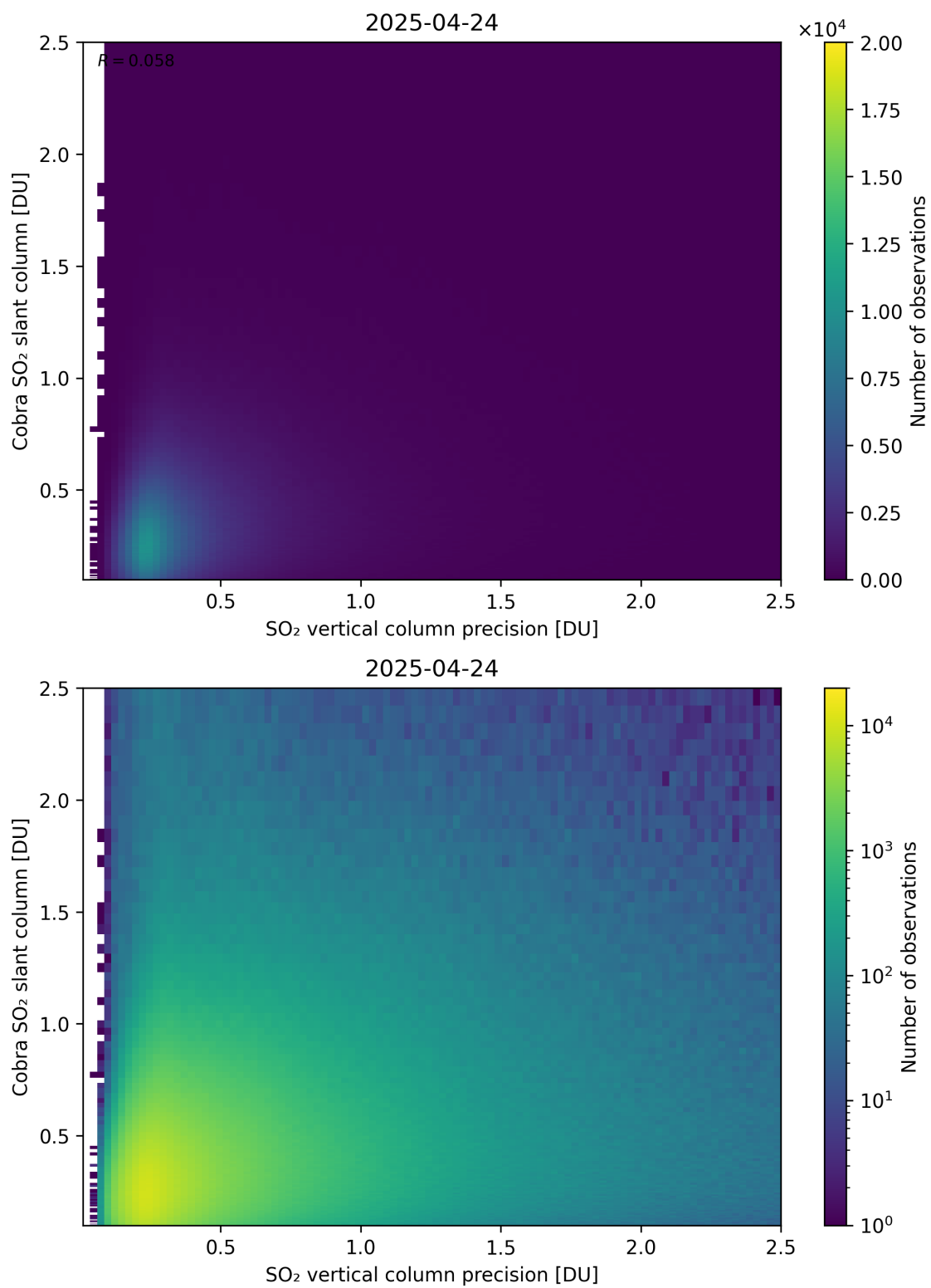
Figure 336: Scatter density plot of “SO 2 vertical column precision” against “Cobra SO 2 slant column” for 2025-04-24 to 2025-04-25.
