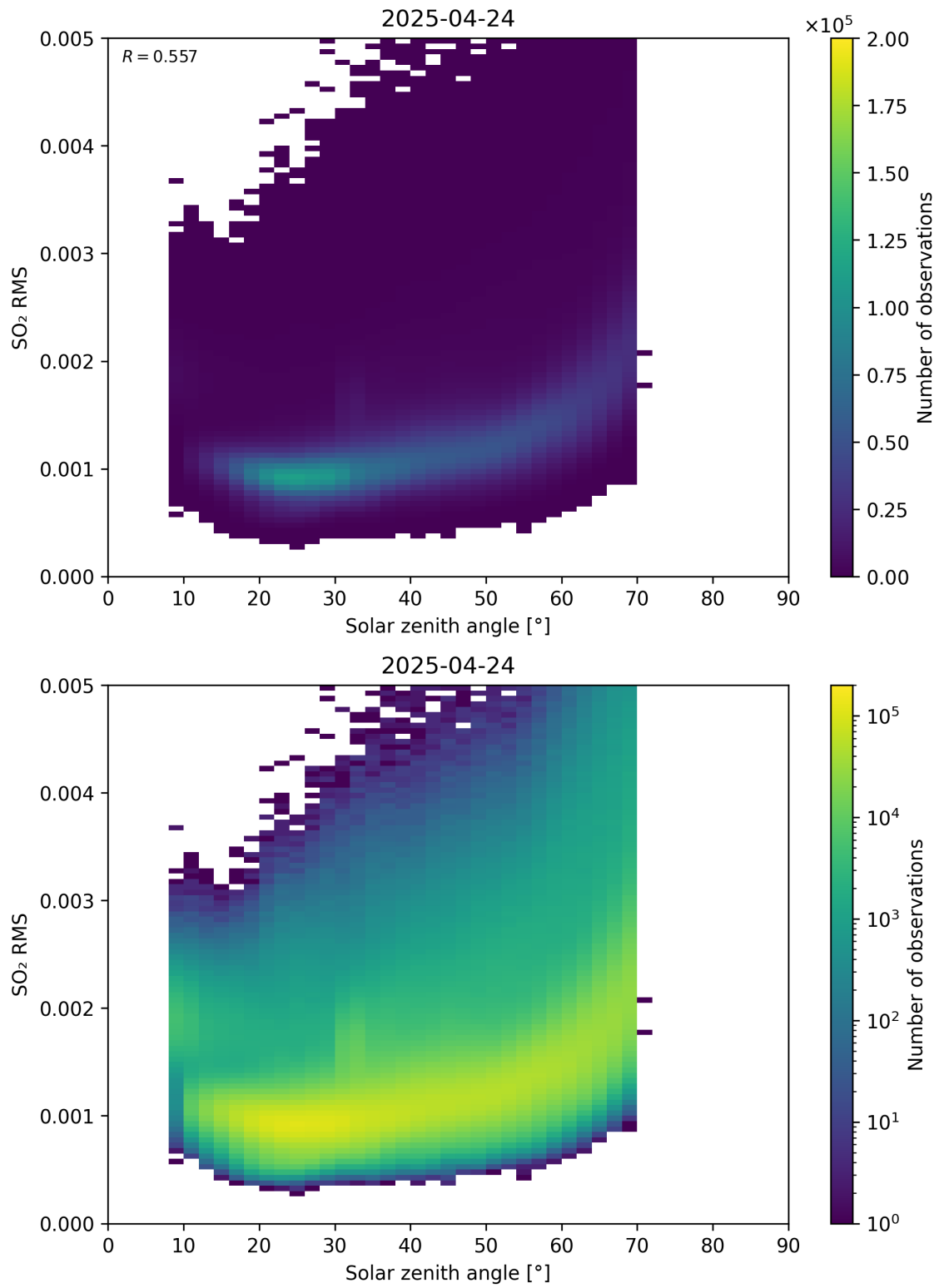
Figure 176: Scatter density plot of “Solar zenith angle” against “SO 2 RMS” for 2025-04-24 to 2025-04-25.
