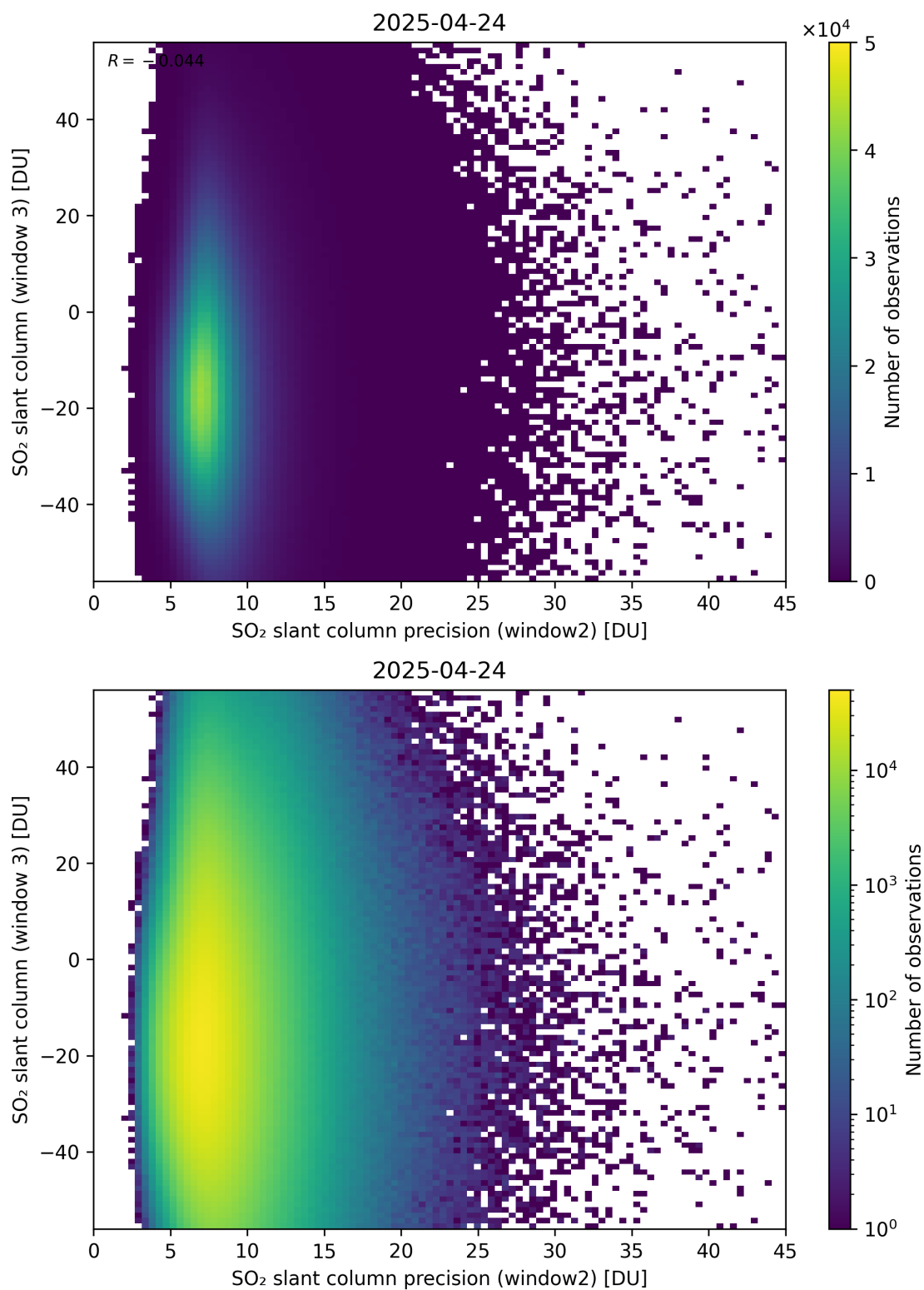
Figure 299: Scatter density plot of “SO 2 slant column precision (window2)” against “SO 2 slant column (window 3)” for 2025-04-24 to 2025-04-25.
