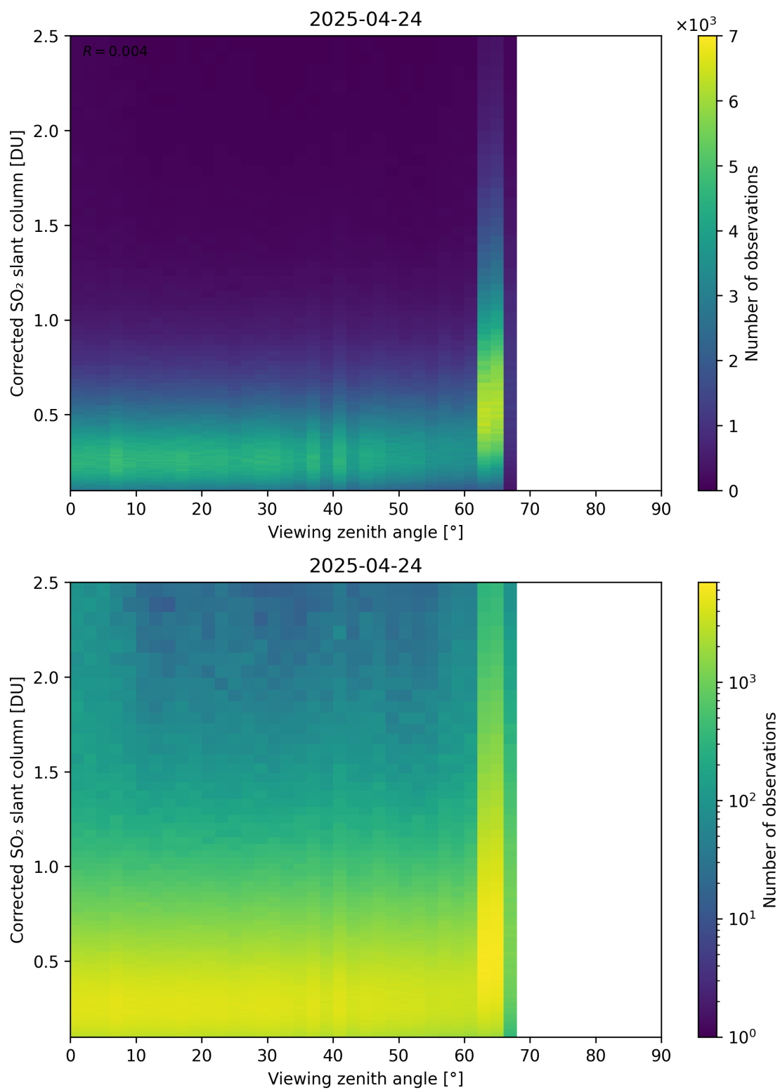
Figure 373: Scatter density plot of “Viewing zenith angle” against “Corrected SO 2 slant column” for 2025-04-24 to 2025-04-25.
