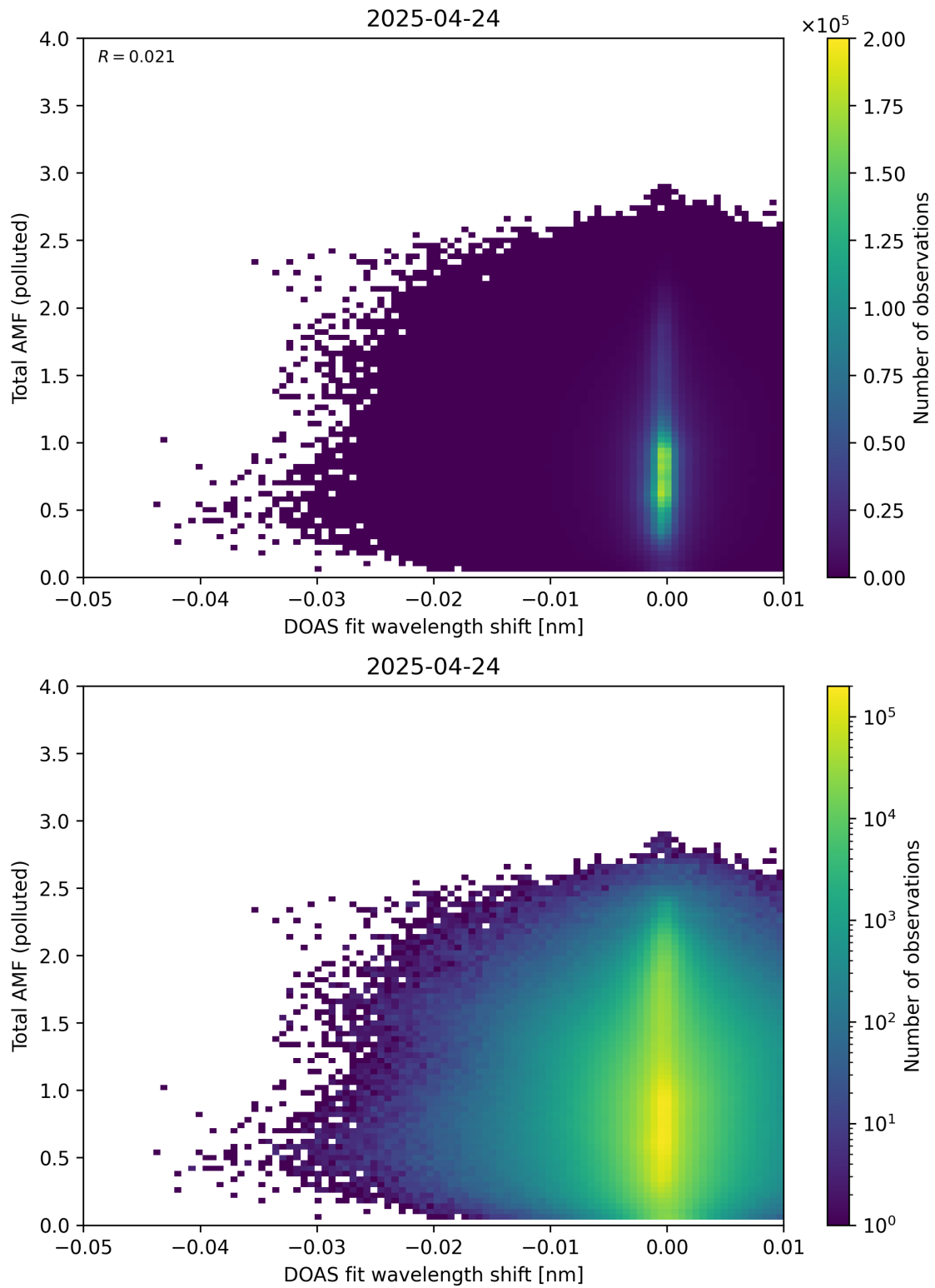
Figure 141: Scatter density plot of “DOAS fit wavelength shift” against “Total AMF (polluted)” for 2025-04-24 to 2025-04-25.
