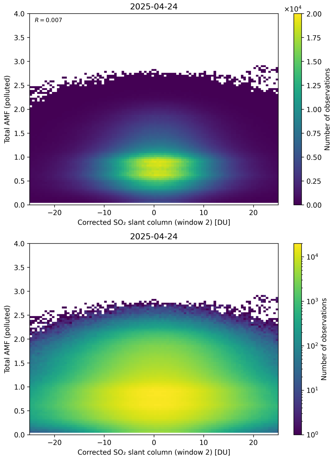
Figure 253: Scatter density plot of “Corrected SO 2 slant column (window 2)” against “Total AMF (polluted)” for 2025-04-24 to 2025-04-25.
