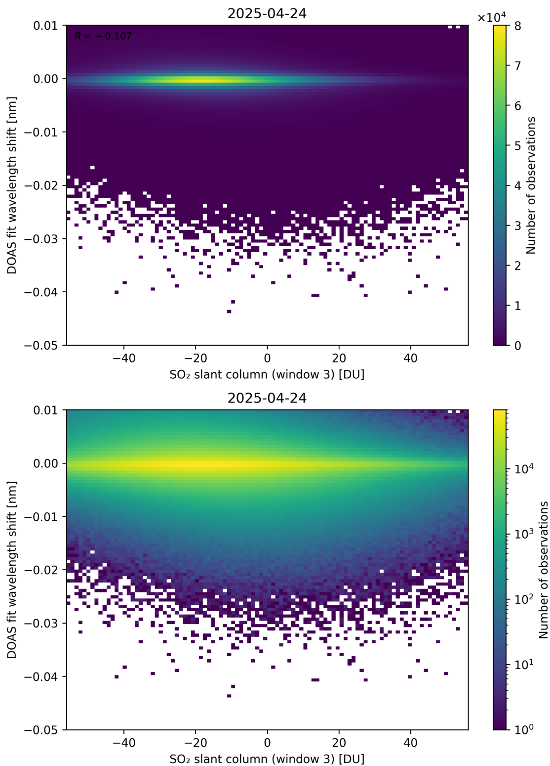
Figure 304: Scatter density plot of “SO 2 slant column (window 3)” against “DOAS fit wavelength shift” for 2025-04-24 to 2025-04-25.
