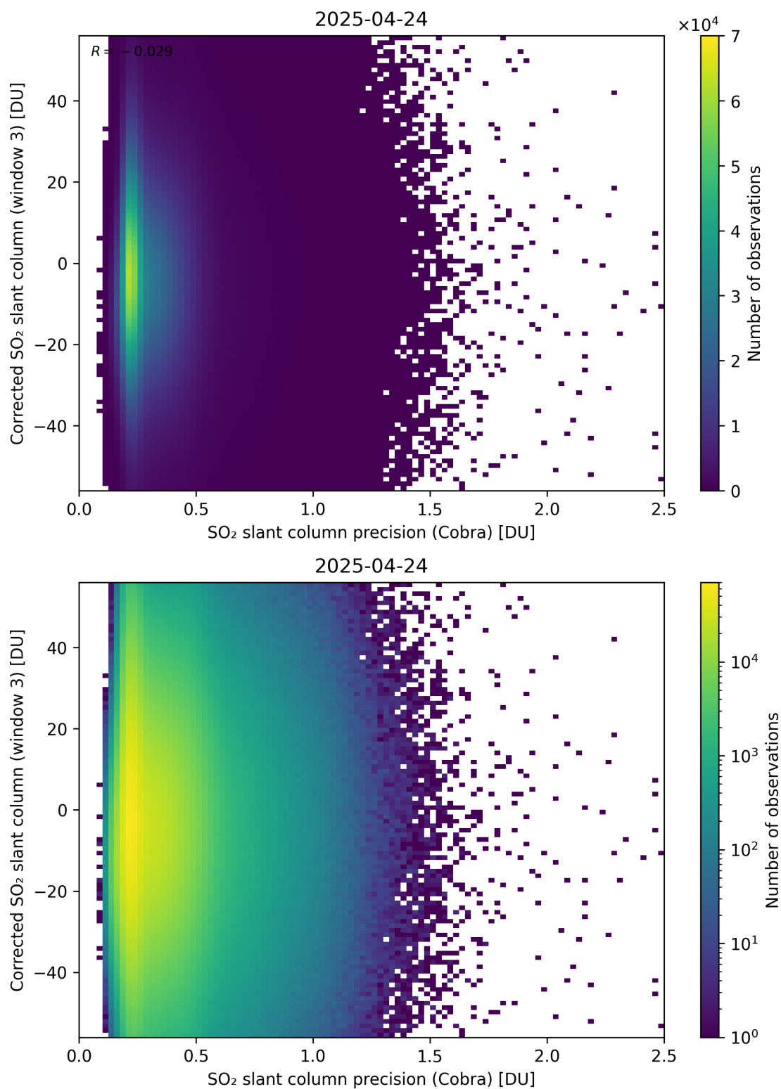
Figure 207: Scatter density plot of “SO 2 slant column precision (Cobra)” against “Corrected SO 2 slant column (window 3)” for 2025-04-24 to 2025-04-25.
