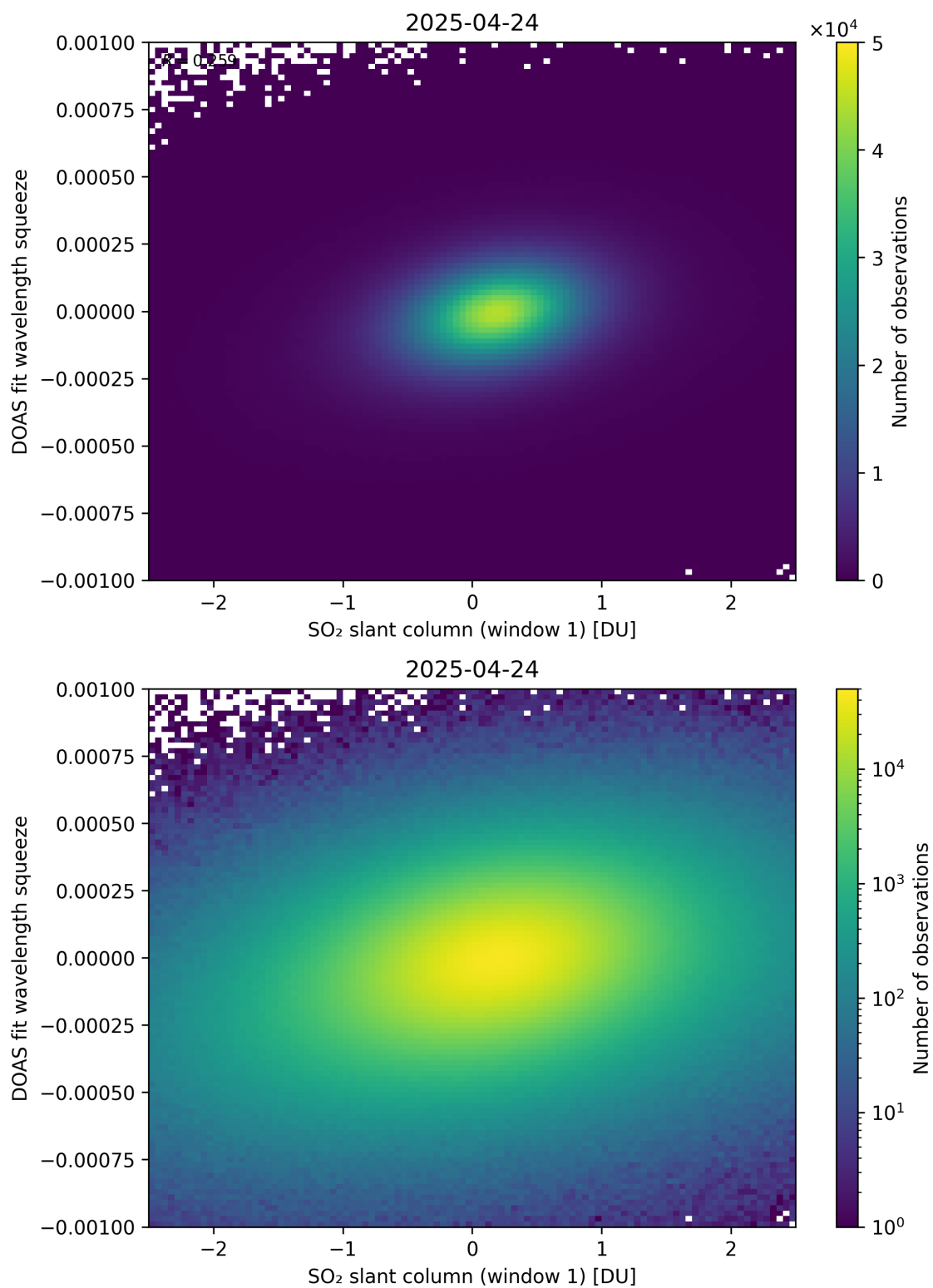
Figure 266: Scatter density plot of “SO 2 slant column (window 1)” against “DOAS fit wavelength squeeze” for 2025-04-24 to 2025-04-25.
