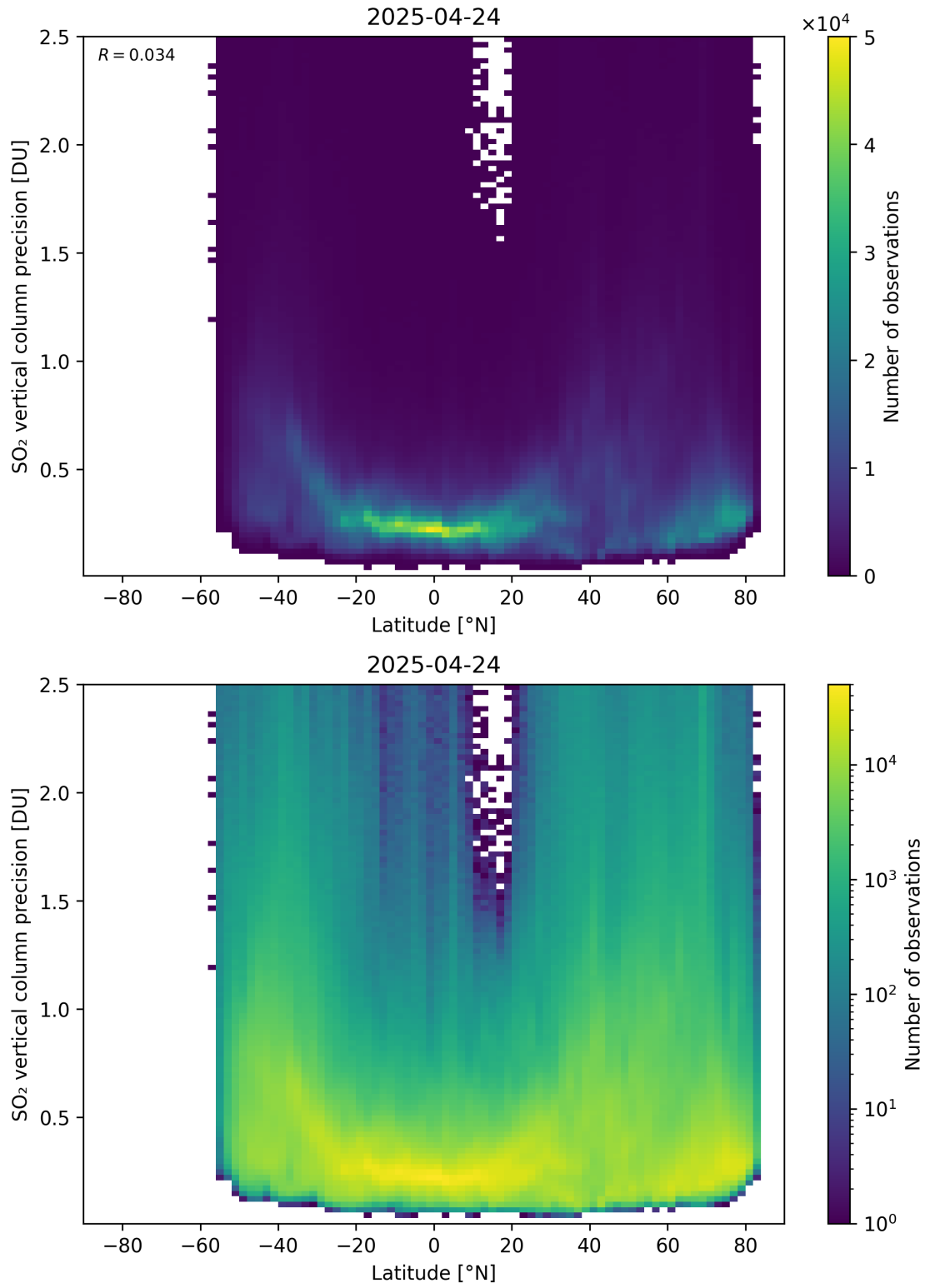
Figure 170: Scatter density plot of “Latitude” against “SO 2 vertical column precision” for 2025-04-24 to 2025-04-25.
