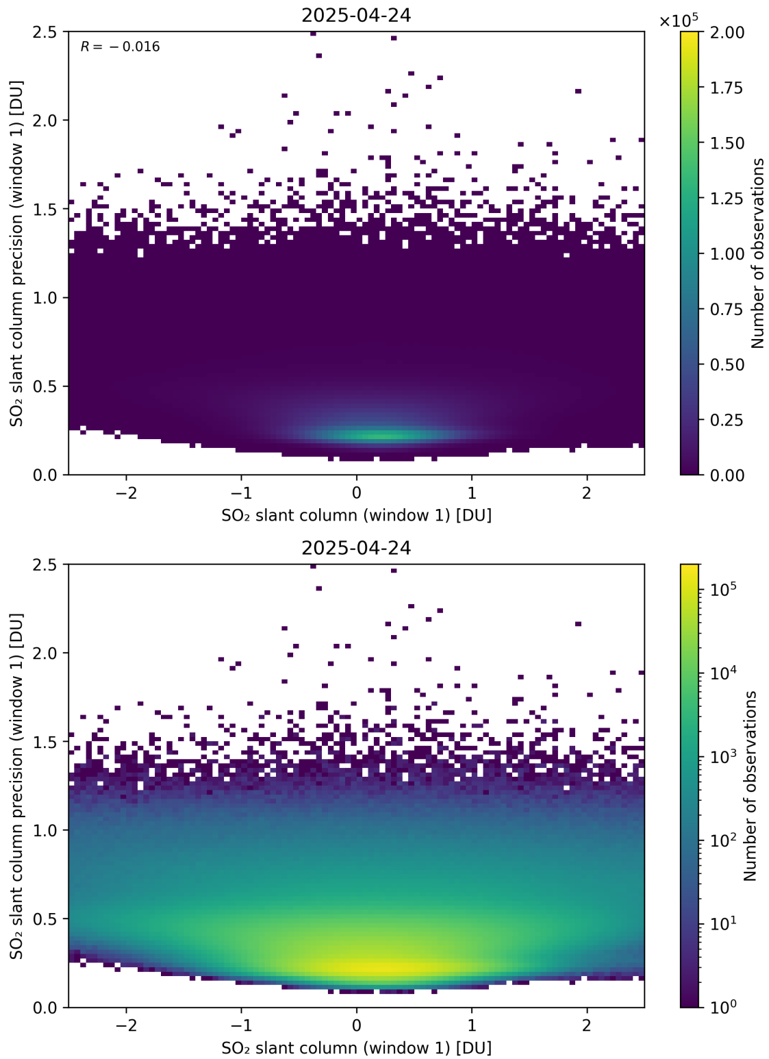
Figure 285: Scatter density plot of “SO 2 slant column (window 1)” against “SO 2 slant column precision (window 1)” for 2025-04-24 to 2025-04-25.
