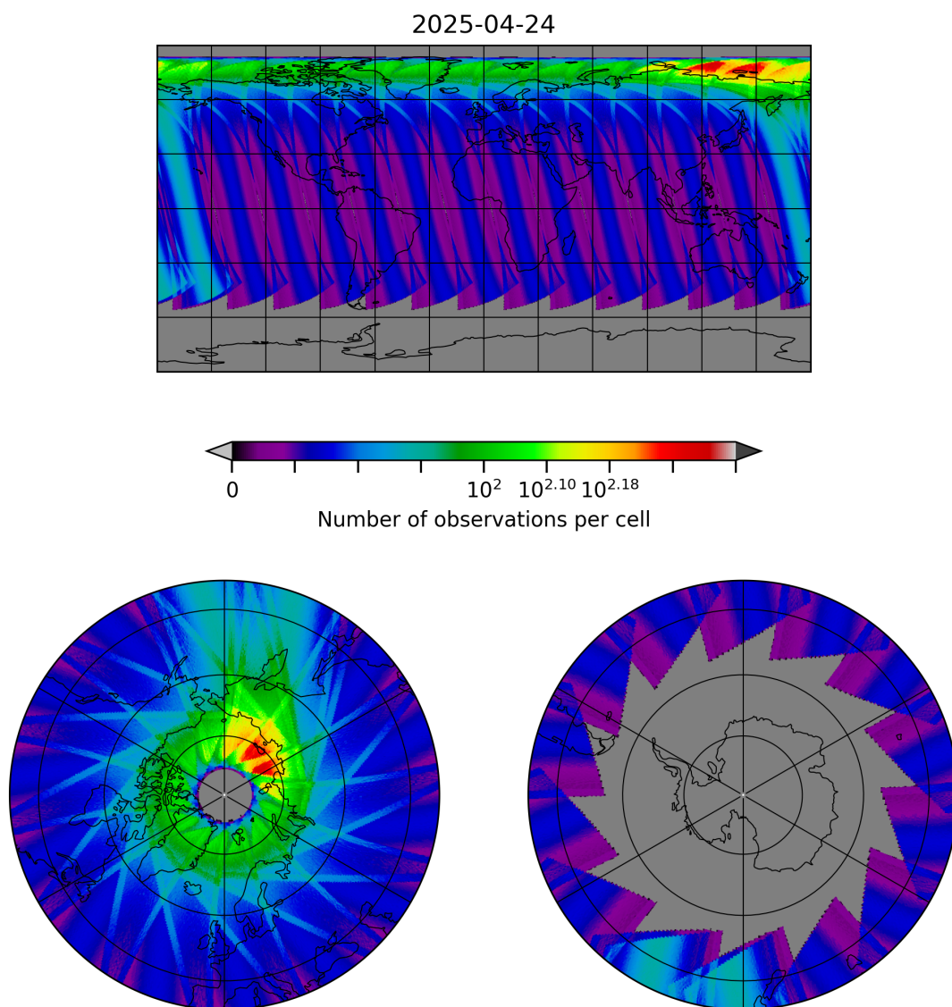
Figure 30: Map of the number of observations for 2025-04-24 to 2025-04-25
