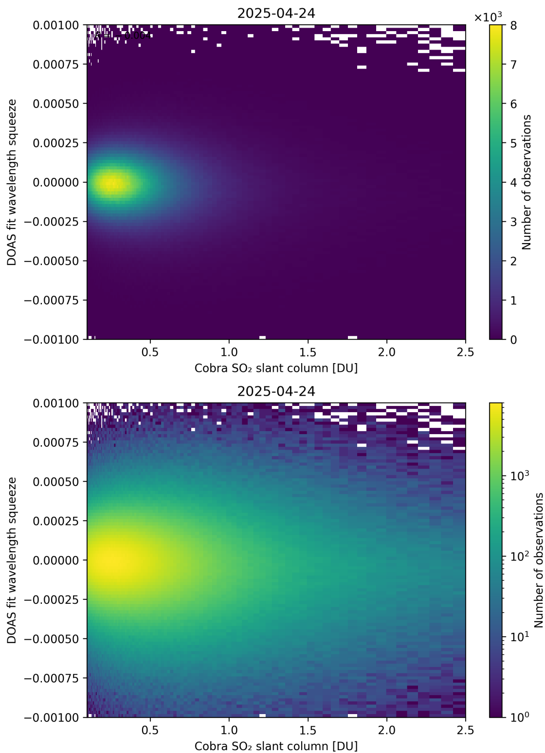
Figure 197: Scatter density plot of “Cobra SO 2 slant column” against “DOAS fit wavelength squeeze” for 2025-04-24 to 2025-04-25.
