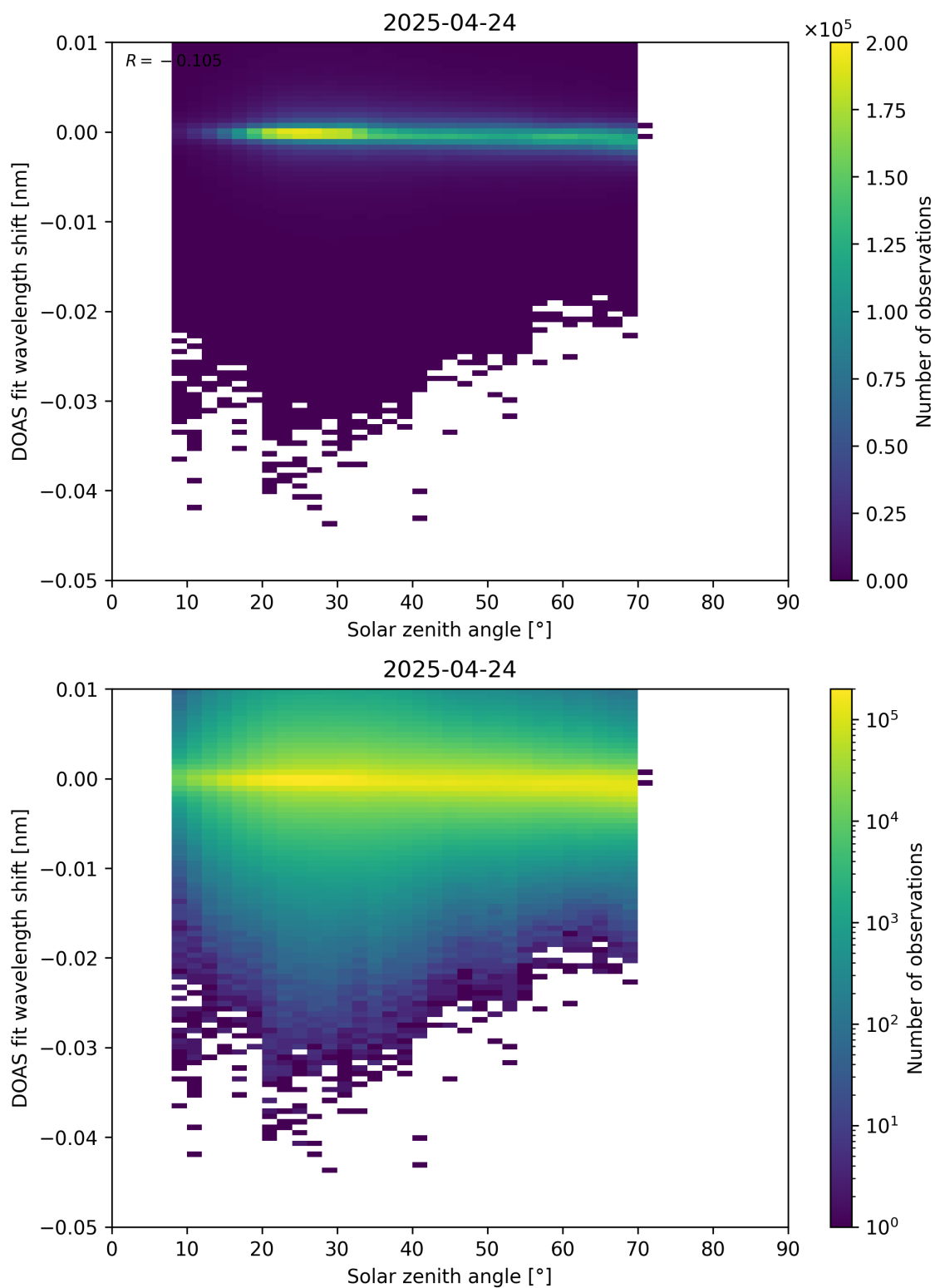
Figure 174: Scatter density plot of “Solar zenith angle” against “DOAS fit wavelength shift” for 2025-04-24 to 2025-04-25.
