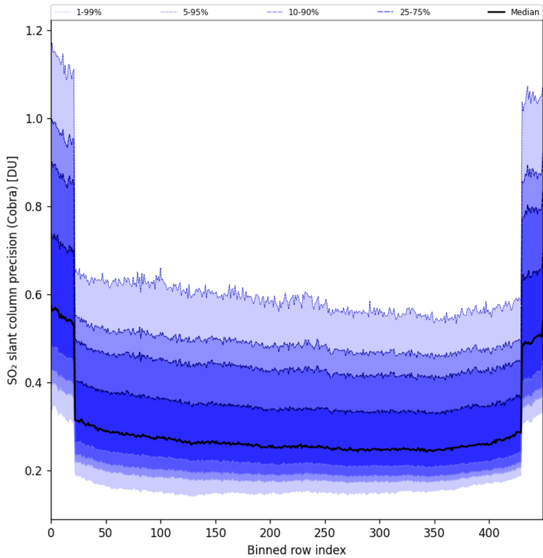
Figure 88: Along track statistics of “SO 2 slant column precision (Cobra)” for 2025-04-24 to 2025-04-25
