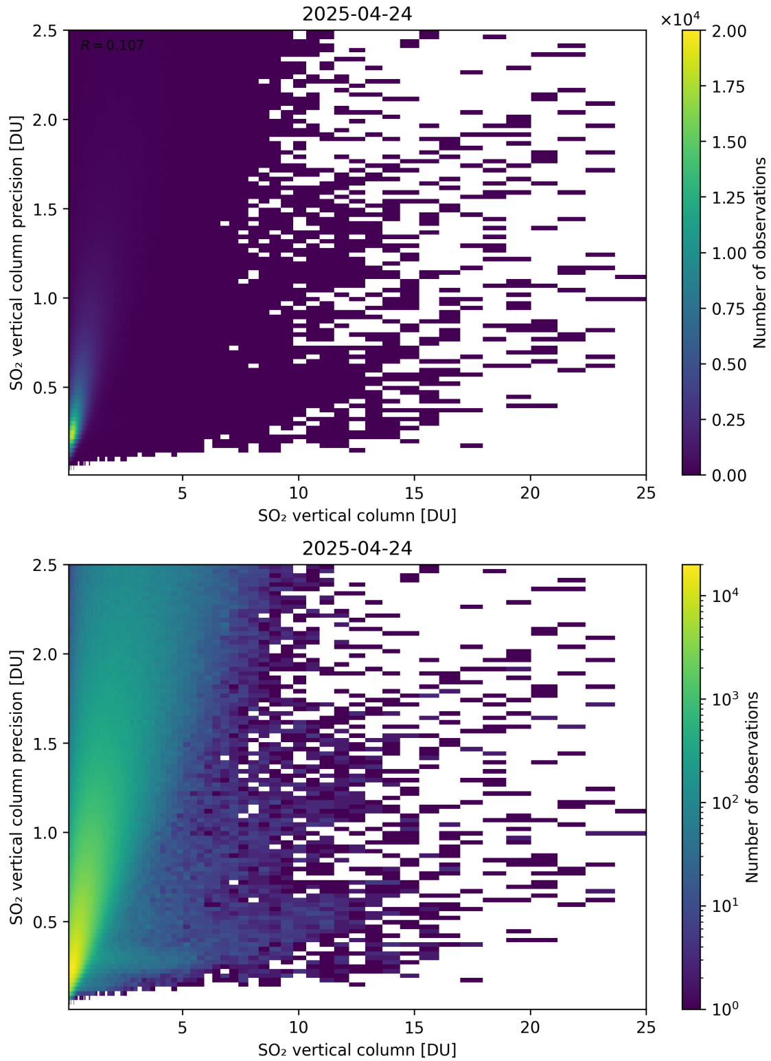
Figure 361: Scatter density plot of “SO 2 vertical column” against “SO 2 vertical column precision” for 2025-04-24 to 2025-04-25.
