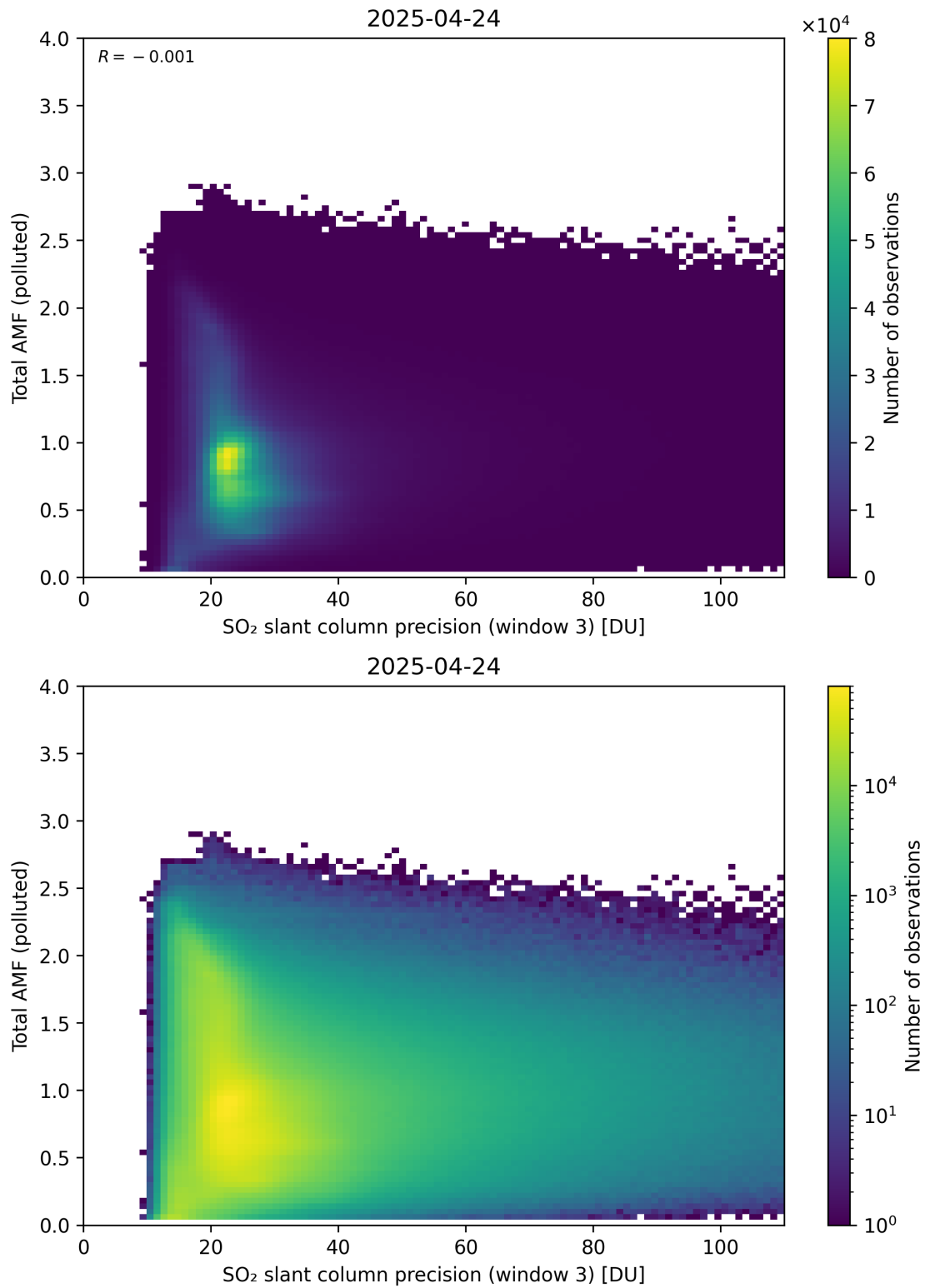
Figure 313: Scatter density plot of “SO 2 slant column precision (window 3)” against “Total AMF (polluted)” for 2025-04-24 to 2025-04-25.
