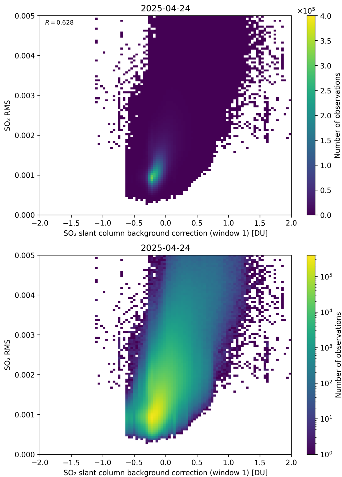
Figure 113: Scatter density plot of “SO 2 slant column background correction (window 1)” against “SO 2 RMS” for 2025-04-24 to 2025-04-25.
