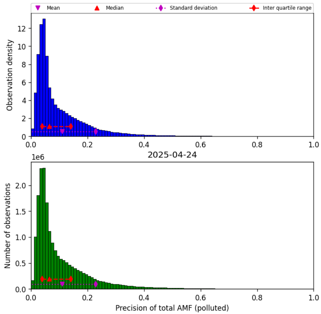
Figure 80: Histogram of “Precision of total AMF (polluted)” for 2025-04-24 to 2025-04-25
