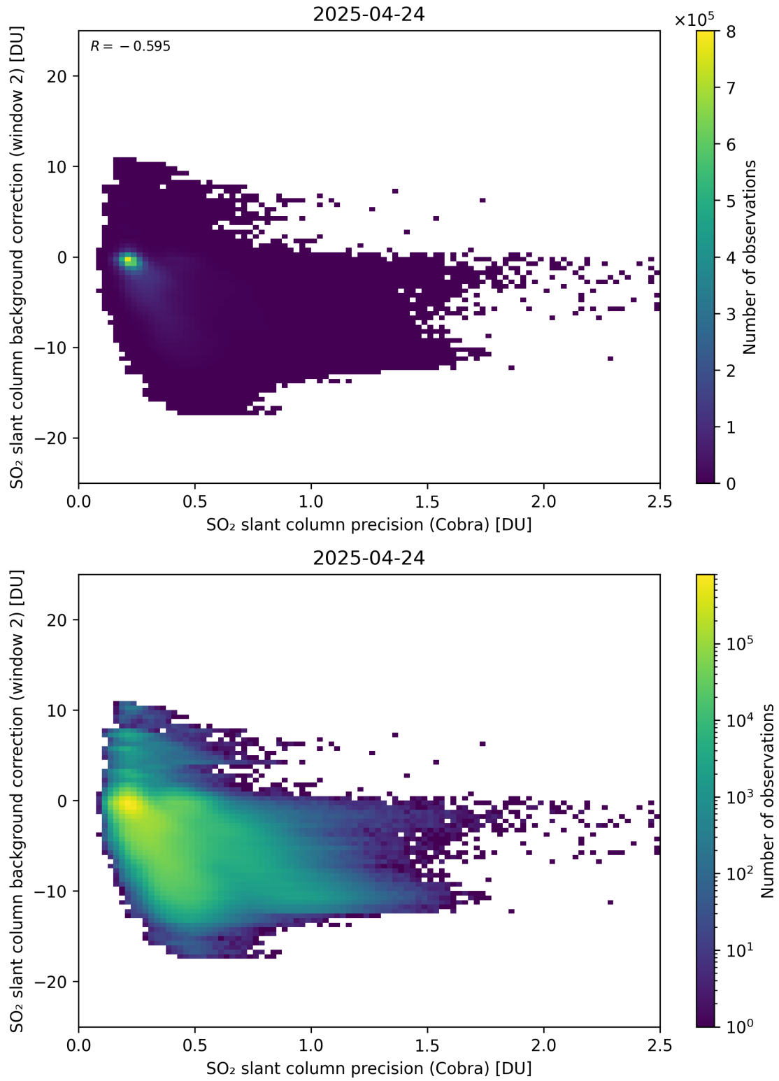
Figure 200: Scatter density plot of “SO 2 slant column precision (Cobra)” against “SO 2 slant column background correction (window 2)” for 2025-04-24 to 2025-04-25.
