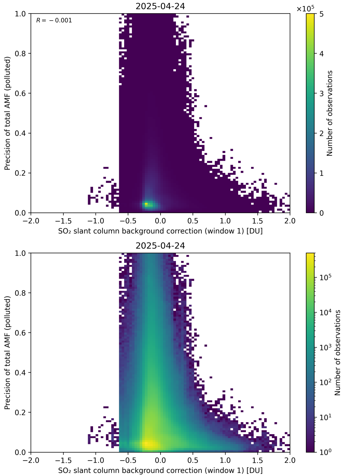
Figure 121: Scatter density plot of “SO 2 slant column background correction (window 1)” against “Precision of total AMF (polluted)” for 2025-04-24 to 2025-04-25.
