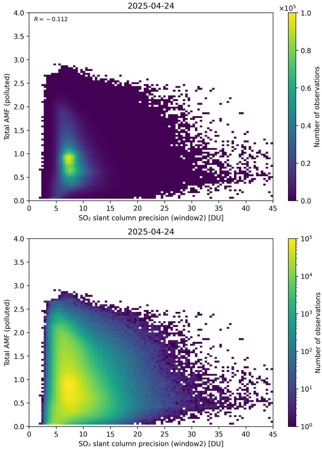
Figure 301: Scatter density plot of “SO 2 slant column precision (window2)” against “Total AMF (polluted)” for 2025-04-24 to 2025-04-25.
