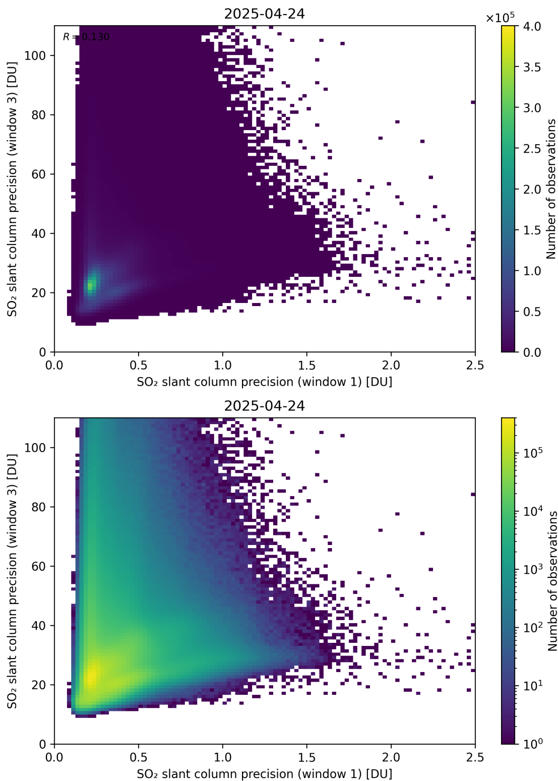
Figure 279: Scatter density plot of “SO 2 slant column precision (window 1)” against “SO 2 slant column precision (window 3)” for 2025-04-24 to 2025-04-25.
