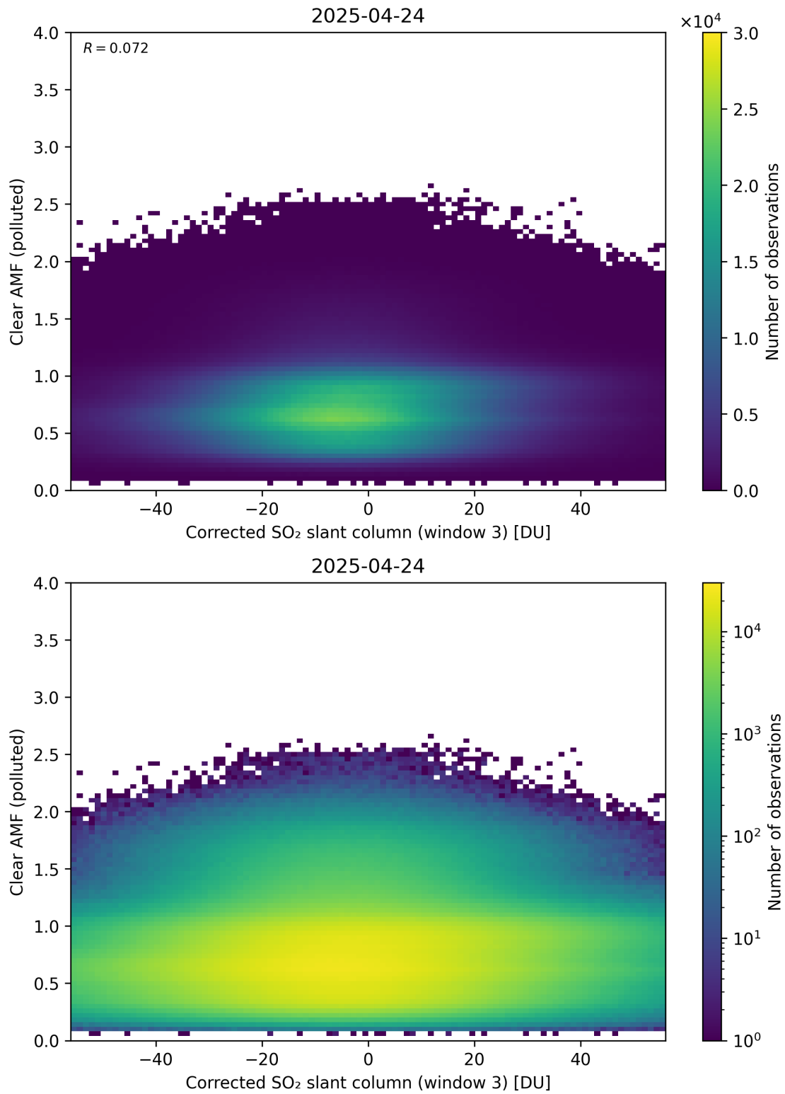
Figure 259: Scatter density plot of “Corrected SO 2 slant column (window 3)” against “Clear AMF (polluted)” for 2025-04-24 to 2025-04-25.
