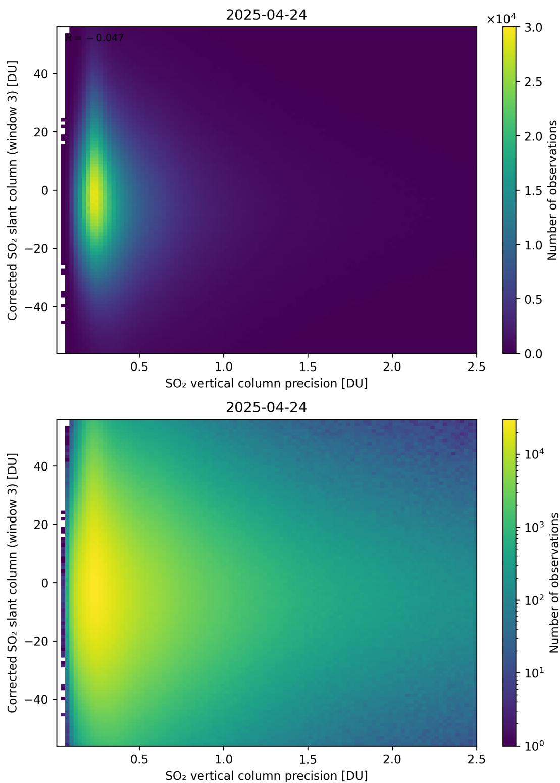
Figure 340: Scatter density plot of “SO 2 vertical column precision” against “Corrected SO 2 slant column (window 3)” for 2025-04-24 to 2025-04-25.
