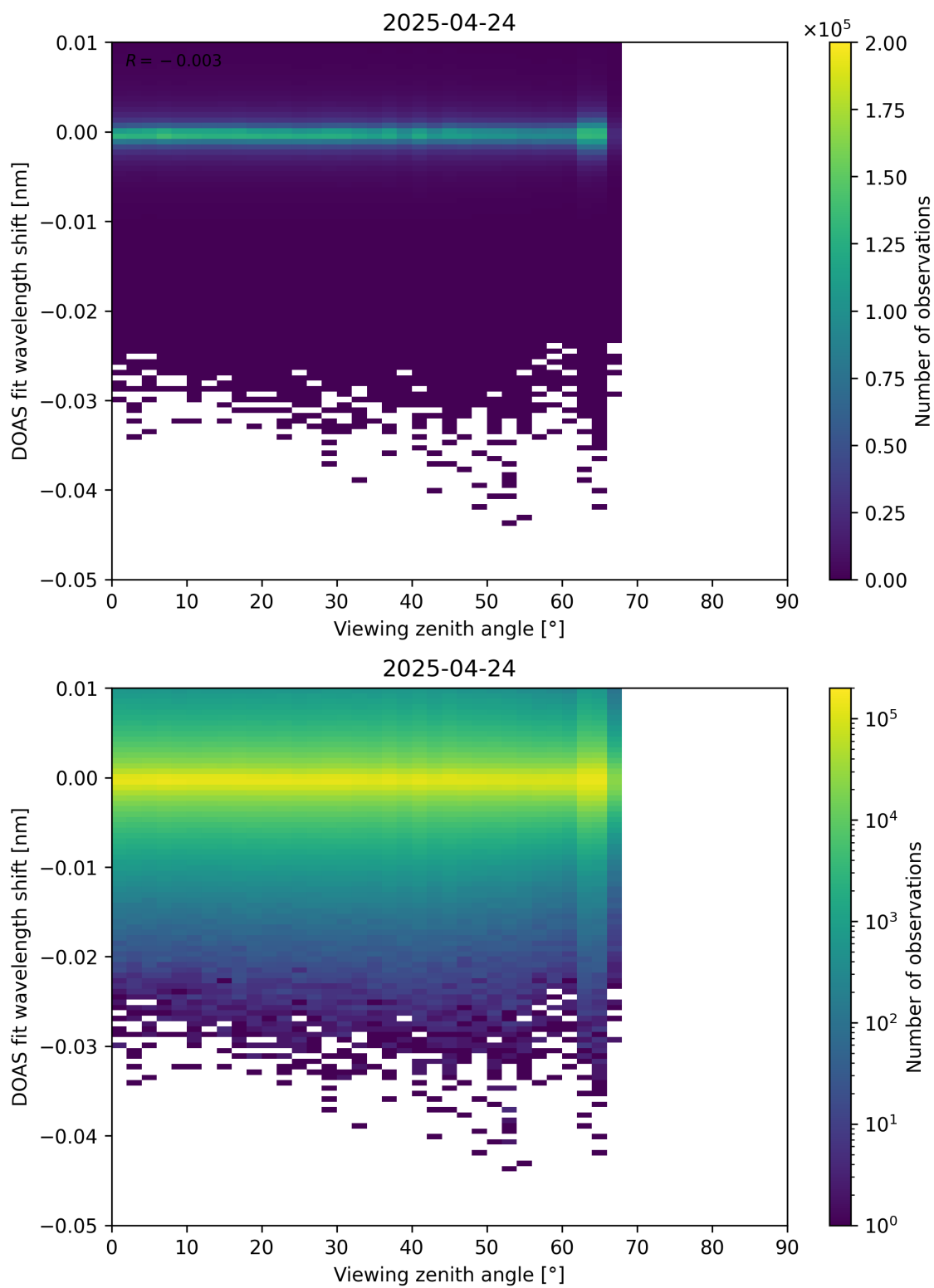
Figure 365: Scatter density plot of “Viewing zenith angle” against “DOAS fit wavelength shift” for 2025-04-24 to 2025-04-25.
