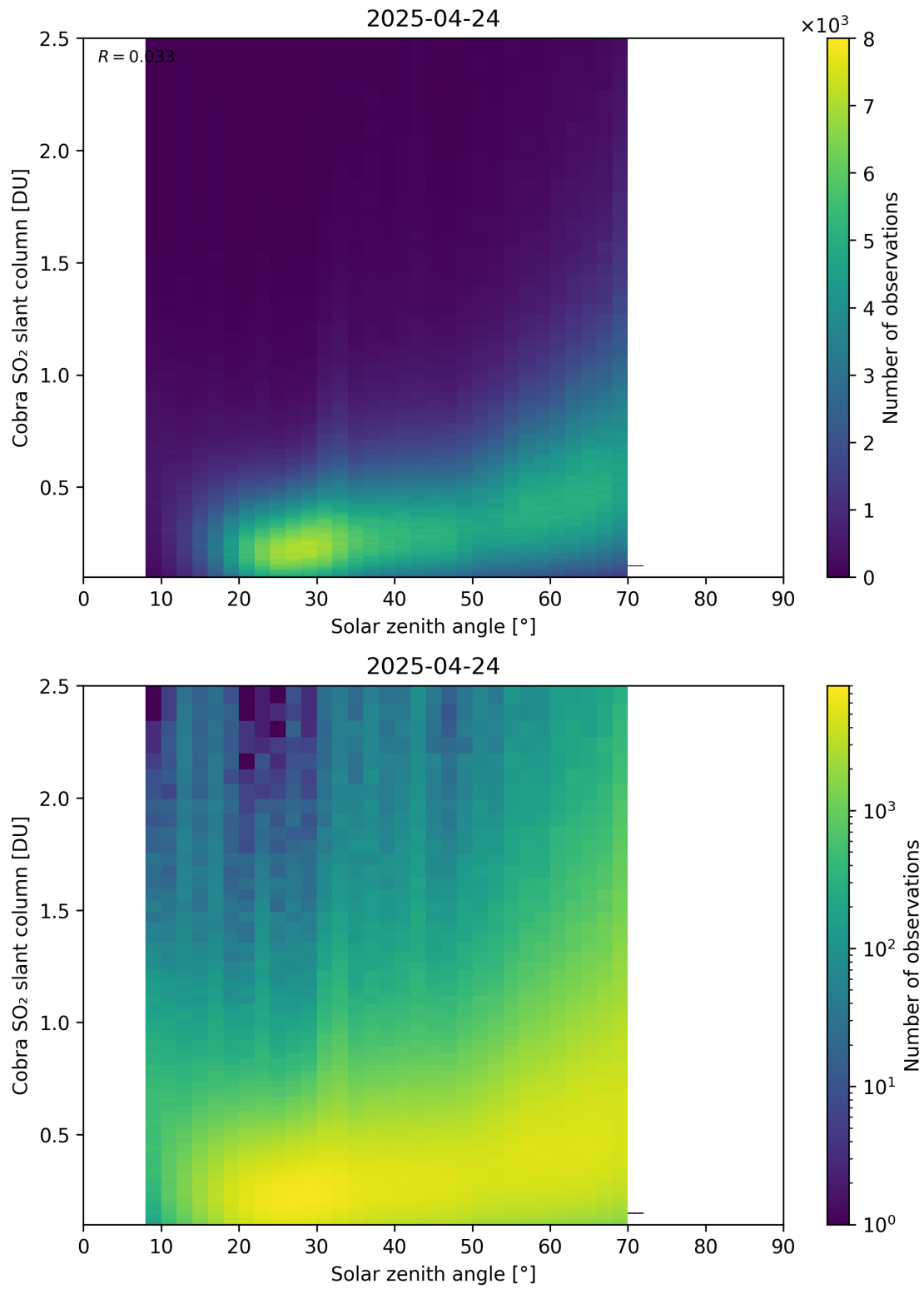
Figure 179: Scatter density plot of “Solar zenith angle” against “Cobra SO 2 slant column” for 2025-04-24 to 2025-04-25.
