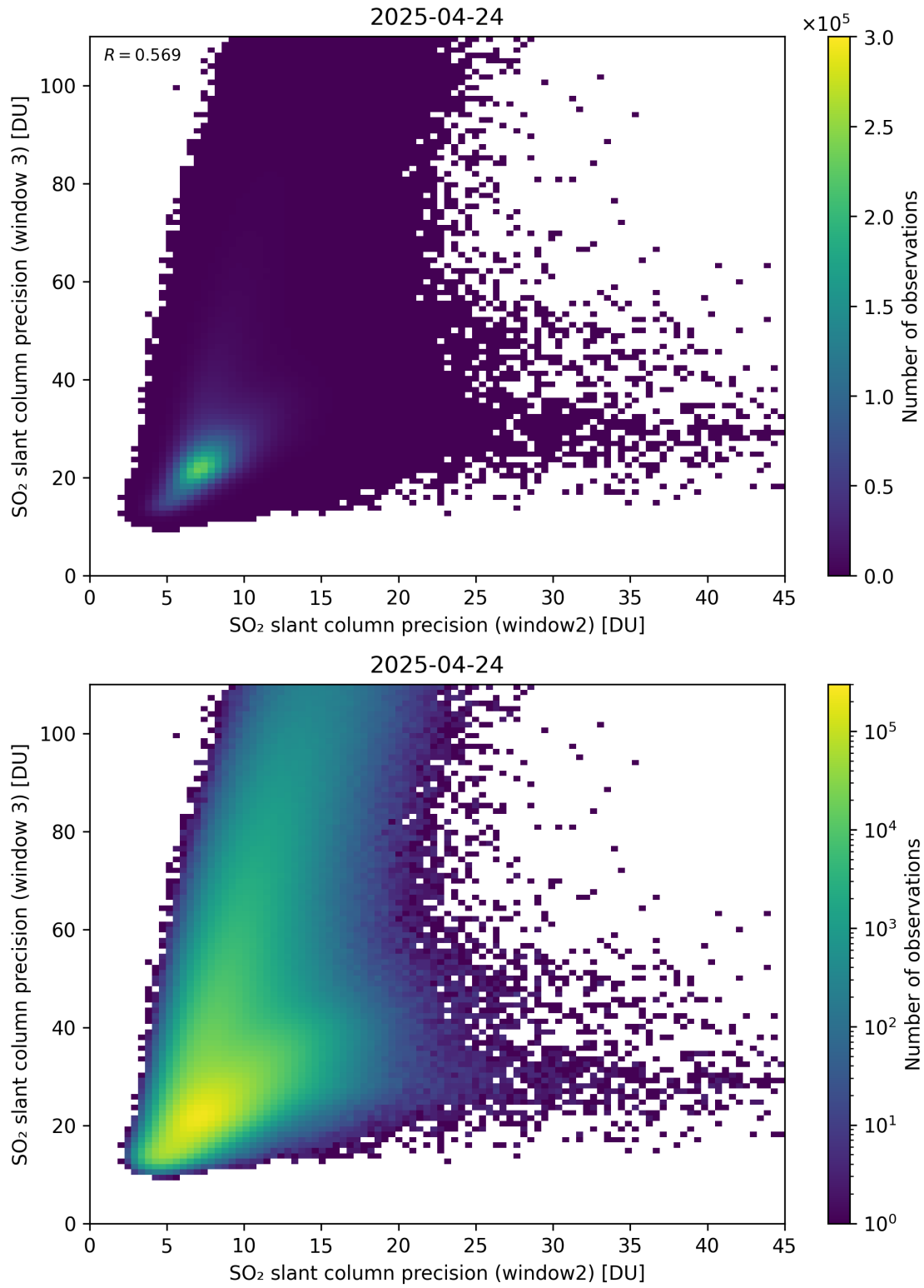
Figure 300: Scatter density plot of “SO 2 slant column precision (window2)” against “SO 2 slant column precision (window 3)” for 2025-04-24 to 2025-04-25.
