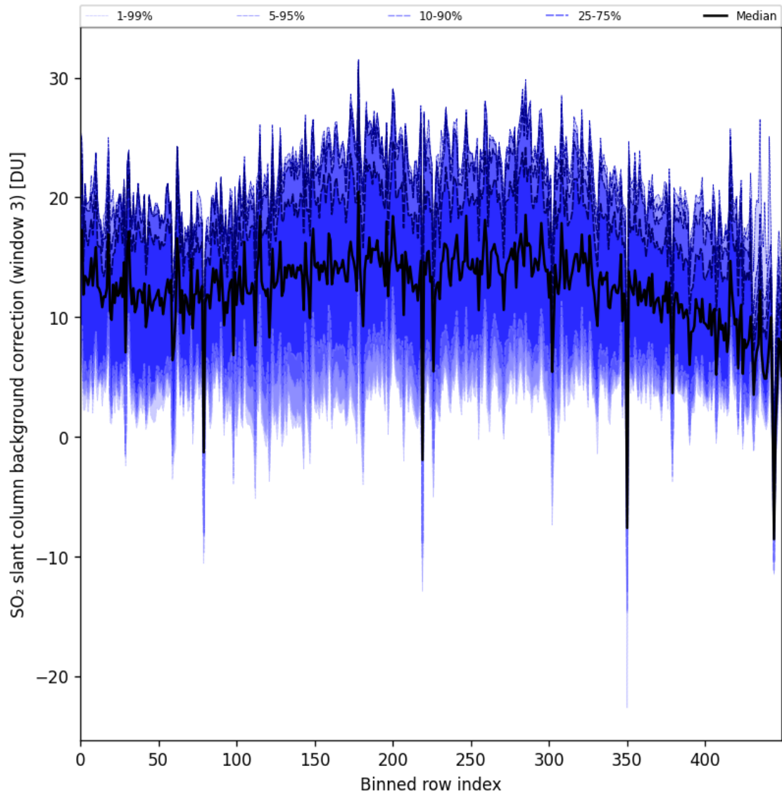
Figure 100: Along track statistics of “SO 2 slant column background correction (window 3)” for 2025-04-24 to 2025-04-25
