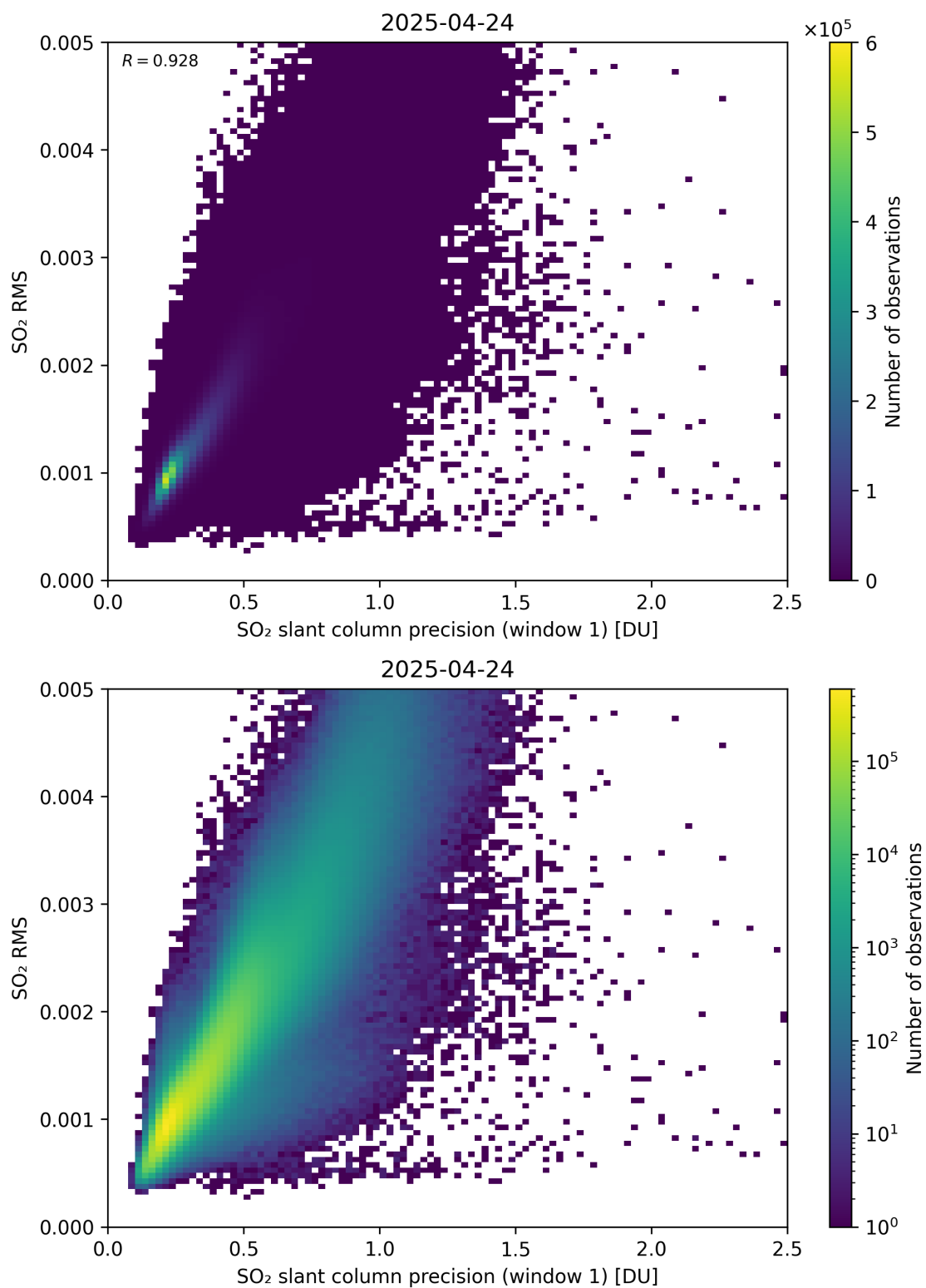
Figure 273: Scatter density plot of “SO 2 slant column precision (window 1)” against “SO 2 RMS” for 2025-04-24 to 2025-04-25.
