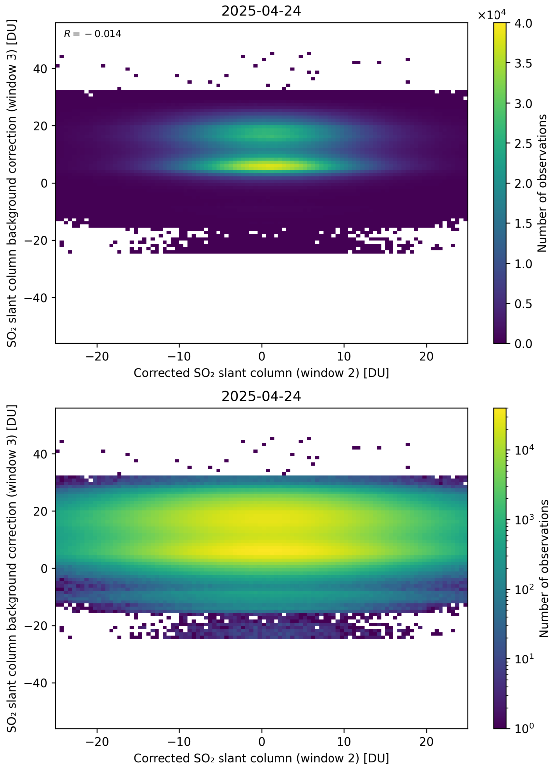
Figure 245: Scatter density plot of “Corrected SO 2 slant column (window 2)” against “SO 2 slant column background correction (window 3)” for 2025-04-24 to 2025-04-25.
