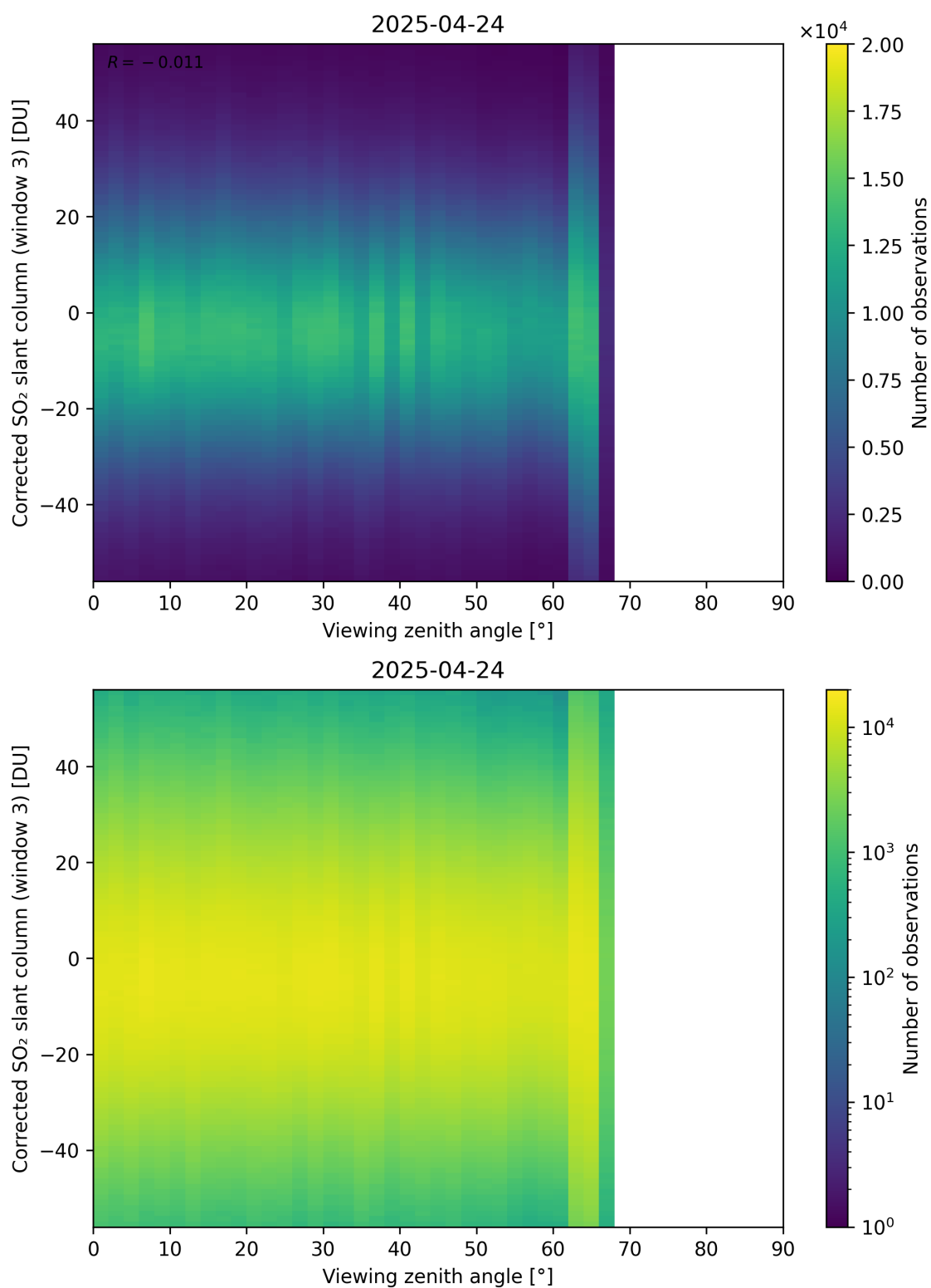
Figure 375: Scatter density plot of “Viewing zenith angle” against “Corrected SO 2 slant column (window 3)” for 2025-04-24 to 2025-04-25.
