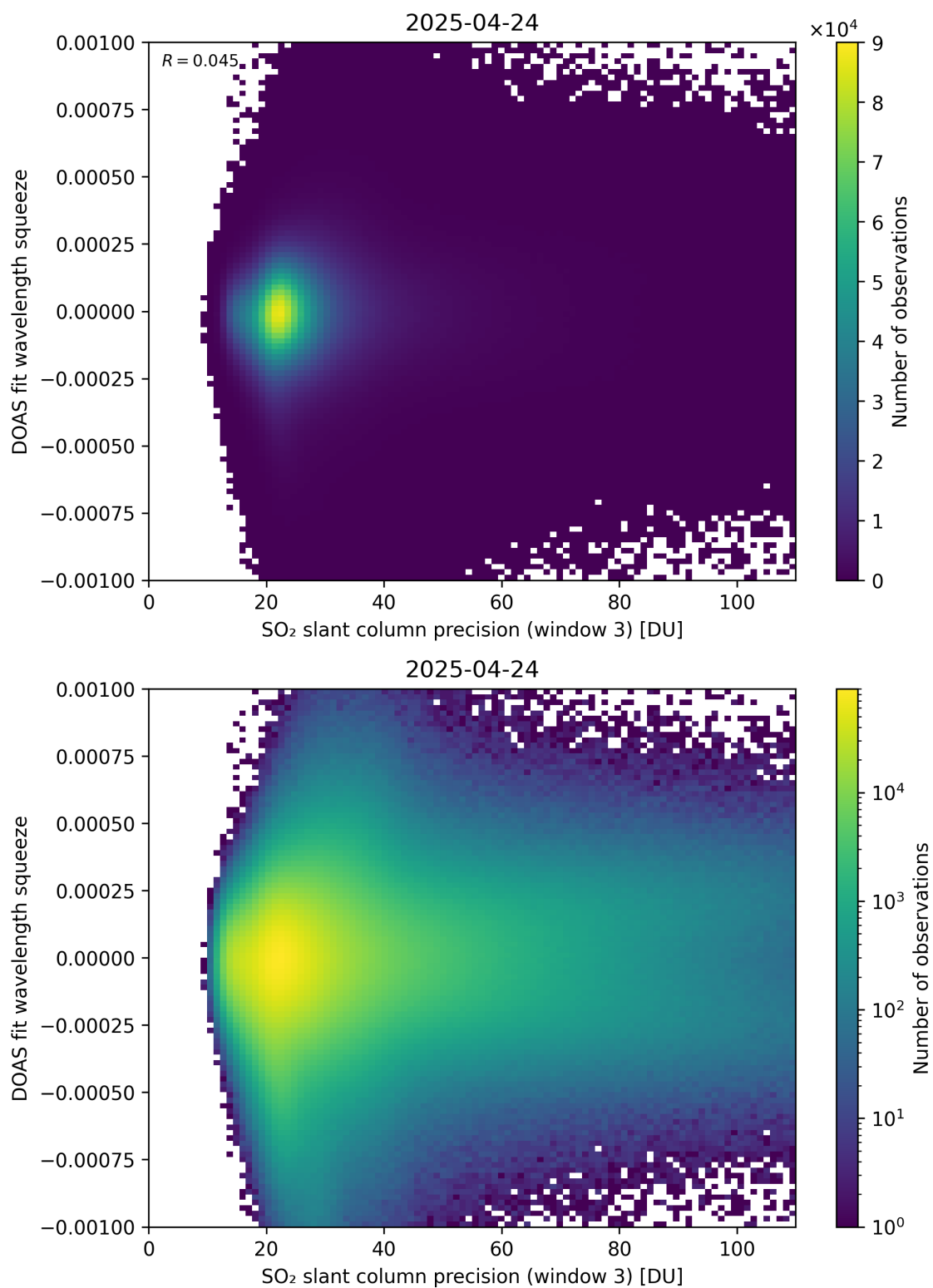
Figure 309: Scatter density plot of “SO 2 slant column precision (window 3)” against “DOAS fit wavelength squeeze” for 2025-04-24 to 2025-04-25.
