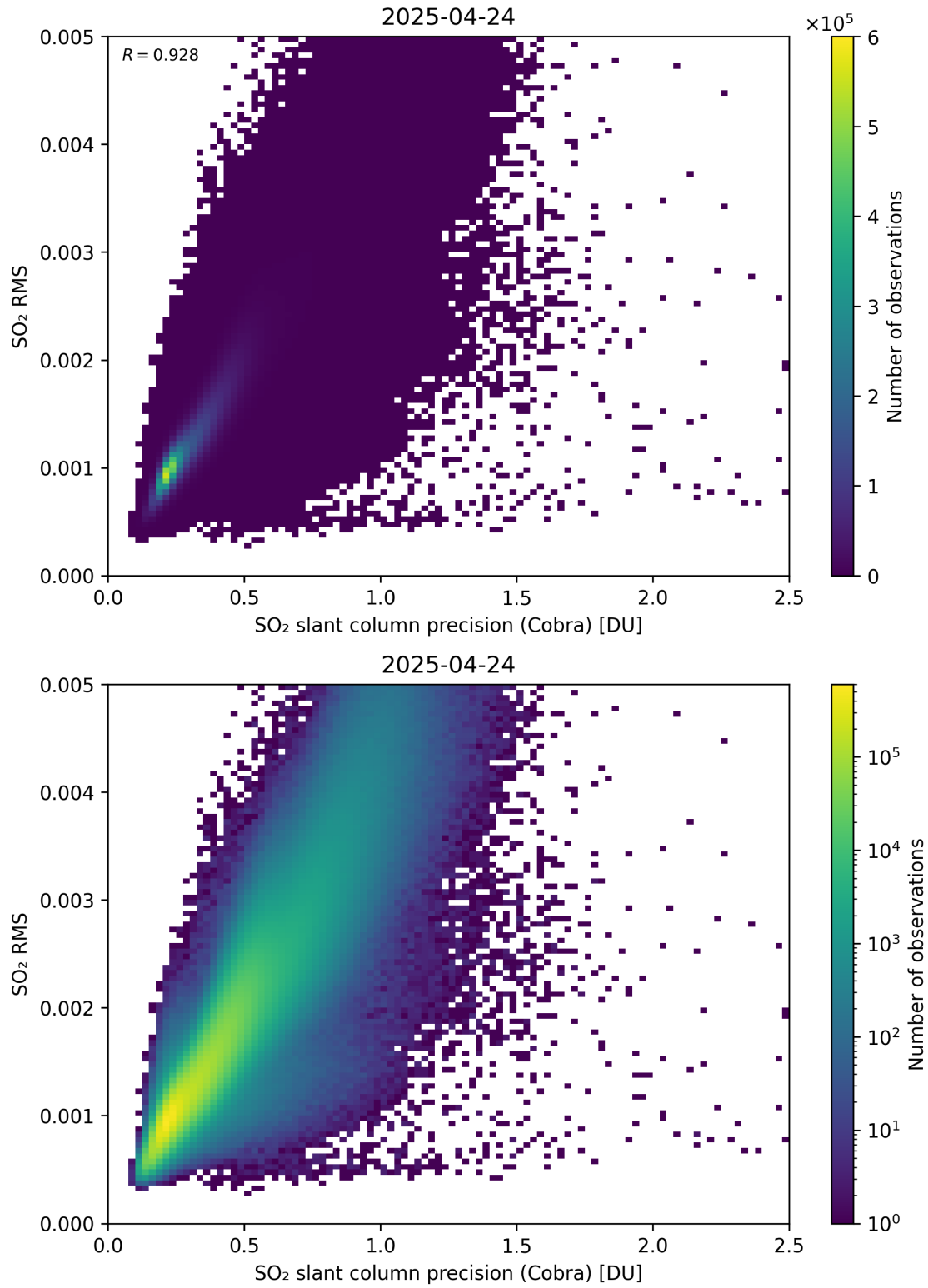
Figure 204: Scatter density plot of “SO 2 slant column precision (Cobra)” against “SO 2 RMS” for 2025-04-24 to 2025-04-25.
