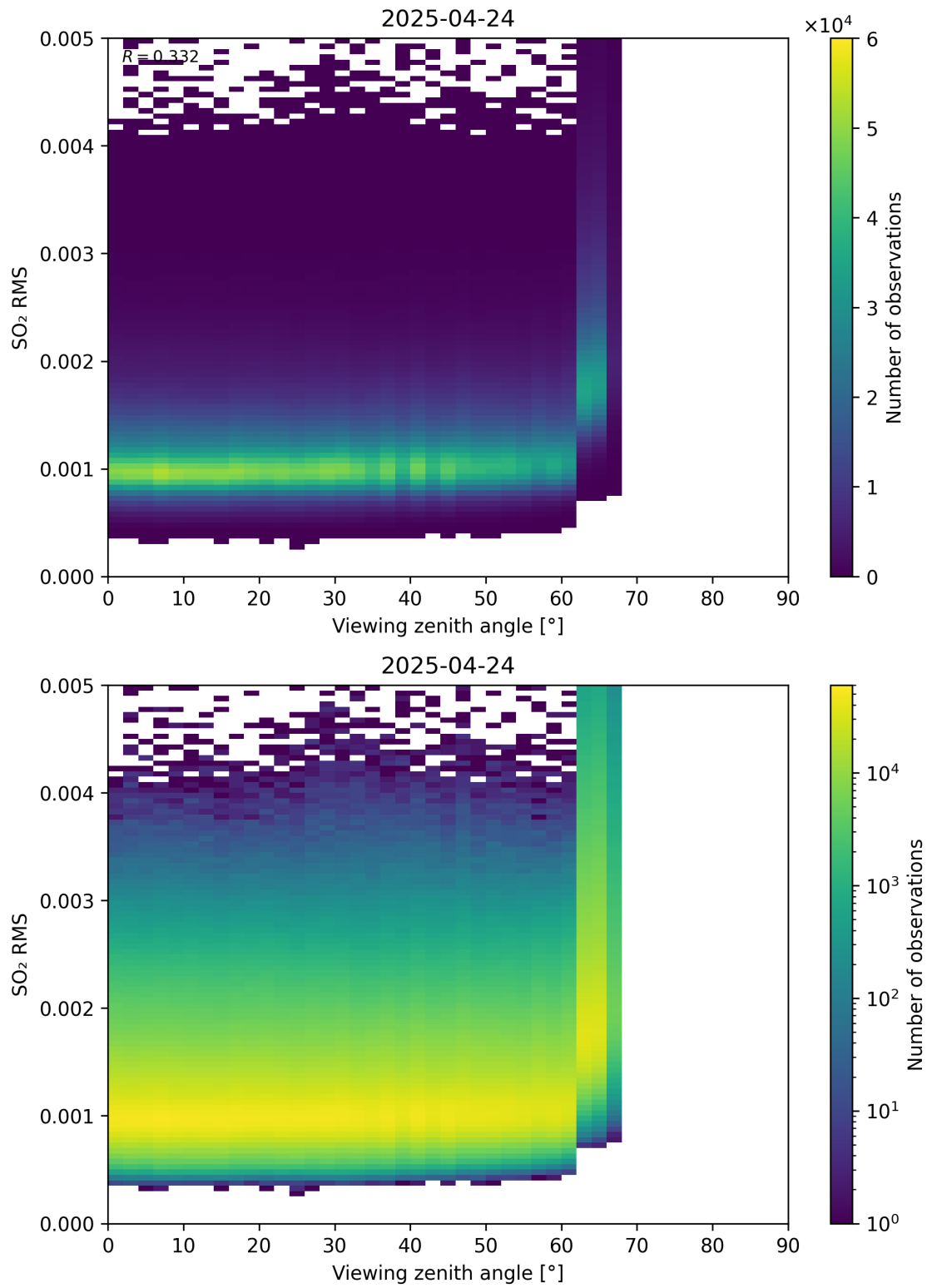
Figure 367: Scatter density plot of “Viewing zenith angle” against “SO 2 RMS” for 2025-04-24 to 2025-04-25.
