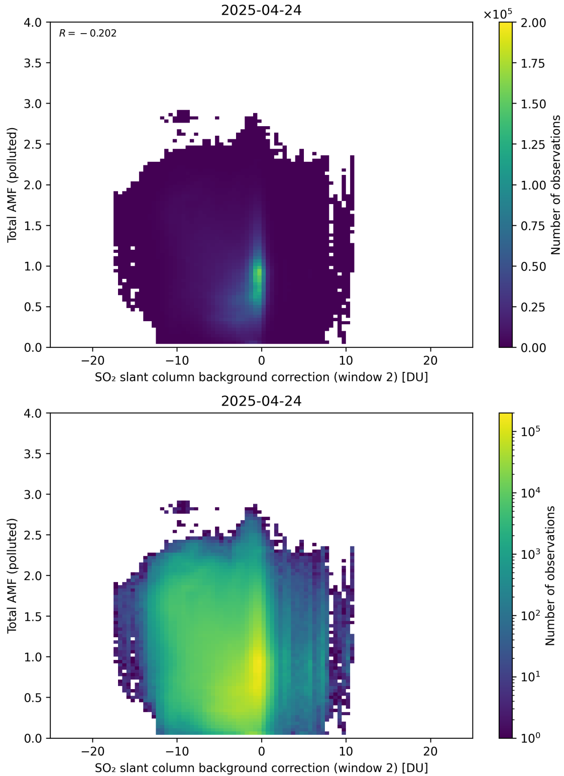
Figure 130: Scatter density plot of “SO 2 slant column background correction (window 2)” against “Total AMF (polluted)” for 2025-04-24 to 2025-04-25.
