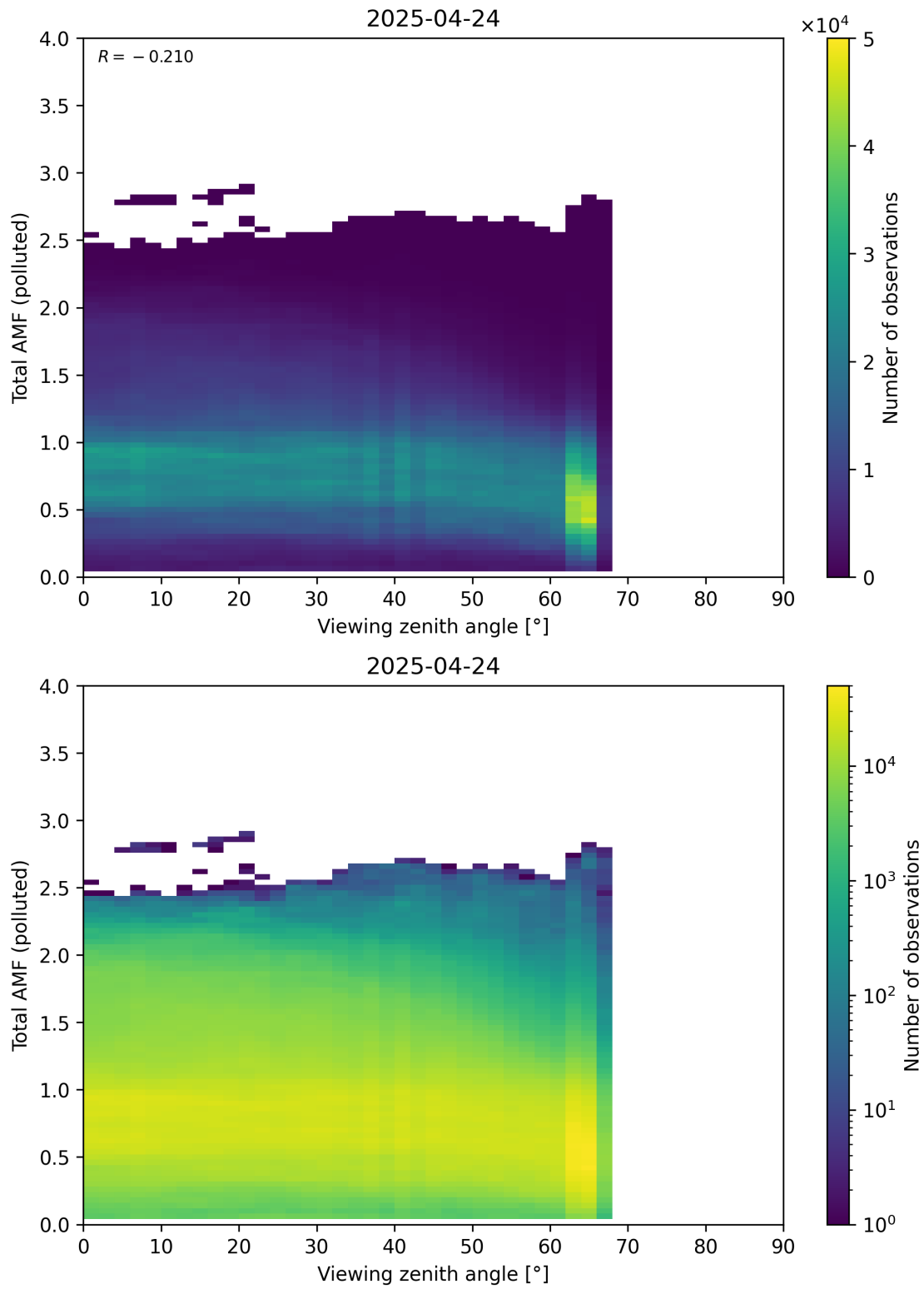
Figure 381: Scatter density plot of “Viewing zenith angle” against “Total AMF (polluted)” for 2025-04-24 to 2025-04-25.
