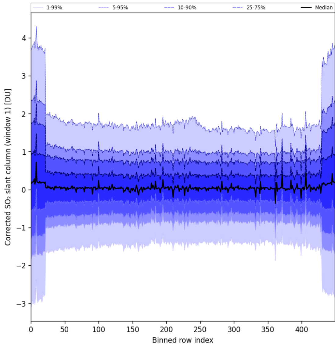
Figure 91: Along track statistics of “Corrected SO 2 slant column (window 1)” for 2025-04-24 to 2025-04-25
