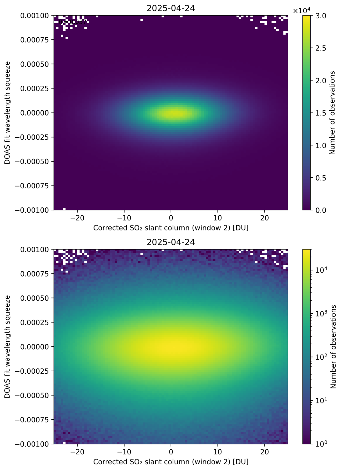
Figure 247: Scatter density plot of “Corrected SO 2 slant column (window 2)” against “DOAS fit wavelength squeeze” for 2025-04-24 to 2025-04-25.
