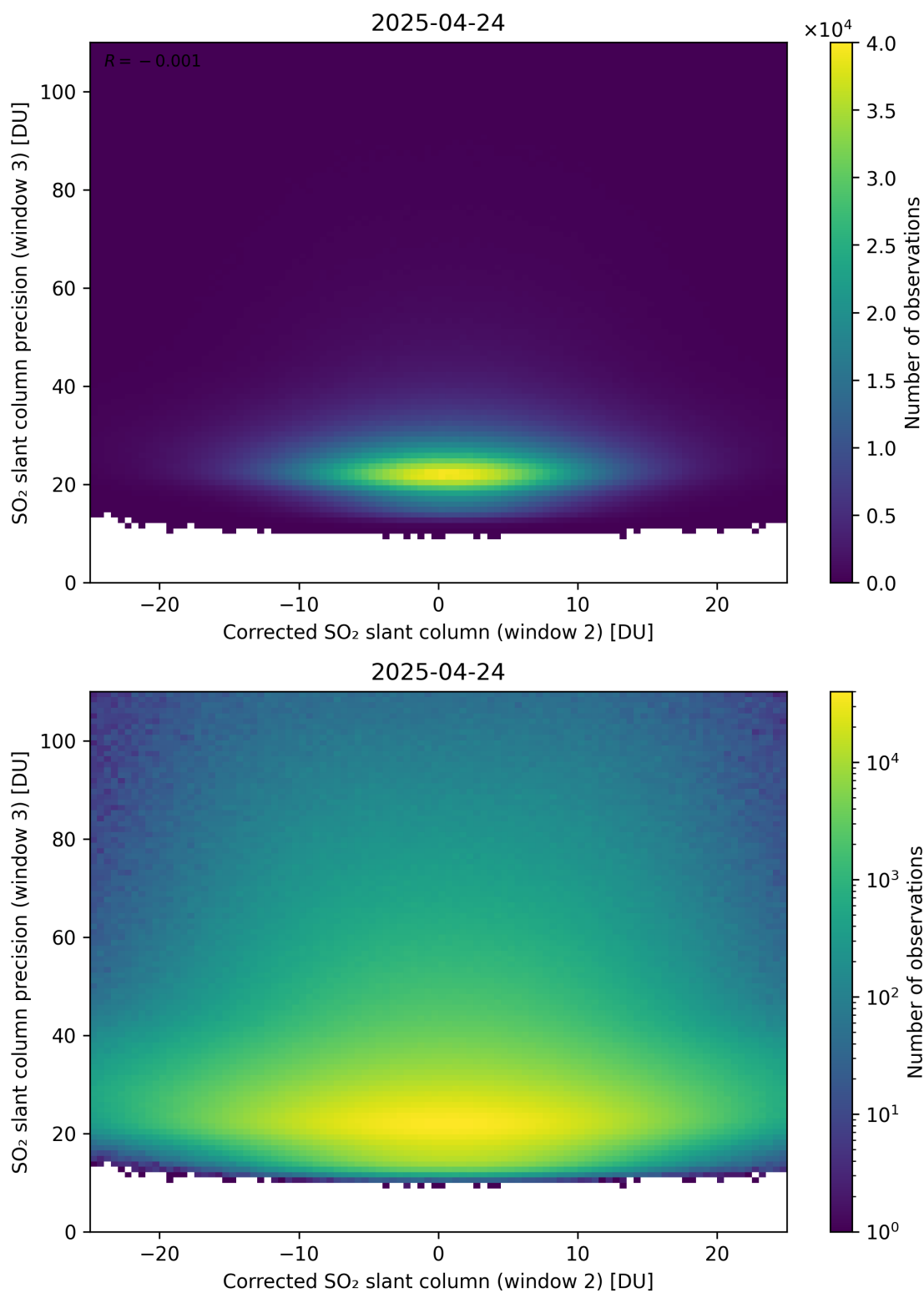
Figure 252: Scatter density plot of “Corrected SO 2 slant column (window 2)” against “SO 2 slant column precision (window 3)” for 2025-04-24 to 2025-04-25.
