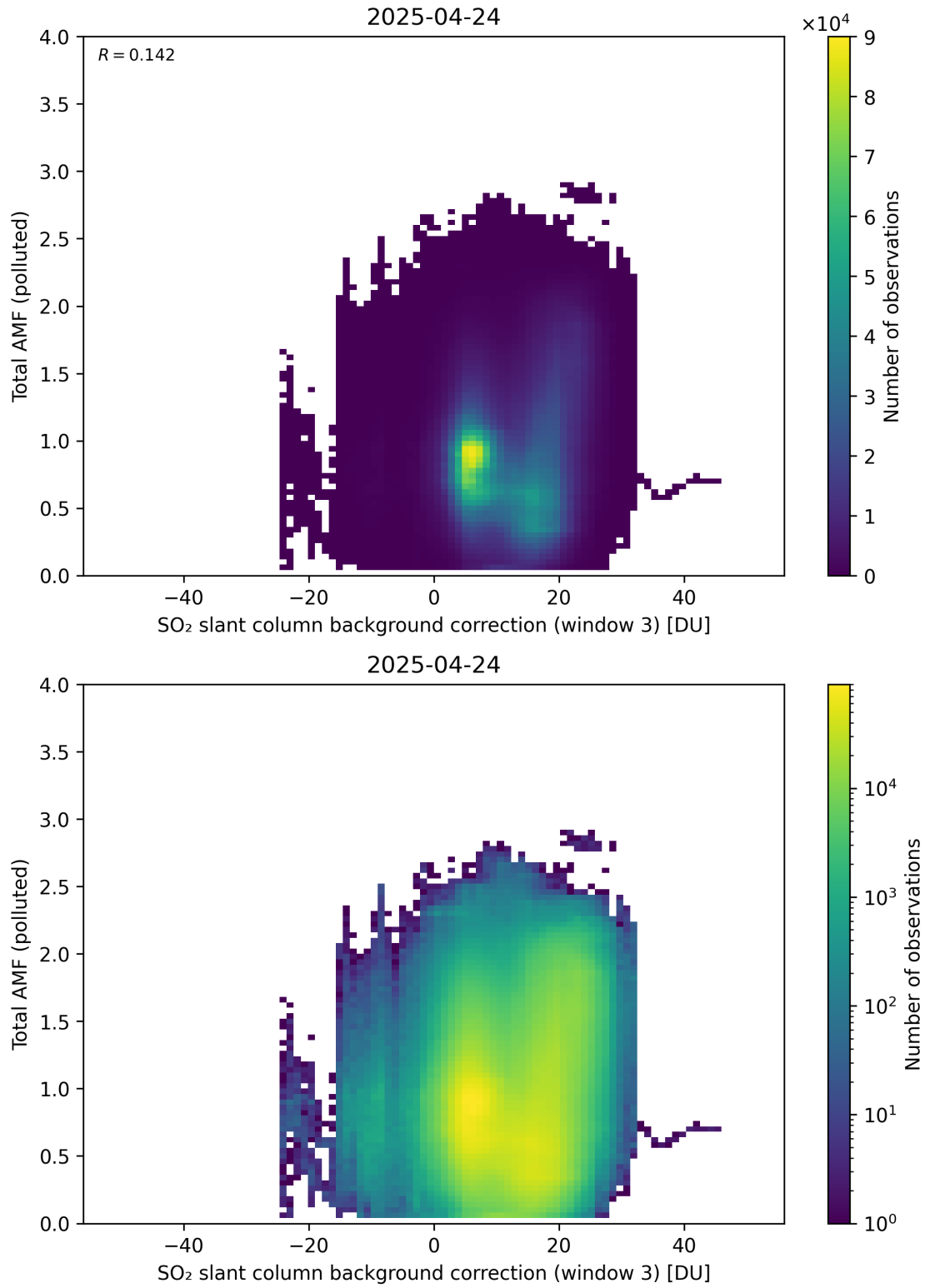
Figure 136: Scatter density plot of “SO 2 slant column background correction (window 3)” against “Total AMF (polluted)” for 2025-04-24 to 2025-04-25.
