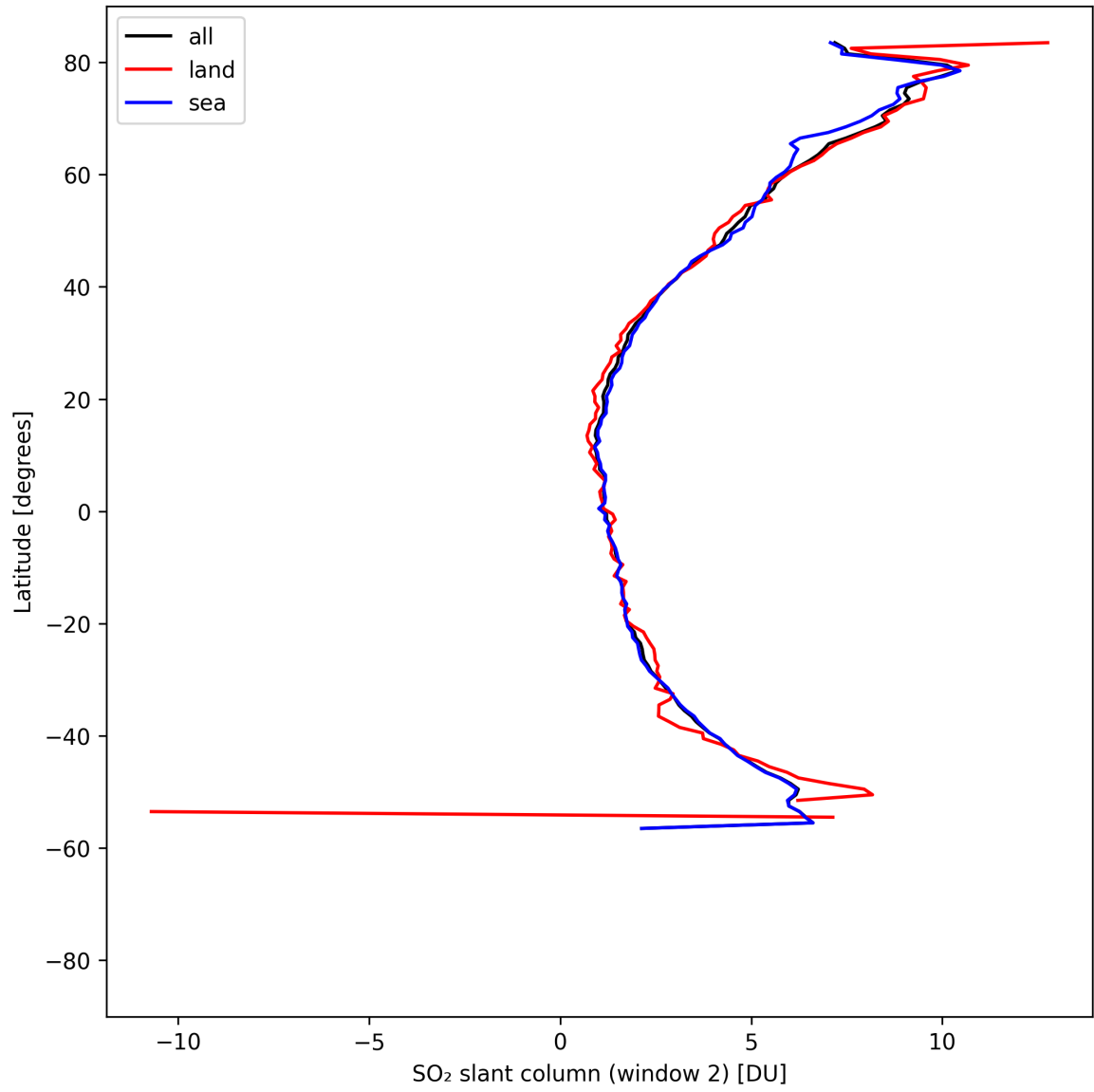
Figure 41: Zonal average of “SO 2 slant column (window 2)” for 2025-04-24 to 2025-04-25.
