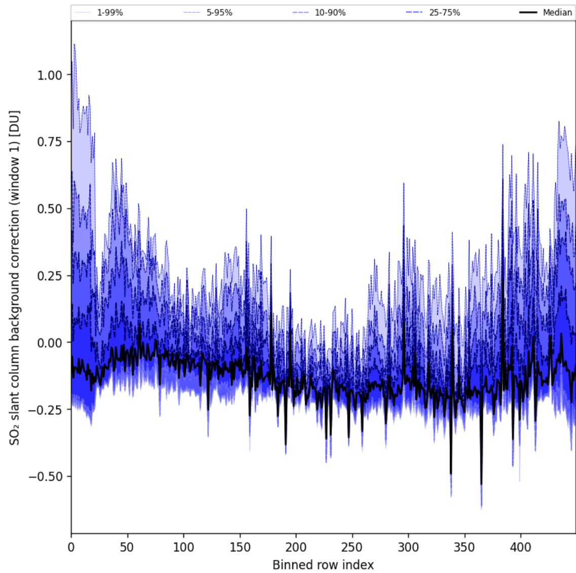
Figure 92: Along track statistics of “SO 2 slant column background correction (window 1)” for 2025-04-24 to 2025-04-25
