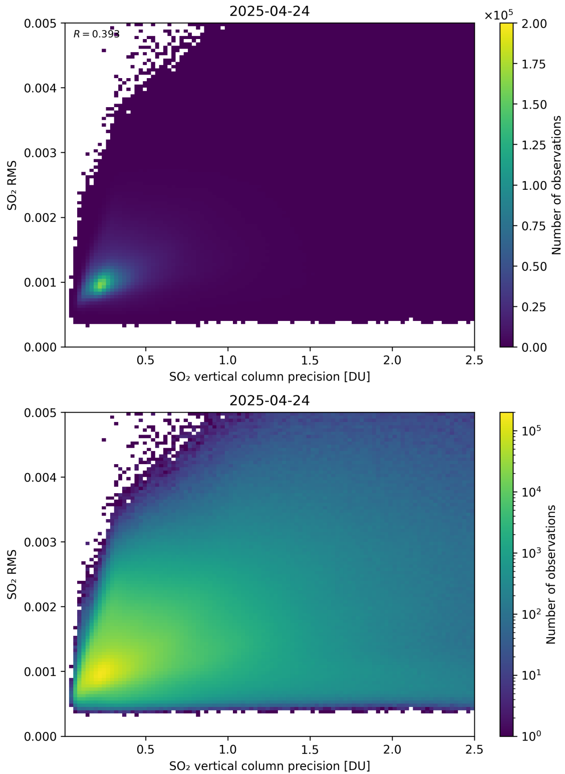
Figure 334: Scatter density plot of “SO 2 vertical column precision” against “SO 2 RMS” for 2025-04-24 to 2025-04-25.
