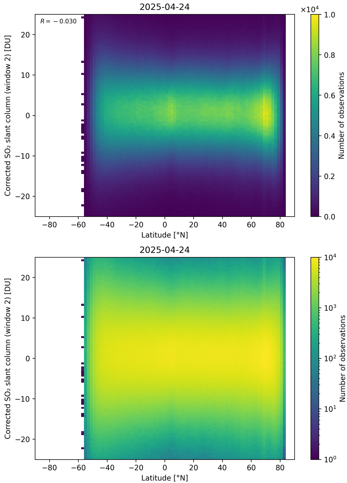
Figure 160: Scatter density plot of “Latitude” against “Corrected SO 2 slant column (window 2)” for 2025-04-24 to 2025-04-25.
