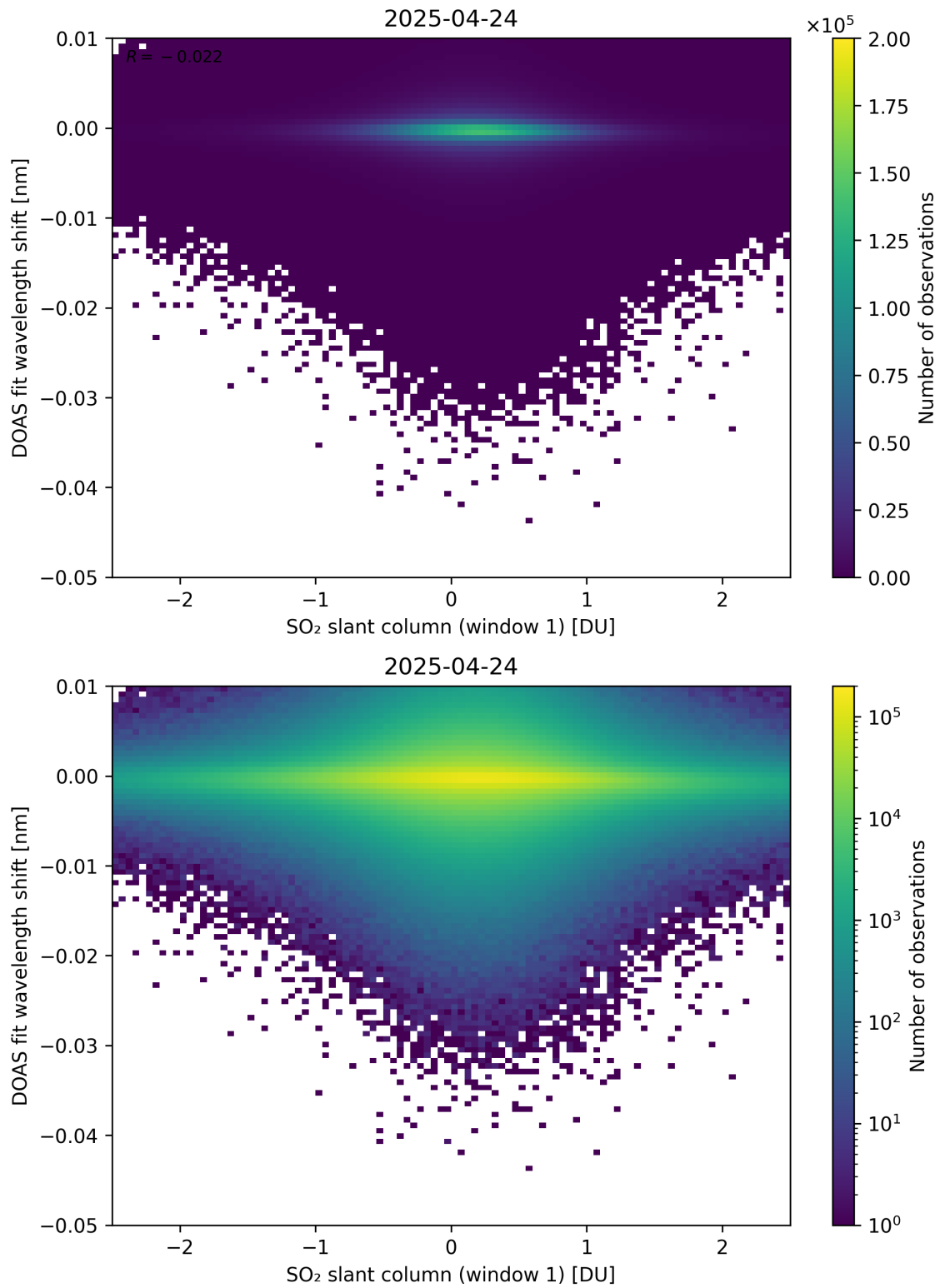
Figure 265: Scatter density plot of “SO 2 slant column (window 1)” against “DOAS fit wavelength shift” for 2025-04-24 to 2025-04-25.
