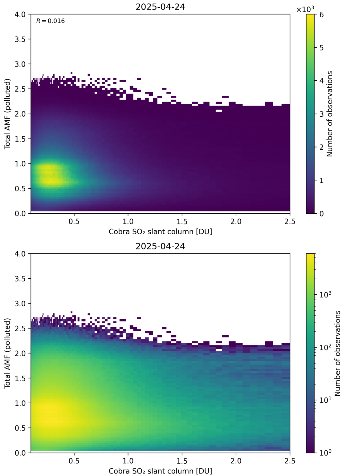
Figure 224: Scatter density plot of “Cobra SO 2 slant column” against “Total AMF (polluted)” for 2025-04-24 to 2025-04-25.
