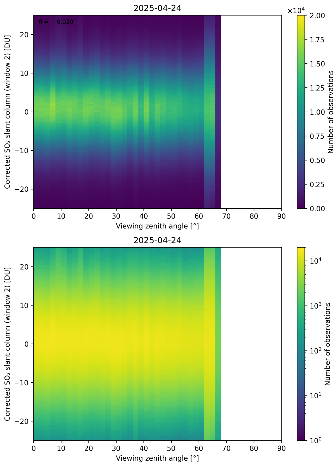
Figure 374: Scatter density plot of “Viewing zenith angle” against “Corrected SO 2 slant column (window 2)” for 2025-04-24 to 2025-04-25.
