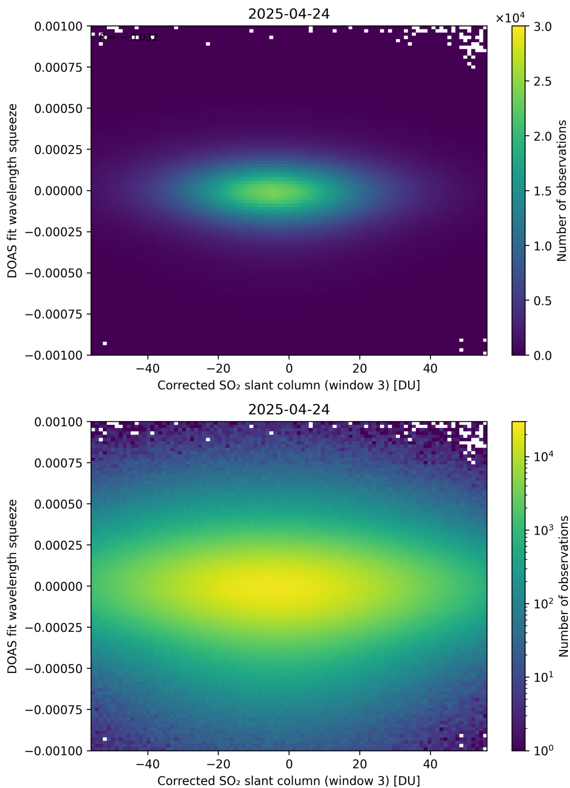
Figure 257: Scatter density plot of “Corrected SO 2 slant column (window 3)” against “DOAS fit wavelength squeeze” for 2025-04-24 to 2025-04-25.
