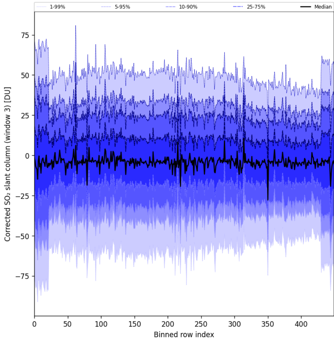
Figure 99: Along track statistics of “Corrected SO 2 slant column (window 3)” for 2025-04-24 to 2025-04-25
