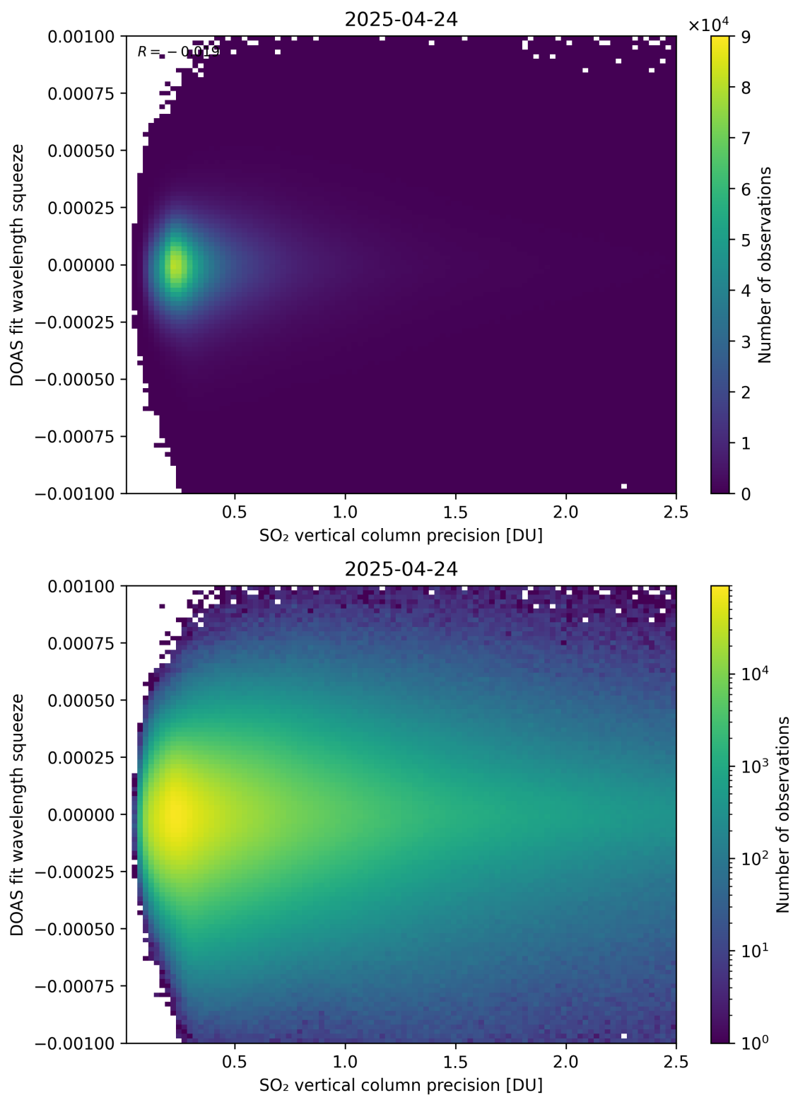
Figure 333: Scatter density plot of “SO 2 vertical column precision” against “DOAS fit wavelength squeeze” for 2025-04-24 to 2025-04-25.
