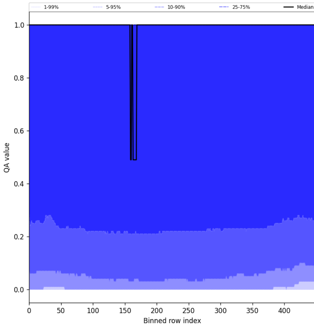
Figure 83: Along track statistics of “QA value” for 2025-04-24 to 2025-04-25
