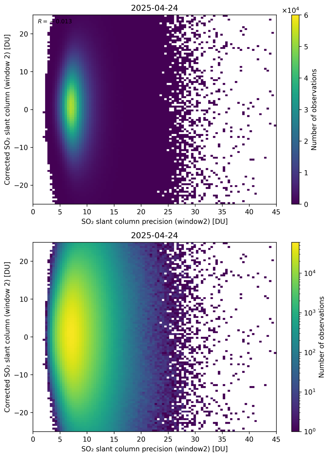
Figure 297: Scatter density plot of “SO 2 slant column precision (window2)” against “Corrected SO 2 slant column (window 2)” for 2025-04-24 to 2025-04-25.
