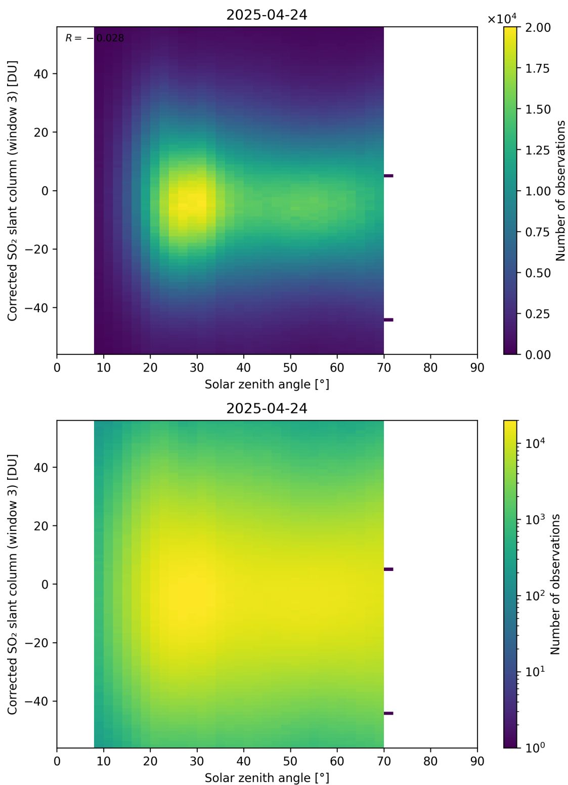
Figure 183: Scatter density plot of “Solar zenith angle” against “Corrected SO 2 slant column (window 3)” for 2025-04-24 to 2025-04-25.
