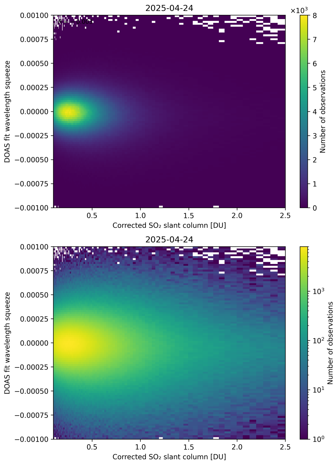
Figure 230: Scatter density plot of "Corrected SO 2 slant column" against "DOAS fit wavelength squeeze" for 2025-04-24 to 2025-04-25.
