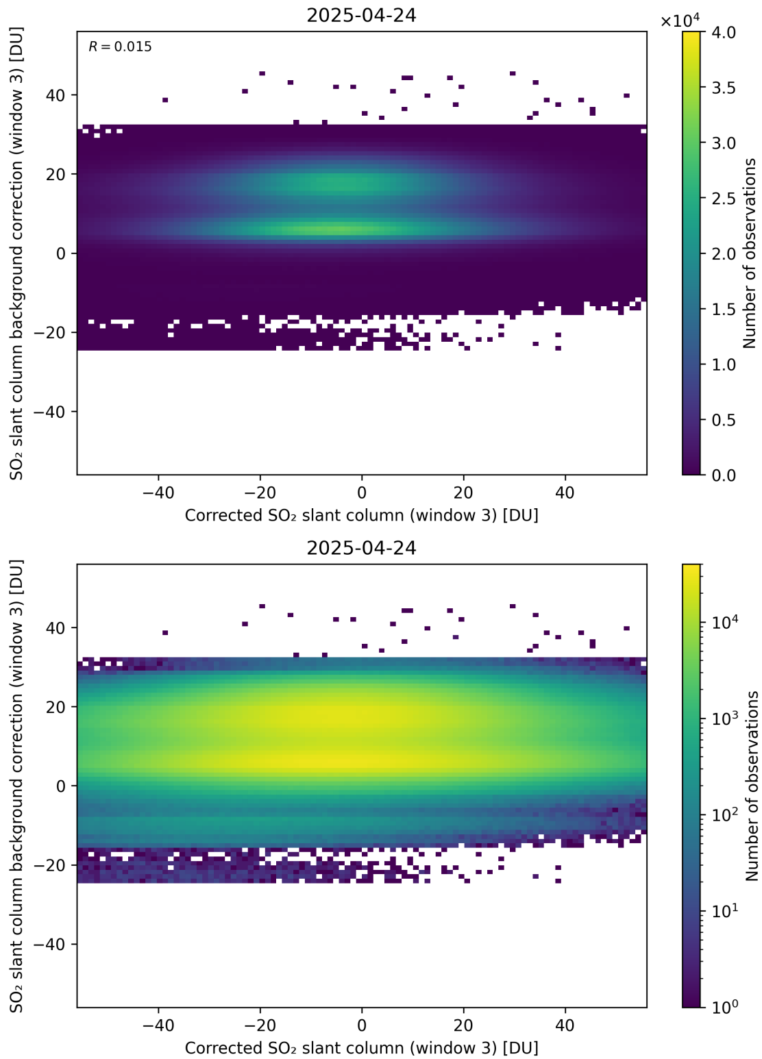
Figure 255: Scatter density plot of “Corrected SO 2 slant column (window 3)” against “SO 2 slant column background correction (window 3)” for 2025-04-24 to 2025-04-25.
