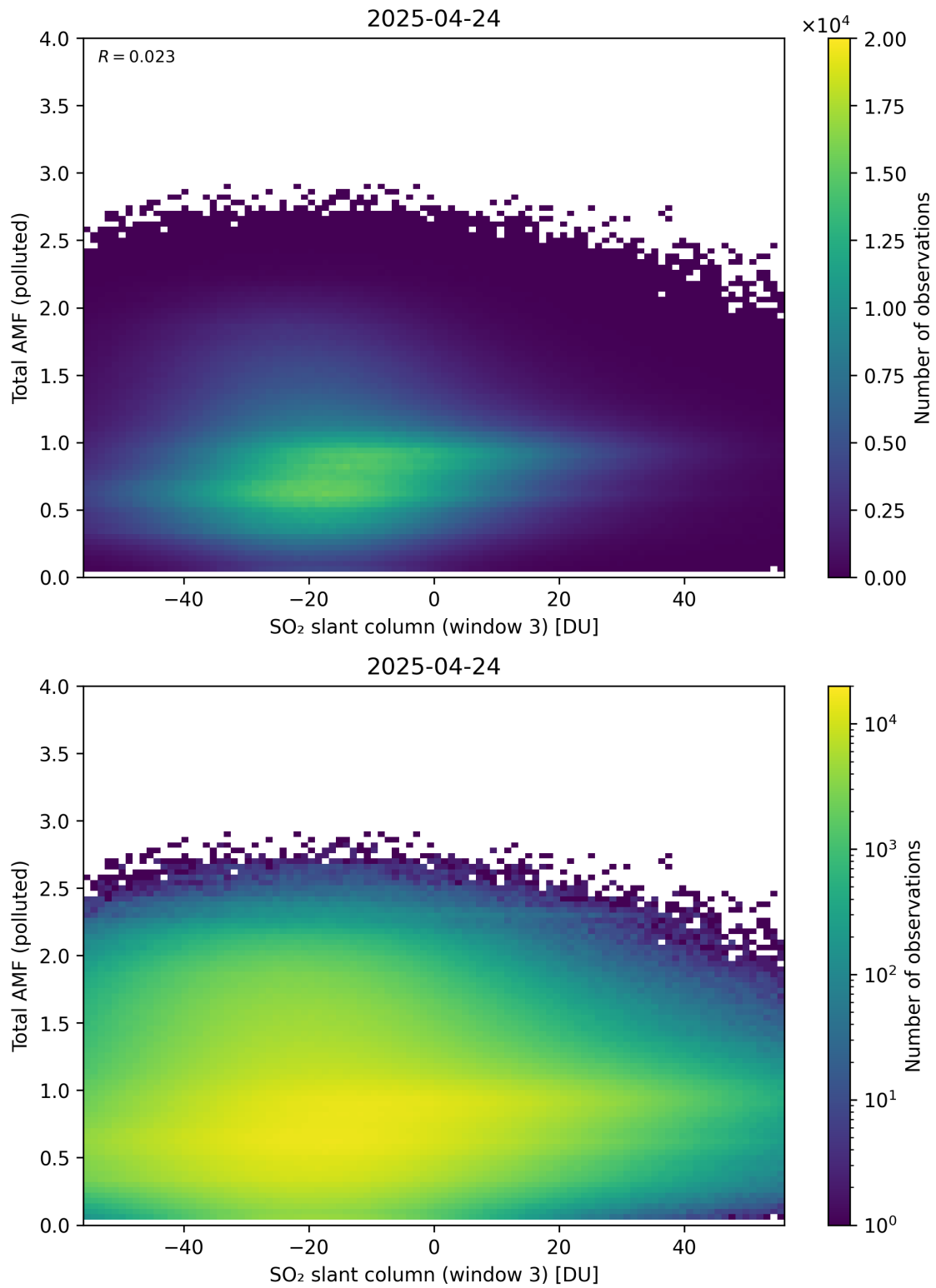
Figure 318: Scatter density plot of “SO 2 slant column (window 3)” against “Total AMF (polluted)” for 2025-04-24 to 2025-04-25.
