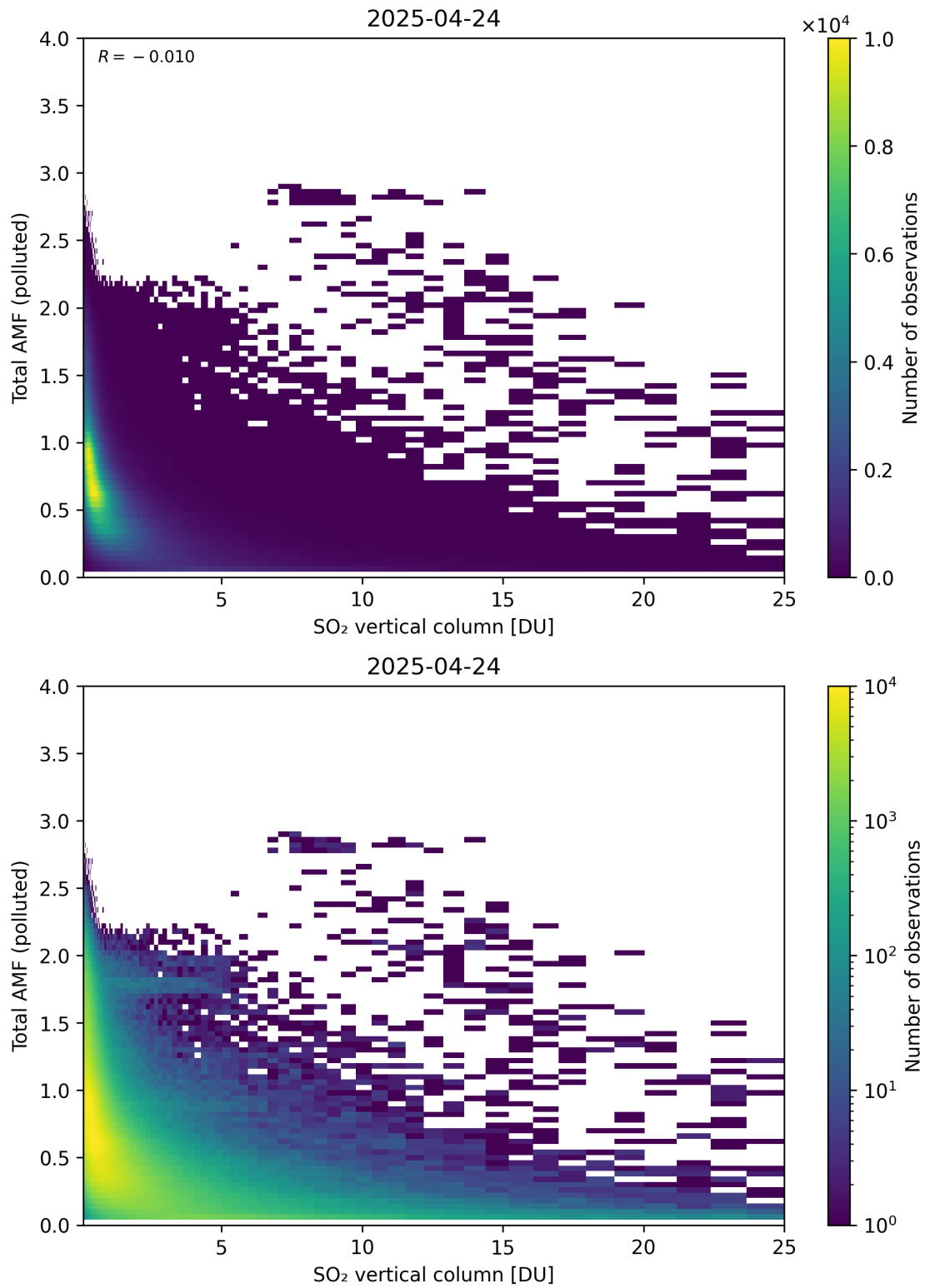
Figure 359: Scatter density plot of “SO 2 vertical column” against “Total AMF (polluted)” for 2025-04-24 to 2025-04-25.
