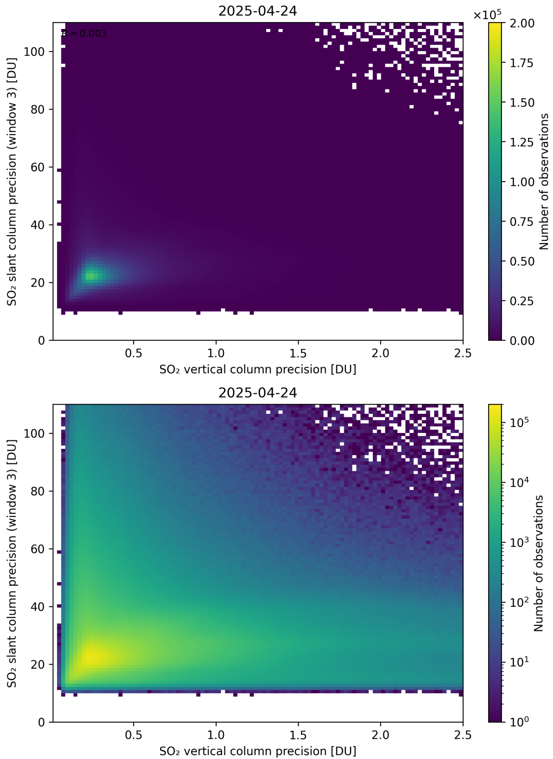
Figure 345: Scatter density plot of “SO 2 vertical column precision” against “SO 2 slant column precision (window 3)” for 2025-04-24 to 2025-04-25.
