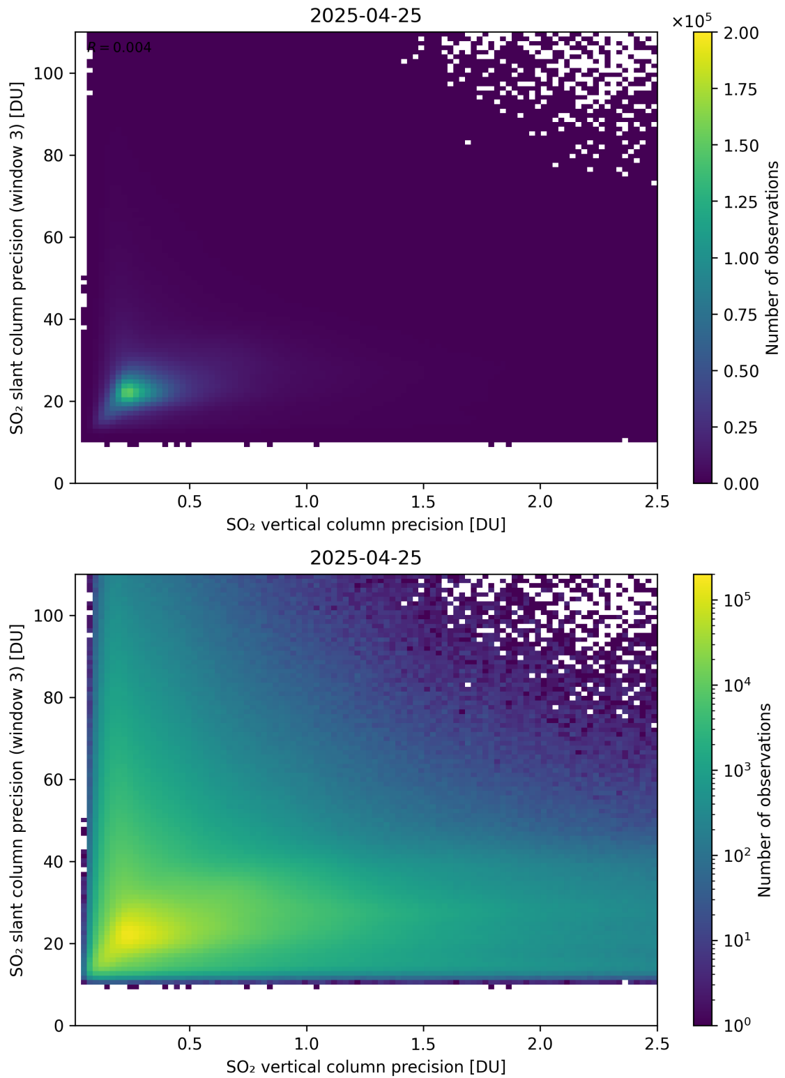
Figure 345: Scatter density plot of “SO 2 vertical column precision” against “SO 2 slant column precision (window 3)” for 2025-04-24 to 2025-04-26.
