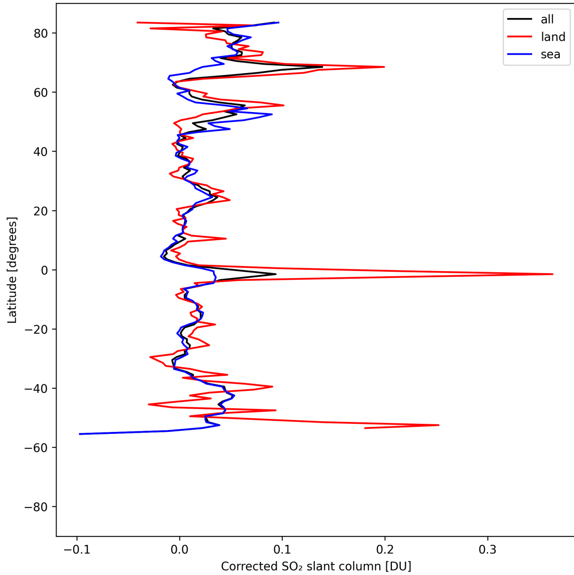
Figure 34: Zonal average of “Corrected SO 2 slant column” for 2025-04-24 to 2025-04-26.
