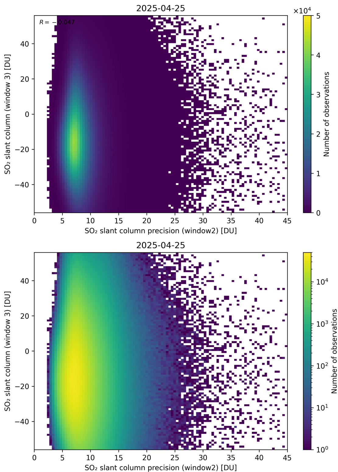
Figure 299: Scatter density plot of “SO 2 slant column precision (window2)” against “SO 2 slant column (window 3)” for 2025-04-24 to 2025-04-26.
