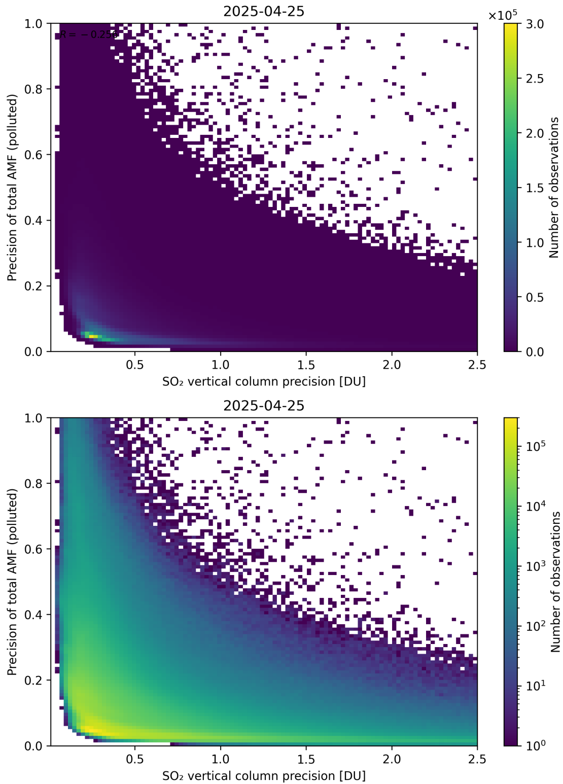
Figure 347: Scatter density plot of “SO 2 vertical column precision” against “Precision of total AMF (polluted)” for 2025-04-24 to 2025-04-26.
