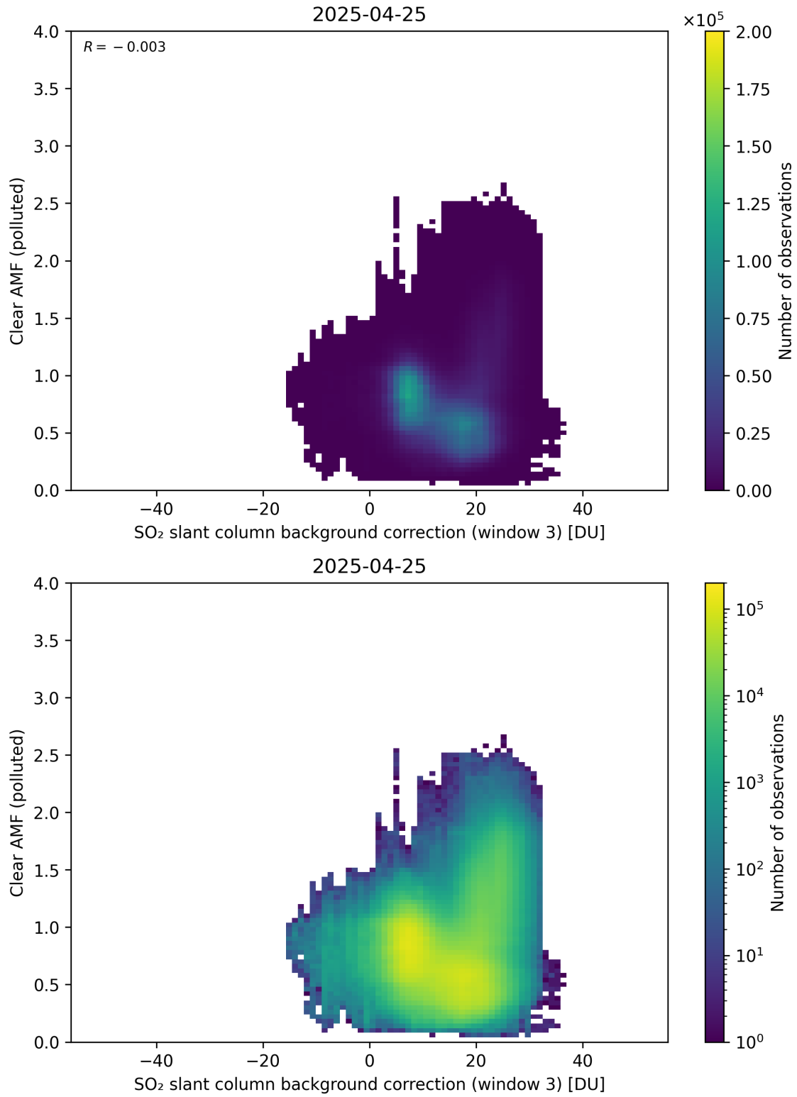
Figure 135: Scatter density plot of “SO 2 slant column background correction (window 3)” against “Clear AMF (polluted)” for 2025-04-24 to 2025-04-26.
