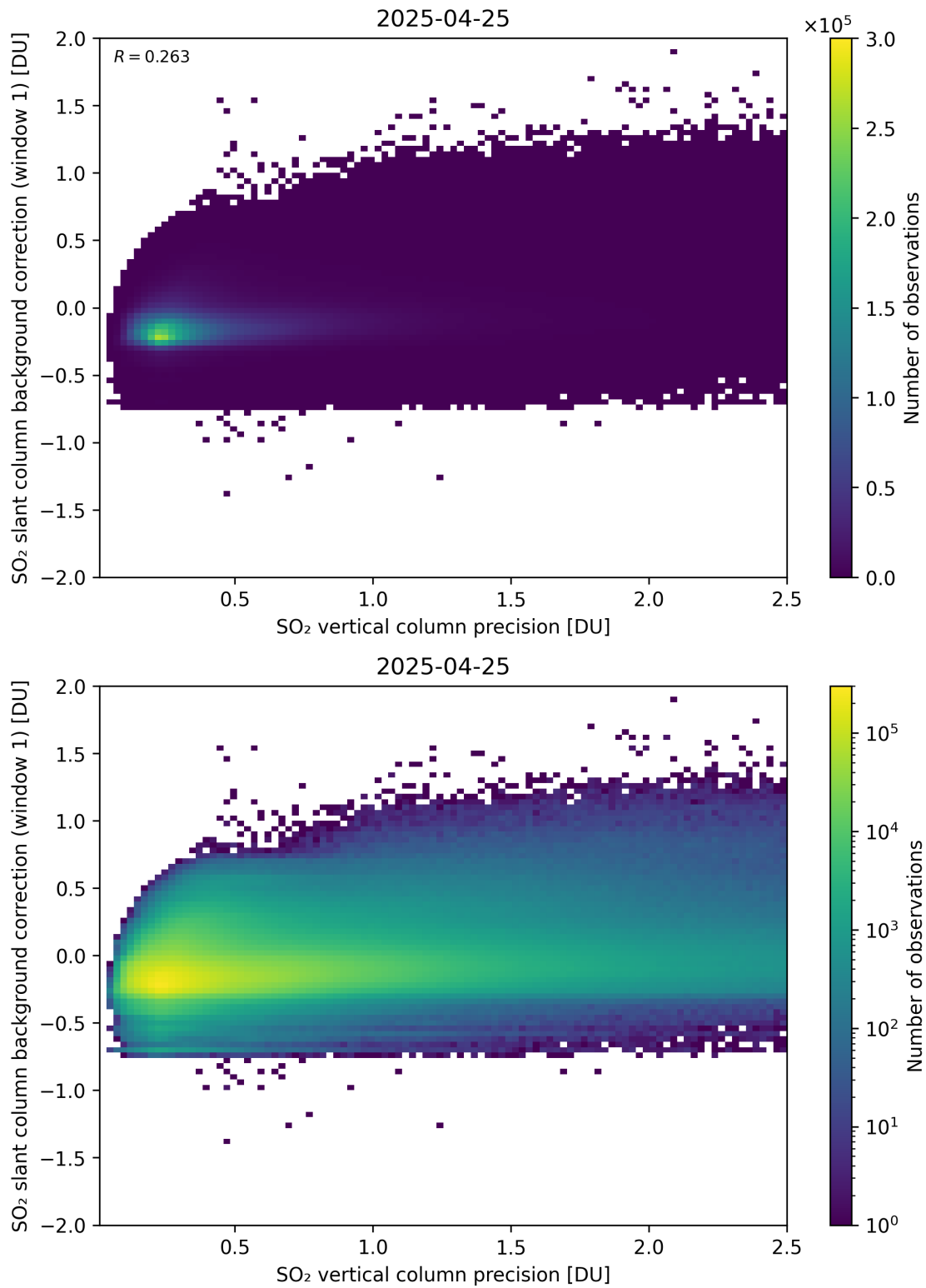
Figure 329: Scatter density plot of “SO 2 vertical column precision” against “SO 2 slant column background correction (window 1)” for 2025-04-24 to 2025-04-26.
