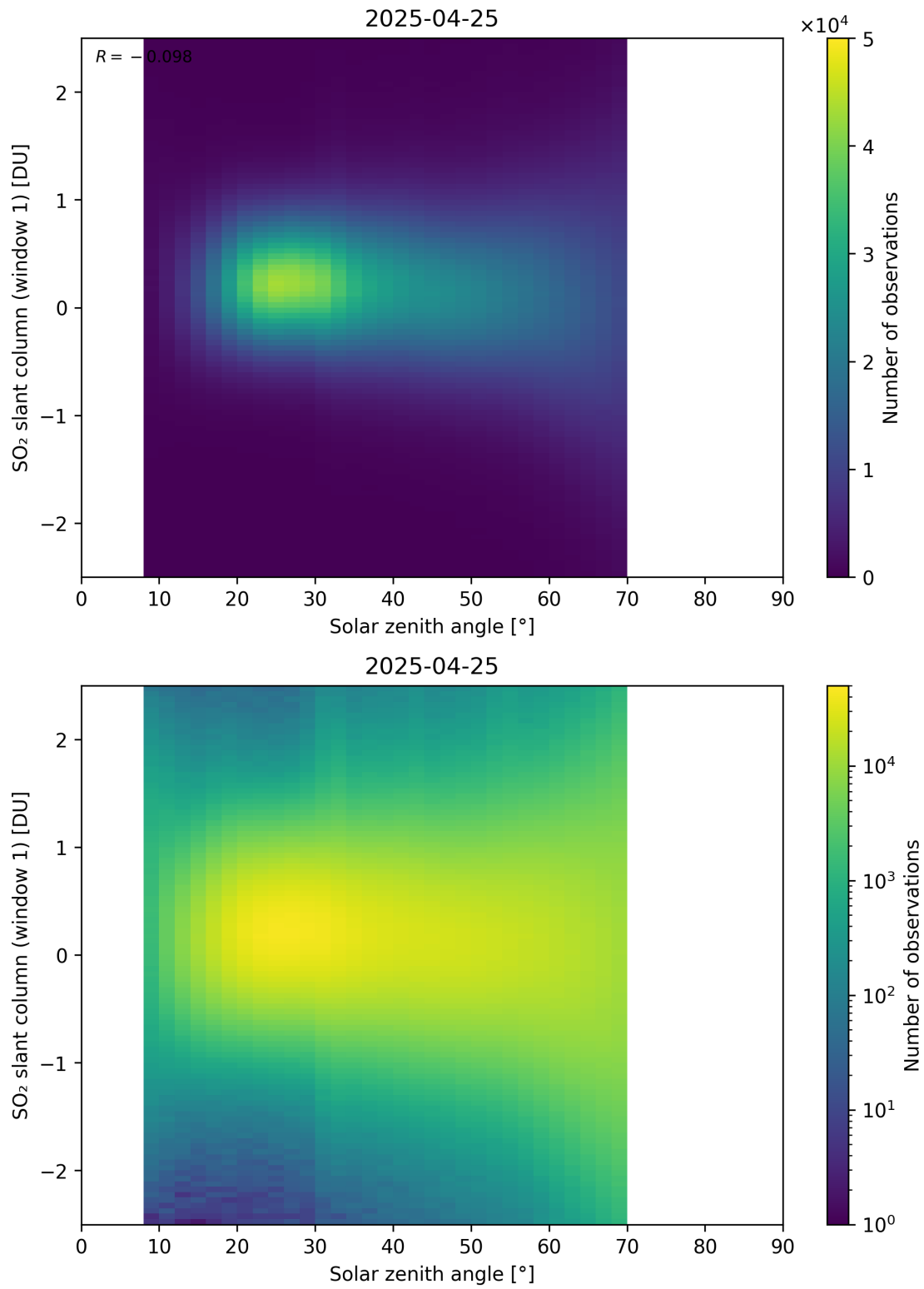
Figure 184: Scatter density plot of “Solar zenith angle” against “SO 2 slant column (window 1)” for 2025-04-24 to 2025-04-26.
