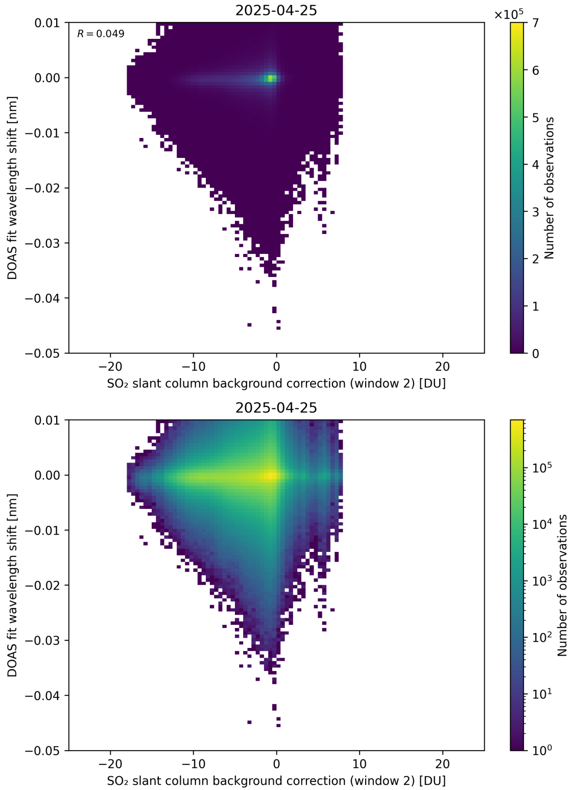
Figure 123: Scatter density plot of “SO 2 slant column background correction (window 2)” against “DOAS fit wavelength shift” for 2025-04-24 to 2025-04-26.
