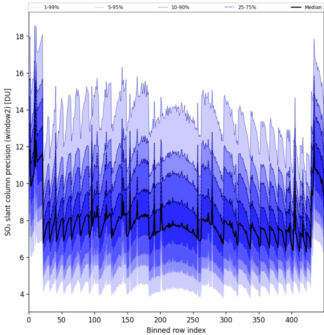
Figure 94: Along track statistics of “SO 2 slant column precision (window2)” for 2025-04-24 to 2025-04-26
