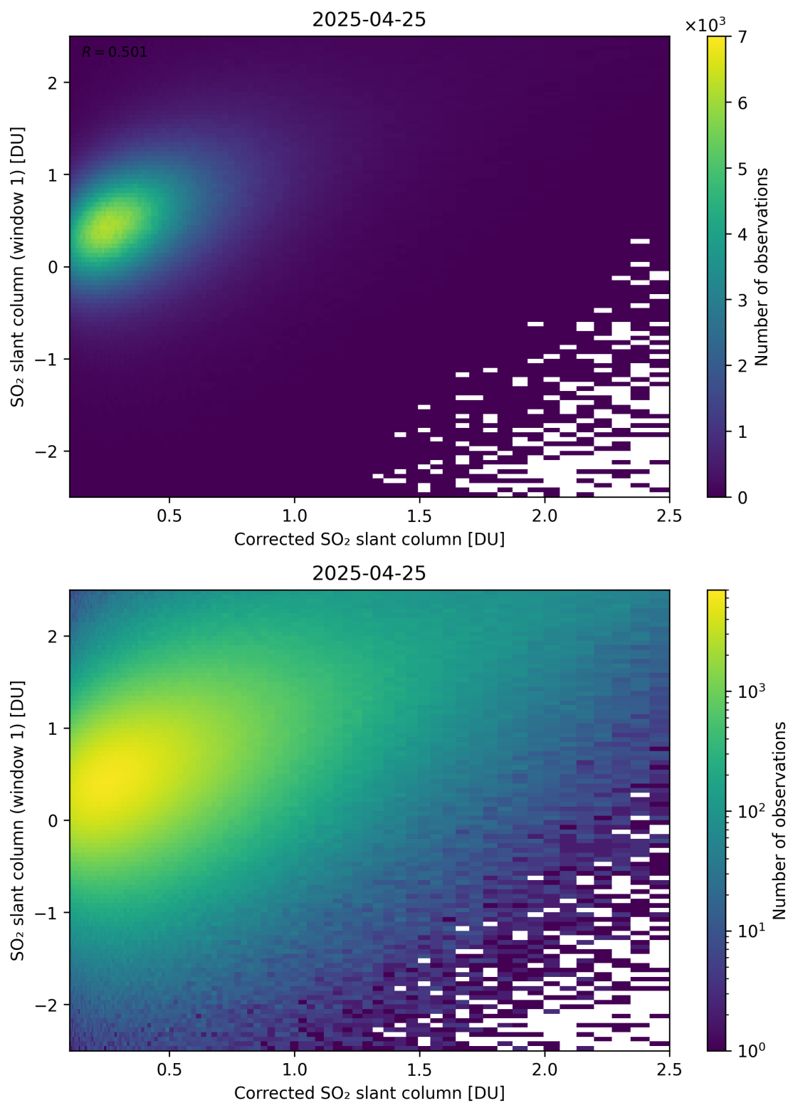
Figure 237: Scatter density plot of “Corrected SO 2 slant column” against “SO 2 slant column (window 1)” for 2025-04-24 to 2025-04-26.
