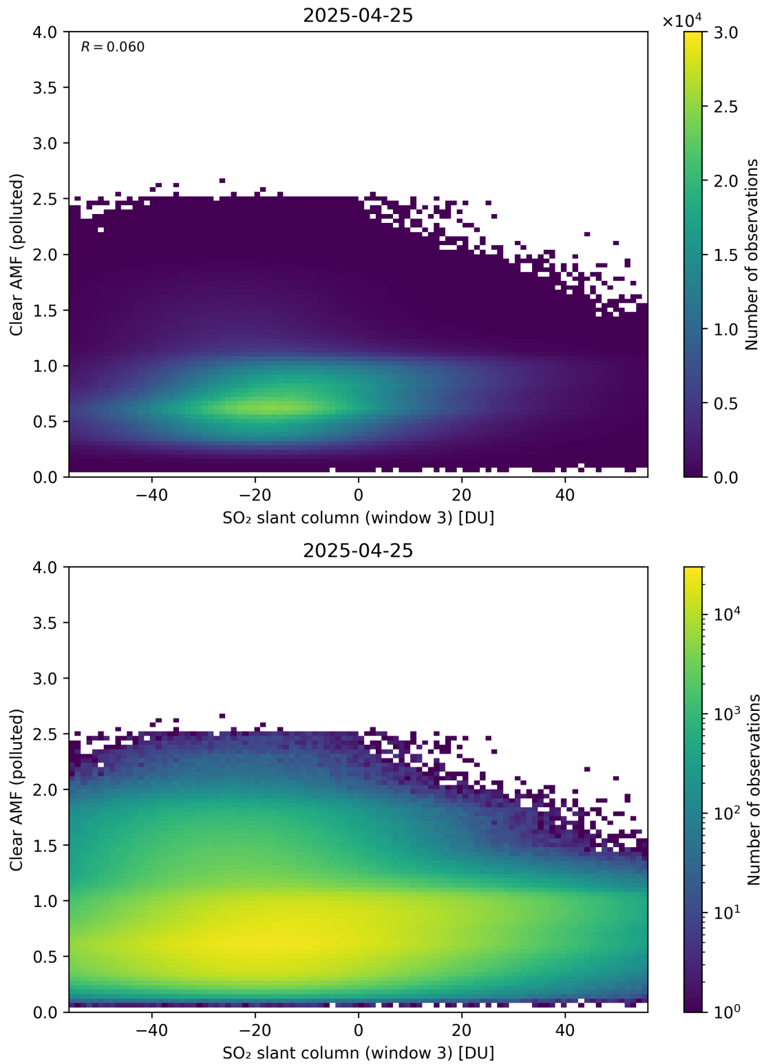
Figure 315: Scatter density plot of “SO 2 slant column (window 3)” against “Clear AMF (polluted)” for 2025-04-24 to 2025-04-26.
