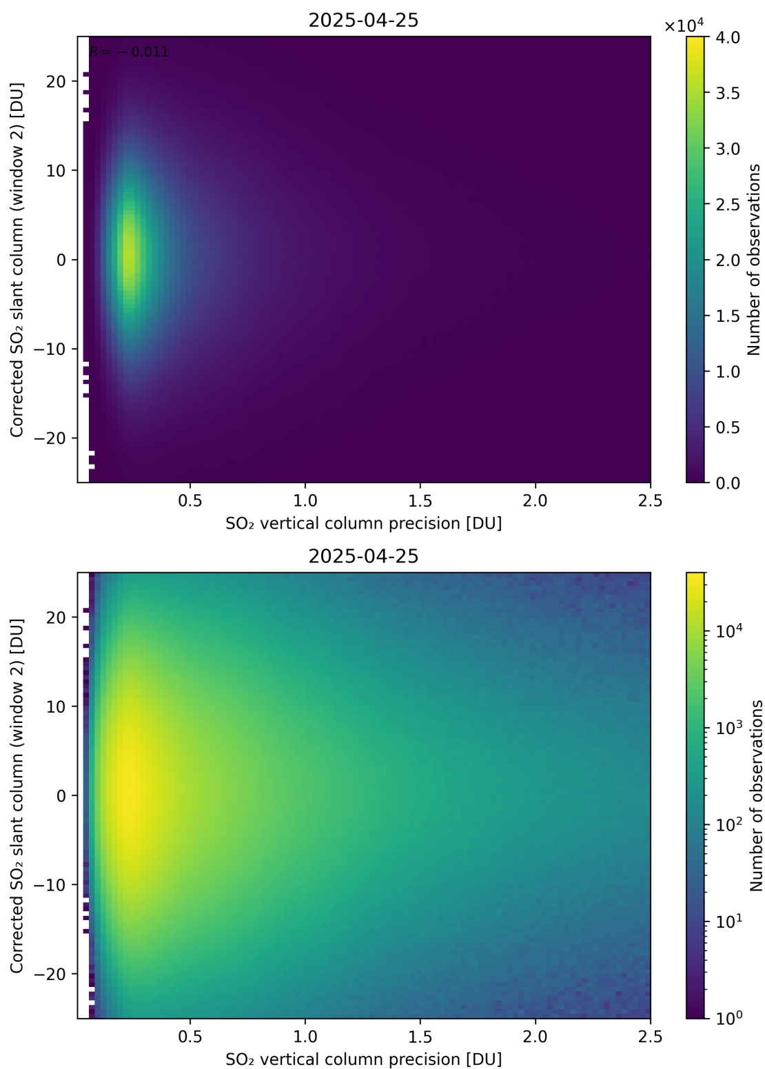
Figure 339: Scatter density plot of “SO 2 vertical column precision” against “Corrected SO 2 slant column (window 2)” for 2025-04-24 to 2025-04-26.
