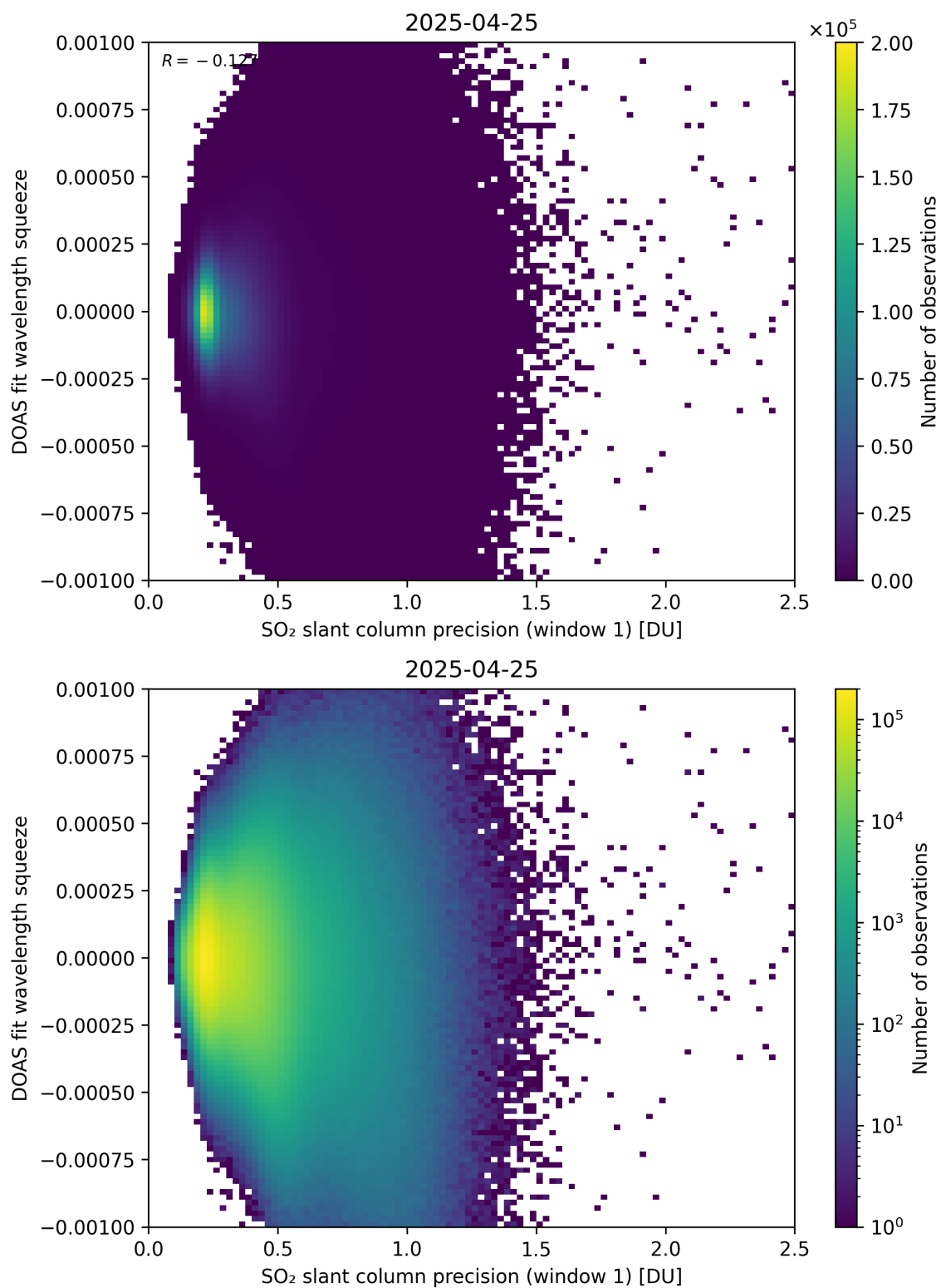
Figure 272: Scatter density plot of “SO 2 slant column precision (window 1)” against “DOAS fit wavelength squeeze” for 2025-04-24 to 2025-04-26.
