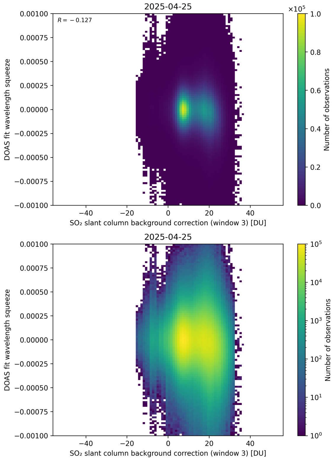
Figure 133: Scatter density plot of “SO 2 slant column background correction (window 3)” against “DOAS fit wavelength squeeze” for 2025-04-24 to 2025-04-26.
