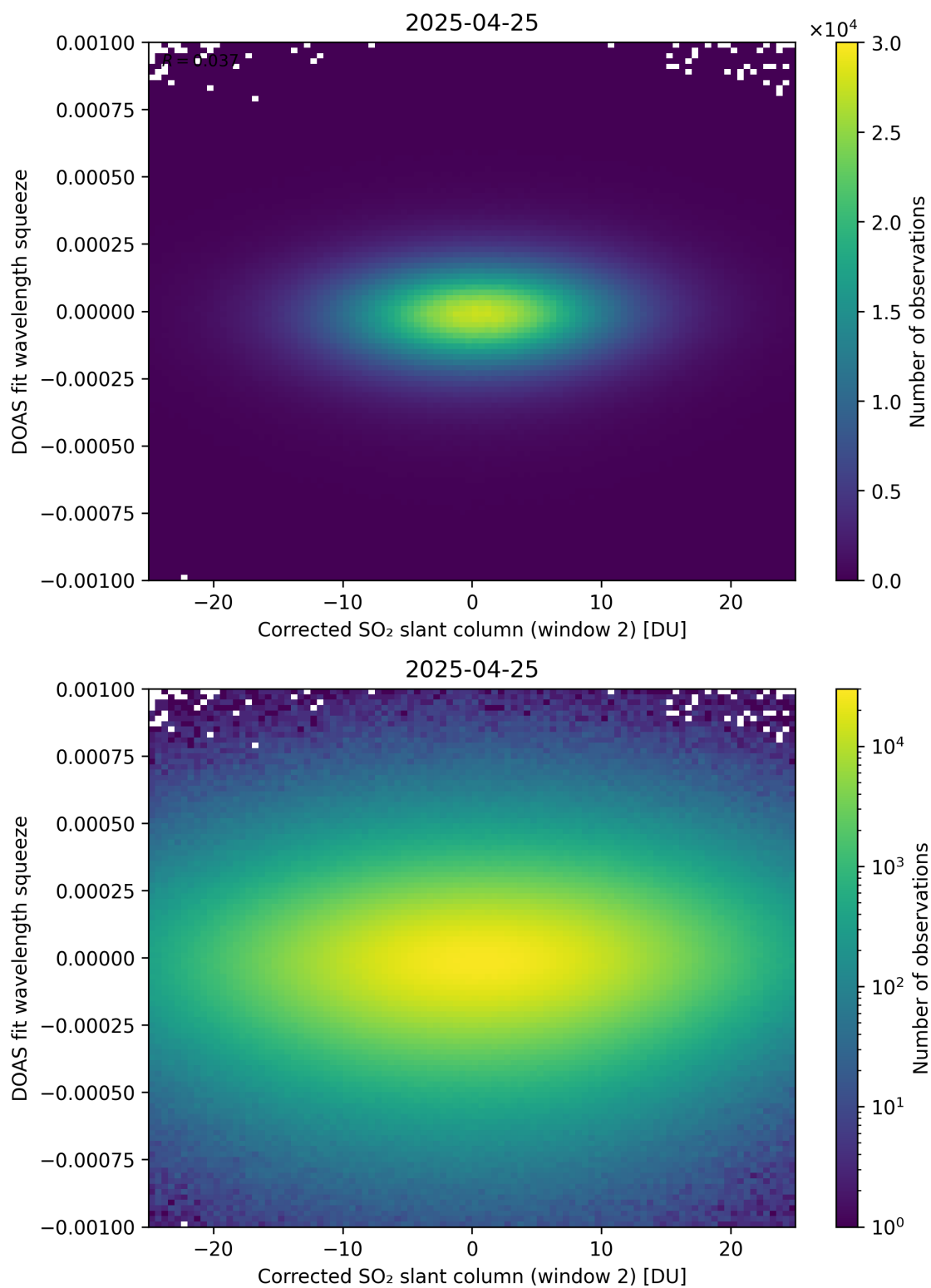
Figure 247: Scatter density plot of “Corrected SO 2 slant column (window 2)” against “DOAS fit wavelength squeeze” for 2025-04-24 to 2025-04-26.
