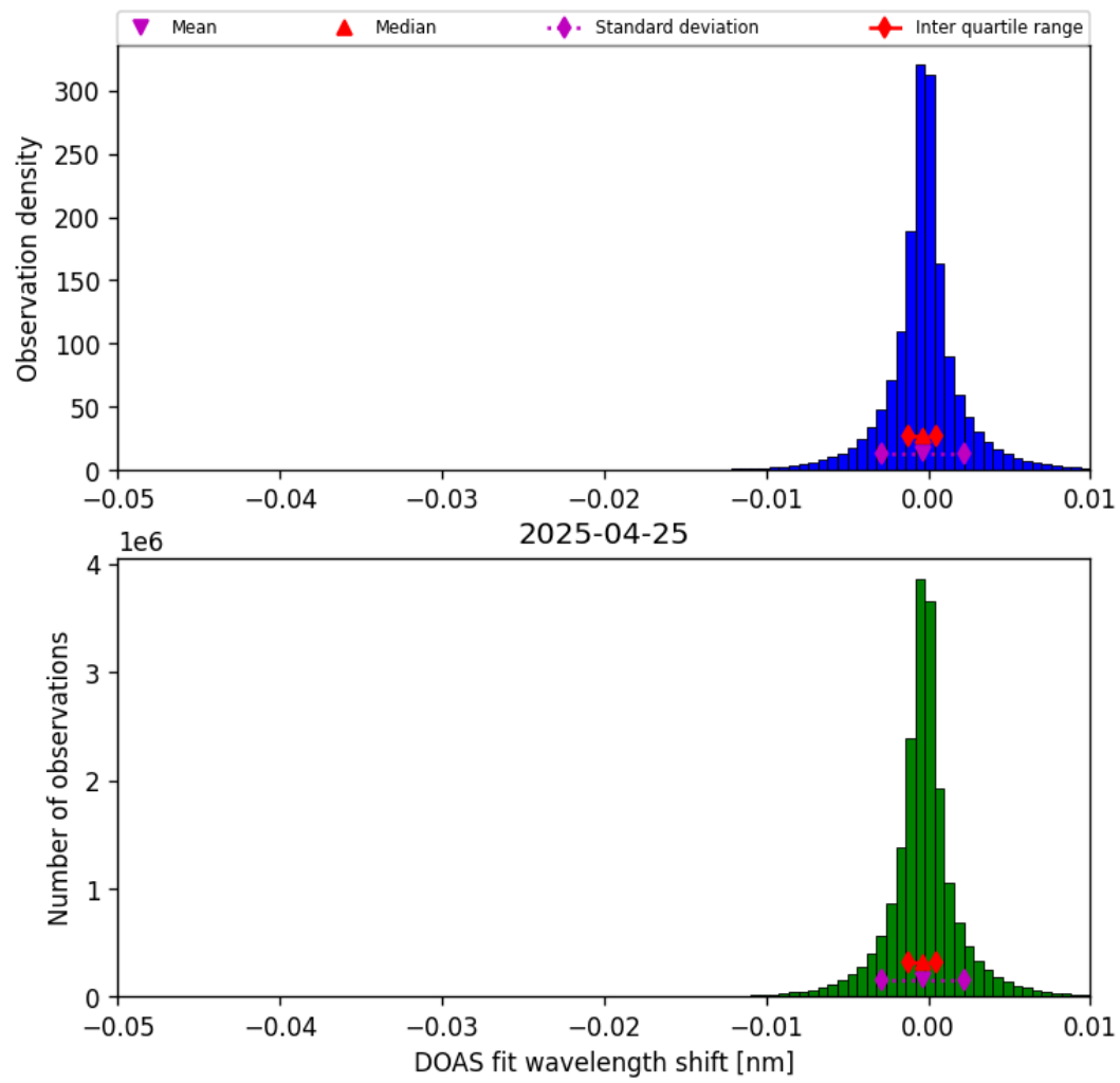
Figure 76: Histogram of “DOAS fit wavelength shift” for 2025-04-24 to 2025-04-26
