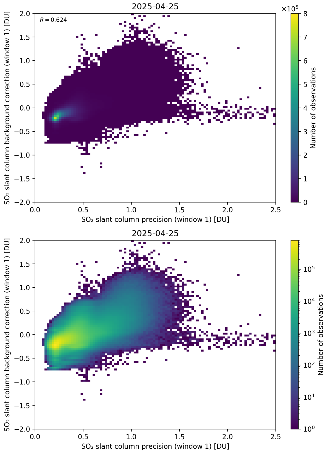
Figure 268: Scatter density plot of “SO 2 slant column precision (window 1)” against “SO 2 slant column background correction (window 1)” for 2025-04-24 to 2025-04-26.
