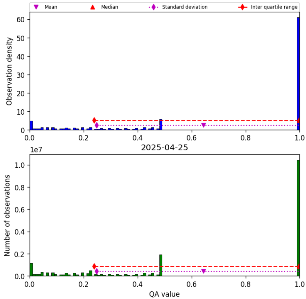
Figure 57: Histogram of “QA value” for 2025-04-24 to 2025-04-26
