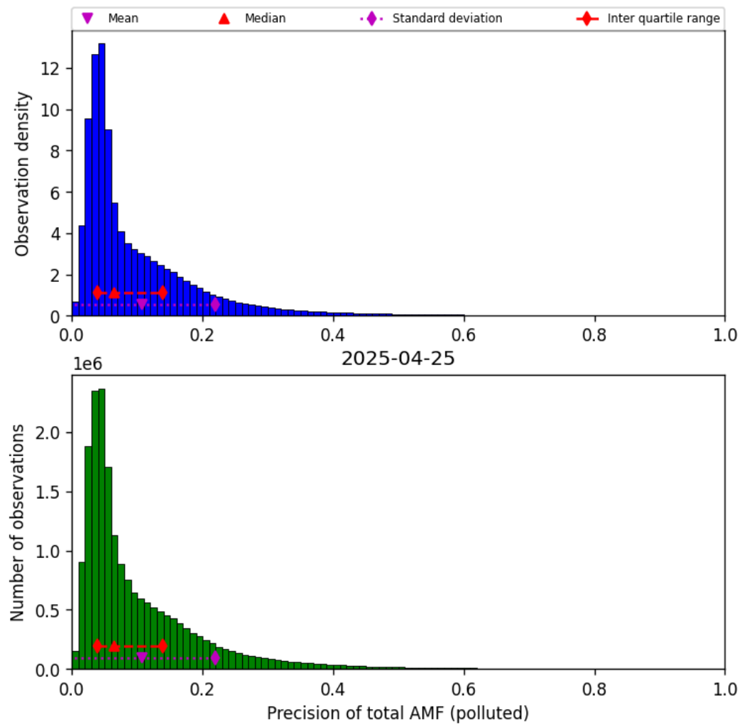
Figure 80: Histogram of “Precision of total AMF (polluted)” for 2025-04-24 to 2025-04-26
