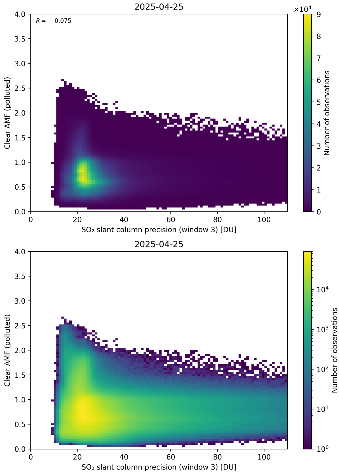
Figure 311: Scatter density plot of “SO 2 slant column precision (window 3)” against “Clear AMF (polluted)” for 2025-04-24 to 2025-04-26.
