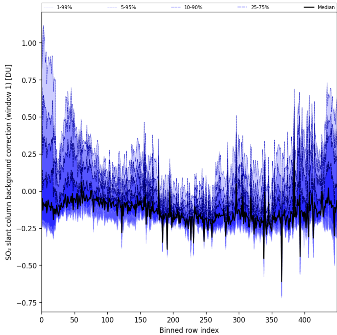
Figure 92: Along track statistics of "SO 2 slant column background correction (window 1)" for 2025-04-24 to 2025-04-26
