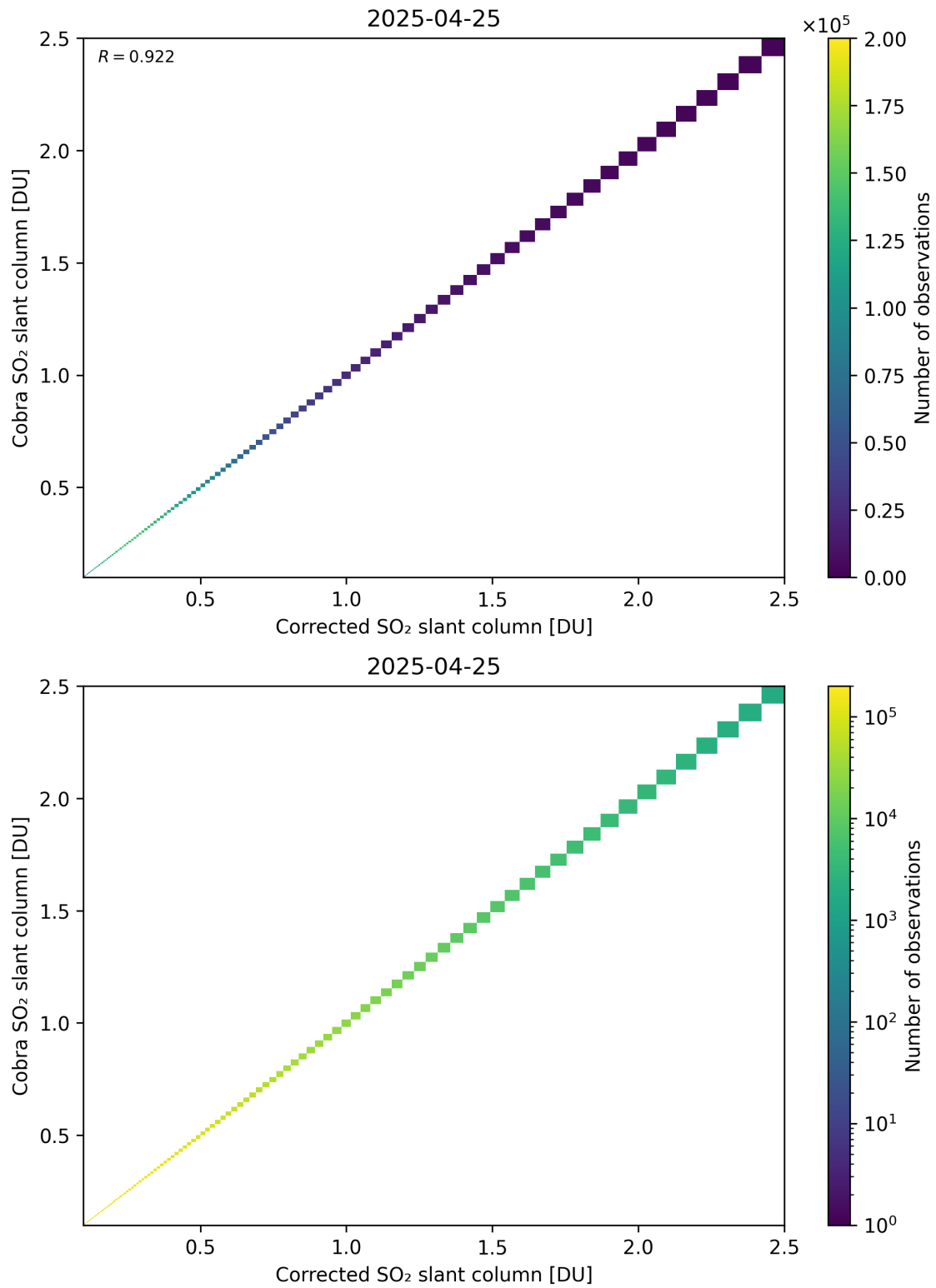
Figure 233: Scatter density plot of “Corrected SO 2 slant column” against “Cobra SO 2 slant column” for 2025-04-24 to 2025-04-26.
