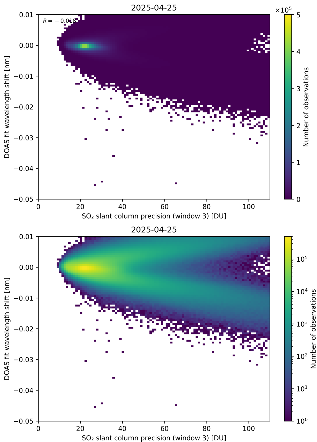
Figure 308: Scatter density plot of “SO 2 slant column precision (window 3)” against “DOAS fit wavelength shift” for 2025-04-24 to 2025-04-26.
