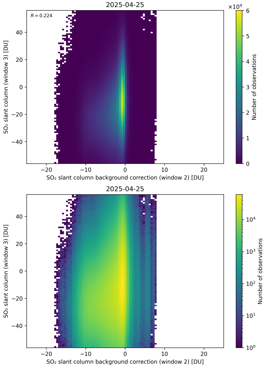
Figure 128: Scatter density plot of “SO 2 slant column background correction (window 2)” against “SO 2 slant column (window 3)” for 2025-04-24 to 2025-04-26.
