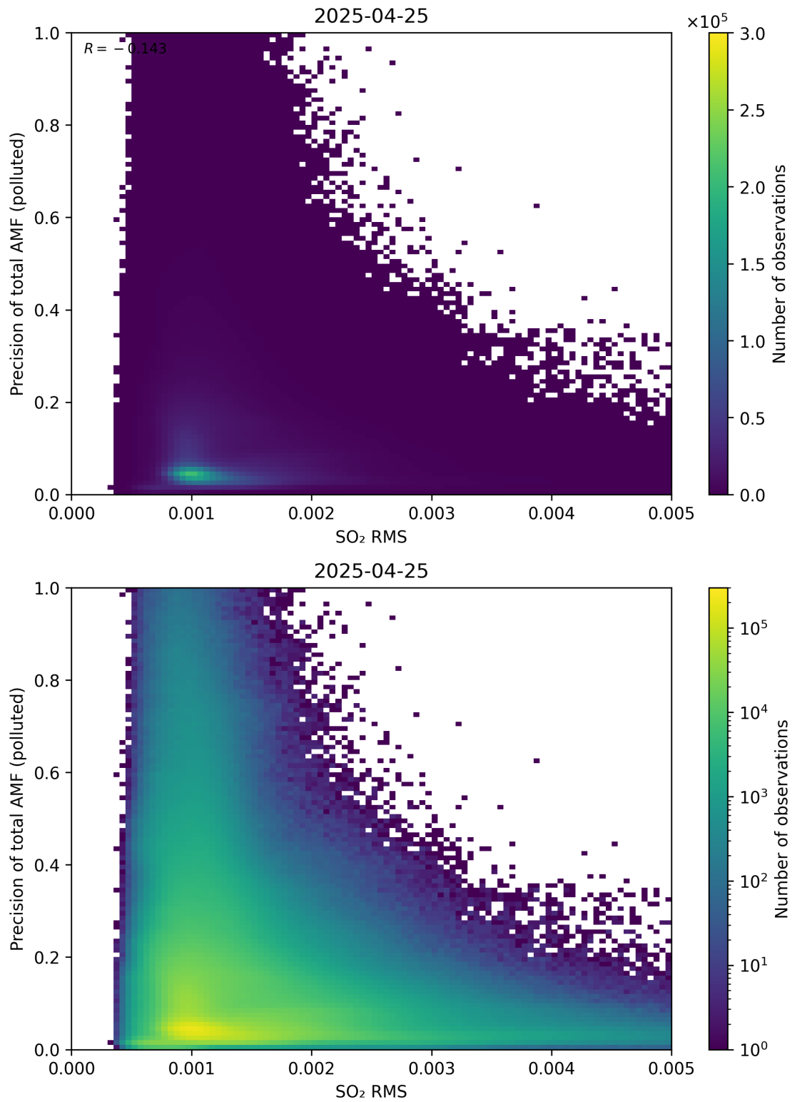
Figure 149: Scatter density plot of “SO 2 RMS” against “Precision of total AMF (polluted)” for 2025-04-24 to 2025-04-26.
