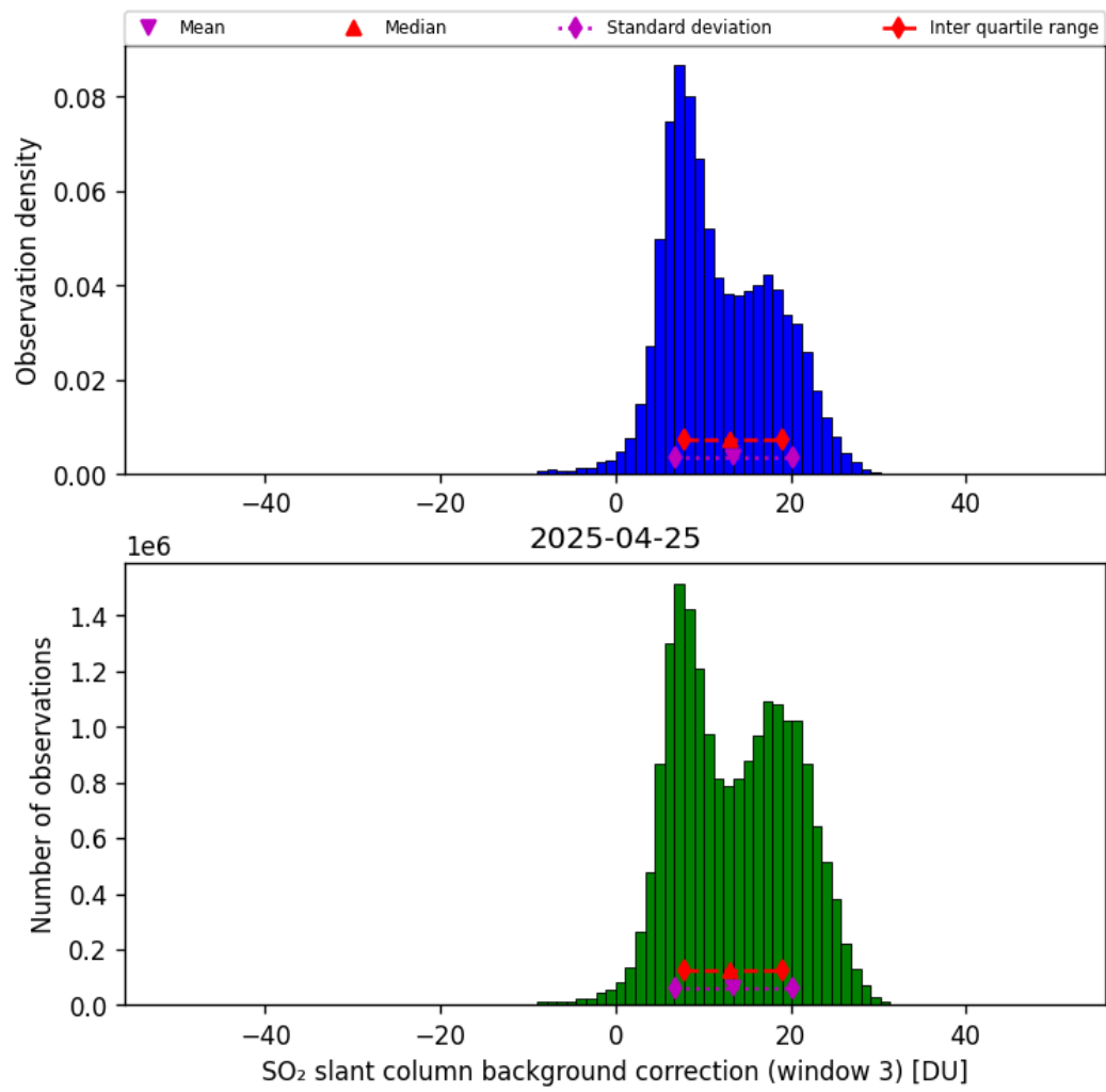
Figure 74: Histogram of “SO 2 slant column background correction (window 3)” for 2025-04-24 to 2025-04-26
