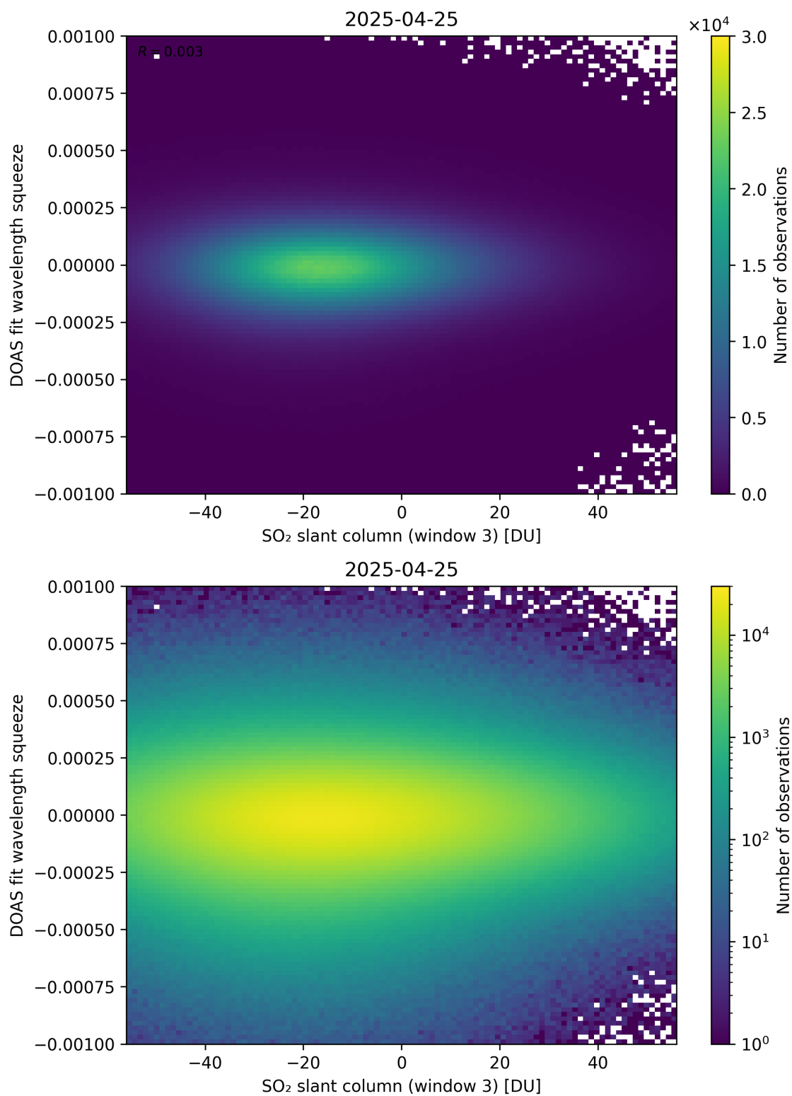
Figure 305: Scatter density plot of “SO 2 slant column (window 3)” against “DOAS fit wavelength squeeze” for 2025-04-24 to 2025-04-26.
