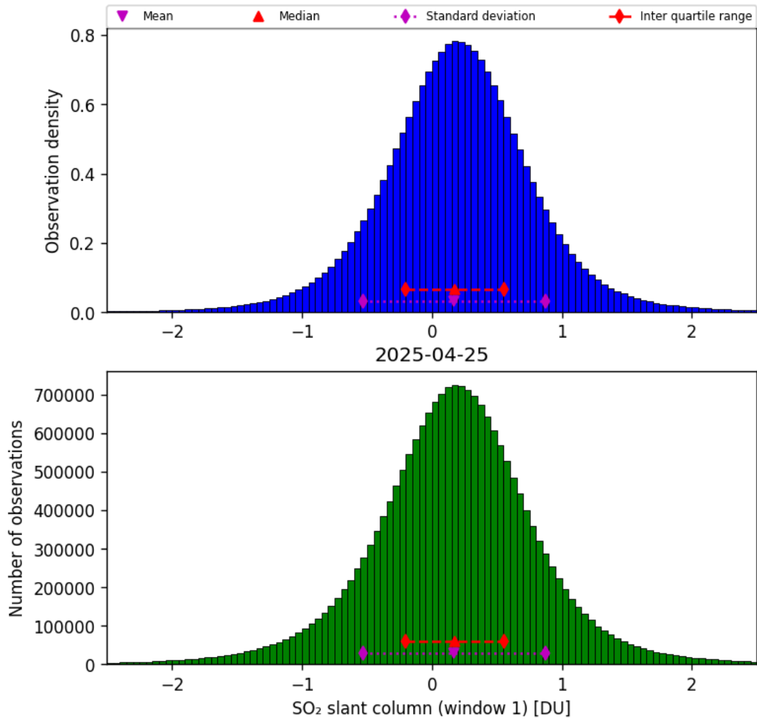
Figure 63: Histogram of “SO 2 slant column (window 1)” for 2025-04-24 to 2025-04-26
