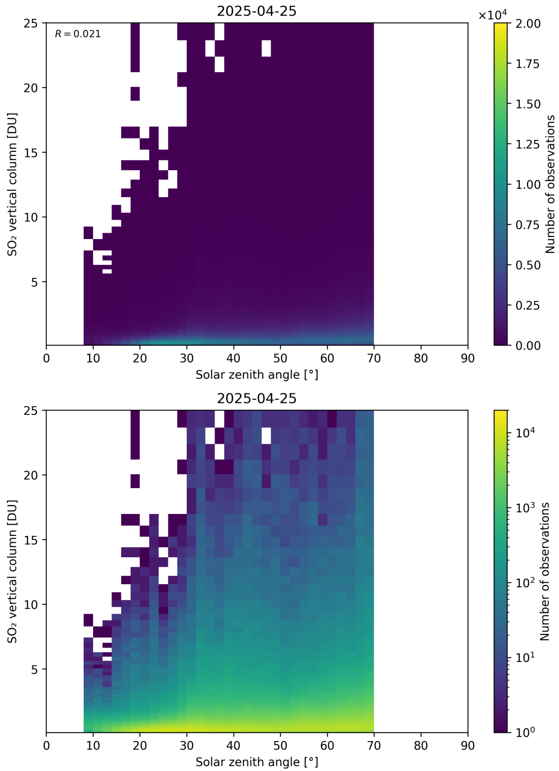
Figure 191: Scatter density plot of “Solar zenith angle” against “SO 2 vertical column” for 2025-04-24 to 2025-04-26.
