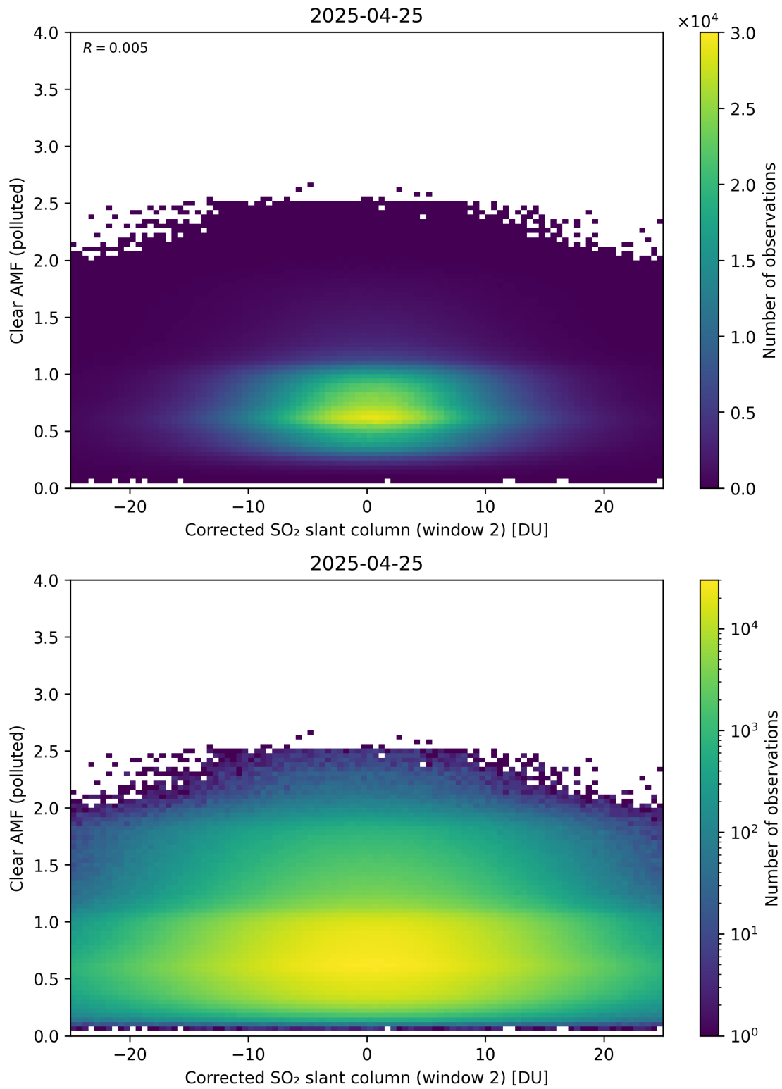
Figure 249: Scatter density plot of “Corrected SO 2 slant column (window 2)” against “Clear AMF (polluted)” for 2025-04-24 to 2025-04-26.
