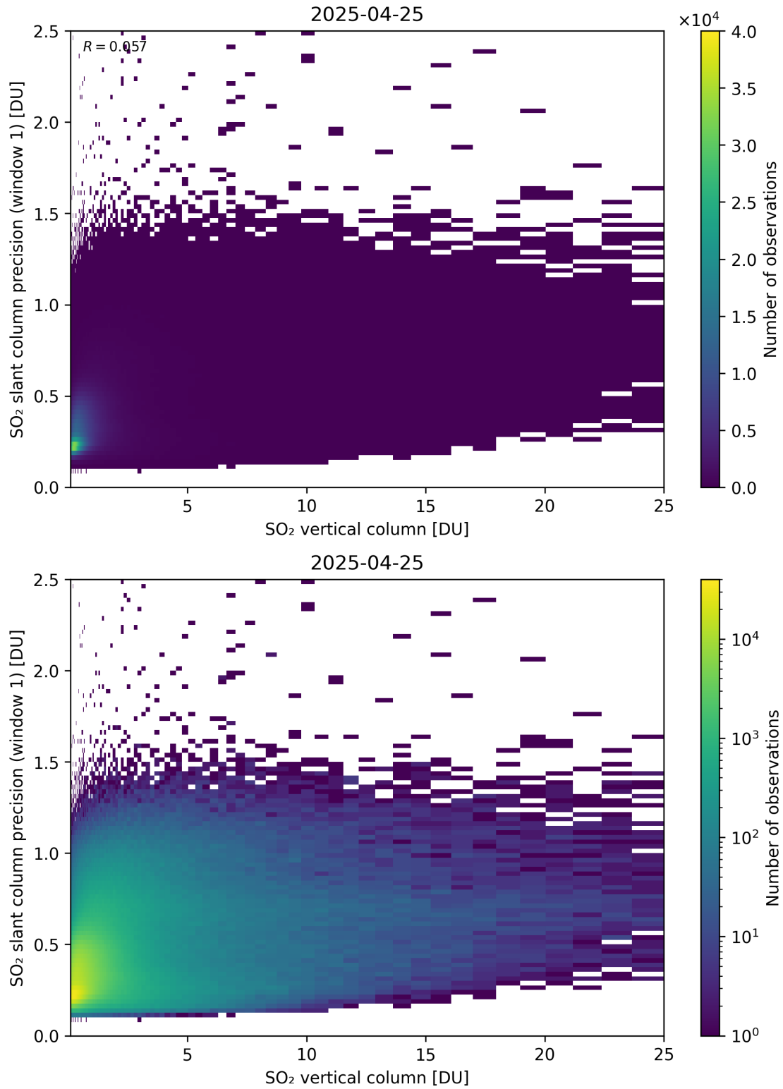
Figure 355: Scatter density plot of “SO 2 vertical column” against “SO 2 slant column precision (window 1)” for 2025-04-24 to 2025-04-26.
