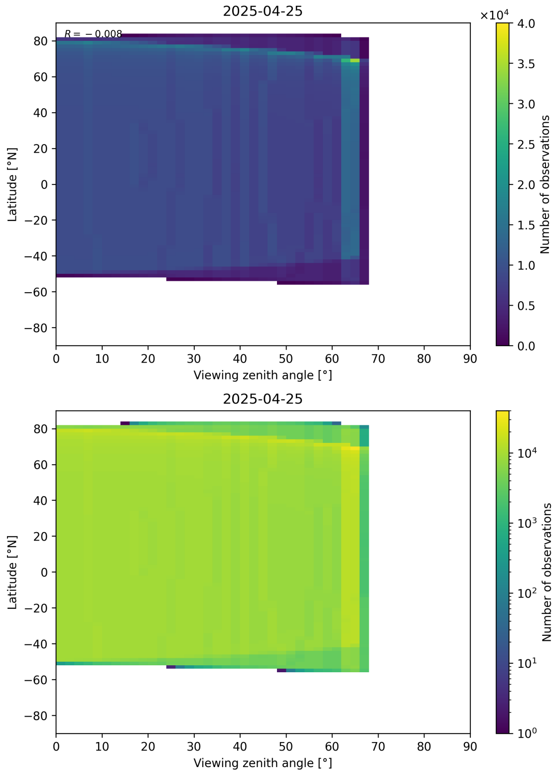
Figure 368: Scatter density plot of “Viewing zenith angle” against “Latitude” for 2025-04-24 to 2025-04-26.
