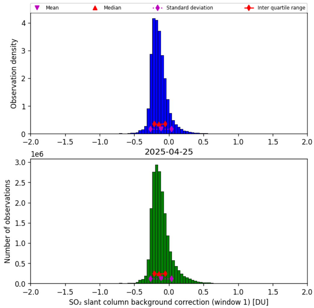
Figure 66: Histogram of “SO 2 slant column background correction (window 1)” for 2025-04-24 to 2025-04-26
