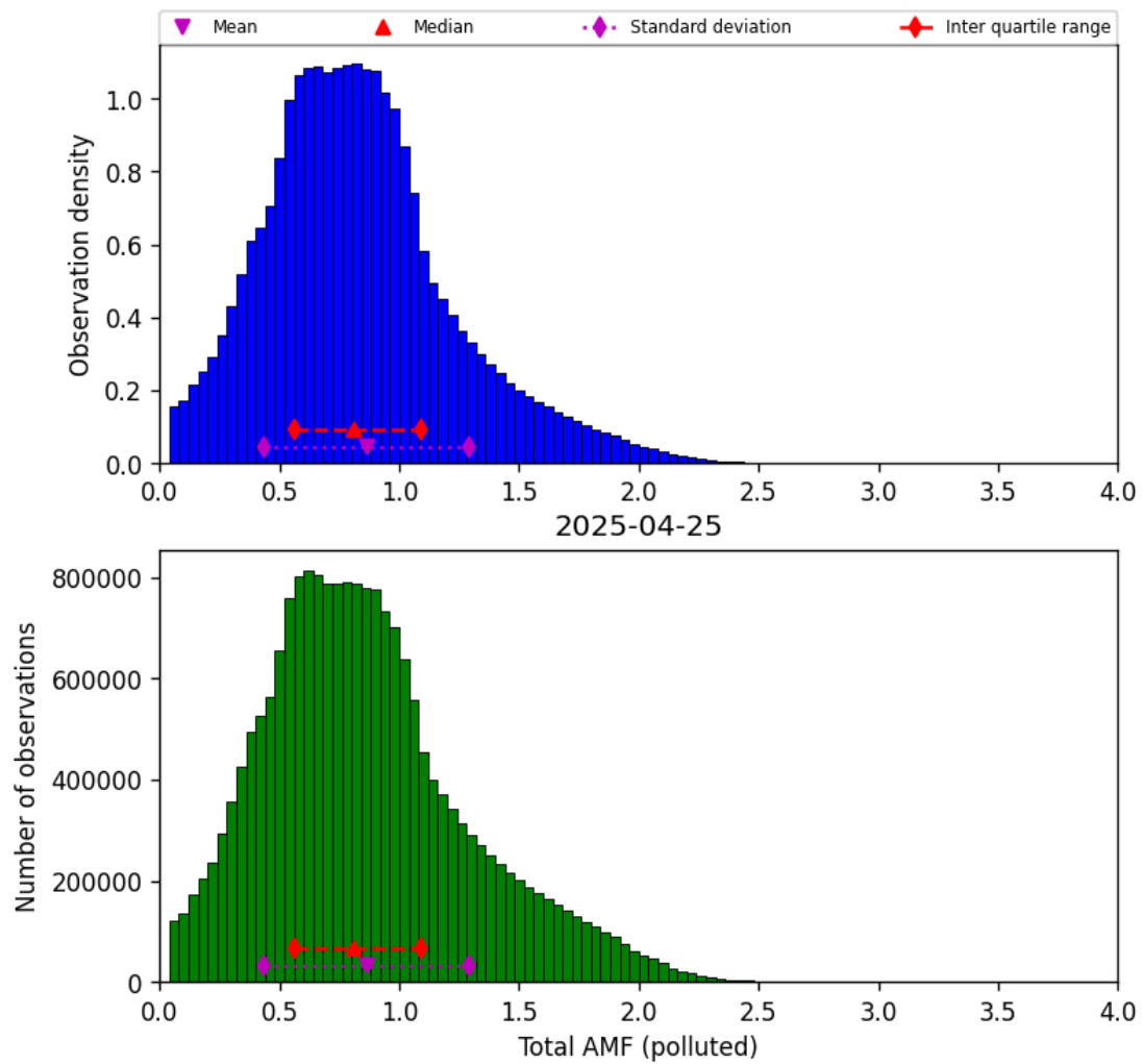
Figure 79: Histogram of “Total AMF (polluted)” for 2025-04-24 to 2025-04-26
