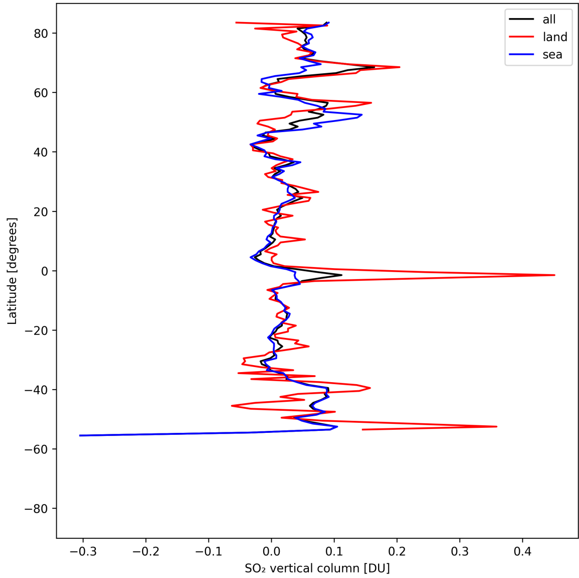
Figure 32: Zonal average of “SO 2 vertical column” for 2025-04-24 to 2025-04-26.
