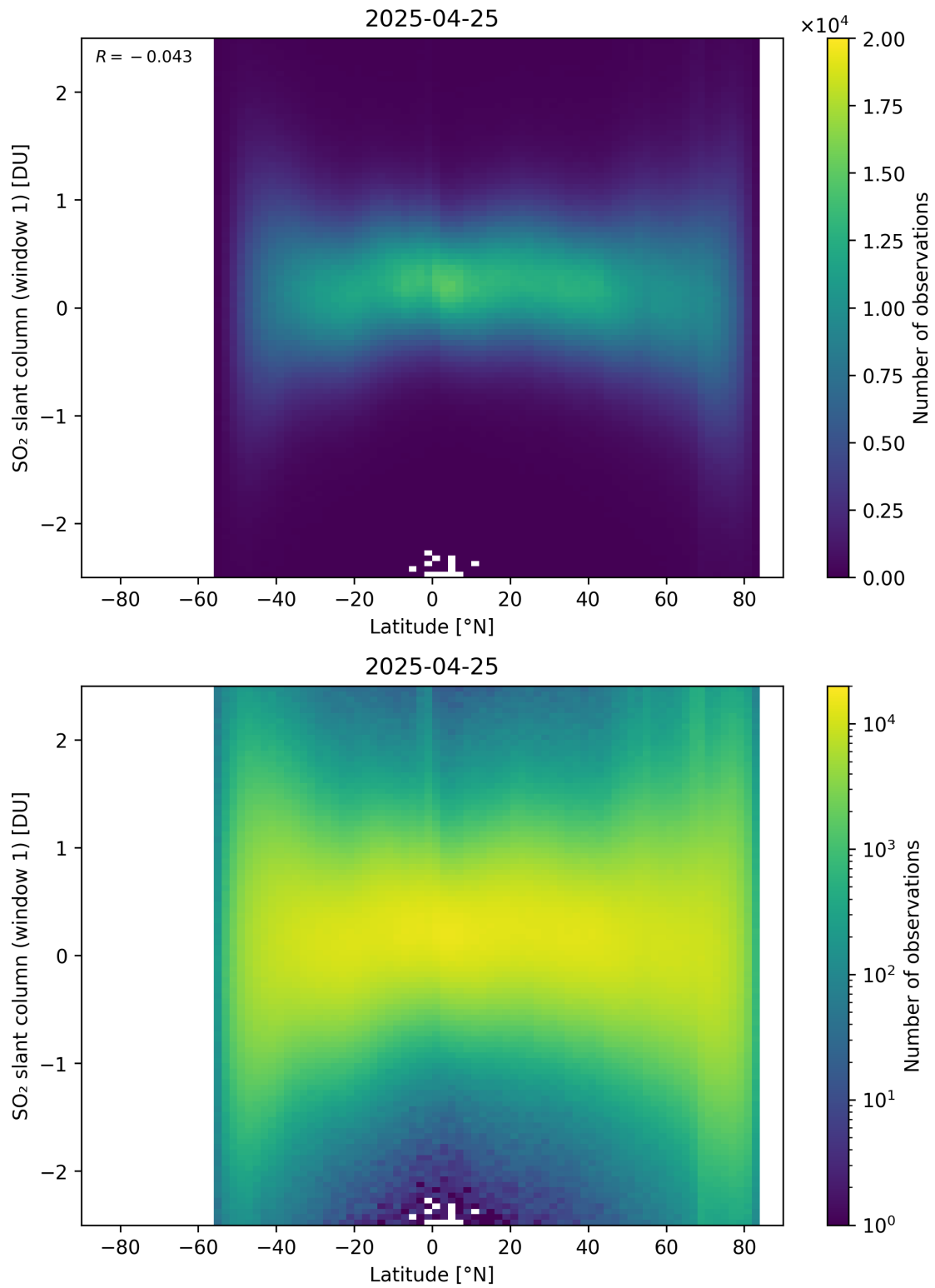
Figure 162: Scatter density plot of “Latitude” against “SO 2 slant column (window 1)” for 2025-04-24 to 2025-04-26.
