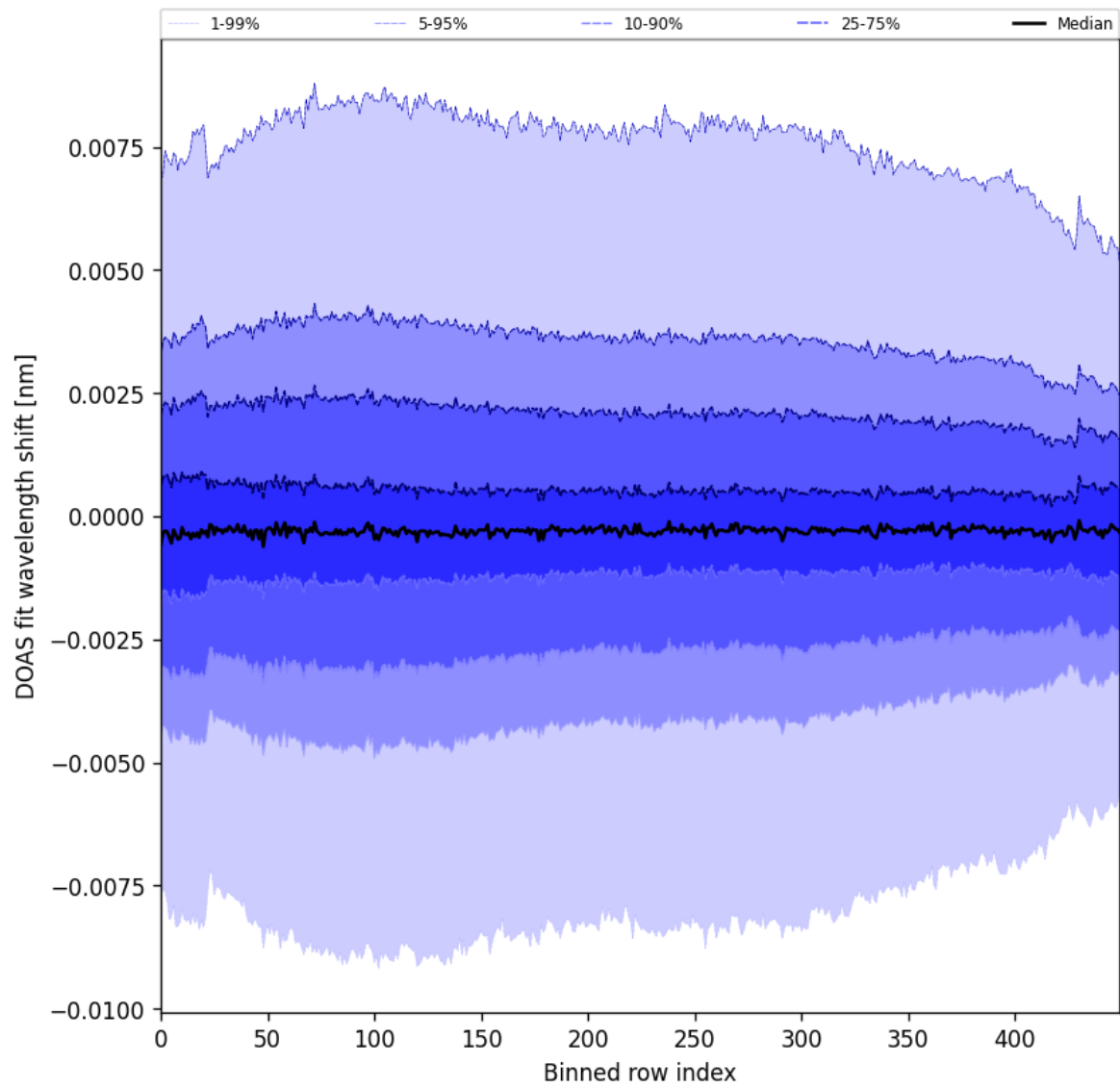
Figure 102: Along track statistics of “DOAS fit wavelength shift” for 2025-04-24 to 2025-04-26
