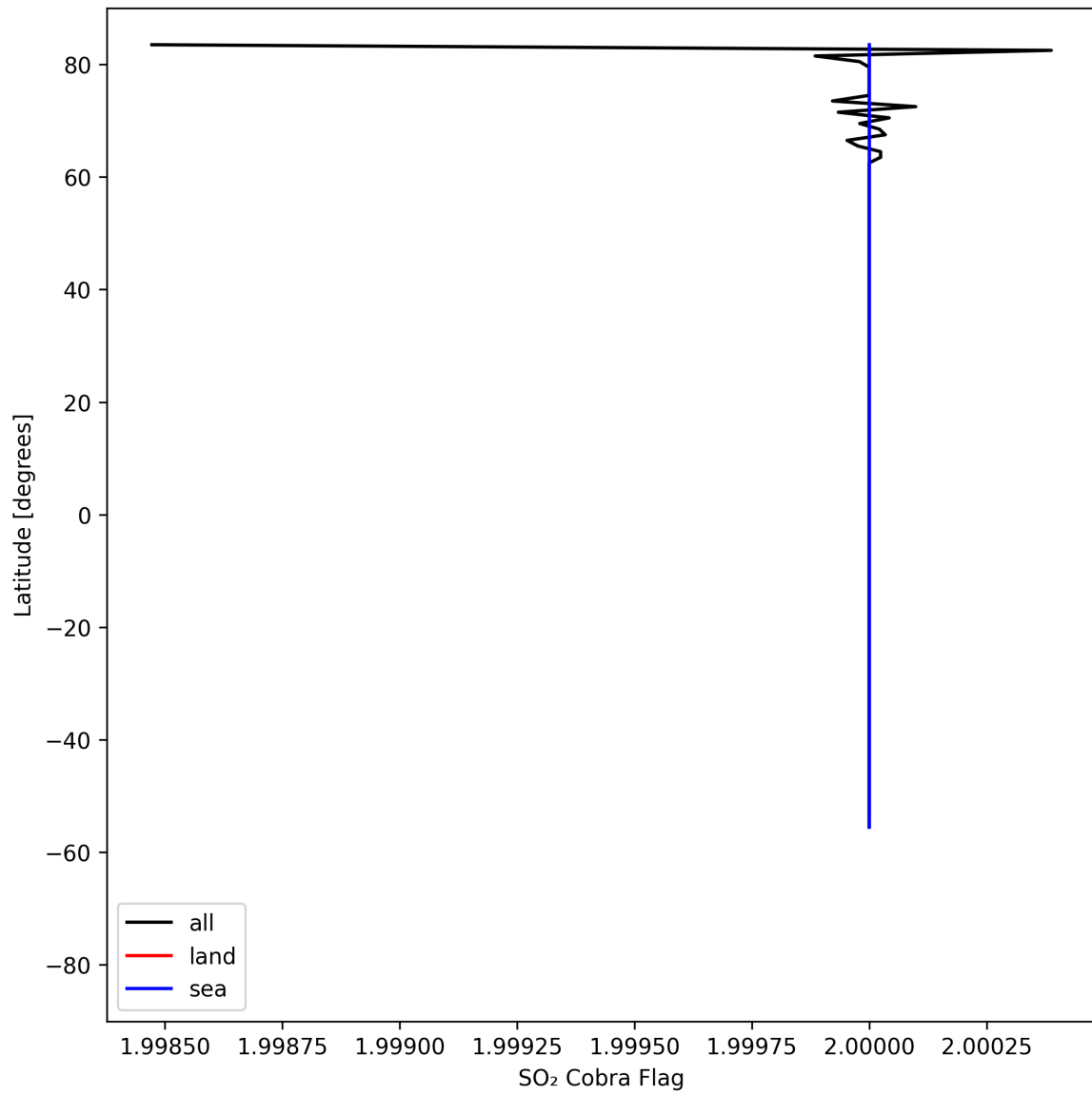
Figure 49: Zonal average of “SO 2 Cobra Flag” for 2025-04-24 to 2025-04-26.
