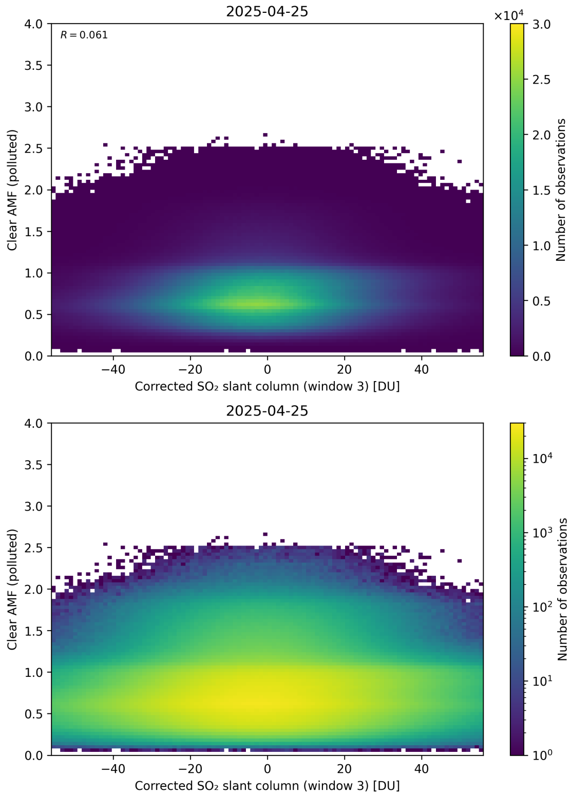
Figure 259: Scatter density plot of “Corrected SO 2 slant column (window 3)” against “Clear AMF (polluted)” for 2025-04-24 to 2025-04-26.
