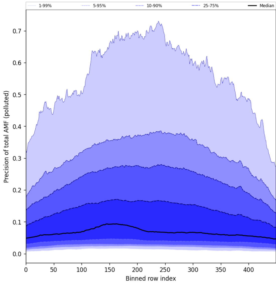
Figure 106: Along track statistics of “Precision of total AMF (polluted)” for 2025-04-24 to 2025-04-26
