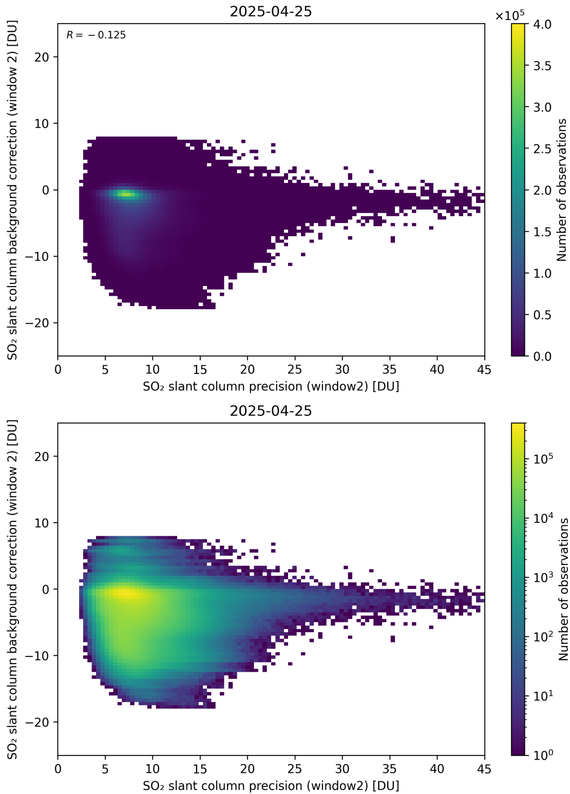
Figure 291: Scatter density plot of “SO 2 slant column precision (window2)” against “SO 2 slant column background correction (window 2)” for 2025-04-24 to 2025-04-26.
