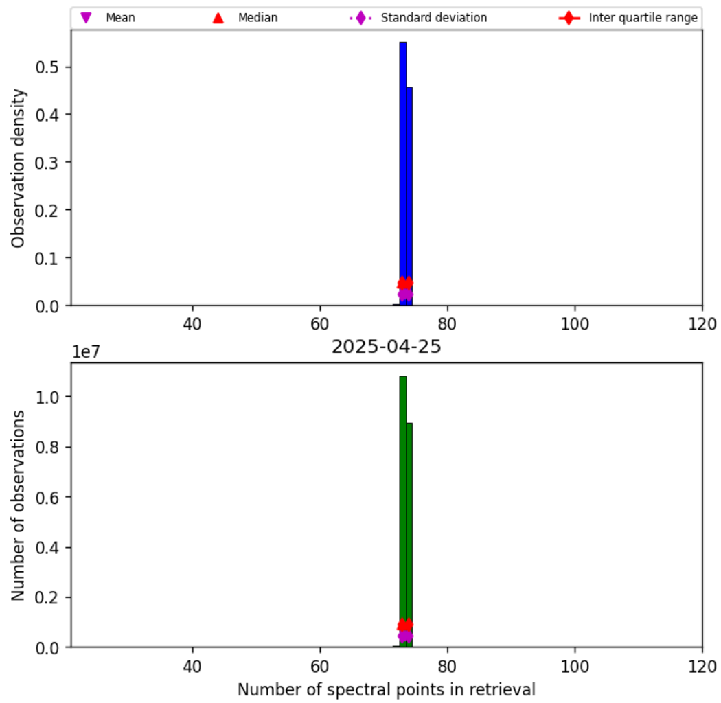
Figure 82: Histogram of “Number of spectral points in retrieval” for 2025-04-24 to 2025-04-26
