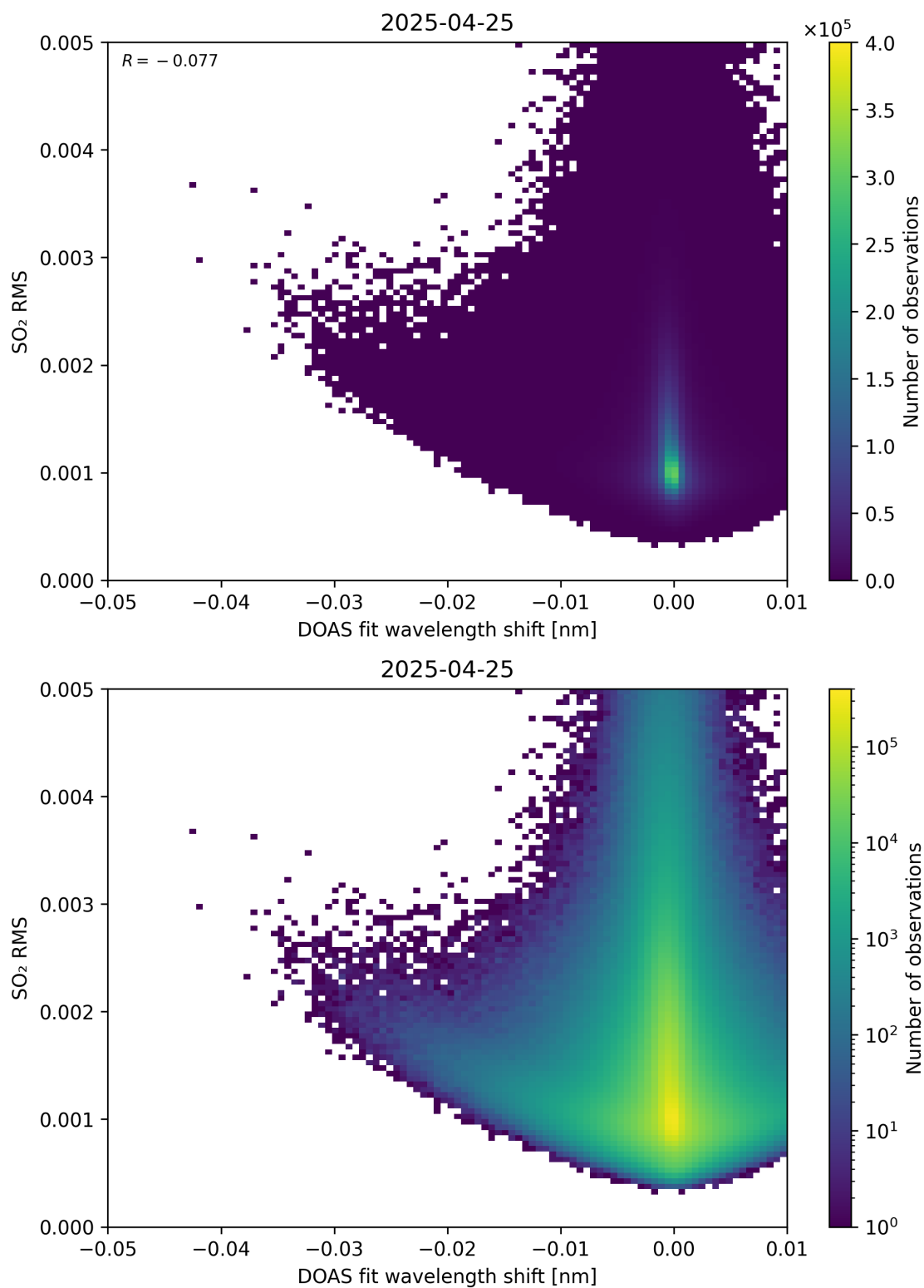
Figure 139: Scatter density plot of “DOAS fit wavelength shift” against “SO 2 RMS” for 2025-04-24 to 2025-04-26.
