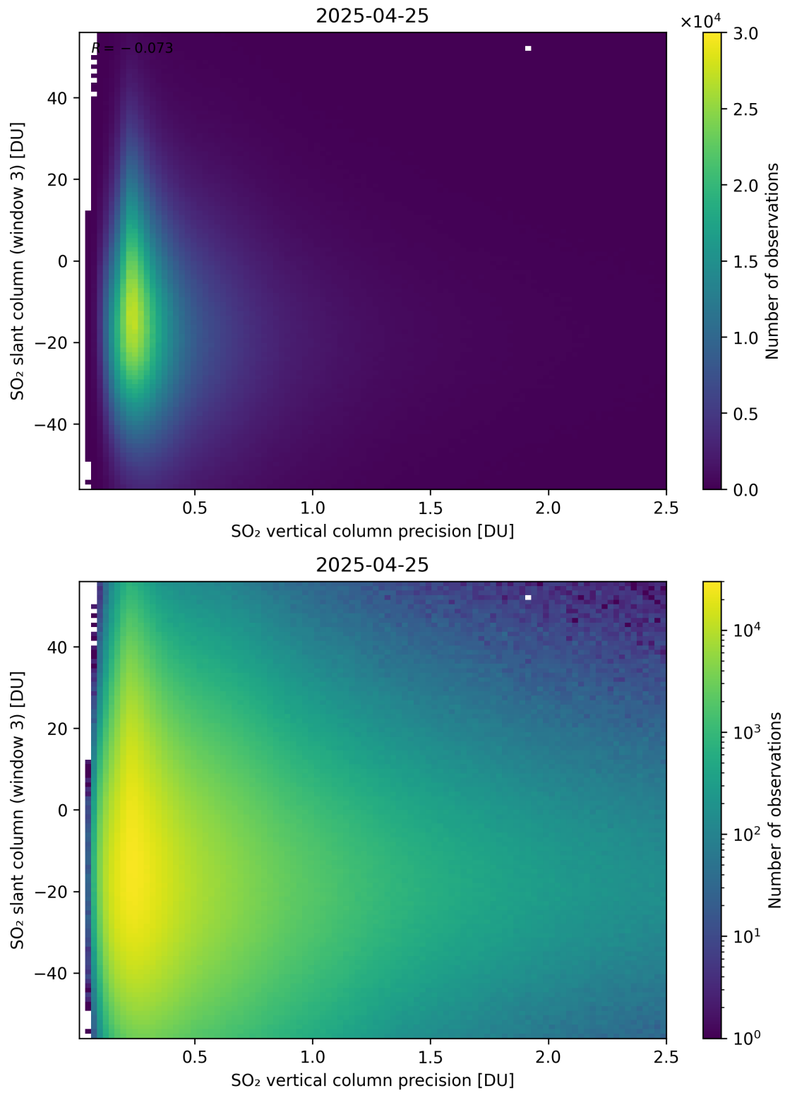
Figure 344: Scatter density plot of “SO 2 vertical column precision” against “SO 2 slant column (window 3)” for 2025-04-24 to 2025-04-26.
