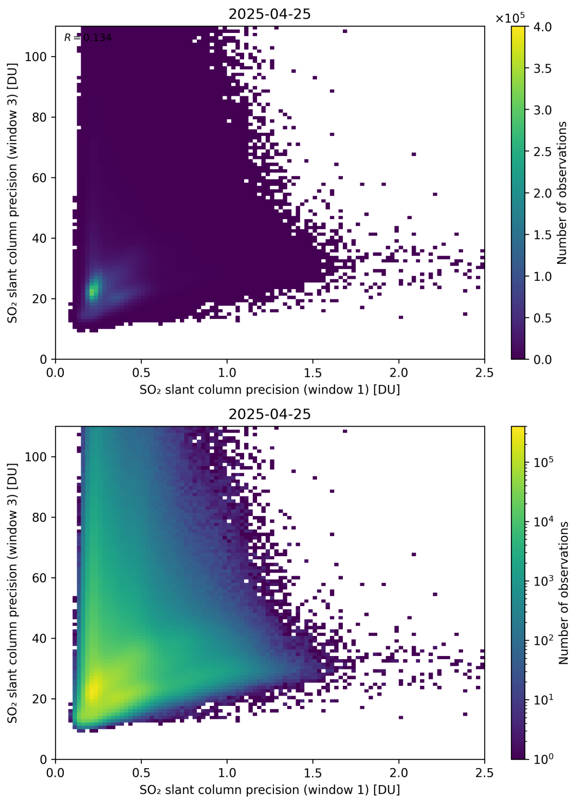
Figure 279: Scatter density plot of “SO 2 slant column precision (window 1)” against “SO 2 slant column precision (window 3)” for 2025-04-24 to 2025-04-26.
