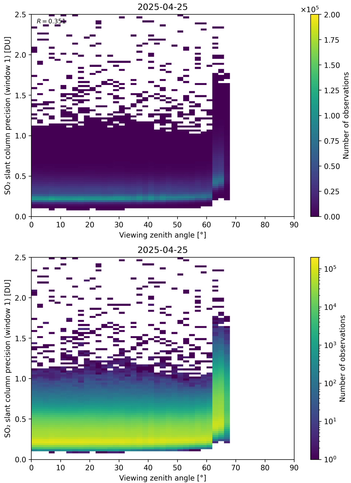
Figure 377: Scatter density plot of “Viewing zenith angle” against “SO 2 slant column precision (window 1)” for 2025-04-24 to 2025-04-26.
