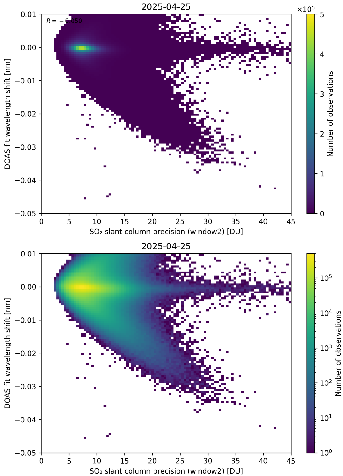
Figure 293: Scatter density plot of “SO 2 slant column precision (window2)” against “DOAS fit wavelength shift” for 2025-04-24 to 2025-04-26.
