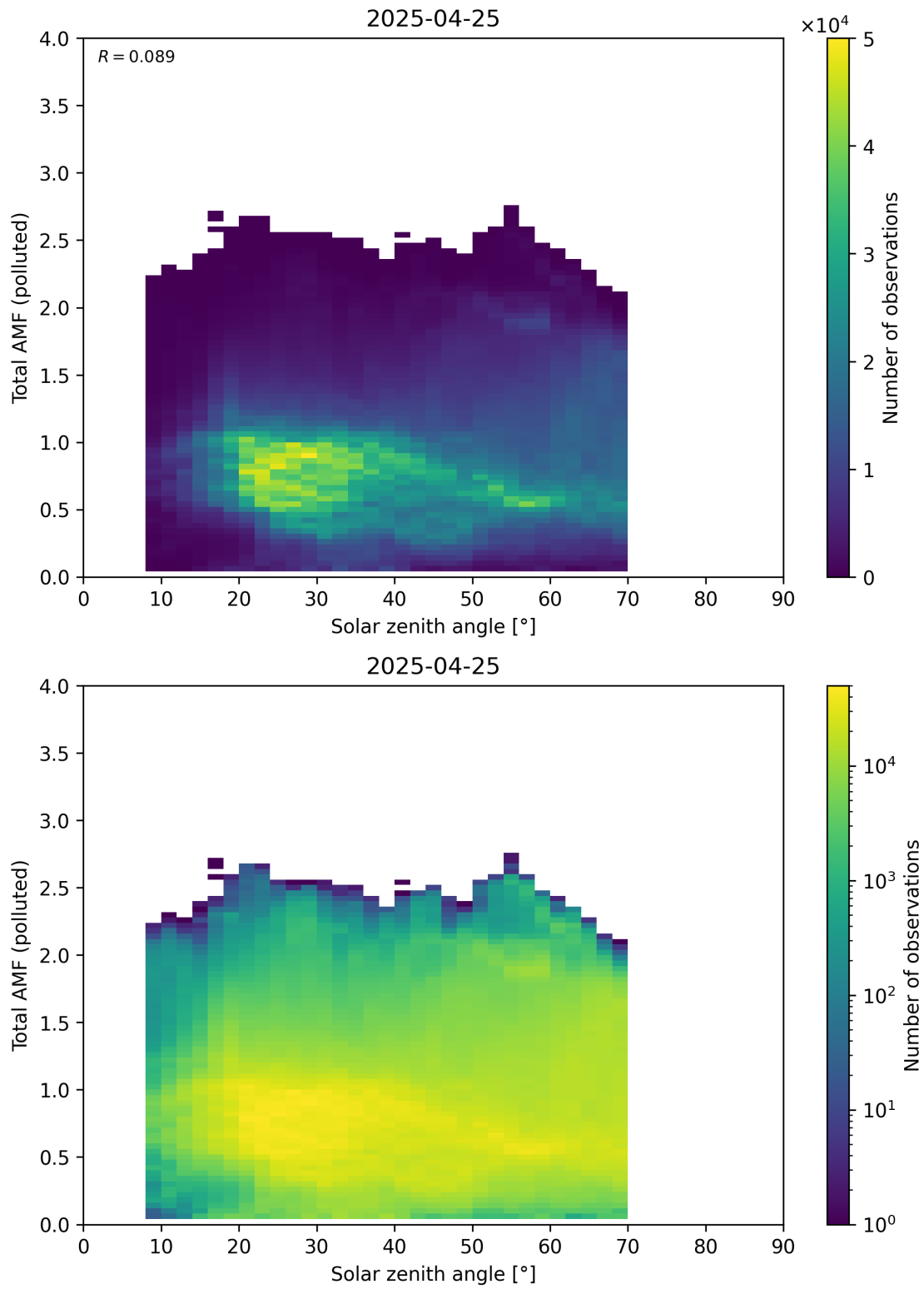
Figure 189: Scatter density plot of “Solar zenith angle” against “Total AMF (polluted)” for 2025-04-24 to 2025-04-26.
