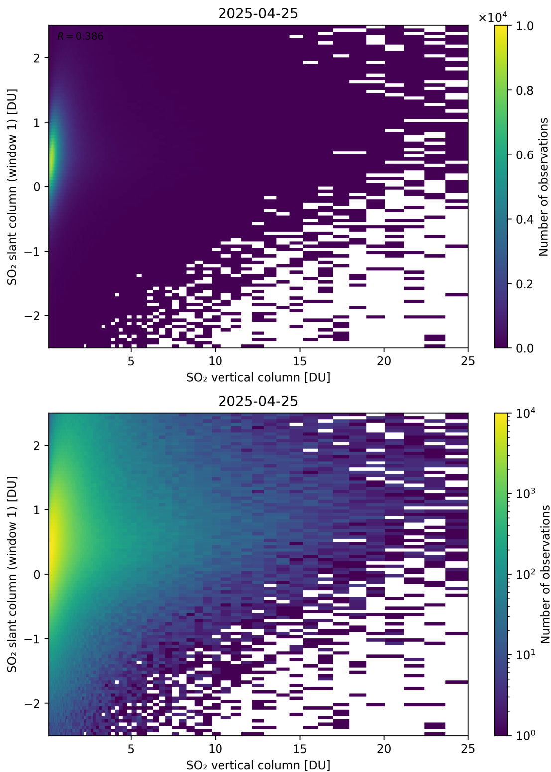
Figure 354: Scatter density plot of “SO 2 vertical column” against “SO 2 slant column (window 1)” for 2025-04-24 to 2025-04-26.
