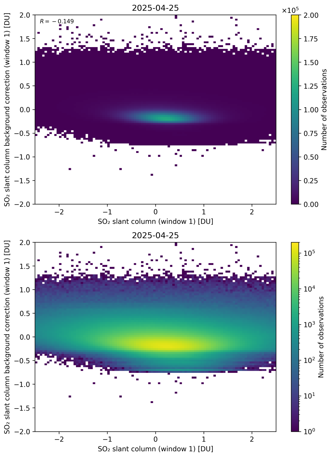
Figure 262: Scatter density plot of “SO 2 slant column (window 1)” against “SO 2 slant column background correction (window 1)” for 2025-04-24 to 2025-04-26.
