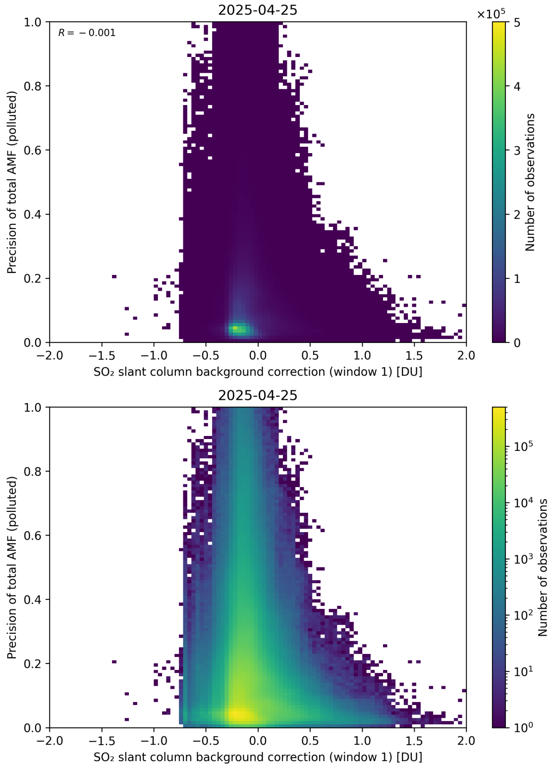
Figure 121: Scatter density plot of “SO 2 slant column background correction (window 1)” against “Precision of total AMF (polluted)” for 2025-04-24 to 2025-04-26.
