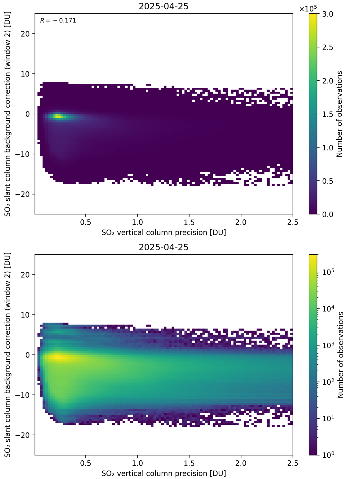
Figure 330: Scatter density plot of “SO 2 vertical column precision” against “SO 2 slant column background correction (window 2)” for 2025-04-24 to 2025-04-26.
