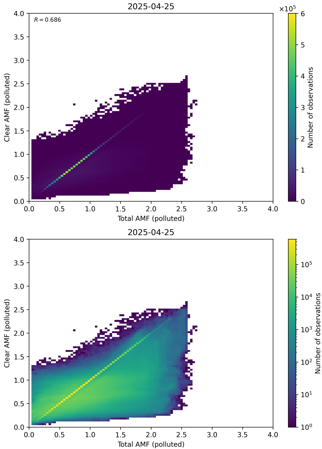
Figure 321: Scatter density plot of “Total AMF (polluted)” against “Clear AMF (polluted)” for 2025-04-24 to 2025-04-26.
