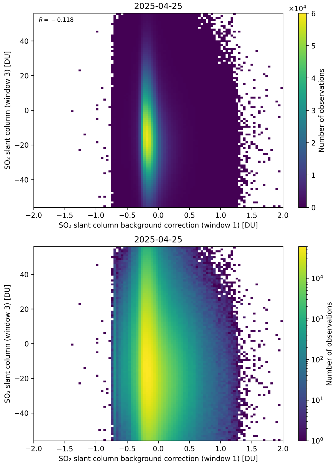
Figure 118: Scatter density plot of “SO 2 slant column background correction (window 1)” against “SO 2 slant column (window 3)” for 2025-04-24 to 2025-04-26.
