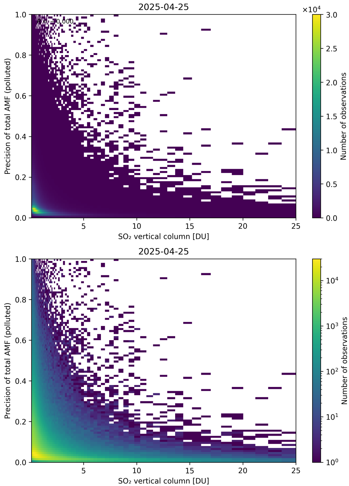
Figure 360: Scatter density plot of “SO 2 vertical column” against “Precision of total AMF (polluted)” for 2025-04-24 to 2025-04-26.
