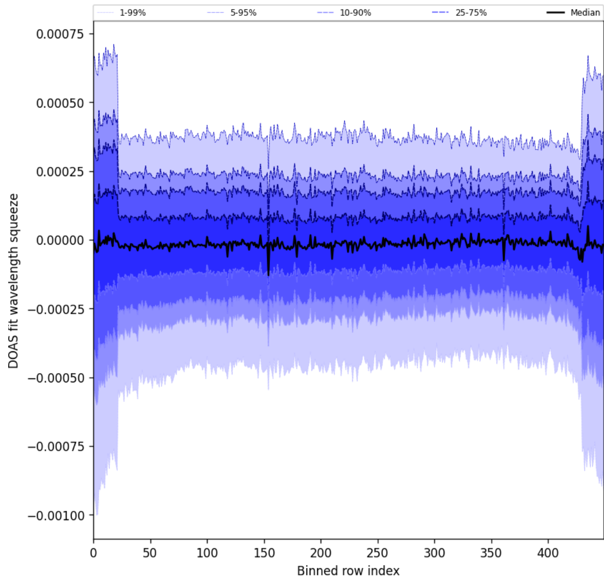
Figure 103: Along track statistics of “DOAS fit wavelength squeeze” for 2025-04-24 to 2025-04-26
