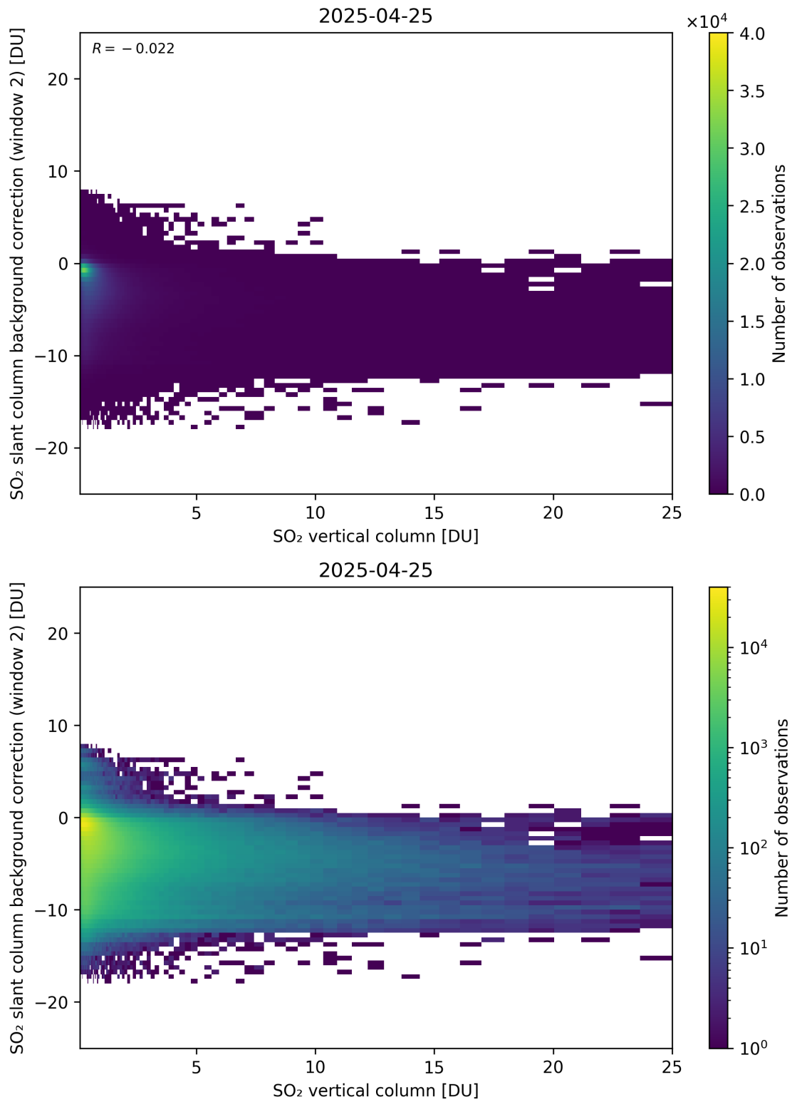
Figure 324: Scatter density plot of “SO 2 vertical column” against “SO 2 slant column background correction (window 2)” for 2025-04-24 to 2025-04-26.
