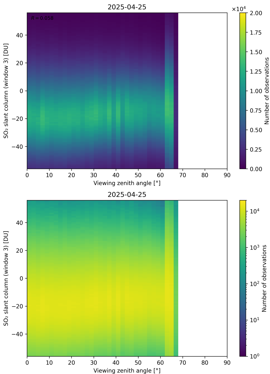
Figure 379: Scatter density plot of “Viewing zenith angle” against “SO 2 slant column (window 3)” for 2025-04-24 to 2025-04-26.
