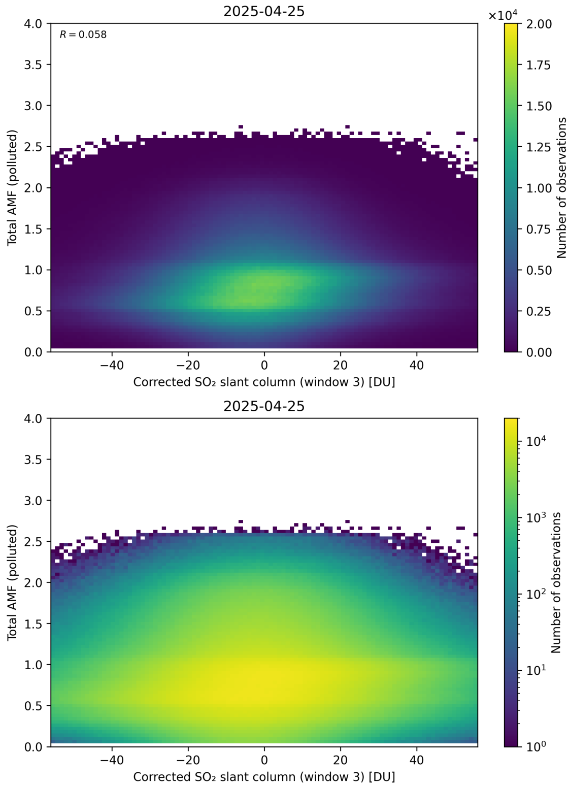
Figure 260: Scatter density plot of “Corrected SO 2 slant column (window 3)” against “Total AMF (polluted)” for 2025-04-24 to 2025-04-26.
