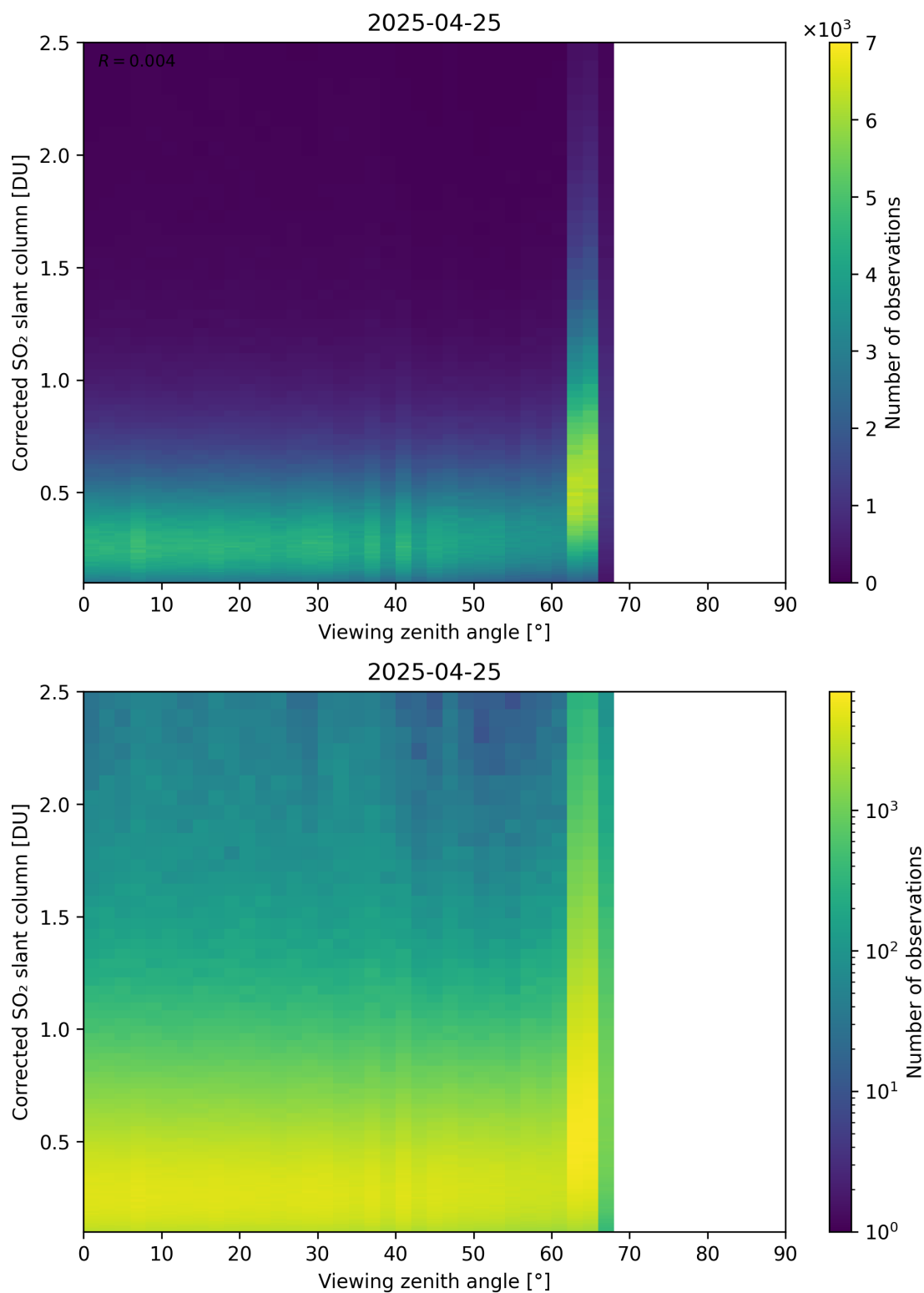
Figure 373: Scatter density plot of “Viewing zenith angle” against “Corrected SO 2 slant column” for 2025-04-24 to 2025-04-26.
