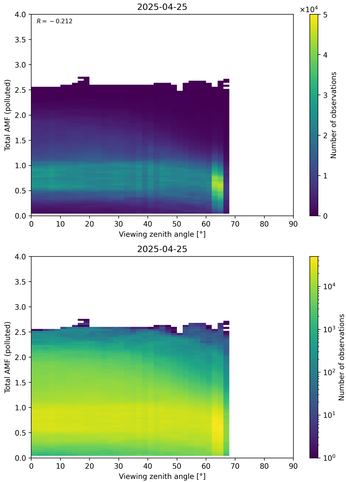
Figure 381: Scatter density plot of “Viewing zenith angle” against “Total AMF (polluted)” for 2025-04-24 to 2025-04-26.
