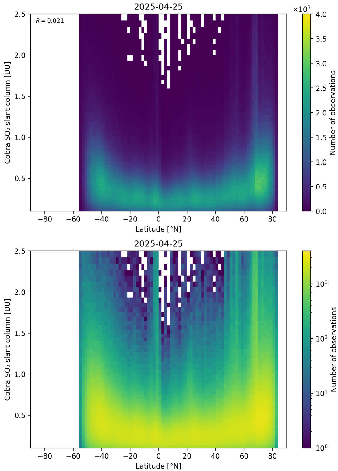
Figure 157: Scatter density plot of “Latitude” against “Cobra SO 2 slant column” for 2025-04-24 to 2025-04-26.
