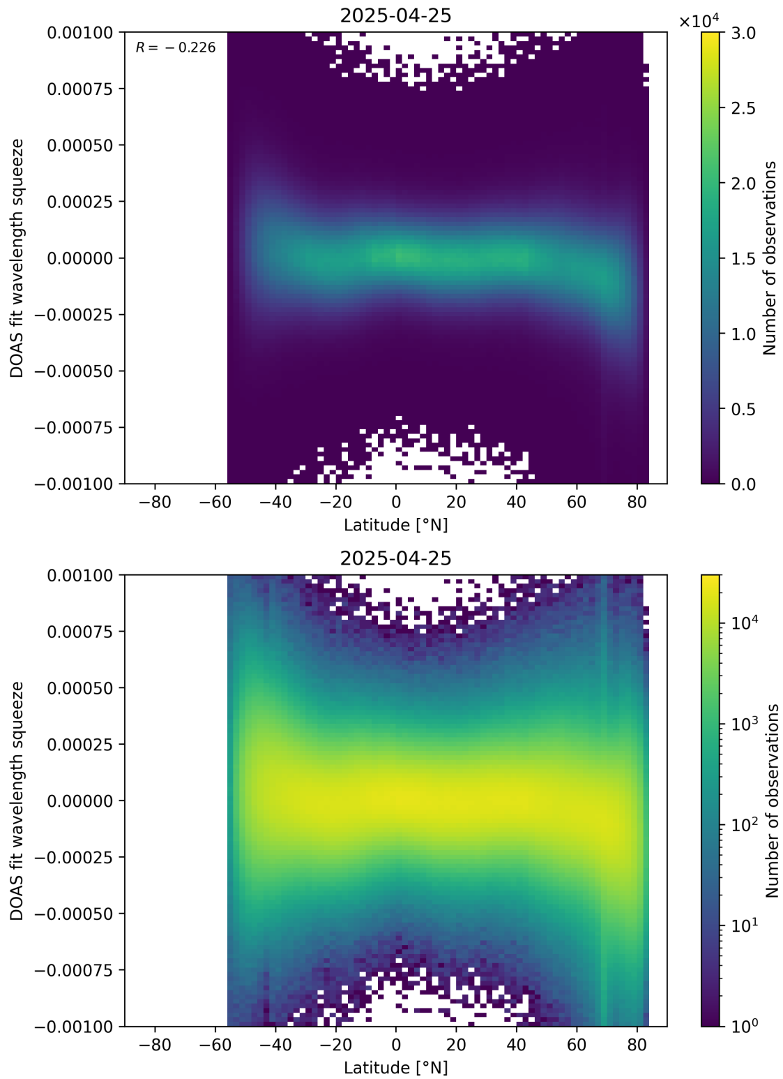
Figure 154: Scatter density plot of “Latitude” against “DOAS fit wavelength squeeze” for 2025-04-24 to 2025-04-26.
