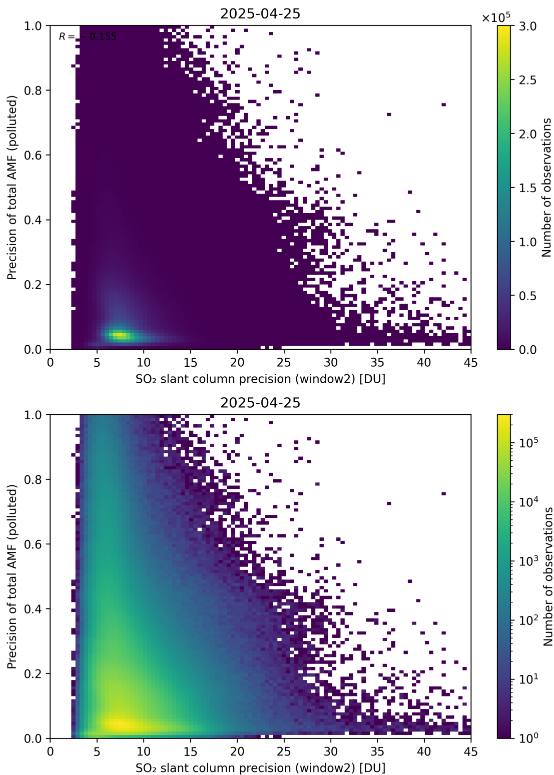
Figure 302: Scatter density plot of “SO 2 slant column precision (window2)” against “Precision of total AMF (polluted)” for 2025-04-24 to 2025-04-26.
