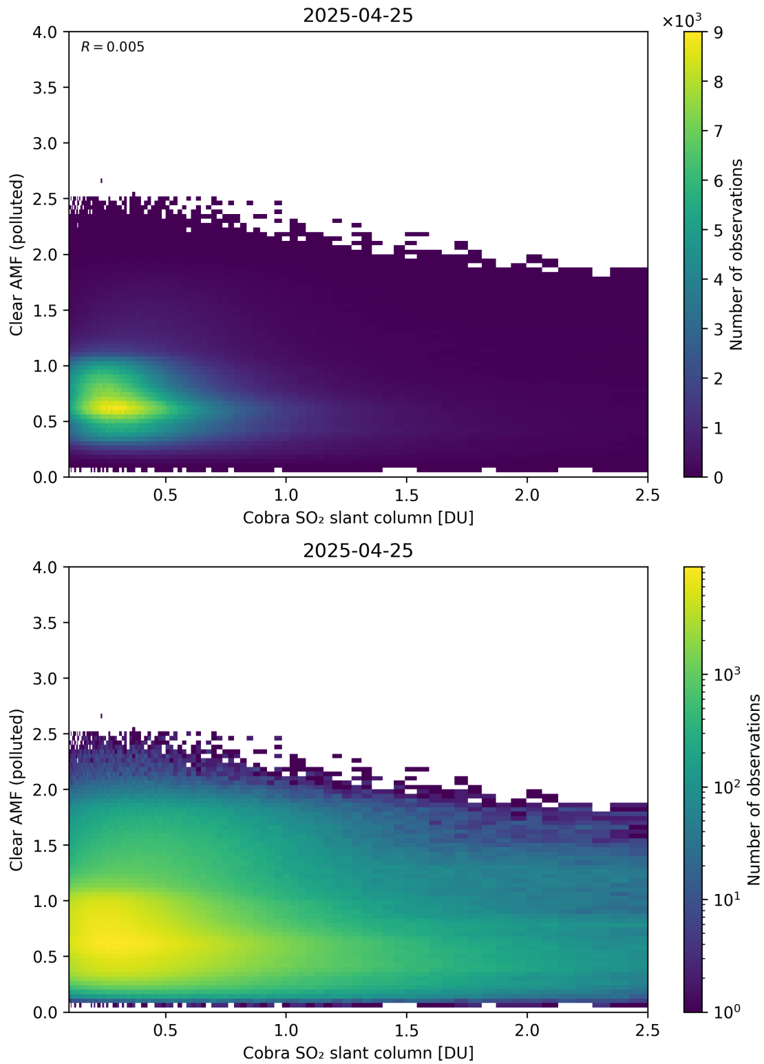
Figure 215: Scatter density plot of “Cobra SO 2 slant column” against “Clear AMF (polluted)” for 2025-04-24 to 2025-04-26.
