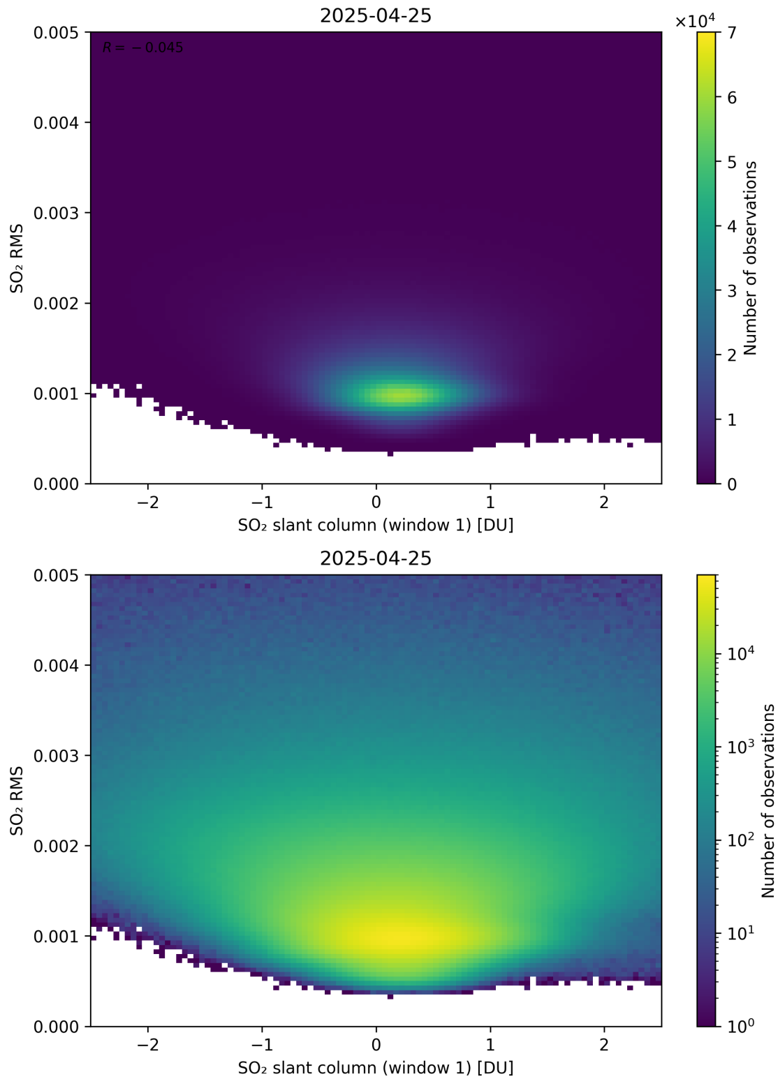
Figure 267: Scatter density plot of “SO 2 slant column (window 1)” against “SO 2 RMS” for 2025-04-24 to 2025-04-26.
