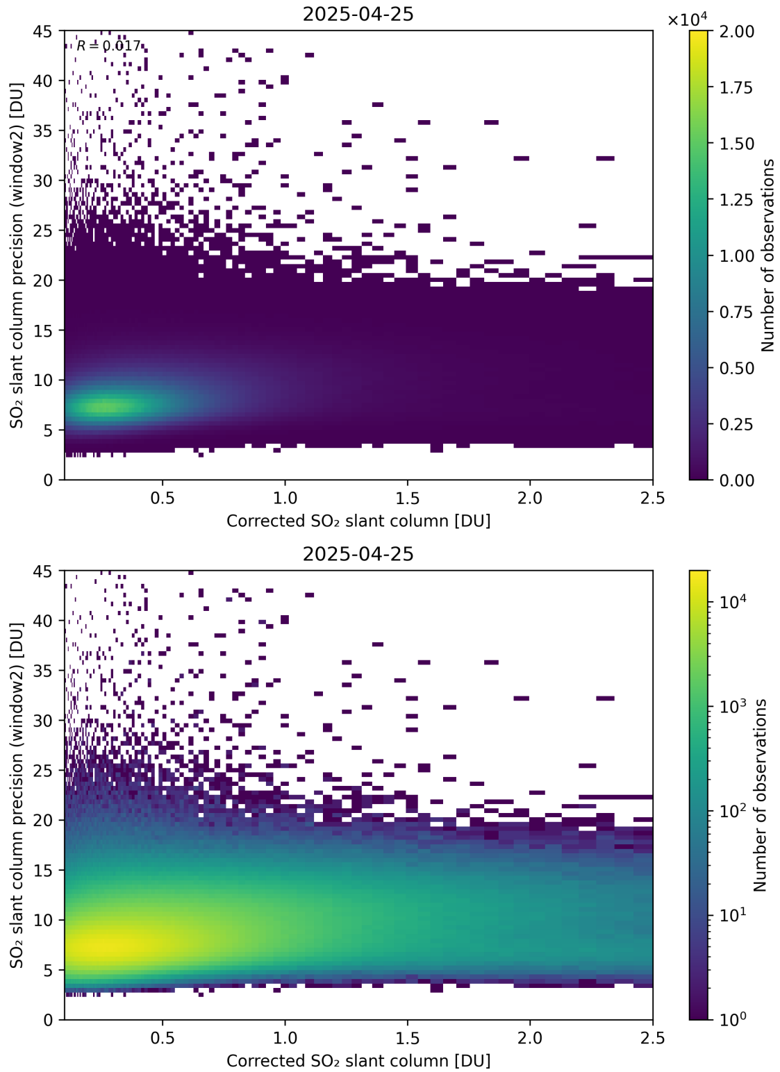
Figure 239: Scatter density plot of “Corrected SO 2 slant column” against “SO 2 slant column precision (window2)” for 2025-04-24 to 2025-04-26.
