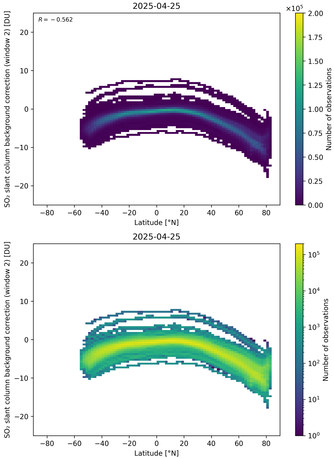
Figure 151: Scatter density plot of “Latitude” against “SO 2 slant column background correction (window 2)” for 2025-04-24 to 2025-04-26.
