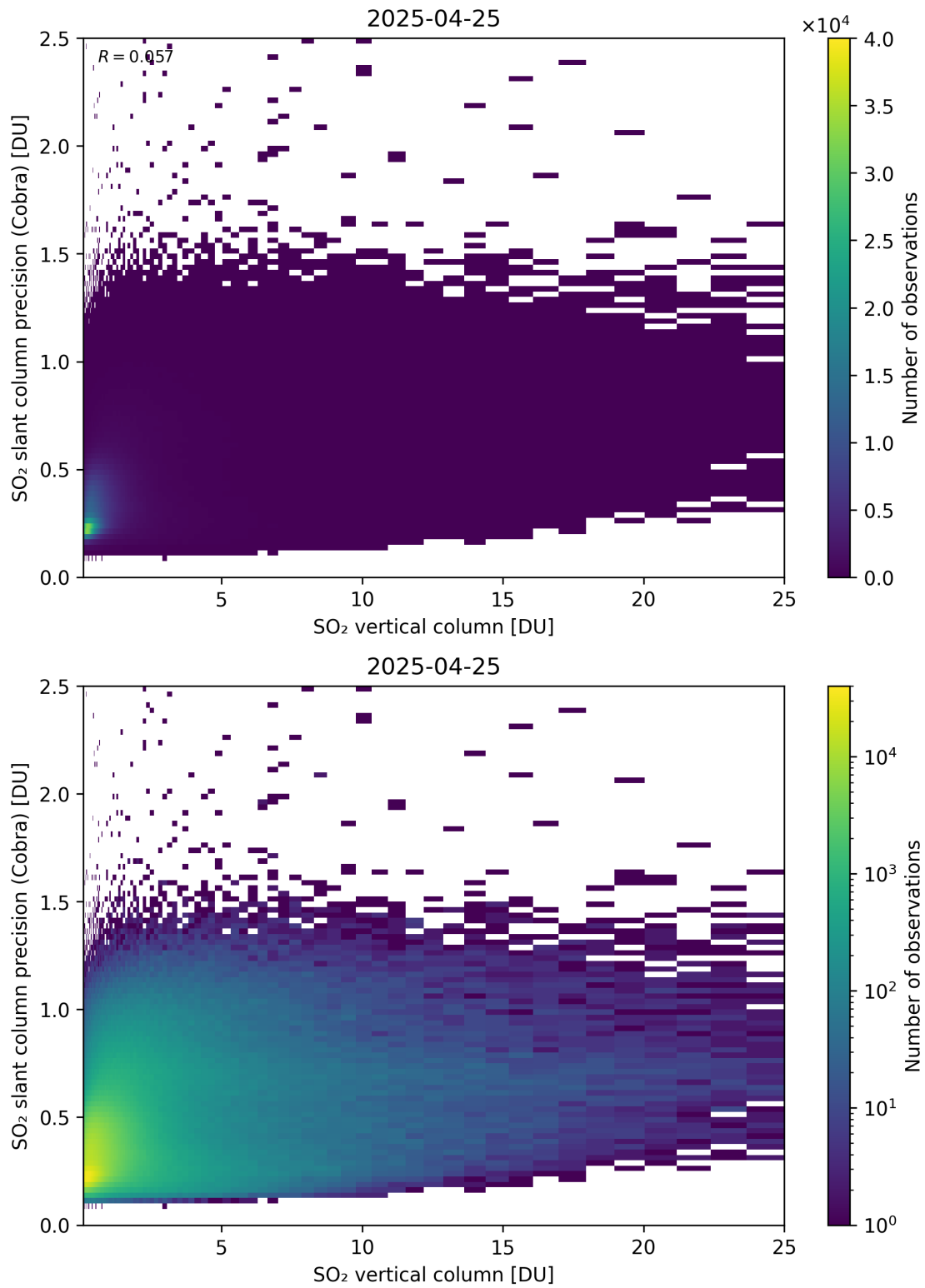
Figure 350: Scatter density plot of “SO 2 vertical column” against “SO 2 slant column precision (Cobra)” for 2025-04-24 to 2025-04-26.
