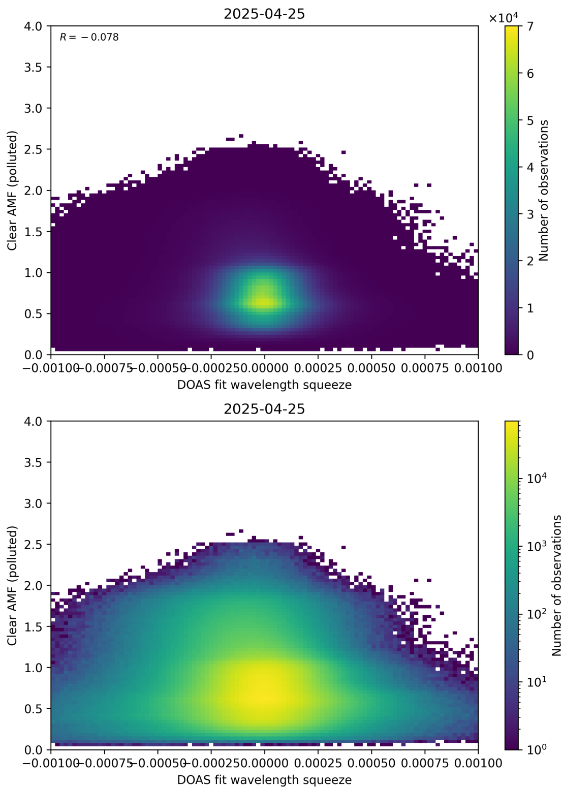
Figure 144: Scatter density plot of “DOAS fit wavelength squeeze” against “Clear AMF (polluted)” for 2025-04-24 to 2025-04-26.
