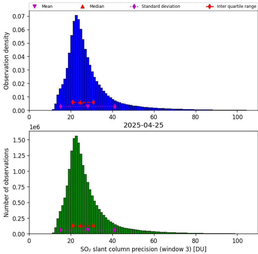
Figure 72: Histogram of “SO 2 slant column precision (window 3)” for 2025-04-24 to 2025-04-26
