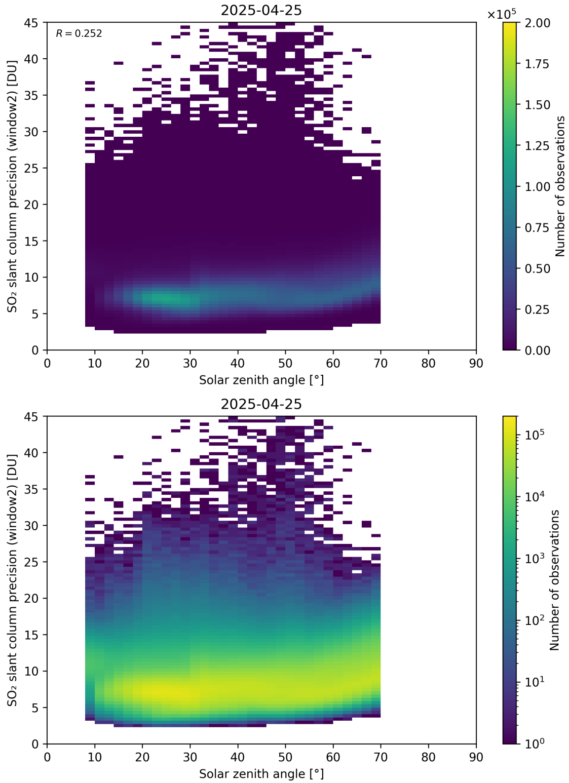
Figure 186: Scatter density plot of “Solar zenith angle” against “SO 2 slant column precision (window2)” for 2025-04-24 to 2025-04-26.
