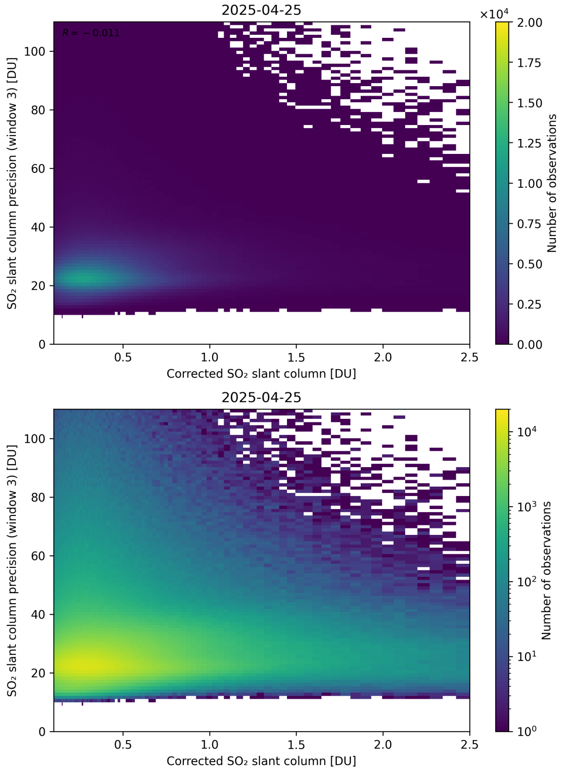
Figure 241: Scatter density plot of “Corrected SO 2 slant column” against “SO 2 slant column precision (window 3)” for 2025-04-24 to 2025-04-26.
