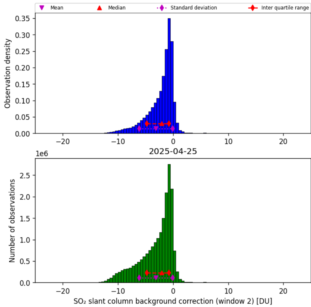
Figure 70: Histogram of “SO 2 slant column background correction (window 2)” for 2025-04-24 to 2025-04-26
