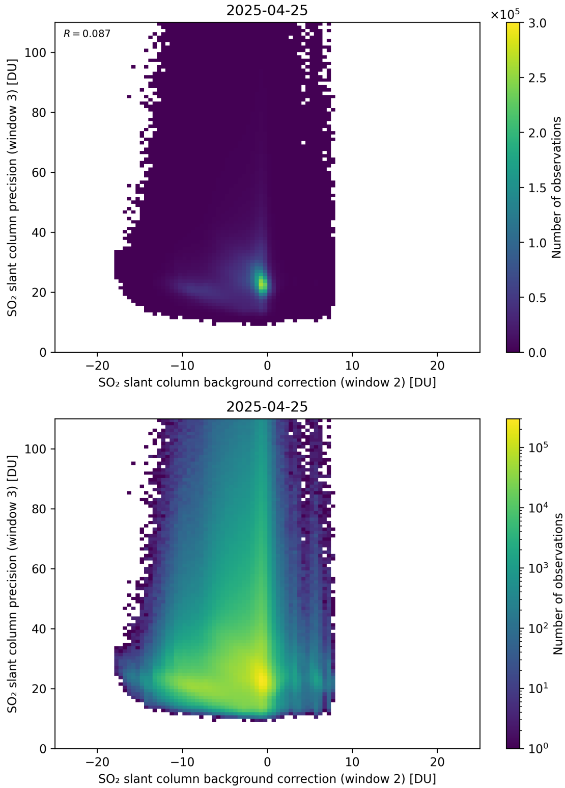
Figure 129: Scatter density plot of “SO 2 slant column background correction (window 2)” against “SO 2 slant column precision (window 3)” for 2025-04-24 to 2025-04-26.
