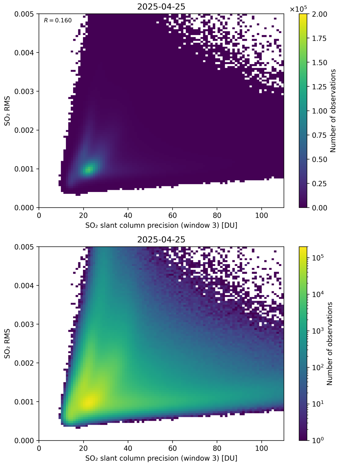
Figure 310: Scatter density plot of “SO 2 slant column precision (window 3)” against “SO 2 RMS” for 2025-04-24 to 2025-04-26.
