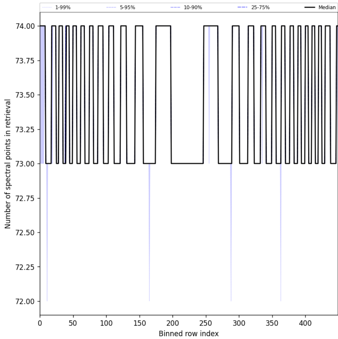
Figure 108: Along track statistics of “Number of spectral points in retrieval” for 2025-04-24 to 2025-04-26
