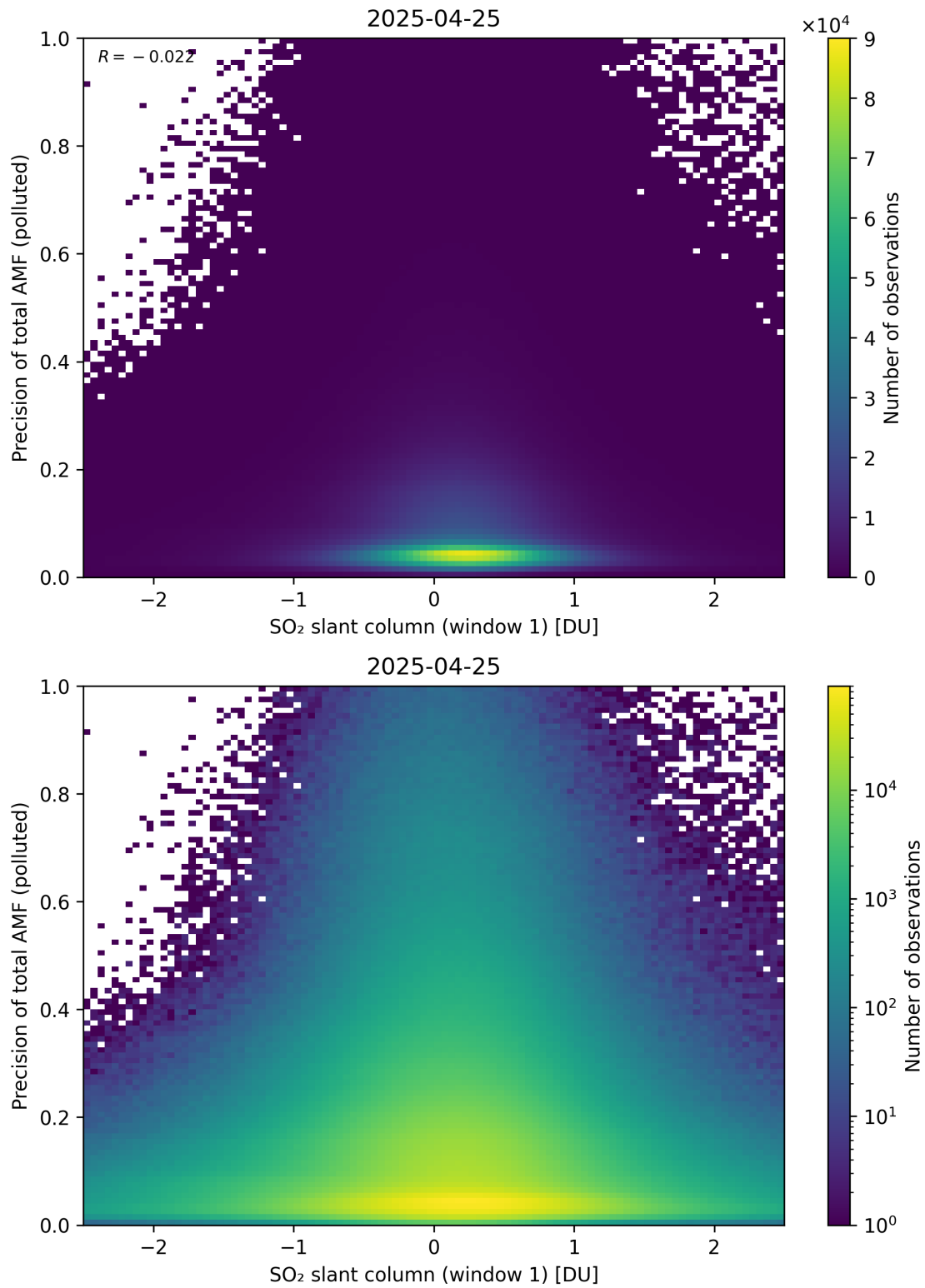
Figure 290: Scatter density plot of “SO 2 slant column (window 1)” against “Precision of total AMF (polluted)” for 2025-04-24 to 2025-04-26.
