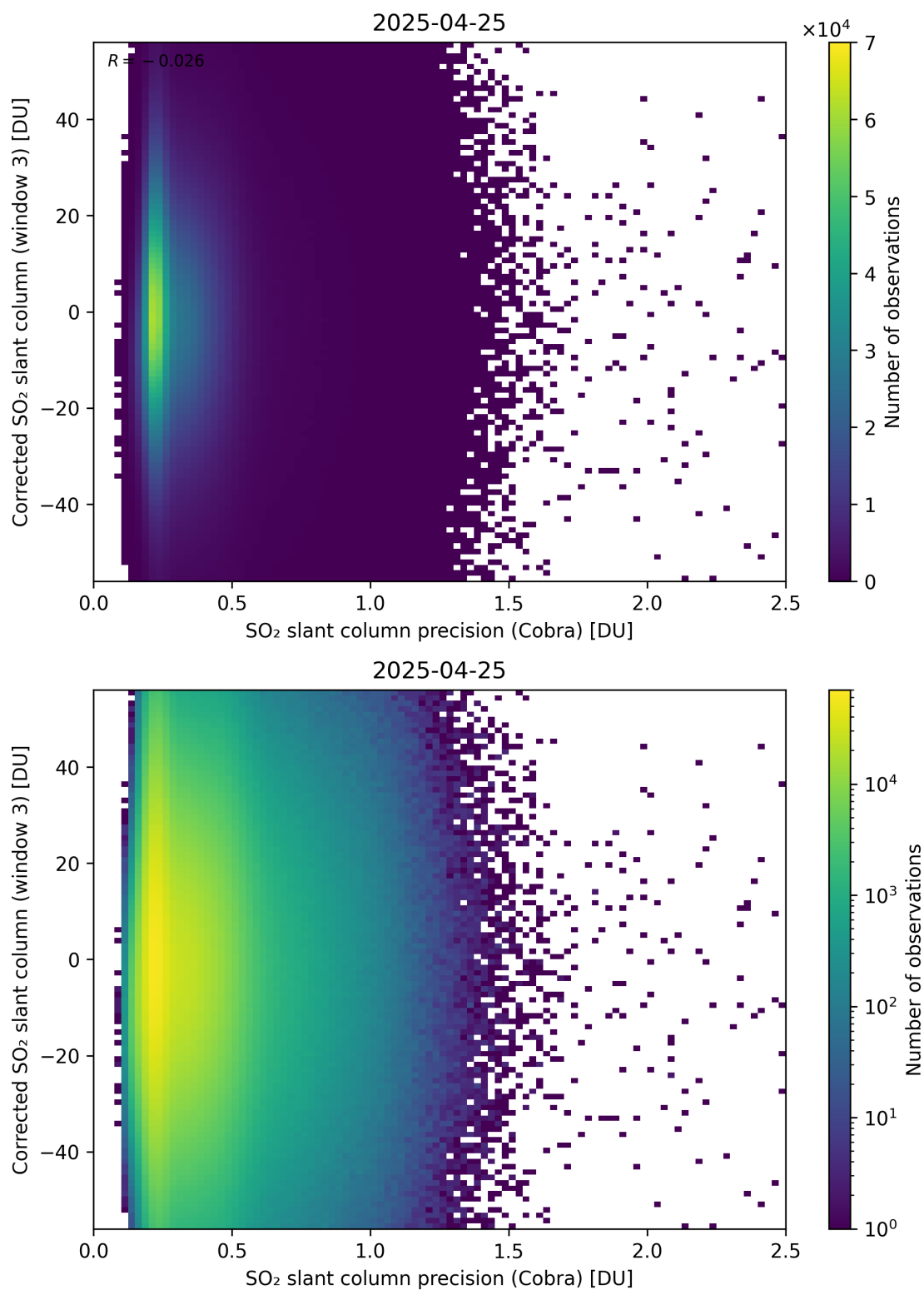
Figure 207: Scatter density plot of “SO 2 slant column precision (Cobra)” against “Corrected SO 2 slant column (window 3)” for 2025-04-24 to 2025-04-26.
