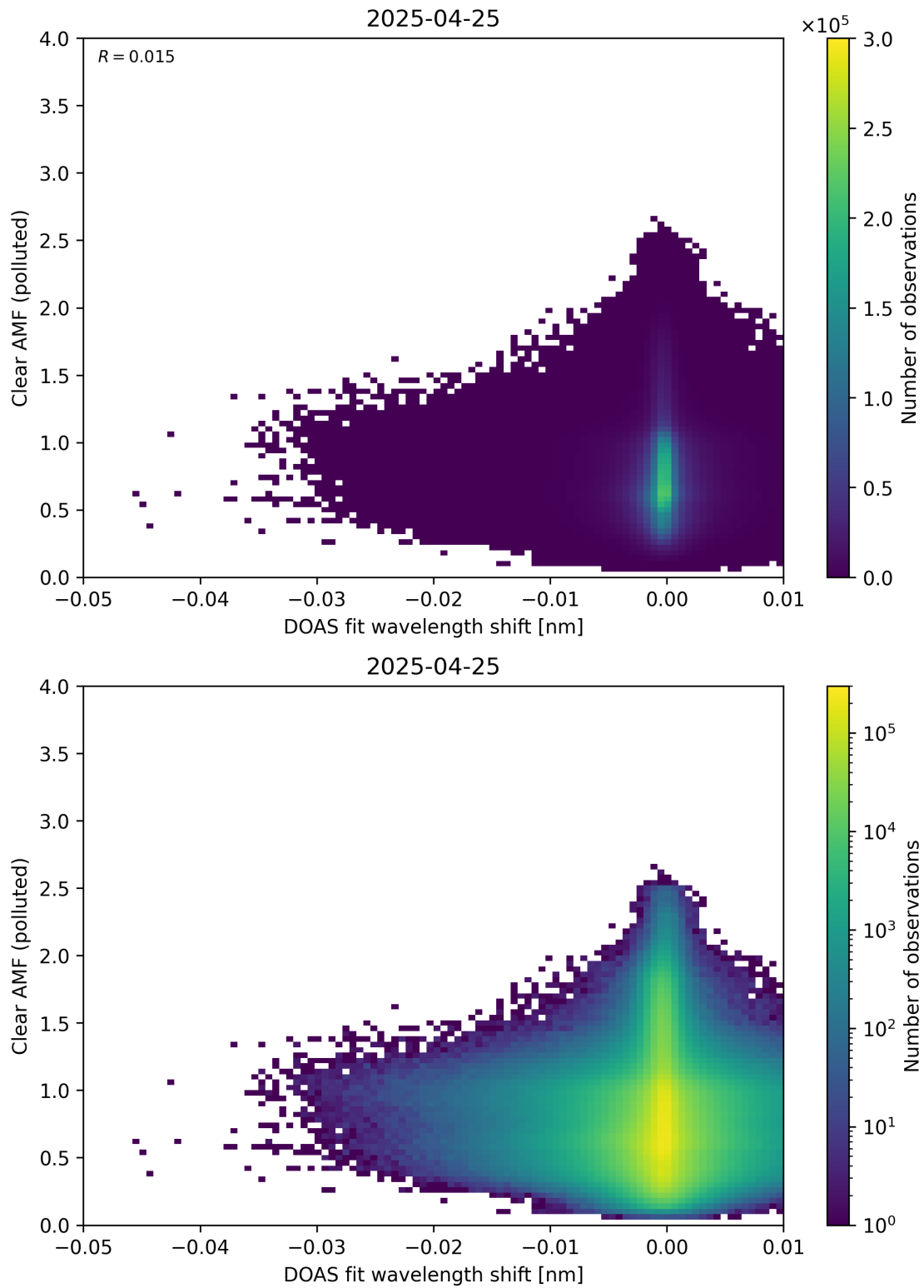
Figure 140: Scatter density plot of “DOAS fit wavelength shift” against “Clear AMF (polluted)” for 2025-04-24 to 2025-04-26.
