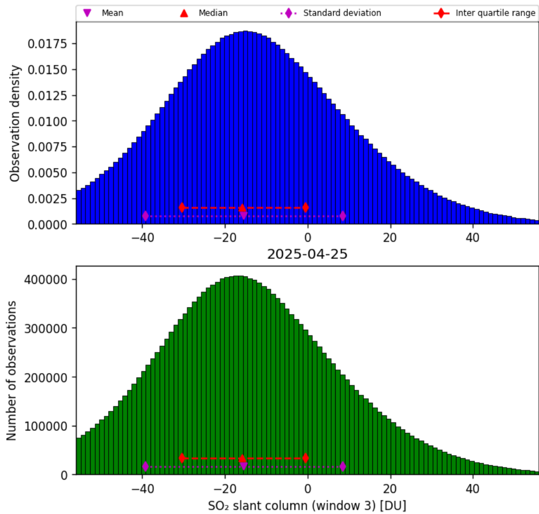
Figure 71: Histogram of “SO 2 slant column (window 3)” for 2025-04-24 to 2025-04-26
