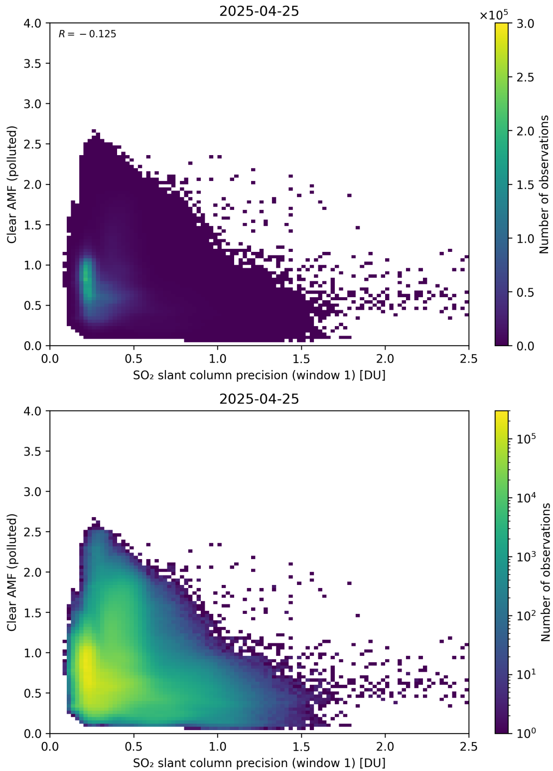
Figure 274: Scatter density plot of “SO 2 slant column precision (window 1)” against “Clear AMF (polluted)” for 2025-04-24 to 2025-04-26.
