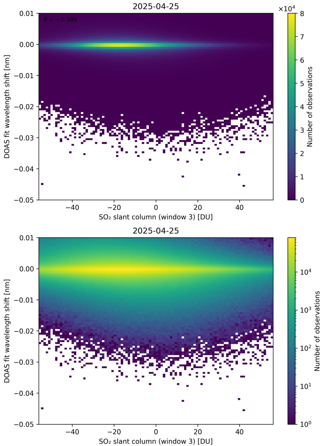
Figure 304: Scatter density plot of “SO 2 slant column (window 3)” against “DOAS fit wavelength shift” for 2025-04-24 to 2025-04-26.
