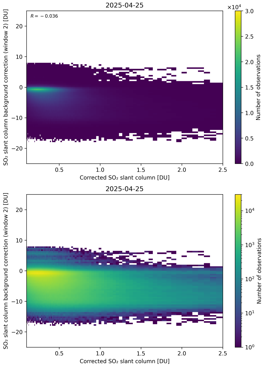
Figure 227: Scatter density plot of “Corrected SO 2 slant column” against “SO 2 slant column background correction (window 2)” for 2025-04-24 to 2025-04-26.
