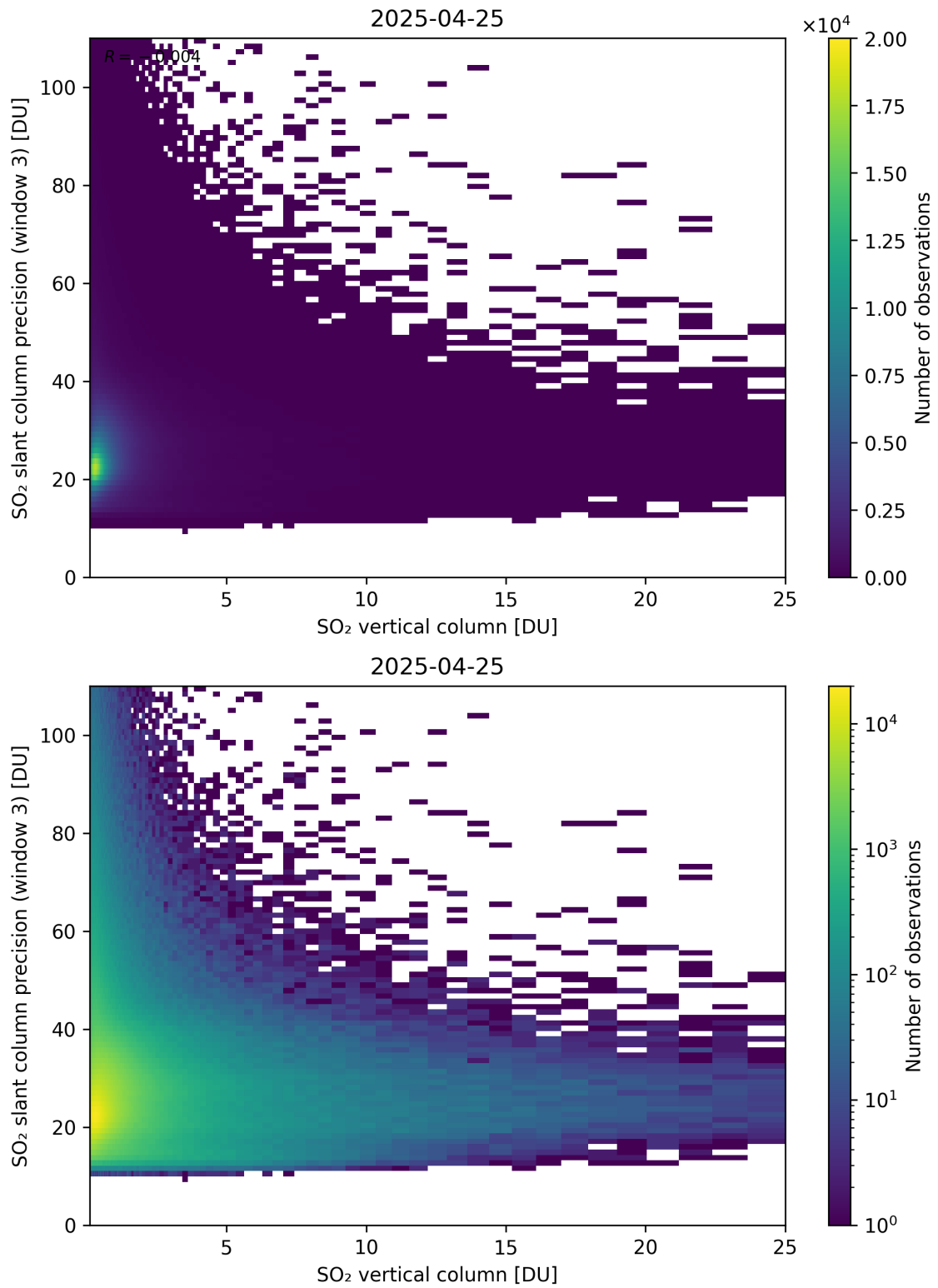
Figure 358: Scatter density plot of “SO 2 vertical column” against “SO 2 slant column precision (window 3)” for 2025-04-24 to 2025-04-26.
