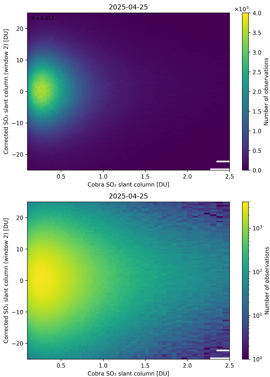
Figure 217: Scatter density plot of “Cobra SO 2 slant column” against “Corrected SO 2 slant column (window 2)” for 2025-04-24 to 2025-04-26.
