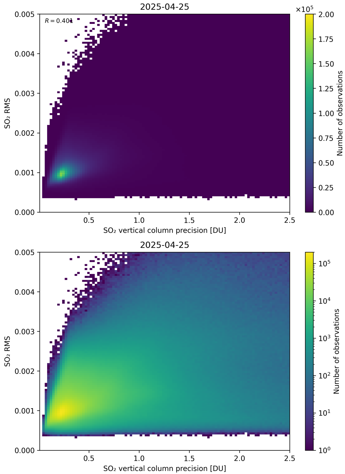
Figure 334: Scatter density plot of “SO 2 vertical column precision” against “SO 2 RMS” for 2025-04-24 to 2025-04-26.
