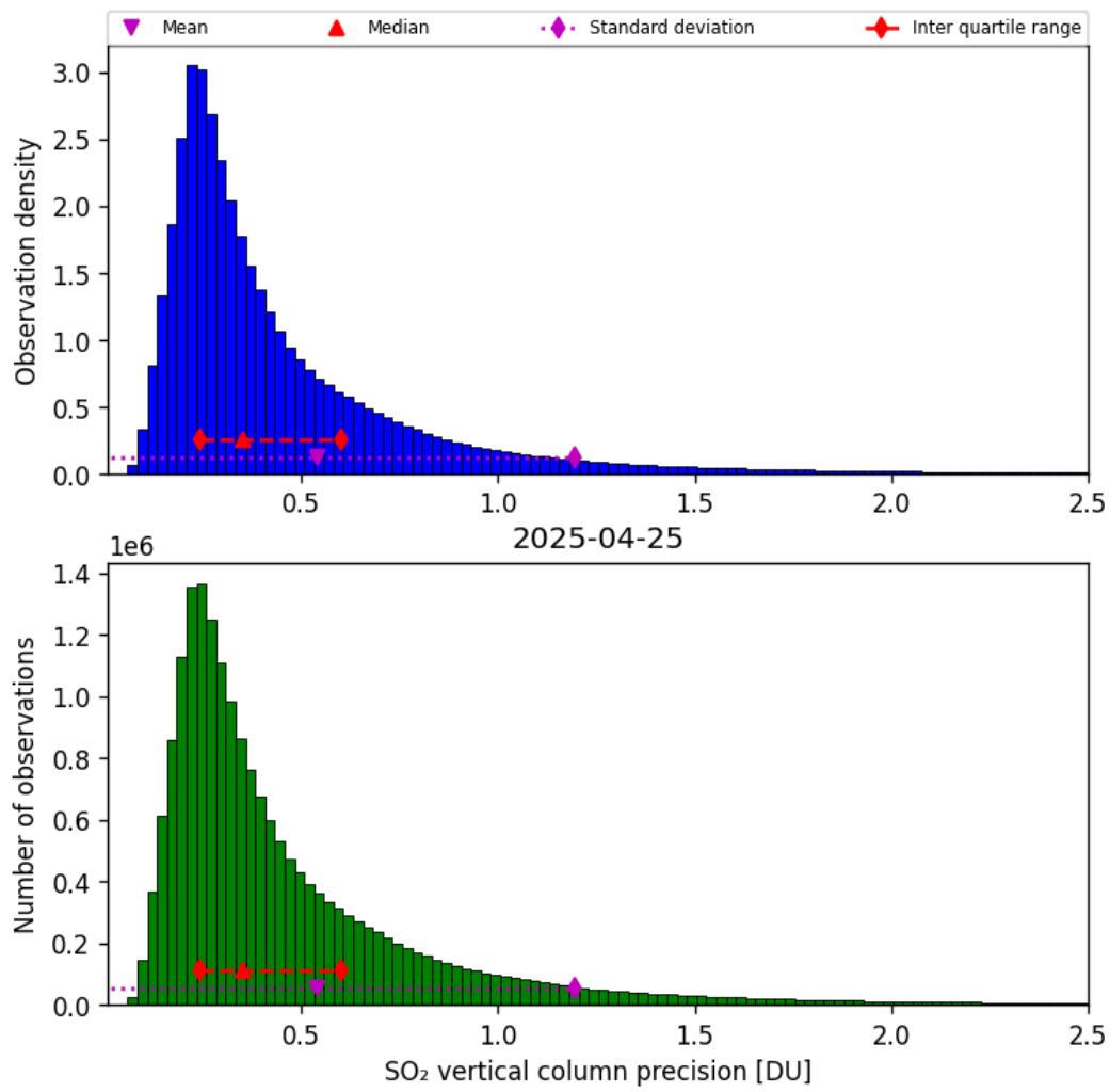
Figure 59: Histogram of “SO 2 vertical column precision” for 2025-04-24 to 2025-04-26
