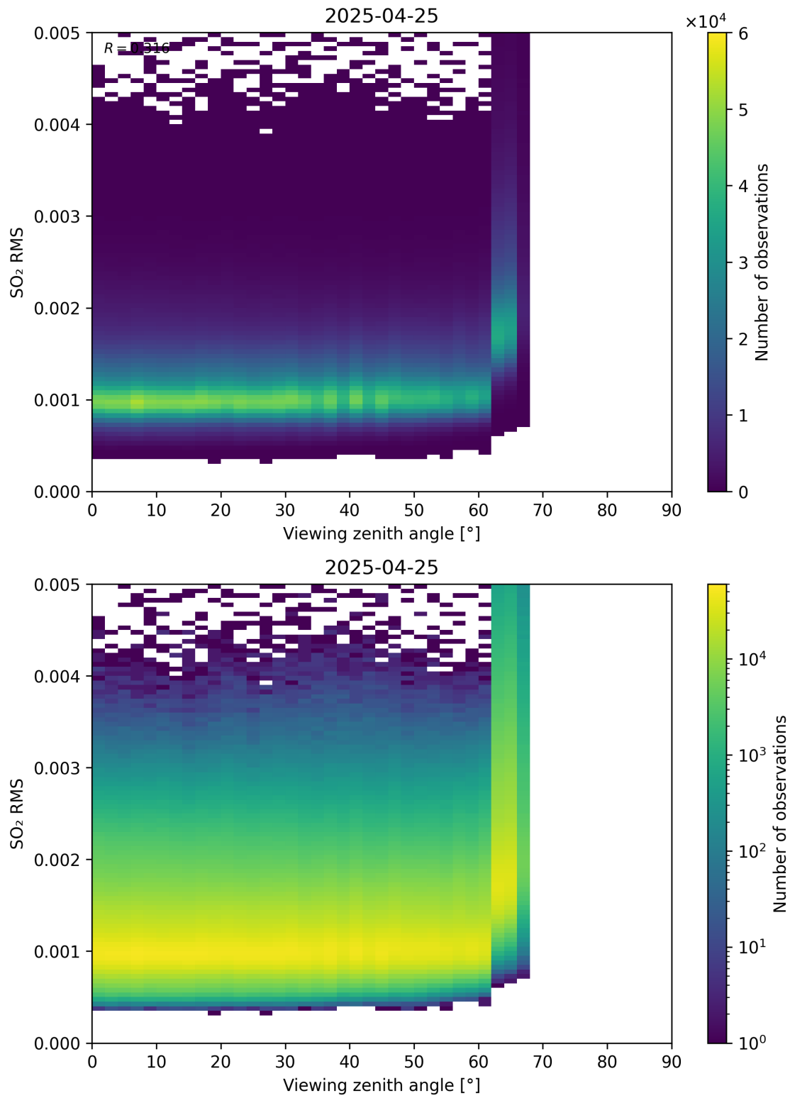
Figure 367: Scatter density plot of “Viewing zenith angle” against “SO 2 RMS” for 2025-04-24 to 2025-04-26.
