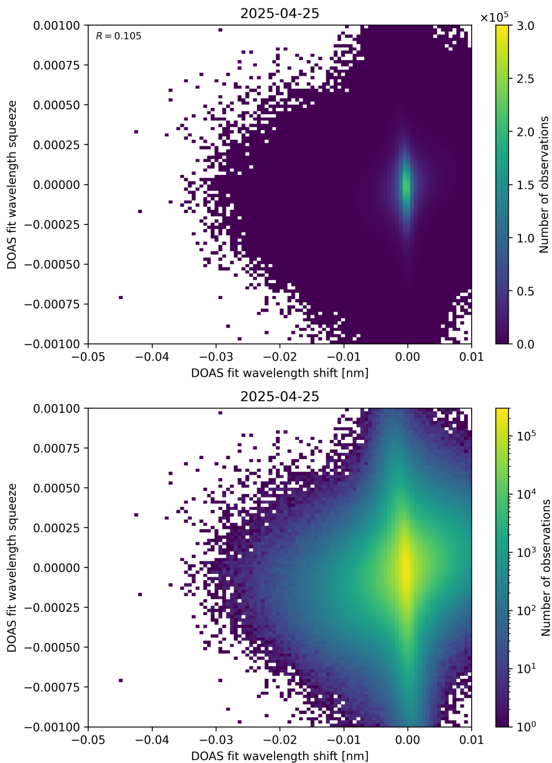
Figure 138: Scatter density plot of “DOAS fit wavelength shift” against “DOAS fit wavelength squeeze” for 2025-04-24 to 2025-04-26.
