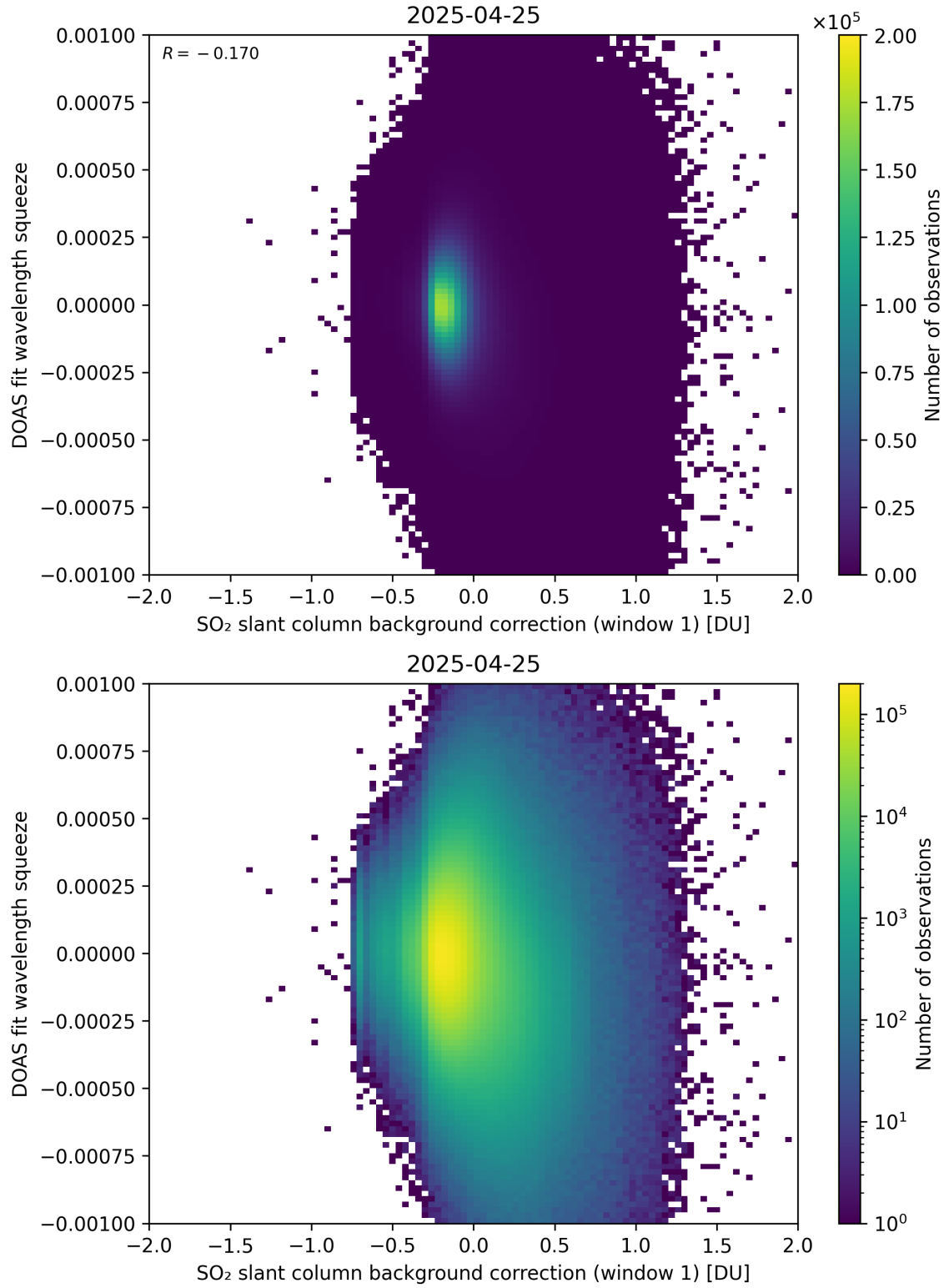
Figure 112: Scatter density plot of “SO 2 slant column background correction (window 1)” against “DOAS fit wavelength squeeze” for 2025-04-24 to 2025-04-26.
