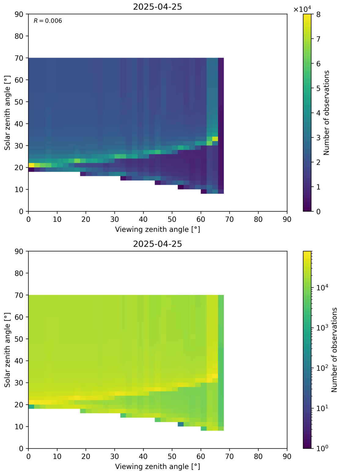
Figure 369: Scatter density plot of “Viewing zenith angle” against “Solar zenith angle” for 2025-04-24 to 2025-04-26.
