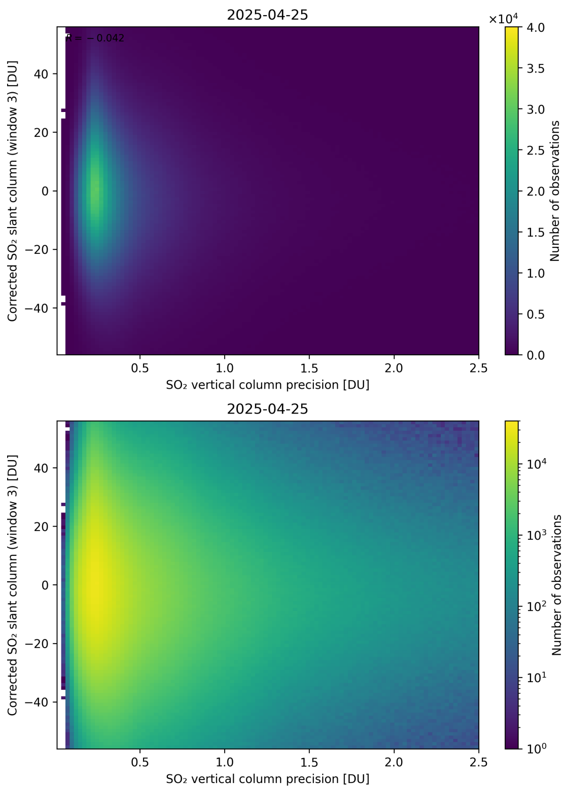
Figure 340: Scatter density plot of “SO 2 vertical column precision” against “Corrected SO 2 slant column (window 3)” for 2025-04-24 to 2025-04-26.
