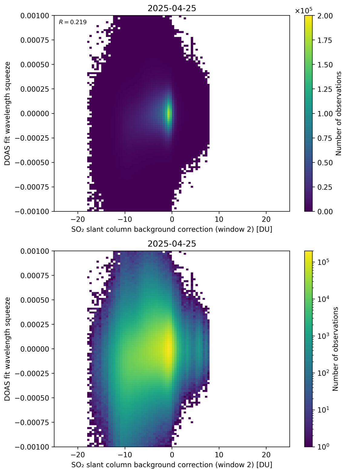
Figure 124: Scatter density plot of “SO 2 slant column background correction (window 2)” against “DOAS fit wavelength squeeze” for 2025-04-24 to 2025-04-26.
