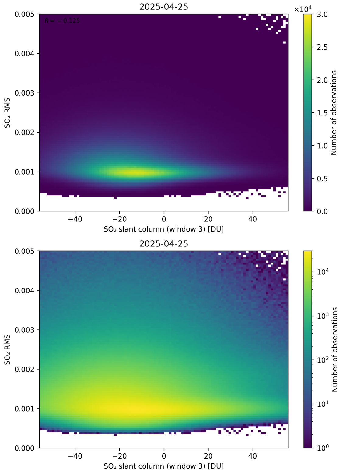
Figure 306: Scatter density plot of “SO 2 slant column (window 3)” against “SO 2 RMS” for 2025-04-24 to 2025-04-26.
