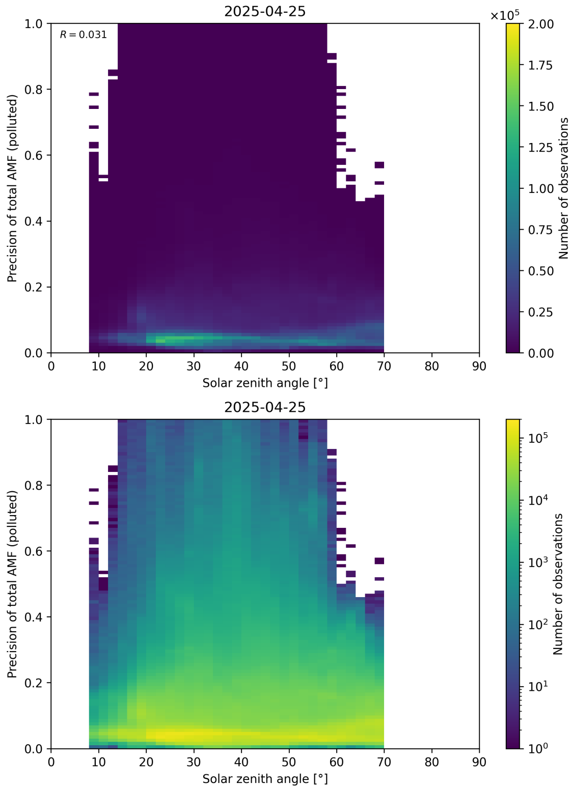
Figure 190: Scatter density plot of “Solar zenith angle” against “Precision of total AMF (polluted)” for 2025-04-24 to 2025-04-26.
