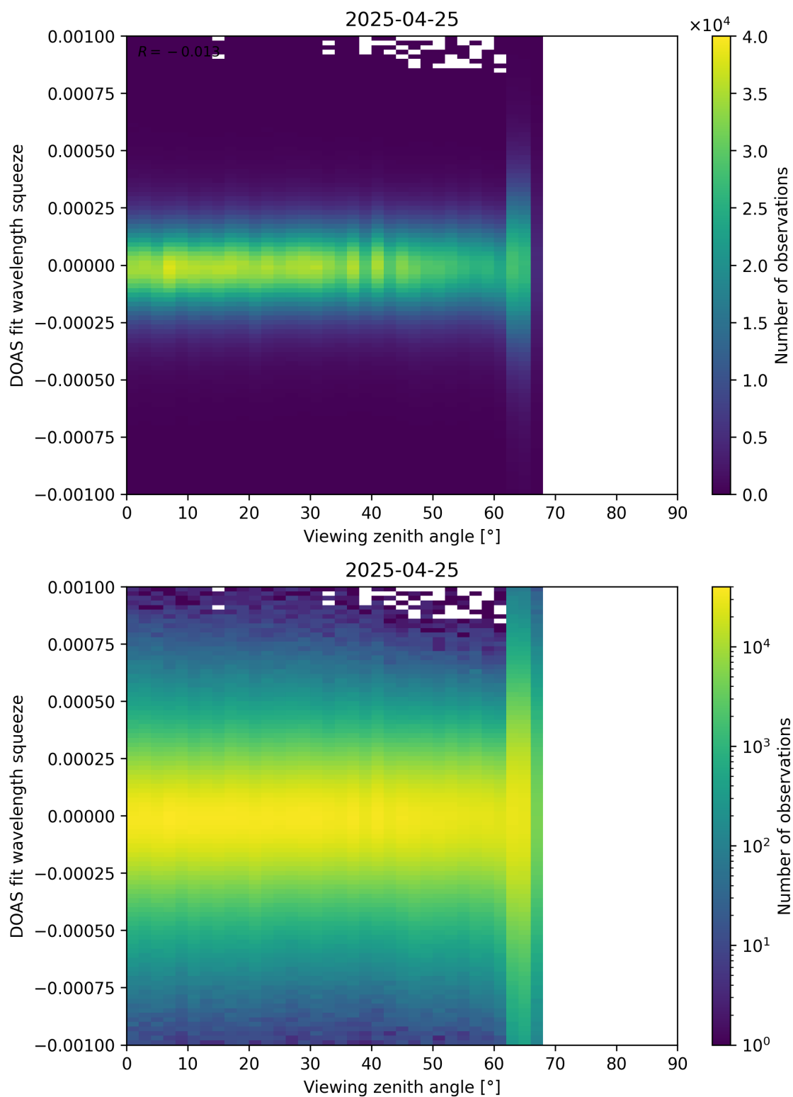
Figure 366: Scatter density plot of “Viewing zenith angle” against “DOAS fit wavelength squeeze” for 2025-04-24 to 2025-04-26.
