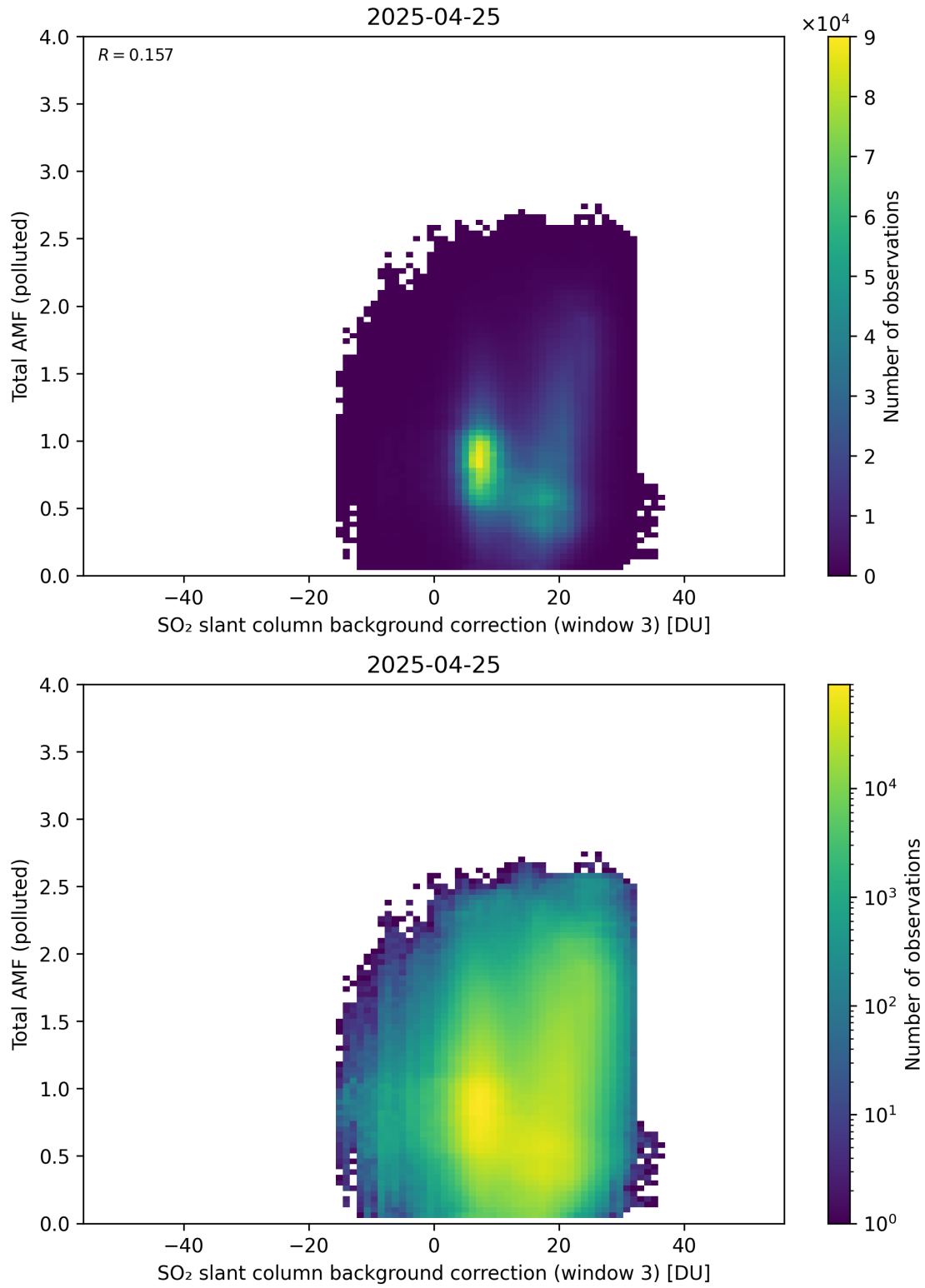
Figure 136: Scatter density plot of “SO 2 slant column background correction (window 3)” against “Total AMF (polluted)” for 2025-04-24 to 2025-04-26.
