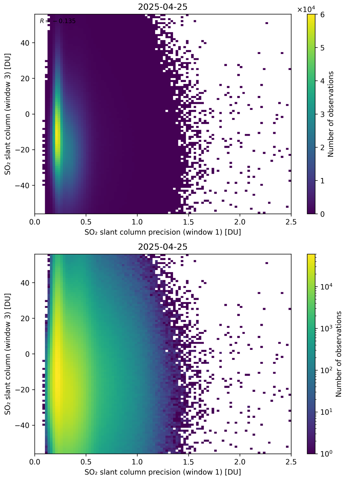
Figure 278: Scatter density plot of “SO 2 slant column precision (window 1)” against “SO 2 slant column (window 3)” for 2025-04-24 to 2025-04-26.
