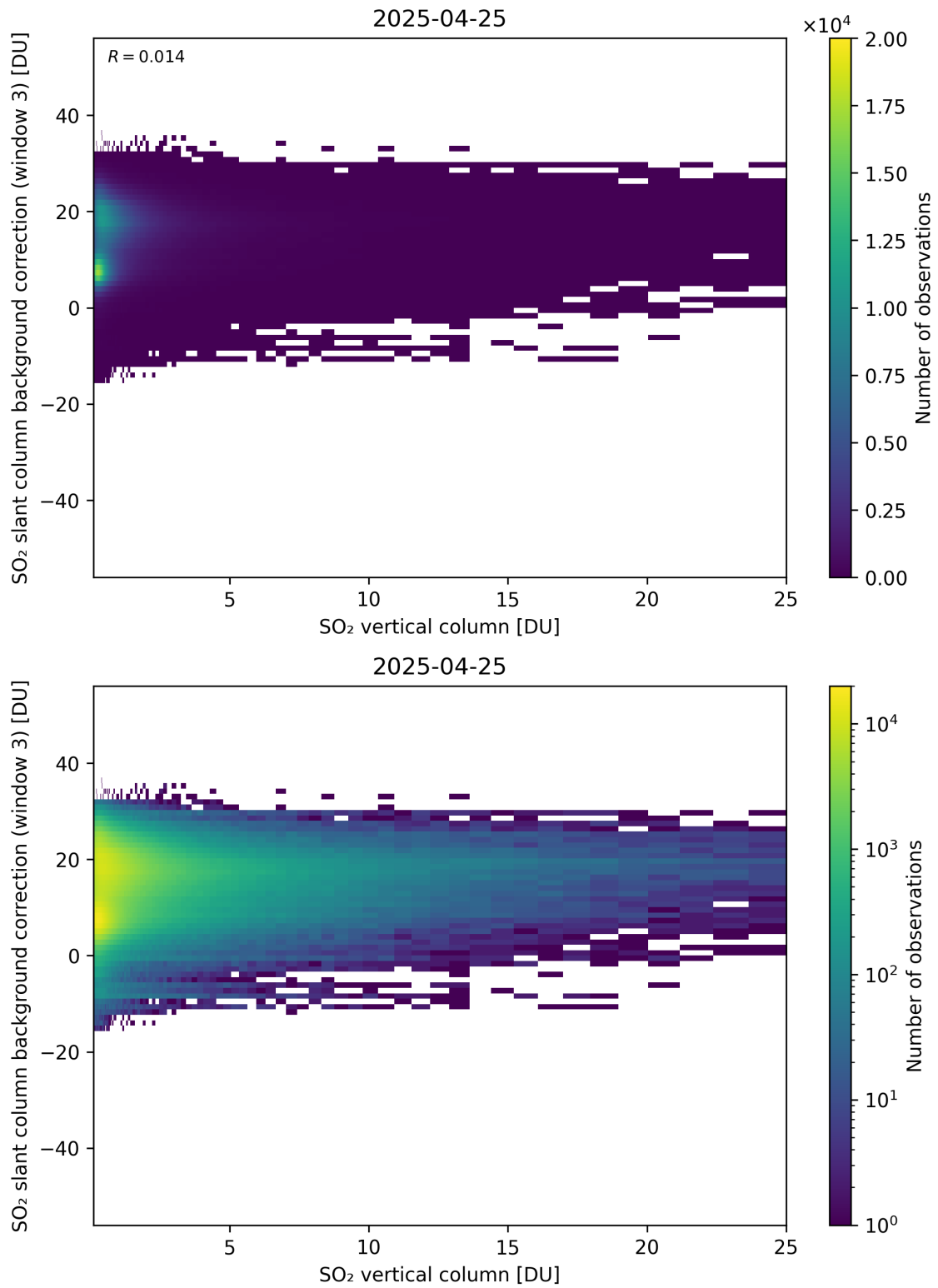
Figure 325: Scatter density plot of “SO 2 vertical column” against “SO 2 slant column background correction (window 3)” for 2025-04-24 to 2025-04-26.
