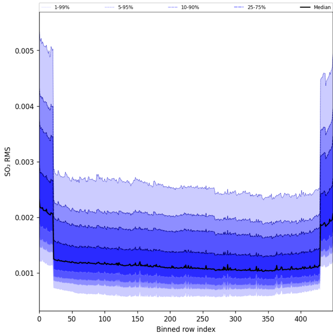
Figure 104: Along track statistics of “SO 2 RMS” for 2025-04-24 to 2025-04-26
