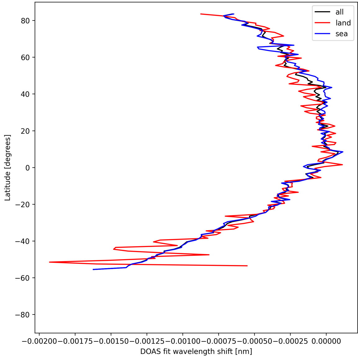
Figure 50: Zonal average of “DOAS fit wavelength shift” for 2025-04-24 to 2025-04-26.
