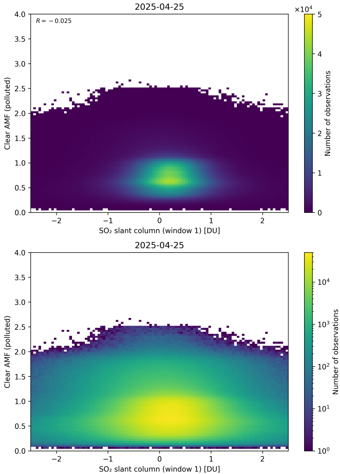
Figure 282: Scatter density plot of “SO 2 slant column (window 1)” against “Clear AMF (polluted)” for 2025-04-24 to 2025-04-26.
