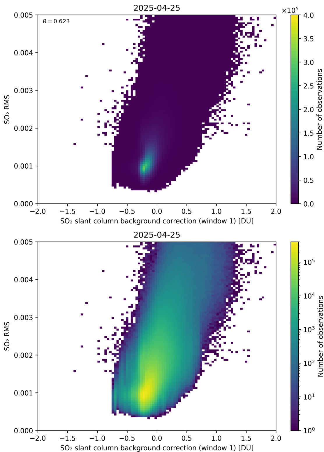
Figure 113: Scatter density plot of “SO 2 slant column background correction (window 1)” against “SO 2 RMS” for 2025-04-24 to 2025-04-26.
