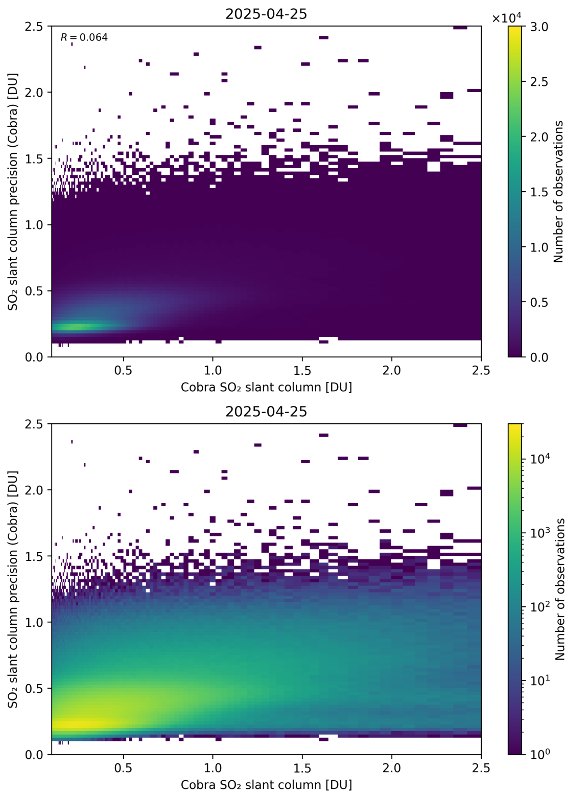
Figure 216: Scatter density plot of “Cobra SO 2 slant column” against “SO 2 slant column precision (Cobra)” for 2025-04-24 to 2025-04-26.
