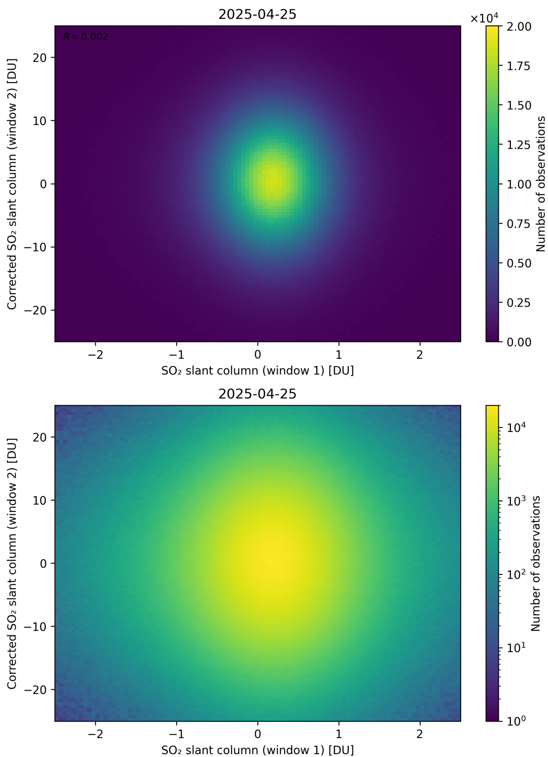
Figure 283: Scatter density plot of “SO 2 slant column (window 1)” against “Corrected SO 2 slant column (window 2)” for 2025-04-24 to 2025-04-26.
