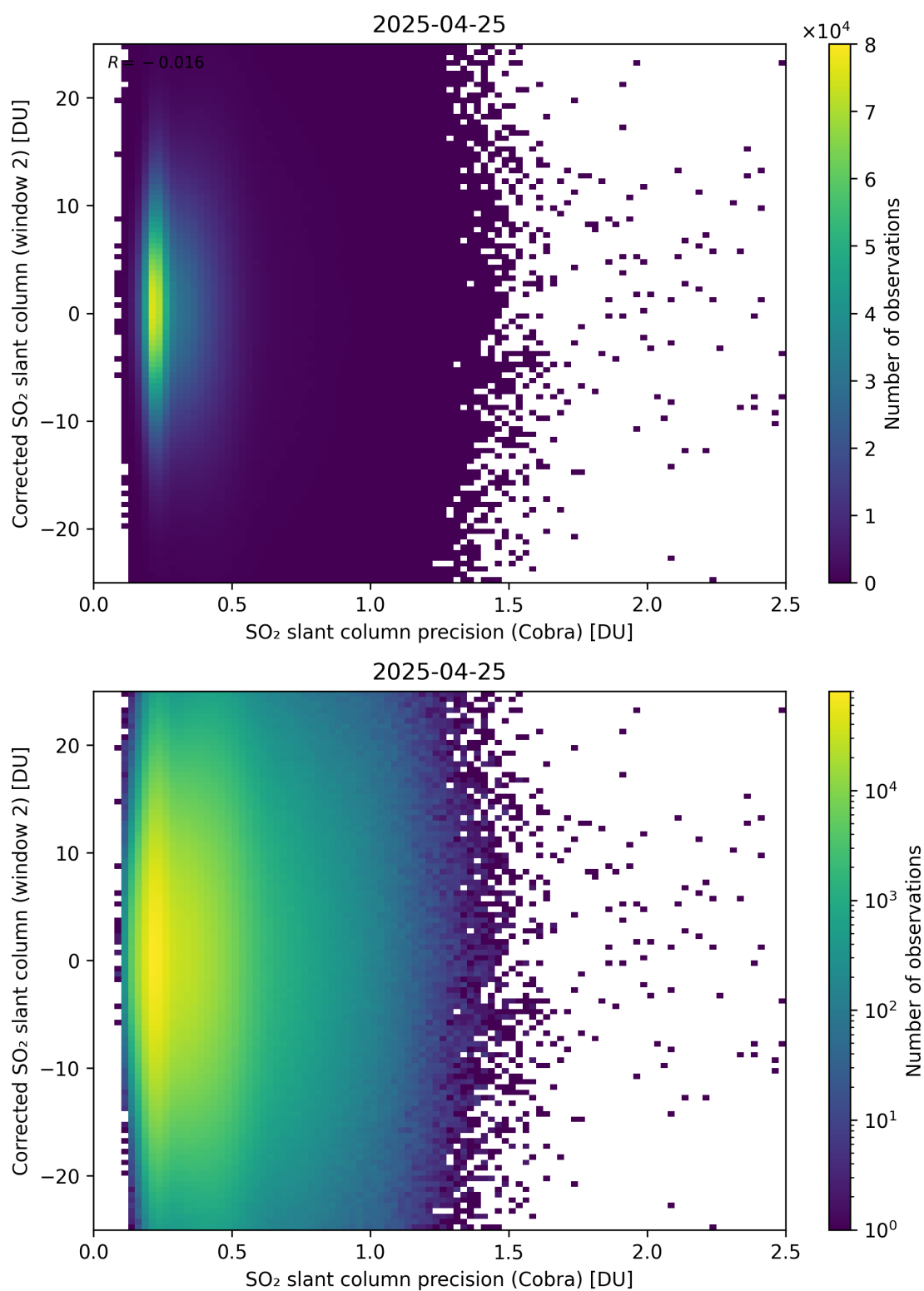
Figure 206: Scatter density plot of “SO 2 slant column precision (Cobra)” against “Corrected SO 2 slant column (window 2)” for 2025-04-24 to 2025-04-26.
