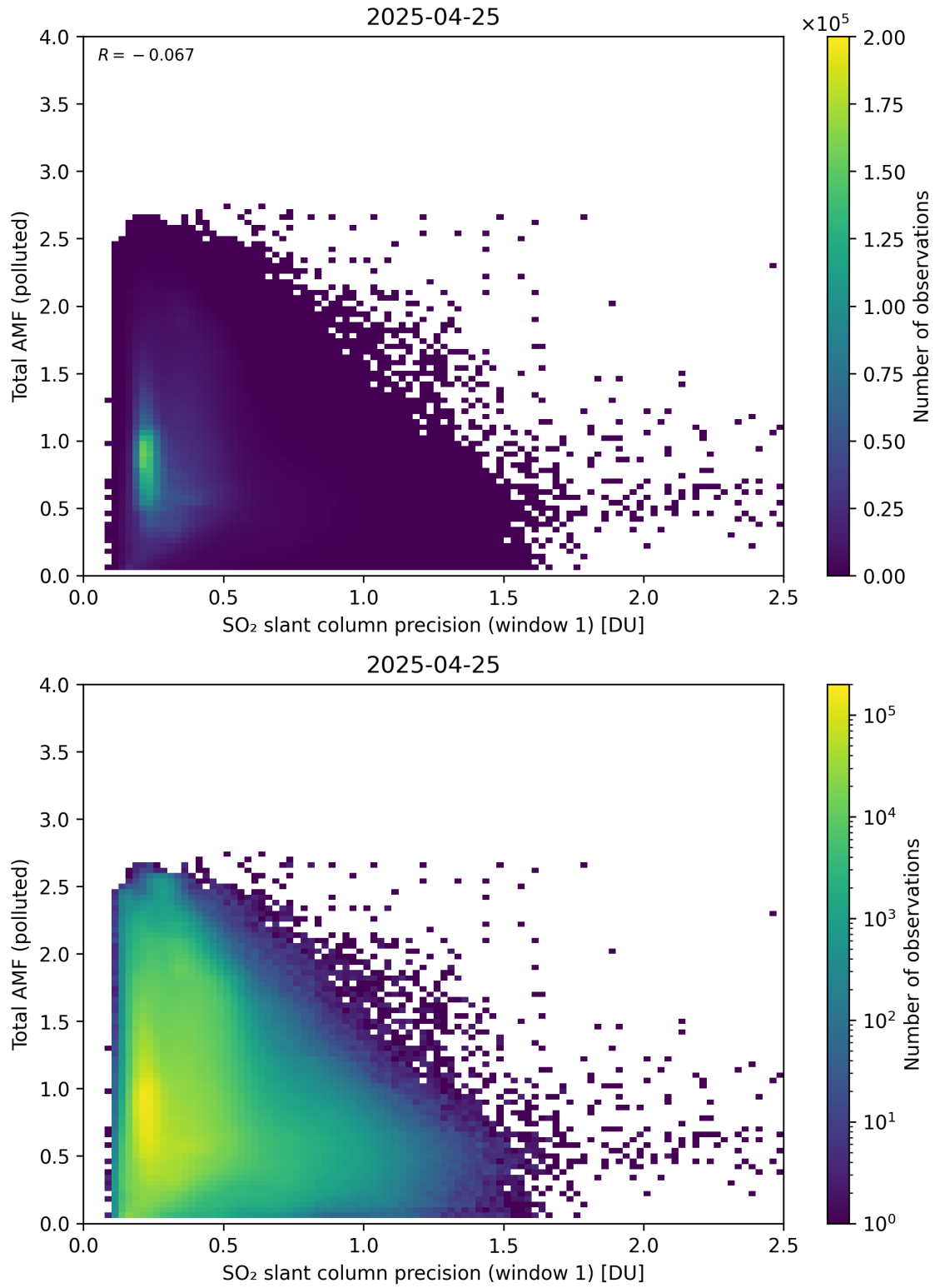
Figure 280: Scatter density plot of “SO 2 slant column precision (window 1)” against “Total AMF (polluted)” for 2025-04-24 to 2025-04-26.
