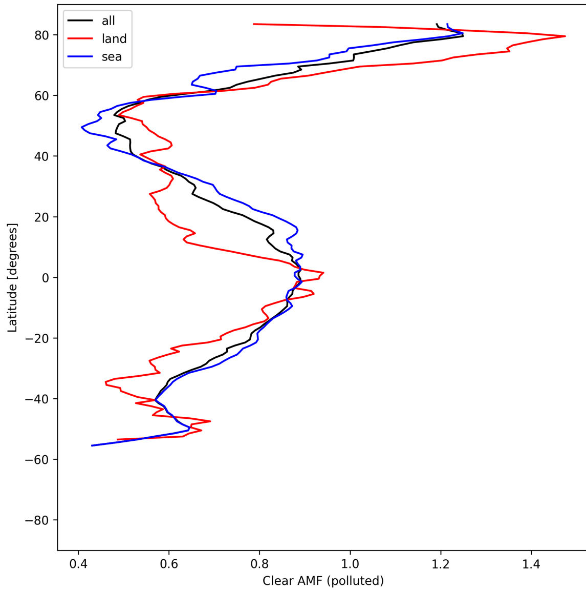
Figure 55: Zonal average of “Clear AMF (polluted)” for 2025-04-24 to 2025-04-26.
