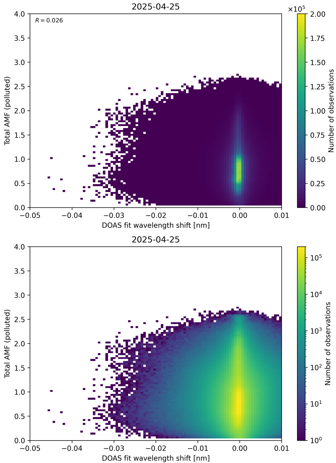
Figure 141: Scatter density plot of “DOAS fit wavelength shift” against “Total AMF (polluted)” for 2025-04-24 to 2025-04-26.
