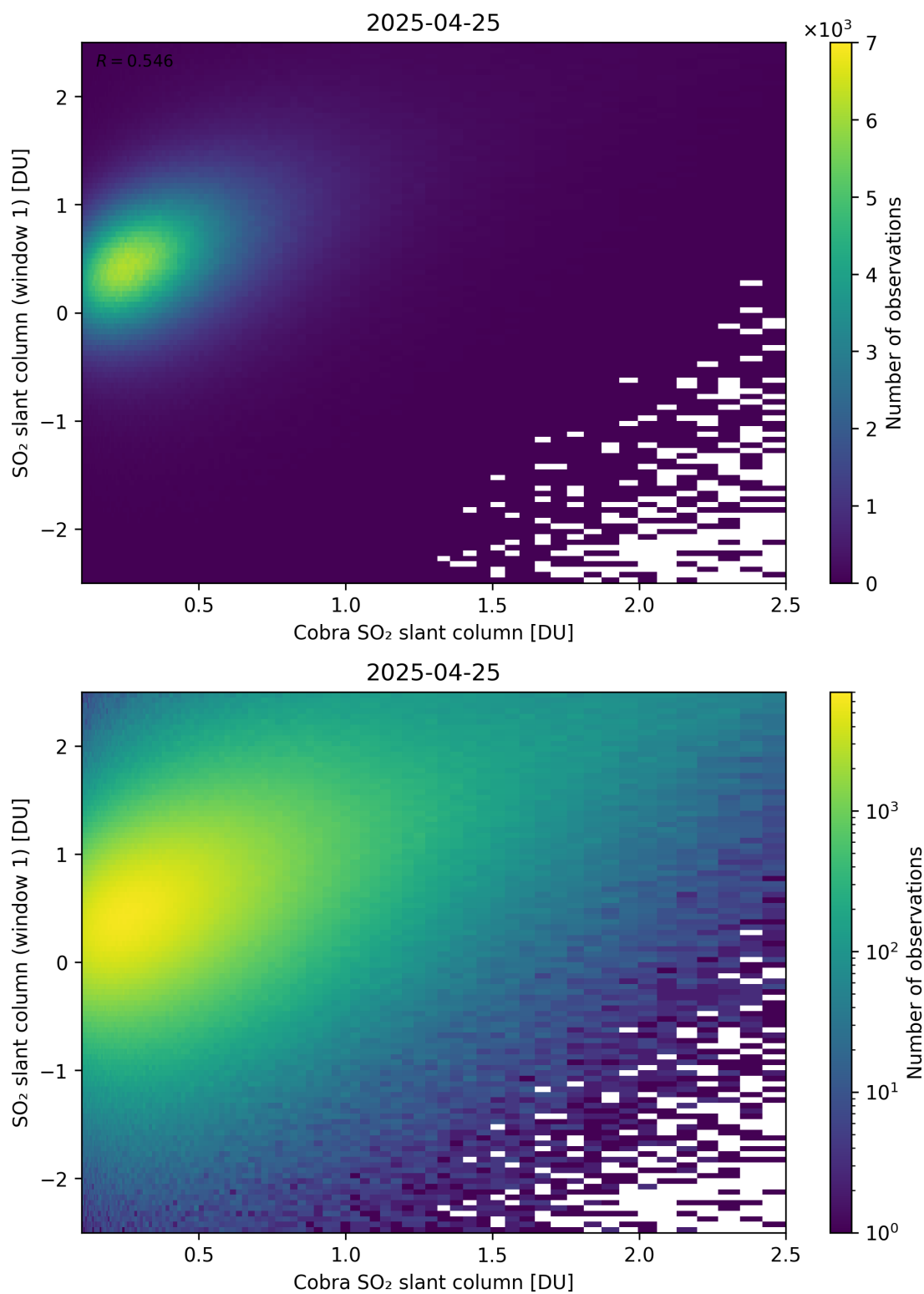
Figure 219: Scatter density plot of “Cobra SO 2 slant column” against “SO 2 slant column (window 1)” for 2025-04-24 to 2025-04-26.
