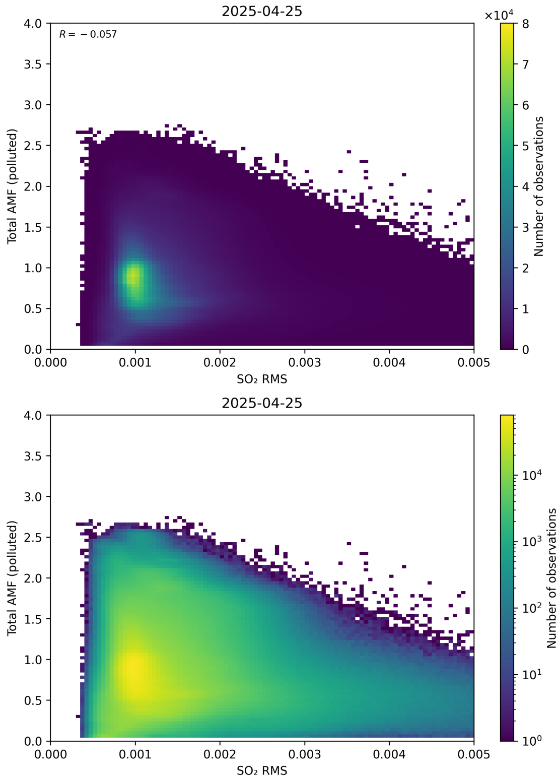
Figure 148: Scatter density plot of “SO 2 RMS” against “Total AMF (polluted)” for 2025-04-24 to 2025-04-26.
