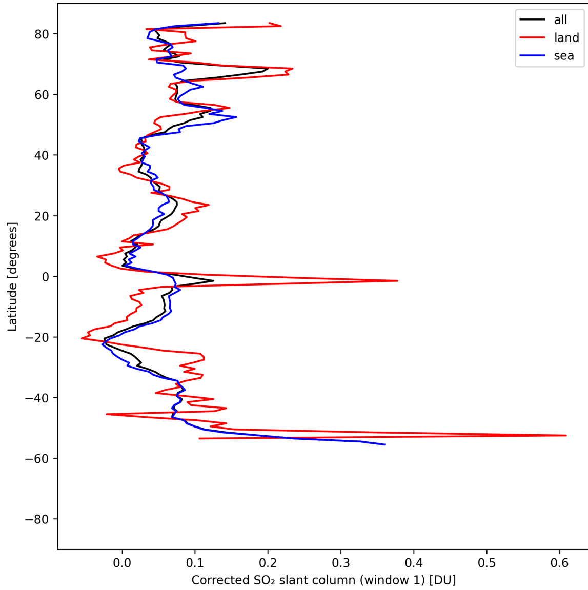
Figure 39: Zonal average of “Corrected SO 2 slant column (window 1)” for 2025-04-24 to 2025-04-26.
