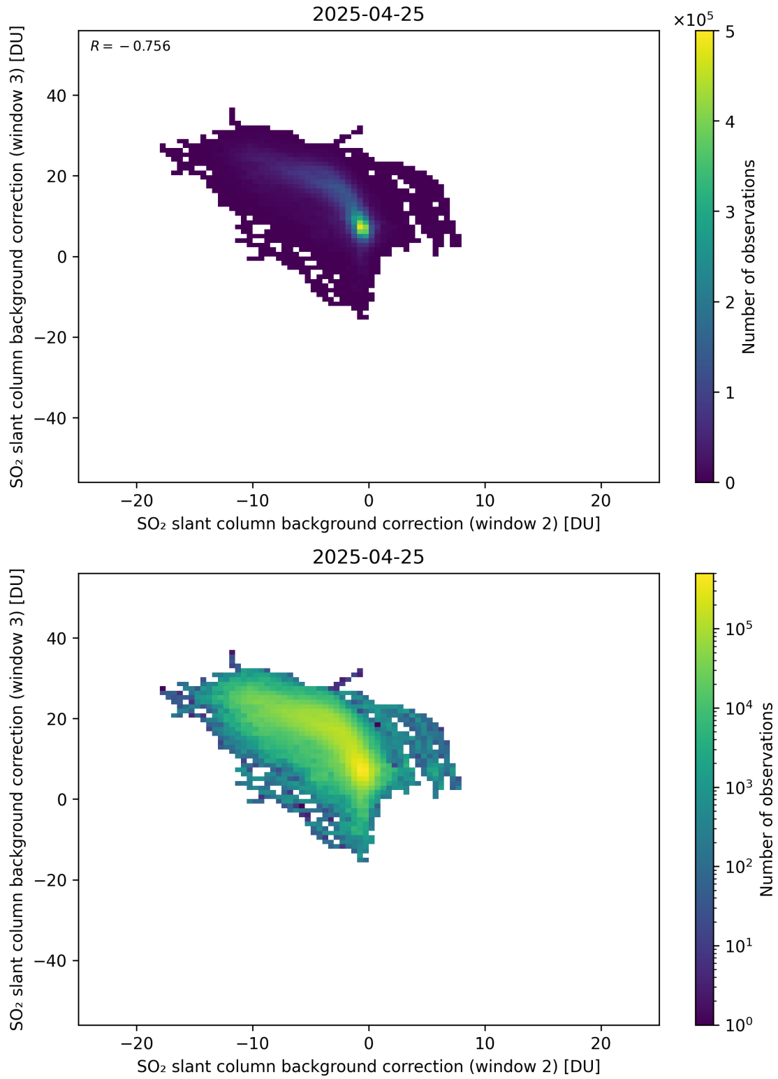
Figure 122: Scatter density plot of “SO 2 slant column background correction (window 2)” against “SO 2 slant column background correction (window 3)” for 2025-04-24 to 2025-04-26.
