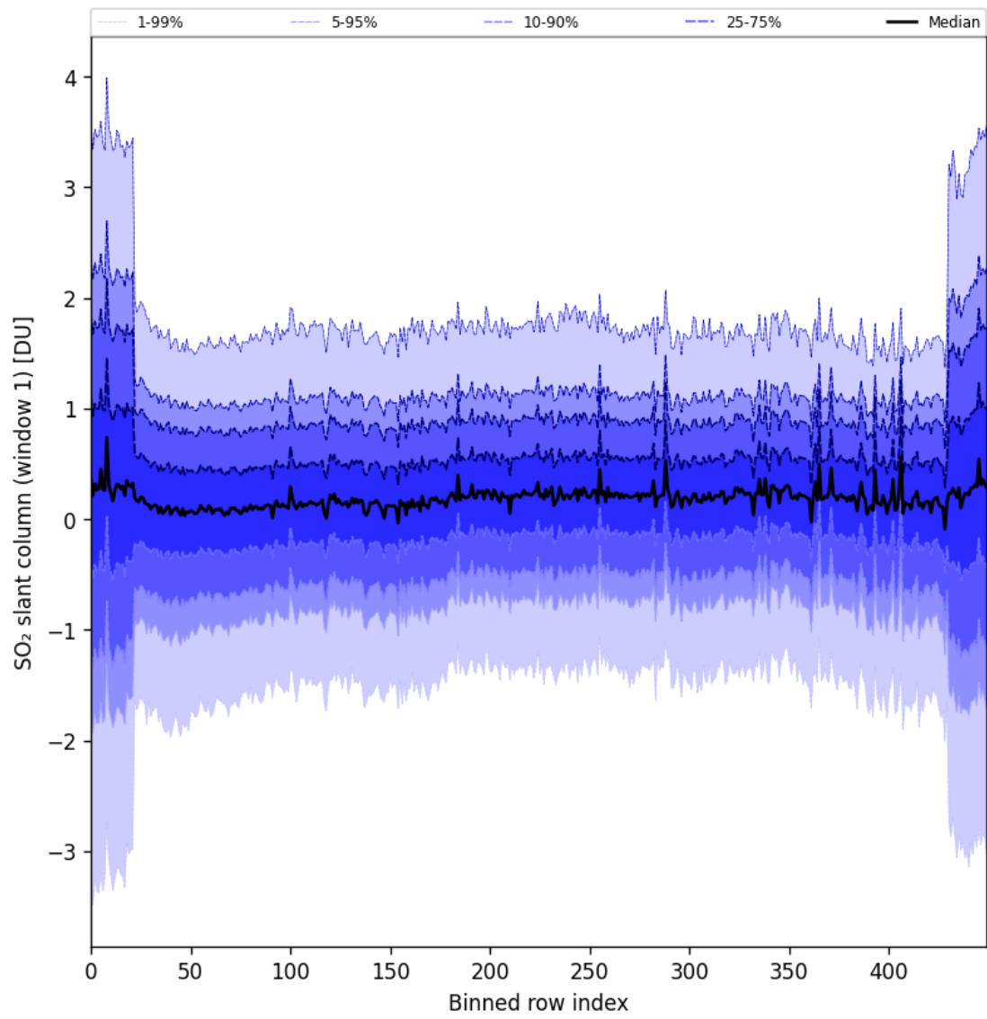
Figure 89: Along track statistics of “SO 2 slant column (window 1)” for 2025-04-24 to 2025-04-26
