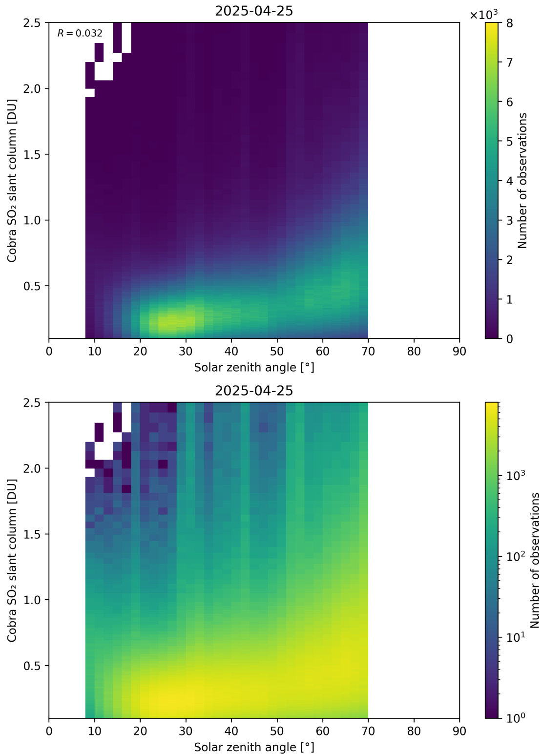
Figure 179: Scatter density plot of “Solar zenith angle” against “Cobra SO 2 slant column” for 2025-04-24 to 2025-04-26.
