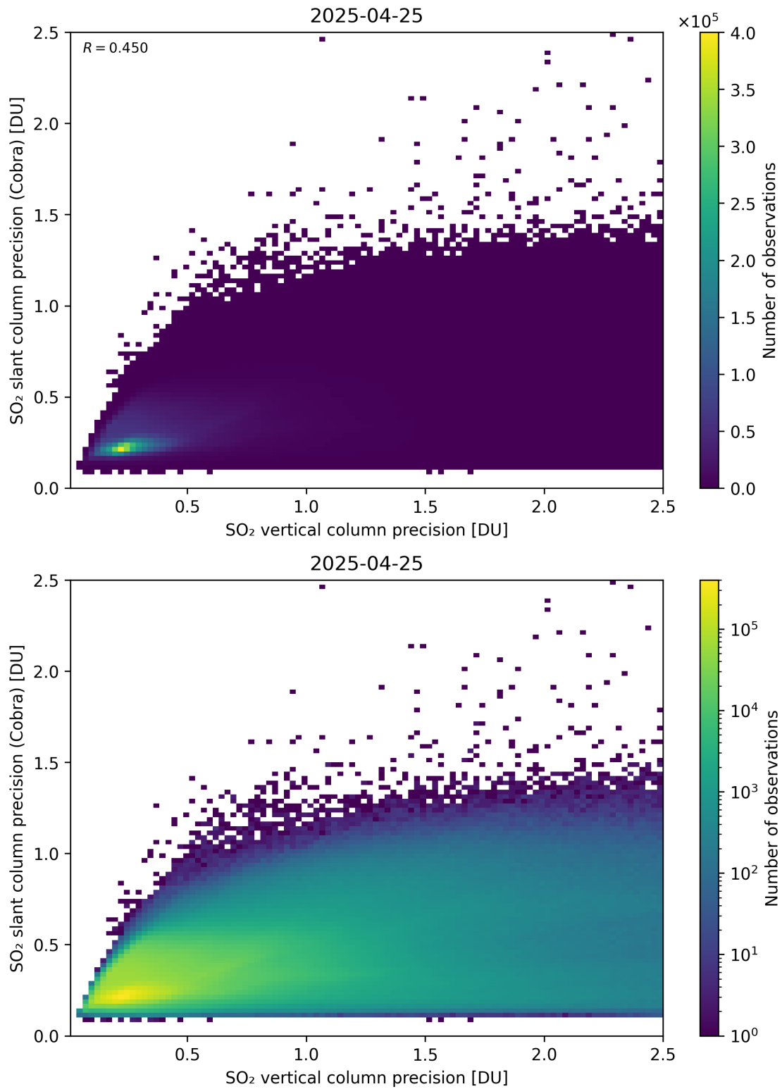
Figure 337: Scatter density plot of “SO 2 vertical column precision” against “SO 2 slant column precision (Cobra)” for 2025-04-24 to 2025-04-26.
