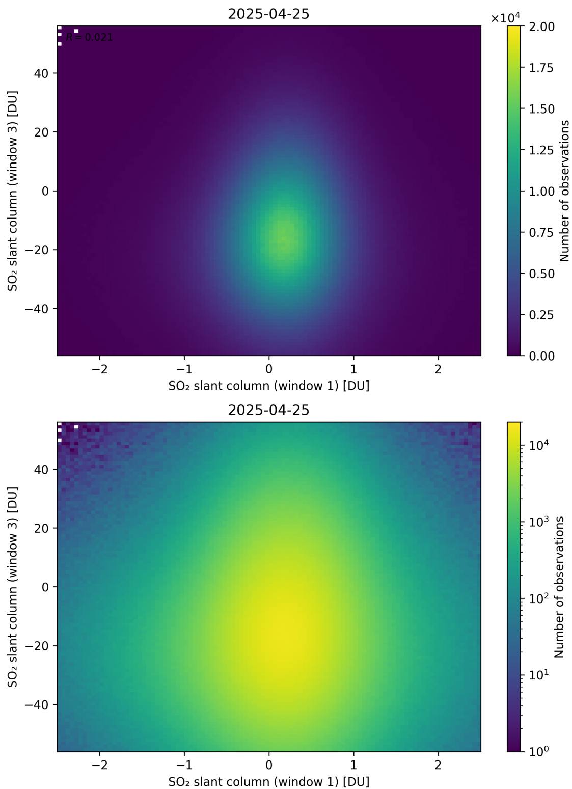
Figure 287: Scatter density plot of “SO 2 slant column (window 1)” against “SO 2 slant column (window 3)” for 2025-04-24 to 2025-04-26.
