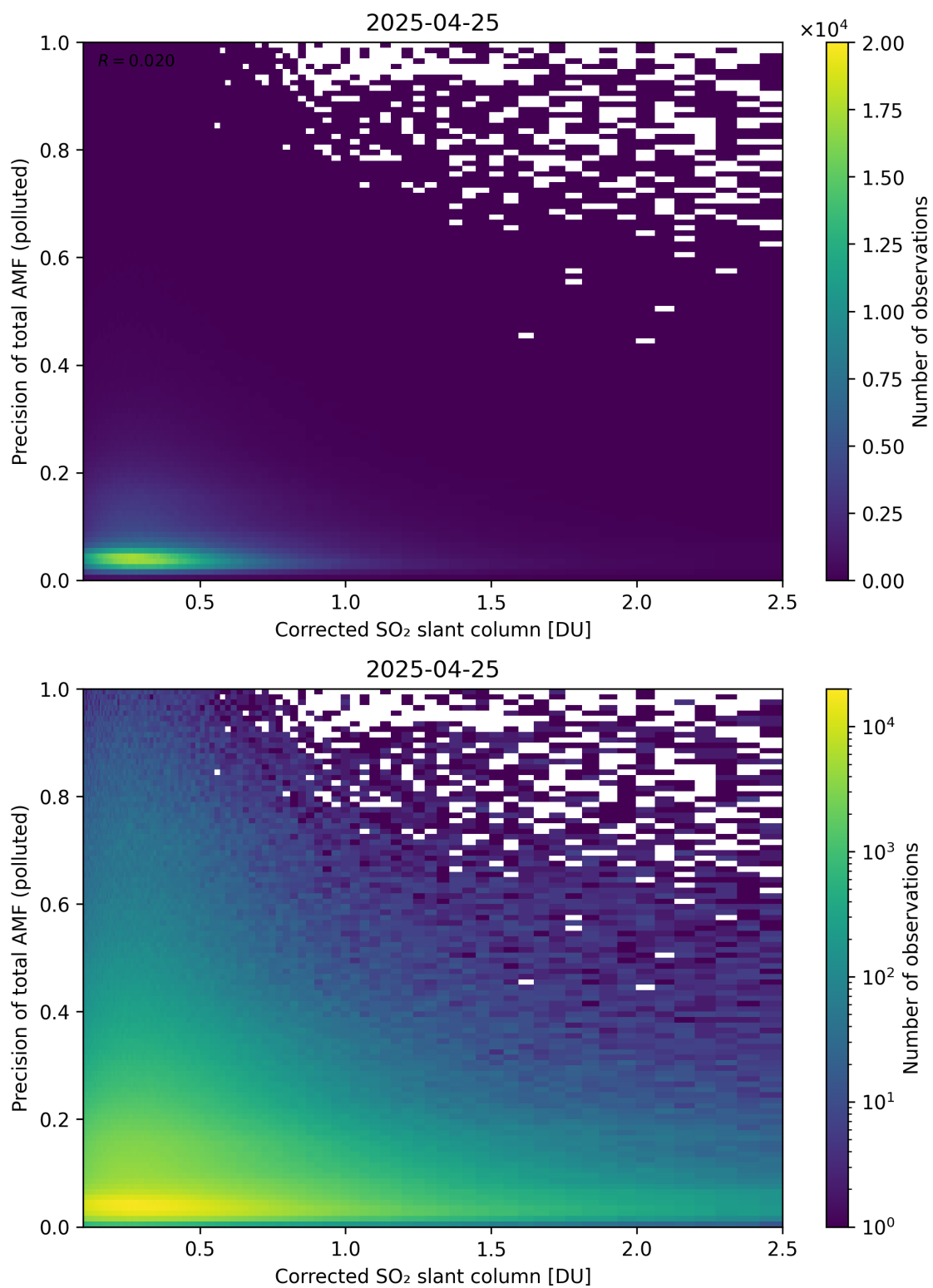
Figure 243: Scatter density plot of “Corrected SO 2 slant column” against “Precision of total AMF (polluted)” for 2025-04-24 to 2025-04-26.
