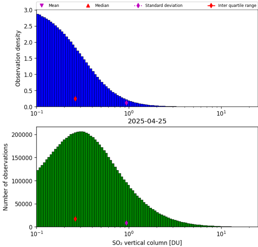
Figure 58: Histogram of “SO 2 vertical column” for 2025-04-24 to 2025-04-26
