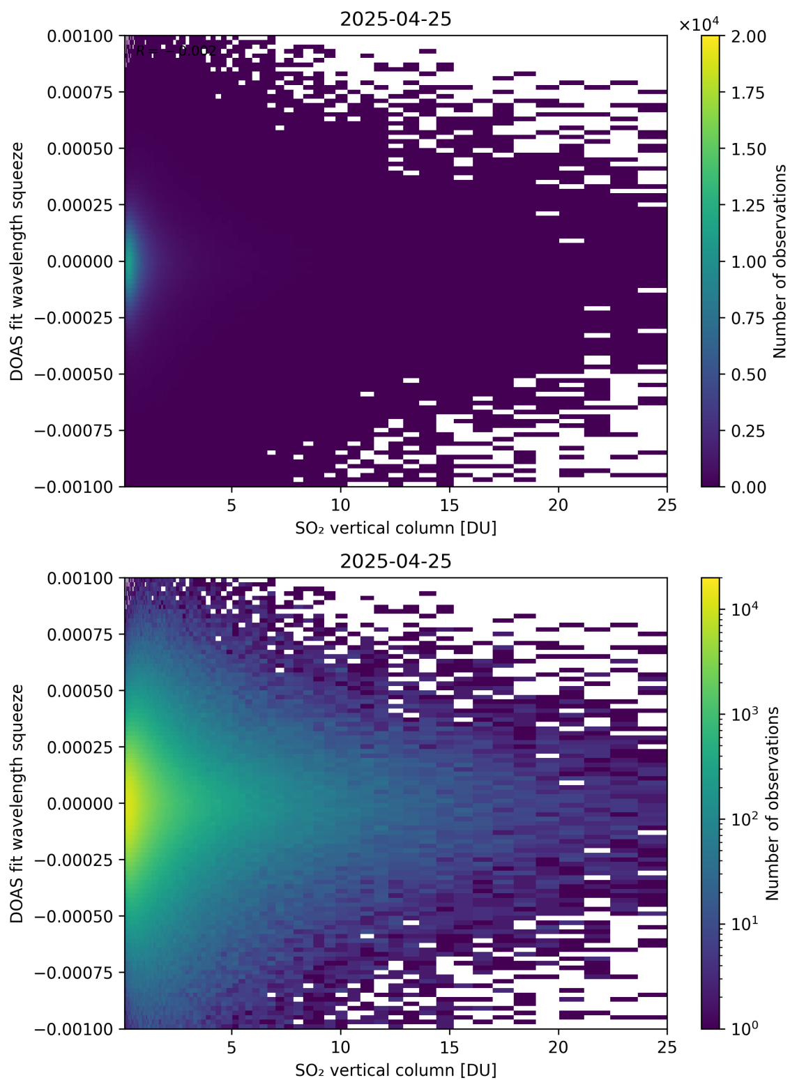
Figure 327: Scatter density plot of “SO 2 vertical column” against “DOAS fit wavelength squeeze” for 2025-04-24 to 2025-04-26.
