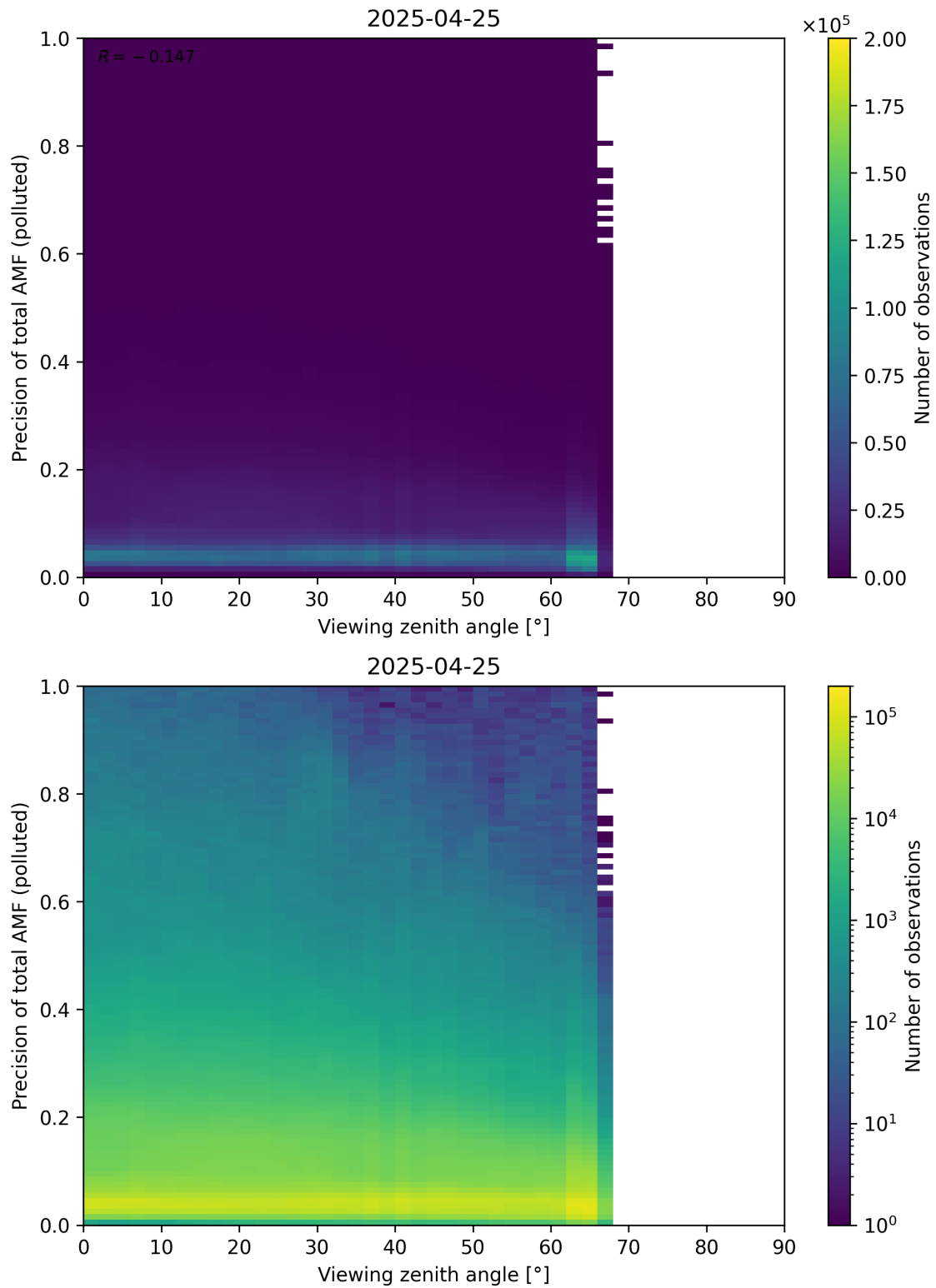
Figure 382: Scatter density plot of “Viewing zenith angle” against “Precision of total AMF (polluted)” for 2025-04-24 to 2025-04-26.
