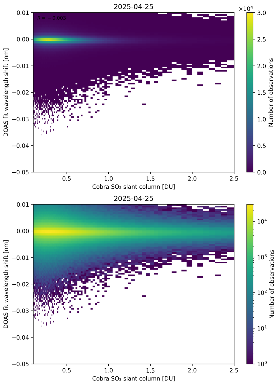
Figure 196: Scatter density plot of “Cobra SO 2 slant column” against “DOAS fit wavelength shift” for 2025-04-24 to 2025-04-26.
