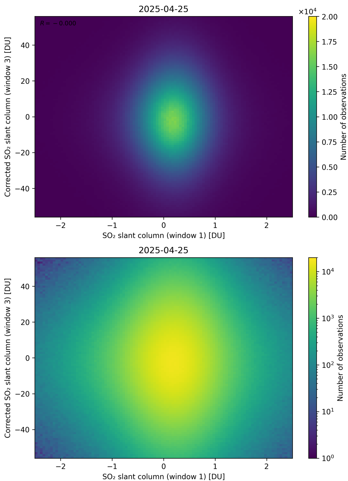
Figure 284: Scatter density plot of “SO 2 slant column (window 1)” against “Corrected SO 2 slant column (window 3)” for 2025-04-24 to 2025-04-26.
