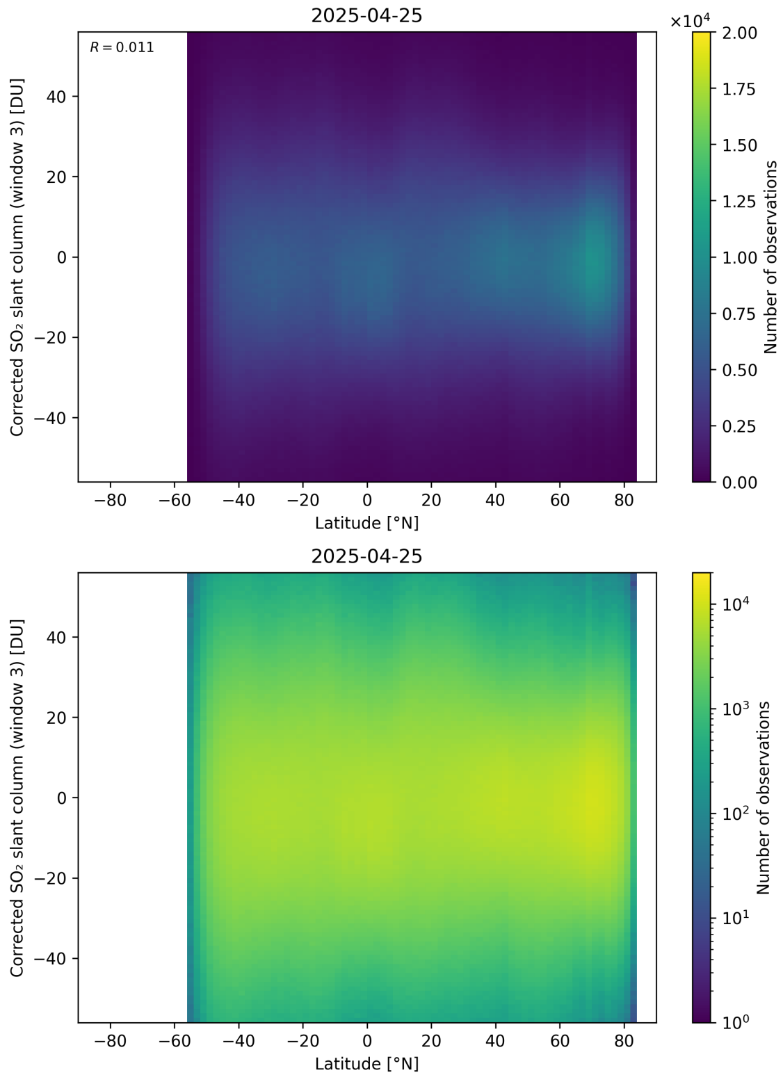
Figure 161: Scatter density plot of “Latitude” against “Corrected SO 2 slant column (window 3)” for 2025-04-24 to 2025-04-26.
