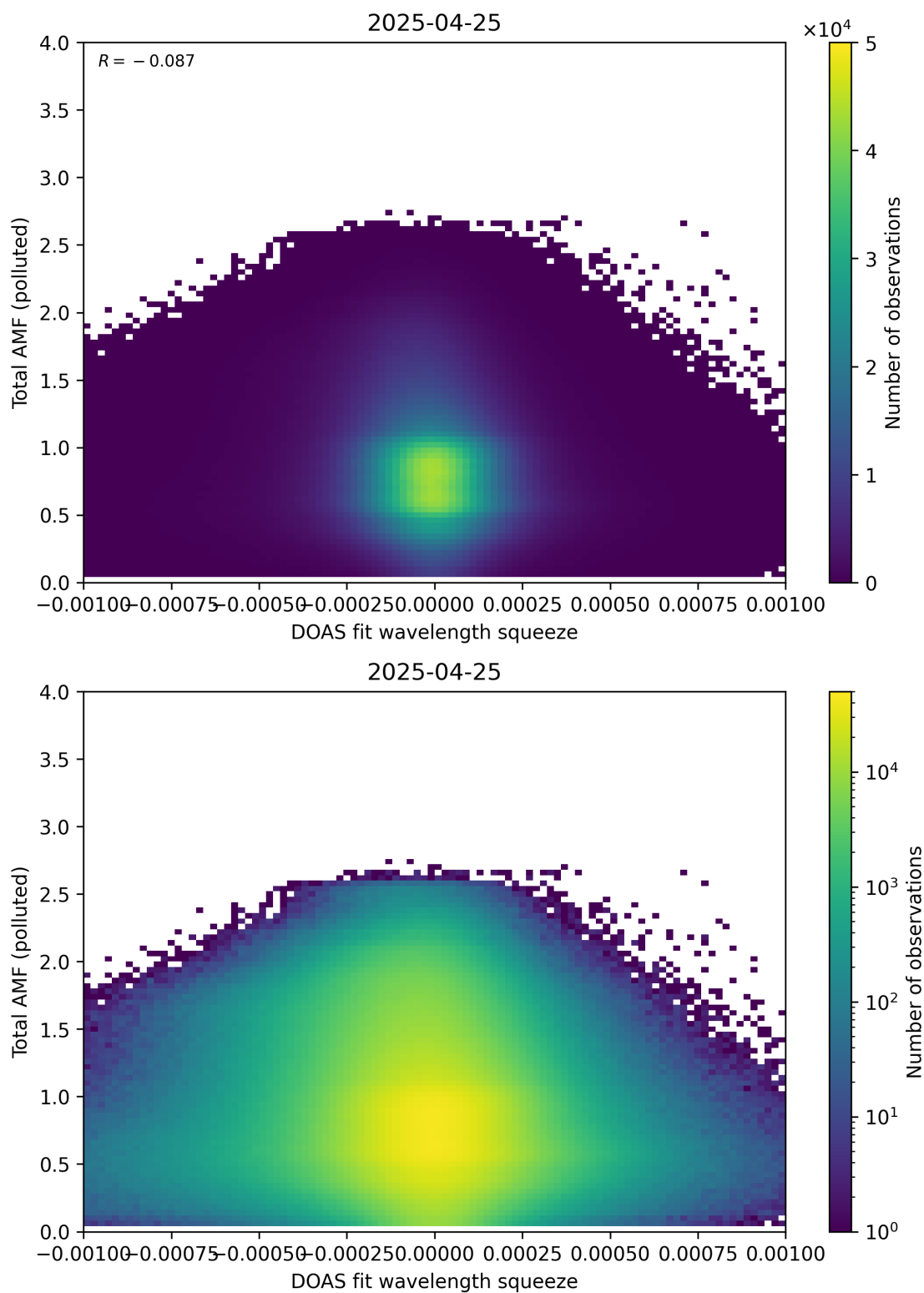
Figure 145: Scatter density plot of “DOAS fit wavelength squeeze” against “Total AMF (polluted)” for 2025-04-24 to 2025-04-26.
