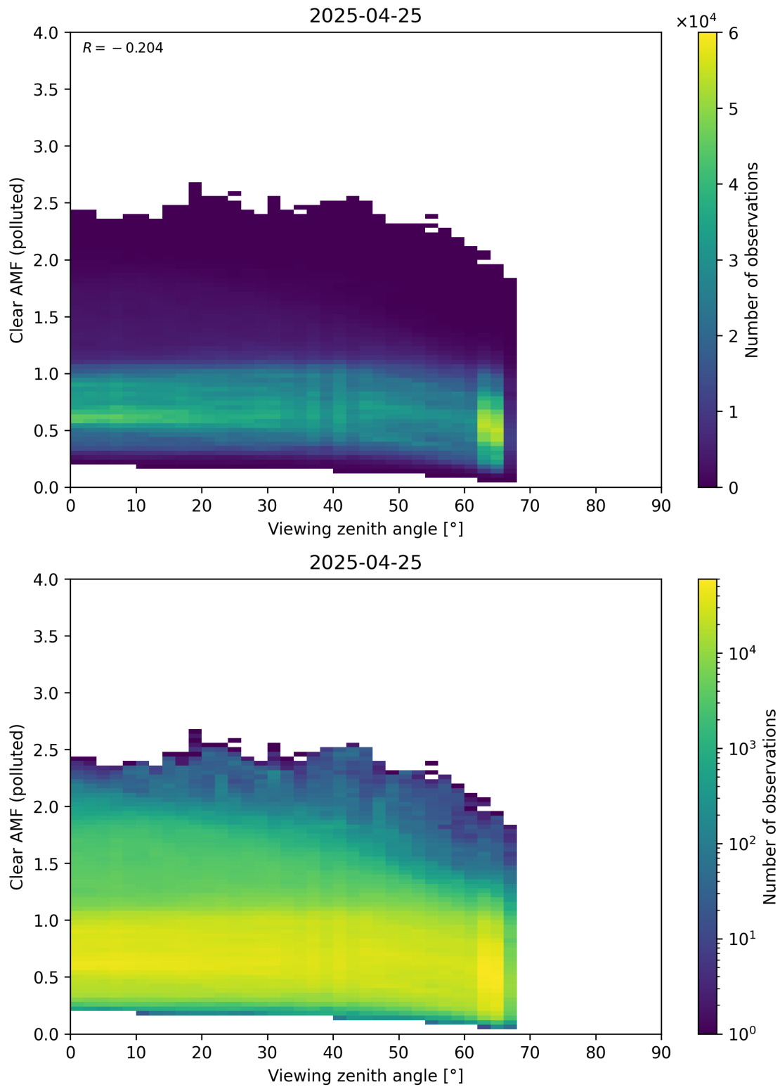
Figure 370: Scatter density plot of “Viewing zenith angle” against “Clear AMF (polluted)” for 2025-04-24 to 2025-04-26.
