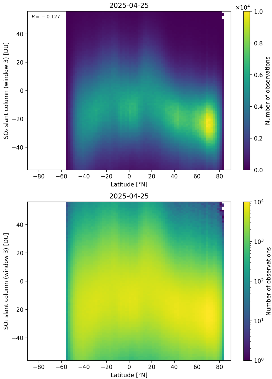
Figure 165: Scatter density plot of “Latitude” against “SO 2 slant column (window 3)” for 2025-04-24 to 2025-04-26.
