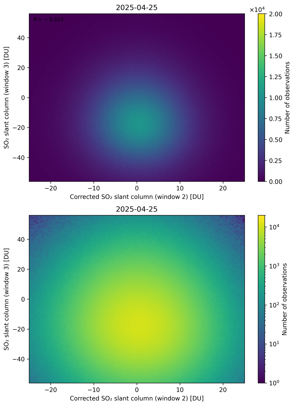
Figure 251: Scatter density plot of “Corrected SO 2 slant column (window 2)” against “SO 2 slant column (window 3)” for 2025-04-24 to 2025-04-26.
