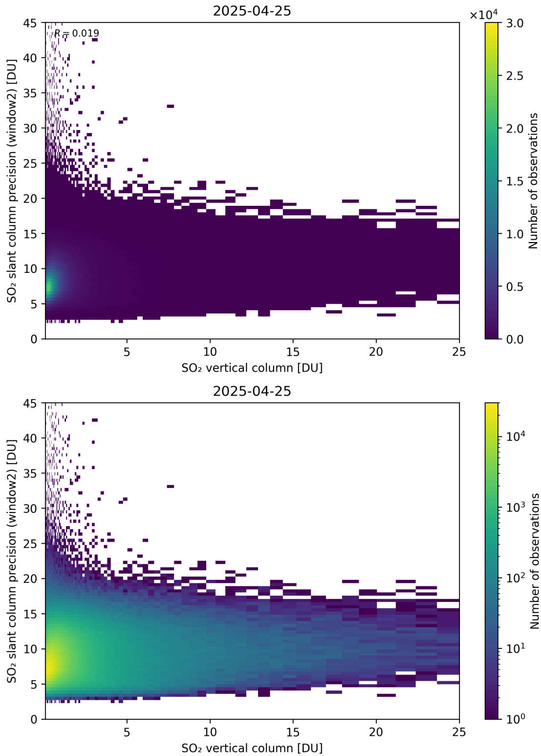
Figure 356: Scatter density plot of “SO 2 vertical column” against “SO 2 slant column precision (window2)” for 2025-04-24 to 2025-04-26.
