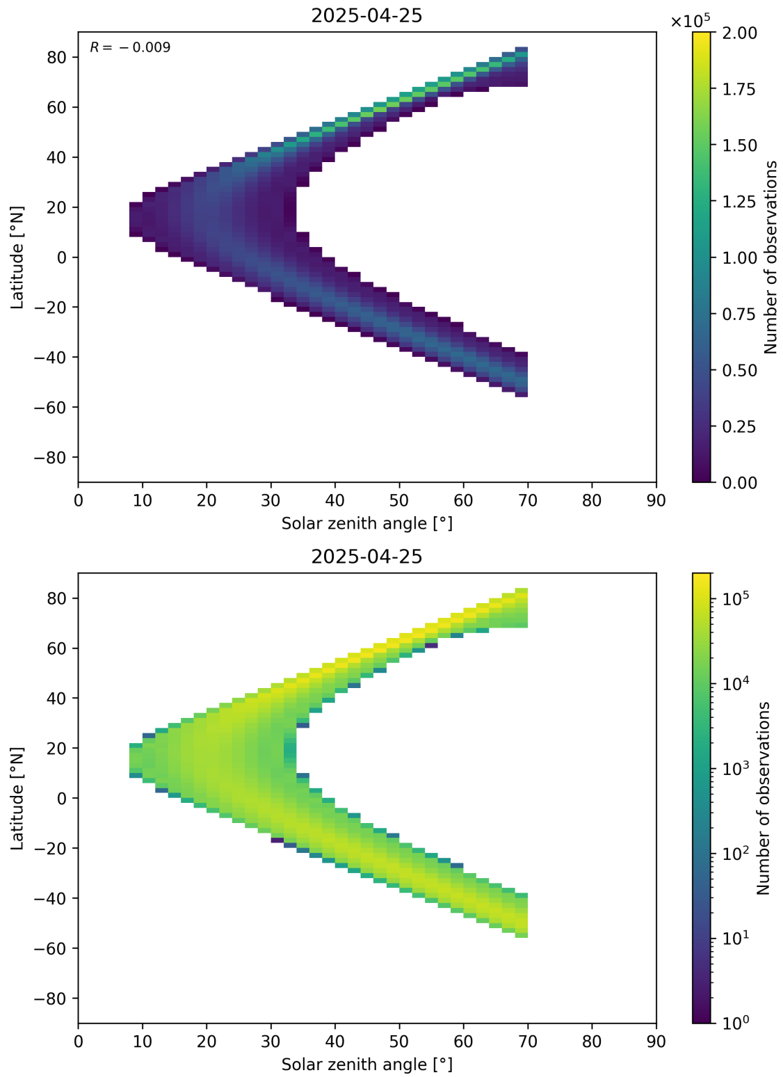
Figure 177: Scatter density plot of “Solar zenith angle” against “Latitude” for 2025-04-24 to 2025-04-26.
