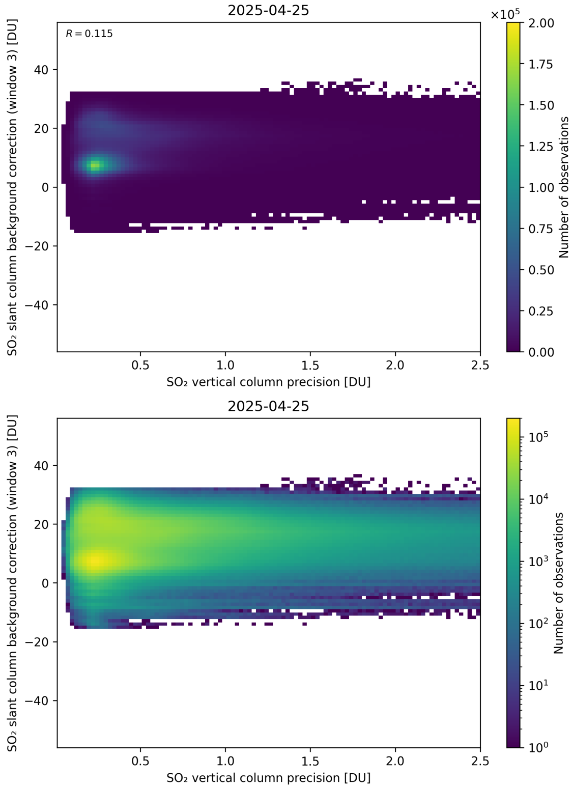
Figure 331: Scatter density plot of “SO 2 vertical column precision” against “SO 2 slant column background correction (window 3)” for 2025-04-24 to 2025-04-26.
