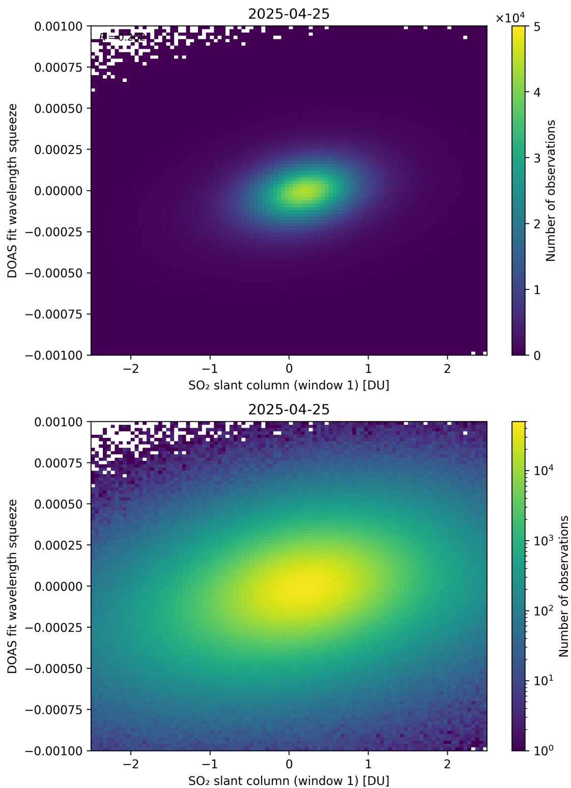
Figure 266: Scatter density plot of “SO 2 slant column (window 1)” against “DOAS fit wavelength squeeze” for 2025-04-24 to 2025-04-26.
