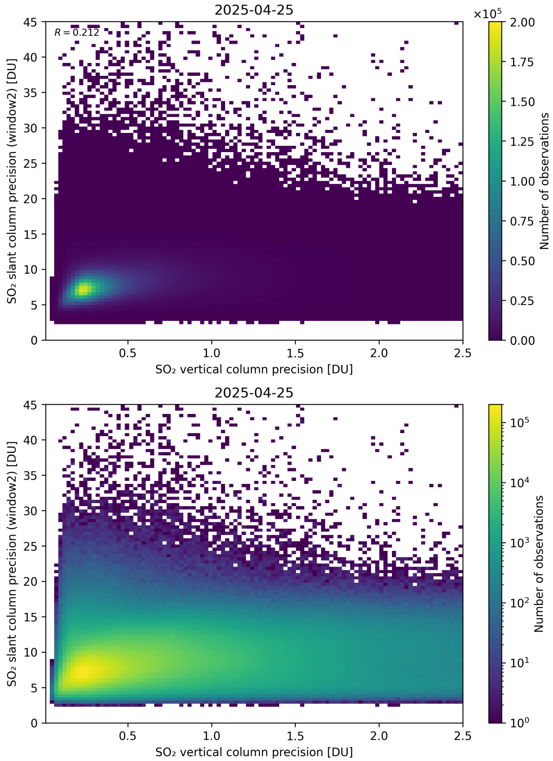
Figure 343: Scatter density plot of “SO 2 vertical column precision” against “SO 2 slant column precision (window2)” for 2025-04-24 to 2025-04-26.
