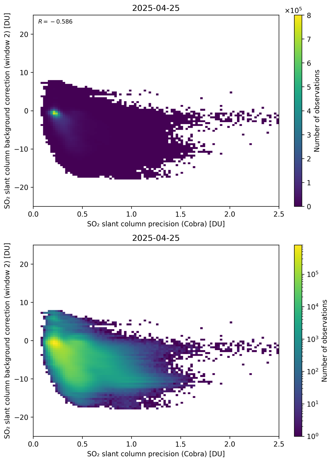
Figure 200: Scatter density plot of “SO 2 slant column precision (Cobra)” against “SO 2 slant column background correction (window 2)” for 2025-04-24 to 2025-04-26.
