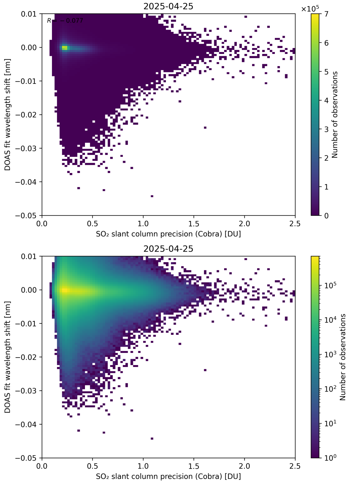
Figure 202: Scatter density plot of “SO 2 slant column precision (Cobra)” against “DOAS fit wavelength shift” for 2025-04-24 to 2025-04-26.
