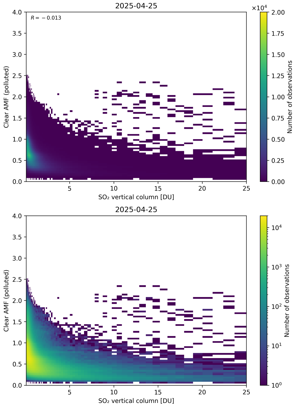
Figure 348: Scatter density plot of “SO 2 vertical column” against “Clear AMF (polluted)” for 2025-04-24 to 2025-04-26.
