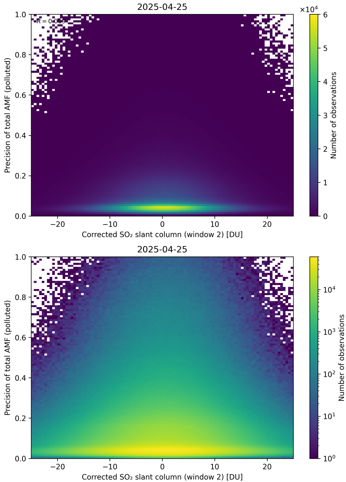
Figure 254: Scatter density plot of “Corrected SO 2 slant column (window 2)” against “Precision of total AMF (polluted)” for 2025-04-24 to 2025-04-26.
