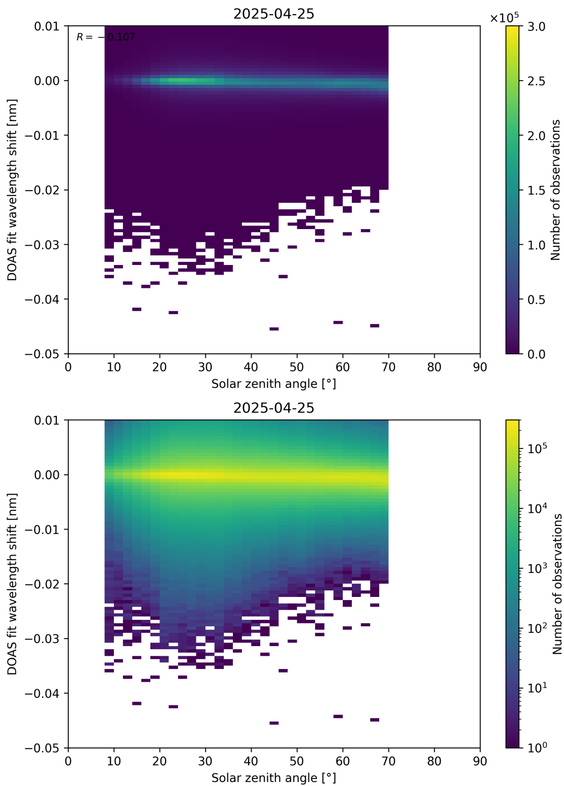
Figure 174: Scatter density plot of “Solar zenith angle” against “DOAS fit wavelength shift” for 2025-04-24 to 2025-04-26.
