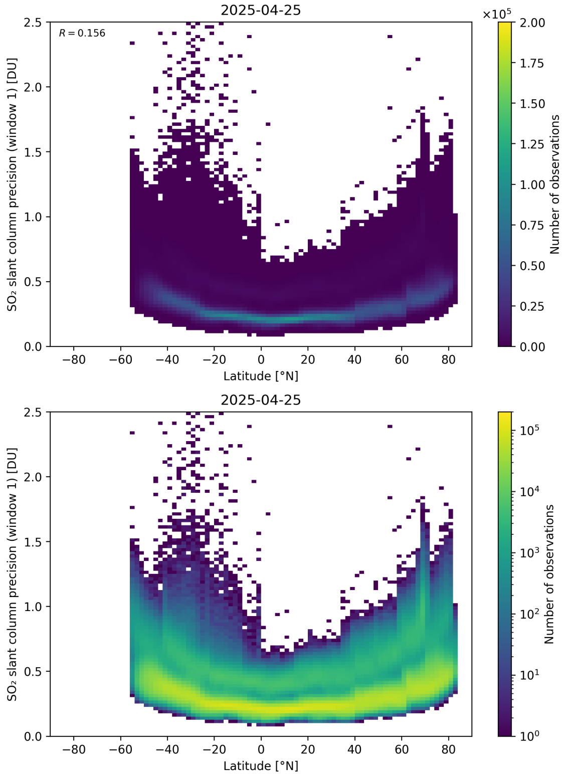
Figure 163: Scatter density plot of “Latitude” against “SO 2 slant column precision (window 1)” for 2025-04-24 to 2025-04-26.
