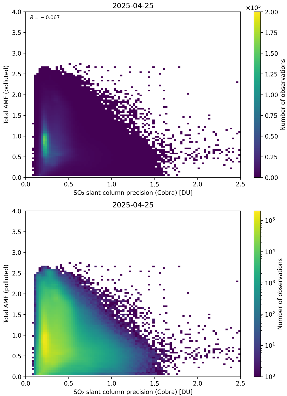
Figure 213: Scatter density plot of “SO 2 slant column precision (Cobra)” against “Total AMF (polluted)” for 2025-04-24 to 2025-04-26.
