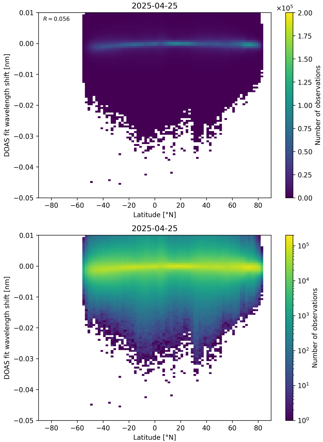
Figure 153: Scatter density plot of “Latitude” against “DOAS fit wavelength shift” for 2025-04-24 to 2025-04-26.
