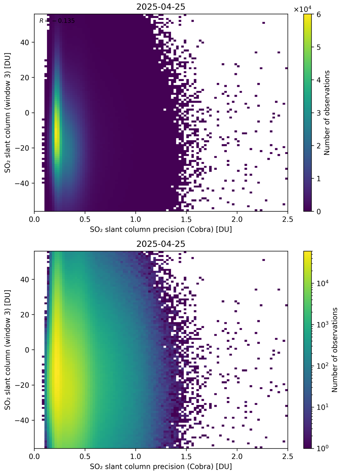
Figure 211: Scatter density plot of “SO 2 slant column precision (Cobra)” against “SO 2 slant column (window 3)” for 2025-04-24 to 2025-04-26.
