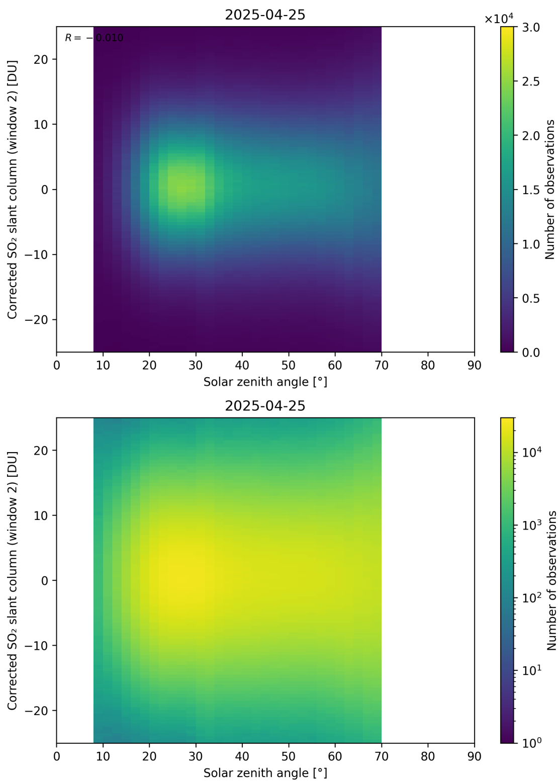
Figure 182: Scatter density plot of “Solar zenith angle” against “Corrected SO 2 slant column (window 2)” for 2025-04-24 to 2025-04-26.
