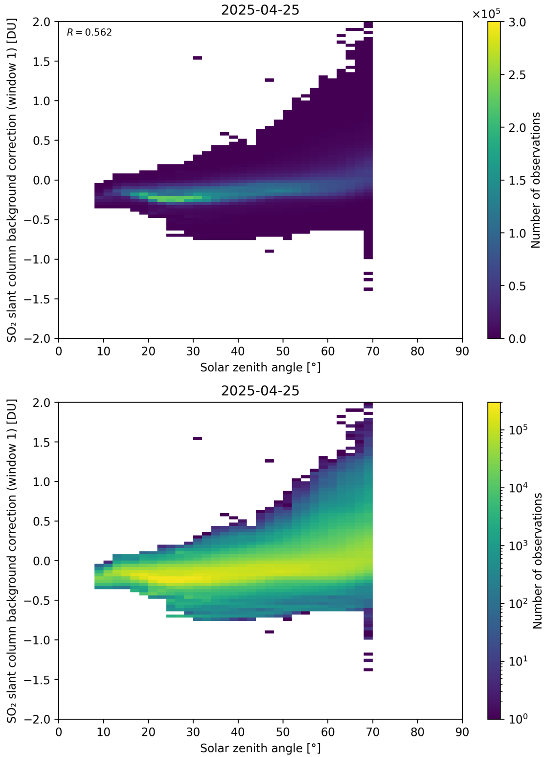
Figure 171: Scatter density plot of “Solar zenith angle” against “SO 2 slant column background correction (window 1)” for 2025-04-24 to 2025-04-26.
