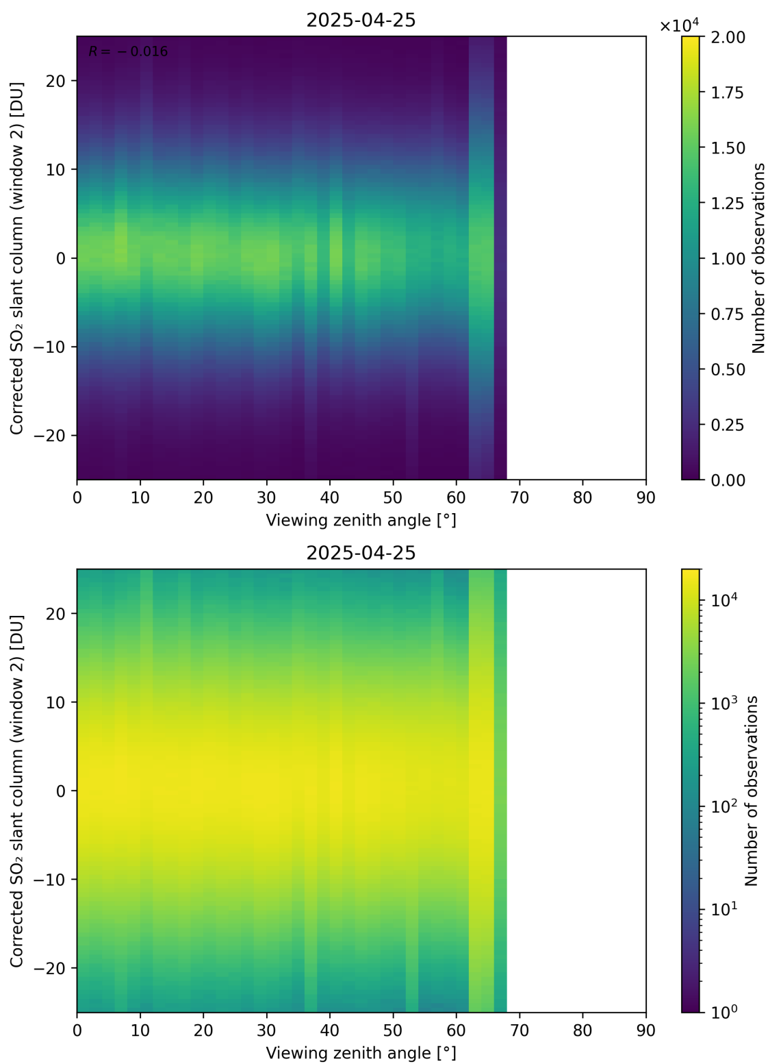
Figure 374: Scatter density plot of “Viewing zenith angle” against “Corrected SO 2 slant column (window 2)” for 2025-04-24 to 2025-04-26.
