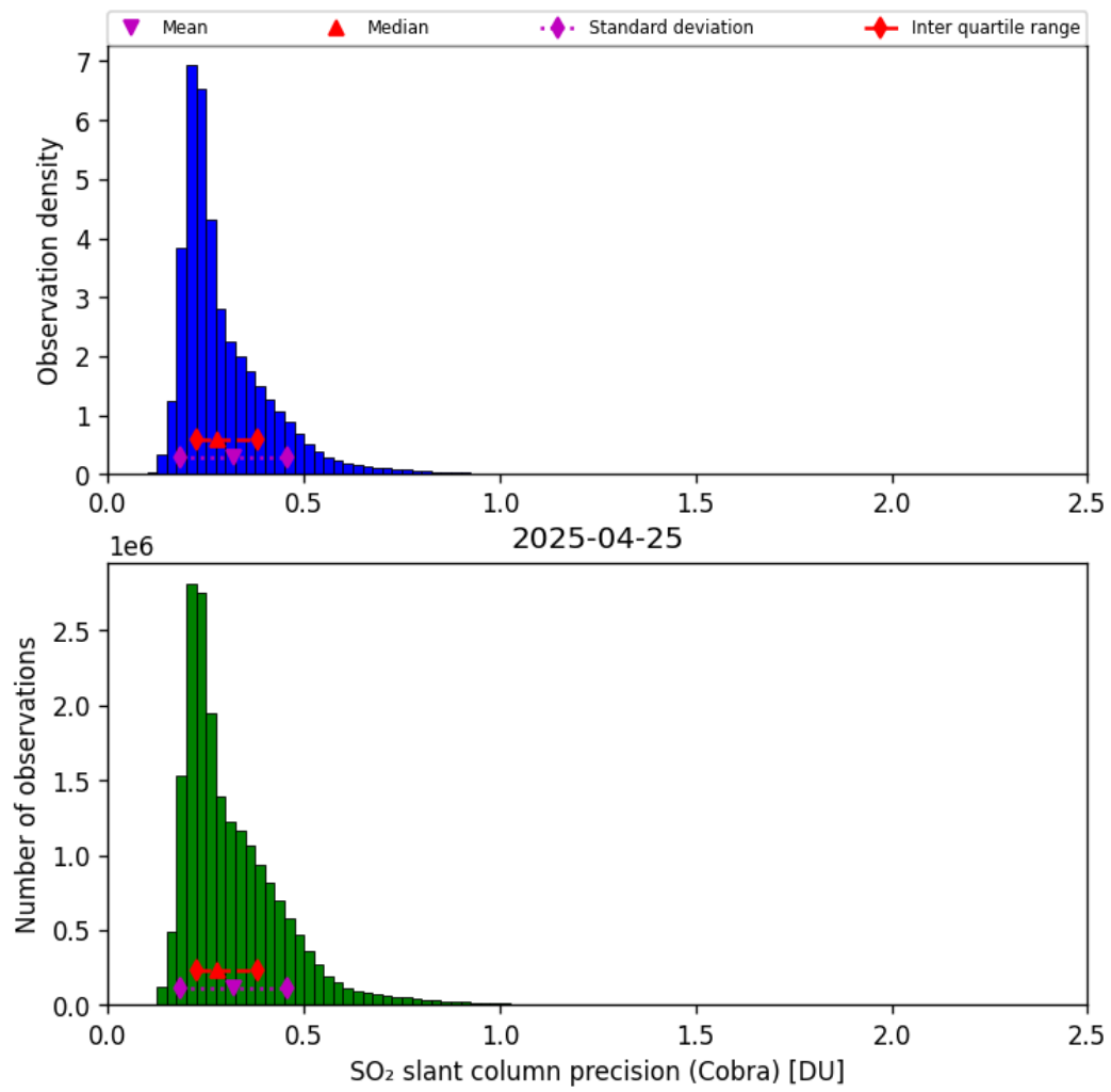
Figure 62: Histogram of “SO 2 slant column precision (Cobra)” for 2025-04-24 to 2025-04-26
