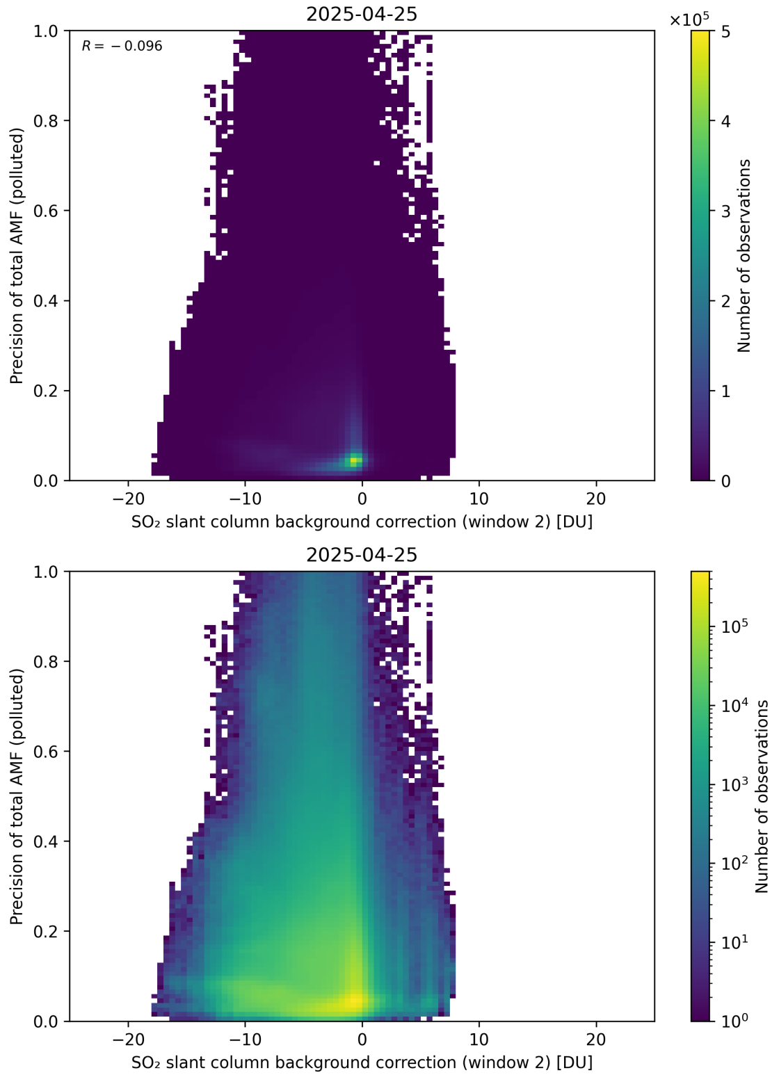
Figure 131: Scatter density plot of “SO 2 slant column background correction (window 2)” against “Precision of total AMF (polluted)” for 2025-04-24 to 2025-04-26.
