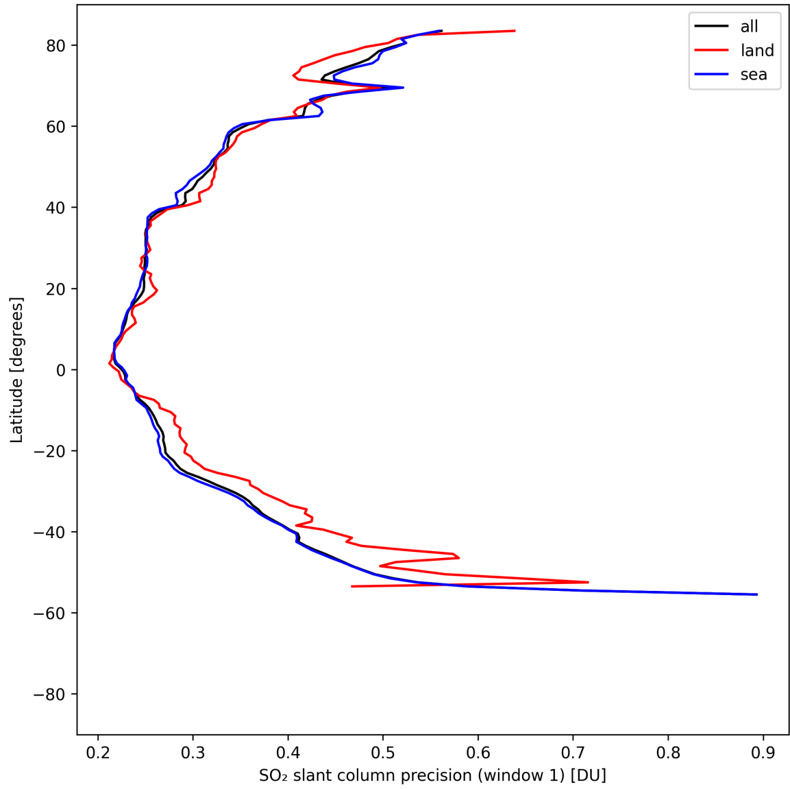
Figure 38: Zonal average of “SO 2 slant column precision (window 1)” for 2025-04-24 to 2025-04-26.
