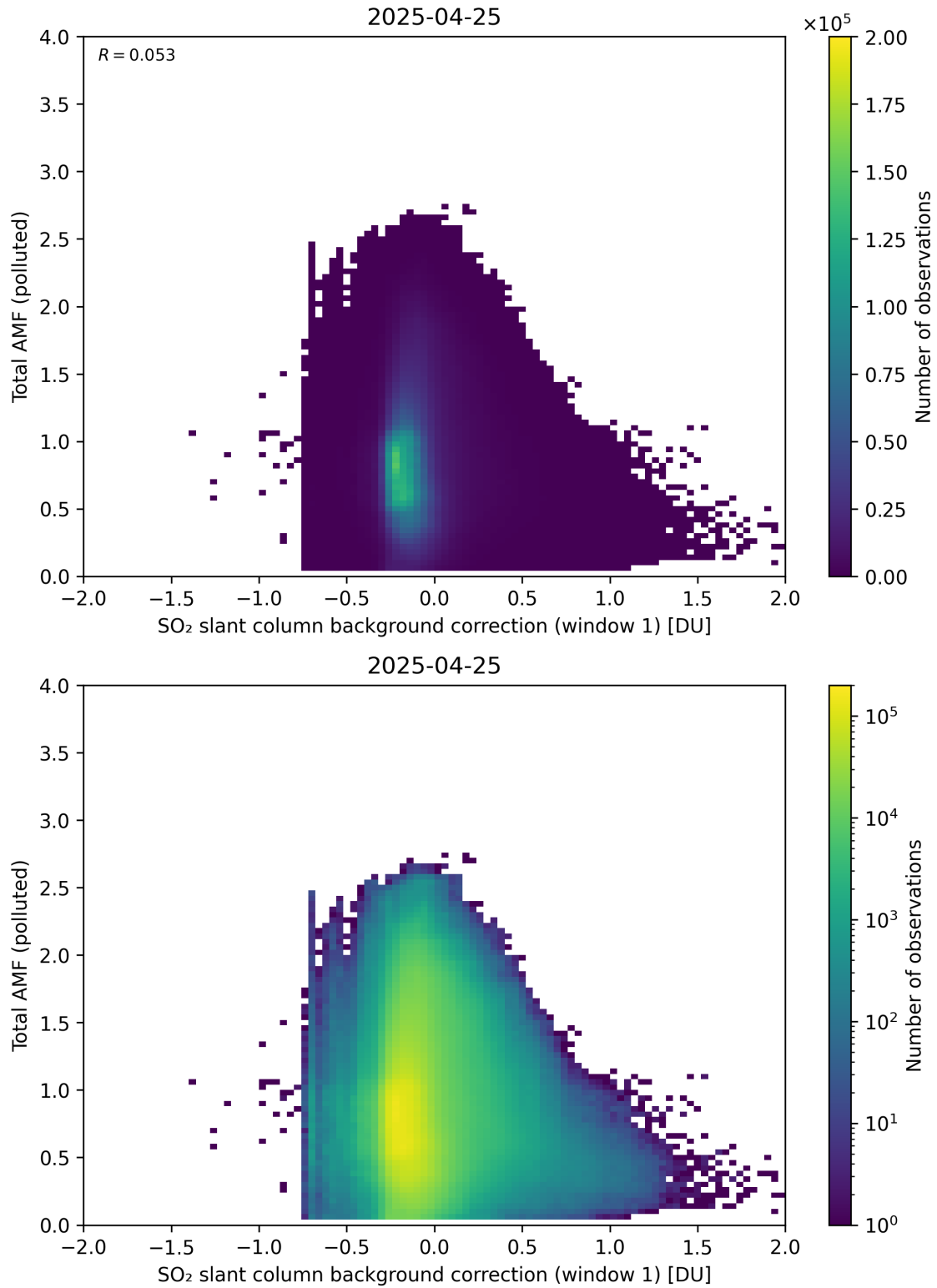
Figure 120: Scatter density plot of “SO 2 slant column background correction (window 1)” against “Total AMF (polluted)” for 2025-04-24 to 2025-04-26.
