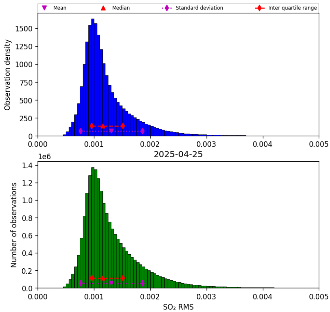
Figure 78: Histogram of "SO 2 RMS" for 2025-04-24 to 2025-04-26
