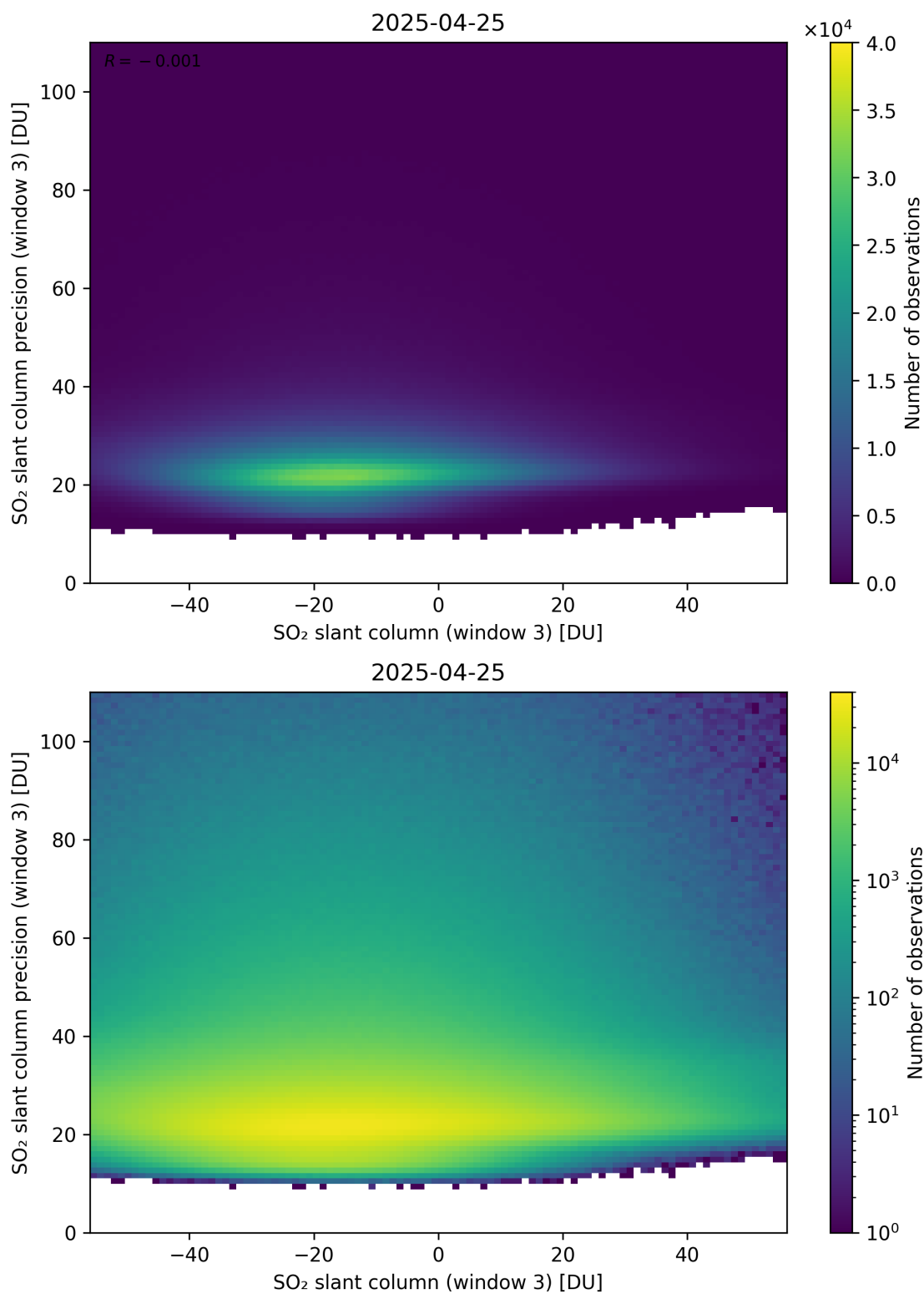
Figure 317: Scatter density plot of “SO 2 slant column (window 3)” against “SO 2 slant column precision (window 3)” for 2025-04-24 to 2025-04-26.
