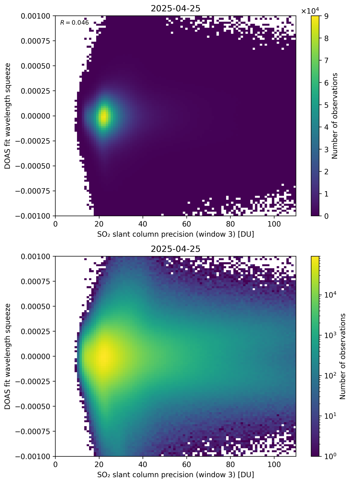
Figure 309: Scatter density plot of “SO 2 slant column precision (window 3)” against “DOAS fit wavelength squeeze” for 2025-04-24 to 2025-04-26.
