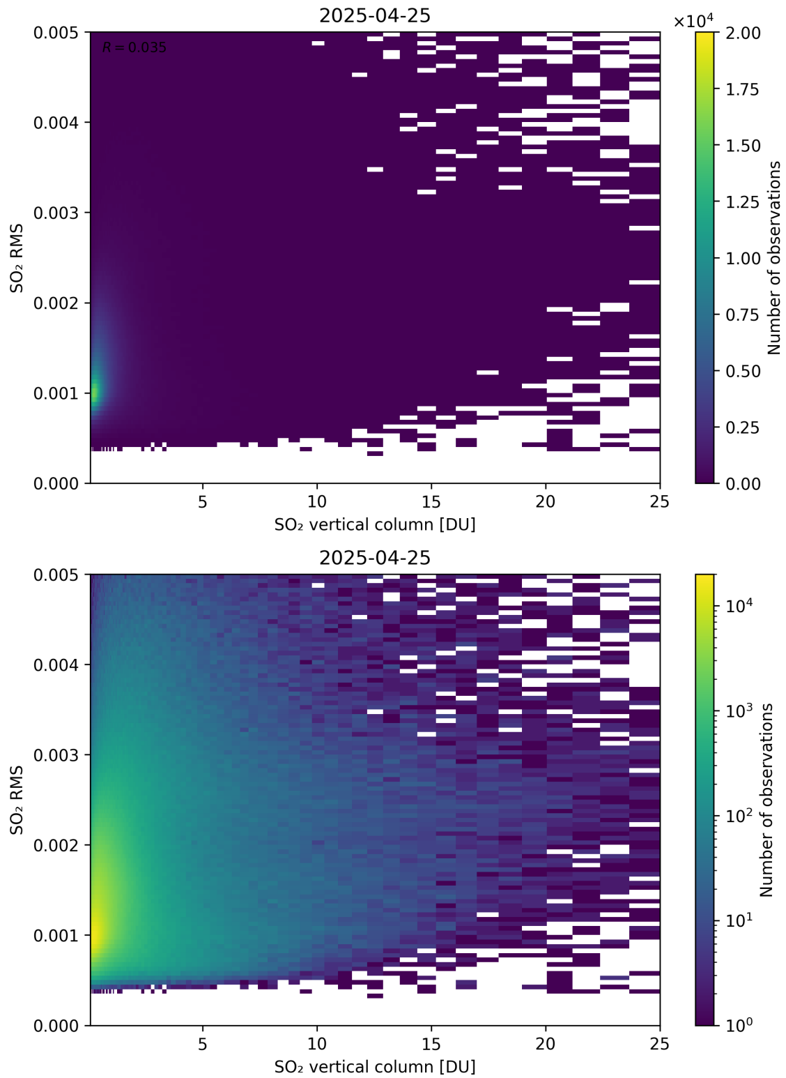
Figure 328: Scatter density plot of “SO 2 vertical column” against “SO 2 RMS” for 2025-04-24 to 2025-04-26.
