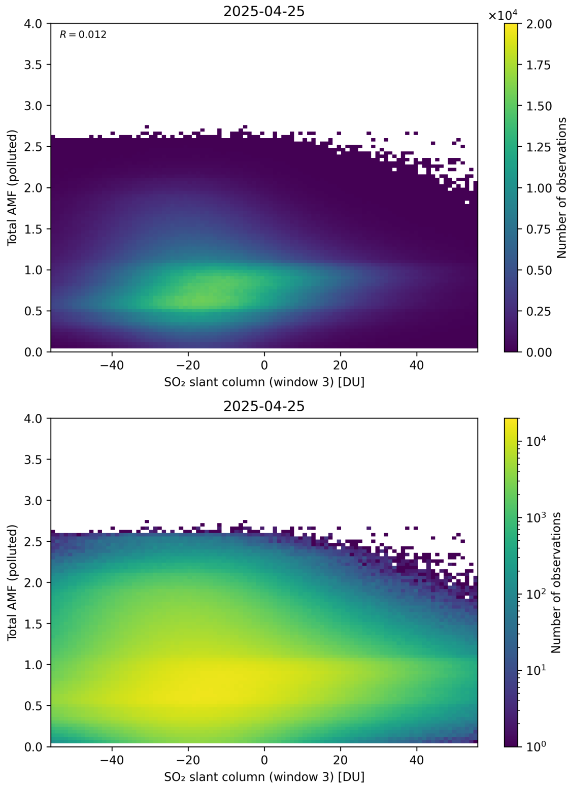
Figure 318: Scatter density plot of “SO 2 slant column (window 3)” against “Total AMF (polluted)” for 2025-04-24 to 2025-04-26.
