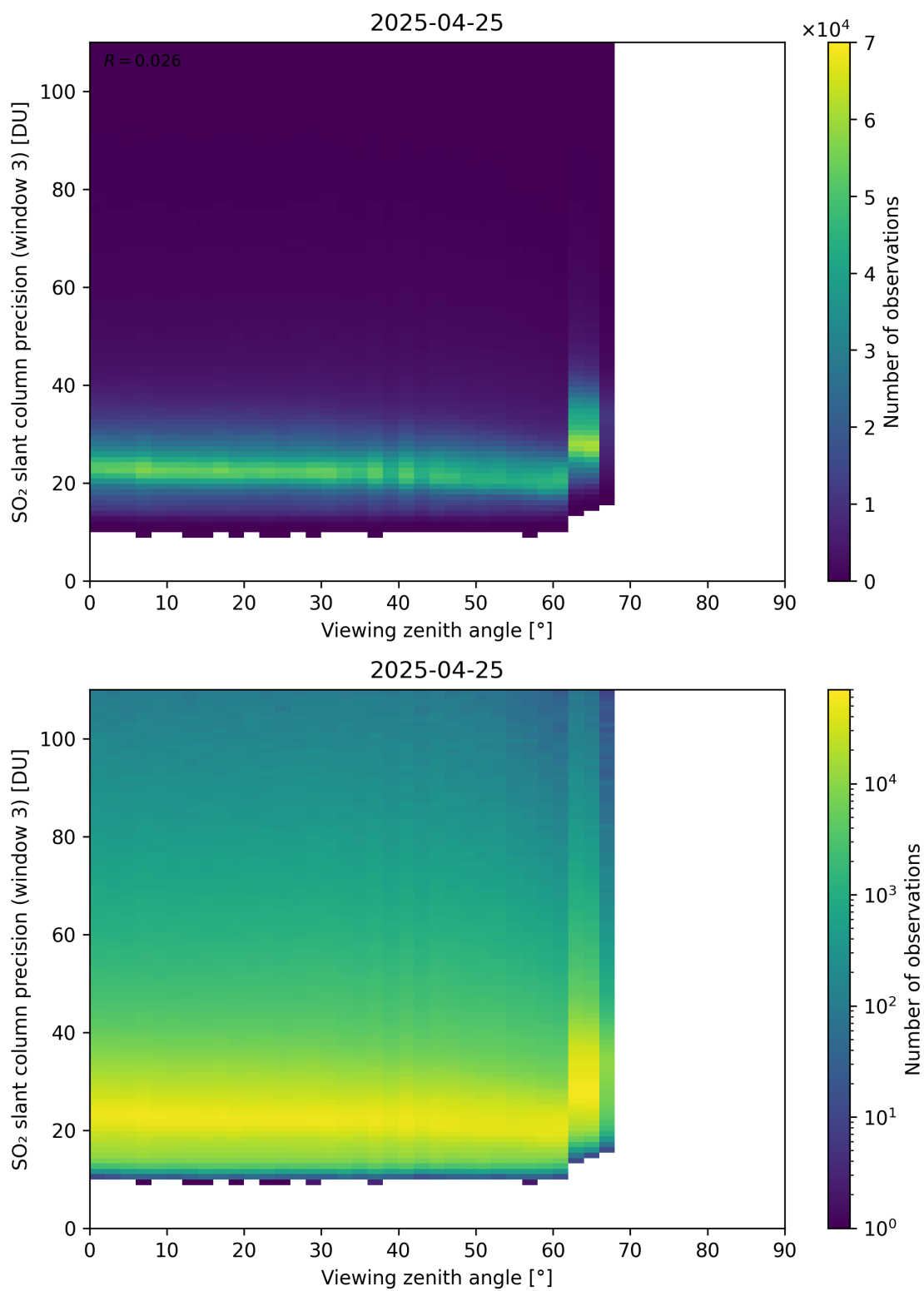
Figure 380: Scatter density plot of “Viewing zenith angle” against “SO 2 slant column precision (window 3)” for 2025-04-24 to 2025-04-26.
