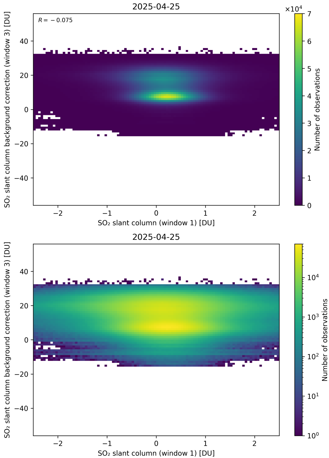
Figure 264: Scatter density plot of “SO 2 slant column (window 1)” against “SO 2 slant column background correction (window 3)” for 2025-04-24 to 2025-04-26.
