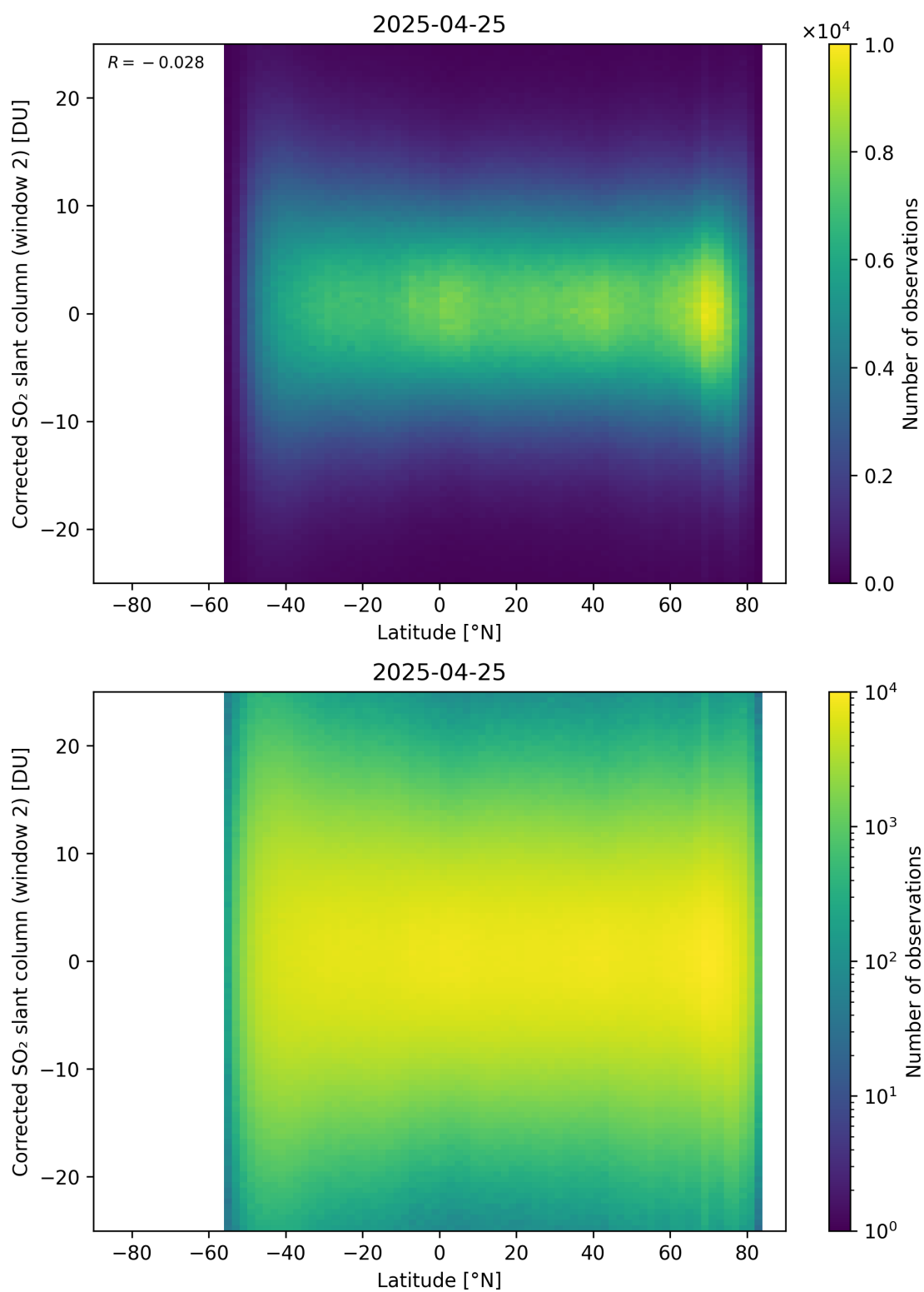
Figure 160: Scatter density plot of “Latitude” against “Corrected SO 2 slant column (window 2)” for 2025-04-24 to 2025-04-26.
