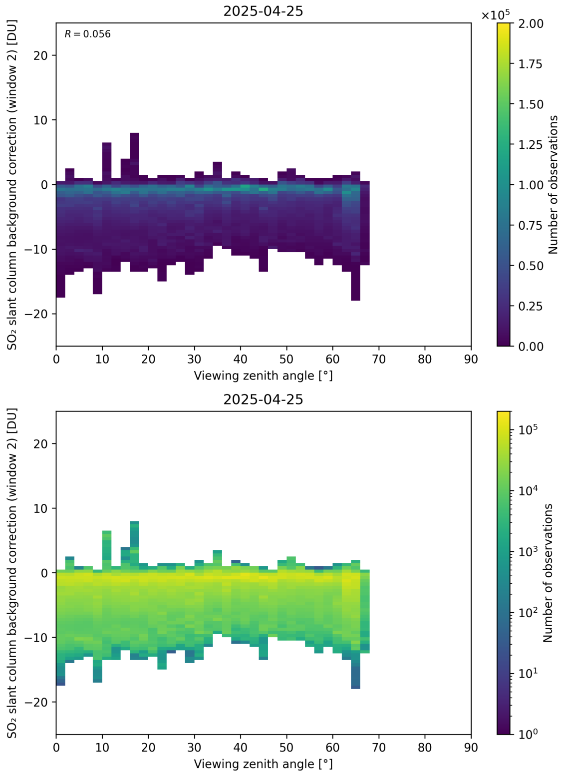
Figure 363: Scatter density plot of “Viewing zenith angle” against “SO 2 slant column background correction (window 2)” for 2025-04-24 to 2025-04-26.
