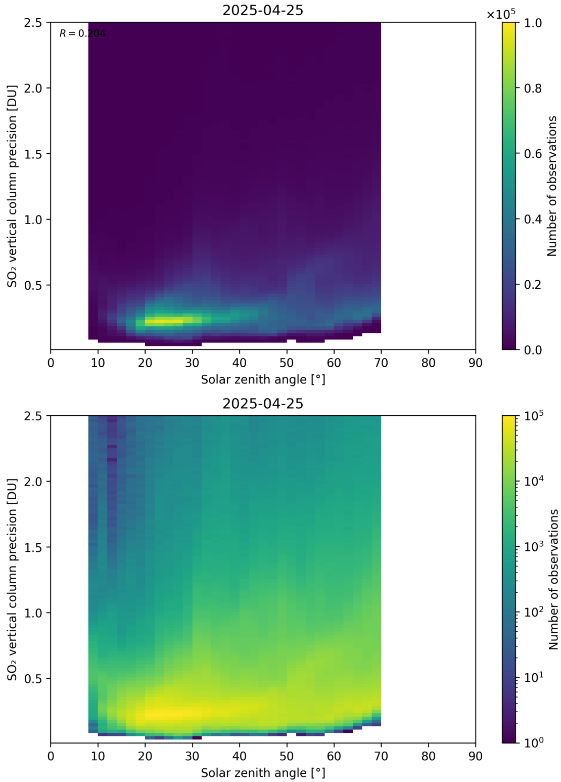
Figure 192: Scatter density plot of “Solar zenith angle” against “SO 2 vertical column precision” for 2025-04-24 to 2025-04-26.
