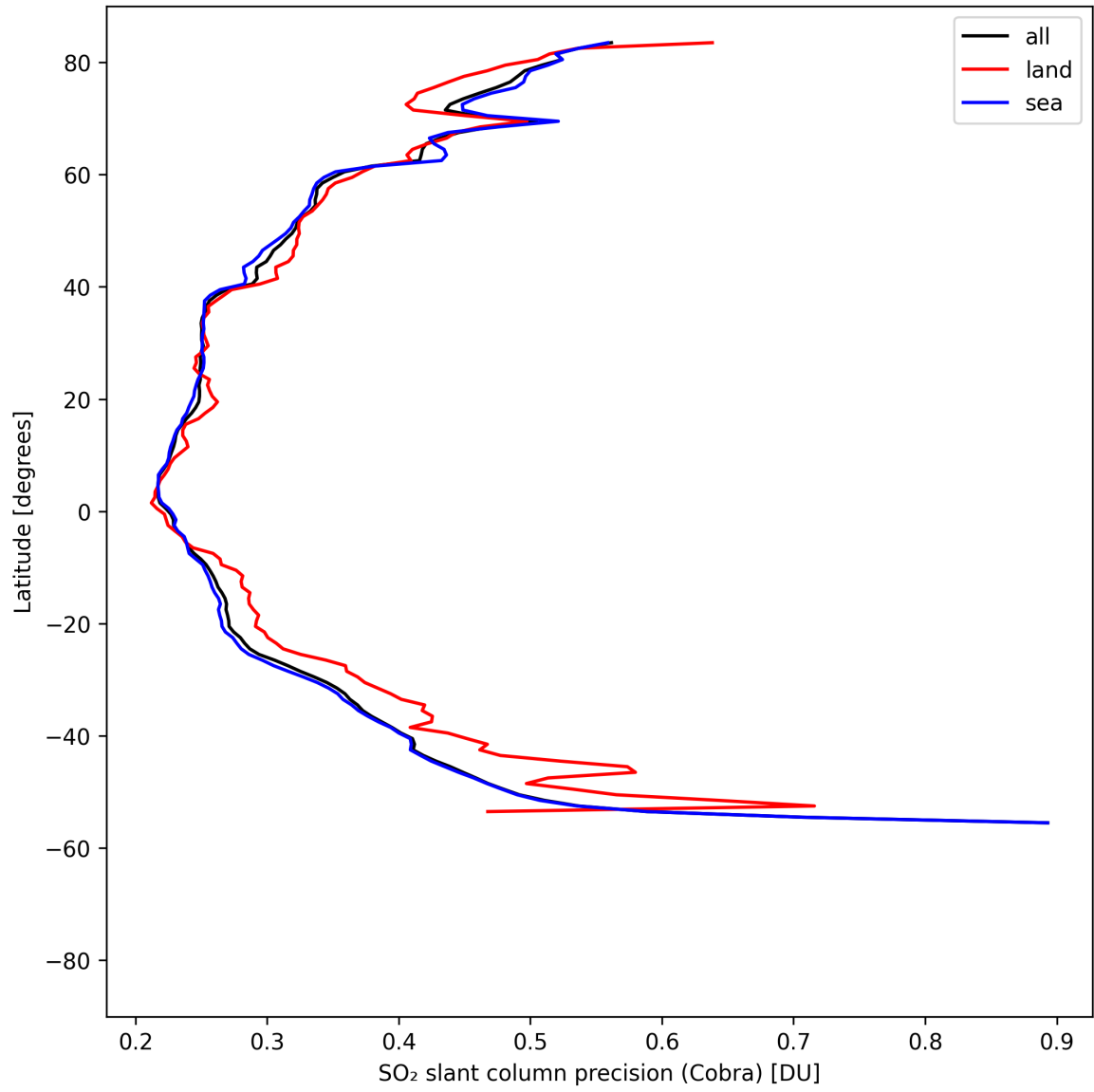
Figure 36: Zonal average of “SO 2 slant column precision (Cobra)” for 2025-04-24 to 2025-04-26.
