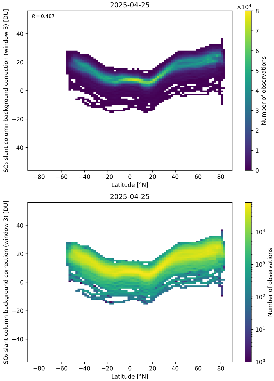
Figure 152: Scatter density plot of “Latitude” against “SO 2 slant column background correction (window 3)” for 2025-04-24 to 2025-04-26.
