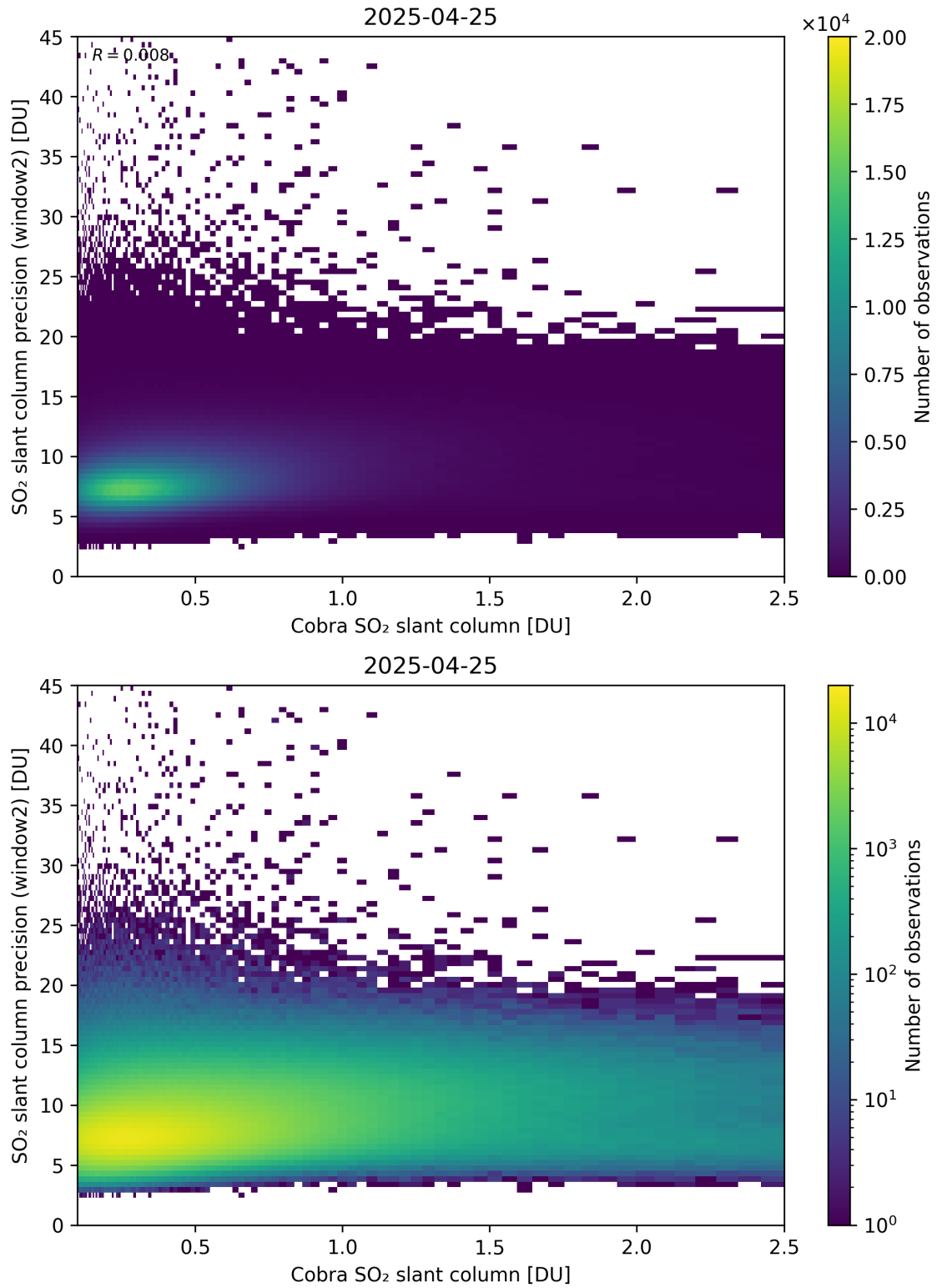
Figure 221: Scatter density plot of “Cobra SO 2 slant column” against “SO 2 slant column precision (window2)” for 2025-04-24 to 2025-04-26.
