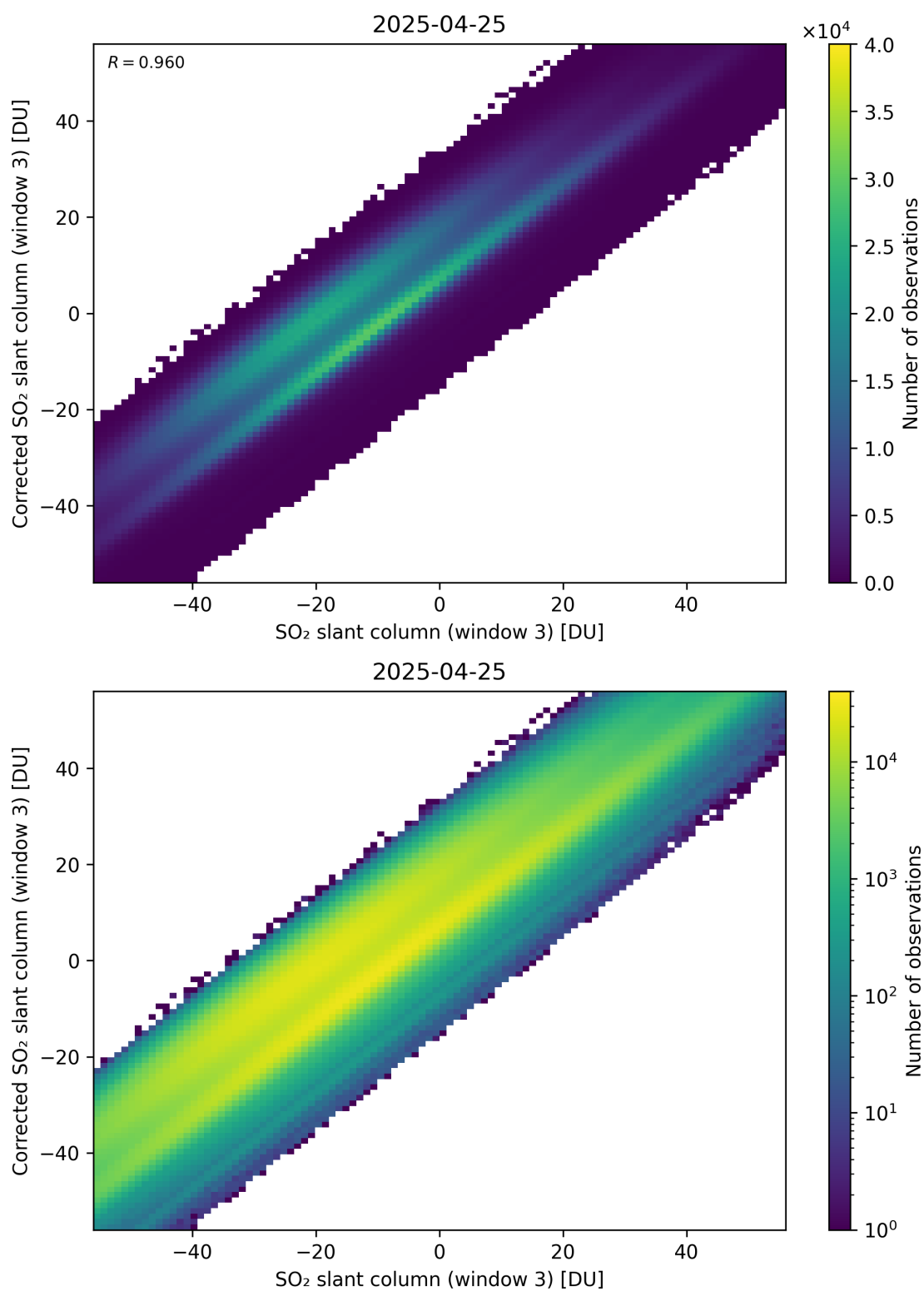
Figure 316: Scatter density plot of “SO 2 slant column (window 3)” against “Corrected SO 2 slant column (window 3)” for 2025-04-24 to 2025-04-26.
