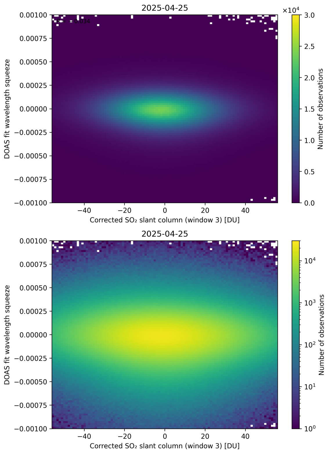
Figure 257: Scatter density plot of “Corrected SO 2 slant column (window 3)” against “DOAS fit wavelength squeeze” for 2025-04-24 to 2025-04-26.
