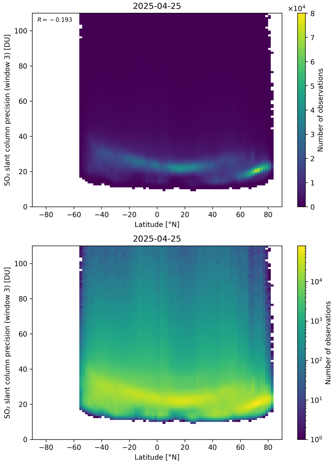
Figure 166: Scatter density plot of “Latitude” against “SO 2 slant column precision (window 3)” for 2025-04-24 to 2025-04-26.
