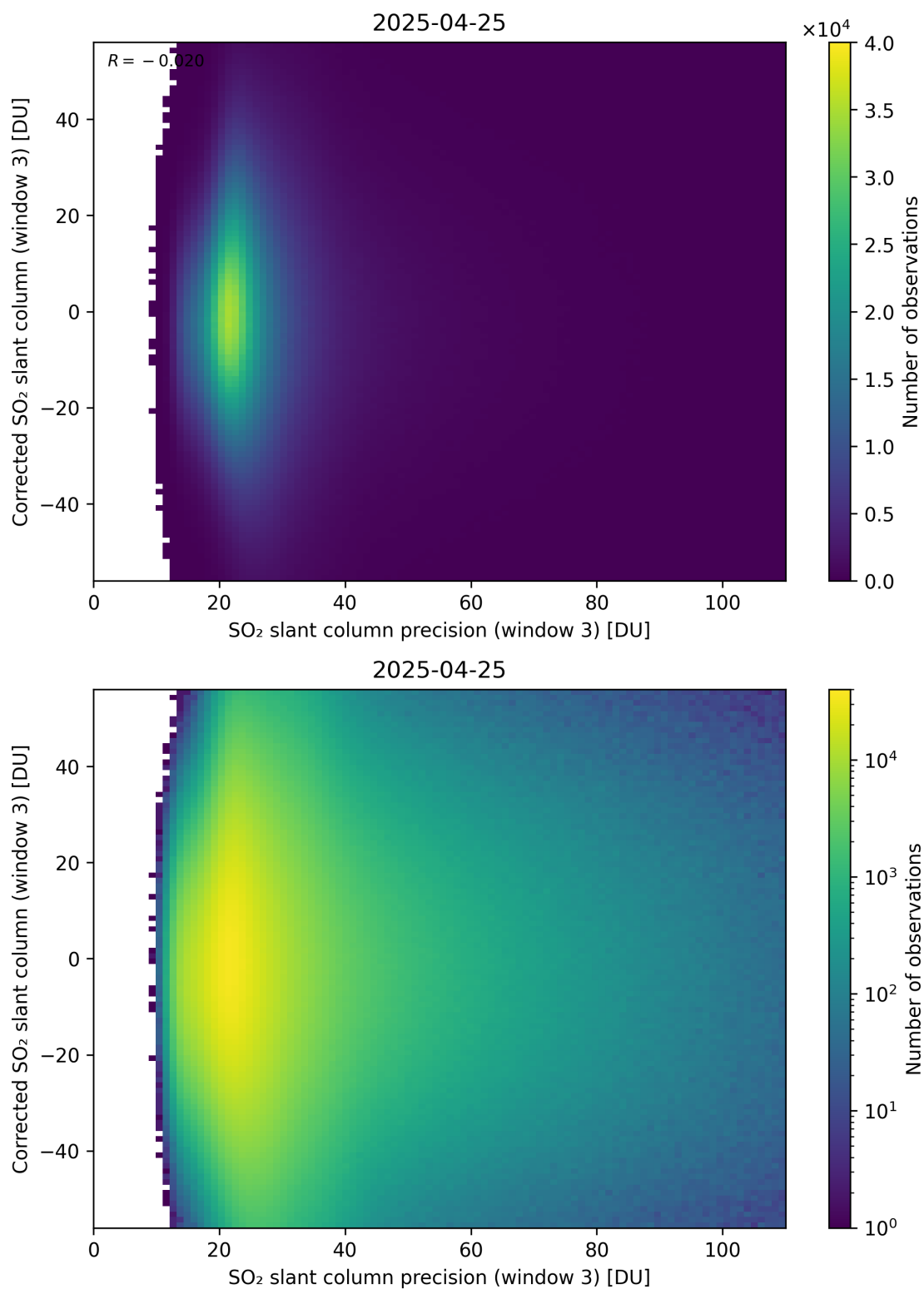
Figure 312: Scatter density plot of “SO 2 slant column precision (window 3)” against “Corrected SO 2 slant column (window 3)” for 2025-04-24 to 2025-04-26.
