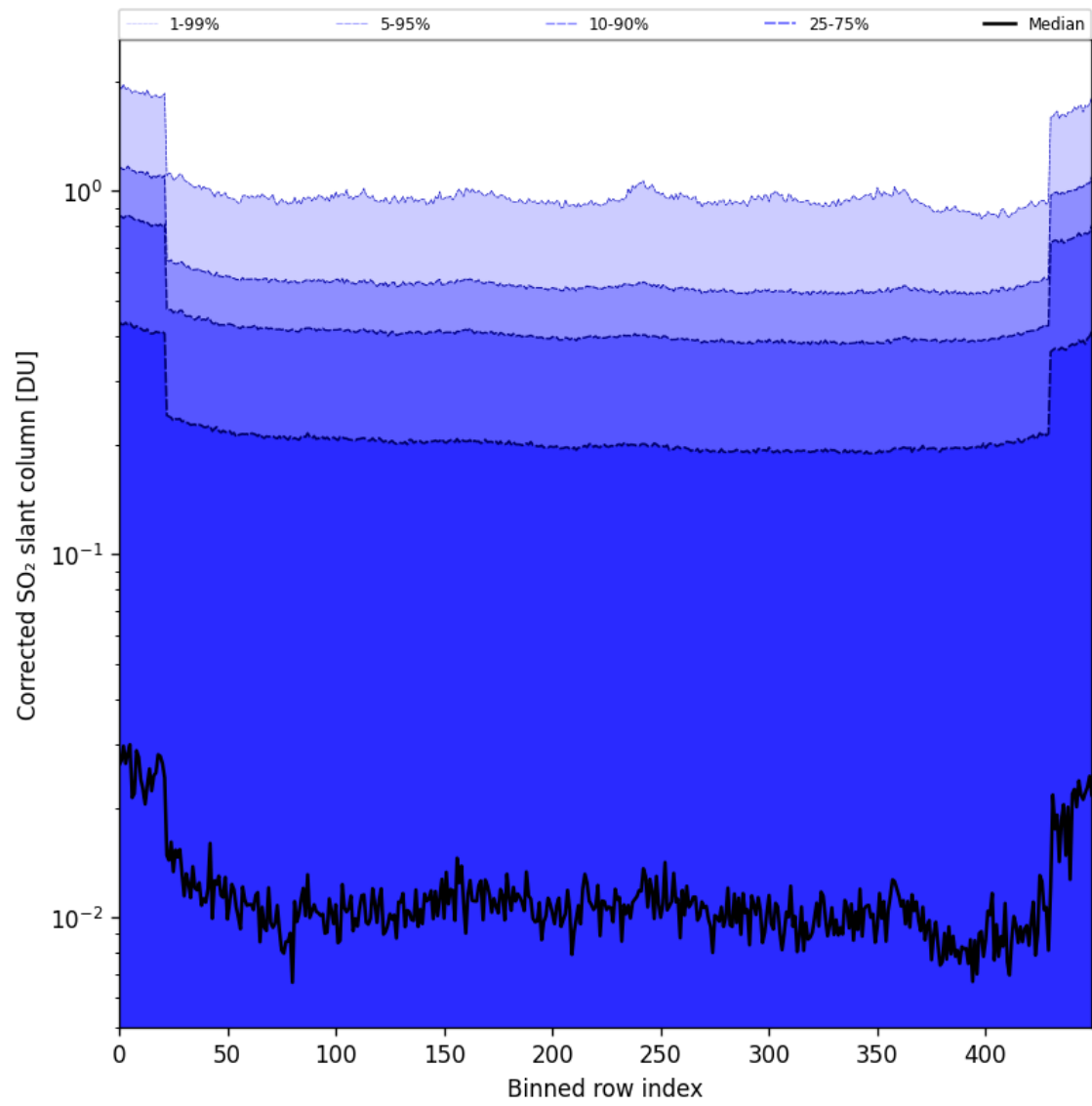
Figure 86: Along track statistics of “Corrected SO 2 slant column” for 2025-04-24 to 2025-04-26
