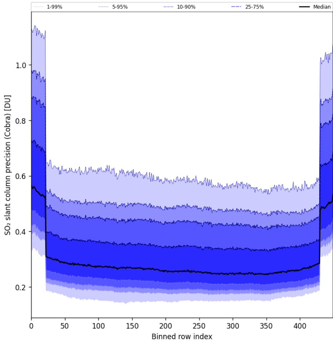
Figure 88: Along track statistics of “SO 2 slant column precision (Cobra)” for 2025-04-24 to 2025-04-26
