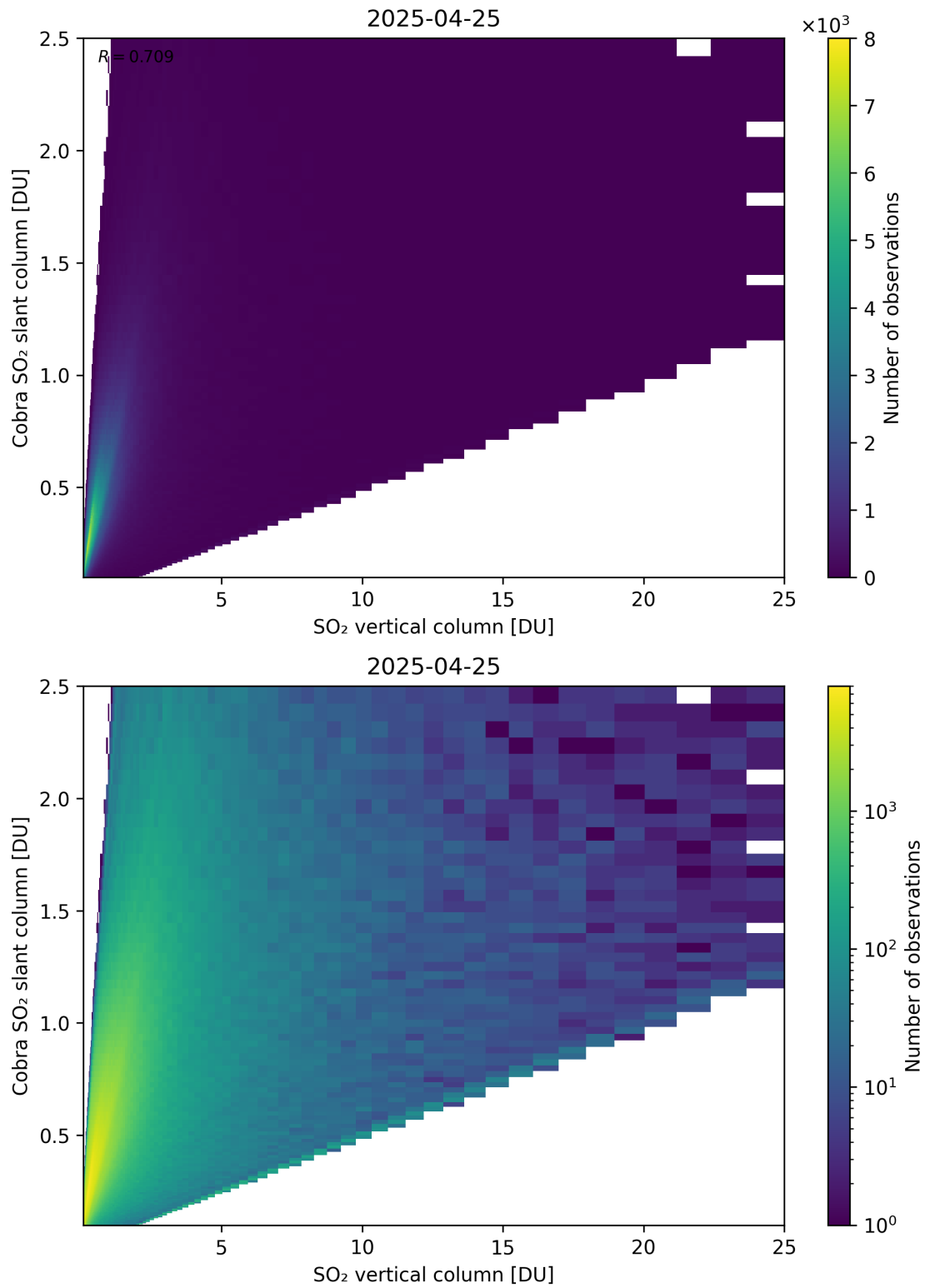
Figure 349: Scatter density plot of “SO 2 vertical column” against “Cobra SO 2 slant column” for 2025-04-24 to 2025-04-26.
