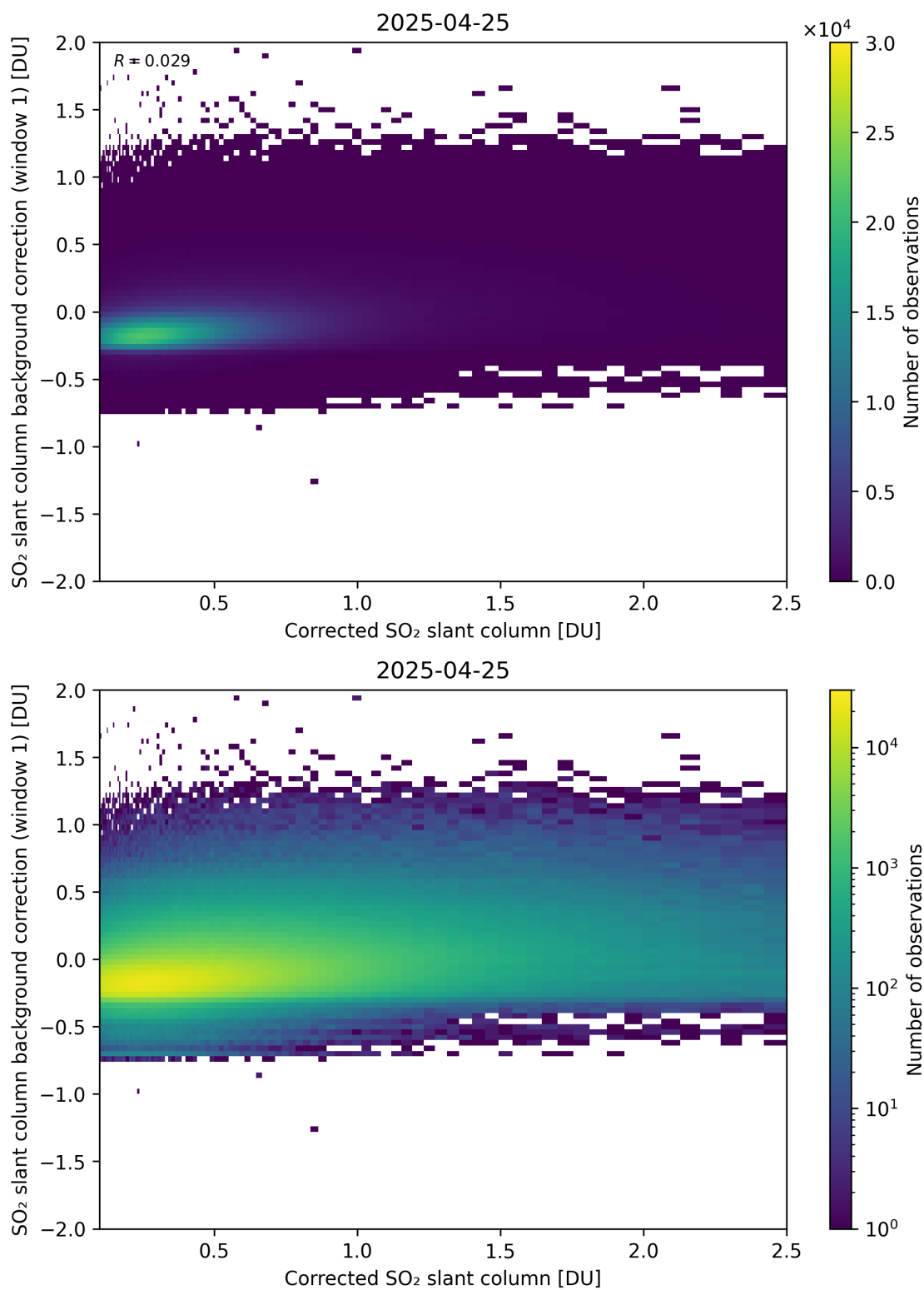
Figure 226: Scatter density plot of “Corrected SO 2 slant column” against “SO 2 slant column background correction (window 1)” for 2025-04-24 to 2025-04-26.
