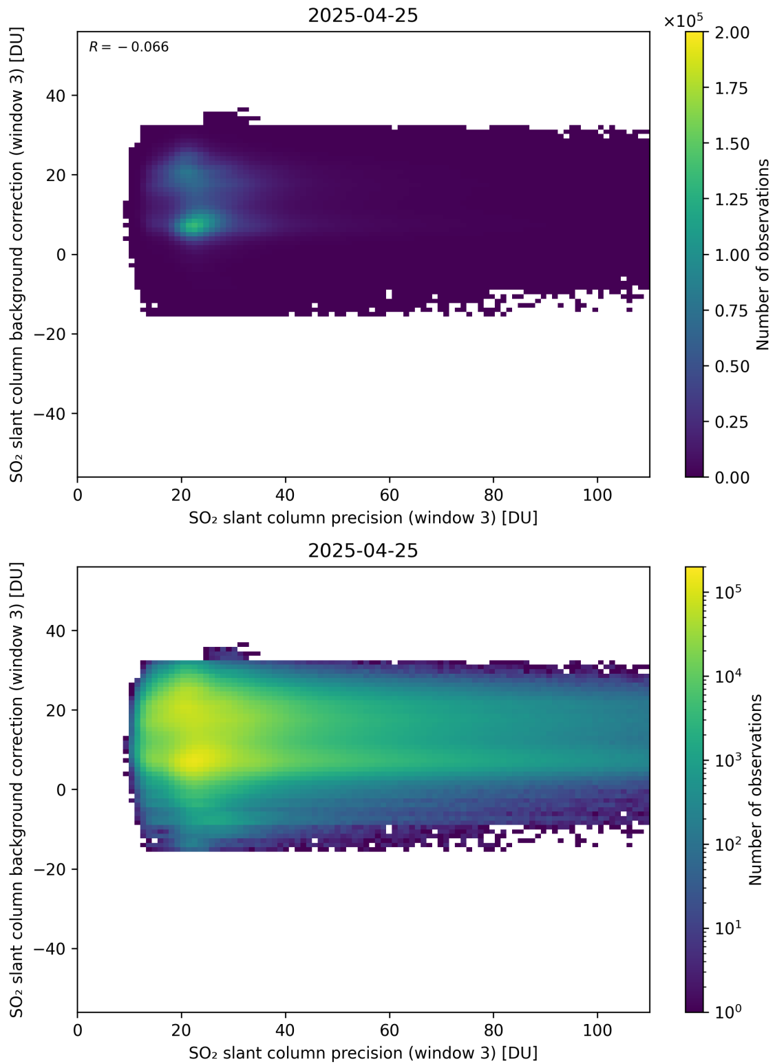
Figure 307: Scatter density plot of “SO 2 slant column precision (window 3)” against “SO 2 slant column background correction (window 3)” for 2025-04-24 to 2025-04-26.
