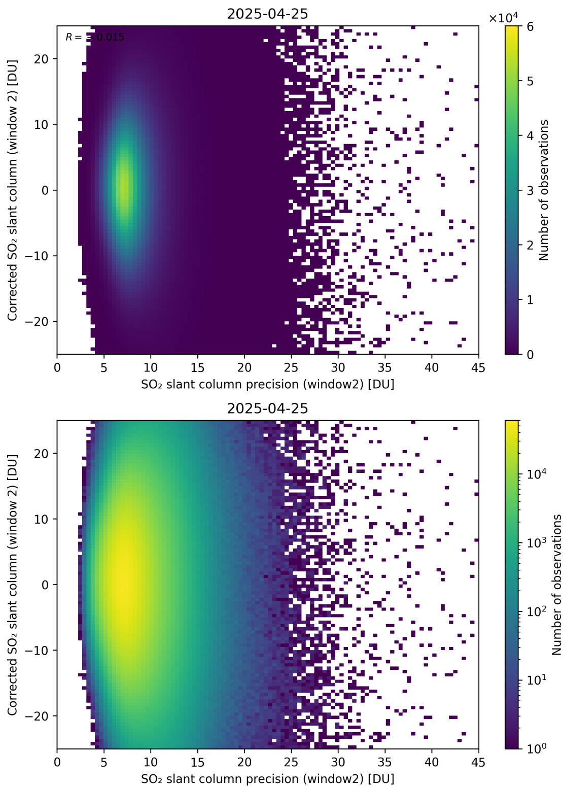
Figure 297: Scatter density plot of “SO 2 slant column precision (window2)” against “Corrected SO 2 slant column (window 2)” for 2025-04-24 to 2025-04-26.
