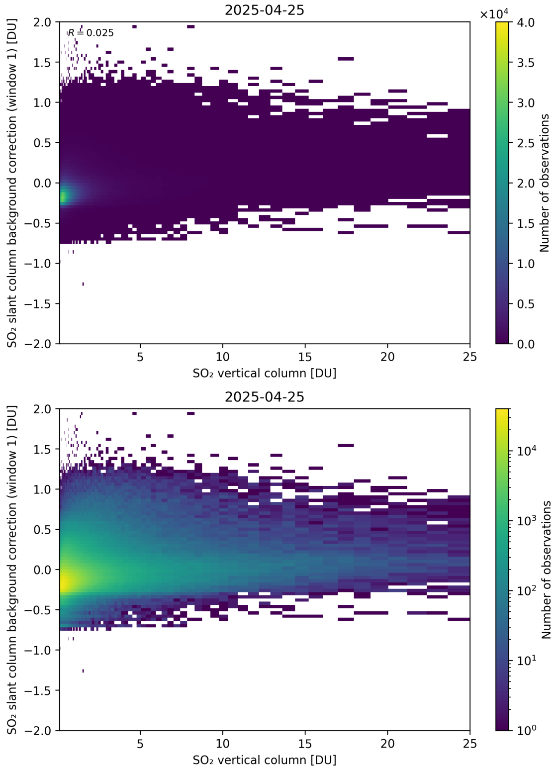
Figure 323: Scatter density plot of “SO 2 vertical column” against “SO 2 slant column background correction (window 1)” for 2025-04-24 to 2025-04-26.
