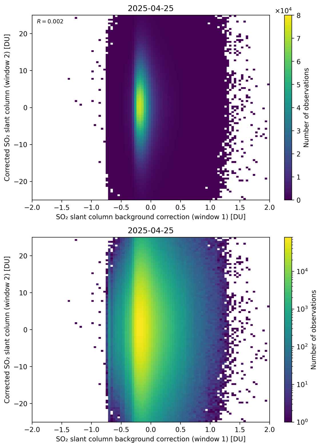
Figure 115: Scatter density plot of “SO 2 slant column background correction (window 1)” against “Corrected SO 2 slant column (window 2)” for 2025-04-24 to 2025-04-26.
