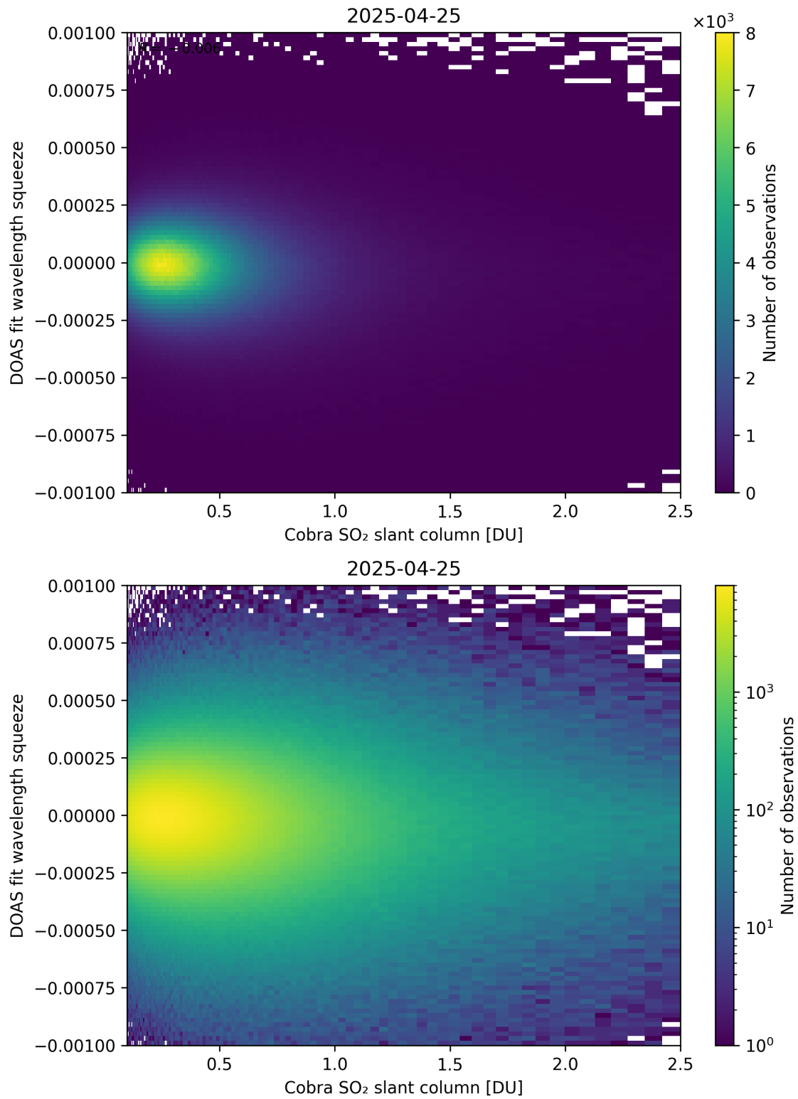
Figure 197: Scatter density plot of “Cobra SO 2 slant column” against “DOAS fit wavelength squeeze” for 2025-04-24 to 2025-04-26.
