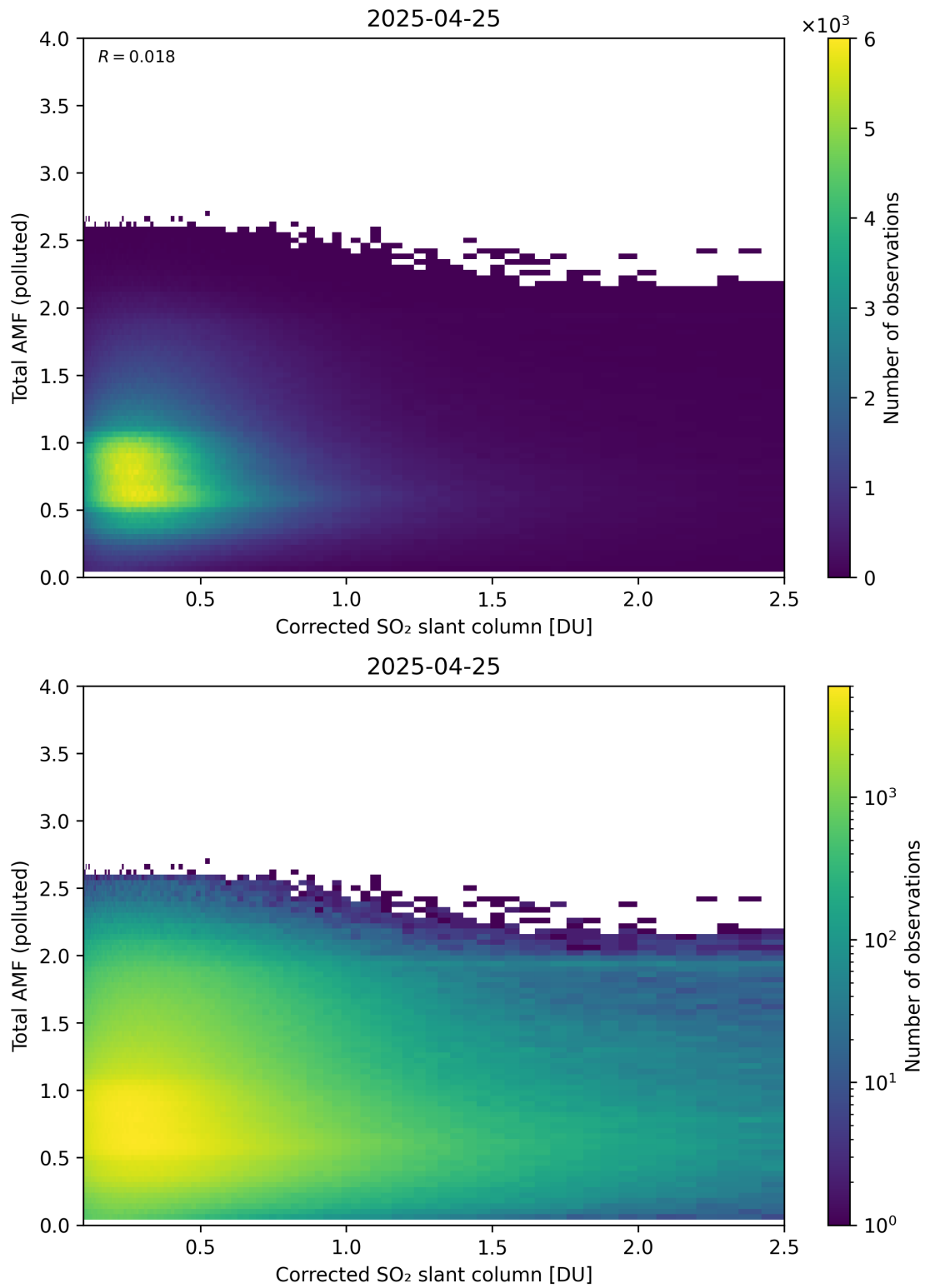
Figure 242: Scatter density plot of “Corrected SO 2 slant column” against “Total AMF (polluted)” for 2025-04-24 to 2025-04-26.
