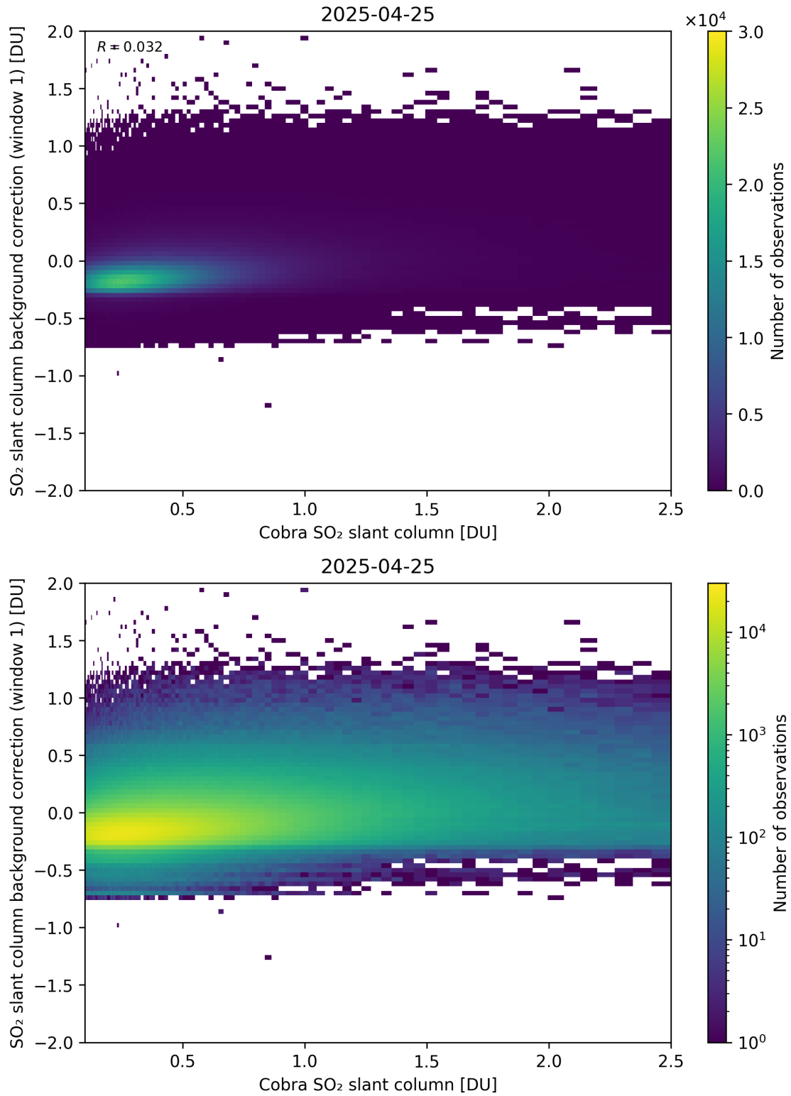
Figure 193: Scatter density plot of “Cobra SO 2 slant column” against “SO 2 slant column background correction (window 1)” for 2025-04-24 to 2025-04-26.
