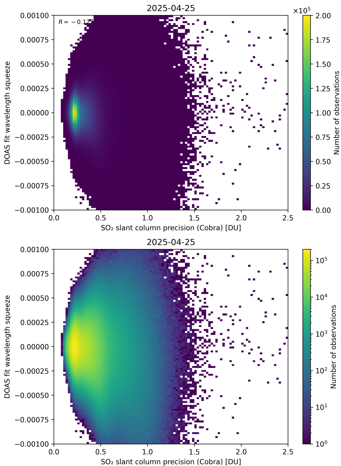
Figure 203: Scatter density plot of “SO 2 slant column precision (Cobra)” against “DOAS fit wavelength squeeze” for 2025-04-24 to 2025-04-26.
