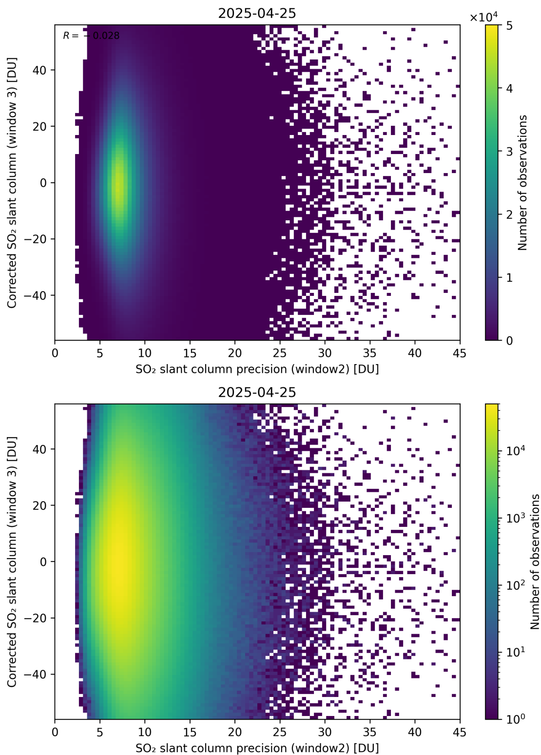
Figure 298: Scatter density plot of “SO 2 slant column precision (window2)” against “Corrected SO 2 slant column (window 3)” for 2025-04-24 to 2025-04-26.
