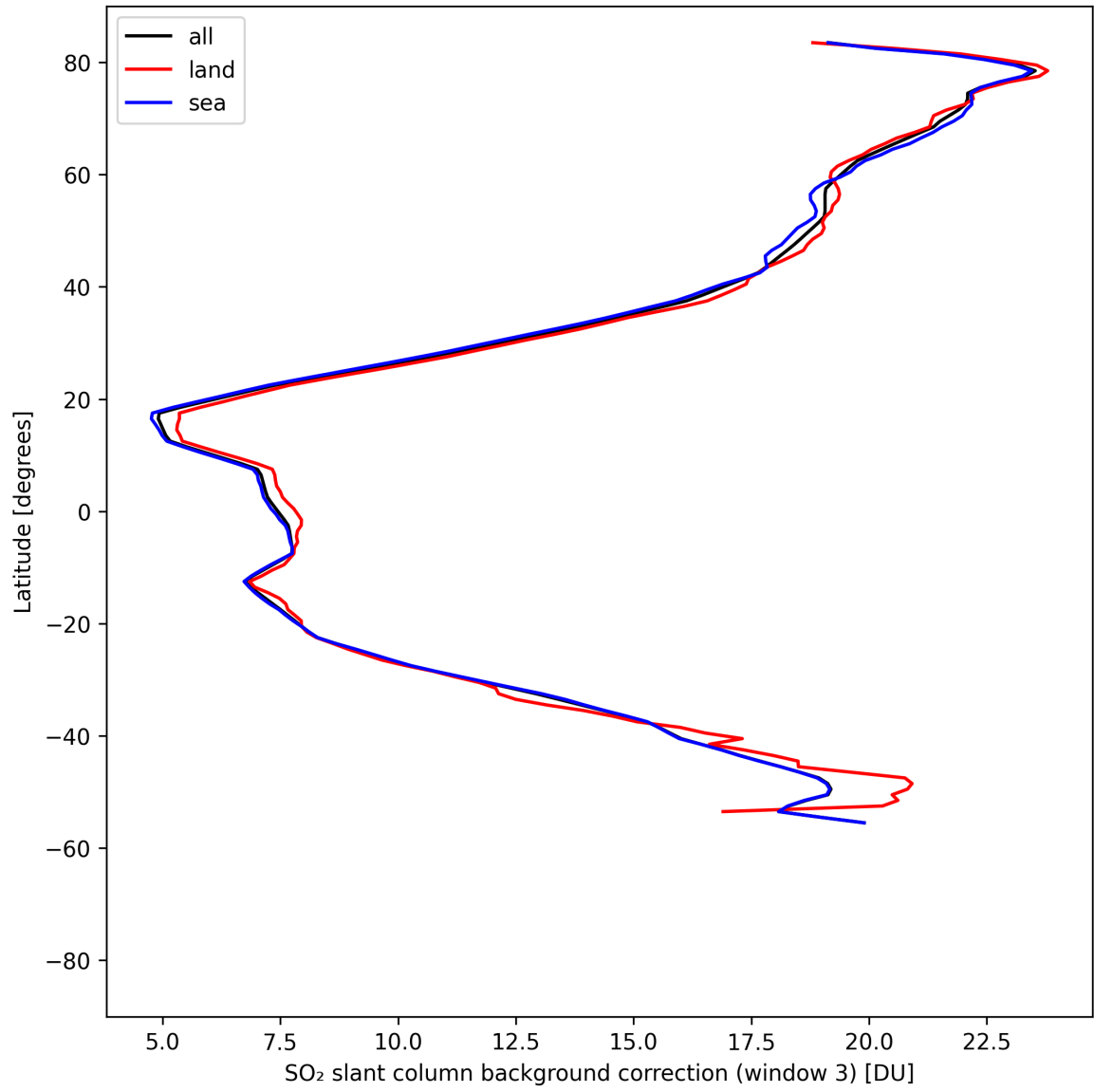
Figure 48: Zonal average of “SO 2 slant column background correction (window 3)” for 2025-04-24 to 2025-04-26.
