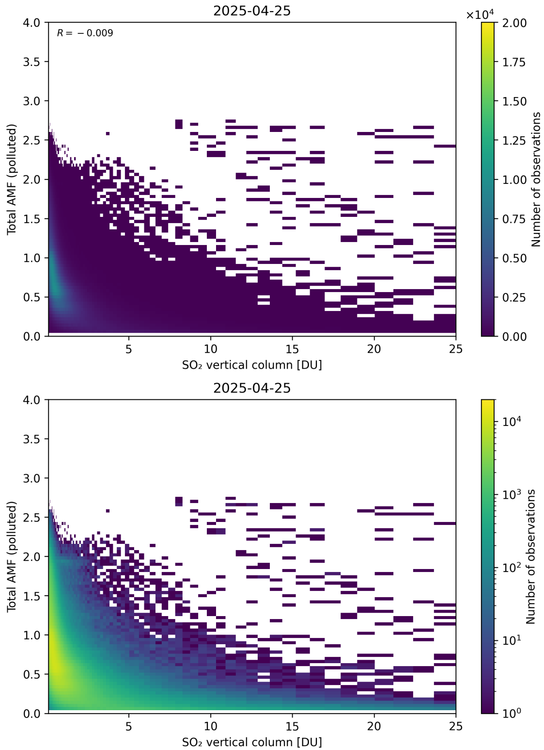
Figure 359: Scatter density plot of “SO 2 vertical column” against “Total AMF (polluted)” for 2025-04-24 to 2025-04-26.
