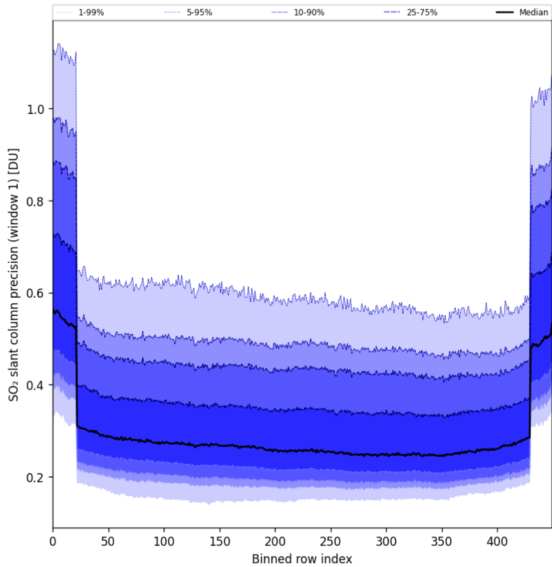
Figure 90: Along track statistics of “SO 2 slant column precision (window 1)” for 2025-04-24 to 2025-04-26
