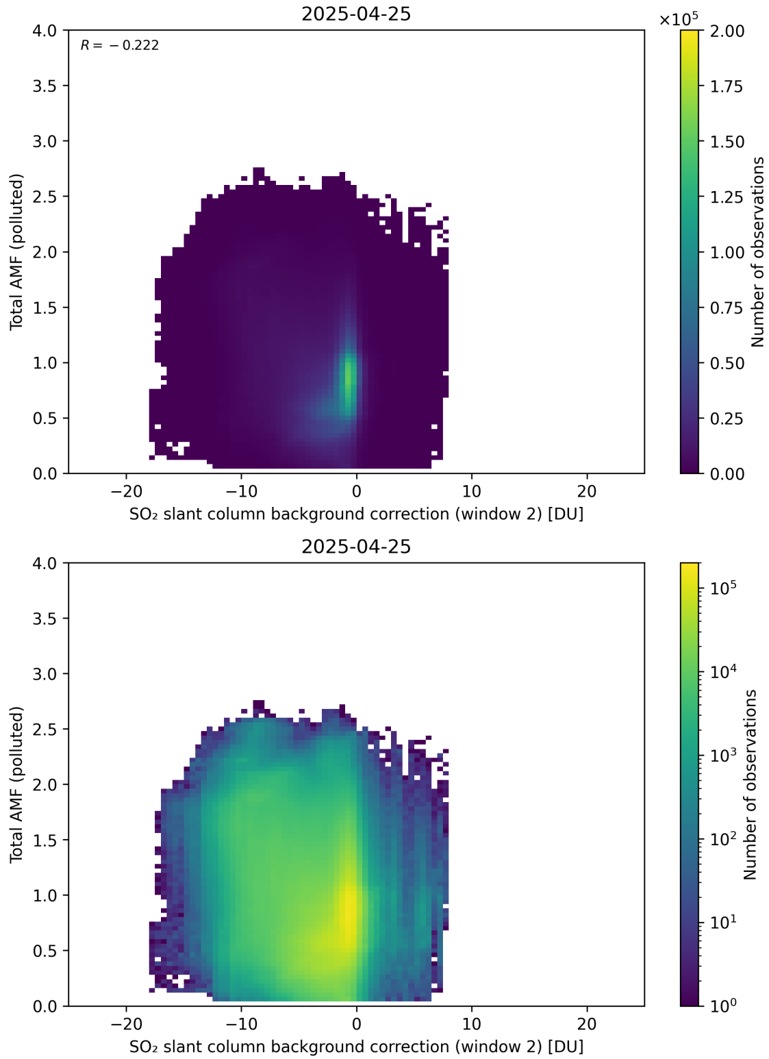
Figure 130: Scatter density plot of “SO 2 slant column background correction (window 2)” against “Total AMF (polluted)” for 2025-04-24 to 2025-04-26.
