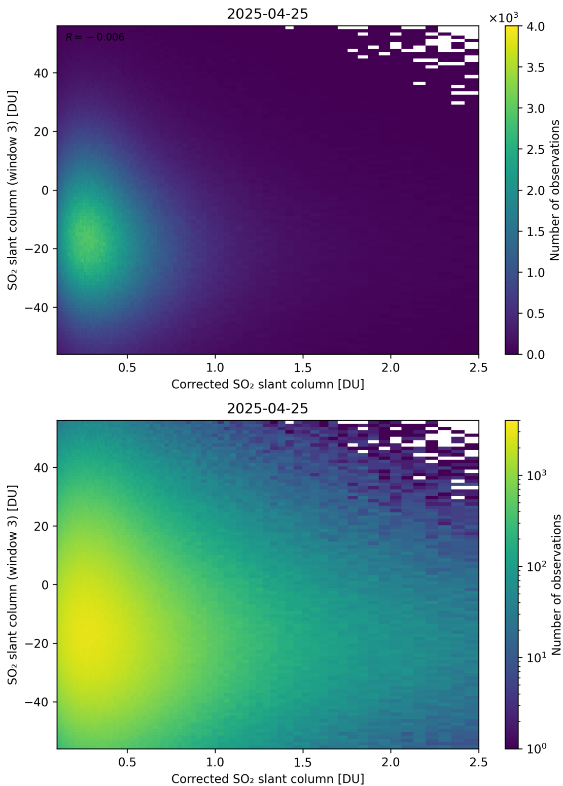
Figure 240: Scatter density plot of “Corrected SO 2 slant column” against “SO 2 slant column (window 3)” for 2025-04-24 to 2025-04-26.
