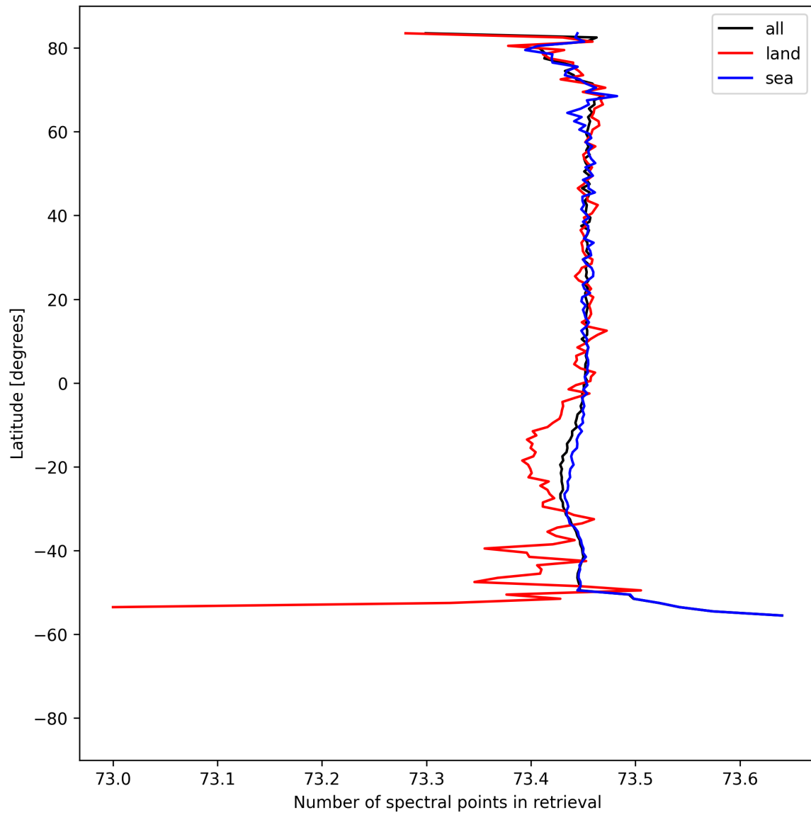
Figure 56: Zonal average of “Number of spectral points in retrieval” for 2025-04-24 to 2025-04-26.
