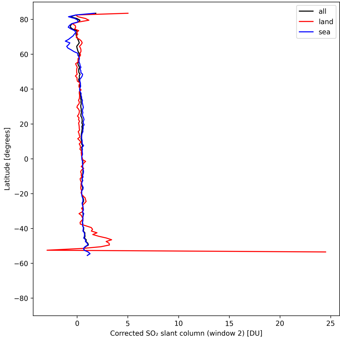
Figure 43: Zonal average of “Corrected SO 2 slant column (window 2)” for 2025-04-24 to 2025-04-26.
