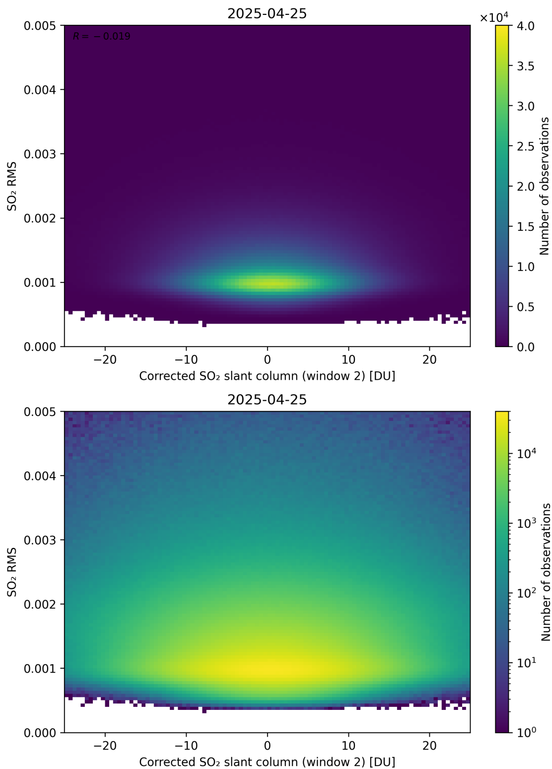
Figure 248: Scatter density plot of “Corrected SO 2 slant column (window 2)” against “SO 2 RMS” for 2025-04-24 to 2025-04-26.
