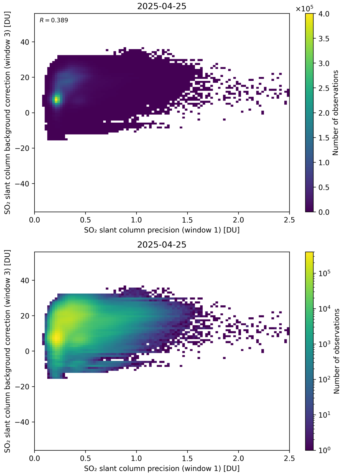
Figure 270: Scatter density plot of “SO 2 slant column precision (window 1)” against “SO 2 slant column background correction (window 3)” for 2025-04-24 to 2025-04-26.
