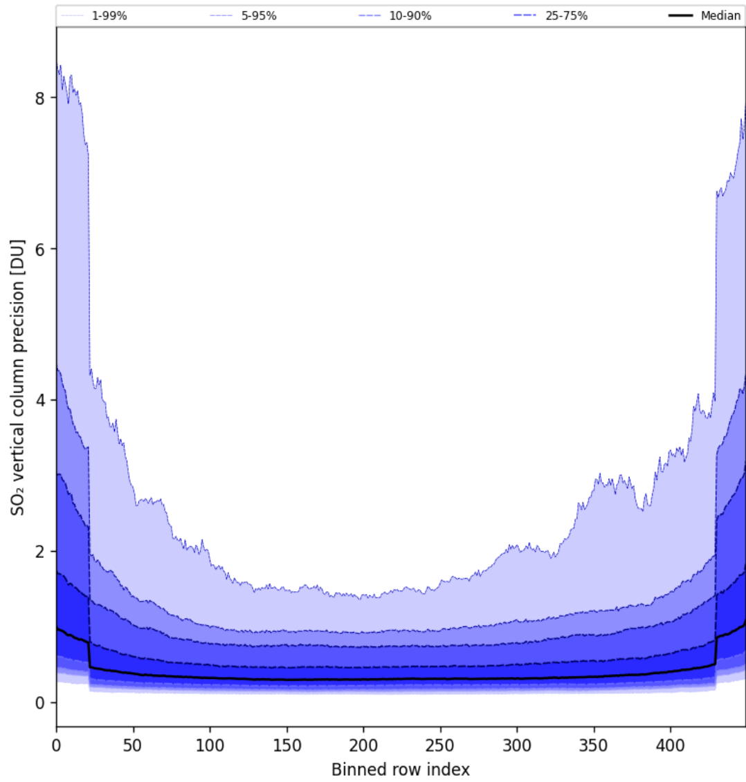
Figure 85: Along track statistics of “SO 2 vertical column precision” for 2025-04-24 to 2025-04-26
