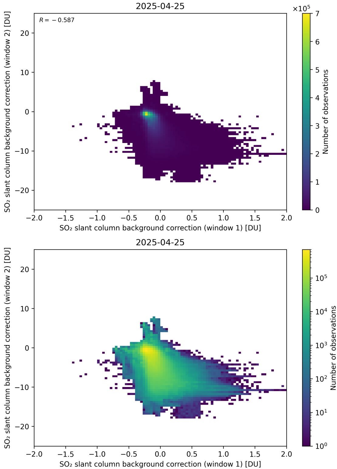
Figure 109: Scatter density plot of “SO 2 slant column background correction (window 1)” against “SO 2 slant column background correction (window 2)” for 2025-04-24 to 2025-04-26.
