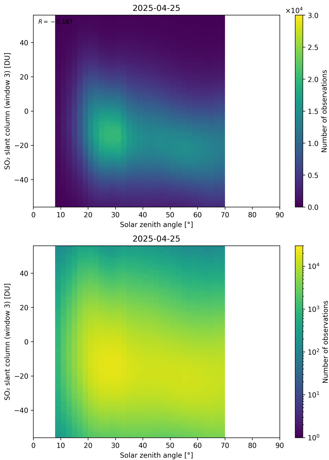
Figure 187: Scatter density plot of “Solar zenith angle” against “SO 2 slant column (window 3)” for 2025-04-24 to 2025-04-26.
