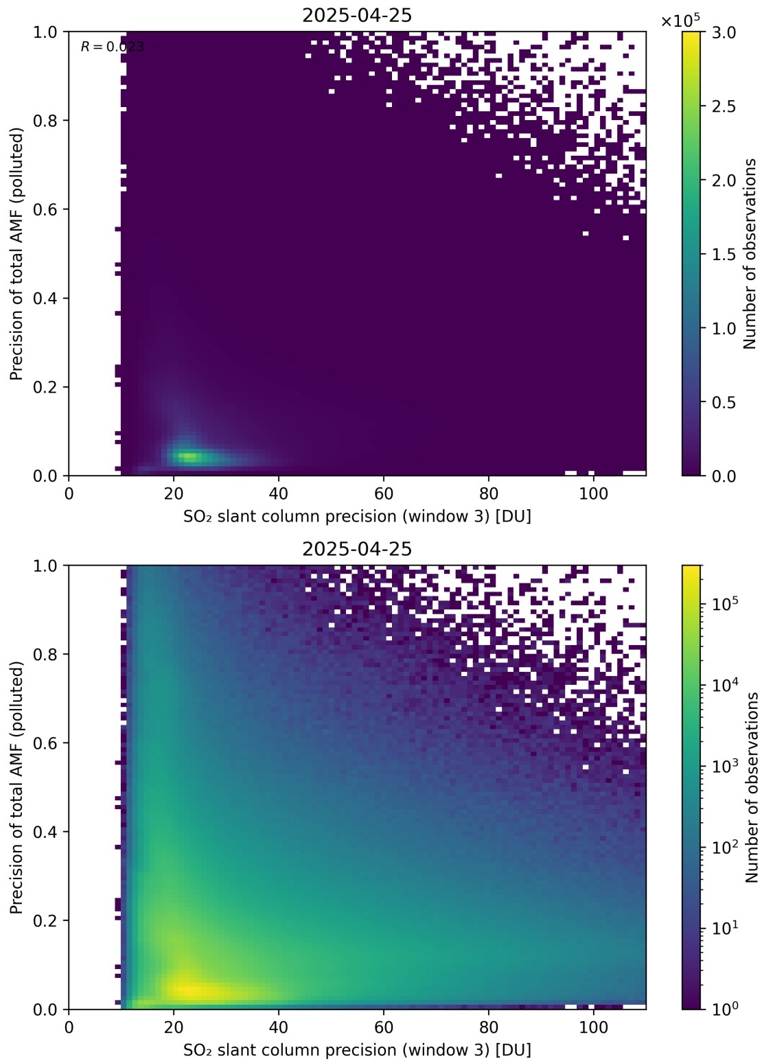
Figure 314: Scatter density plot of “SO 2 slant column precision (window 3)” against “Precision of total AMF (polluted)” for 2025-04-24 to 2025-04-26.
