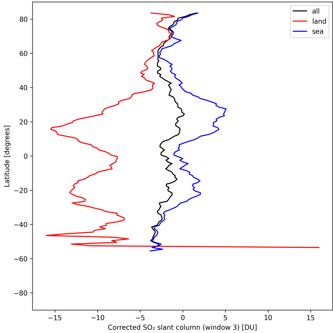
Figure 47: Zonal average of “Corrected SO 2 slant column (window 3)” for 2025-04-24 to 2025-04-26.
