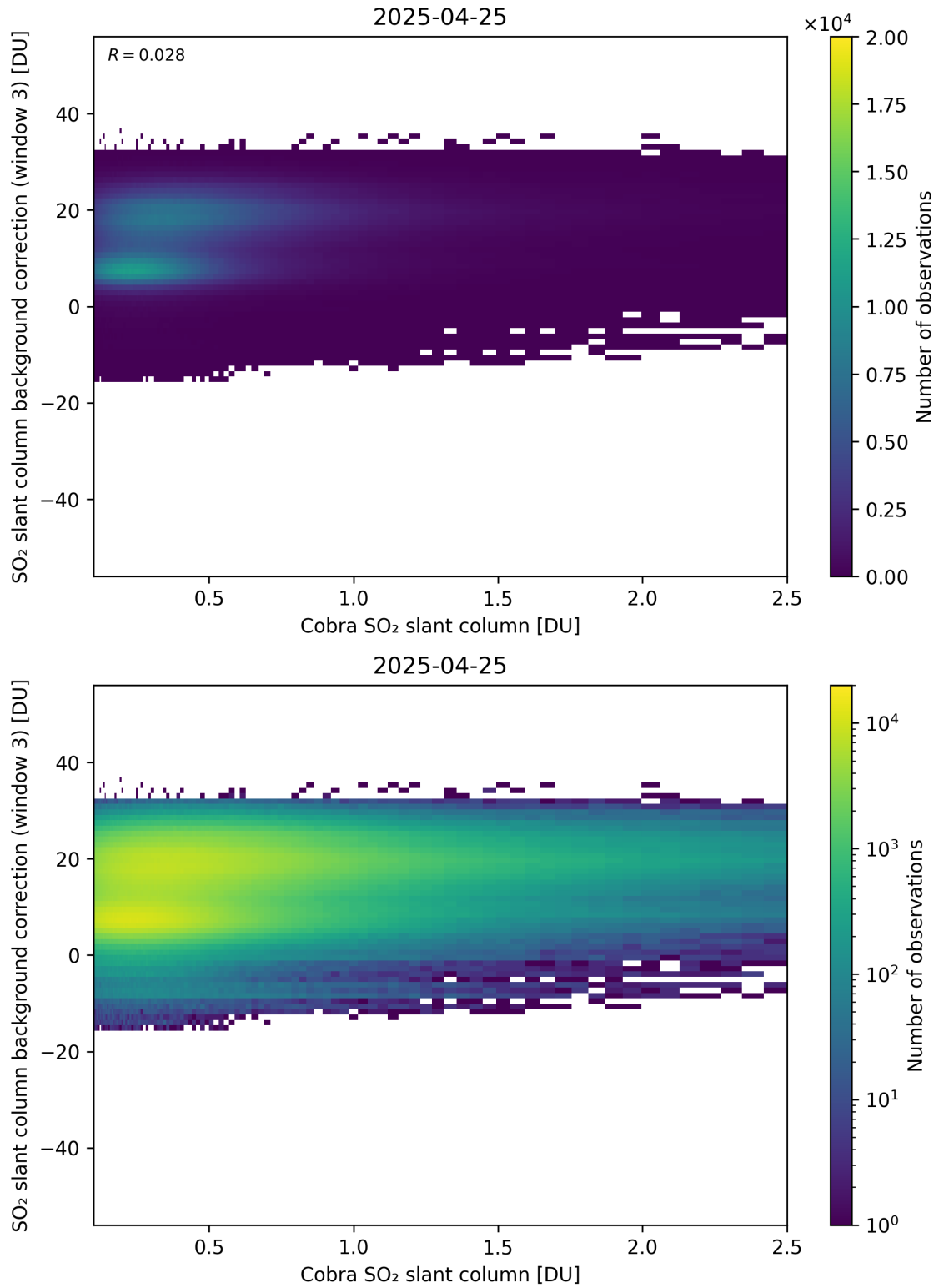
Figure 195: Scatter density plot of “Cobra SO 2 slant column” against “SO 2 slant column background correction (window 3)” for 2025-04-24 to 2025-04-26.
