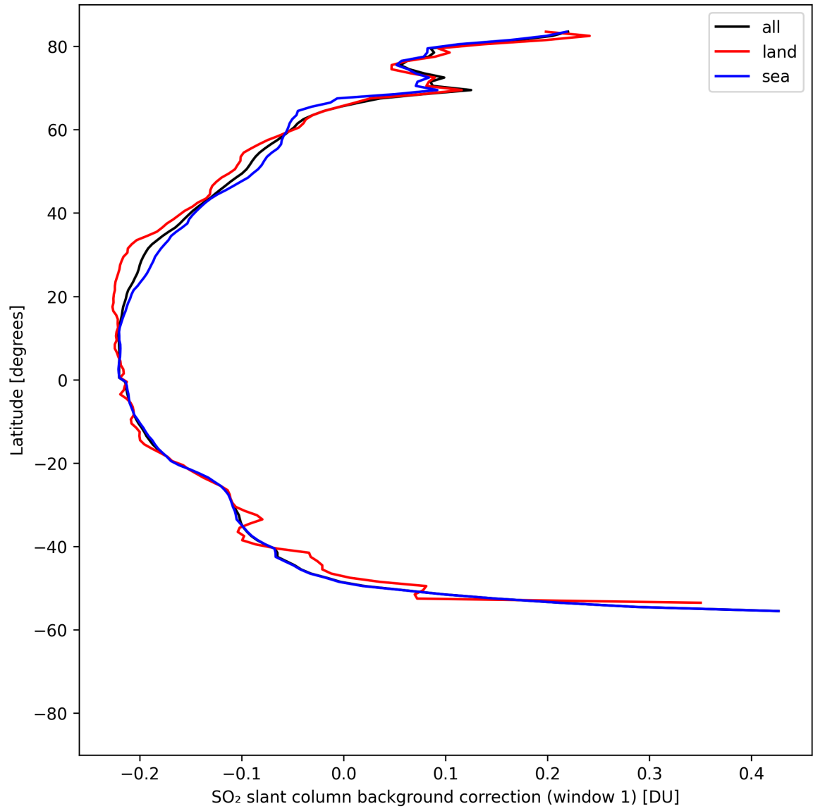
Figure 40: Zonal average of “SO 2 slant column background correction (window 1)” for 2025-04-24 to 2025-04-26.
