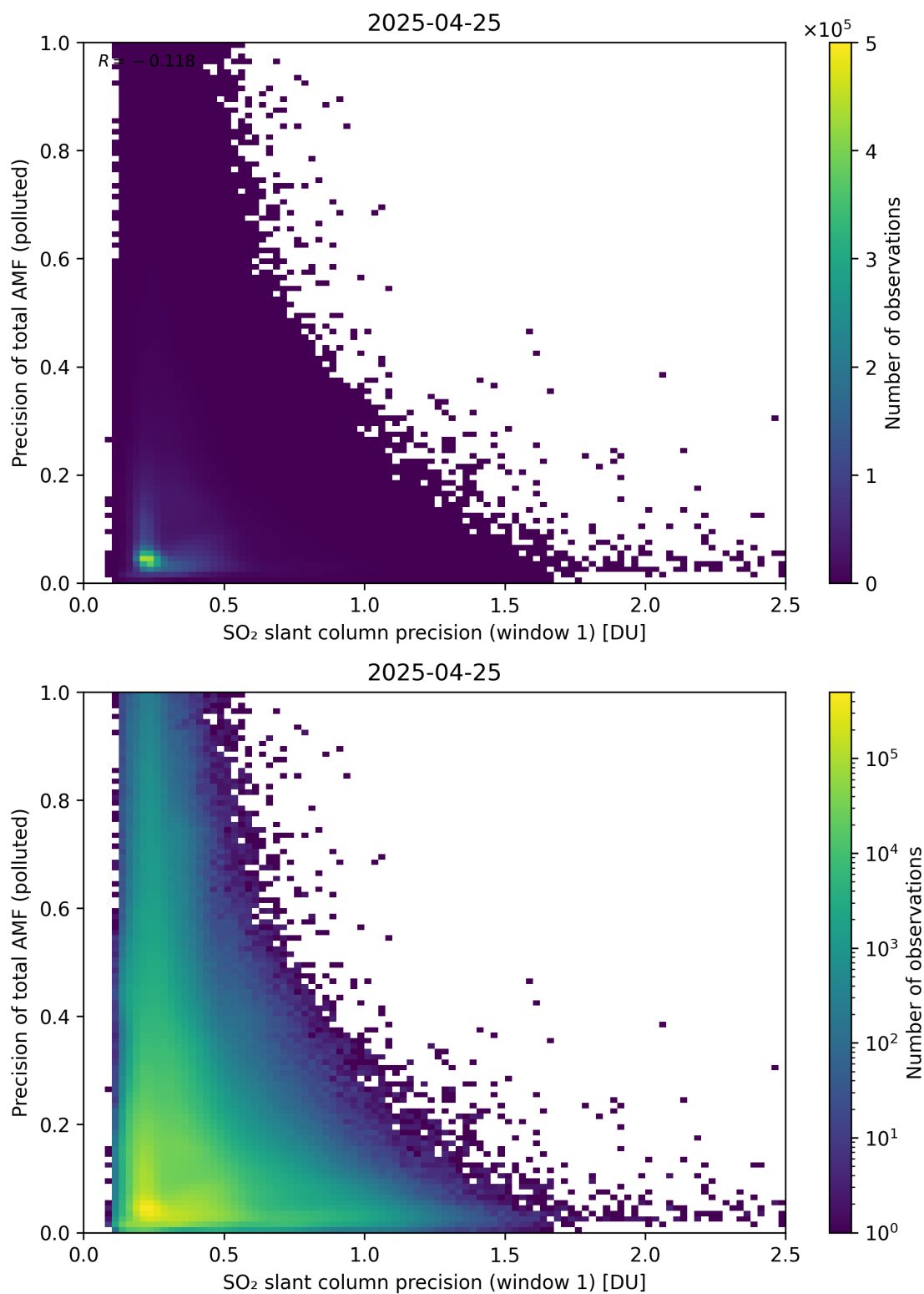
Figure 281: Scatter density plot of “SO 2 slant column precision (window 1)” against “Precision of total AMF (polluted)” for 2025-04-24 to 2025-04-26.
