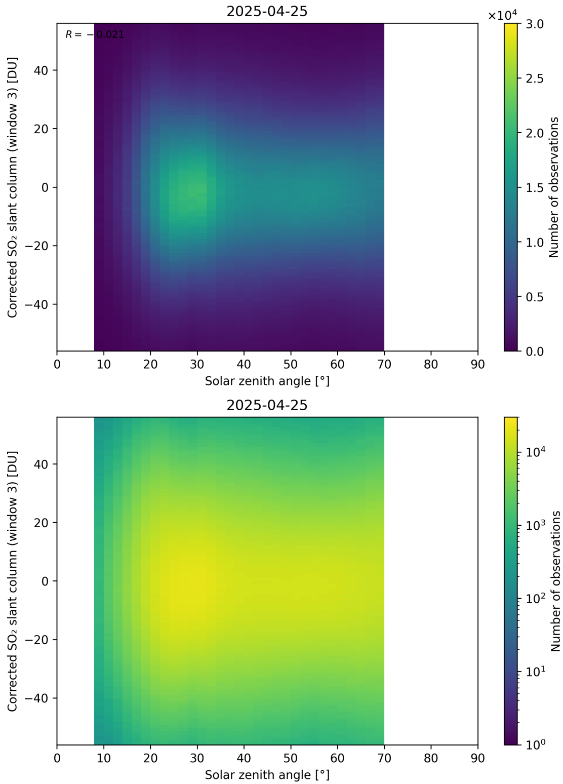
Figure 183: Scatter density plot of “Solar zenith angle” against “Corrected SO 2 slant column (window 3)” for 2025-04-24 to 2025-04-26.
