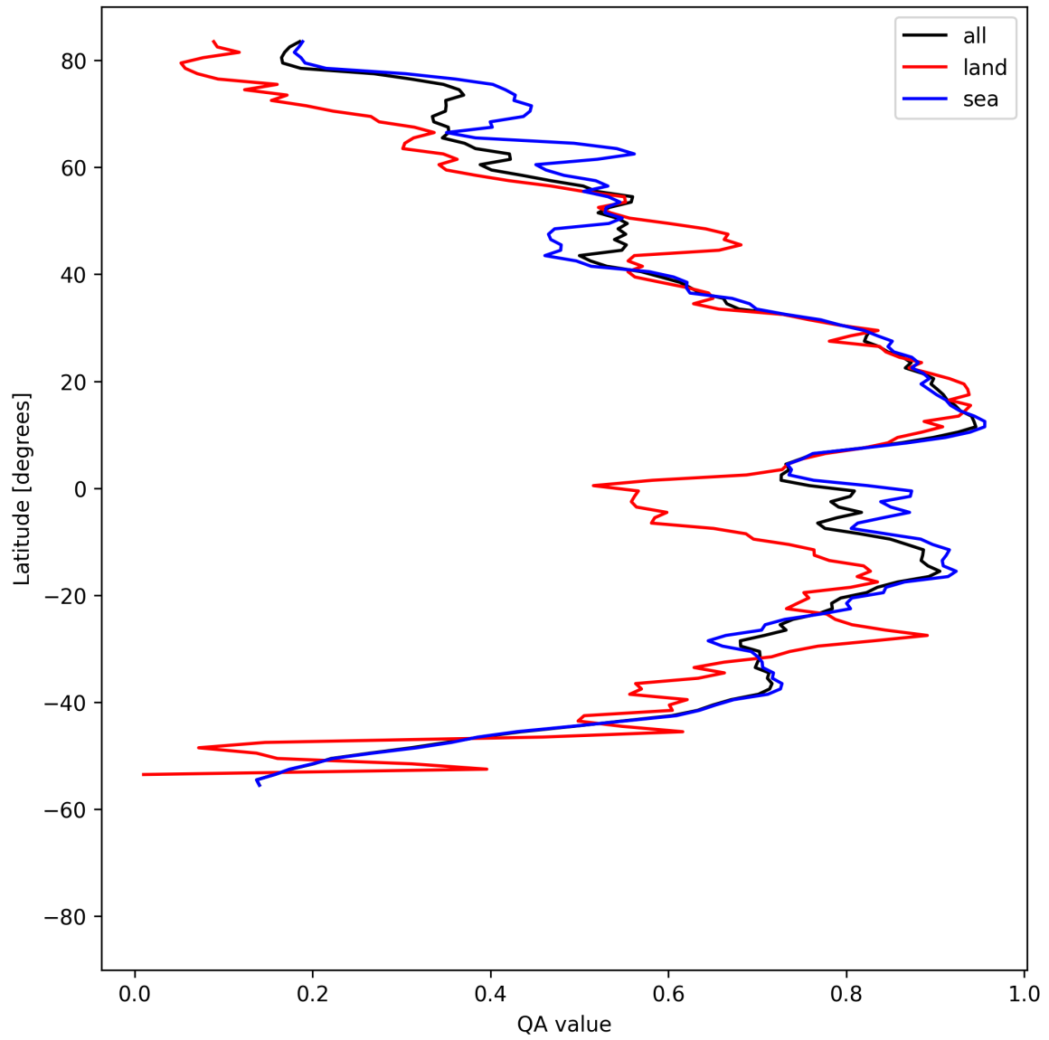
Figure 31: Zonal average of “QA value” for 2025-04-24 to 2025-04-26.
