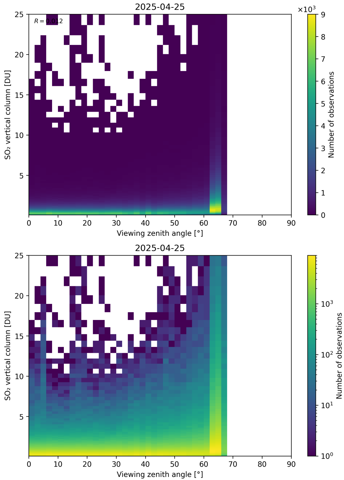
Figure 383: Scatter density plot of “Viewing zenith angle” against “SO 2 vertical column” for 2025-04-24 to 2025-04-26.
