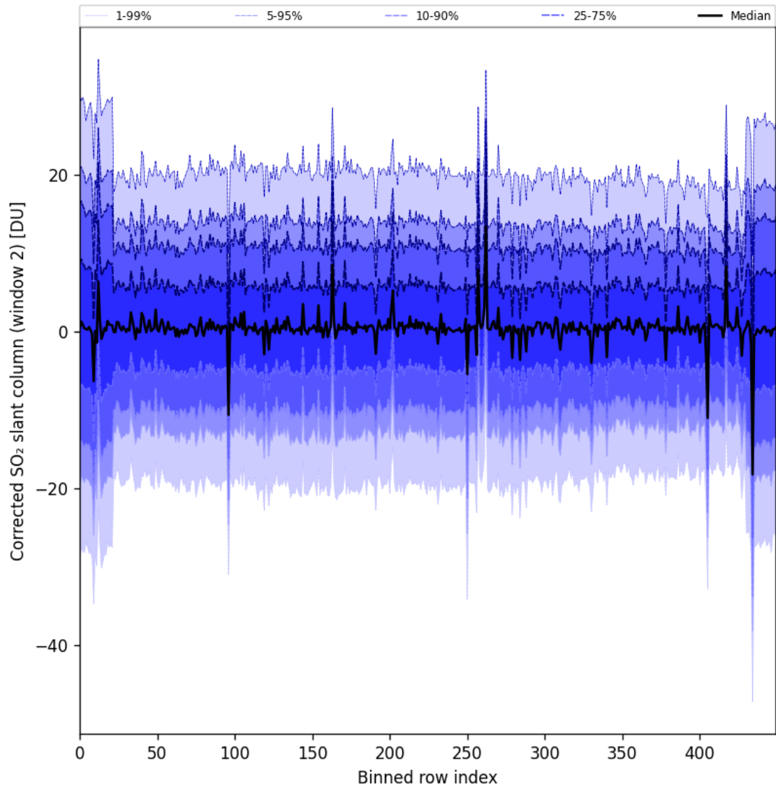
Figure 95: Along track statistics of “Corrected SO 2 slant column (window 2)” for 2025-04-24 to 2025-04-26
