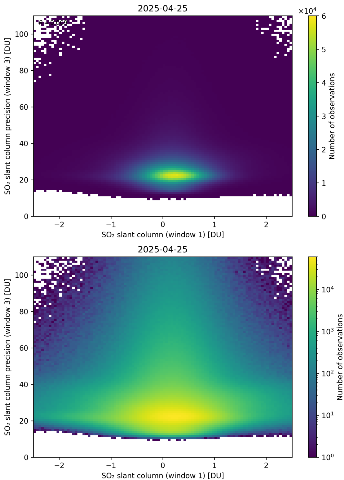
Figure 288: Scatter density plot of “SO 2 slant column (window 1)” against “SO 2 slant column precision (window 3)” for 2025-04-24 to 2025-04-26.
