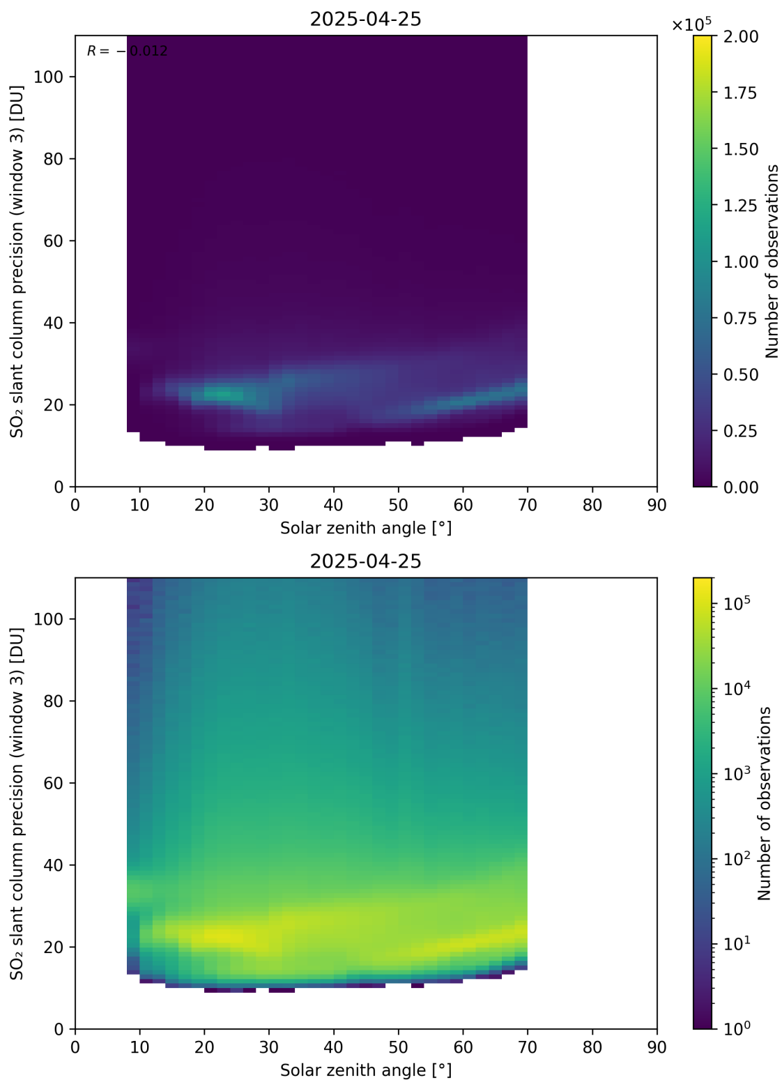
Figure 188: Scatter density plot of “Solar zenith angle” against “SO 2 slant column precision (window 3)” for 2025-04-24 to 2025-04-26.
