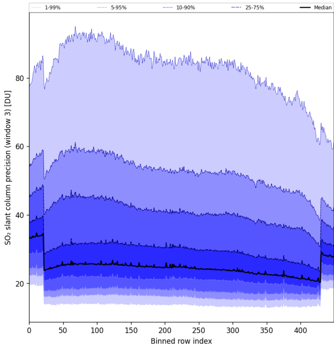
Figure 98: Along track statistics of “SO 2 slant column precision (window 3)” for 2025-04-24 to 2025-04-26
