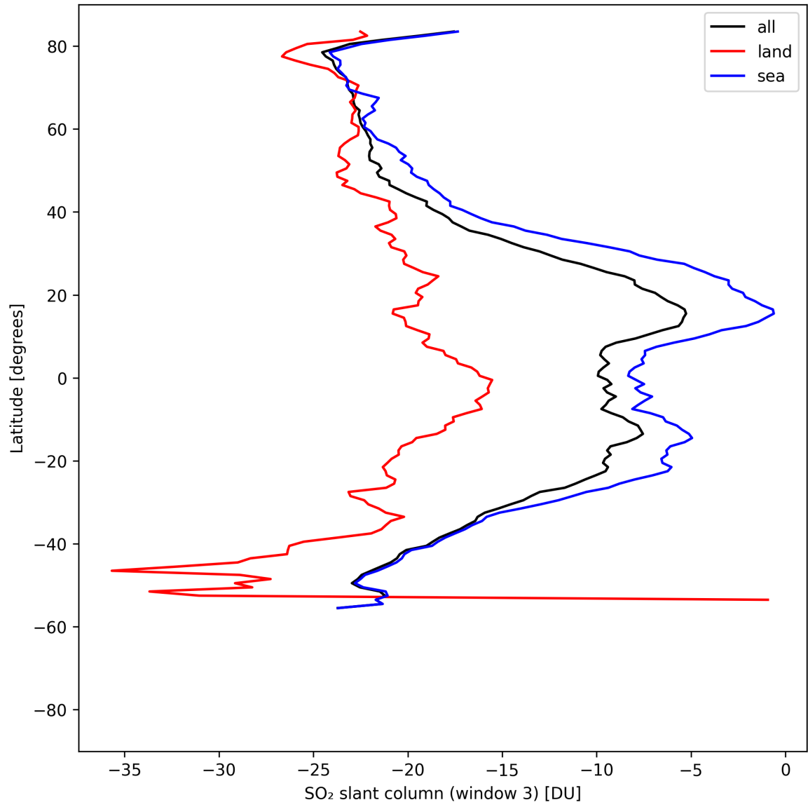
Figure 45: Zonal average of “SO 2 slant column (window 3)” for 2025-04-24 to 2025-04-26.
