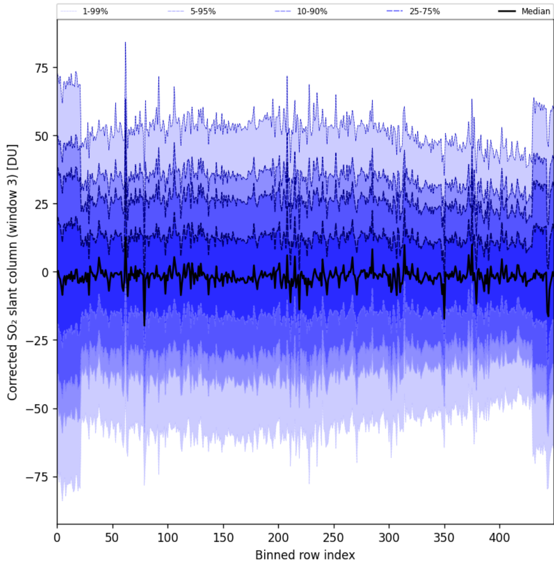
Figure 99: Along track statistics of “Corrected SO 2 slant column (window 3)” for 2025-04-24 to 2025-04-26
