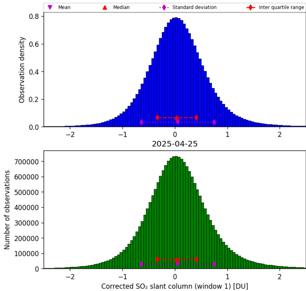
Figure 65: Histogram of “Corrected SO 2 slant column (window 1)” for 2025-04-24 to 2025-04-26
