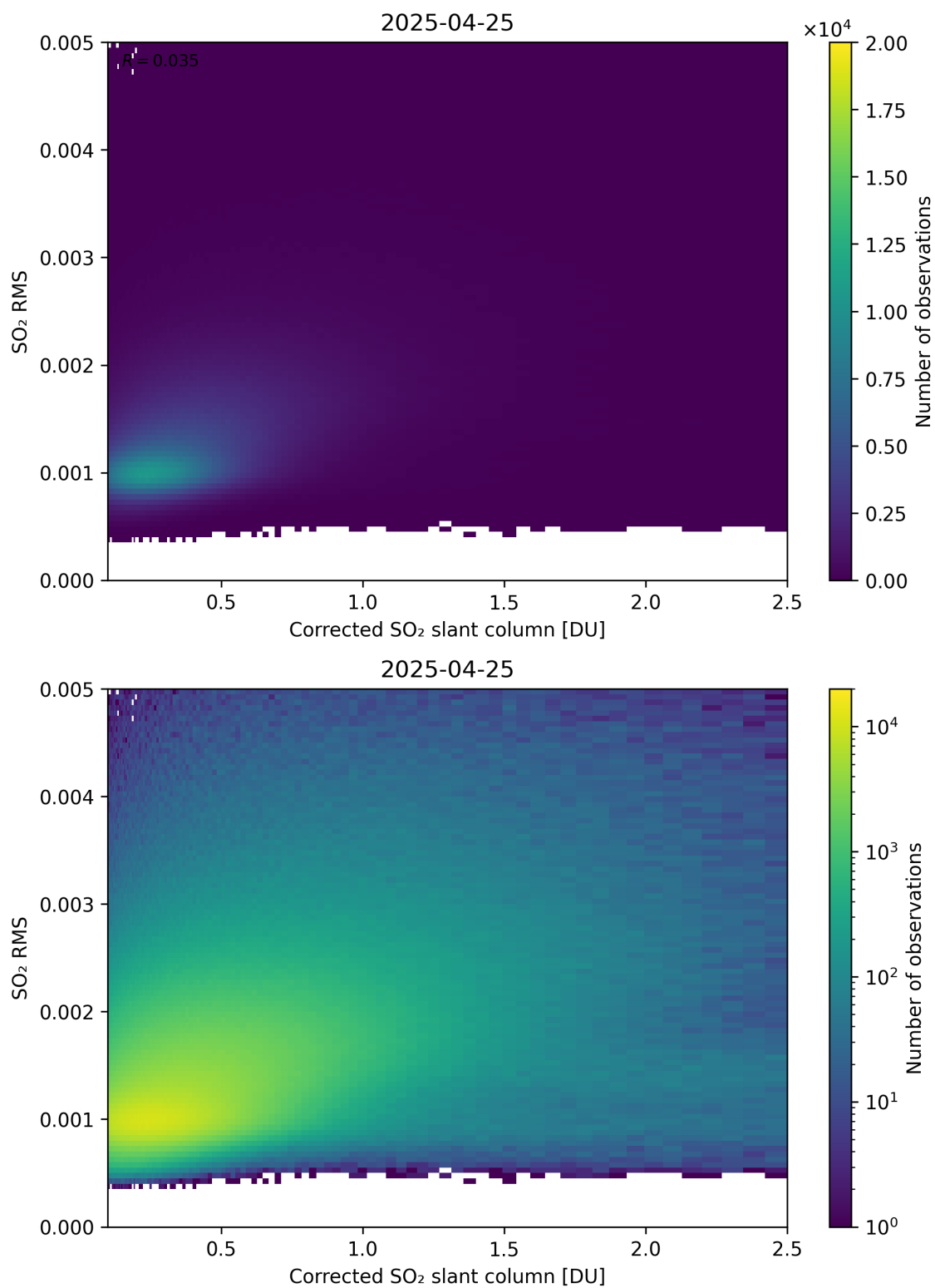
Figure 231: Scatter density plot of “Corrected SO 2 slant column” against “SO 2 RMS” for 2025-04-24 to 2025-04-26.
