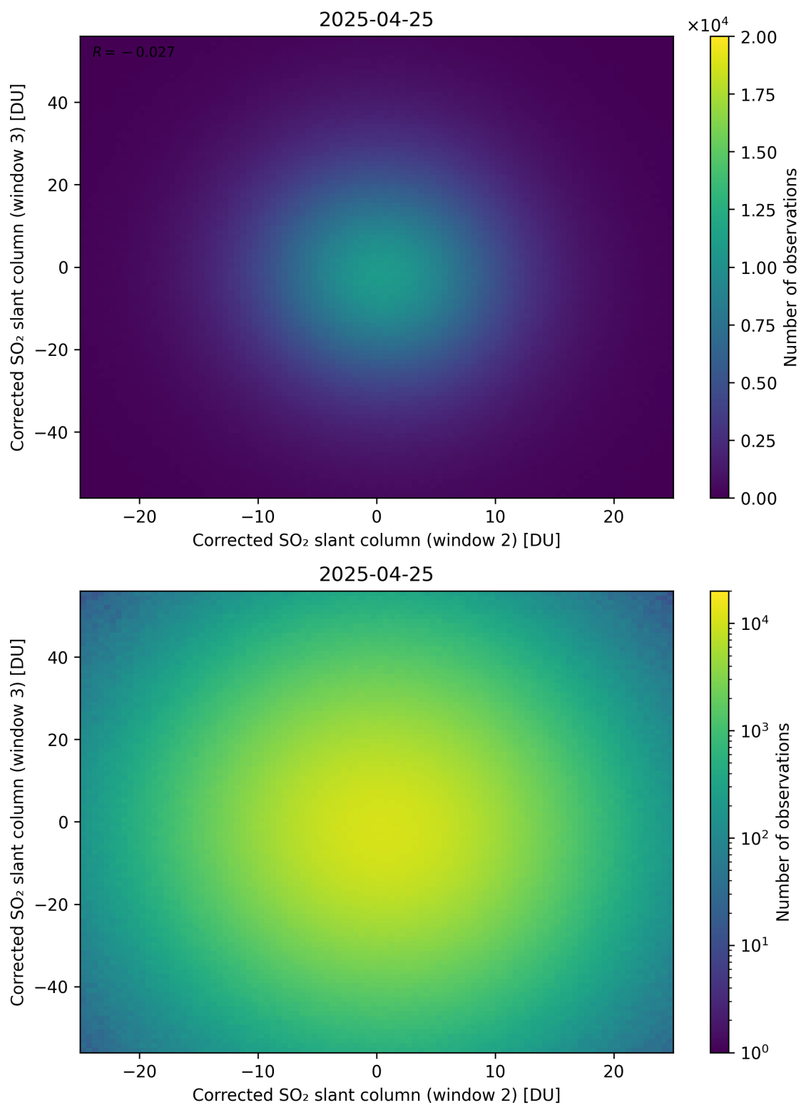
Figure 250: Scatter density plot of “Corrected SO 2 slant column (window 2)” against “Corrected SO 2 slant column (window 3)” for 2025-04-24 to 2025-04-26.
