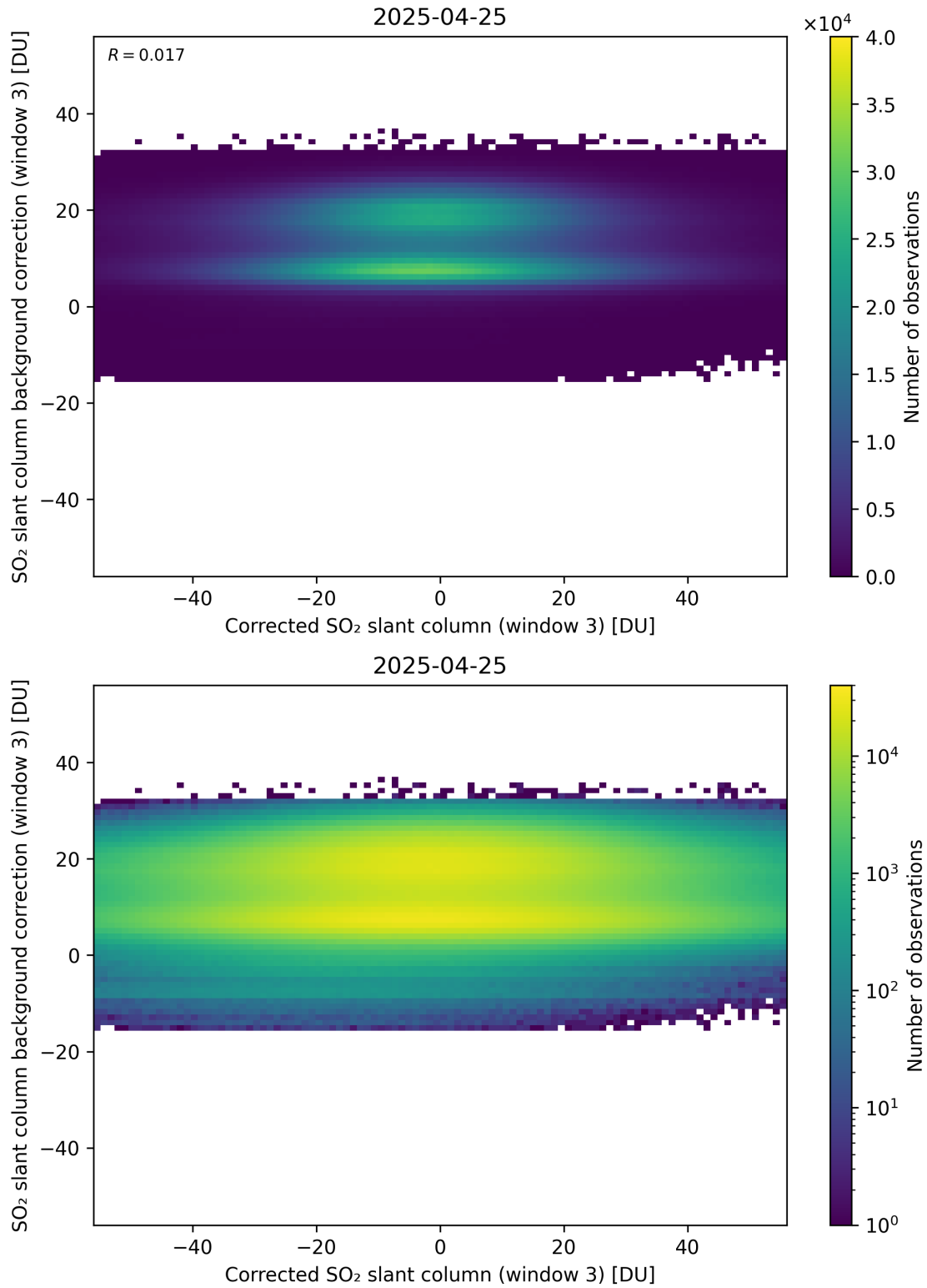
Figure 255: Scatter density plot of “Corrected SO 2 slant column (window 3)” against “SO 2 slant column background correction (window 3)” for 2025-04-24 to 2025-04-26.
