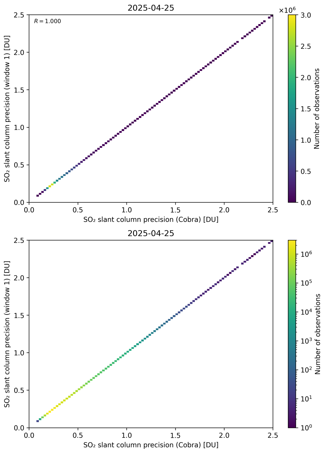
Figure 209: Scatter density plot of “SO 2 slant column precision (Cobra)” against “SO 2 slant column precision (window 1)” for 2025-04-24 to 2025-04-26.
