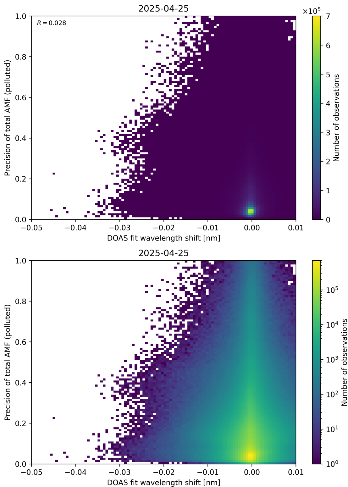
Figure 142: Scatter density plot of “DOAS fit wavelength shift” against “Precision of total AMF (polluted)” for 2025-04-24 to 2025-04-26.
