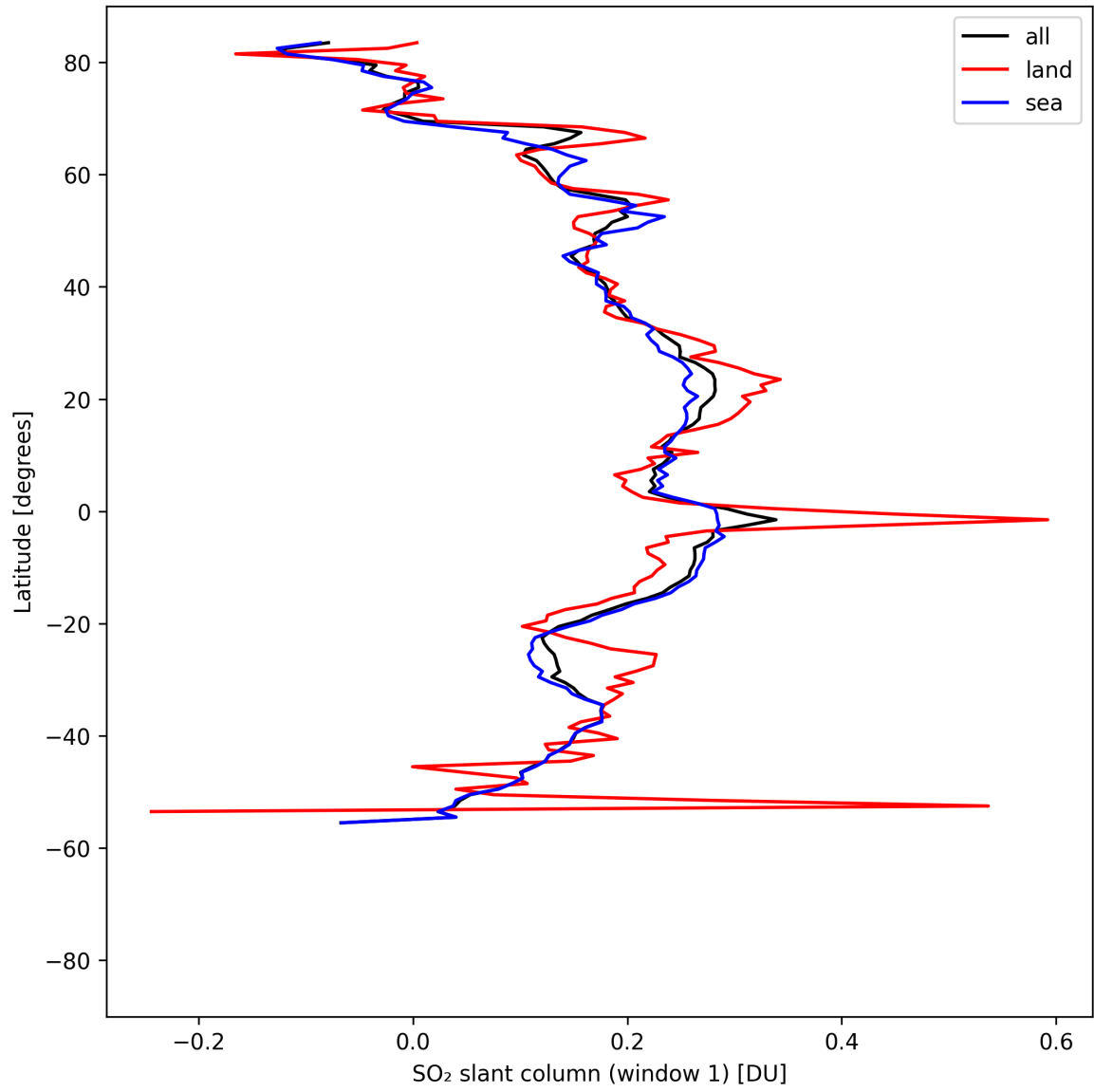
Figure 37: Zonal average of “SO 2 slant column (window 1)” for 2025-04-24 to 2025-04-26.
