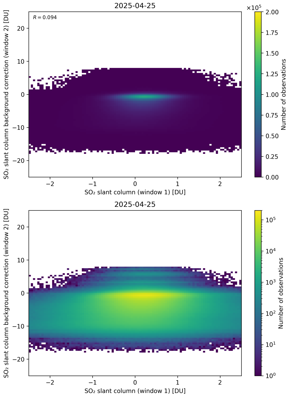
Figure 263: Scatter density plot of “SO 2 slant column (window 1)” against “SO 2 slant column background correction (window 2)” for 2025-04-24 to 2025-04-26.
