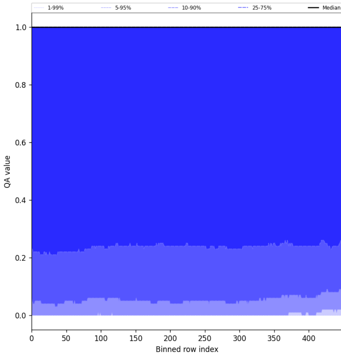
Figure 83: Along track statistics of “QA value” for 2025-04-24 to 2025-04-26
