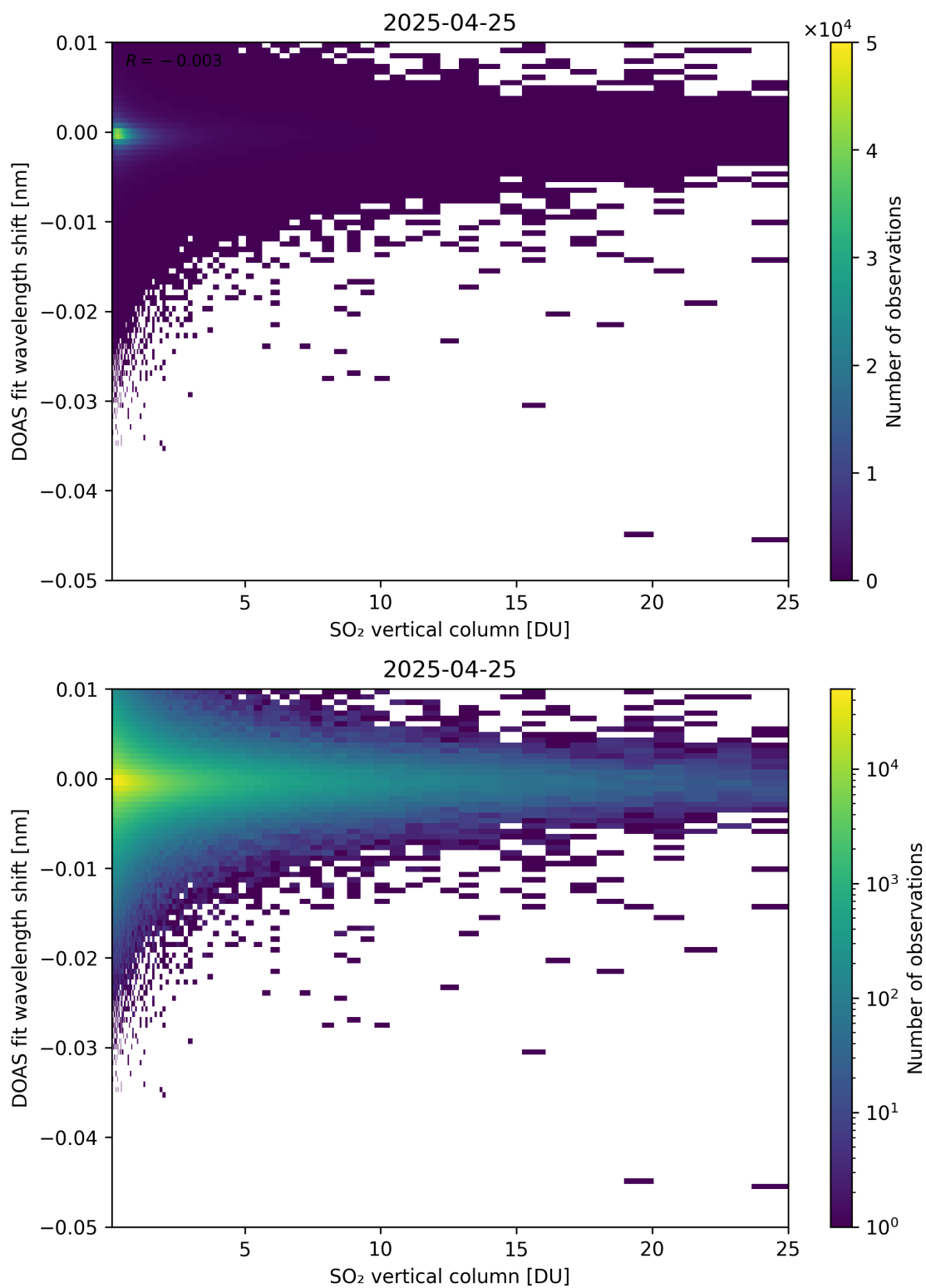
Figure 326: Scatter density plot of “SO 2 vertical column” against “DOAS fit wavelength shift” for 2025-04-24 to 2025-04-26.
