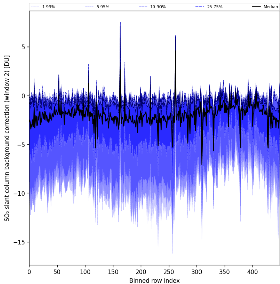
Figure 96: Along track statistics of “SO 2 slant column background correction (window 2)” for 2025-04-24 to 2025-04-26
