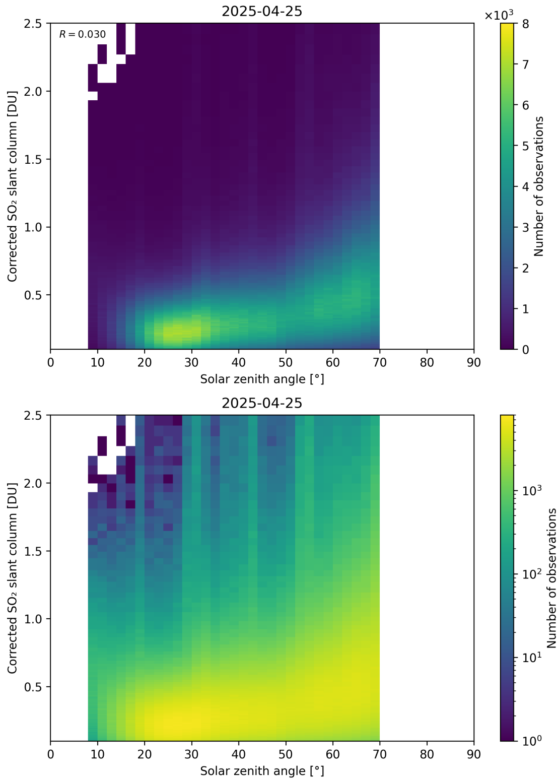
Figure 181: Scatter density plot of “Solar zenith angle” against “Corrected SO 2 slant column” for 2025-04-24 to 2025-04-26.
