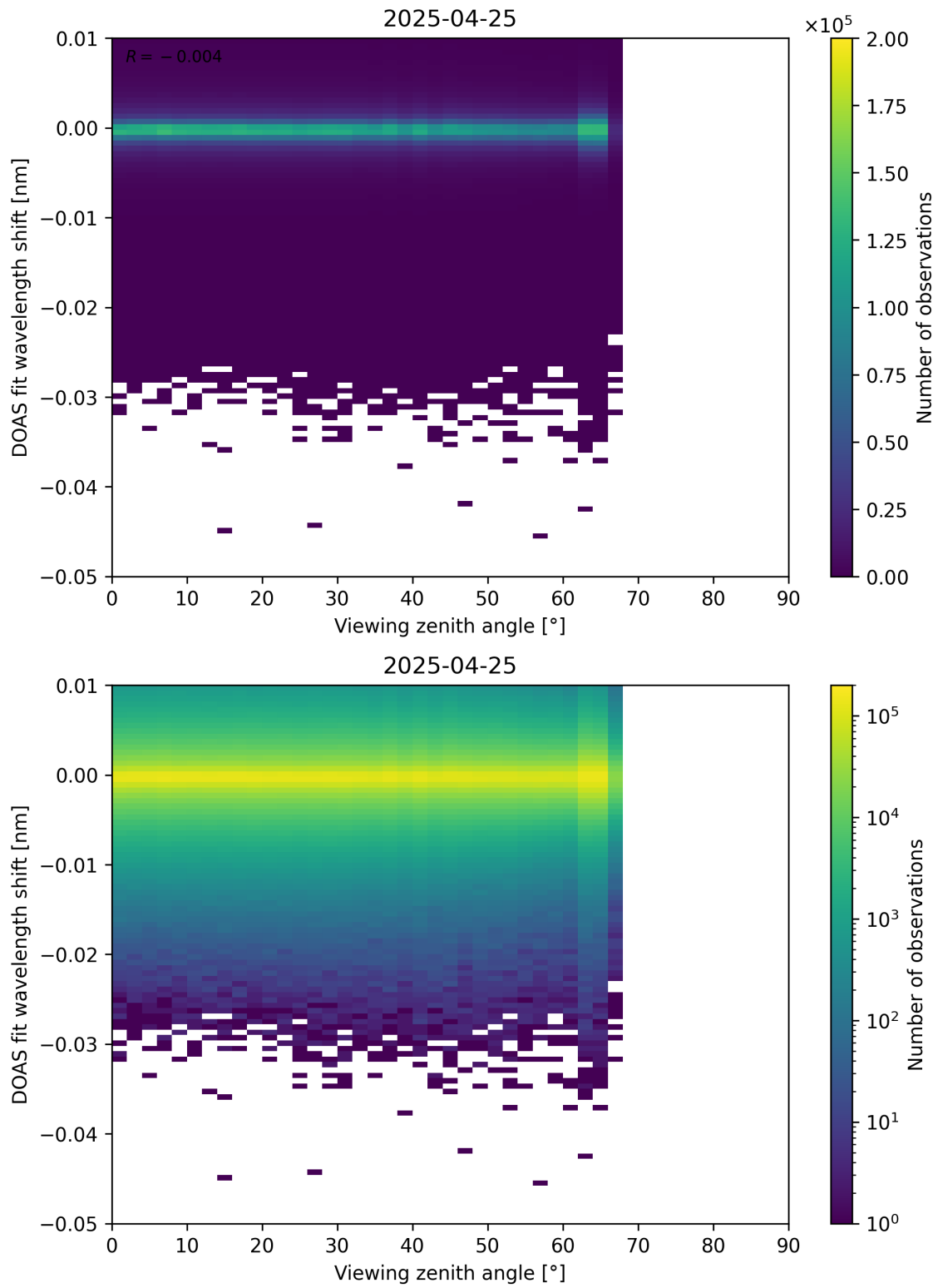
Figure 365: Scatter density plot of “Viewing zenith angle” against “DOAS fit wavelength shift” for 2025-04-24 to 2025-04-26.
