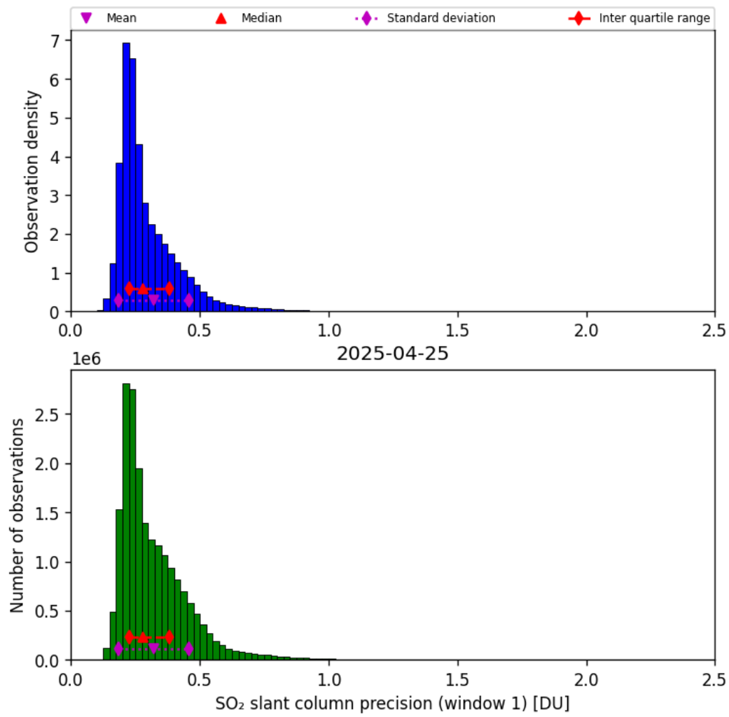
Figure 64: Histogram of “SO 2 slant column precision (window 1)” for 2025-04-24 to 2025-04-26
