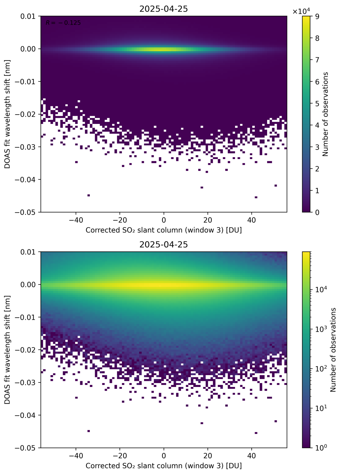
Figure 256: Scatter density plot of “Corrected SO 2 slant column (window 3)” against “DOAS fit wavelength shift” for 2025-04-24 to 2025-04-26.
