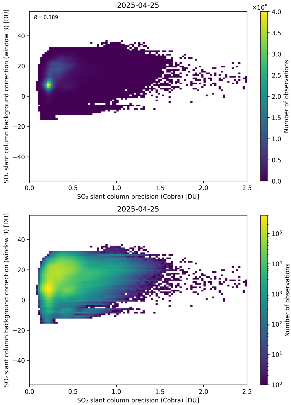
Figure 201: Scatter density plot of “SO 2 slant column precision (Cobra)” against “SO 2 slant column background correction (window 3)” for 2025-04-24 to 2025-04-26.
