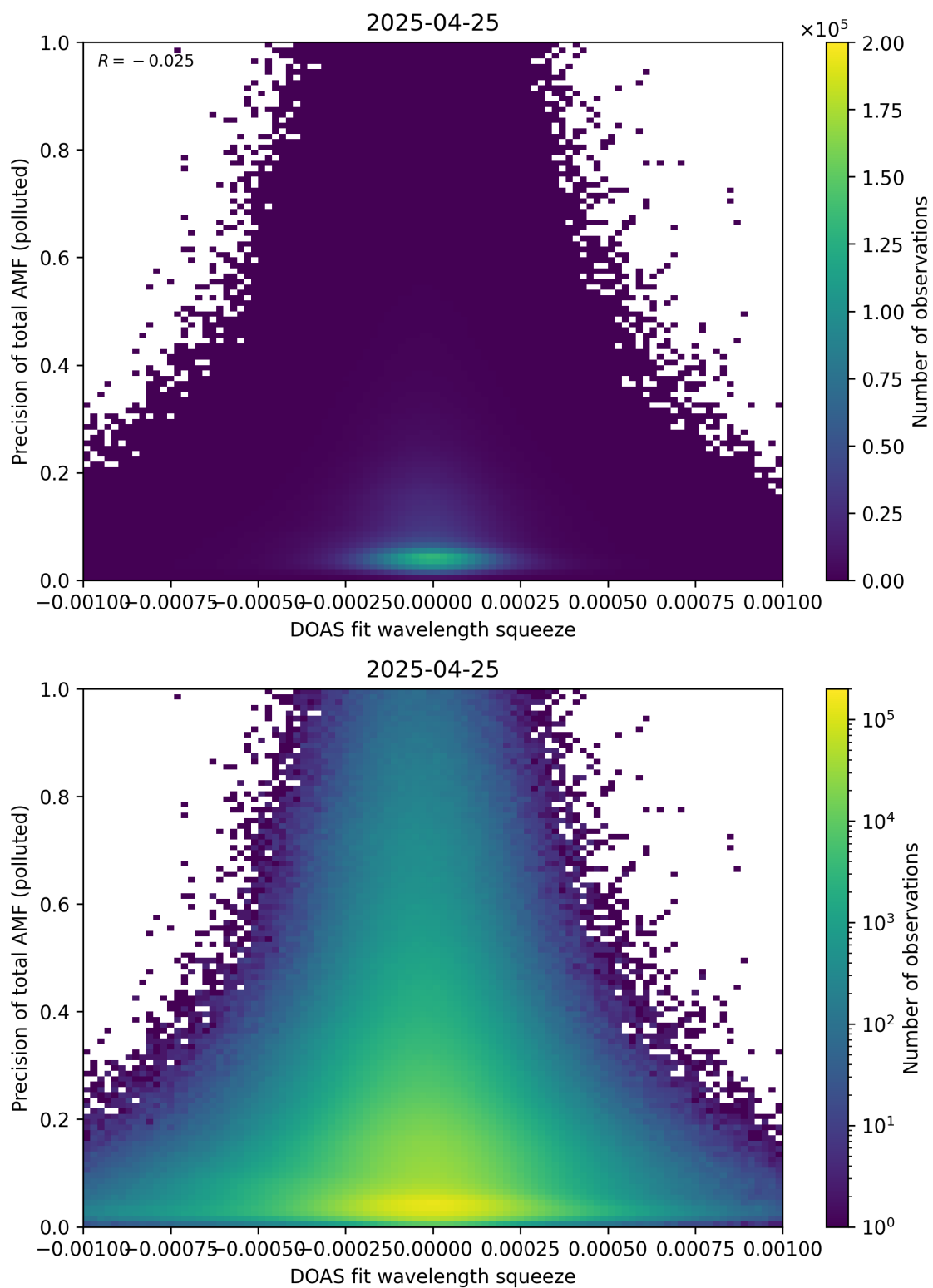
Figure 146: Scatter density plot of “DOAS fit wavelength squeeze” against “Precision of total AMF (polluted)” for 2025-04-24 to 2025-04-26.
