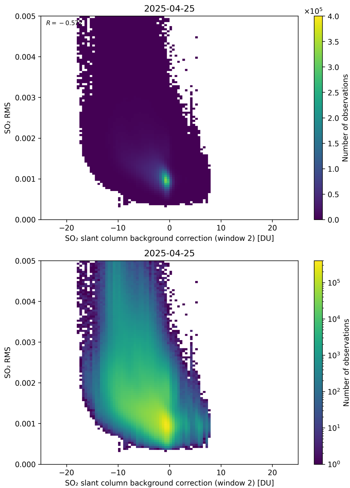
Figure 125: Scatter density plot of “SO 2 slant column background correction (window 2)” against “SO 2 RMS” for 2025-04-24 to 2025-04-26.
