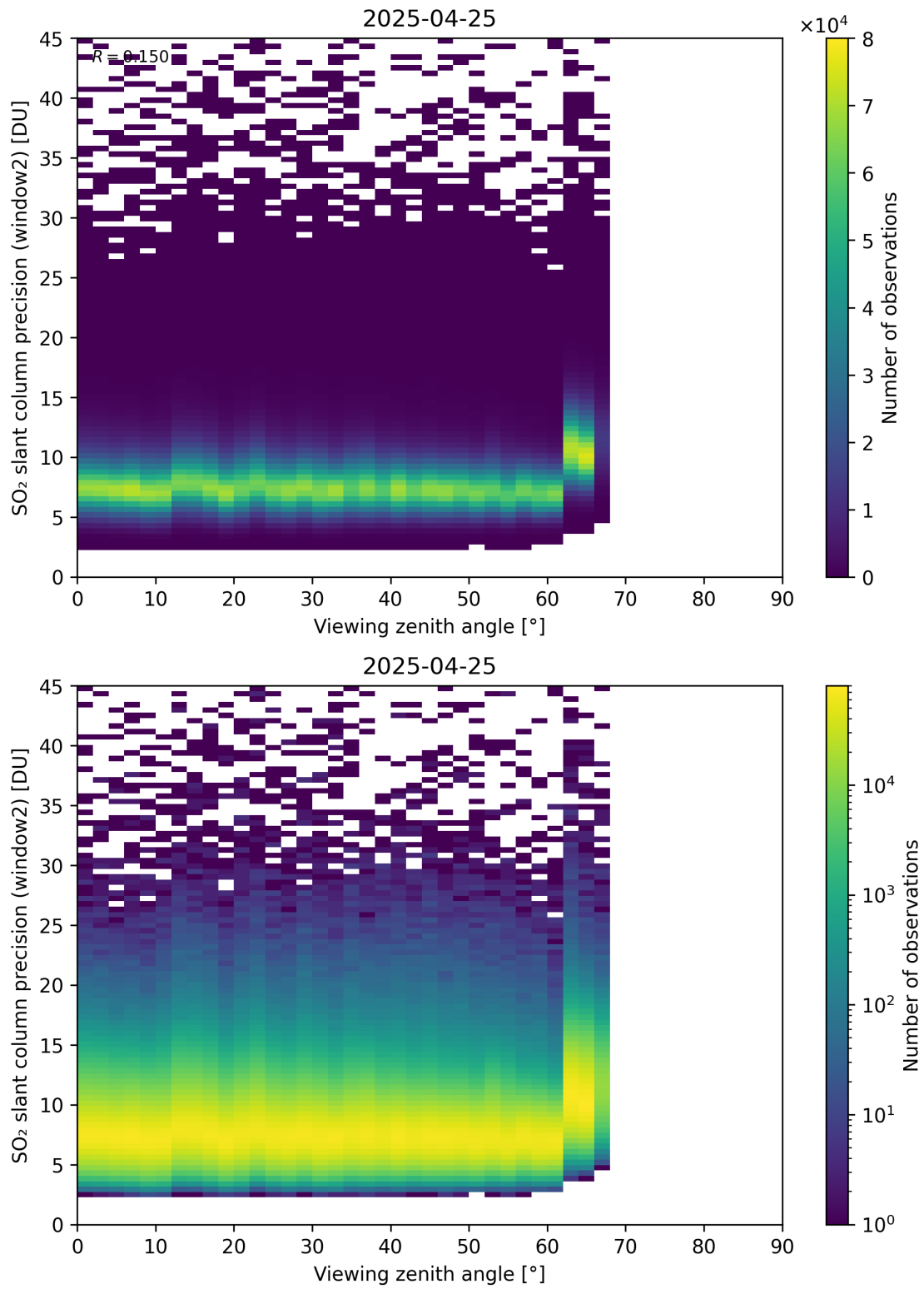
Figure 378: Scatter density plot of “Viewing zenith angle” against “SO 2 slant column precision (window2)” for 2025-04-24 to 2025-04-26.
