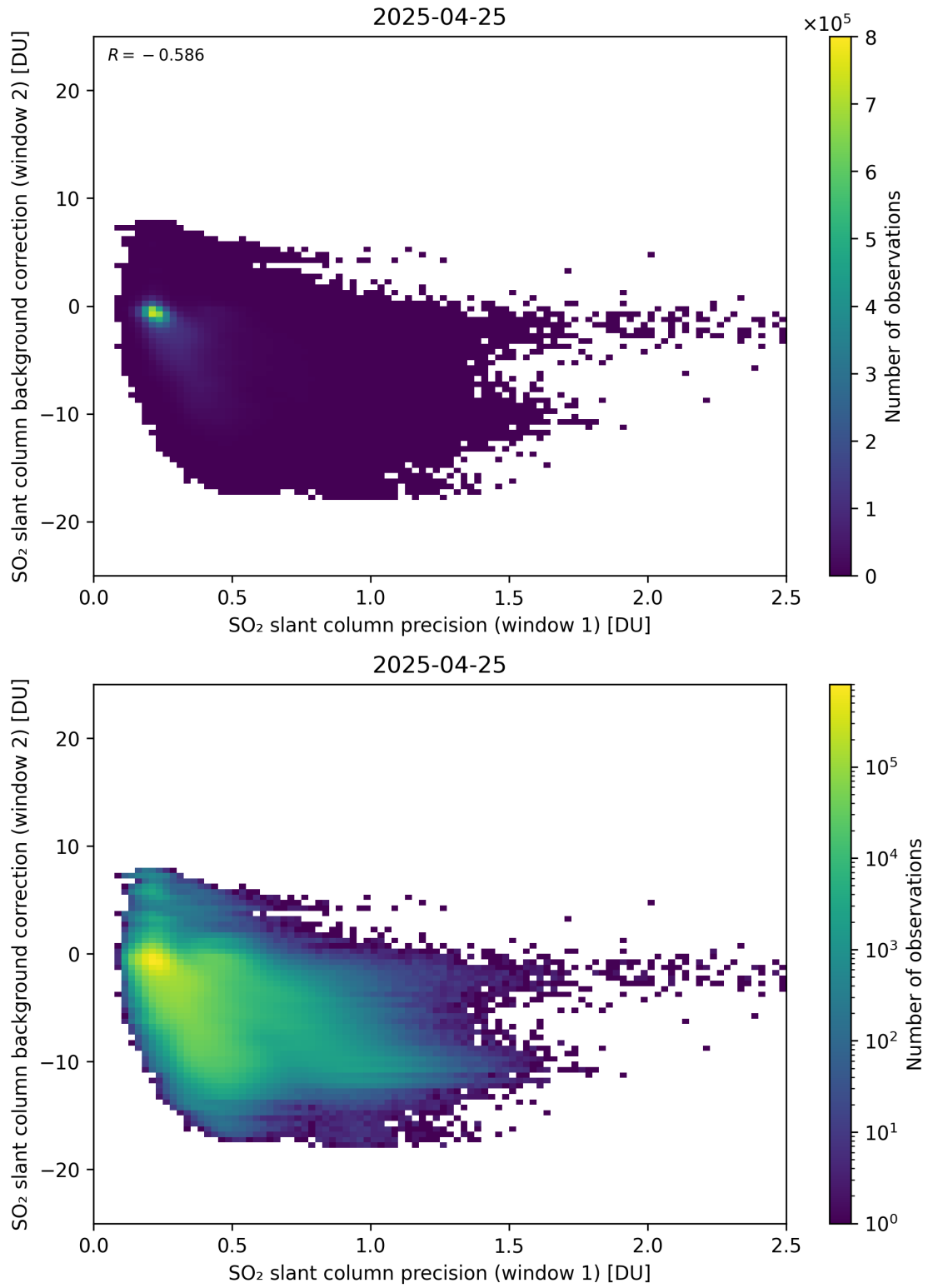
Figure 269: Scatter density plot of “SO 2 slant column precision (window 1)” against “SO 2 slant column background correction (window 2)” for 2025-04-24 to 2025-04-26.
