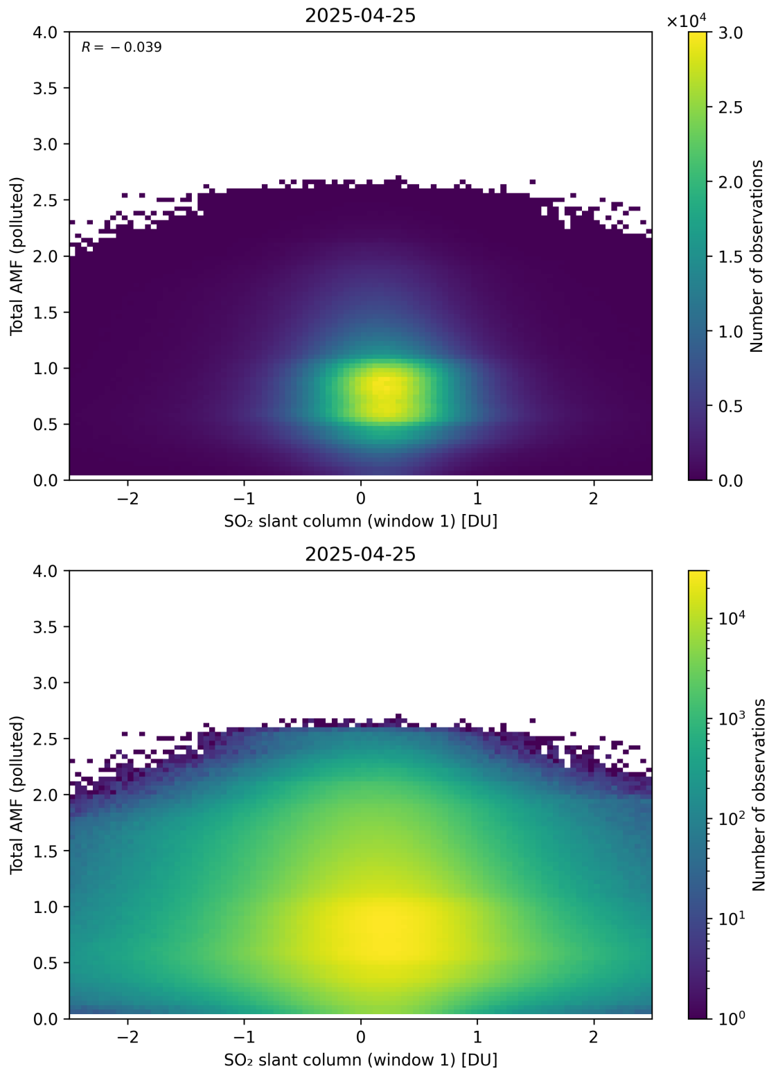
Figure 289: Scatter density plot of “SO 2 slant column (window 1)” against “Total AMF (polluted)” for 2025-04-24 to 2025-04-26.
