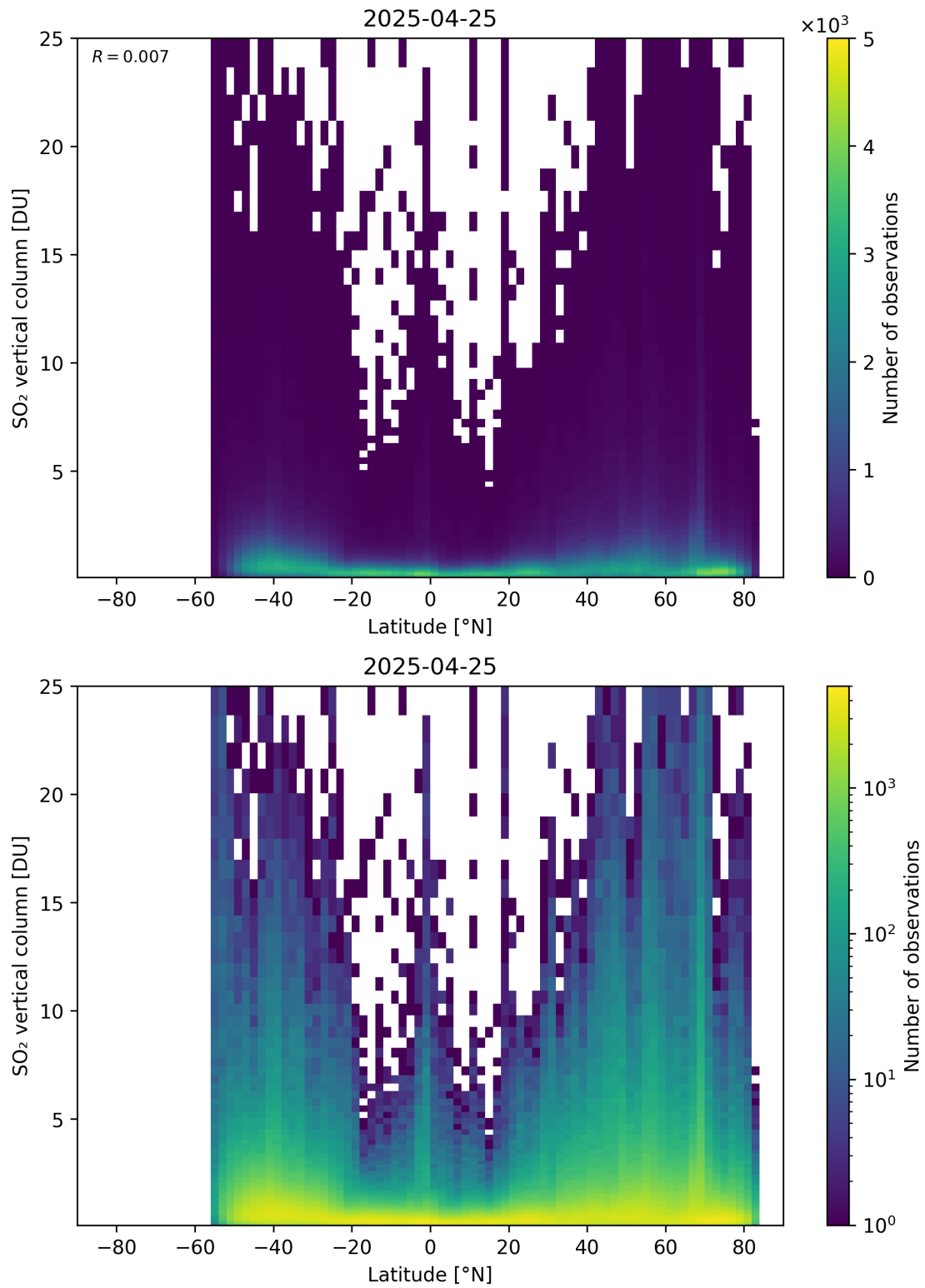
Figure 169: Scatter density plot of “Latitude” against “SO 2 vertical column” for 2025-04-24 to 2025-04-26.
