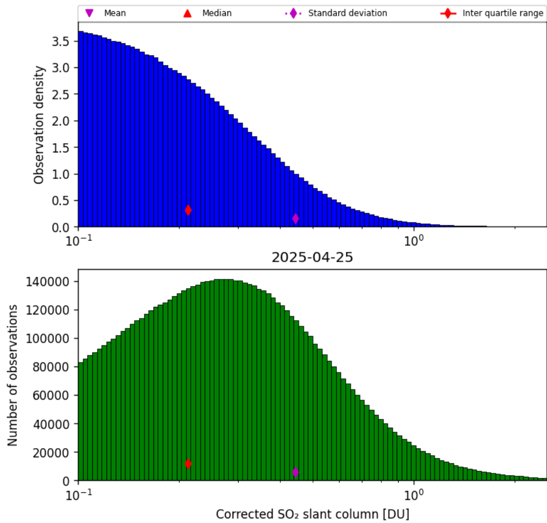
Figure 60: Histogram of “Corrected SO 2 slant column” for 2025-04-24 to 2025-04-26
