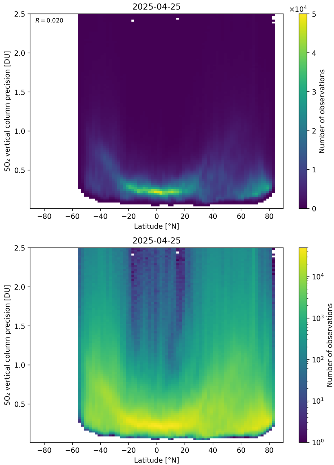
Figure 170: Scatter density plot of “Latitude” against “SO 2 vertical column precision” for 2025-04-24 to 2025-04-26.
