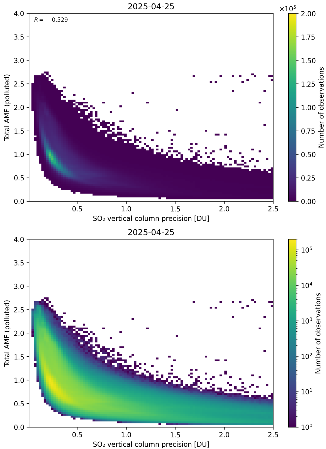
Figure 346: Scatter density plot of “SO 2 vertical column precision” against “Total AMF (polluted)” for 2025-04-24 to 2025-04-26.
