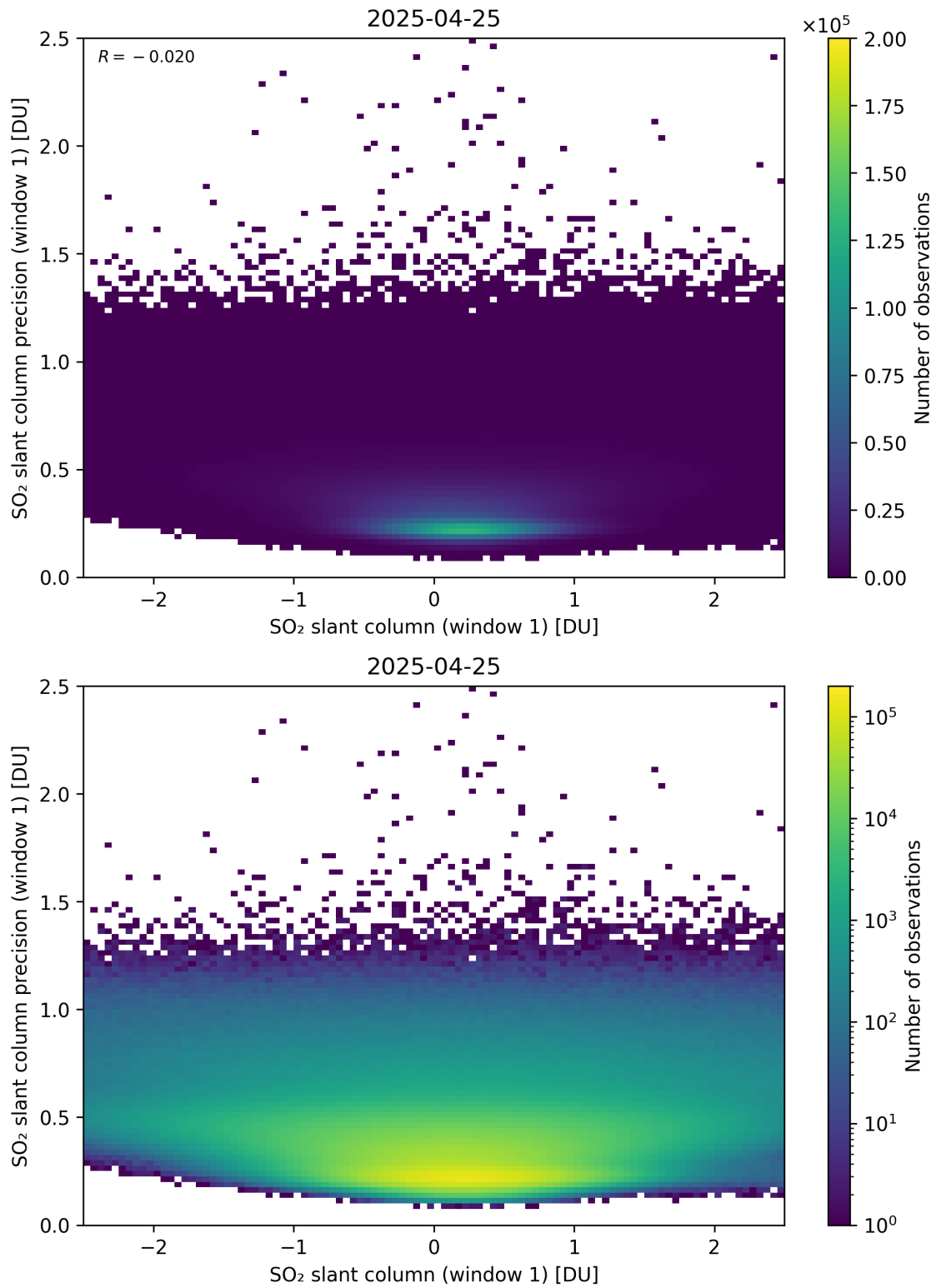
Figure 285: Scatter density plot of “SO 2 slant column (window 1)” against “SO 2 slant column precision (window 1)” for 2025-04-24 to 2025-04-26.
