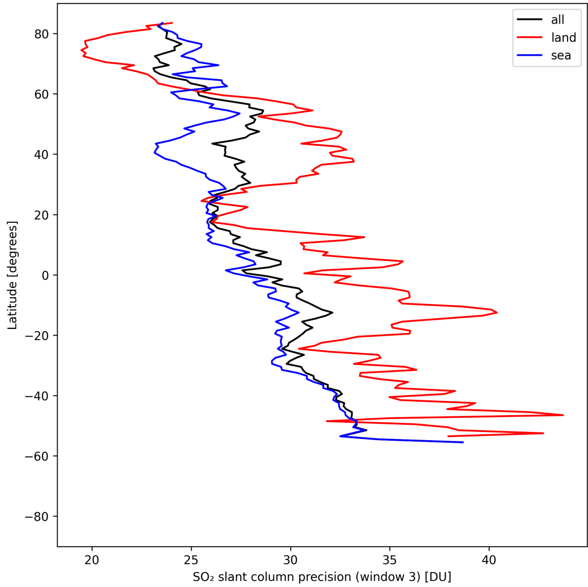
Figure 46: Zonal average of “SO 2 slant column precision (window 3)” for 2025-04-24 to 2025-04-26.
