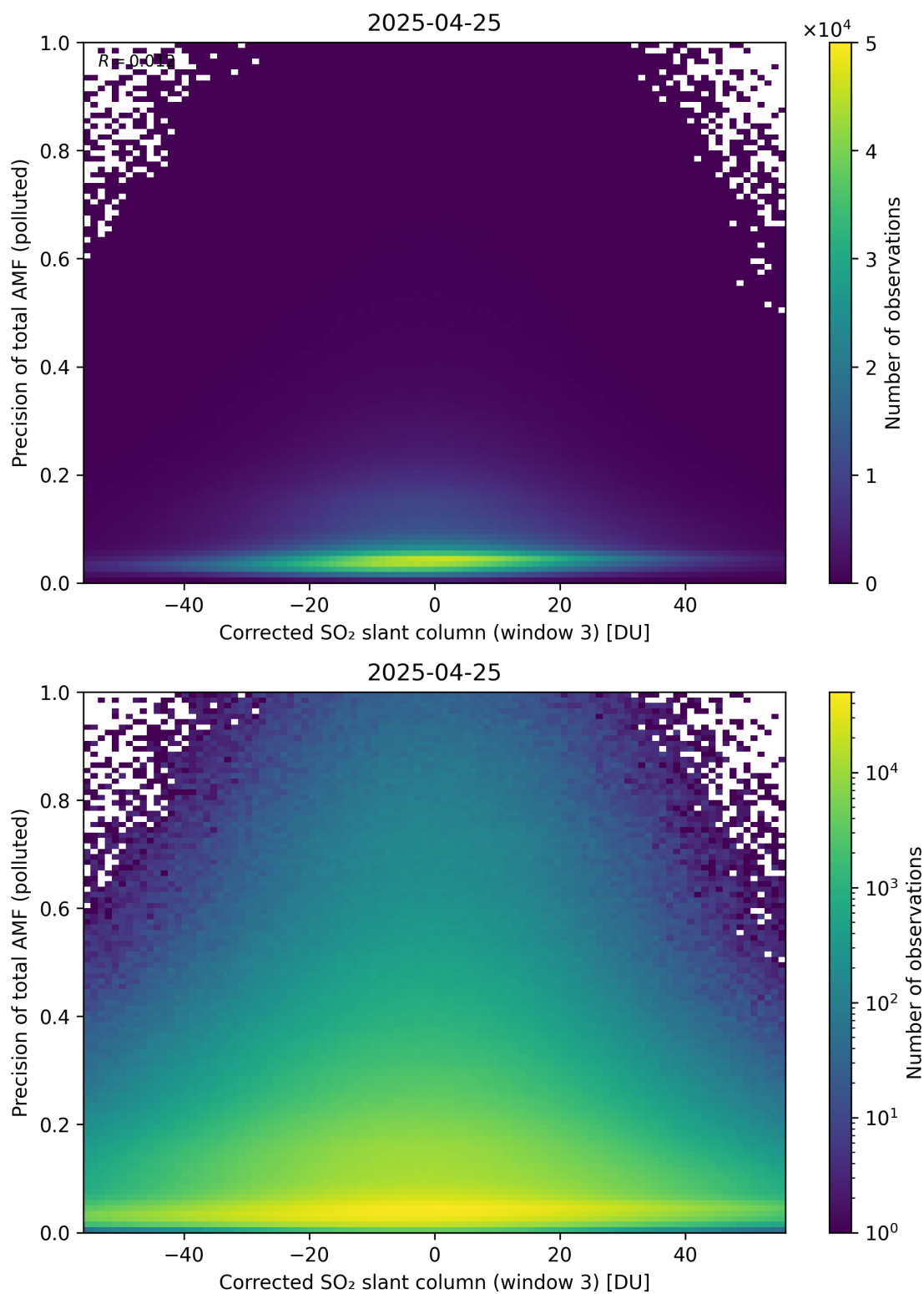
Figure 261: Scatter density plot of “Corrected SO 2 slant column (window 3)” against “Precision of total AMF (polluted)” for 2025-04-24 to 2025-04-26.
