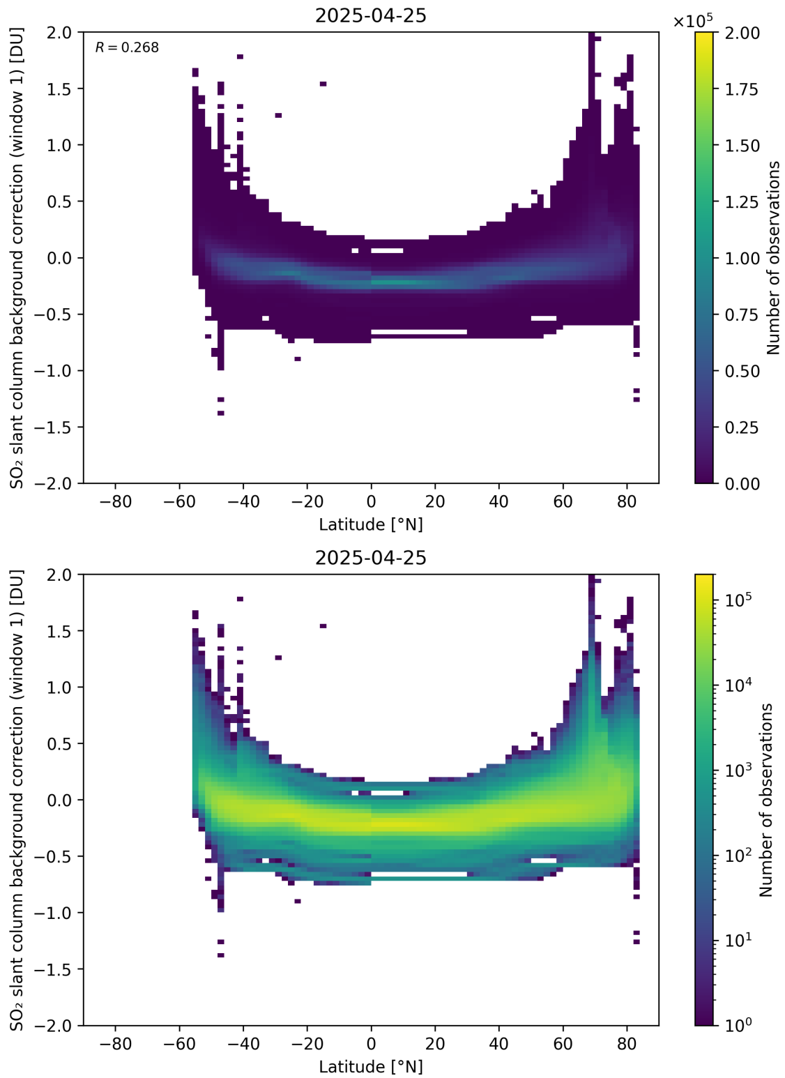
Figure 150: Scatter density plot of “Latitude” against “SO 2 slant column background correction (window 1)” for 2025-04-24 to 2025-04-26.
