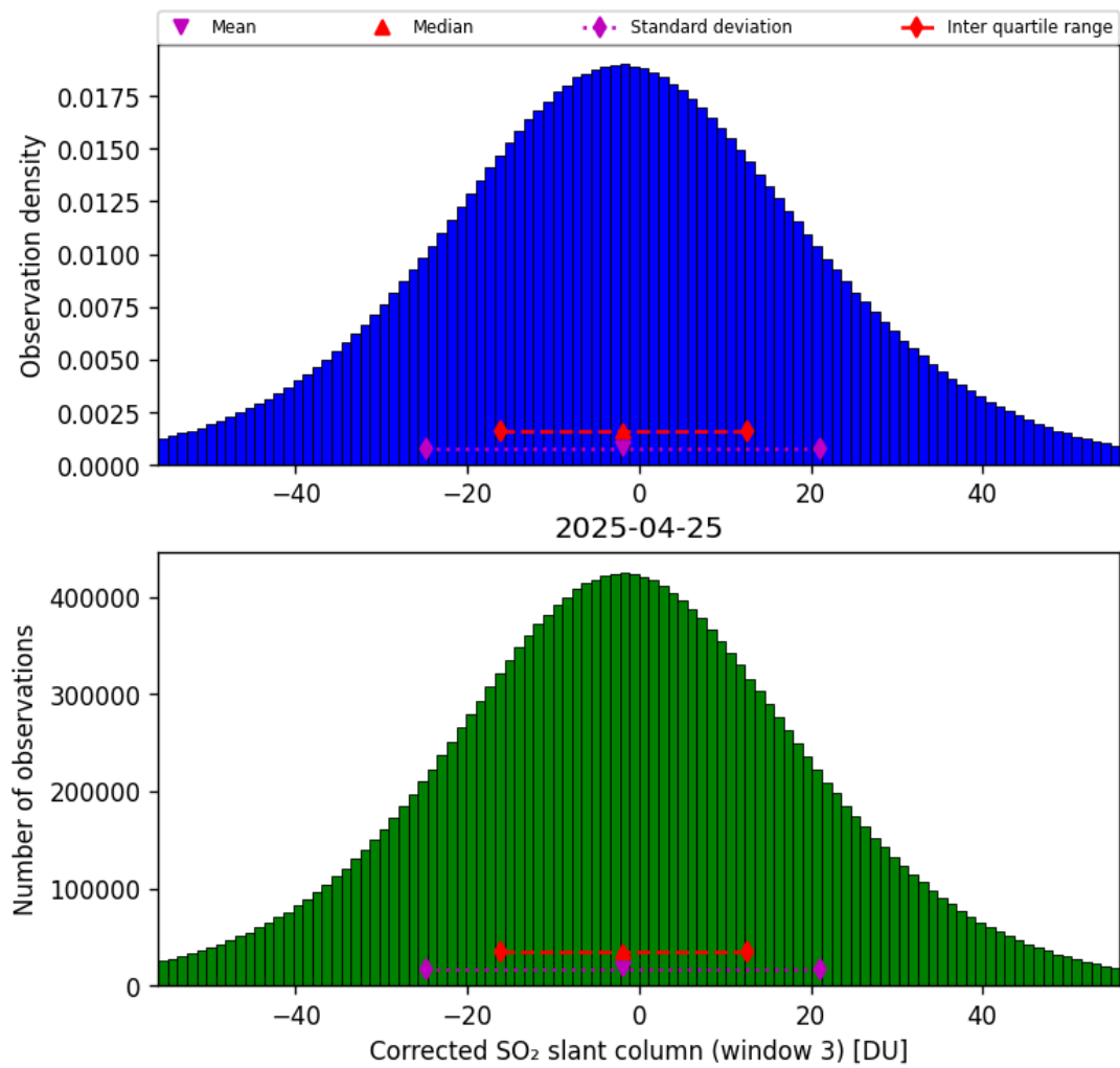
Figure 73: Histogram of “Corrected SO 2 slant column (window 3)” for 2025-04-24 to 2025-04-26
