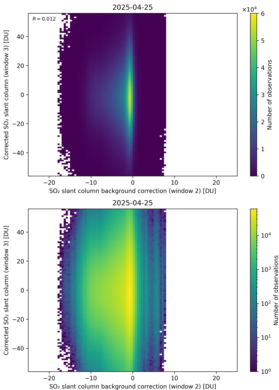
Figure 127: Scatter density plot of “SO 2 slant column background correction (window 2)” against “Corrected SO 2 slant column (window 3)” for 2025-04-24 to 2025-04-26.
