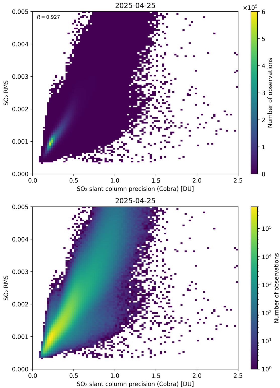
Figure 204: Scatter density plot of “SO 2 slant column precision (Cobra)” against “SO 2 RMS” for 2025-04-24 to 2025-04-26.
