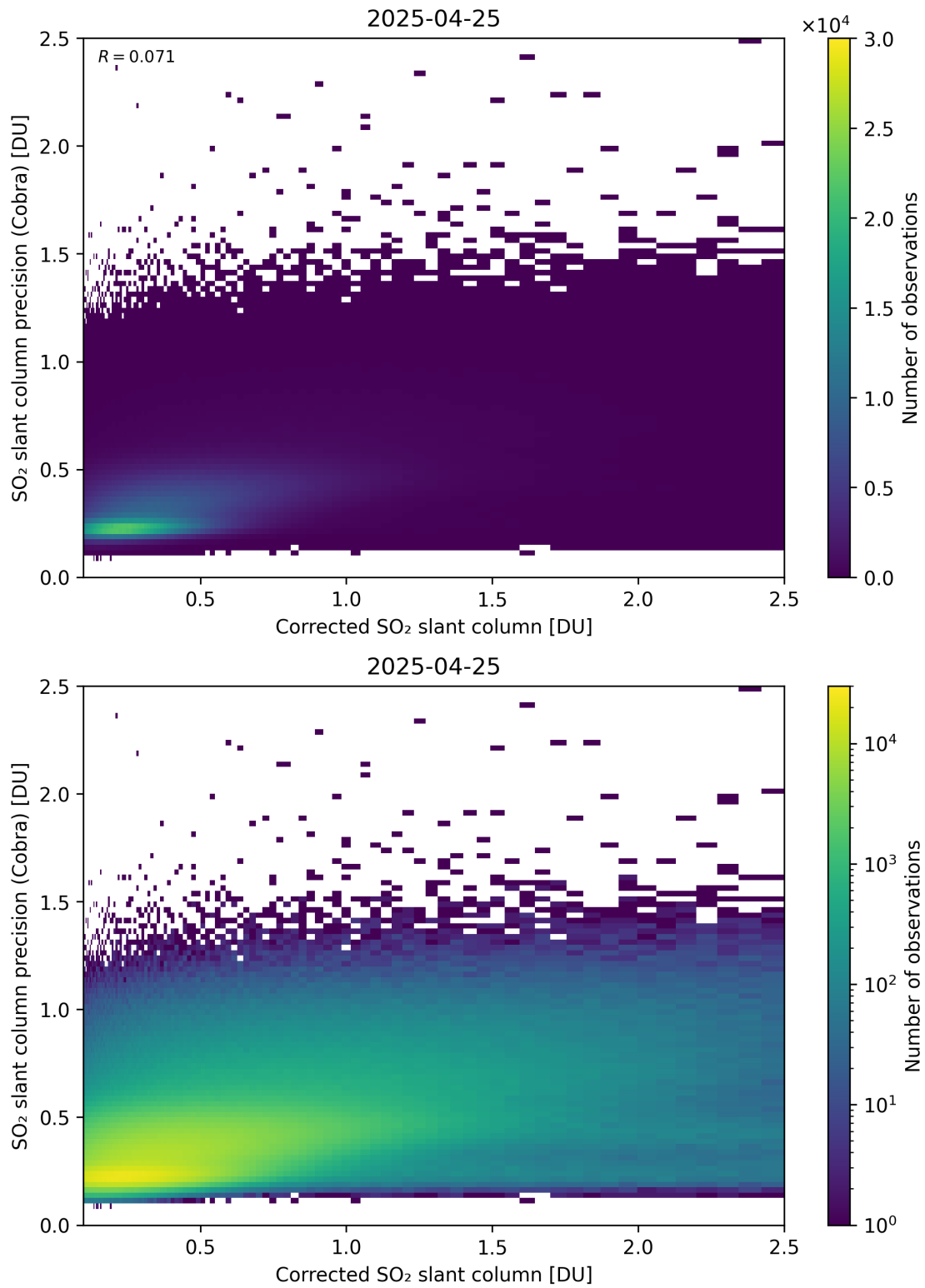
Figure 234: Scatter density plot of “Corrected SO 2 slant column” against “SO 2 slant column precision (Cobra)” for 2025-04-24 to 2025-04-26.
