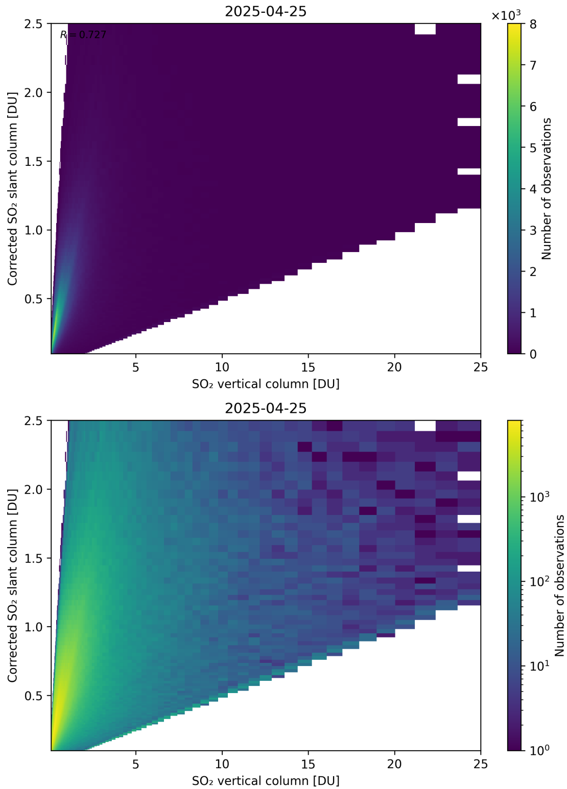
Figure 351: Scatter density plot of “SO 2 vertical column” against “Corrected SO 2 slant column” for 2025-04-24 to 2025-04-26.
