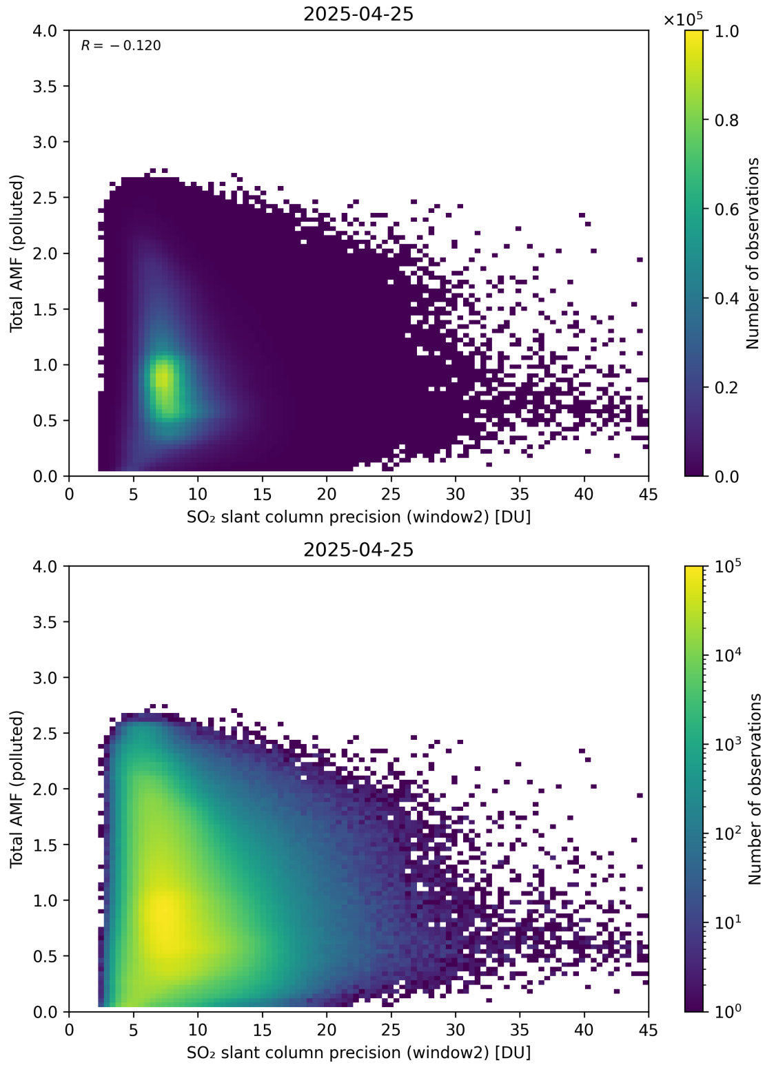
Figure 301: Scatter density plot of “SO 2 slant column precision (window2)” against “Total AMF (polluted)” for 2025-04-24 to 2025-04-26.
