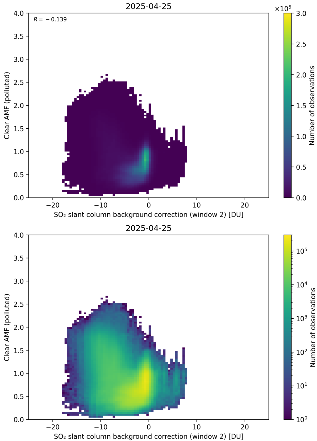
Figure 126: Scatter density plot of “SO 2 slant column background correction (window 2)” against “Clear AMF (polluted)” for 2025-04-24 to 2025-04-26.
