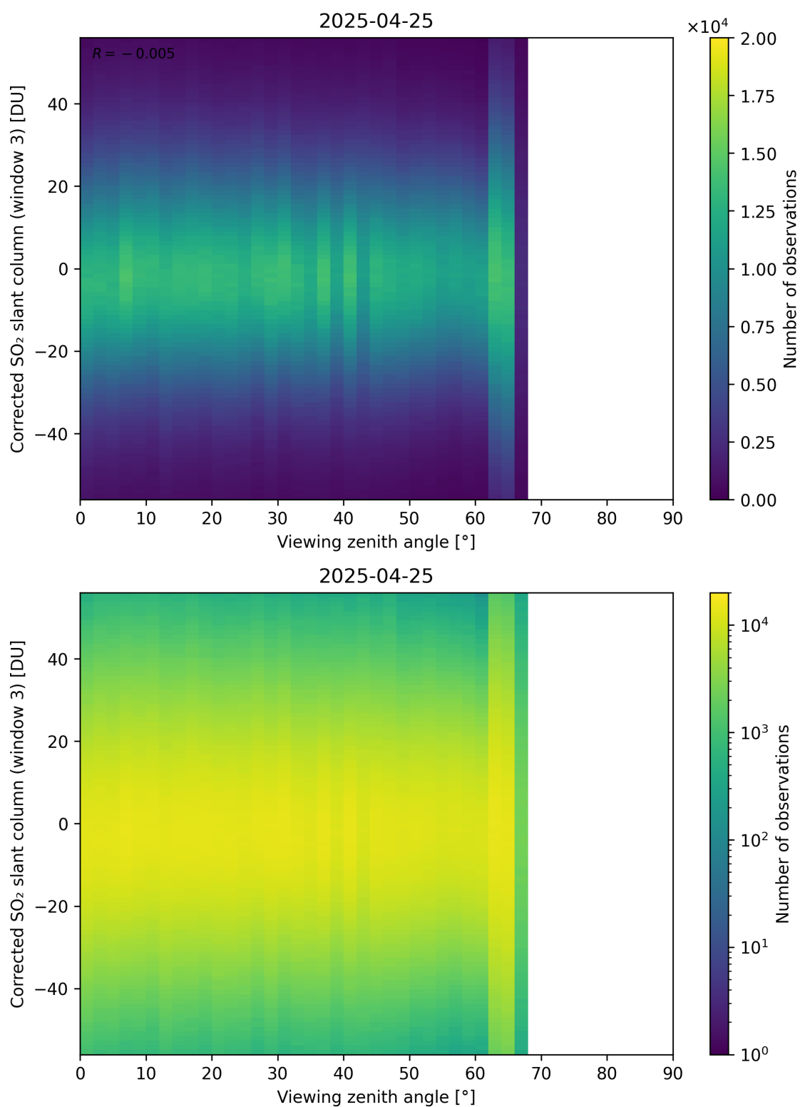
Figure 375: Scatter density plot of “Viewing zenith angle” against “Corrected SO 2 slant column (window 3)” for 2025-04-24 to 2025-04-26.
