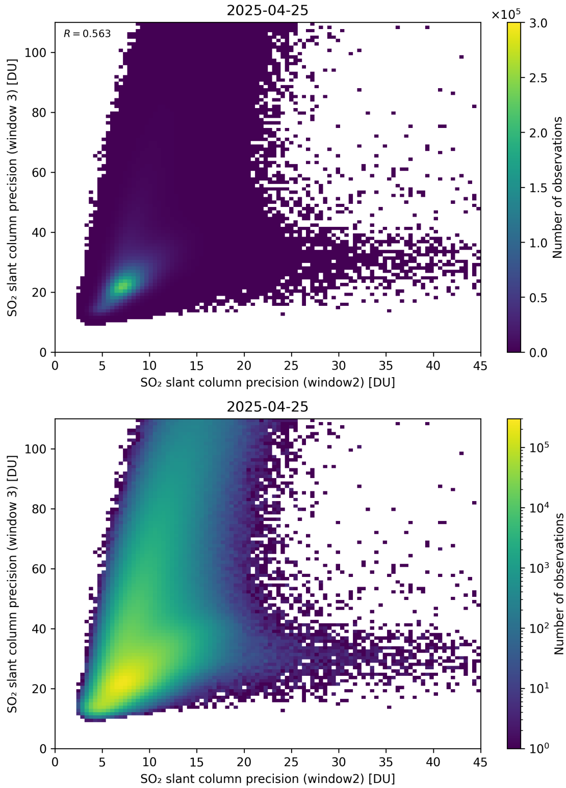
Figure 300: Scatter density plot of “SO 2 slant column precision (window2)” against “SO 2 slant column precision (window 3)” for 2025-04-24 to 2025-04-26.
