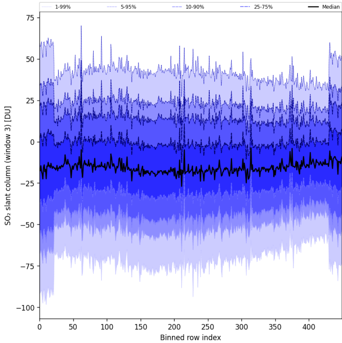
Figure 97: Along track statistics of “SO 2 slant column (window 3)” for 2025-04-24 to 2025-04-26
