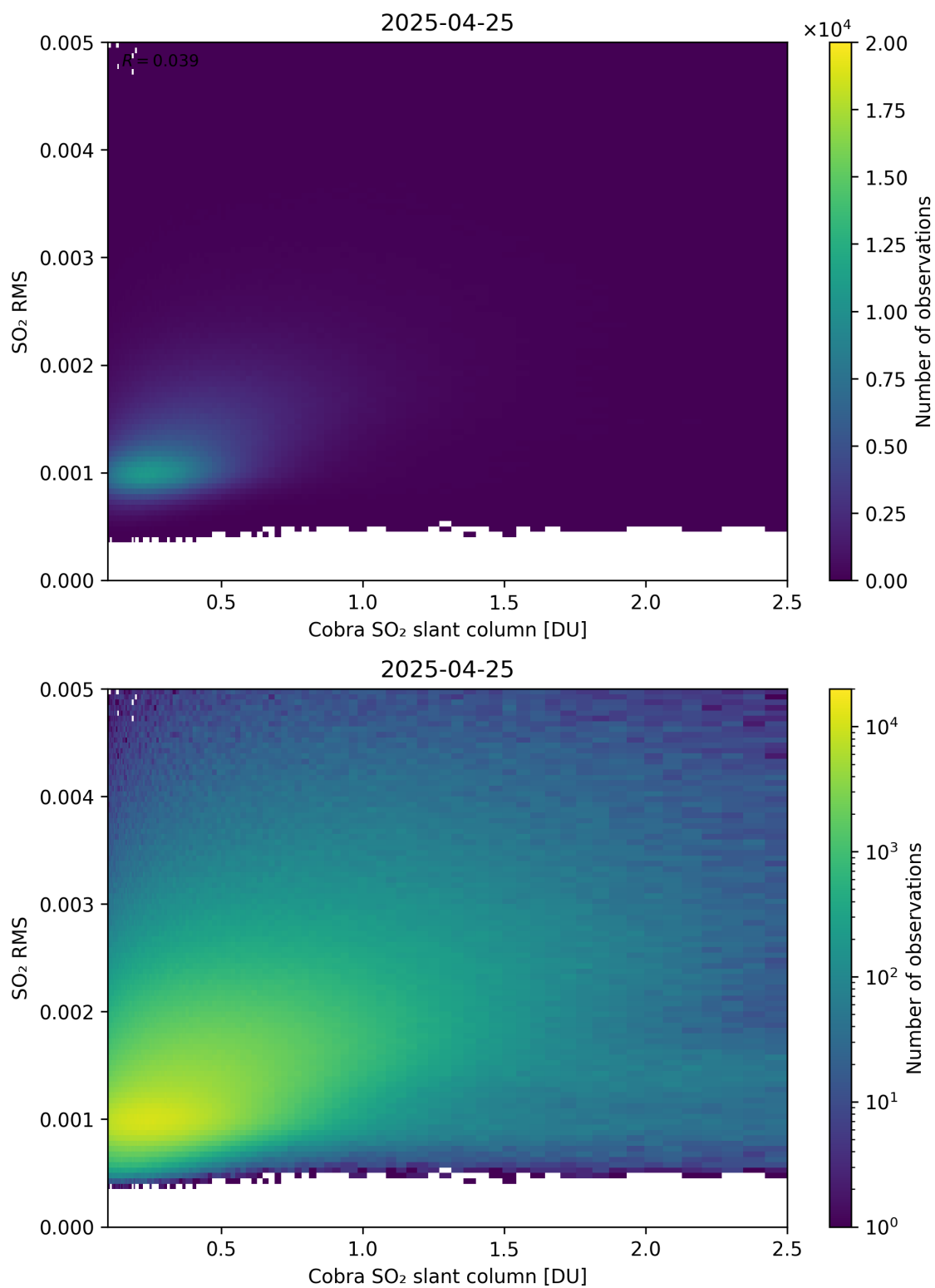
Figure 198: Scatter density plot of “Cobra SO 2 slant column” against “SO 2 RMS” for 2025-04-24 to 2025-04-26.
