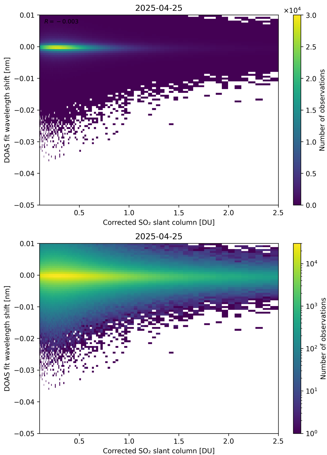
Figure 229: Scatter density plot of “Corrected SO 2 slant column” against “DOAS fit wavelength shift” for 2025-04-24 to 2025-04-26.
