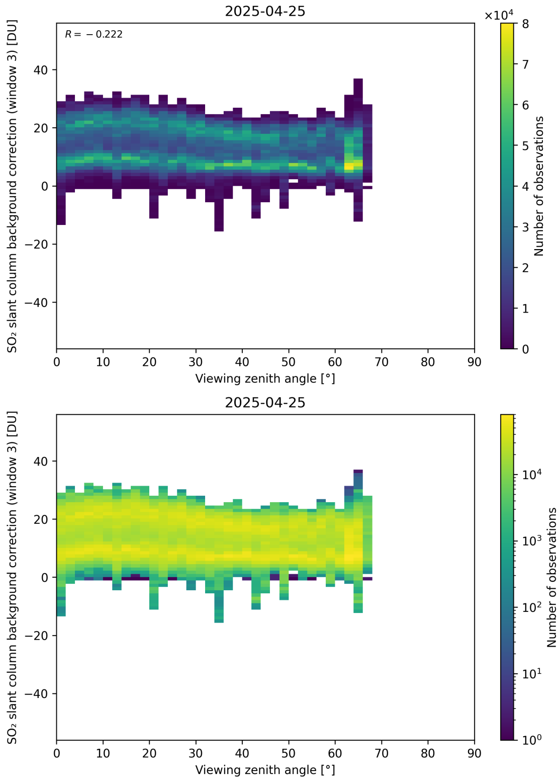
Figure 364: Scatter density plot of “Viewing zenith angle” against “SO 2 slant column background correction (window 3)” for 2025-04-24 to 2025-04-26.
