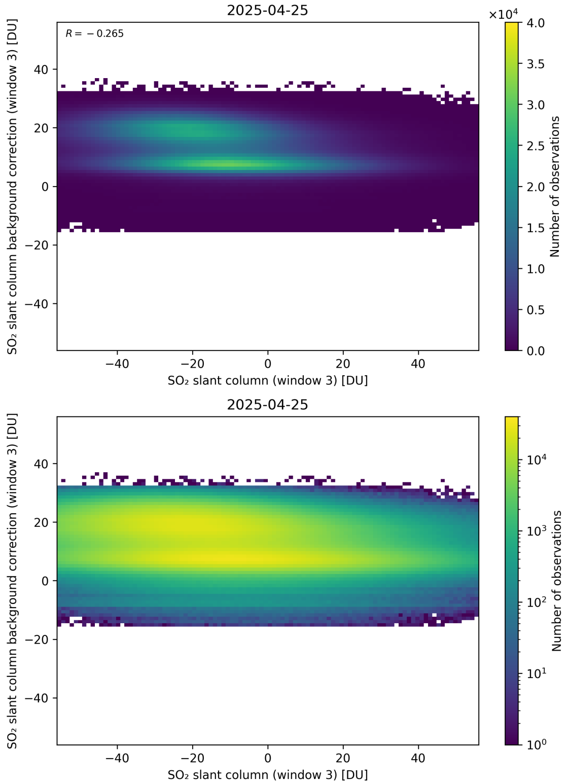
Figure 303: Scatter density plot of “SO 2 slant column (window 3)” against “SO 2 slant column background correction (window 3)” for 2025-04-24 to 2025-04-26.
