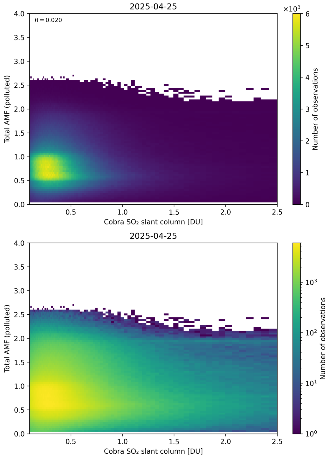
Figure 224: Scatter density plot of “Cobra SO 2 slant column” against “Total AMF (polluted)” for 2025-04-24 to 2025-04-26.
