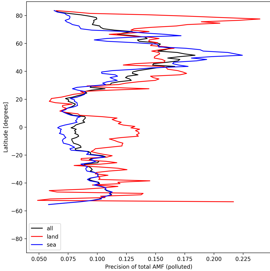
Figure 54: Zonal average of “Precision of total AMF (polluted)” for 2025-04-24 to 2025-04-26.
