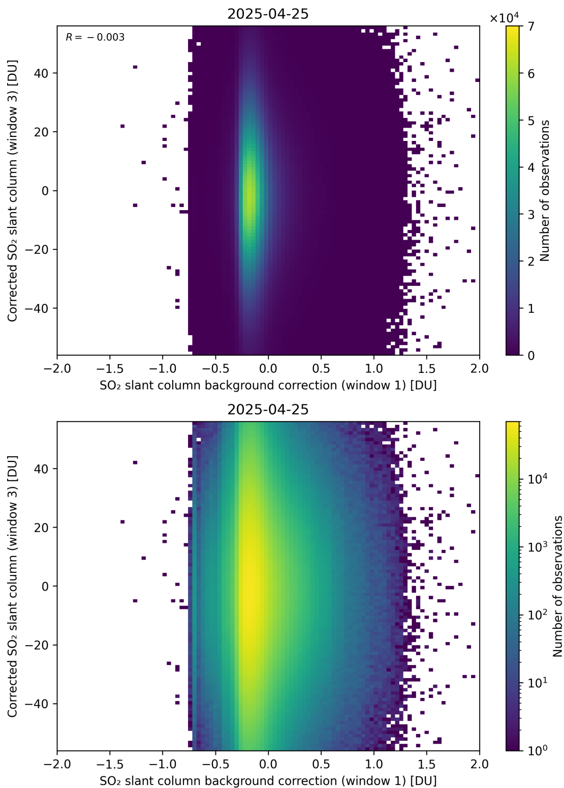
Figure 116: Scatter density plot of “SO 2 slant column background correction (window 1)” against “Corrected SO 2 slant column (window 3)” for 2025-04-24 to 2025-04-26.
