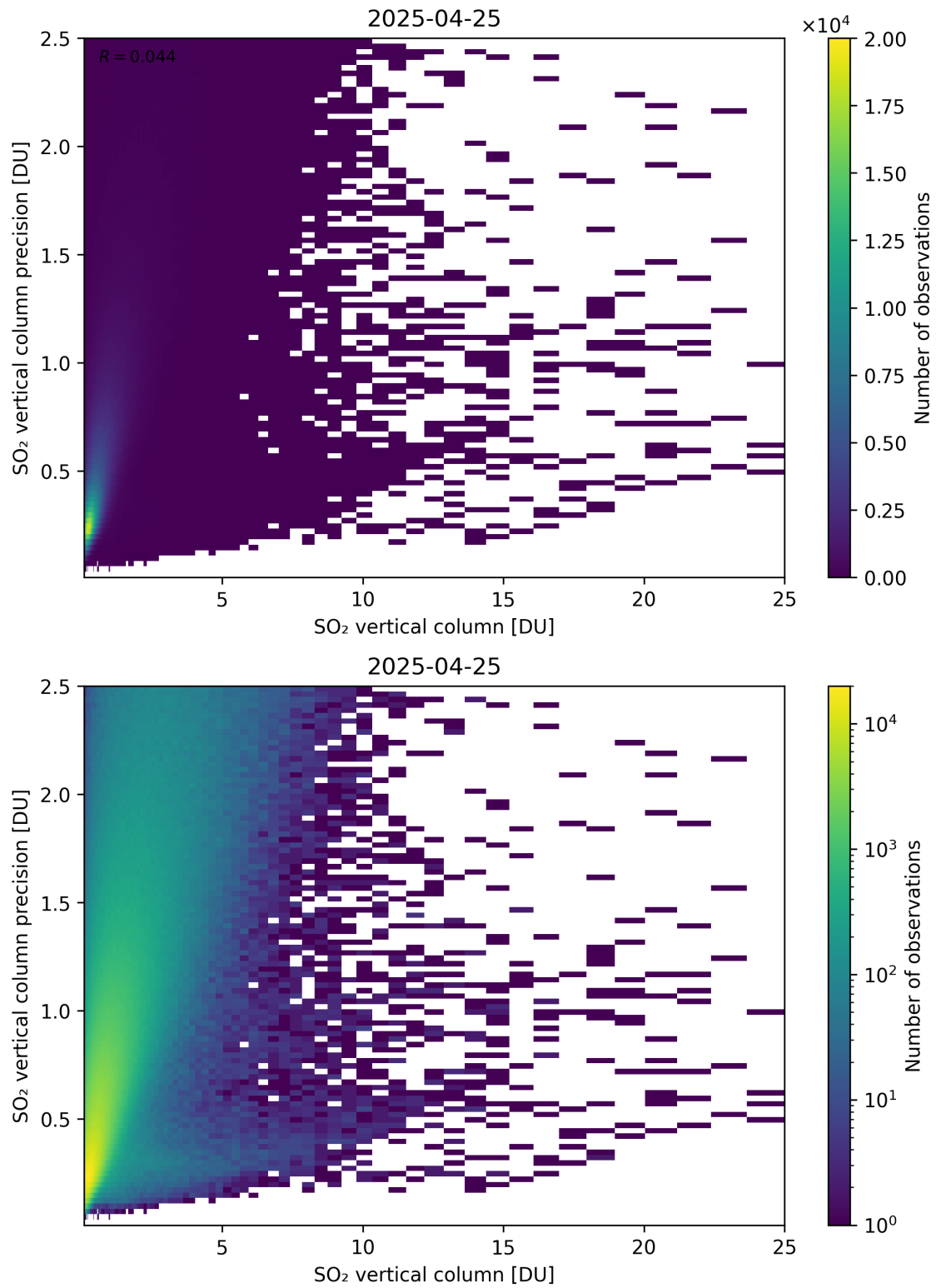
Figure 361: Scatter density plot of “SO 2 vertical column” against “SO 2 vertical column precision” for 2025-04-24 to 2025-04-26.
