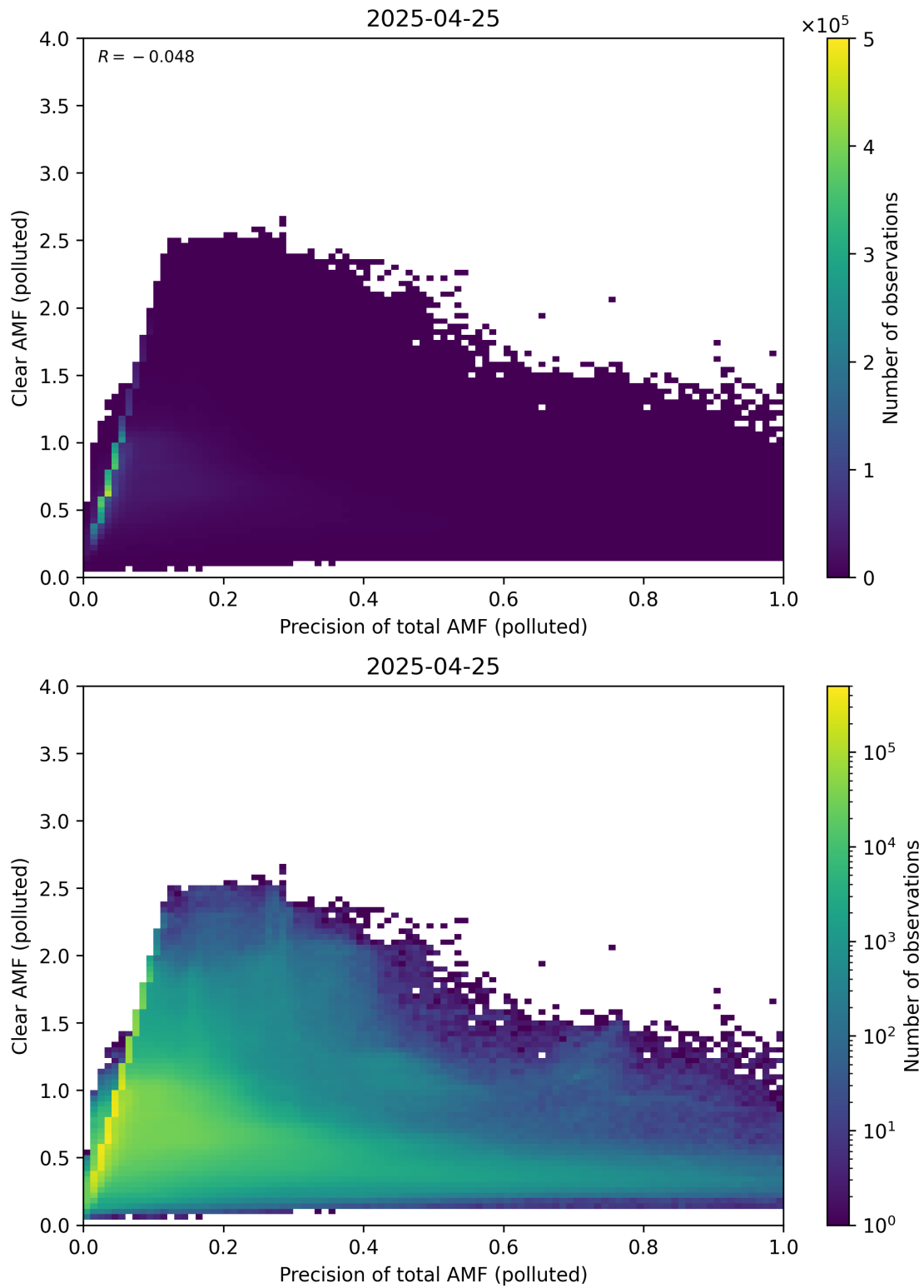
Figure 320: Scatter density plot of “Precision of total AMF (polluted)” against “Clear AMF (polluted)” for 2025-04-24 to 2025-04-26.
