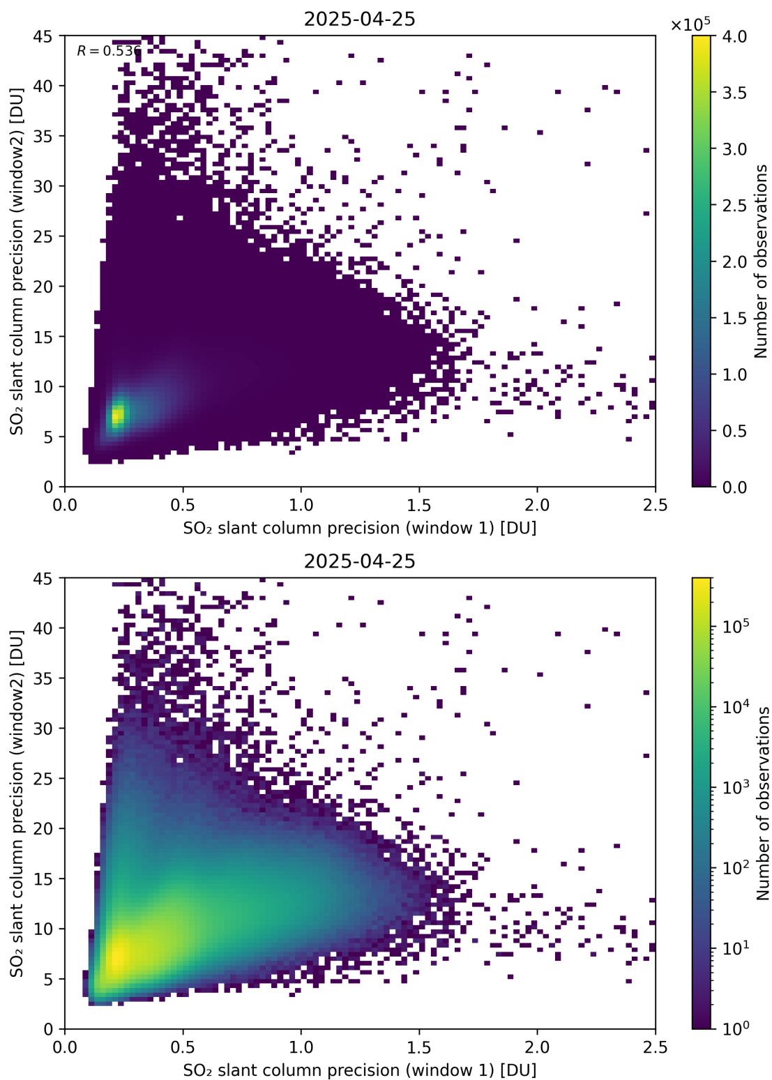
Figure 277: Scatter density plot of “SO 2 slant column precision (window 1)” against “SO 2 slant column precision (window2)” for 2025-04-24 to 2025-04-26.
