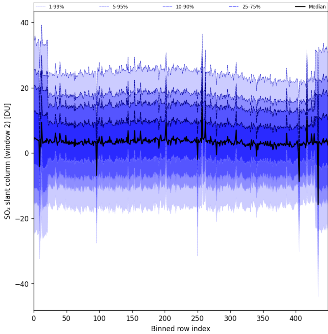
Figure 93: Along track statistics of “SO 2 slant column (window 2)” for 2025-04-24 to 2025-04-26
