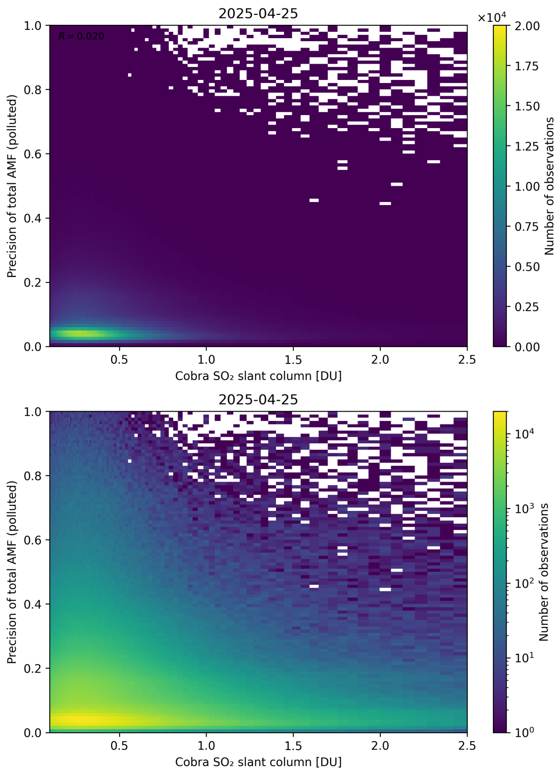
Figure 225: Scatter density plot of “Cobra SO 2 slant column” against “Precision of total AMF (polluted)” for 2025-04-24 to 2025-04-26.
