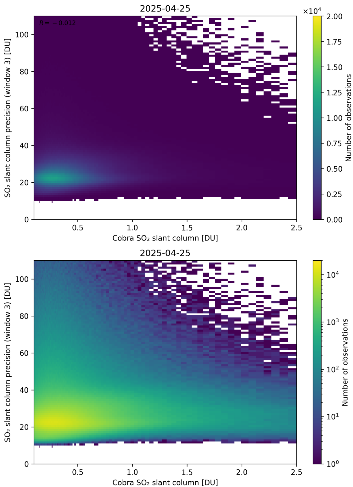
Figure 223: Scatter density plot of “Cobra SO 2 slant column” against “SO 2 slant column precision (window 3)” for 2025-04-24 to 2025-04-26.
