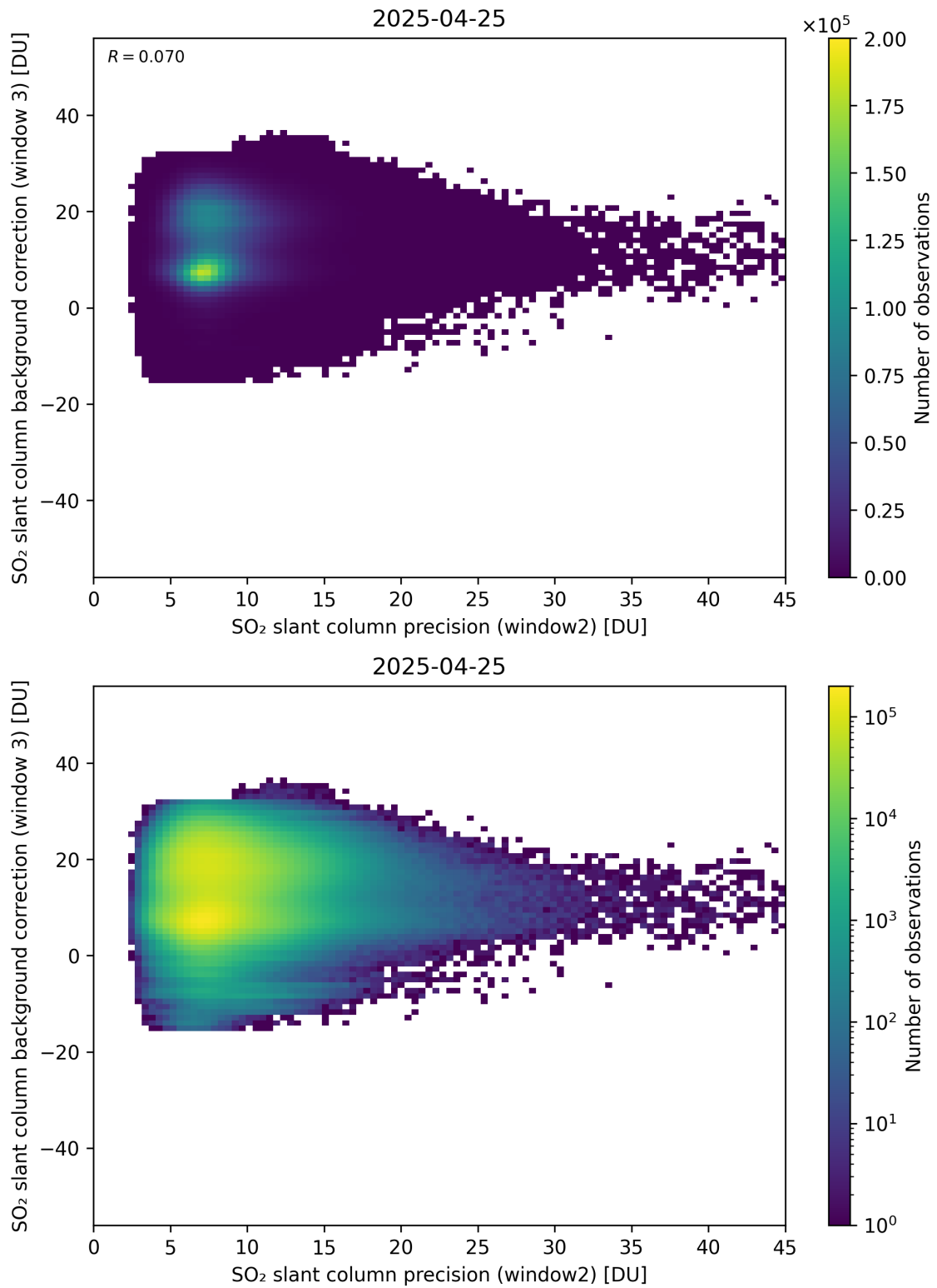
Figure 292: Scatter density plot of “SO 2 slant column precision (window2)” against “SO 2 slant column background correction (window 3)” for 2025-04-24 to 2025-04-26.
