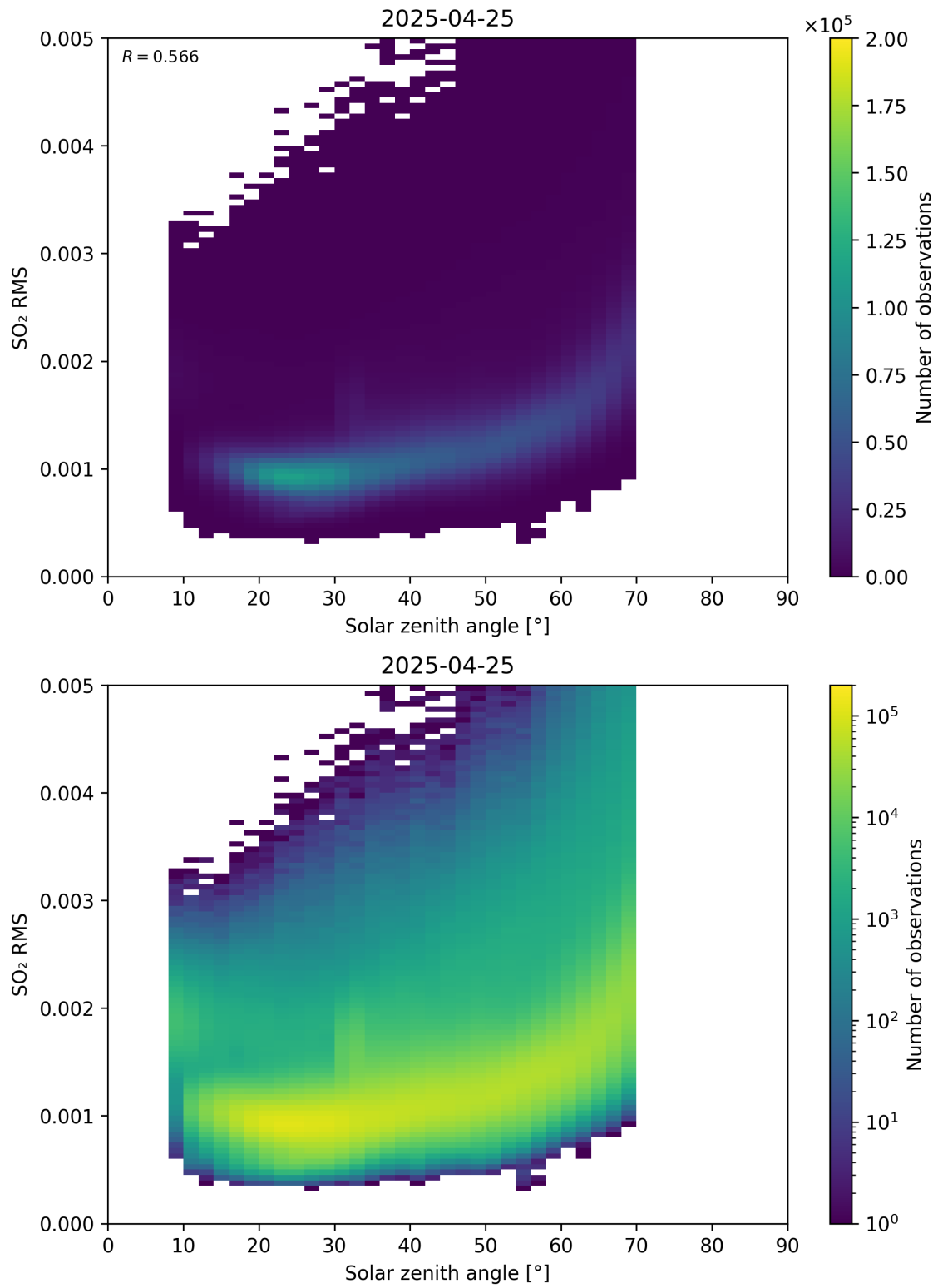
Figure 176: Scatter density plot of “Solar zenith angle” against “SO 2 RMS” for 2025-04-24 to 2025-04-26.
