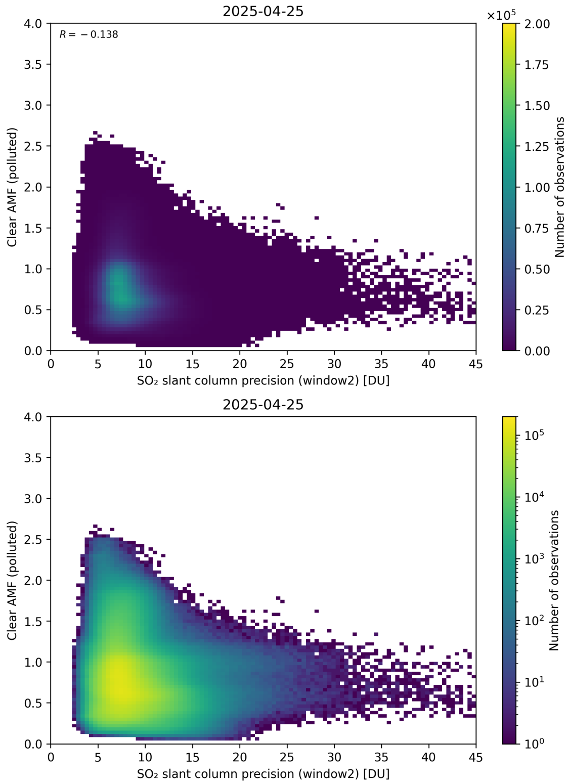
Figure 296: Scatter density plot of “SO 2 slant column precision (window2)” against “Clear AMF (polluted)” for 2025-04-24 to 2025-04-26.
