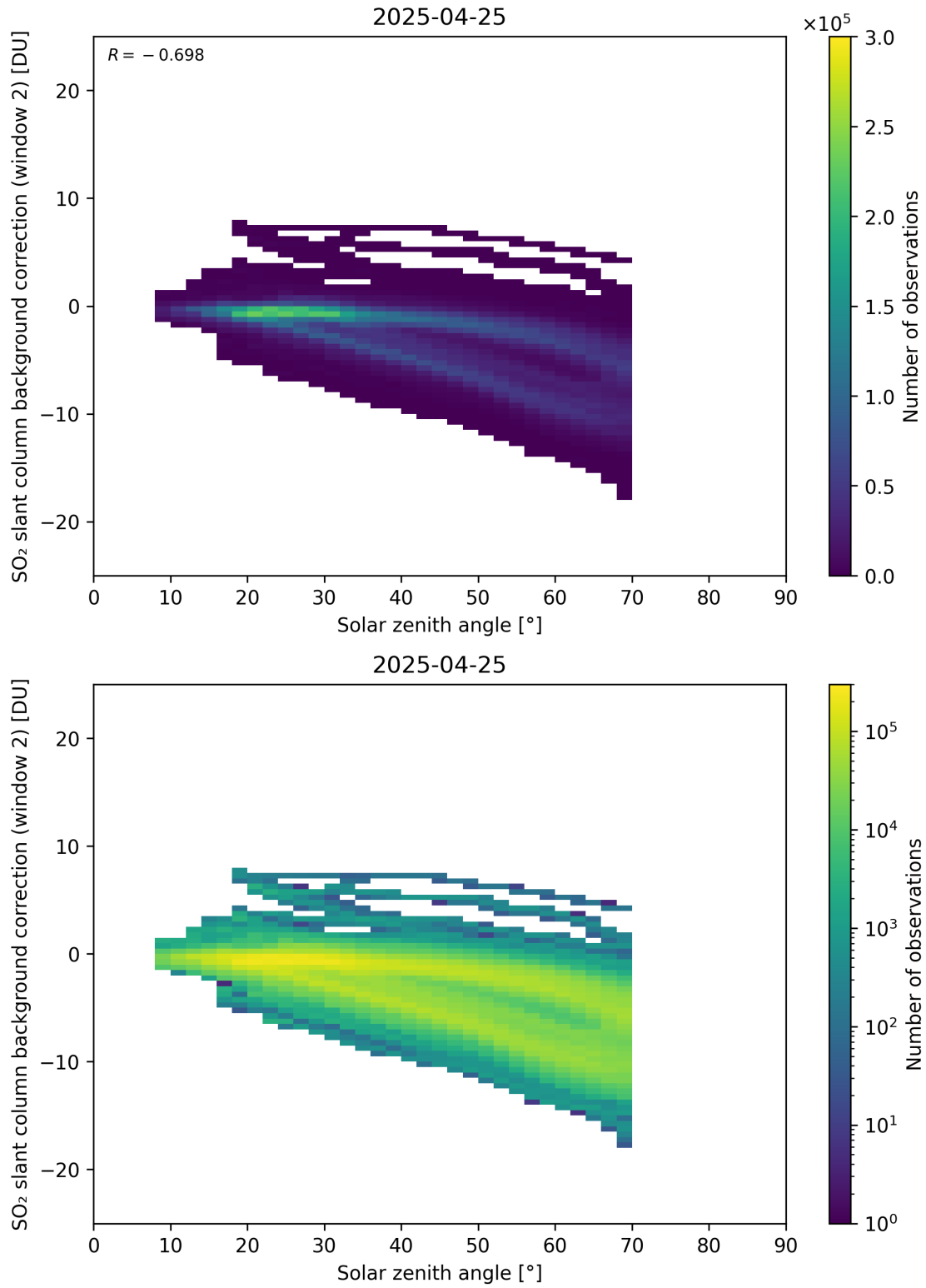
Figure 172: Scatter density plot of “Solar zenith angle” against “SO 2 slant column background correction (window 2)” for 2025-04-24 to 2025-04-26.
