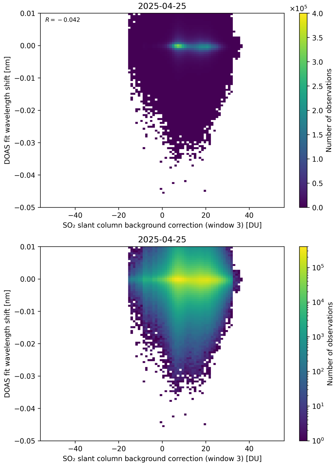
Figure 132: Scatter density plot of “SO 2 slant column background correction (window 3)” against “DOAS fit wavelength shift” for 2025-04-24 to 2025-04-26.
