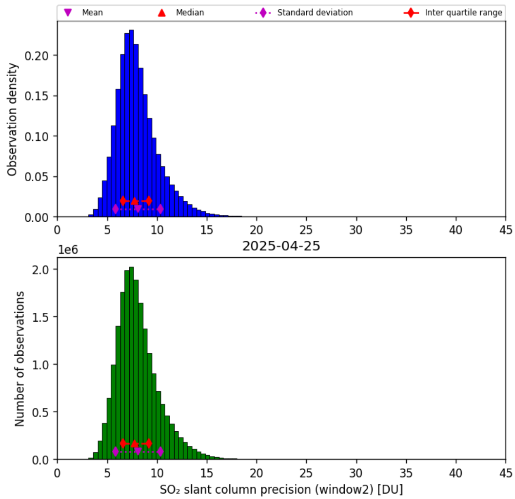
Figure 68: Histogram of “SO 2 slant column precision (window2)” for 2025-04-24 to 2025-04-26
