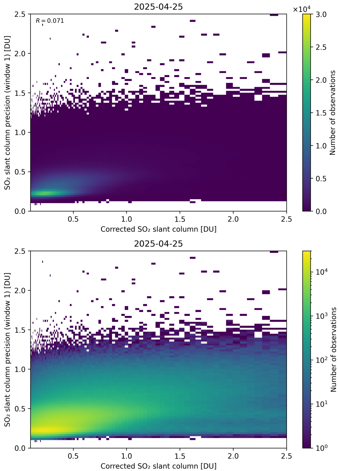
Figure 238: Scatter density plot of “Corrected SO 2 slant column” against “SO 2 slant column precision (window 1)” for 2025-04-24 to 2025-04-26.
