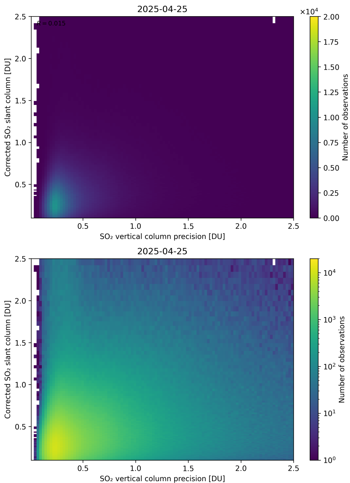
Figure 338: Scatter density plot of “SO 2 vertical column precision” against “Corrected SO 2 slant column” for 2025-04-24 to 2025-04-26.
