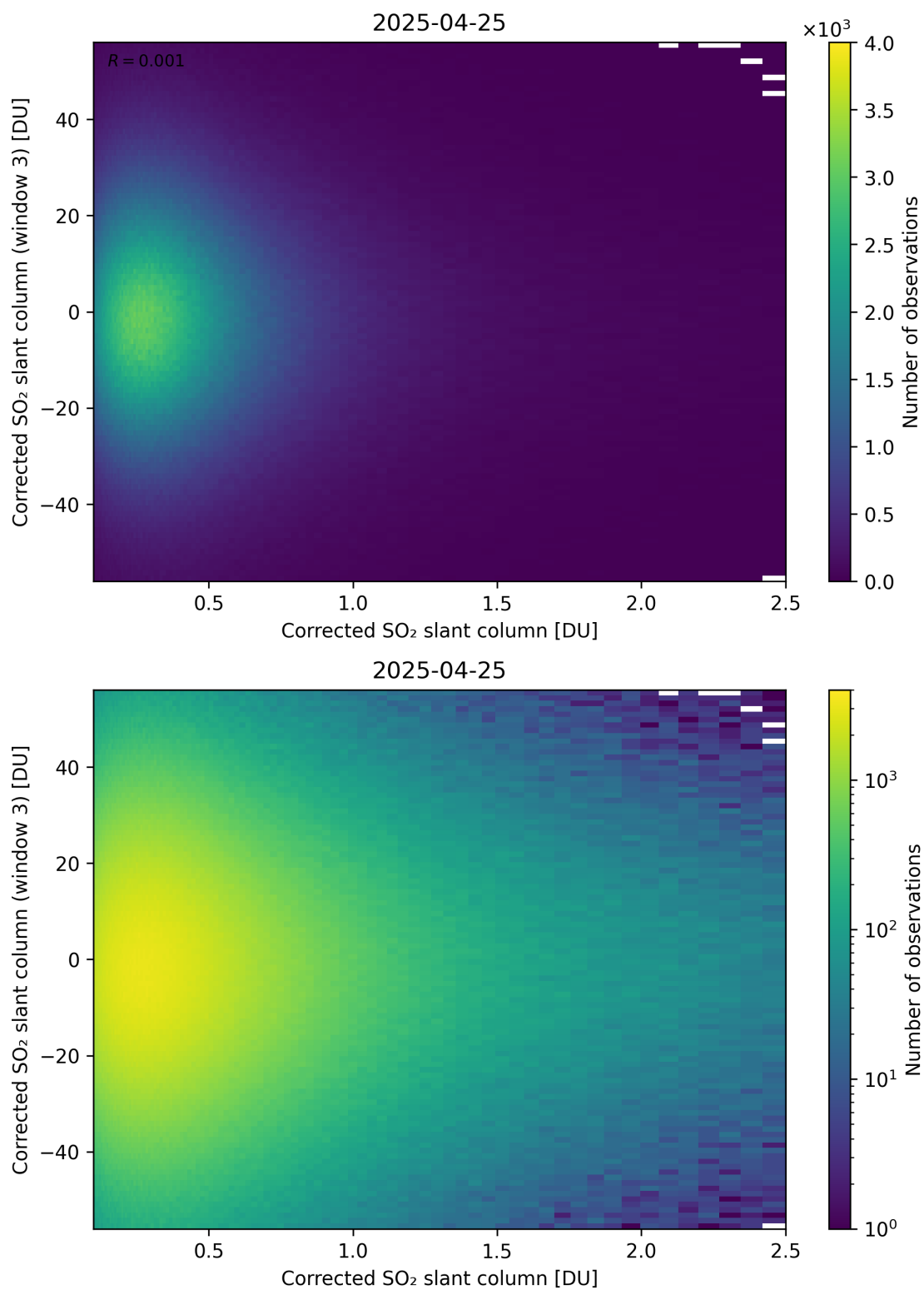
Figure 236: Scatter density plot of “Corrected SO 2 slant column” against “Corrected SO 2 slant column (window 3)” for 2025-04-24 to 2025-04-26.
