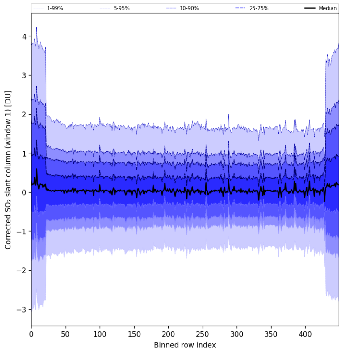
Figure 91: Along track statistics of “Corrected SO 2 slant column (window 1)” for 2025-04-24 to 2025-04-26
