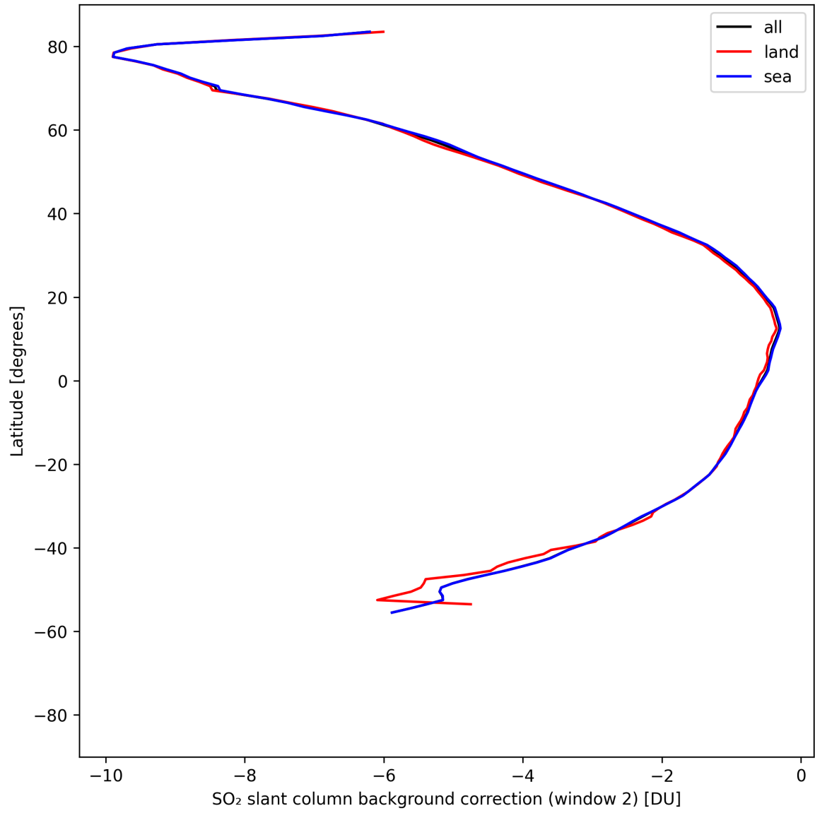
Figure 44: Zonal average of “SO 2 slant column background correction (window 2)” for 2025-04-24 to 2025-04-26.
