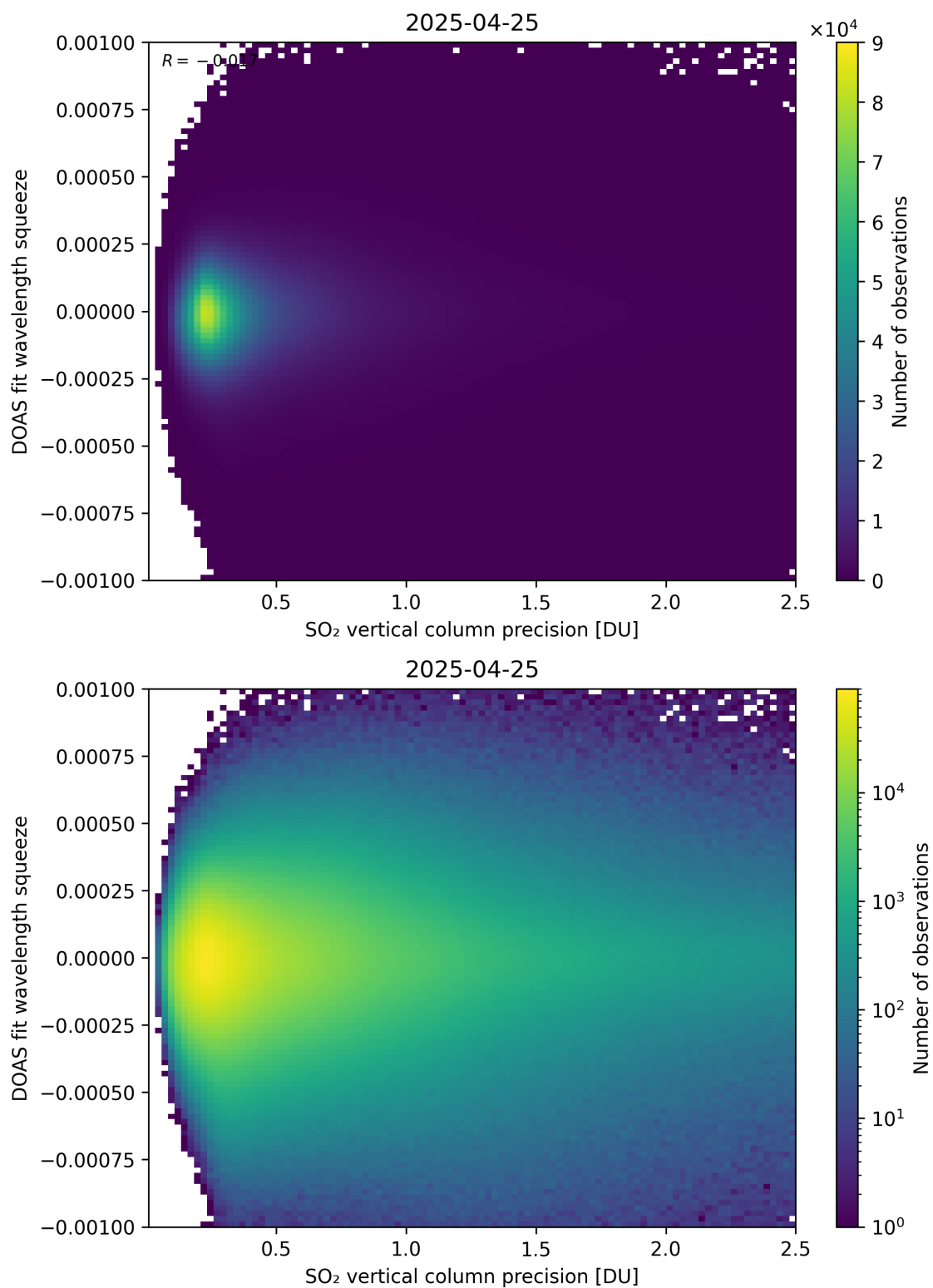
Figure 333: Scatter density plot of “SO 2 vertical column precision” against “DOAS fit wavelength squeeze” for 2025-04-24 to 2025-04-26.
