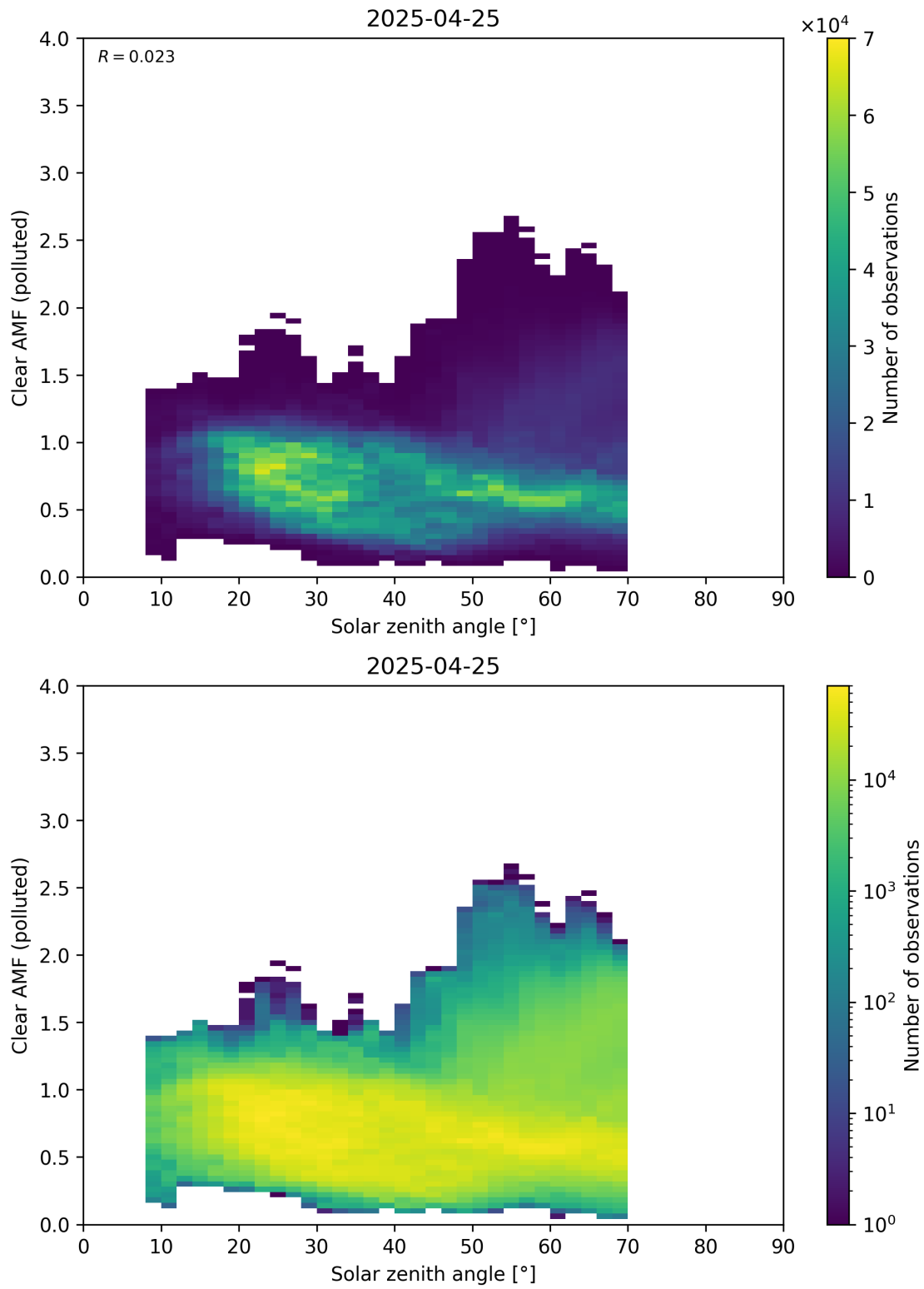
Figure 178: Scatter density plot of “Solar zenith angle” against “Clear AMF (polluted)” for 2025-04-24 to 2025-04-26.
