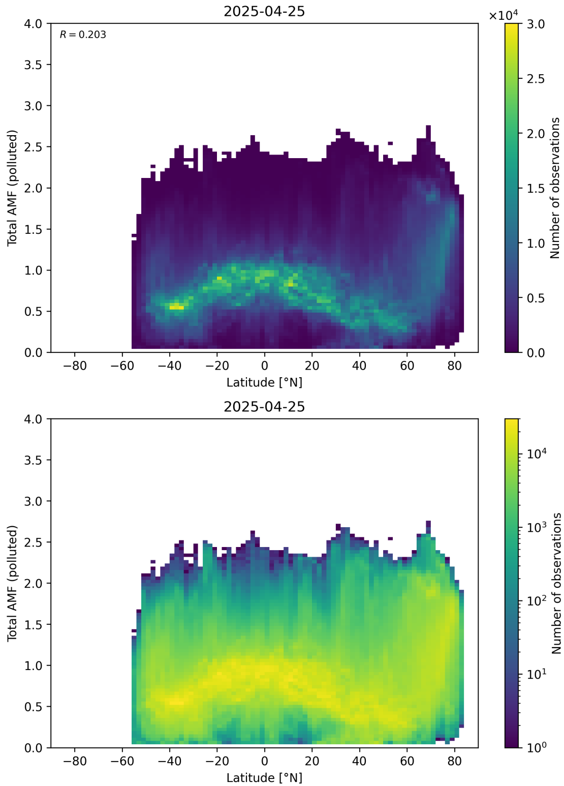
Figure 167: Scatter density plot of “Latitude” against “Total AMF (polluted)” for 2025-04-24 to 2025-04-26.
