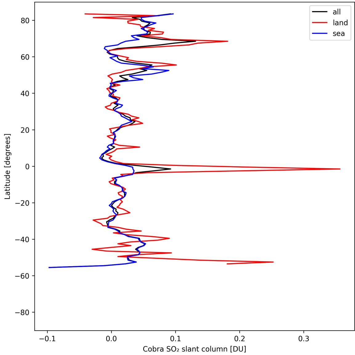
Figure 35: Zonal average of “Cobra SO 2 slant column” for 2025-04-24 to 2025-04-26.
