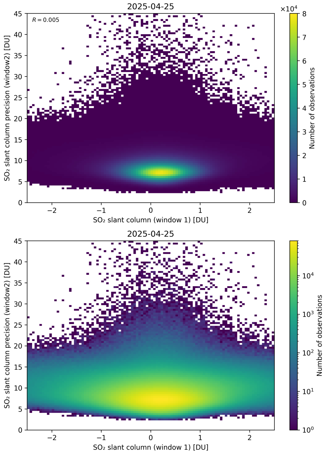
Figure 286: Scatter density plot of “SO 2 slant column (window 1)” against “SO 2 slant column precision (window2)” for 2025-04-24 to 2025-04-26.
