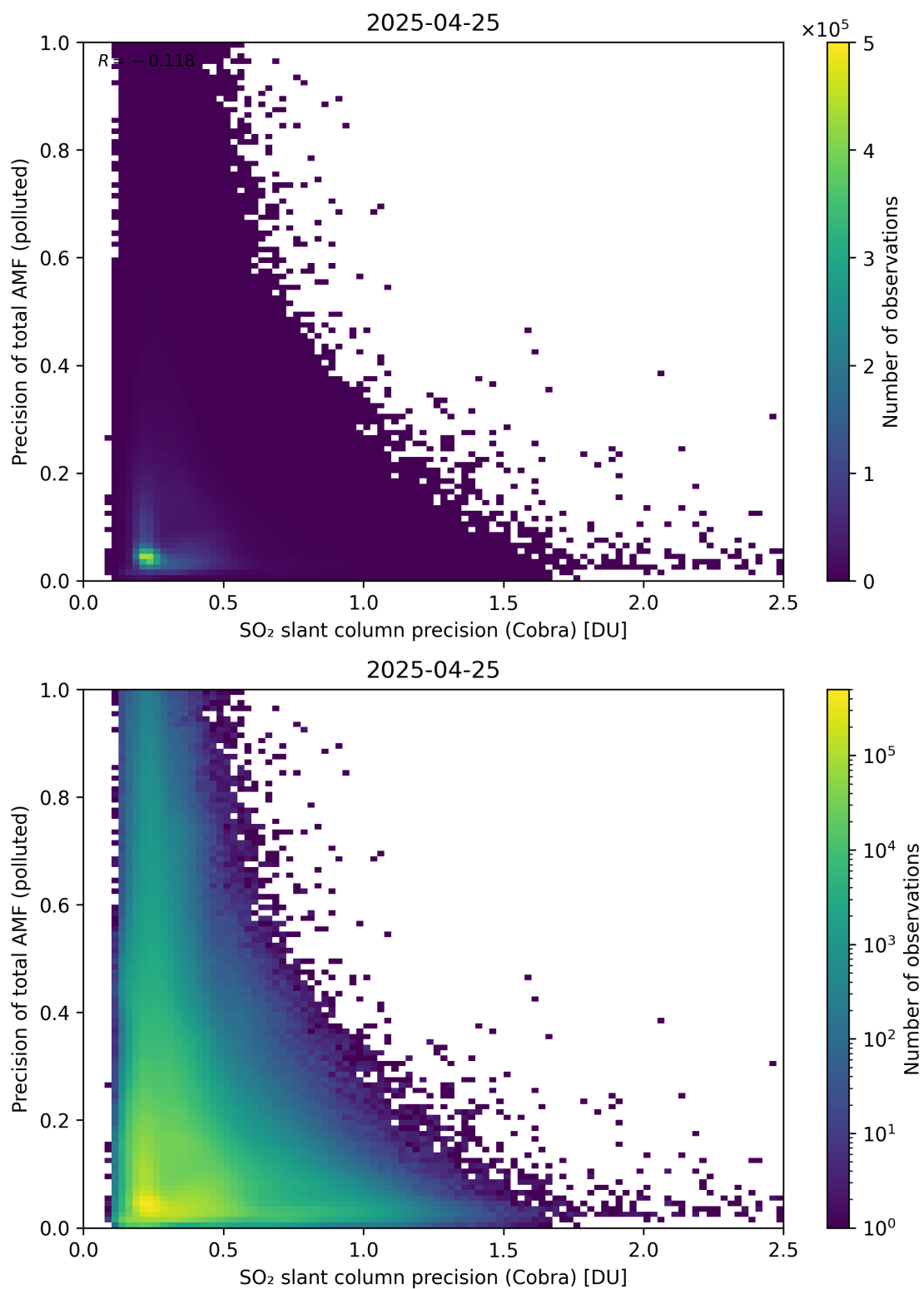
Figure 214: Scatter density plot of “SO 2 slant column precision (Cobra)” against “Precision of total AMF (polluted)” for 2025-04-24 to 2025-04-26.
