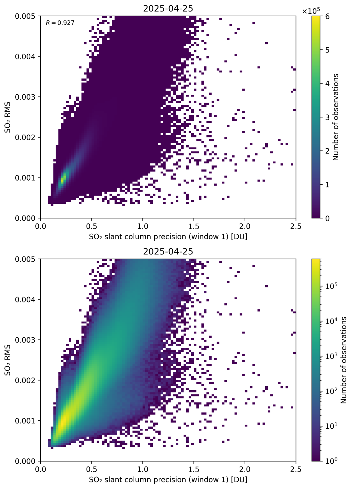
Figure 273: Scatter density plot of “SO 2 slant column precision (window 1)” against “SO 2 RMS” for 2025-04-24 to 2025-04-26.
