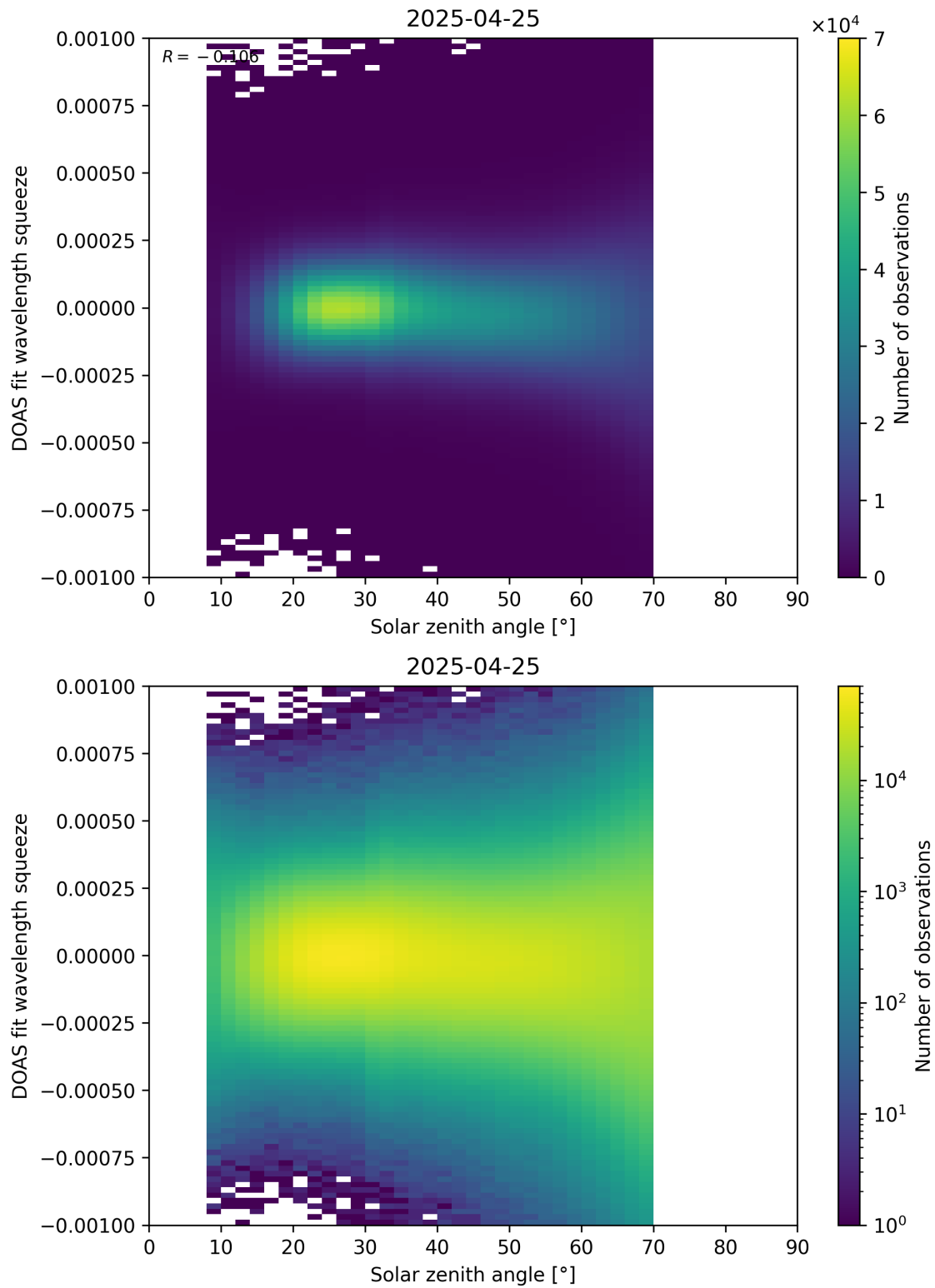
Figure 175: Scatter density plot of “Solar zenith angle” against “DOAS fit wavelength squeeze” for 2025-04-24 to 2025-04-26.
