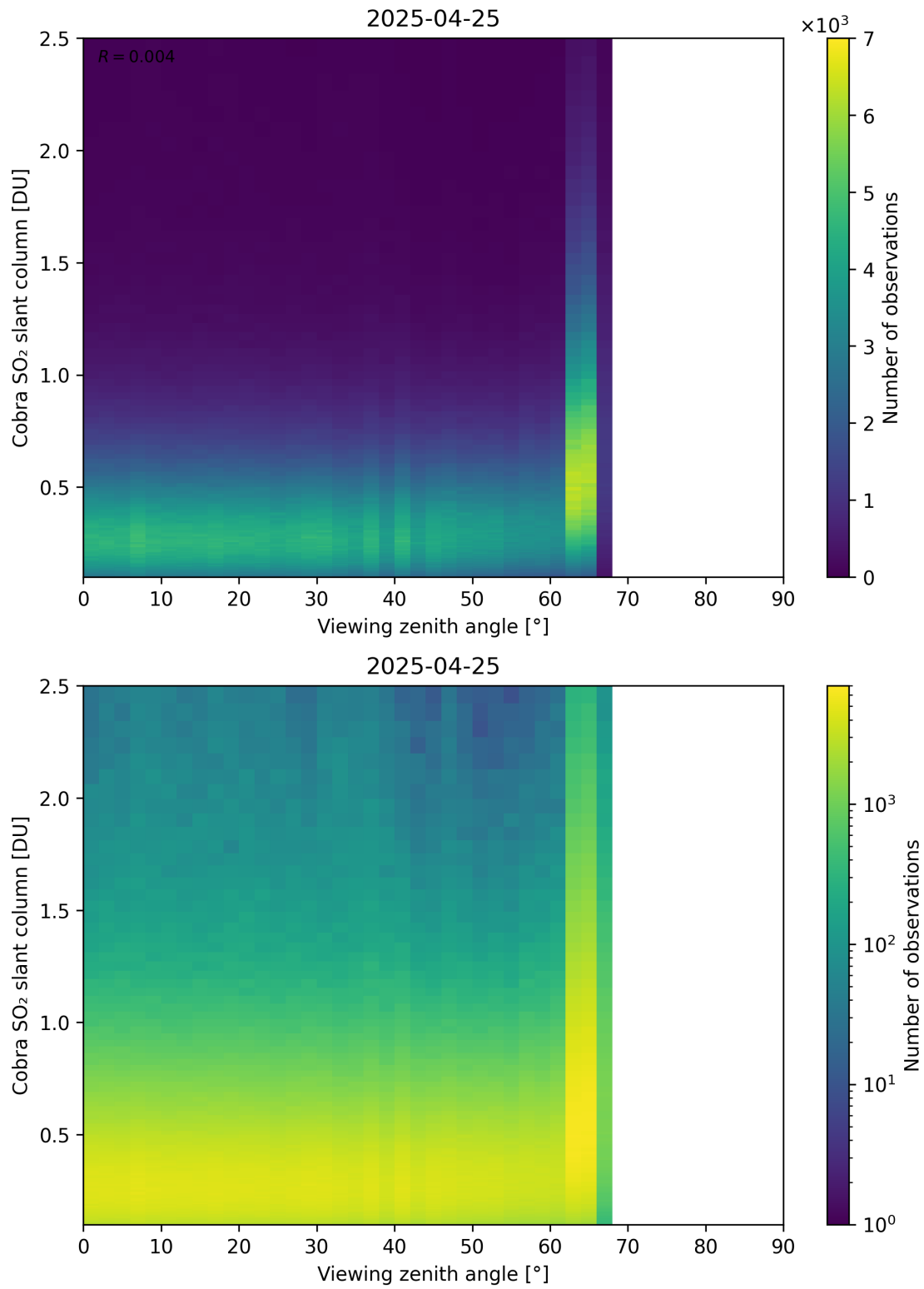
Figure 371: Scatter density plot of “Viewing zenith angle” against “Cobra SO 2 slant column” for 2025-04-24 to 2025-04-26.
