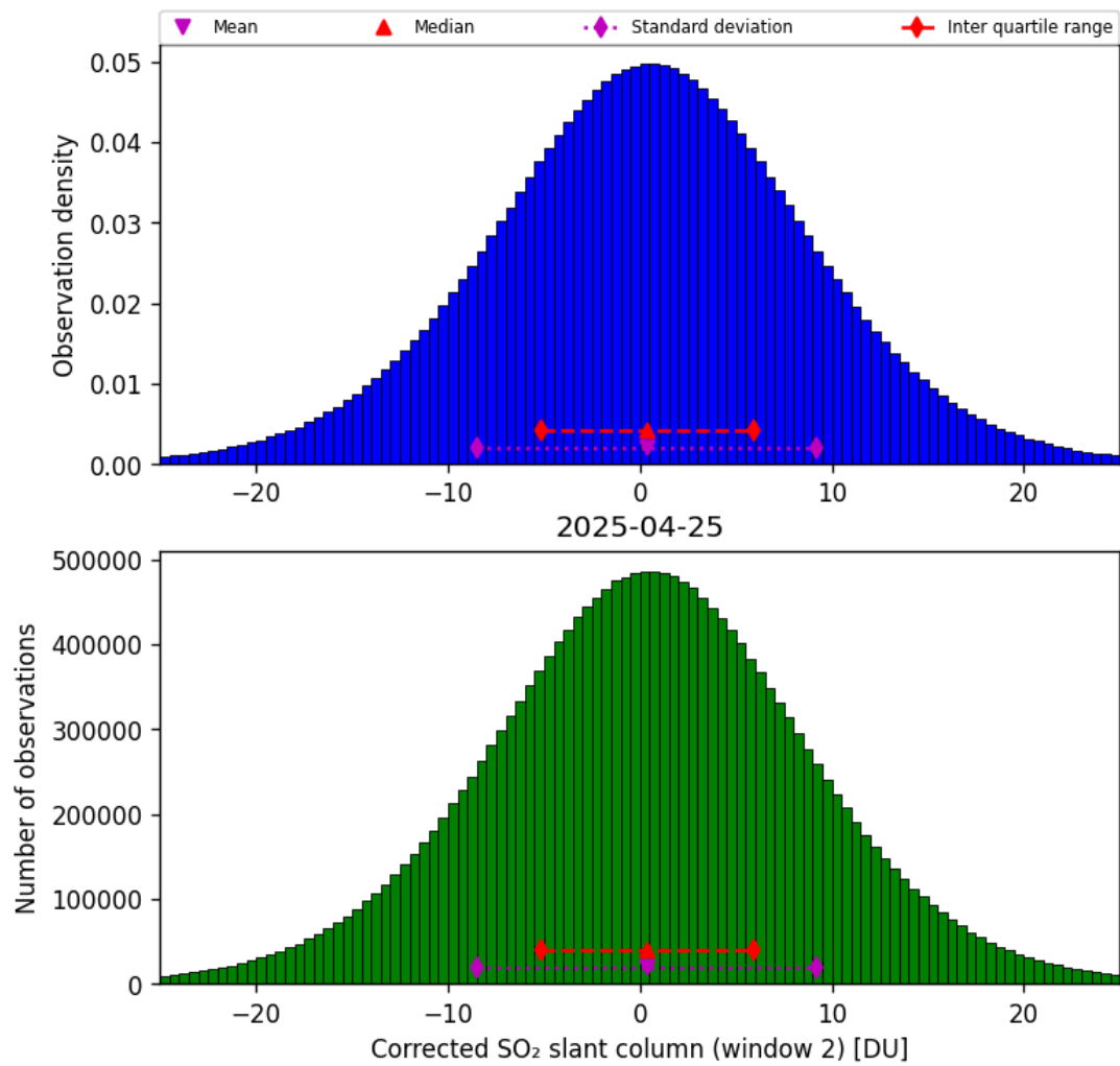
Figure 69: Histogram of “Corrected SO 2 slant column (window 2)” for 2025-04-24 to 2025-04-26
