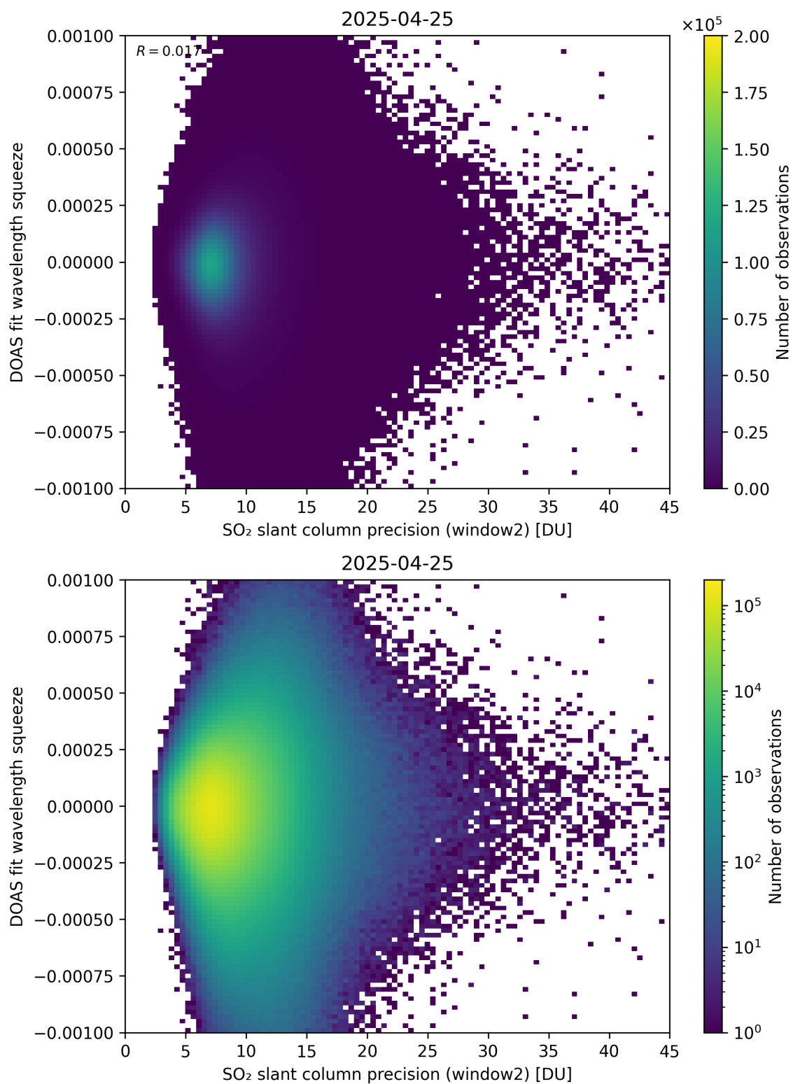
Figure 294: Scatter density plot of “SO 2 slant column precision (window2)” against “DOAS fit wavelength squeeze” for 2025-04-24 to 2025-04-26.
