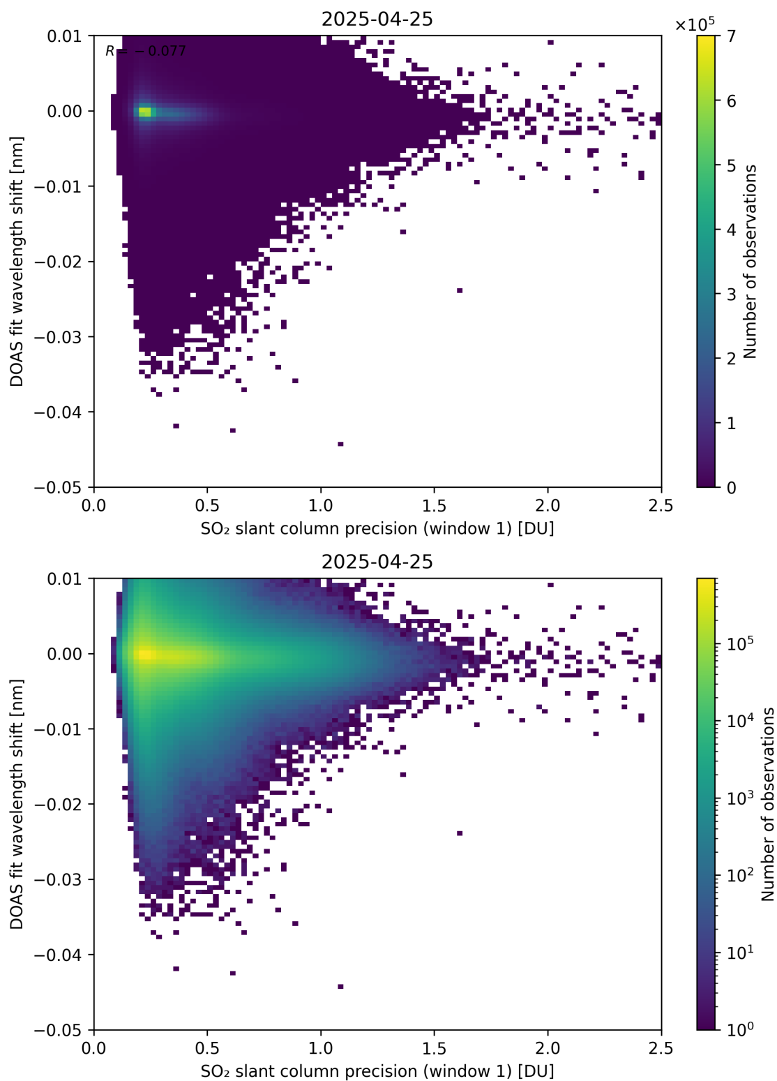
Figure 271: Scatter density plot of “SO 2 slant column precision (window 1)” against “DOAS fit wavelength shift” for 2025-04-24 to 2025-04-26.
