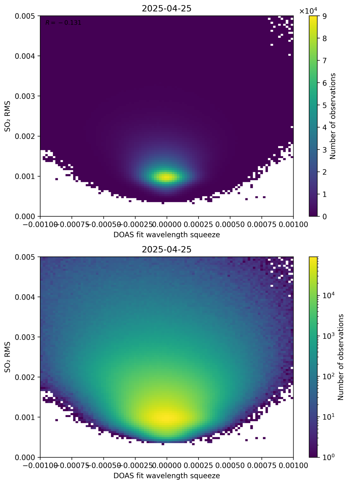
Figure 143: Scatter density plot of “DOAS fit wavelength squeeze” against “SO 2 RMS” for 2025-04-24 to 2025-04-26.
