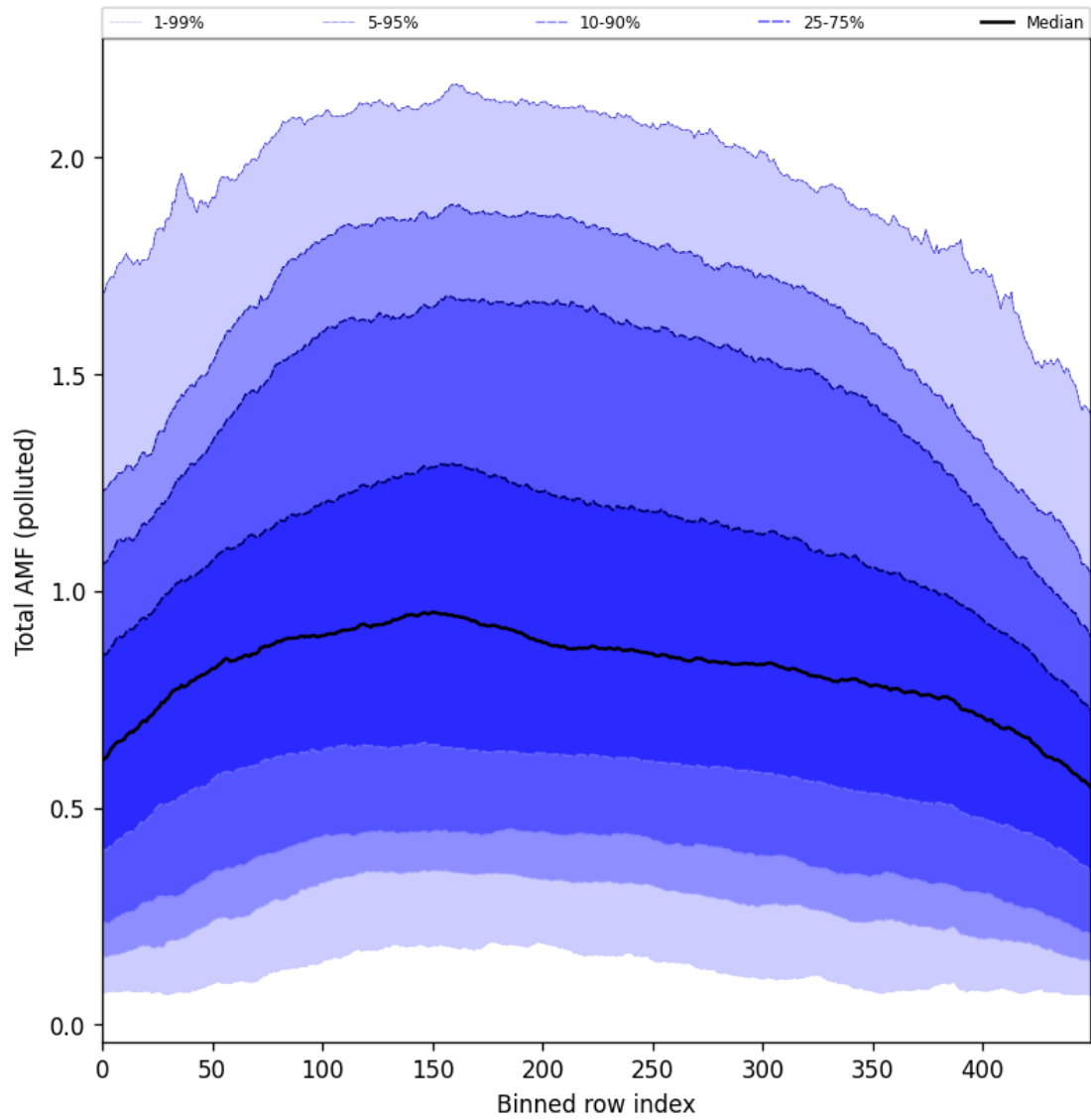
Figure 105: Along track statistics of “Total AMF (polluted)” for 2025-04-24 to 2025-04-26
