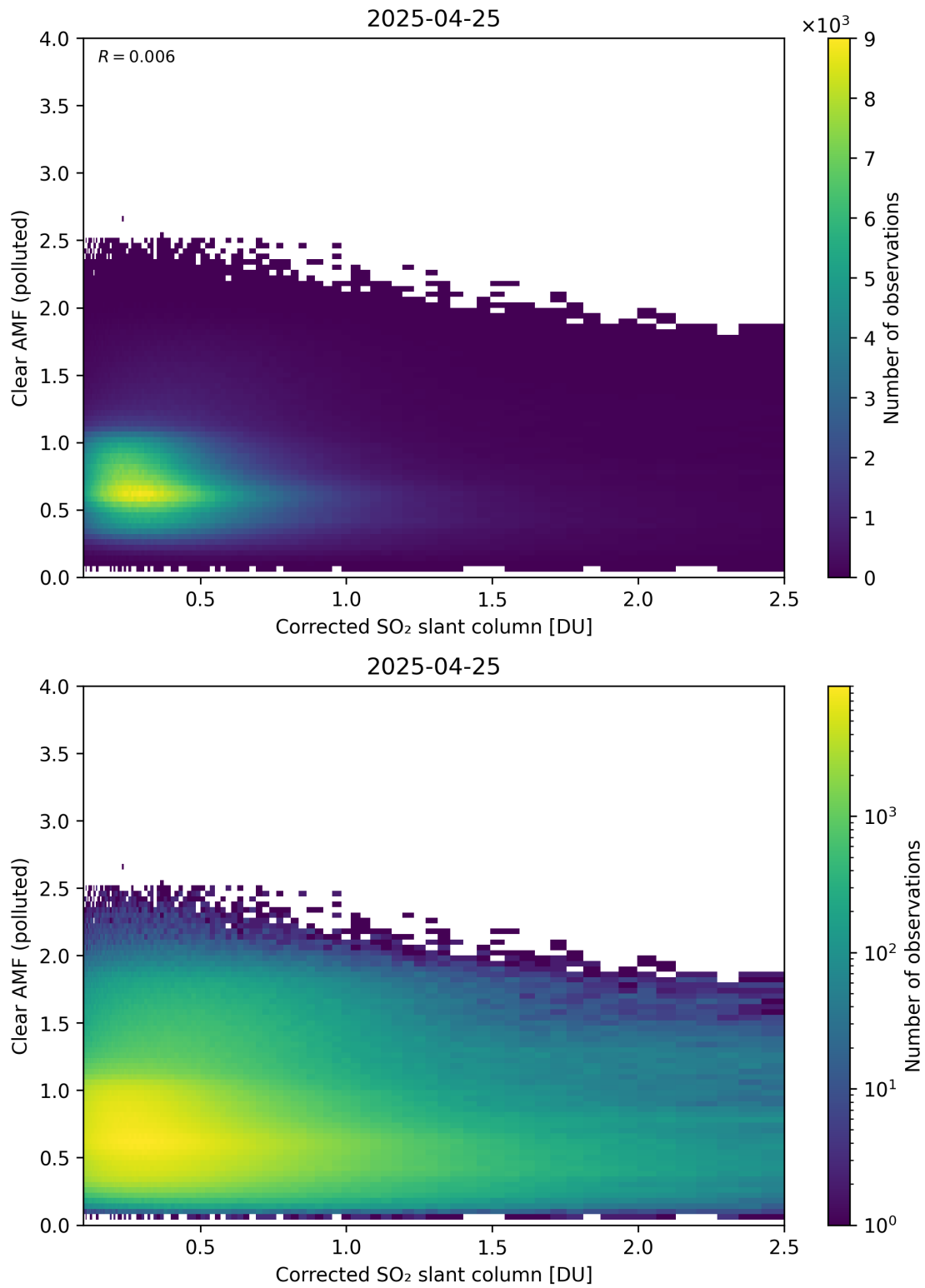
Figure 232: Scatter density plot of “Corrected SO 2 slant column” against “Clear AMF (polluted)” for 2025-04-24 to 2025-04-26.
