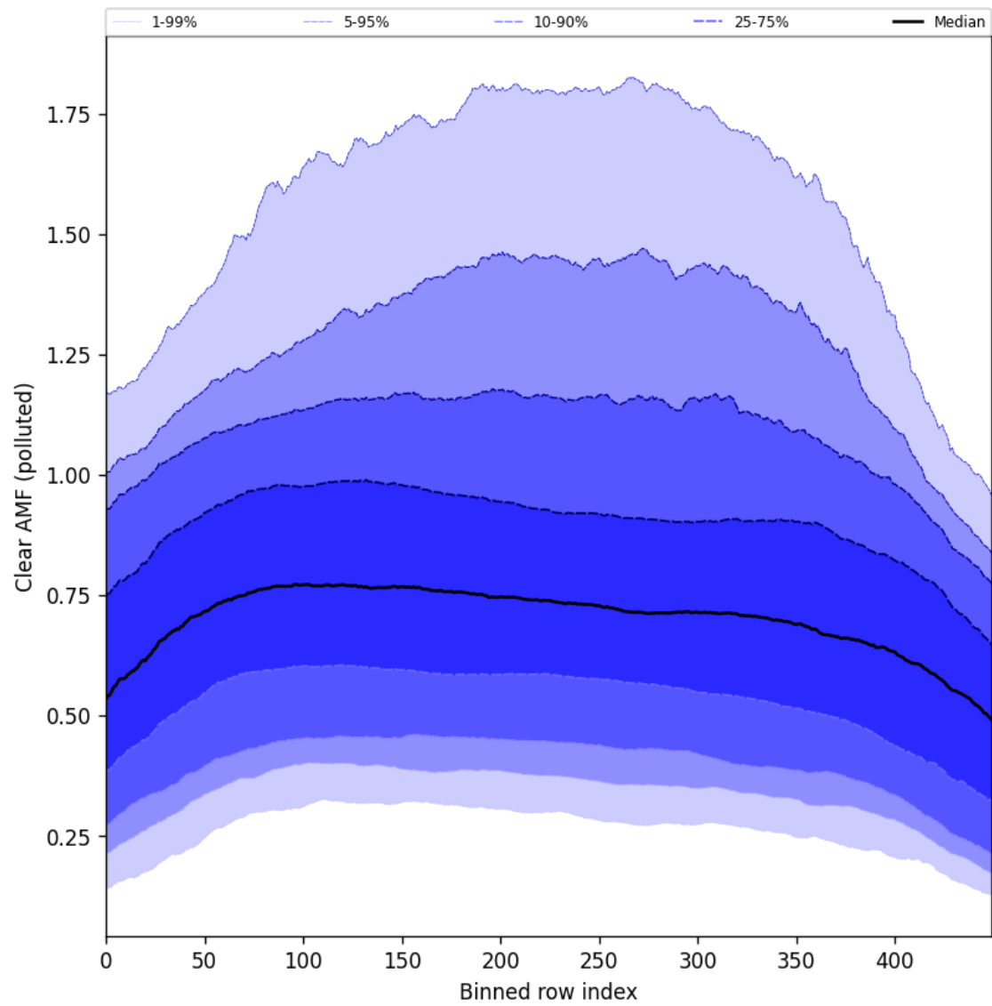
Figure 107: Along track statistics of “Clear AMF (polluted)” for 2025-04-24 to 2025-04-26
