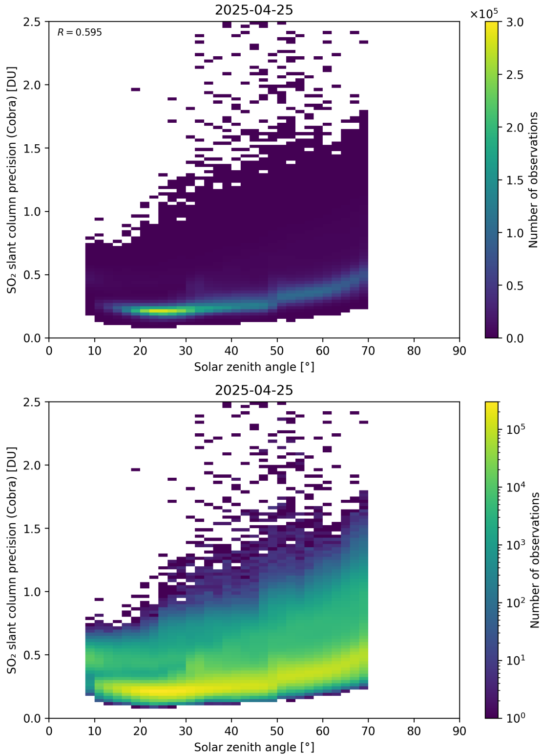
Figure 180: Scatter density plot of “Solar zenith angle” against “SO 2 slant column precision (Cobra)” for 2025-04-24 to 2025-04-26.
