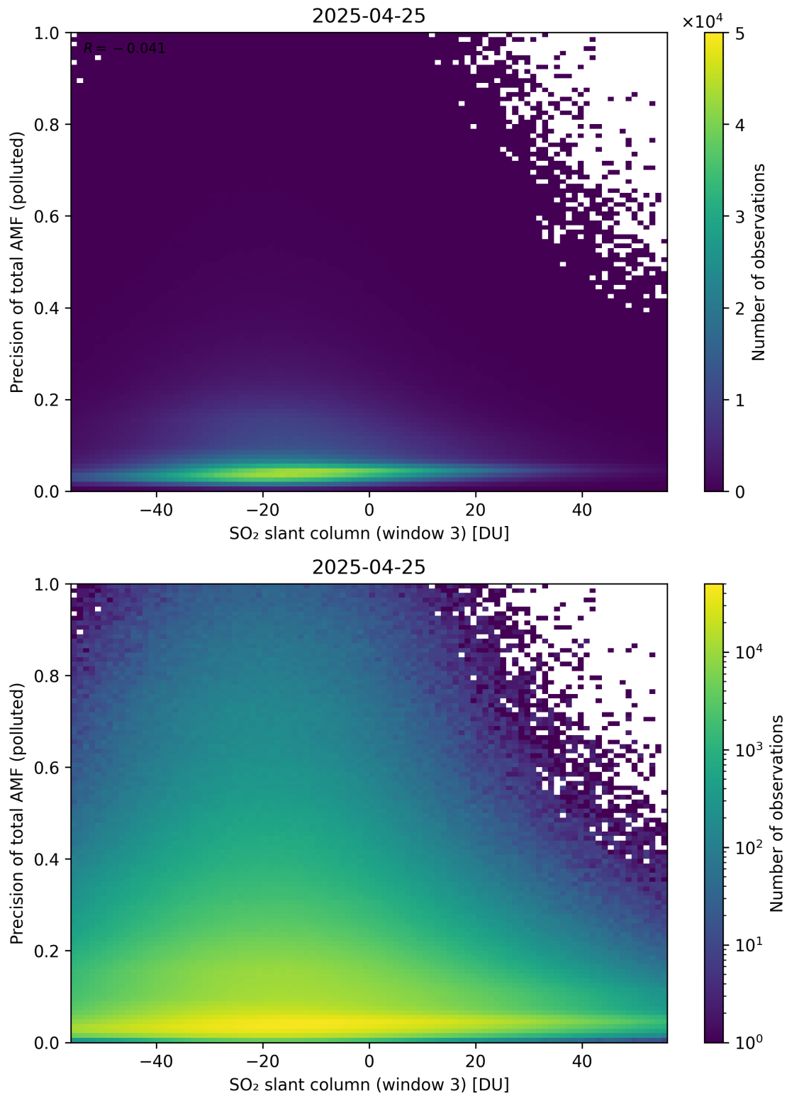
Figure 319: Scatter density plot of “SO 2 slant column (window 3)” against “Precision of total AMF (polluted)” for 2025-04-24 to 2025-04-26.
