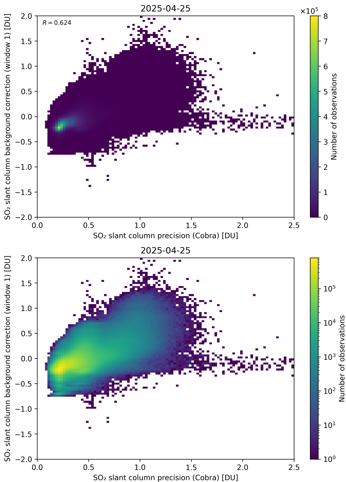
Figure 199: Scatter density plot of “SO 2 slant column precision (Cobra)” against “SO 2 slant column background correction (window 1)” for 2025-04-24 to 2025-04-26.
