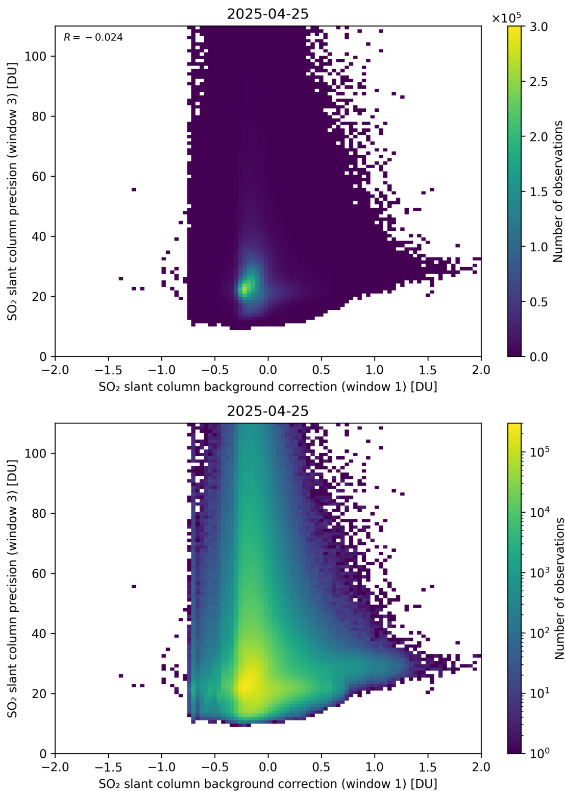
Figure 119: Scatter density plot of “SO 2 slant column background correction (window 1)” against “SO 2 slant column precision (window 3)” for 2025-04-24 to 2025-04-26.
