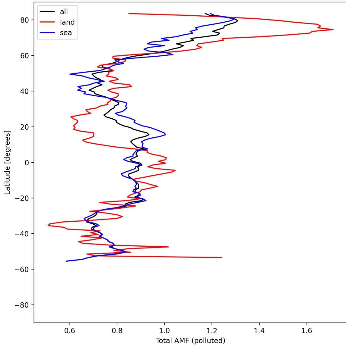
Figure 53: Zonal average of “Total AMF (polluted)” for 2025-04-24 to 2025-04-26.
