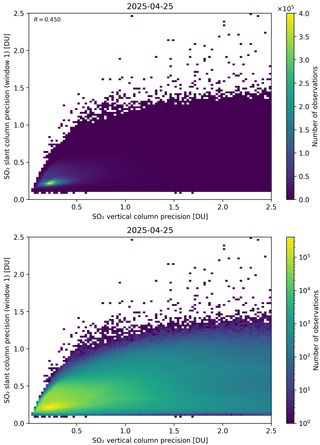
Figure 342: Scatter density plot of “SO 2 vertical column precision” against “SO 2 slant column precision (window 1)” for 2025-04-24 to 2025-04-26.
