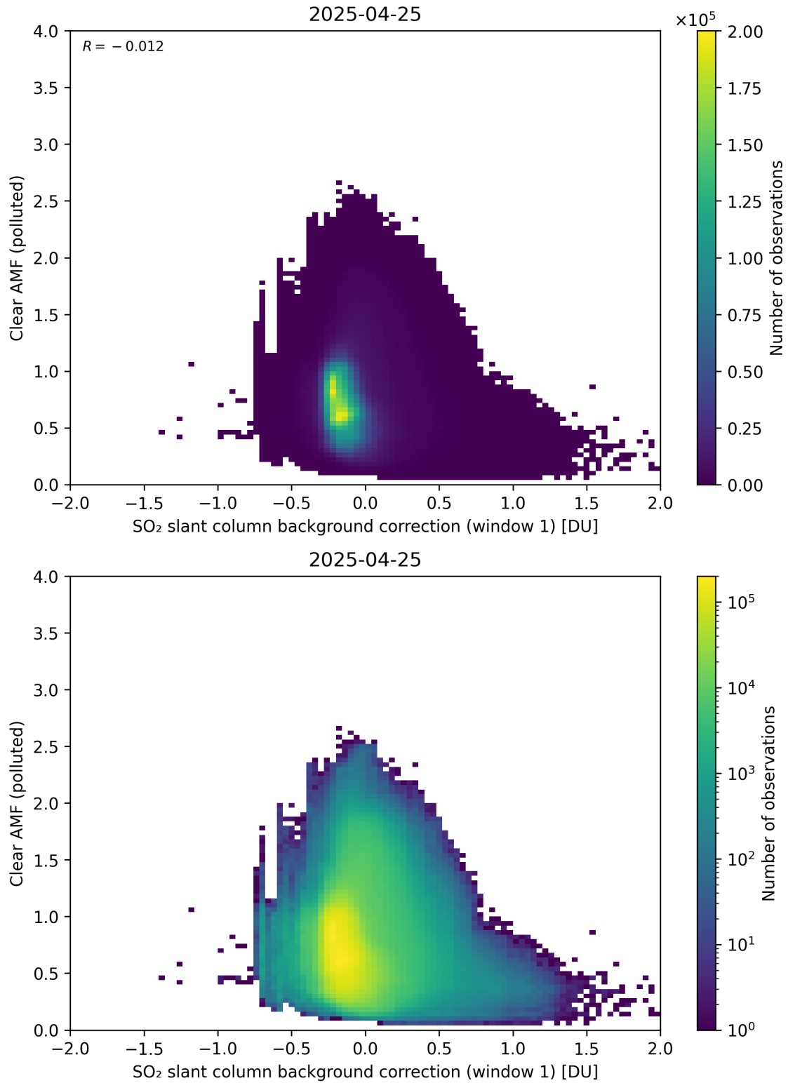
Figure 114: Scatter density plot of “SO 2 slant column background correction (window 1)” against “Clear AMF (polluted)” for 2025-04-24 to 2025-04-26.
