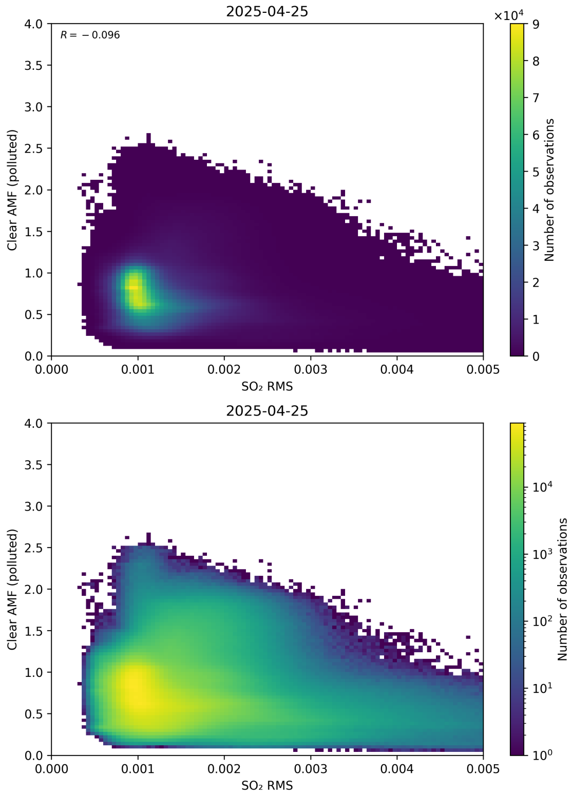
Figure 147: Scatter density plot of “SO 2 RMS” against “Clear AMF (polluted)” for 2025-04-24 to 2025-04-26.
