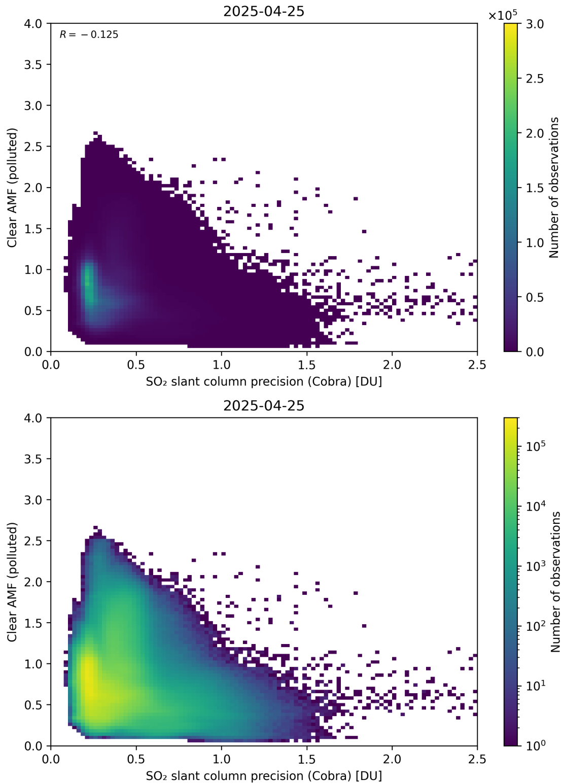
Figure 205: Scatter density plot of “SO 2 slant column precision (Cobra)” against “Clear AMF (polluted)” for 2025-04-24 to 2025-04-26.
