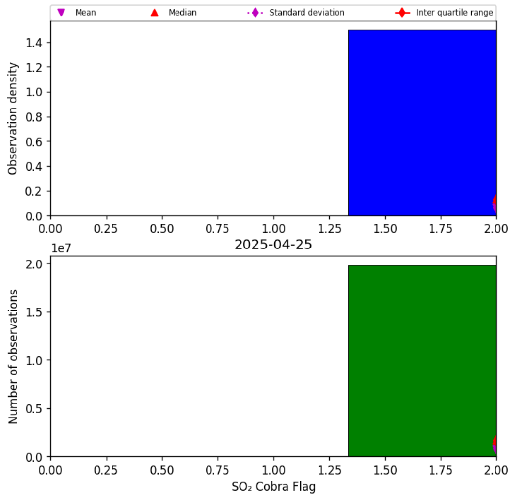
Figure 75: Histogram of “SO 2 Cobra Flag” for 2025-04-24 to 2025-04-26
