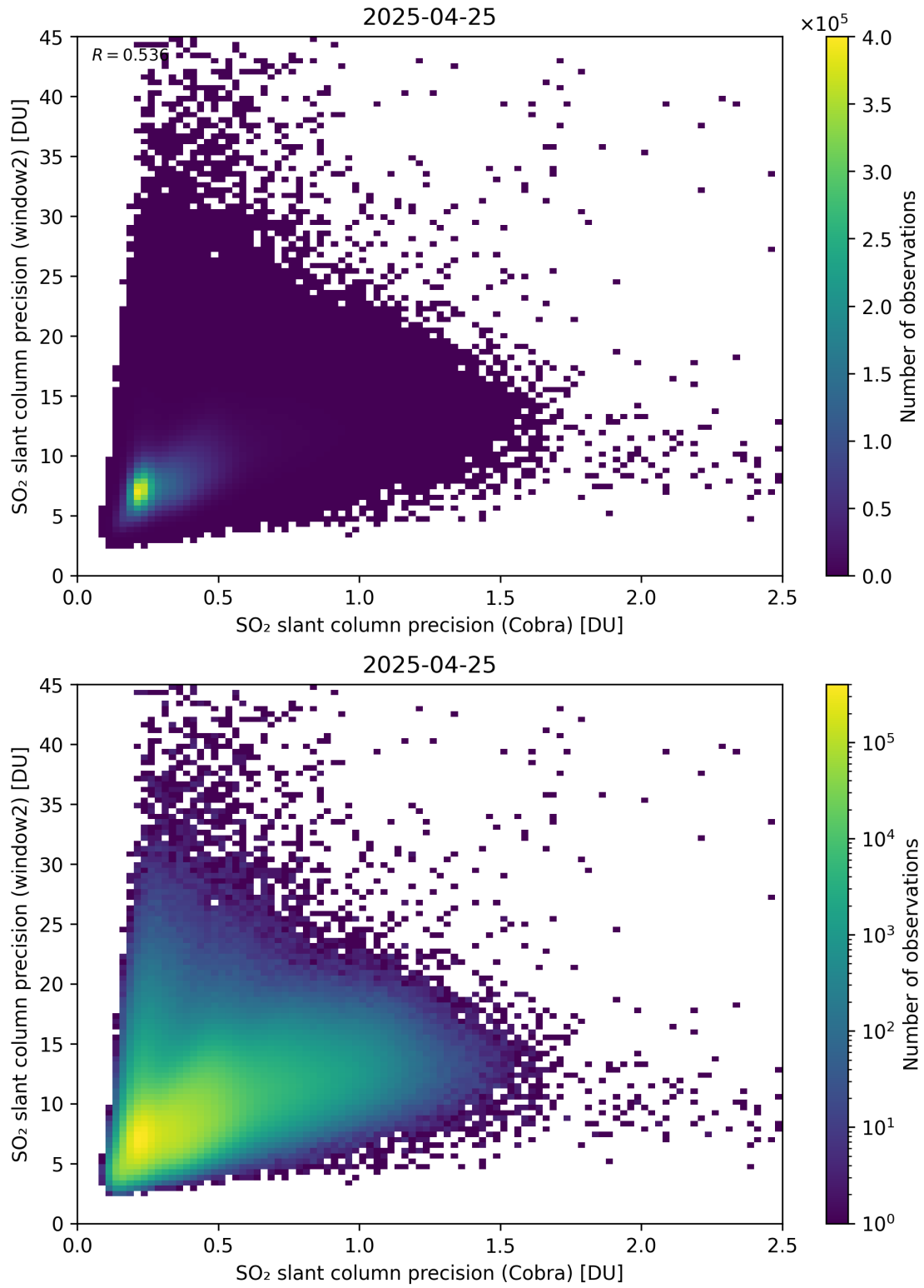
Figure 210: Scatter density plot of “SO 2 slant column precision (Cobra)” against “SO 2 slant column precision (window2)” for 2025-04-24 to 2025-04-26.
