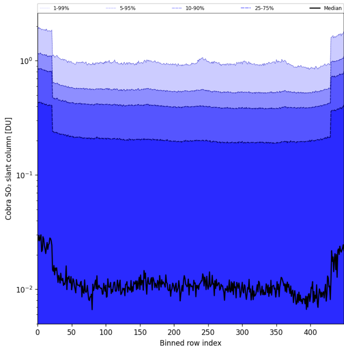
Figure 87: Along track statistics of “Cobra SO 2 slant column” for 2025-04-24 to 2025-04-26
