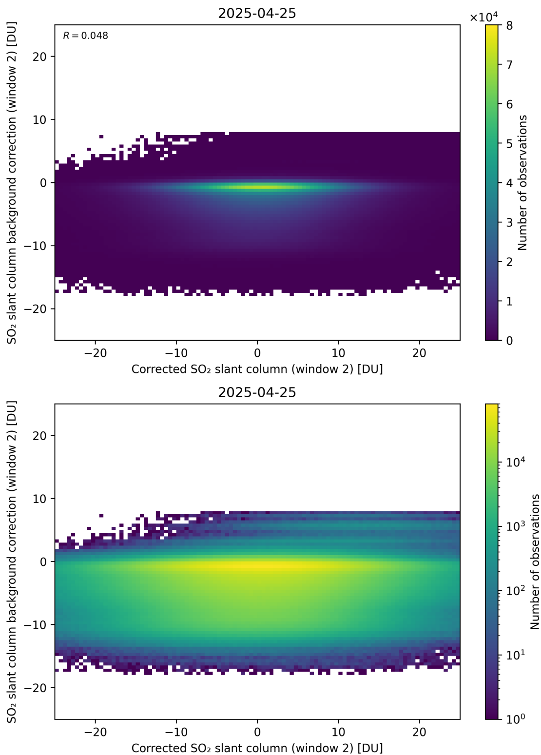
Figure 244: Scatter density plot of “Corrected SO 2 slant column (window 2)” against “SO 2 slant column background correction (window 2)” for 2025-04-24 to 2025-04-26.
