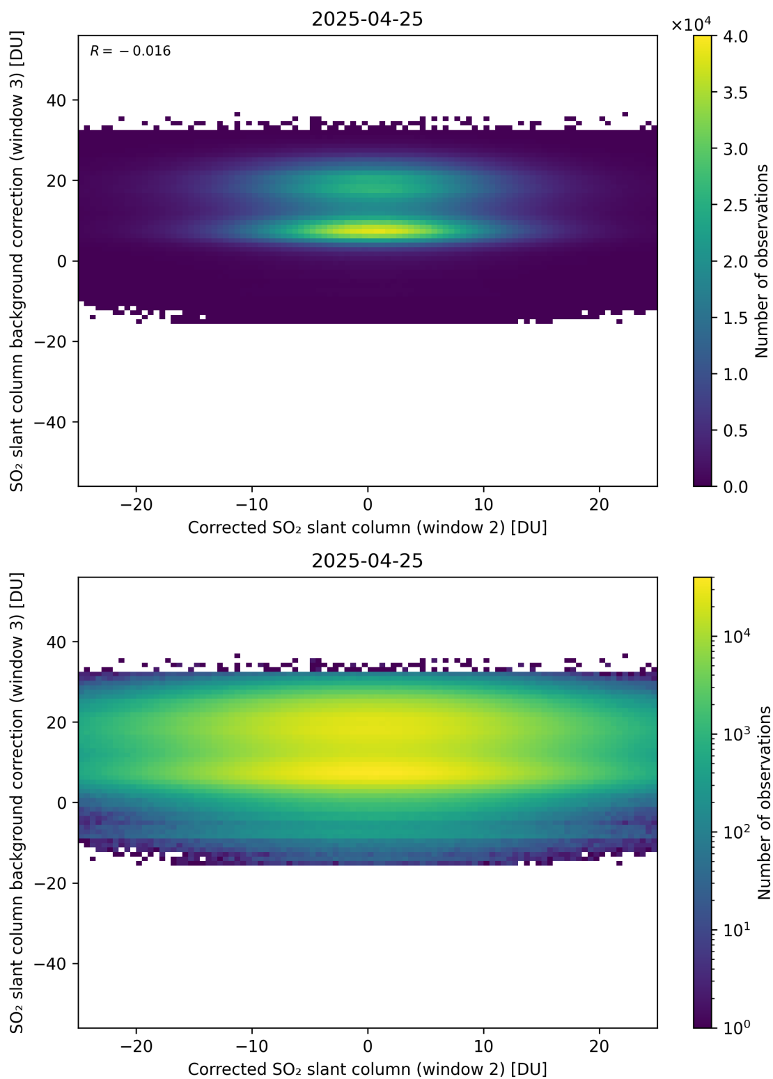
Figure 245: Scatter density plot of “Corrected SO 2 slant column (window 2)” against “SO 2 slant column background correction (window 3)” for 2025-04-24 to 2025-04-26.
