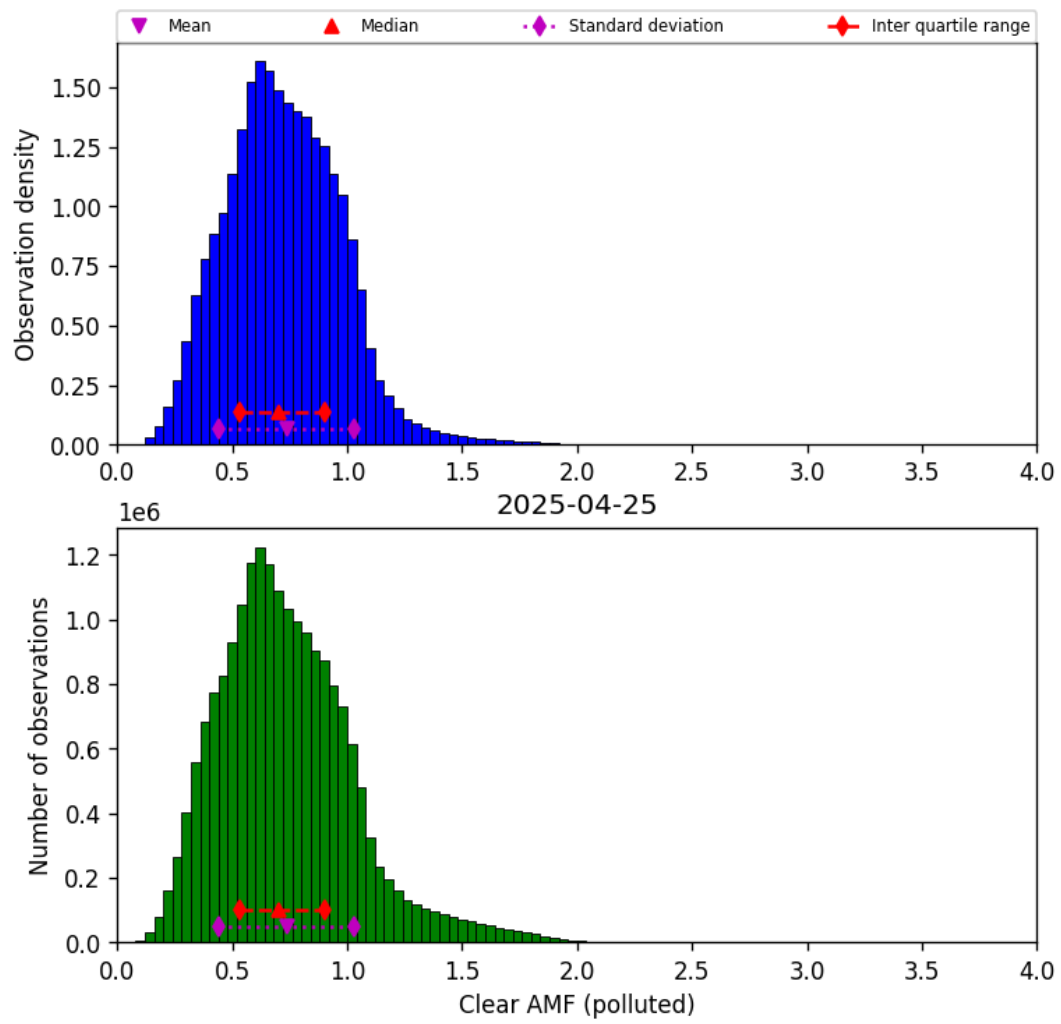
Figure 81: Histogram of “Clear AMF (polluted)” for 2025-04-24 to 2025-04-26
