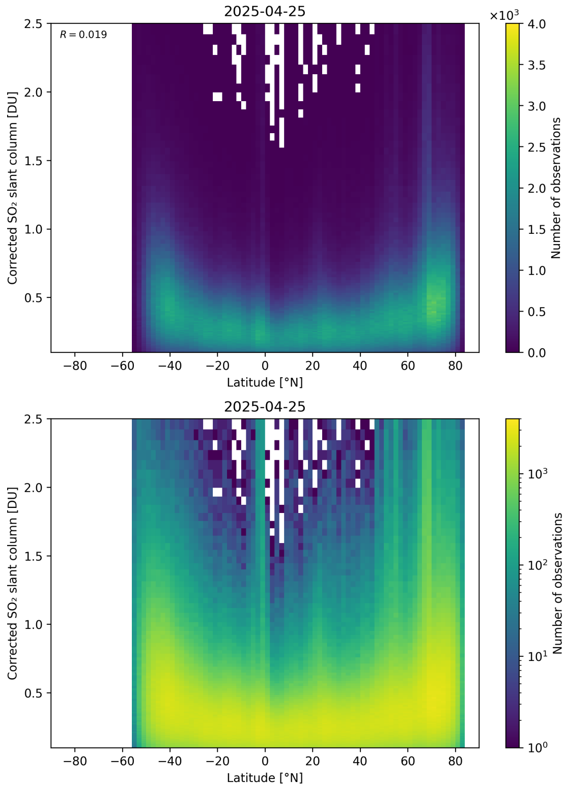
Figure 159: Scatter density plot of “Latitude” against “Corrected SO 2 slant column” for 2025-04-24 to 2025-04-26.
