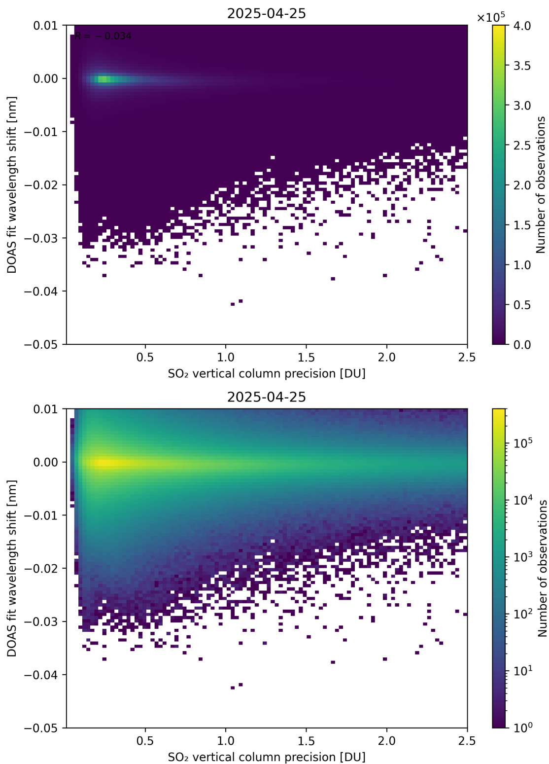
Figure 332: Scatter density plot of “SO 2 vertical column precision” against “DOAS fit wavelength shift” for 2025-04-24 to 2025-04-26.
