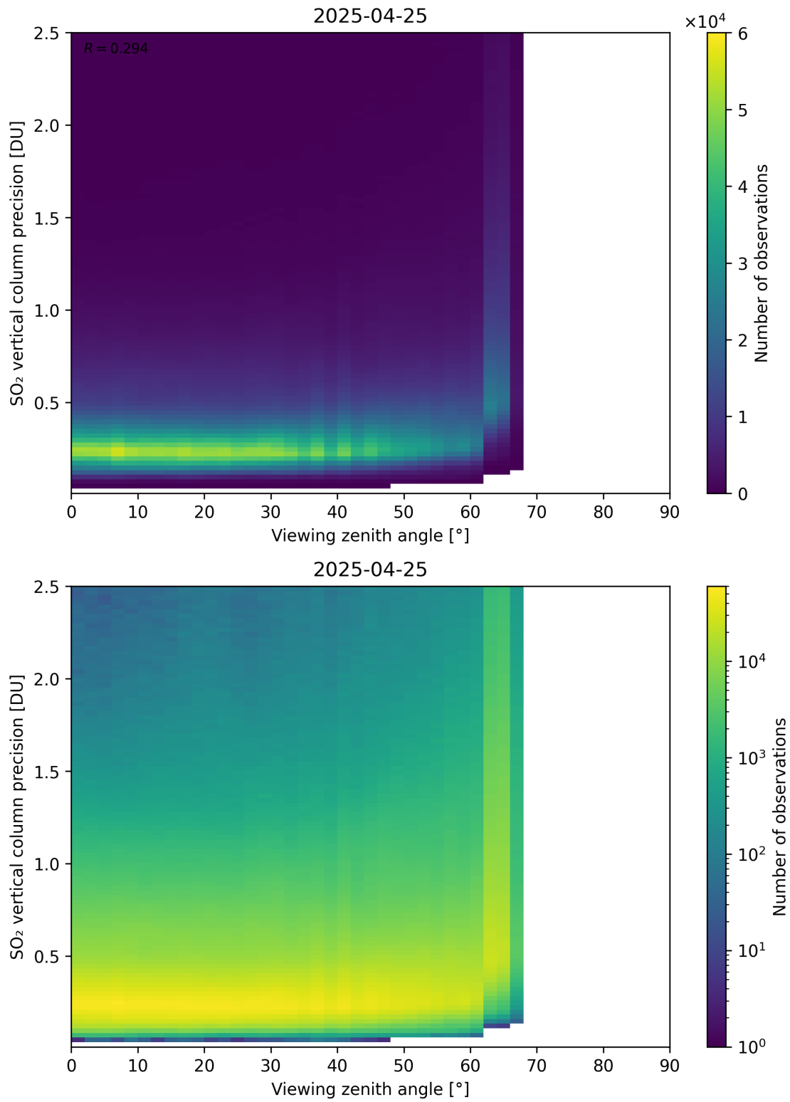
Figure 384: Scatter density plot of “Viewing zenith angle” against “SO 2 vertical column precision” for 2025-04-24 to 2025-04-26.
