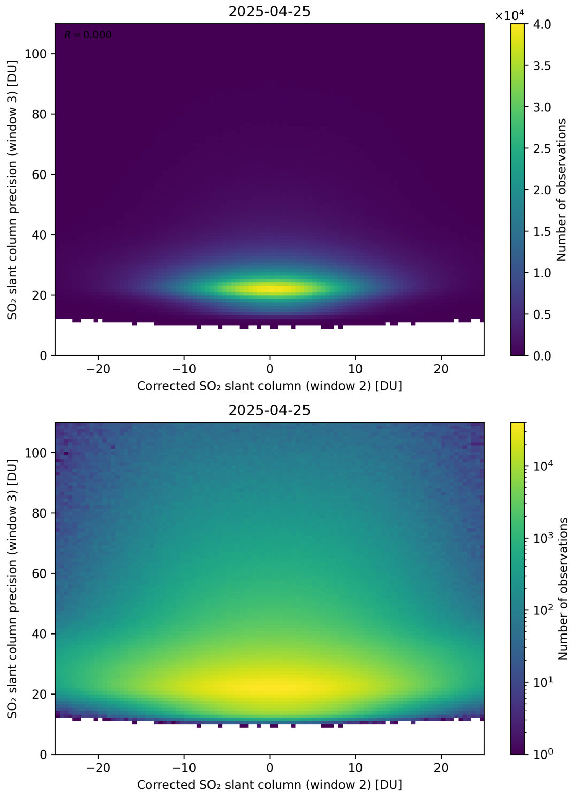
Figure 252: Scatter density plot of “Corrected SO 2 slant column (window 2)” against “SO 2 slant column precision (window 3)” for 2025-04-24 to 2025-04-26.
