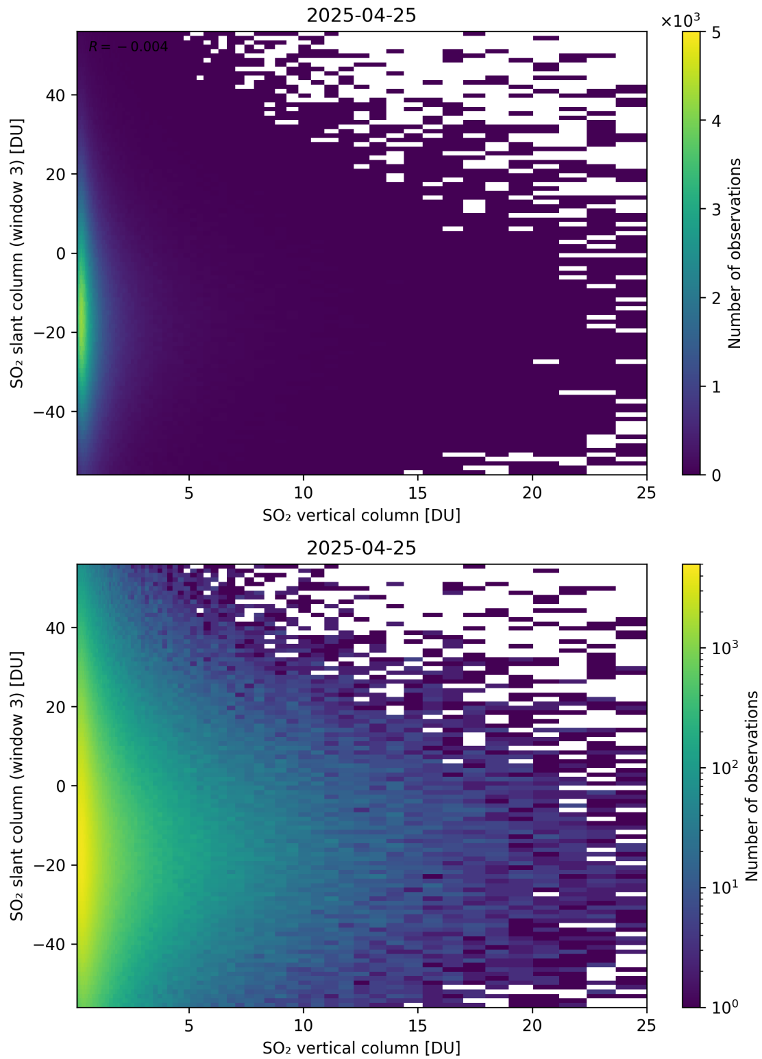
Figure 357: Scatter density plot of “SO 2 vertical column” against “SO 2 slant column (window 3)” for 2025-04-24 to 2025-04-26.
