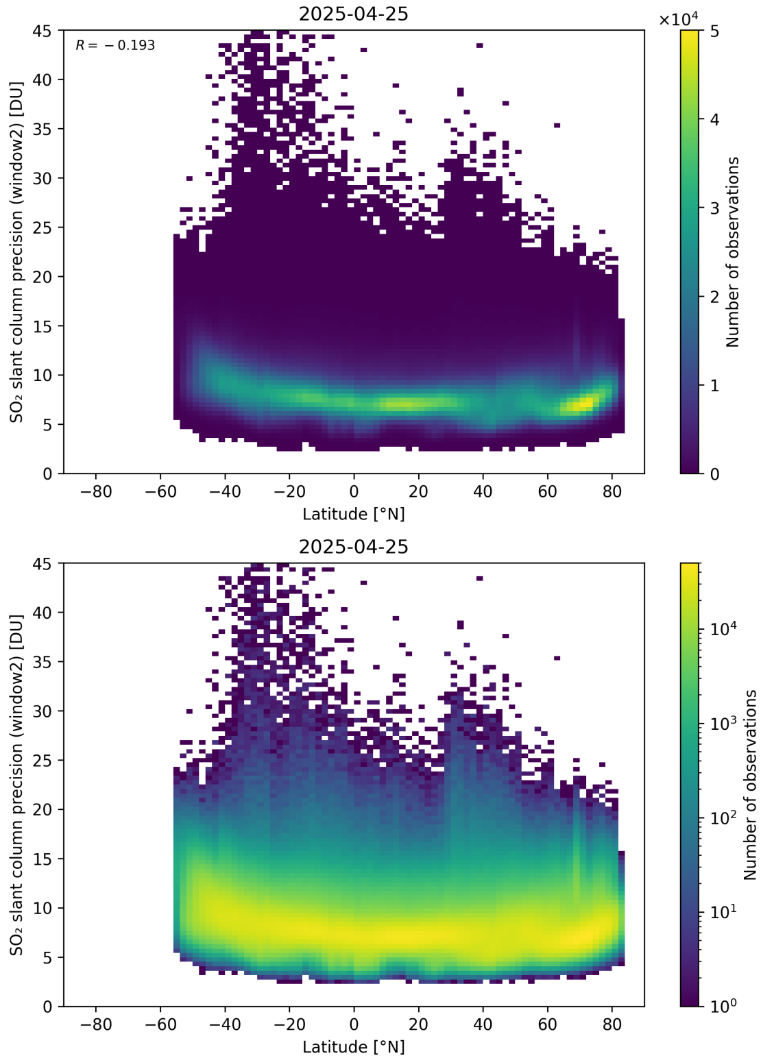
Figure 164: Scatter density plot of “Latitude” against “SO 2 slant column precision (window2)” for 2025-04-24 to 2025-04-26.
