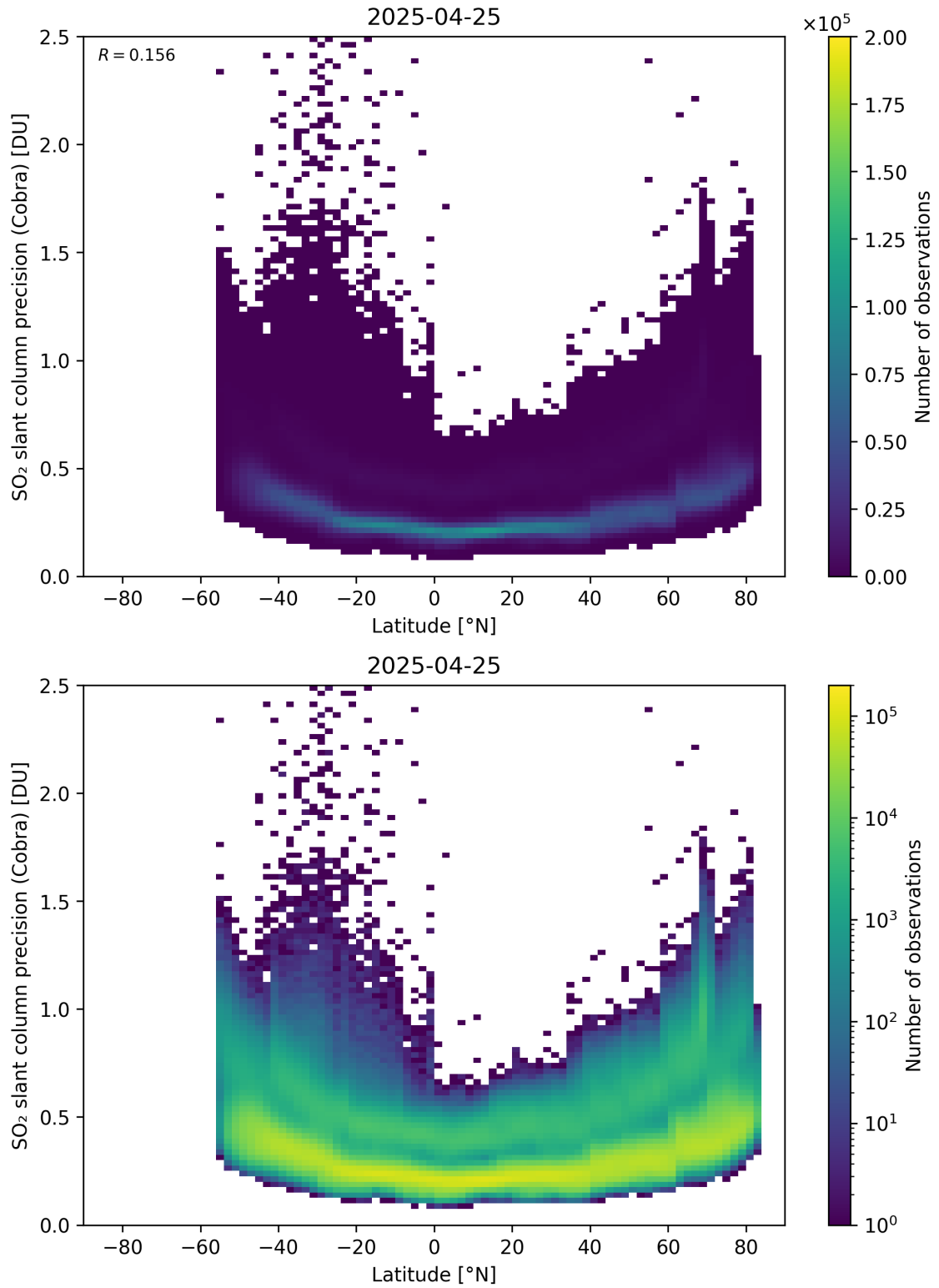
Figure 158: Scatter density plot of “Latitude” against “SO 2 slant column precision (Cobra)” for 2025-04-24 to 2025-04-26.
