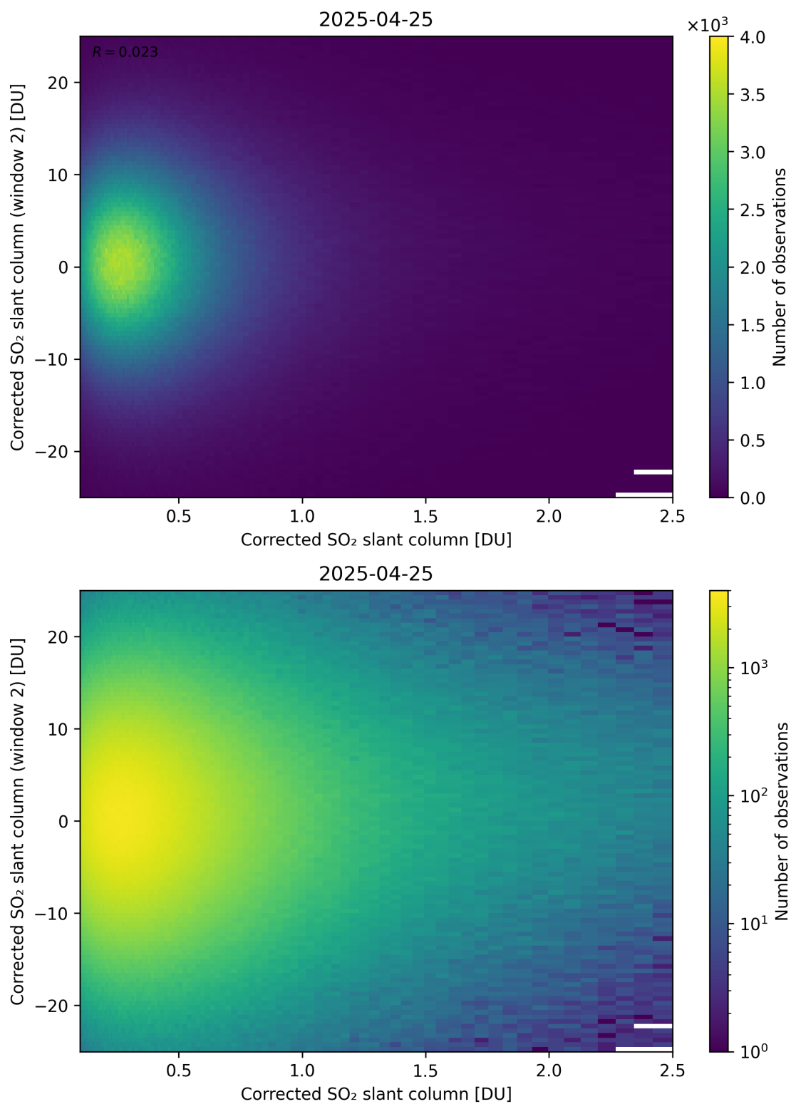
Figure 235: Scatter density plot of “Corrected SO 2 slant column” against “Corrected SO 2 slant column (window 2)” for 2025-04-24 to 2025-04-26.
