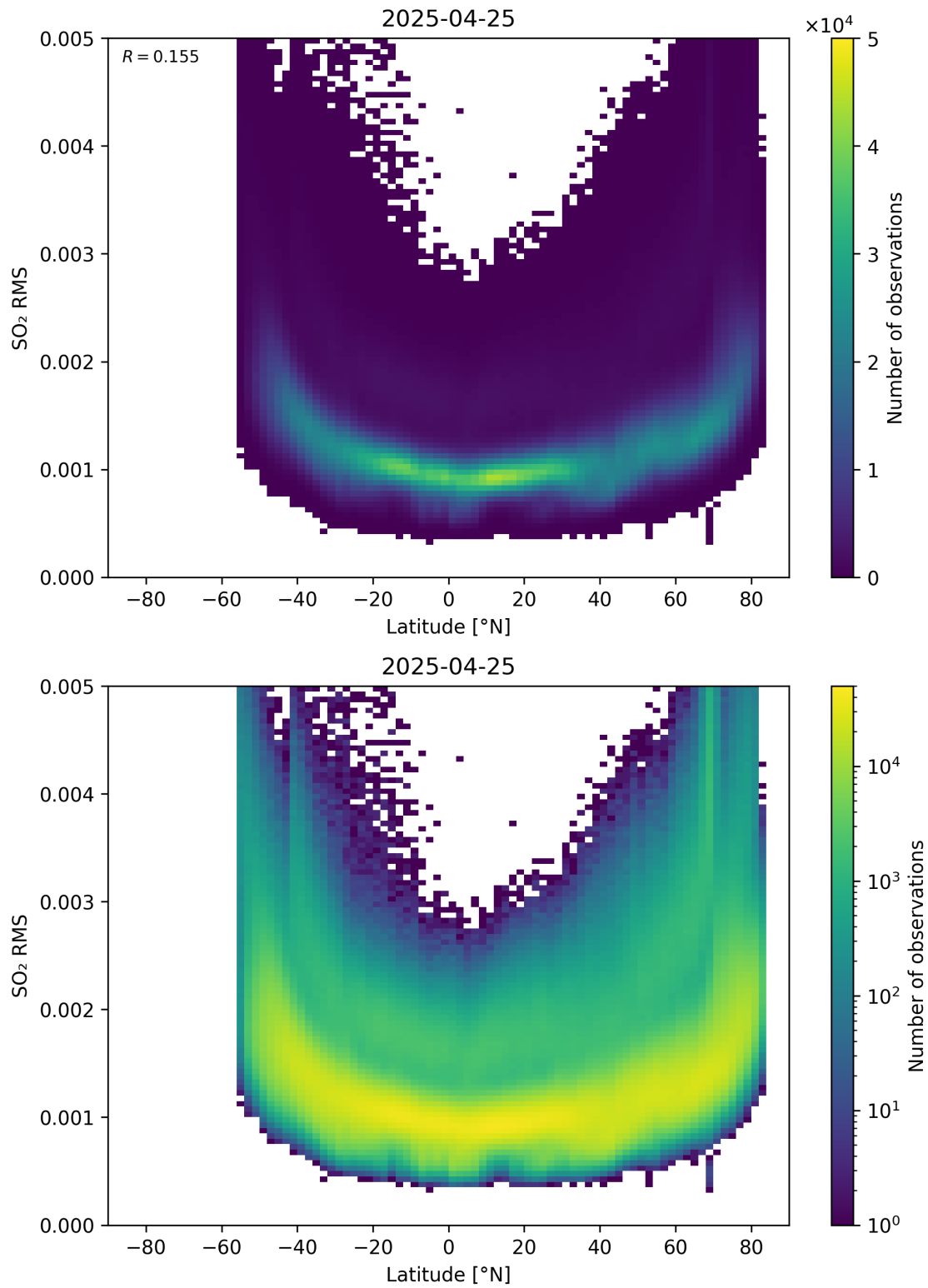
Figure 155: Scatter density plot of “Latitude” against “SO 2 RMS” for 2025-04-24 to 2025-04-26.
