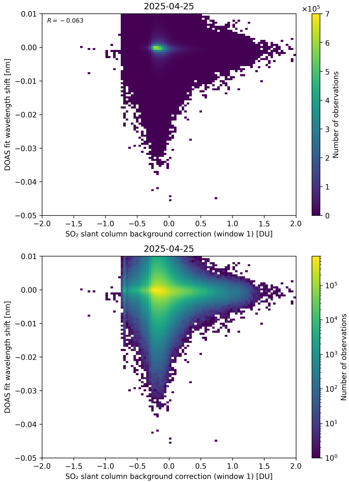
Figure 111: Scatter density plot of “SO 2 slant column background correction (window 1)” against “DOAS fit wavelength shift” for 2025-04-24 to 2025-04-26.
