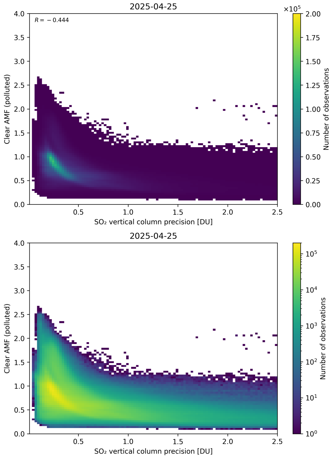
Figure 335: Scatter density plot of “SO 2 vertical column precision” against “Clear AMF (polluted)” for 2025-04-24 to 2025-04-26.
