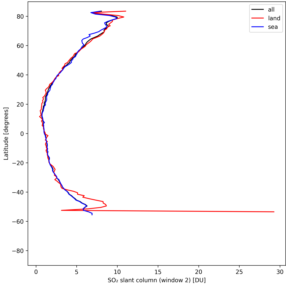
Figure 41: Zonal average of “SO 2 slant column (window 2)” for 2025-04-24 to 2025-04-26.
