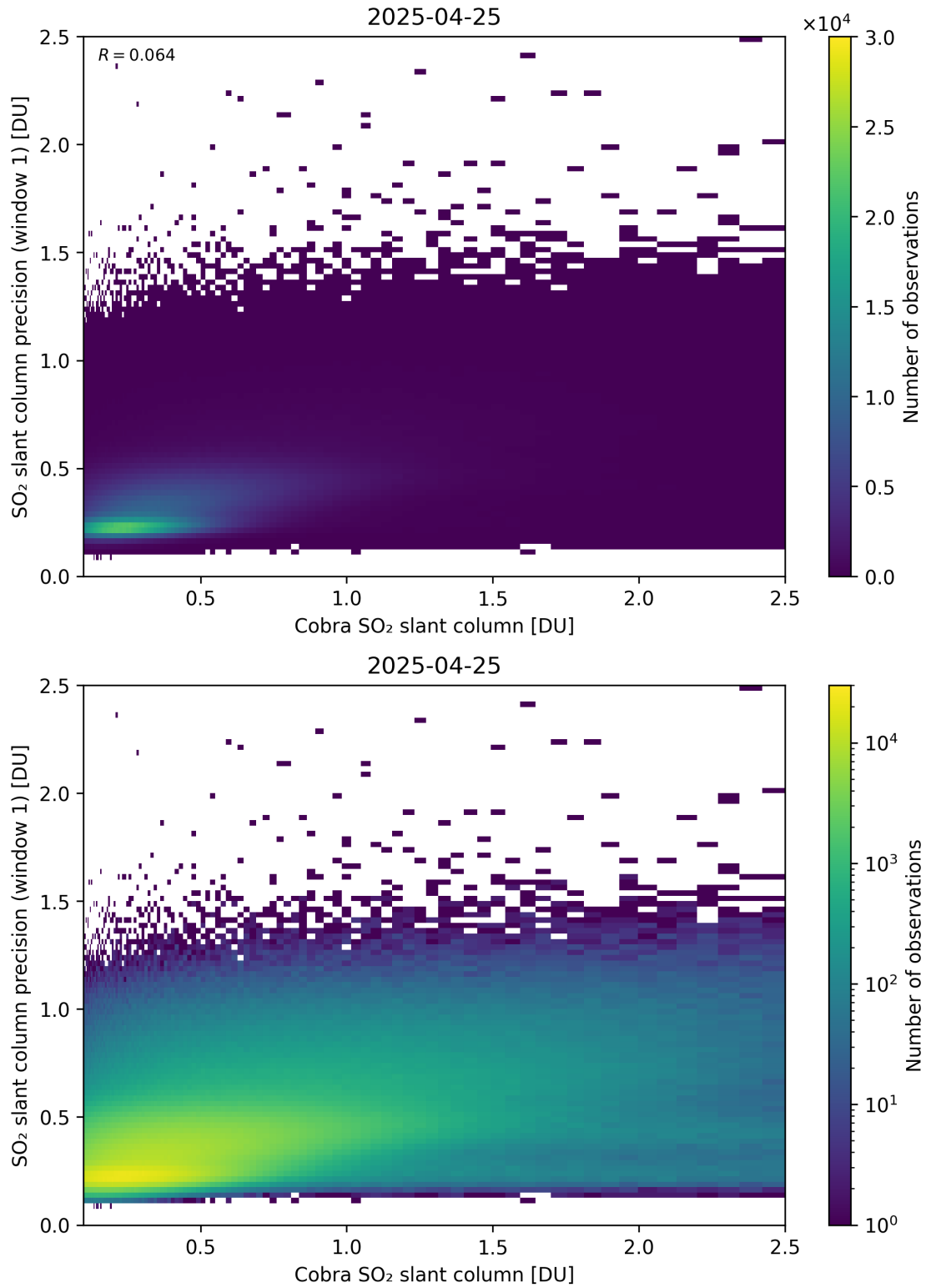
Figure 220: Scatter density plot of “Cobra SO 2 slant column” against “SO 2 slant column precision (window 1)” for 2025-04-24 to 2025-04-26.
