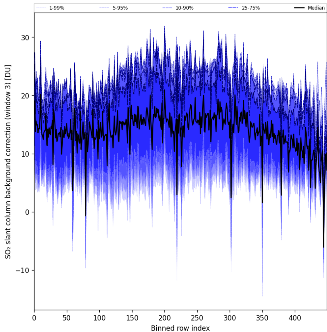
Figure 100: Along track statistics of “SO 2 slant column background correction (window 3)” for 2025-04-24 to 2025-04-26
