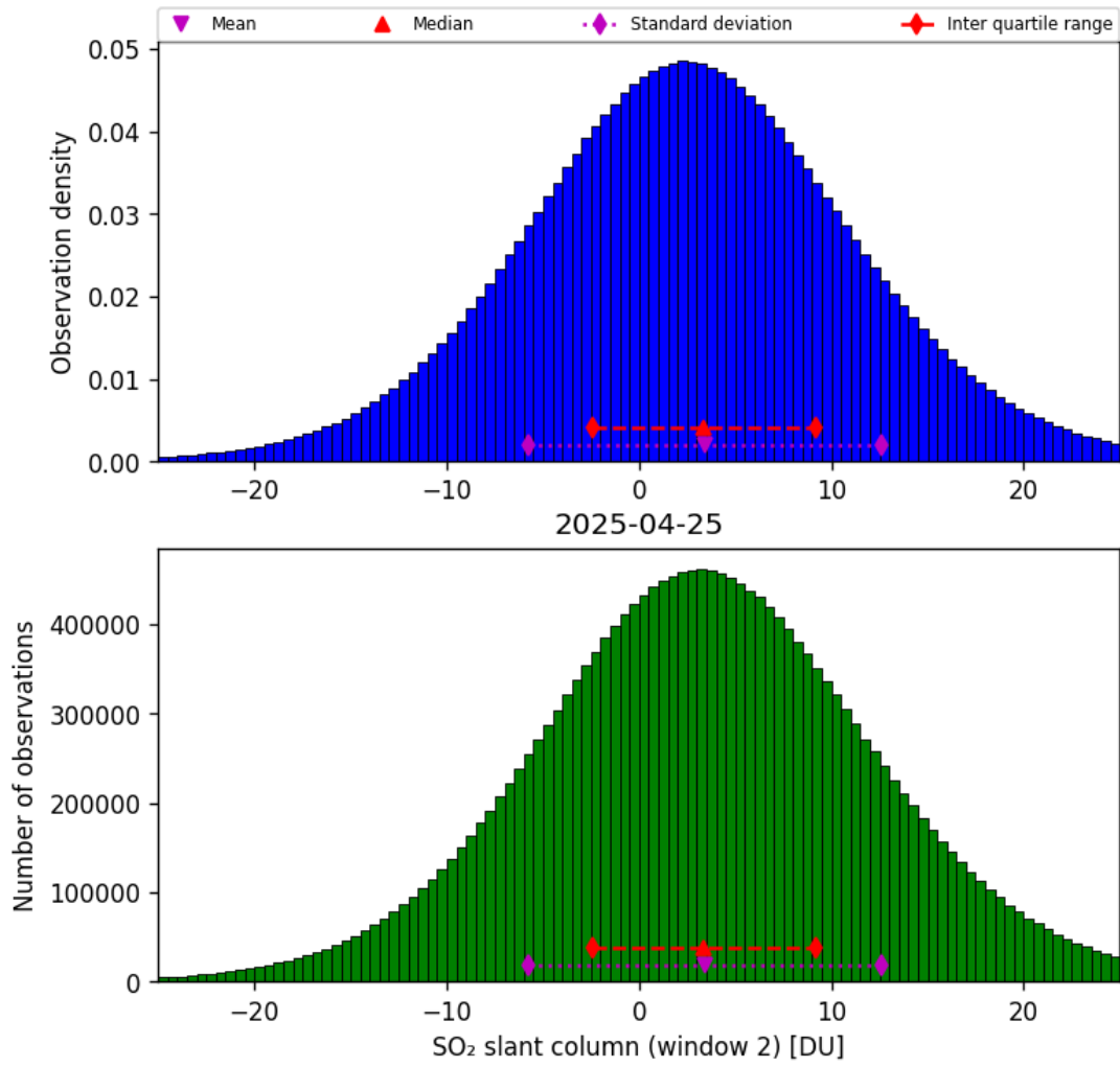
Figure 67: Histogram of “SO 2 slant column (window 2)” for 2025-04-24 to 2025-04-26
