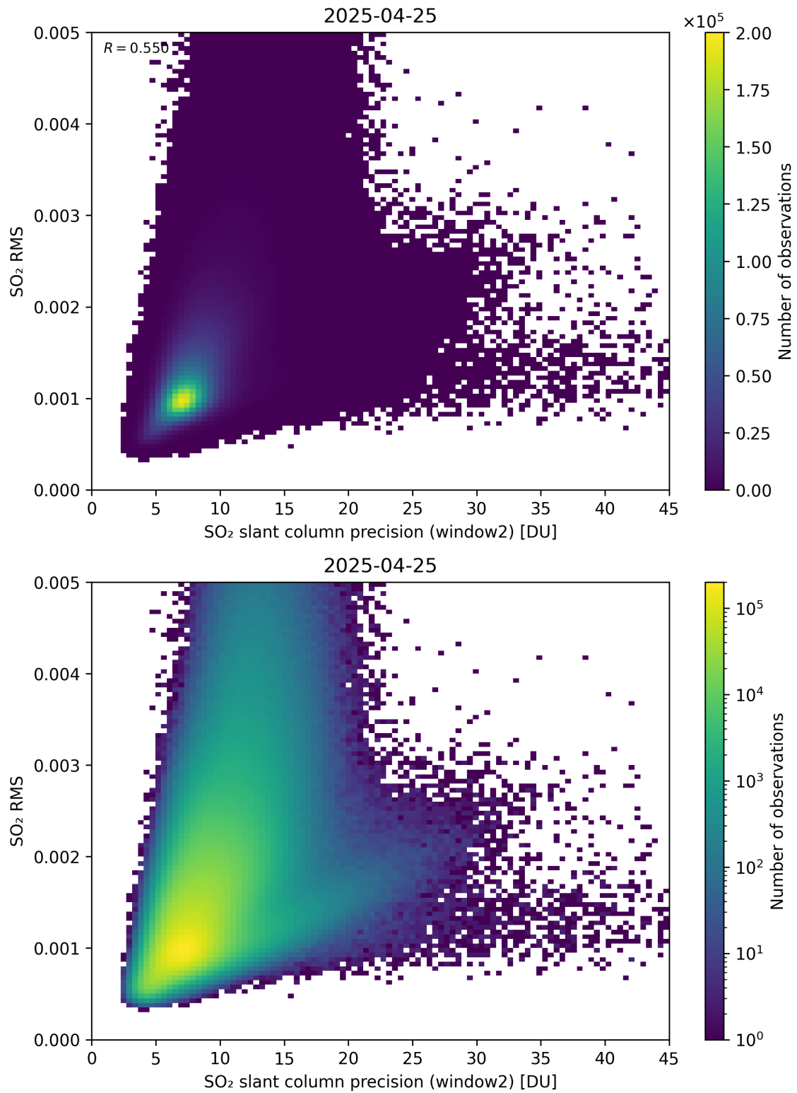
Figure 295: Scatter density plot of “SO 2 slant column precision (window2)” against “SO 2 RMS” for 2025-04-24 to 2025-04-26.
