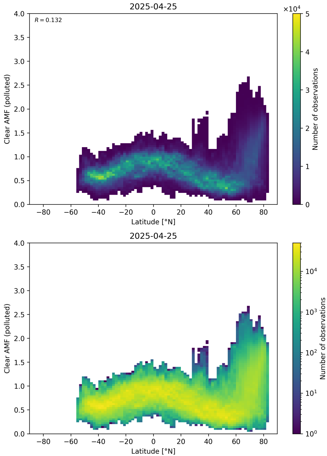
Figure 156: Scatter density plot of “Latitude” against “Clear AMF (polluted)” for 2025-04-24 to 2025-04-26.
