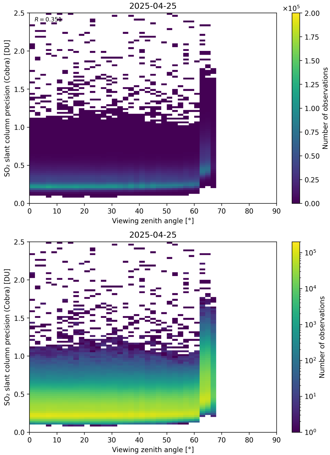
Figure 372: Scatter density plot of “Viewing zenith angle” against “SO 2 slant column precision (Cobra)” for 2025-04-24 to 2025-04-26.
