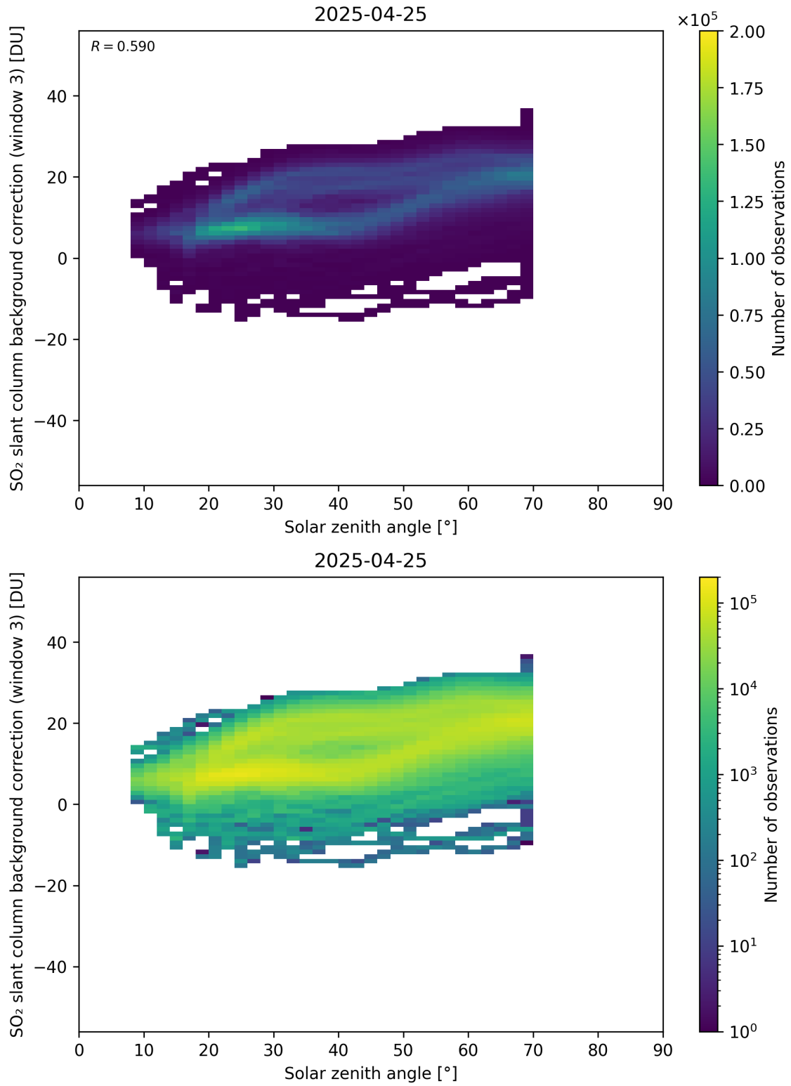
Figure 173: Scatter density plot of “Solar zenith angle” against “SO 2 slant column background correction (window 3)” for 2025-04-24 to 2025-04-26.
