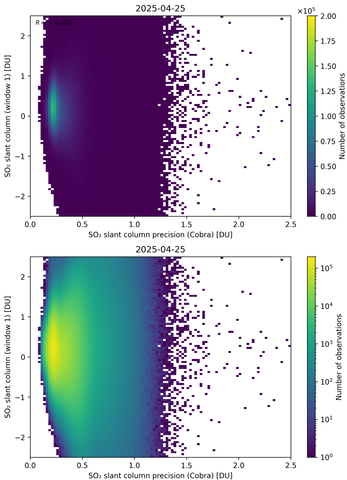
Figure 208: Scatter density plot of “SO 2 slant column precision (Cobra)” against “SO 2 slant column (window 1)” for 2025-04-24 to 2025-04-26.
