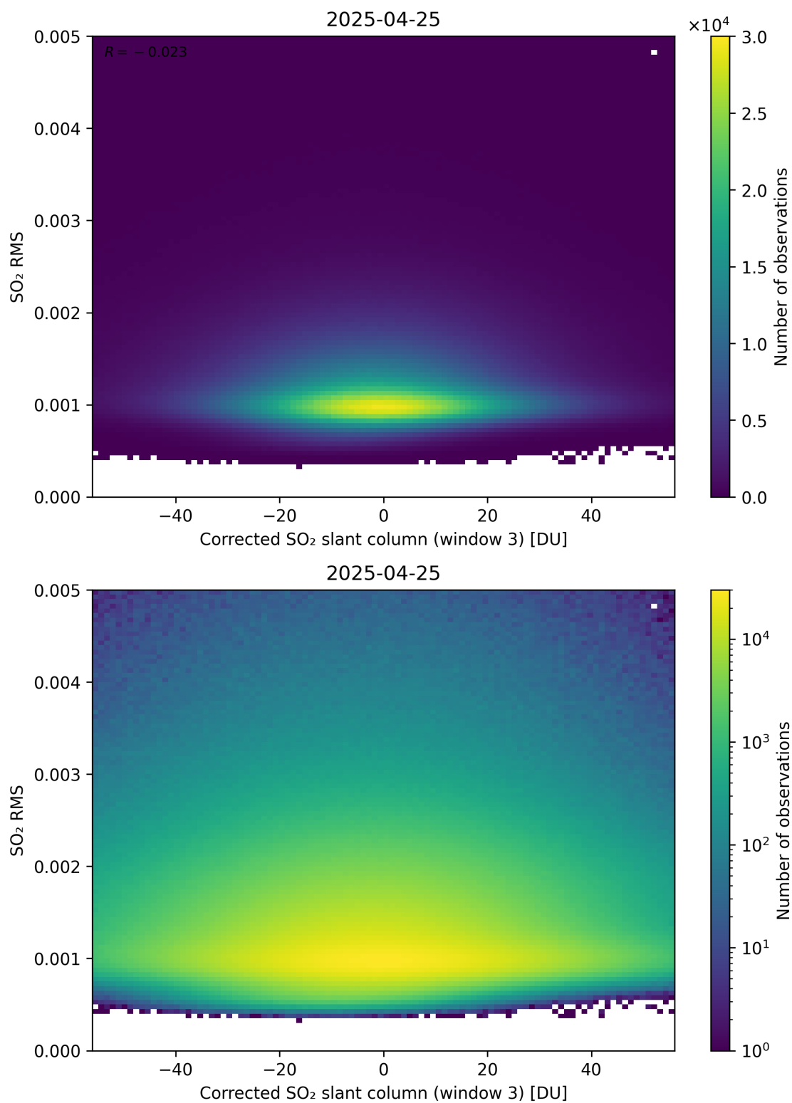
Figure 258: Scatter density plot of “Corrected SO 2 slant column (window 3)” against “SO 2 RMS” for 2025-04-24 to 2025-04-26.
