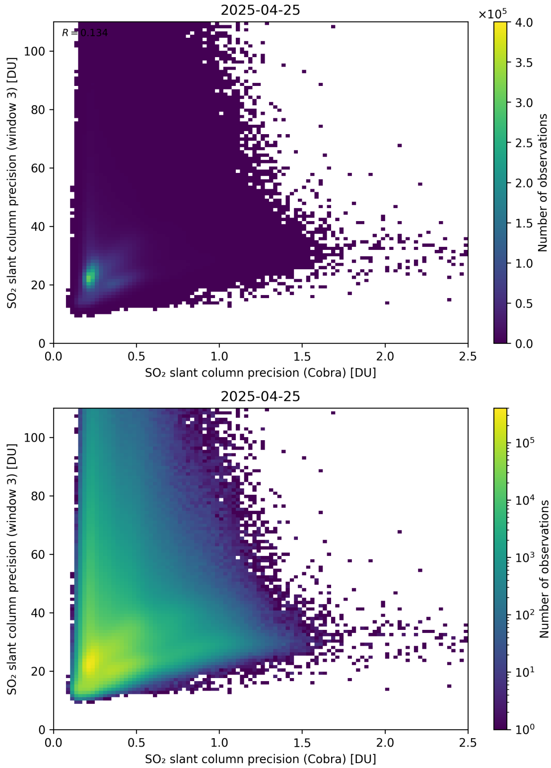
Figure 212: Scatter density plot of “SO 2 slant column precision (Cobra)” against “SO 2 slant column precision (window 3)” for 2025-04-24 to 2025-04-26.
