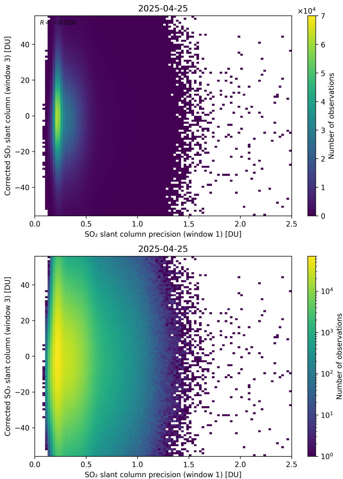
Figure 276: Scatter density plot of “SO 2 slant column precision (window 1)” against “Corrected SO 2 slant column (window 3)” for 2025-04-24 to 2025-04-26.
