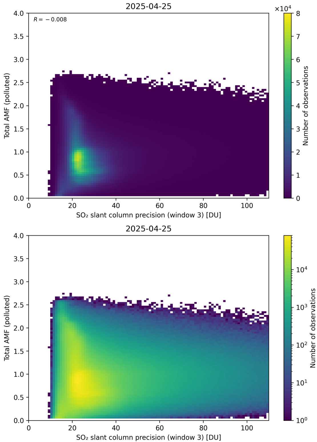
Figure 313: Scatter density plot of “SO 2 slant column precision (window 3)” against “Total AMF (polluted)” for 2025-04-24 to 2025-04-26.
