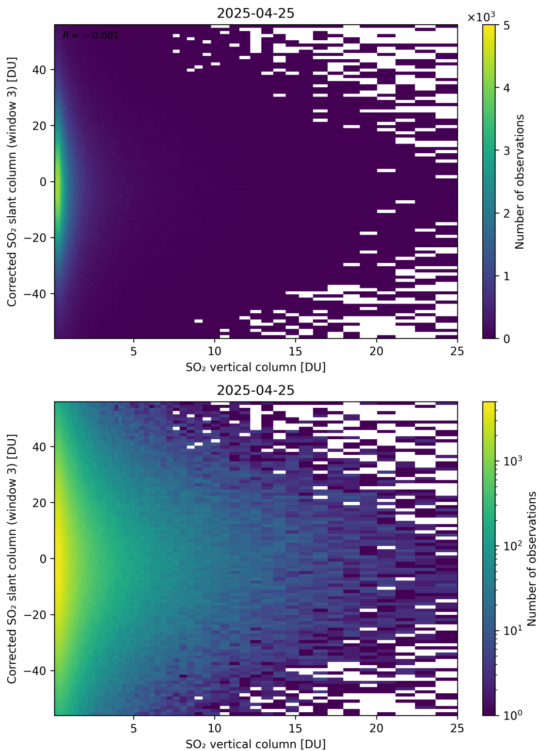
Figure 353: Scatter density plot of “SO 2 vertical column” against “Corrected SO 2 slant column (window 3)” for 2025-04-24 to 2025-04-26.
