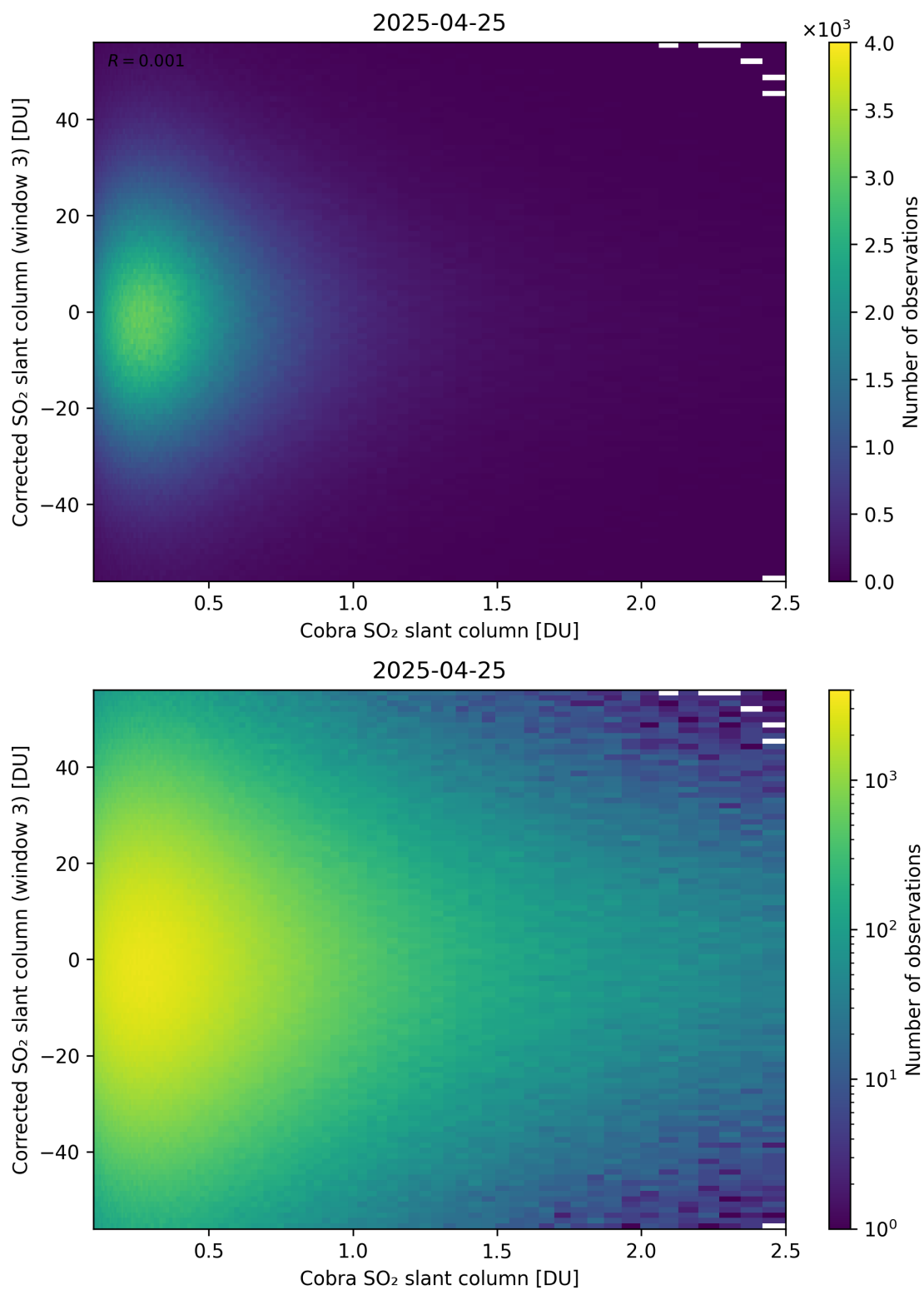
Figure 218: Scatter density plot of “Cobra SO 2 slant column” against “Corrected SO 2 slant column (window 3)” for 2025-04-24 to 2025-04-26.
