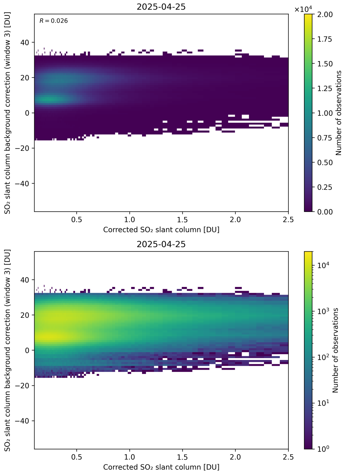
Figure 228: Scatter density plot of “Corrected SO 2 slant column” against “SO 2 slant column background correction (window 3)” for 2025-04-24 to 2025-04-26.
