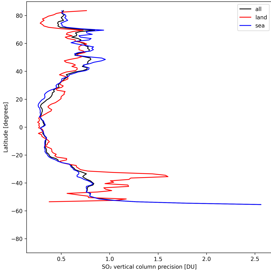
Figure 33: Zonal average of “SO 2 vertical column precision” for 2025-04-24 to 2025-04-26.
