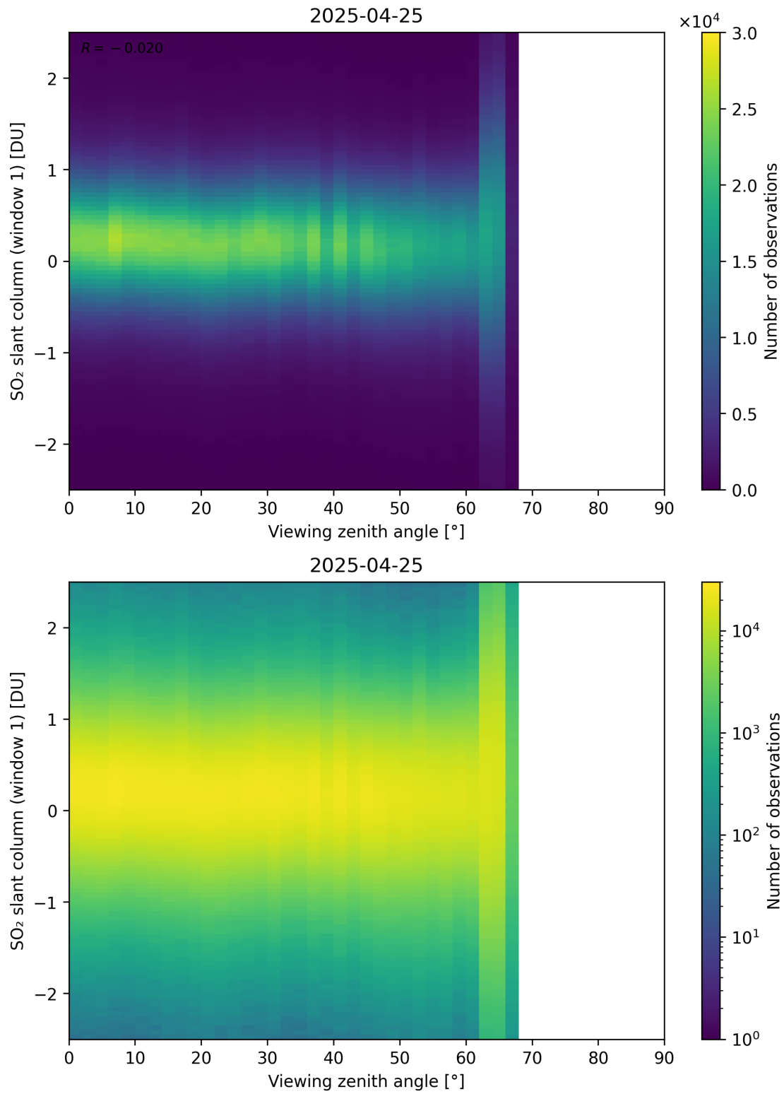
Figure 376: Scatter density plot of “Viewing zenith angle” against “SO 2 slant column (window 1)” for 2025-04-24 to 2025-04-26.
