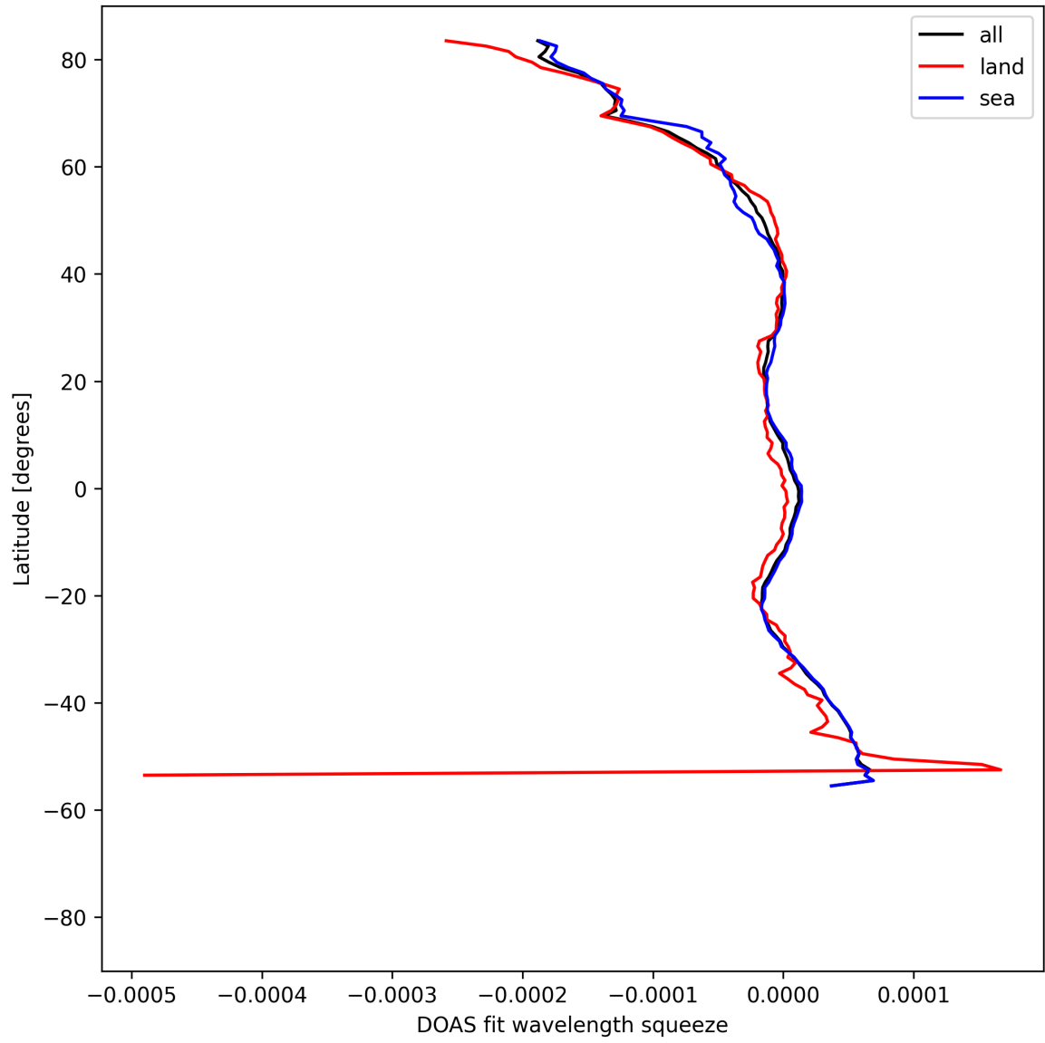
Figure 51: Zonal average of “DOAS fit wavelength squeeze” for 2025-04-24 to 2025-04-26.
