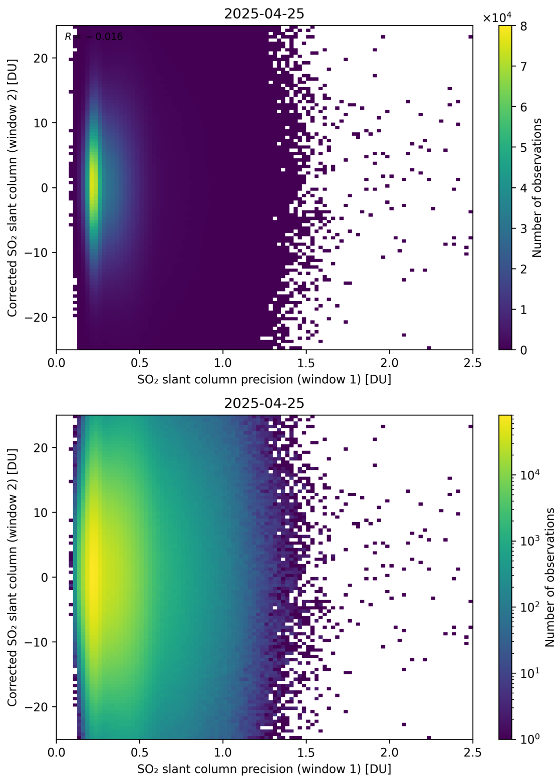
Figure 275: Scatter density plot of “SO 2 slant column precision (window 1)” against “Corrected SO 2 slant column (window 2)” for 2025-04-24 to 2025-04-26.
