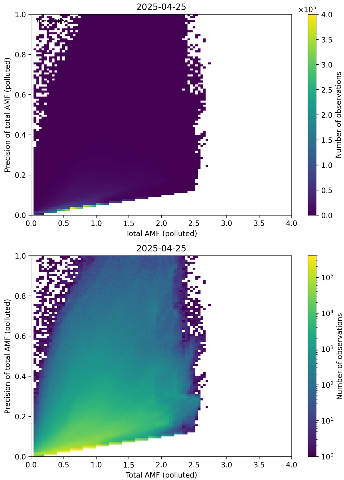
Figure 322: Scatter density plot of “Total AMF (polluted)” against “Precision of total AMF (polluted)” for 2025-04-24 to 2025-04-26.
