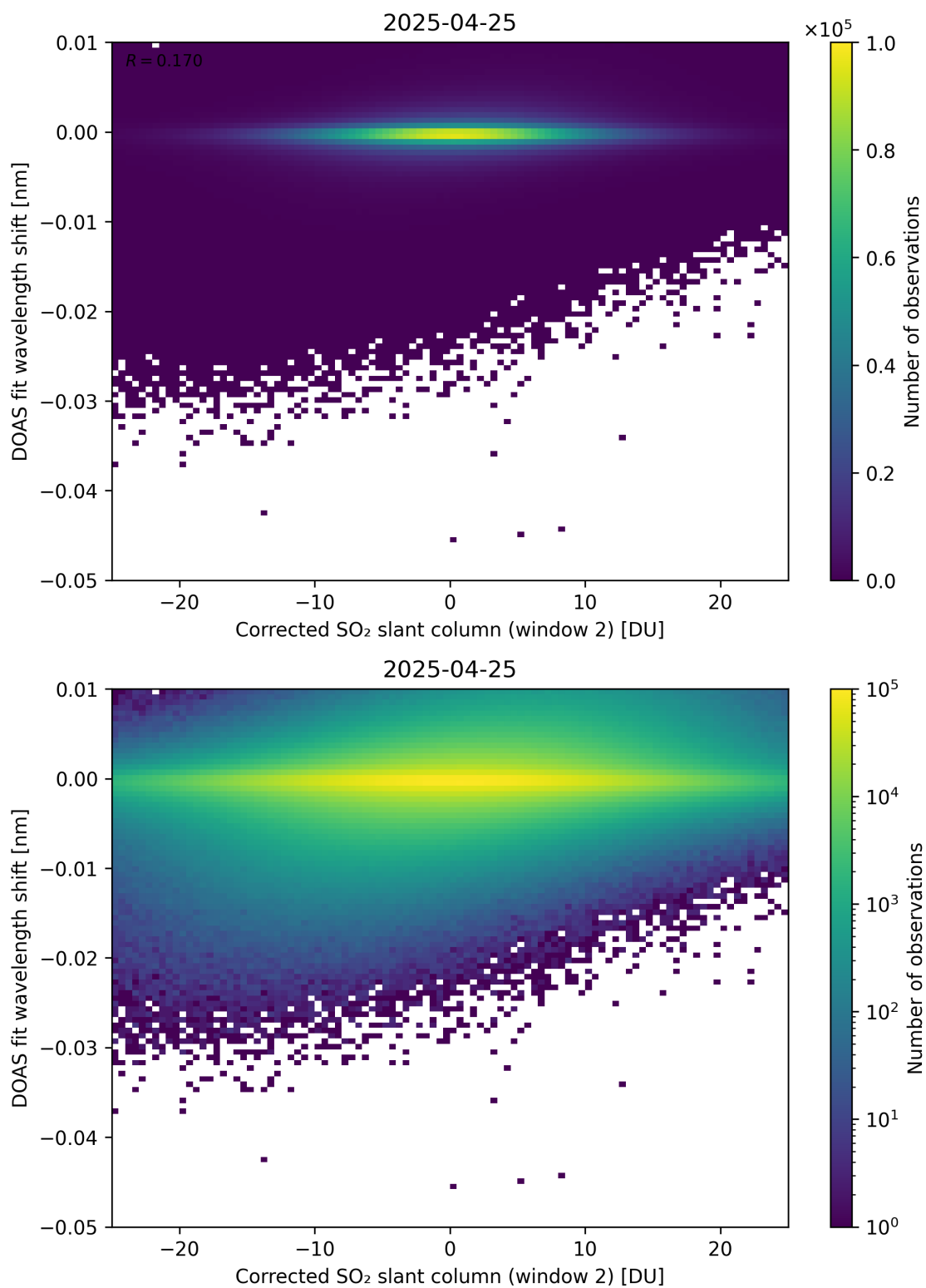
Figure 246: Scatter density plot of “Corrected SO 2 slant column (window 2)” against “DOAS fit wavelength shift” for 2025-04-24 to 2025-04-26.
