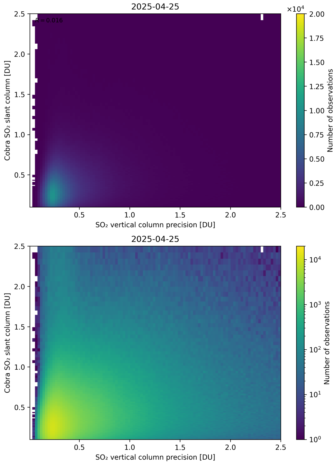
Figure 336: Scatter density plot of “SO 2 vertical column precision” against “Cobra SO 2 slant column” for 2025-04-24 to 2025-04-26.
