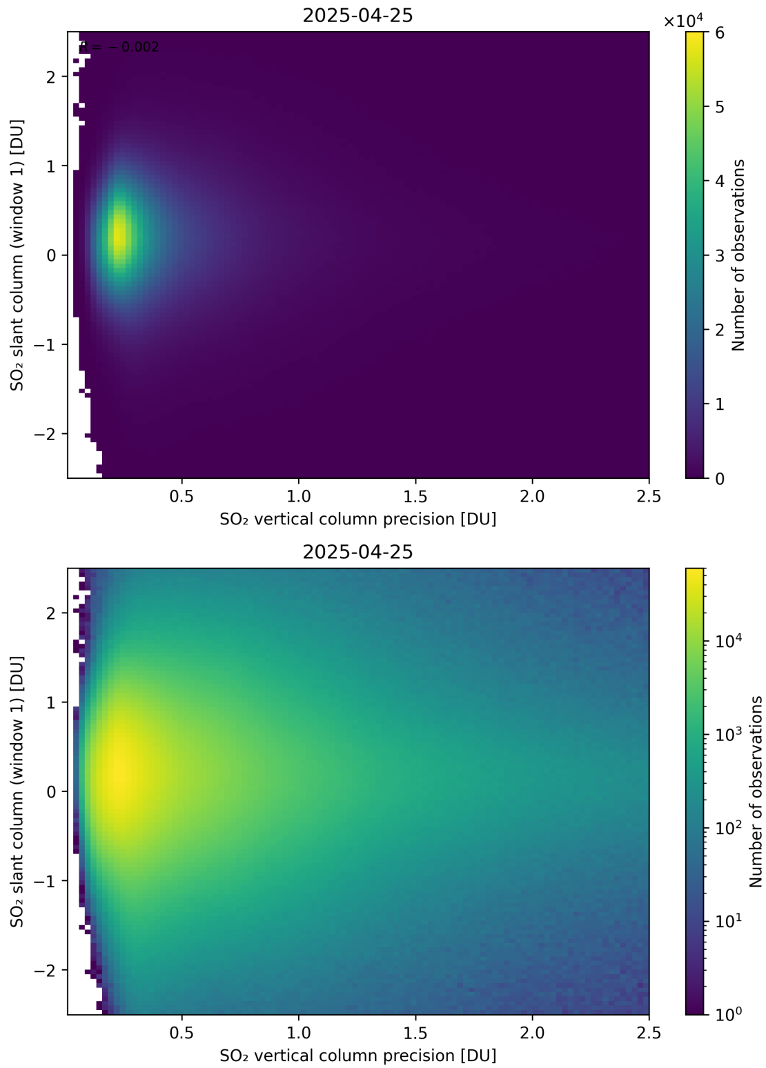
Figure 341: Scatter density plot of “SO 2 vertical column precision” against “SO 2 slant column (window 1)” for 2025-04-24 to 2025-04-26.
