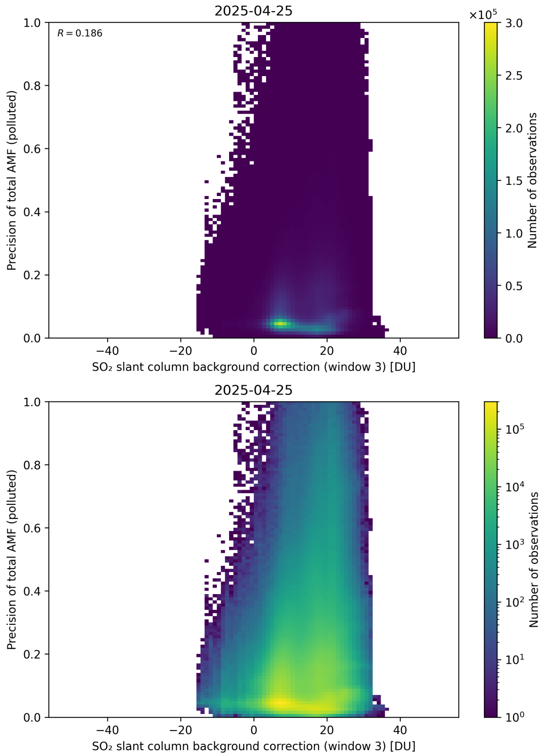
Figure 137: Scatter density plot of “SO 2 slant column background correction (window 3)” against “Precision of total AMF (polluted)” for 2025-04-24 to 2025-04-26.
