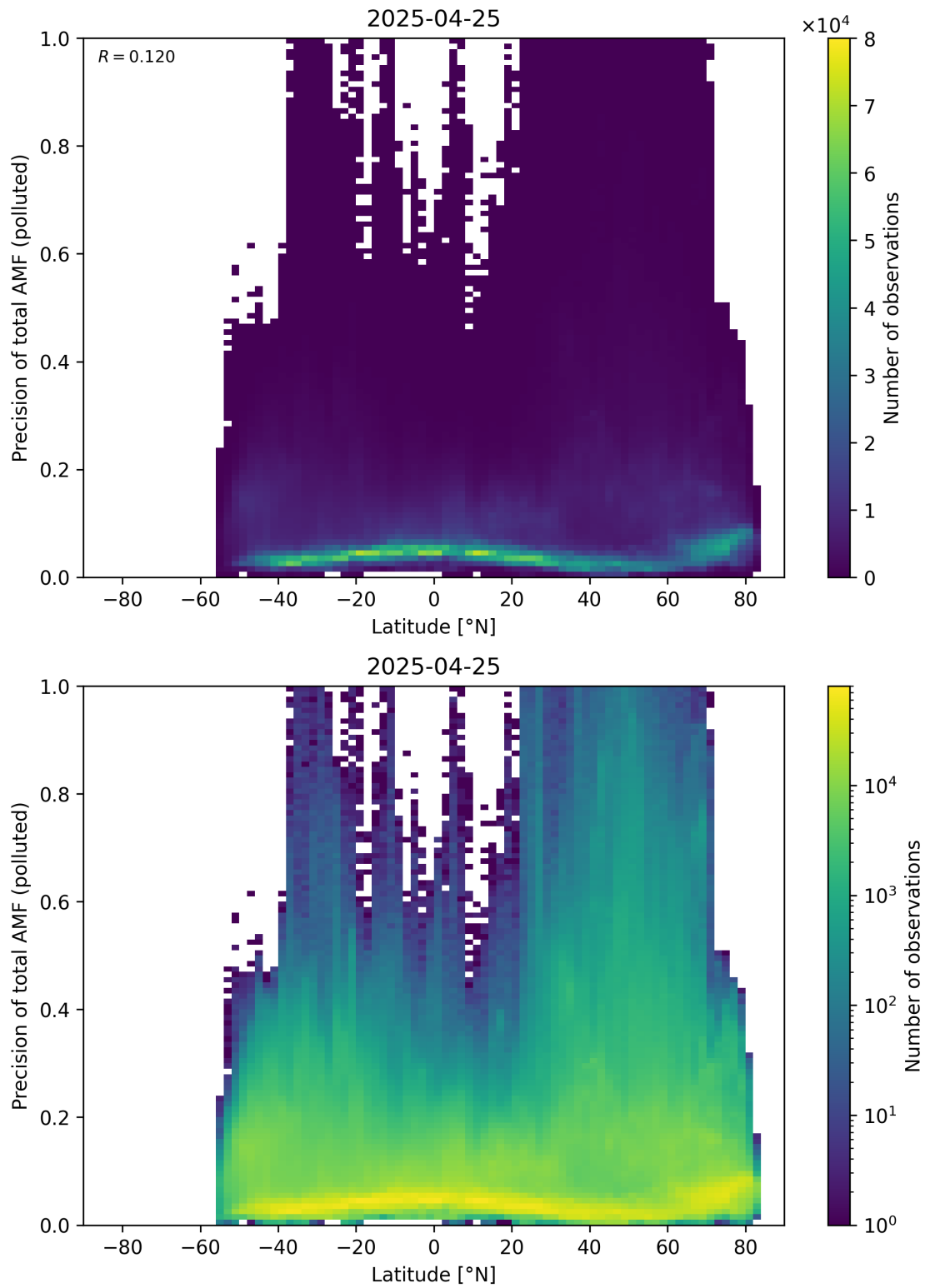
Figure 168: Scatter density plot of “Latitude” against “Precision of total AMF (polluted)” for 2025-04-24 to 2025-04-26.
