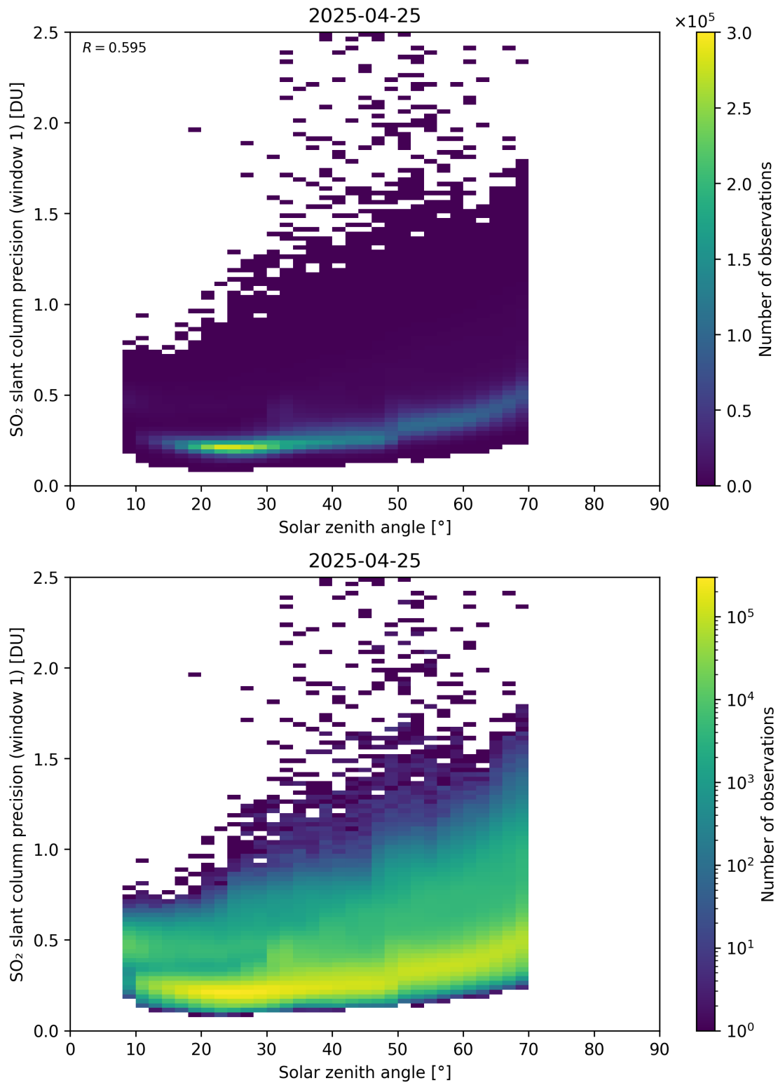
Figure 185: Scatter density plot of “Solar zenith angle” against “SO 2 slant column precision (window 1)” for 2025-04-24 to 2025-04-26.
