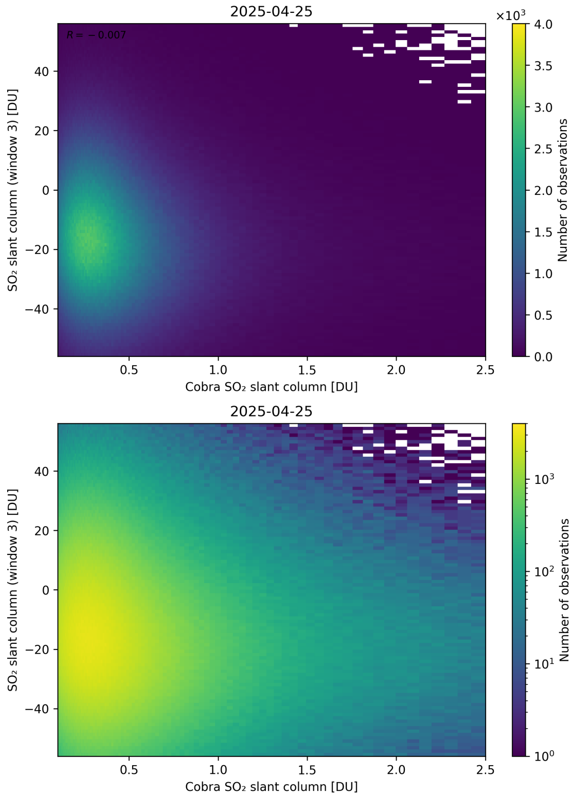
Figure 222: Scatter density plot of “Cobra SO 2 slant column” against “SO 2 slant column (window 3)” for 2025-04-24 to 2025-04-26.
