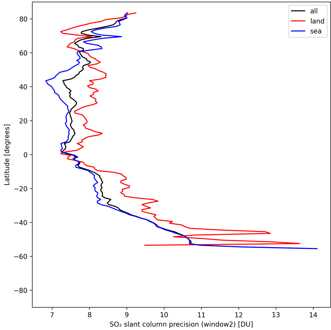
Figure 42: Zonal average of “SO 2 slant column precision (window2)” for 2025-04-24 to 2025-04-26.
