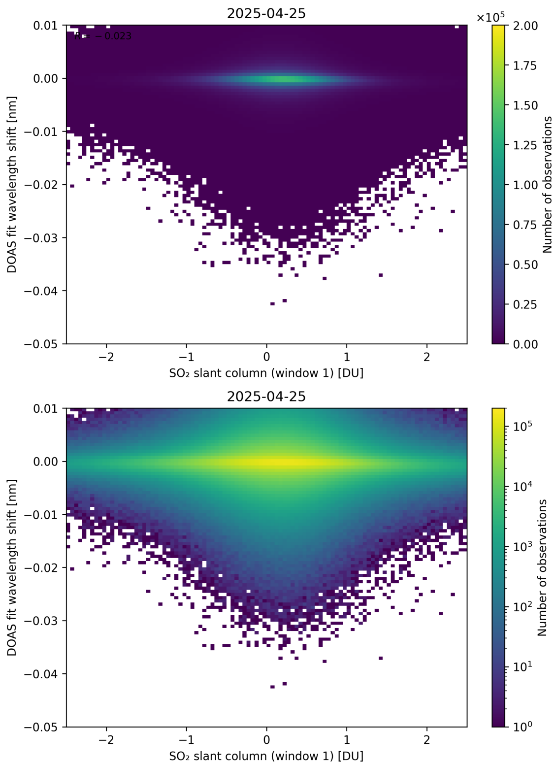
Figure 265: Scatter density plot of “SO 2 slant column (window 1)” against “DOAS fit wavelength shift” for 2025-04-24 to 2025-04-26.
