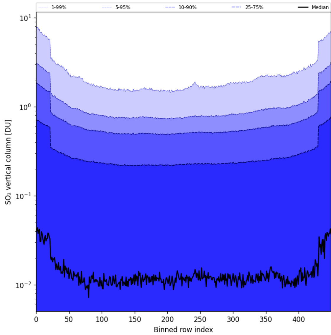
Figure 84: Along track statistics of “SO 2 vertical column” for 2025-04-24 to 2025-04-26
