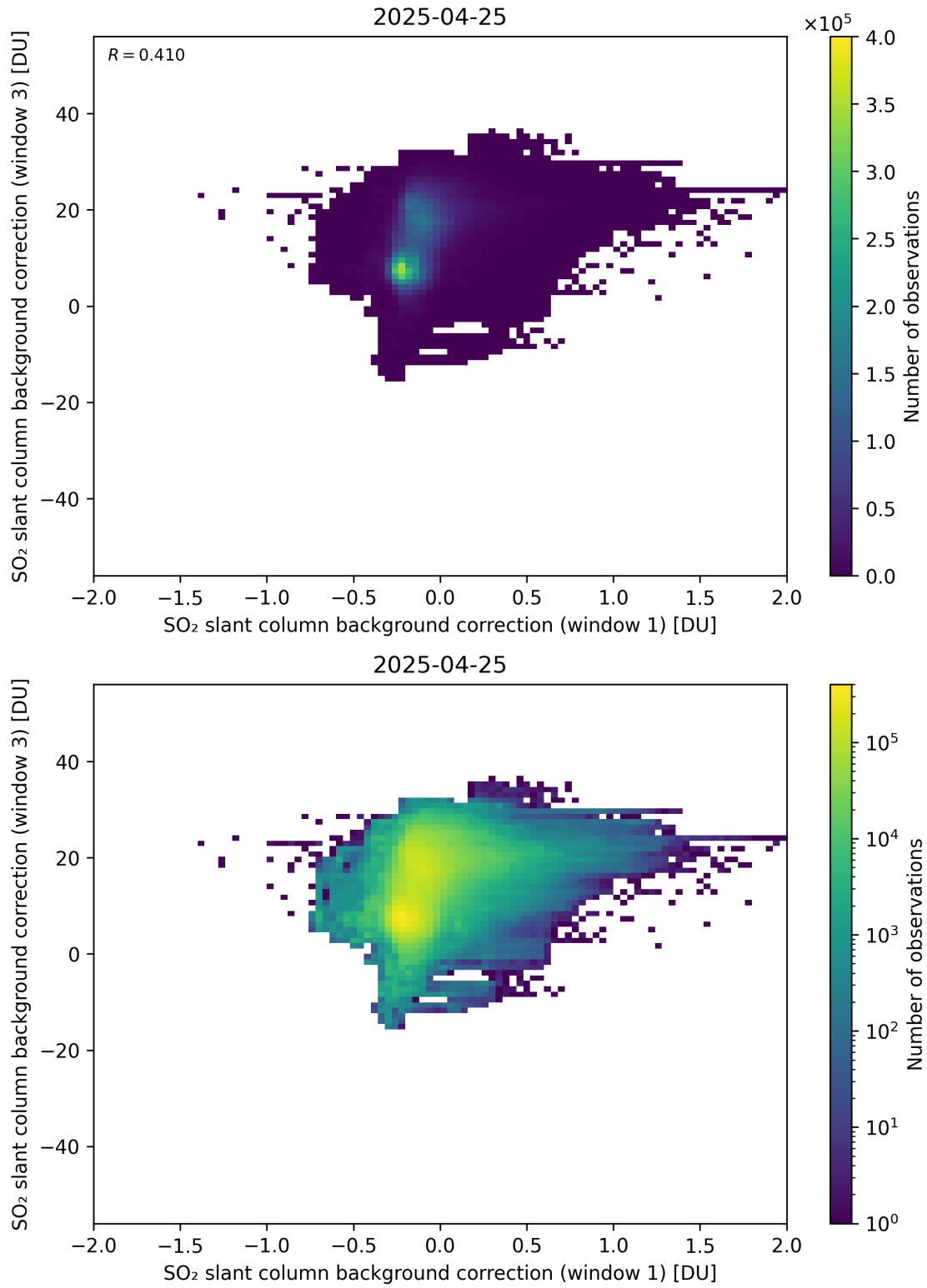
Figure 110: Scatter density plot of “SO 2 slant column background correction (window 1)” against “SO 2 slant column background correction (window 3)” for 2025-04-24 to 2025-04-26.
