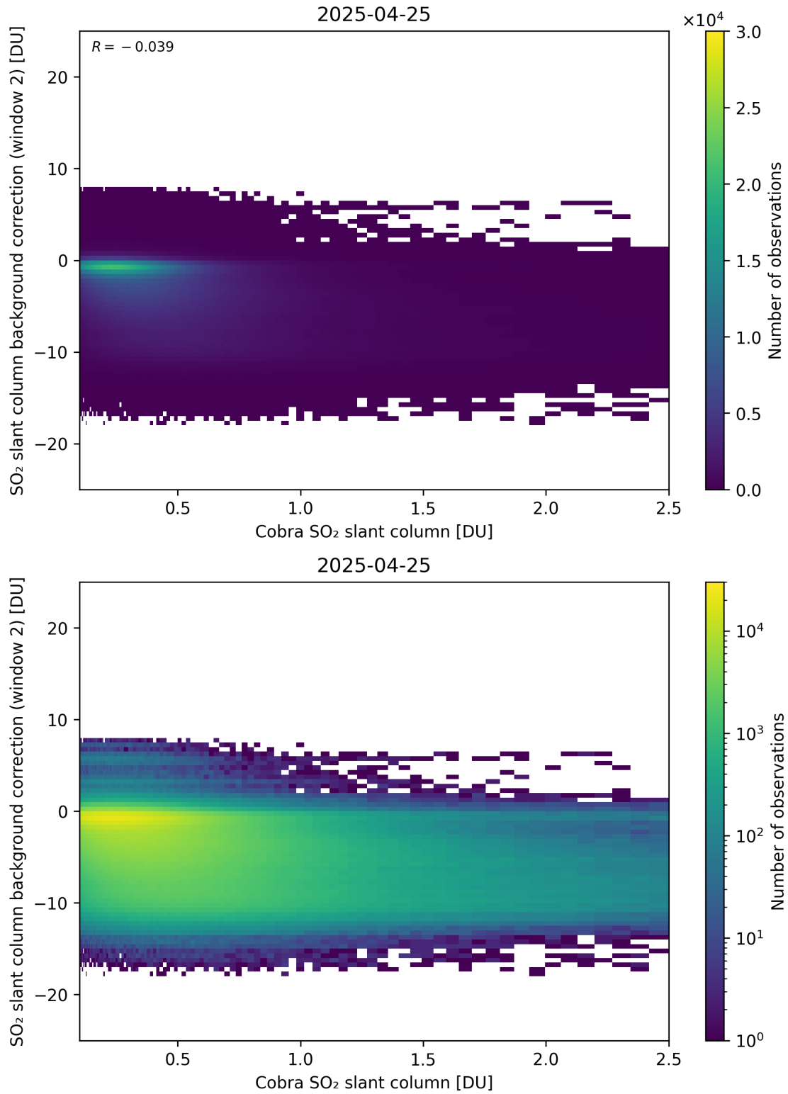
Figure 194: Scatter density plot of “Cobra SO 2 slant column” against “SO 2 slant column background correction (window 2)” for 2025-04-24 to 2025-04-26.
