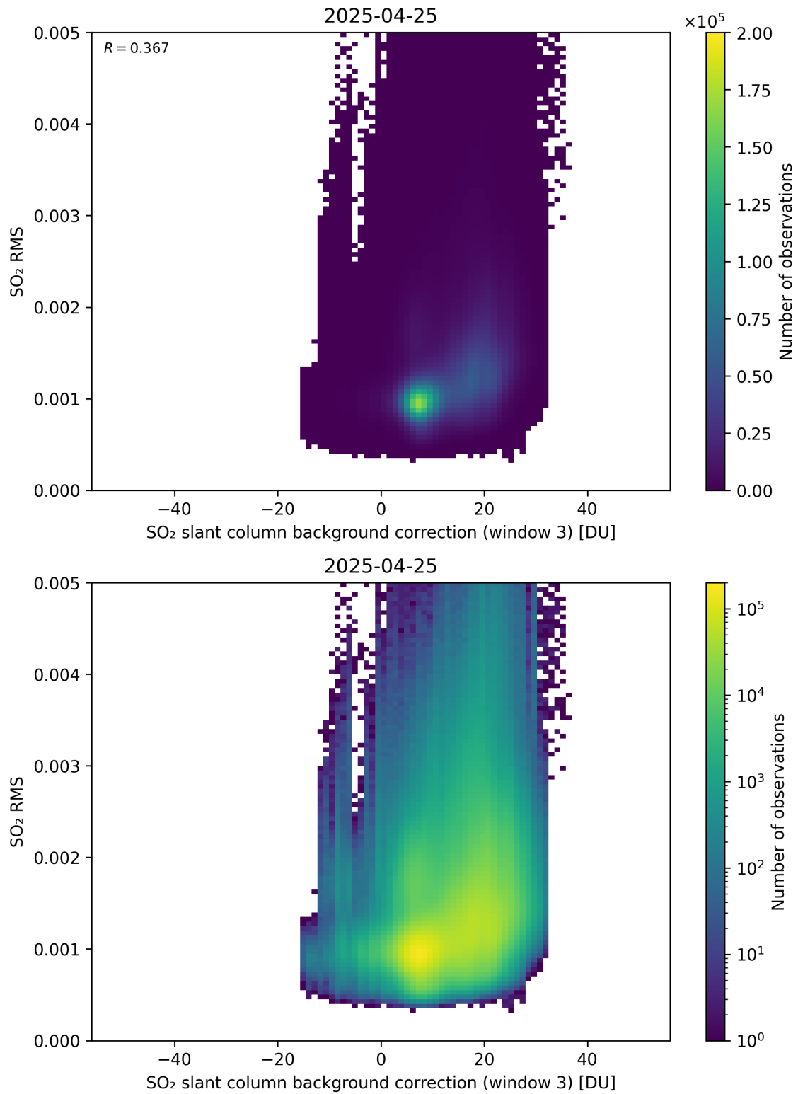
Figure 134: Scatter density plot of “SO 2 slant column background correction (window 3)” against “SO 2 RMS” for 2025-04-24 to 2025-04-26.
