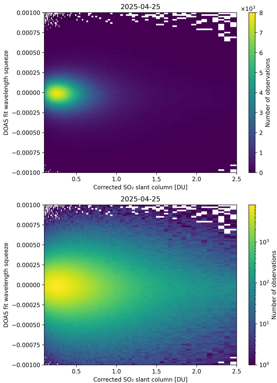
Figure 230: Scatter density plot of "Corrected SO 2 slant column" against "DOAS fit wavelength squeeze" for 2025-04-24 to 2025-04-26.
