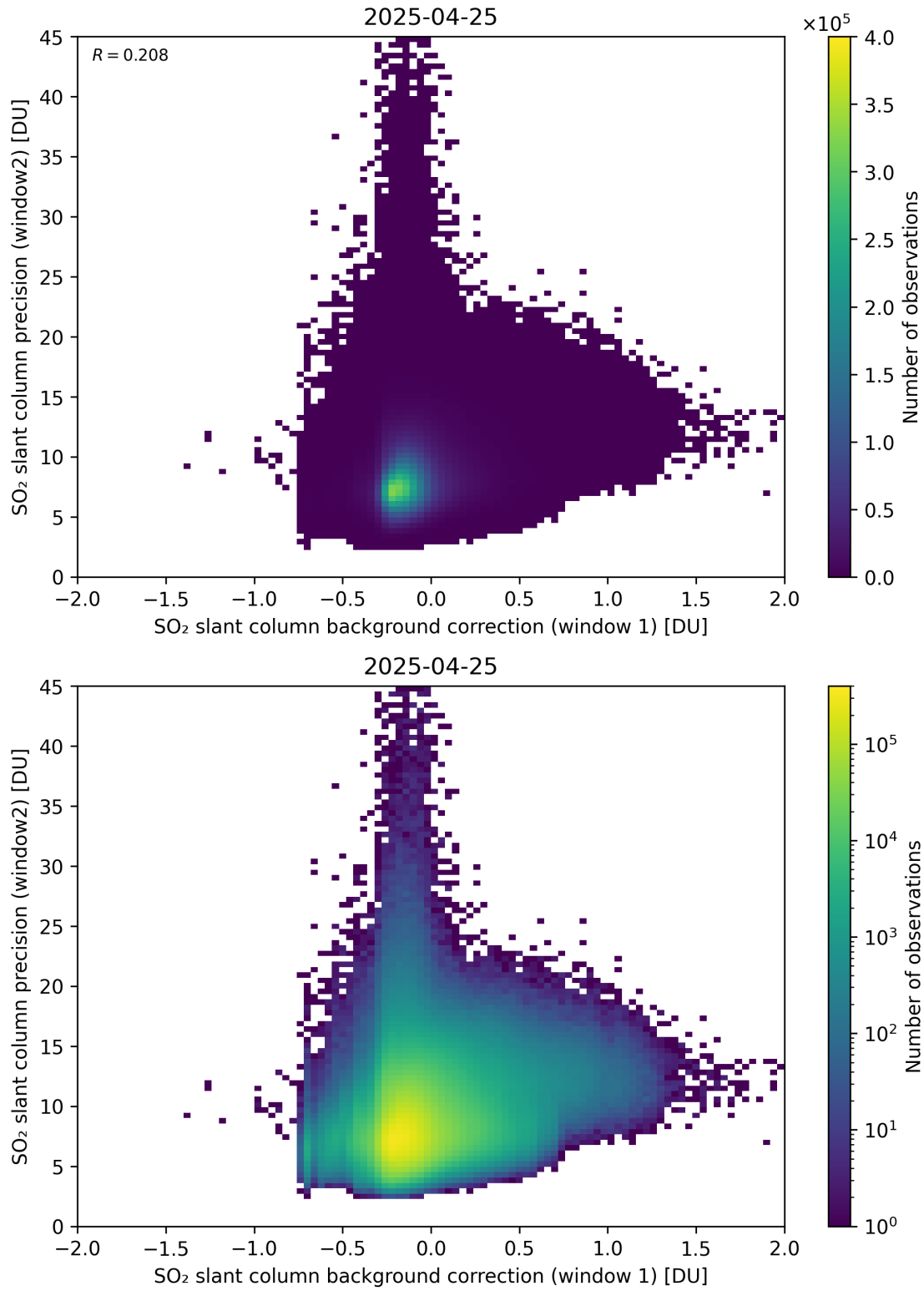
Figure 117: Scatter density plot of “SO 2 slant column background correction (window 1)” against “SO 2 slant column precision (window2)” for 2025-04-24 to 2025-04-26.
