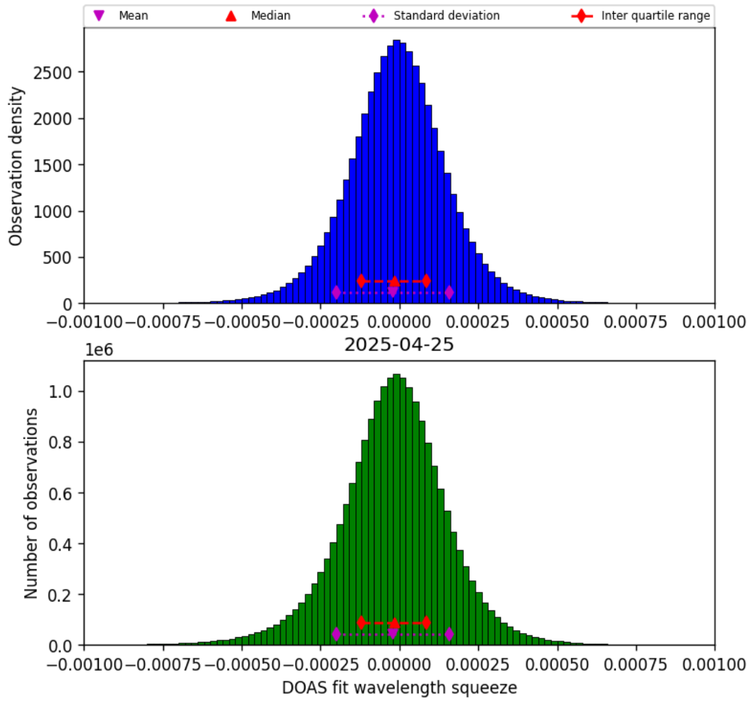
Figure 77: Histogram of “DOAS fit wavelength squeeze” for 2025-04-24 to 2025-04-26
