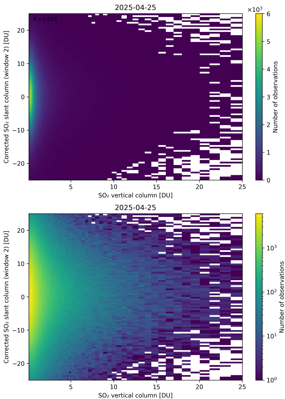
Figure 352: Scatter density plot of “SO 2 vertical column” against “Corrected SO 2 slant column (window 2)” for 2025-04-24 to 2025-04-26.
