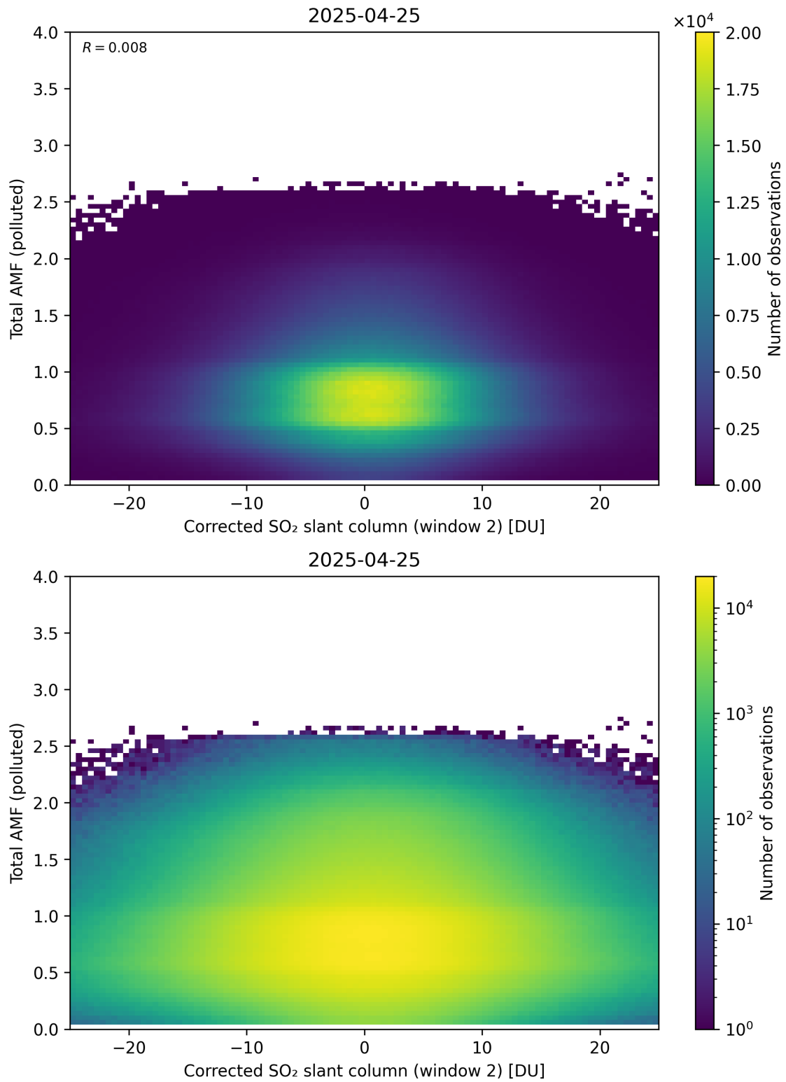
Figure 253: Scatter density plot of “Corrected SO 2 slant column (window 2)” against “Total AMF (polluted)” for 2025-04-24 to 2025-04-26.
