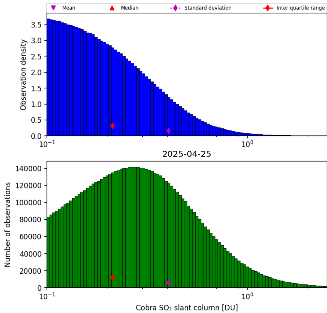
Figure 61: Histogram of “Cobra SO 2 slant column” for 2025-04-24 to 2025-04-26
