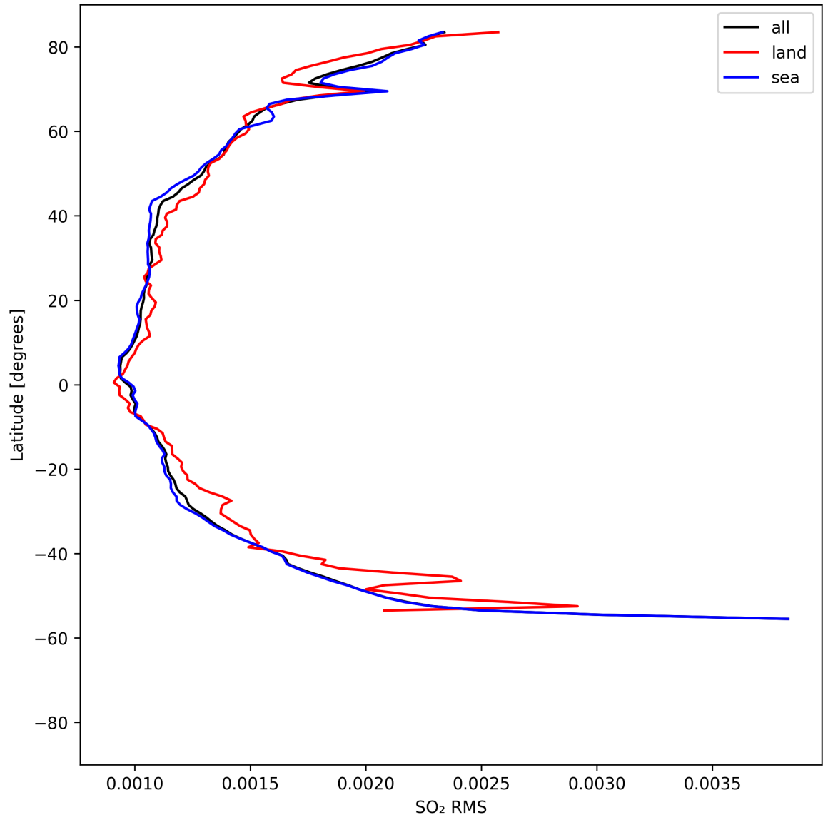
Figure 52: Zonal average of “SO 2 RMS” for 2025-04-24 to 2025-04-26.
