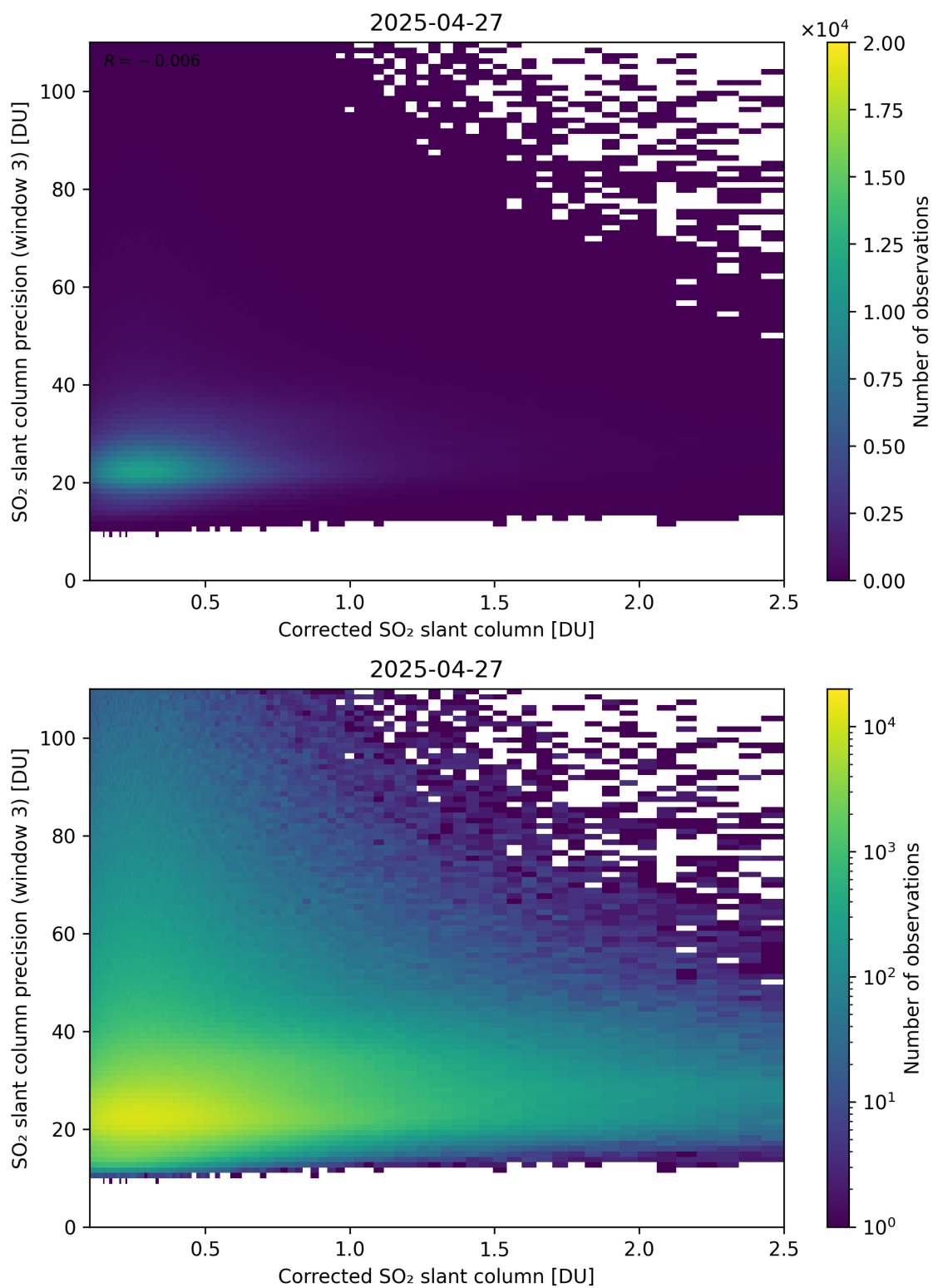
Figure 241: Scatter density plot of “Corrected SO 2 slant column” against “SO 2 slant column precision (window 3)” for 2025-04-26 to 2025-04-28.
