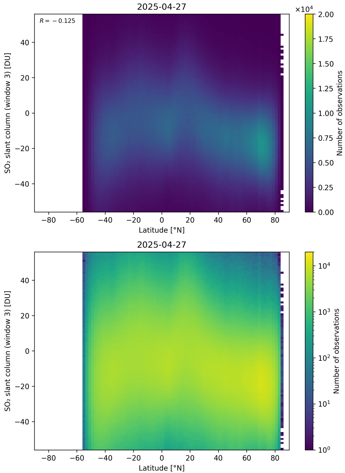
Figure 165: Scatter density plot of “Latitude” against “SO 2 slant column (window 3)” for 2025-04-26 to 2025-04-28.
