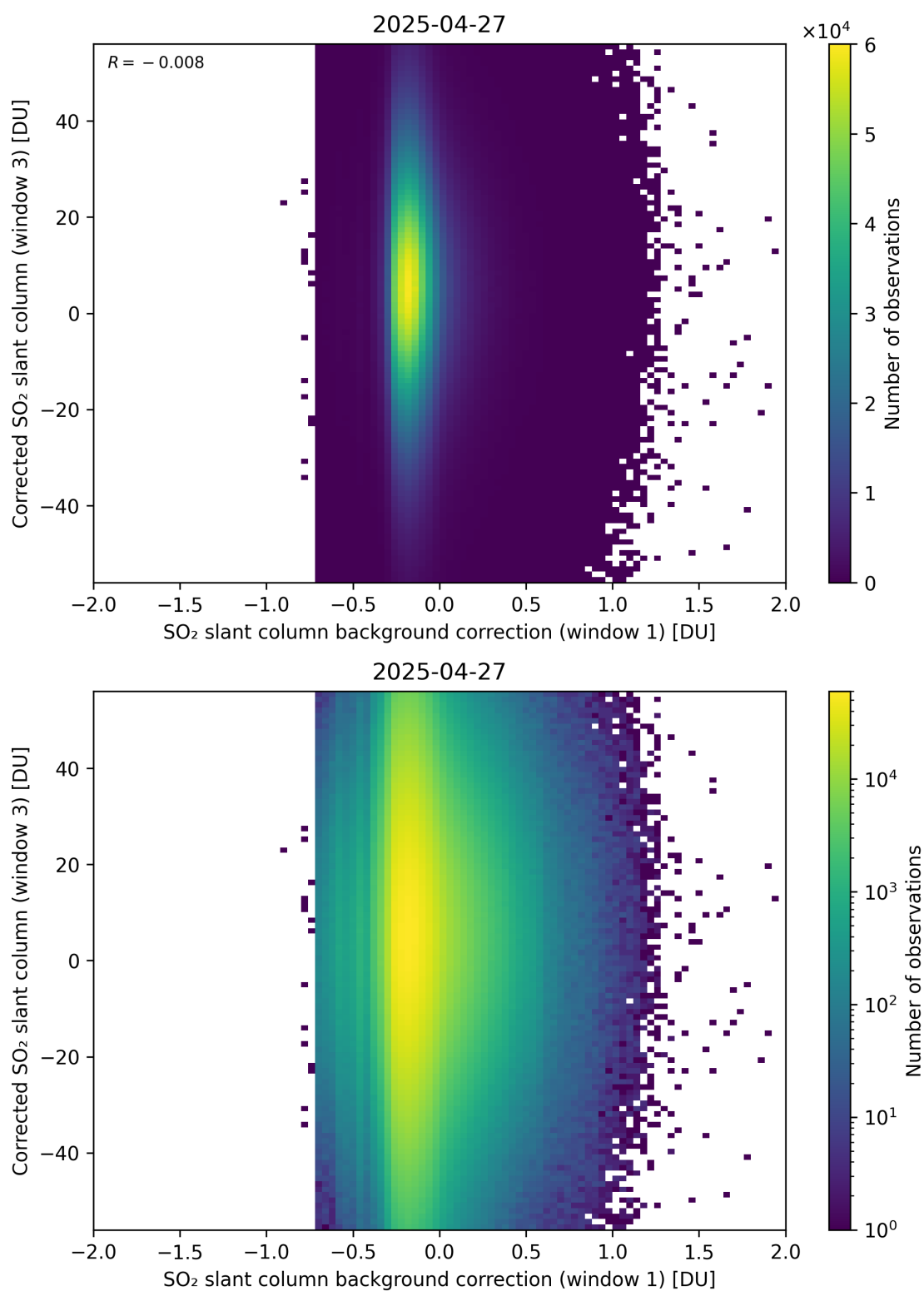
Figure 116: Scatter density plot of “SO 2 slant column background correction (window 1)” against “Corrected SO 2 slant column (window 3)” for 2025-04-26 to 2025-04-28.
