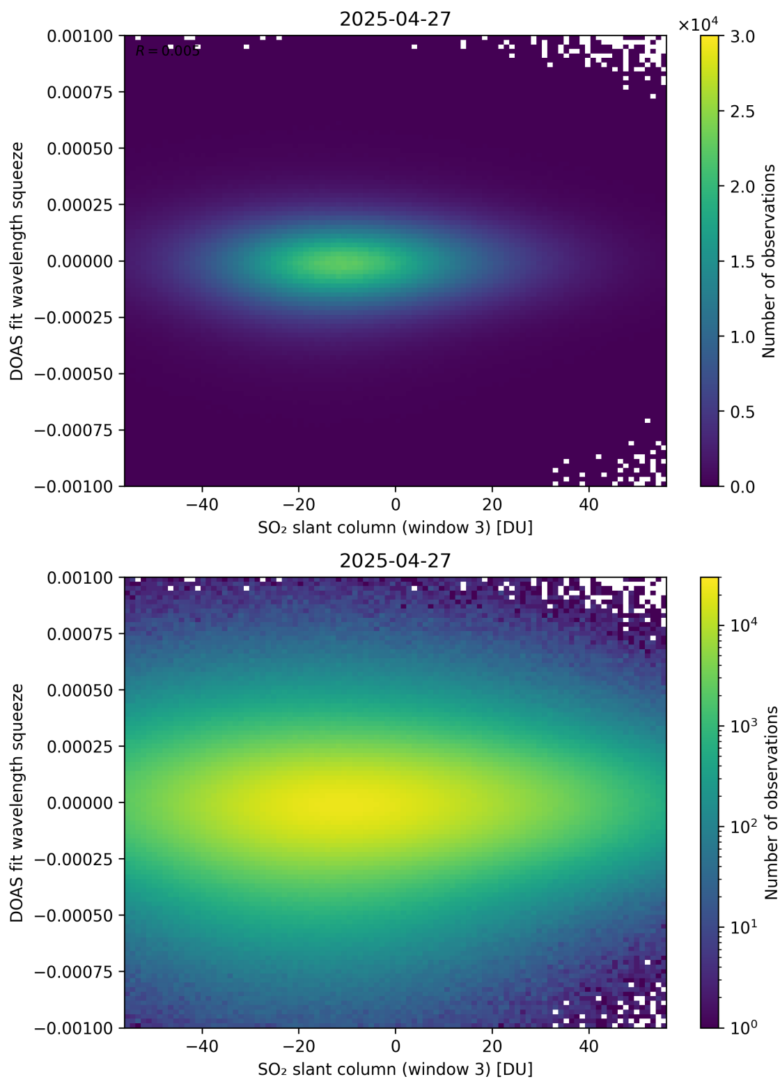
Figure 305: Scatter density plot of “SO 2 slant column (window 3)” against “DOAS fit wavelength squeeze” for 2025-04-26 to 2025-04-28.
