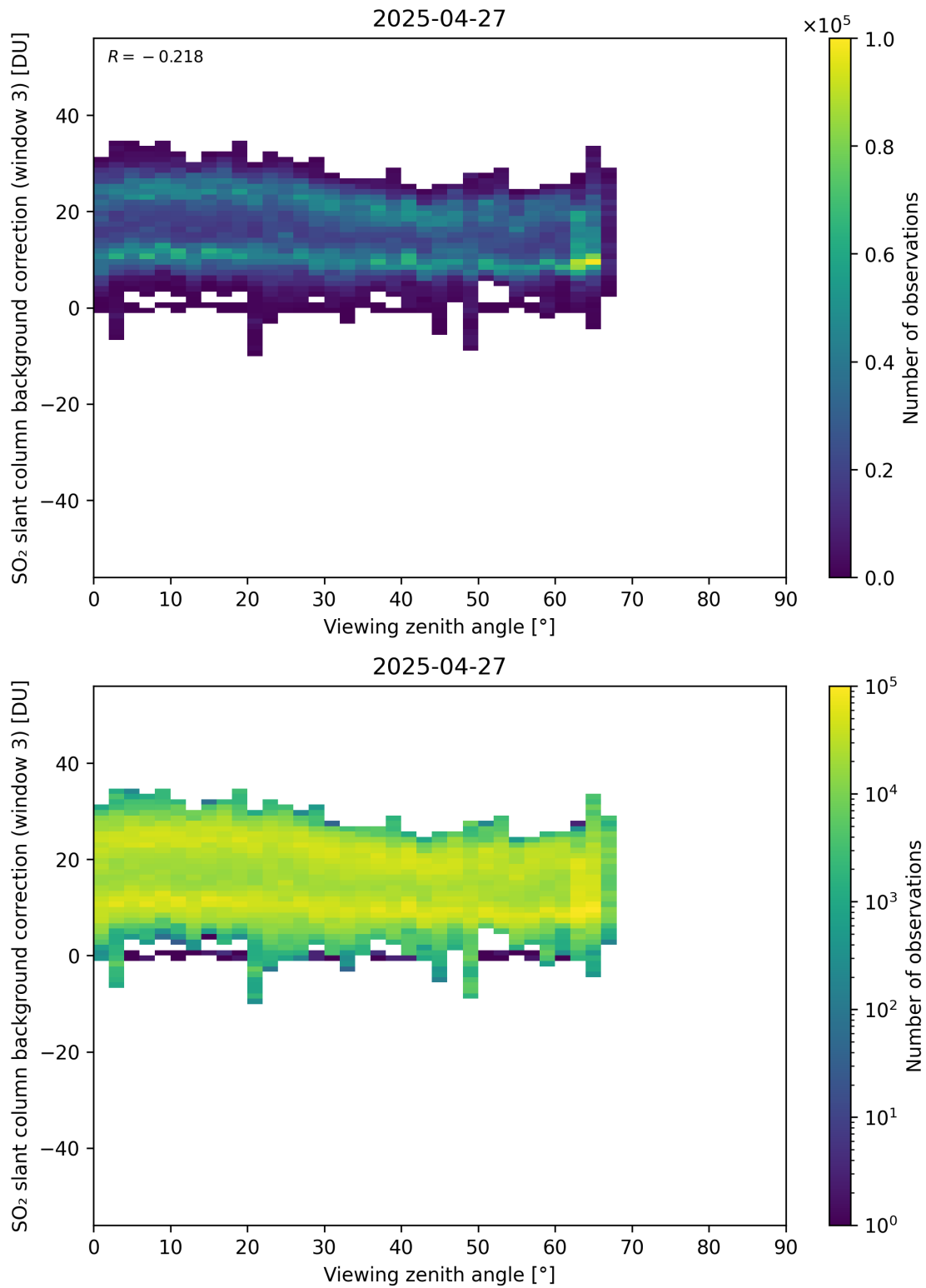
Figure 364: Scatter density plot of “Viewing zenith angle” against “SO 2 slant column background correction (window 3)” for 2025-04-26 to 2025-04-28.
