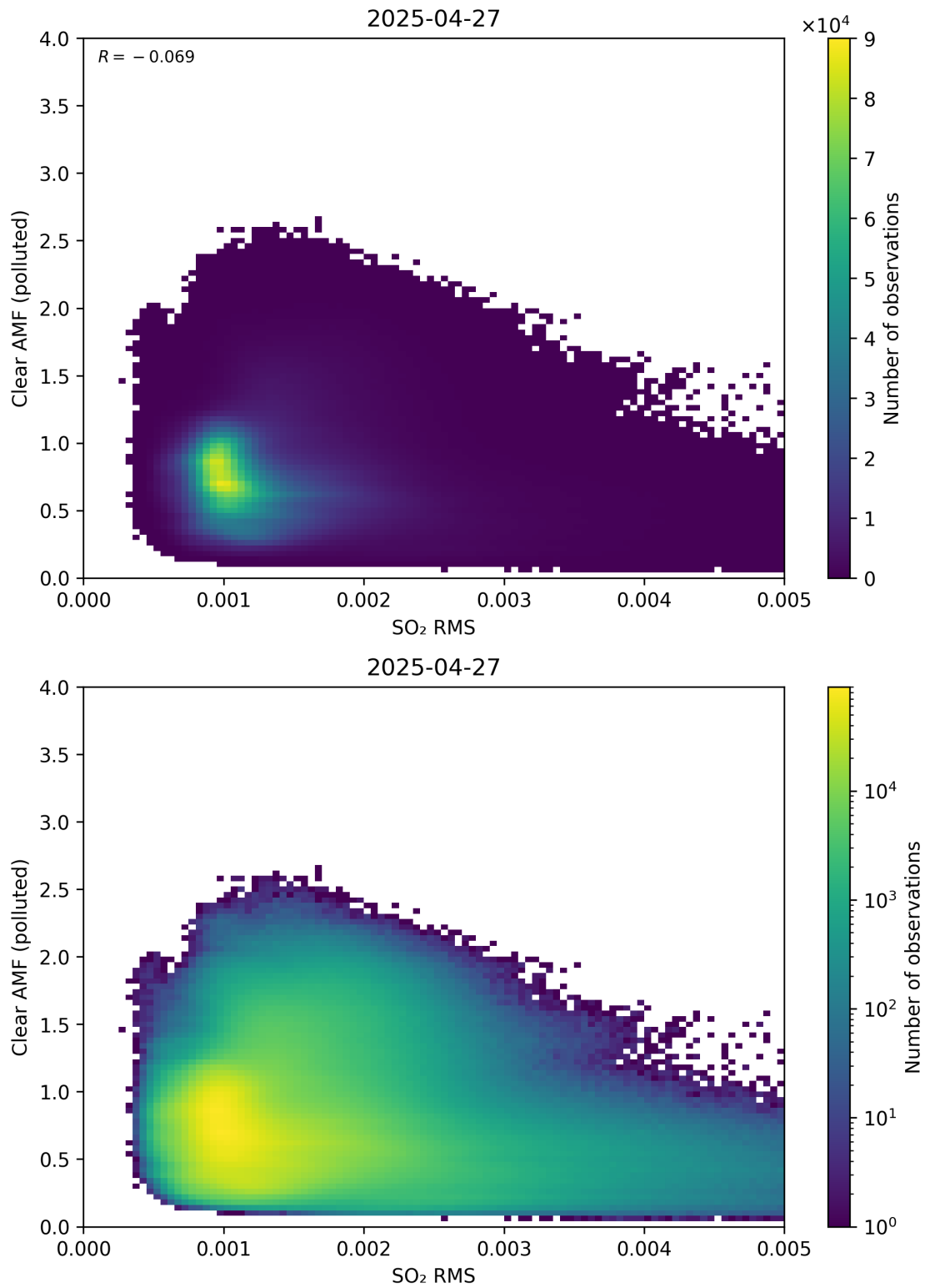
Figure 147: Scatter density plot of “SO 2 RMS” against “Clear AMF (polluted)” for 2025-04-26 to 2025-04-28.
