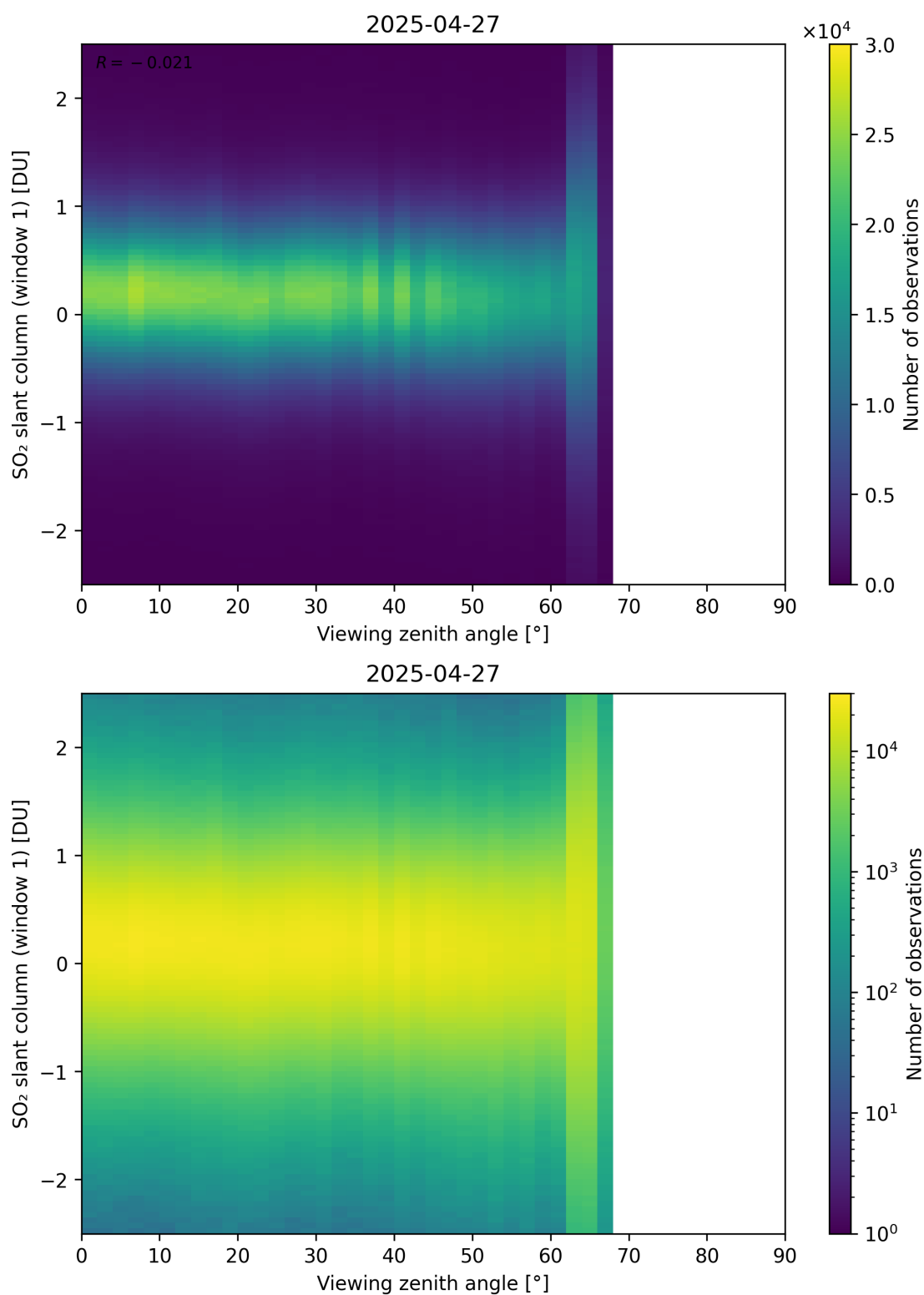
Figure 376: Scatter density plot of “Viewing zenith angle” against “SO 2 slant column (window 1)” for 2025-04-26 to 2025-04-28.
