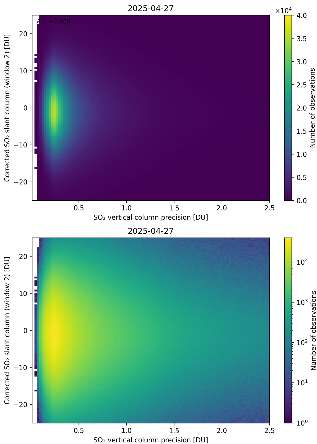
Figure 339: Scatter density plot of “SO 2 vertical column precision” against “Corrected SO 2 slant column (window 2)” for 2025-04-26 to 2025-04-28.
