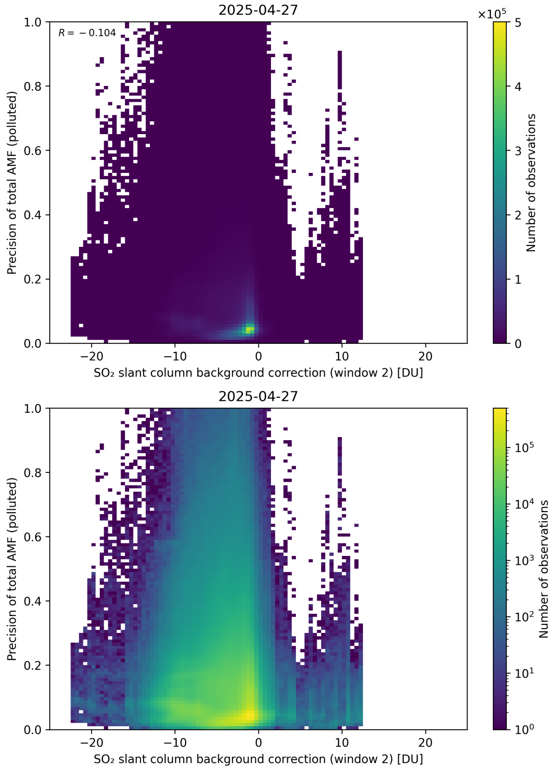
Figure 131: Scatter density plot of “SO 2 slant column background correction (window 2)” against “Precision of total AMF (polluted)” for 2025-04-26 to 2025-04-28.
