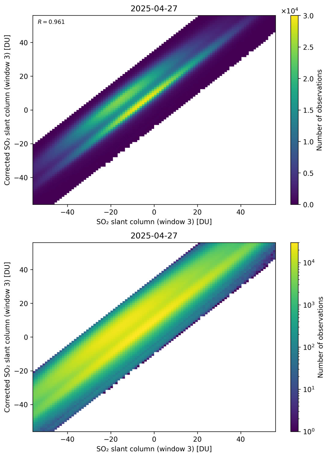
Figure 316: Scatter density plot of “SO 2 slant column (window 3)” against “Corrected SO 2 slant column (window 3)” for 2025-04-26 to 2025-04-28.
