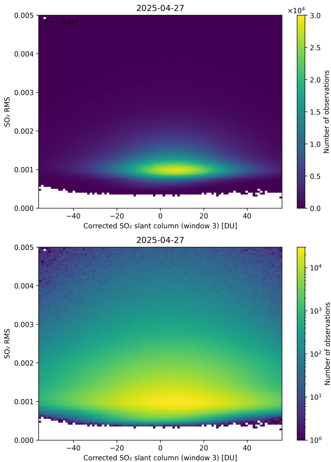
Figure 258: Scatter density plot of “Corrected SO 2 slant column (window 3)” against “SO 2 RMS” for 2025-04-26 to 2025-04-28.
