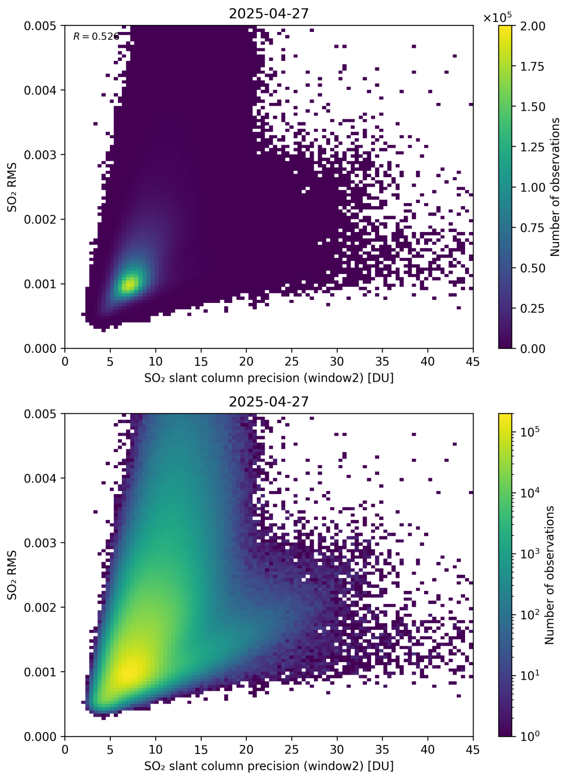
Figure 295: Scatter density plot of “SO 2 slant column precision (window2)” against “SO 2 RMS” for 2025-04-26 to 2025-04-28.
