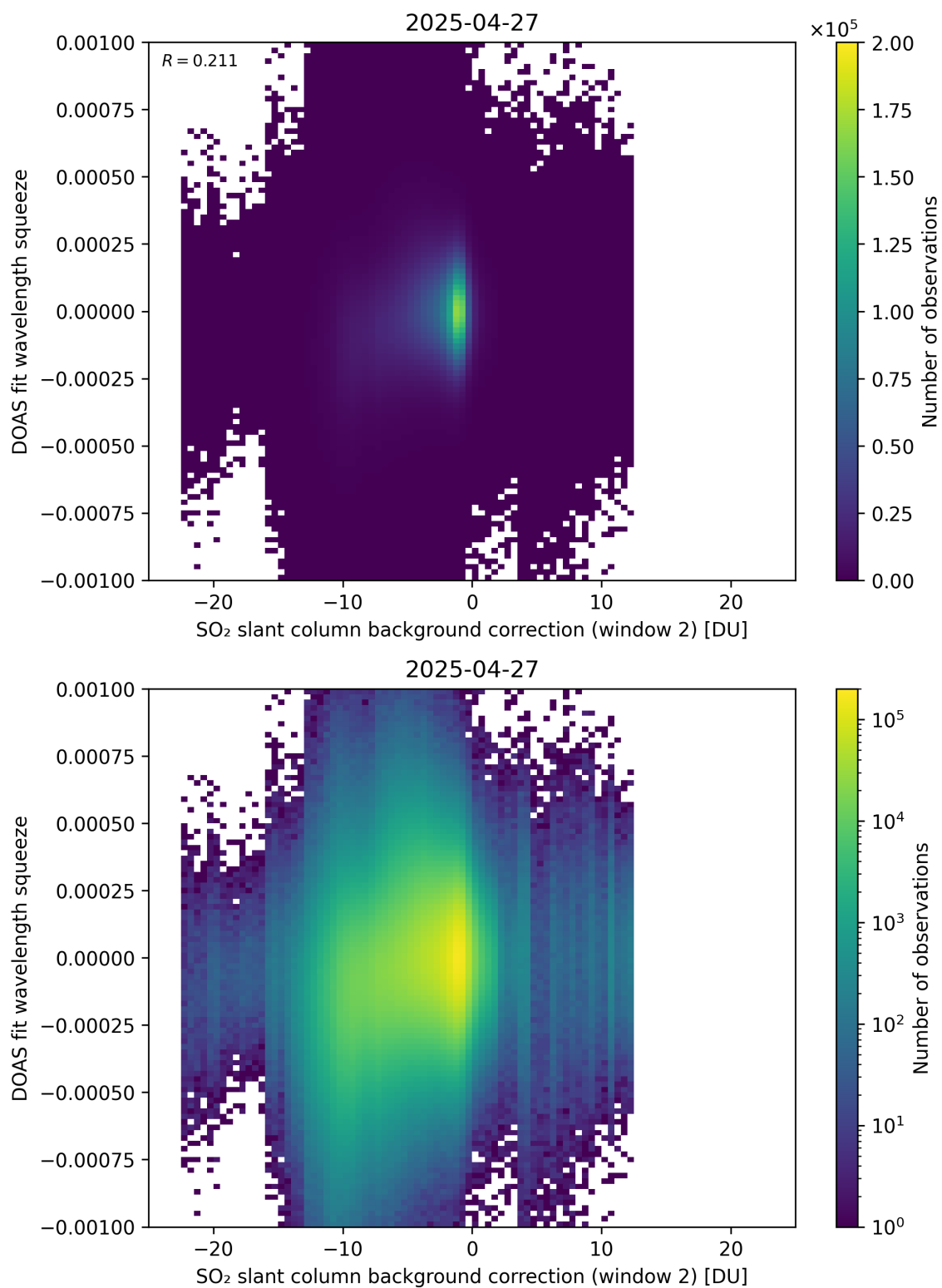
Figure 124: Scatter density plot of “SO 2 slant column background correction (window 2)” against “DOAS fit wavelength squeeze” for 2025-04-26 to 2025-04-28.
