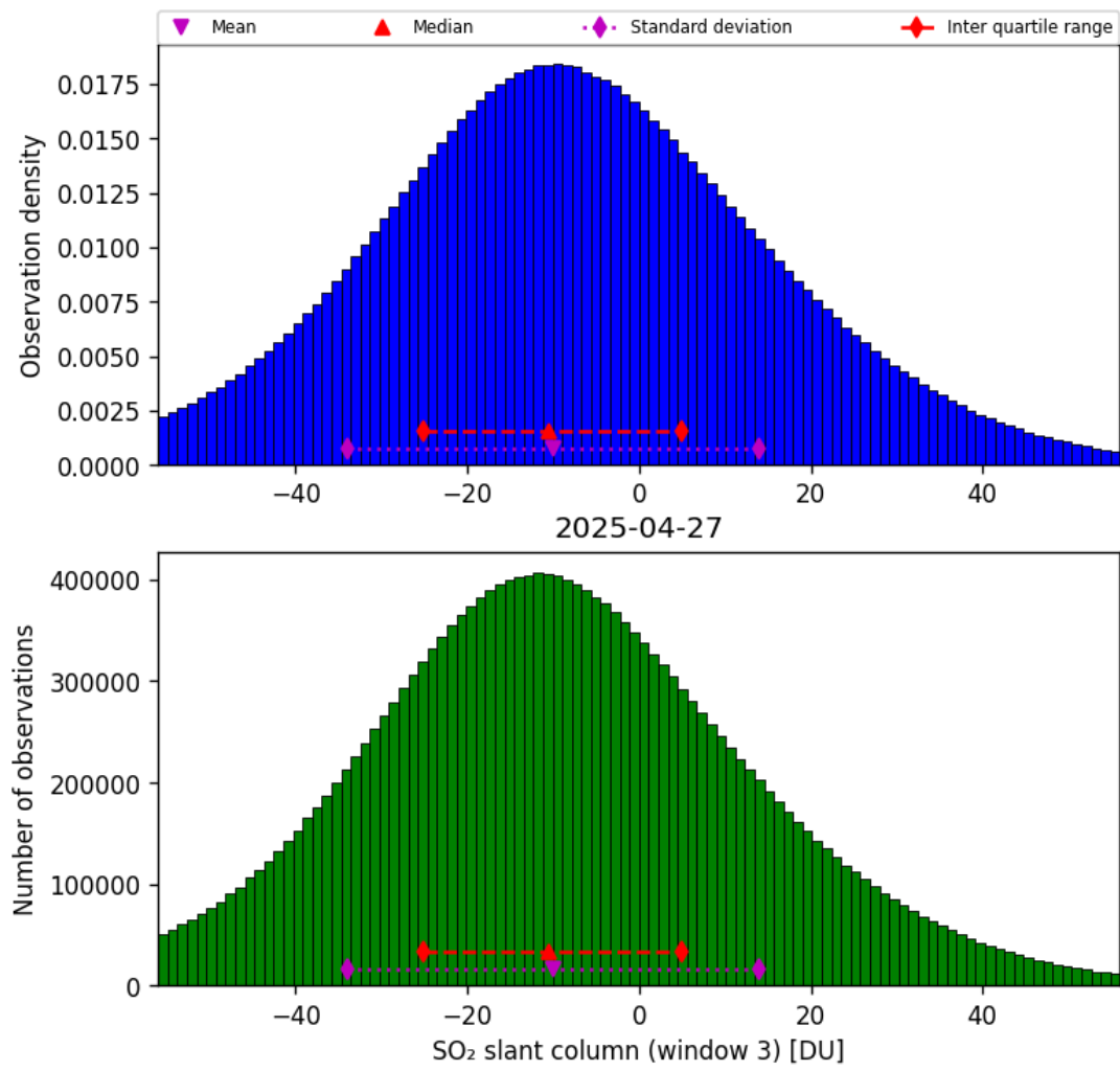
Figure 71: Histogram of “SO 2 slant column (window 3)” for 2025-04-26 to 2025-04-28
