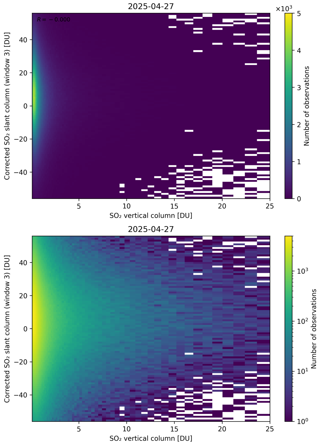
Figure 353: Scatter density plot of “SO 2 vertical column” against “Corrected SO 2 slant column (window 3)” for 2025-04-26 to 2025-04-28.
