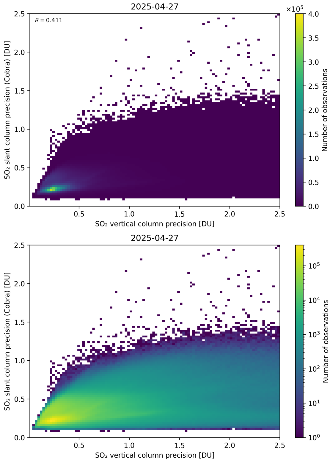
Figure 337: Scatter density plot of “SO 2 vertical column precision” against “SO 2 slant column precision (Cobra)” for 2025-04-26 to 2025-04-28.
