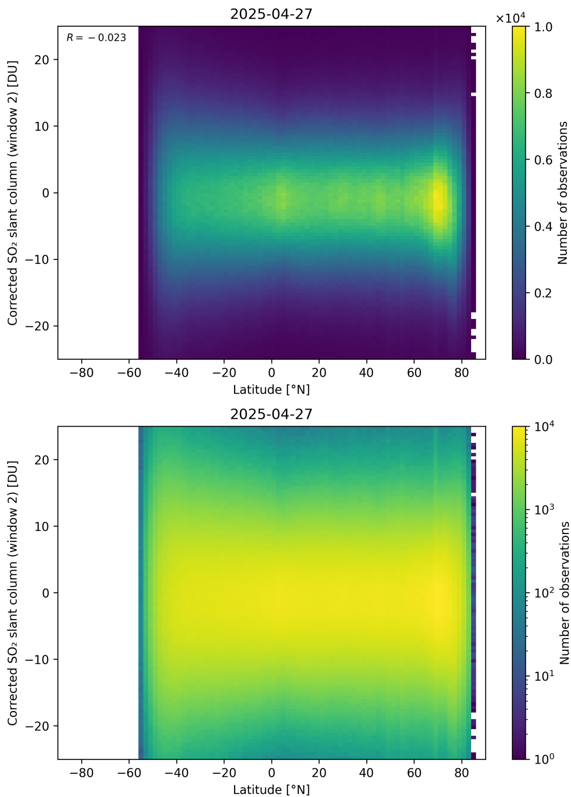
Figure 160: Scatter density plot of “Latitude” against “Corrected SO 2 slant column (window 2)” for 2025-04-26 to 2025-04-28.
