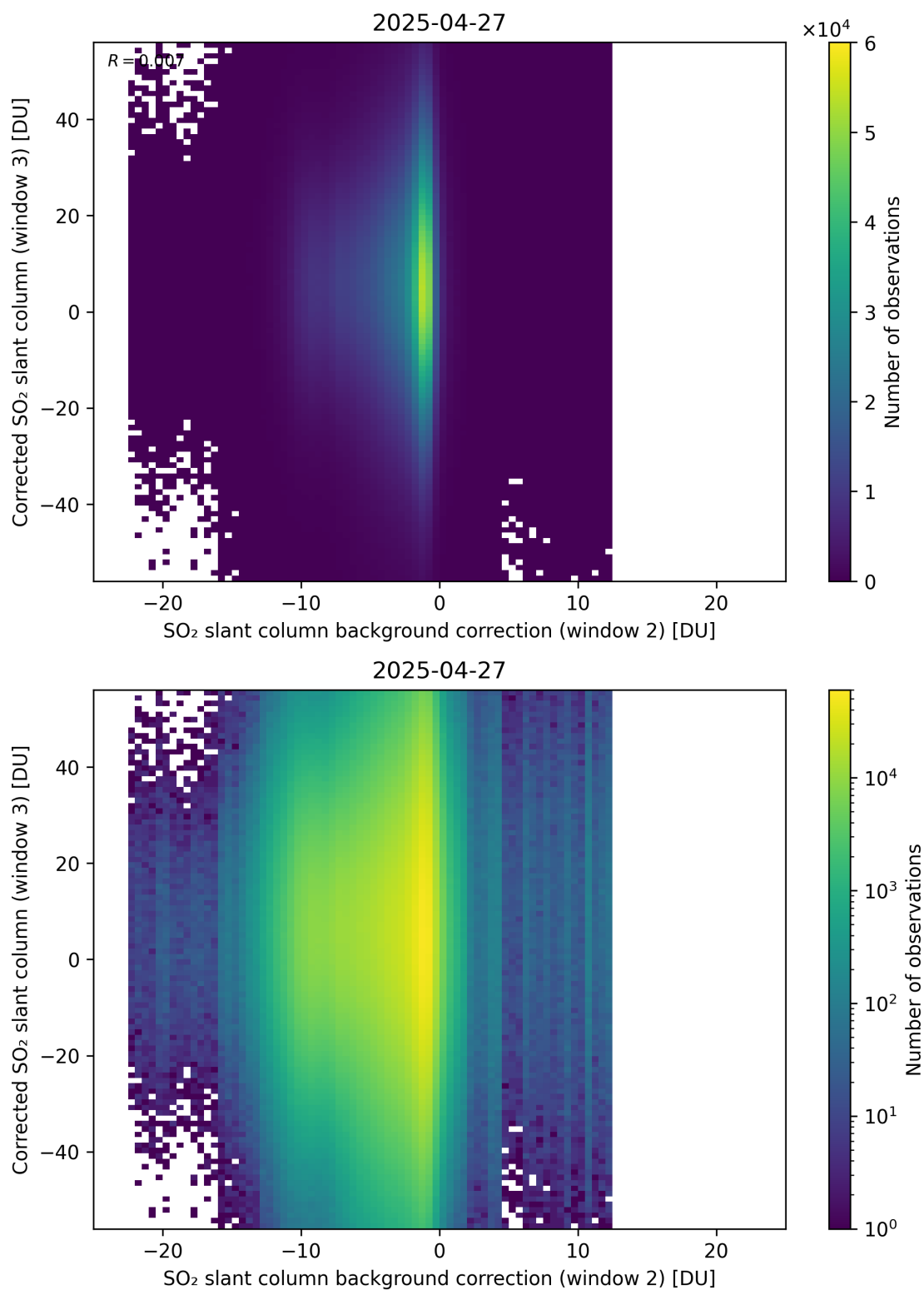
Figure 127: Scatter density plot of “SO 2 slant column background correction (window 2)” against “Corrected SO 2 slant column (window 3)” for 2025-04-26 to 2025-04-28.
