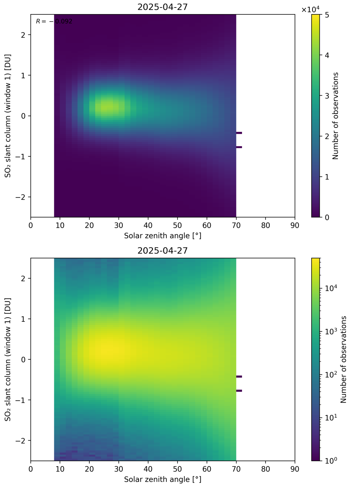
Figure 184: Scatter density plot of “Solar zenith angle” against “SO 2 slant column (window 1)” for 2025-04-26 to 2025-04-28.
