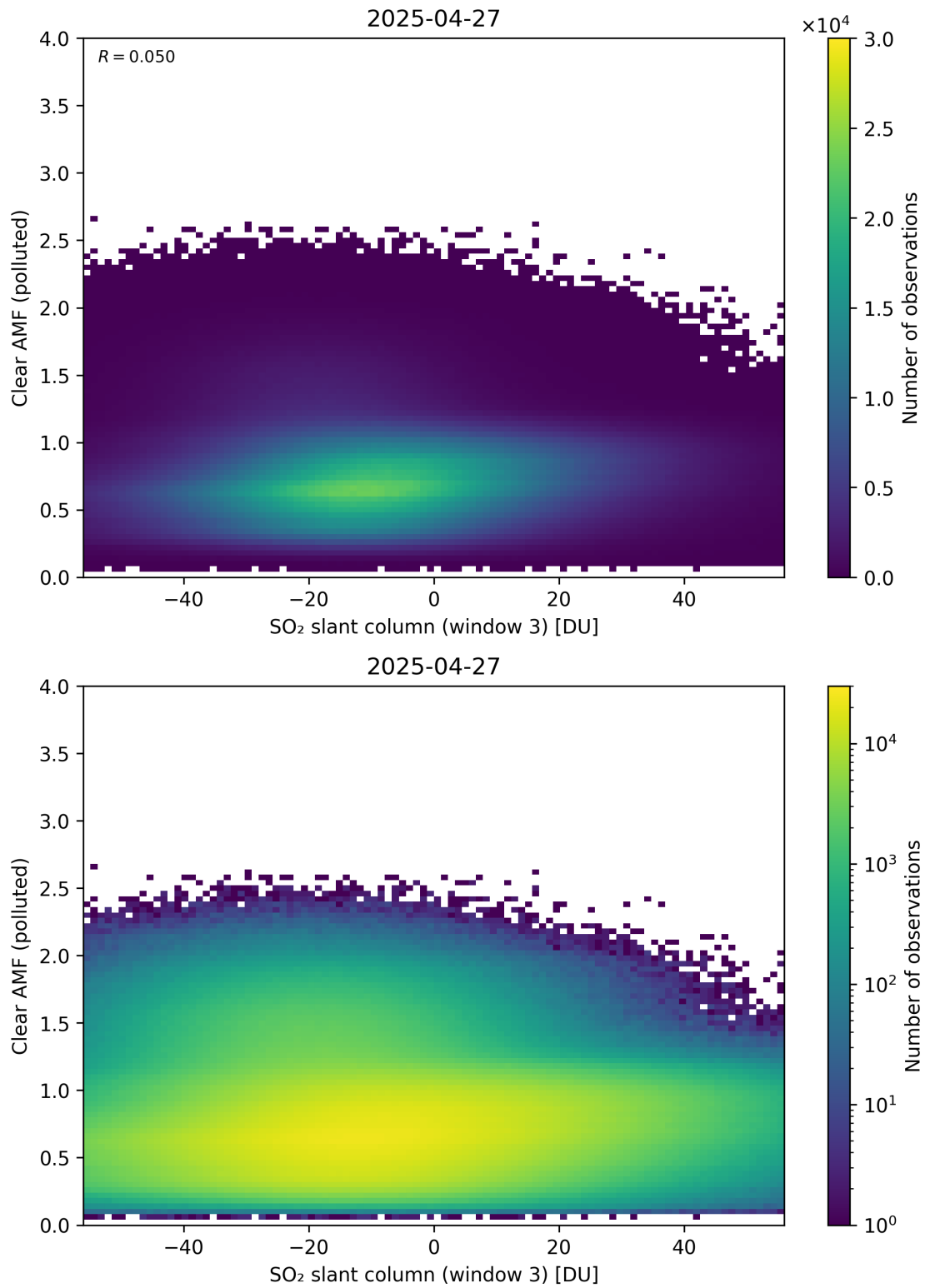
Figure 315: Scatter density plot of “SO 2 slant column (window 3)” against “Clear AMF (polluted)” for 2025-04-26 to 2025-04-28.
