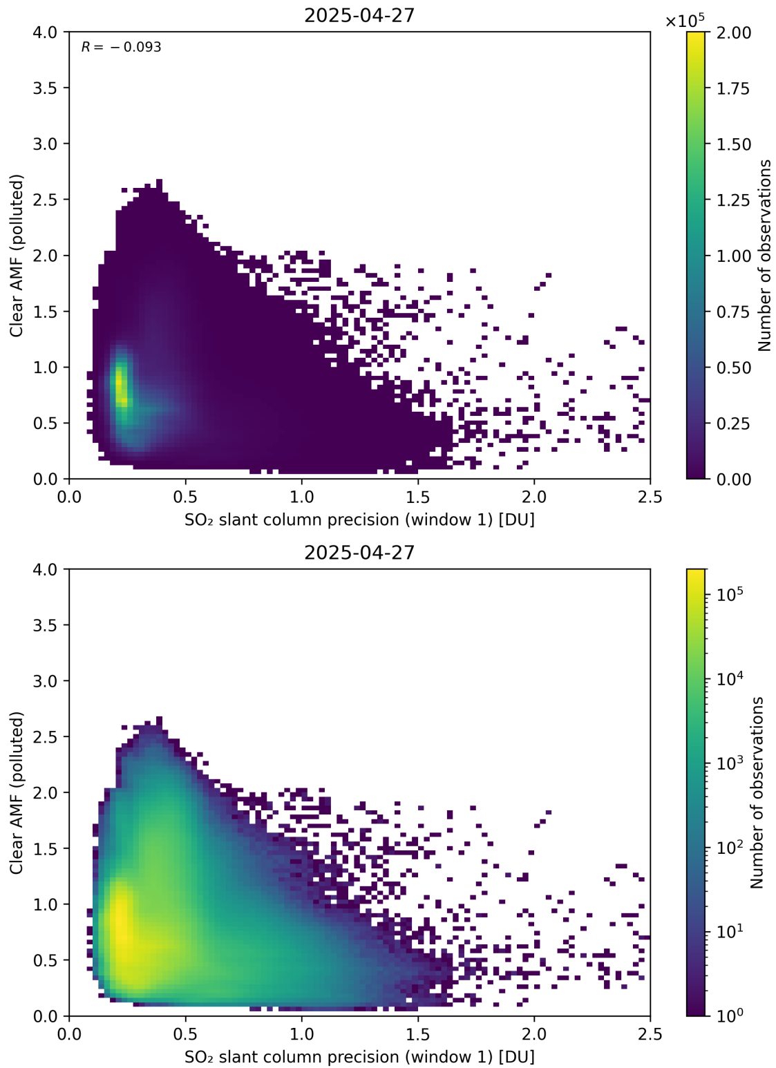
Figure 274: Scatter density plot of “SO 2 slant column precision (window 1)” against “Clear AMF (polluted)” for 2025-04-26 to 2025-04-28.
