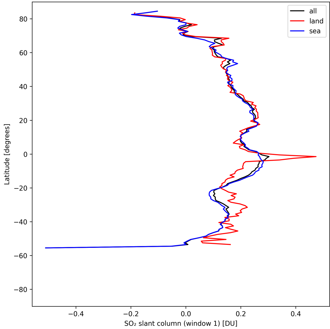
Figure 37: Zonal average of “SO 2 slant column (window 1)” for 2025-04-26 to 2025-04-28.
