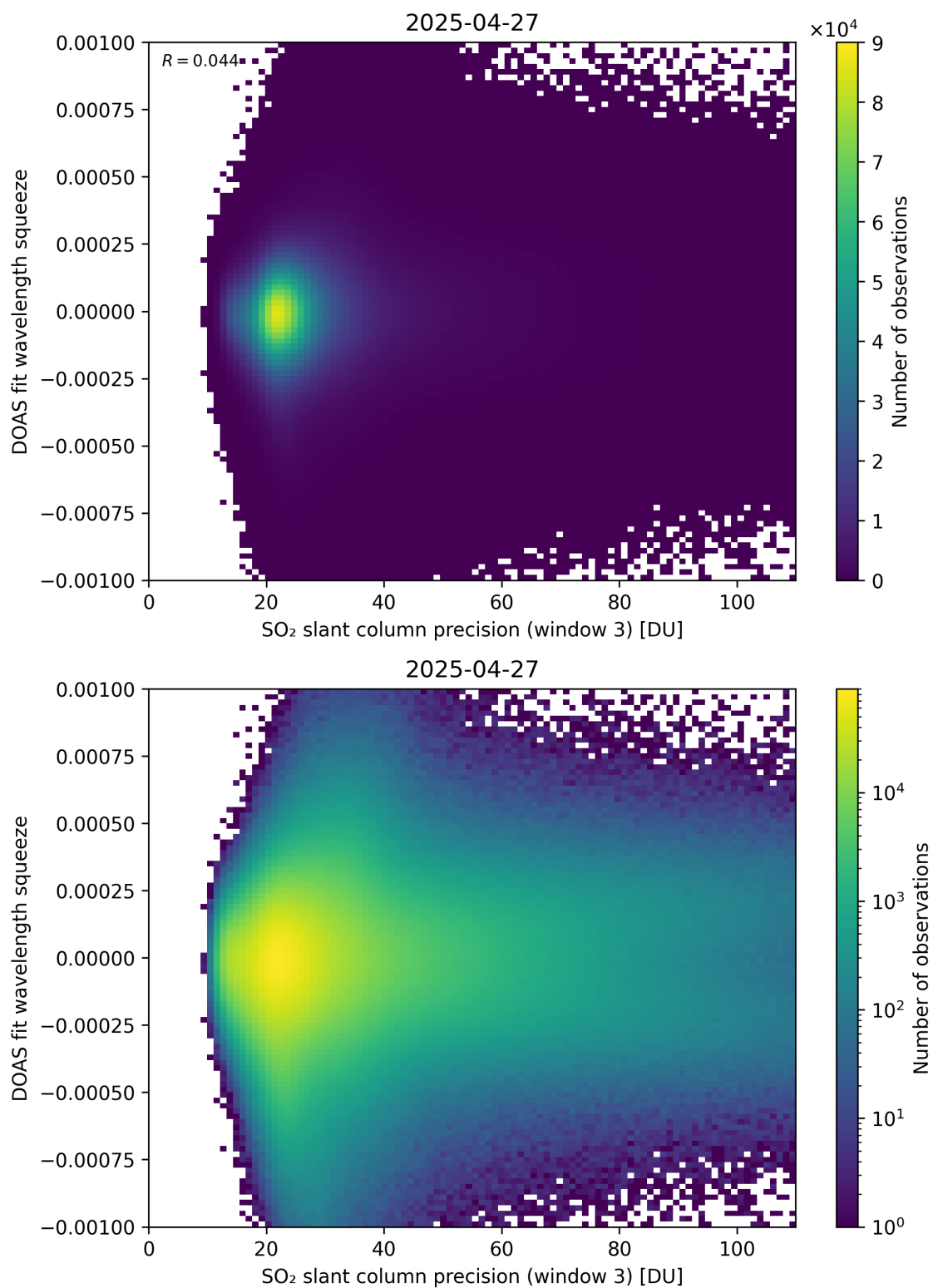
Figure 309: Scatter density plot of “SO 2 slant column precision (window 3)” against “DOAS fit wavelength squeeze” for 2025-04-26 to 2025-04-28.
