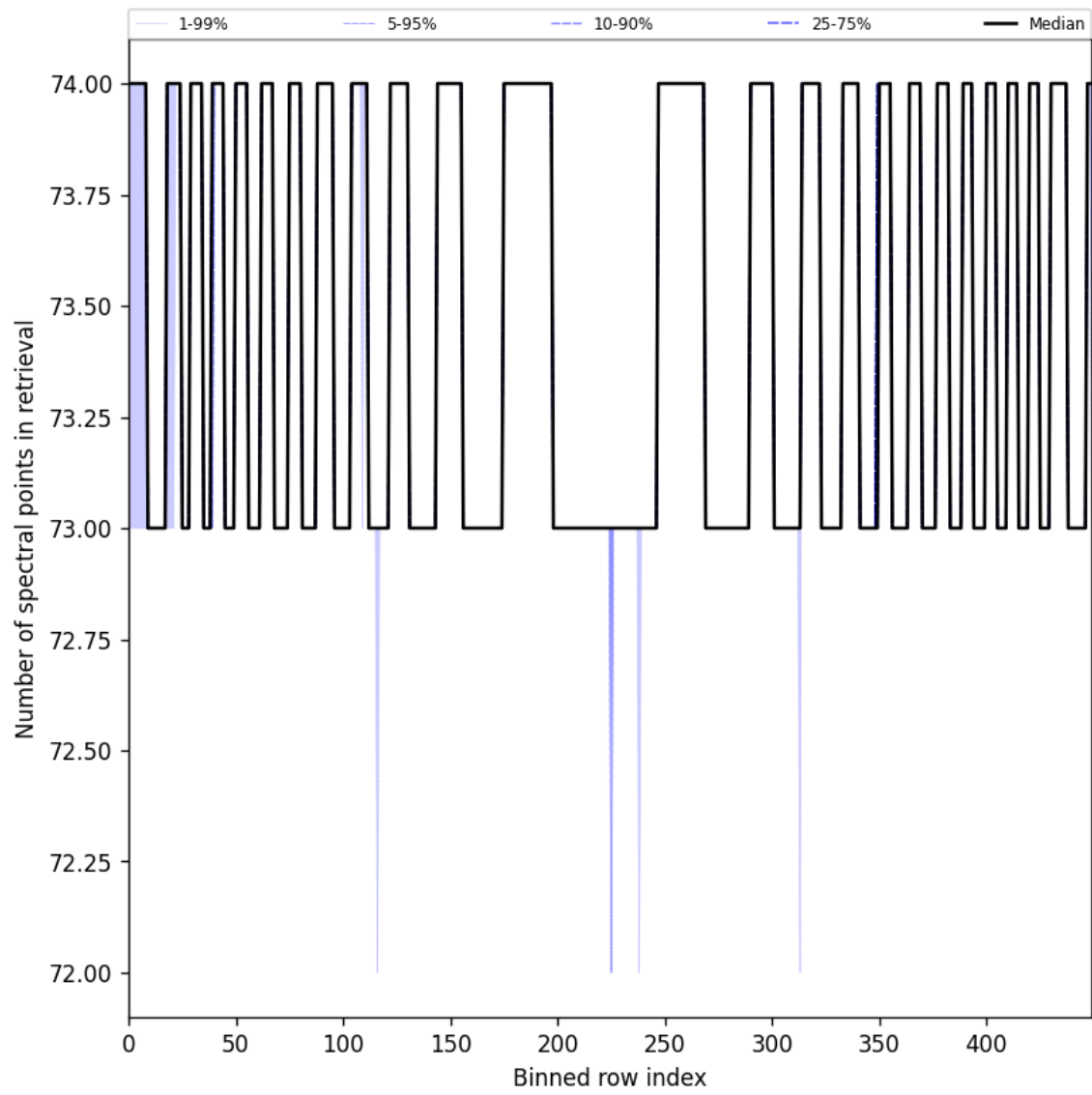
Figure 108: Along track statistics of “Number of spectral points in retrieval” for 2025-04-26 to 2025-04-28
