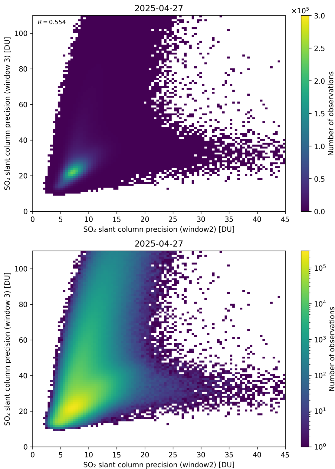
Figure 300: Scatter density plot of “SO 2 slant column precision (window2)” against “SO 2 slant column precision (window 3)” for 2025-04-26 to 2025-04-28.
