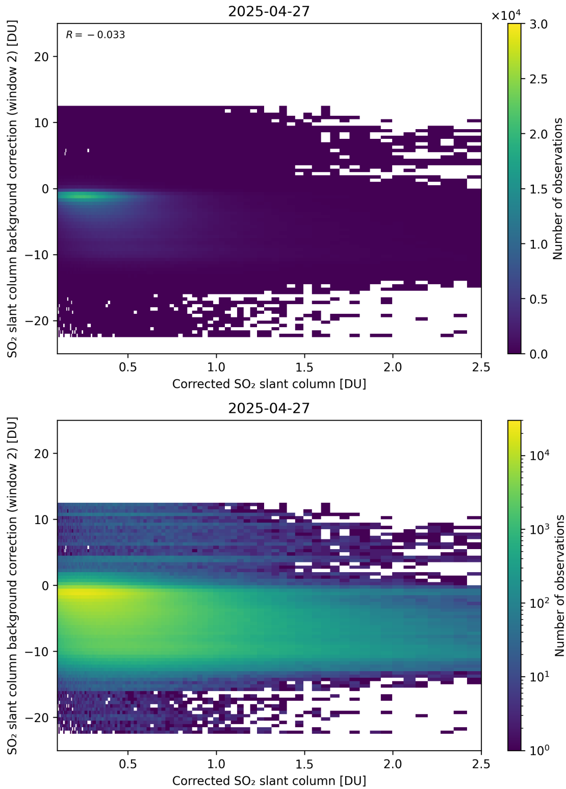
Figure 227: Scatter density plot of “Corrected SO 2 slant column” against “SO 2 slant column background correction (window 2)” for 2025-04-26 to 2025-04-28.
