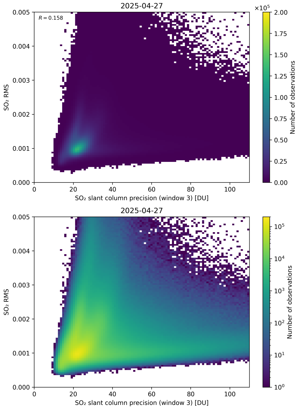
Figure 310: Scatter density plot of “SO 2 slant column precision (window 3)” against “SO 2 RMS” for 2025-04-26 to 2025-04-28.
