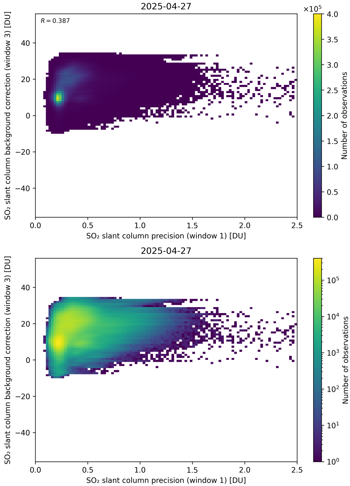
Figure 270: Scatter density plot of “SO 2 slant column precision (window 1)” against “SO 2 slant column background correction (window 3)” for 2025-04-26 to 2025-04-28.
