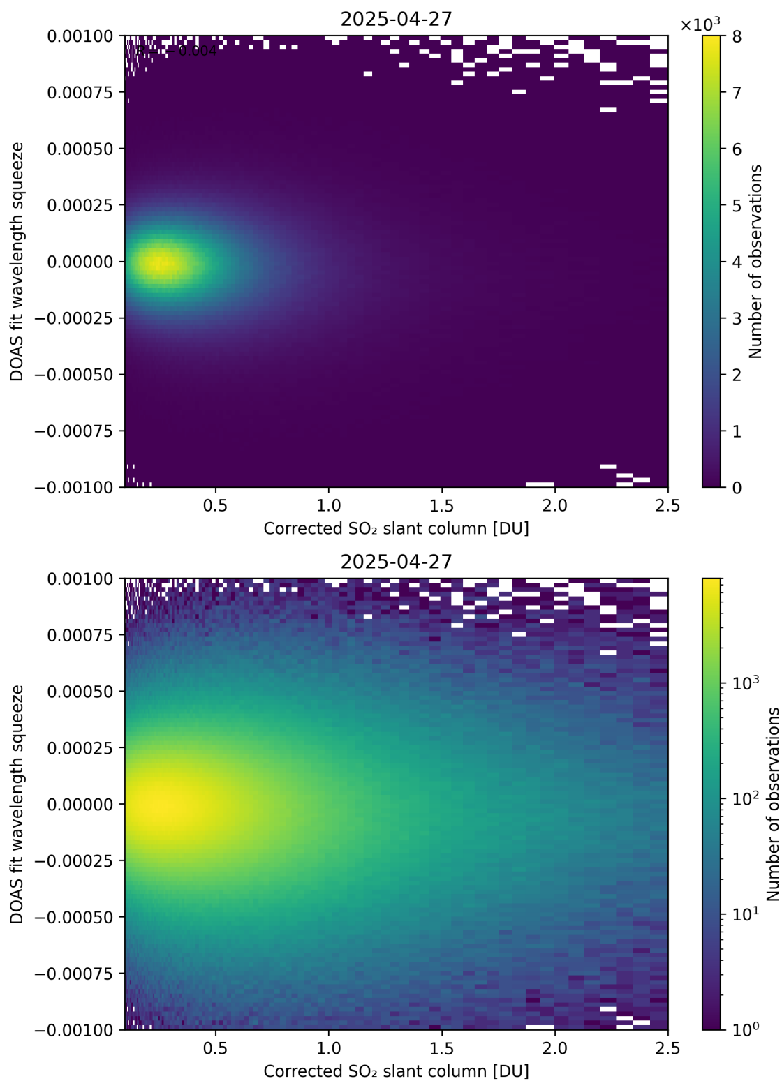
Figure 230: Scatter density plot of “Corrected SO 2 slant column” against “DOAS fit wavelength squeeze” for 2025-04-26 to 2025-04-28.
