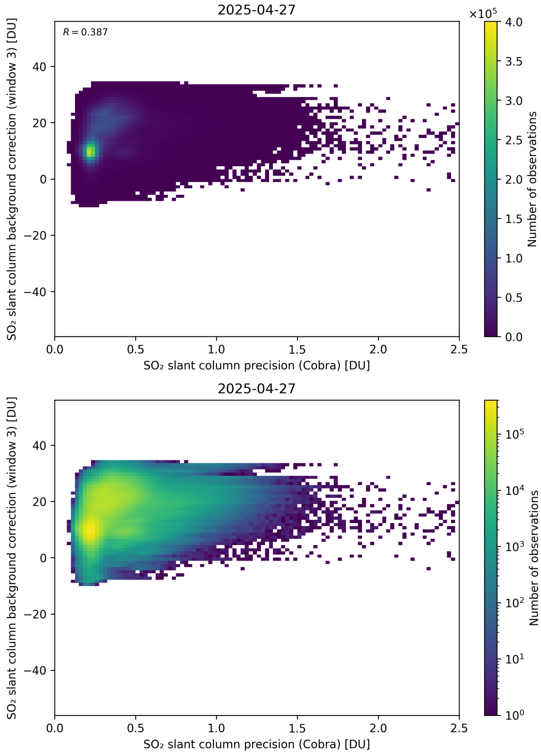
Figure 201: Scatter density plot of “SO 2 slant column precision (Cobra)” against “SO 2 slant column background correction (window 3)” for 2025-04-26 to 2025-04-28.
