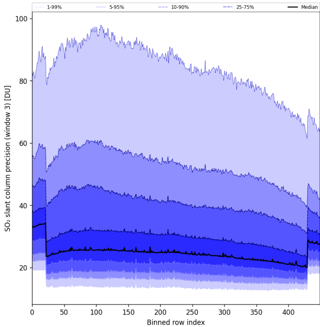
Figure 98: Along track statistics of “SO 2 slant column precision (window 3)” for 2025-04-26 to 2025-04-28
