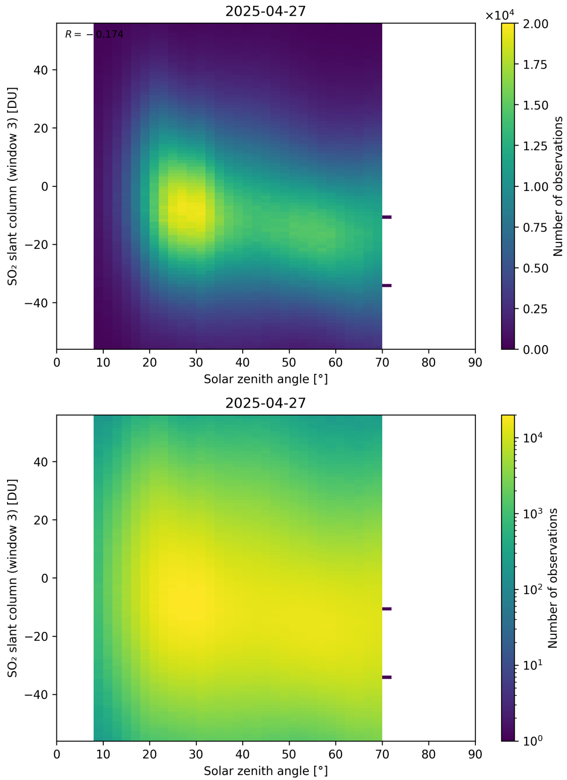
Figure 187: Scatter density plot of “Solar zenith angle” against “SO 2 slant column (window 3)” for 2025-04-26 to 2025-04-28.
