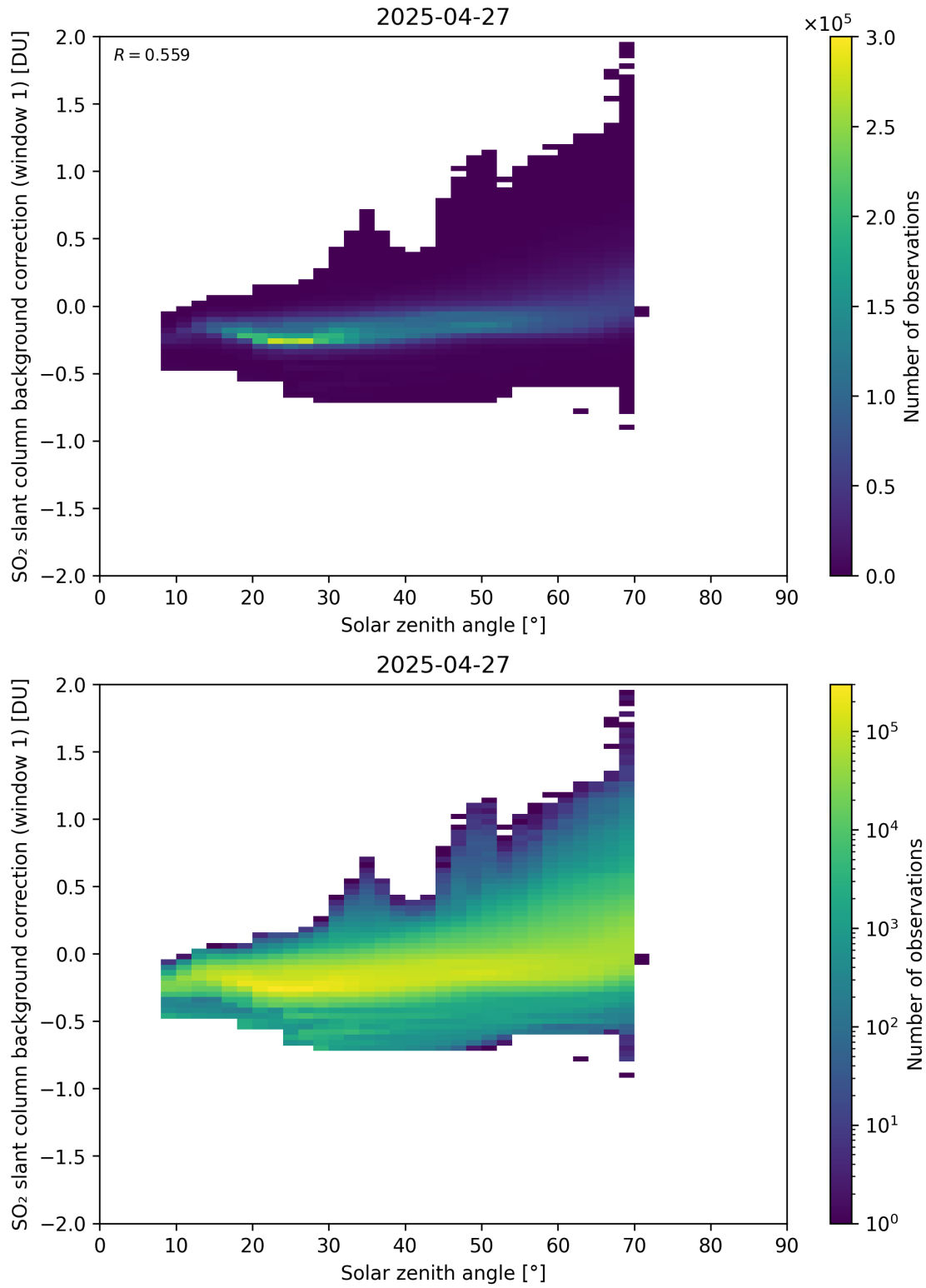
Figure 171: Scatter density plot of “Solar zenith angle” against “SO 2 slant column background correction (window 1)” for 2025-04-26 to 2025-04-28.
