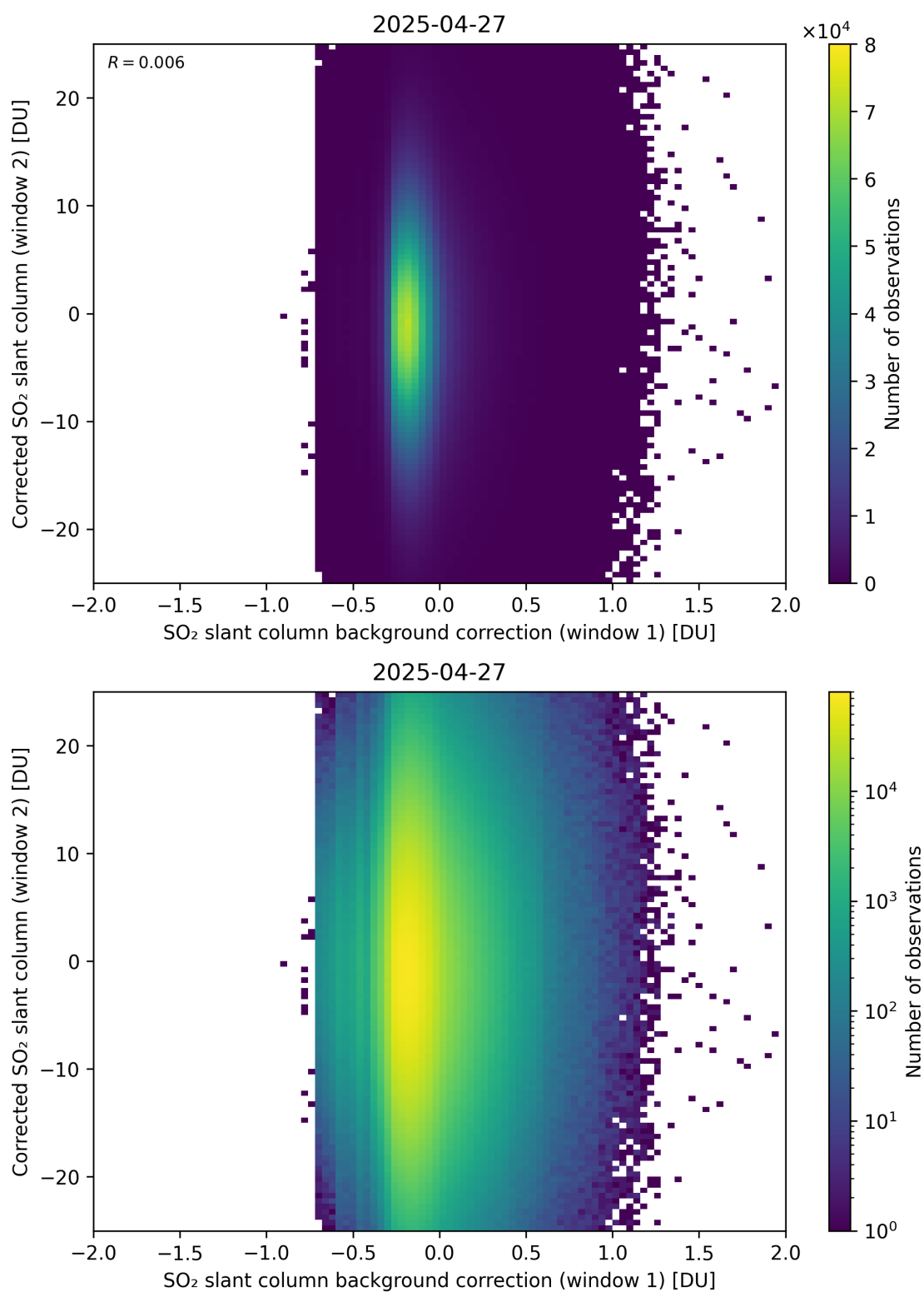
Figure 115: Scatter density plot of “SO 2 slant column background correction (window 1)” against “Corrected SO 2 slant column (window 2)” for 2025-04-26 to 2025-04-28.
