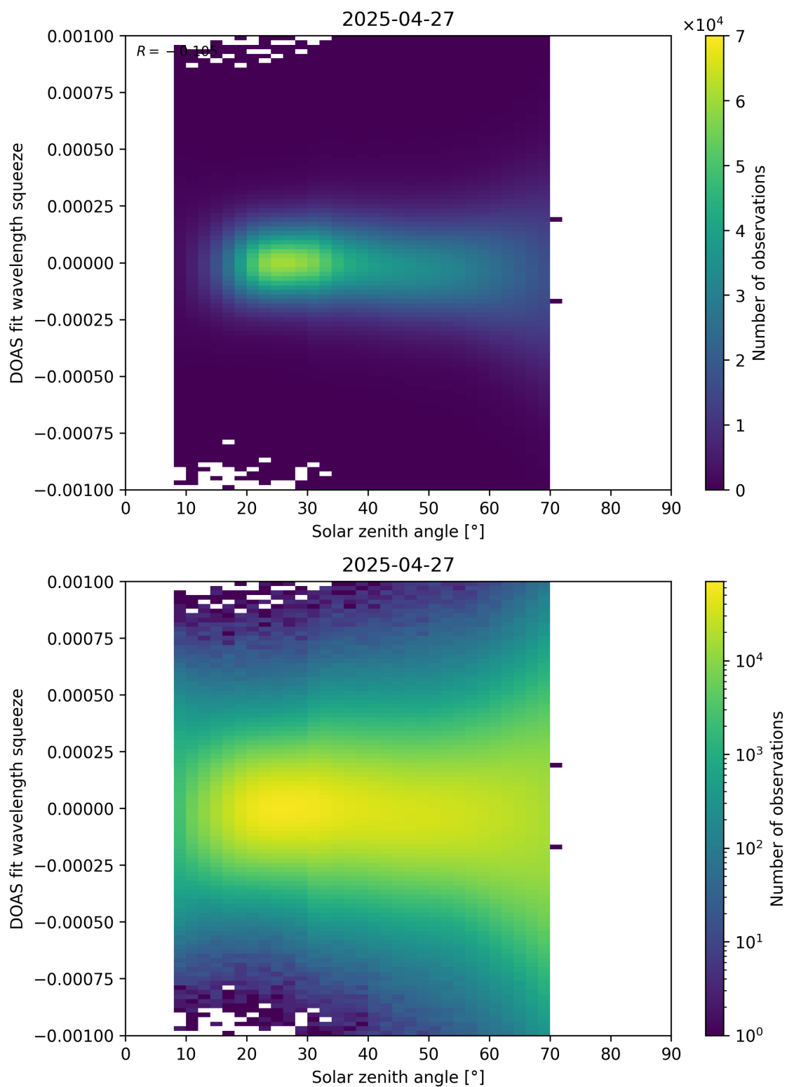
Figure 175: Scatter density plot of “Solar zenith angle” against “DOAS fit wavelength squeeze” for 2025-04-26 to 2025-04-28.
