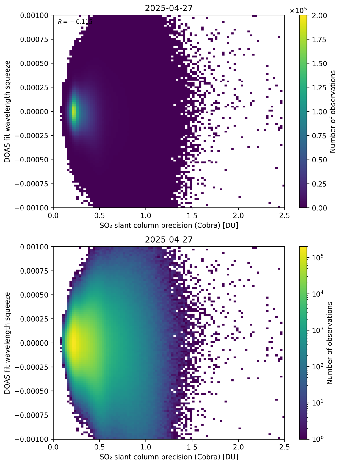
Figure 203: Scatter density plot of “SO 2 slant column precision (Cobra)” against “DOAS fit wavelength squeeze” for 2025-04-26 to 2025-04-28.
