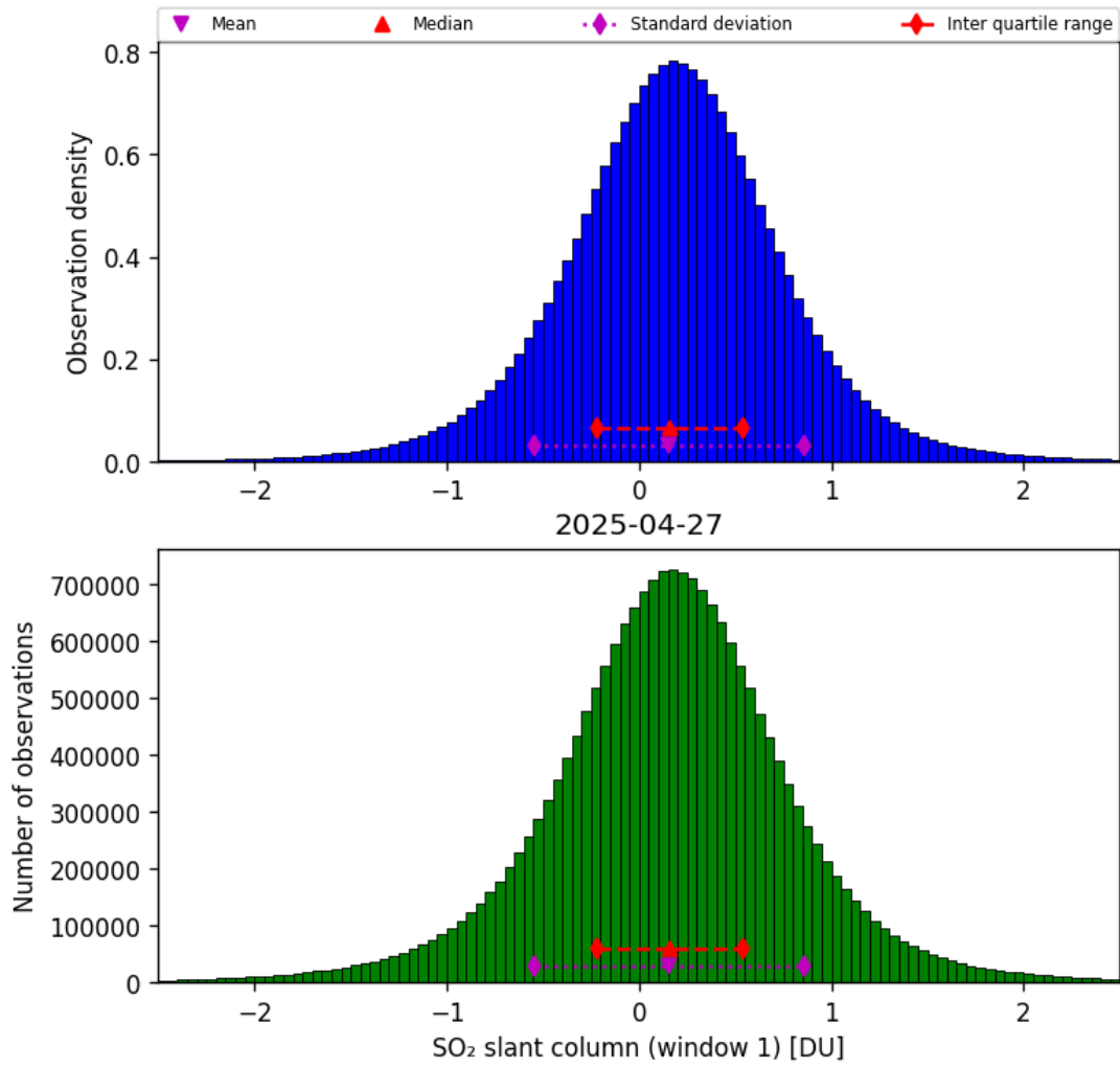
Figure 63: Histogram of “SO 2 slant column (window 1)” for 2025-04-26 to 2025-04-28
