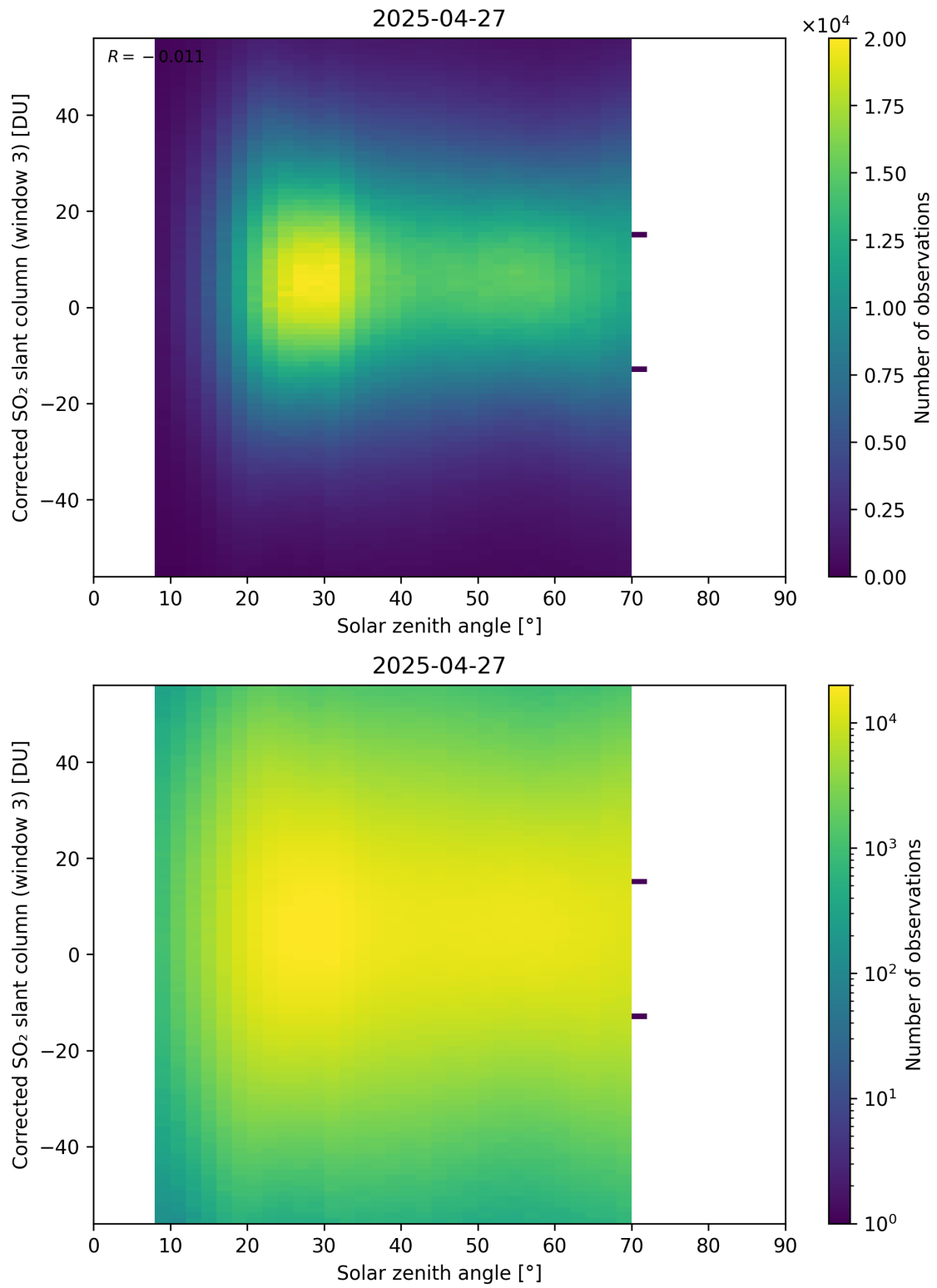
Figure 183: Scatter density plot of “Solar zenith angle” against “Corrected SO 2 slant column (window 3)” for 2025-04-26 to 2025-04-28.
