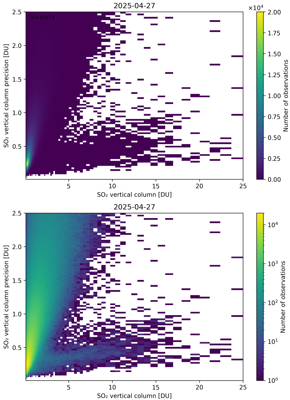
Figure 361: Scatter density plot of “SO 2 vertical column” against “SO 2 vertical column precision” for 2025-04-26 to 2025-04-28.
