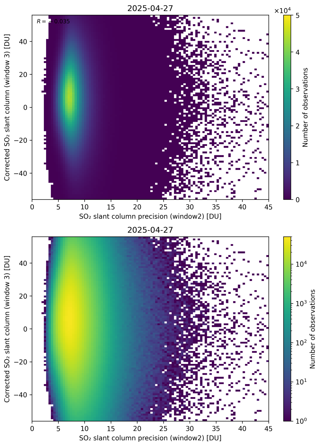
Figure 298: Scatter density plot of “SO 2 slant column precision (window2)” against “Corrected SO 2 slant column (window 3)” for 2025-04-26 to 2025-04-28.
