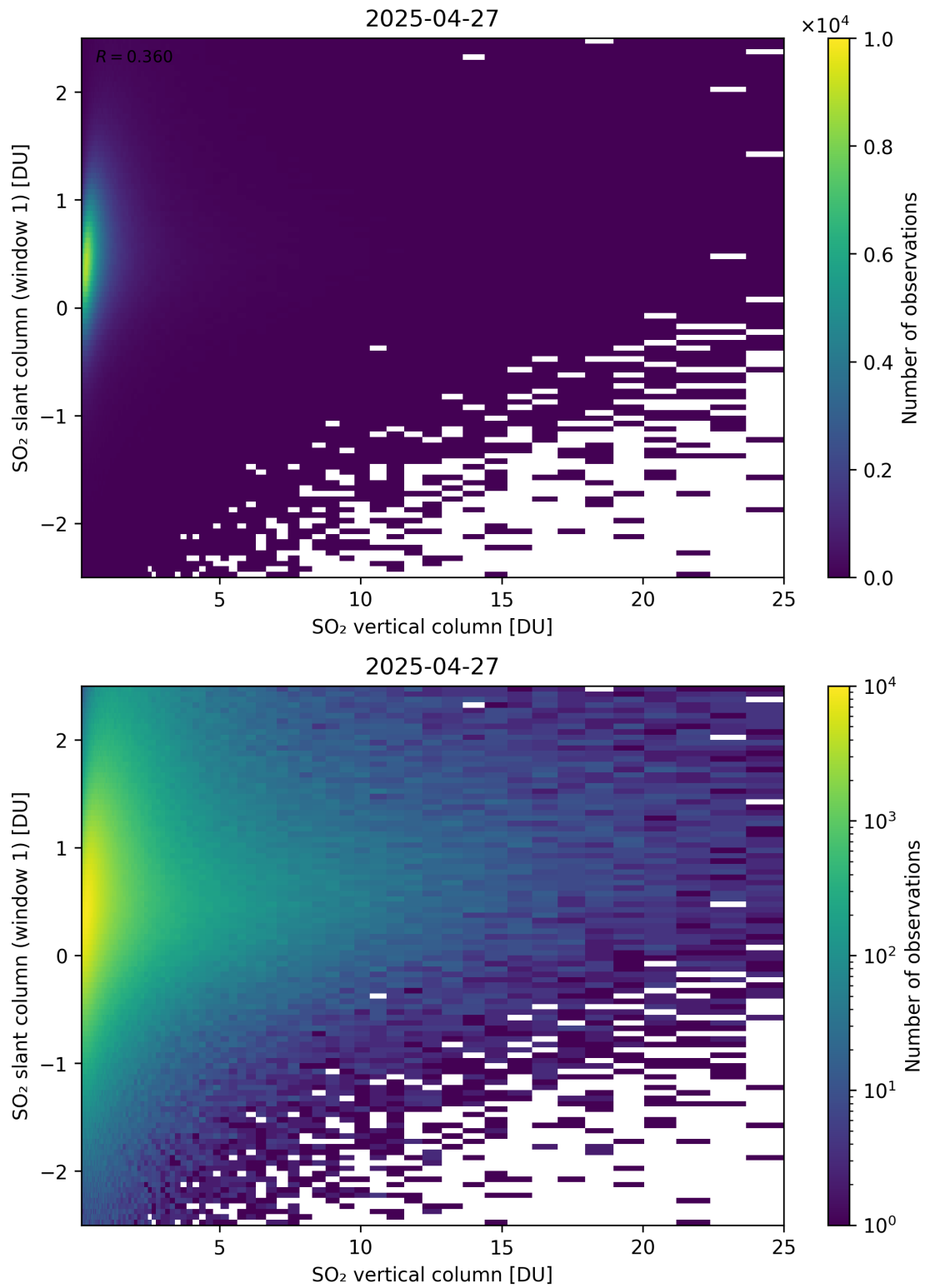
Figure 354: Scatter density plot of “SO 2 vertical column” against “SO 2 slant column (window 1)” for 2025-04-26 to 2025-04-28.
