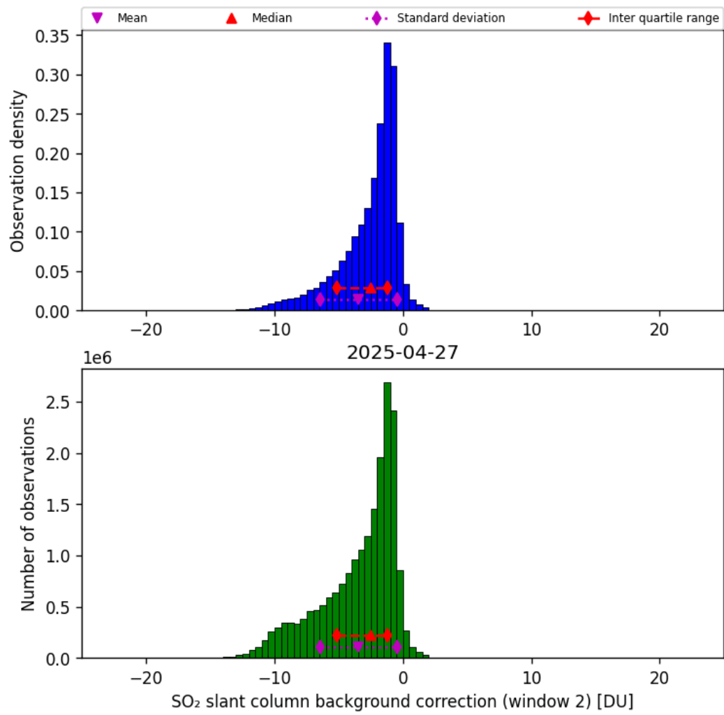
Figure 70: Histogram of “SO 2 slant column background correction (window 2)” for 2025-04-26 to 2025-04-28
