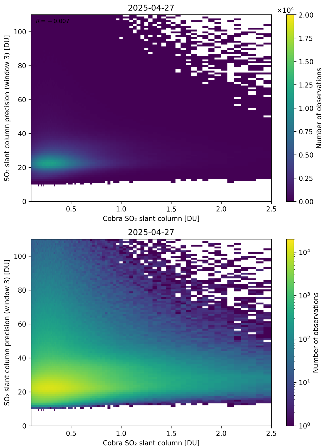
Figure 223: Scatter density plot of “Cobra SO 2 slant column” against “SO 2 slant column precision (window 3)” for 2025-04-26 to 2025-04-28.
