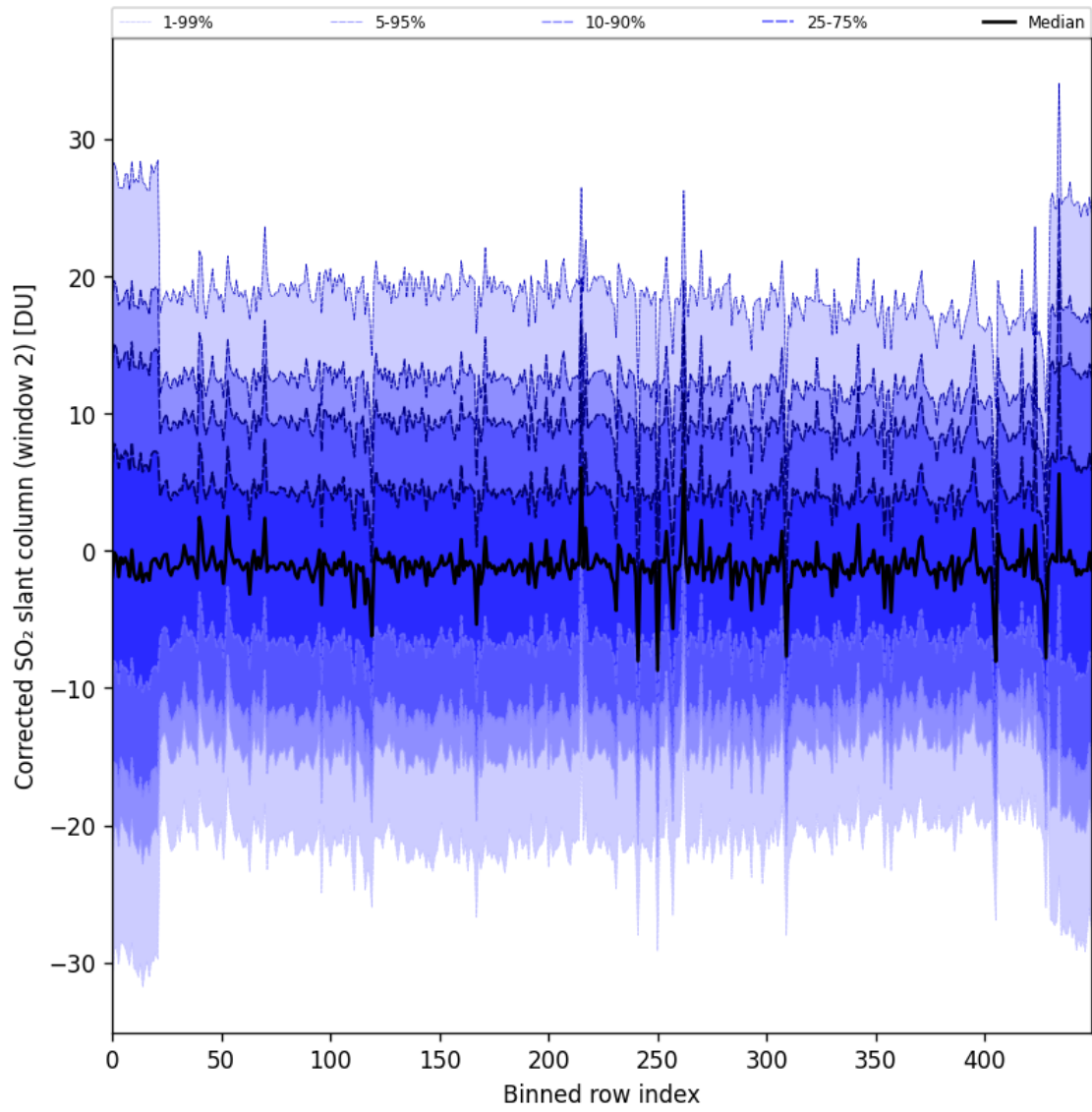
Figure 95: Along track statistics of “Corrected SO 2 slant column (window 2)” for 2025-04-26 to 2025-04-28
