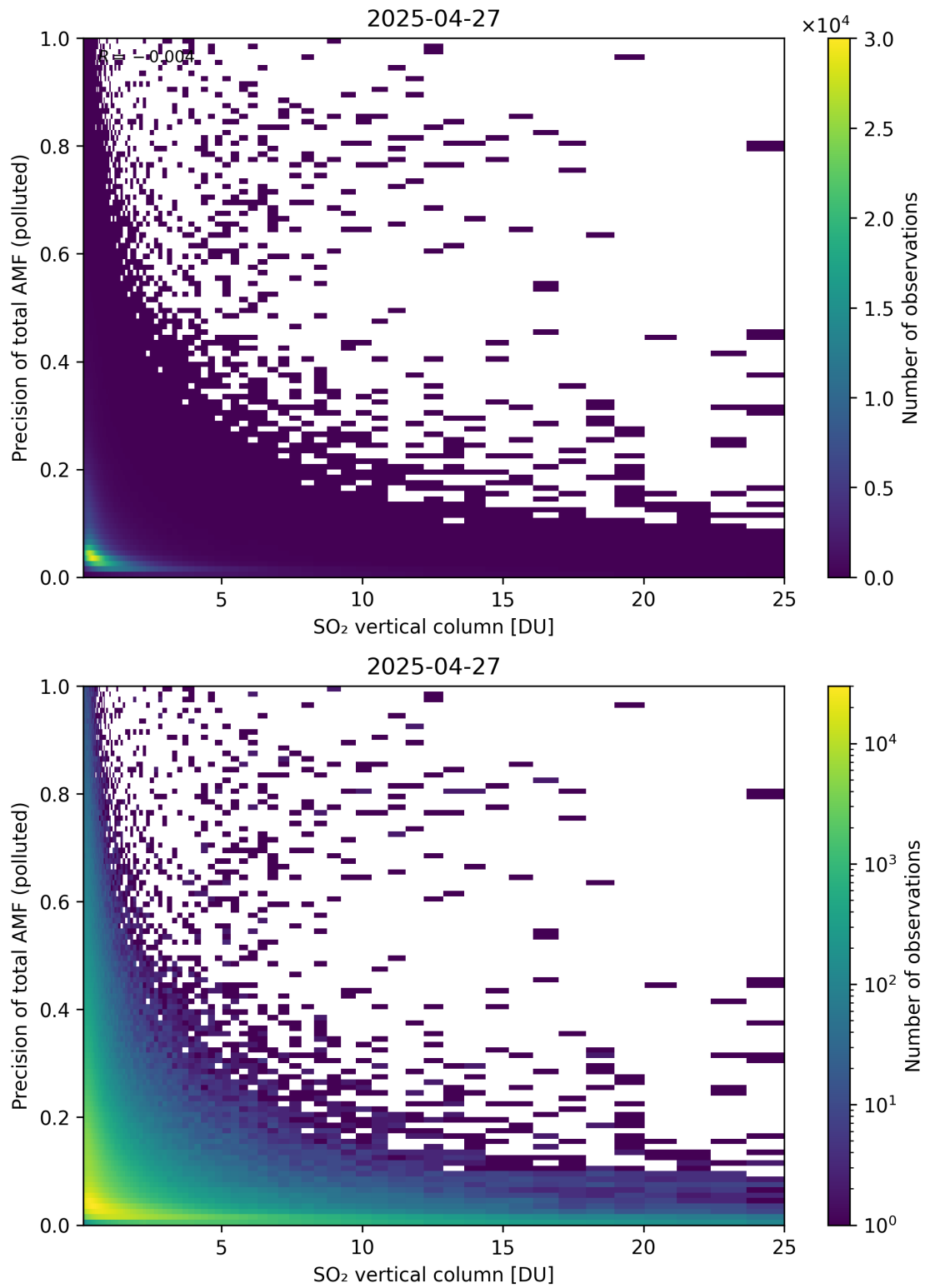
Figure 360: Scatter density plot of “SO 2 vertical column” against “Precision of total AMF (polluted)” for 2025-04-26 to 2025-04-28.
