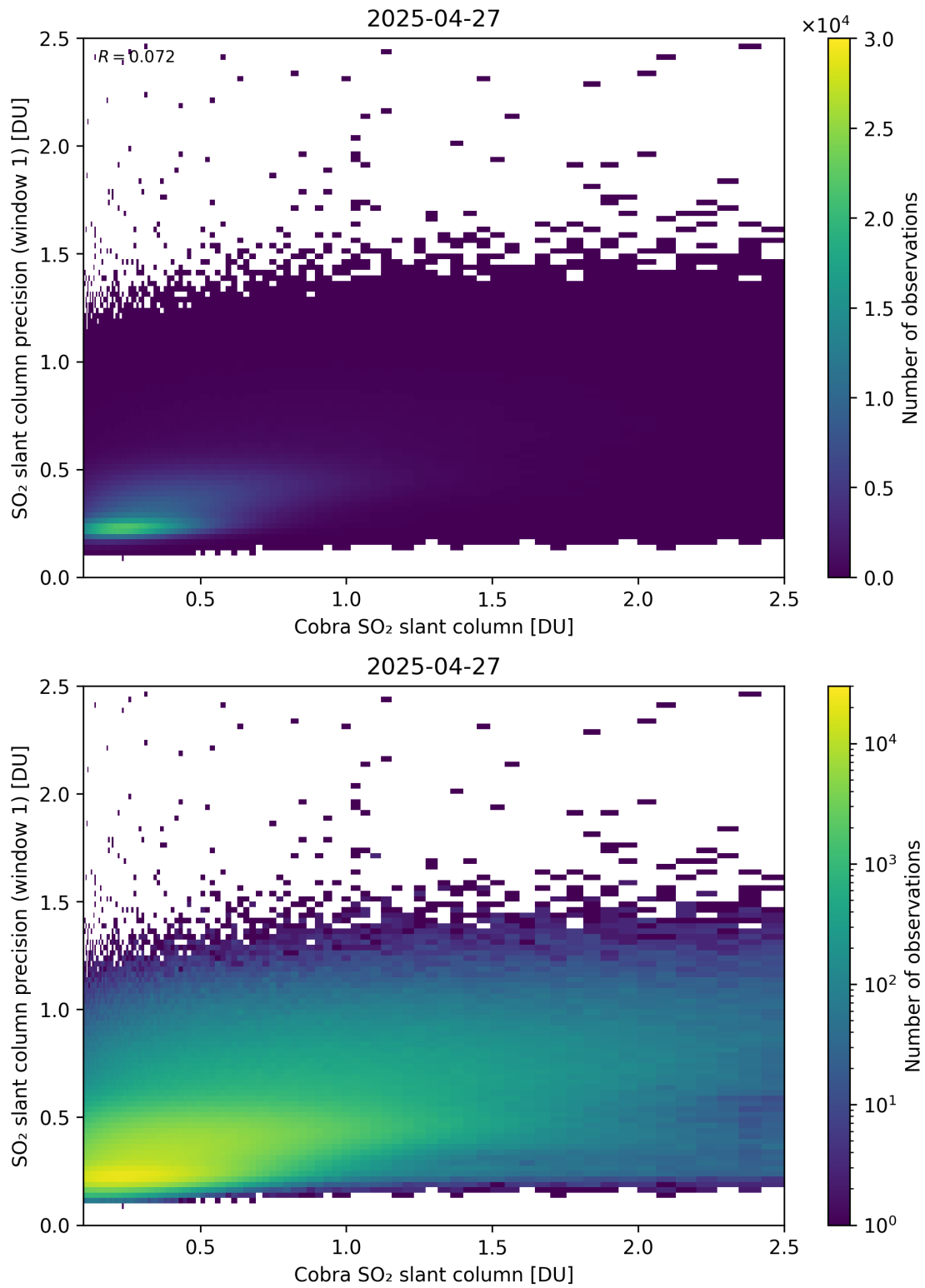
Figure 220: Scatter density plot of “Cobra SO 2 slant column” against “SO 2 slant column precision (window 1)” for 2025-04-26 to 2025-04-28.
