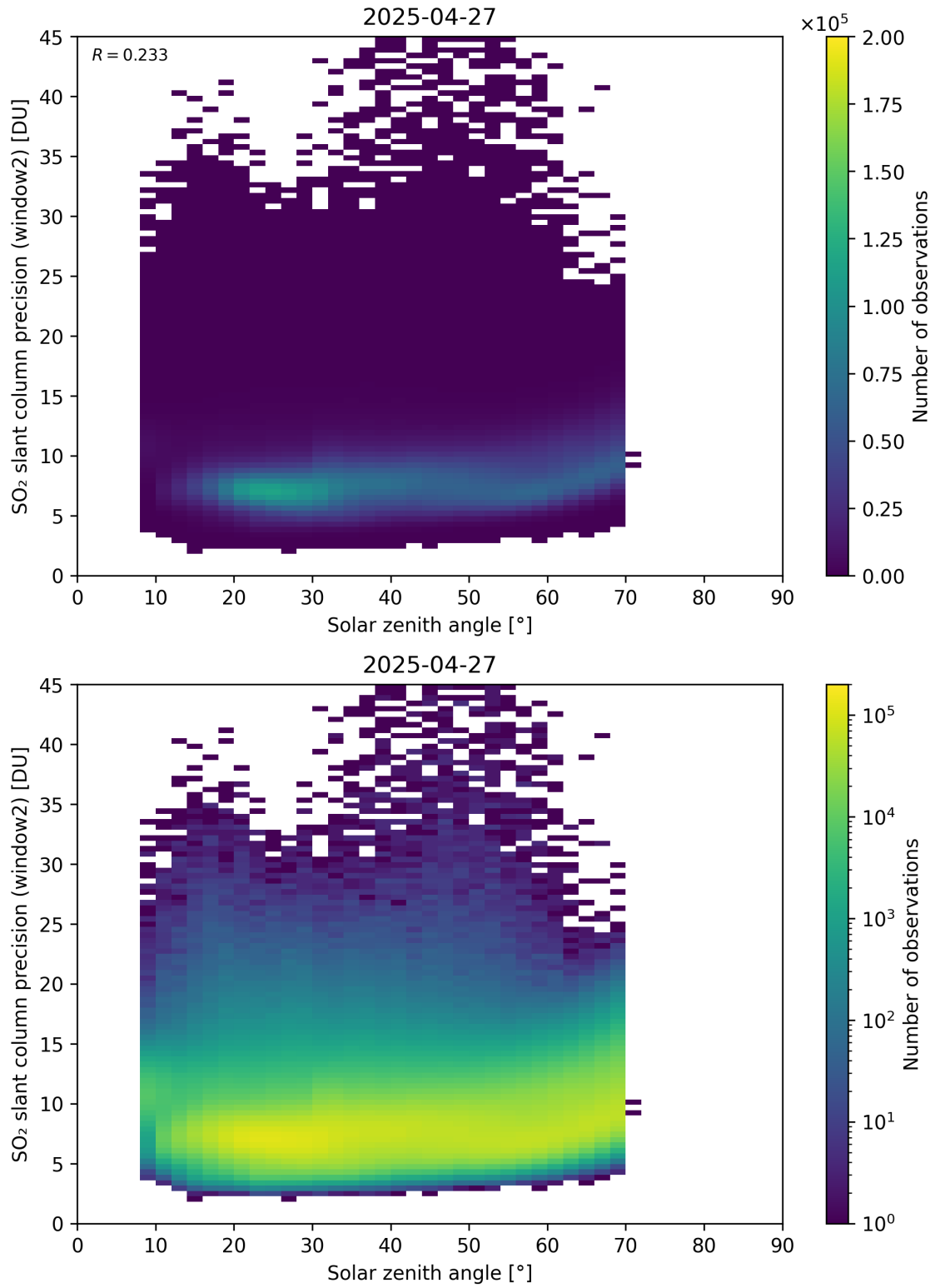
Figure 186: Scatter density plot of “Solar zenith angle” against “SO 2 slant column precision (window2)” for 2025-04-26 to 2025-04-28.
