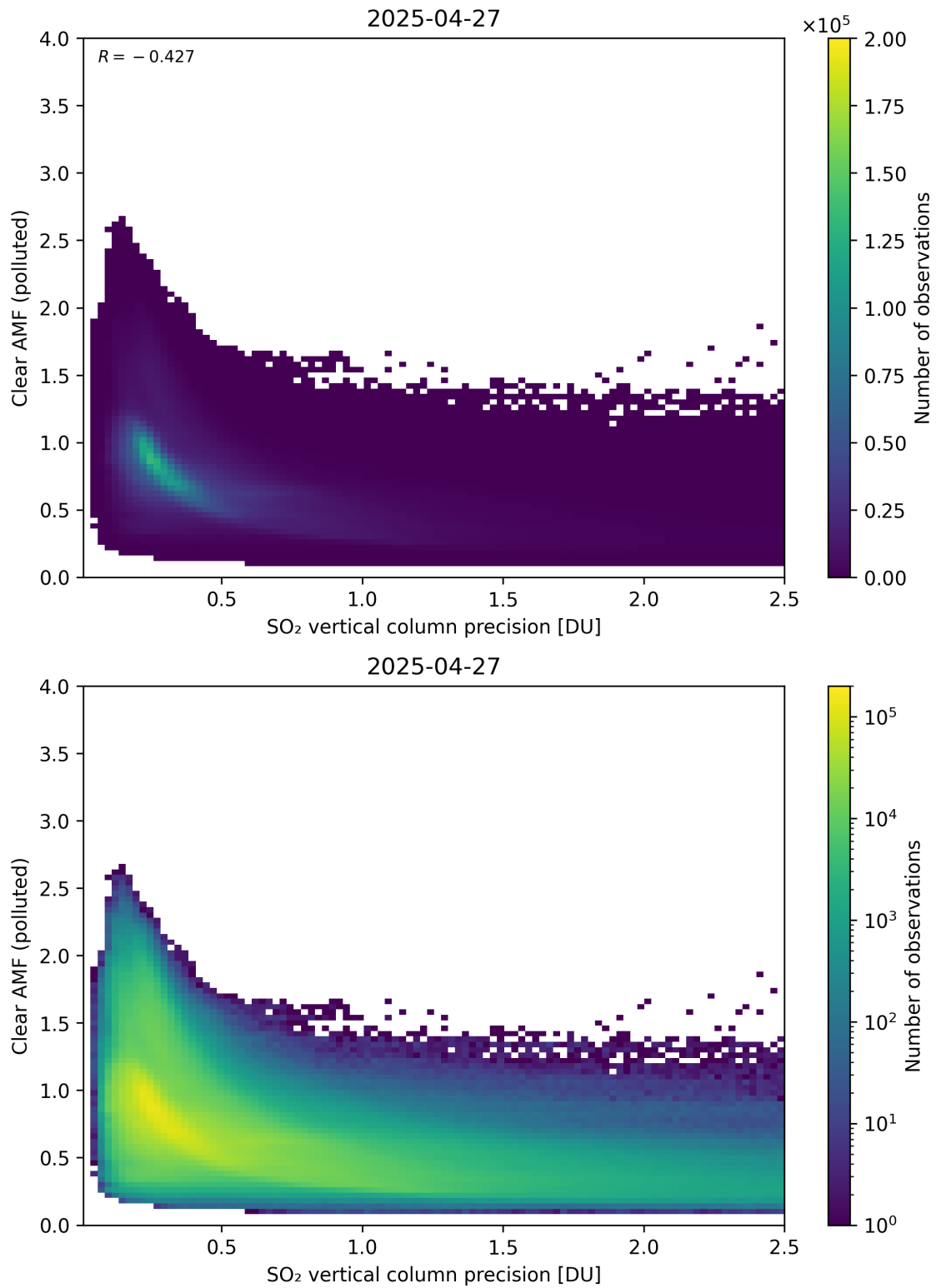
Figure 335: Scatter density plot of “SO 2 vertical column precision” against “Clear AMF (polluted)” for 2025-04-26 to 2025-04-28.
