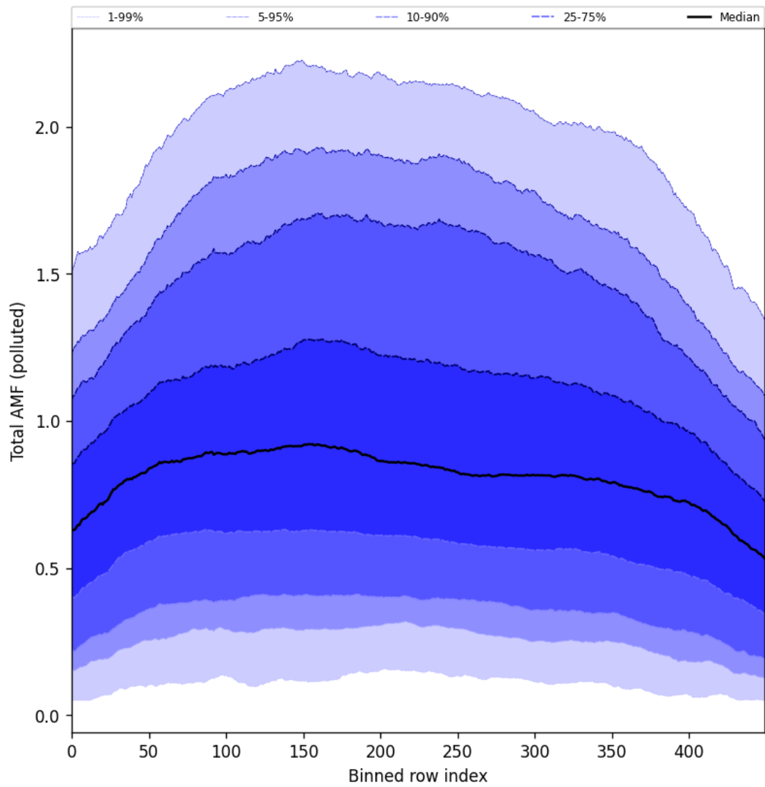
Figure 105: Along track statistics of “Total AMF (polluted)” for 2025-04-26 to 2025-04-28
