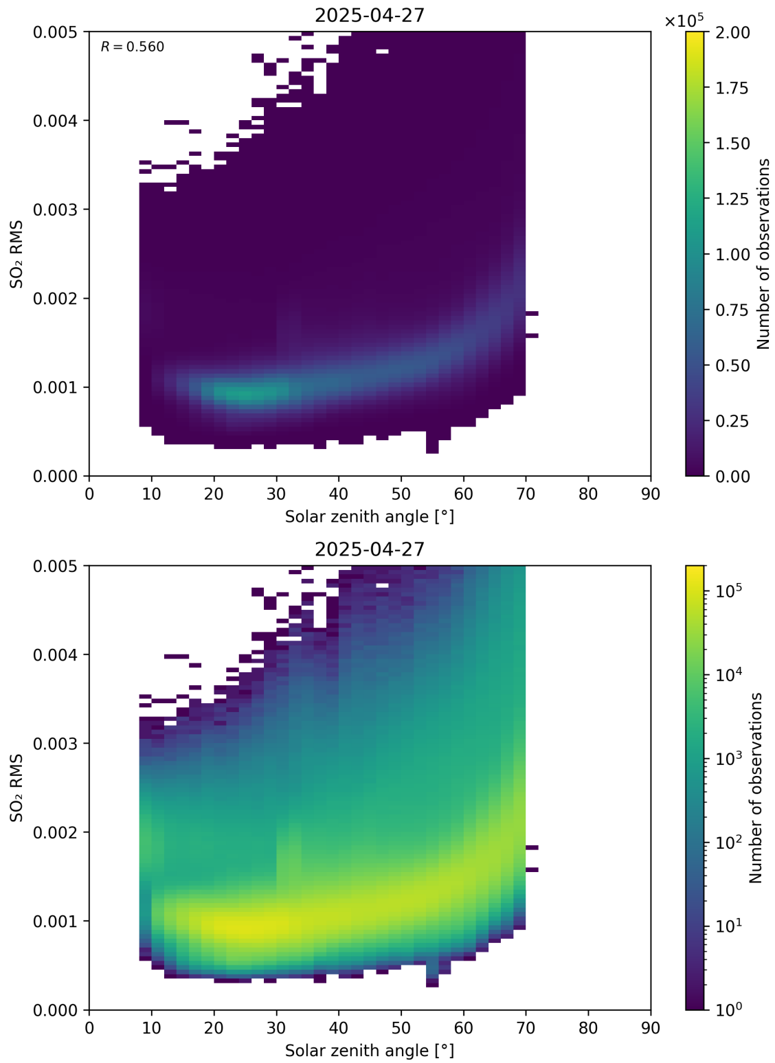
Figure 176: Scatter density plot of “Solar zenith angle” against “SO 2 RMS” for 2025-04-26 to 2025-04-28.
