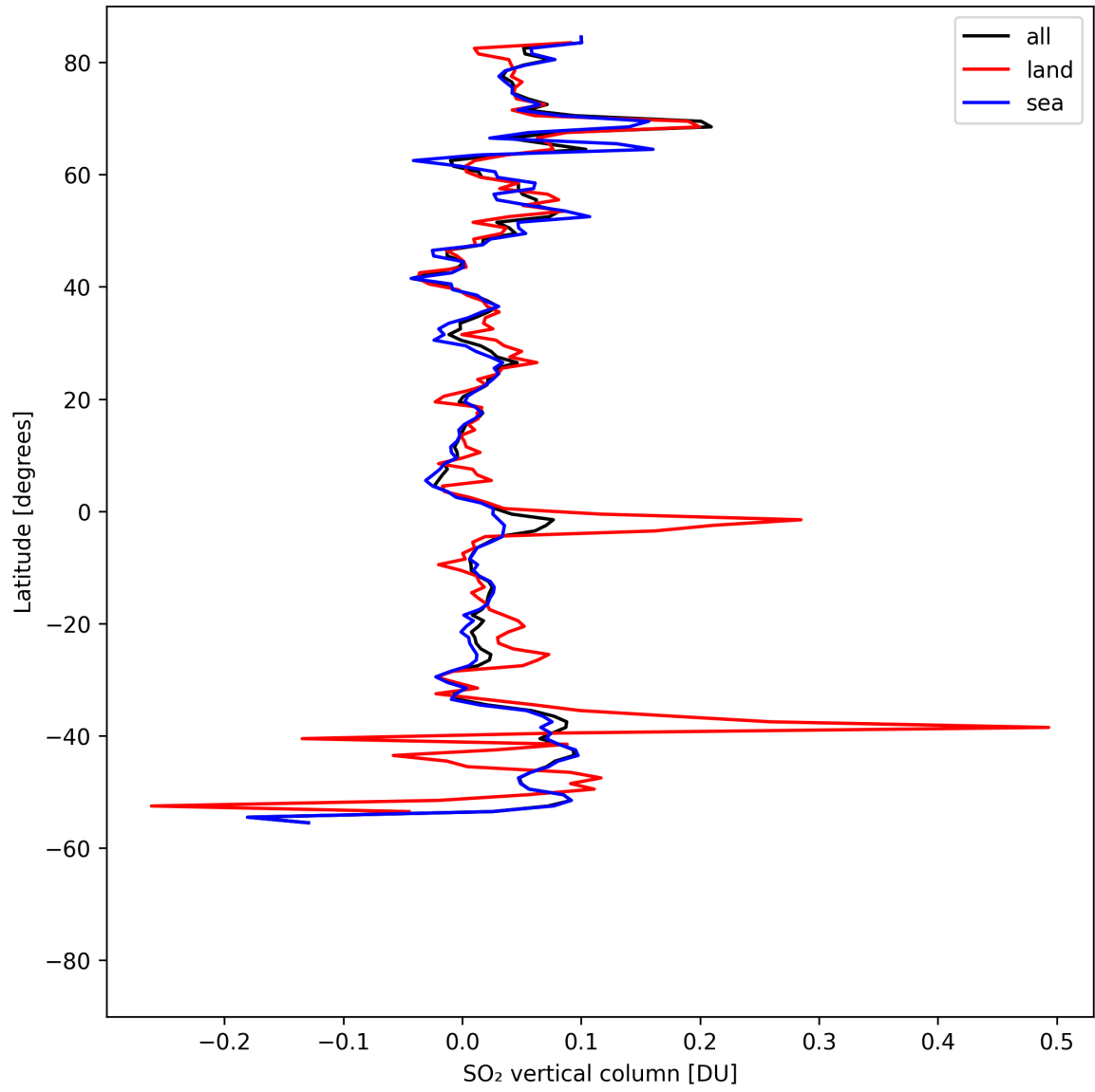
Figure 32: Zonal average of “SO 2 vertical column” for 2025-04-26 to 2025-04-28.
