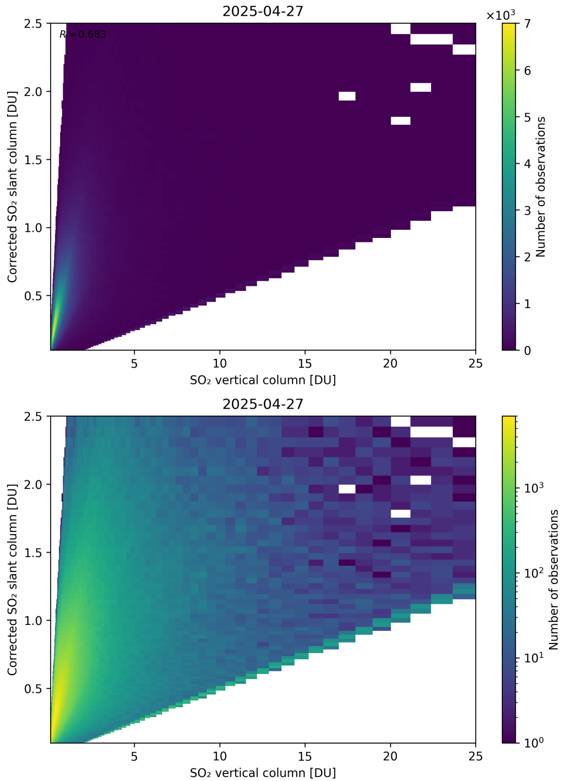
Figure 351: Scatter density plot of “SO 2 vertical column” against “Corrected SO 2 slant column” for 2025-04-26 to 2025-04-28.
