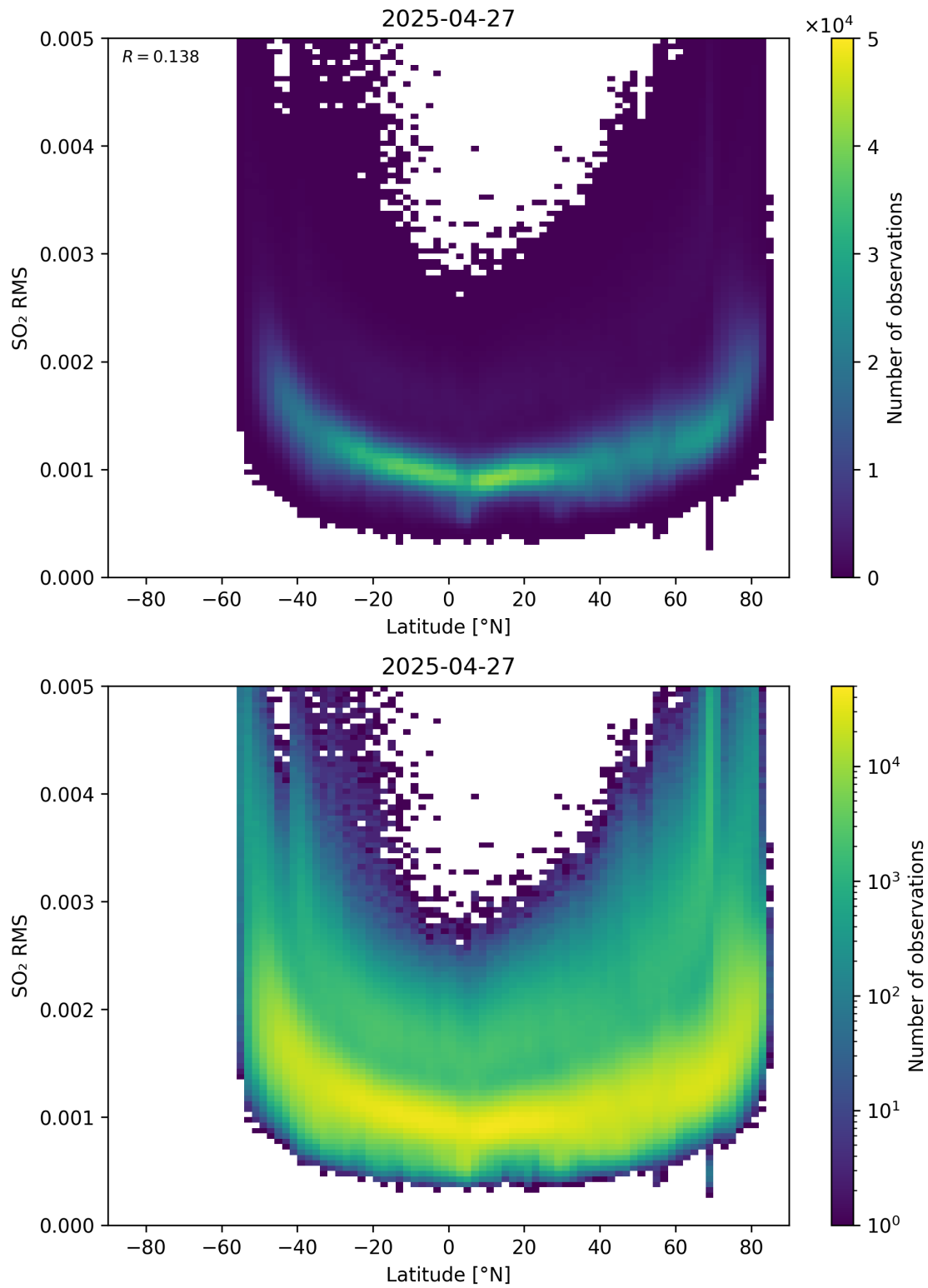
Figure 155: Scatter density plot of “Latitude” against “SO 2 RMS” for 2025-04-26 to 2025-04-28.
