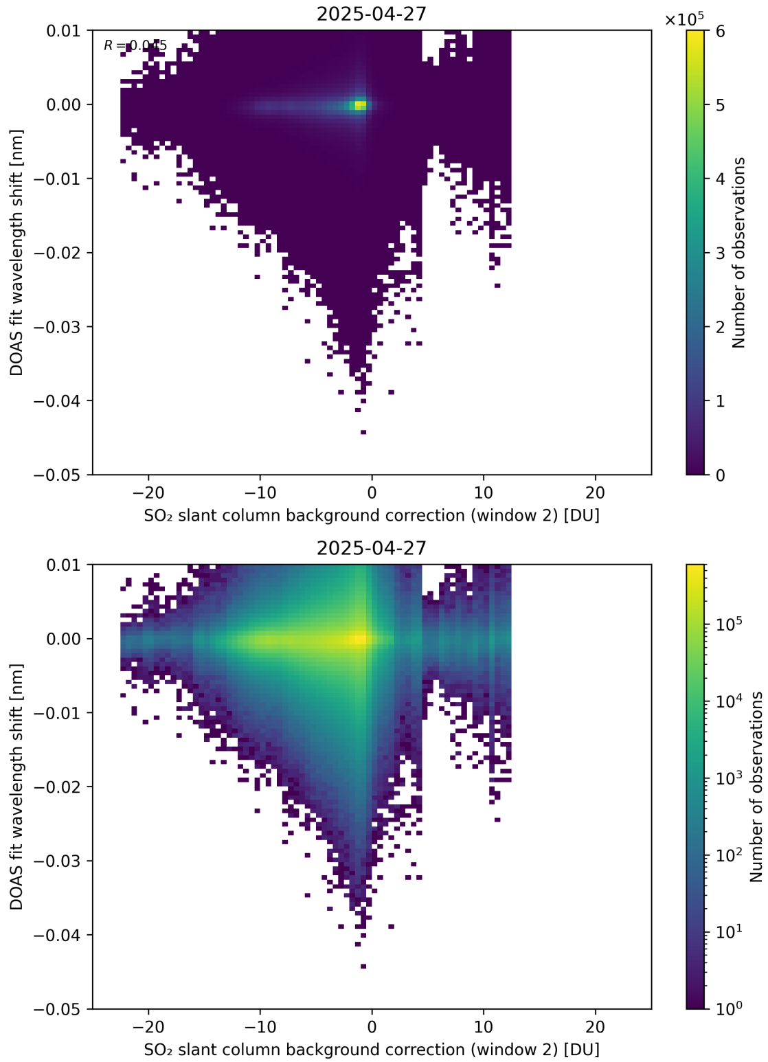
Figure 123: Scatter density plot of “SO 2 slant column background correction (window 2)” against “DOAS fit wavelength shift” for 2025-04-26 to 2025-04-28.
