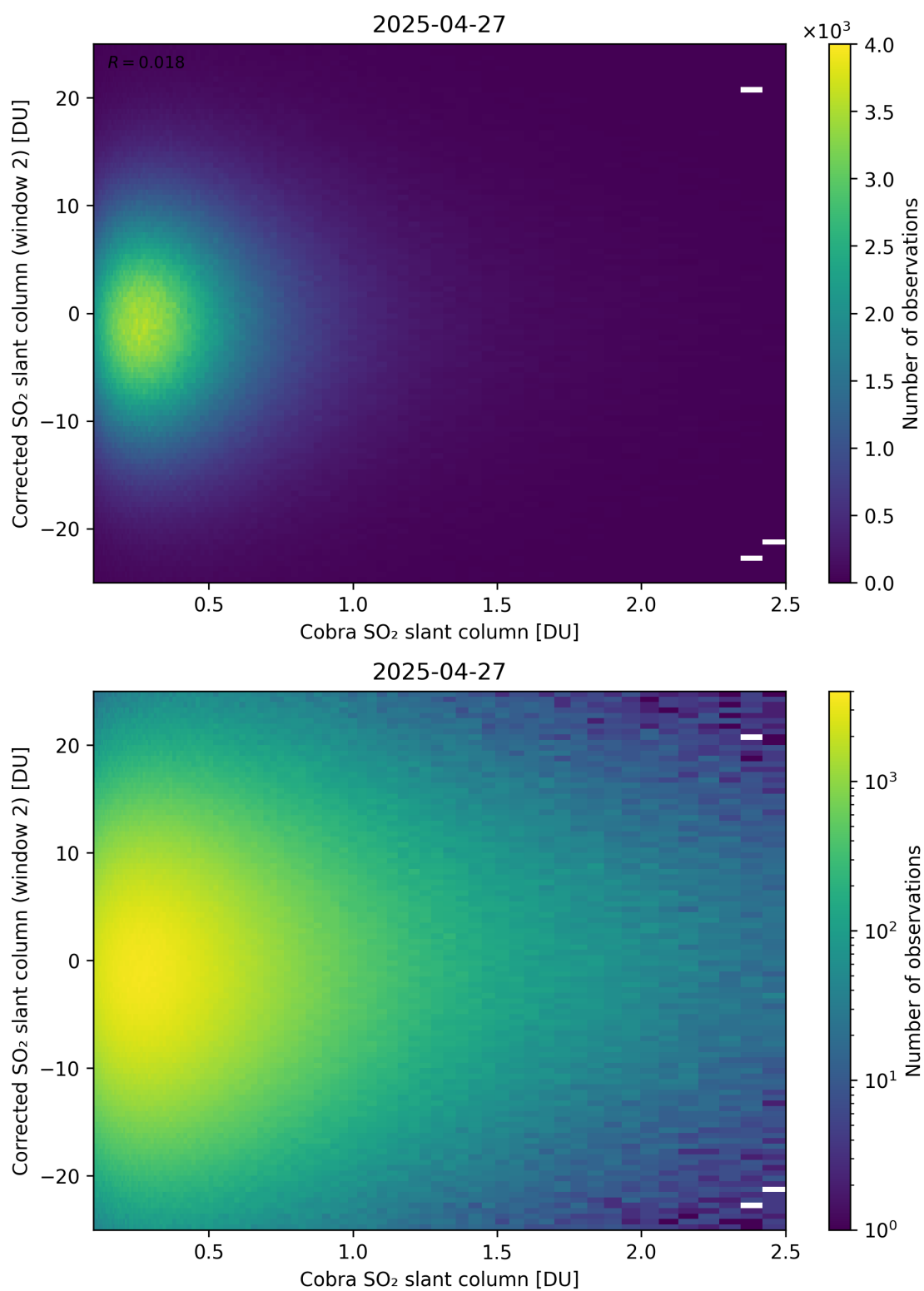
Figure 217: Scatter density plot of “Cobra SO 2 slant column” against “Corrected SO 2 slant column (window 2)” for 2025-04-26 to 2025-04-28.
