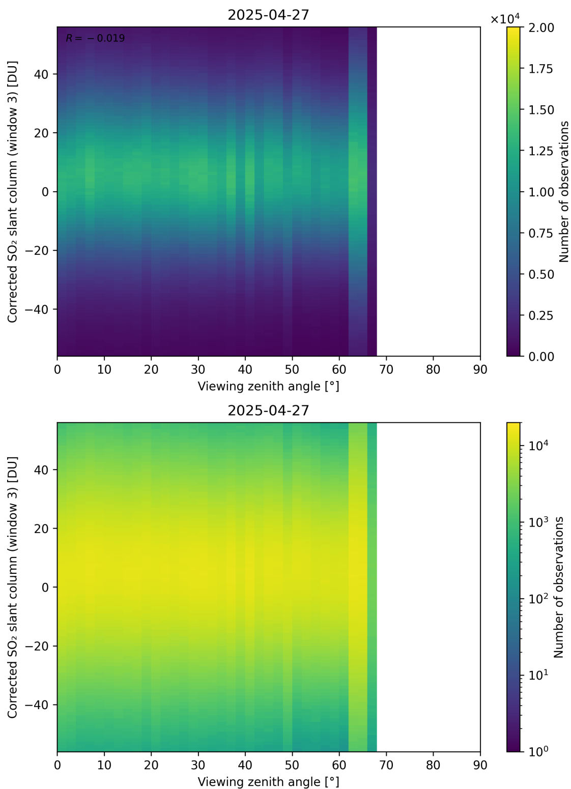
Figure 375: Scatter density plot of “Viewing zenith angle” against “Corrected SO 2 slant column (window 3)” for 2025-04-26 to 2025-04-28.
