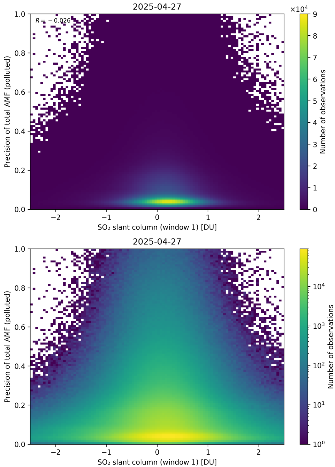
Figure 290: Scatter density plot of “SO 2 slant column (window 1)” against “Precision of total AMF (polluted)” for 2025-04-26 to 2025-04-28.
