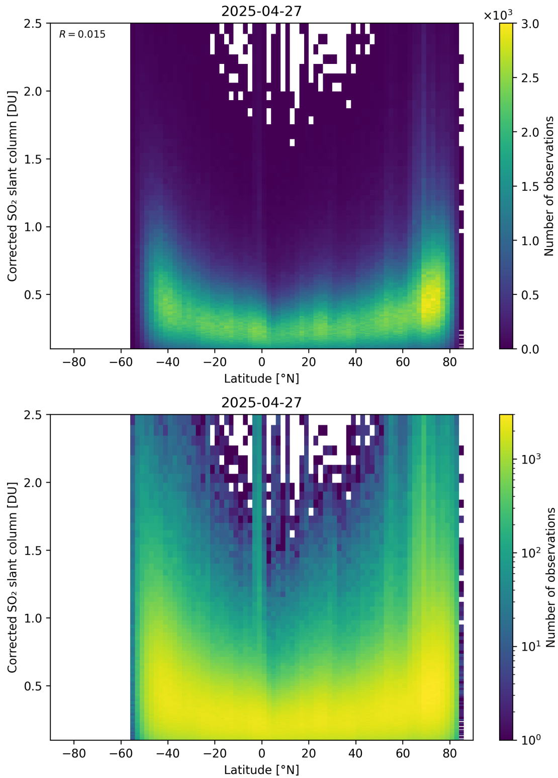
Figure 159: Scatter density plot of “Latitude” against “Corrected SO 2 slant column” for 2025-04-26 to 2025-04-28.
