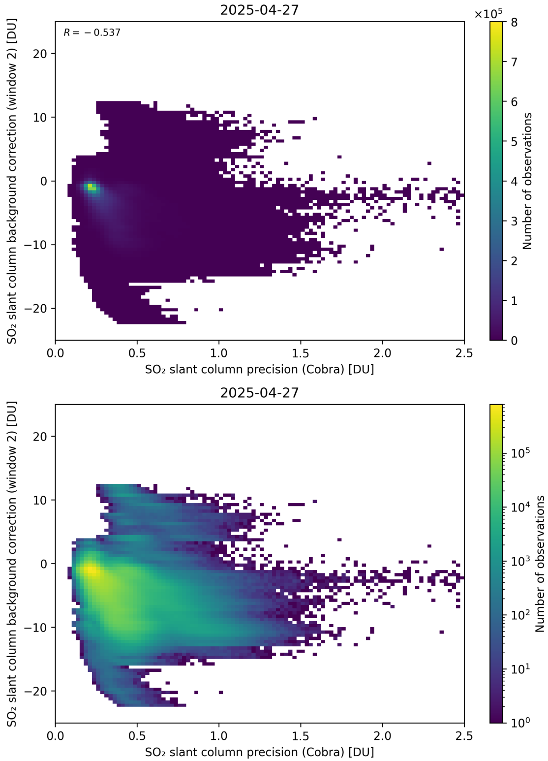
Figure 200: Scatter density plot of “SO 2 slant column precision (Cobra)” against “SO 2 slant column background correction (window 2)” for 2025-04-26 to 2025-04-28.
