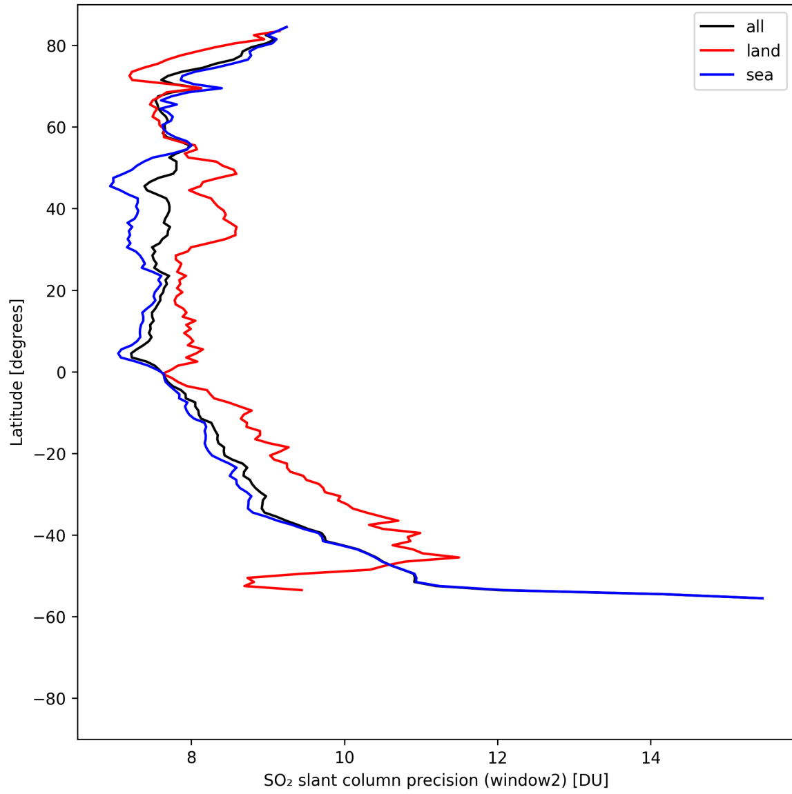
Figure 42: Zonal average of “SO 2 slant column precision (window2)” for 2025-04-26 to 2025-04-28.
