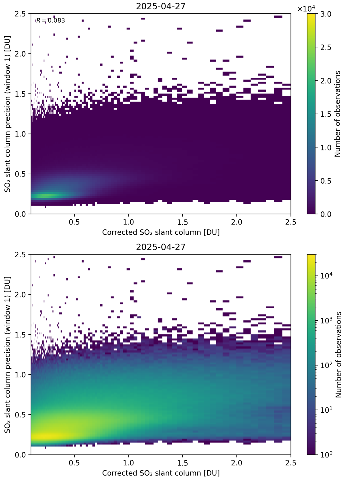
Figure 238: Scatter density plot of “Corrected SO 2 slant column” against “SO 2 slant column precision (window 1)” for 2025-04-26 to 2025-04-28.
