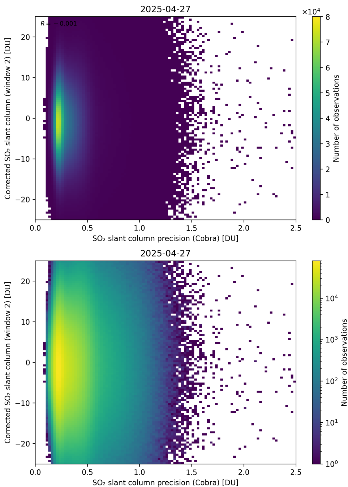
Figure 206: Scatter density plot of “SO 2 slant column precision (Cobra)” against “Corrected SO 2 slant column (window 2)” for 2025-04-26 to 2025-04-28.
