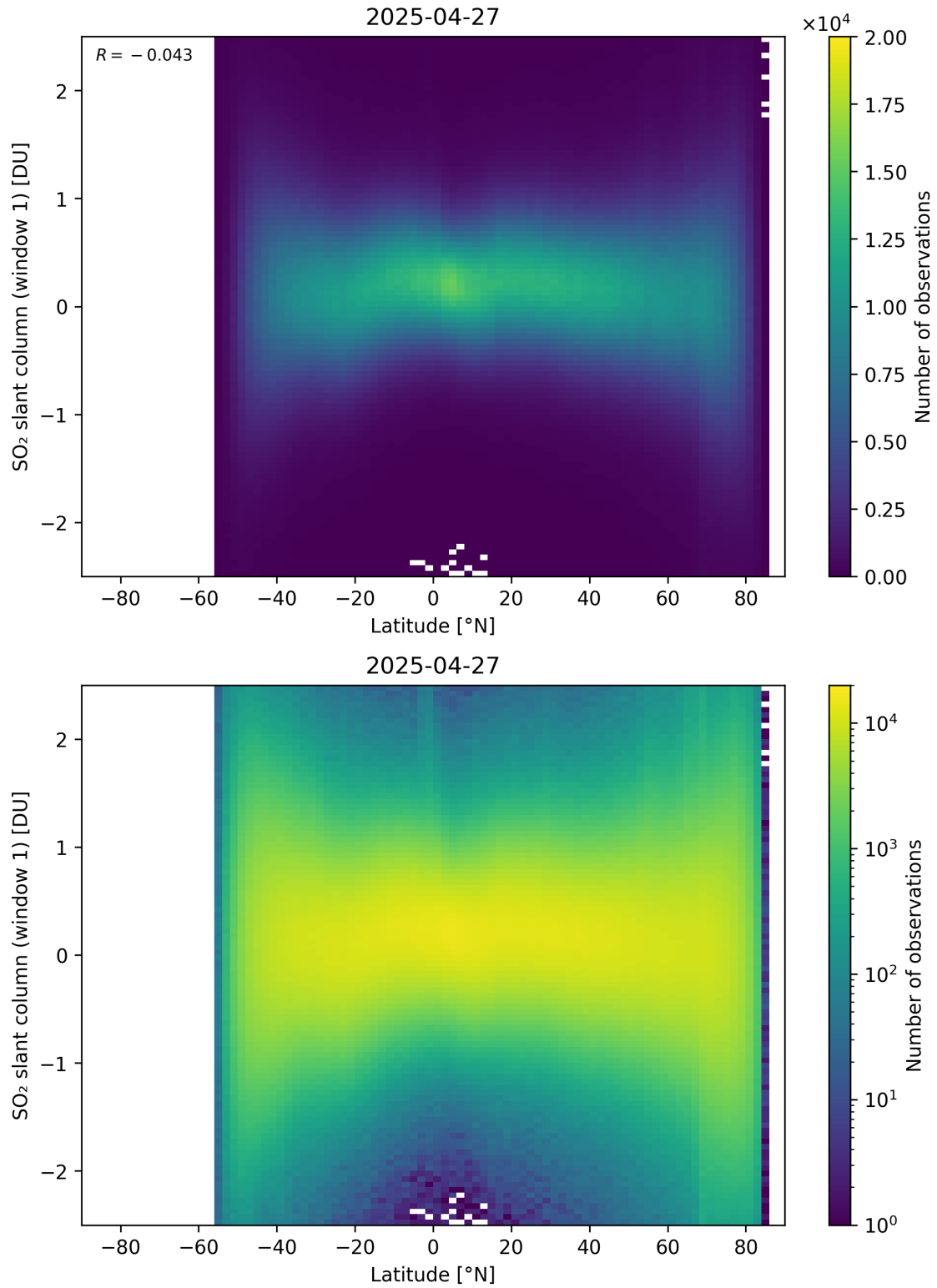
Figure 162: Scatter density plot of “Latitude” against “SO 2 slant column (window 1)” for 2025-04-26 to 2025-04-28.
