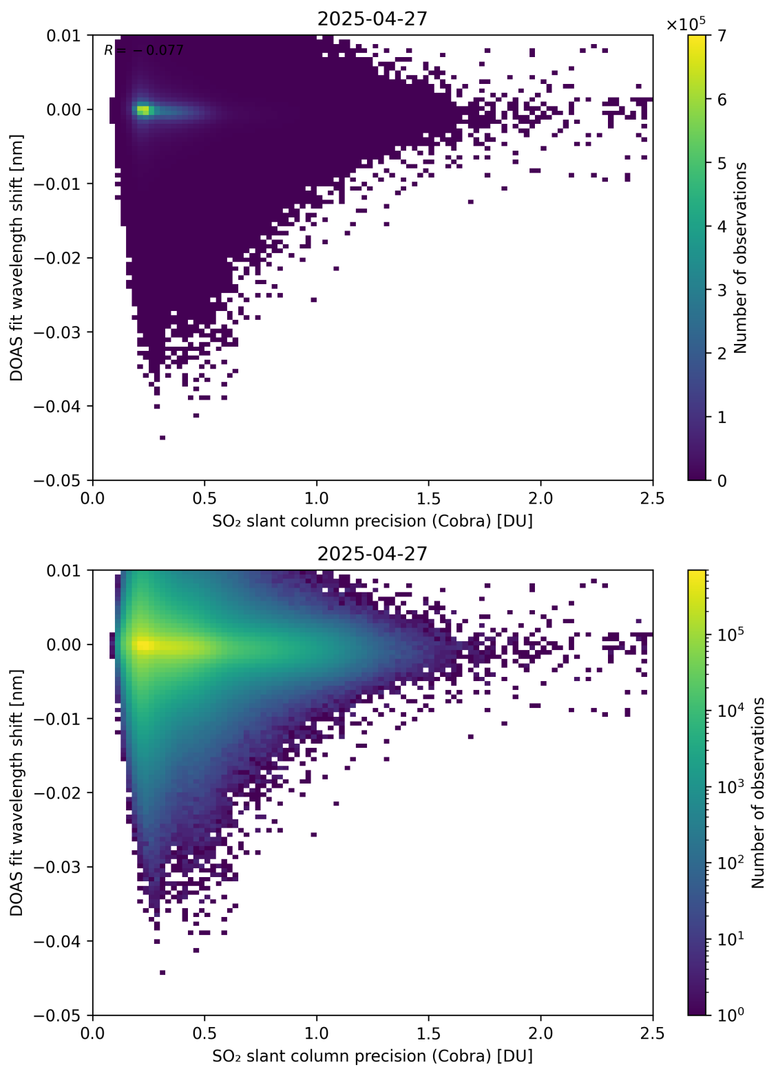
Figure 202: Scatter density plot of “SO 2 slant column precision (Cobra)” against “DOAS fit wavelength shift” for 2025-04-26 to 2025-04-28.
