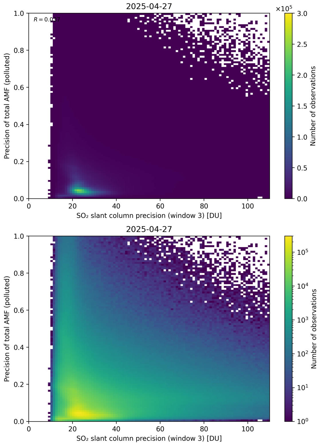
Figure 314: Scatter density plot of “SO 2 slant column precision (window 3)” against “Precision of total AMF (polluted)” for 2025-04-26 to 2025-04-28.
