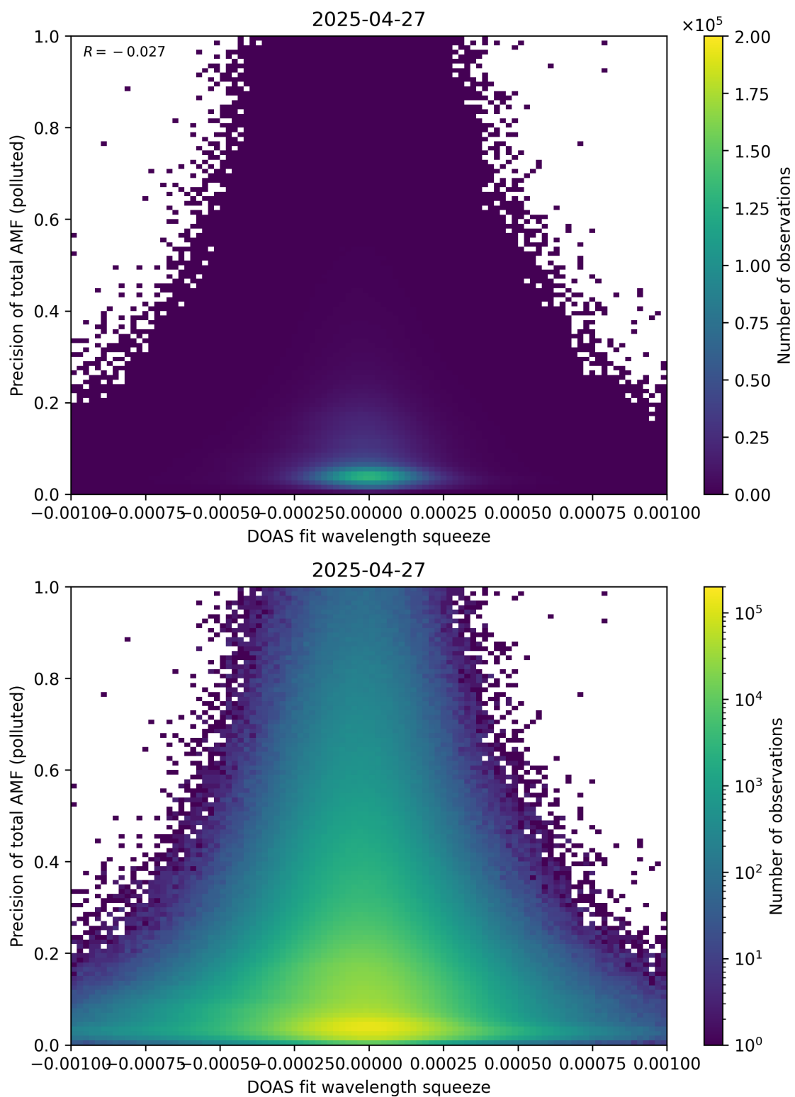
Figure 146: Scatter density plot of “DOAS fit wavelength squeeze” against “Precision of total AMF (polluted)” for 2025-04-26 to 2025-04-28.
