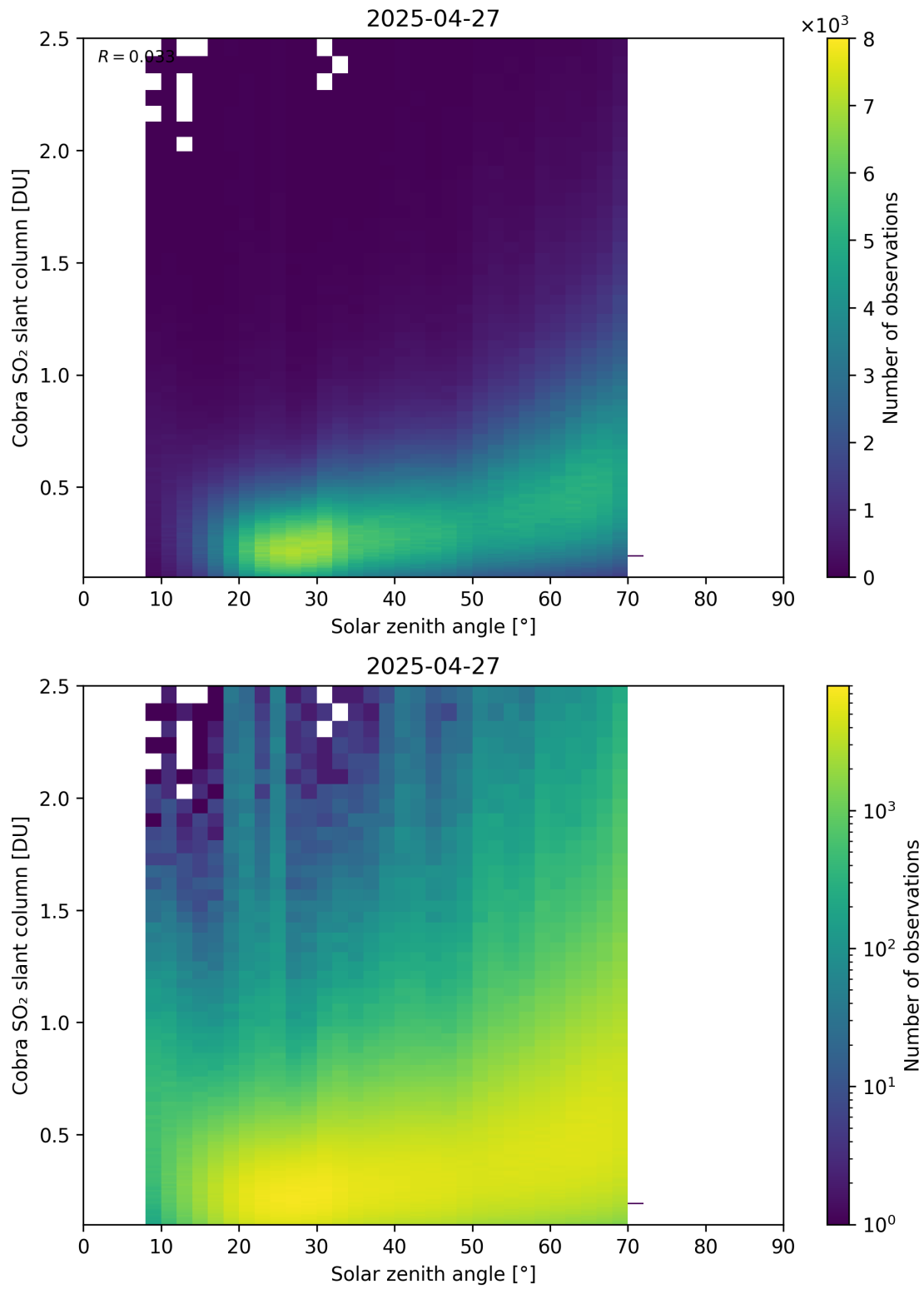
Figure 179: Scatter density plot of “Solar zenith angle” against “Cobra SO 2 slant column” for 2025-04-26 to 2025-04-28.
