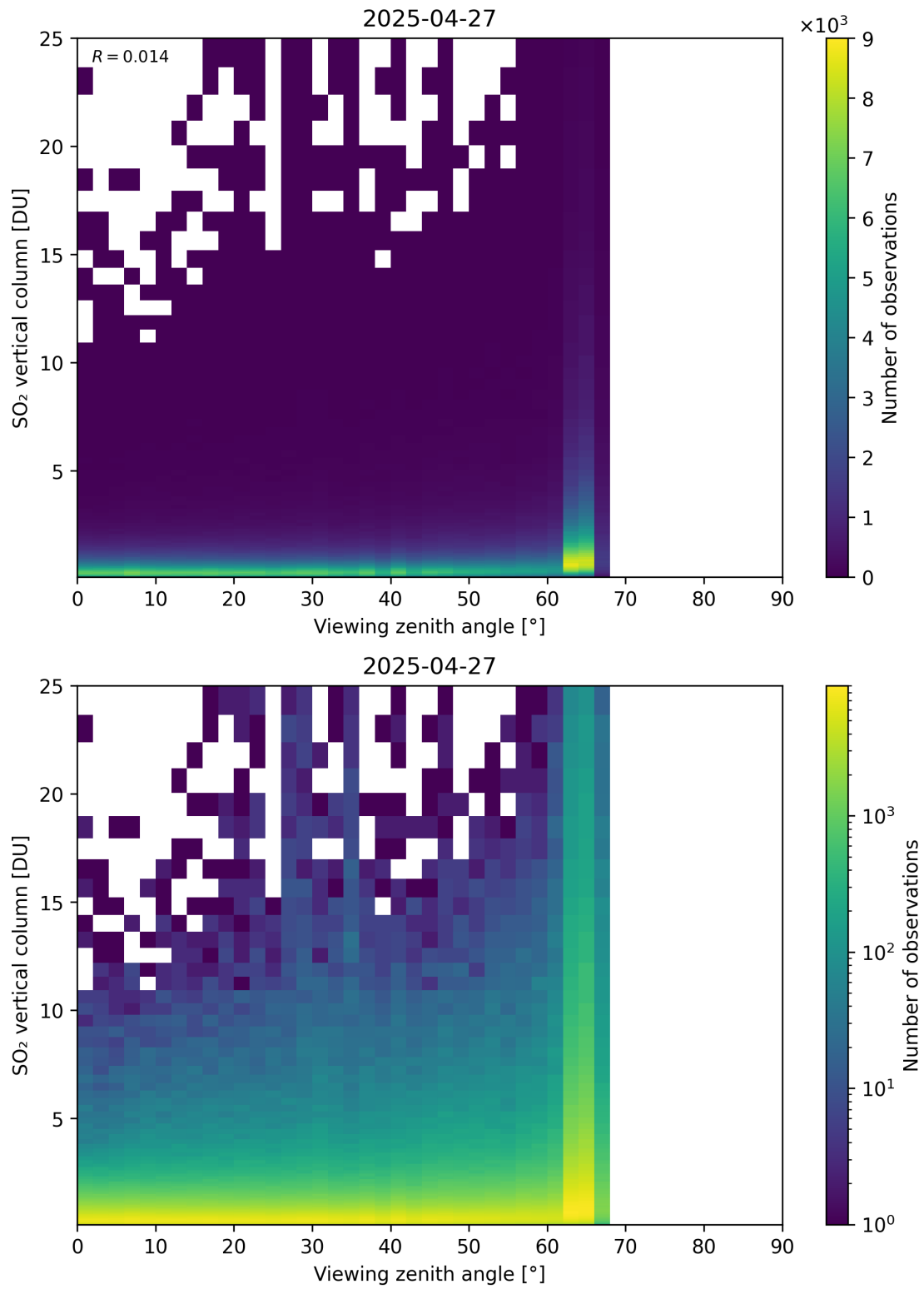
Figure 383: Scatter density plot of “Viewing zenith angle” against “SO 2 vertical column” for 2025-04-26 to 2025-04-28.
