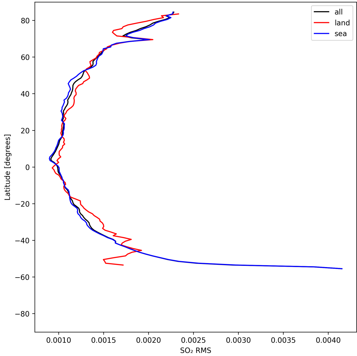
Figure 52: Zonal average of “SO 2 RMS” for 2025-04-26 to 2025-04-28.
