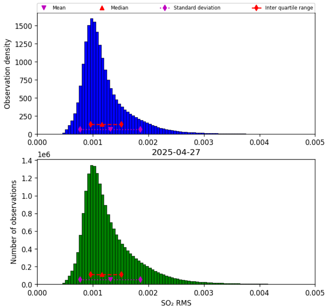
Figure 78: Histogram of “SO 2 RMS” for 2025-04-26 to 2025-04-28
