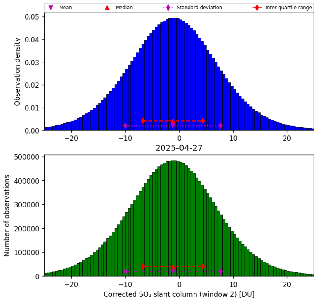
Figure 69: Histogram of “Corrected SO 2 slant column (window 2)” for 2025-04-26 to 2025-04-28
