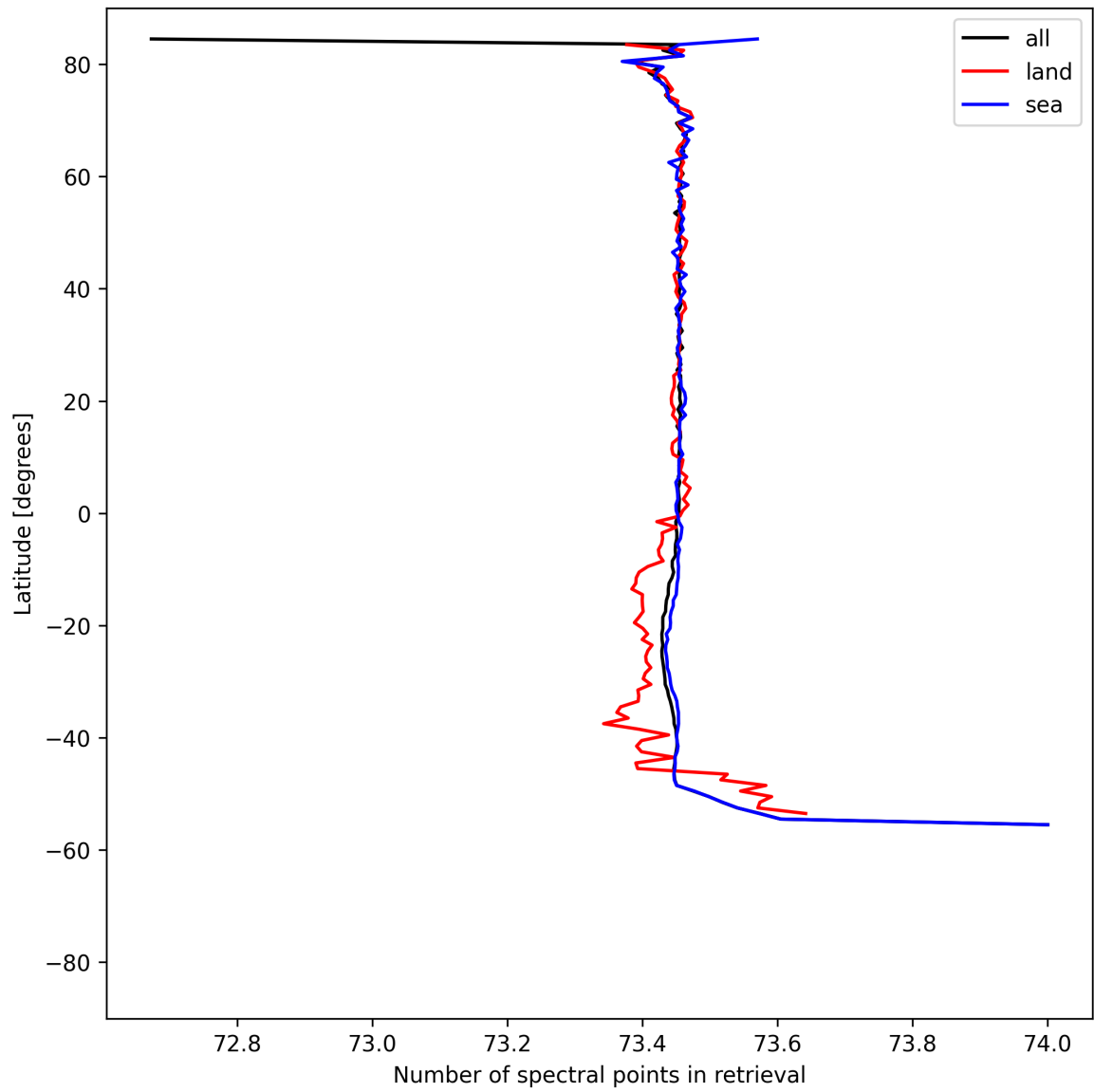
Figure 56: Zonal average of “Number of spectral points in retrieval” for 2025-04-26 to 2025-04-28.
