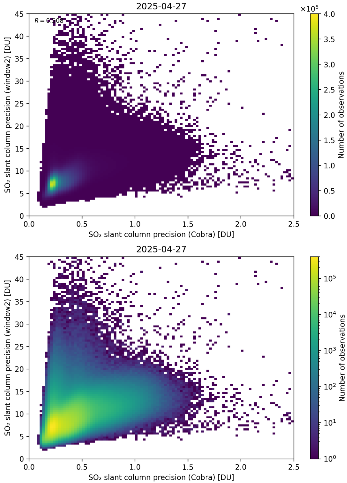
Figure 210: Scatter density plot of “SO 2 slant column precision (Cobra)” against “SO 2 slant column precision (window2)” for 2025-04-26 to 2025-04-28.
