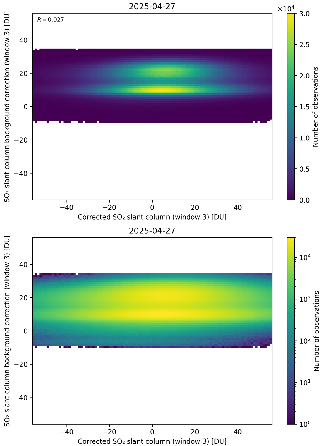
Figure 255: Scatter density plot of “Corrected SO 2 slant column (window 3)” against “SO 2 slant column background correction (window 3)” for 2025-04-26 to 2025-04-28.
