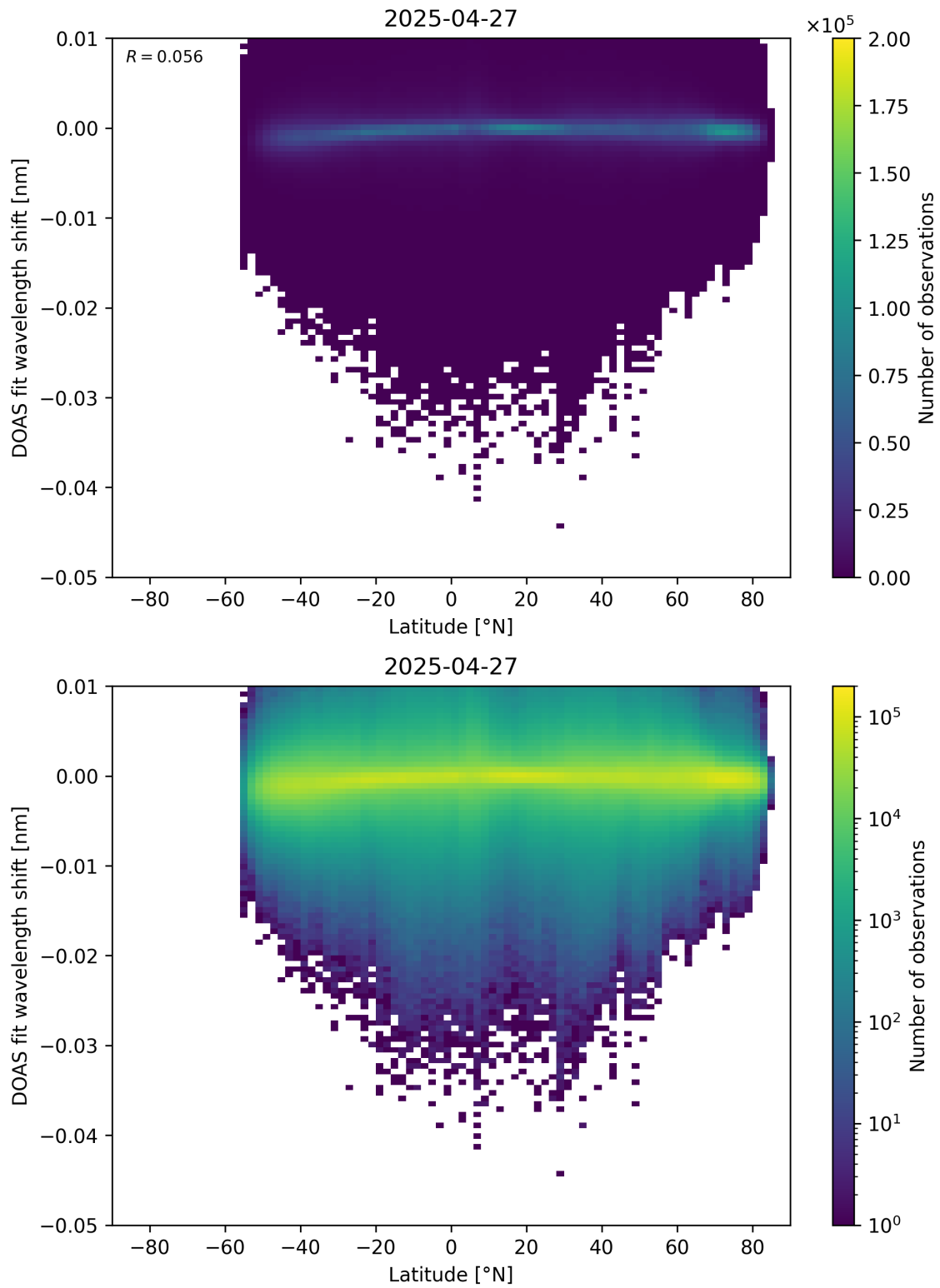
Figure 153: Scatter density plot of “Latitude” against “DOAS fit wavelength shift” for 2025-04-26 to 2025-04-28.
