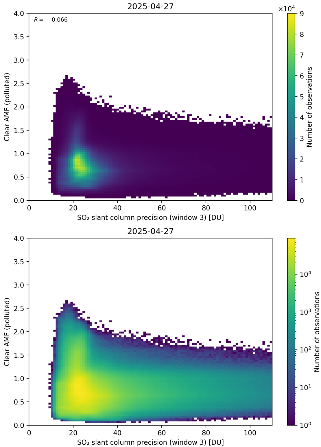
Figure 311: Scatter density plot of “SO 2 slant column precision (window 3)” against “Clear AMF (polluted)” for 2025-04-26 to 2025-04-28.
