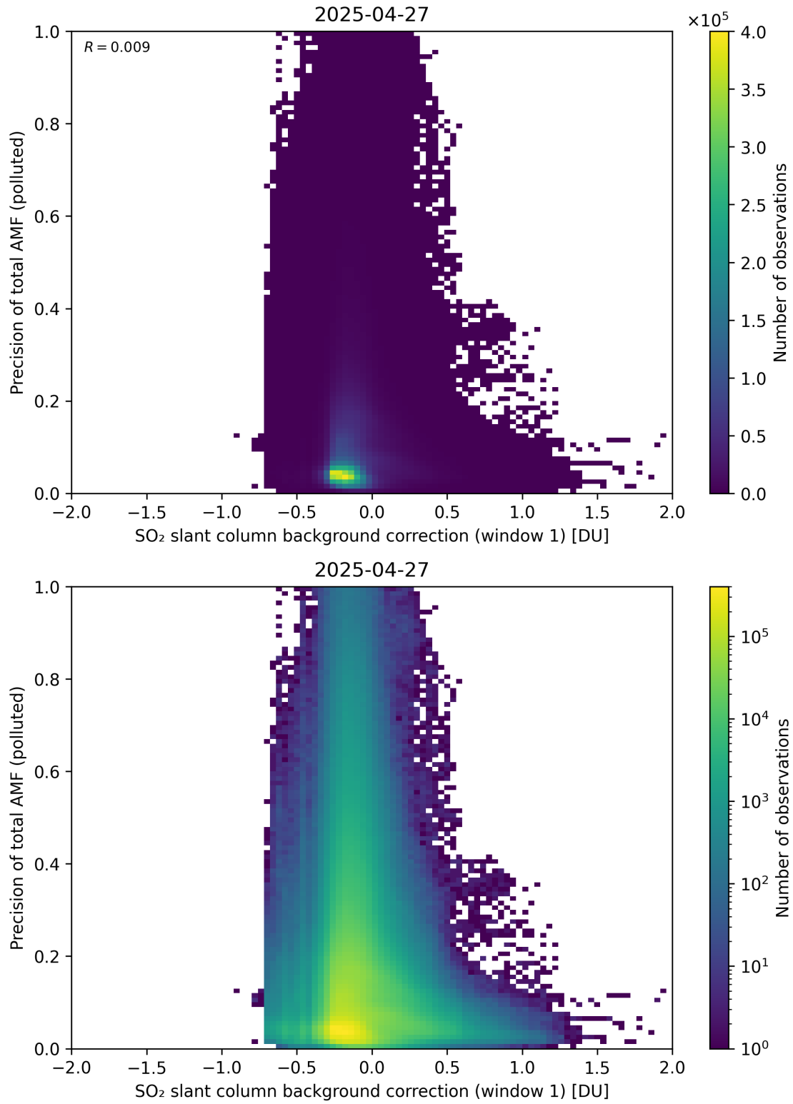
Figure 121: Scatter density plot of “SO 2 slant column background correction (window 1)” against “Precision of total AMF (polluted)” for 2025-04-26 to 2025-04-28.
