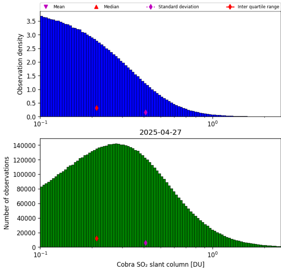
Figure 61: Histogram of “Cobra SO 2 slant column” for 2025-04-26 to 2025-04-28
