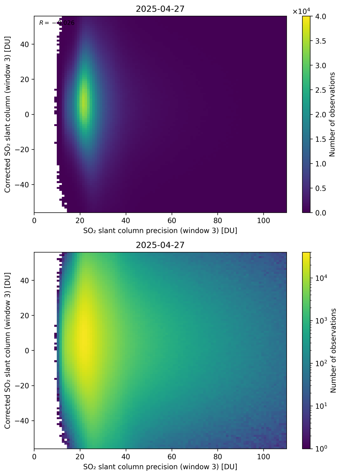
Figure 312: Scatter density plot of “SO 2 slant column precision (window 3)” against “Corrected SO 2 slant column (window 3)” for 2025-04-26 to 2025-04-28.
