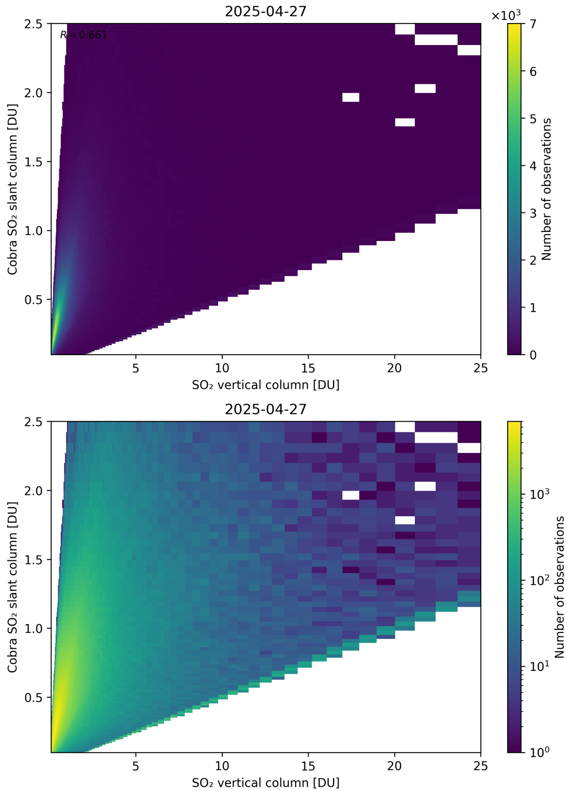
Figure 349: Scatter density plot of “SO 2 vertical column” against “Cobra SO 2 slant column” for 2025-04-26 to 2025-04-28.
