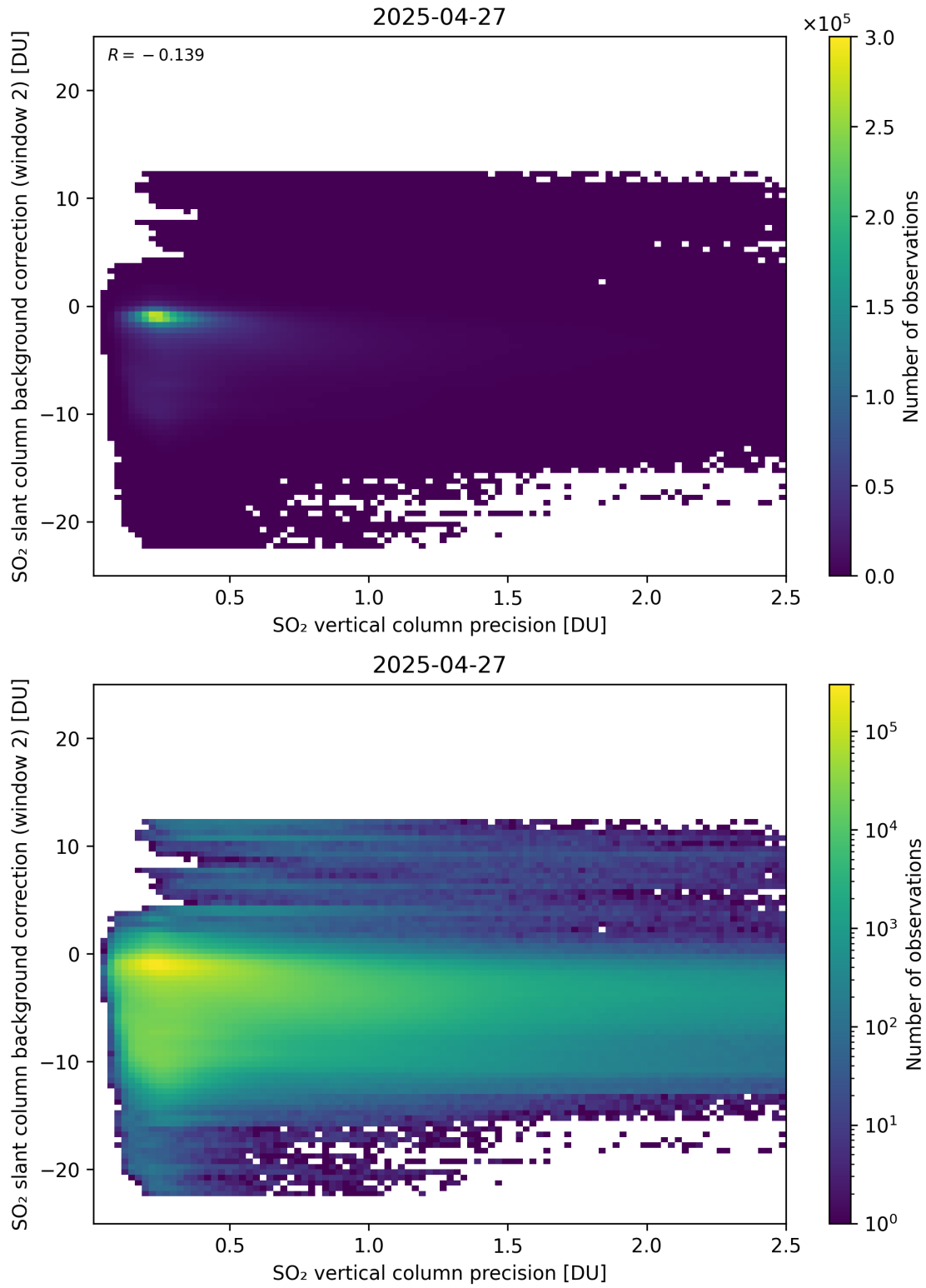
Figure 330: Scatter density plot of “SO 2 vertical column precision” against “SO 2 slant column background correction (window 2)” for 2025-04-26 to 2025-04-28.
