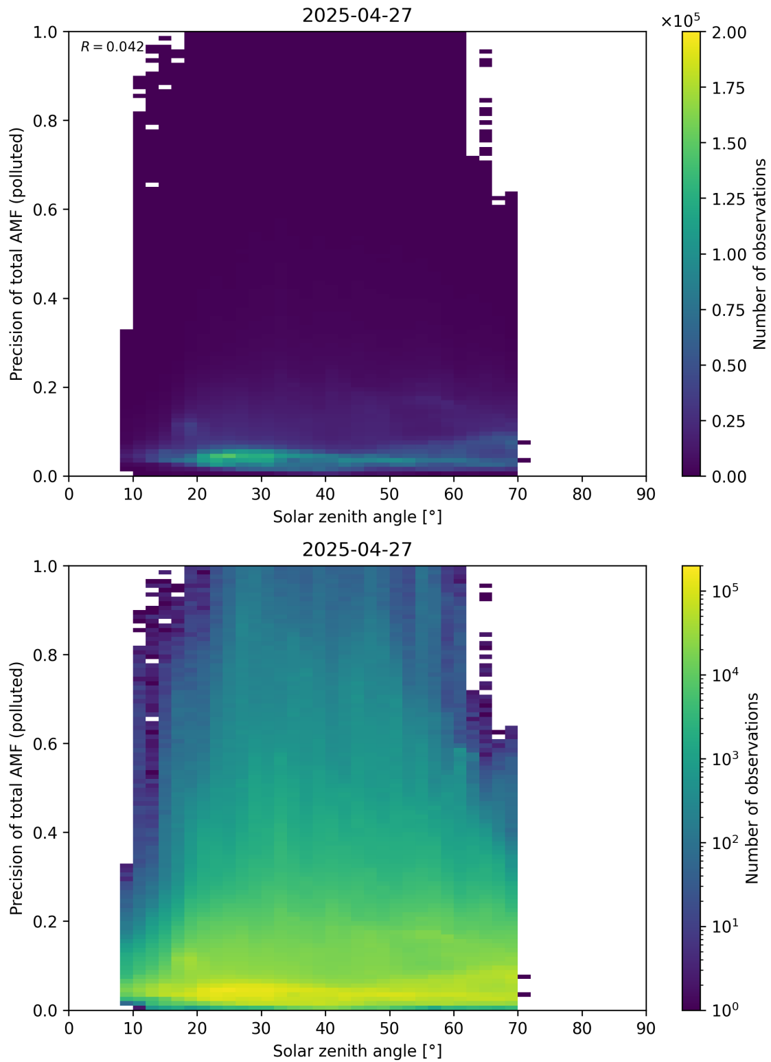
Figure 190: Scatter density plot of “Solar zenith angle” against “Precision of total AMF (polluted)” for 2025-04-26 to 2025-04-28.
