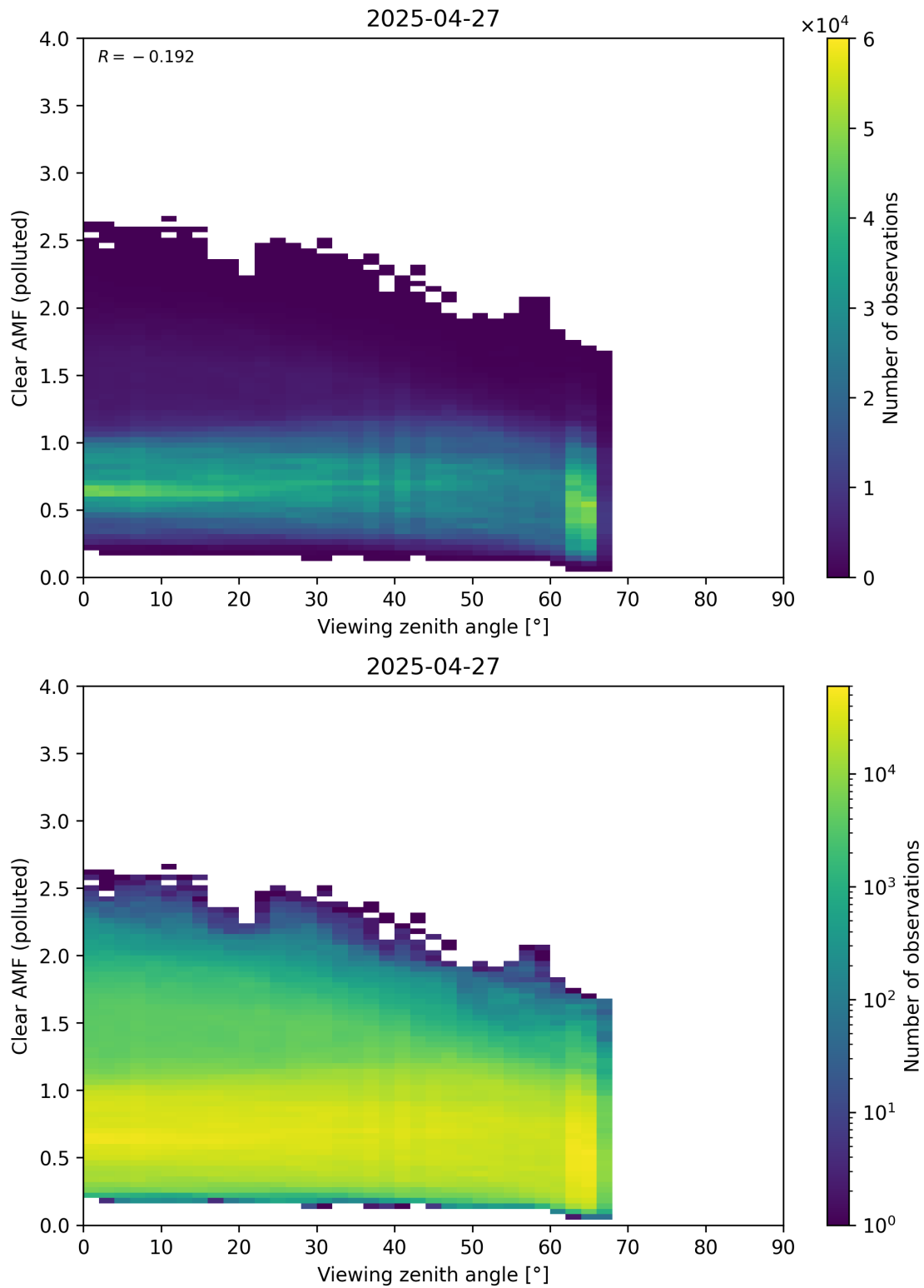
Figure 370: Scatter density plot of “Viewing zenith angle” against “Clear AMF (polluted)” for 2025-04-26 to 2025-04-28.
