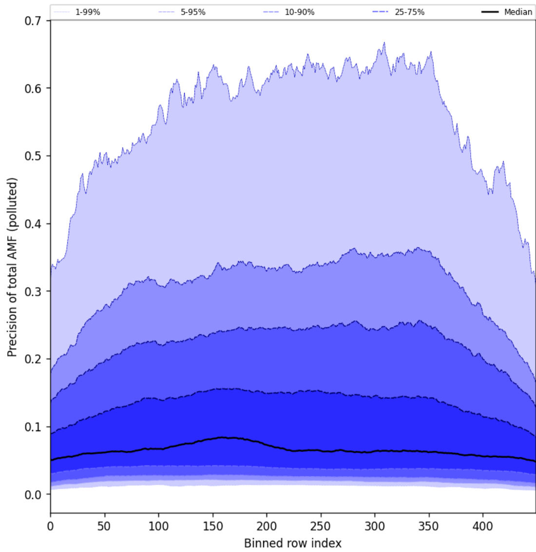
Figure 106: Along track statistics of “Precision of total AMF (polluted)” for 2025-04-26 to 2025-04-28
