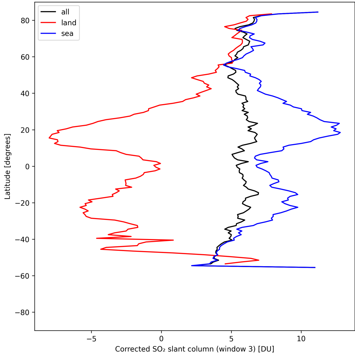
Figure 47: Zonal average of “Corrected SO 2 slant column (window 3)” for 2025-04-26 to 2025-04-28.
