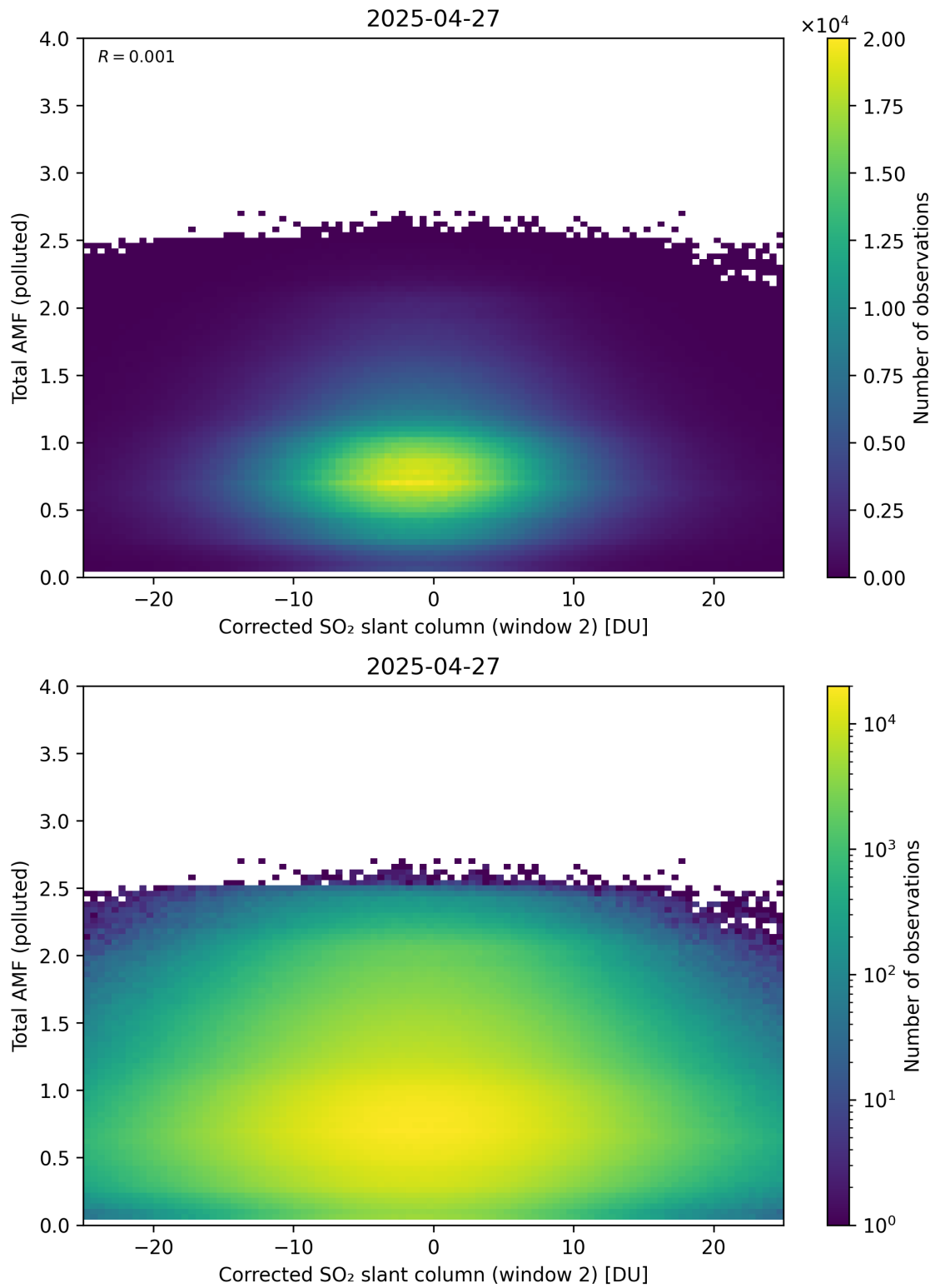
Figure 253: Scatter density plot of “Corrected SO 2 slant column (window 2)” against “Total AMF (polluted)” for 2025-04-26 to 2025-04-28.
