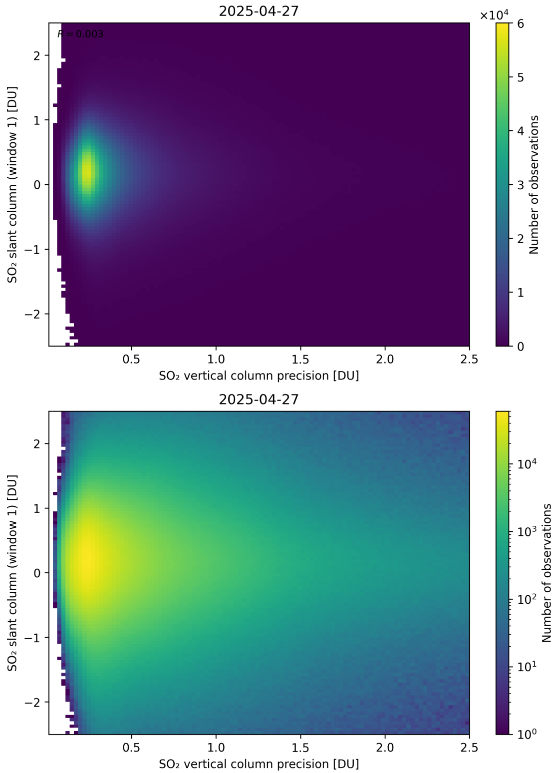
Figure 341: Scatter density plot of “SO 2 vertical column precision” against “SO 2 slant column (window 1)” for 2025-04-26 to 2025-04-28.
