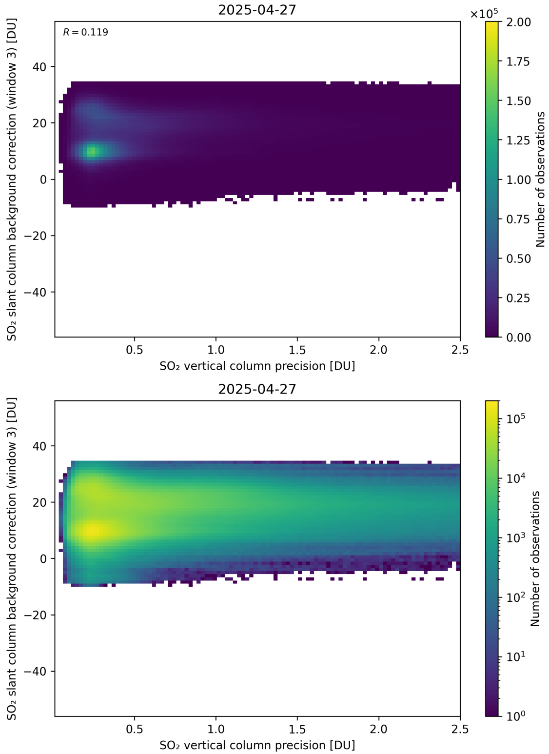
Figure 331: Scatter density plot of “SO 2 vertical column precision” against “SO 2 slant column background correction (window 3)” for 2025-04-26 to 2025-04-28.
