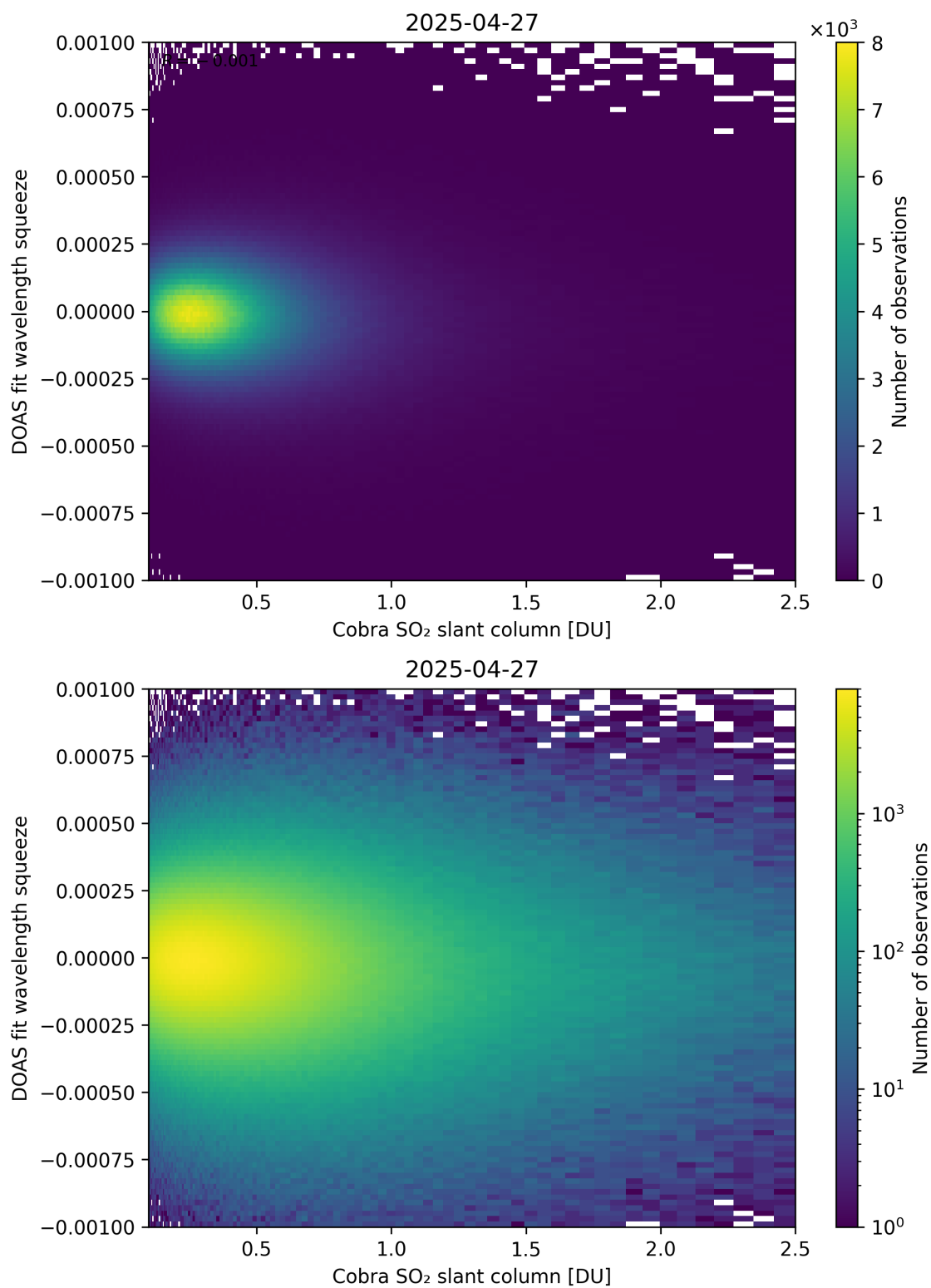
Figure 197: Scatter density plot of “Cobra SO 2 slant column” against “DOAS fit wavelength squeeze” for 2025-04-26 to 2025-04-28.
