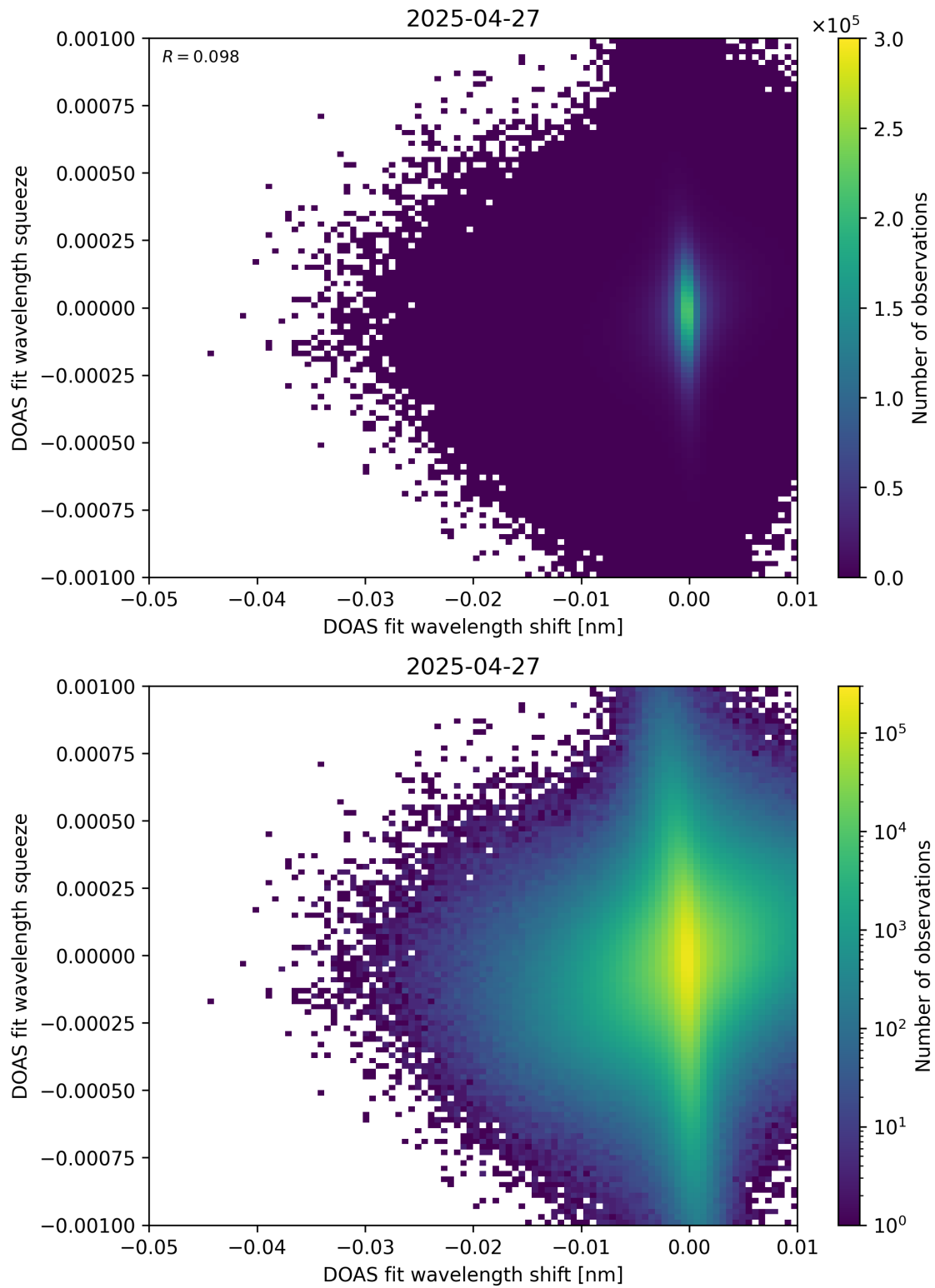
Figure 138: Scatter density plot of “DOAS fit wavelength shift” against “DOAS fit wavelength squeeze” for 2025-04-26 to 2025-04-28.
