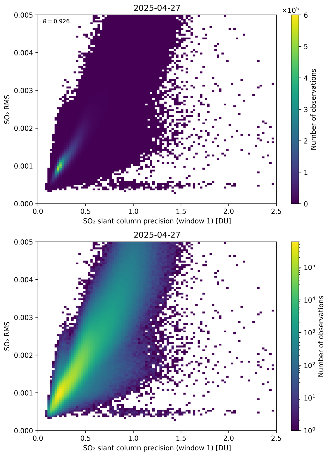
Figure 273: Scatter density plot of “SO 2 slant column precision (window 1)” against “SO 2 RMS” for 2025-04-26 to 2025-04-28.
