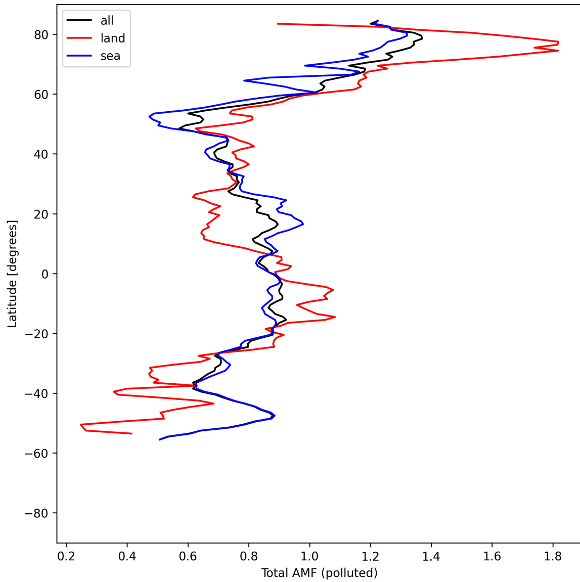
Figure 53: Zonal average of “Total AMF (polluted)” for 2025-04-26 to 2025-04-28.
