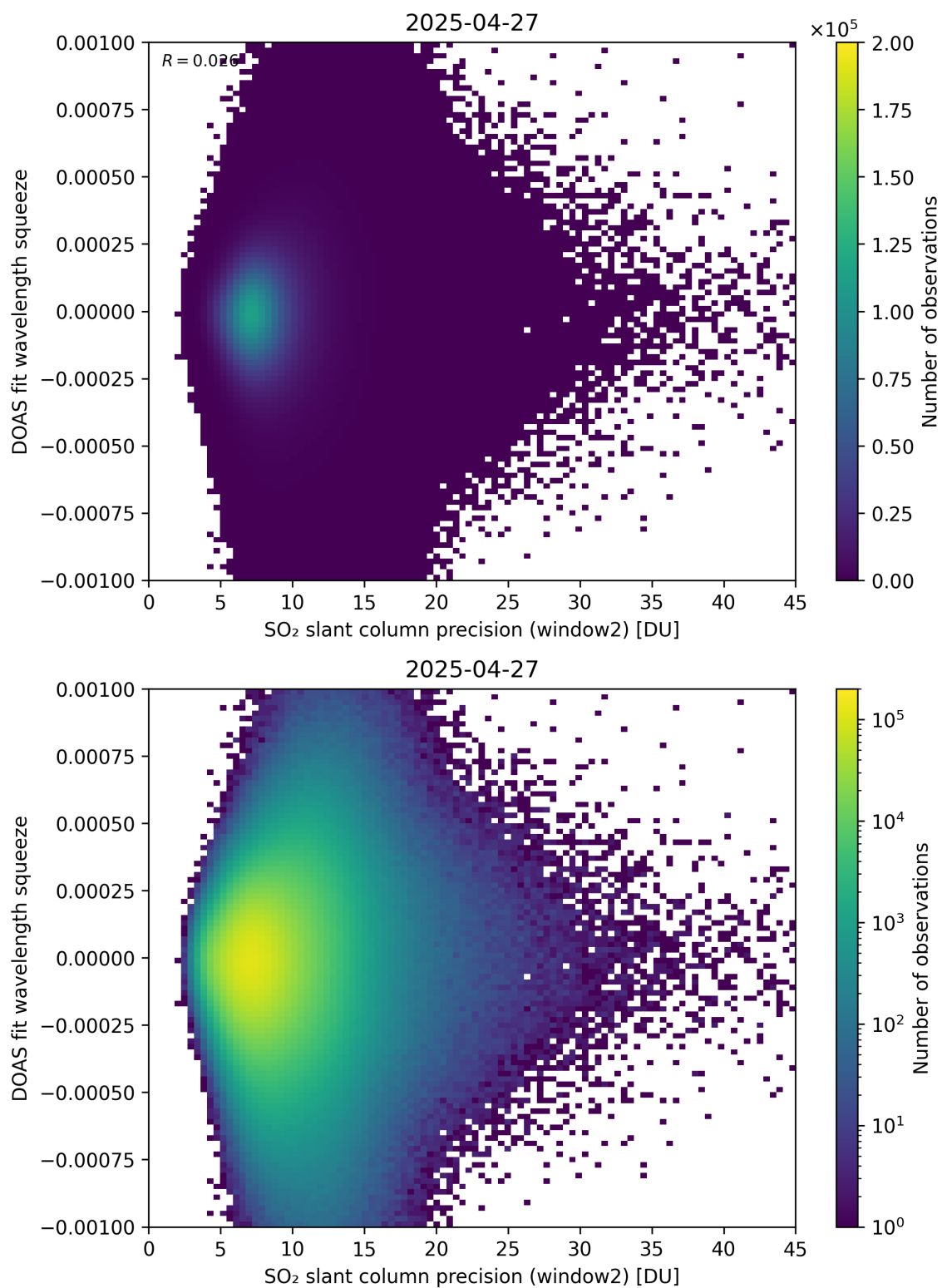
Figure 294: Scatter density plot of “SO 2 slant column precision (window2)” against “DOAS fit wavelength squeeze” for 2025-04-26 to 2025-04-28.
