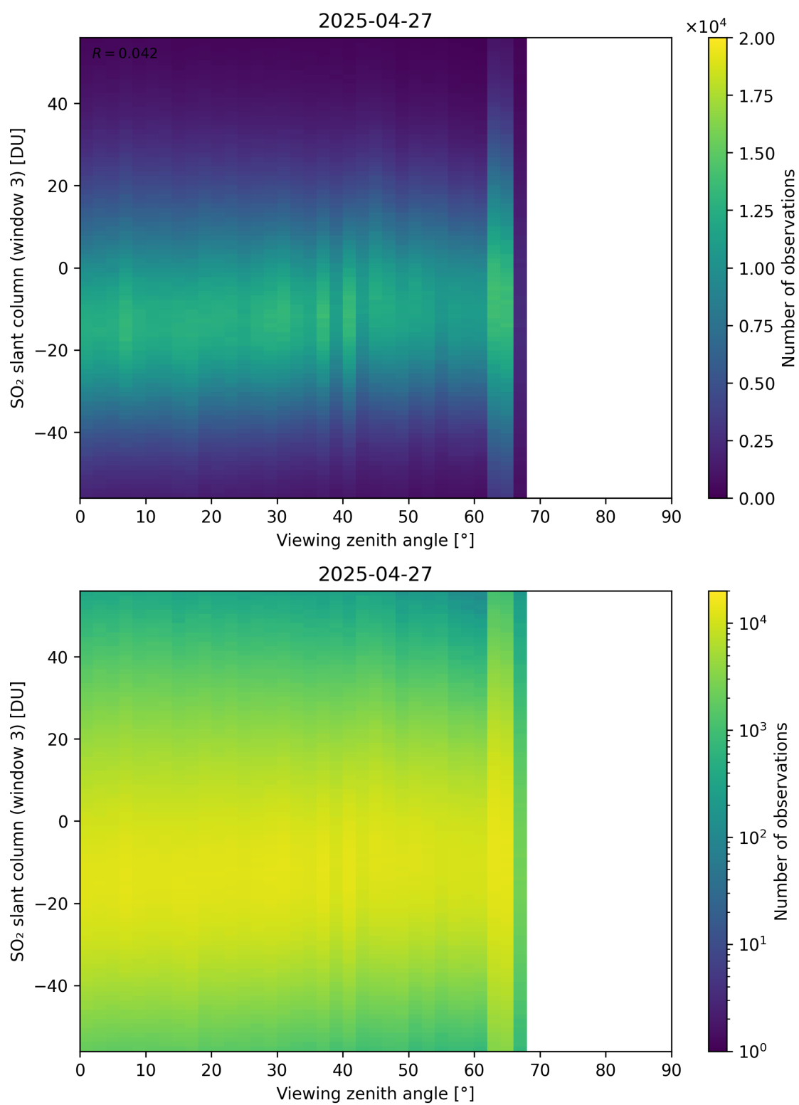
Figure 379: Scatter density plot of “Viewing zenith angle” against “SO 2 slant column (window 3)” for 2025-04-26 to 2025-04-28.
