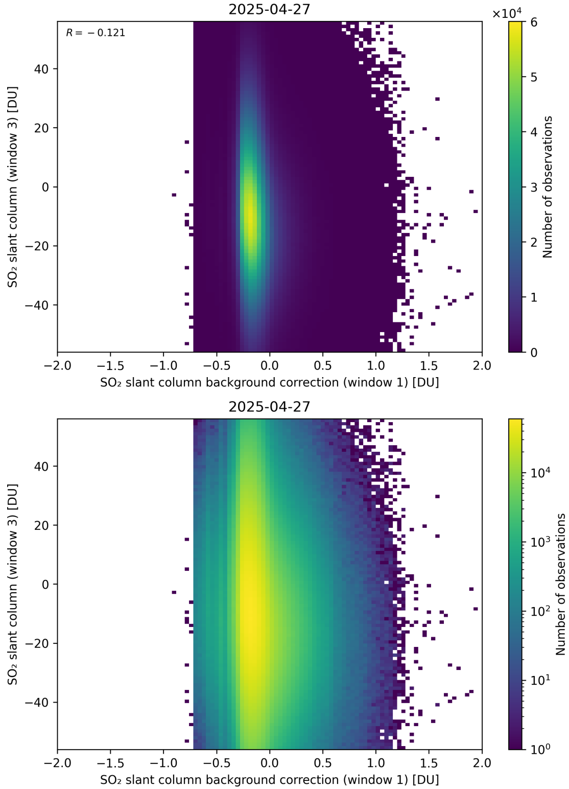
Figure 118: Scatter density plot of “SO 2 slant column background correction (window 1)” against “SO 2 slant column (window 3)” for 2025-04-26 to 2025-04-28.
