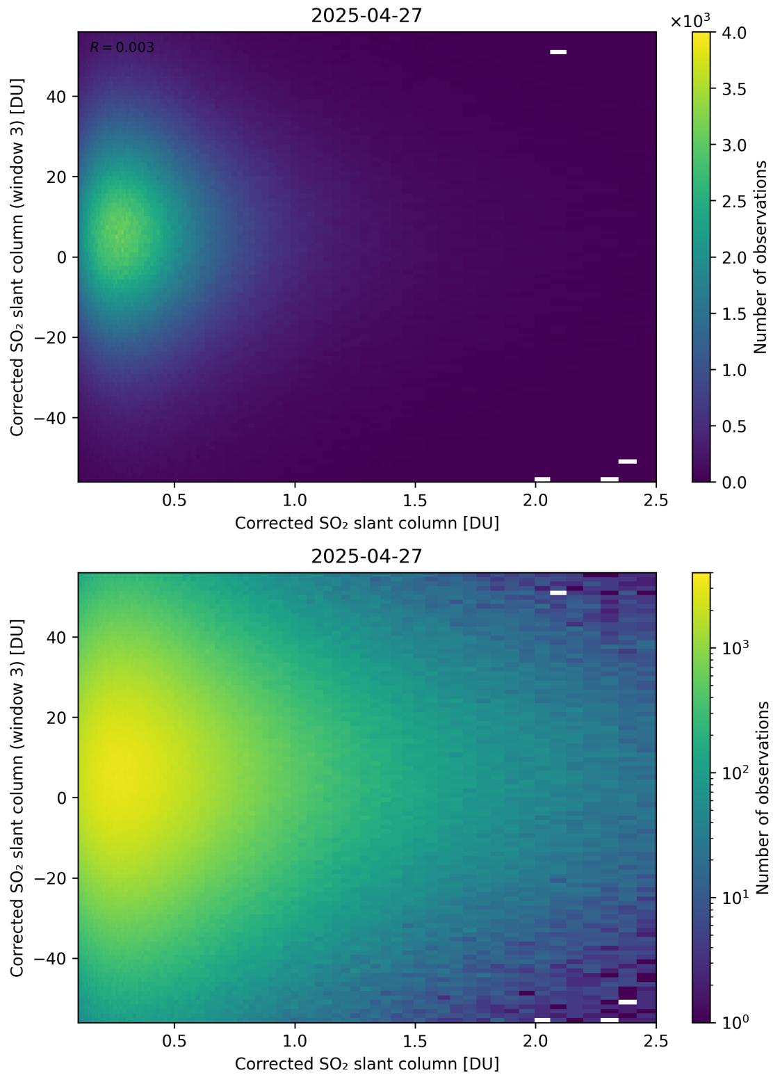
Figure 236: Scatter density plot of “Corrected SO 2 slant column” against “Corrected SO 2 slant column (window 3)” for 2025-04-26 to 2025-04-28.
