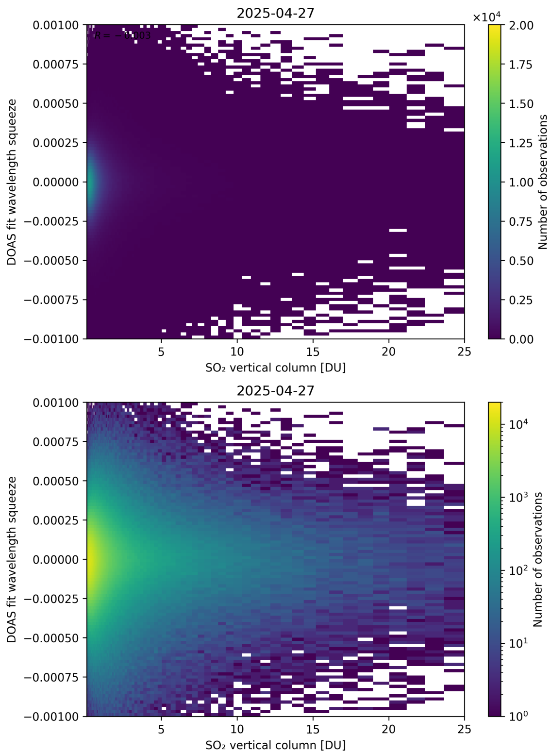
Figure 327: Scatter density plot of “SO 2 vertical column” against “DOAS fit wavelength squeeze” for 2025-04-26 to 2025-04-28.
