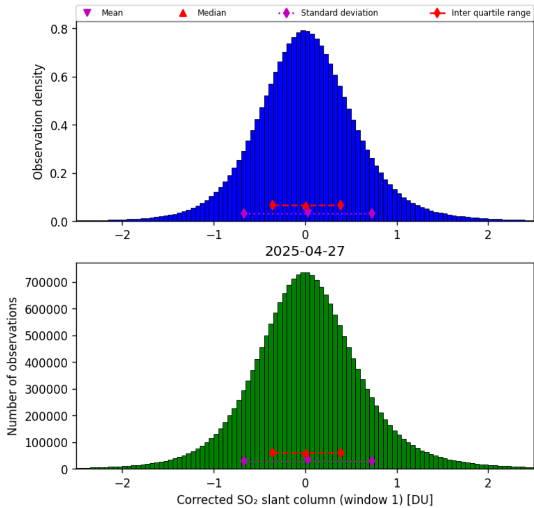
Figure 65: Histogram of “Corrected SO 2 slant column (window 1)” for 2025-04-26 to 2025-04-28
