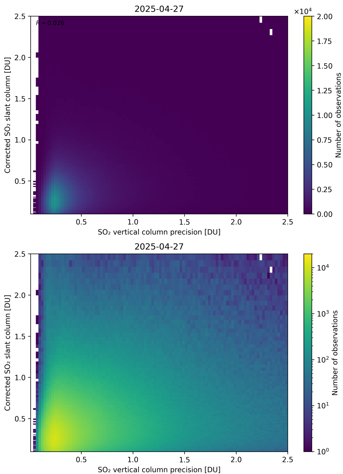
Figure 338: Scatter density plot of “SO 2 vertical column precision” against “Corrected SO 2 slant column” for 2025-04-26 to 2025-04-28.
