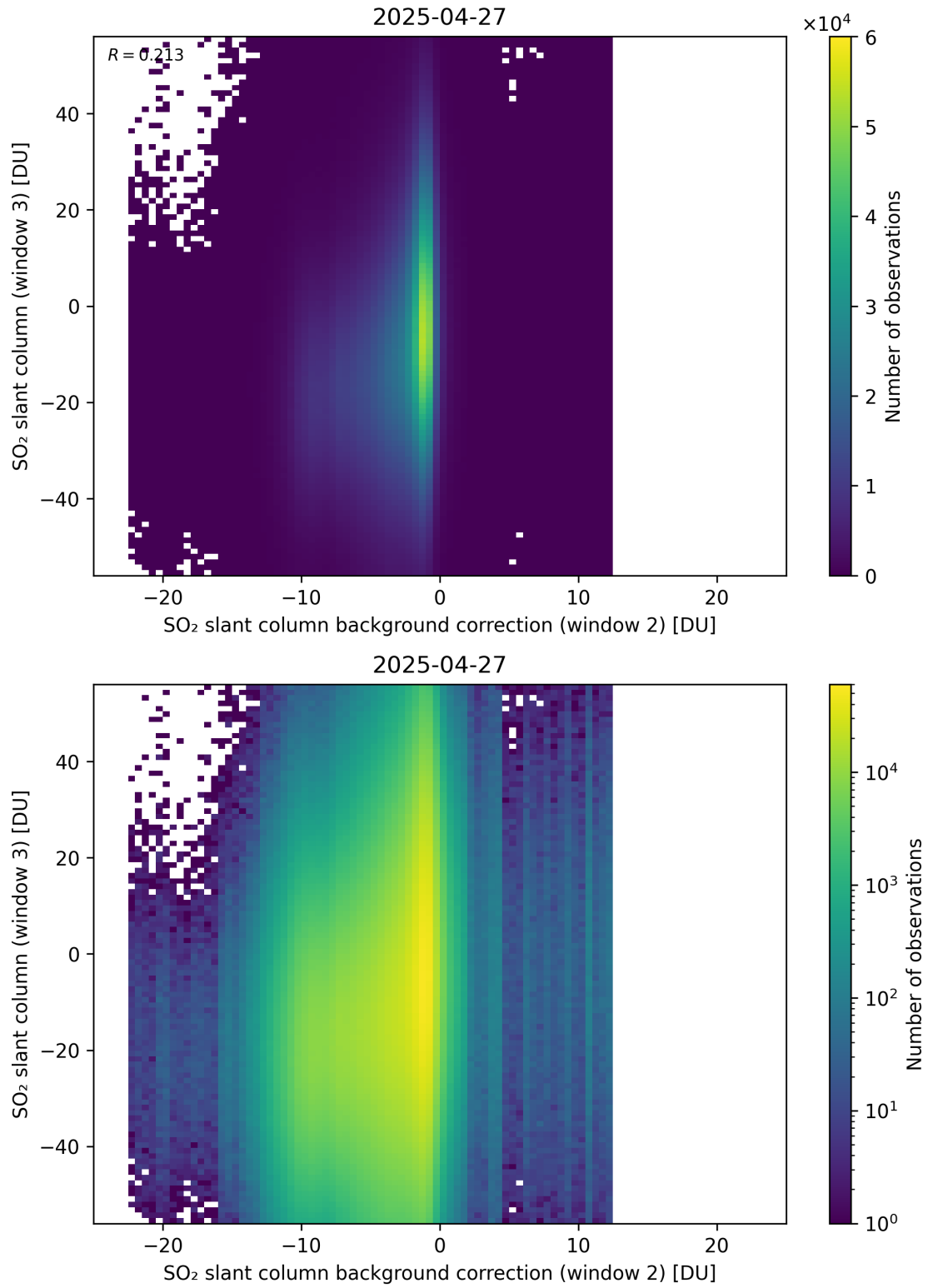
Figure 128: Scatter density plot of “SO 2 slant column background correction (window 2)” against “SO 2 slant column (window 3)” for 2025-04-26 to 2025-04-28.
