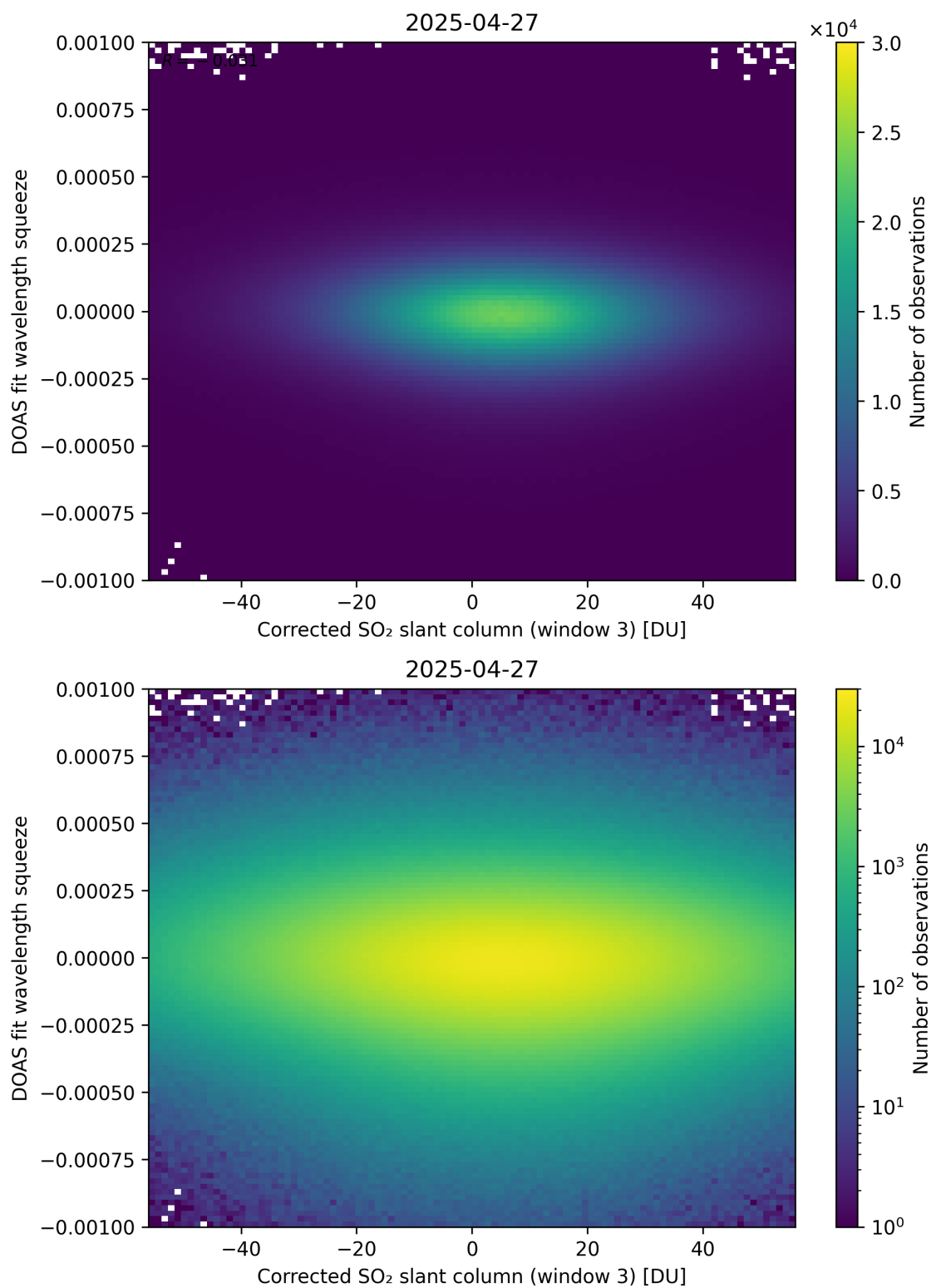
Figure 257: Scatter density plot of “Corrected SO 2 slant column (window 3)” against “DOAS fit wavelength squeeze” for 2025-04-26 to 2025-04-28.
