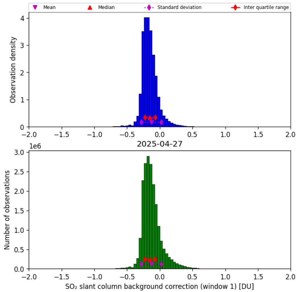
Figure 66: Histogram of “SO 2 slant column background correction (window 1)” for 2025-04-26 to 2025-04-28
