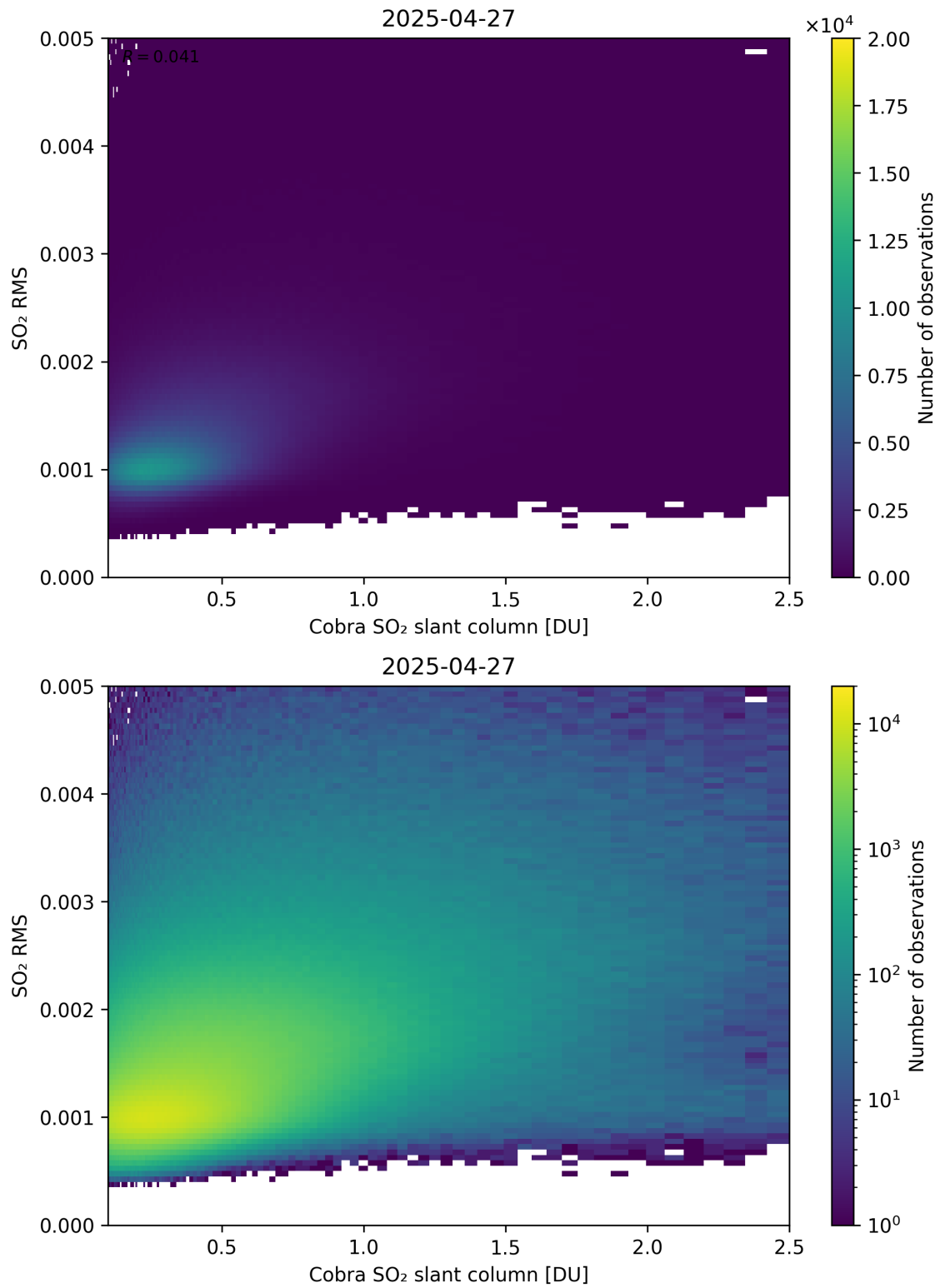
Figure 198: Scatter density plot of “Cobra SO 2 slant column” against “SO 2 RMS” for 2025-04-26 to 2025-04-28.
