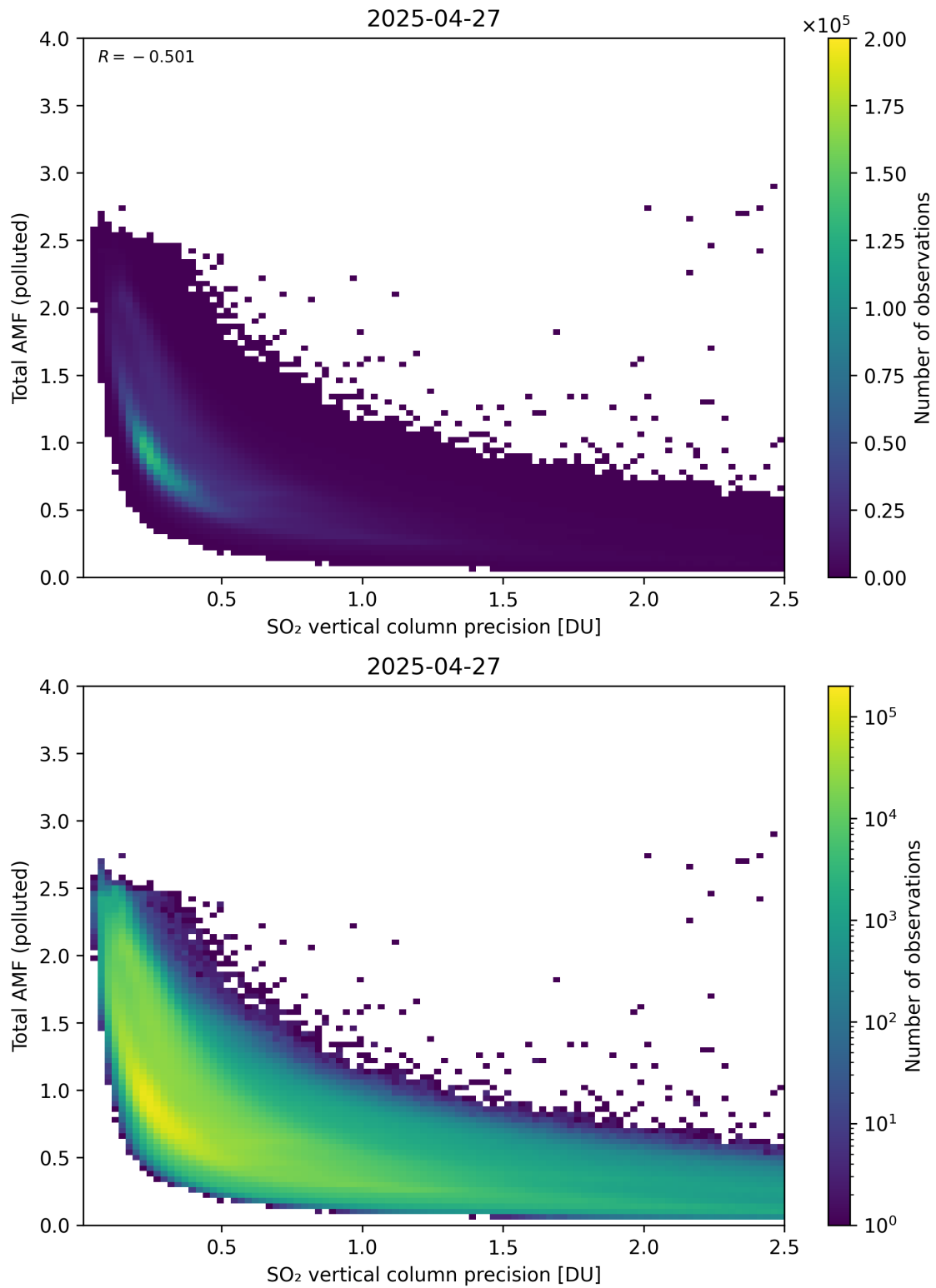
Figure 346: Scatter density plot of “SO 2 vertical column precision” against “Total AMF (polluted)” for 2025-04-26 to 2025-04-28.
