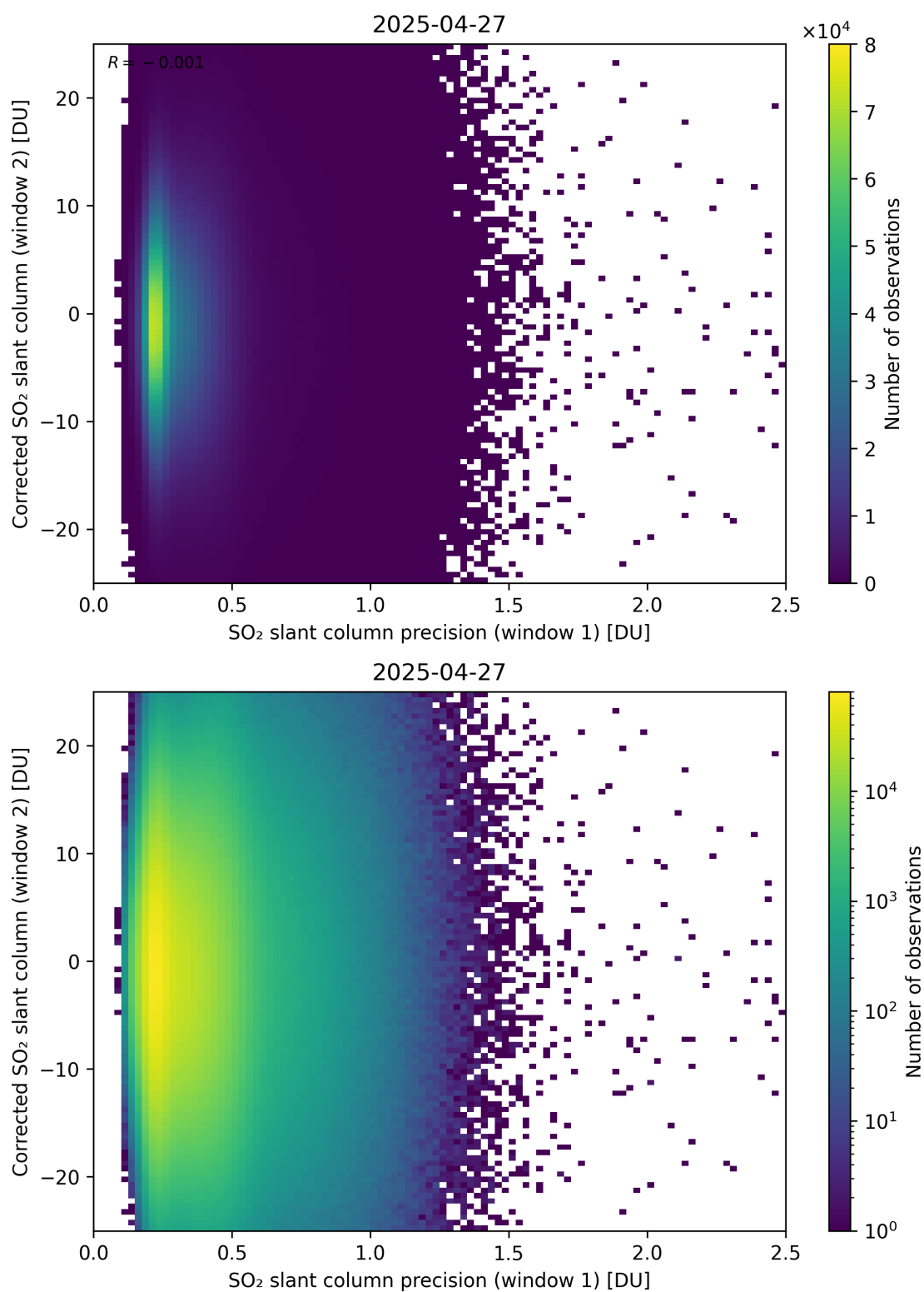
Figure 275: Scatter density plot of “SO 2 slant column precision (window 1)” against “Corrected SO 2 slant column (window 2)” for 2025-04-26 to 2025-04-28.
