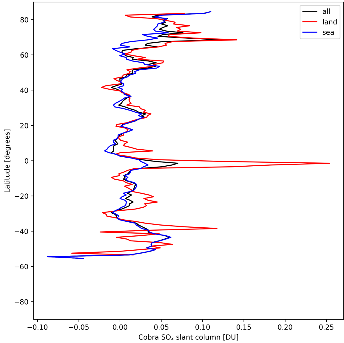
Figure 35: Zonal average of “Cobra SO 2 slant column” for 2025-04-26 to 2025-04-28.
