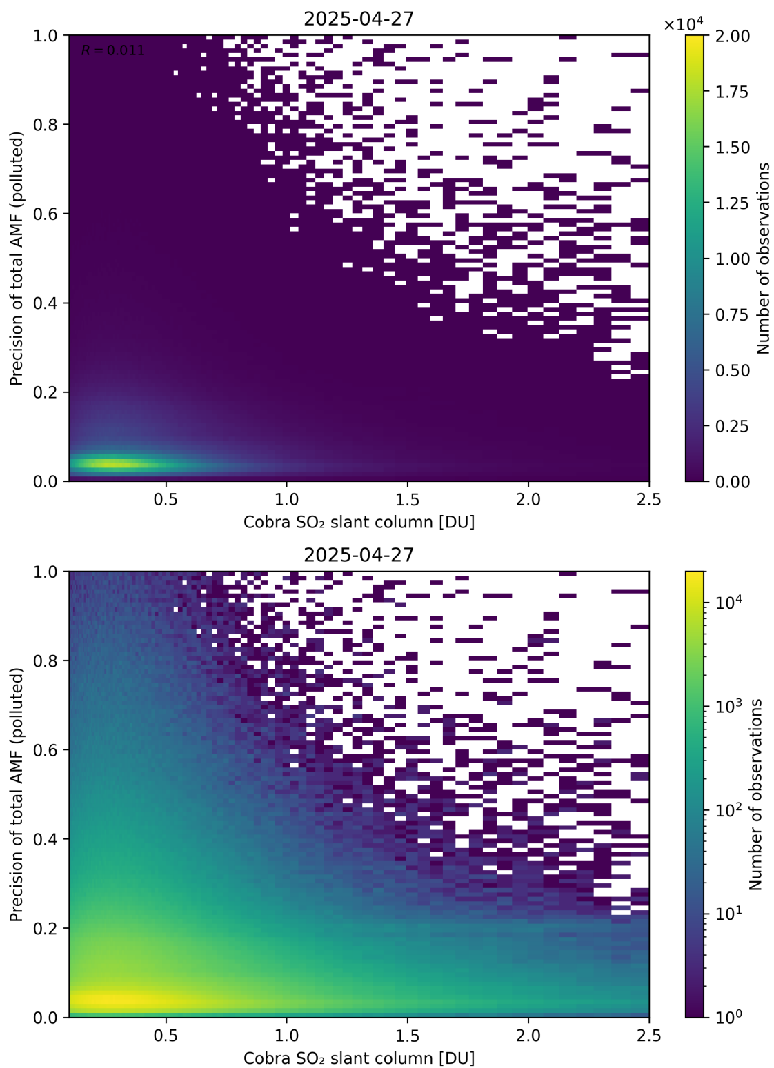
Figure 225: Scatter density plot of “Cobra SO 2 slant column” against “Precision of total AMF (polluted)” for 2025-04-26 to 2025-04-28.
