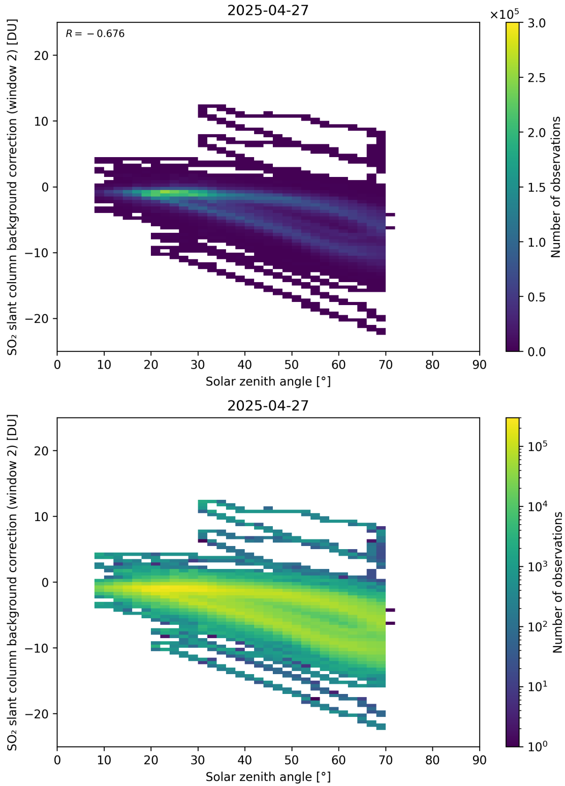
Figure 172: Scatter density plot of “Solar zenith angle” against “SO 2 slant column background correction (window 2)” for 2025-04-26 to 2025-04-28.
