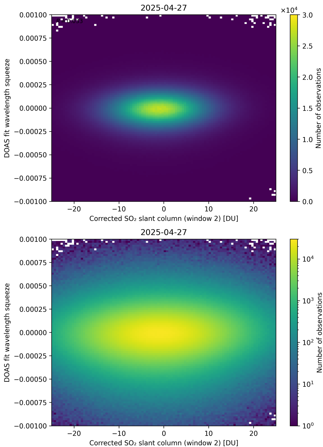
Figure 247: Scatter density plot of “Corrected SO 2 slant column (window 2)” against “DOAS fit wavelength squeeze” for 2025-04-26 to 2025-04-28.
