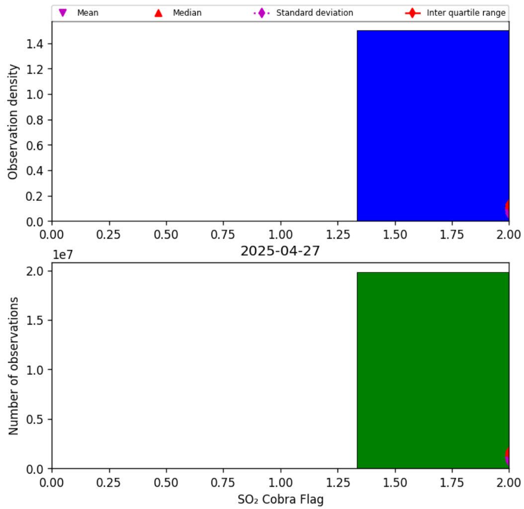
Figure 75: Histogram of “SO 2 Cobra Flag” for 2025-04-26 to 2025-04-28
