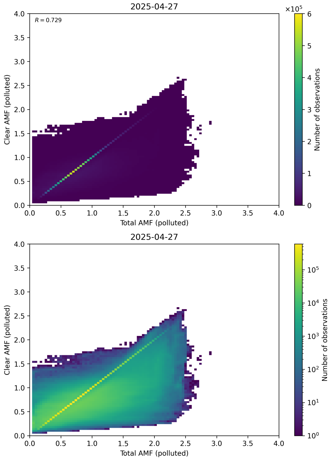
Figure 321: Scatter density plot of “Total AMF (polluted)” against “Clear AMF (polluted)” for 2025-04-26 to 2025-04-28.
