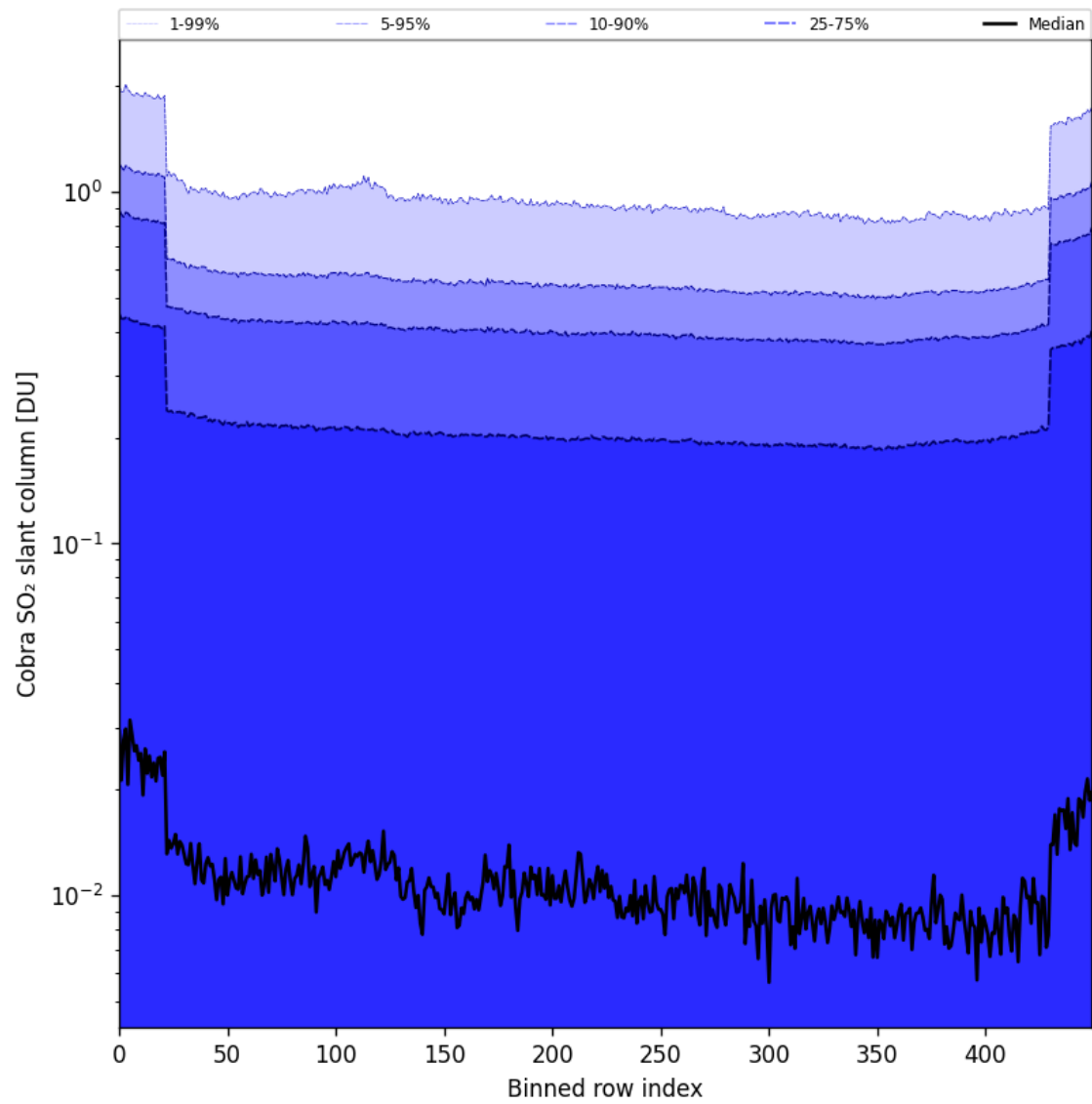
Figure 87: Along track statistics of “Cobra SO 2 slant column” for 2025-04-26 to 2025-04-28
