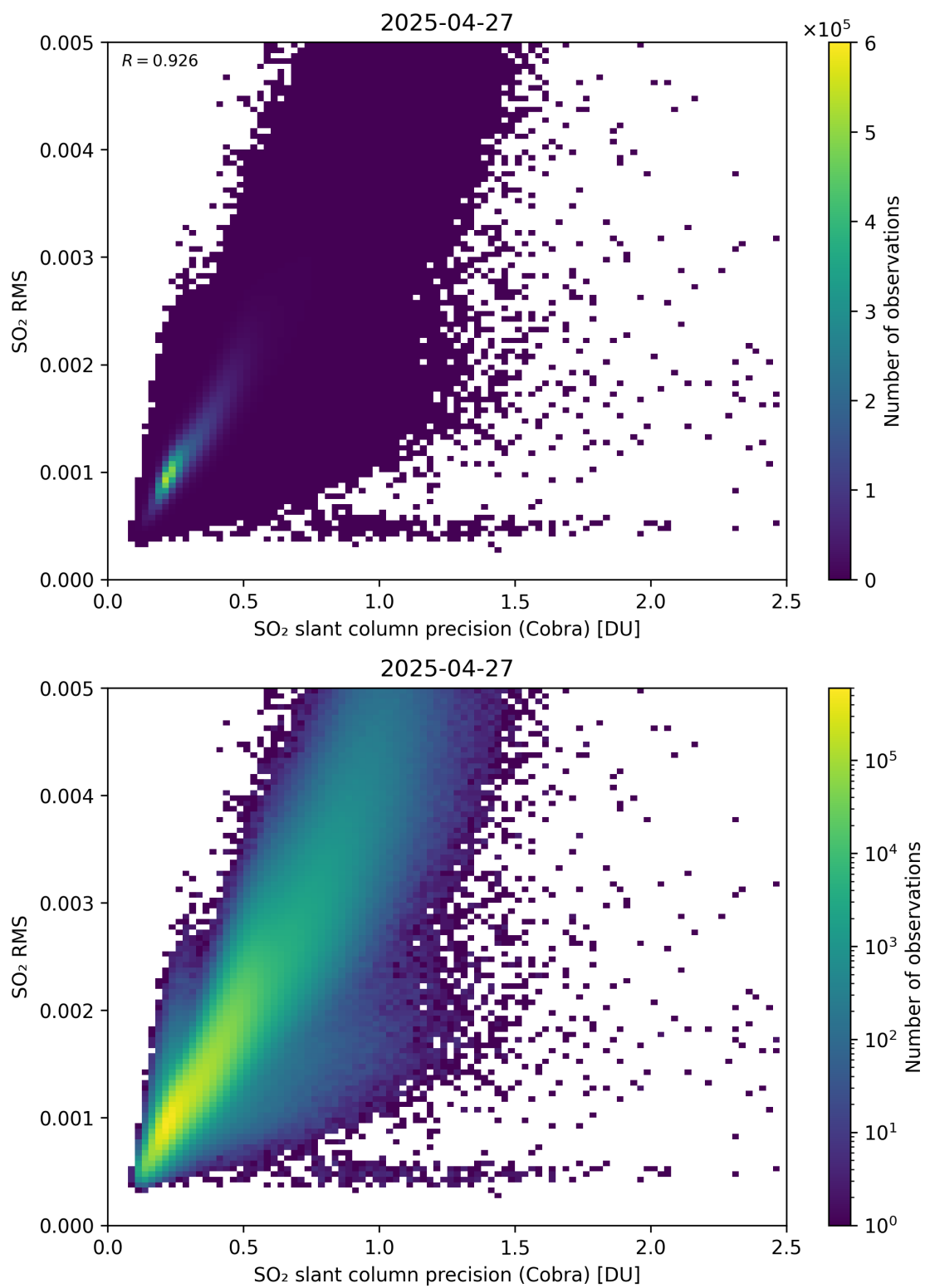
Figure 204: Scatter density plot of “SO 2 slant column precision (Cobra)” against “SO 2 RMS” for 2025-04-26 to 2025-04-28.
