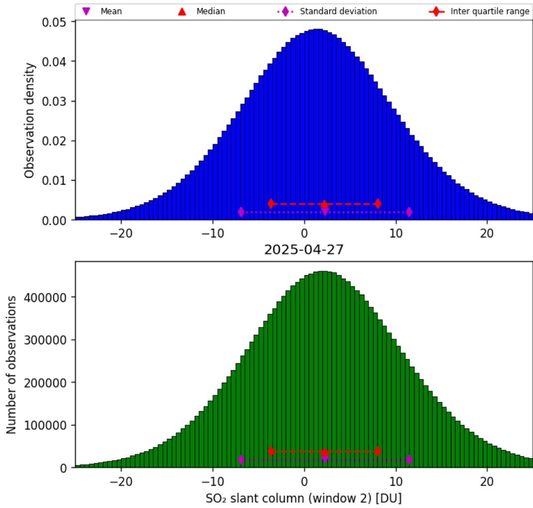
Figure 67: Histogram of “SO 2 slant column (window 2)” for 2025-04-26 to 2025-04-28
