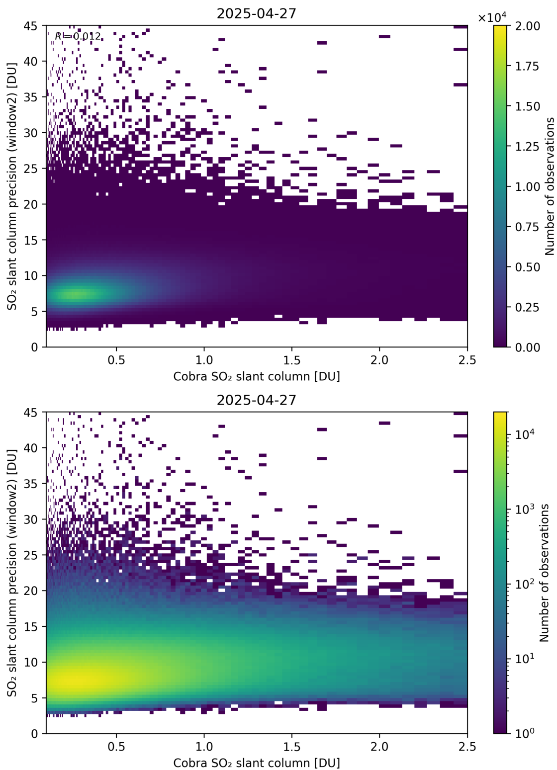
Figure 221: Scatter density plot of “Cobra SO 2 slant column” against “SO 2 slant column precision (window2)” for 2025-04-26 to 2025-04-28.
