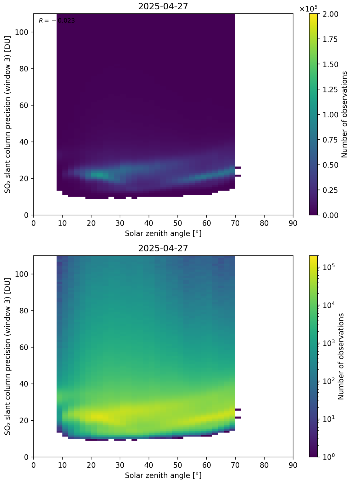
Figure 188: Scatter density plot of “Solar zenith angle” against “SO 2 slant column precision (window 3)” for 2025-04-26 to 2025-04-28.
