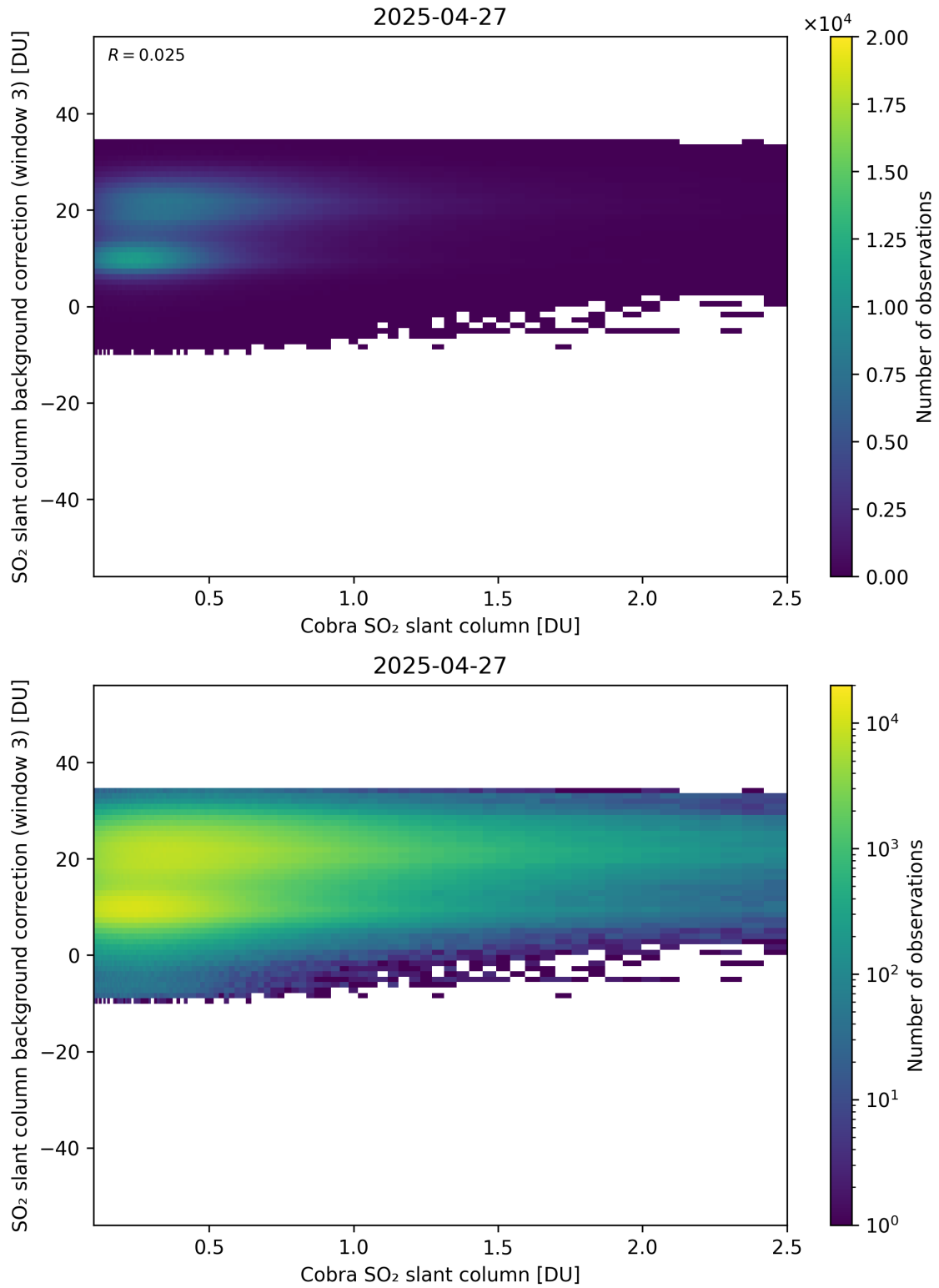
Figure 195: Scatter density plot of “Cobra SO 2 slant column” against “SO 2 slant column background correction (window 3)” for 2025-04-26 to 2025-04-28.
