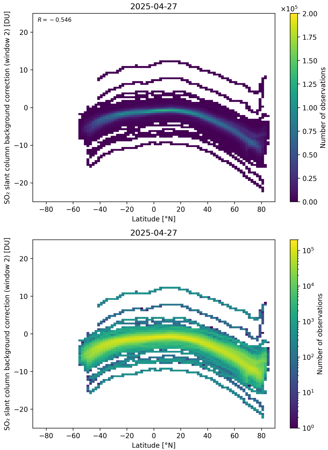
Figure 151: Scatter density plot of “Latitude” against “SO 2 slant column background correction (window 2)” for 2025-04-26 to 2025-04-28.
