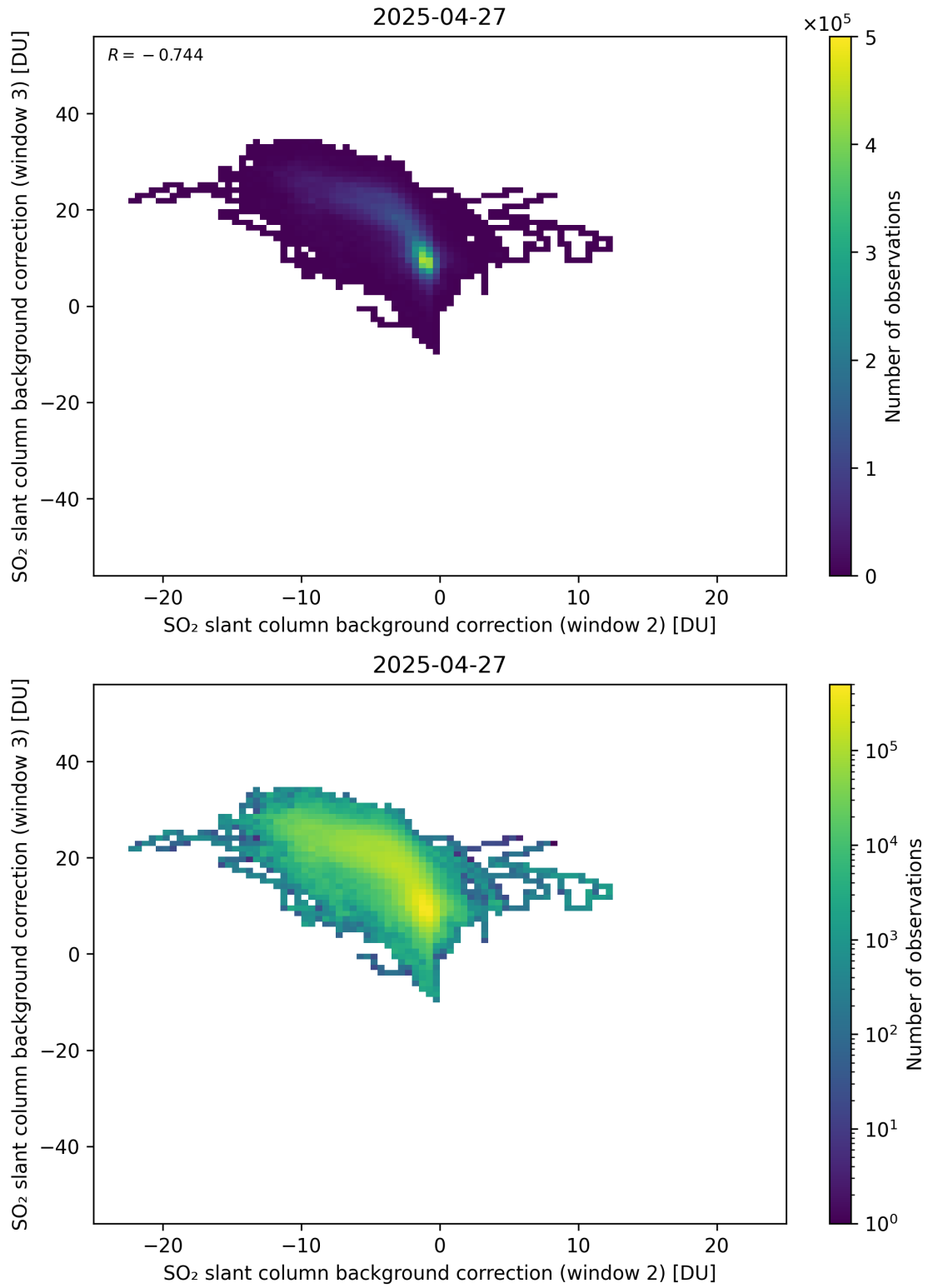
Figure 122: Scatter density plot of “SO 2 slant column background correction (window 2)” against “SO 2 slant column background correction (window 3)” for 2025-04-26 to 2025-04-28.
