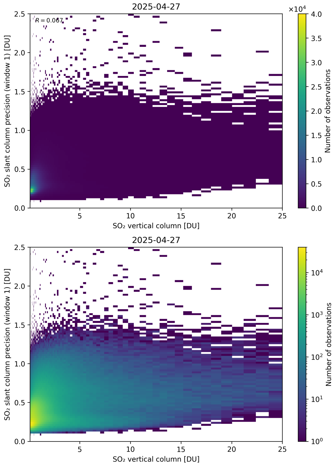
Figure 355: Scatter density plot of “SO 2 vertical column” against “SO 2 slant column precision (window 1)” for 2025-04-26 to 2025-04-28.
