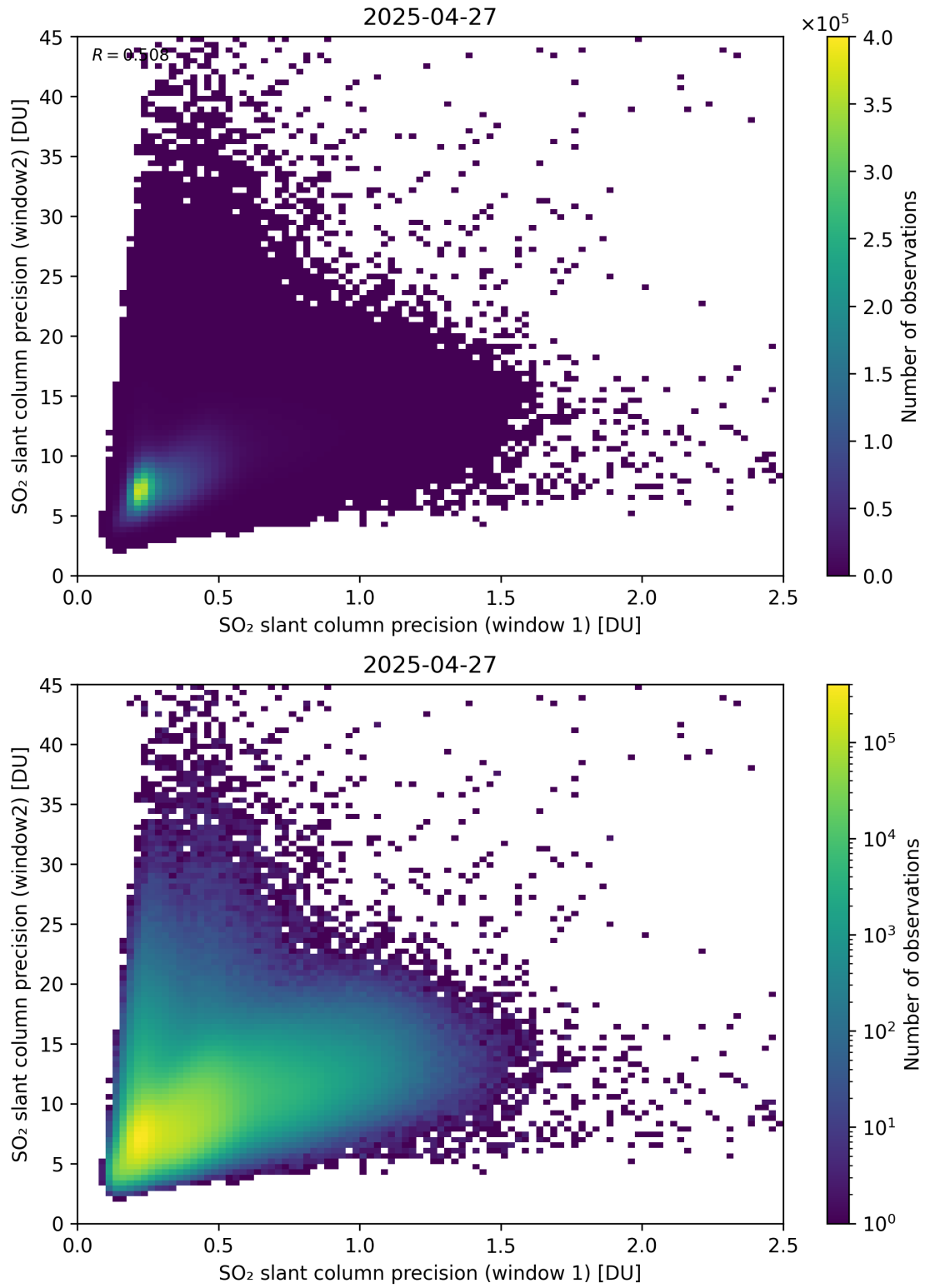
Figure 277: Scatter density plot of “SO 2 slant column precision (window 1)” against “SO 2 slant column precision (window2)” for 2025-04-26 to 2025-04-28.
