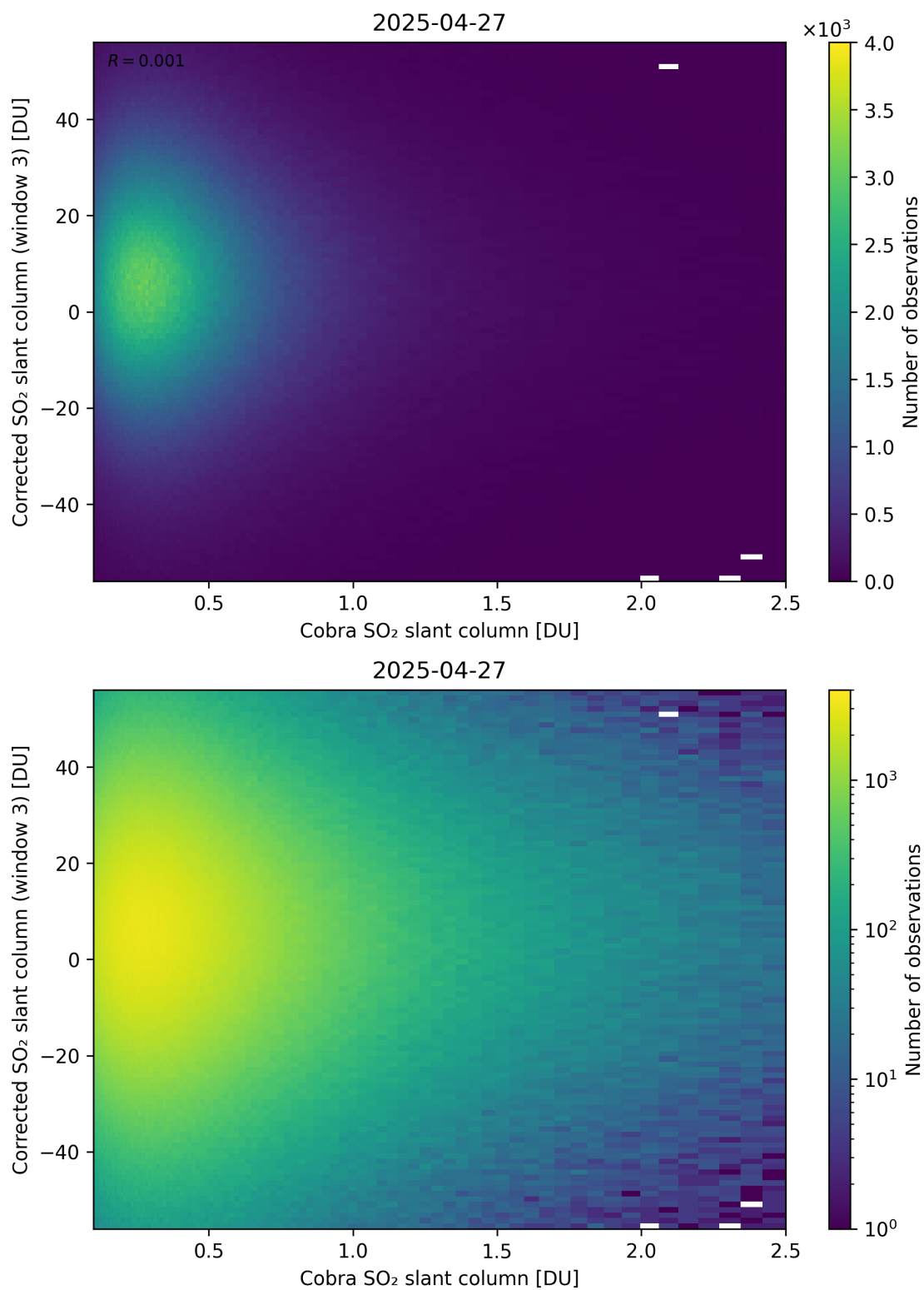
Figure 218: Scatter density plot of “Cobra SO 2 slant column” against “Corrected SO 2 slant column (window 3)” for 2025-04-26 to 2025-04-28.
