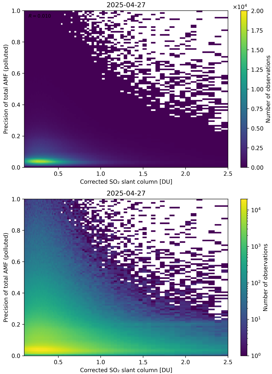
Figure 243: Scatter density plot of “Corrected SO 2 slant column” against “Precision of total AMF (polluted)” for 2025-04-26 to 2025-04-28.
