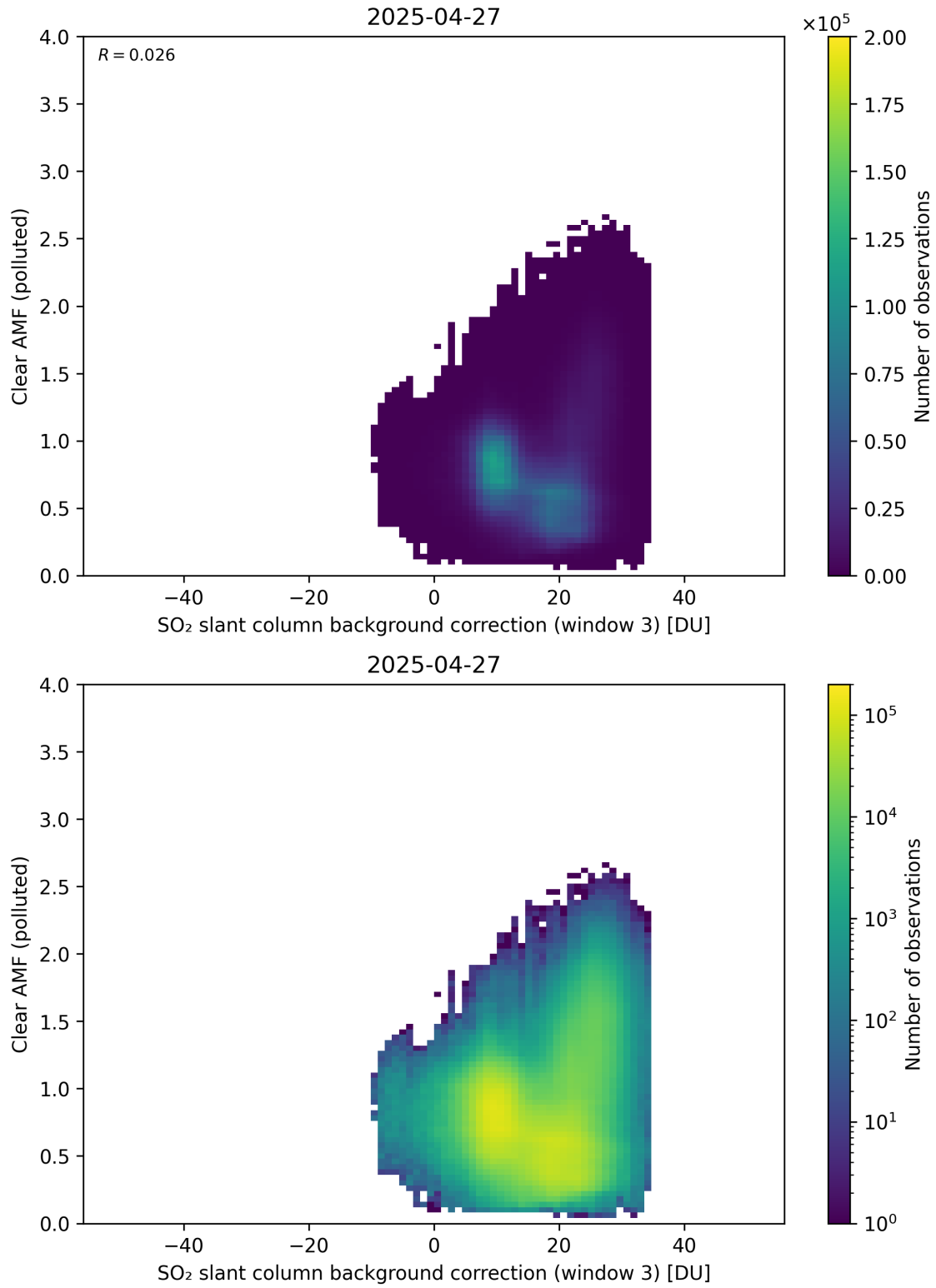
Figure 135: Scatter density plot of “SO 2 slant column background correction (window 3)” against “Clear AMF (polluted)” for 2025-04-26 to 2025-04-28.
