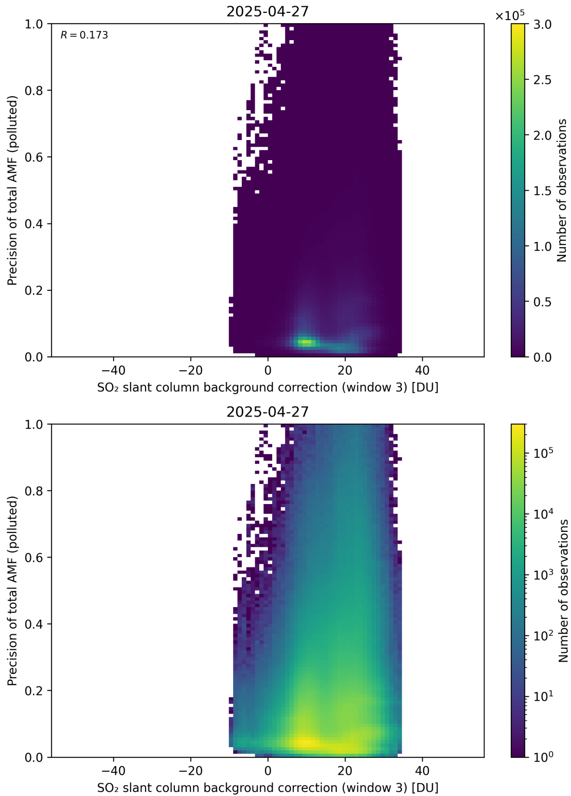
Figure 137: Scatter density plot of “SO 2 slant column background correction (window 3)” against “Precision of total AMF (polluted)” for 2025-04-26 to 2025-04-28.
