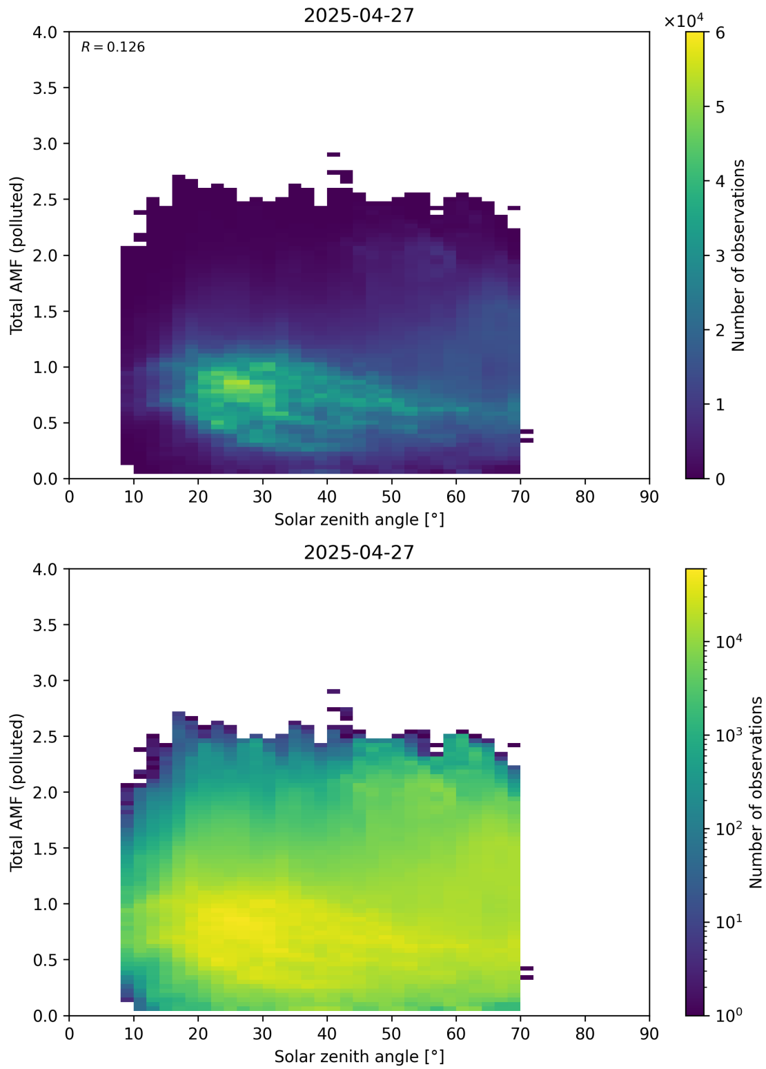
Figure 189: Scatter density plot of “Solar zenith angle” against “Total AMF (polluted)” for 2025-04-26 to 2025-04-28.
