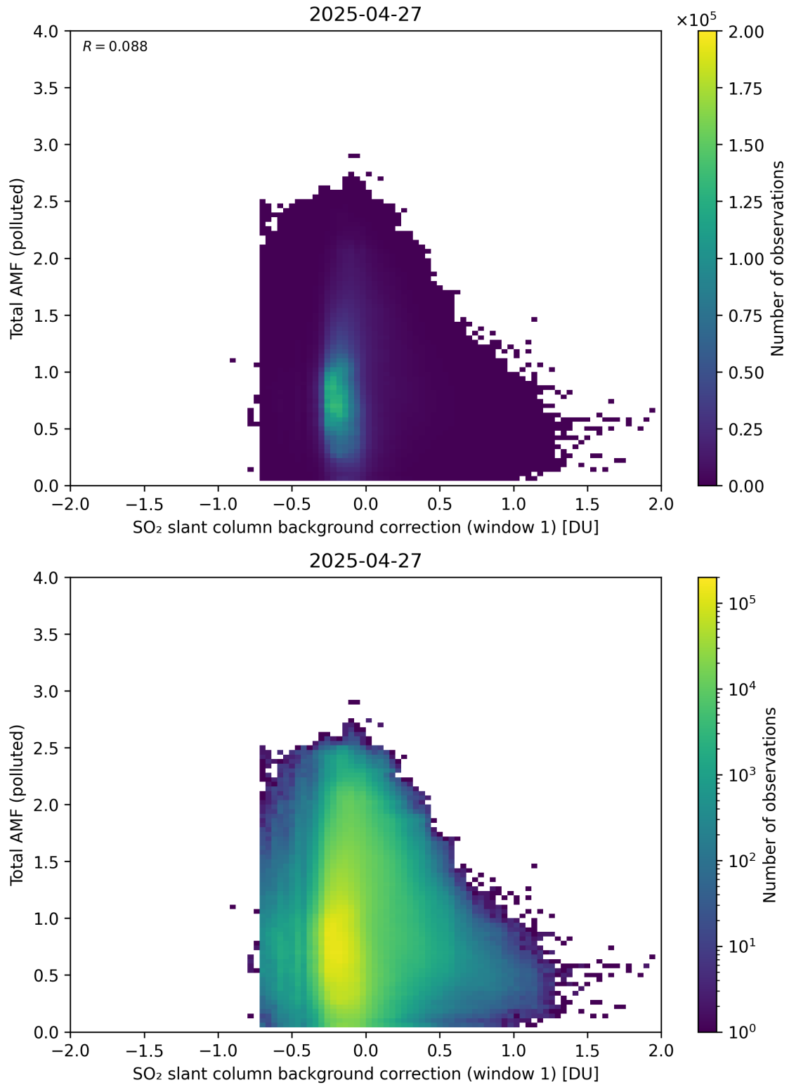
Figure 120: Scatter density plot of “SO 2 slant column background correction (window 1)” against “Total AMF (polluted)” for 2025-04-26 to 2025-04-28.
