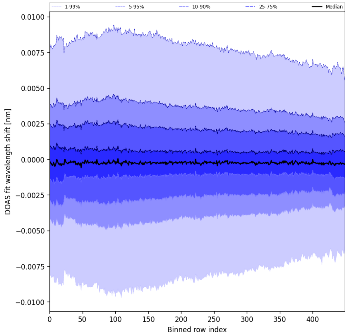
Figure 102: Along track statistics of “DOAS fit wavelength shift” for 2025-04-26 to 2025-04-28
