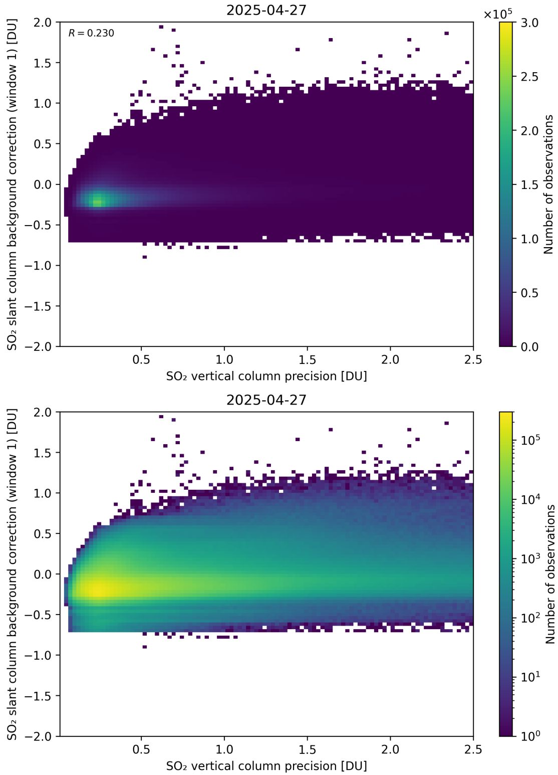
Figure 329: Scatter density plot of “SO 2 vertical column precision” against “SO 2 slant column background correction (window 1)” for 2025-04-26 to 2025-04-28.
