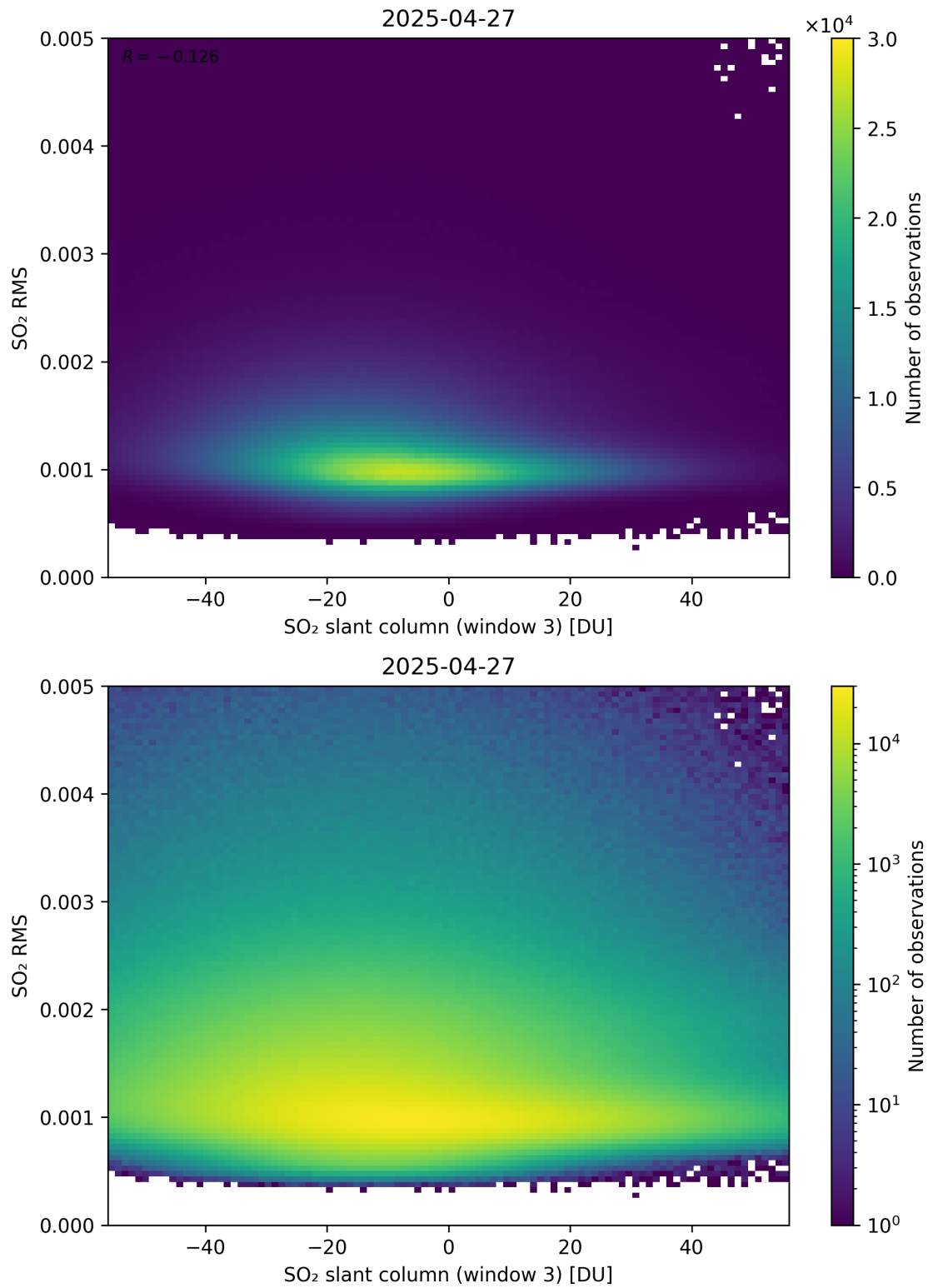
Figure 306: Scatter density plot of “SO 2 slant column (window 3)” against “SO 2 RMS” for 2025-04-26 to 2025-04-28.
