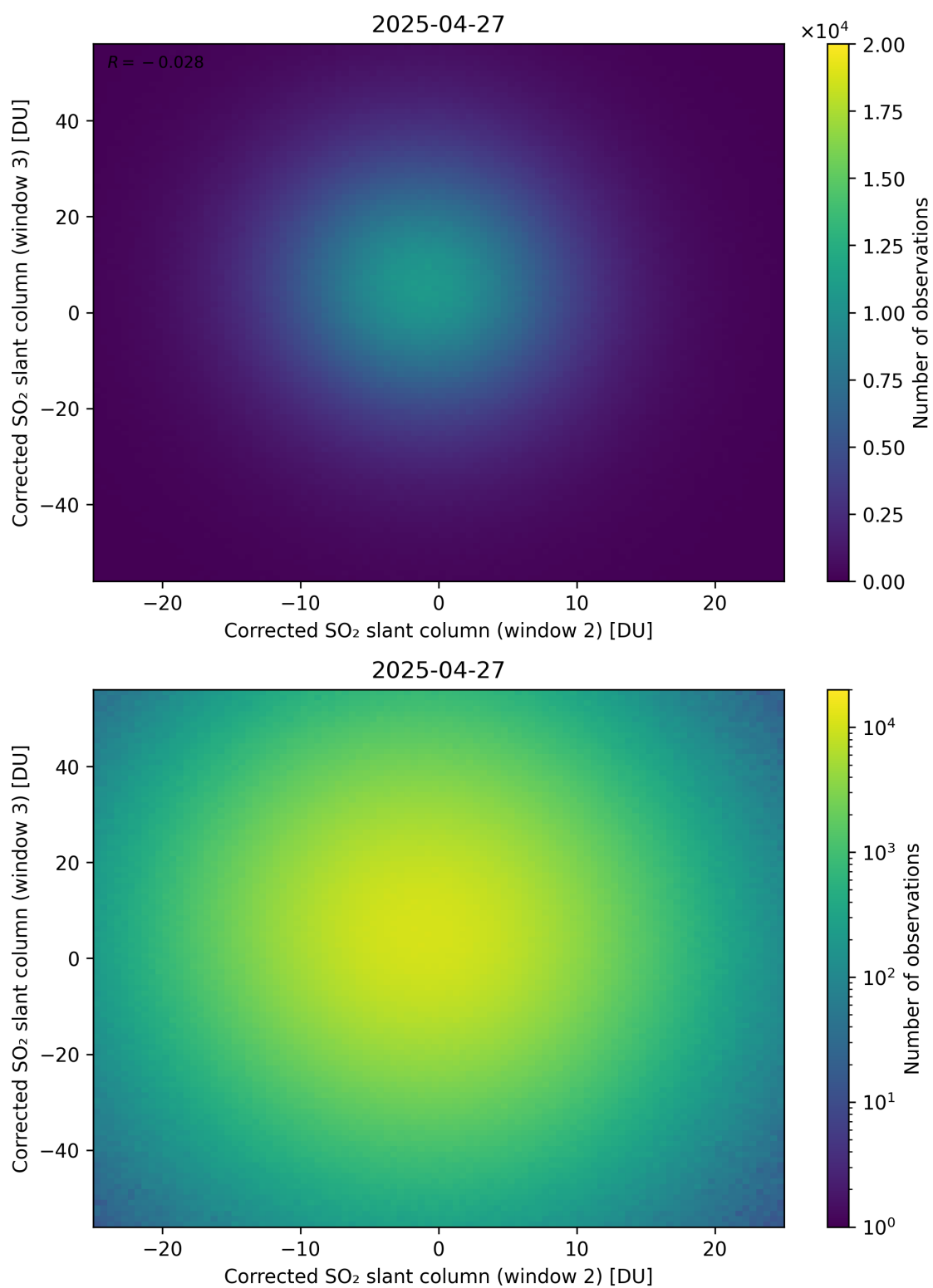
Figure 250: Scatter density plot of “Corrected SO 2 slant column (window 2)” against “Corrected SO 2 slant column (window 3)” for 2025-04-26 to 2025-04-28.
