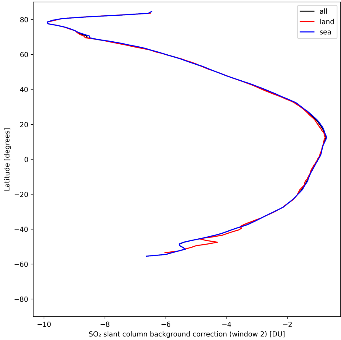
Figure 44: Zonal average of “SO 2 slant column background correction (window 2)” for 2025-04-26 to 2025-04-28.
