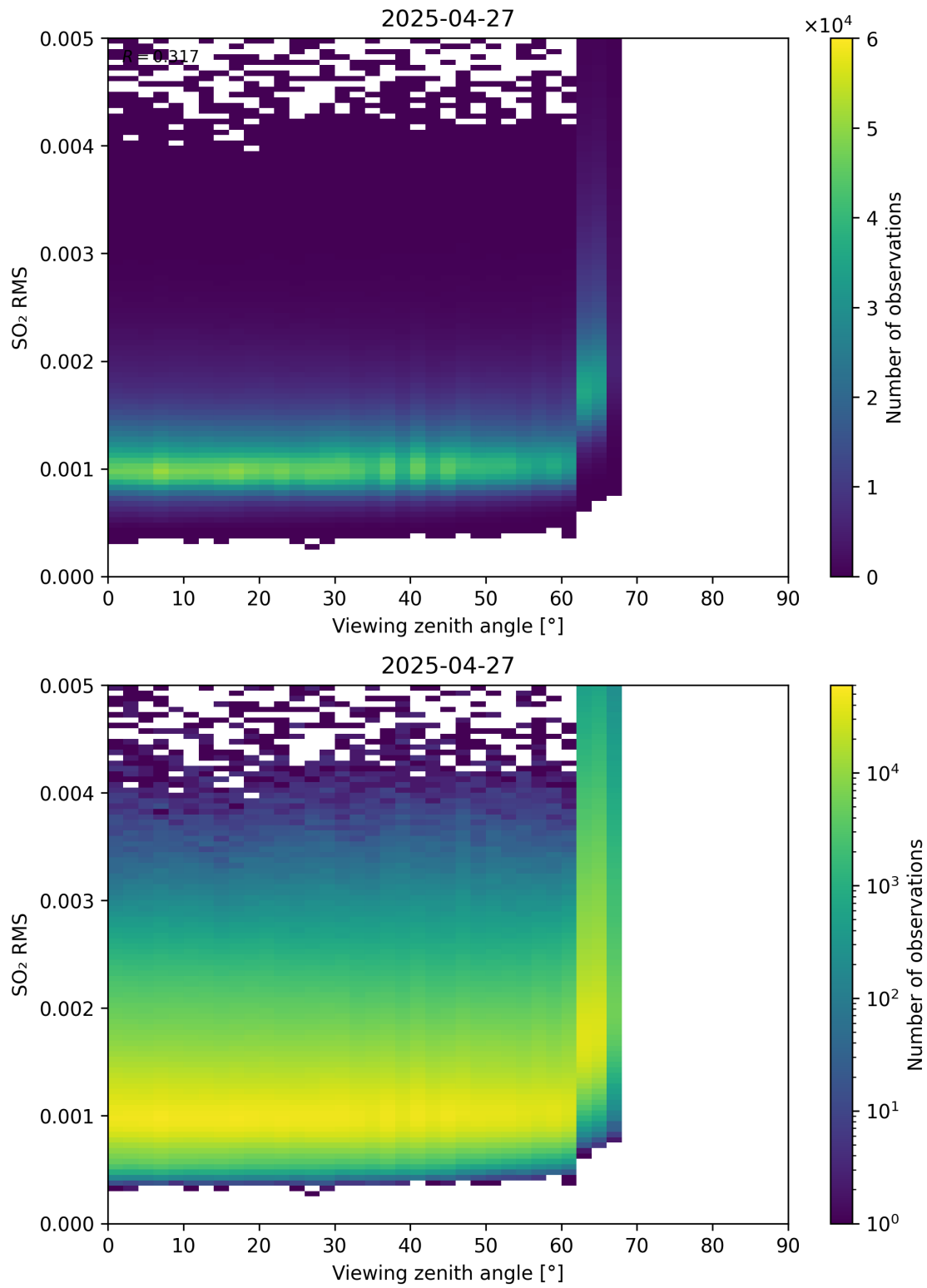
Figure 367: Scatter density plot of “Viewing zenith angle” against “SO 2 RMS” for 2025-04-26 to 2025-04-28.
