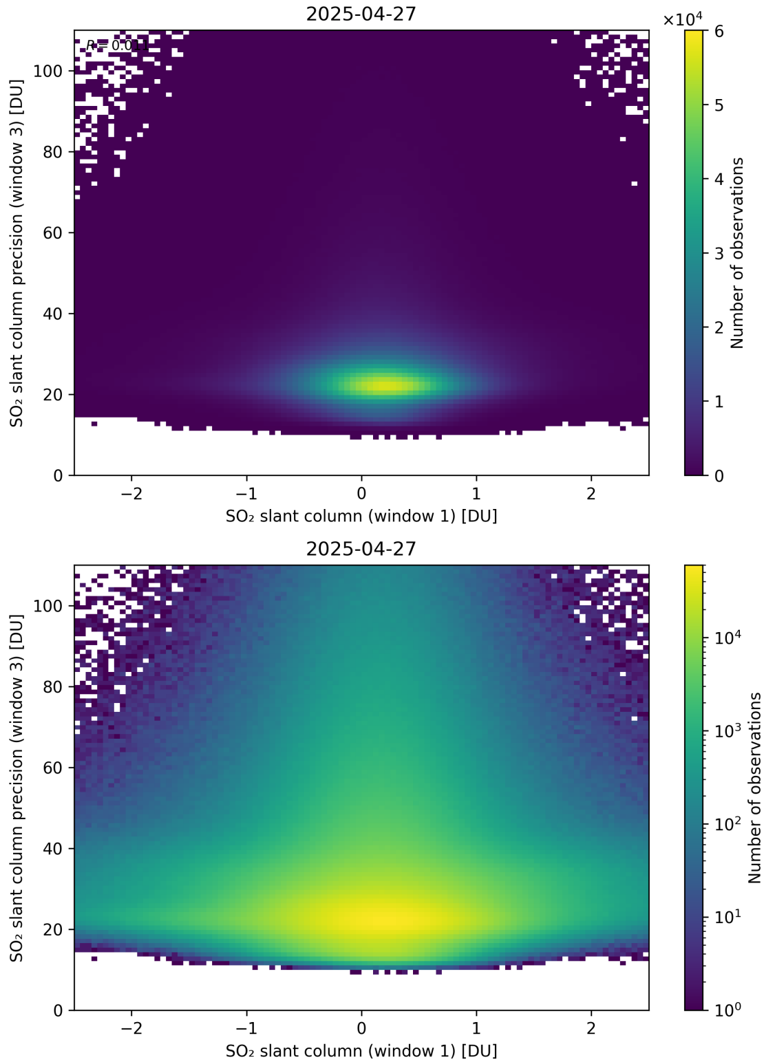
Figure 288: Scatter density plot of “SO 2 slant column (window 1)” against “SO 2 slant column precision (window 3)” for 2025-04-26 to 2025-04-28.
