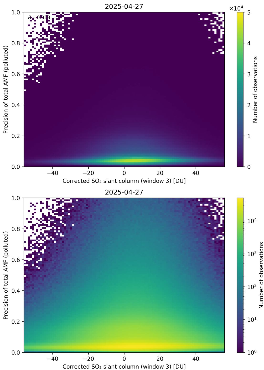
Figure 261: Scatter density plot of “Corrected SO 2 slant column (window 3)” against “Precision of total AMF (polluted)” for 2025-04-26 to 2025-04-28.
