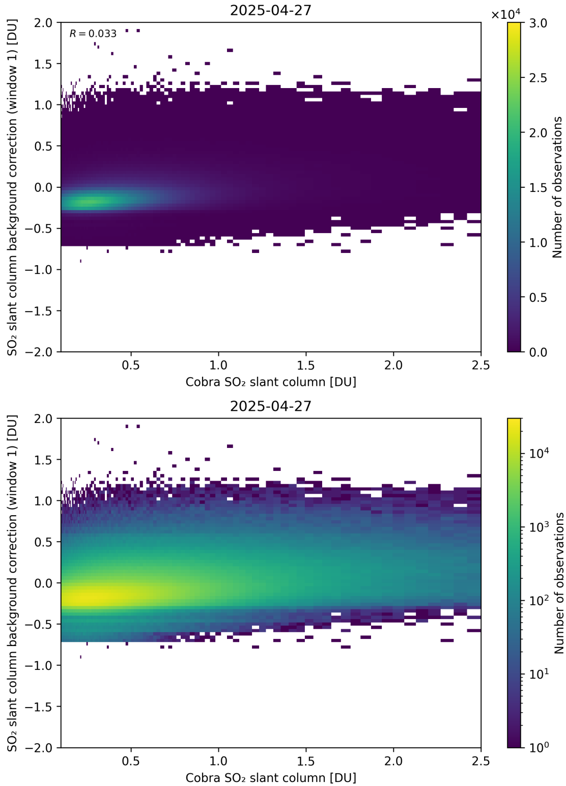
Figure 193: Scatter density plot of “Cobra SO 2 slant column” against “SO 2 slant column background correction (window 1)” for 2025-04-26 to 2025-04-28.
