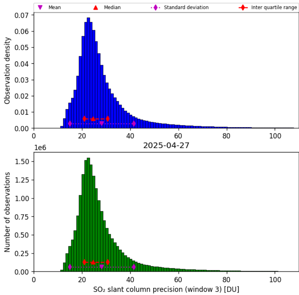
Figure 72: Histogram of “SO 2 slant column precision (window 3)” for 2025-04-26 to 2025-04-28
