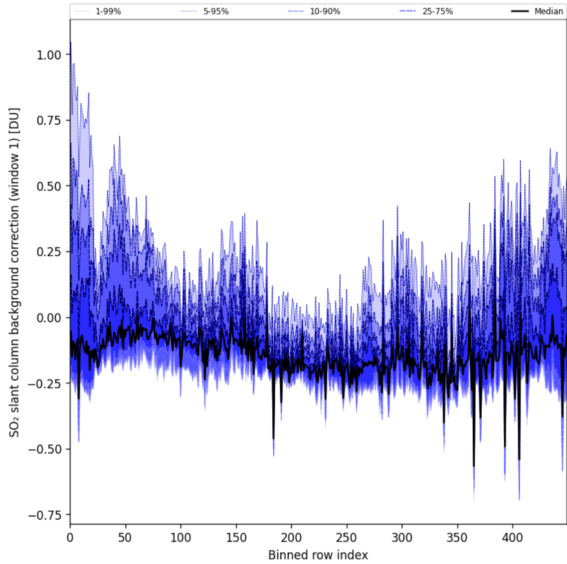
Figure 92: Along track statistics of “SO 2 slant column background correction (window 1)” for 2025-04-26 to 2025-04-28
