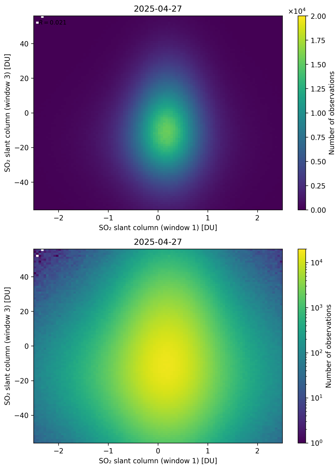
Figure 287: Scatter density plot of “SO 2 slant column (window 1)” against “SO 2 slant column (window 3)” for 2025-04-26 to 2025-04-28.
