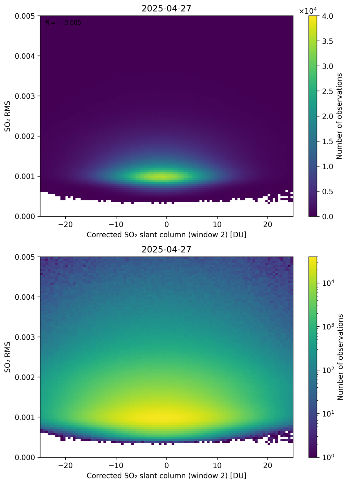
Figure 248: Scatter density plot of “Corrected SO 2 slant column (window 2)” against “SO 2 RMS” for 2025-04-26 to 2025-04-28.
