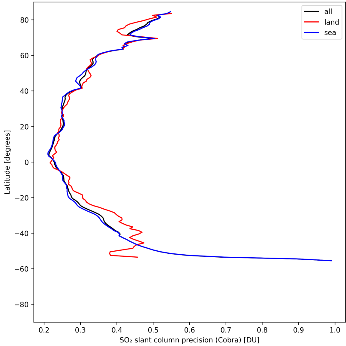
Figure 36: Zonal average of “SO 2 slant column precision (Cobra)” for 2025-04-26 to 2025-04-28.
