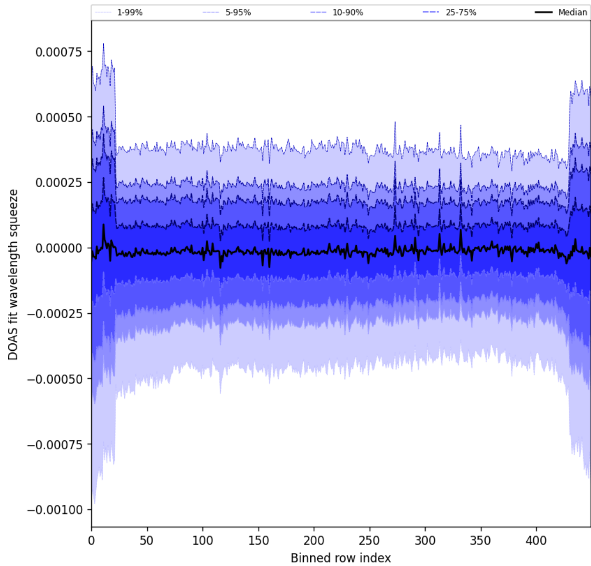
Figure 103: Along track statistics of “DOAS fit wavelength squeeze” for 2025-04-26 to 2025-04-28
