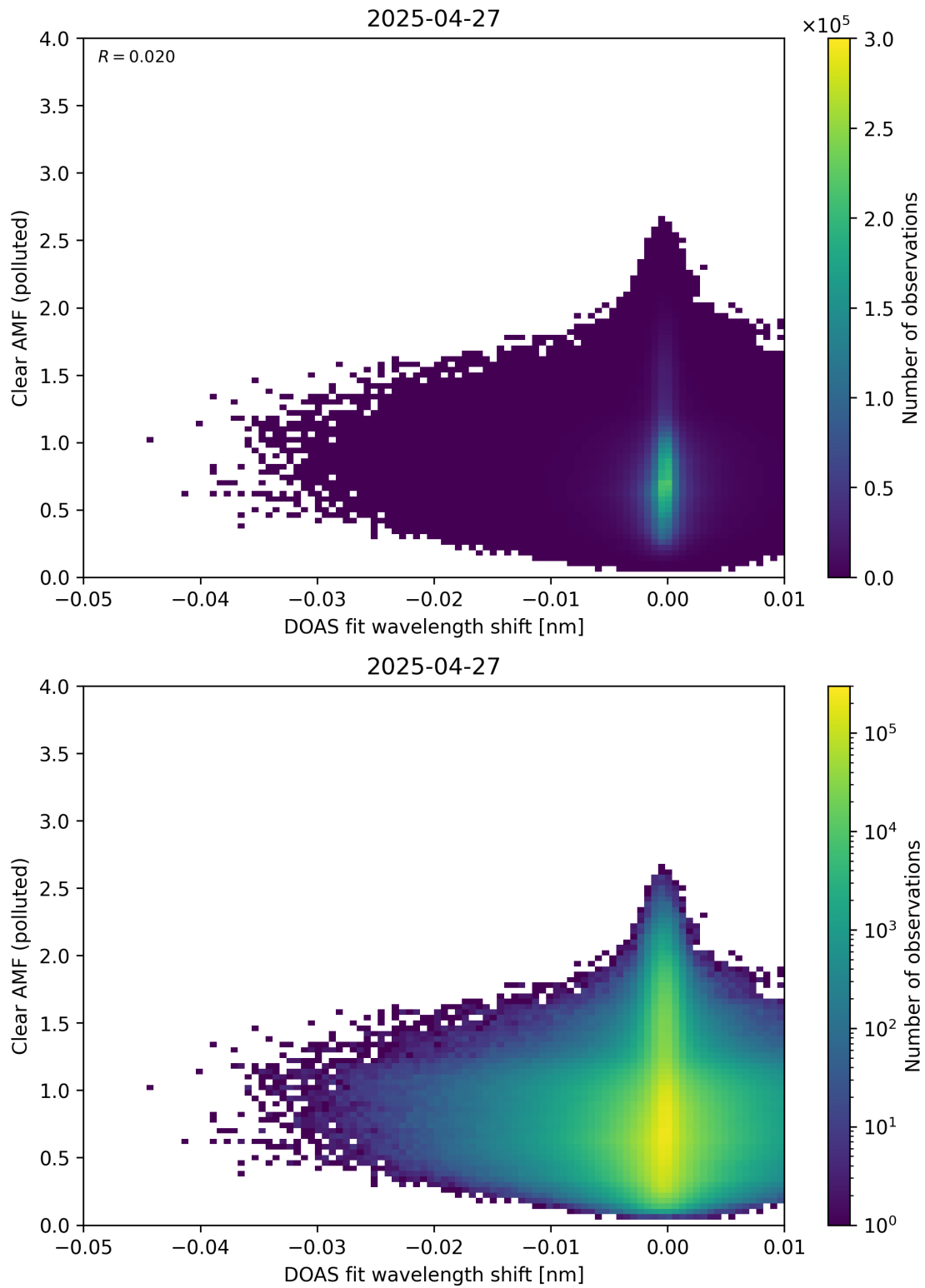
Figure 140: Scatter density plot of “DOAS fit wavelength shift” against “Clear AMF (polluted)” for 2025-04-26 to 2025-04-28.
