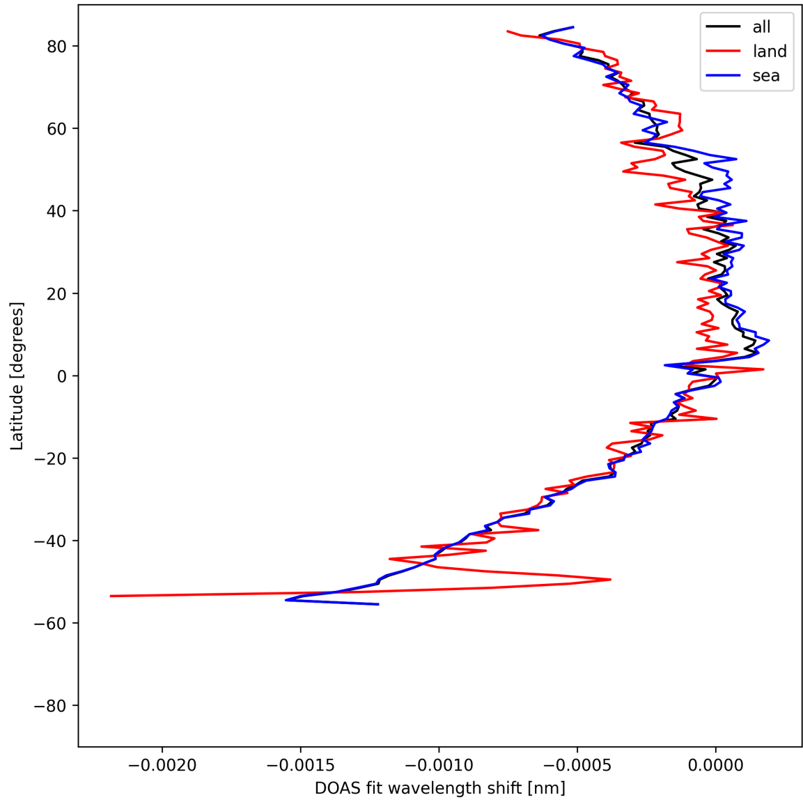
Figure 50: Zonal average of “DOAS fit wavelength shift” for 2025-04-26 to 2025-04-28.
