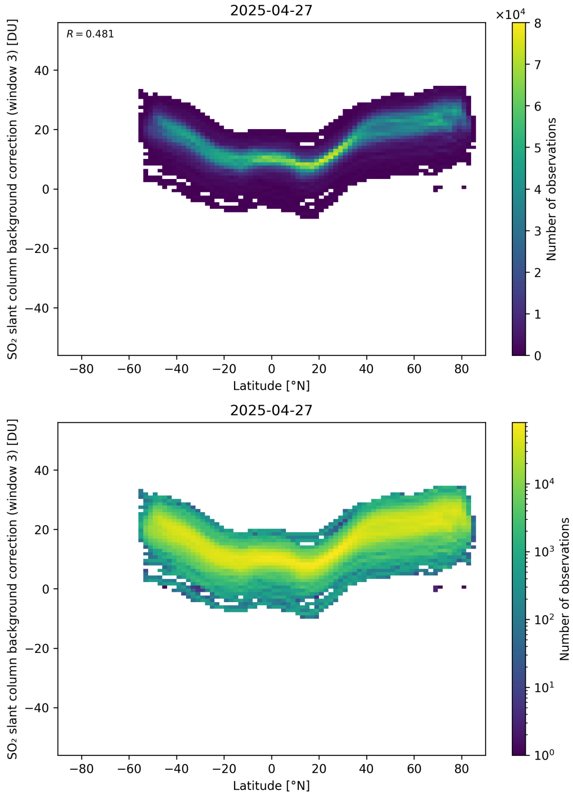
Figure 152: Scatter density plot of “Latitude” against “SO 2 slant column background correction (window 3)” for 2025-04-26 to 2025-04-28.
