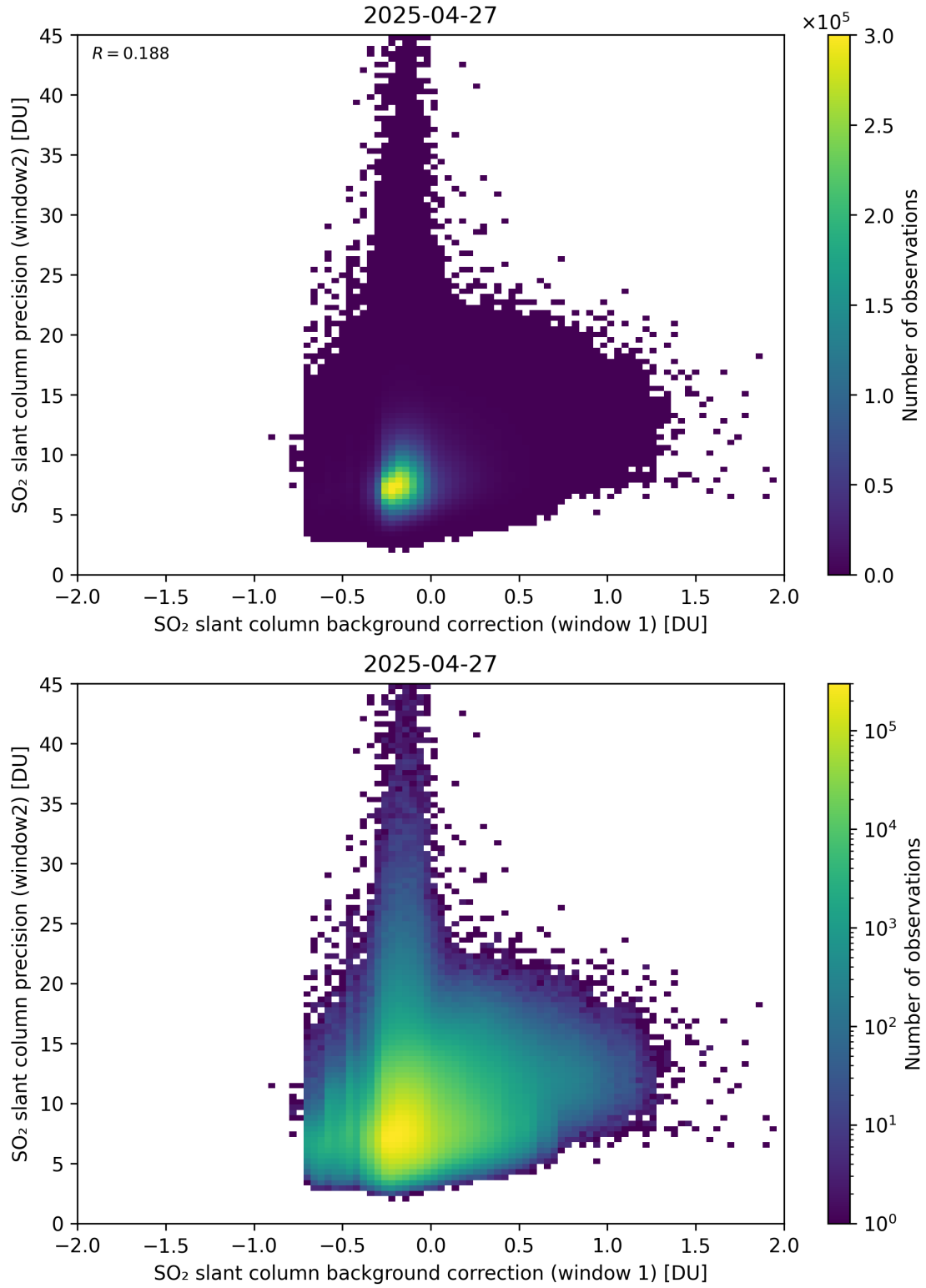
Figure 117: Scatter density plot of “SO 2 slant column background correction (window 1)” against “SO 2 slant column precision (window2)” for 2025-04-26 to 2025-04-28.
