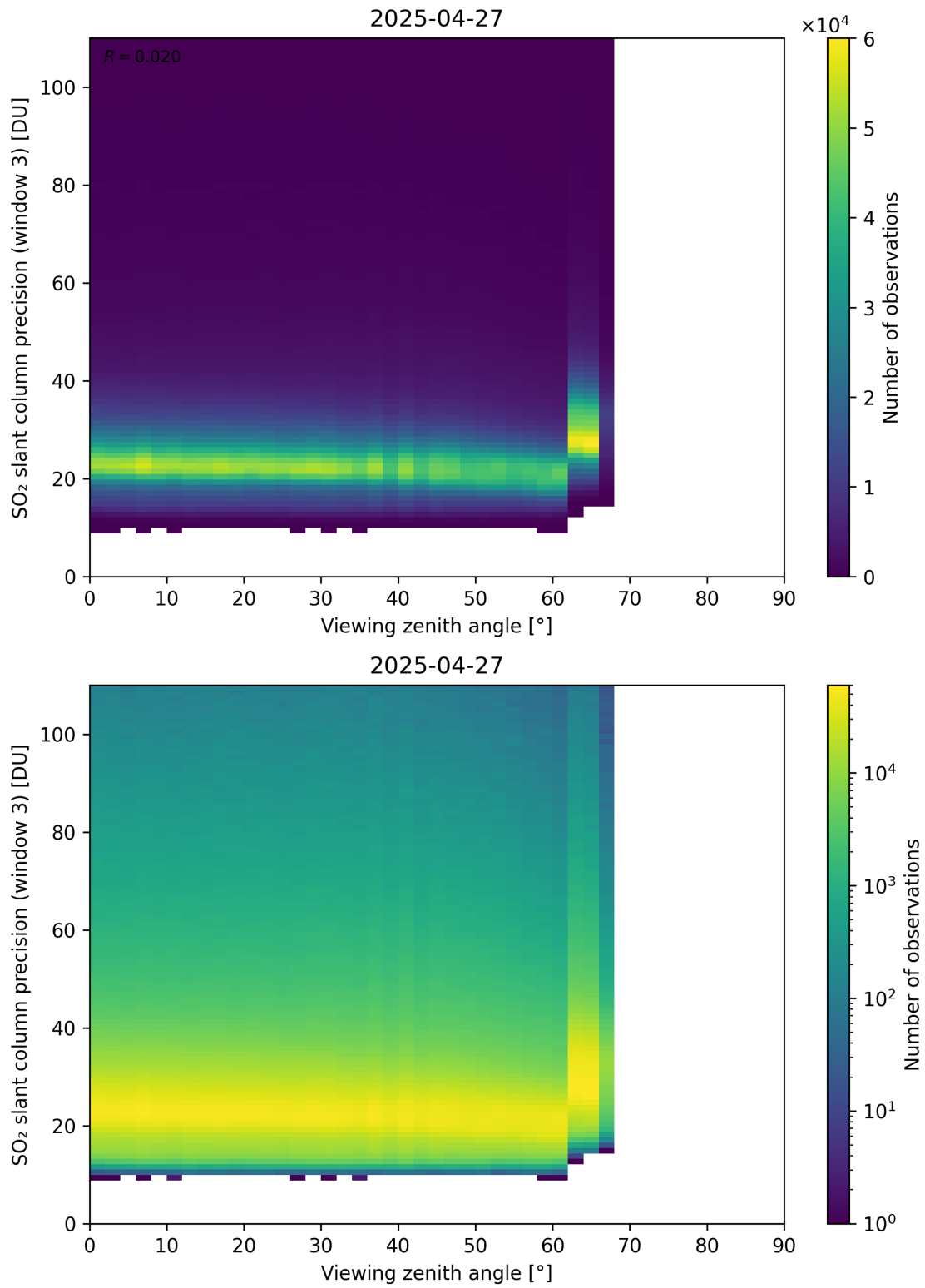
Figure 380: Scatter density plot of “Viewing zenith angle” against “SO 2 slant column precision (window 3)” for 2025-04-26 to 2025-04-28.
