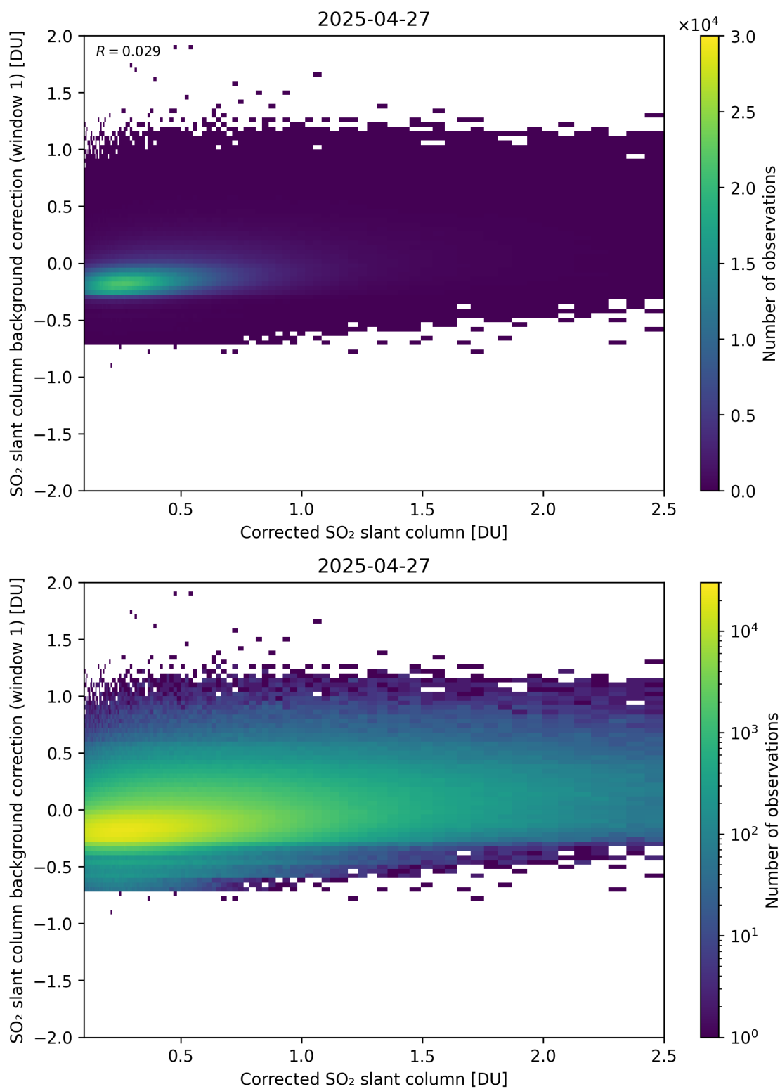
Figure 226: Scatter density plot of “Corrected SO 2 slant column” against “SO 2 slant column background correction (window 1)” for 2025-04-26 to 2025-04-28.
