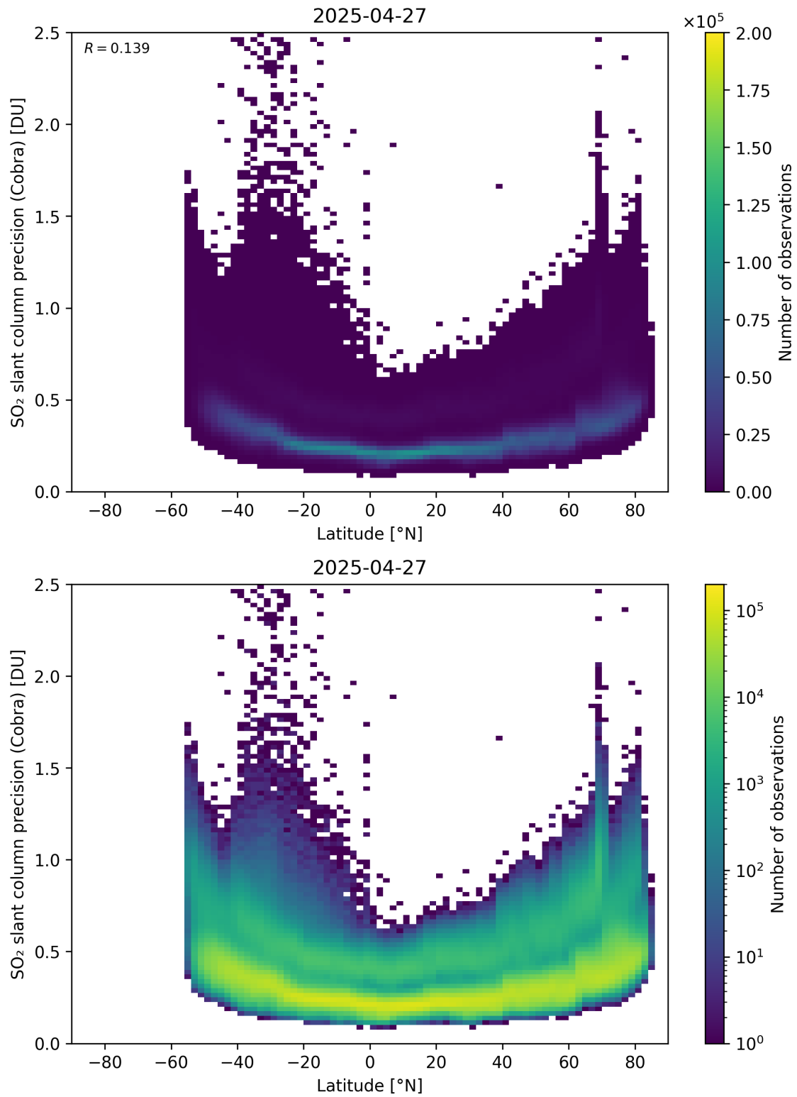
Figure 158: Scatter density plot of “Latitude” against “SO 2 slant column precision (Cobra)” for 2025-04-26 to 2025-04-28.
