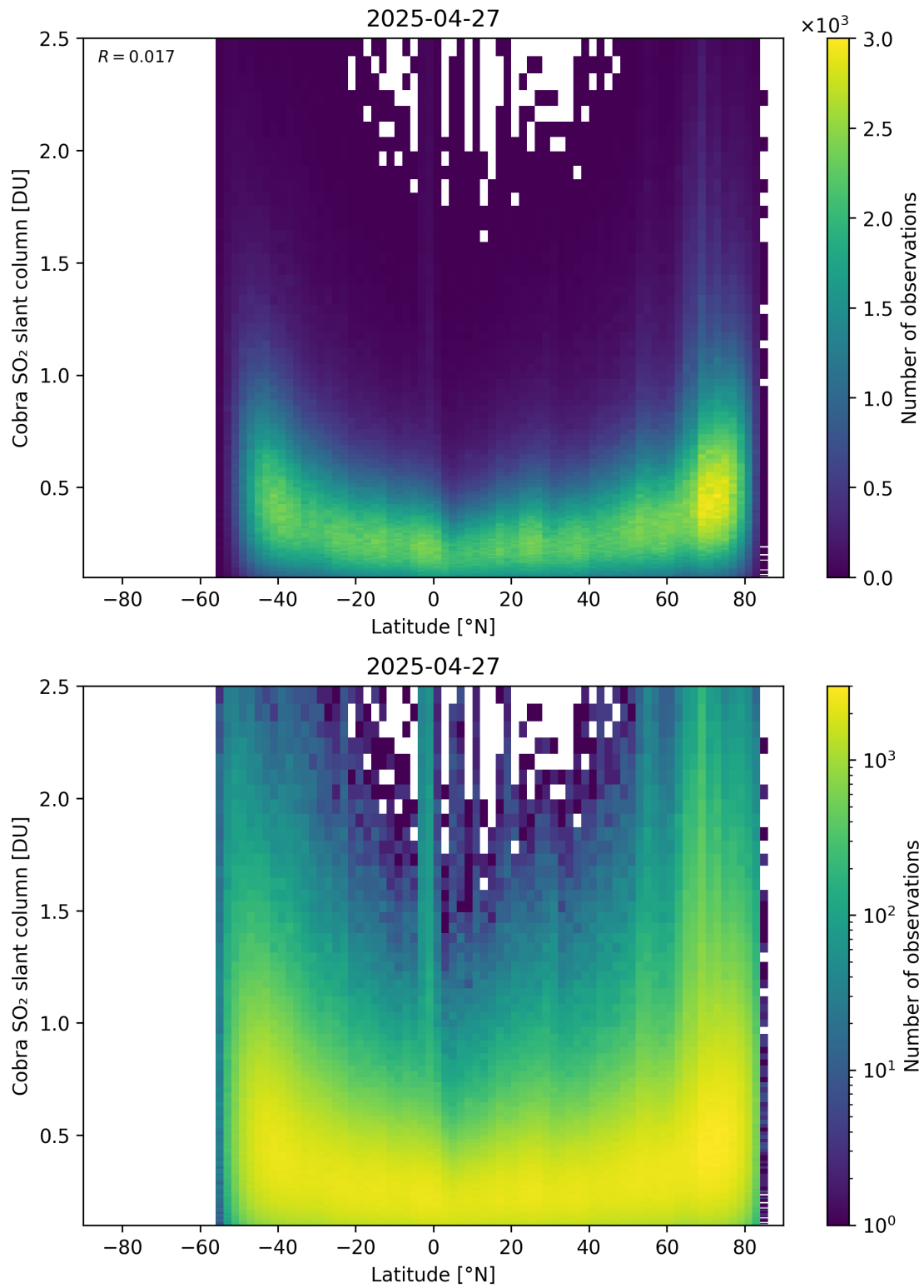
Figure 157: Scatter density plot of “Latitude” against “Cobra SO 2 slant column” for 2025-04-26 to 2025-04-28.
