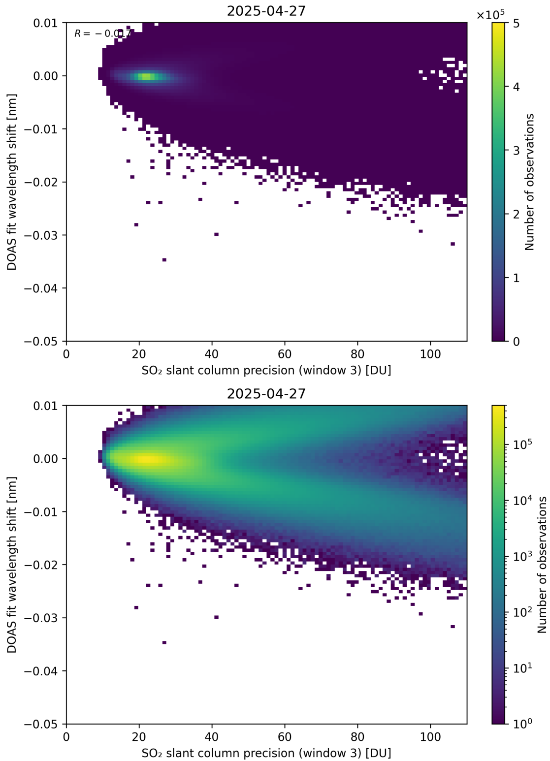
Figure 308: Scatter density plot of “SO 2 slant column precision (window 3)” against “DOAS fit wavelength shift” for 2025-04-26 to 2025-04-28.
