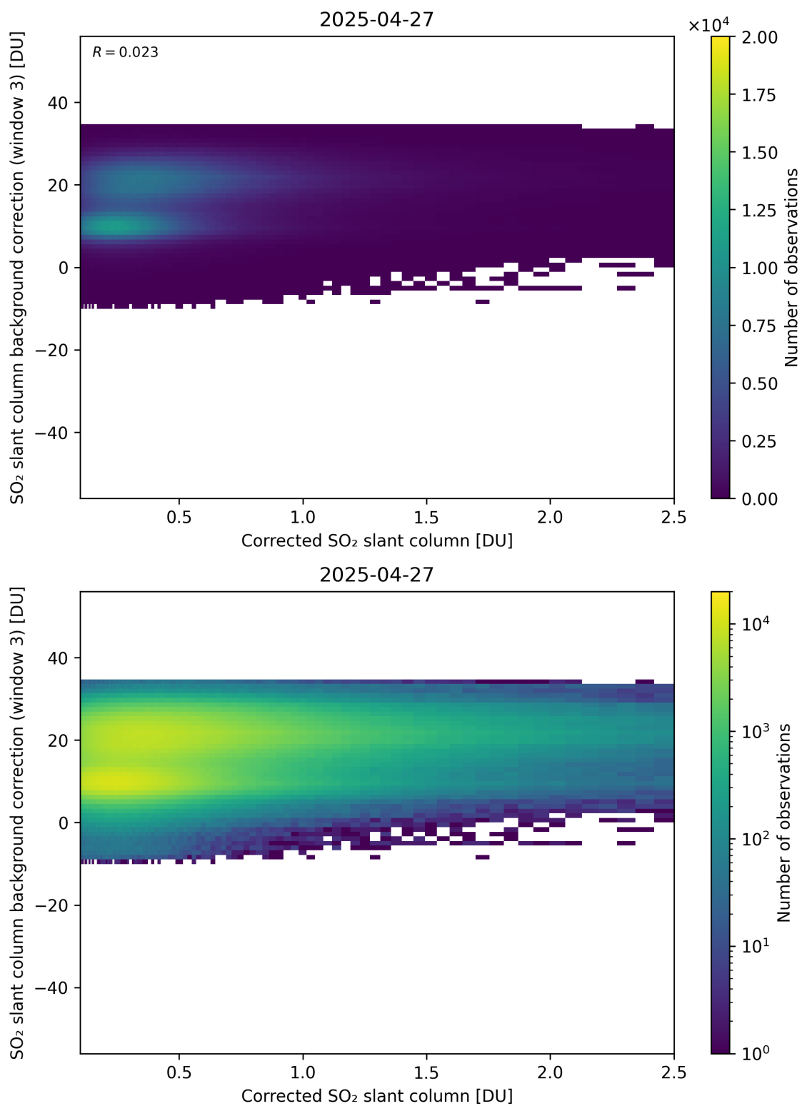
Figure 228: Scatter density plot of “Corrected SO 2 slant column” against “SO 2 slant column background correction (window 3)” for 2025-04-26 to 2025-04-28.
