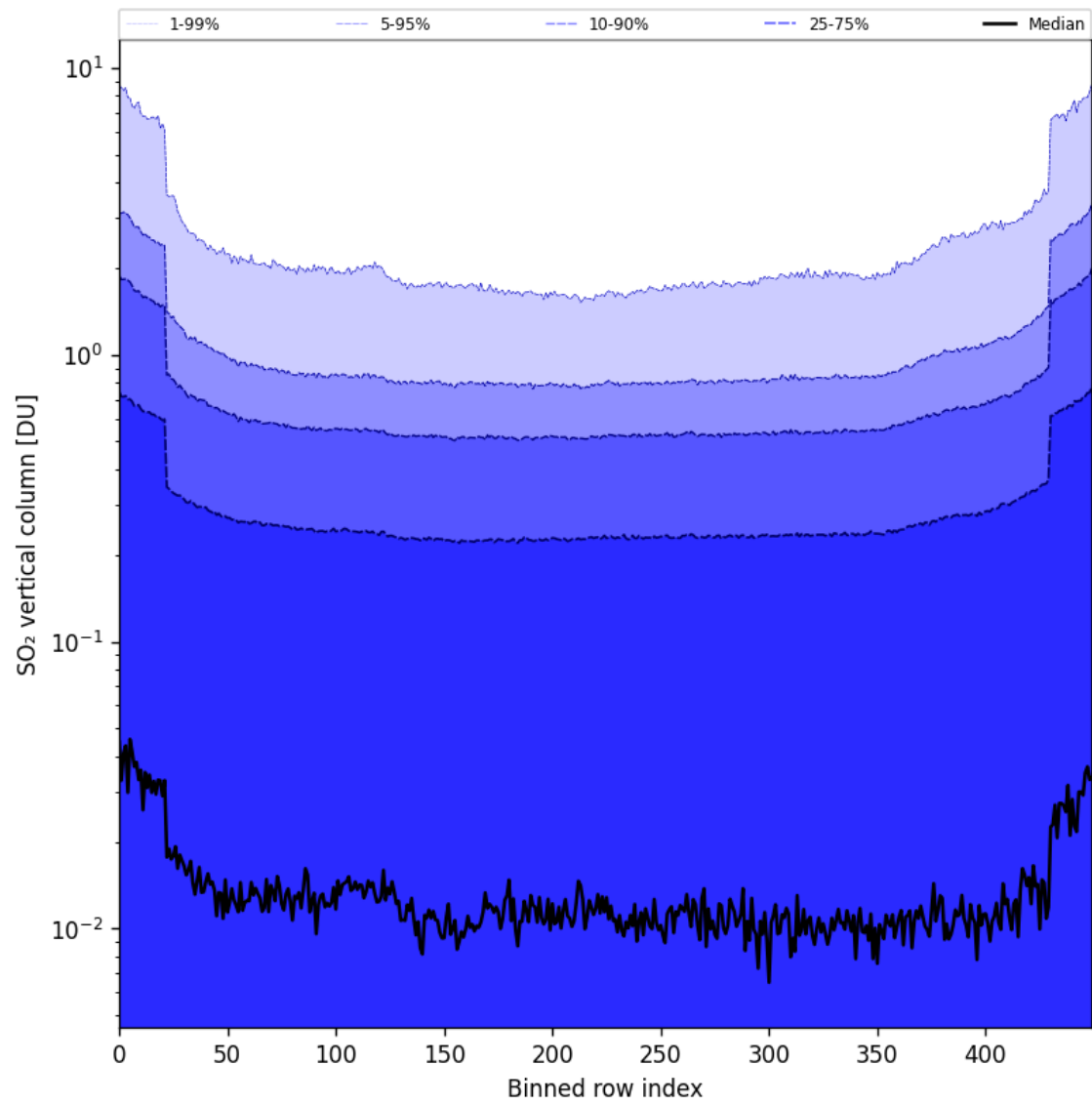
Figure 84: Along track statistics of “SO 2 vertical column” for 2025-04-26 to 2025-04-28
