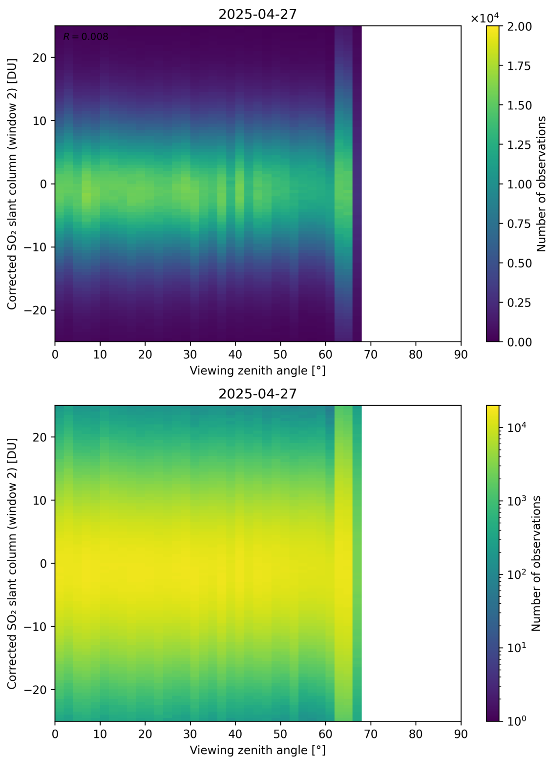
Figure 374: Scatter density plot of “Viewing zenith angle” against “Corrected SO 2 slant column (window 2)” for 2025-04-26 to 2025-04-28.
