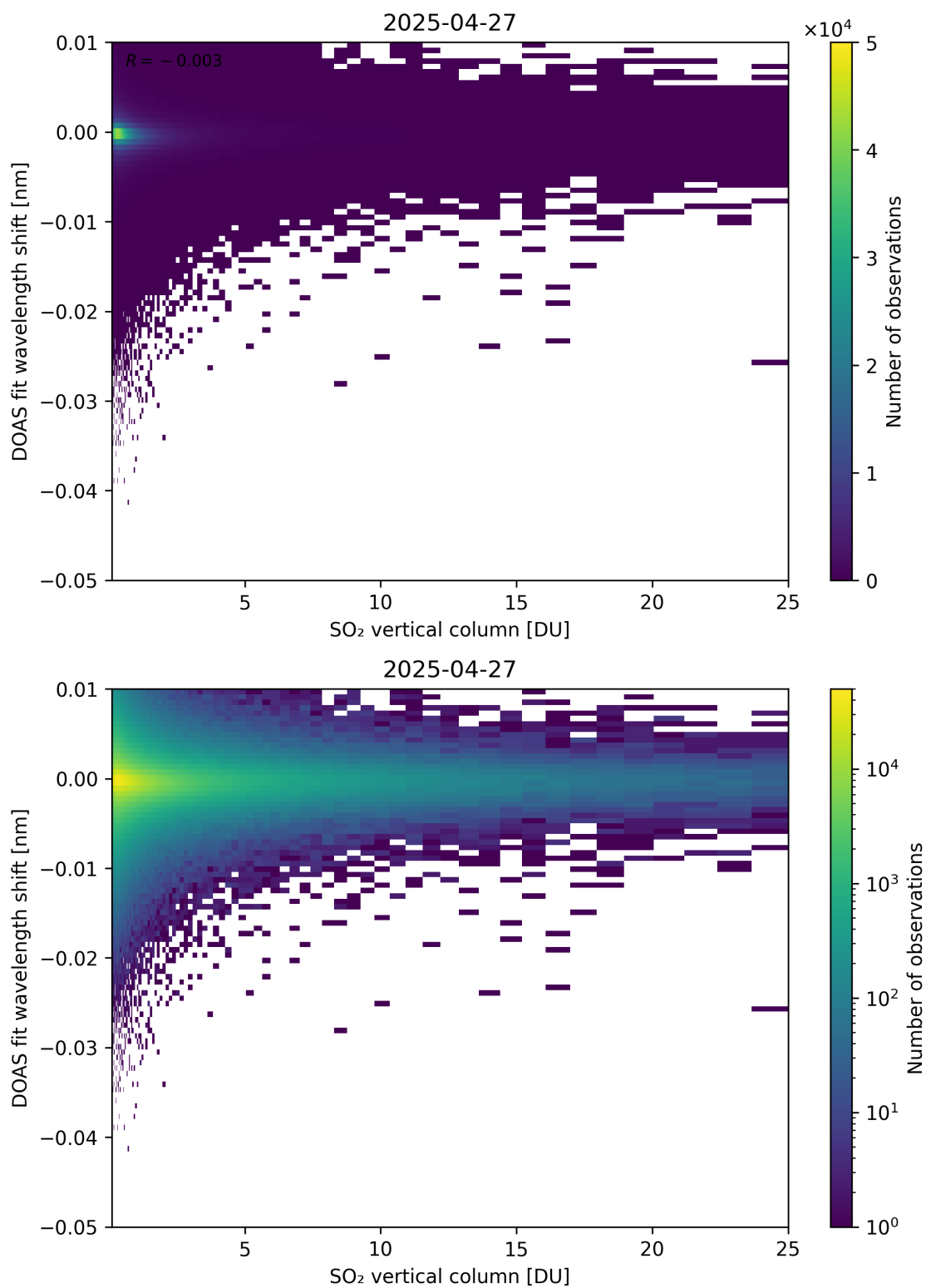
Figure 326: Scatter density plot of “SO 2 vertical column” against “DOAS fit wavelength shift” for 2025-04-26 to 2025-04-28.
