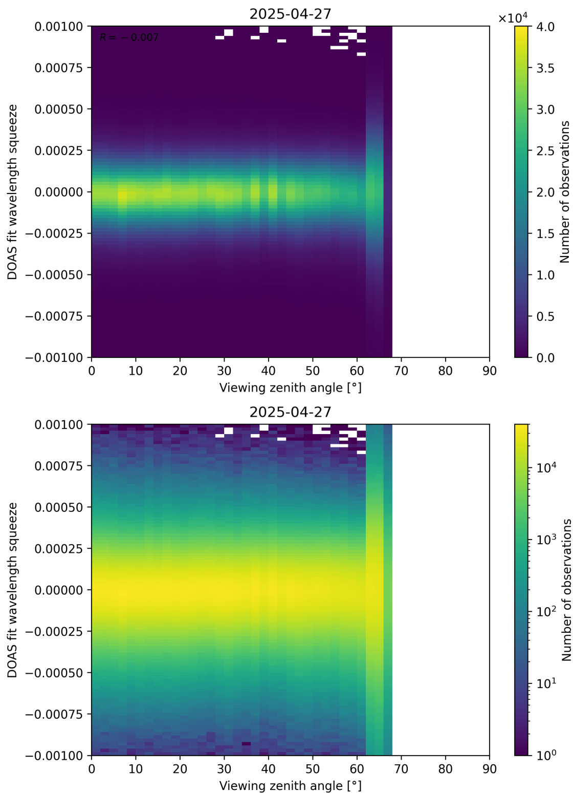
Figure 366: Scatter density plot of “Viewing zenith angle” against “DOAS fit wavelength squeeze” for 2025-04-26 to 2025-04-28.
