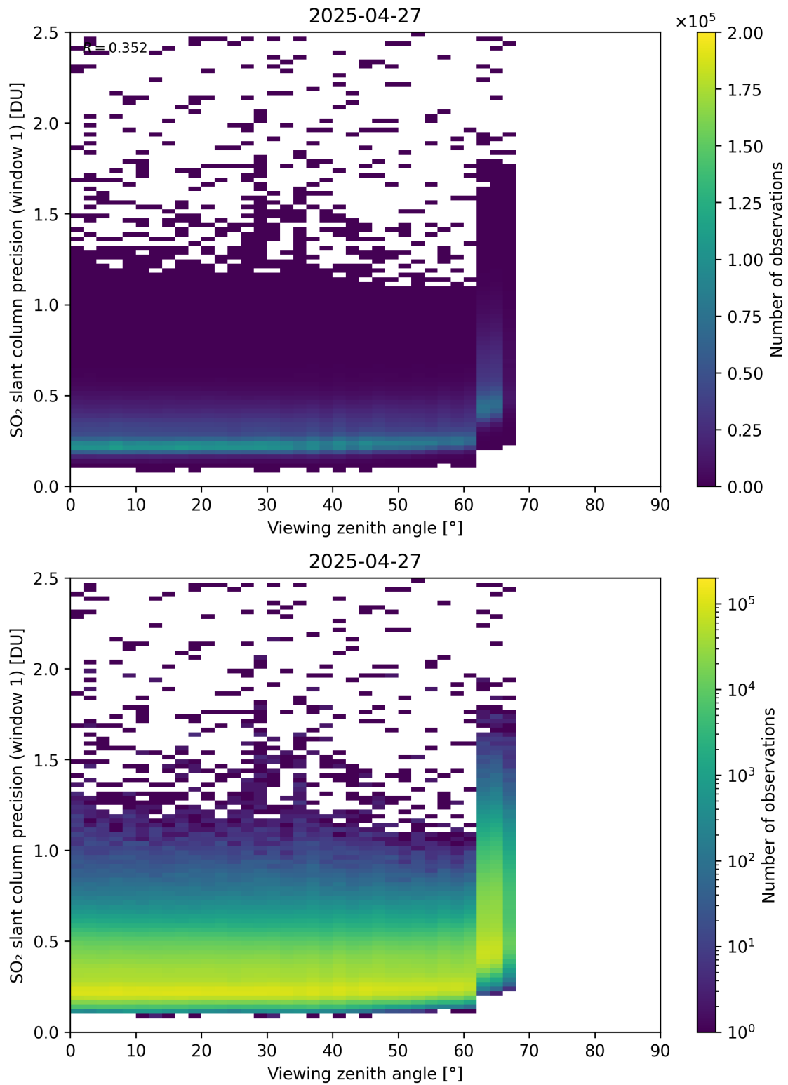
Figure 377: Scatter density plot of “Viewing zenith angle” against “SO 2 slant column precision (window 1)” for 2025-04-26 to 2025-04-28.
