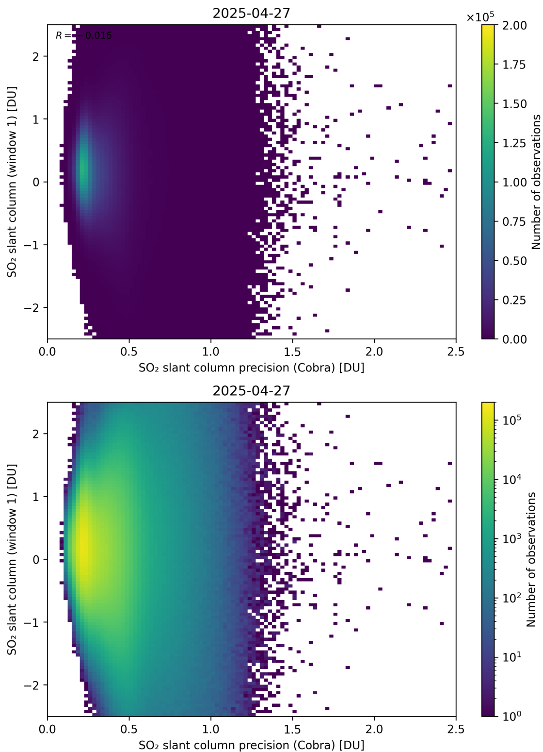
Figure 208: Scatter density plot of “SO 2 slant column precision (Cobra)” against “SO 2 slant column (window 1)” for 2025-04-26 to 2025-04-28.
