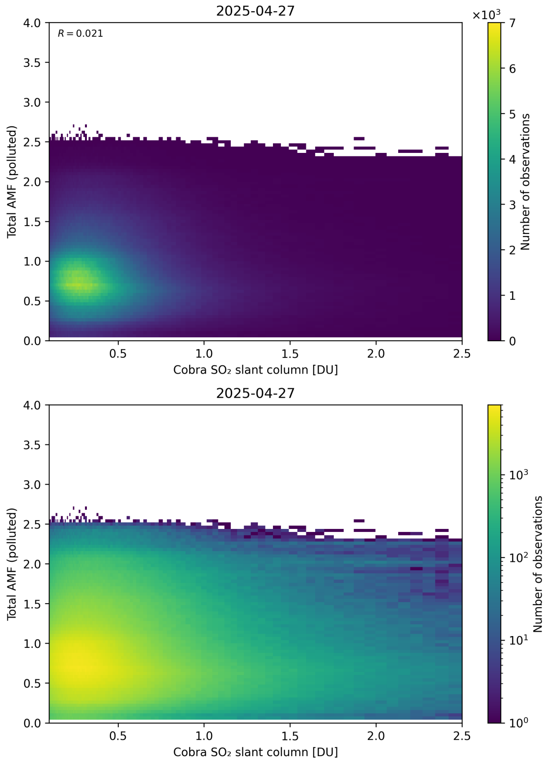
Figure 224: Scatter density plot of “Cobra SO 2 slant column” against “Total AMF (polluted)” for 2025-04-26 to 2025-04-28.
