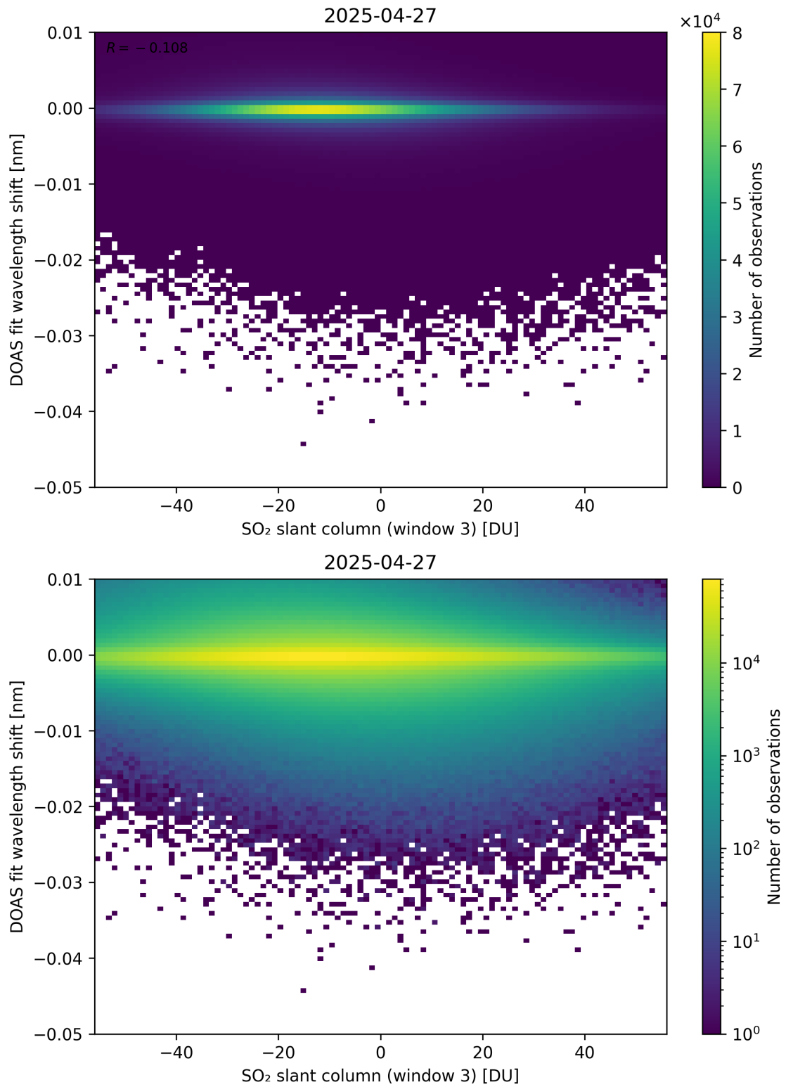
Figure 304: Scatter density plot of “SO 2 slant column (window 3)” against “DOAS fit wavelength shift” for 2025-04-26 to 2025-04-28.
