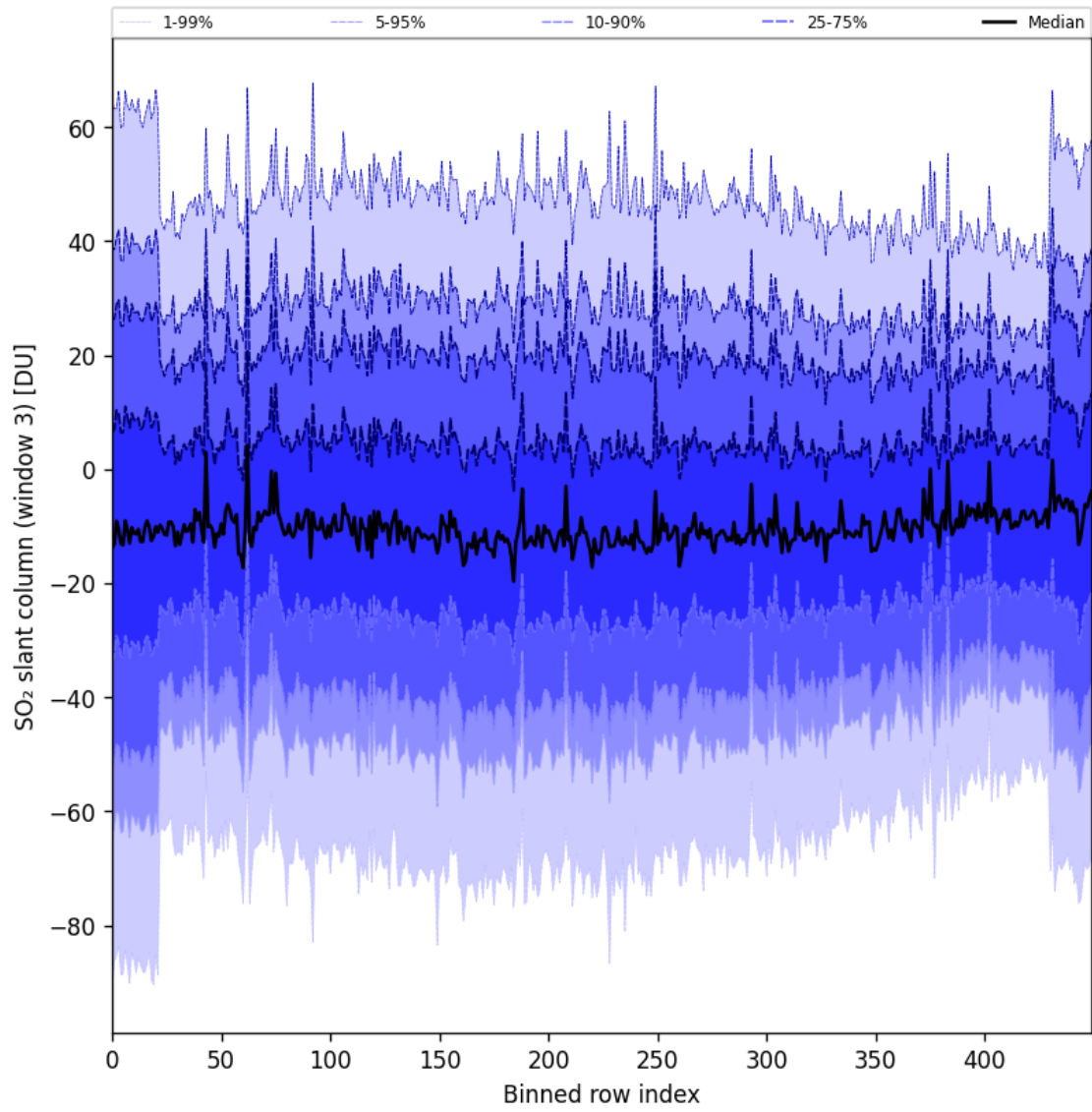
Figure 97: Along track statistics of “SO 2 slant column (window 3)” for 2025-04-26 to 2025-04-28
