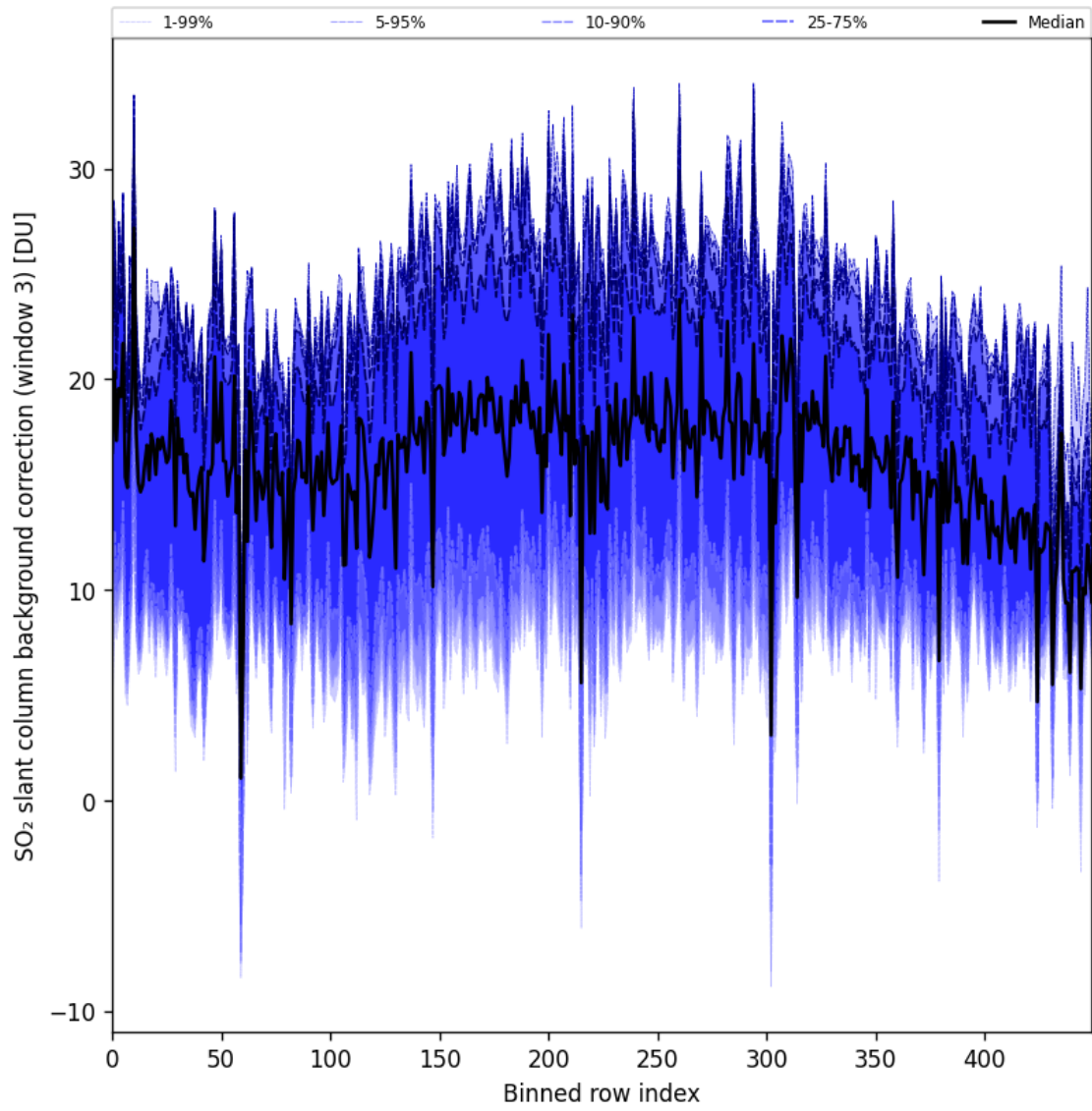
Figure 100: Along track statistics of “SO 2 slant column background correction (window 3)” for 2025-04-26 to 2025-04-28
