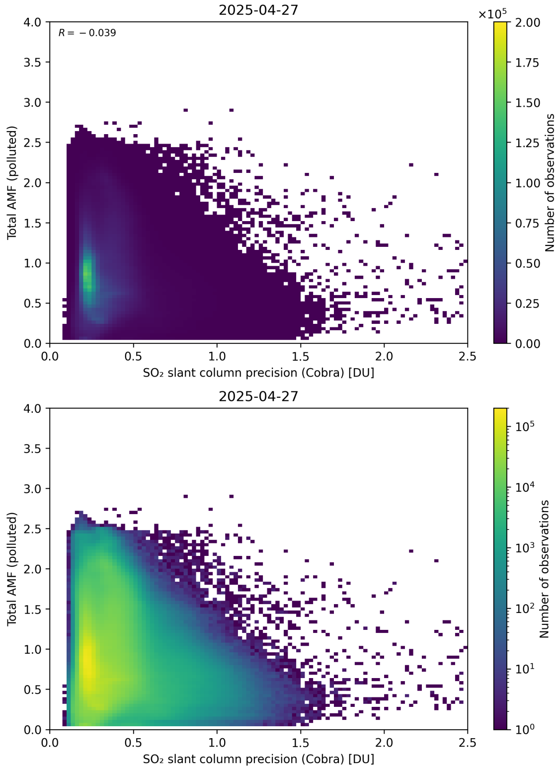
Figure 213: Scatter density plot of “SO 2 slant column precision (Cobra)” against “Total AMF (polluted)” for 2025-04-26 to 2025-04-28.
