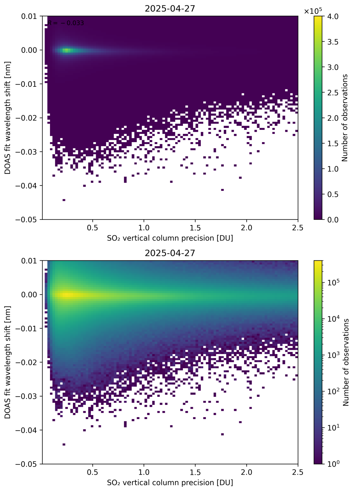
Figure 332: Scatter density plot of “SO 2 vertical column precision” against “DOAS fit wavelength shift” for 2025-04-26 to 2025-04-28.
