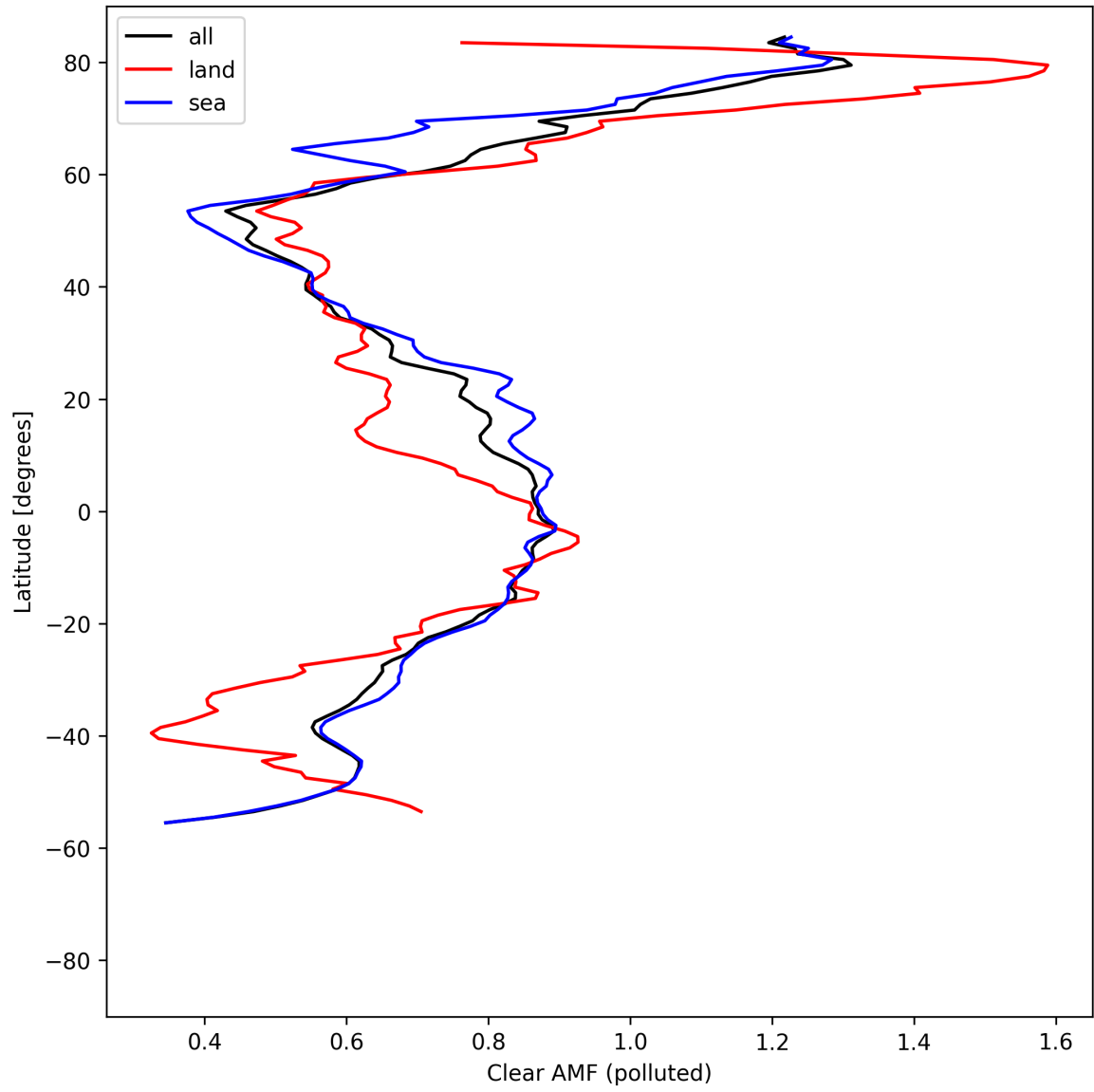
Figure 55: Zonal average of “Clear AMF (polluted)” for 2025-04-26 to 2025-04-28.
