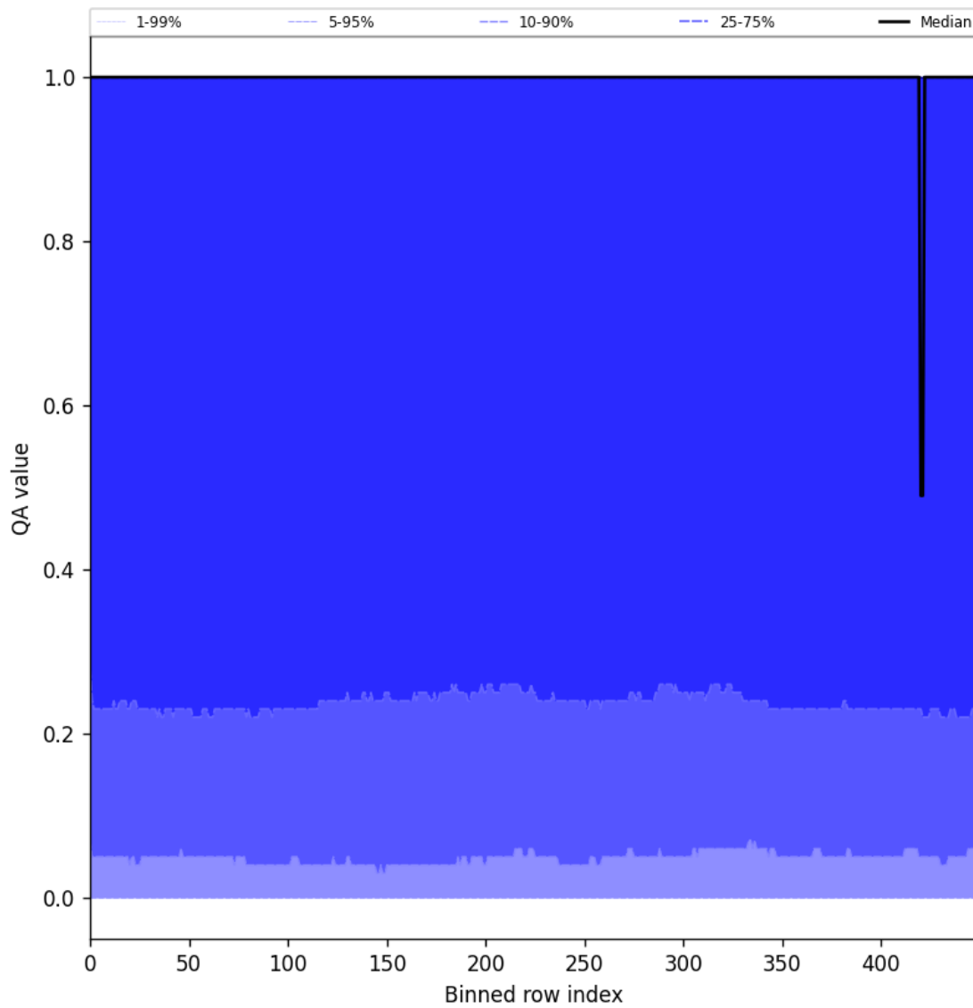
Figure 83: Along track statistics of “QA value” for 2025-04-26 to 2025-04-28
