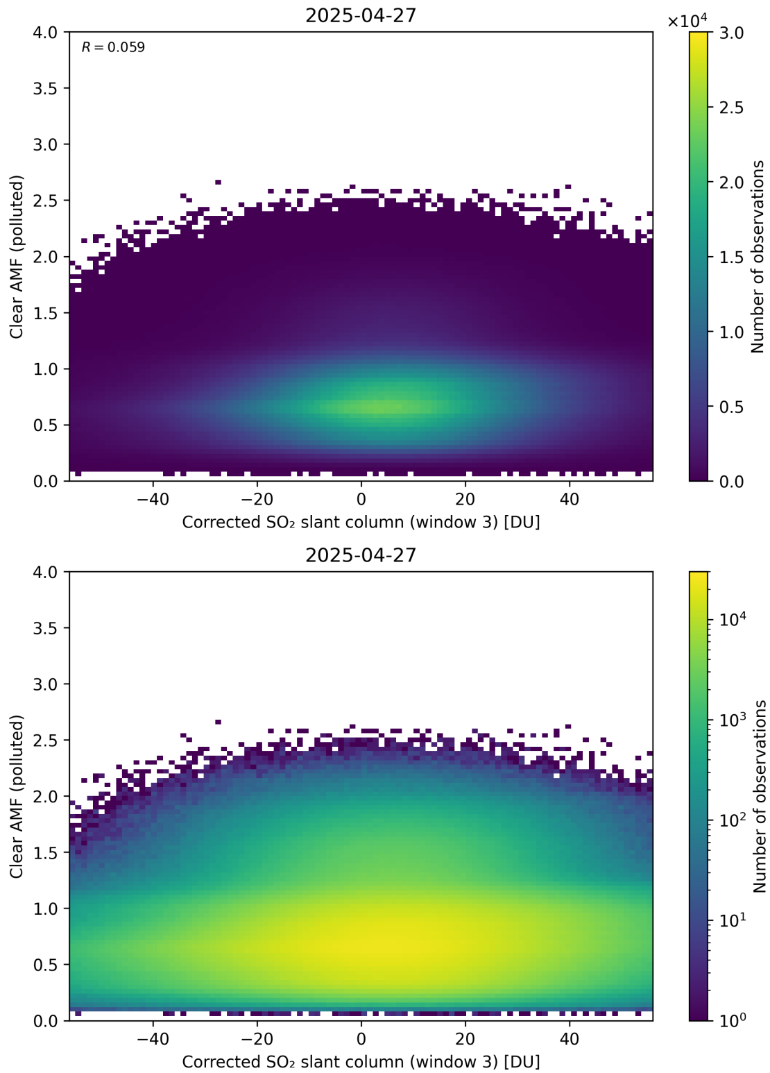
Figure 259: Scatter density plot of “Corrected SO 2 slant column (window 3)” against “Clear AMF (polluted)” for 2025-04-26 to 2025-04-28.
