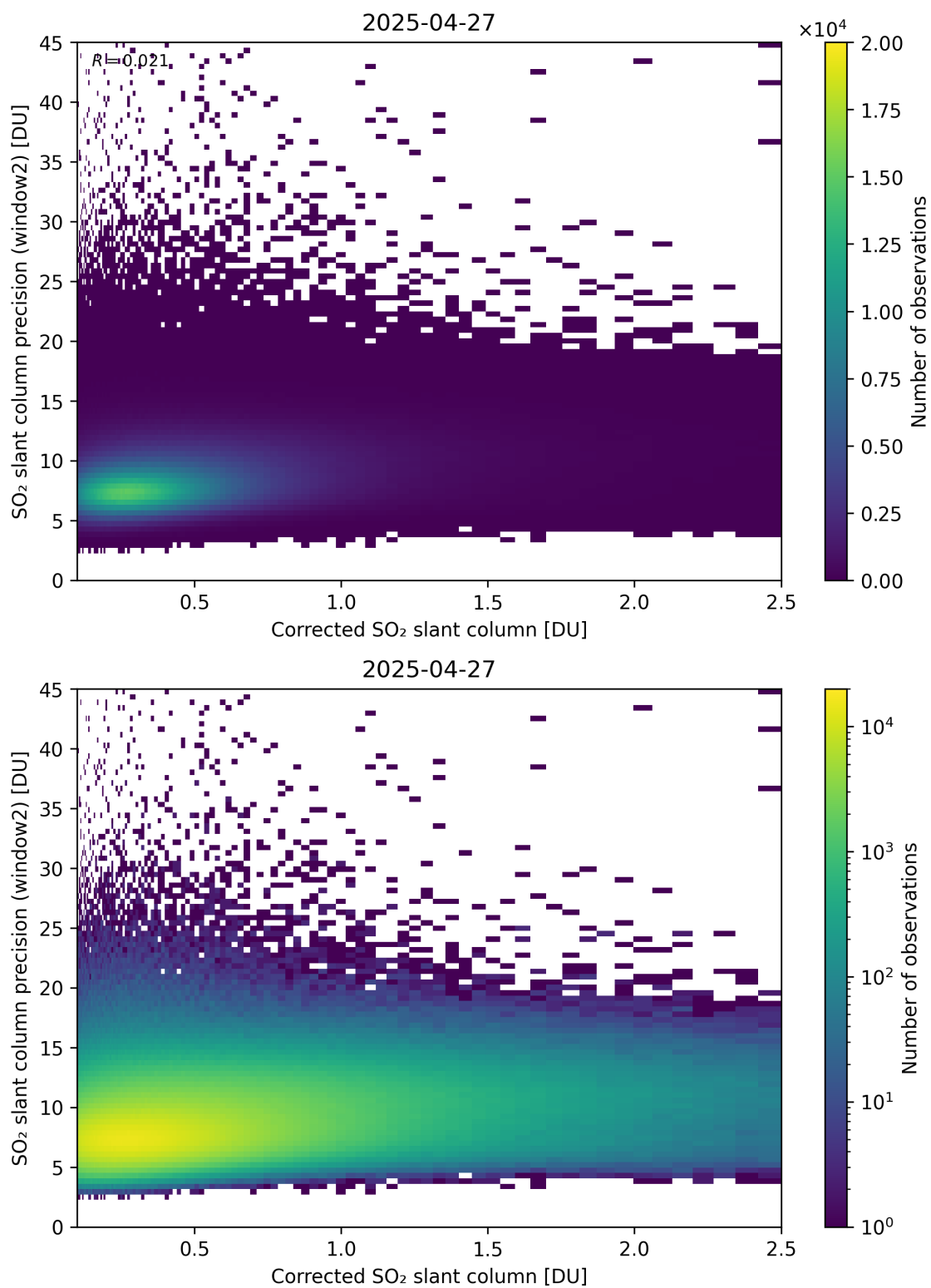
Figure 239: Scatter density plot of “Corrected SO 2 slant column” against “SO 2 slant column precision (window2)” for 2025-04-26 to 2025-04-28.
