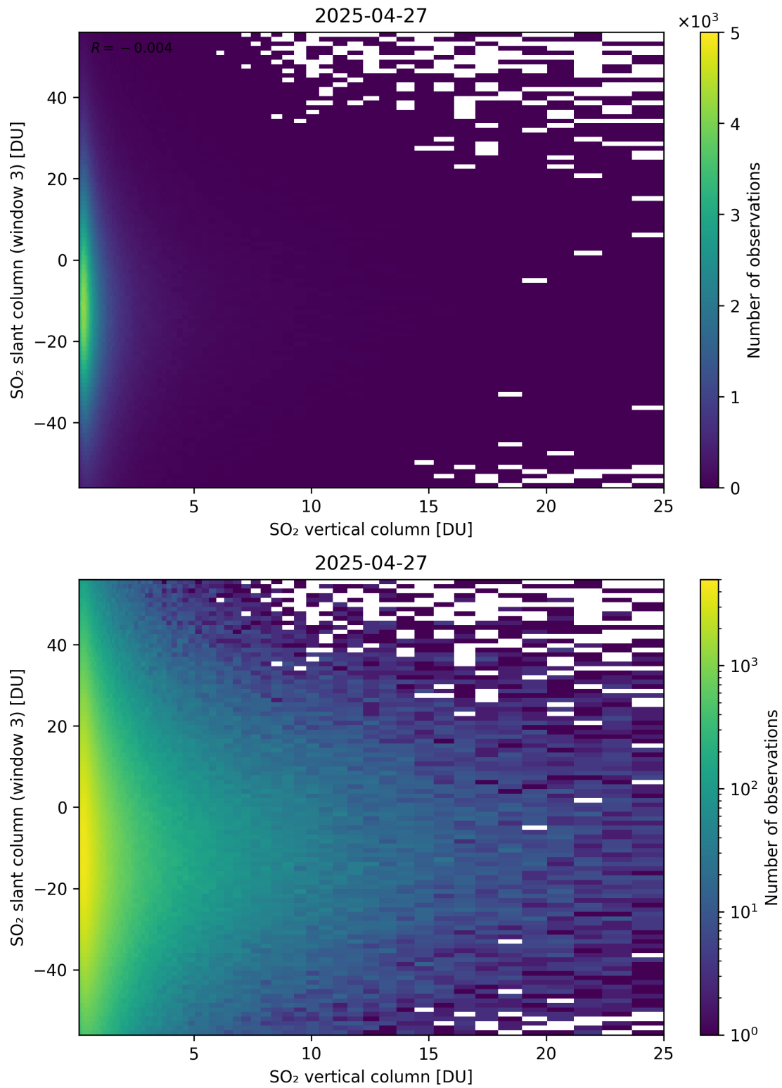
Figure 357: Scatter density plot of “SO 2 vertical column” against “SO 2 slant column (window 3)” for 2025-04-26 to 2025-04-28.
