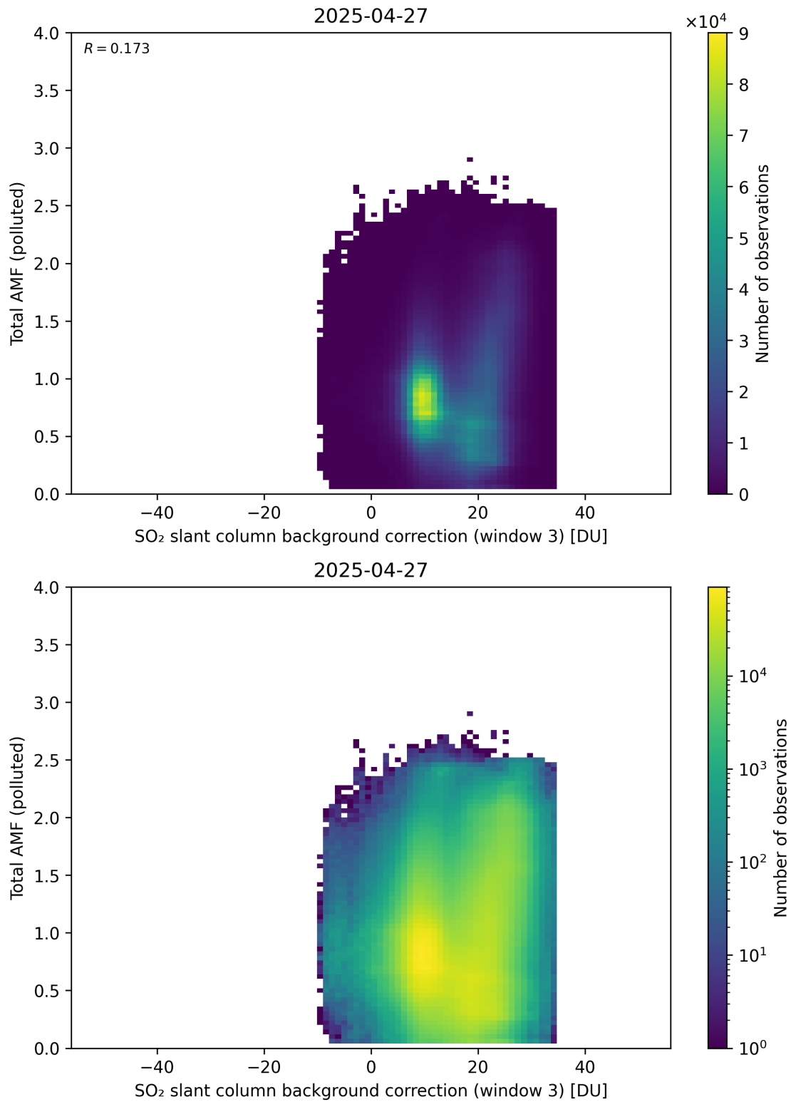
Figure 136: Scatter density plot of “SO 2 slant column background correction (window 3)” against “Total AMF (polluted)” for 2025-04-26 to 2025-04-28.
