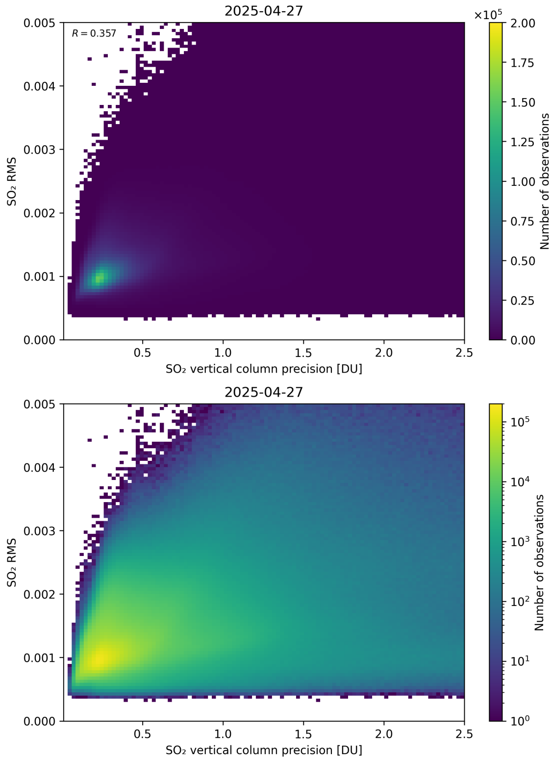
Figure 334: Scatter density plot of “SO 2 vertical column precision” against “SO 2 RMS” for 2025-04-26 to 2025-04-28.
