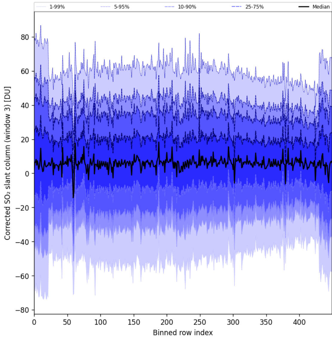
Figure 99: Along track statistics of “Corrected SO 2 slant column (window 3)” for 2025-04-26 to 2025-04-28
