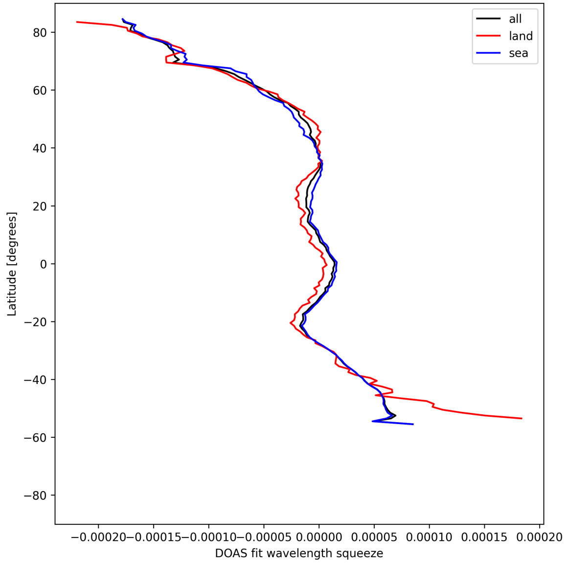
Figure 51: Zonal average of “DOAS fit wavelength squeeze” for 2025-04-26 to 2025-04-28.
