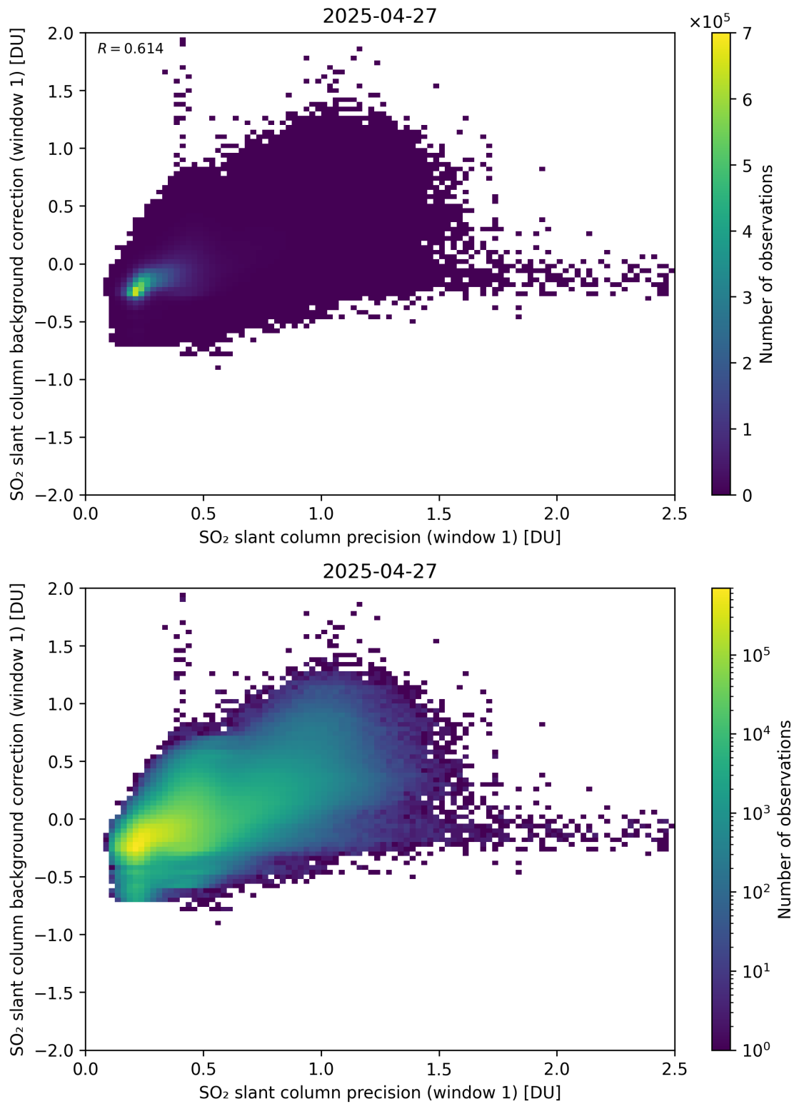
Figure 268: Scatter density plot of “SO 2 slant column precision (window 1)” against “SO 2 slant column background correction (window 1)” for 2025-04-26 to 2025-04-28.
