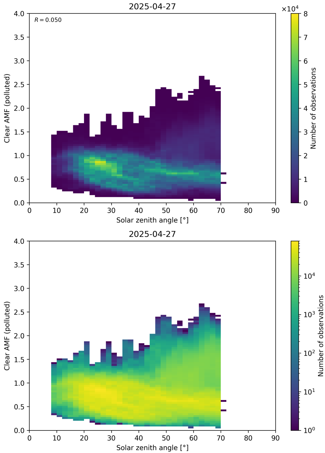
Figure 178: Scatter density plot of “Solar zenith angle” against “Clear AMF (polluted)” for 2025-04-26 to 2025-04-28.
