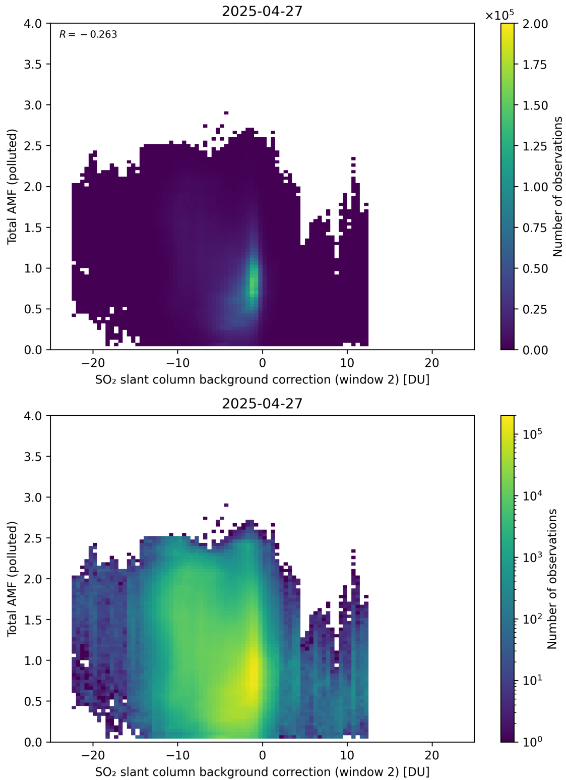
Figure 130: Scatter density plot of “SO 2 slant column background correction (window 2)” against “Total AMF (polluted)” for 2025-04-26 to 2025-04-28.
