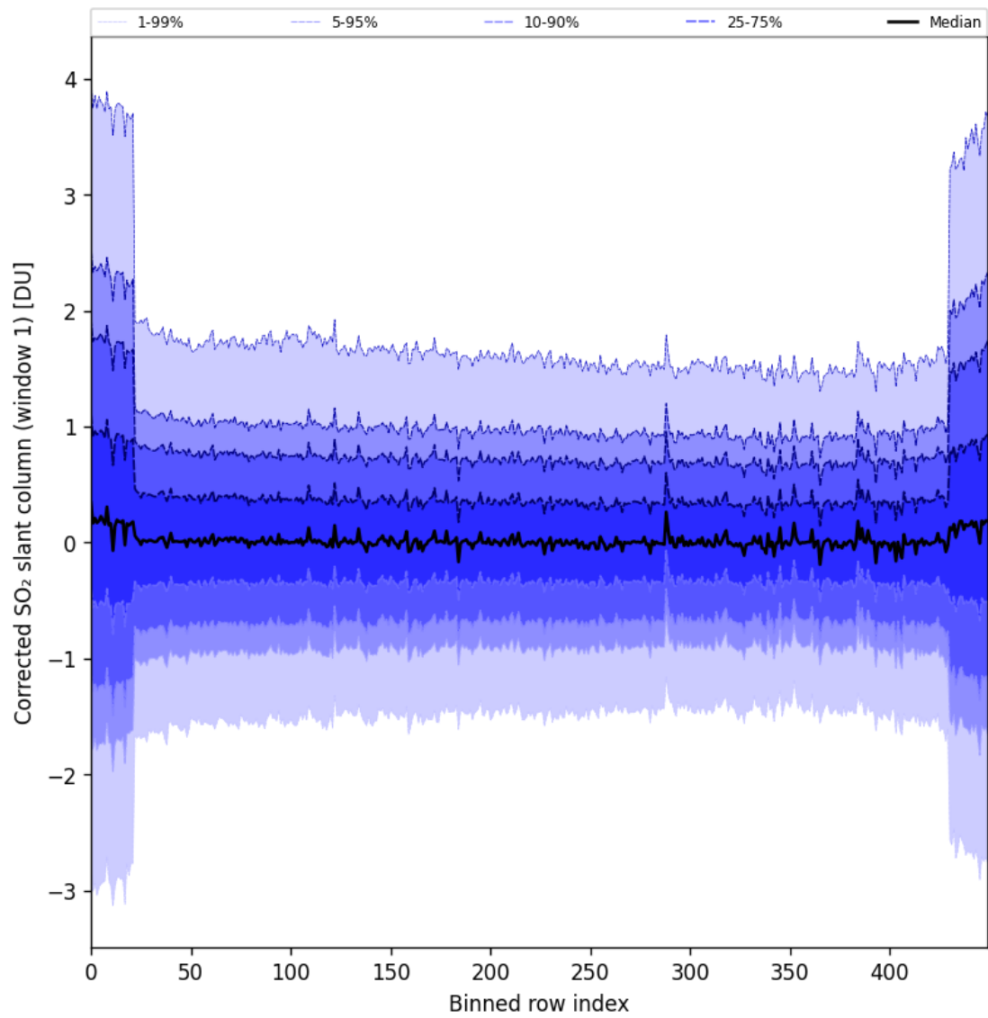
Figure 91: Along track statistics of “Corrected SO 2 slant column (window 1)” for 2025-04-26 to 2025-04-28
