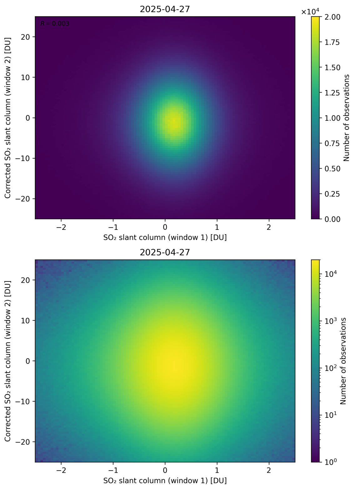
Figure 283: Scatter density plot of “SO 2 slant column (window 1)” against “Corrected SO 2 slant column (window 2)” for 2025-04-26 to 2025-04-28.
