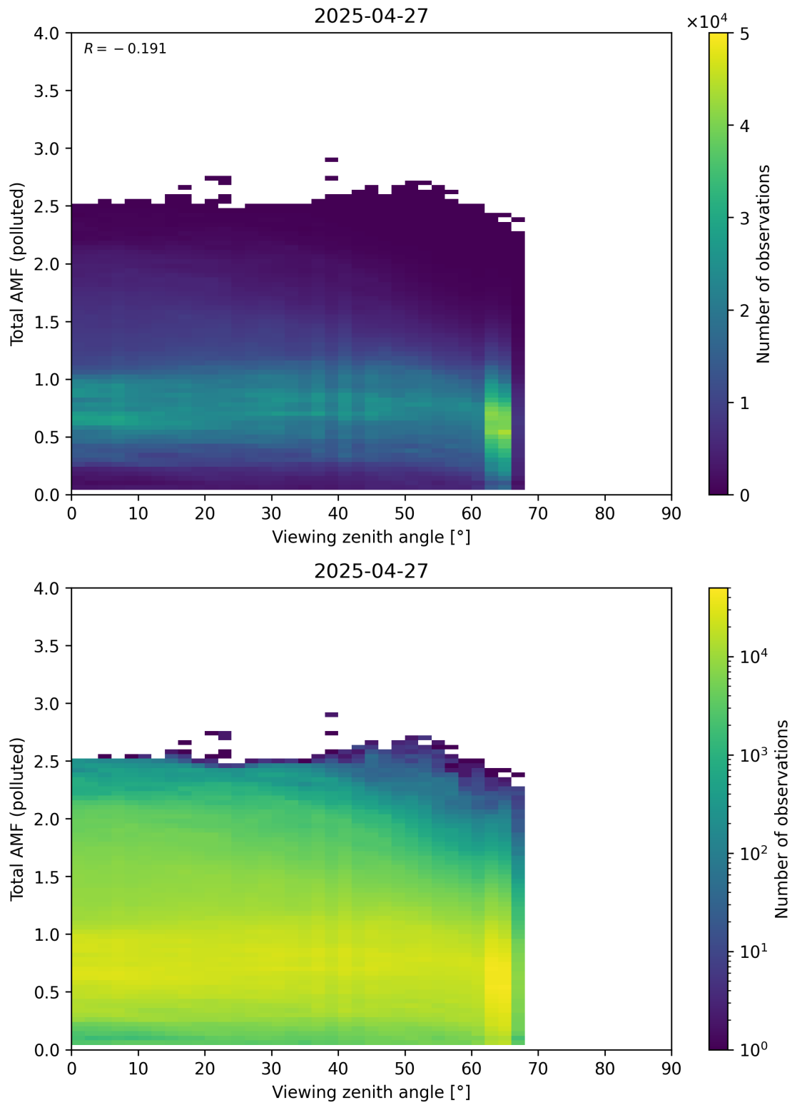
Figure 381: Scatter density plot of “Viewing zenith angle” against “Total AMF (polluted)” for 2025-04-26 to 2025-04-28.
