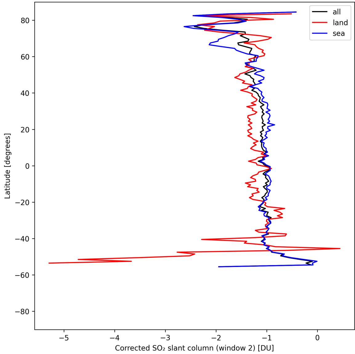
Figure 43: Zonal average of “Corrected SO 2 slant column (window 2)” for 2025-04-26 to 2025-04-28.
