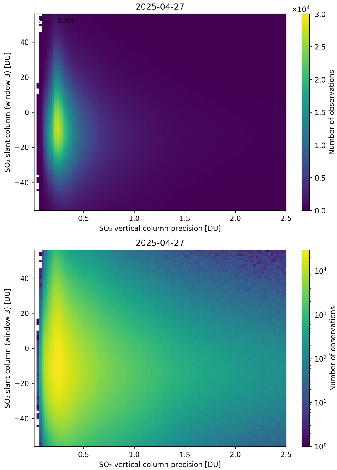
Figure 344: Scatter density plot of “SO 2 vertical column precision” against “SO 2 slant column (window 3)” for 2025-04-26 to 2025-04-28.
