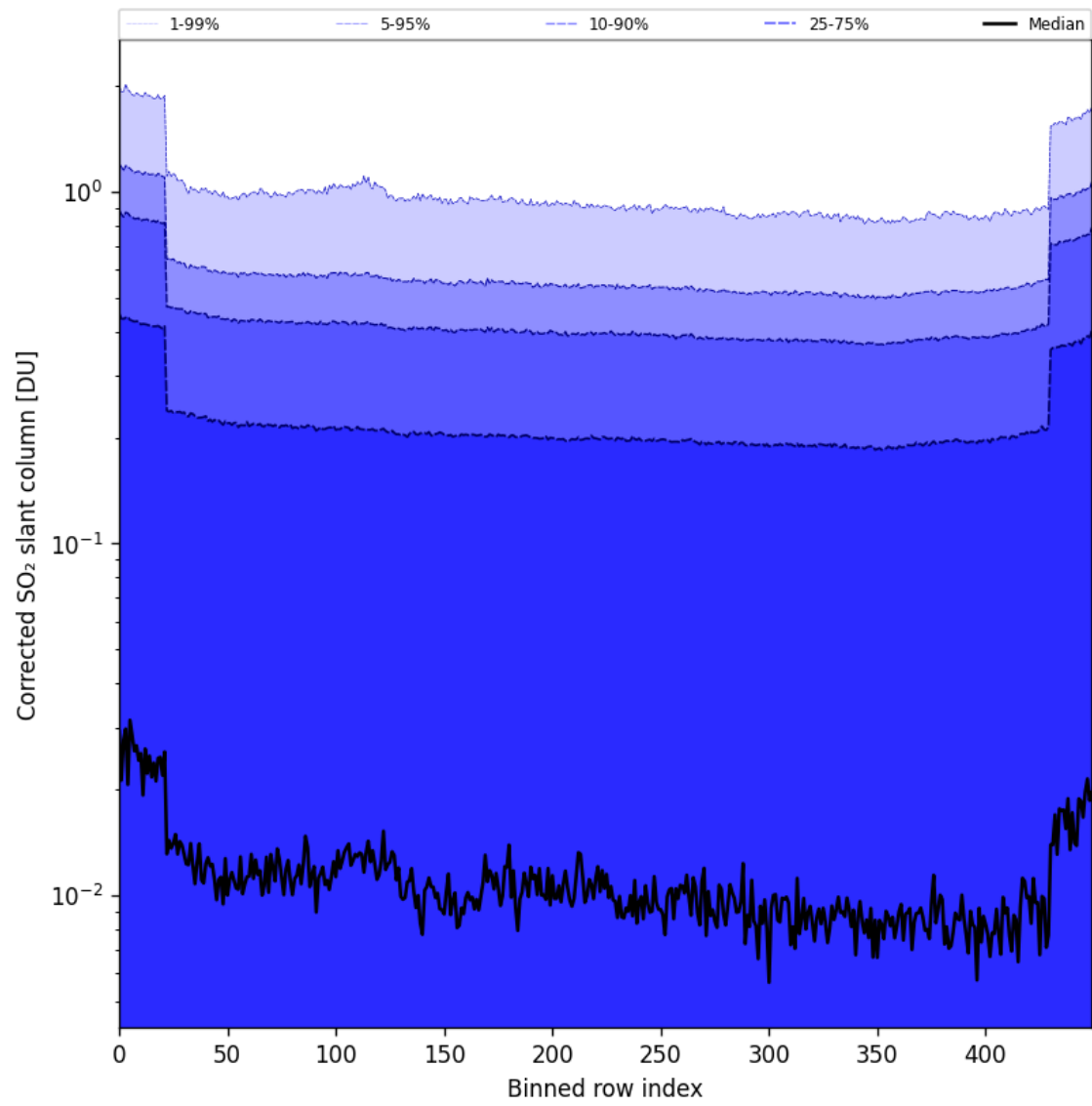
Figure 86: Along track statistics of “Corrected SO 2 slant column” for 2025-04-26 to 2025-04-28
