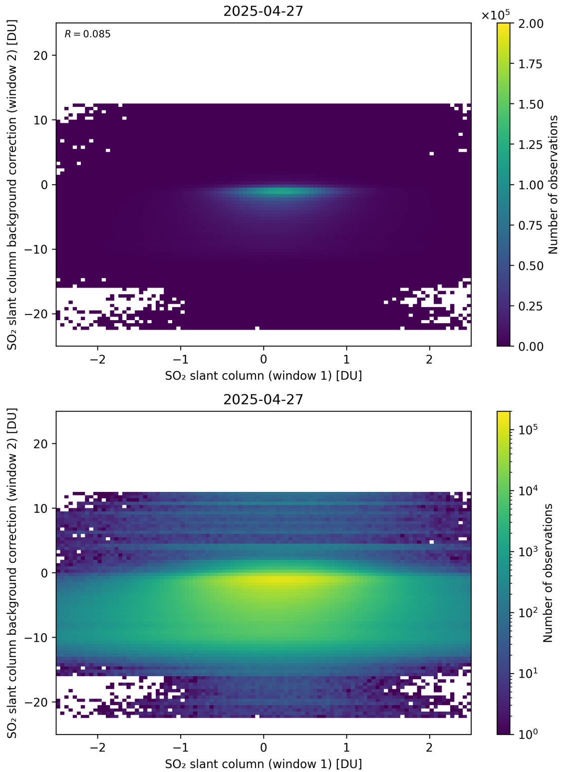
Figure 263: Scatter density plot of “SO 2 slant column (window 1)” against “SO 2 slant column background correction (window 2)” for 2025-04-26 to 2025-04-28.
