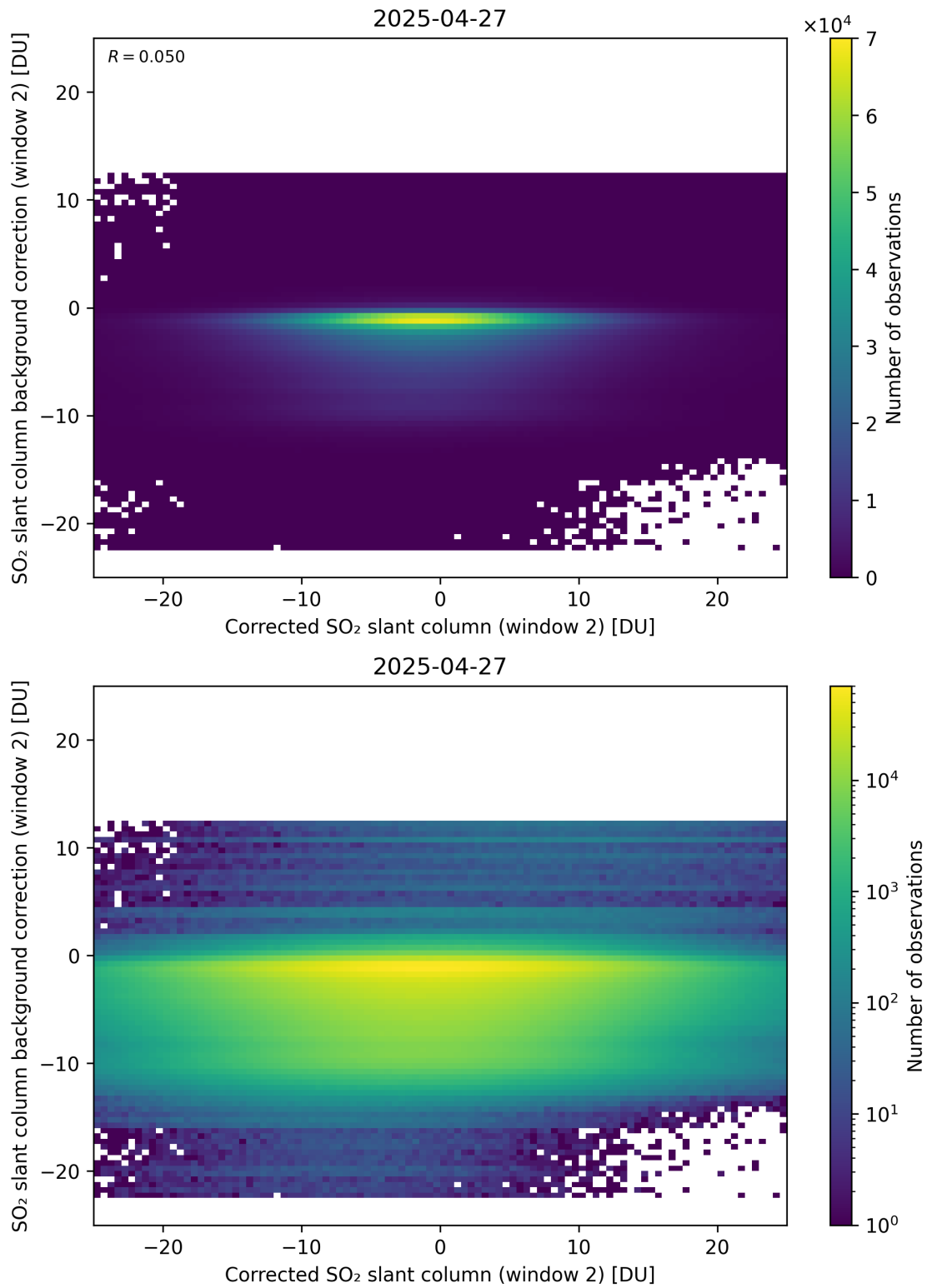
Figure 244: Scatter density plot of “Corrected SO 2 slant column (window 2)” against “SO 2 slant column background correction (window 2)” for 2025-04-26 to 2025-04-28.
