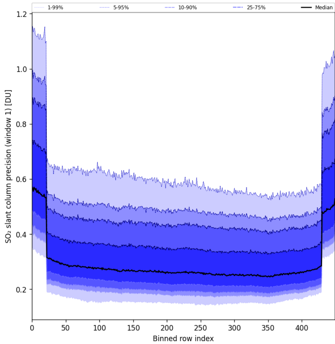
Figure 90: Along track statistics of “SO 2 slant column precision (window 1)” for 2025-04-26 to 2025-04-28
