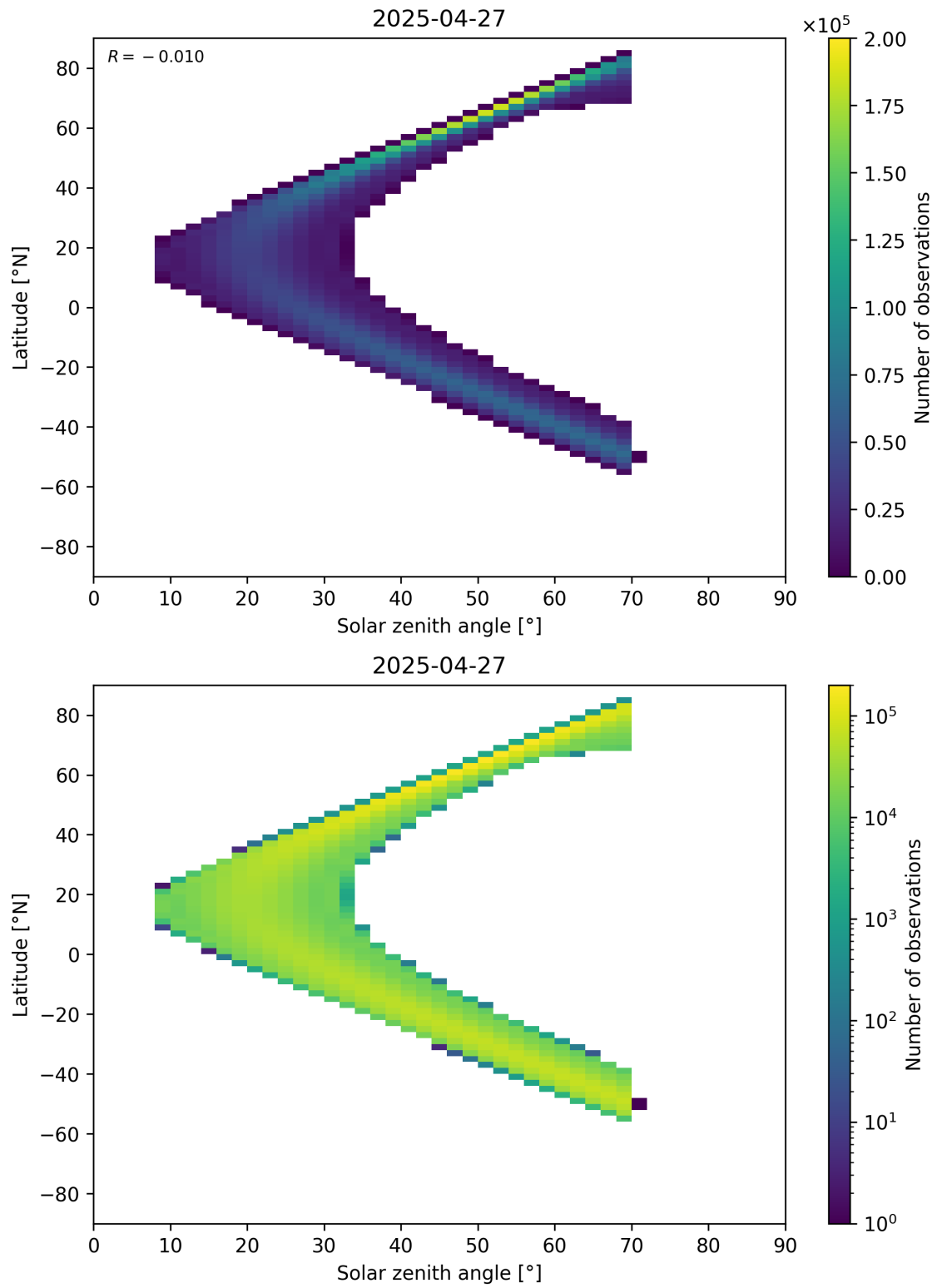
Figure 177: Scatter density plot of “Solar zenith angle” against “Latitude” for 2025-04-26 to 2025-04-28.
