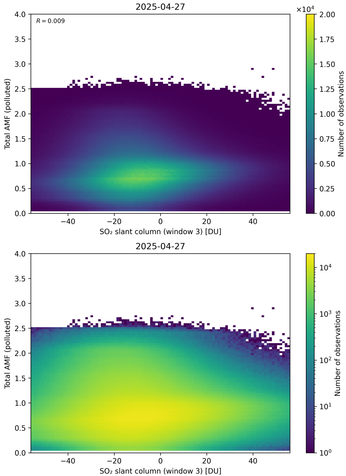
Figure 318: Scatter density plot of “SO 2 slant column (window 3)” against “Total AMF (polluted)” for 2025-04-26 to 2025-04-28.
