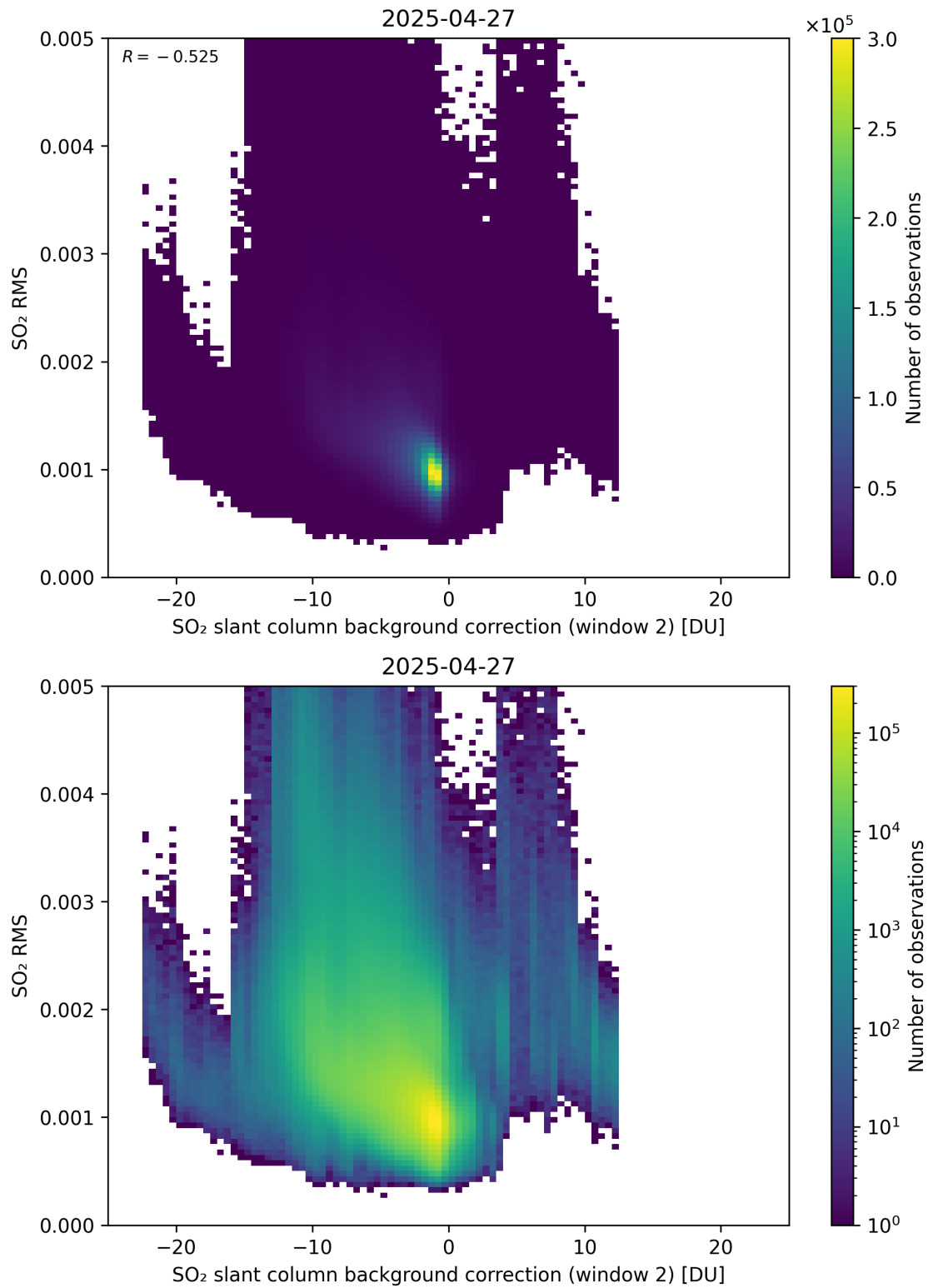
Figure 125: Scatter density plot of “SO 2 slant column background correction (window 2)” against “SO 2 RMS” for 2025-04-26 to 2025-04-28.
