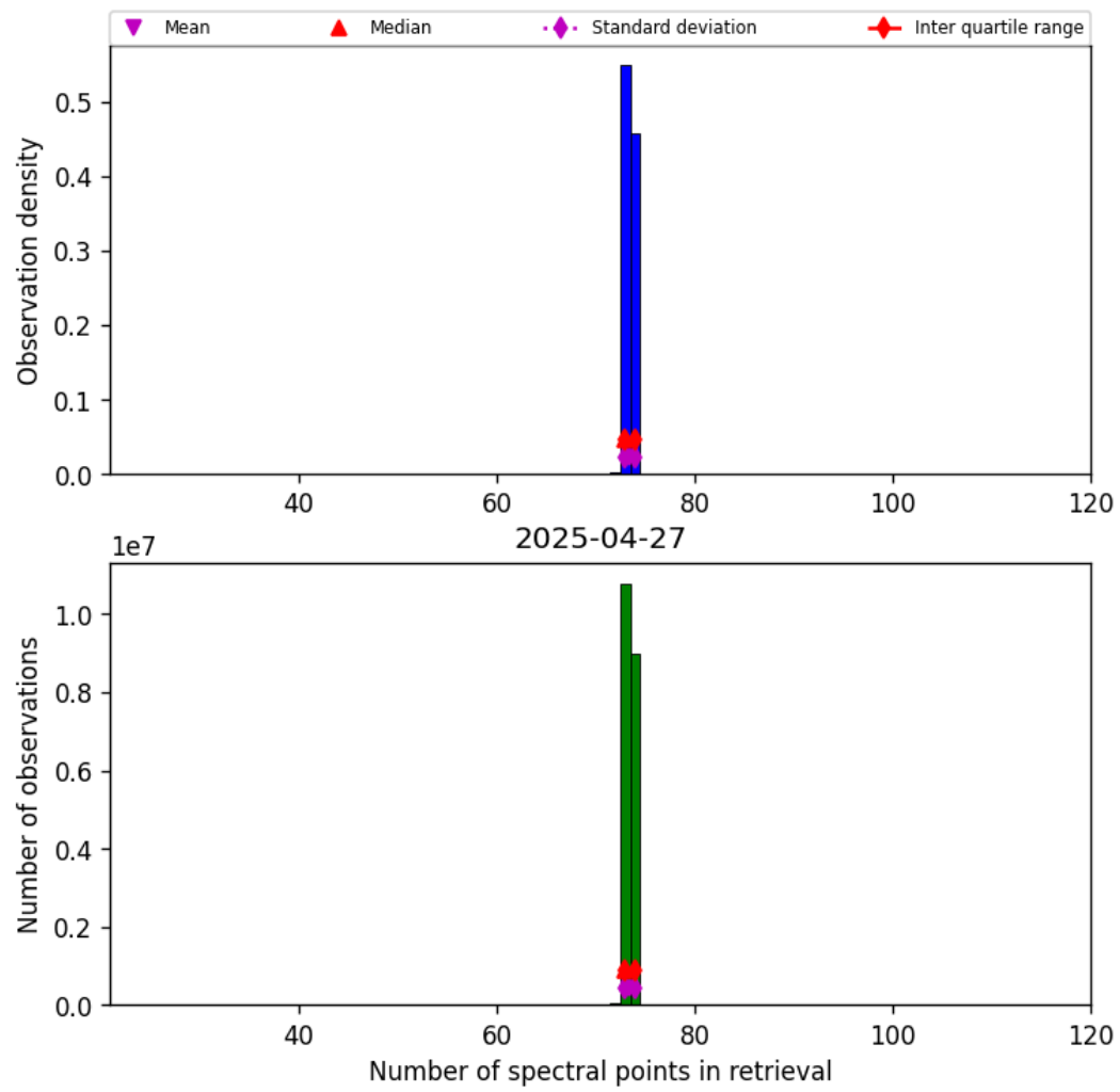
Figure 82: Histogram of “Number of spectral points in retrieval” for 2025-04-26 to 2025-04-28
