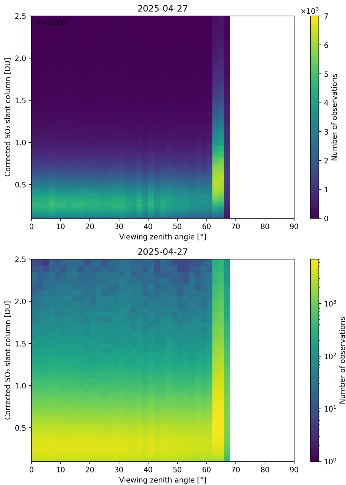
Figure 373: Scatter density plot of “Viewing zenith angle” against “Corrected SO 2 slant column” for 2025-04-26 to 2025-04-28.
