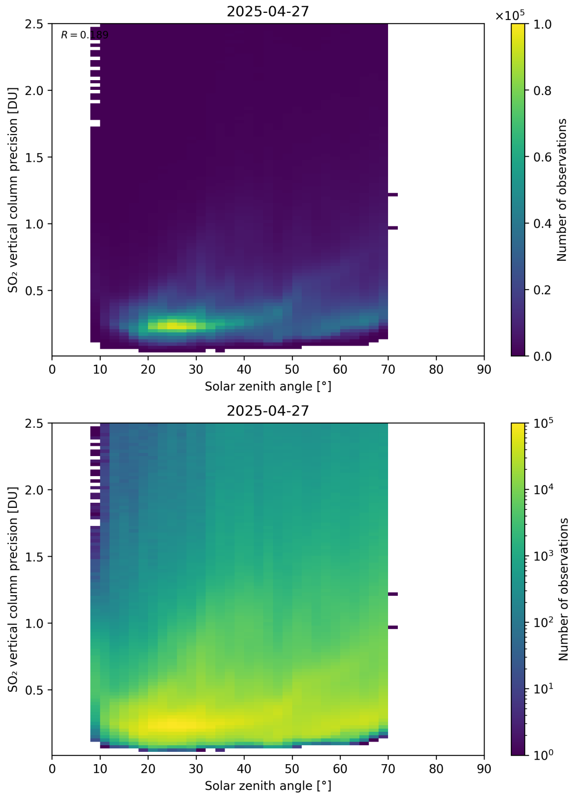
Figure 192: Scatter density plot of “Solar zenith angle” against “SO 2 vertical column precision” for 2025-04-26 to 2025-04-28.
