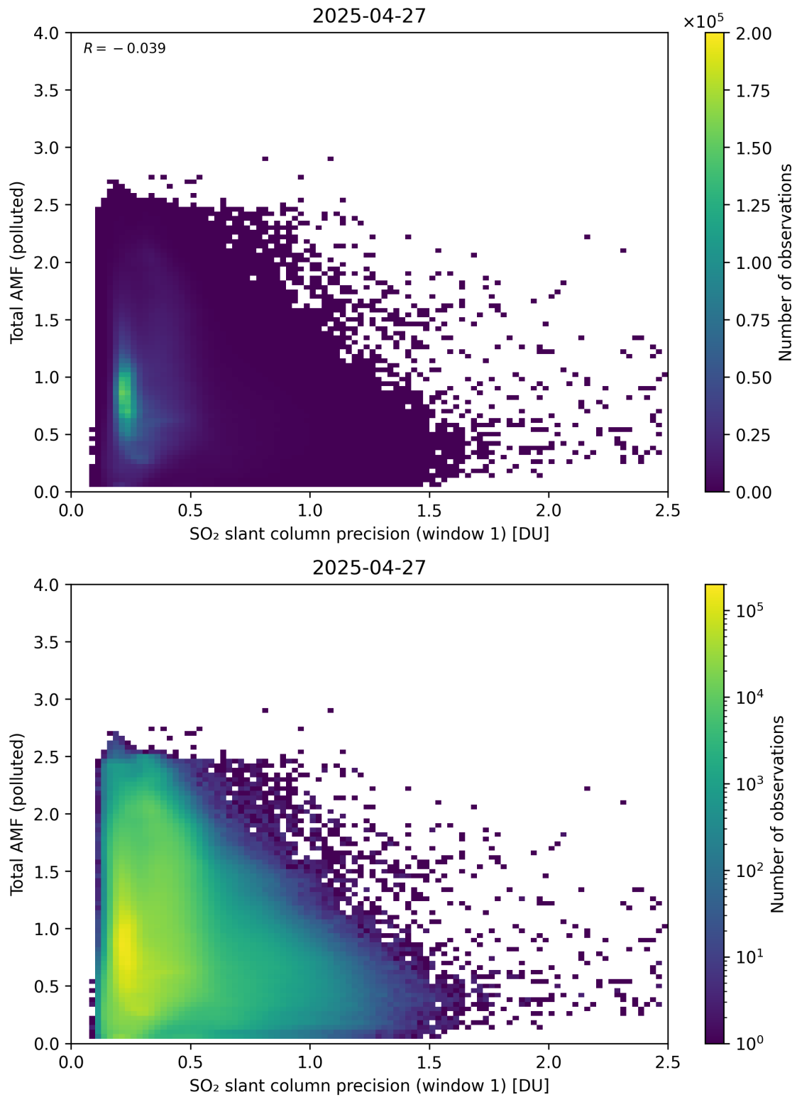
Figure 280: Scatter density plot of “SO 2 slant column precision (window 1)” against “Total AMF (polluted)” for 2025-04-26 to 2025-04-28.
