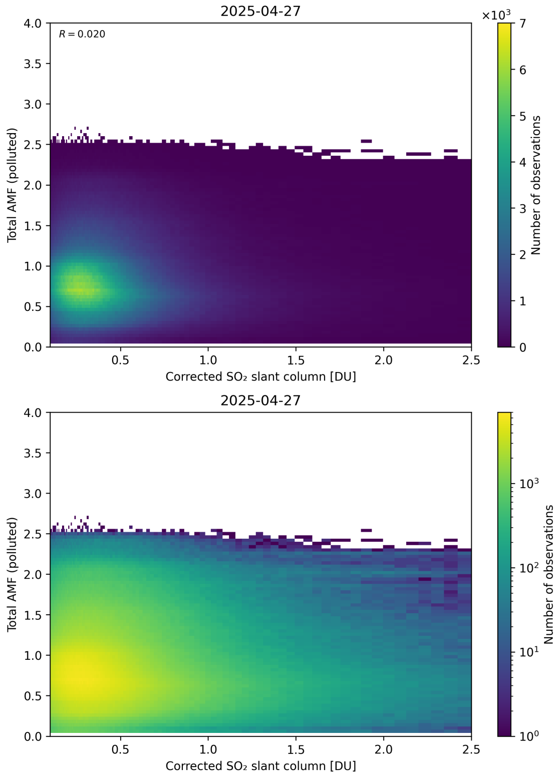
Figure 242: Scatter density plot of “Corrected SO 2 slant column” against “Total AMF (polluted)” for 2025-04-26 to 2025-04-28.
