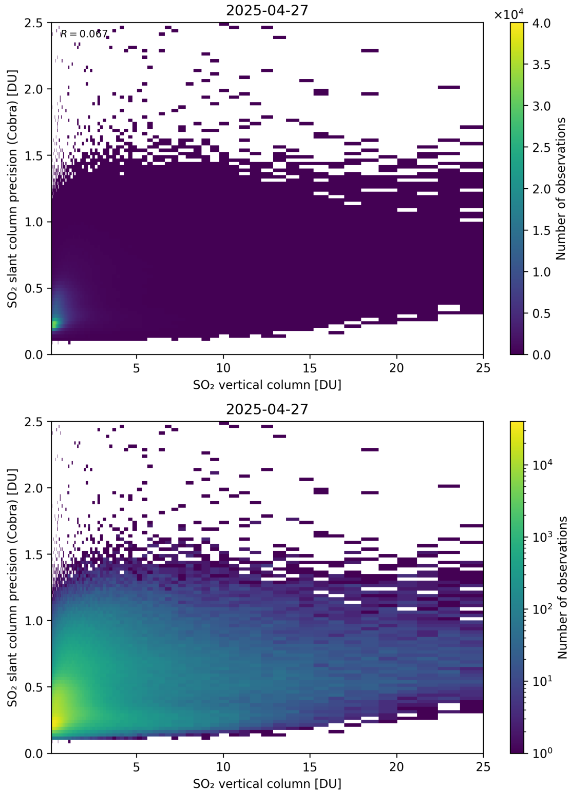
Figure 350: Scatter density plot of “SO 2 vertical column” against “SO 2 slant column precision (Cobra)” for 2025-04-26 to 2025-04-28.
