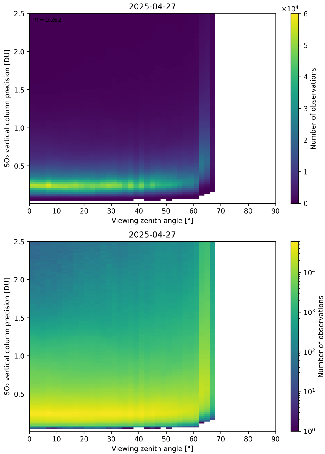
Figure 384: Scatter density plot of “Viewing zenith angle” against “SO 2 vertical column precision” for 2025-04-26 to 2025-04-28.
