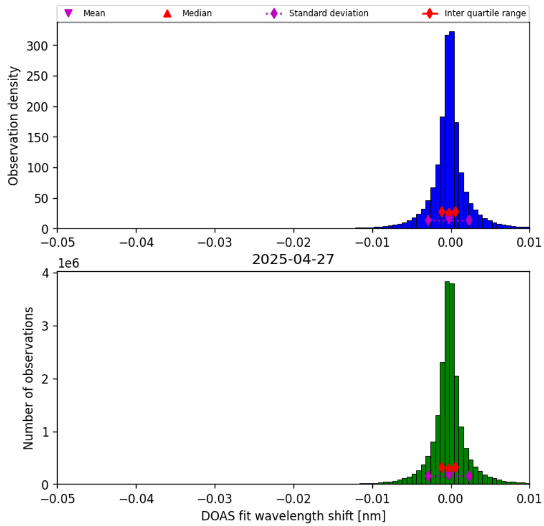
Figure 76: Histogram of “DOAS fit wavelength shift” for 2025-04-26 to 2025-04-28
