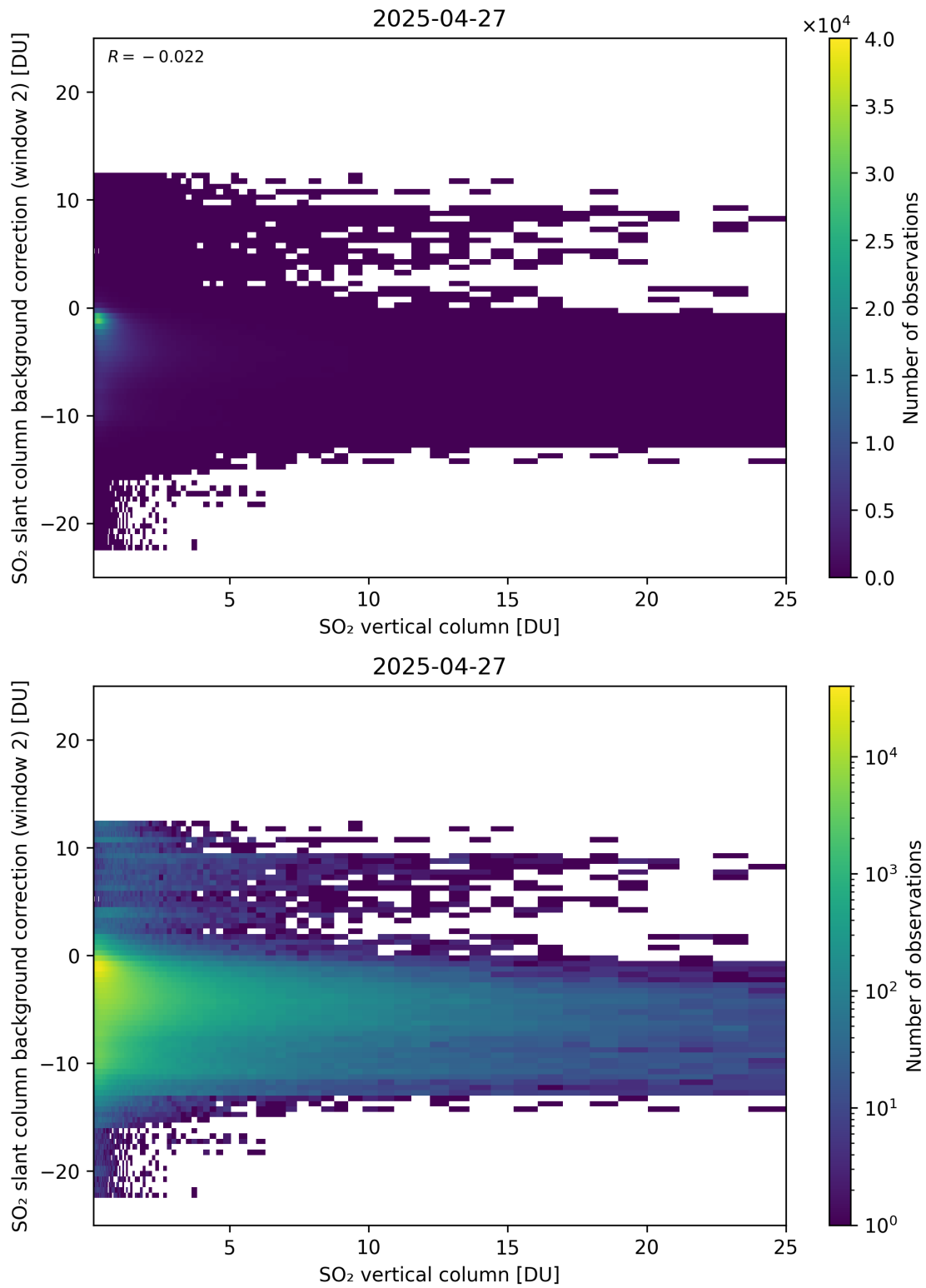
Figure 324: Scatter density plot of “SO 2 vertical column” against “SO 2 slant column background correction (window 2)” for 2025-04-26 to 2025-04-28.
