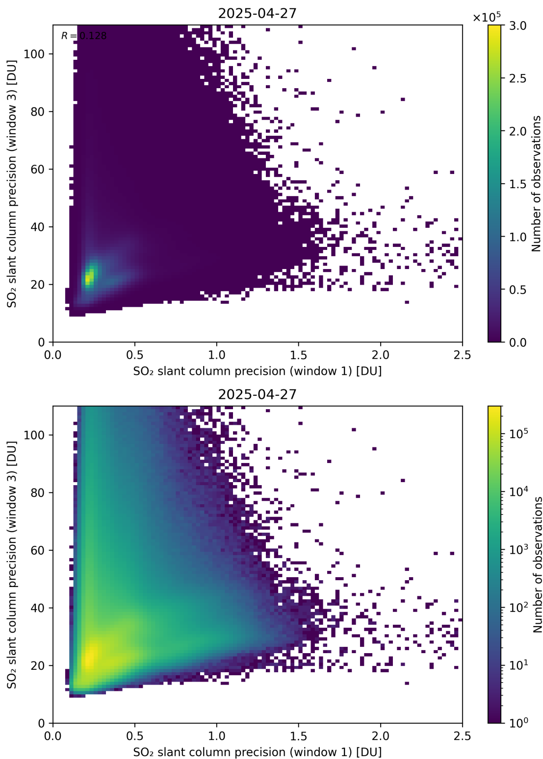
Figure 279: Scatter density plot of “SO 2 slant column precision (window 1)” against “SO 2 slant column precision (window 3)” for 2025-04-26 to 2025-04-28.
