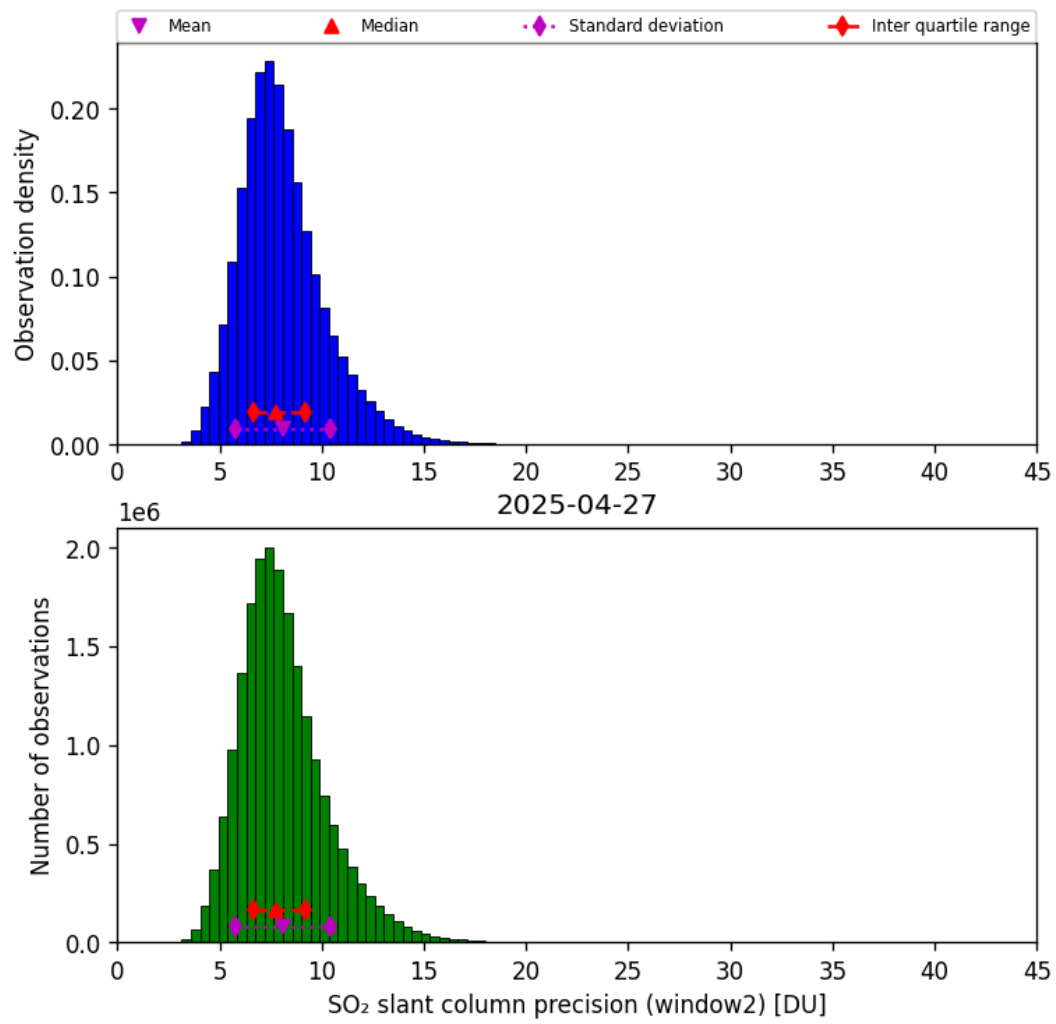
Figure 68: Histogram of “SO 2 slant column precision (window2)” for 2025-04-26 to 2025-04-28
