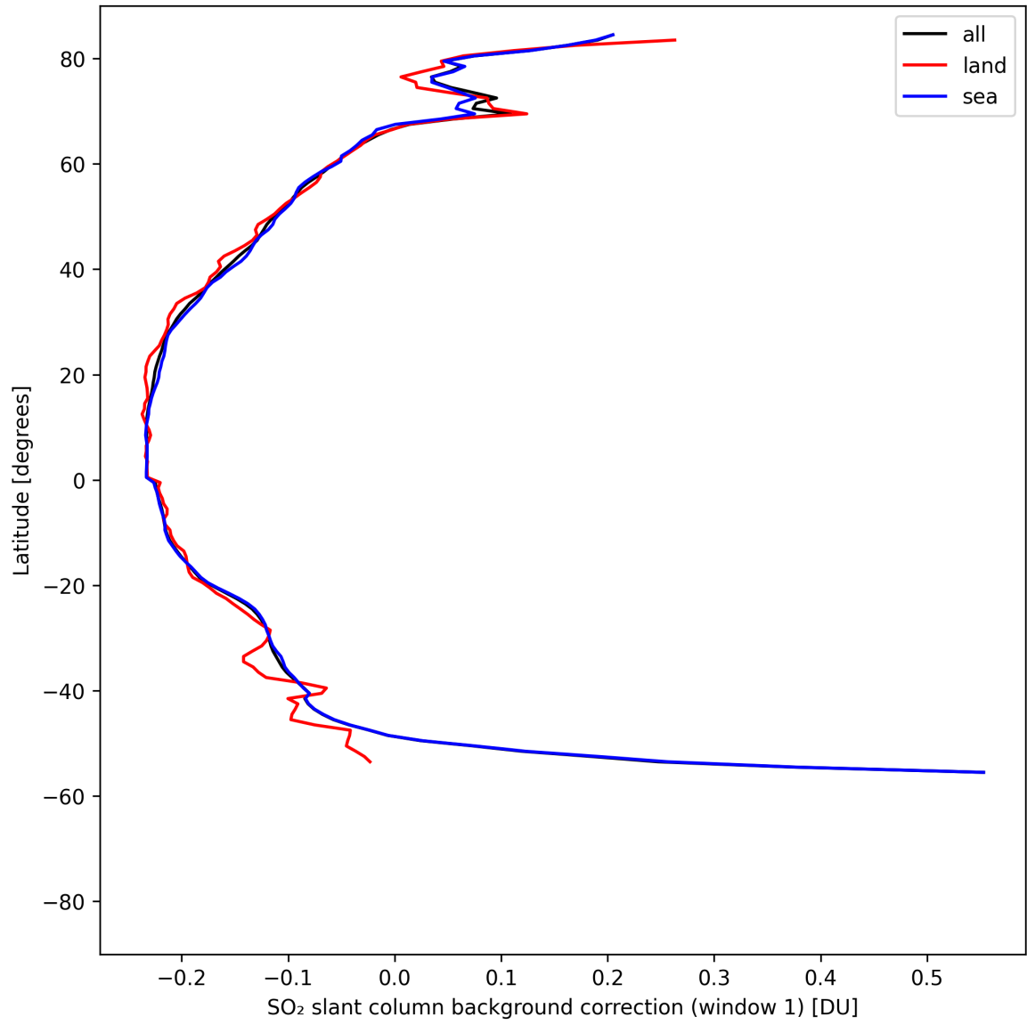
Figure 40: Zonal average of “SO 2 slant column background correction (window 1)” for 2025-04-26 to 2025-04-28.
