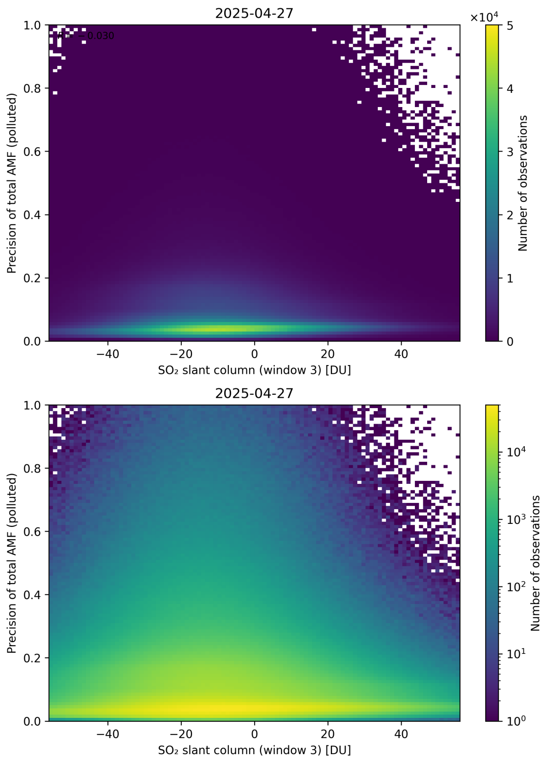
Figure 319: Scatter density plot of “SO 2 slant column (window 3)” against “Precision of total AMF (polluted)” for 2025-04-26 to 2025-04-28.
