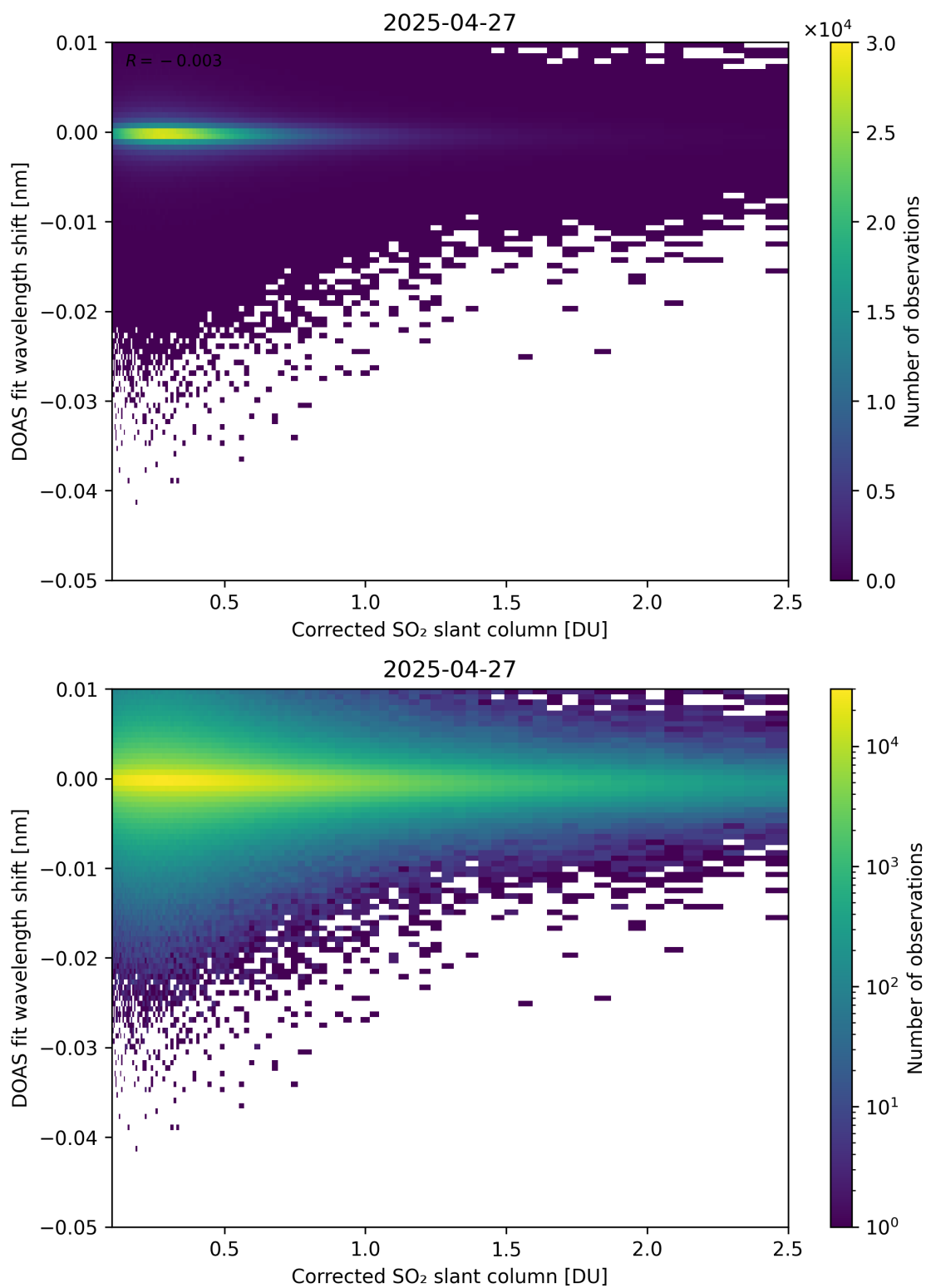
Figure 229: Scatter density plot of “Corrected SO 2 slant column” against “DOAS fit wavelength shift” for 2025-04-26 to 2025-04-28.
