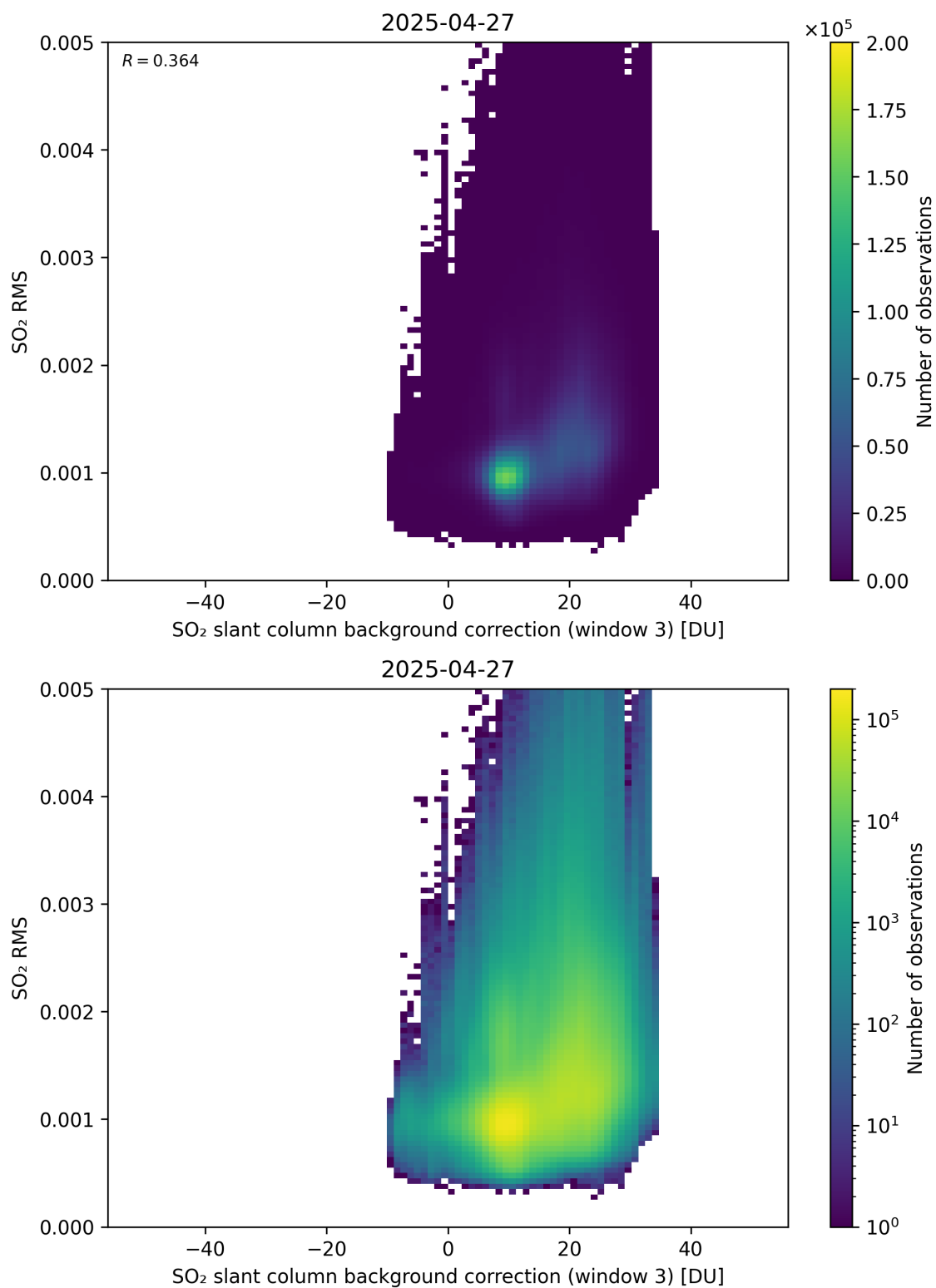
Figure 134: Scatter density plot of “SO 2 slant column background correction (window 3)” against “SO 2 RMS” for 2025-04-26 to 2025-04-28.
