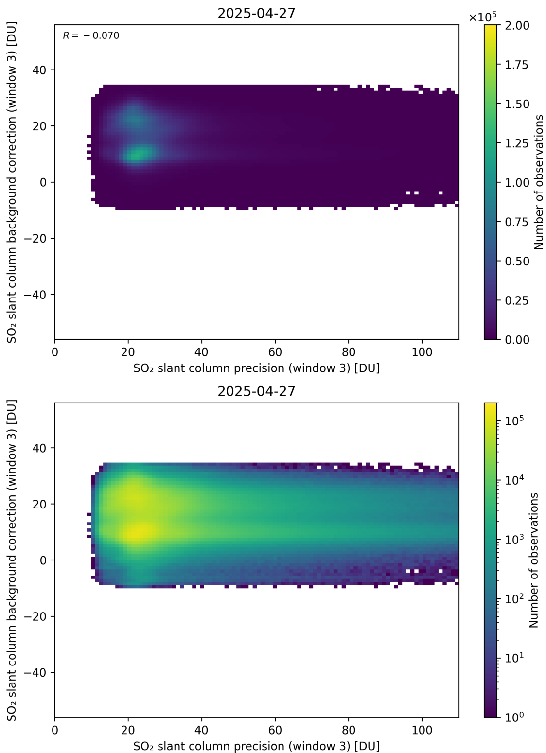
Figure 307: Scatter density plot of “SO 2 slant column precision (window 3)” against “SO 2 slant column background correction (window 3)” for 2025-04-26 to 2025-04-28.
