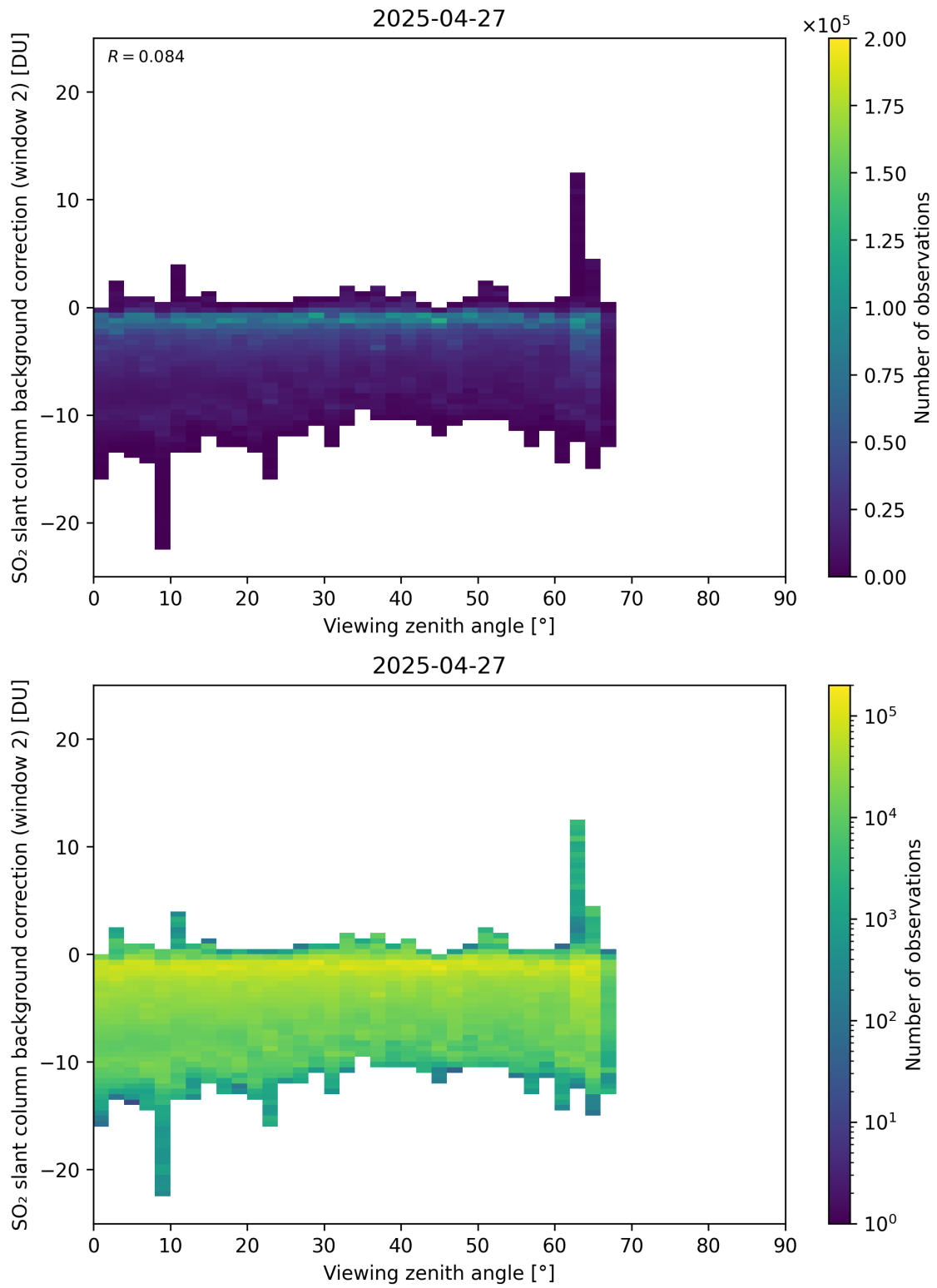
Figure 363: Scatter density plot of “Viewing zenith angle” against “SO 2 slant column background correction (window 2)” for 2025-04-26 to 2025-04-28.
