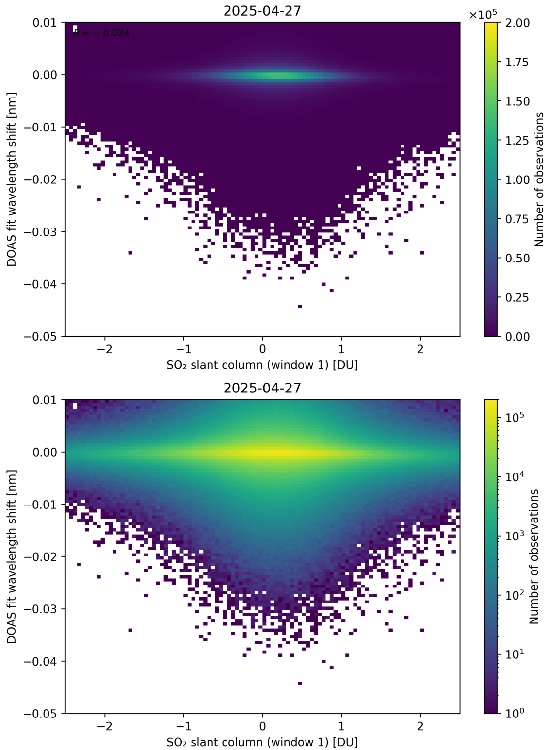
Figure 265: Scatter density plot of “SO 2 slant column (window 1)” against “DOAS fit wavelength shift” for 2025-04-26 to 2025-04-28.
