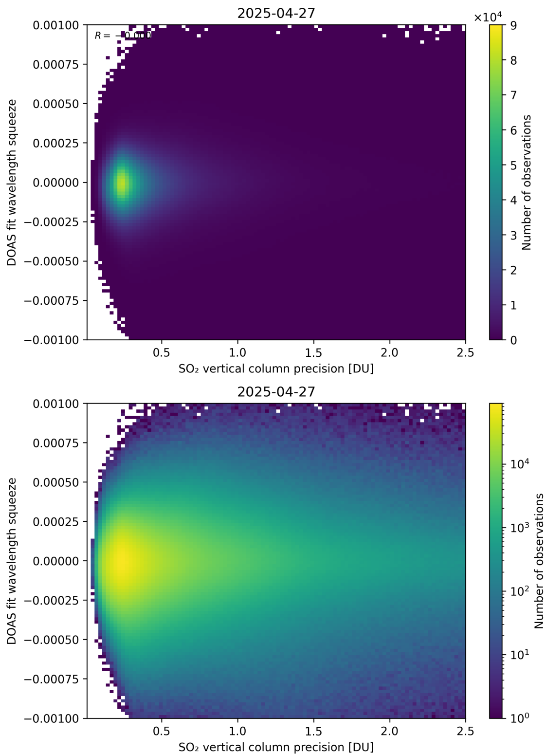
Figure 333: Scatter density plot of “SO 2 vertical column precision” against “DOAS fit wavelength squeeze” for 2025-04-26 to 2025-04-28.
