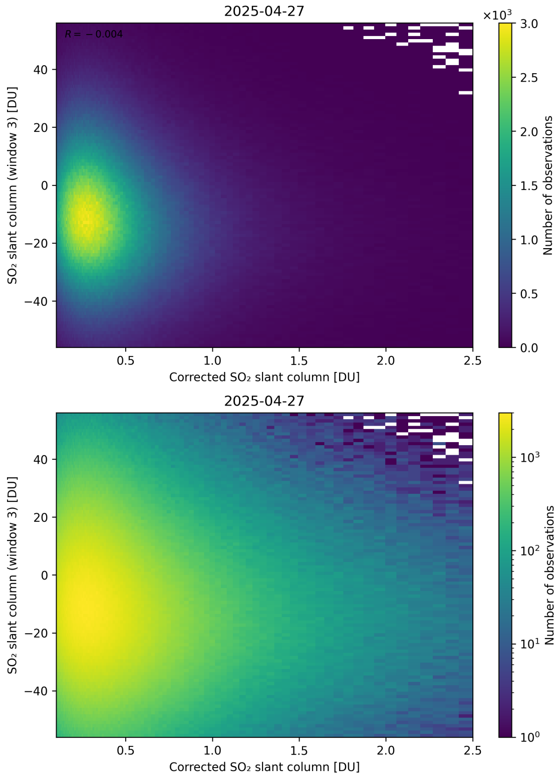
Figure 240: Scatter density plot of “Corrected SO 2 slant column” against “SO 2 slant column (window 3)” for 2025-04-26 to 2025-04-28.
