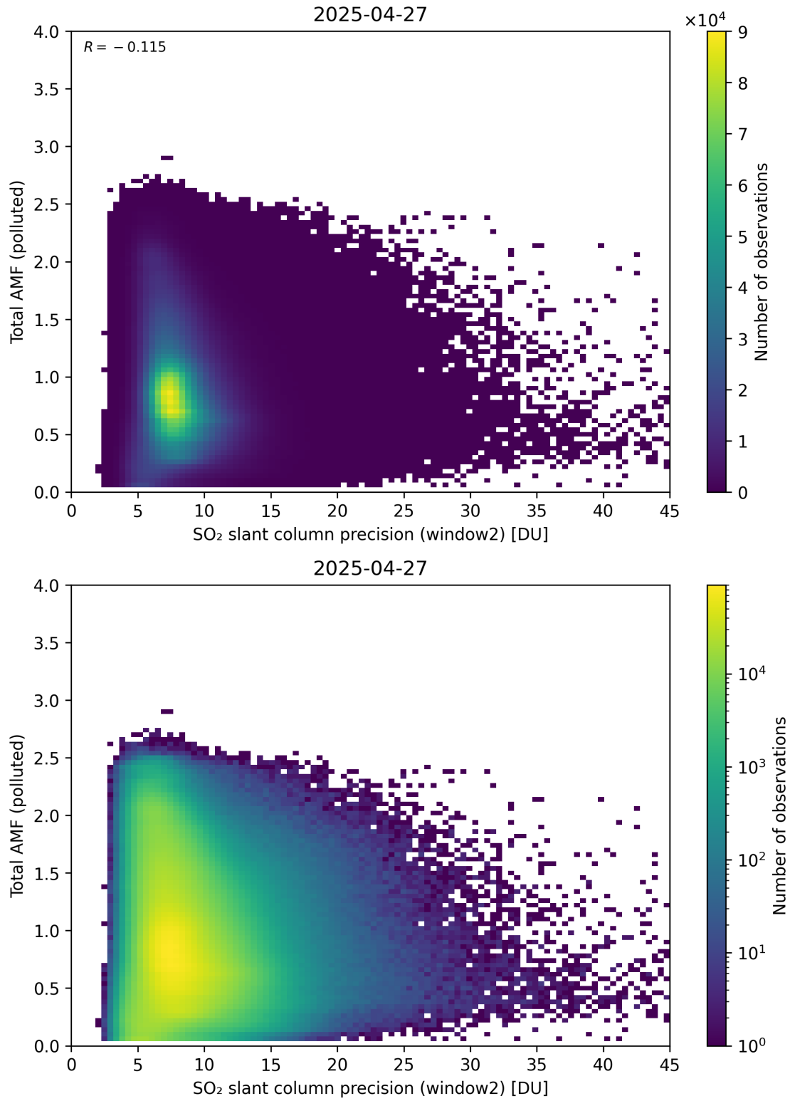
Figure 301: Scatter density plot of “SO 2 slant column precision (window2)” against “Total AMF (polluted)” for 2025-04-26 to 2025-04-28.
