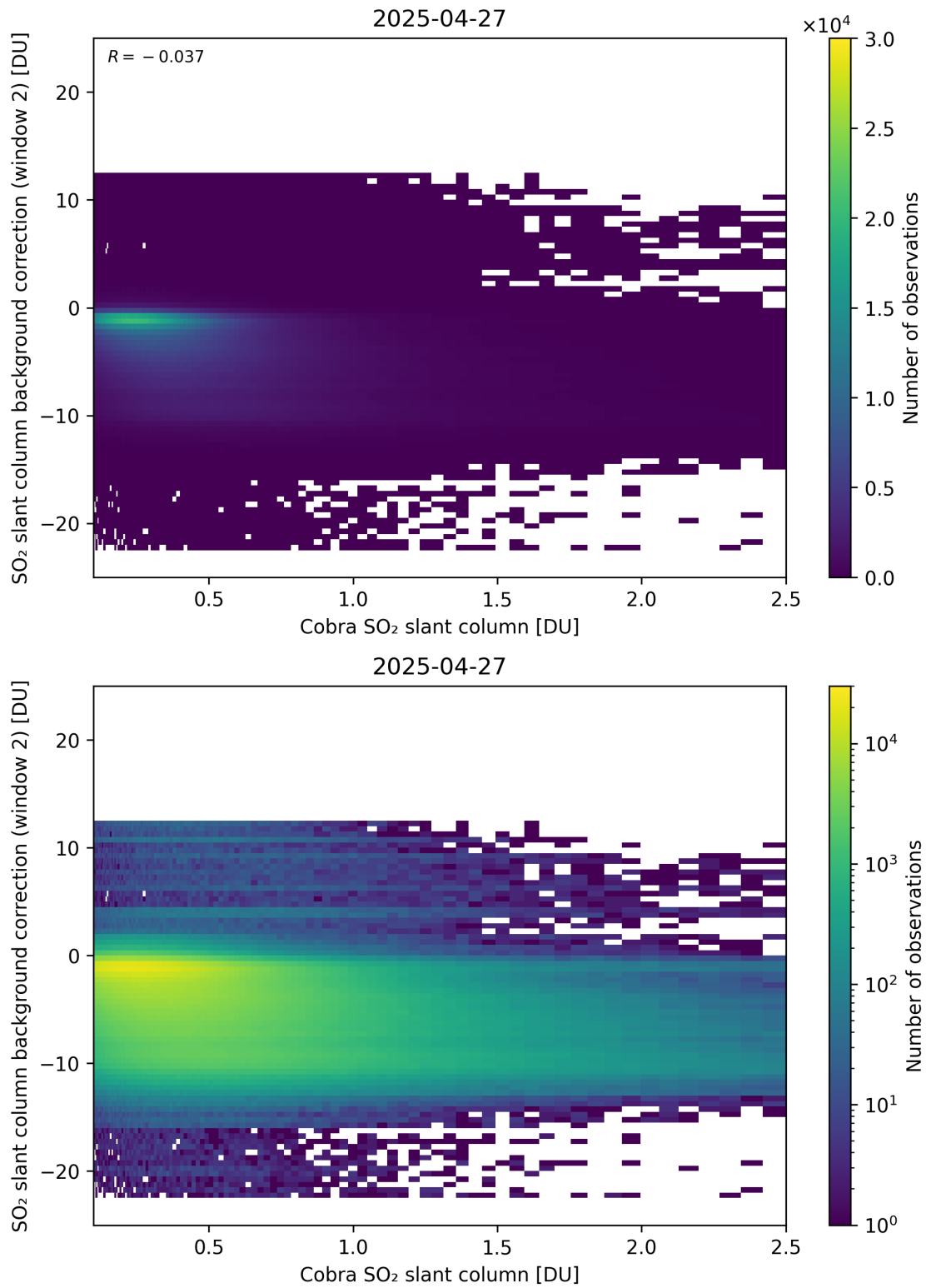
Figure 194: Scatter density plot of “Cobra SO 2 slant column” against “SO 2 slant column background correction (window 2)” for 2025-04-26 to 2025-04-28.
