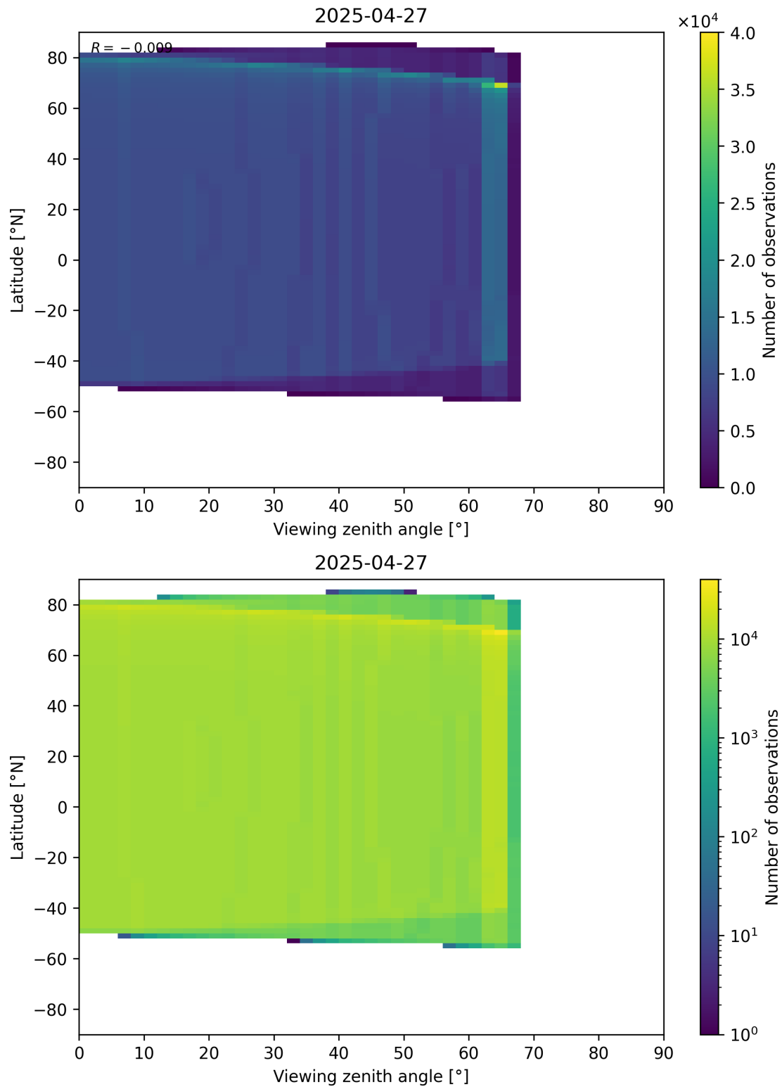
Figure 368: Scatter density plot of “Viewing zenith angle” against “Latitude” for 2025-04-26 to 2025-04-28.
