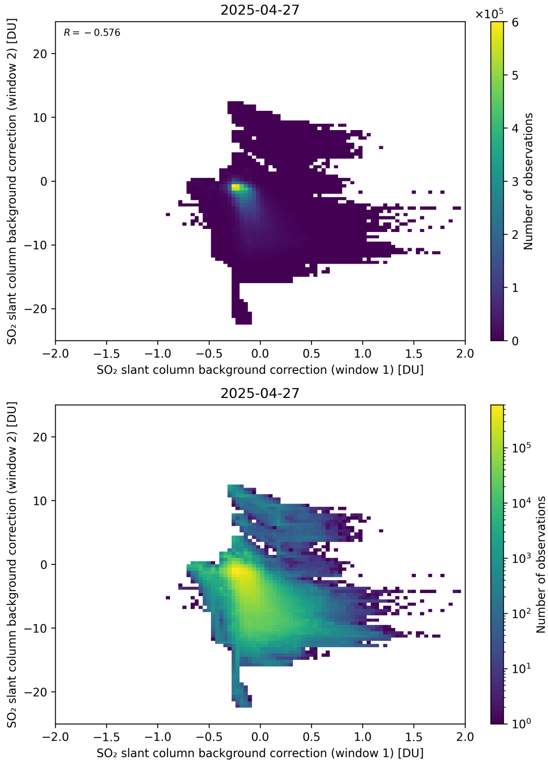
Figure 109: Scatter density plot of “SO 2 slant column background correction (window 1)” against “SO 2 slant column background correction (window 2)” for 2025-04-26 to 2025-04-28.
