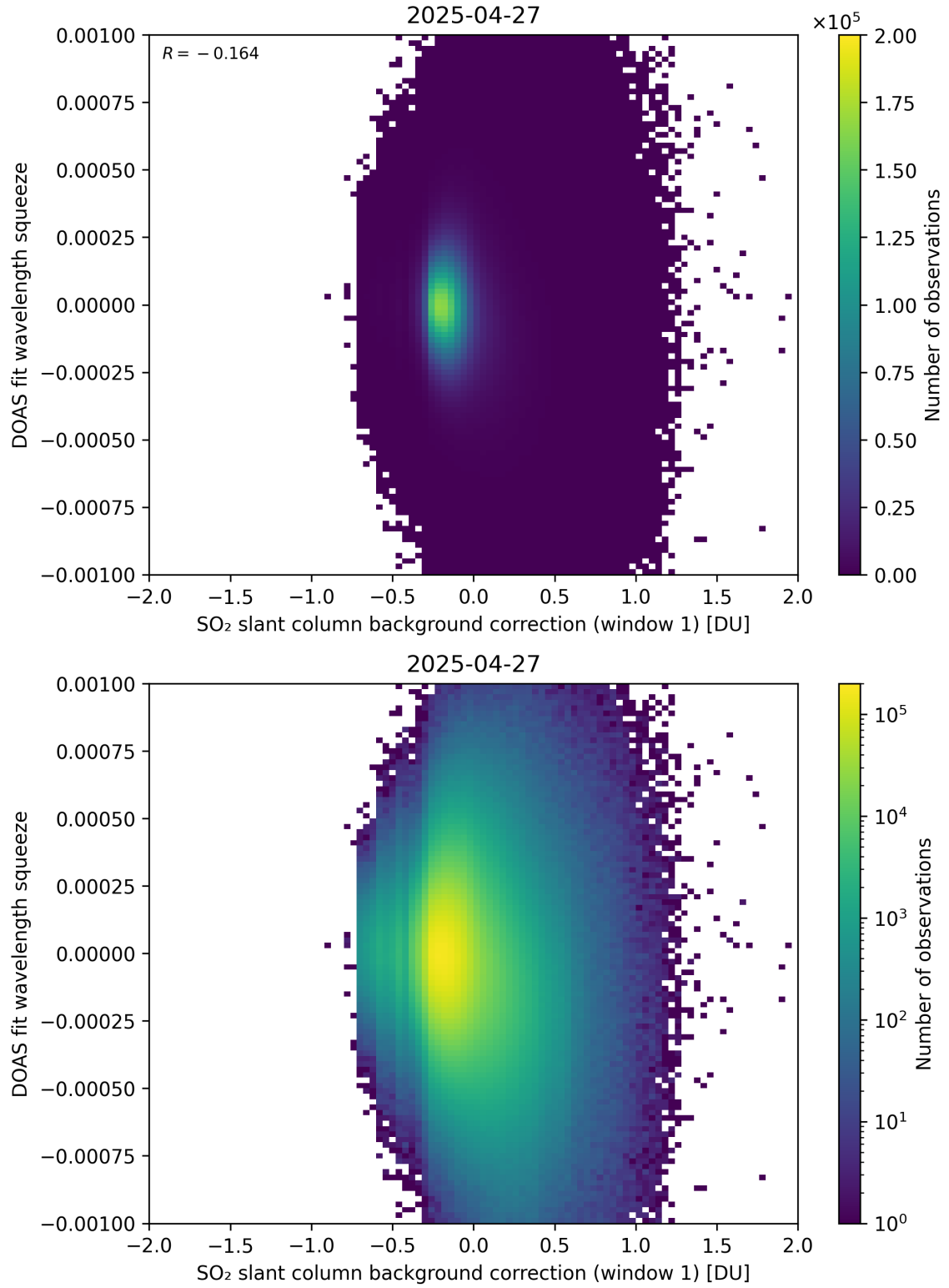
Figure 112: Scatter density plot of “SO 2 slant column background correction (window 1)” against “DOAS fit wavelength squeeze” for 2025-04-26 to 2025-04-28.
