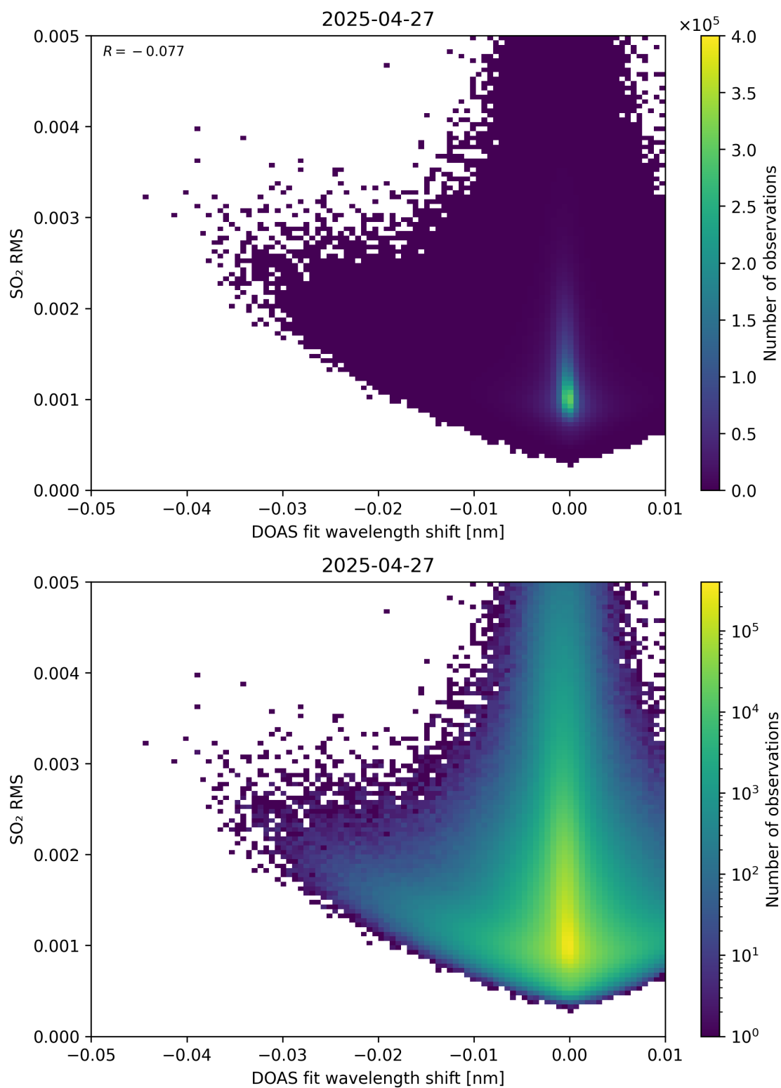
Figure 139: Scatter density plot of “DOAS fit wavelength shift” against “SO 2 RMS” for 2025-04-26 to 2025-04-28.
