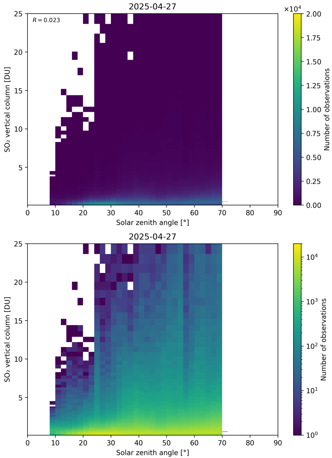
Figure 191: Scatter density plot of “Solar zenith angle” against “SO 2 vertical column” for 2025-04-26 to 2025-04-28.
