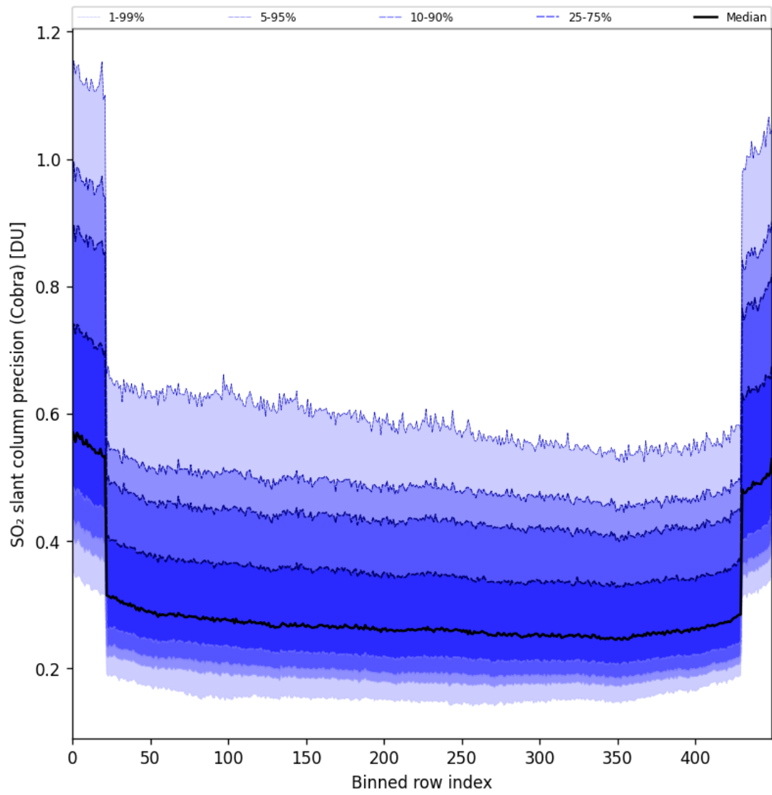
Figure 88: Along track statistics of “SO 2 slant column precision (Cobra)” for 2025-04-26 to 2025-04-28
