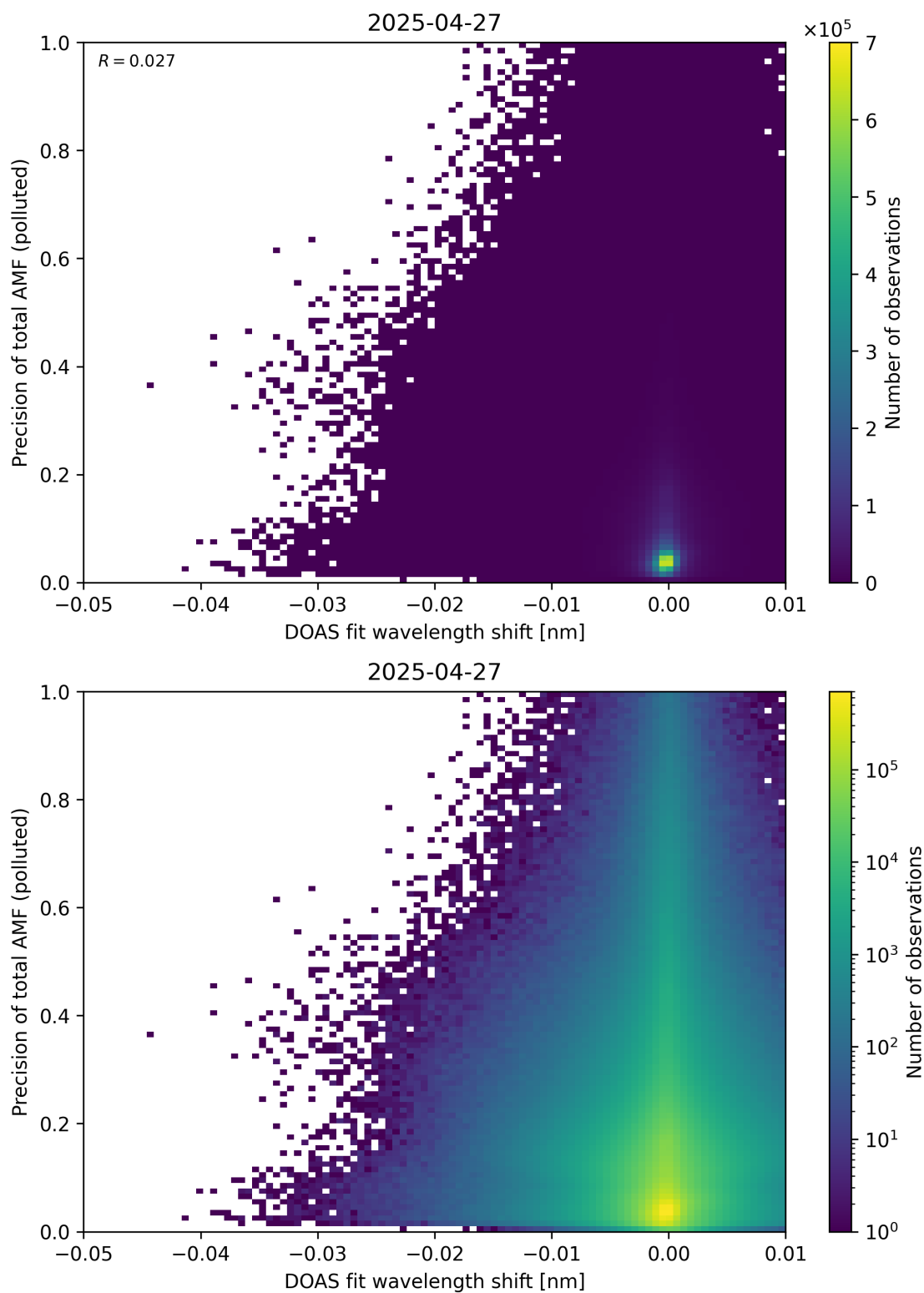
Figure 142: Scatter density plot of “DOAS fit wavelength shift” against “Precision of total AMF (polluted)” for 2025-04-26 to 2025-04-28.
