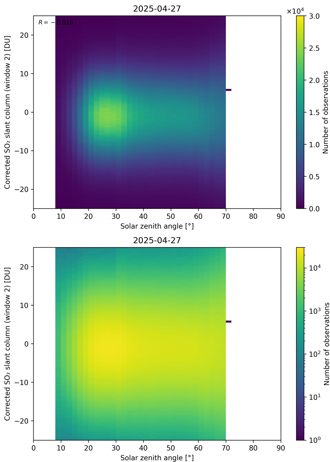
Figure 182: Scatter density plot of “Solar zenith angle” against “Corrected SO 2 slant column (window 2)” for 2025-04-26 to 2025-04-28.
