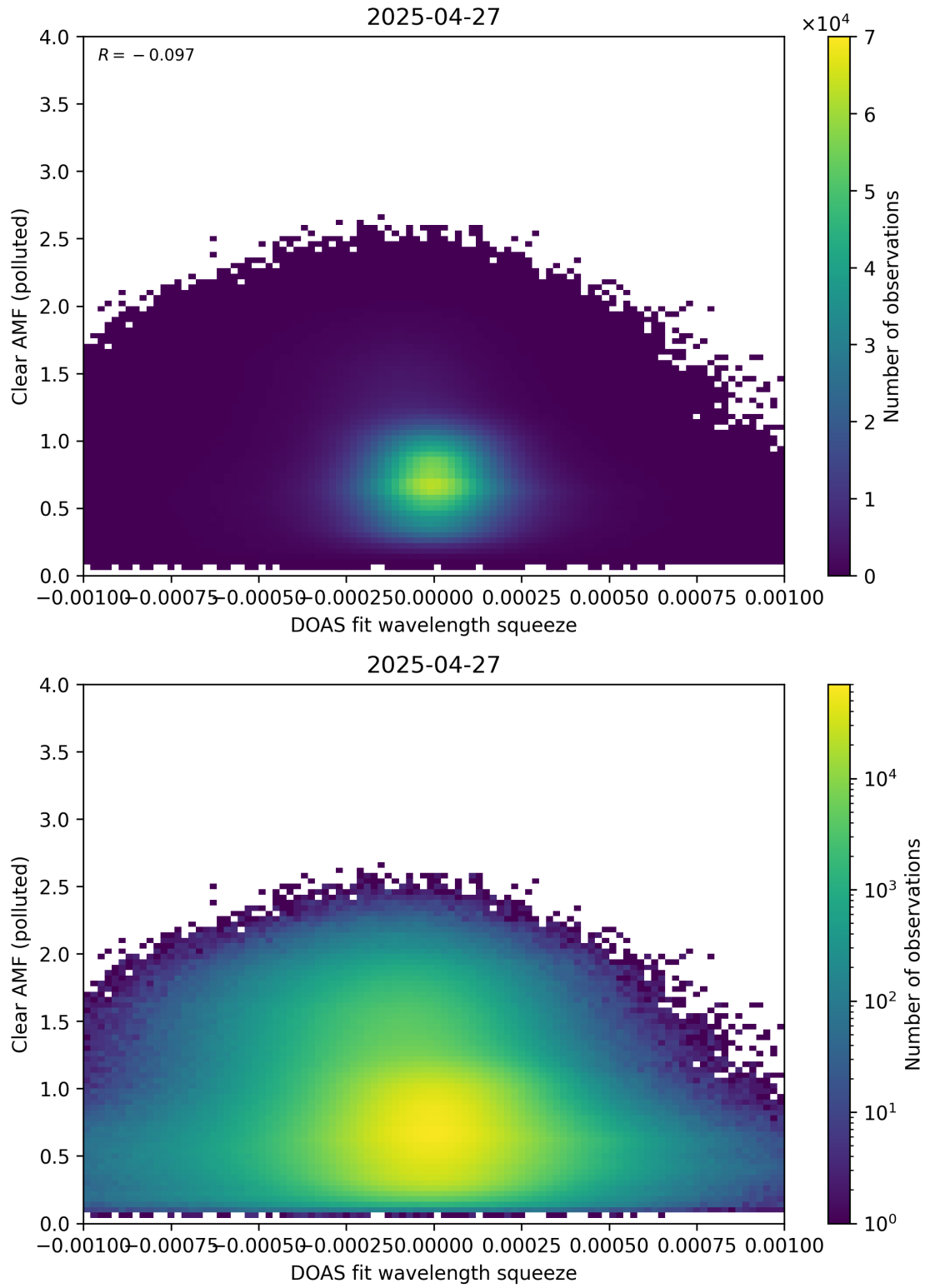
Figure 144: Scatter density plot of “DOAS fit wavelength squeeze” against “Clear AMF (polluted)” for 2025-04-26 to 2025-04-28.
