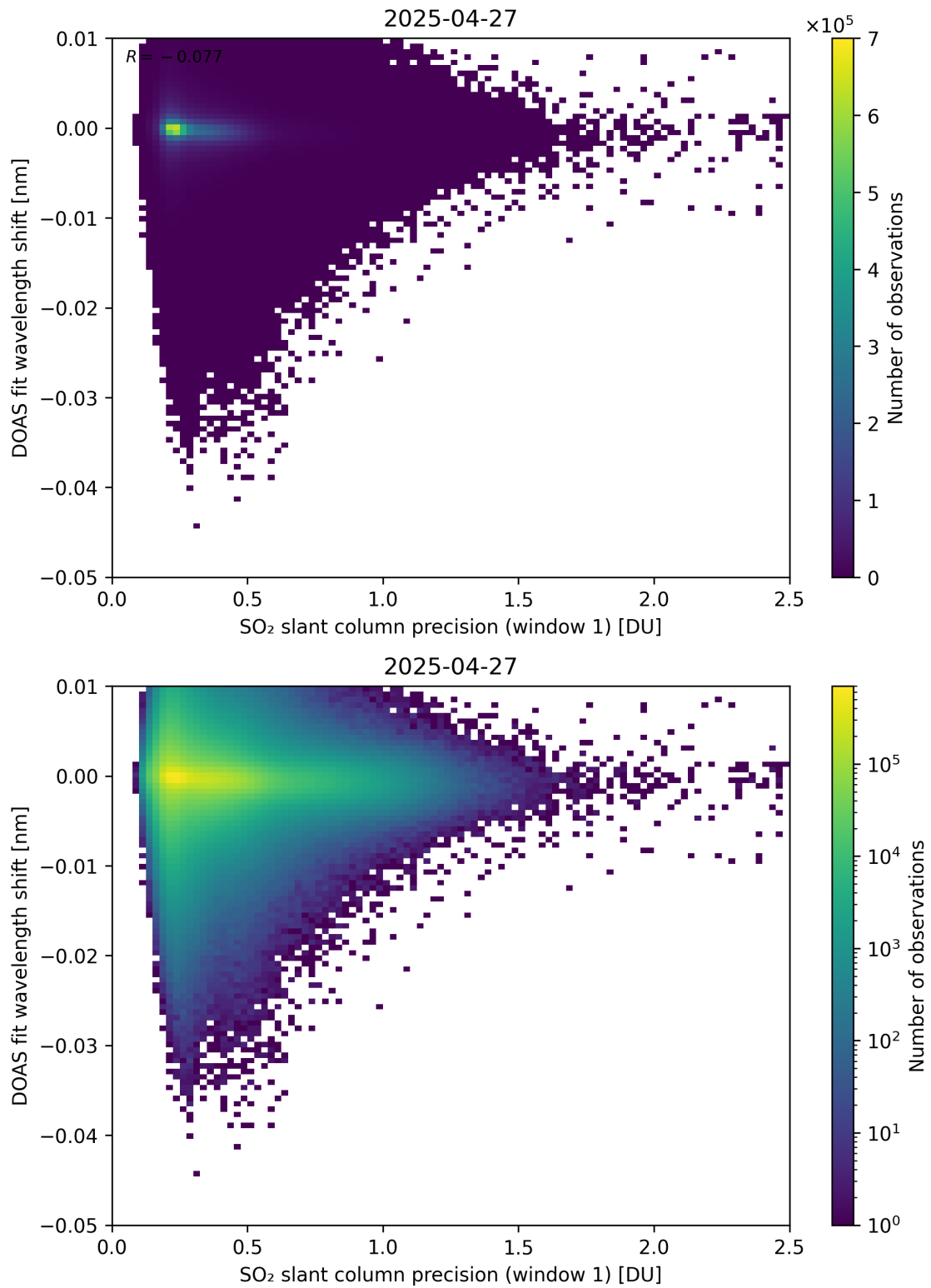
Figure 271: Scatter density plot of “SO 2 slant column precision (window 1)” against “DOAS fit wavelength shift” for 2025-04-26 to 2025-04-28.
