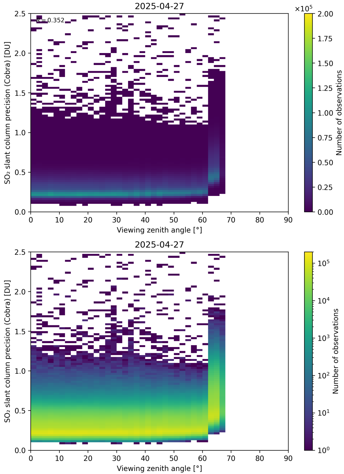
Figure 372: Scatter density plot of “Viewing zenith angle” against “SO 2 slant column precision (Cobra)” for 2025-04-26 to 2025-04-28.
