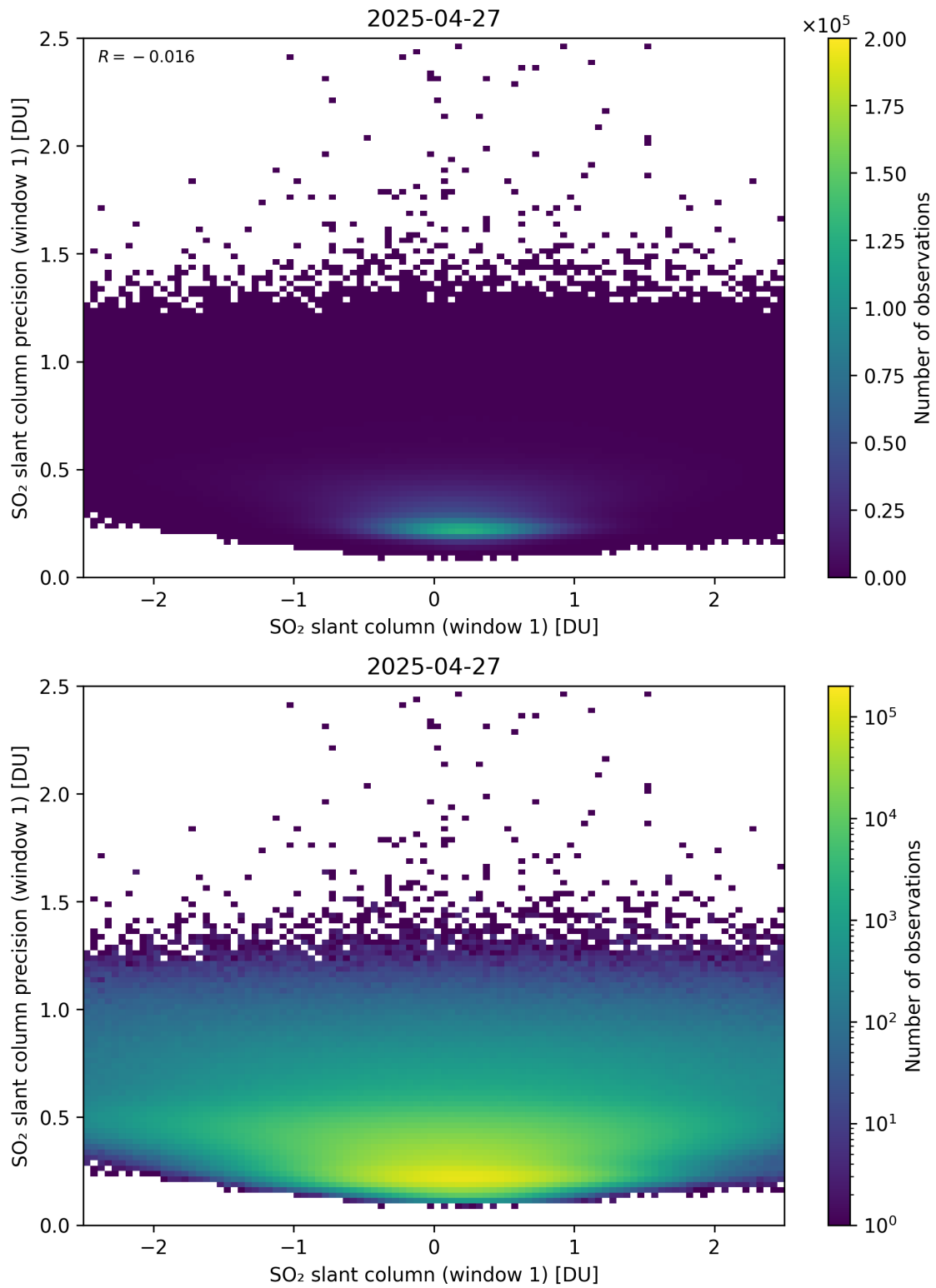
Figure 285: Scatter density plot of “SO 2 slant column (window 1)” against “SO 2 slant column precision (window 1)” for 2025-04-26 to 2025-04-28.
