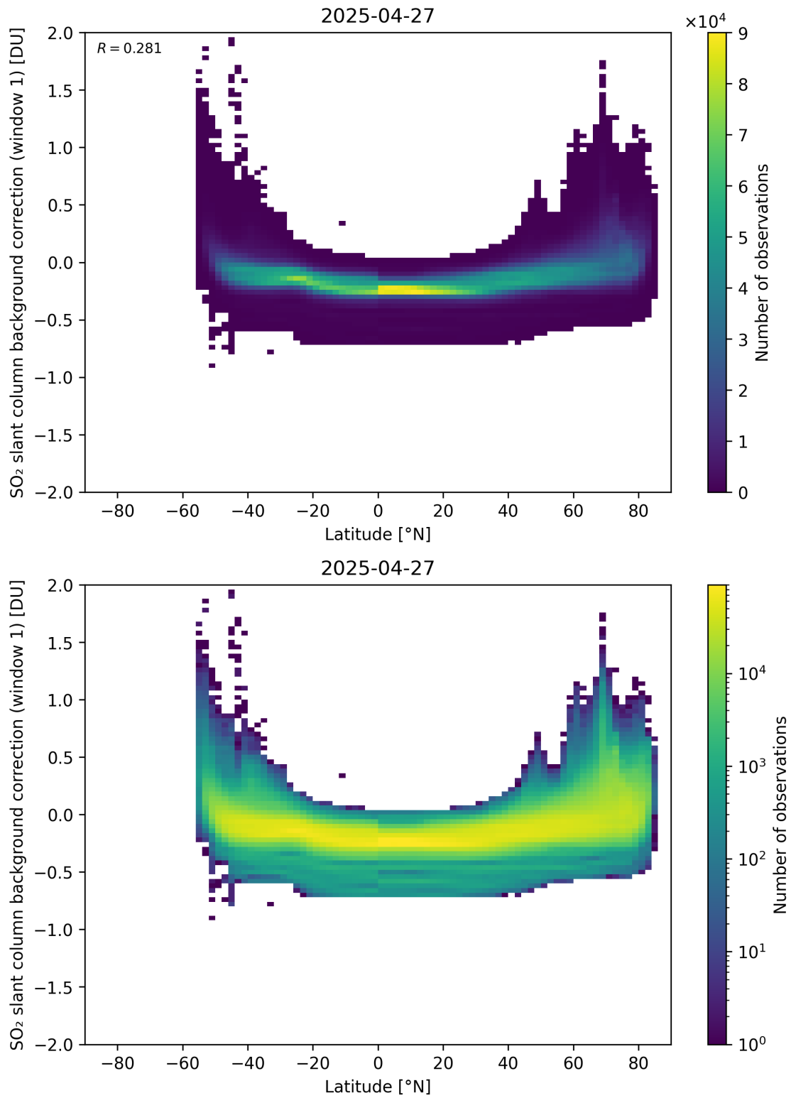
Figure 150: Scatter density plot of “Latitude” against “SO 2 slant column background correction (window 1)” for 2025-04-26 to 2025-04-28.
