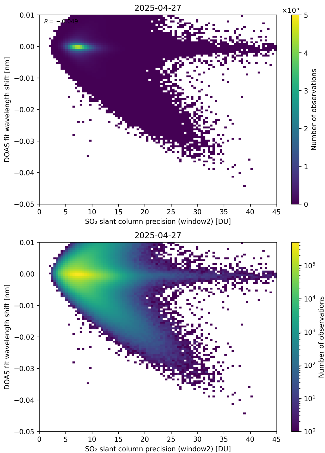
Figure 293: Scatter density plot of “SO 2 slant column precision (window2)” against “DOAS fit wavelength shift” for 2025-04-26 to 2025-04-28.
