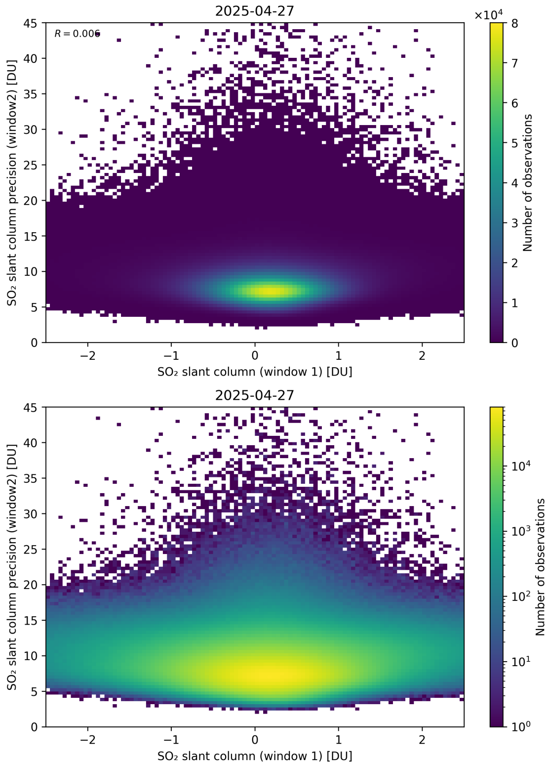
Figure 286: Scatter density plot of “SO 2 slant column (window 1)” against “SO 2 slant column precision (window2)” for 2025-04-26 to 2025-04-28.
