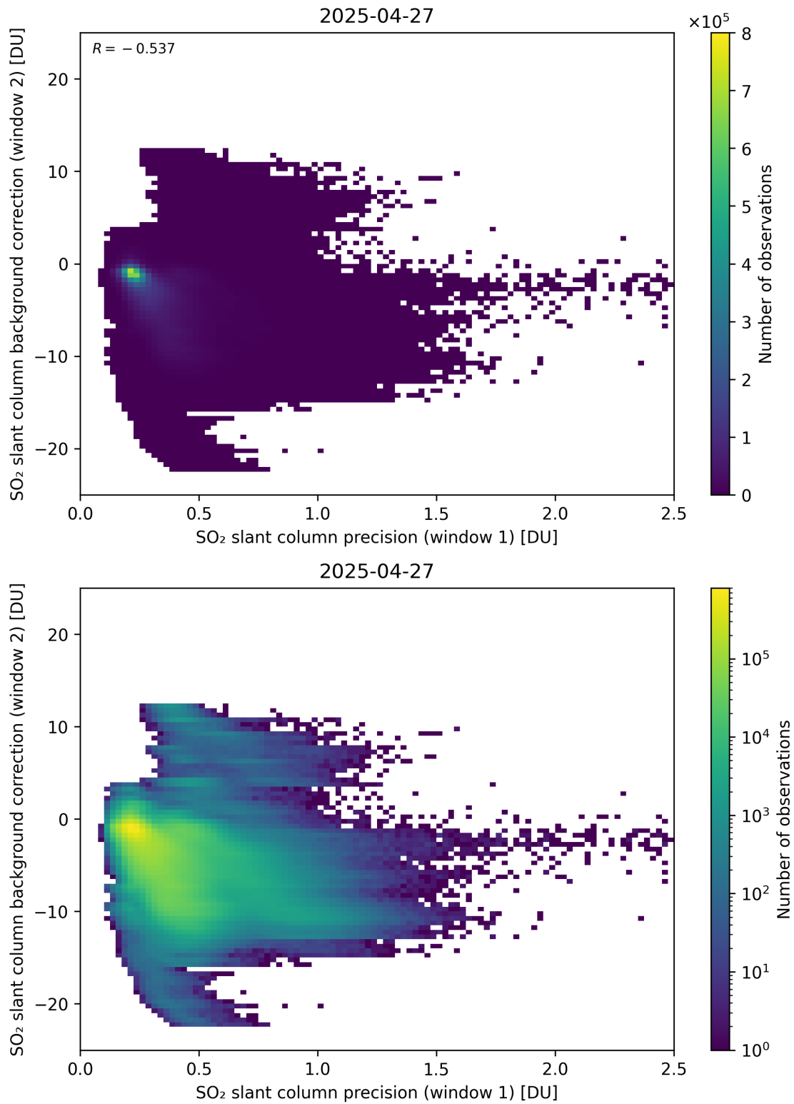
Figure 269: Scatter density plot of “SO 2 slant column precision (window 1)” against “SO 2 slant column background correction (window 2)” for 2025-04-26 to 2025-04-28.
