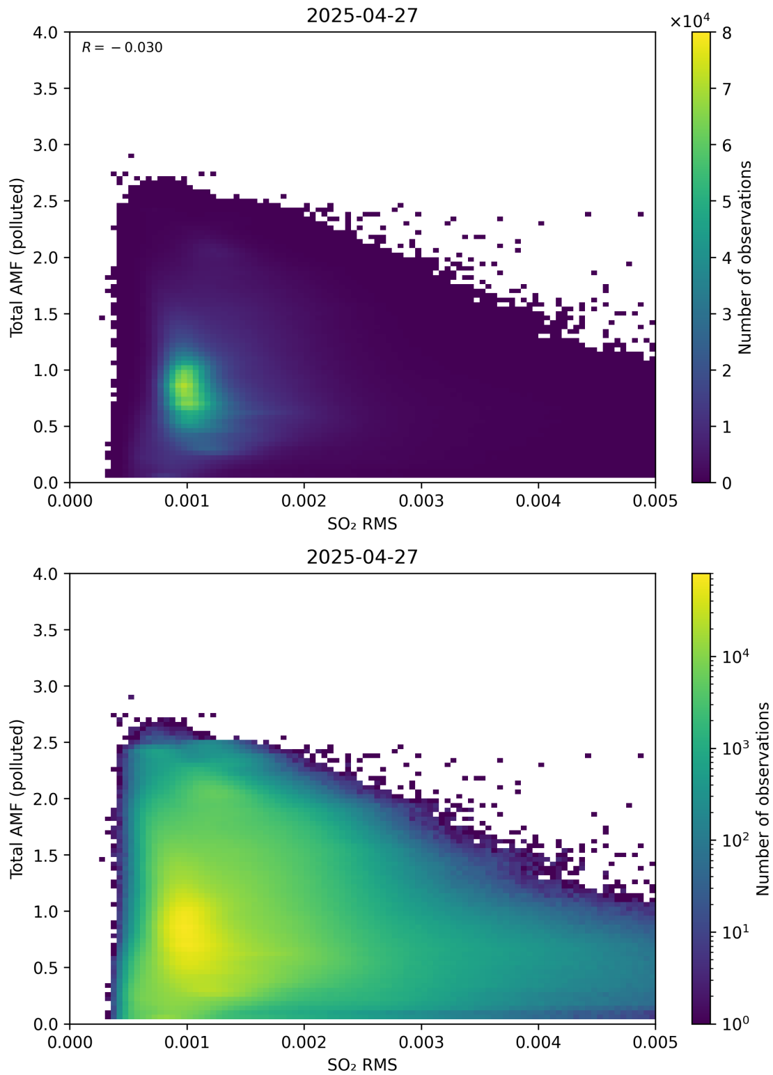
Figure 148: Scatter density plot of “SO 2 RMS” against “Total AMF (polluted)” for 2025-04-26 to 2025-04-28.
