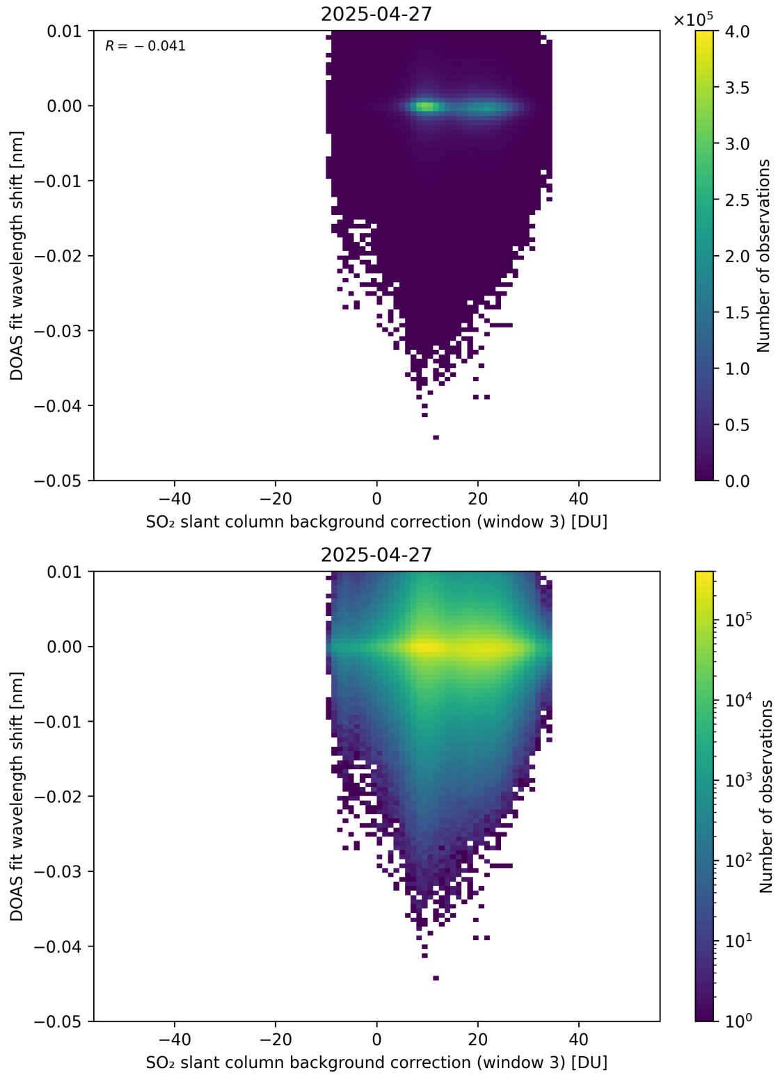
Figure 132: Scatter density plot of “SO 2 slant column background correction (window 3)” against “DOAS fit wavelength shift” for 2025-04-26 to 2025-04-28.
