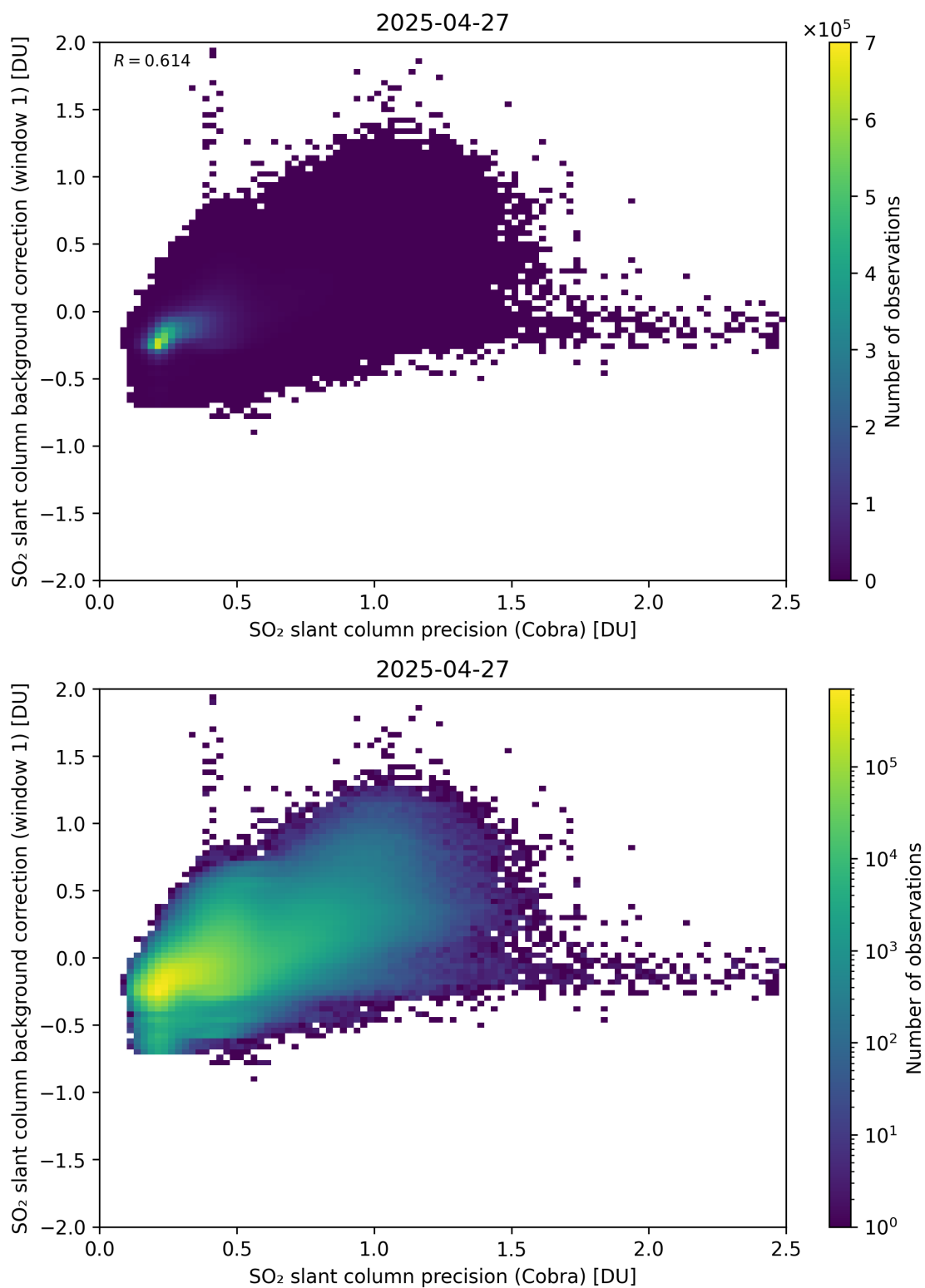
Figure 199: Scatter density plot of “SO 2 slant column precision (Cobra)” against “SO 2 slant column background correction (window 1)” for 2025-04-26 to 2025-04-28.
