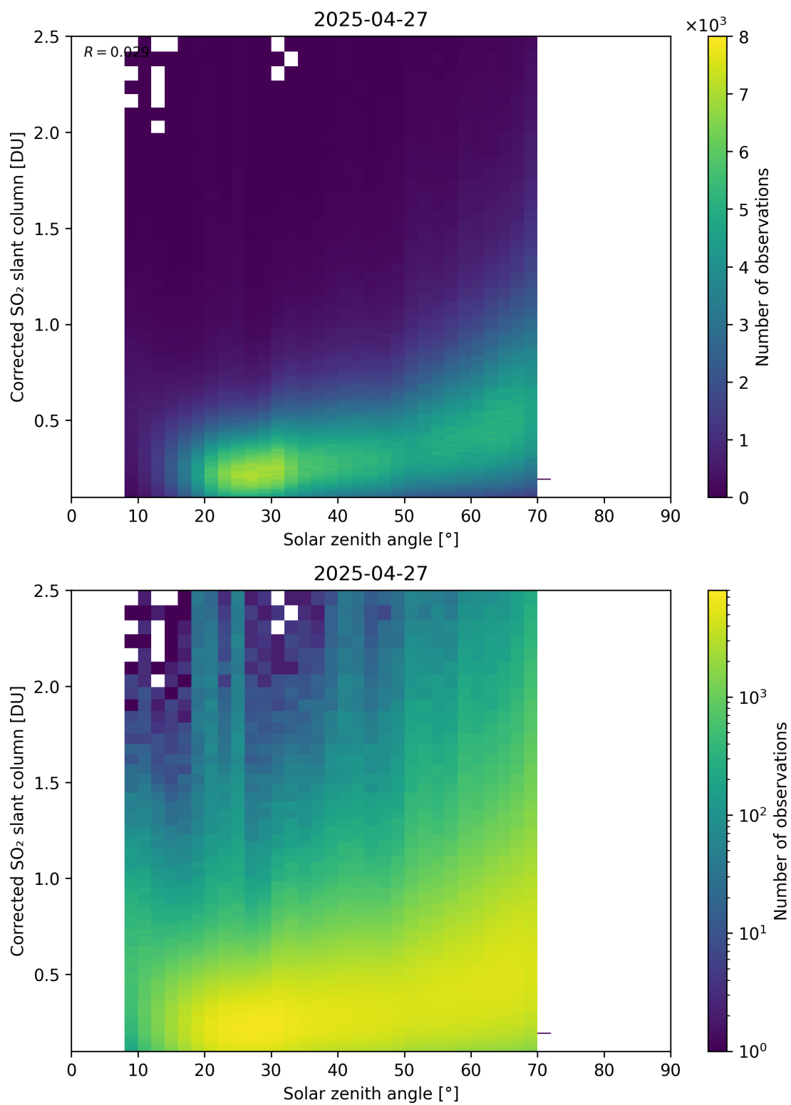
Figure 181: Scatter density plot of “Solar zenith angle” against “Corrected SO 2 slant column” for 2025-04-26 to 2025-04-28.
