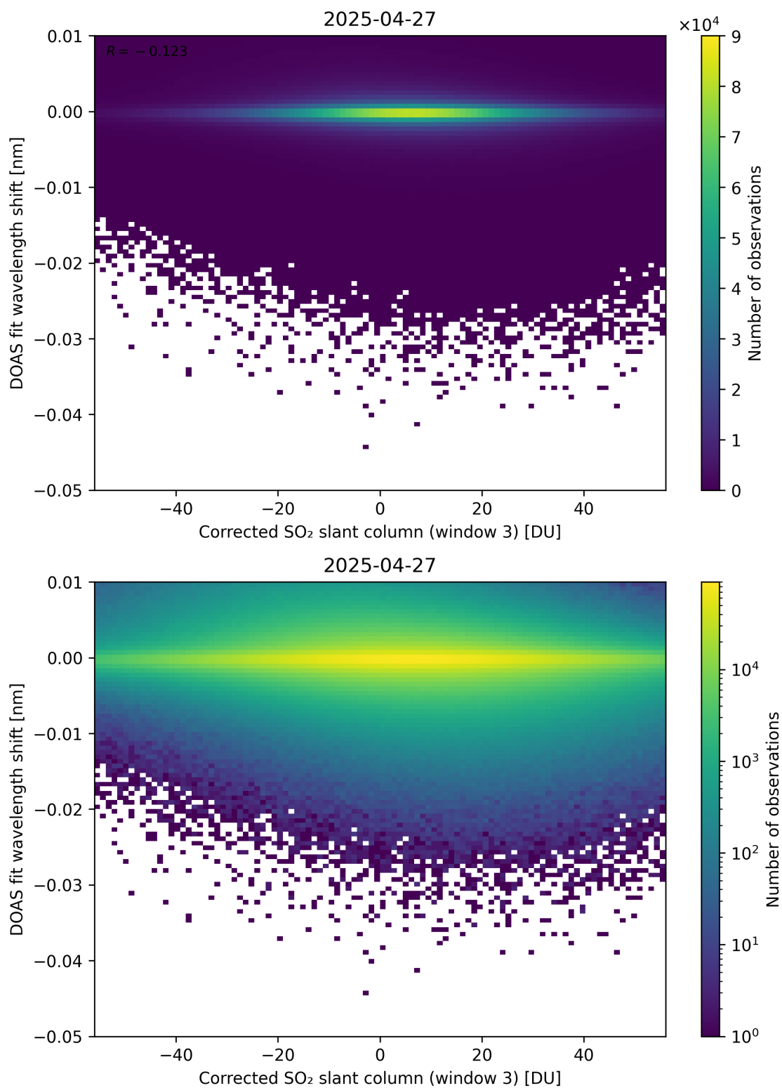
Figure 256: Scatter density plot of “Corrected SO 2 slant column (window 3)” against “DOAS fit wavelength shift” for 2025-04-26 to 2025-04-28.
