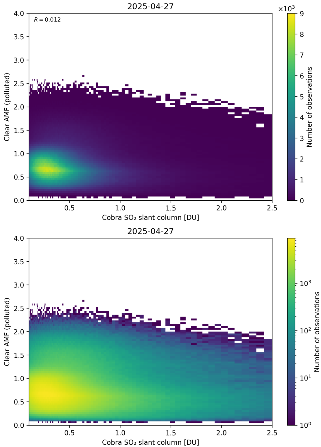
Figure 215: Scatter density plot of “Cobra SO 2 slant column” against “Clear AMF (polluted)” for 2025-04-26 to 2025-04-28.
