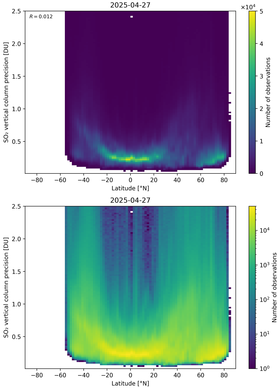
Figure 170: Scatter density plot of “Latitude” against “SO 2 vertical column precision” for 2025-04-26 to 2025-04-28.
