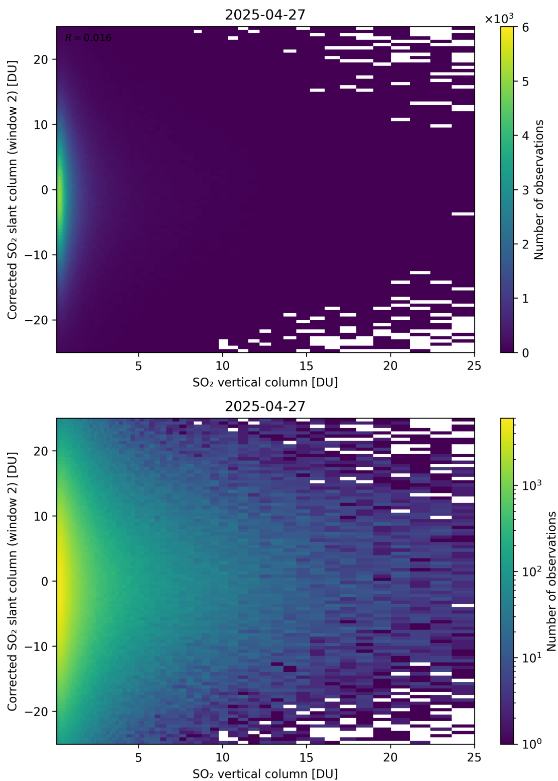
Figure 352: Scatter density plot of “SO 2 vertical column” against “Corrected SO 2 slant column (window 2)” for 2025-04-26 to 2025-04-28.
