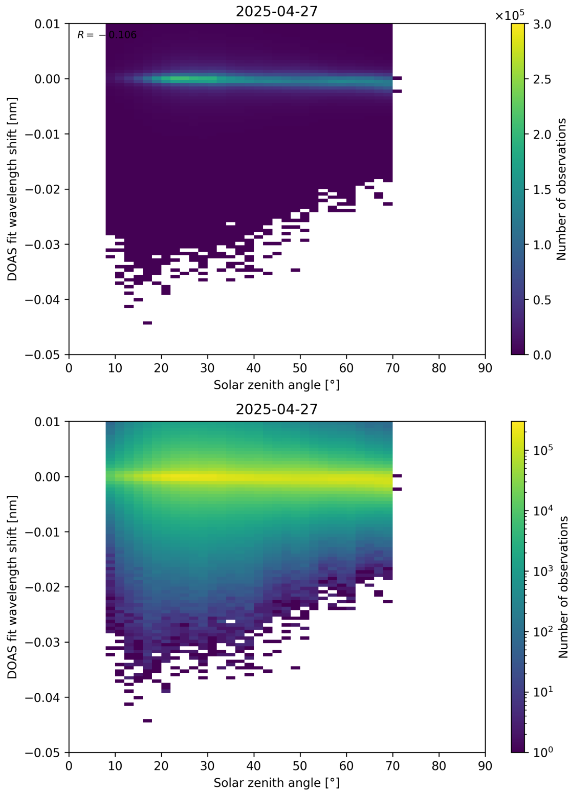
Figure 174: Scatter density plot of “Solar zenith angle” against “DOAS fit wavelength shift” for 2025-04-26 to 2025-04-28.
