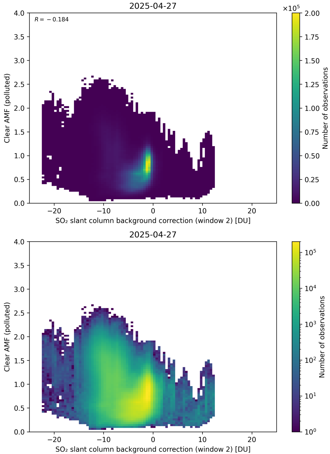
Figure 126: Scatter density plot of “SO 2 slant column background correction (window 2)” against “Clear AMF (polluted)” for 2025-04-26 to 2025-04-28.
