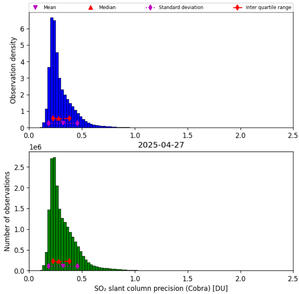
Figure 62: Histogram of “SO 2 slant column precision (Cobra)” for 2025-04-26 to 2025-04-28
