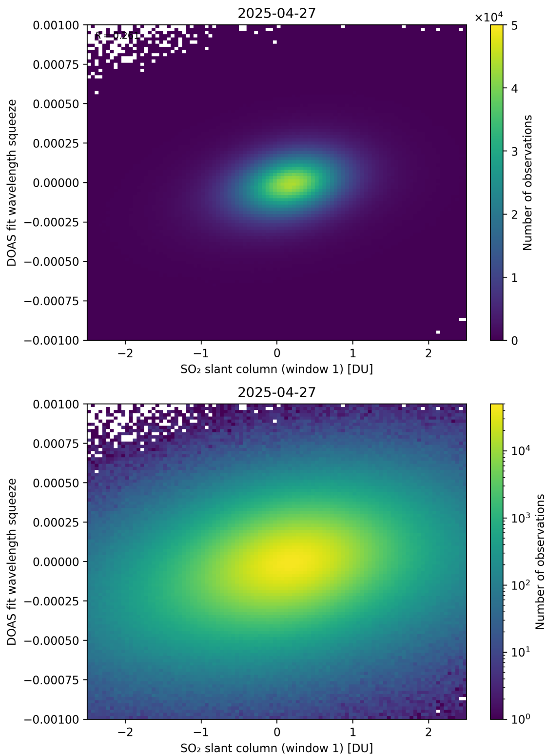
Figure 266: Scatter density plot of “SO 2 slant column (window 1)” against “DOAS fit wavelength squeeze” for 2025-04-26 to 2025-04-28.
