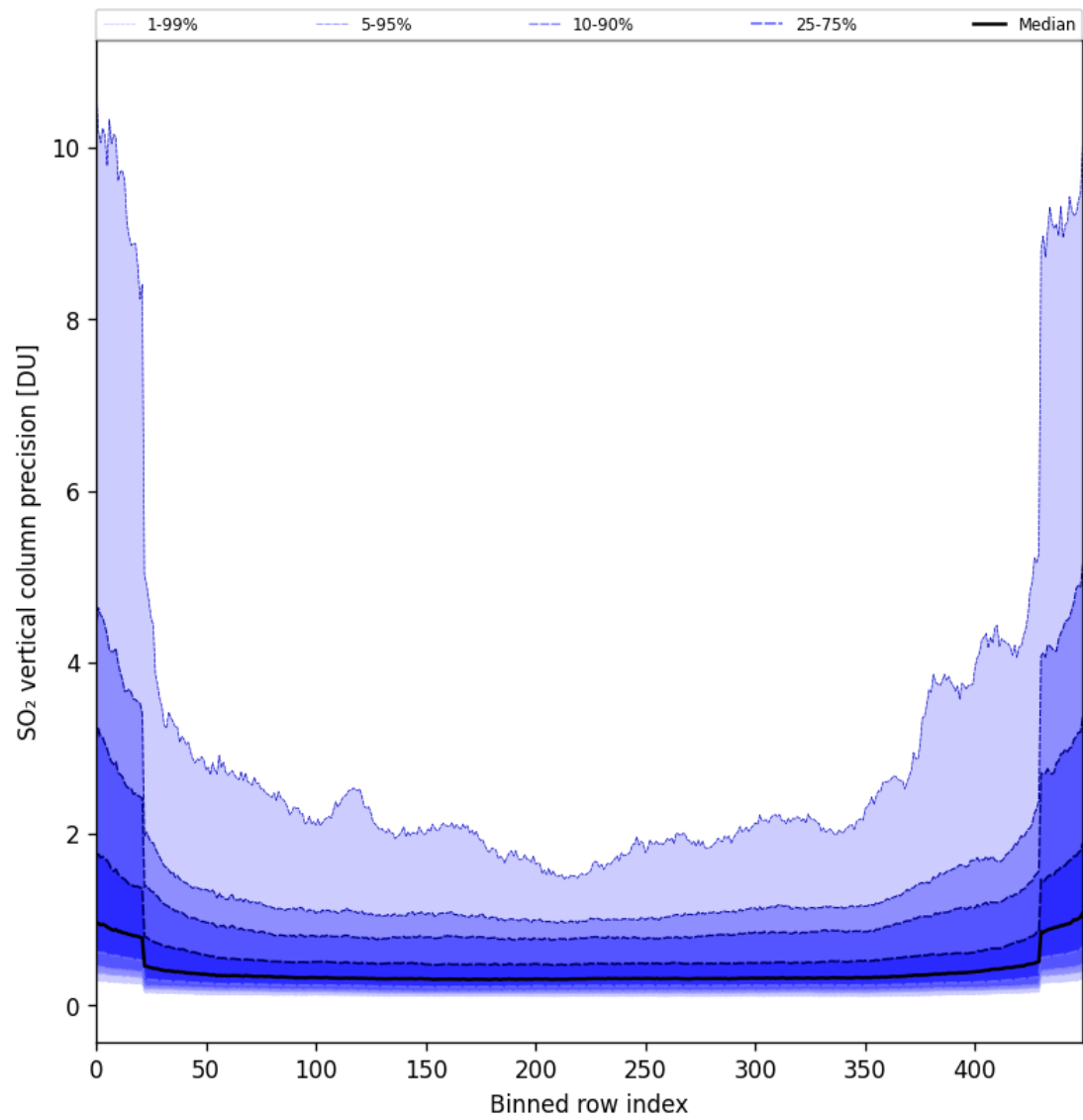
Figure 85: Along track statistics of “SO 2 vertical column precision” for 2025-04-26 to 2025-04-28
