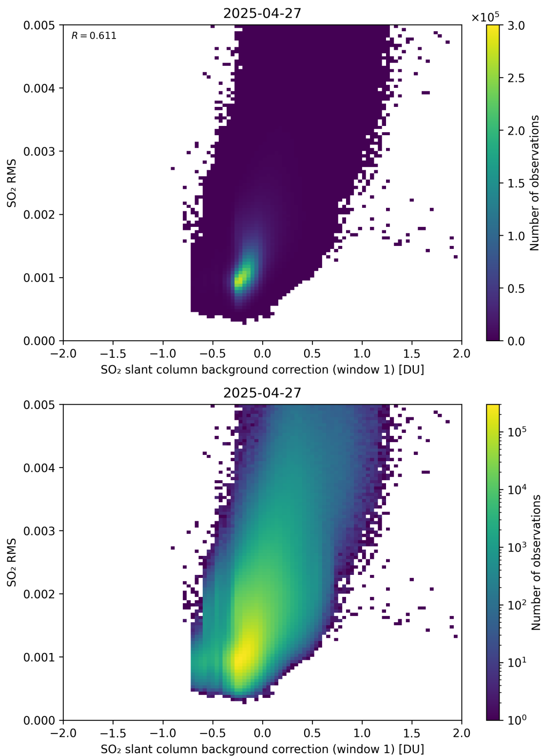
Figure 113: Scatter density plot of “SO 2 slant column background correction (window 1)” against “SO 2 RMS” for 2025-04-26 to 2025-04-28.
