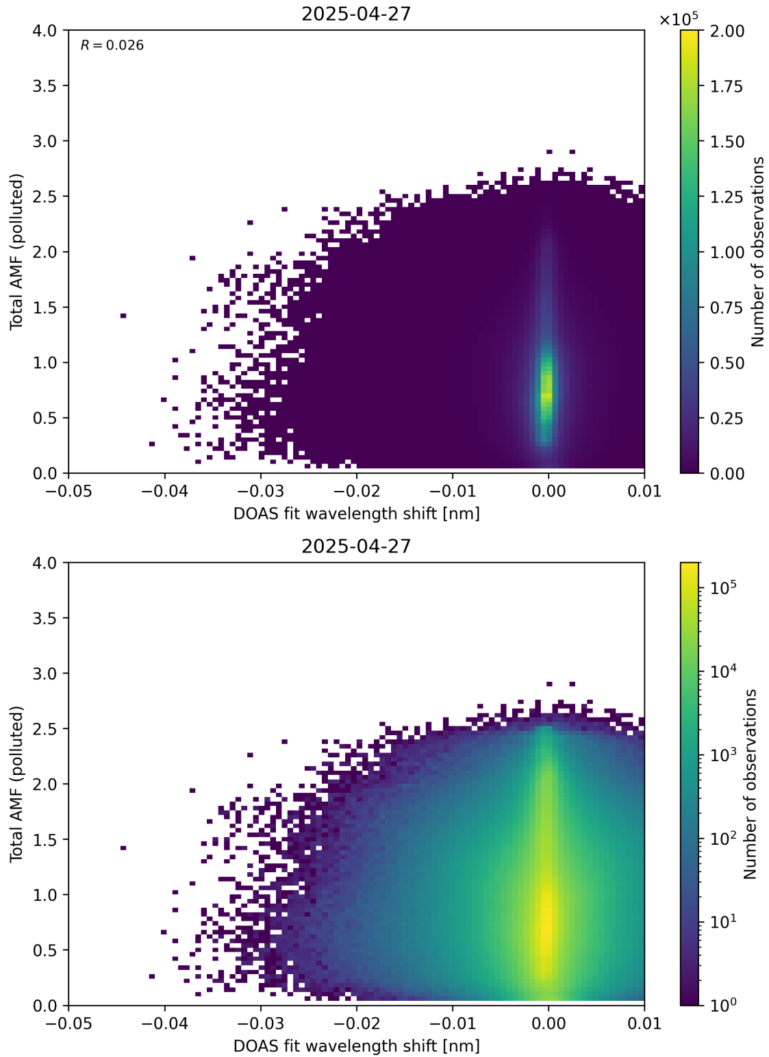
Figure 141: Scatter density plot of “DOAS fit wavelength shift” against “Total AMF (polluted)” for 2025-04-26 to 2025-04-28.
