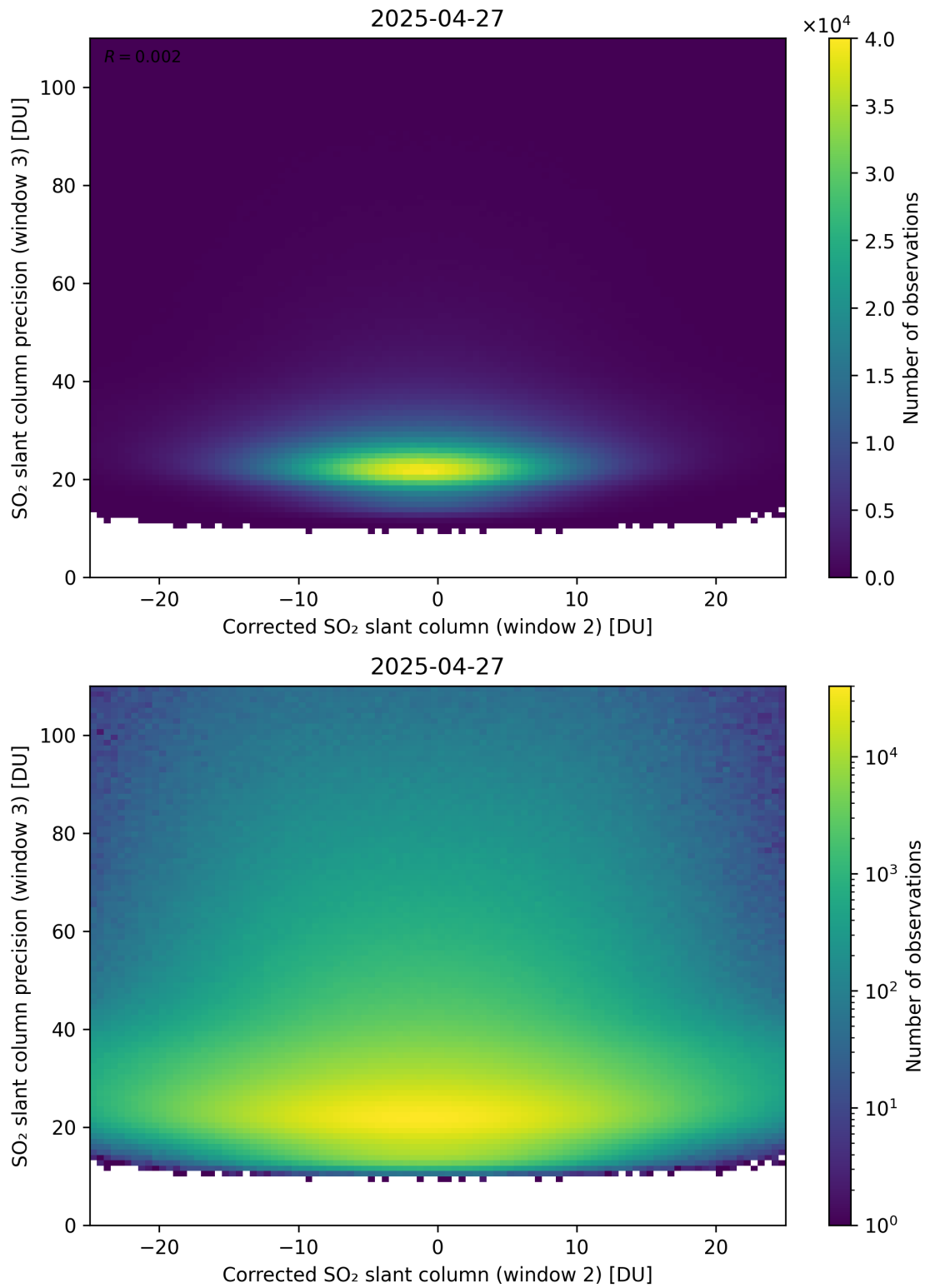
Figure 252: Scatter density plot of “Corrected SO 2 slant column (window 2)” against “SO 2 slant column precision (window 3)” for 2025-04-26 to 2025-04-28.
