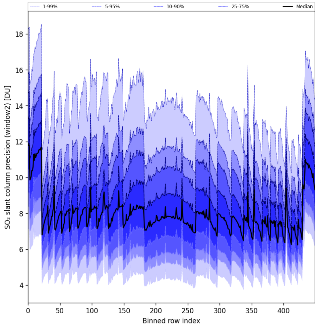
Figure 94: Along track statistics of “SO 2 slant column precision (window2)” for 2025-04-26 to 2025-04-28
