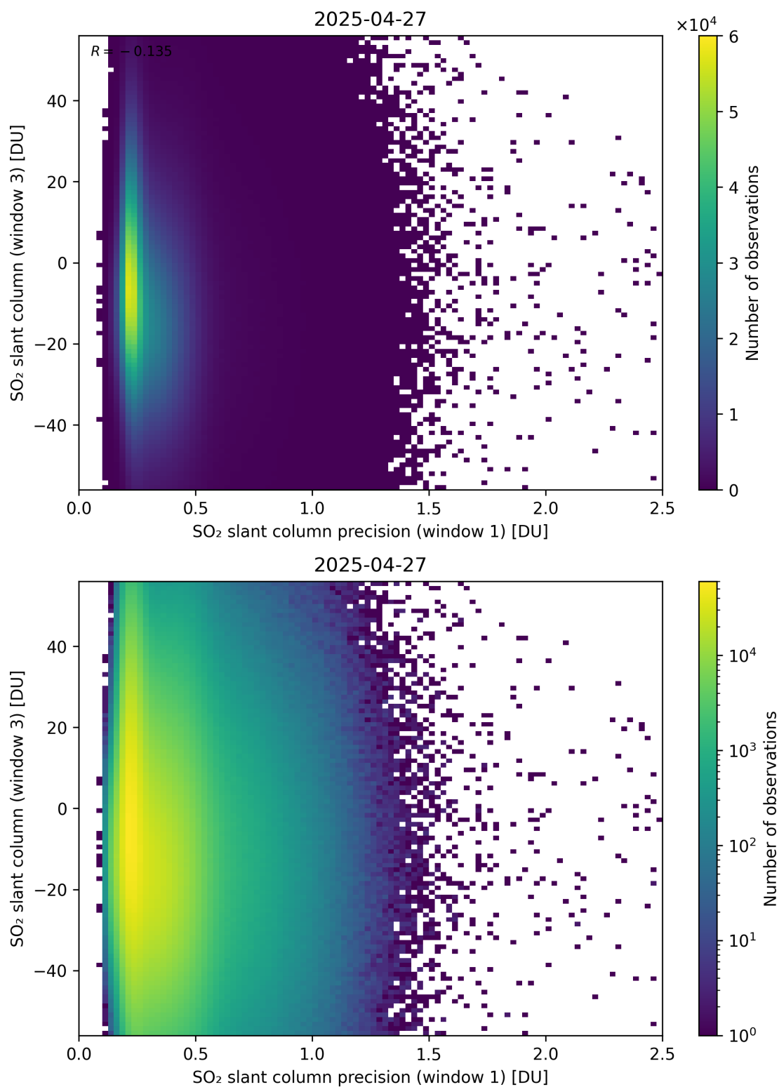
Figure 278: Scatter density plot of “SO 2 slant column precision (window 1)” against “SO 2 slant column (window 3)” for 2025-04-26 to 2025-04-28.
