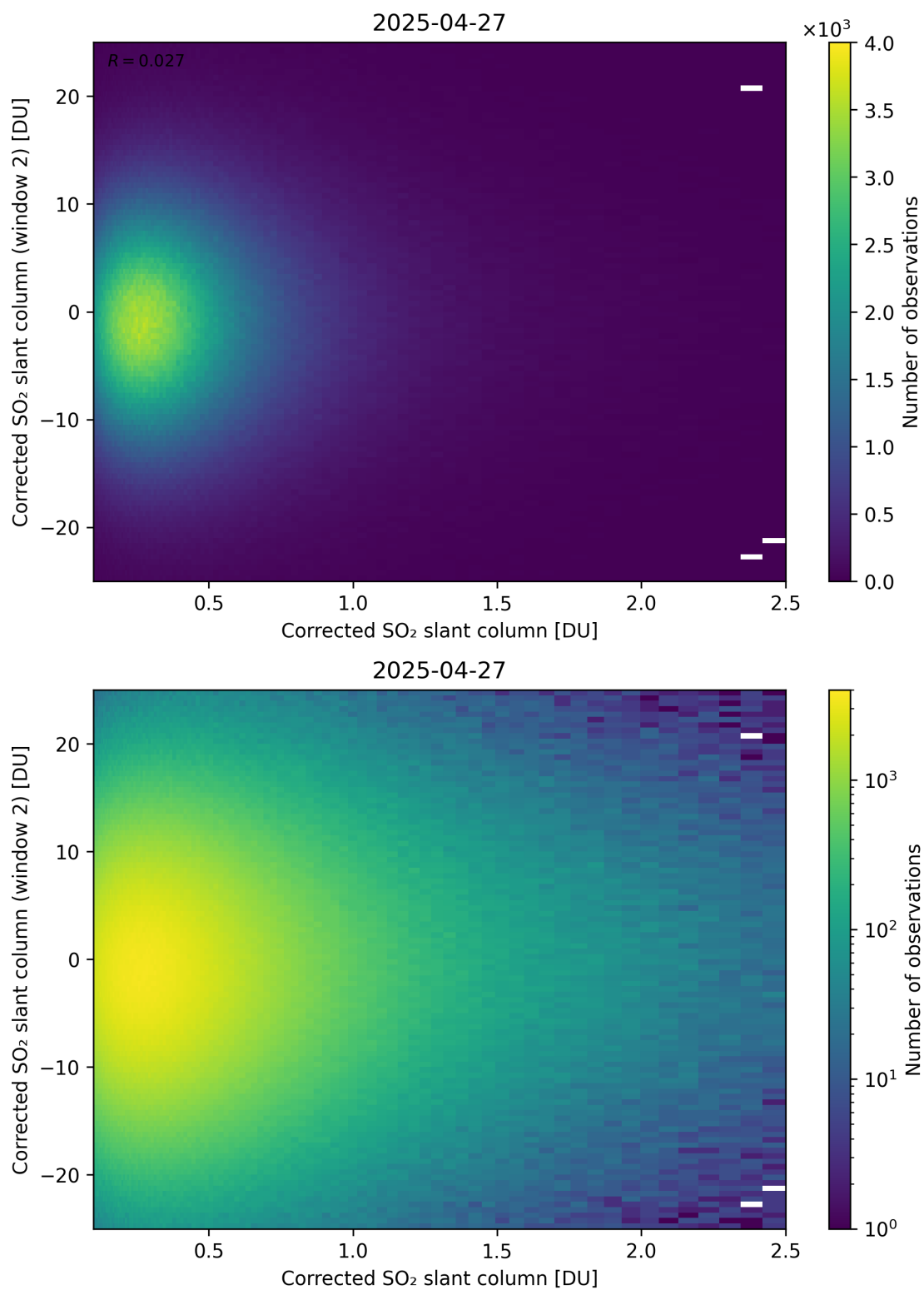
Figure 235: Scatter density plot of “Corrected SO 2 slant column” against “Corrected SO 2 slant column (window 2)” for 2025-04-26 to 2025-04-28.
