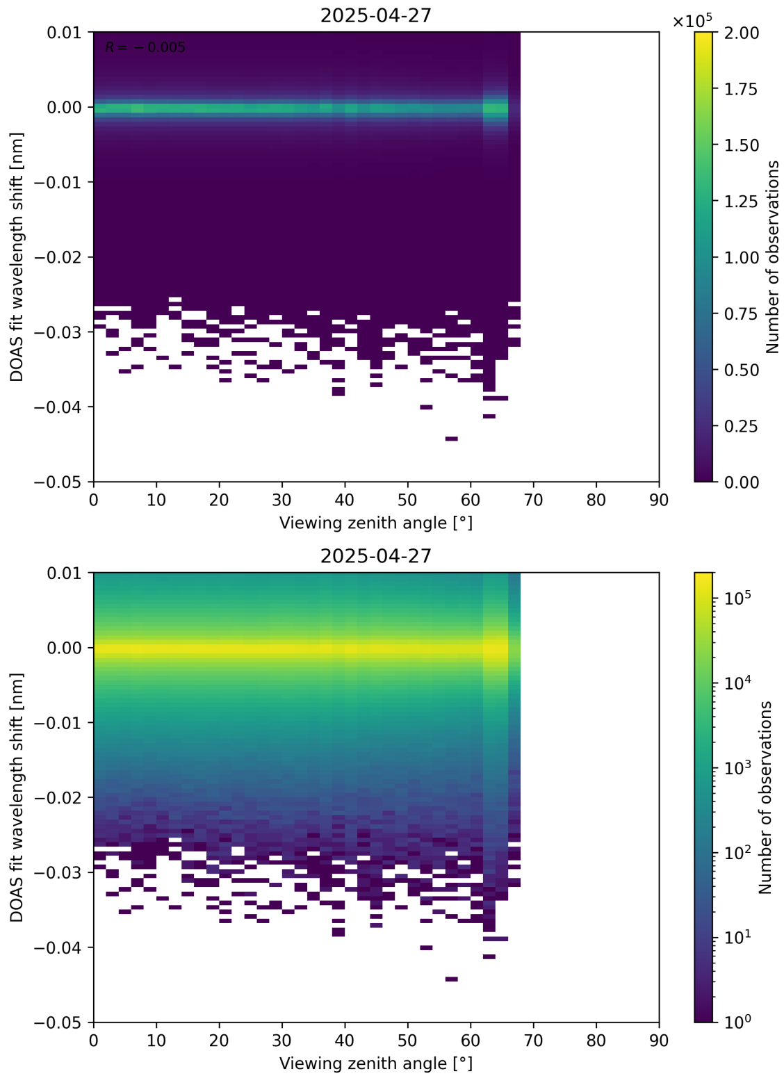
Figure 365: Scatter density plot of “Viewing zenith angle” against “DOAS fit wavelength shift” for 2025-04-26 to 2025-04-28.
