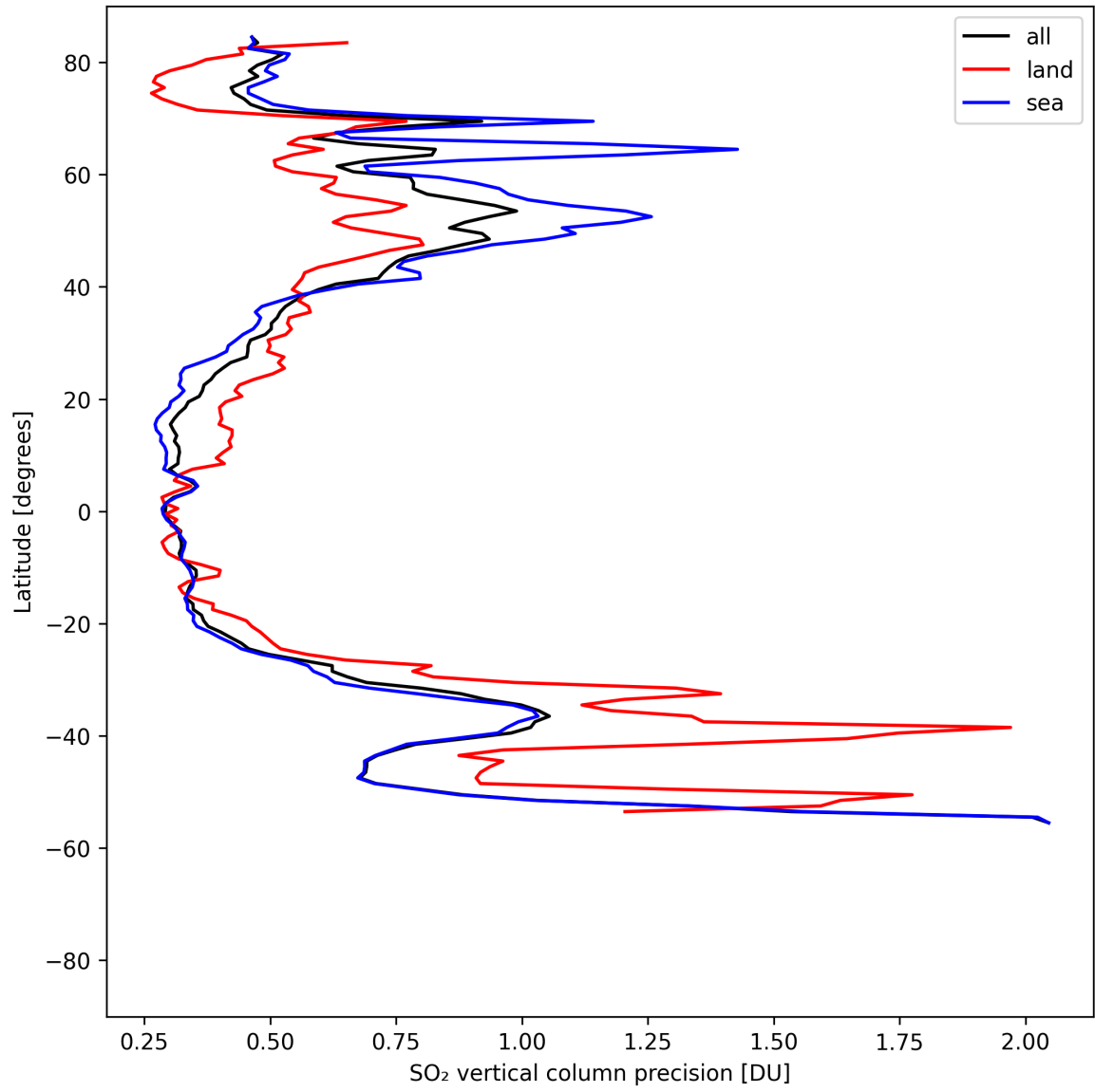
Figure 33: Zonal average of “SO 2 vertical column precision” for 2025-04-26 to 2025-04-28.
