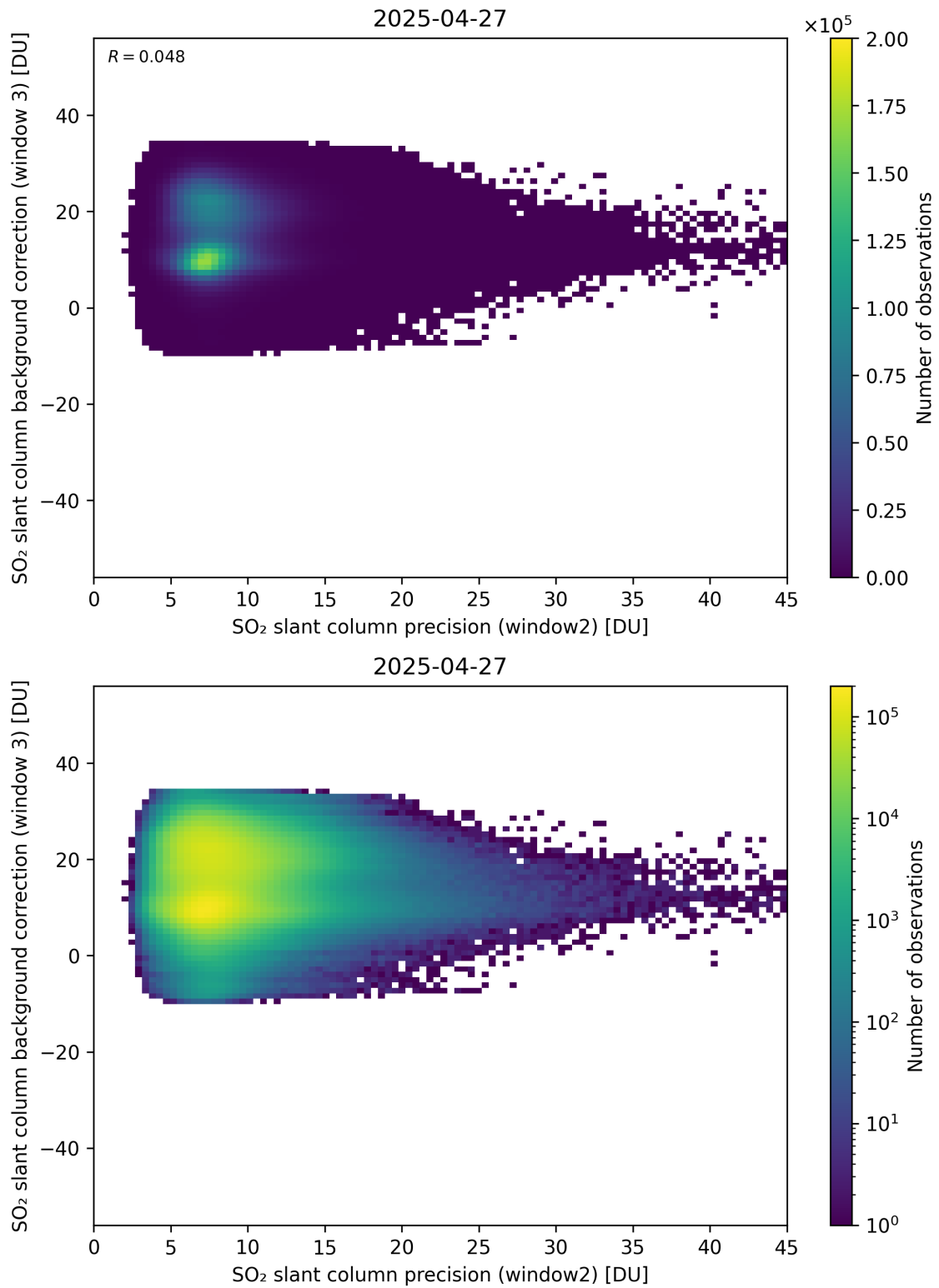
Figure 292: Scatter density plot of “SO 2 slant column precision (window2)” against “SO 2 slant column background correction (window 3)” for 2025-04-26 to 2025-04-28.
