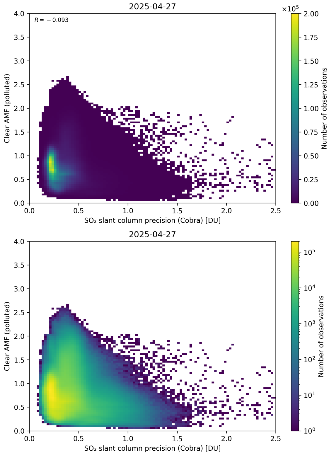
Figure 205: Scatter density plot of “SO 2 slant column precision (Cobra)” against “Clear AMF (polluted)” for 2025-04-26 to 2025-04-28.
