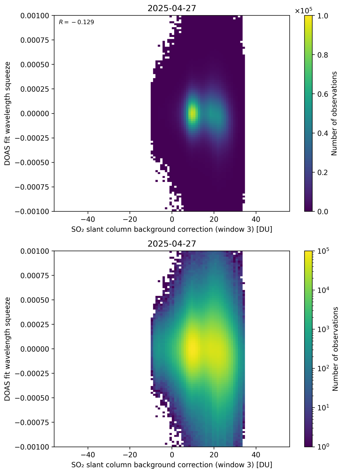
Figure 133: Scatter density plot of “SO 2 slant column background correction (window 3)” against “DOAS fit wavelength squeeze” for 2025-04-26 to 2025-04-28.
