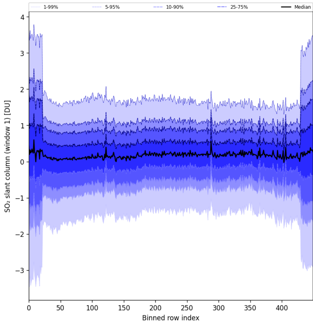
Figure 89: Along track statistics of “SO 2 slant column (window 1)” for 2025-04-26 to 2025-04-28
