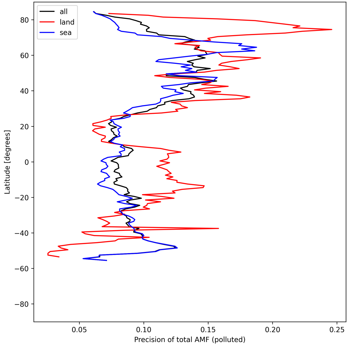
Figure 54: Zonal average of “Precision of total AMF (polluted)” for 2025-04-26 to 2025-04-28.
