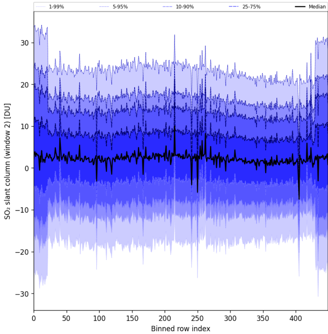
Figure 93: Along track statistics of “SO 2 slant column (window 2)” for 2025-04-26 to 2025-04-28
