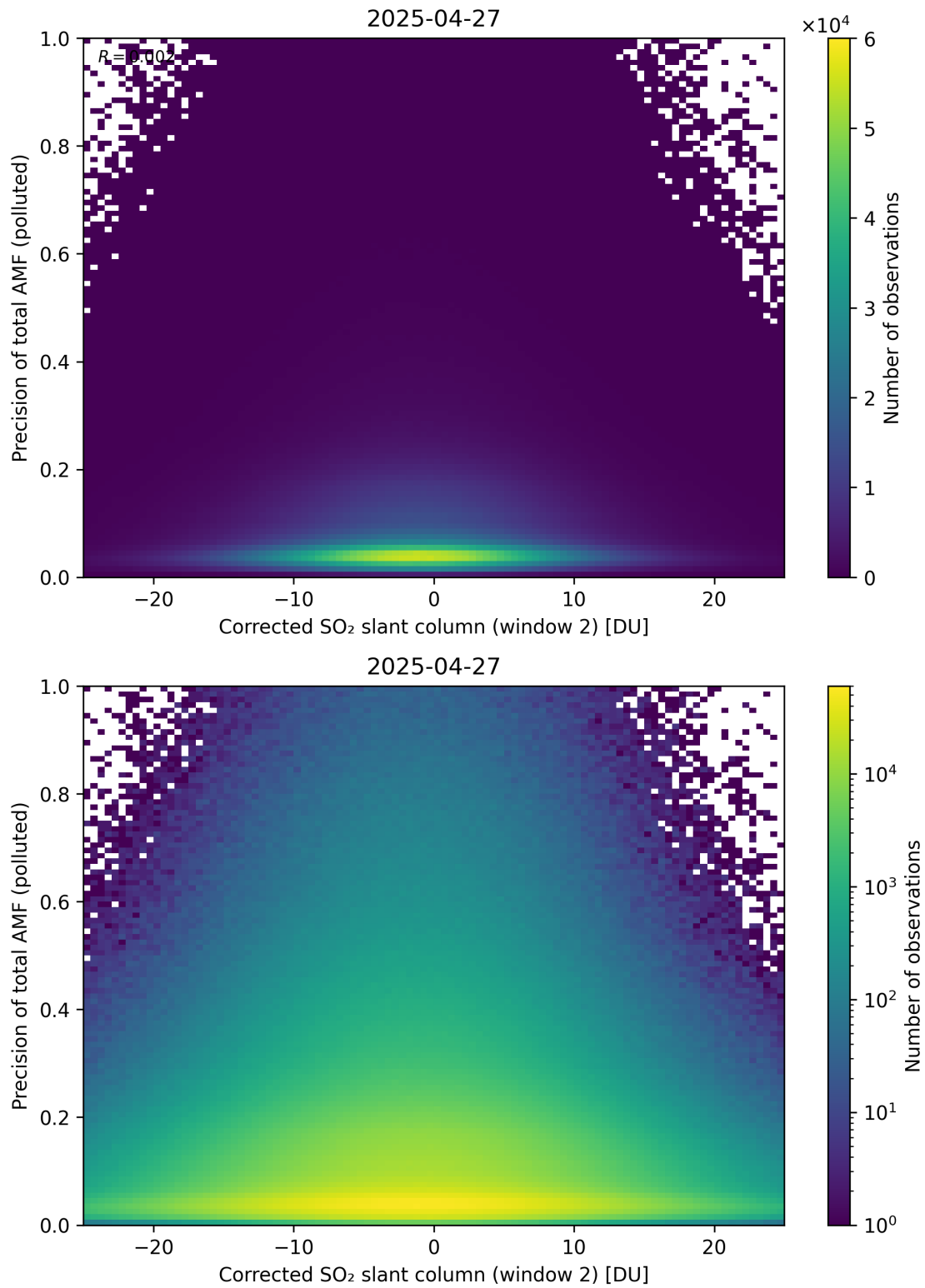
Figure 254: Scatter density plot of “Corrected SO 2 slant column (window 2)” against “Precision of total AMF (polluted)” for 2025-04-26 to 2025-04-28.
