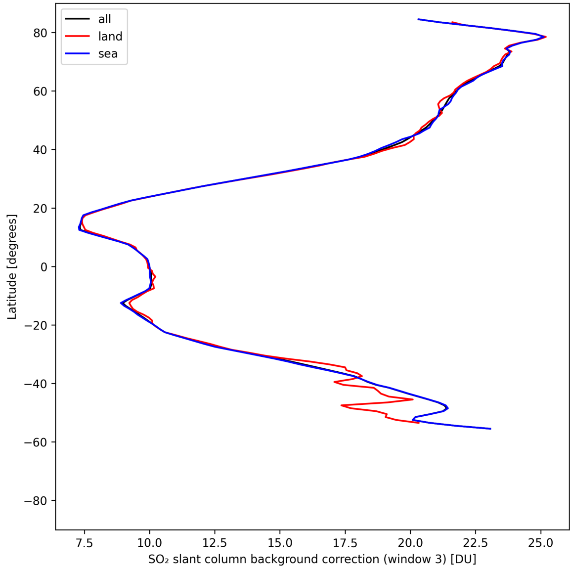
Figure 48: Zonal average of “SO 2 slant column background correction (window 3)” for 2025-04-26 to 2025-04-28.
