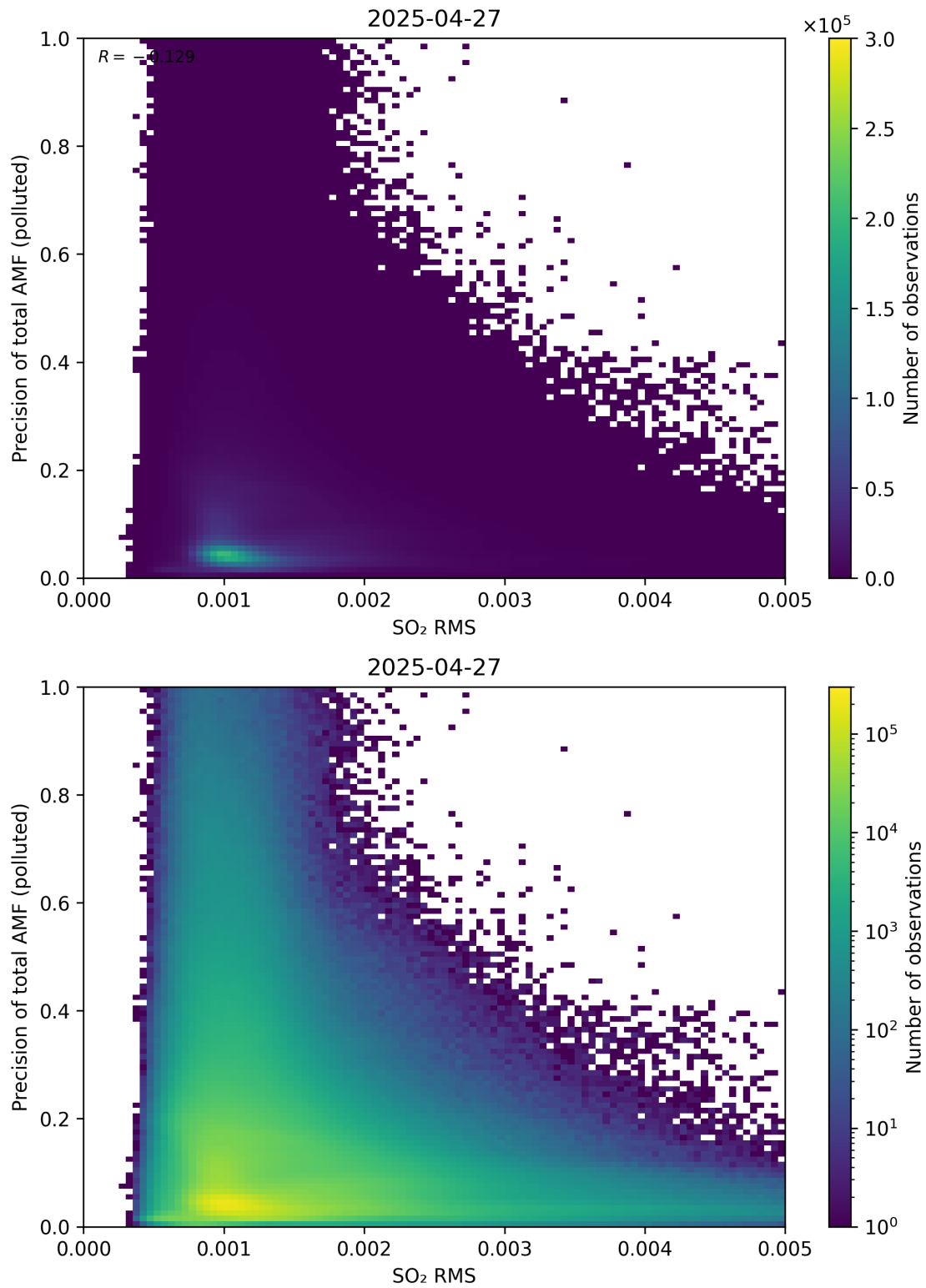
Figure 149: Scatter density plot of “SO 2 RMS” against “Precision of total AMF (polluted)” for 2025-04-26 to 2025-04-28.
