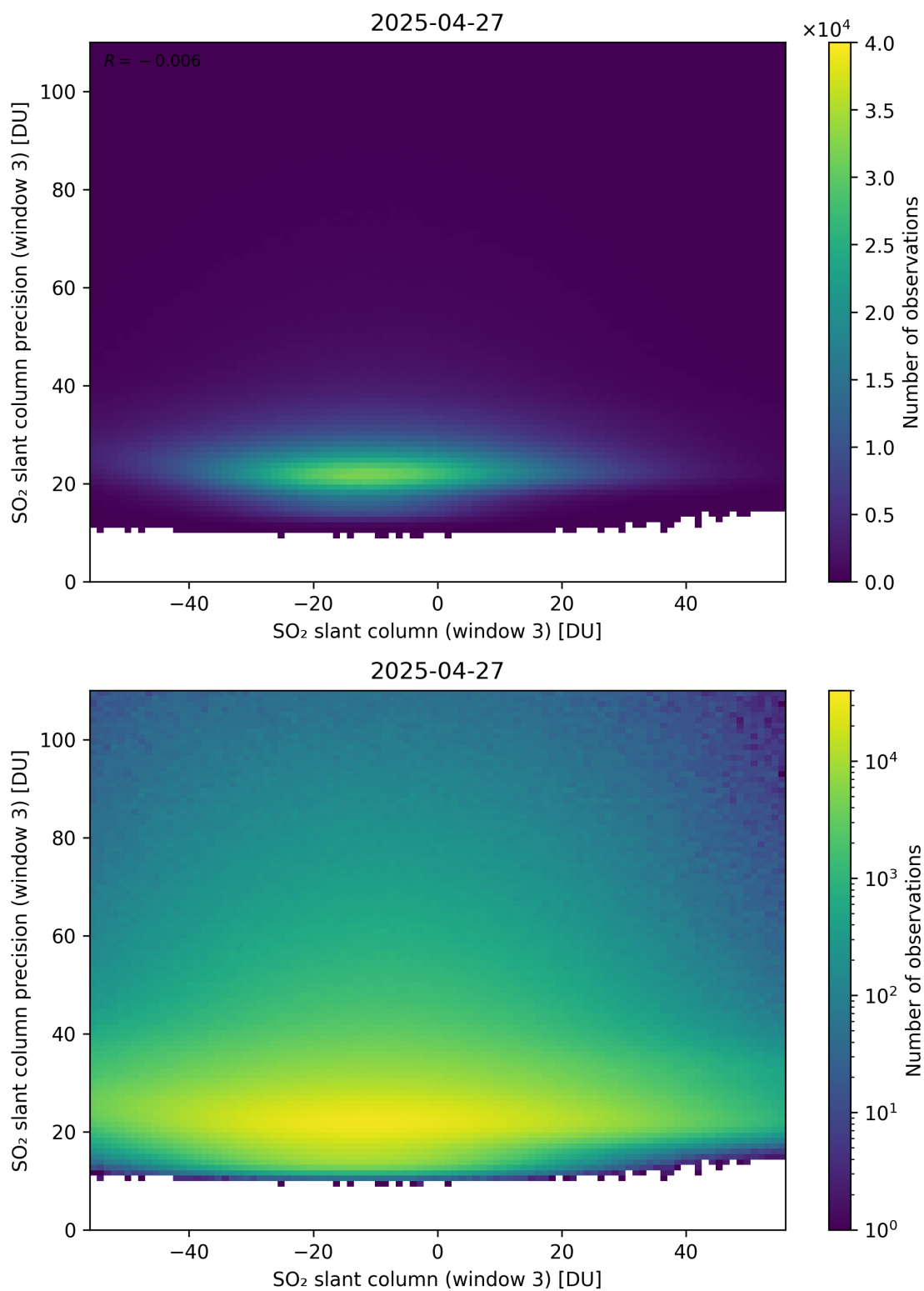
Figure 317: Scatter density plot of “SO 2 slant column (window 3)” against “SO 2 slant column precision (window 3)” for 2025-04-26 to 2025-04-28.
