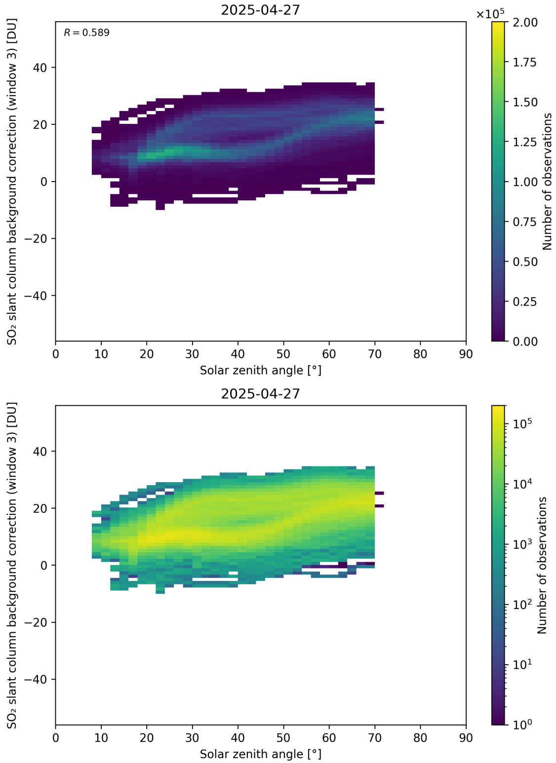
Figure 173: Scatter density plot of “Solar zenith angle” against “SO 2 slant column background correction (window 3)” for 2025-04-26 to 2025-04-28.
