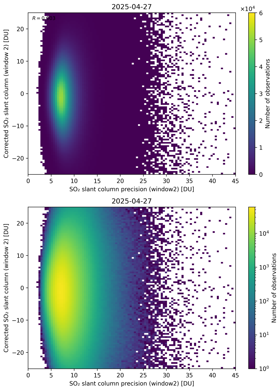
Figure 297: Scatter density plot of “SO 2 slant column precision (window2)” against “Corrected SO 2 slant column (window 2)” for 2025-04-26 to 2025-04-28.
