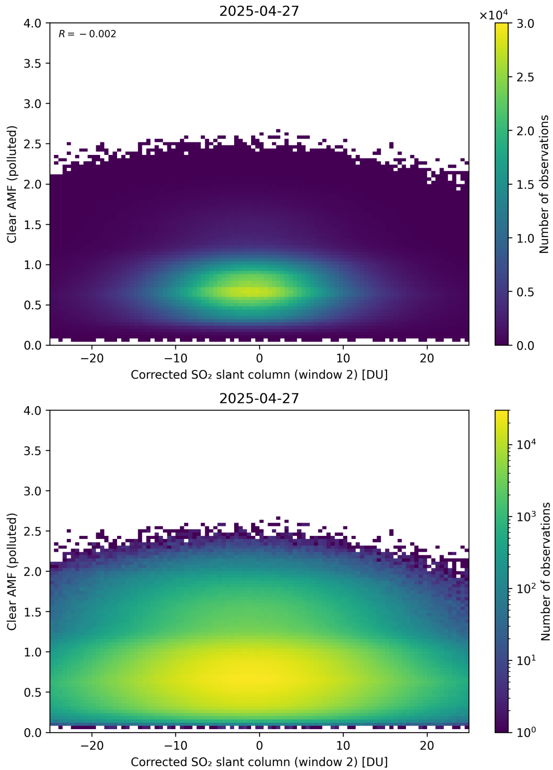
Figure 249: Scatter density plot of “Corrected SO 2 slant column (window 2)” against “Clear AMF (polluted)” for 2025-04-26 to 2025-04-28.
