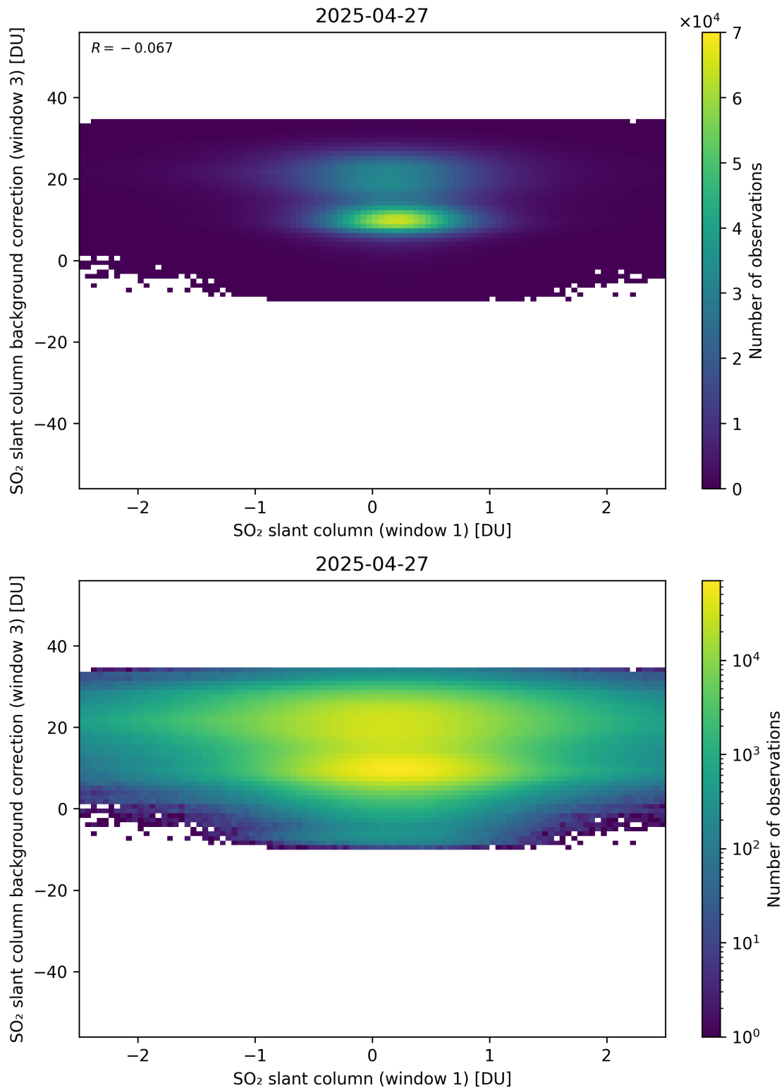
Figure 264: Scatter density plot of “SO 2 slant column (window 1)” against “SO 2 slant column background correction (window 3)” for 2025-04-26 to 2025-04-28.
