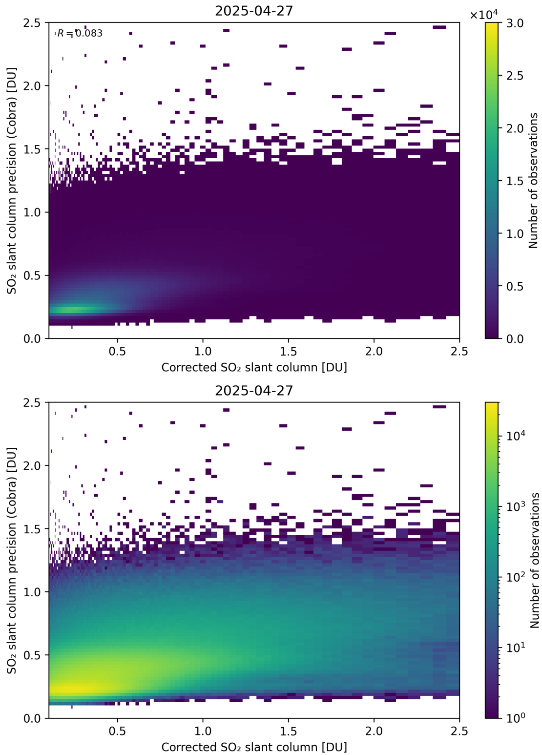
Figure 234: Scatter density plot of “Corrected SO 2 slant column” against “SO 2 slant column precision (Cobra)” for 2025-04-26 to 2025-04-28.
