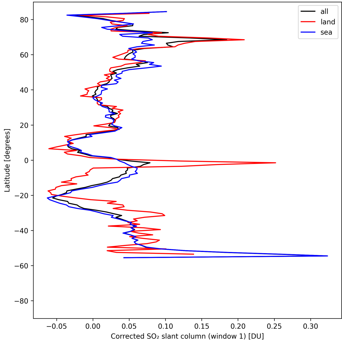
Figure 39: Zonal average of “Corrected SO 2 slant column (window 1)” for 2025-04-26 to 2025-04-28.
