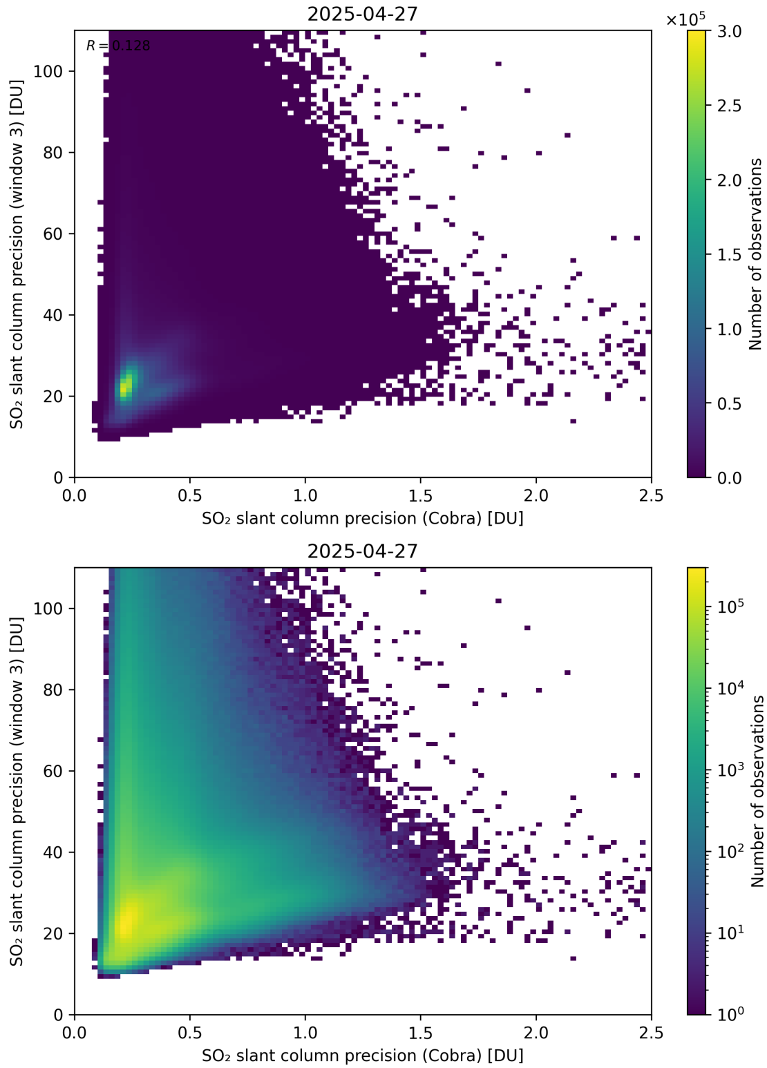
Figure 212: Scatter density plot of “SO 2 slant column precision (Cobra)” against “SO 2 slant column precision (window 3)” for 2025-04-26 to 2025-04-28.
