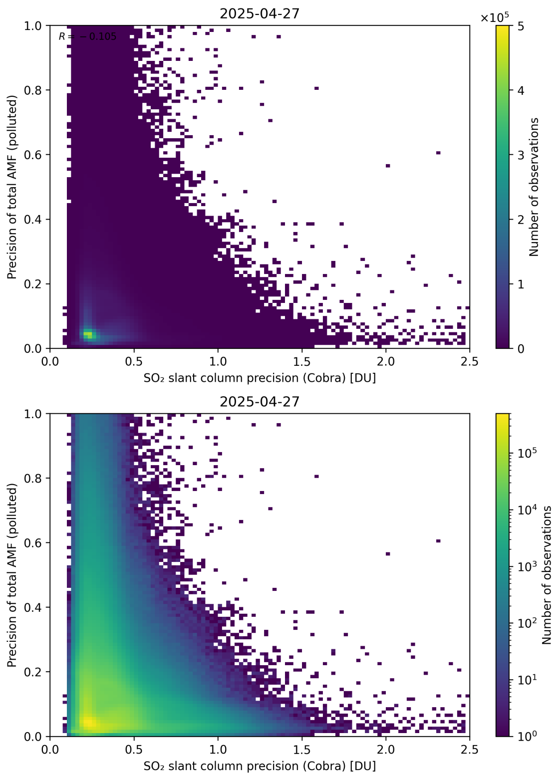
Figure 214: Scatter density plot of “SO 2 slant column precision (Cobra)” against “Precision of total AMF (polluted)” for 2025-04-26 to 2025-04-28.
