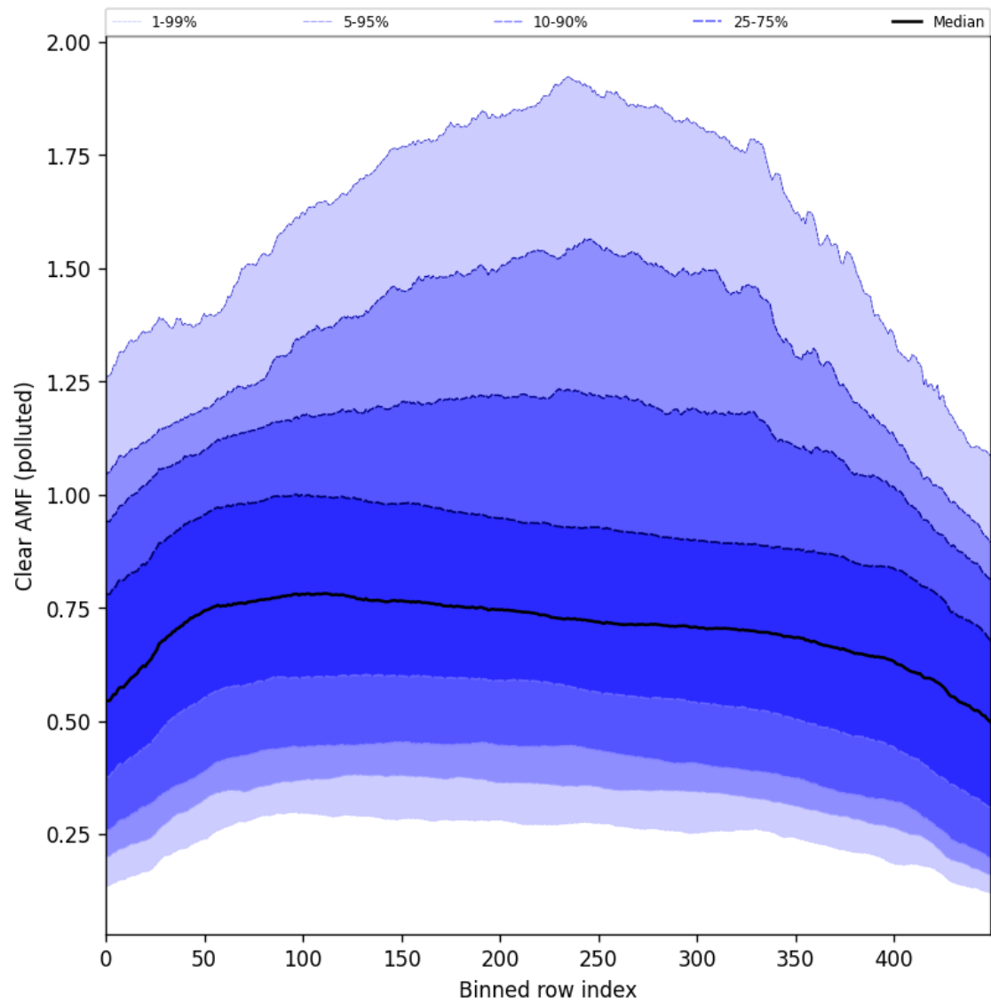
Figure 107: Along track statistics of “Clear AMF (polluted)” for 2025-04-26 to 2025-04-28
