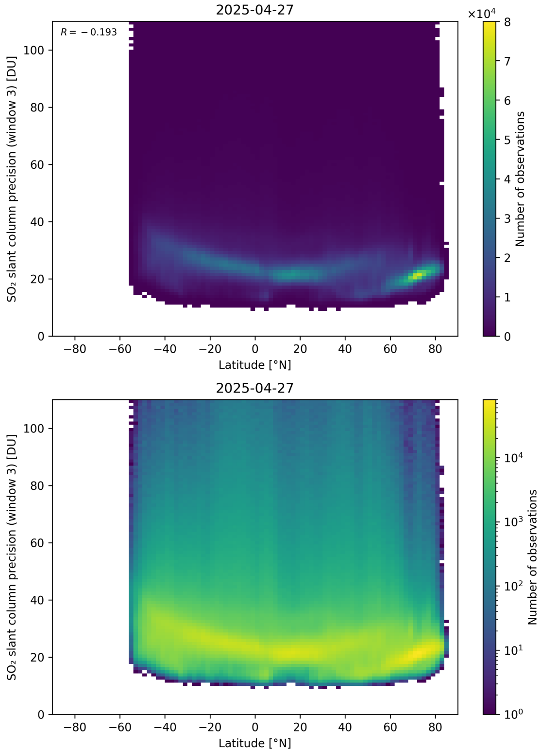
Figure 166: Scatter density plot of “Latitude” against “SO 2 slant column precision (window 3)” for 2025-04-26 to 2025-04-28.
