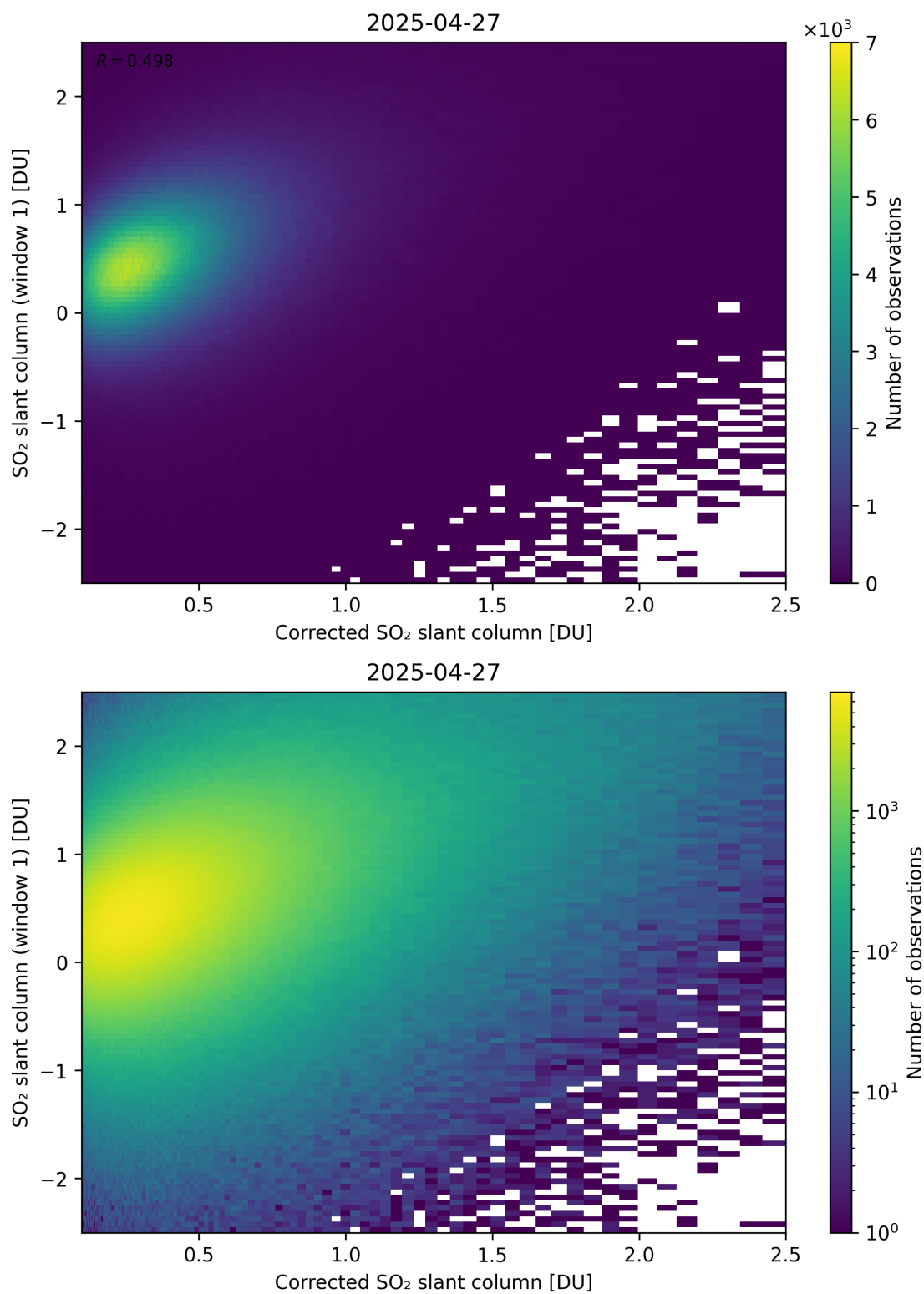
Figure 237: Scatter density plot of “Corrected SO 2 slant column” against “SO 2 slant column (window 1)” for 2025-04-26 to 2025-04-28.
