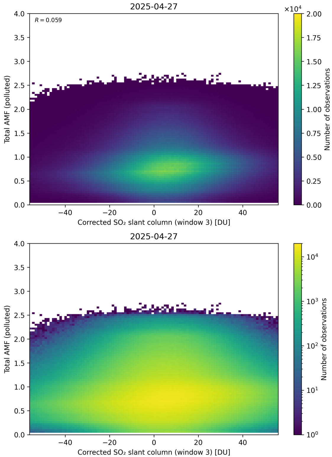
Figure 260: Scatter density plot of “Corrected SO 2 slant column (window 3)” against “Total AMF (polluted)” for 2025-04-26 to 2025-04-28.
