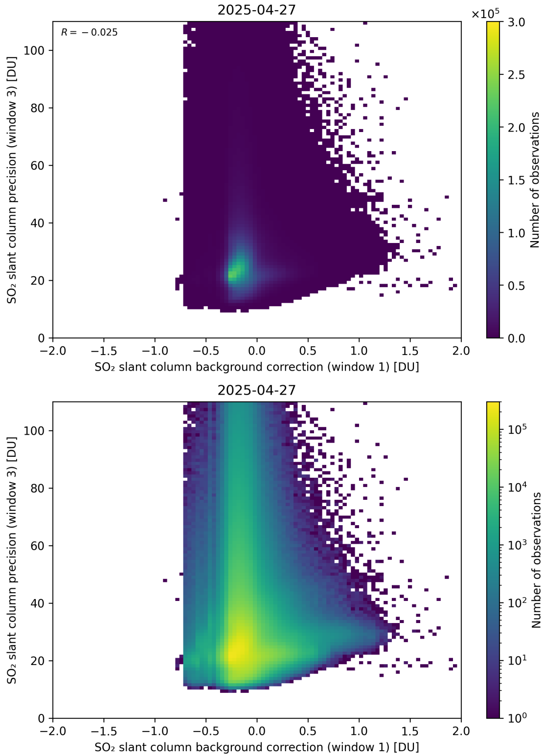
Figure 119: Scatter density plot of “SO 2 slant column background correction (window 1)” against “SO 2 slant column precision (window 3)” for 2025-04-26 to 2025-04-28.
