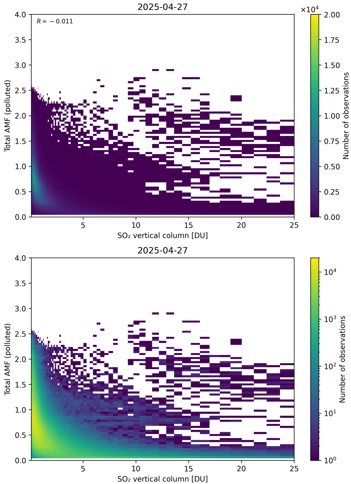
Figure 359: Scatter density plot of “SO 2 vertical column” against “Total AMF (polluted)” for 2025-04-26 to 2025-04-28.
