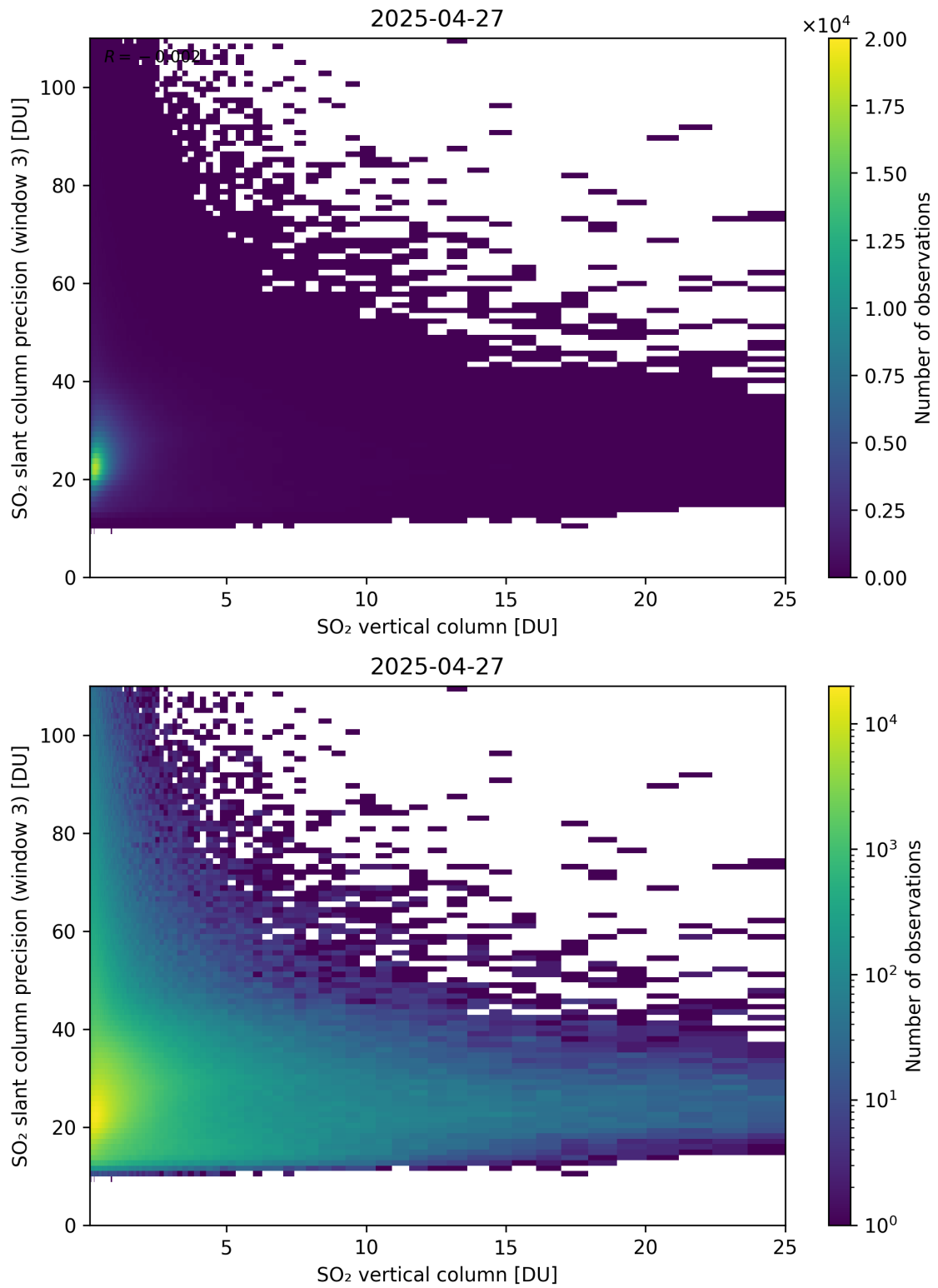
Figure 358: Scatter density plot of “SO 2 vertical column” against “SO 2 slant column precision (window 3)” for 2025-04-26 to 2025-04-28.
