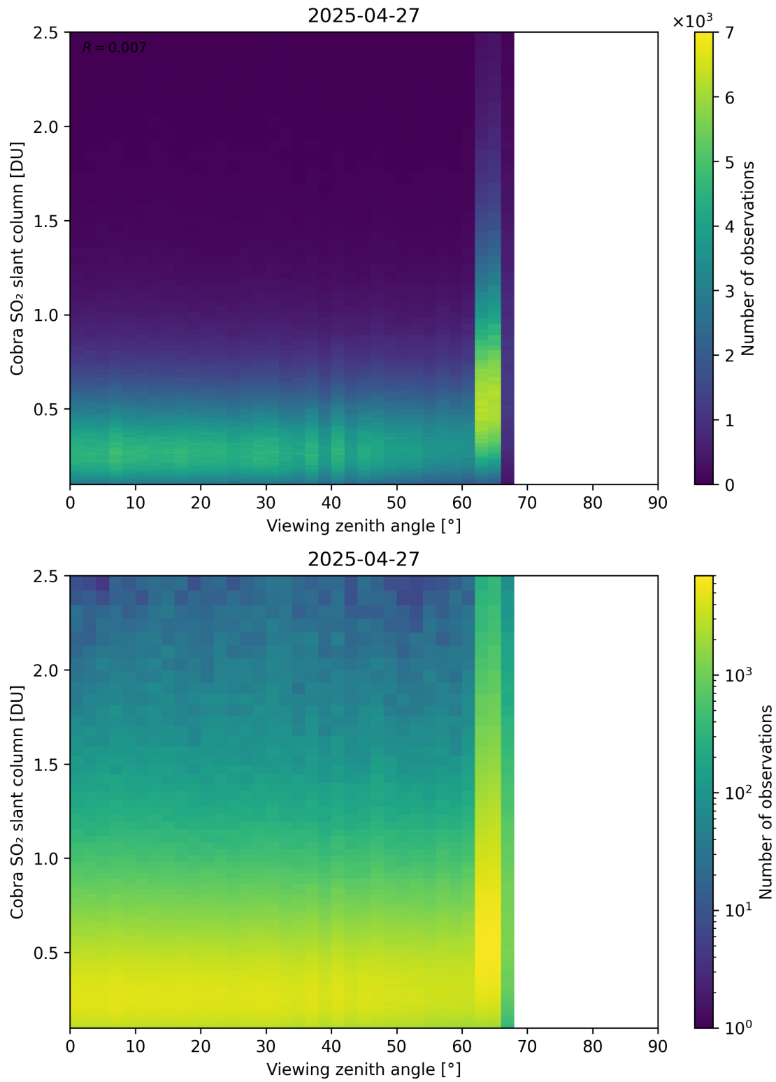
Figure 371: Scatter density plot of “Viewing zenith angle” against “Cobra SO 2 slant column” for 2025-04-26 to 2025-04-28.
