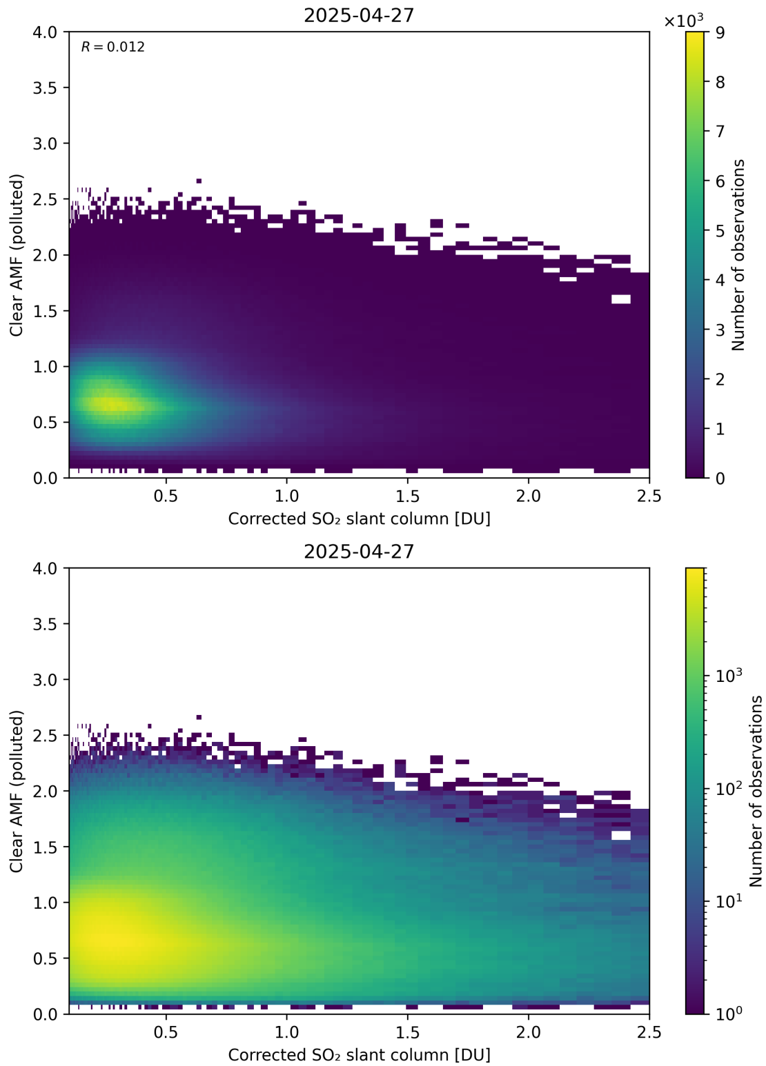
Figure 232: Scatter density plot of “Corrected SO 2 slant column” against “Clear AMF (polluted)” for 2025-04-26 to 2025-04-28.
