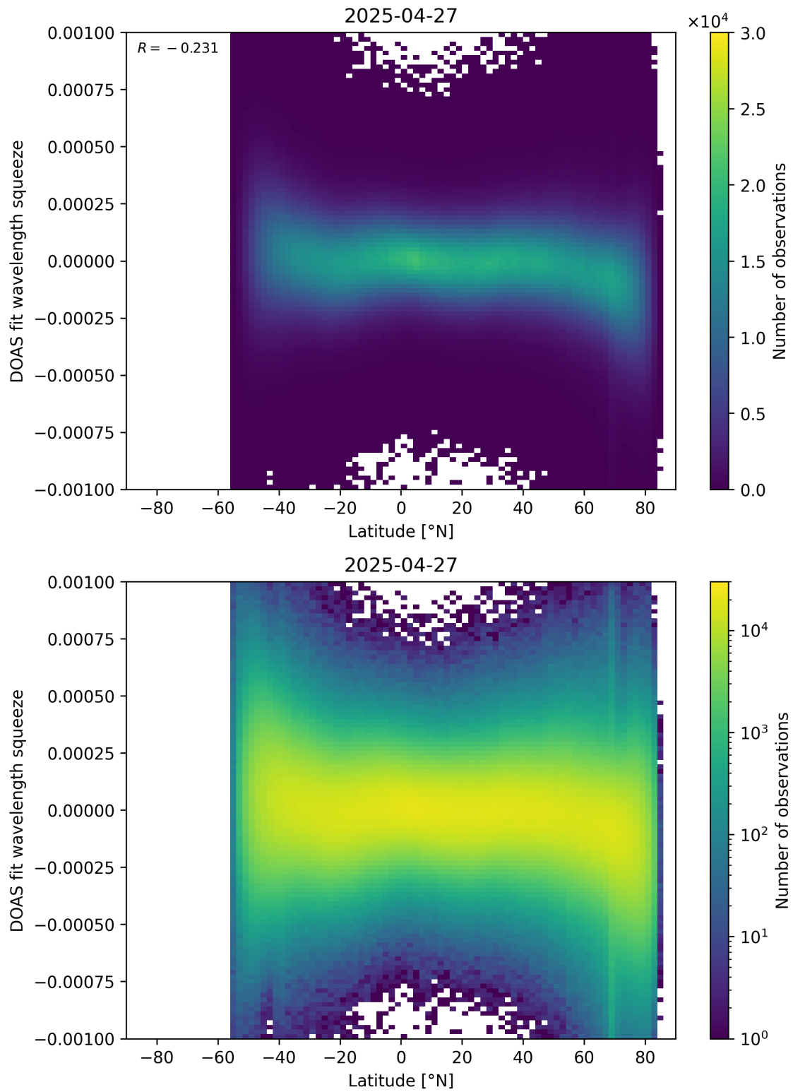
Figure 154: Scatter density plot of “Latitude” against “DOAS fit wavelength squeeze” for 2025-04-26 to 2025-04-28.
