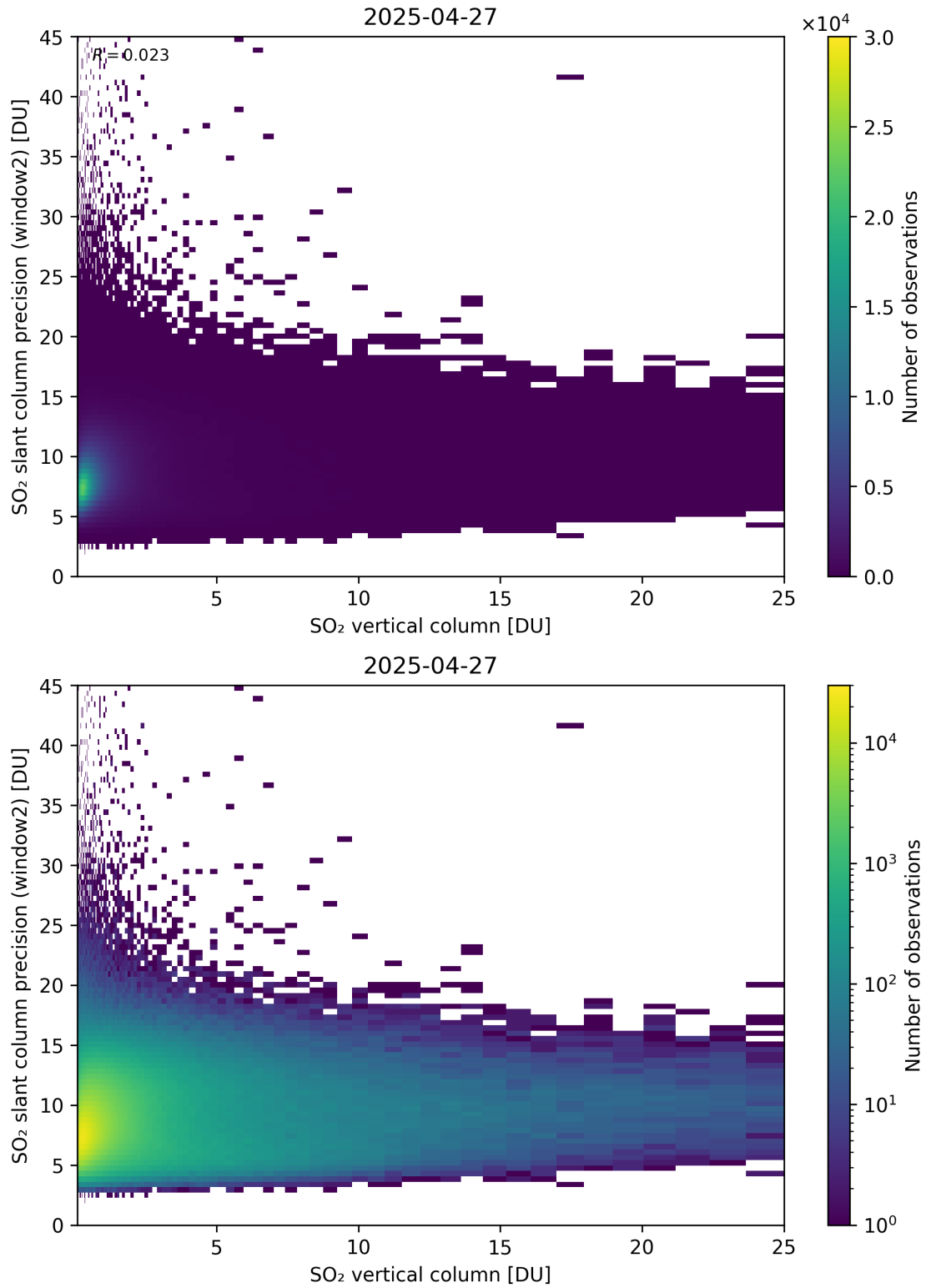
Figure 356: Scatter density plot of “SO 2 vertical column” against “SO 2 slant column precision (window2)” for 2025-04-26 to 2025-04-28.
