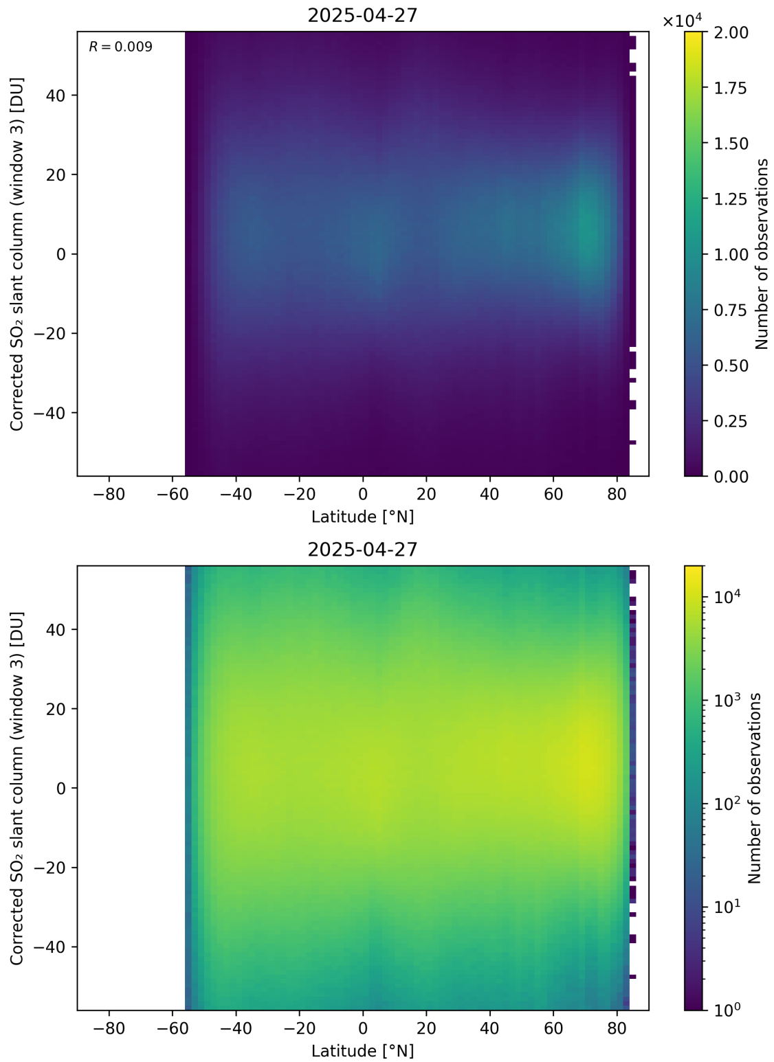
Figure 161: Scatter density plot of “Latitude” against “Corrected SO 2 slant column (window 3)” for 2025-04-26 to 2025-04-28.
