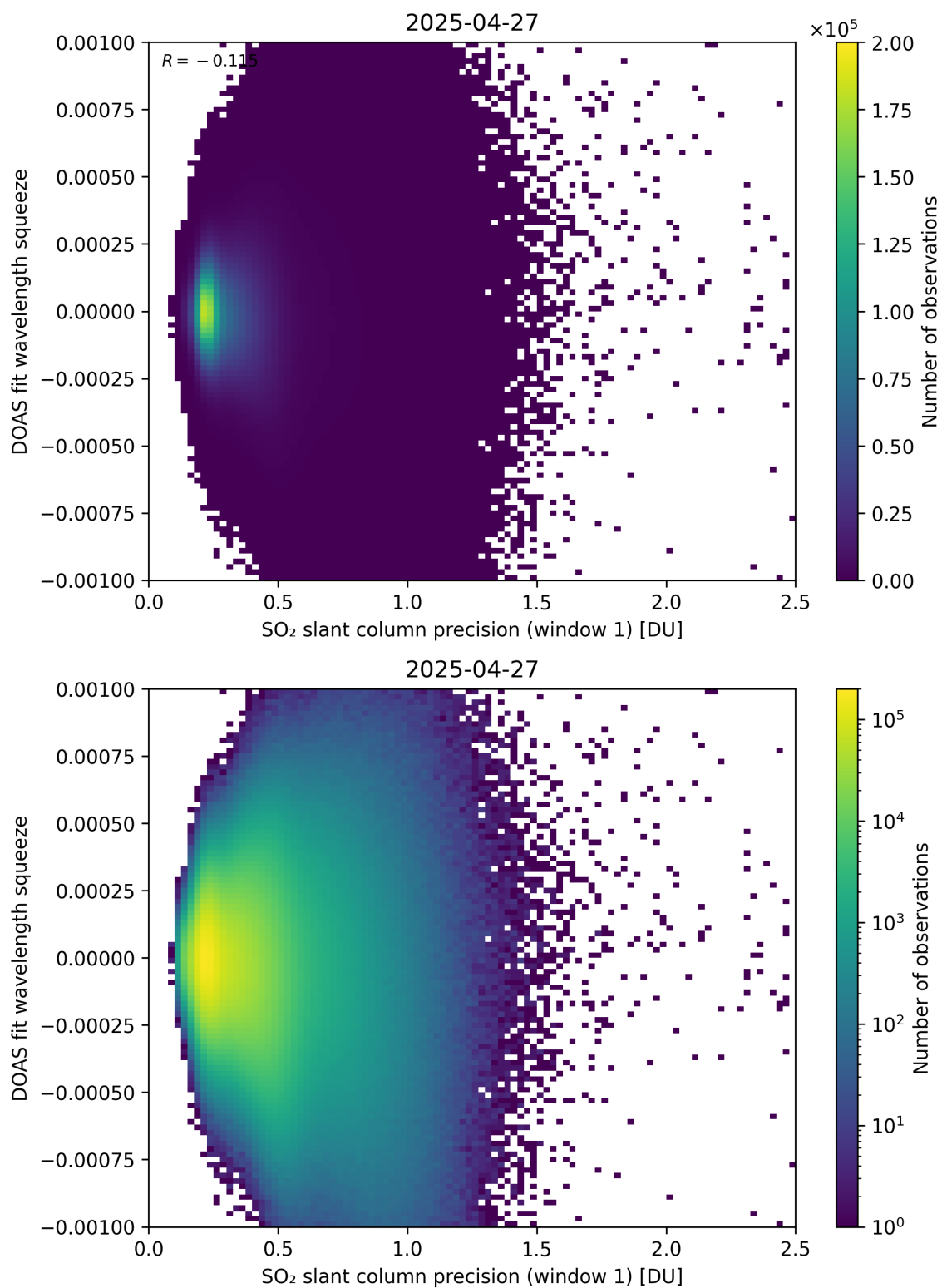
Figure 272: Scatter density plot of “SO 2 slant column precision (window 1)” against “DOAS fit wavelength squeeze” for 2025-04-26 to 2025-04-28.
