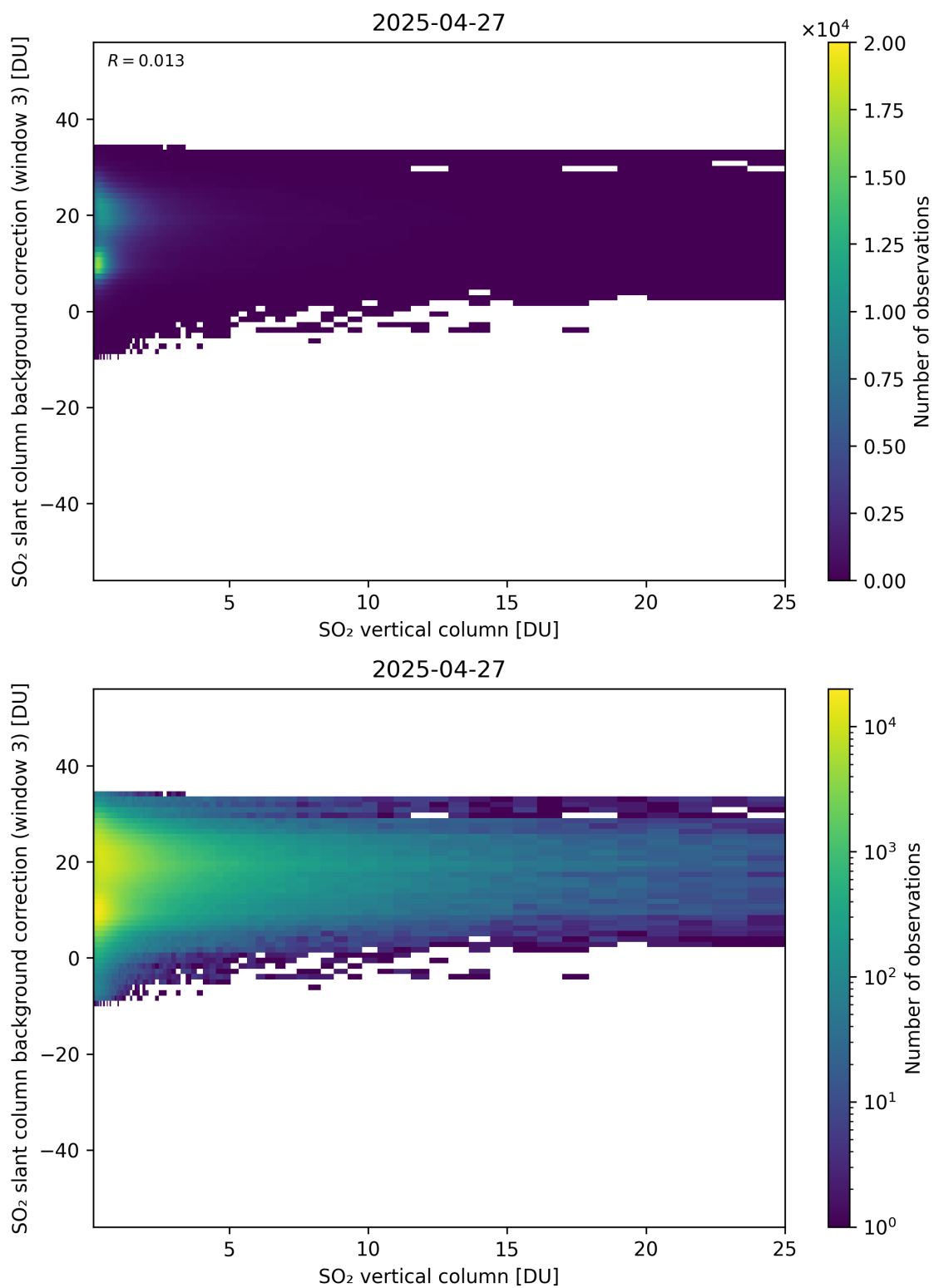
Figure 325: Scatter density plot of “SO 2 vertical column” against “SO 2 slant column background correction (window 3)” for 2025-04-26 to 2025-04-28.
