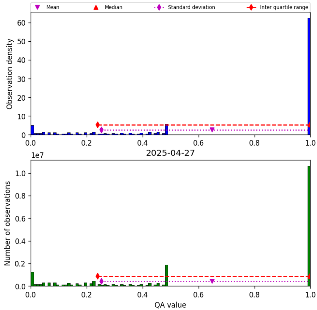
Figure 57: Histogram of “QA value” for 2025-04-26 to 2025-04-28
