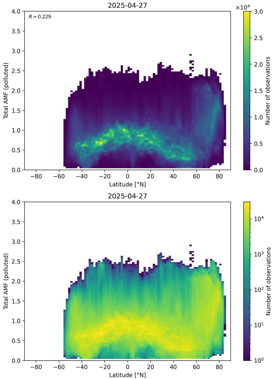
Figure 167: Scatter density plot of “Latitude” against “Total AMF (polluted)” for 2025-04-26 to 2025-04-28.
