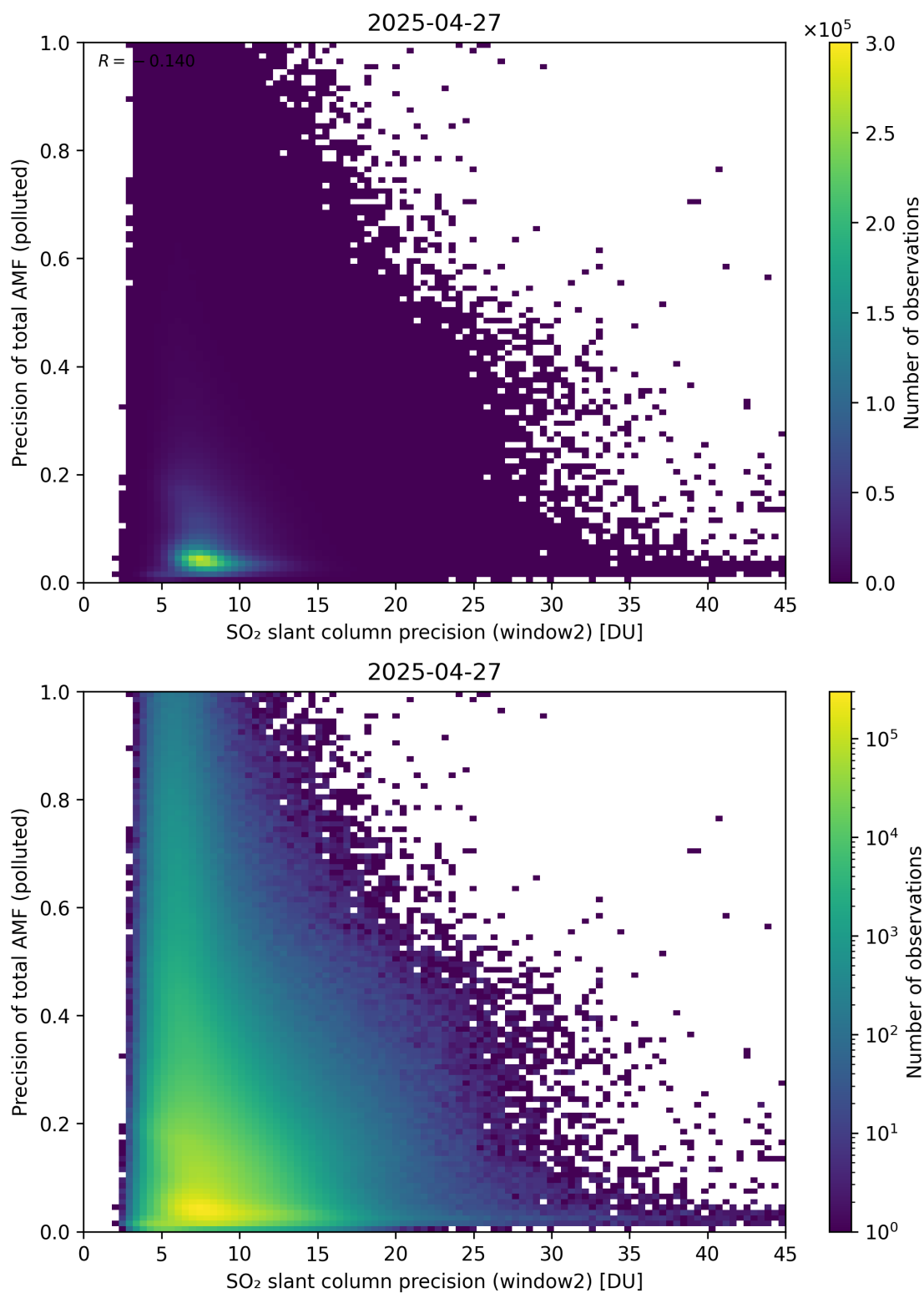
Figure 302: Scatter density plot of “SO 2 slant column precision (window2)” against “Precision of total AMF (polluted)” for 2025-04-26 to 2025-04-28.
