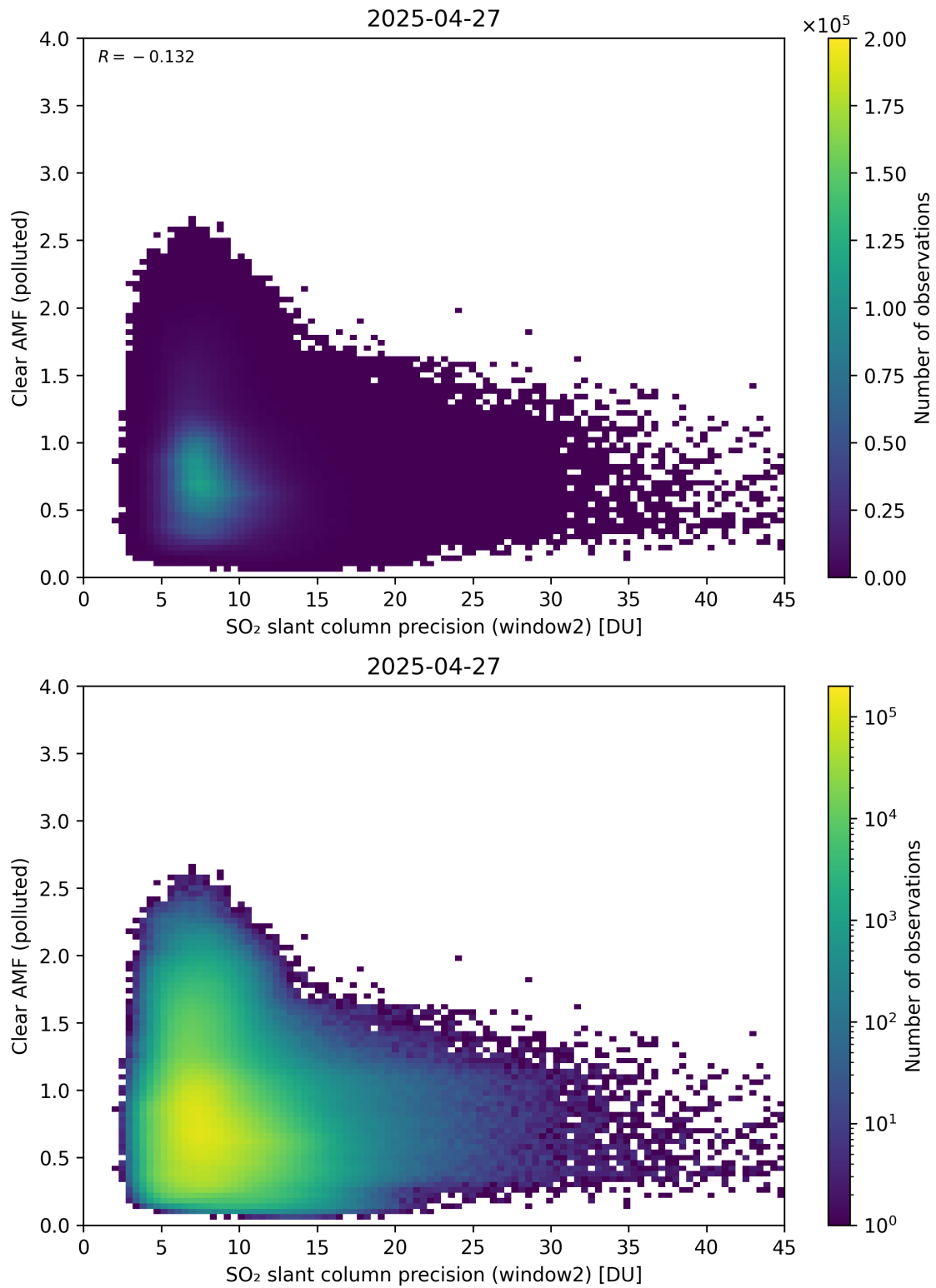
Figure 296: Scatter density plot of “SO 2 slant column precision (window2)” against “Clear AMF (polluted)” for 2025-04-26 to 2025-04-28.
