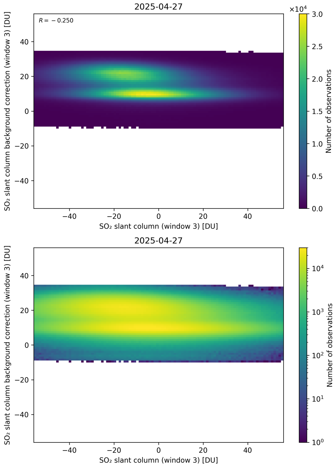
Figure 303: Scatter density plot of “SO 2 slant column (window 3)” against “SO 2 slant column background correction (window 3)” for 2025-04-26 to 2025-04-28.
