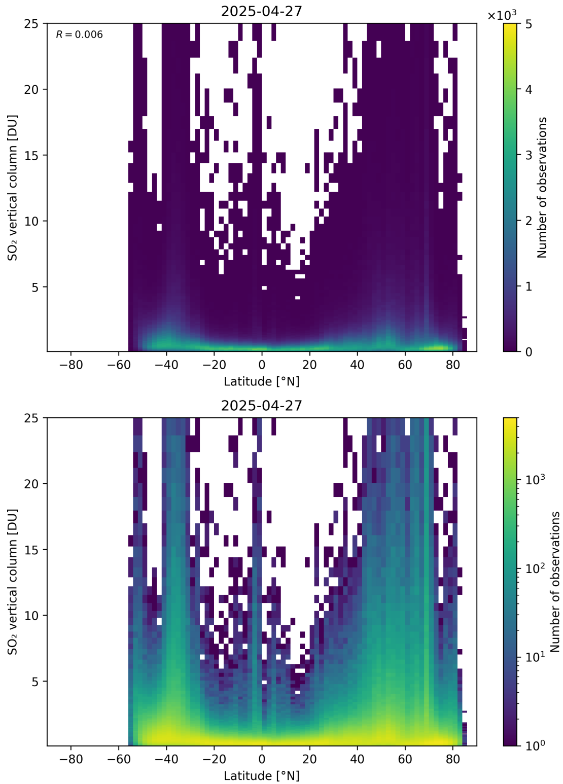
Figure 169: Scatter density plot of “Latitude” against “SO 2 vertical column” for 2025-04-26 to 2025-04-28.
