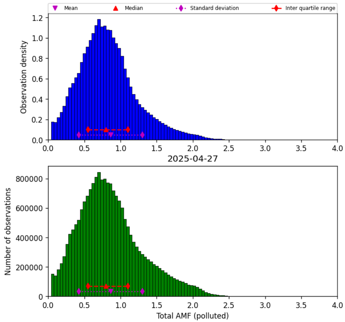
Figure 79: Histogram of “Total AMF (polluted)” for 2025-04-26 to 2025-04-28
