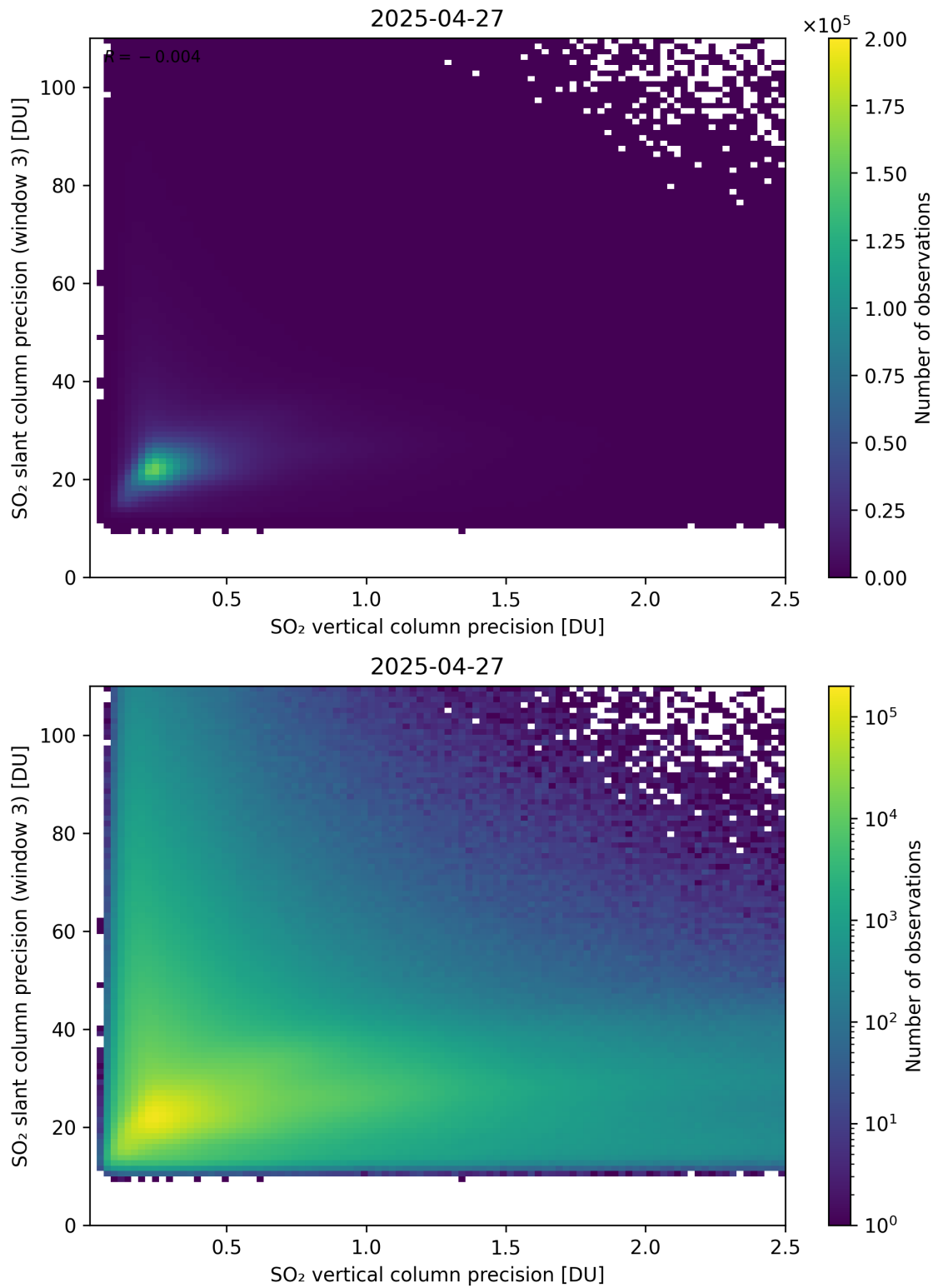
Figure 345: Scatter density plot of “SO 2 vertical column precision” against “SO 2 slant column precision (window 3)” for 2025-04-26 to 2025-04-28.
