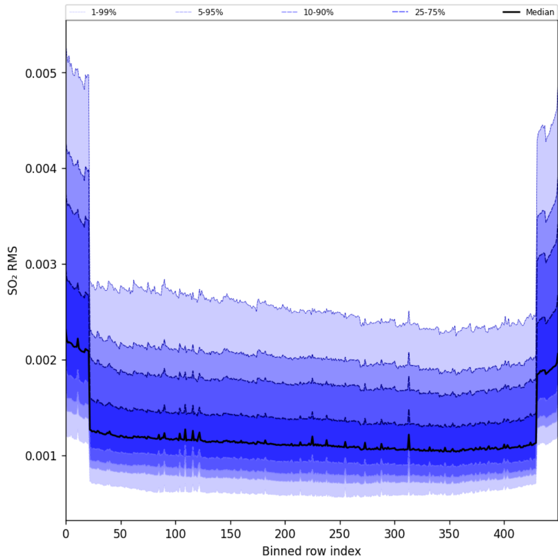
Figure 104: Along track statistics of “SO 2 RMS” for 2025-04-26 to 2025-04-28
