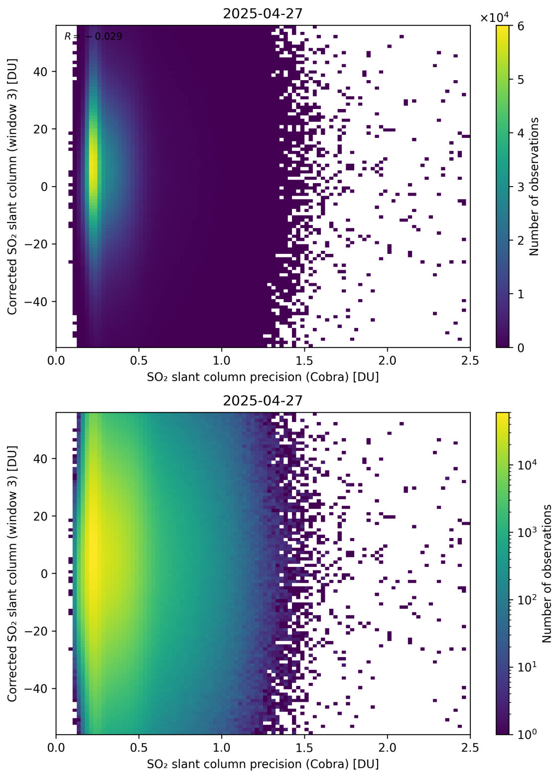
Figure 207: Scatter density plot of “SO 2 slant column precision (Cobra)” against “Corrected SO 2 slant column (window 3)” for 2025-04-26 to 2025-04-28.
