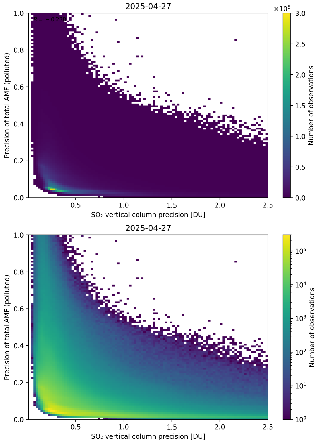
Figure 347: Scatter density plot of “SO 2 vertical column precision” against “Precision of total AMF (polluted)” for 2025-04-26 to 2025-04-28.
