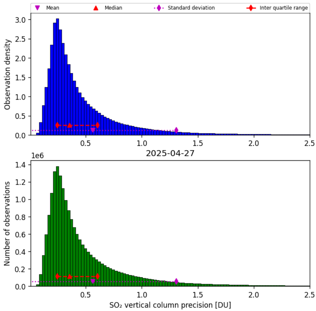
Figure 59: Histogram of “SO 2 vertical column precision” for 2025-04-26 to 2025-04-28
