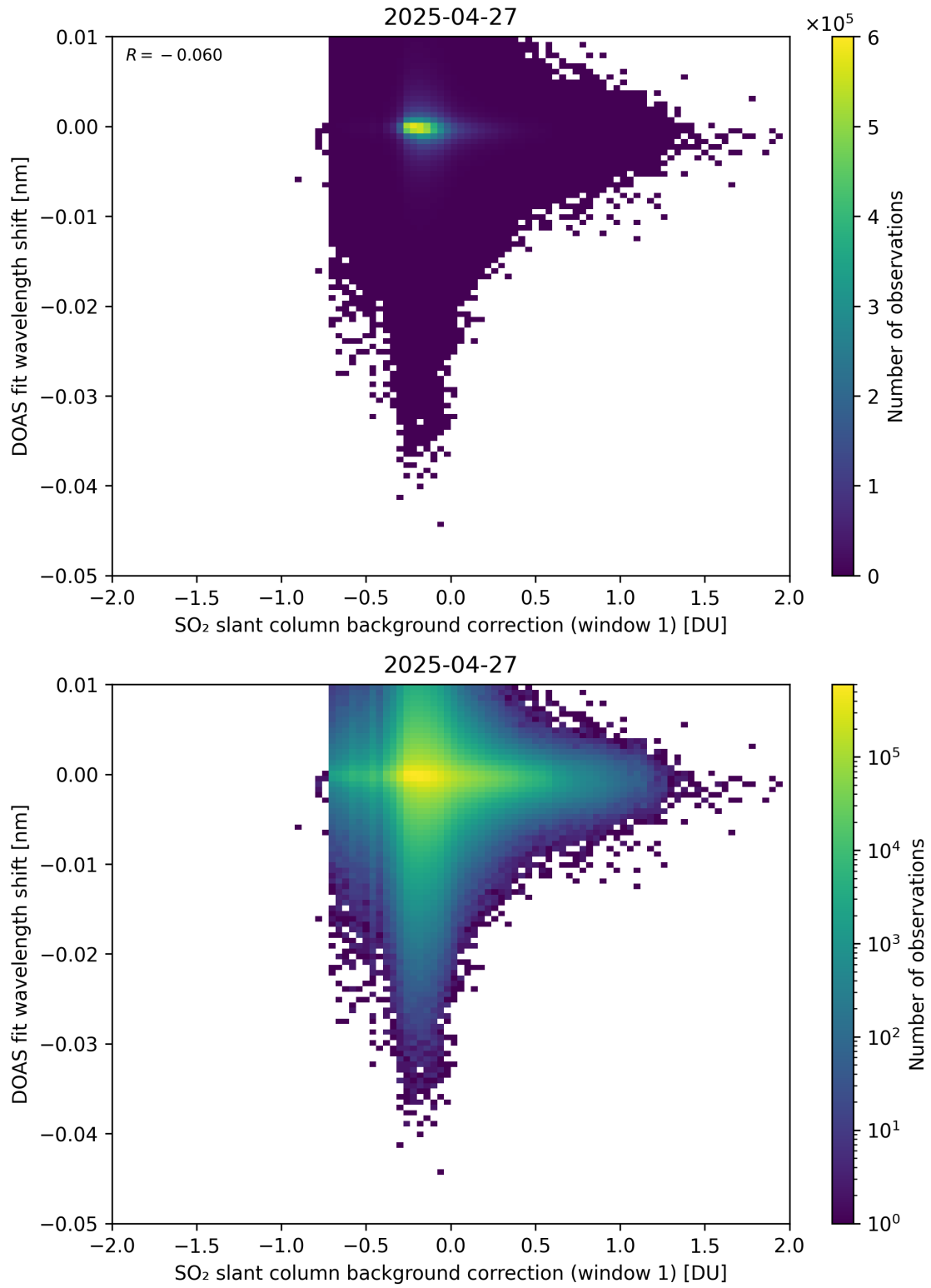
Figure 111: Scatter density plot of “SO 2 slant column background correction (window 1)” against “DOAS fit wavelength shift” for 2025-04-26 to 2025-04-28.
