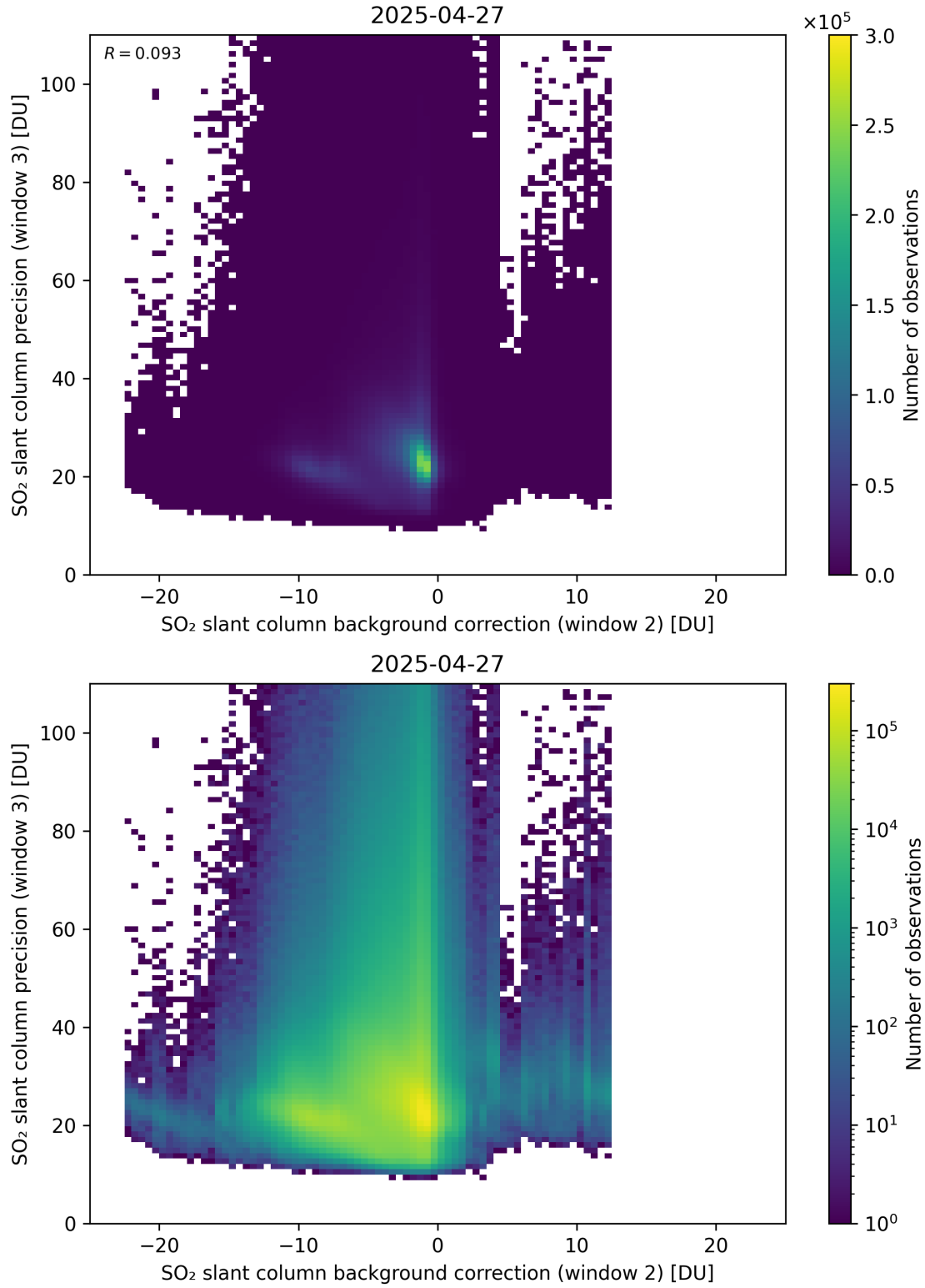
Figure 129: Scatter density plot of “SO 2 slant column background correction (window 2)” against “SO 2 slant column precision (window 3)” for 2025-04-26 to 2025-04-28.
