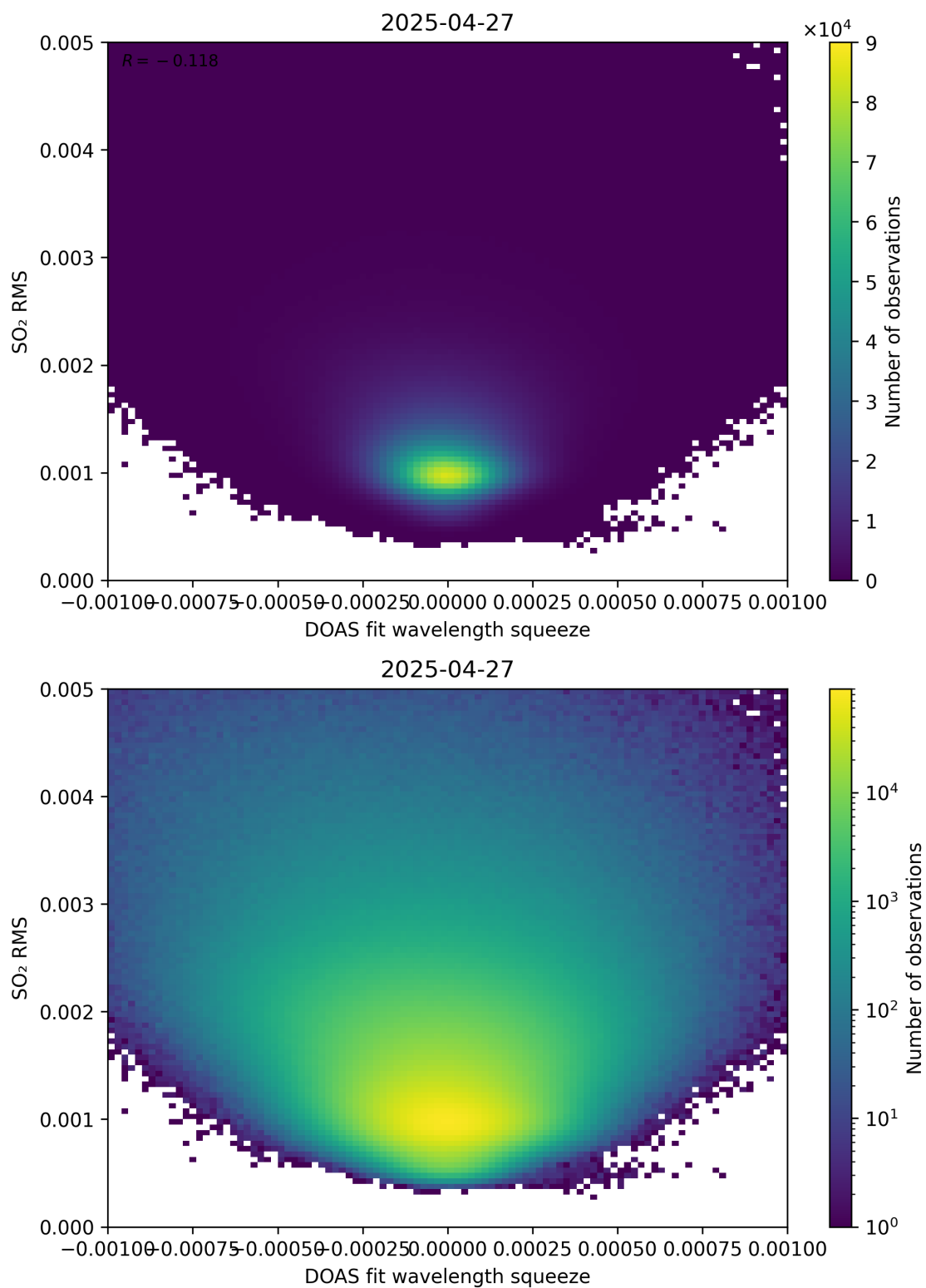
Figure 143: Scatter density plot of “DOAS fit wavelength squeeze” against “SO 2 RMS” for 2025-04-26 to 2025-04-28.
