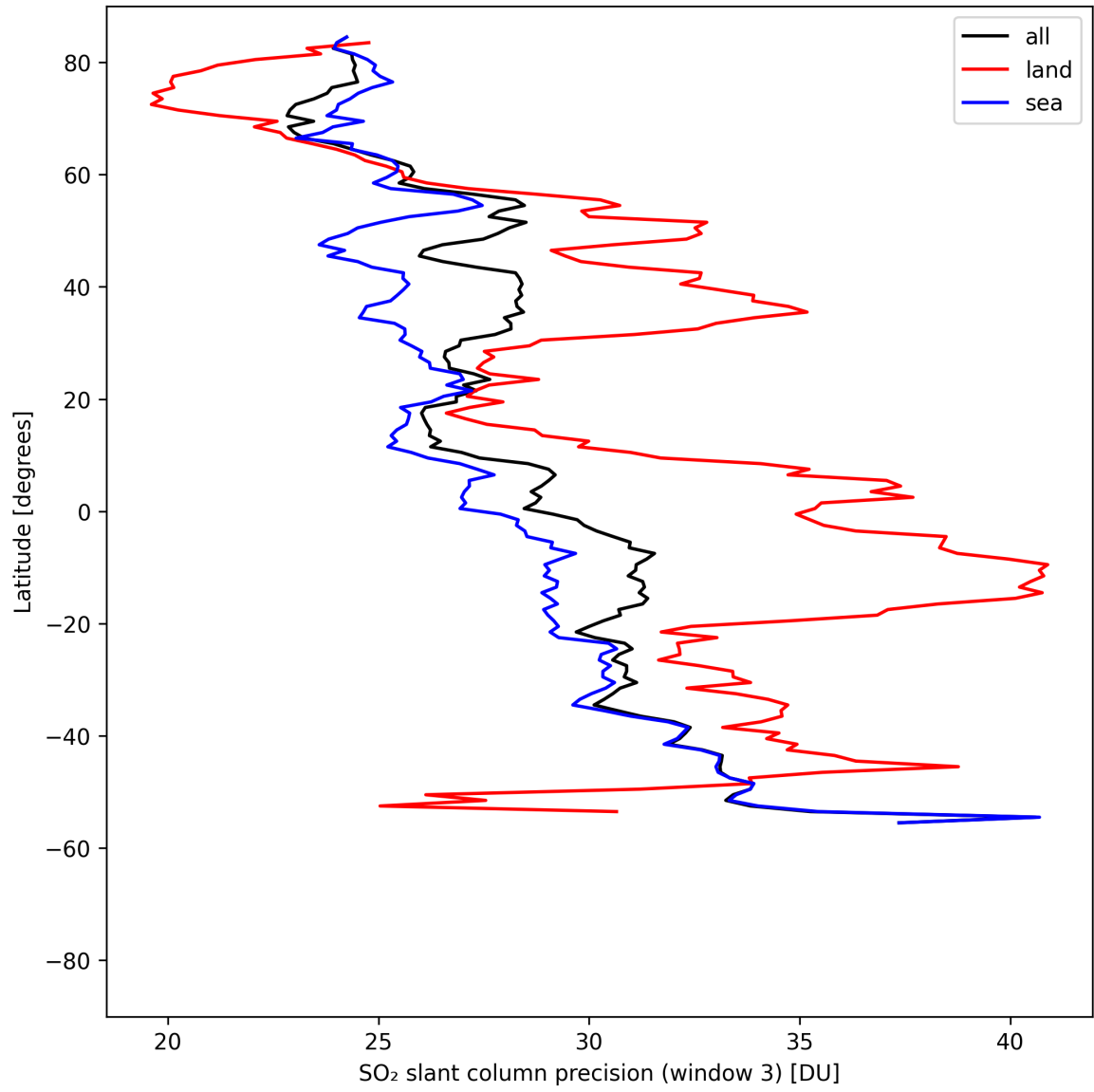
Figure 46: Zonal average of “SO 2 slant column precision (window 3)” for 2025-04-26 to 2025-04-28.
