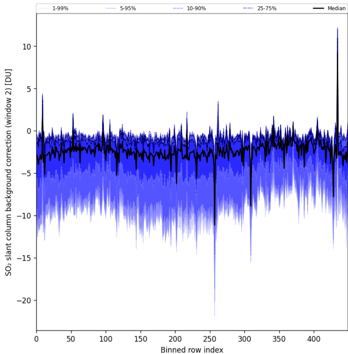
Figure 96: Along track statistics of “SO 2 slant column background correction (window 2)” for 2025-04-26 to 2025-04-28
