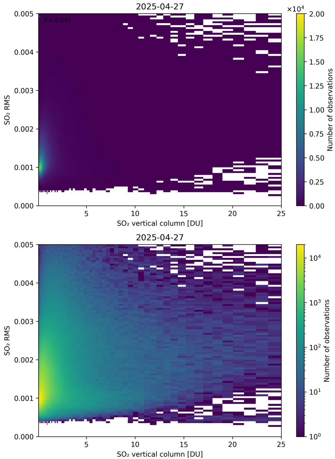
Figure 328: Scatter density plot of “SO 2 vertical column” against “SO 2 RMS” for 2025-04-26 to 2025-04-28.
