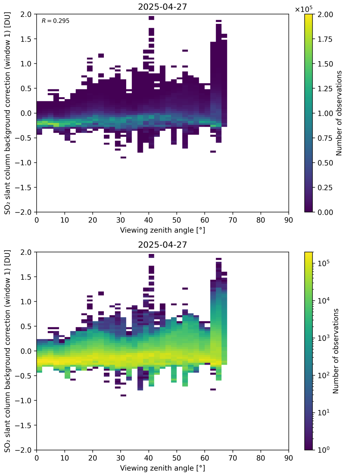
Figure 362: Scatter density plot of “Viewing zenith angle” against “SO 2 slant column background correction (window 1)” for 2025-04-26 to 2025-04-28.
