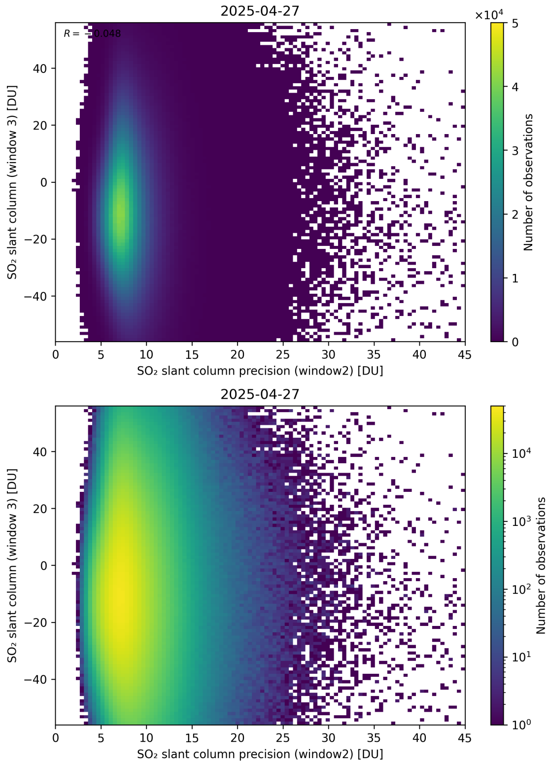
Figure 299: Scatter density plot of “SO 2 slant column precision (window2)” against “SO 2 slant column (window 3)” for 2025-04-26 to 2025-04-28.
