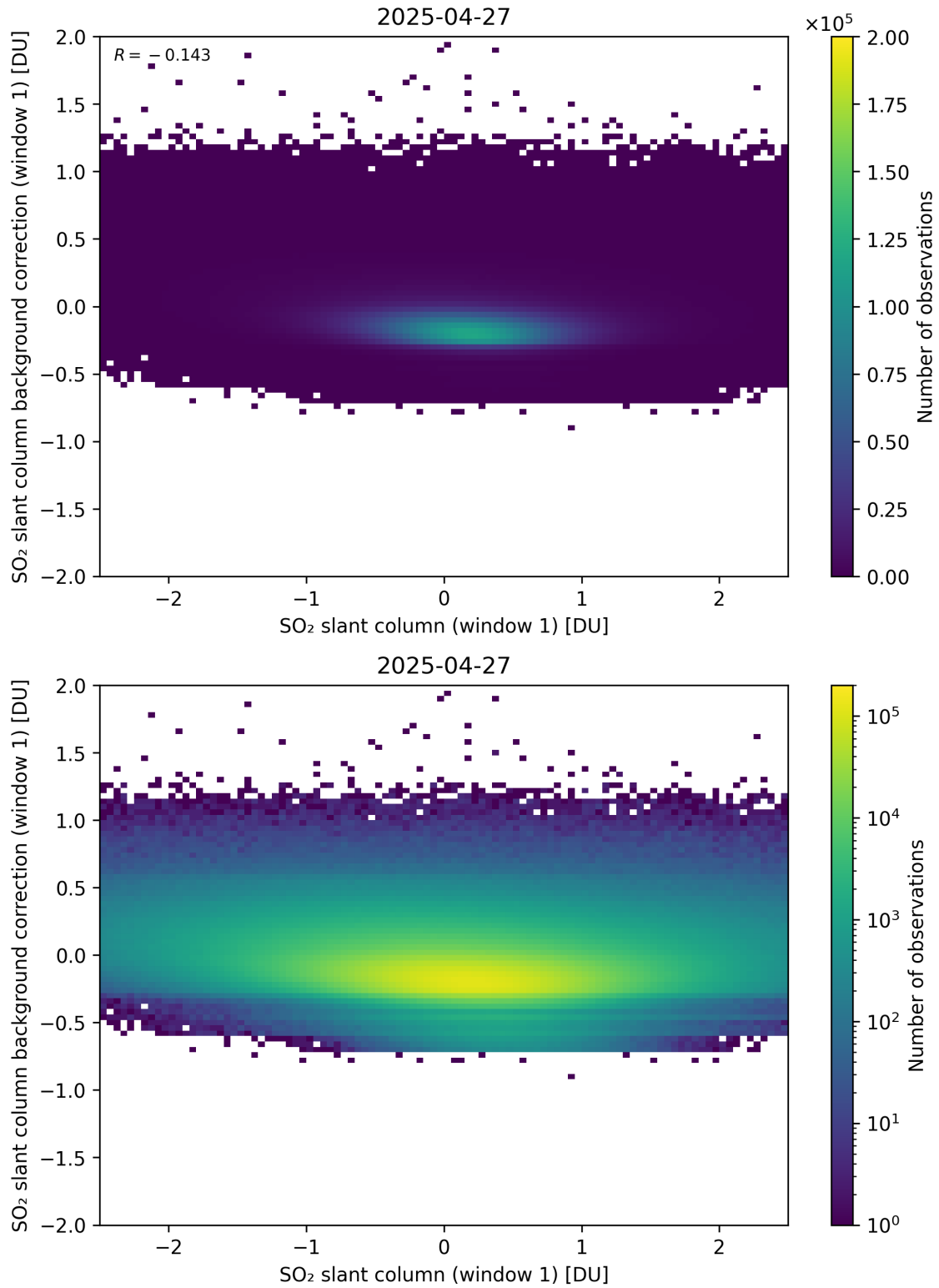
Figure 262: Scatter density plot of “SO 2 slant column (window 1)” against “SO 2 slant column background correction (window 1)” for 2025-04-26 to 2025-04-28.
