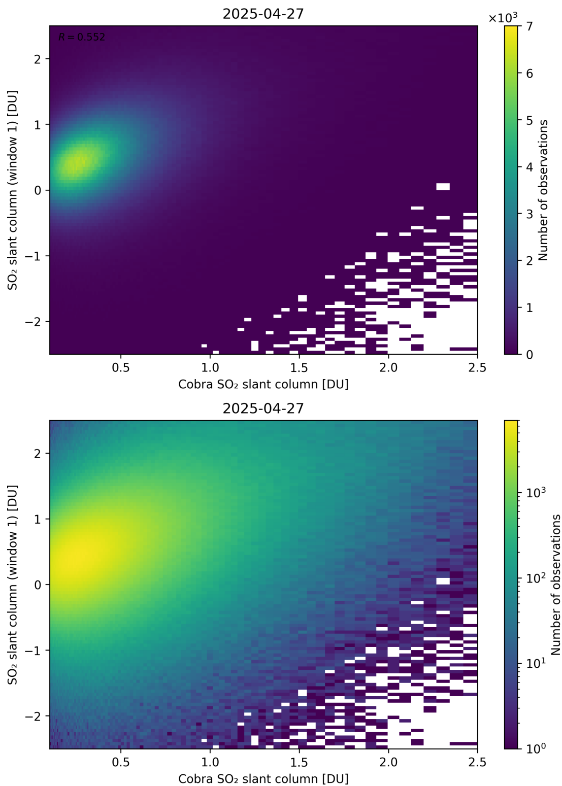
Figure 219: Scatter density plot of “Cobra SO 2 slant column” against “SO 2 slant column (window 1)” for 2025-04-26 to 2025-04-28.
