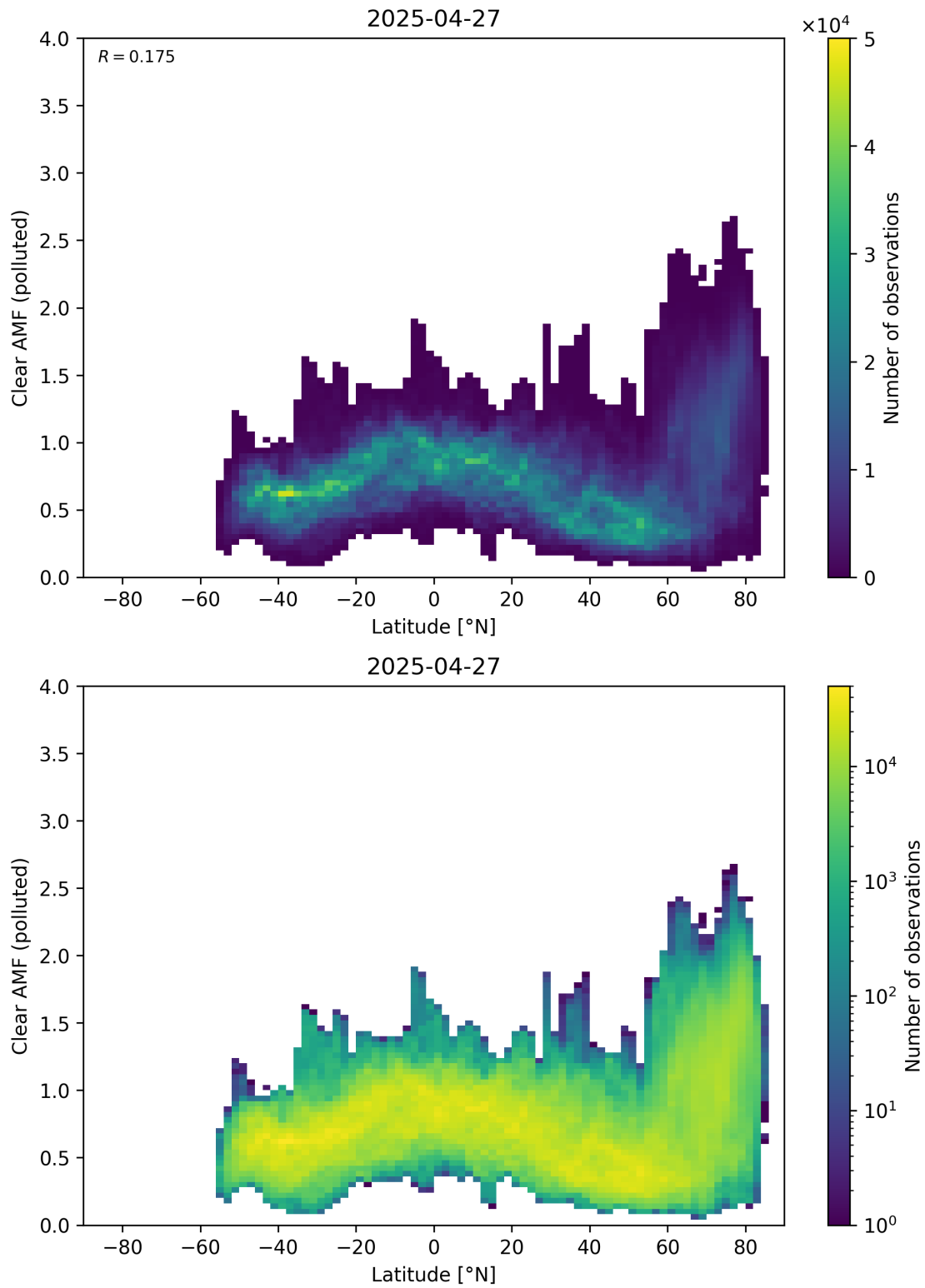
Figure 156: Scatter density plot of “Latitude” against “Clear AMF (polluted)” for 2025-04-26 to 2025-04-28.
