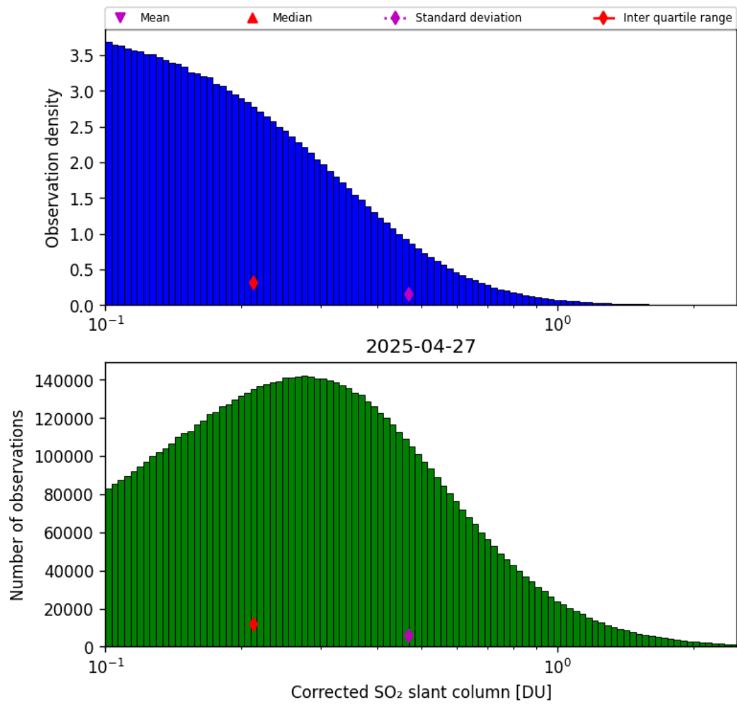
Figure 60: Histogram of “Corrected SO 2 slant column” for 2025-04-26 to 2025-04-28
