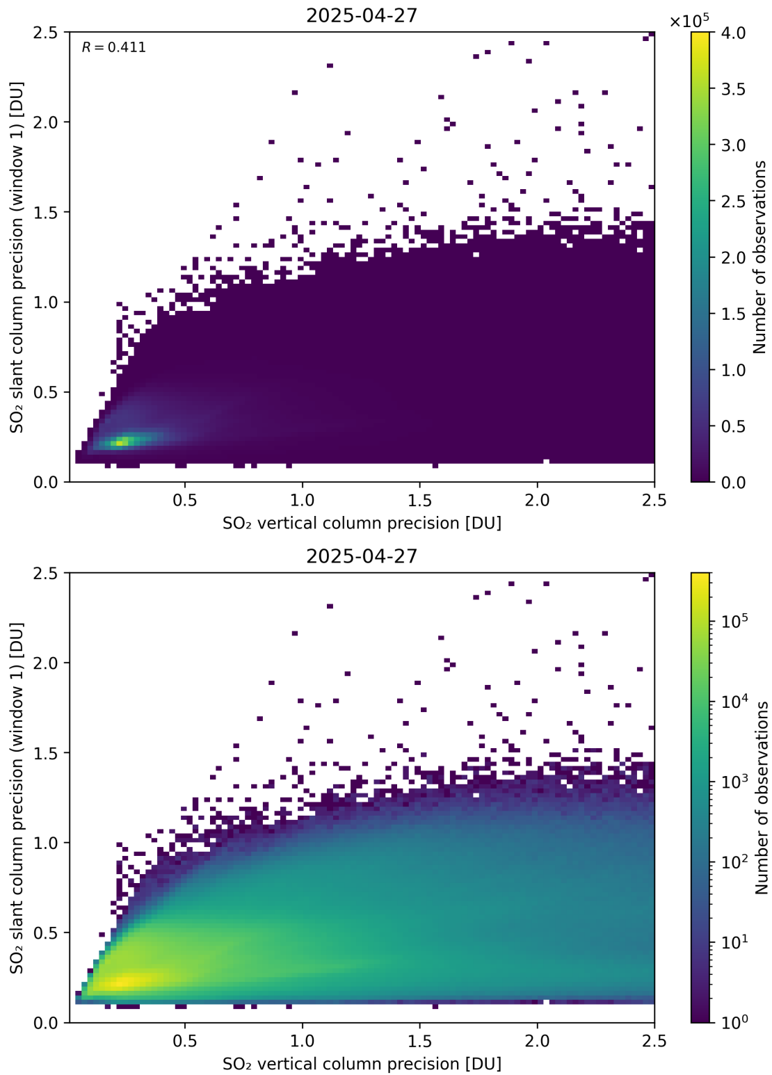
Figure 342: Scatter density plot of “SO 2 vertical column precision” against “SO 2 slant column precision (window 1)” for 2025-04-26 to 2025-04-28.
