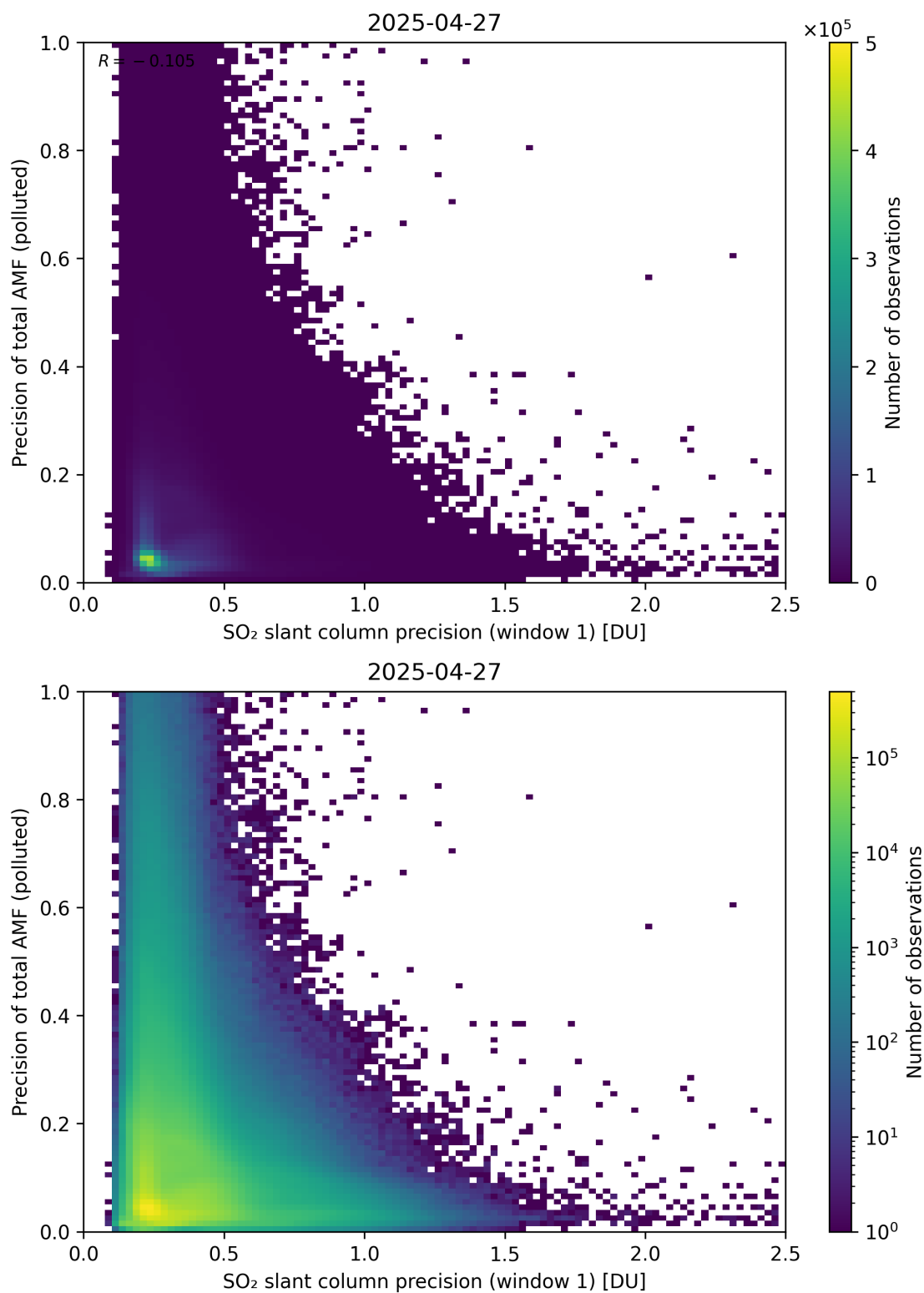
Figure 281: Scatter density plot of “SO 2 slant column precision (window 1)” against “Precision of total AMF (polluted)” for 2025-04-26 to 2025-04-28.
