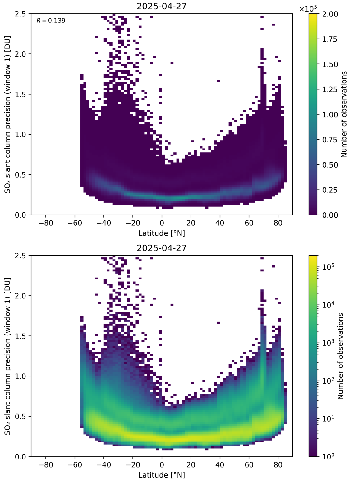
Figure 163: Scatter density plot of “Latitude” against “SO 2 slant column precision (window 1)” for 2025-04-26 to 2025-04-28.
