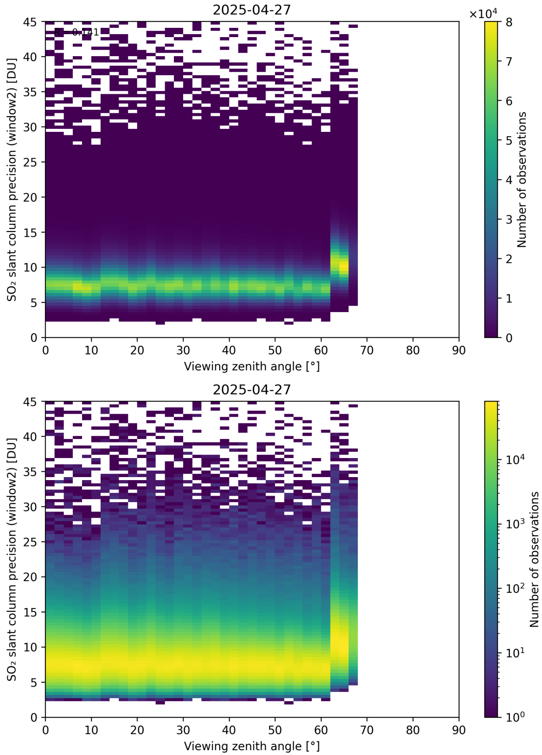
Figure 378: Scatter density plot of “Viewing zenith angle” against “SO 2 slant column precision (window2)” for 2025-04-26 to 2025-04-28.
