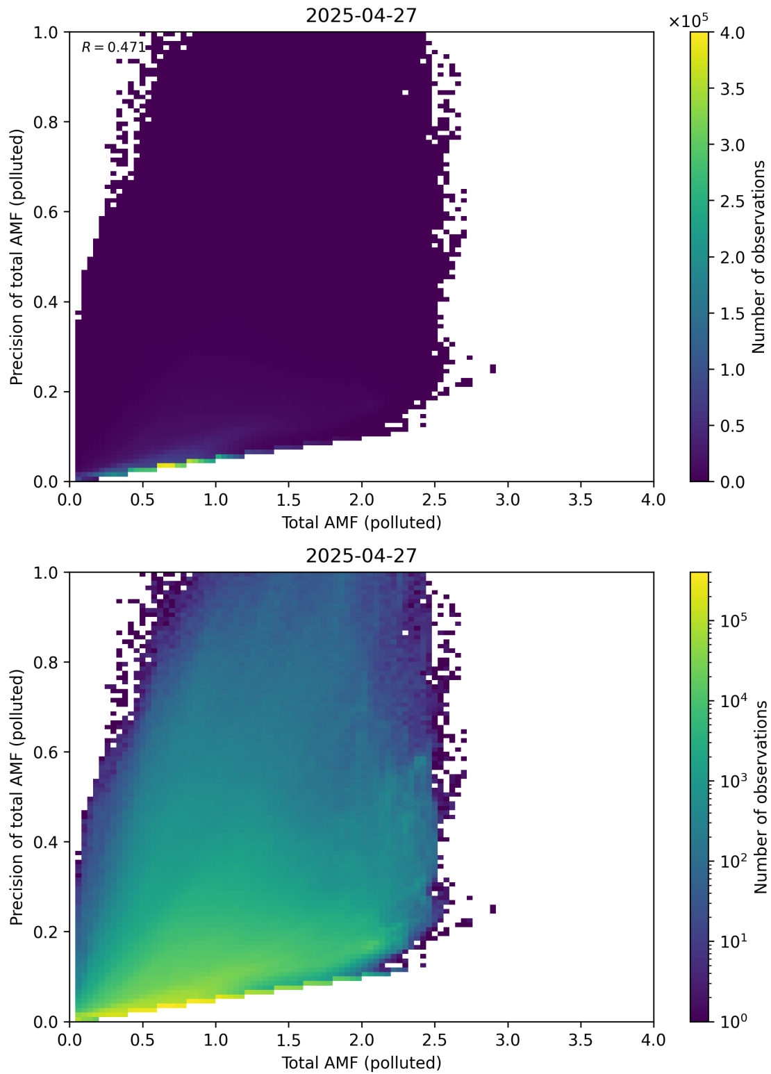
Figure 322: Scatter density plot of “Total AMF (polluted)” against “Precision of total AMF (polluted)” for 2025-04-26 to 2025-04-28.
