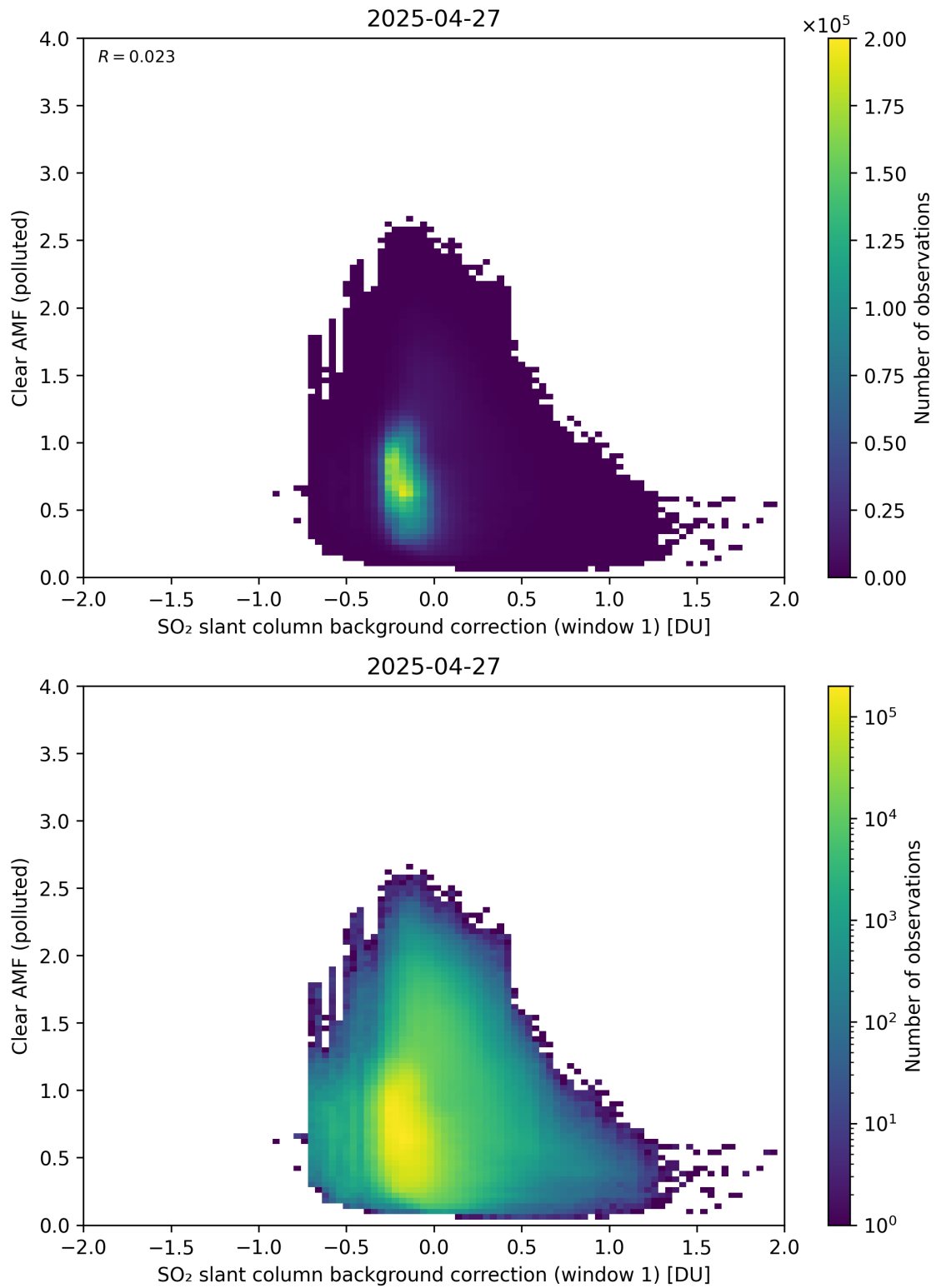
Figure 114: Scatter density plot of “SO 2 slant column background correction (window 1)” against “Clear AMF (polluted)” for 2025-04-26 to 2025-04-28.
