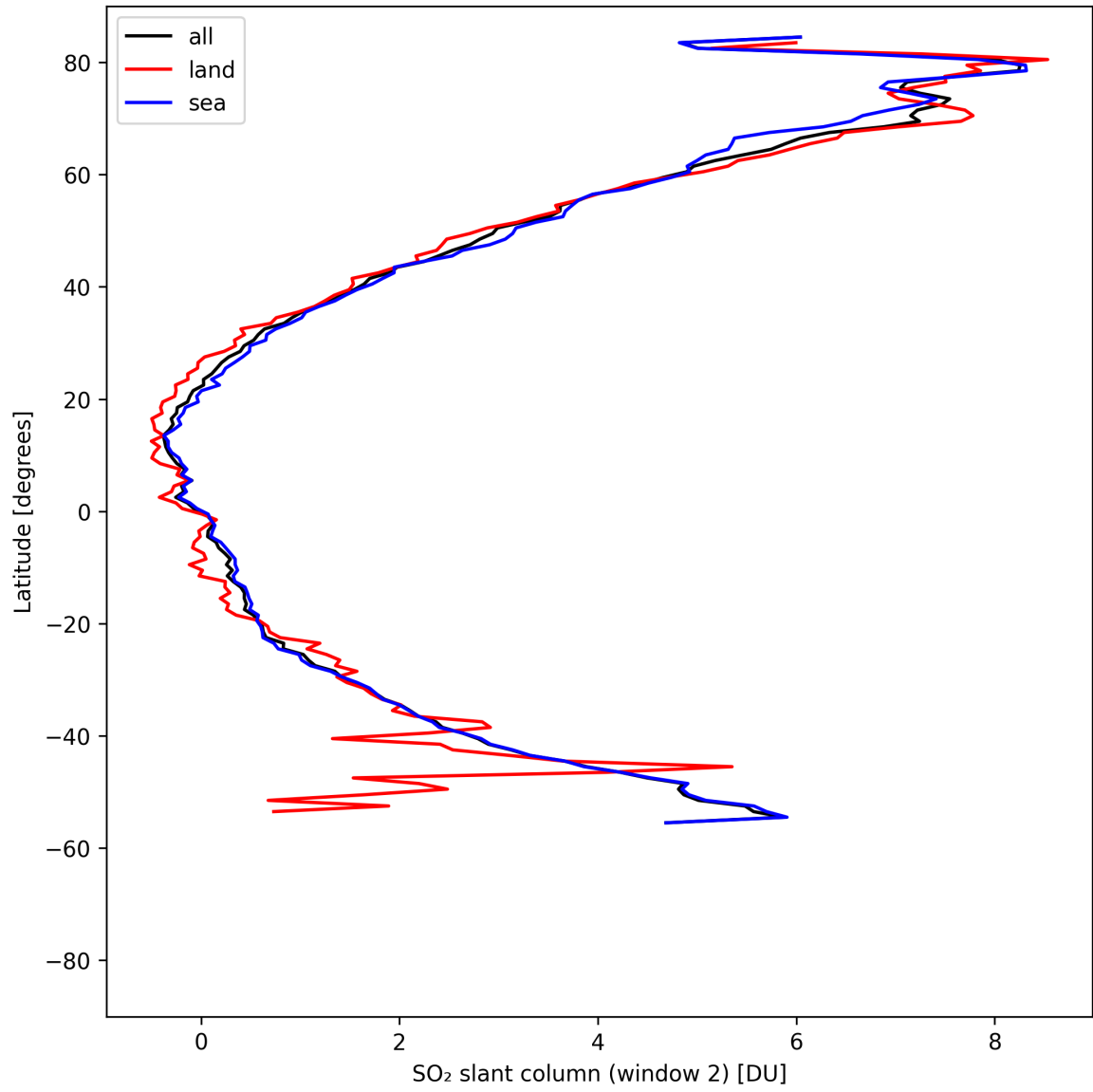
Figure 41: Zonal average of “SO 2 slant column (window 2)” for 2025-04-26 to 2025-04-28.
