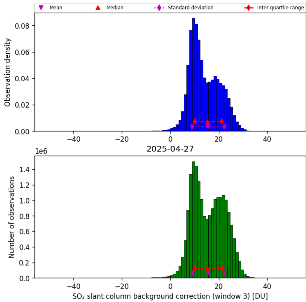
Figure 74: Histogram of “SO 2 slant column background correction (window 3)” for 2025-04-26 to 2025-04-28
