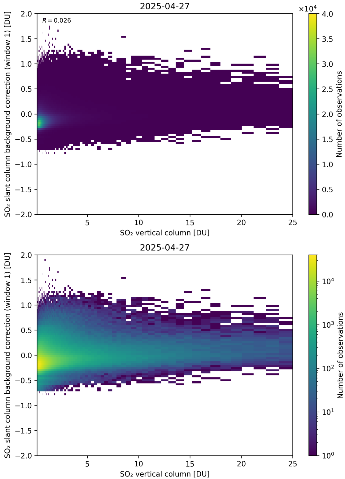
Figure 323: Scatter density plot of “SO 2 vertical column” against “SO 2 slant column background correction (window 1)” for 2025-04-26 to 2025-04-28.
