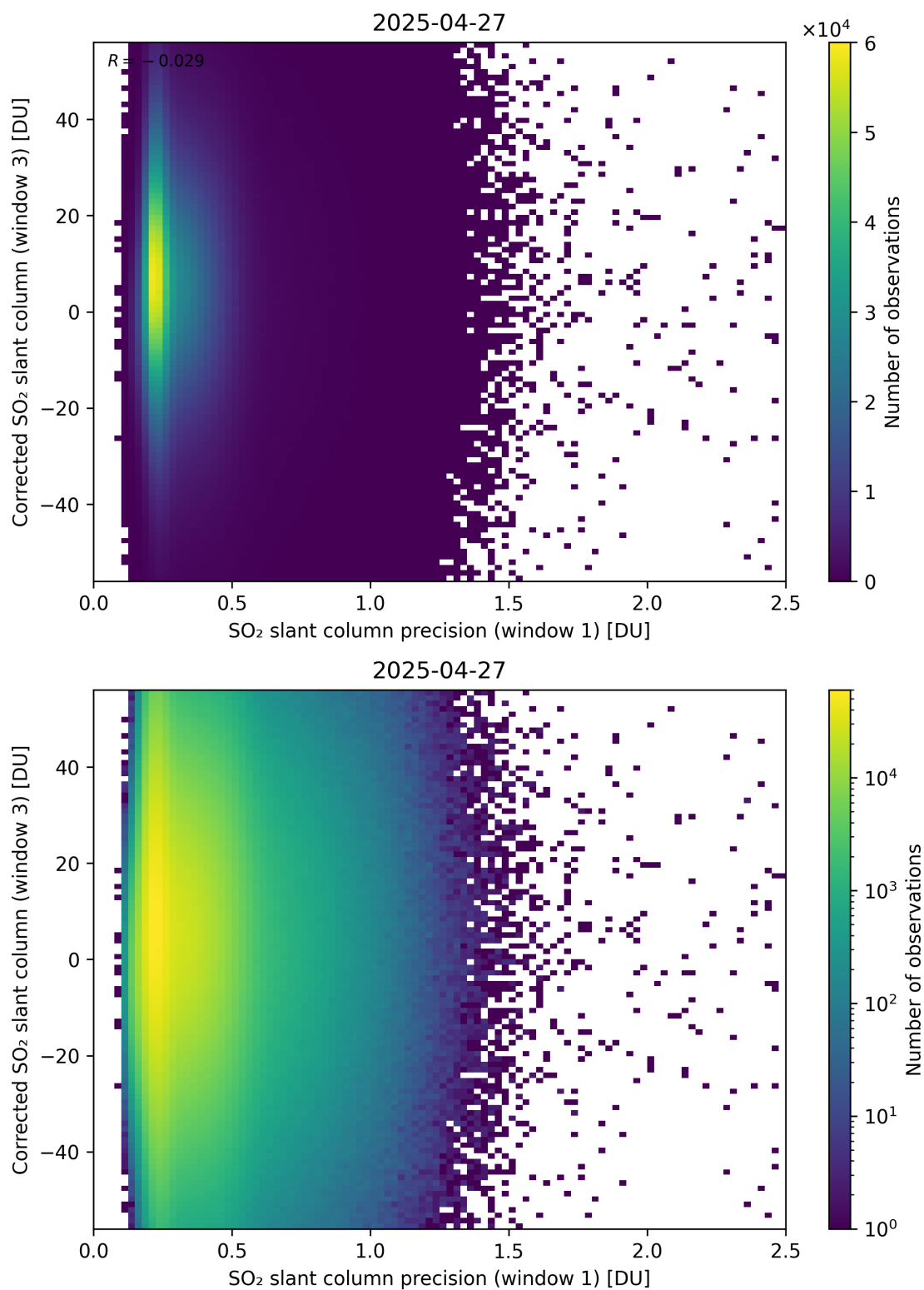
Figure 276: Scatter density plot of “SO 2 slant column precision (window 1)” against “Corrected SO 2 slant column (window 3)” for 2025-04-26 to 2025-04-28.
