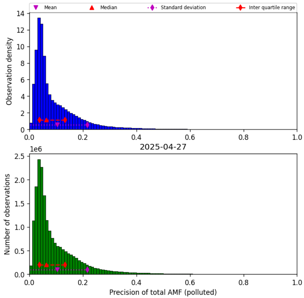
Figure 80: Histogram of “Precision of total AMF (polluted)” for 2025-04-26 to 2025-04-28
