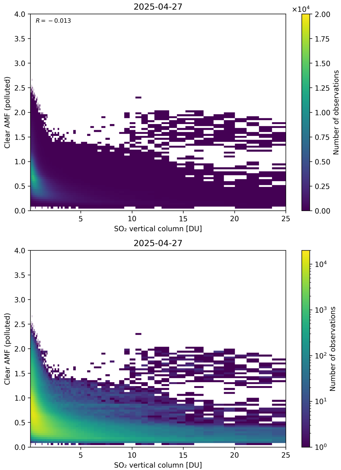
Figure 348: Scatter density plot of “SO 2 vertical column” against “Clear AMF (polluted)” for 2025-04-26 to 2025-04-28.
