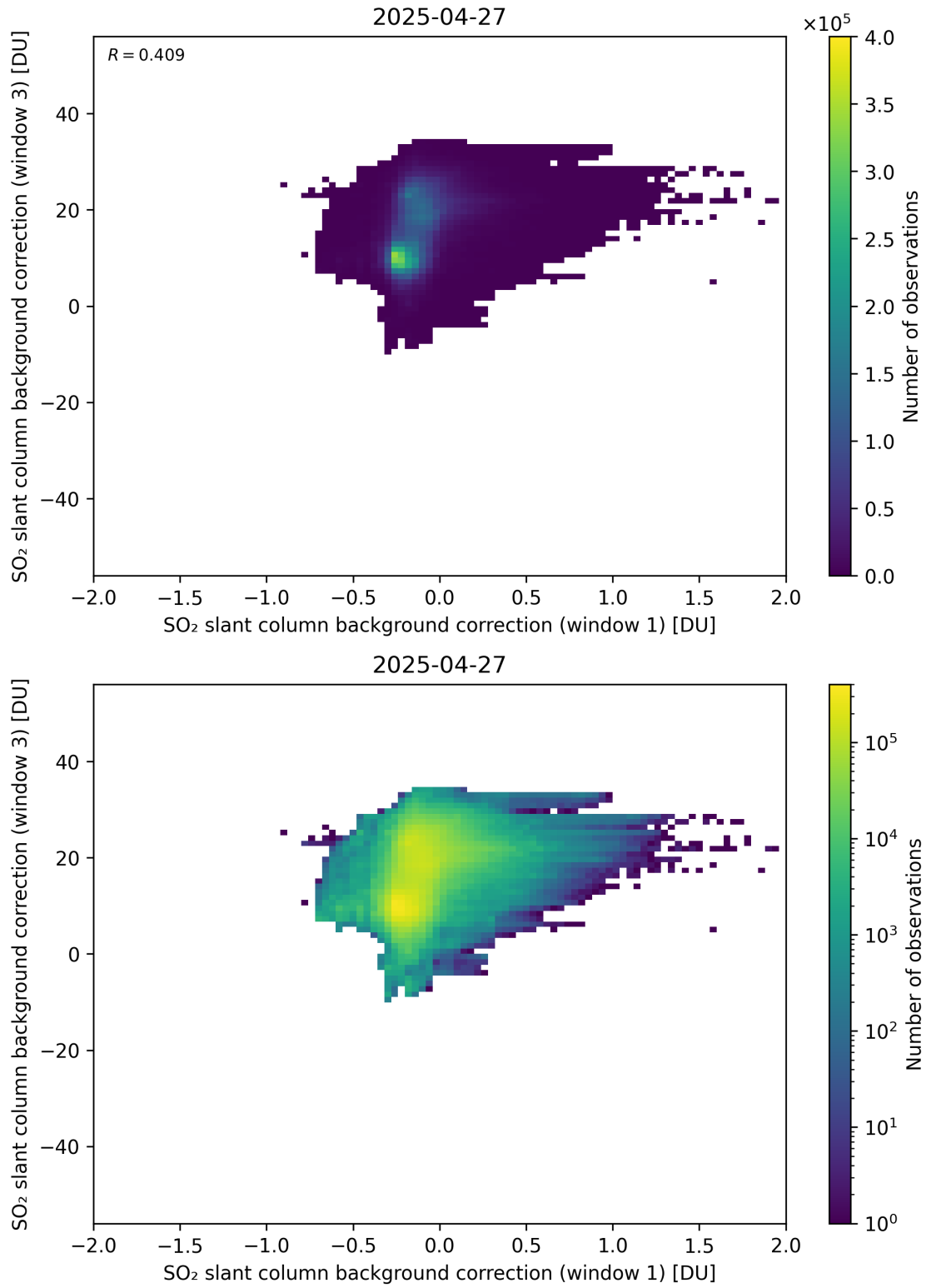
Figure 110: Scatter density plot of “SO 2 slant column background correction (window 1)” against “SO 2 slant column background correction (window 3)” for 2025-04-26 to 2025-04-28.
