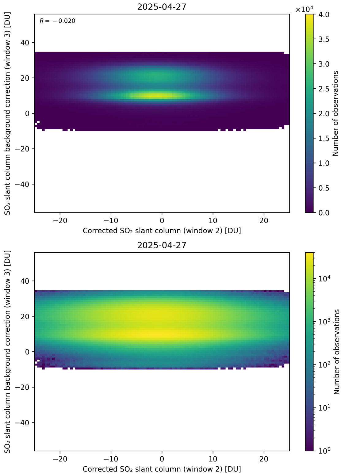
Figure 245: Scatter density plot of “Corrected SO 2 slant column (window 2)” against “SO 2 slant column background correction (window 3)” for 2025-04-26 to 2025-04-28.
