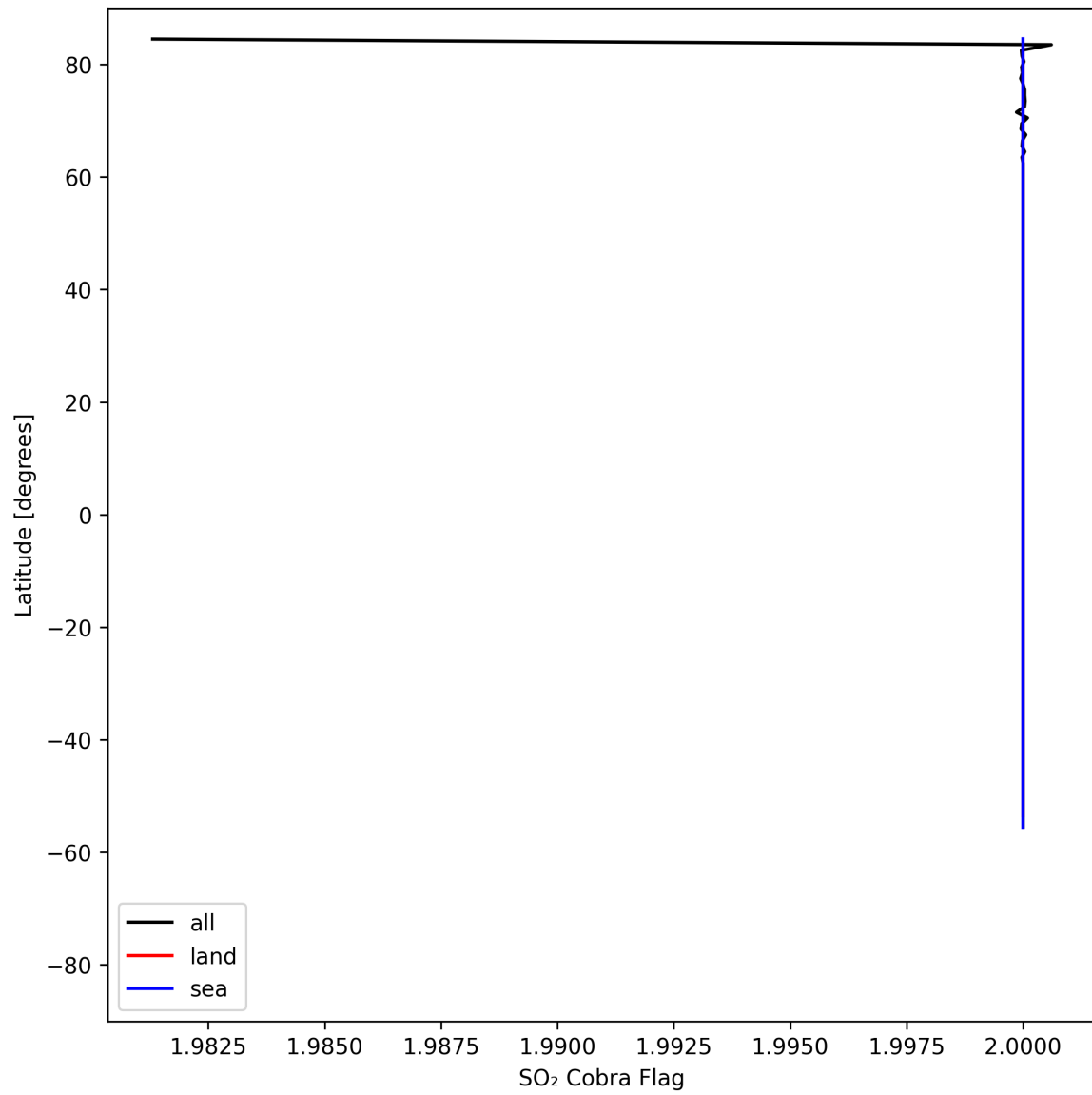
Figure 49: Zonal average of "SO 2 Cobra Flag" for 2025-04-26 to 2025-04-28.
