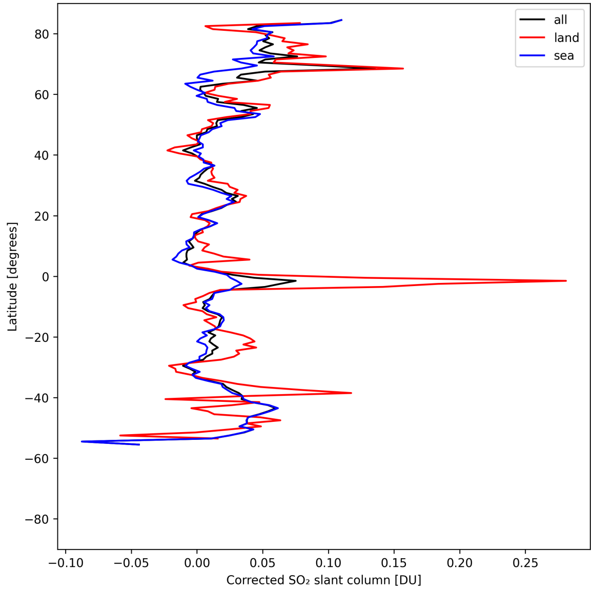
Figure 34: Zonal average of “Corrected SO 2 slant column” for 2025-04-26 to 2025-04-28.
