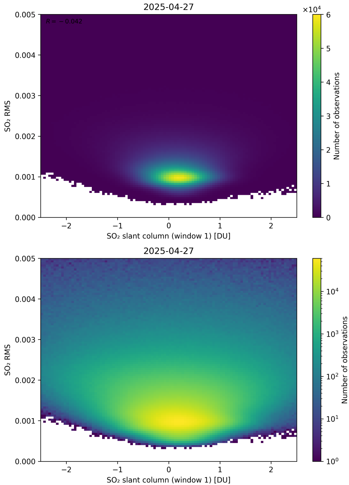
Figure 267: Scatter density plot of “SO 2 slant column (window 1)” against “SO 2 RMS” for 2025-04-26 to 2025-04-28.
