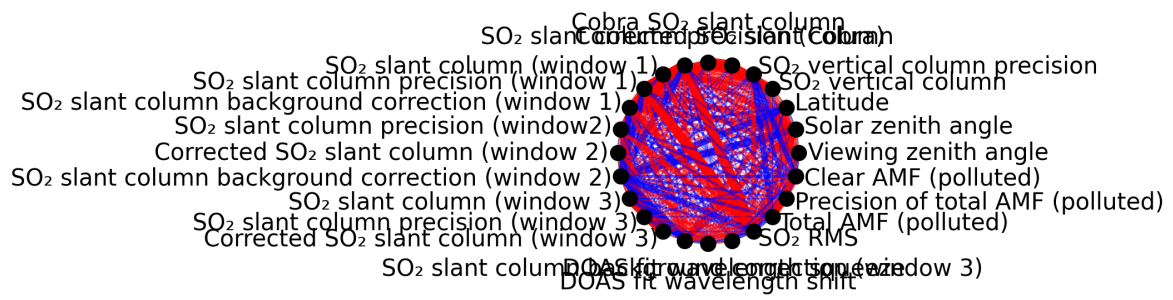
Figure 1: Map of correlation graph for 2025-04-26 to 2025-04-28.
