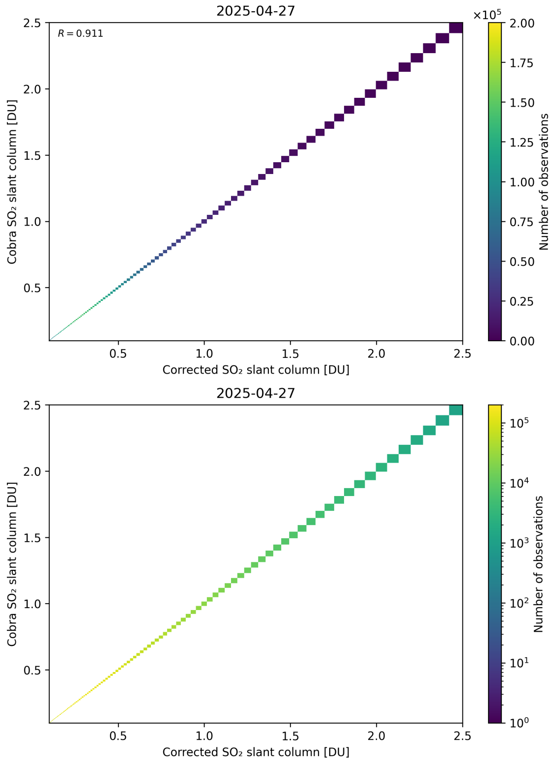
Figure 233: Scatter density plot of “Corrected SO 2 slant column” against “Cobra SO 2 slant column” for 2025-04-26 to 2025-04-28.
