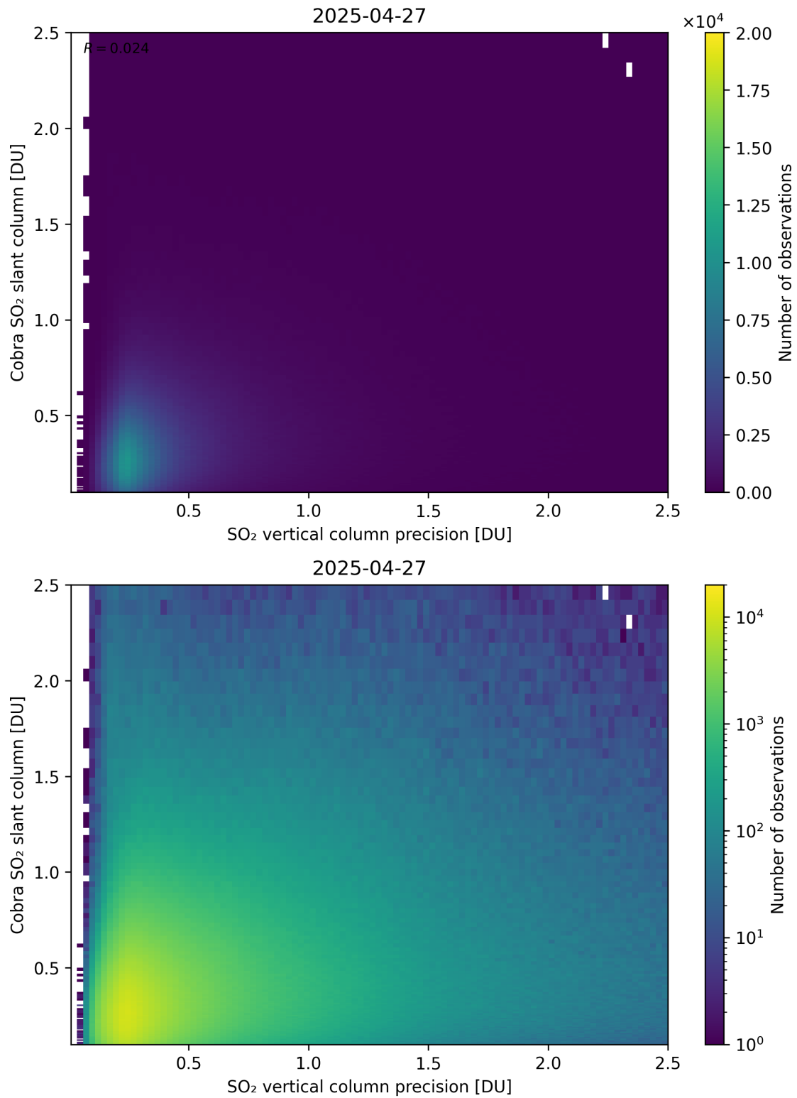
Figure 336: Scatter density plot of “SO 2 vertical column precision” against “Cobra SO 2 slant column” for 2025-04-26 to 2025-04-28.
