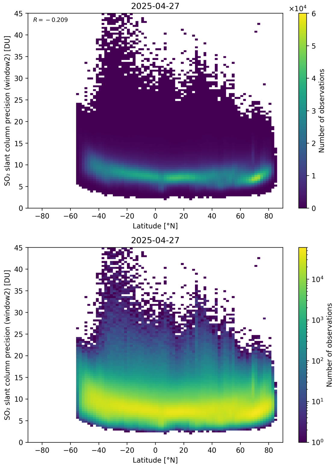
Figure 164: Scatter density plot of “Latitude” against “SO 2 slant column precision (window2)” for 2025-04-26 to 2025-04-28.
