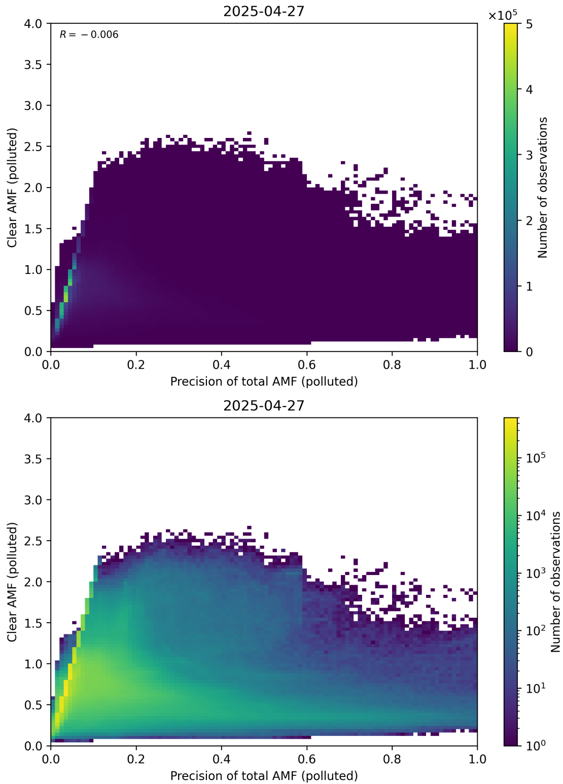
Figure 320: Scatter density plot of “Precision of total AMF (polluted)” against “Clear AMF (polluted)” for 2025-04-26 to 2025-04-28.
