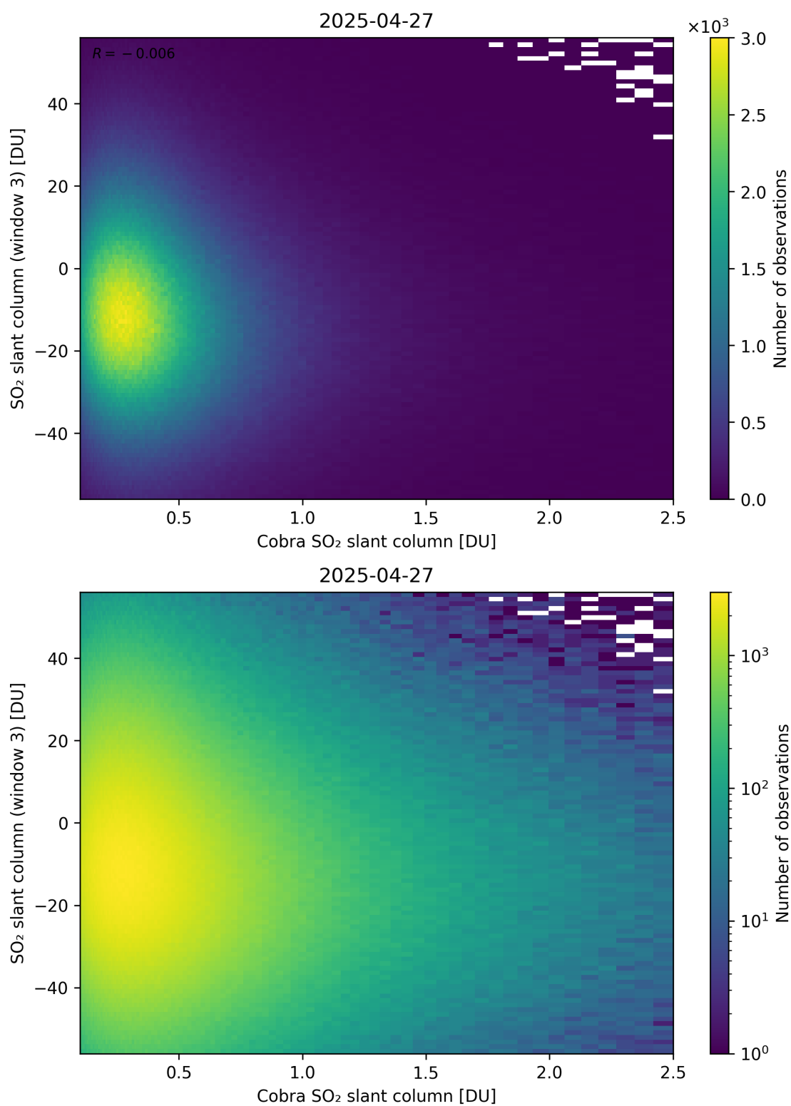
Figure 222: Scatter density plot of “Cobra SO 2 slant column” against “SO 2 slant column (window 3)” for 2025-04-26 to 2025-04-28.
