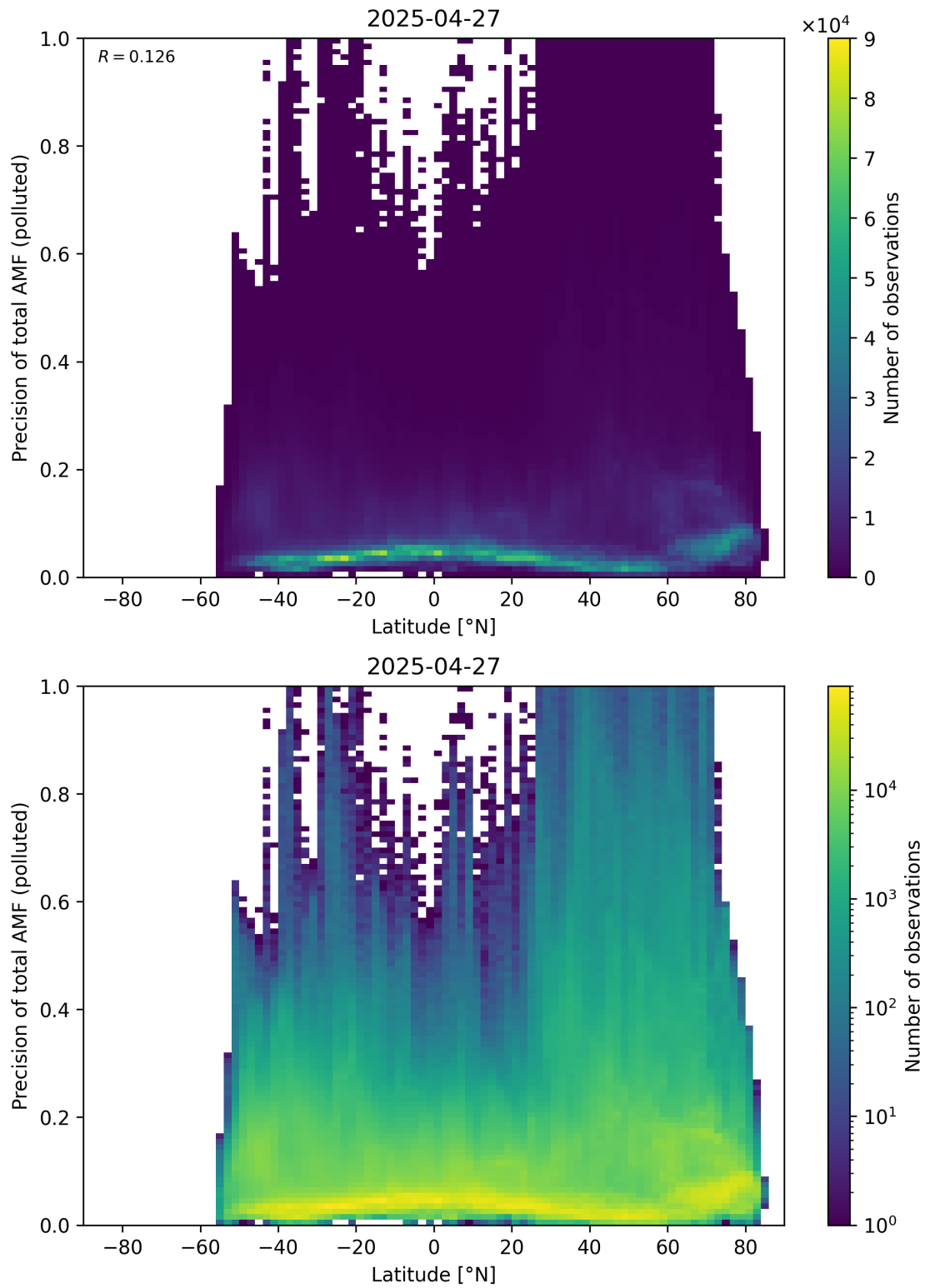
Figure 168: Scatter density plot of “Latitude” against “Precision of total AMF (polluted)” for 2025-04-26 to 2025-04-28.
