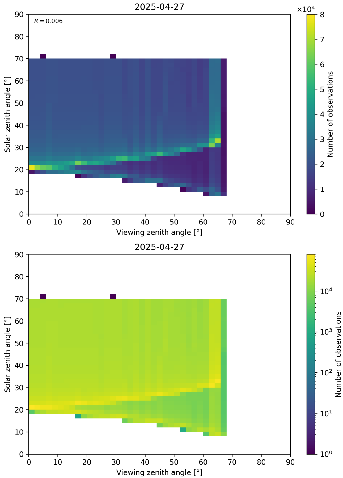
Figure 369: Scatter density plot of “Viewing zenith angle” against “Solar zenith angle” for 2025-04-26 to 2025-04-28.
