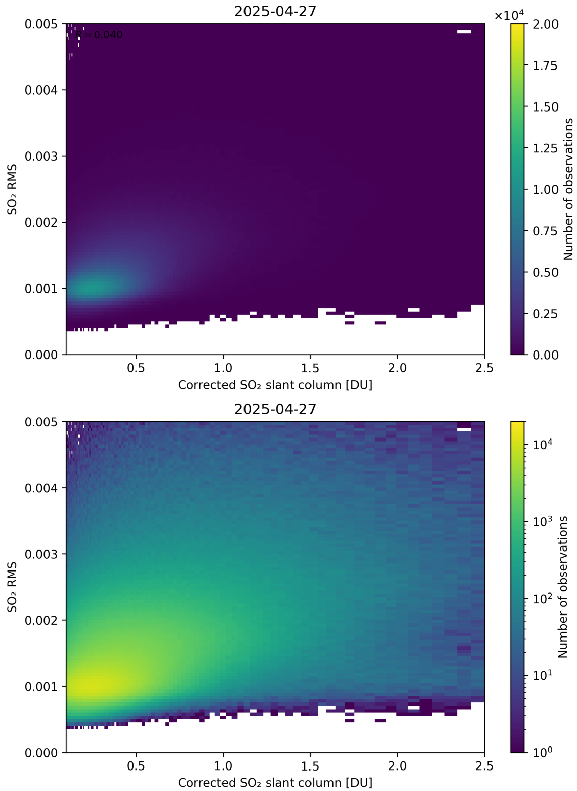
Figure 231: Scatter density plot of “Corrected SO 2 slant column” against “SO 2 RMS” for 2025-04-26 to 2025-04-28.
