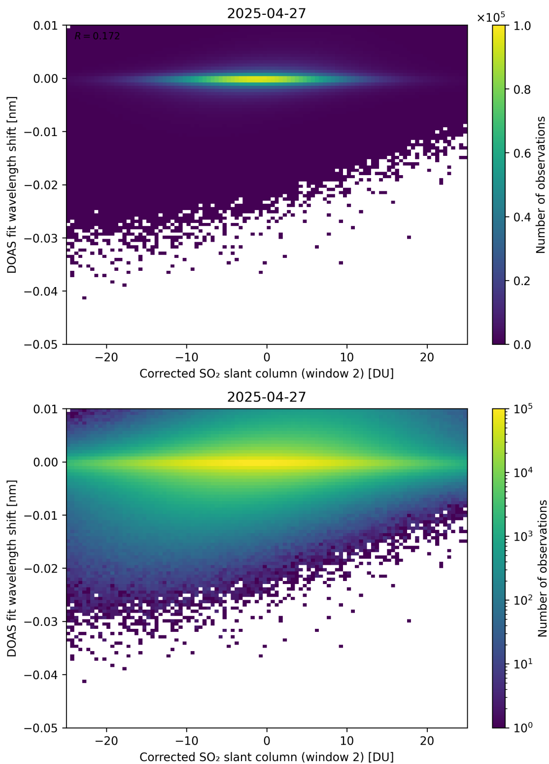
Figure 246: Scatter density plot of “Corrected SO 2 slant column (window 2)” against “DOAS fit wavelength shift” for 2025-04-26 to 2025-04-28.
