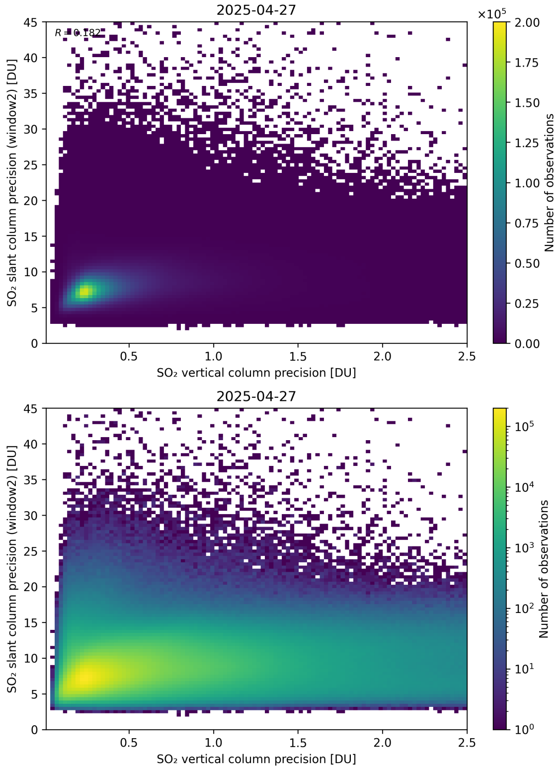
Figure 343: Scatter density plot of “SO 2 vertical column precision” against “SO 2 slant column precision (window2)” for 2025-04-26 to 2025-04-28.
