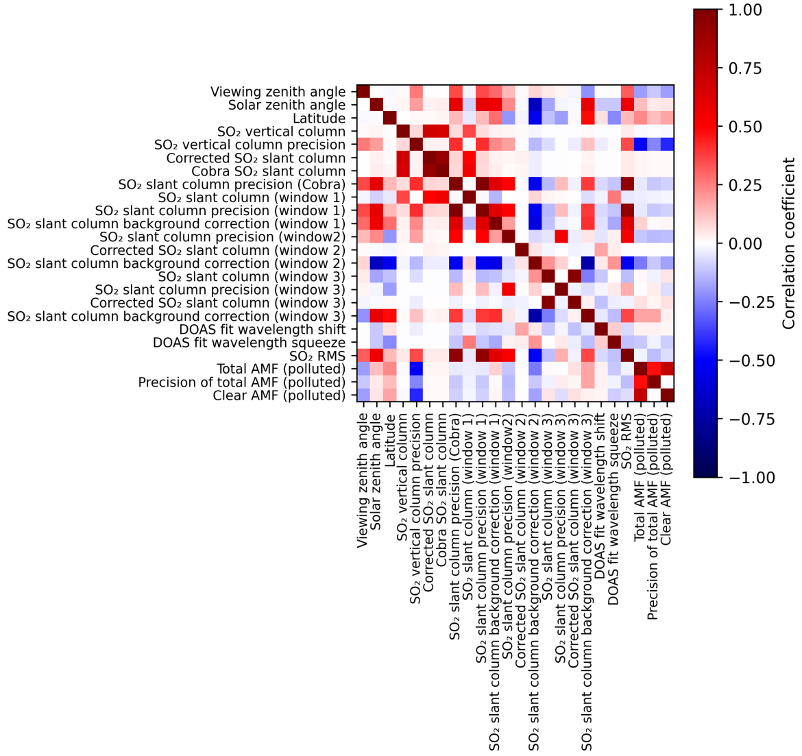
Figure 2: Map of correlation matrix for 2025-04-26 to 2025-04-28.
