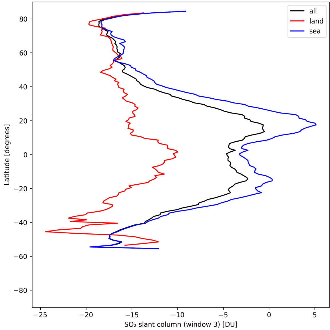
Figure 45: Zonal average of “SO 2 slant column (window 3)” for 2025-04-26 to 2025-04-28.
