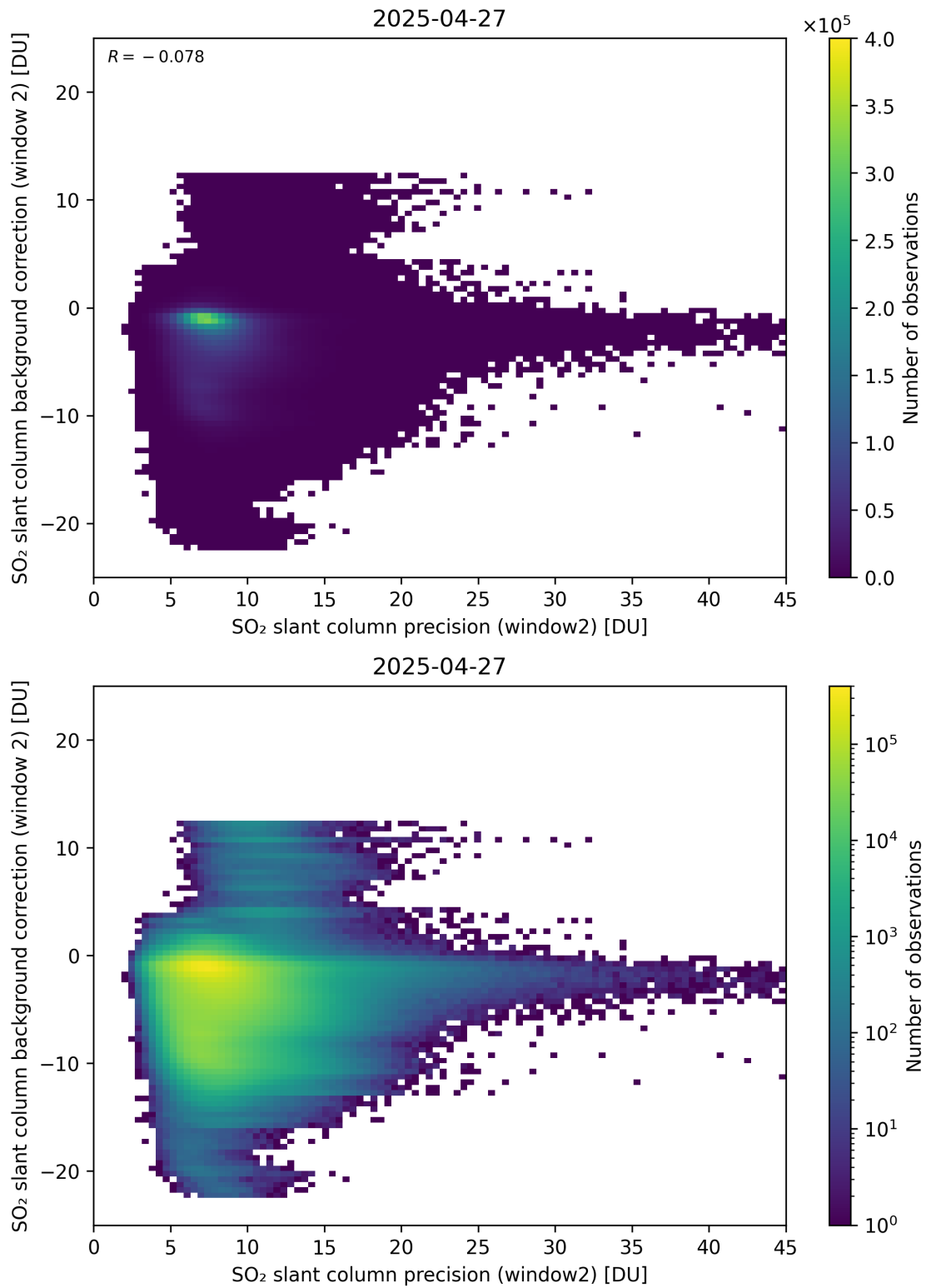
Figure 291: Scatter density plot of “SO 2 slant column precision (window2)” against “SO 2 slant column background correction (window 2)” for 2025-04-26 to 2025-04-28.
