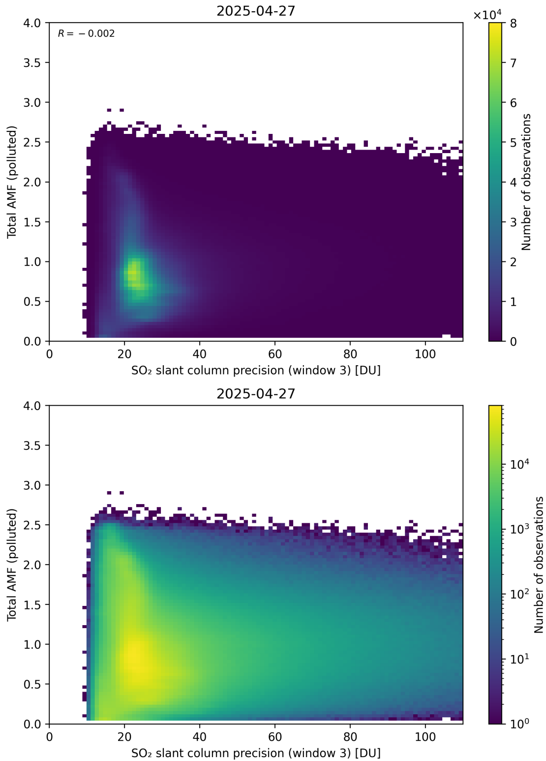
Figure 313: Scatter density plot of “SO 2 slant column precision (window 3)” against “Total AMF (polluted)” for 2025-04-26 to 2025-04-28.
