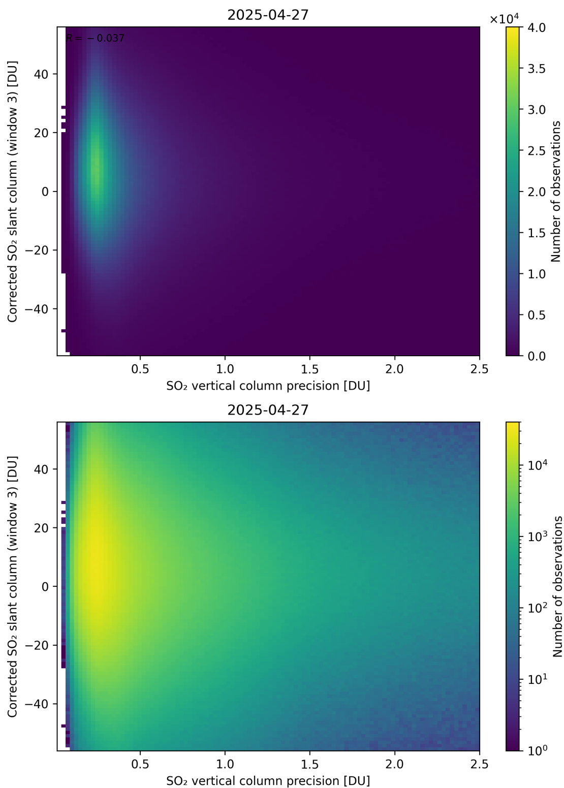
Figure 340: Scatter density plot of “SO 2 vertical column precision” against “Corrected SO 2 slant column (window 3)” for 2025-04-26 to 2025-04-28.
