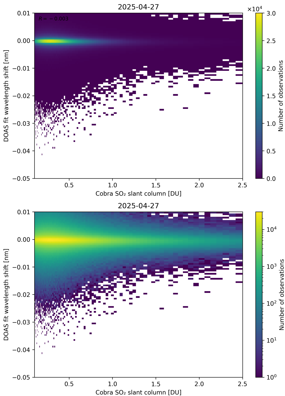
Figure 196: Scatter density plot of “Cobra SO 2 slant column” against “DOAS fit wavelength shift” for 2025-04-26 to 2025-04-28.
