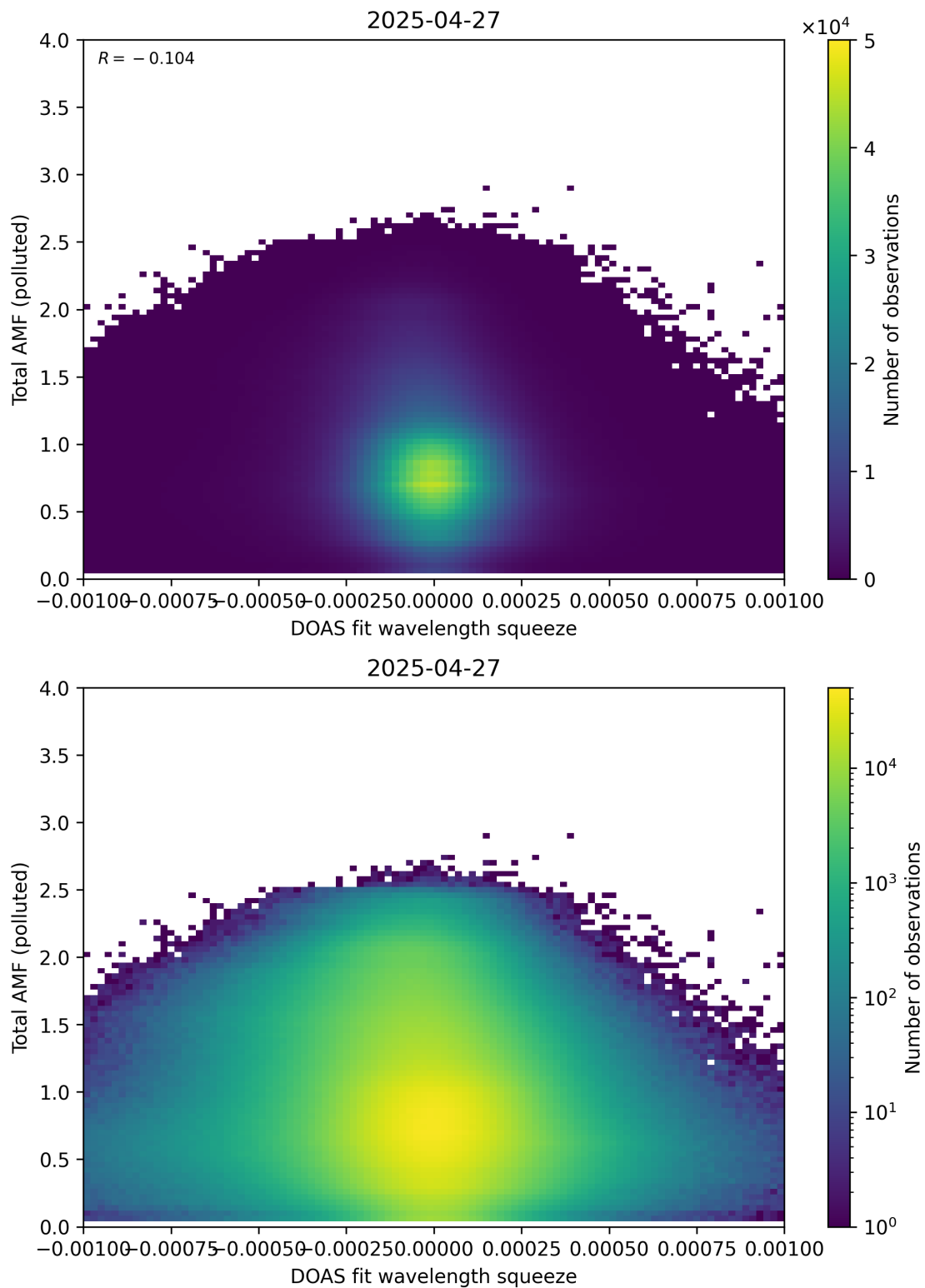
Figure 145: Scatter density plot of “DOAS fit wavelength squeeze” against “Total AMF (polluted)” for 2025-04-26 to 2025-04-28.
