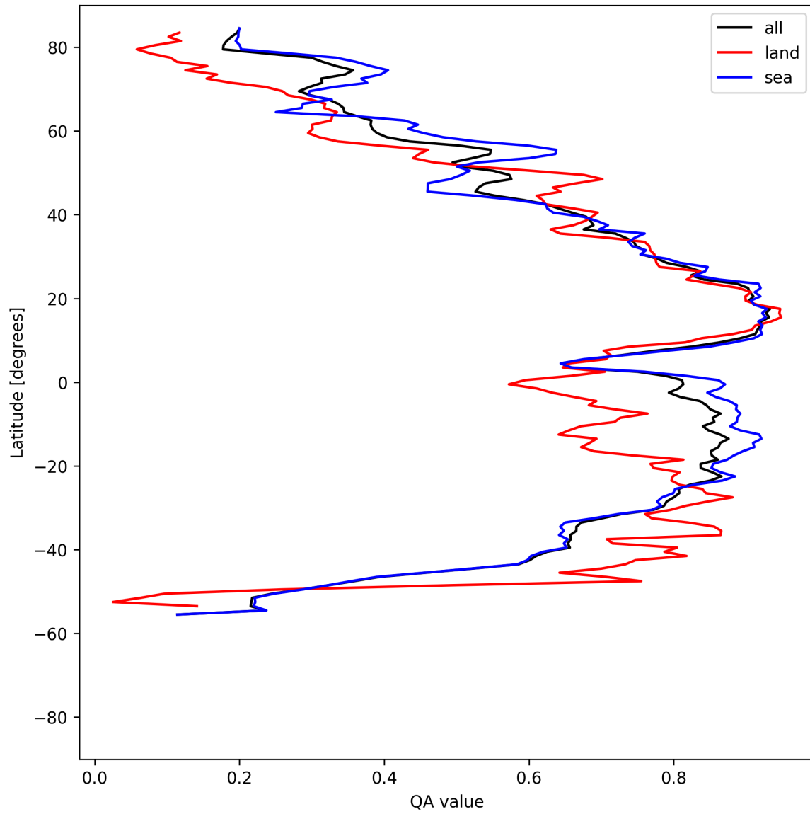
Figure 31: Zonal average of “QA value” for 2025-04-26 to 2025-04-28.
