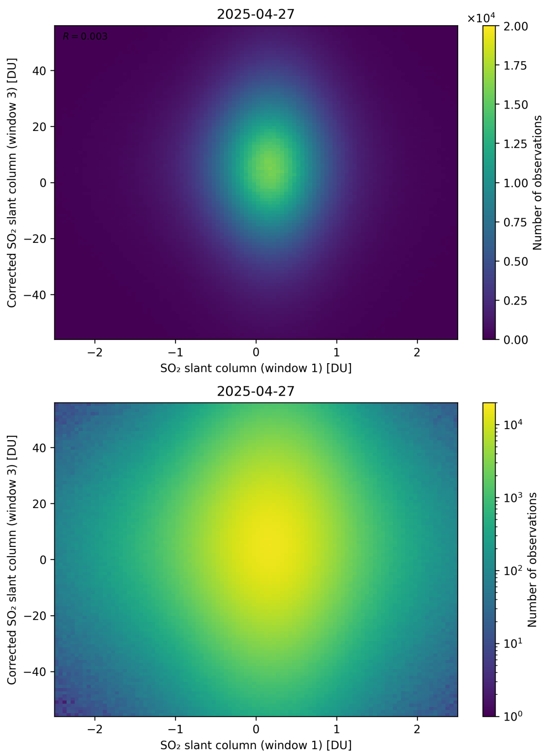
Figure 284: Scatter density plot of “SO 2 slant column (window 1)” against “Corrected SO 2 slant column (window 3)” for 2025-04-26 to 2025-04-28.
