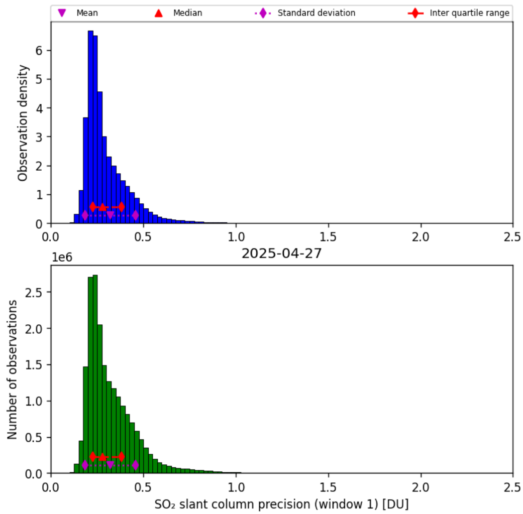
Figure 64: Histogram of “SO 2 slant column precision (window 1)” for 2025-04-26 to 2025-04-28
