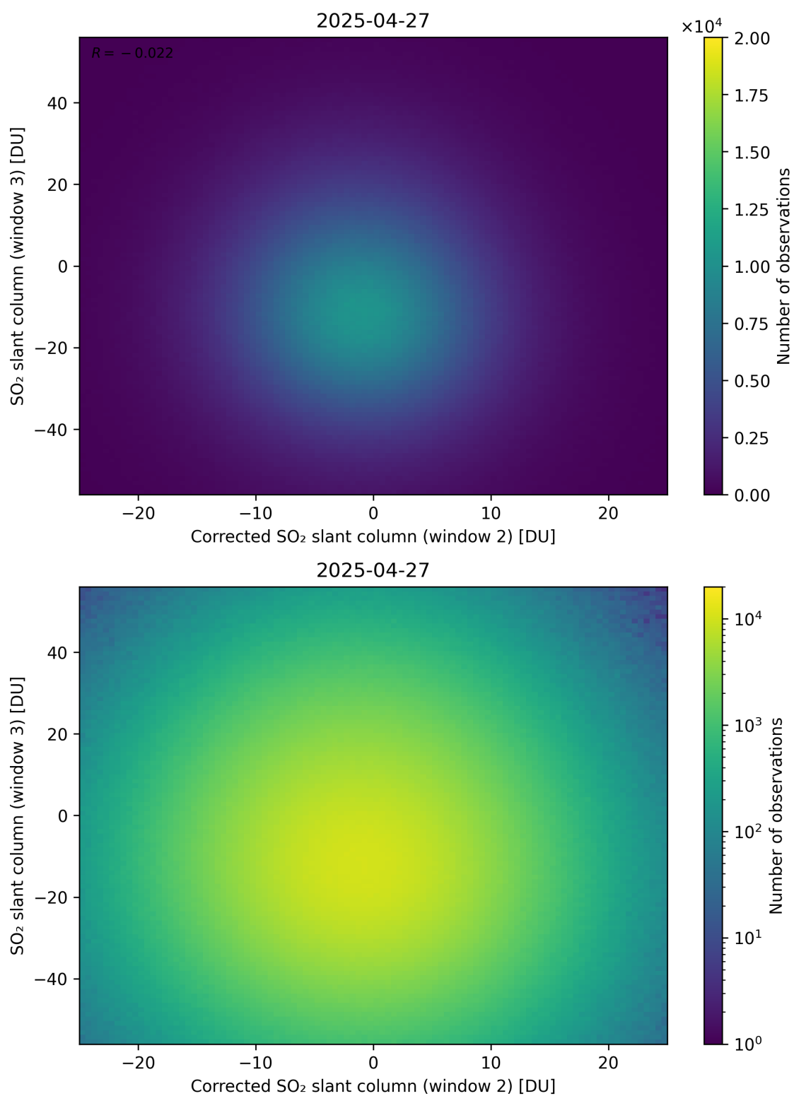
Figure 251: Scatter density plot of “Corrected SO 2 slant column (window 2)” against “SO 2 slant column (window 3)” for 2025-04-26 to 2025-04-28.
