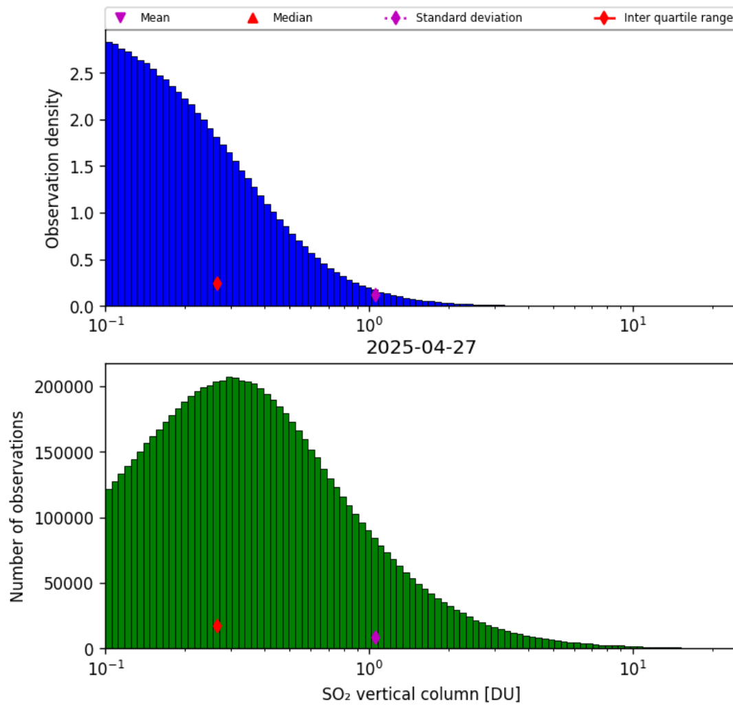
Figure 58: Histogram of “SO 2 vertical column” for 2025-04-26 to 2025-04-28
