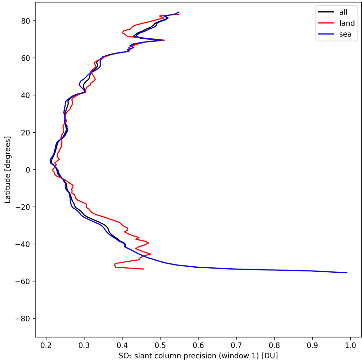
Figure 38: Zonal average of “SO 2 slant column precision (window 1)” for 2025-04-26 to 2025-04-28.
