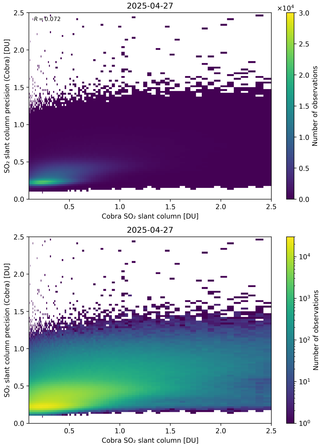
Figure 216: Scatter density plot of “Cobra SO 2 slant column” against “SO 2 slant column precision (Cobra)” for 2025-04-26 to 2025-04-28.
