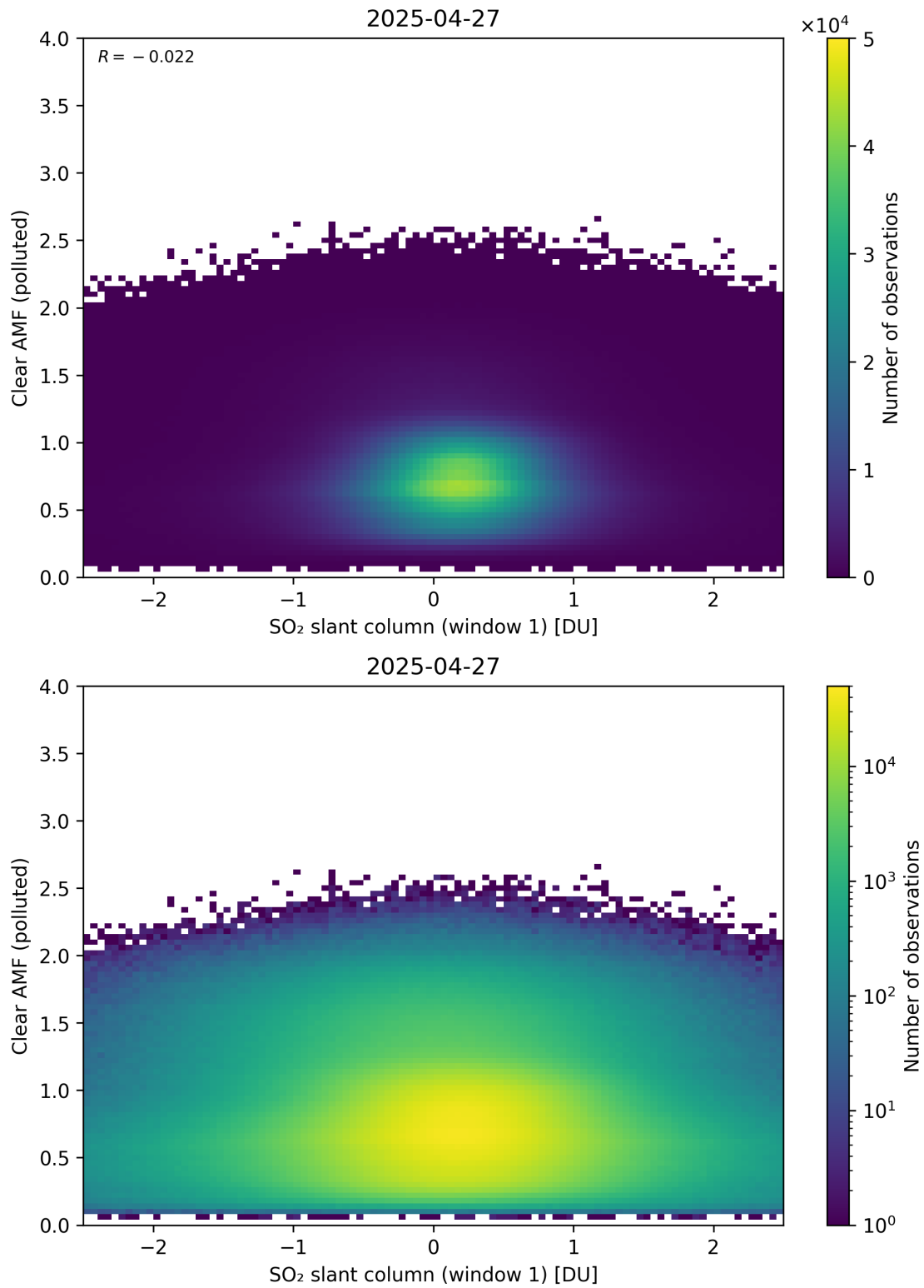
Figure 282: Scatter density plot of “SO 2 slant column (window 1)” against “Clear AMF (polluted)” for 2025-04-26 to 2025-04-28.
