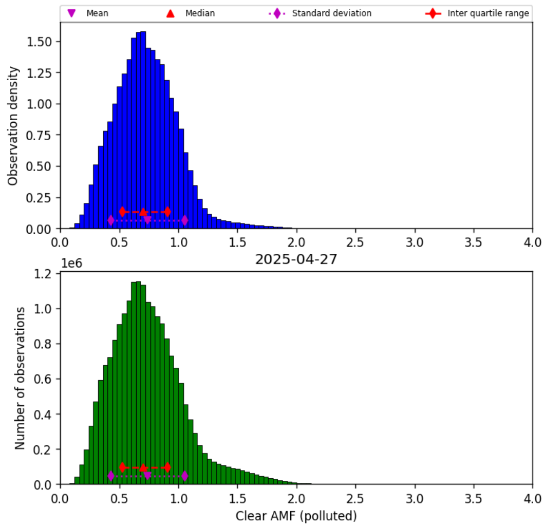
Figure 81: Histogram of “Clear AMF (polluted)” for 2025-04-26 to 2025-04-28
