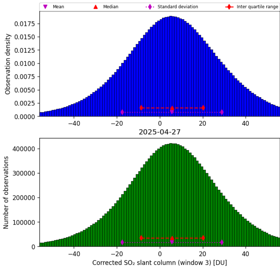
Figure 73: Histogram of “Corrected SO 2 slant column (window 3)” for 2025-04-26 to 2025-04-28
