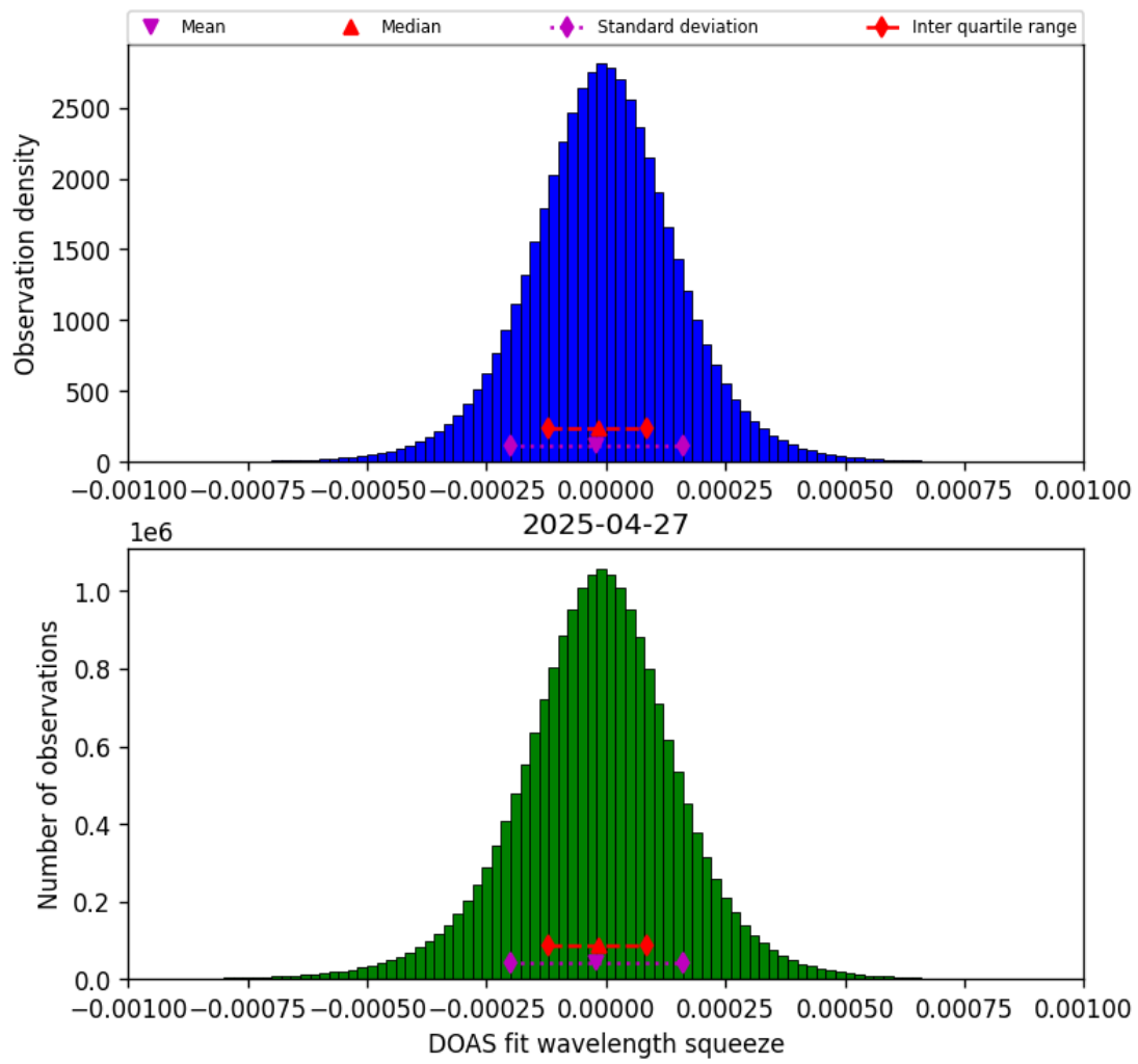
Figure 77: Histogram of “DOAS fit wavelength squeeze” for 2025-04-26 to 2025-04-28
