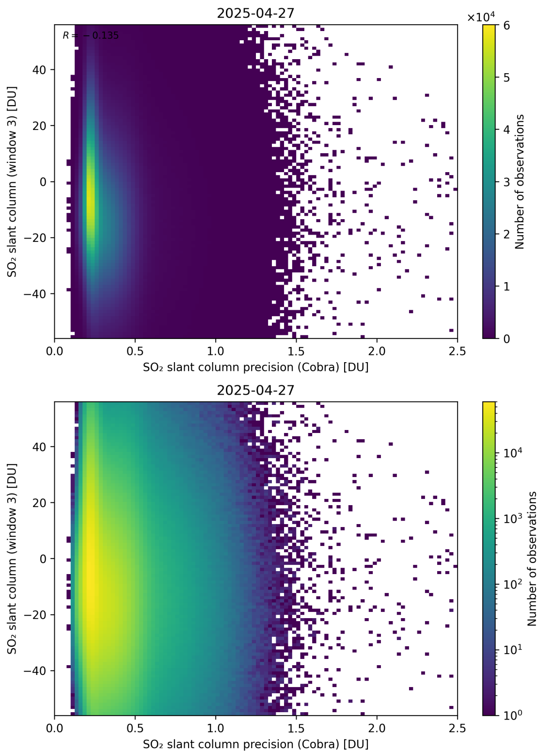
Figure 211: Scatter density plot of “SO 2 slant column precision (Cobra)” against “SO 2 slant column (window 3)” for 2025-04-26 to 2025-04-28.
