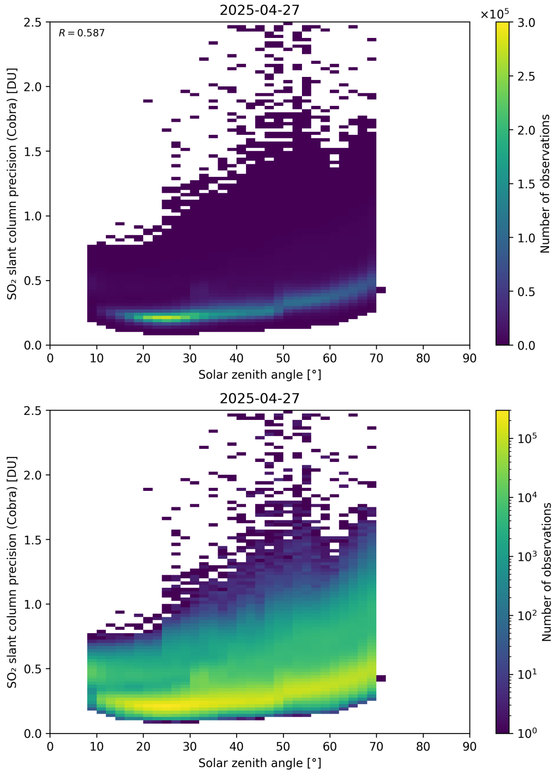
Figure 180: Scatter density plot of “Solar zenith angle” against “SO 2 slant column precision (Cobra)” for 2025-04-26 to 2025-04-28.
