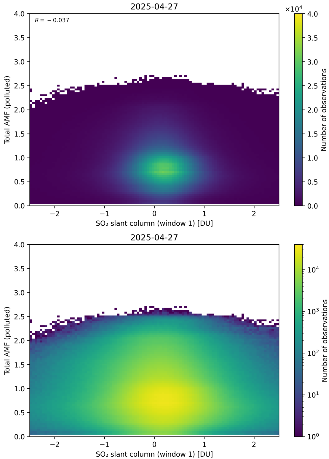
Figure 289: Scatter density plot of “SO 2 slant column (window 1)” against “Total AMF (polluted)” for 2025-04-26 to 2025-04-28.
