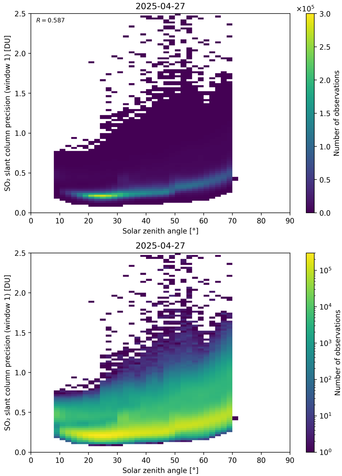
Figure 185: Scatter density plot of “Solar zenith angle” against “SO 2 slant column precision (window 1)” for 2025-04-26 to 2025-04-28.
