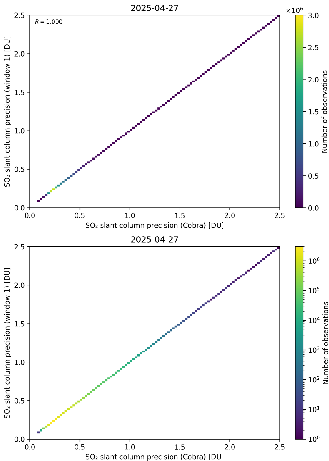
Figure 209: Scatter density plot of “SO 2 slant column precision (Cobra)” against “SO 2 slant column precision (window 1)” for 2025-04-26 to 2025-04-28.
