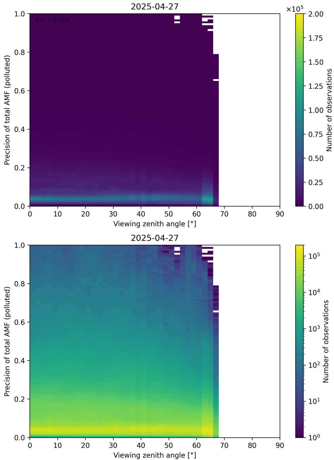
Figure 382: Scatter density plot of “Viewing zenith angle” against “Precision of total AMF (polluted)” for 2025-04-26 to 2025-04-28.
