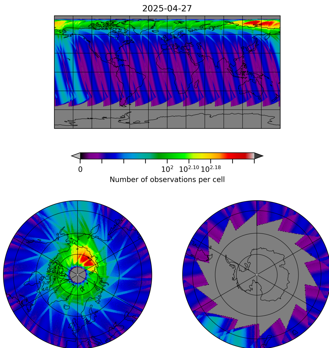
Figure 30: Map of the number of observations for 2025-04-26 to 2025-04-28
