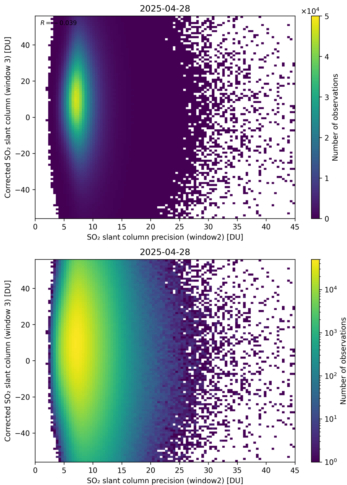
Figure 298: Scatter density plot of “SO 2 slant column precision (window2)” against “Corrected SO 2 slant column (window 3)” for 2025-04-27 to 2025-04-29.
