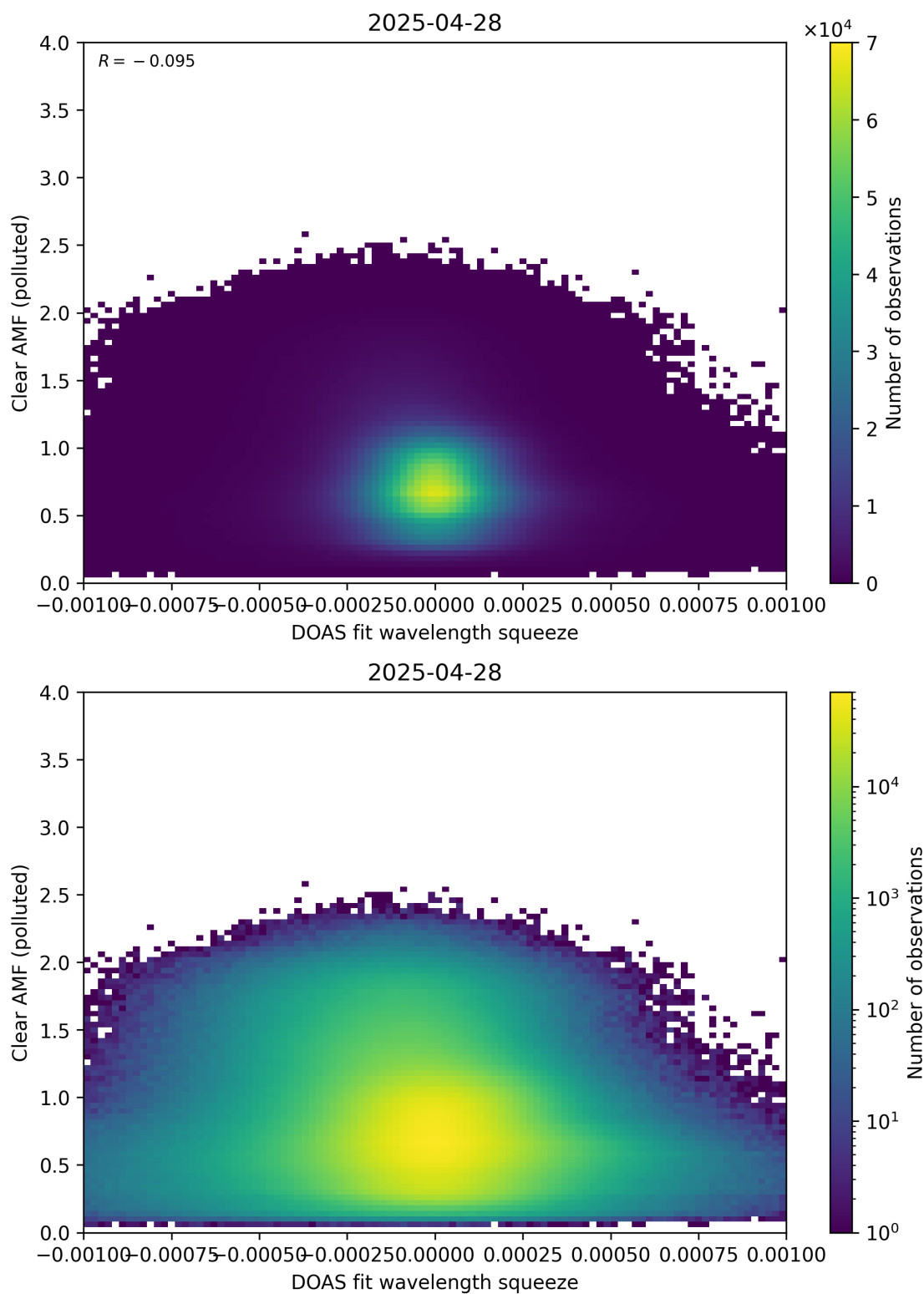
Figure 144: Scatter density plot of “DOAS fit wavelength squeeze” against “Clear AMF (polluted)” for 2025-04-27 to 2025-04-29.
