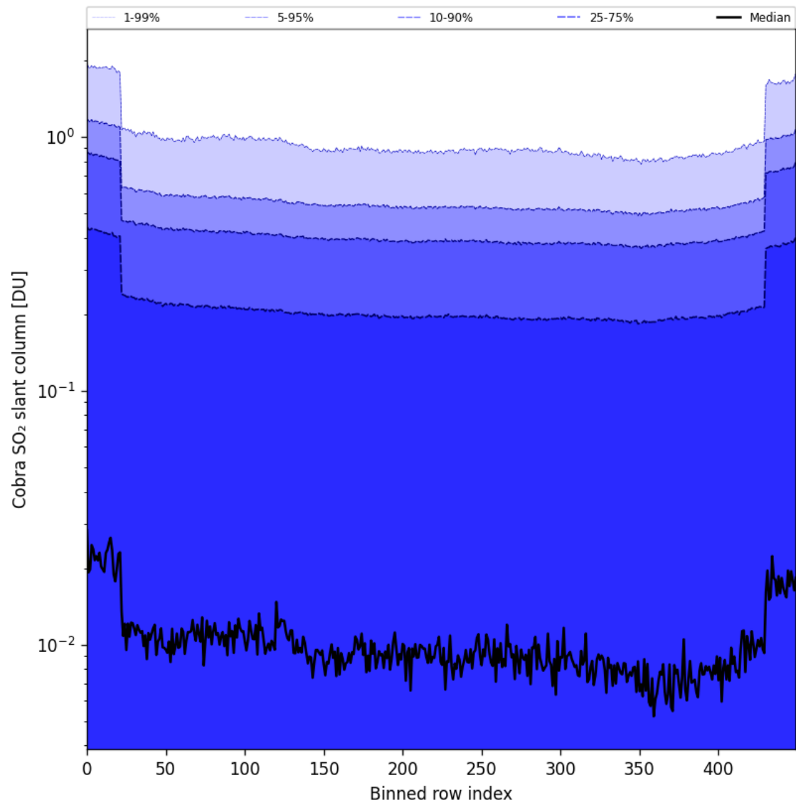
Figure 87: Along track statistics of "Cobra SO 2 slant column" for 2025-04-27 to 2025-04-29
