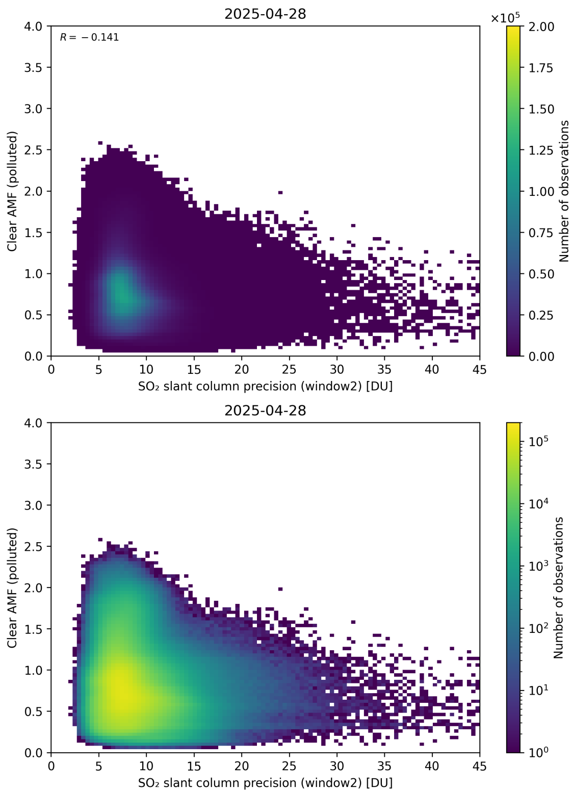
Figure 296: Scatter density plot of “SO 2 slant column precision (window2)” against “Clear AMF (polluted)” for 2025-04-27 to 2025-04-29.
