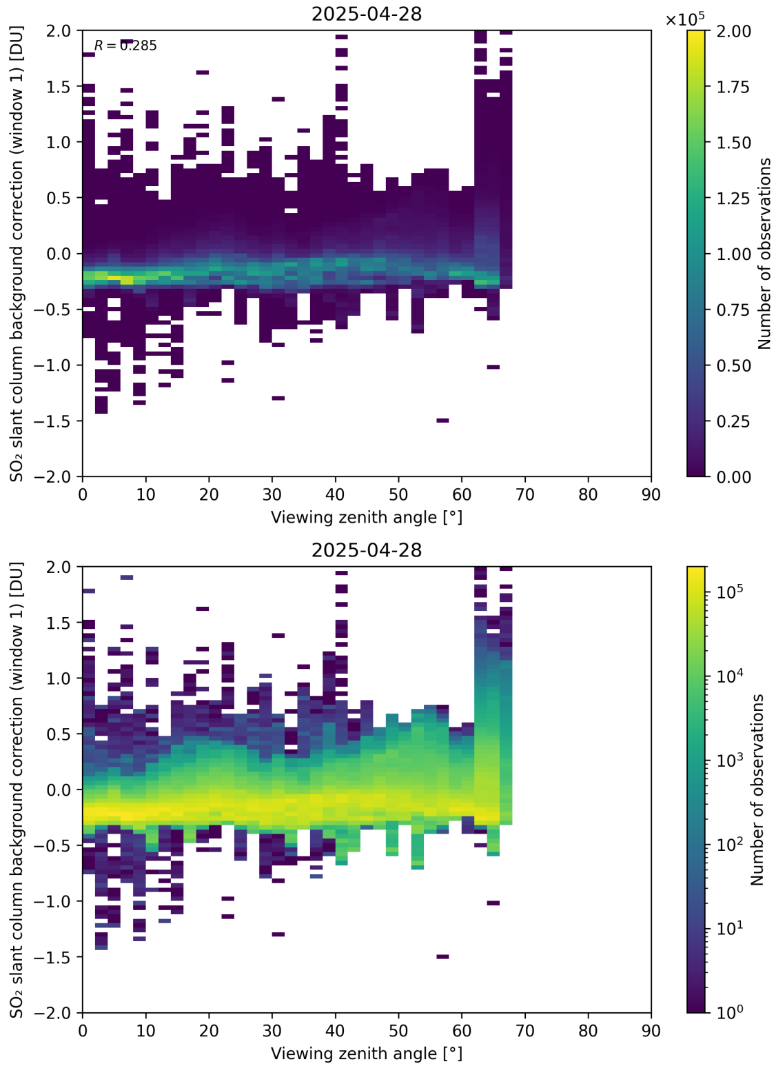
Figure 362: Scatter density plot of “Viewing zenith angle” against “SO 2 slant column background correction (window 1)” for 2025-04-27 to 2025-04-29.
