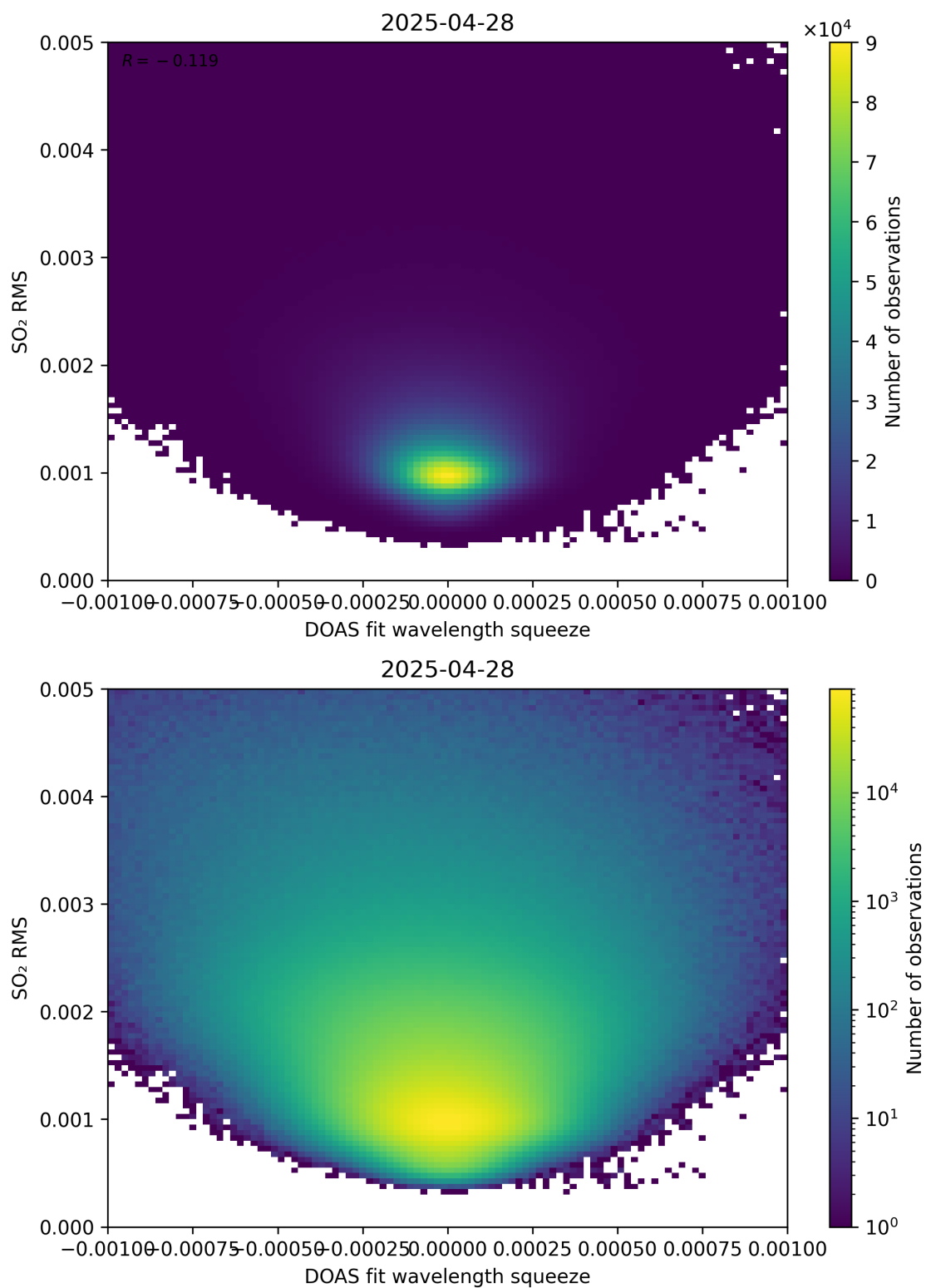
Figure 143: Scatter density plot of “DOAS fit wavelength squeeze” against “SO 2 RMS” for 2025-04-27 to 2025-04-29.
