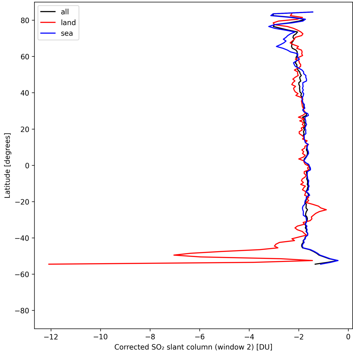
Figure 43: Zonal average of “Corrected SO 2 slant column (window 2)” for 2025-04-27 to 2025-04-29.
