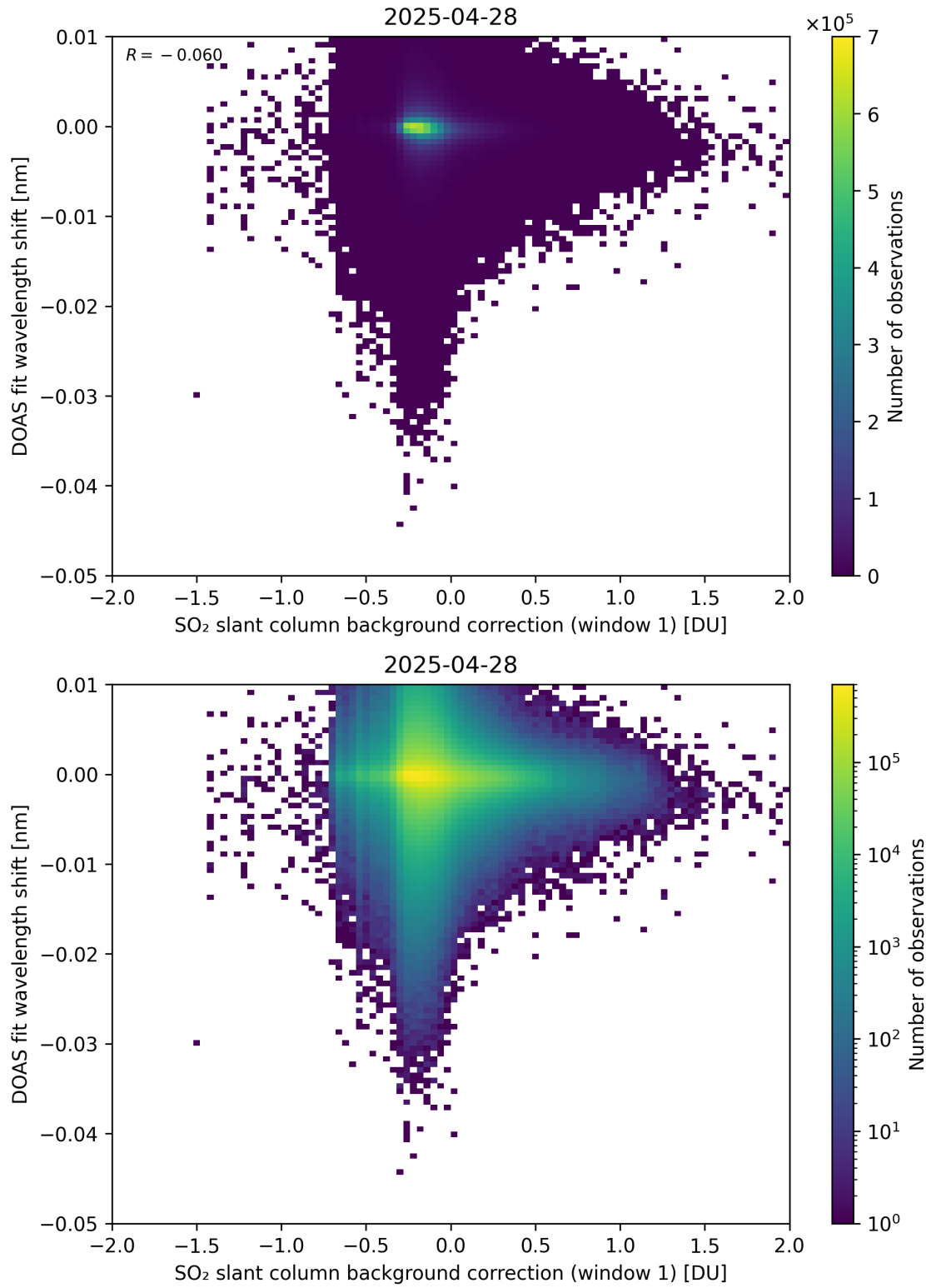
Figure 111: Scatter density plot of “SO 2 slant column background correction (window 1)” against “DOAS fit wavelength shift” for 2025-04-27 to 2025-04-29.
