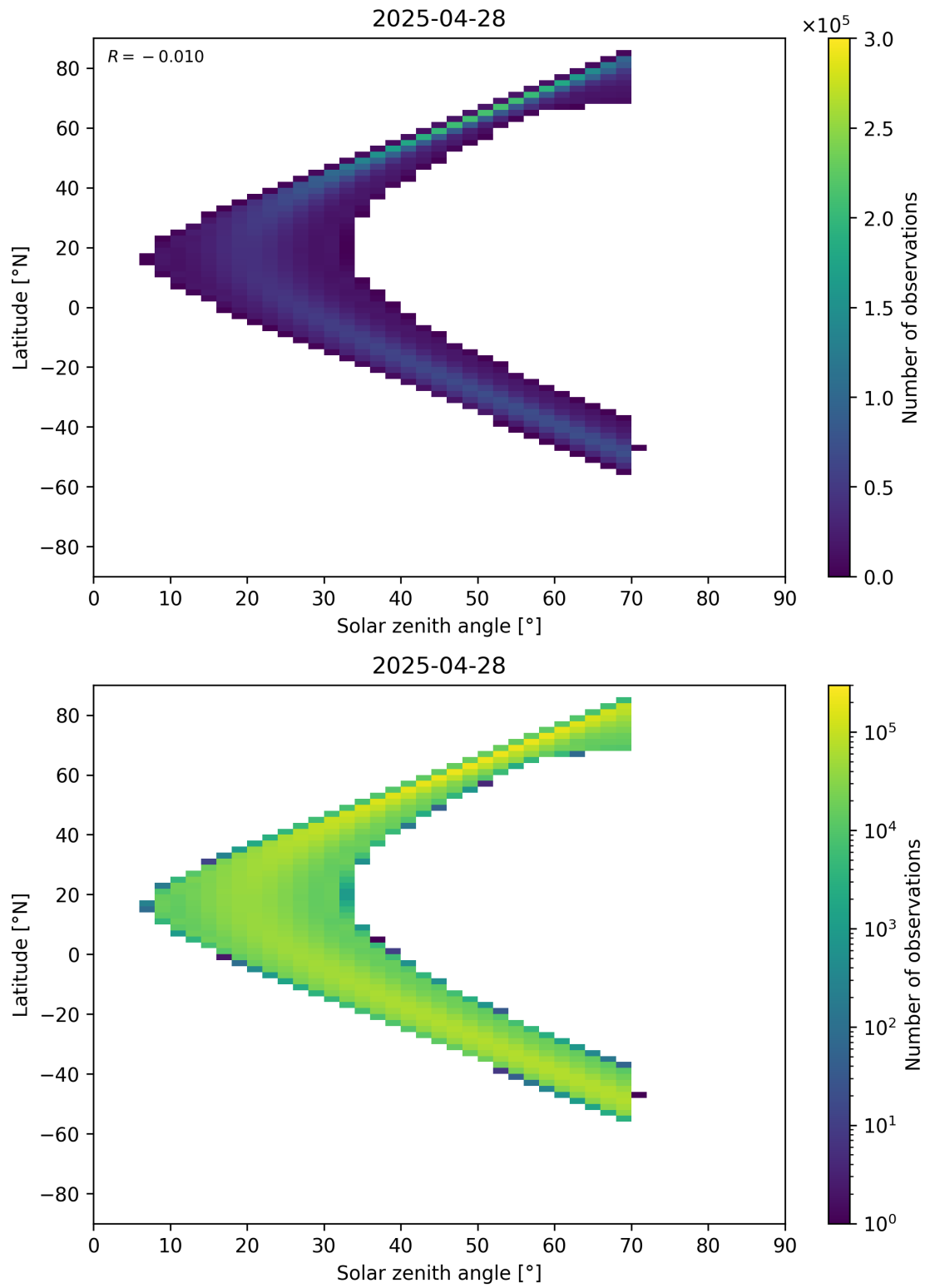
Figure 177: Scatter density plot of “Solar zenith angle” against “Latitude” for 2025-04-27 to 2025-04-29.
