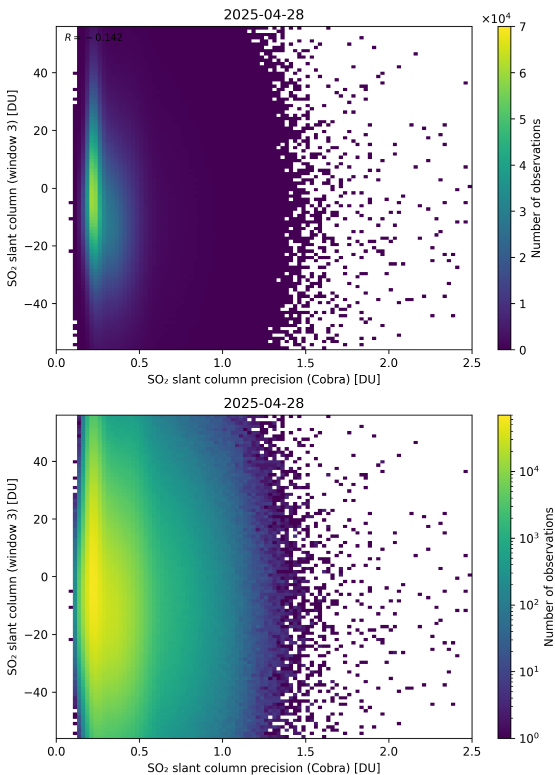
Figure 211: Scatter density plot of “SO 2 slant column precision (Cobra)” against “SO 2 slant column (window 3)” for 2025-04-27 to 2025-04-29.
