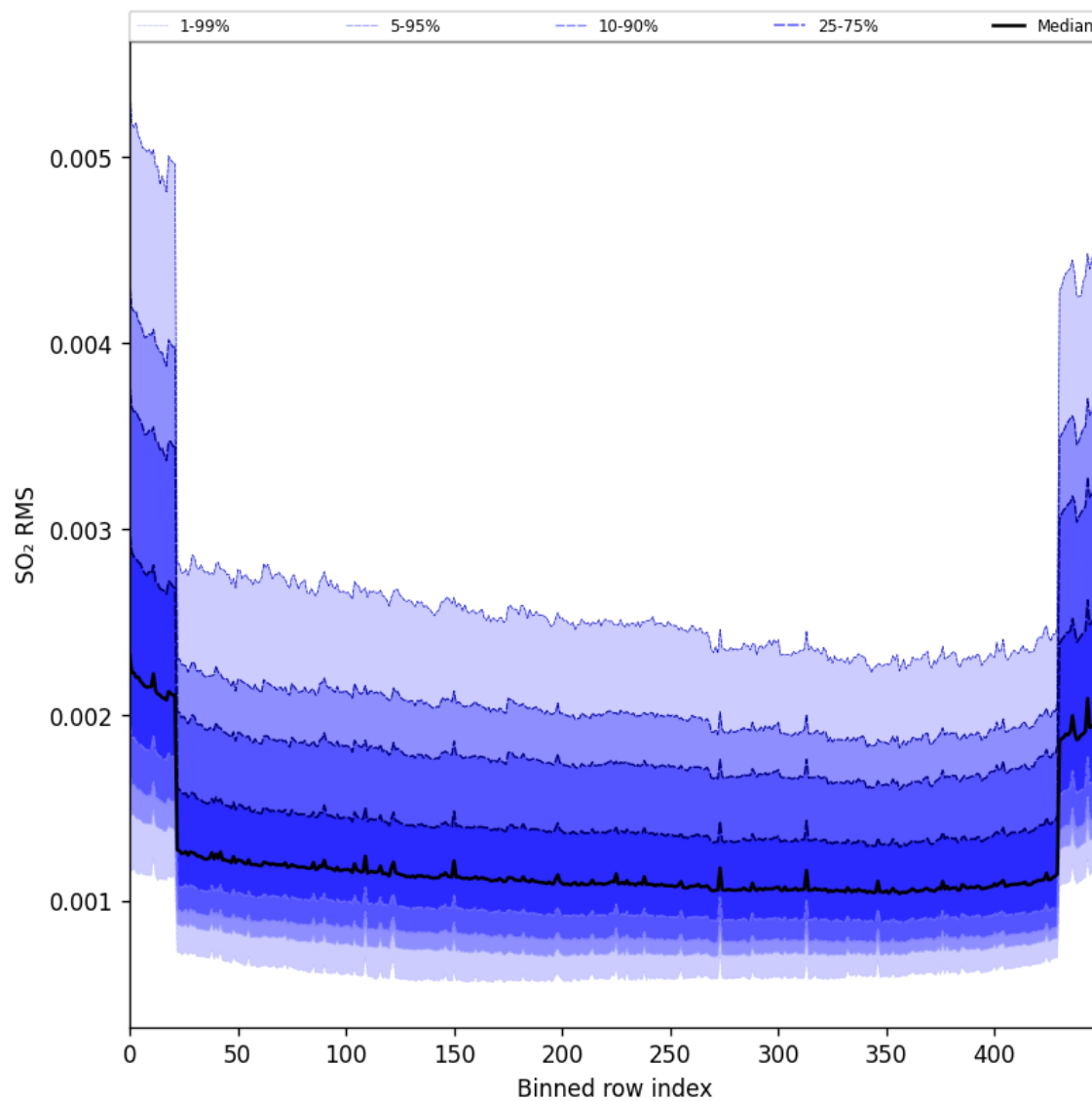
Figure 104: Along track statistics of “SO 2 RMS” for 2025-04-27 to 2025-04-29
