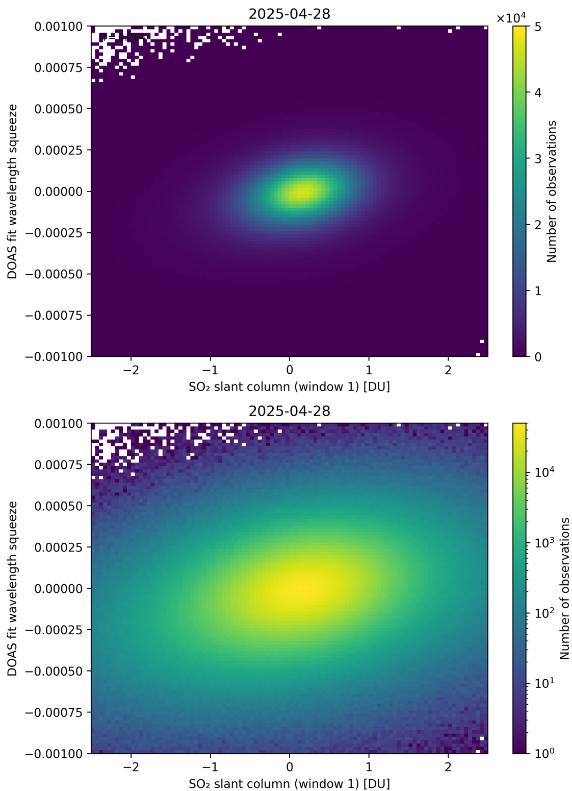
Figure 266: Scatter density plot of “SO 2 slant column (window 1)” against “DOAS fit wavelength squeeze” for 2025-04-27 to 2025-04-29.
