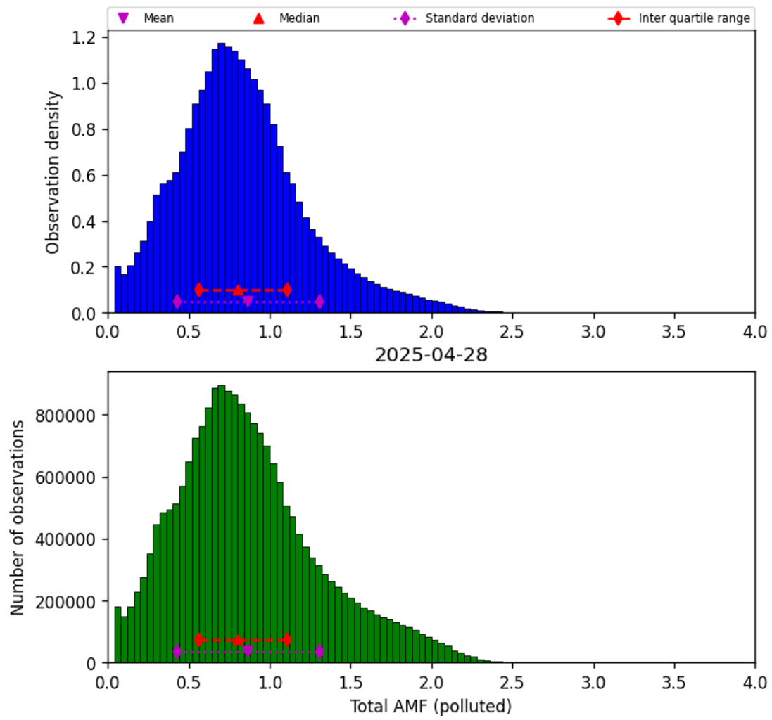
Figure 79: Histogram of “Total AMF (polluted)” for 2025-04-27 to 2025-04-29
