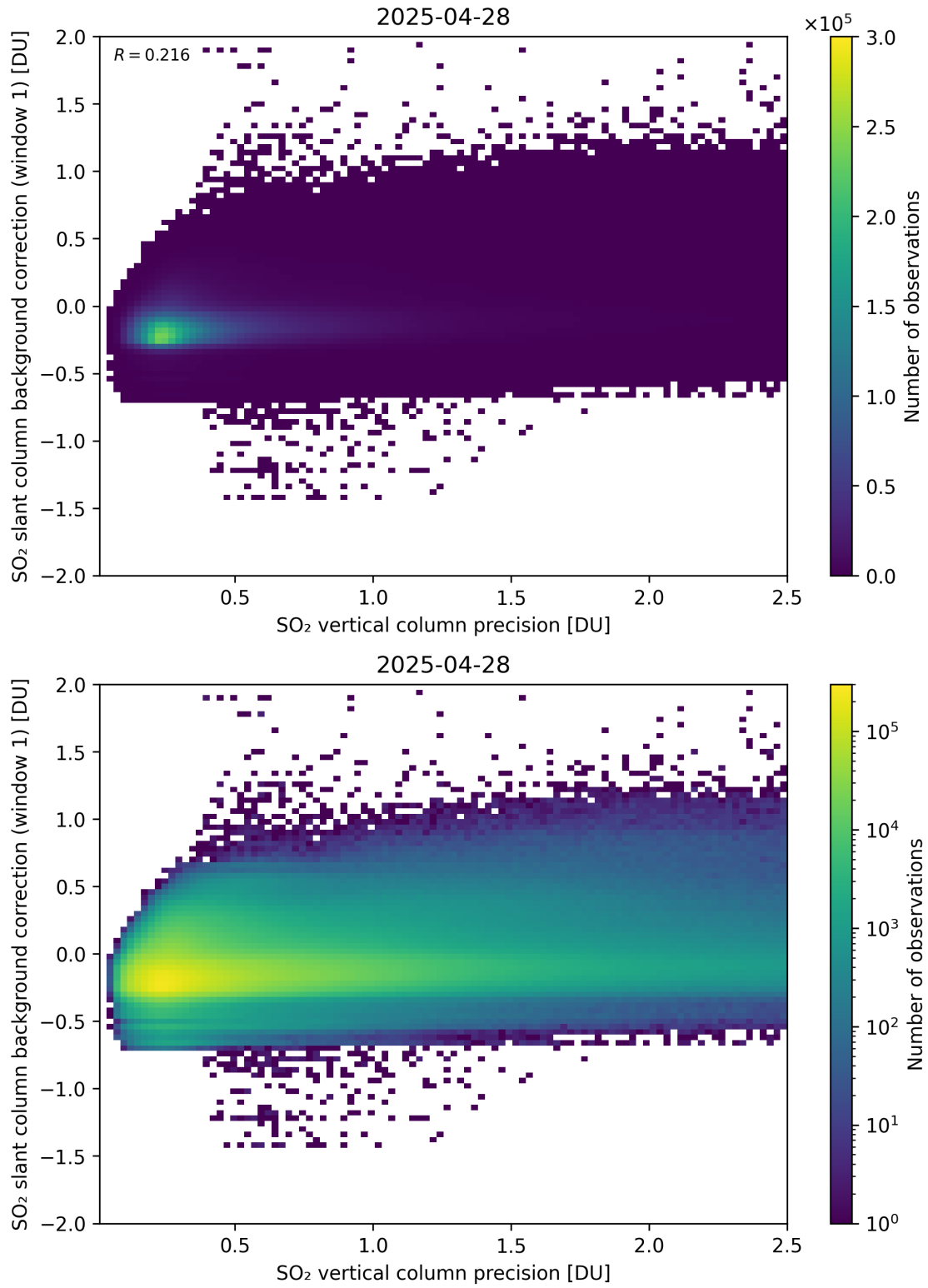
Figure 329: Scatter density plot of “SO 2 vertical column precision” against “SO 2 slant column background correction (window 1)” for 2025-04-27 to 2025-04-29.
