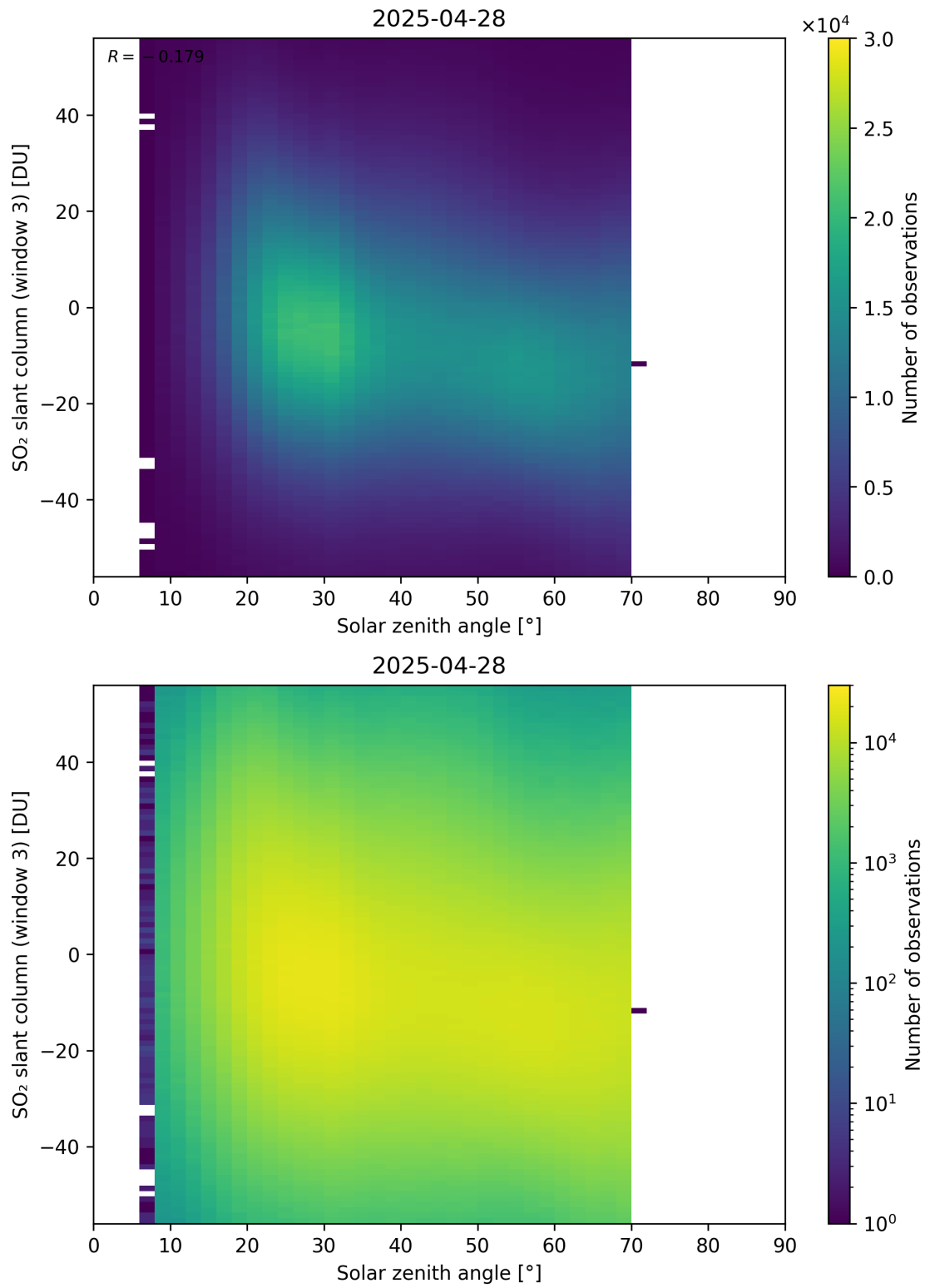
Figure 187: Scatter density plot of “Solar zenith angle” against “SO 2 slant column (window 3)” for 2025-04-27 to 2025-04-29.
