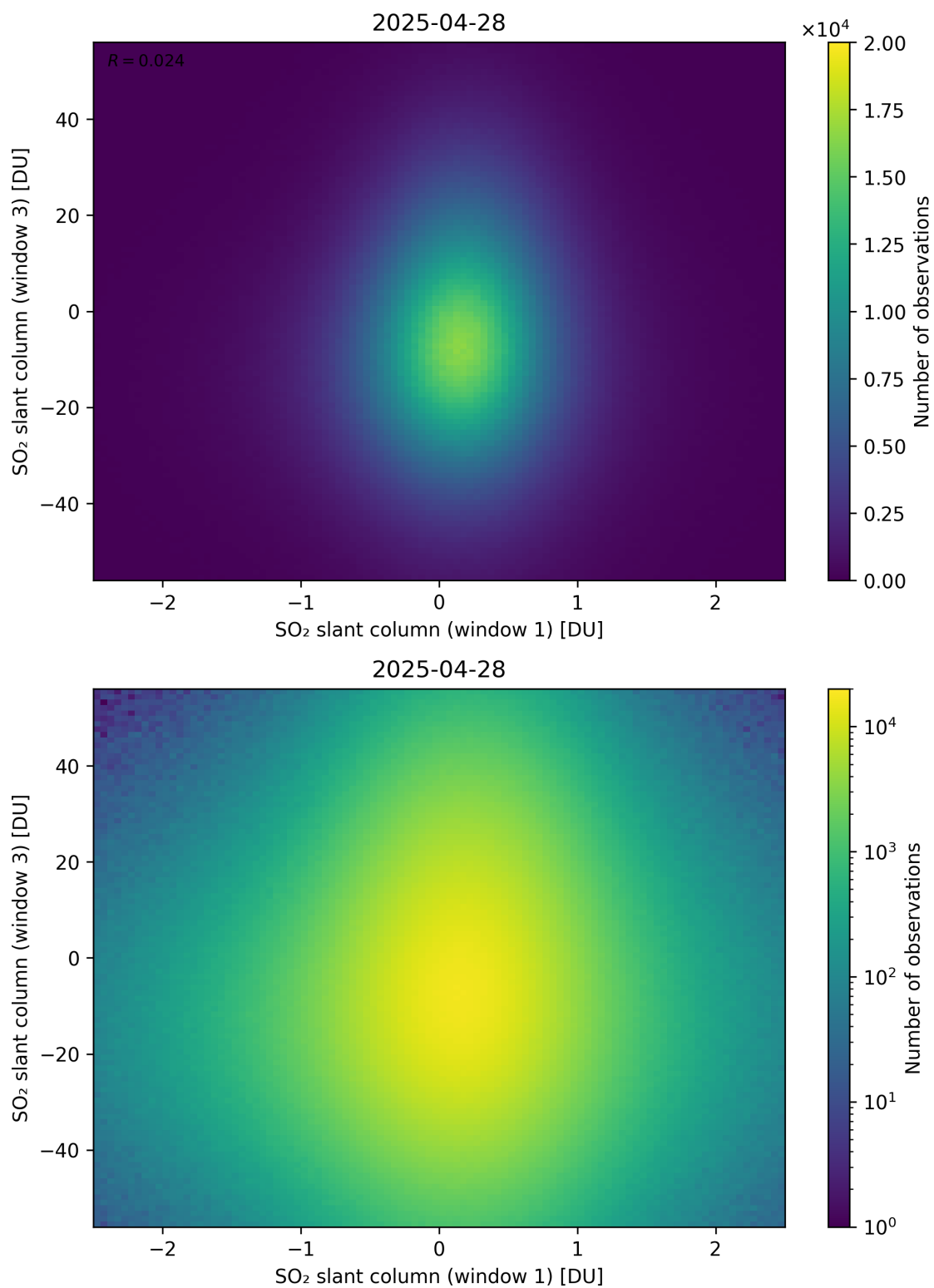
Figure 287: Scatter density plot of “SO 2 slant column (window 1)” against “SO 2 slant column (window 3)” for 2025-04-27 to 2025-04-29.
