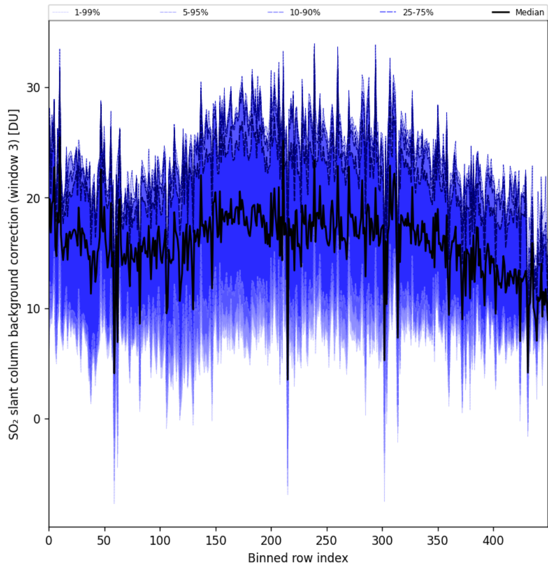
Figure 100: Along track statistics of “SO 2 slant column background correction (window 3)” for 2025-04-27 to 2025-04-29
