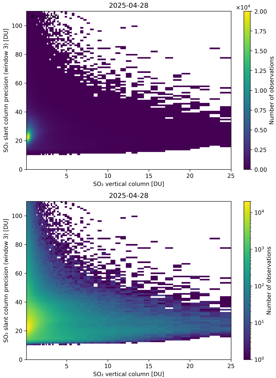
Figure 358: Scatter density plot of “SO 2 vertical column” against “SO 2 slant column precision (window 3)” for 2025-04-27 to 2025-04-29.
