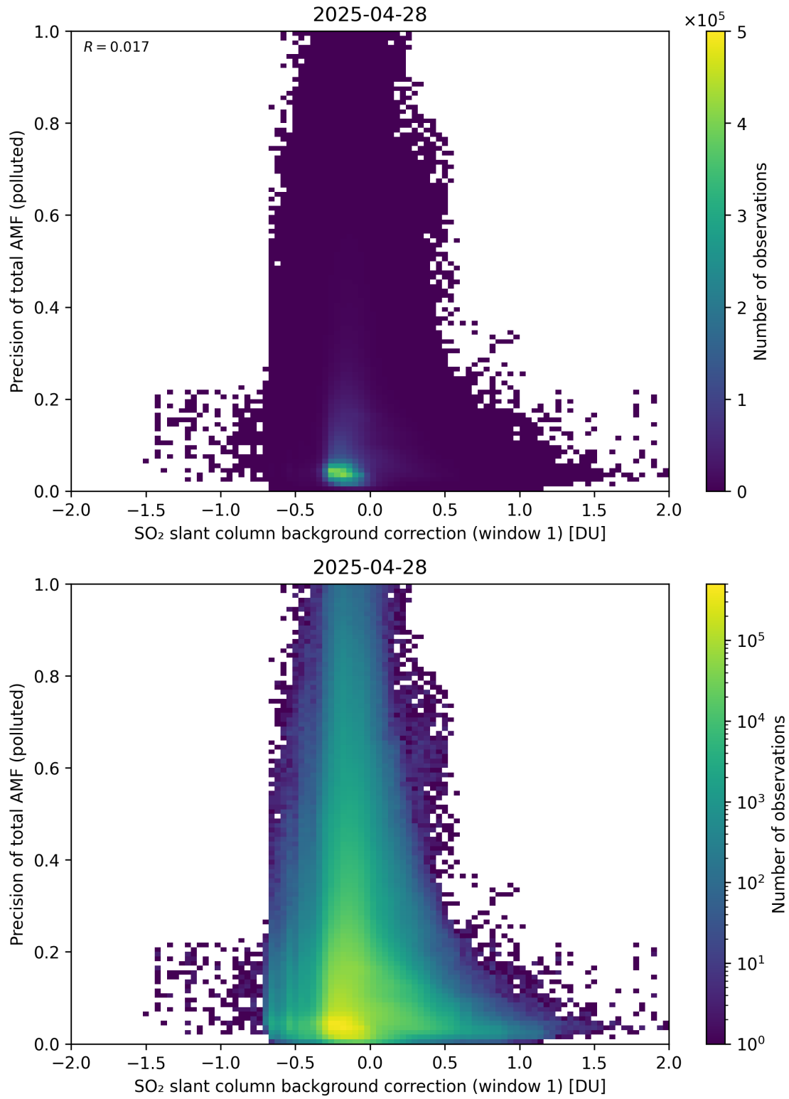
Figure 121: Scatter density plot of “SO 2 slant column background correction (window 1)” against “Precision of total AMF (polluted)” for 2025-04-27 to 2025-04-29.
