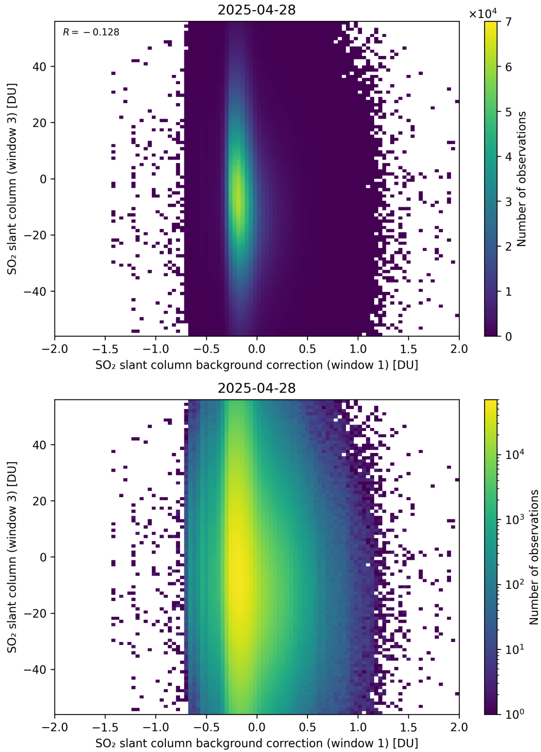
Figure 118: Scatter density plot of “SO 2 slant column background correction (window 1)” against “SO 2 slant column (window 3)” for 2025-04-27 to 2025-04-29.
