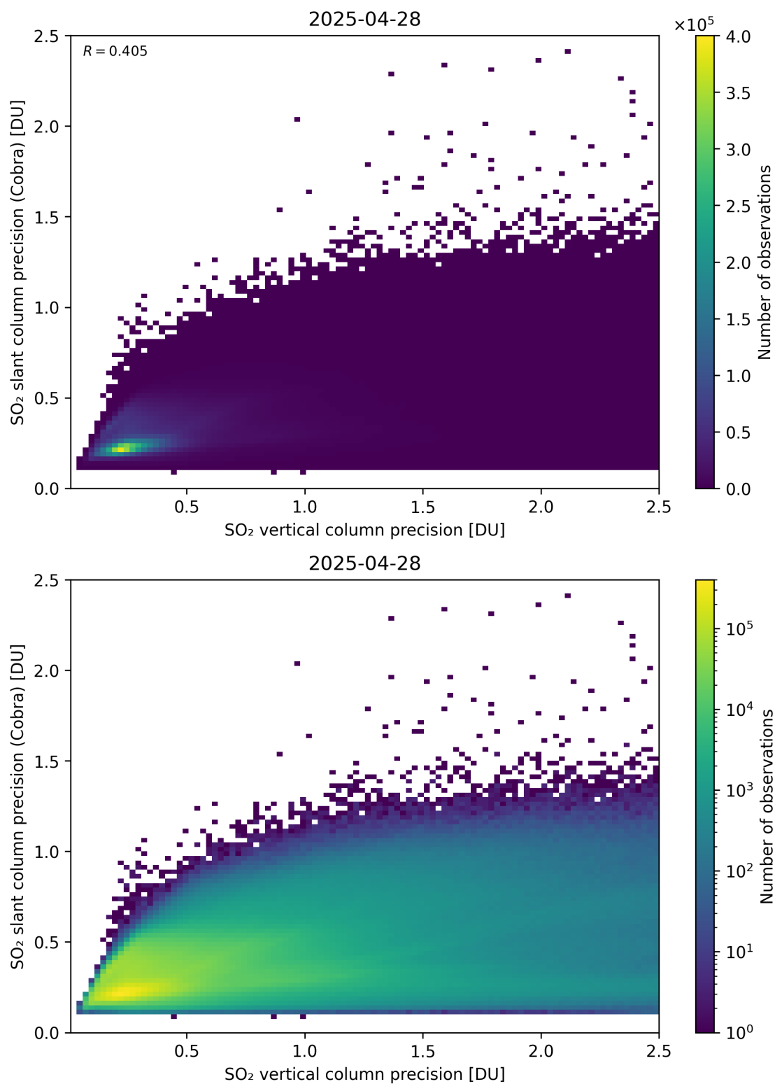
Figure 337: Scatter density plot of “SO 2 vertical column precision” against “SO 2 slant column precision (Cobra)” for 2025-04-27 to 2025-04-29.
