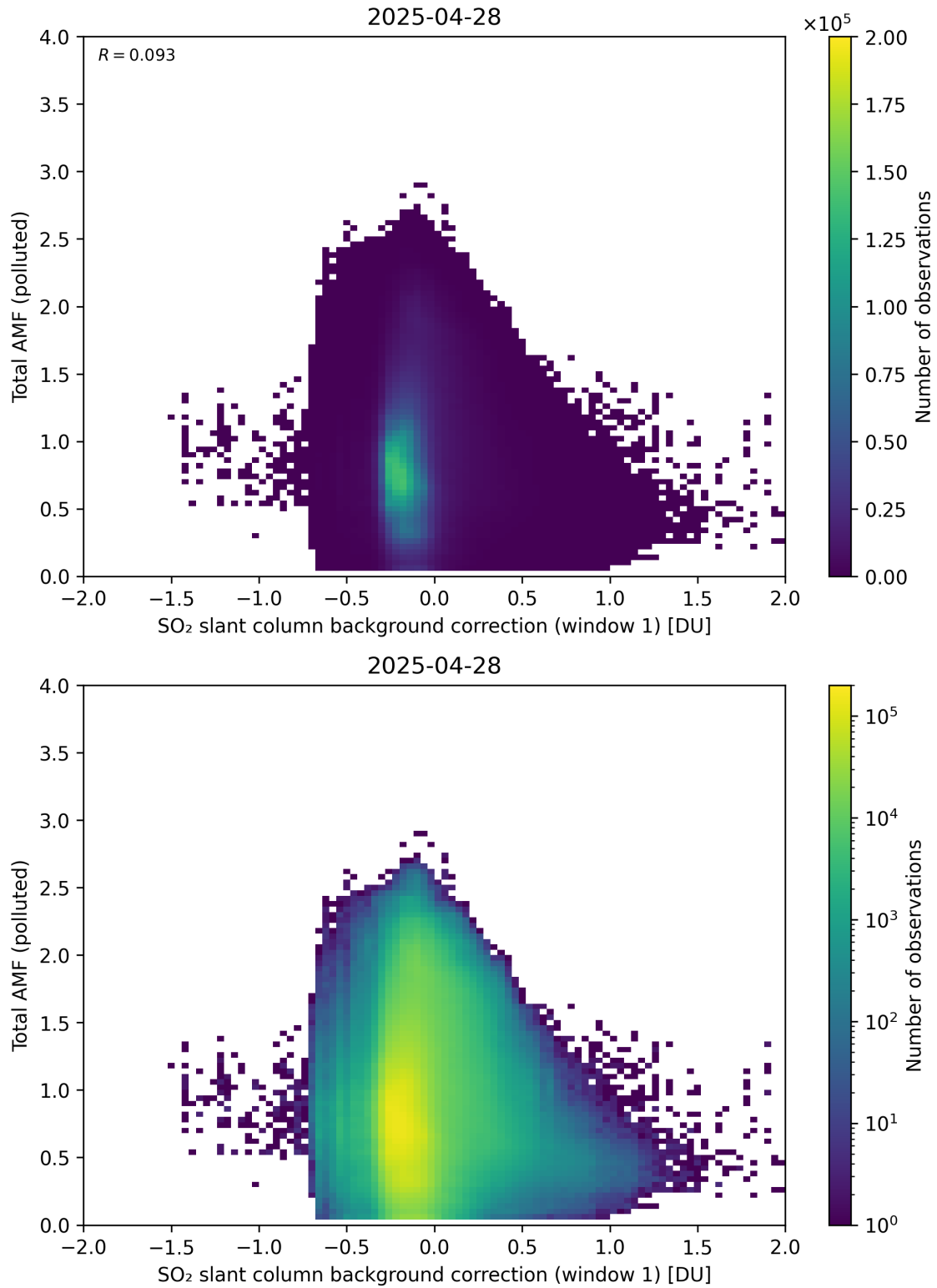
Figure 120: Scatter density plot of “SO 2 slant column background correction (window 1)” against “Total AMF (polluted)” for 2025-04-27 to 2025-04-29.
