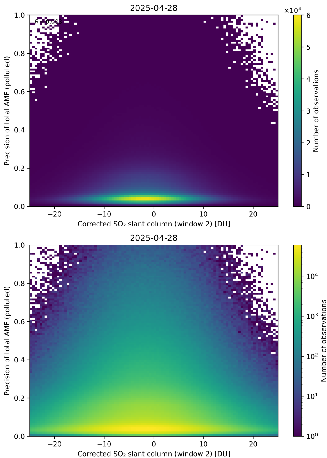
Figure 254: Scatter density plot of “Corrected SO 2 slant column (window 2)” against “Precision of total AMF (polluted)” for 2025-04-27 to 2025-04-29.
