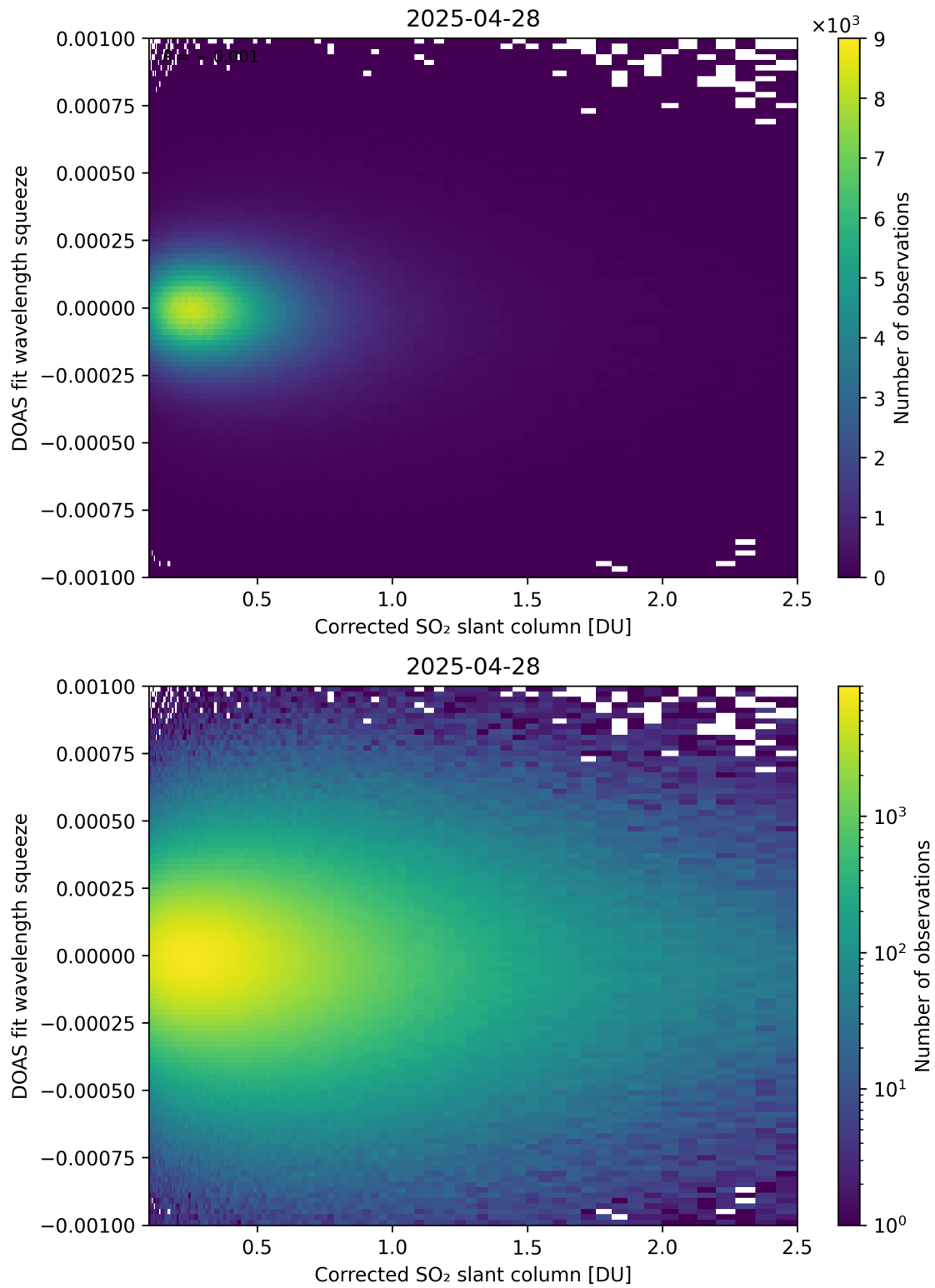
Figure 230: Scatter density plot of “Corrected SO 2 slant column” against “DOAS fit wavelength squeeze” for 2025-04-27 to 2025-04-29.
