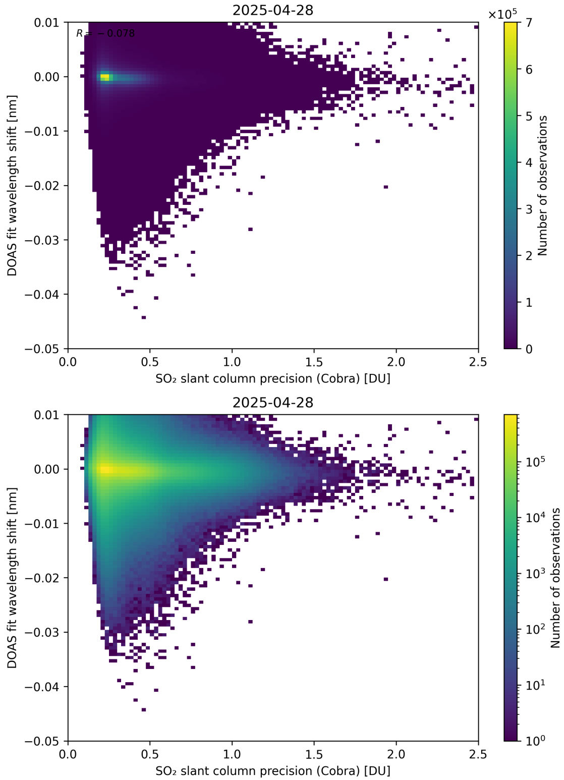
Figure 202: Scatter density plot of “SO 2 slant column precision (Cobra)” against “DOAS fit wavelength shift” for 2025-04-27 to 2025-04-29.
