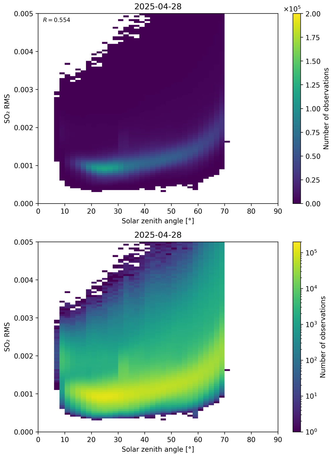
Figure 176: Scatter density plot of “Solar zenith angle” against “SO 2 RMS” for 2025-04-27 to 2025-04-29.
