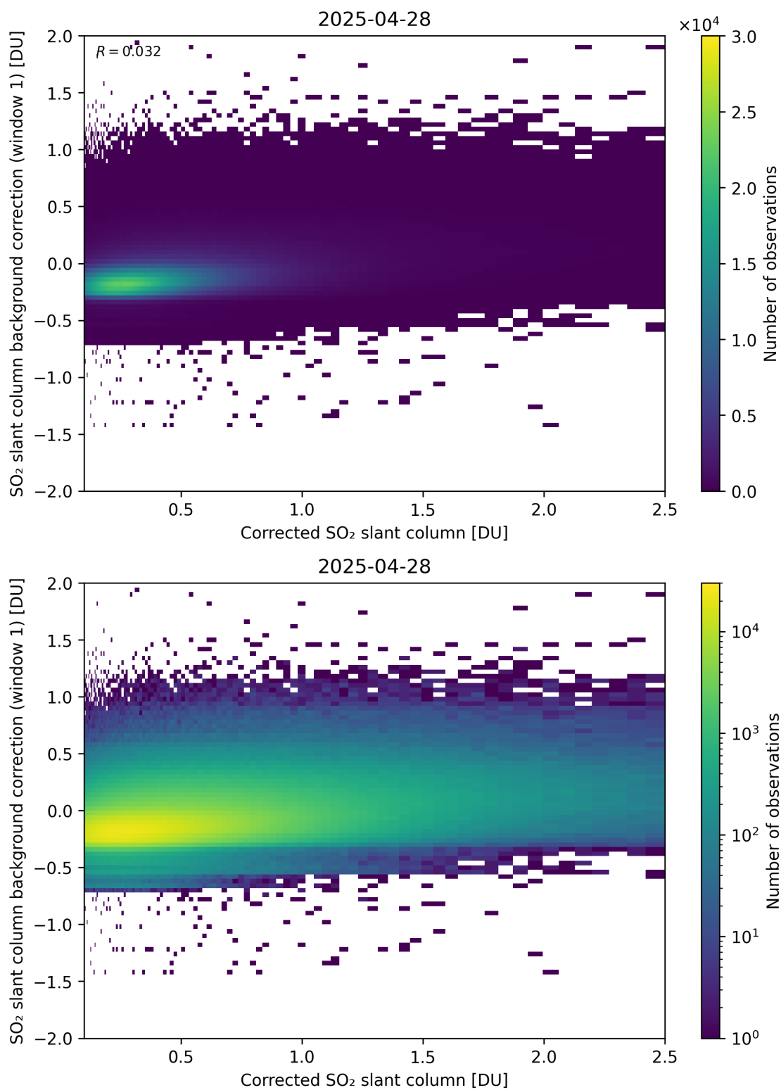
Figure 226: Scatter density plot of “Corrected SO 2 slant column” against “SO 2 slant column background correction (window 1)” for 2025-04-27 to 2025-04-29.
