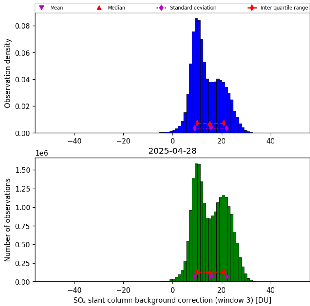
Figure 74: Histogram of “SO 2 slant column background correction (window 3)” for 2025-04-27 to 2025-04-29
