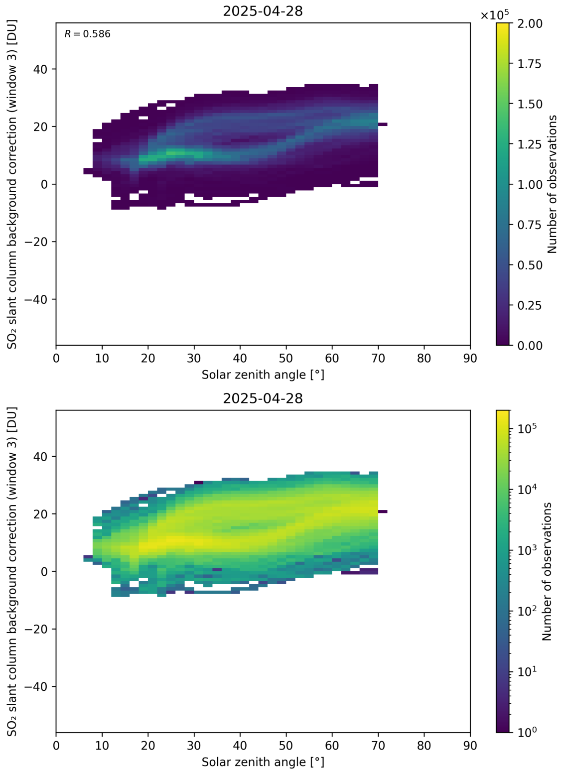
Figure 173: Scatter density plot of “Solar zenith angle” against “SO 2 slant column background correction (window 3)” for 2025-04-27 to 2025-04-29.
