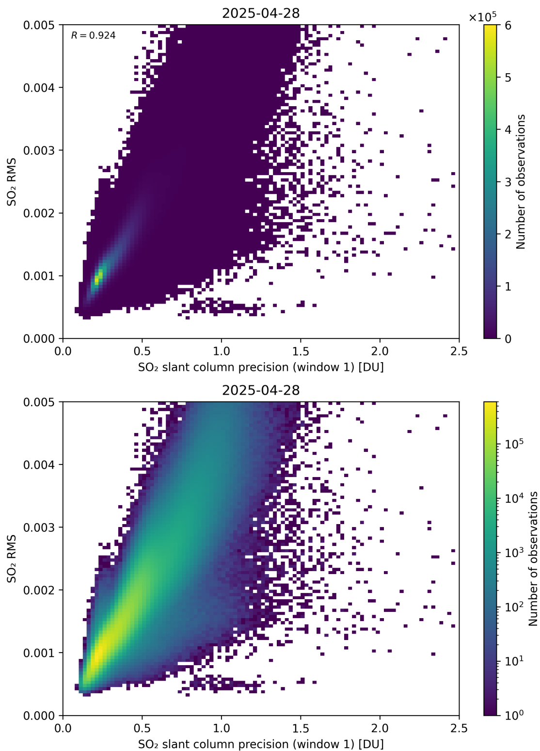
Figure 273: Scatter density plot of “SO 2 slant column precision (window 1)” against “SO 2 RMS” for 2025-04-27 to 2025-04-29.
