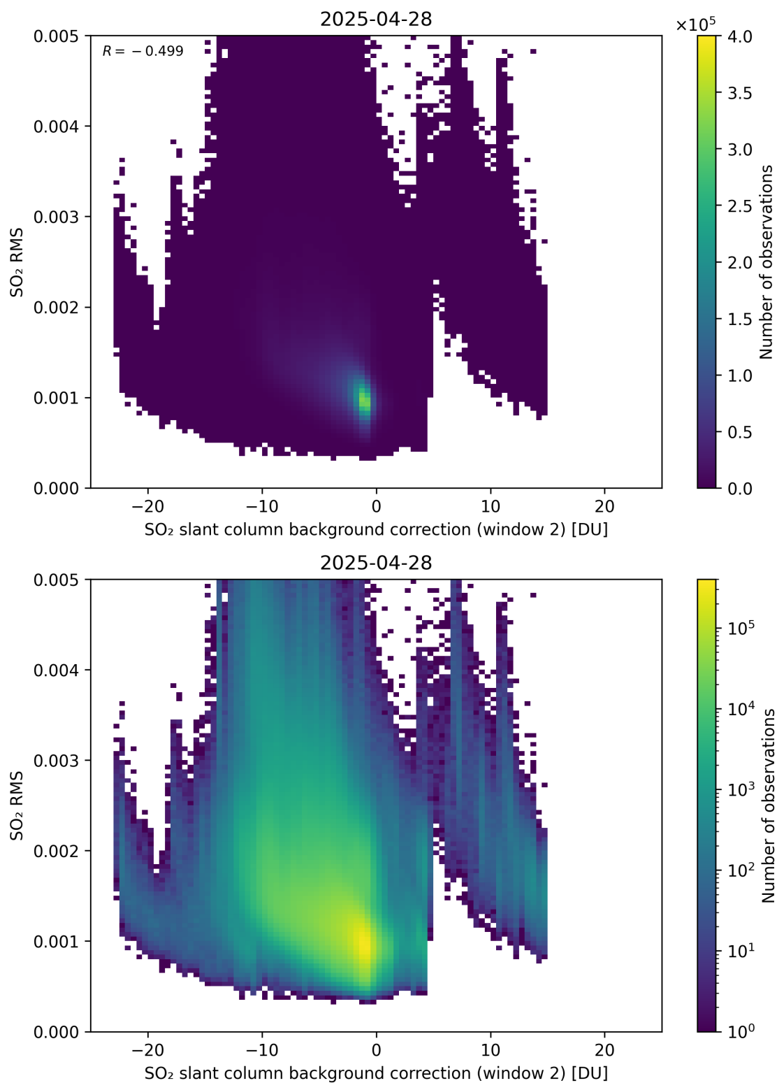
Figure 125: Scatter density plot of “SO 2 slant column background correction (window 2)” against “SO 2 RMS” for 2025-04-27 to 2025-04-29.
