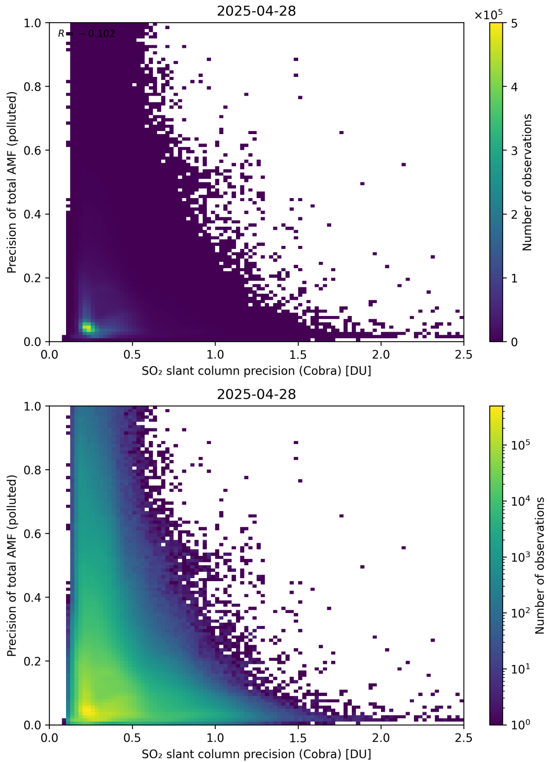
Figure 214: Scatter density plot of “SO 2 slant column precision (Cobra)” against “Precision of total AMF (polluted)” for 2025-04-27 to 2025-04-29.
