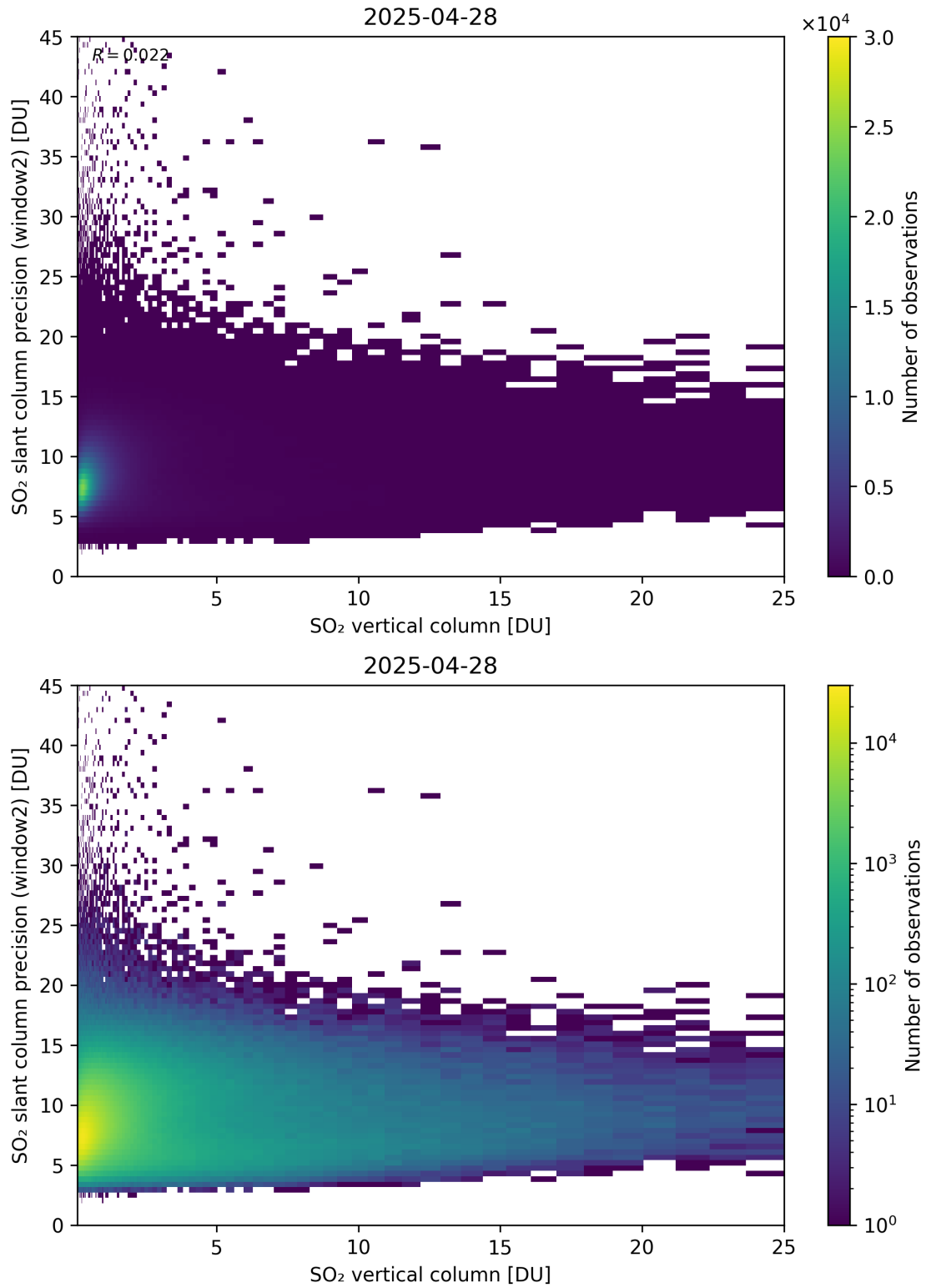
Figure 356: Scatter density plot of “SO 2 vertical column” against “SO 2 slant column precision (window2)” for 2025-04-27 to 2025-04-29.
