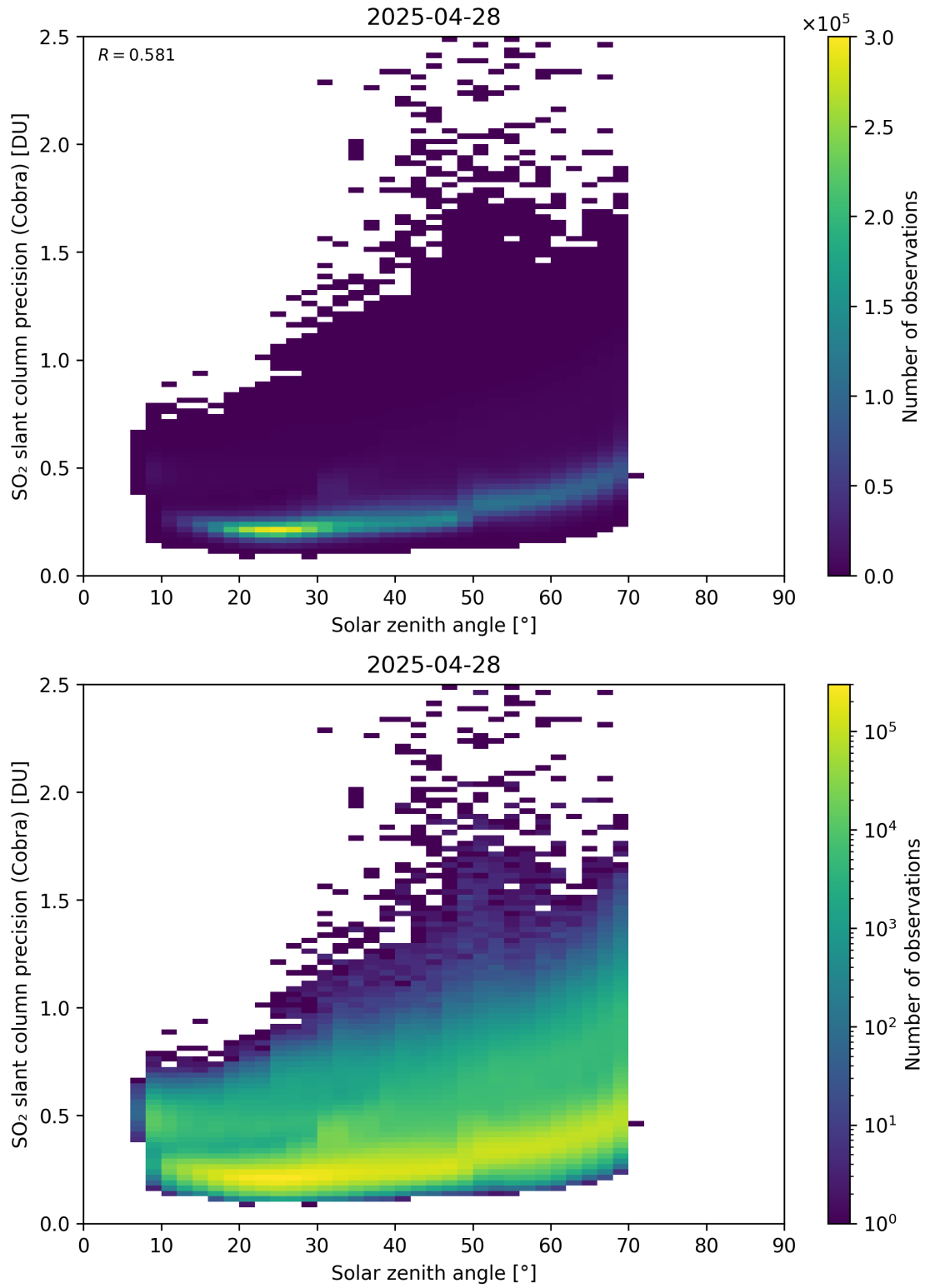
Figure 180: Scatter density plot of “Solar zenith angle” against “SO 2 slant column precision (Cobra)” for 2025-04-27 to 2025-04-29.
