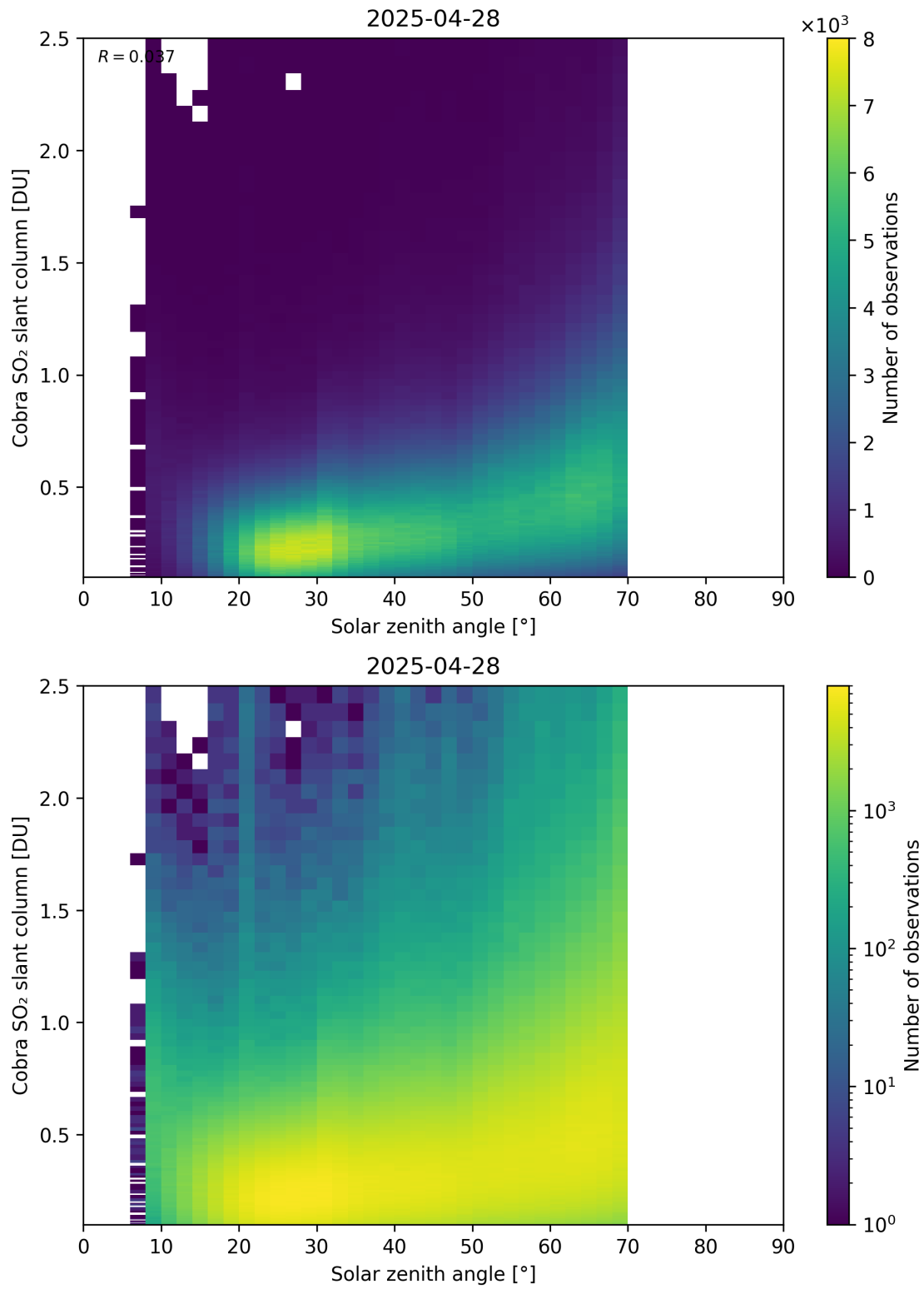
Figure 179: Scatter density plot of “Solar zenith angle” against “Cobra SO 2 slant column” for 2025-04-27 to 2025-04-29.
