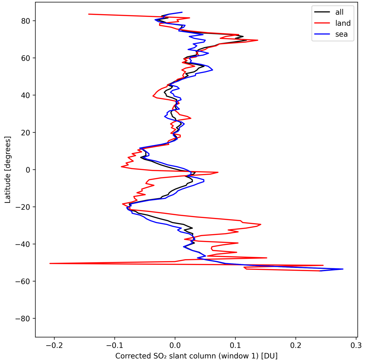
Figure 39: Zonal average of “Corrected SO 2 slant column (window 1)” for 2025-04-27 to 2025-04-29.
