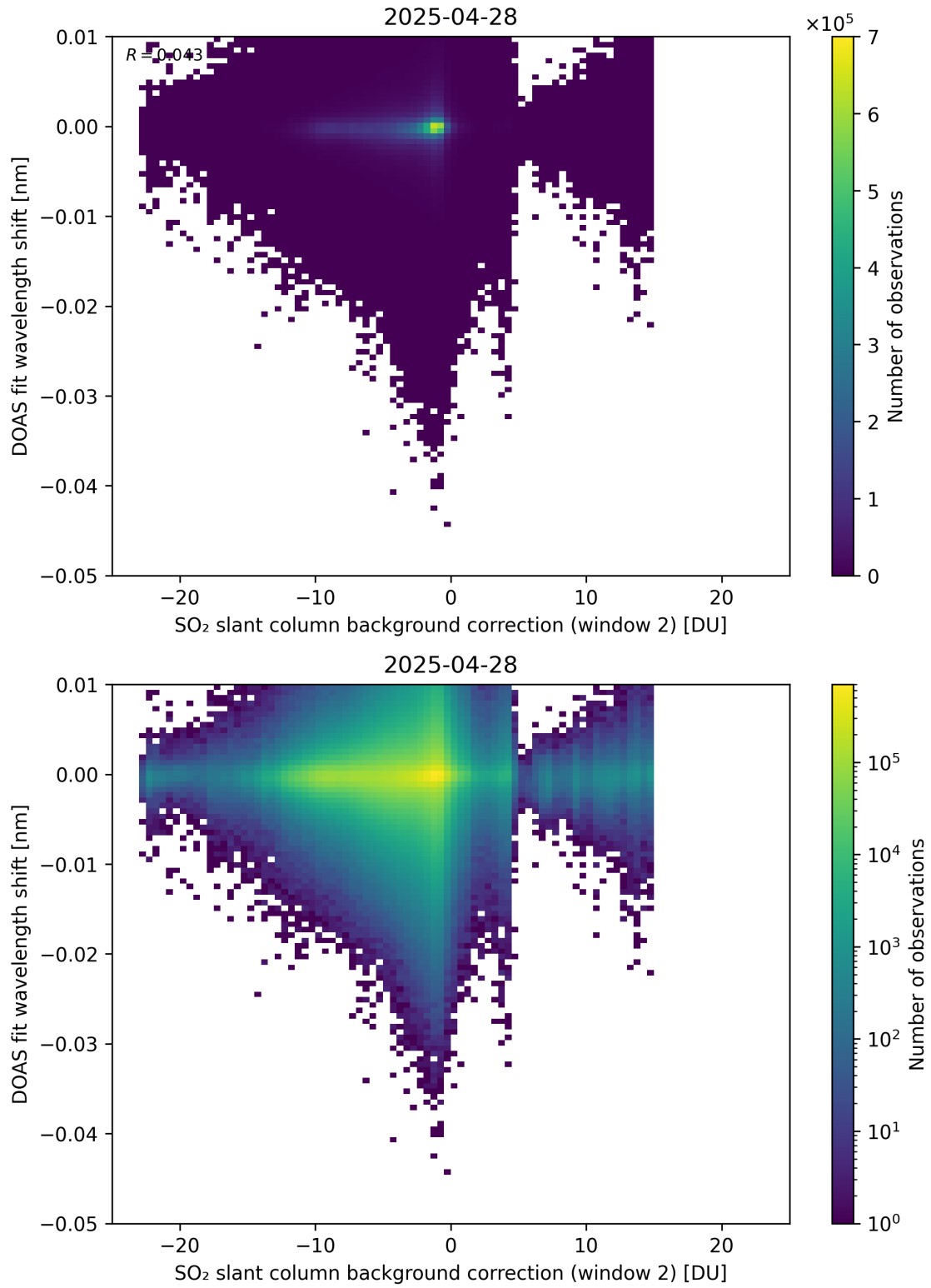
Figure 123: Scatter density plot of “SO 2 slant column background correction (window 2)” against “DOAS fit wavelength shift” for 2025-04-27 to 2025-04-29.
