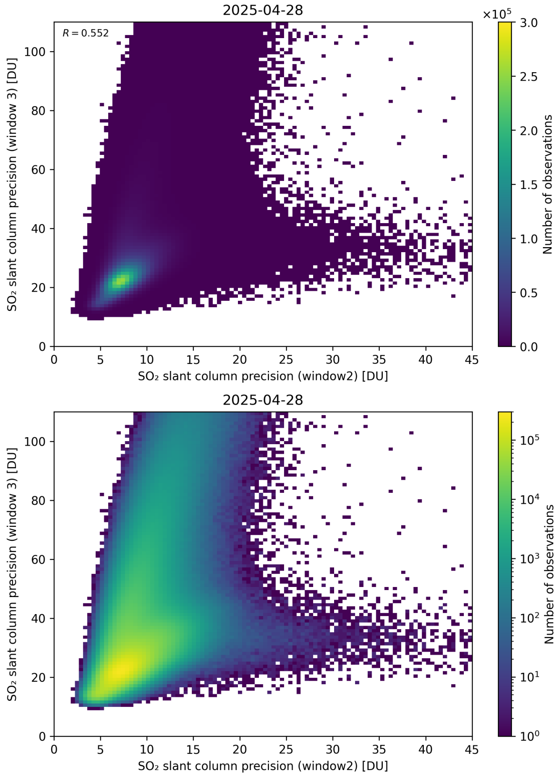
Figure 300: Scatter density plot of “SO 2 slant column precision (window2)” against “SO 2 slant column precision (window 3)” for 2025-04-27 to 2025-04-29.
