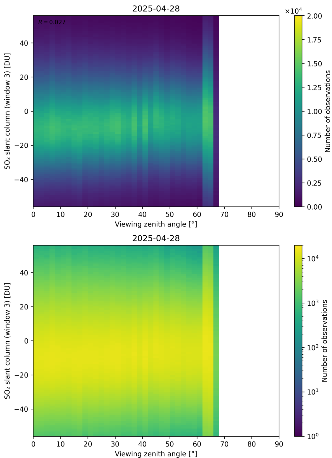
Figure 379: Scatter density plot of “Viewing zenith angle” against “SO 2 slant column (window 3)” for 2025-04-27 to 2025-04-29.
