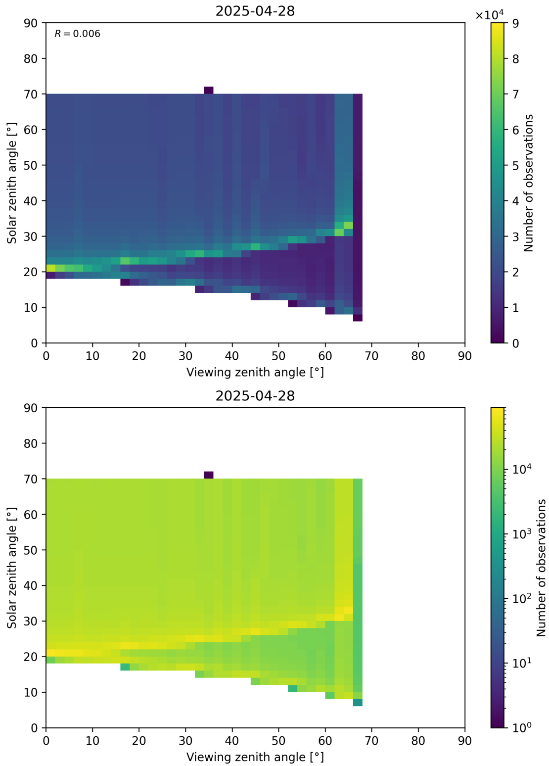
Figure 369: Scatter density plot of “Viewing zenith angle” against “Solar zenith angle” for 2025-04-27 to 2025-04-29.
