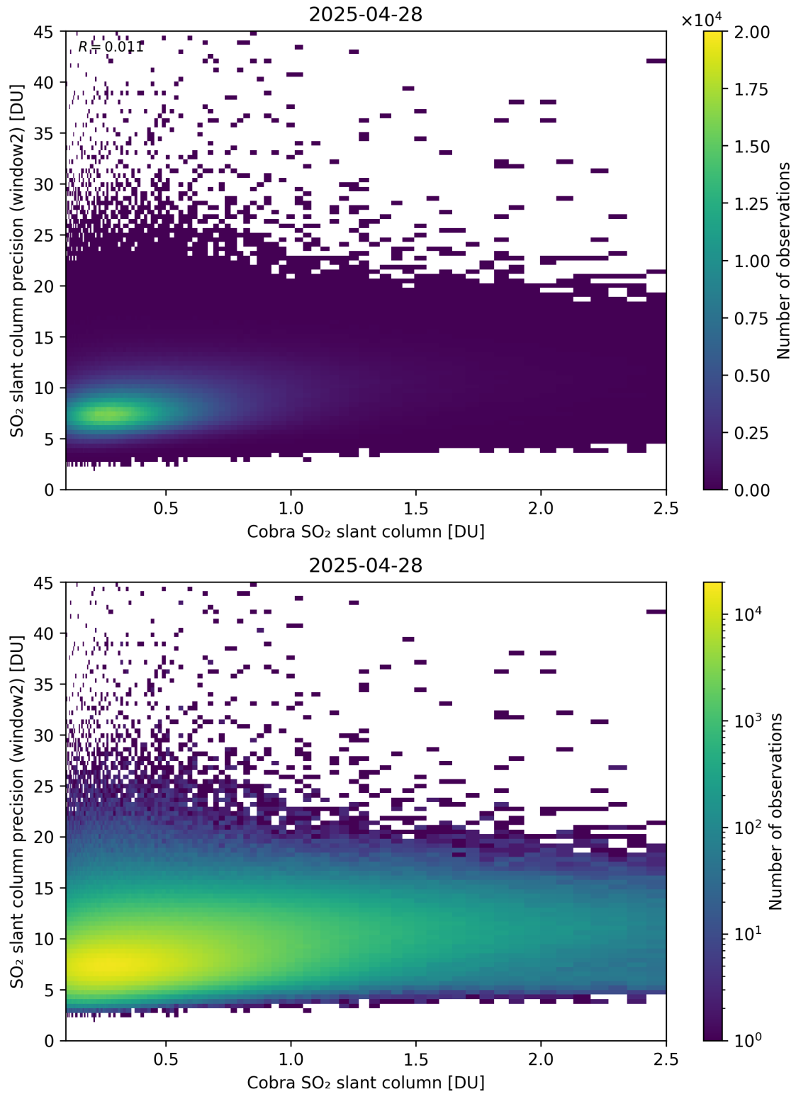
Figure 221: Scatter density plot of “Cobra SO 2 slant column” against “SO 2 slant column precision (window2)” for 2025-04-27 to 2025-04-29.
