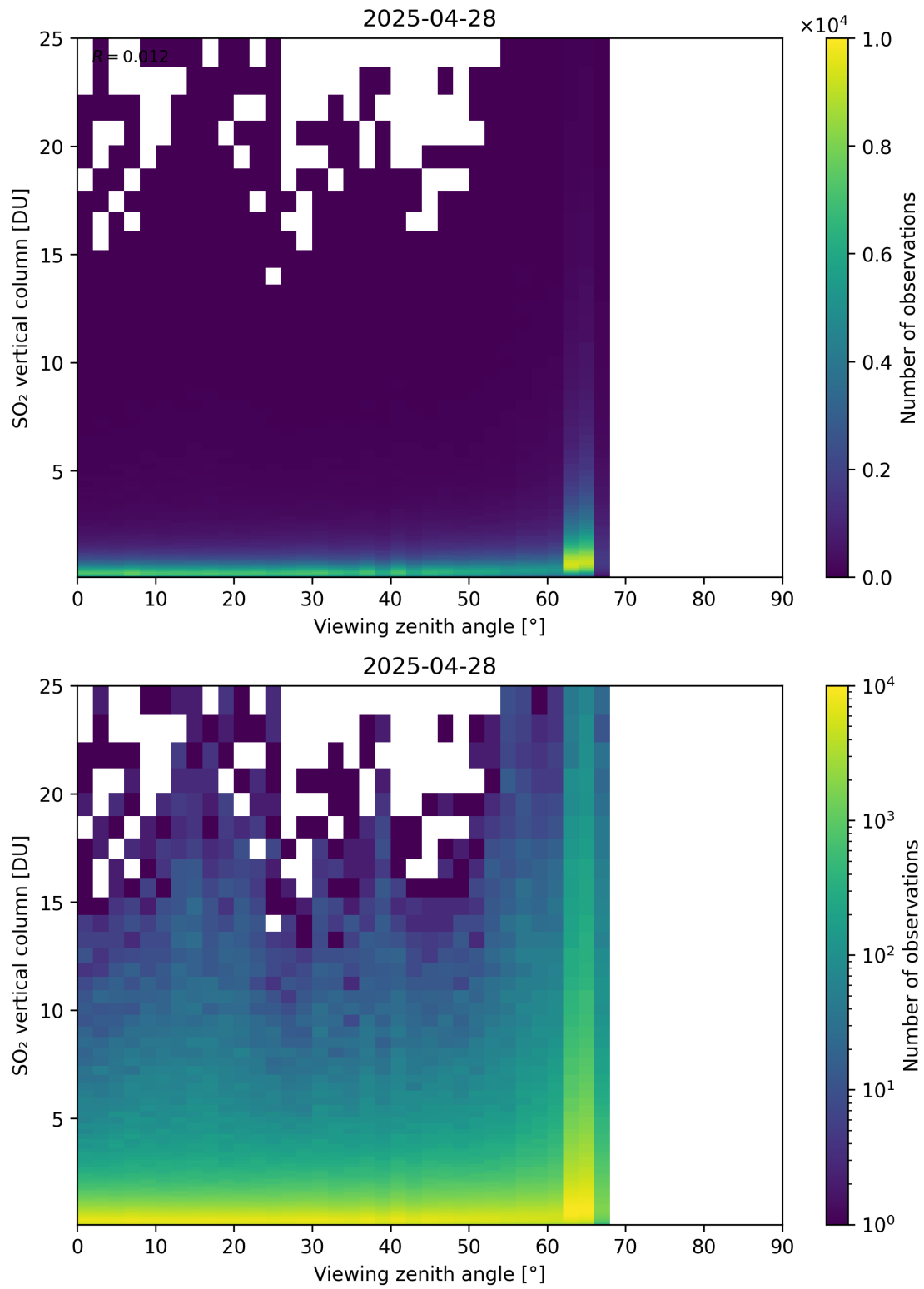
Figure 383: Scatter density plot of “Viewing zenith angle” against “SO 2 vertical column” for 2025-04-27 to 2025-04-29.
