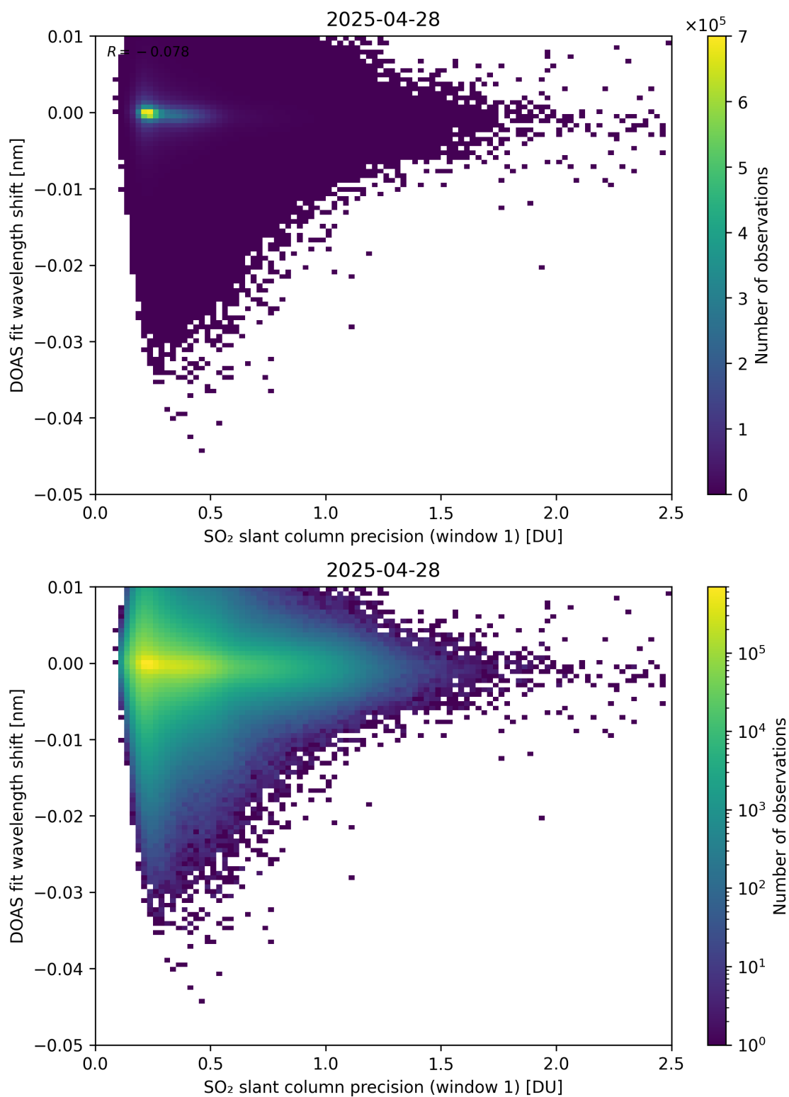
Figure 271: Scatter density plot of “SO 2 slant column precision (window 1)” against “DOAS fit wavelength shift” for 2025-04-27 to 2025-04-29.
