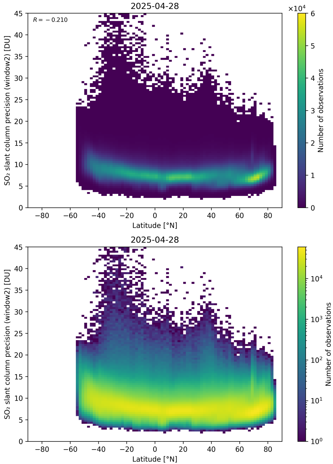
Figure 164: Scatter density plot of “Latitude” against “SO 2 slant column precision (window2)” for 2025-04-27 to 2025-04-29.
