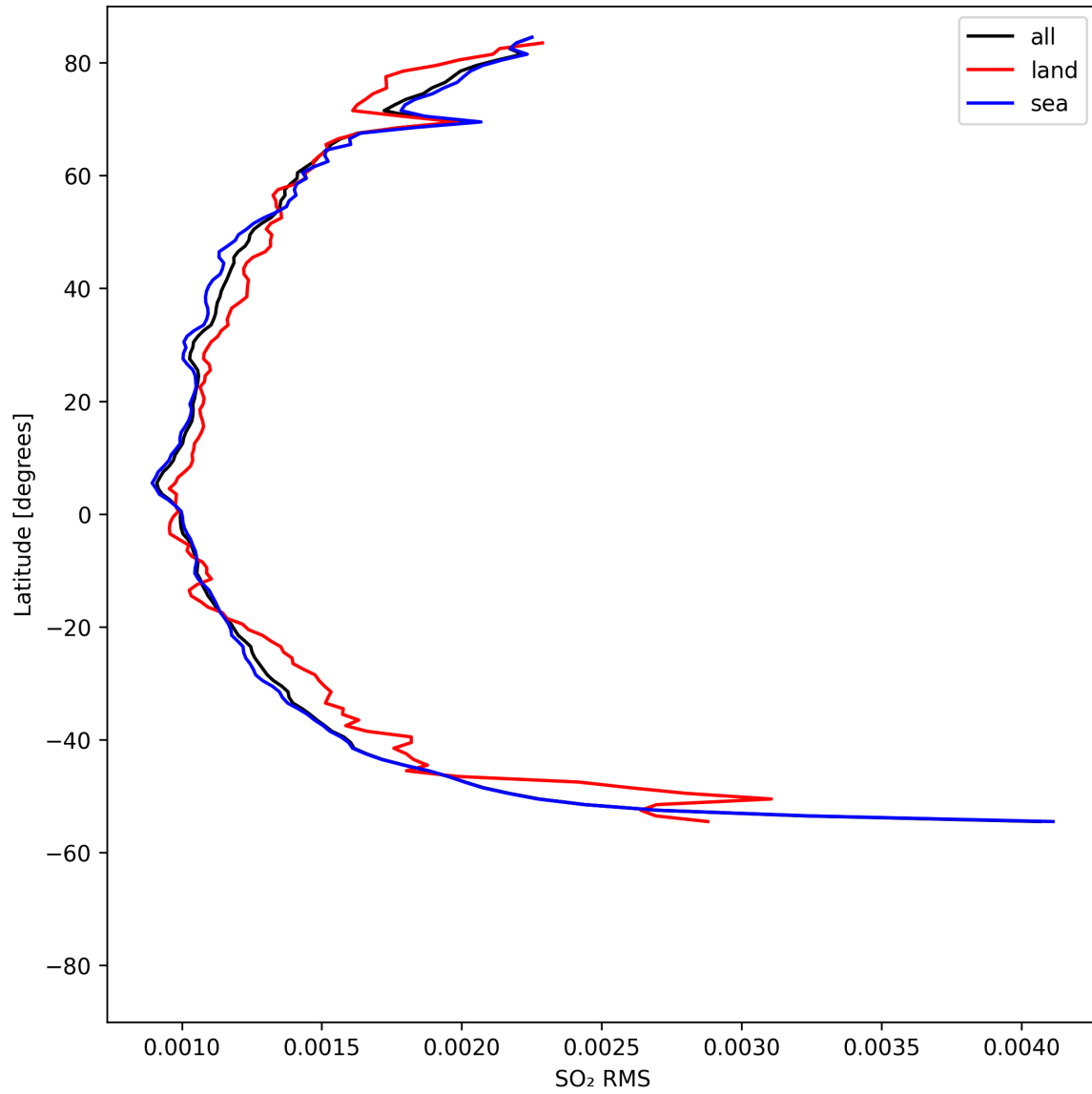
Figure 52: Zonal average of “SO 2 RMS” for 2025-04-27 to 2025-04-29.
