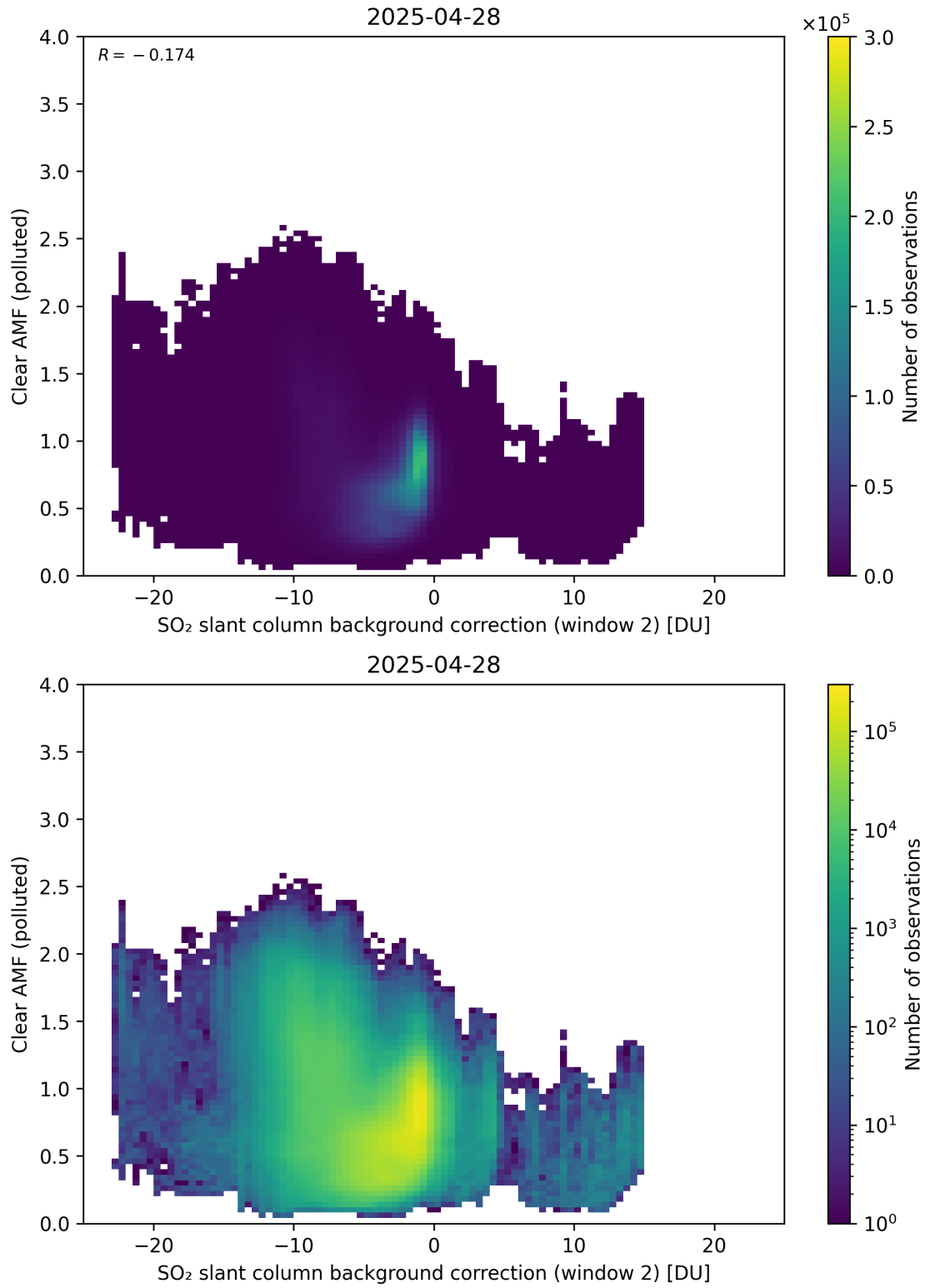
Figure 126: Scatter density plot of “SO 2 slant column background correction (window 2)” against “Clear AMF (polluted)” for 2025-04-27 to 2025-04-29.
