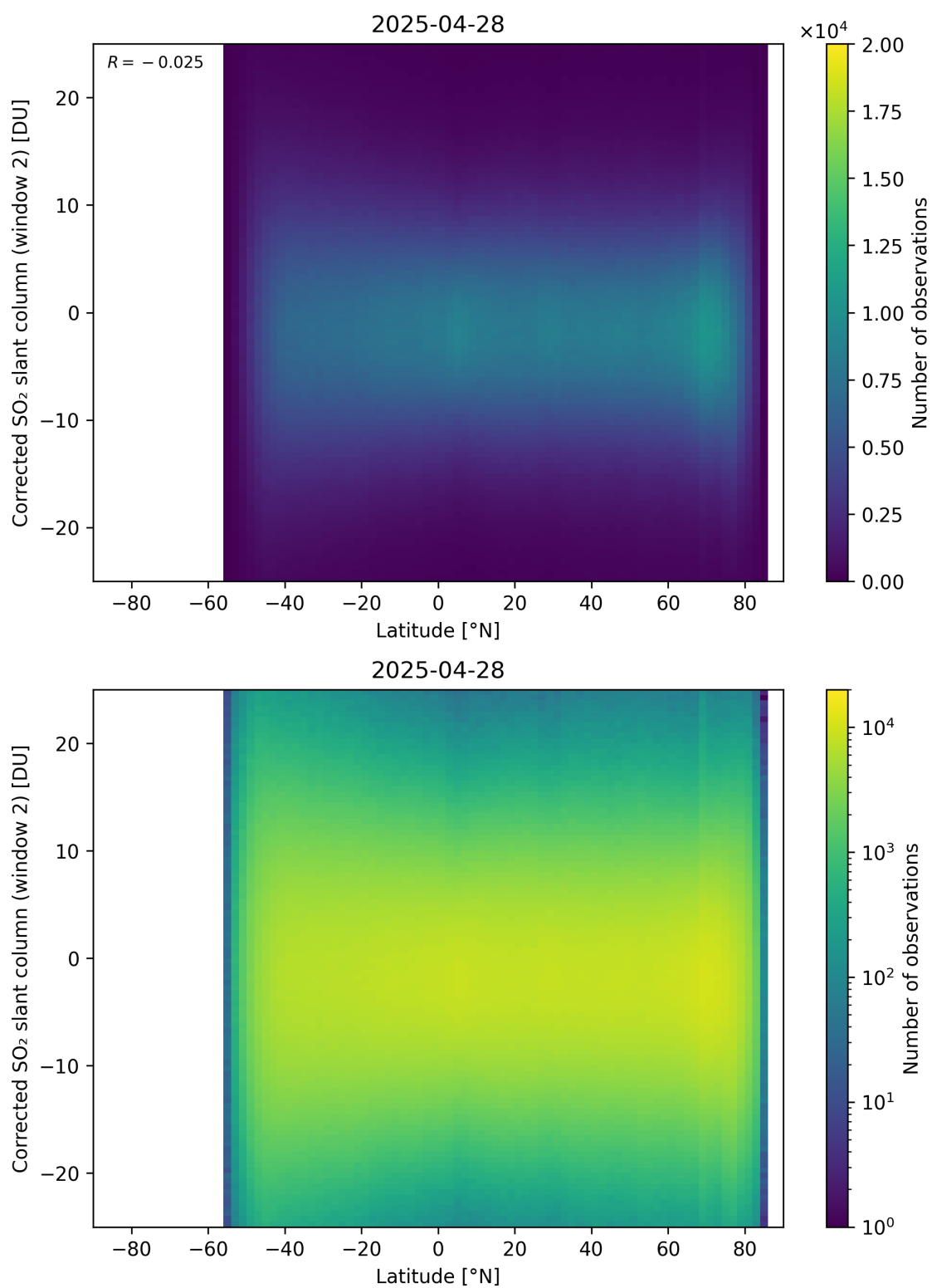
Figure 160: Scatter density plot of “Latitude” against “Corrected SO 2 slant column (window 2)” for 2025-04-27 to 2025-04-29.
