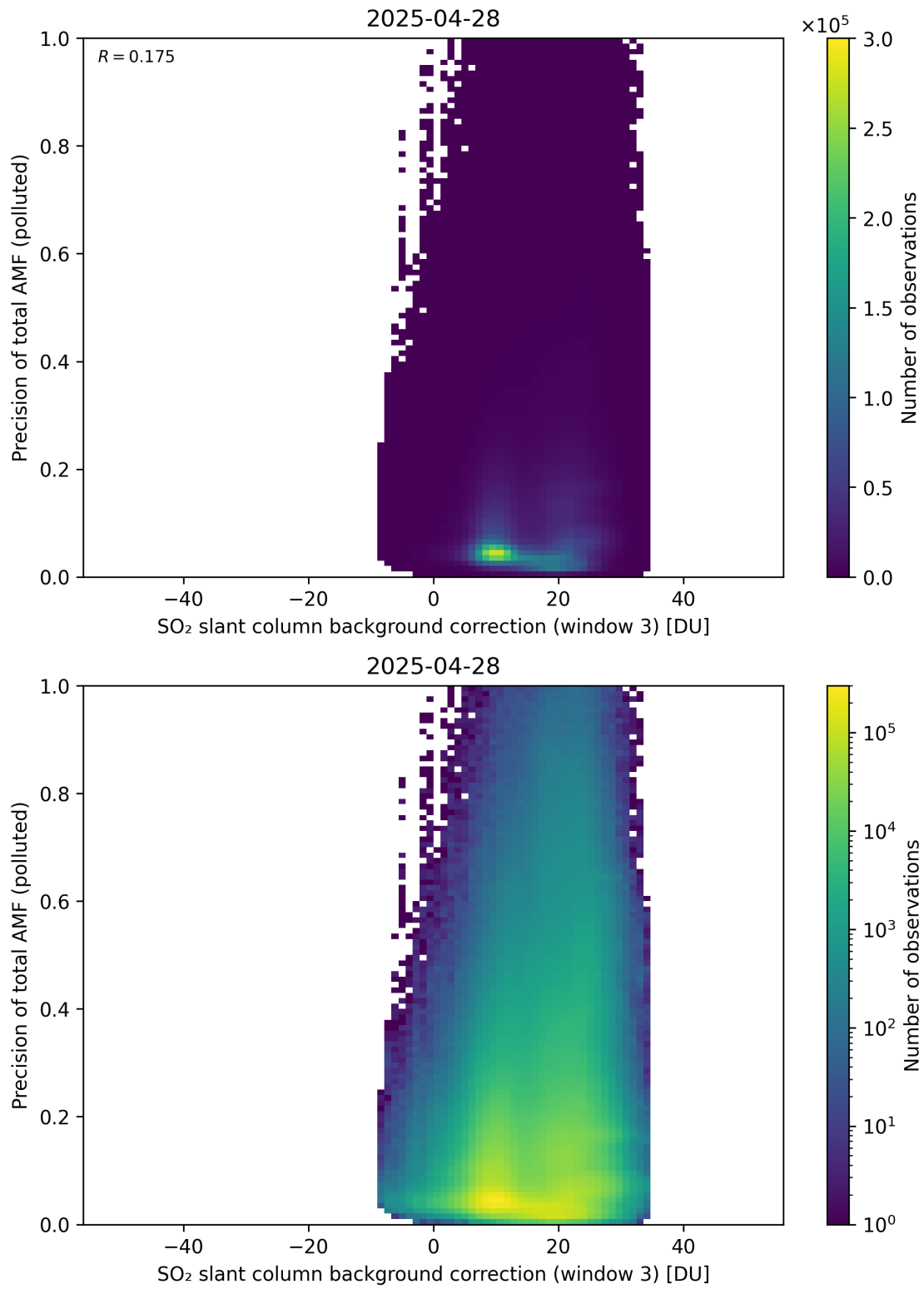
Figure 137: Scatter density plot of “SO 2 slant column background correction (window 3)” against “Precision of total AMF (polluted)” for 2025-04-27 to 2025-04-29.
