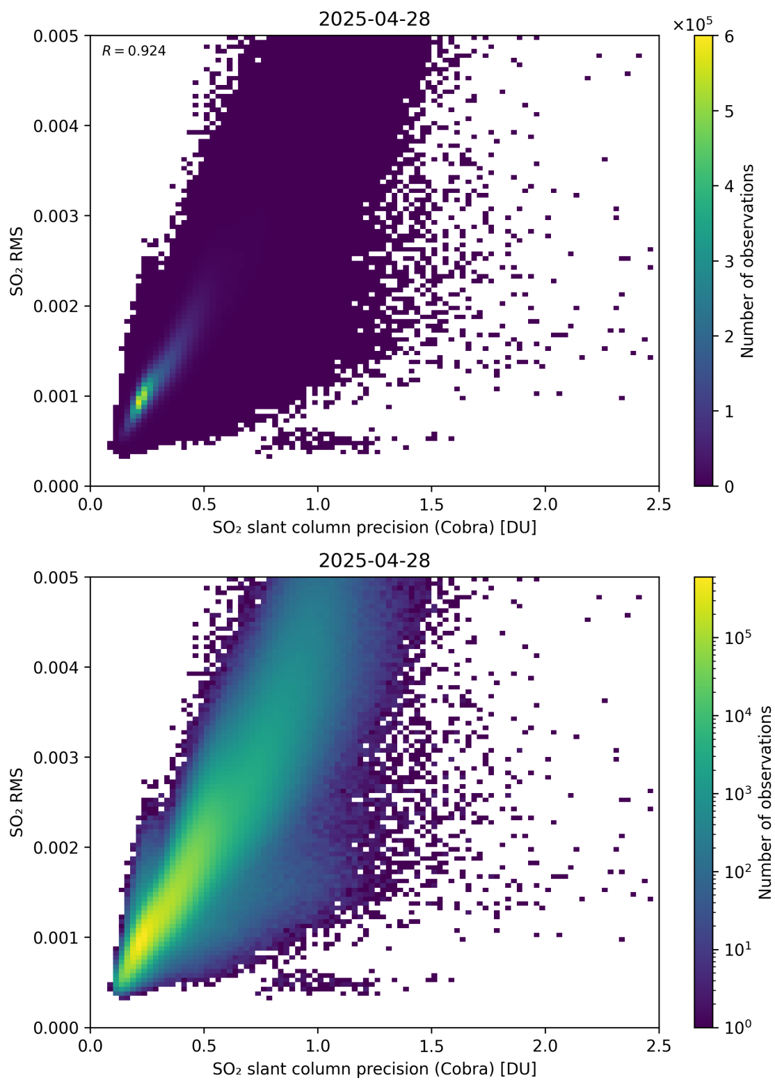
Figure 204: Scatter density plot of “SO 2 slant column precision (Cobra)” against “SO 2 RMS” for 2025-04-27 to 2025-04-29.
