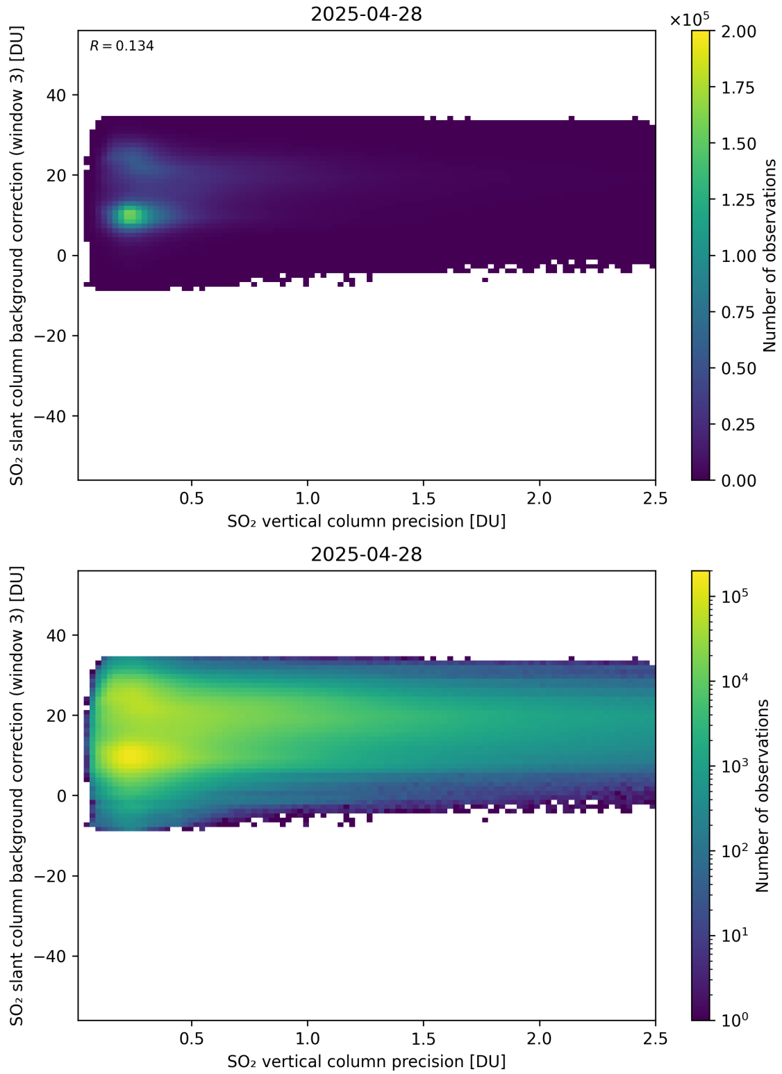
Figure 331: Scatter density plot of “SO 2 vertical column precision” against “SO 2 slant column background correction (window 3)” for 2025-04-27 to 2025-04-29.
