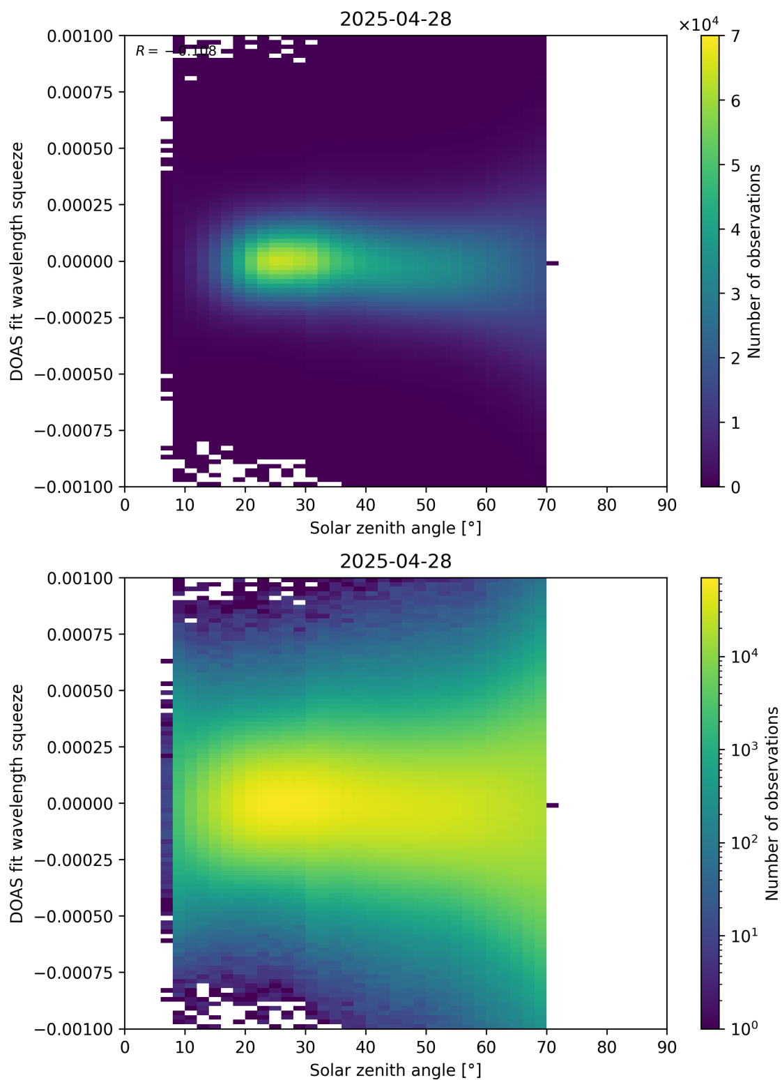
Figure 175: Scatter density plot of “Solar zenith angle” against “DOAS fit wavelength squeeze” for 2025-04-27 to 2025-04-29.
