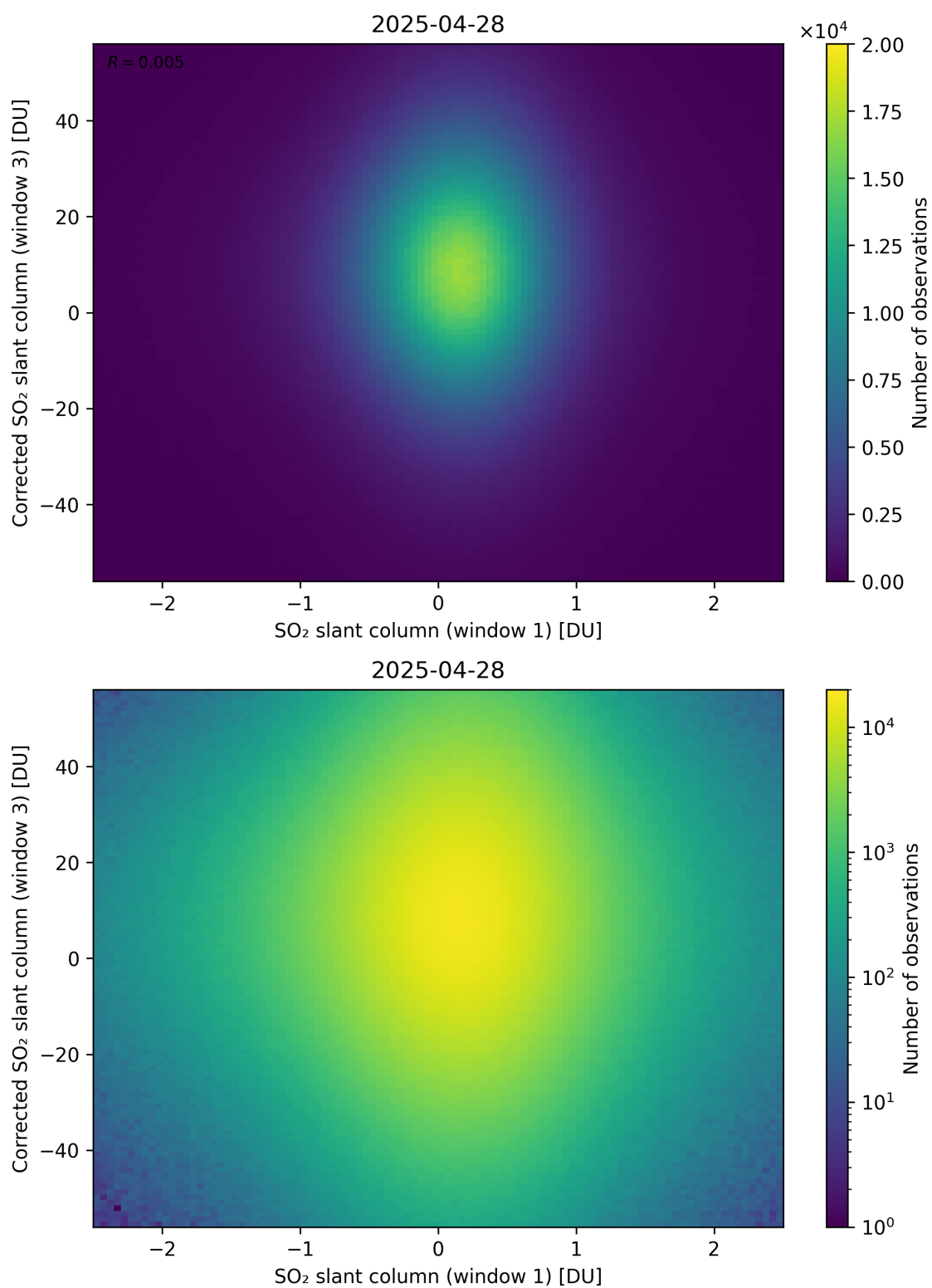
Figure 284: Scatter density plot of “SO 2 slant column (window 1)” against “Corrected SO 2 slant column (window 3)” for 2025-04-27 to 2025-04-29.
