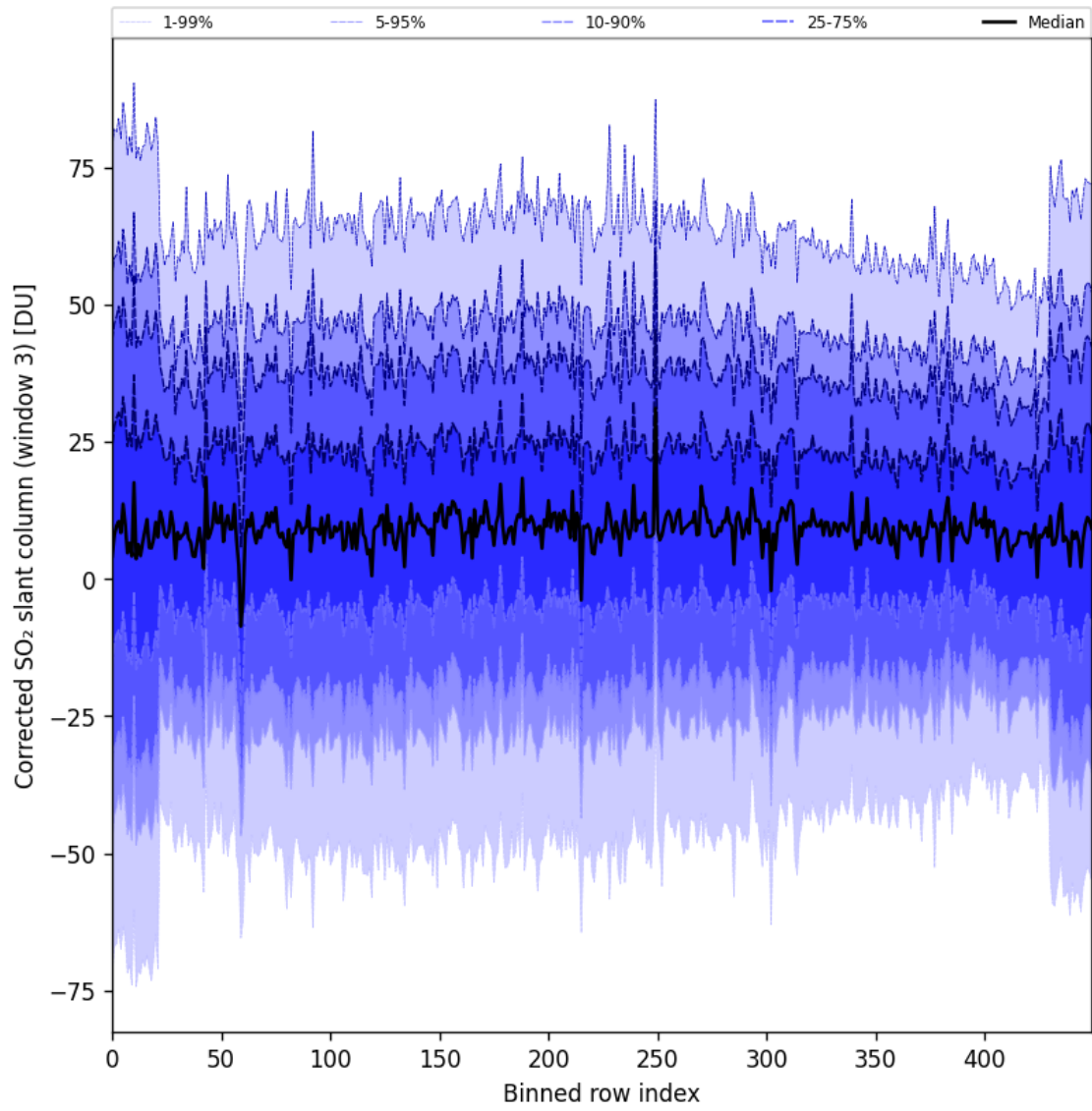
Figure 99: Along track statistics of “Corrected SO 2 slant column (window 3)” for 2025-04-27 to 2025-04-29
