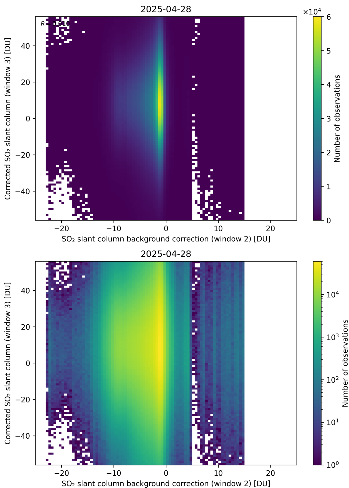
Figure 127: Scatter density plot of “SO 2 slant column background correction (window 2)” against “Corrected SO 2 slant column (window 3)” for 2025-04-27 to 2025-04-29.
