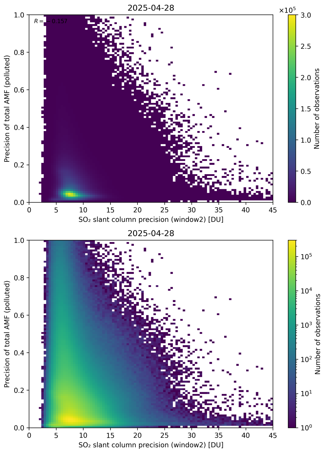
Figure 302: Scatter density plot of “SO 2 slant column precision (window2)” against “Precision of total AMF (polluted)” for 2025-04-27 to 2025-04-29.
