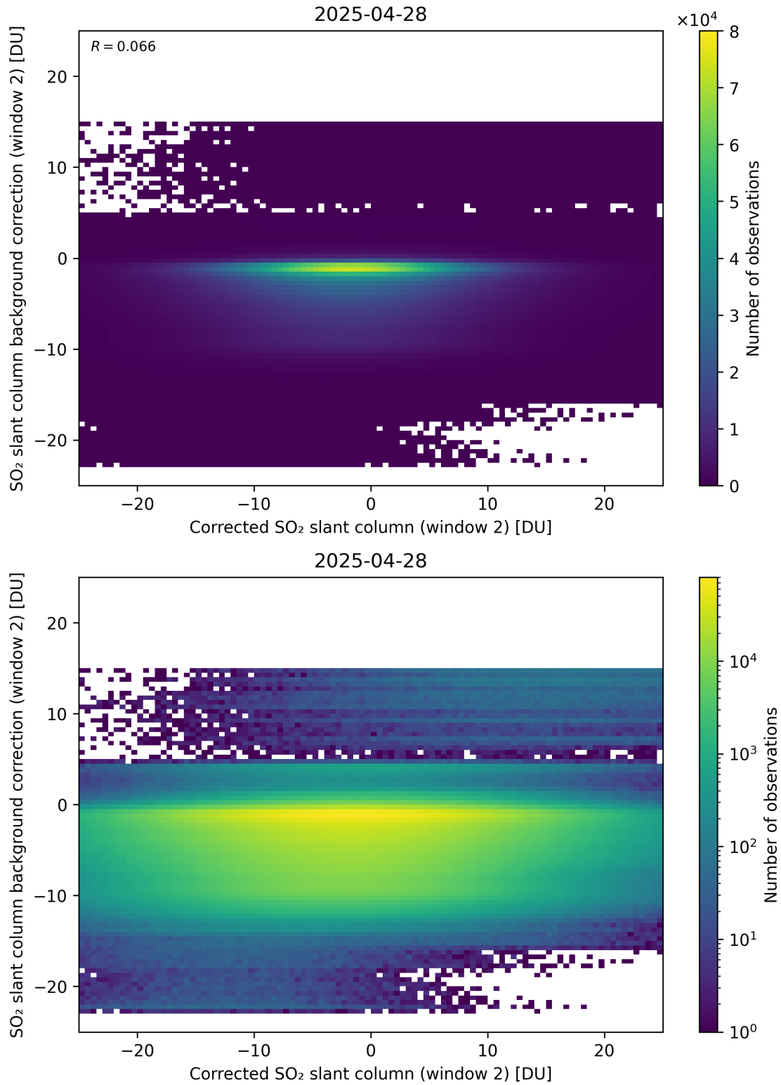
Figure 244: Scatter density plot of “Corrected SO 2 slant column (window 2)” against “SO 2 slant column background correction (window 2)” for 2025-04-27 to 2025-04-29.
