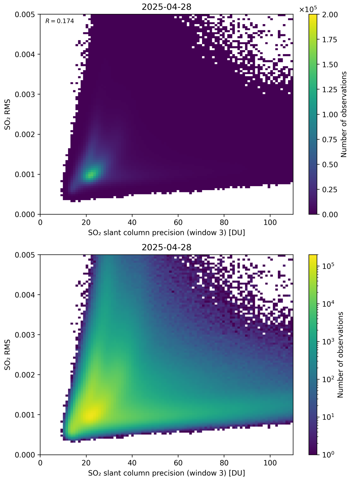
Figure 310: Scatter density plot of “SO 2 slant column precision (window 3)” against “SO 2 RMS” for 2025-04-27 to 2025-04-29.
