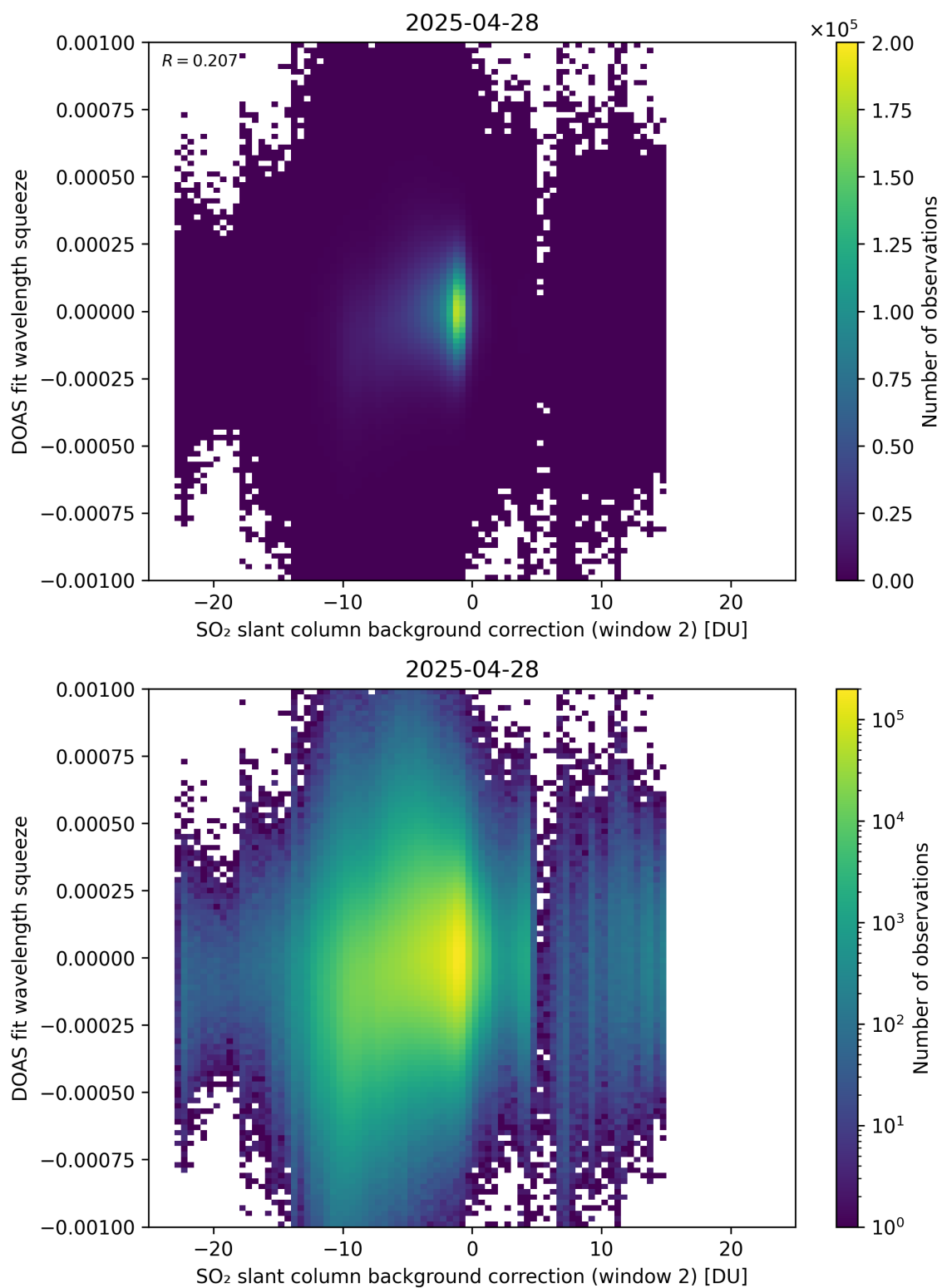
Figure 124: Scatter density plot of “SO 2 slant column background correction (window 2)” against “DOAS fit wavelength squeeze” for 2025-04-27 to 2025-04-29.
