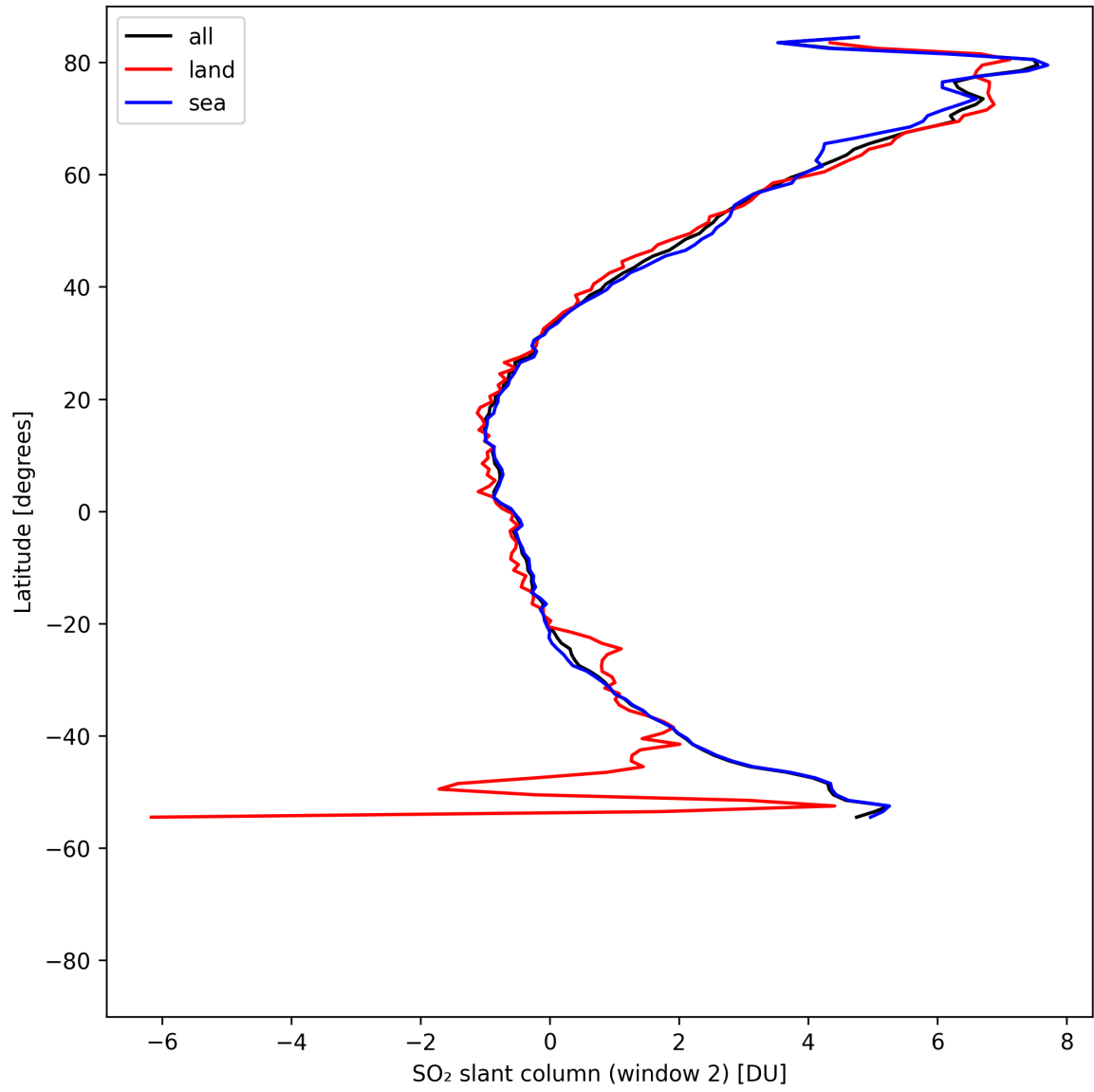
Figure 41: Zonal average of “SO 2 slant column (window 2)” for 2025-04-27 to 2025-04-29.
