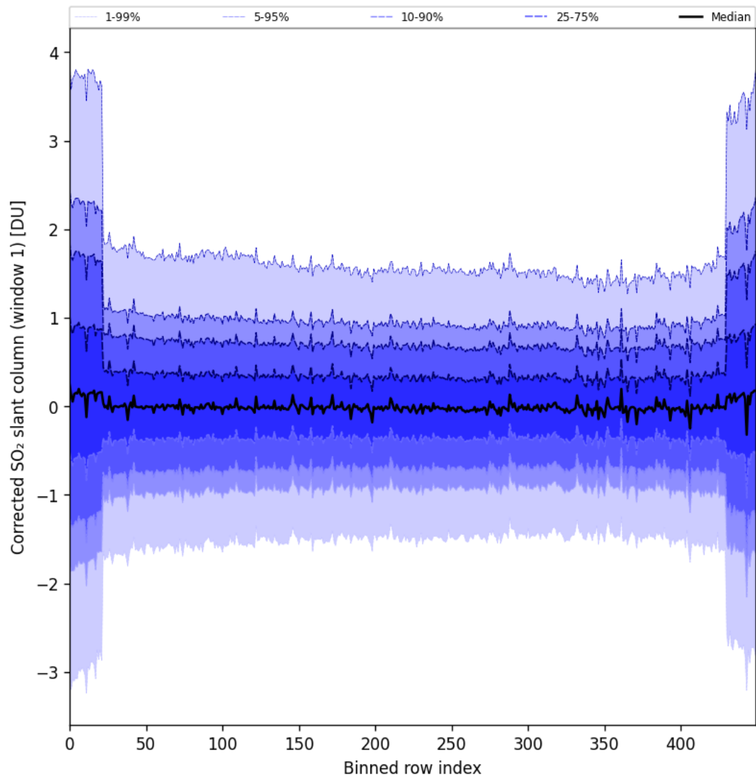
Figure 91: Along track statistics of “Corrected SO 2 slant column (window 1)” for 2025-04-27 to 2025-04-29
