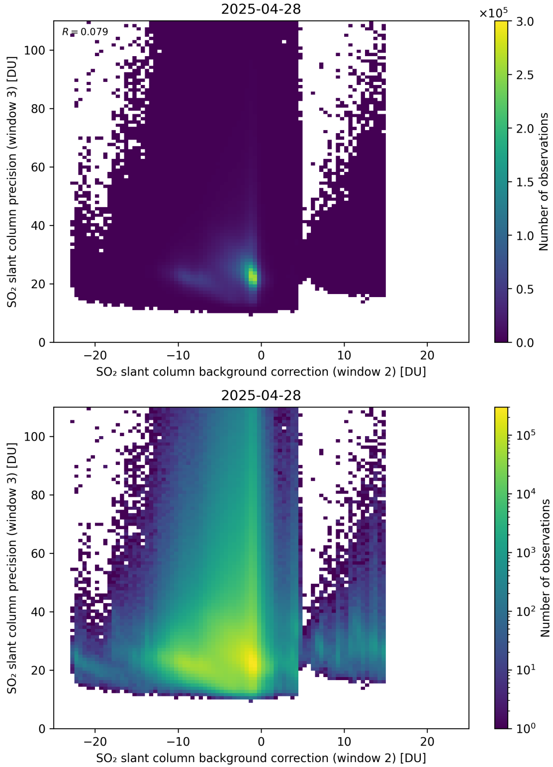
Figure 129: Scatter density plot of “SO 2 slant column background correction (window 2)” against “SO 2 slant column precision (window 3)” for 2025-04-27 to 2025-04-29.
