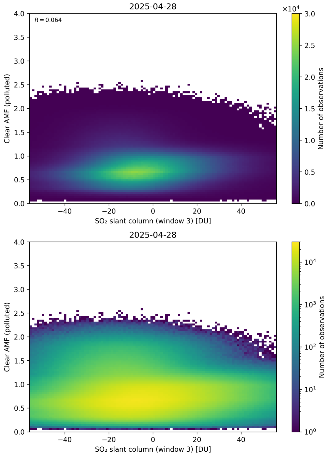
Figure 315: Scatter density plot of “SO 2 slant column (window 3)” against “Clear AMF (polluted)” for 2025-04-27 to 2025-04-29.
