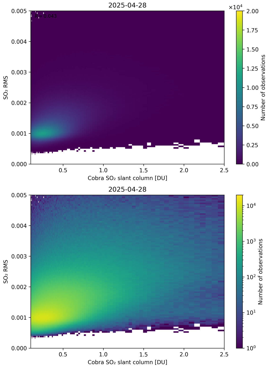
Figure 198: Scatter density plot of “Cobra SO 2 slant column” against “SO 2 RMS” for 2025-04-27 to 2025-04-29.
