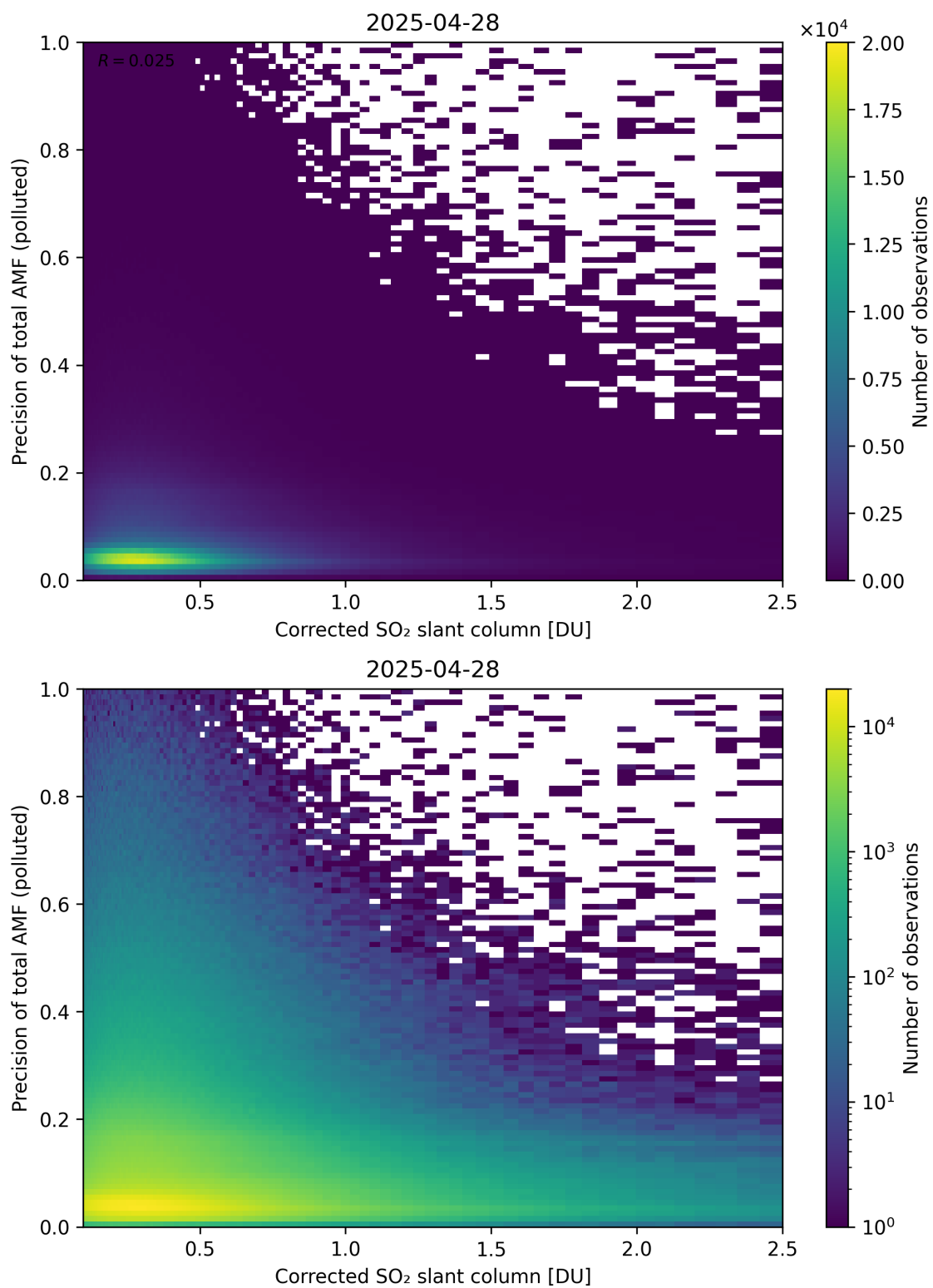
Figure 243: Scatter density plot of “Corrected SO 2 slant column” against “Precision of total AMF (polluted)” for 2025-04-27 to 2025-04-29.
