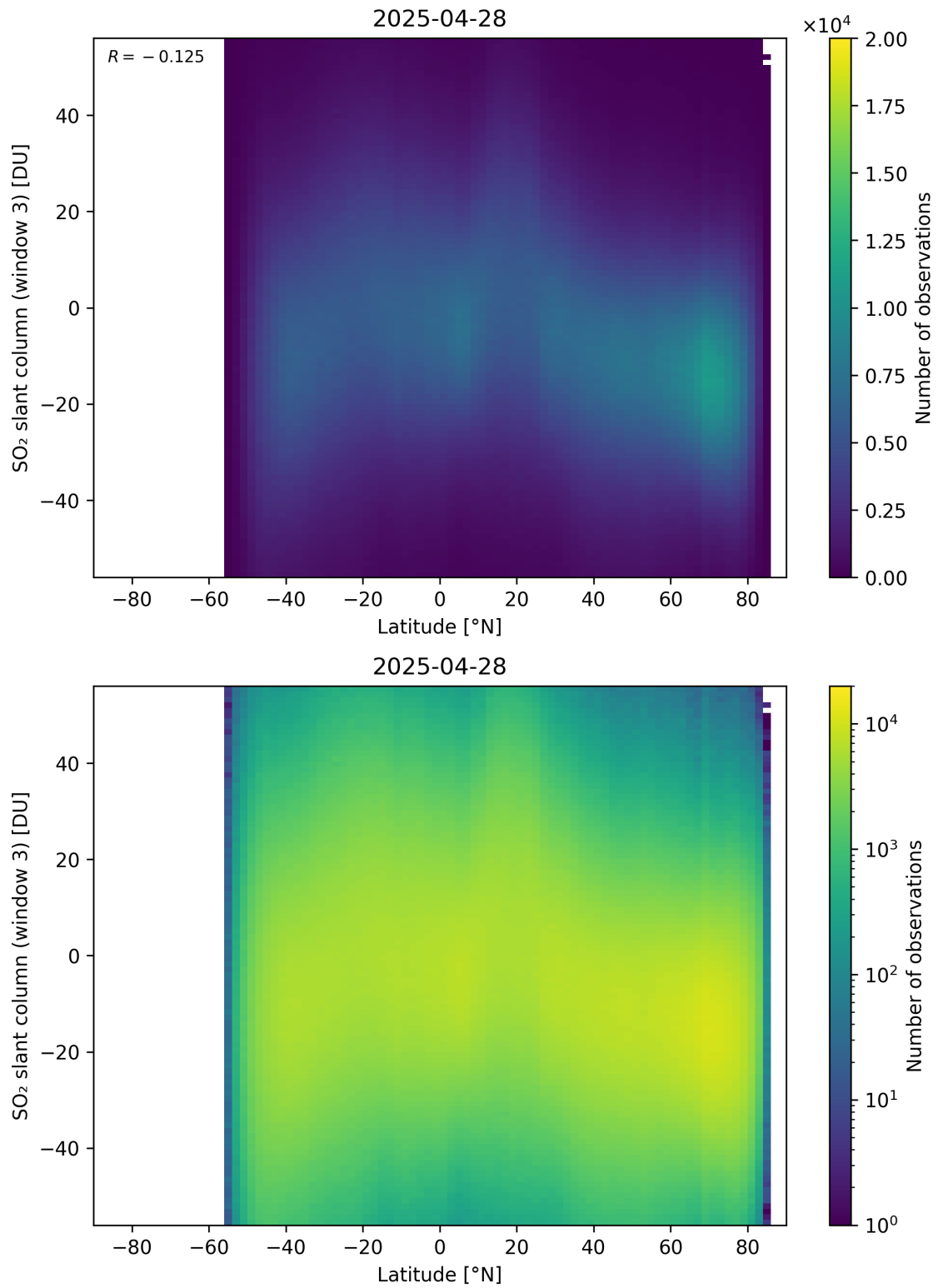
Figure 165: Scatter density plot of “Latitude” against “SO 2 slant column (window 3)” for 2025-04-27 to 2025-04-29.
