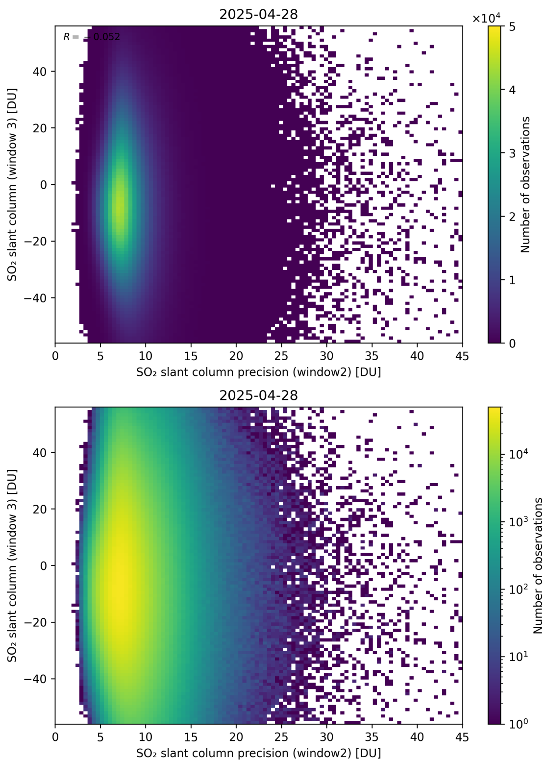
Figure 299: Scatter density plot of “SO 2 slant column precision (window2)” against “SO 2 slant column (window 3)” for 2025-04-27 to 2025-04-29.
