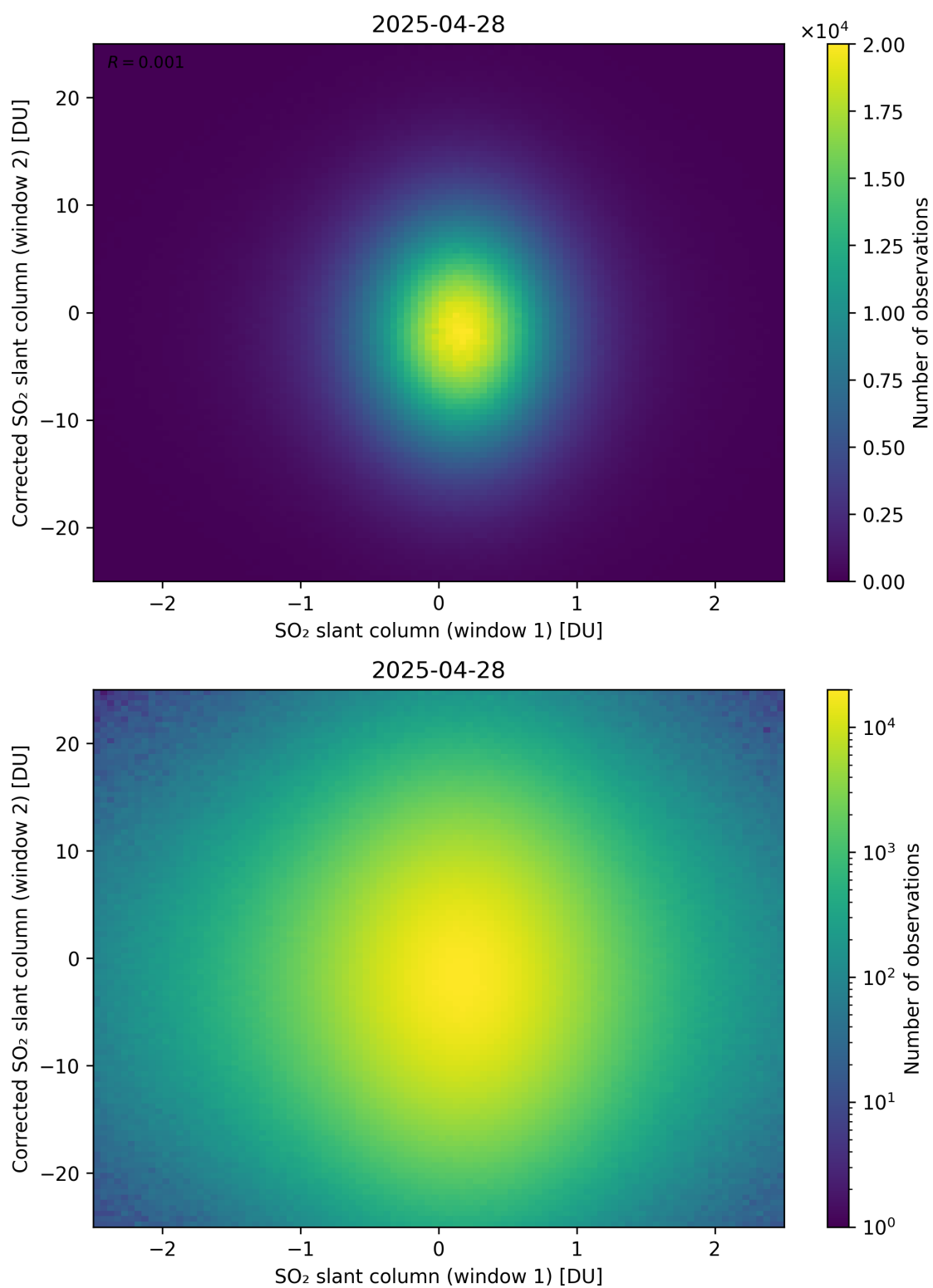
Figure 283: Scatter density plot of “SO 2 slant column (window 1)” against “Corrected SO 2 slant column (window 2)” for 2025-04-27 to 2025-04-29.
