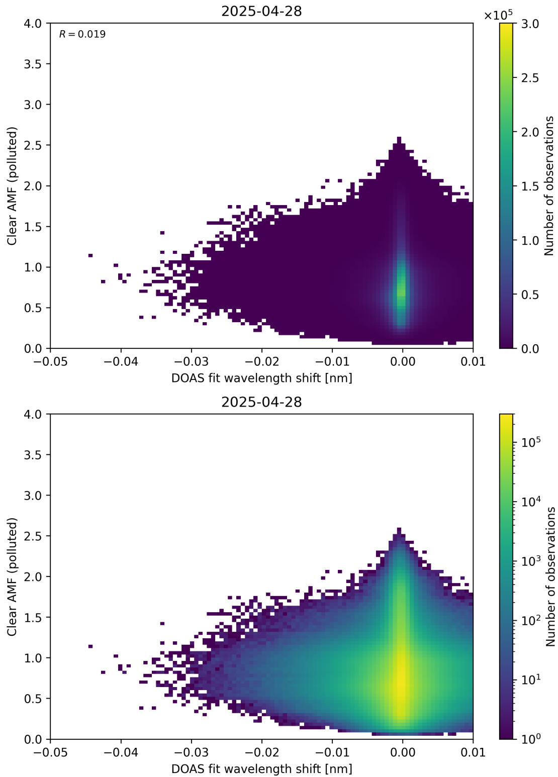
Figure 140: Scatter density plot of “DOAS fit wavelength shift” against “Clear AMF (polluted)” for 2025-04-27 to 2025-04-29.
