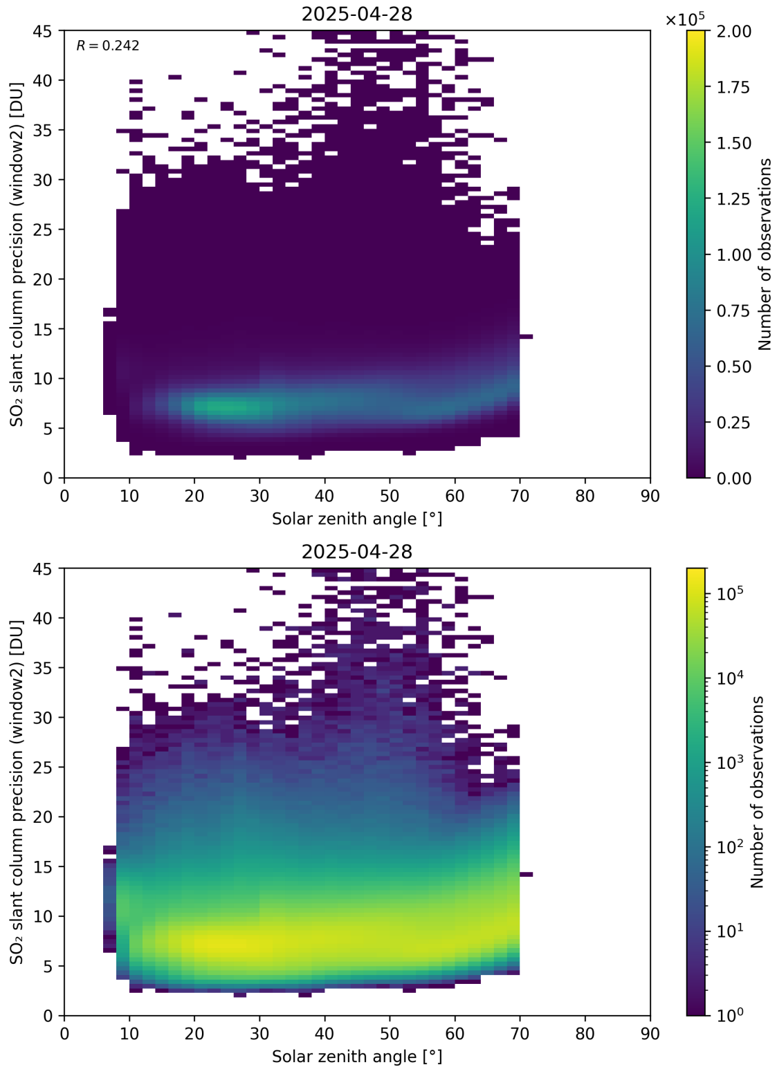
Figure 186: Scatter density plot of “Solar zenith angle” against “SO 2 slant column precision (window2)” for 2025-04-27 to 2025-04-29.
