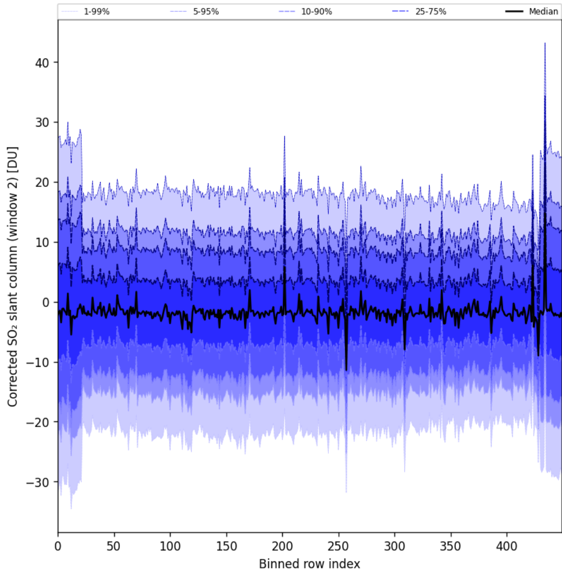
Figure 95: Along track statistics of “Corrected SO 2 slant column (window 2)” for 2025-04-27 to 2025-04-29
