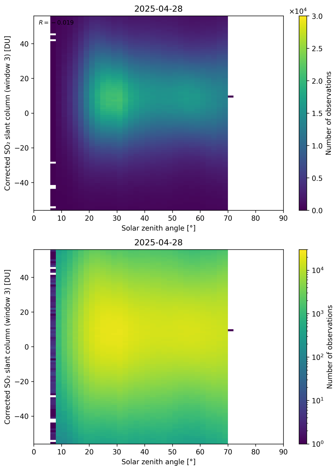
Figure 183: Scatter density plot of “Solar zenith angle” against “Corrected SO 2 slant column (window 3)” for 2025-04-27 to 2025-04-29.
