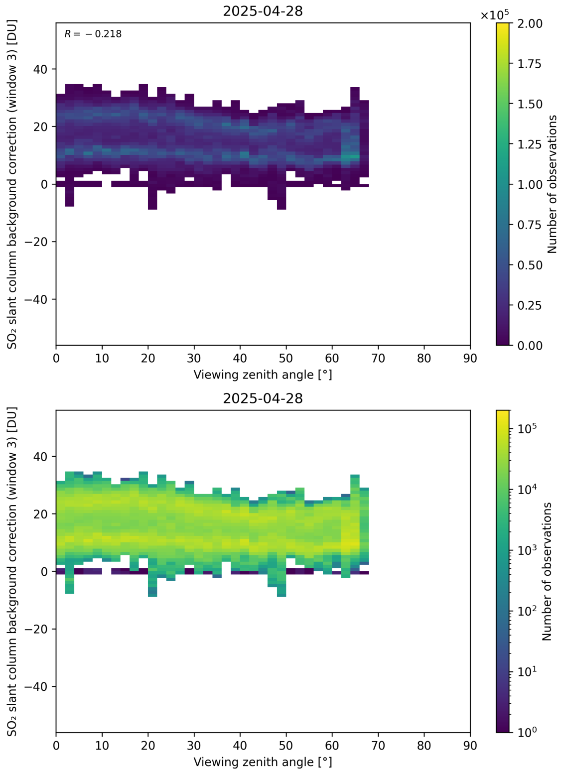
Figure 364: Scatter density plot of “Viewing zenith angle” against “SO 2 slant column background correction (window 3)” for 2025-04-27 to 2025-04-29.
