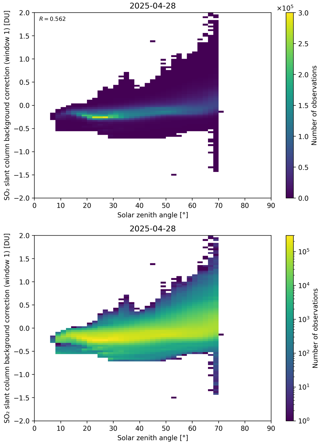
Figure 171: Scatter density plot of “Solar zenith angle” against “SO 2 slant column background correction (window 1)” for 2025-04-27 to 2025-04-29.
