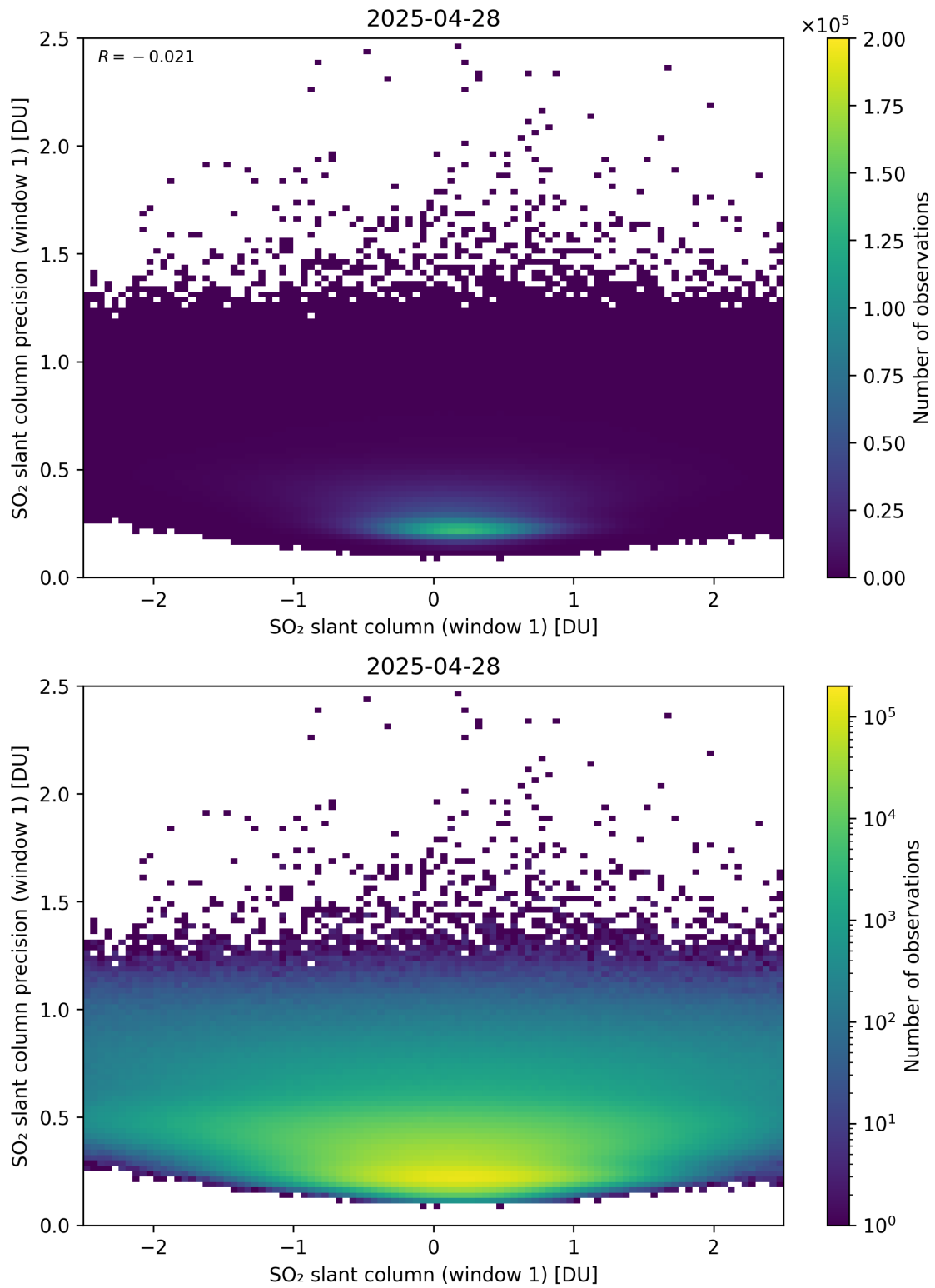
Figure 285: Scatter density plot of “SO 2 slant column (window 1)” against “SO 2 slant column precision (window 1)” for 2025-04-27 to 2025-04-29.
