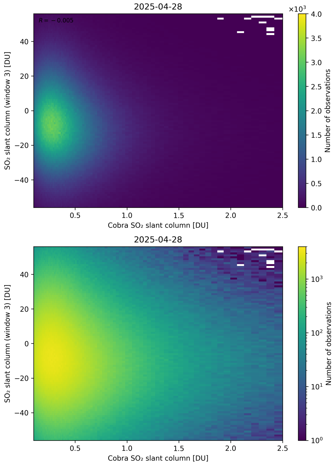
Figure 222: Scatter density plot of “Cobra SO 2 slant column” against “SO 2 slant column (window 3)” for 2025-04-27 to 2025-04-29.
