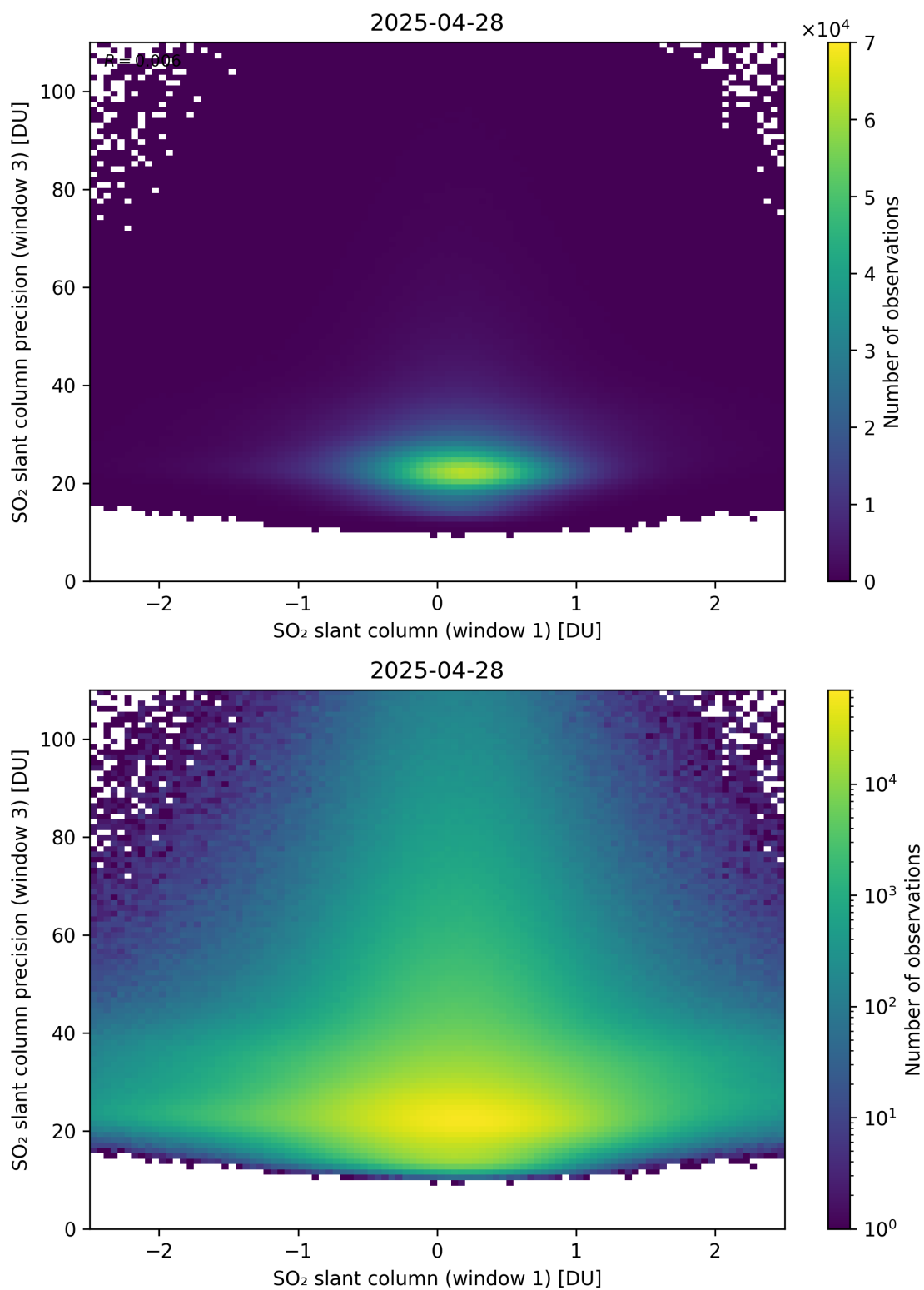
Figure 288: Scatter density plot of “SO 2 slant column (window 1)” against “SO 2 slant column precision (window 3)” for 2025-04-27 to 2025-04-29.
