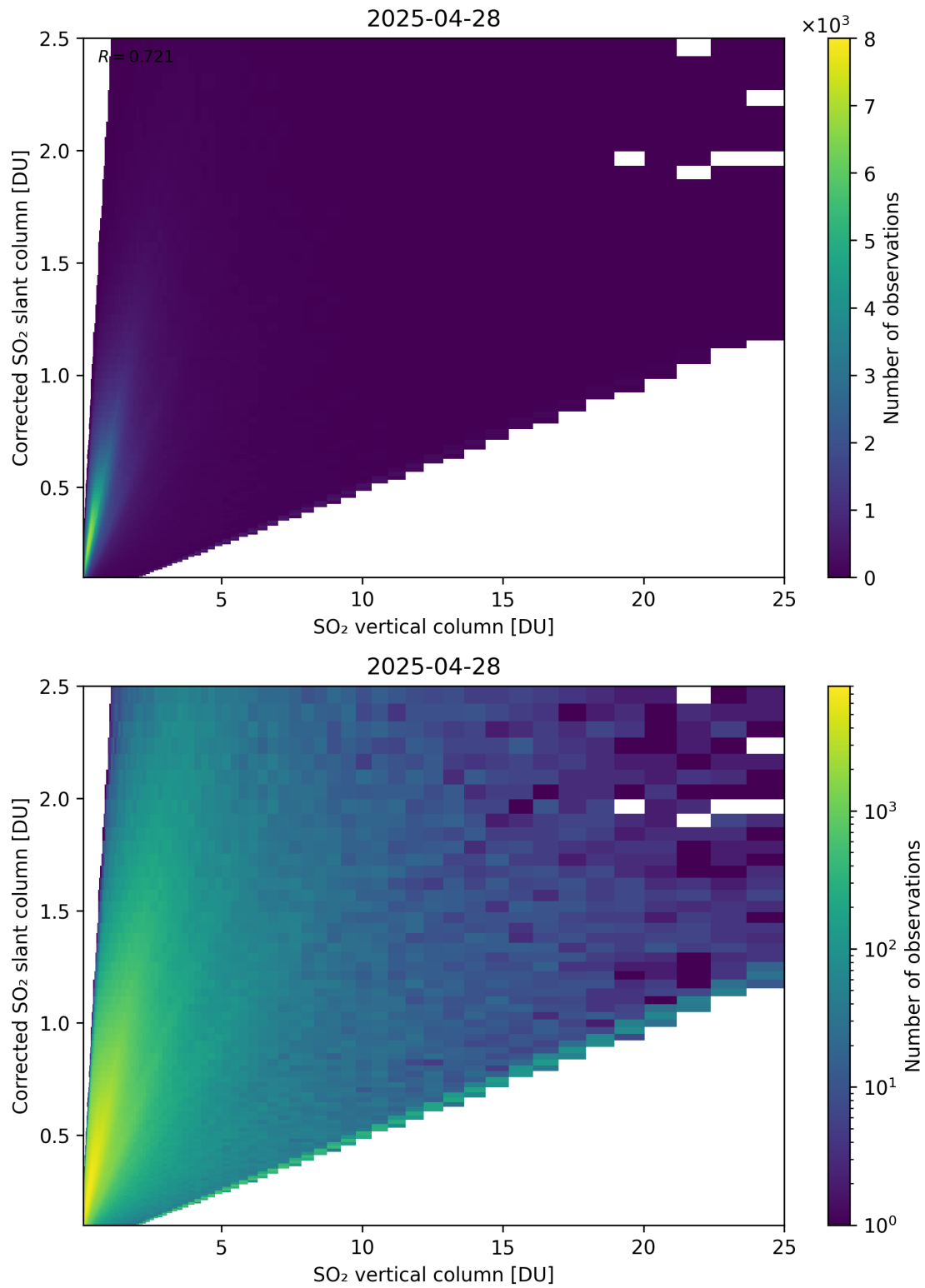
Figure 351: Scatter density plot of “SO 2 vertical column” against “Corrected SO 2 slant column” for 2025-04-27 to 2025-04-29.
