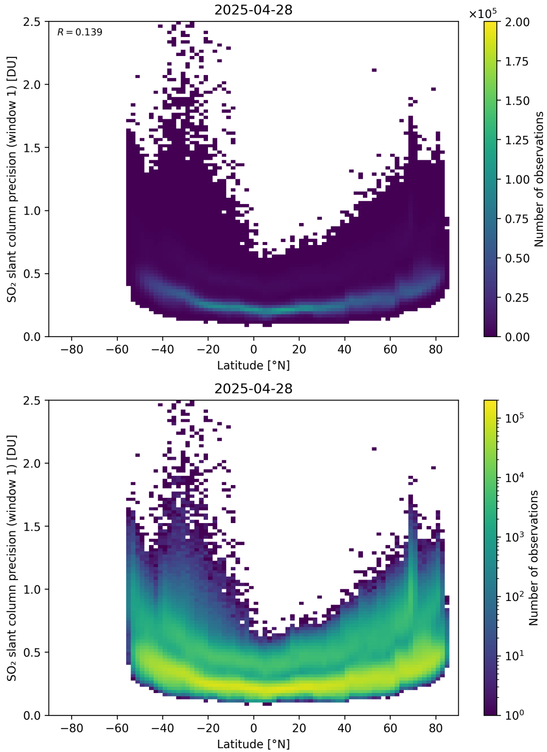
Figure 163: Scatter density plot of “Latitude” against “SO 2 slant column precision (window 1)” for 2025-04-27 to 2025-04-29.
