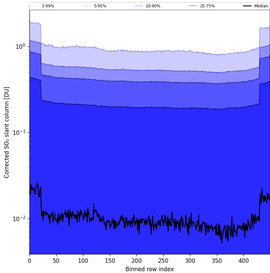
Figure 86: Along track statistics of “Corrected SO 2 slant column” for 2025-04-27 to 2025-04-29
