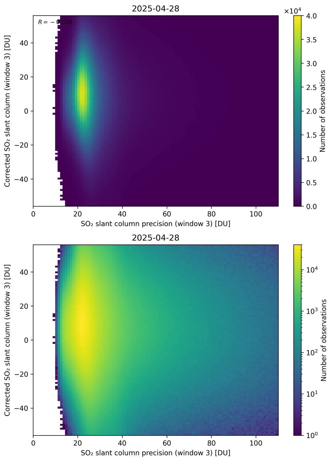
Figure 312: Scatter density plot of “SO 2 slant column precision (window 3)” against “Corrected SO 2 slant column (window 3)” for 2025-04-27 to 2025-04-29.
