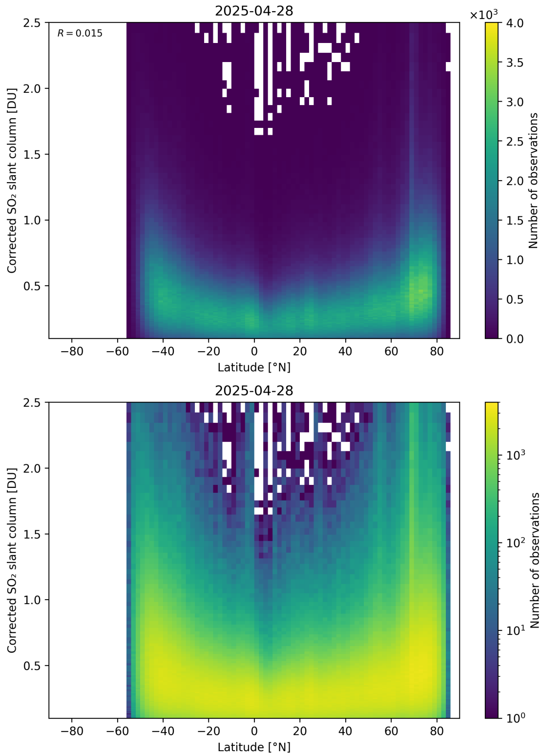
Figure 159: Scatter density plot of “Latitude” against “Corrected SO 2 slant column” for 2025-04-27 to 2025-04-29.
