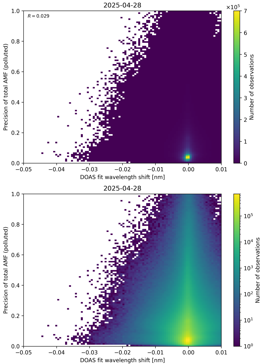
Figure 142: Scatter density plot of “DOAS fit wavelength shift” against “Precision of total AMF (polluted)” for 2025-04-27 to 2025-04-29.
