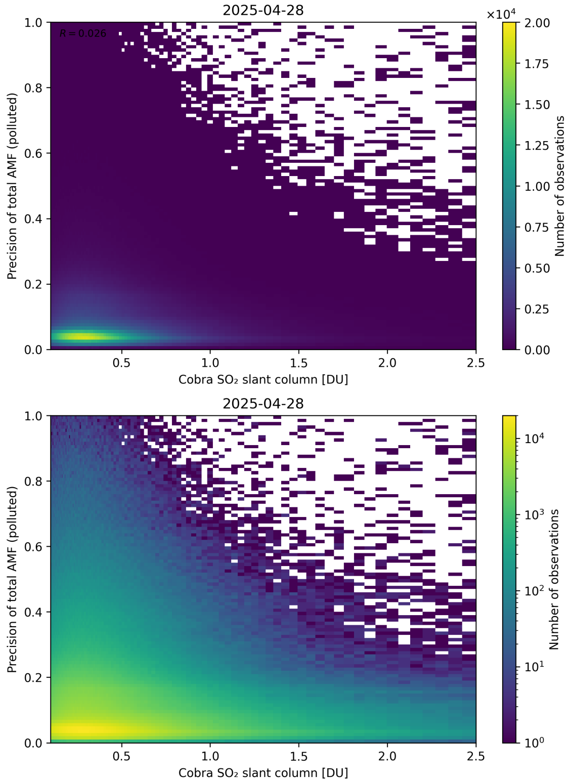
Figure 225: Scatter density plot of “Cobra SO 2 slant column” against “Precision of total AMF (polluted)” for 2025-04-27 to 2025-04-29.
