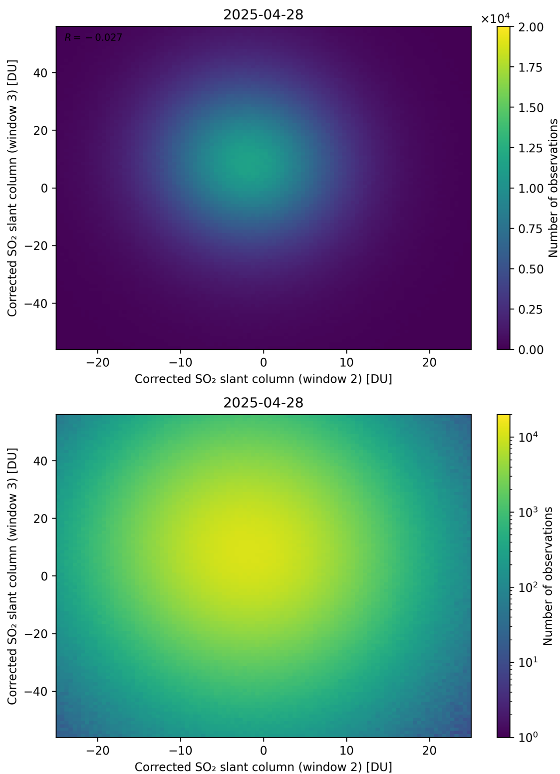
Figure 250: Scatter density plot of “Corrected SO 2 slant column (window 2)” against “Corrected SO 2 slant column (window 3)” for 2025-04-27 to 2025-04-29.
