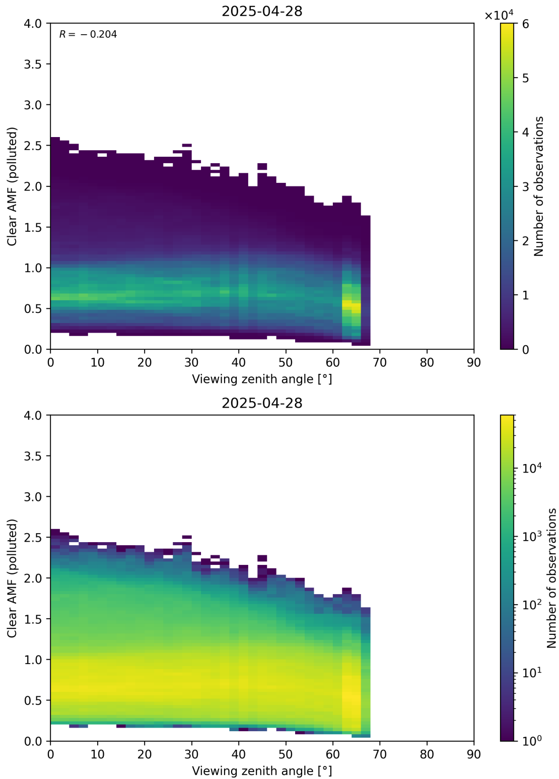
Figure 370: Scatter density plot of “Viewing zenith angle” against “Clear AMF (polluted)” for 2025-04-27 to 2025-04-29.
