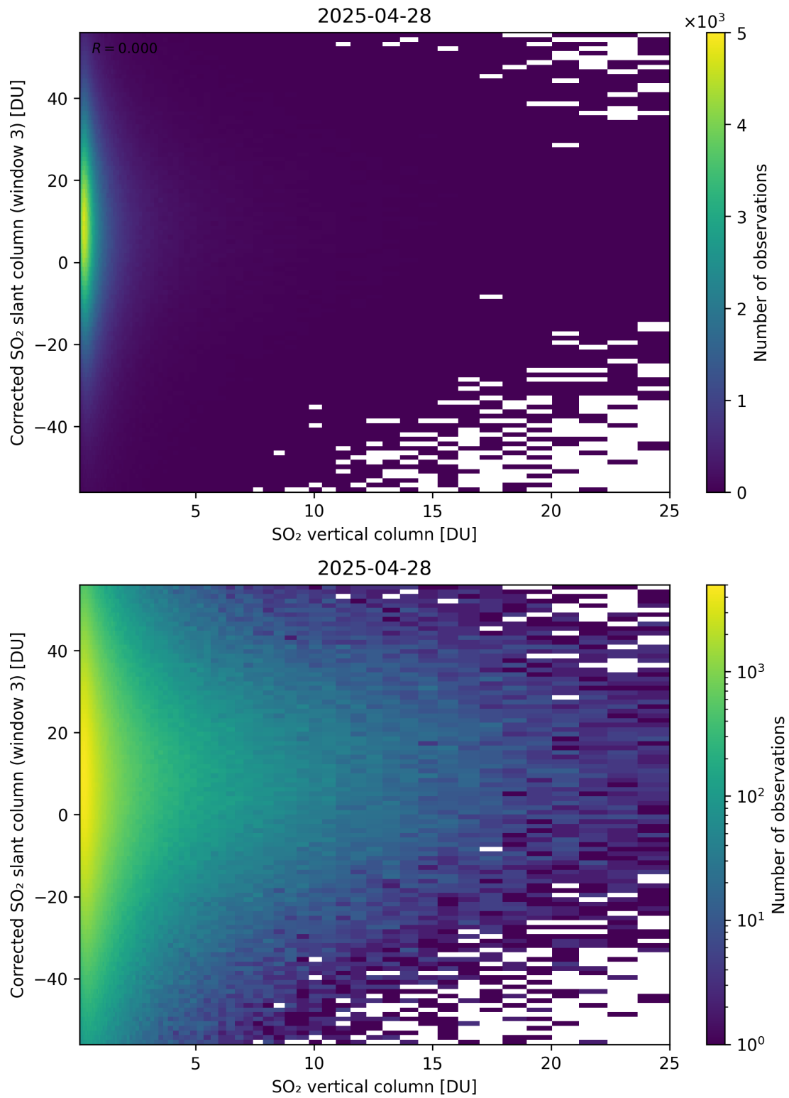
Figure 353: Scatter density plot of “SO 2 vertical column” against “Corrected SO 2 slant column (window 3)” for 2025-04-27 to 2025-04-29.
