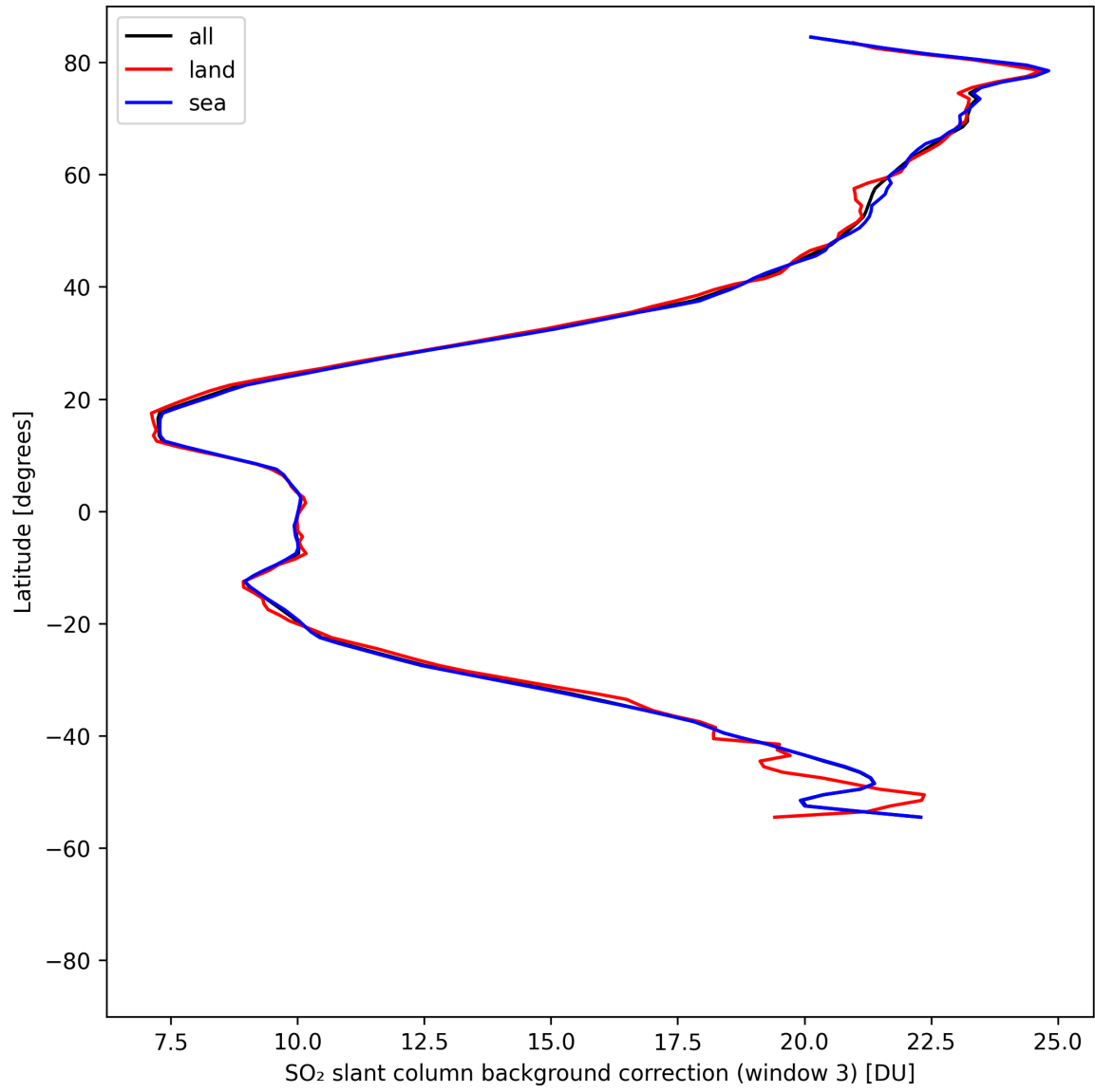
Figure 48: Zonal average of “SO 2 slant column background correction (window 3)” for 2025-04-27 to 2025-04-29.
