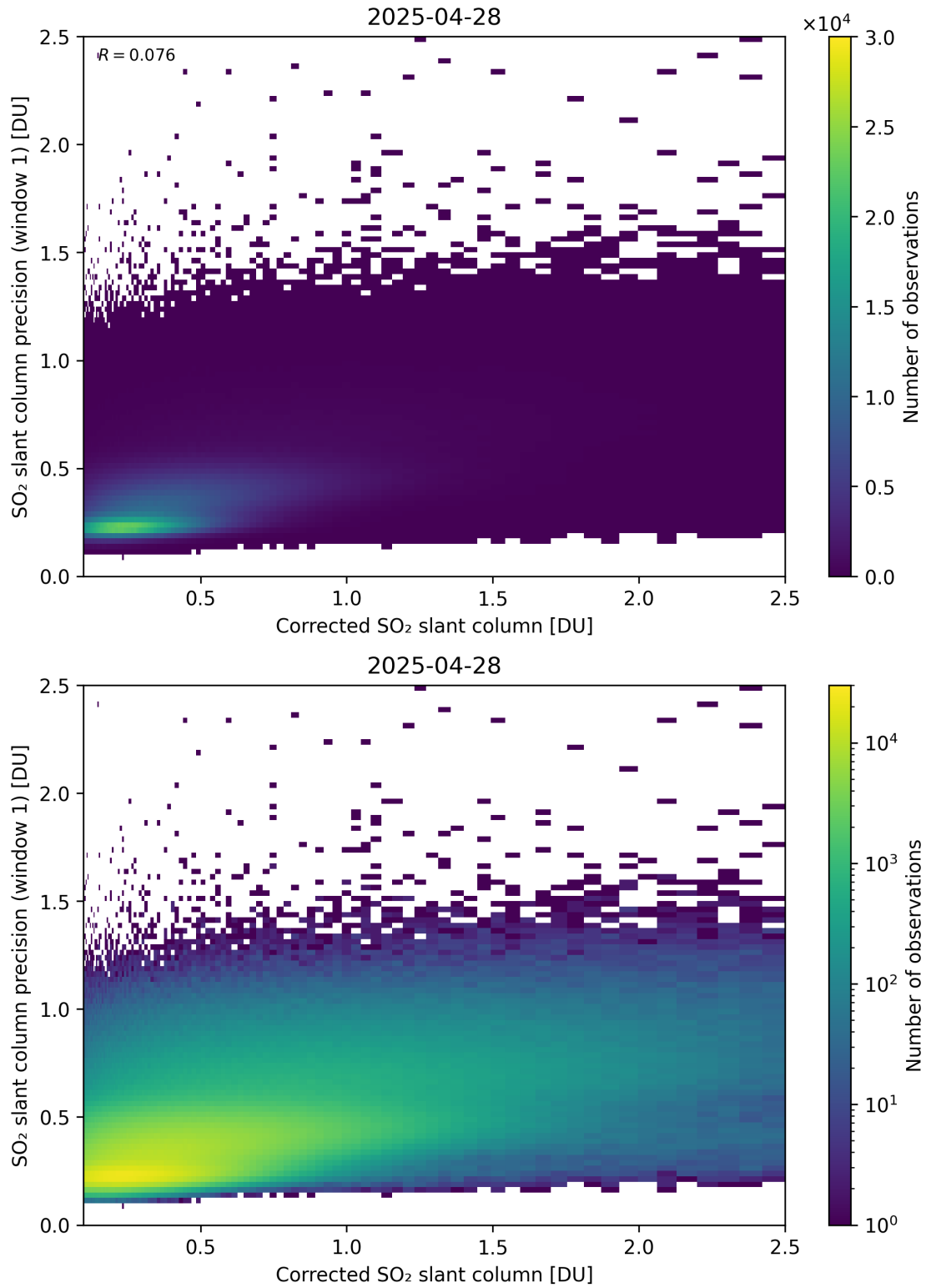
Figure 238: Scatter density plot of “Corrected SO 2 slant column” against “SO 2 slant column precision (window 1)” for 2025-04-27 to 2025-04-29.
