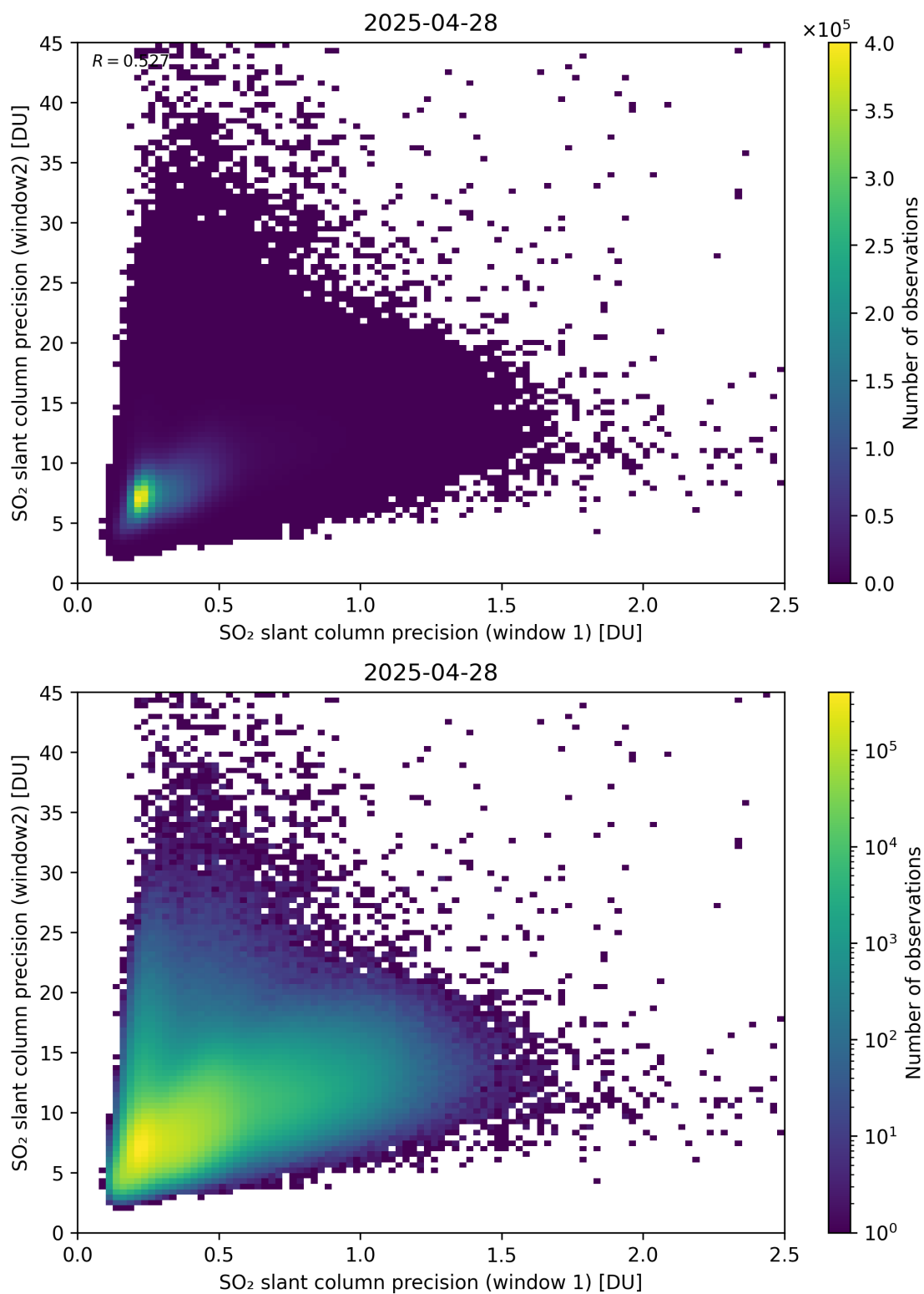
Figure 277: Scatter density plot of “SO 2 slant column precision (window 1)” against “SO 2 slant column precision (window2)” for 2025-04-27 to 2025-04-29.
