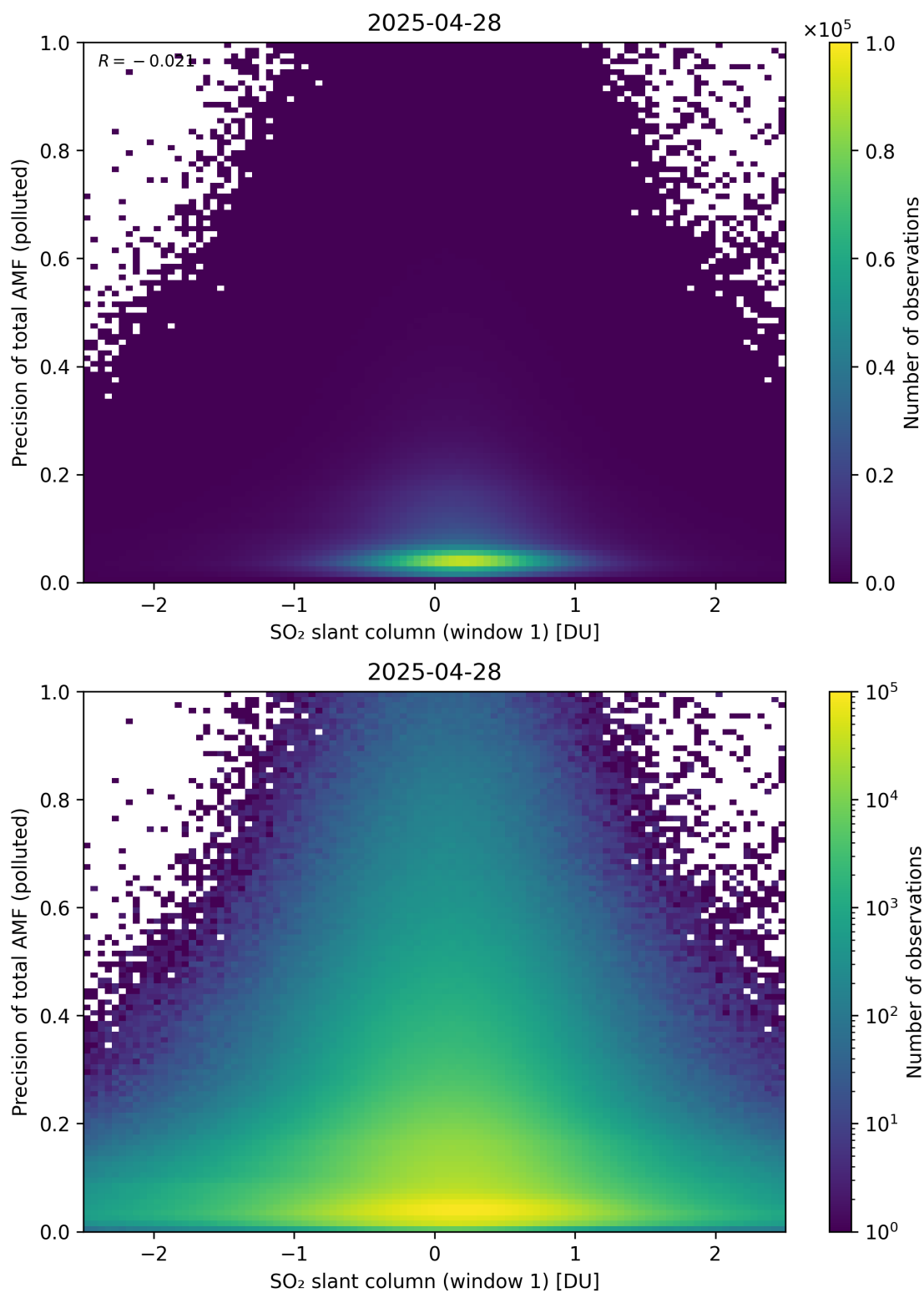
Figure 290: Scatter density plot of “SO 2 slant column (window 1)” against “Precision of total AMF (polluted)” for 2025-04-27 to 2025-04-29.
