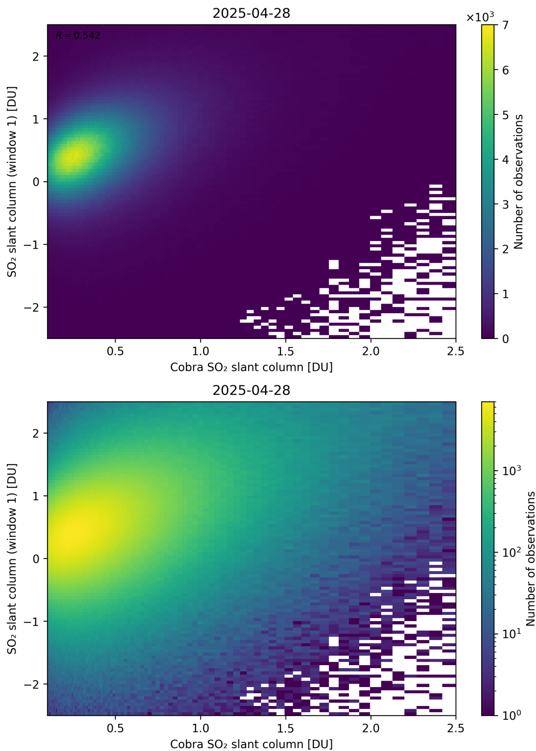
Figure 219: Scatter density plot of “Cobra SO 2 slant column” against “SO 2 slant column (window 1)” for 2025-04-27 to 2025-04-29.
