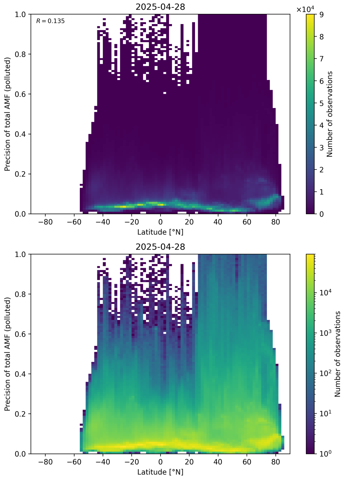
Figure 168: Scatter density plot of “Latitude” against “Precision of total AMF (polluted)” for 2025-04-27 to 2025-04-29.
