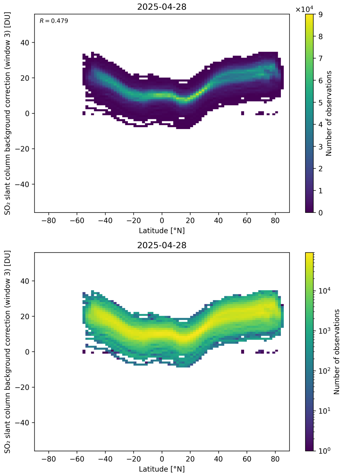
Figure 152: Scatter density plot of “Latitude” against “SO 2 slant column background correction (window 3)” for 2025-04-27 to 2025-04-29.
