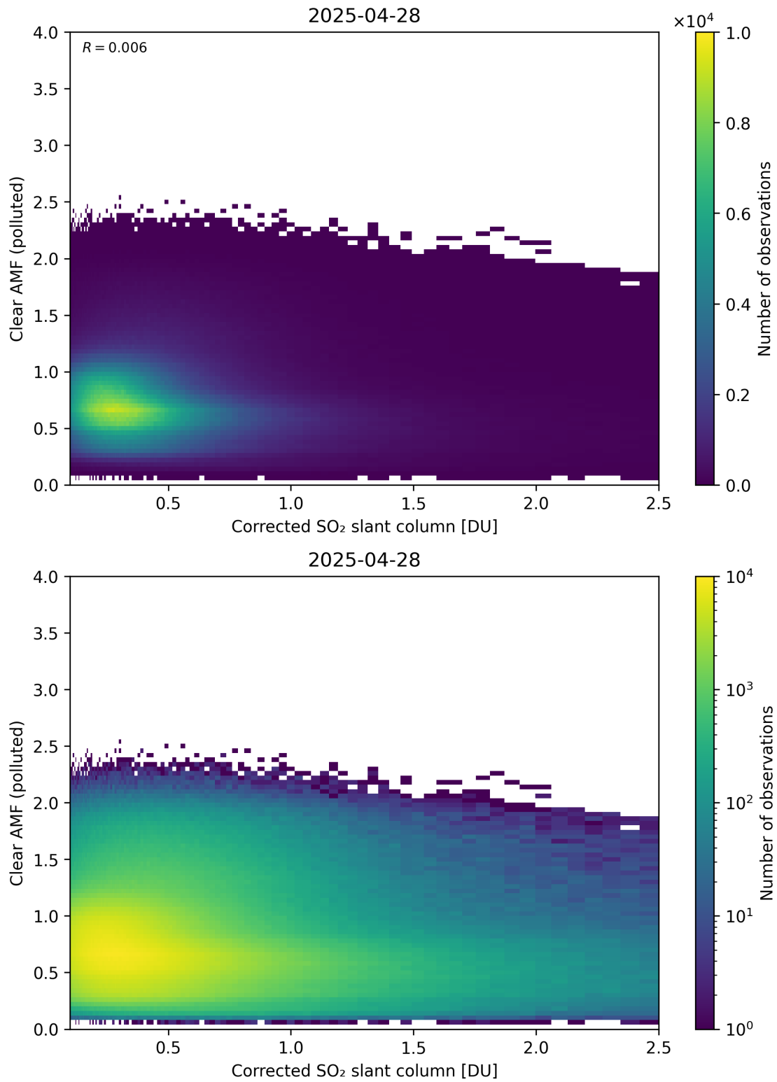
Figure 232: Scatter density plot of “Corrected SO 2 slant column” against “Clear AMF (polluted)” for 2025-04-27 to 2025-04-29.
