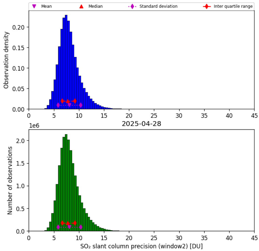
Figure 68: Histogram of “SO 2 slant column precision (window2)” for 2025-04-27 to 2025-04-29
