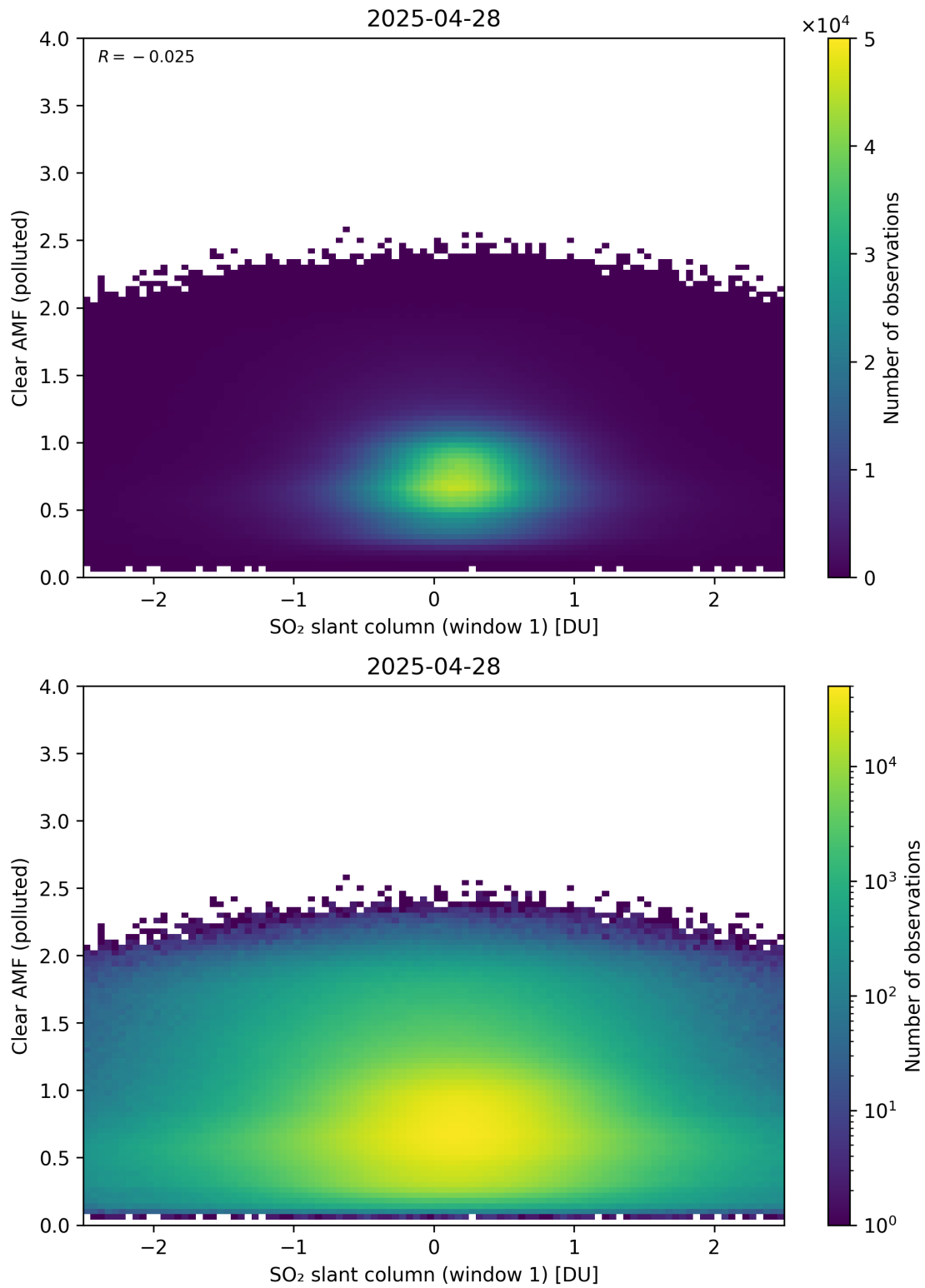
Figure 282: Scatter density plot of “SO 2 slant column (window 1)” against “Clear AMF (polluted)” for 2025-04-27 to 2025-04-29.
