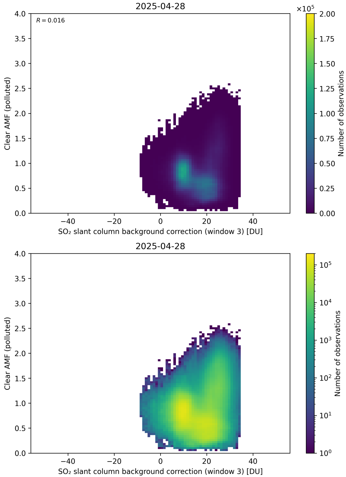
Figure 135: Scatter density plot of “SO 2 slant column background correction (window 3)” against “Clear AMF (polluted)” for 2025-04-27 to 2025-04-29.
