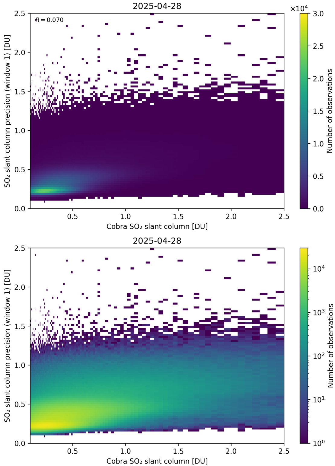
Figure 220: Scatter density plot of “Cobra SO 2 slant column” against “SO 2 slant column precision (window 1)” for 2025-04-27 to 2025-04-29.
