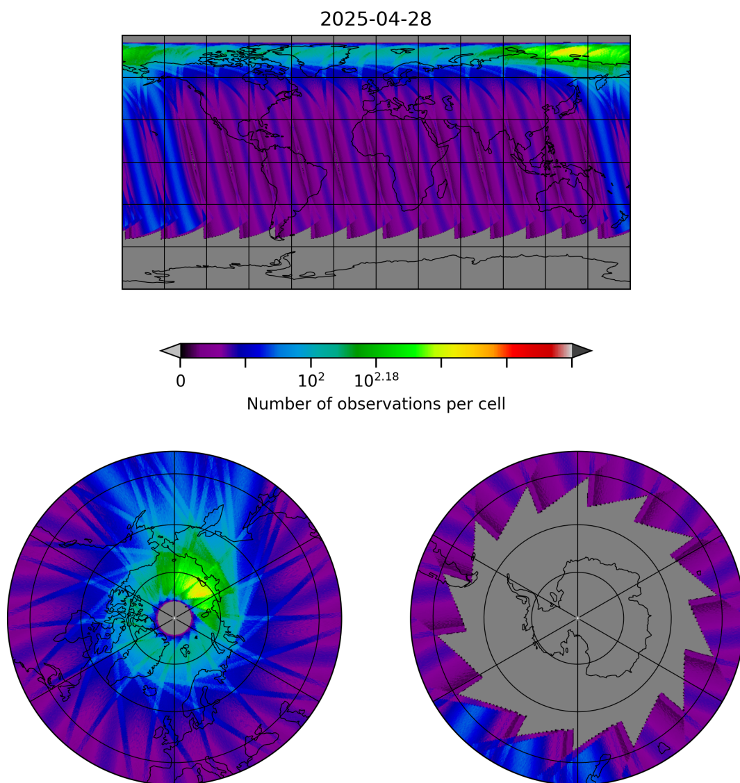
Figure 30: Map of the number of observations for 2025-04-27 to 2025-04-29
