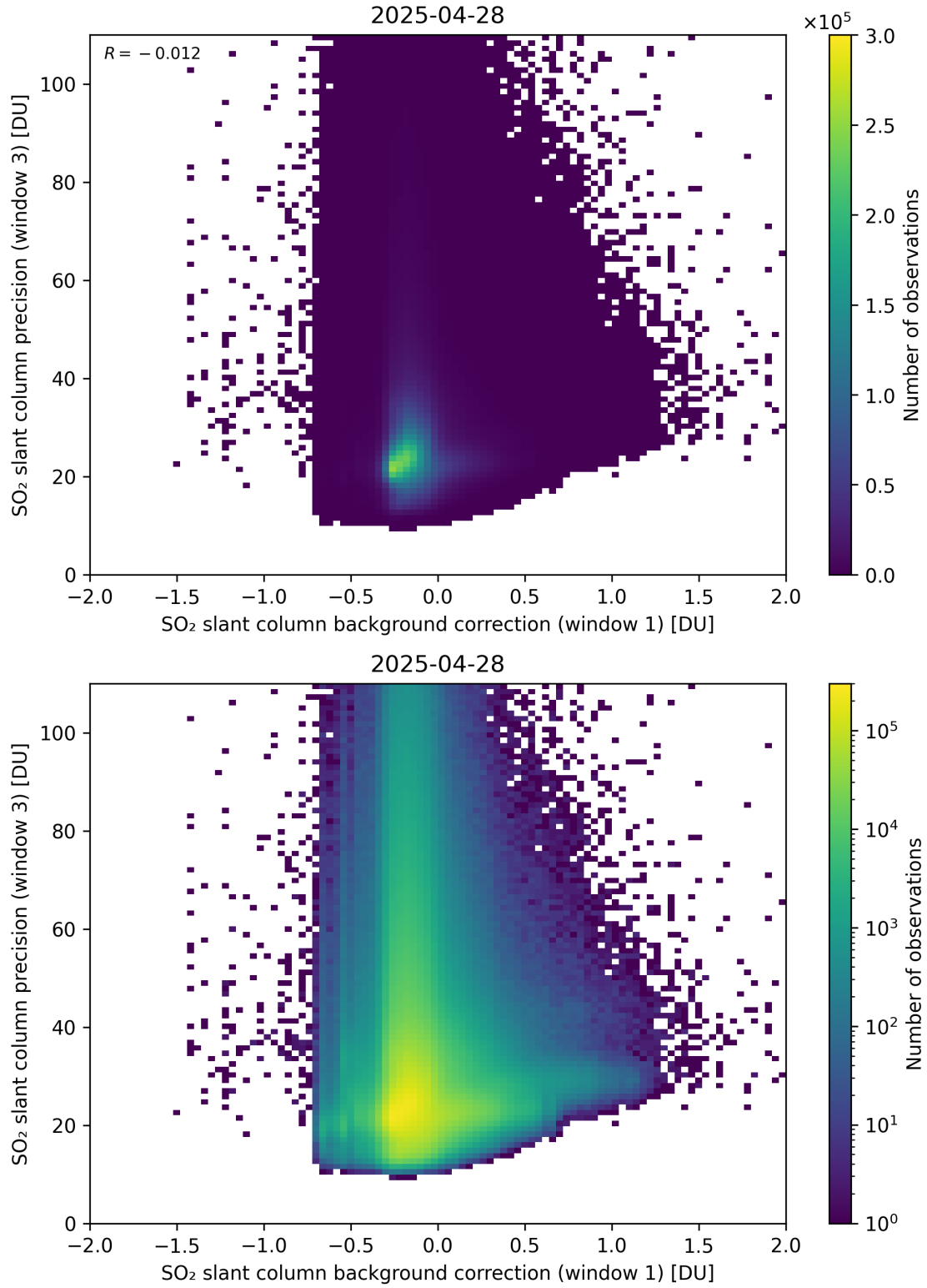
Figure 119: Scatter density plot of “SO 2 slant column background correction (window 1)” against “SO 2 slant column precision (window 3)” for 2025-04-27 to 2025-04-29.
