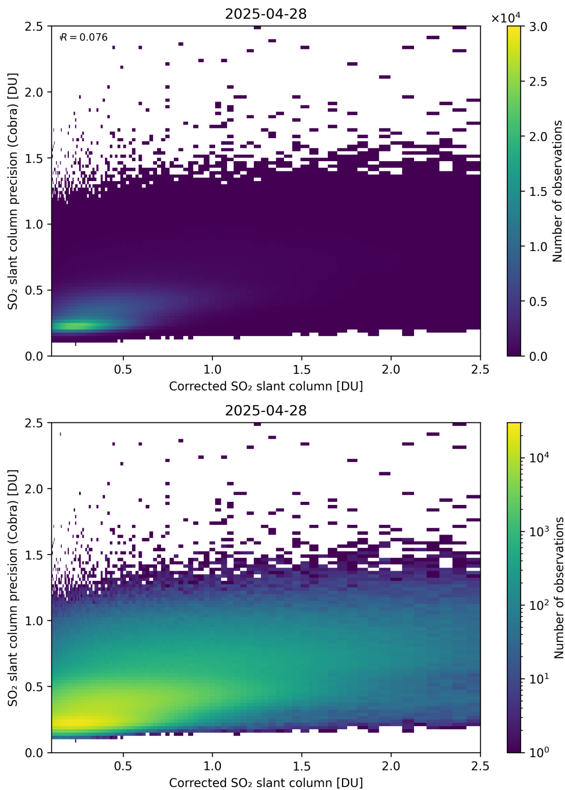
Figure 234: Scatter density plot of “Corrected SO 2 slant column” against “SO 2 slant column precision (Cobra)” for 2025-04-27 to 2025-04-29.
