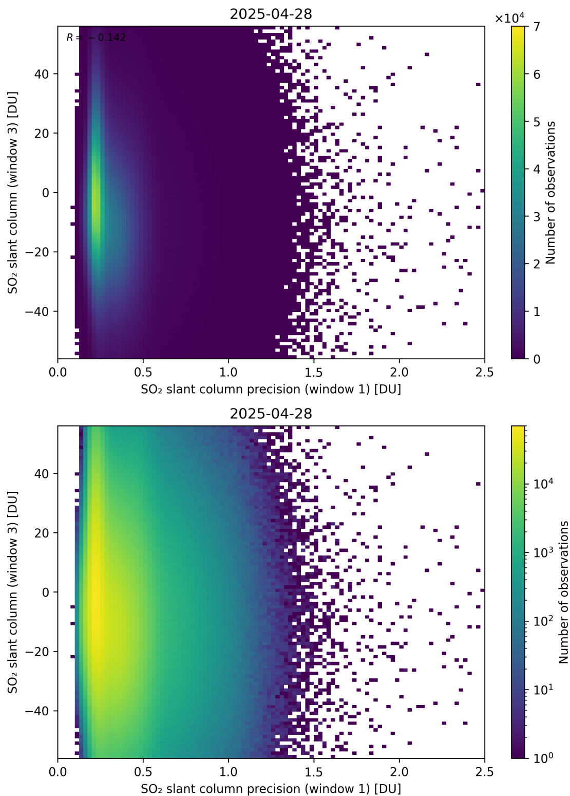
Figure 278: Scatter density plot of “SO 2 slant column precision (window 1)” against “SO 2 slant column (window 3)” for 2025-04-27 to 2025-04-29.
