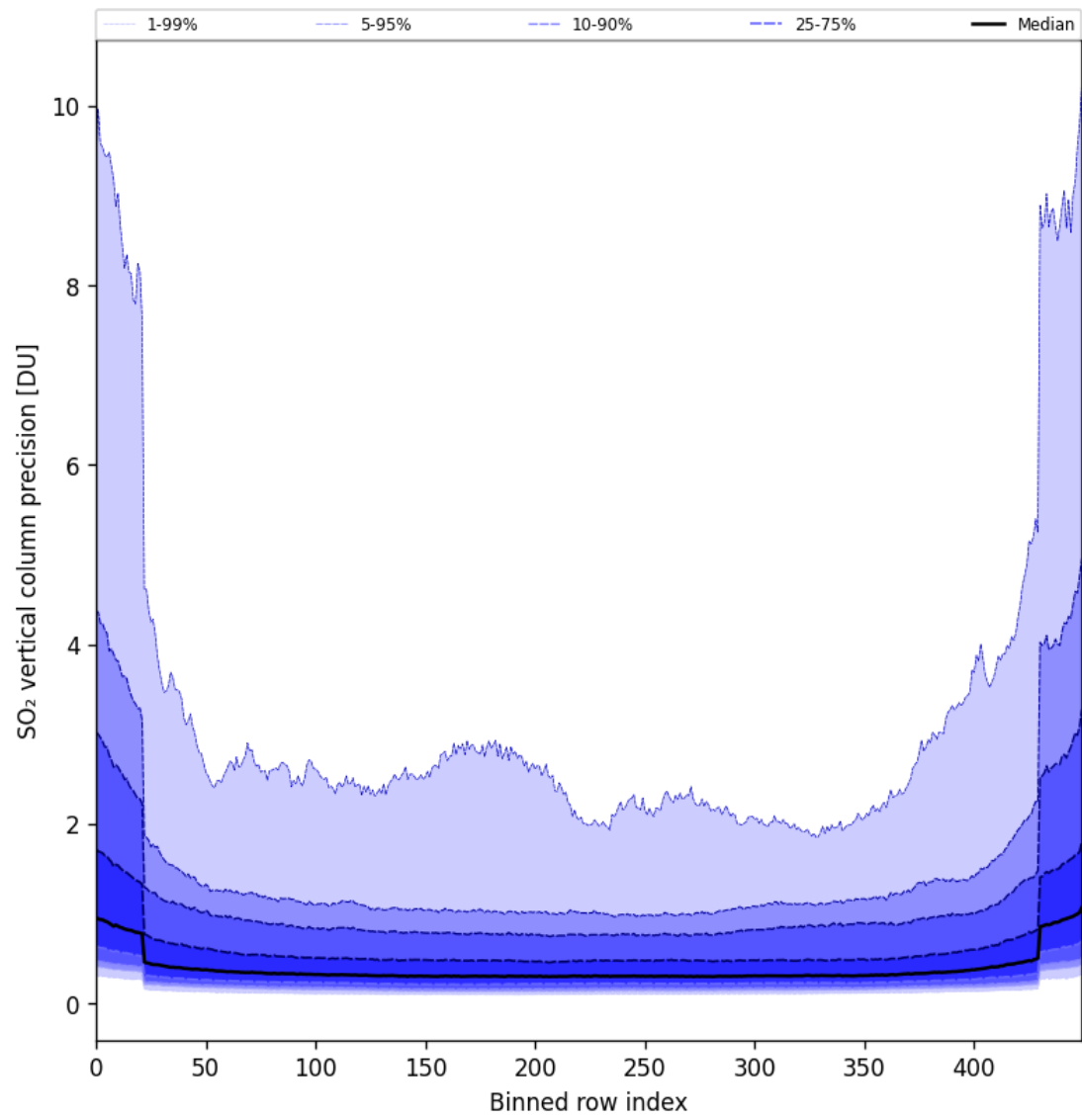
Figure 85: Along track statistics of “SO 2 vertical column precision” for 2025-04-27 to 2025-04-29
