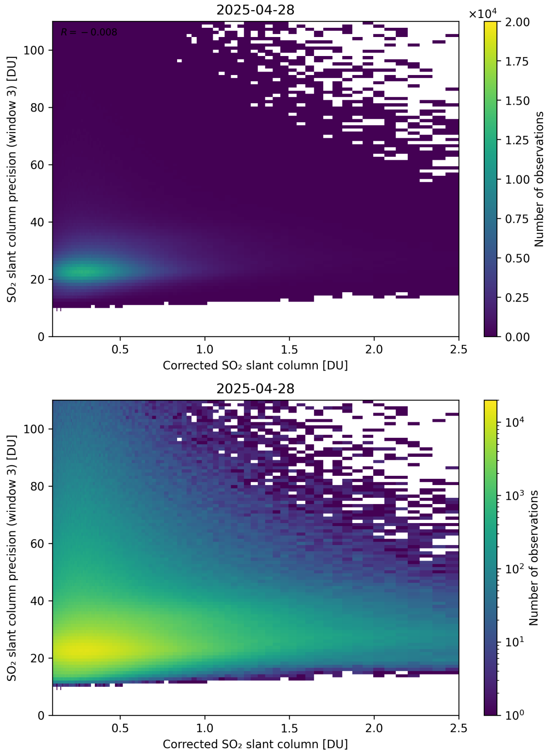
Figure 241: Scatter density plot of “Corrected SO 2 slant column” against “SO 2 slant column precision (window 3)” for 2025-04-27 to 2025-04-29.
