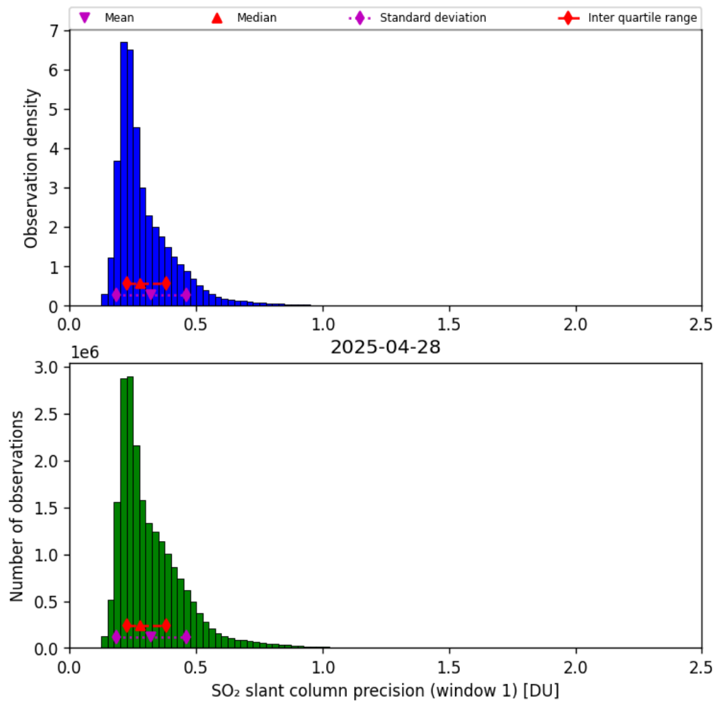
Figure 64: Histogram of “SO 2 slant column precision (window 1)” for 2025-04-27 to 2025-04-29
