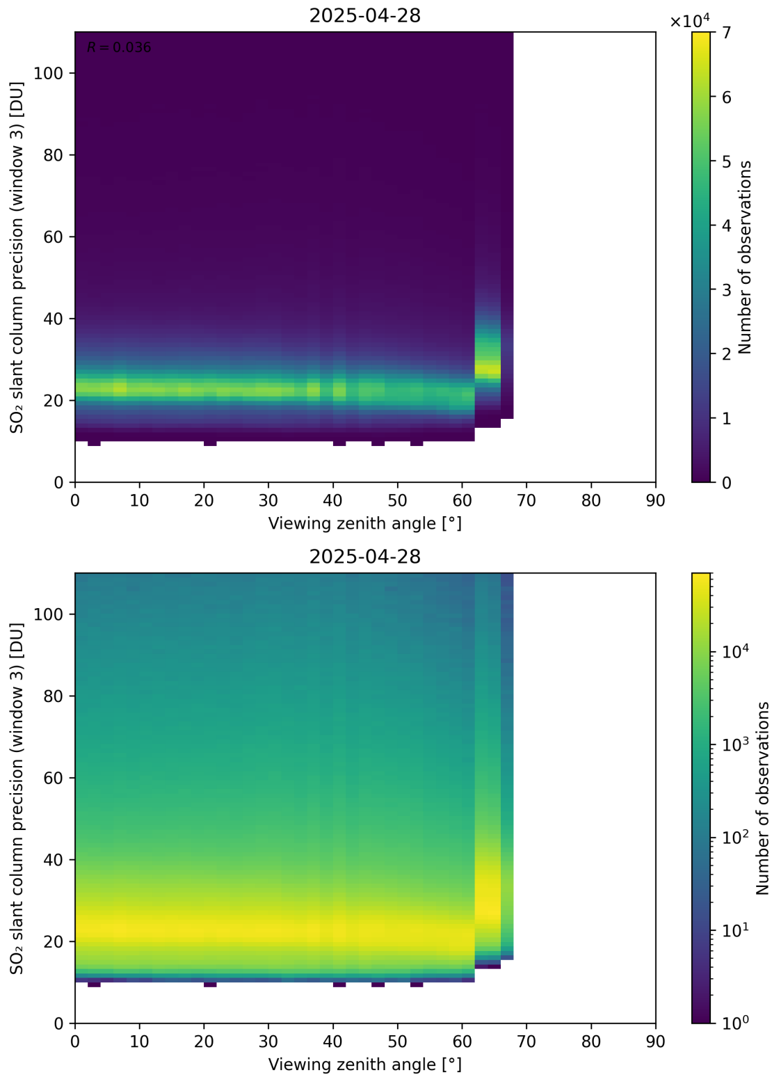
Figure 380: Scatter density plot of “Viewing zenith angle” against “SO 2 slant column precision (window 3)” for 2025-04-27 to 2025-04-29.
