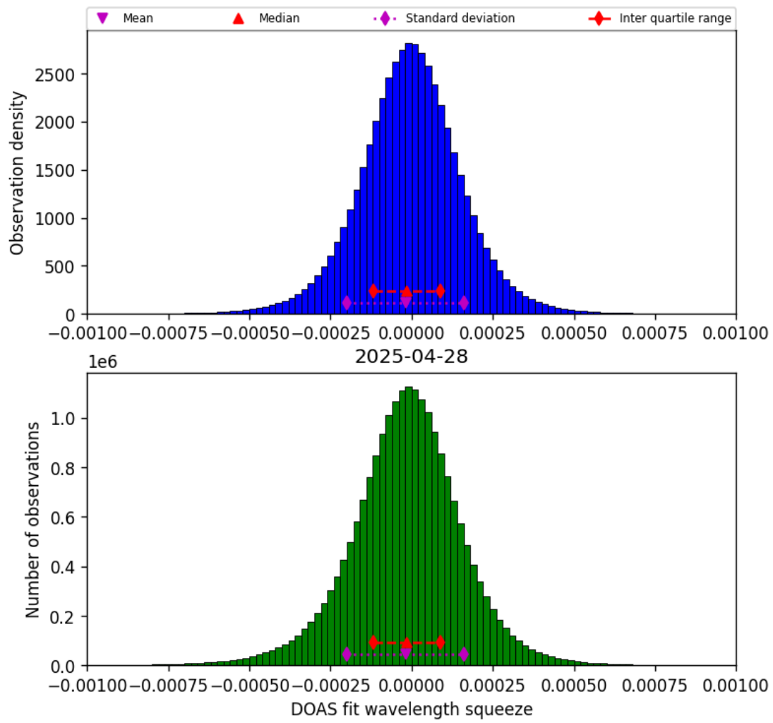
Figure 77: Histogram of “DOAS fit wavelength squeeze” for 2025-04-27 to 2025-04-29
