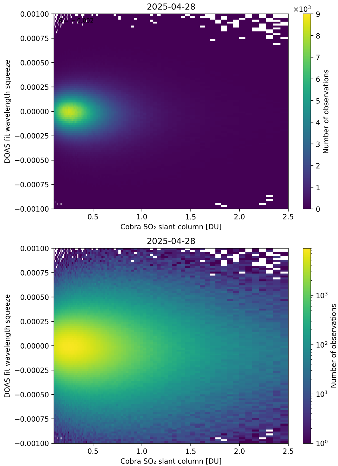
Figure 197: Scatter density plot of “Cobra SO 2 slant column” against “DOAS fit wavelength squeeze” for 2025-04-27 to 2025-04-29.
