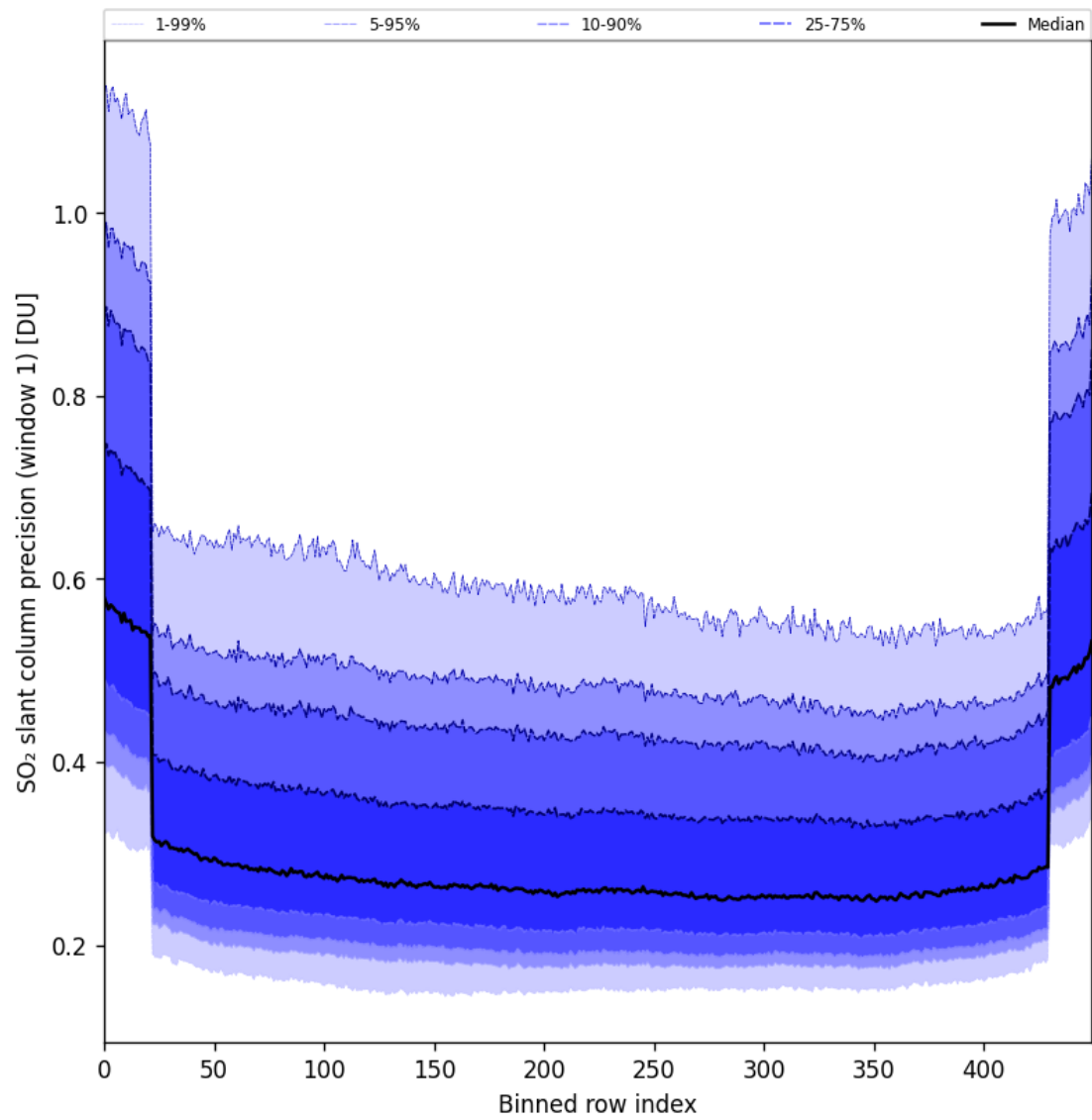
Figure 90: Along track statistics of “SO 2 slant column precision (window 1)” for 2025-04-27 to 2025-04-29
