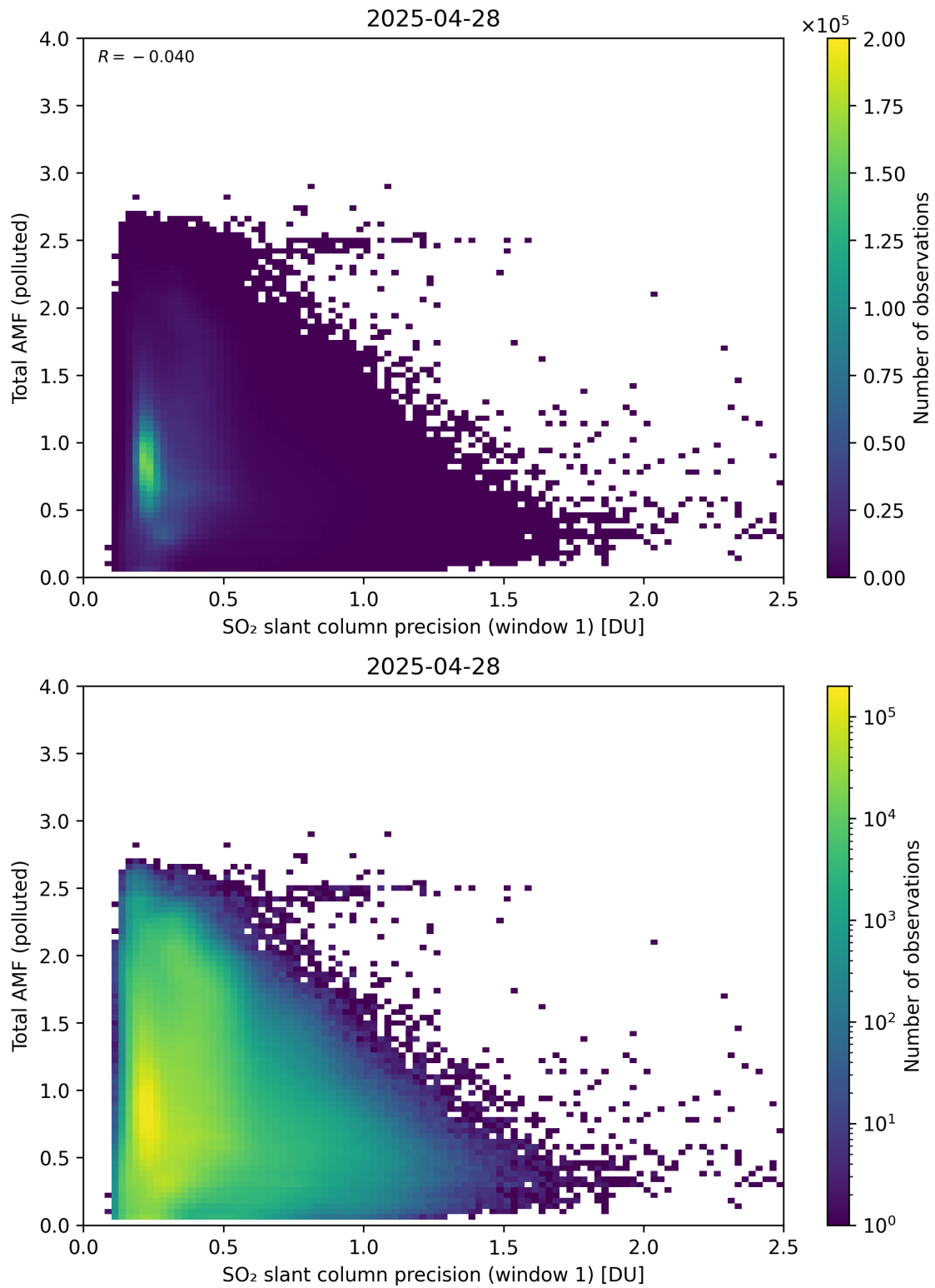
Figure 280: Scatter density plot of “SO 2 slant column precision (window 1)” against “Total AMF (polluted)” for 2025-04-27 to 2025-04-29.
