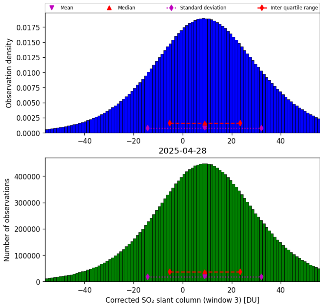
Figure 73: Histogram of “Corrected SO 2 slant column (window 3)” for 2025-04-27 to 2025-04-29
