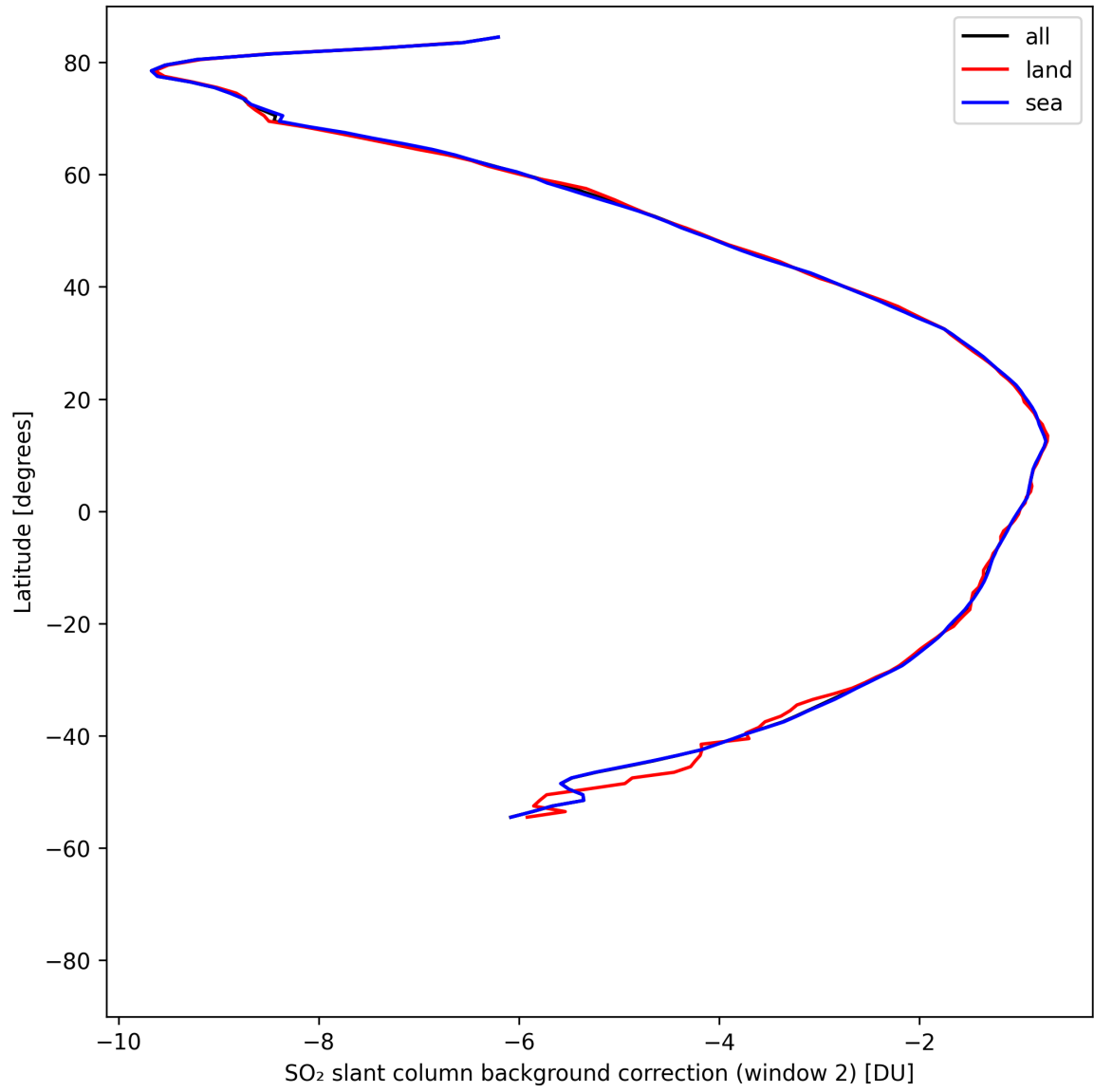
Figure 44: Zonal average of “SO 2 slant column background correction (window 2)” for 2025-04-27 to 2025-04-29.
