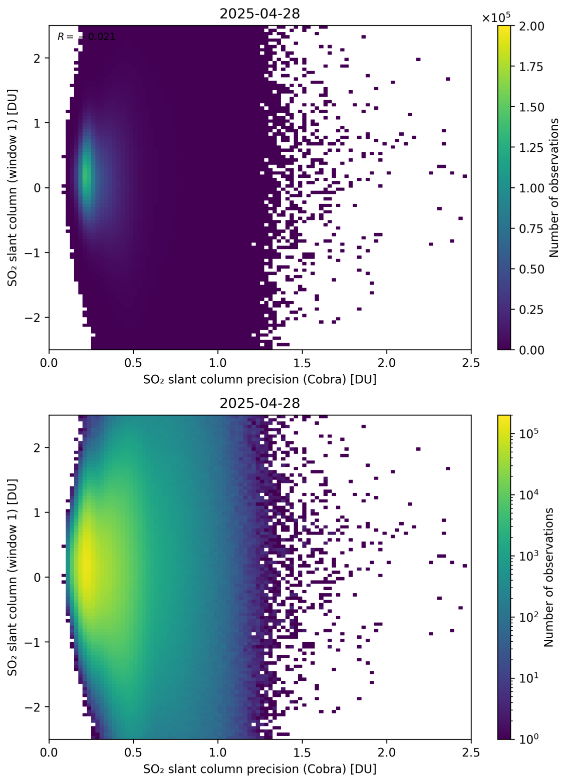
Figure 208: Scatter density plot of “SO 2 slant column precision (Cobra)” against “SO 2 slant column (window 1)” for 2025-04-27 to 2025-04-29.
