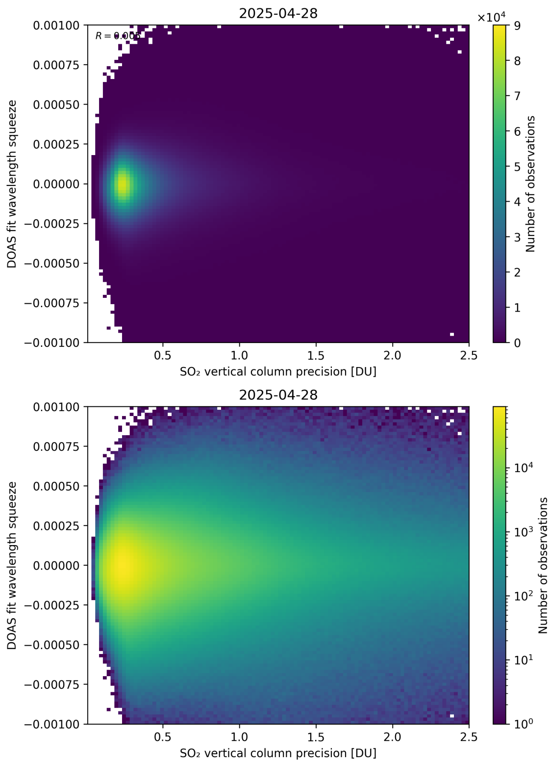
Figure 333: Scatter density plot of “SO 2 vertical column precision” against “DOAS fit wavelength squeeze” for 2025-04-27 to 2025-04-29.
