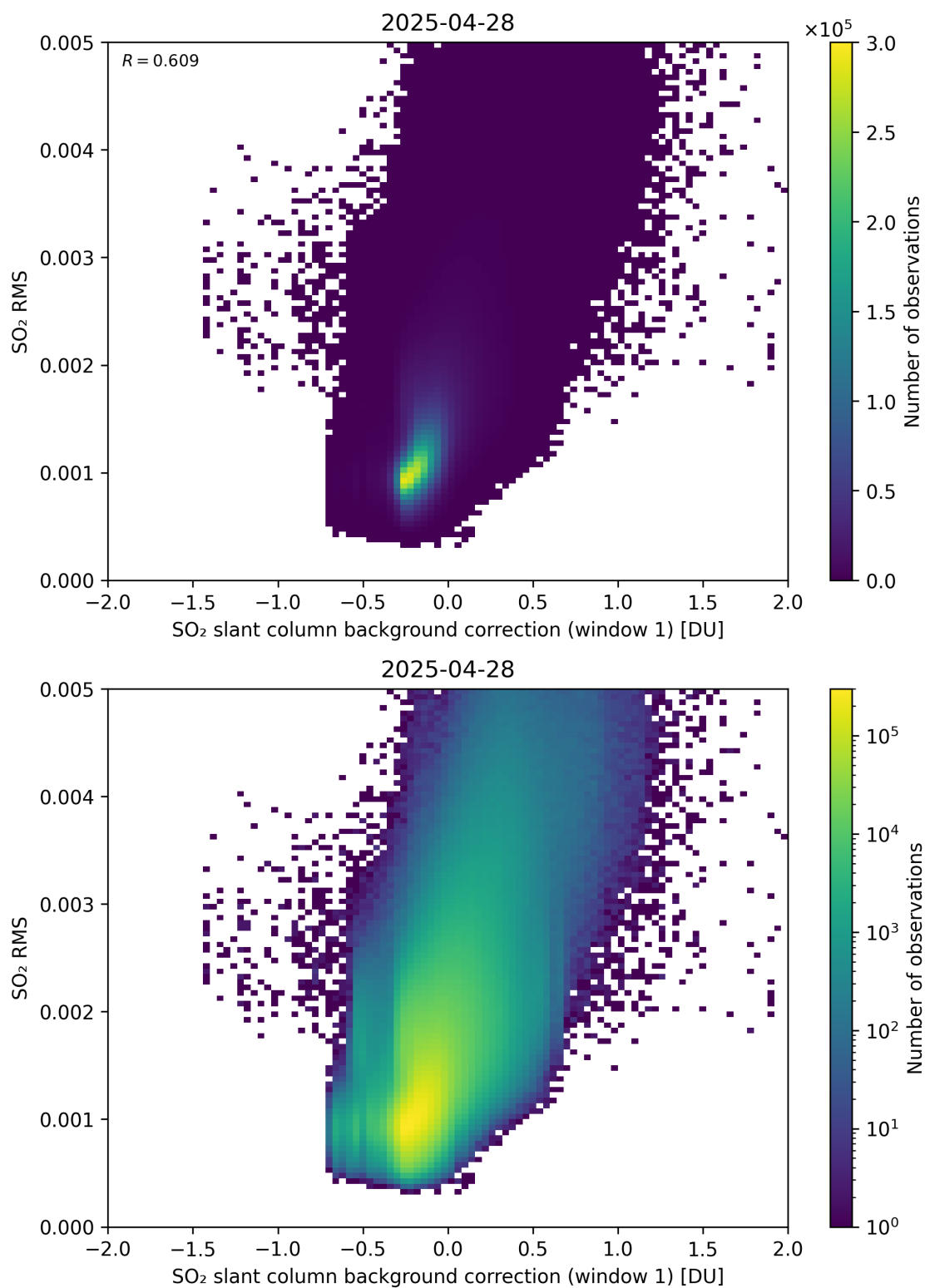
Figure 113: Scatter density plot of “SO 2 slant column background correction (window 1)” against “SO 2 RMS” for 2025-04-27 to 2025-04-29.
