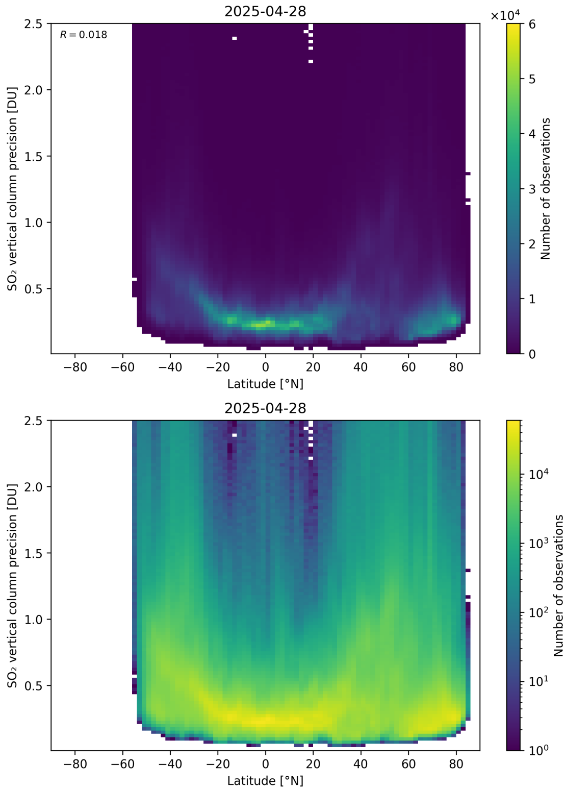
Figure 170: Scatter density plot of “Latitude” against “SO 2 vertical column precision” for 2025-04-27 to 2025-04-29.
