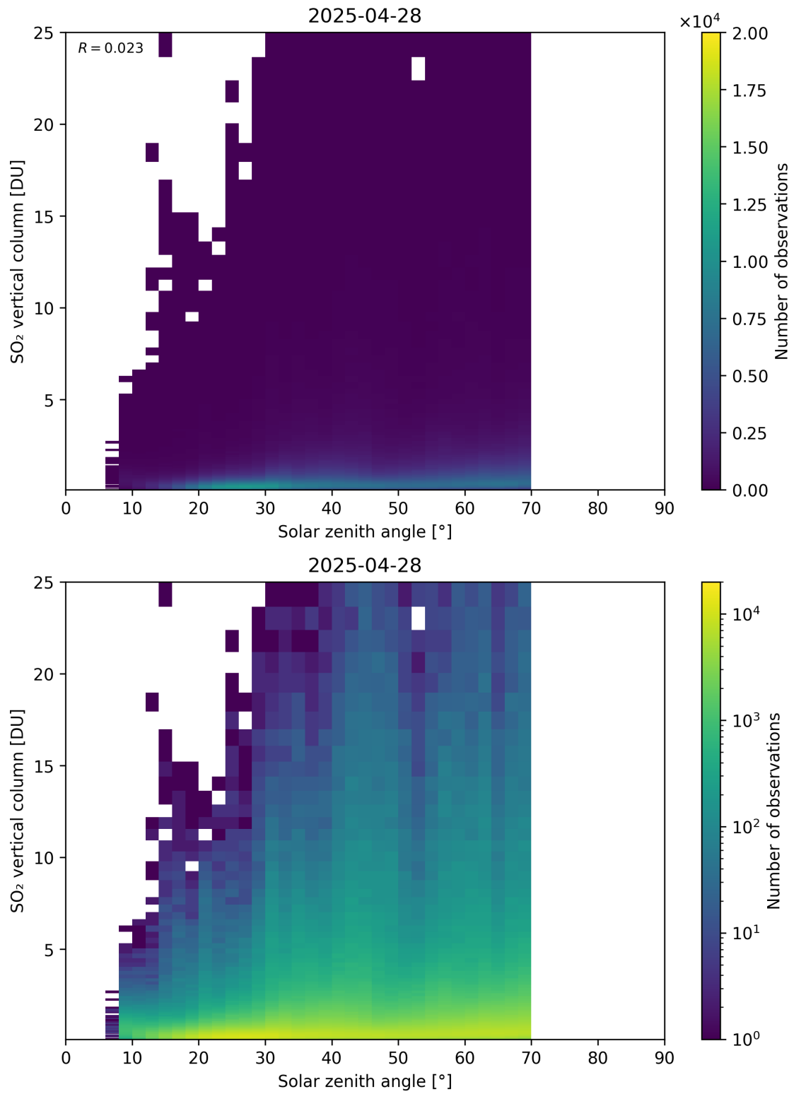
Figure 191: Scatter density plot of “Solar zenith angle” against “SO 2 vertical column” for 2025-04-27 to 2025-04-29.
