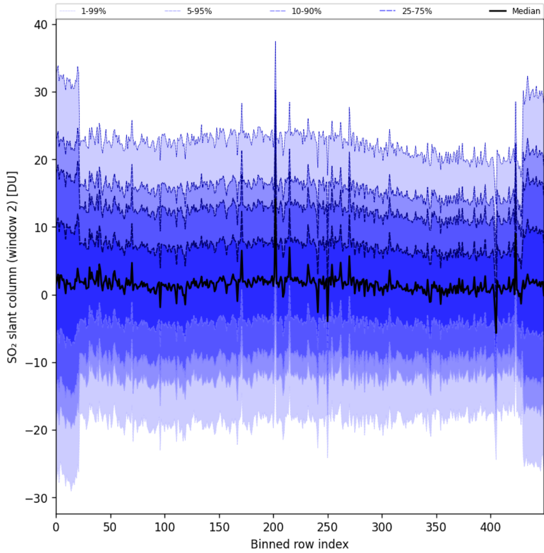
Figure 93: Along track statistics of “SO 2 slant column (window 2)” for 2025-04-27 to 2025-04-29
