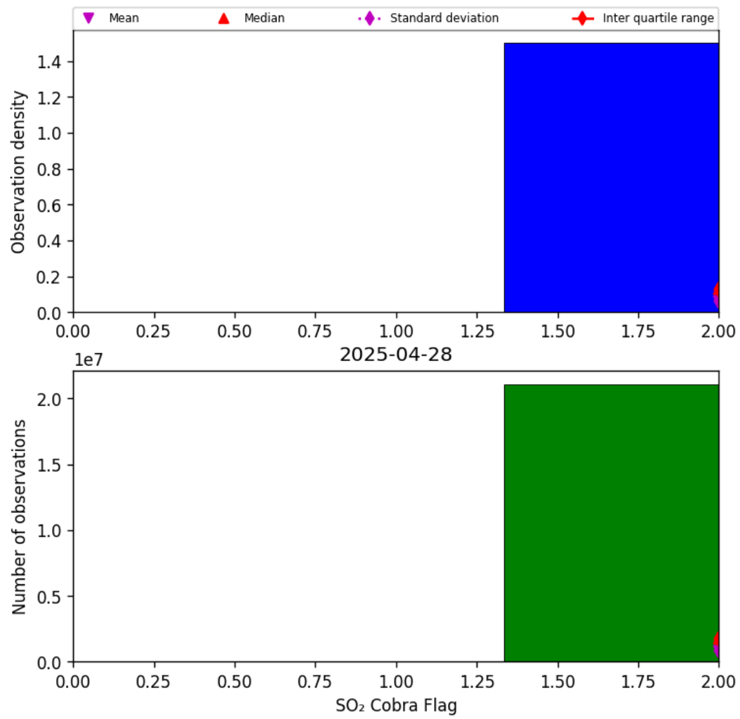
Figure 75: Histogram of “SO 2 Cobra Flag” for 2025-04-27 to 2025-04-29
