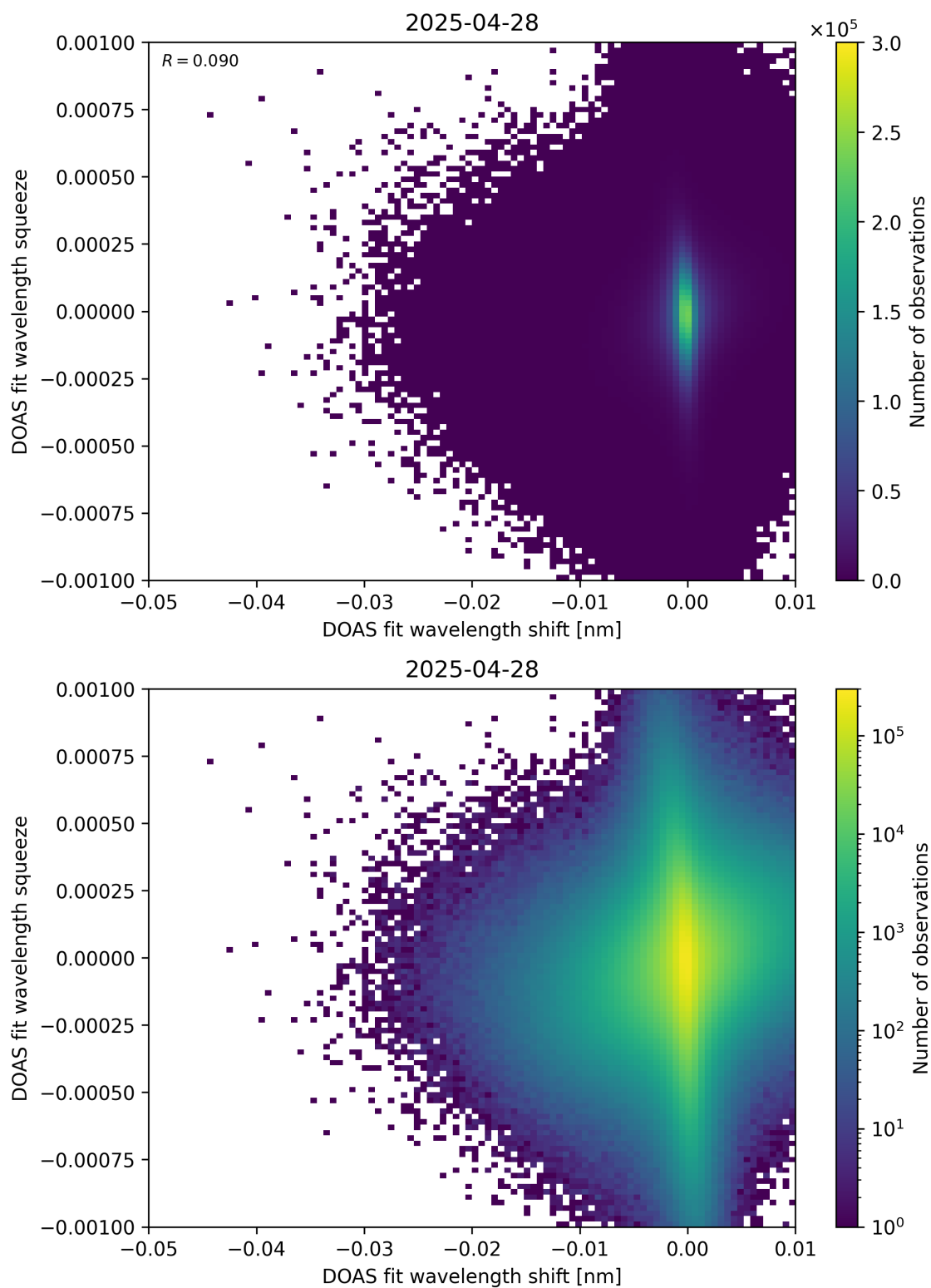
Figure 138: Scatter density plot of “DOAS fit wavelength shift” against “DOAS fit wavelength squeeze” for 2025-04-27 to 2025-04-29.
