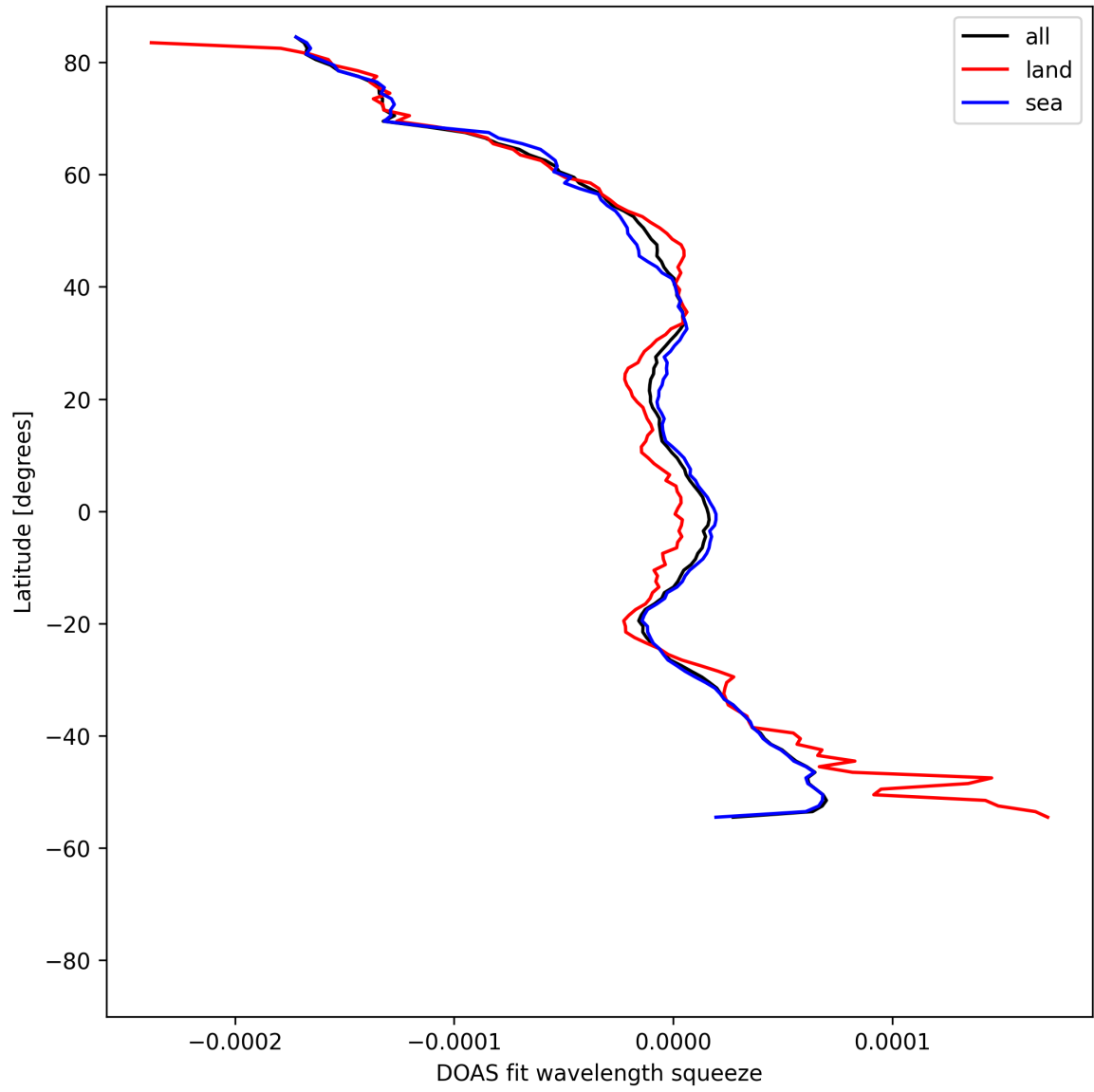
Figure 51: Zonal average of “DOAS fit wavelength squeeze” for 2025-04-27 to 2025-04-29.
