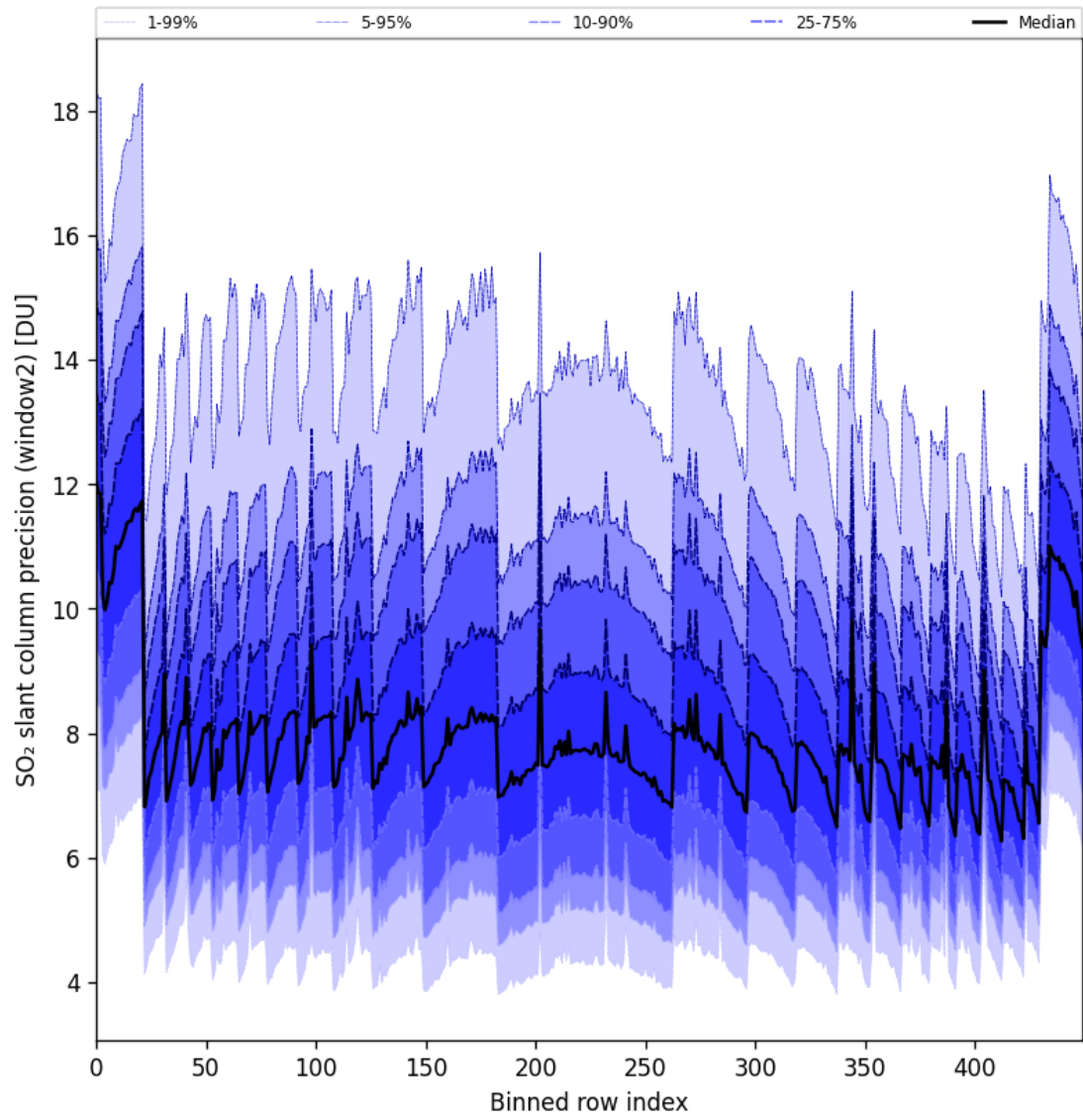
Figure 94: Along track statistics of “SO 2 slant column precision (window2)” for 2025-04-27 to 2025-04-29
