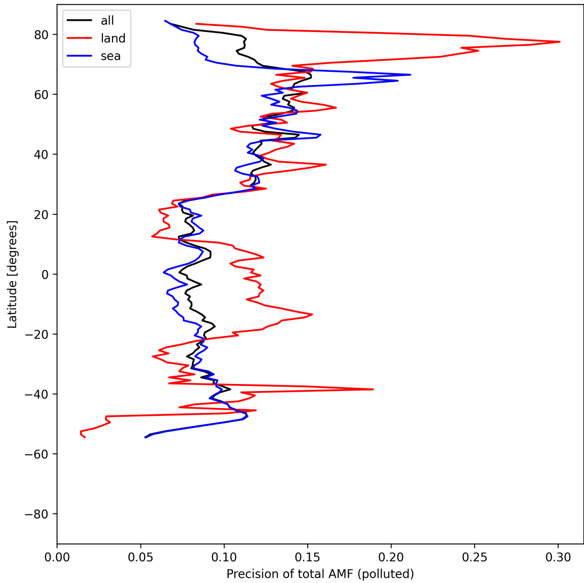
Figure 54: Zonal average of “Precision of total AMF (polluted)” for 2025-04-27 to 2025-04-29.
