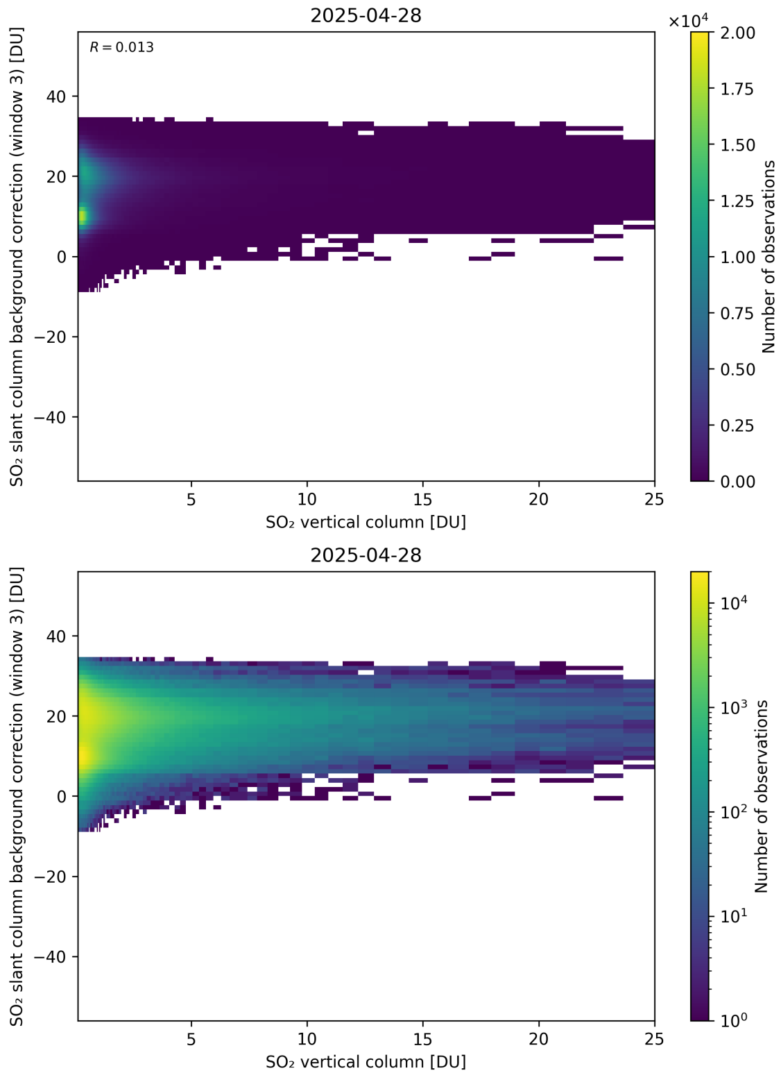
Figure 325: Scatter density plot of “SO 2 vertical column” against “SO 2 slant column background correction (window 3)” for 2025-04-27 to 2025-04-29.
