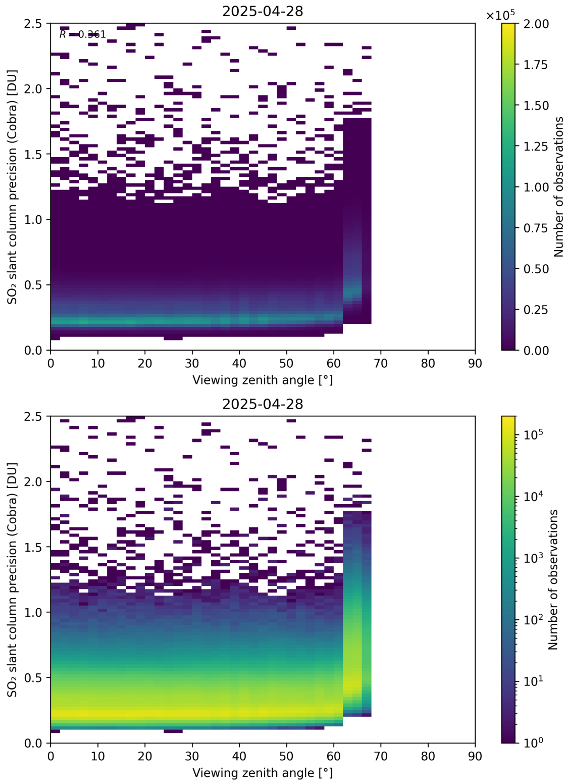
Figure 372: Scatter density plot of “Viewing zenith angle” against “SO 2 slant column precision (Cobra)” for 2025-04-27 to 2025-04-29.
