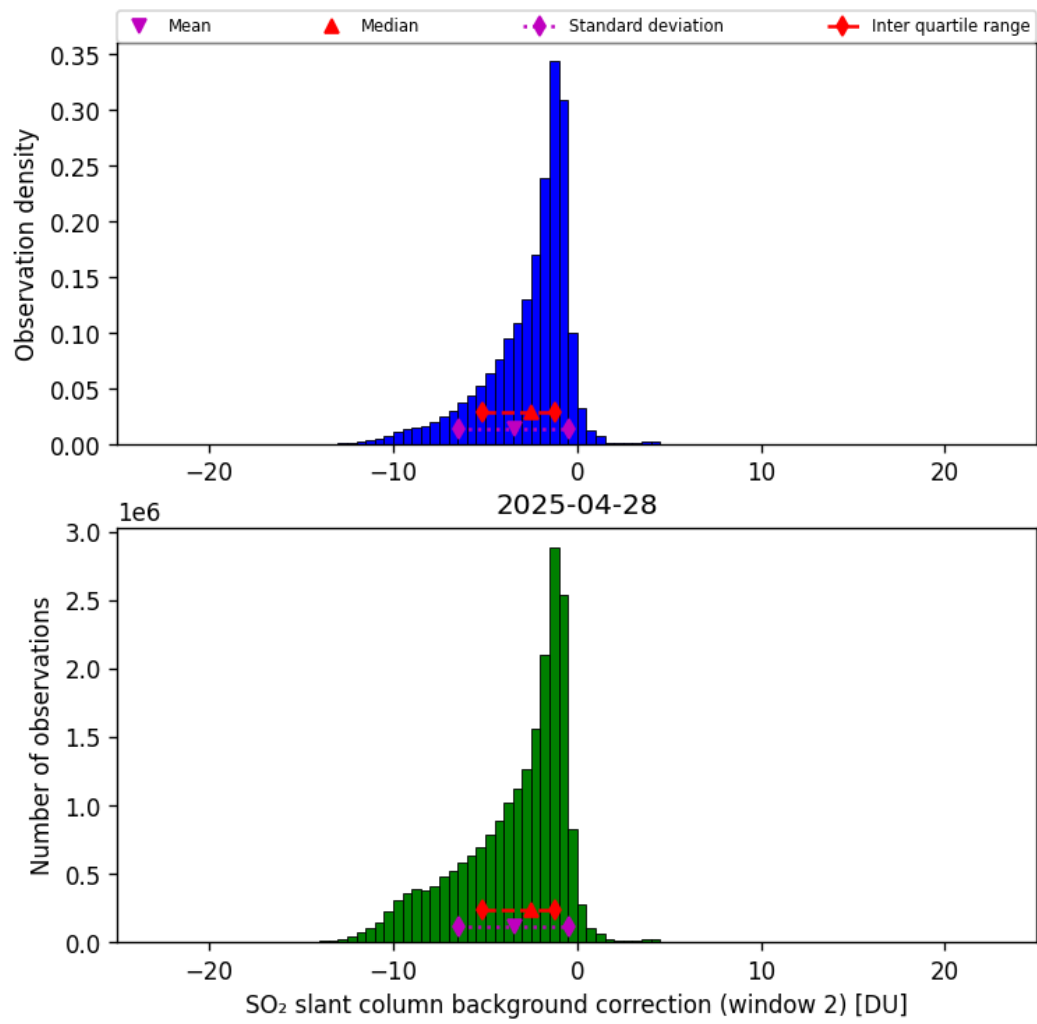
Figure 70: Histogram of “SO 2 slant column background correction (window 2)” for 2025-04-27 to 2025-04-29
