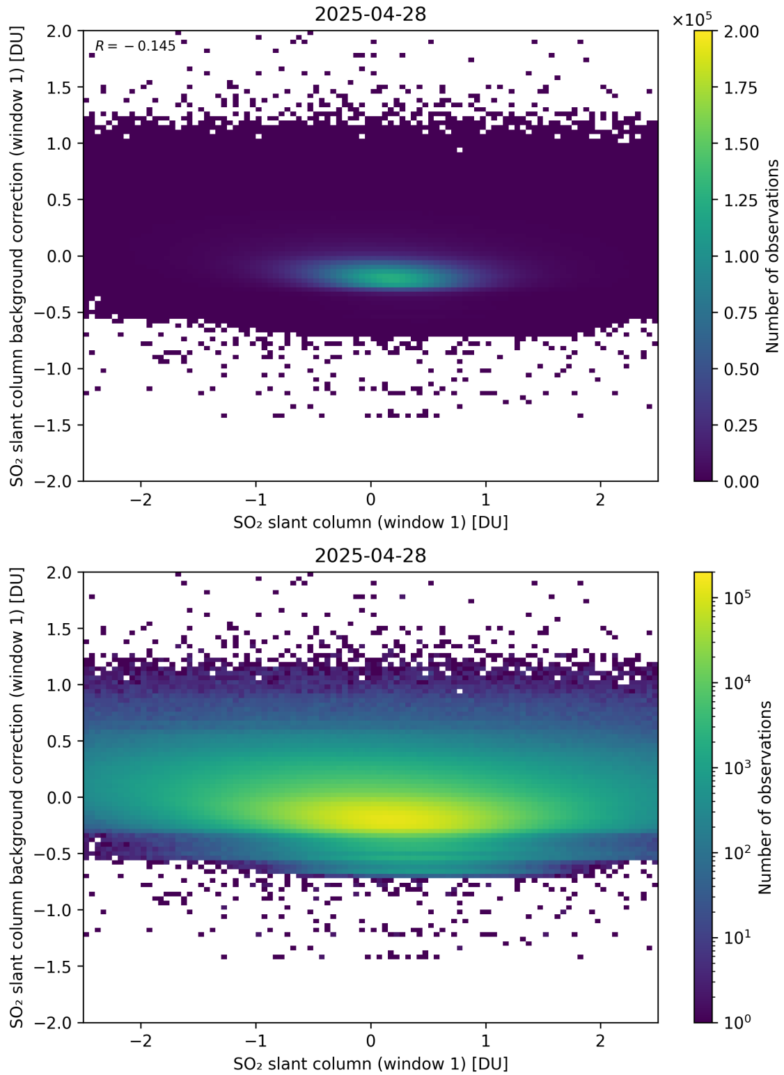
Figure 262: Scatter density plot of “SO 2 slant column (window 1)” against “SO 2 slant column background correction (window 1)” for 2025-04-27 to 2025-04-29.
