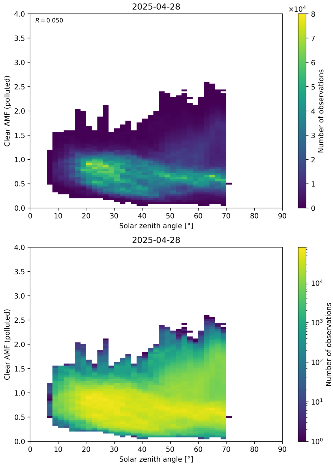
Figure 178: Scatter density plot of “Solar zenith angle” against “Clear AMF (polluted)” for 2025-04-27 to 2025-04-29.
