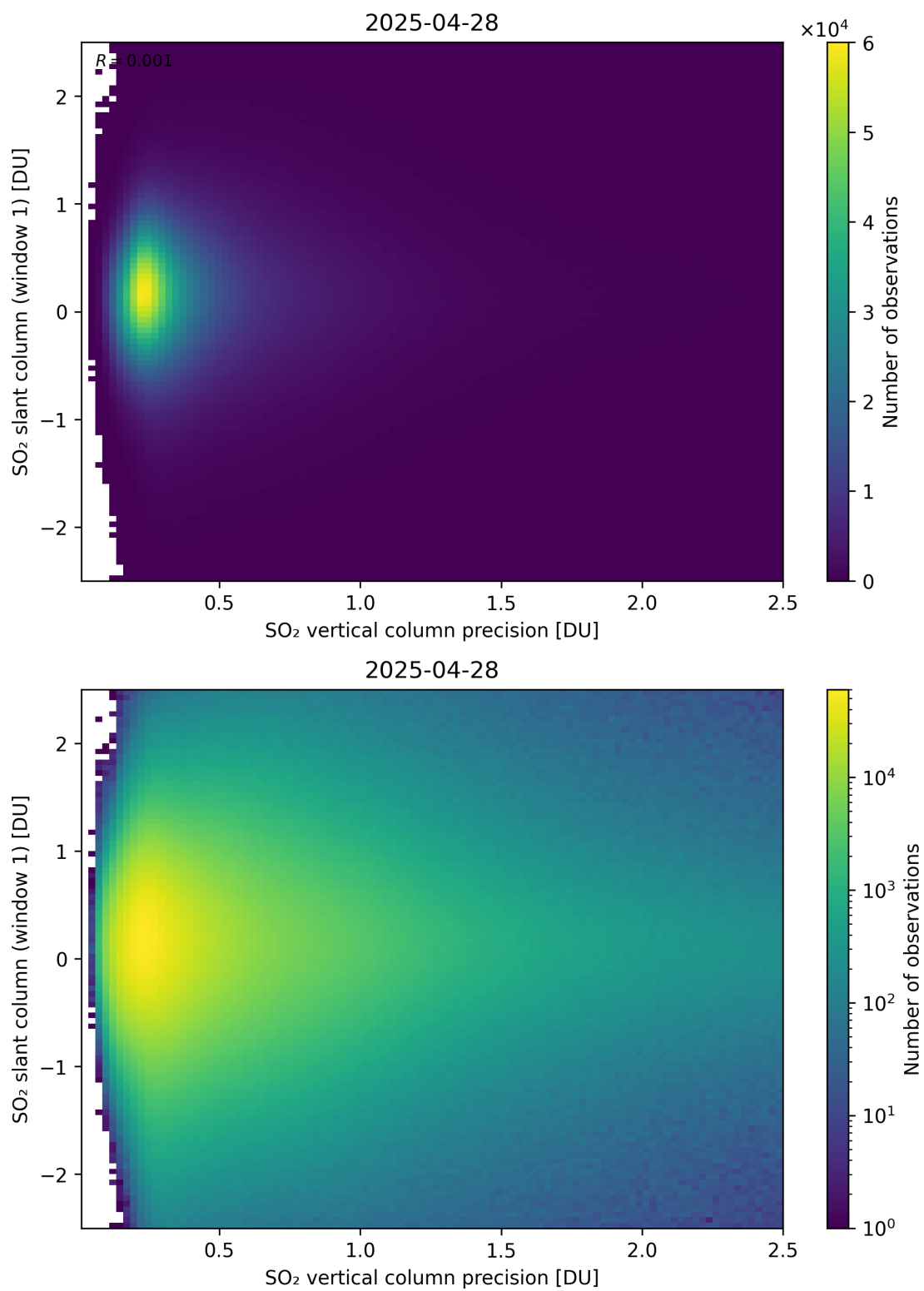
Figure 341: Scatter density plot of “SO 2 vertical column precision” against “SO 2 slant column (window 1)” for 2025-04-27 to 2025-04-29.
