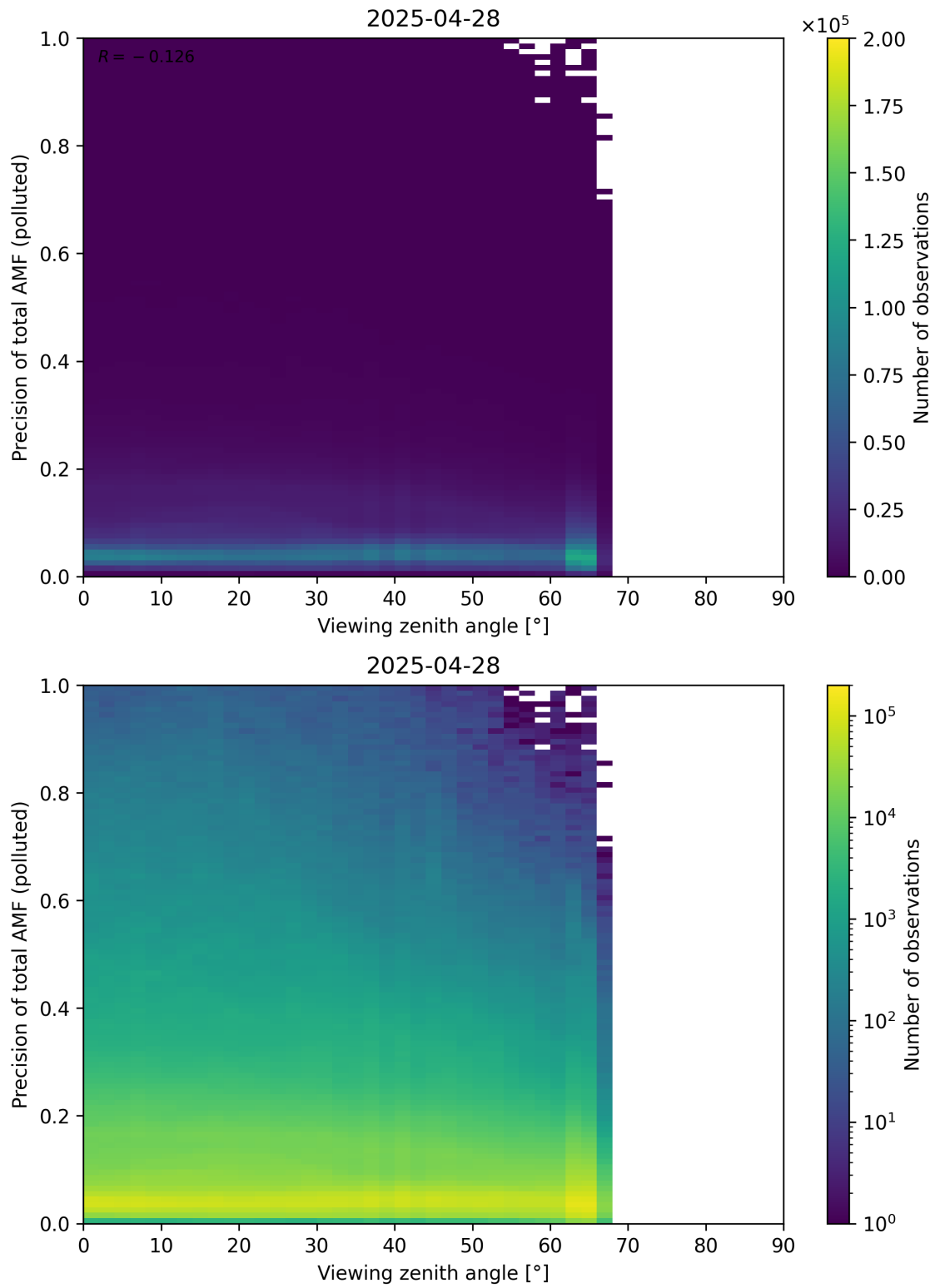
Figure 382: Scatter density plot of “Viewing zenith angle” against “Precision of total AMF (polluted)” for 2025-04-27 to 2025-04-29.
