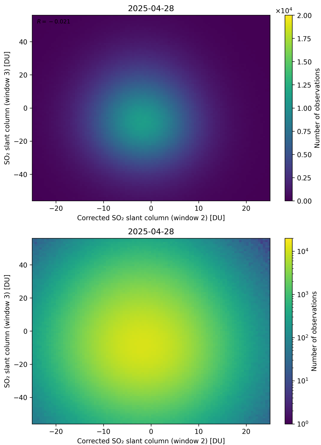
Figure 251: Scatter density plot of “Corrected SO 2 slant column (window 2)” against “SO 2 slant column (window 3)” for 2025-04-27 to 2025-04-29.
