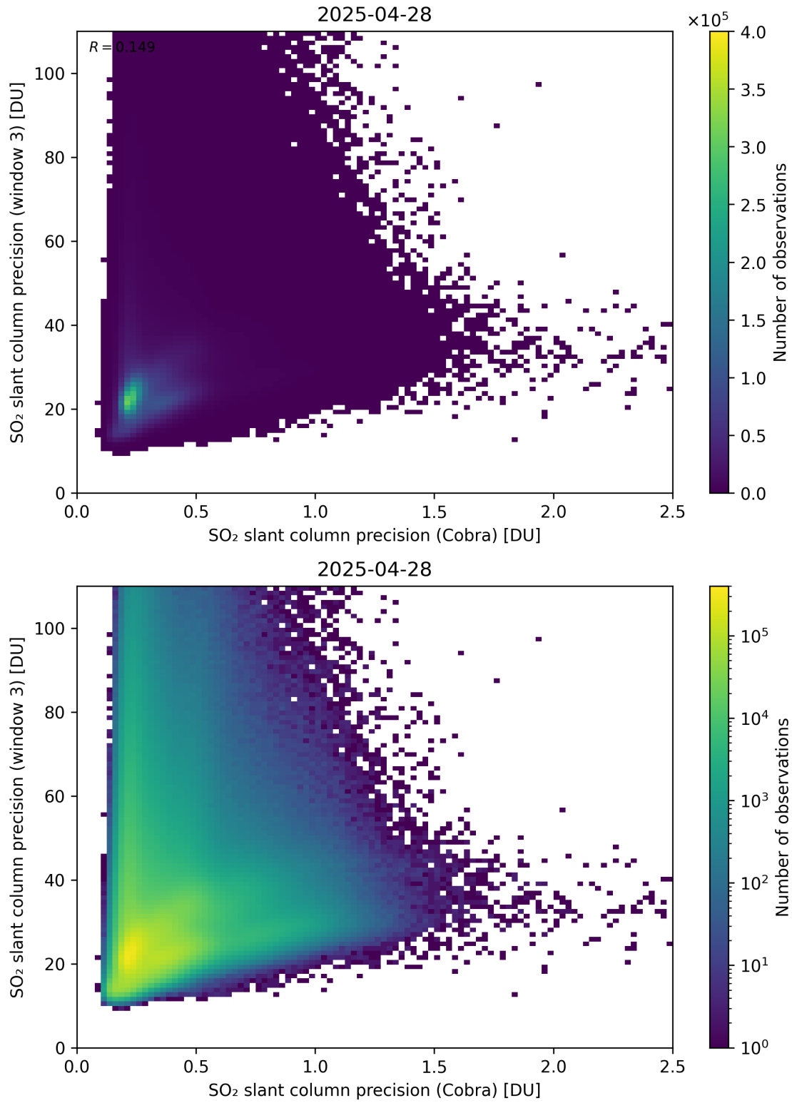
Figure 212: Scatter density plot of “SO 2 slant column precision (Cobra)” against “SO 2 slant column precision (window 3)” for 2025-04-27 to 2025-04-29.
