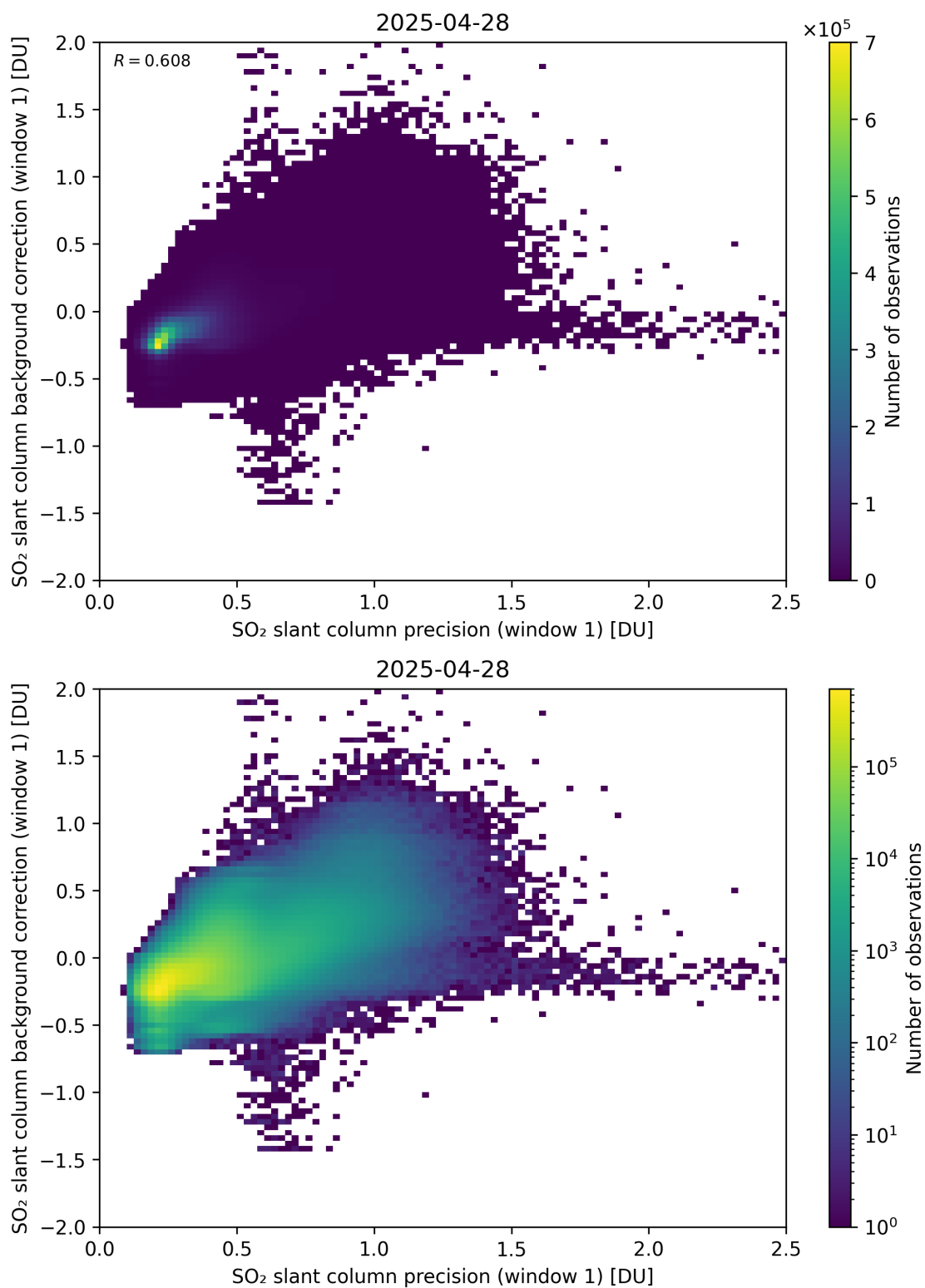
Figure 268: Scatter density plot of “SO 2 slant column precision (window 1)” against “SO 2 slant column background correction (window 1)” for 2025-04-27 to 2025-04-29.
