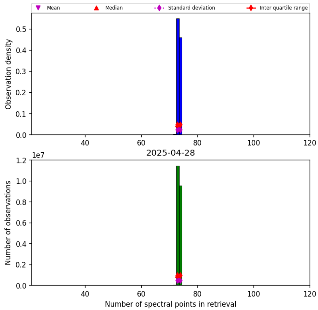
Figure 82: Histogram of “Number of spectral points in retrieval” for 2025-04-27 to 2025-04-29
