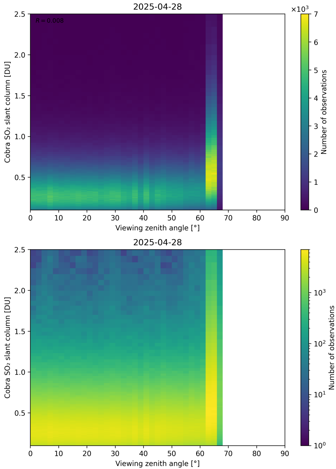
Figure 371: Scatter density plot of “Viewing zenith angle” against “Cobra SO 2 slant column” for 2025-04-27 to 2025-04-29.
