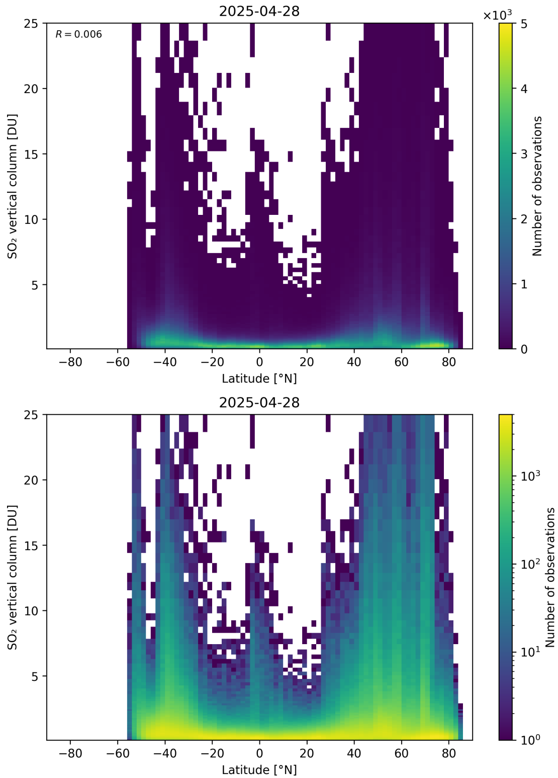
Figure 169: Scatter density plot of “Latitude” against “SO 2 vertical column” for 2025-04-27 to 2025-04-29.
