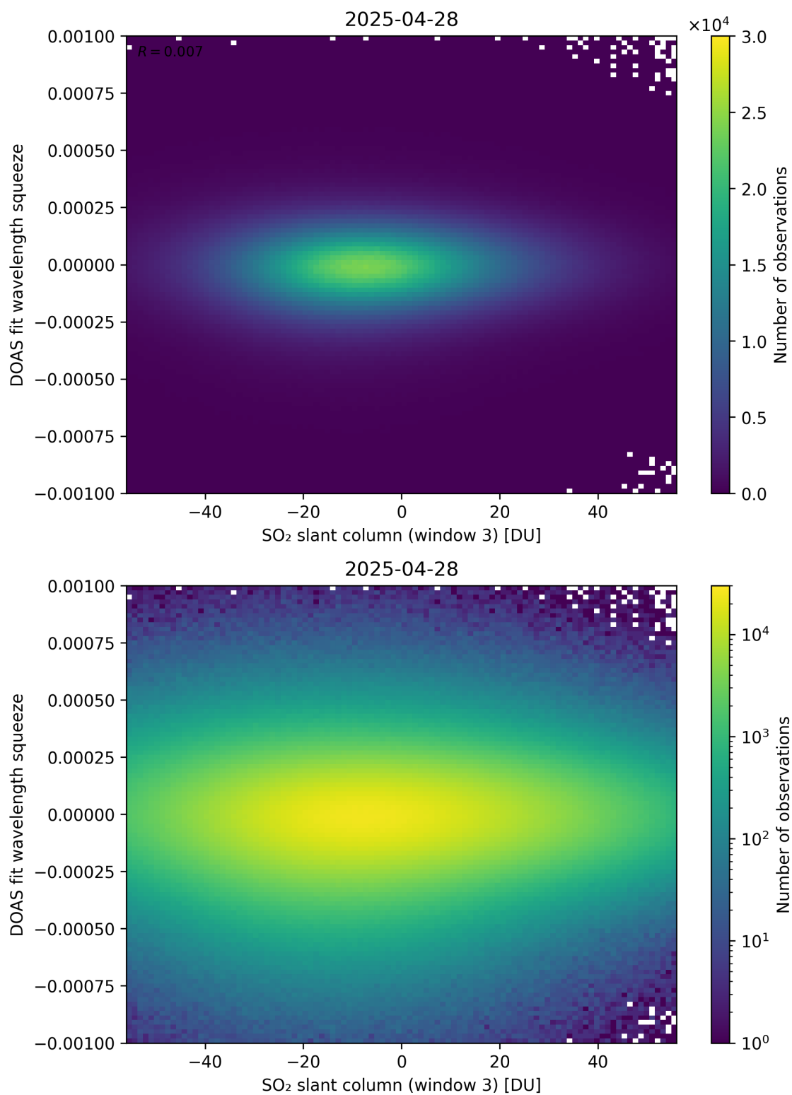
Figure 305: Scatter density plot of “SO 2 slant column (window 3)” against “DOAS fit wavelength squeeze” for 2025-04-27 to 2025-04-29.
