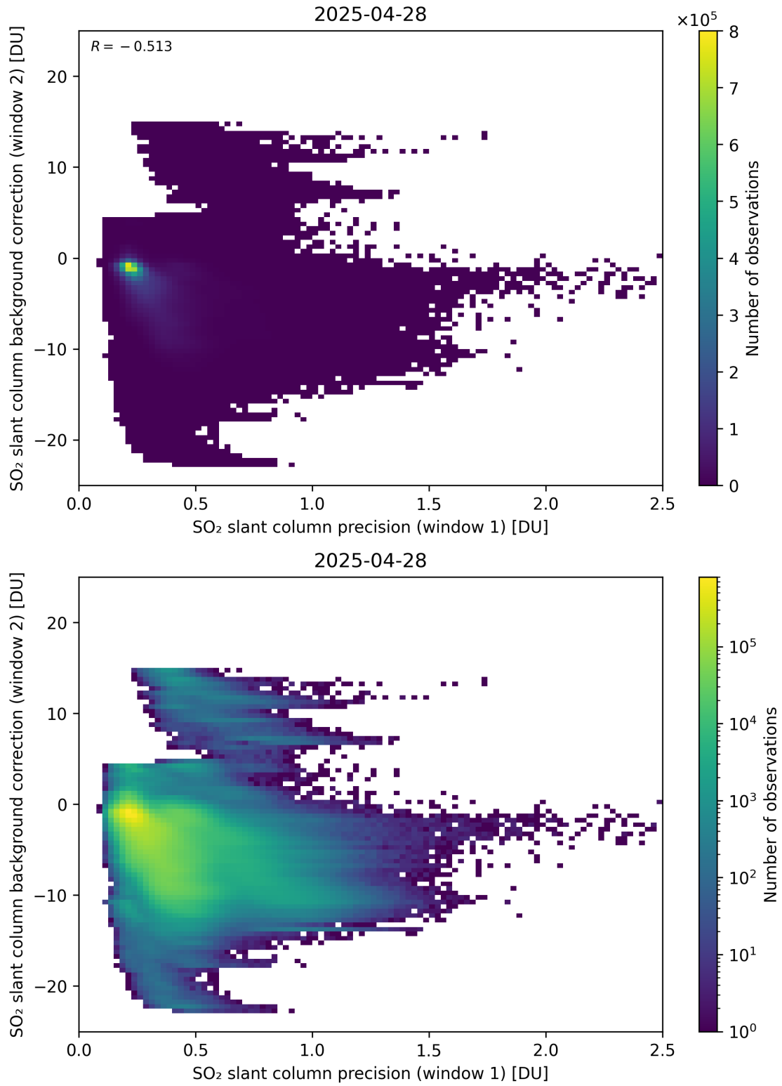
Figure 269: Scatter density plot of “SO 2 slant column precision (window 1)” against “SO 2 slant column background correction (window 2)” for 2025-04-27 to 2025-04-29.
