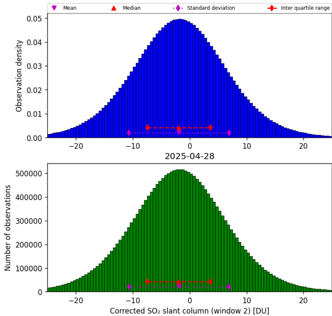
Figure 69: Histogram of “Corrected SO 2 slant column (window 2)” for 2025-04-27 to 2025-04-29
