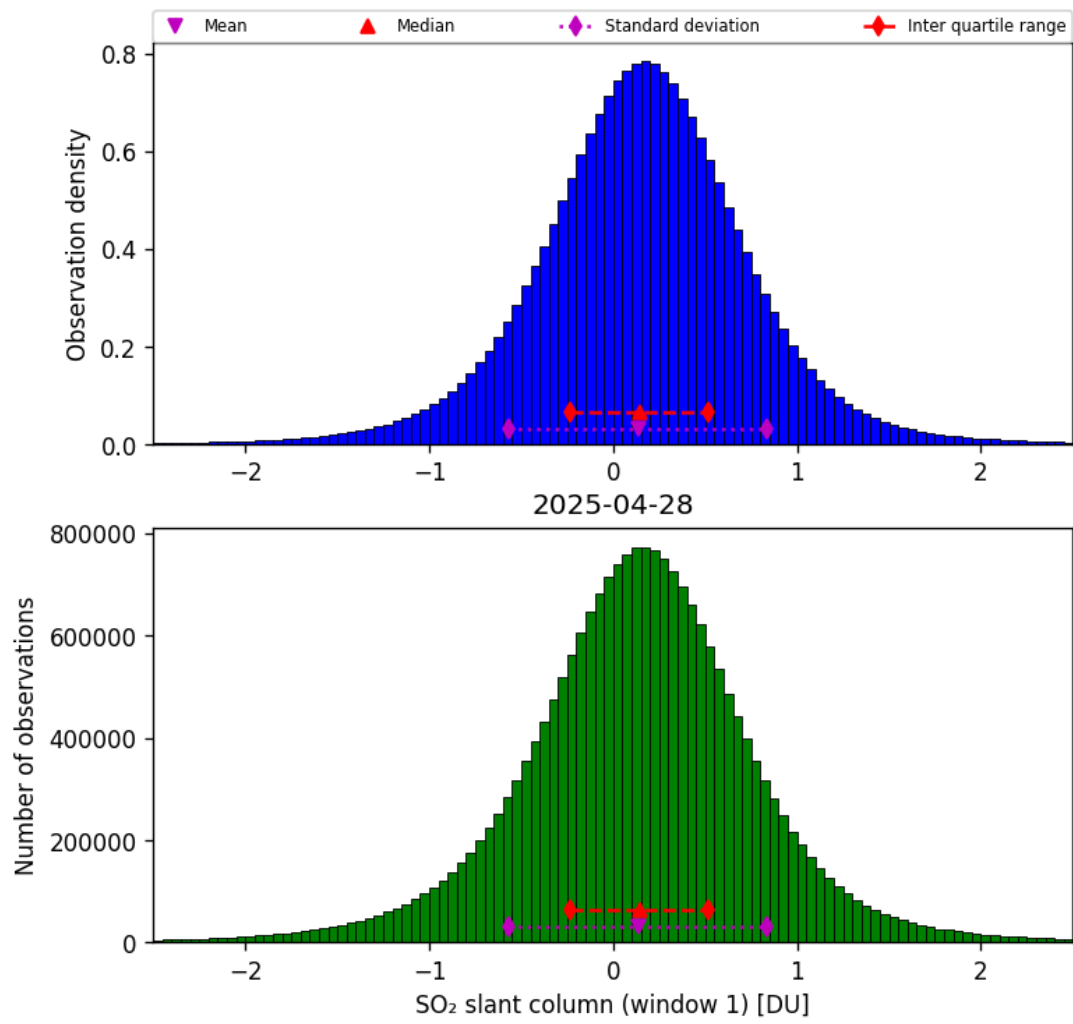
Figure 63: Histogram of “SO 2 slant column (window 1)” for 2025-04-27 to 2025-04-29
