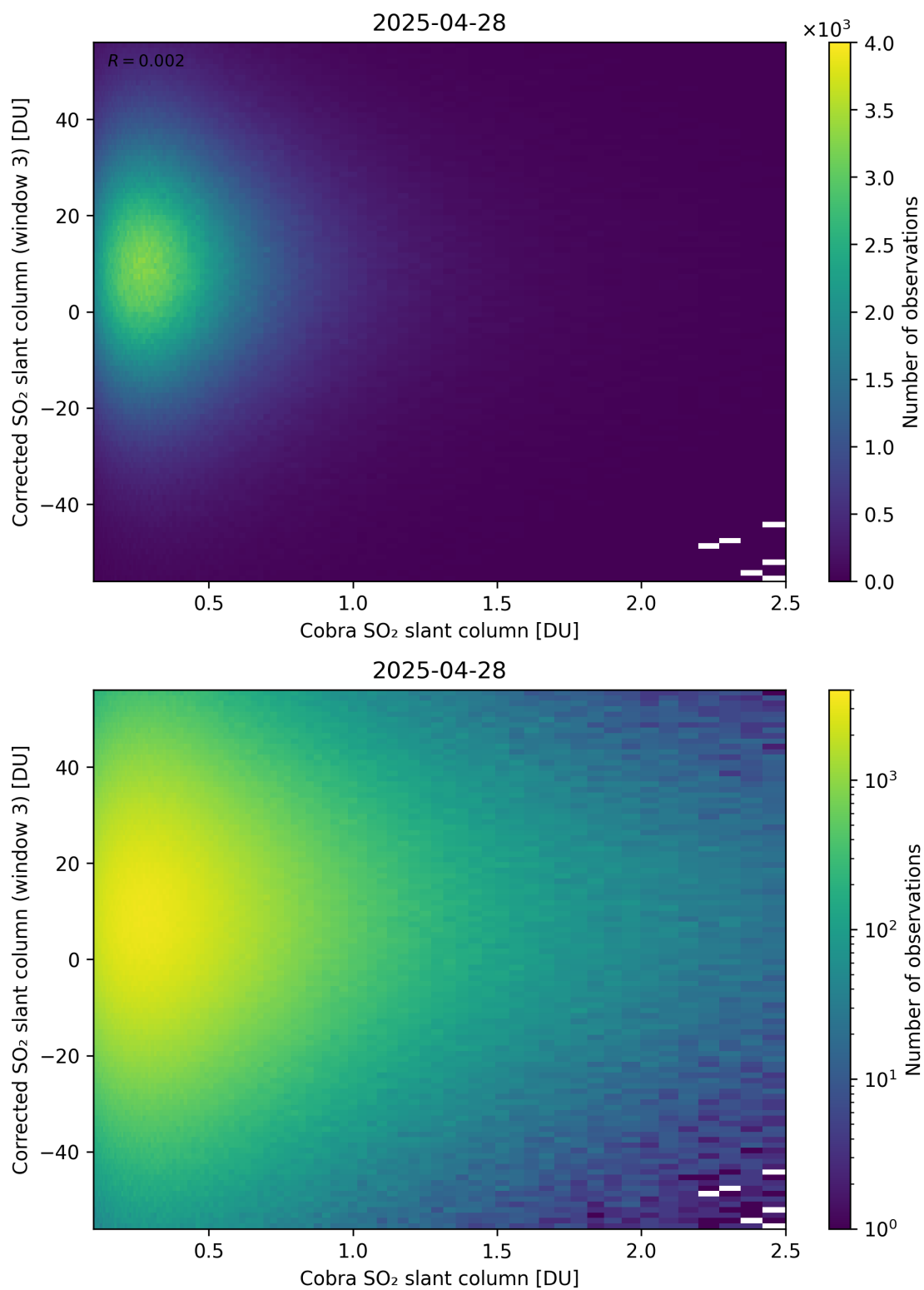
Figure 218: Scatter density plot of “Cobra SO 2 slant column” against “Corrected SO 2 slant column (window 3)” for 2025-04-27 to 2025-04-29.
