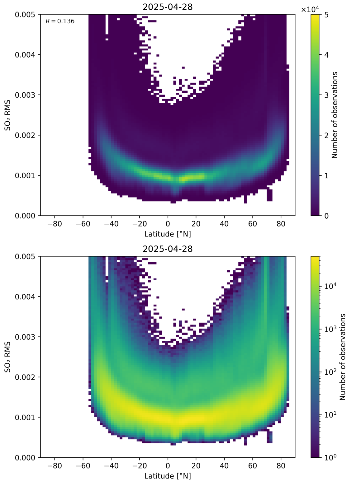
Figure 155: Scatter density plot of “Latitude” against “SO 2 RMS” for 2025-04-27 to 2025-04-29.
