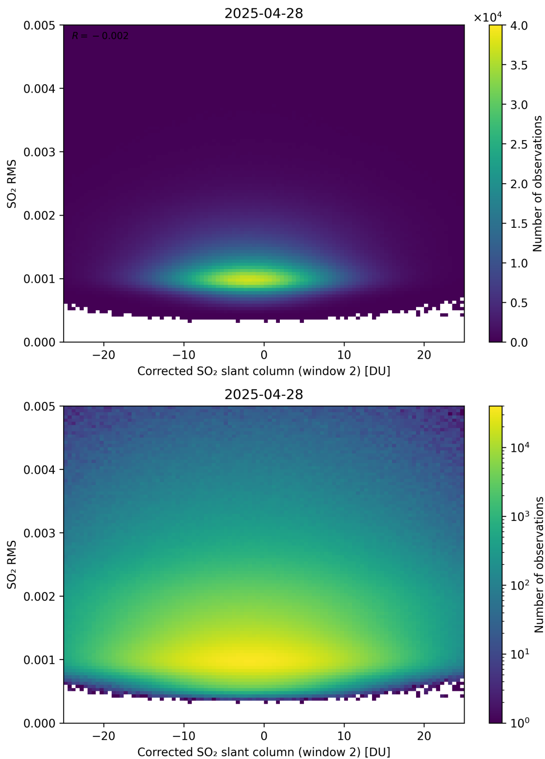
Figure 248: Scatter density plot of “Corrected SO 2 slant column (window 2)” against “SO 2 RMS” for 2025-04-27 to 2025-04-29.
