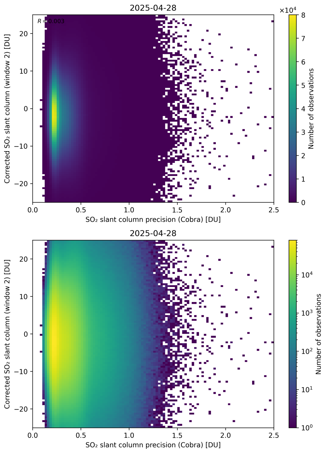
Figure 206: Scatter density plot of “SO 2 slant column precision (Cobra)” against “Corrected SO 2 slant column (window 2)” for 2025-04-27 to 2025-04-29.
