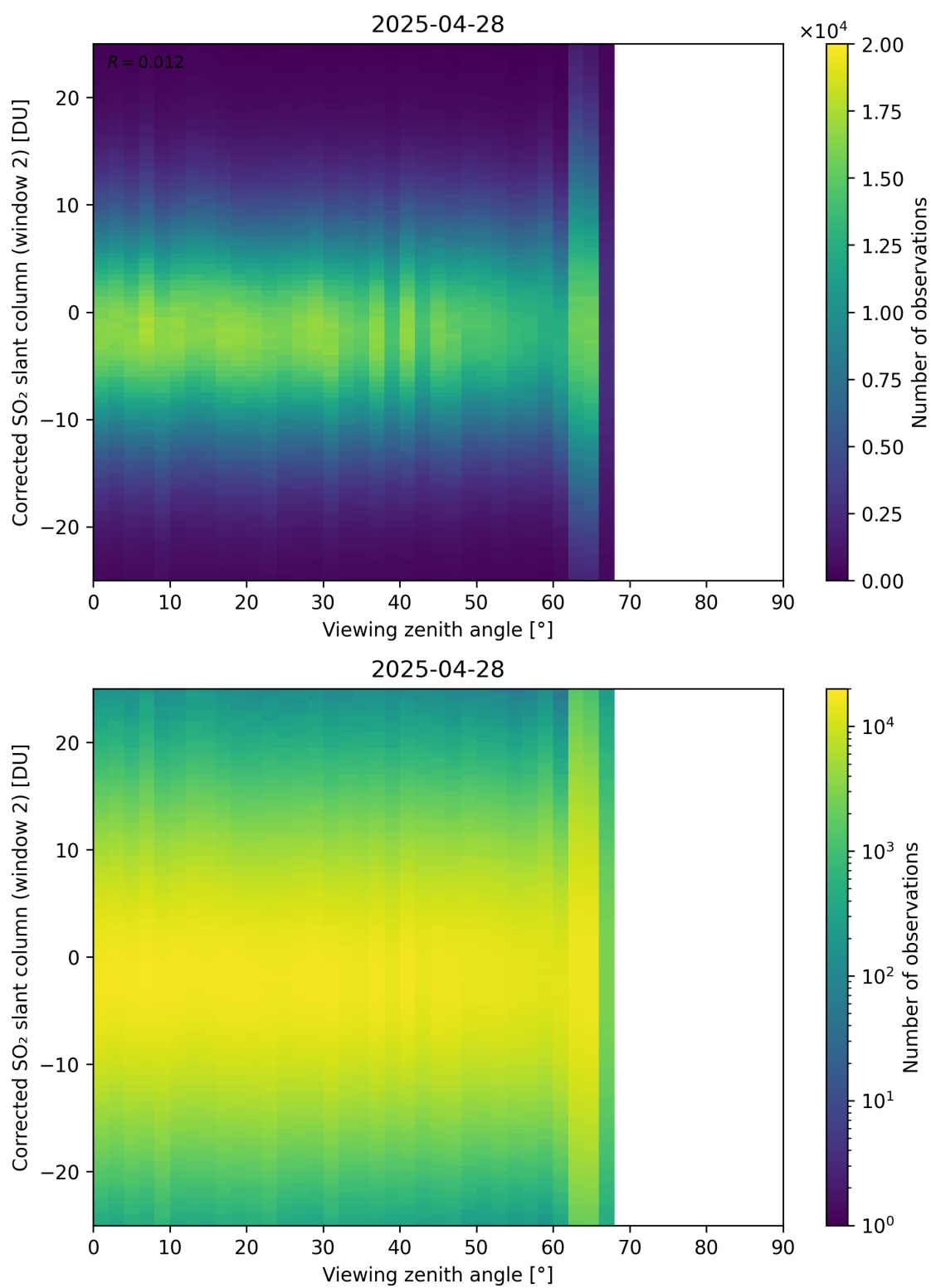
Figure 374: Scatter density plot of “Viewing zenith angle” against “Corrected SO 2 slant column (window 2)” for 2025-04-27 to 2025-04-29.
