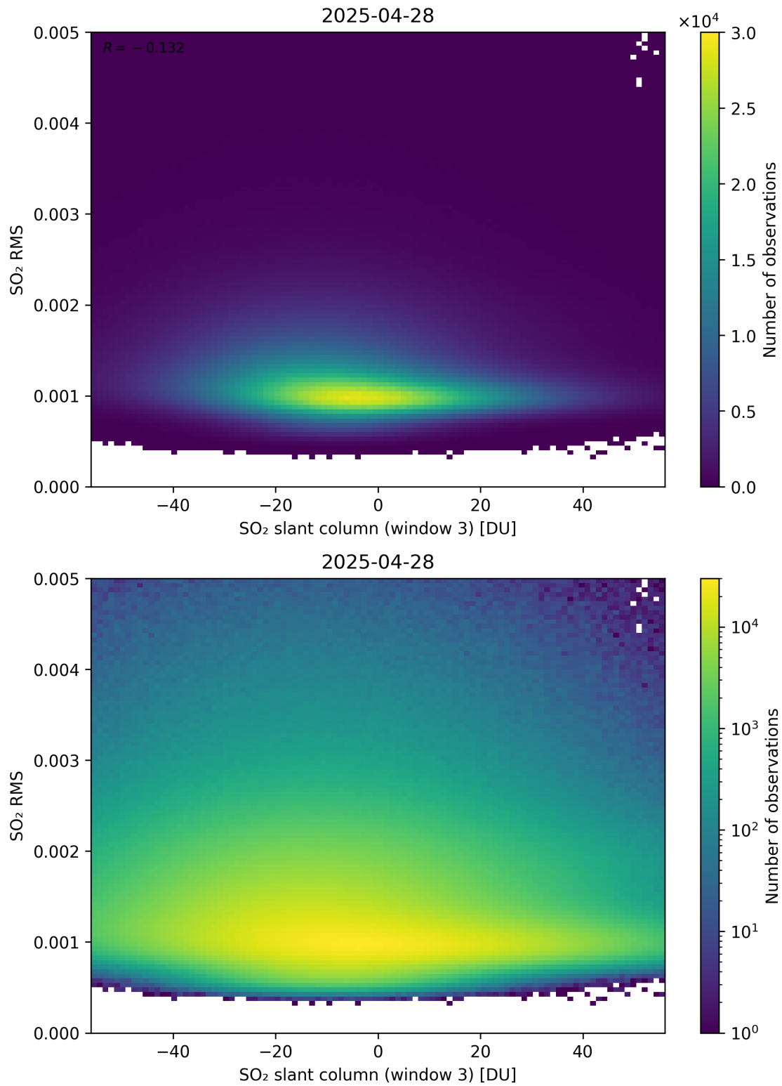
Figure 306: Scatter density plot of “SO 2 slant column (window 3)” against “SO 2 RMS” for 2025-04-27 to 2025-04-29.
