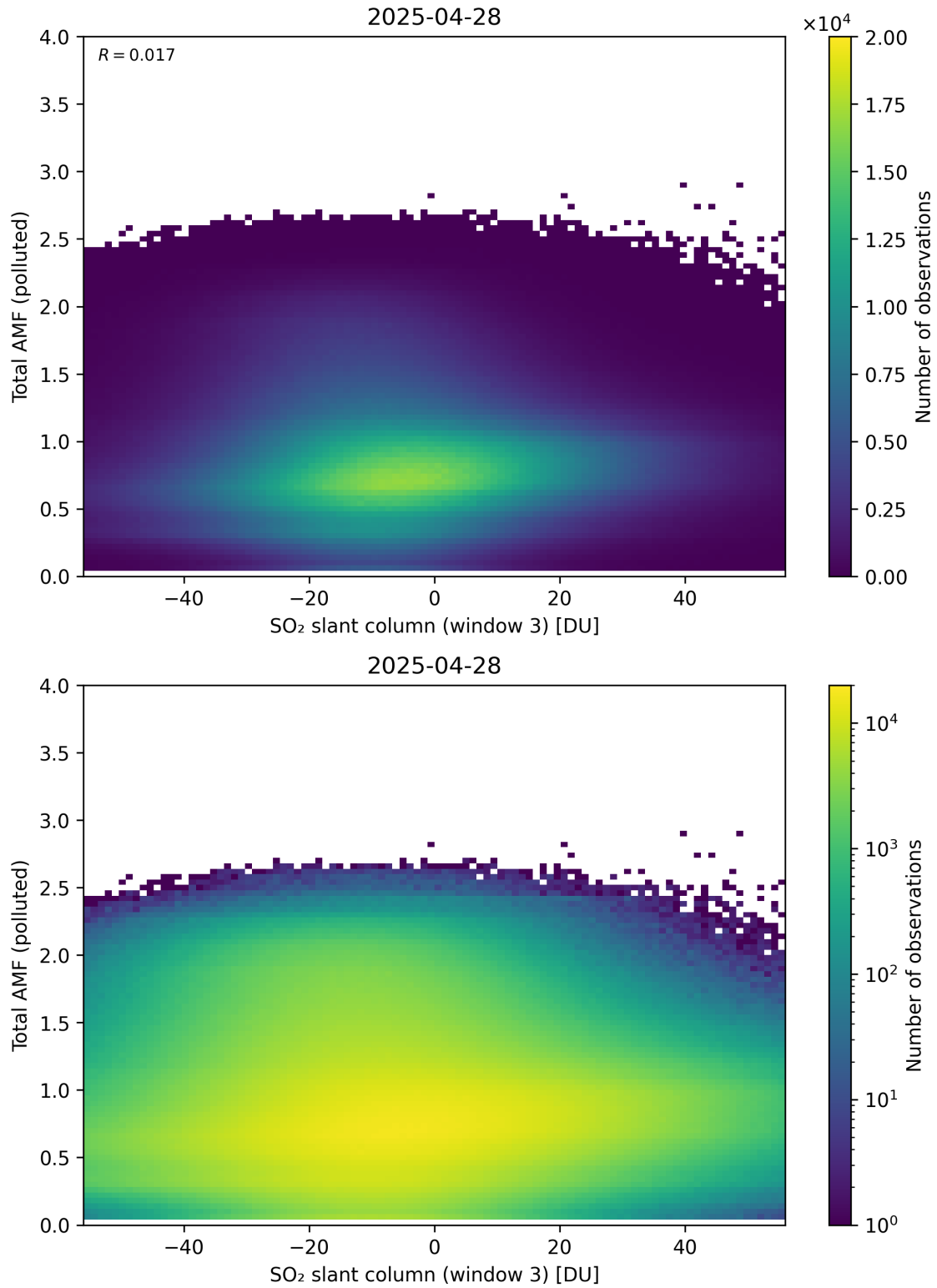
Figure 318: Scatter density plot of “SO 2 slant column (window 3)” against “Total AMF (polluted)” for 2025-04-27 to 2025-04-29.
