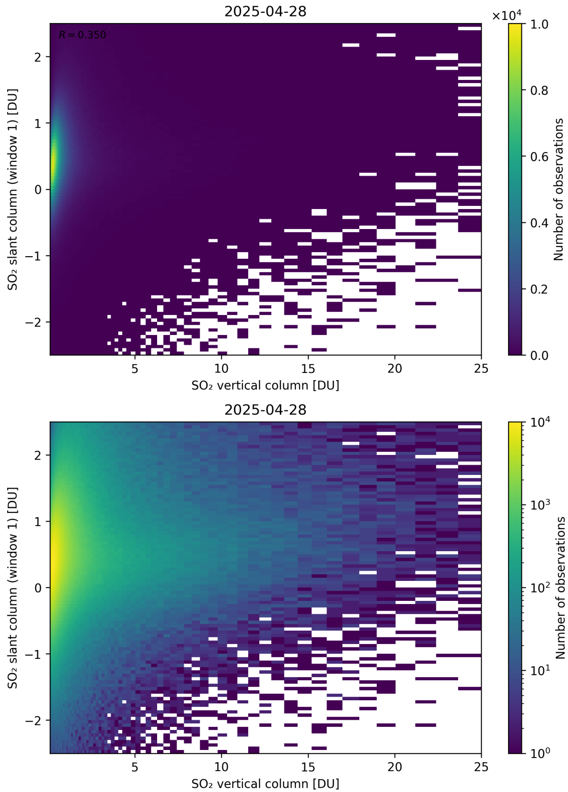
Figure 354: Scatter density plot of “SO 2 vertical column” against “SO 2 slant column (window 1)” for 2025-04-27 to 2025-04-29.
