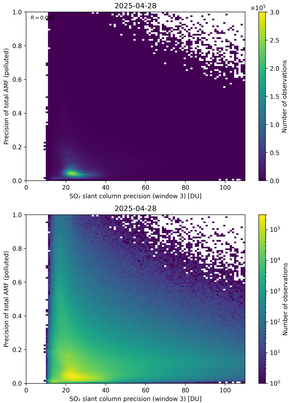
Figure 314: Scatter density plot of “SO 2 slant column precision (window 3)” against “Precision of total AMF (polluted)” for 2025-04-27 to 2025-04-29.
