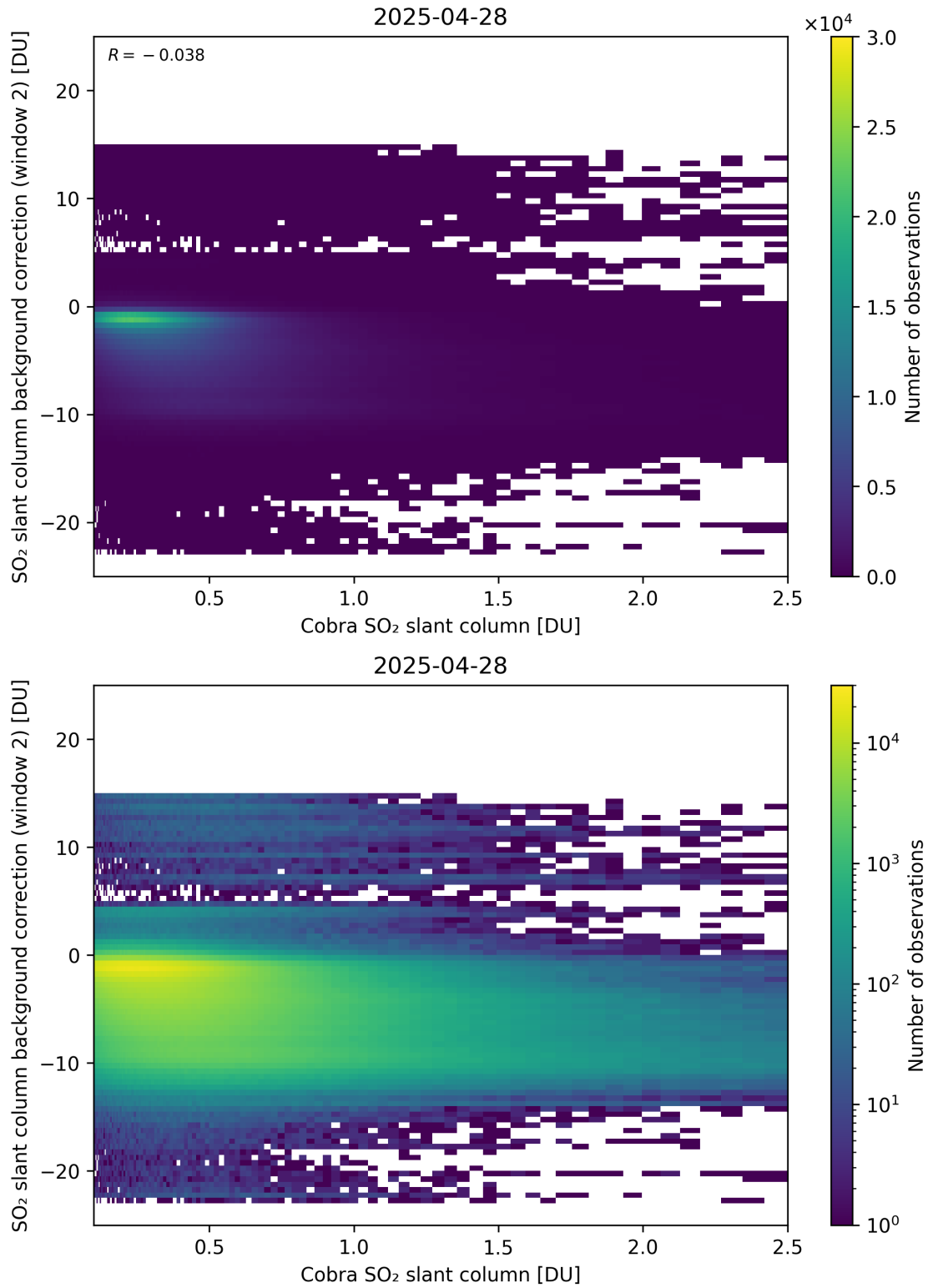
Figure 194: Scatter density plot of “Cobra SO 2 slant column” against “SO 2 slant column background correction (window 2)” for 2025-04-27 to 2025-04-29.
