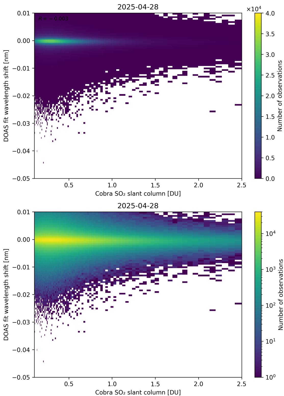
Figure 196: Scatter density plot of “Cobra SO 2 slant column” against “DOAS fit wavelength shift” for 2025-04-27 to 2025-04-29.
