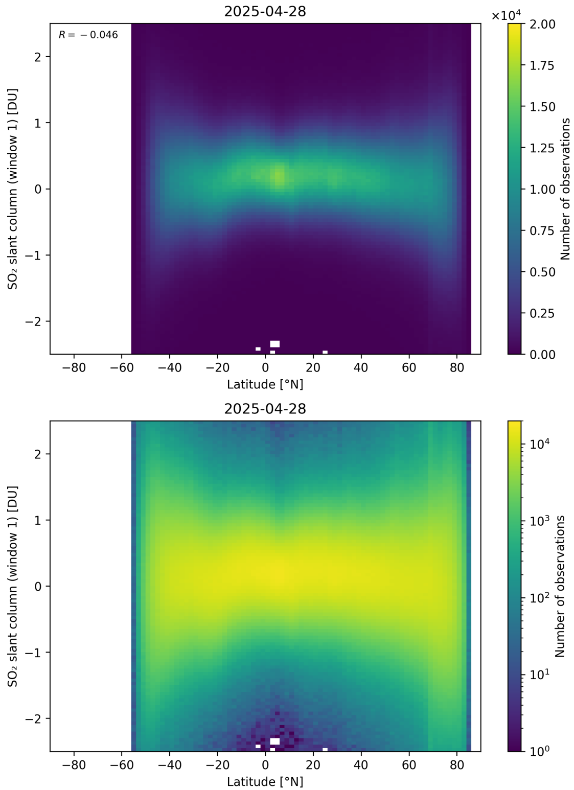
Figure 162: Scatter density plot of “Latitude” against “SO 2 slant column (window 1)” for 2025-04-27 to 2025-04-29.
