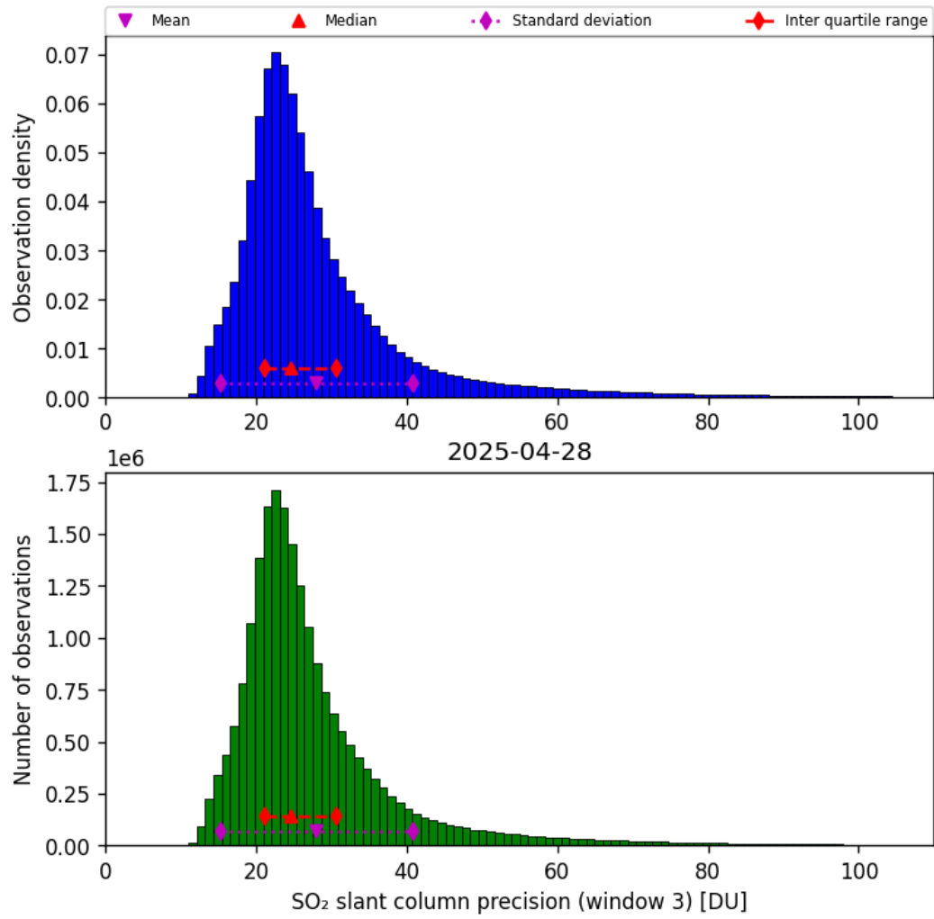
Figure 72: Histogram of “SO 2 slant column precision (window 3)” for 2025-04-27 to 2025-04-29
