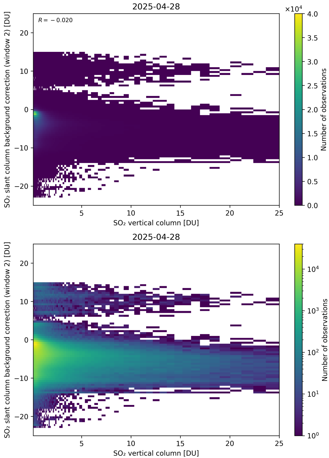
Figure 324: Scatter density plot of “SO 2 vertical column” against “SO 2 slant column background correction (window 2)” for 2025-04-27 to 2025-04-29.
