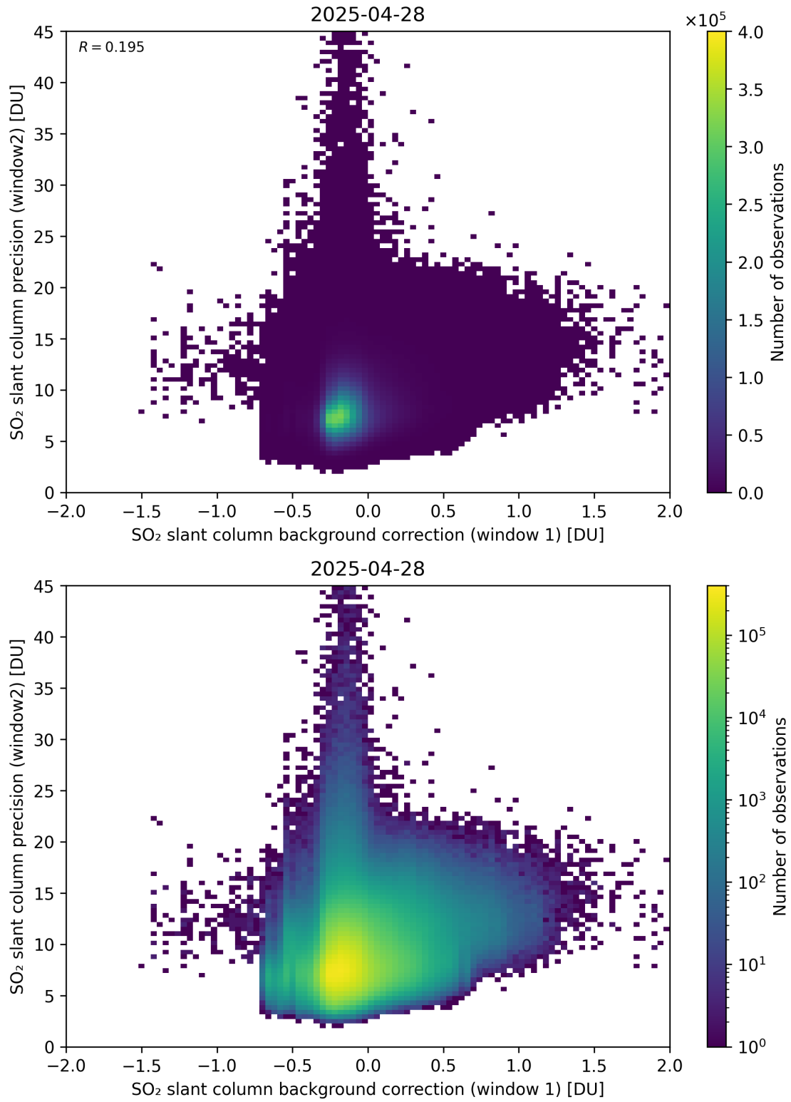
Figure 117: Scatter density plot of “SO 2 slant column background correction (window 1)” against “SO 2 slant column precision (window2)” for 2025-04-27 to 2025-04-29.
