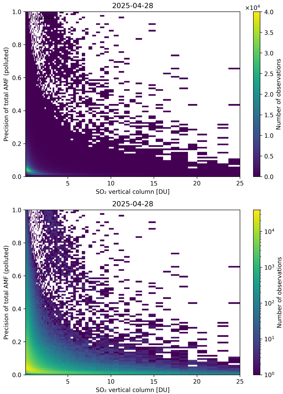
Figure 360: Scatter density plot of “SO 2 vertical column” against “Precision of total AMF (polluted)” for 2025-04-27 to 2025-04-29.
