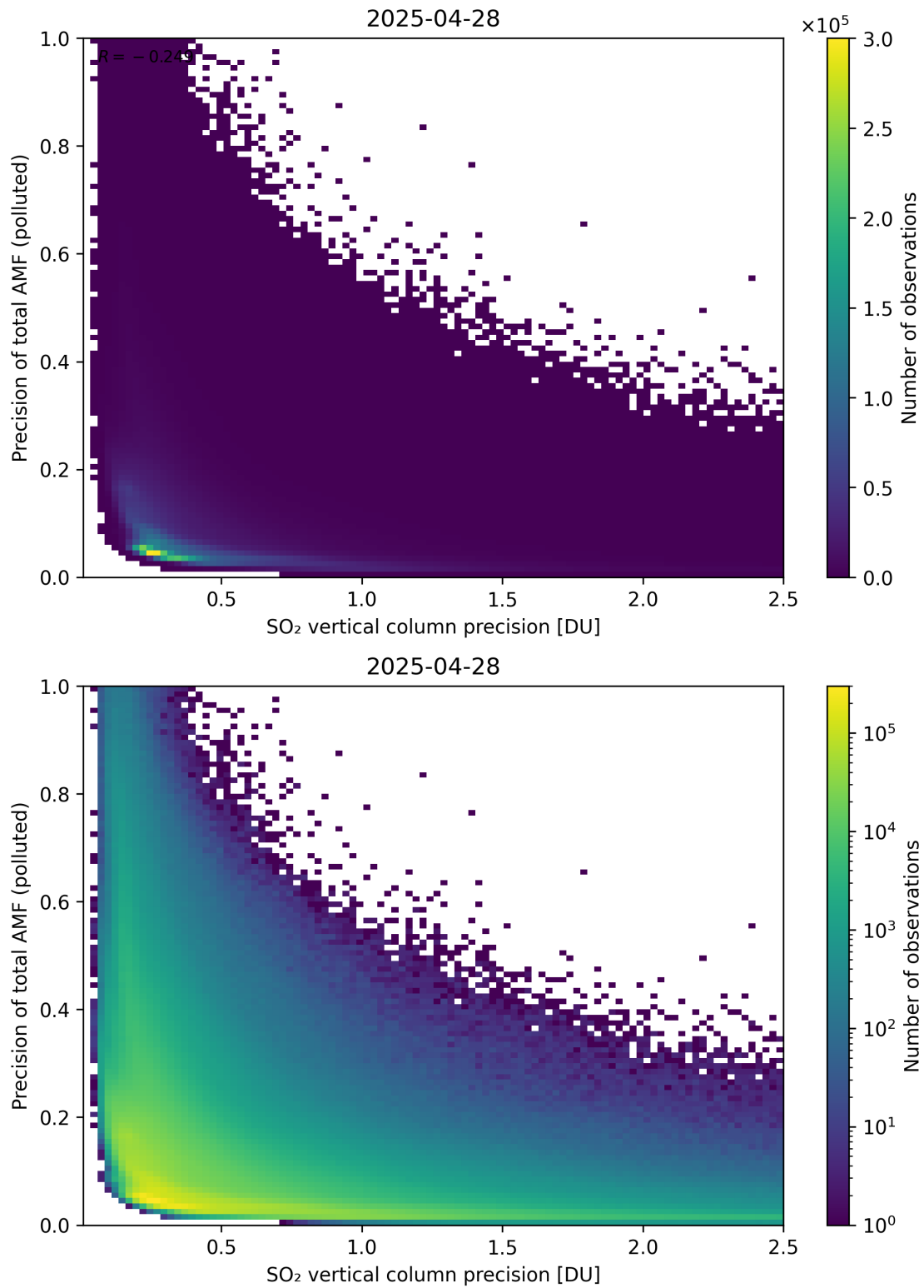
Figure 347: Scatter density plot of “SO 2 vertical column precision” against “Precision of total AMF (polluted)” for 2025-04-27 to 2025-04-29.
