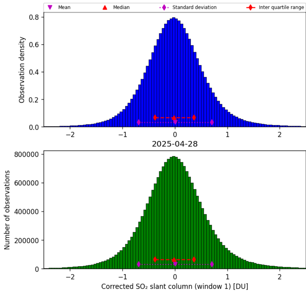
Figure 65: Histogram of “Corrected SO 2 slant column (window 1)” for 2025-04-27 to 2025-04-29
