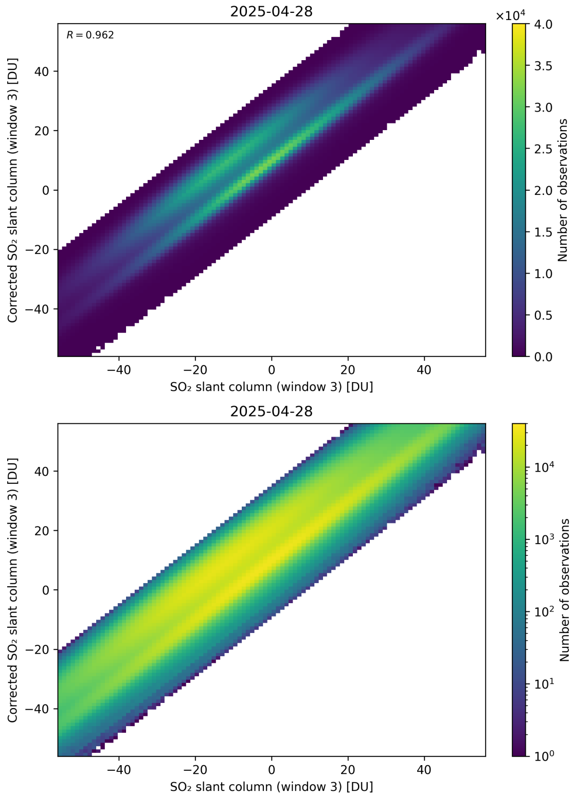
Figure 316: Scatter density plot of “SO 2 slant column (window 3)” against “Corrected SO 2 slant column (window 3)” for 2025-04-27 to 2025-04-29.
