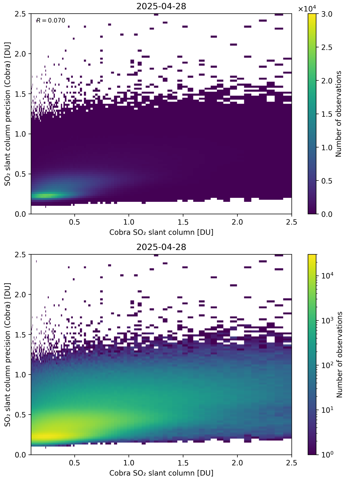
Figure 216: Scatter density plot of “Cobra SO 2 slant column” against “SO 2 slant column precision (Cobra)” for 2025-04-27 to 2025-04-29.
