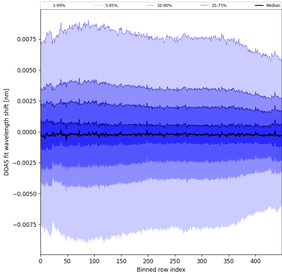
Figure 102: Along track statistics of “DOAS fit wavelength shift” for 2025-04-27 to 2025-04-29
