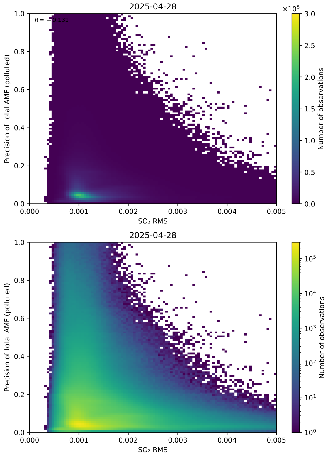
Figure 149: Scatter density plot of “SO 2 RMS” against “Precision of total AMF (polluted)” for 2025-04-27 to 2025-04-29.
