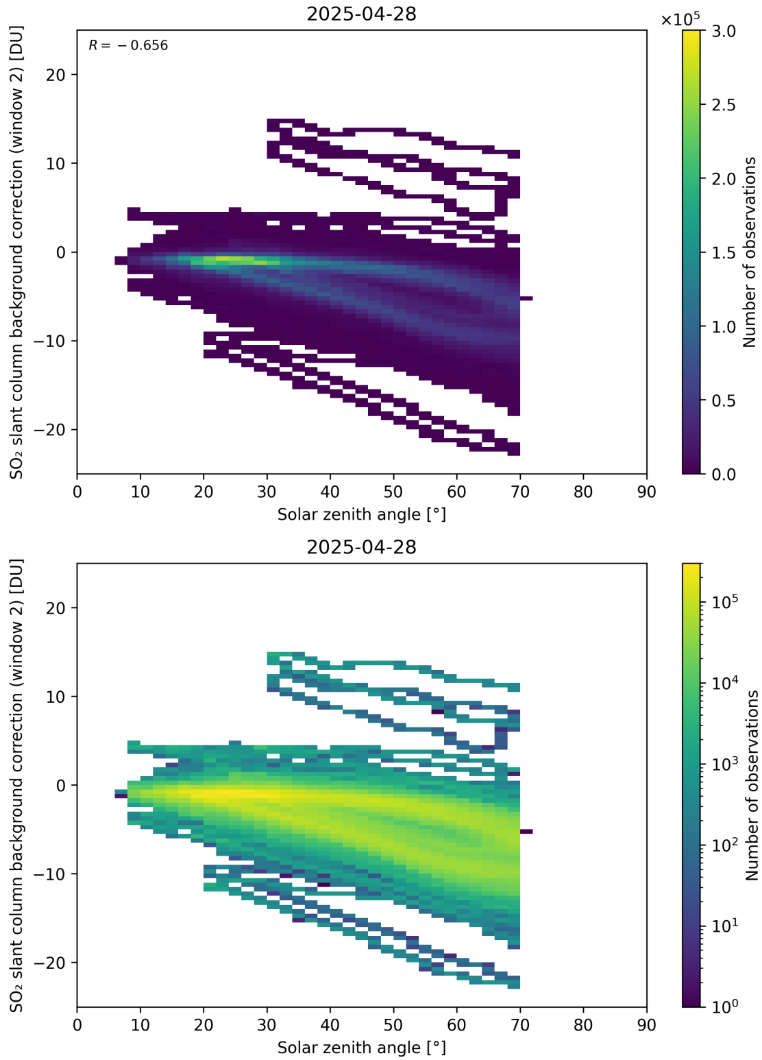
Figure 172: Scatter density plot of “Solar zenith angle” against “SO 2 slant column background correction (window 2)” for 2025-04-27 to 2025-04-29.
