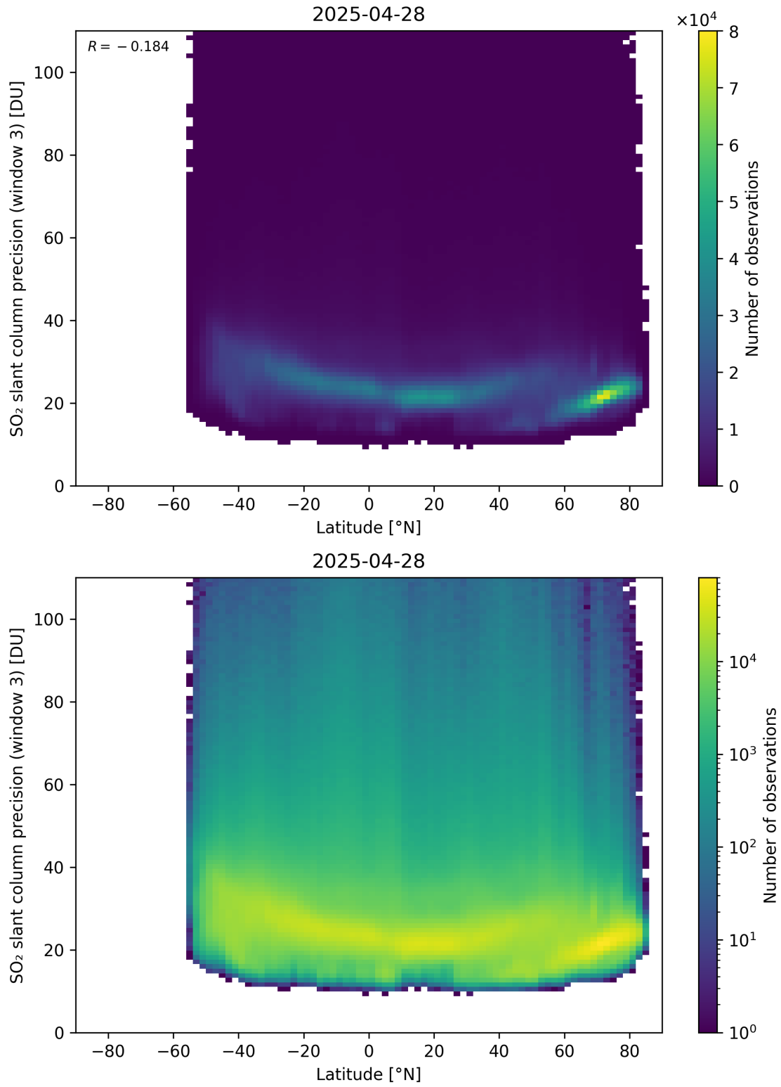
Figure 166: Scatter density plot of “Latitude” against “SO 2 slant column precision (window 3)” for 2025-04-27 to 2025-04-29.
