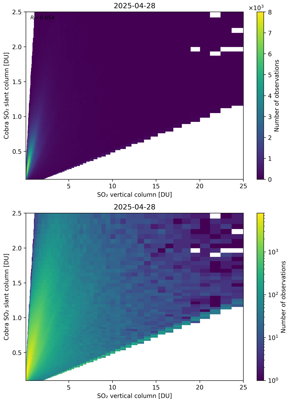
Figure 349: Scatter density plot of “SO 2 vertical column” against “Cobra SO 2 slant column” for 2025-04-27 to 2025-04-29.
