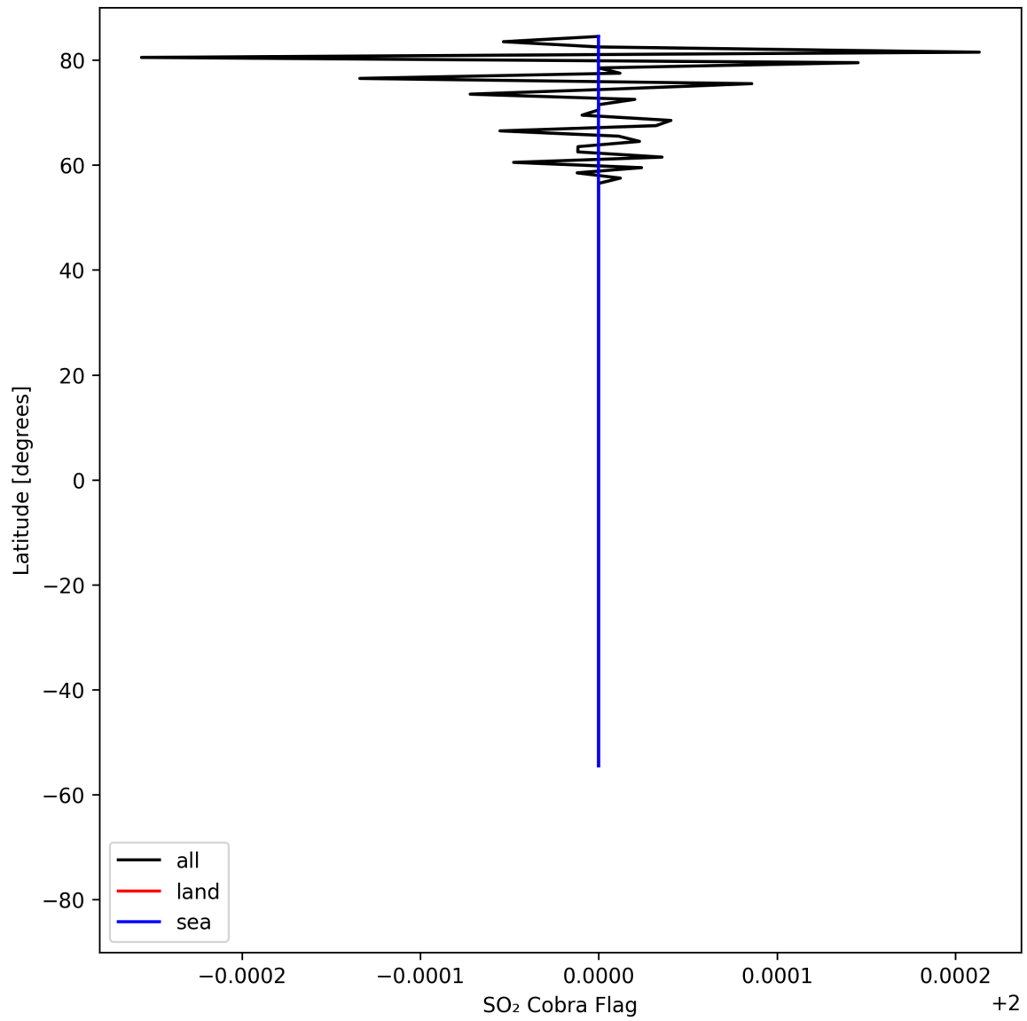
Figure 49: Zonal average of “SO 2 Cobra Flag” for 2025-04-27 to 2025-04-29.
