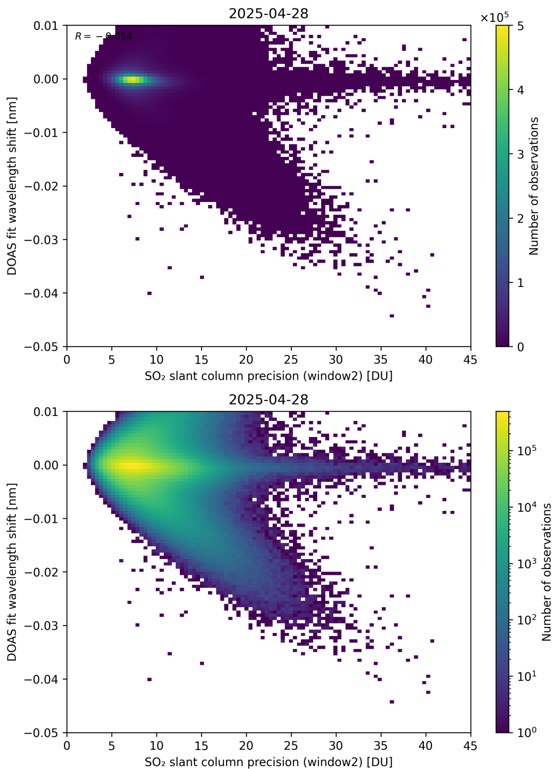
Figure 293: Scatter density plot of “SO 2 slant column precision (window2)” against “DOAS fit wavelength shift” for 2025-04-27 to 2025-04-29.
