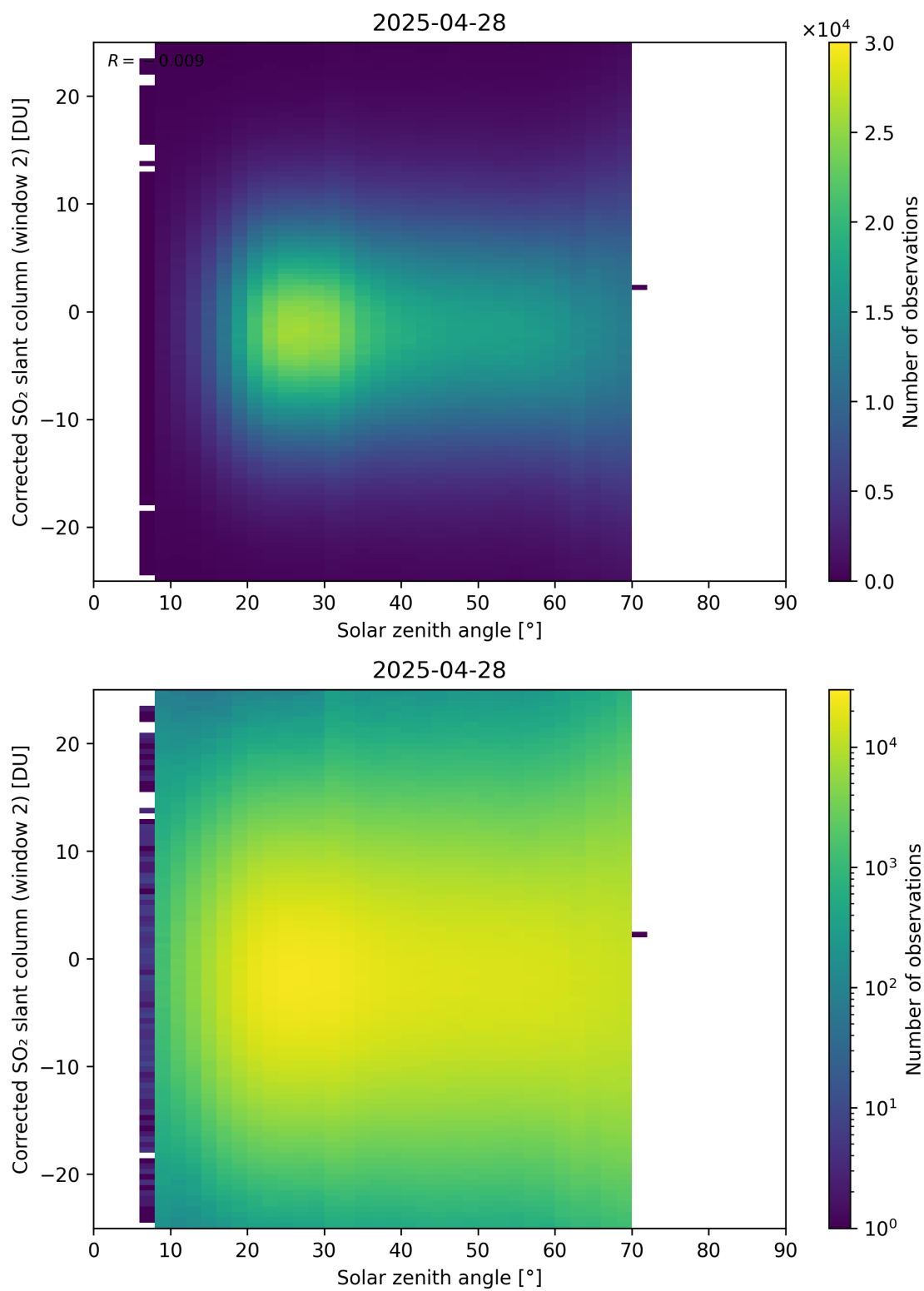
Figure 182: Scatter density plot of “Solar zenith angle” against “Corrected SO 2 slant column (window 2)” for 2025-04-27 to 2025-04-29.
