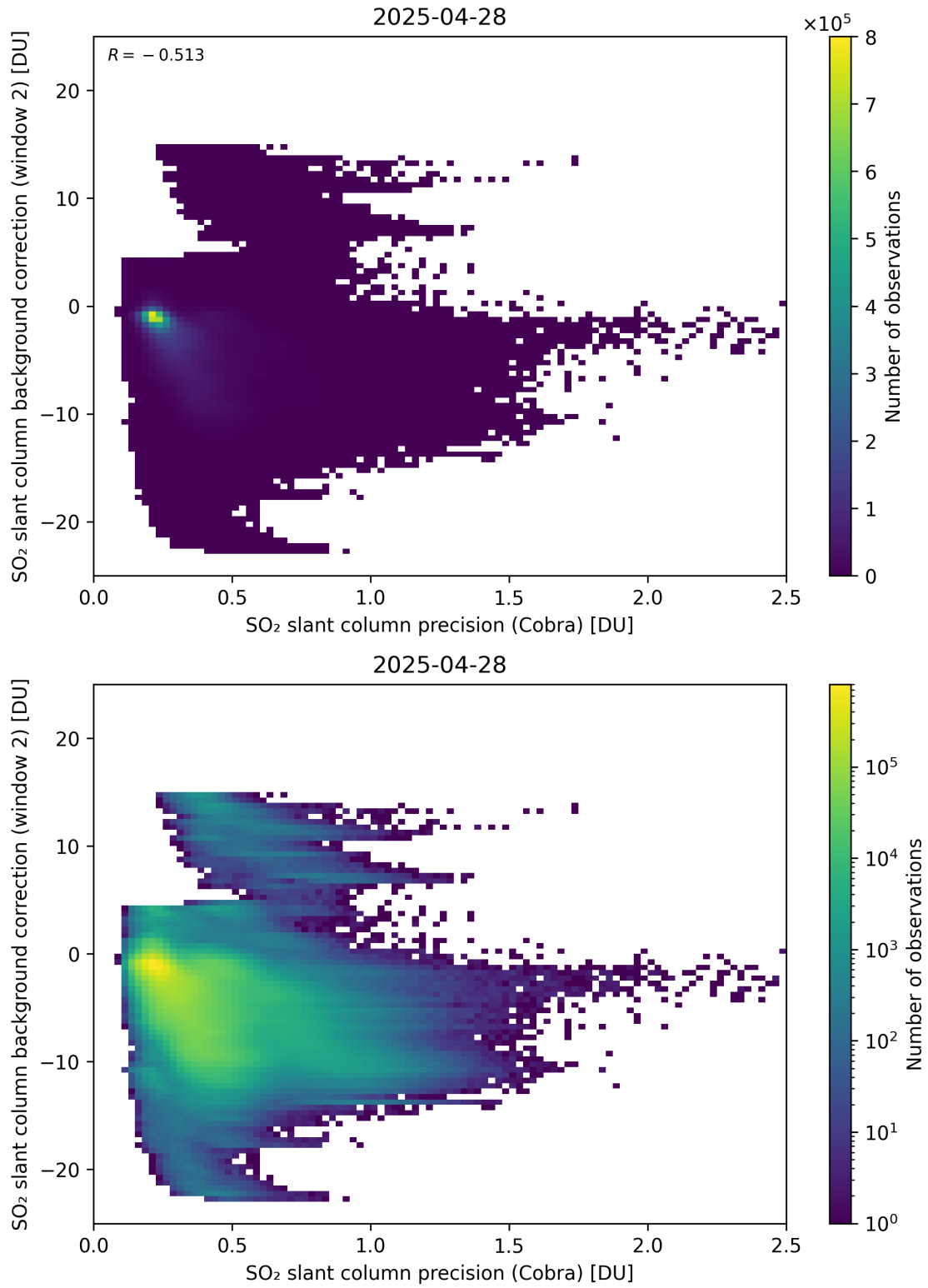
Figure 200: Scatter density plot of “SO 2 slant column precision (Cobra)” against “SO 2 slant column background correction (window 2)” for 2025-04-27 to 2025-04-29.
