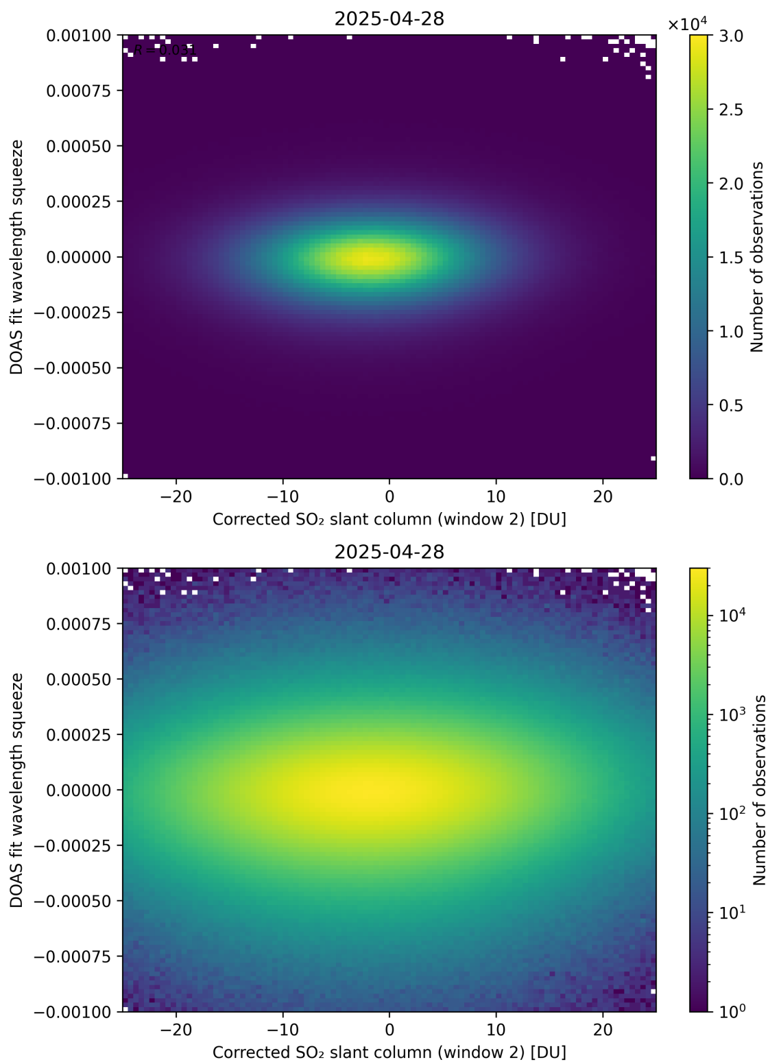
Figure 247: Scatter density plot of “Corrected SO 2 slant column (window 2)” against “DOAS fit wavelength squeeze” for 2025-04-27 to 2025-04-29.
