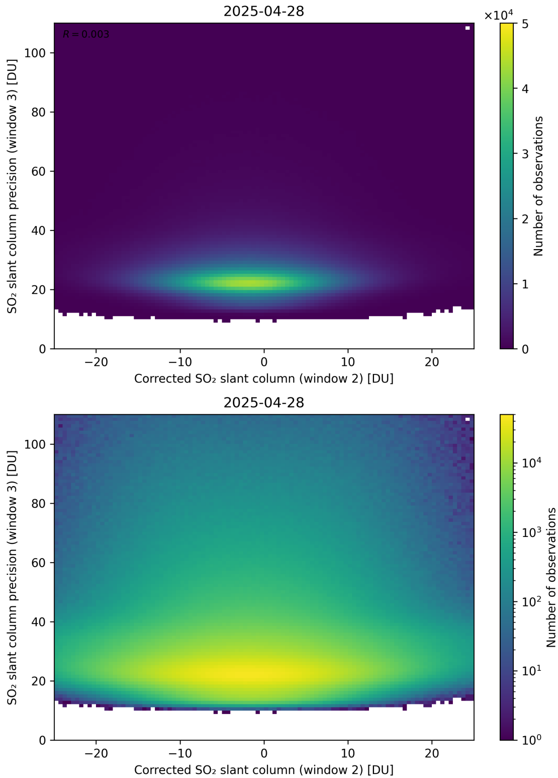
Figure 252: Scatter density plot of “Corrected SO 2 slant column (window 2)” against “SO 2 slant column precision (window 3)” for 2025-04-27 to 2025-04-29.
