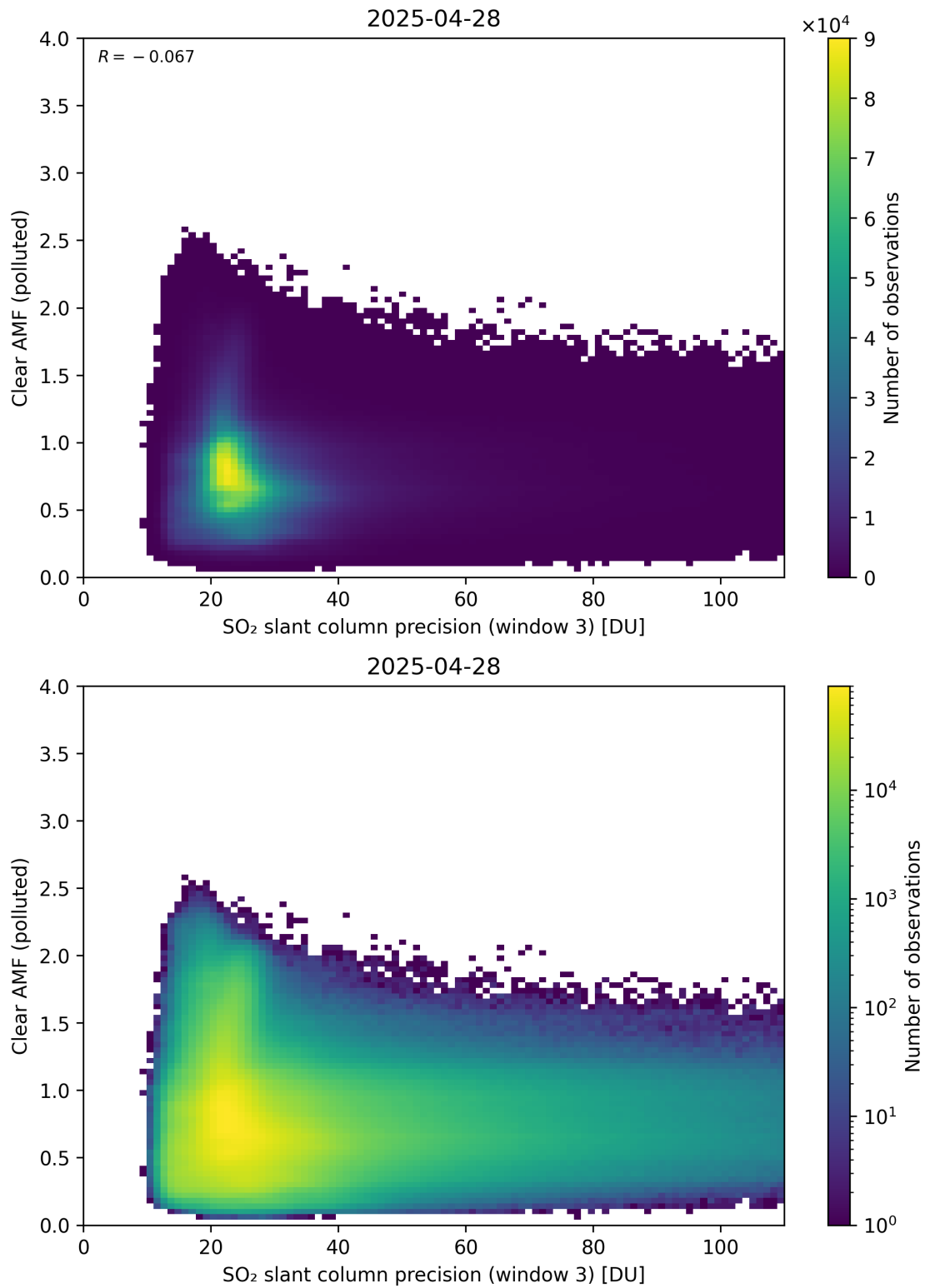
Figure 311: Scatter density plot of “SO 2 slant column precision (window 3)” against “Clear AMF (polluted)” for 2025-04-27 to 2025-04-29.
