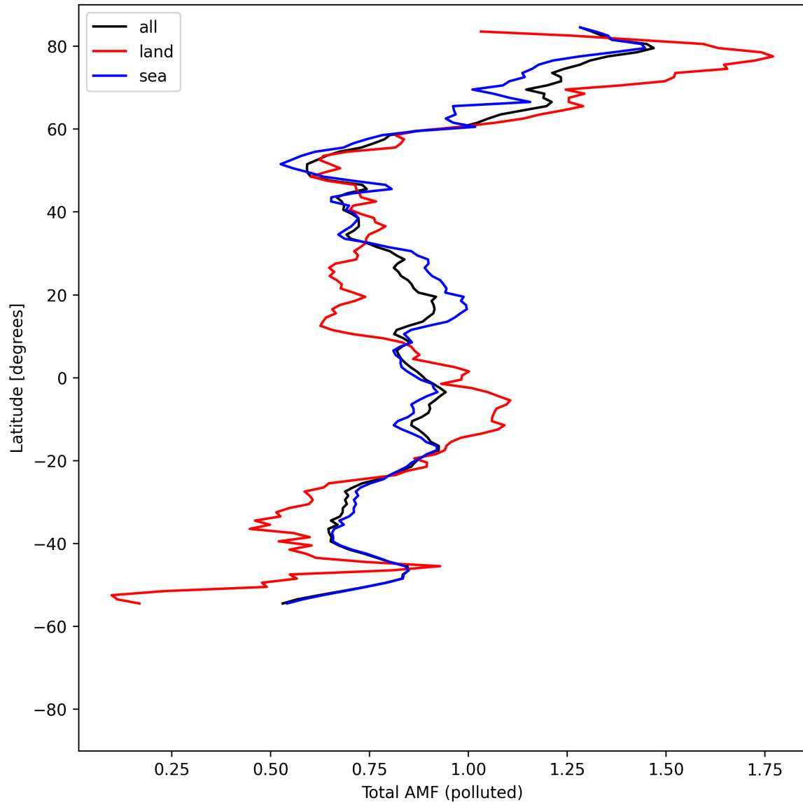
Figure 53: Zonal average of “Total AMF (polluted)” for 2025-04-27 to 2025-04-29.
