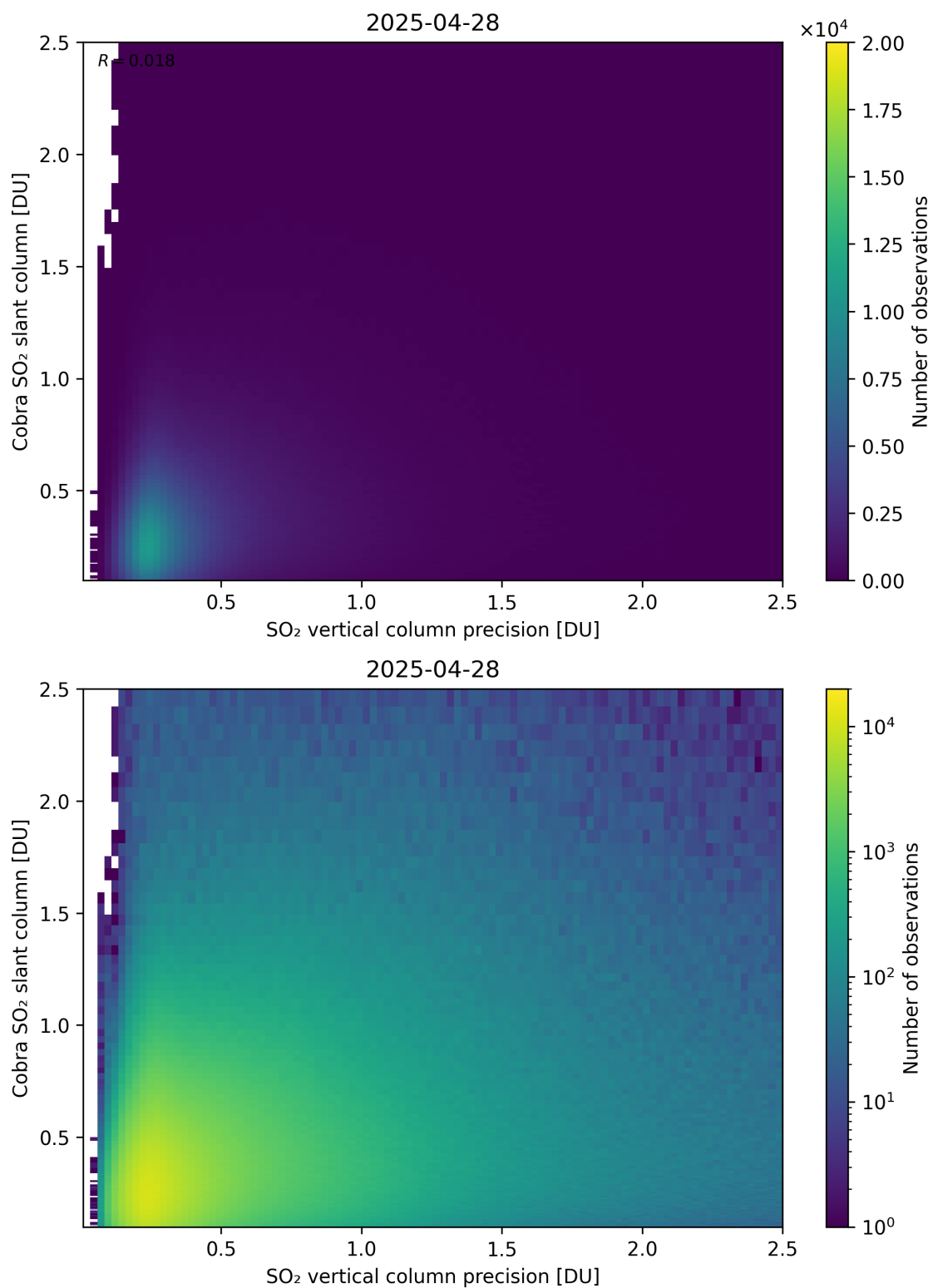
Figure 336: Scatter density plot of “SO 2 vertical column precision” against “Cobra SO 2 slant column” for 2025-04-27 to 2025-04-29.
