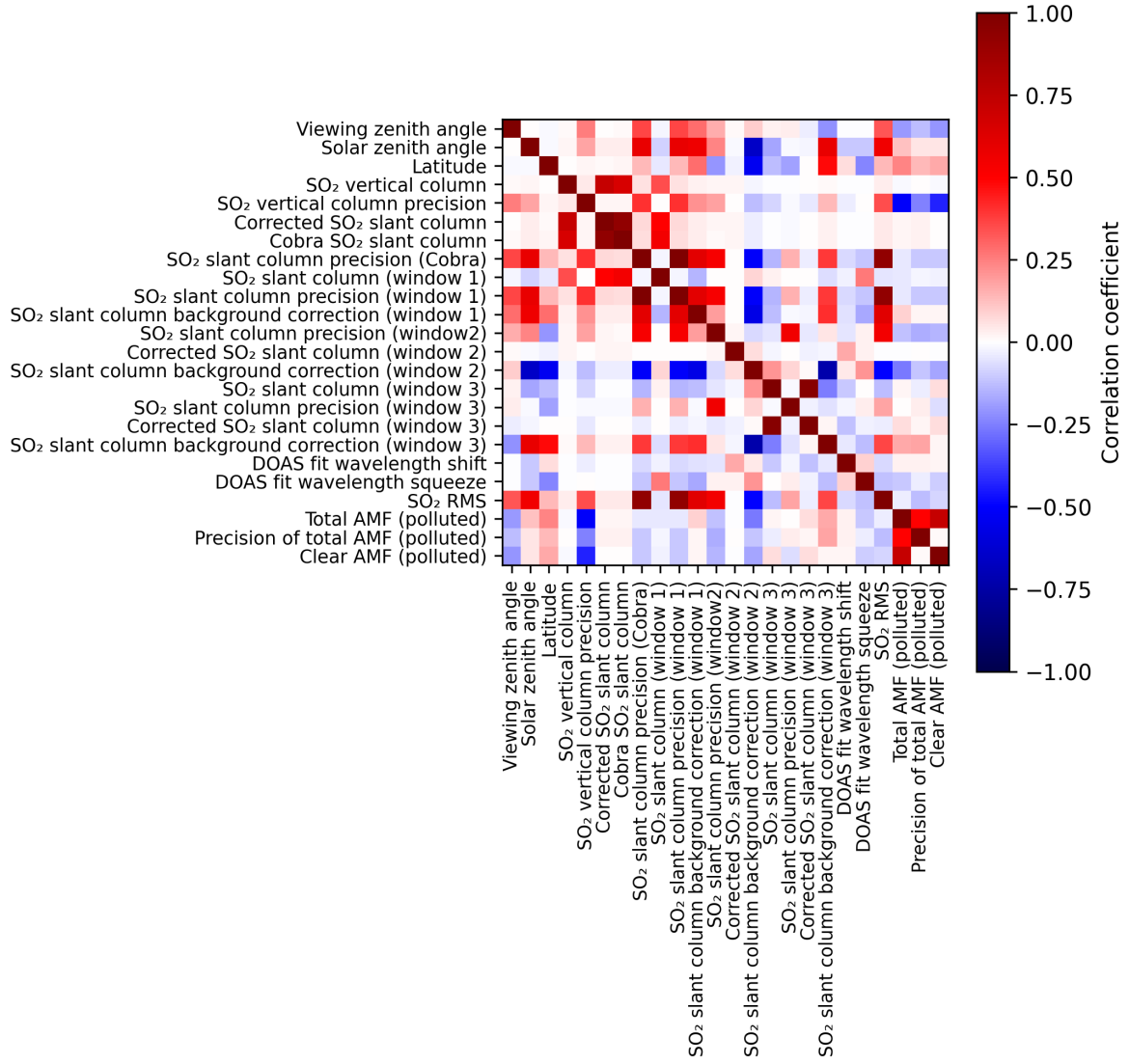
Figure 2: Map of correlation matrix for 2025-04-27 to 2025-04-29.
