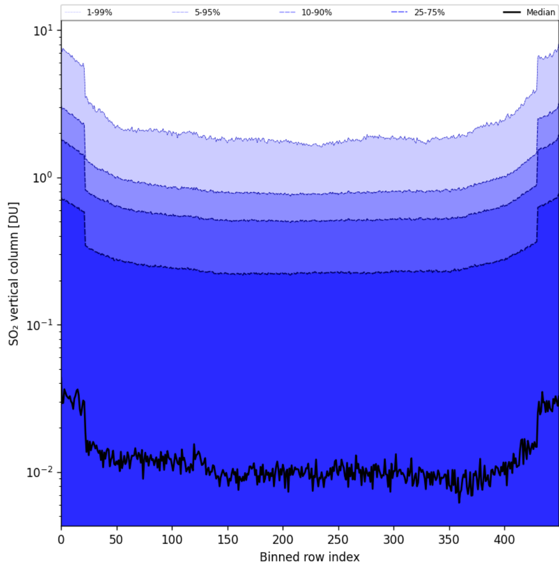
Figure 84: Along track statistics of “SO 2 vertical column” for 2025-04-27 to 2025-04-29
