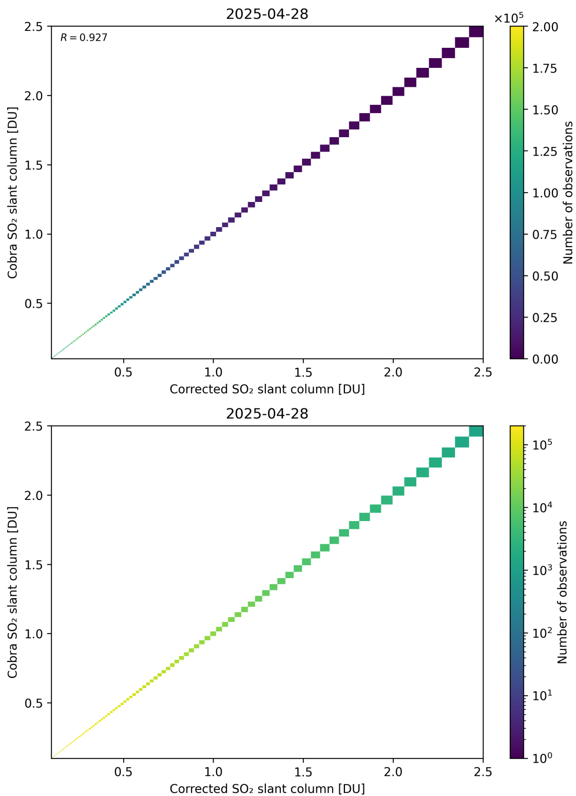
Figure 233: Scatter density plot of “Corrected SO 2 slant column” against “Cobra SO 2 slant column” for 2025-04-27 to 2025-04-29.
