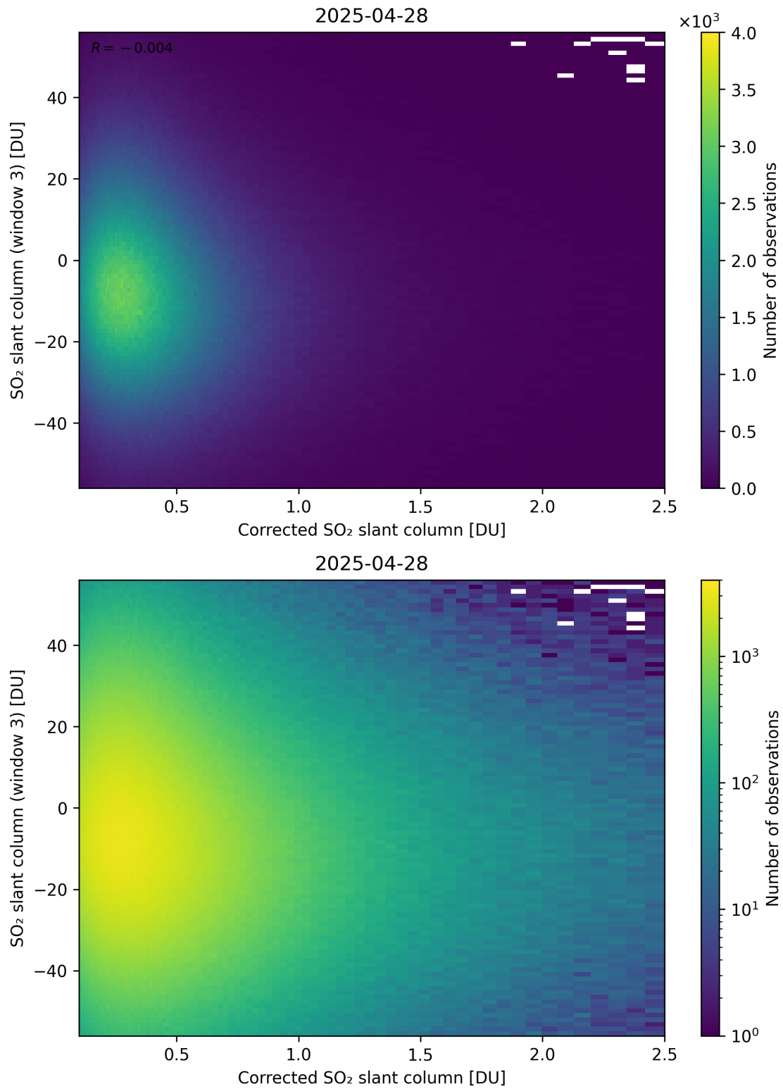
Figure 240: Scatter density plot of “Corrected SO 2 slant column” against “SO 2 slant column (window 3)” for 2025-04-27 to 2025-04-29.
