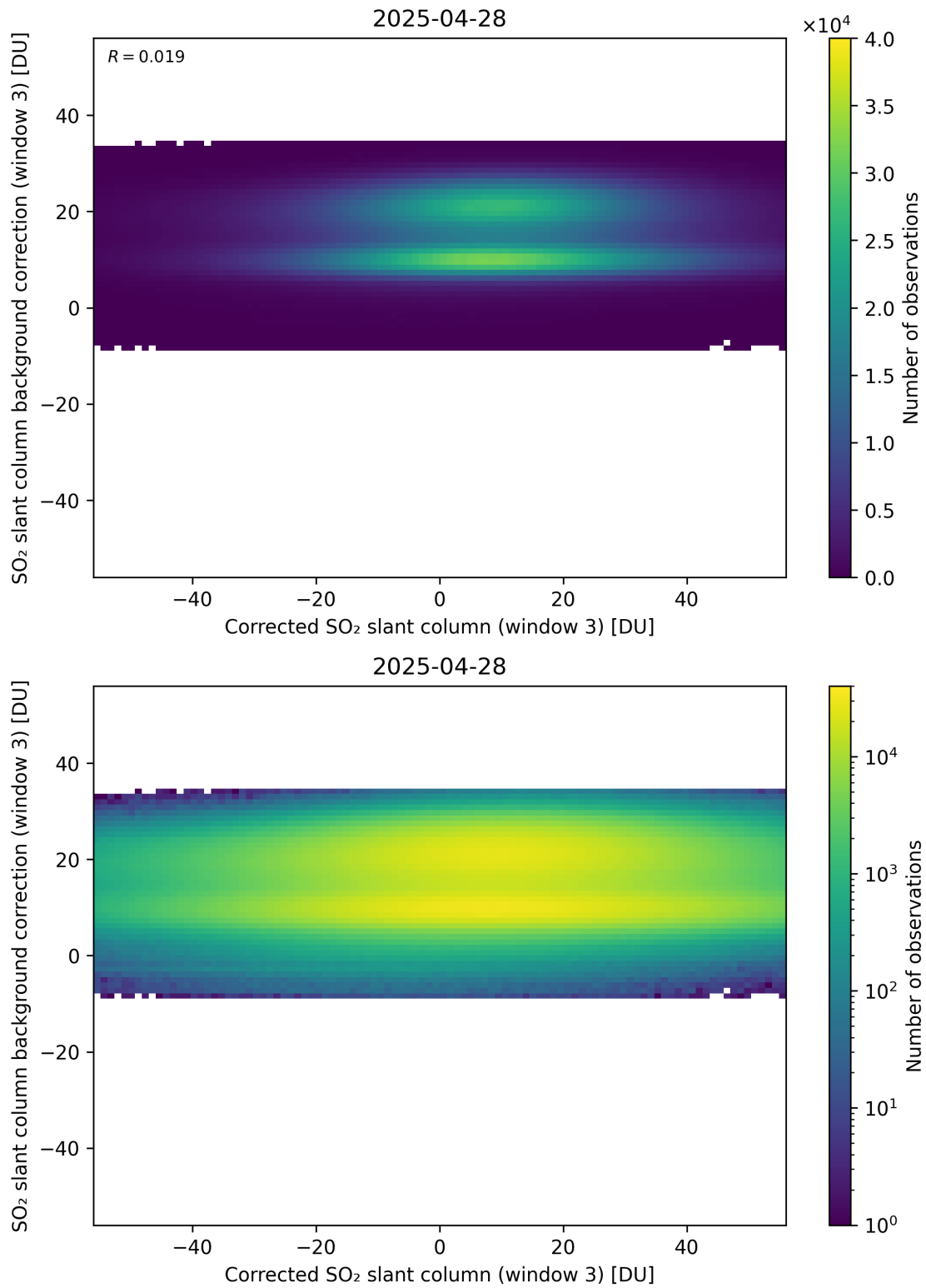
Figure 255: Scatter density plot of “Corrected SO 2 slant column (window 3)” against “SO 2 slant column background correction (window 3)” for 2025-04-27 to 2025-04-29.
