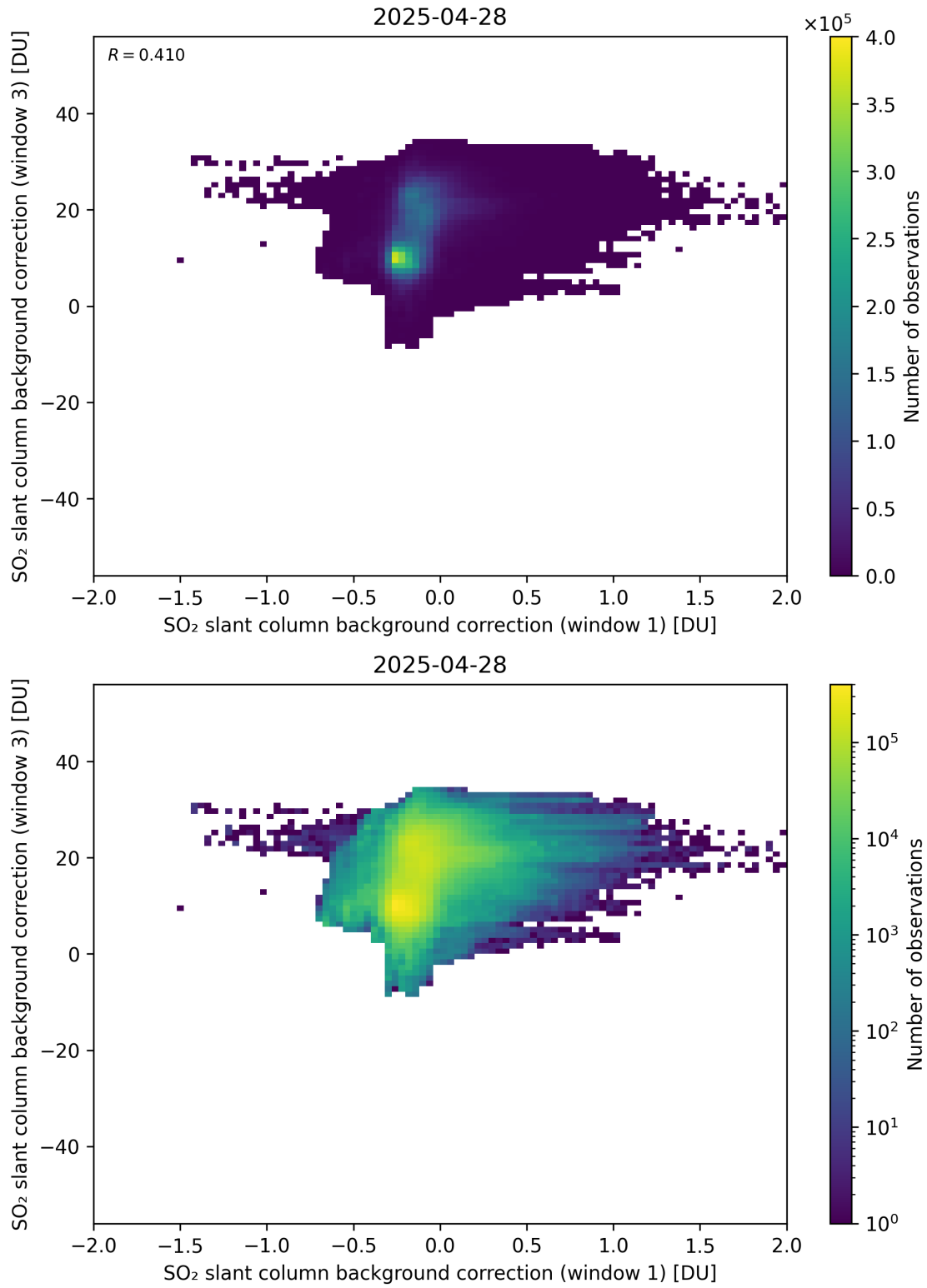
Figure 110: Scatter density plot of “SO 2 slant column background correction (window 1)” against “SO 2 slant column background correction (window 3)” for 2025-04-27 to 2025-04-29.
