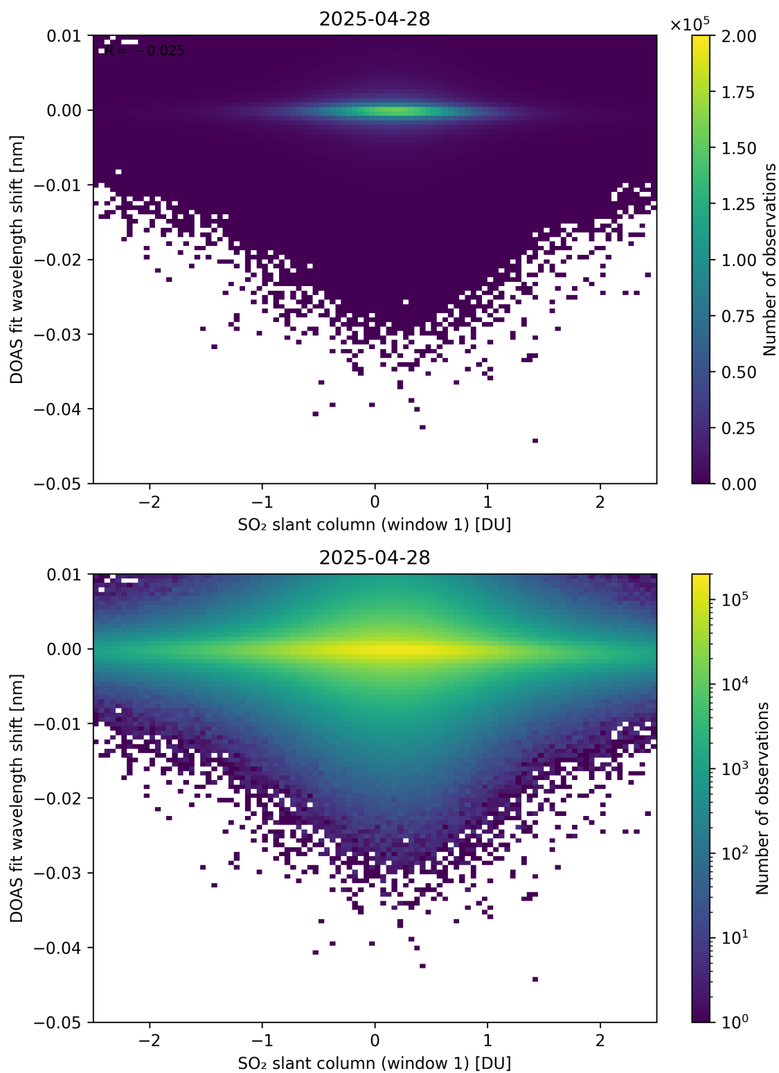
Figure 265: Scatter density plot of “SO 2 slant column (window 1)” against “DOAS fit wavelength shift” for 2025-04-27 to 2025-04-29.
