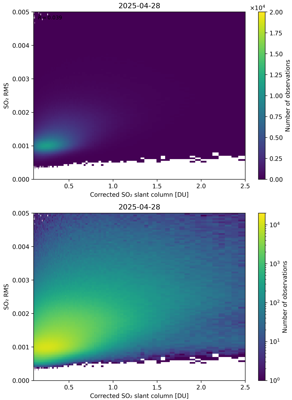
Figure 231: Scatter density plot of “Corrected SO 2 slant column” against “SO 2 RMS” for 2025-04-27 to 2025-04-29.
