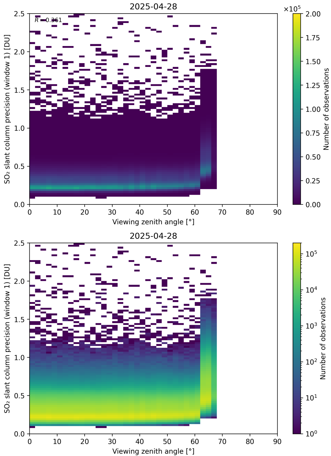
Figure 377: Scatter density plot of “Viewing zenith angle” against “SO 2 slant column precision (window 1)” for 2025-04-27 to 2025-04-29.
