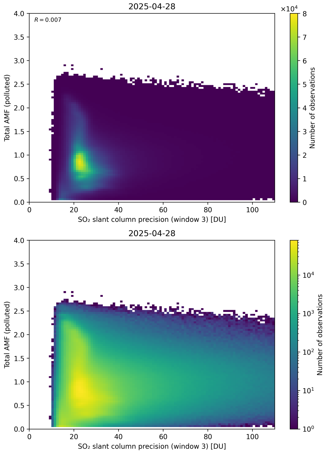
Figure 313: Scatter density plot of “SO 2 slant column precision (window 3)” against “Total AMF (polluted)” for 2025-04-27 to 2025-04-29.
