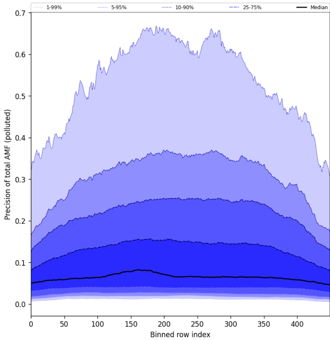
Figure 106: Along track statistics of “Precision of total AMF (polluted)” for 2025-04-27 to 2025-04-29
