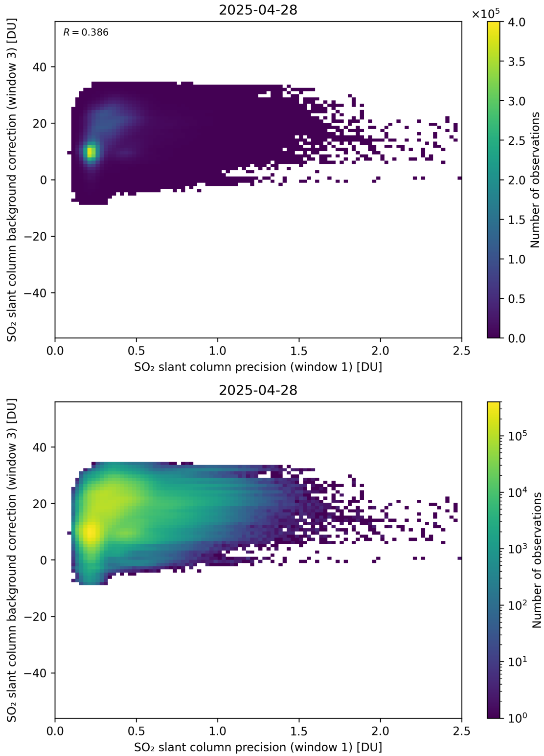
Figure 270: Scatter density plot of “SO 2 slant column precision (window 1)” against “SO 2 slant column background correction (window 3)” for 2025-04-27 to 2025-04-29.
