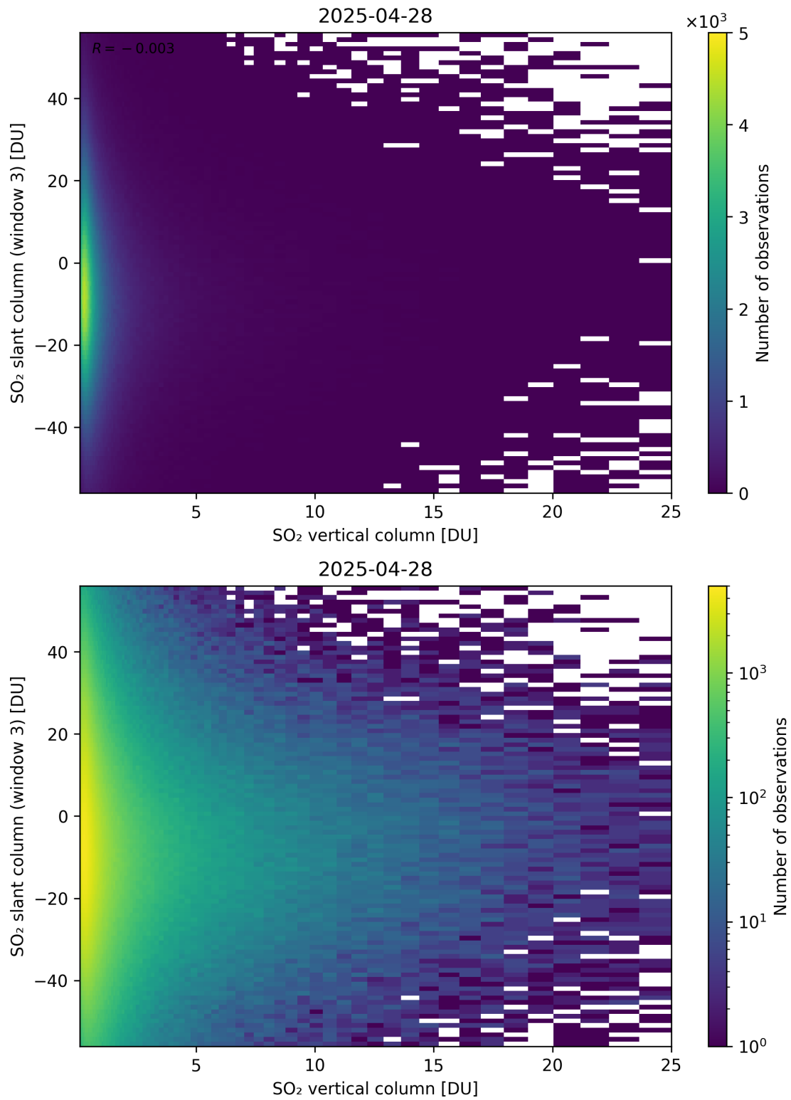
Figure 357: Scatter density plot of “SO 2 vertical column” against “SO 2 slant column (window 3)” for 2025-04-27 to 2025-04-29.
