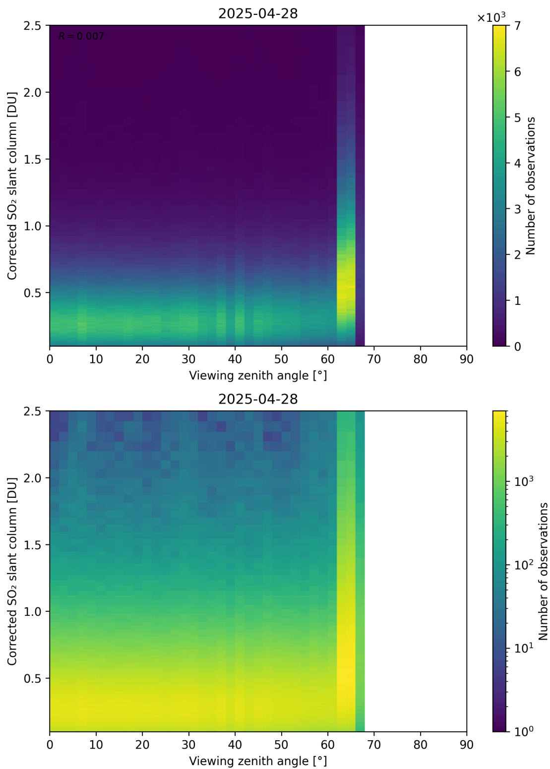
Figure 373: Scatter density plot of “Viewing zenith angle” against “Corrected SO 2 slant column” for 2025-04-27 to 2025-04-29.
