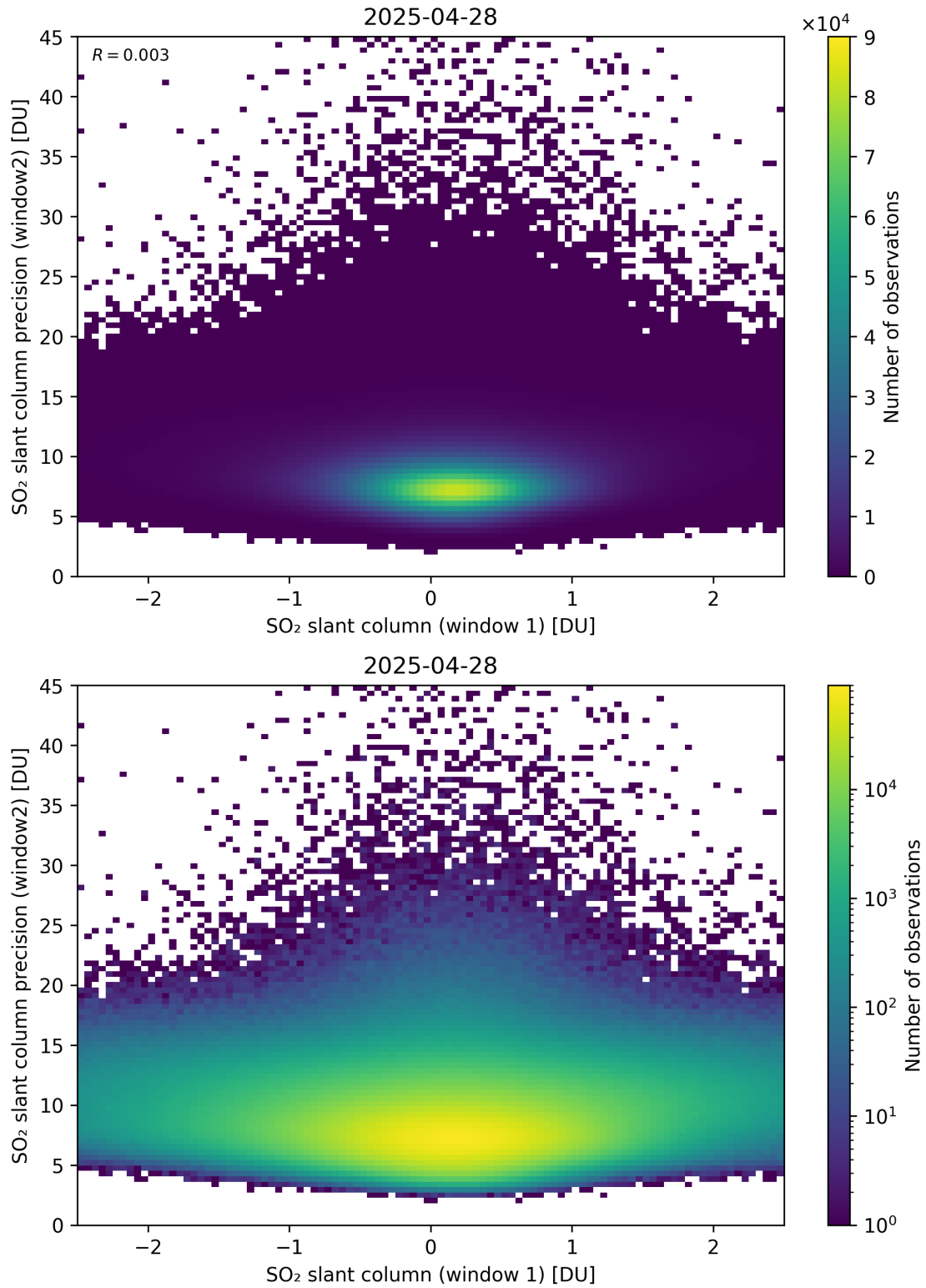
Figure 286: Scatter density plot of “SO 2 slant column (window 1)” against “SO 2 slant column precision (window2)” for 2025-04-27 to 2025-04-29.
