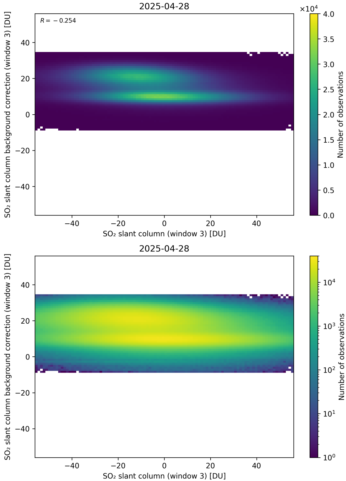
Figure 303: Scatter density plot of “SO 2 slant column (window 3)” against “SO 2 slant column background correction (window 3)” for 2025-04-27 to 2025-04-29.
