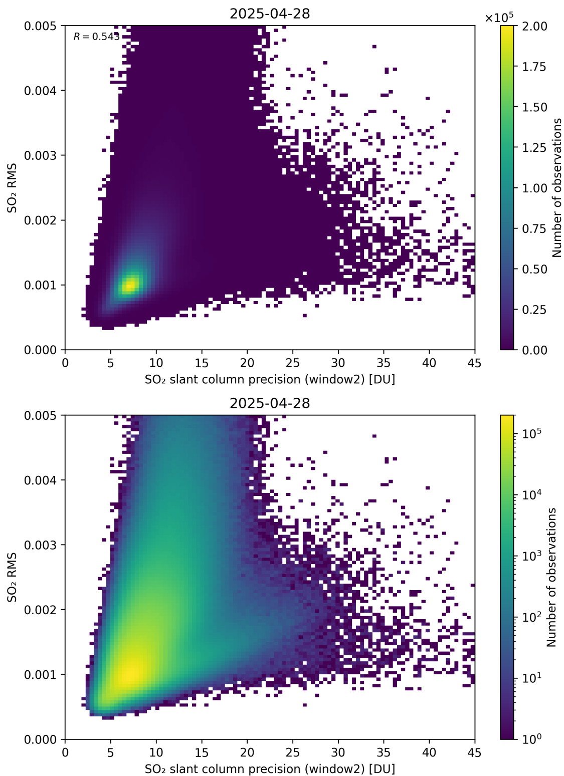
Figure 295: Scatter density plot of “SO 2 slant column precision (window2)” against “SO 2 RMS” for 2025-04-27 to 2025-04-29.
