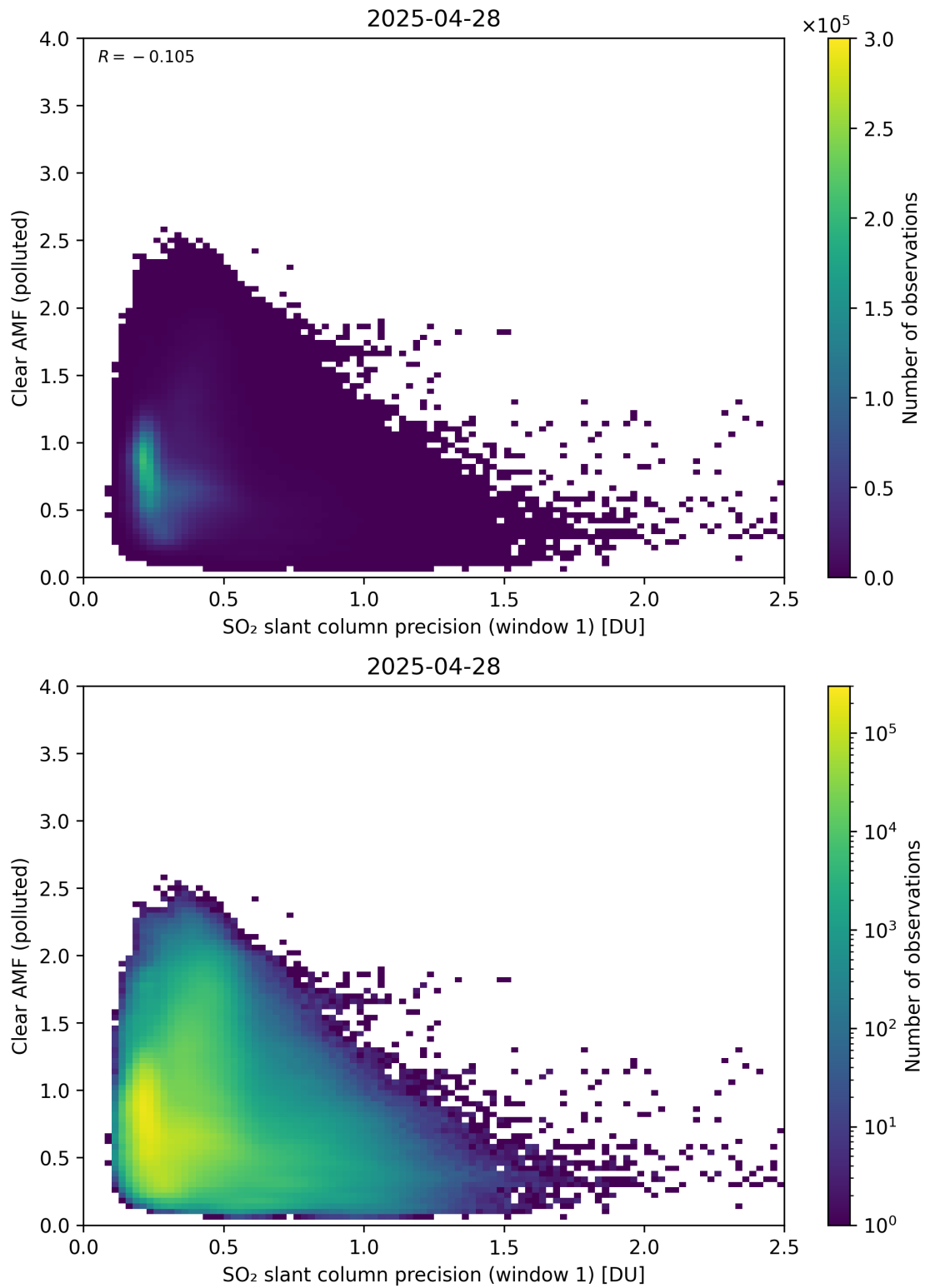
Figure 274: Scatter density plot of “SO 2 slant column precision (window 1)” against “Clear AMF (polluted)” for 2025-04-27 to 2025-04-29.
