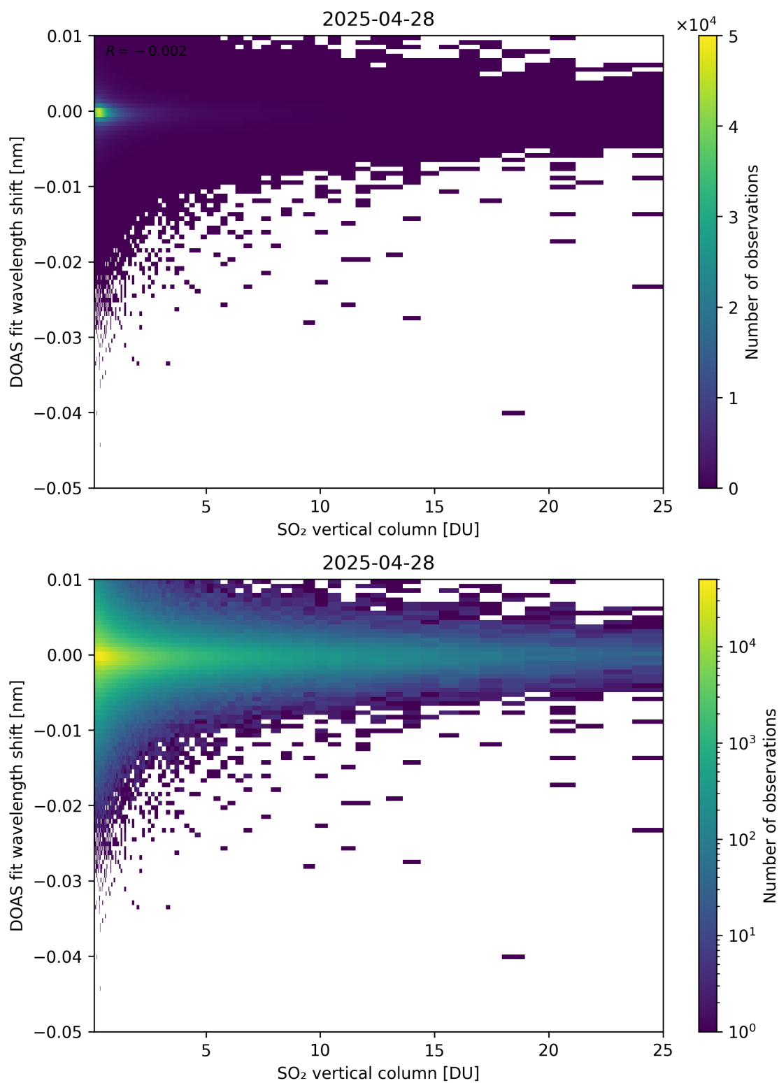
Figure 326: Scatter density plot of “SO 2 vertical column” against “DOAS fit wavelength shift” for 2025-04-27 to 2025-04-29.
