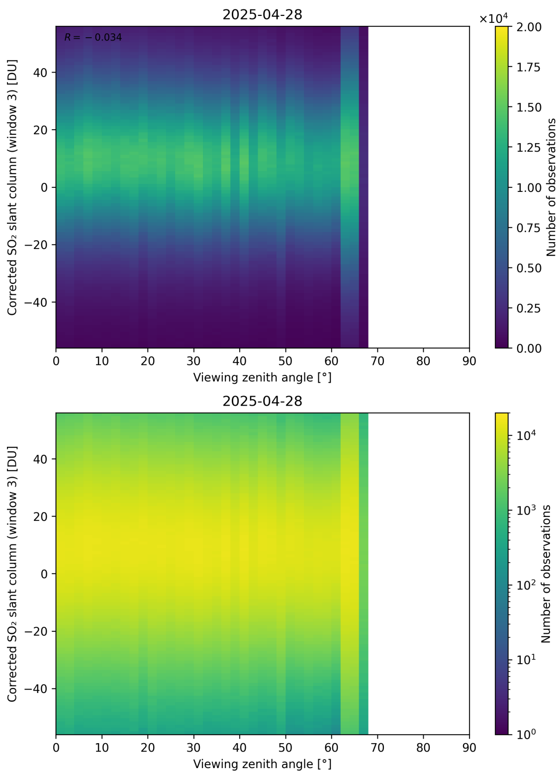
Figure 375: Scatter density plot of “Viewing zenith angle” against “Corrected SO 2 slant column (window 3)” for 2025-04-27 to 2025-04-29.
