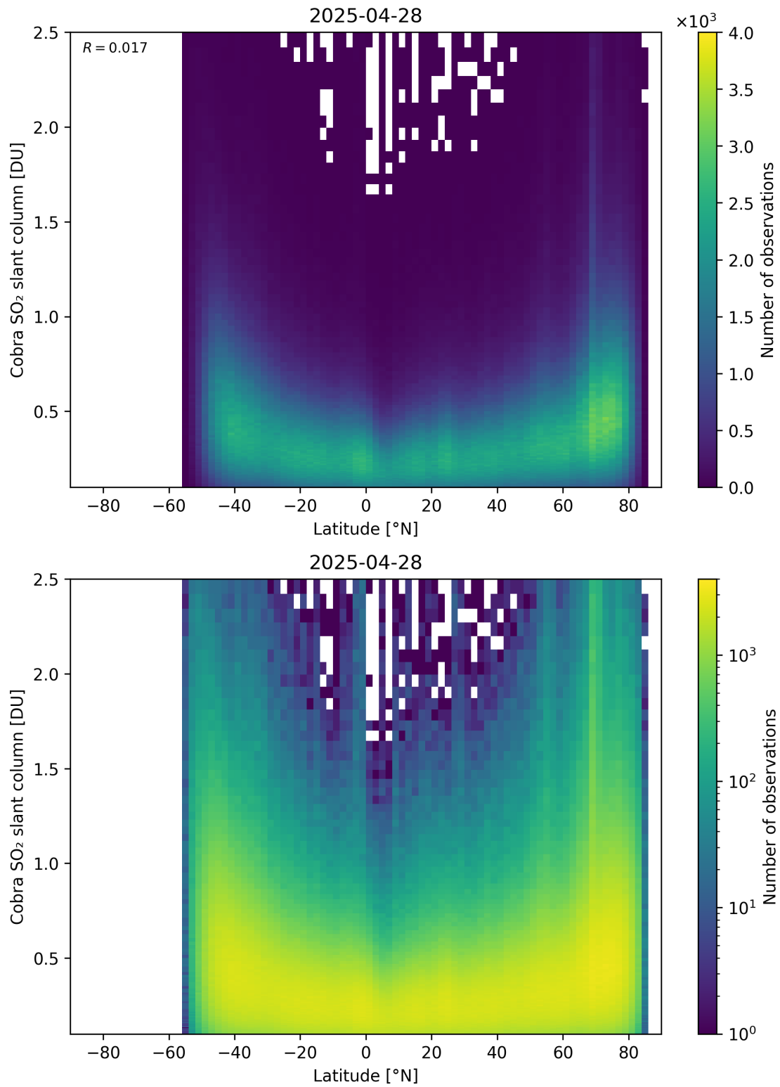
Figure 157: Scatter density plot of “Latitude” against “Cobra SO 2 slant column” for 2025-04-27 to 2025-04-29.
