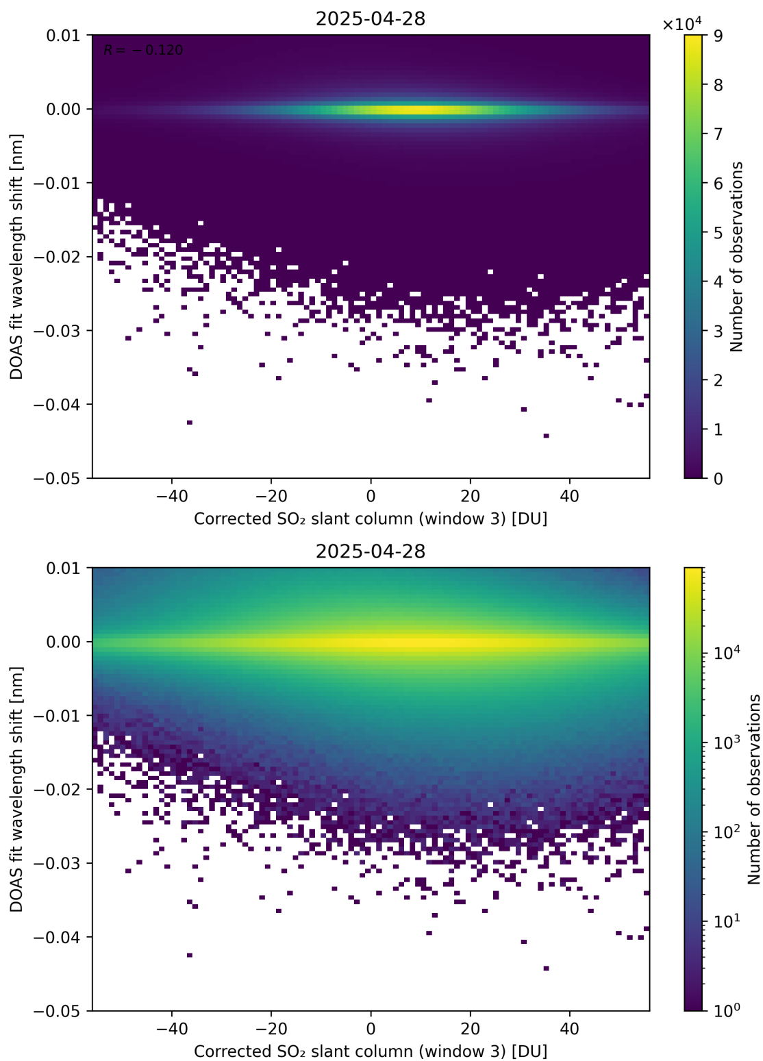
Figure 256: Scatter density plot of “Corrected SO 2 slant column (window 3)” against “DOAS fit wavelength shift” for 2025-04-27 to 2025-04-29.
