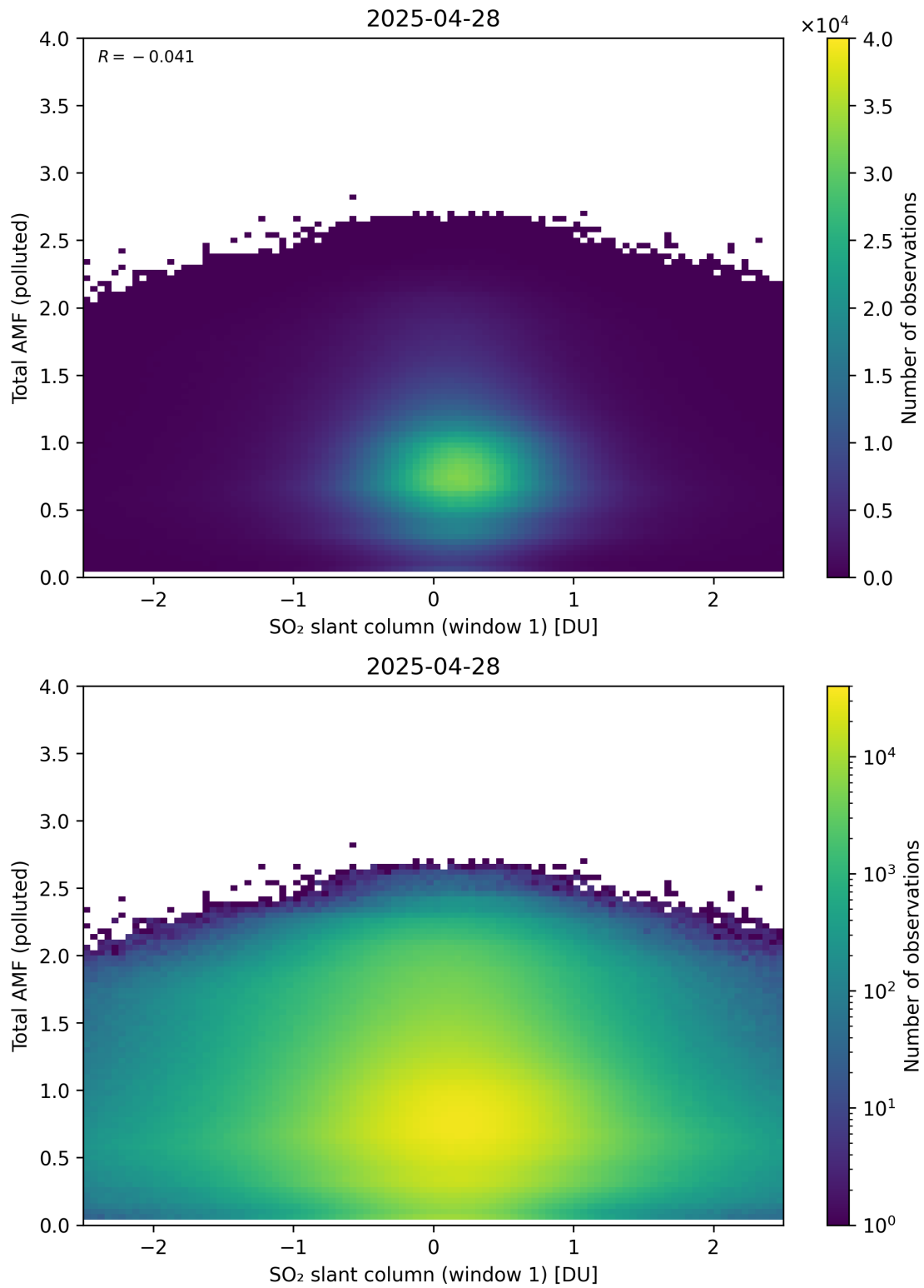
Figure 289: Scatter density plot of “SO 2 slant column (window 1)” against “Total AMF (polluted)” for 2025-04-27 to 2025-04-29.
