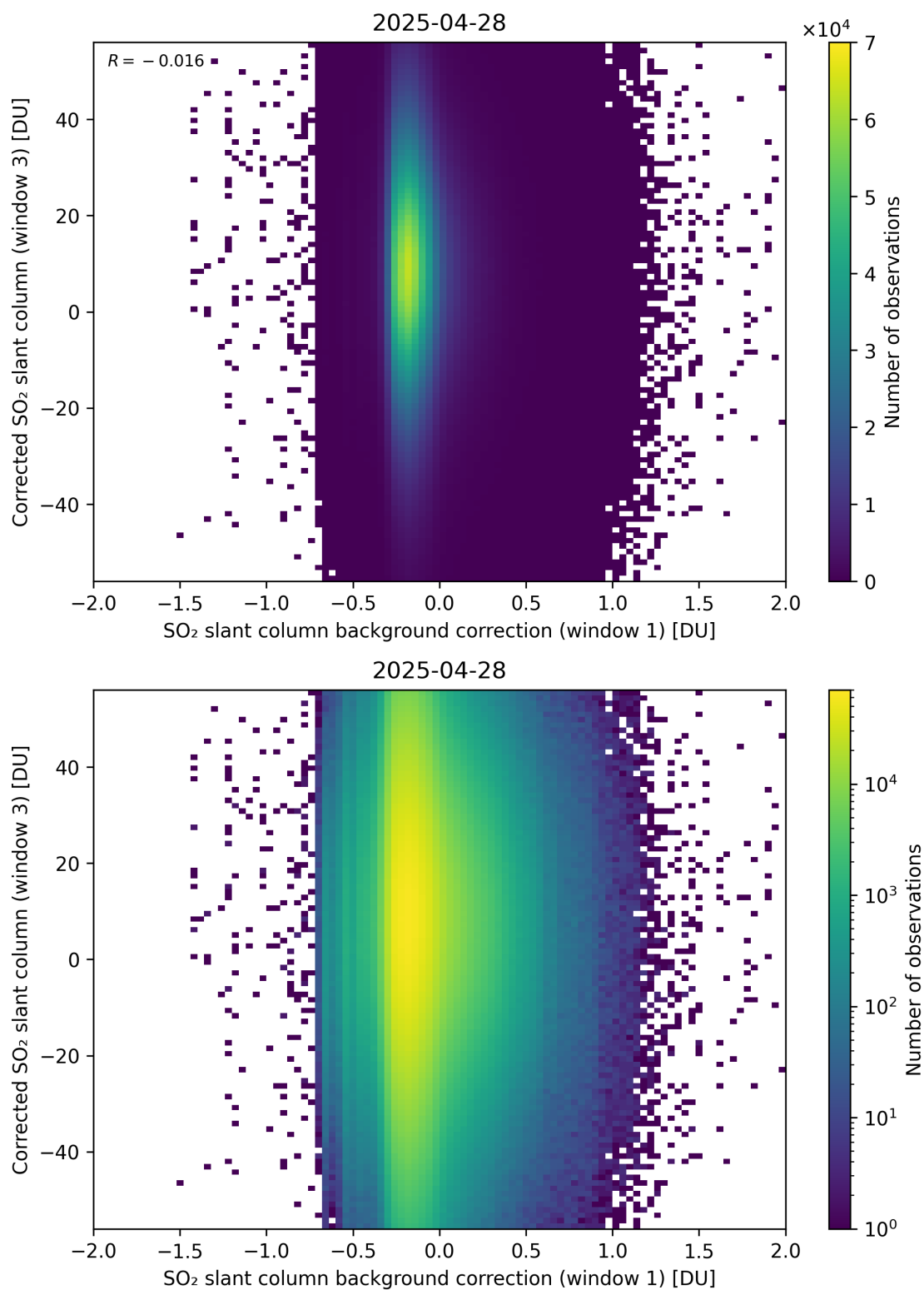
Figure 116: Scatter density plot of “SO 2 slant column background correction (window 1)” against “Corrected SO 2 slant column (window 3)” for 2025-04-27 to 2025-04-29.
