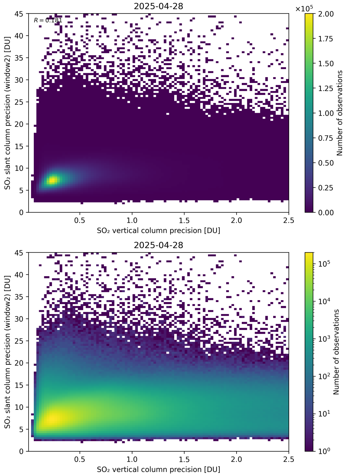
Figure 343: Scatter density plot of “SO 2 vertical column precision” against “SO 2 slant column precision (window2)” for 2025-04-27 to 2025-04-29.
