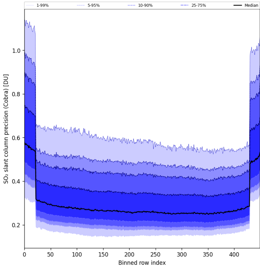
Figure 88: Along track statistics of “SO 2 slant column precision (Cobra)” for 2025-04-27 to 2025-04-29
