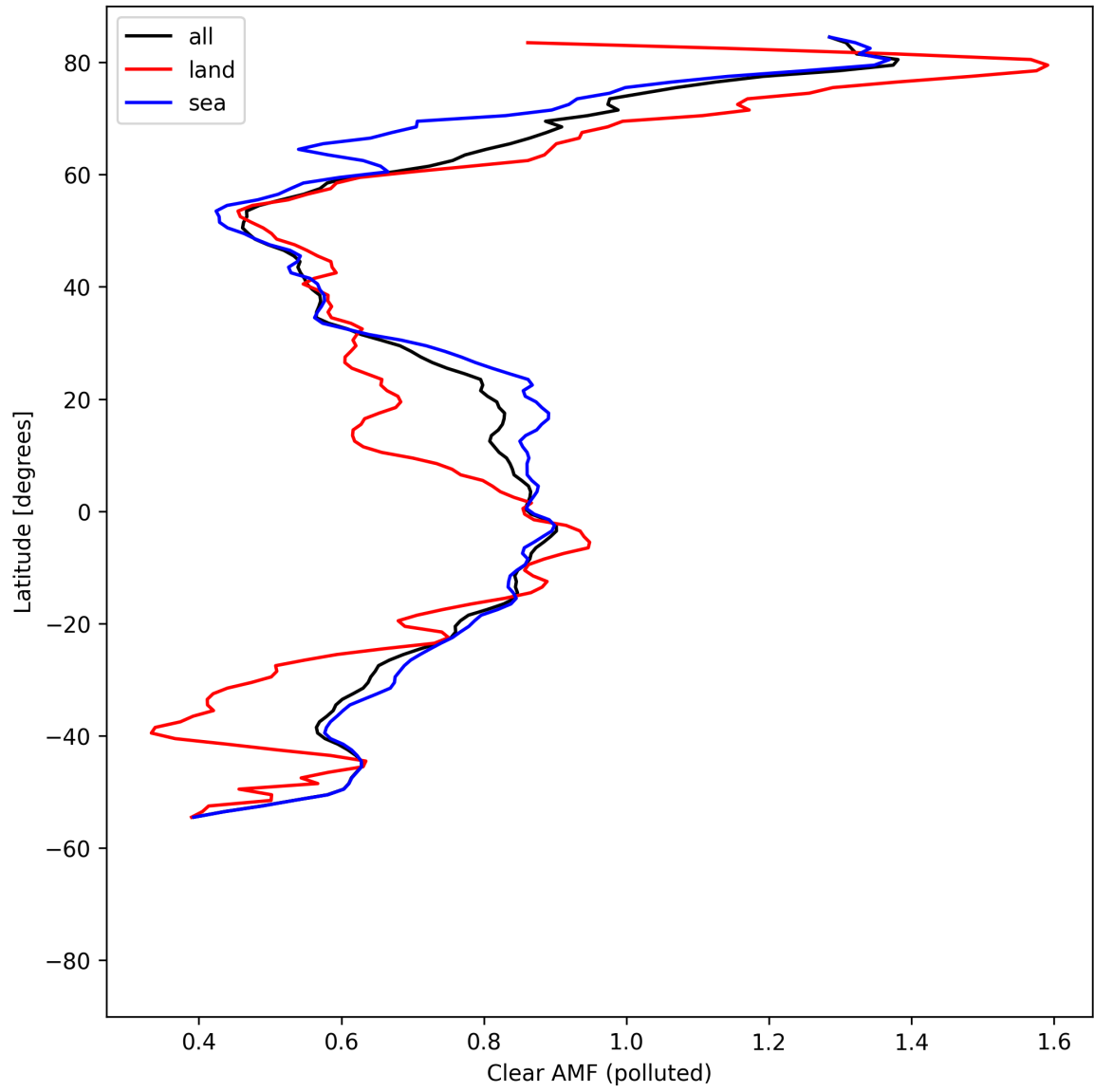
Figure 55: Zonal average of “Clear AMF (polluted)” for 2025-04-27 to 2025-04-29.
