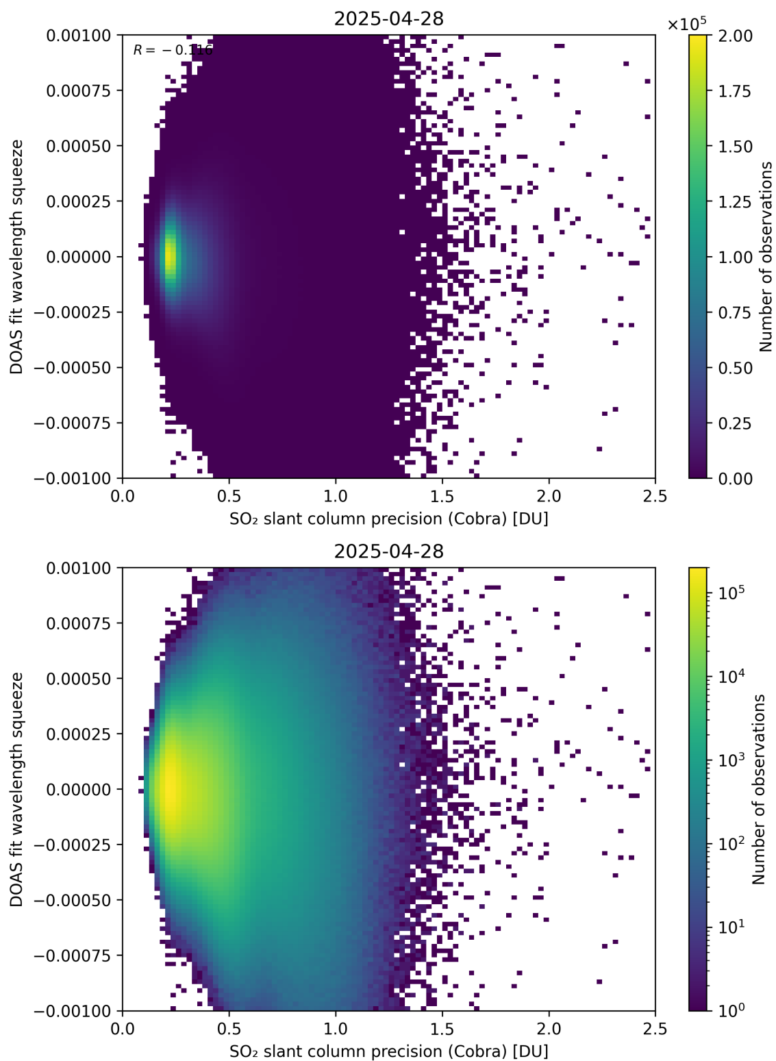
Figure 203: Scatter density plot of “SO 2 slant column precision (Cobra)” against “DOAS fit wavelength squeeze” for 2025-04-27 to 2025-04-29.
