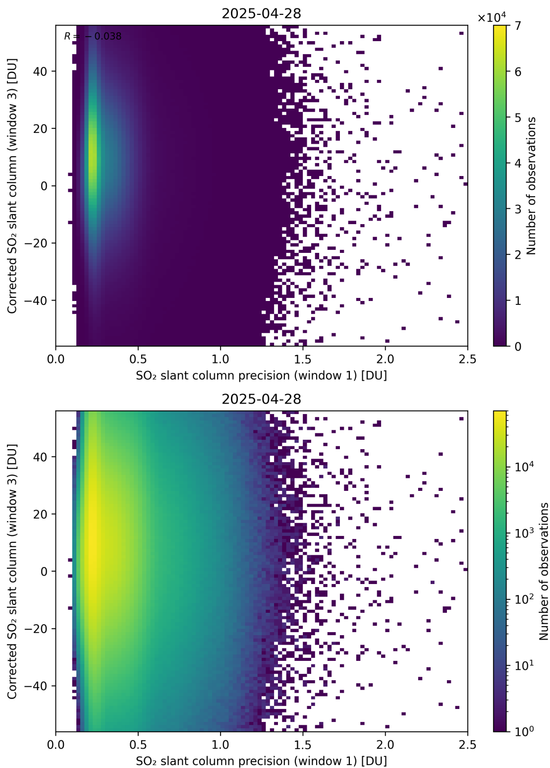
Figure 276: Scatter density plot of “SO 2 slant column precision (window 1)” against “Corrected SO 2 slant column (window 3)” for 2025-04-27 to 2025-04-29.
