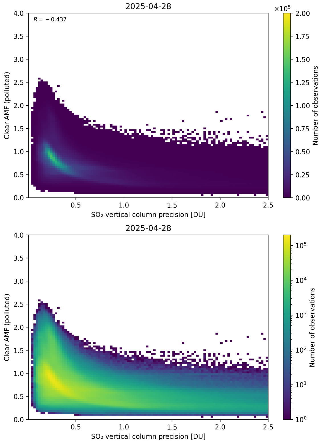
Figure 335: Scatter density plot of “SO 2 vertical column precision” against “Clear AMF (polluted)” for 2025-04-27 to 2025-04-29.
