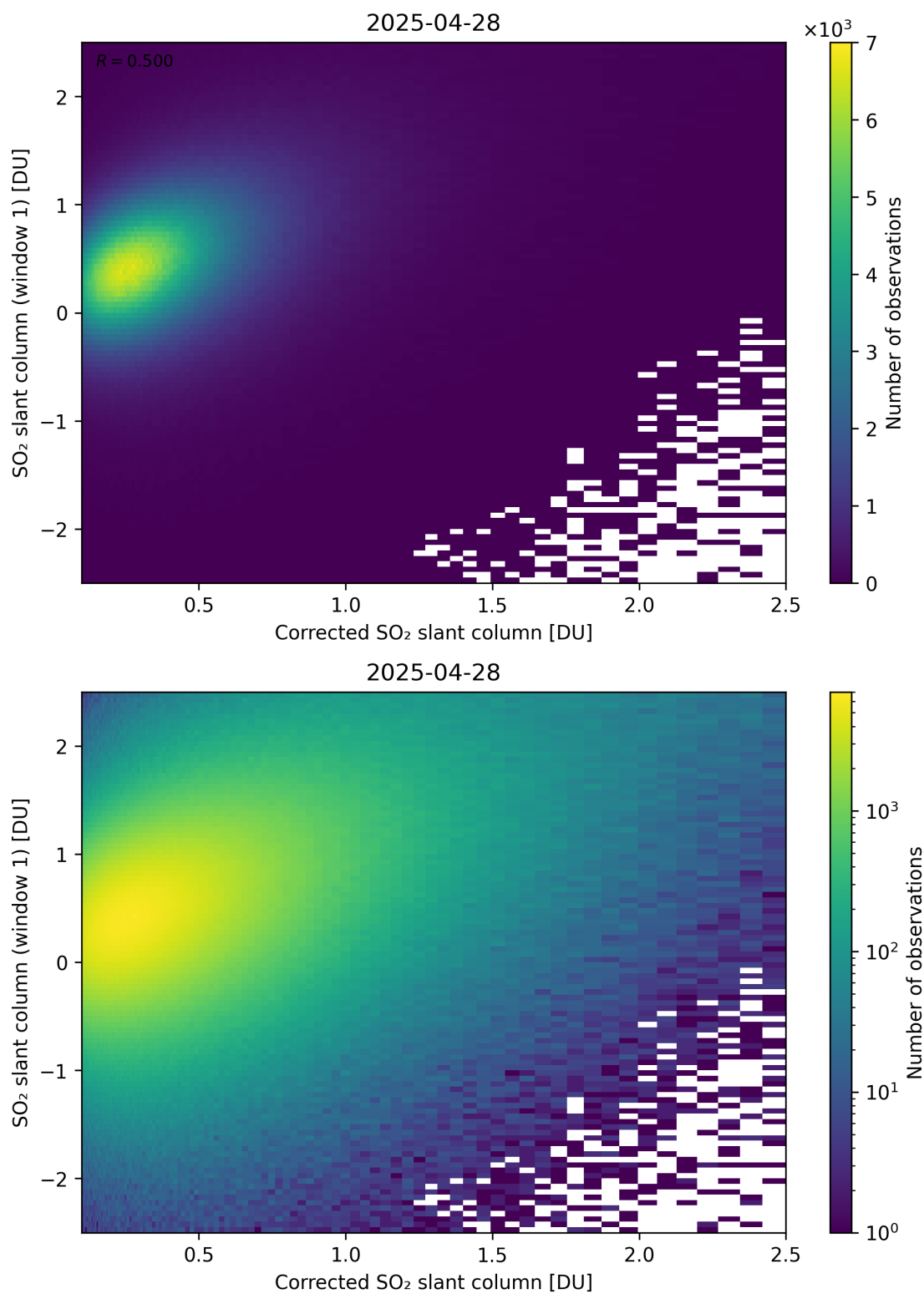
Figure 237: Scatter density plot of “Corrected SO 2 slant column” against “SO 2 slant column (window 1)” for 2025-04-27 to 2025-04-29.
