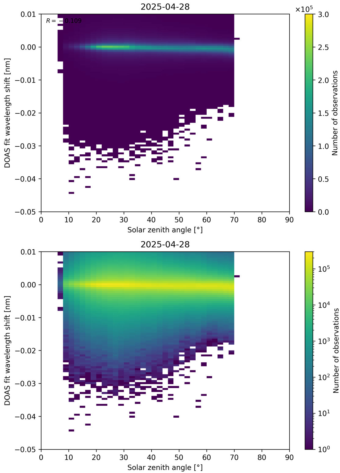
Figure 174: Scatter density plot of “Solar zenith angle” against “DOAS fit wavelength shift” for 2025-04-27 to 2025-04-29.
