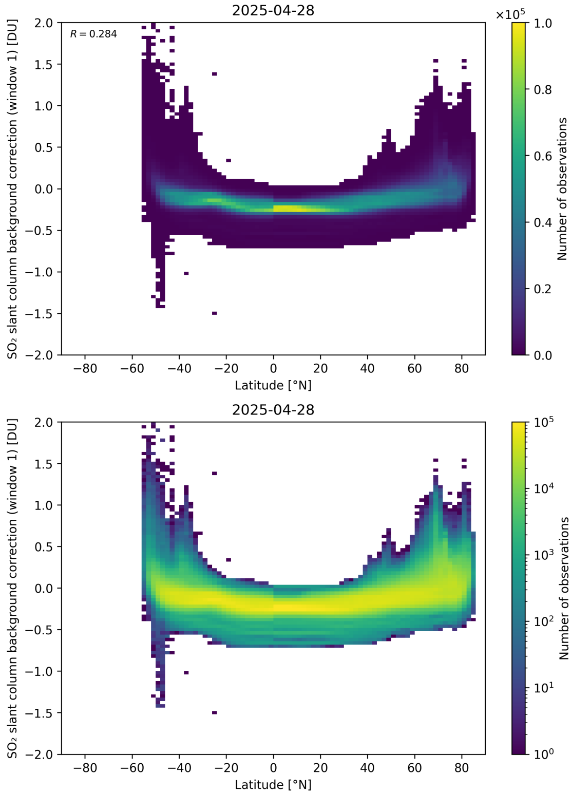
Figure 150: Scatter density plot of “Latitude” against “SO 2 slant column background correction (window 1)” for 2025-04-27 to 2025-04-29.
