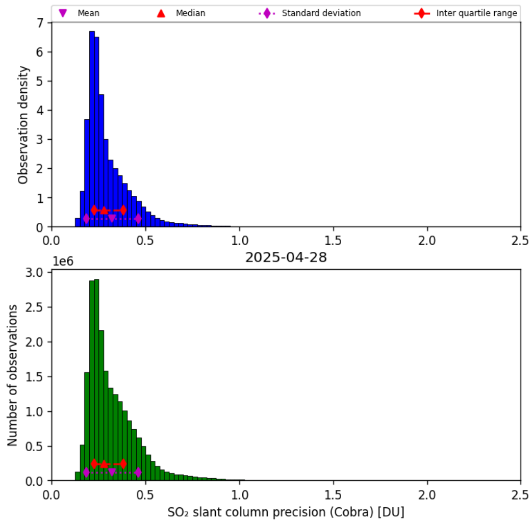
Figure 62: Histogram of “SO 2 slant column precision (Cobra)” for 2025-04-27 to 2025-04-29
