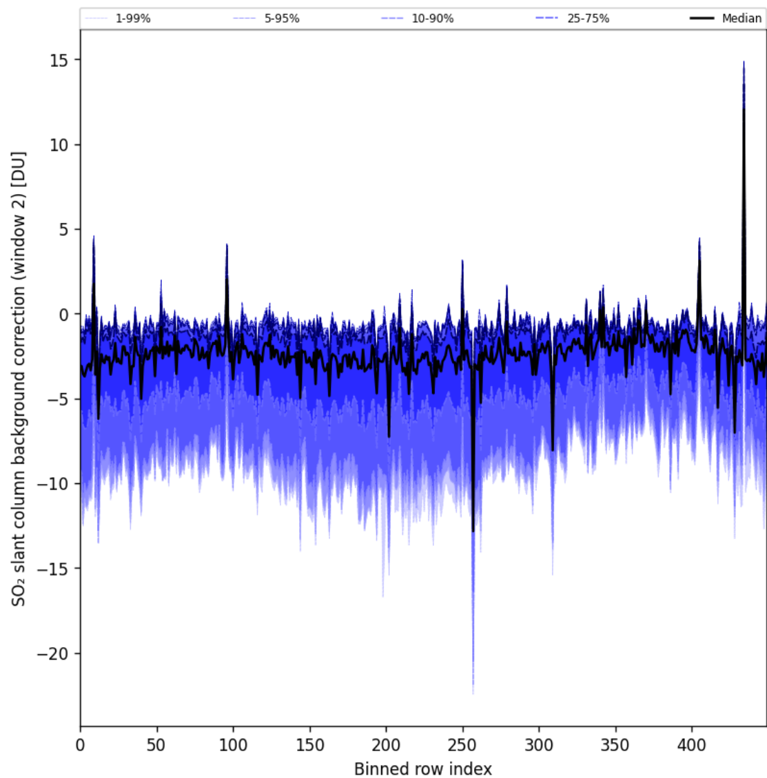
Figure 96: Along track statistics of “SO 2 slant column background correction (window 2)” for 2025-04-27 to 2025-04-29
