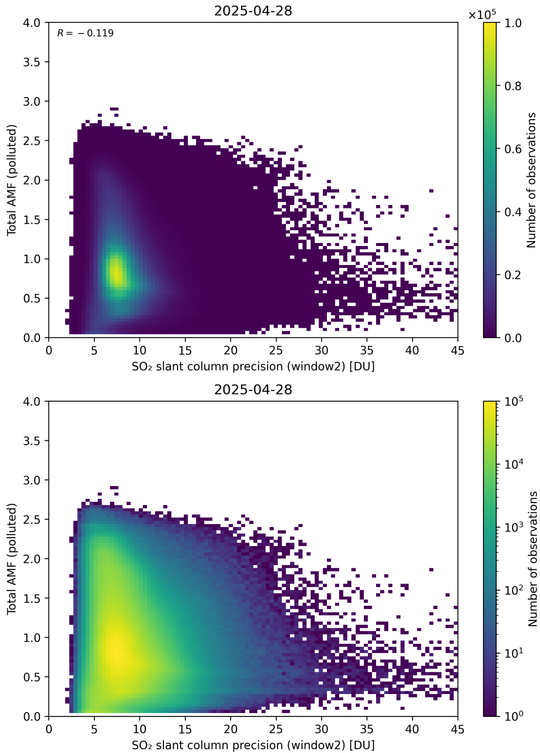
Figure 301: Scatter density plot of “SO 2 slant column precision (window2)” against “Total AMF (polluted)” for 2025-04-27 to 2025-04-29.
