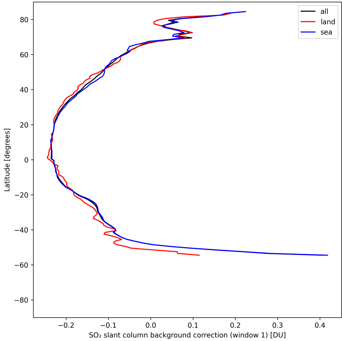
Figure 40: Zonal average of "SO 2 slant column background correction (window 1)" for 2025-04-27 to 2025-04-29.
