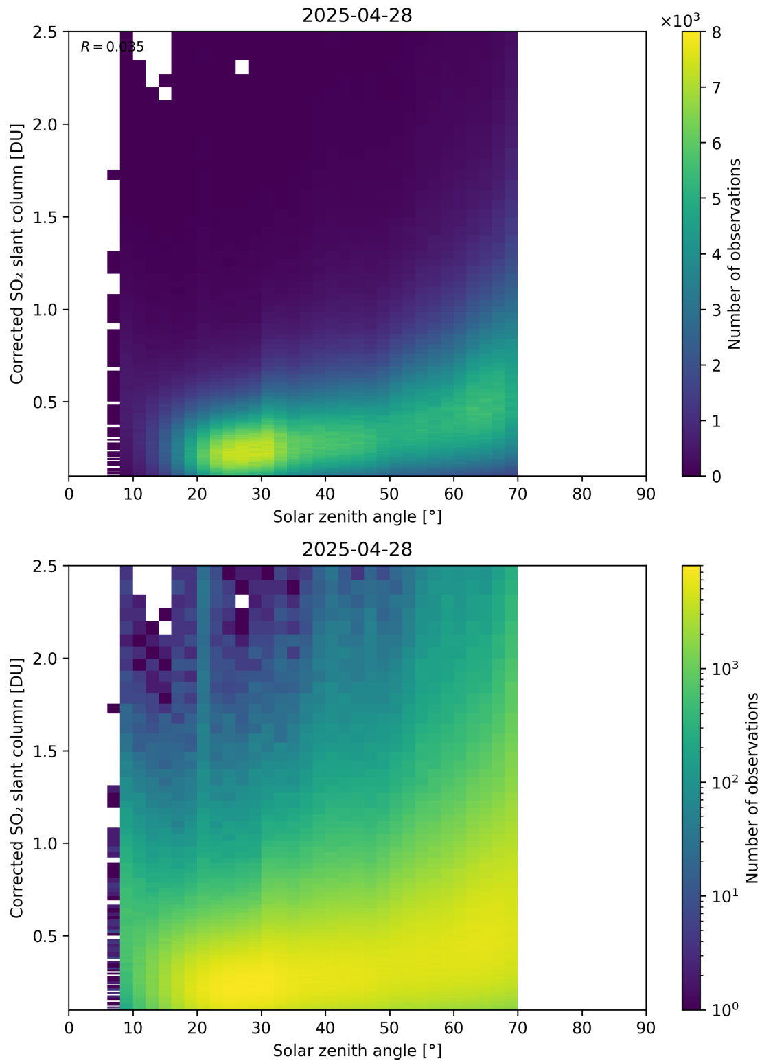
Figure 181: Scatter density plot of “Solar zenith angle” against “Corrected SO 2 slant column” for 2025-04-27 to 2025-04-29.
