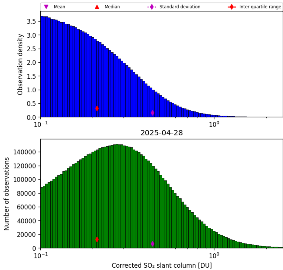
Figure 60: Histogram of “Corrected SO 2 slant column” for 2025-04-27 to 2025-04-29
