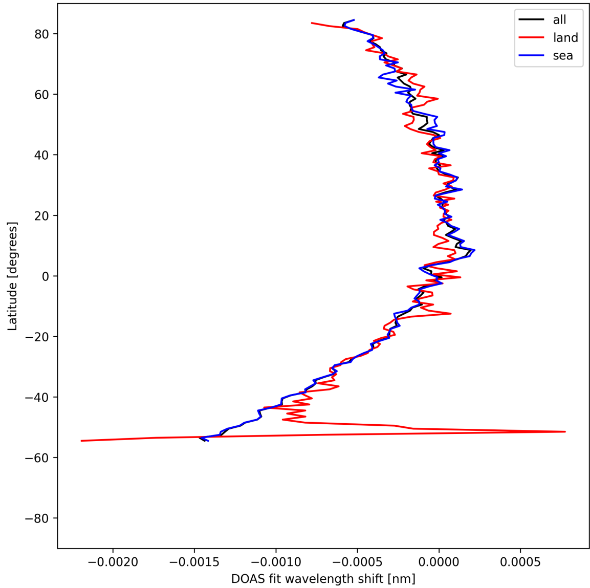
Figure 50: Zonal average of “DOAS fit wavelength shift” for 2025-04-27 to 2025-04-29.
