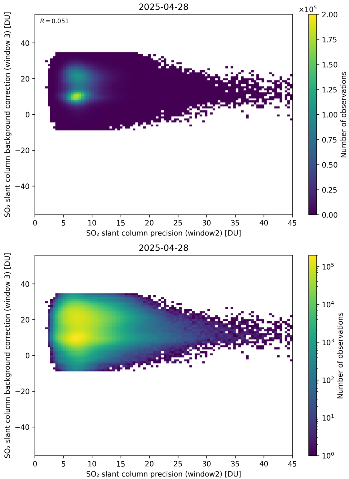
Figure 292: Scatter density plot of “SO 2 slant column precision (window2)” against “SO 2 slant column background correction (window 3)” for 2025-04-27 to 2025-04-29.
