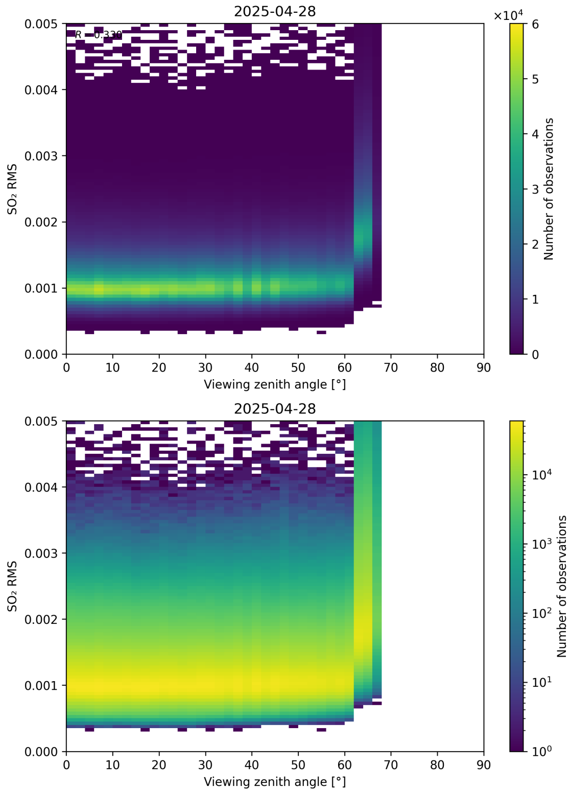
Figure 367: Scatter density plot of “Viewing zenith angle” against “SO 2 RMS” for 2025-04-27 to 2025-04-29.
