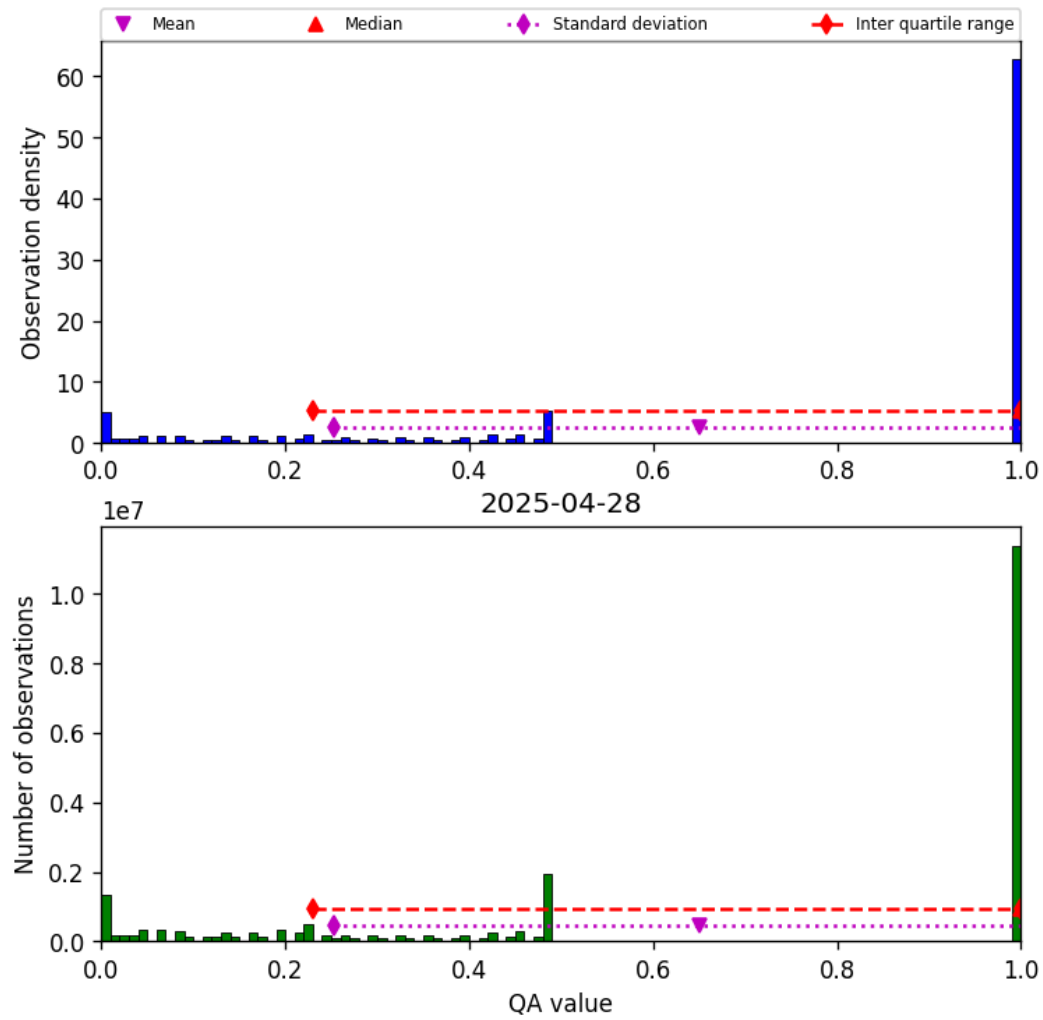
Figure 57: Histogram of “QA value” for 2025-04-27 to 2025-04-29
