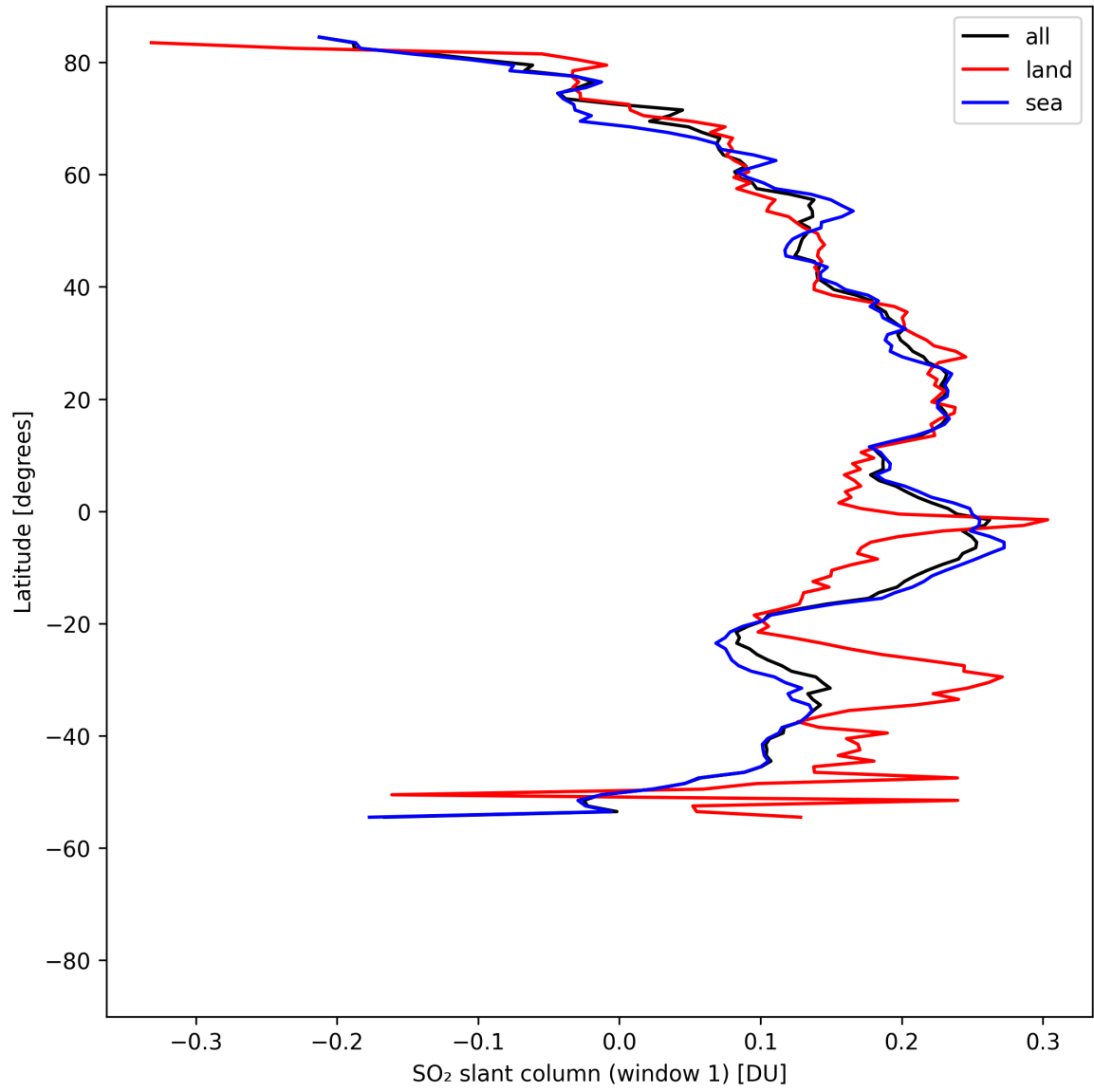
Figure 37: Zonal average of “SO 2 slant column (window 1)” for 2025-04-27 to 2025-04-29.
