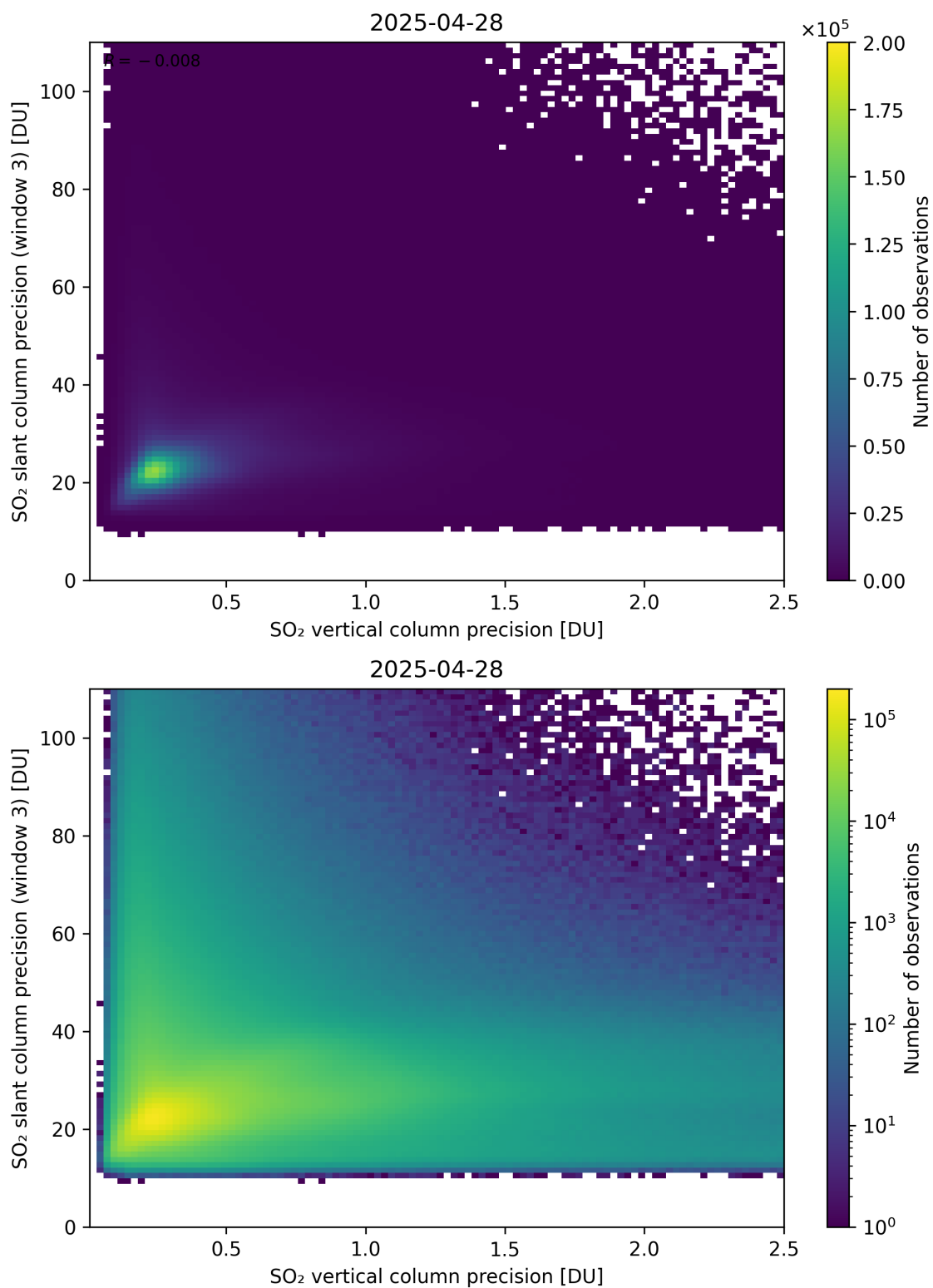
Figure 345: Scatter density plot of “SO 2 vertical column precision” against “SO 2 slant column precision (window 3)” for 2025-04-27 to 2025-04-29.
