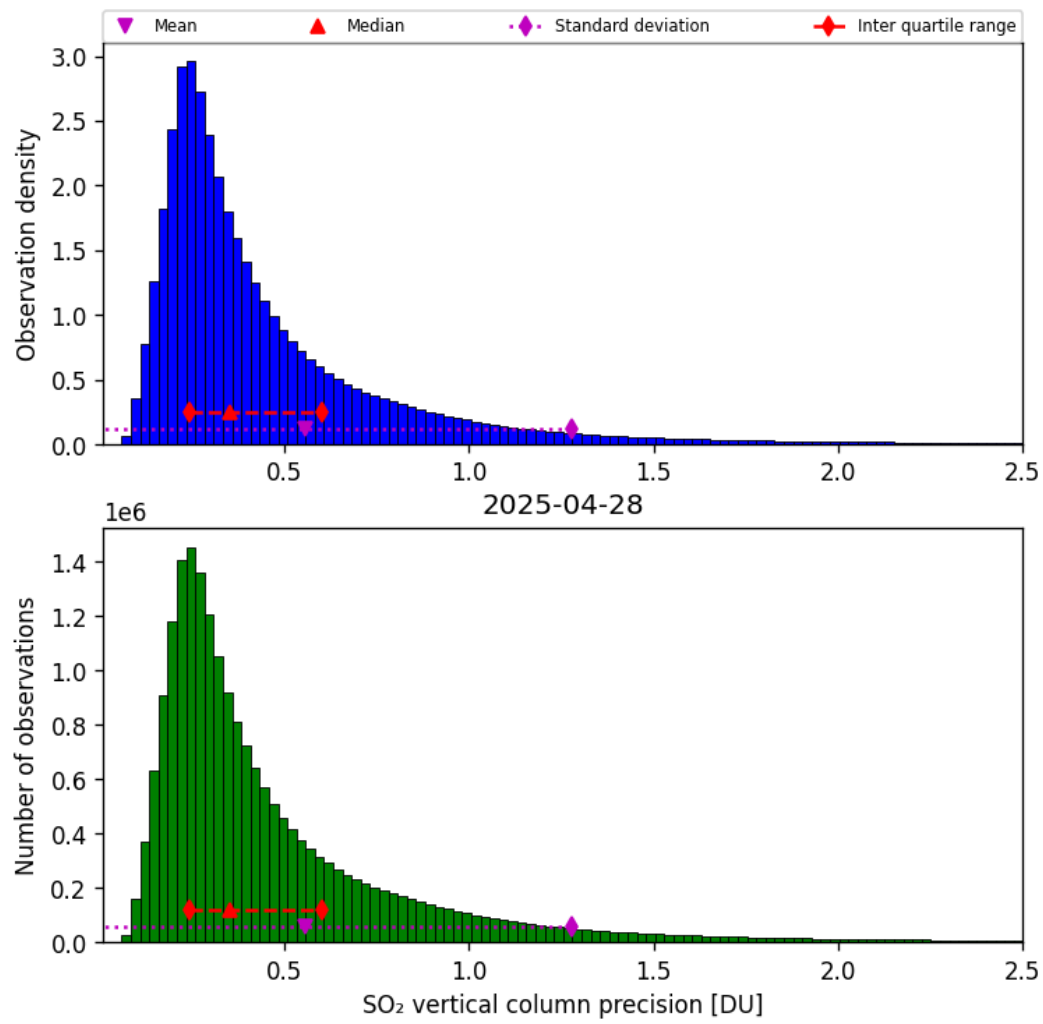
Figure 59: Histogram of “SO 2 vertical column precision” for 2025-04-27 to 2025-04-29
