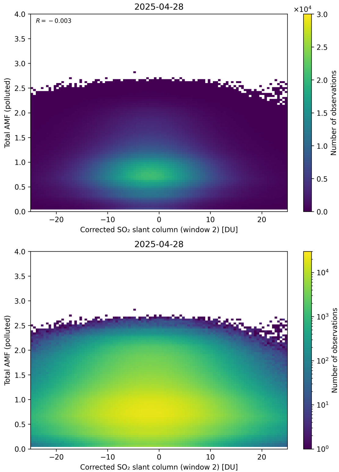
Figure 253: Scatter density plot of “Corrected SO 2 slant column (window 2)” against “Total AMF (polluted)” for 2025-04-27 to 2025-04-29.
