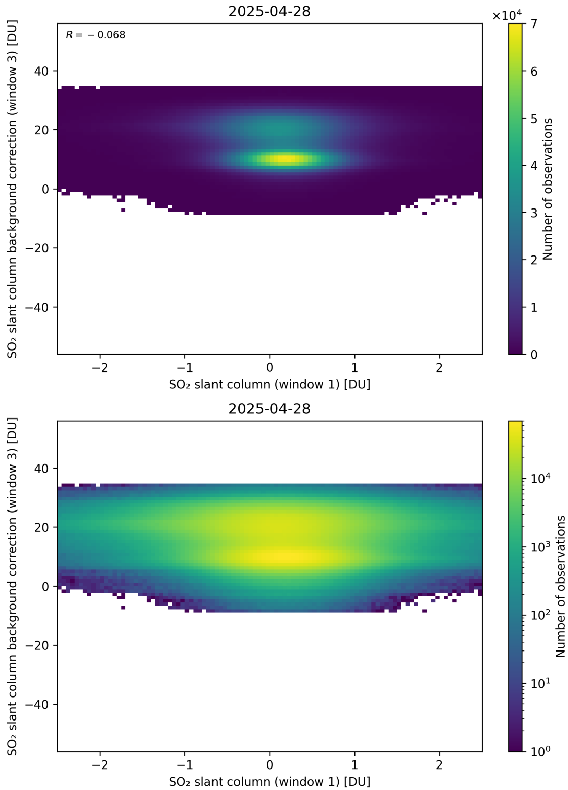
Figure 264: Scatter density plot of “SO 2 slant column (window 1)” against “SO 2 slant column background correction (window 3)” for 2025-04-27 to 2025-04-29.
