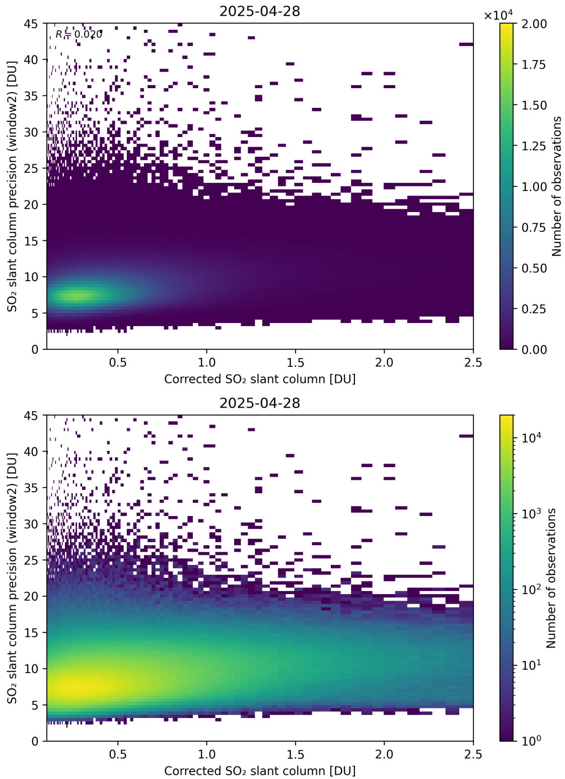
Figure 239: Scatter density plot of “Corrected SO 2 slant column” against “SO 2 slant column precision (window2)” for 2025-04-27 to 2025-04-29.
