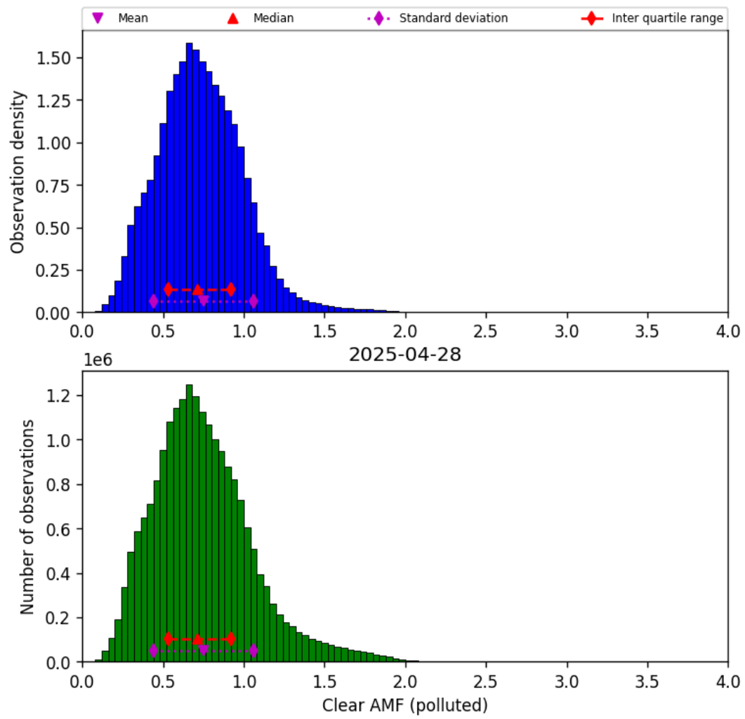
Figure 81: Histogram of “Clear AMF (polluted)” for 2025-04-27 to 2025-04-29
