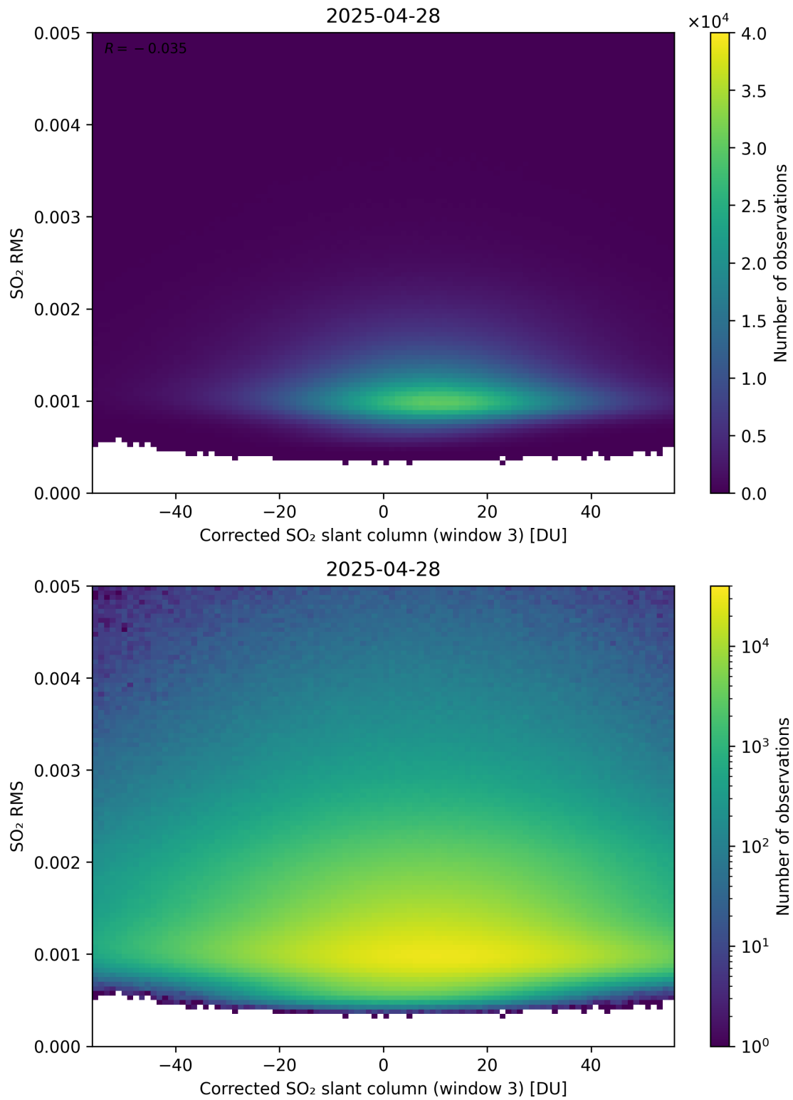
Figure 258: Scatter density plot of “Corrected SO 2 slant column (window 3)” against “SO 2 RMS” for 2025-04-27 to 2025-04-29.
