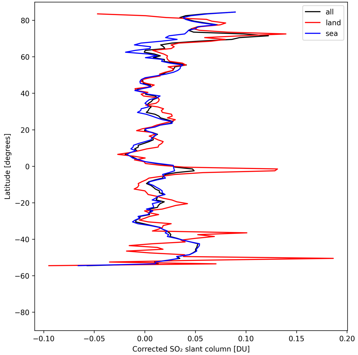
Figure 34: Zonal average of “Corrected SO 2 slant column” for 2025-04-27 to 2025-04-29.
