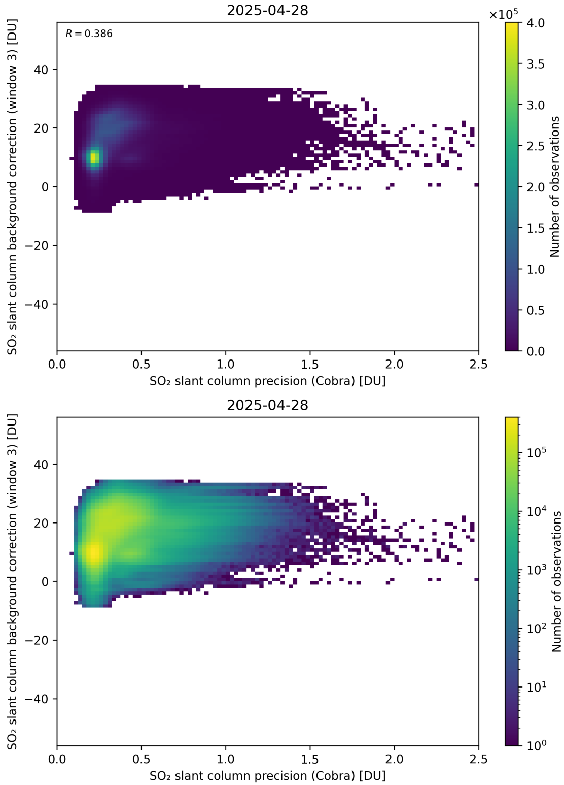
Figure 201: Scatter density plot of “SO 2 slant column precision (Cobra)” against “SO 2 slant column background correction (window 3)” for 2025-04-27 to 2025-04-29.
