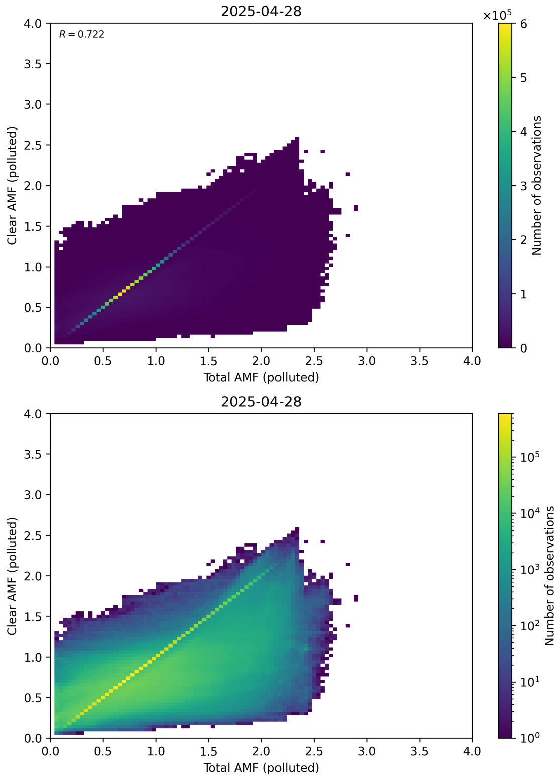
Figure 321: Scatter density plot of “Total AMF (polluted)” against “Clear AMF (polluted)” for 2025-04-27 to 2025-04-29.
