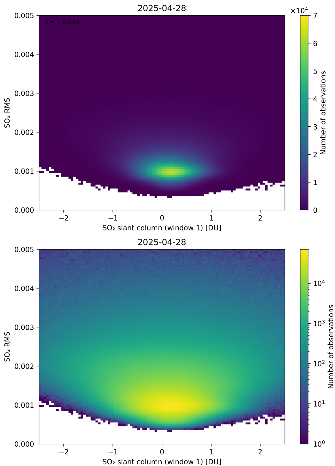
Figure 267: Scatter density plot of “SO 2 slant column (window 1)” against “SO 2 RMS” for 2025-04-27 to 2025-04-29.
