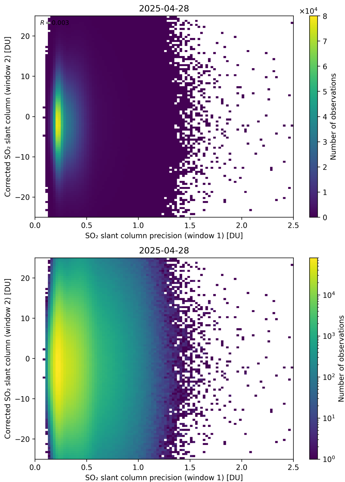
Figure 275: Scatter density plot of “SO 2 slant column precision (window 1)” against “Corrected SO 2 slant column (window 2)” for 2025-04-27 to 2025-04-29.
