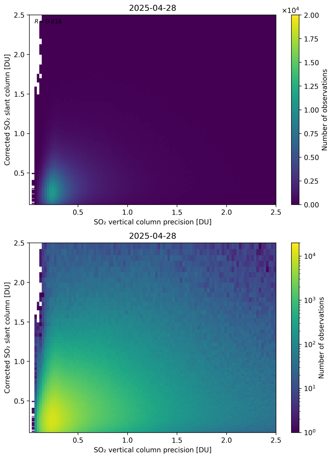
Figure 338: Scatter density plot of “SO 2 vertical column precision” against “Corrected SO 2 slant column” for 2025-04-27 to 2025-04-29.
