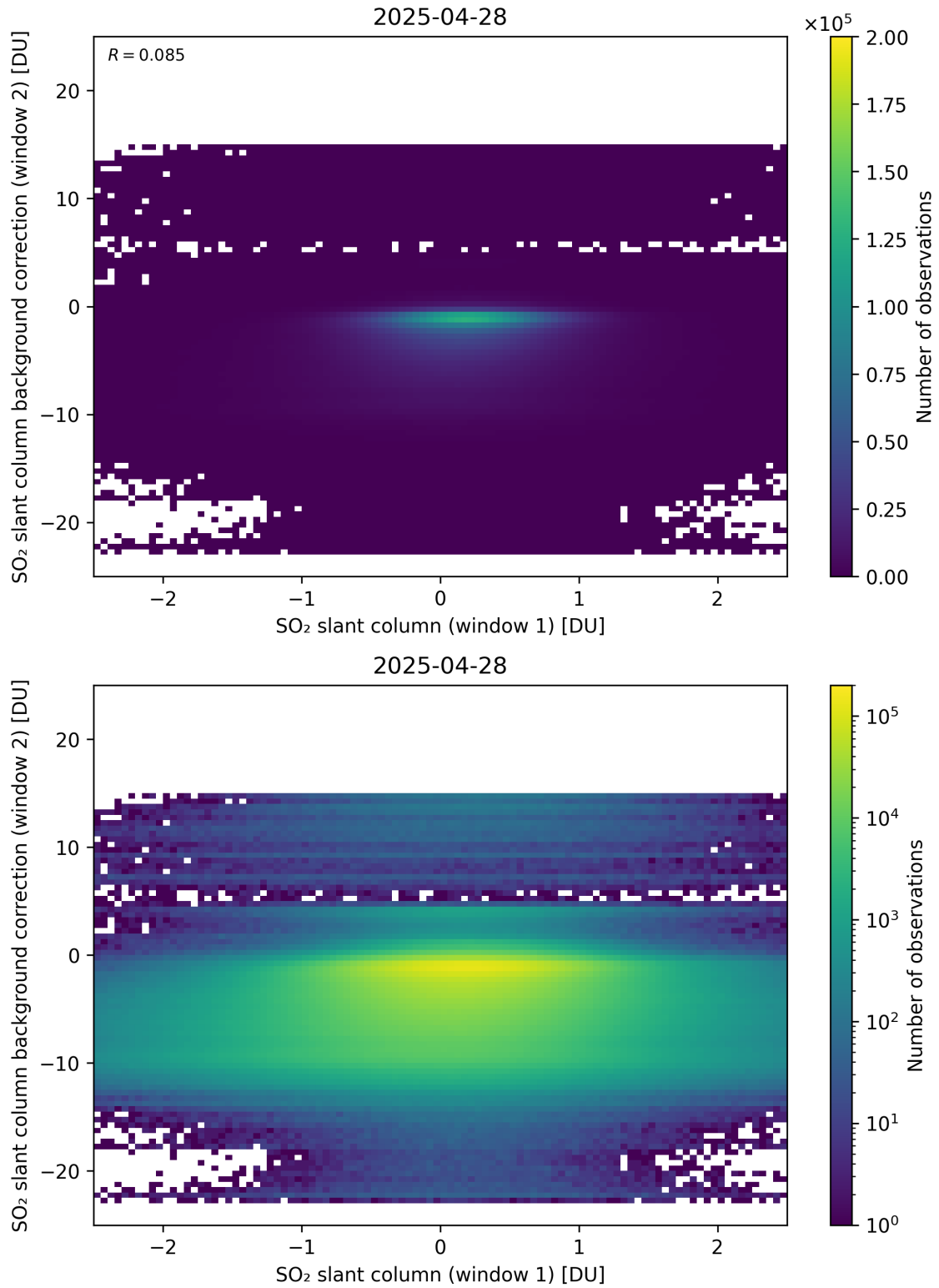
Figure 263: Scatter density plot of “SO 2 slant column (window 1)” against “SO 2 slant column background correction (window 2)” for 2025-04-27 to 2025-04-29.
