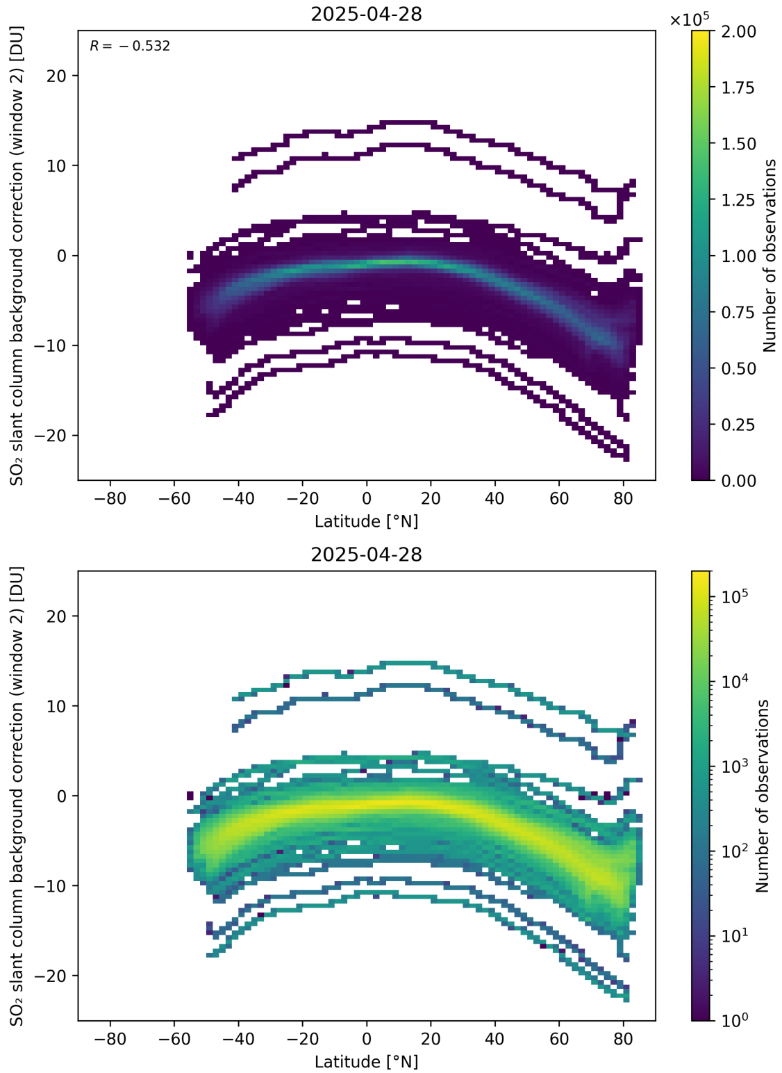
Figure 151: Scatter density plot of “Latitude” against “SO 2 slant column background correction (window 2)” for 2025-04-27 to 2025-04-29.
