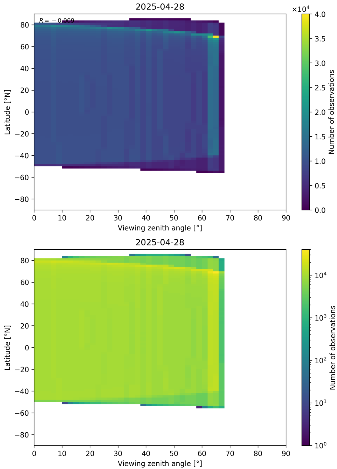
Figure 368: Scatter density plot of “Viewing zenith angle” against “Latitude” for 2025-04-27 to 2025-04-29.
