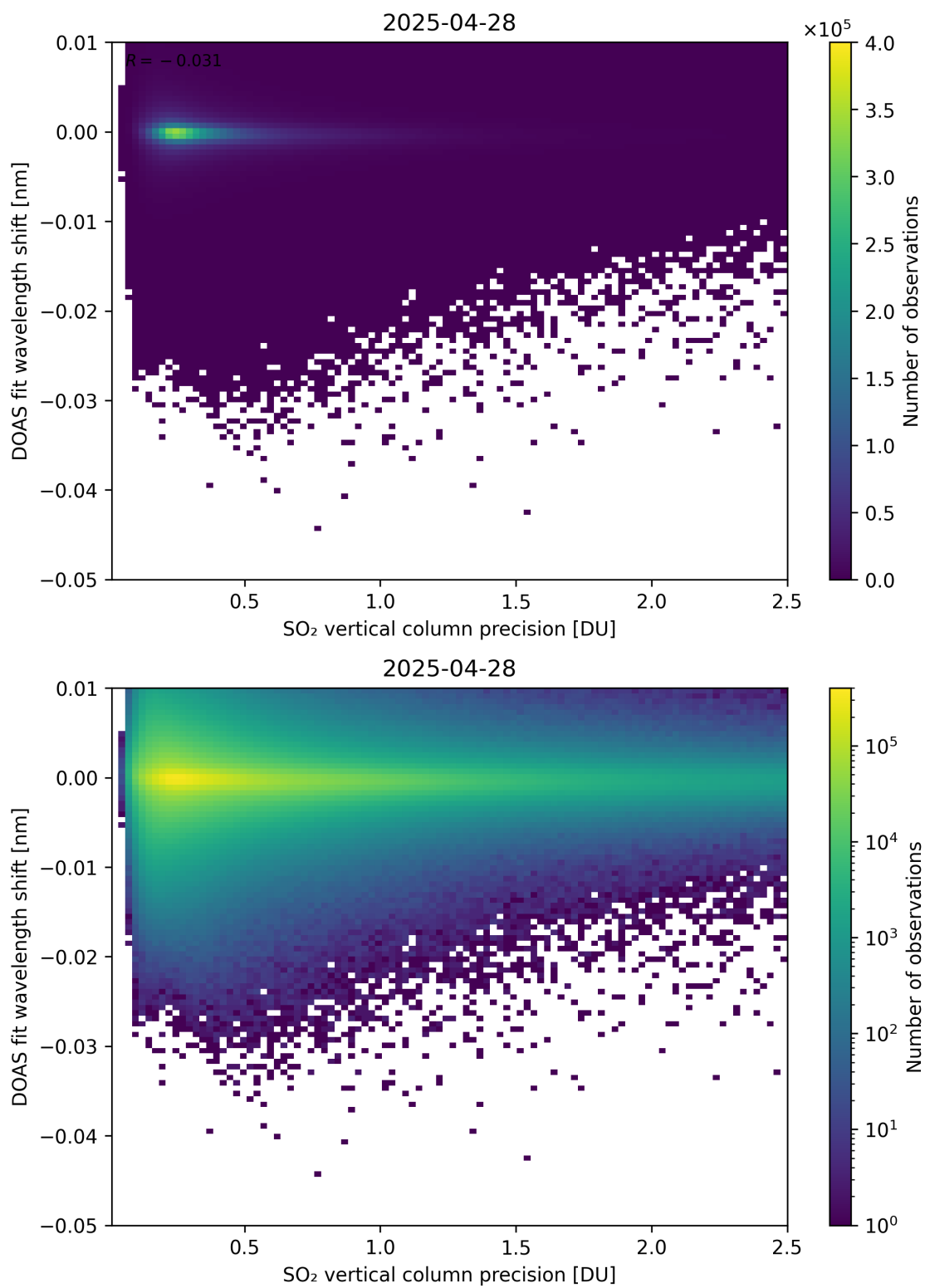
Figure 332: Scatter density plot of “SO 2 vertical column precision” against “DOAS fit wavelength shift” for 2025-04-27 to 2025-04-29.
