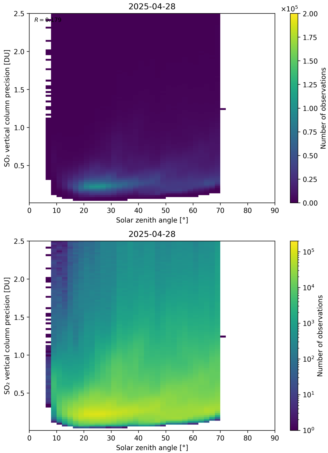
Figure 192: Scatter density plot of “Solar zenith angle” against “SO 2 vertical column precision” for 2025-04-27 to 2025-04-29.
