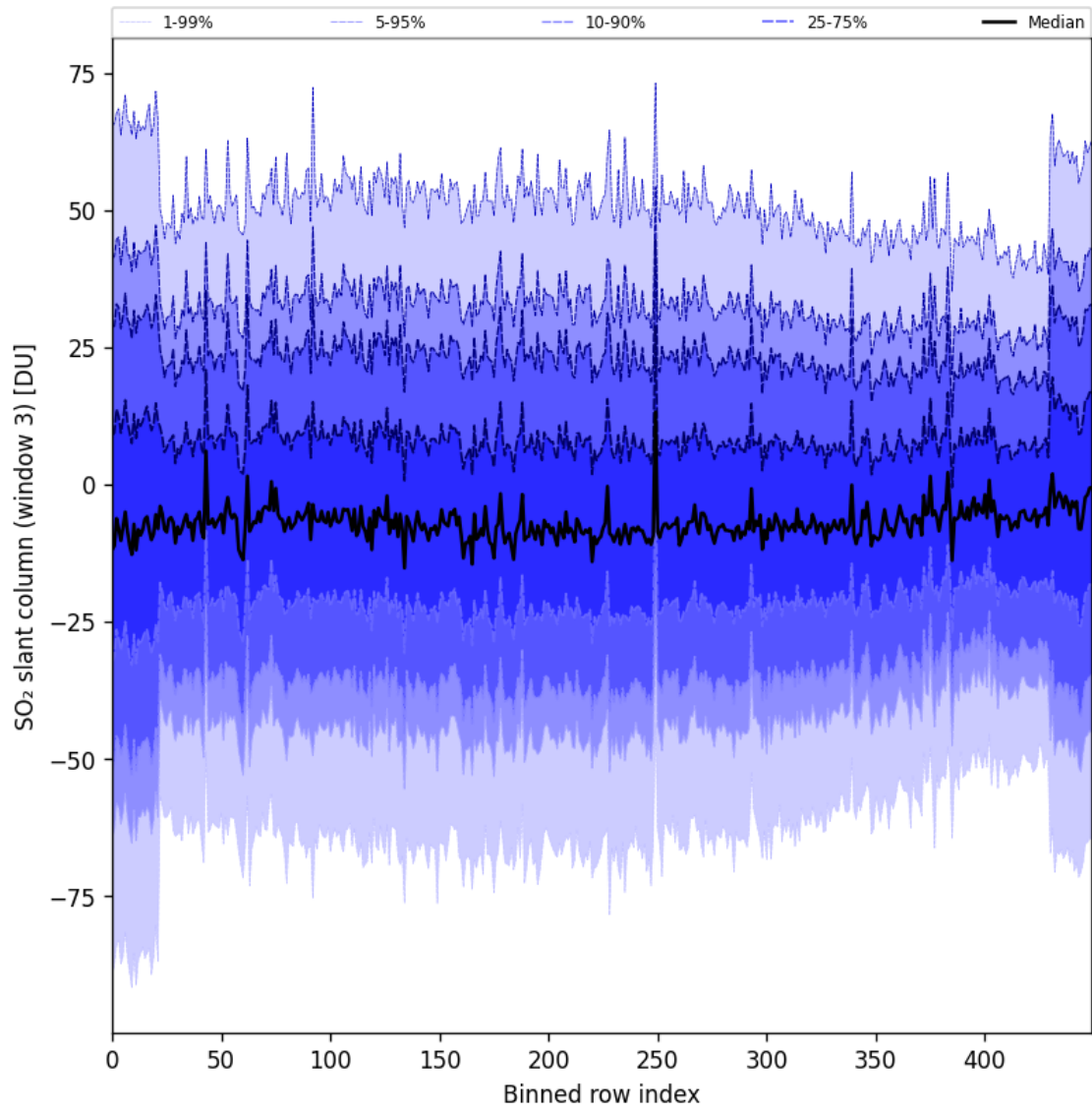
Figure 97: Along track statistics of “SO 2 slant column (window 3)” for 2025-04-27 to 2025-04-29
