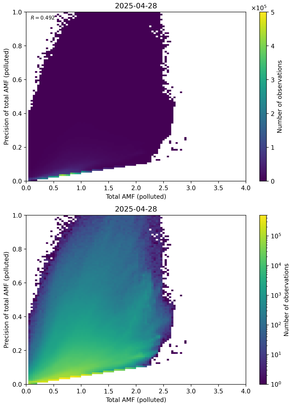
Figure 322: Scatter density plot of “Total AMF (polluted)” against “Precision of total AMF (polluted)” for 2025-04-27 to 2025-04-29.
