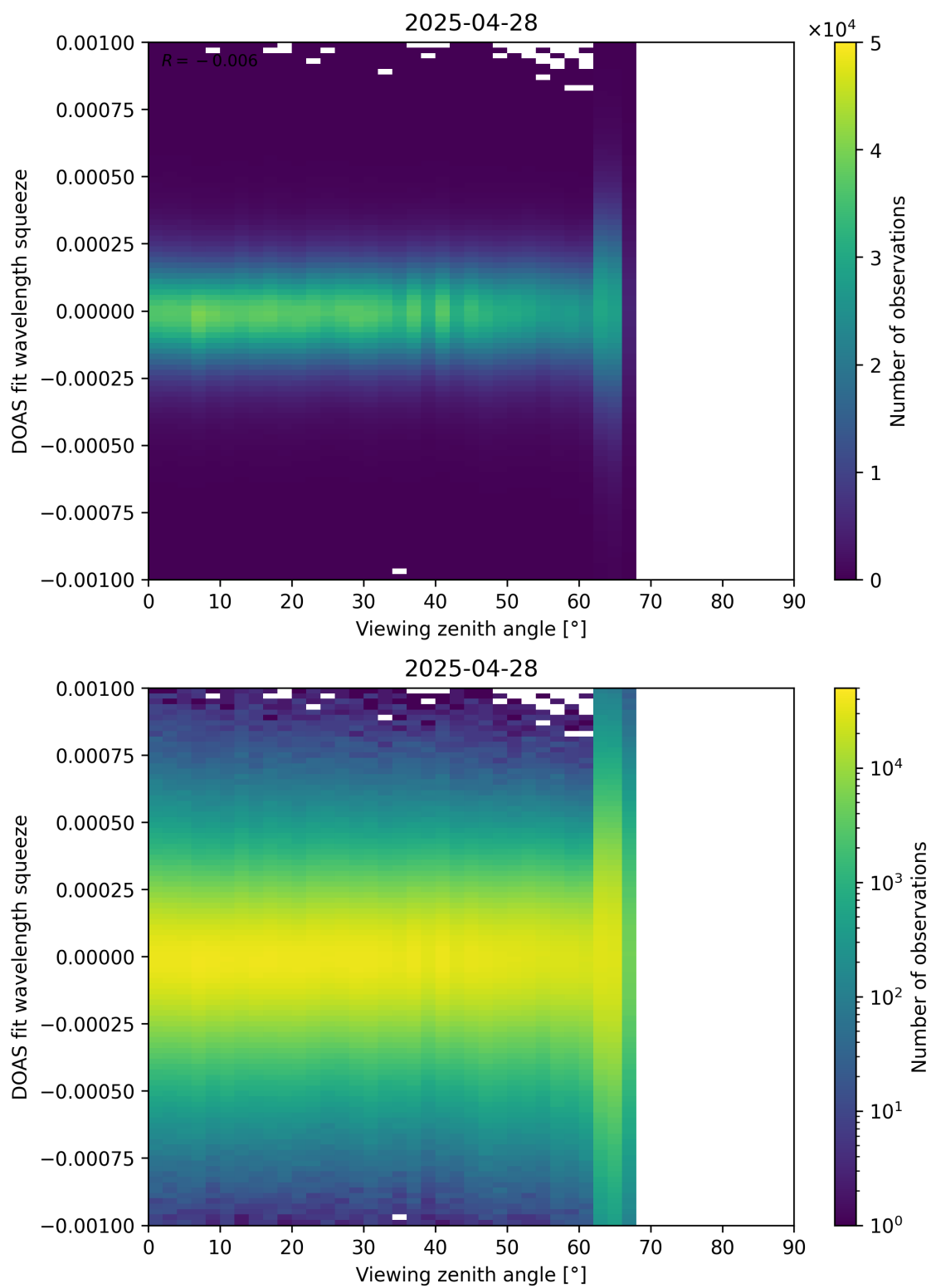
Figure 366: Scatter density plot of “Viewing zenith angle” against “DOAS fit wavelength squeeze” for 2025-04-27 to 2025-04-29.
