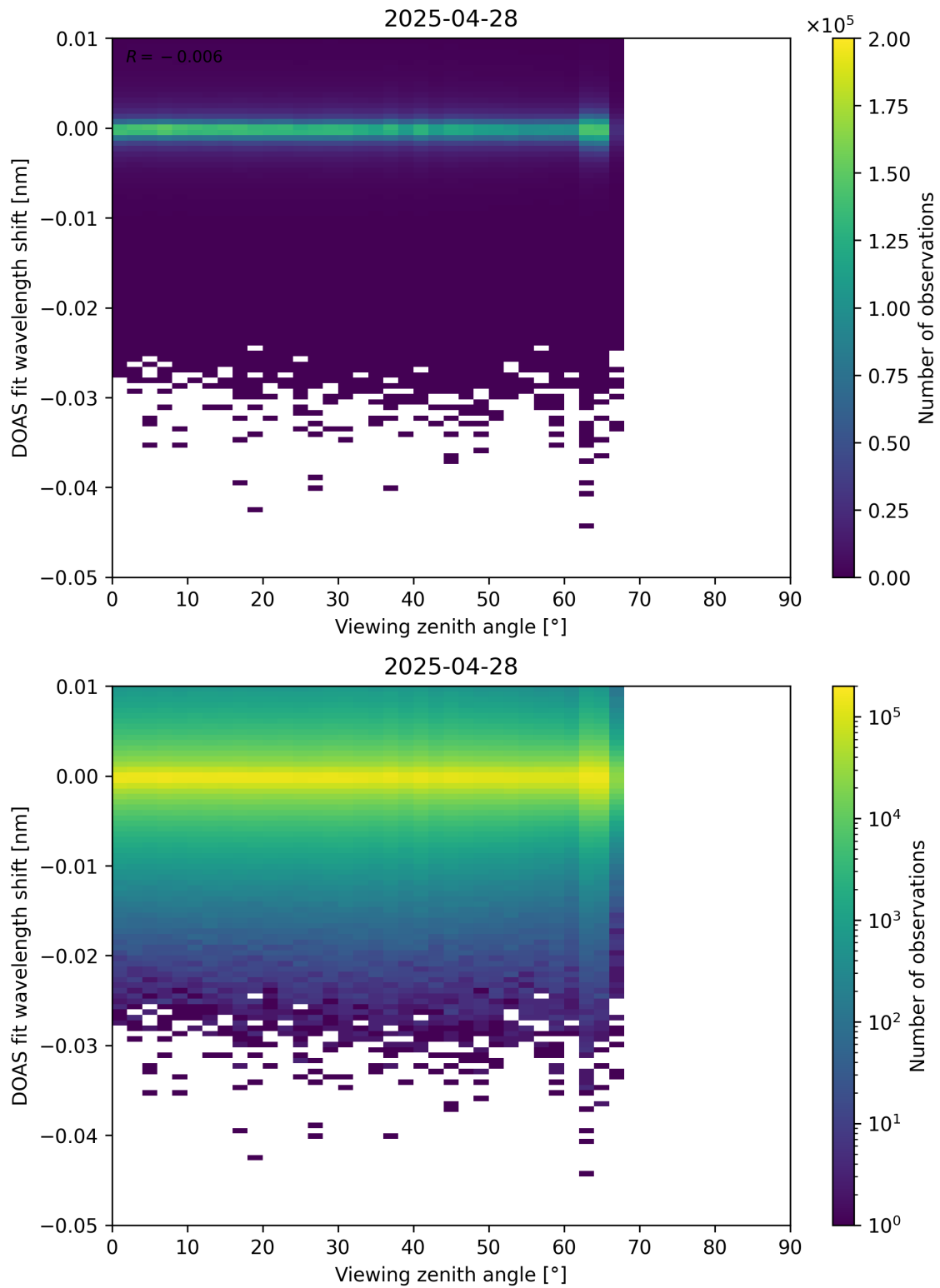
Figure 365: Scatter density plot of “Viewing zenith angle” against “DOAS fit wavelength shift” for 2025-04-27 to 2025-04-29.
