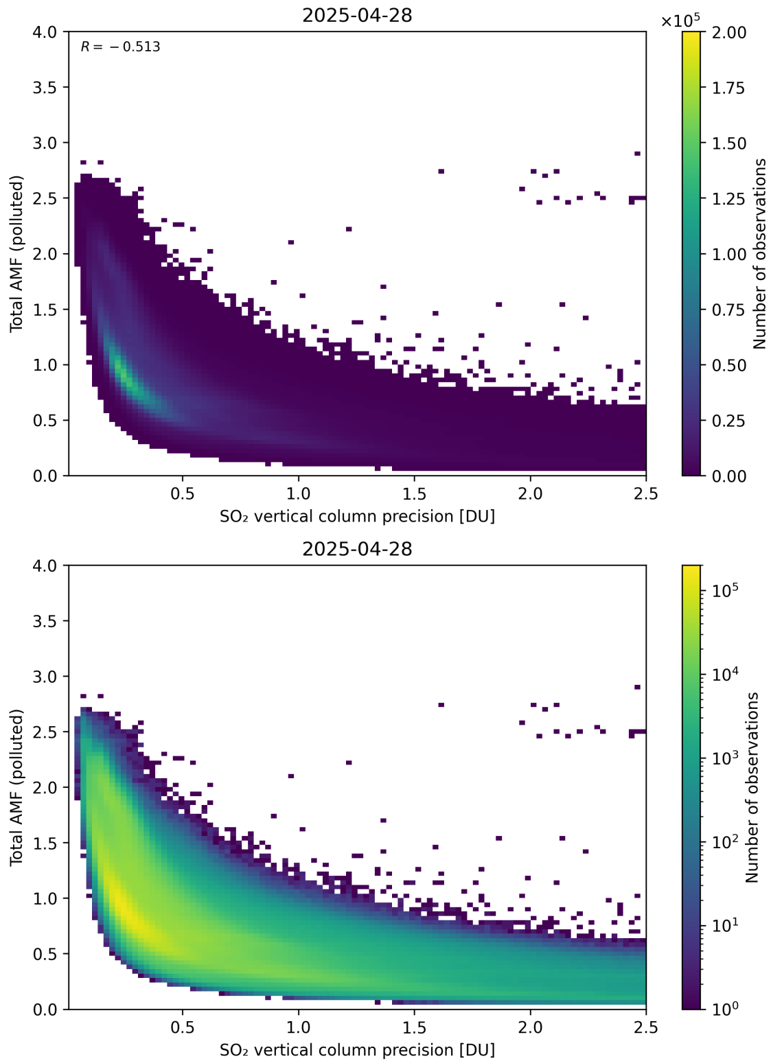
Figure 346: Scatter density plot of “SO 2 vertical column precision” against “Total AMF (polluted)” for 2025-04-27 to 2025-04-29.
