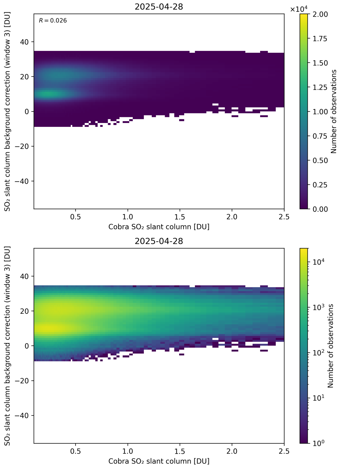
Figure 195: Scatter density plot of “Cobra SO 2 slant column” against “SO 2 slant column background correction (window 3)” for 2025-04-27 to 2025-04-29.
