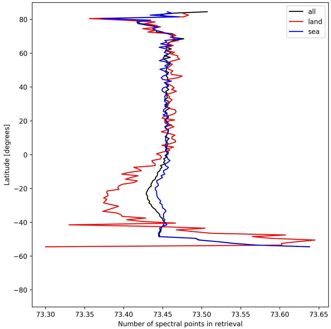
Figure 56: Zonal average of “Number of spectral points in retrieval” for 2025-04-27 to 2025-04-29.
