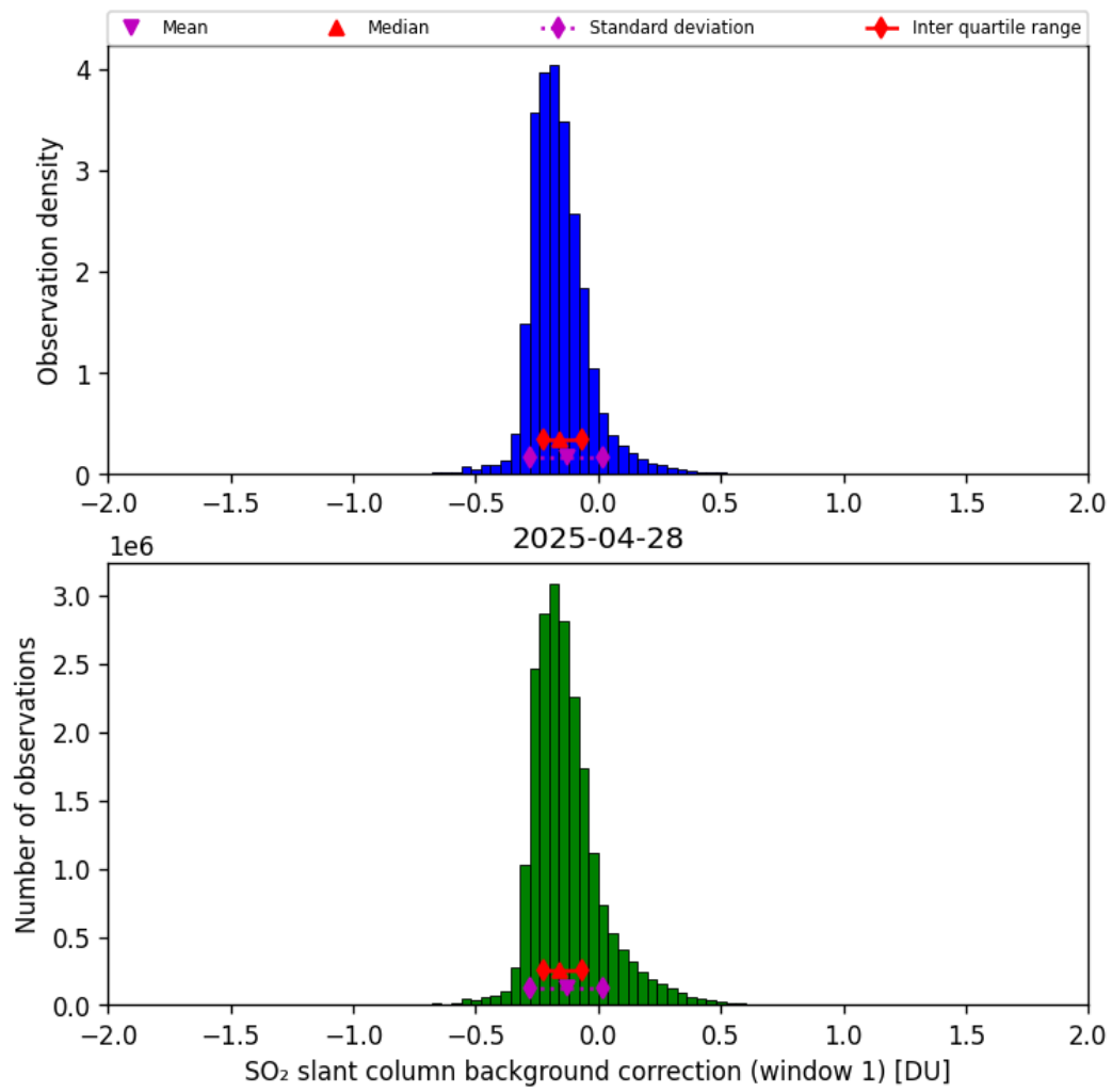
Figure 66: Histogram of “SO 2 slant column background correction (window 1)” for 2025-04-27 to 2025-04-29
