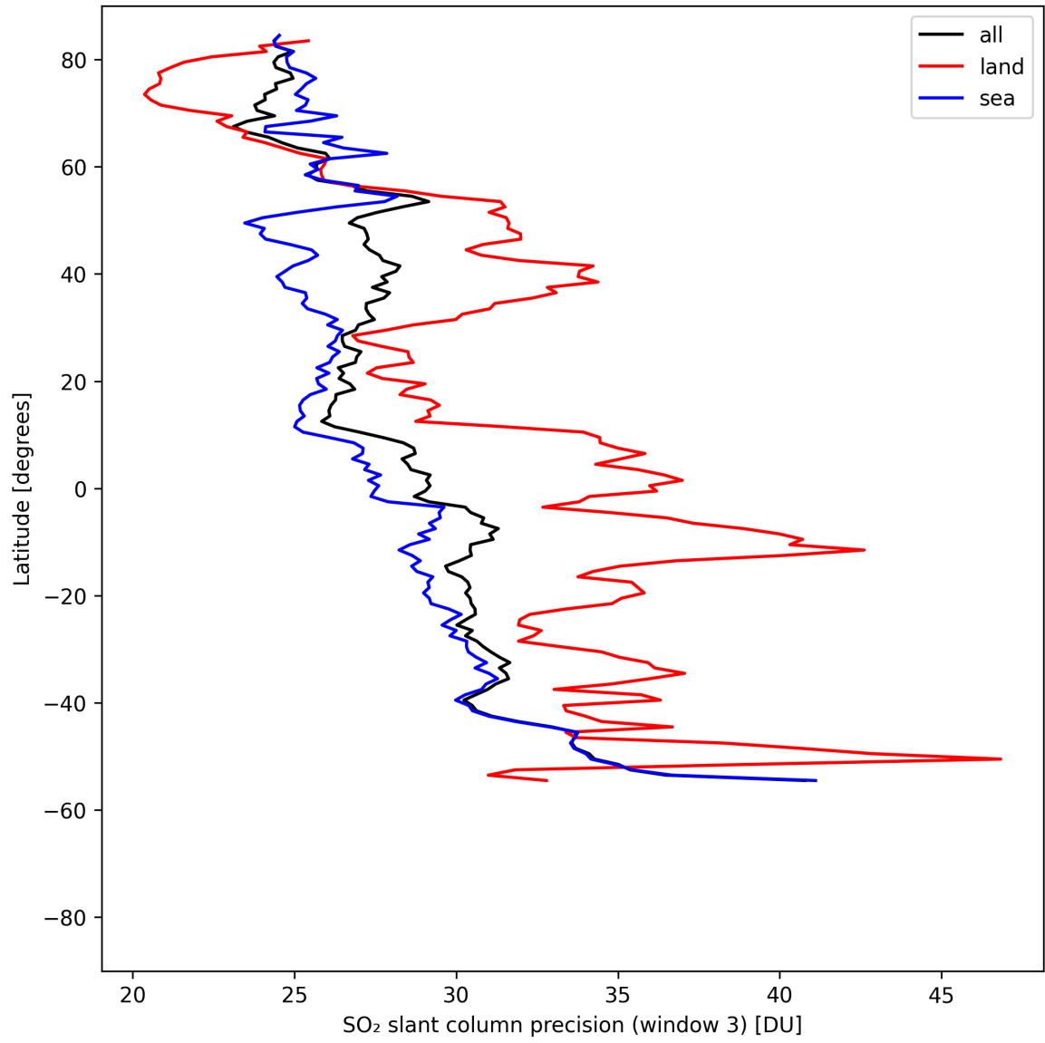
Figure 46: Zonal average of “SO 2 slant column precision (window 3)” for 2025-04-27 to 2025-04-29.
