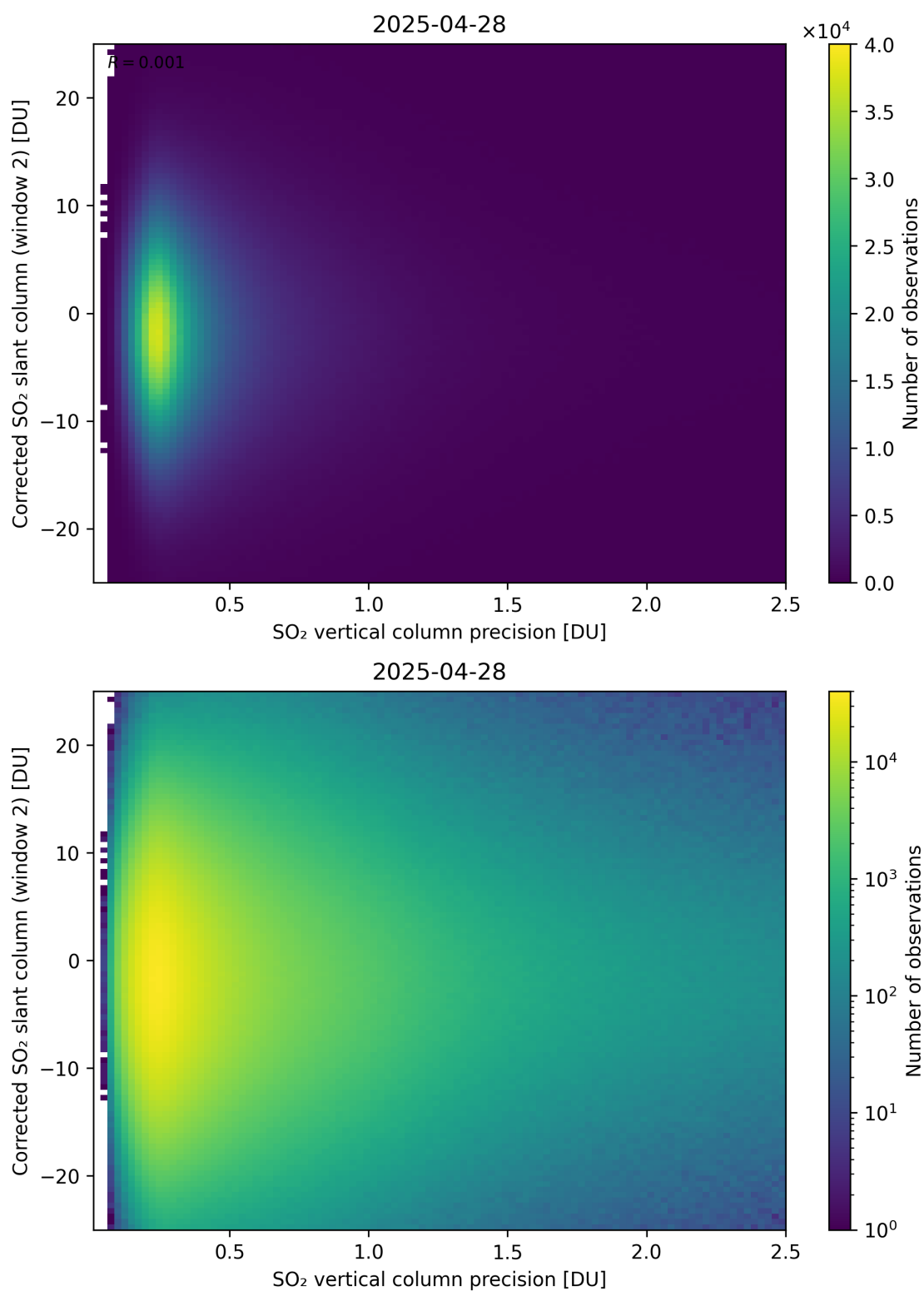
Figure 339: Scatter density plot of “SO 2 vertical column precision” against “Corrected SO 2 slant column (window 2)” for 2025-04-27 to 2025-04-29.
