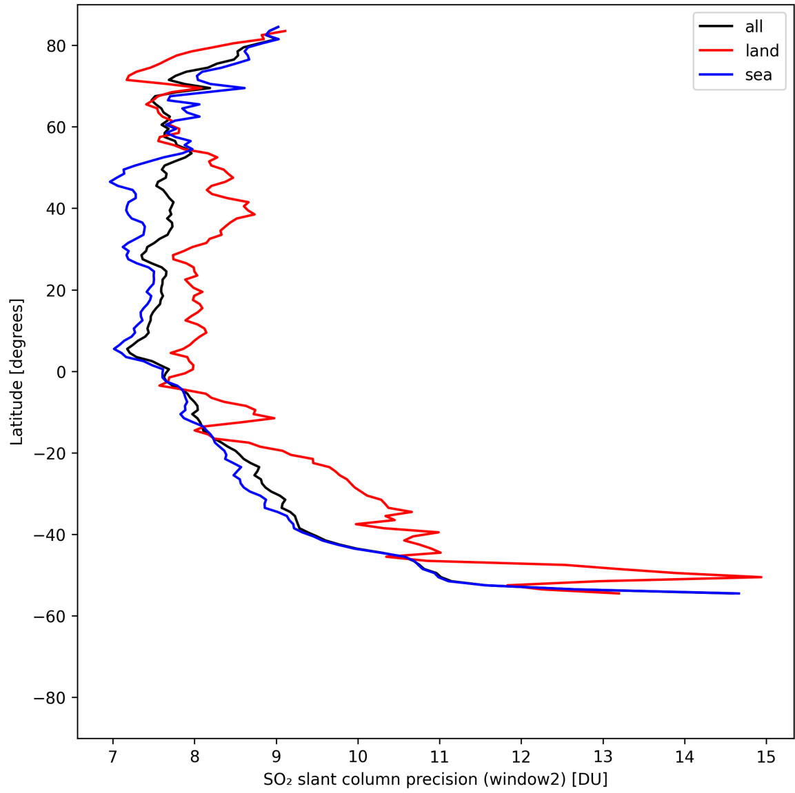
Figure 42: Zonal average of “SO 2 slant column precision (window2)” for 2025-04-27 to 2025-04-29.
