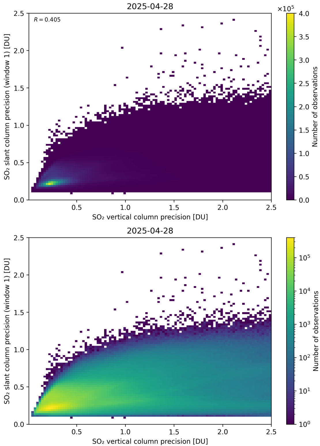
Figure 342: Scatter density plot of “SO 2 vertical column precision” against “SO 2 slant column precision (window 1)” for 2025-04-27 to 2025-04-29.
