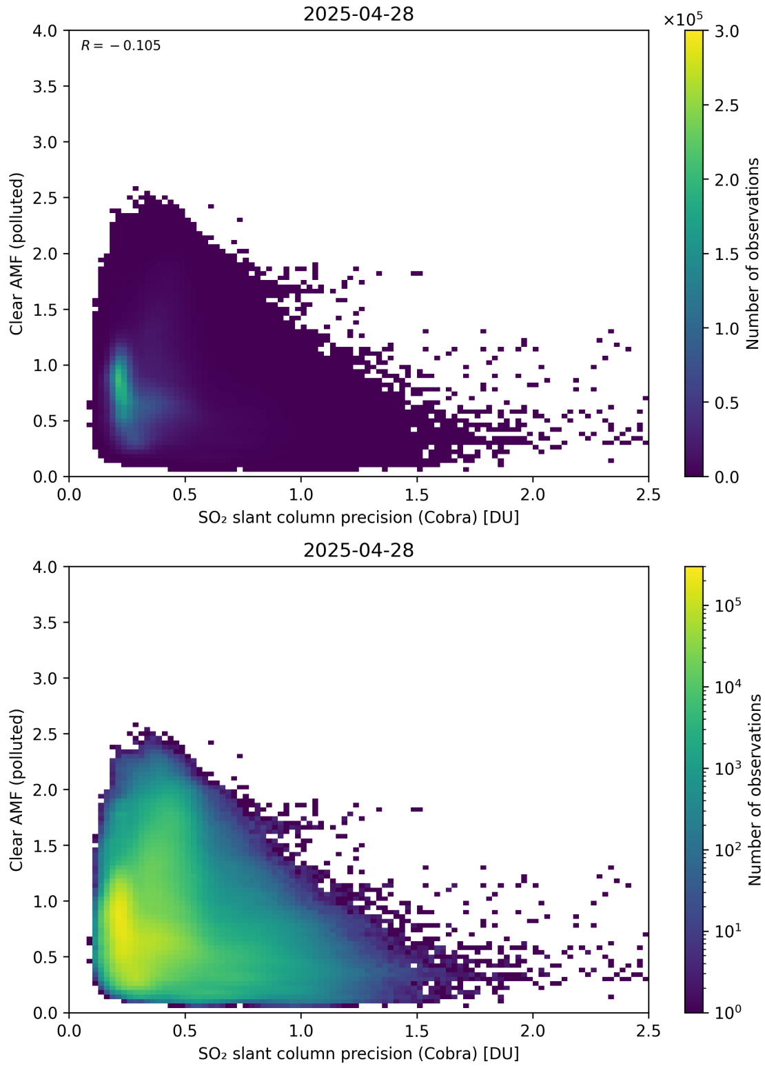
Figure 205: Scatter density plot of “SO 2 slant column precision (Cobra)” against “Clear AMF (polluted)” for 2025-04-27 to 2025-04-29.
