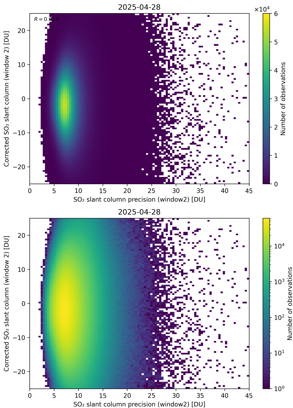
Figure 297: Scatter density plot of “SO 2 slant column precision (window2)” against “Corrected SO 2 slant column (window 2)” for 2025-04-27 to 2025-04-29.
