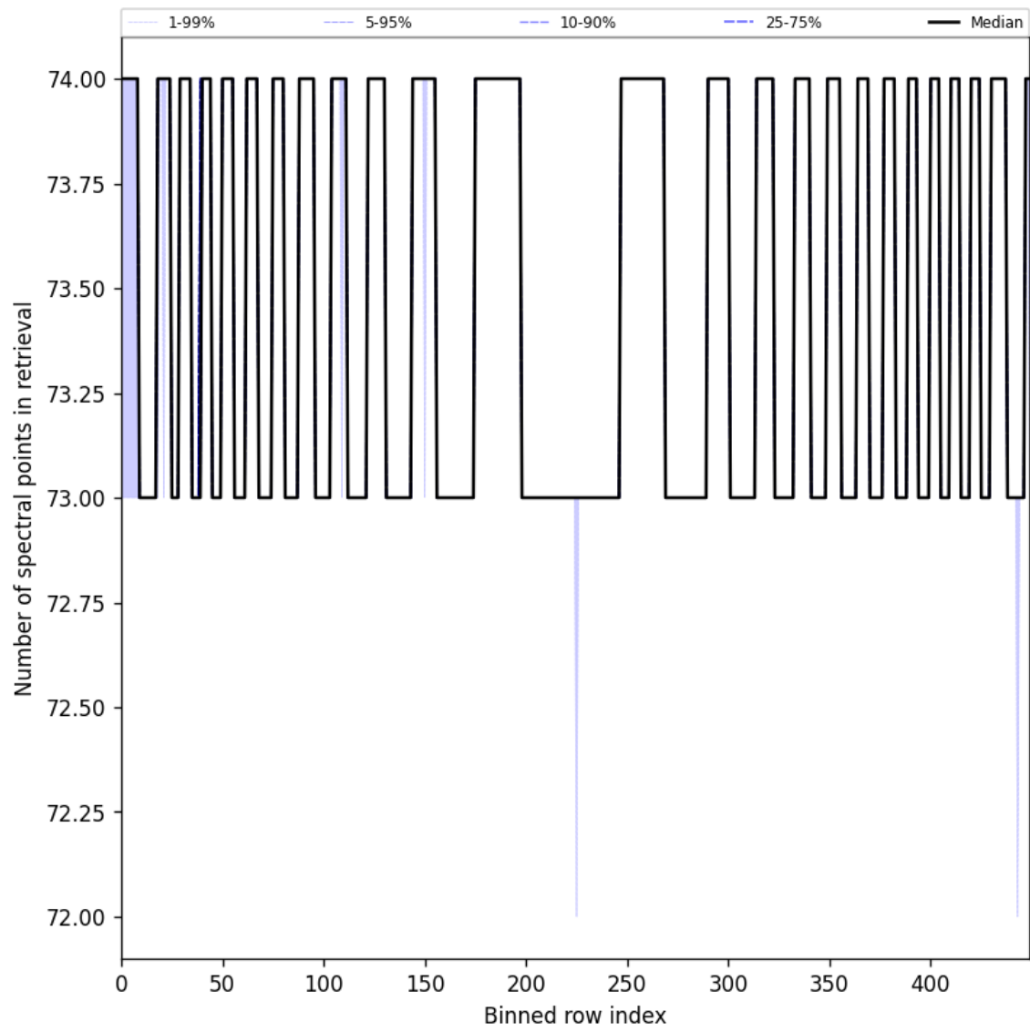
Figure 108: Along track statistics of “Number of spectral points in retrieval” for 2025-04-27 to 2025-04-29
