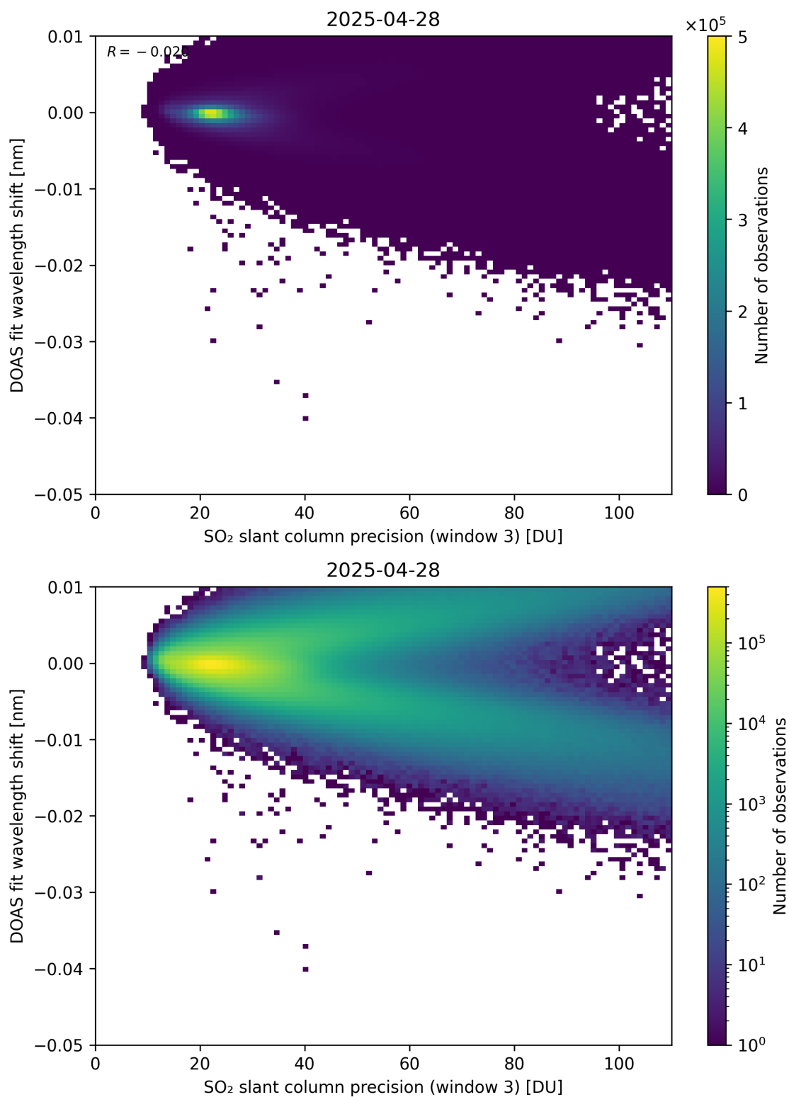
Figure 308: Scatter density plot of “SO 2 slant column precision (window 3)” against “DOAS fit wavelength shift” for 2025-04-27 to 2025-04-29.
