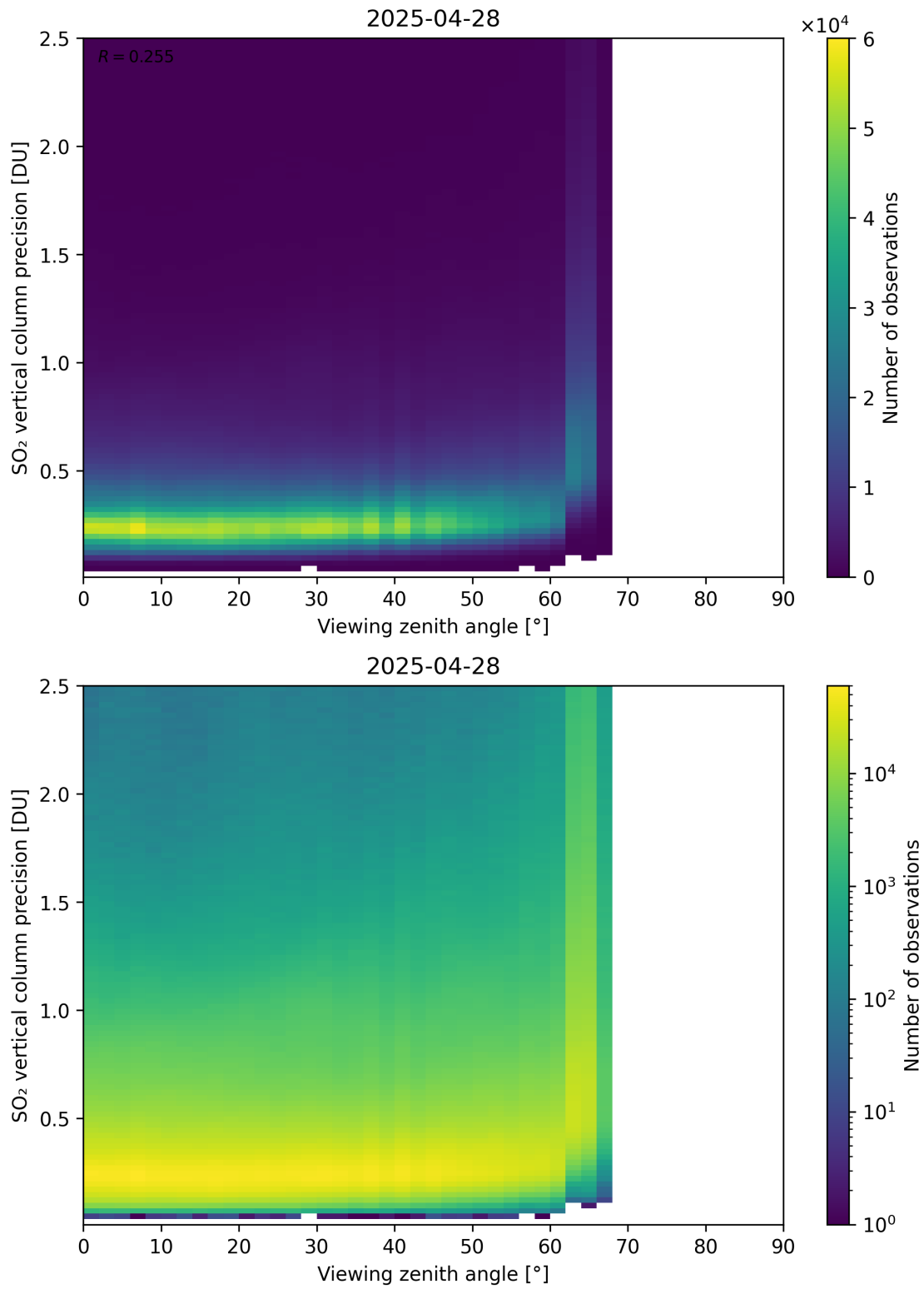
Figure 384: Scatter density plot of “Viewing zenith angle” against “SO 2 vertical column precision” for 2025-04-27 to 2025-04-29.
