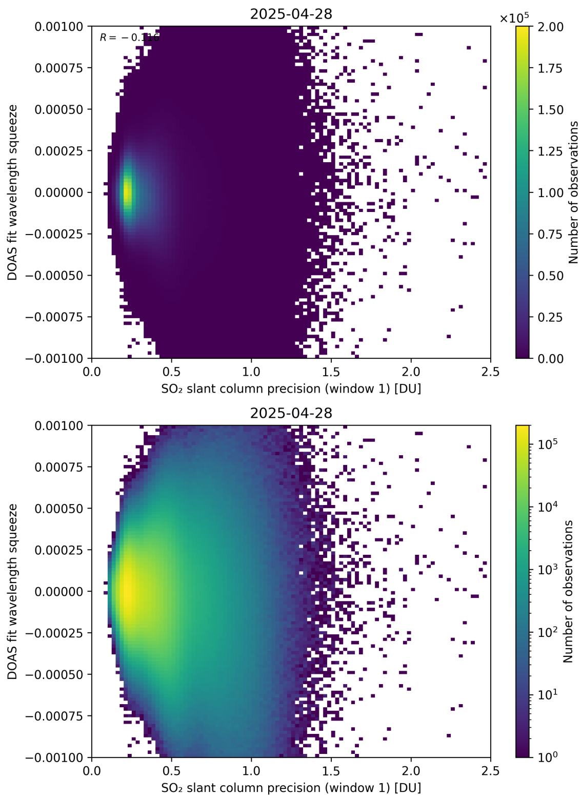
Figure 272: Scatter density plot of “SO 2 slant column precision (window 1)” against “DOAS fit wavelength squeeze” for 2025-04-27 to 2025-04-29.
