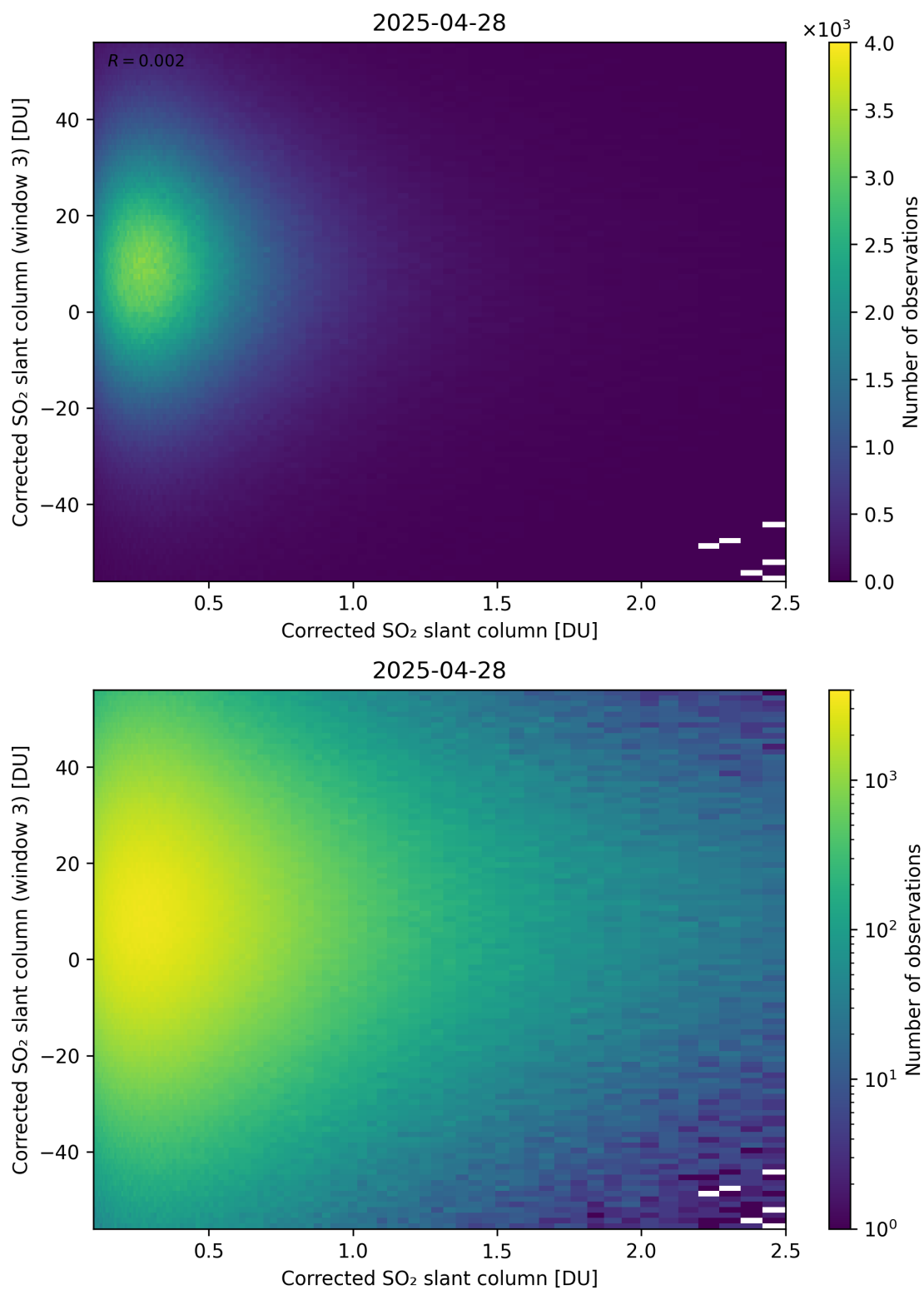
Figure 236: Scatter density plot of “Corrected SO 2 slant column” against “Corrected SO 2 slant column (window 3)” for 2025-04-27 to 2025-04-29.
