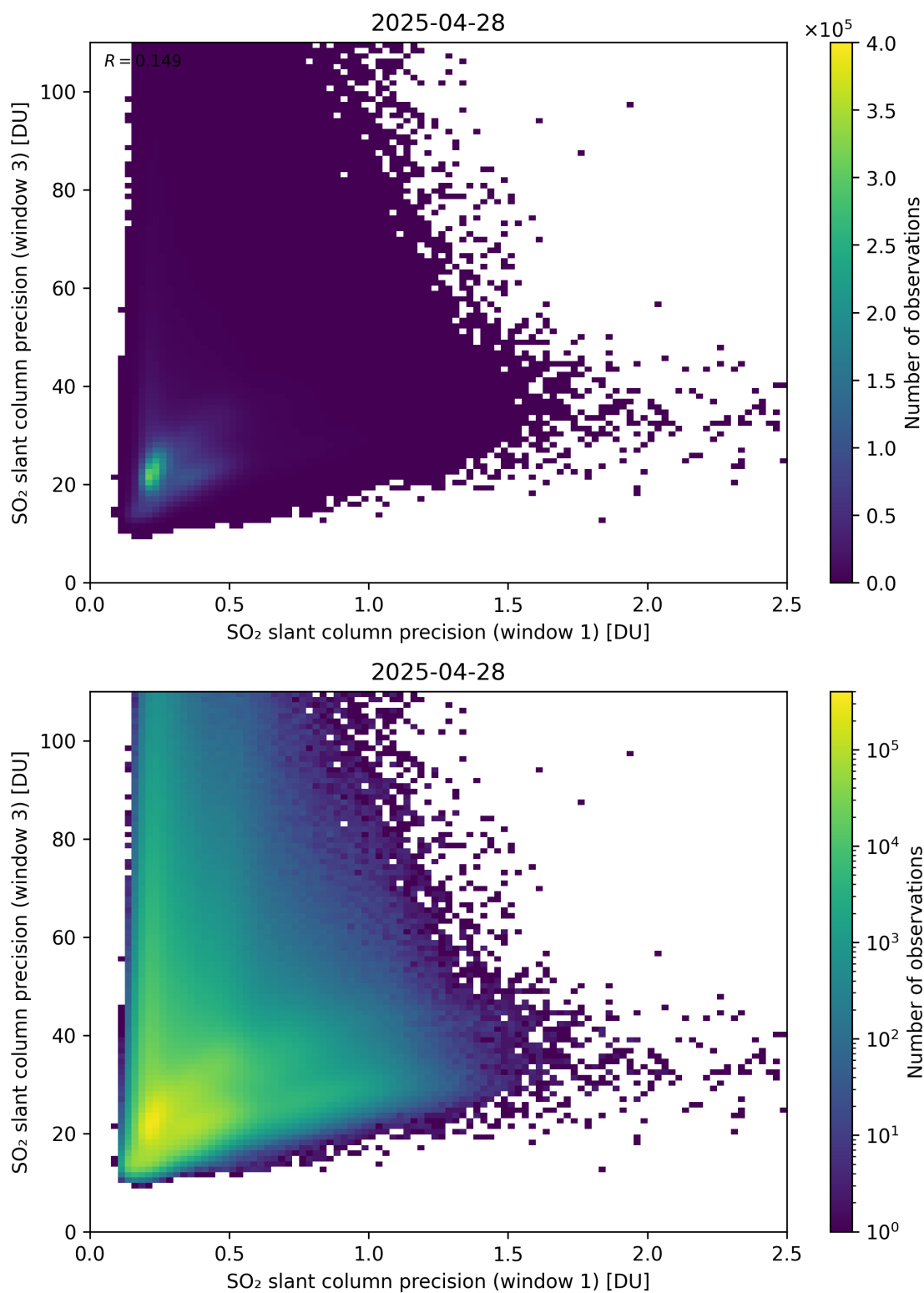
Figure 279: Scatter density plot of “SO 2 slant column precision (window 1)” against “SO 2 slant column precision (window 3)” for 2025-04-27 to 2025-04-29.
