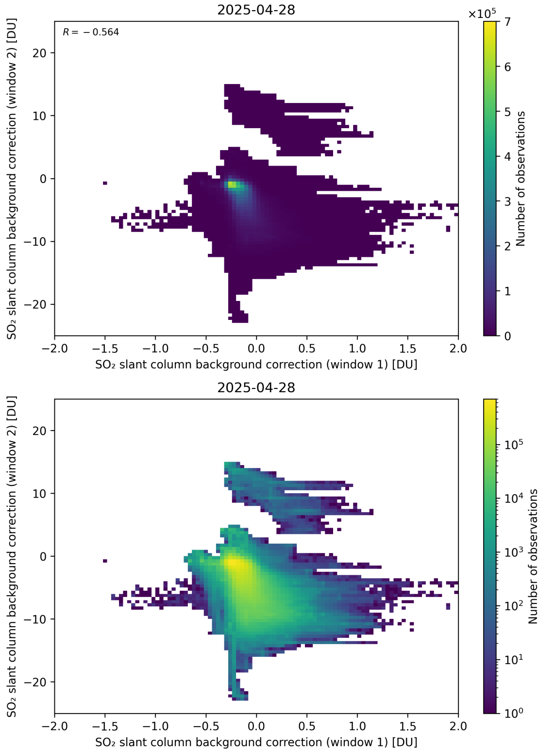
Figure 109: Scatter density plot of “SO 2 slant column background correction (window 1)” against “SO 2 slant column background correction (window 2)” for 2025-04-27 to 2025-04-29.
