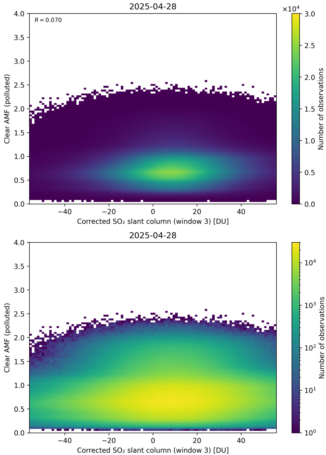
Figure 259: Scatter density plot of “Corrected SO 2 slant column (window 3)” against “Clear AMF (polluted)” for 2025-04-27 to 2025-04-29.
