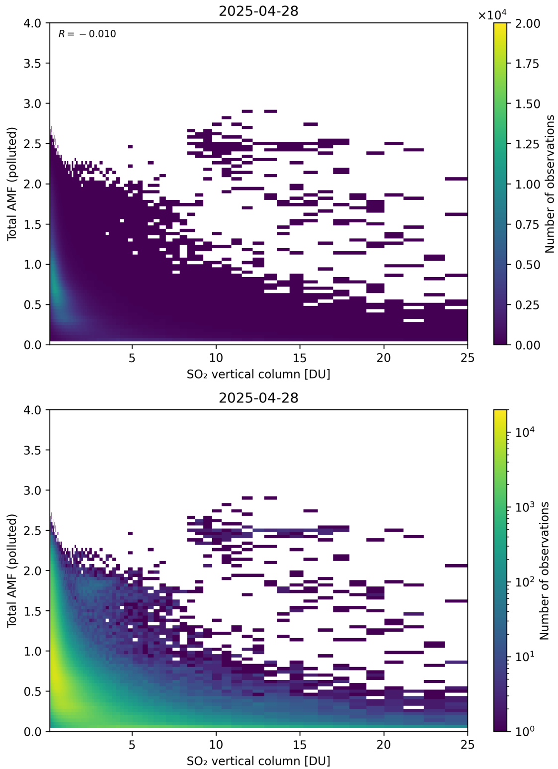
Figure 359: Scatter density plot of “SO 2 vertical column” against “Total AMF (polluted)” for 2025-04-27 to 2025-04-29.
