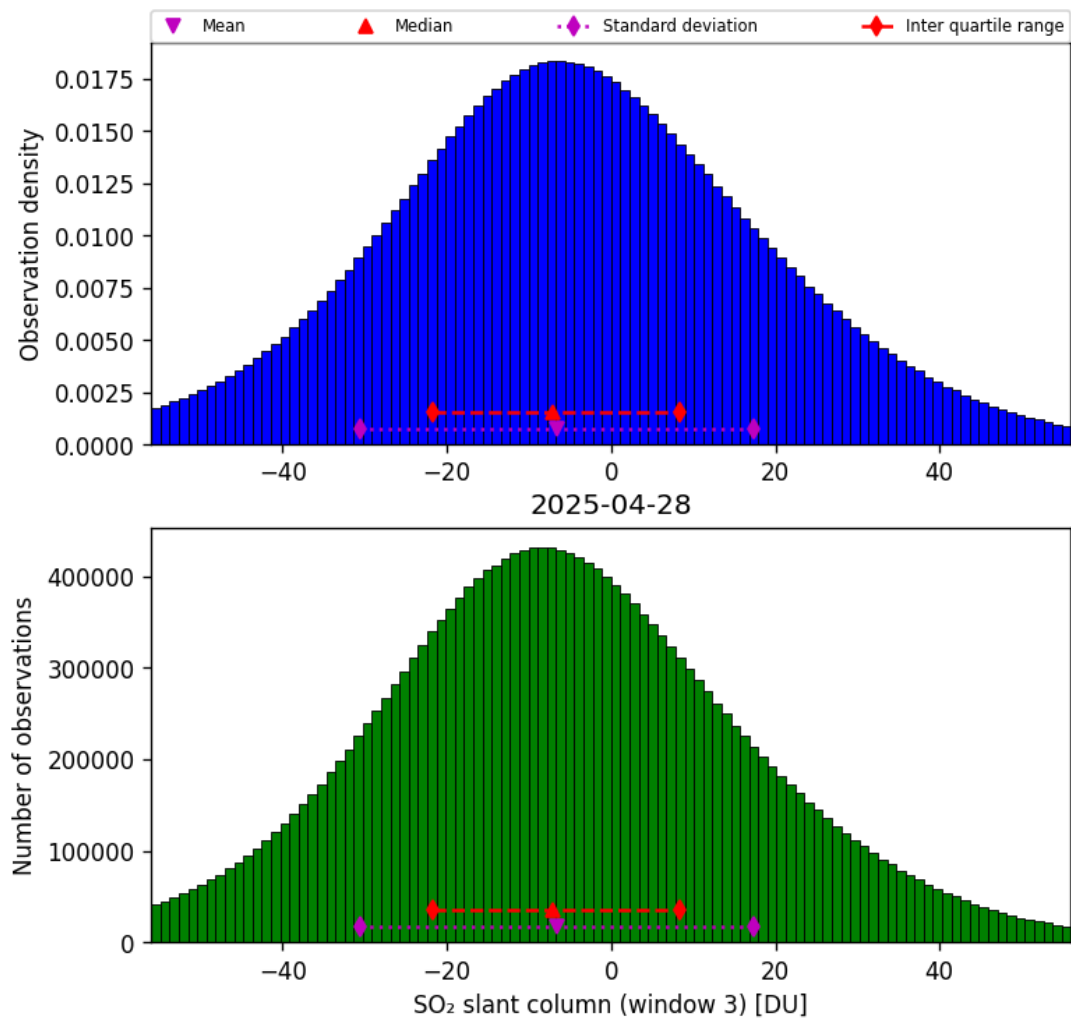
Figure 71: Histogram of “SO 2 slant column (window 3)” for 2025-04-27 to 2025-04-29
