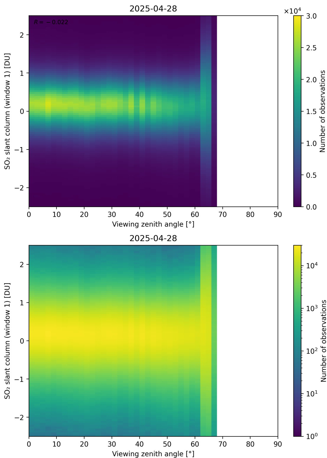
Figure 376: Scatter density plot of “Viewing zenith angle” against “SO 2 slant column (window 1)” for 2025-04-27 to 2025-04-29.
