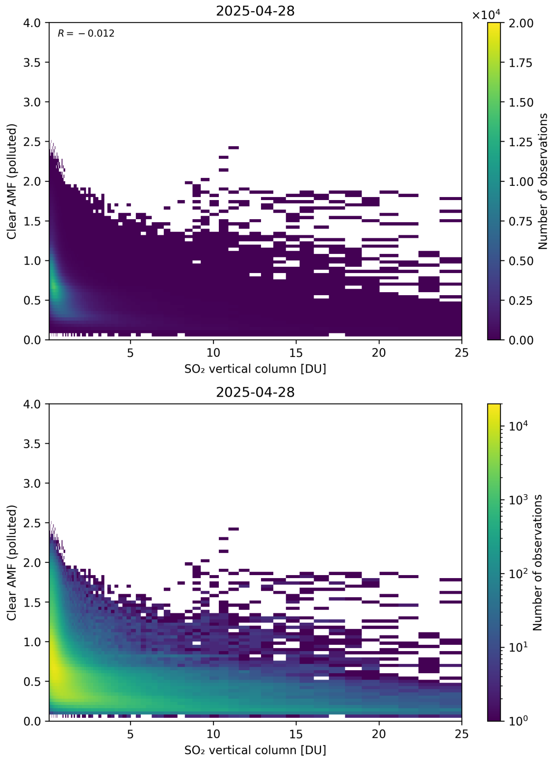
Figure 348: Scatter density plot of “SO 2 vertical column” against “Clear AMF (polluted)” for 2025-04-27 to 2025-04-29.
