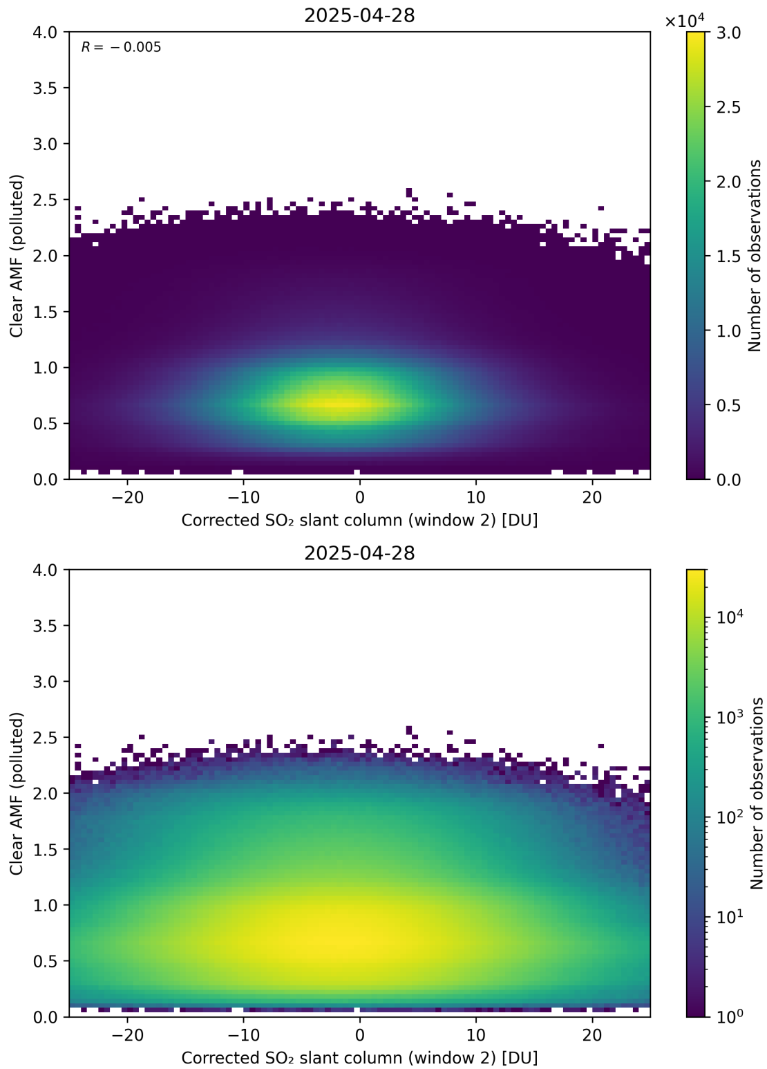
Figure 249: Scatter density plot of “Corrected SO 2 slant column (window 2)” against “Clear AMF (polluted)” for 2025-04-27 to 2025-04-29.
