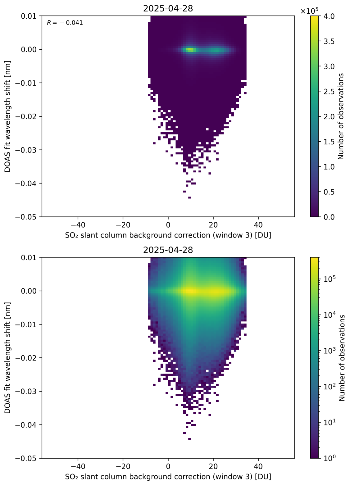
Figure 132: Scatter density plot of “SO 2 slant column background correction (window 3)” against “DOAS fit wavelength shift” for 2025-04-27 to 2025-04-29.
