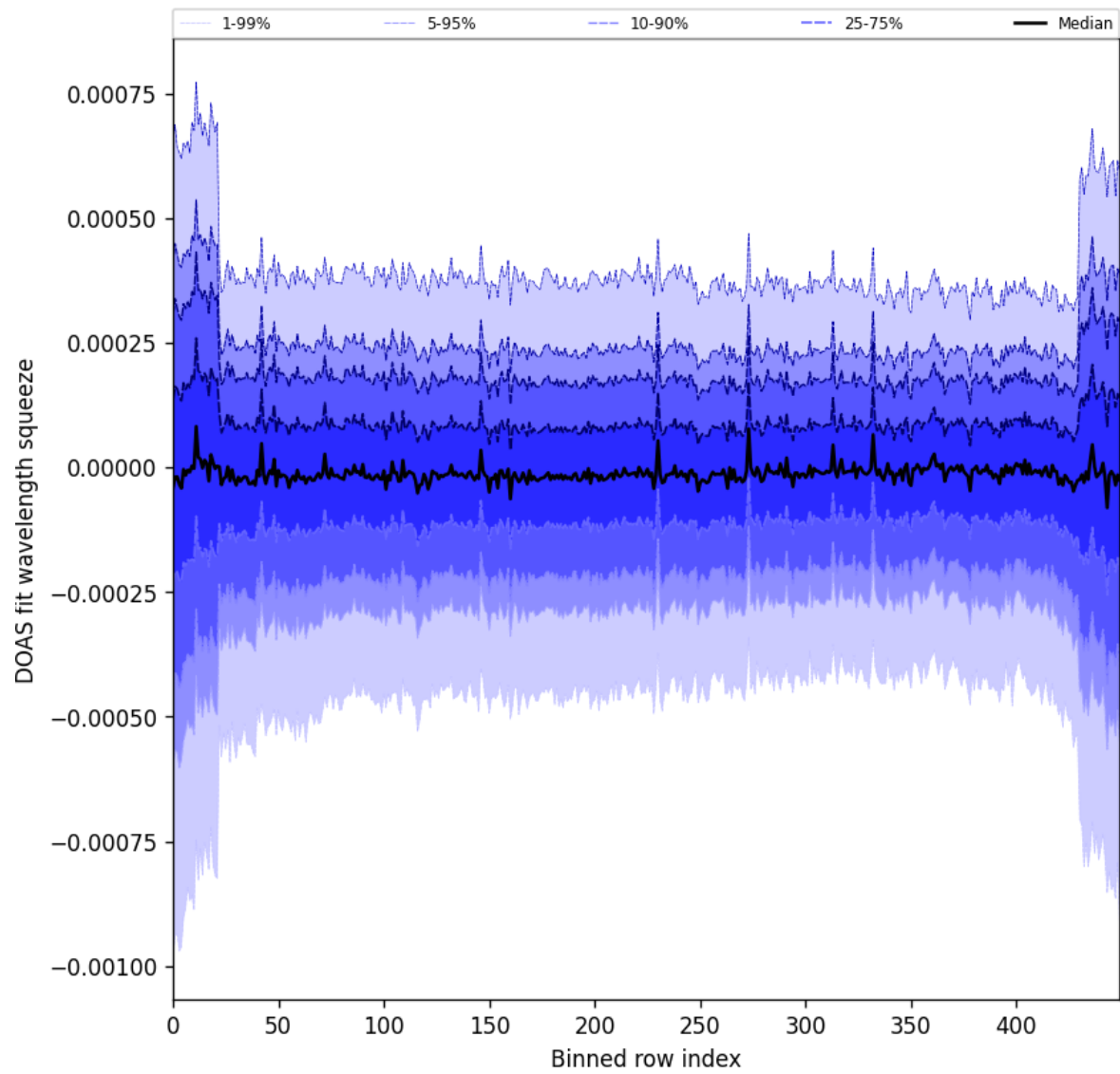
Figure 103: Along track statistics of “DOAS fit wavelength squeeze” for 2025-04-27 to 2025-04-29
