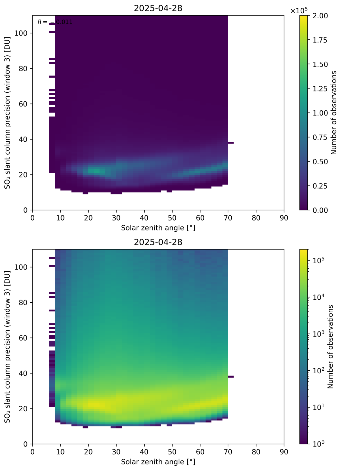
Figure 188: Scatter density plot of “Solar zenith angle” against “SO 2 slant column precision (window 3)” for 2025-04-27 to 2025-04-29.
