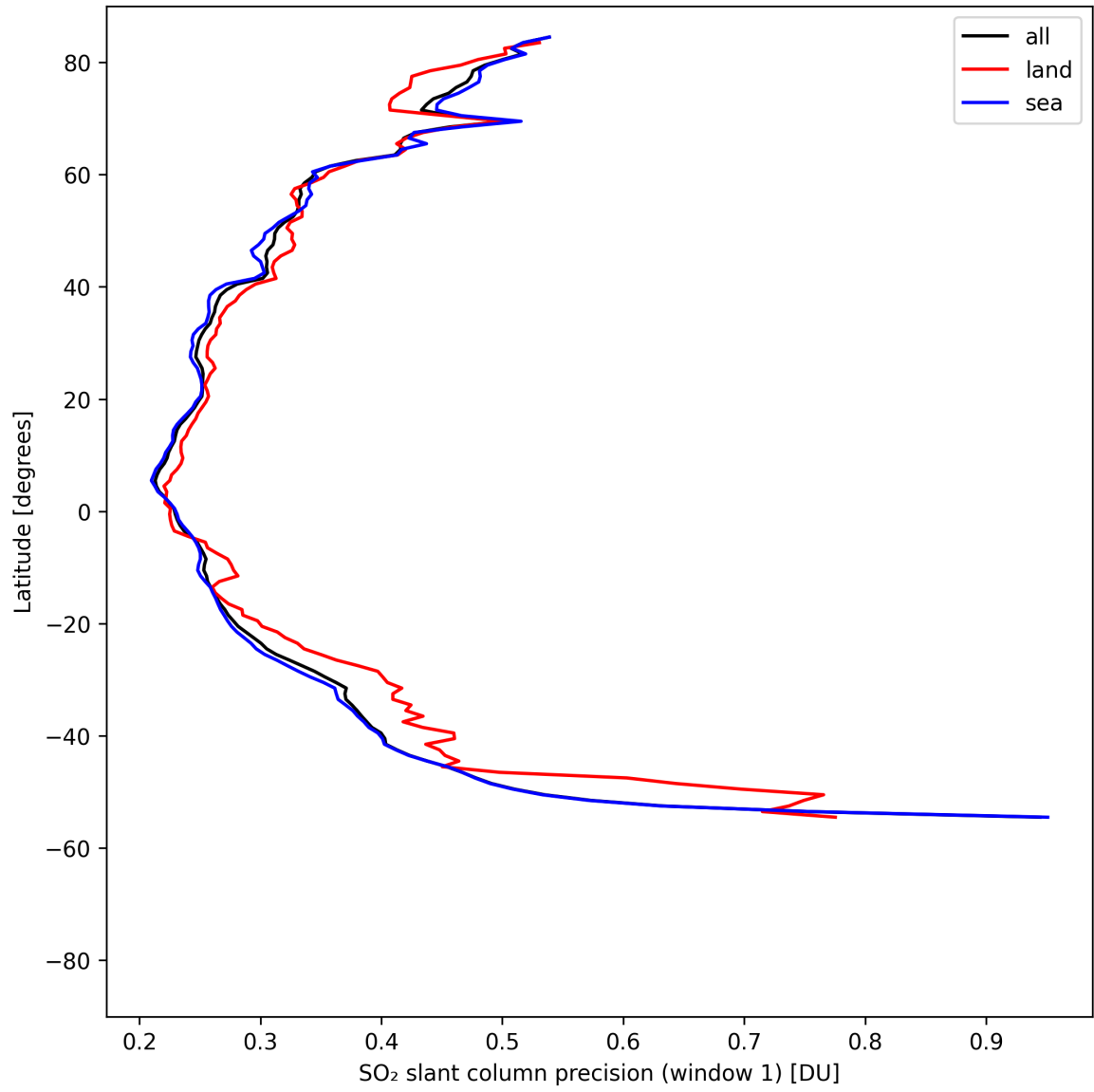
Figure 38: Zonal average of “SO 2 slant column precision (window 1)” for 2025-04-27 to 2025-04-29.
