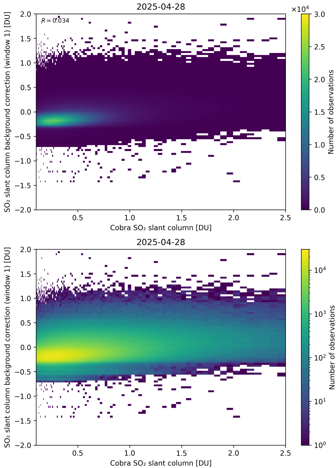
Figure 193: Scatter density plot of “Cobra SO 2 slant column” against “SO 2 slant column background correction (window 1)” for 2025-04-27 to 2025-04-29.
