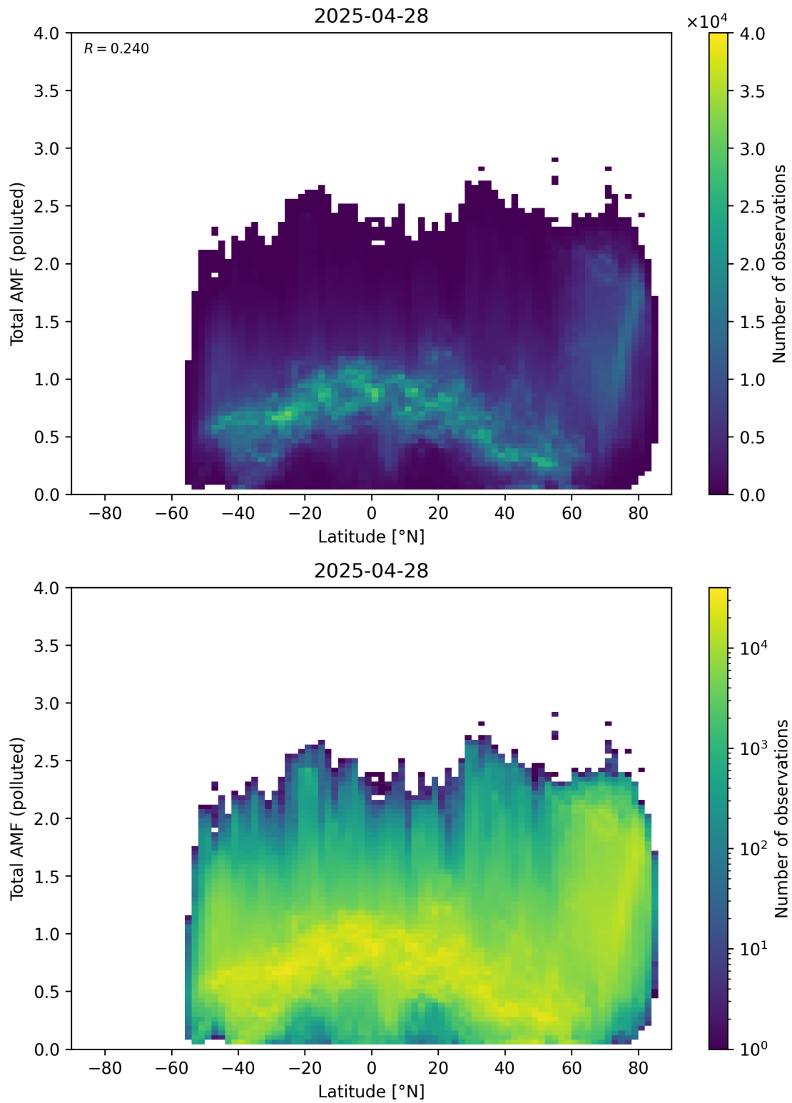
Figure 167: Scatter density plot of “Latitude” against “Total AMF (polluted)” for 2025-04-27 to 2025-04-29.
