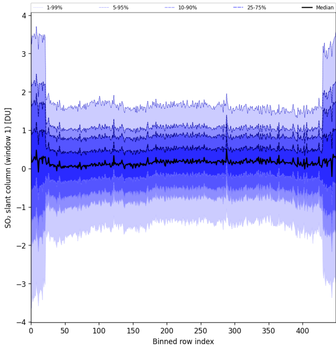
Figure 89: Along track statistics of “SO 2 slant column (window 1)” for 2025-04-27 to 2025-04-29
