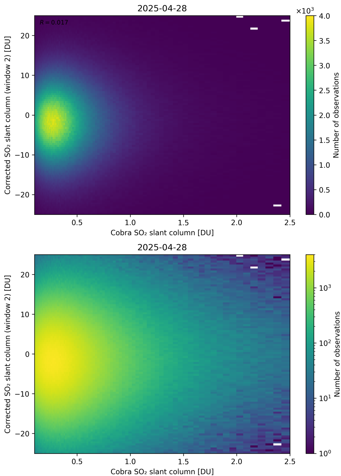
Figure 217: Scatter density plot of “Cobra SO 2 slant column” against “Corrected SO 2 slant column (window 2)” for 2025-04-27 to 2025-04-29.
