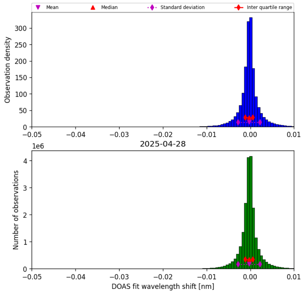
Figure 76: Histogram of “DOAS fit wavelength shift” for 2025-04-27 to 2025-04-29
