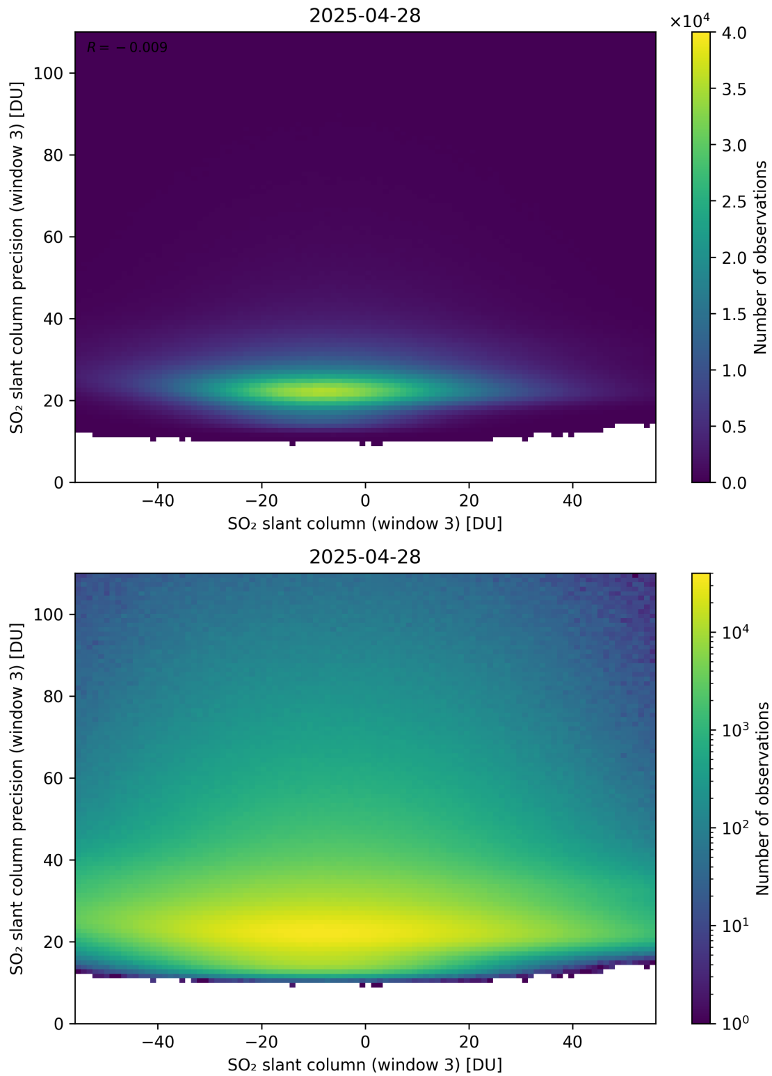
Figure 317: Scatter density plot of “SO 2 slant column (window 3)” against “SO 2 slant column precision (window 3)” for 2025-04-27 to 2025-04-29.
