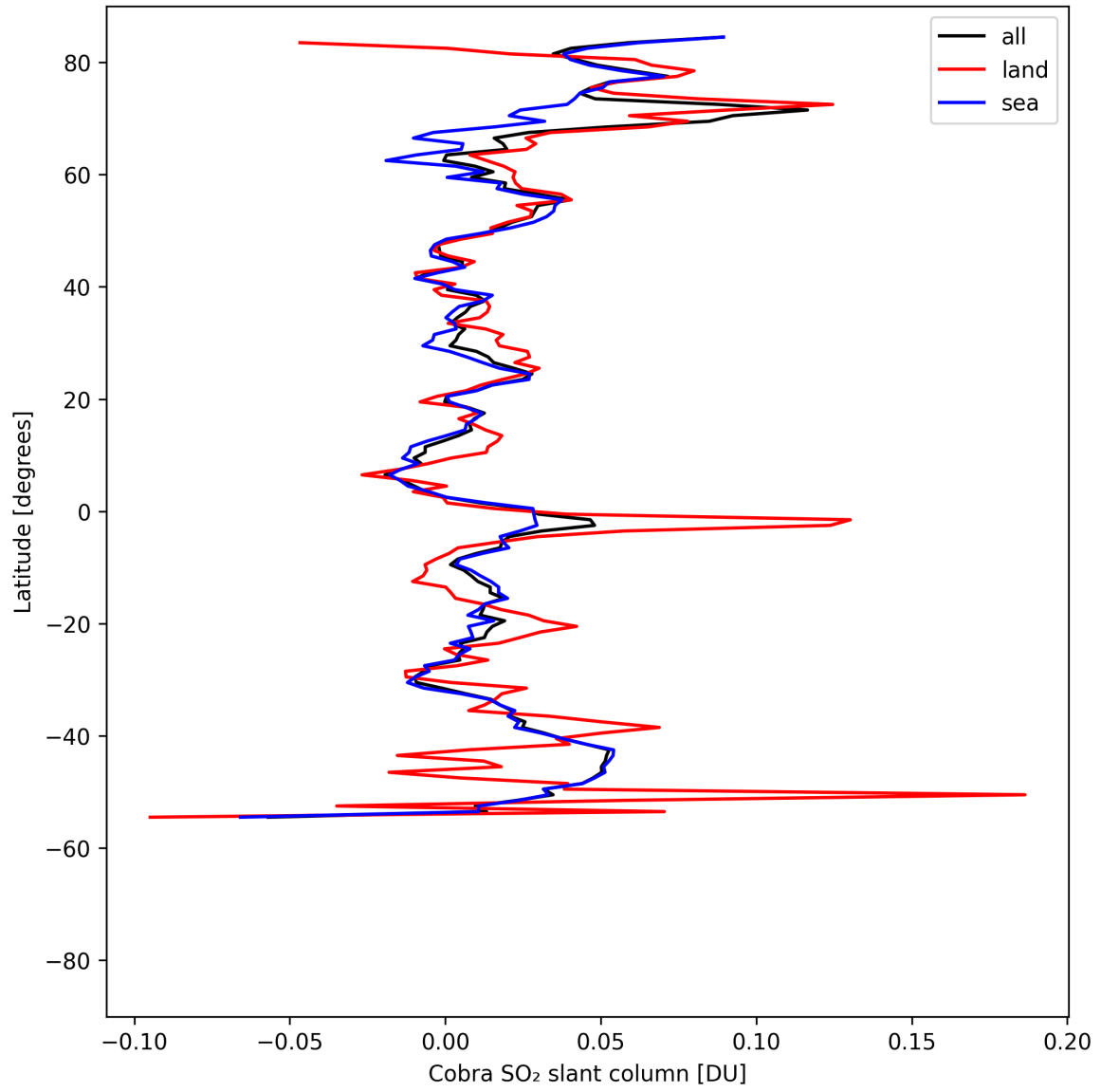
Figure 35: Zonal average of “Cobra SO 2 slant column” for 2025-04-27 to 2025-04-29.
