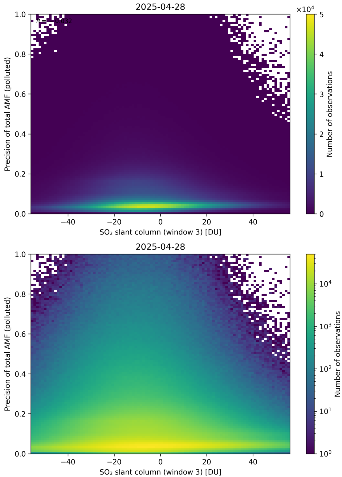
Figure 319: Scatter density plot of “SO 2 slant column (window 3)” against “Precision of total AMF (polluted)” for 2025-04-27 to 2025-04-29.
