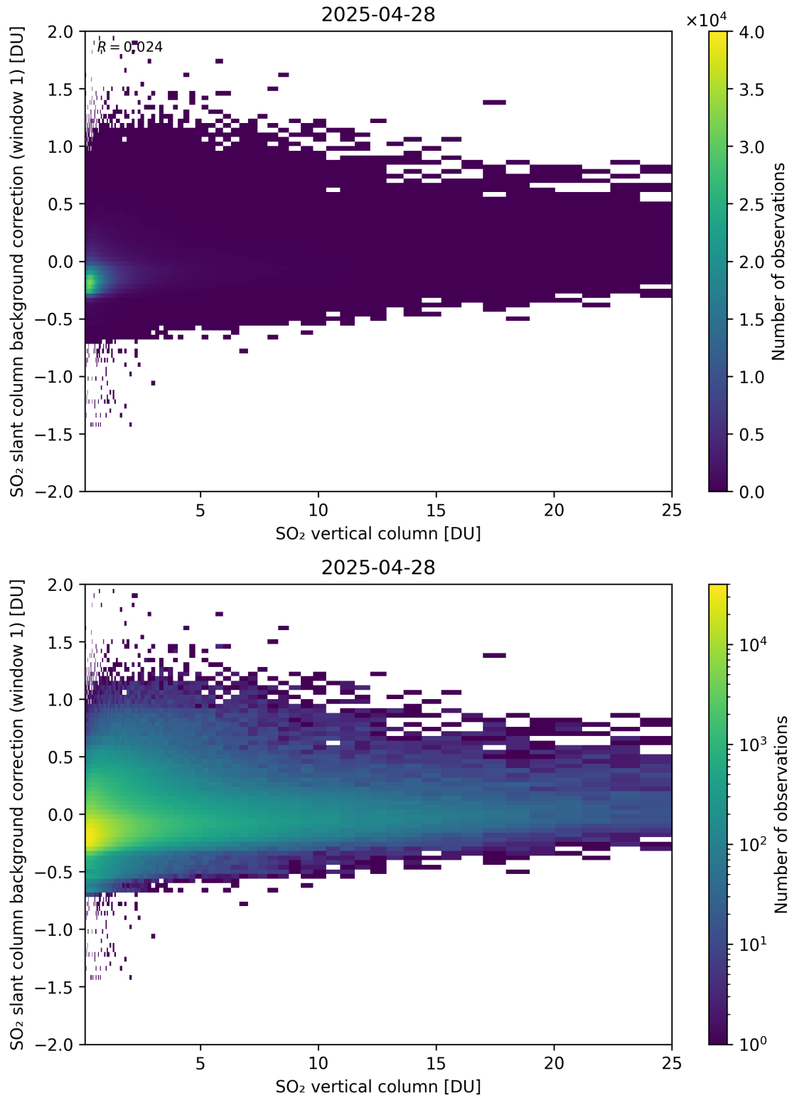
Figure 323: Scatter density plot of “SO 2 vertical column” against “SO 2 slant column background correction (window 1)” for 2025-04-27 to 2025-04-29.
