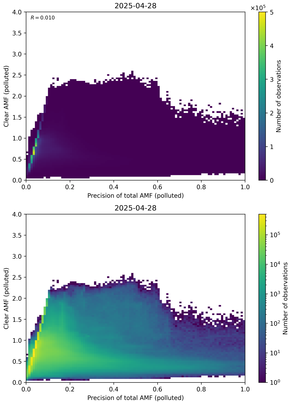
Figure 320: Scatter density plot of “Precision of total AMF (polluted)” against “Clear AMF (polluted)” for 2025-04-27 to 2025-04-29.
