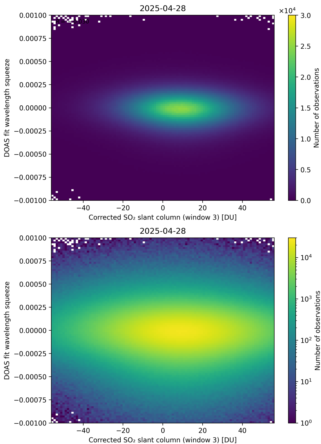
Figure 257: Scatter density plot of “Corrected SO 2 slant column (window 3)” against “DOAS fit wavelength squeeze” for 2025-04-27 to 2025-04-29.
