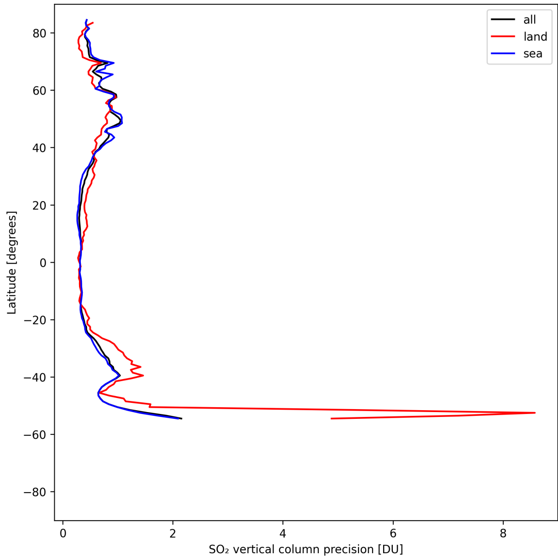
Figure 33: Zonal average of “SO 2 vertical column precision” for 2025-04-27 to 2025-04-29.
