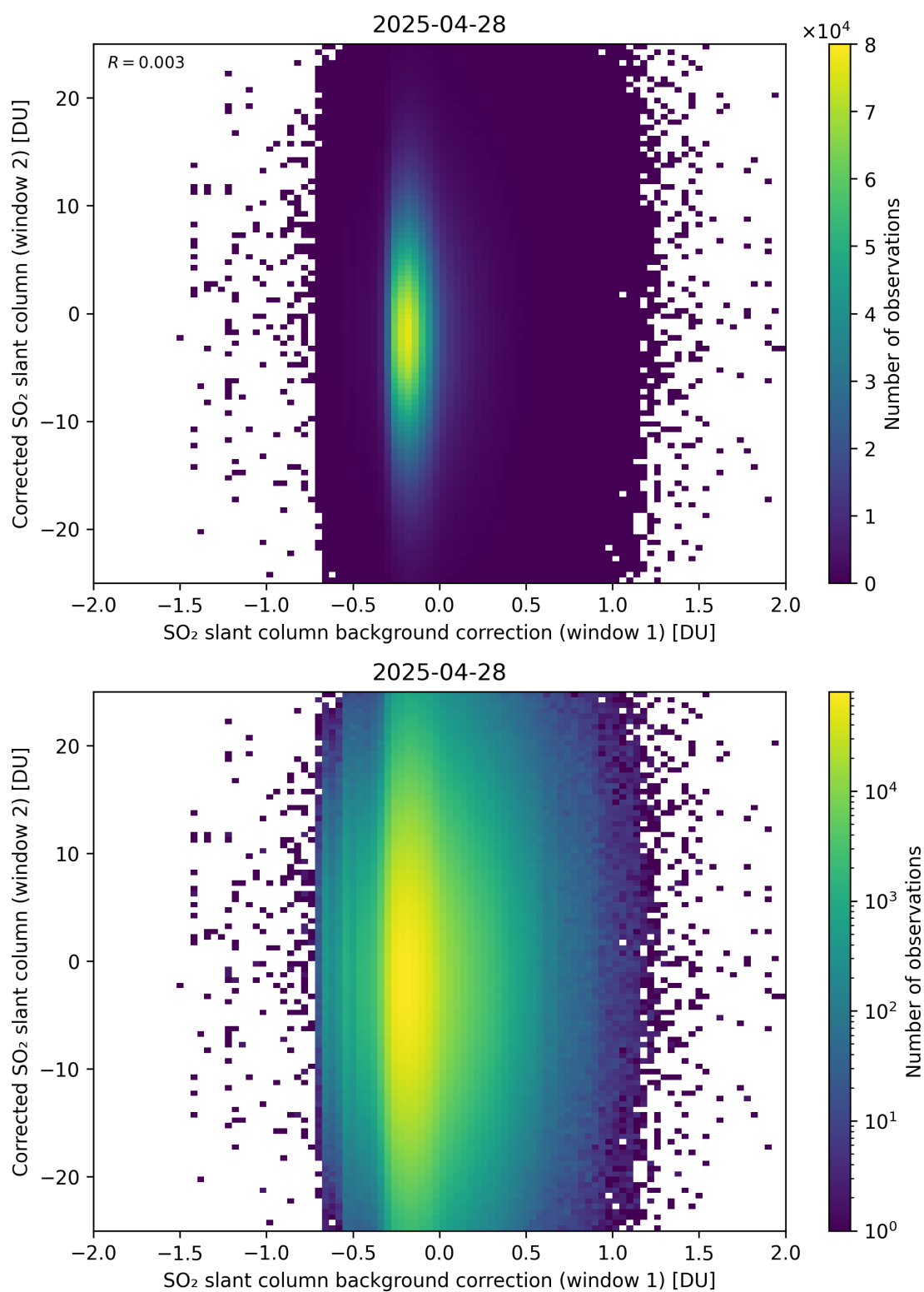
Figure 115: Scatter density plot of “SO 2 slant column background correction (window 1)” against “Corrected SO 2 slant column (window 2)” for 2025-04-27 to 2025-04-29.
