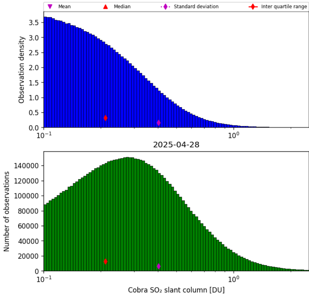
Figure 61: Histogram of “Cobra SO 2 slant column” for 2025-04-27 to 2025-04-29
