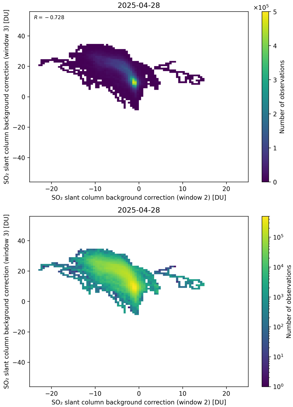
Figure 122: Scatter density plot of “SO 2 slant column background correction (window 2)” against “SO 2 slant column background correction (window 3)” for 2025-04-27 to 2025-04-29.
