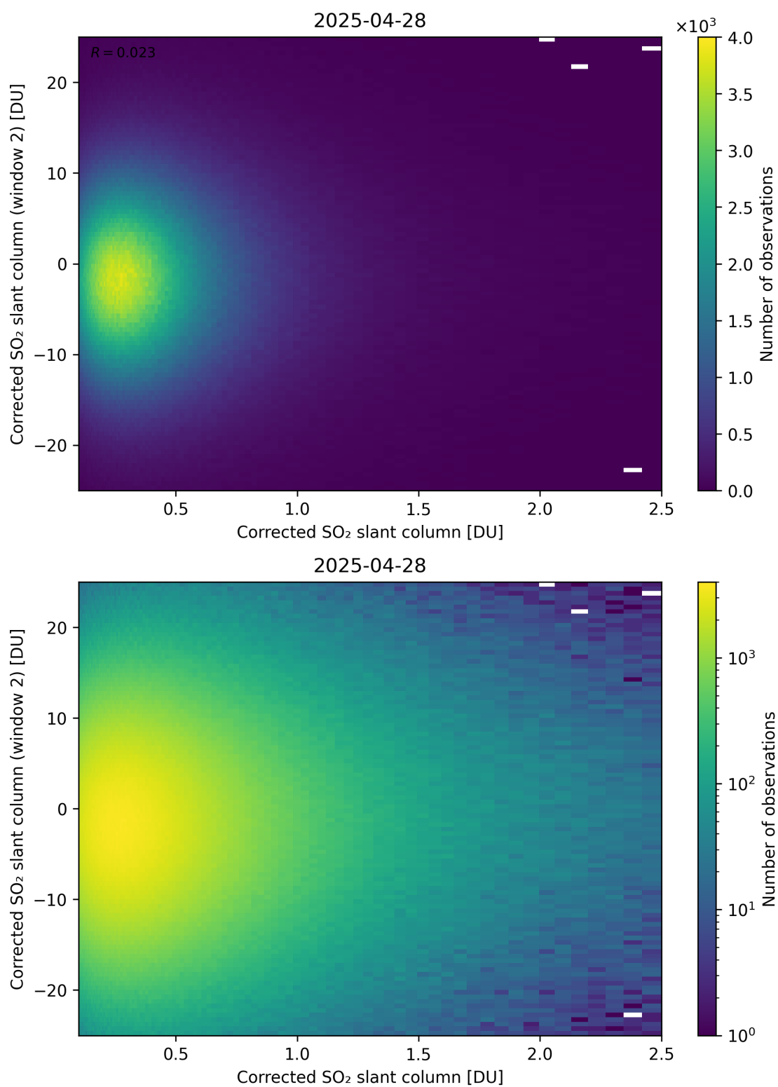
Figure 235: Scatter density plot of “Corrected SO 2 slant column” against “Corrected SO 2 slant column (window 2)” for 2025-04-27 to 2025-04-29.
