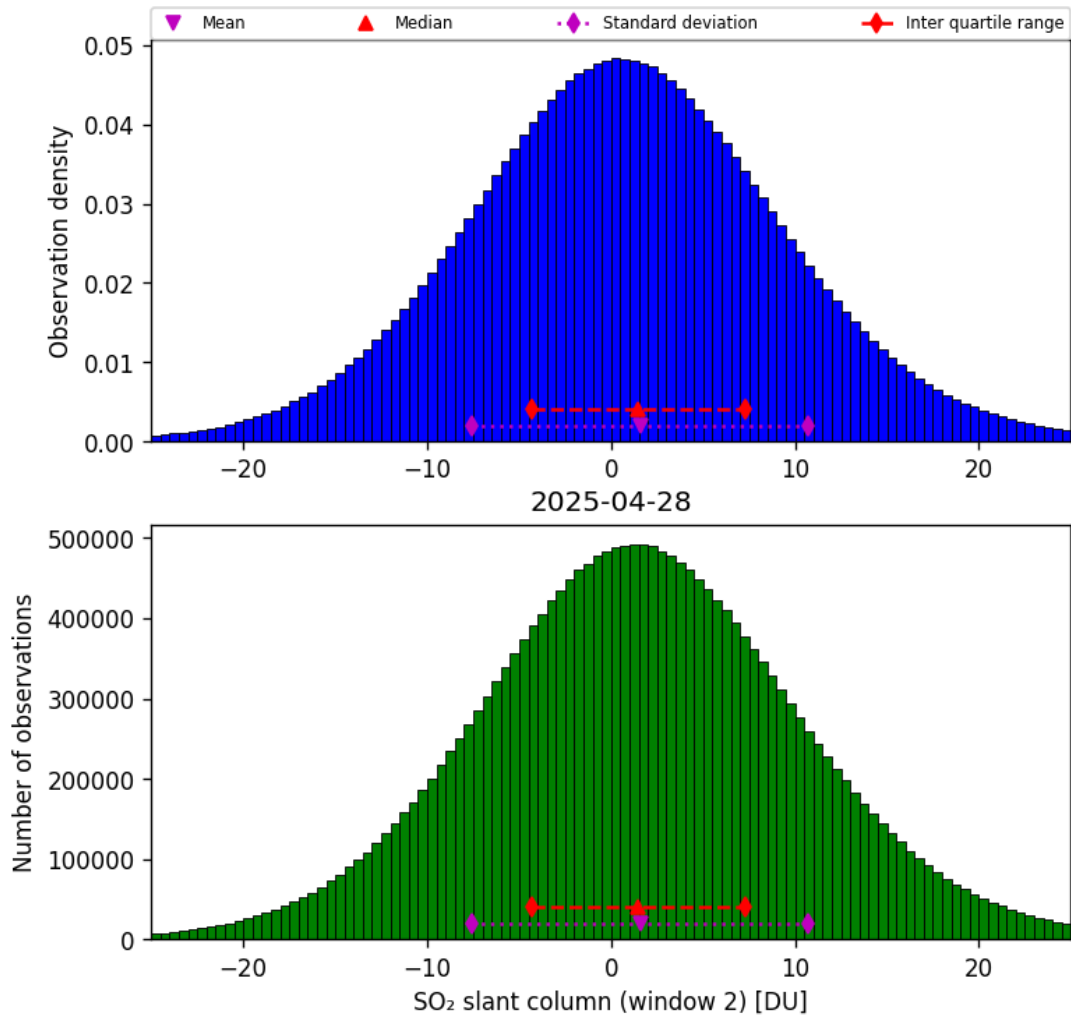
Figure 67: Histogram of “SO 2 slant column (window 2)” for 2025-04-27 to 2025-04-29
