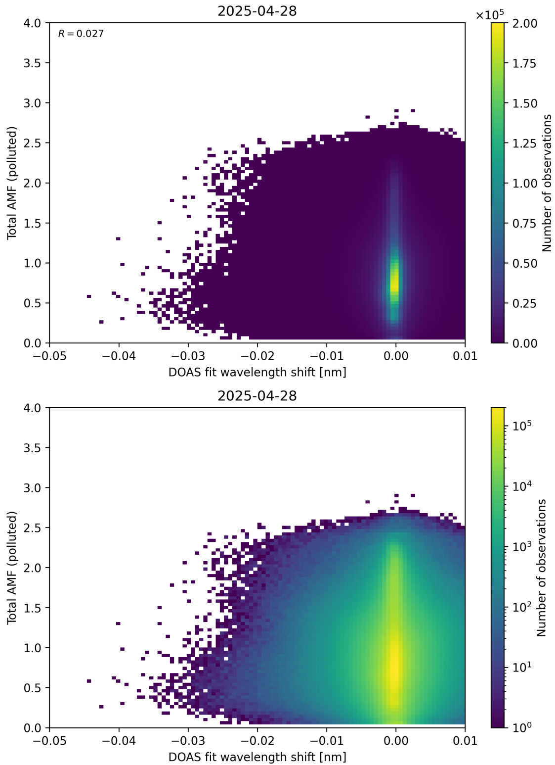
Figure 141: Scatter density plot of “DOAS fit wavelength shift” against “Total AMF (polluted)” for 2025-04-27 to 2025-04-29.
