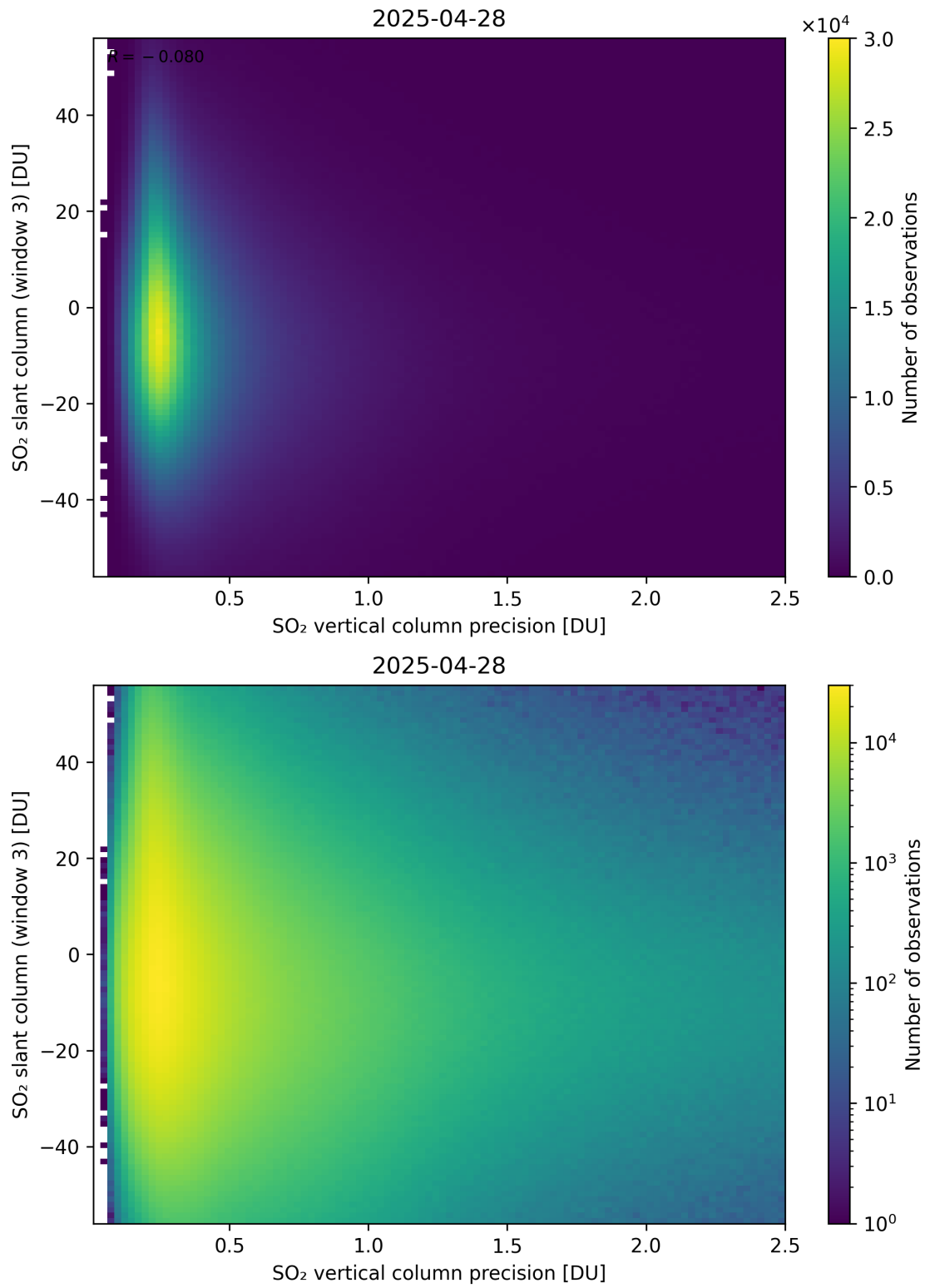
Figure 344: Scatter density plot of “SO 2 vertical column precision” against “SO 2 slant column (window 3)” for 2025-04-27 to 2025-04-29.
