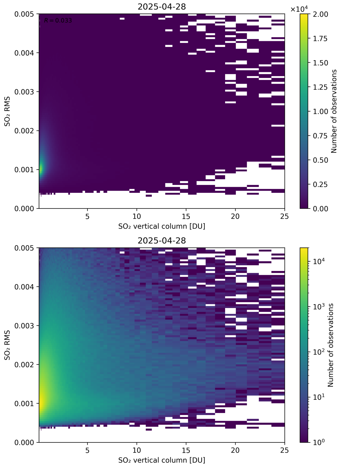
Figure 328: Scatter density plot of “SO 2 vertical column” against “SO 2 RMS” for 2025-04-27 to 2025-04-29.
