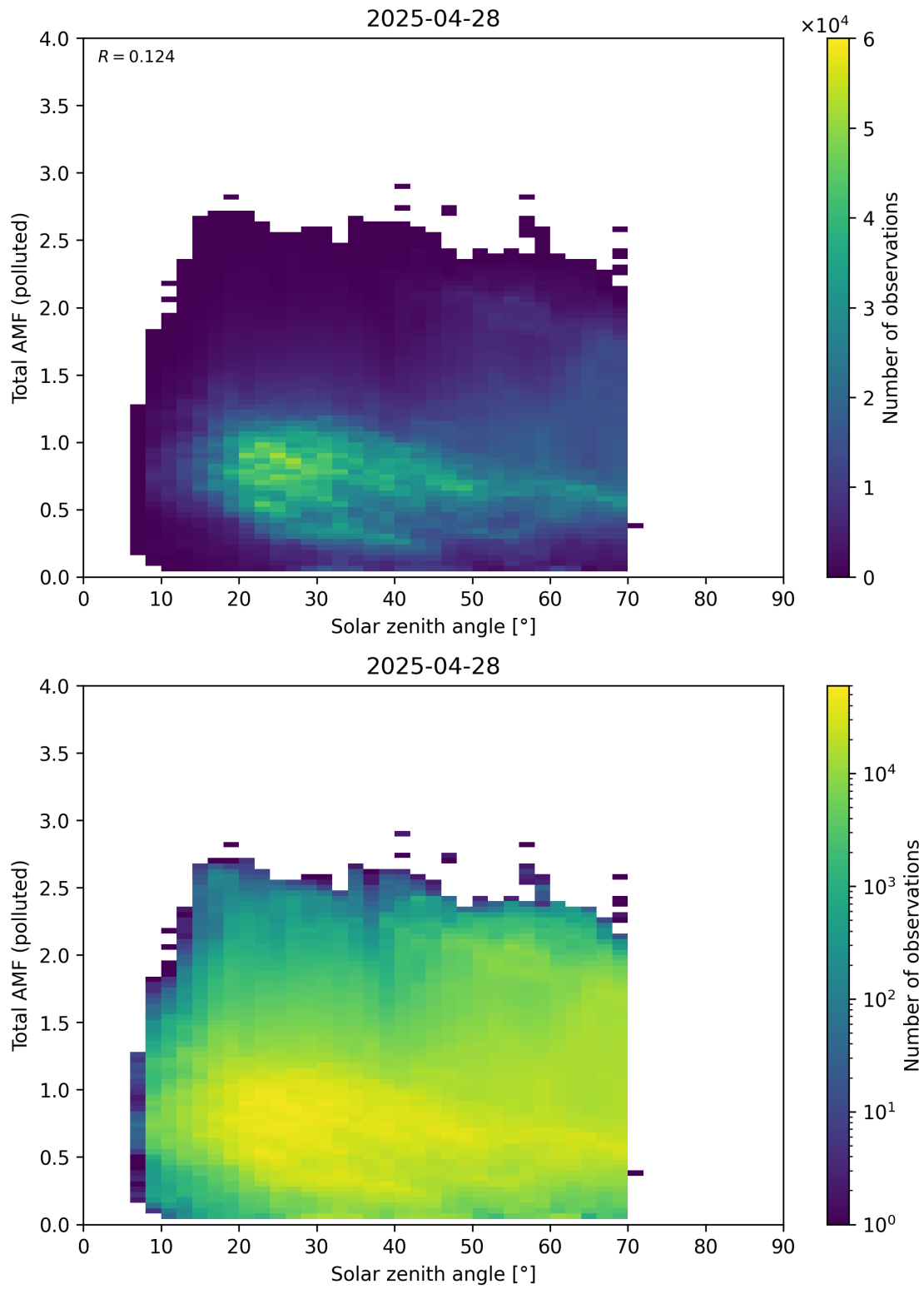
Figure 189: Scatter density plot of “Solar zenith angle” against “Total AMF (polluted)” for 2025-04-27 to 2025-04-29.
