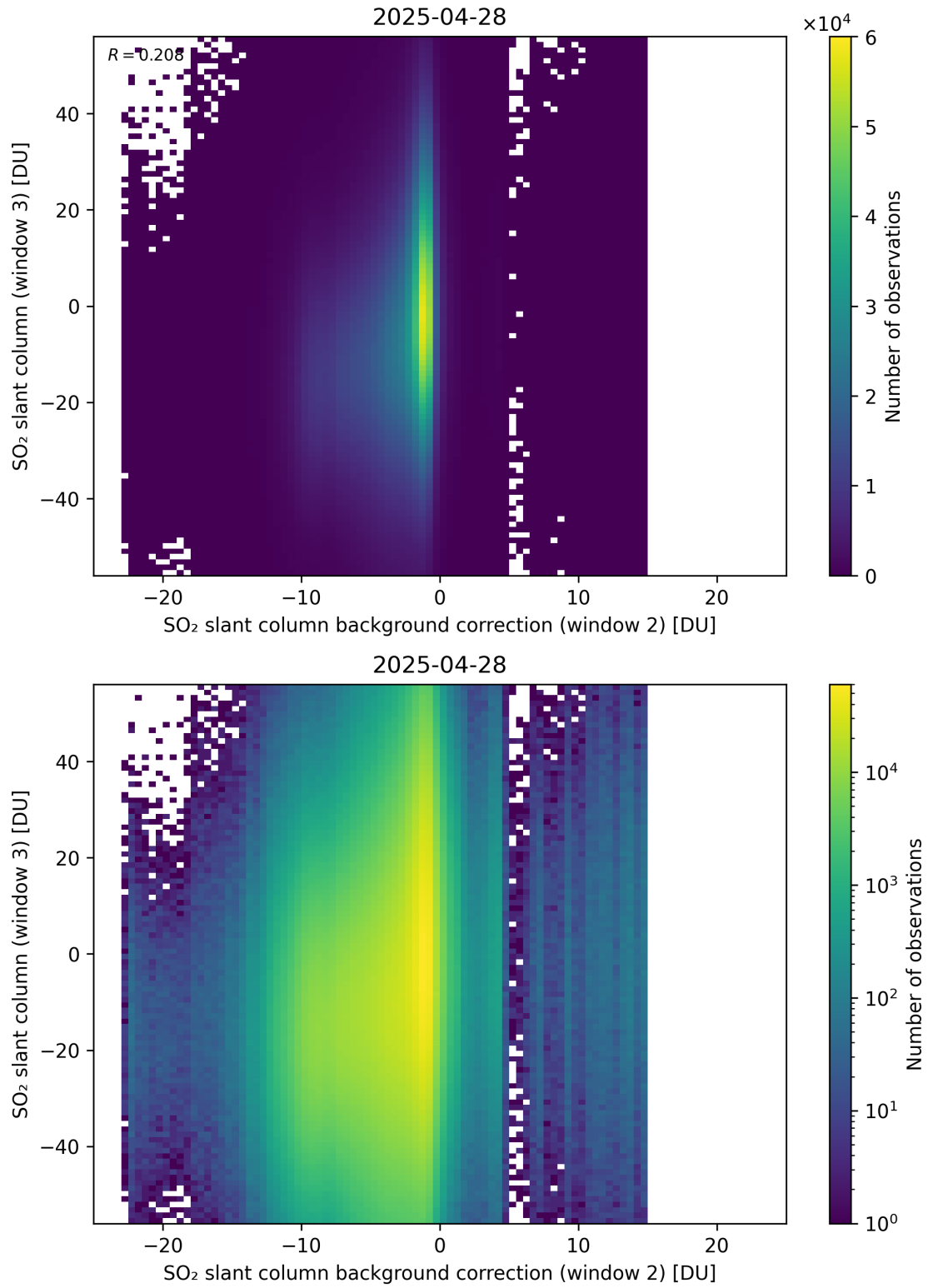
Figure 128: Scatter density plot of “SO 2 slant column background correction (window 2)” against “SO 2 slant column (window 3)” for 2025-04-27 to 2025-04-29.
