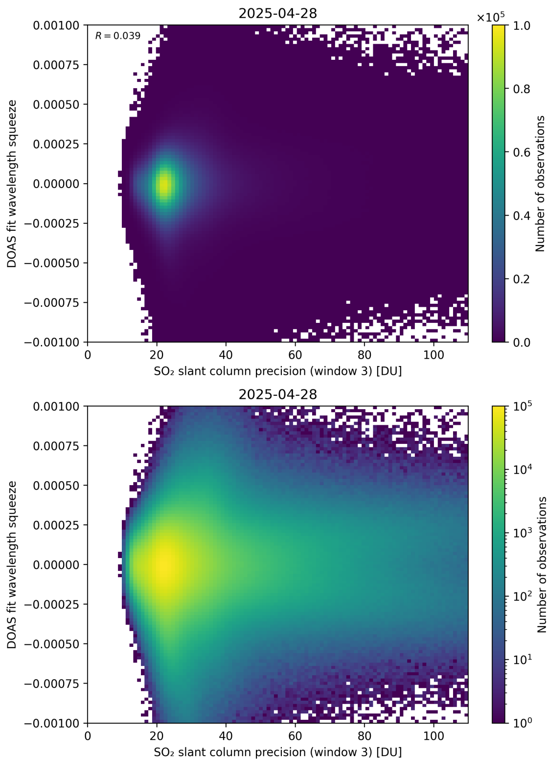
Figure 309: Scatter density plot of “SO 2 slant column precision (window 3)” against “DOAS fit wavelength squeeze” for 2025-04-27 to 2025-04-29.
