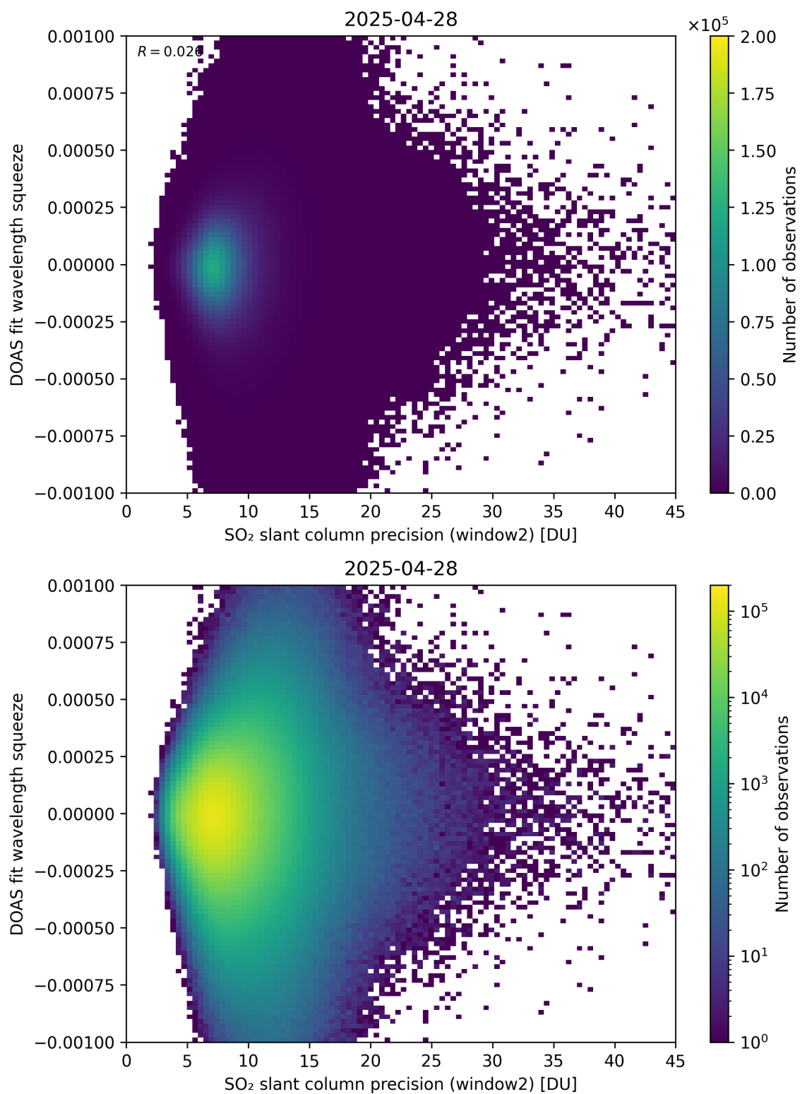
Figure 294: Scatter density plot of “SO 2 slant column precision (window2)” against “DOAS fit wavelength squeeze” for 2025-04-27 to 2025-04-29.
