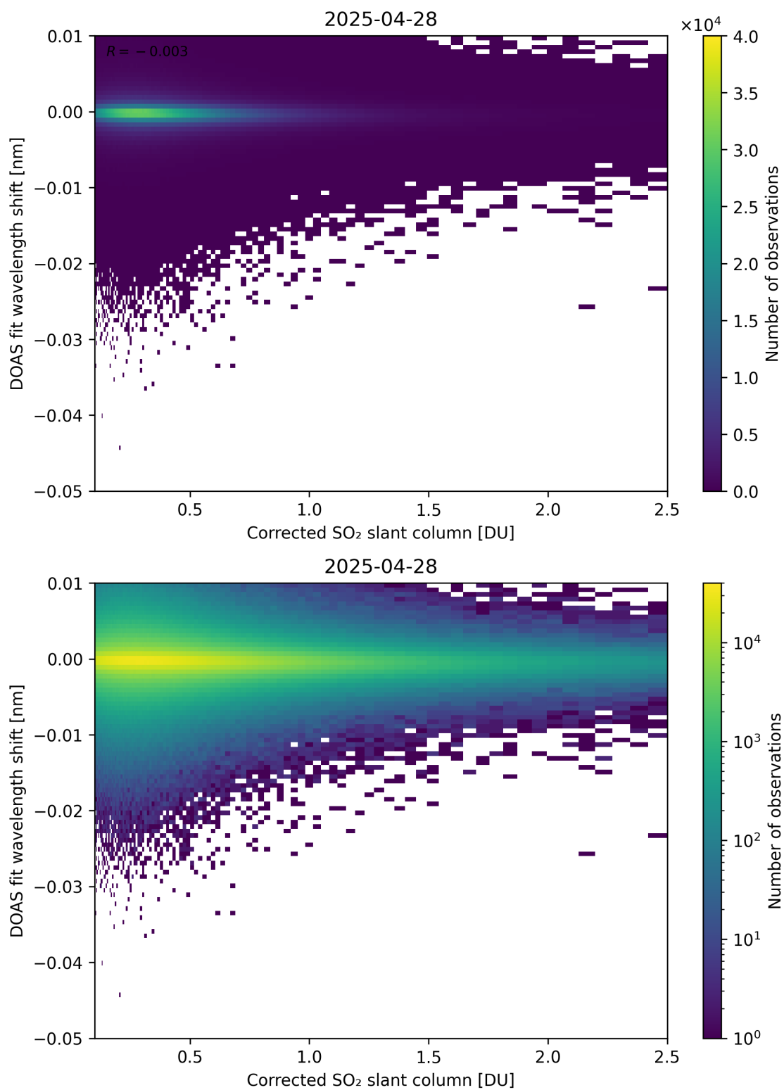
Figure 229: Scatter density plot of “Corrected SO 2 slant column” against “DOAS fit wavelength shift” for 2025-04-27 to 2025-04-29.
