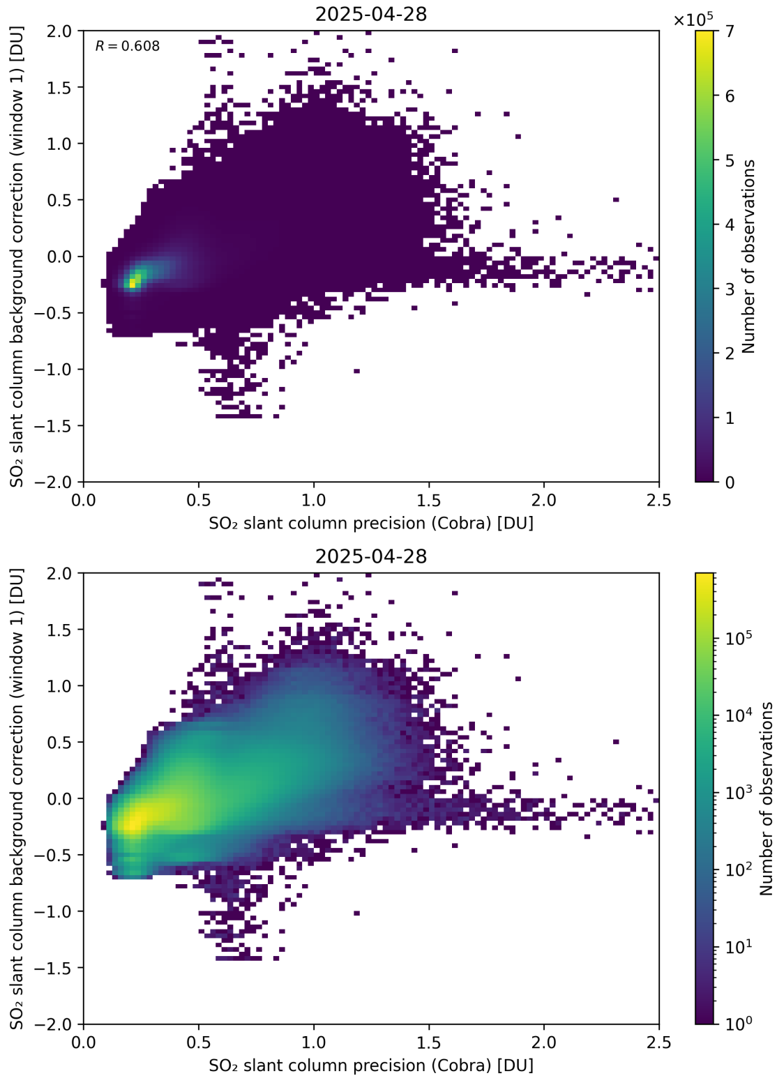
Figure 199: Scatter density plot of “SO 2 slant column precision (Cobra)” against “SO 2 slant column background correction (window 1)” for 2025-04-27 to 2025-04-29.
