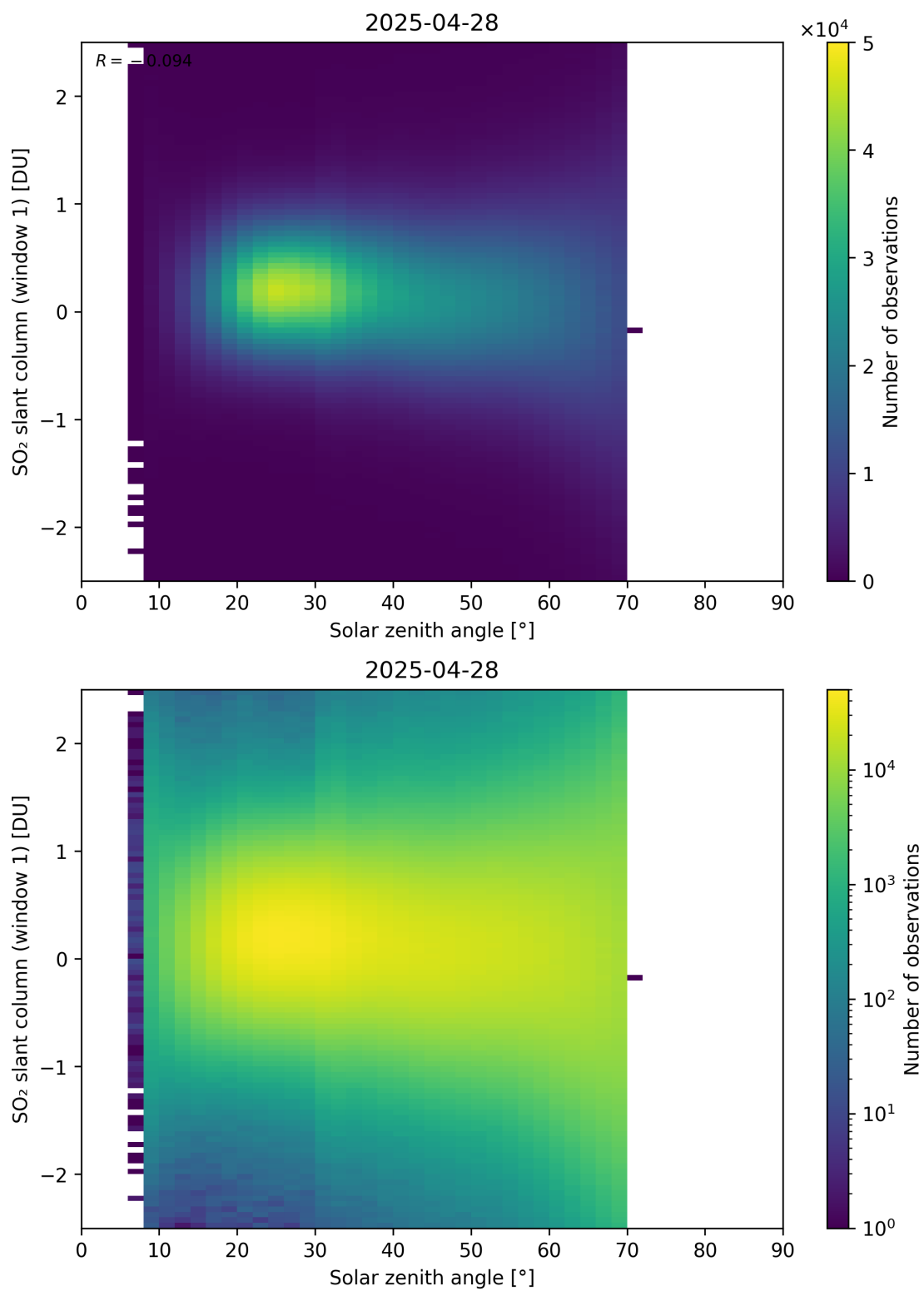
Figure 184: Scatter density plot of “Solar zenith angle” against “SO 2 slant column (window 1)” for 2025-04-27 to 2025-04-29.
