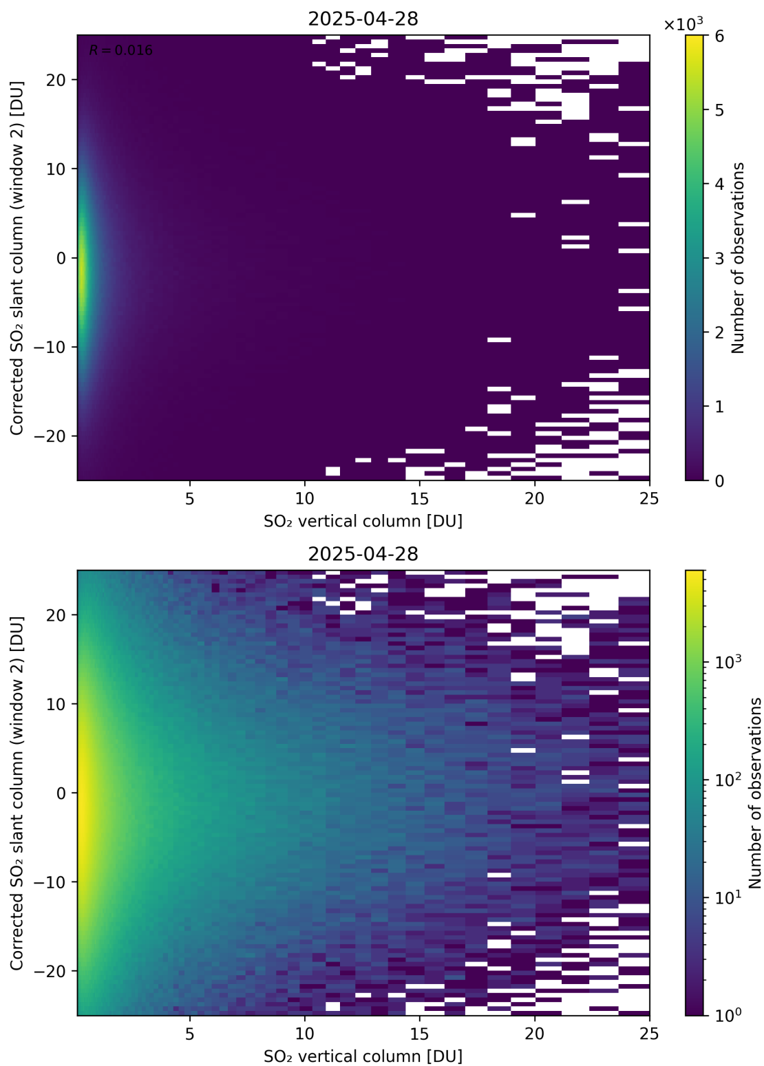
Figure 352: Scatter density plot of “SO 2 vertical column” against “Corrected SO 2 slant column (window 2)” for 2025-04-27 to 2025-04-29.
