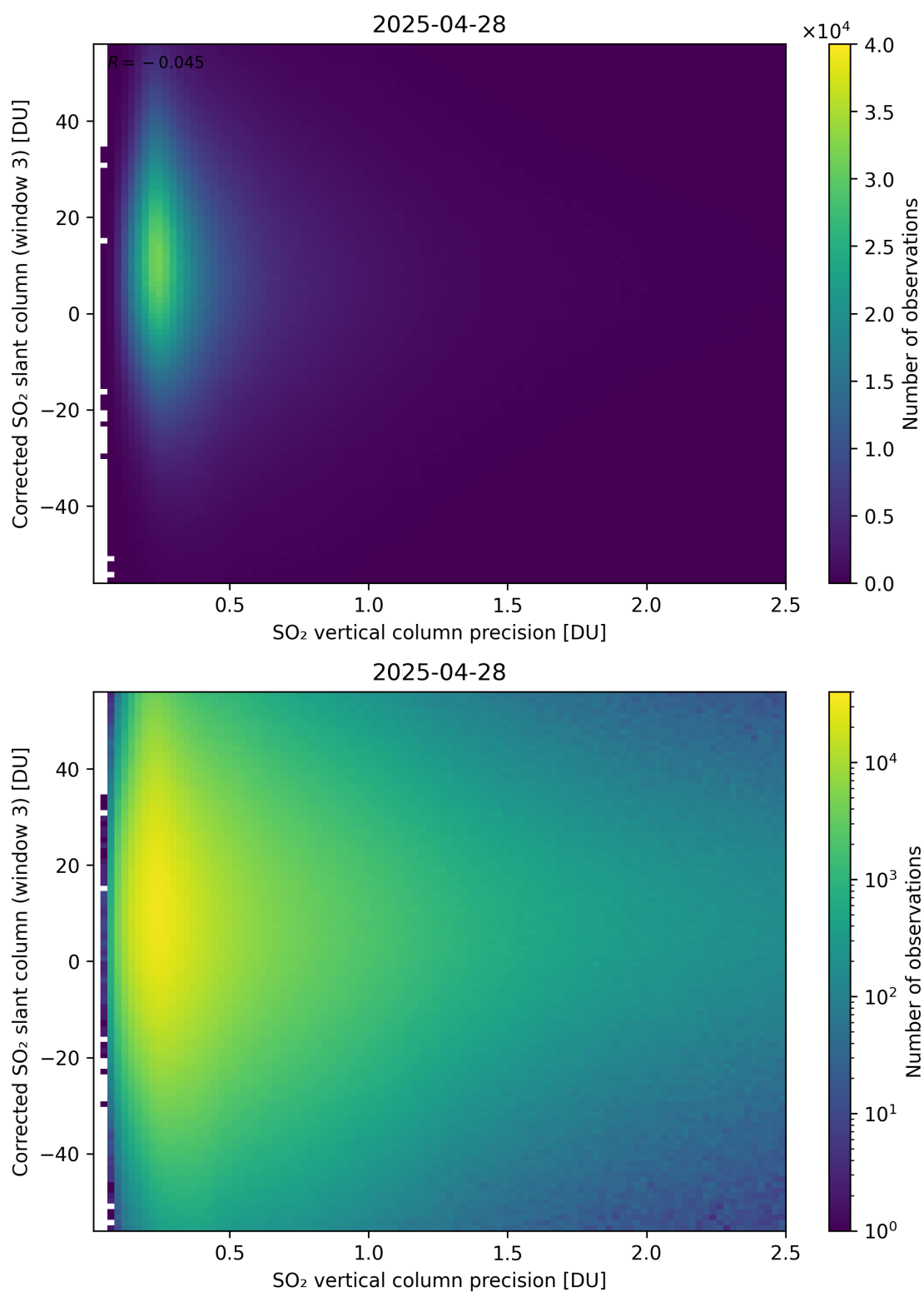
Figure 340: Scatter density plot of “SO 2 vertical column precision” against “Corrected SO 2 slant column (window 3)” for 2025-04-27 to 2025-04-29.
