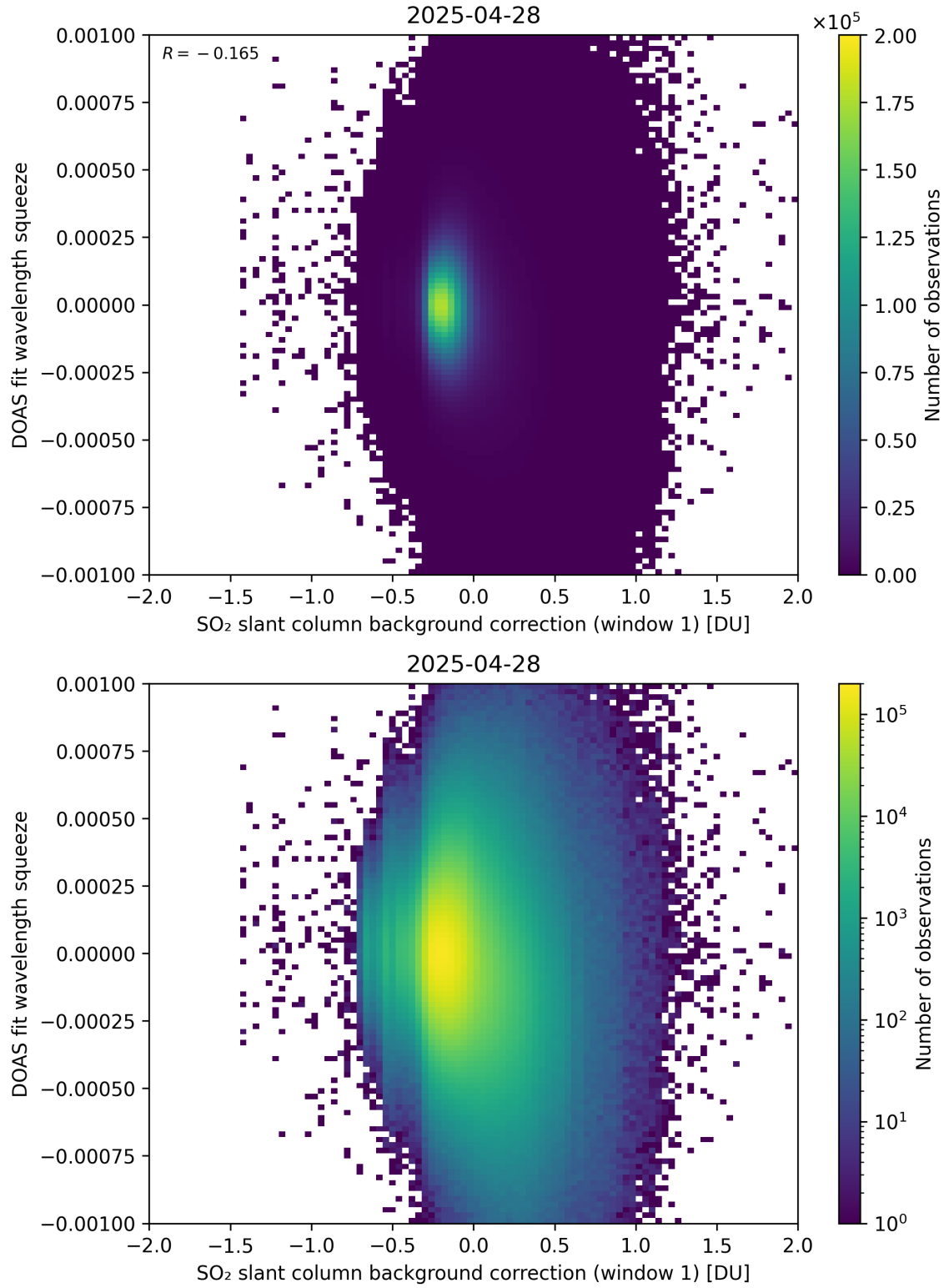
Figure 112: Scatter density plot of “SO 2 slant column background correction (window 1)” against “DOAS fit wavelength squeeze” for 2025-04-27 to 2025-04-29.
