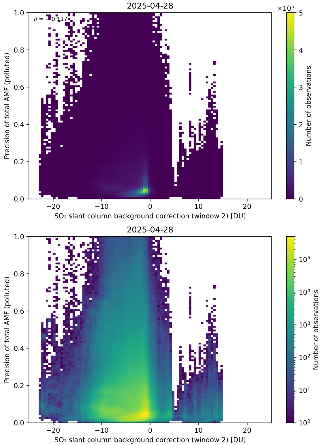
Figure 131: Scatter density plot of “SO 2 slant column background correction (window 2)” against “Precision of total AMF (polluted)” for 2025-04-27 to 2025-04-29.
