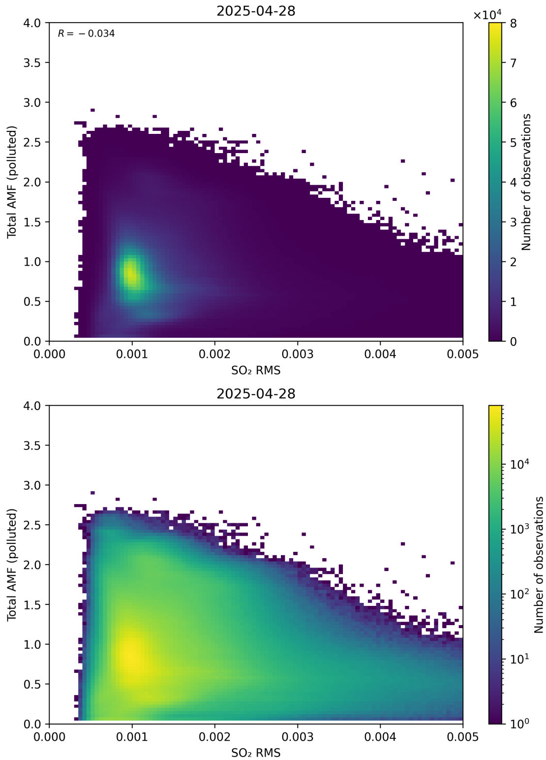
Figure 148: Scatter density plot of “SO 2 RMS” against “Total AMF (polluted)” for 2025-04-27 to 2025-04-29.
