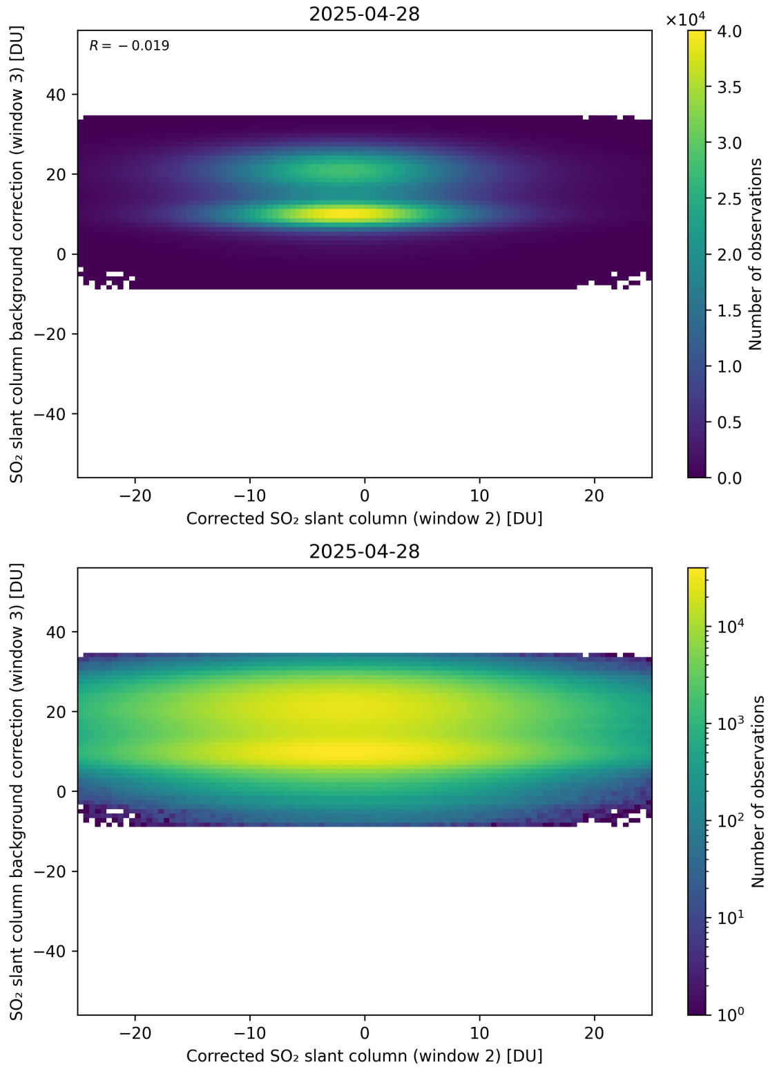
Figure 245: Scatter density plot of “Corrected SO 2 slant column (window 2)” against “SO 2 slant column background correction (window 3)” for 2025-04-27 to 2025-04-29.
