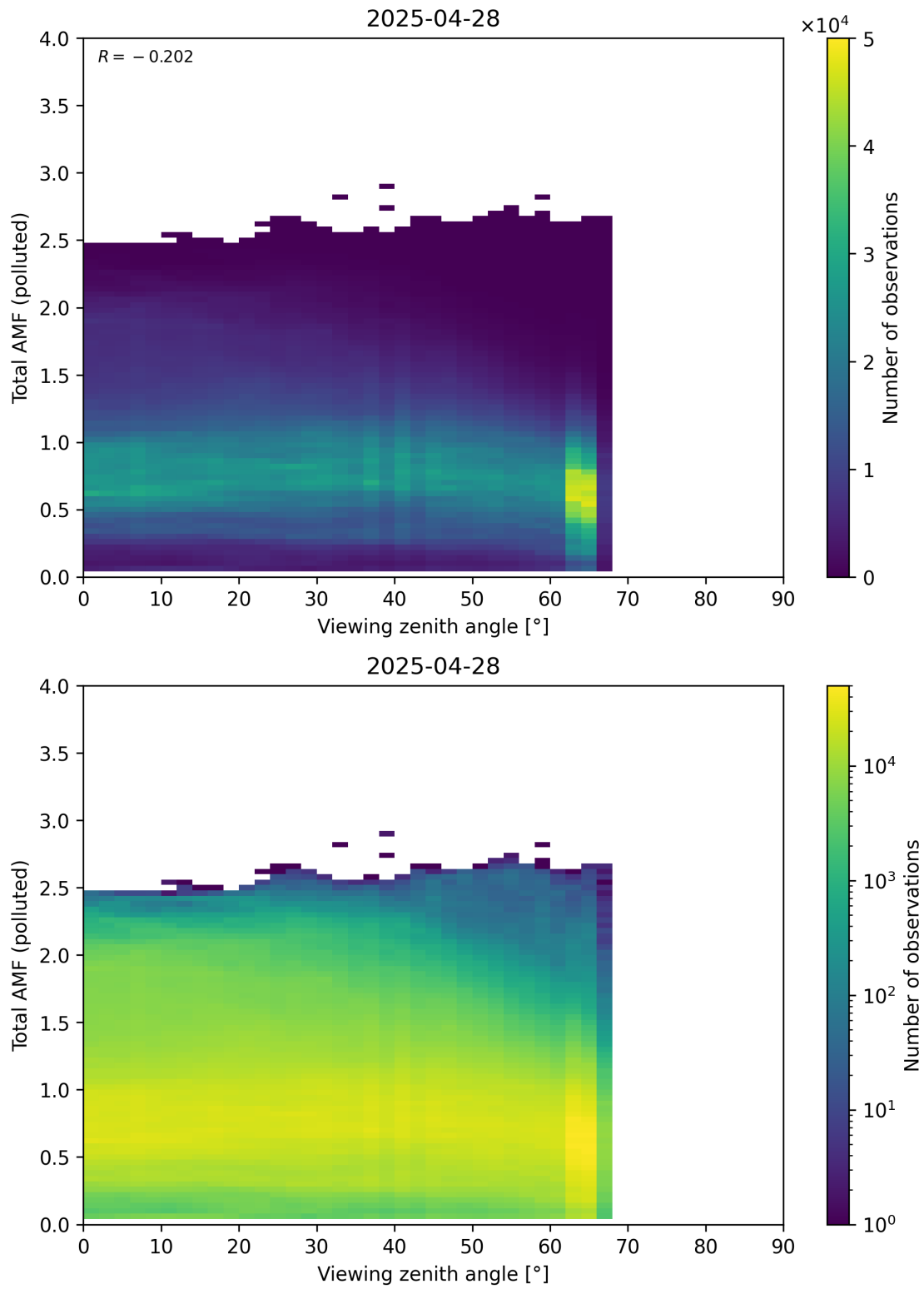
Figure 381: Scatter density plot of “Viewing zenith angle” against “Total AMF (polluted)” for 2025-04-27 to 2025-04-29.
