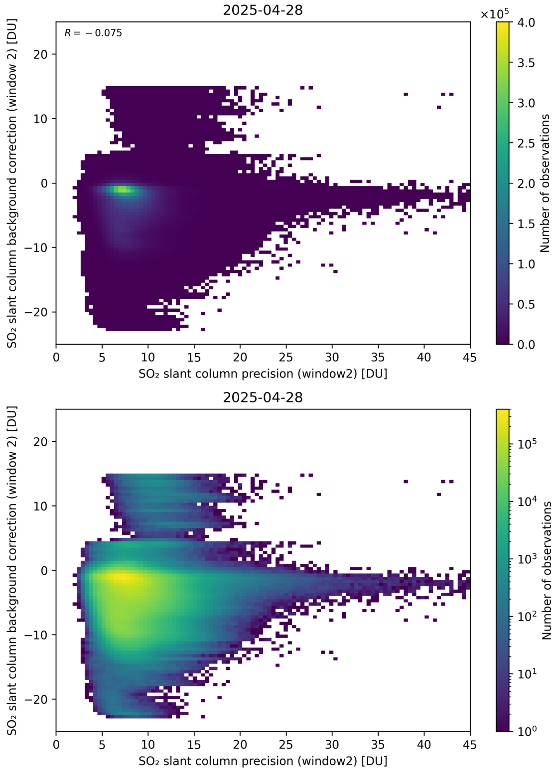
Figure 291: Scatter density plot of “SO 2 slant column precision (window2)” against “SO 2 slant column background correction (window 2)” for 2025-04-27 to 2025-04-29.
