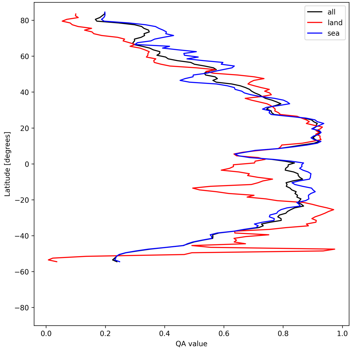
Figure 31: Zonal average of “QA value” for 2025-04-27 to 2025-04-29.
