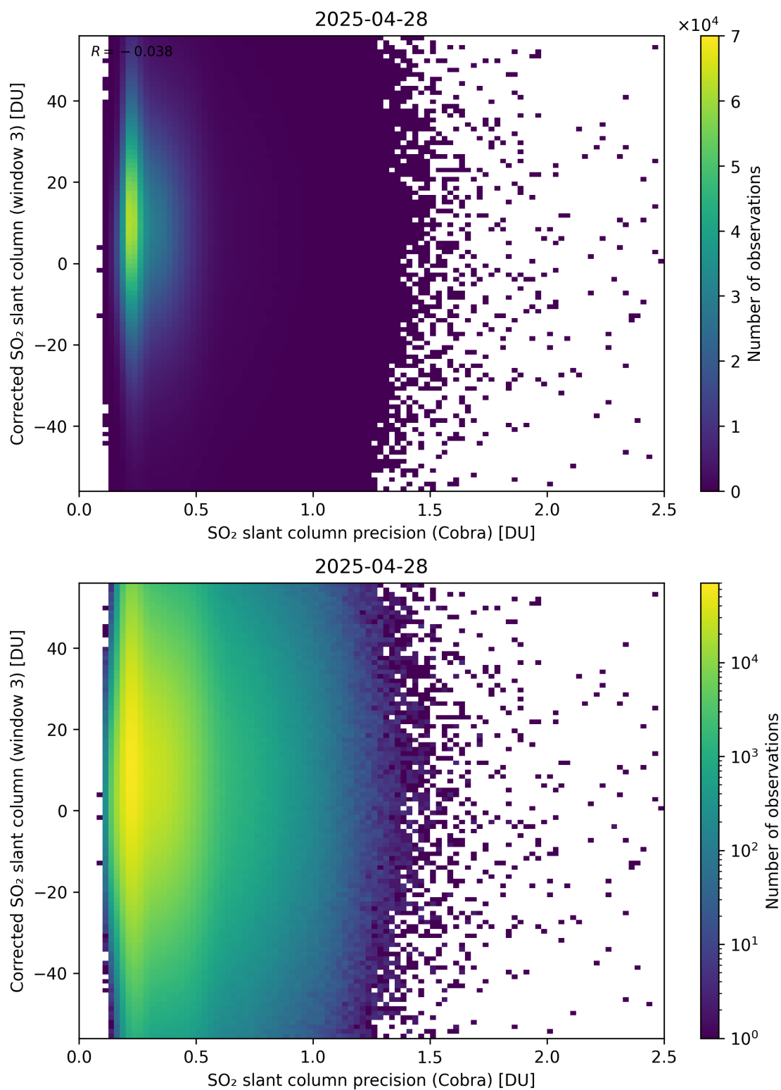
Figure 207: Scatter density plot of “SO 2 slant column precision (Cobra)” against “Corrected SO 2 slant column (window 3)” for 2025-04-27 to 2025-04-29.
