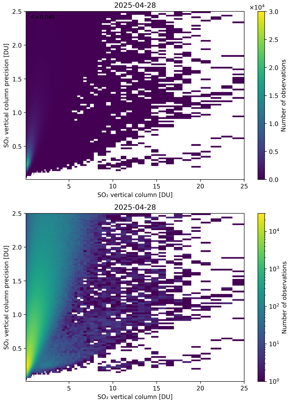
Figure 361: Scatter density plot of “SO 2 vertical column” against “SO 2 vertical column precision” for 2025-04-27 to 2025-04-29.
