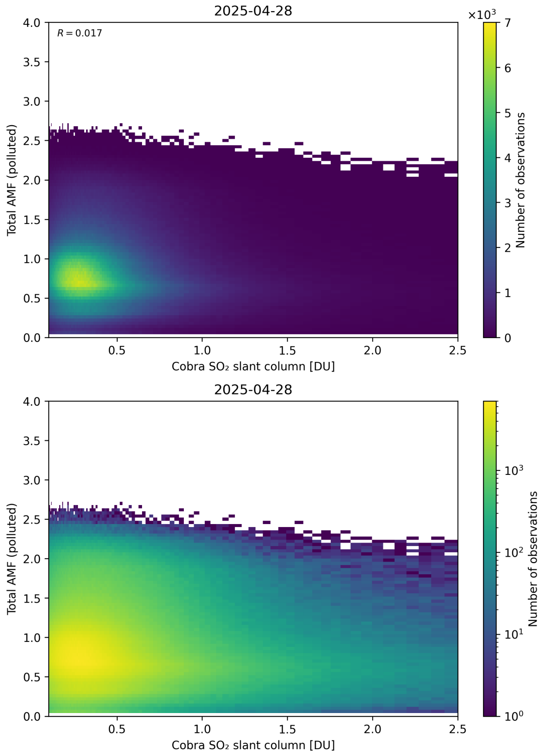
Figure 224: Scatter density plot of “Cobra SO 2 slant column” against “Total AMF (polluted)” for 2025-04-27 to 2025-04-29.
