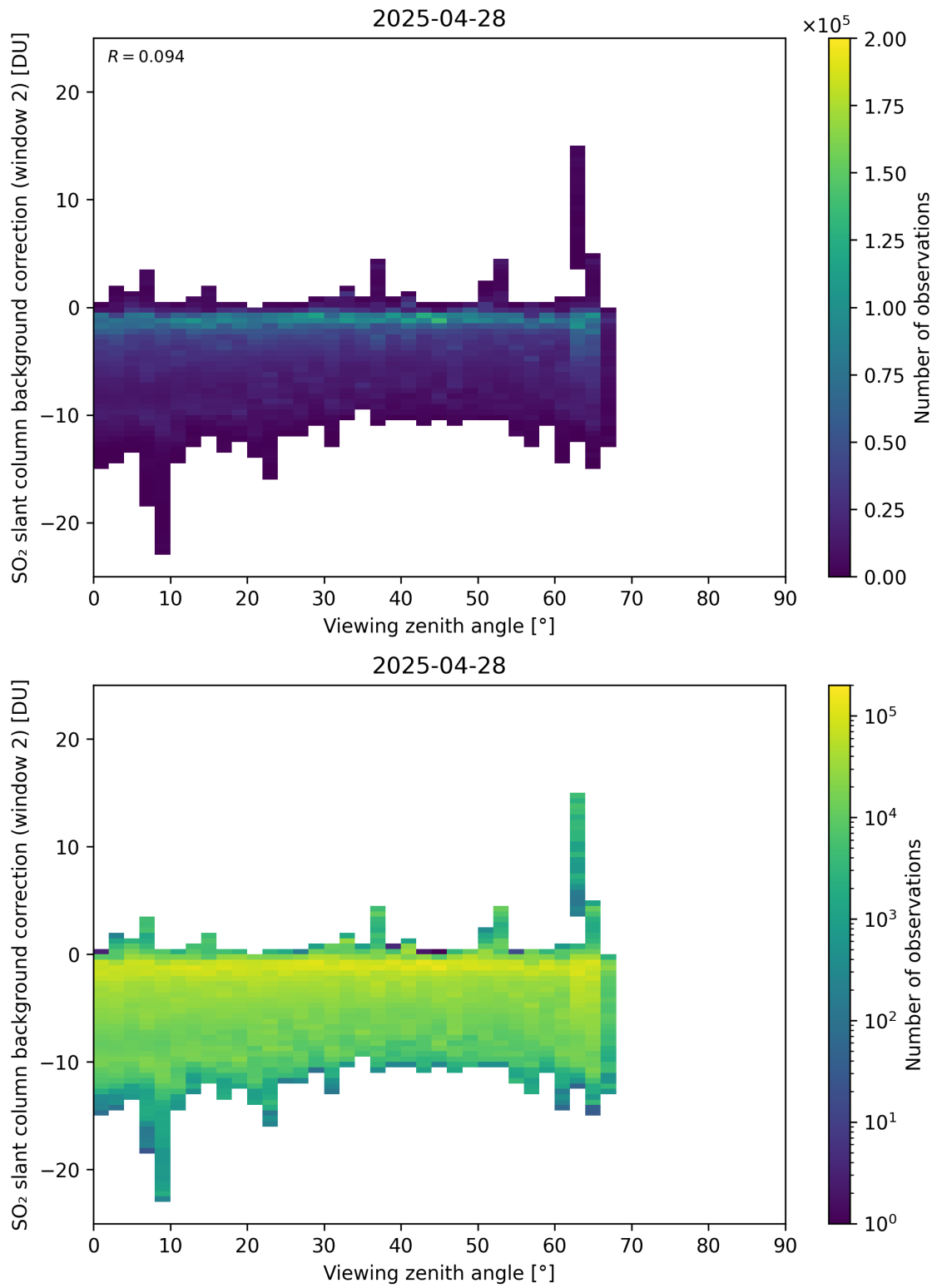
Figure 363: Scatter density plot of “Viewing zenith angle” against “SO 2 slant column background correction (window 2)” for 2025-04-27 to 2025-04-29.
