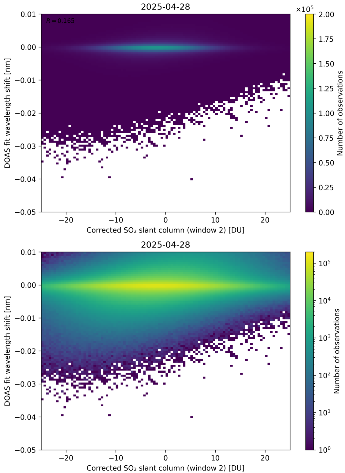
Figure 246: Scatter density plot of “Corrected SO 2 slant column (window 2)” against “DOAS fit wavelength shift” for 2025-04-27 to 2025-04-29.
