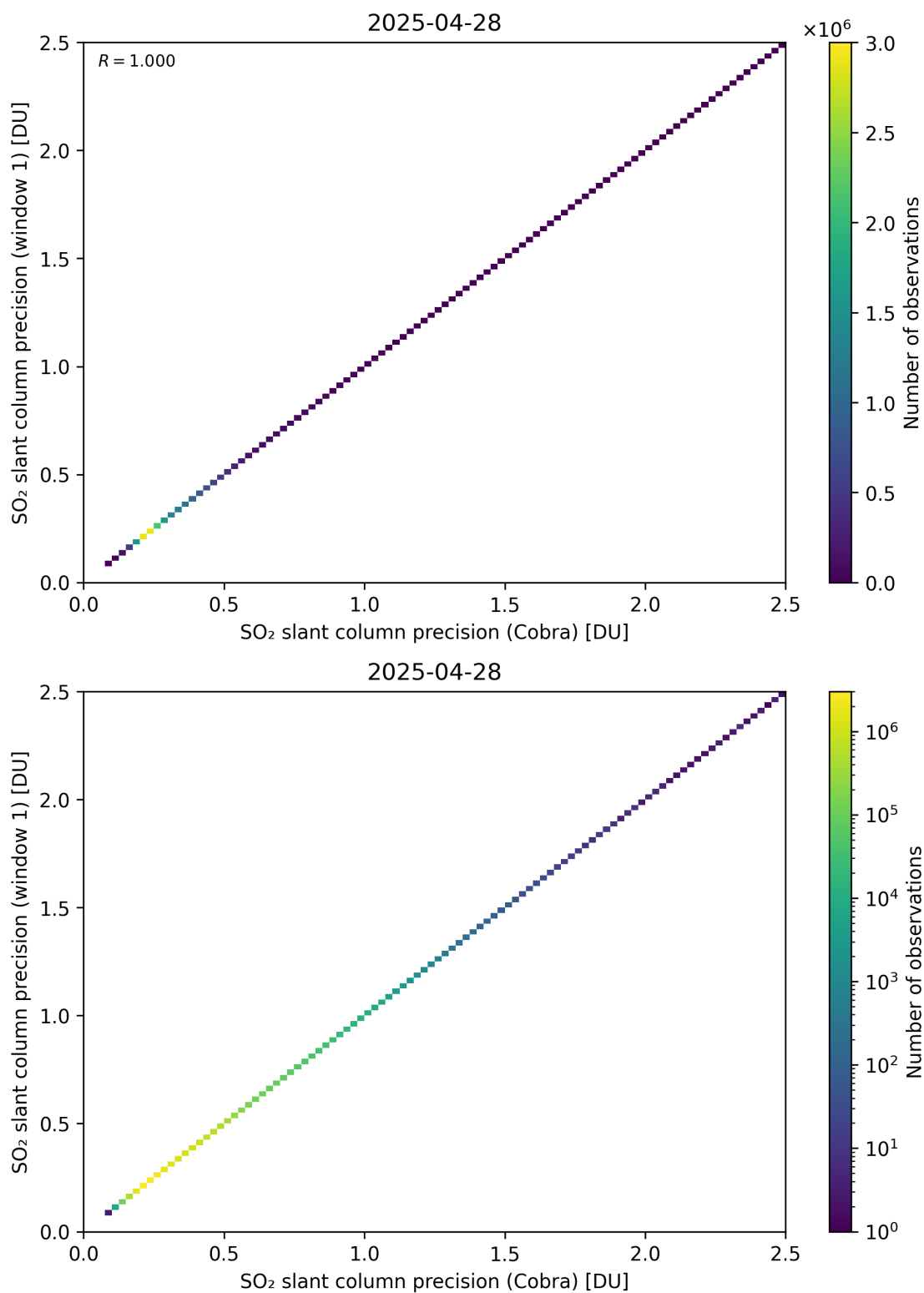
Figure 209: Scatter density plot of “SO 2 slant column precision (Cobra)” against “SO 2 slant column precision (window 1)” for 2025-04-27 to 2025-04-29.
