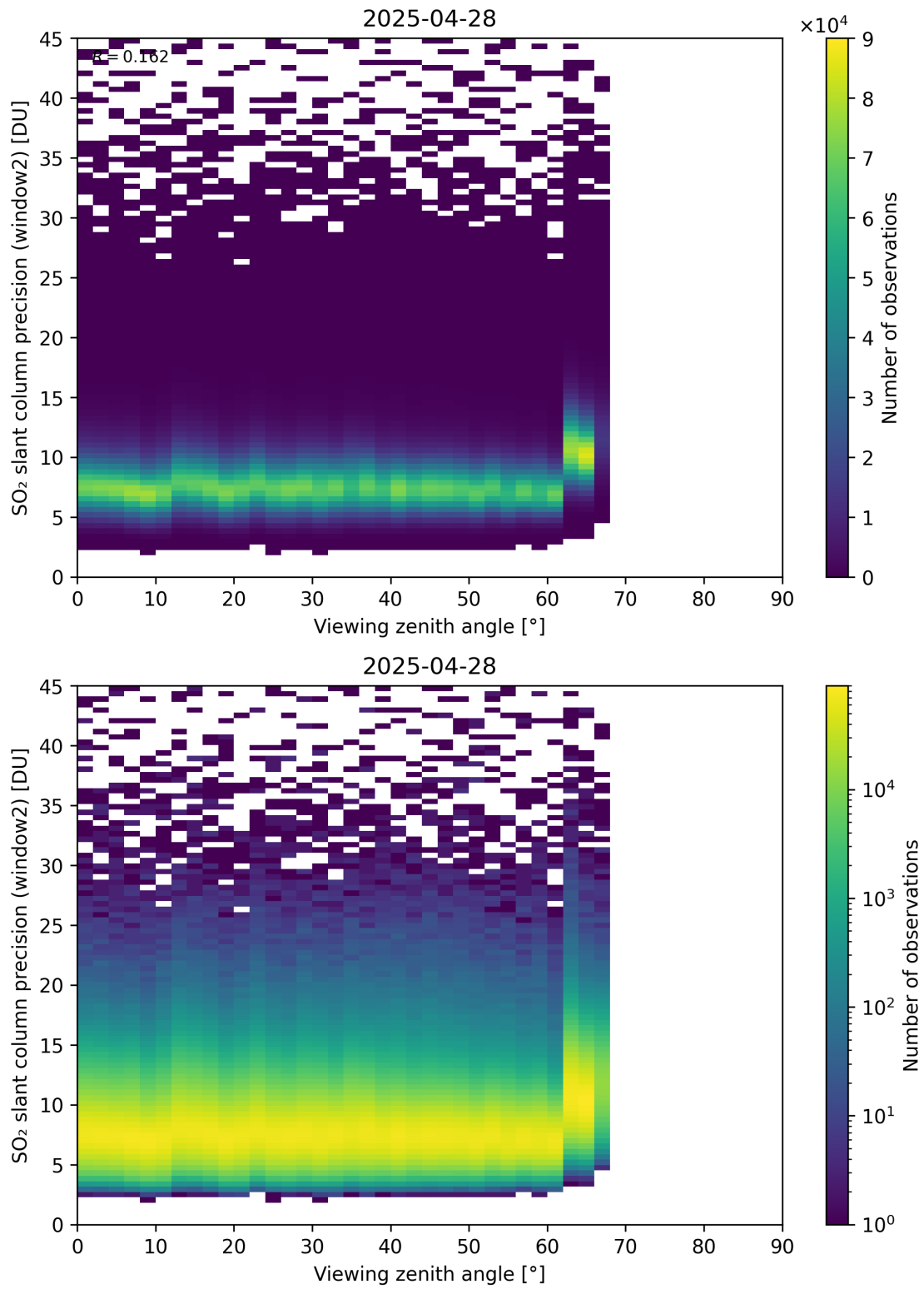
Figure 378: Scatter density plot of “Viewing zenith angle” against “SO 2 slant column precision (window2)” for 2025-04-27 to 2025-04-29.
