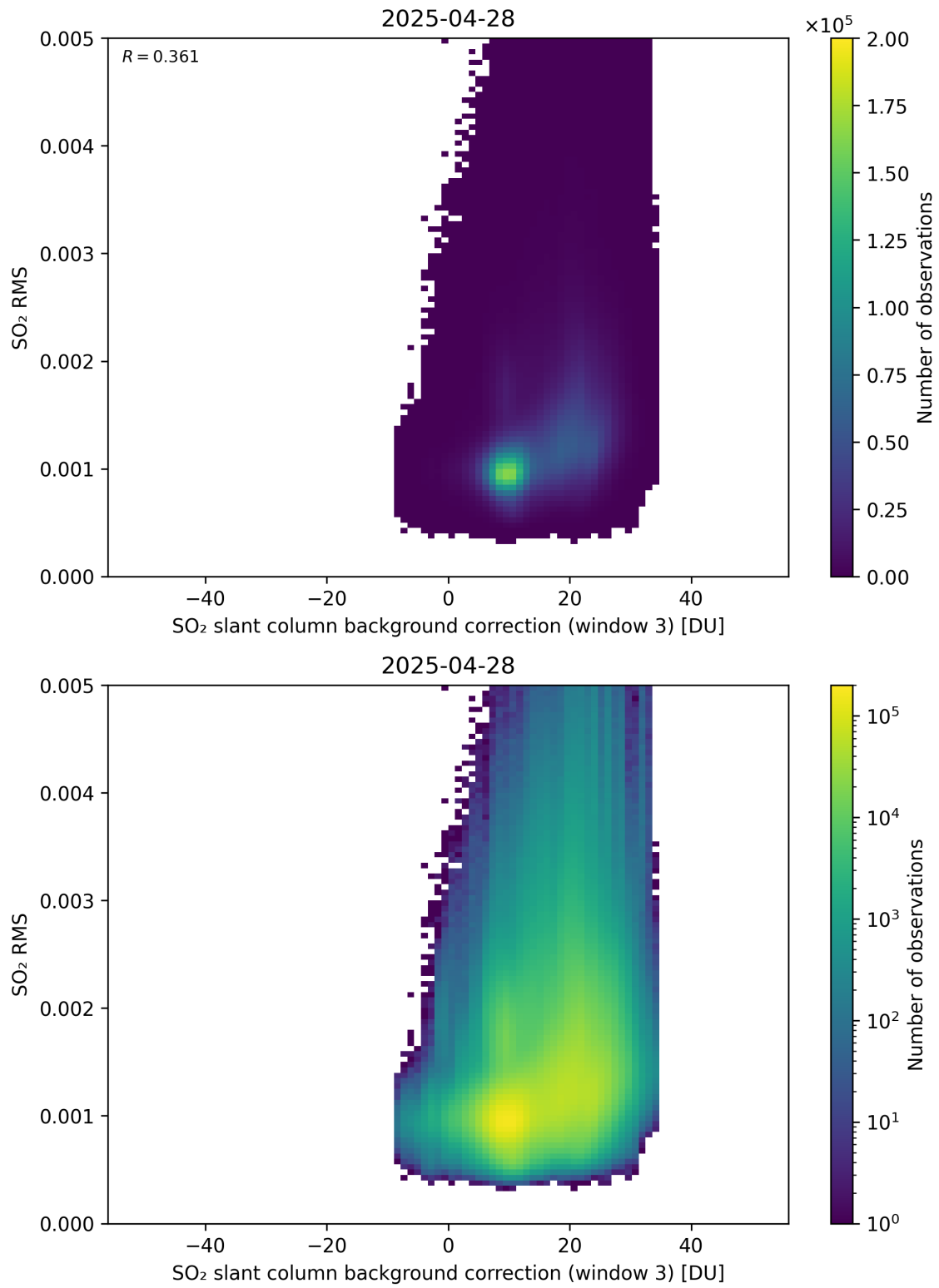
Figure 134: Scatter density plot of “SO 2 slant column background correction (window 3)” against “SO 2 RMS” for 2025-04-27 to 2025-04-29.
