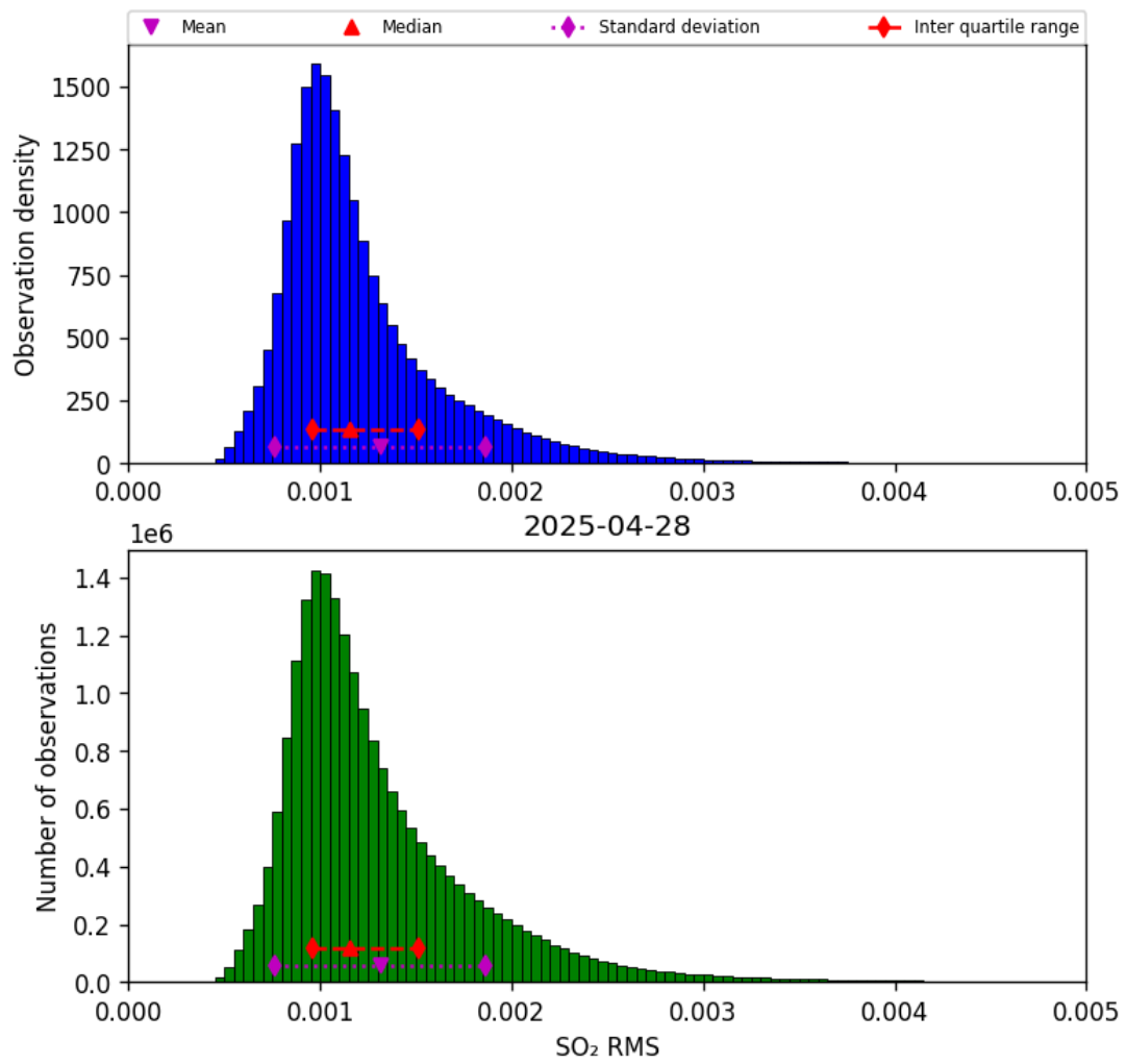
Figure 78: Histogram of “SO 2 RMS” for 2025-04-27 to 2025-04-29
