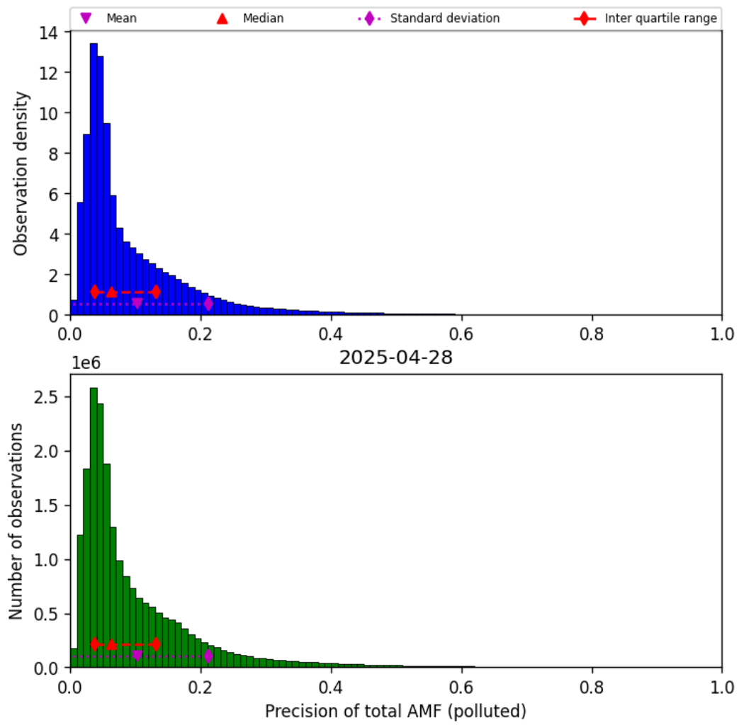
Figure 80: Histogram of “Precision of total AMF (polluted)” for 2025-04-27 to 2025-04-29
