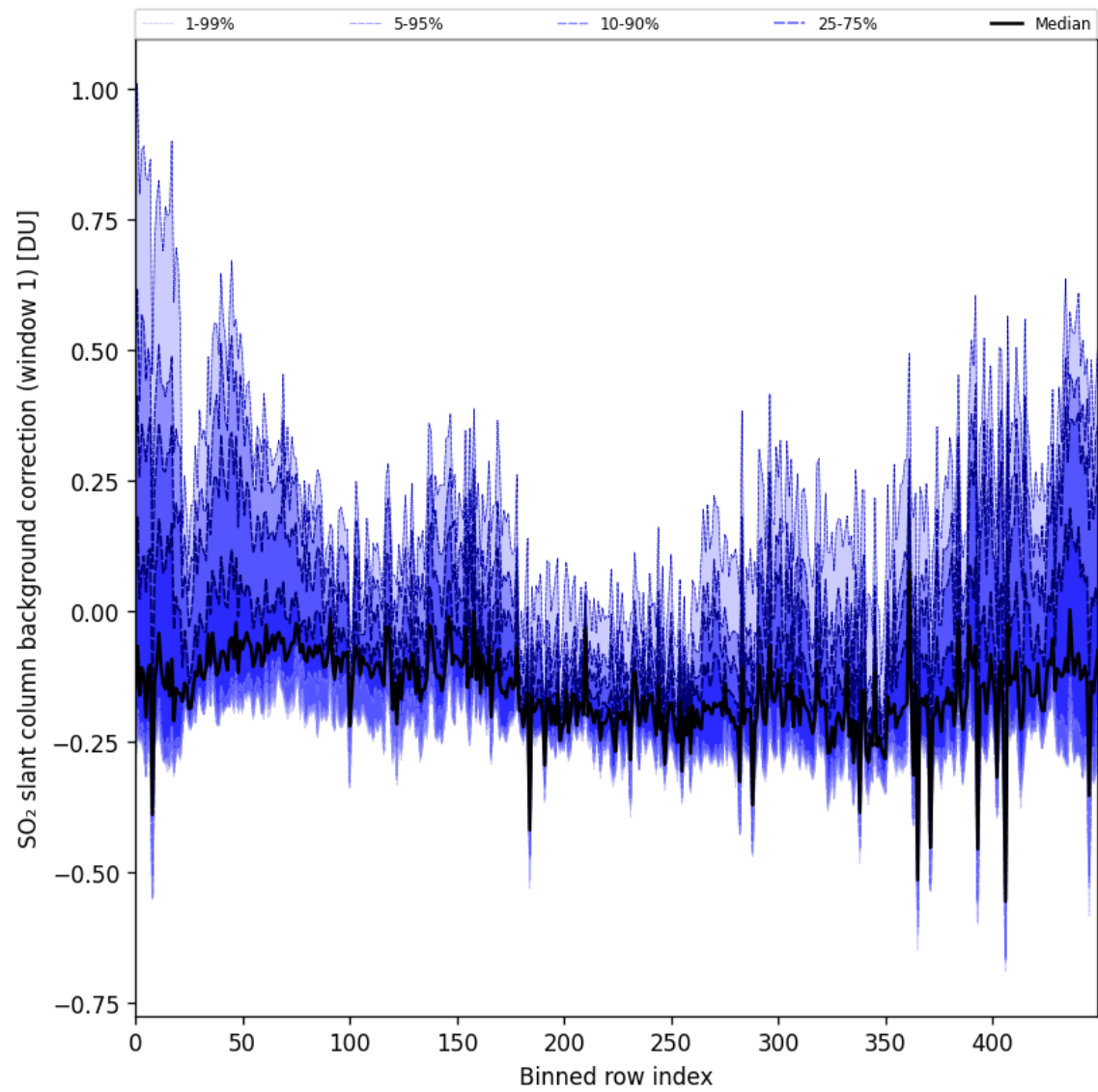
Figure 92: Along track statistics of “SO 2 slant column background correction (window 1)” for 2025-04-27 to 2025-04-29
