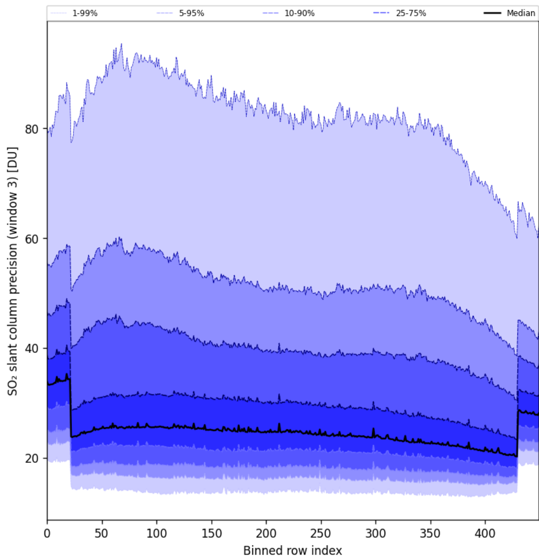
Figure 98: Along track statistics of “SO 2 slant column precision (window 3)” for 2025-04-27 to 2025-04-29
