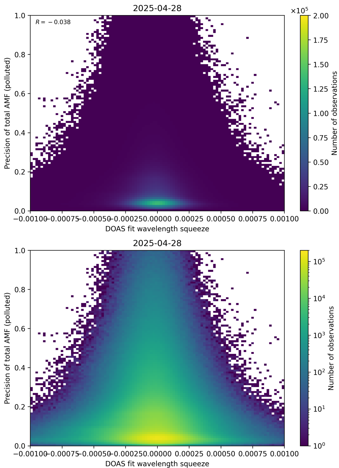
Figure 146: Scatter density plot of “DOAS fit wavelength squeeze” against “Precision of total AMF (polluted)” for 2025-04-27 to 2025-04-29.
