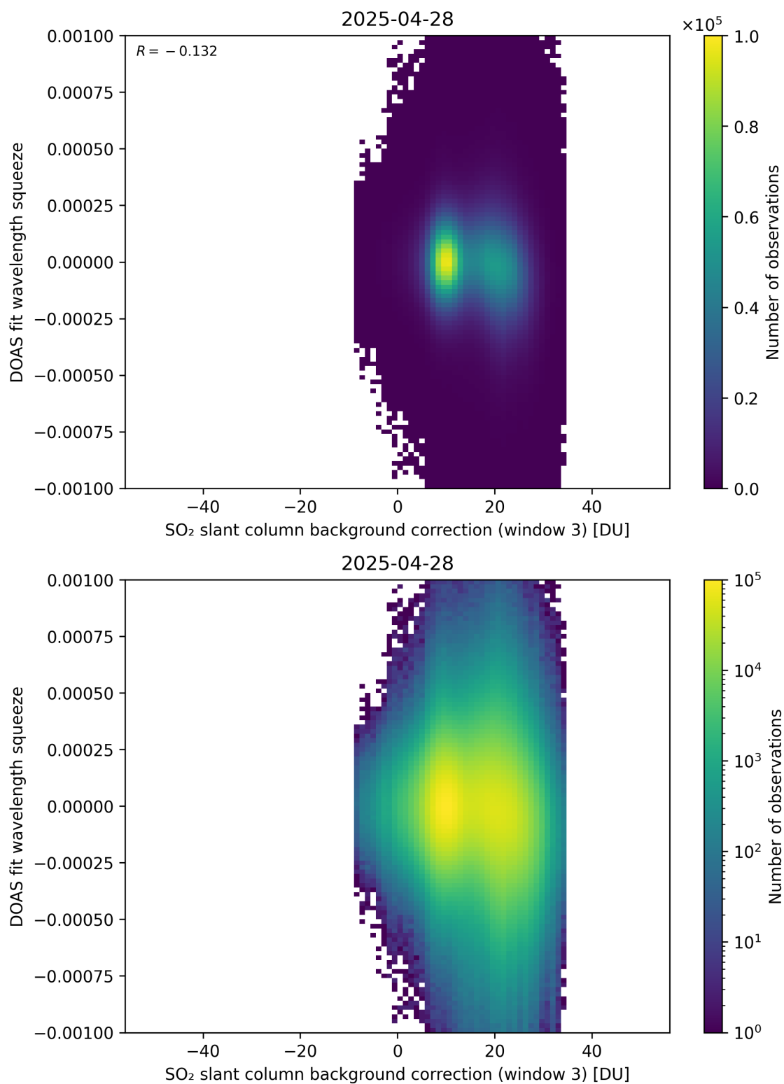
Figure 133: Scatter density plot of “SO 2 slant column background correction (window 3)” against “DOAS fit wavelength squeeze” for 2025-04-27 to 2025-04-29.
