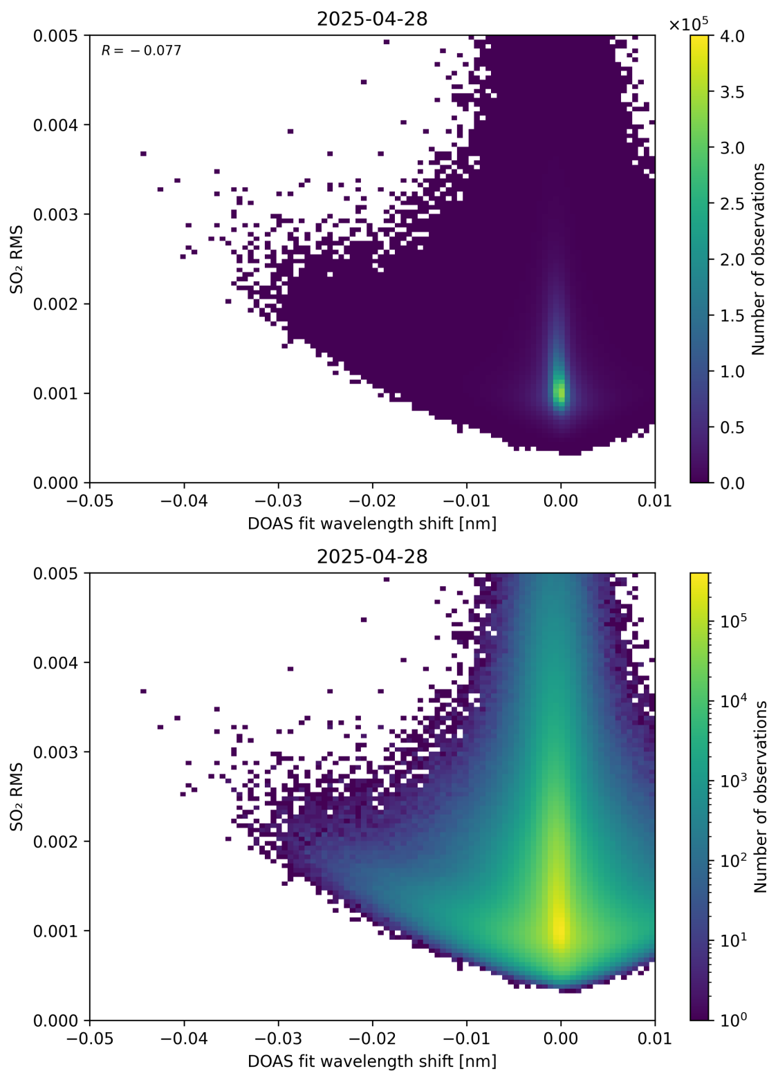
Figure 139: Scatter density plot of “DOAS fit wavelength shift” against “SO 2 RMS” for 2025-04-27 to 2025-04-29.
