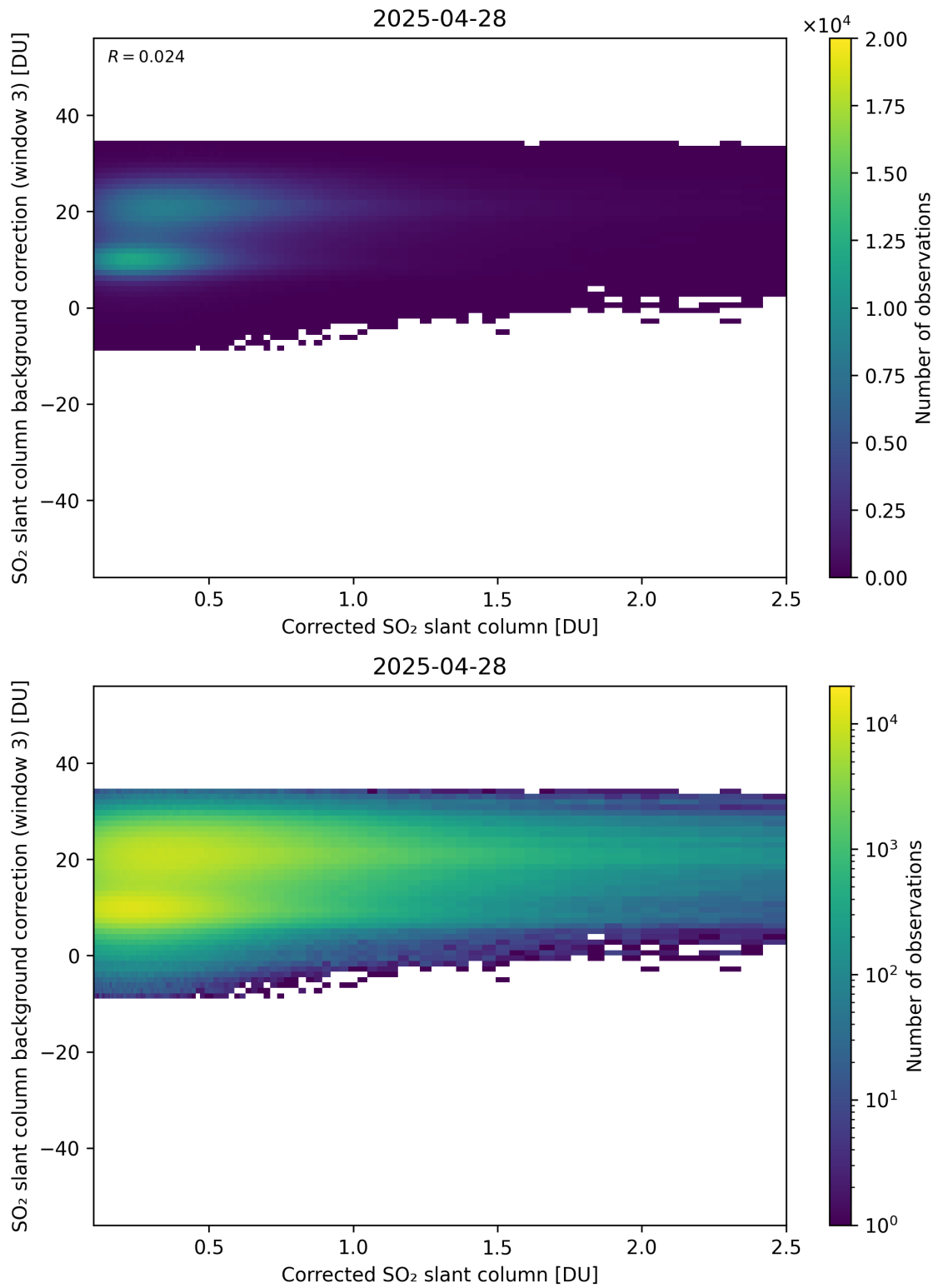
Figure 228: Scatter density plot of “Corrected SO 2 slant column” against “SO 2 slant column background correction (window 3)” for 2025-04-27 to 2025-04-29.
