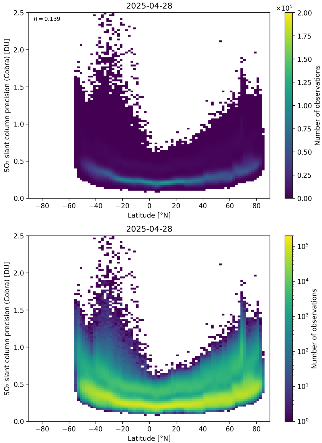
Figure 158: Scatter density plot of “Latitude” against “SO 2 slant column precision (Cobra)” for 2025-04-27 to 2025-04-29.
