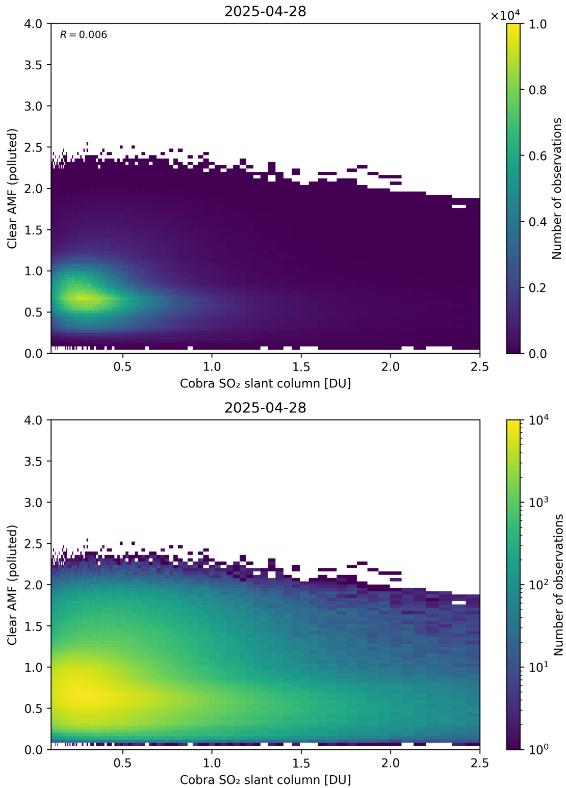
Figure 215: Scatter density plot of “Cobra SO 2 slant column” against “Clear AMF (polluted)” for 2025-04-27 to 2025-04-29.
