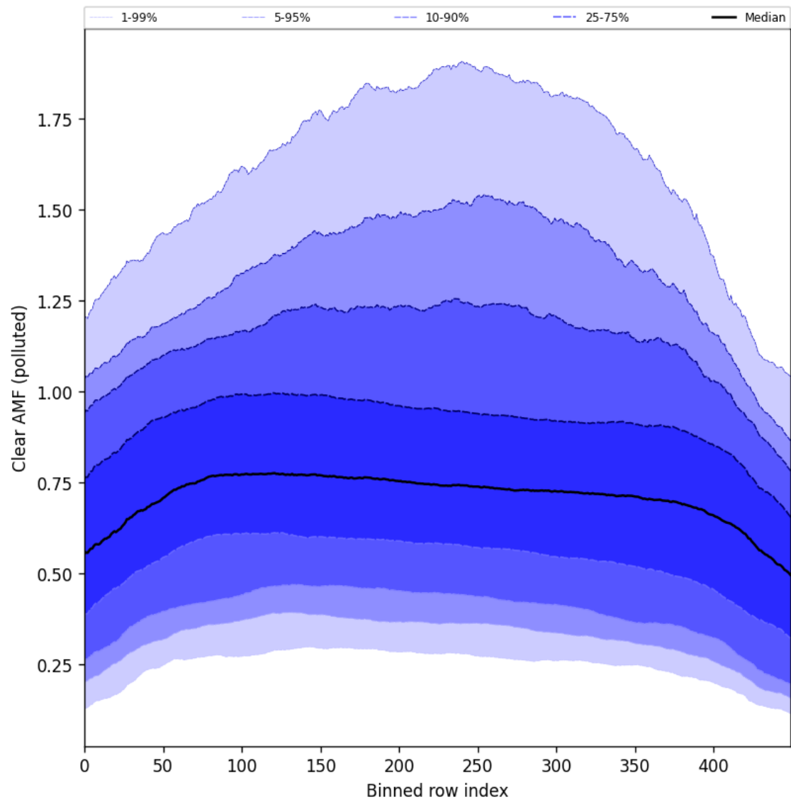
Figure 107: Along track statistics of “Clear AMF (polluted)” for 2025-04-27 to 2025-04-29
