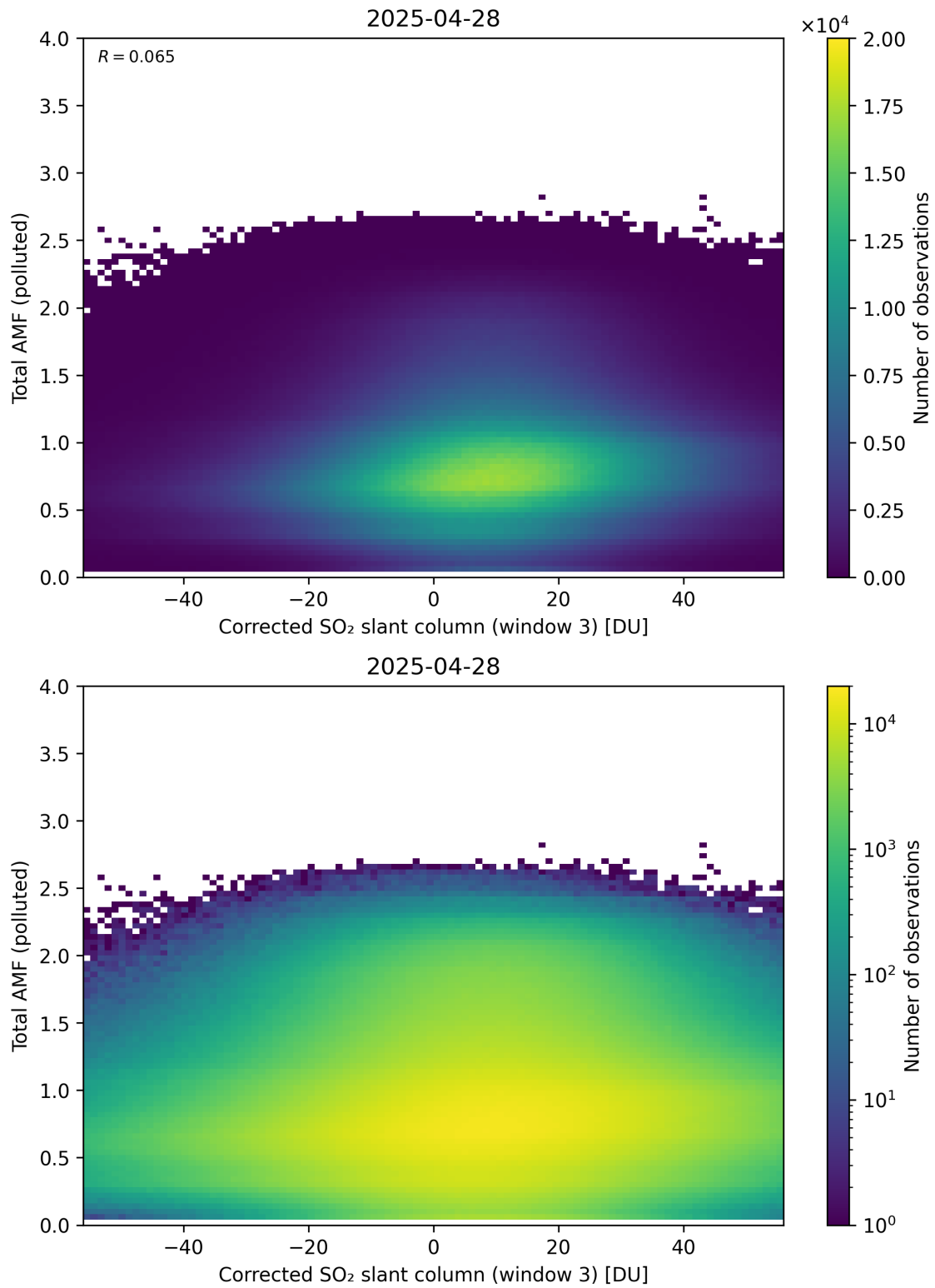
Figure 260: Scatter density plot of “Corrected SO 2 slant column (window 3)” against “Total AMF (polluted)” for 2025-04-27 to 2025-04-29.
