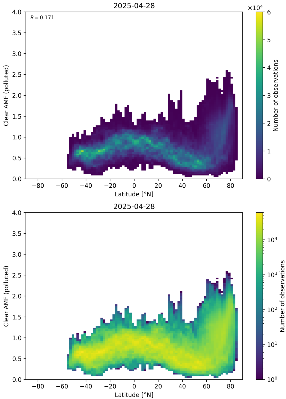
Figure 156: Scatter density plot of “Latitude” against “Clear AMF (polluted)” for 2025-04-27 to 2025-04-29.
