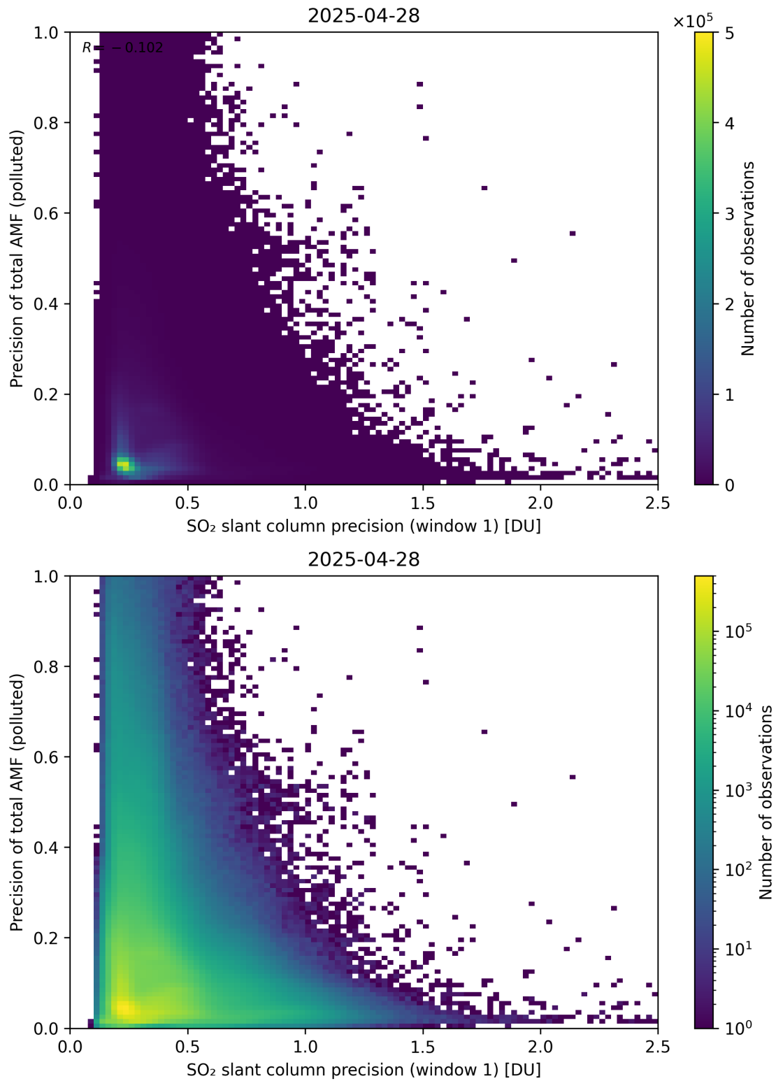
Figure 281: Scatter density plot of “SO 2 slant column precision (window 1)” against “Precision of total AMF (polluted)” for 2025-04-27 to 2025-04-29.
