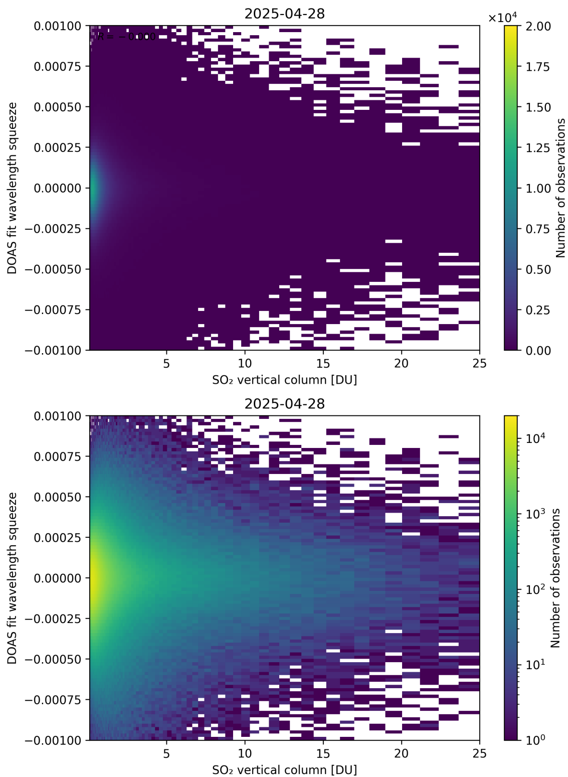
Figure 327: Scatter density plot of “SO 2 vertical column” against “DOAS fit wavelength squeeze” for 2025-04-27 to 2025-04-29.
