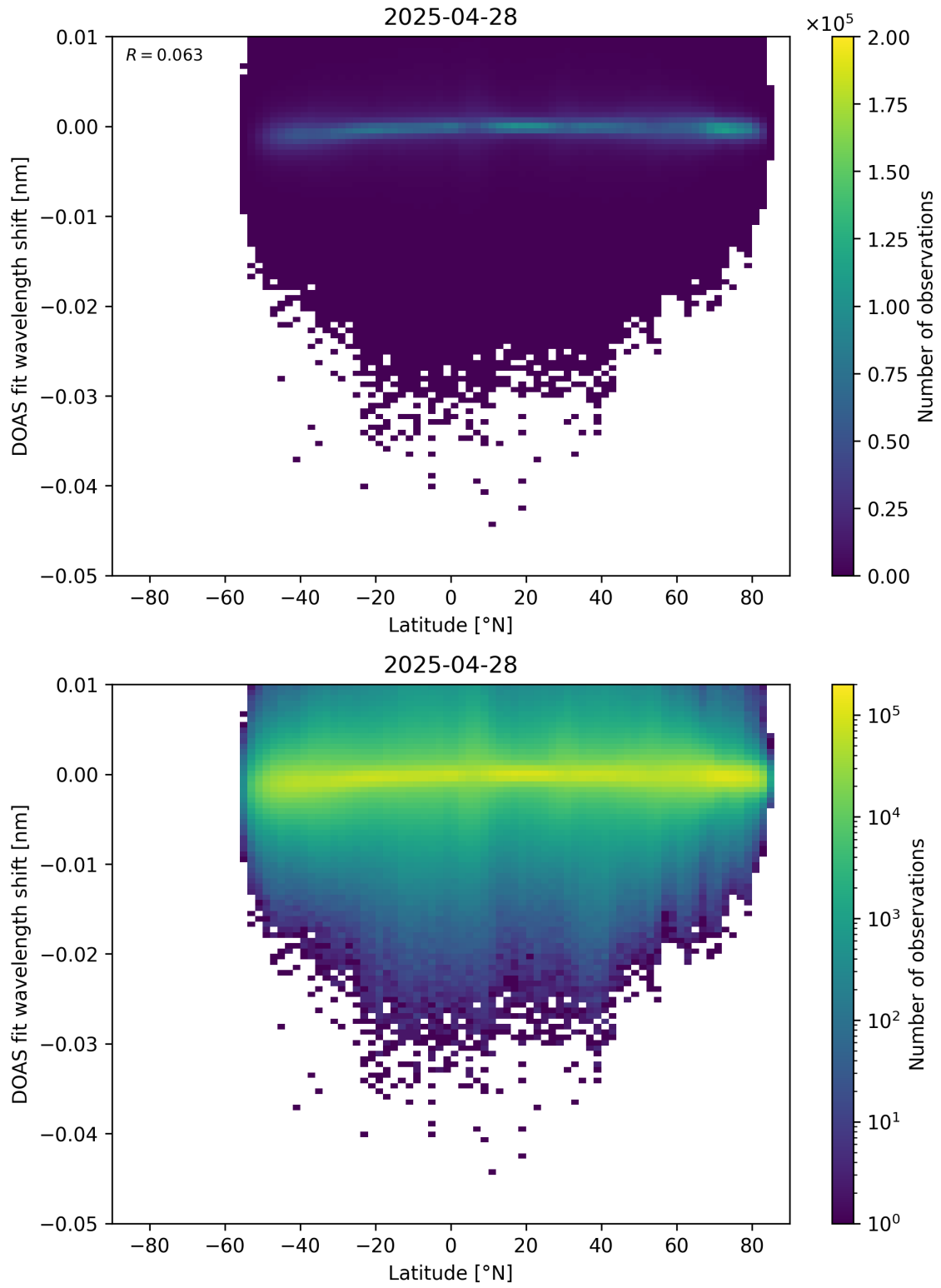
Figure 153: Scatter density plot of “Latitude” against “DOAS fit wavelength shift” for 2025-04-27 to 2025-04-29.
