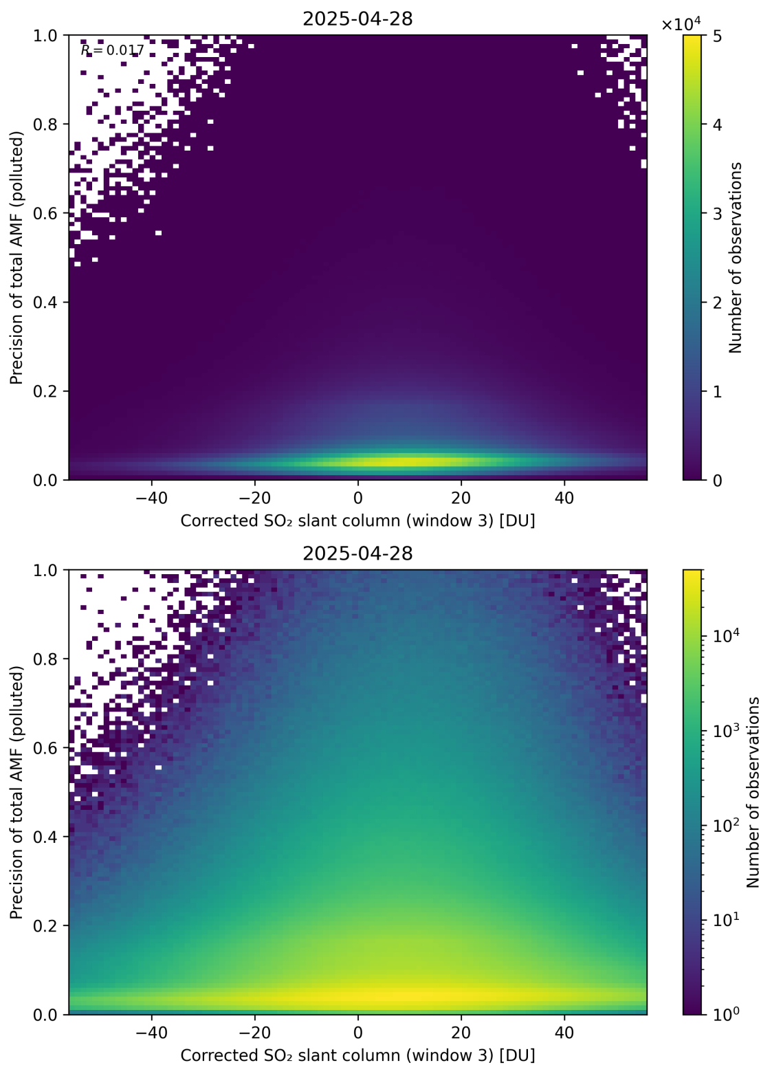
Figure 261: Scatter density plot of “Corrected SO 2 slant column (window 3)” against “Precision of total AMF (polluted)” for 2025-04-27 to 2025-04-29.
