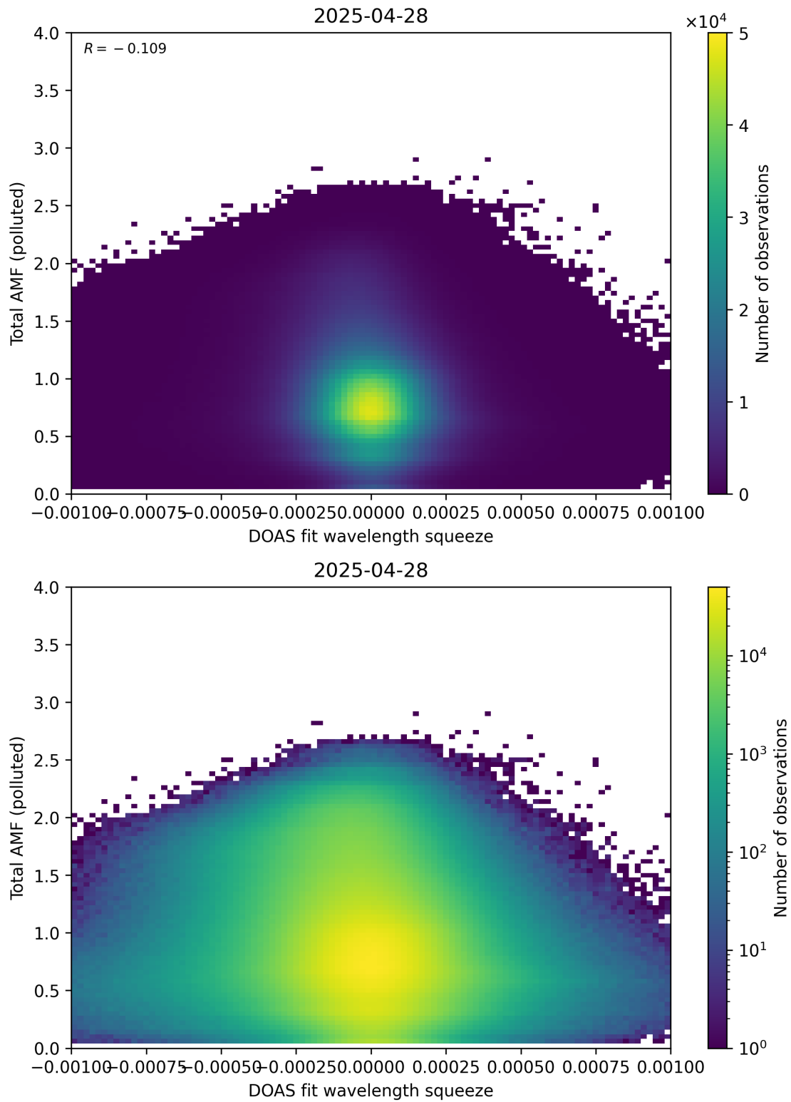
Figure 145: Scatter density plot of “DOAS fit wavelength squeeze” against “Total AMF (polluted)” for 2025-04-27 to 2025-04-29.
