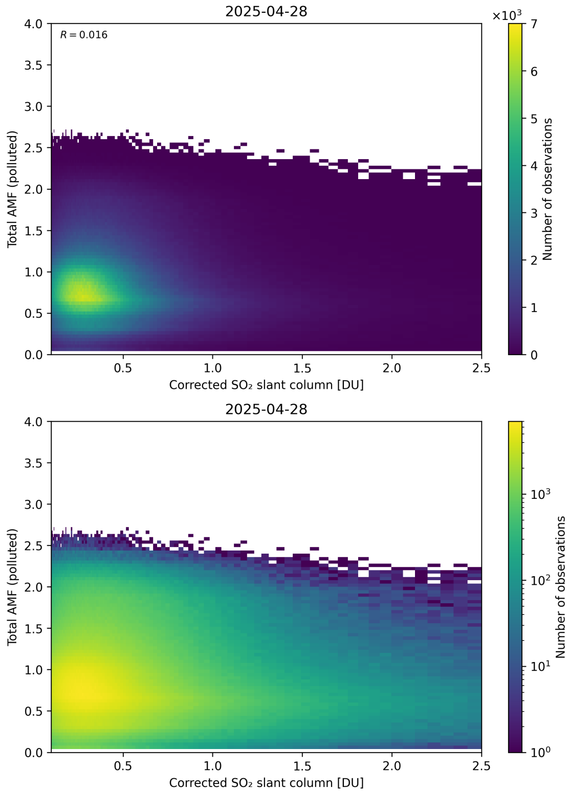
Figure 242: Scatter density plot of “Corrected SO 2 slant column” against “Total AMF (polluted)” for 2025-04-27 to 2025-04-29.
