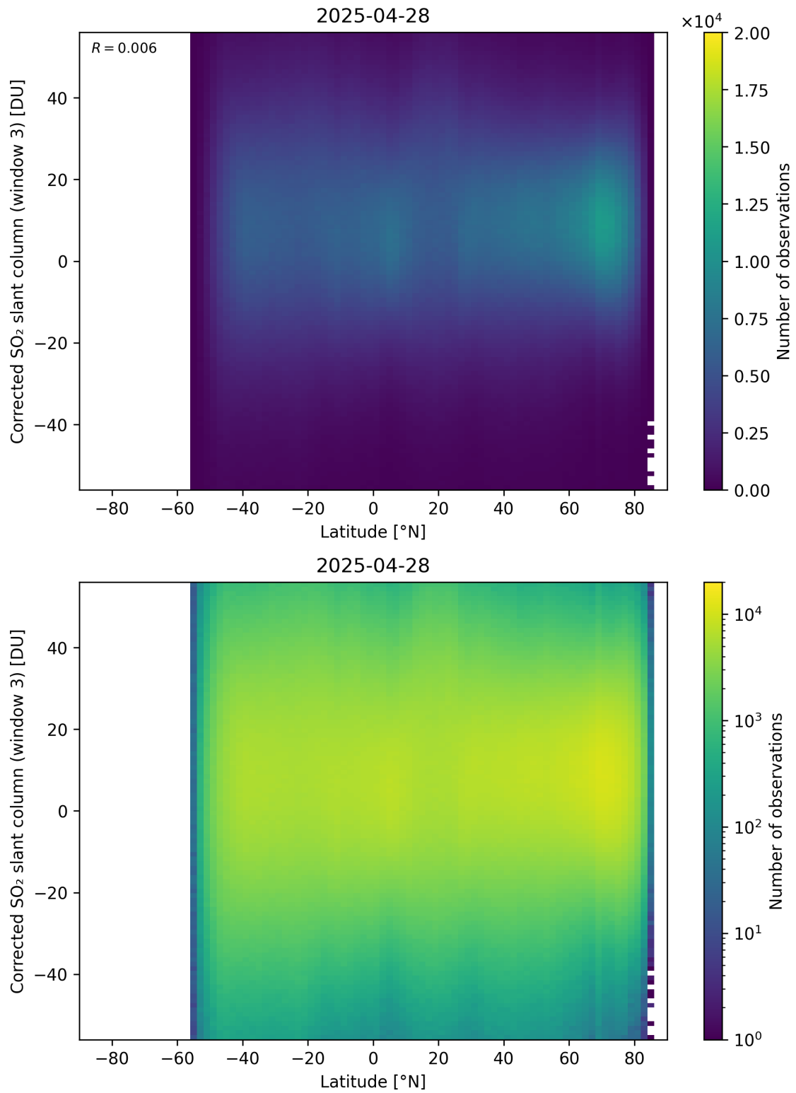
Figure 161: Scatter density plot of “Latitude” against “Corrected SO 2 slant column (window 3)” for 2025-04-27 to 2025-04-29.
