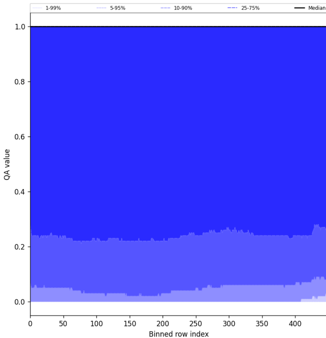
Figure 83: Along track statistics of “QA value” for 2025-04-27 to 2025-04-29
