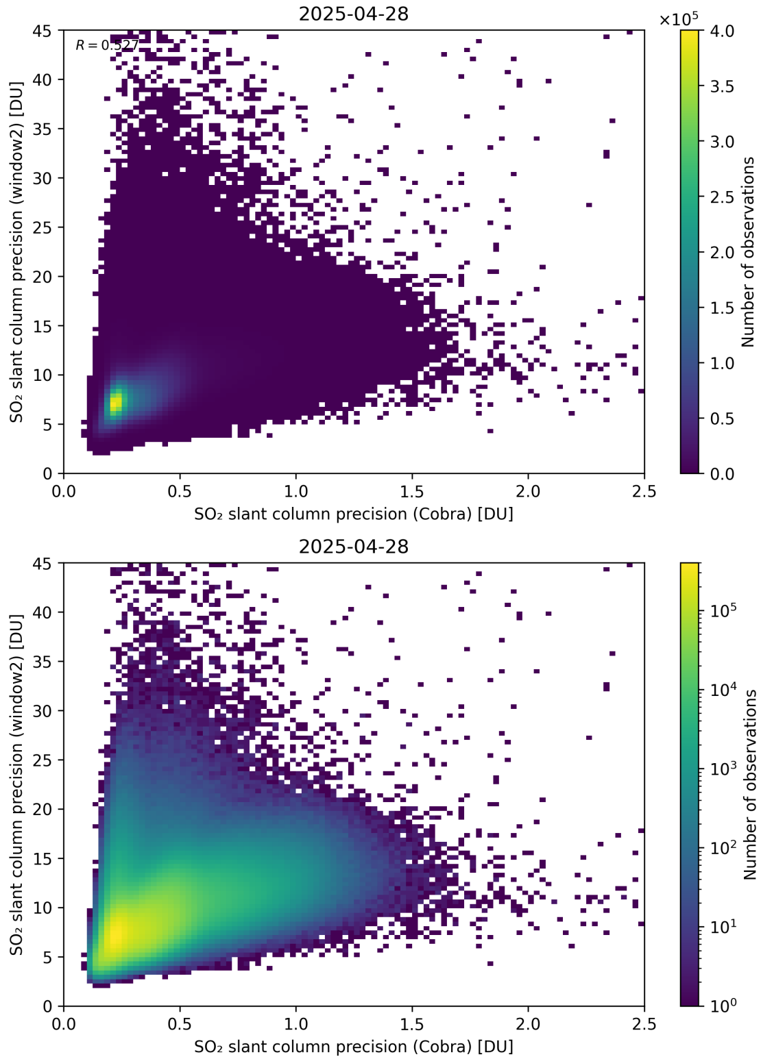
Figure 210: Scatter density plot of “SO 2 slant column precision (Cobra)” against “SO 2 slant column precision (window2)” for 2025-04-27 to 2025-04-29.
