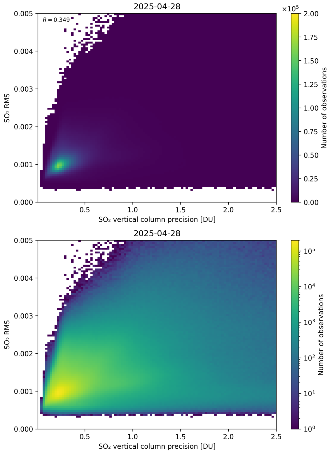
Figure 334: Scatter density plot of “SO 2 vertical column precision” against “SO 2 RMS” for 2025-04-27 to 2025-04-29.
