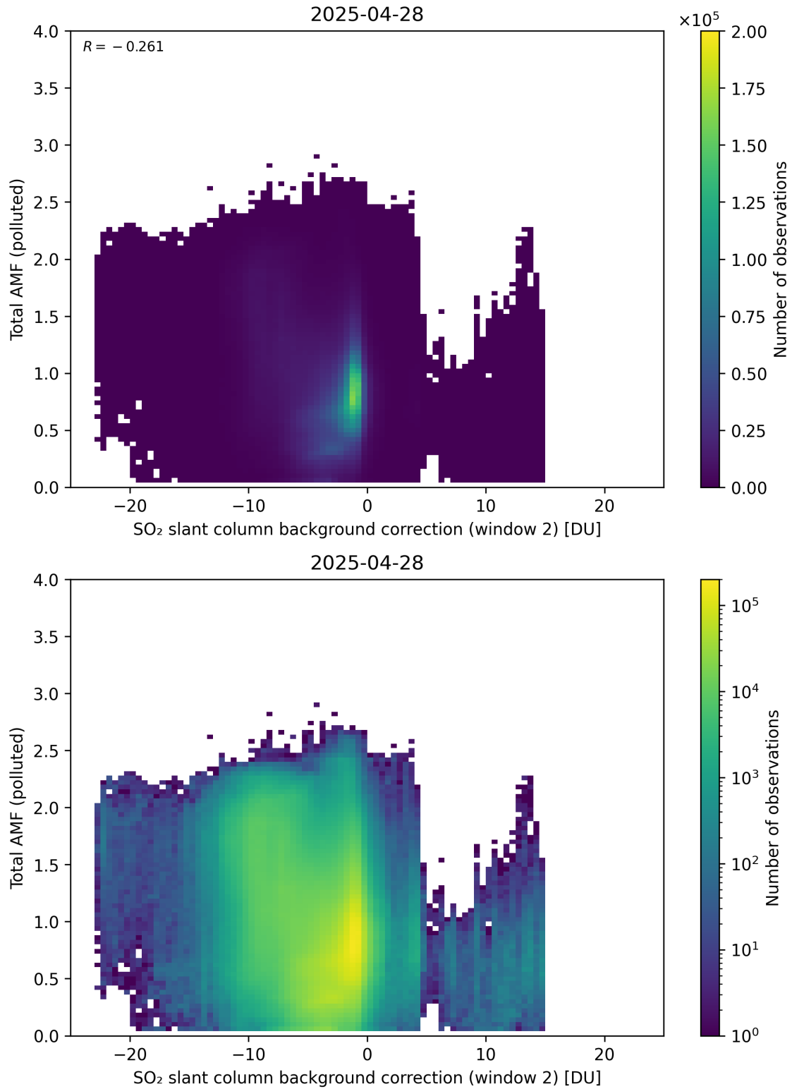
Figure 130: Scatter density plot of “SO 2 slant column background correction (window 2)” against “Total AMF (polluted)” for 2025-04-27 to 2025-04-29.
