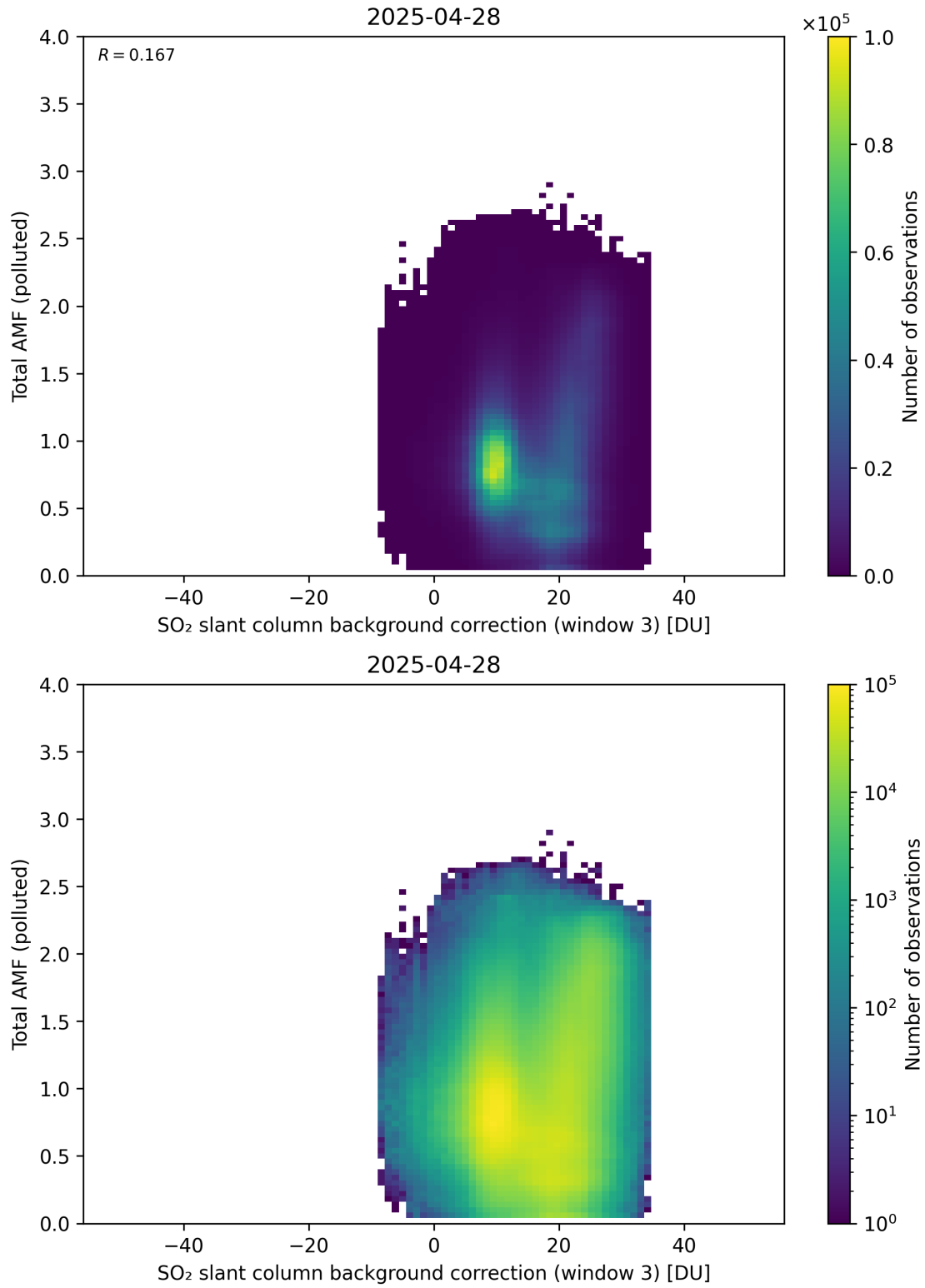
Figure 136: Scatter density plot of “SO 2 slant column background correction (window 3)” against “Total AMF (polluted)” for 2025-04-27 to 2025-04-29.
