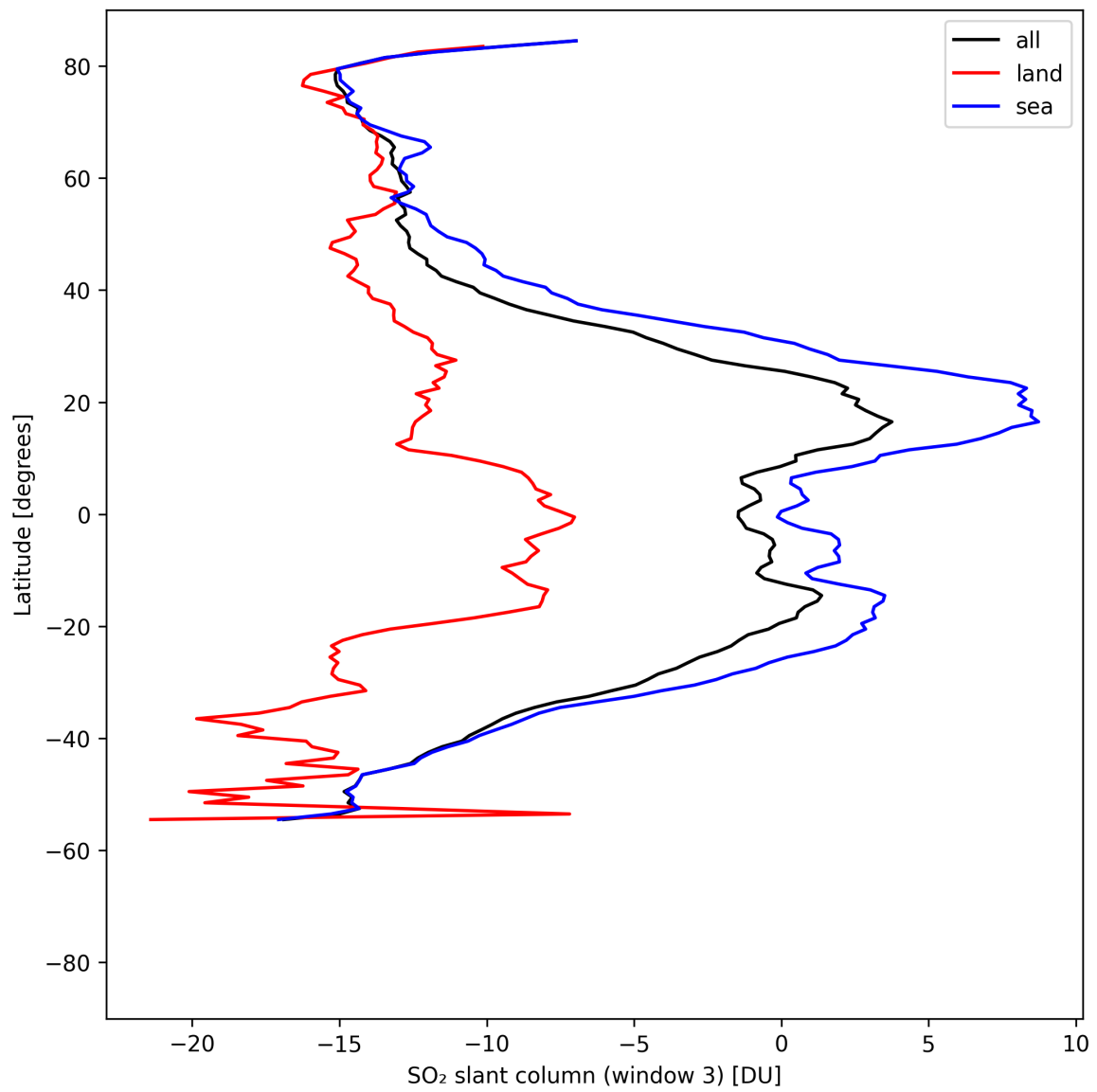
Figure 45: Zonal average of “SO 2 slant column (window 3)” for 2025-04-27 to 2025-04-29.
