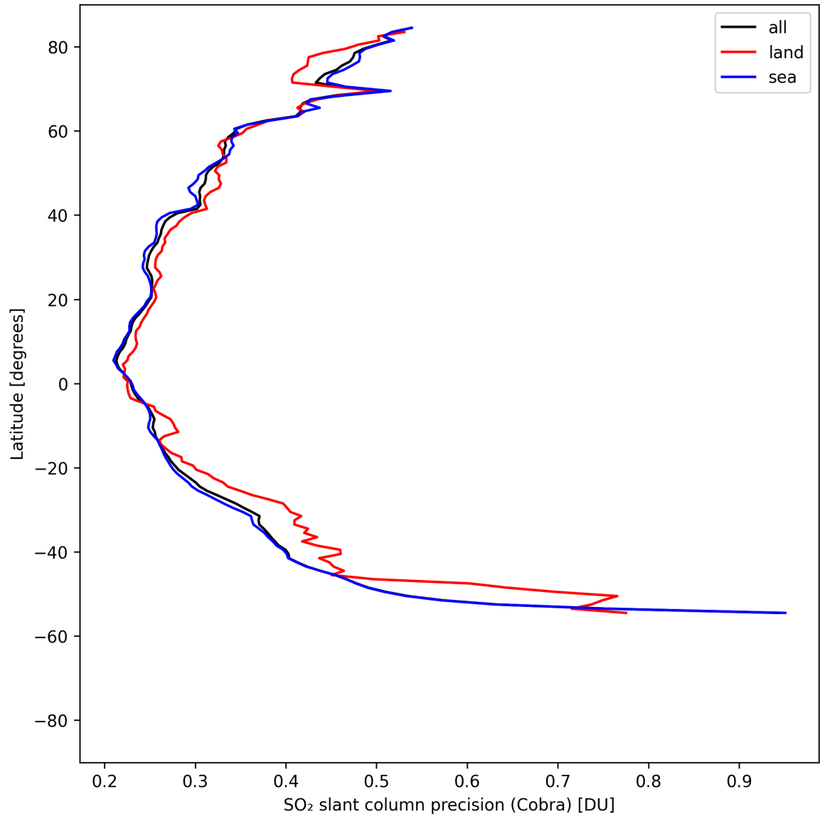
Figure 36: Zonal average of "SO 2 slant column precision (Cobra)" for 2025-04-27 to 2025-04-29.
