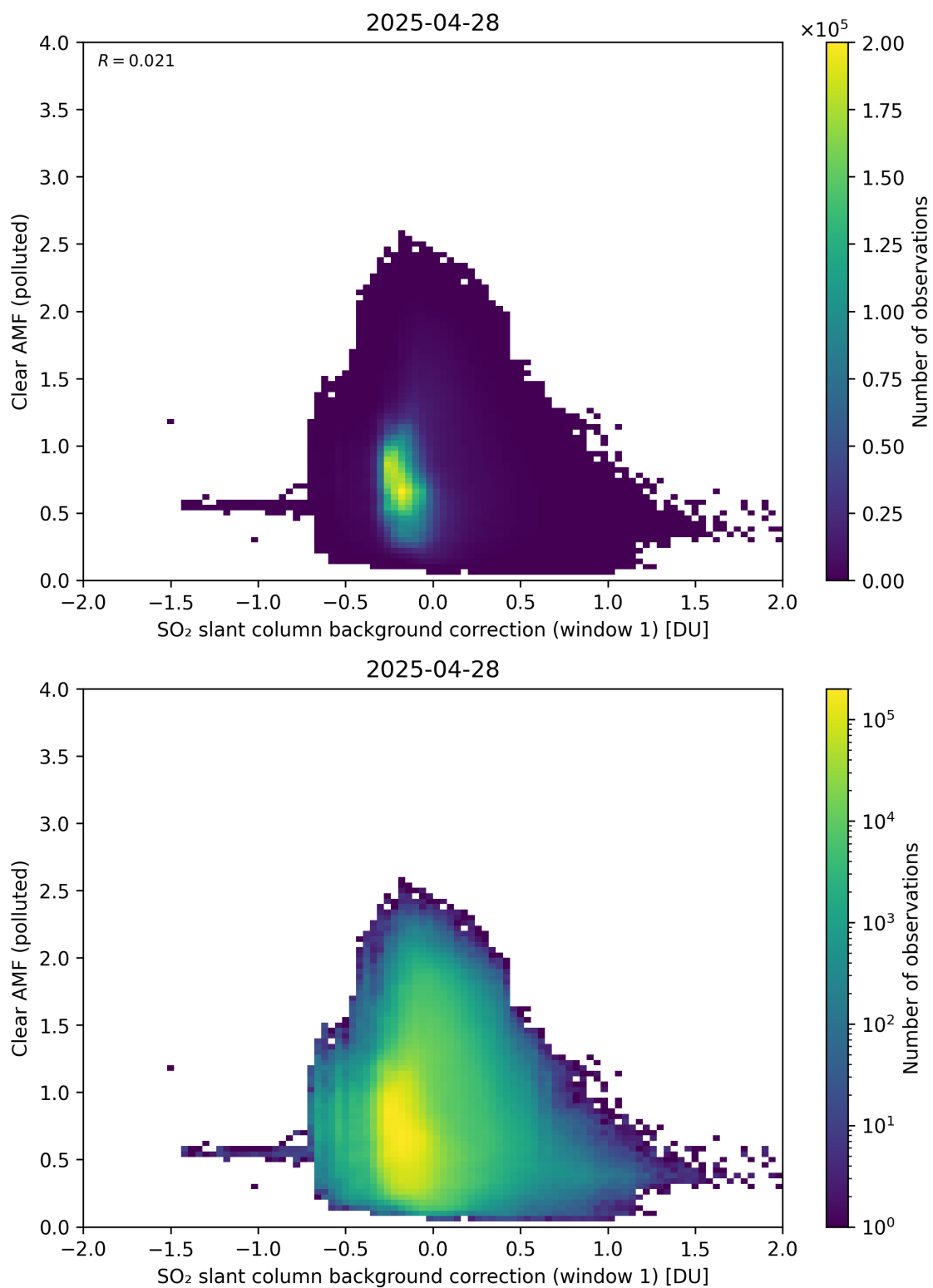
Figure 114: Scatter density plot of “SO 2 slant column background correction (window 1)” against “Clear AMF (polluted)” for 2025-04-27 to 2025-04-29.
