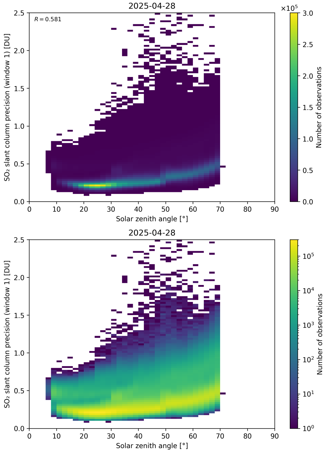
Figure 185: Scatter density plot of “Solar zenith angle” against “SO 2 slant column precision (window 1)” for 2025-04-27 to 2025-04-29.
