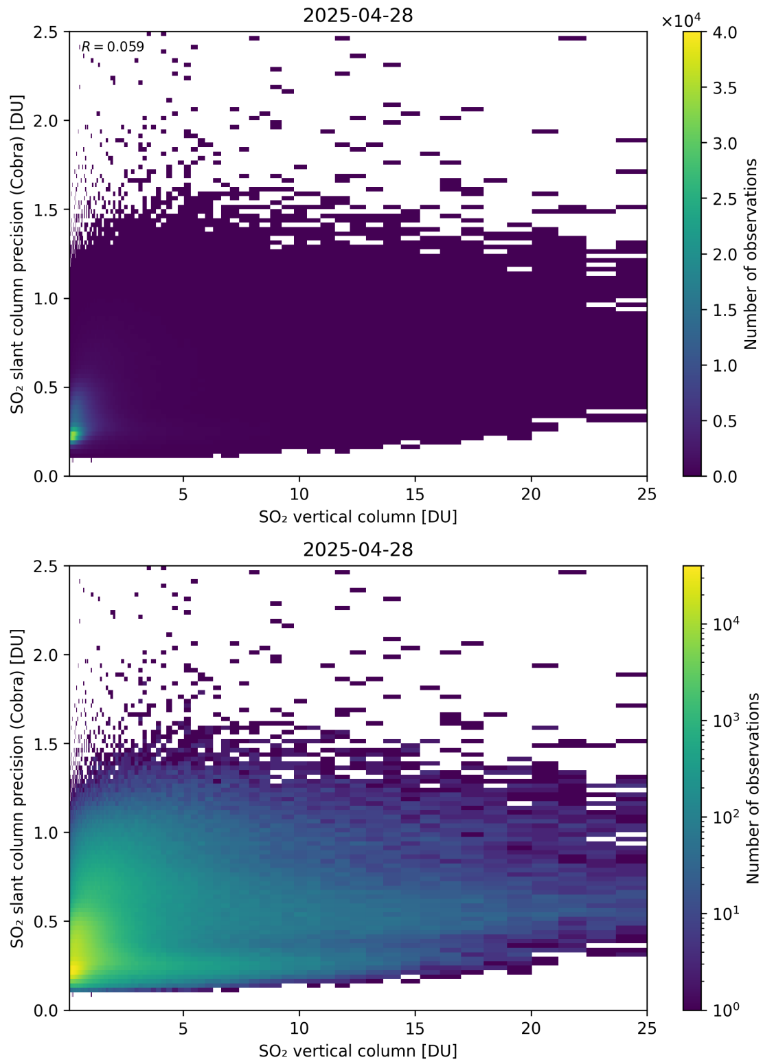
Figure 350: Scatter density plot of “SO 2 vertical column” against “SO 2 slant column precision (Cobra)” for 2025-04-27 to 2025-04-29.
