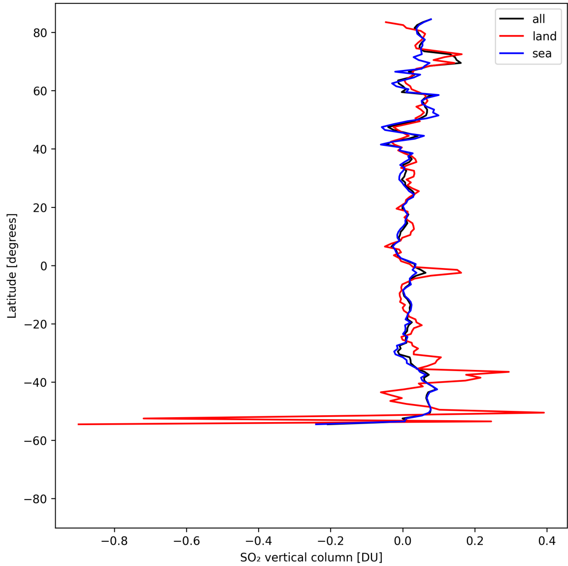
Figure 32: Zonal average of “SO 2 vertical column” for 2025-04-27 to 2025-04-29.
