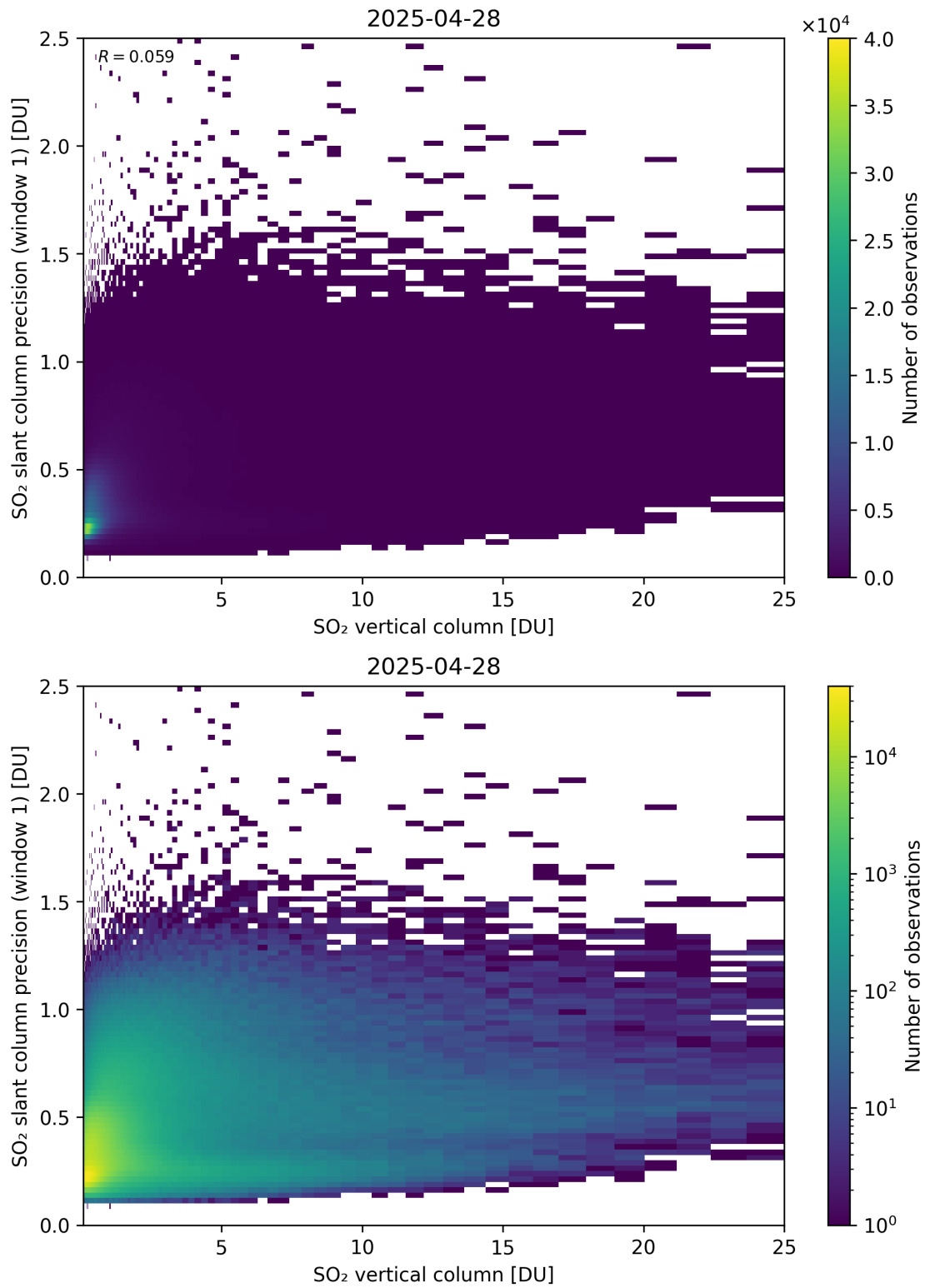
Figure 355: Scatter density plot of “SO 2 vertical column” against “SO 2 slant column precision (window 1)” for 2025-04-27 to 2025-04-29.
