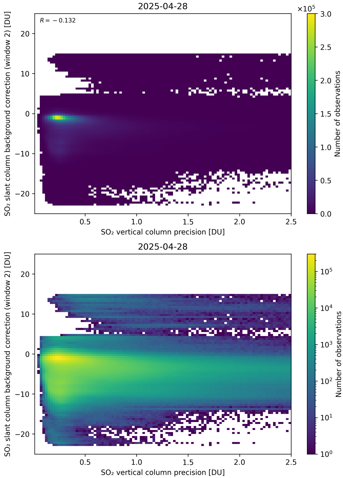
Figure 330: Scatter density plot of “SO 2 vertical column precision” against “SO 2 slant column background correction (window 2)” for 2025-04-27 to 2025-04-29.
