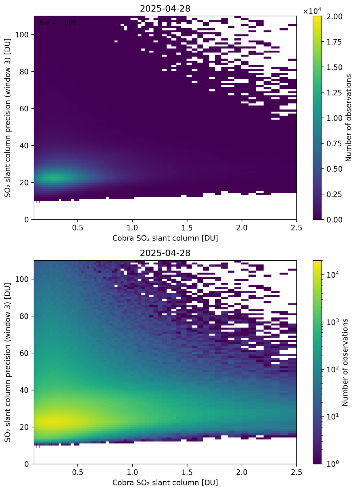
Figure 223: Scatter density plot of “Cobra SO 2 slant column” against “SO 2 slant column precision (window 3)” for 2025-04-27 to 2025-04-29.
