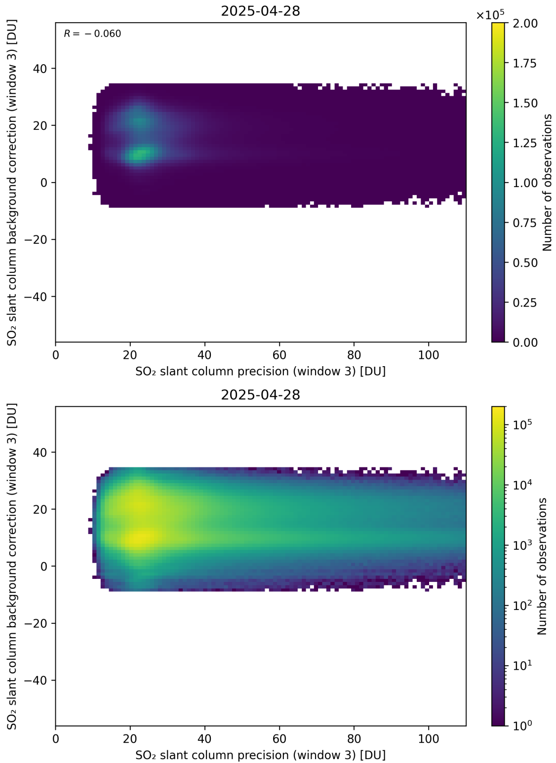
Figure 307: Scatter density plot of “SO 2 slant column precision (window 3)” against “SO 2 slant column background correction (window 3)” for 2025-04-27 to 2025-04-29.
