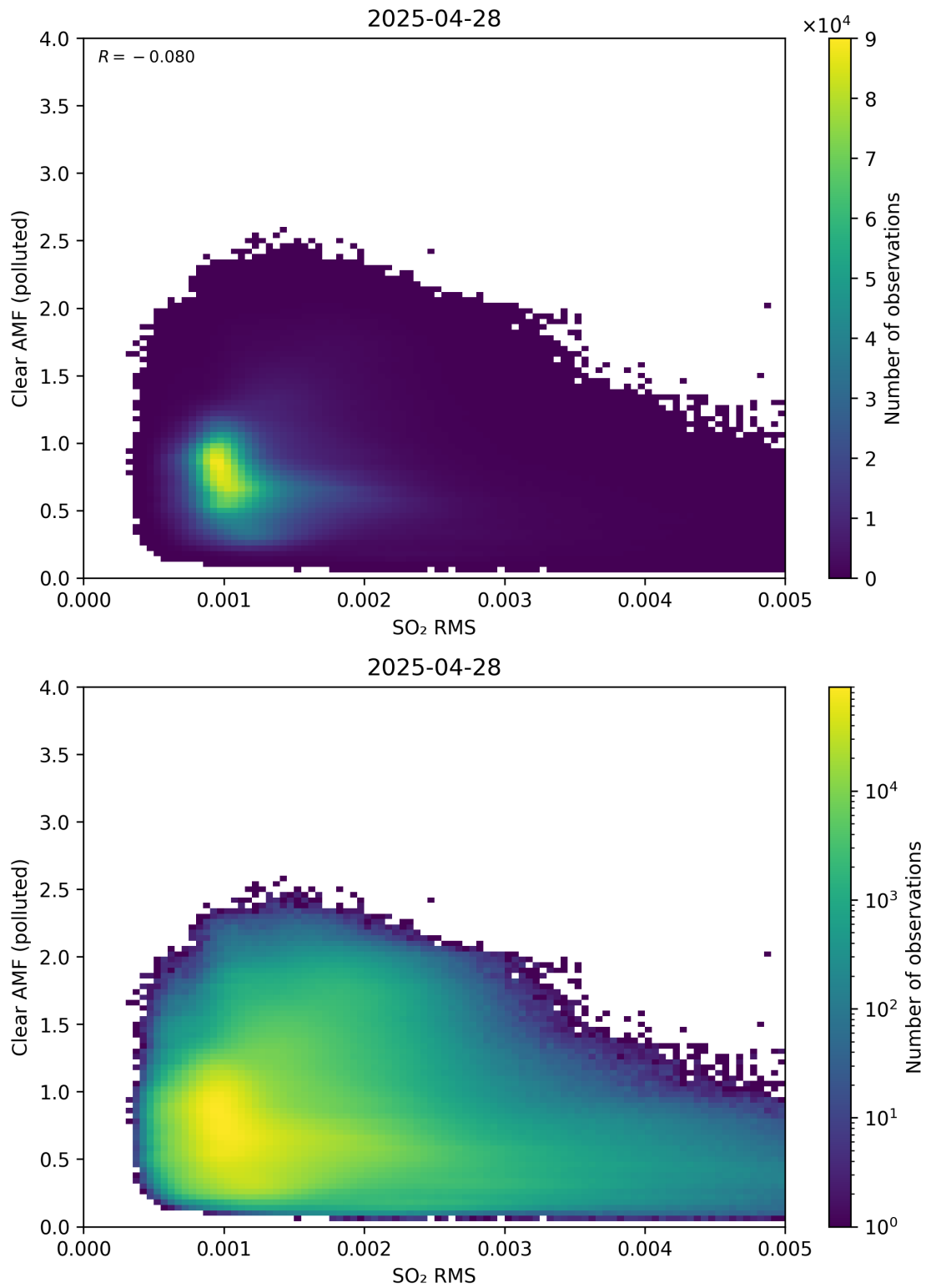
Figure 147: Scatter density plot of “SO 2 RMS” against “Clear AMF (polluted)” for 2025-04-27 to 2025-04-29.
