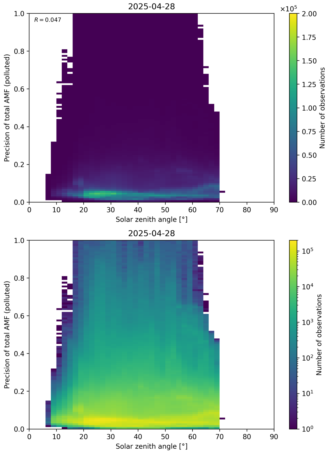
Figure 190: Scatter density plot of “Solar zenith angle” against “Precision of total AMF (polluted)” for 2025-04-27 to 2025-04-29.
