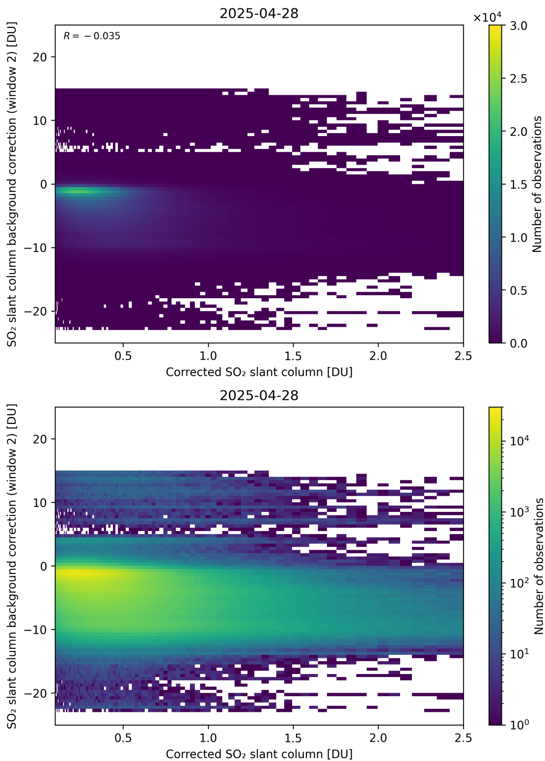
Figure 227: Scatter density plot of “Corrected SO 2 slant column” against “SO 2 slant column background correction (window 2)” for 2025-04-27 to 2025-04-29.
