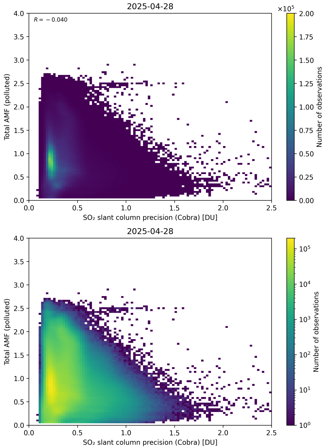
Figure 213: Scatter density plot of “SO 2 slant column precision (Cobra)” against “Total AMF (polluted)” for 2025-04-27 to 2025-04-29.
