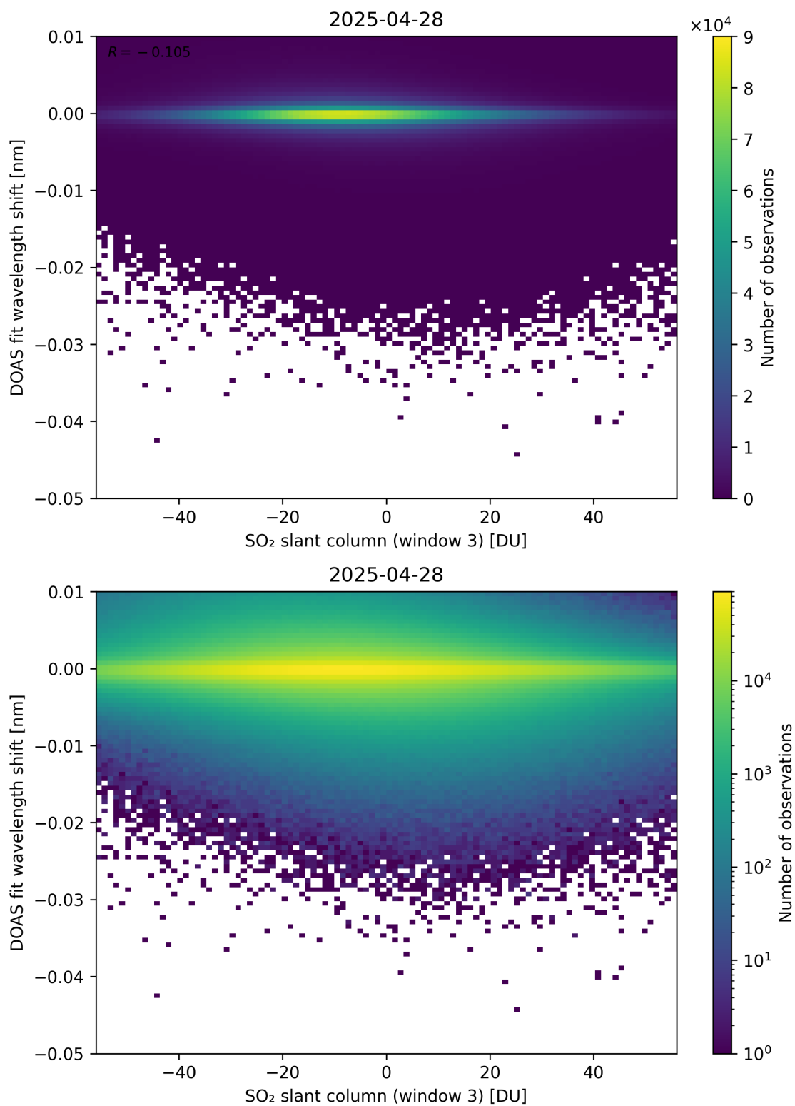
Figure 304: Scatter density plot of “SO 2 slant column (window 3)” against “DOAS fit wavelength shift” for 2025-04-27 to 2025-04-29.
