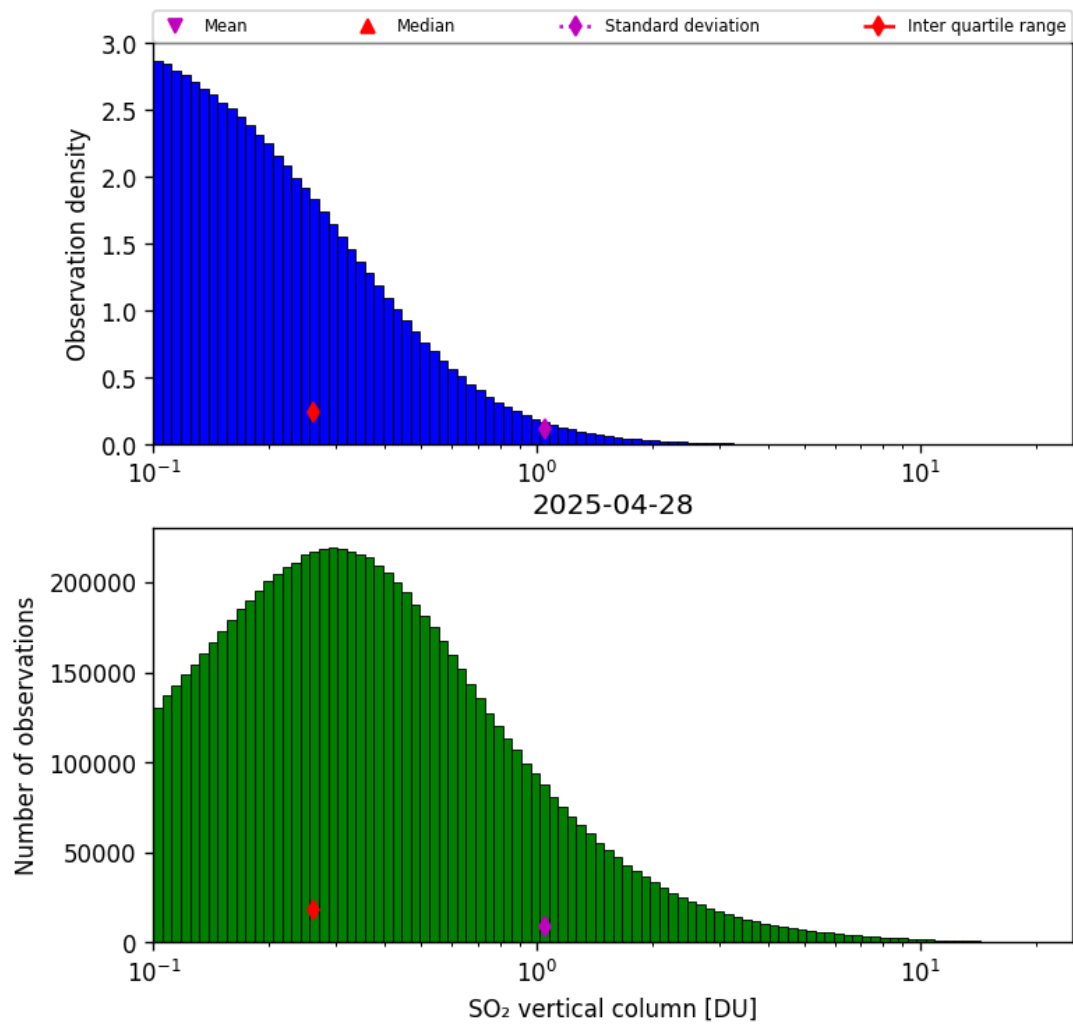
Figure 58: Histogram of “SO 2 vertical column” for 2025-04-27 to 2025-04-29
