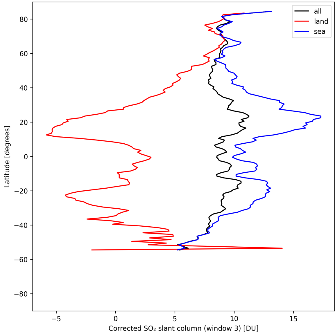
Figure 47: Zonal average of “Corrected SO 2 slant column (window 3)” for 2025-04-27 to 2025-04-29.
