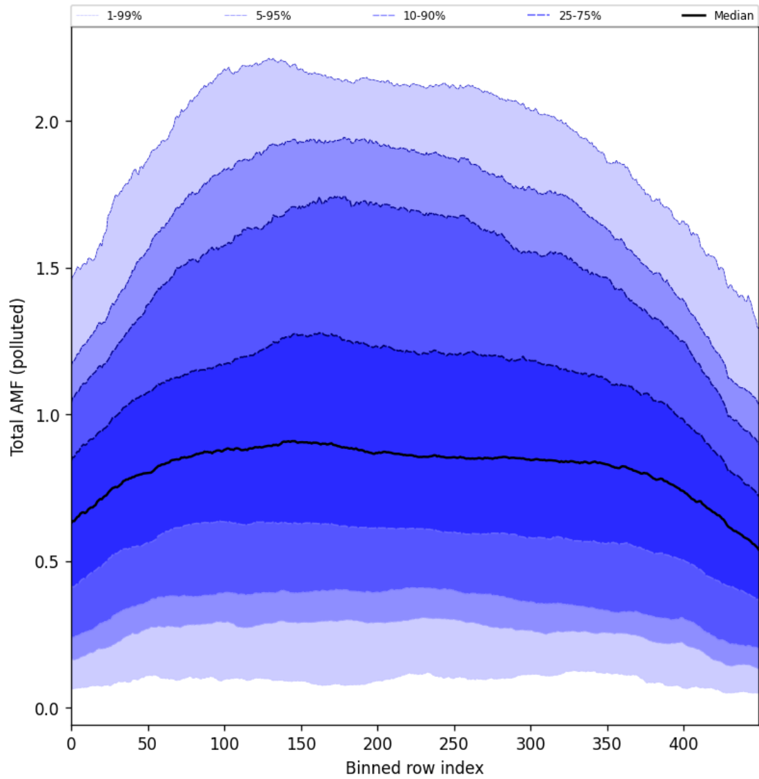
Figure 105: Along track statistics of “Total AMF (polluted)” for 2025-04-27 to 2025-04-29
