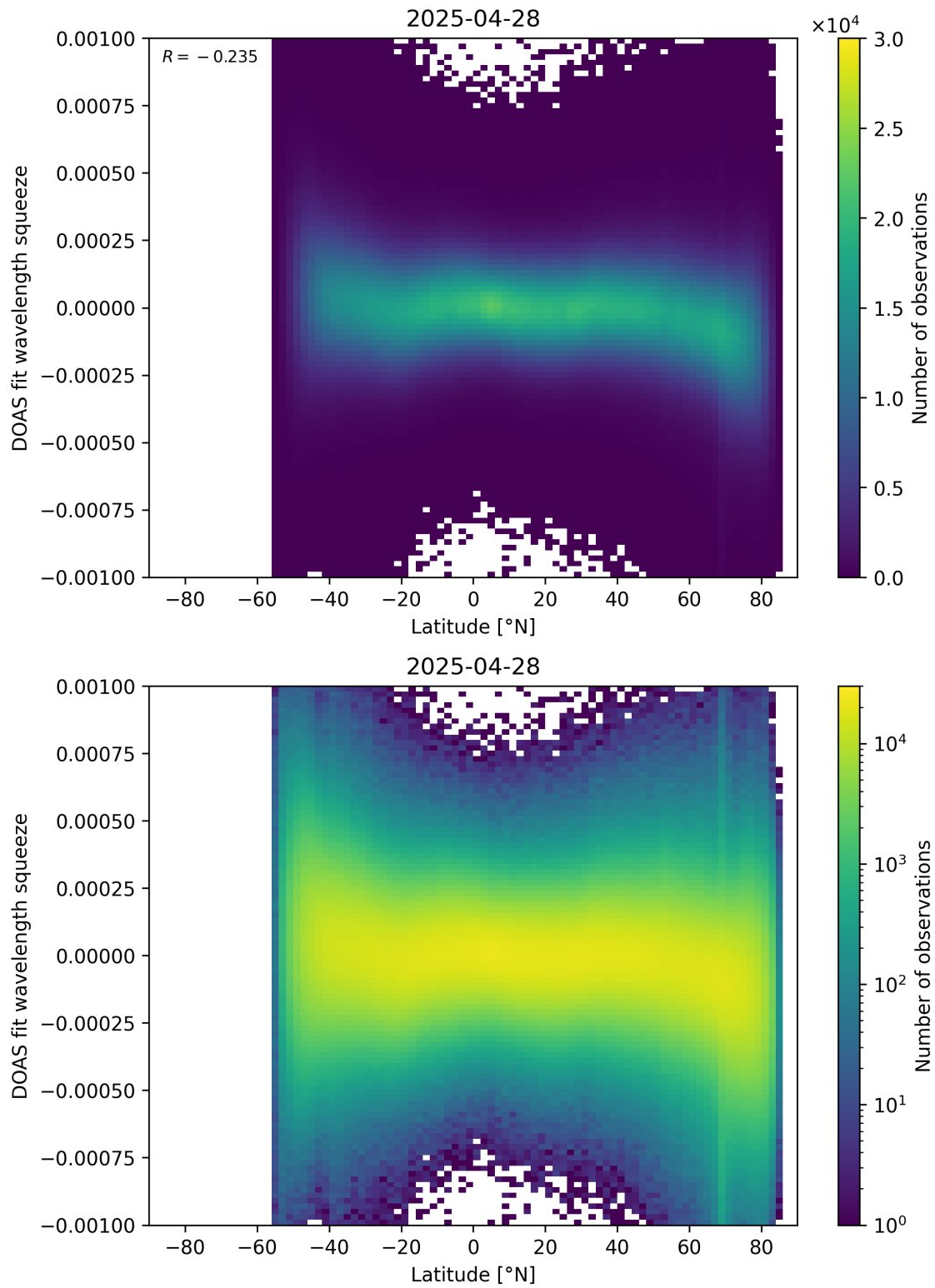
Figure 154: Scatter density plot of “Latitude” against “DOAS fit wavelength squeeze” for 2025-04-27 to 2025-04-29.
