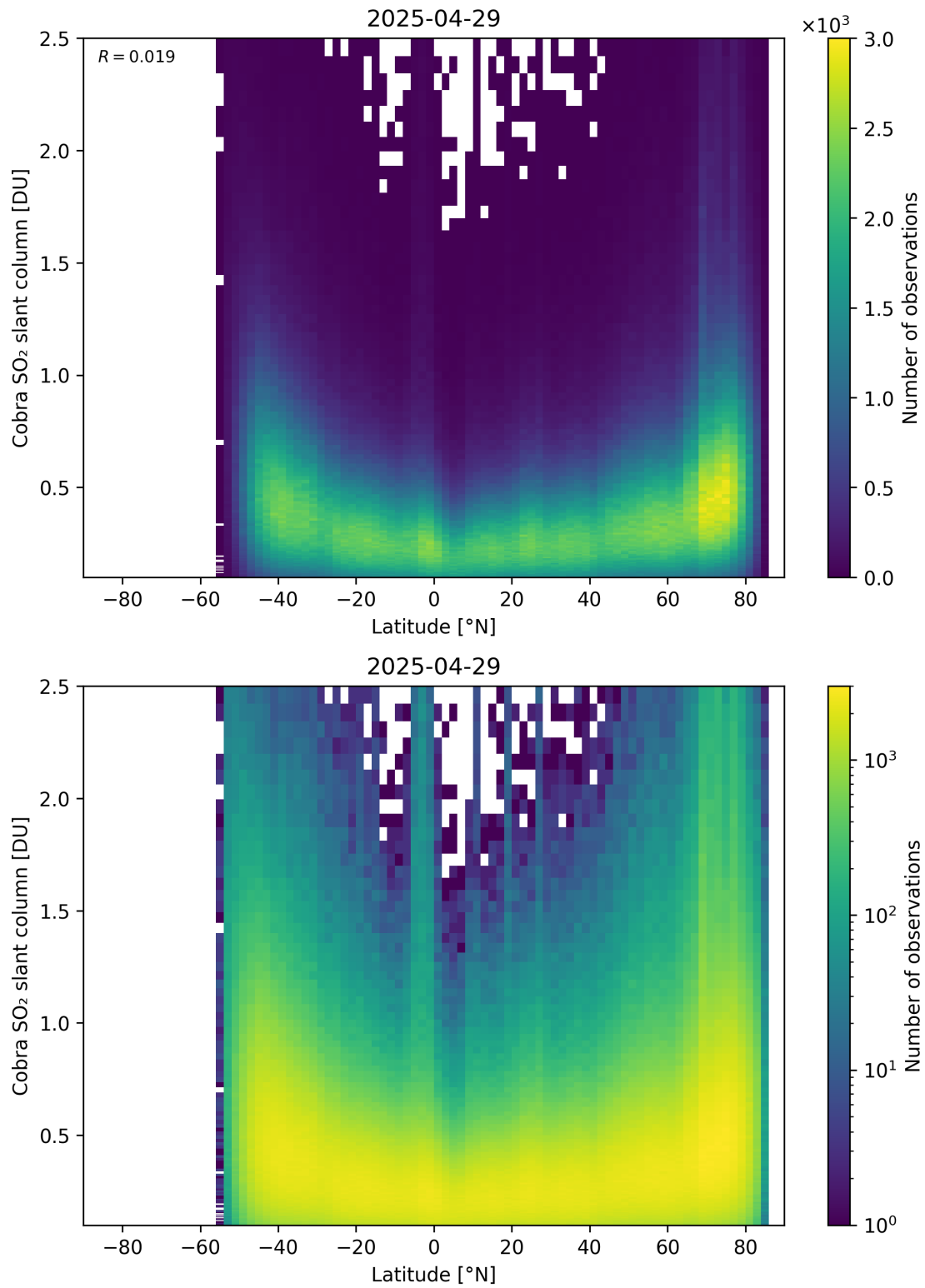
Figure 157: Scatter density plot of “Latitude” against “Cobra SO 2 slant column” for 2025-04-29 to 2025-04-30.
