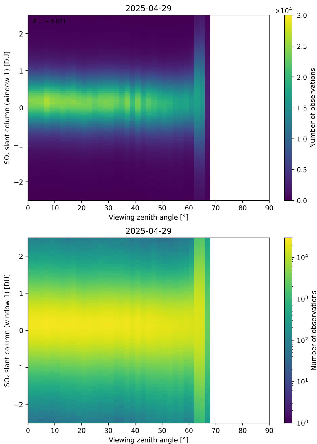
Figure 376: Scatter density plot of “Viewing zenith angle” against “SO 2 slant column (window 1)” for 2025-04-29 to 2025-04-30.
