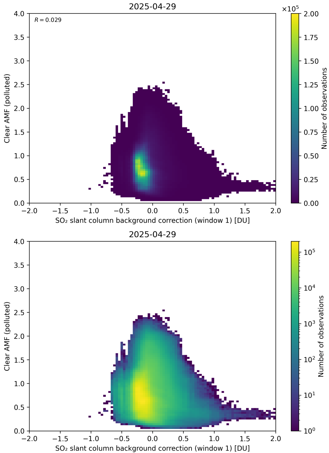
Figure 114: Scatter density plot of “SO 2 slant column background correction (window 1)” against “Clear AMF (polluted)” for 2025-04-29 to 2025-04-30.
