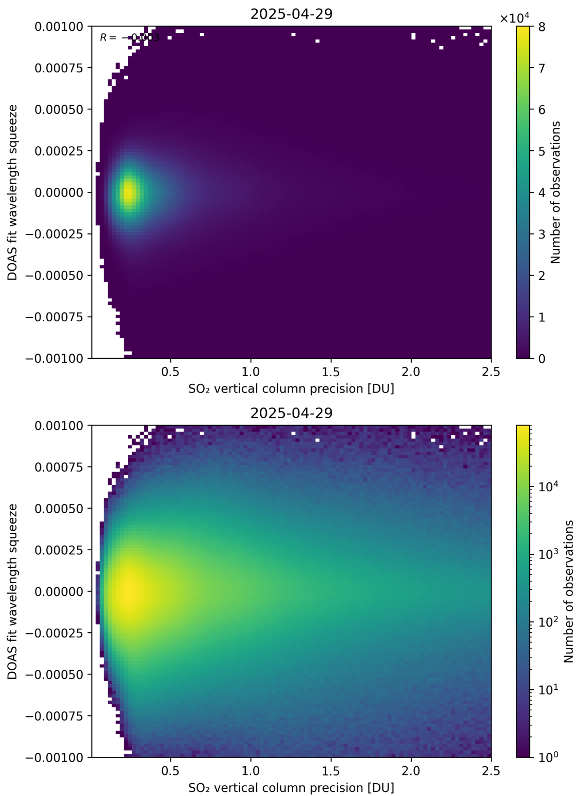
Figure 333: Scatter density plot of “SO 2 vertical column precision” against “DOAS fit wavelength squeeze” for 2025-04-29 to 2025-04-30.
