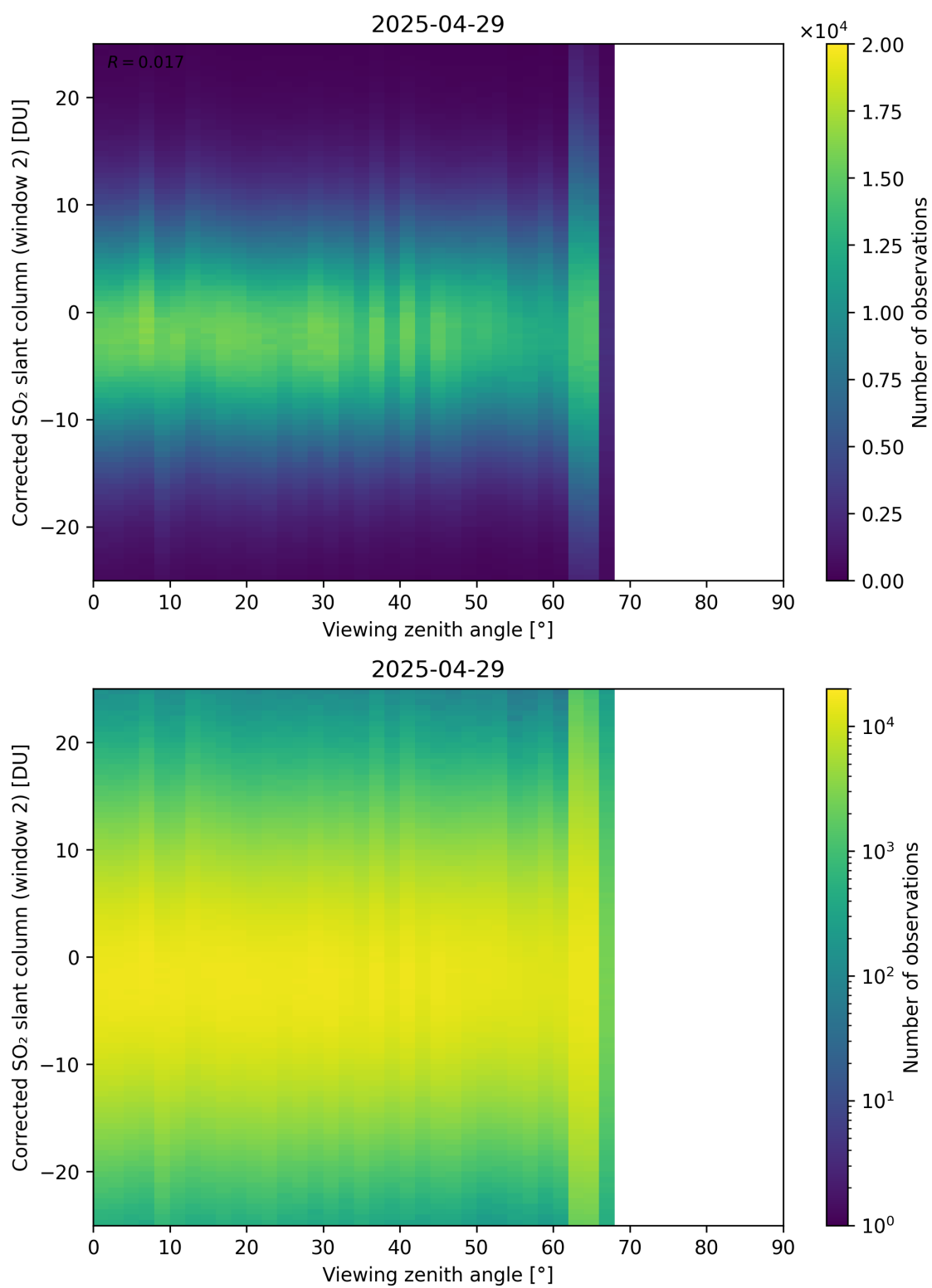
Figure 374: Scatter density plot of “Viewing zenith angle” against “Corrected SO 2 slant column (window 2)” for 2025-04-29 to 2025-04-30.
