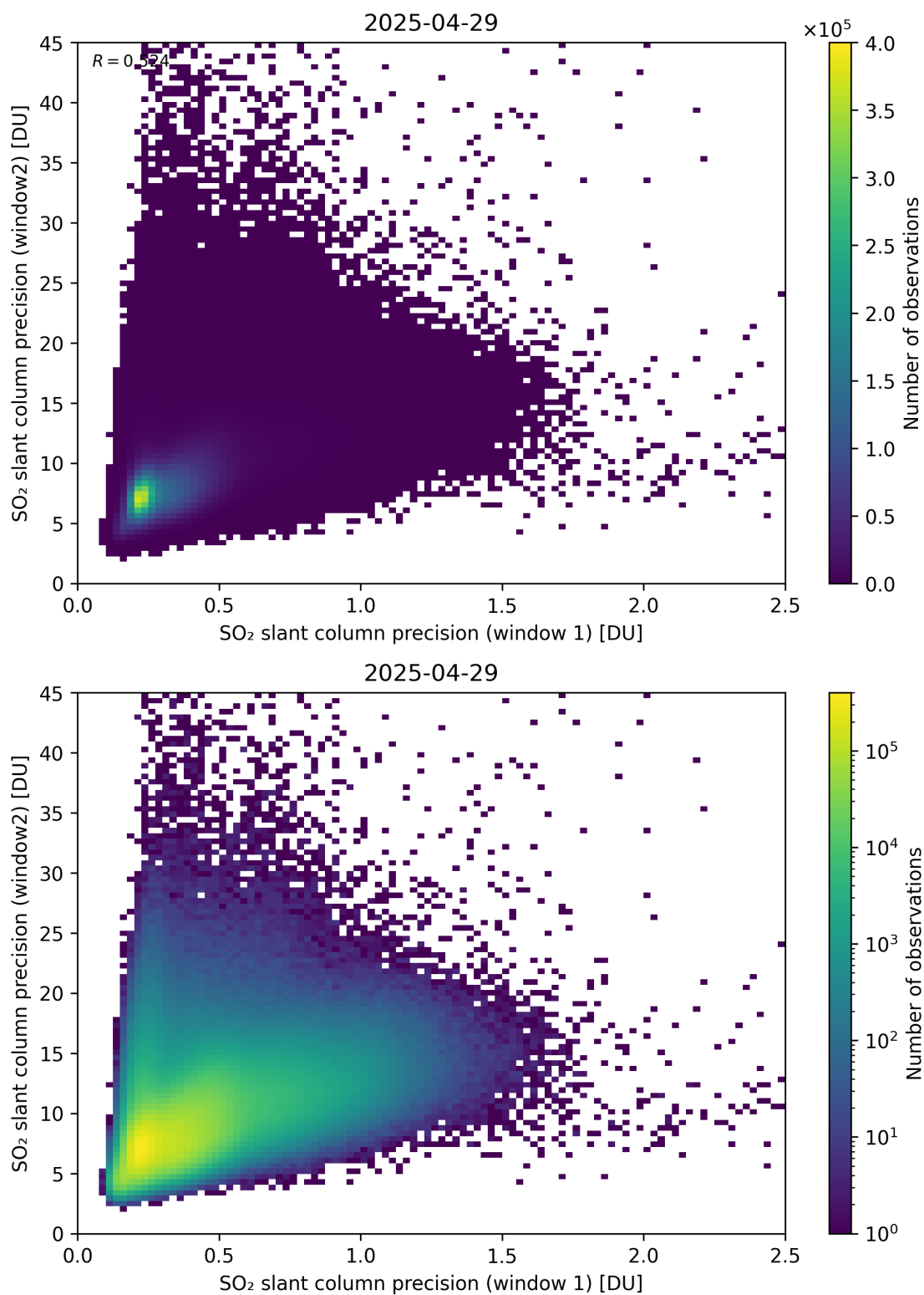
Figure 277: Scatter density plot of “SO 2 slant column precision (window 1)” against “SO 2 slant column precision (window2)” for 2025-04-29 to 2025-04-30.
