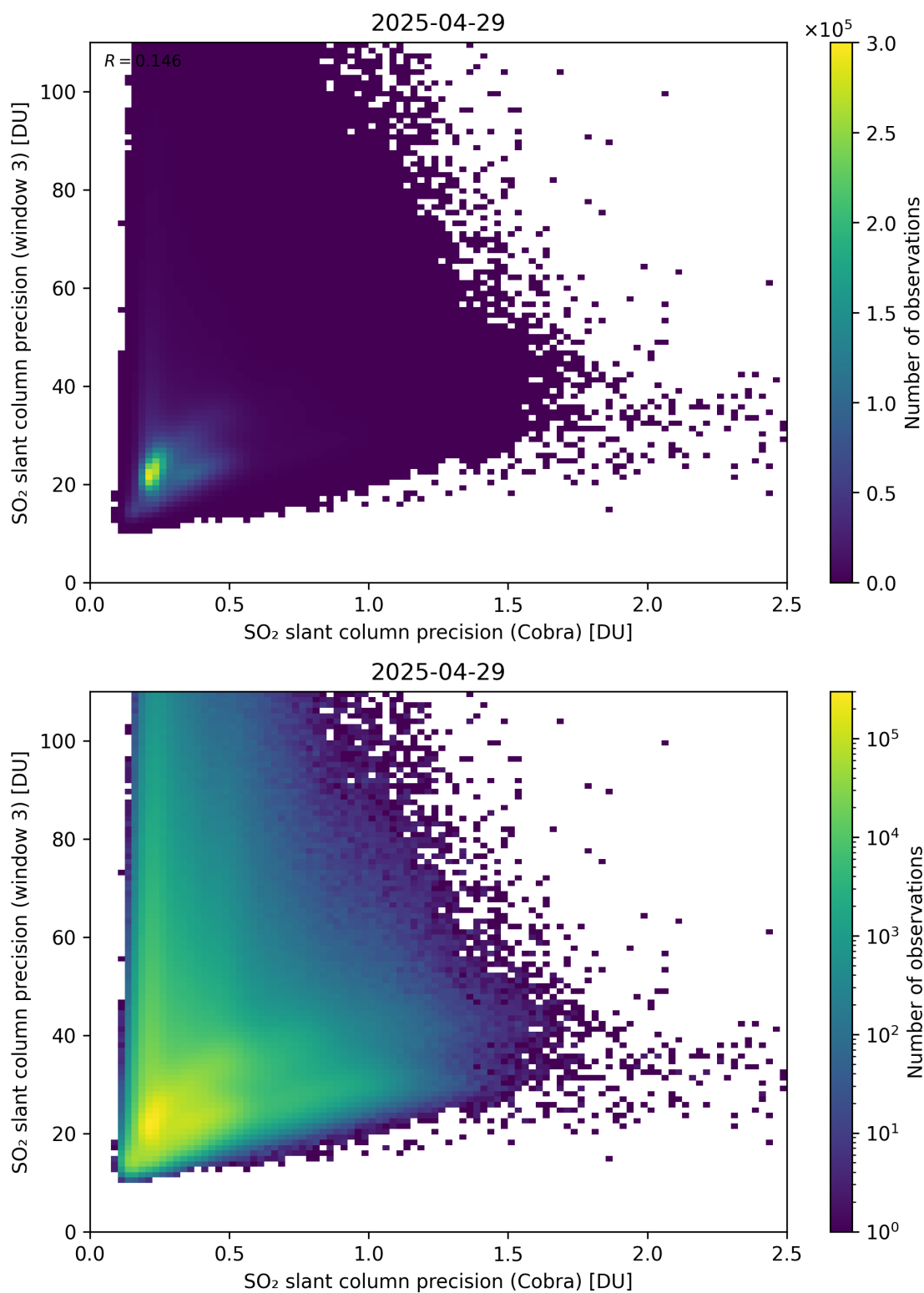
Figure 212: Scatter density plot of “SO 2 slant column precision (Cobra)” against “SO 2 slant column precision (window 3)” for 2025-04-29 to 2025-04-30.
