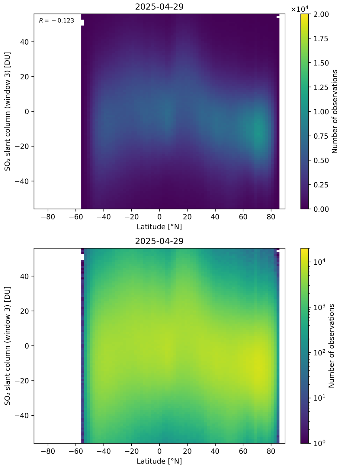
Figure 165: Scatter density plot of “Latitude” against “SO 2 slant column (window 3)” for 2025-04-29 to 2025-04-30.
