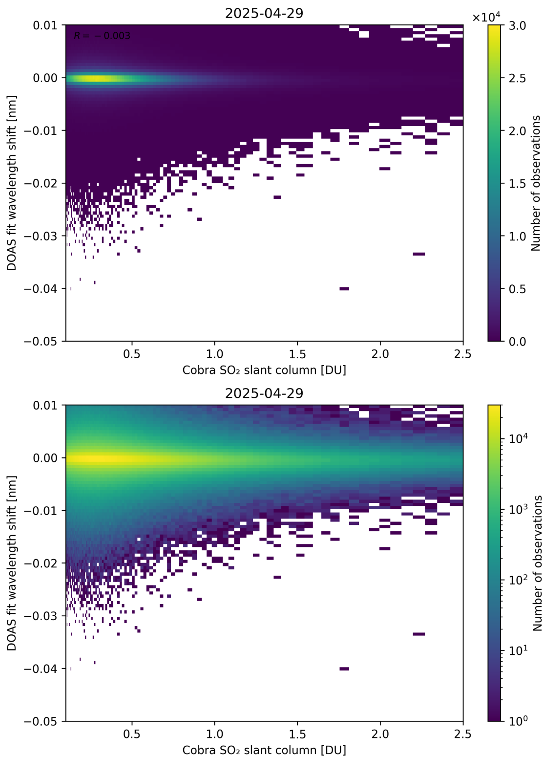
Figure 196: Scatter density plot of “Cobra SO 2 slant column” against “DOAS fit wavelength shift” for 2025-04-29 to 2025-04-30.
