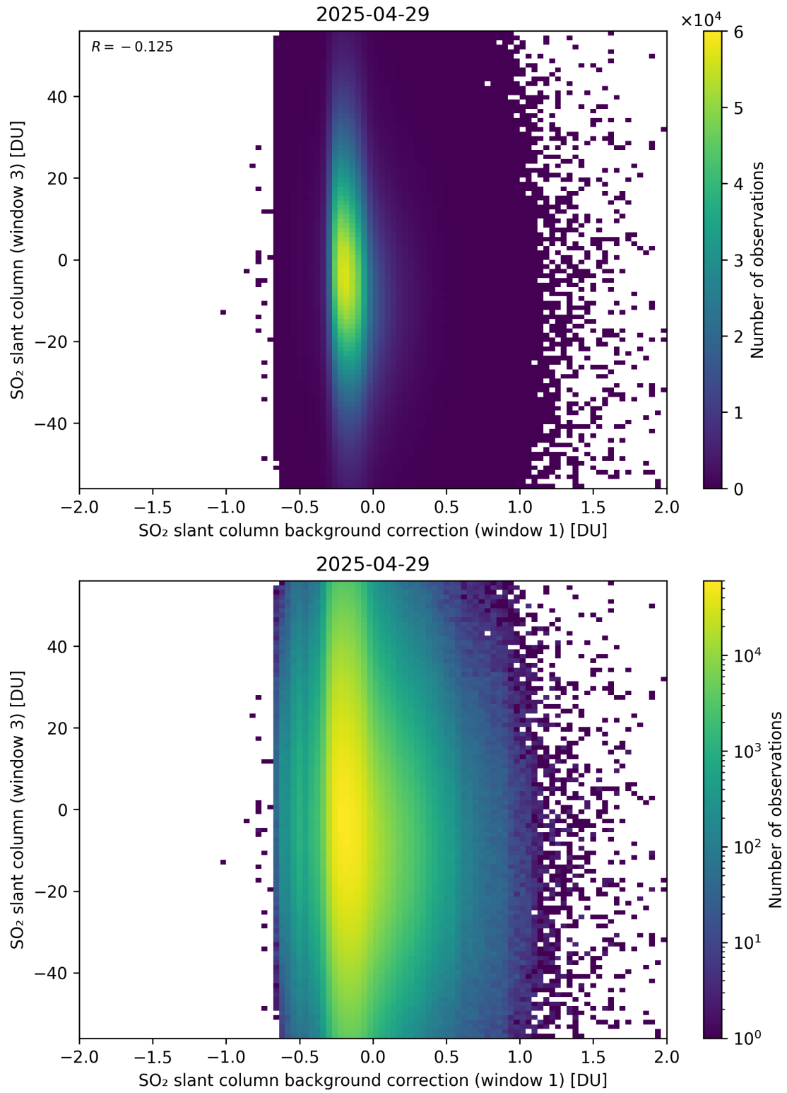
Figure 118: Scatter density plot of “SO 2 slant column background correction (window 1)” against “SO 2 slant column (window 3)” for 2025-04-29 to 2025-04-30.
