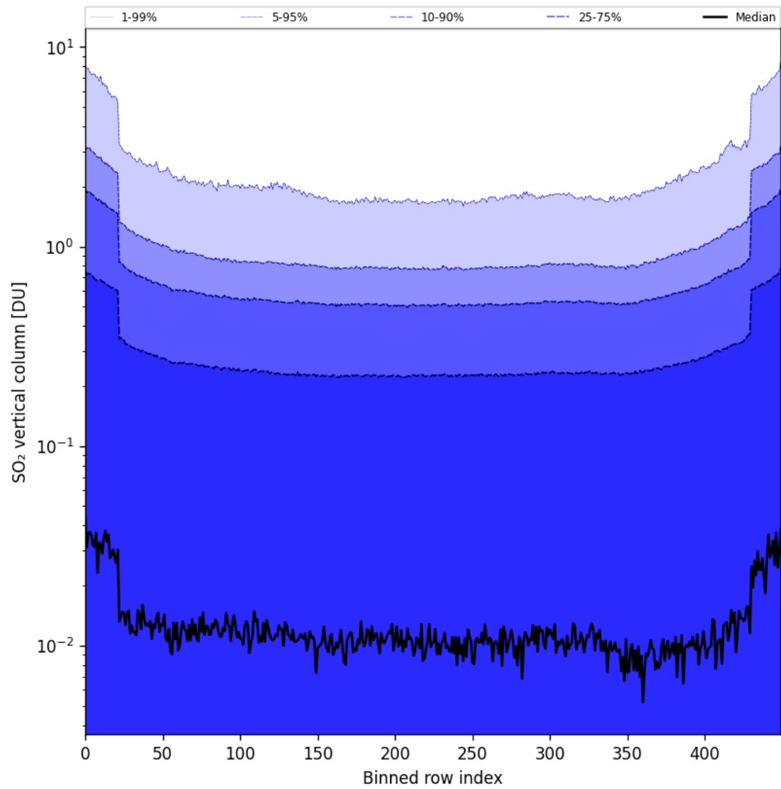
Figure 84: Along track statistics of “SO 2 vertical column” for 2025-04-29 to 2025-04-30
