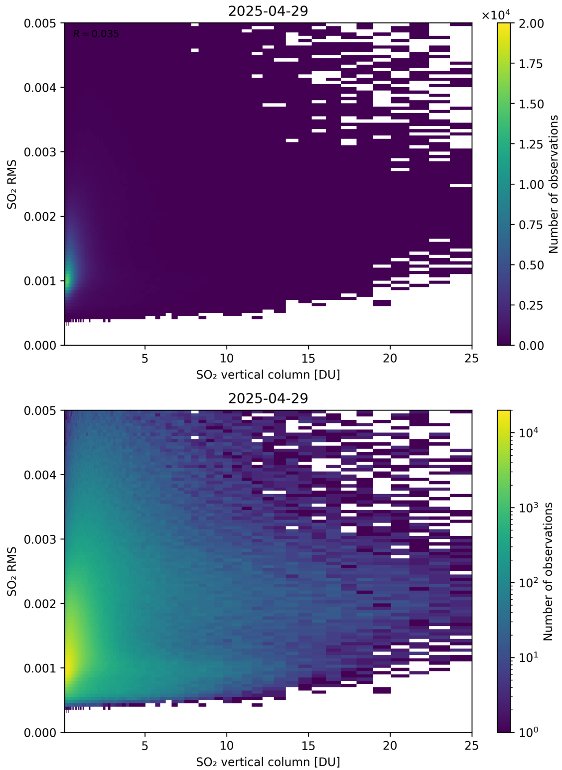
Figure 328: Scatter density plot of “SO 2 vertical column” against “SO 2 RMS” for 2025-04-29 to 2025-04-30.
