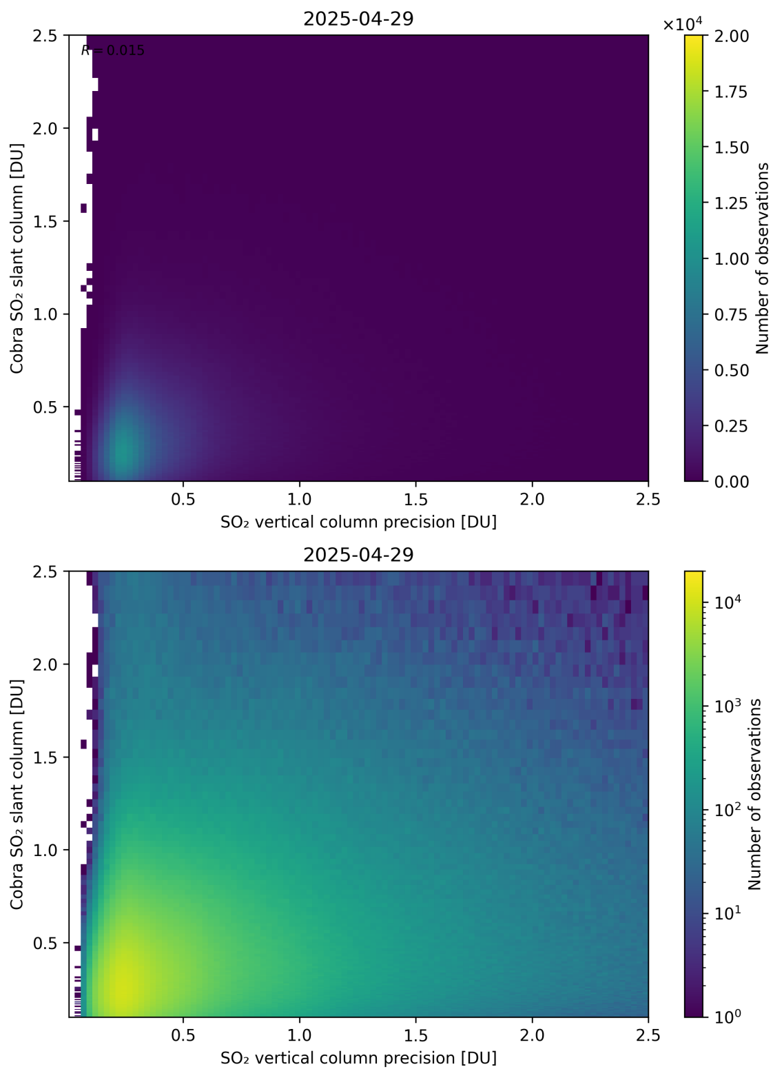
Figure 336: Scatter density plot of “SO 2 vertical column precision” against “Cobra SO 2 slant column” for 2025-04-29 to 2025-04-30.
