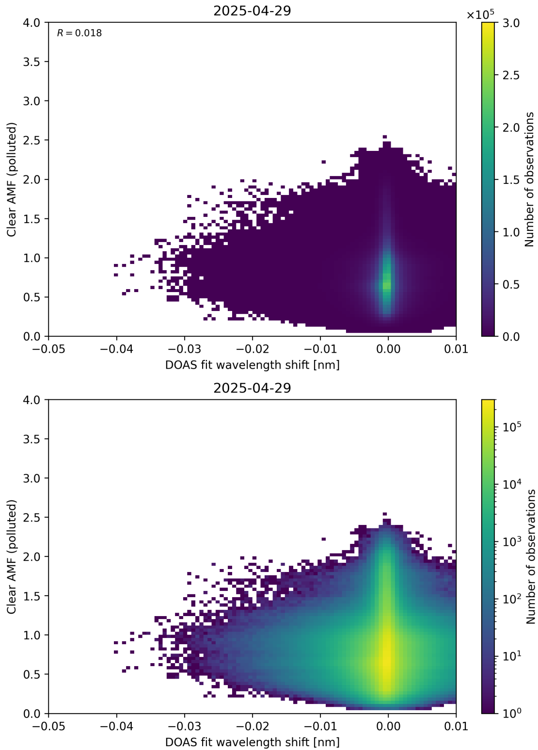
Figure 140: Scatter density plot of “DOAS fit wavelength shift” against “Clear AMF (polluted)” for 2025-04-29 to 2025-04-30.
