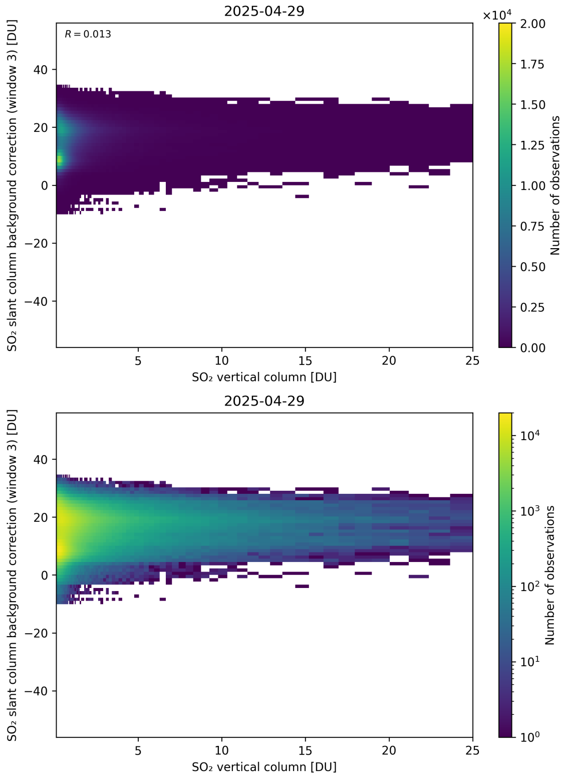
Figure 325: Scatter density plot of “SO 2 vertical column” against “SO 2 slant column background correction (window 3)” for 2025-04-29 to 2025-04-30.
