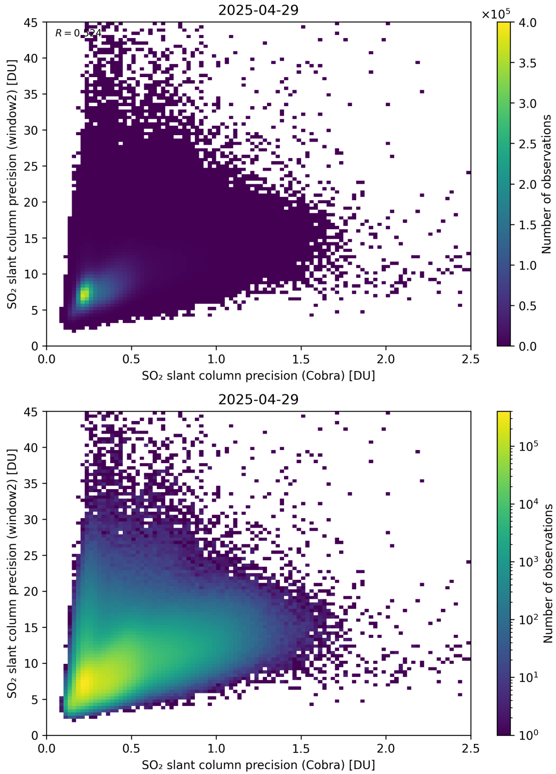
Figure 210: Scatter density plot of “SO 2 slant column precision (Cobra)” against “SO 2 slant column precision (window2)” for 2025-04-29 to 2025-04-30.
