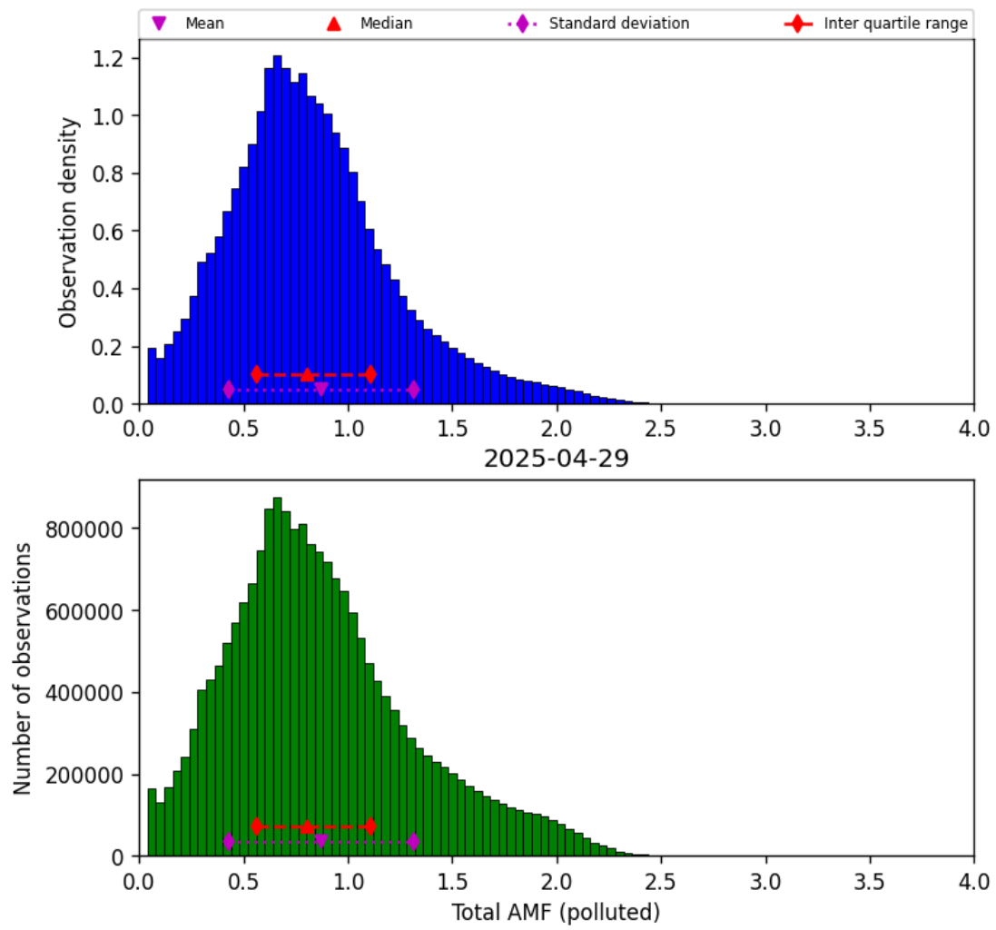
Figure 79: Histogram of “Total AMF (polluted)” for 2025-04-29 to 2025-04-30
