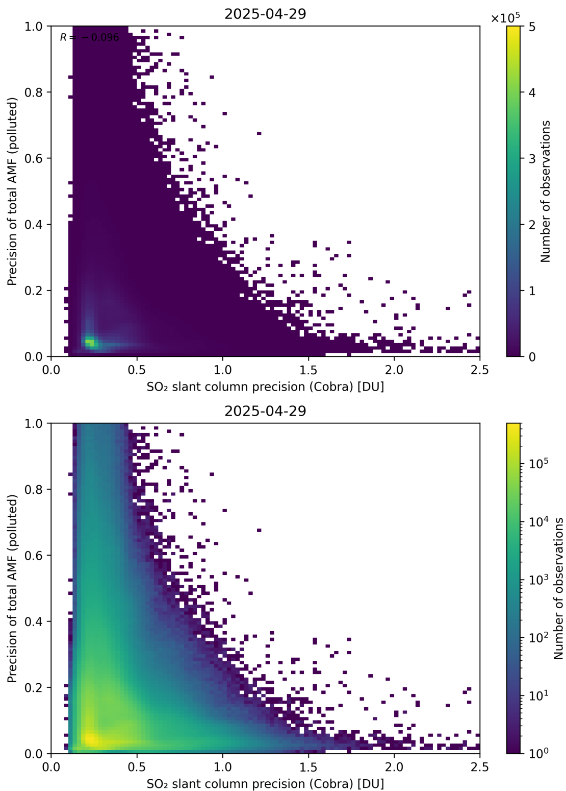
Figure 214: Scatter density plot of “SO 2 slant column precision (Cobra)” against “Precision of total AMF (polluted)” for 2025-04-29 to 2025-04-30.
