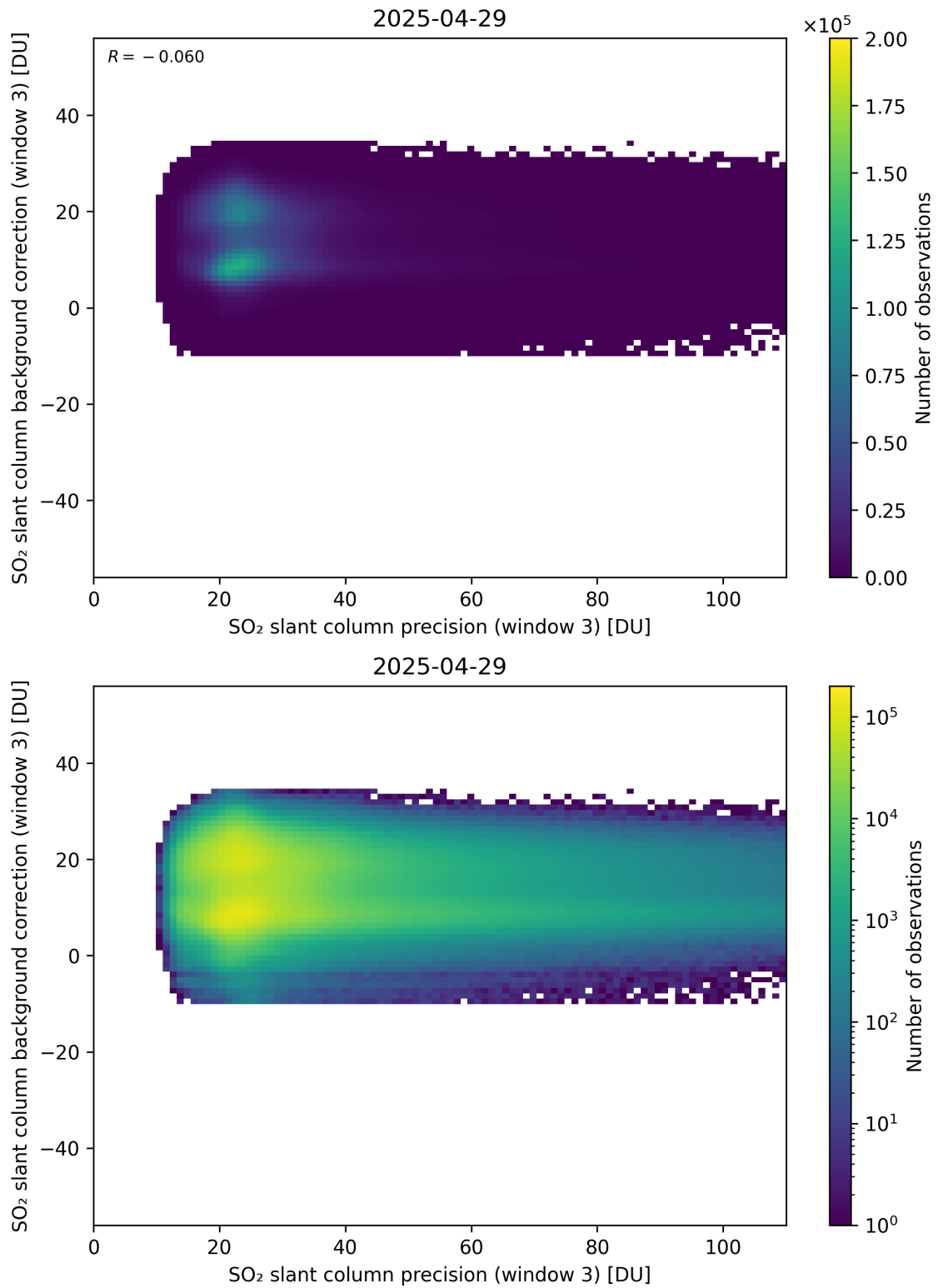
Figure 307: Scatter density plot of “SO 2 slant column precision (window 3)” against “SO 2 slant column background correction (window 3)” for 2025-04-29 to 2025-04-30.
