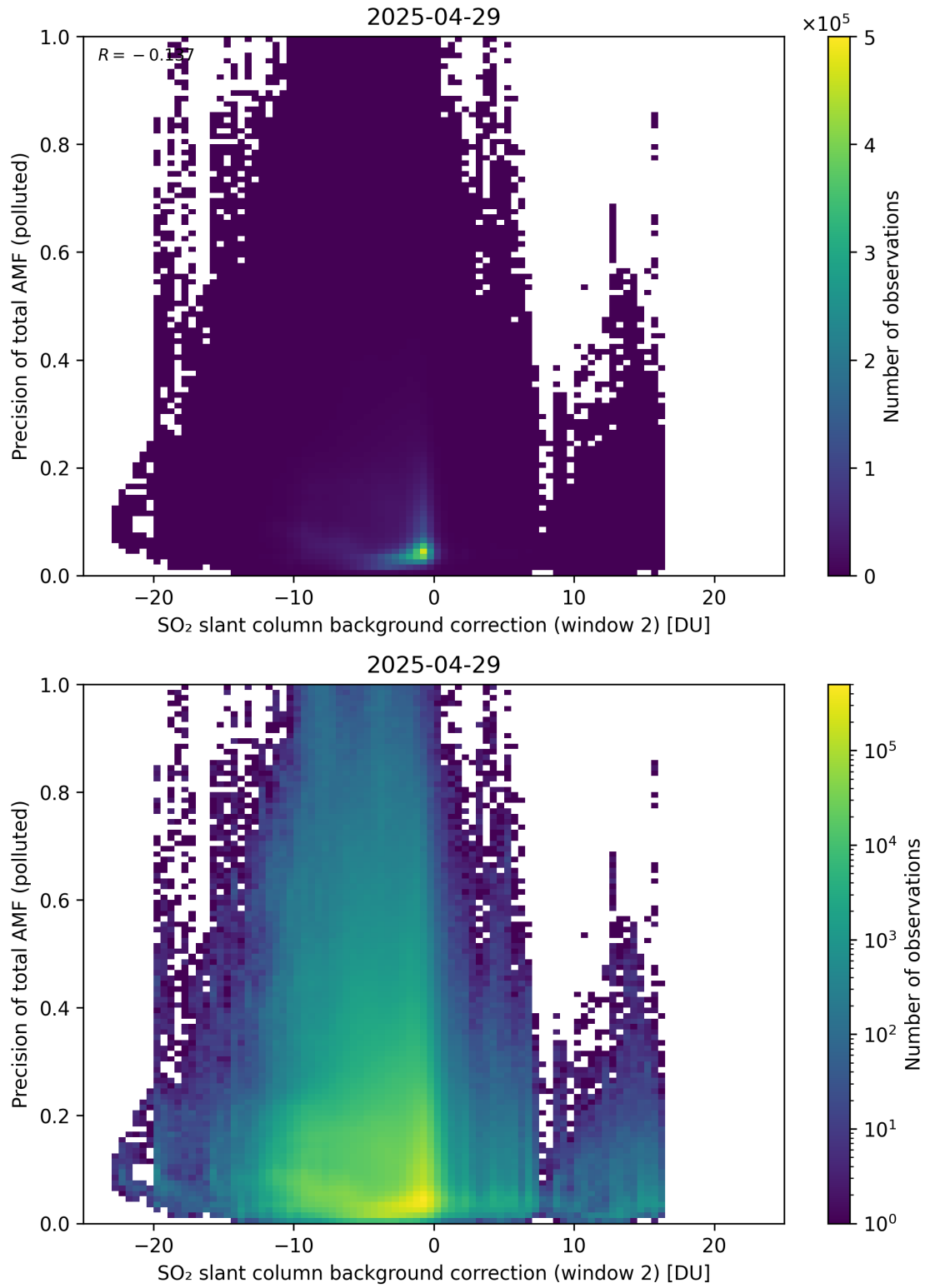
Figure 131: Scatter density plot of “SO 2 slant column background correction (window 2)” against “Precision of total AMF (polluted)” for 2025-04-29 to 2025-04-30.
