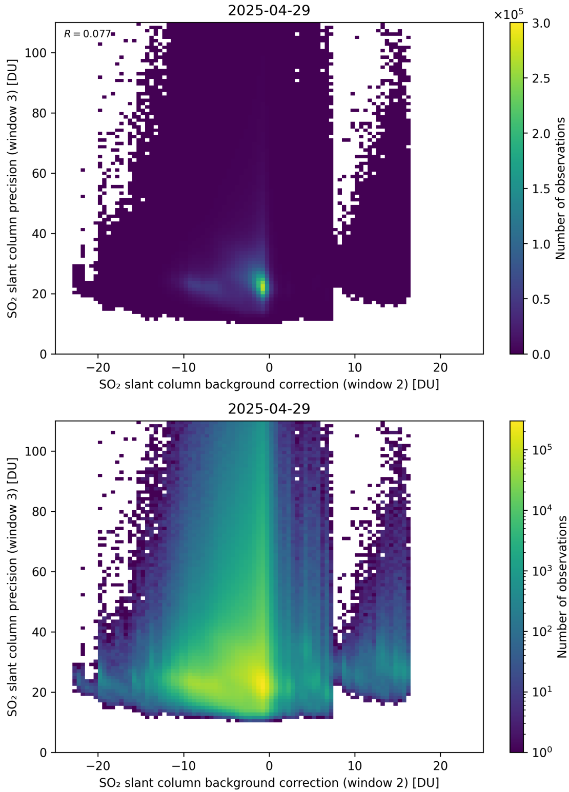
Figure 129: Scatter density plot of “SO 2 slant column background correction (window 2)” against “SO 2 slant column precision (window 3)” for 2025-04-29 to 2025-04-30.
