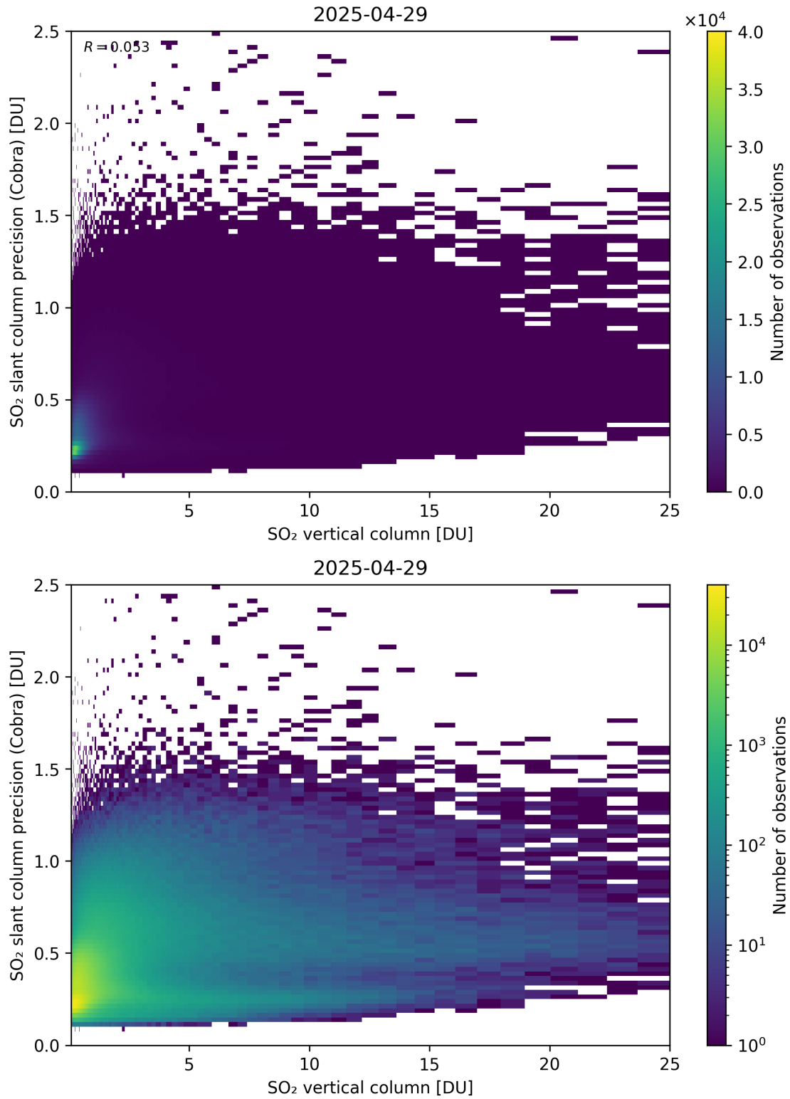
Figure 350: Scatter density plot of “SO 2 vertical column” against “SO 2 slant column precision (Cobra)” for 2025-04-29 to 2025-04-30.
