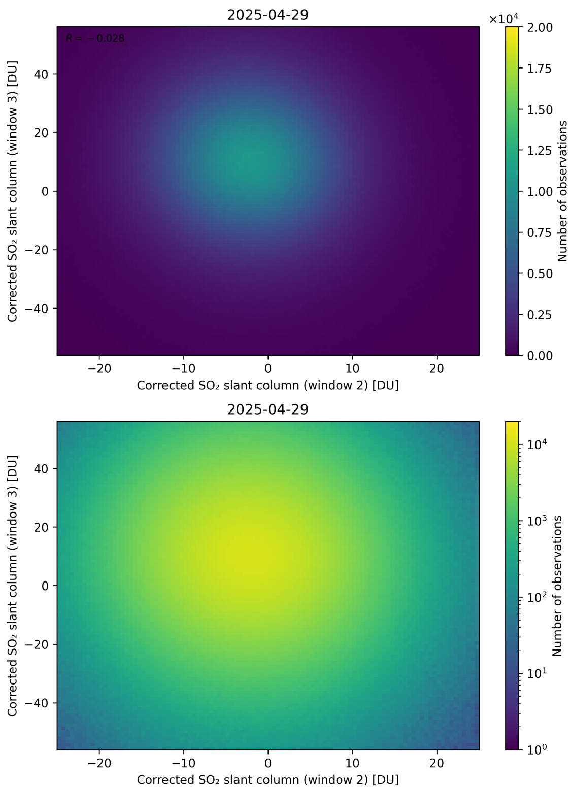
Figure 250: Scatter density plot of “Corrected SO 2 slant column (window 2)” against “Corrected SO 2 slant column (window 3)” for 2025-04-29 to 2025-04-30.
