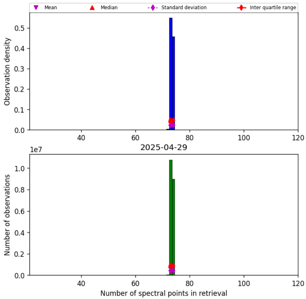
Figure 82: Histogram of “Number of spectral points in retrieval” for 2025-04-29 to 2025-04-30
