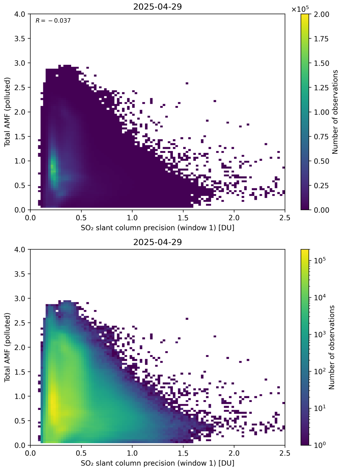
Figure 280: Scatter density plot of “SO 2 slant column precision (window 1)” against “Total AMF (polluted)” for 2025-04-29 to 2025-04-30.
