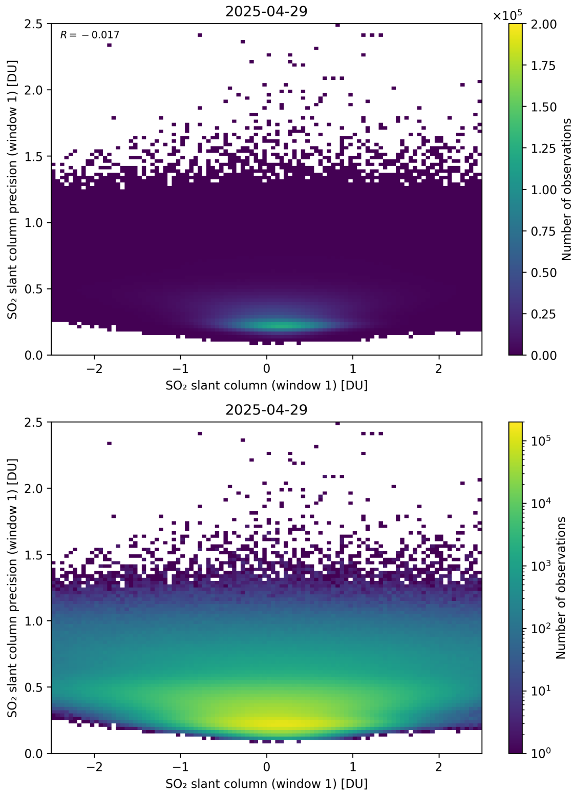
Figure 285: Scatter density plot of “SO 2 slant column (window 1)” against “SO 2 slant column precision (window 1)” for 2025-04-29 to 2025-04-30.
