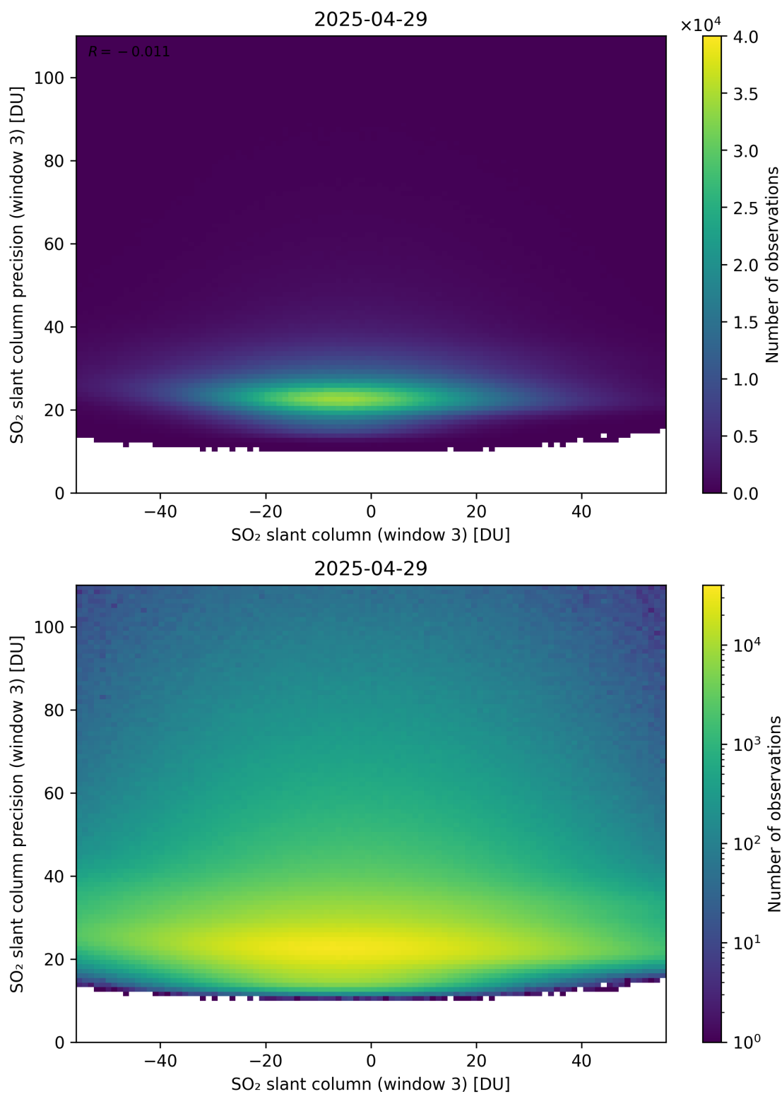
Figure 317: Scatter density plot of “SO 2 slant column (window 3)” against “SO 2 slant column precision (window 3)” for 2025-04-29 to 2025-04-30.
