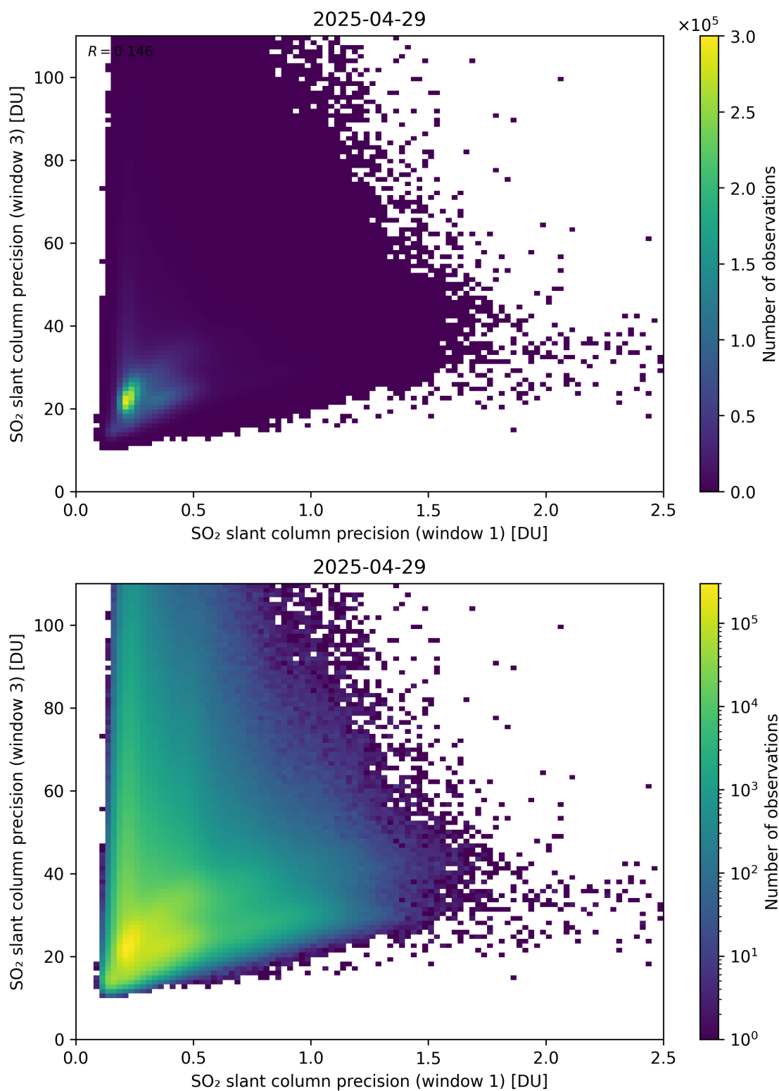
Figure 279: Scatter density plot of “SO 2 slant column precision (window 1)” against “SO 2 slant column precision (window 3)” for 2025-04-29 to 2025-04-30.
