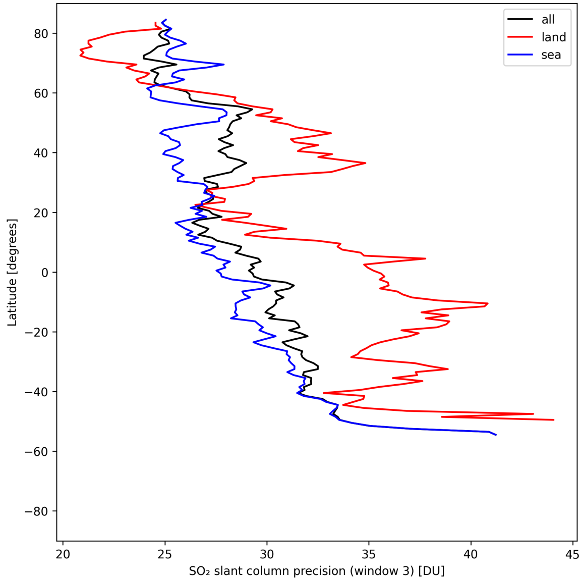
Figure 46: Zonal average of “SO 2 slant column precision (window 3)” for 2025-04-29 to 2025-04-30.
