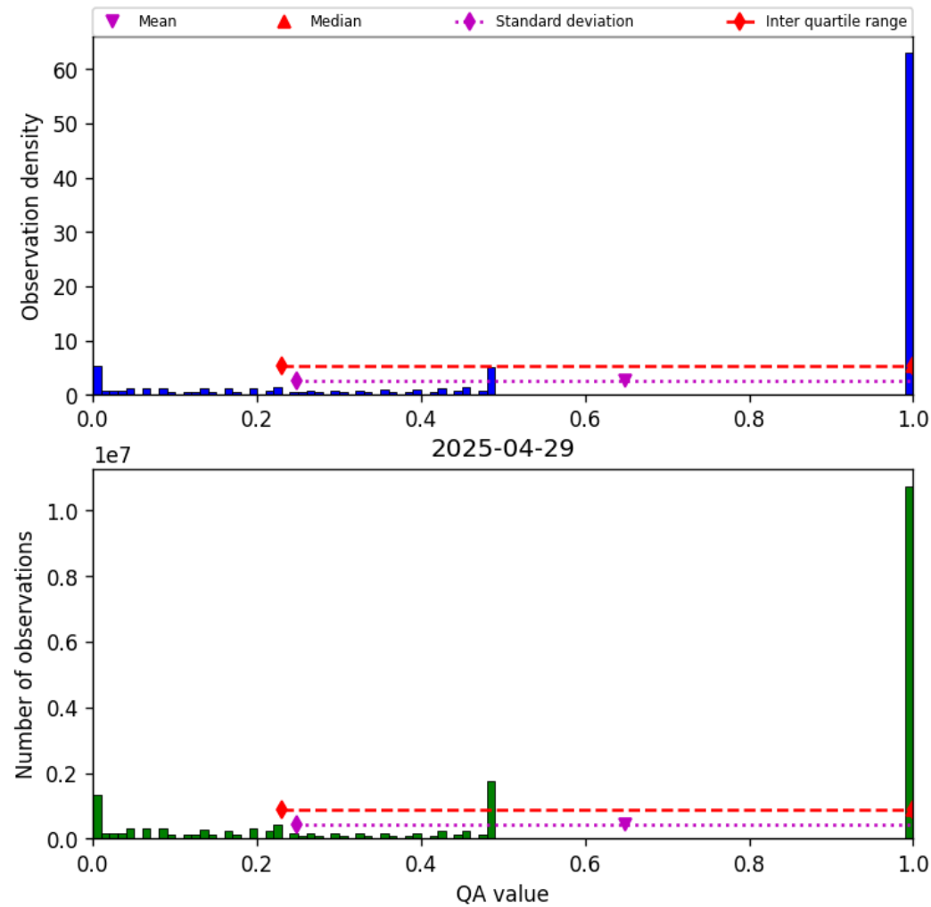
Figure 57: Histogram of “QA value” for 2025-04-29 to 2025-04-30
