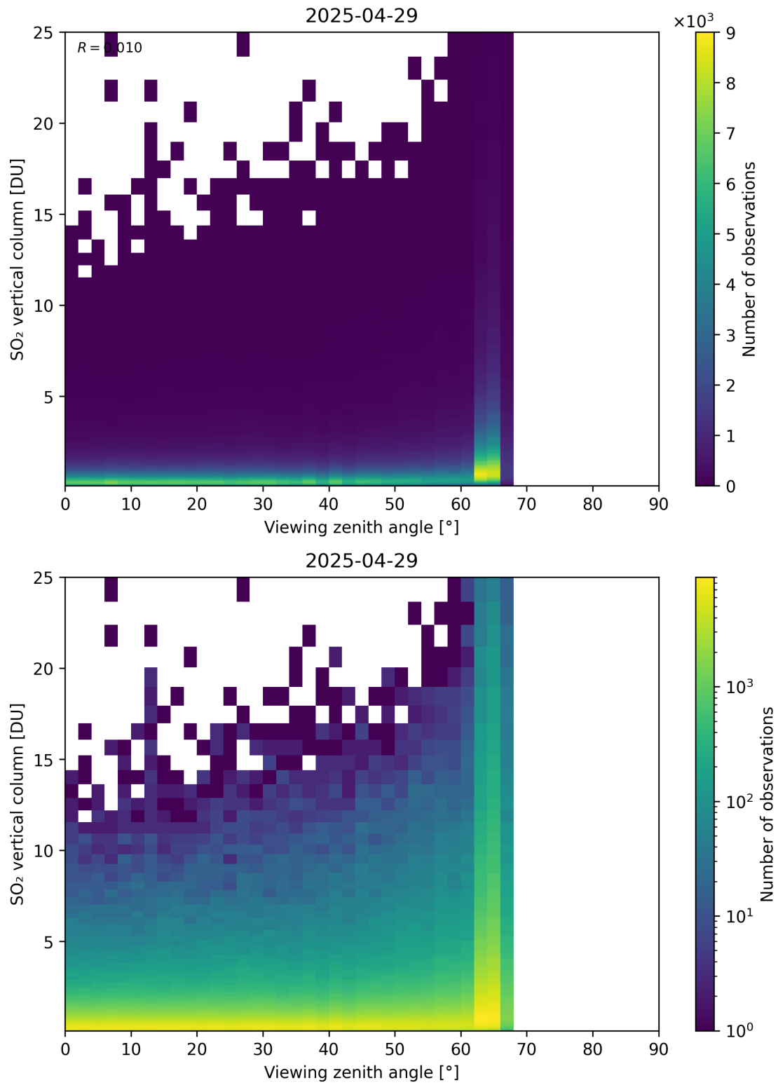
Figure 383: Scatter density plot of “Viewing zenith angle” against “SO 2 vertical column” for 2025-04-29 to 2025-04-30.
