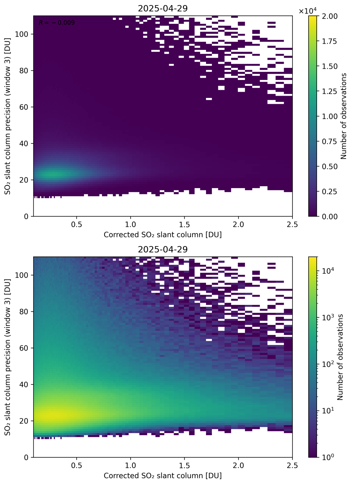
Figure 241: Scatter density plot of “Corrected SO 2 slant column” against “SO 2 slant column precision (window 3)” for 2025-04-29 to 2025-04-30.
