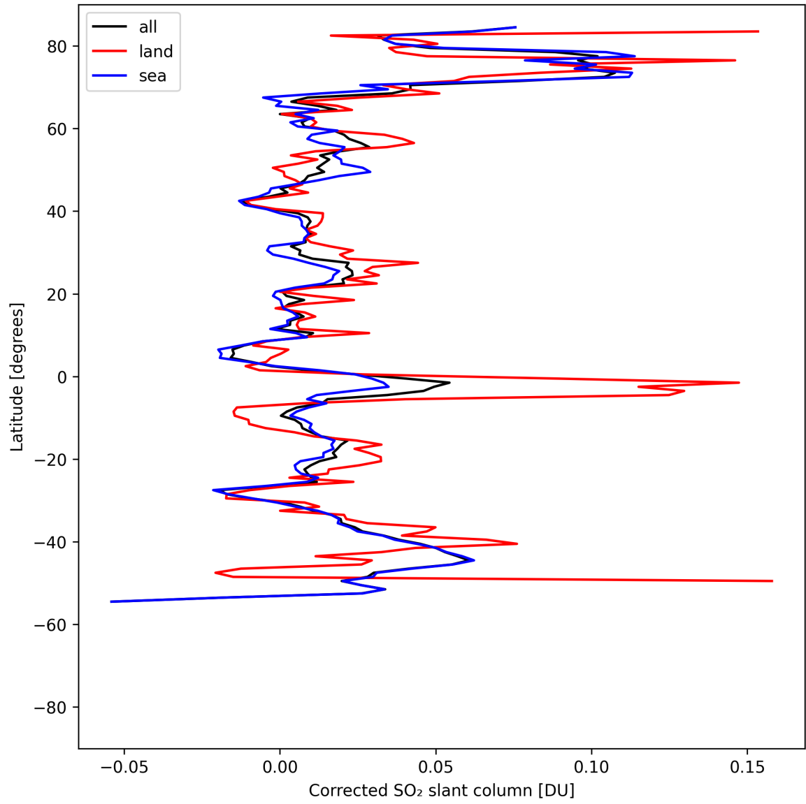
Figure 34: Zonal average of “Corrected SO 2 slant column” for 2025-04-29 to 2025-04-30.
