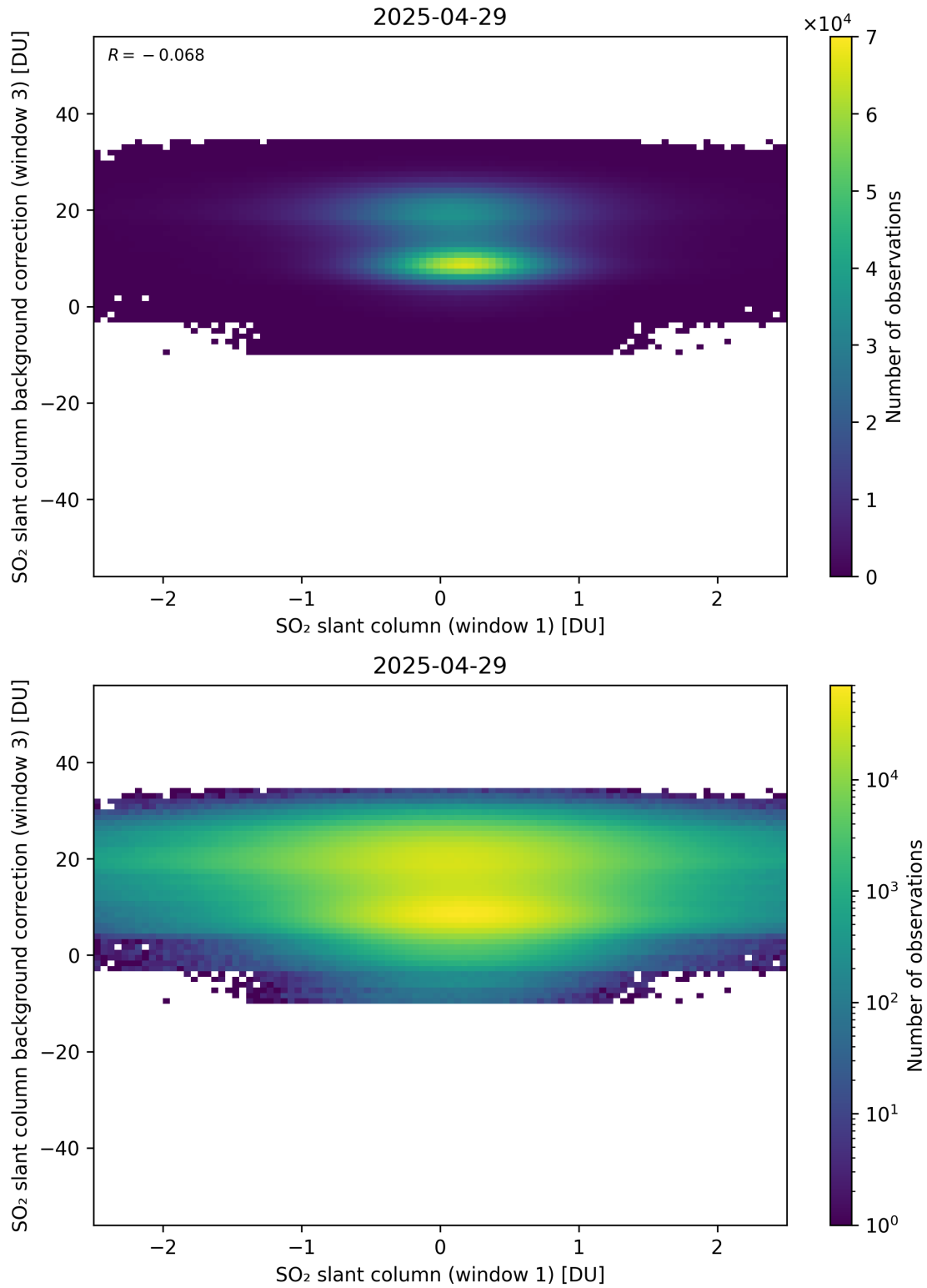
Figure 264: Scatter density plot of “SO 2 slant column (window 1)” against “SO 2 slant column background correction (window 3)” for 2025-04-29 to 2025-04-30.
