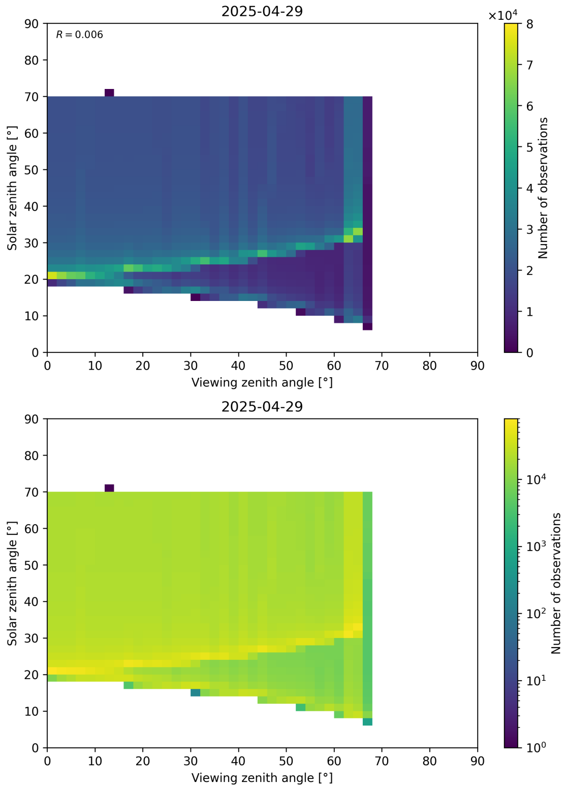
Figure 369: Scatter density plot of “Viewing zenith angle” against “Solar zenith angle” for 2025-04-29 to 2025-04-30.
