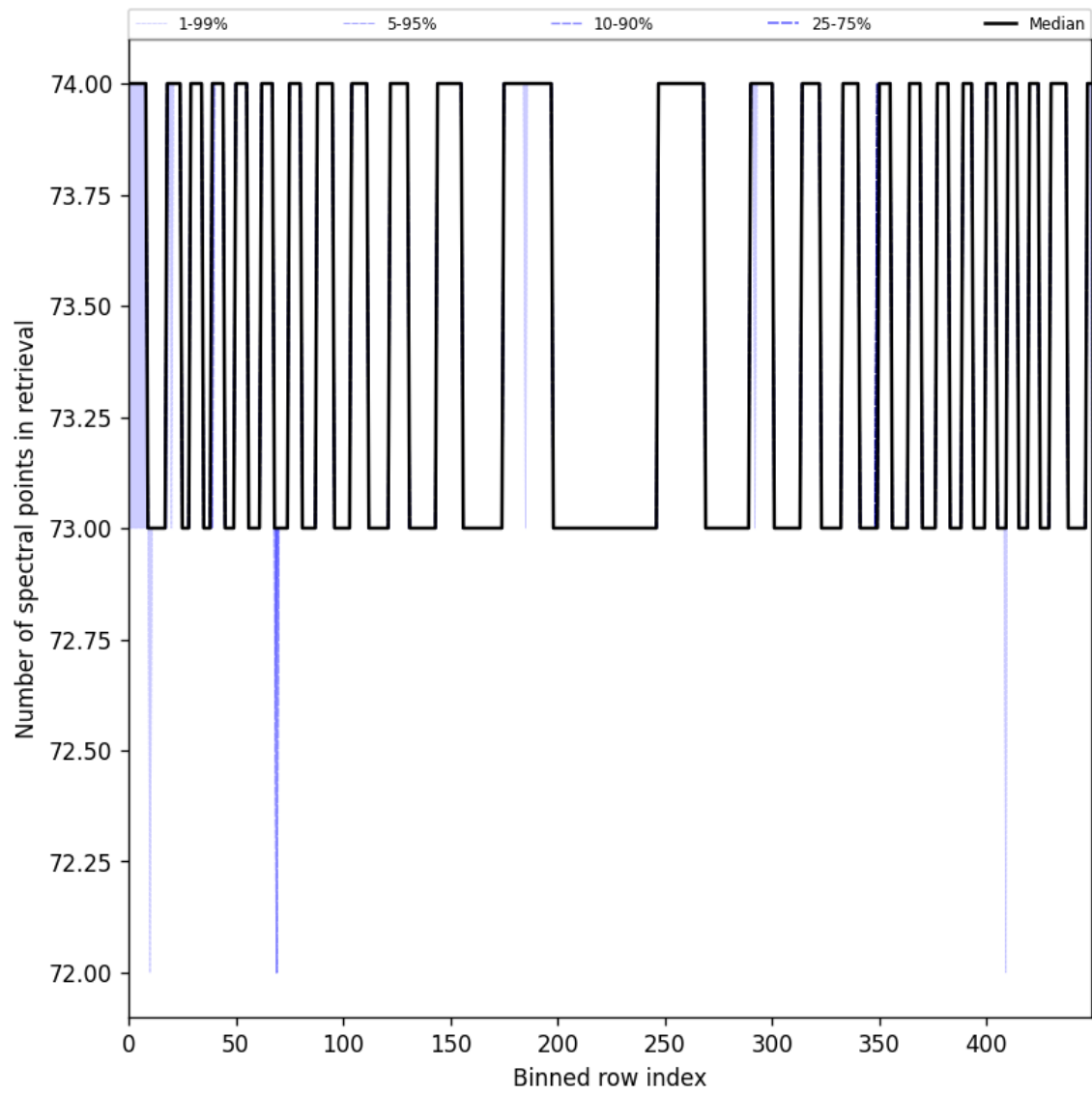
Figure 108: Along track statistics of “Number of spectral points in retrieval” for 2025-04-29 to 2025-04-30
