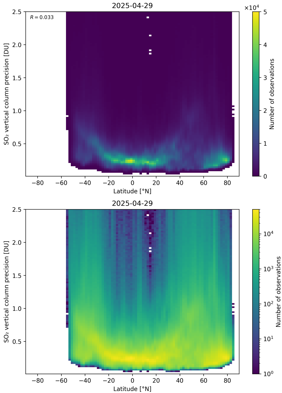
Figure 170: Scatter density plot of “Latitude” against “SO 2 vertical column precision” for 2025-04-29 to 2025-04-30.
