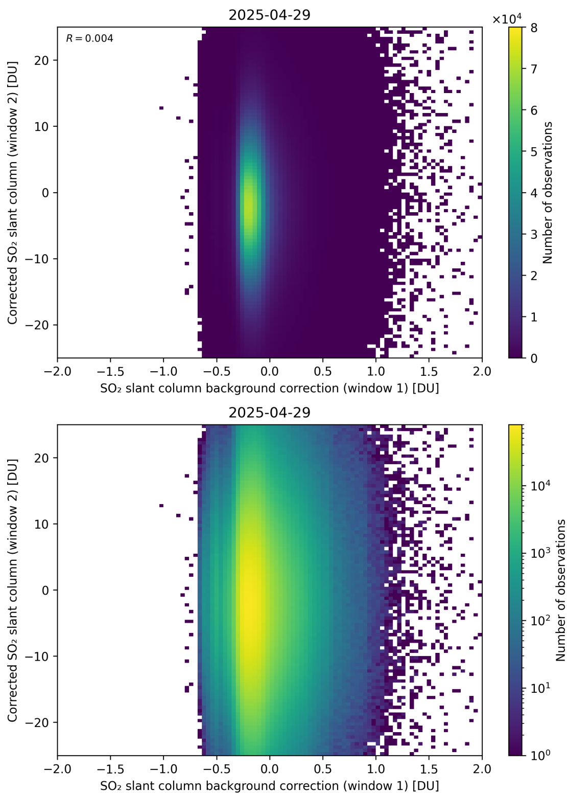
Figure 115: Scatter density plot of “SO 2 slant column background correction (window 1)” against “Corrected SO 2 slant column (window 2)” for 2025-04-29 to 2025-04-30.
