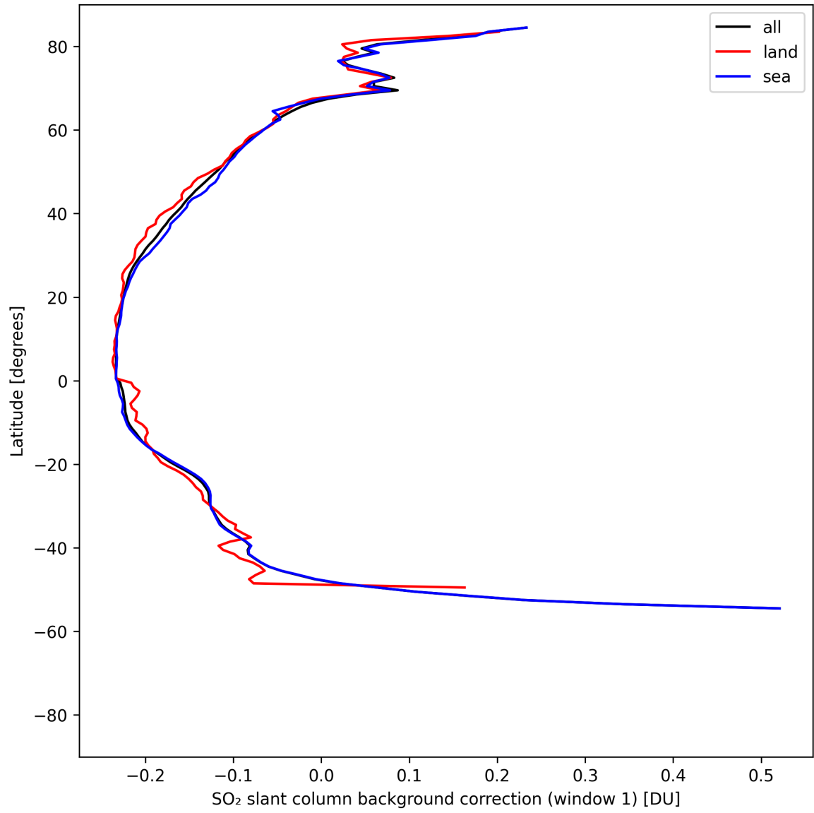
Figure 40: Zonal average of “SO 2 slant column background correction (window 1)” for 2025-04-29 to 2025-04-30.
