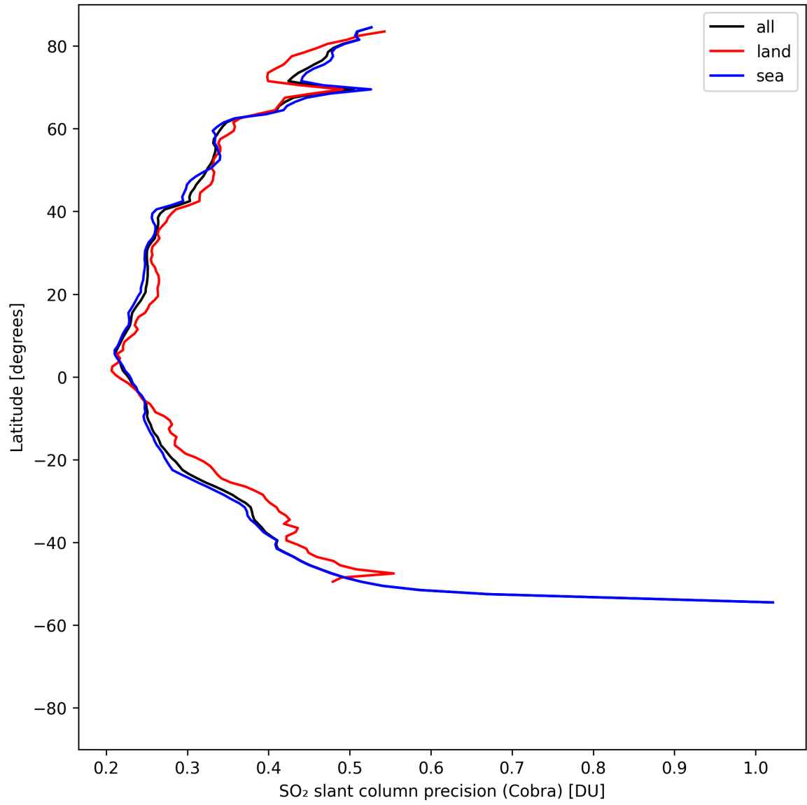
Figure 36: Zonal average of “SO 2 slant column precision (Cobra)” for 2025-04-29 to 2025-04-30.
