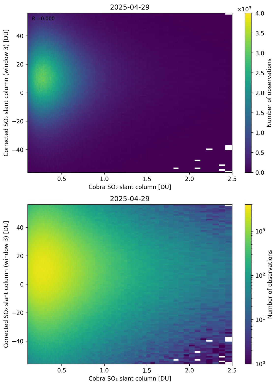
Figure 218: Scatter density plot of “Cobra SO 2 slant column” against “Corrected SO 2 slant column (window 3)” for 2025-04-29 to 2025-04-30.
