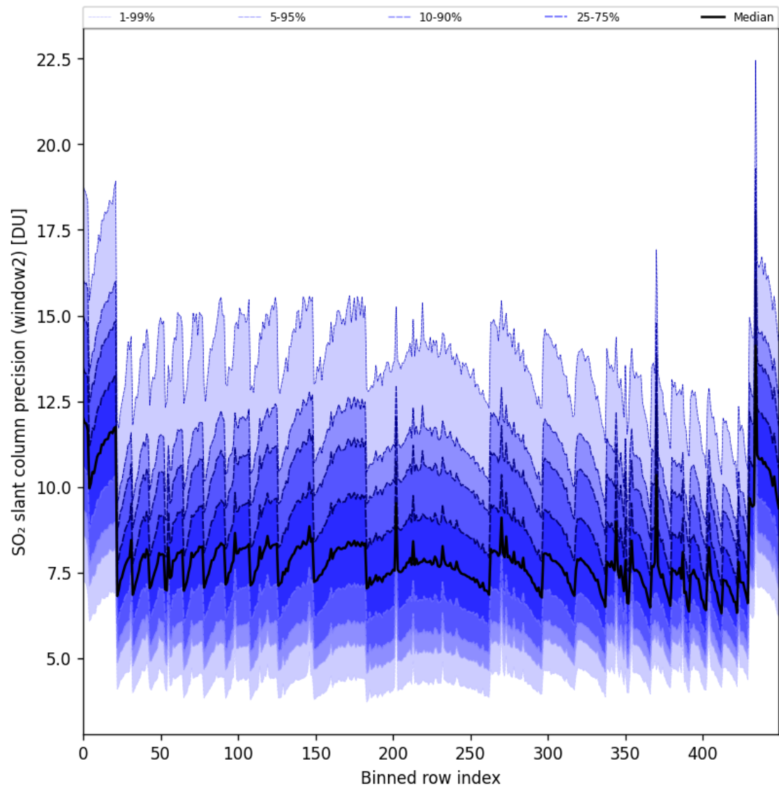
Figure 94: Along track statistics of “SO 2 slant column precision (window2)” for 2025-04-29 to 2025-04-30
