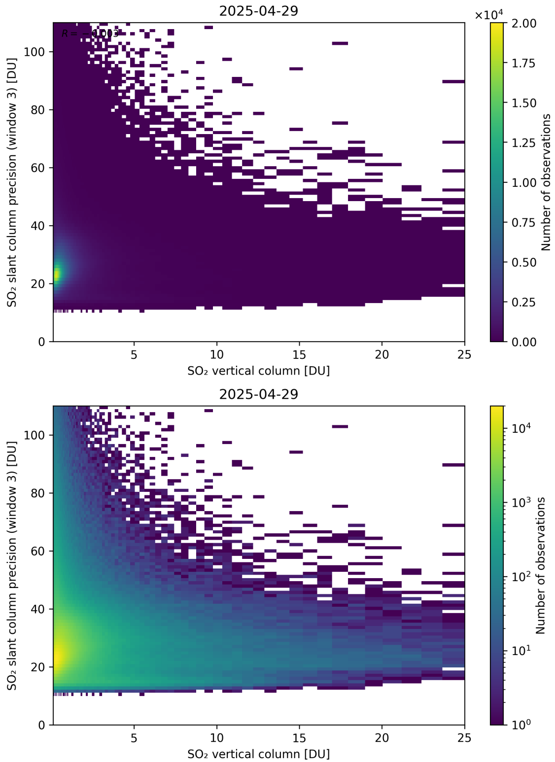
Figure 358: Scatter density plot of “SO 2 vertical column” against “SO 2 slant column precision (window 3)” for 2025-04-29 to 2025-04-30.
