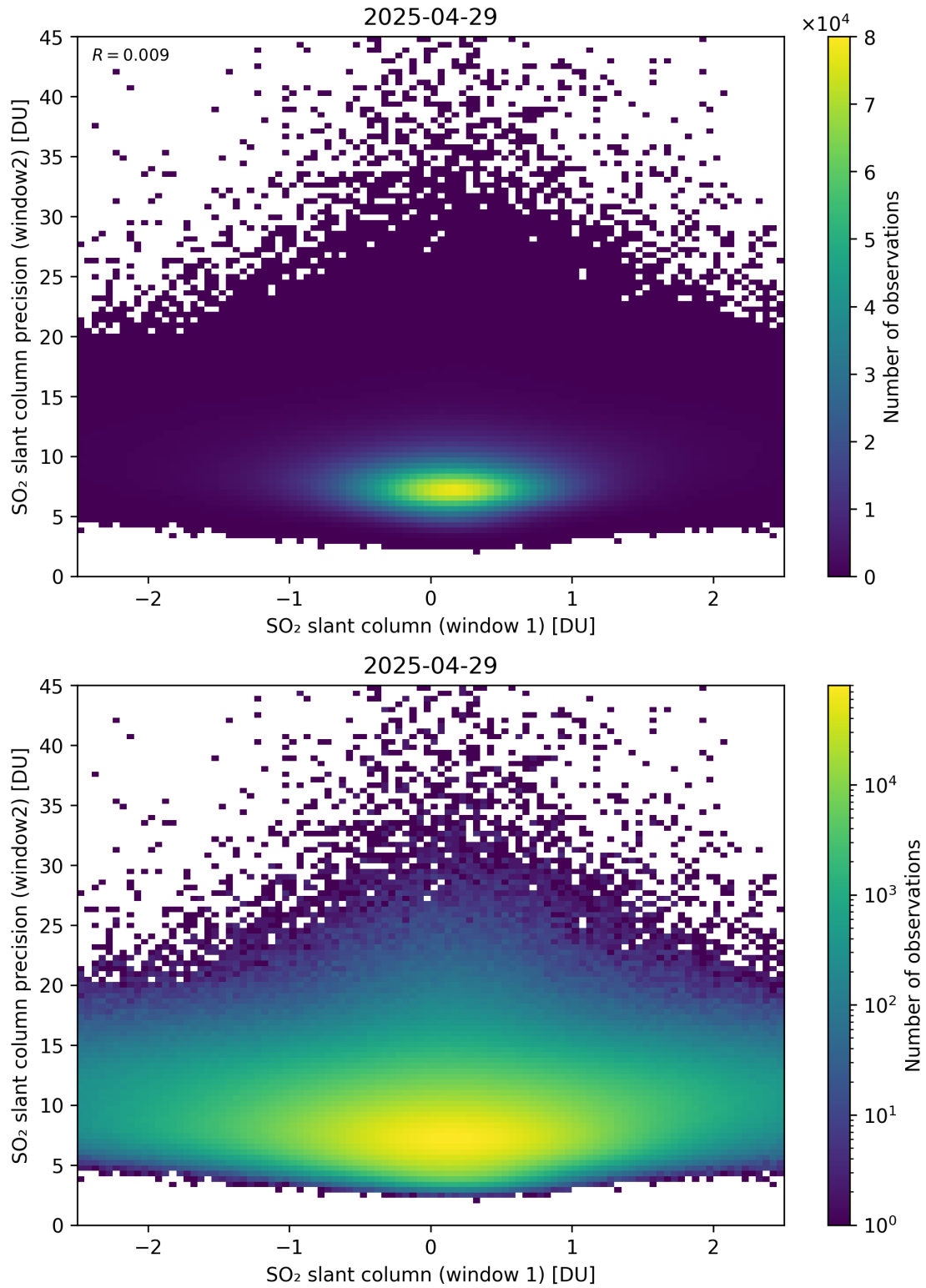
Figure 286: Scatter density plot of “SO 2 slant column (window 1)” against “SO 2 slant column precision (window2)” for 2025-04-29 to 2025-04-30.
