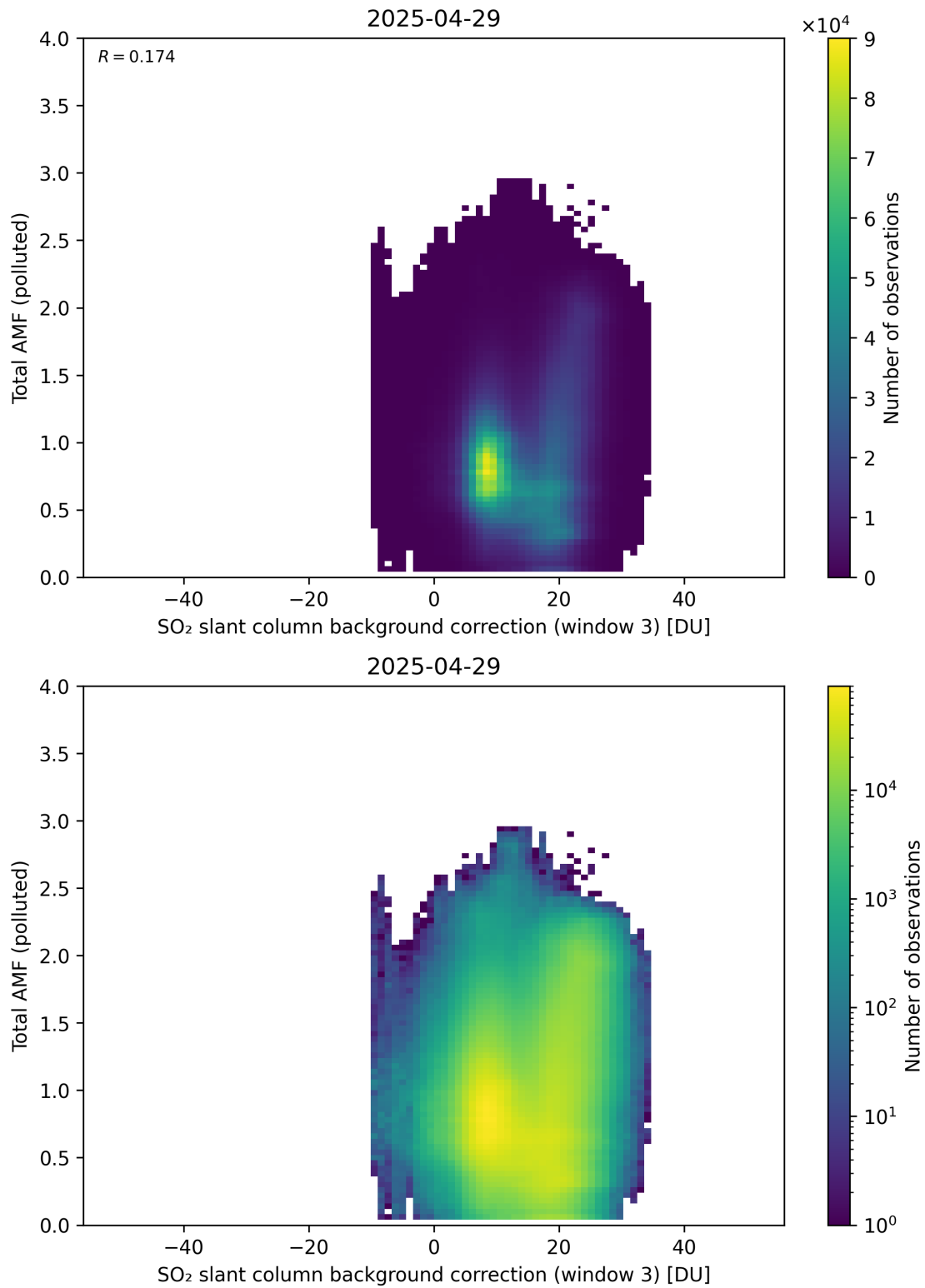
Figure 136: Scatter density plot of “SO 2 slant column background correction (window 3)” against “Total AMF (polluted)” for 2025-04-29 to 2025-04-30.
