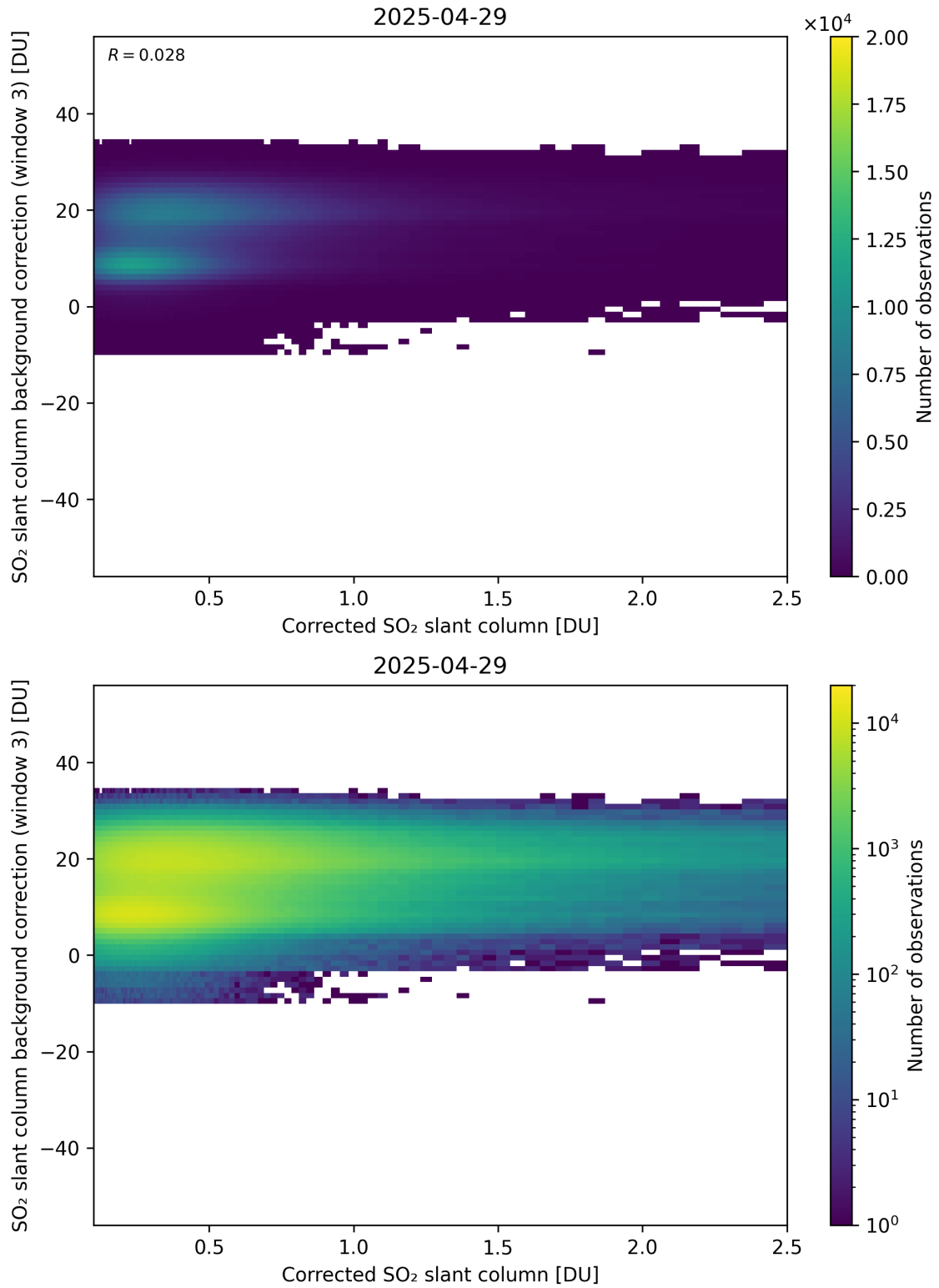
Figure 228: Scatter density plot of “Corrected SO 2 slant column” against “SO 2 slant column background correction (window 3)” for 2025-04-29 to 2025-04-30.
