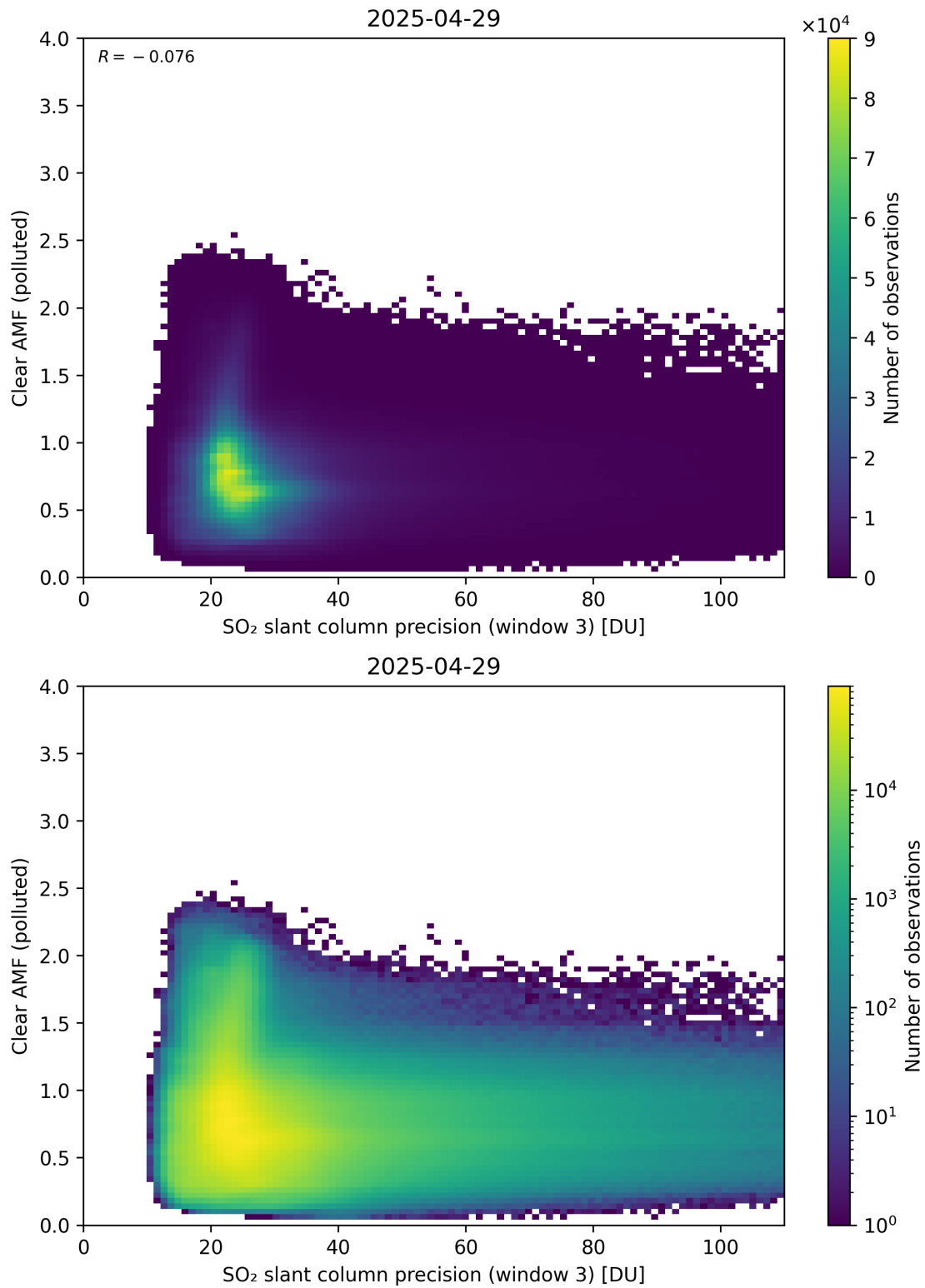
Figure 311: Scatter density plot of “SO 2 slant column precision (window 3)” against “Clear AMF (polluted)” for 2025-04-29 to 2025-04-30.
