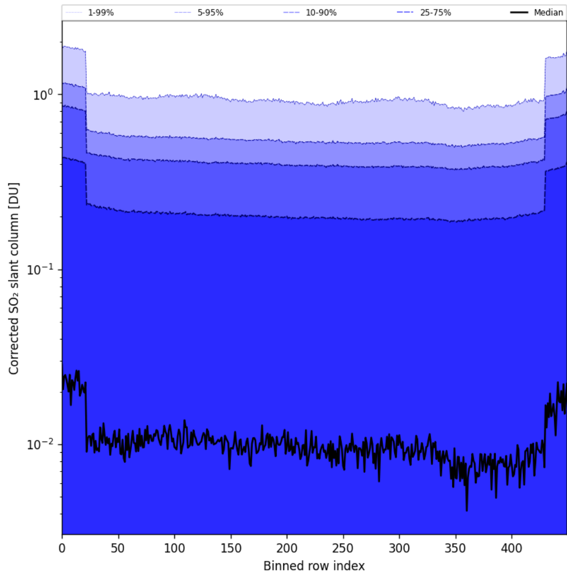
Figure 86: Along track statistics of “Corrected SO 2 slant column” for 2025-04-29 to 2025-04-30
