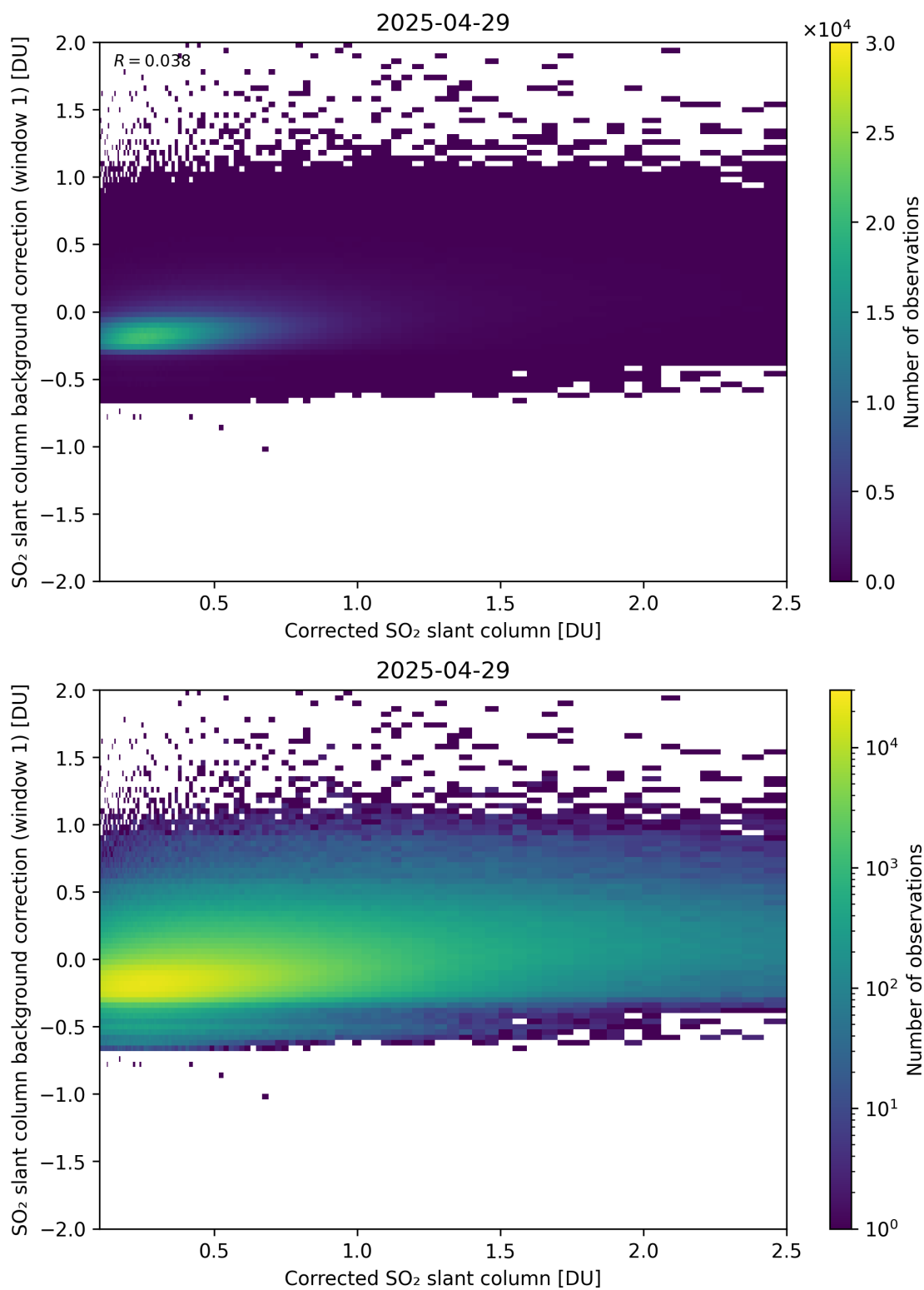
Figure 226: Scatter density plot of “Corrected SO 2 slant column” against “SO 2 slant column background correction (window 1)” for 2025-04-29 to 2025-04-30.
