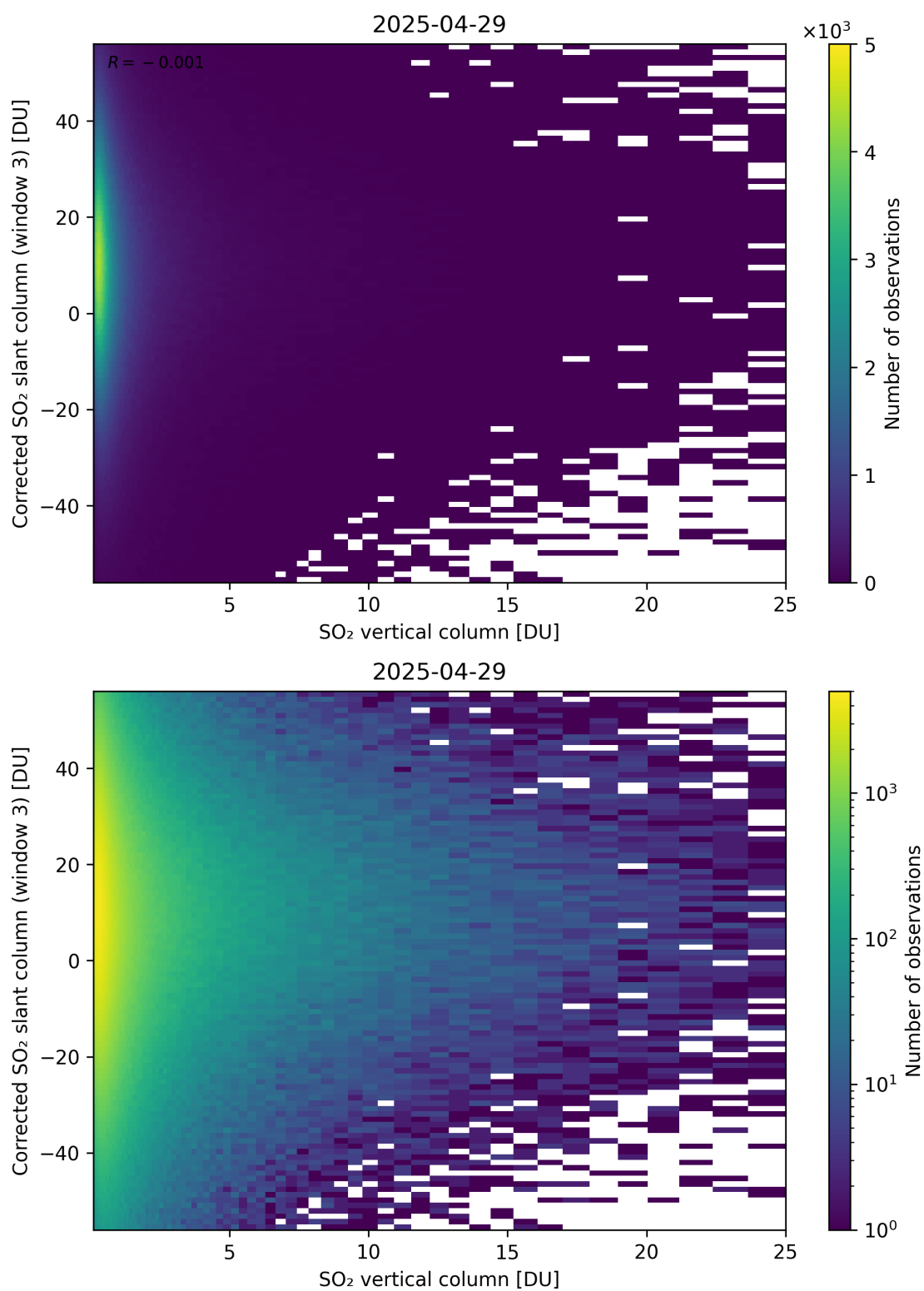
Figure 353: Scatter density plot of “SO 2 vertical column” against “Corrected SO 2 slant column (window 3)” for 2025-04-29 to 2025-04-30.
