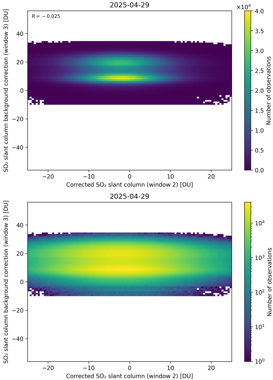
Figure 245: Scatter density plot of “Corrected SO 2 slant column (window 2)” against “SO 2 slant column background correction (window 3)” for 2025-04-29 to 2025-04-30.
