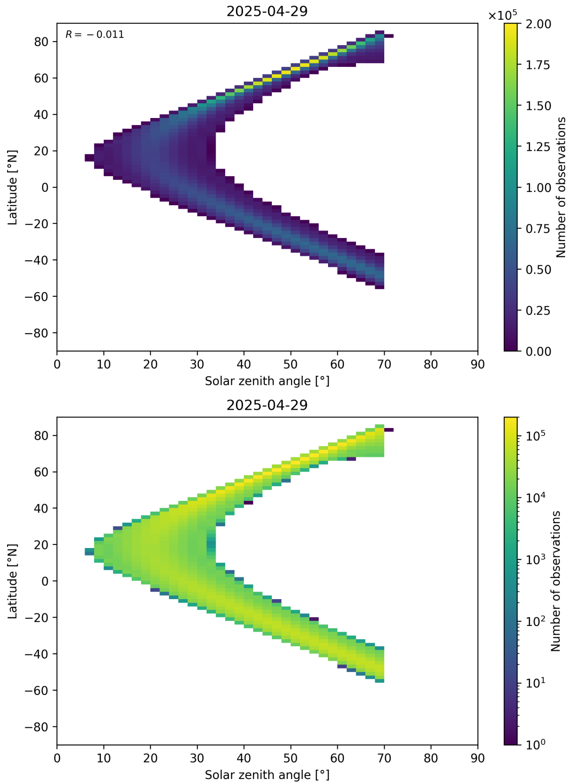
Figure 177: Scatter density plot of “Solar zenith angle” against “Latitude” for 2025-04-29 to 2025-04-30.
