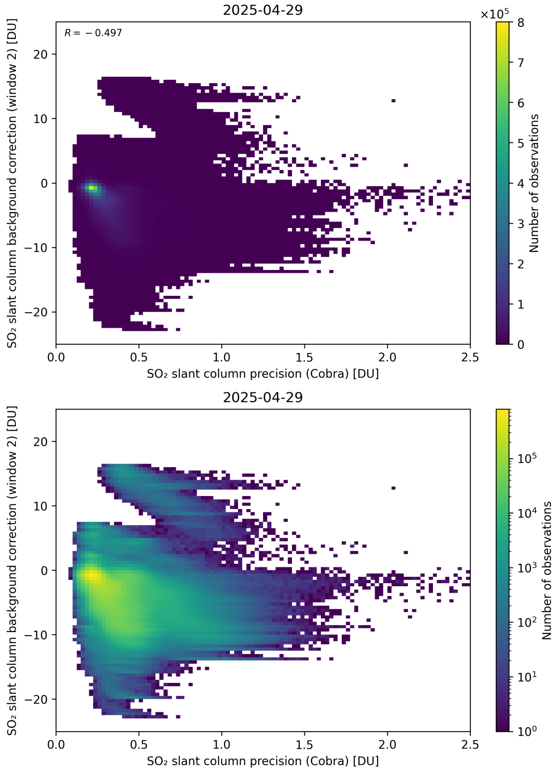
Figure 200: Scatter density plot of “SO 2 slant column precision (Cobra)” against “SO 2 slant column background correction (window 2)” for 2025-04-29 to 2025-04-30.
