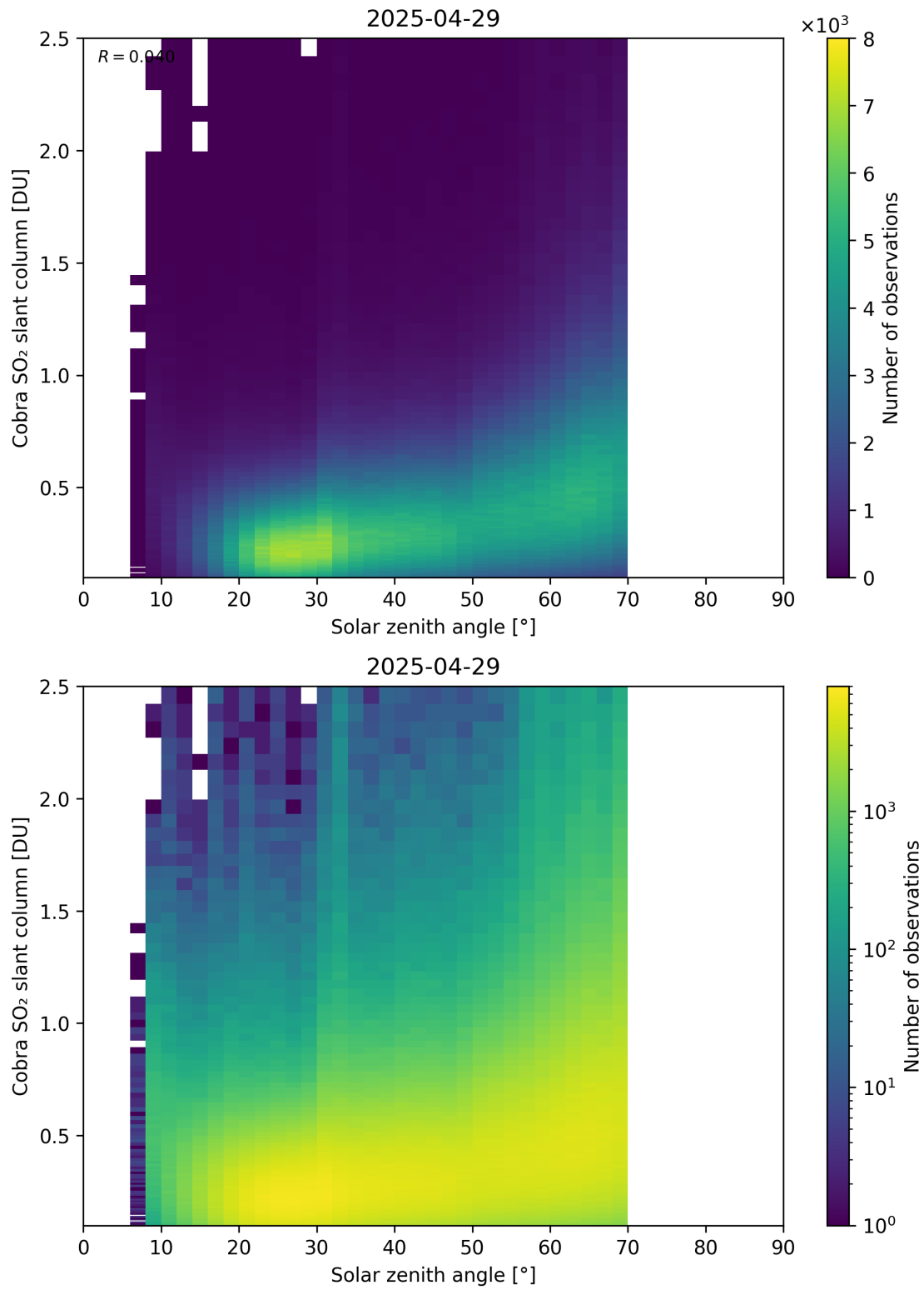
Figure 179: Scatter density plot of “Solar zenith angle” against “Cobra SO 2 slant column” for 2025-04-29 to 2025-04-30.
