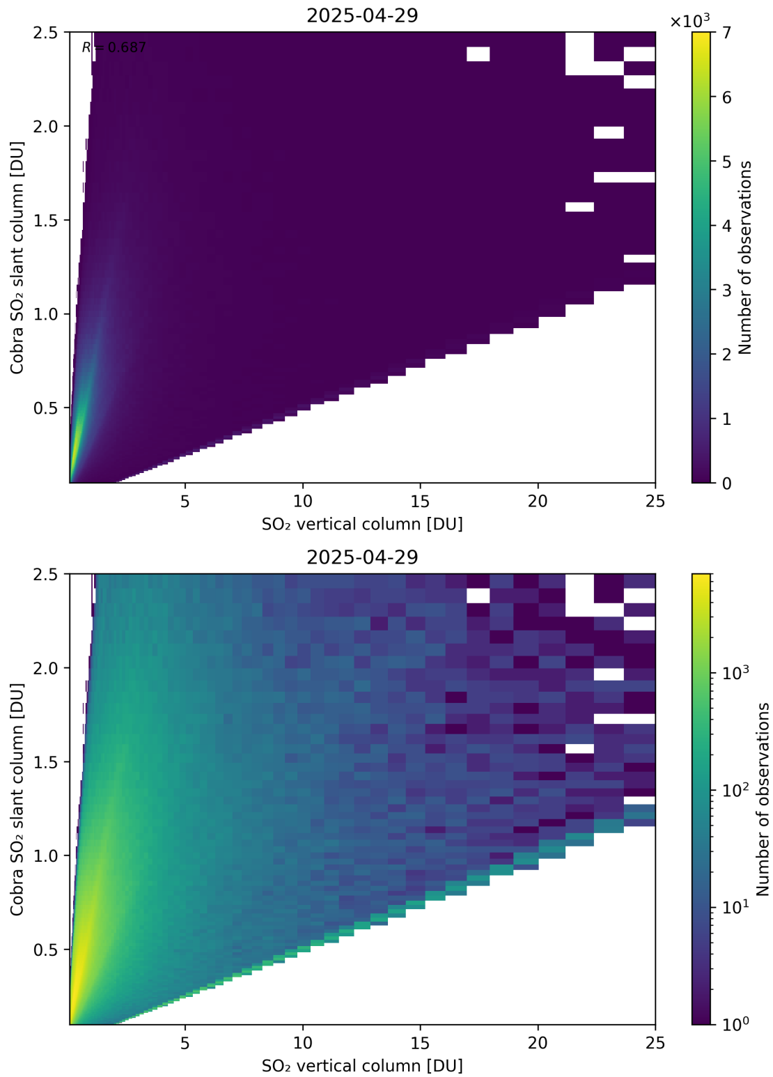
Figure 349: Scatter density plot of “SO 2 vertical column” against “Cobra SO 2 slant column” for 2025-04-29 to 2025-04-30.
