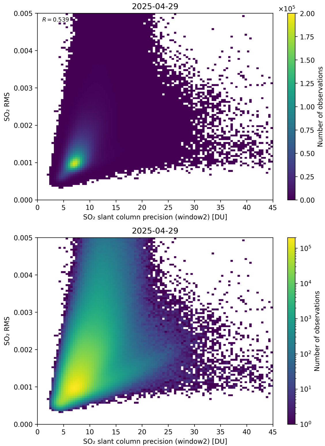
Figure 295: Scatter density plot of “SO 2 slant column precision (window2)” against “SO 2 RMS” for 2025-04-29 to 2025-04-30.
