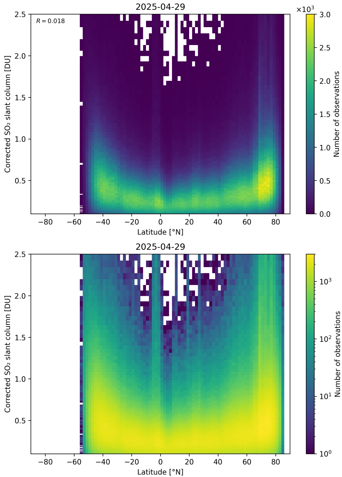
Figure 159: Scatter density plot of “Latitude” against “Corrected SO 2 slant column” for 2025-04-29 to 2025-04-30.
