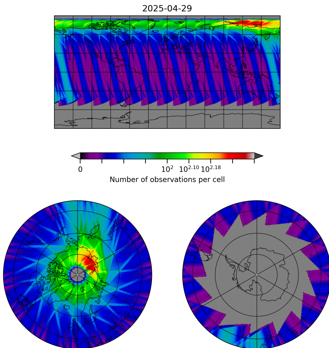
Figure 30: Map of the number of observations for 2025-04-29 to 2025-04-30
