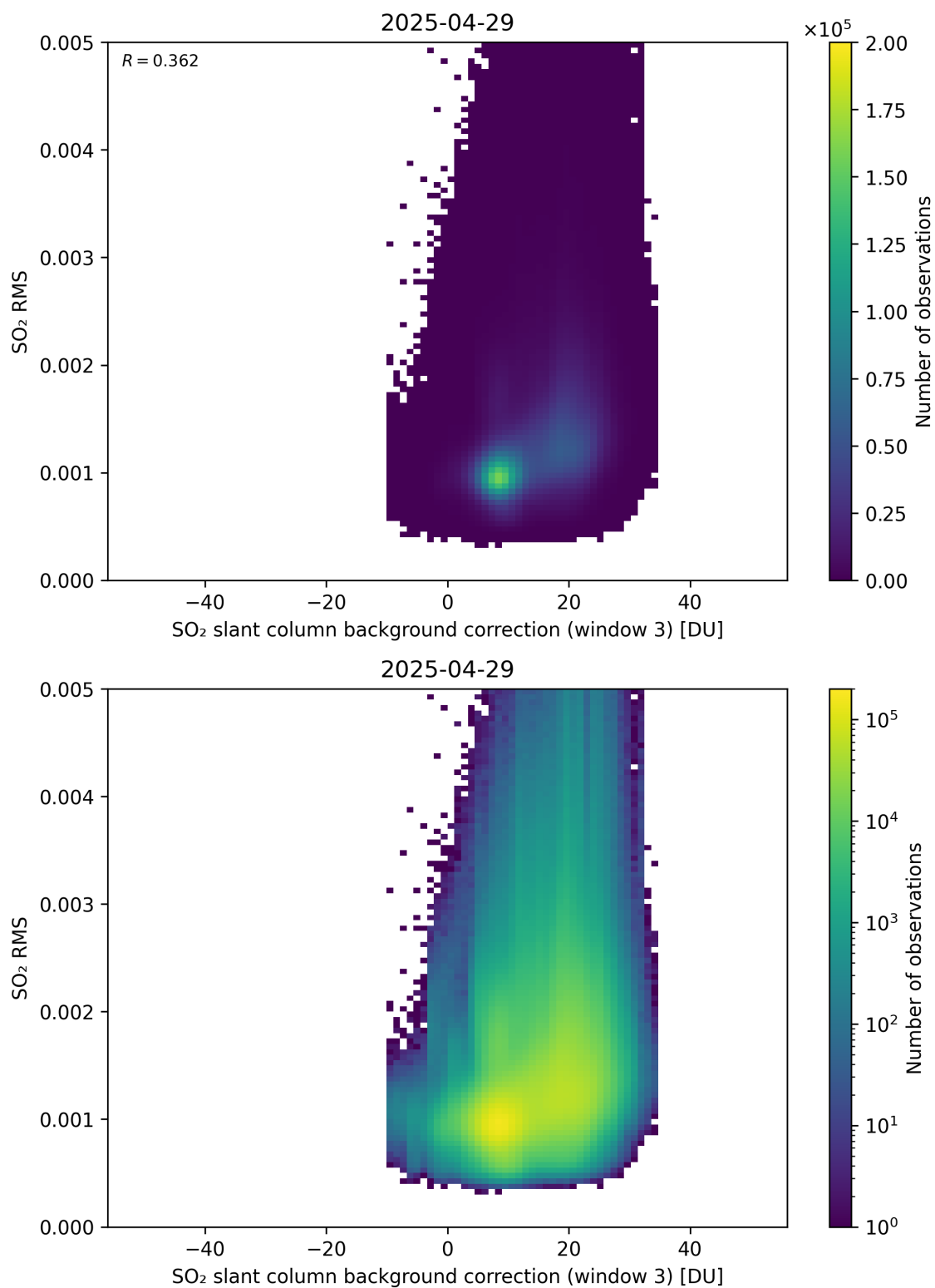
Figure 134: Scatter density plot of “SO 2 slant column background correction (window 3)” against “SO 2 RMS” for 2025-04-29 to 2025-04-30.
