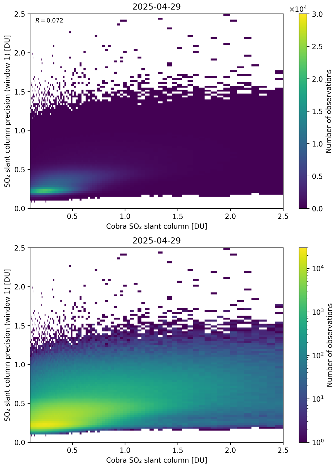
Figure 220: Scatter density plot of “Cobra SO 2 slant column” against “SO 2 slant column precision (window 1)” for 2025-04-29 to 2025-04-30.
