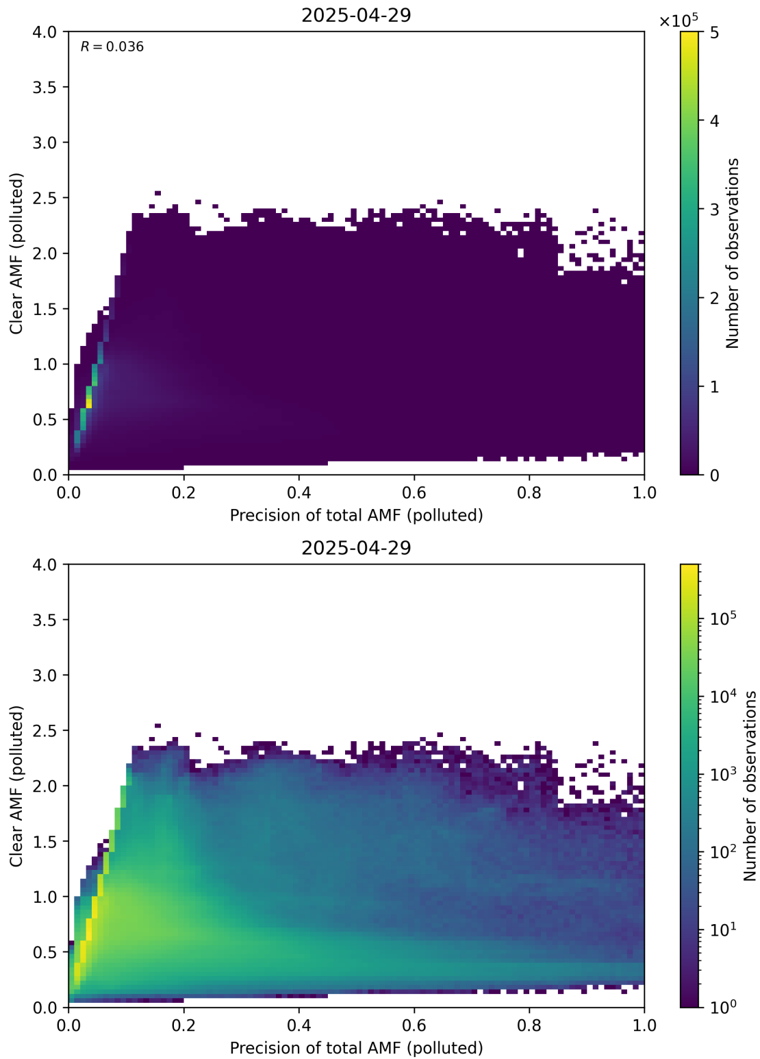
Figure 320: Scatter density plot of “Precision of total AMF (polluted)” against “Clear AMF (polluted)” for 2025-04-29 to 2025-04-30.
