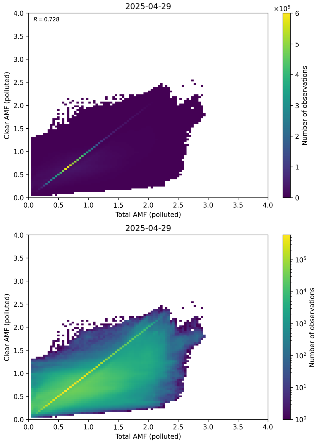
Figure 321: Scatter density plot of “Total AMF (polluted)” against “Clear AMF (polluted)” for 2025-04-29 to 2025-04-30.
