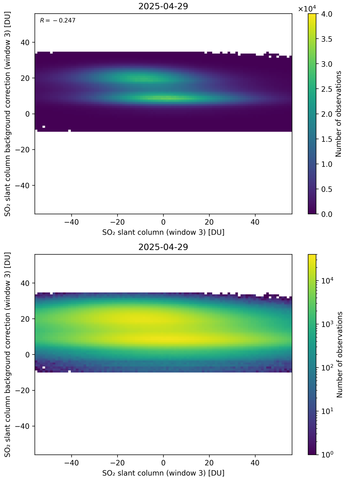
Figure 303: Scatter density plot of “SO 2 slant column (window 3)” against “SO 2 slant column background correction (window 3)” for 2025-04-29 to 2025-04-30.
