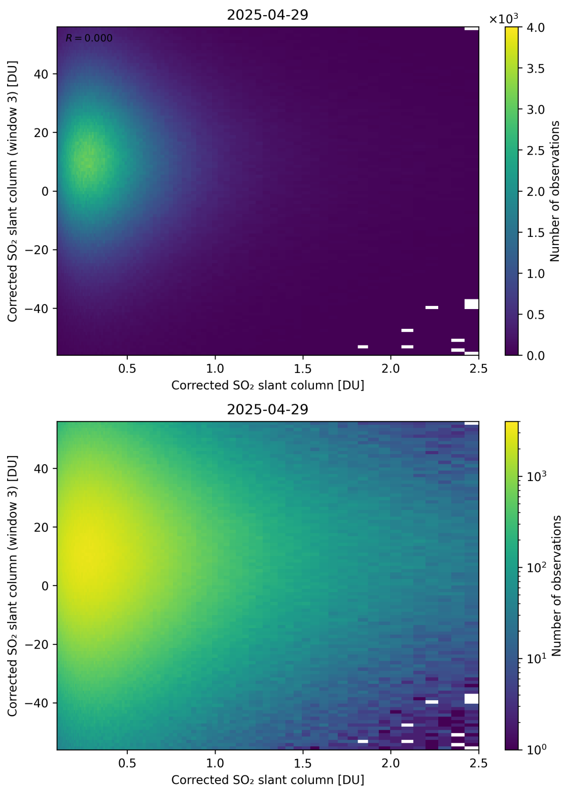
Figure 236: Scatter density plot of “Corrected SO 2 slant column” against “Corrected SO 2 slant column (window 3)” for 2025-04-29 to 2025-04-30.
