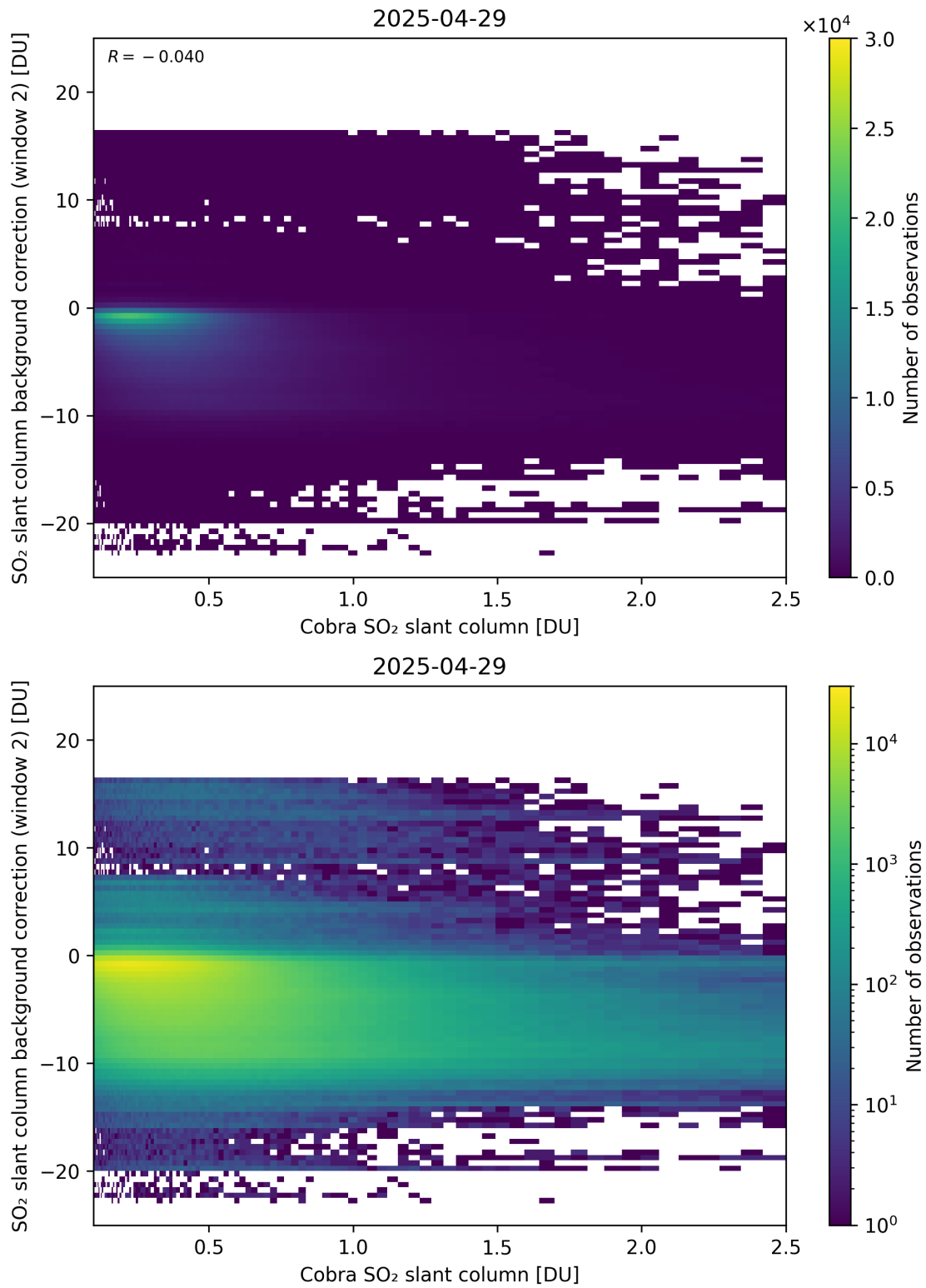
Figure 194: Scatter density plot of “Cobra SO 2 slant column” against “SO 2 slant column background correction (window 2)” for 2025-04-29 to 2025-04-30.
