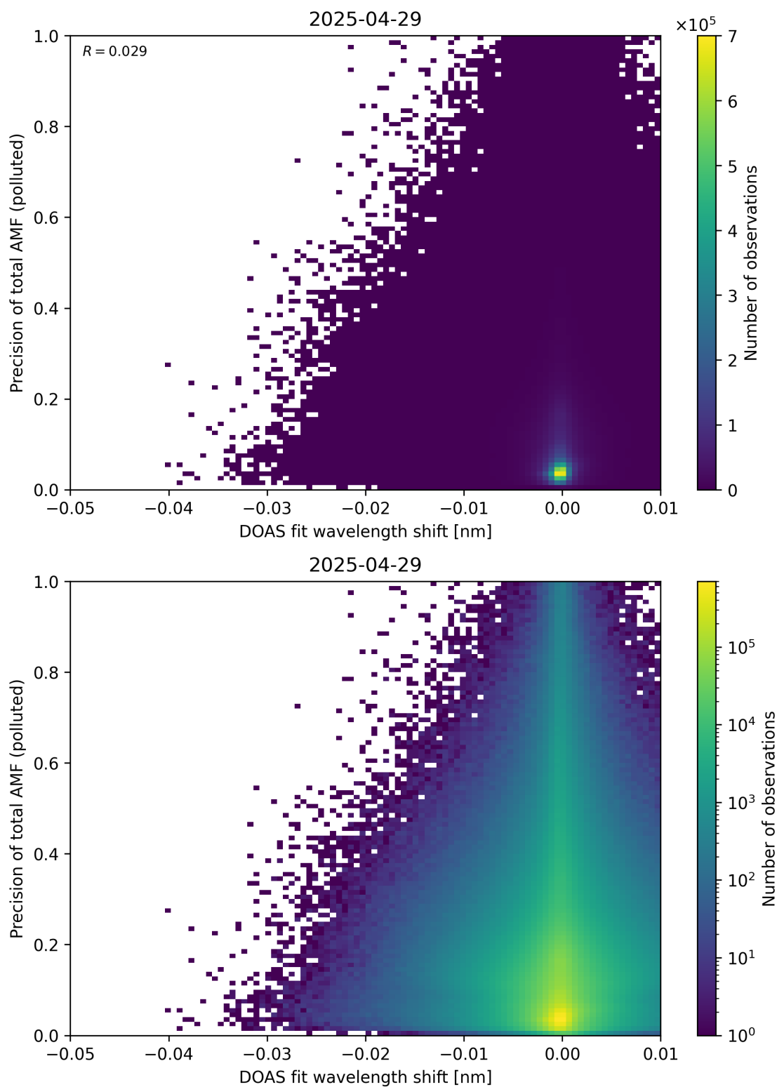
Figure 142: Scatter density plot of “DOAS fit wavelength shift” against “Precision of total AMF (polluted)” for 2025-04-29 to 2025-04-30.
