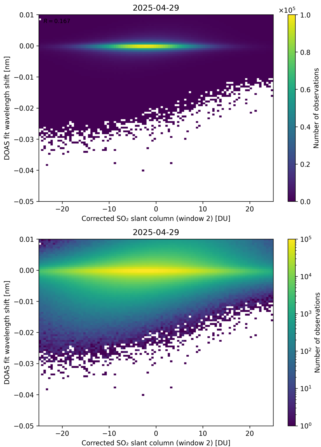
Figure 246: Scatter density plot of “Corrected SO 2 slant column (window 2)” against “DOAS fit wavelength shift” for 2025-04-29 to 2025-04-30.
