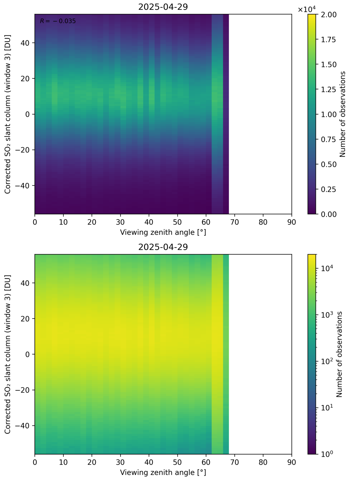
Figure 375: Scatter density plot of “Viewing zenith angle” against “Corrected SO 2 slant column (window 3)” for 2025-04-29 to 2025-04-30.
