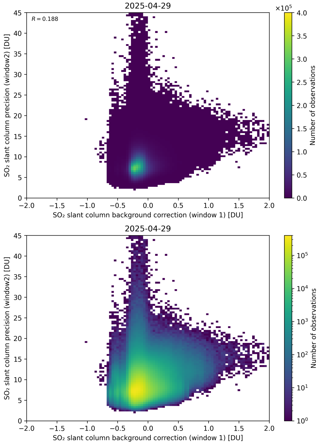
Figure 117: Scatter density plot of “SO 2 slant column background correction (window 1)” against “SO 2 slant column precision (window2)” for 2025-04-29 to 2025-04-30.
