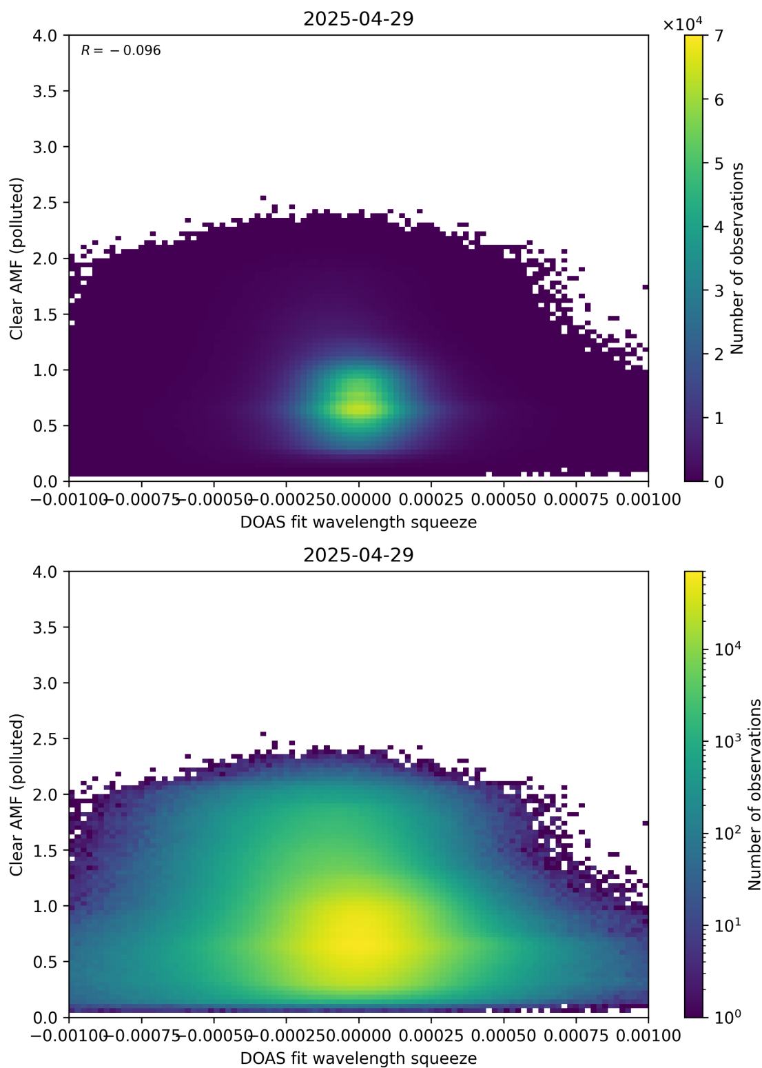
Figure 144: Scatter density plot of “DOAS fit wavelength squeeze” against “Clear AMF (polluted)” for 2025-04-29 to 2025-04-30.
