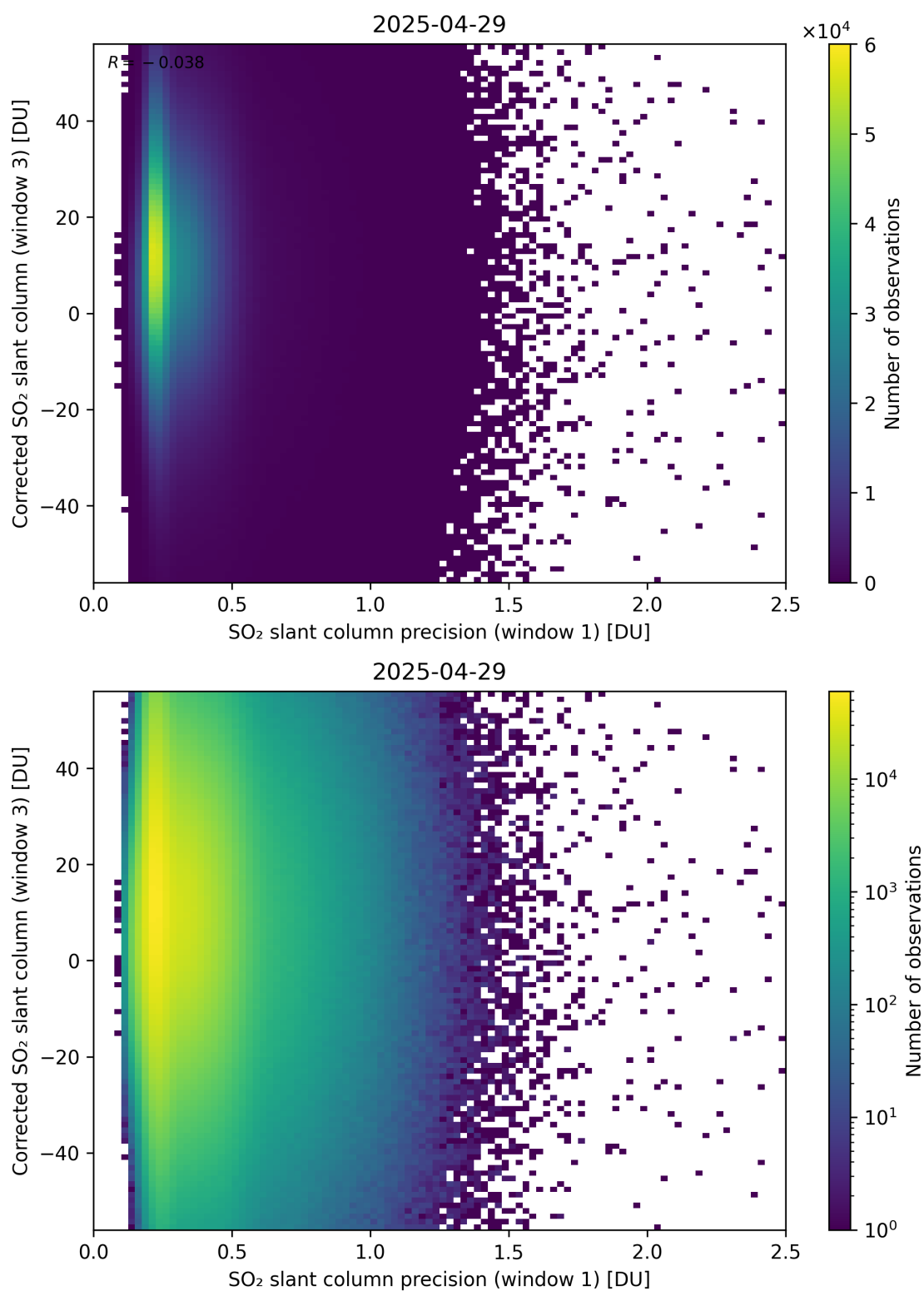
Figure 276: Scatter density plot of “SO 2 slant column precision (window 1)” against “Corrected SO 2 slant column (window 3)” for 2025-04-29 to 2025-04-30.
