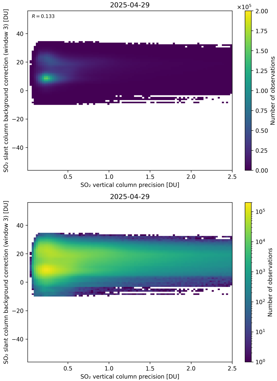
Figure 331: Scatter density plot of “SO 2 vertical column precision” against “SO 2 slant column background correction (window 3)” for 2025-04-29 to 2025-04-30.
