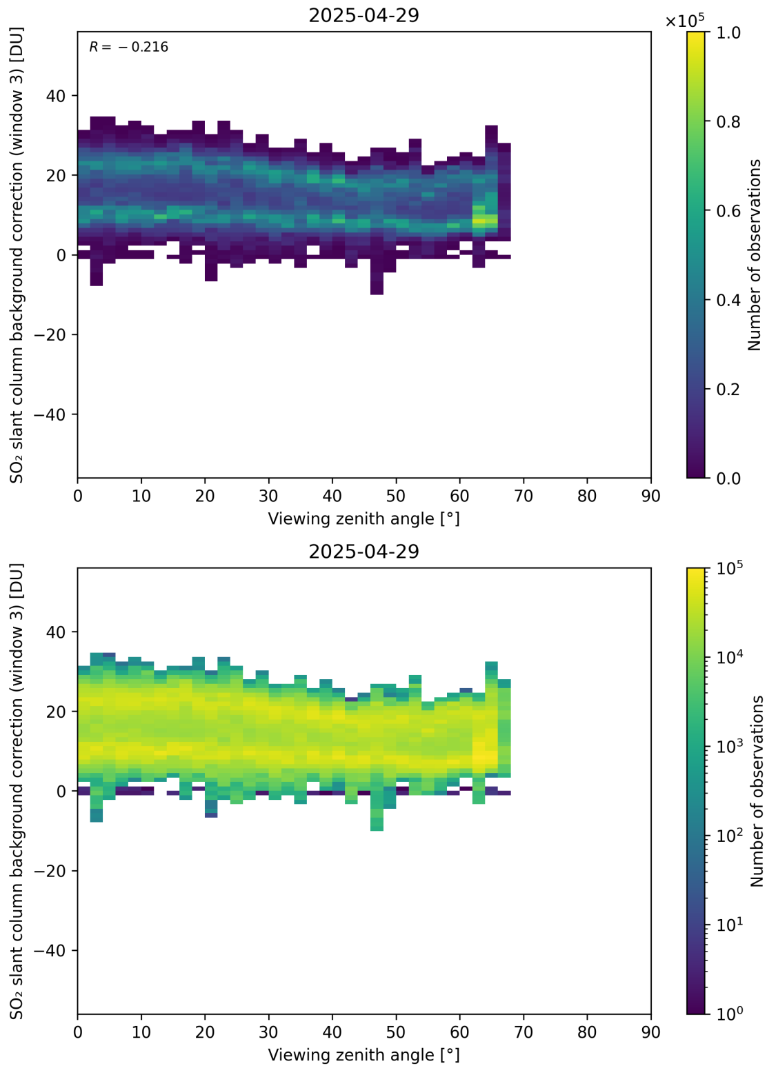
Figure 364: Scatter density plot of “Viewing zenith angle” against “SO 2 slant column background correction (window 3)” for 2025-04-29 to 2025-04-30.
