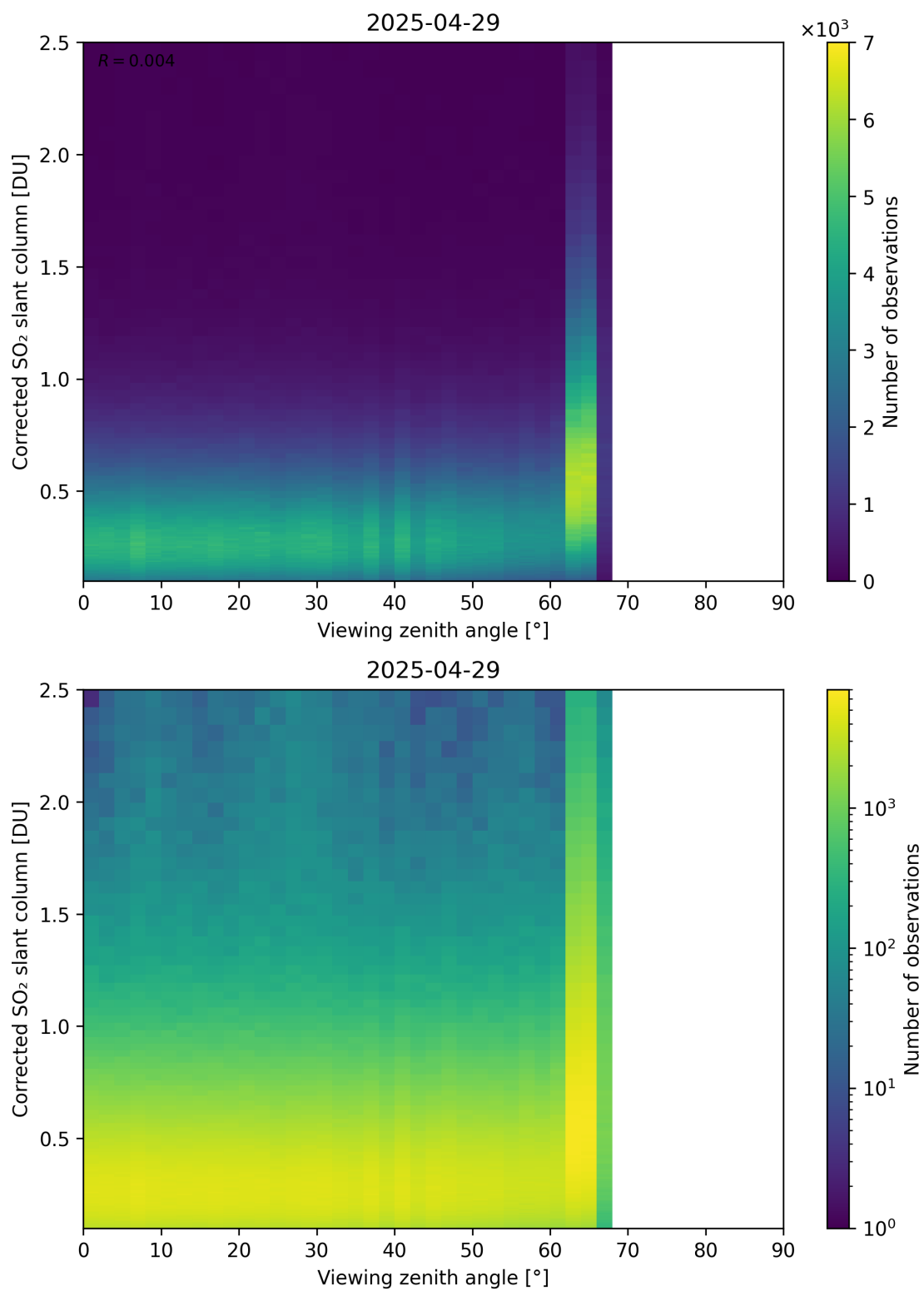
Figure 373: Scatter density plot of “Viewing zenith angle” against “Corrected SO 2 slant column” for 2025-04-29 to 2025-04-30.
