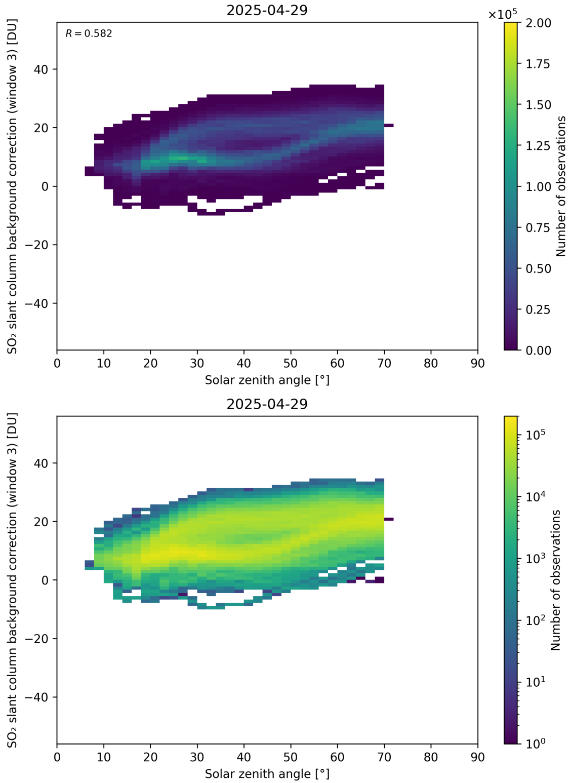
Figure 173: Scatter density plot of “Solar zenith angle” against “SO 2 slant column background correction (window 3)” for 2025-04-29 to 2025-04-30.
