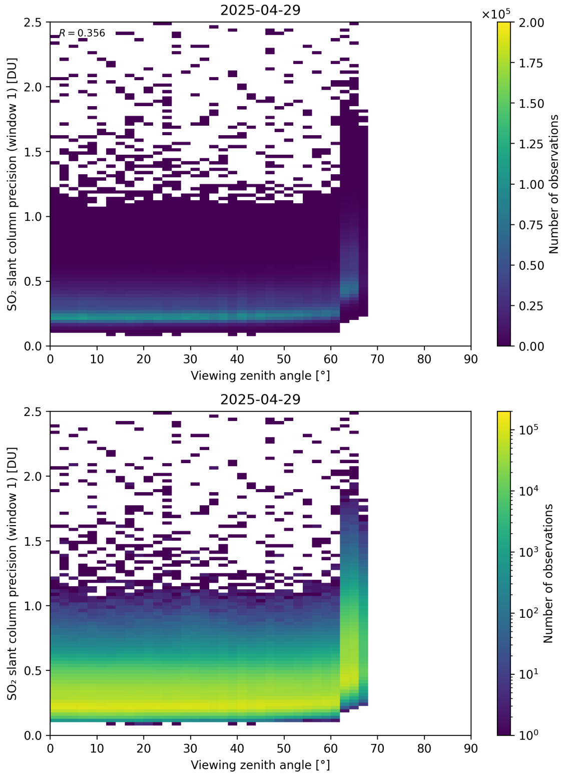
Figure 377: Scatter density plot of “Viewing zenith angle” against “SO 2 slant column precision (window 1)” for 2025-04-29 to 2025-04-30.
