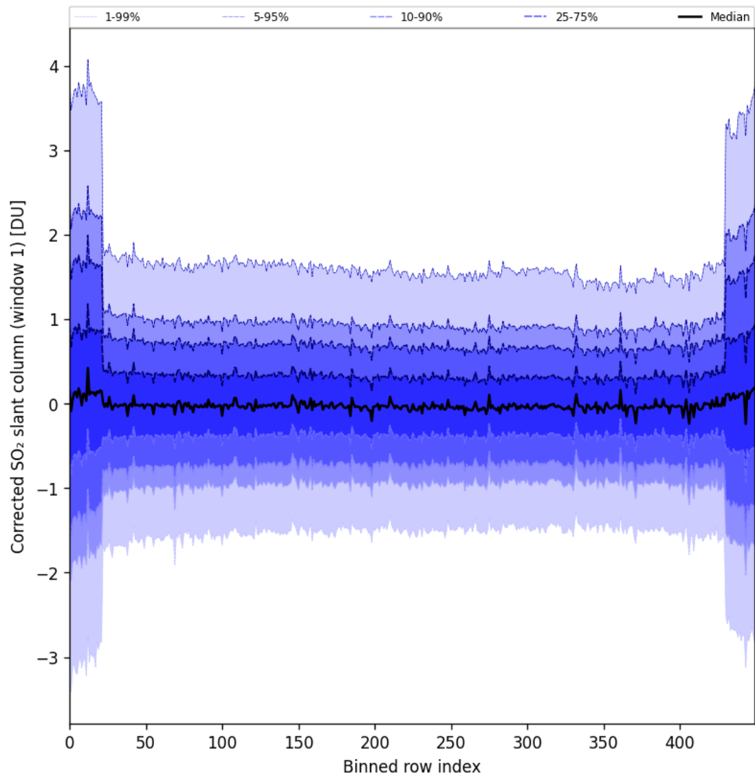
Figure 91: Along track statistics of “Corrected SO 2 slant column (window 1)” for 2025-04-29 to 2025-04-30
