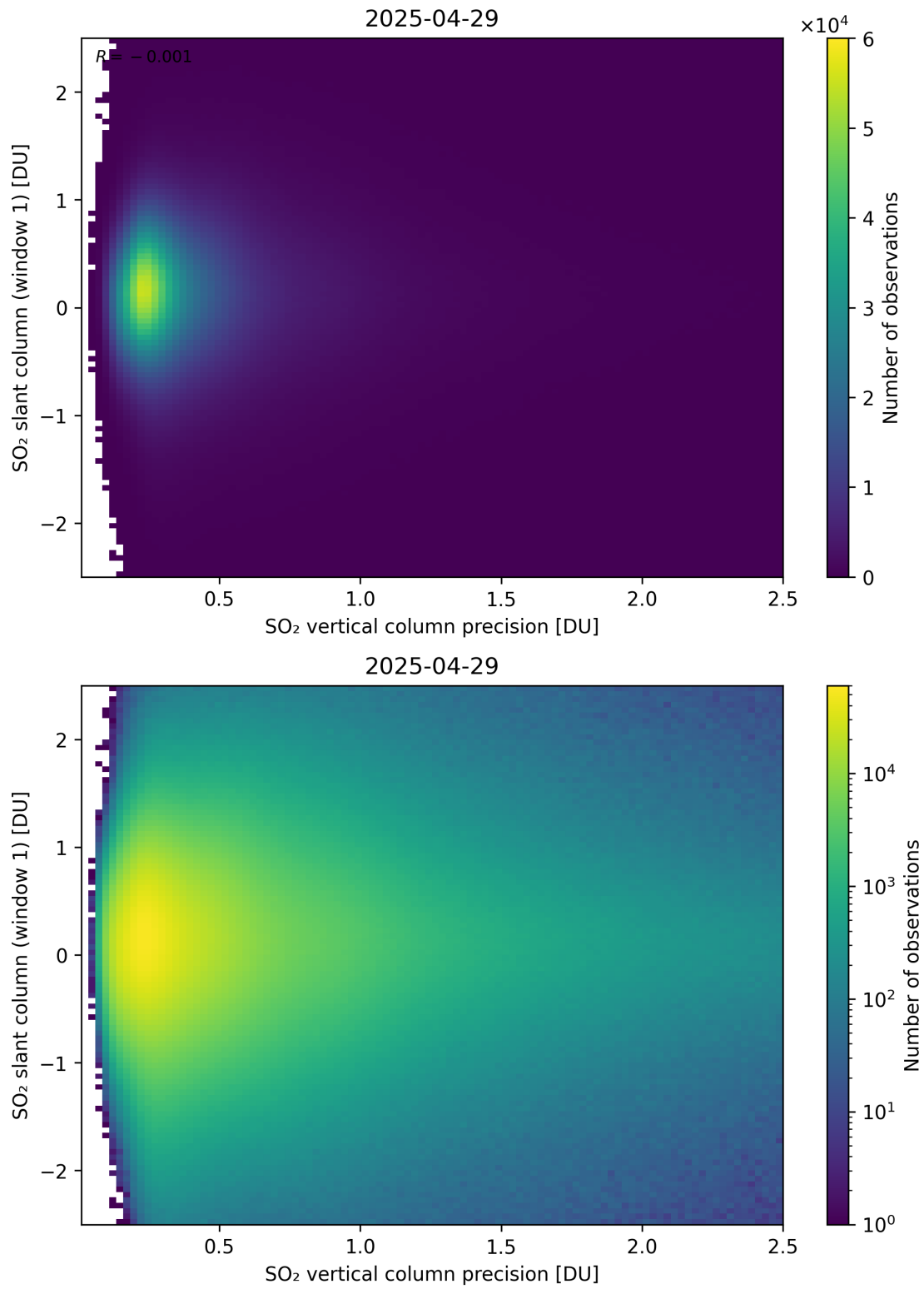
Figure 341: Scatter density plot of “SO 2 vertical column precision” against “SO 2 slant column (window 1)” for 2025-04-29 to 2025-04-30.
