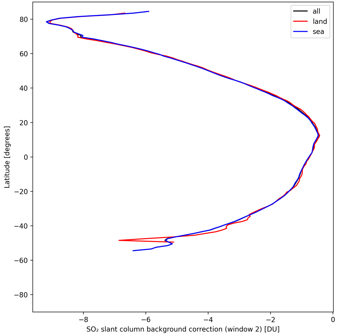
Figure 44: Zonal average of “SO 2 slant column background correction (window 2)” for 2025-04-29 to 2025-04-30.
