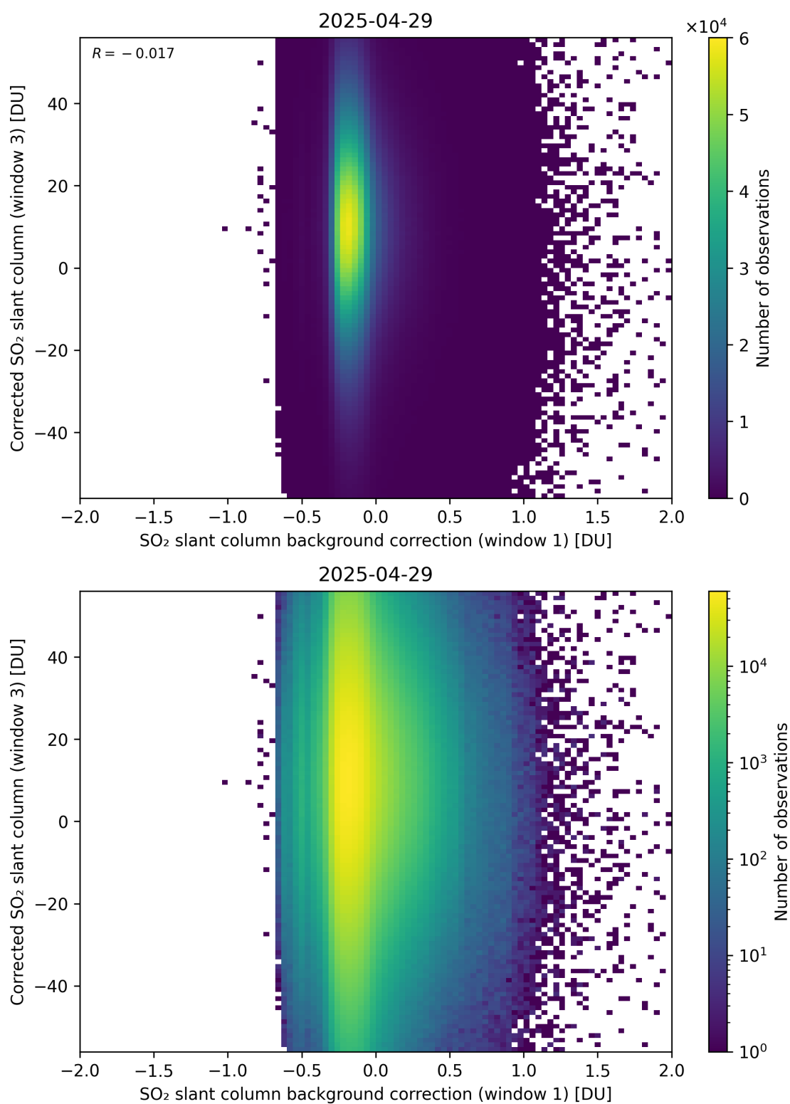
Figure 116: Scatter density plot of “SO 2 slant column background correction (window 1)” against “Corrected SO 2 slant column (window 3)” for 2025-04-29 to 2025-04-30.
