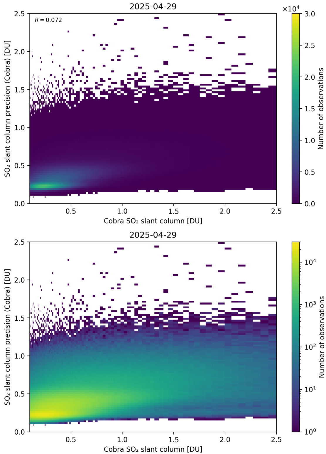
Figure 216: Scatter density plot of “Cobra SO 2 slant column” against “SO 2 slant column precision (Cobra)” for 2025-04-29 to 2025-04-30.
