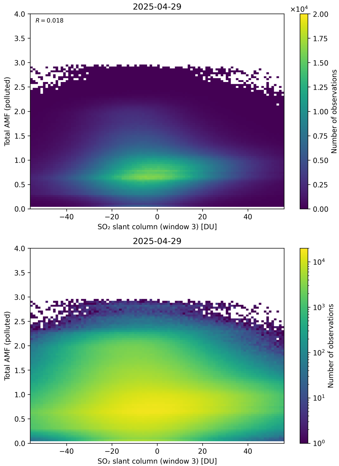
Figure 318: Scatter density plot of “SO 2 slant column (window 3)” against “Total AMF (polluted)” for 2025-04-29 to 2025-04-30.
