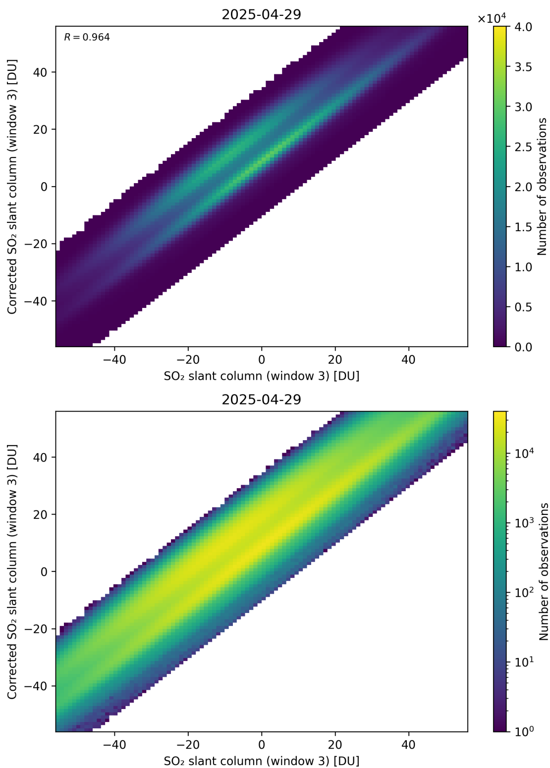
Figure 316: Scatter density plot of “SO 2 slant column (window 3)” against “Corrected SO 2 slant column (window 3)” for 2025-04-29 to 2025-04-30.
