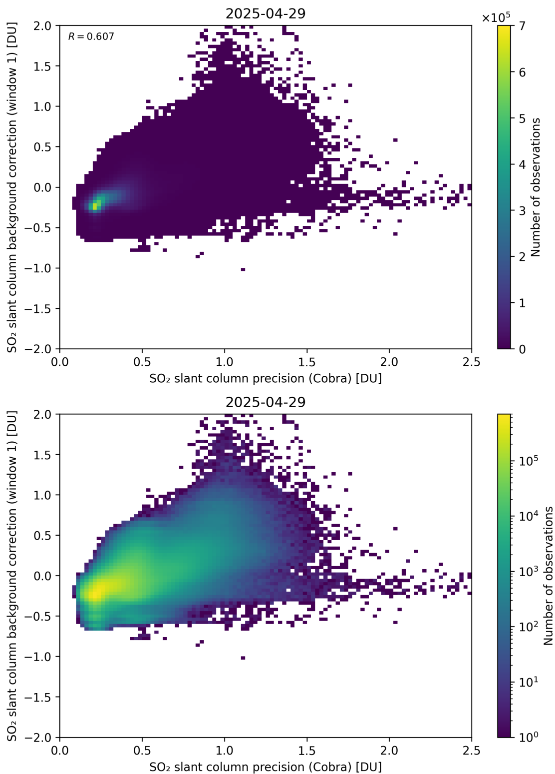
Figure 199: Scatter density plot of “SO 2 slant column precision (Cobra)” against “SO 2 slant column background correction (window 1)” for 2025-04-29 to 2025-04-30.
