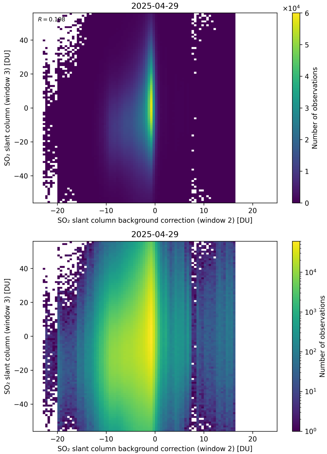
Figure 128: Scatter density plot of “SO 2 slant column background correction (window 2)” against “SO 2 slant column (window 3)” for 2025-04-29 to 2025-04-30.
