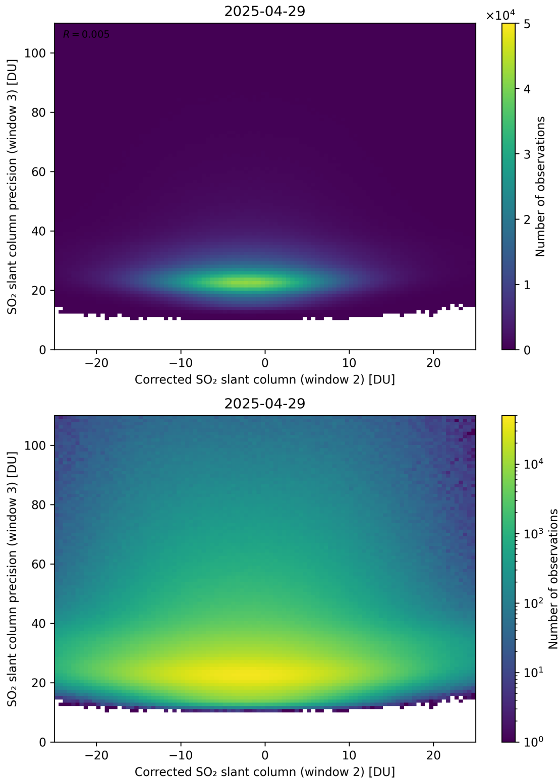
Figure 252: Scatter density plot of “Corrected SO 2 slant column (window 2)” against “SO 2 slant column precision (window 3)” for 2025-04-29 to 2025-04-30.
