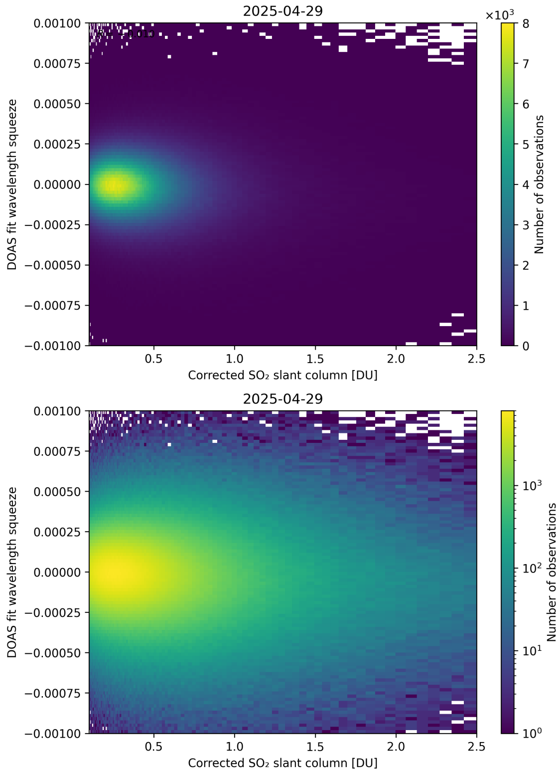
Figure 230: Scatter density plot of “Corrected SO 2 slant column” against “DOAS fit wavelength squeeze” for 2025-04-29 to 2025-04-30.
