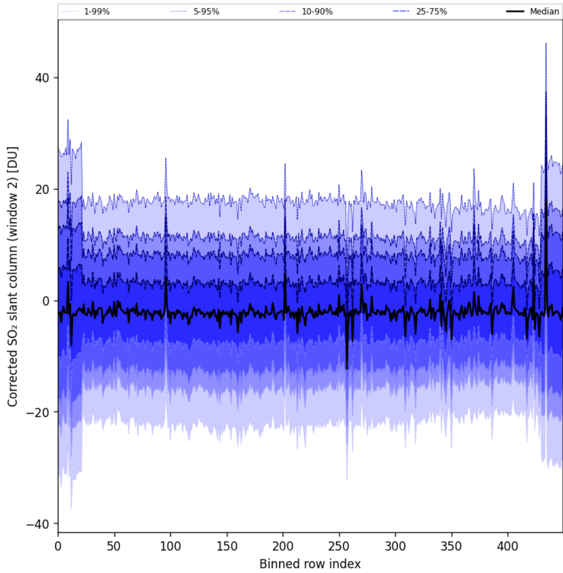
Figure 95: Along track statistics of “Corrected SO 2 slant column (window 2)” for 2025-04-29 to 2025-04-30
