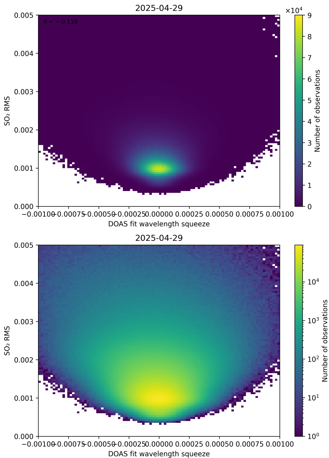
Figure 143: Scatter density plot of “DOAS fit wavelength squeeze” against “SO 2 RMS” for 2025-04-29 to 2025-04-30.
