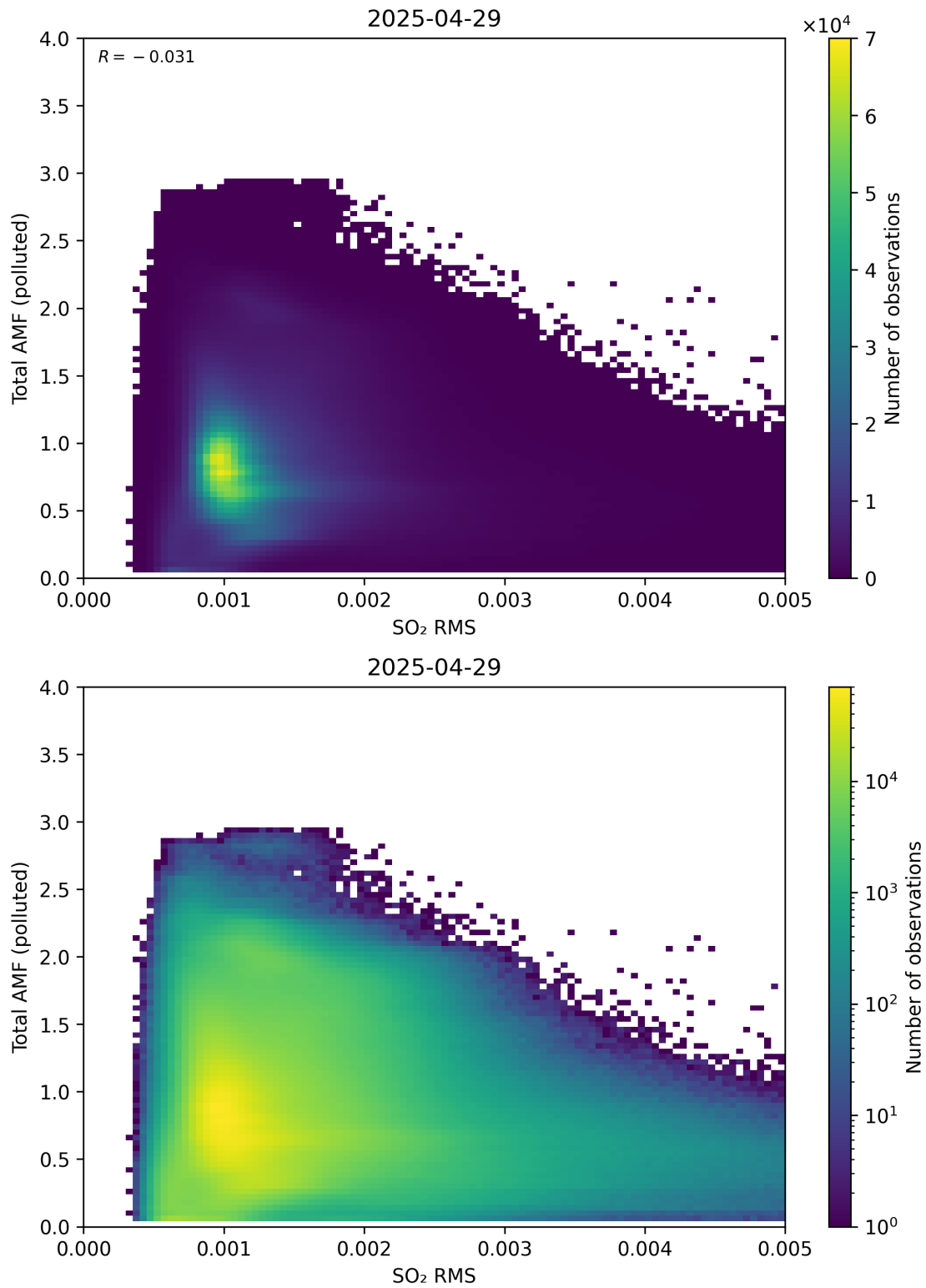
Figure 148: Scatter density plot of “SO 2 RMS” against “Total AMF (polluted)” for 2025-04-29 to 2025-04-30.
