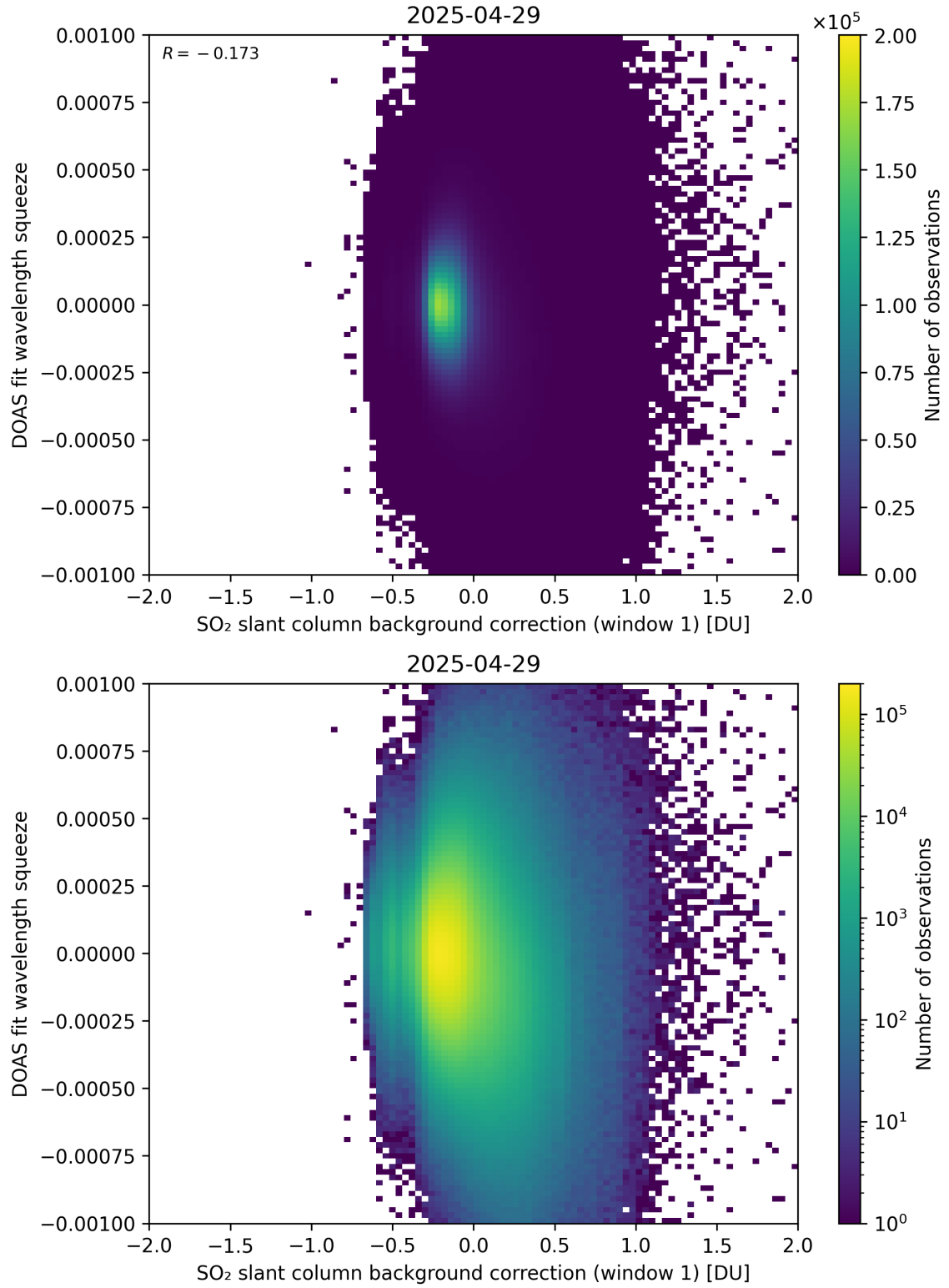
Figure 112: Scatter density plot of “SO 2 slant column background correction (window 1)” against “DOAS fit wavelength squeeze” for 2025-04-29 to 2025-04-30.
