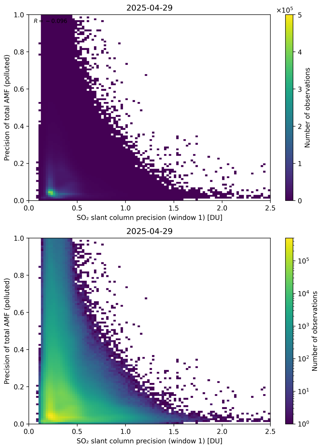
Figure 281: Scatter density plot of “SO 2 slant column precision (window 1)” against “Precision of total AMF (polluted)” for 2025-04-29 to 2025-04-30.
