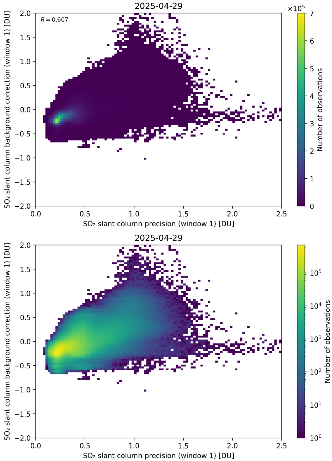
Figure 268: Scatter density plot of “SO 2 slant column precision (window 1)” against “SO 2 slant column background correction (window 1)” for 2025-04-29 to 2025-04-30.
