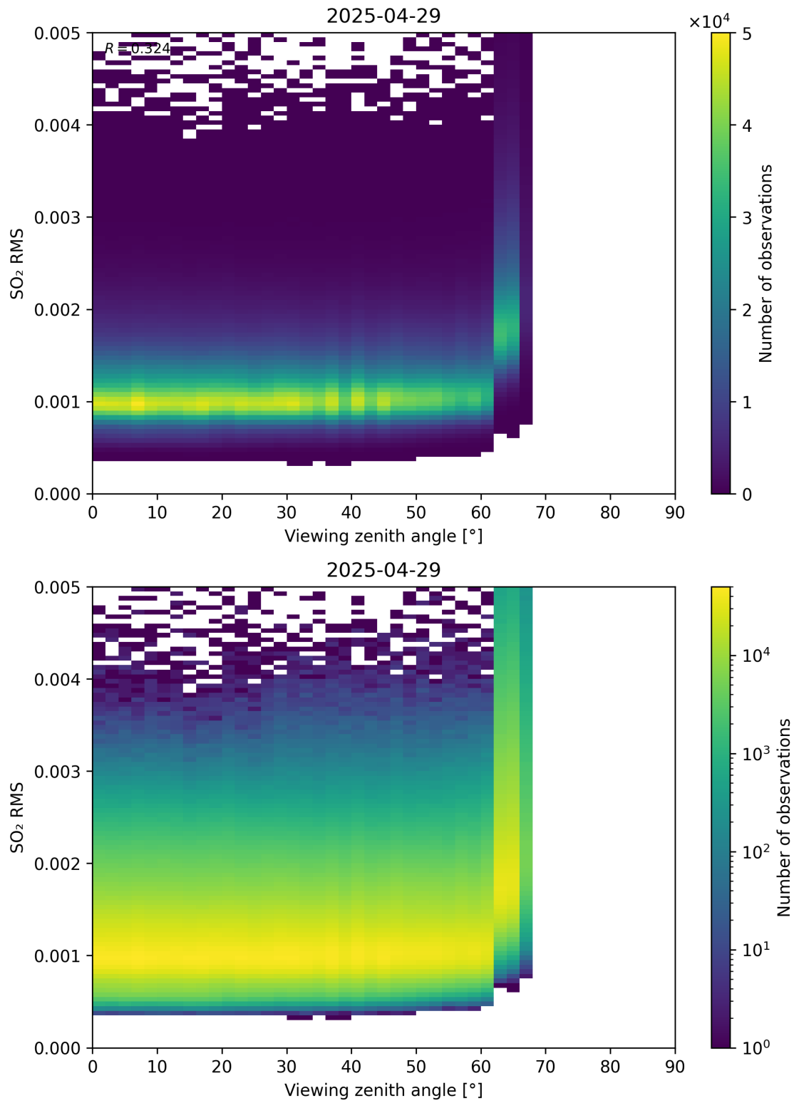
Figure 367: Scatter density plot of “Viewing zenith angle” against “SO 2 RMS” for 2025-04-29 to 2025-04-30.
