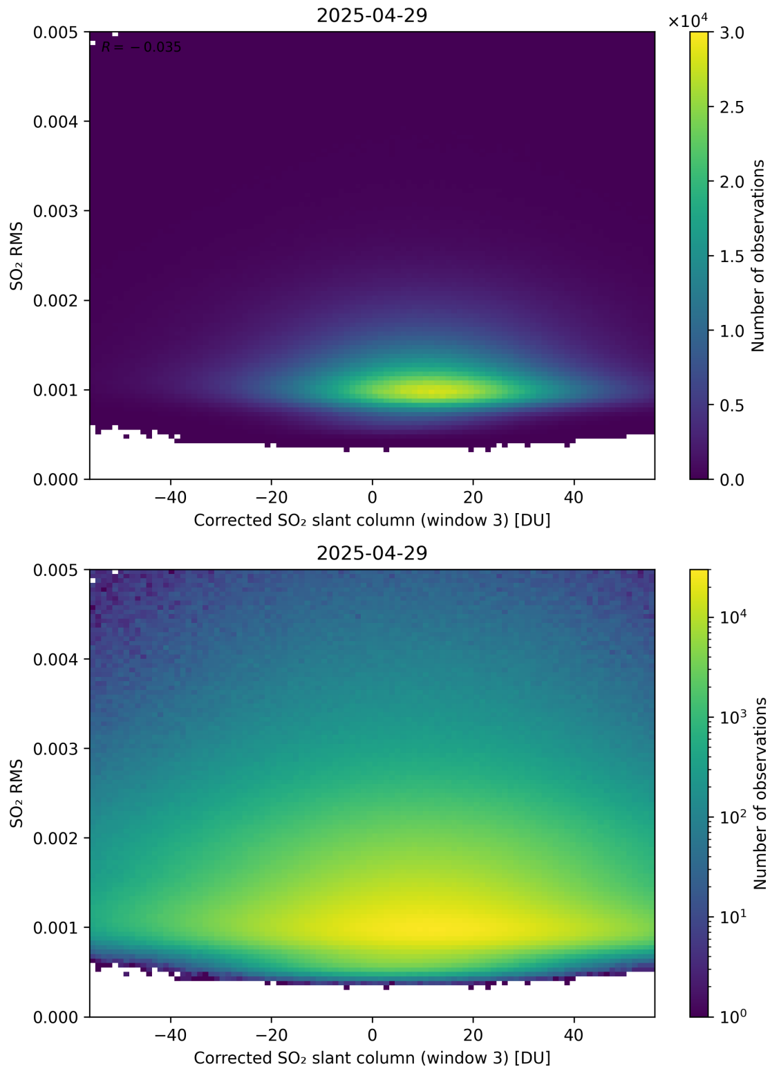
Figure 258: Scatter density plot of “Corrected SO 2 slant column (window 3)” against “SO 2 RMS” for 2025-04-29 to 2025-04-30.
