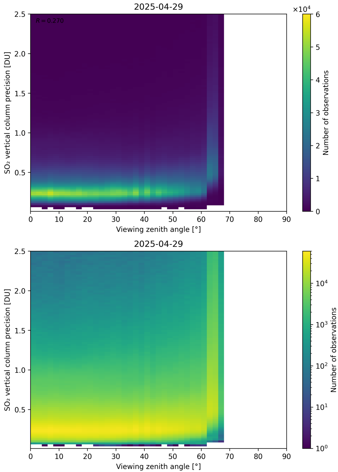
Figure 384: Scatter density plot of “Viewing zenith angle” against “SO 2 vertical column precision” for 2025-04-29 to 2025-04-30.
