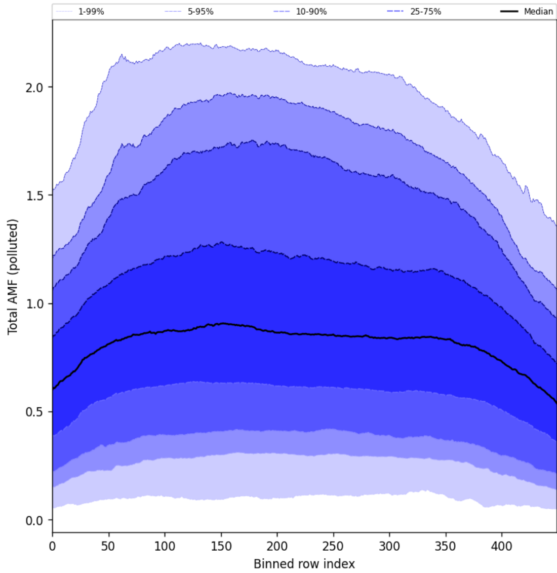
Figure 105: Along track statistics of “Total AMF (polluted)” for 2025-04-29 to 2025-04-30
