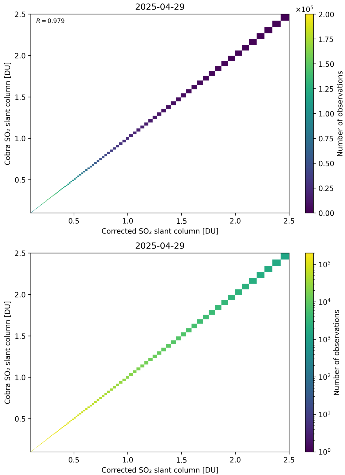
Figure 233: Scatter density plot of “Corrected SO 2 slant column” against “Cobra SO 2 slant column” for 2025-04-29 to 2025-04-30.
