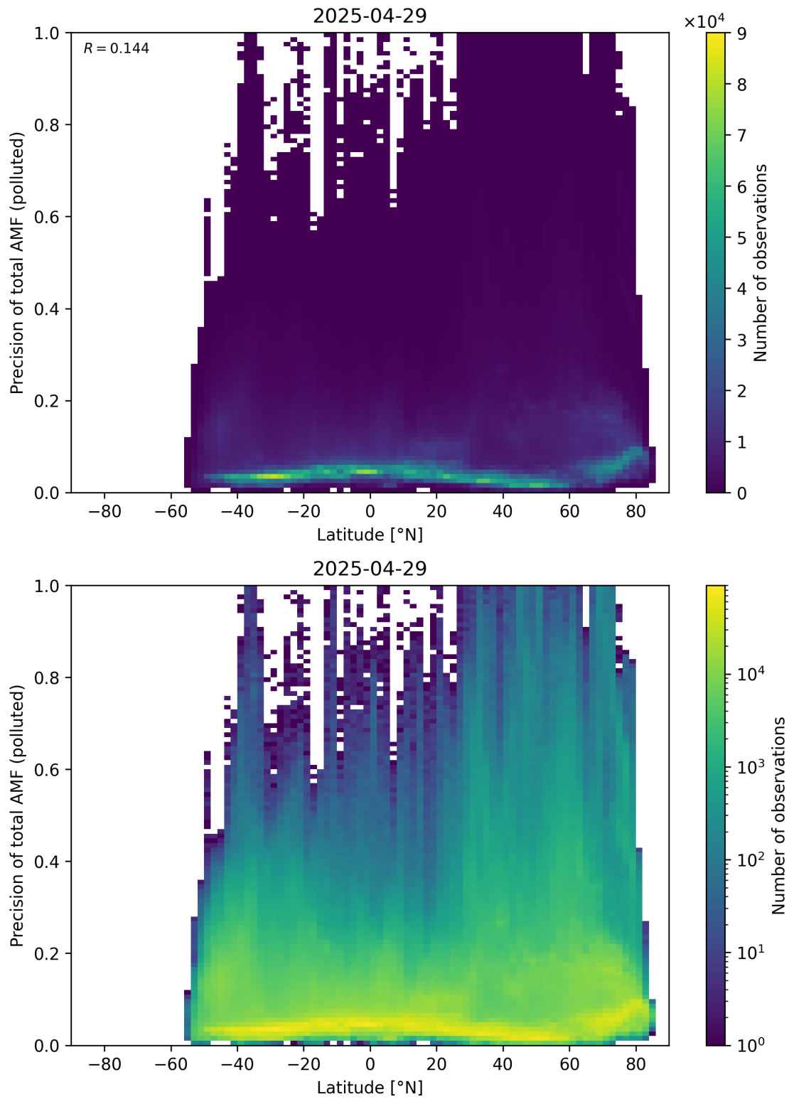
Figure 168: Scatter density plot of “Latitude” against “Precision of total AMF (polluted)” for 2025-04-29 to 2025-04-30.
