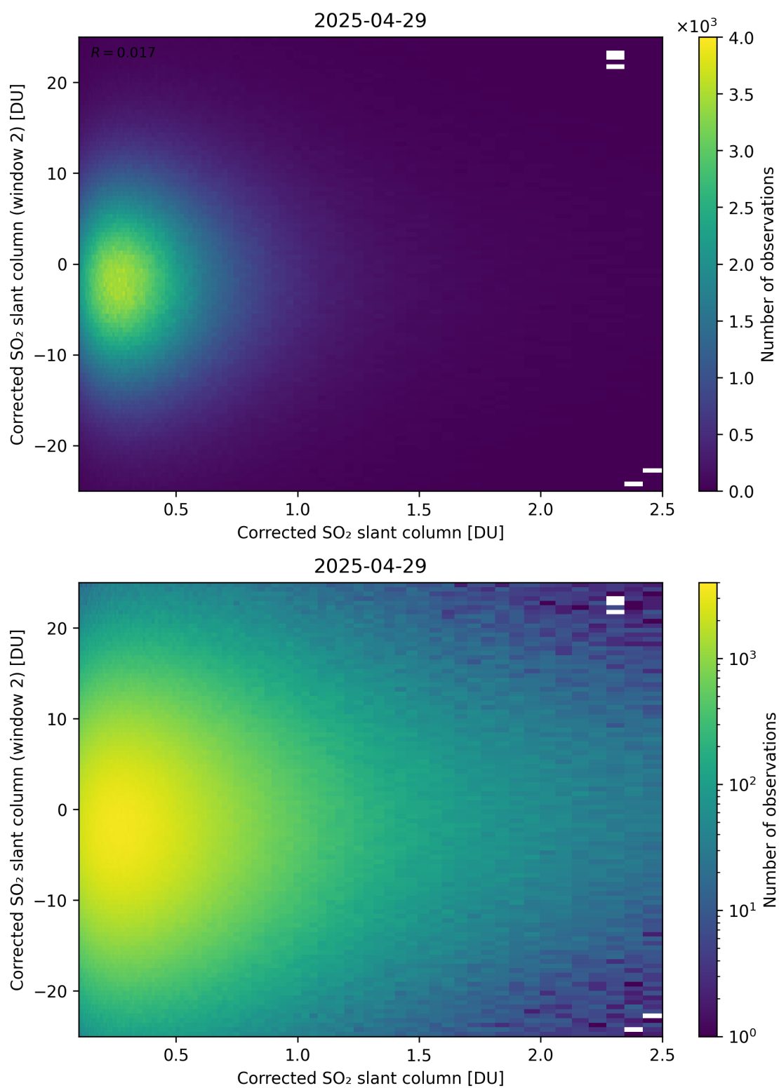
Figure 235: Scatter density plot of “Corrected SO 2 slant column” against “Corrected SO 2 slant column (window 2)” for 2025-04-29 to 2025-04-30.
