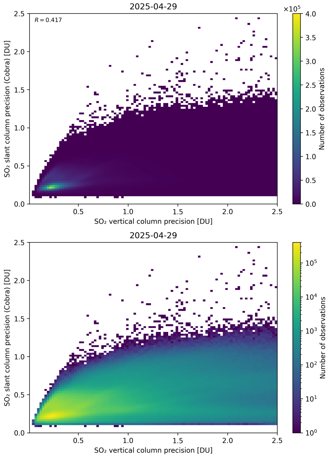
Figure 337: Scatter density plot of “SO 2 vertical column precision” against “SO 2 slant column precision (Cobra)” for 2025-04-29 to 2025-04-30.
