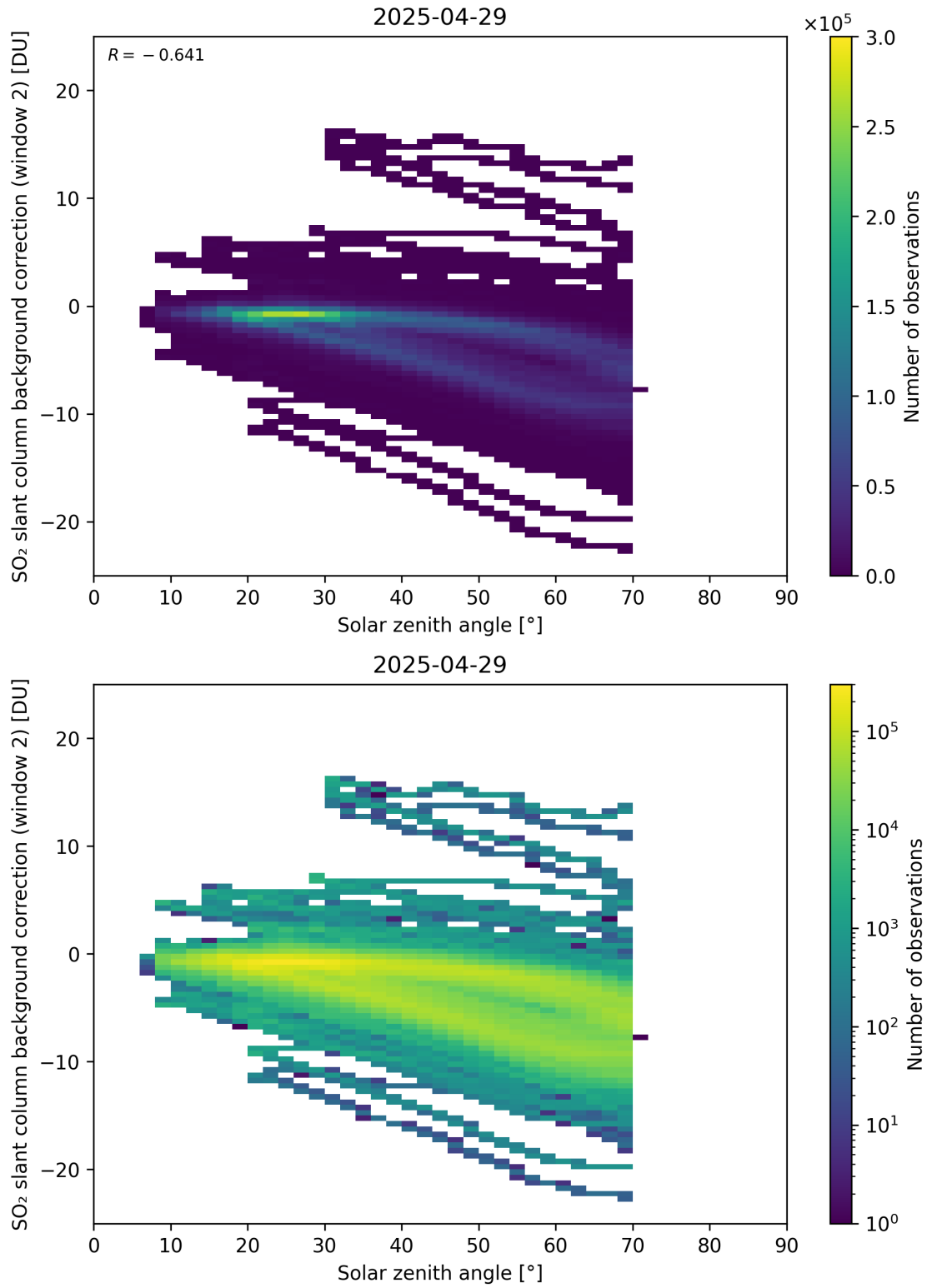
Figure 172: Scatter density plot of “Solar zenith angle” against “SO 2 slant column background correction (window 2)” for 2025-04-29 to 2025-04-30.
