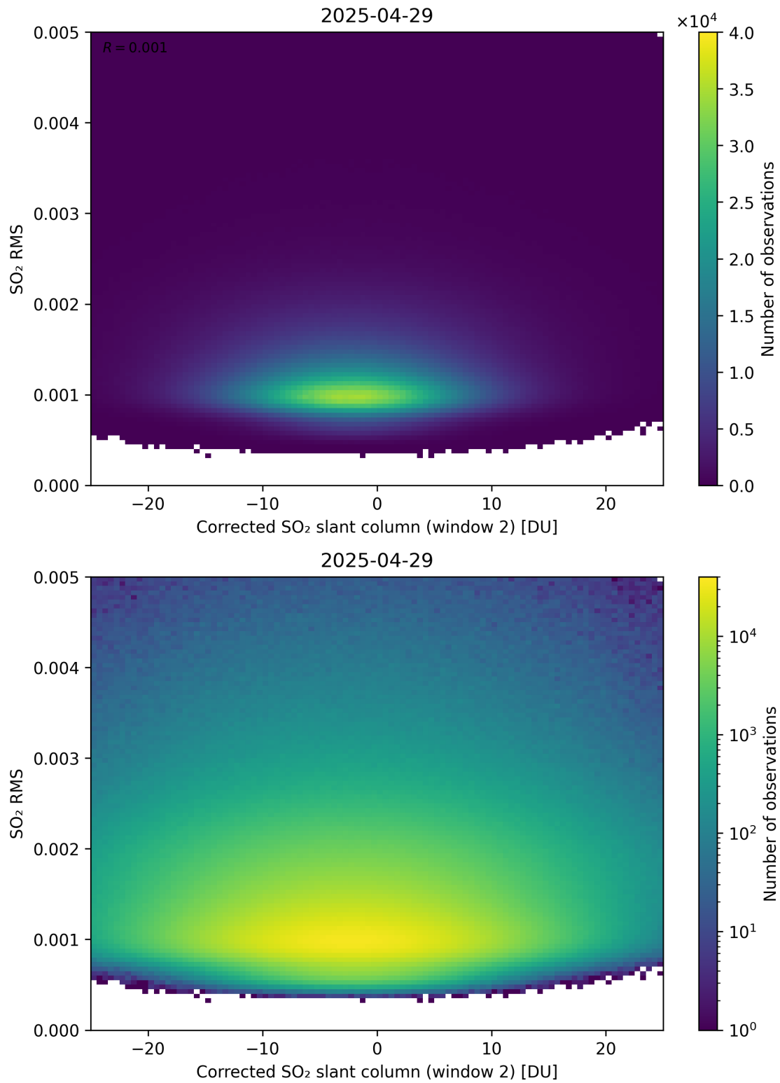
Figure 248: Scatter density plot of “Corrected SO 2 slant column (window 2)” against “SO 2 RMS” for 2025-04-29 to 2025-04-30.
