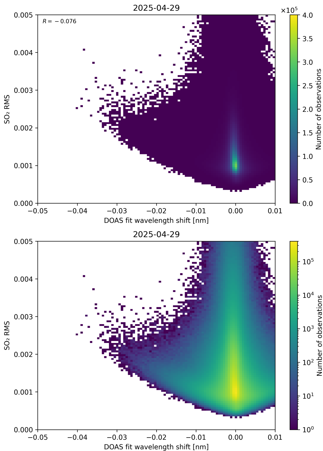
Figure 139: Scatter density plot of “DOAS fit wavelength shift” against “SO 2 RMS” for 2025-04-29 to 2025-04-30.
