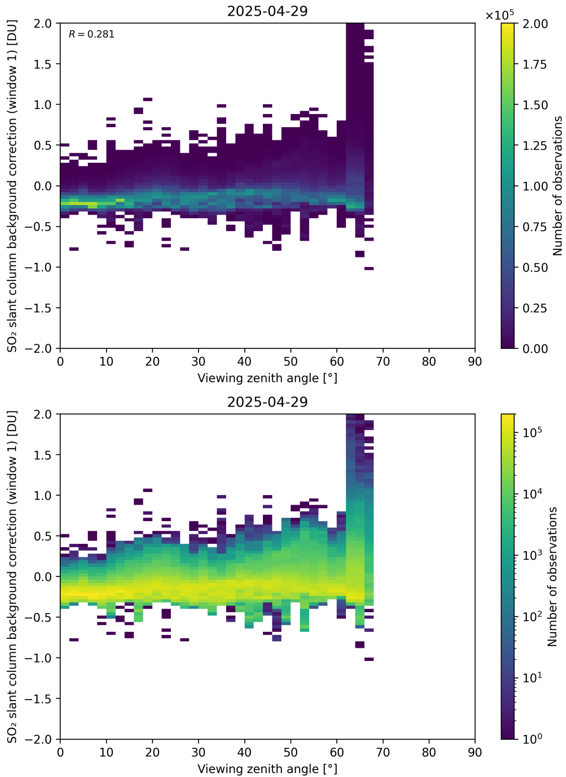
Figure 362: Scatter density plot of “Viewing zenith angle” against “SO 2 slant column background correction (window 1)” for 2025-04-29 to 2025-04-30.
