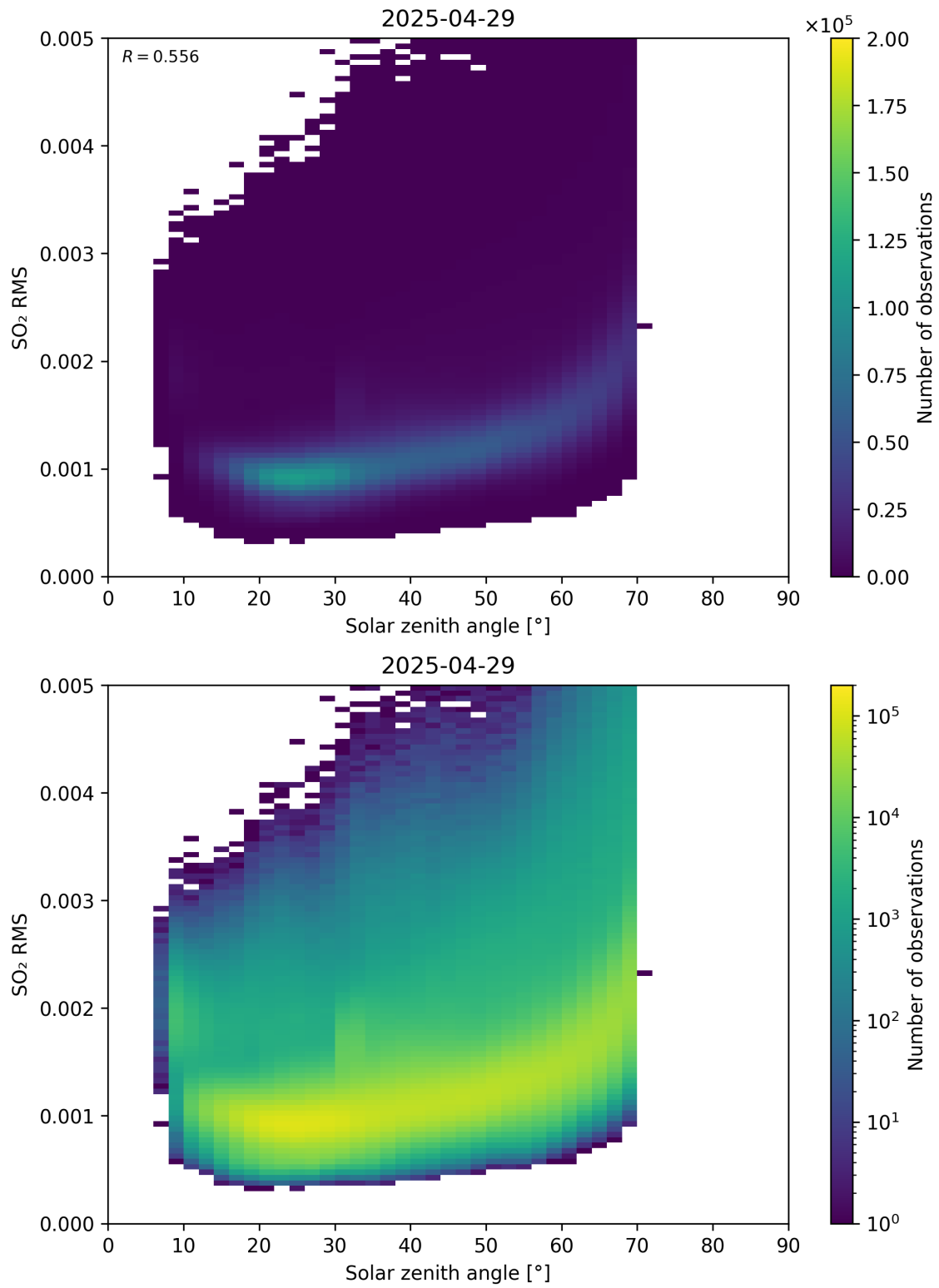
Figure 176: Scatter density plot of “Solar zenith angle” against “SO 2 RMS” for 2025-04-29 to 2025-04-30.
