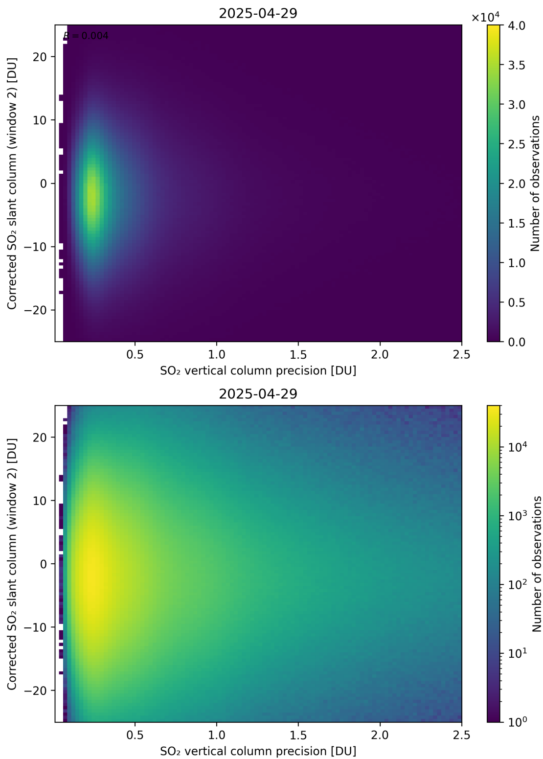
Figure 339: Scatter density plot of “SO 2 vertical column precision” against “Corrected SO 2 slant column (window 2)” for 2025-04-29 to 2025-04-30.
