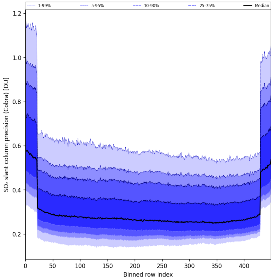
Figure 88: Along track statistics of “SO 2 slant column precision (Cobra)” for 2025-04-29 to 2025-04-30
