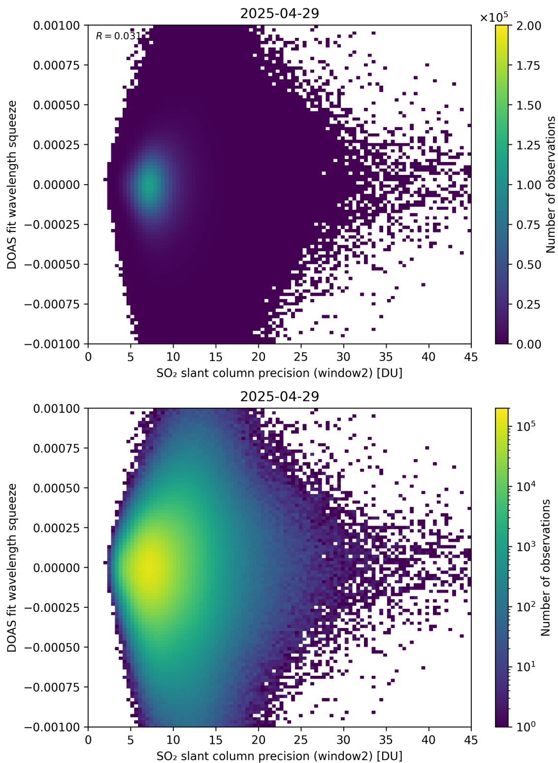
Figure 294: Scatter density plot of “SO 2 slant column precision (window2)” against “DOAS fit wavelength squeeze” for 2025-04-29 to 2025-04-30.
