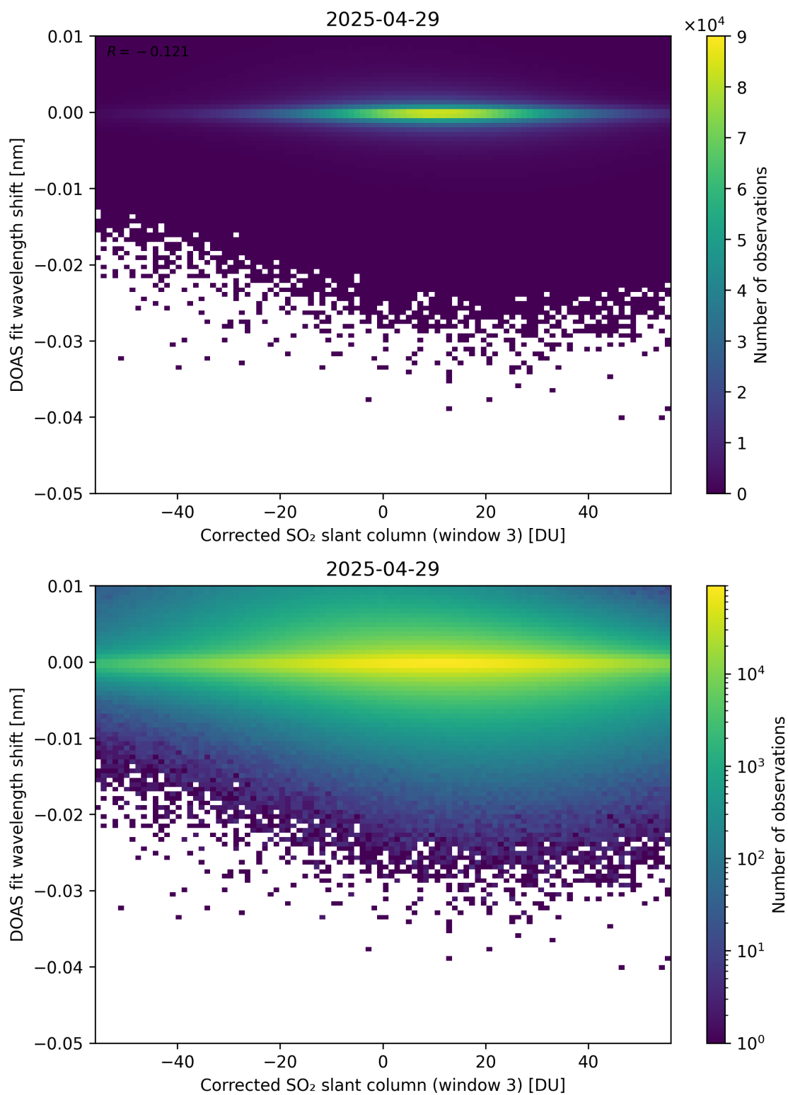
Figure 256: Scatter density plot of “Corrected SO 2 slant column (window 3)” against “DOAS fit wavelength shift” for 2025-04-29 to 2025-04-30.
