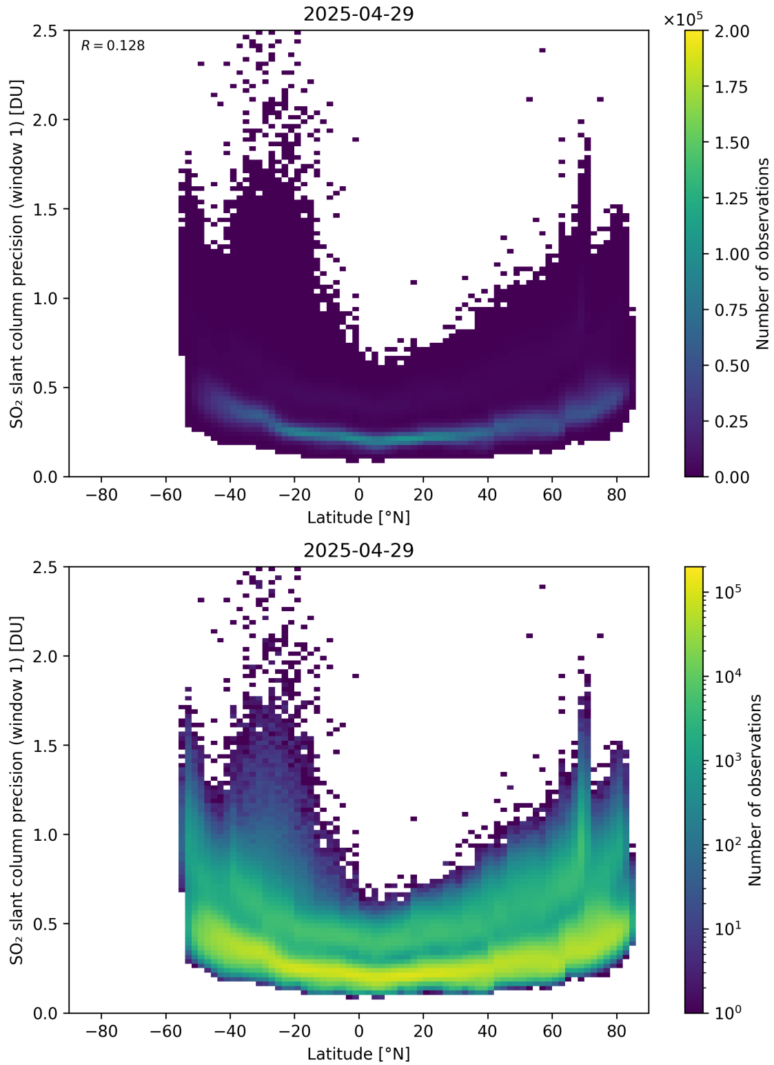
Figure 163: Scatter density plot of “Latitude” against “SO 2 slant column precision (window 1)” for 2025-04-29 to 2025-04-30.
