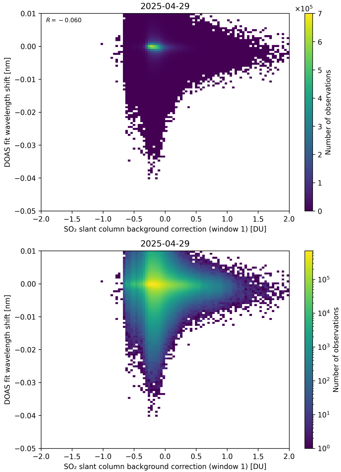
Figure 111: Scatter density plot of “SO 2 slant column background correction (window 1)” against “DOAS fit wavelength shift” for 2025-04-29 to 2025-04-30.
