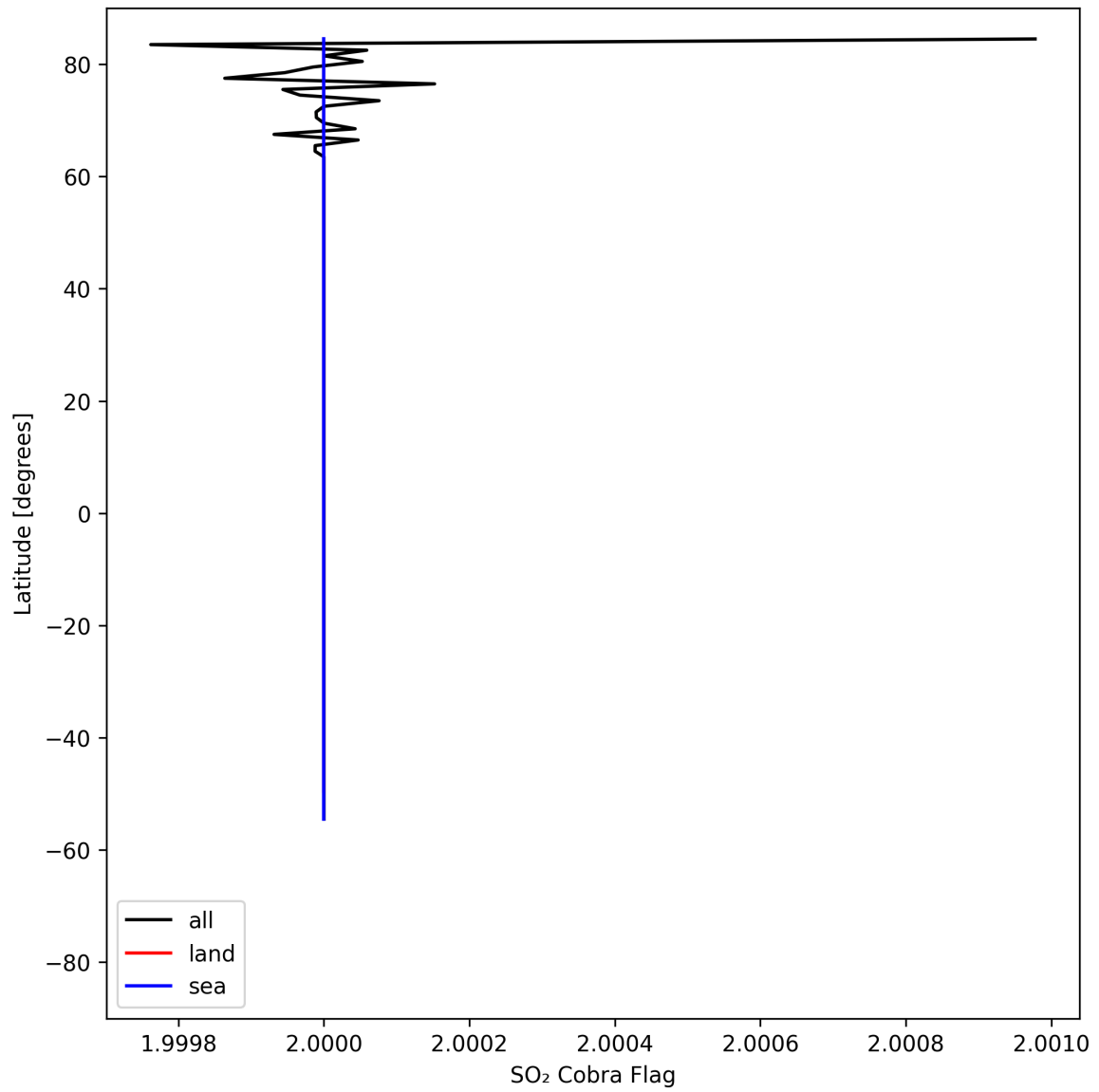
Figure 49: Zonal average of “SO 2 Cobra Flag” for 2025-04-29 to 2025-04-30.
