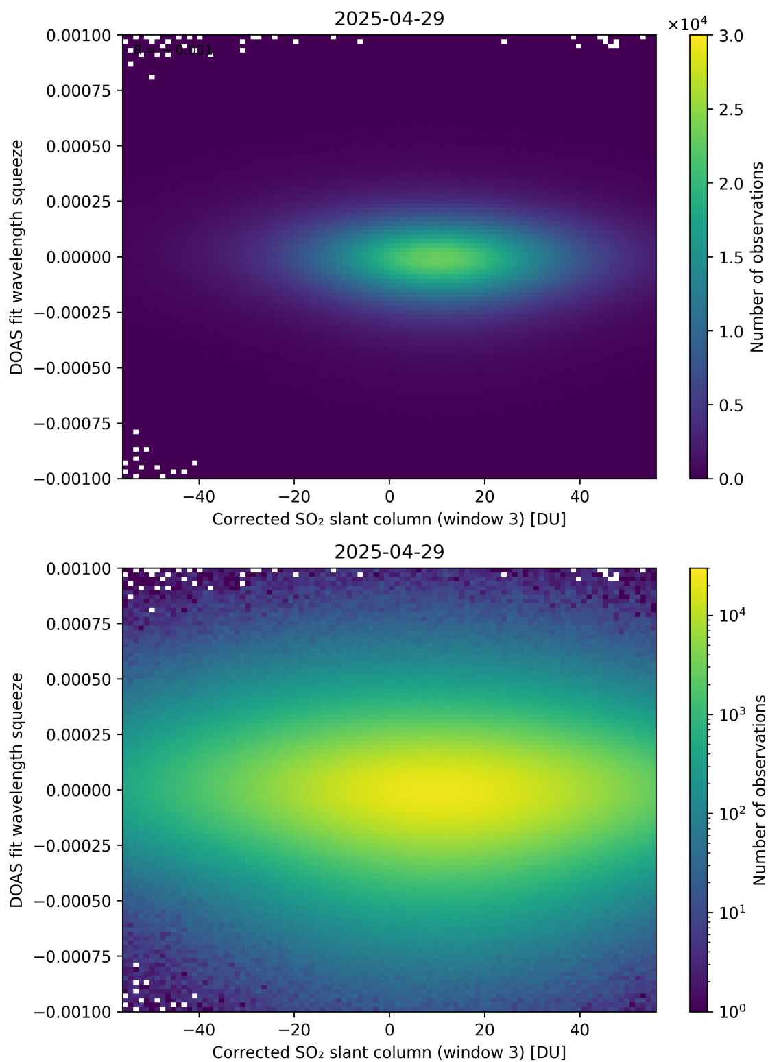
Figure 257: Scatter density plot of “Corrected SO 2 slant column (window 3)” against “DOAS fit wavelength squeeze” for 2025-04-29 to 2025-04-30.
