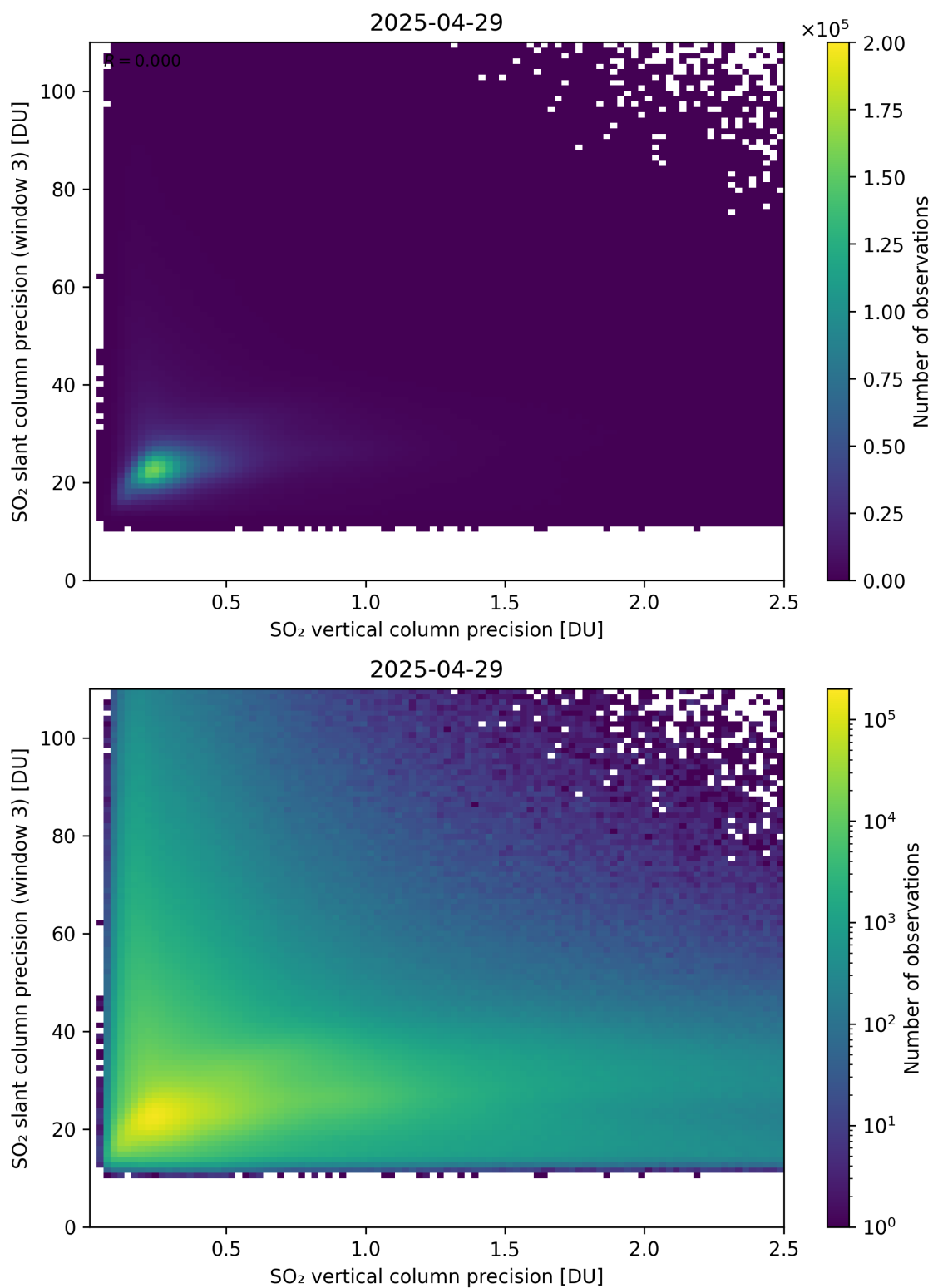
Figure 345: Scatter density plot of “SO 2 vertical column precision” against “SO 2 slant column precision (window 3)” for 2025-04-29 to 2025-04-30.
