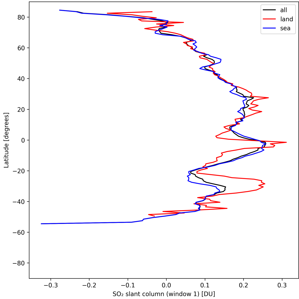
Figure 37: Zonal average of “SO 2 slant column (window 1)” for 2025-04-29 to 2025-04-30.
