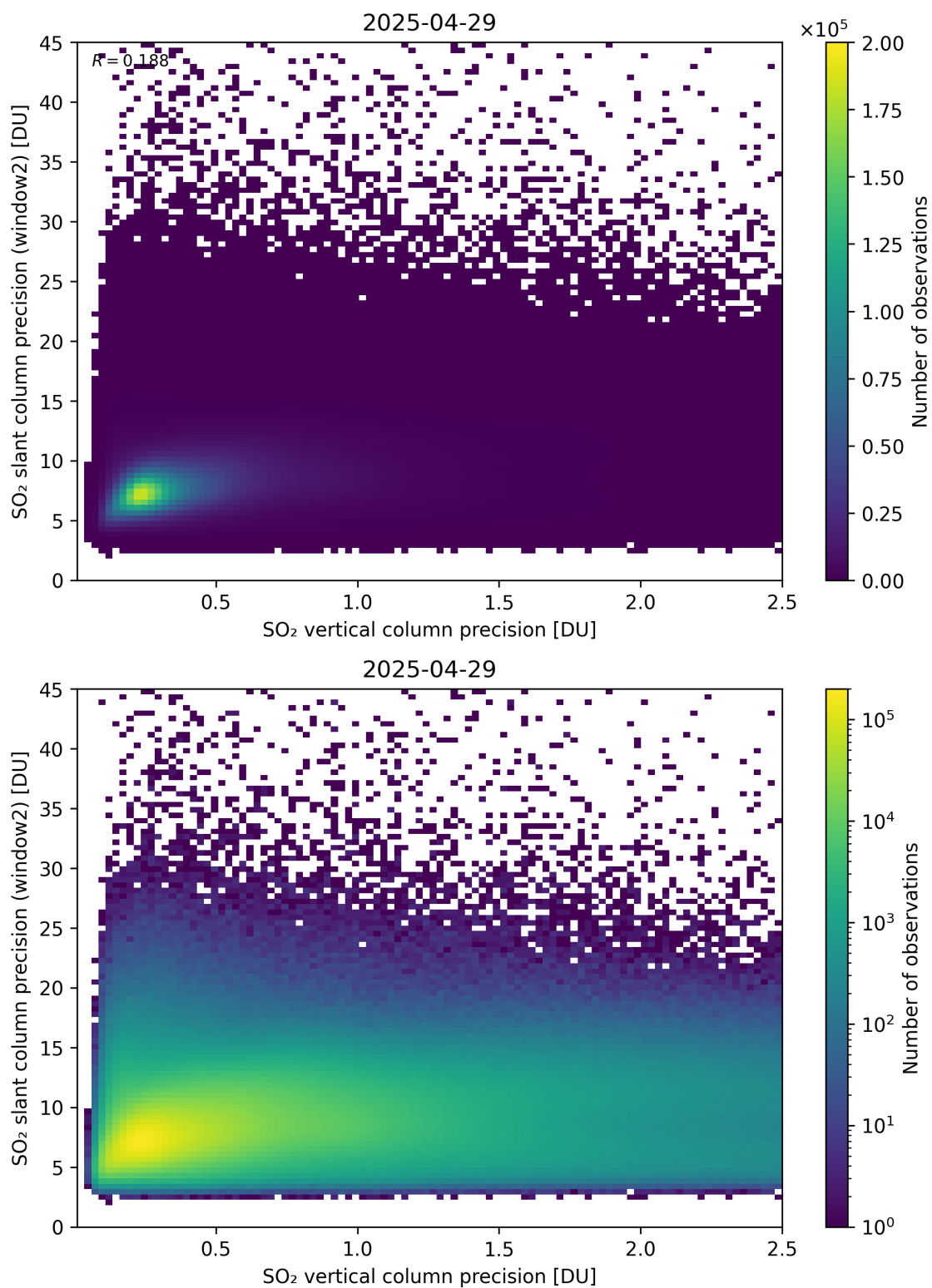
Figure 343: Scatter density plot of “SO 2 vertical column precision” against “SO 2 slant column precision (window2)” for 2025-04-29 to 2025-04-30.
