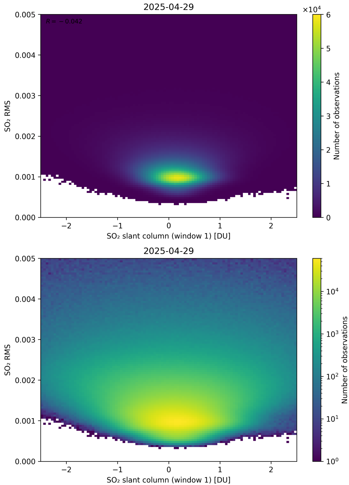
Figure 267: Scatter density plot of “SO 2 slant column (window 1)” against “SO 2 RMS” for 2025-04-29 to 2025-04-30.
