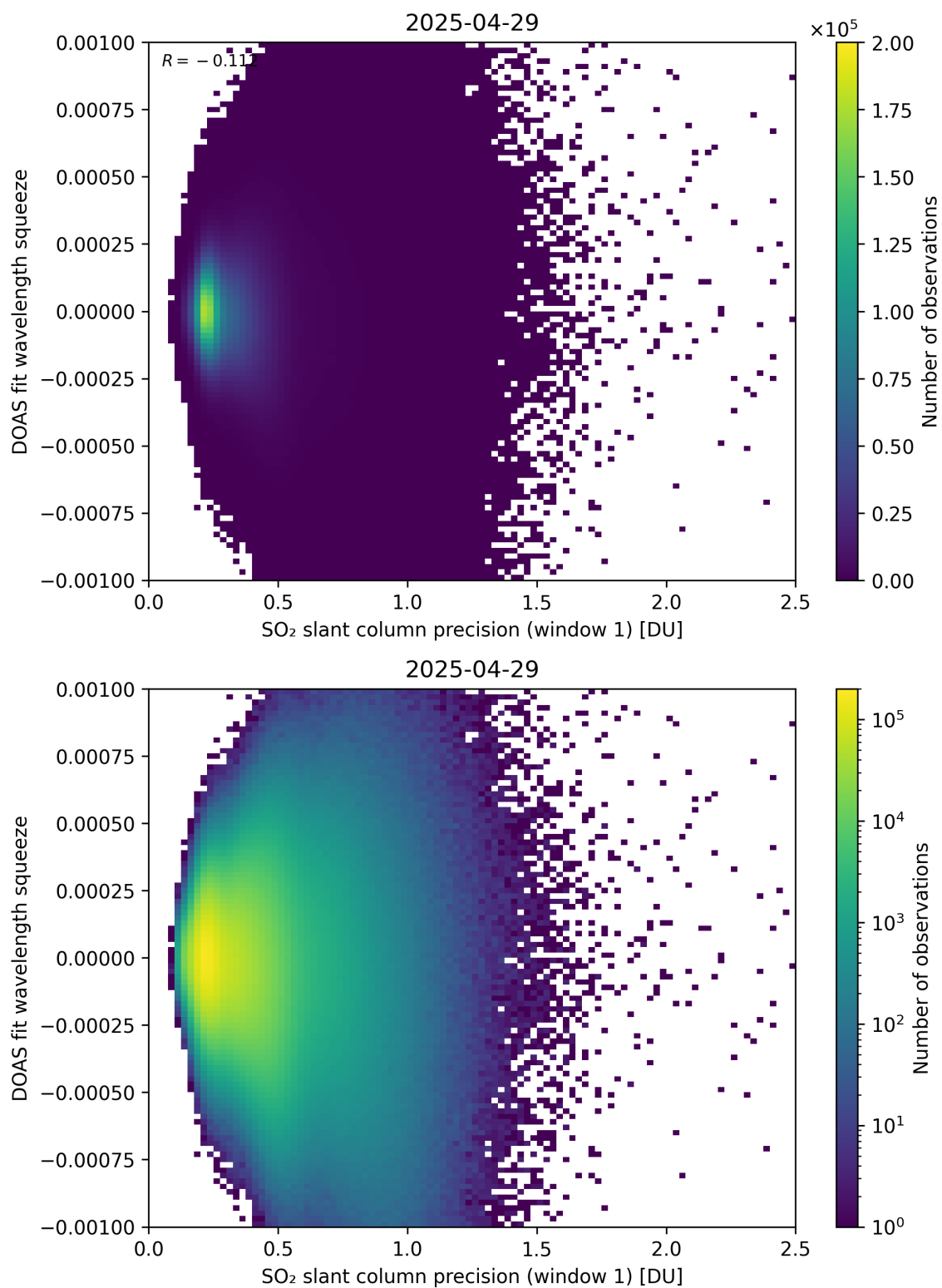
Figure 272: Scatter density plot of “SO 2 slant column precision (window 1)” against “DOAS fit wavelength squeeze” for 2025-04-29 to 2025-04-30.
