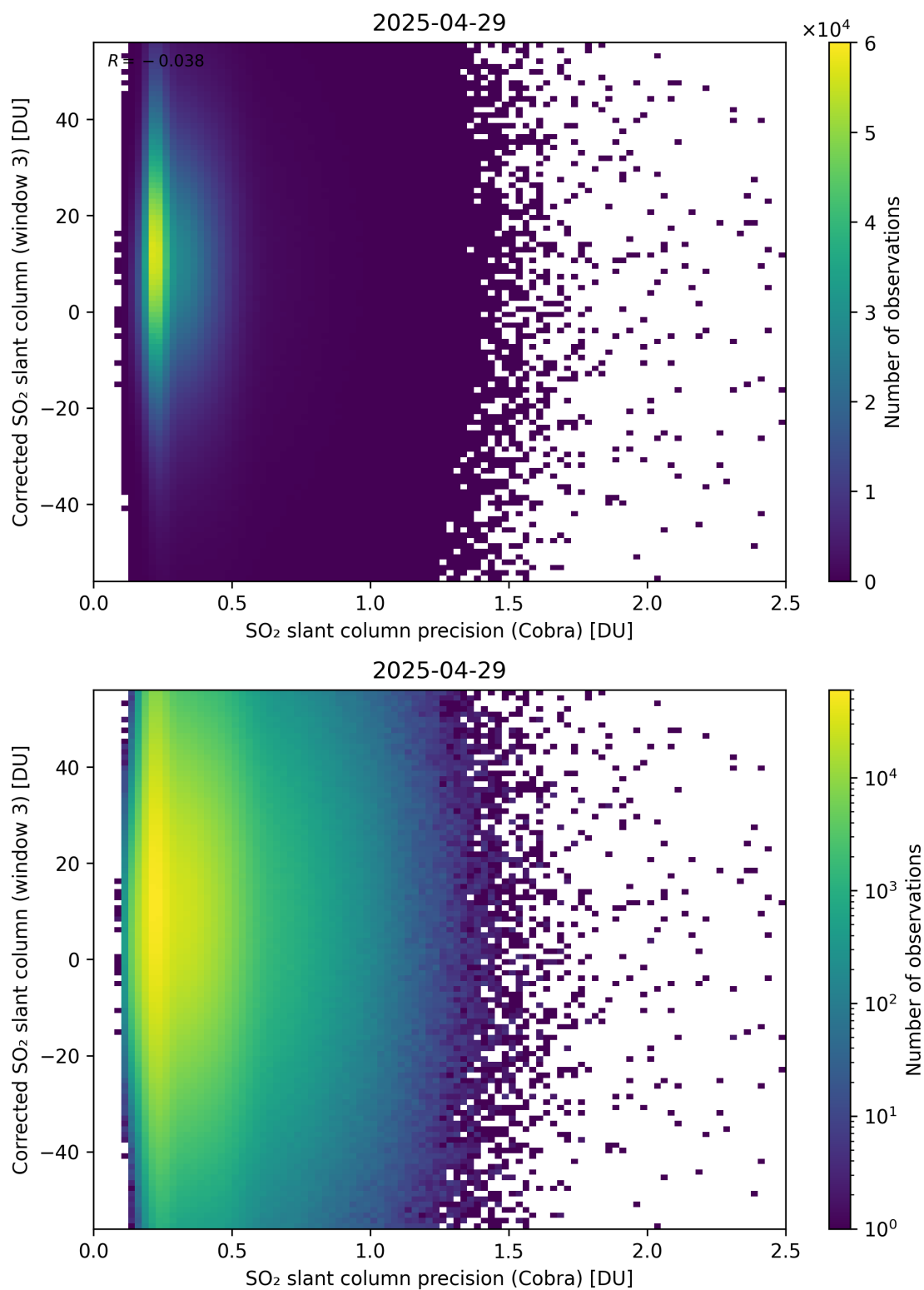
Figure 207: Scatter density plot of “SO 2 slant column precision (Cobra)” against “Corrected SO 2 slant column (window 3)” for 2025-04-29 to 2025-04-30.
