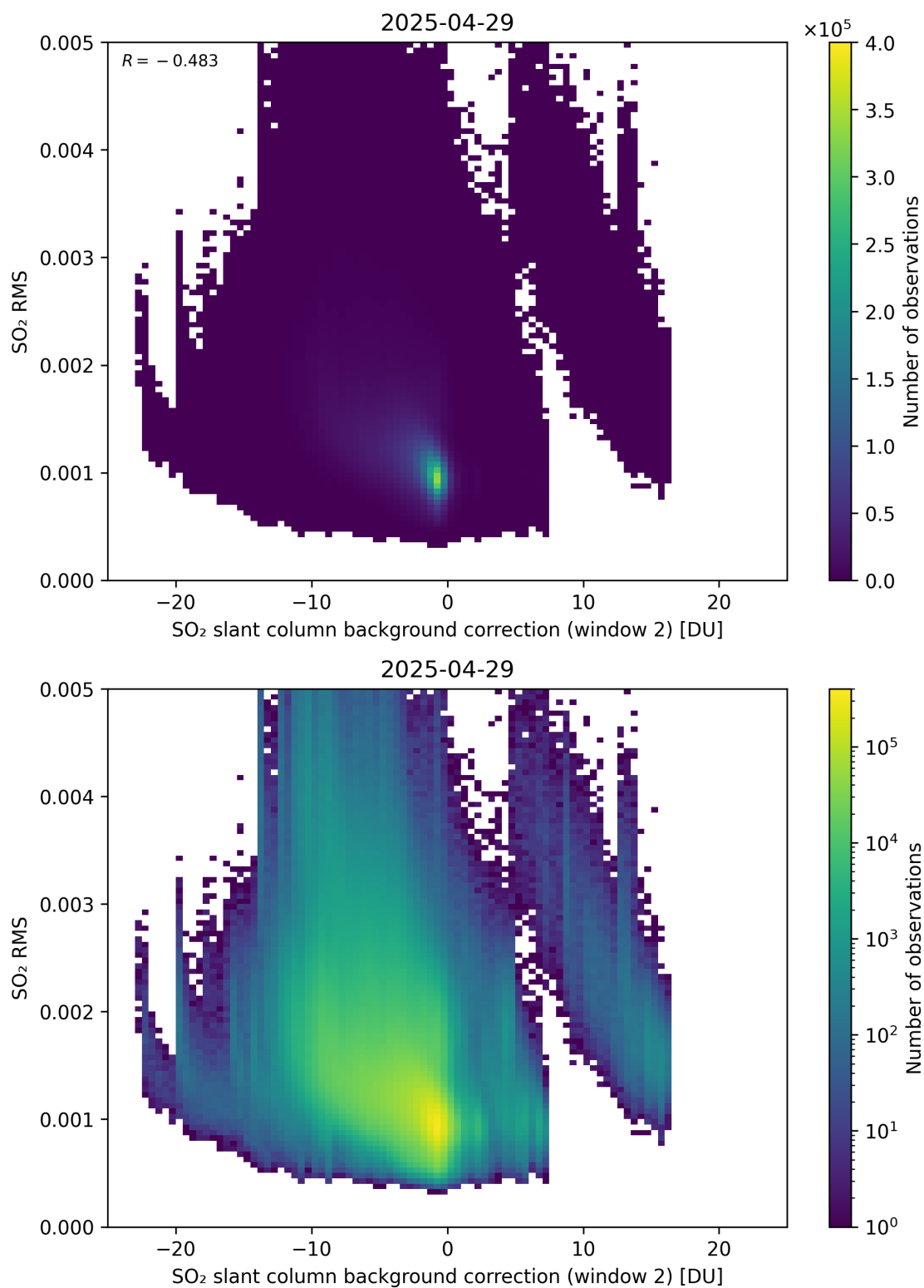
Figure 125: Scatter density plot of “SO 2 slant column background correction (window 2)” against “SO 2 RMS” for 2025-04-29 to 2025-04-30.
