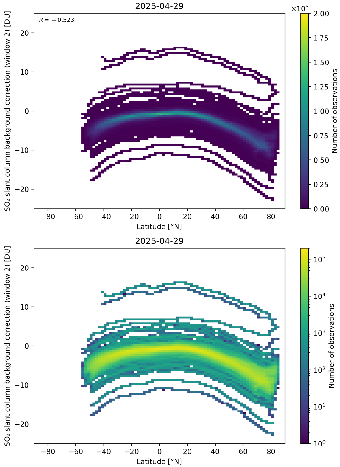
Figure 151: Scatter density plot of “Latitude” against “SO 2 slant column background correction (window 2)” for 2025-04-29 to 2025-04-30.
