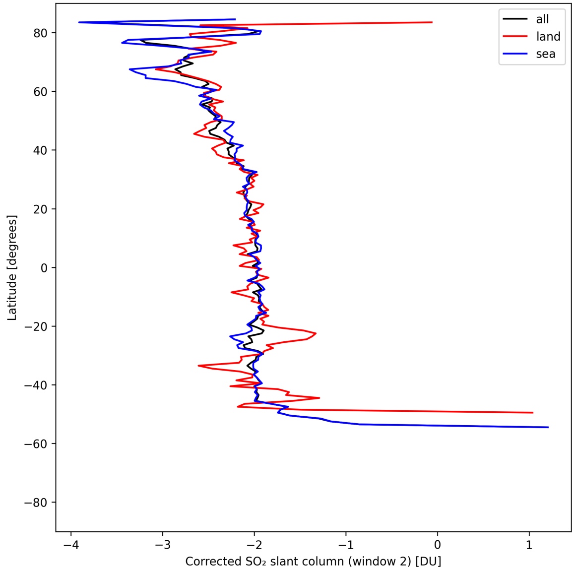
Figure 43: Zonal average of “Corrected SO 2 slant column (window 2)” for 2025-04-29 to 2025-04-30.
