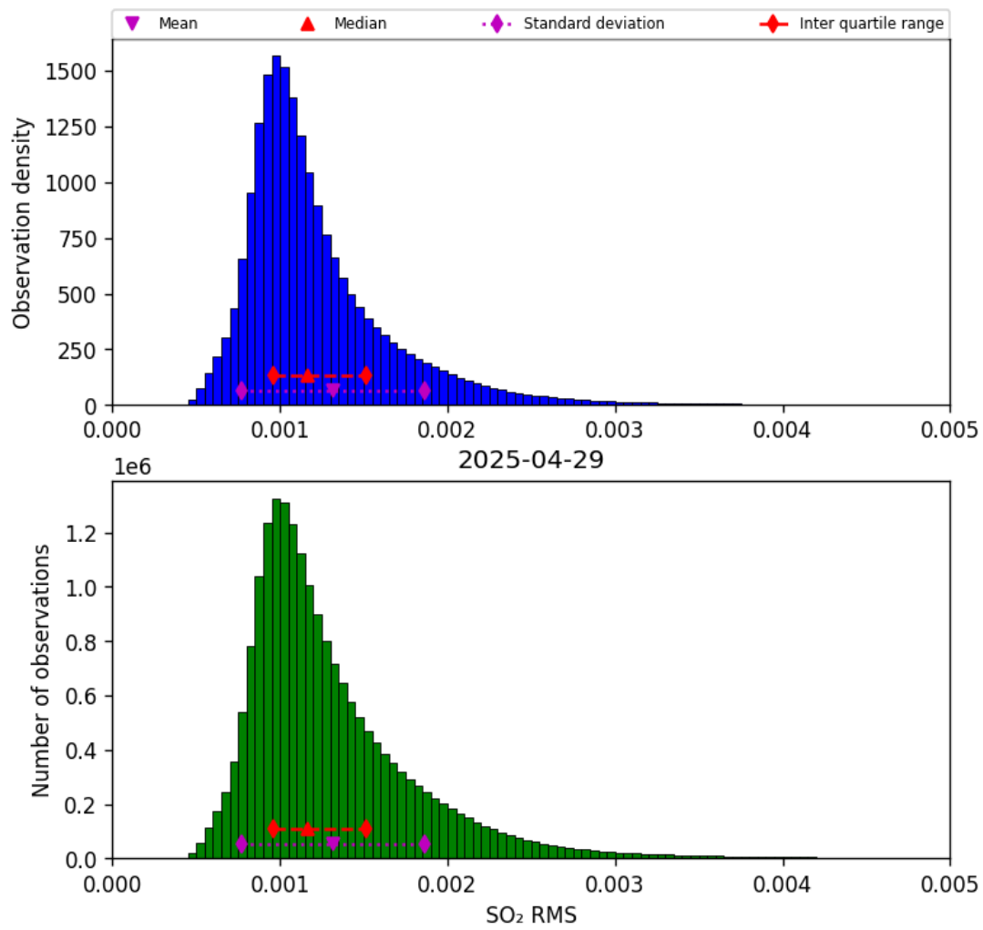
Figure 78: Histogram of “SO 2 RMS” for 2025-04-29 to 2025-04-30
