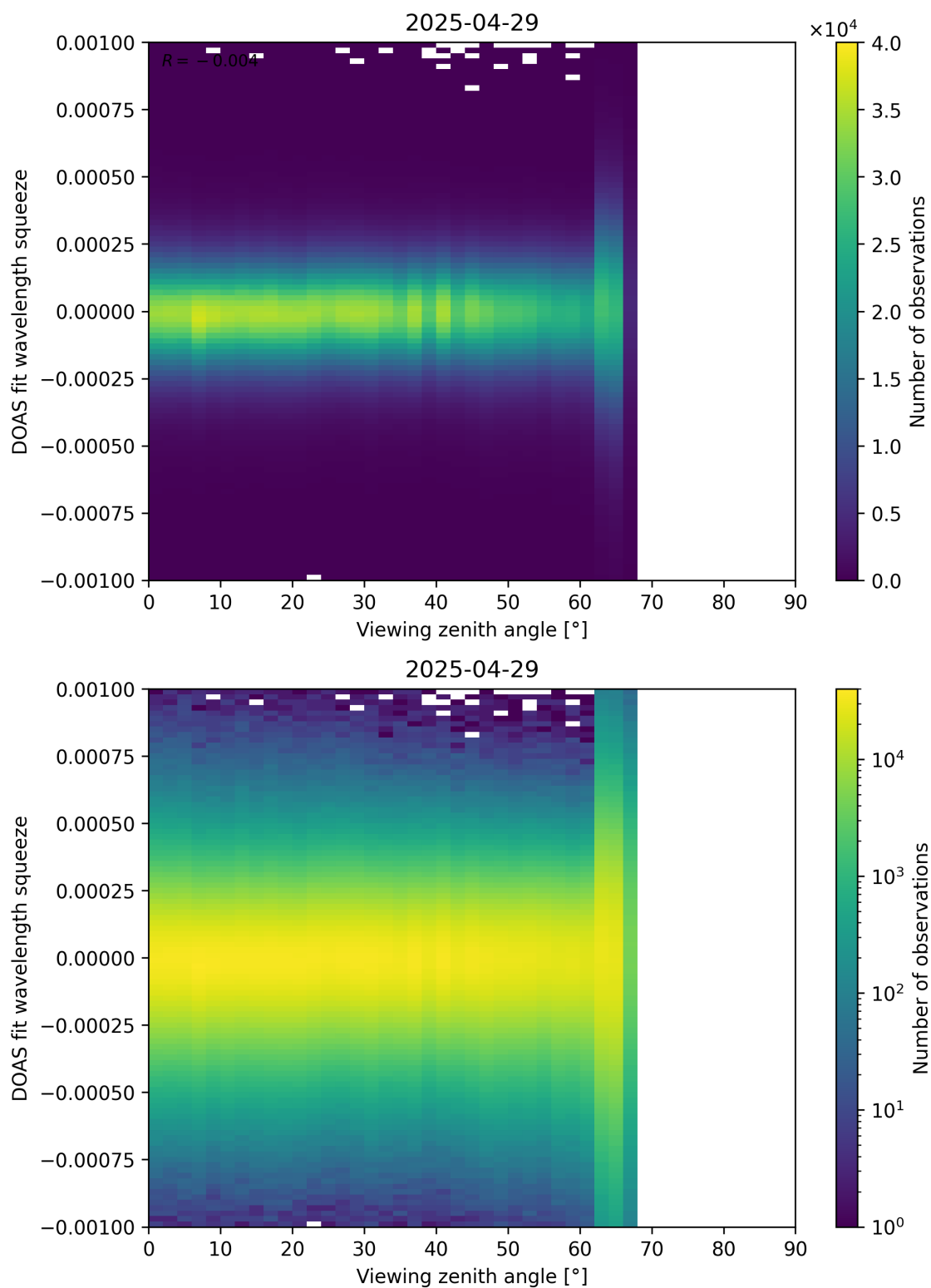
Figure 366: Scatter density plot of “Viewing zenith angle” against “DOAS fit wavelength squeeze” for 2025-04-29 to 2025-04-30.
