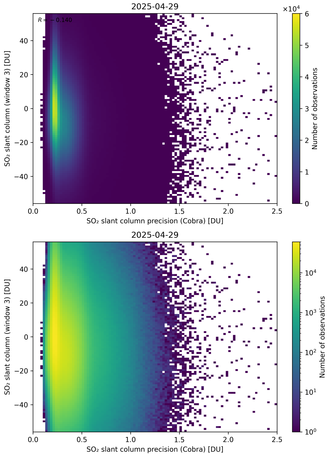
Figure 211: Scatter density plot of “SO 2 slant column precision (Cobra)” against “SO 2 slant column (window 3)” for 2025-04-29 to 2025-04-30.
