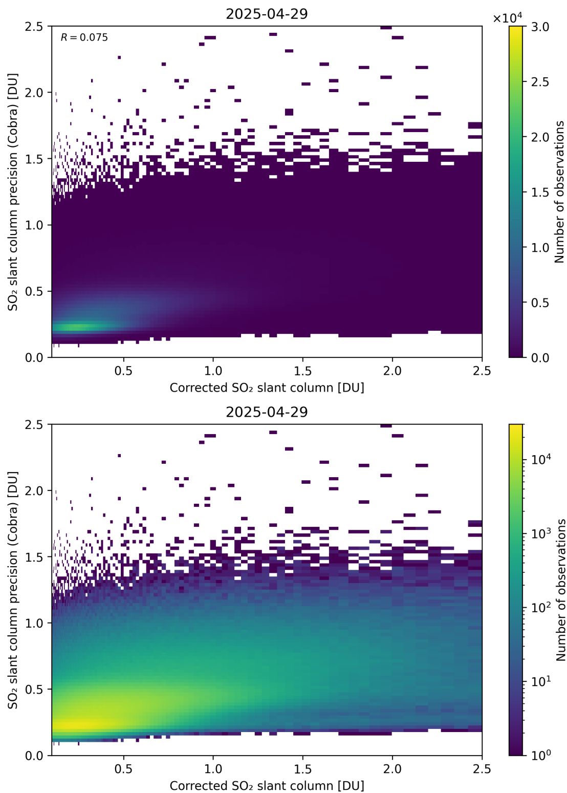
Figure 234: Scatter density plot of “Corrected SO 2 slant column” against “SO 2 slant column precision (Cobra)” for 2025-04-29 to 2025-04-30.
