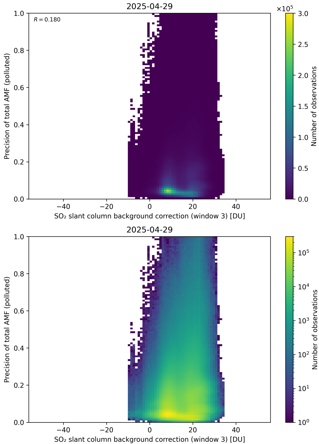
Figure 137: Scatter density plot of “SO 2 slant column background correction (window 3)” against “Precision of total AMF (polluted)” for 2025-04-29 to 2025-04-30.
