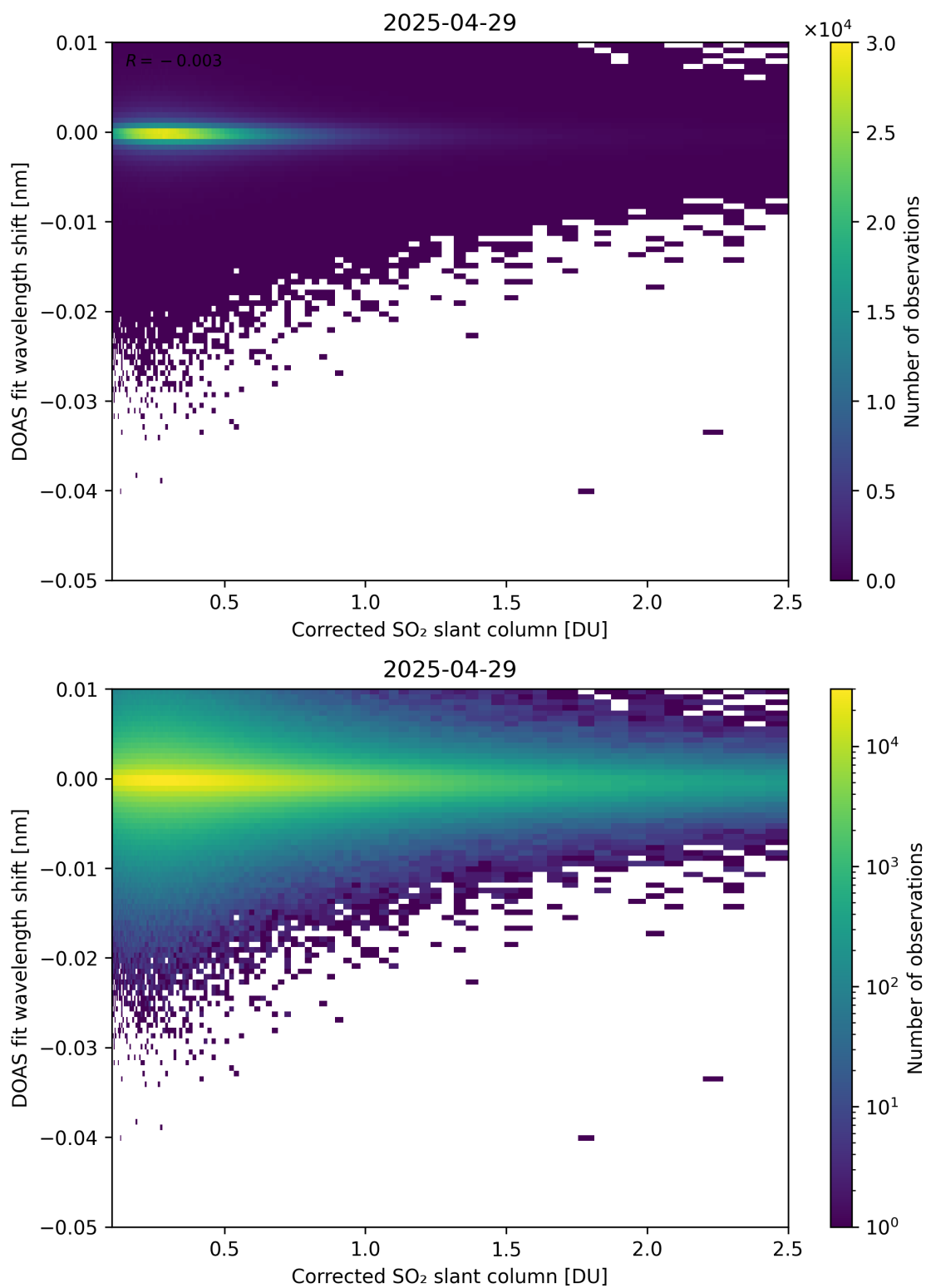
Figure 229: Scatter density plot of “Corrected SO 2 slant column” against “DOAS fit wavelength shift” for 2025-04-29 to 2025-04-30.
