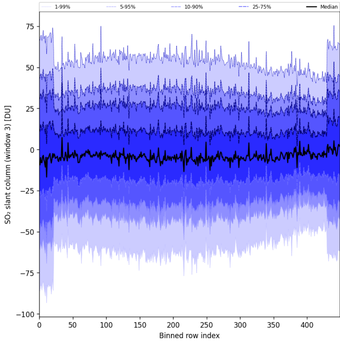
Figure 97: Along track statistics of “SO 2 slant column (window 3)” for 2025-04-29 to 2025-04-30
