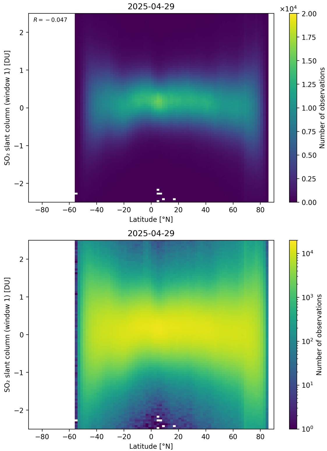
Figure 162: Scatter density plot of “Latitude” against “SO 2 slant column (window 1)” for 2025-04-29 to 2025-04-30.
