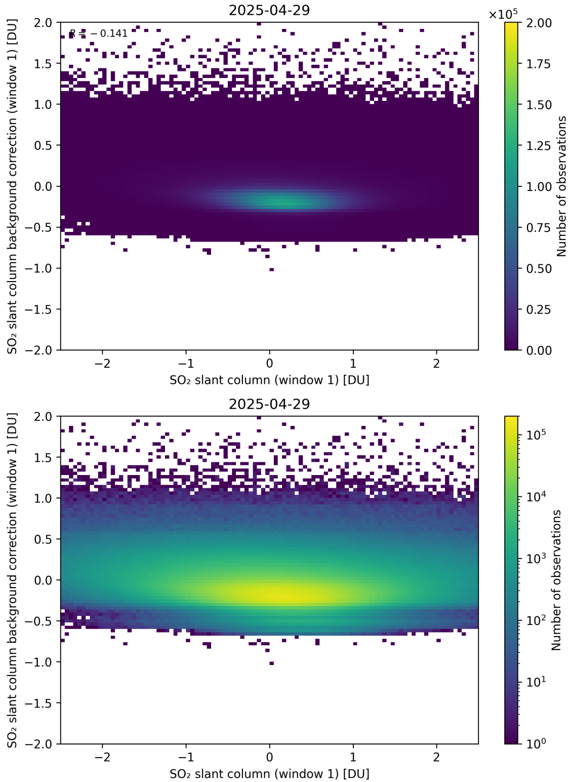
Figure 262: Scatter density plot of “SO 2 slant column (window 1)” against “SO 2 slant column background correction (window 1)” for 2025-04-29 to 2025-04-30.
