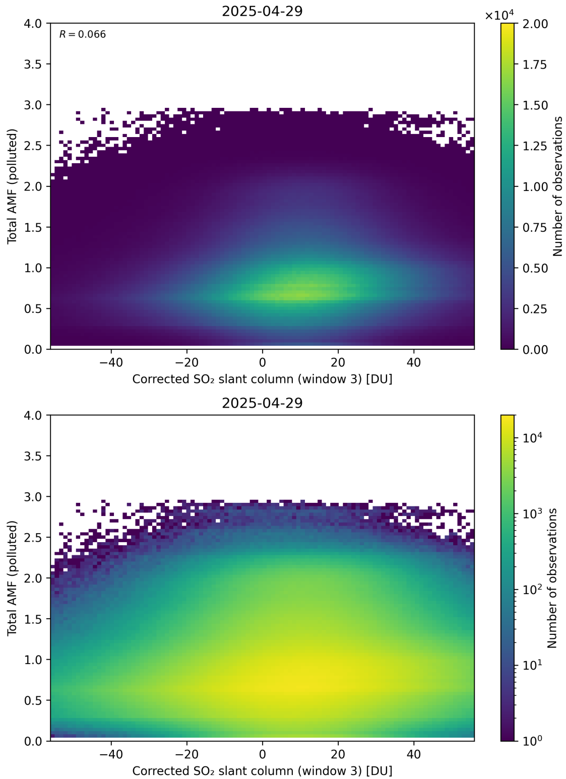
Figure 260: Scatter density plot of “Corrected SO 2 slant column (window 3)” against “Total AMF (polluted)” for 2025-04-29 to 2025-04-30.
