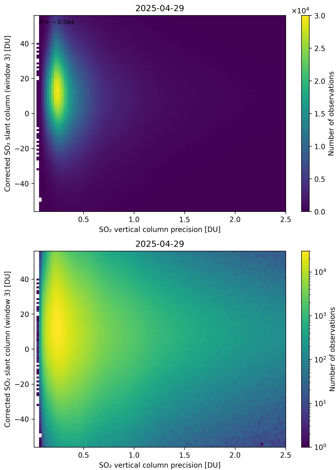
Figure 340: Scatter density plot of “SO 2 vertical column precision” against “Corrected SO 2 slant column (window 3)” for 2025-04-29 to 2025-04-30.
