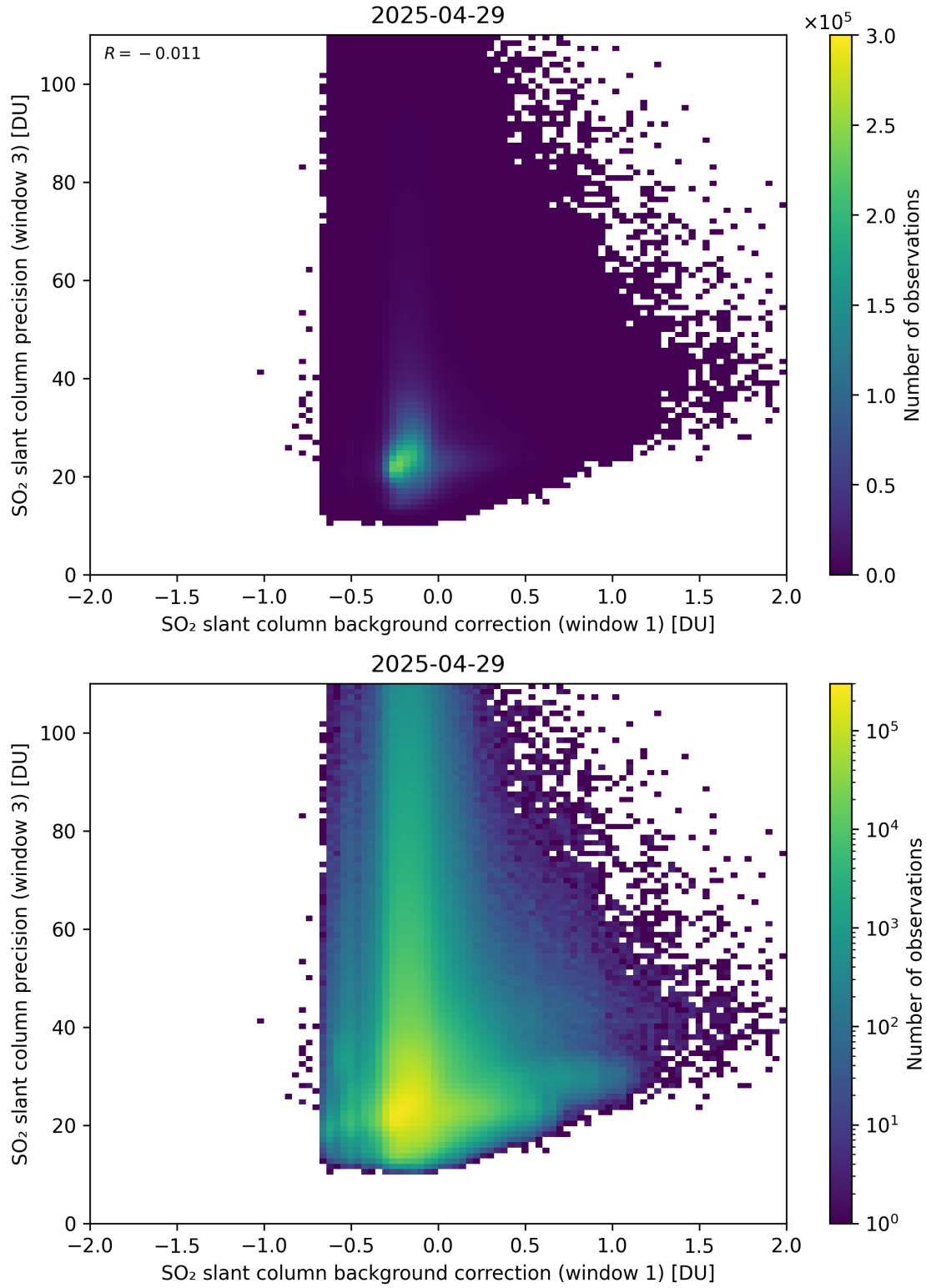
Figure 119: Scatter density plot of “SO 2 slant column background correction (window 1)” against “SO 2 slant column precision (window 3)” for 2025-04-29 to 2025-04-30.
