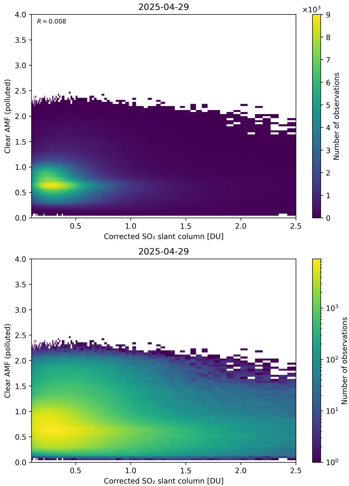
Figure 232: Scatter density plot of “Corrected SO 2 slant column” against “Clear AMF (polluted)” for 2025-04-29 to 2025-04-30.
