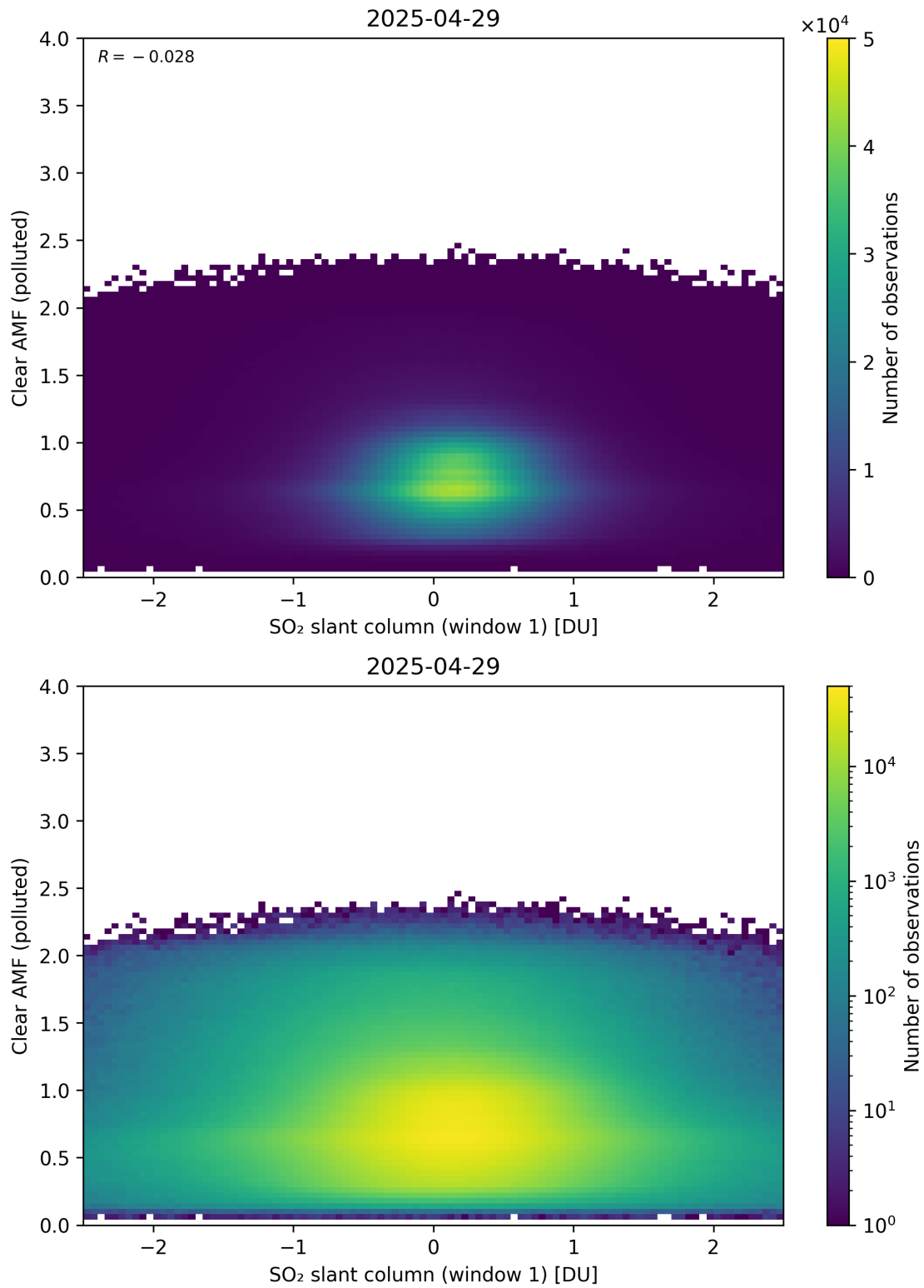
Figure 282: Scatter density plot of “SO 2 slant column (window 1)” against “Clear AMF (polluted)” for 2025-04-29 to 2025-04-30.
