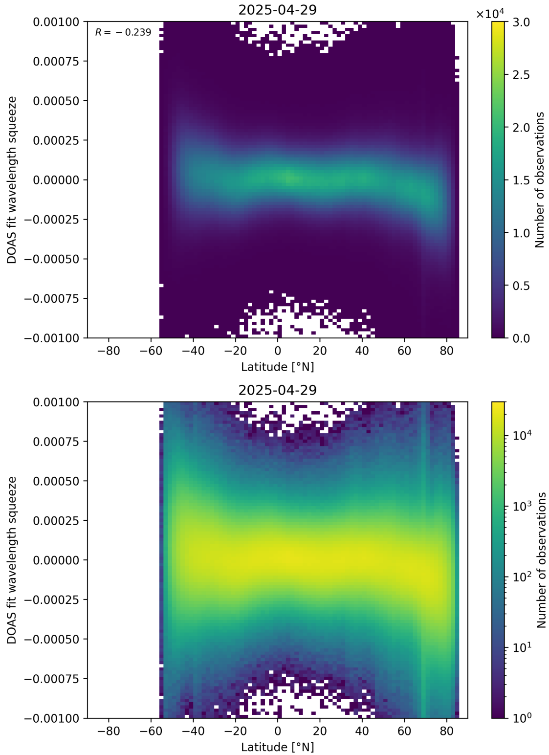
Figure 154: Scatter density plot of “Latitude” against “DOAS fit wavelength squeeze” for 2025-04-29 to 2025-04-30.
