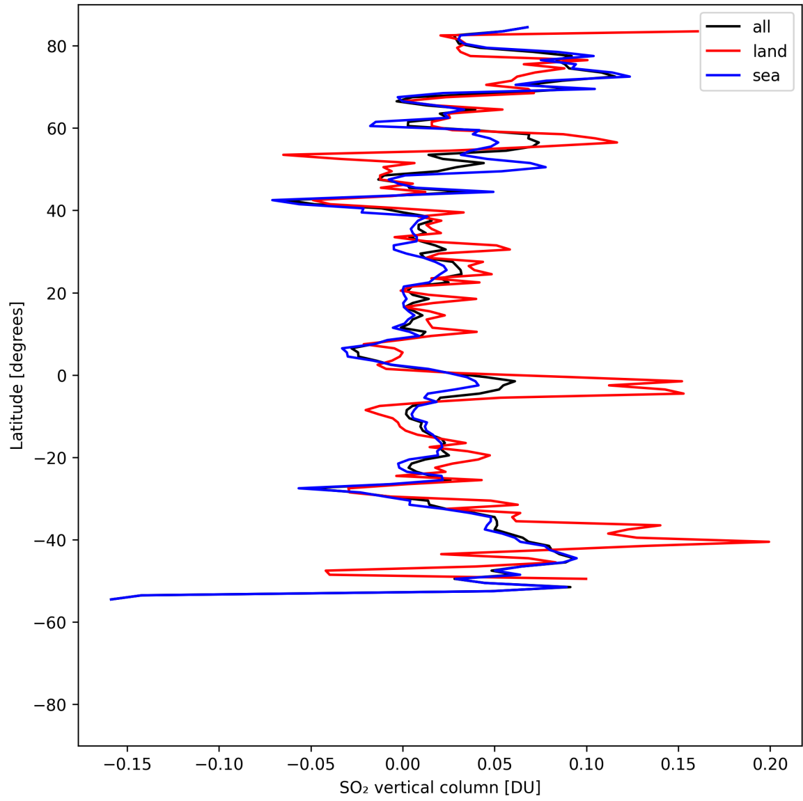
Figure 32: Zonal average of “SO 2 vertical column” for 2025-04-29 to 2025-04-30.
