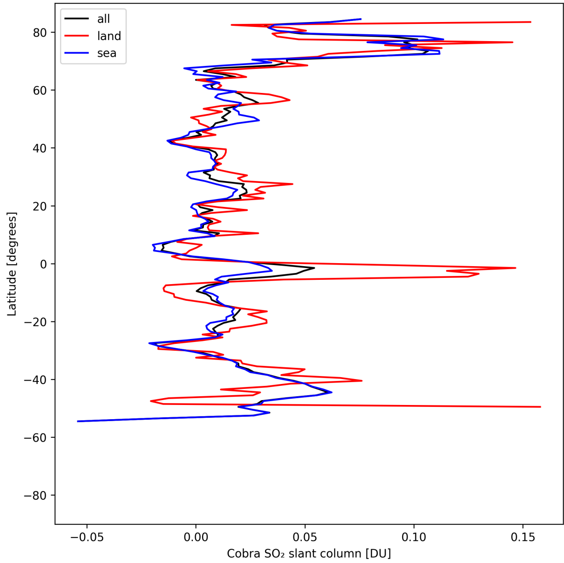
Figure 35: Zonal average of “Cobra SO 2 slant column” for 2025-04-29 to 2025-04-30.
