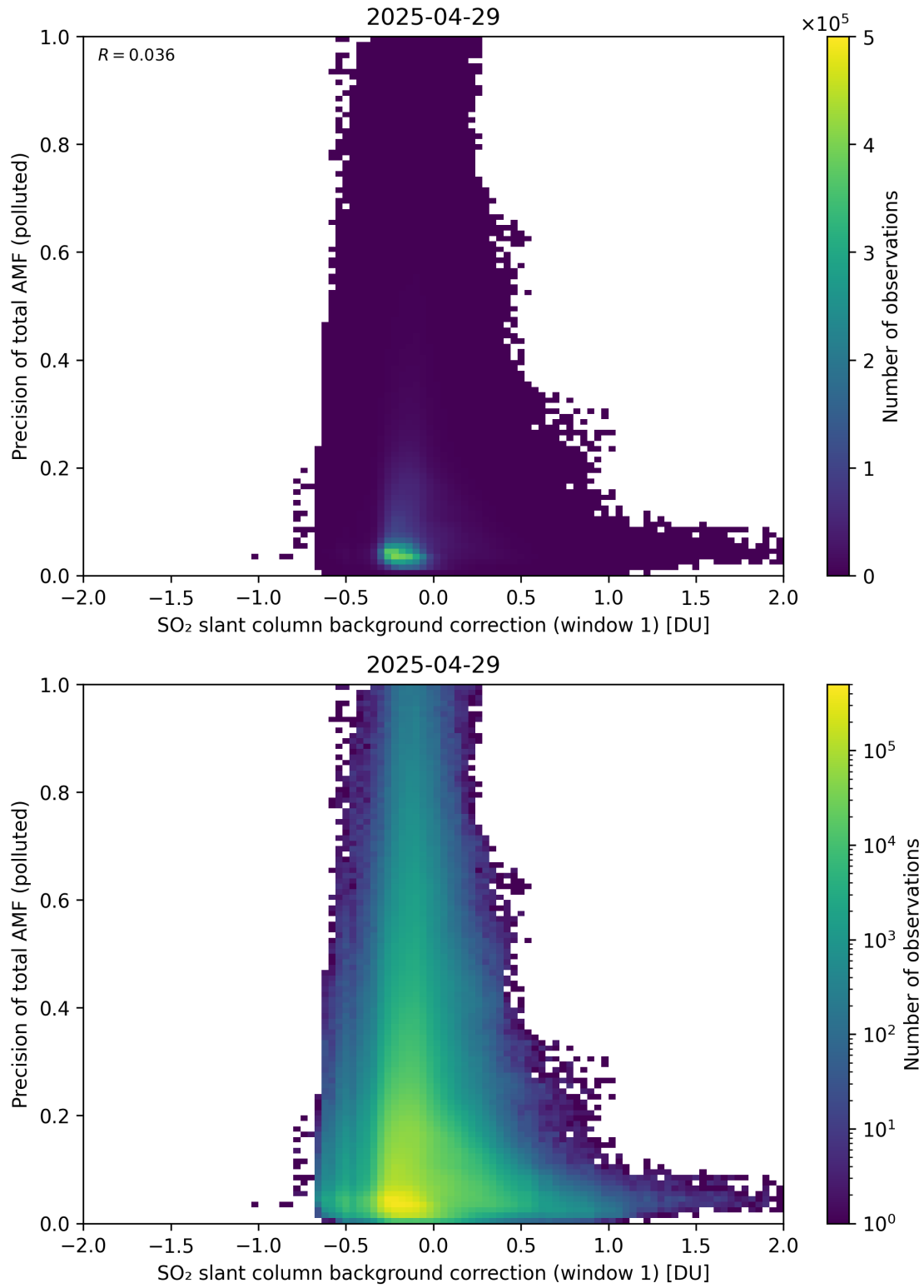
Figure 121: Scatter density plot of “SO 2 slant column background correction (window 1)” against “Precision of total AMF (polluted)” for 2025-04-29 to 2025-04-30.
