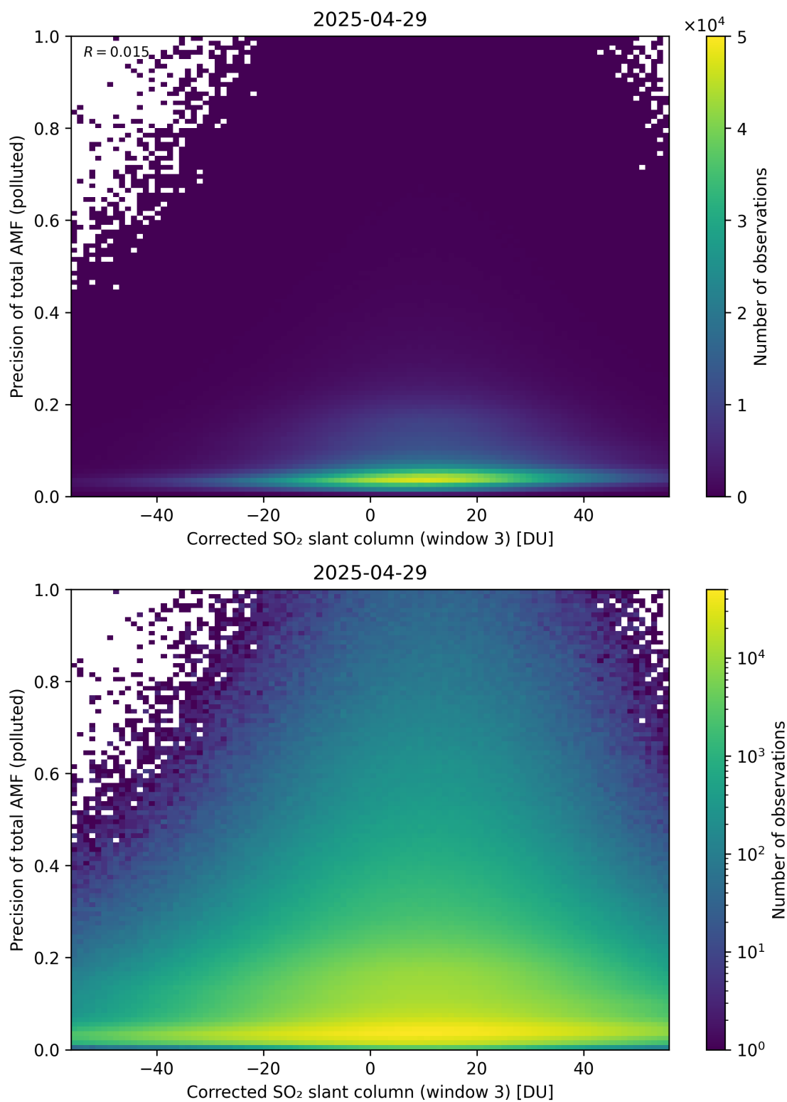
Figure 261: Scatter density plot of “Corrected SO 2 slant column (window 3)” against “Precision of total AMF (polluted)” for 2025-04-29 to 2025-04-30.
