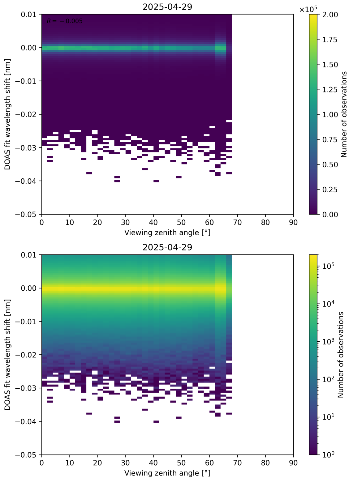
Figure 365: Scatter density plot of “Viewing zenith angle” against “DOAS fit wavelength shift” for 2025-04-29 to 2025-04-30.
