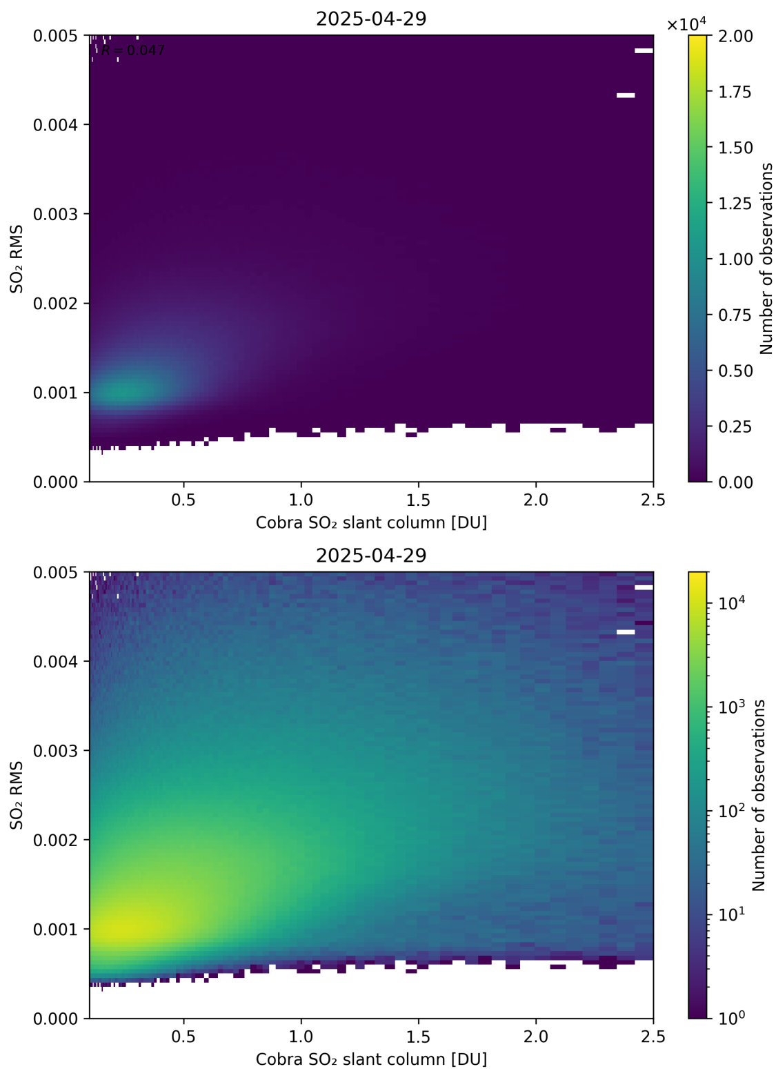
Figure 198: Scatter density plot of “Cobra SO 2 slant column” against “SO 2 RMS” for 2025-04-29 to 2025-04-30.
