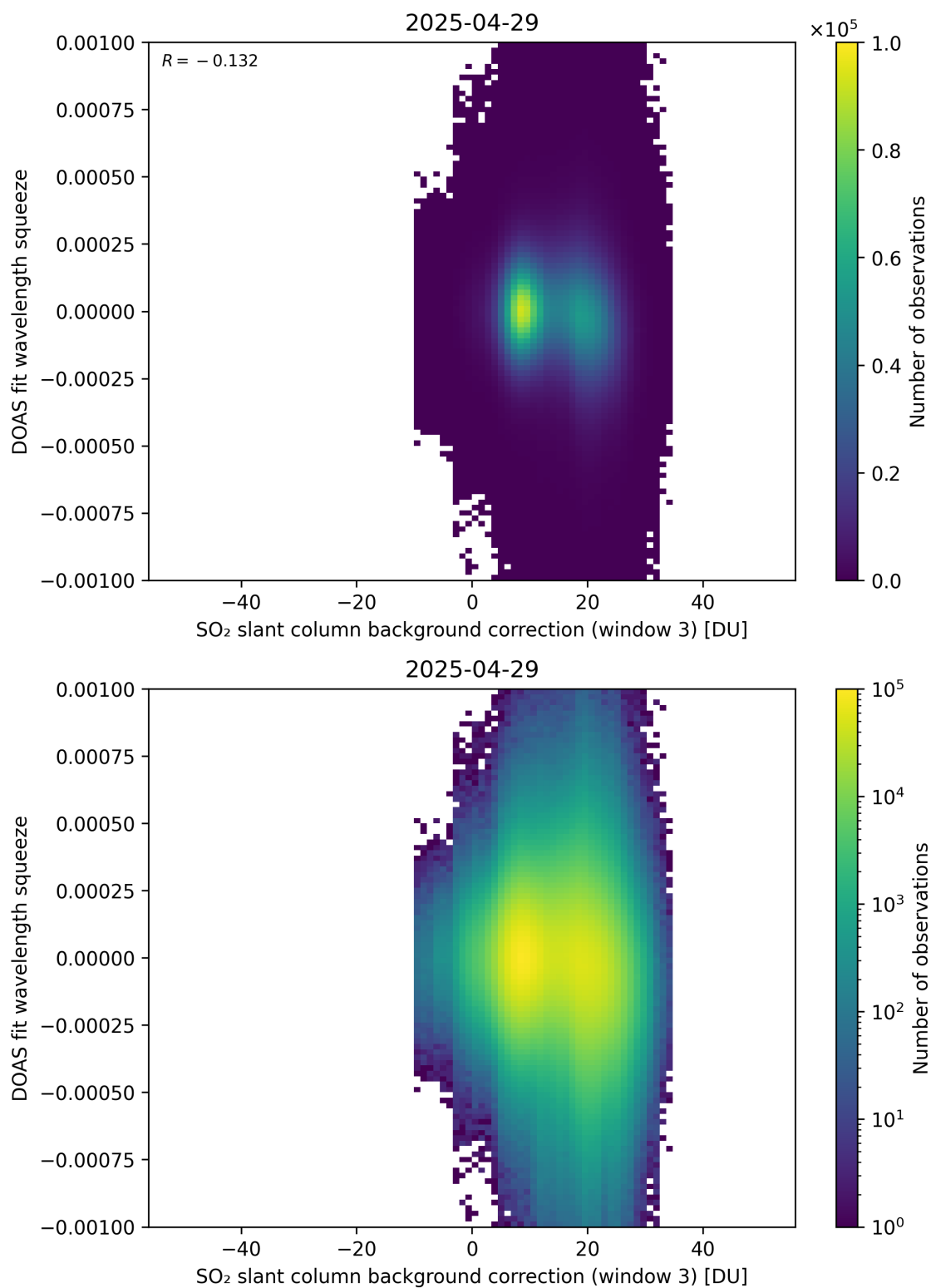
Figure 133: Scatter density plot of “SO 2 slant column background correction (window 3)” against “DOAS fit wavelength squeeze” for 2025-04-29 to 2025-04-30.
