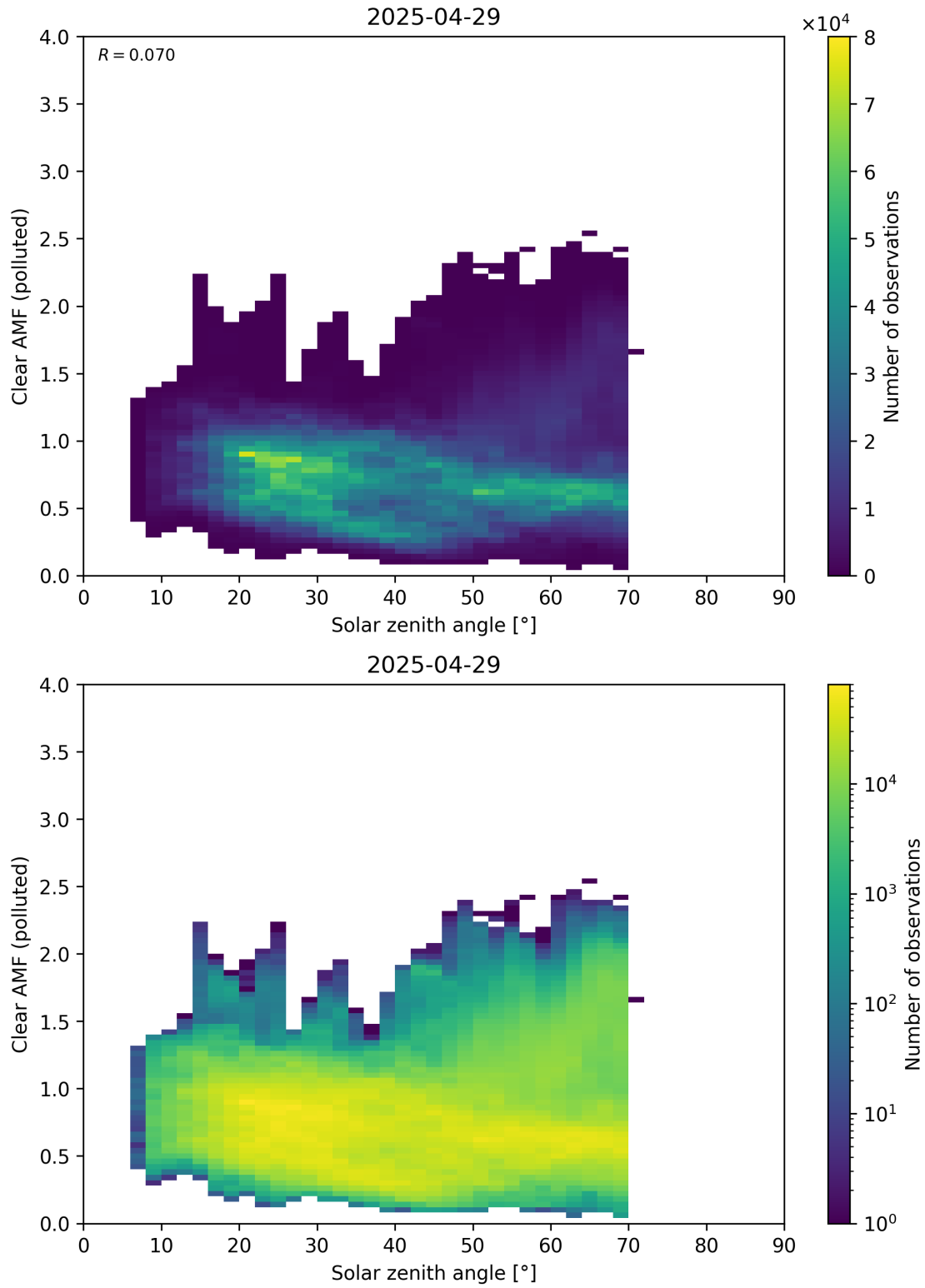
Figure 178: Scatter density plot of “Solar zenith angle” against “Clear AMF (polluted)” for 2025-04-29 to 2025-04-30.
