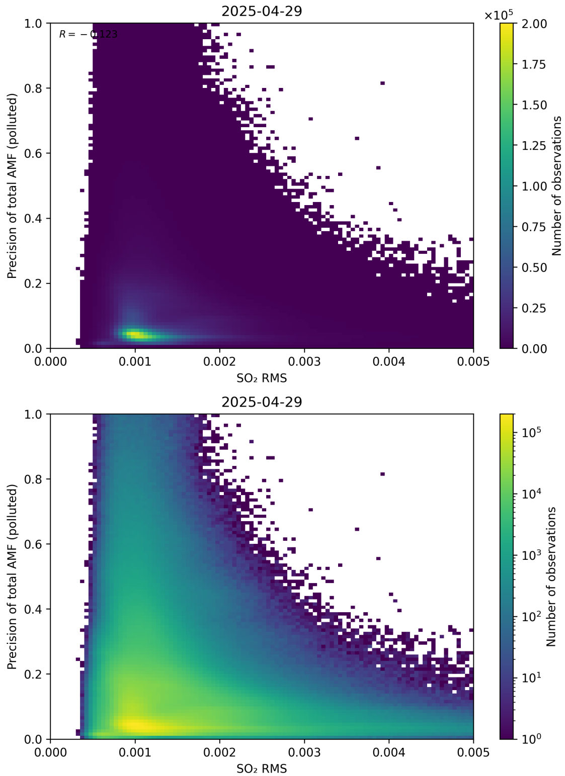
Figure 149: Scatter density plot of “SO 2 RMS” against “Precision of total AMF (polluted)” for 2025-04-29 to 2025-04-30.
