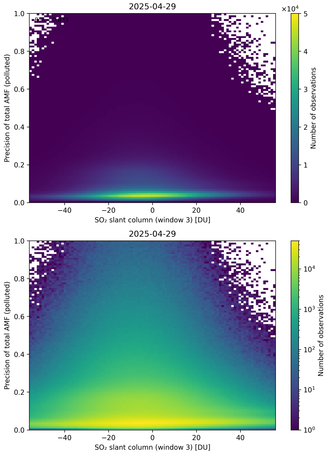
Figure 319: Scatter density plot of “SO 2 slant column (window 3)” against “Precision of total AMF (polluted)” for 2025-04-29 to 2025-04-30.
