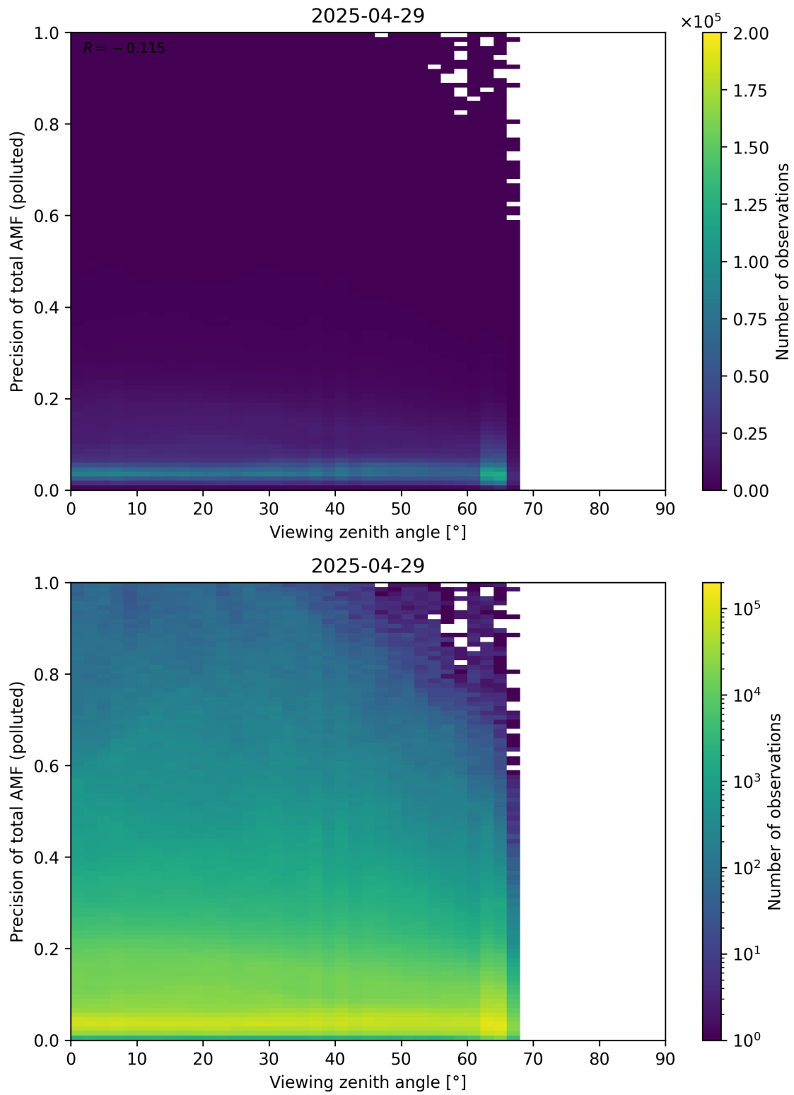
Figure 382: Scatter density plot of “Viewing zenith angle” against “Precision of total AMF (polluted)” for 2025-04-29 to 2025-04-30.
