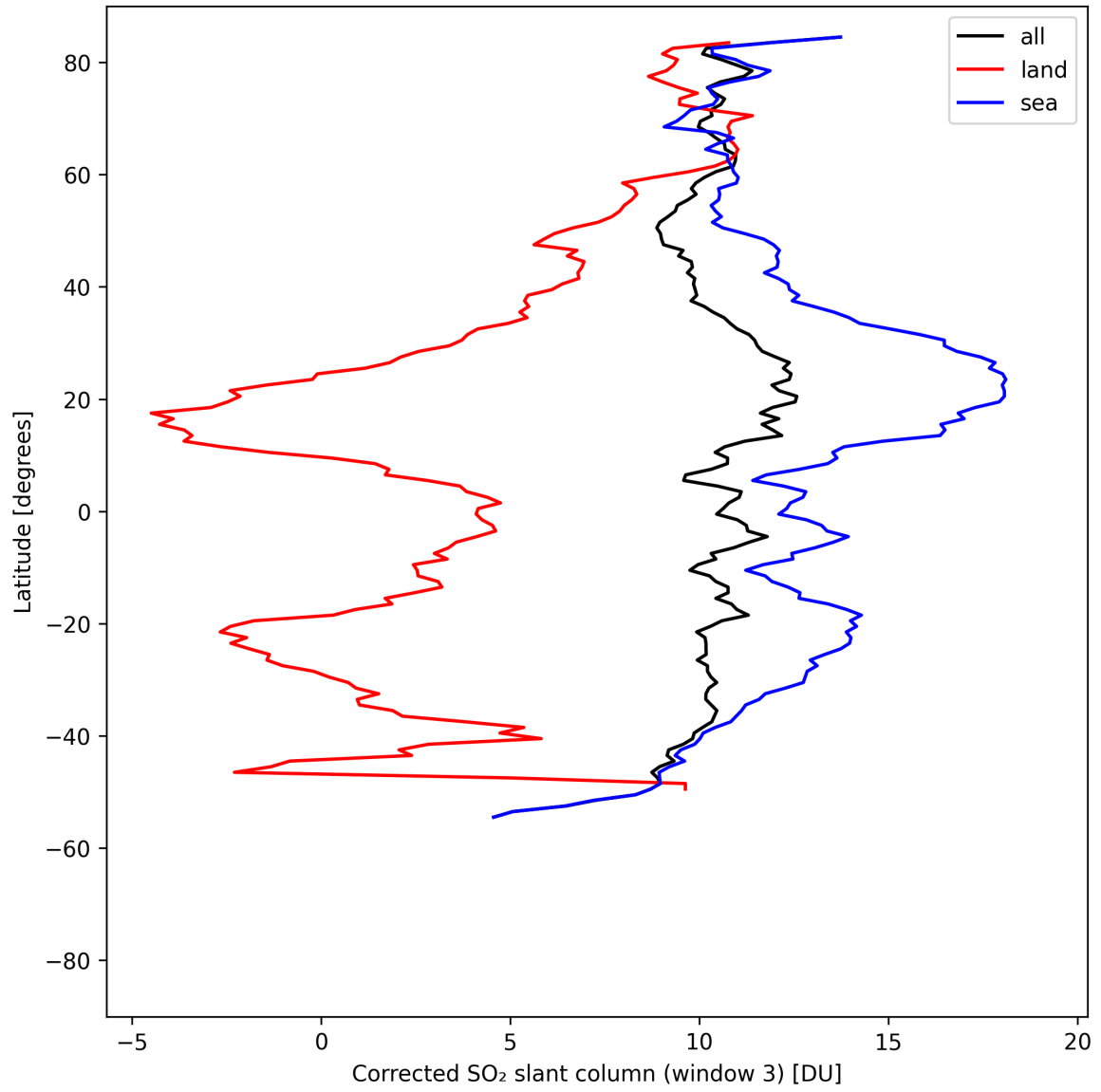
Figure 47: Zonal average of “Corrected SO 2 slant column (window 3)” for 2025-04-29 to 2025-04-30.
