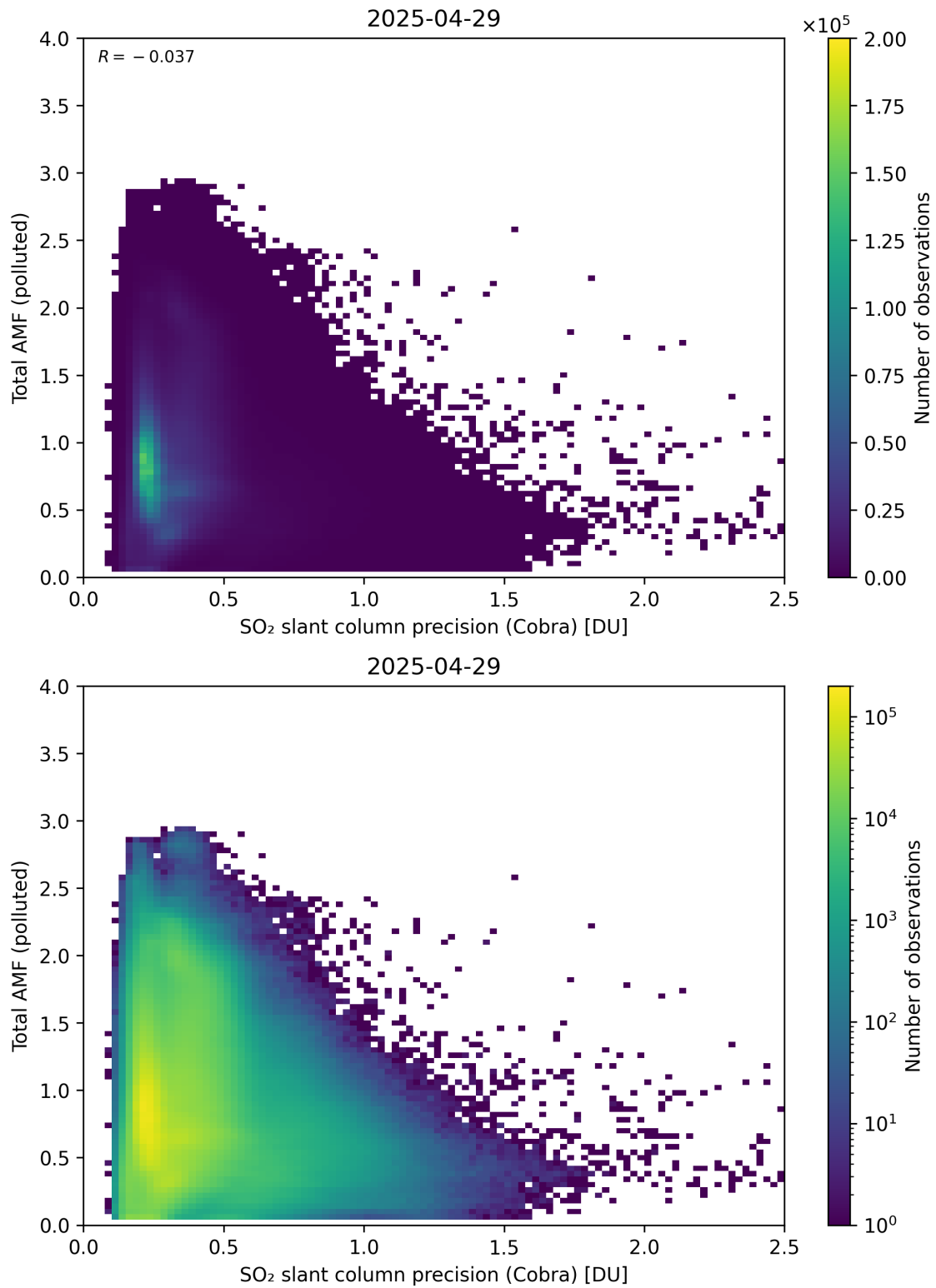
Figure 213: Scatter density plot of “SO 2 slant column precision (Cobra)” against “Total AMF (polluted)” for 2025-04-29 to 2025-04-30.
