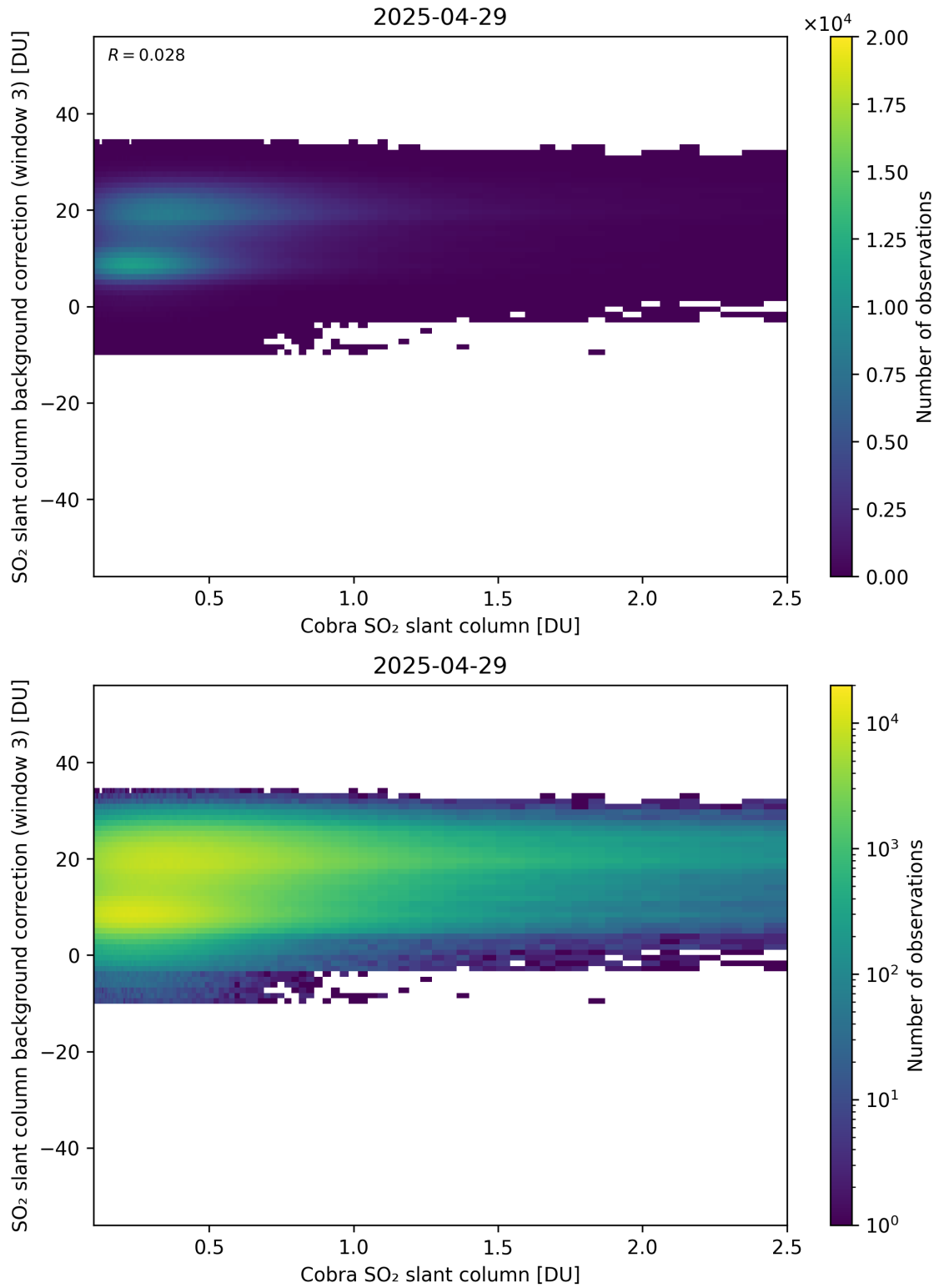
Figure 195: Scatter density plot of “Cobra SO 2 slant column” against “SO 2 slant column background correction (window 3)” for 2025-04-29 to 2025-04-30.
