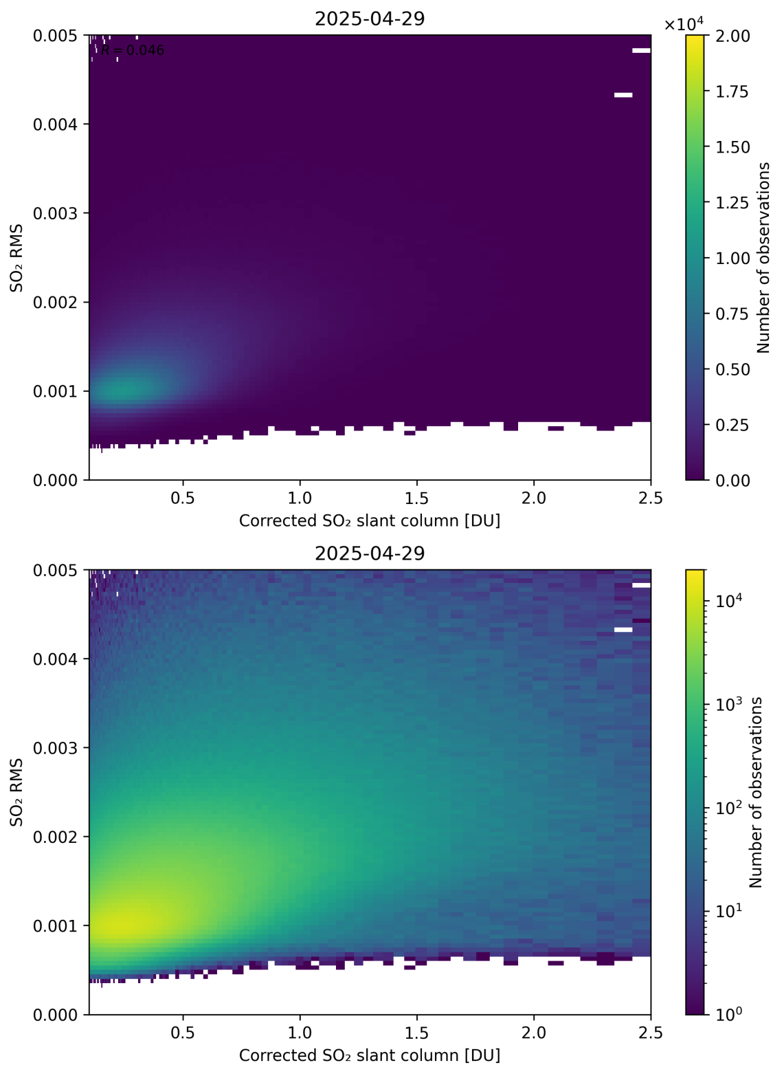
Figure 231: Scatter density plot of “Corrected SO 2 slant column” against “SO 2 RMS” for 2025-04-29 to 2025-04-30.
