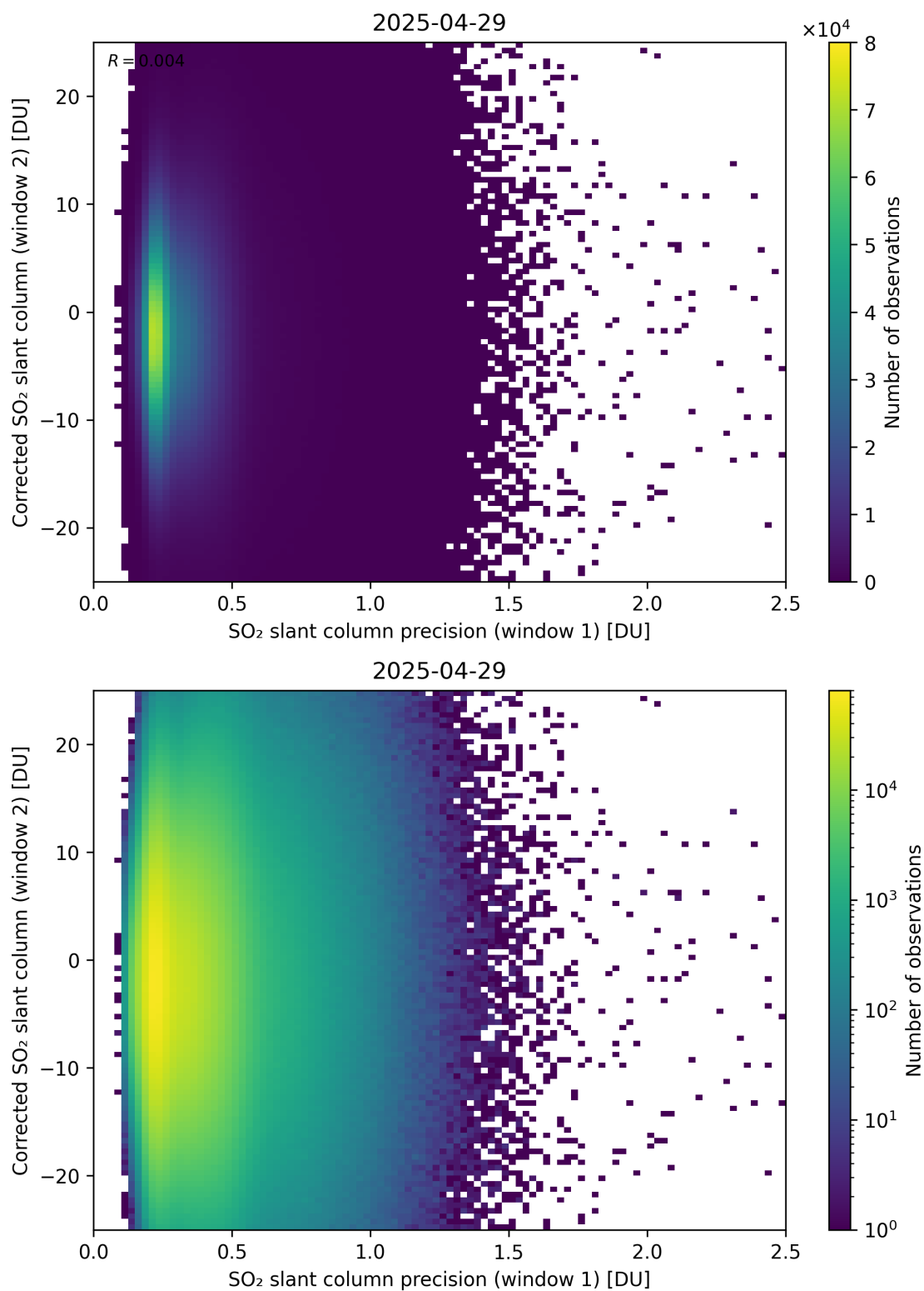
Figure 275: Scatter density plot of “SO 2 slant column precision (window 1)” against “Corrected SO 2 slant column (window 2)” for 2025-04-29 to 2025-04-30.
