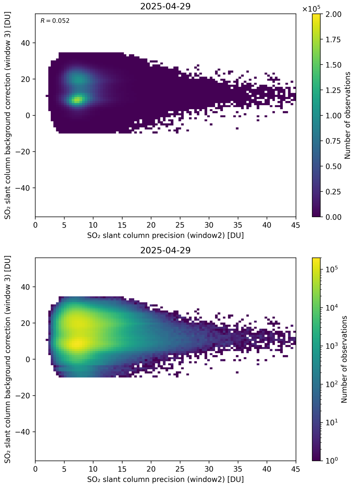
Figure 292: Scatter density plot of “SO 2 slant column precision (window2)” against “SO 2 slant column background correction (window 3)” for 2025-04-29 to 2025-04-30.
