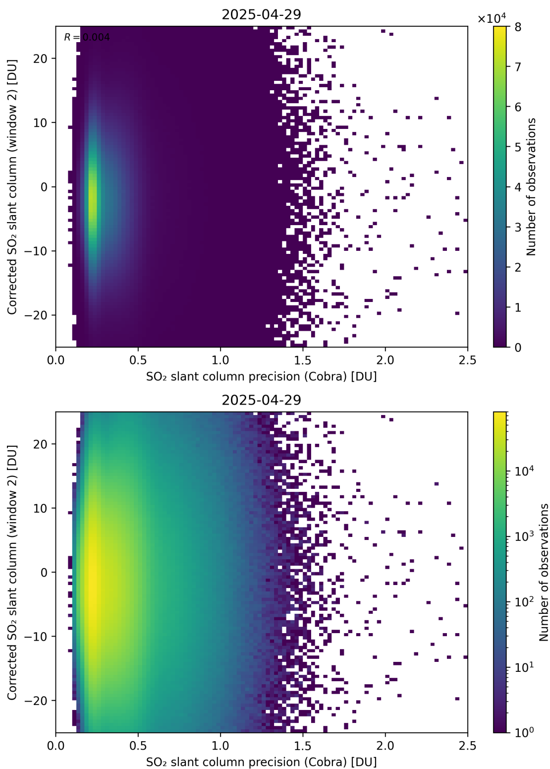
Figure 206: Scatter density plot of “SO 2 slant column precision (Cobra)” against “Corrected SO 2 slant column (window 2)” for 2025-04-29 to 2025-04-30.
