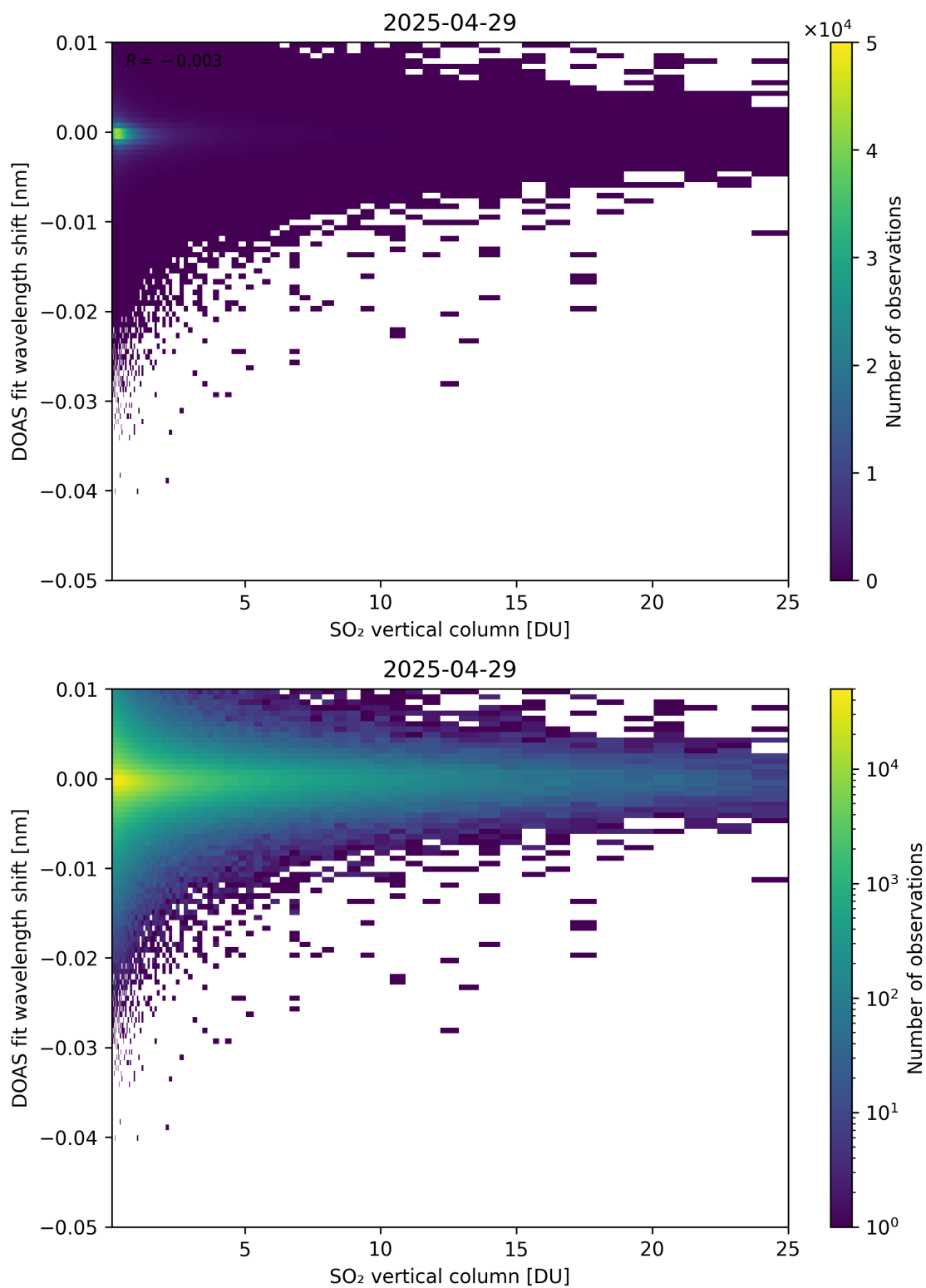
Figure 326: Scatter density plot of “SO 2 vertical column” against “DOAS fit wavelength shift” for 2025-04-29 to 2025-04-30.
