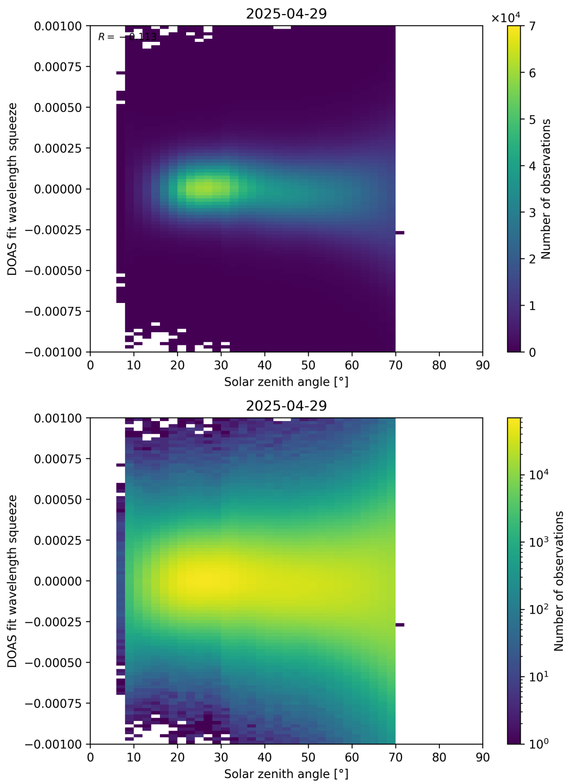
Figure 175: Scatter density plot of “Solar zenith angle” against “DOAS fit wavelength squeeze” for 2025-04-29 to 2025-04-30.
