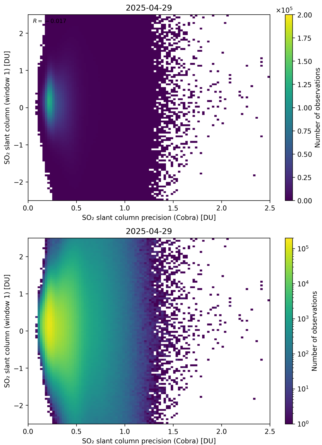
Figure 208: Scatter density plot of “SO 2 slant column precision (Cobra)” against “SO 2 slant column (window 1)” for 2025-04-29 to 2025-04-30.
