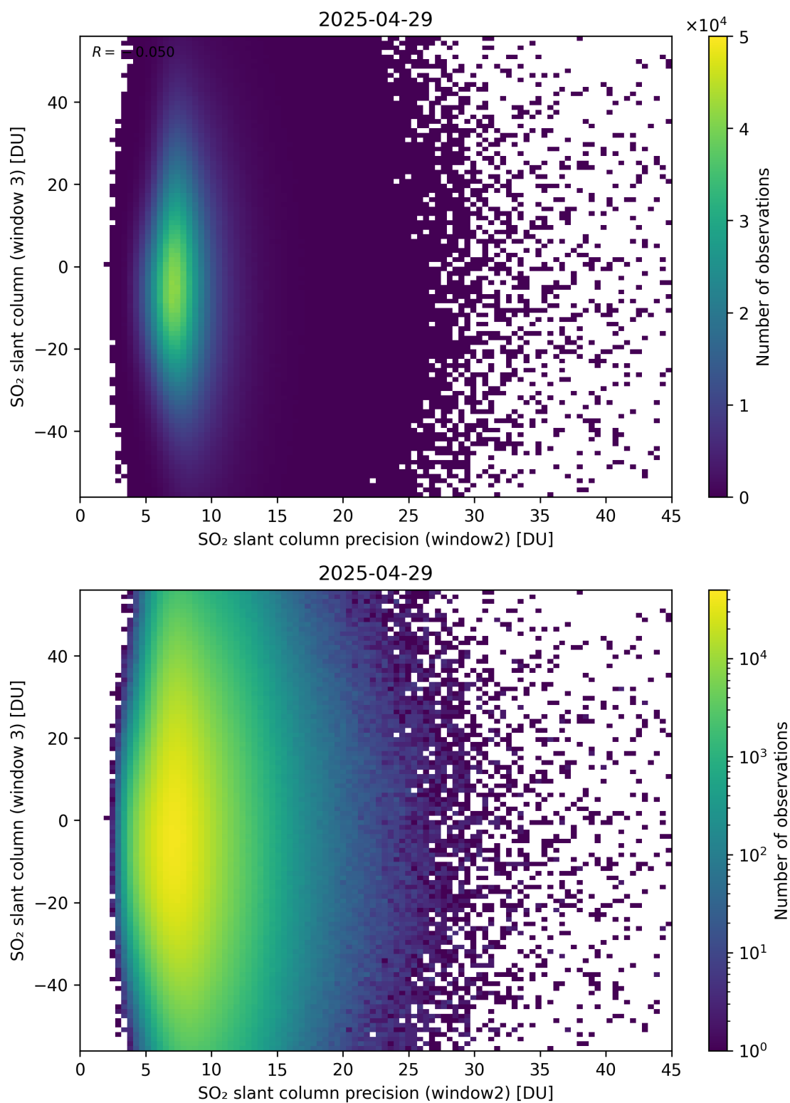
Figure 299: Scatter density plot of “SO 2 slant column precision (window2)” against “SO 2 slant column (window 3)” for 2025-04-29 to 2025-04-30.
