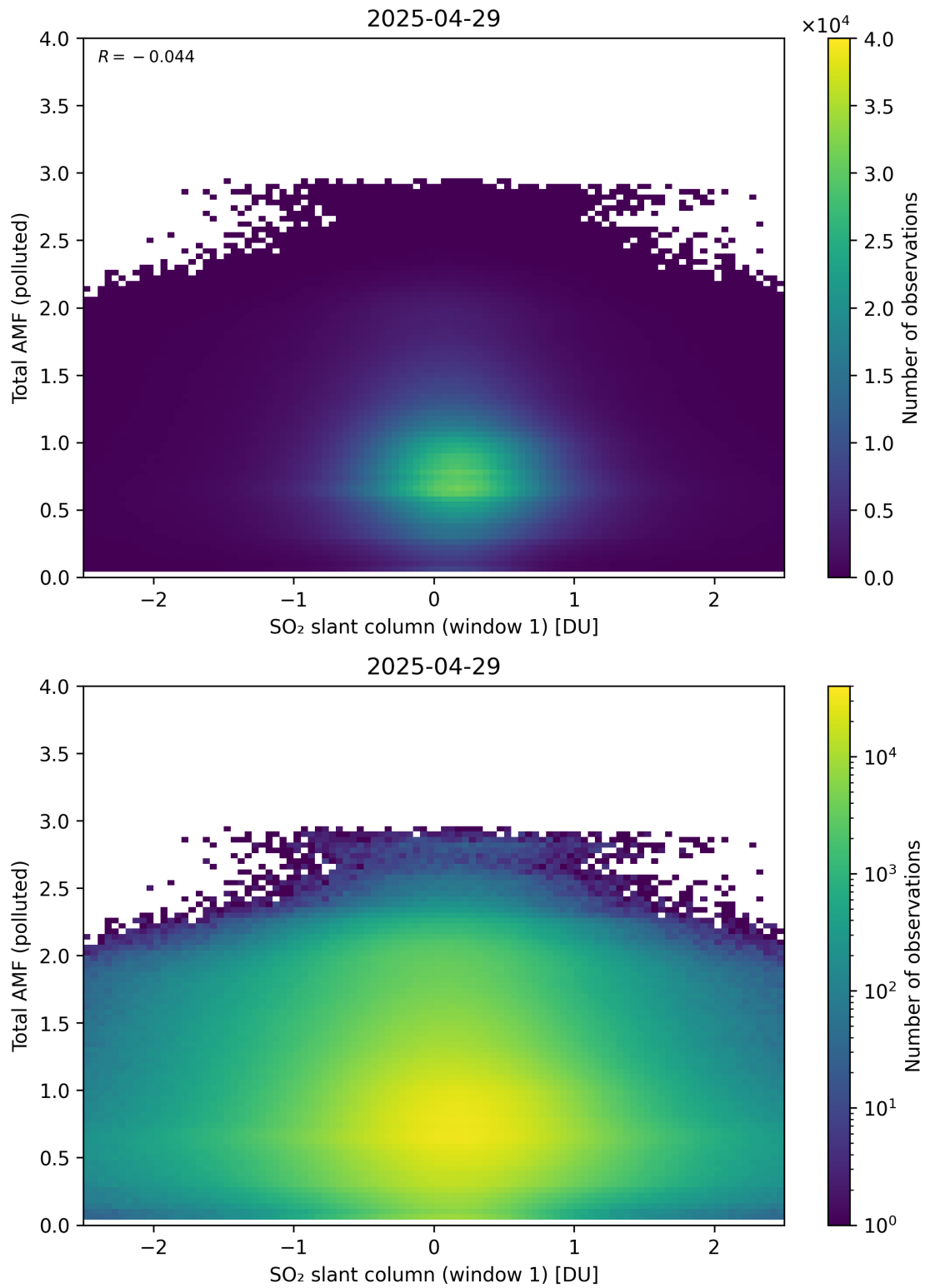
Figure 289: Scatter density plot of “SO 2 slant column (window 1)” against “Total AMF (polluted)” for 2025-04-29 to 2025-04-30.
