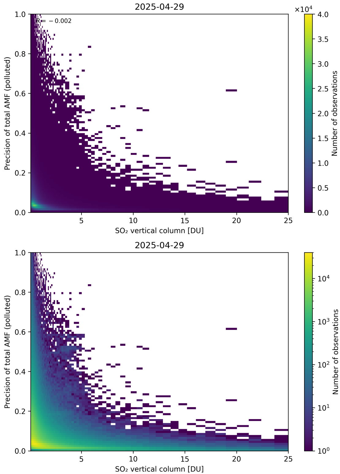
Figure 360: Scatter density plot of “SO 2 vertical column” against “Precision of total AMF (polluted)” for 2025-04-29 to 2025-04-30.
