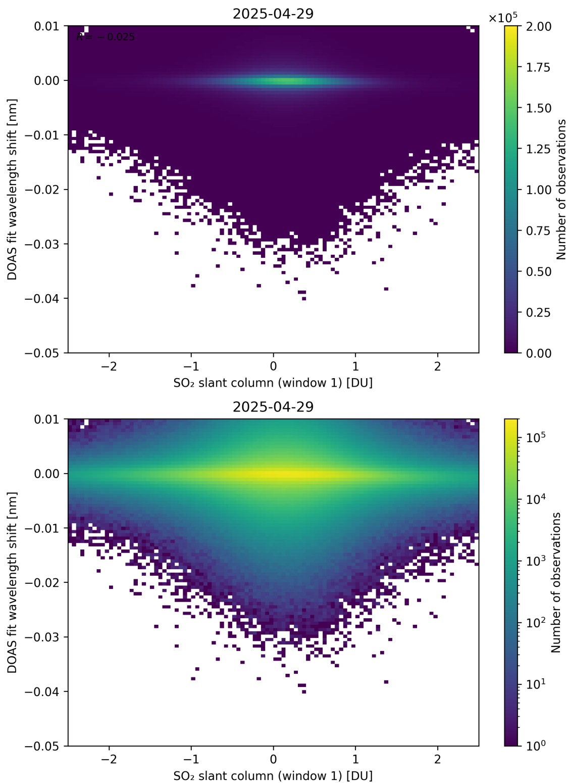
Figure 265: Scatter density plot of “SO 2 slant column (window 1)” against “DOAS fit wavelength shift” for 2025-04-29 to 2025-04-30.
