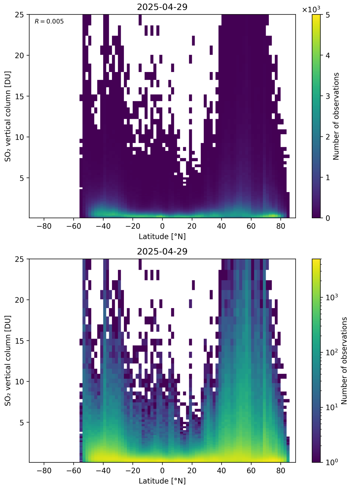
Figure 169: Scatter density plot of “Latitude” against “SO 2 vertical column” for 2025-04-29 to 2025-04-30.
