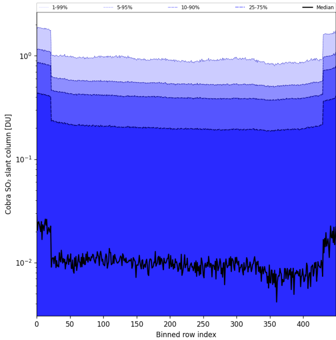
Figure 87: Along track statistics of “Cobra SO 2 slant column” for 2025-04-29 to 2025-04-30
