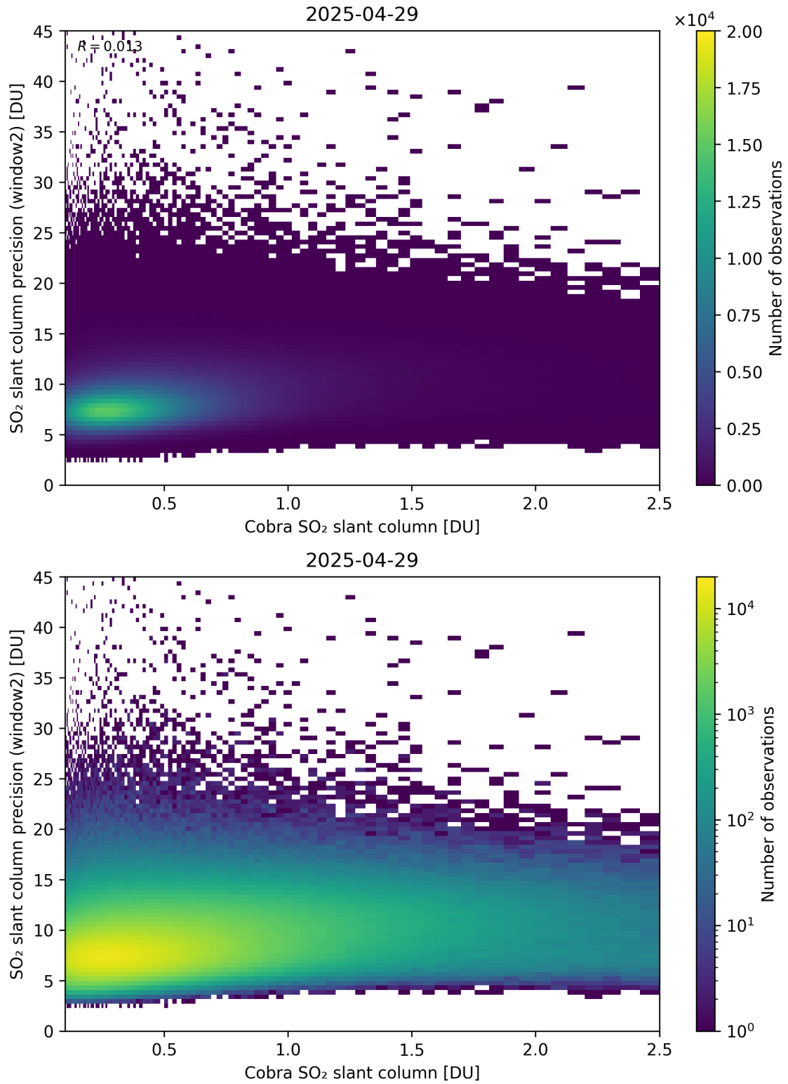
Figure 221: Scatter density plot of “Cobra SO 2 slant column” against “SO 2 slant column precision (window2)” for 2025-04-29 to 2025-04-30.
