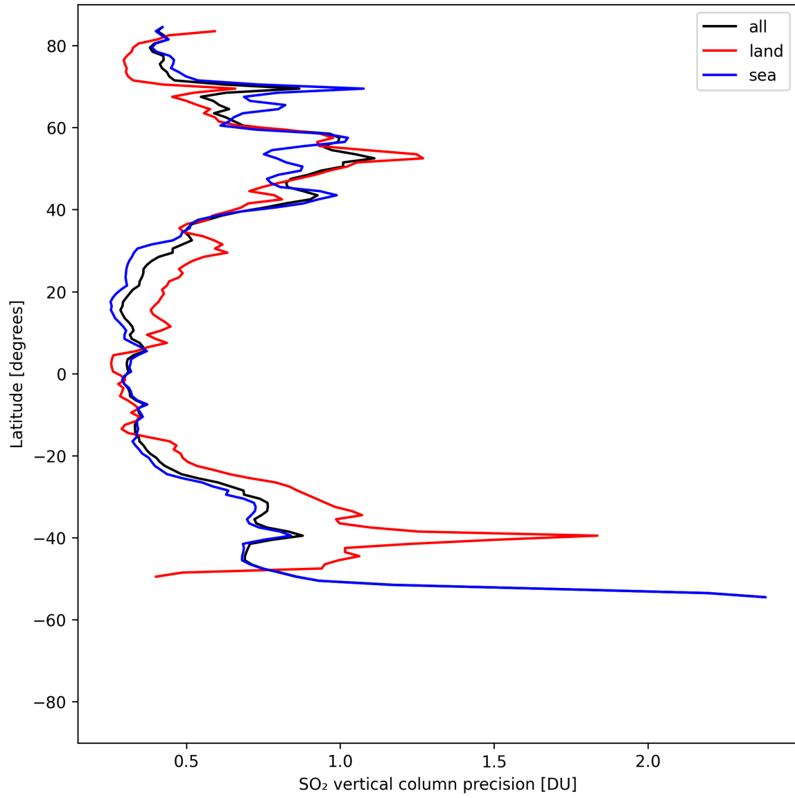
Figure 33: Zonal average of “SO 2 vertical column precision” for 2025-04-29 to 2025-04-30.
