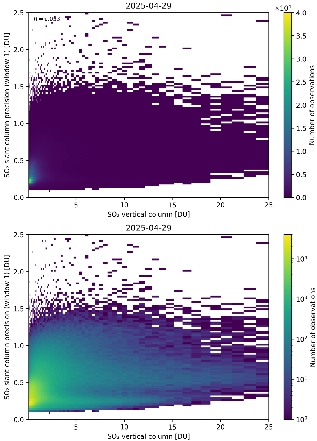
Figure 355: Scatter density plot of “SO 2 vertical column” against “SO 2 slant column precision (window 1)” for 2025-04-29 to 2025-04-30.
