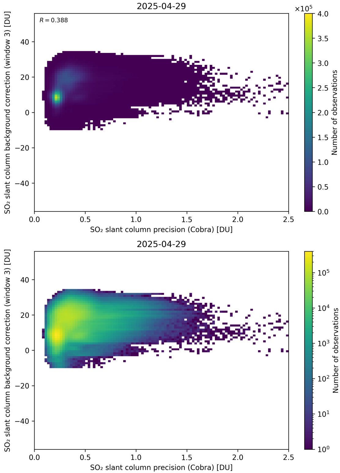
Figure 201: Scatter density plot of “SO 2 slant column precision (Cobra)” against “SO 2 slant column background correction (window 3)” for 2025-04-29 to 2025-04-30.
