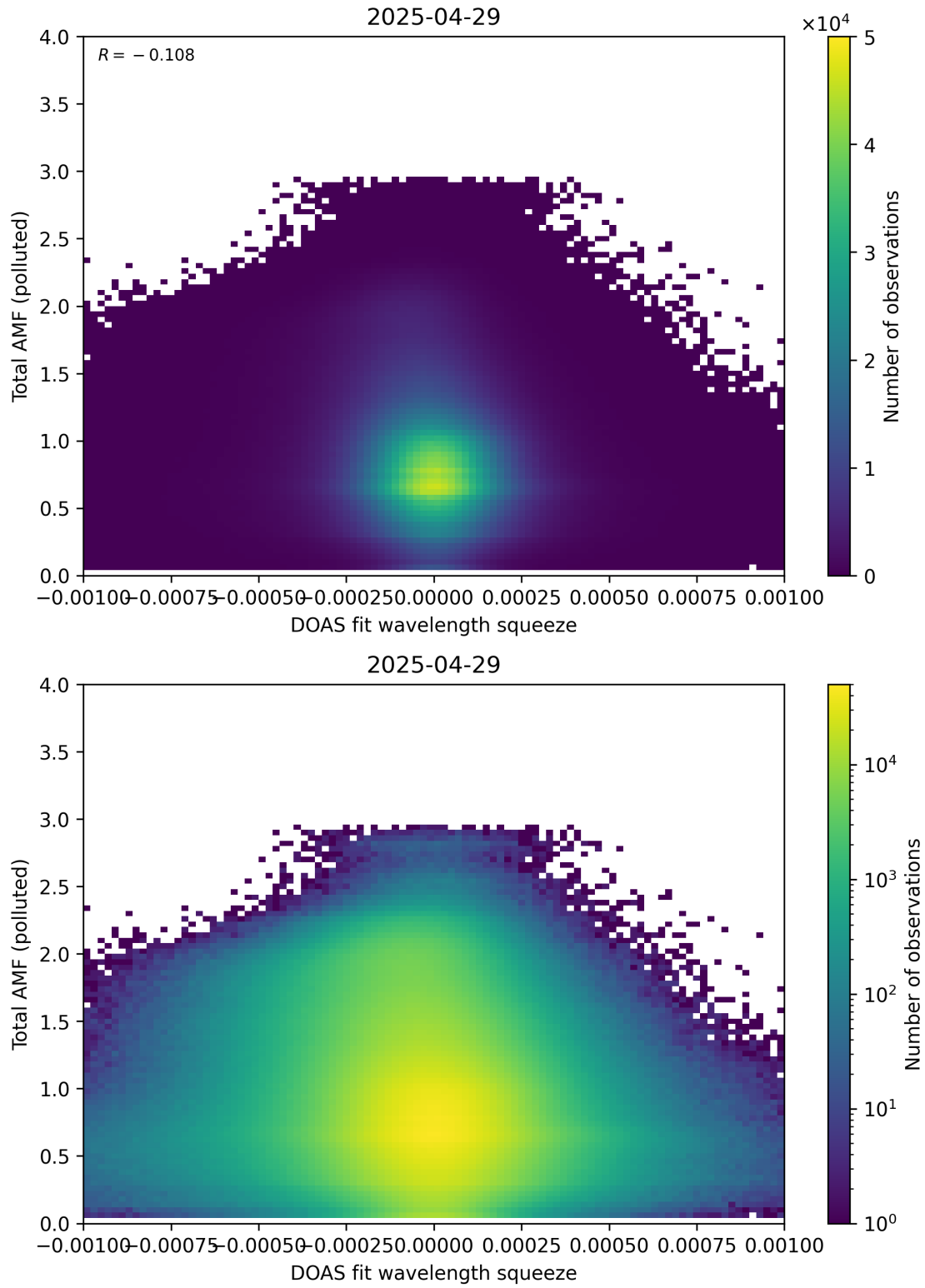
Figure 145: Scatter density plot of “DOAS fit wavelength squeeze” against “Total AMF (polluted)” for 2025-04-29 to 2025-04-30.
