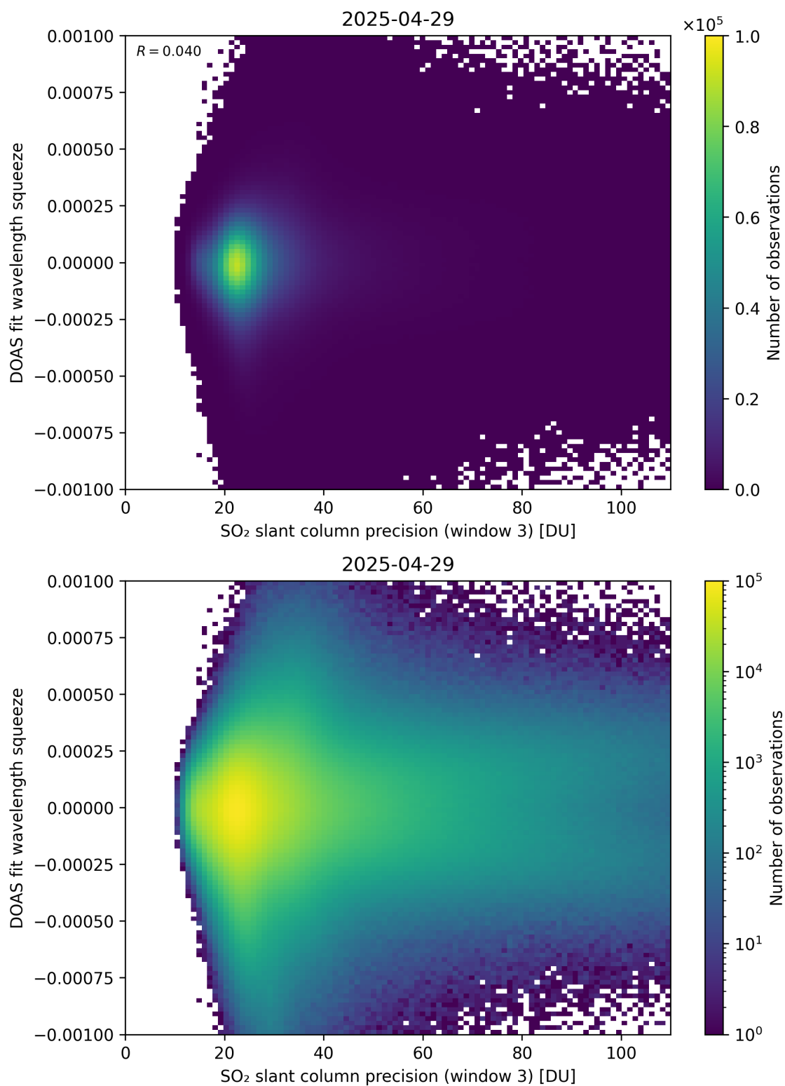
Figure 309: Scatter density plot of “SO 2 slant column precision (window 3)” against “DOAS fit wavelength squeeze” for 2025-04-29 to 2025-04-30.
