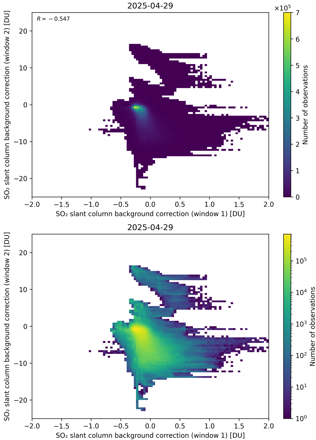
Figure 109: Scatter density plot of “SO 2 slant column background correction (window 1)” against “SO 2 slant column background correction (window 2)” for 2025-04-29 to 2025-04-30.
