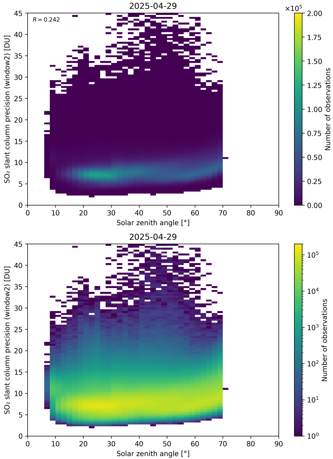
Figure 186: Scatter density plot of “Solar zenith angle” against “SO 2 slant column precision (window2)” for 2025-04-29 to 2025-04-30.
