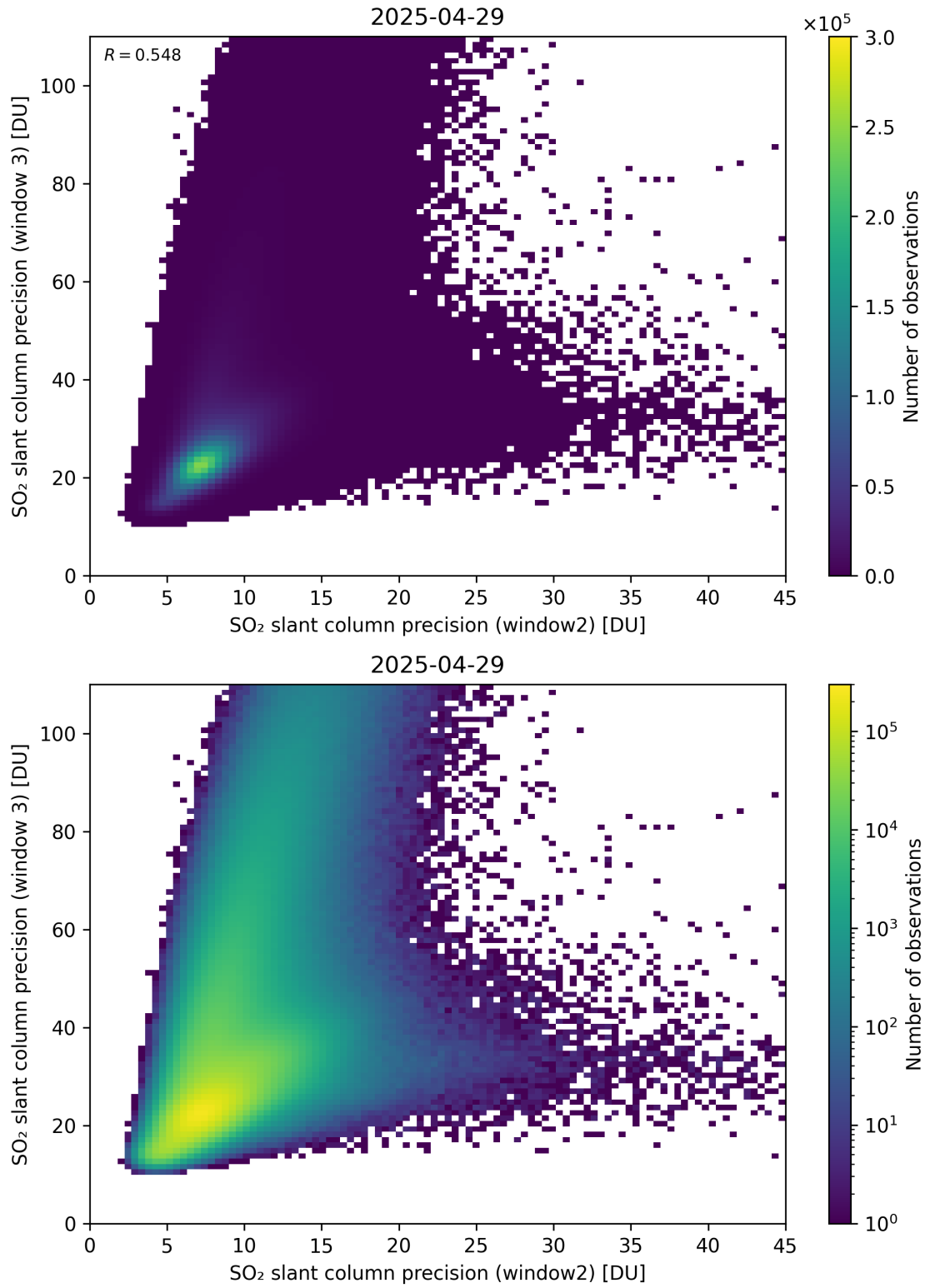
Figure 300: Scatter density plot of “SO 2 slant column precision (window2)” against “SO 2 slant column precision (window 3)” for 2025-04-29 to 2025-04-30.
