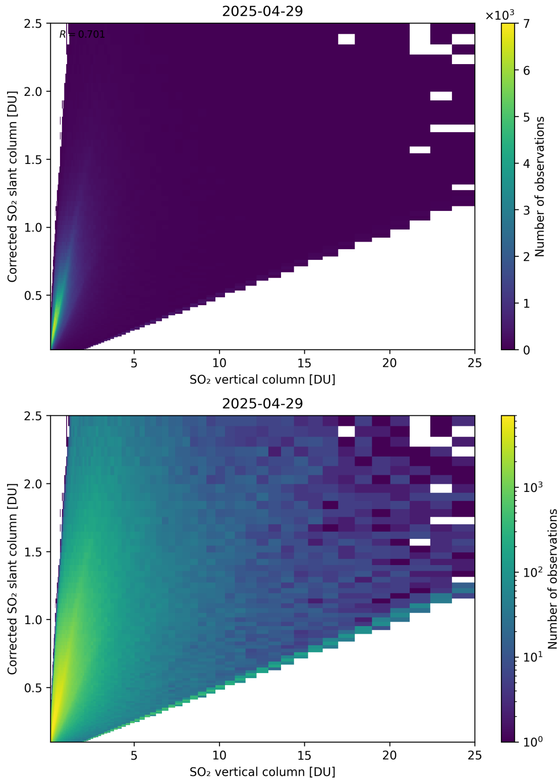
Figure 351: Scatter density plot of “SO 2 vertical column” against “Corrected SO 2 slant column” for 2025-04-29 to 2025-04-30.
