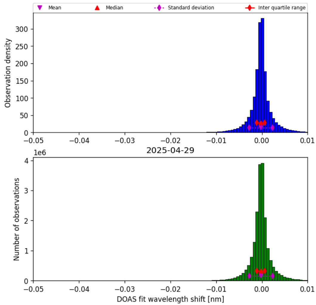
Figure 76: Histogram of “DOAS fit wavelength shift” for 2025-04-29 to 2025-04-30
