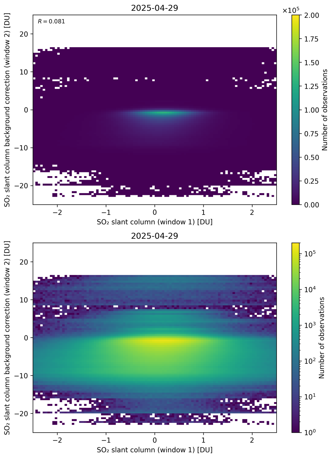
Figure 263: Scatter density plot of “SO 2 slant column (window 1)” against “SO 2 slant column background correction (window 2)” for 2025-04-29 to 2025-04-30.
