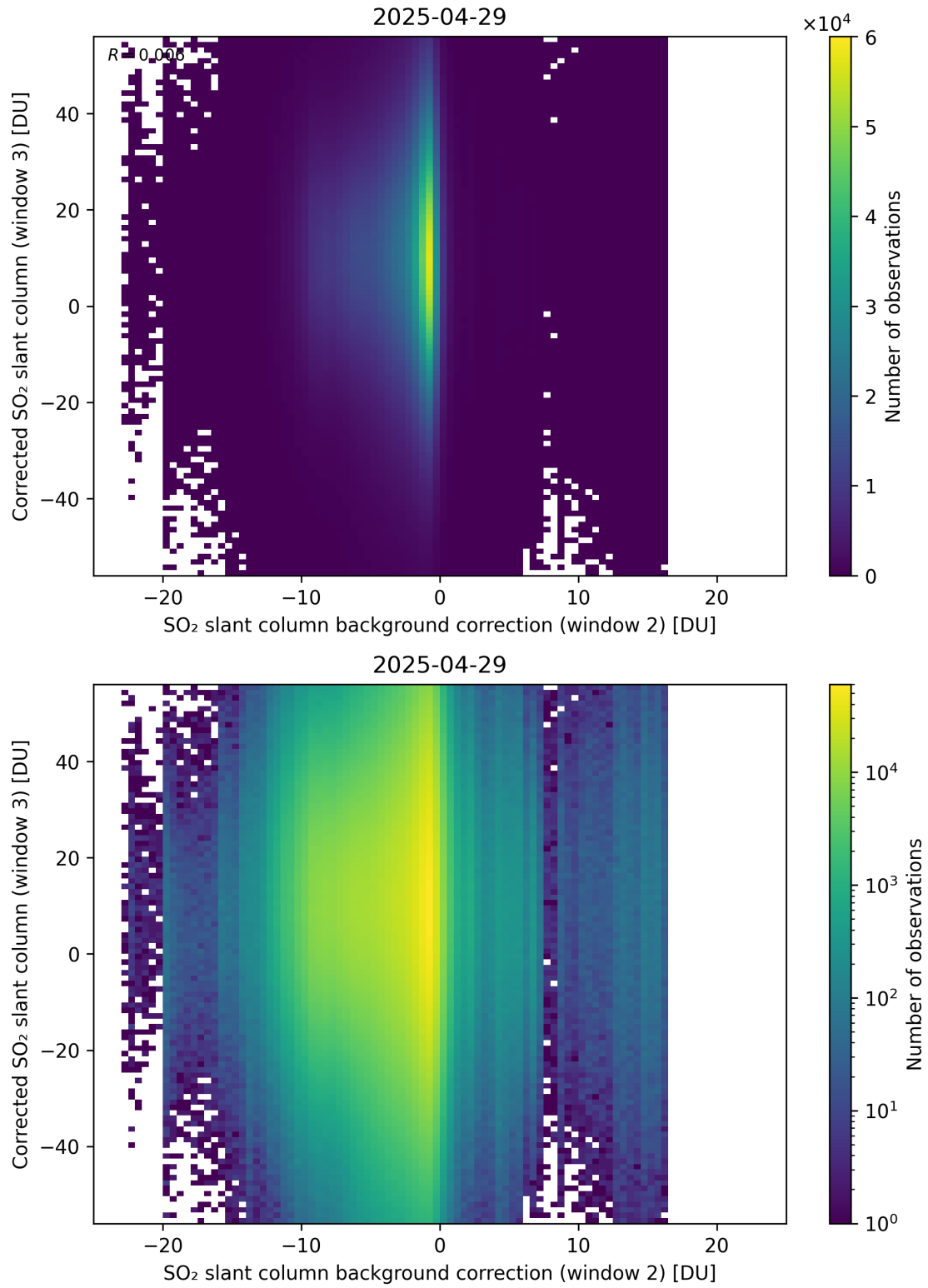
Figure 127: Scatter density plot of “SO 2 slant column background correction (window 2)” against “Corrected SO 2 slant column (window 3)” for 2025-04-29 to 2025-04-30.
