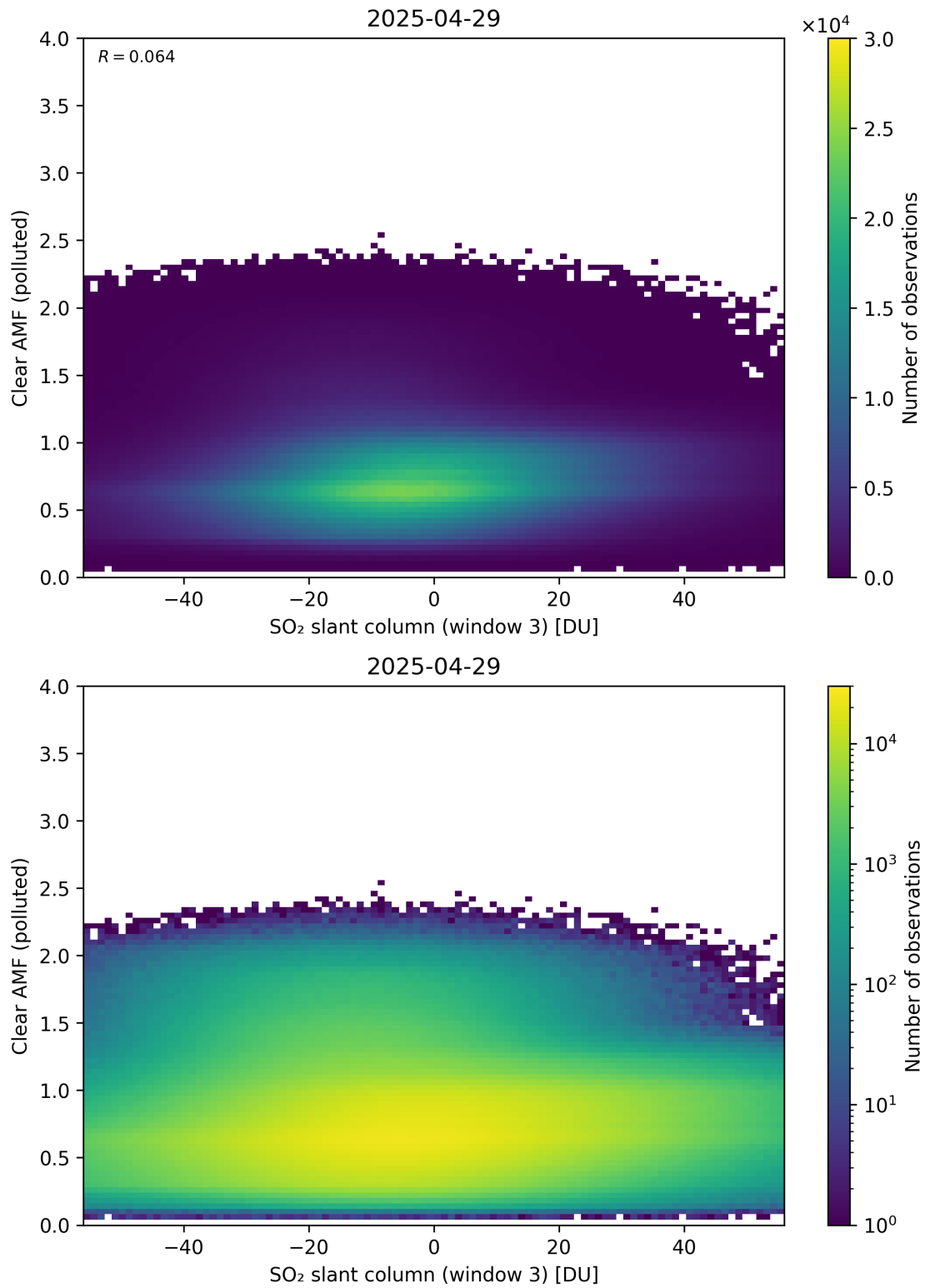
Figure 315: Scatter density plot of “SO 2 slant column (window 3)” against “Clear AMF (polluted)” for 2025-04-29 to 2025-04-30.
