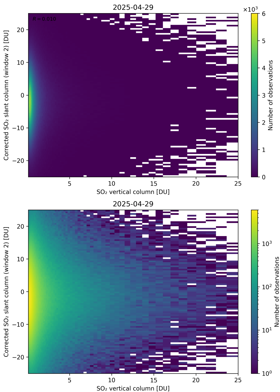
Figure 352: Scatter density plot of “SO 2 vertical column” against “Corrected SO 2 slant column (window 2)” for 2025-04-29 to 2025-04-30.
