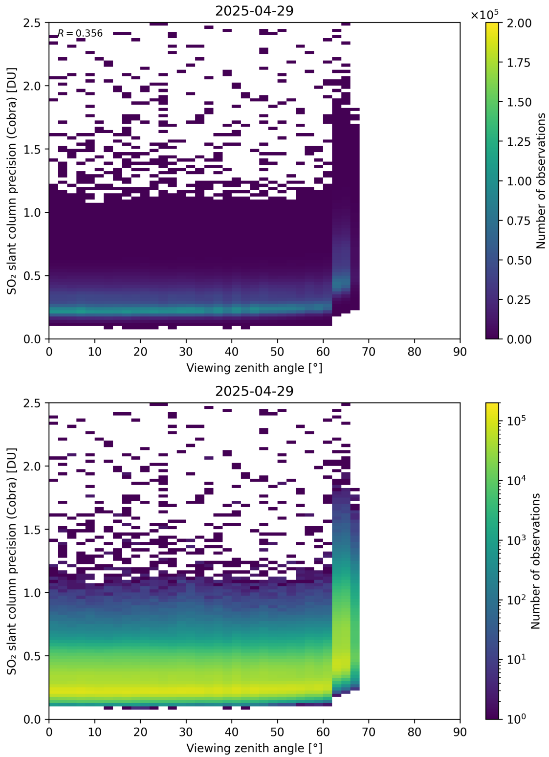
Figure 372: Scatter density plot of “Viewing zenith angle” against “SO 2 slant column precision (Cobra)” for 2025-04-29 to 2025-04-30.
