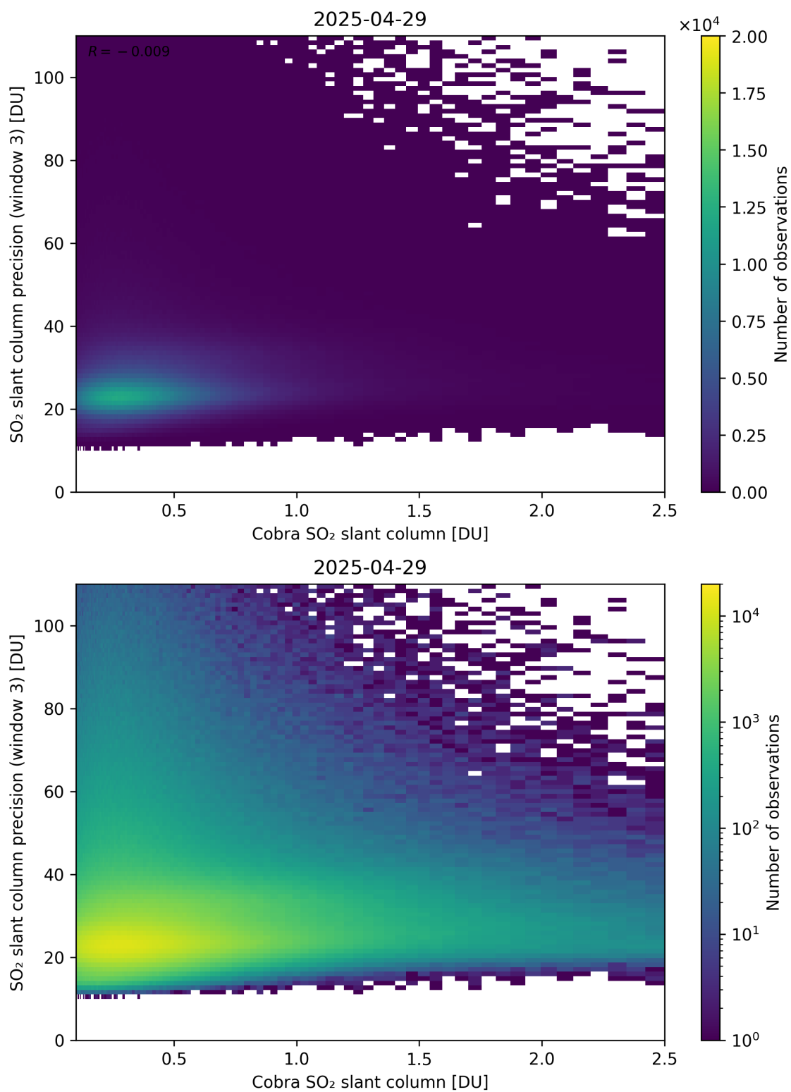
Figure 223: Scatter density plot of “Cobra SO 2 slant column” against “SO 2 slant column precision (window 3)” for 2025-04-29 to 2025-04-30.
