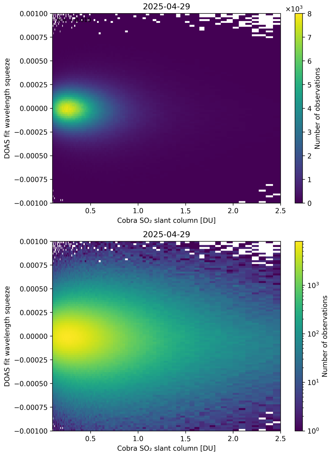
Figure 197: Scatter density plot of “Cobra SO 2 slant column” against “DOAS fit wavelength squeeze” for 2025-04-29 to 2025-04-30.
