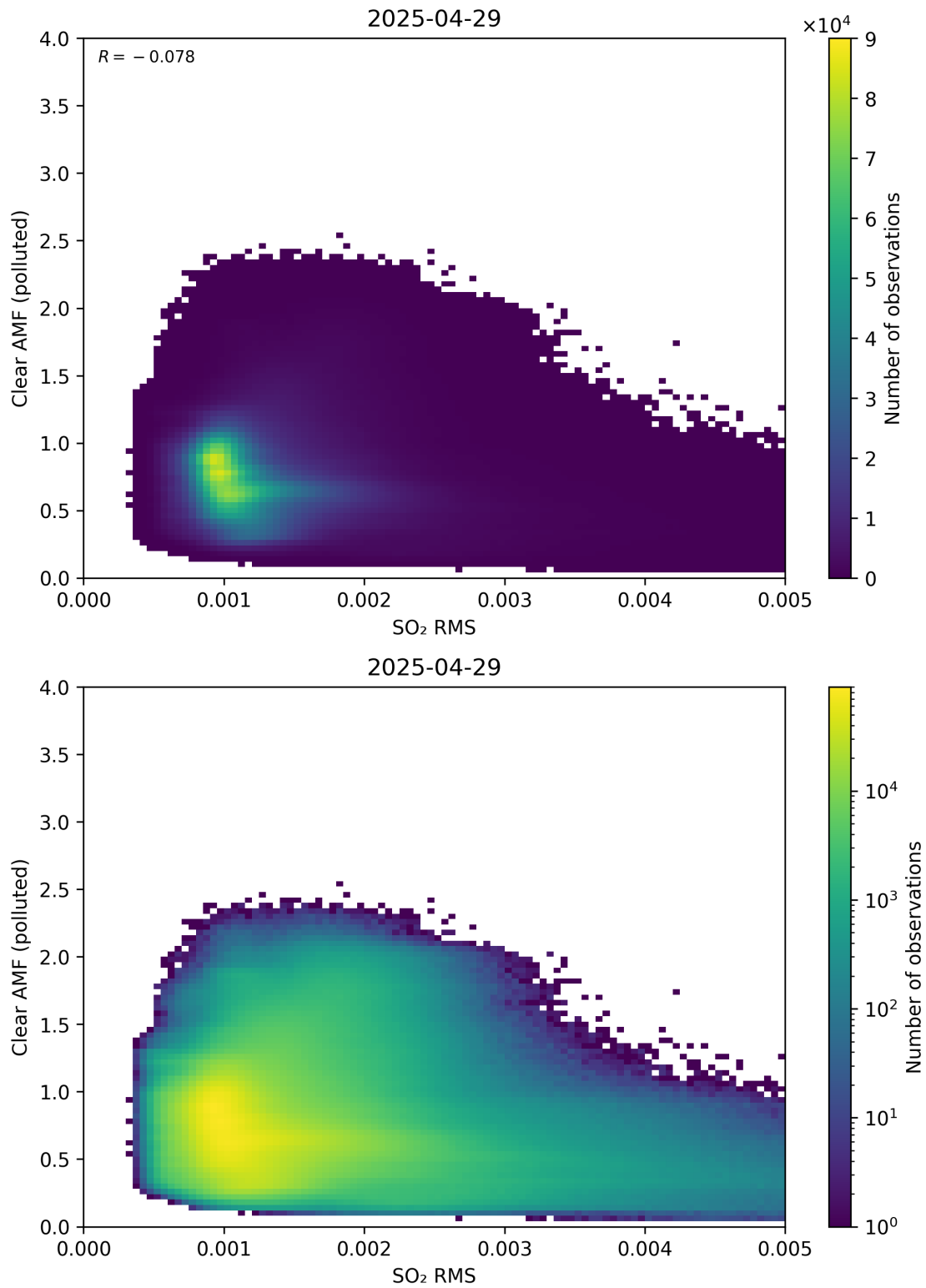
Figure 147: Scatter density plot of “SO 2 RMS” against “Clear AMF (polluted)” for 2025-04-29 to 2025-04-30.
