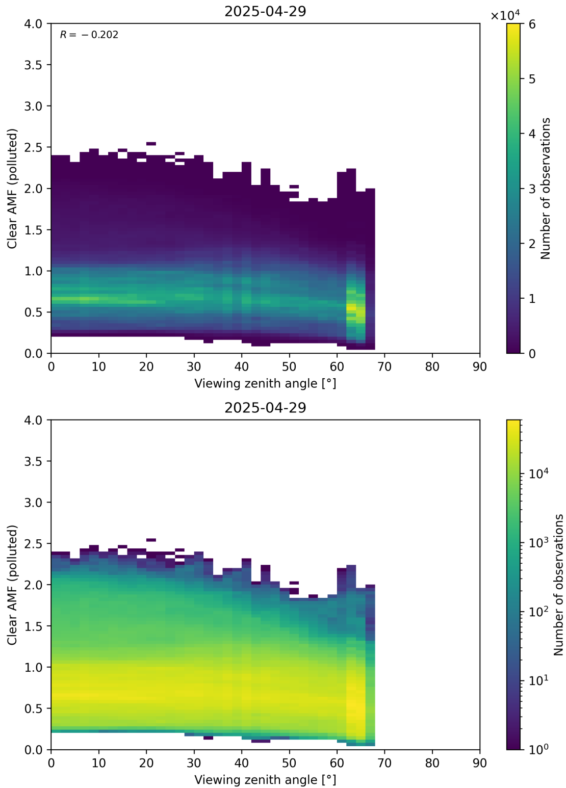
Figure 370: Scatter density plot of “Viewing zenith angle” against “Clear AMF (polluted)” for 2025-04-29 to 2025-04-30.
