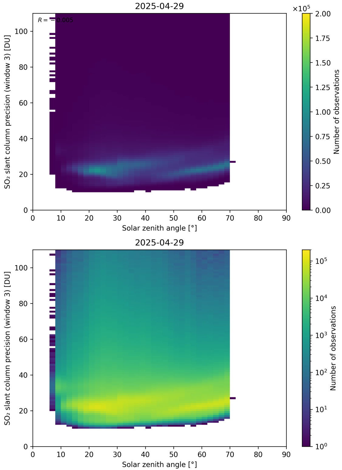
Figure 188: Scatter density plot of “Solar zenith angle” against “SO 2 slant column precision (window 3)” for 2025-04-29 to 2025-04-30.
