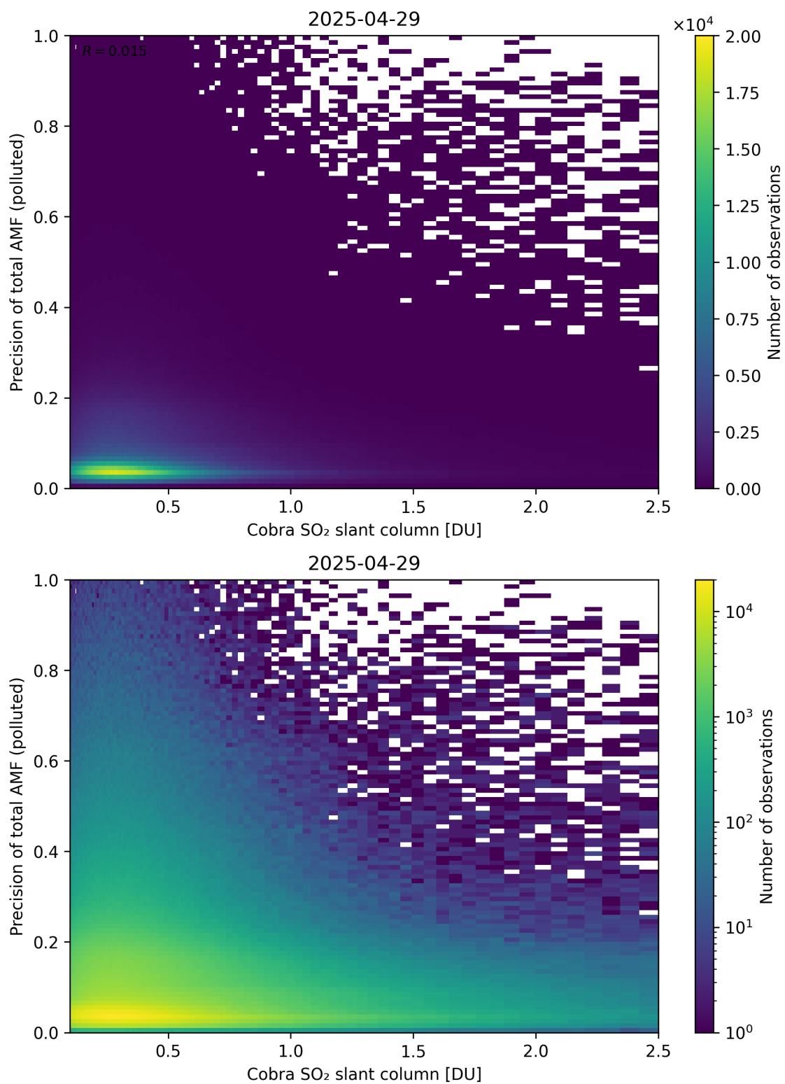
Figure 225: Scatter density plot of “Cobra SO 2 slant column” against “Precision of total AMF (polluted)” for 2025-04-29 to 2025-04-30.
