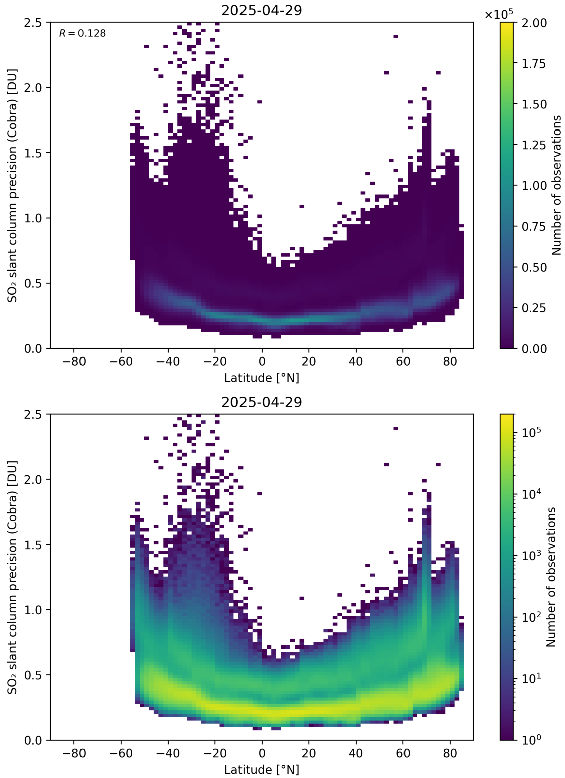
Figure 158: Scatter density plot of “Latitude” against “SO 2 slant column precision (Cobra)” for 2025-04-29 to 2025-04-30.
