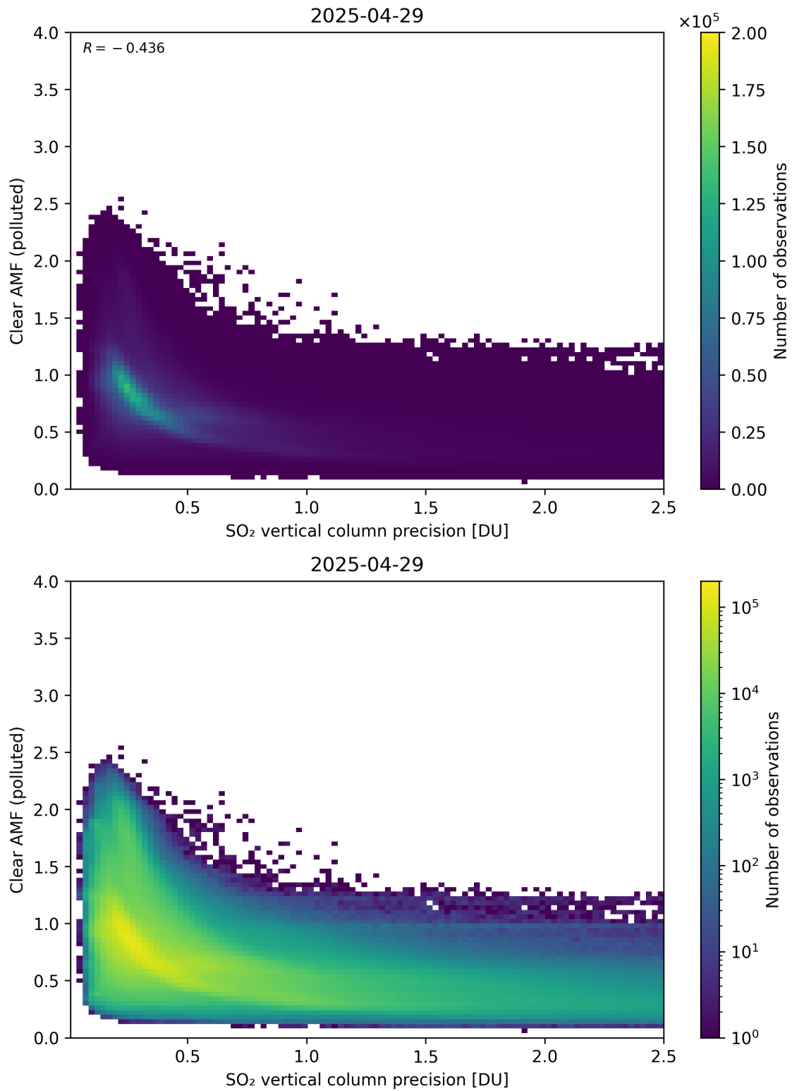
Figure 335: Scatter density plot of “SO 2 vertical column precision” against “Clear AMF (polluted)” for 2025-04-29 to 2025-04-30.
