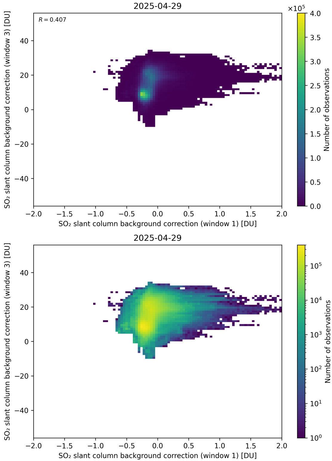
Figure 110: Scatter density plot of “SO 2 slant column background correction (window 1)” against “SO 2 slant column background correction (window 3)” for 2025-04-29 to 2025-04-30.
