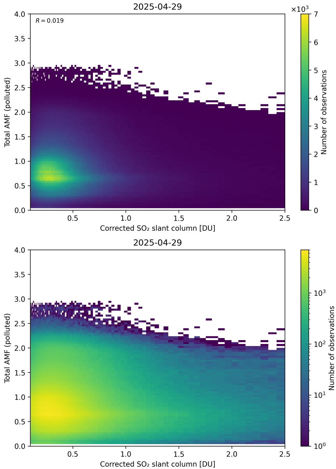
Figure 242: Scatter density plot of “Corrected SO 2 slant column” against “Total AMF (polluted)” for 2025-04-29 to 2025-04-30.
