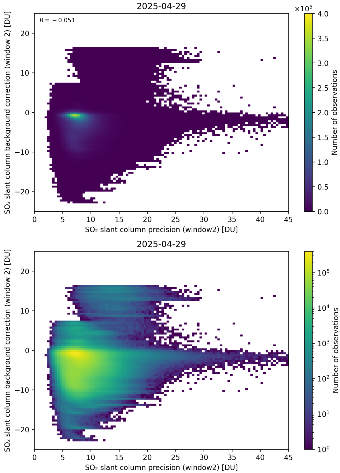
Figure 291: Scatter density plot of “SO 2 slant column precision (window2)” against “SO 2 slant column background correction (window 2)” for 2025-04-29 to 2025-04-30.
