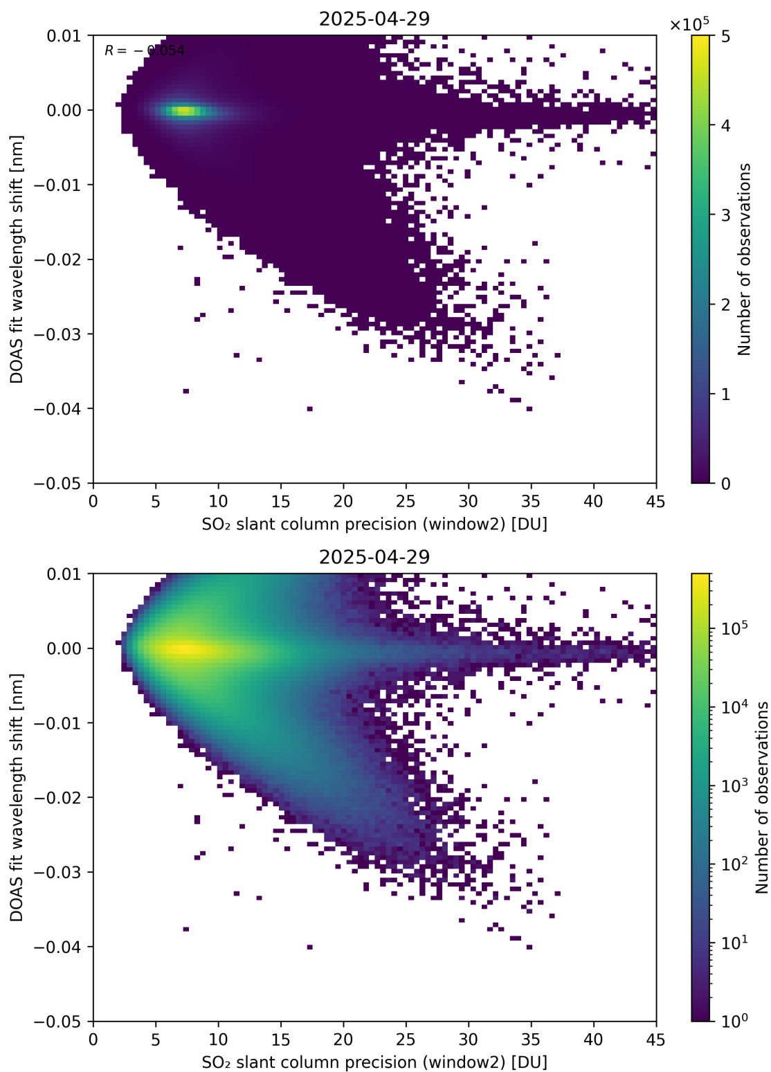
Figure 293: Scatter density plot of “SO 2 slant column precision (window2)” against “DOAS fit wavelength shift” for 2025-04-29 to 2025-04-30.
