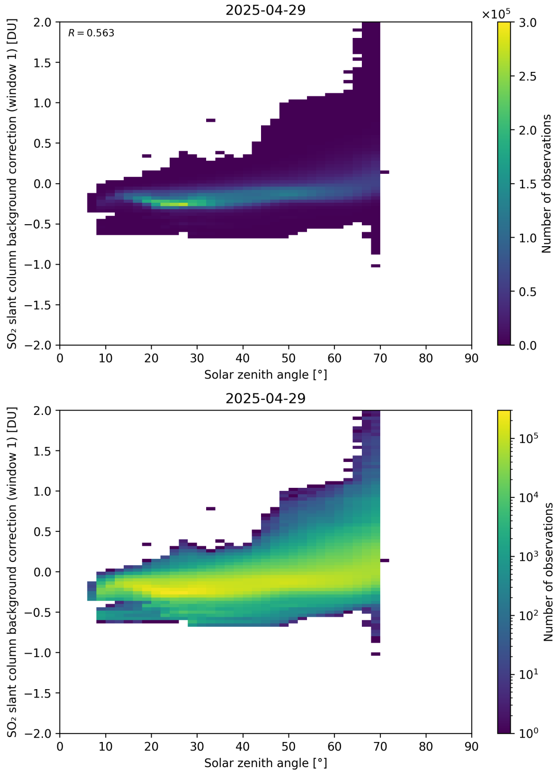
Figure 171: Scatter density plot of “Solar zenith angle” against “SO 2 slant column background correction (window 1)” for 2025-04-29 to 2025-04-30.
