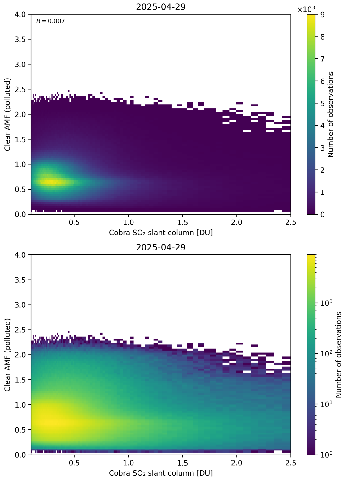
Figure 215: Scatter density plot of “Cobra SO 2 slant column” against “Clear AMF (polluted)” for 2025-04-29 to 2025-04-30.
