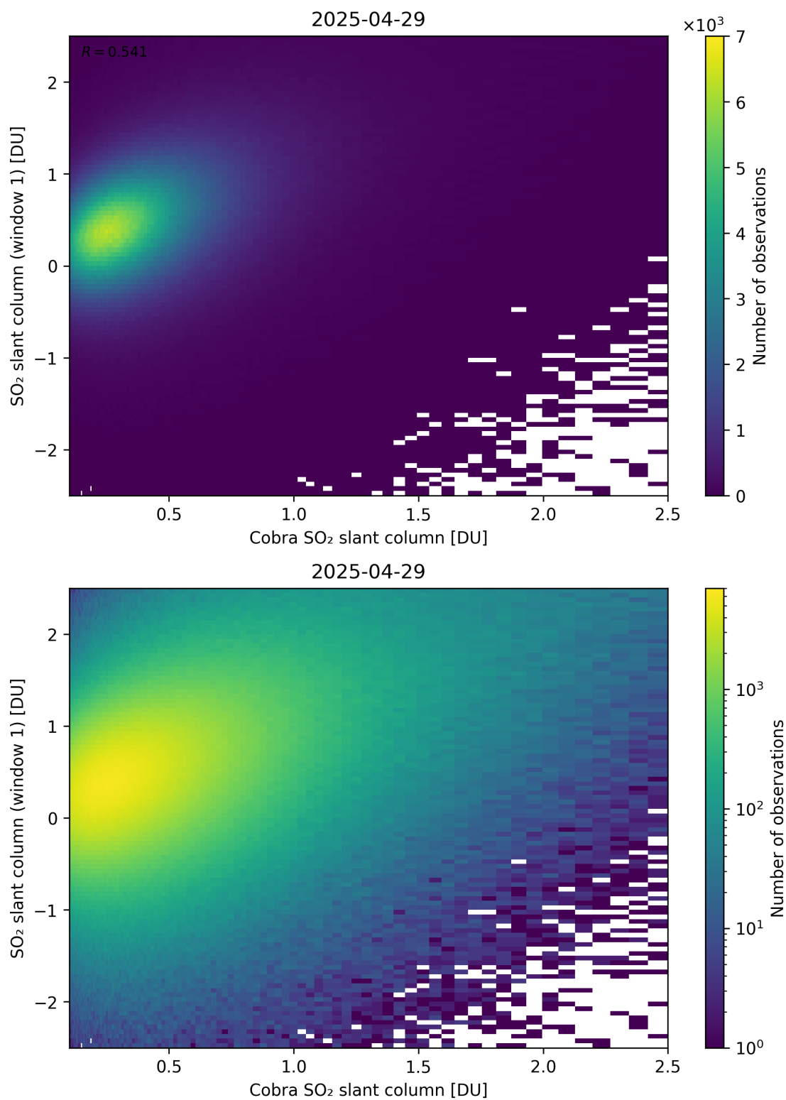
Figure 219: Scatter density plot of “Cobra SO 2 slant column” against “SO 2 slant column (window 1)” for 2025-04-29 to 2025-04-30.
