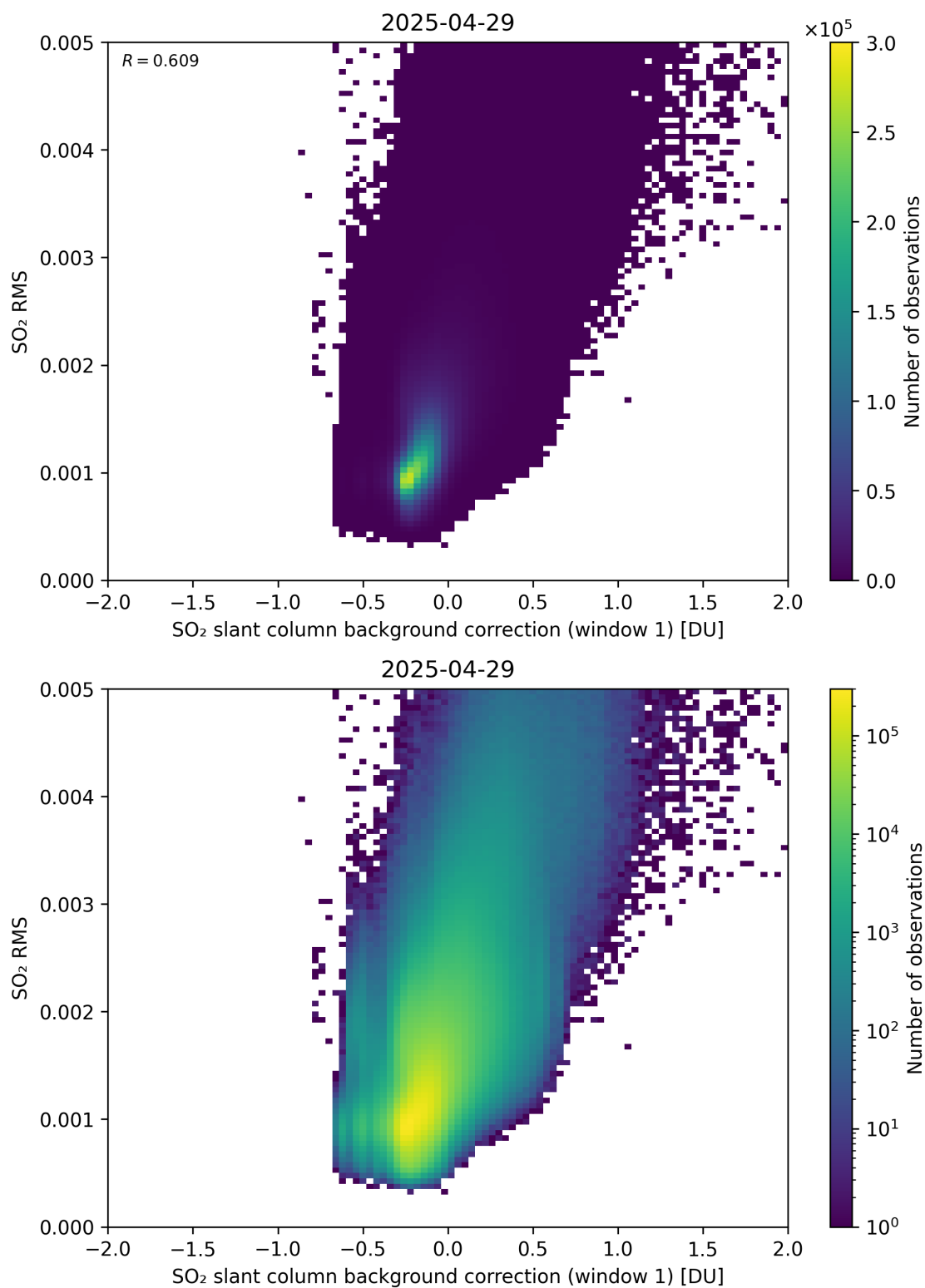
Figure 113: Scatter density plot of “SO 2 slant column background correction (window 1)” against “SO 2 RMS” for 2025-04-29 to 2025-04-30.
