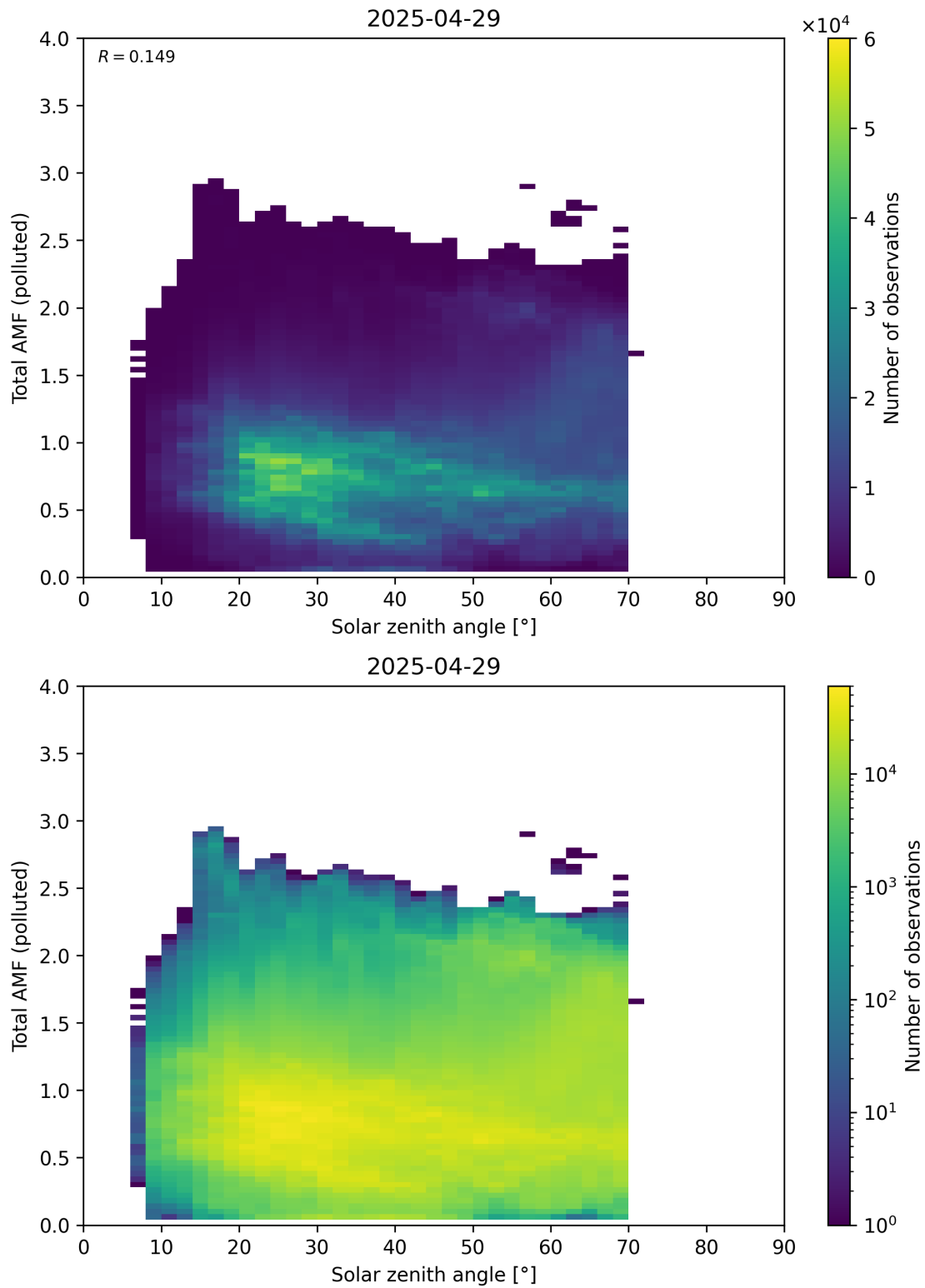
Figure 189: Scatter density plot of “Solar zenith angle” against “Total AMF (polluted)” for 2025-04-29 to 2025-04-30.
