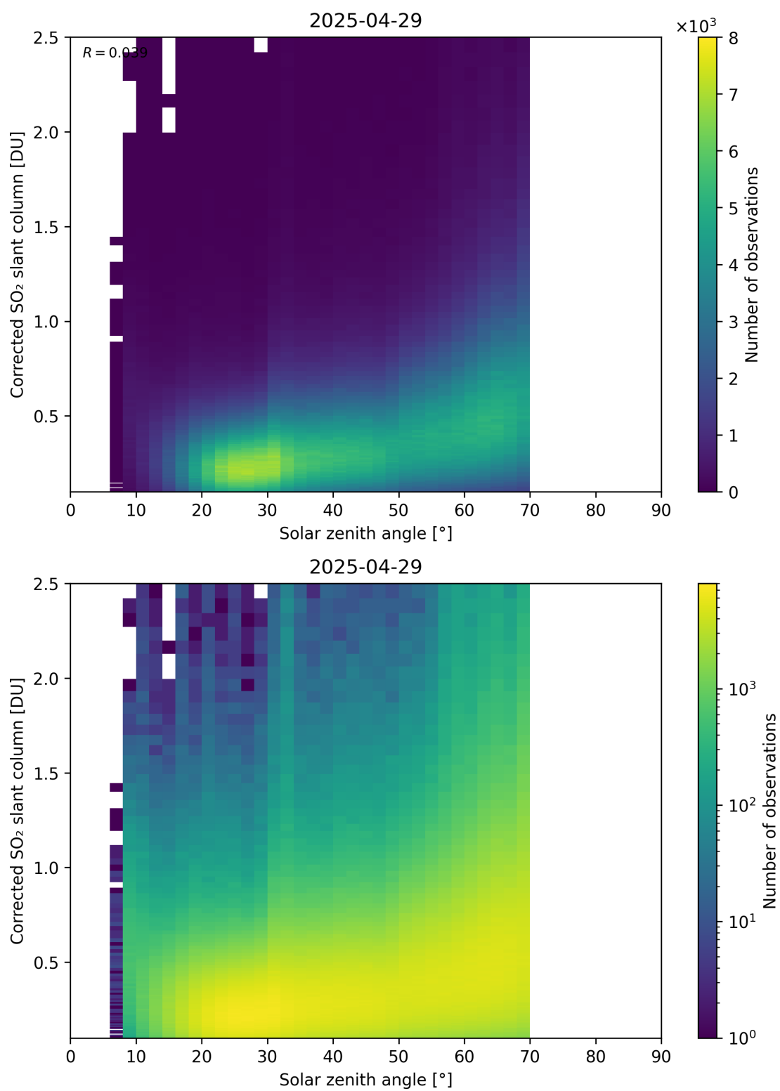
Figure 181: Scatter density plot of “Solar zenith angle” against “Corrected SO 2 slant column” for 2025-04-29 to 2025-04-30.
