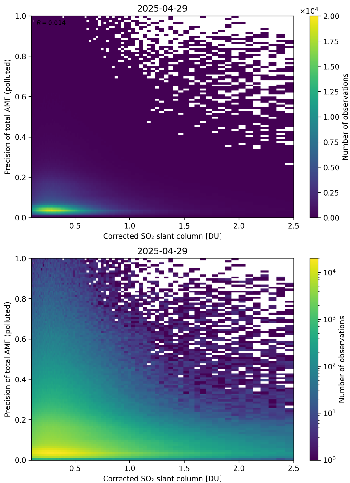
Figure 243: Scatter density plot of “Corrected SO 2 slant column” against “Precision of total AMF (polluted)” for 2025-04-29 to 2025-04-30.
