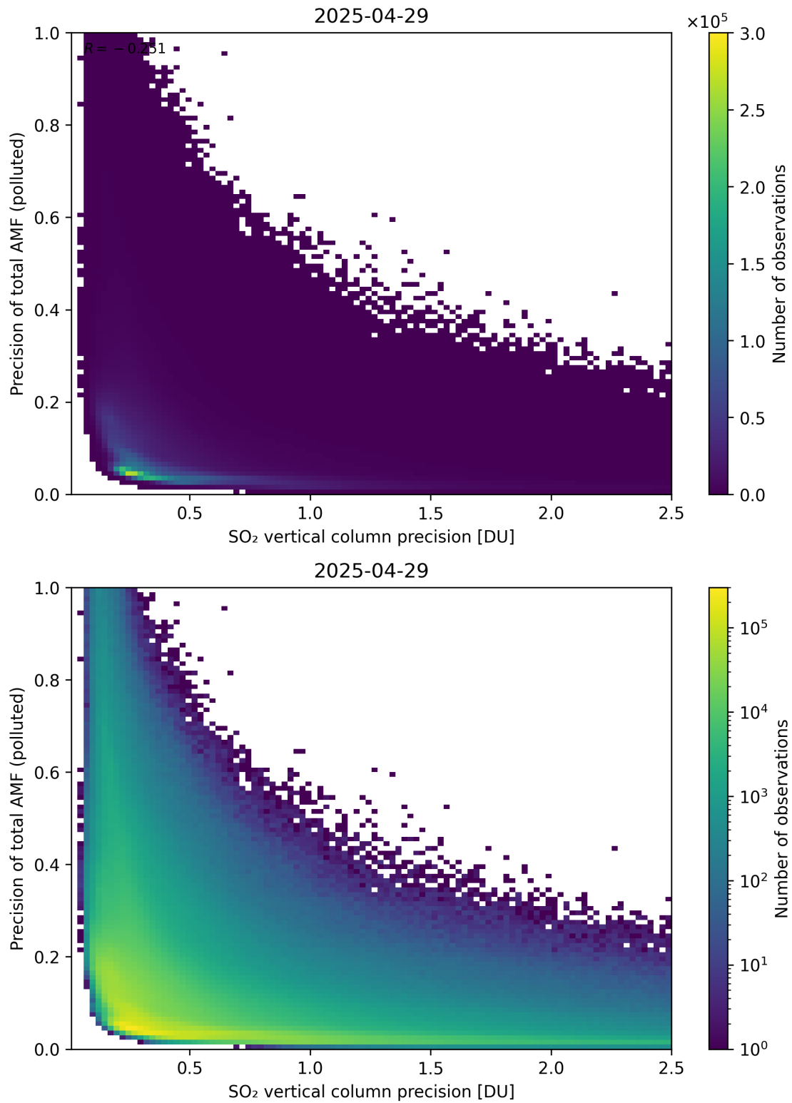
Figure 347: Scatter density plot of “SO 2 vertical column precision” against “Precision of total AMF (polluted)” for 2025-04-29 to 2025-04-30.
