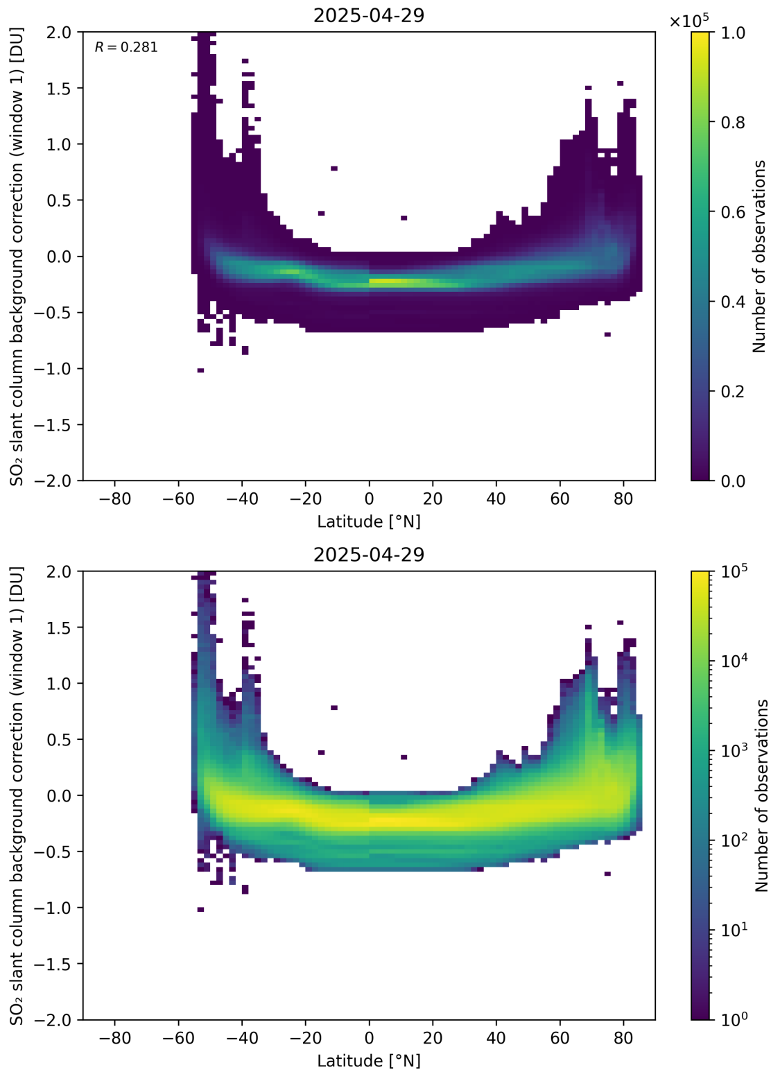
Figure 150: Scatter density plot of “Latitude” against “SO 2 slant column background correction (window 1)” for 2025-04-29 to 2025-04-30.
