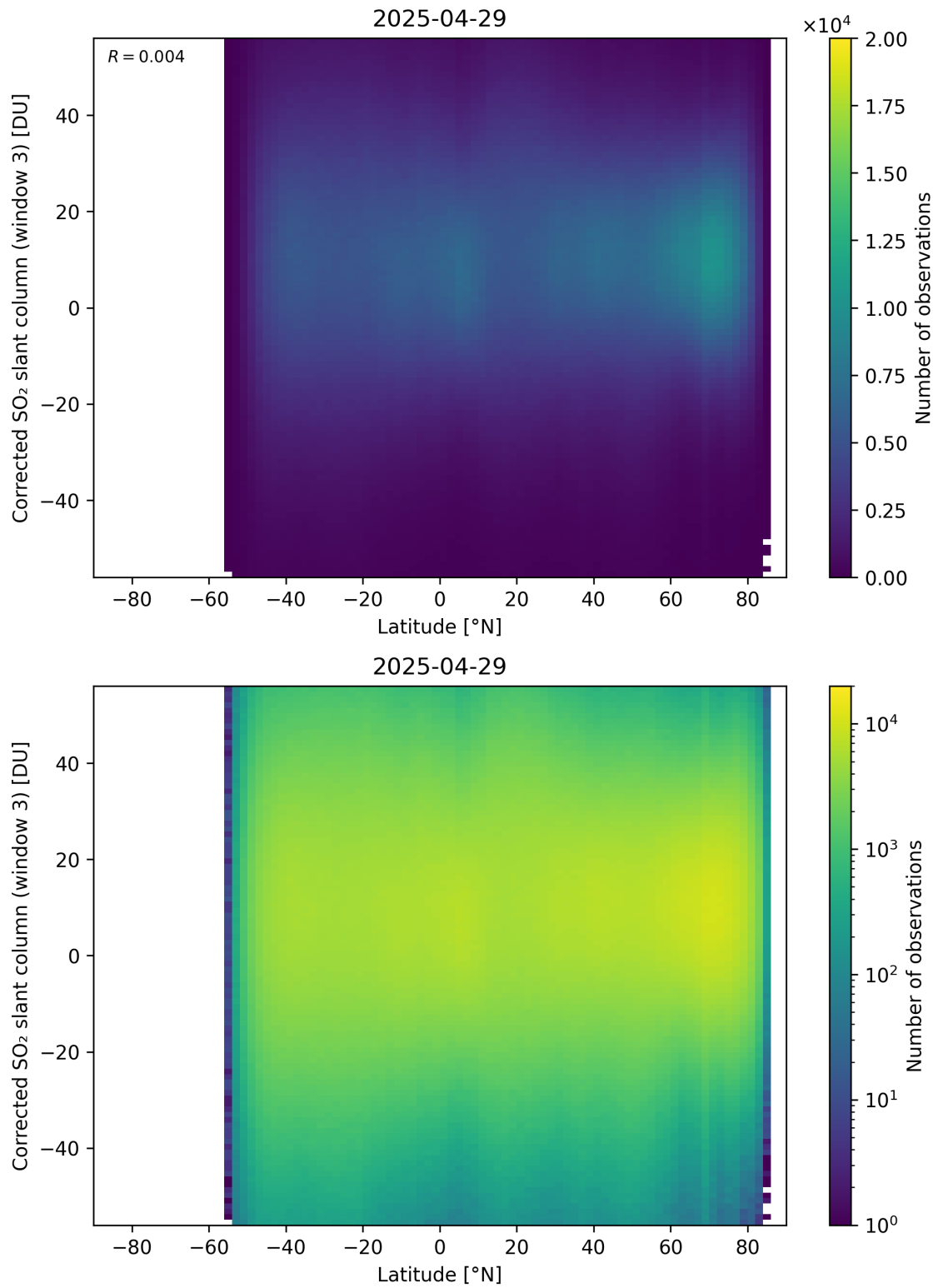
Figure 161: Scatter density plot of “Latitude” against “Corrected SO 2 slant column (window 3)” for 2025-04-29 to 2025-04-30.
