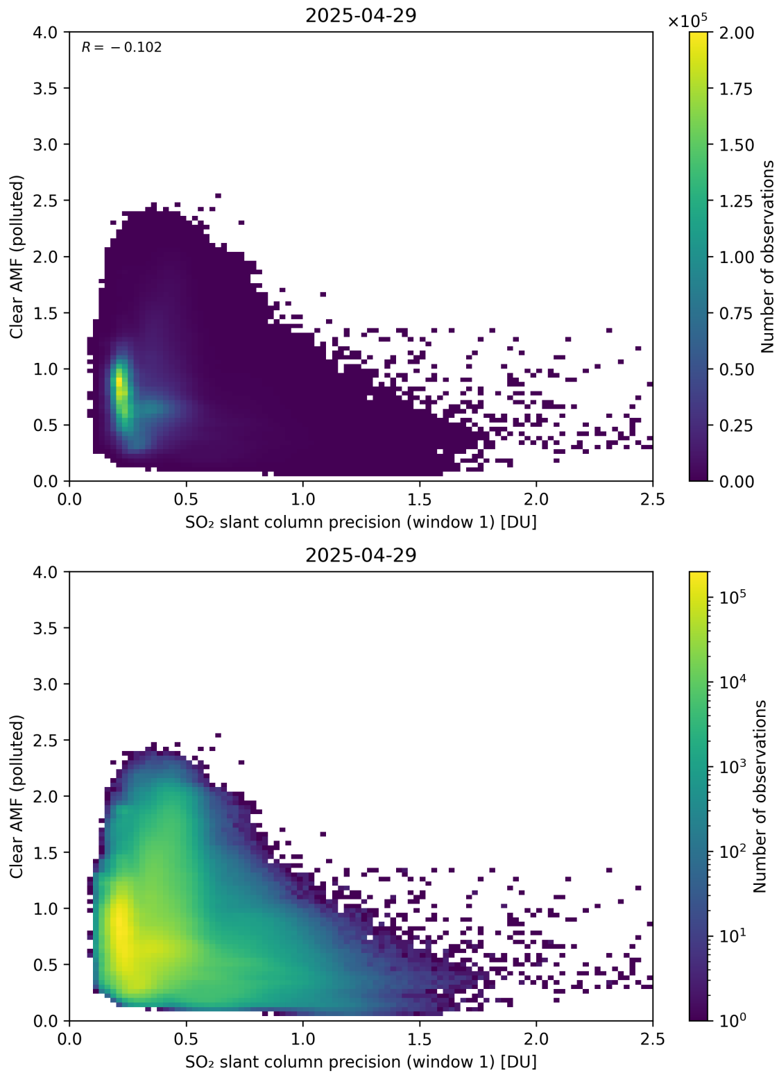
Figure 274: Scatter density plot of “SO 2 slant column precision (window 1)” against “Clear AMF (polluted)” for 2025-04-29 to 2025-04-30.
