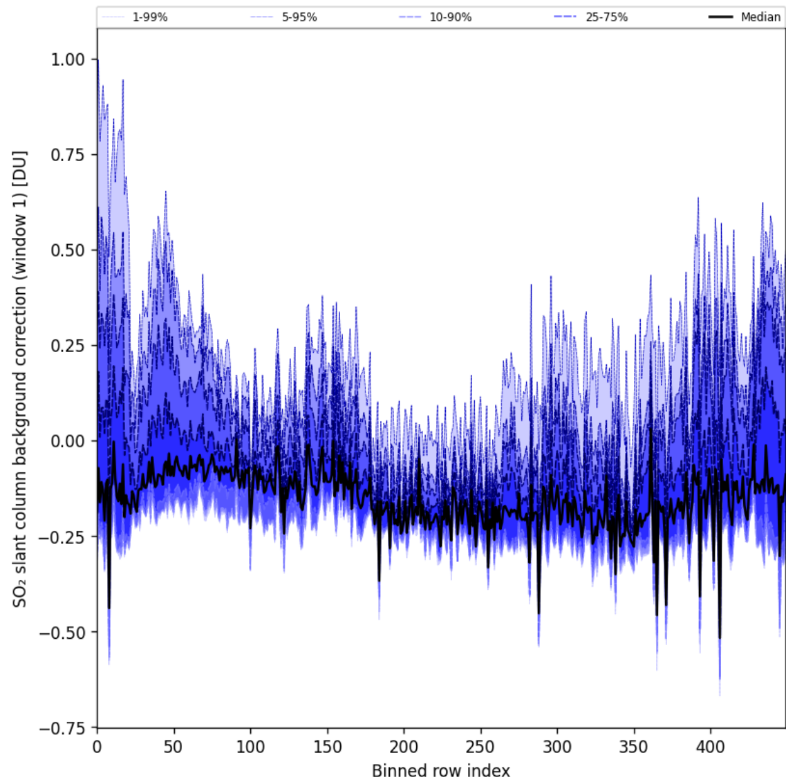
Figure 92: Along track statistics of “SO 2 slant column background correction (window 1)” for 2025-04-29 to 2025-04-30
