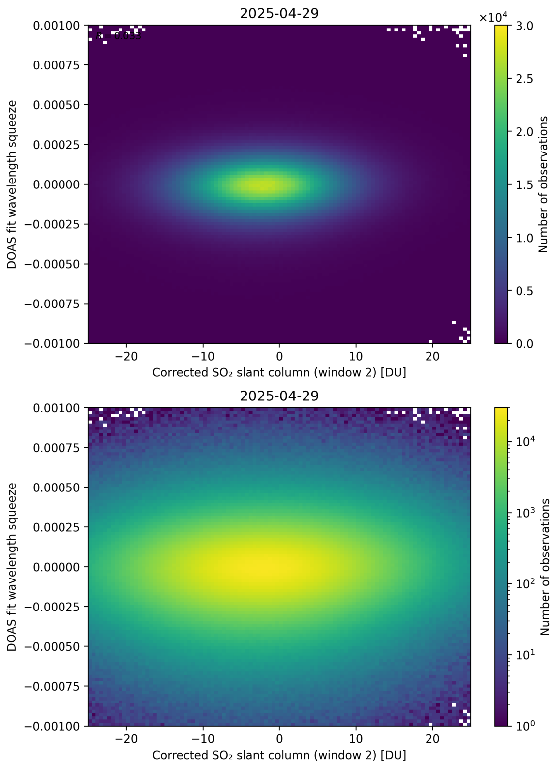
Figure 247: Scatter density plot of “Corrected SO 2 slant column (window 2)” against “DOAS fit wavelength squeeze” for 2025-04-29 to 2025-04-30.
