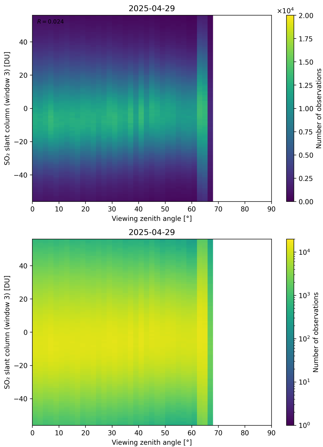
Figure 379: Scatter density plot of “Viewing zenith angle” against “SO 2 slant column (window 3)” for 2025-04-29 to 2025-04-30.
