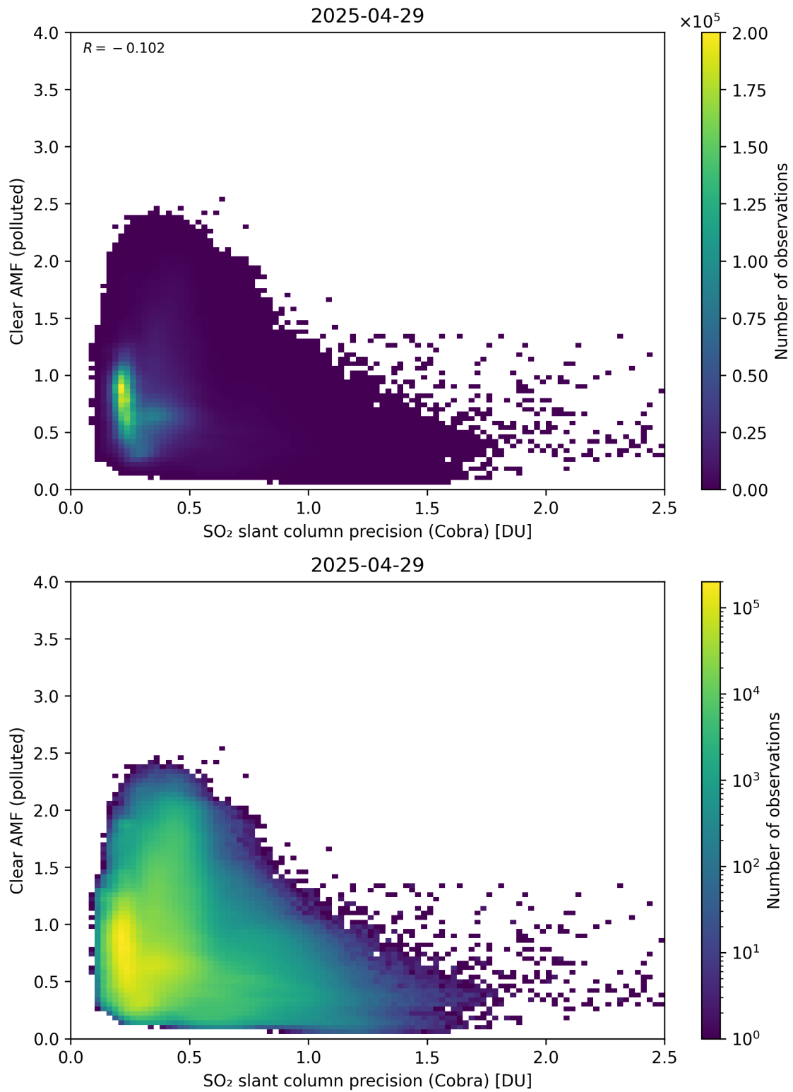
Figure 205: Scatter density plot of “SO 2 slant column precision (Cobra)” against “Clear AMF (polluted)” for 2025-04-29 to 2025-04-30.
