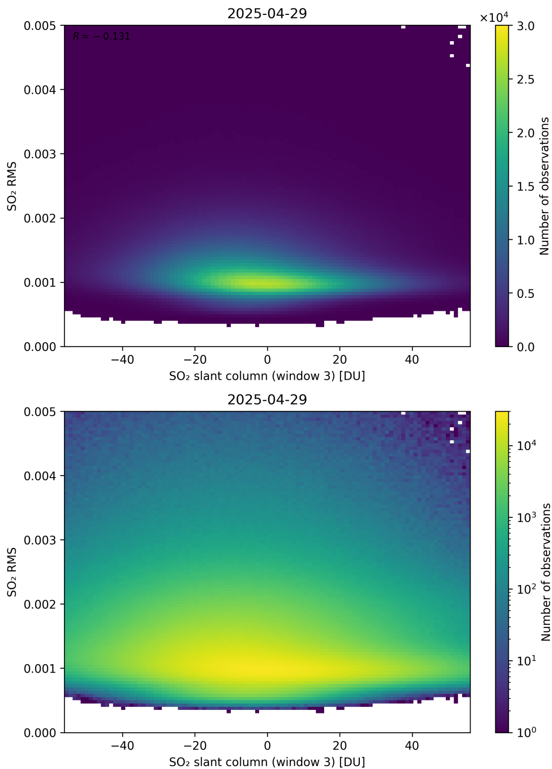
Figure 306: Scatter density plot of “SO 2 slant column (window 3)” against “SO 2 RMS” for 2025-04-29 to 2025-04-30.
