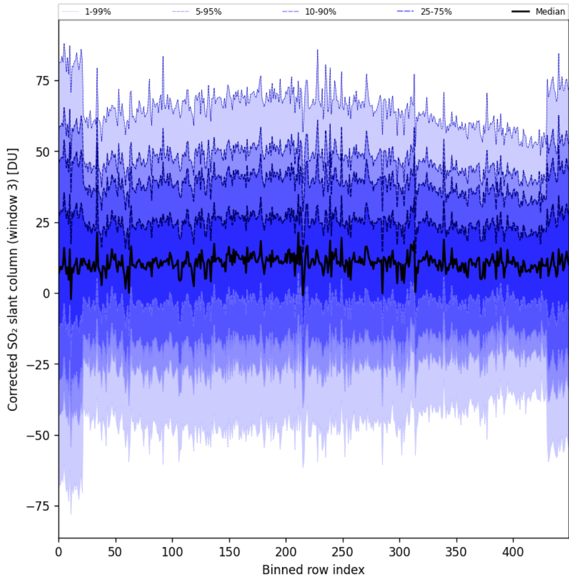
Figure 99: Along track statistics of “Corrected SO 2 slant column (window 3)” for 2025-04-29 to 2025-04-30
