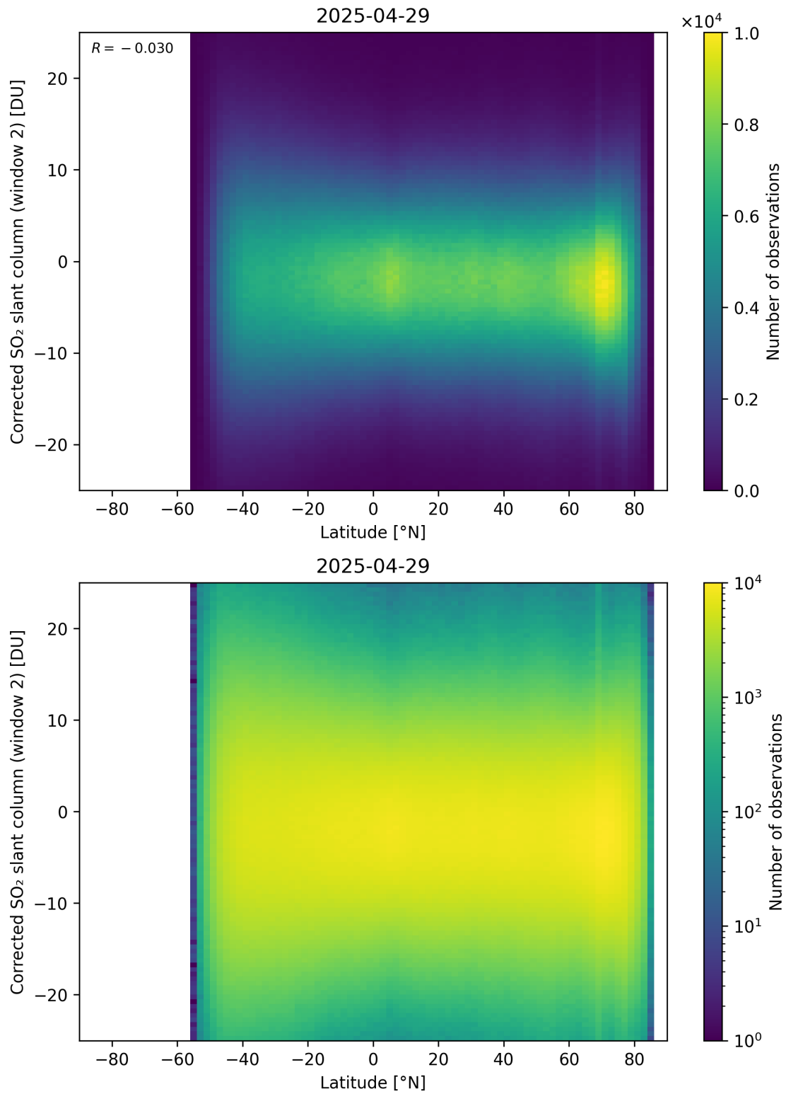
Figure 160: Scatter density plot of “Latitude” against “Corrected SO 2 slant column (window 2)” for 2025-04-29 to 2025-04-30.
