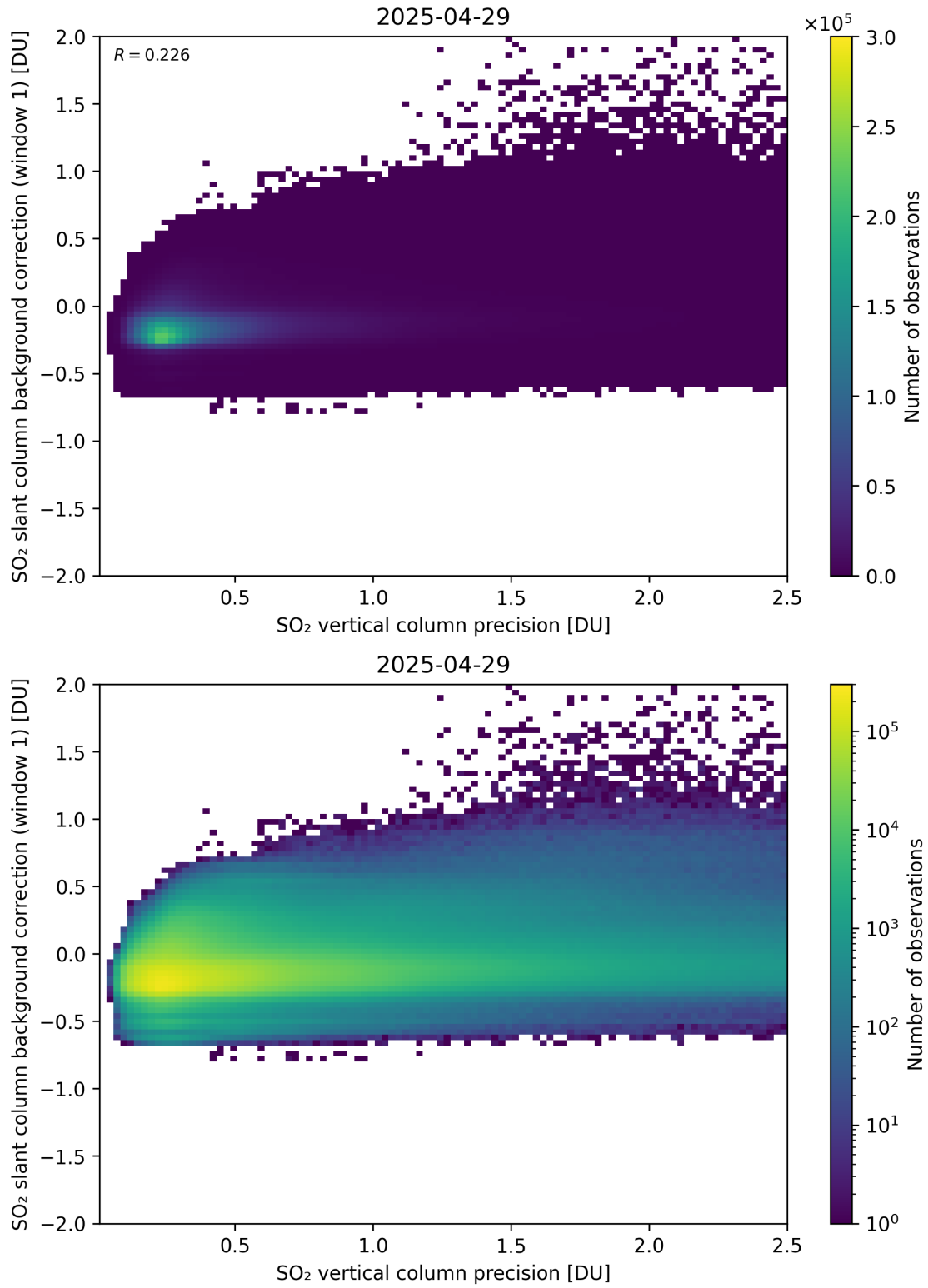
Figure 329: Scatter density plot of “SO 2 vertical column precision” against “SO 2 slant column background correction (window 1)” for 2025-04-29 to 2025-04-30.
