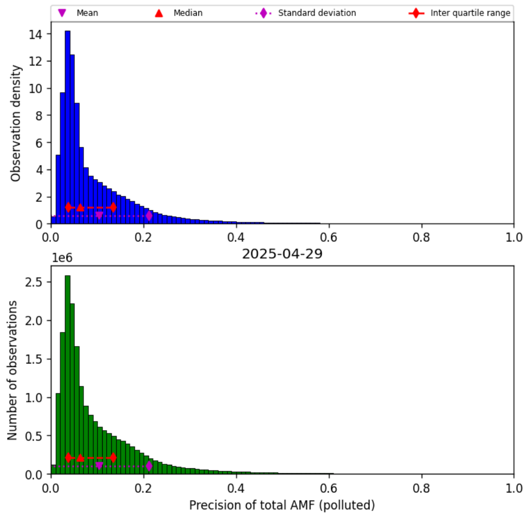
Figure 80: Histogram of “Precision of total AMF (polluted)” for 2025-04-29 to 2025-04-30
