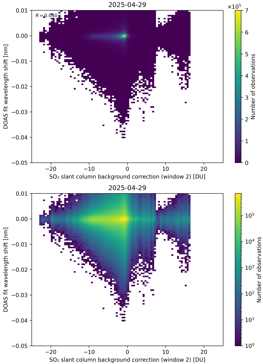
Figure 123: Scatter density plot of “SO 2 slant column background correction (window 2)” against “DOAS fit wavelength shift” for 2025-04-29 to 2025-04-30.
