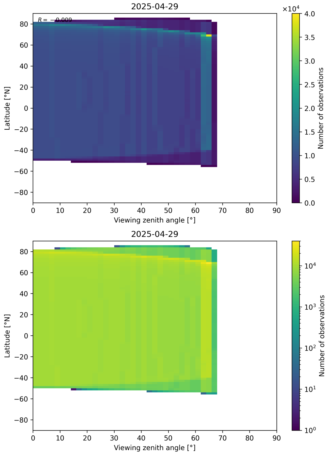
Figure 368: Scatter density plot of “Viewing zenith angle” against “Latitude” for 2025-04-29 to 2025-04-30.
