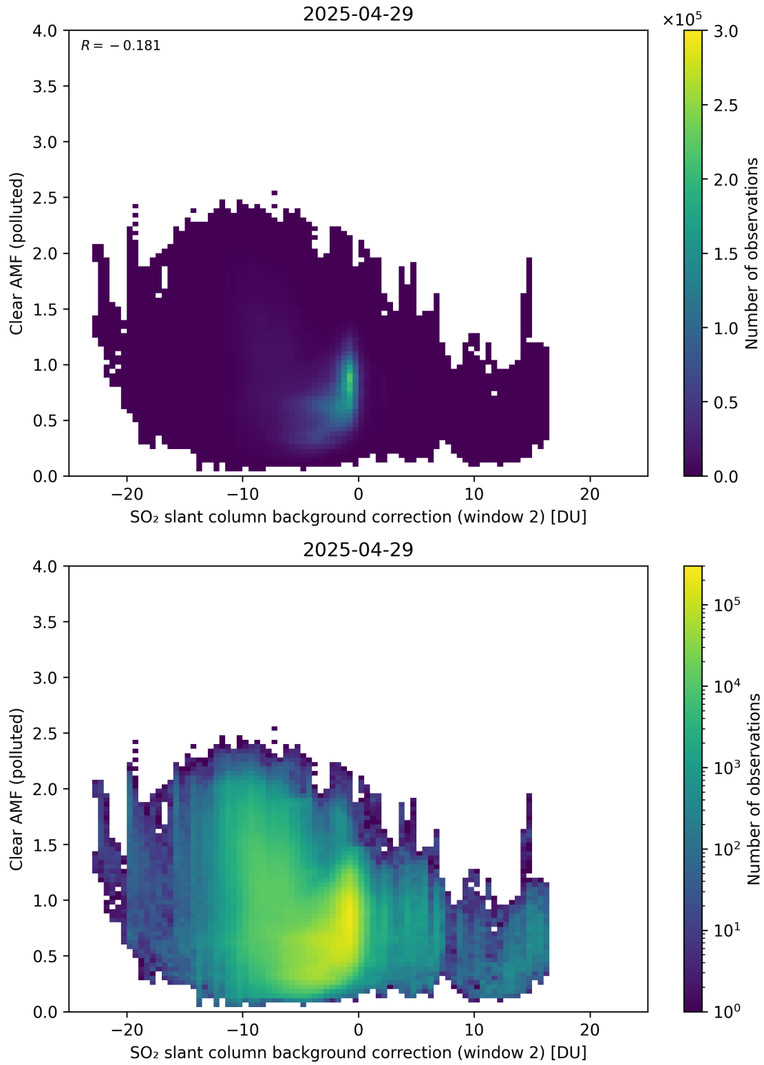
Figure 126: Scatter density plot of “SO 2 slant column background correction (window 2)” against “Clear AMF (polluted)” for 2025-04-29 to 2025-04-30.
