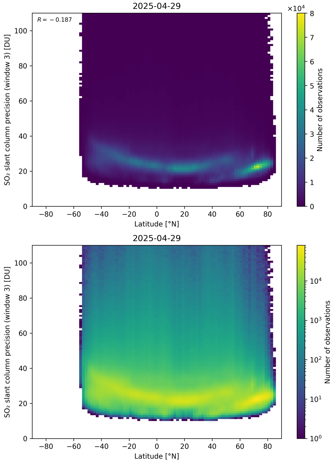
Figure 166: Scatter density plot of “Latitude” against “SO 2 slant column precision (window 3)” for 2025-04-29 to 2025-04-30.
