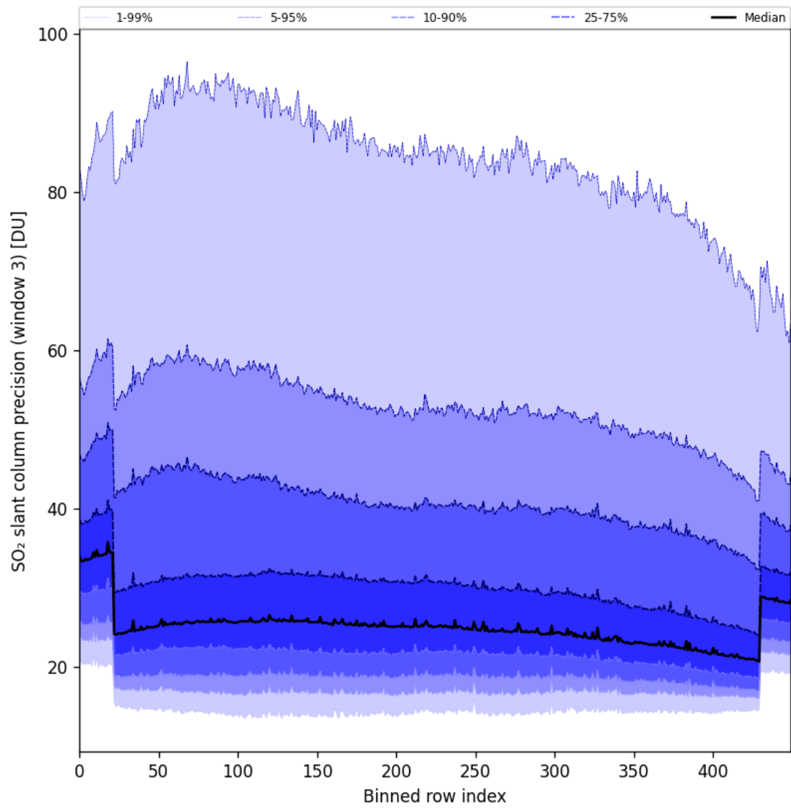
Figure 98: Along track statistics of “SO 2 slant column precision (window 3)” for 2025-04-29 to 2025-04-30
