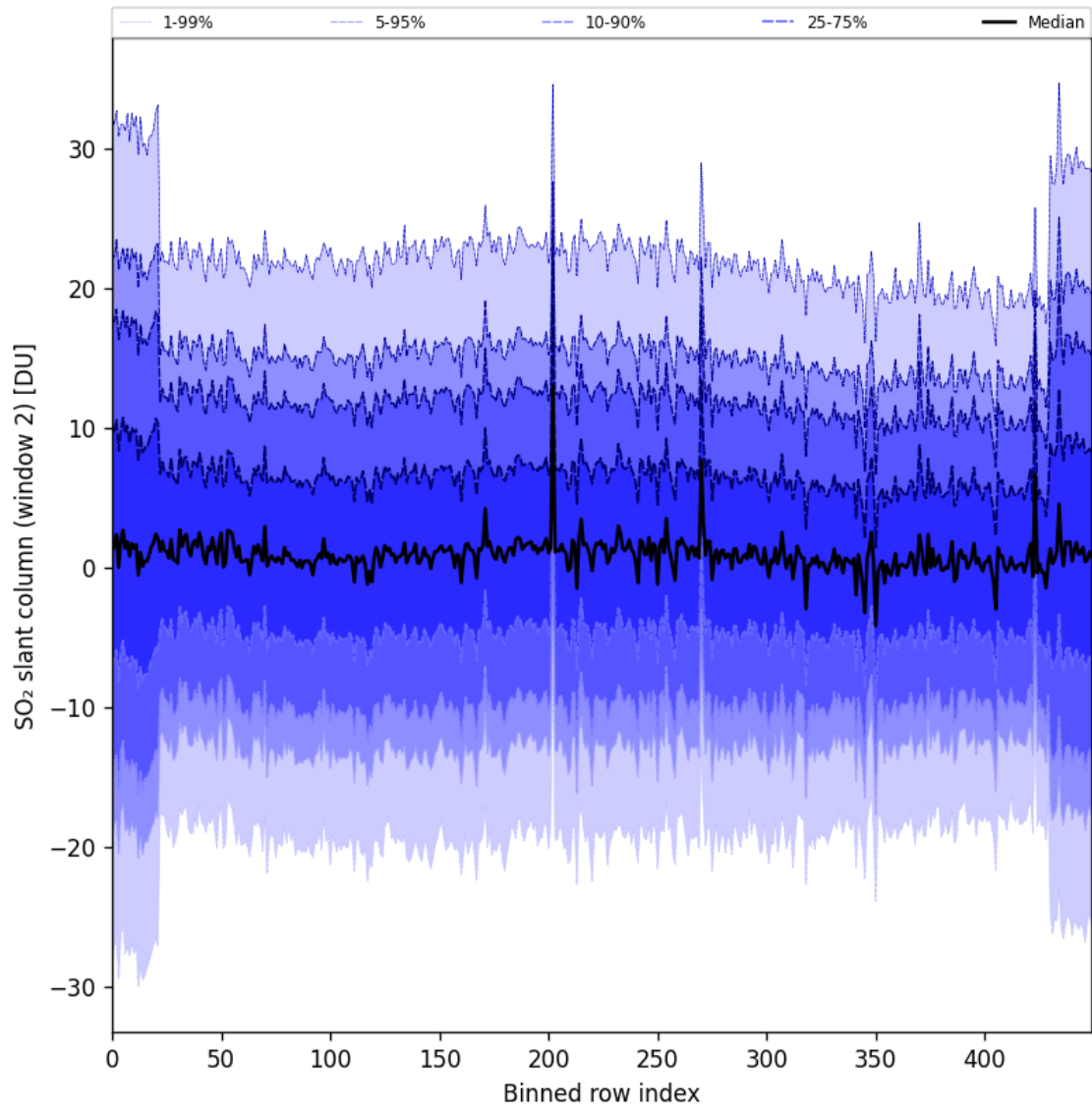
Figure 93: Along track statistics of “SO 2 slant column (window 2)” for 2025-04-29 to 2025-04-30
