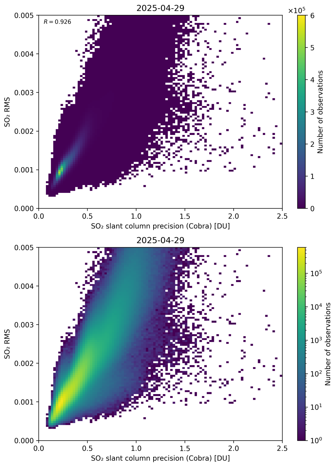
Figure 204: Scatter density plot of “SO 2 slant column precision (Cobra)” against “SO 2 RMS” for 2025-04-29 to 2025-04-30.
