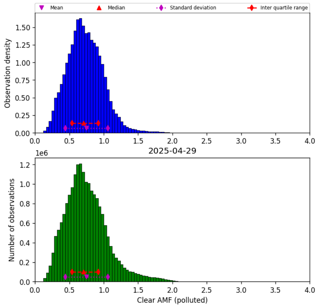
Figure 81: Histogram of “Clear AMF (polluted)” for 2025-04-29 to 2025-04-30
