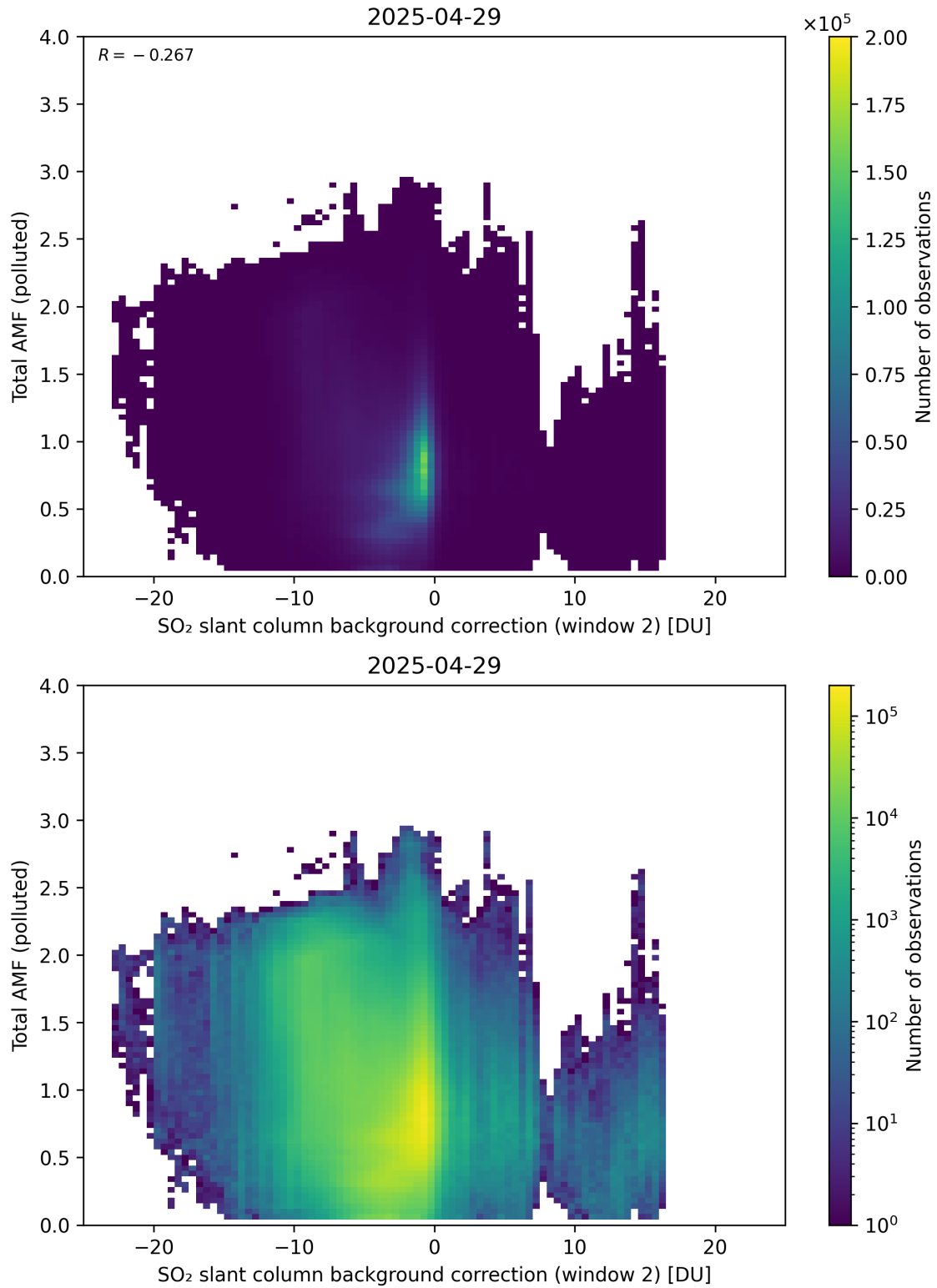
Figure 130: Scatter density plot of “SO 2 slant column background correction (window 2)” against “Total AMF (polluted)” for 2025-04-29 to 2025-04-30.
