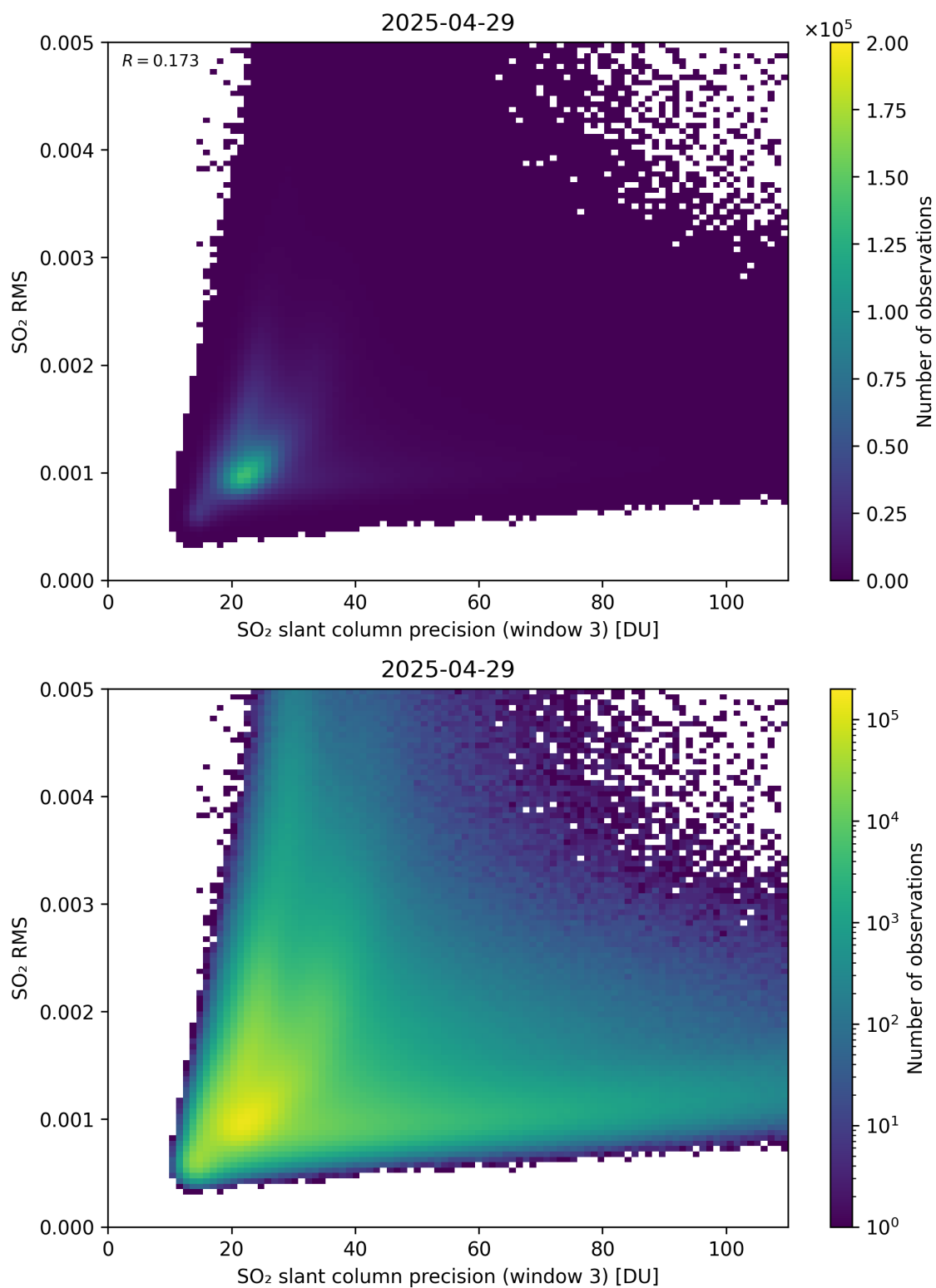
Figure 310: Scatter density plot of “SO 2 slant column precision (window 3)” against “SO 2 RMS” for 2025-04-29 to 2025-04-30.
