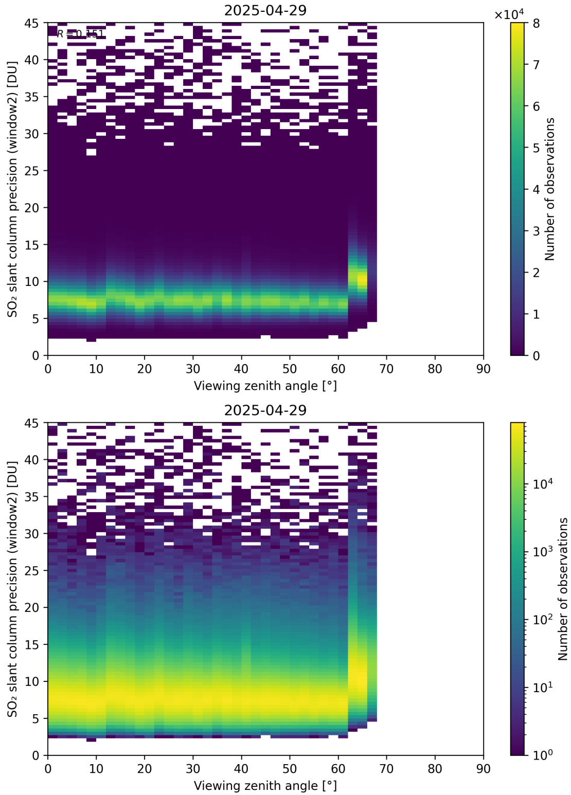
Figure 378: Scatter density plot of “Viewing zenith angle” against “SO 2 slant column precision (window2)” for 2025-04-29 to 2025-04-30.
