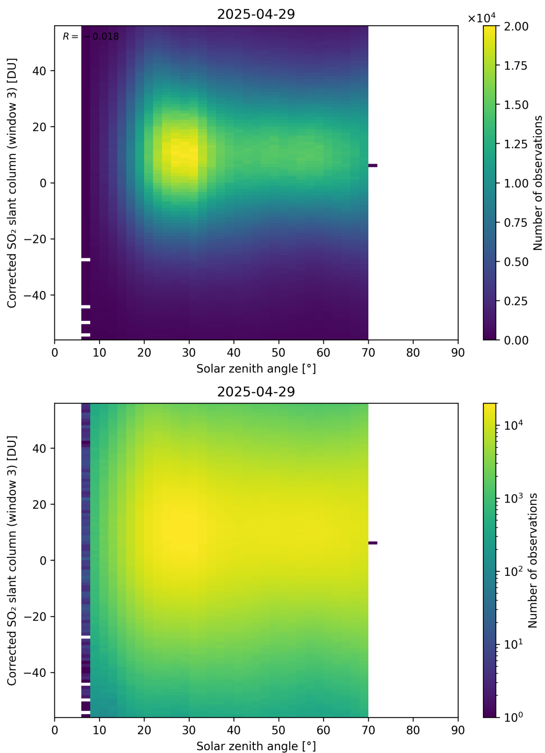
Figure 183: Scatter density plot of “Solar zenith angle” against “Corrected SO 2 slant column (window 3)” for 2025-04-29 to 2025-04-30.
