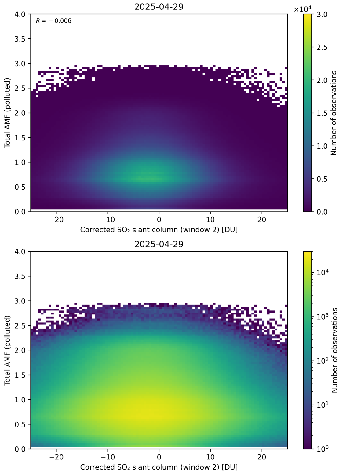
Figure 253: Scatter density plot of “Corrected SO 2 slant column (window 2)” against “Total AMF (polluted)” for 2025-04-29 to 2025-04-30.
