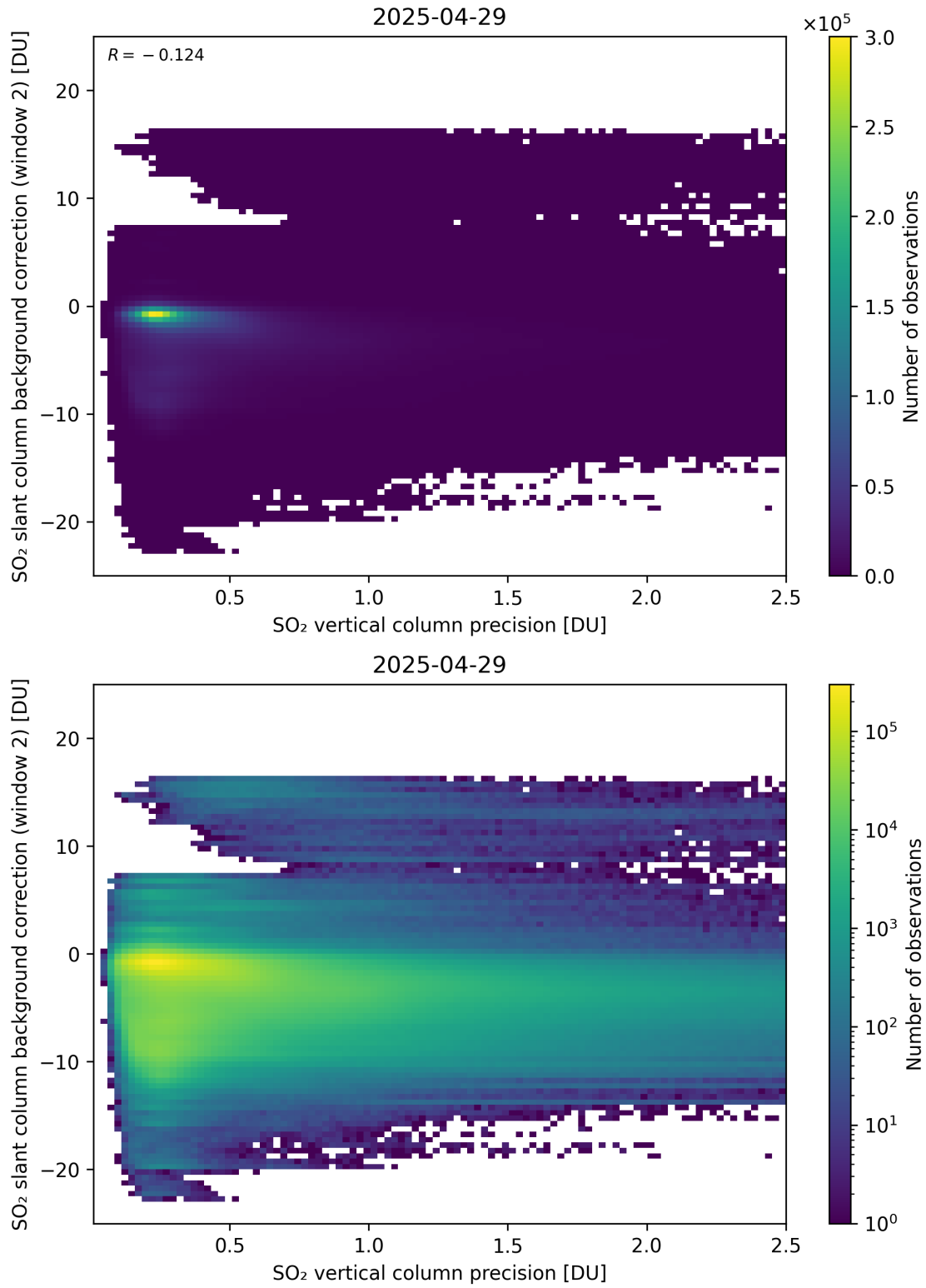
Figure 330: Scatter density plot of “SO 2 vertical column precision” against “SO 2 slant column background correction (window 2)” for 2025-04-29 to 2025-04-30.
