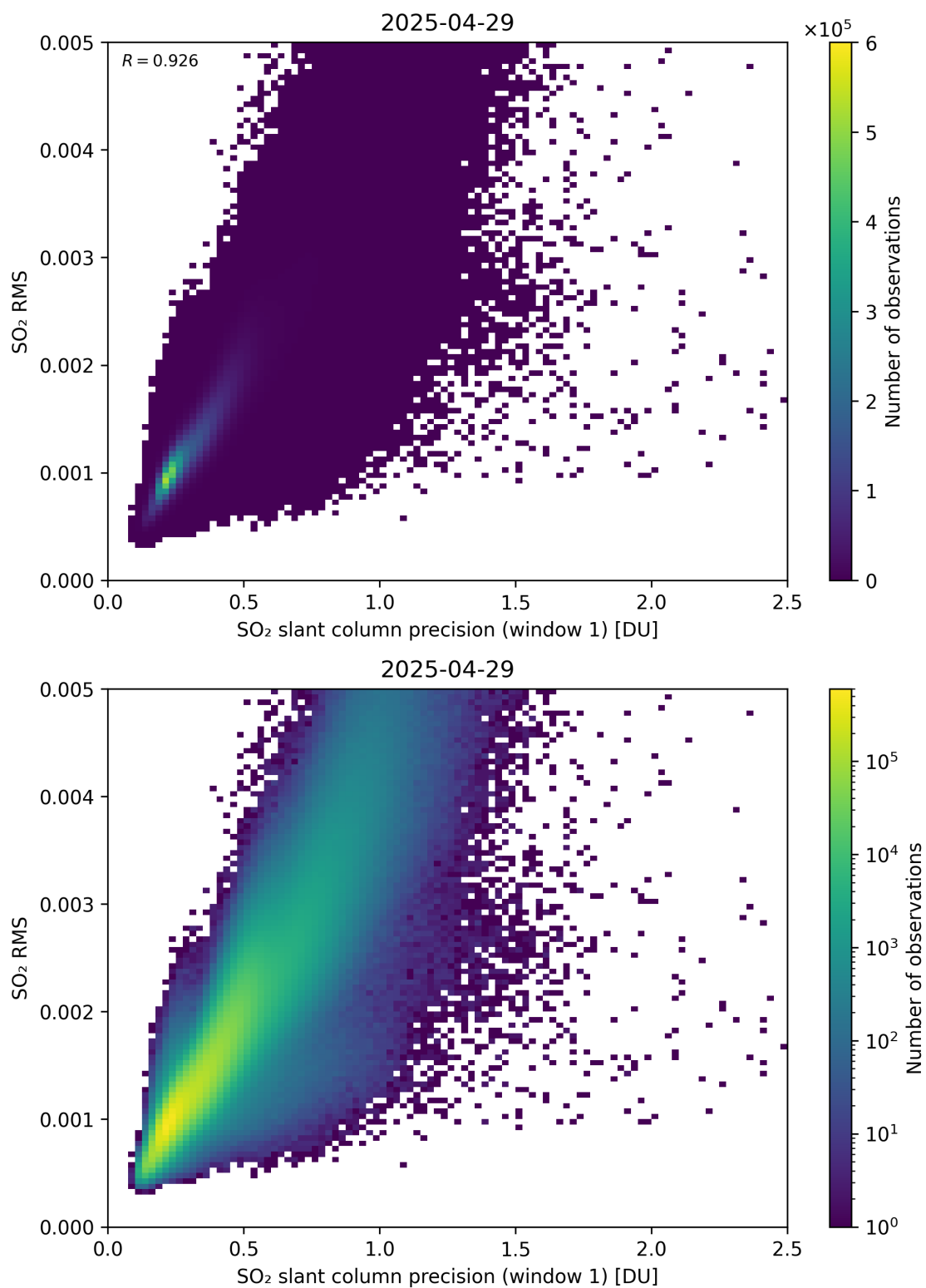
Figure 273: Scatter density plot of “SO 2 slant column precision (window 1)” against “SO 2 RMS” for 2025-04-29 to 2025-04-30.
