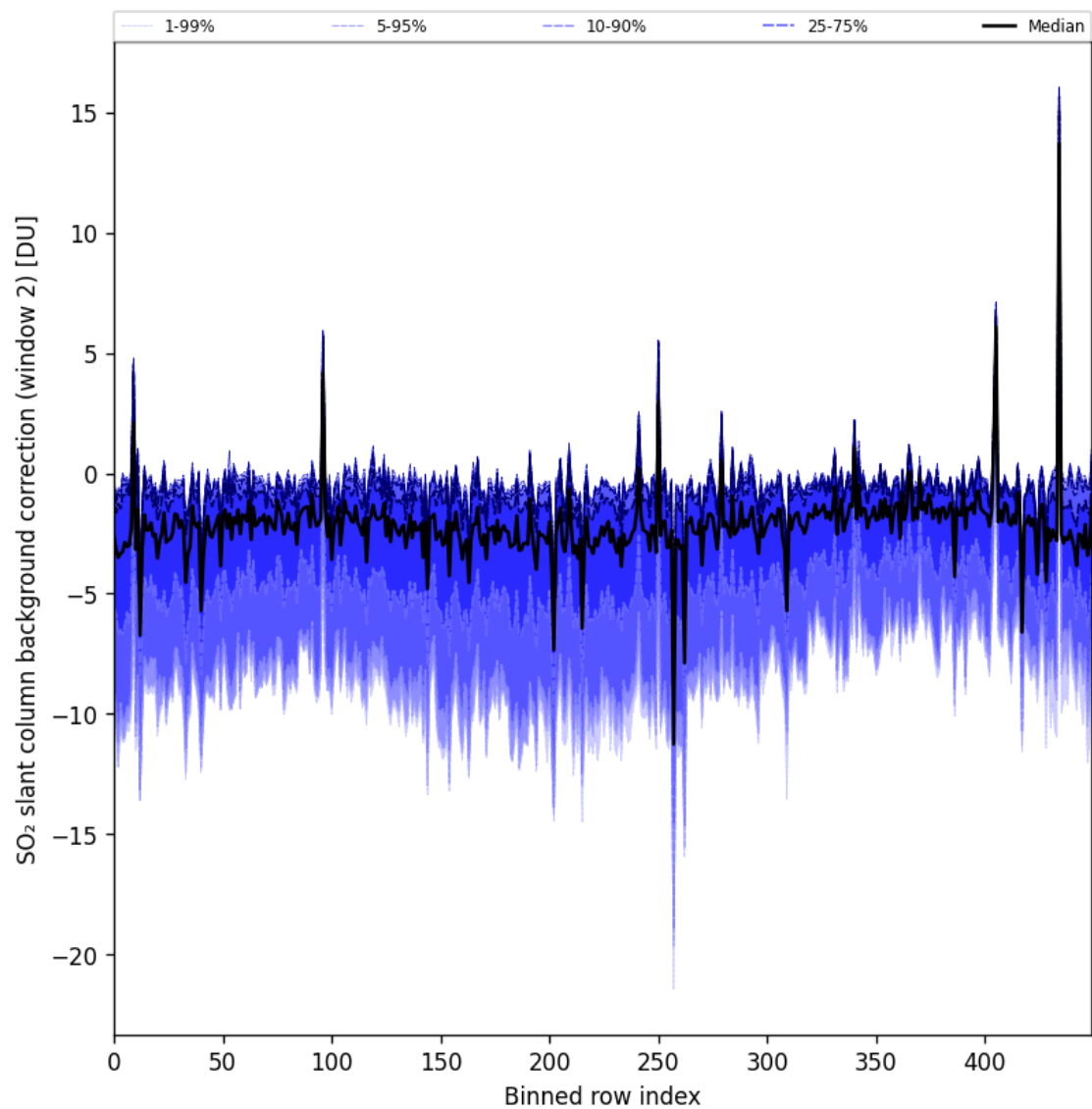
Figure 96: Along track statistics of “SO 2 slant column background correction (window 2)” for 2025-04-29 to 2025-04-30
