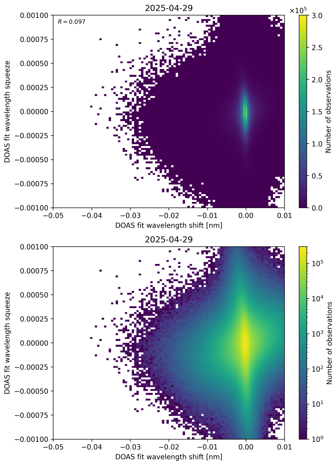
Figure 138: Scatter density plot of “DOAS fit wavelength shift” against “DOAS fit wavelength squeeze” for 2025-04-29 to 2025-04-30.
