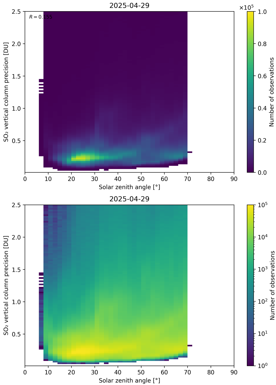
Figure 192: Scatter density plot of “Solar zenith angle” against “SO 2 vertical column precision” for 2025-04-29 to 2025-04-30.
