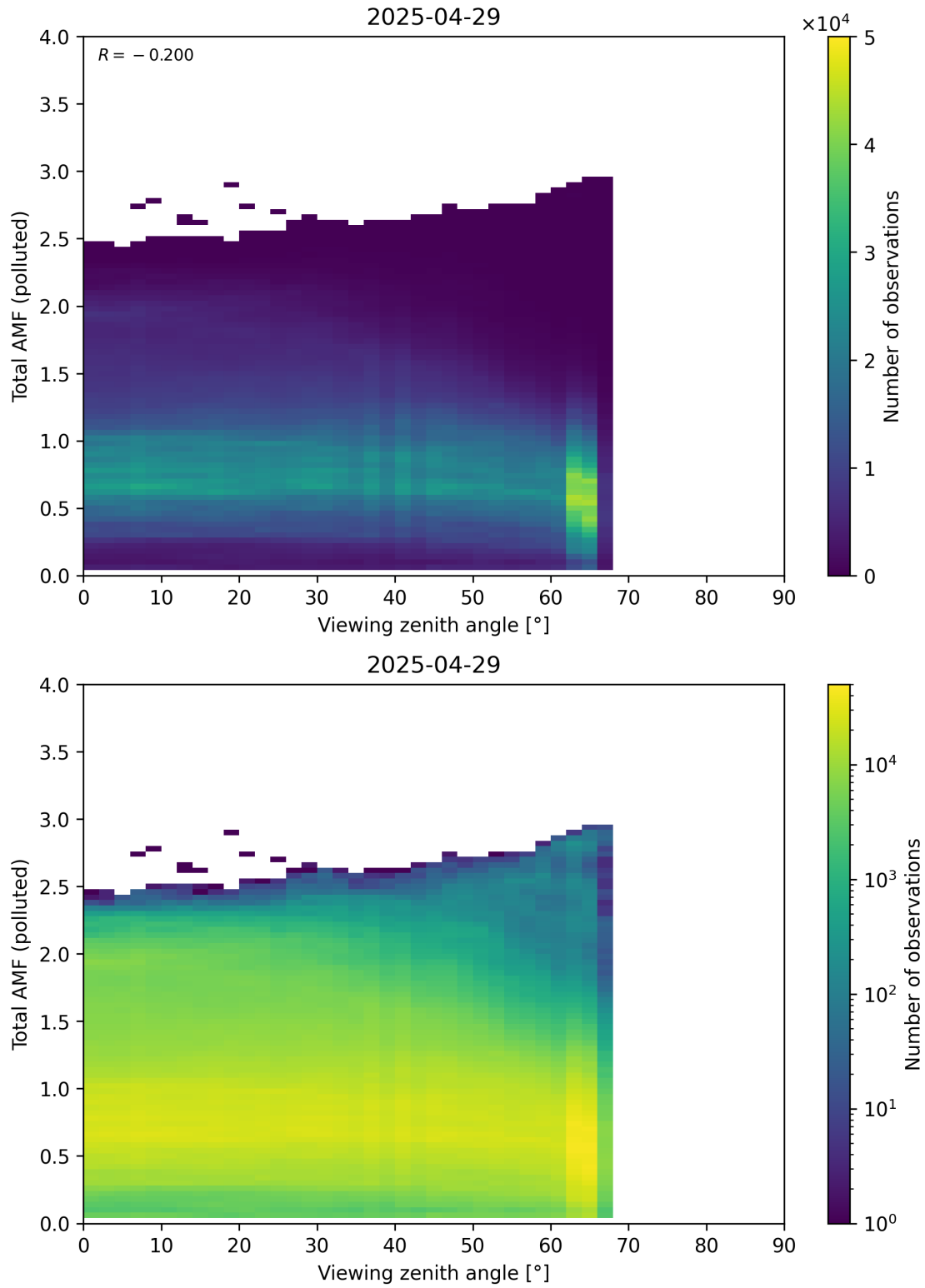
Figure 381: Scatter density plot of “Viewing zenith angle” against “Total AMF (polluted)” for 2025-04-29 to 2025-04-30.
