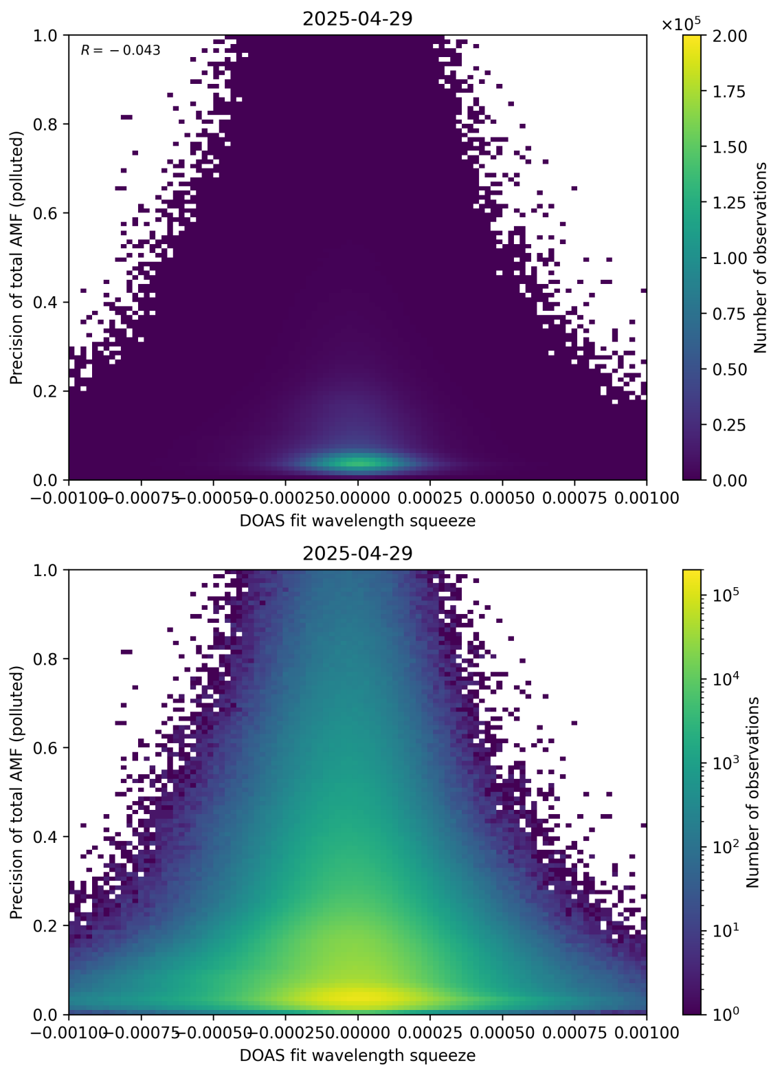
Figure 146: Scatter density plot of “DOAS fit wavelength squeeze” against “Precision of total AMF (polluted)” for 2025-04-29 to 2025-04-30.
