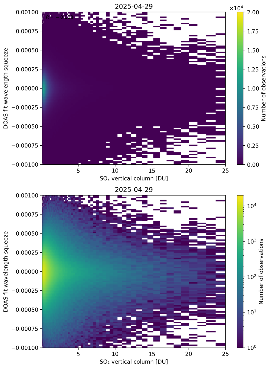
Figure 327: Scatter density plot of “SO 2 vertical column” against “DOAS fit wavelength squeeze” for 2025-04-29 to 2025-04-30.
