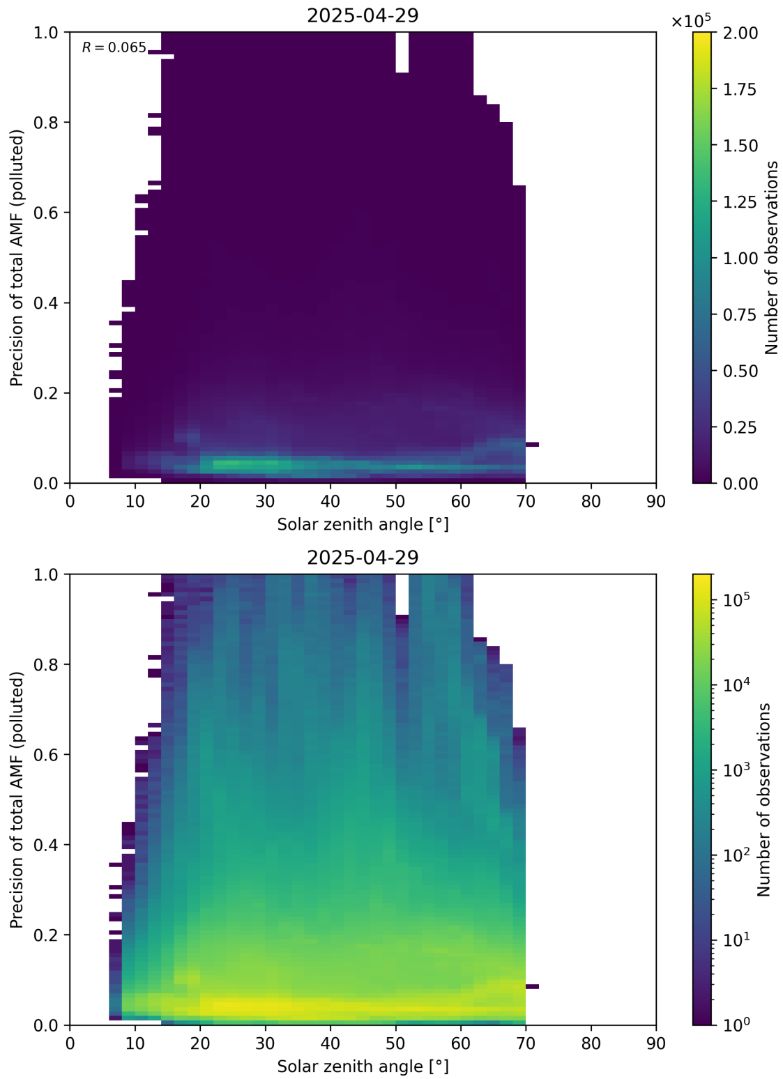
Figure 190: Scatter density plot of “Solar zenith angle” against “Precision of total AMF (polluted)” for 2025-04-29 to 2025-04-30.
