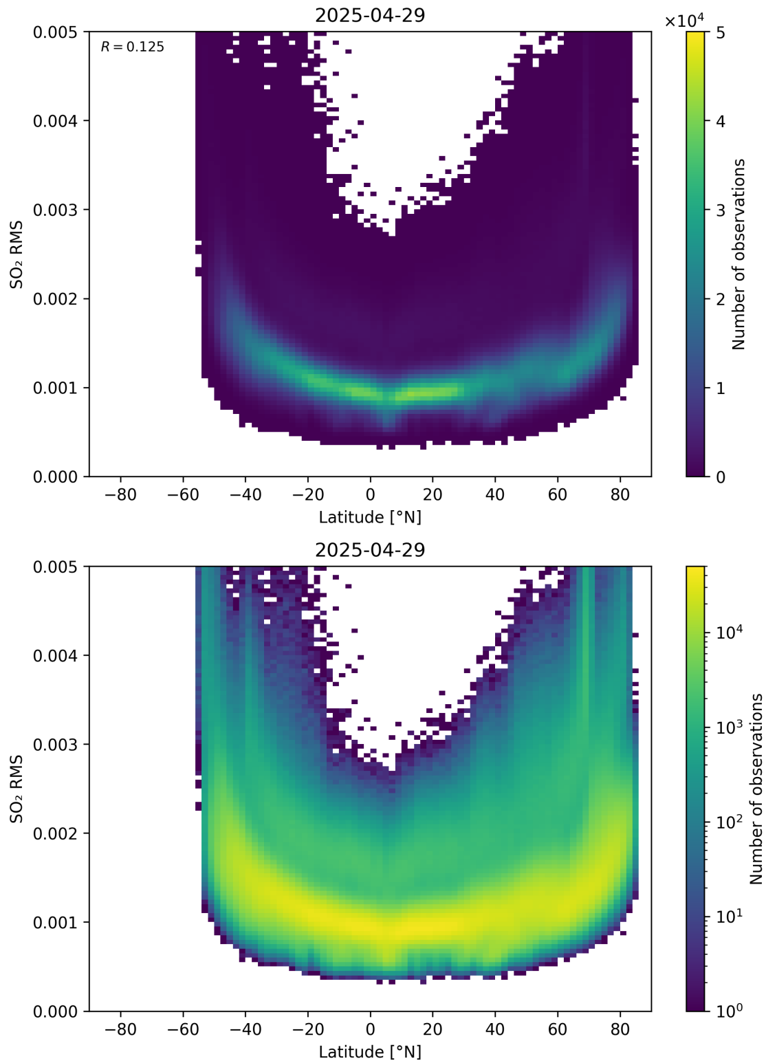
Figure 155: Scatter density plot of “Latitude” against “SO 2 RMS” for 2025-04-29 to 2025-04-30.
