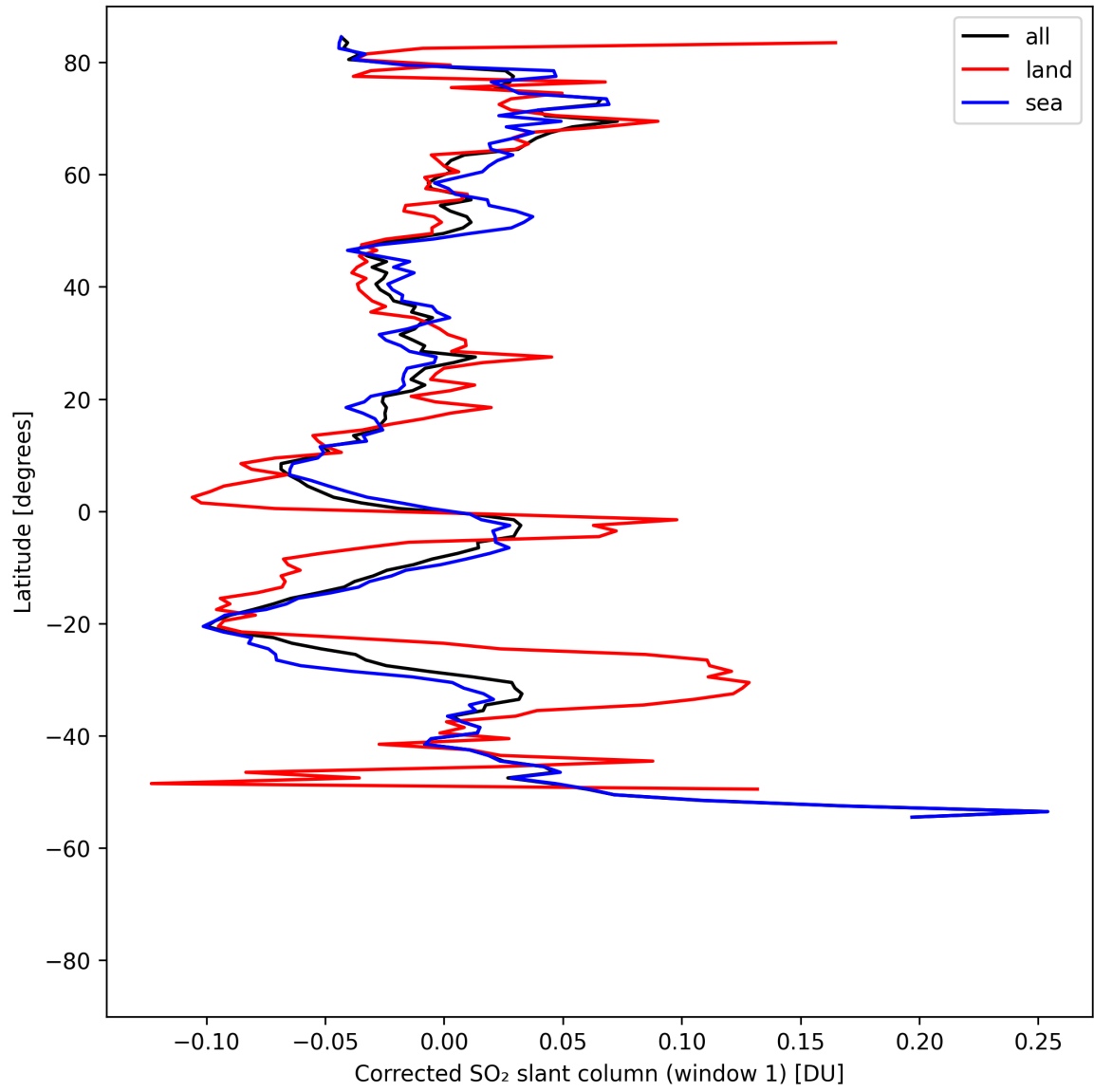
Figure 39: Zonal average of “Corrected SO 2 slant column (window 1)” for 2025-04-29 to 2025-04-30.
