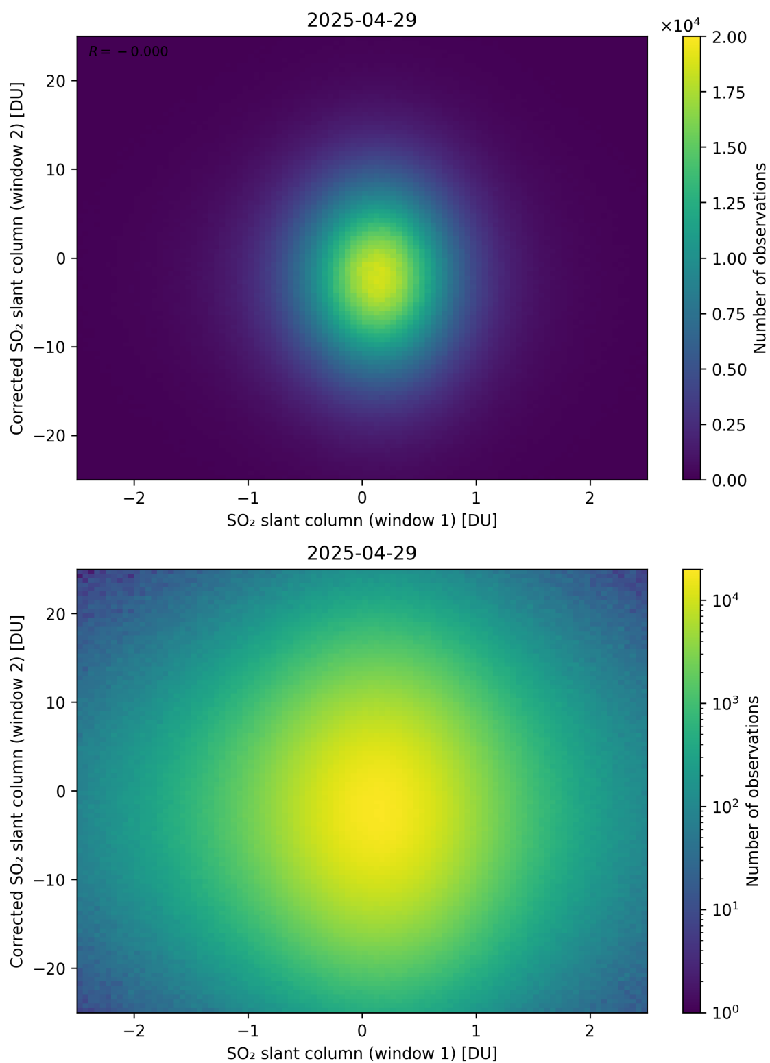
Figure 283: Scatter density plot of “SO 2 slant column (window 1)” against “Corrected SO 2 slant column (window 2)” for 2025-04-29 to 2025-04-30.
