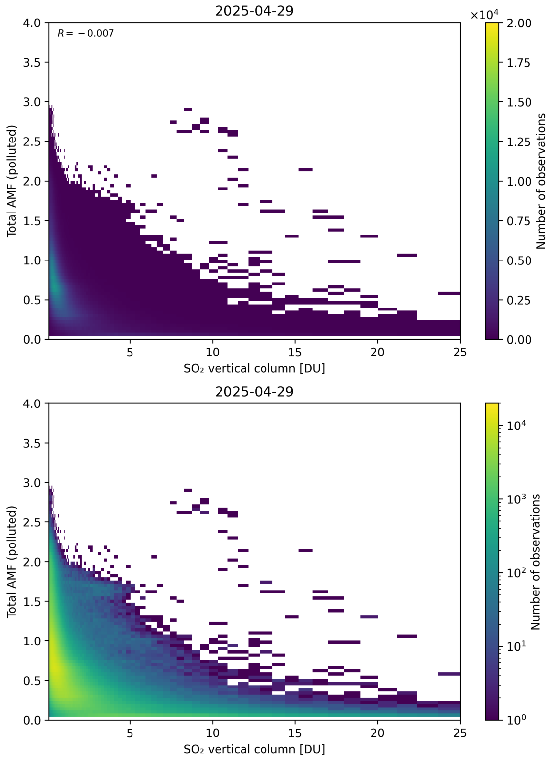
Figure 359: Scatter density plot of “SO 2 vertical column” against “Total AMF (polluted)” for 2025-04-29 to 2025-04-30.
