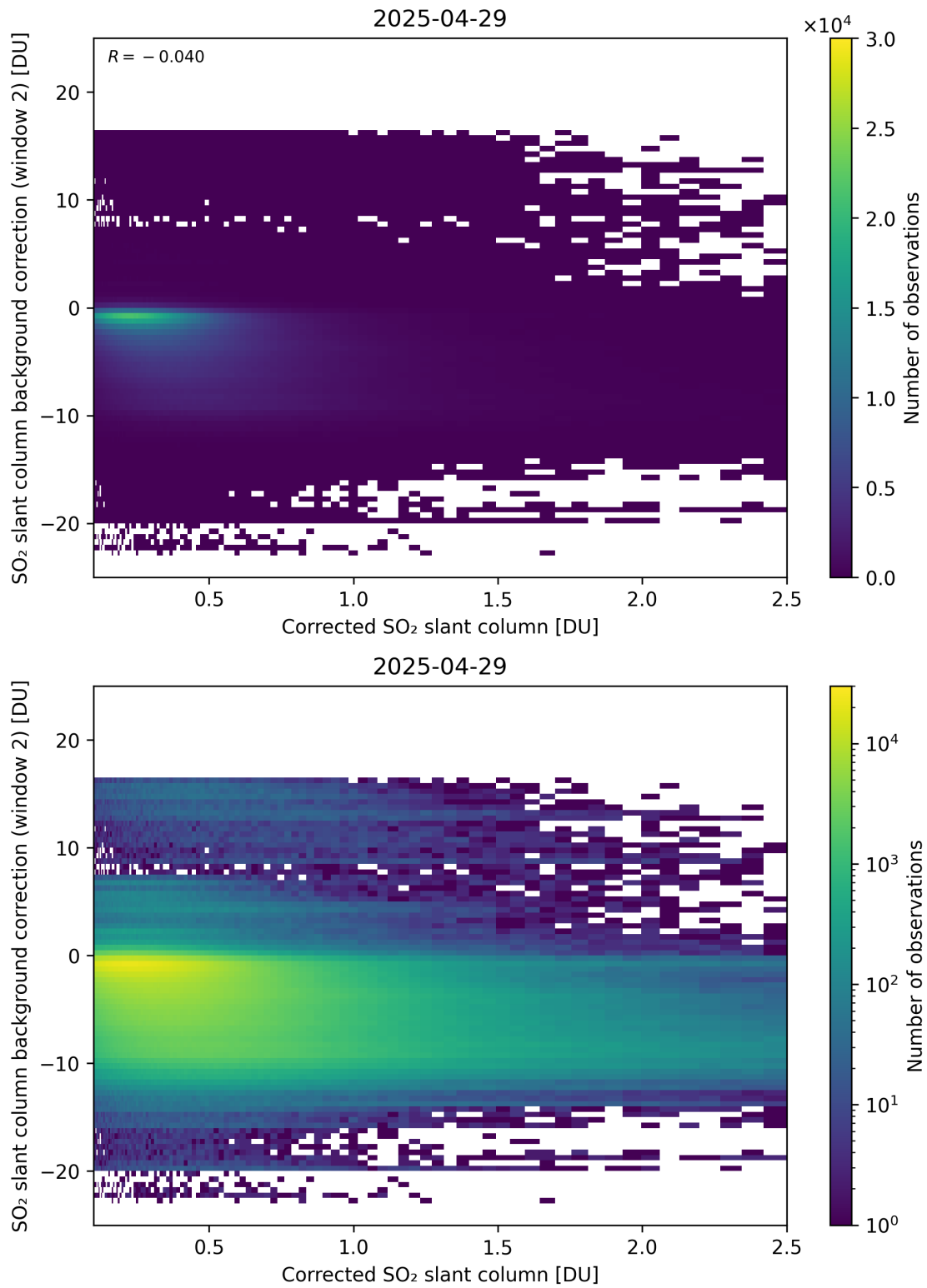
Figure 227: Scatter density plot of “Corrected SO 2 slant column” against “SO 2 slant column background correction (window 2)” for 2025-04-29 to 2025-04-30.
