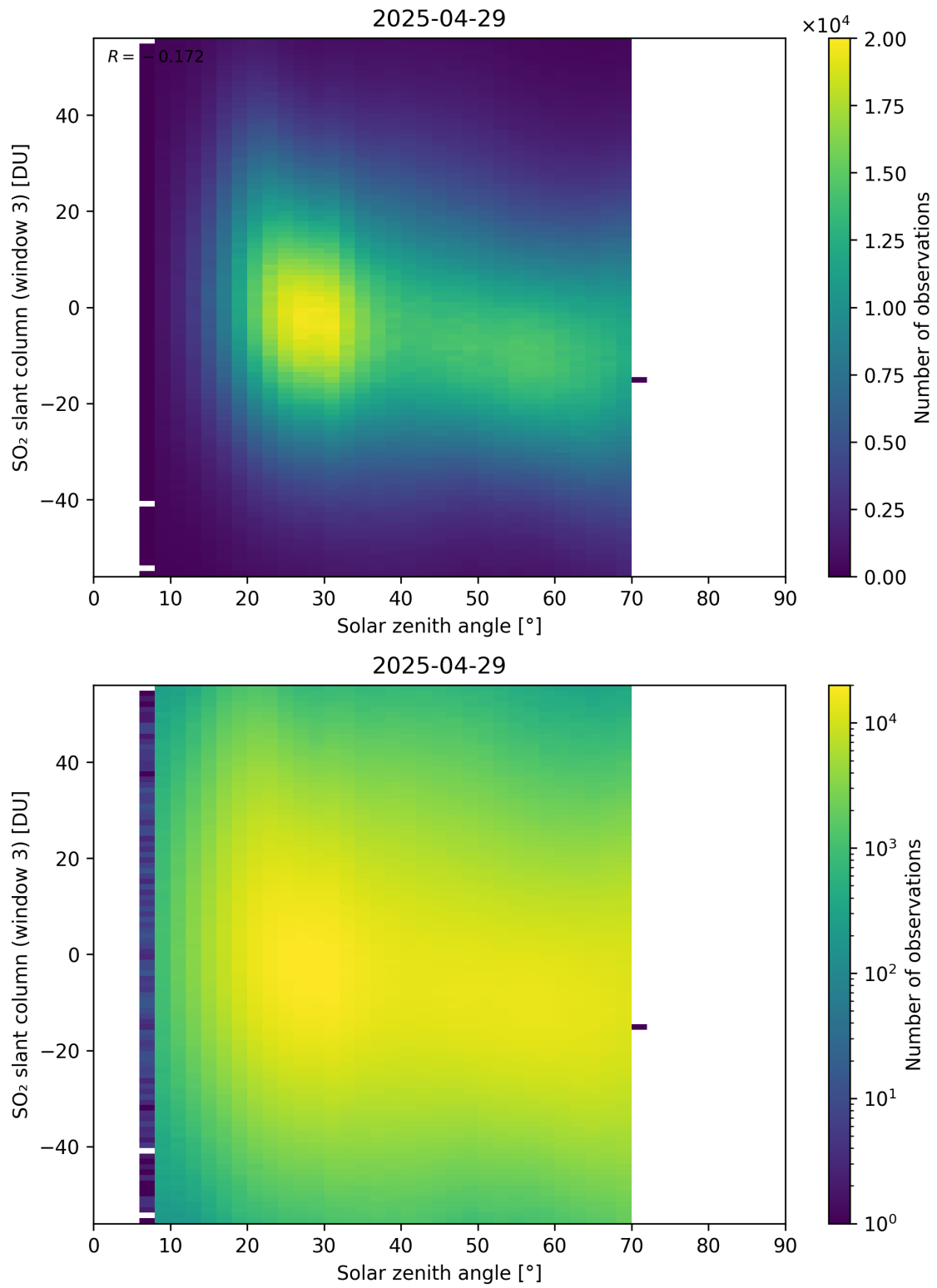
Figure 187: Scatter density plot of “Solar zenith angle” against “SO 2 slant column (window 3)” for 2025-04-29 to 2025-04-30.
