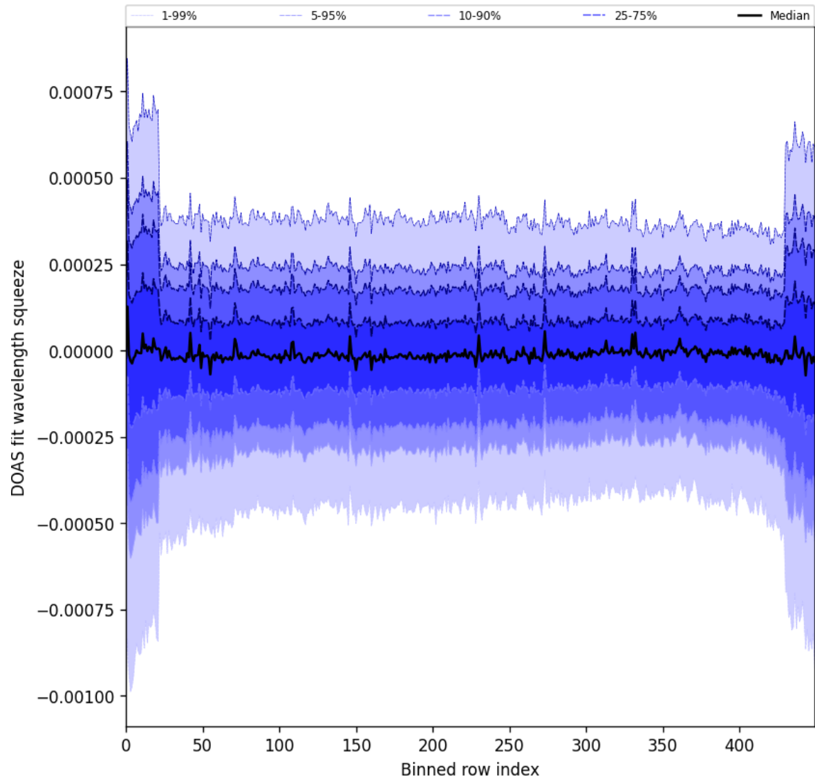
Figure 103: Along track statistics of “DOAS fit wavelength squeeze” for 2025-04-29 to 2025-04-30
