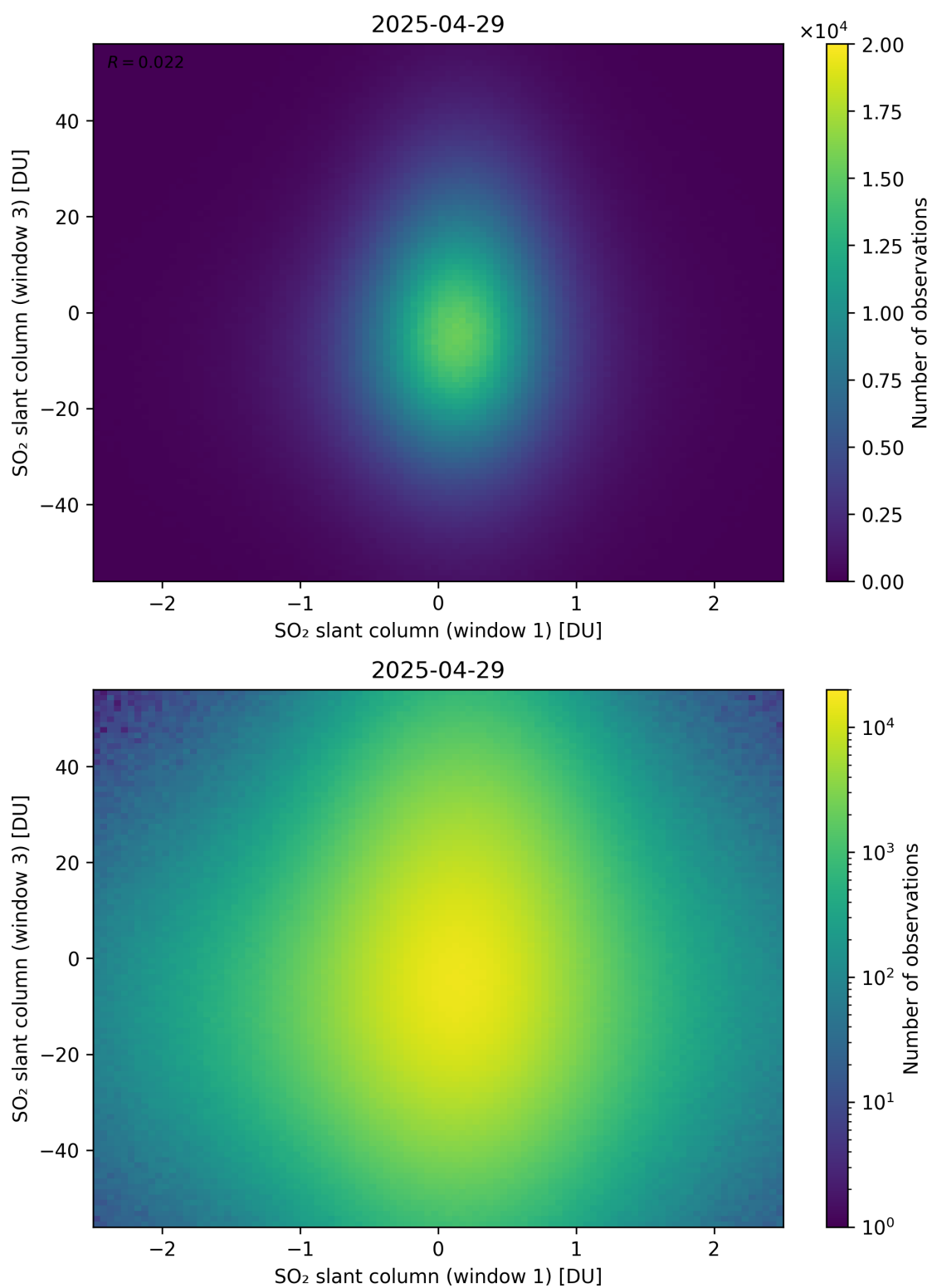
Figure 287: Scatter density plot of “SO 2 slant column (window 1)” against “SO 2 slant column (window 3)” for 2025-04-29 to 2025-04-30.
