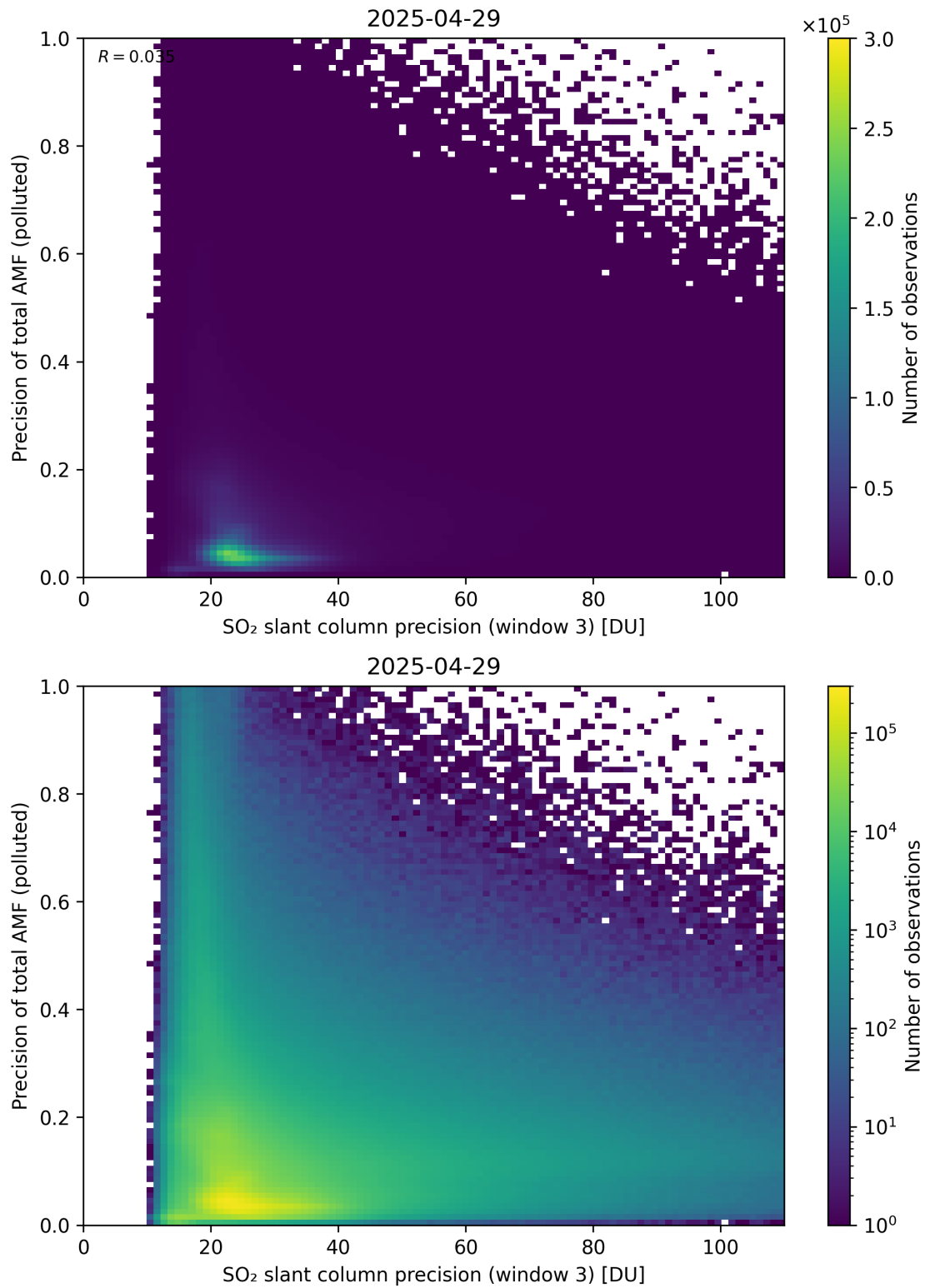
Figure 314: Scatter density plot of “SO 2 slant column precision (window 3)” against “Precision of total AMF (polluted)” for 2025-04-29 to 2025-04-30.
