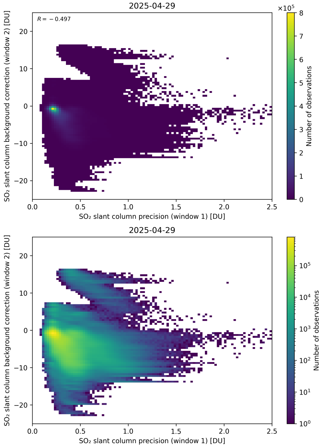
Figure 269: Scatter density plot of “SO 2 slant column precision (window 1)” against “SO 2 slant column background correction (window 2)” for 2025-04-29 to 2025-04-30.
