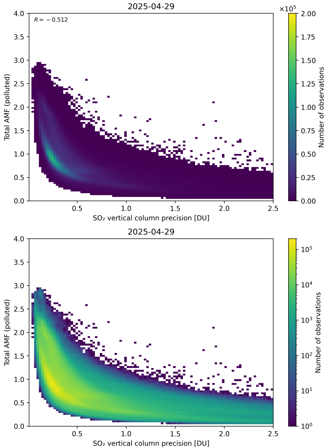
Figure 346: Scatter density plot of “SO 2 vertical column precision” against “Total AMF (polluted)” for 2025-04-29 to 2025-04-30.
