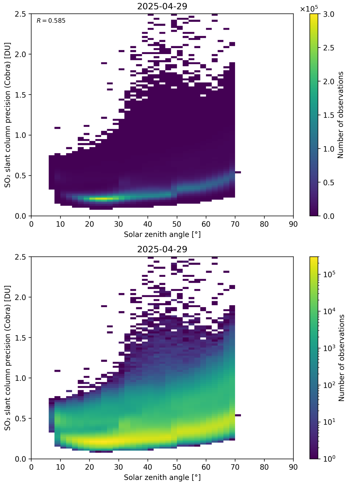
Figure 180: Scatter density plot of “Solar zenith angle” against “SO 2 slant column precision (Cobra)” for 2025-04-29 to 2025-04-30.
