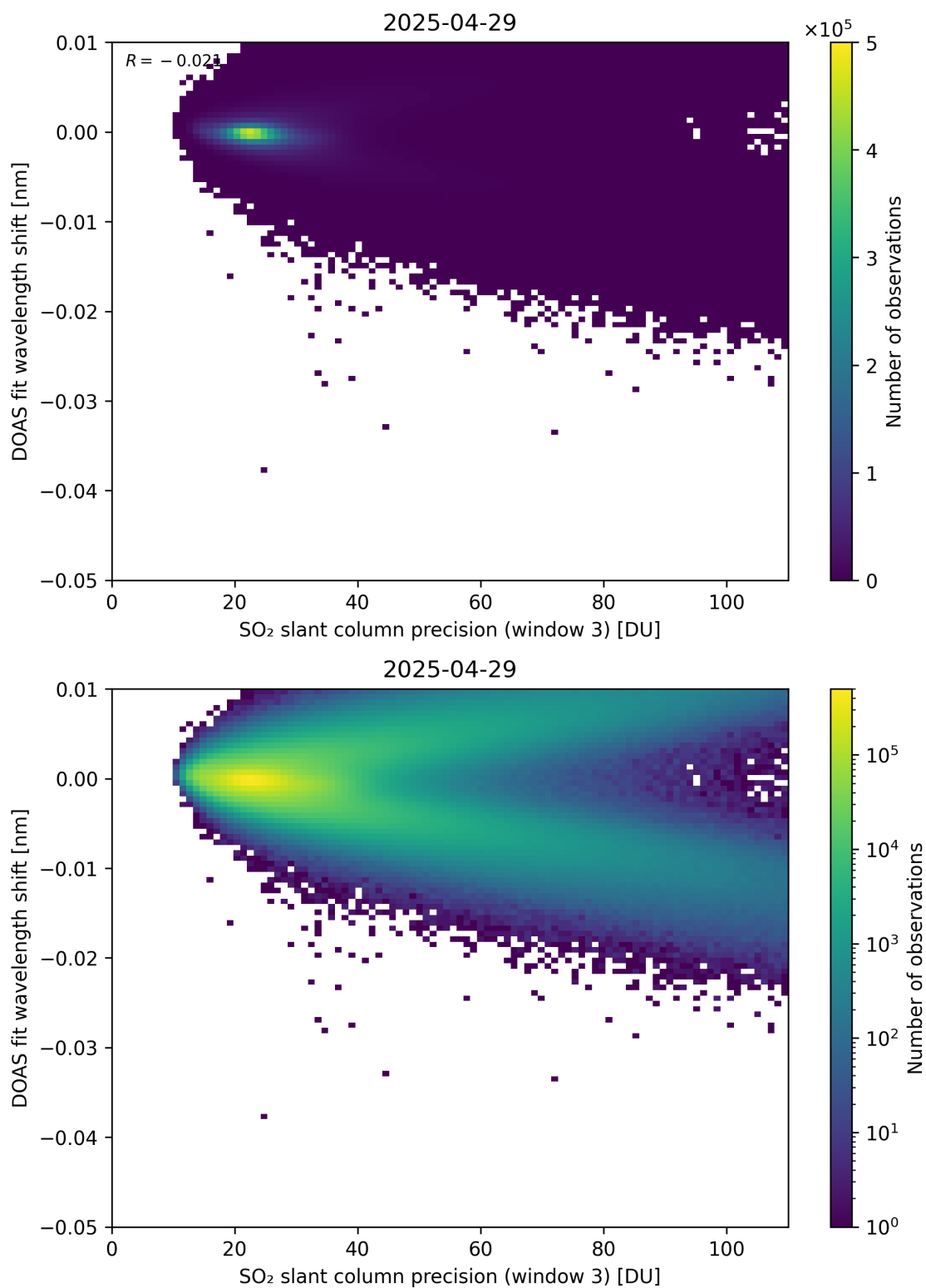
Figure 308: Scatter density plot of “SO 2 slant column precision (window 3)” against “DOAS fit wavelength shift” for 2025-04-29 to 2025-04-30.
