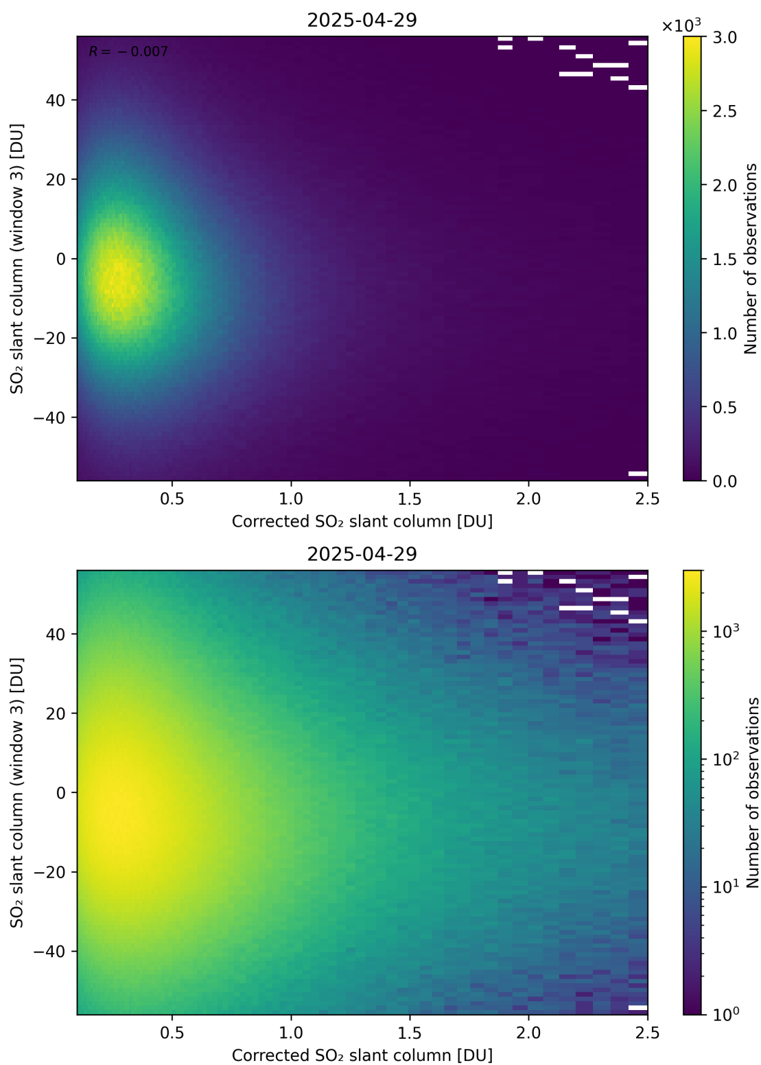
Figure 240: Scatter density plot of “Corrected SO 2 slant column” against “SO 2 slant column (window 3)” for 2025-04-29 to 2025-04-30.
