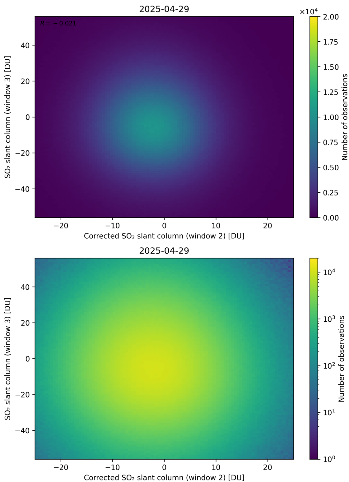
Figure 251: Scatter density plot of “Corrected SO 2 slant column (window 2)” against “SO 2 slant column (window 3)” for 2025-04-29 to 2025-04-30.
