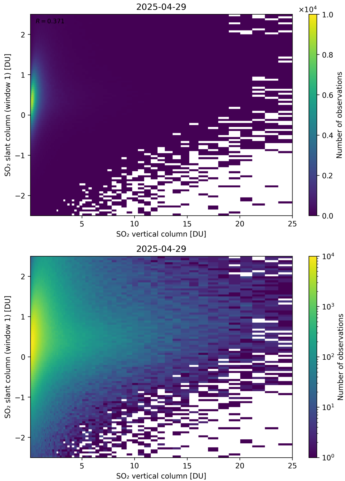
Figure 354: Scatter density plot of “SO 2 vertical column” against “SO 2 slant column (window 1)” for 2025-04-29 to 2025-04-30.
