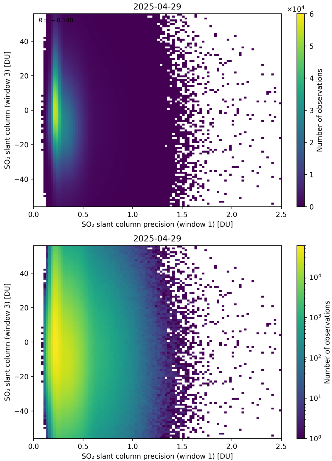
Figure 278: Scatter density plot of “SO 2 slant column precision (window 1)” against “SO 2 slant column (window 3)” for 2025-04-29 to 2025-04-30.
