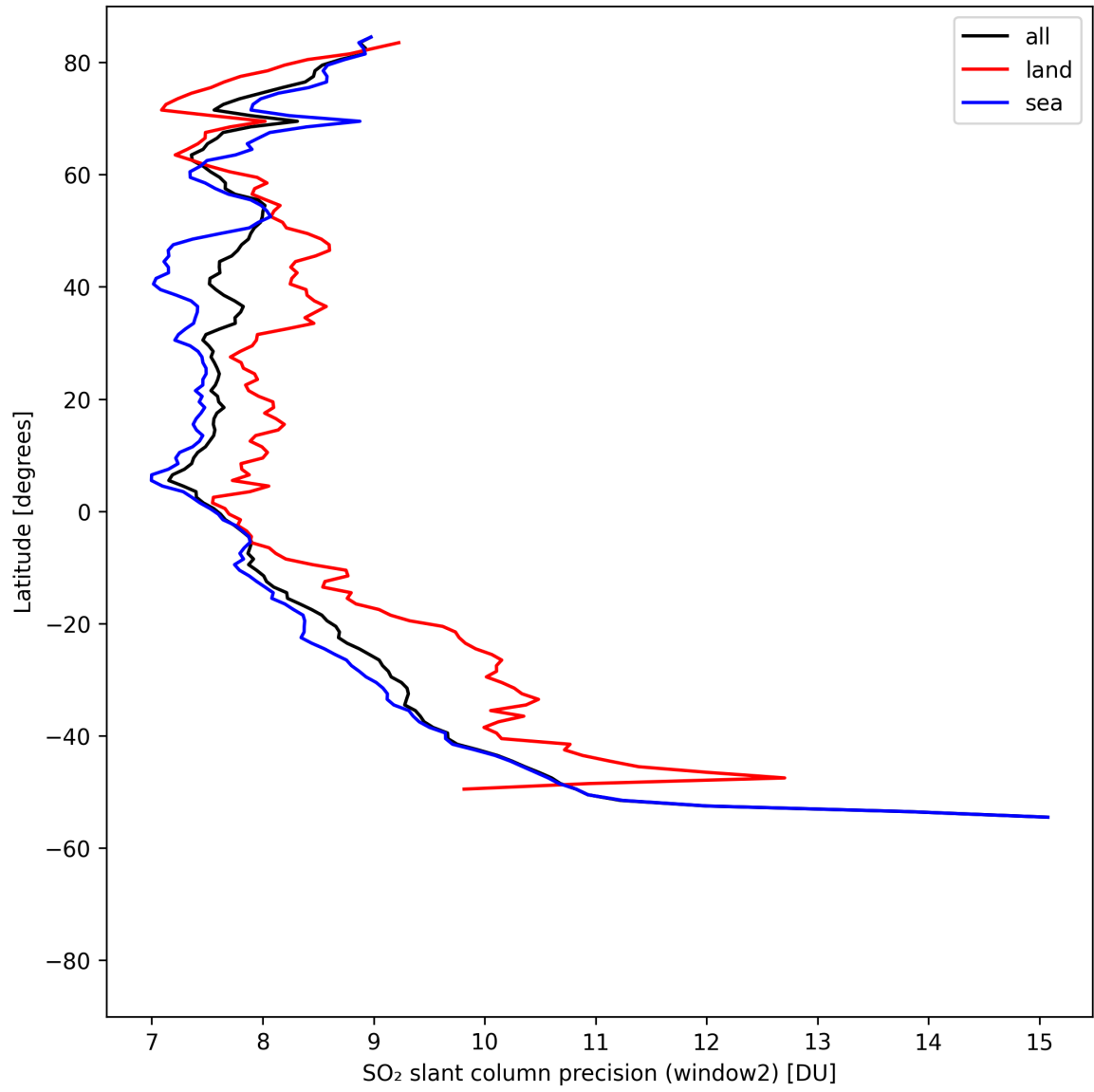
Figure 42: Zonal average of “SO 2 slant column precision (window2)” for 2025-04-29 to 2025-04-30.
