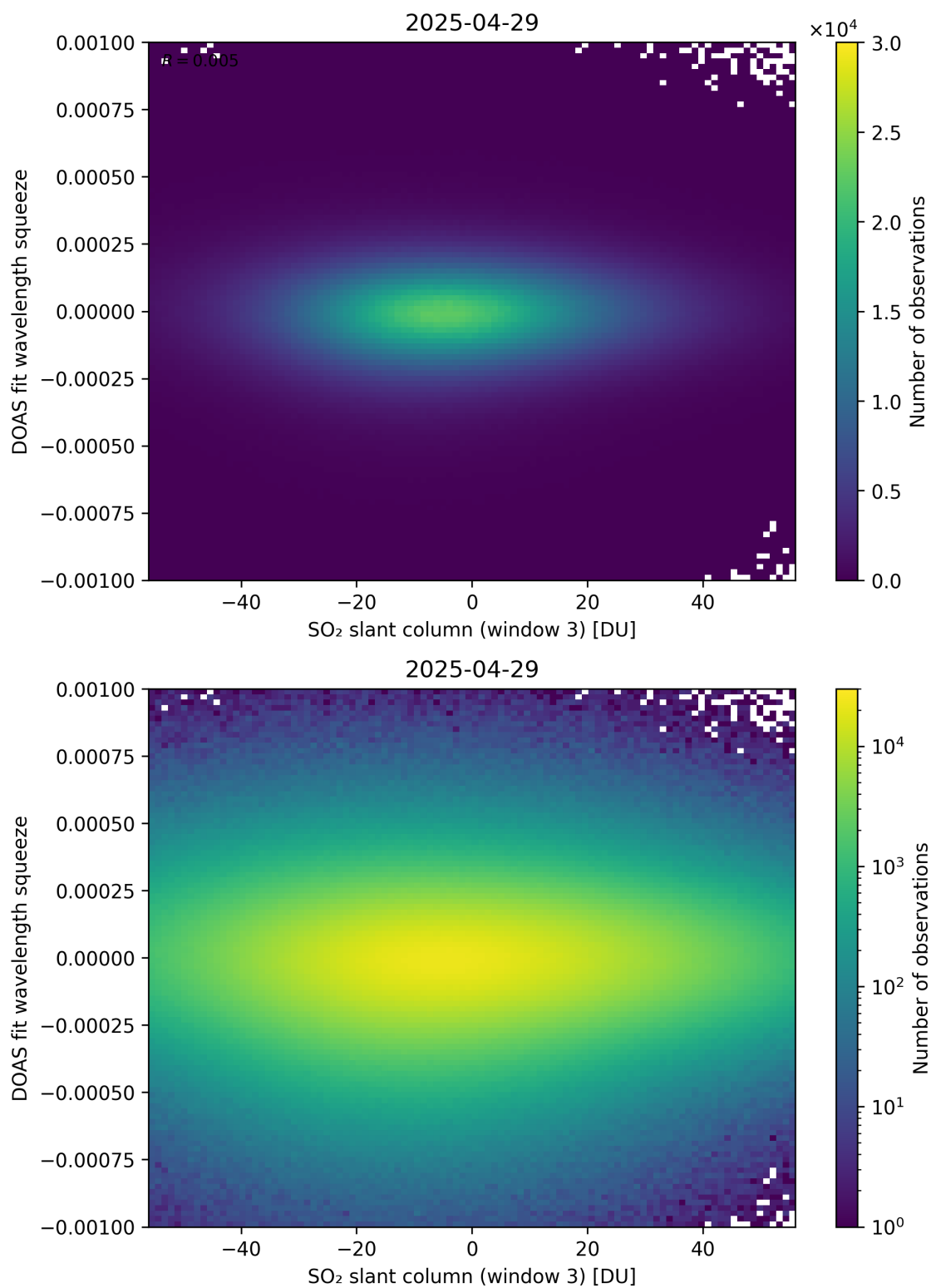
Figure 305: Scatter density plot of “SO 2 slant column (window 3)” against “DOAS fit wavelength squeeze” for 2025-04-29 to 2025-04-30.
