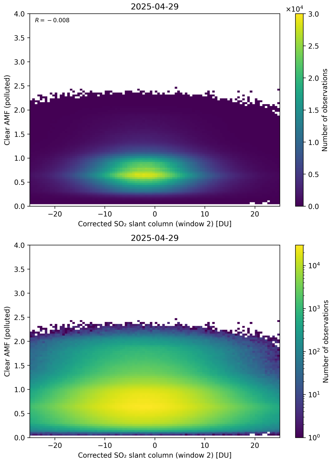
Figure 249: Scatter density plot of “Corrected SO 2 slant column (window 2)” against “Clear AMF (polluted)” for 2025-04-29 to 2025-04-30.
