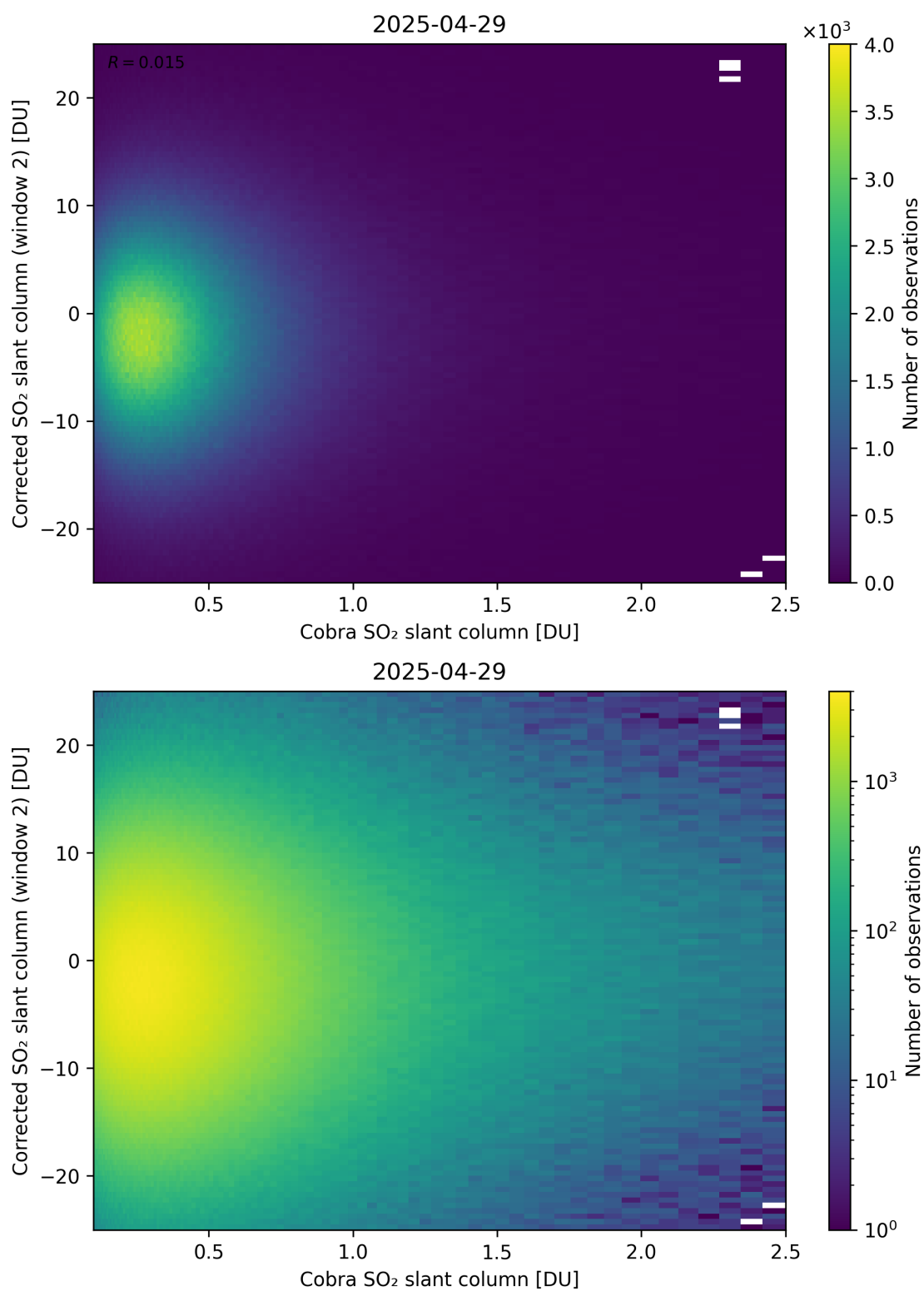
Figure 217: Scatter density plot of “Cobra SO 2 slant column” against “Corrected SO 2 slant column (window 2)” for 2025-04-29 to 2025-04-30.
