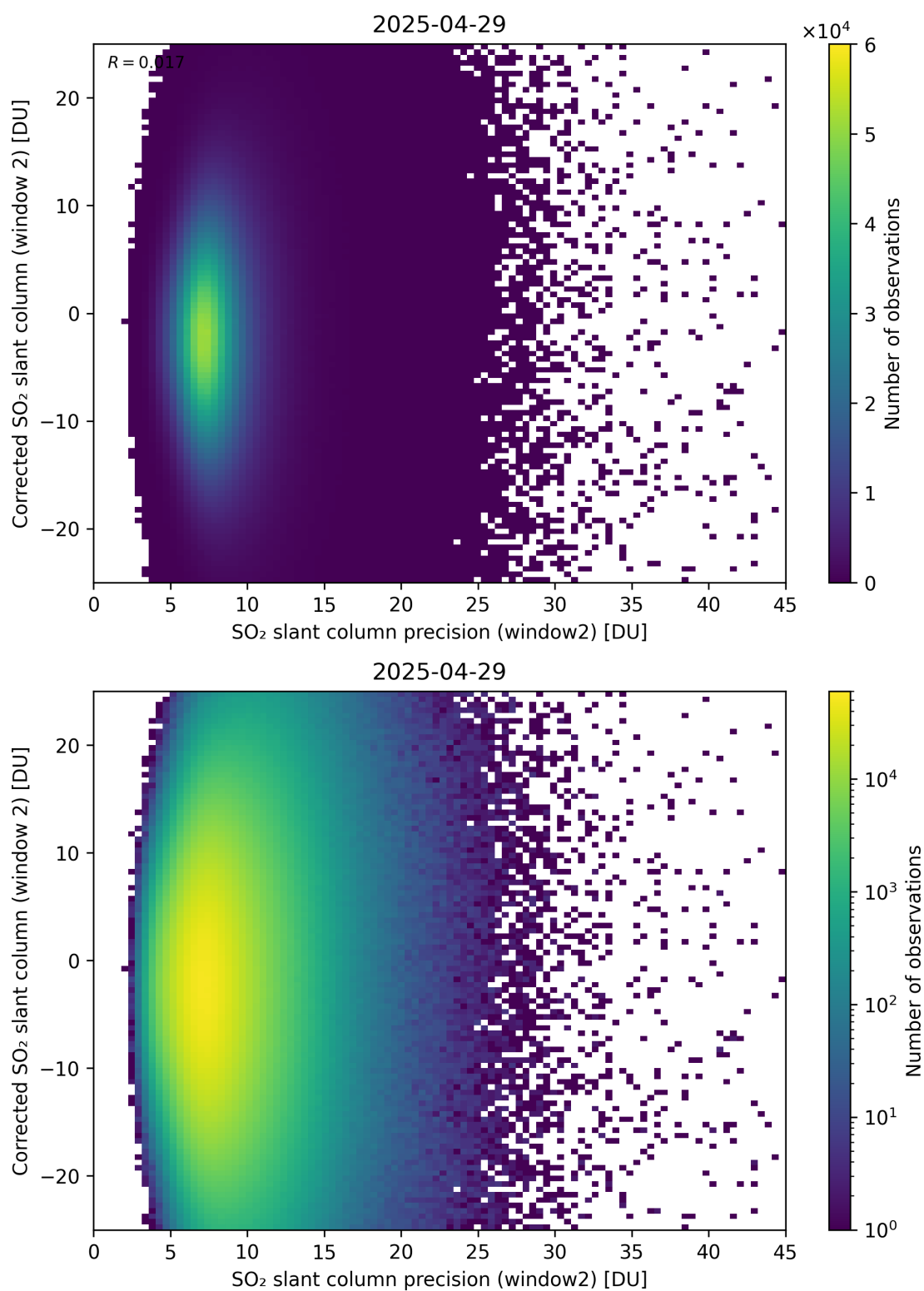
Figure 297: Scatter density plot of “SO 2 slant column precision (window2)” against “Corrected SO 2 slant column (window 2)” for 2025-04-29 to 2025-04-30.
