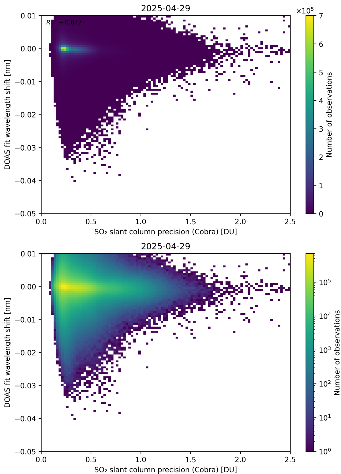
Figure 202: Scatter density plot of “SO 2 slant column precision (Cobra)” against “DOAS fit wavelength shift” for 2025-04-29 to 2025-04-30.
