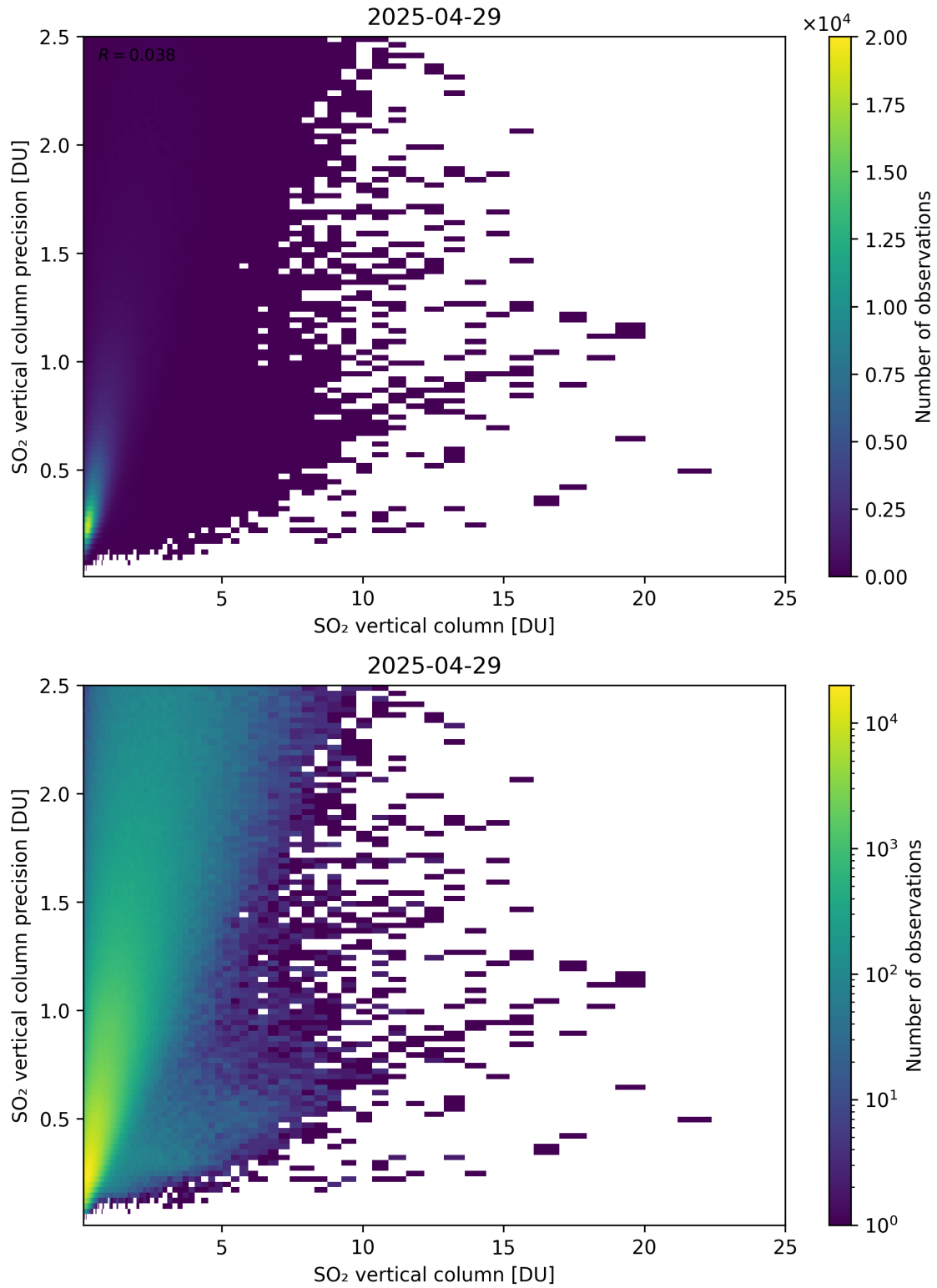
Figure 361: Scatter density plot of “SO 2 vertical column” against “SO 2 vertical column precision” for 2025-04-29 to 2025-04-30.
