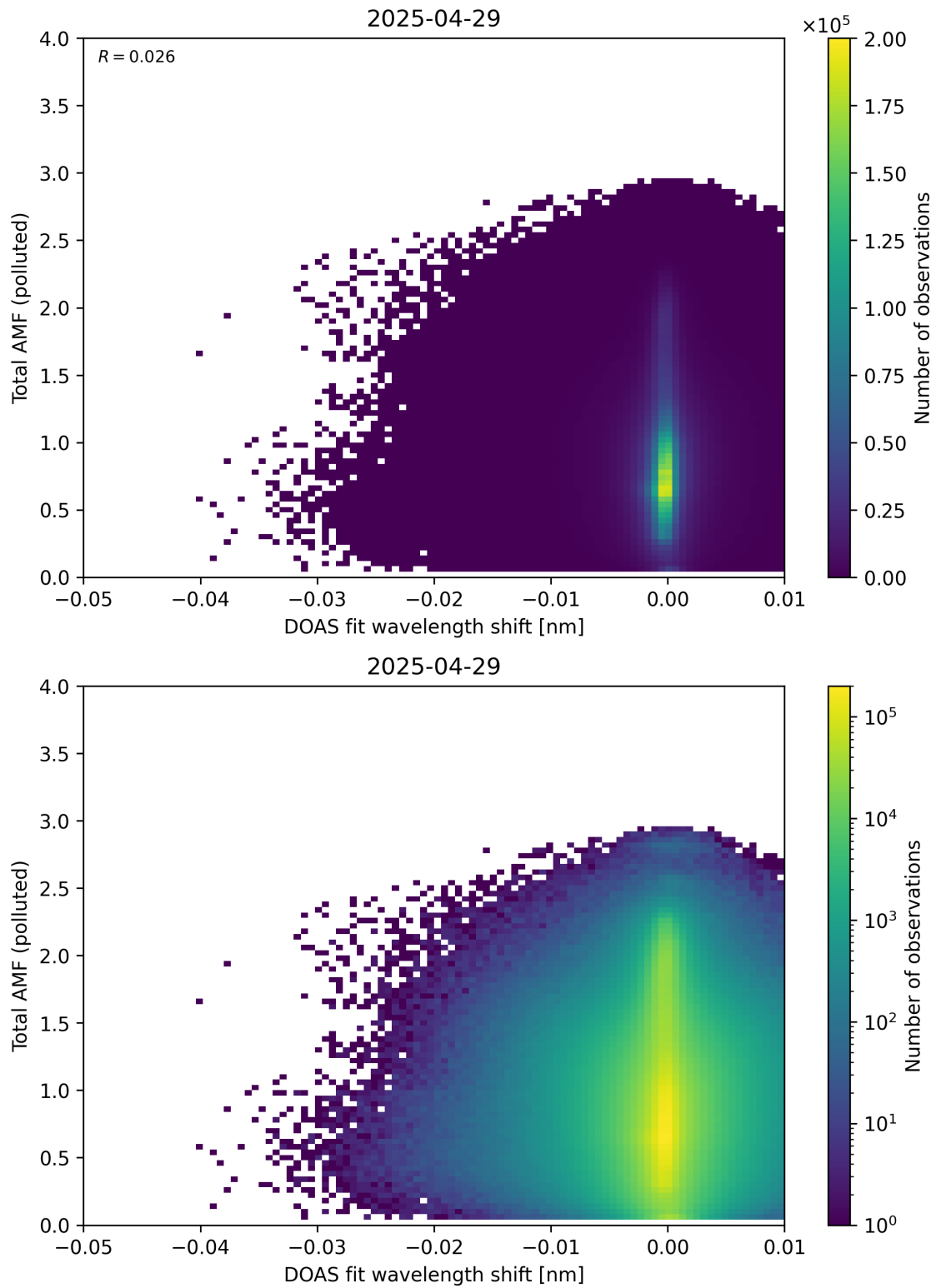
Figure 141: Scatter density plot of “DOAS fit wavelength shift” against “Total AMF (polluted)” for 2025-04-29 to 2025-04-30.
