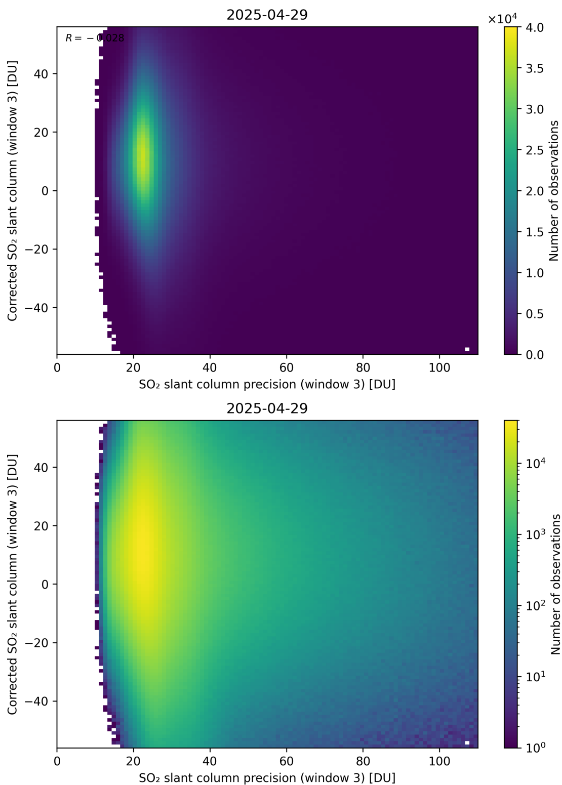
Figure 312: Scatter density plot of “SO 2 slant column precision (window 3)” against “Corrected SO 2 slant column (window 3)” for 2025-04-29 to 2025-04-30.
