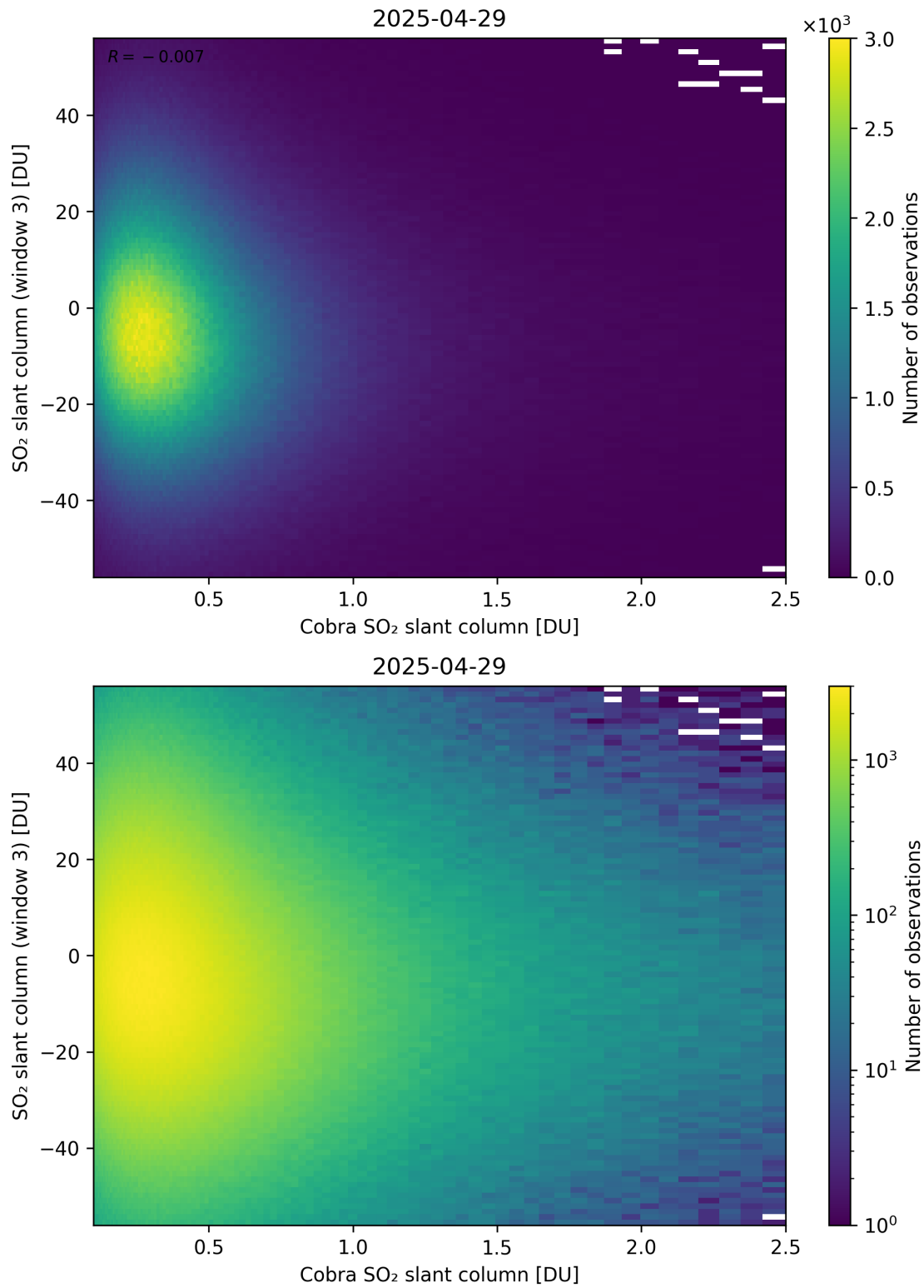
Figure 222: Scatter density plot of “Cobra SO 2 slant column” against “SO 2 slant column (window 3)” for 2025-04-29 to 2025-04-30.
