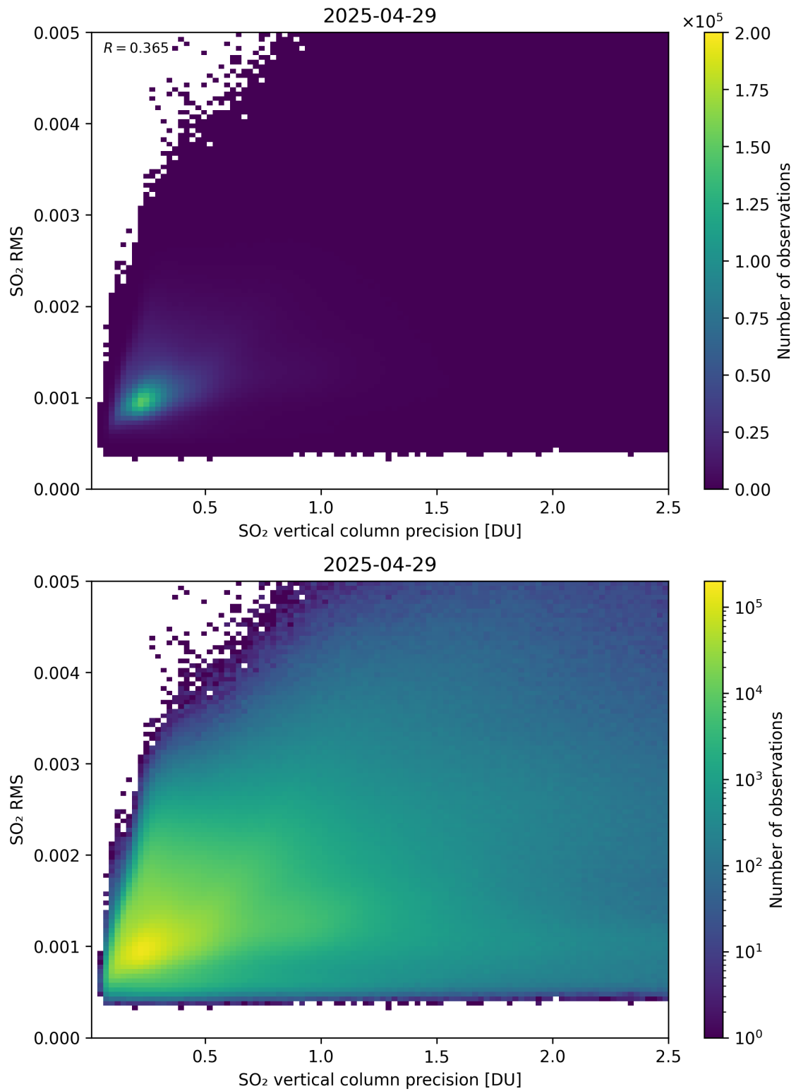
Figure 334: Scatter density plot of “SO 2 vertical column precision” against “SO 2 RMS” for 2025-04-29 to 2025-04-30.
