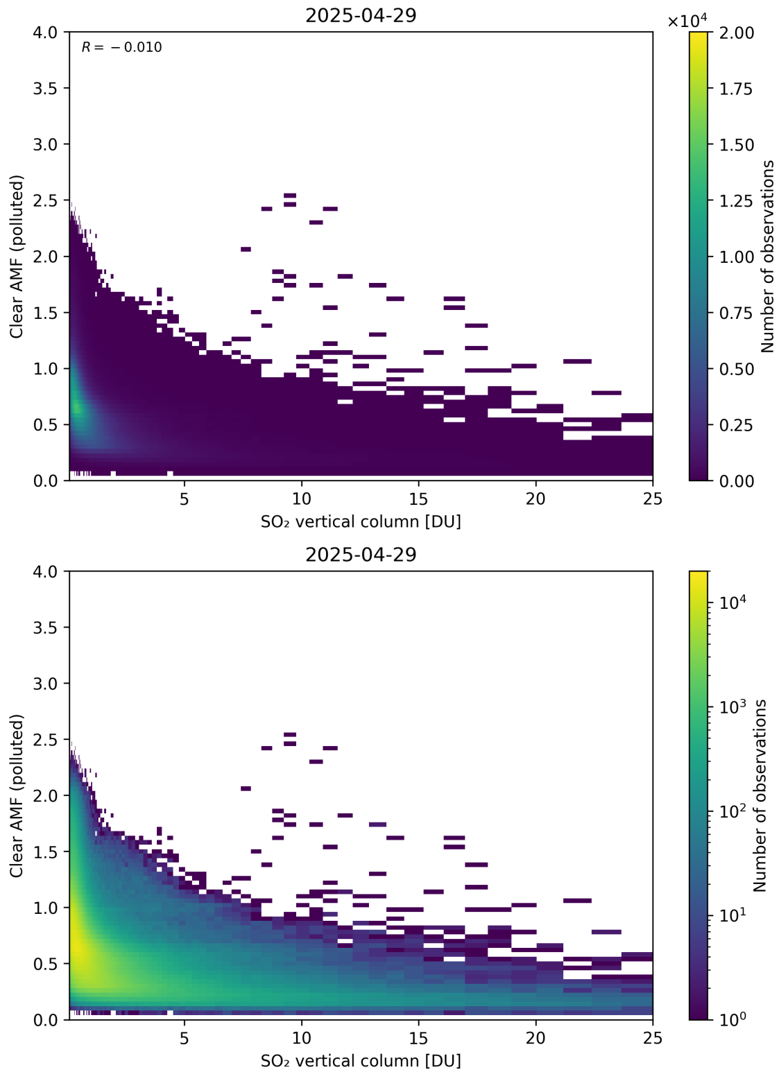
Figure 348: Scatter density plot of “SO 2 vertical column” against “Clear AMF (polluted)” for 2025-04-29 to 2025-04-30.
