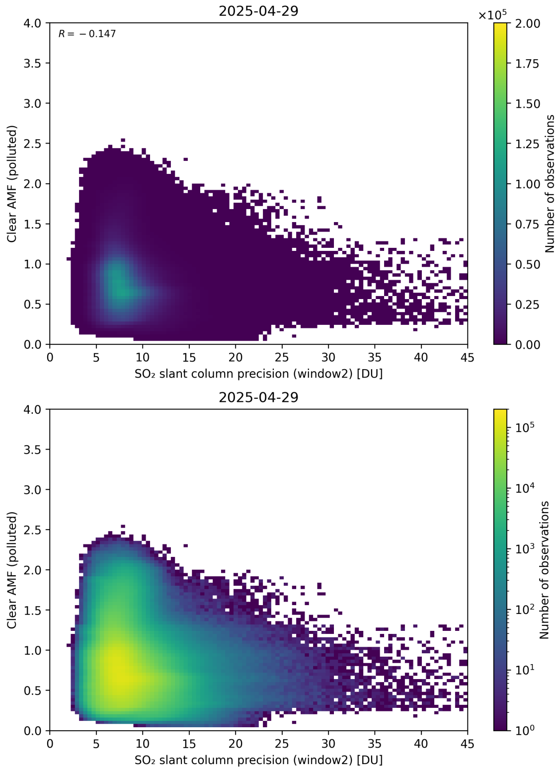
Figure 296: Scatter density plot of “SO 2 slant column precision (window2)” against “Clear AMF (polluted)” for 2025-04-29 to 2025-04-30.
