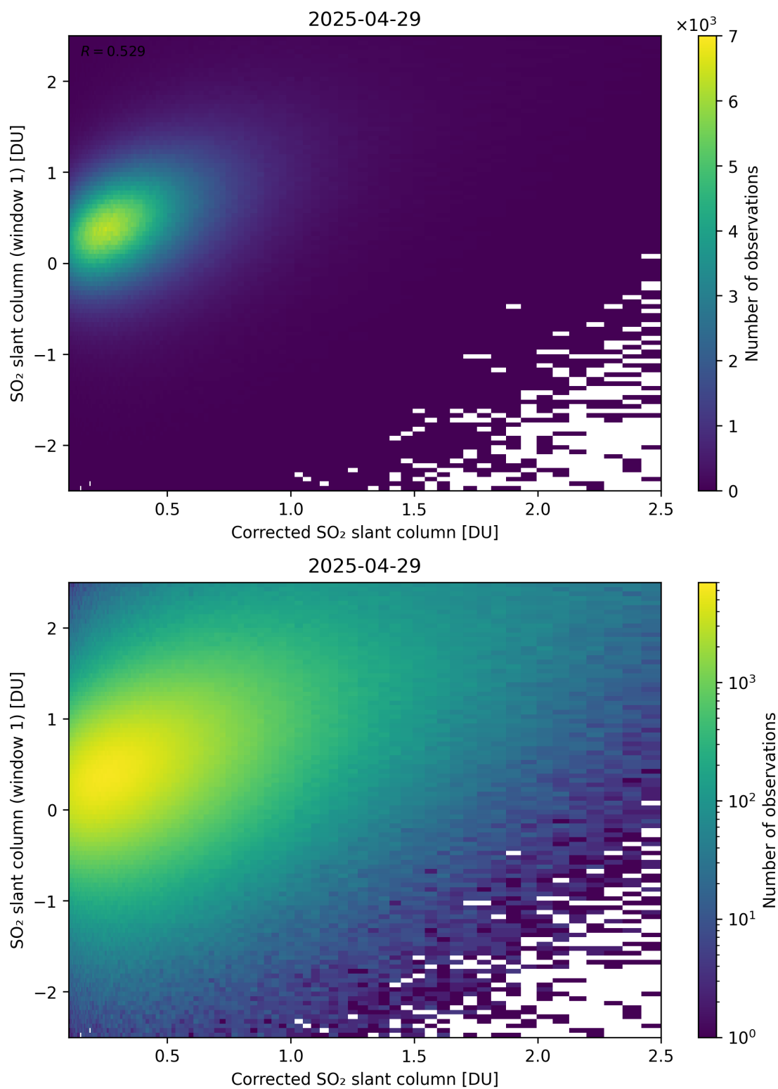
Figure 237: Scatter density plot of “Corrected SO 2 slant column” against “SO 2 slant column (window 1)” for 2025-04-29 to 2025-04-30.
