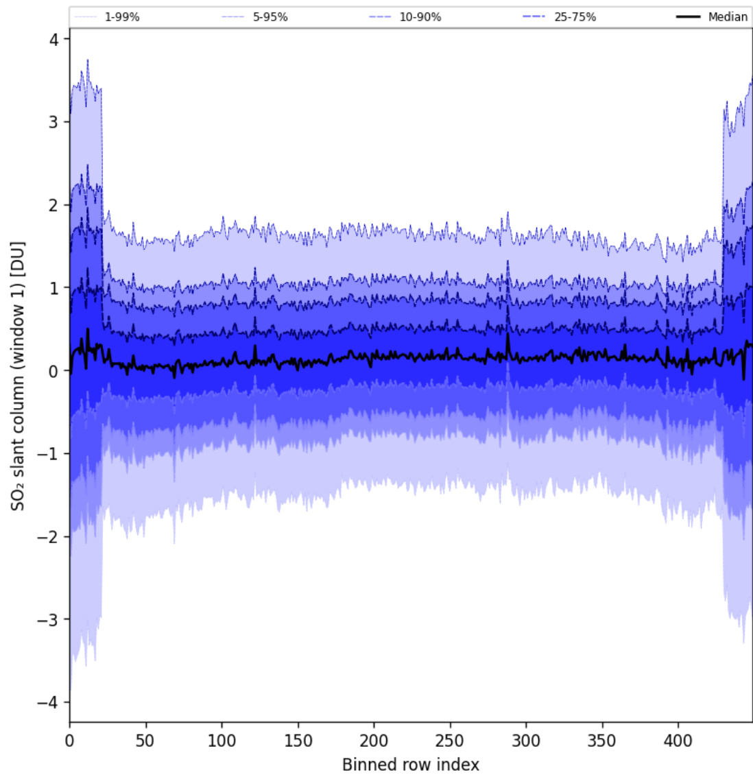
Figure 89: Along track statistics of “SO 2 slant column (window 1)” for 2025-04-29 to 2025-04-30
