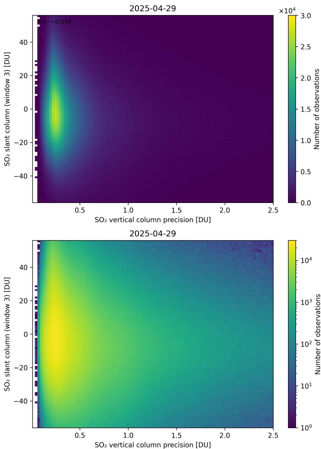
Figure 344: Scatter density plot of “SO 2 vertical column precision” against “SO 2 slant column (window 3)” for 2025-04-29 to 2025-04-30.
