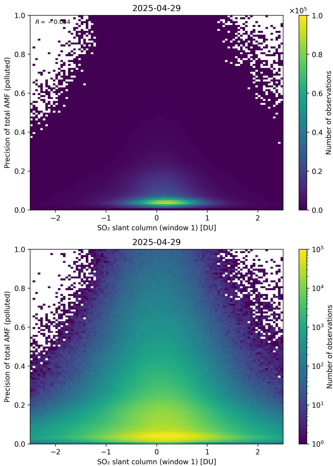
Figure 290: Scatter density plot of “SO 2 slant column (window 1)” against “Precision of total AMF (polluted)” for 2025-04-29 to 2025-04-30.
