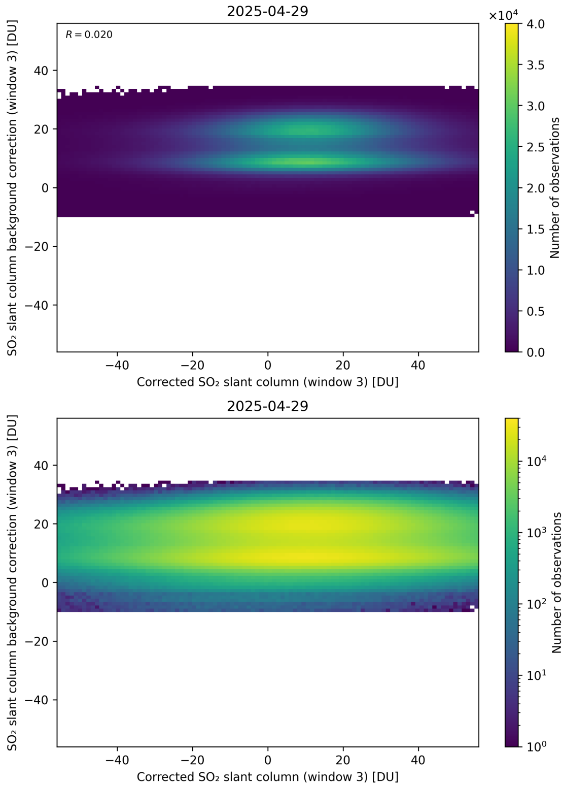
Figure 255: Scatter density plot of “Corrected SO 2 slant column (window 3)” against “SO 2 slant column background correction (window 3)” for 2025-04-29 to 2025-04-30.
