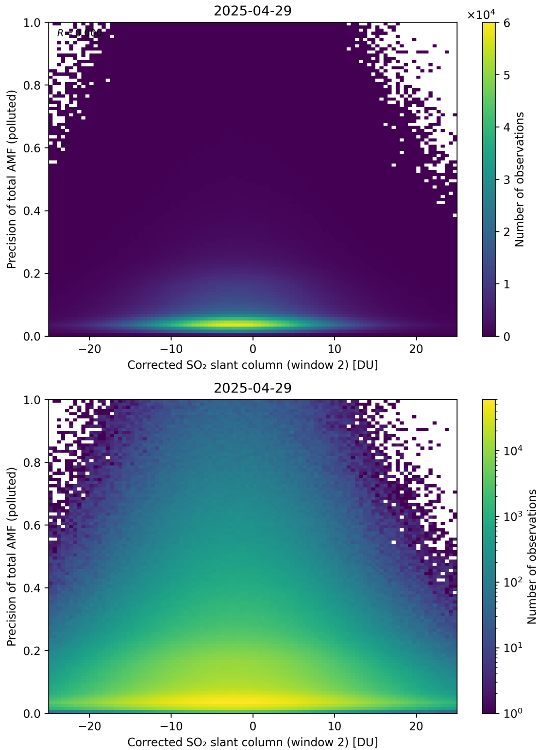
Figure 254: Scatter density plot of “Corrected SO 2 slant column (window 2)” against “Precision of total AMF (polluted)” for 2025-04-29 to 2025-04-30.
