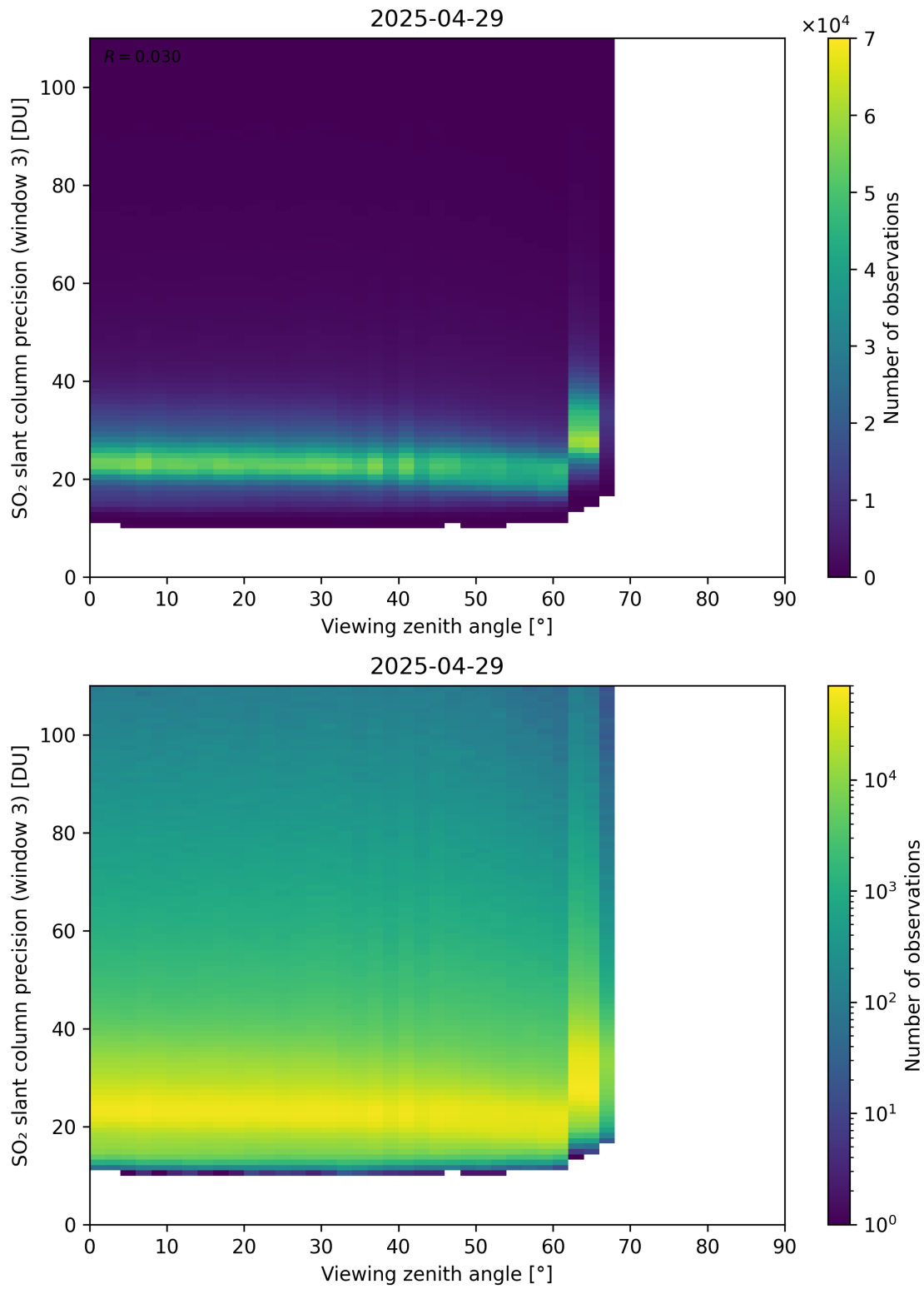
Figure 380: Scatter density plot of “Viewing zenith angle” against “SO 2 slant column precision (window 3)” for 2025-04-29 to 2025-04-30.
