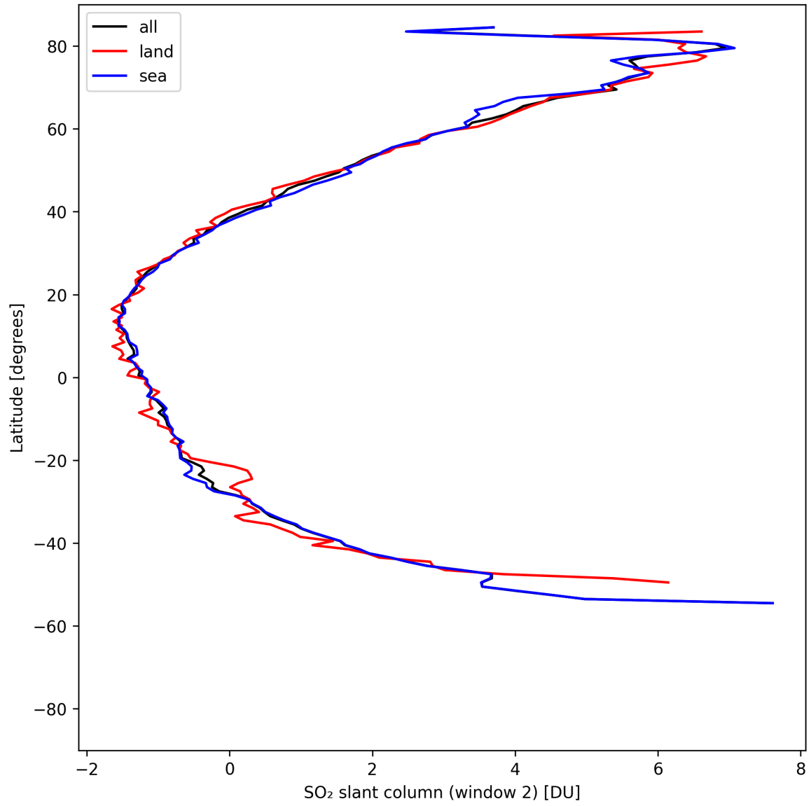
Figure 41: Zonal average of “SO 2 slant column (window 2)” for 2025-04-29 to 2025-04-30.
