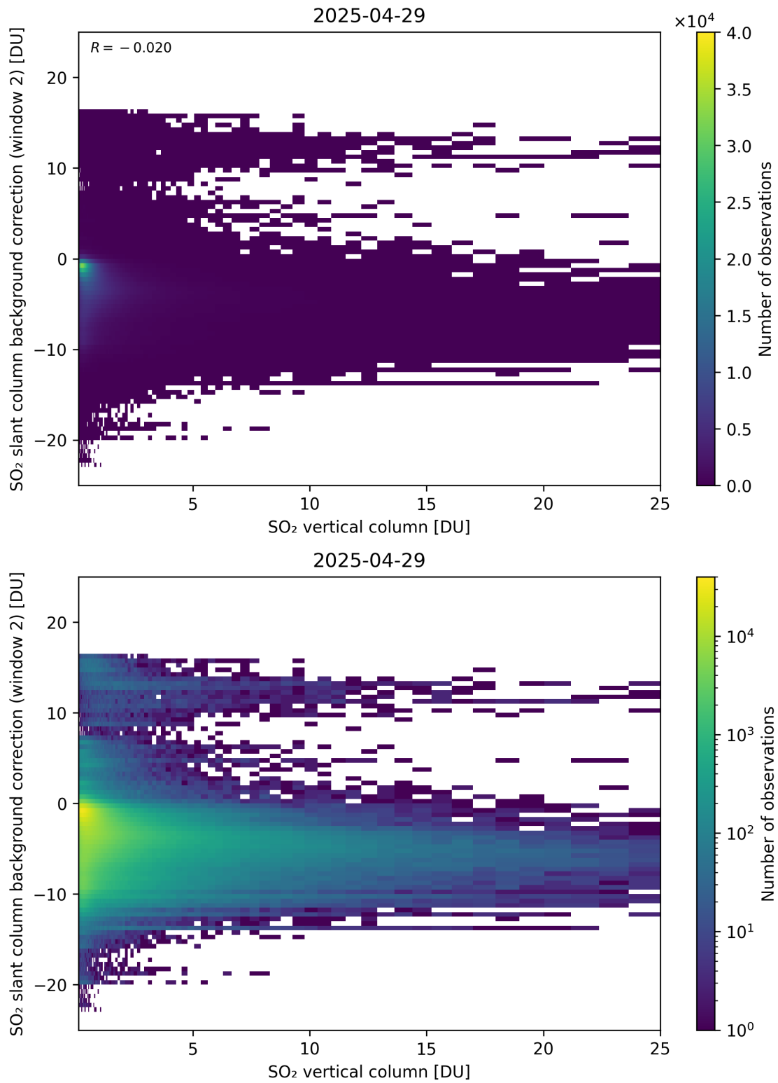
Figure 324: Scatter density plot of “SO 2 vertical column” against “SO 2 slant column background correction (window 2)” for 2025-04-29 to 2025-04-30.
