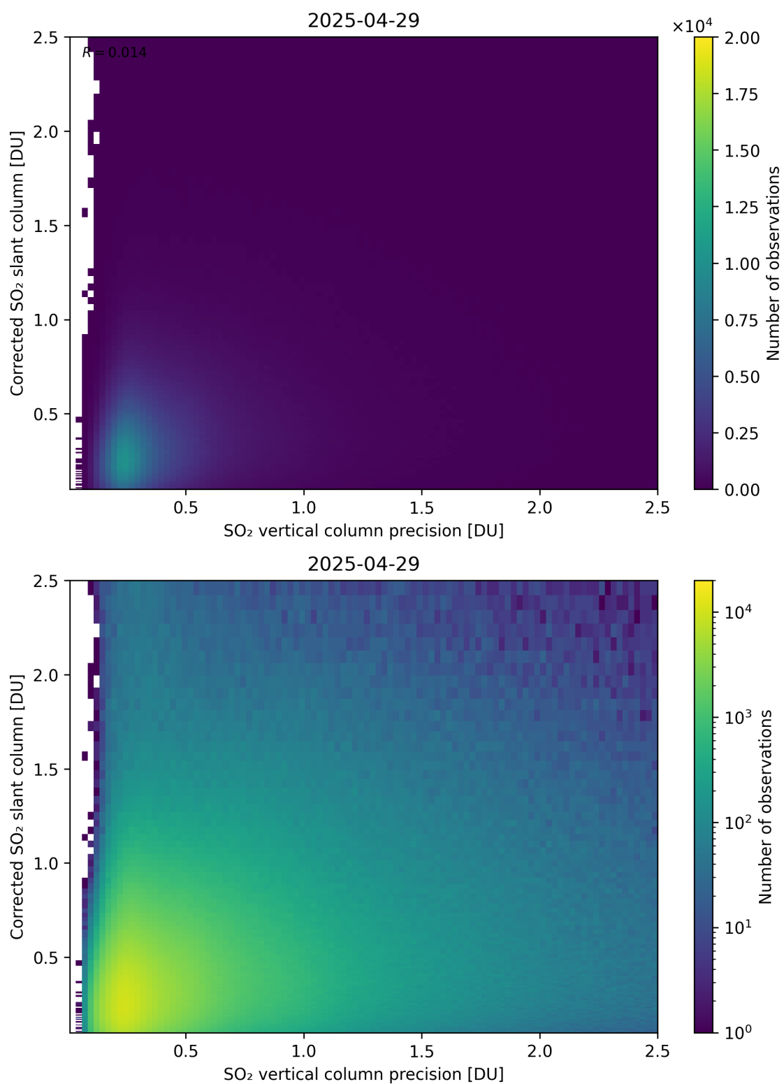
Figure 338: Scatter density plot of “SO 2 vertical column precision” against “Corrected SO 2 slant column” for 2025-04-29 to 2025-04-30.
