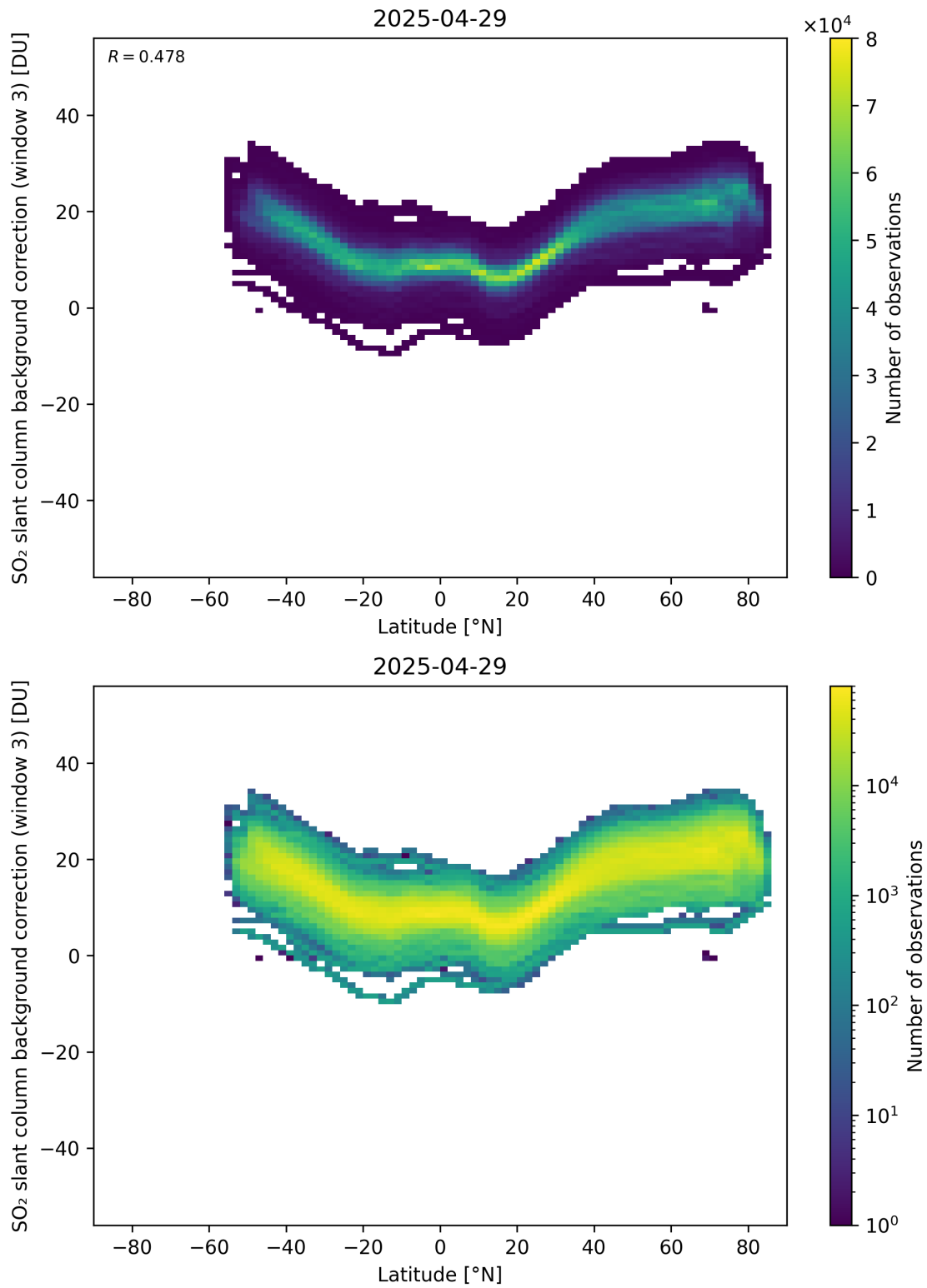
Figure 152: Scatter density plot of “Latitude” against “SO 2 slant column background correction (window 3)” for 2025-04-29 to 2025-04-30.
