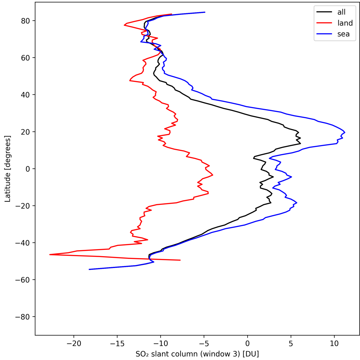
Figure 45: Zonal average of “SO 2 slant column (window 3)” for 2025-04-29 to 2025-04-30.
