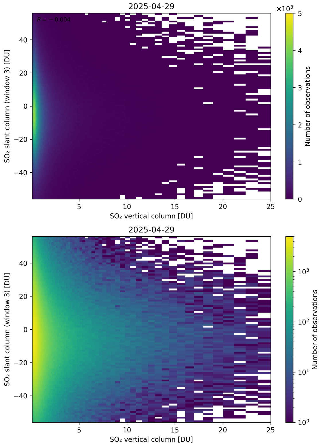
Figure 357: Scatter density plot of “SO 2 vertical column” against “SO 2 slant column (window 3)” for 2025-04-29 to 2025-04-30.
