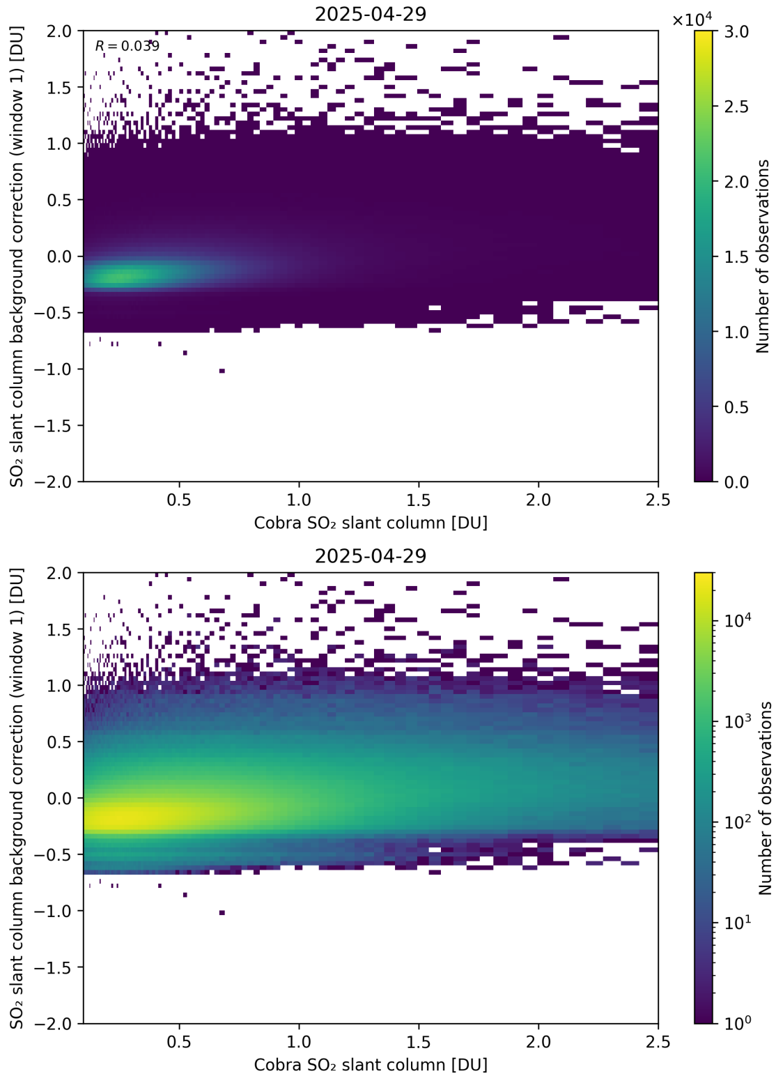
Figure 193: Scatter density plot of “Cobra SO 2 slant column” against “SO 2 slant column background correction (window 1)” for 2025-04-29 to 2025-04-30.
