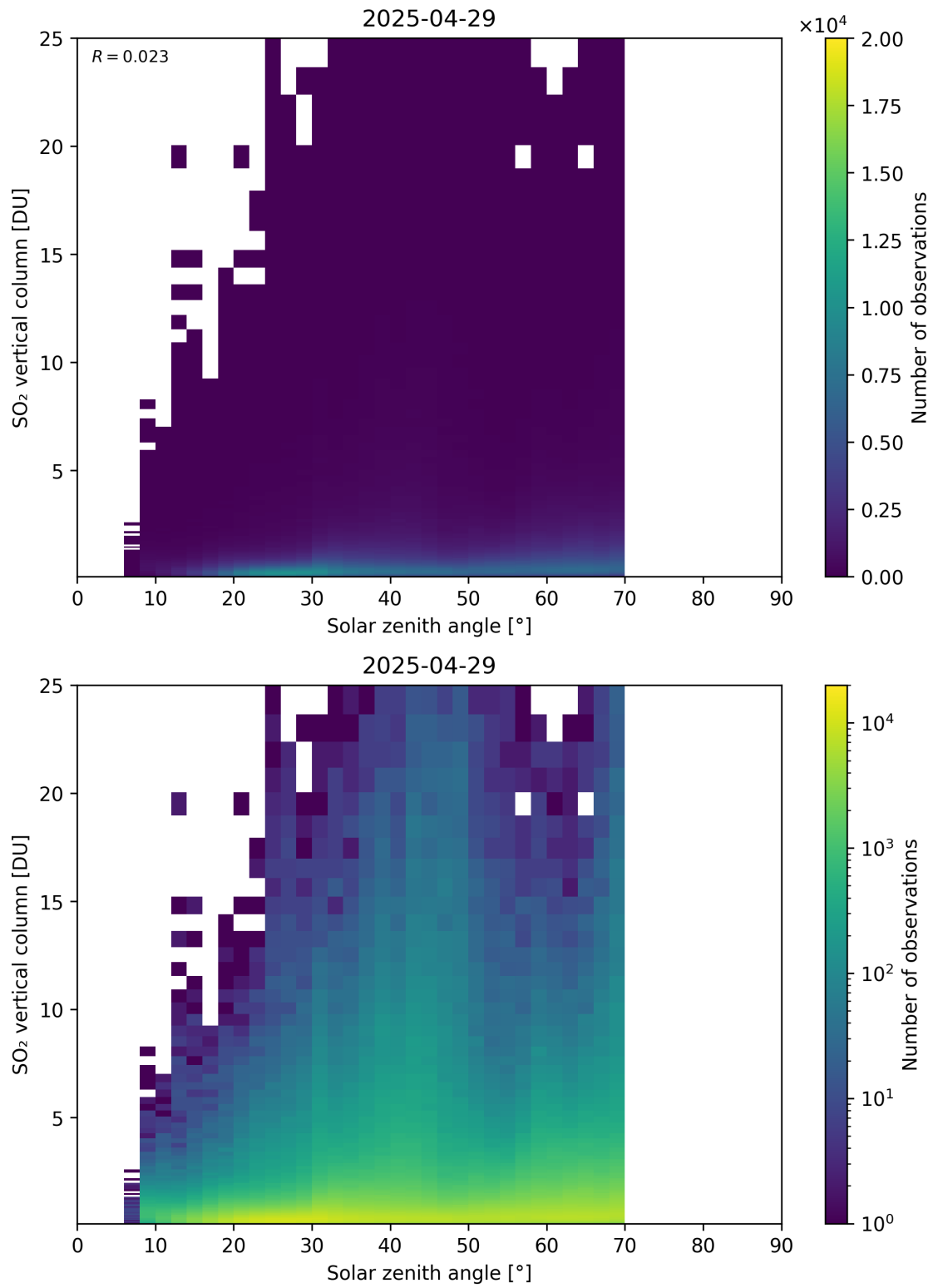
Figure 191: Scatter density plot of “Solar zenith angle” against “SO 2 vertical column” for 2025-04-29 to 2025-04-30.
