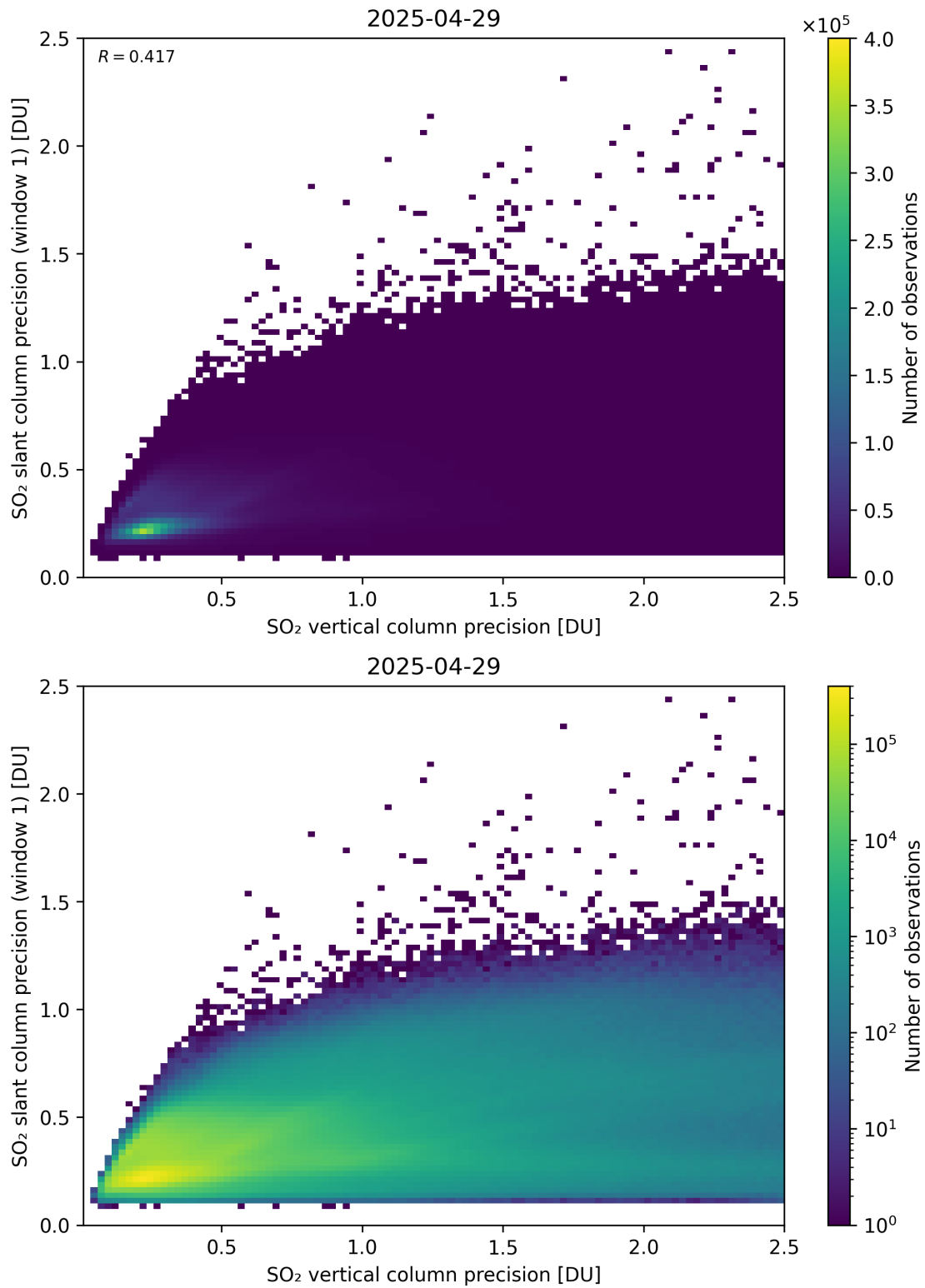
Figure 342: Scatter density plot of “SO 2 vertical column precision” against “SO 2 slant column precision (window 1)” for 2025-04-29 to 2025-04-30.
