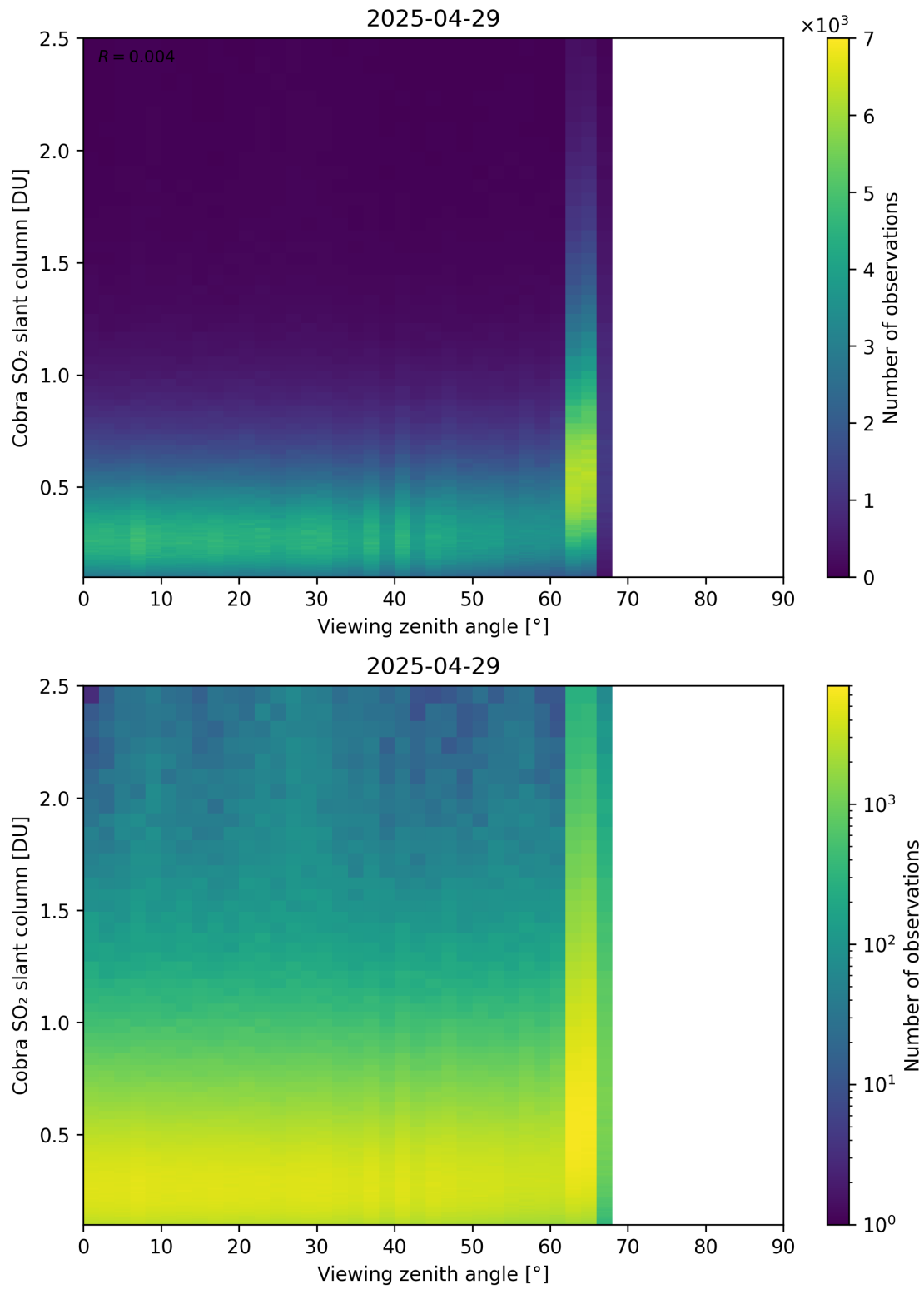
Figure 371: Scatter density plot of “Viewing zenith angle” against “Cobra SO 2 slant column” for 2025-04-29 to 2025-04-30.
