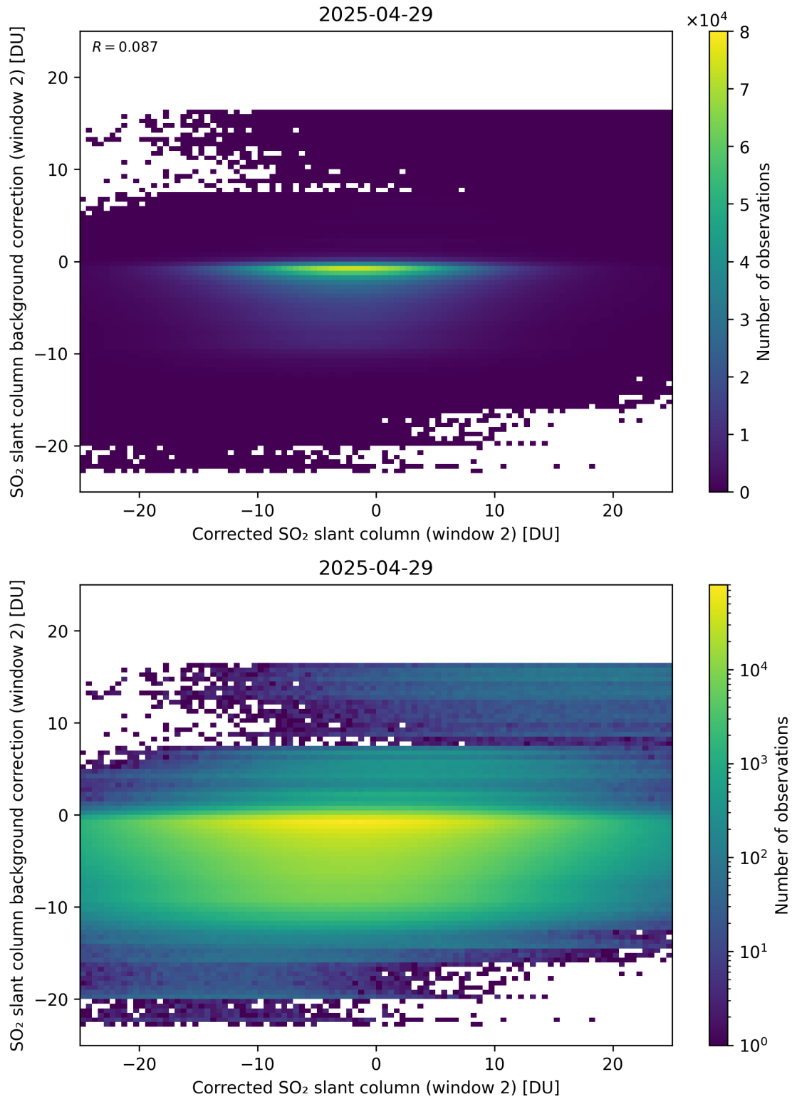
Figure 244: Scatter density plot of “Corrected SO 2 slant column (window 2)” against “SO 2 slant column background correction (window 2)” for 2025-04-29 to 2025-04-30.
