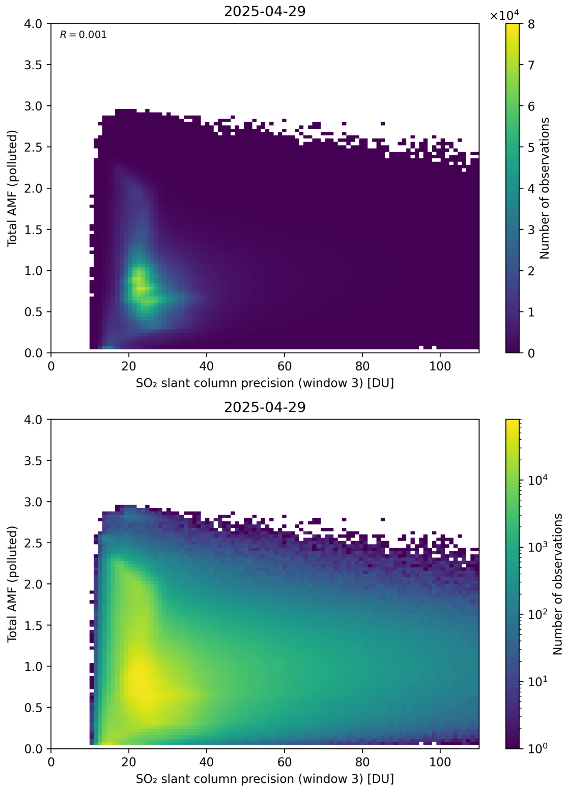
Figure 313: Scatter density plot of “SO 2 slant column precision (window 3)” against “Total AMF (polluted)” for 2025-04-29 to 2025-04-30.
