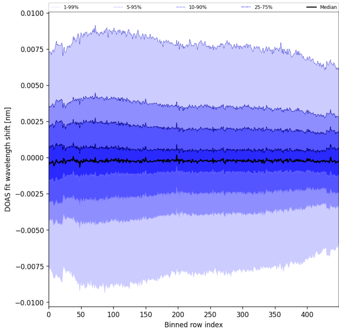
Figure 102: Along track statistics of “DOAS fit wavelength shift” for 2025-04-29 to 2025-04-30
