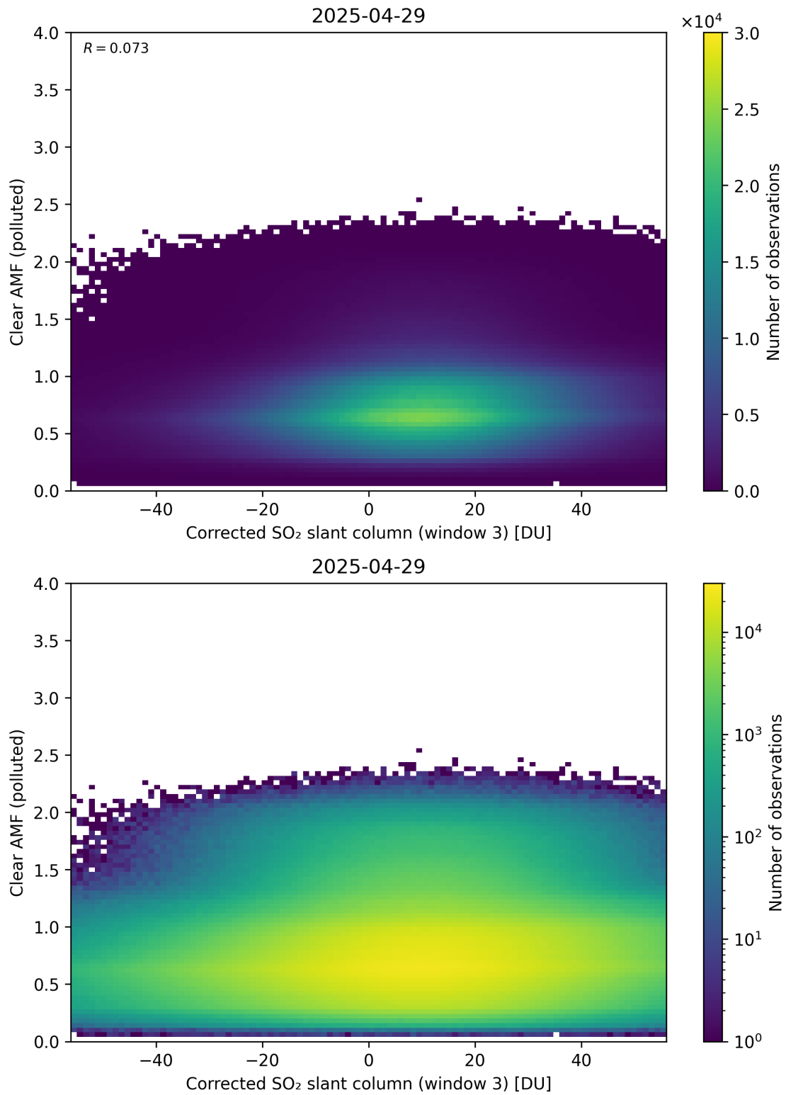
Figure 259: Scatter density plot of “Corrected SO 2 slant column (window 3)” against “Clear AMF (polluted)” for 2025-04-29 to 2025-04-30.
