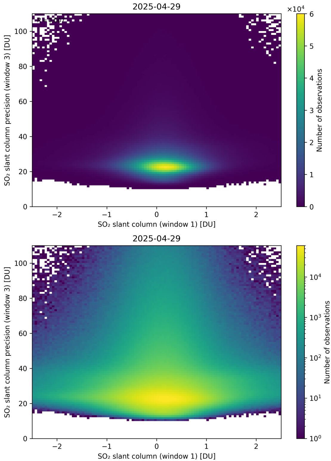
Figure 288: Scatter density plot of “SO 2 slant column (window 1)” against “SO 2 slant column precision (window 3)” for 2025-04-29 to 2025-04-30.
