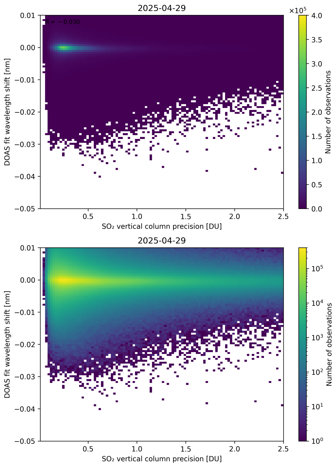
Figure 332: Scatter density plot of “SO 2 vertical column precision” against “DOAS fit wavelength shift” for 2025-04-29 to 2025-04-30.
