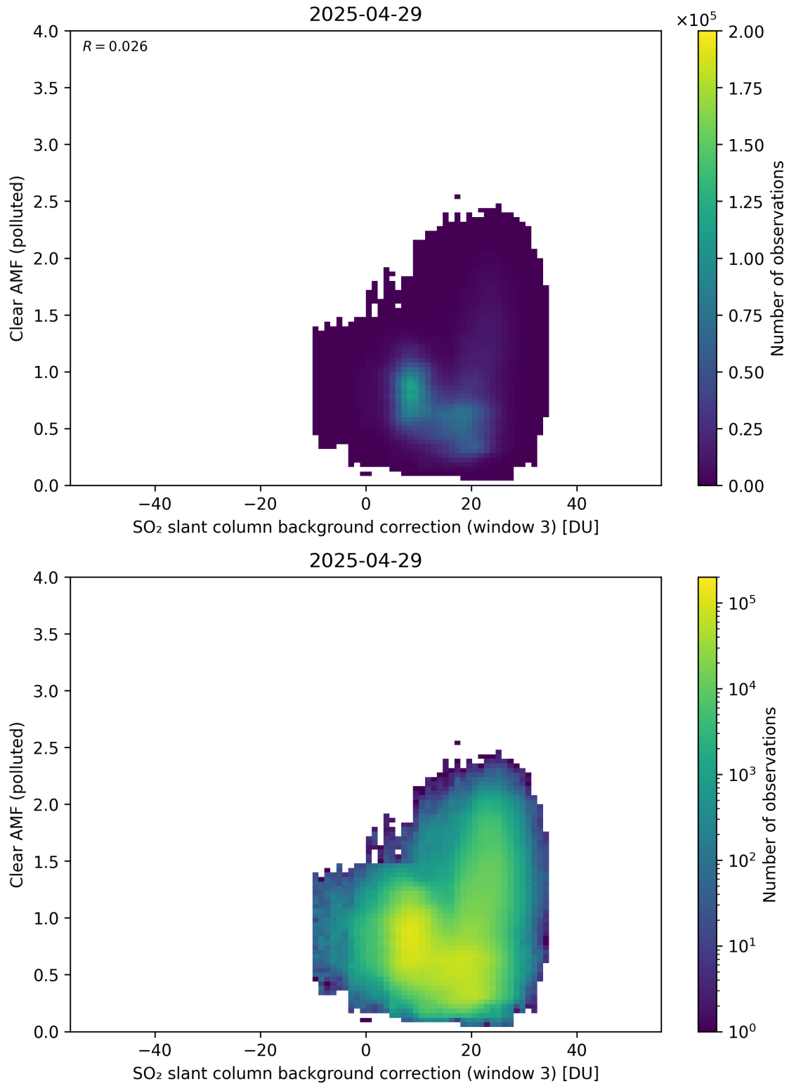
Figure 135: Scatter density plot of “SO 2 slant column background correction (window 3)” against “Clear AMF (polluted)” for 2025-04-29 to 2025-04-30.
