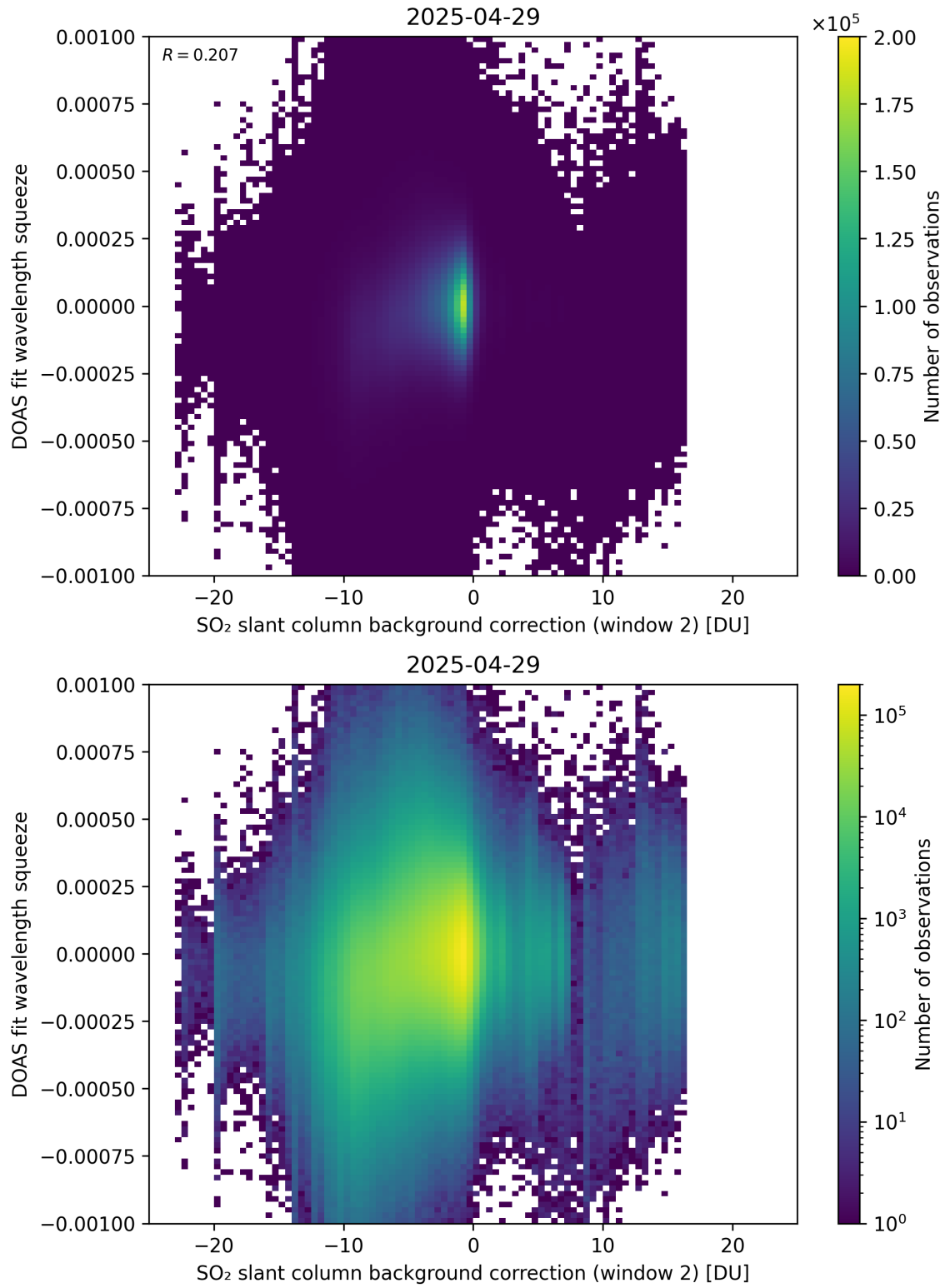
Figure 124: Scatter density plot of “SO 2 slant column background correction (window 2)” against “DOAS fit wavelength squeeze” for 2025-04-29 to 2025-04-30.
