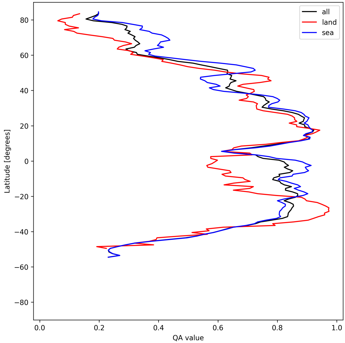
Figure 31: Zonal average of “QA value” for 2025-04-29 to 2025-04-30.
