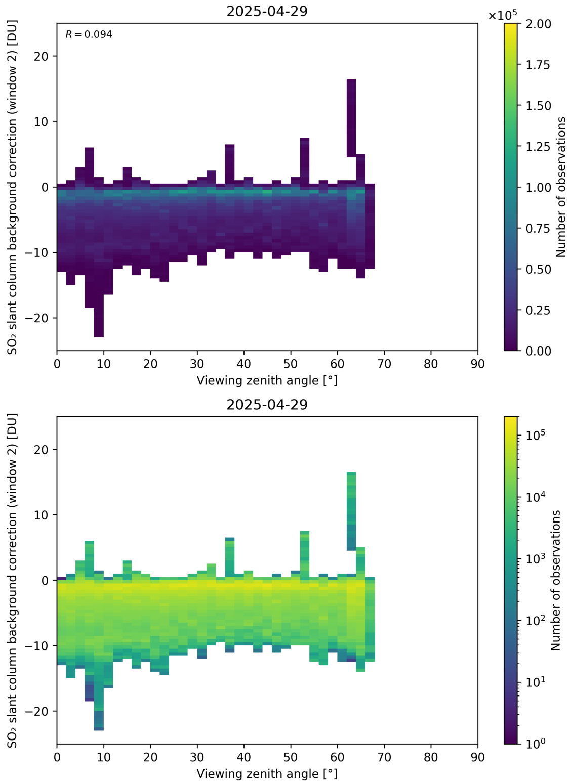
Figure 363: Scatter density plot of “Viewing zenith angle” against “SO 2 slant column background correction (window 2)” for 2025-04-29 to 2025-04-30.
