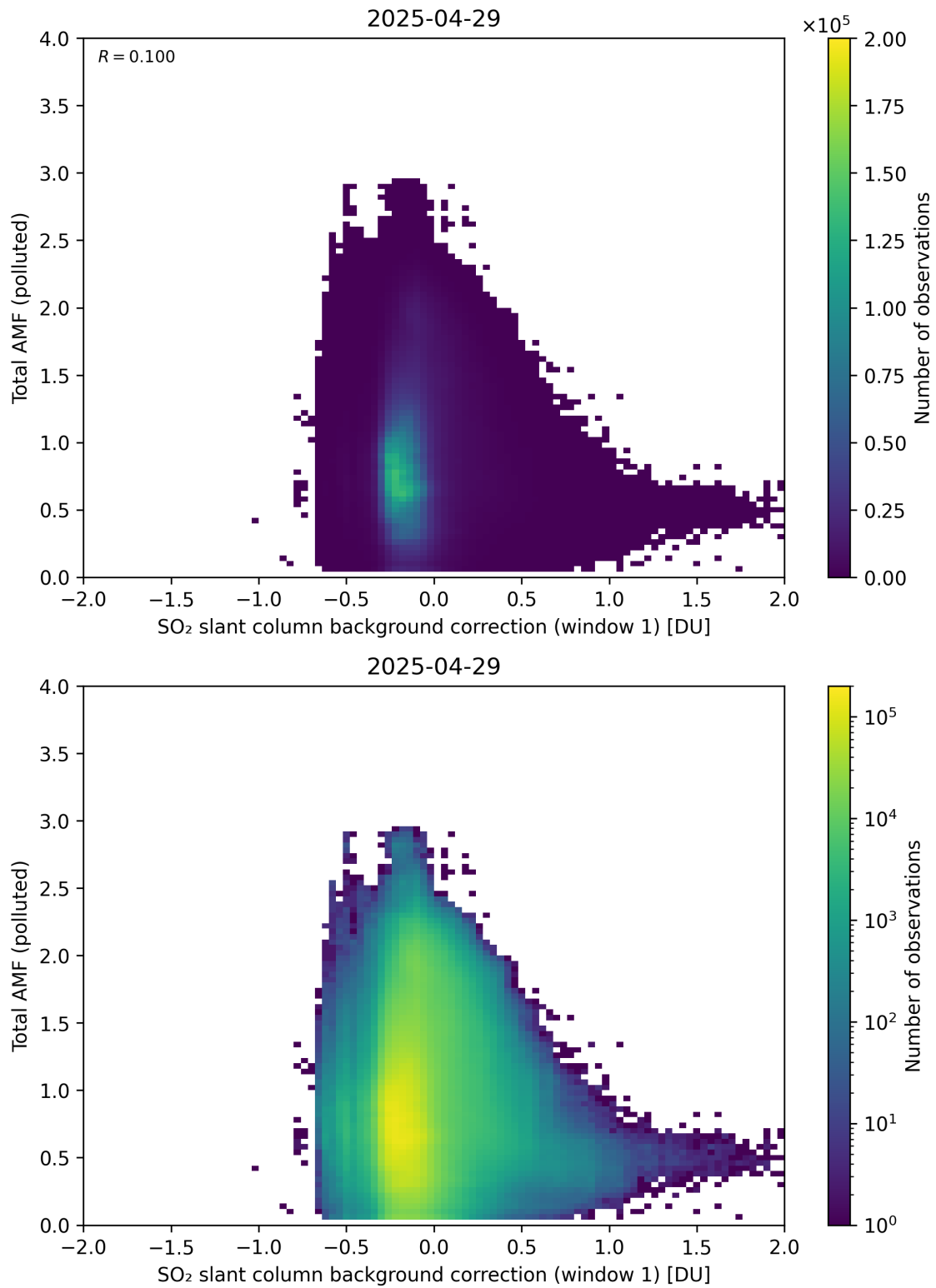
Figure 120: Scatter density plot of “SO 2 slant column background correction (window 1)” against “Total AMF (polluted)” for 2025-04-29 to 2025-04-30.
