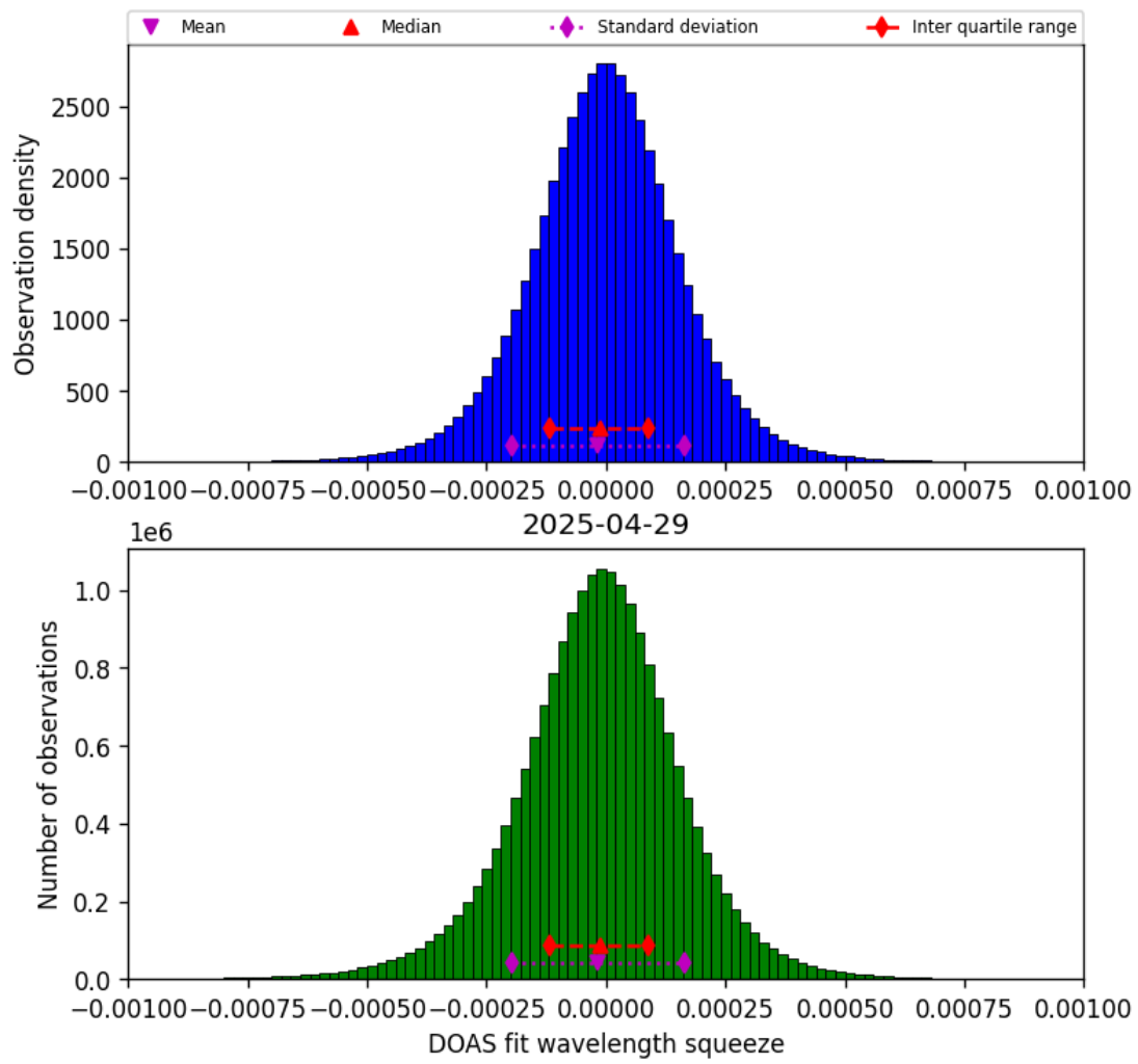
Figure 77: Histogram of “DOAS fit wavelength squeeze” for 2025-04-29 to 2025-04-30
