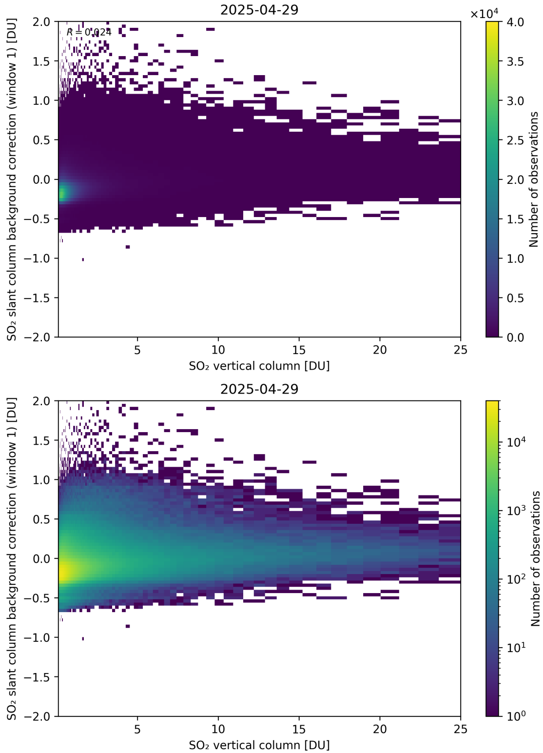
Figure 323: Scatter density plot of “SO 2 vertical column” against “SO 2 slant column background correction (window 1)” for 2025-04-29 to 2025-04-30.
