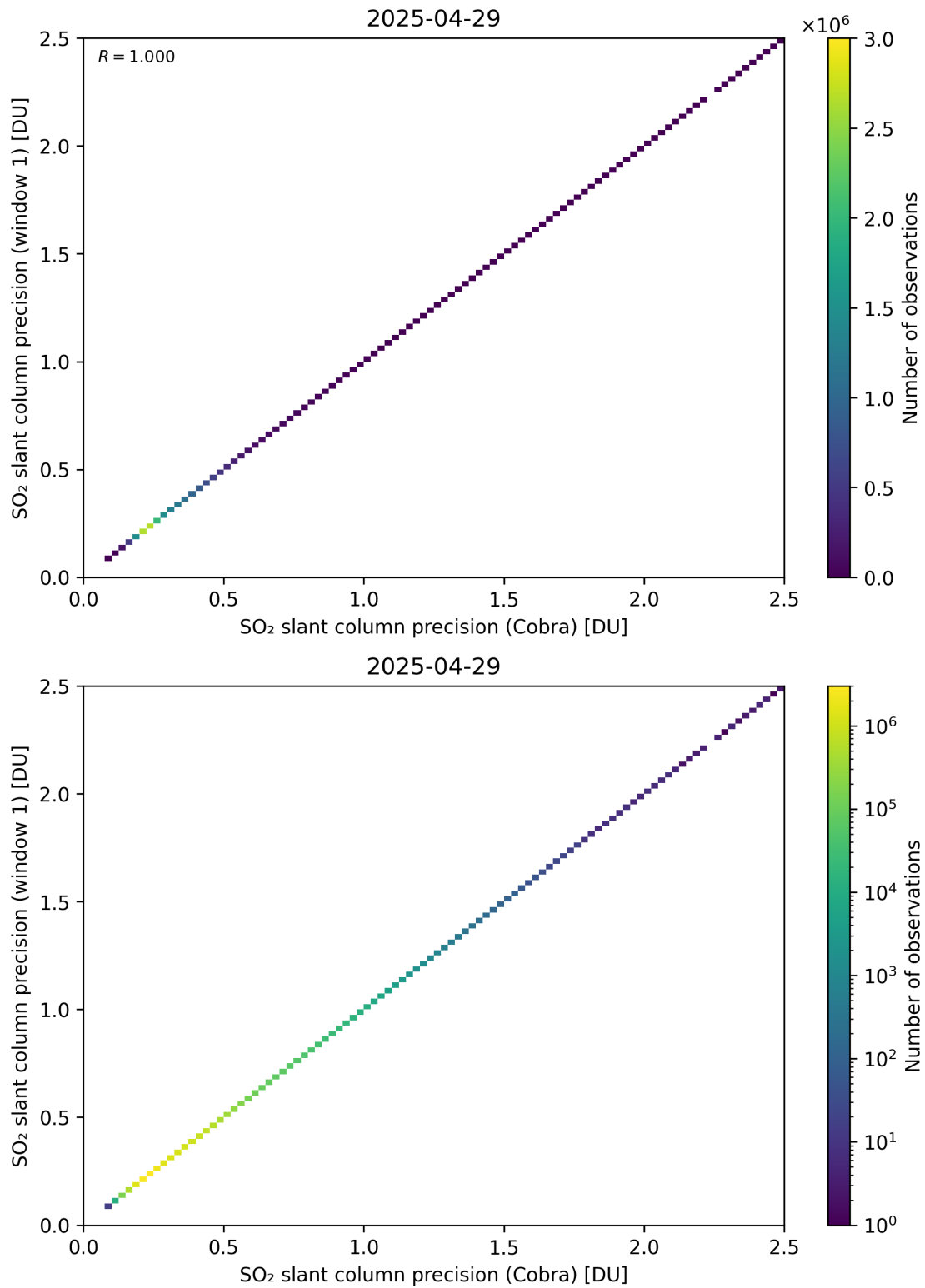
Figure 209: Scatter density plot of “SO 2 slant column precision (Cobra)” against “SO 2 slant column precision (window 1)” for 2025-04-29 to 2025-04-30.
