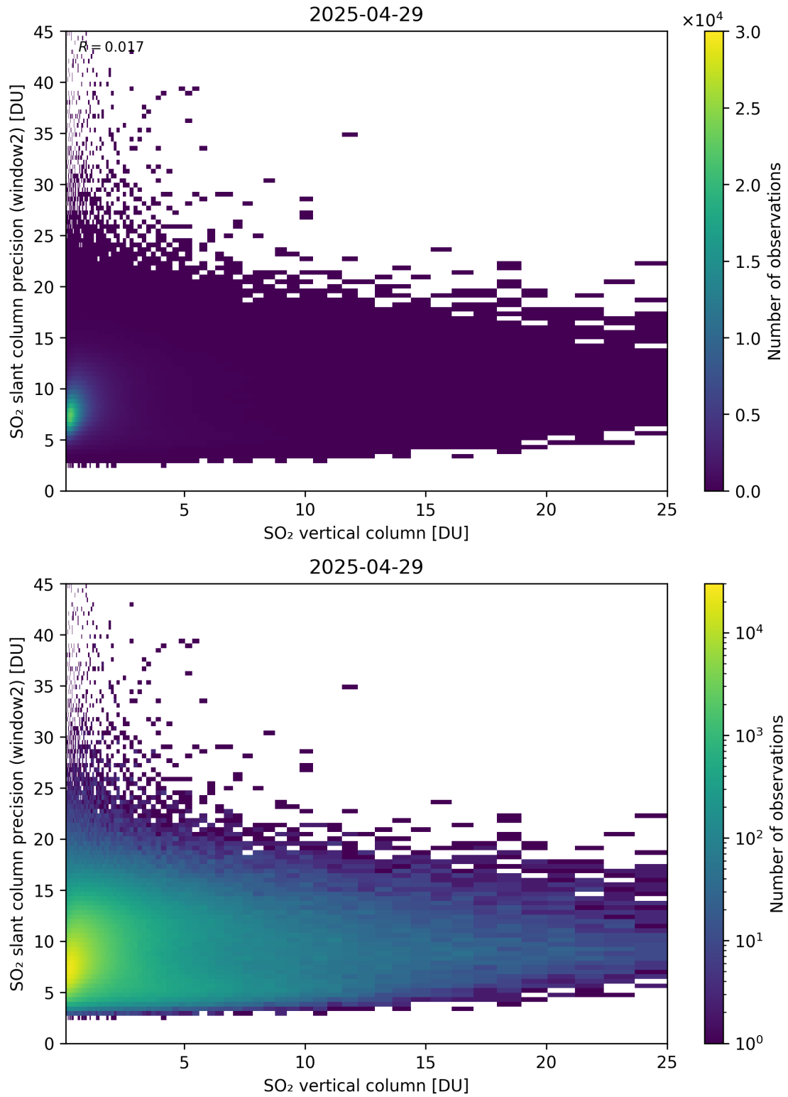
Figure 356: Scatter density plot of “SO 2 vertical column” against “SO 2 slant column precision (window2)” for 2025-04-29 to 2025-04-30.
