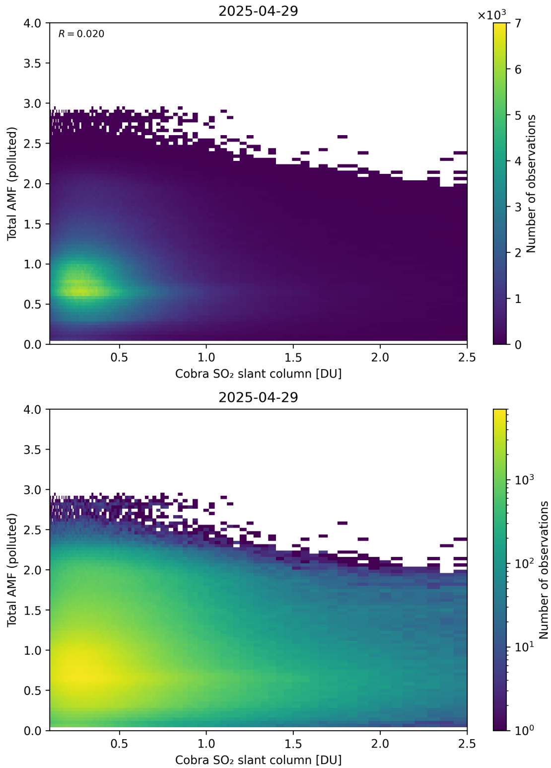
Figure 224: Scatter density plot of “Cobra SO 2 slant column” against “Total AMF (polluted)” for 2025-04-29 to 2025-04-30.
