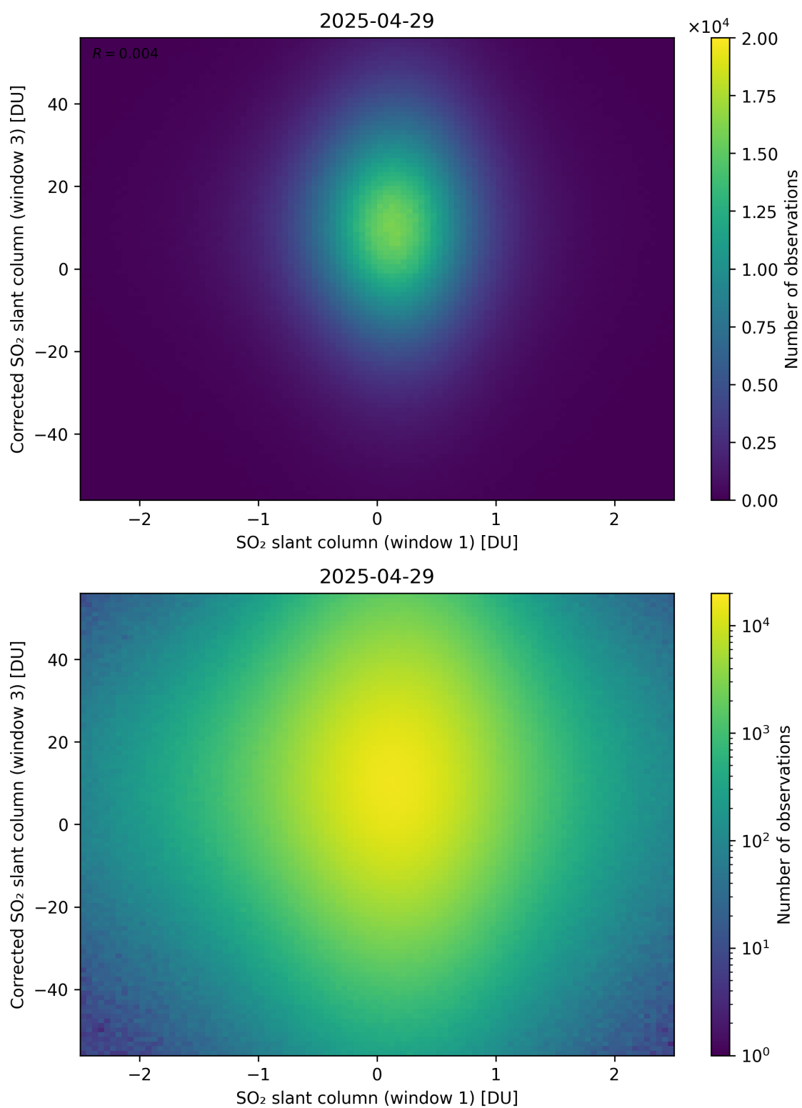
Figure 284: Scatter density plot of “SO 2 slant column (window 1)” against “Corrected SO 2 slant column (window 3)” for 2025-04-29 to 2025-04-30.
