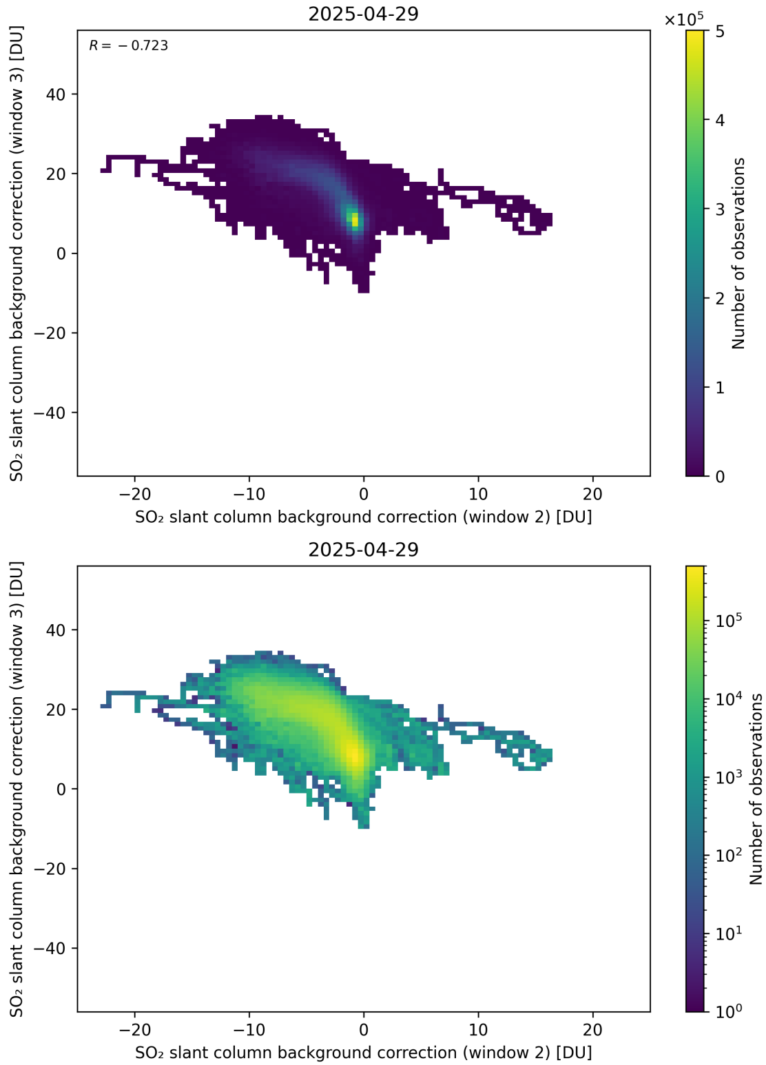
Figure 122: Scatter density plot of “SO 2 slant column background correction (window 2)” against “SO 2 slant column background correction (window 3)” for 2025-04-29 to 2025-04-30.
