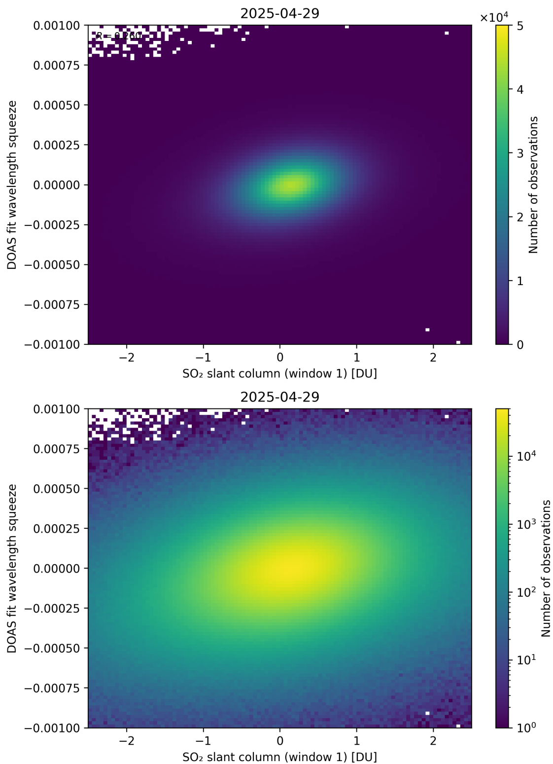
Figure 266: Scatter density plot of “SO 2 slant column (window 1)” against “DOAS fit wavelength squeeze” for 2025-04-29 to 2025-04-30.
