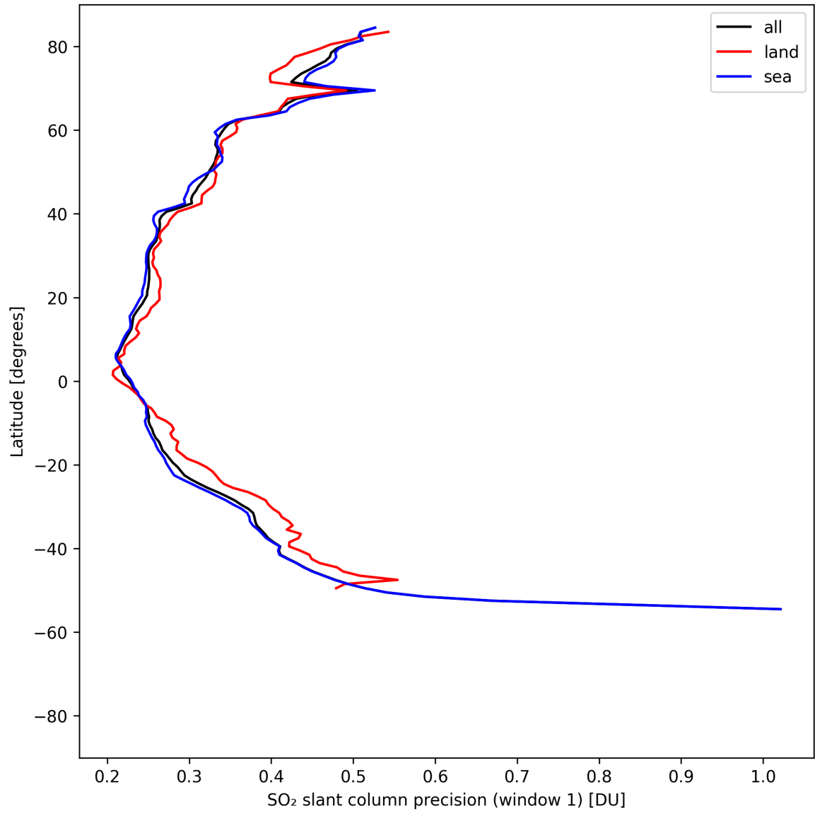
Figure 38: Zonal average of “SO 2 slant column precision (window 1)” for 2025-04-29 to 2025-04-30.
