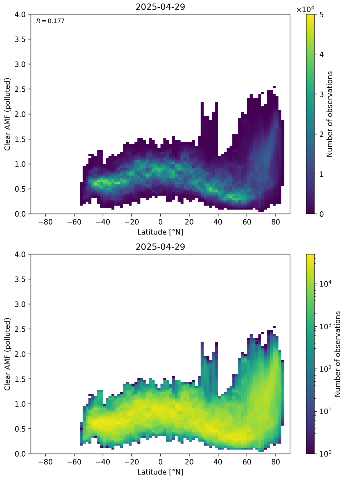
Figure 156: Scatter density plot of “Latitude” against “Clear AMF (polluted)” for 2025-04-29 to 2025-04-30.
