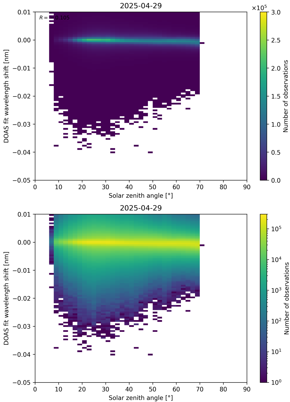
Figure 174: Scatter density plot of “Solar zenith angle” against “DOAS fit wavelength shift” for 2025-04-29 to 2025-04-30.
