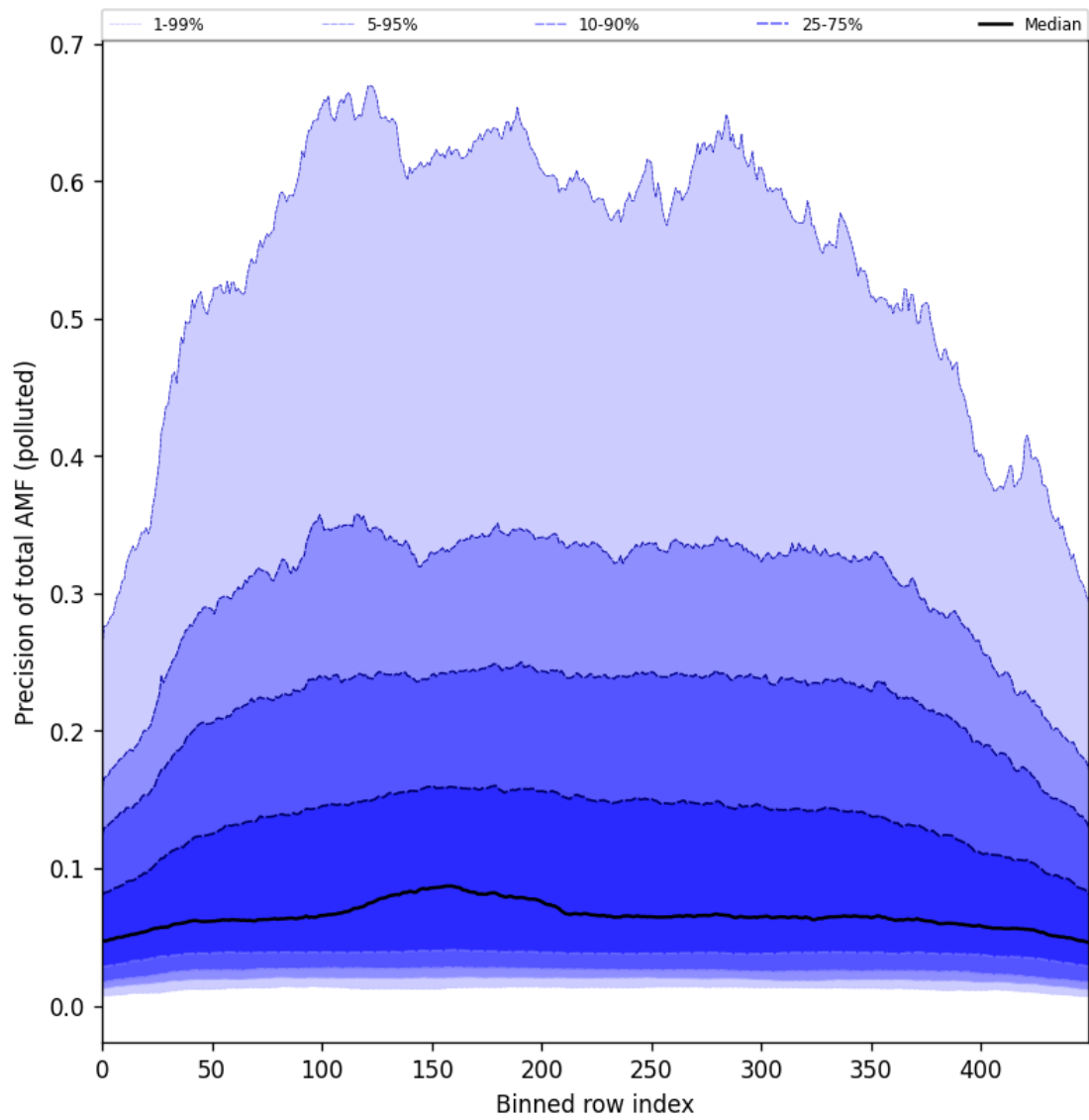
Figure 106: Along track statistics of “Precision of total AMF (polluted)” for 2025-04-29 to 2025-04-30
