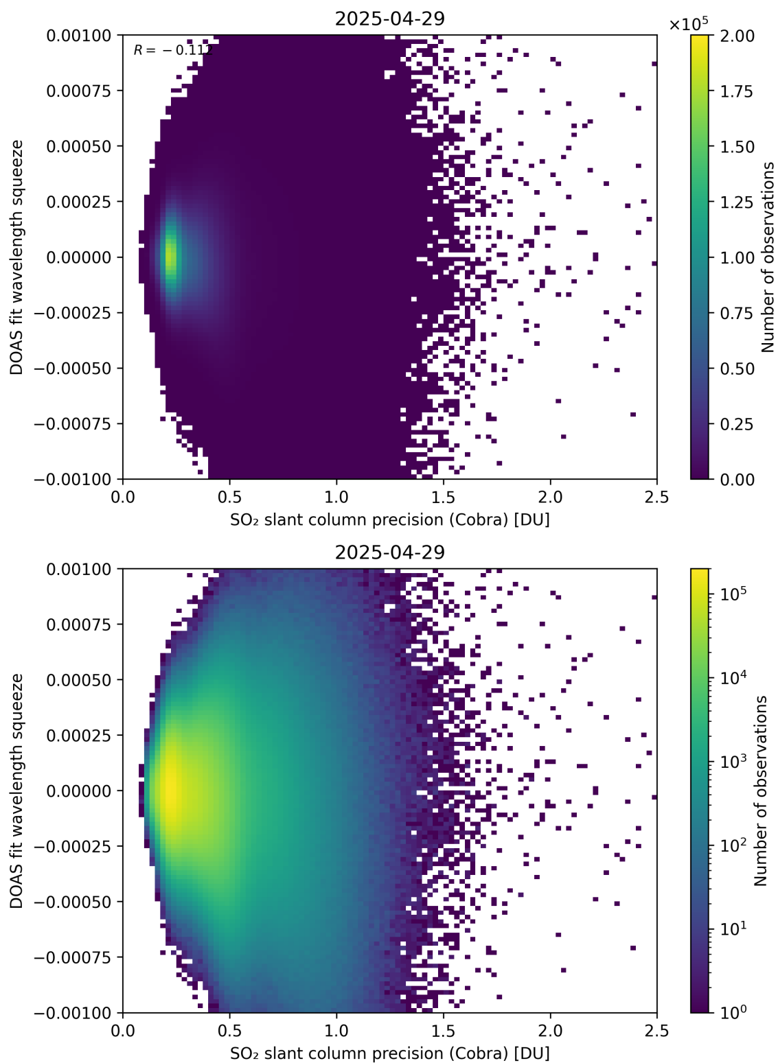
Figure 203: Scatter density plot of “SO 2 slant column precision (Cobra)” against “DOAS fit wavelength squeeze” for 2025-04-29 to 2025-04-30.
