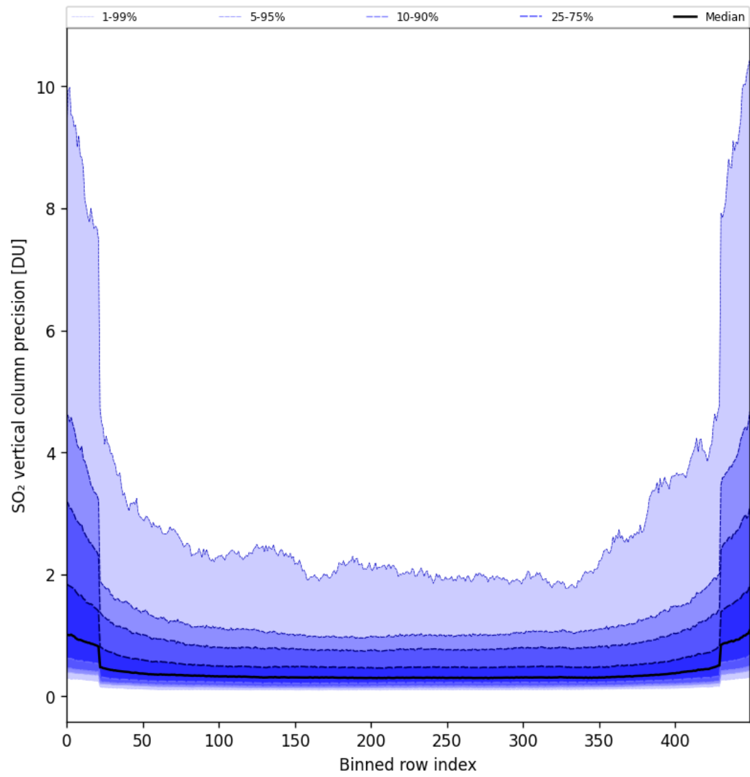
Figure 85: Along track statistics of “SO 2 vertical column precision” for 2025-04-29 to 2025-04-30
