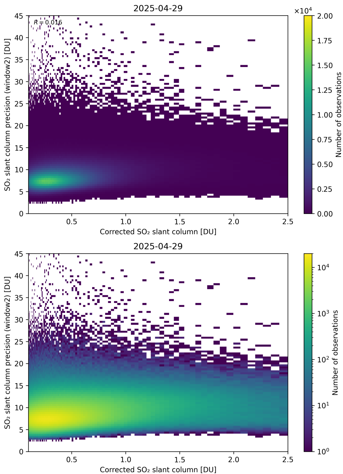
Figure 239: Scatter density plot of “Corrected SO 2 slant column” against “SO 2 slant column precision (window2)” for 2025-04-29 to 2025-04-30.
