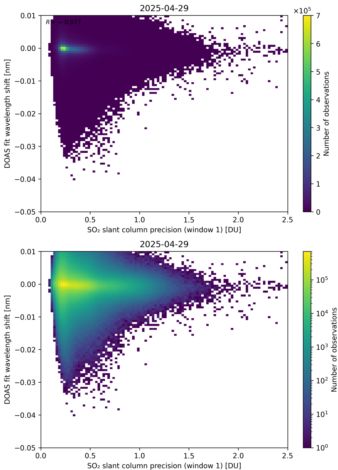
Figure 271: Scatter density plot of “SO 2 slant column precision (window 1)” against “DOAS fit wavelength shift” for 2025-04-29 to 2025-04-30.
