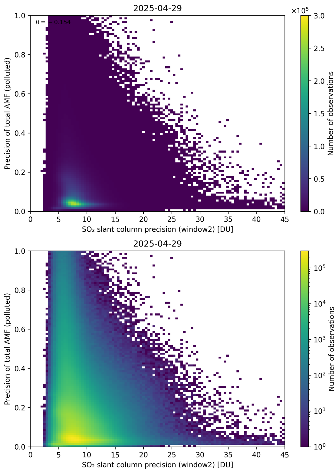
Figure 302: Scatter density plot of “SO 2 slant column precision (window2)” against “Precision of total AMF (polluted)” for 2025-04-29 to 2025-04-30.
