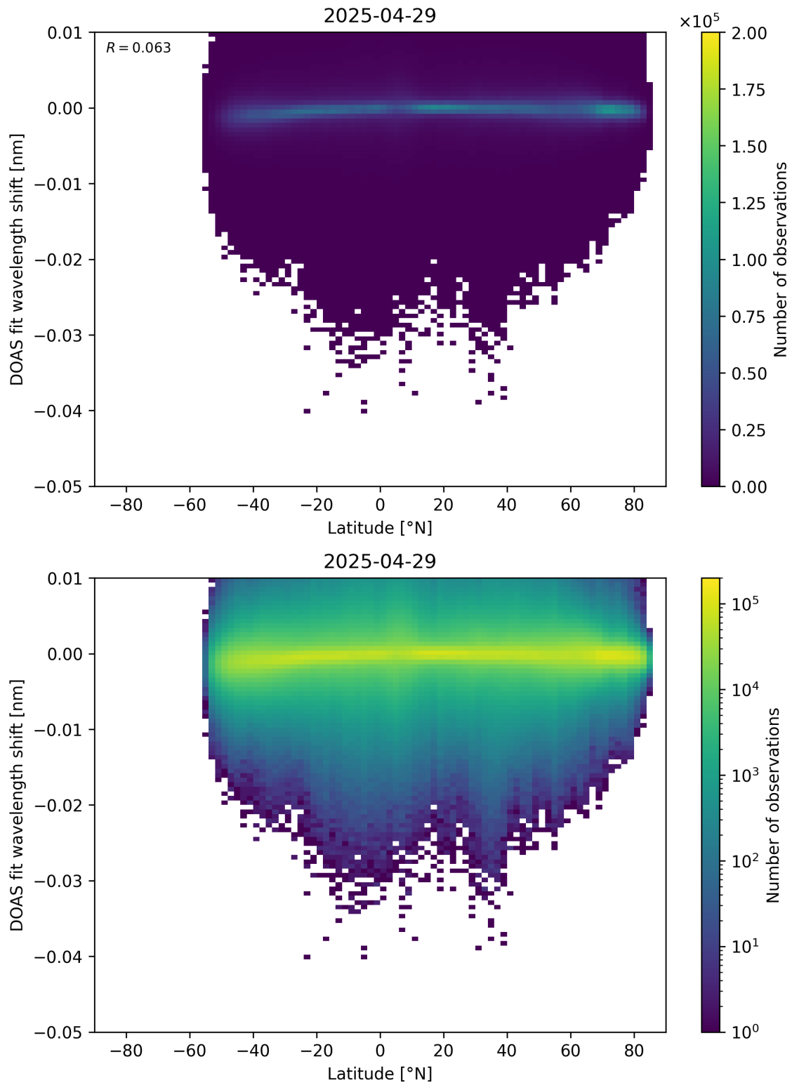
Figure 153: Scatter density plot of “Latitude” against “DOAS fit wavelength shift” for 2025-04-29 to 2025-04-30.
