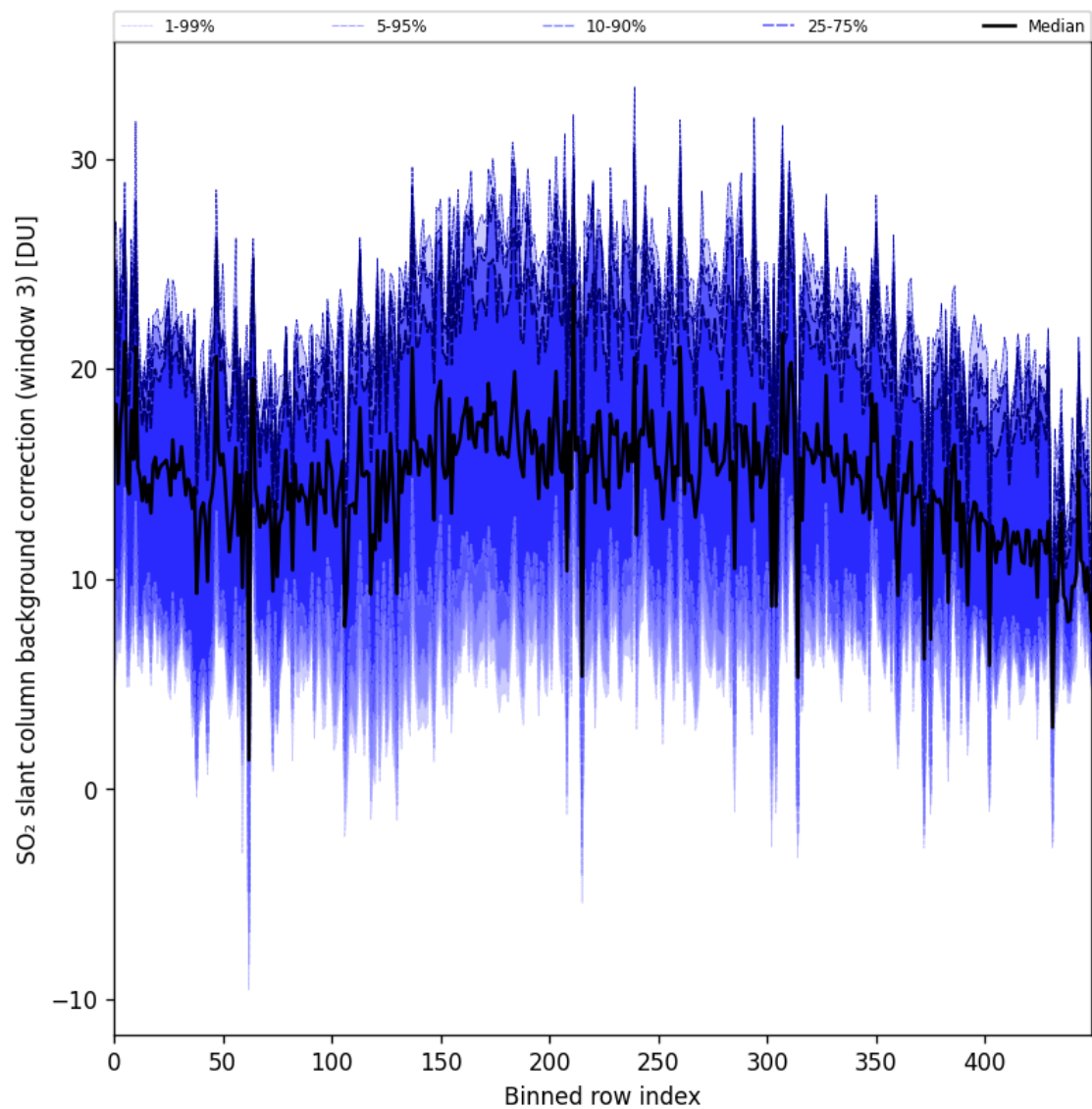
Figure 100: Along track statistics of “SO 2 slant column background correction (window 3)” for 2025-04-29 to 2025-04-30
