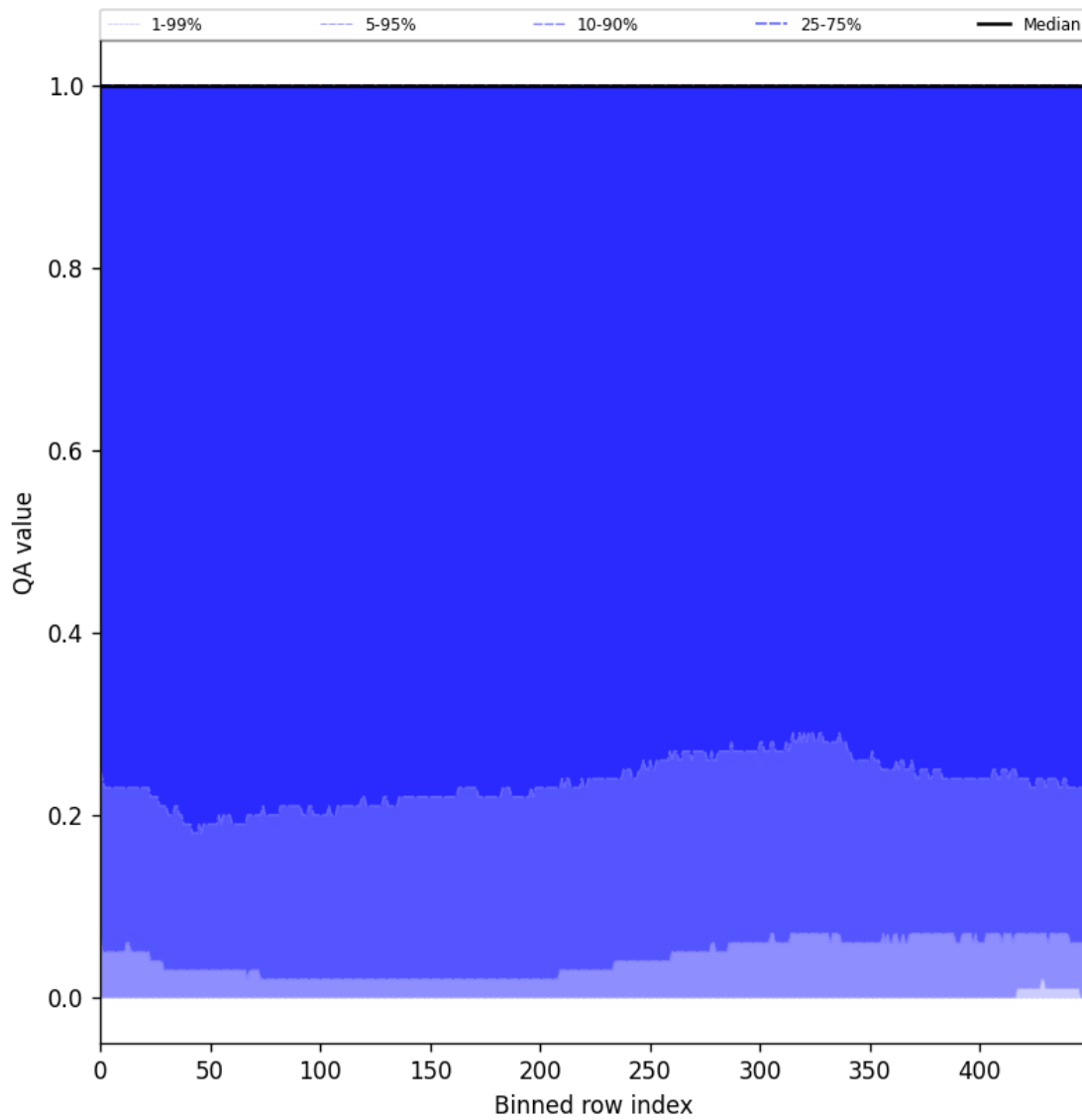
Figure 83: Along track statistics of “QA value” for 2025-04-29 to 2025-04-30
