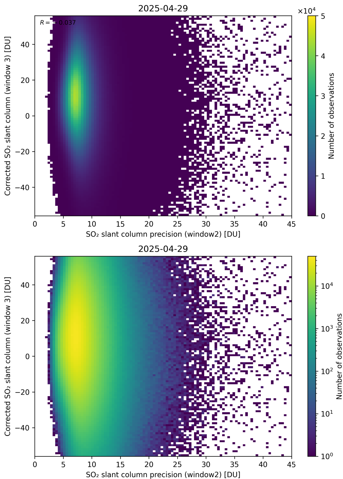
Figure 298: Scatter density plot of “SO 2 slant column precision (window2)” against “Corrected SO 2 slant column (window 3)” for 2025-04-29 to 2025-04-30.
