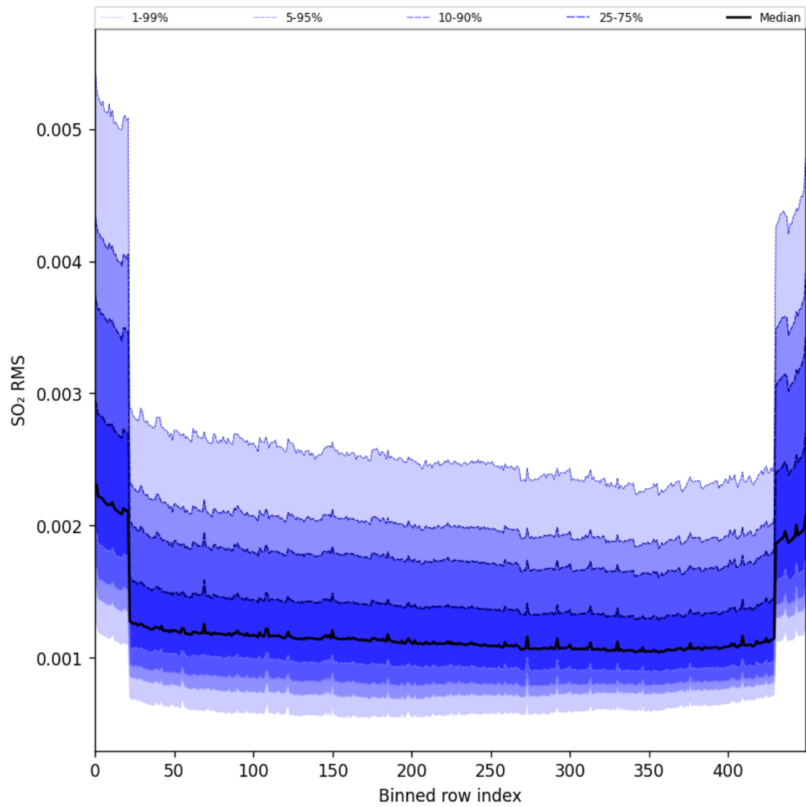
Figure 104: Along track statistics of “SO 2 RMS” for 2025-04-29 to 2025-04-30
