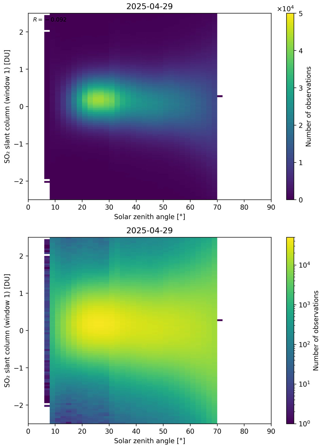
Figure 184: Scatter density plot of “Solar zenith angle” against “SO 2 slant column (window 1)” for 2025-04-29 to 2025-04-30.
