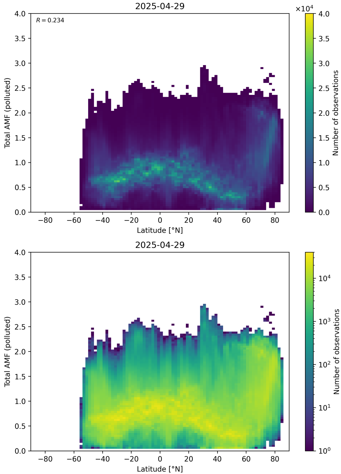
Figure 167: Scatter density plot of “Latitude” against “Total AMF (polluted)” for 2025-04-29 to 2025-04-30.
