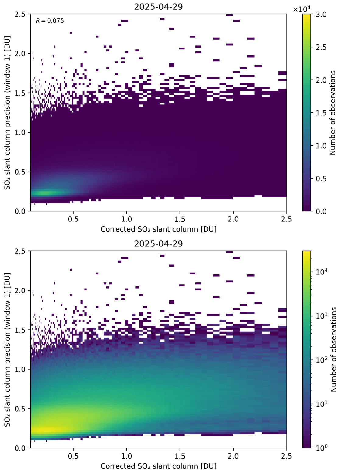
Figure 238: Scatter density plot of “Corrected SO 2 slant column” against “SO 2 slant column precision (window 1)” for 2025-04-29 to 2025-04-30.
