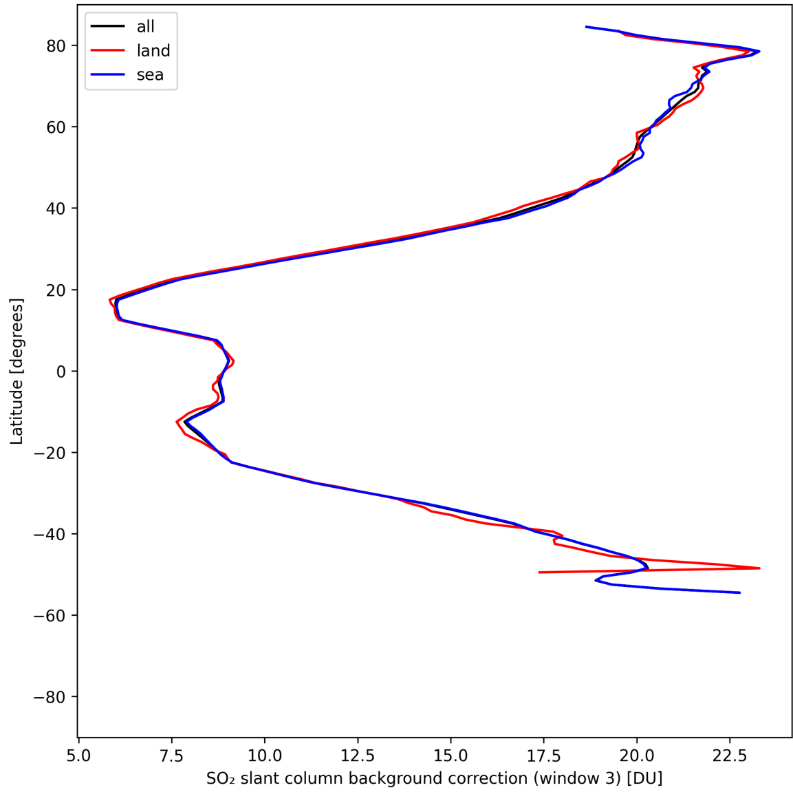
Figure 48: Zonal average of “SO 2 slant column background correction (window 3)” for 2025-04-29 to 2025-04-30.
