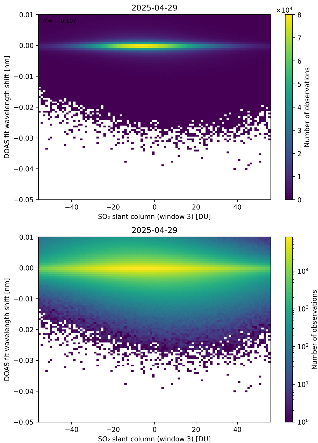
Figure 304: Scatter density plot of “SO 2 slant column (window 3)” against “DOAS fit wavelength shift” for 2025-04-29 to 2025-04-30.
