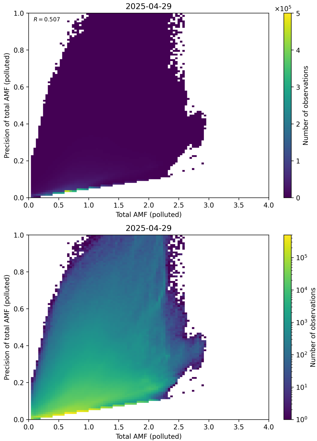
Figure 322: Scatter density plot of “Total AMF (polluted)” against “Precision of total AMF (polluted)” for 2025-04-29 to 2025-04-30.
