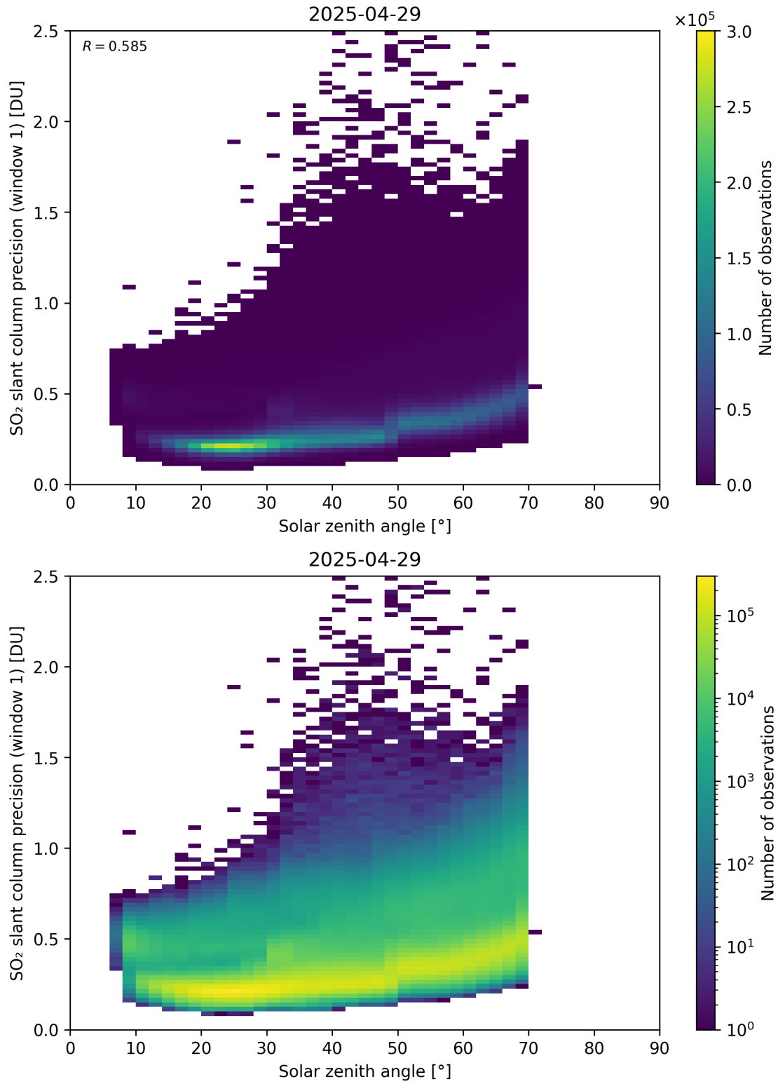
Figure 185: Scatter density plot of “Solar zenith angle” against “SO 2 slant column precision (window 1)” for 2025-04-29 to 2025-04-30.
