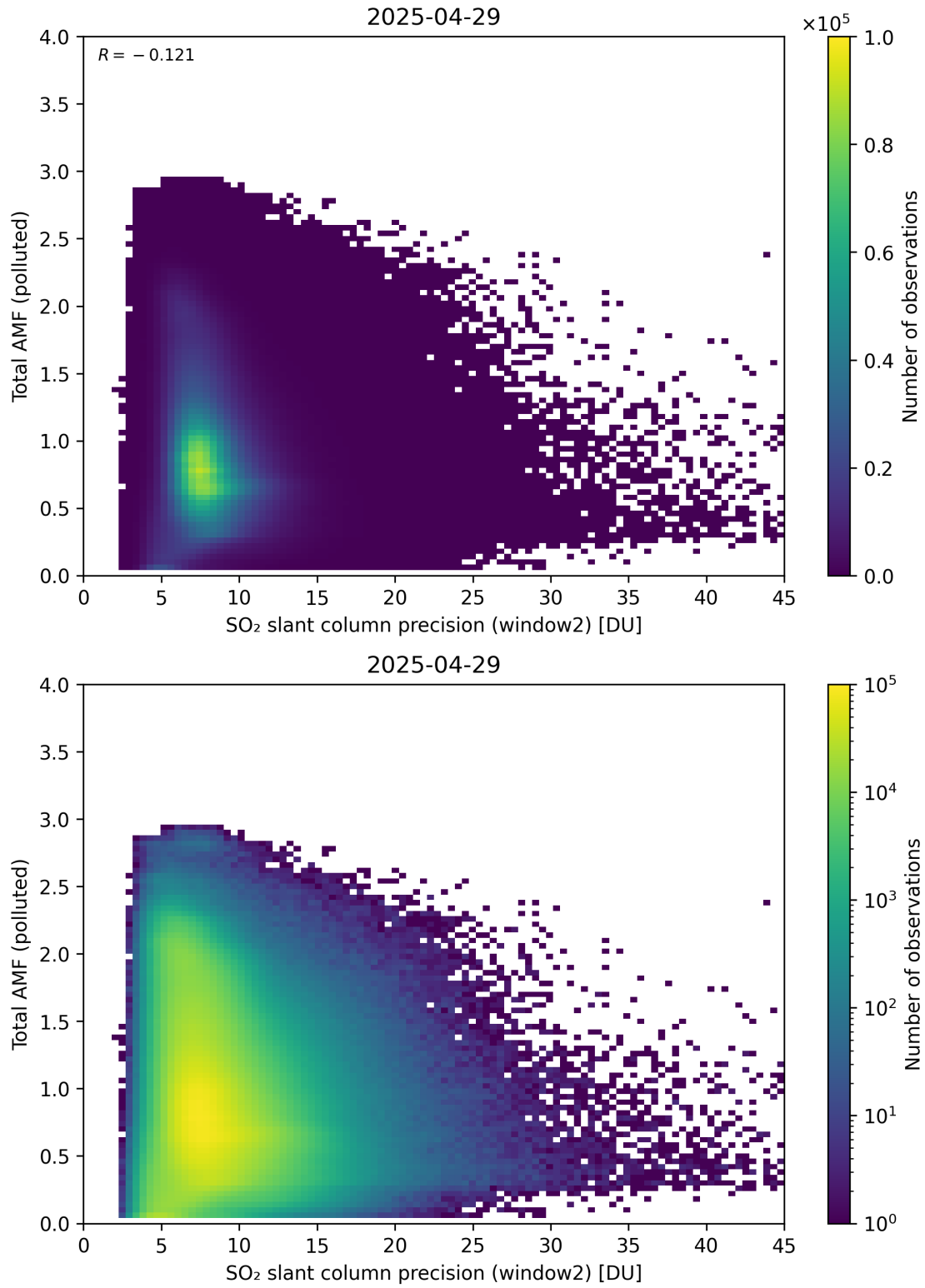
Figure 301: Scatter density plot of “SO 2 slant column precision (window2)” against “Total AMF (polluted)” for 2025-04-29 to 2025-04-30.
