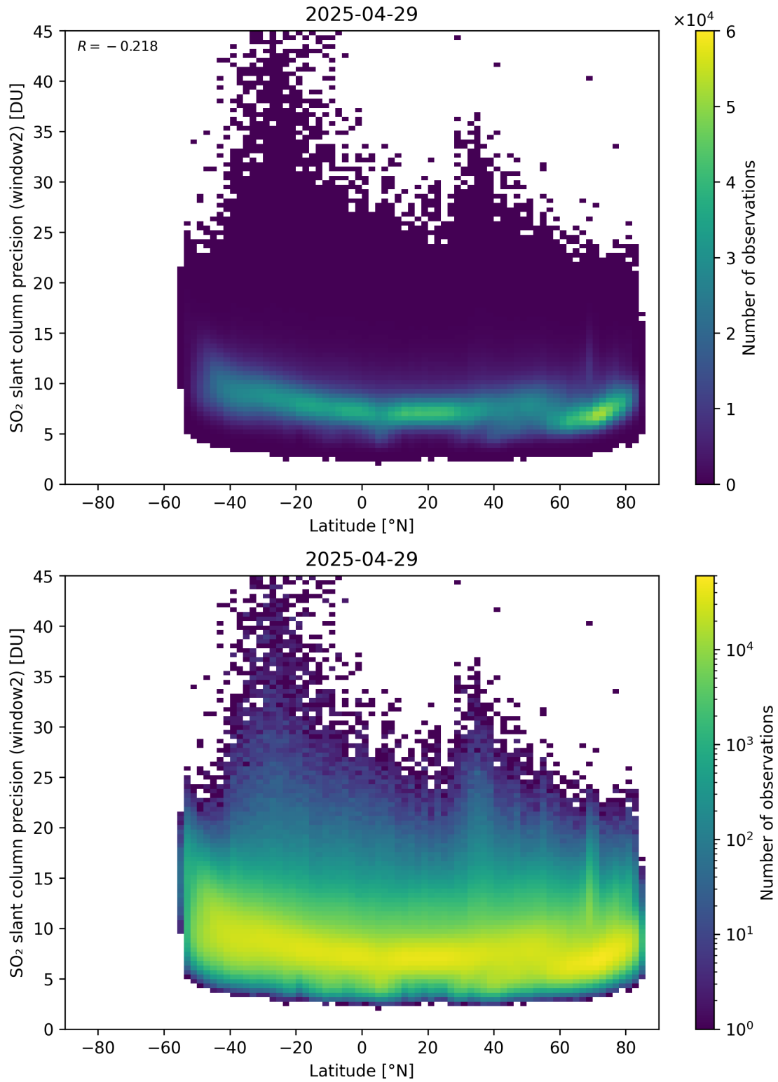
Figure 164: Scatter density plot of “Latitude” against “SO 2 slant column precision (window2)” for 2025-04-29 to 2025-04-30.
