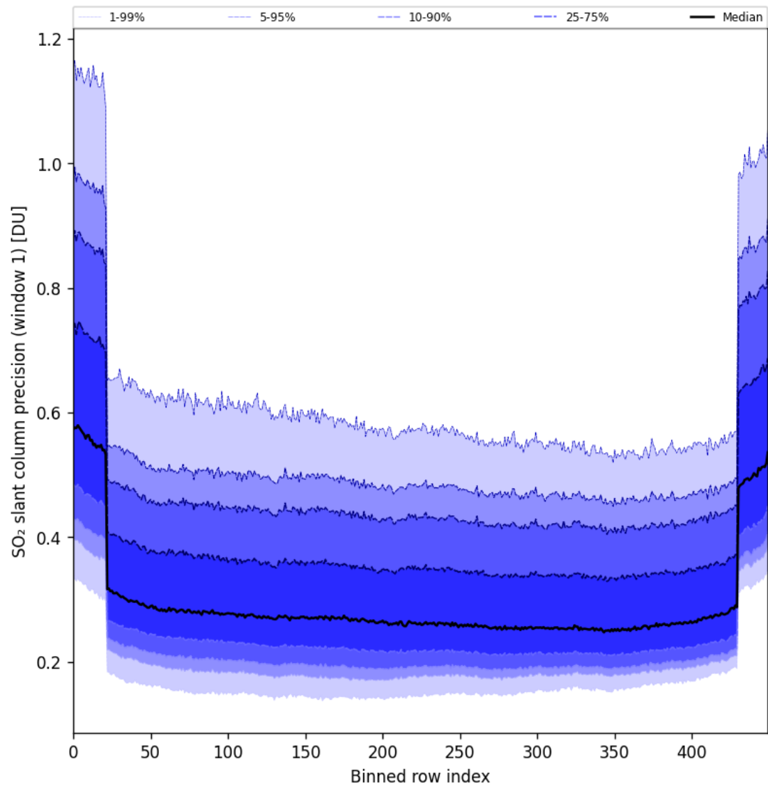
Figure 90: Along track statistics of “SO 2 slant column precision (window 1)” for 2025-04-29 to 2025-04-30
