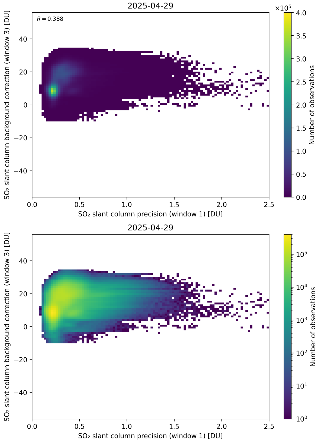
Figure 270: Scatter density plot of “SO 2 slant column precision (window 1)” against “SO 2 slant column background correction (window 3)” for 2025-04-29 to 2025-04-30.
