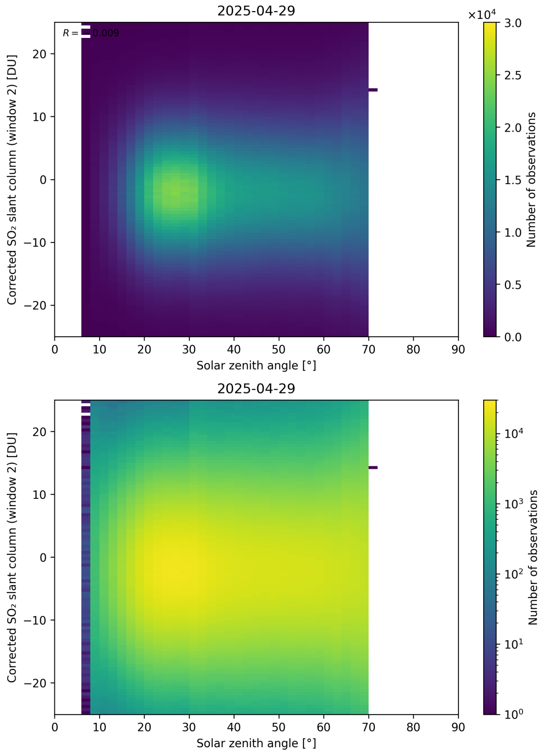
Figure 182: Scatter density plot of “Solar zenith angle” against “Corrected SO 2 slant column (window 2)” for 2025-04-29 to 2025-04-30.
