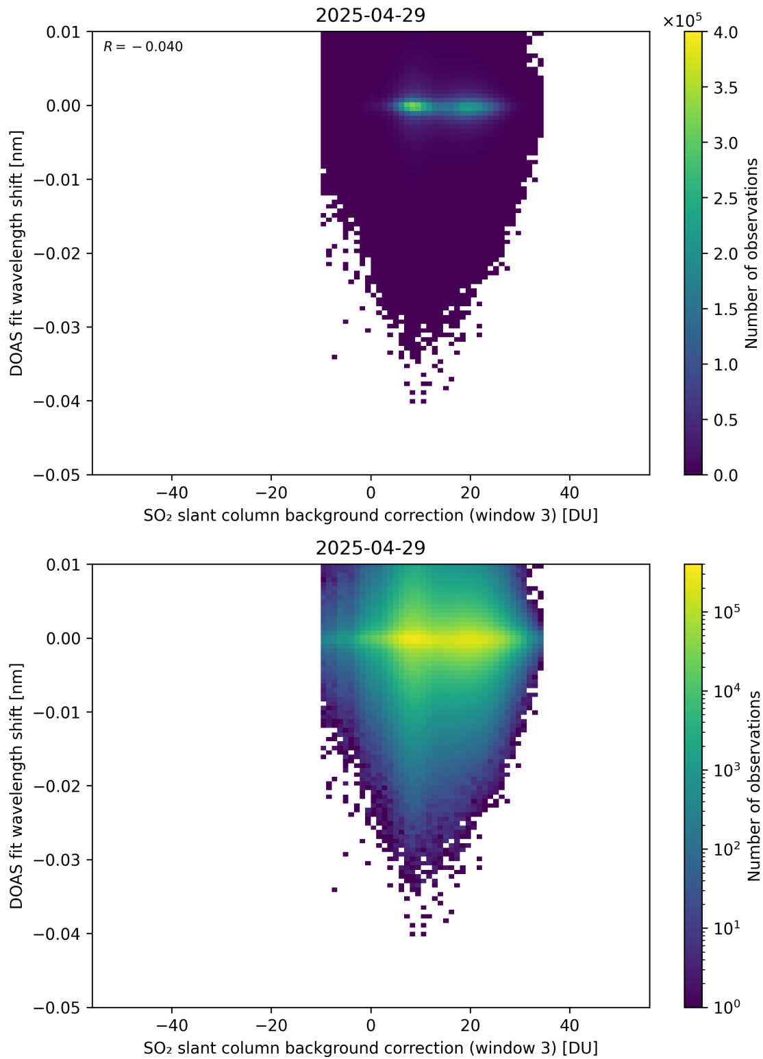
Figure 132: Scatter density plot of “SO 2 slant column background correction (window 3)” against “DOAS fit wavelength shift” for 2025-04-29 to 2025-04-30.
