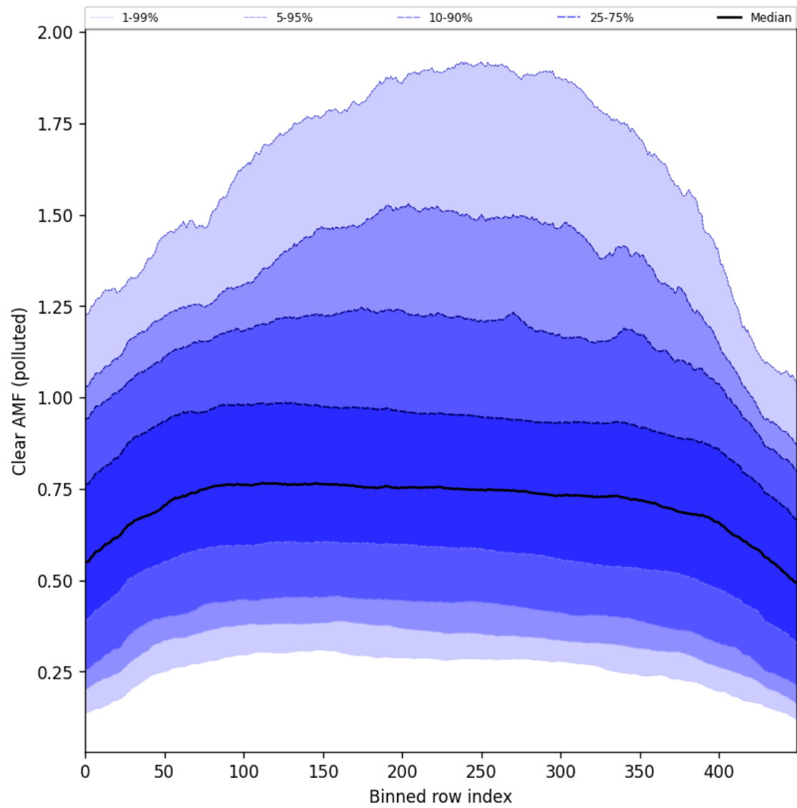
Figure 107: Along track statistics of “Clear AMF (polluted)” for 2025-04-29 to 2025-04-30
