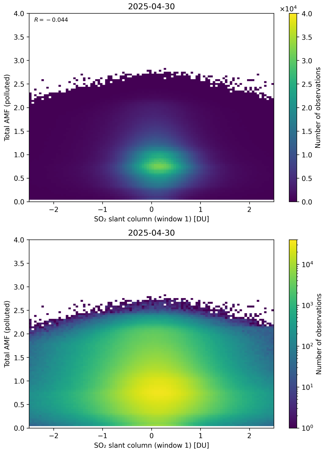
Figure 289: Scatter density plot of “SO 2 slant column (window 1)” against “Total AMF (polluted)” for 2025-04-29 to 2025-05-01.
