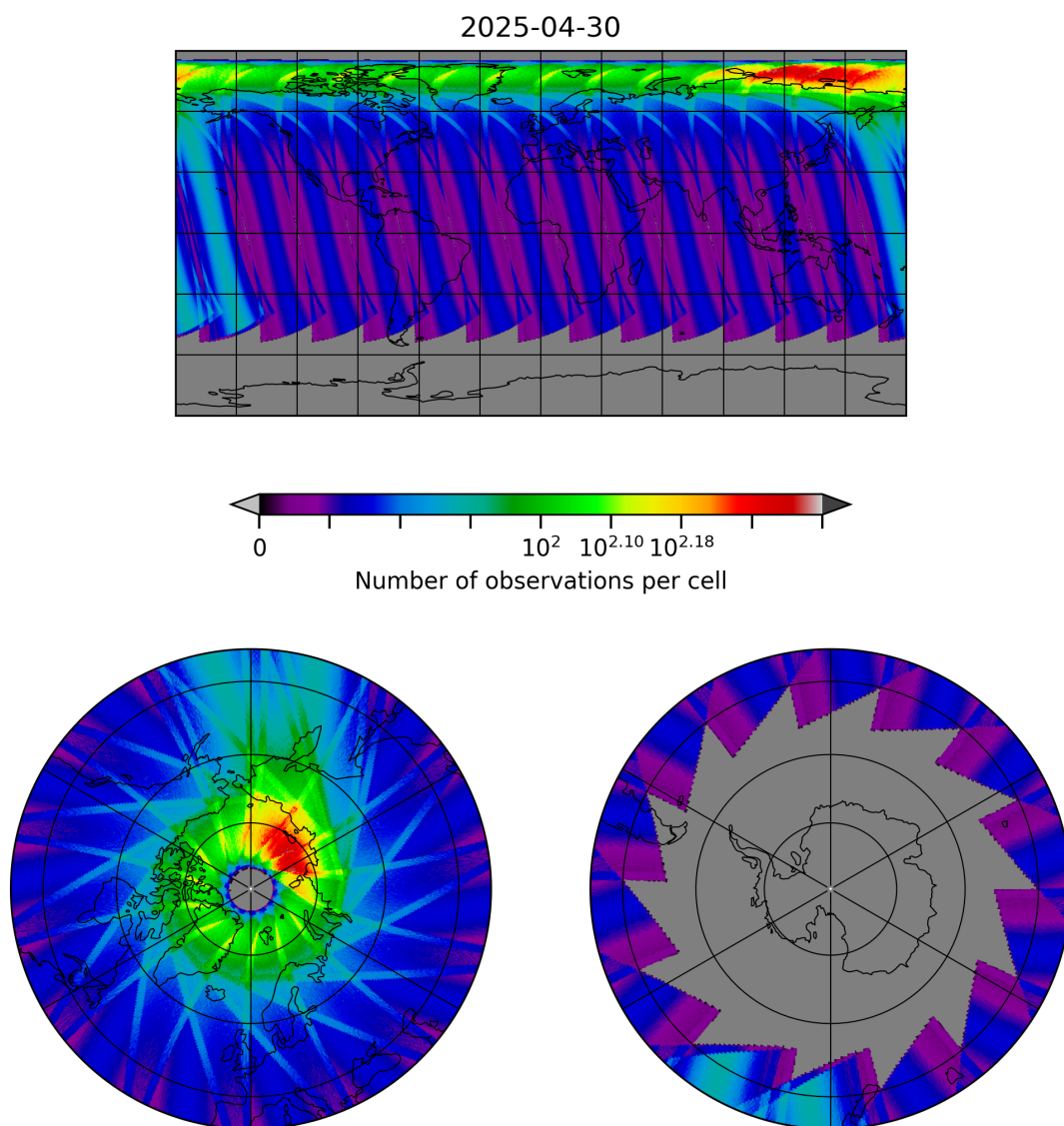
Figure 30: Map of the number of observations for 2025-04-29 to 2025-05-01
