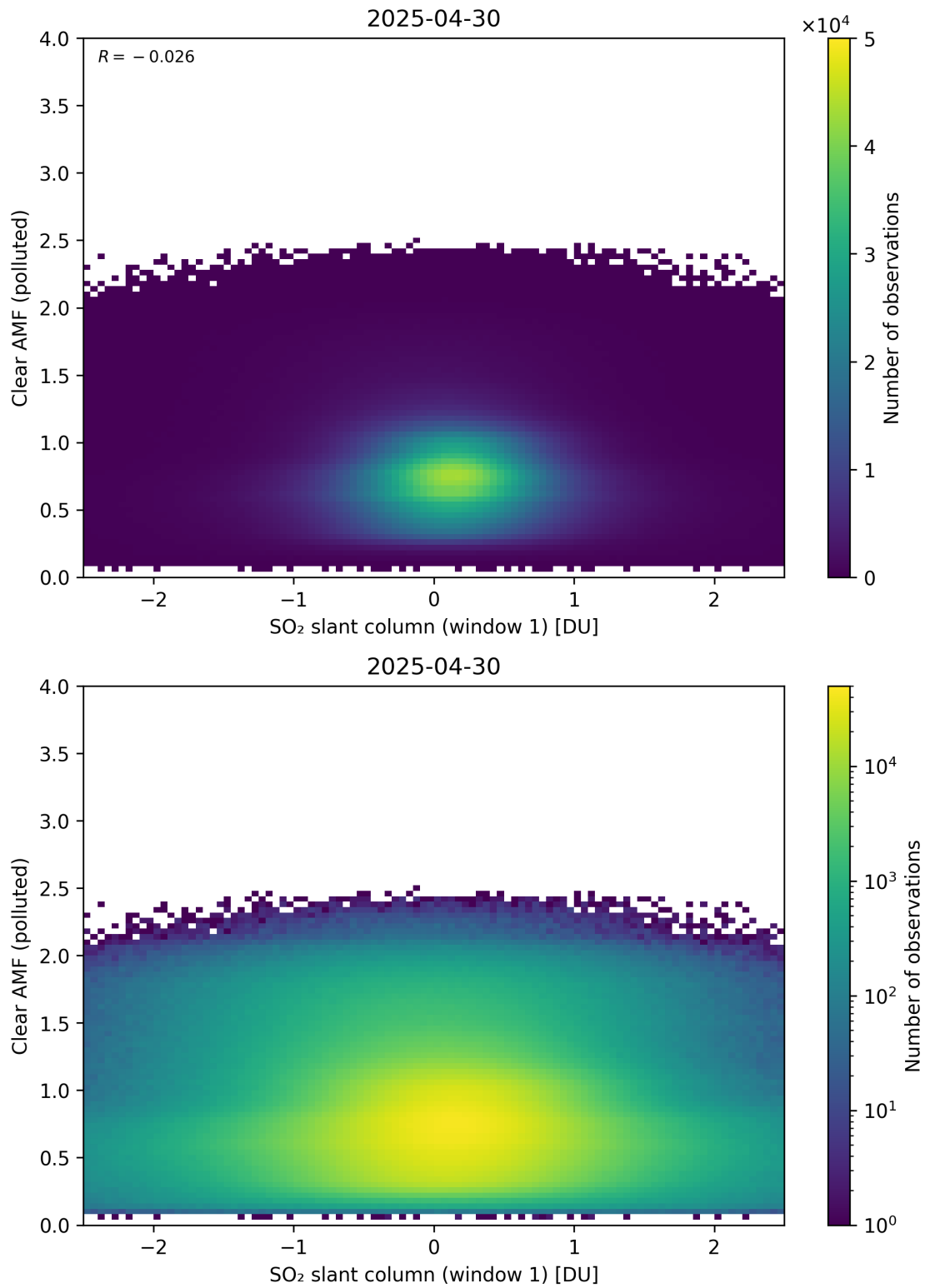
Figure 282: Scatter density plot of “SO 2 slant column (window 1)” against “Clear AMF (polluted)” for 2025-04-29 to 2025-05-01.
