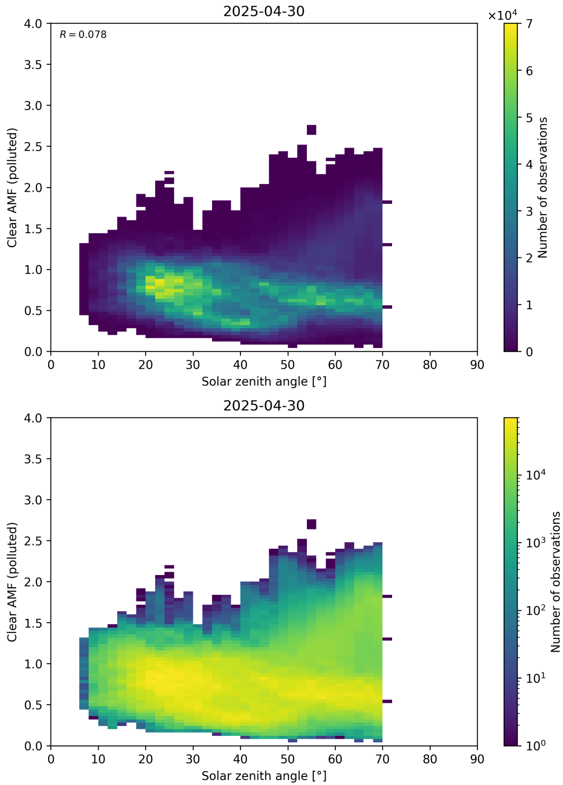
Figure 178: Scatter density plot of “Solar zenith angle” against “Clear AMF (polluted)” for 2025-04-29 to 2025-05-01.
