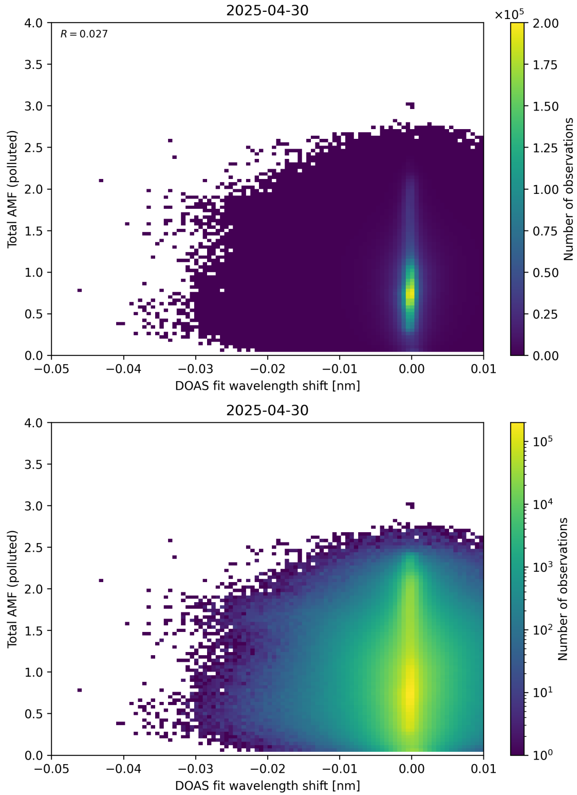
Figure 141: Scatter density plot of “DOAS fit wavelength shift” against “Total AMF (polluted)” for 2025-04-29 to 2025-05-01.
