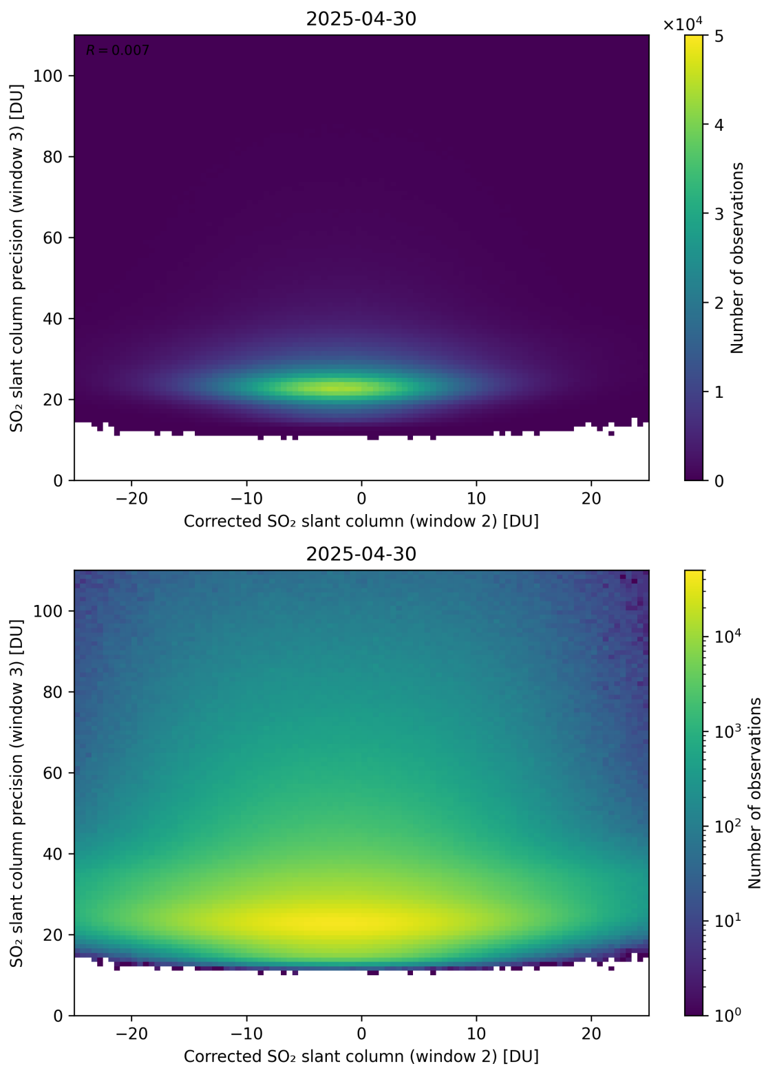
Figure 252: Scatter density plot of “Corrected SO 2 slant column (window 2)” against “SO 2 slant column precision (window 3)” for 2025-04-29 to 2025-05-01.
