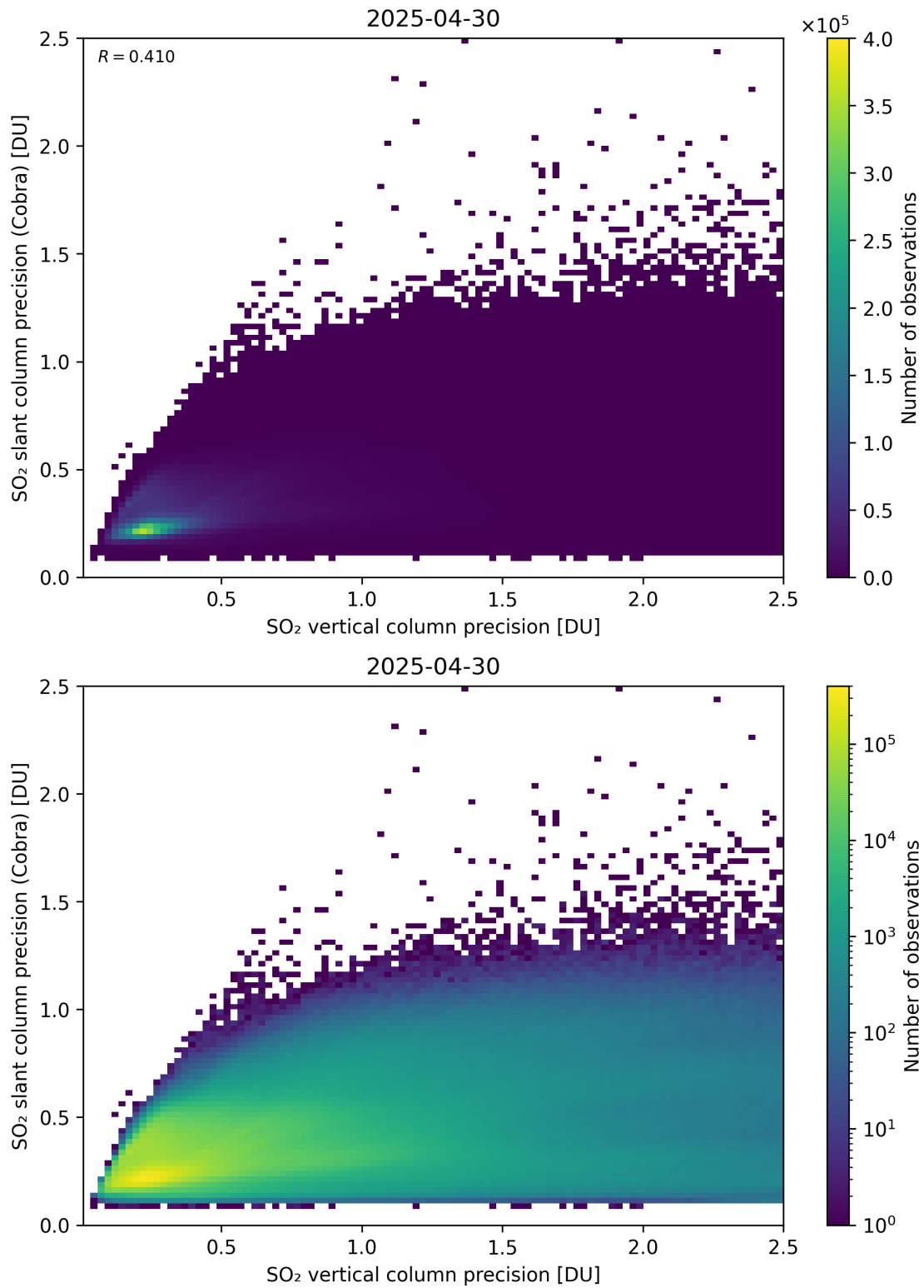
Figure 337: Scatter density plot of “SO 2 vertical column precision” against “SO 2 slant column precision (Cobra)” for 2025-04-29 to 2025-05-01.
