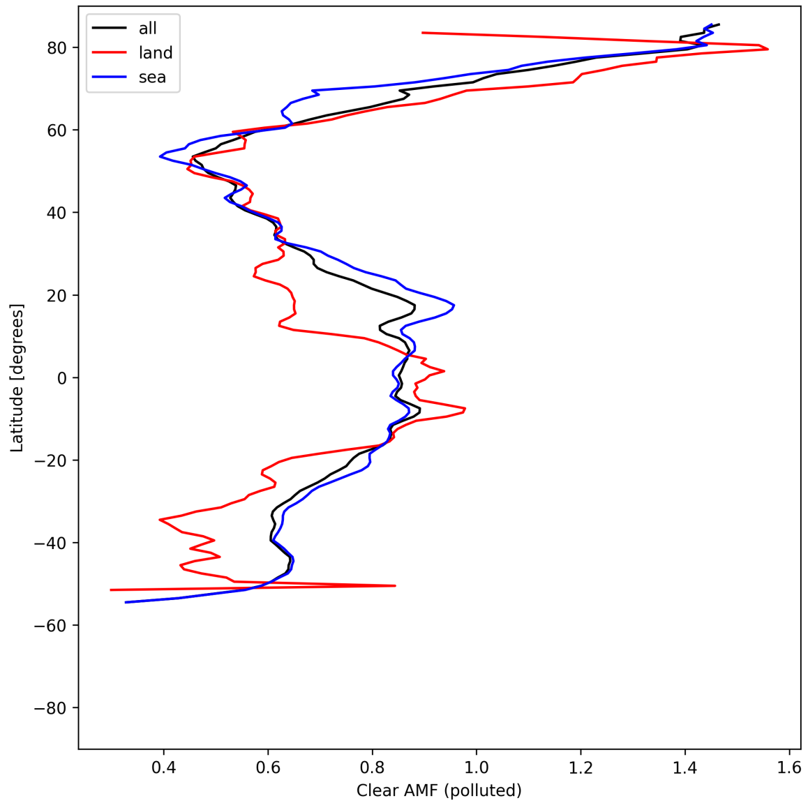
Figure 55: Zonal average of “Clear AMF (polluted)” for 2025-04-29 to 2025-05-01.
