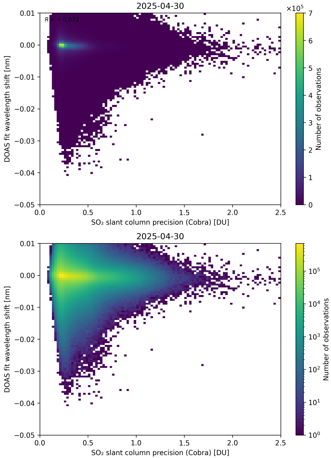
Figure 202: Scatter density plot of “SO 2 slant column precision (Cobra)” against “DOAS fit wavelength shift” for 2025-04-29 to 2025-05-01.
