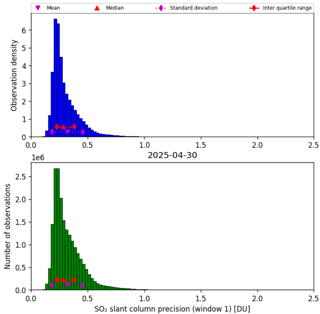
Figure 64: Histogram of “SO 2 slant column precision (window 1)” for 2025-04-29 to 2025-05-01
