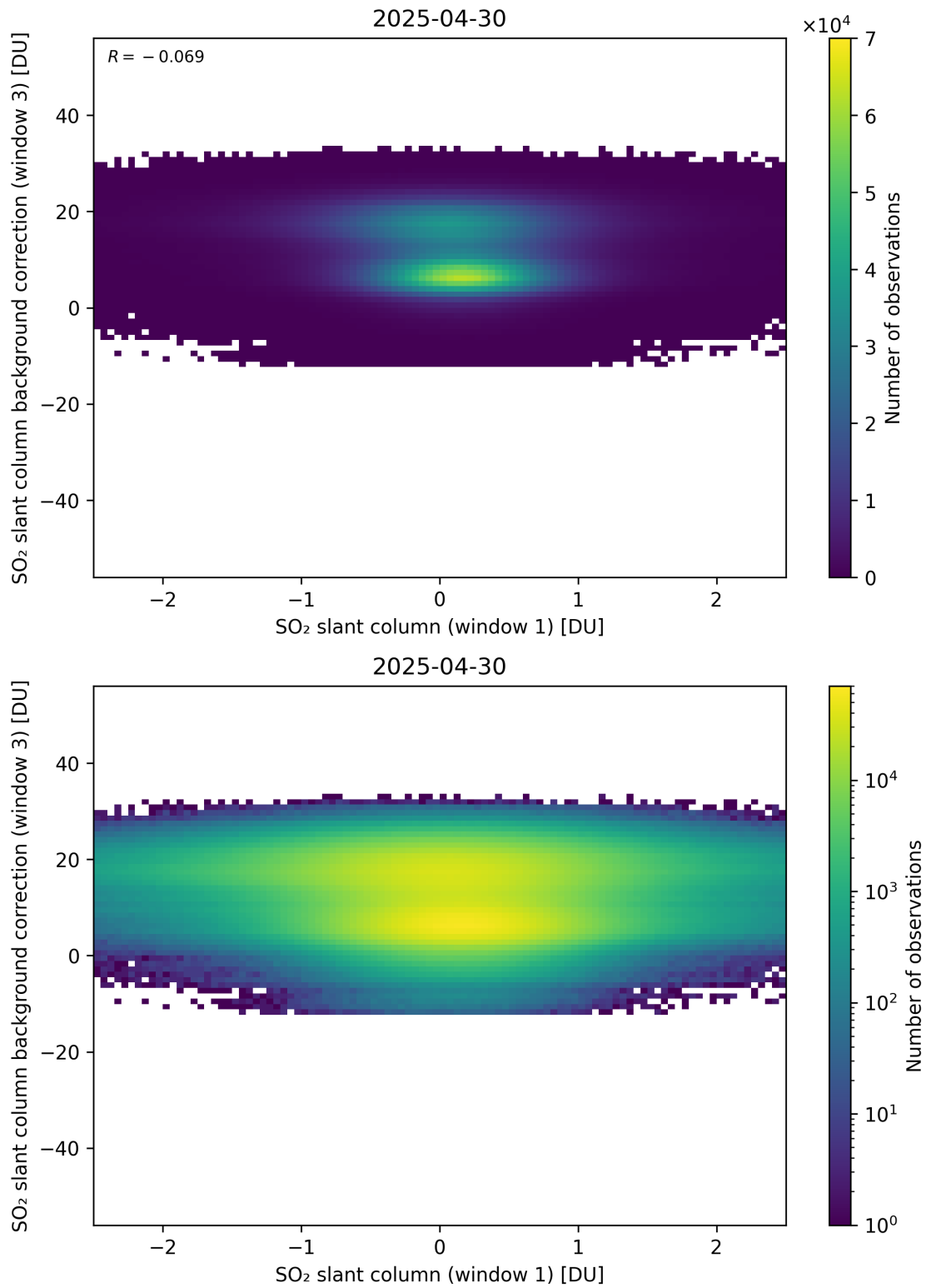
Figure 264: Scatter density plot of “SO 2 slant column (window 1)” against “SO 2 slant column background correction (window 3)” for 2025-04-29 to 2025-05-01.
