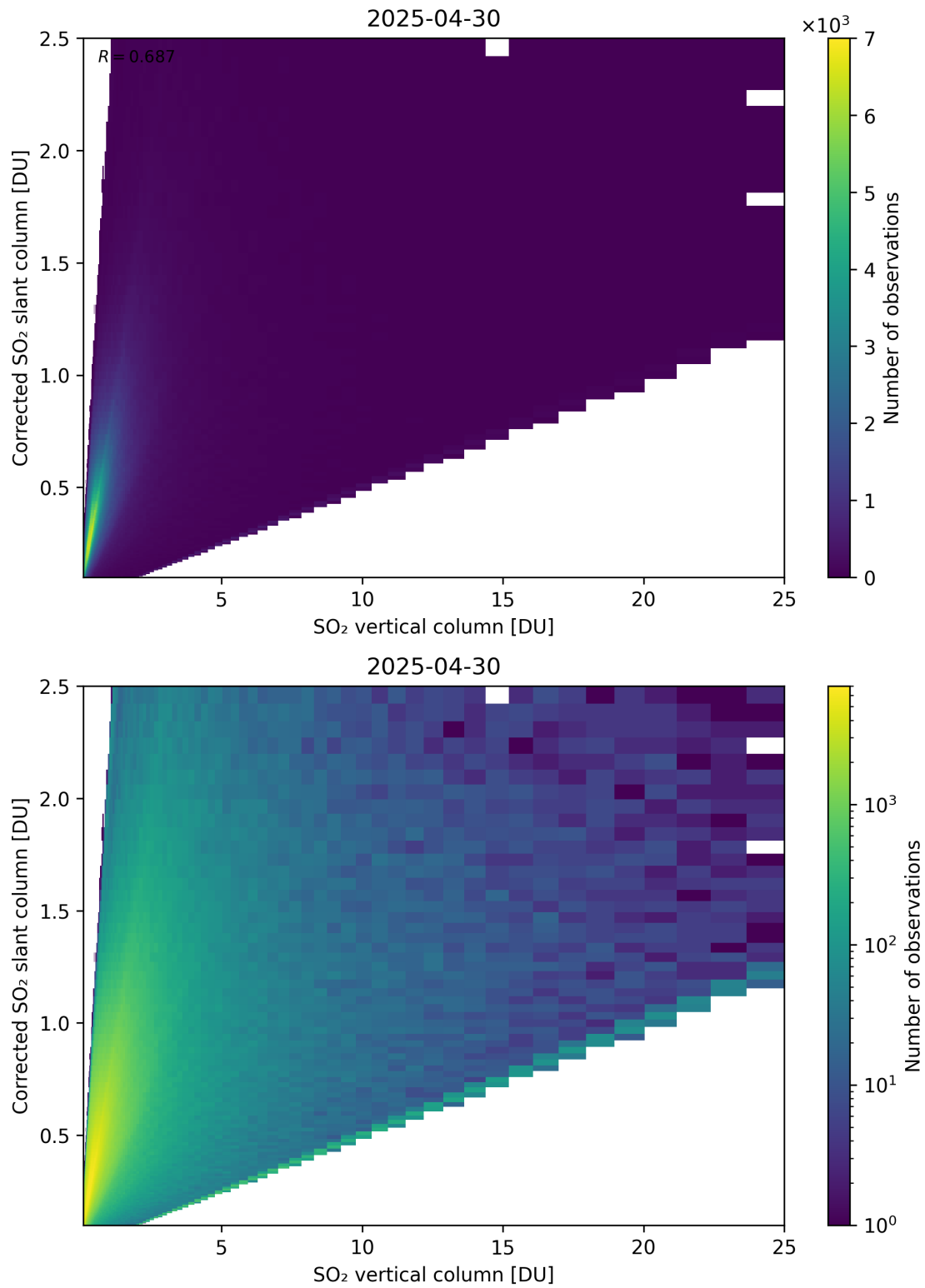
Figure 351: Scatter density plot of “SO 2 vertical column” against “Corrected SO 2 slant column” for 2025-04-29 to 2025-05-01.
