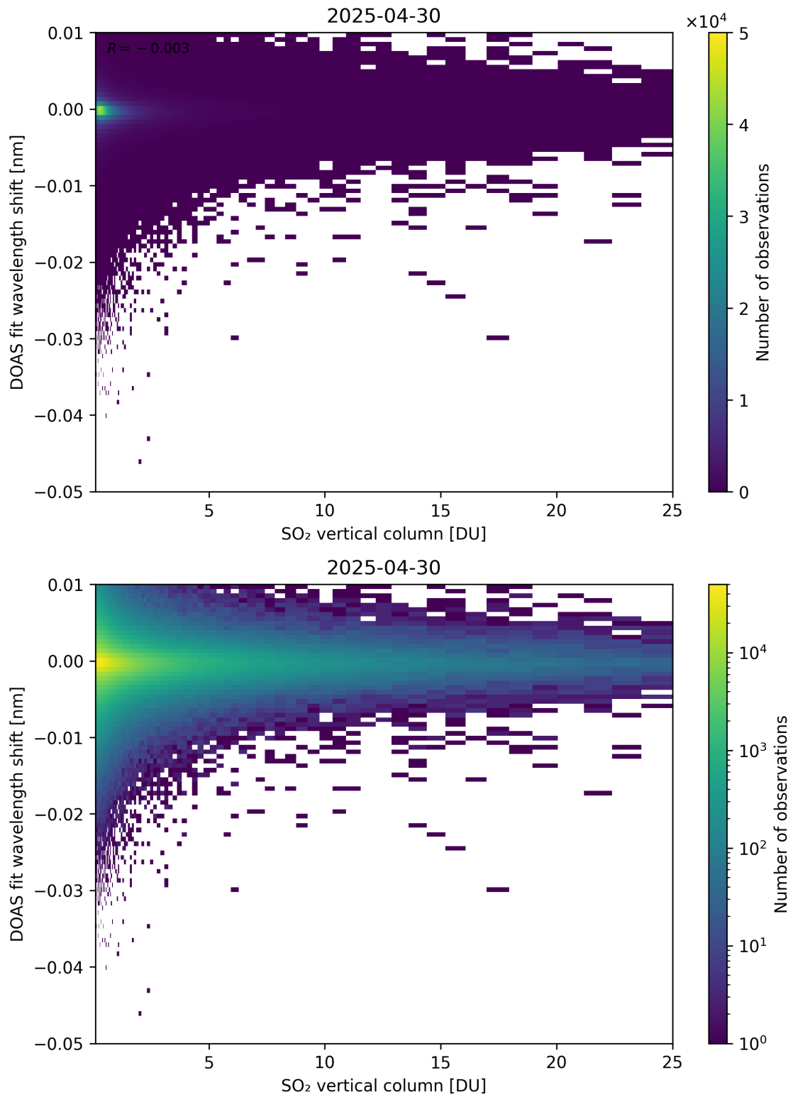
Figure 326: Scatter density plot of “SO 2 vertical column” against “DOAS fit wavelength shift” for 2025-04-29 to 2025-05-01.
