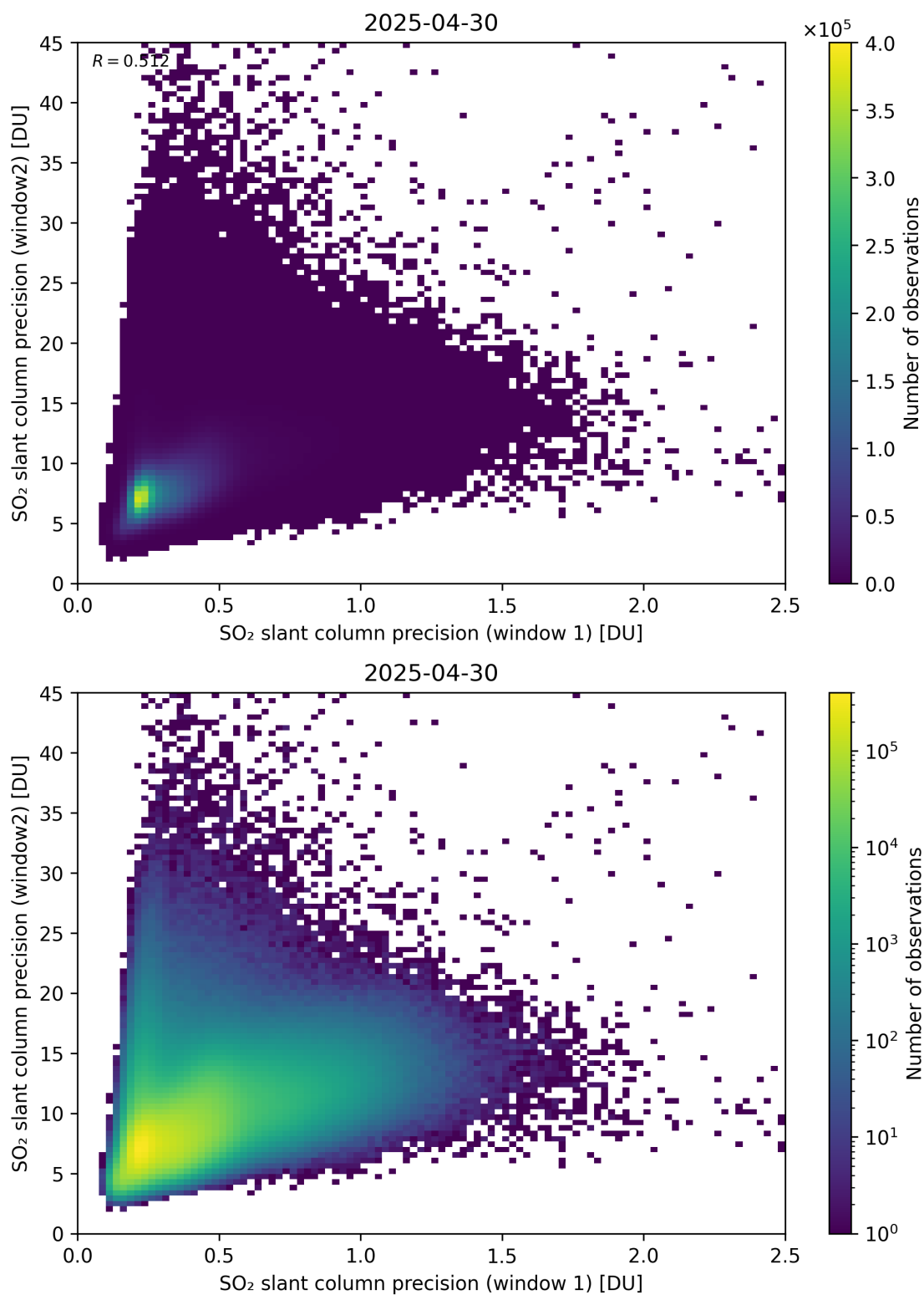
Figure 277: Scatter density plot of “SO 2 slant column precision (window 1)” against “SO 2 slant column precision (window2)” for 2025-04-29 to 2025-05-01.
