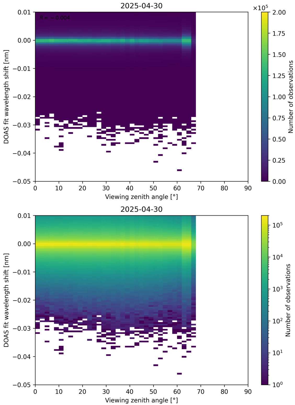
Figure 365: Scatter density plot of “Viewing zenith angle” against “DOAS fit wavelength shift” for 2025-04-29 to 2025-05-01.
