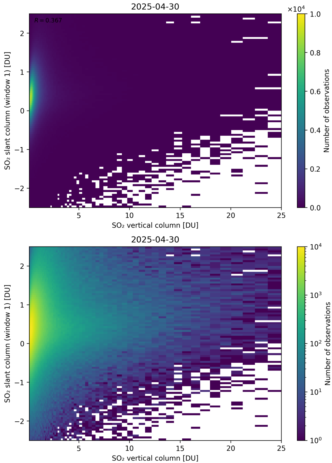
Figure 354: Scatter density plot of “SO 2 vertical column” against “SO 2 slant column (window 1)” for 2025-04-29 to 2025-05-01.
