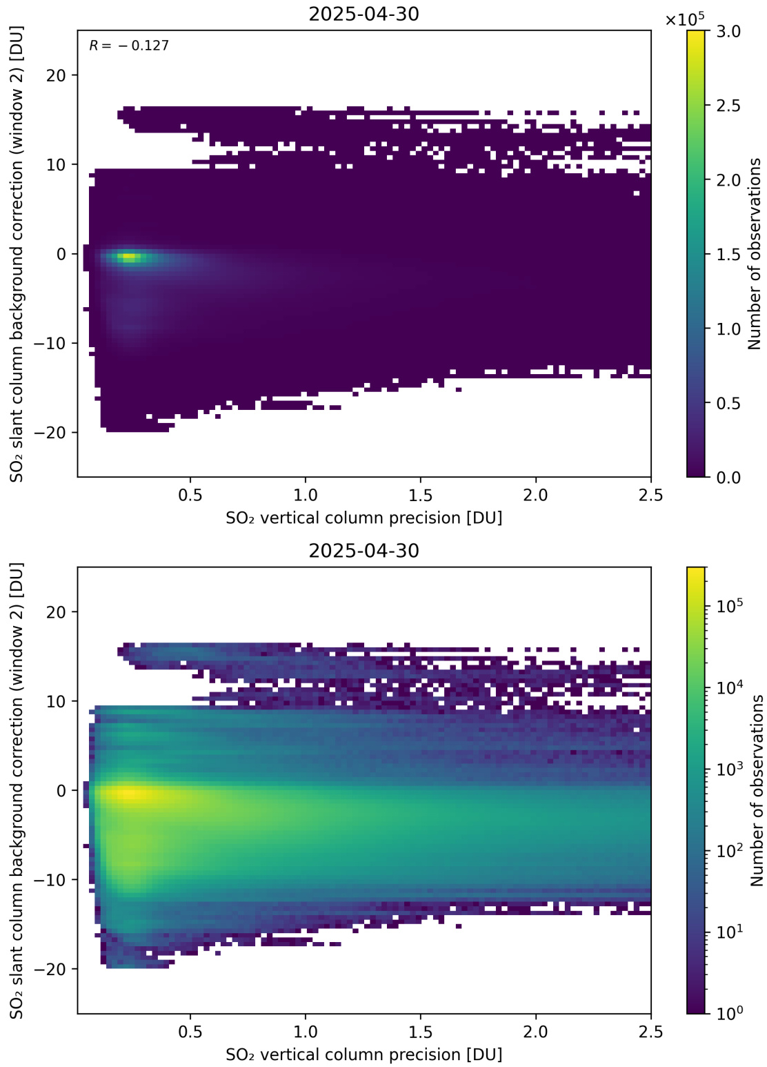
Figure 330: Scatter density plot of “SO 2 vertical column precision” against “SO 2 slant column background correction (window 2)” for 2025-04-29 to 2025-05-01.
