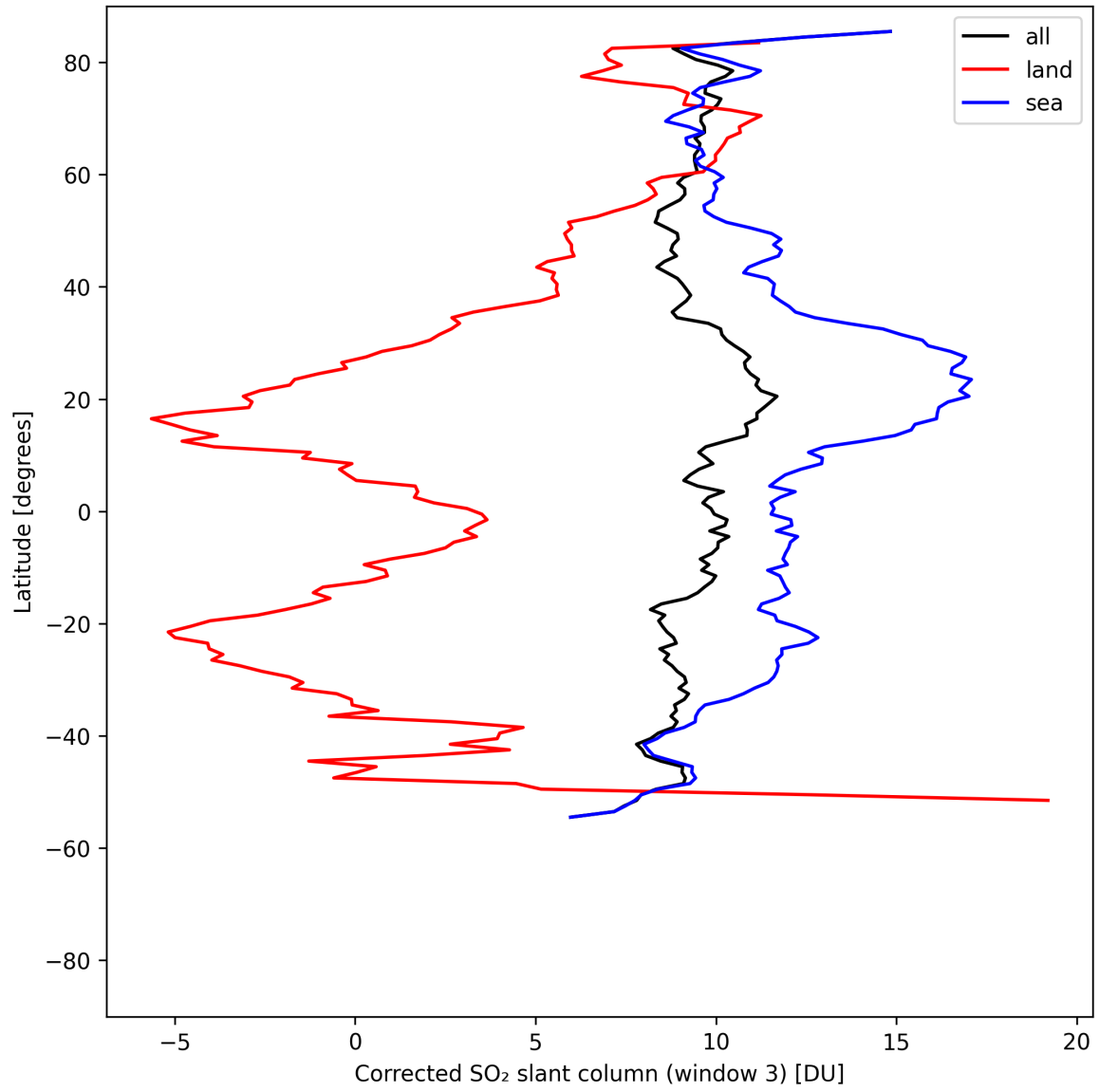
Figure 47: Zonal average of “Corrected SO 2 slant column (window 3)” for 2025-04-29 to 2025-05-01.
