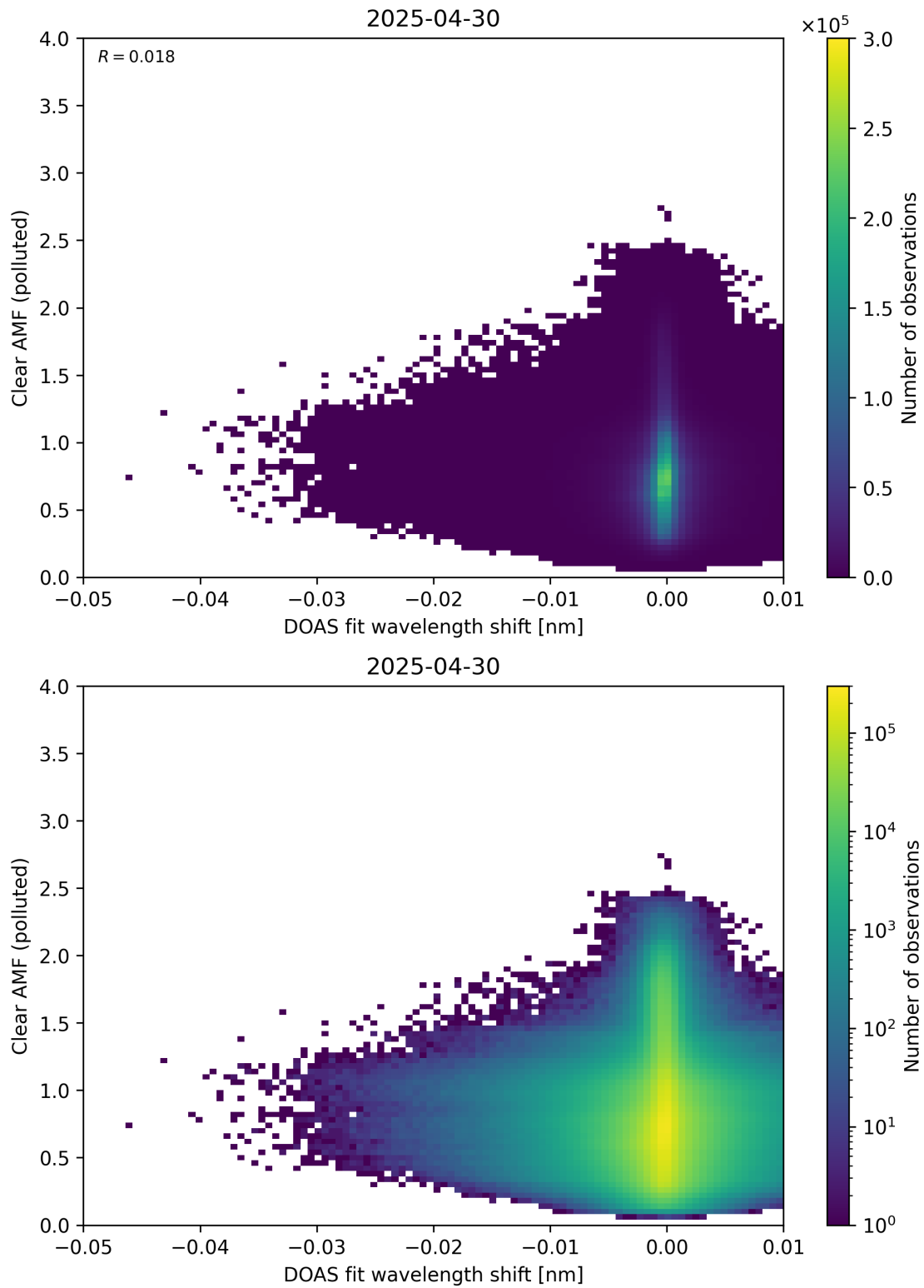
Figure 140: Scatter density plot of “DOAS fit wavelength shift” against “Clear AMF (polluted)” for 2025-04-29 to 2025-05-01.
