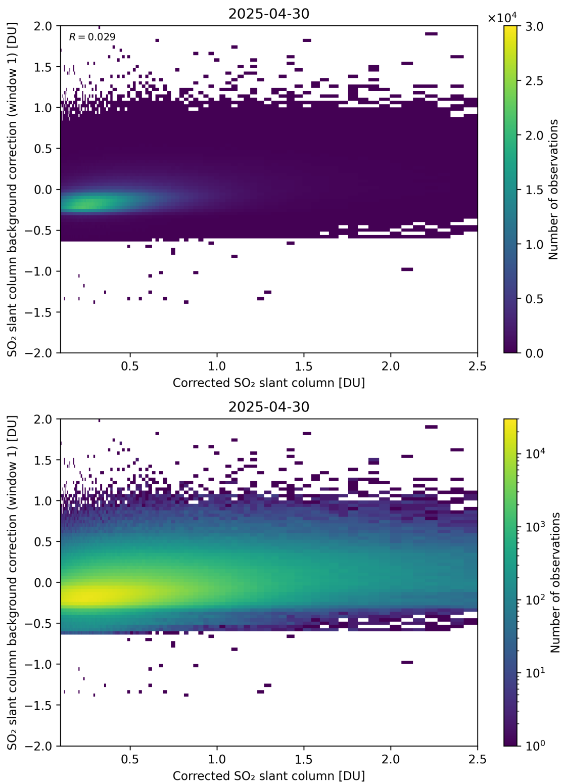
Figure 226: Scatter density plot of “Corrected SO 2 slant column” against “SO 2 slant column background correction (window 1)” for 2025-04-29 to 2025-05-01.
