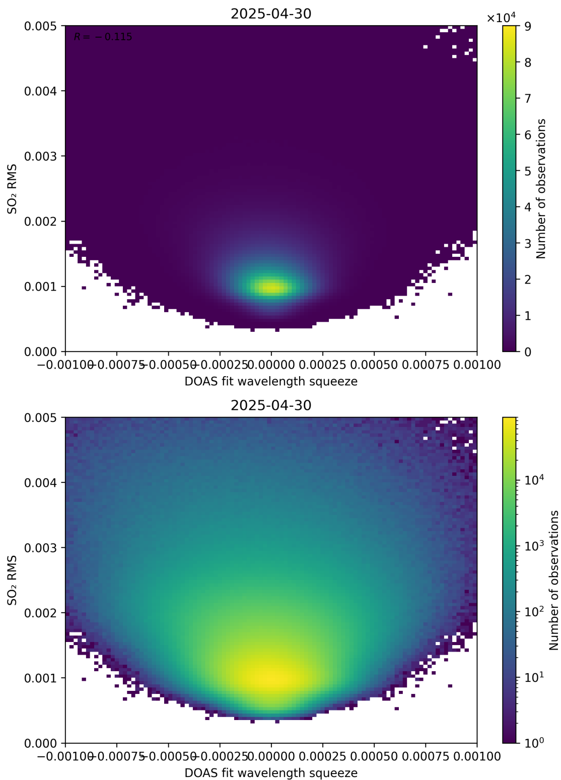
Figure 143: Scatter density plot of “DOAS fit wavelength squeeze” against “SO 2 RMS” for 2025-04-29 to 2025-05-01.
