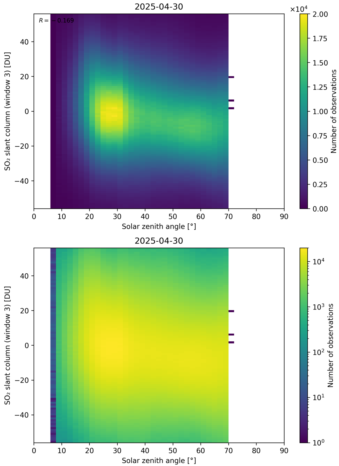
Figure 187: Scatter density plot of “Solar zenith angle” against “SO 2 slant column (window 3)” for 2025-04-29 to 2025-05-01.
