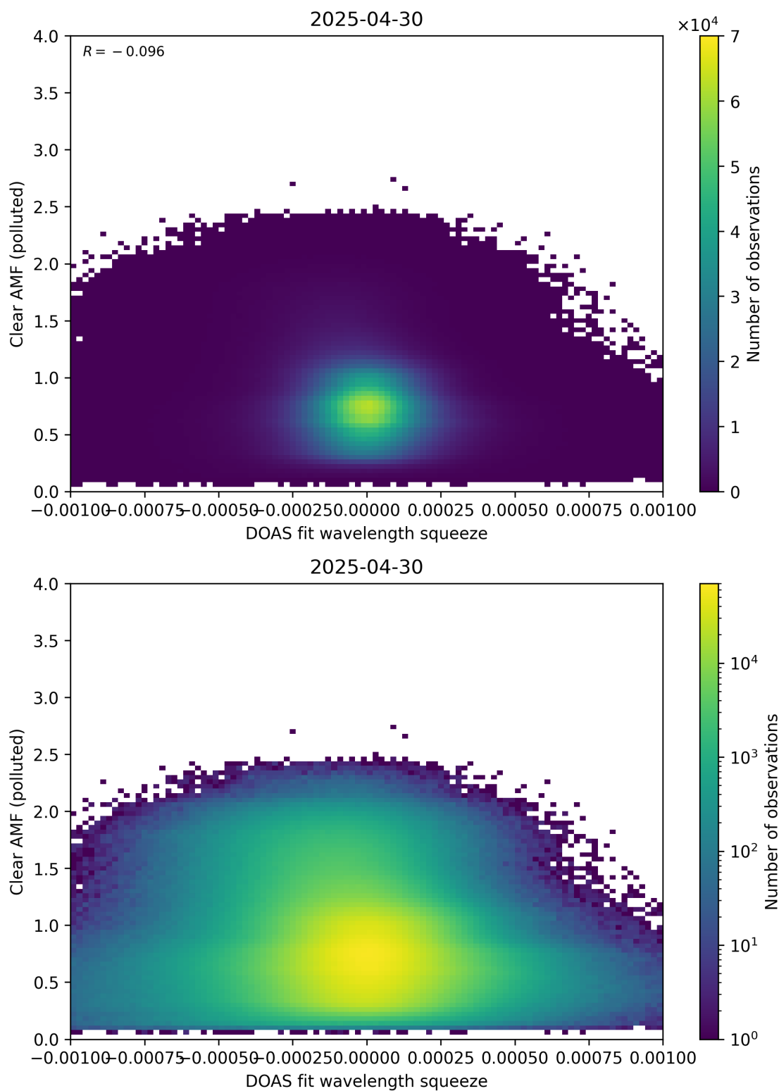
Figure 144: Scatter density plot of “DOAS fit wavelength squeeze” against “Clear AMF (polluted)” for 2025-04-29 to 2025-05-01.
