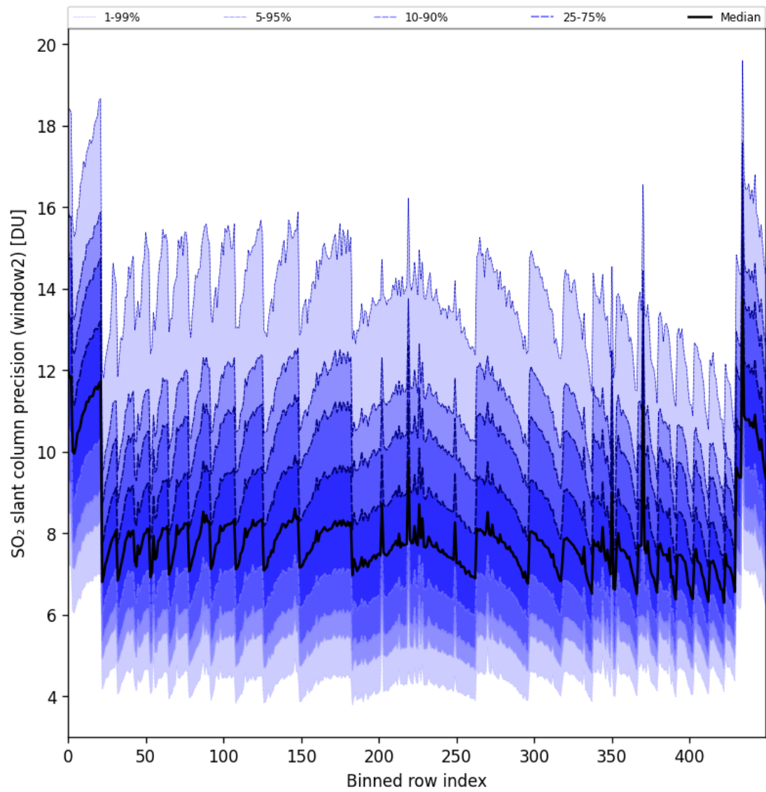
Figure 94: Along track statistics of “SO 2 slant column precision (window2)” for 2025-04-29 to 2025-05-01
