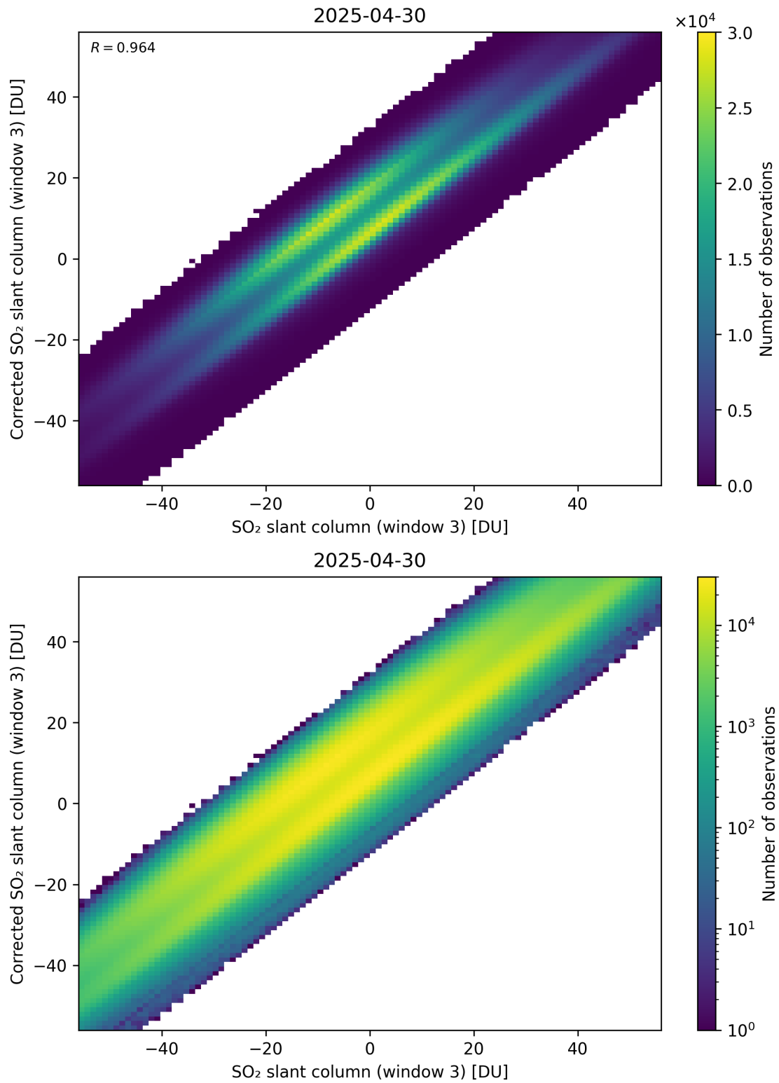
Figure 316: Scatter density plot of “SO 2 slant column (window 3)” against “Corrected SO 2 slant column (window 3)” for 2025-04-29 to 2025-05-01.
