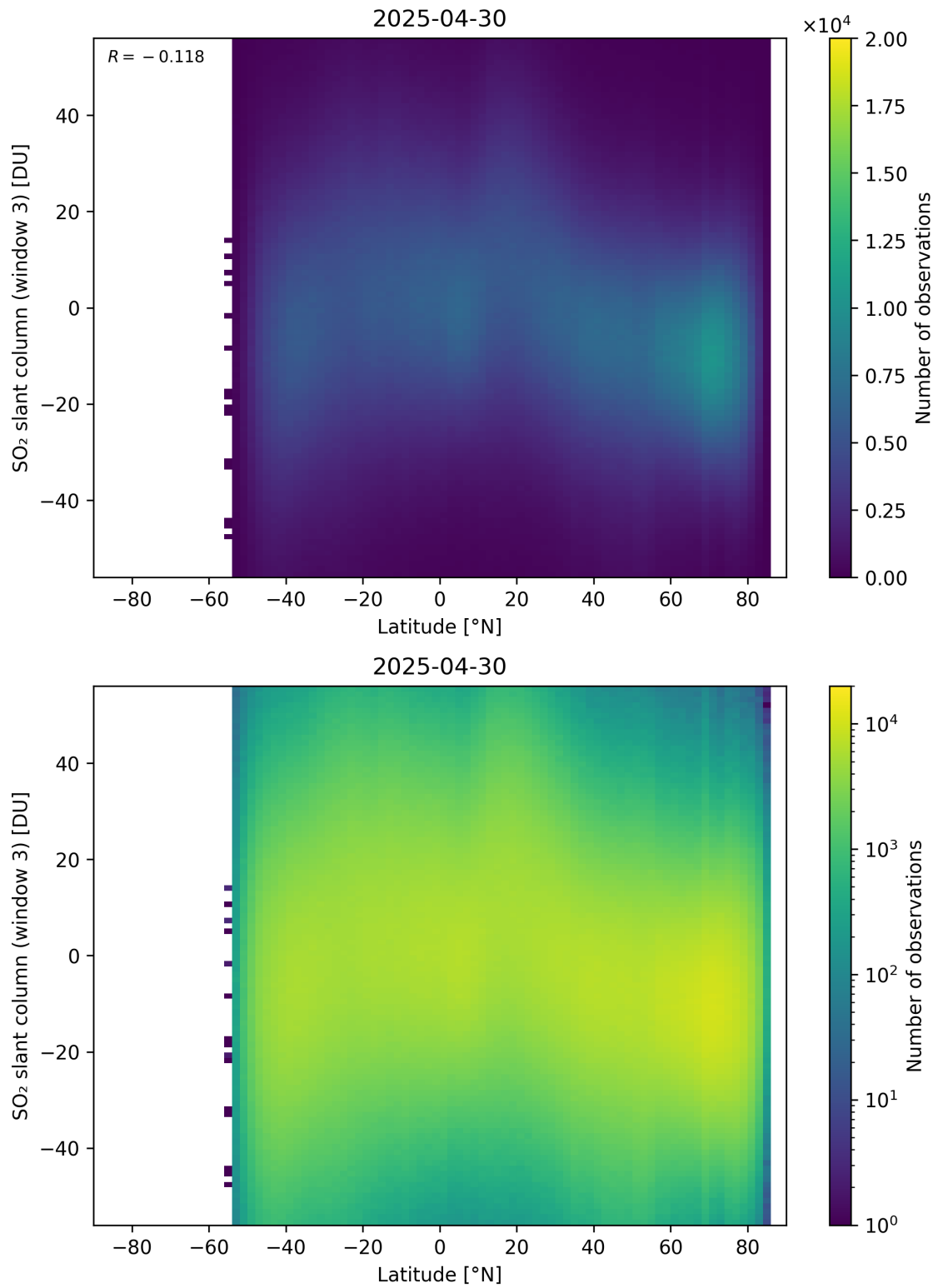
Figure 165: Scatter density plot of “Latitude” against “SO 2 slant column (window 3)” for 2025-04-29 to 2025-05-01.
