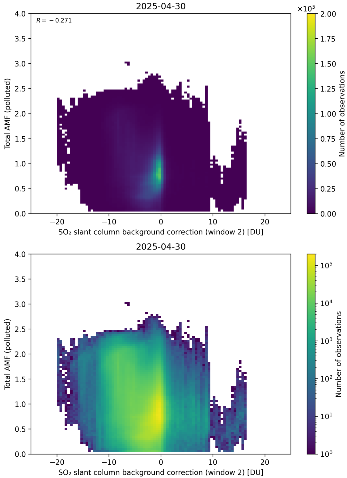
Figure 130: Scatter density plot of “SO 2 slant column background correction (window 2)” against “Total AMF (polluted)” for 2025-04-29 to 2025-05-01.
