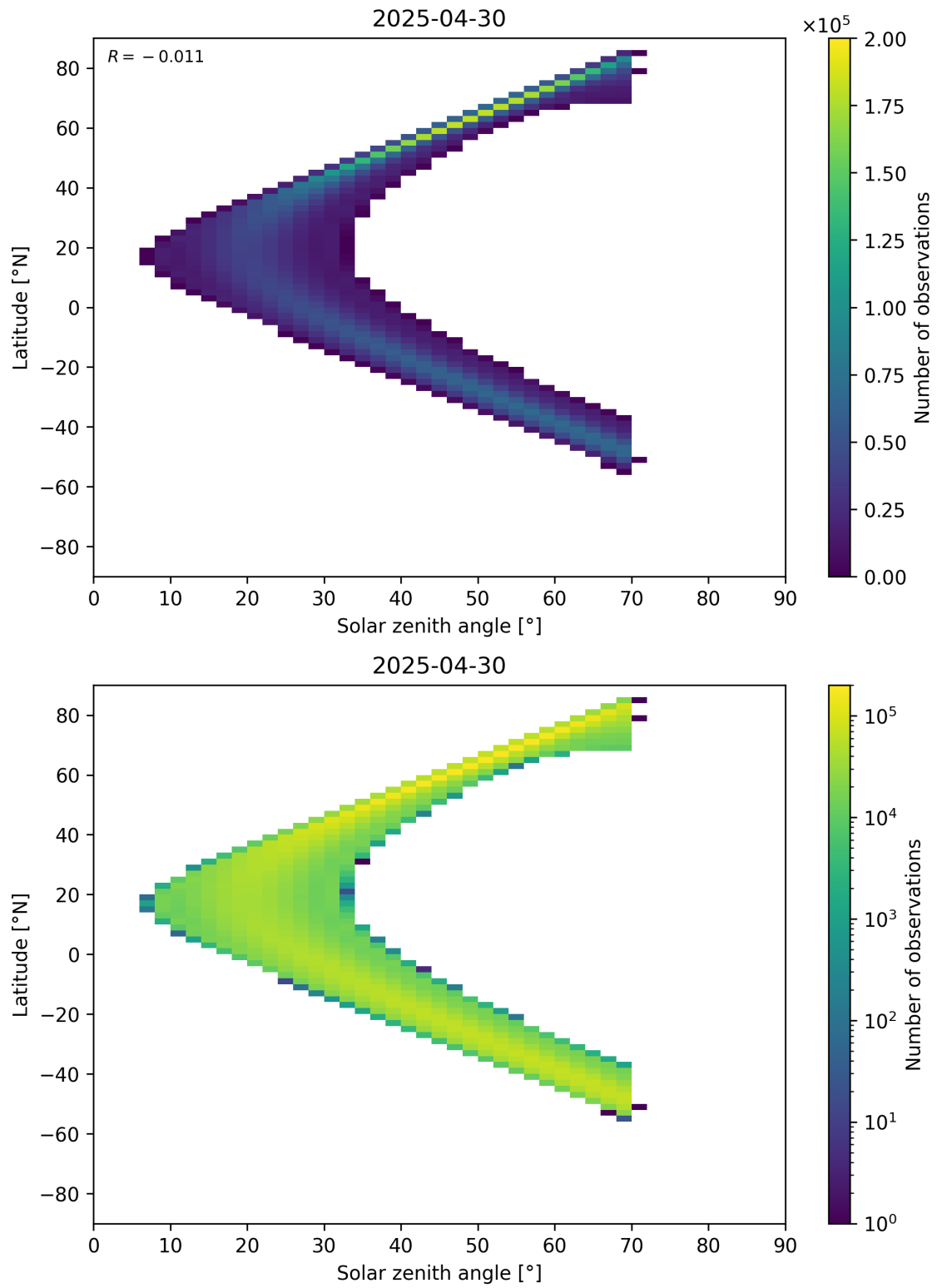
Figure 177: Scatter density plot of “Solar zenith angle” against “Latitude” for 2025-04-29 to 2025-05-01.
