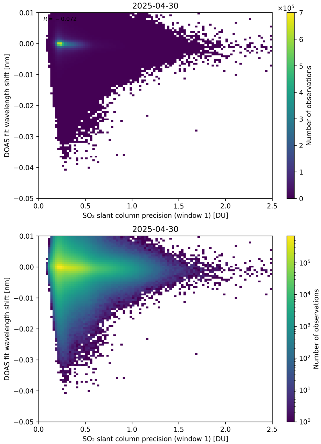
Figure 271: Scatter density plot of “SO 2 slant column precision (window 1)” against “DOAS fit wavelength shift” for 2025-04-29 to 2025-05-01.
