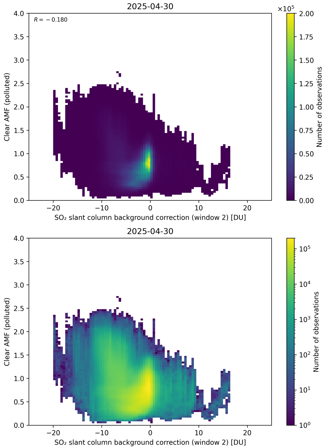
Figure 126: Scatter density plot of “SO 2 slant column background correction (window 2)” against “Clear AMF (polluted)” for 2025-04-29 to 2025-05-01.
