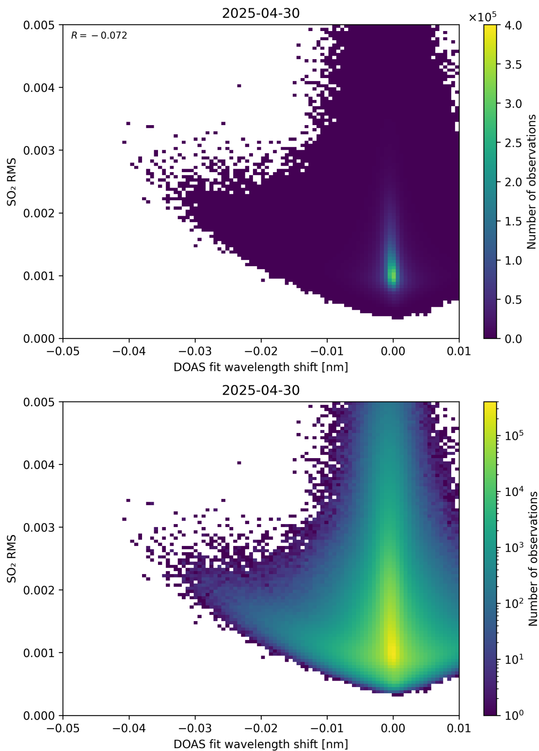
Figure 139: Scatter density plot of “DOAS fit wavelength shift” against “SO 2 RMS” for 2025-04-29 to 2025-05-01.
