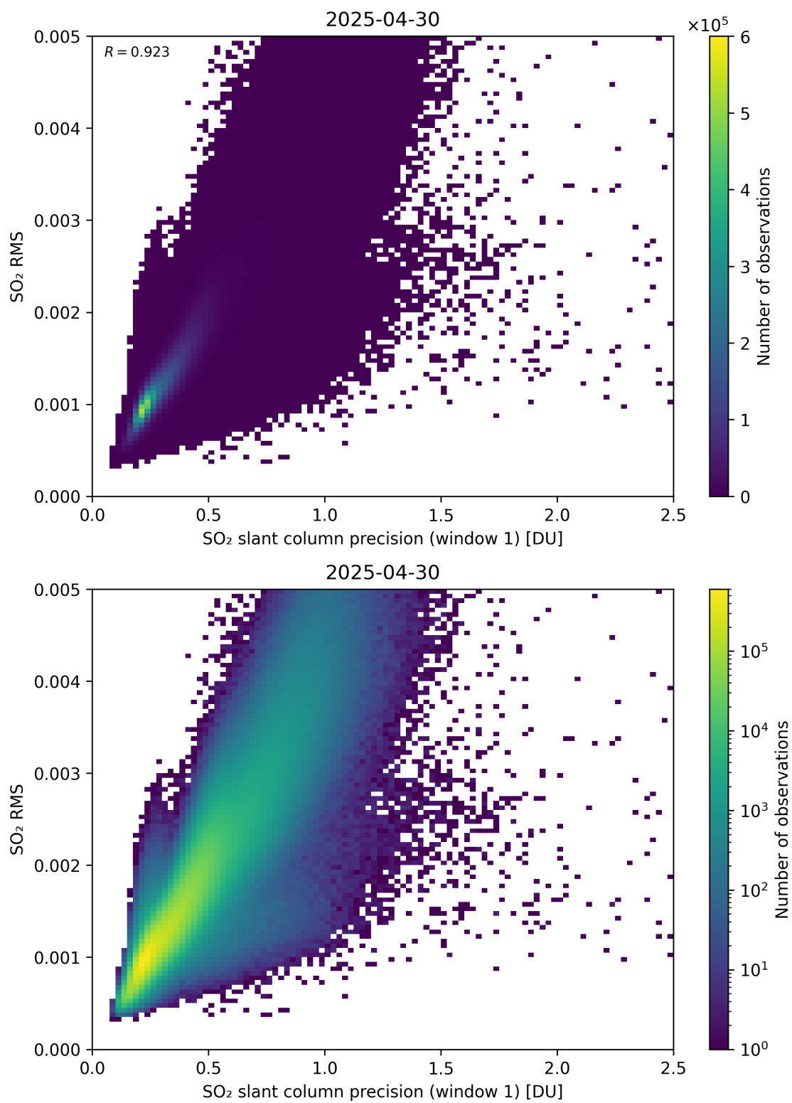
Figure 273: Scatter density plot of “SO 2 slant column precision (window 1)” against “SO 2 RMS” for 2025-04-29 to 2025-05-01.
