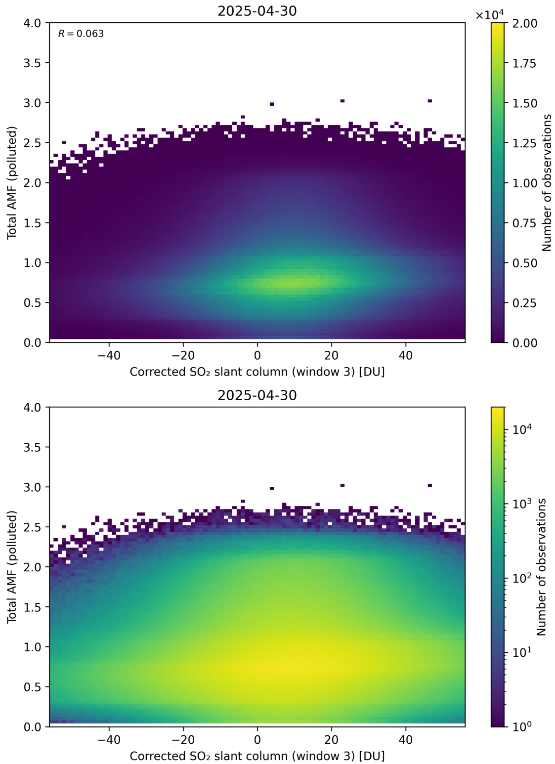
Figure 260: Scatter density plot of “Corrected SO 2 slant column (window 3)” against “Total AMF (polluted)” for 2025-04-29 to 2025-05-01.
