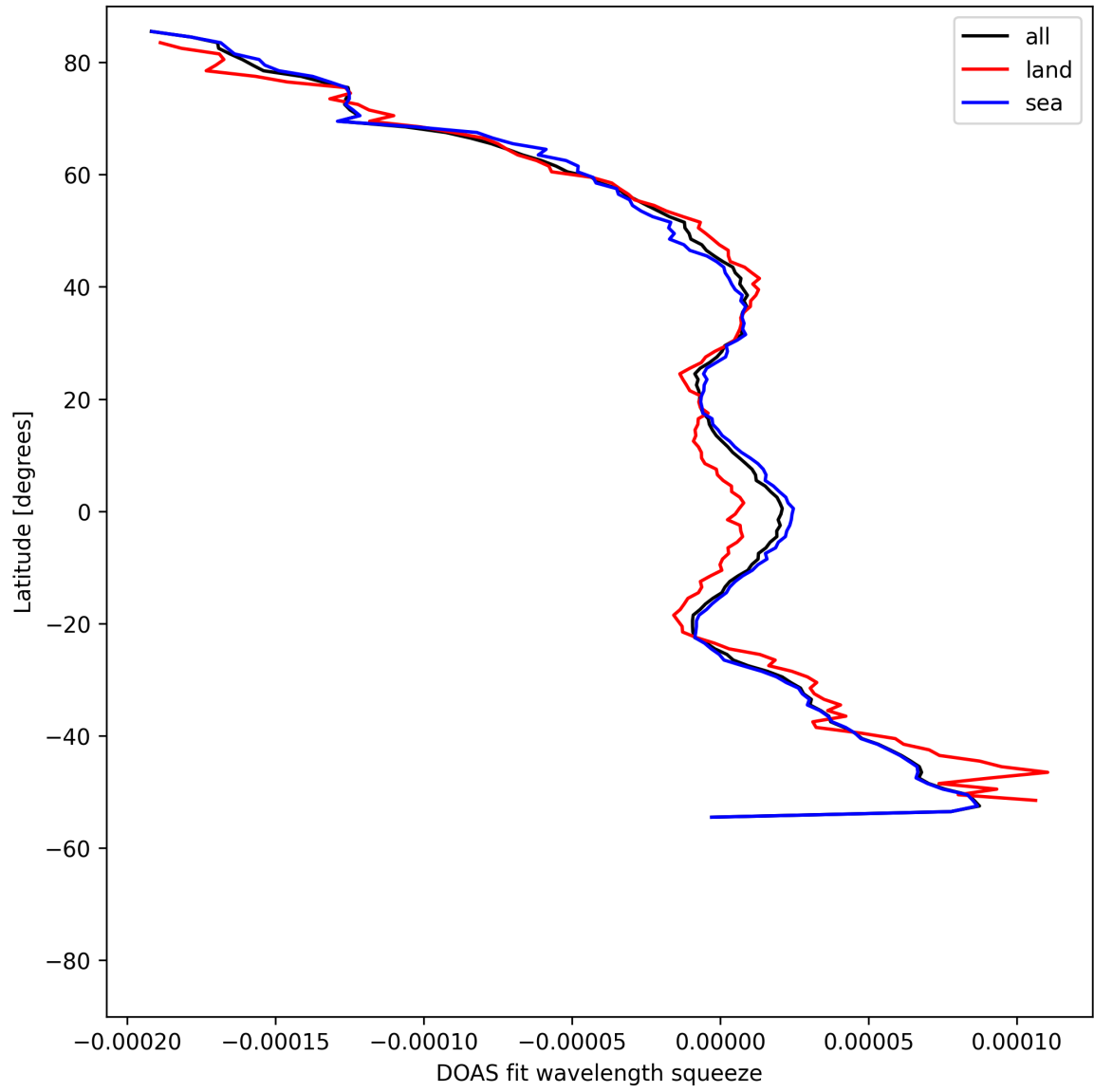
Figure 51: Zonal average of “DOAS fit wavelength squeeze” for 2025-04-29 to 2025-05-01.
