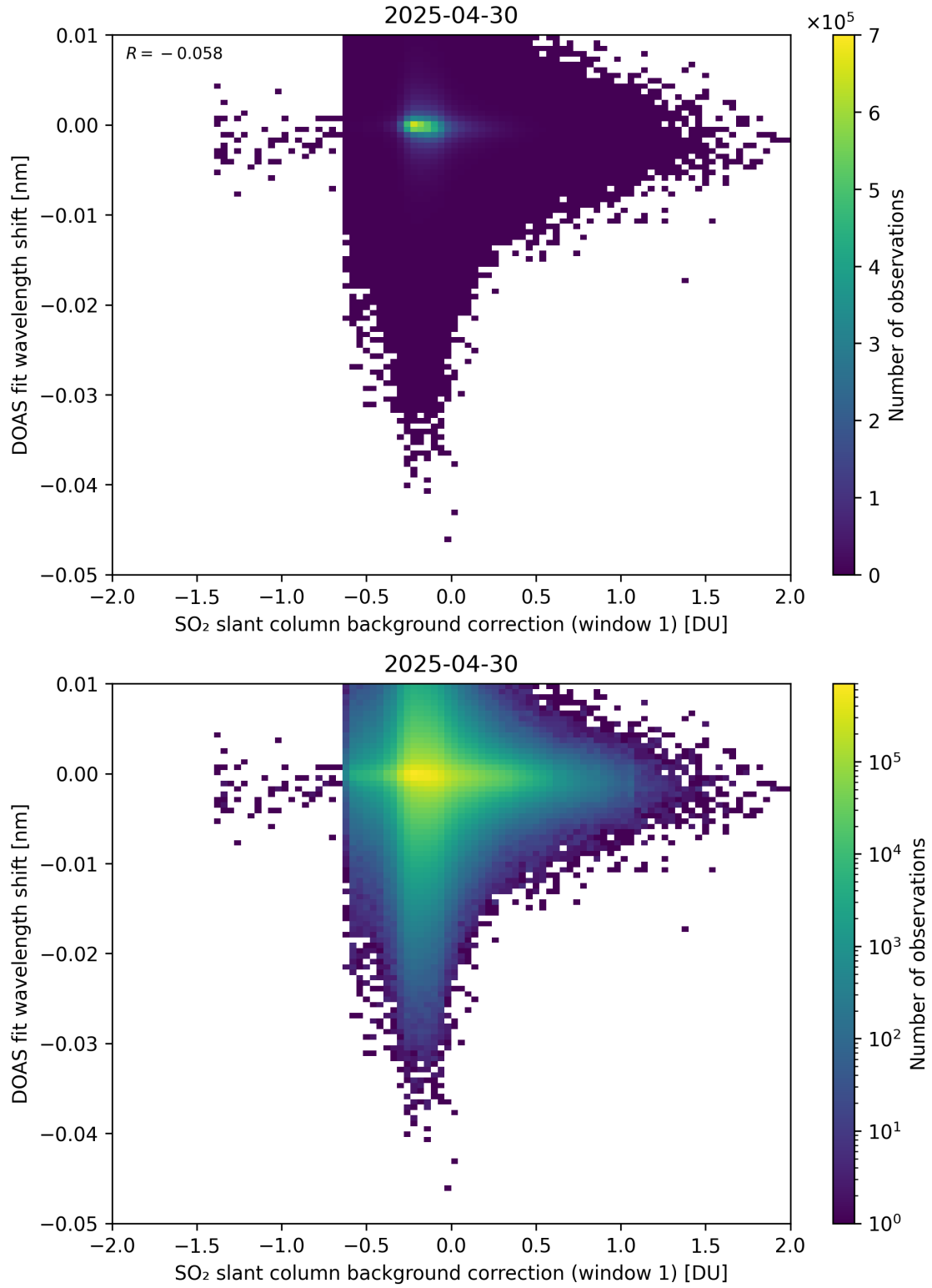
Figure 111: Scatter density plot of “SO 2 slant column background correction (window 1)” against “DOAS fit wavelength shift” for 2025-04-29 to 2025-05-01.
