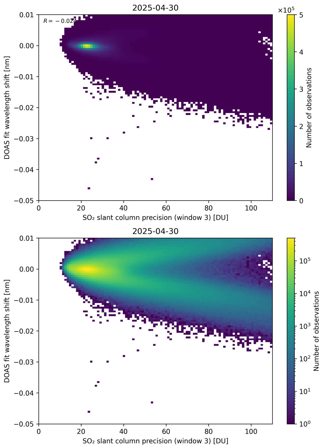
Figure 308: Scatter density plot of “SO 2 slant column precision (window 3)” against “DOAS fit wavelength shift” for 2025-04-29 to 2025-05-01.
