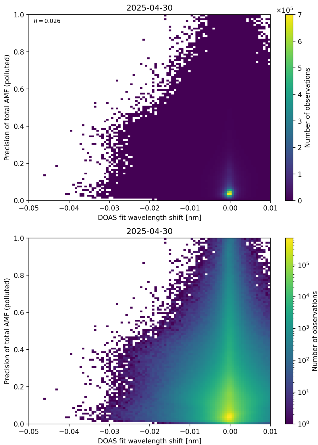
Figure 142: Scatter density plot of “DOAS fit wavelength shift” against “Precision of total AMF (polluted)” for 2025-04-29 to 2025-05-01.
