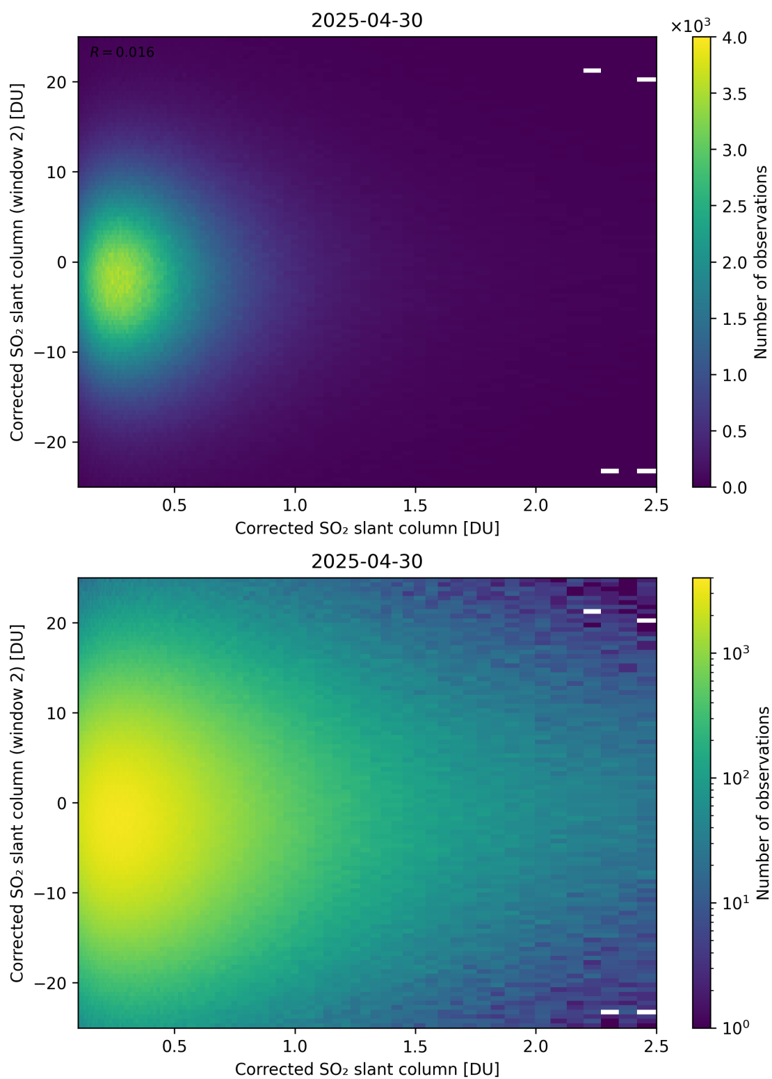
Figure 235: Scatter density plot of “Corrected SO 2 slant column” against “Corrected SO 2 slant column (window 2)” for 2025-04-29 to 2025-05-01.
