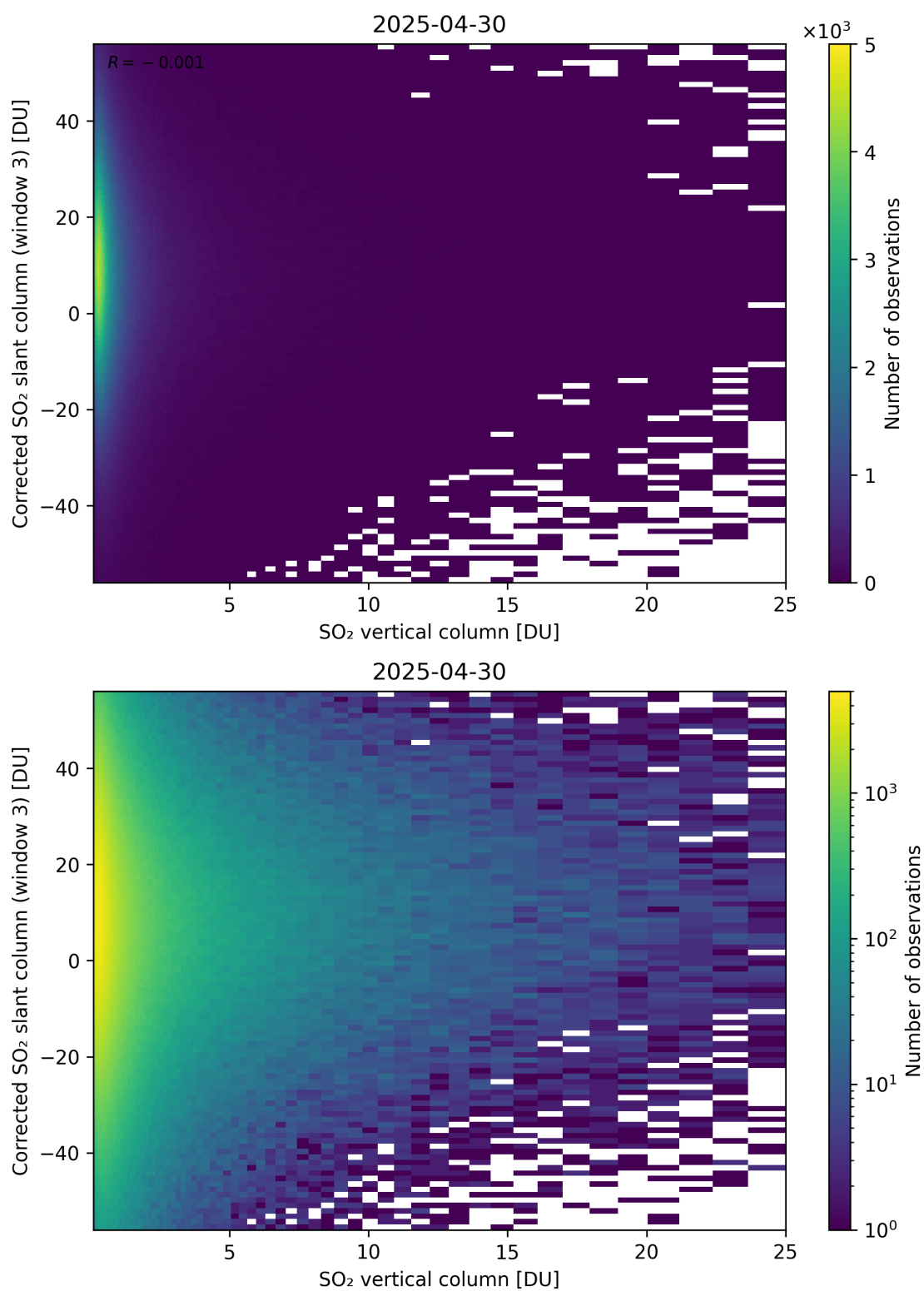
Figure 353: Scatter density plot of “SO 2 vertical column” against “Corrected SO 2 slant column (window 3)” for 2025-04-29 to 2025-05-01.
