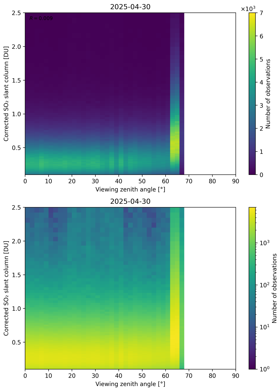
Figure 373: Scatter density plot of “Viewing zenith angle” against “Corrected SO 2 slant column” for 2025-04-29 to 2025-05-01.
