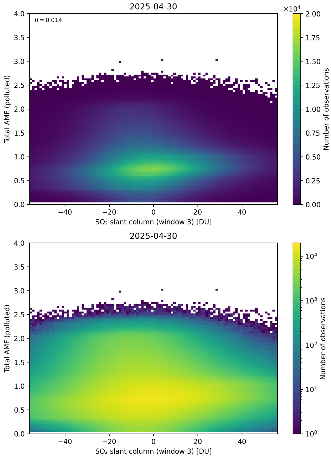
Figure 318: Scatter density plot of “SO 2 slant column (window 3)” against “Total AMF (polluted)” for 2025-04-29 to 2025-05-01.
