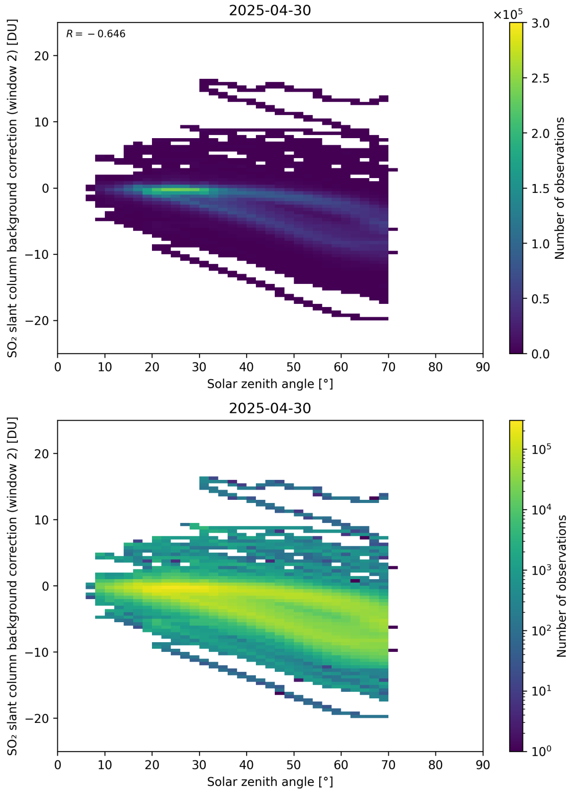
Figure 172: Scatter density plot of “Solar zenith angle” against “SO 2 slant column background correction (window 2)” for 2025-04-29 to 2025-05-01.
