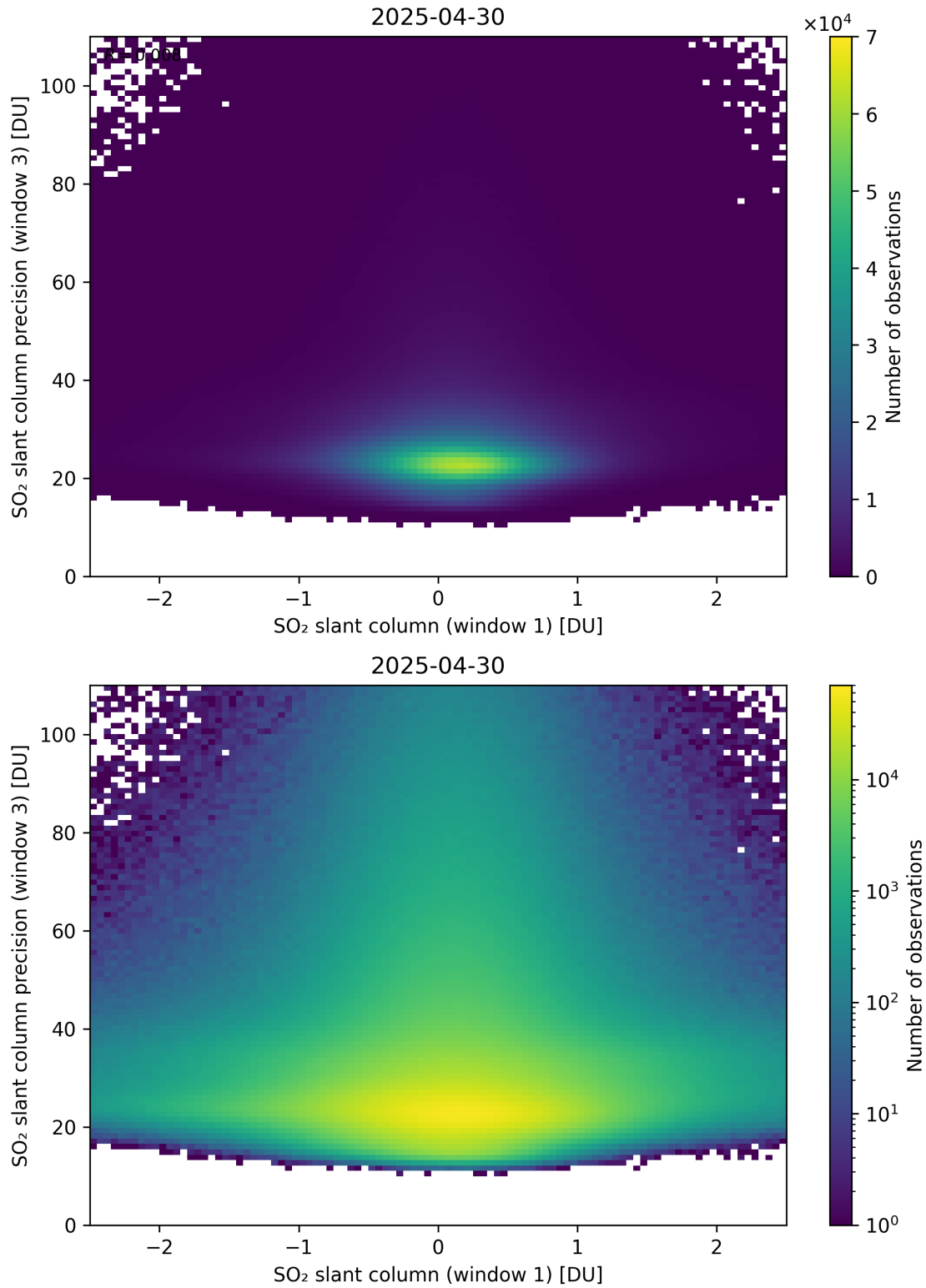
Figure 288: Scatter density plot of “SO 2 slant column (window 1)” against “SO 2 slant column precision (window 3)” for 2025-04-29 to 2025-05-01.
