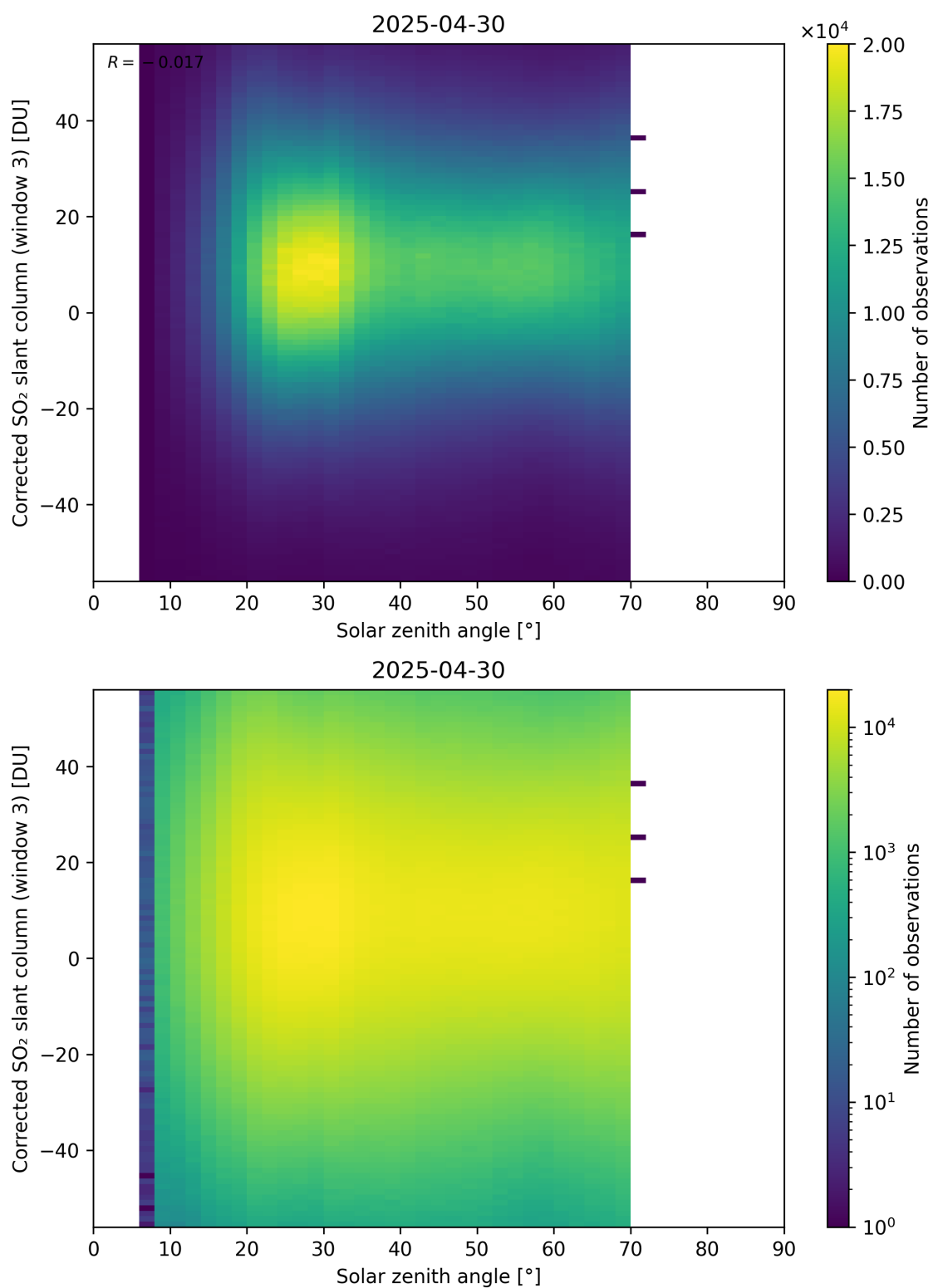
Figure 183: Scatter density plot of “Solar zenith angle” against “Corrected SO 2 slant column (window 3)” for 2025-04-29 to 2025-05-01.
