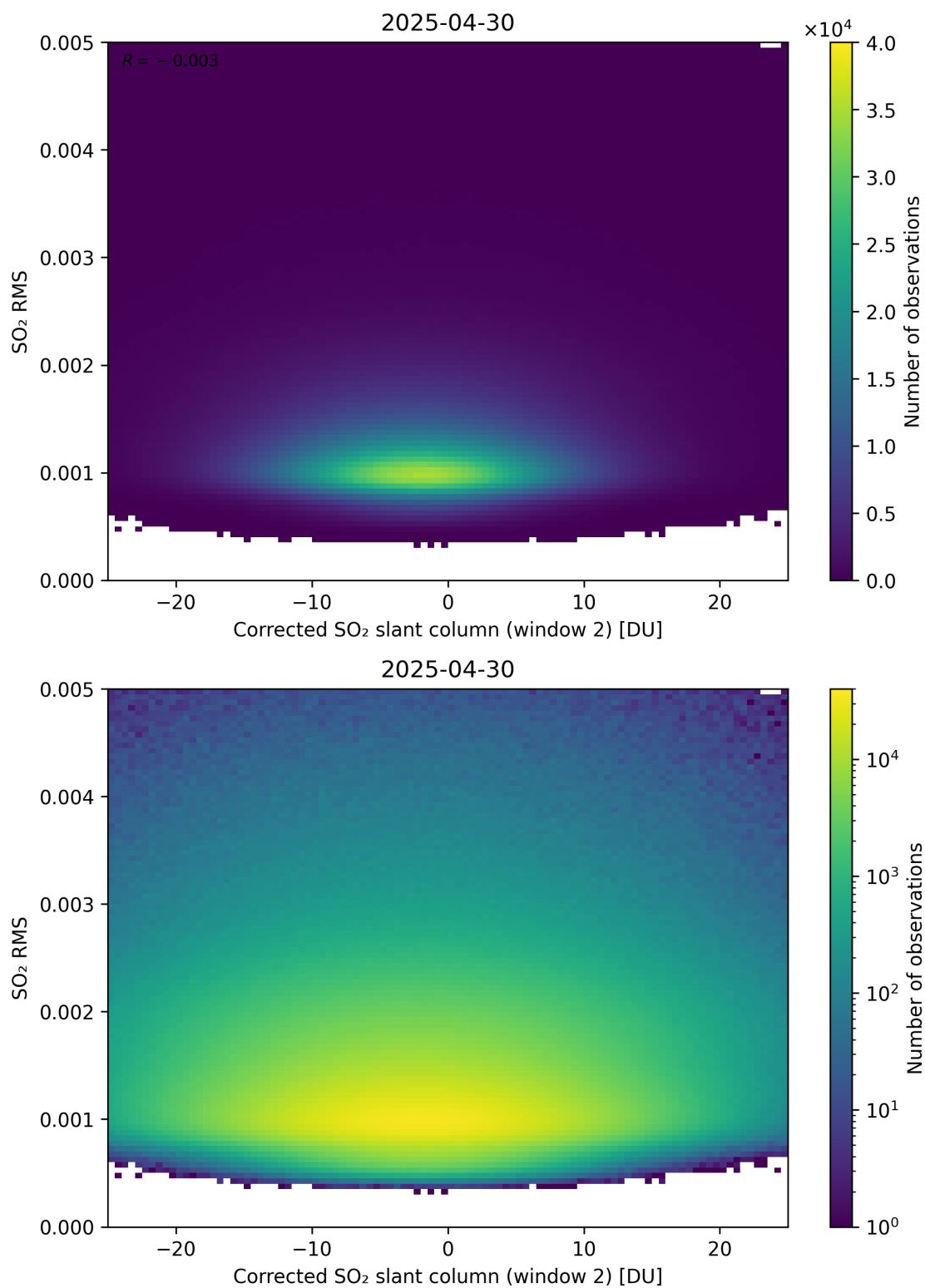
Figure 248: Scatter density plot of “Corrected SO 2 slant column (window 2)” against “SO 2 RMS” for 2025-04-29 to 2025-05-01.
