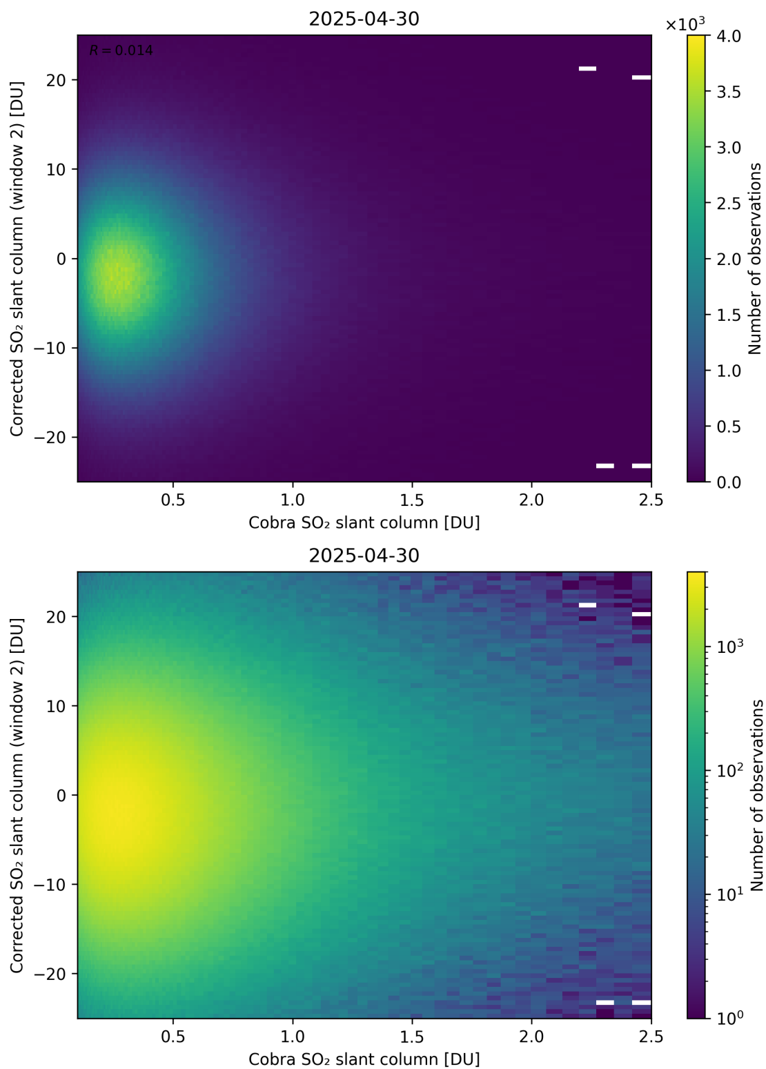
Figure 217: Scatter density plot of “Cobra SO 2 slant column” against “Corrected SO 2 slant column (window 2)” for 2025-04-29 to 2025-05-01.
