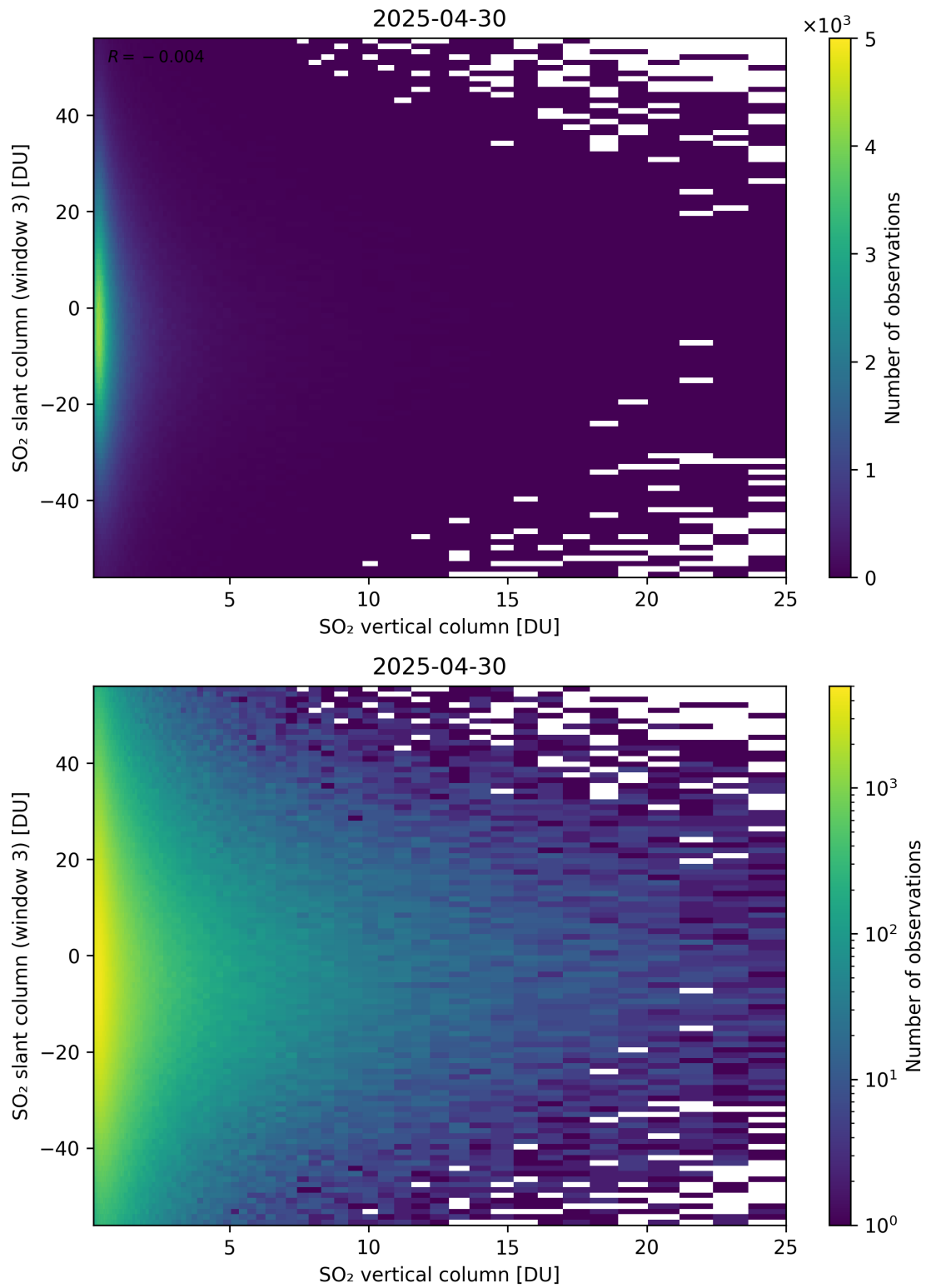
Figure 357: Scatter density plot of “SO 2 vertical column” against “SO 2 slant column (window 3)” for 2025-04-29 to 2025-05-01.
