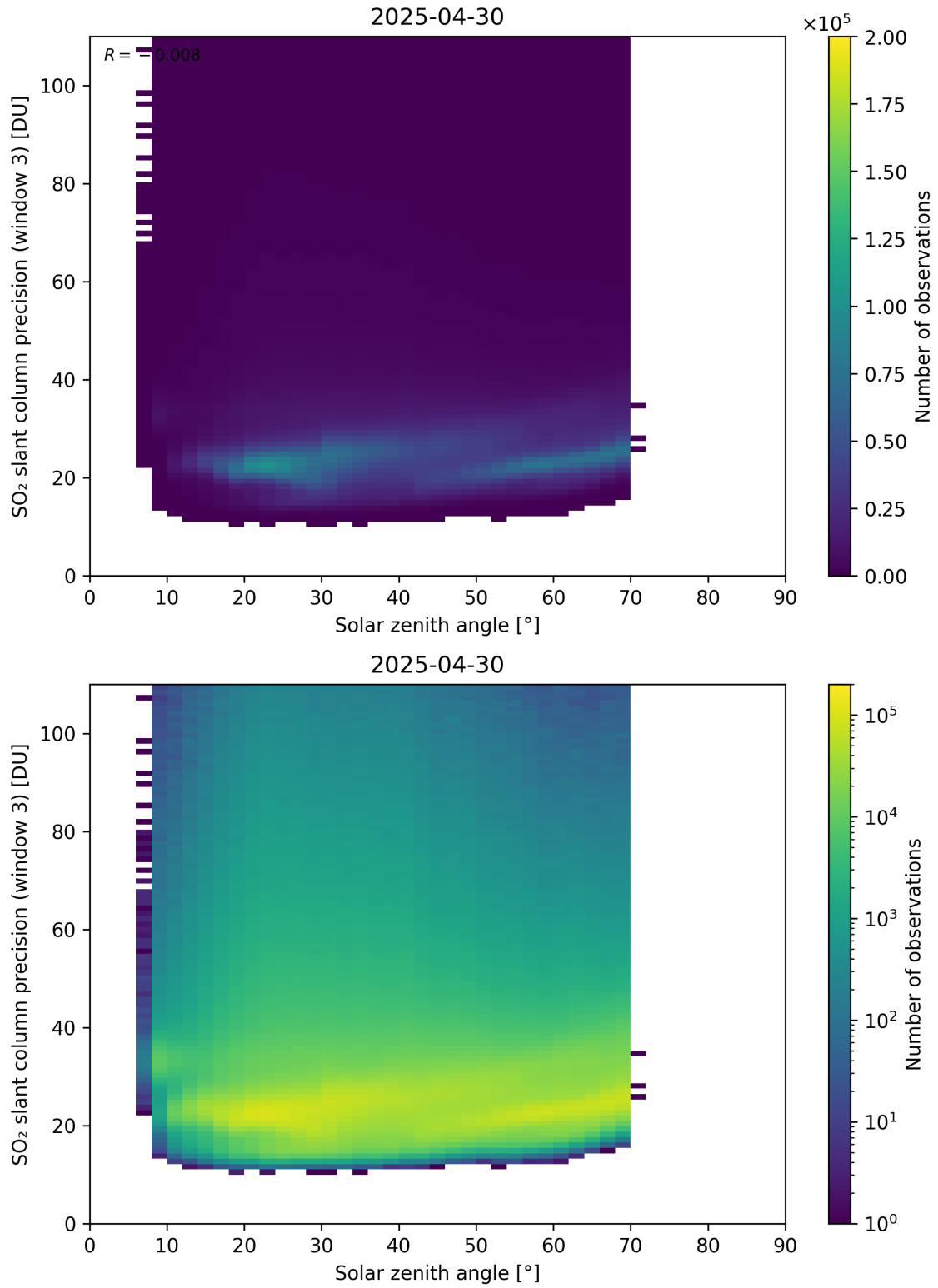
Figure 188: Scatter density plot of “Solar zenith angle” against “SO 2 slant column precision (window 3)” for 2025-04-29 to 2025-05-01.
