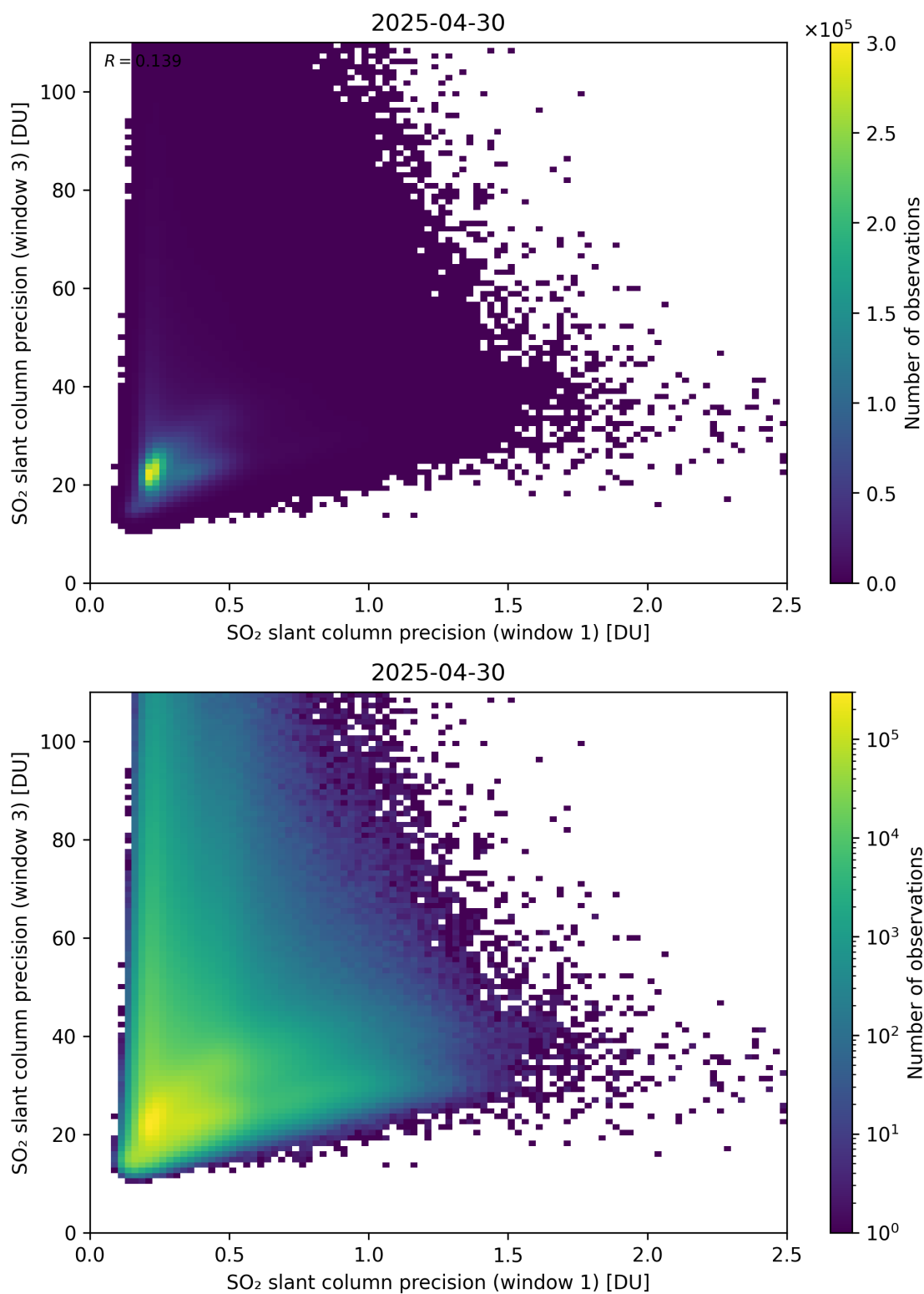
Figure 279: Scatter density plot of “SO 2 slant column precision (window 1)” against “SO 2 slant column precision (window 3)” for 2025-04-29 to 2025-05-01.
