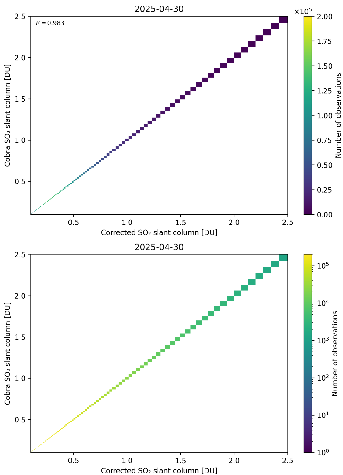
Figure 233: Scatter density plot of “Corrected SO 2 slant column” against “Cobra SO 2 slant column” for 2025-04-29 to 2025-05-01.
