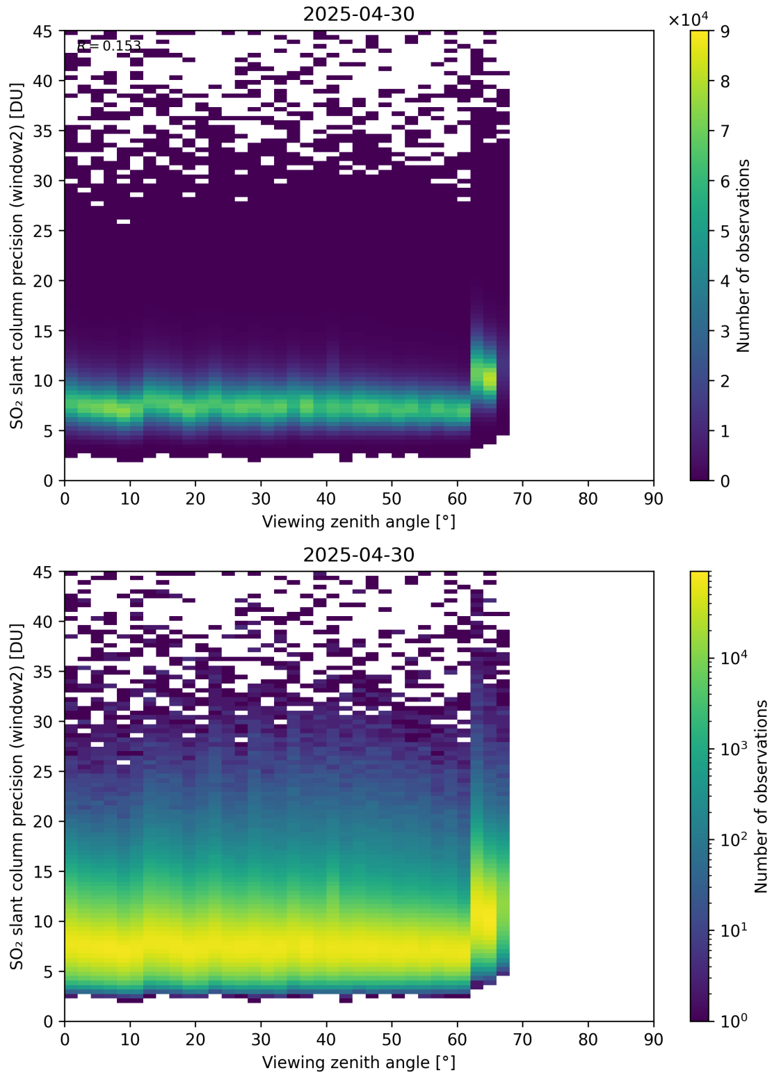
Figure 378: Scatter density plot of “Viewing zenith angle” against “SO 2 slant column precision (window2)” for 2025-04-29 to 2025-05-01.
