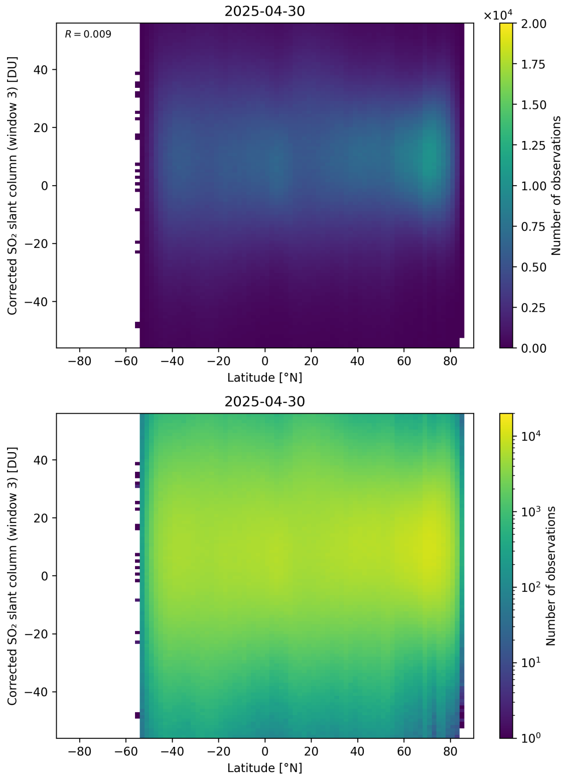
Figure 161: Scatter density plot of “Latitude” against “Corrected SO 2 slant column (window 3)” for 2025-04-29 to 2025-05-01.
