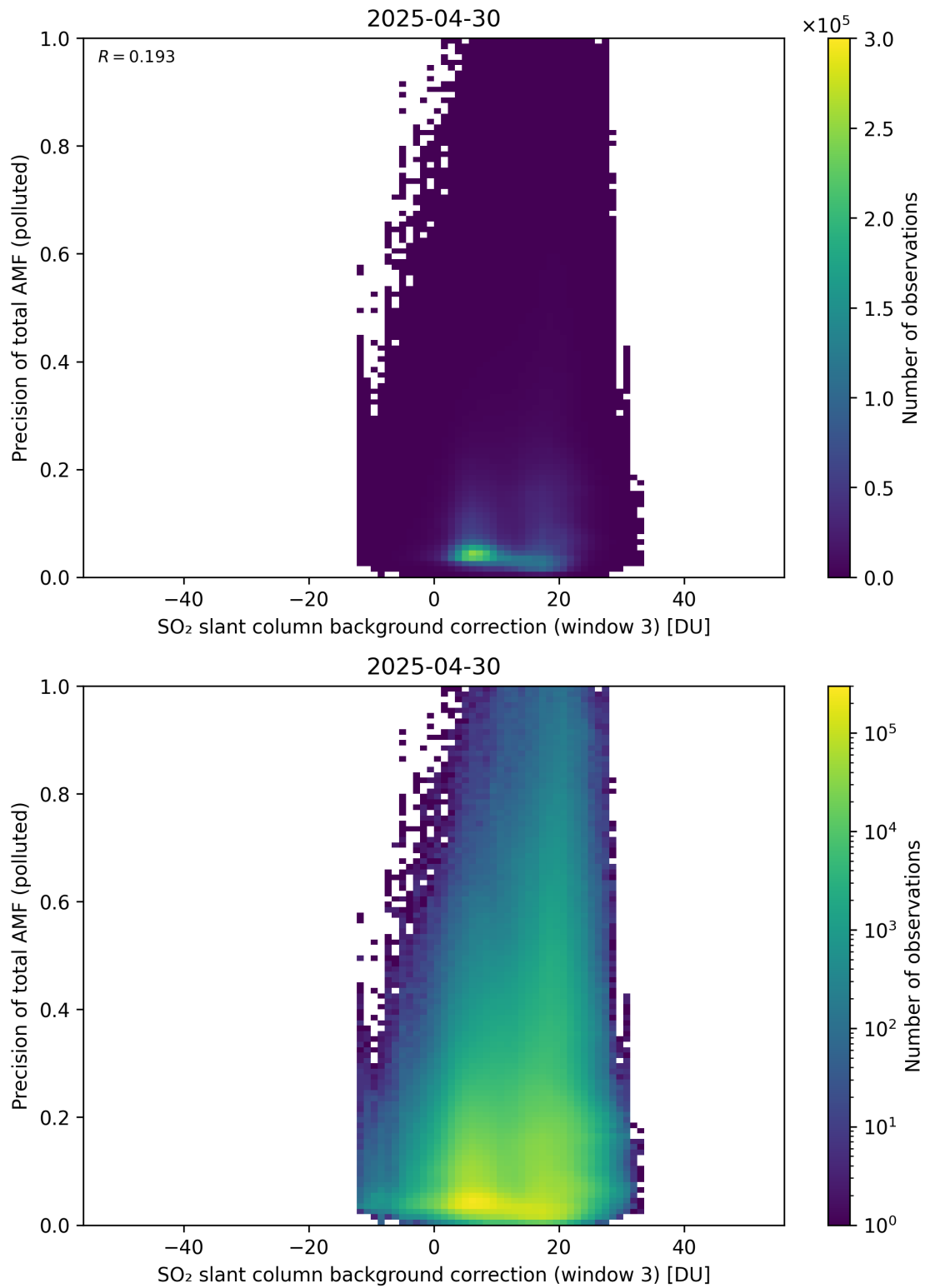
Figure 137: Scatter density plot of “SO 2 slant column background correction (window 3)” against “Precision of total AMF (polluted)” for 2025-04-29 to 2025-05-01.
