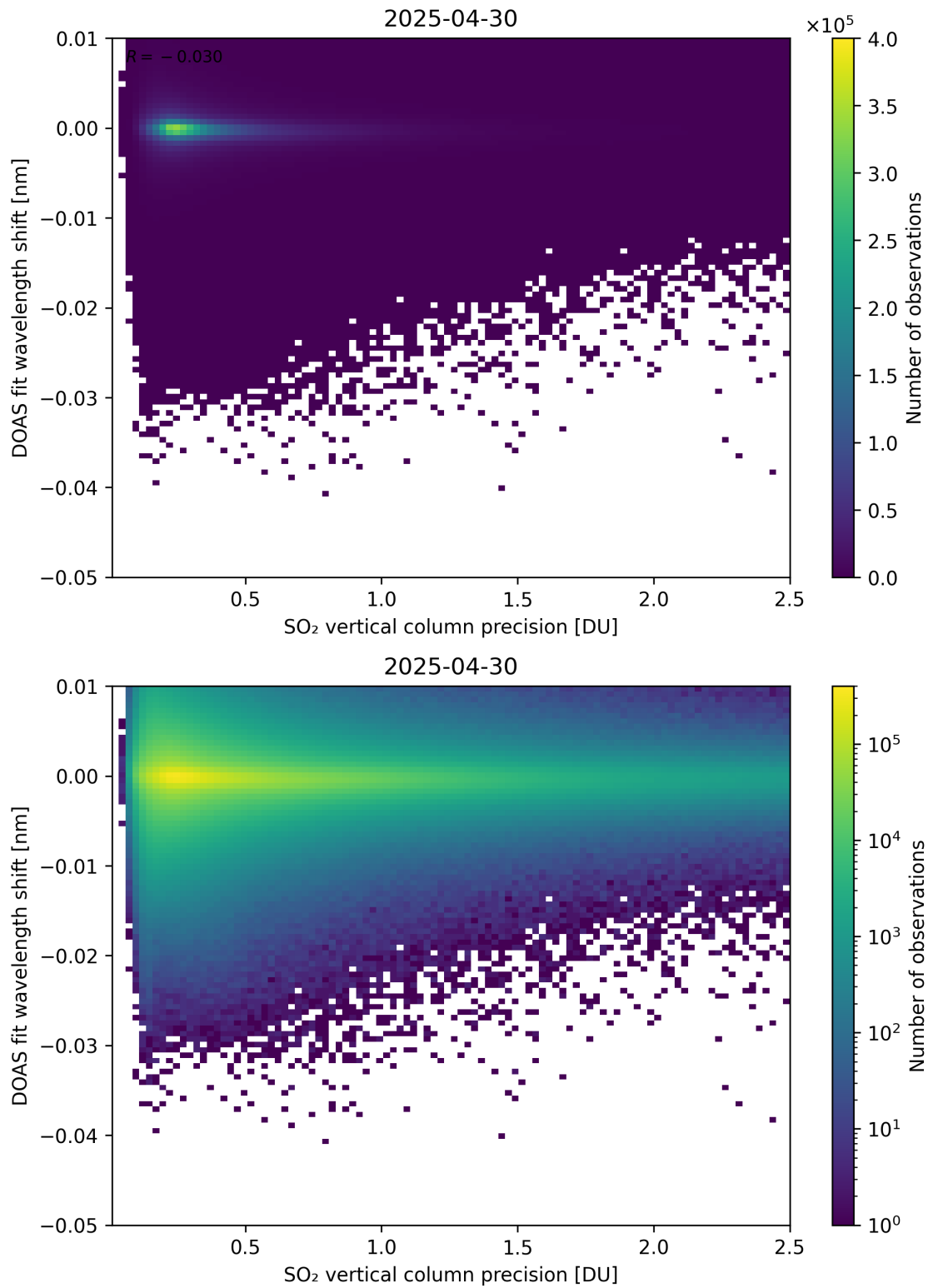
Figure 332: Scatter density plot of “SO 2 vertical column precision” against “DOAS fit wavelength shift” for 2025-04-29 to 2025-05-01.
