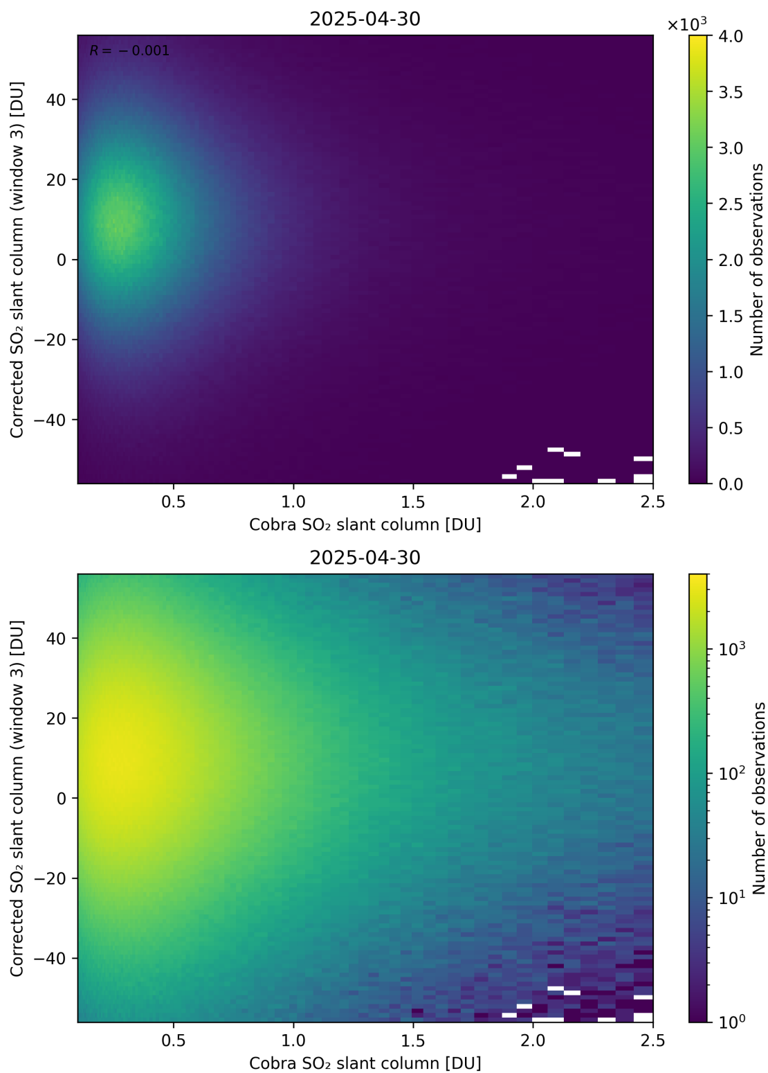
Figure 218: Scatter density plot of “Cobra SO 2 slant column” against “Corrected SO 2 slant column (window 3)” for 2025-04-29 to 2025-05-01.
