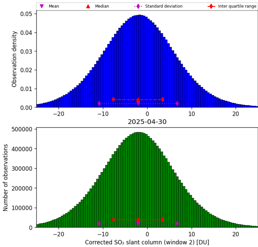
Figure 69: Histogram of “Corrected SO 2 slant column (window 2)” for 2025-04-29 to 2025-05-01
