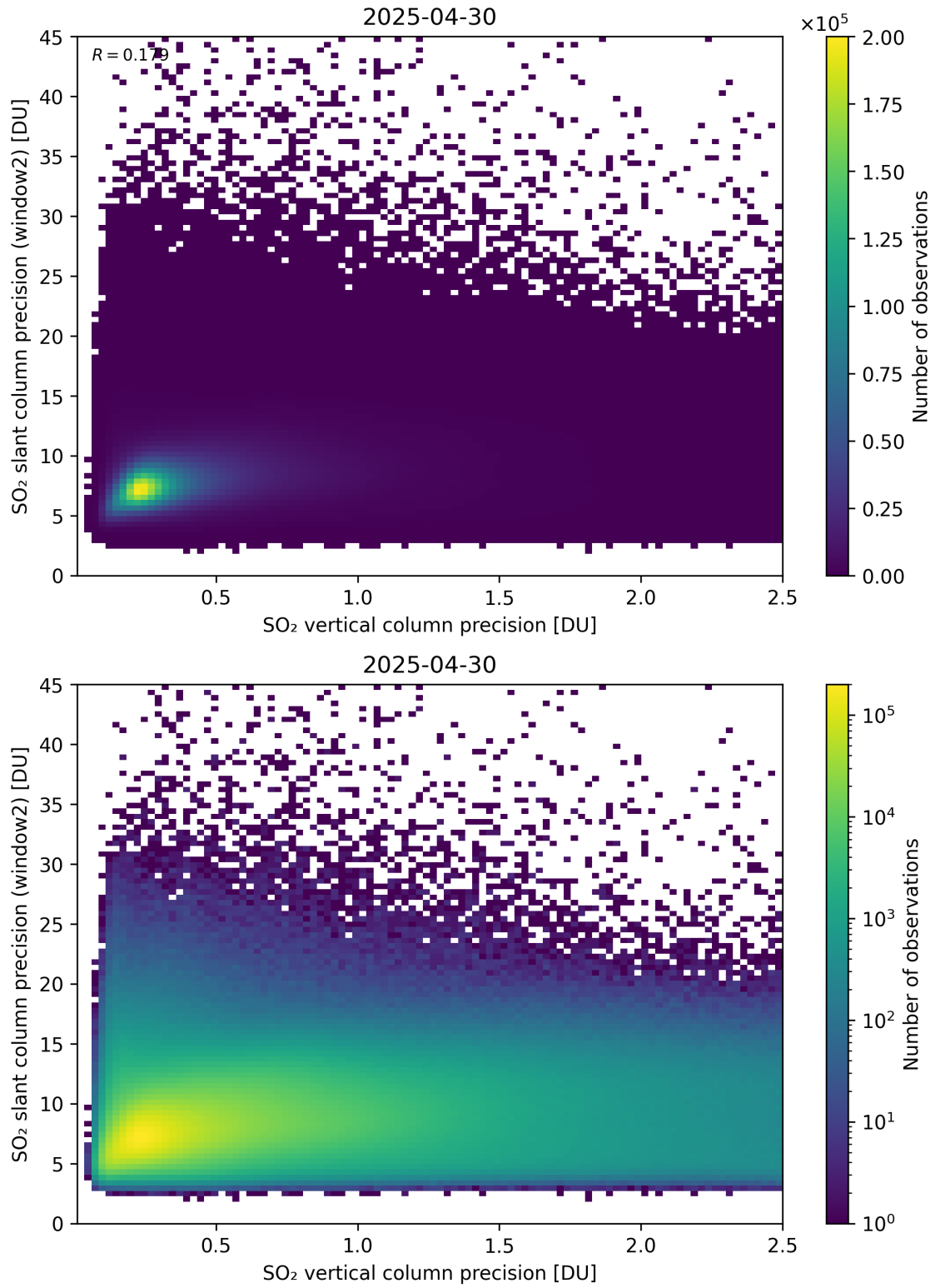
Figure 343: Scatter density plot of “SO 2 vertical column precision” against “SO 2 slant column precision (window2)” for 2025-04-29 to 2025-05-01.
