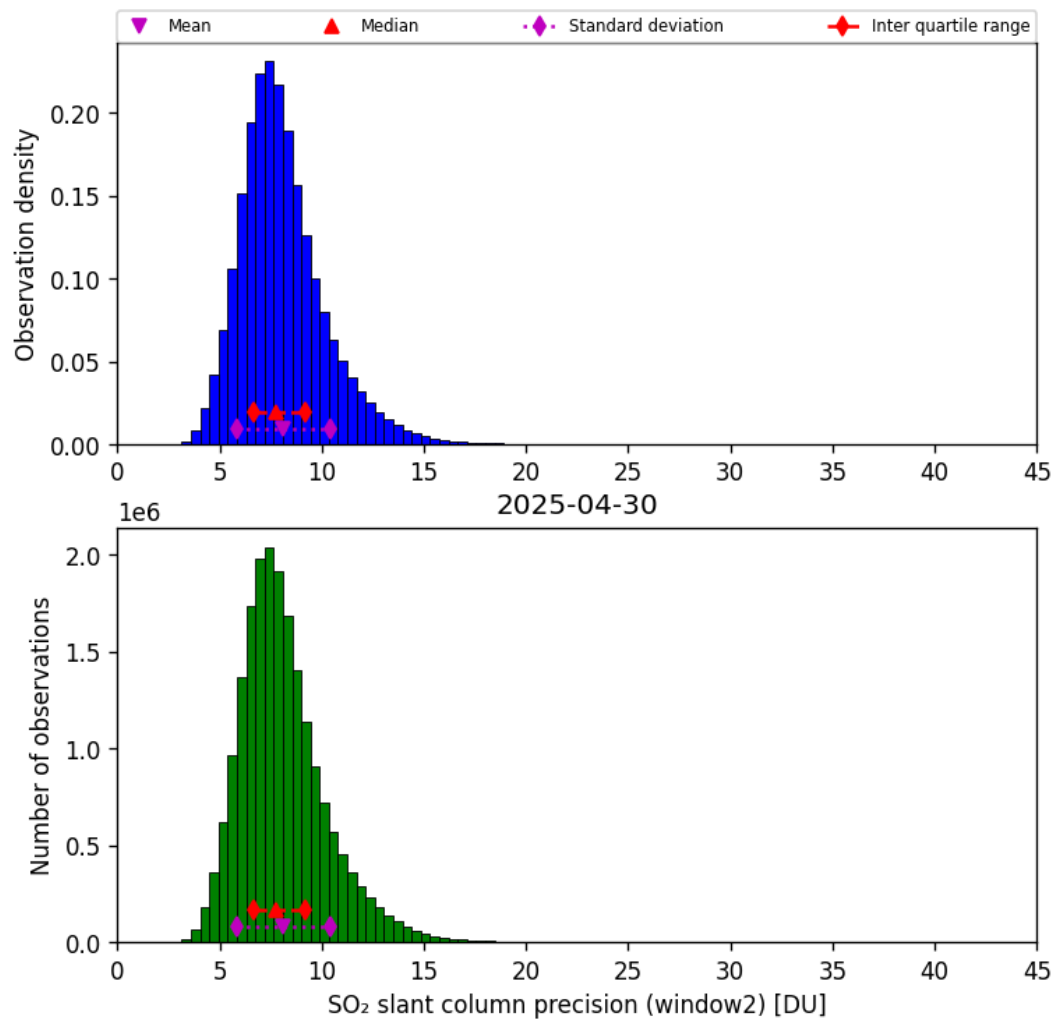
Figure 68: Histogram of “SO 2 slant column precision (window2)” for 2025-04-29 to 2025-05-01
