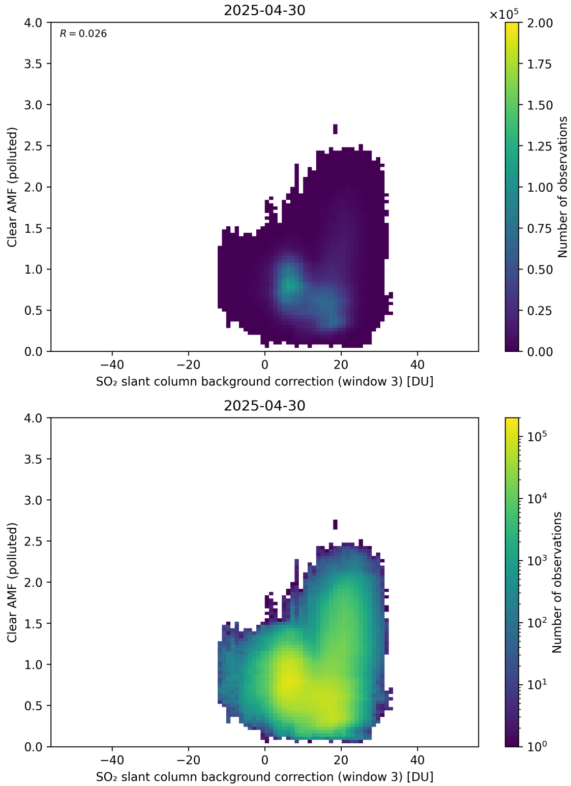
Figure 135: Scatter density plot of “SO 2 slant column background correction (window 3)” against “Clear AMF (polluted)” for 2025-04-29 to 2025-05-01.
