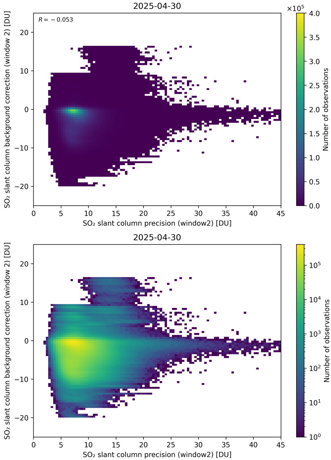
Figure 291: Scatter density plot of “SO 2 slant column precision (window2)” against “SO 2 slant column background correction (window 2)” for 2025-04-29 to 2025-05-01.
