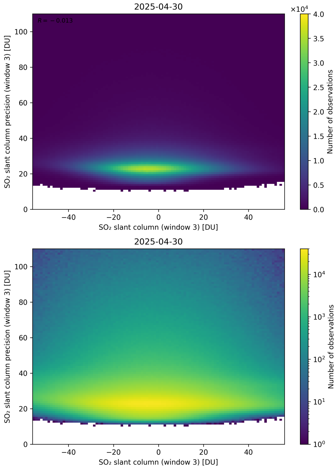
Figure 317: Scatter density plot of “SO 2 slant column (window 3)” against “SO 2 slant column precision (window 3)” for 2025-04-29 to 2025-05-01.
