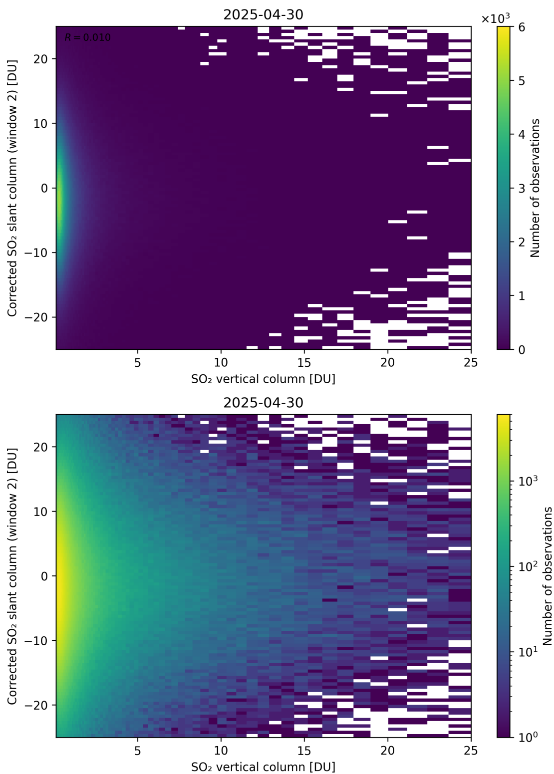
Figure 352: Scatter density plot of “SO 2 vertical column” against “Corrected SO 2 slant column (window 2)” for 2025-04-29 to 2025-05-01.
