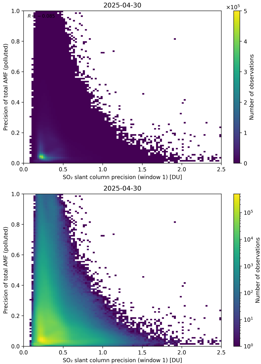
Figure 281: Scatter density plot of “SO 2 slant column precision (window 1)” against “Precision of total AMF (polluted)” for 2025-04-29 to 2025-05-01.
