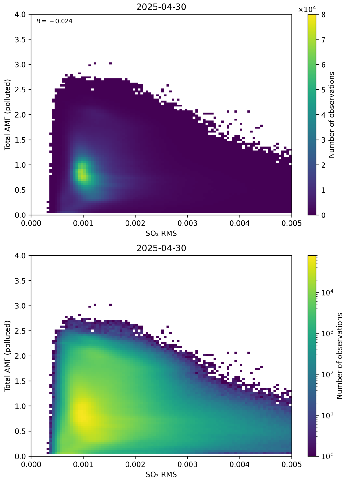
Figure 148: Scatter density plot of “SO 2 RMS” against “Total AMF (polluted)” for 2025-04-29 to 2025-05-01.
