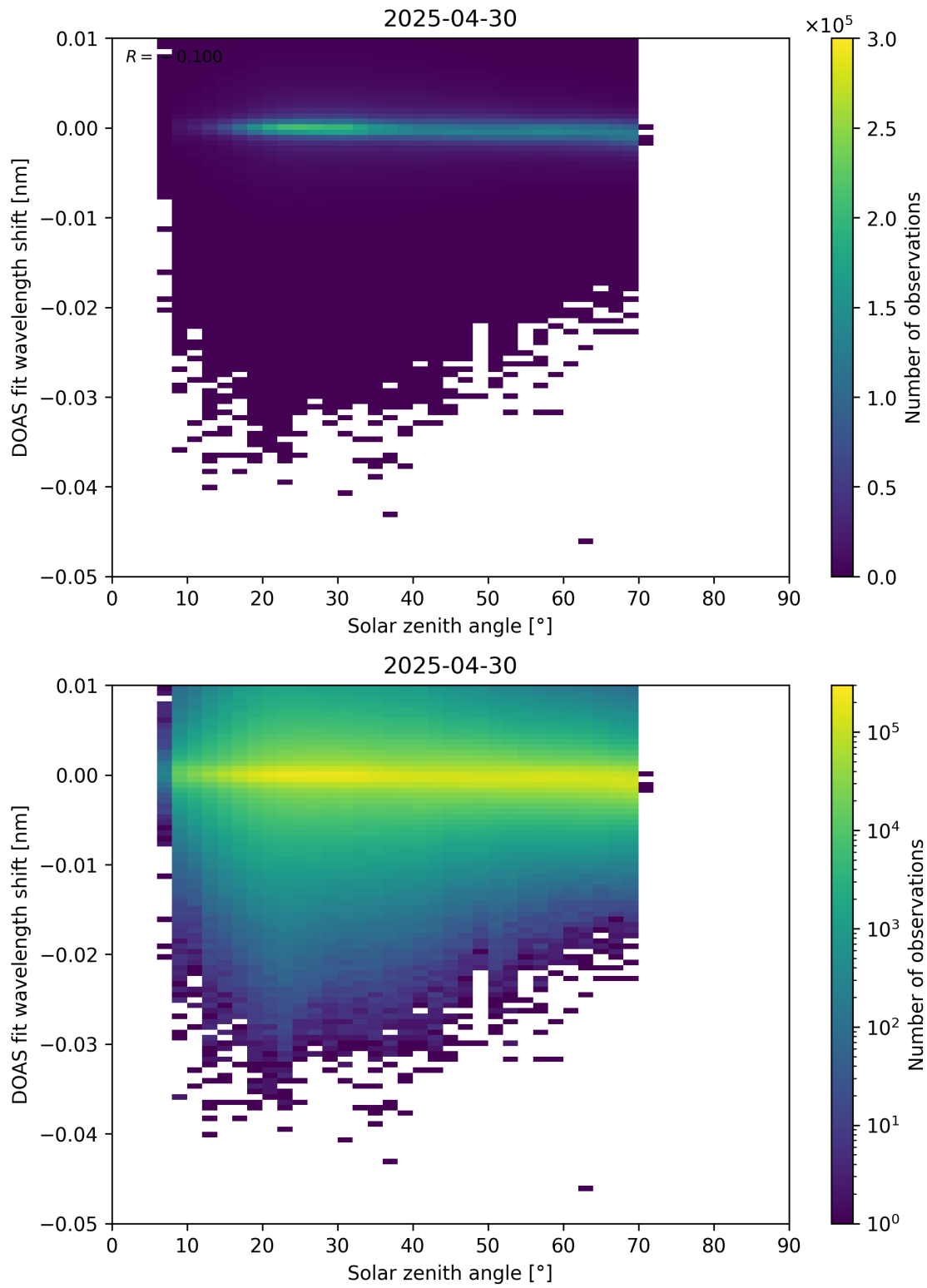
Figure 174: Scatter density plot of “Solar zenith angle” against “DOAS fit wavelength shift” for 2025-04-29 to 2025-05-01.
