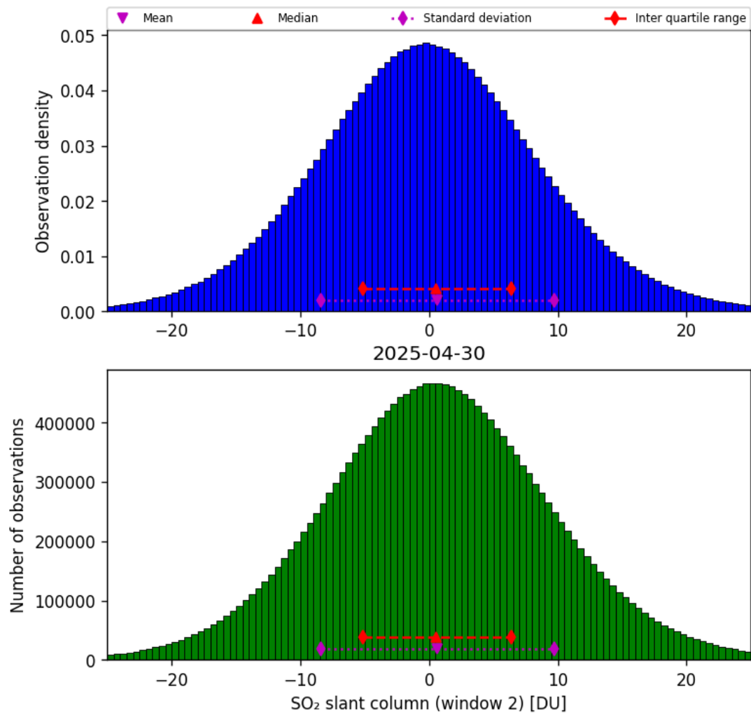
Figure 67: Histogram of “SO 2 slant column (window 2)” for 2025-04-29 to 2025-05-01
