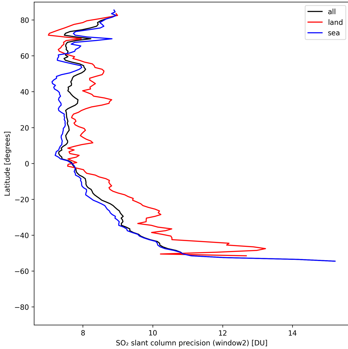
Figure 42: Zonal average of “SO 2 slant column precision (window2)” for 2025-04-29 to 2025-05-01.
