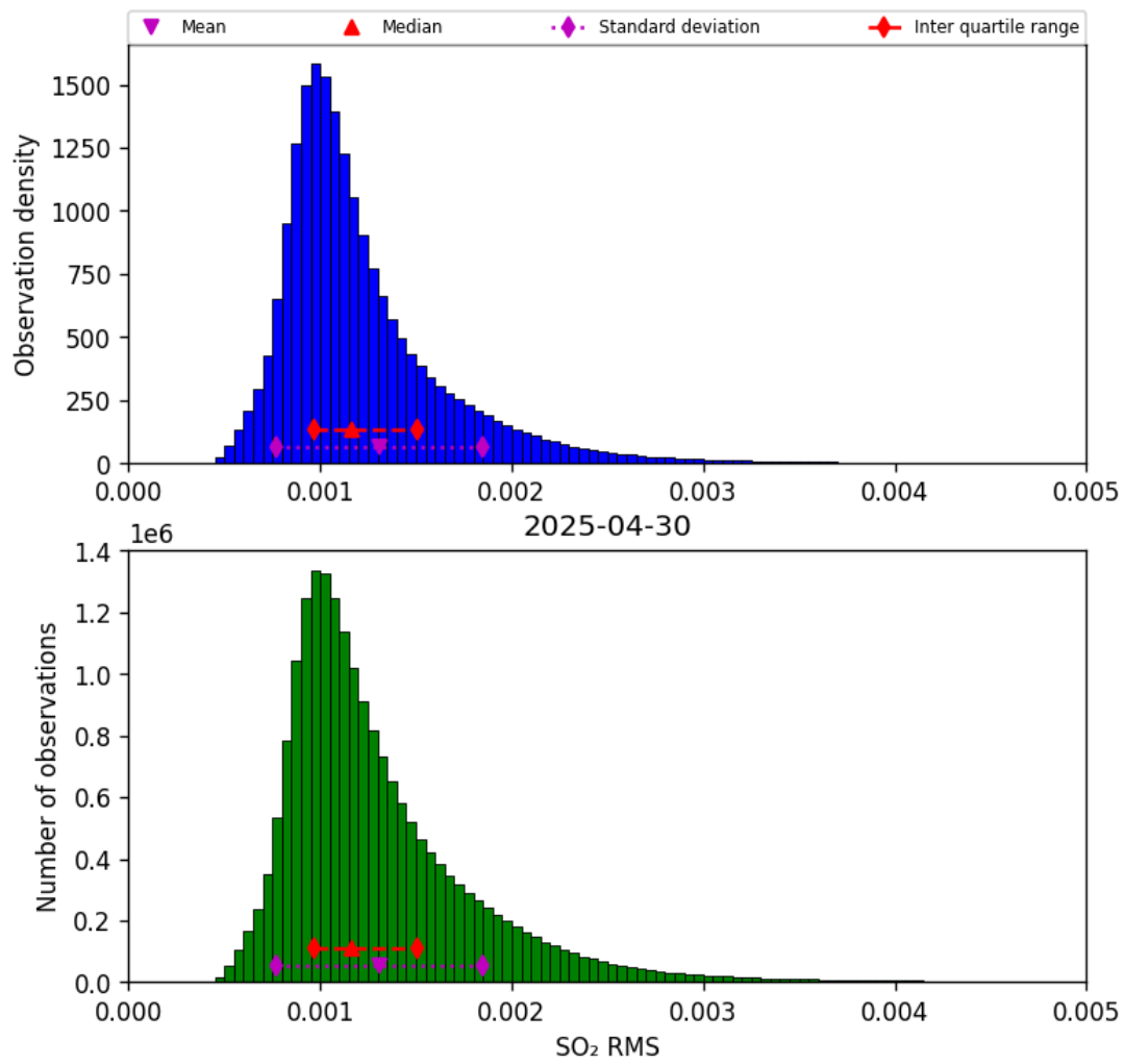
Figure 78: Histogram of “SO 2 RMS” for 2025-04-29 to 2025-05-01
