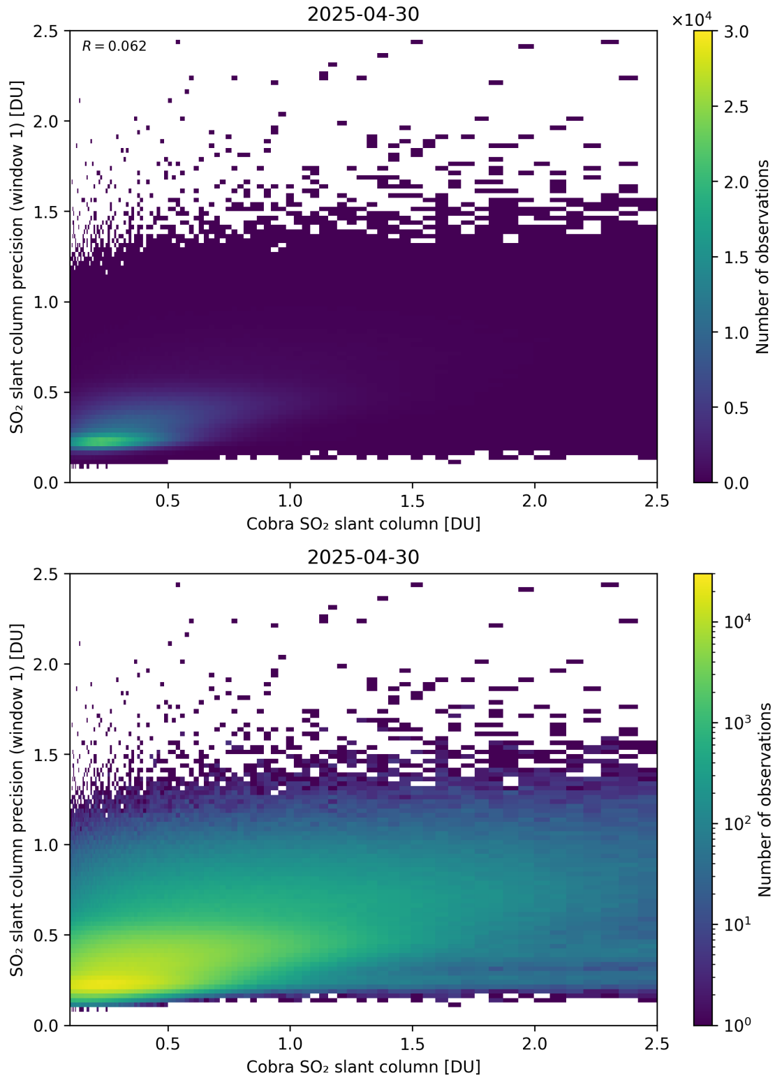
Figure 220: Scatter density plot of “Cobra SO 2 slant column” against “SO 2 slant column precision (window 1)” for 2025-04-29 to 2025-05-01.
