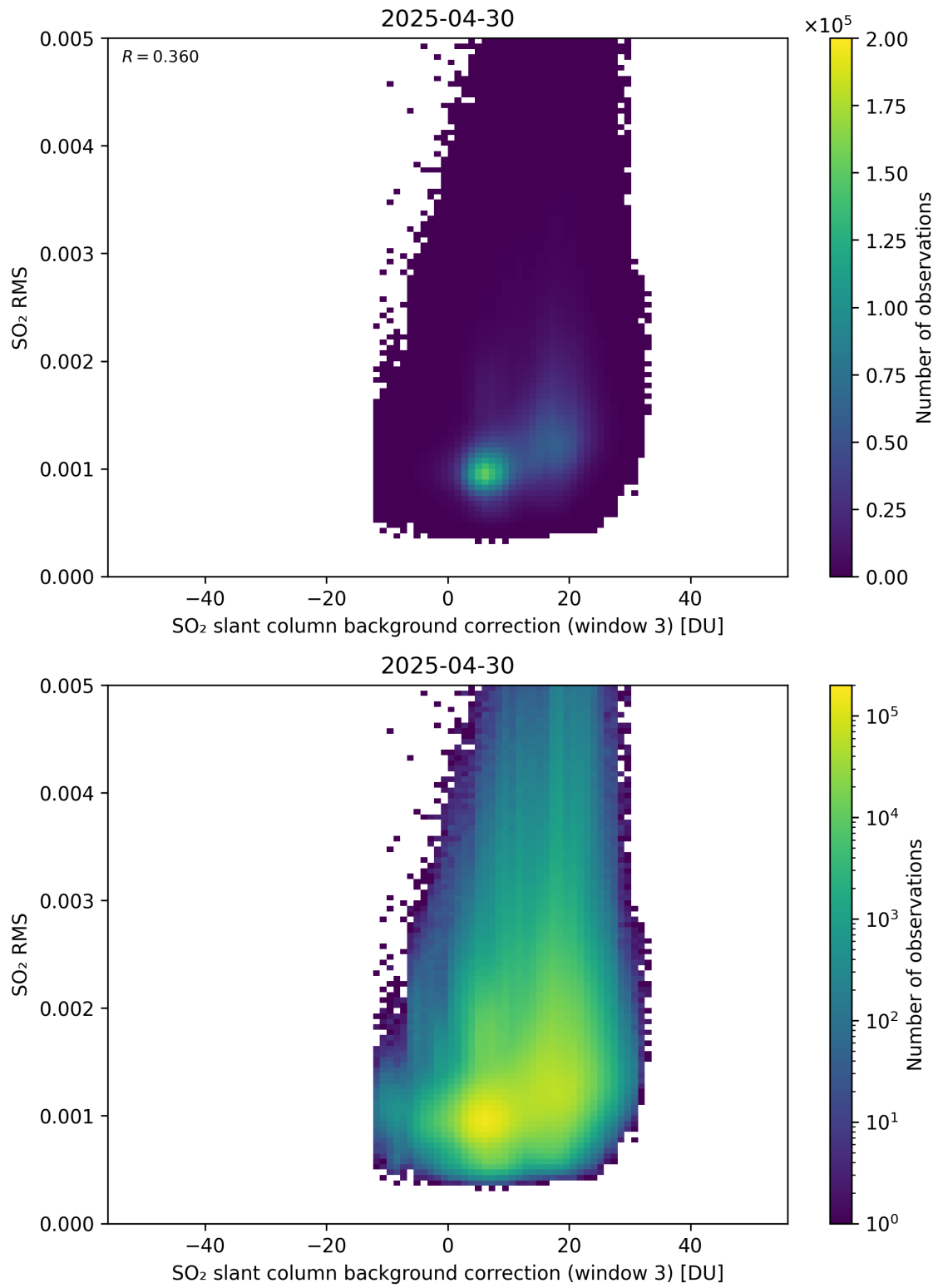
Figure 134: Scatter density plot of “SO 2 slant column background correction (window 3)” against “SO 2 RMS” for 2025-04-29 to 2025-05-01.
