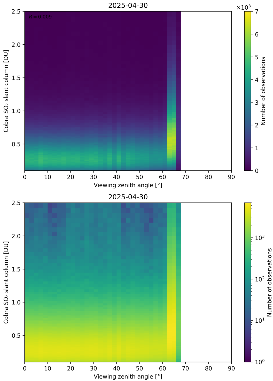
Figure 371: Scatter density plot of “Viewing zenith angle” against “Cobra SO 2 slant column” for 2025-04-29 to 2025-05-01.
