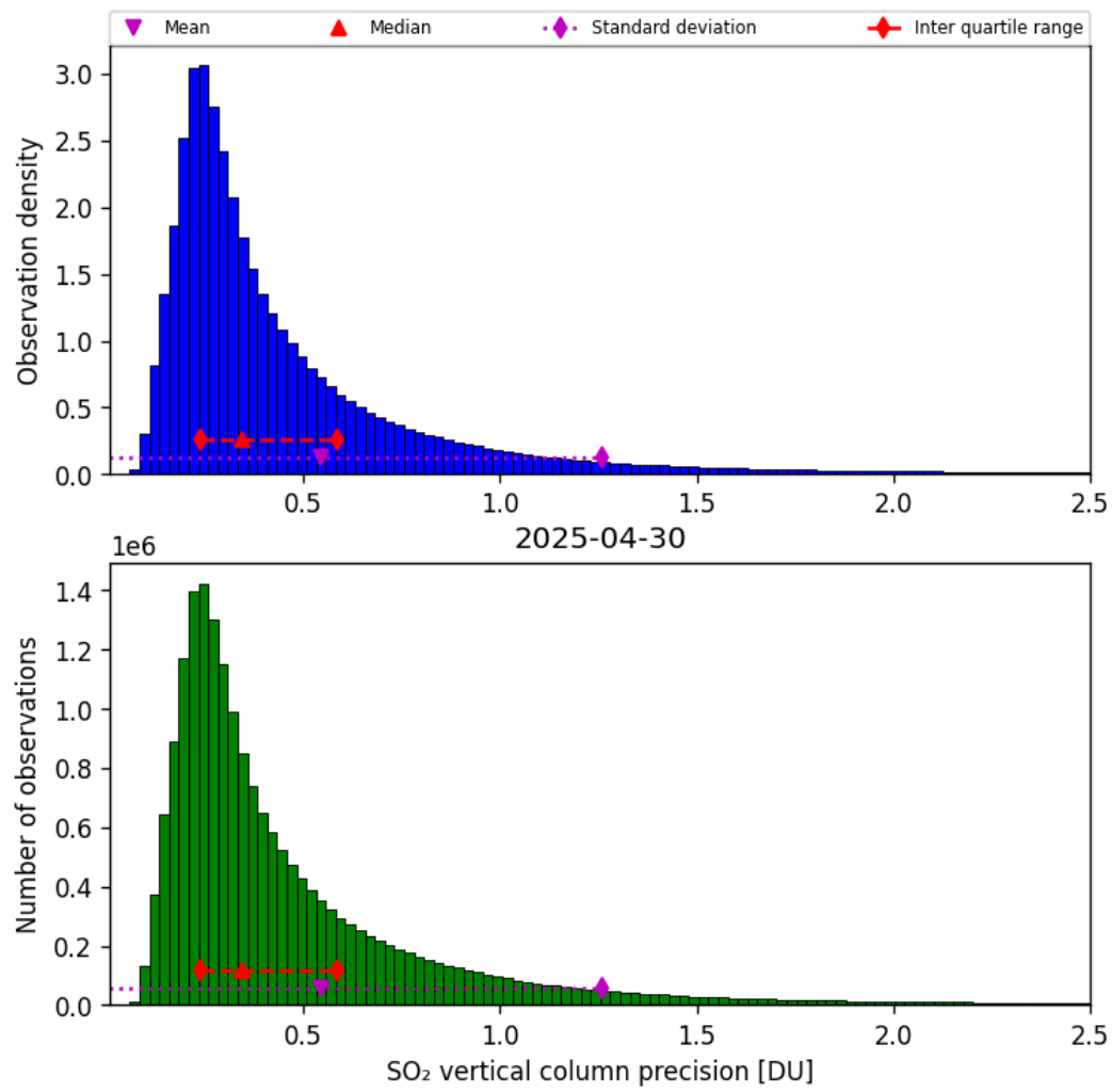
Figure 59: Histogram of “SO 2 vertical column precision” for 2025-04-29 to 2025-05-01
