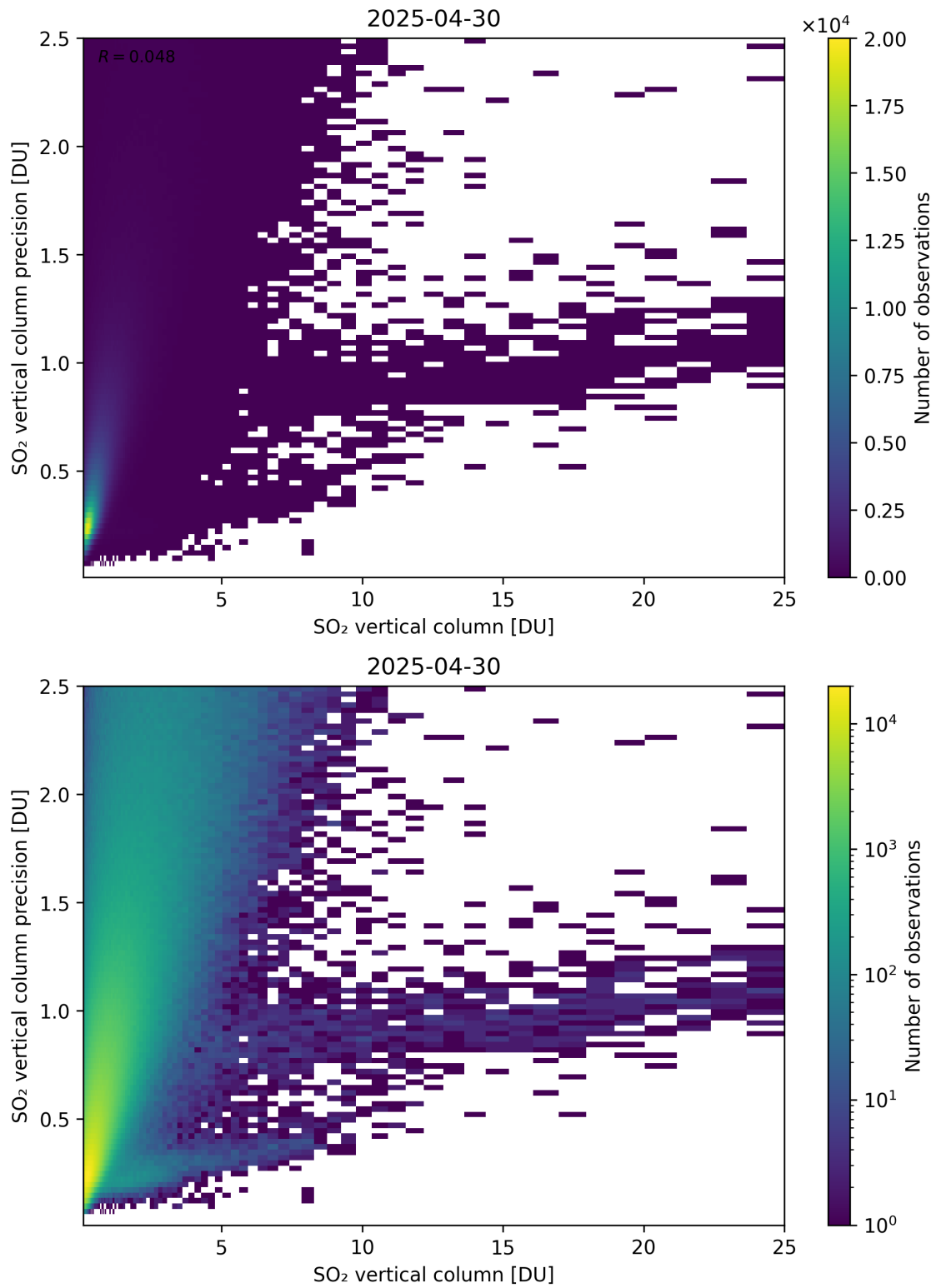
Figure 361: Scatter density plot of “SO 2 vertical column” against “SO 2 vertical column precision” for 2025-04-29 to 2025-05-01.
