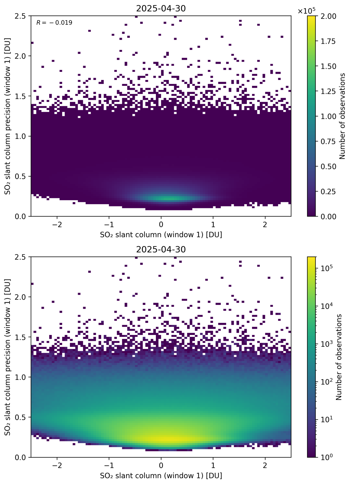
Figure 285: Scatter density plot of “SO 2 slant column (window 1)” against “SO 2 slant column precision (window 1)” for 2025-04-29 to 2025-05-01.
