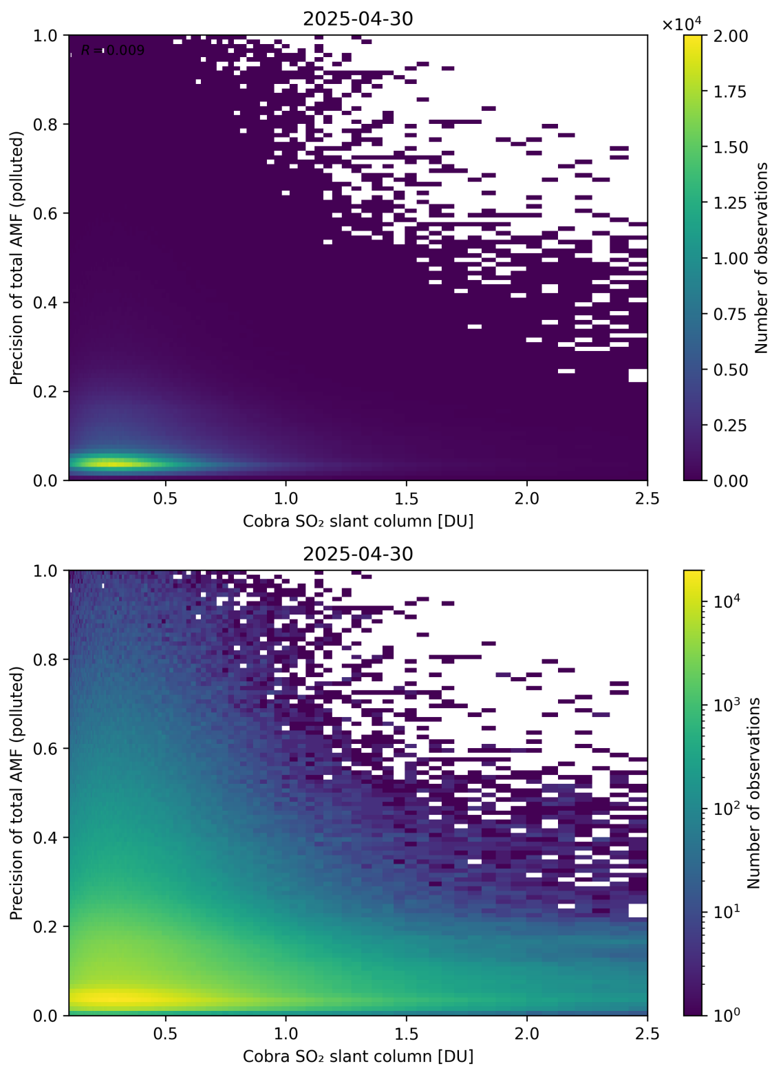
Figure 225: Scatter density plot of “Cobra SO 2 slant column” against “Precision of total AMF (polluted)” for 2025-04-29 to 2025-05-01.
