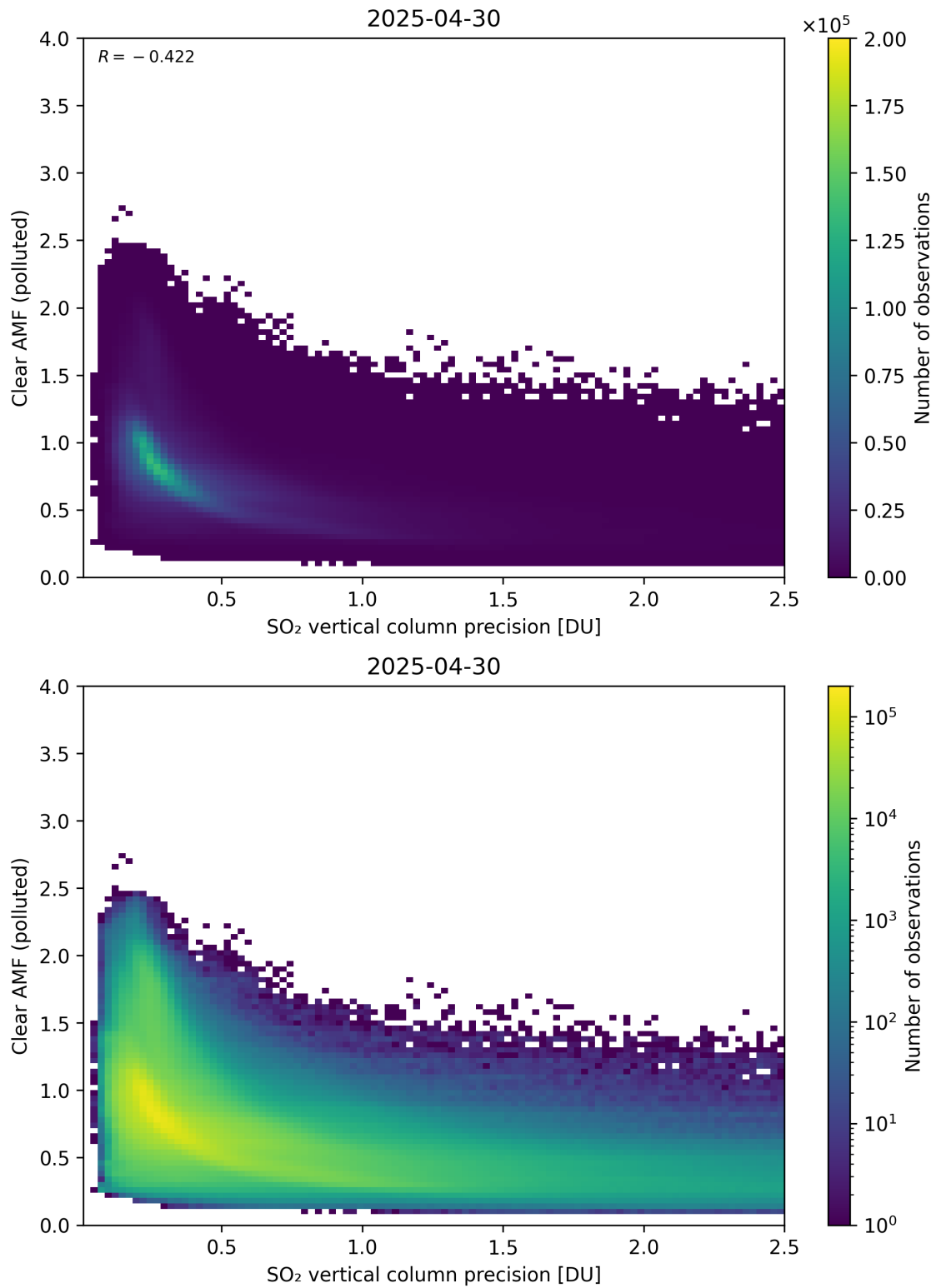
Figure 335: Scatter density plot of “SO 2 vertical column precision” against “Clear AMF (polluted)” for 2025-04-29 to 2025-05-01.
