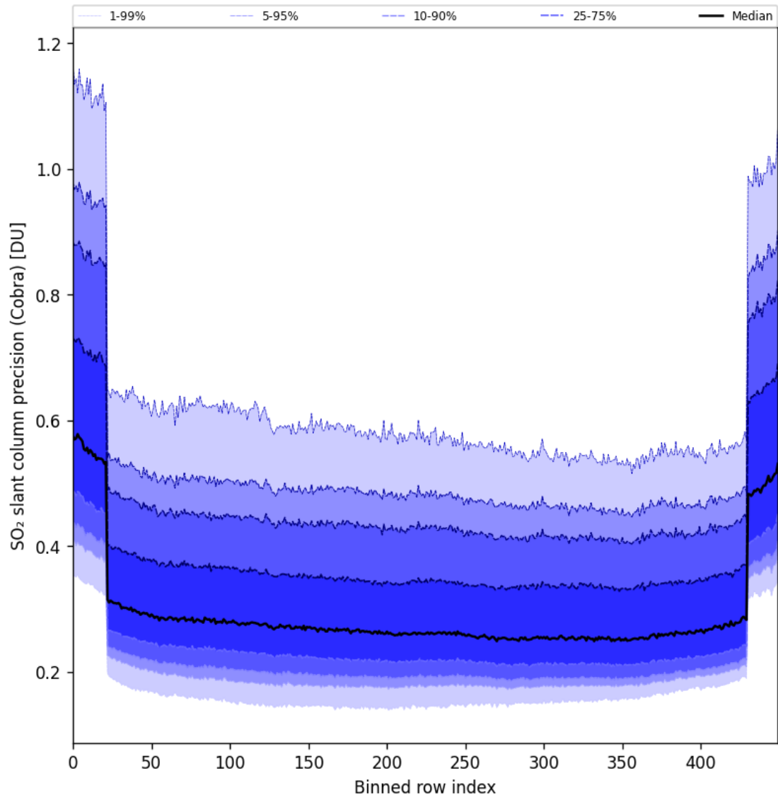
Figure 88: Along track statistics of “SO 2 slant column precision (Cobra)” for 2025-04-29 to 2025-05-01
