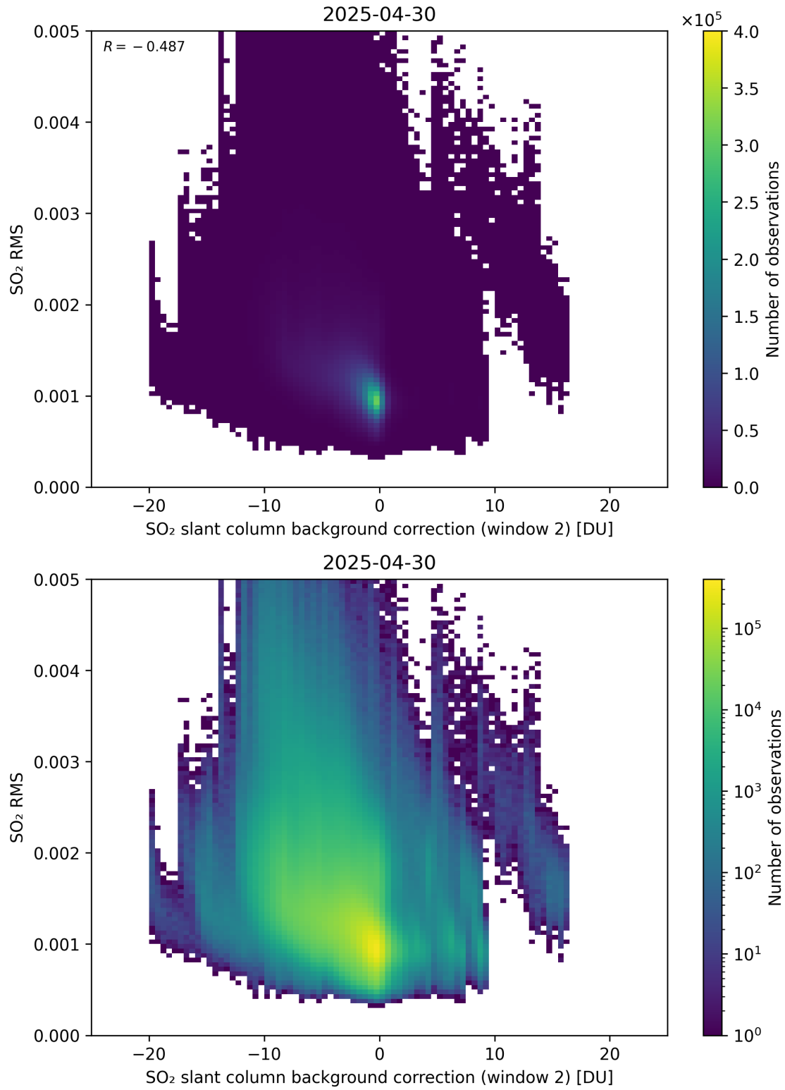
Figure 125: Scatter density plot of “SO 2 slant column background correction (window 2)” against “SO 2 RMS” for 2025-04-29 to 2025-05-01.
