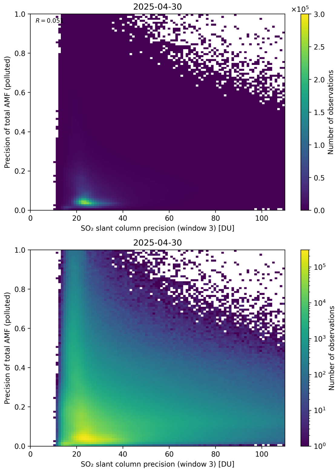
Figure 314: Scatter density plot of “SO 2 slant column precision (window 3)” against “Precision of total AMF (polluted)” for 2025-04-29 to 2025-05-01.
