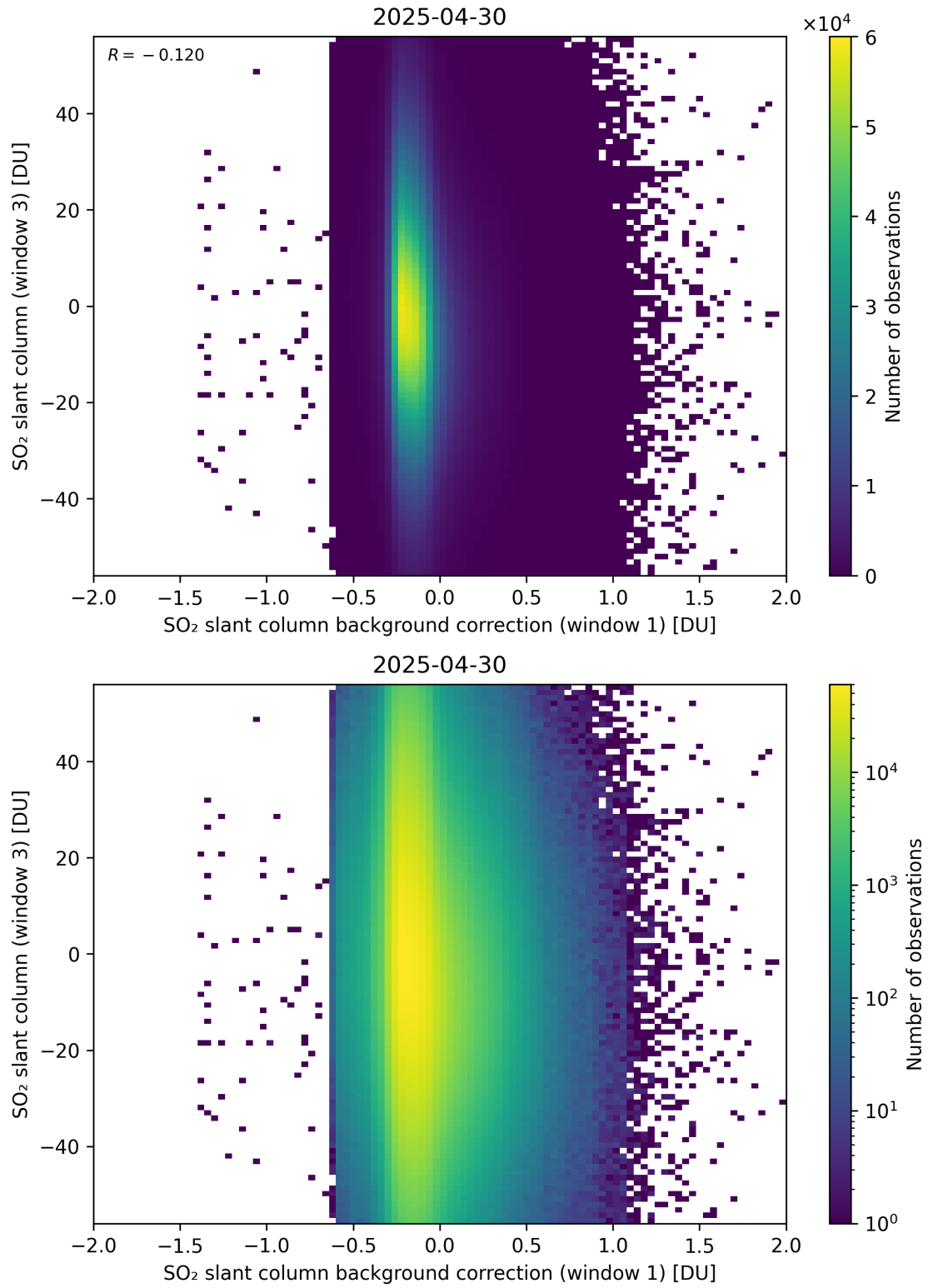
Figure 118: Scatter density plot of “SO 2 slant column background correction (window 1)” against “SO 2 slant column (window 3)” for 2025-04-29 to 2025-05-01.
