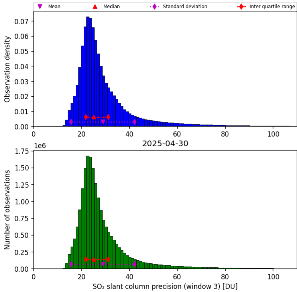
Figure 72: Histogram of “SO 2 slant column precision (window 3)” for 2025-04-29 to 2025-05-01
