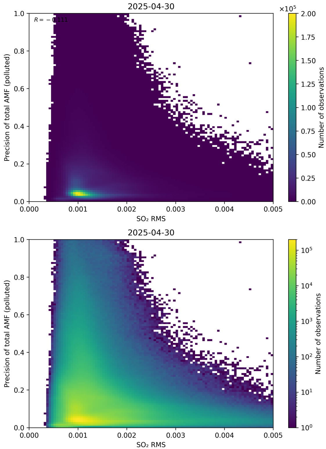
Figure 149: Scatter density plot of “SO 2 RMS” against “Precision of total AMF (polluted)” for 2025-04-29 to 2025-05-01.
