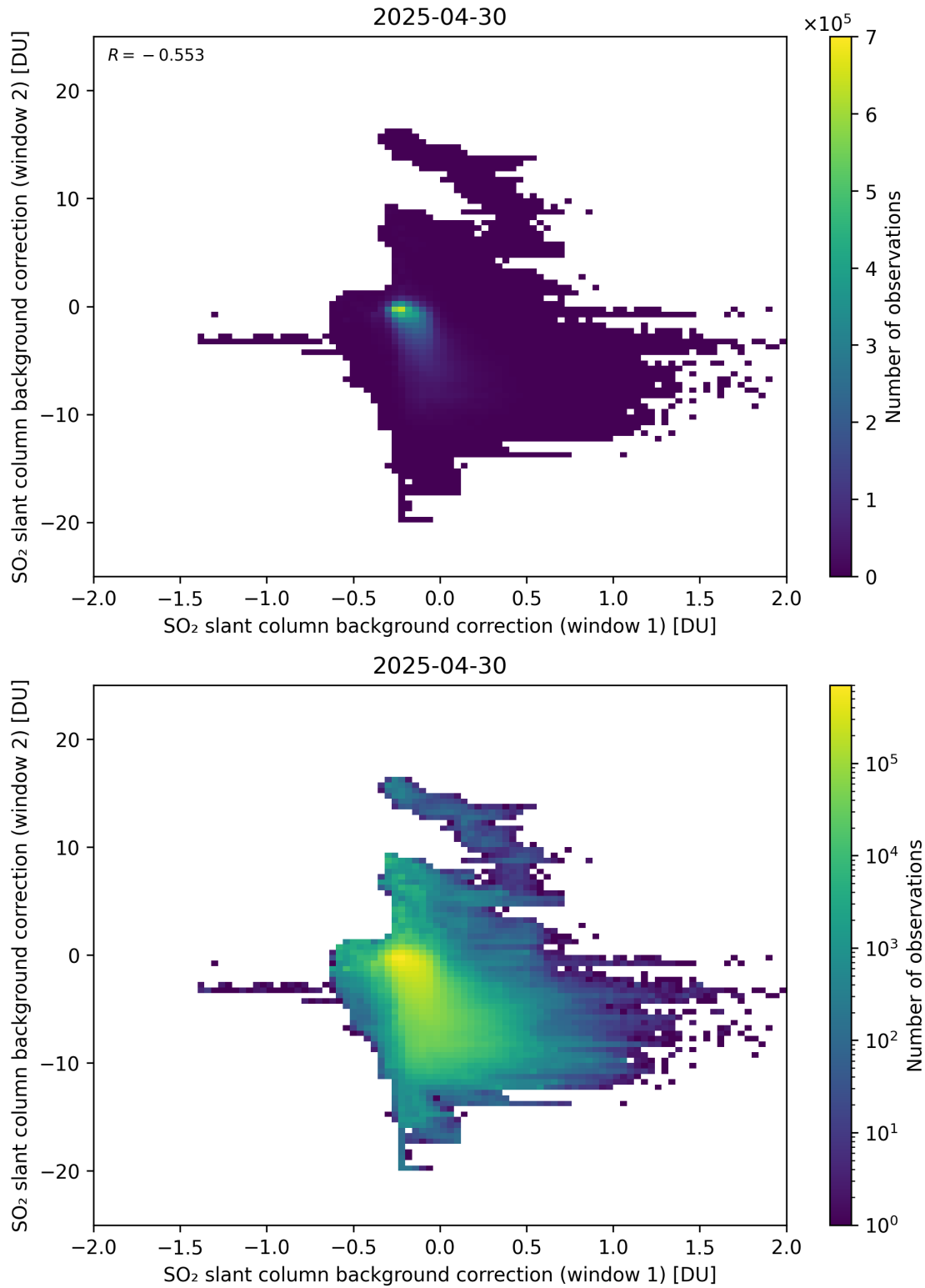
Figure 109: Scatter density plot of “SO 2 slant column background correction (window 1)” against “SO 2 slant column background correction (window 2)” for 2025-04-29 to 2025-05-01.
