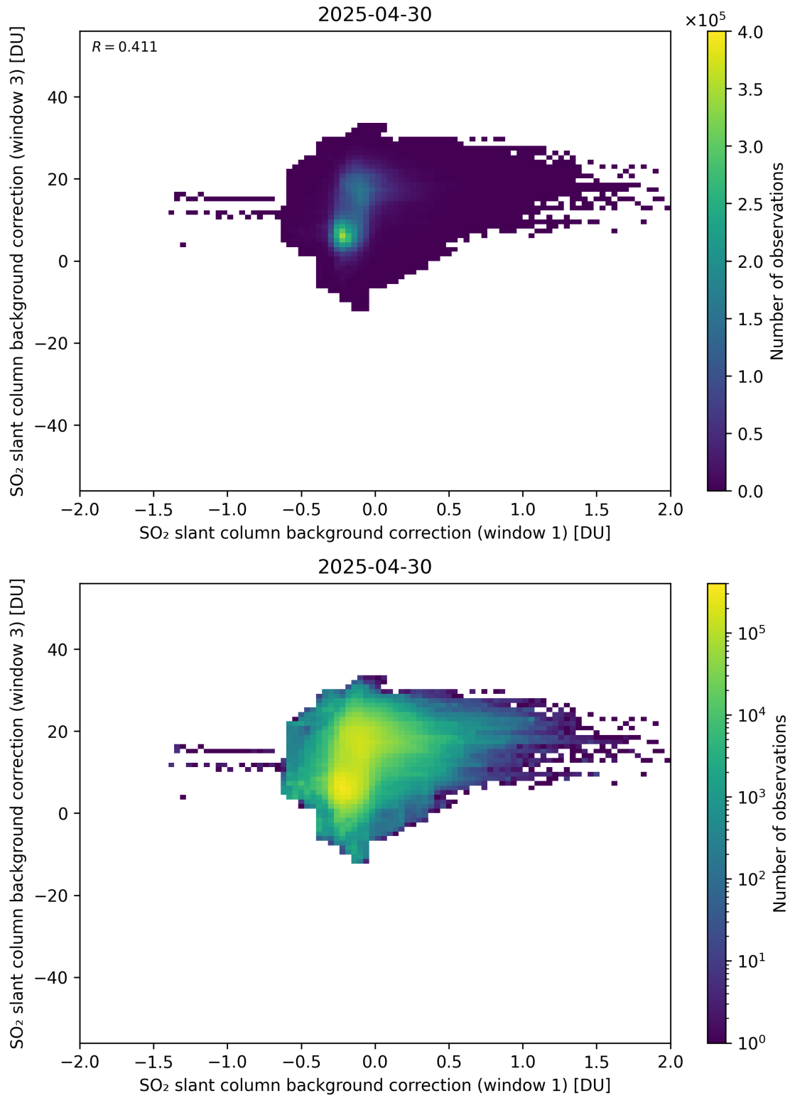
Figure 110: Scatter density plot of “SO 2 slant column background correction (window 1)” against “SO 2 slant column background correction (window 3)” for 2025-04-29 to 2025-05-01.
