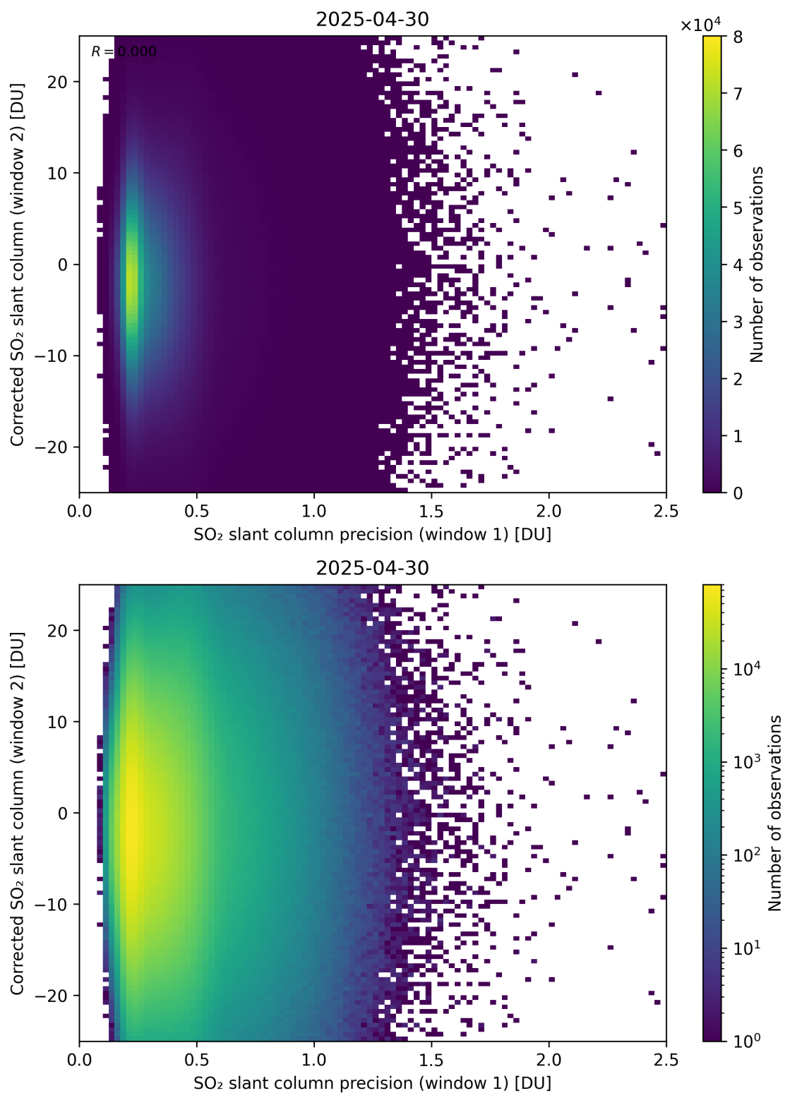
Figure 275: Scatter density plot of “SO 2 slant column precision (window 1)” against “Corrected SO 2 slant column (window 2)” for 2025-04-29 to 2025-05-01.
