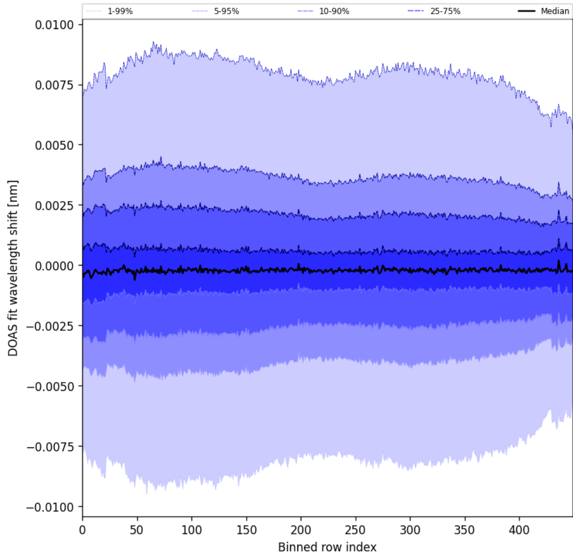
Figure 102: Along track statistics of “DOAS fit wavelength shift” for 2025-04-29 to 2025-05-01
