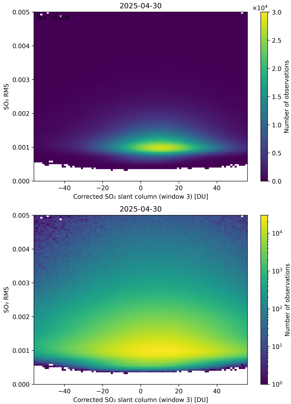
Figure 258: Scatter density plot of “Corrected SO 2 slant column (window 3)” against “SO 2 RMS” for 2025-04-29 to 2025-05-01.
