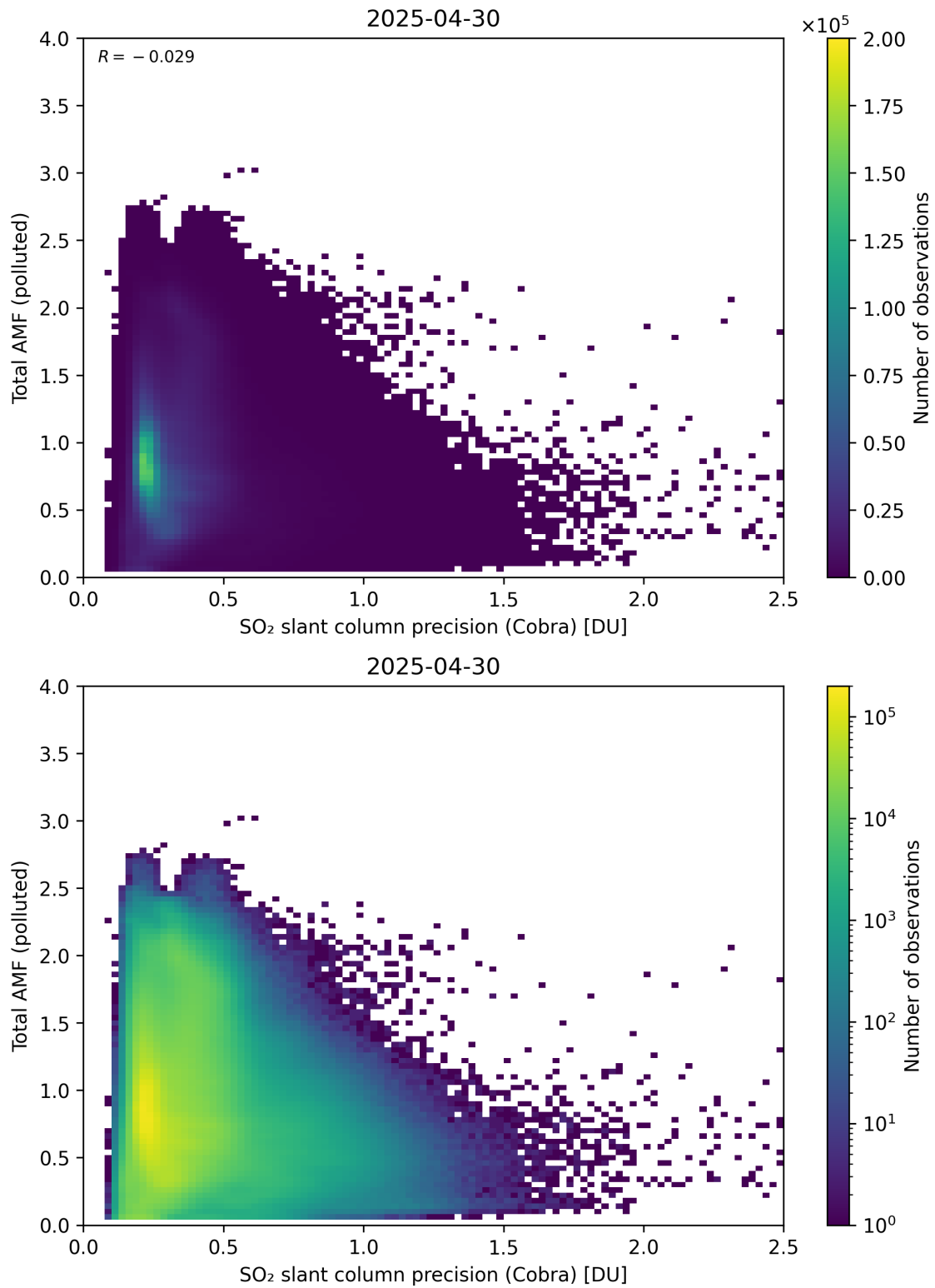
Figure 213: Scatter density plot of “SO 2 slant column precision (Cobra)” against “Total AMF (polluted)” for 2025-04-29 to 2025-05-01.
