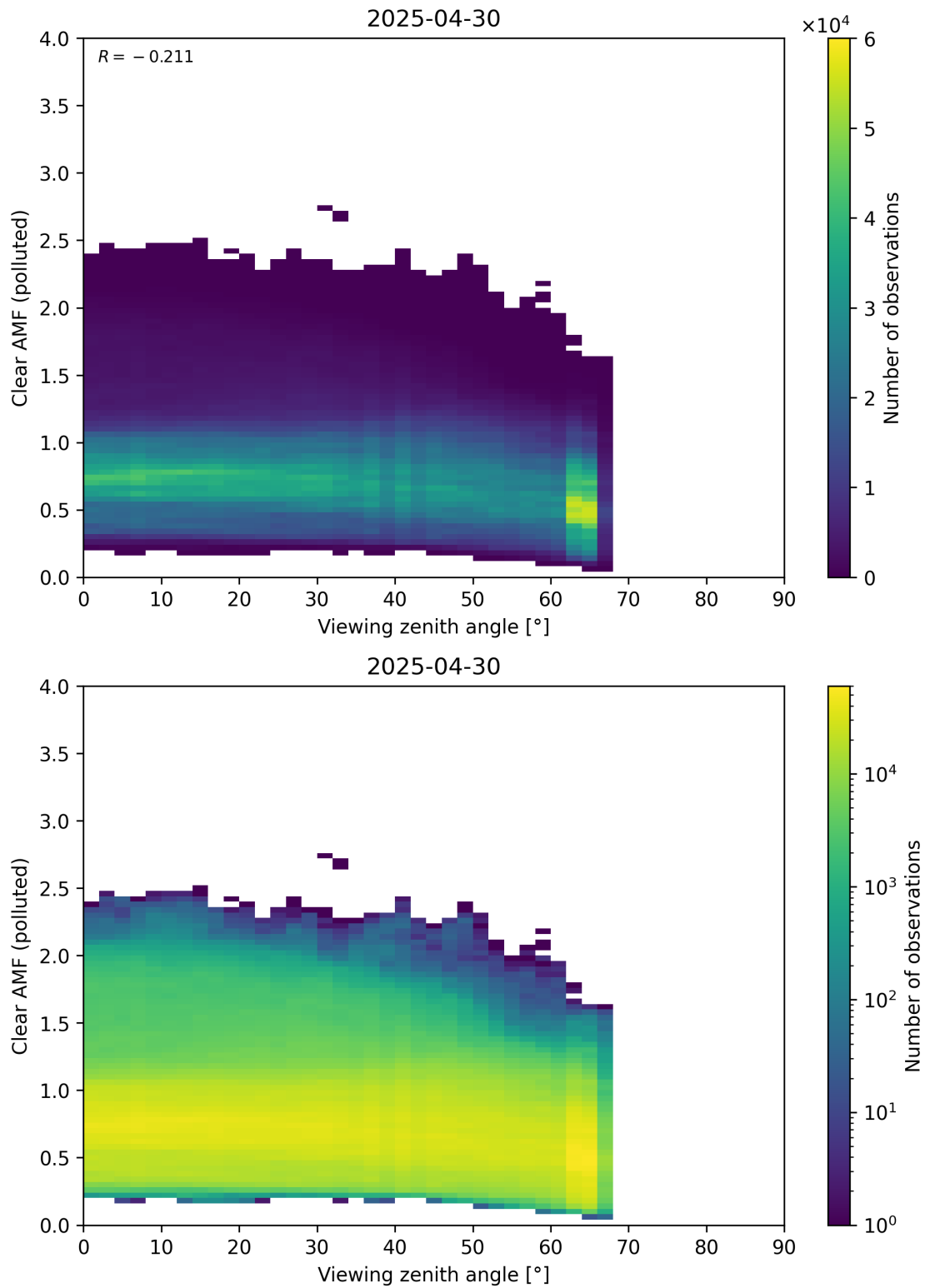
Figure 370: Scatter density plot of “Viewing zenith angle” against “Clear AMF (polluted)” for 2025-04-29 to 2025-05-01.
