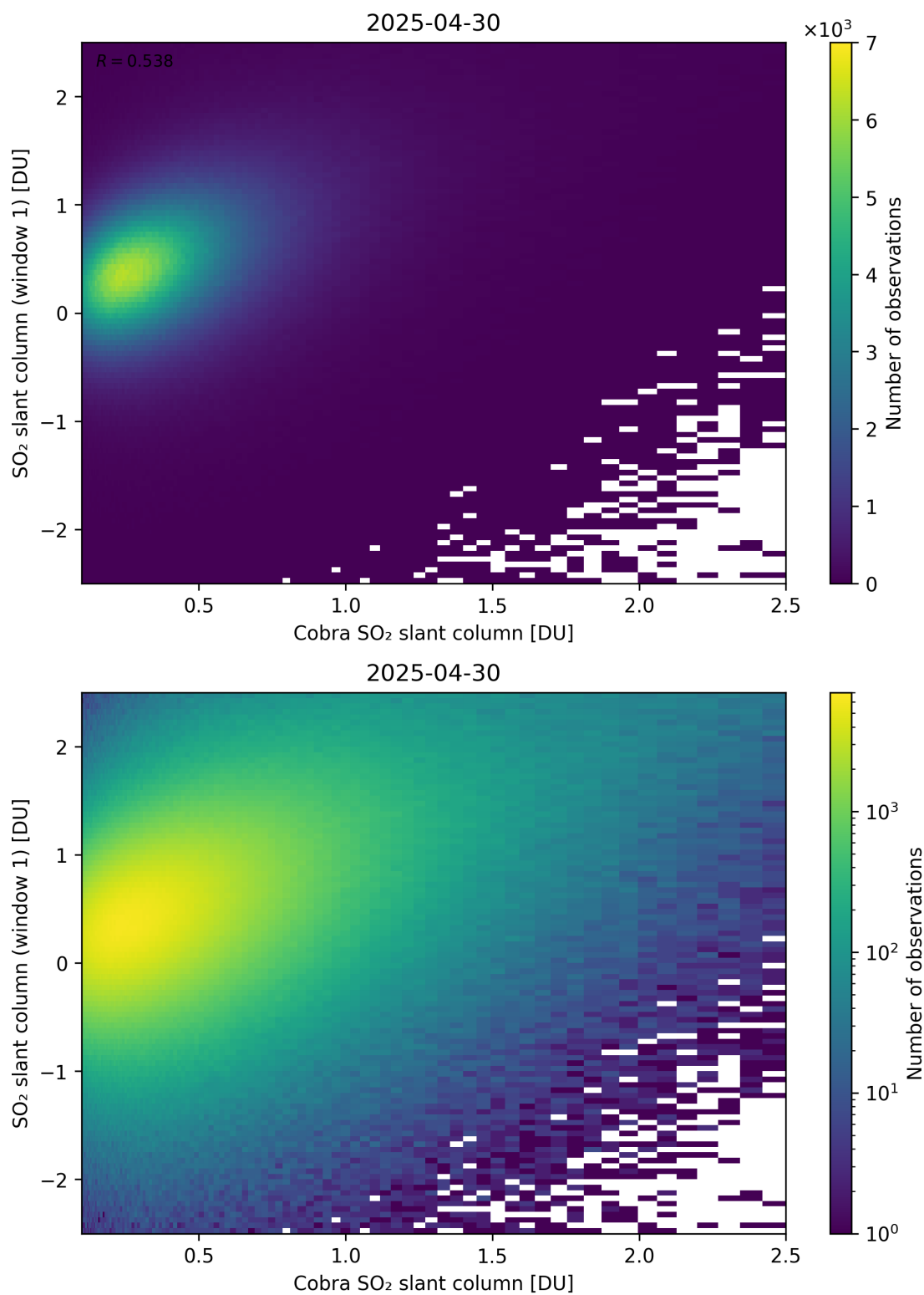
Figure 219: Scatter density plot of “Cobra SO 2 slant column” against “SO 2 slant column (window 1)” for 2025-04-29 to 2025-05-01.
