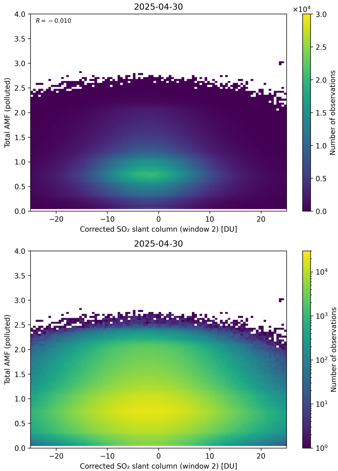
Figure 253: Scatter density plot of “Corrected SO 2 slant column (window 2)” against “Total AMF (polluted)” for 2025-04-29 to 2025-05-01.
