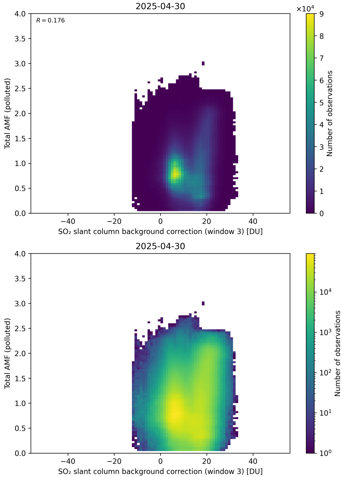
Figure 136: Scatter density plot of “SO 2 slant column background correction (window 3)” against “Total AMF (polluted)” for 2025-04-29 to 2025-05-01.
