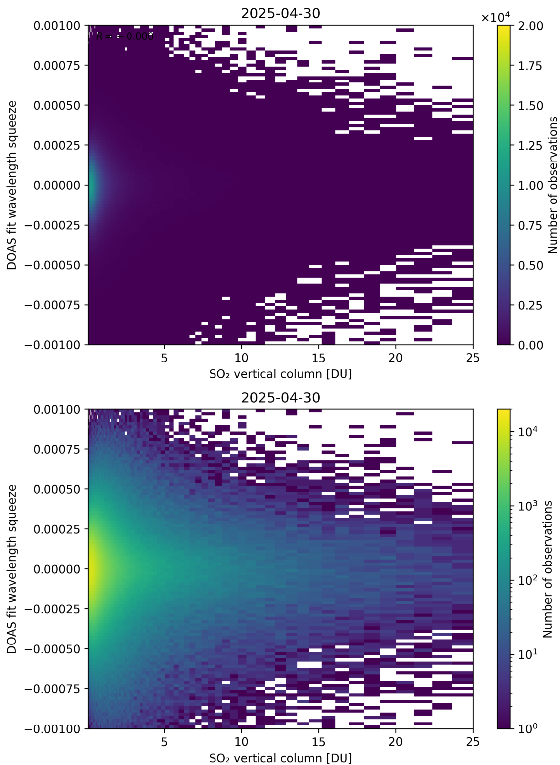
Figure 327: Scatter density plot of “SO 2 vertical column” against “DOAS fit wavelength squeeze” for 2025-04-29 to 2025-05-01.
