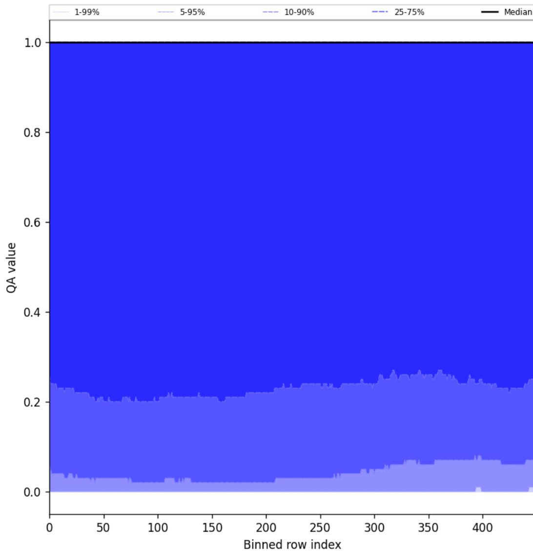
Figure 83: Along track statistics of “QA value” for 2025-04-29 to 2025-05-01
