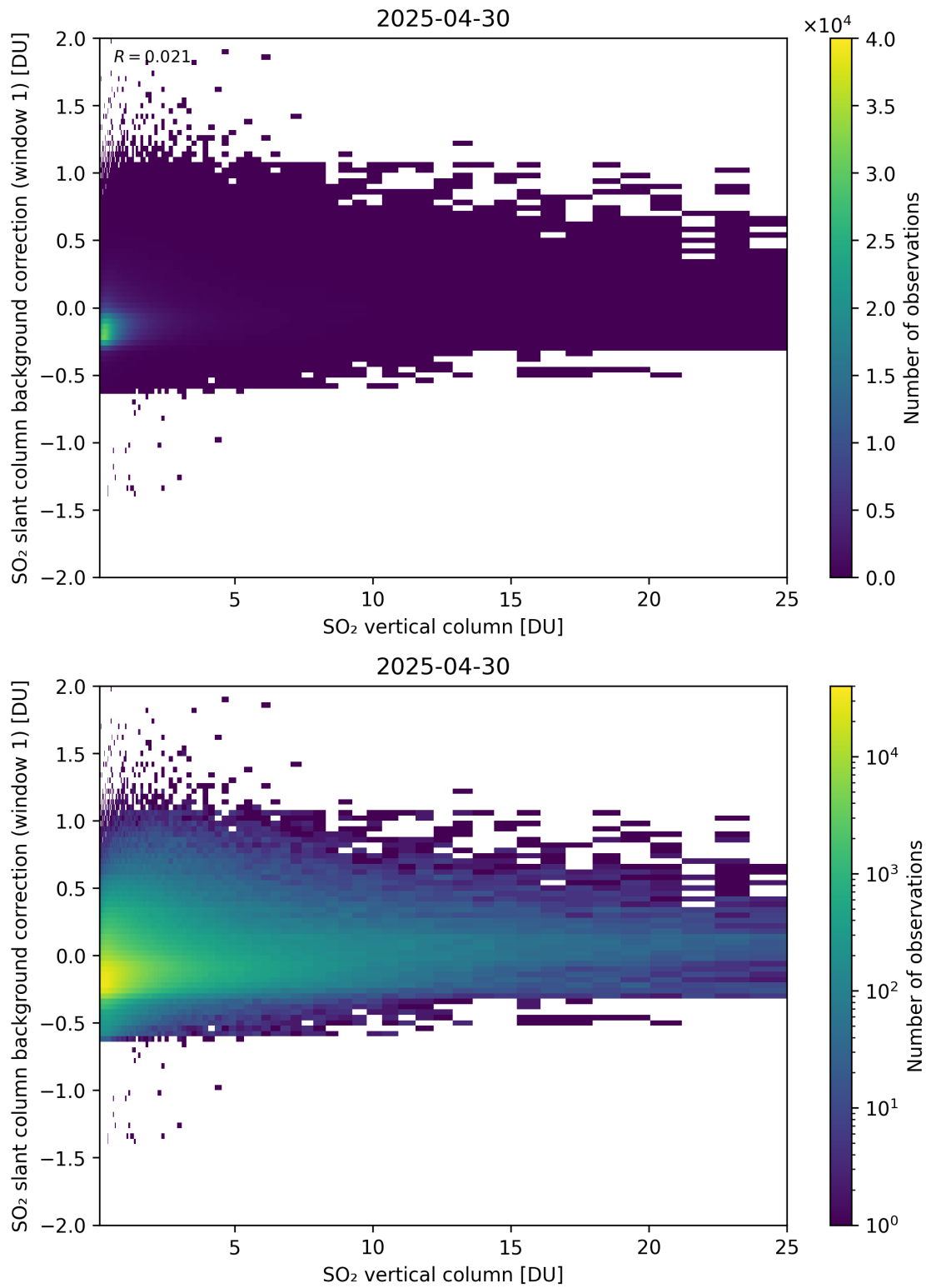
Figure 323: Scatter density plot of “SO 2 vertical column” against “SO 2 slant column background correction (window 1)” for 2025-04-29 to 2025-05-01.
