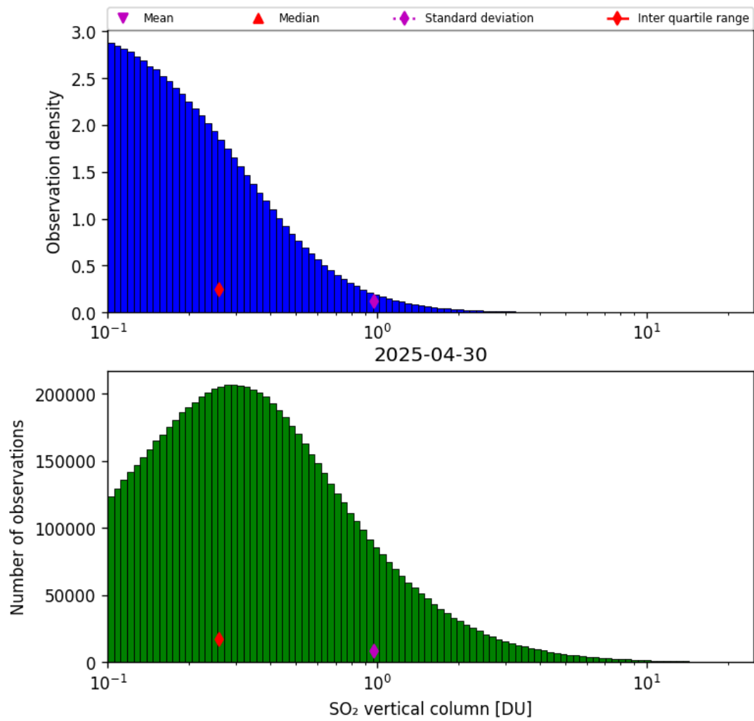
Figure 58: Histogram of “SO 2 vertical column” for 2025-04-29 to 2025-05-01
