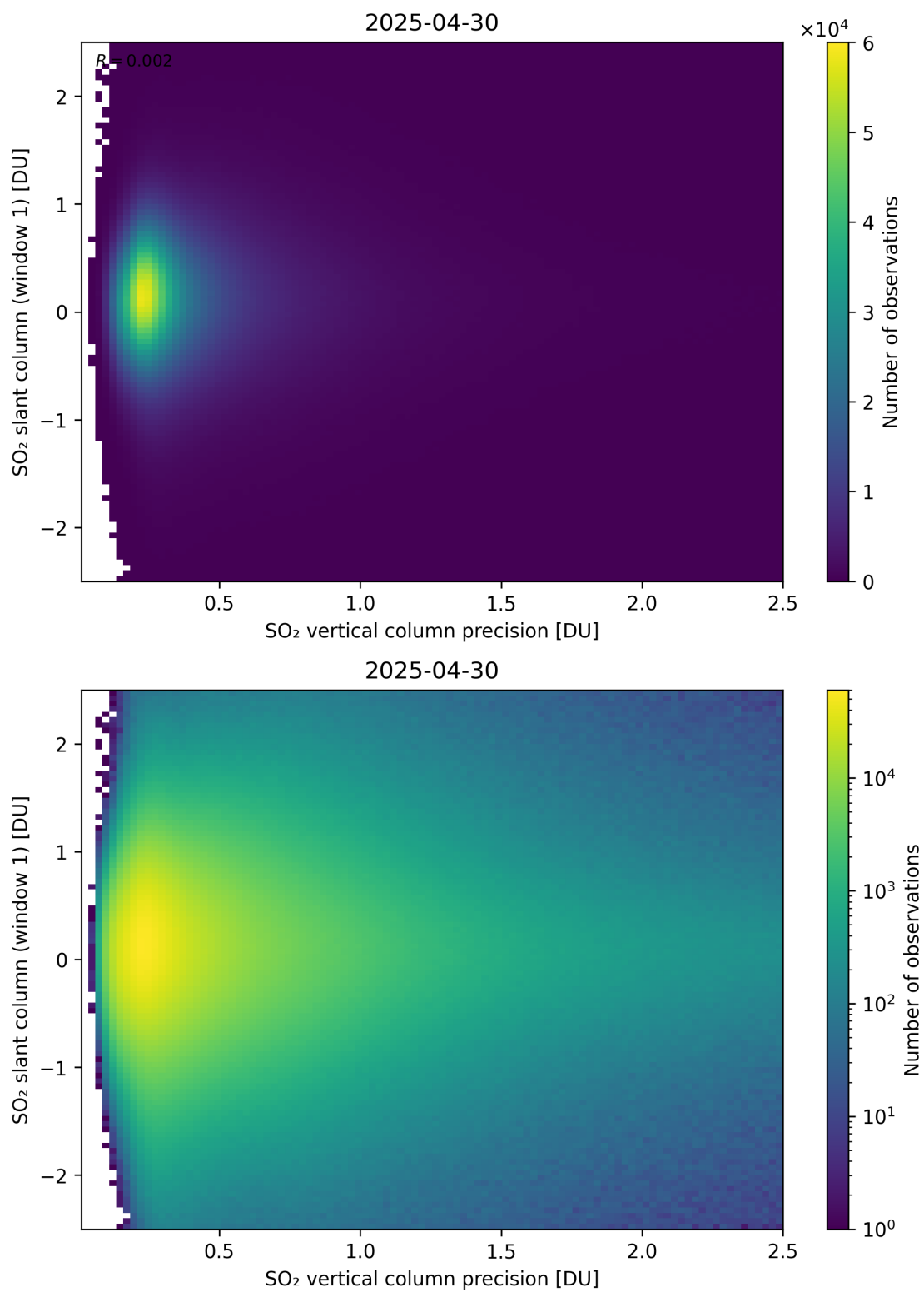
Figure 341: Scatter density plot of “SO 2 vertical column precision” against “SO 2 slant column (window 1)” for 2025-04-29 to 2025-05-01.
