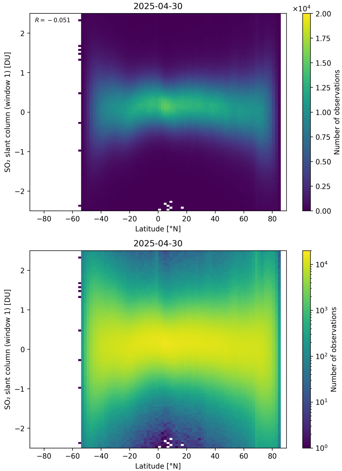
Figure 162: Scatter density plot of “Latitude” against “SO 2 slant column (window 1)” for 2025-04-29 to 2025-05-01.
