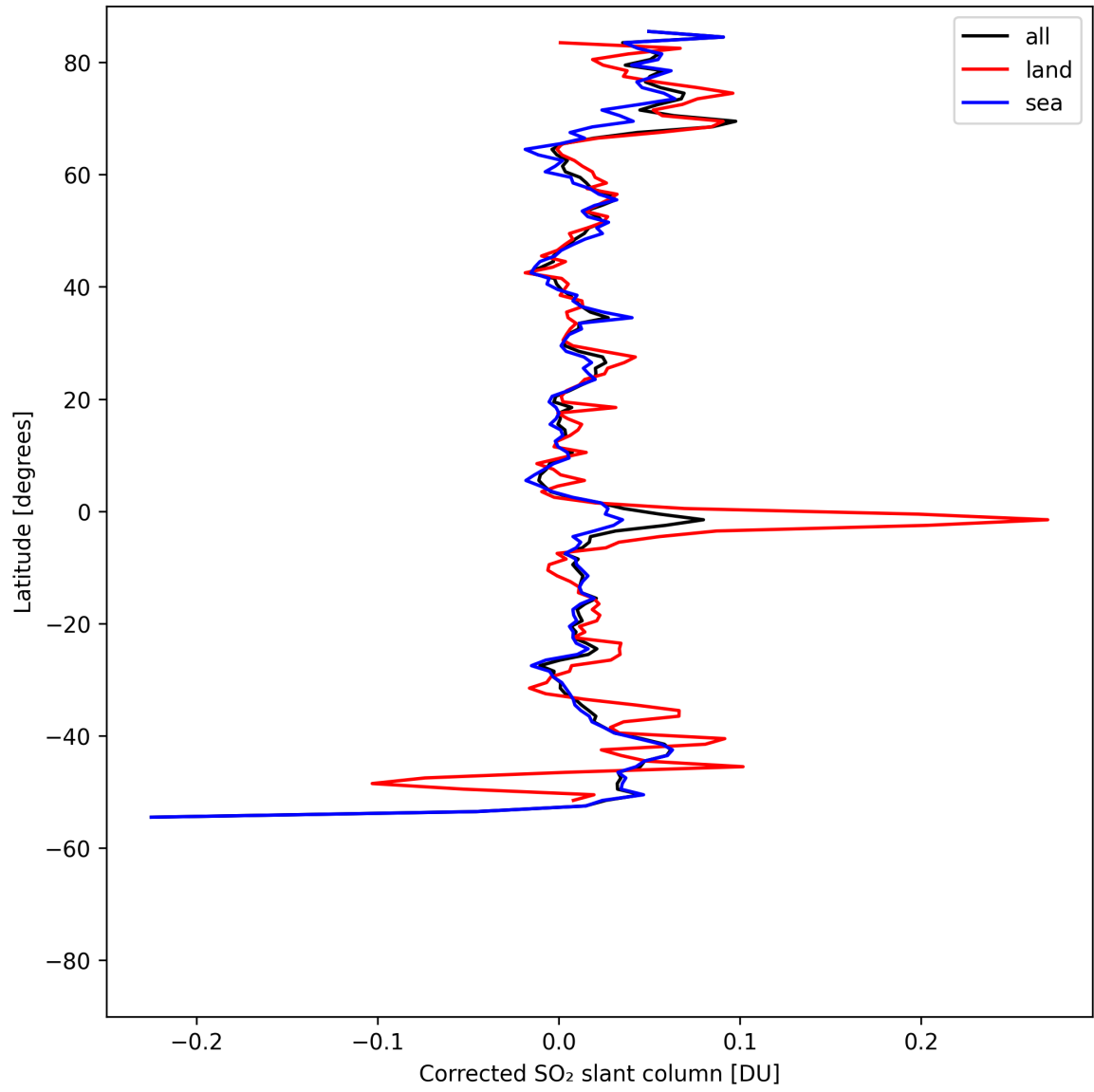
Figure 34: Zonal average of “Corrected SO 2 slant column” for 2025-04-29 to 2025-05-01.
