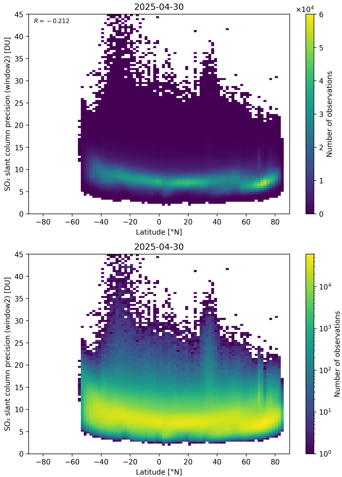
Figure 164: Scatter density plot of “Latitude” against “SO 2 slant column precision (window2)” for 2025-04-29 to 2025-05-01.
