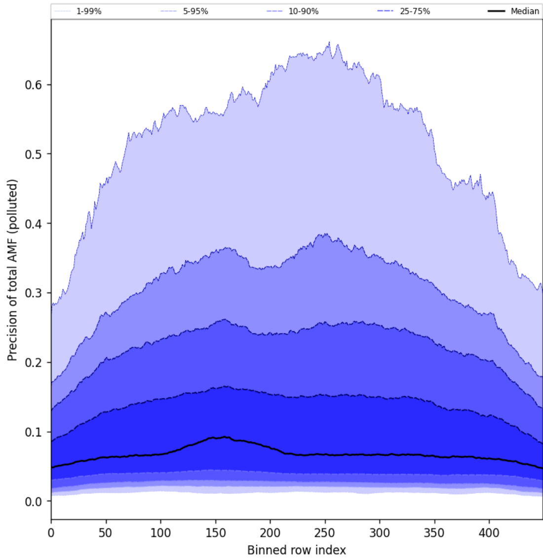
Figure 106: Along track statistics of “Precision of total AMF (polluted)” for 2025-04-29 to 2025-05-01
