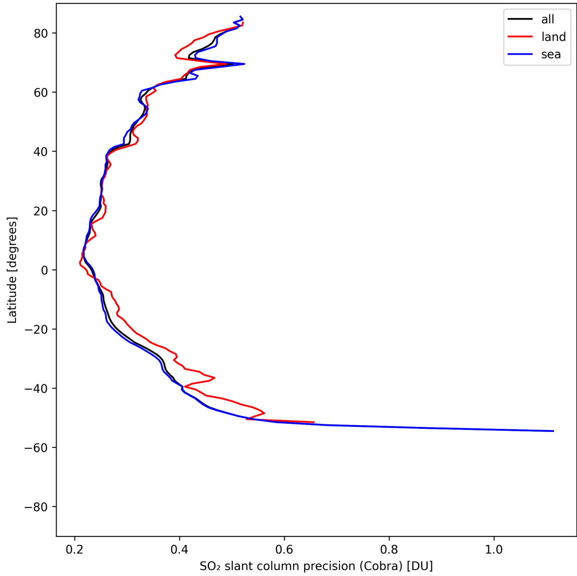
Figure 36: Zonal average of “SO 2 slant column precision (Cobra)” for 2025-04-29 to 2025-05-01.
