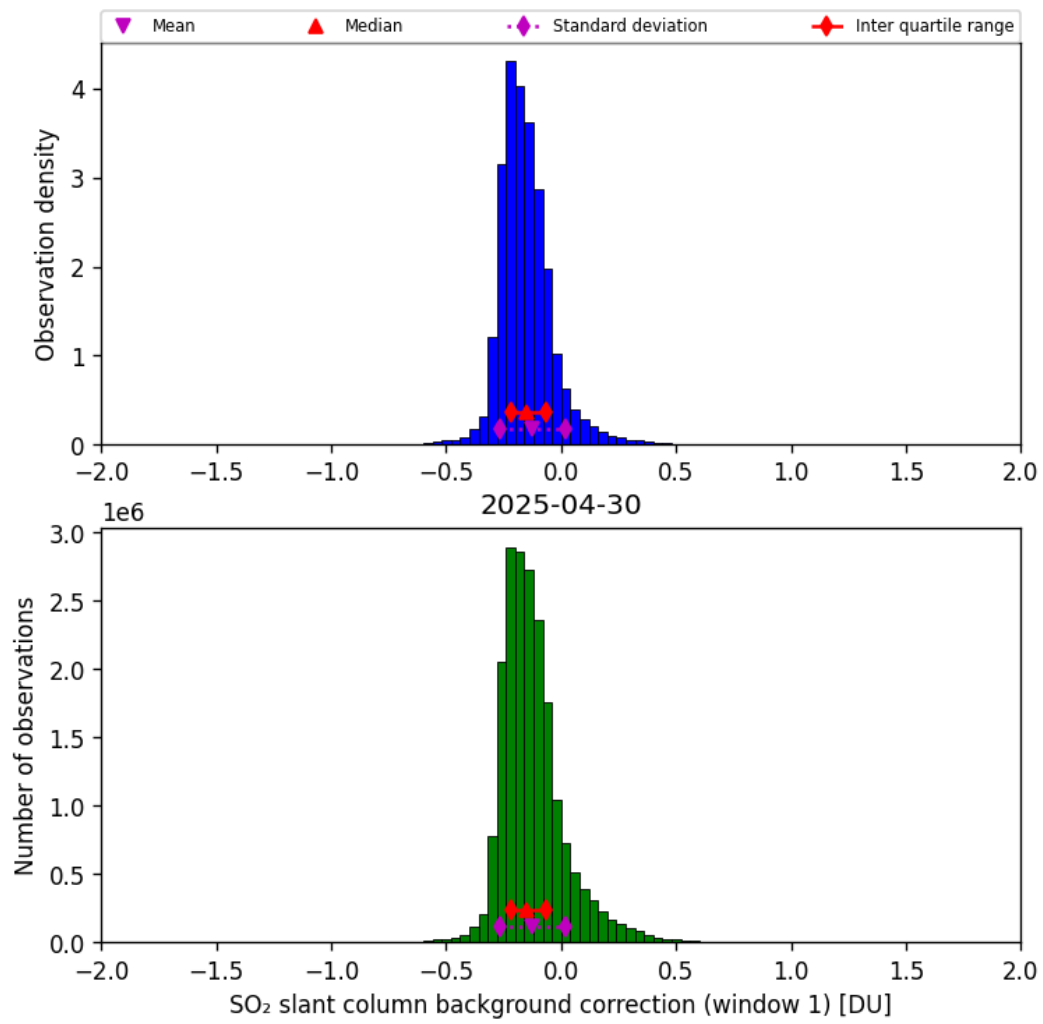
Figure 66: Histogram of “SO 2 slant column background correction (window 1)” for 2025-04-29 to 2025-05-01
