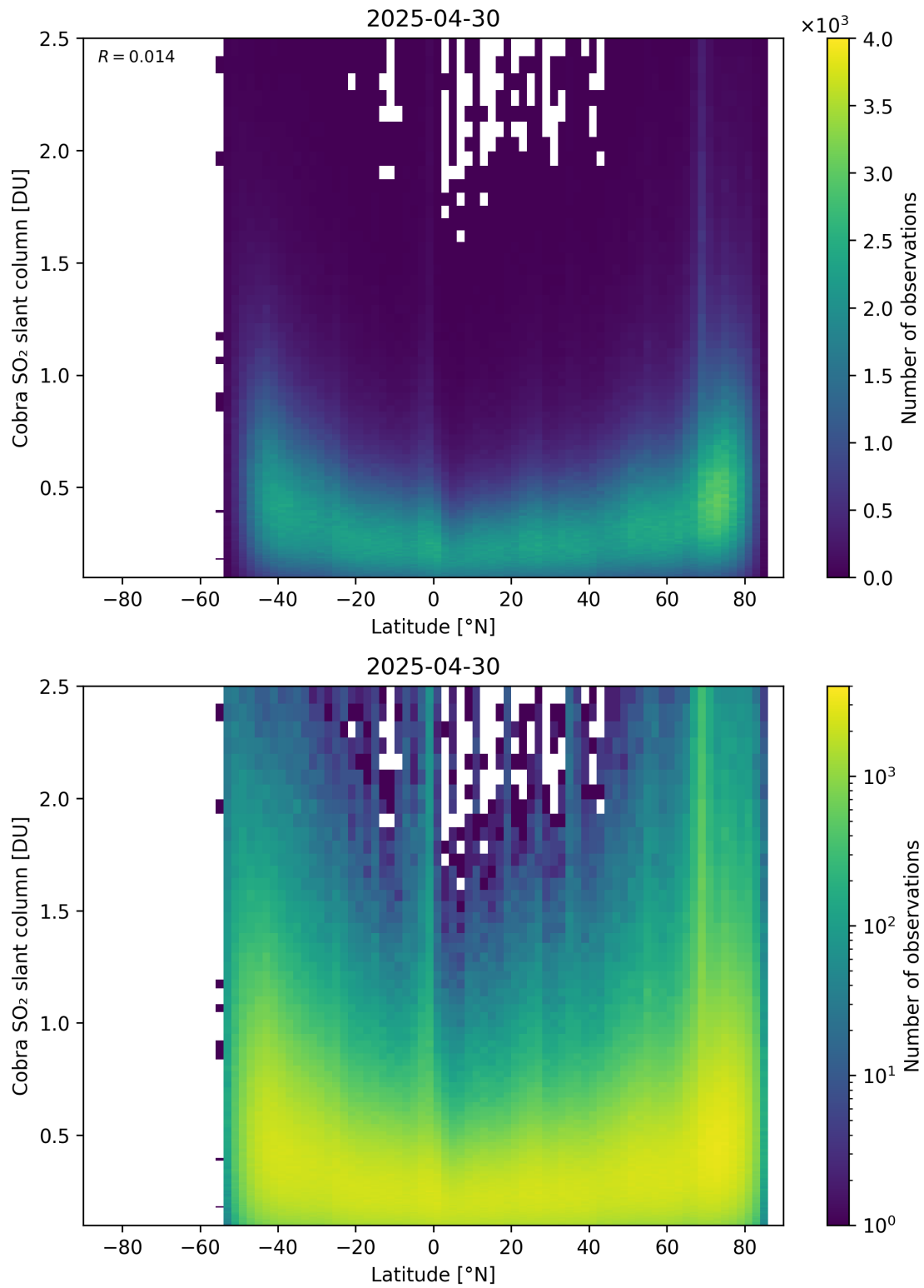
Figure 157: Scatter density plot of “Latitude” against “Cobra SO 2 slant column” for 2025-04-29 to 2025-05-01.
