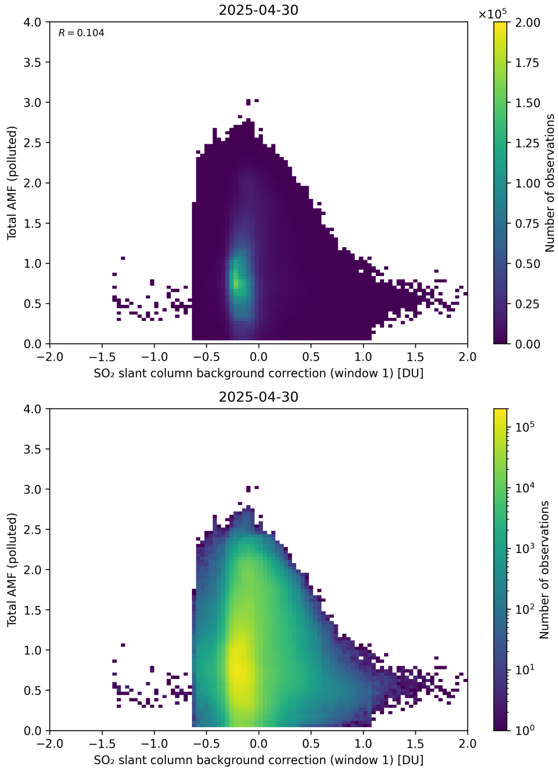
Figure 120: Scatter density plot of “SO 2 slant column background correction (window 1)” against “Total AMF (polluted)” for 2025-04-29 to 2025-05-01.
