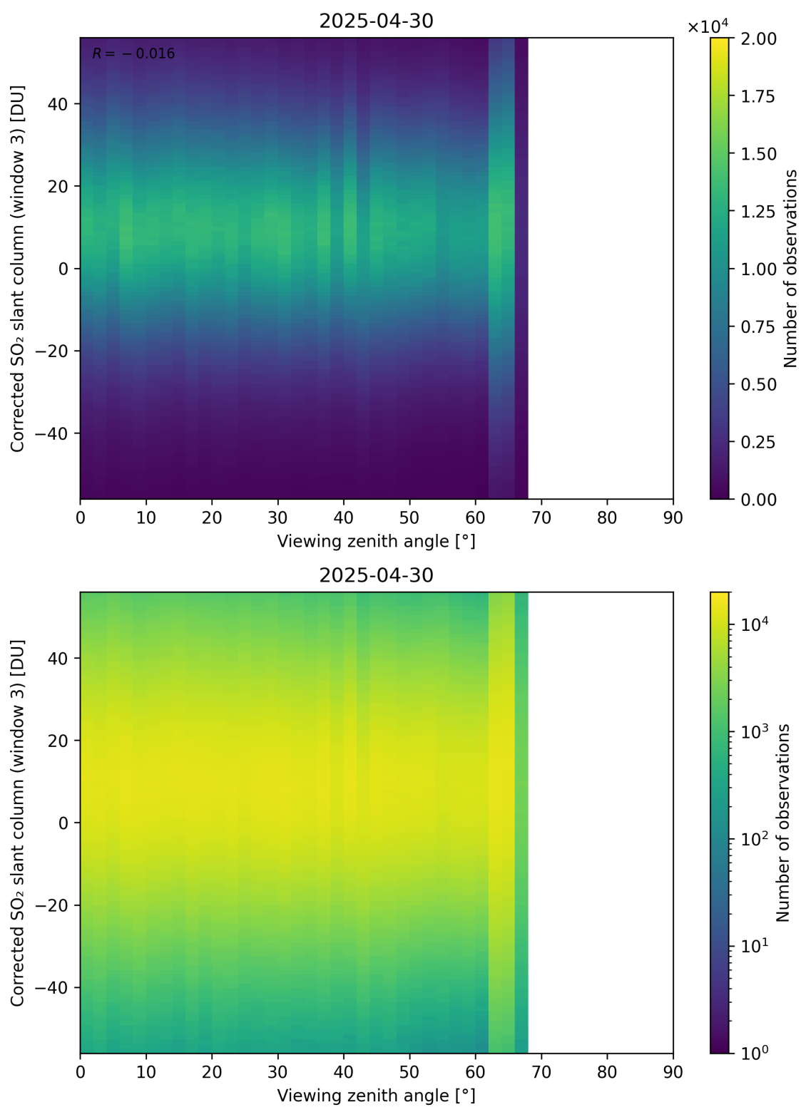
Figure 375: Scatter density plot of “Viewing zenith angle” against “Corrected SO 2 slant column (window 3)” for 2025-04-29 to 2025-05-01.
