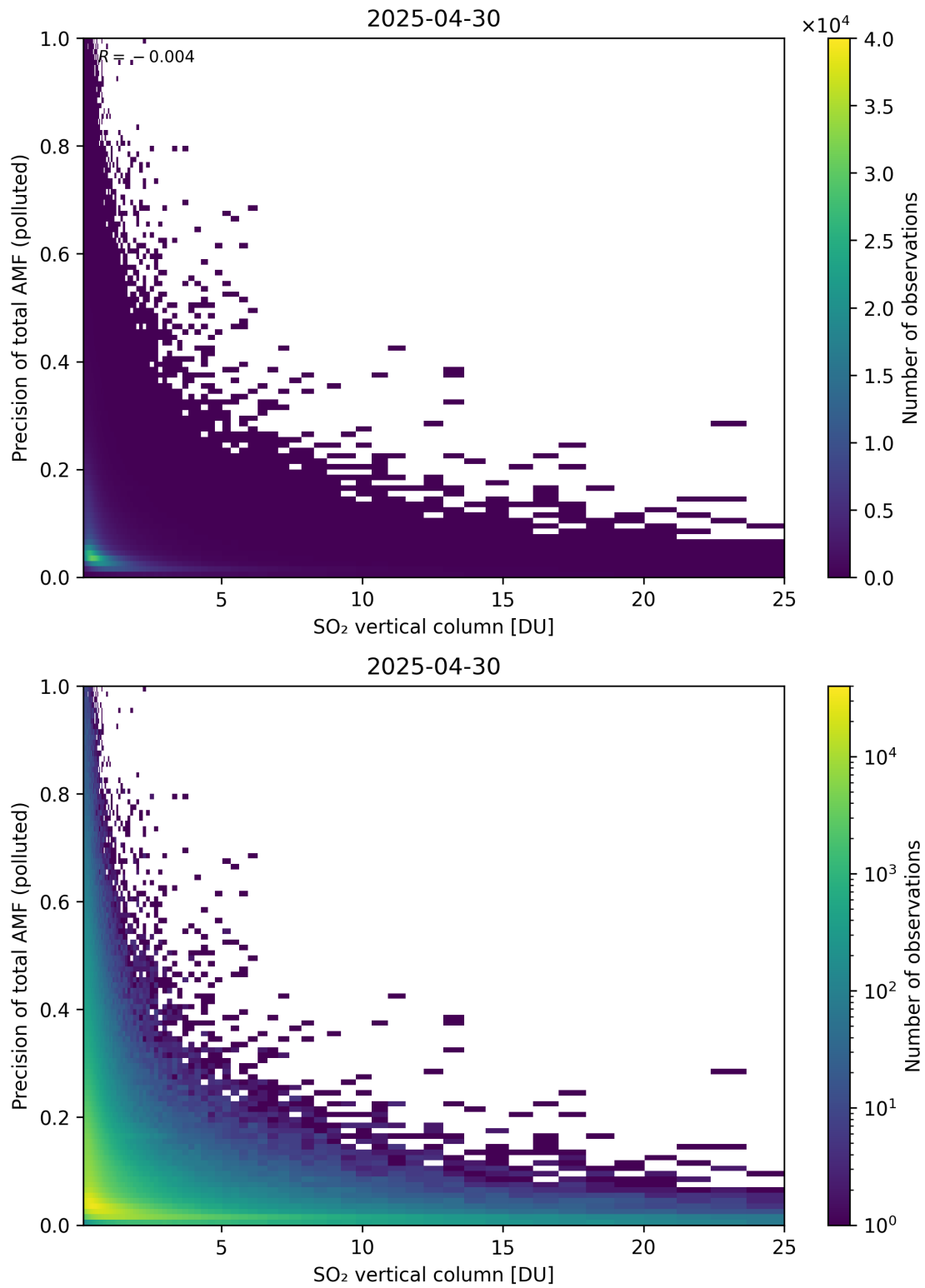
Figure 360: Scatter density plot of “SO 2 vertical column” against “Precision of total AMF (polluted)” for 2025-04-29 to 2025-05-01.
