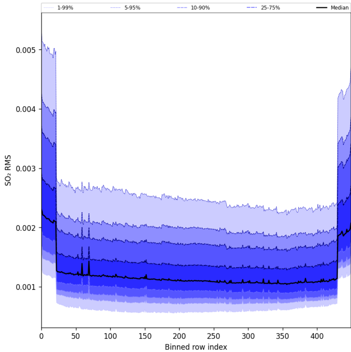
Figure 104: Along track statistics of “SO 2 RMS” for 2025-04-29 to 2025-05-01
