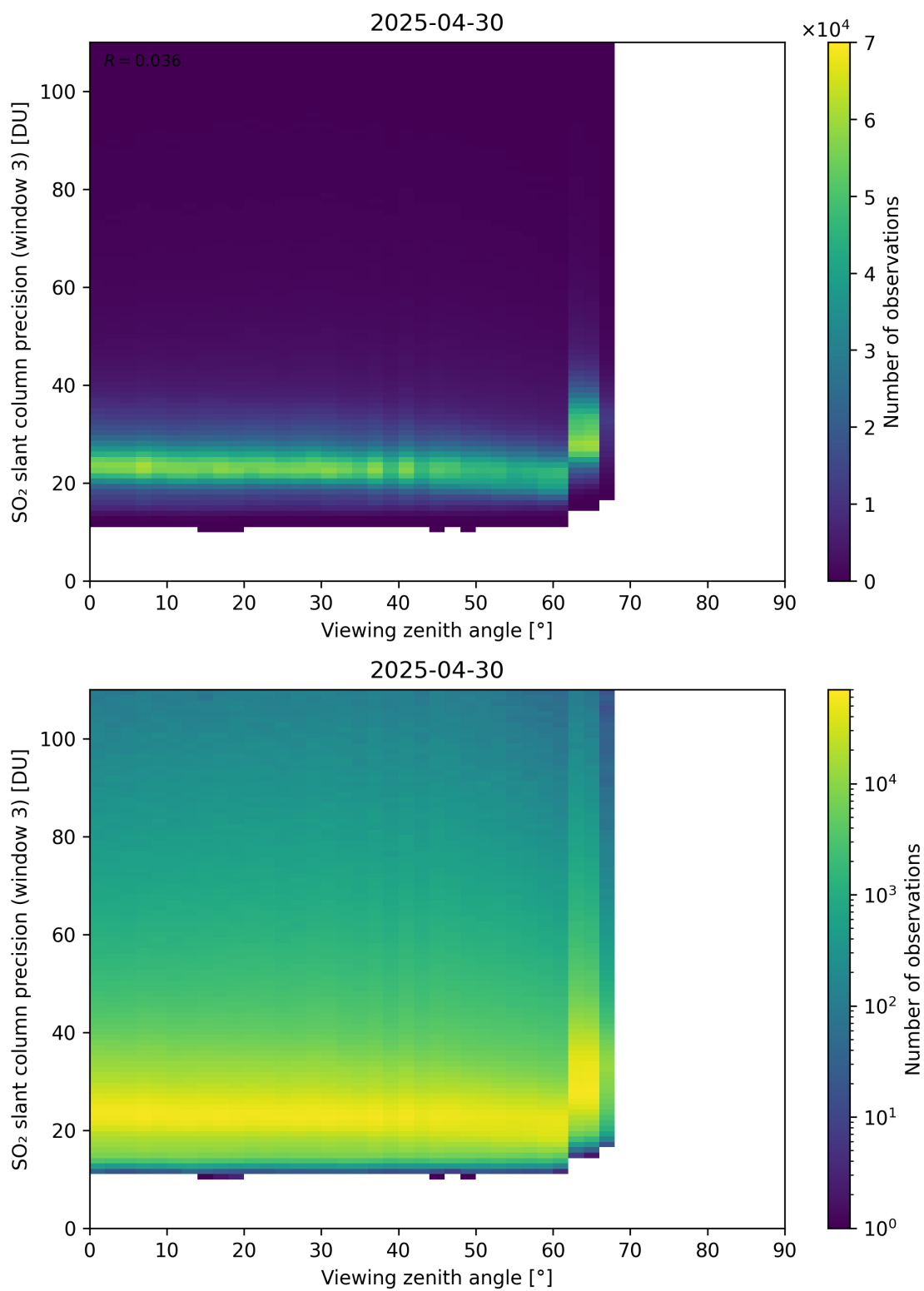
Figure 380: Scatter density plot of “Viewing zenith angle” against “SO 2 slant column precision (window 3)” for 2025-04-29 to 2025-05-01.
