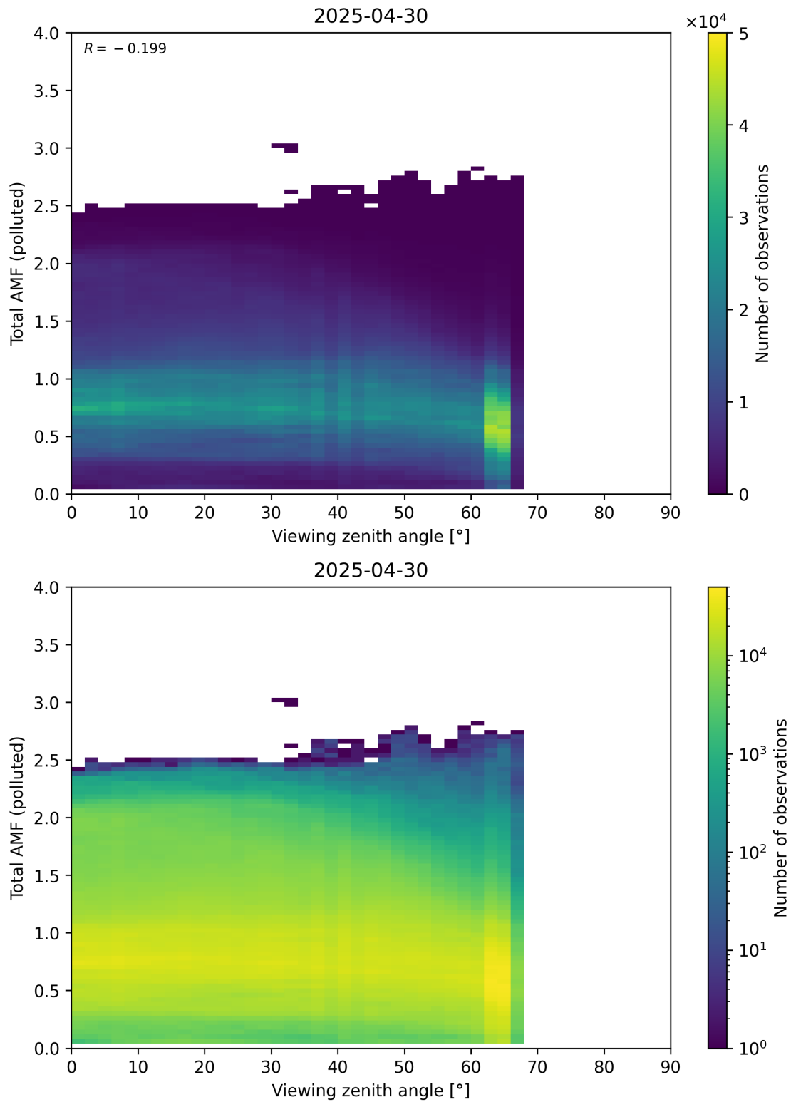
Figure 381: Scatter density plot of “Viewing zenith angle” against “Total AMF (polluted)” for 2025-04-29 to 2025-05-01.
