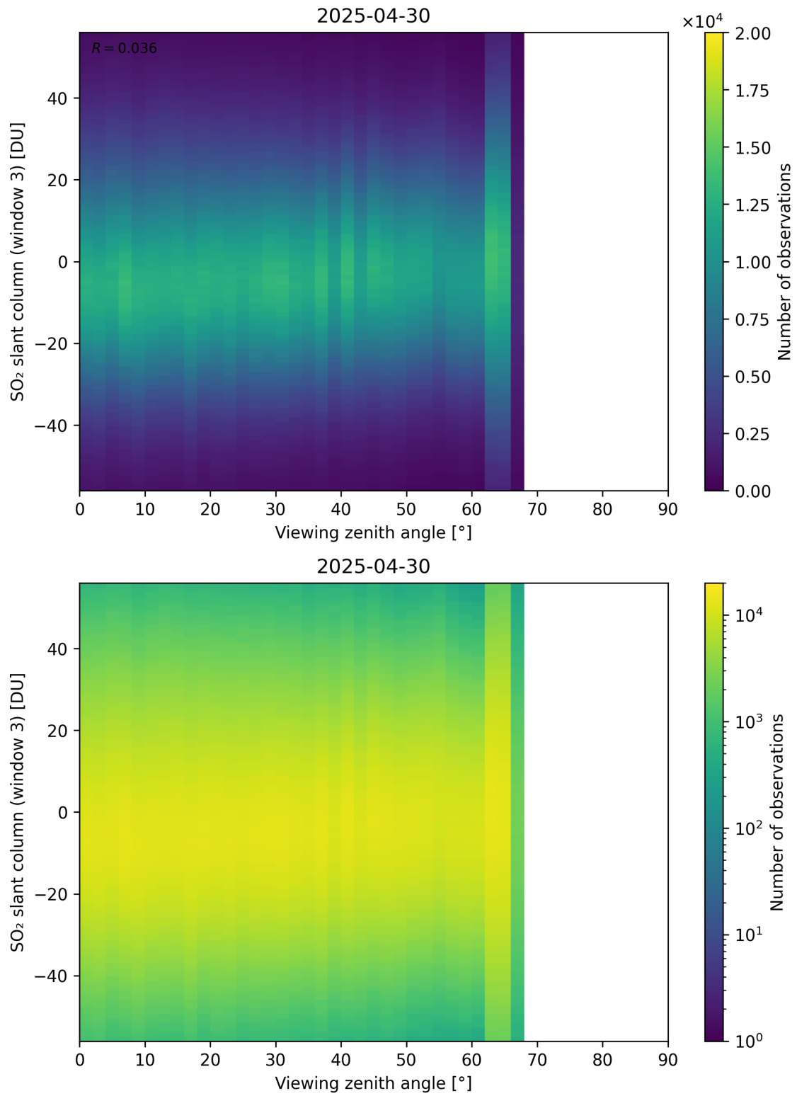
Figure 379: Scatter density plot of “Viewing zenith angle” against “SO 2 slant column (window 3)” for 2025-04-29 to 2025-05-01.
