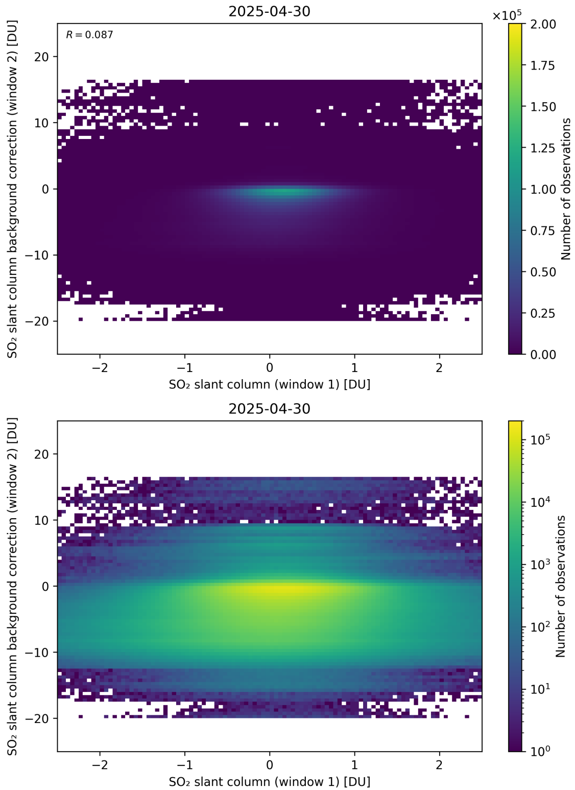
Figure 263: Scatter density plot of “SO 2 slant column (window 1)” against “SO 2 slant column background correction (window 2)” for 2025-04-29 to 2025-05-01.
