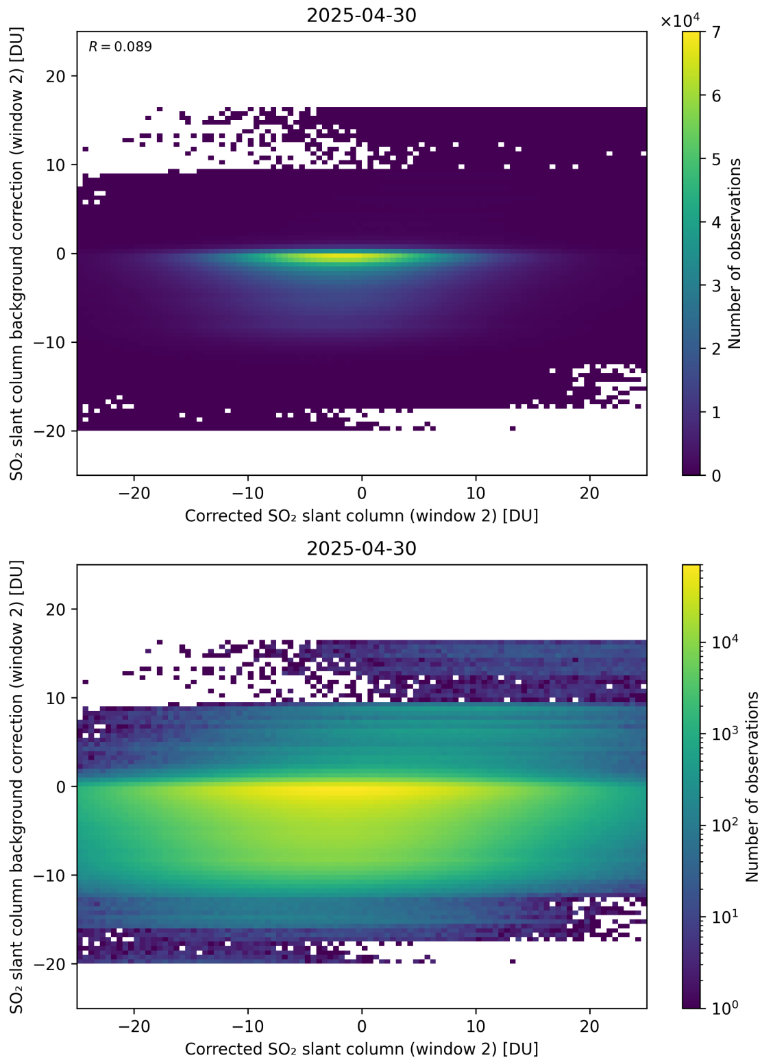
Figure 244: Scatter density plot of “Corrected SO 2 slant column (window 2)” against “SO 2 slant column background correction (window 2)” for 2025-04-29 to 2025-05-01.
