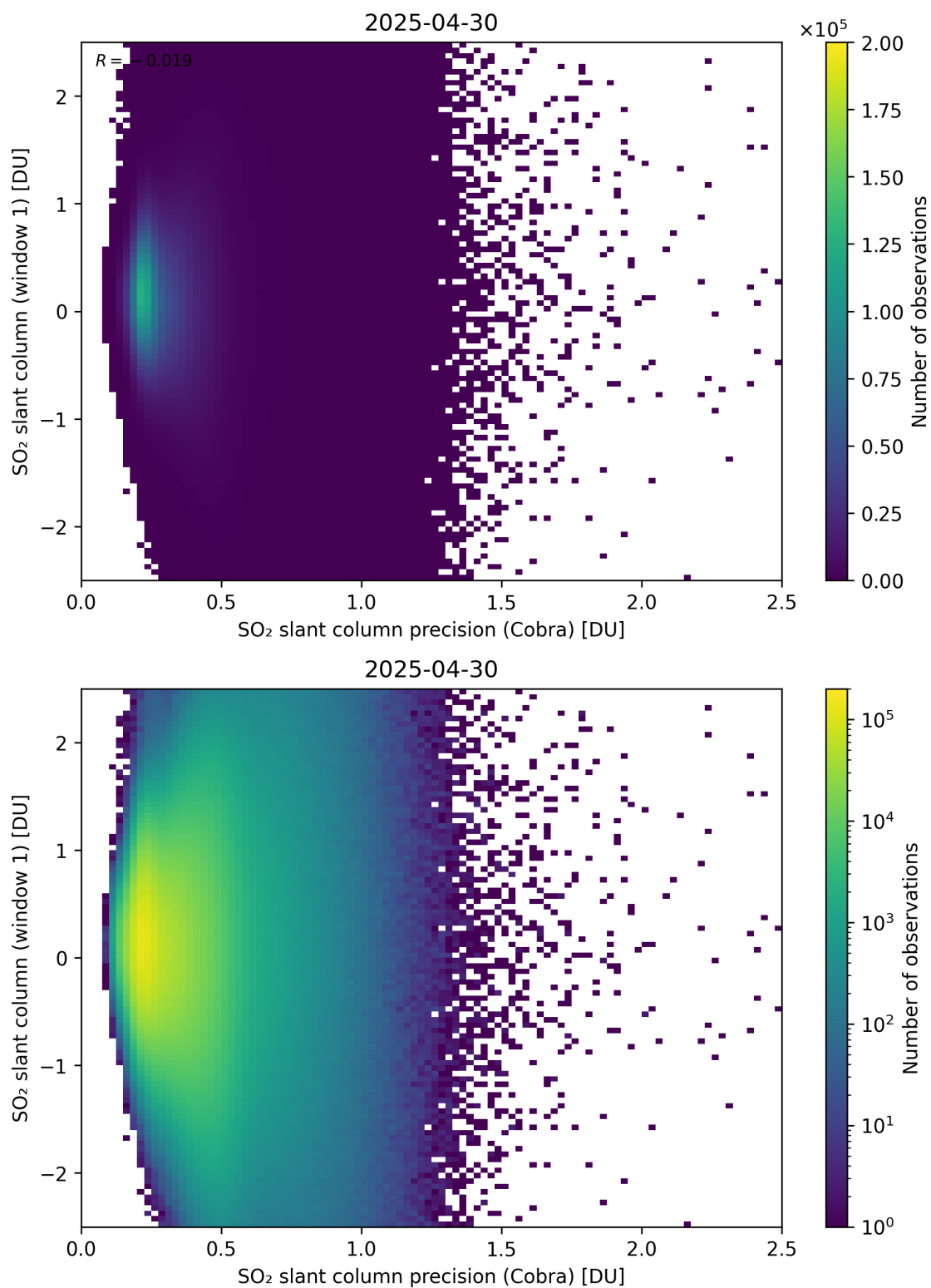
Figure 208: Scatter density plot of “SO 2 slant column precision (Cobra)” against “SO 2 slant column (window 1)” for 2025-04-29 to 2025-05-01.
