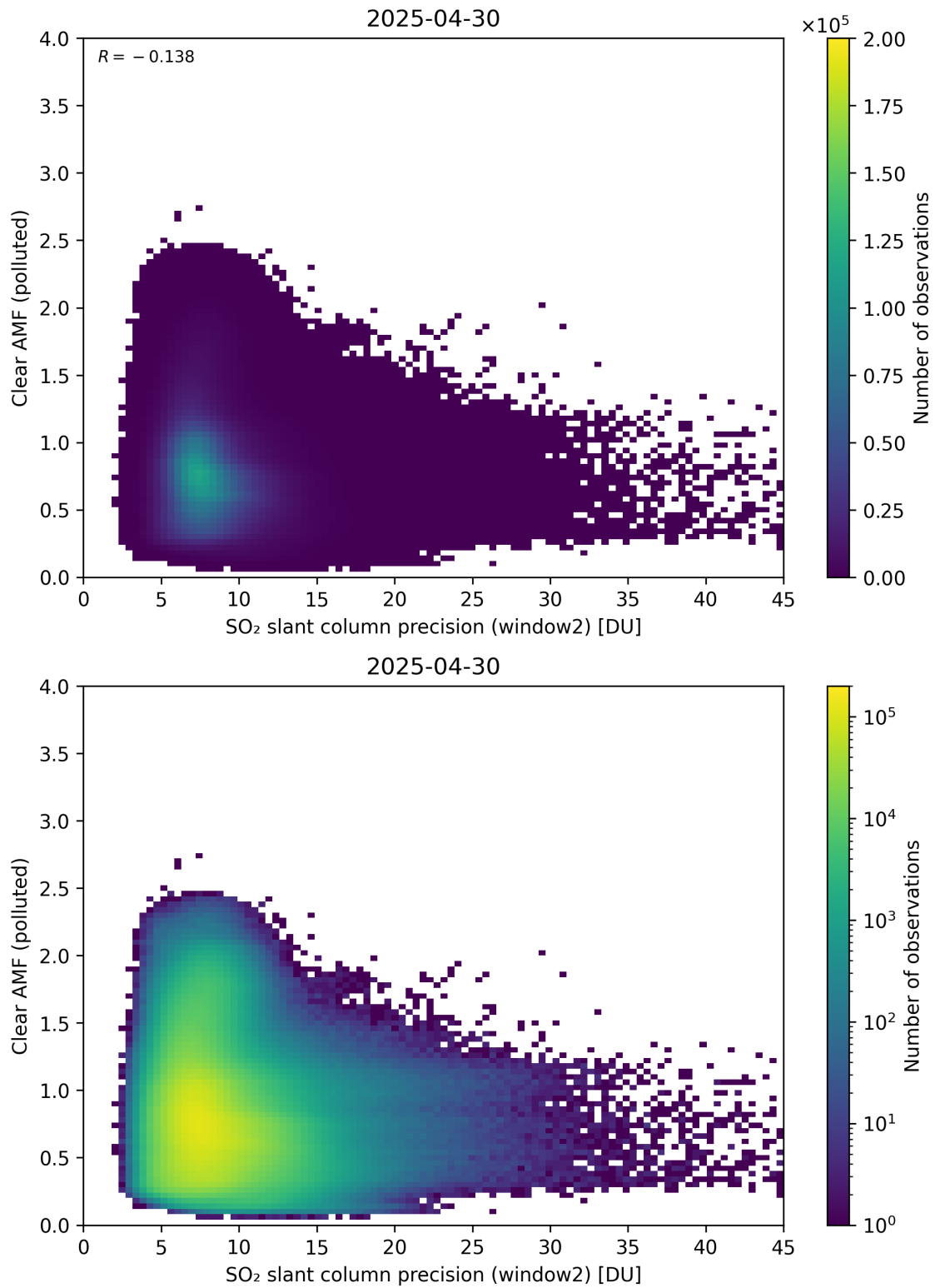
Figure 296: Scatter density plot of “SO 2 slant column precision (window2)” against “Clear AMF (polluted)” for 2025-04-29 to 2025-05-01.
