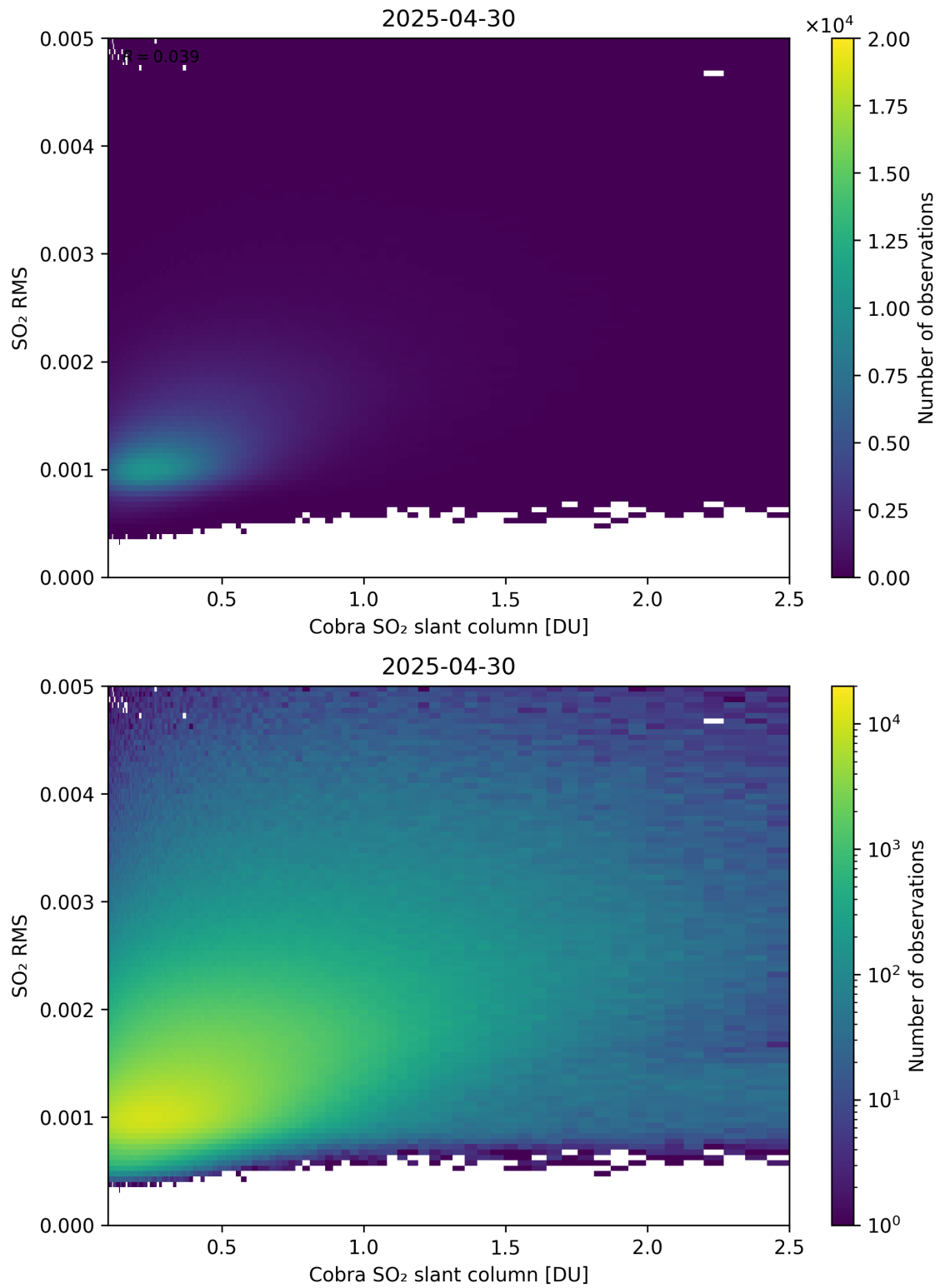
Figure 198: Scatter density plot of “Cobra SO 2 slant column” against “SO 2 RMS” for 2025-04-29 to 2025-05-01.
