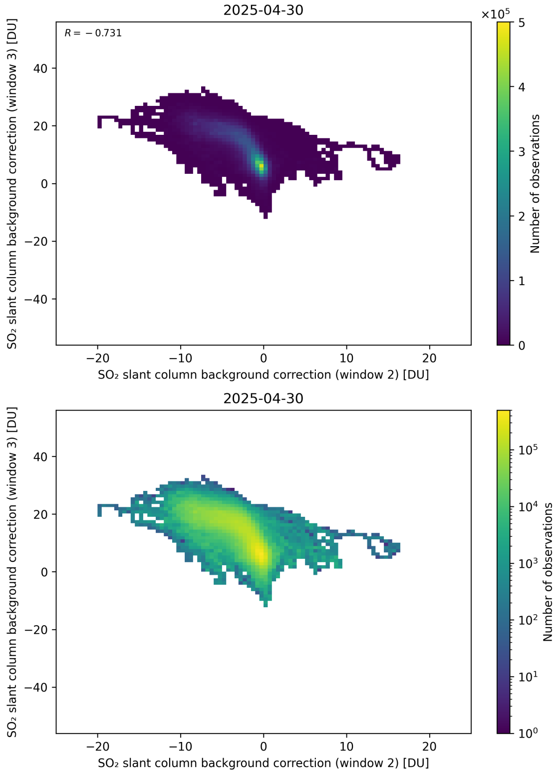
Figure 122: Scatter density plot of “SO 2 slant column background correction (window 2)” against “SO 2 slant column background correction (window 3)” for 2025-04-29 to 2025-05-01.
