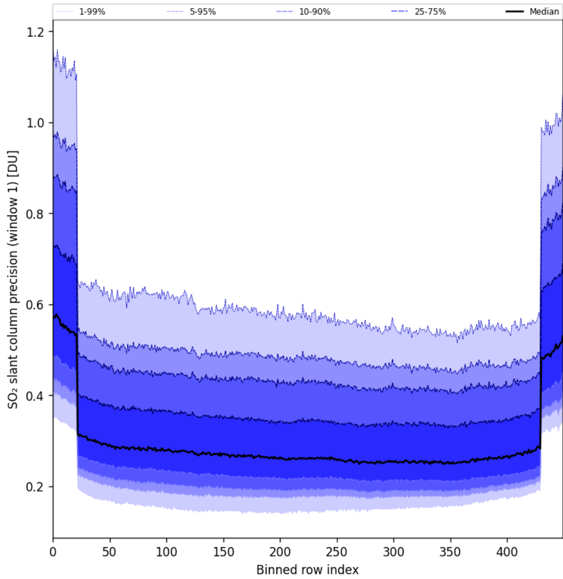
Figure 90: Along track statistics of “SO 2 slant column precision (window 1)” for 2025-04-29 to 2025-05-01
