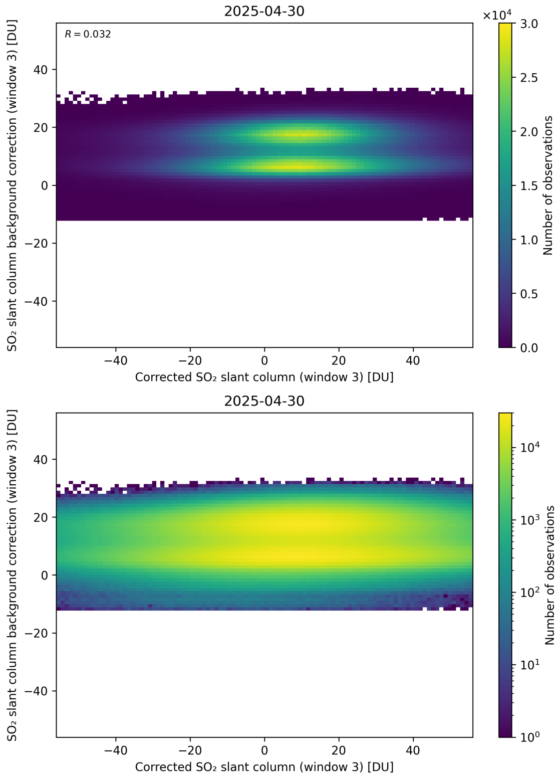
Figure 255: Scatter density plot of “Corrected SO 2 slant column (window 3)” against “SO 2 slant column background correction (window 3)” for 2025-04-29 to 2025-05-01.
