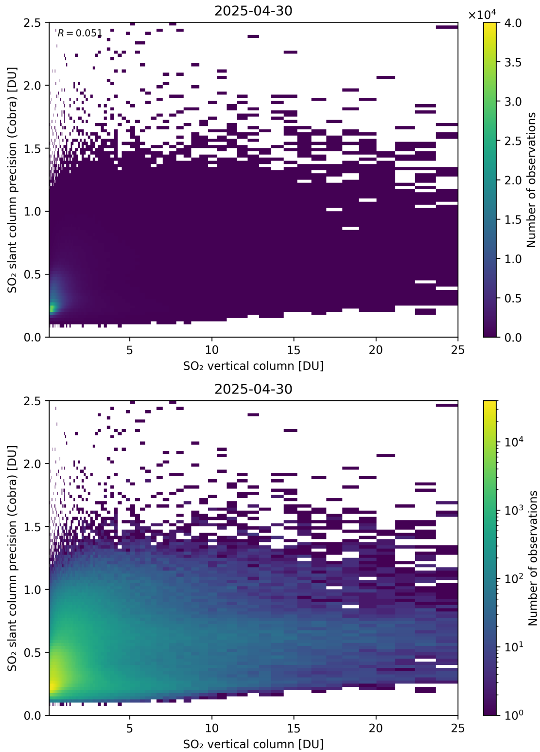
Figure 350: Scatter density plot of “SO 2 vertical column” against “SO 2 slant column precision (Cobra)” for 2025-04-29 to 2025-05-01.
