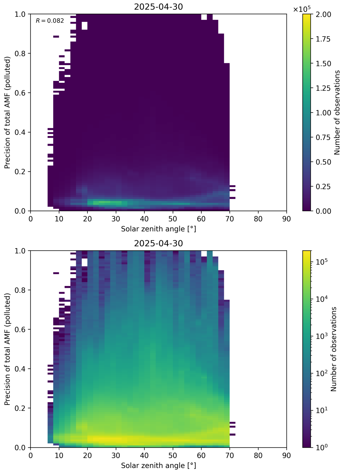
Figure 190: Scatter density plot of “Solar zenith angle” against “Precision of total AMF (polluted)” for 2025-04-29 to 2025-05-01.
