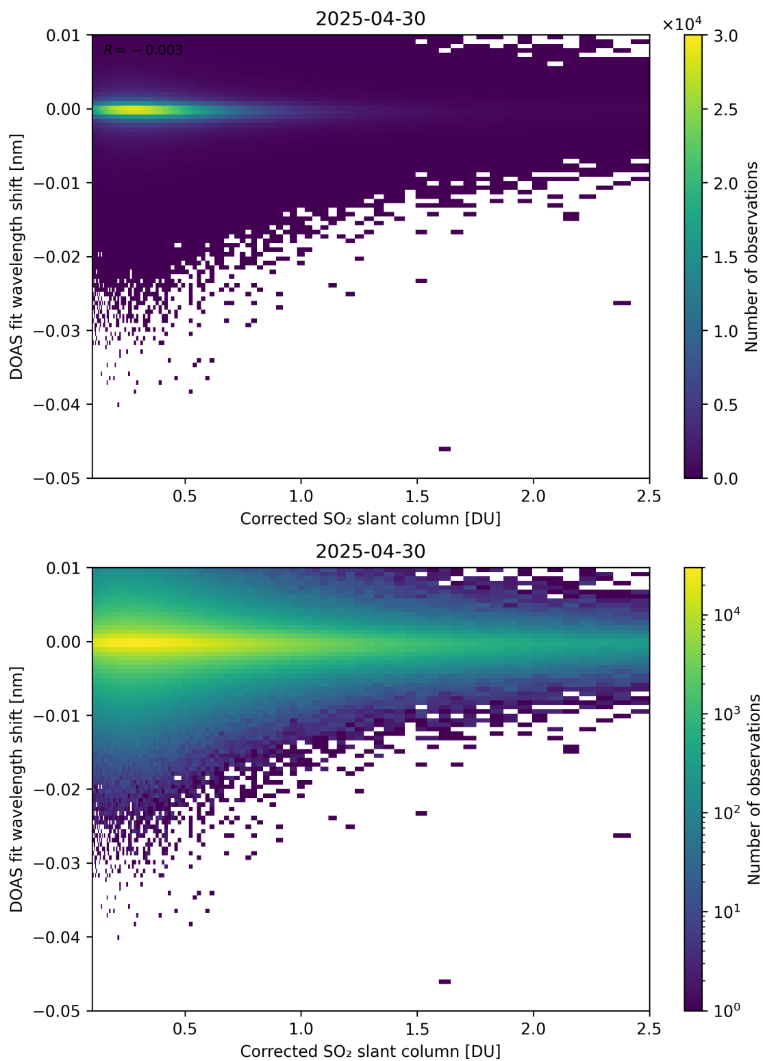
Figure 229: Scatter density plot of “Corrected SO 2 slant column” against “DOAS fit wavelength shift” for 2025-04-29 to 2025-05-01.
