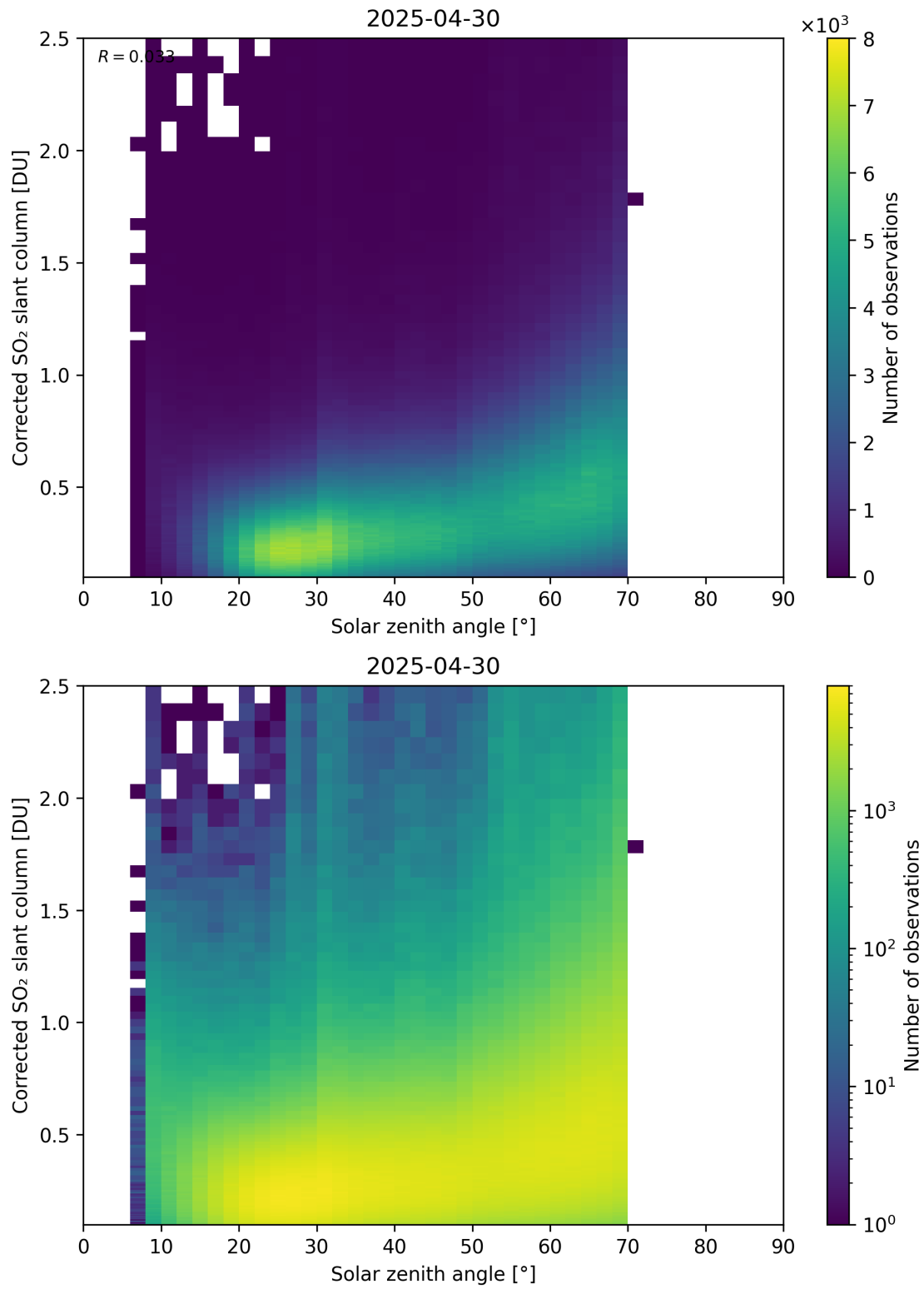
Figure 181: Scatter density plot of “Solar zenith angle” against “Corrected SO 2 slant column” for 2025-04-29 to 2025-05-01.
