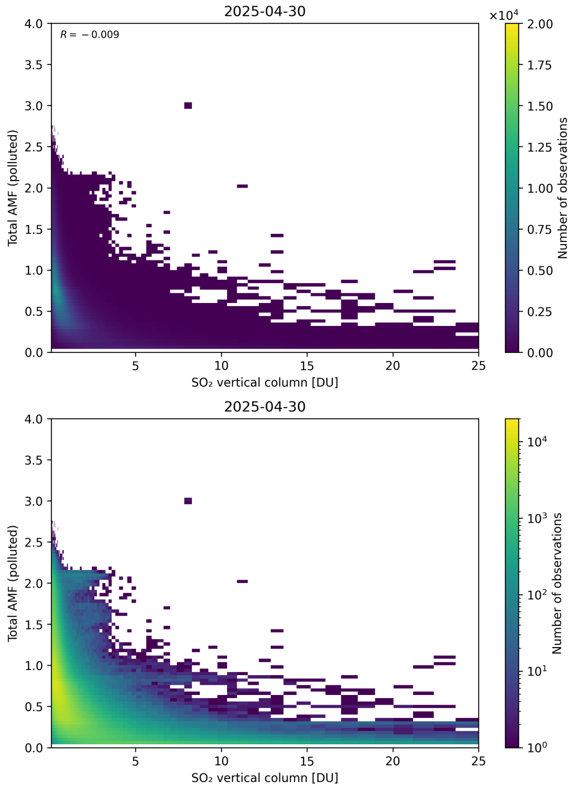
Figure 359: Scatter density plot of “SO 2 vertical column” against “Total AMF (polluted)” for 2025-04-29 to 2025-05-01.
