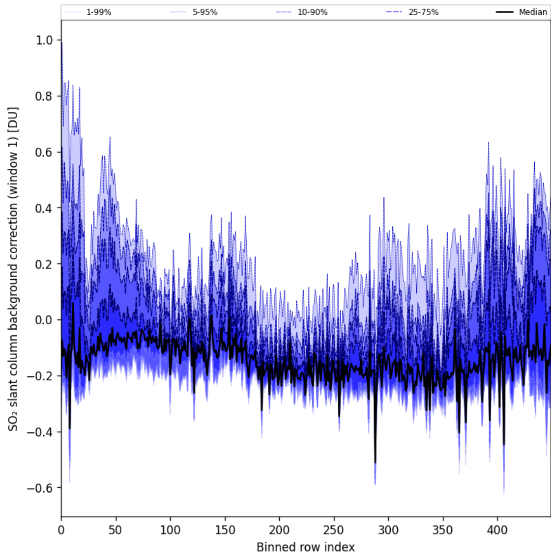
Figure 92: Along track statistics of “SO 2 slant column background correction (window 1)” for 2025-04-29 to 2025-05-01
