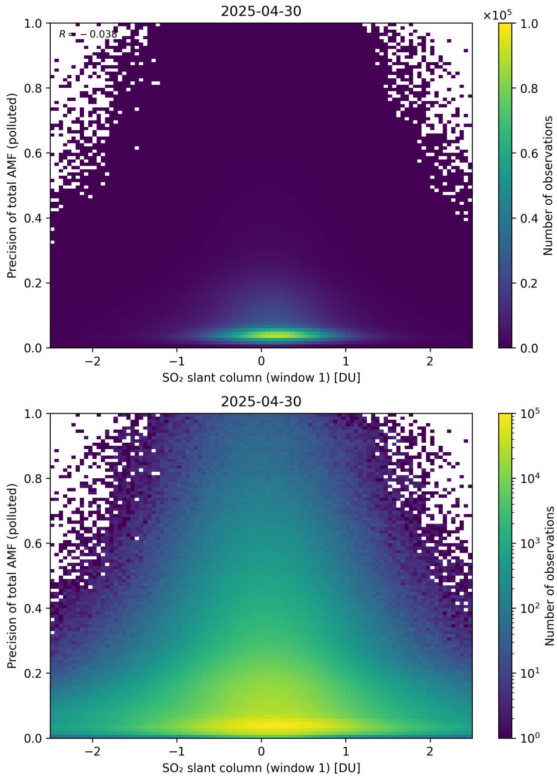
Figure 290: Scatter density plot of “SO 2 slant column (window 1)” against “Precision of total AMF (polluted)” for 2025-04-29 to 2025-05-01.
