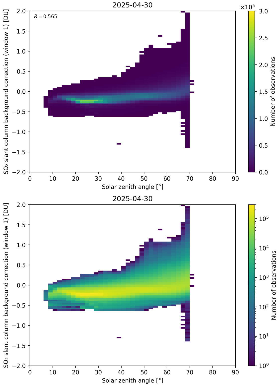
Figure 171: Scatter density plot of “Solar zenith angle” against “SO 2 slant column background correction (window 1)” for 2025-04-29 to 2025-05-01.
