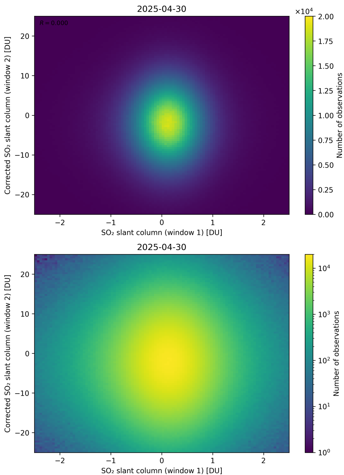
Figure 283: Scatter density plot of “SO 2 slant column (window 1)” against “Corrected SO 2 slant column (window 2)” for 2025-04-29 to 2025-05-01.
