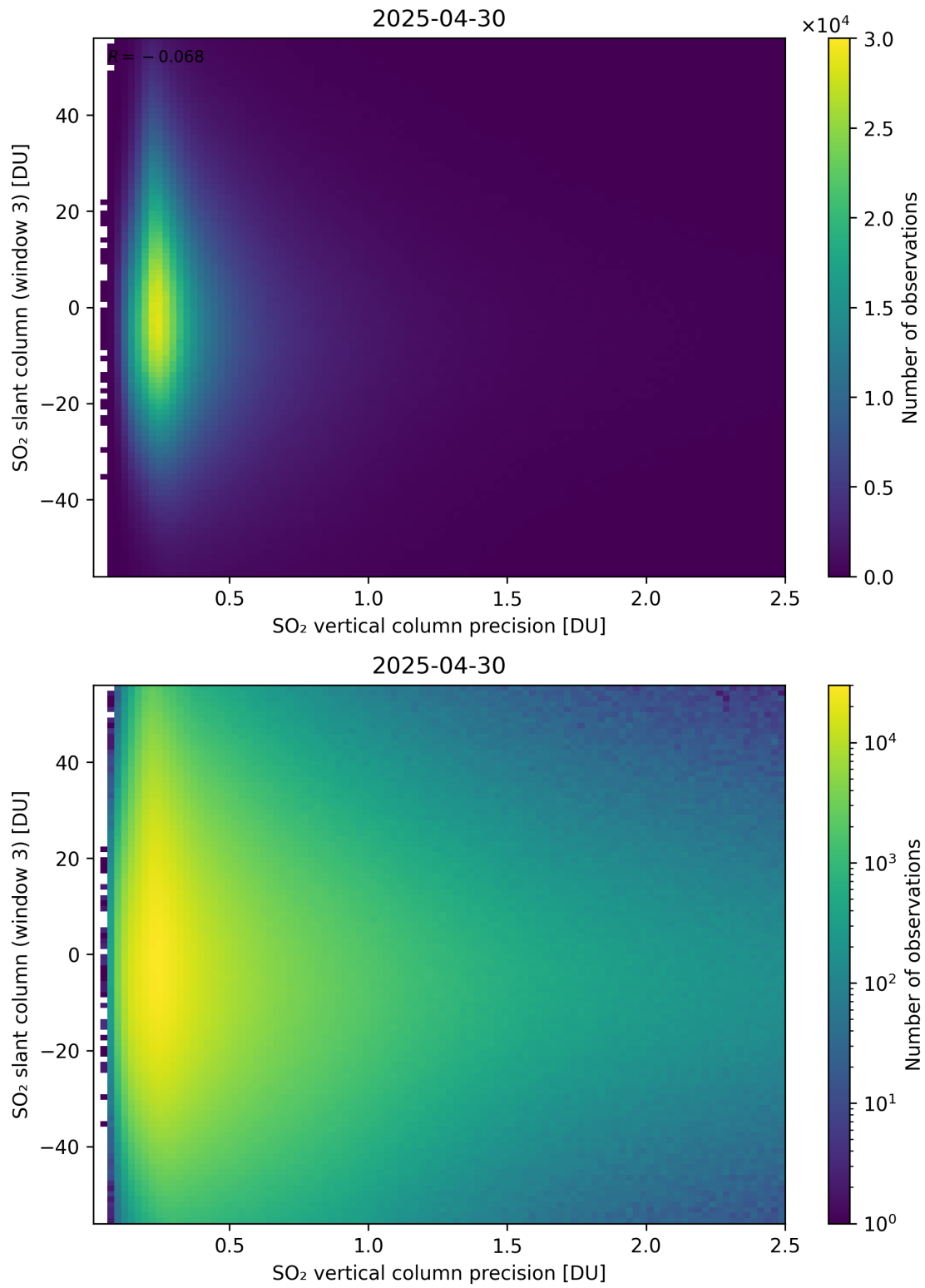
Figure 344: Scatter density plot of “SO 2 vertical column precision” against “SO 2 slant column (window 3)” for 2025-04-29 to 2025-05-01.
