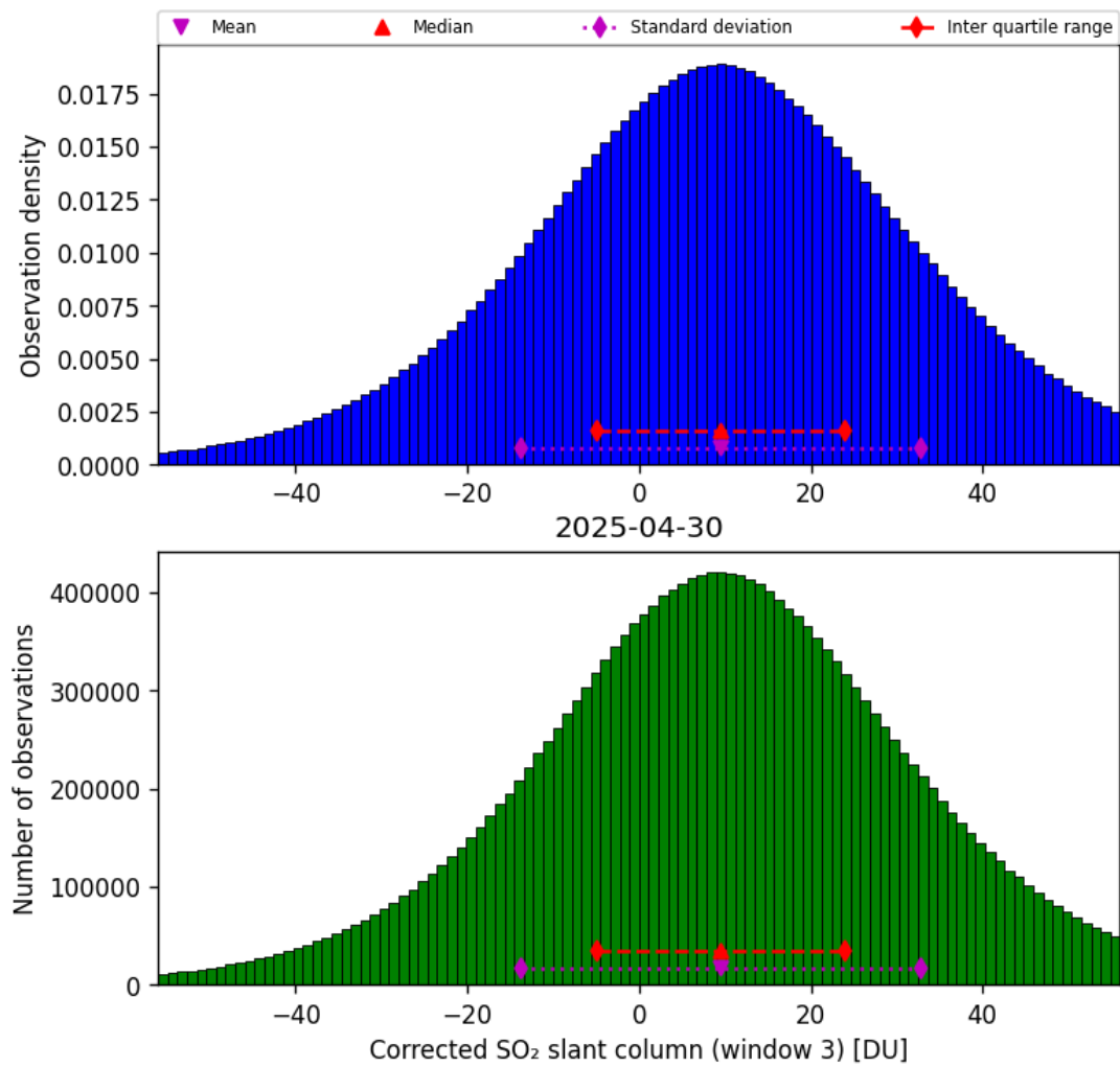
Figure 73: Histogram of “Corrected SO 2 slant column (window 3)” for 2025-04-29 to 2025-05-01
