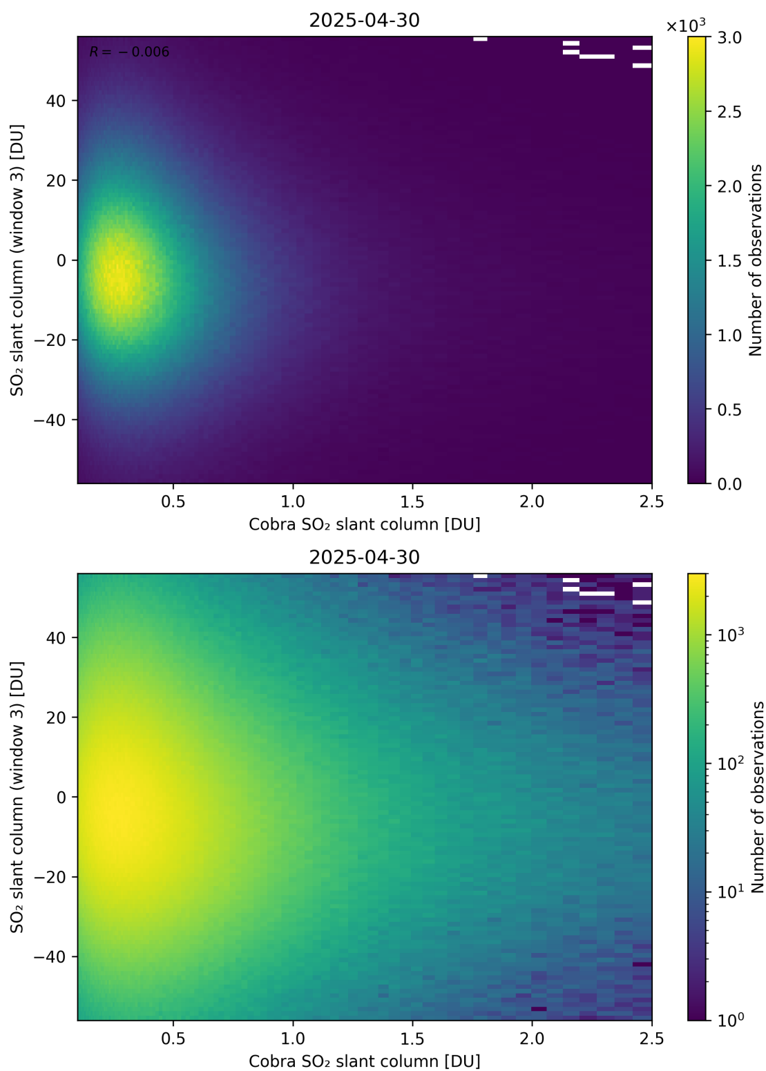
Figure 222: Scatter density plot of “Cobra SO 2 slant column” against “SO 2 slant column (window 3)” for 2025-04-29 to 2025-05-01.
