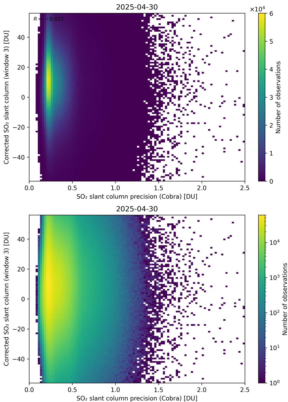
Figure 207: Scatter density plot of “SO 2 slant column precision (Cobra)” against “Corrected SO 2 slant column (window 3)” for 2025-04-29 to 2025-05-01.
