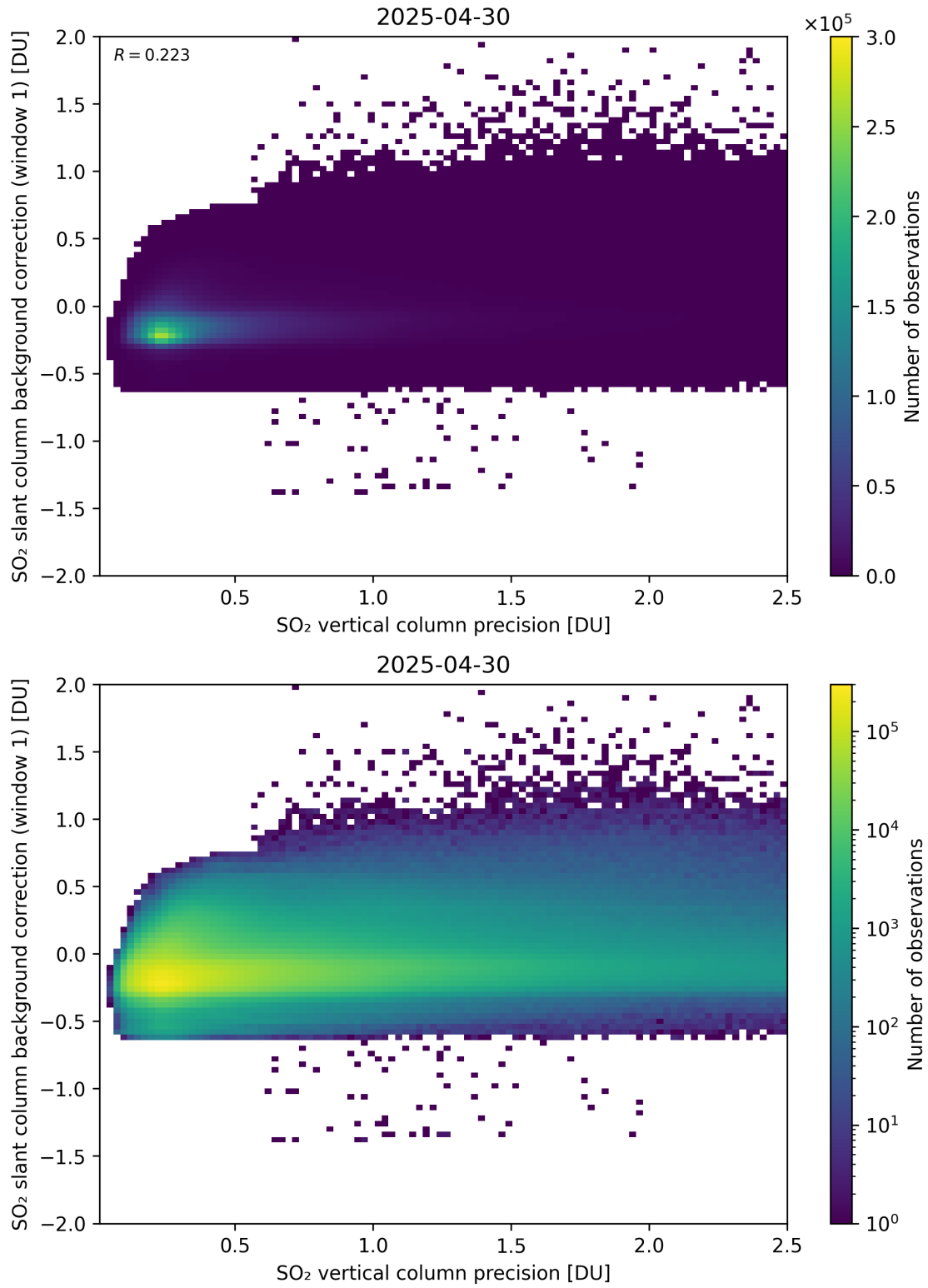
Figure 329: Scatter density plot of “SO 2 vertical column precision” against “SO 2 slant column background correction (window 1)” for 2025-04-29 to 2025-05-01.
