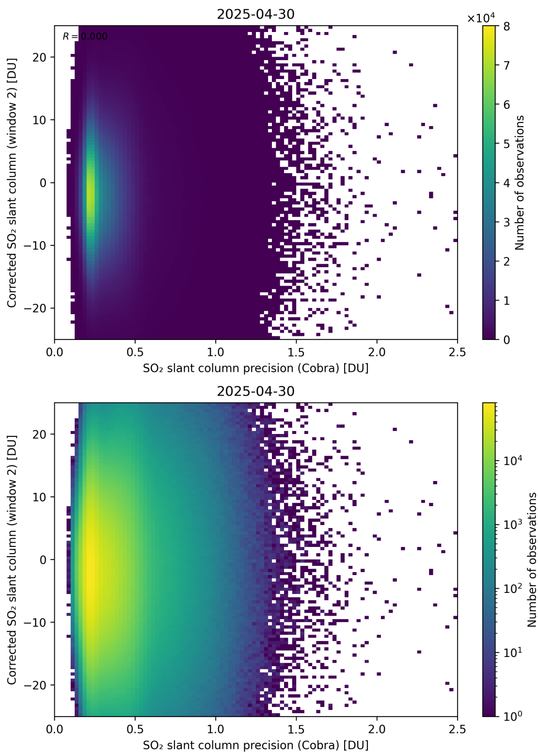
Figure 206: Scatter density plot of “SO 2 slant column precision (Cobra)” against “Corrected SO 2 slant column (window 2)” for 2025-04-29 to 2025-05-01.
