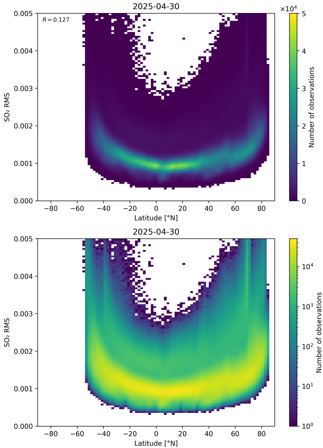
Figure 155: Scatter density plot of “Latitude” against “SO 2 RMS” for 2025-04-29 to 2025-05-01.
