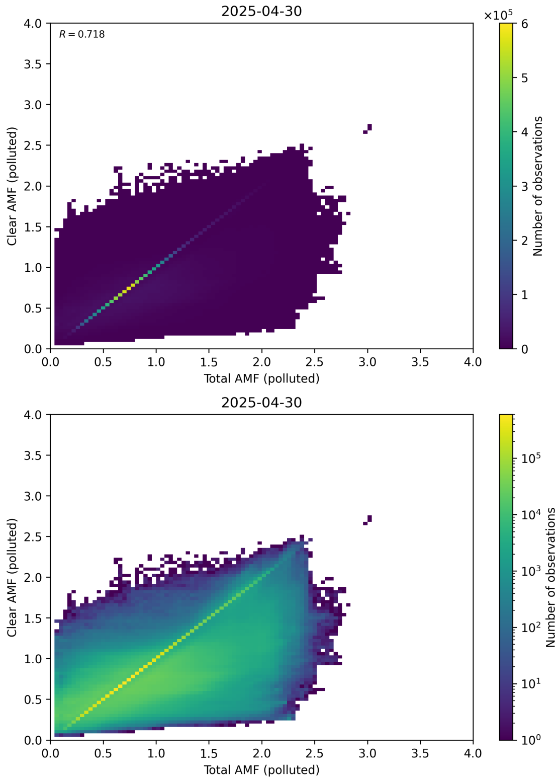
Figure 321: Scatter density plot of “Total AMF (polluted)” against “Clear AMF (polluted)” for 2025-04-29 to 2025-05-01.
