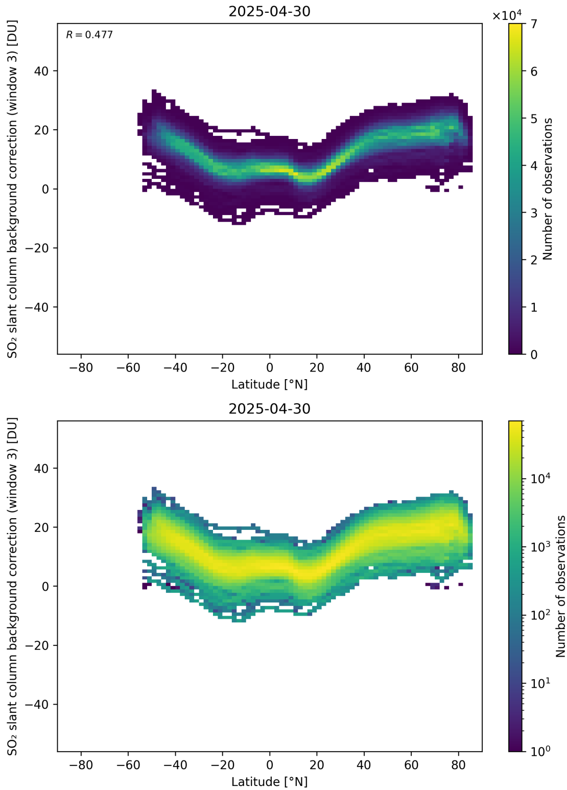
Figure 152: Scatter density plot of “Latitude” against “SO 2 slant column background correction (window 3)” for 2025-04-29 to 2025-05-01.
