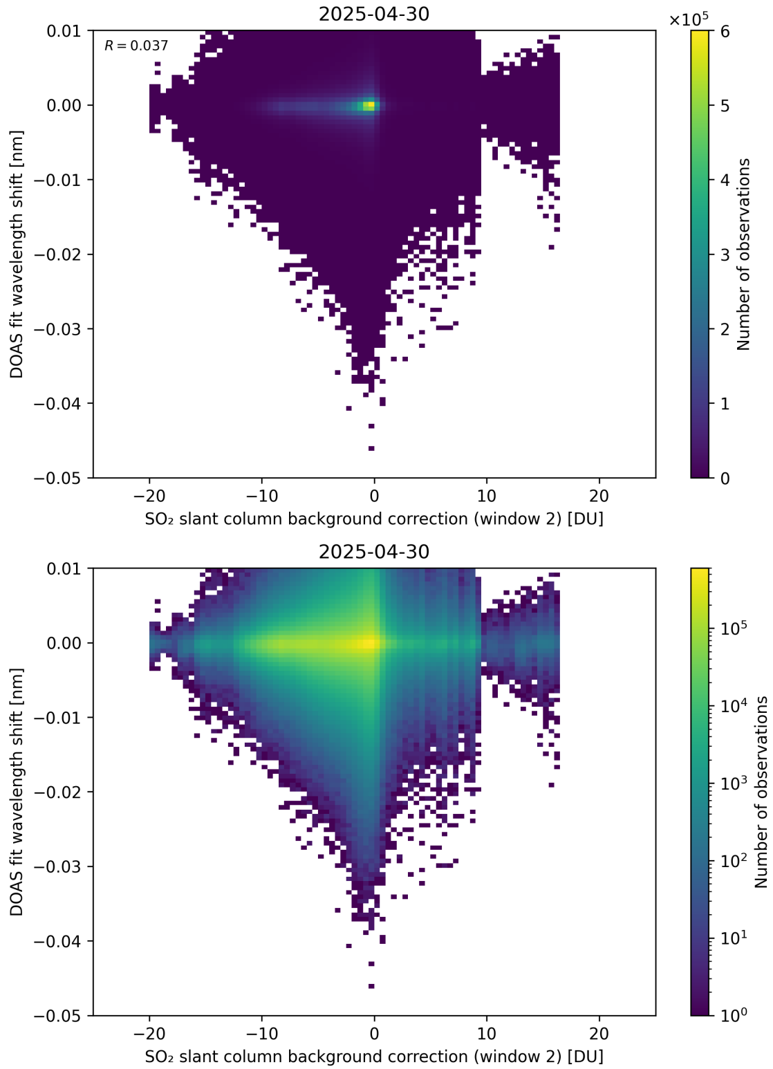
Figure 123: Scatter density plot of “SO 2 slant column background correction (window 2)” against “DOAS fit wavelength shift” for 2025-04-29 to 2025-05-01.
