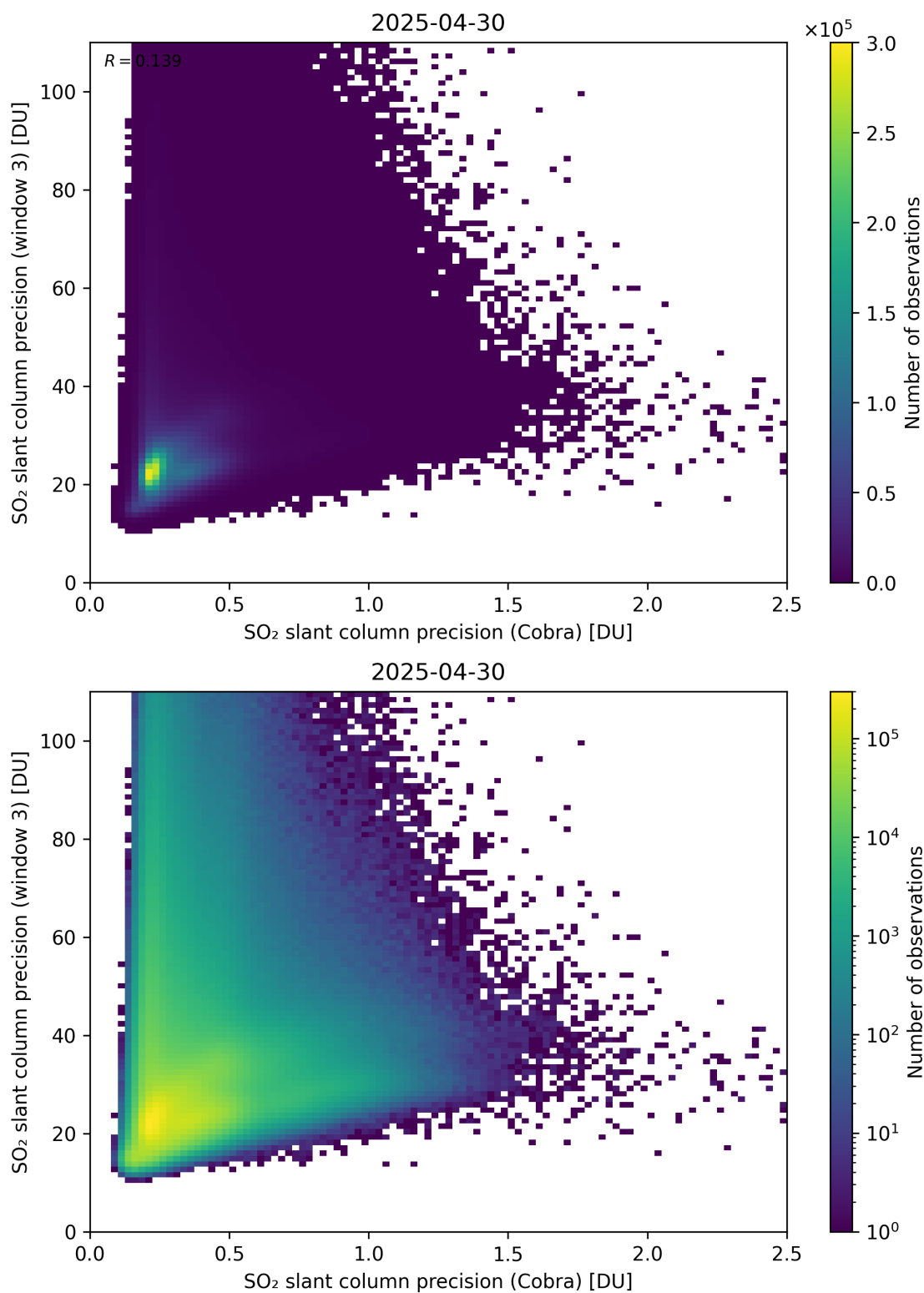
Figure 212: Scatter density plot of “SO 2 slant column precision (Cobra)” against “SO 2 slant column precision (window 3)” for 2025-04-29 to 2025-05-01.
