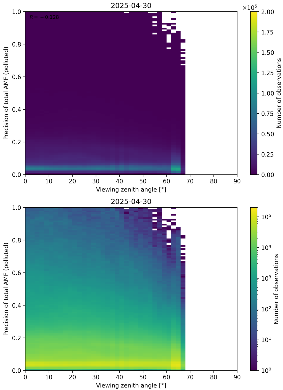
Figure 382: Scatter density plot of “Viewing zenith angle” against “Precision of total AMF (polluted)” for 2025-04-29 to 2025-05-01.
