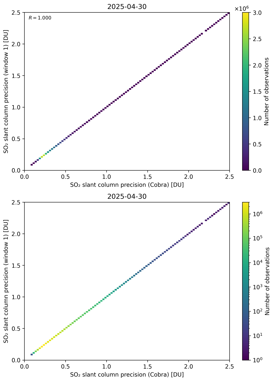
Figure 209: Scatter density plot of “SO 2 slant column precision (Cobra)” against “SO 2 slant column precision (window 1)” for 2025-04-29 to 2025-05-01.
