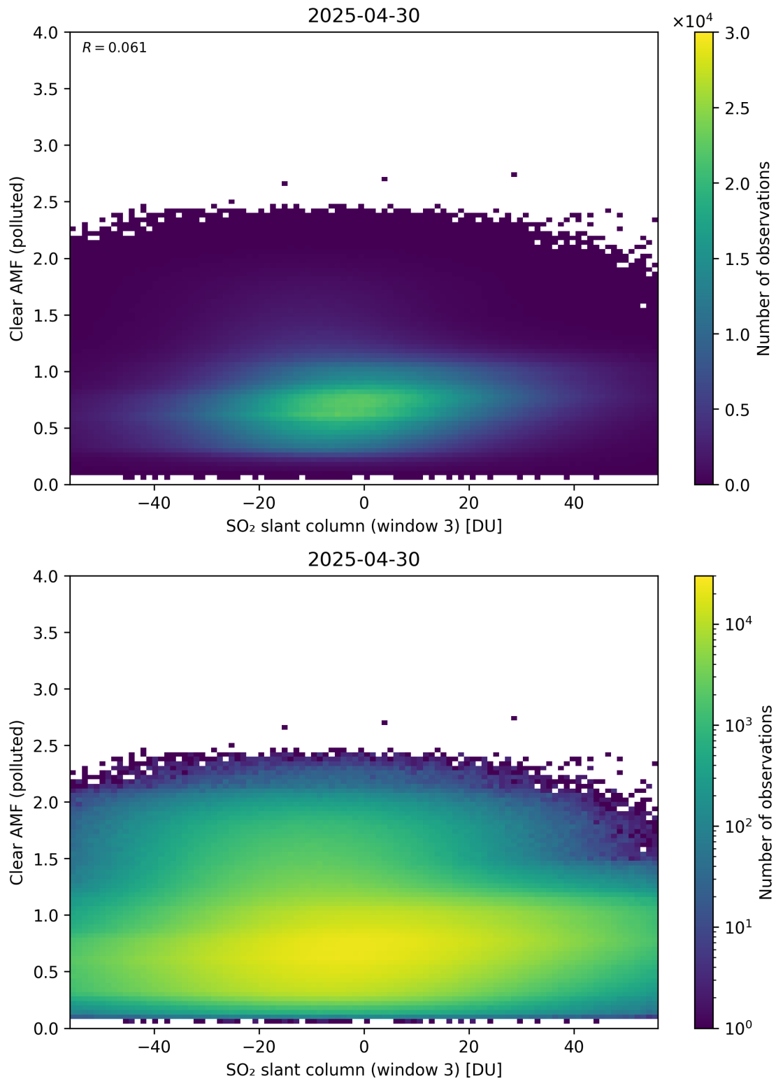
Figure 315: Scatter density plot of “SO 2 slant column (window 3)” against “Clear AMF (polluted)” for 2025-04-29 to 2025-05-01.
