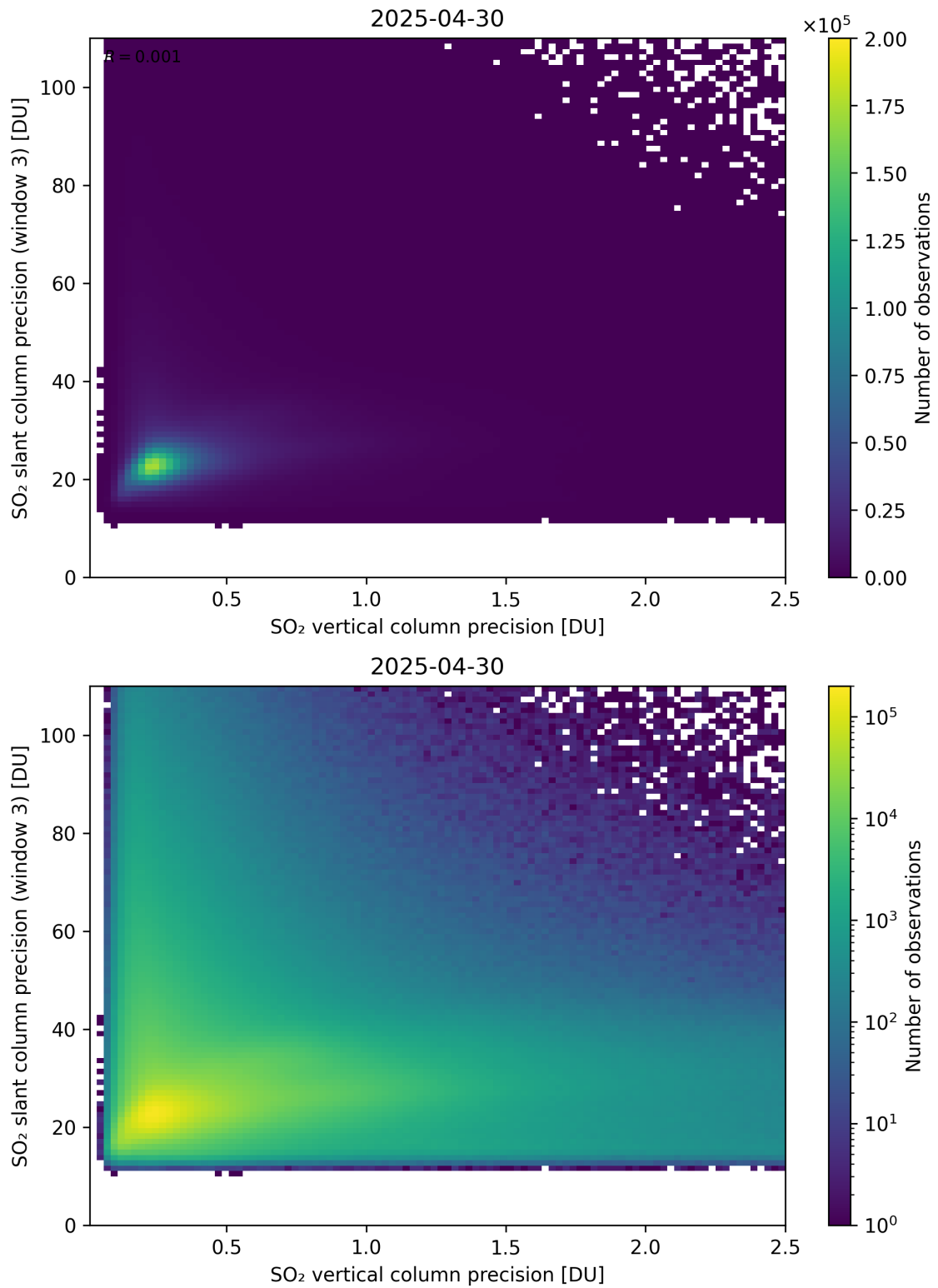
Figure 345: Scatter density plot of “SO 2 vertical column precision” against “SO 2 slant column precision (window 3)” for 2025-04-29 to 2025-05-01.
