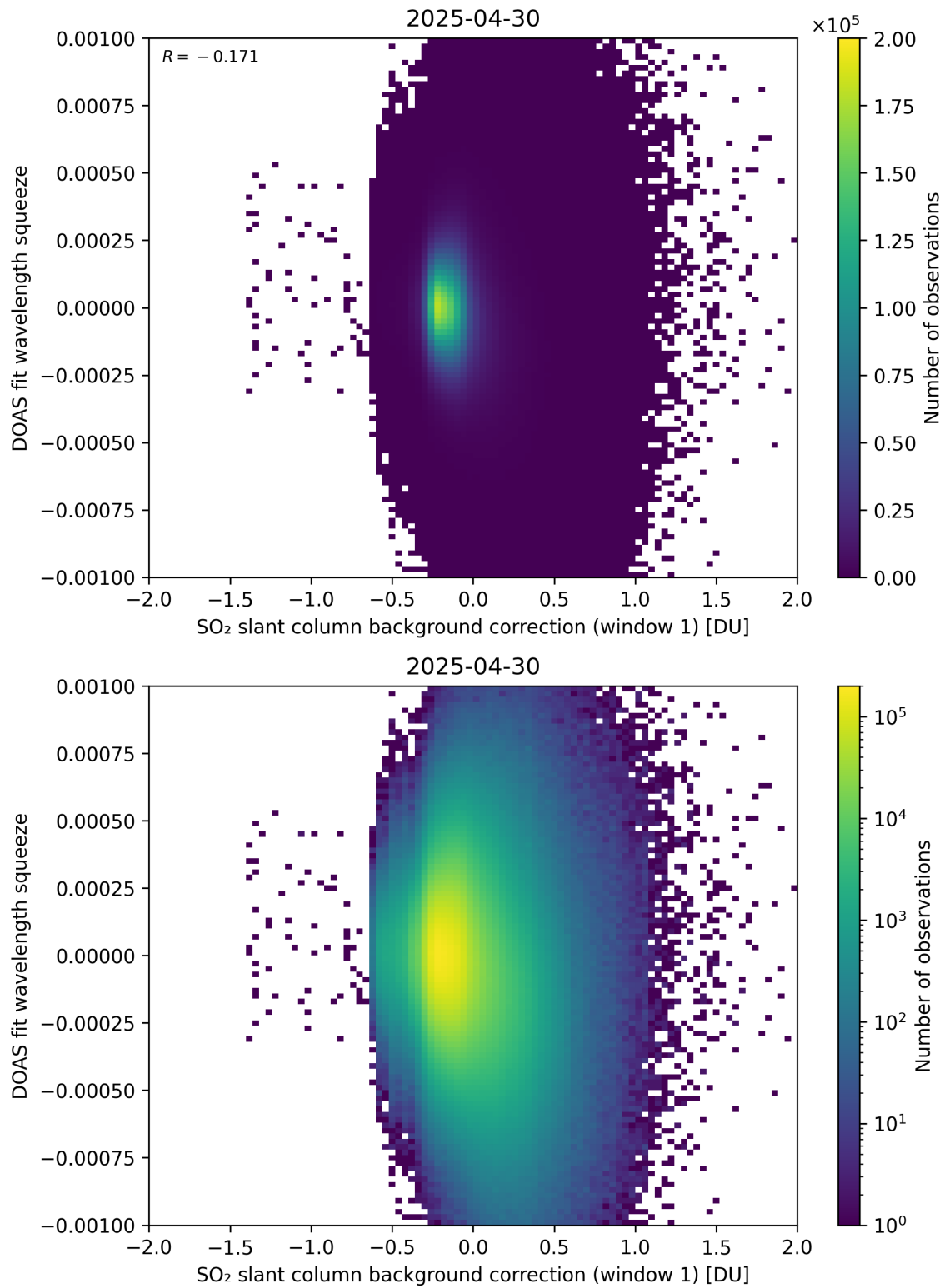
Figure 112: Scatter density plot of “SO 2 slant column background correction (window 1)” against “DOAS fit wavelength squeeze” for 2025-04-29 to 2025-05-01.
