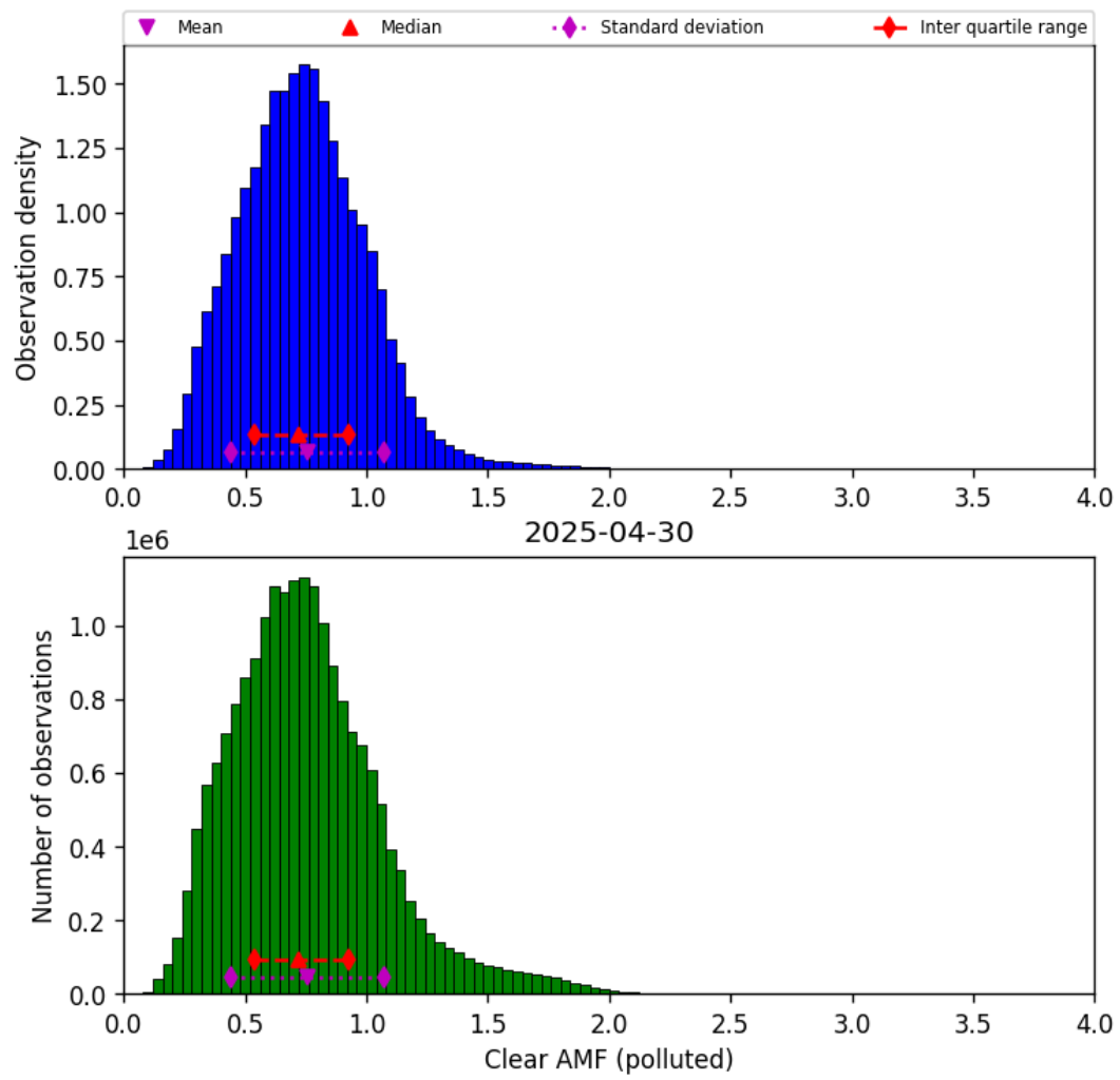
Figure 81: Histogram of “Clear AMF (polluted)” for 2025-04-29 to 2025-05-01
