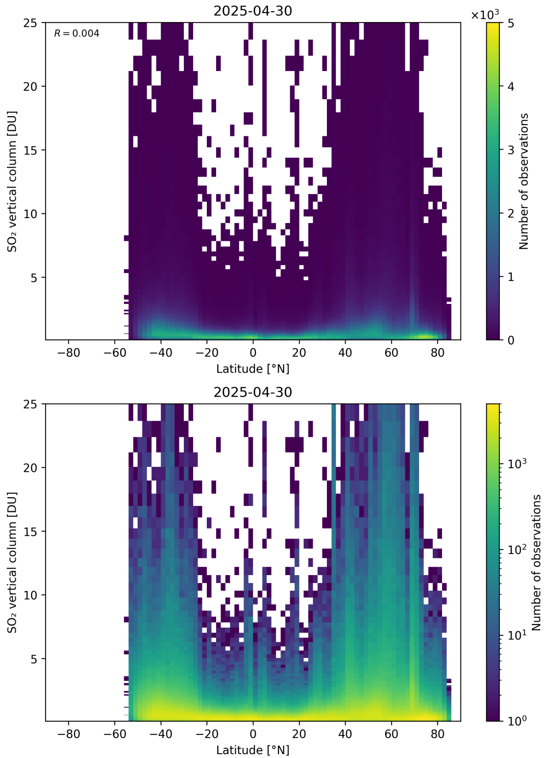
Figure 169: Scatter density plot of “Latitude” against “SO 2 vertical column” for 2025-04-29 to 2025-05-01.
