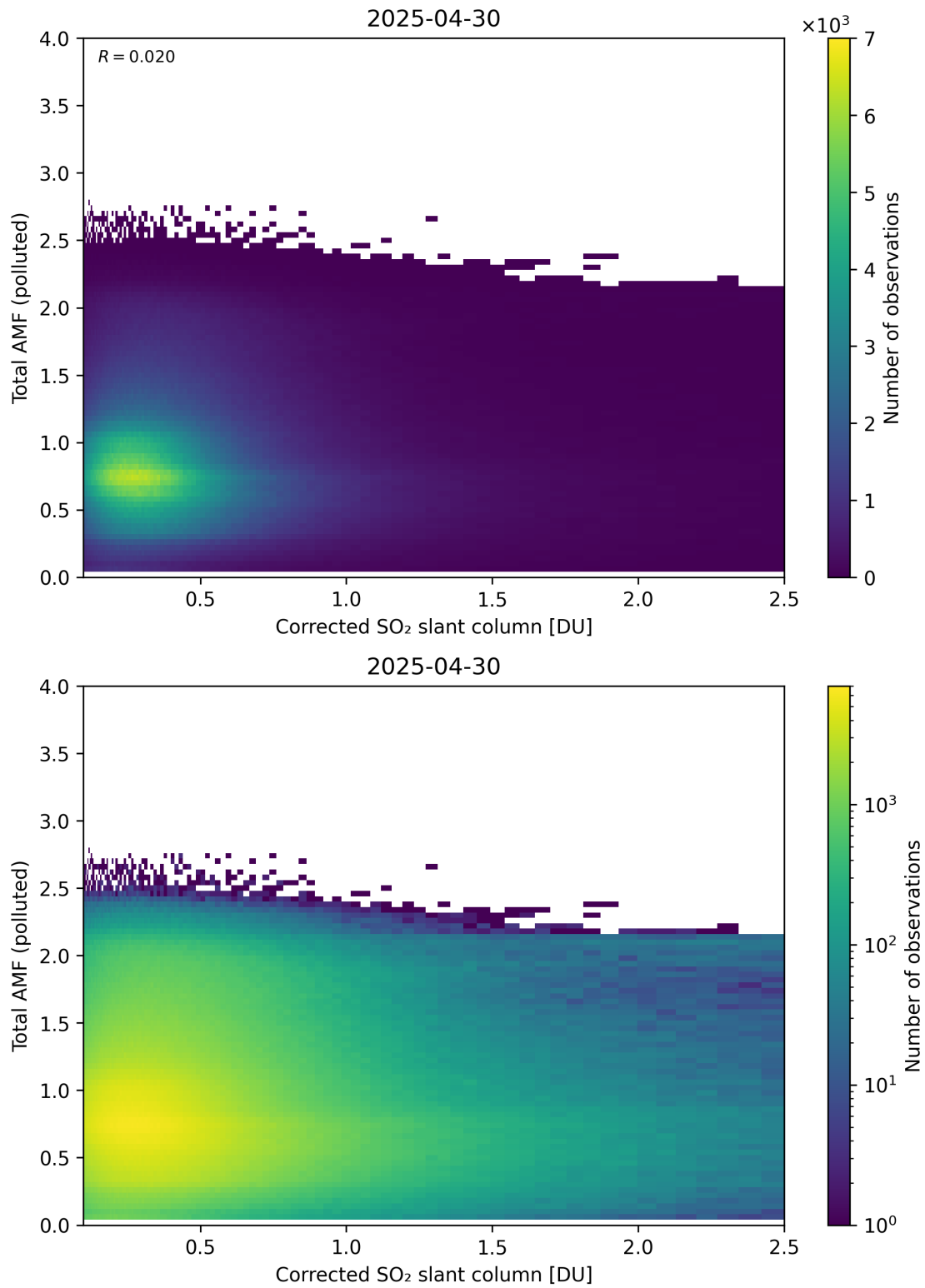
Figure 242: Scatter density plot of “Corrected SO 2 slant column” against “Total AMF (polluted)” for 2025-04-29 to 2025-05-01.
