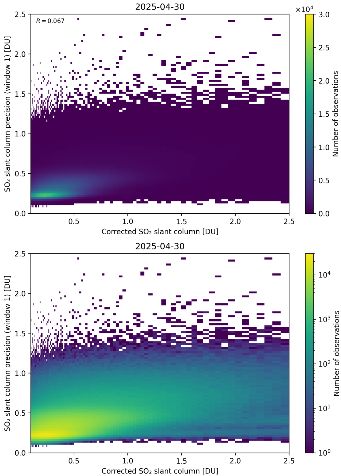
Figure 238: Scatter density plot of “Corrected SO 2 slant column” against “SO 2 slant column precision (window 1)” for 2025-04-29 to 2025-05-01.
