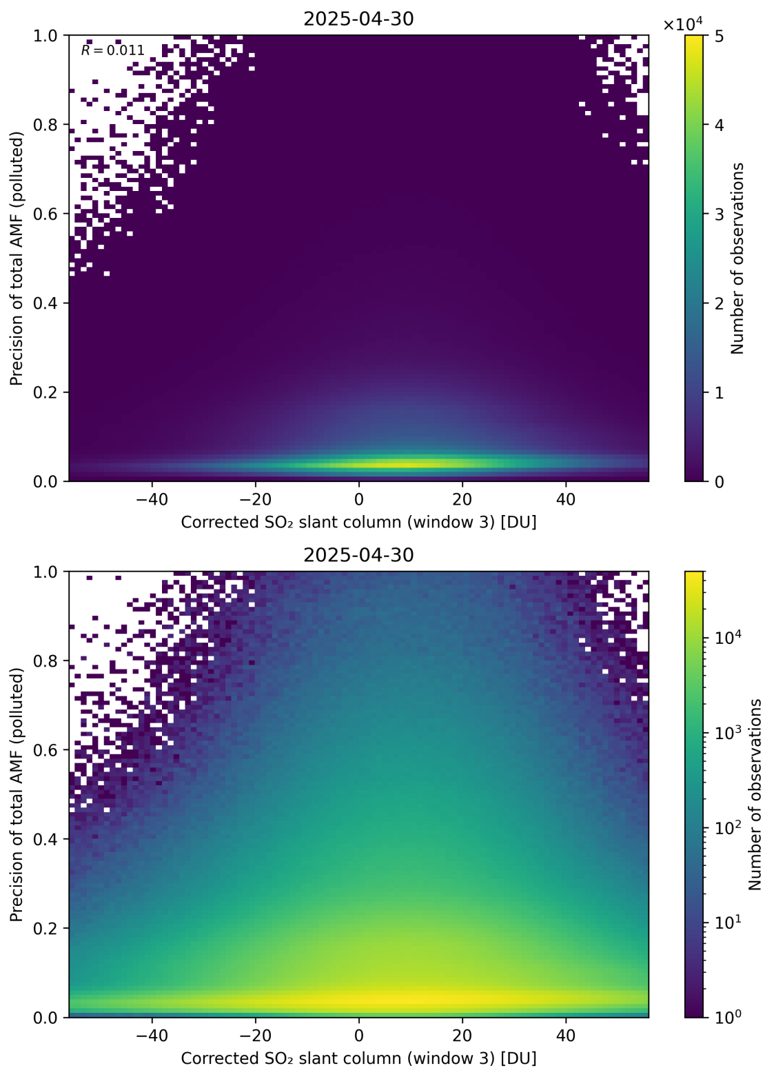
Figure 261: Scatter density plot of “Corrected SO 2 slant column (window 3)” against “Precision of total AMF (polluted)” for 2025-04-29 to 2025-05-01.
