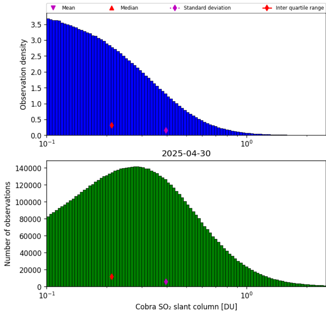
Figure 61: Histogram of “Cobra SO 2 slant column” for 2025-04-29 to 2025-05-01
