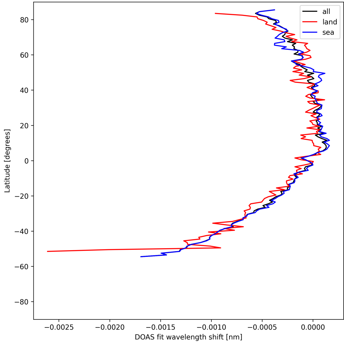
Figure 50: Zonal average of “DOAS fit wavelength shift” for 2025-04-29 to 2025-05-01.
