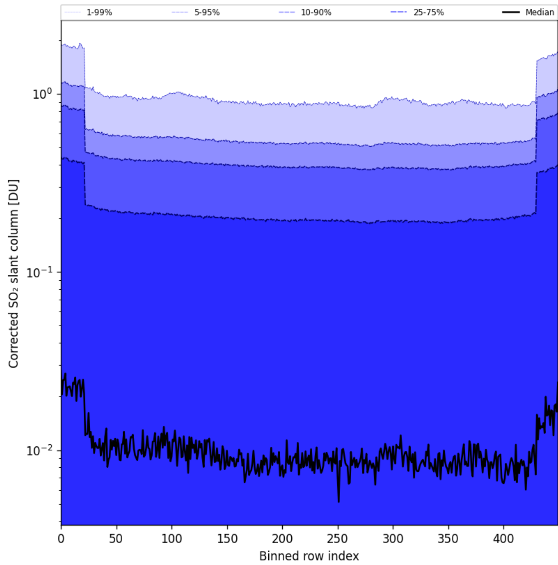
Figure 86: Along track statistics of "Corrected SO 2 slant column" for 2025-04-29 to 2025-05-01
