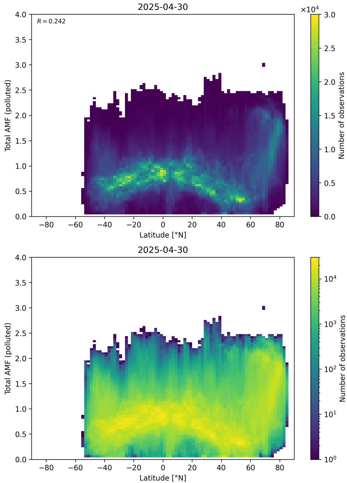
Figure 167: Scatter density plot of “Latitude” against “Total AMF (polluted)” for 2025-04-29 to 2025-05-01.
