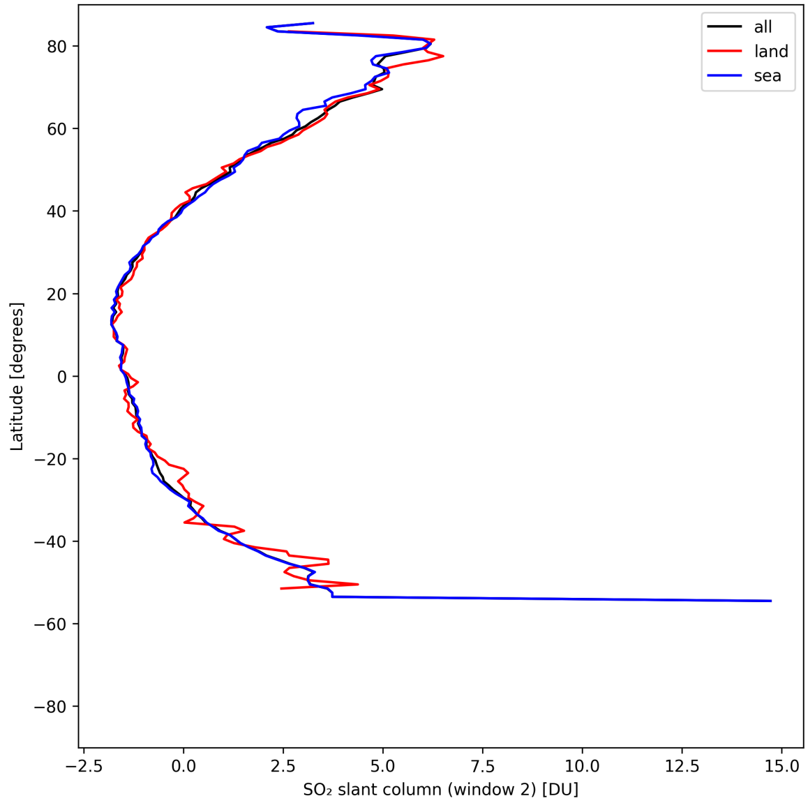
Figure 41: Zonal average of “SO 2 slant column (window 2)” for 2025-04-29 to 2025-05-01.
