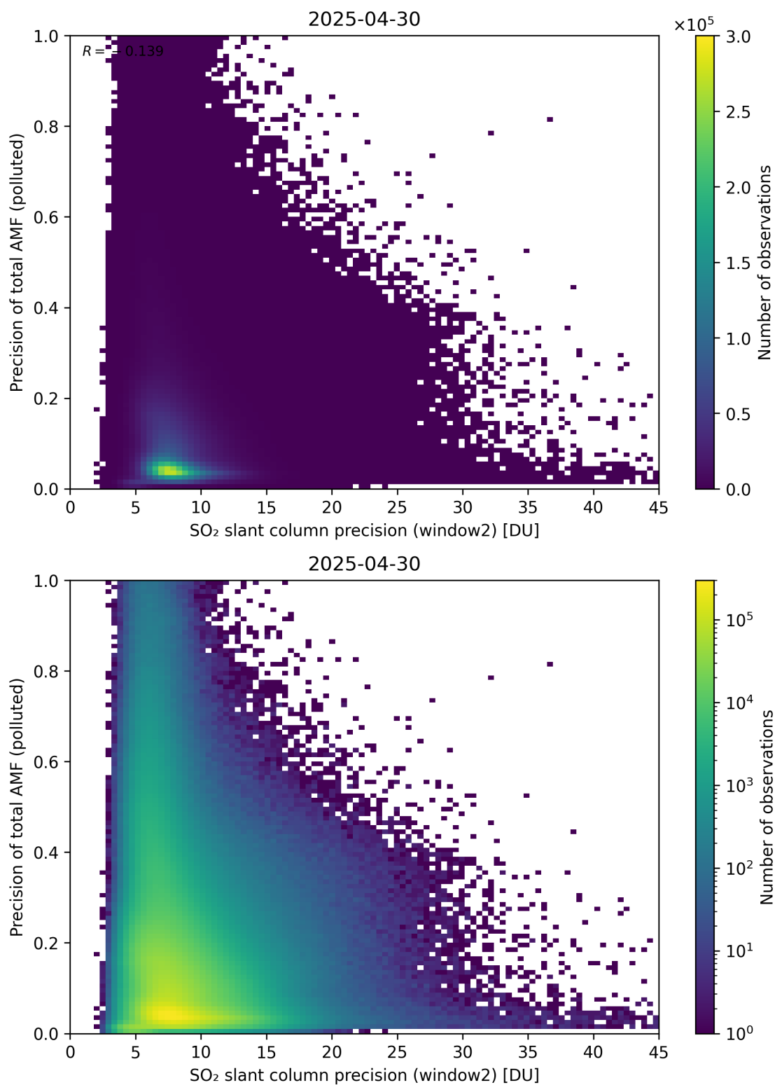
Figure 302: Scatter density plot of “SO 2 slant column precision (window2)” against “Precision of total AMF (polluted)” for 2025-04-29 to 2025-05-01.
