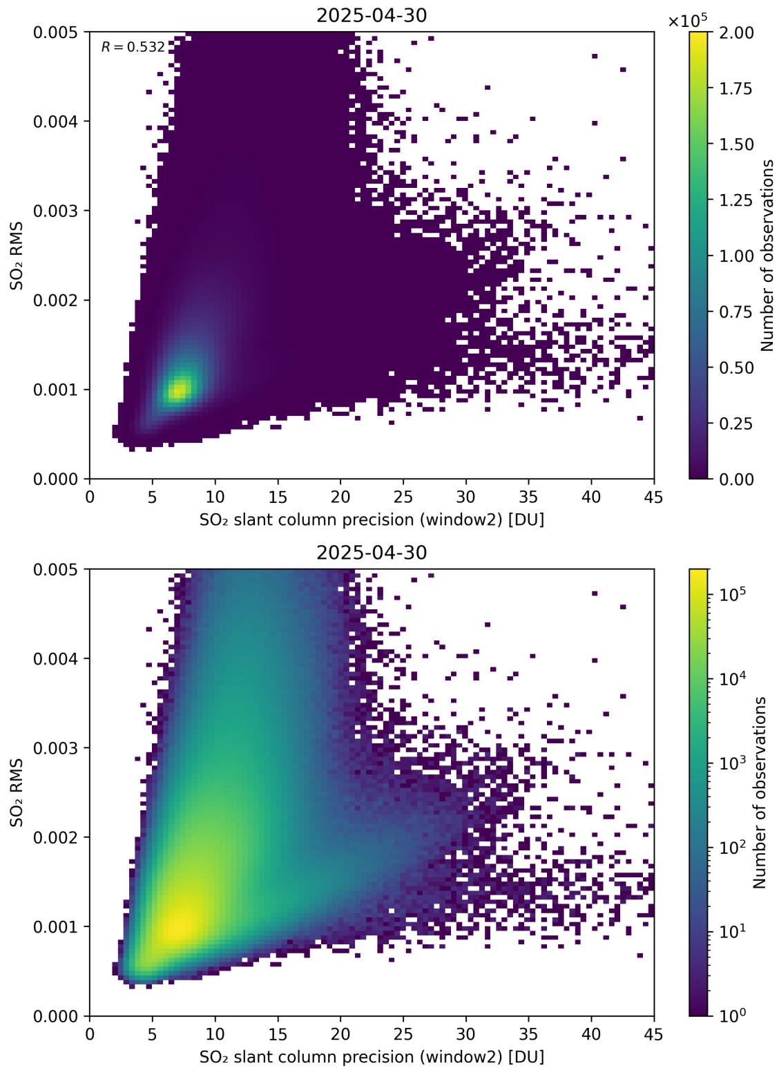
Figure 295: Scatter density plot of “SO 2 slant column precision (window2)” against “SO 2 RMS” for 2025-04-29 to 2025-05-01.
