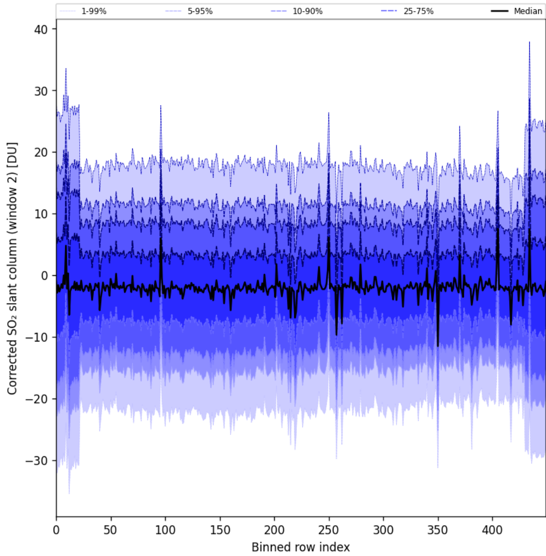
Figure 95: Along track statistics of "Corrected SO 2 slant column (window 2)" for 2025-04-29 to 2025-05-01
