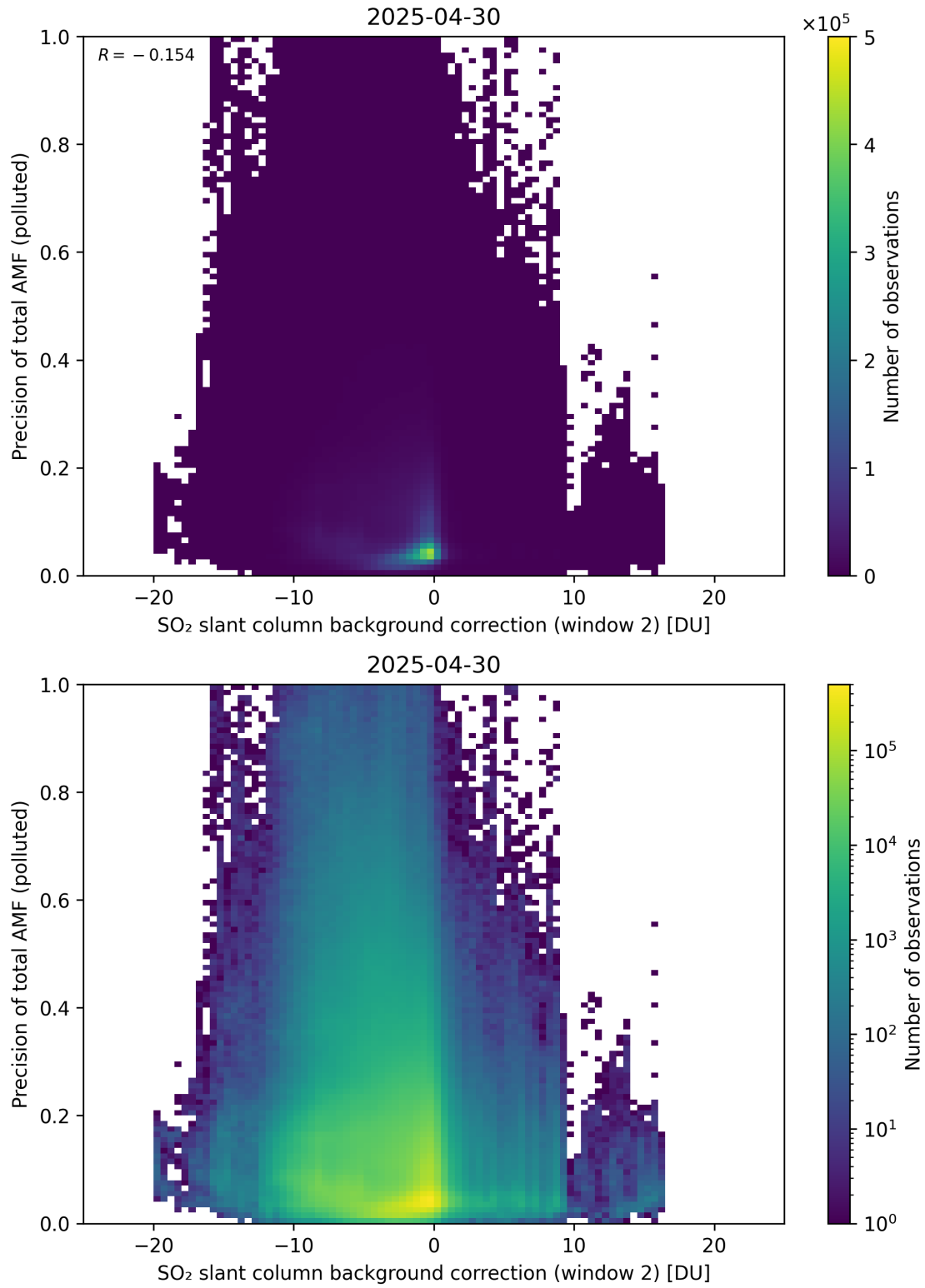
Figure 131: Scatter density plot of “SO 2 slant column background correction (window 2)” against “Precision of total AMF (polluted)” for 2025-04-29 to 2025-05-01.
