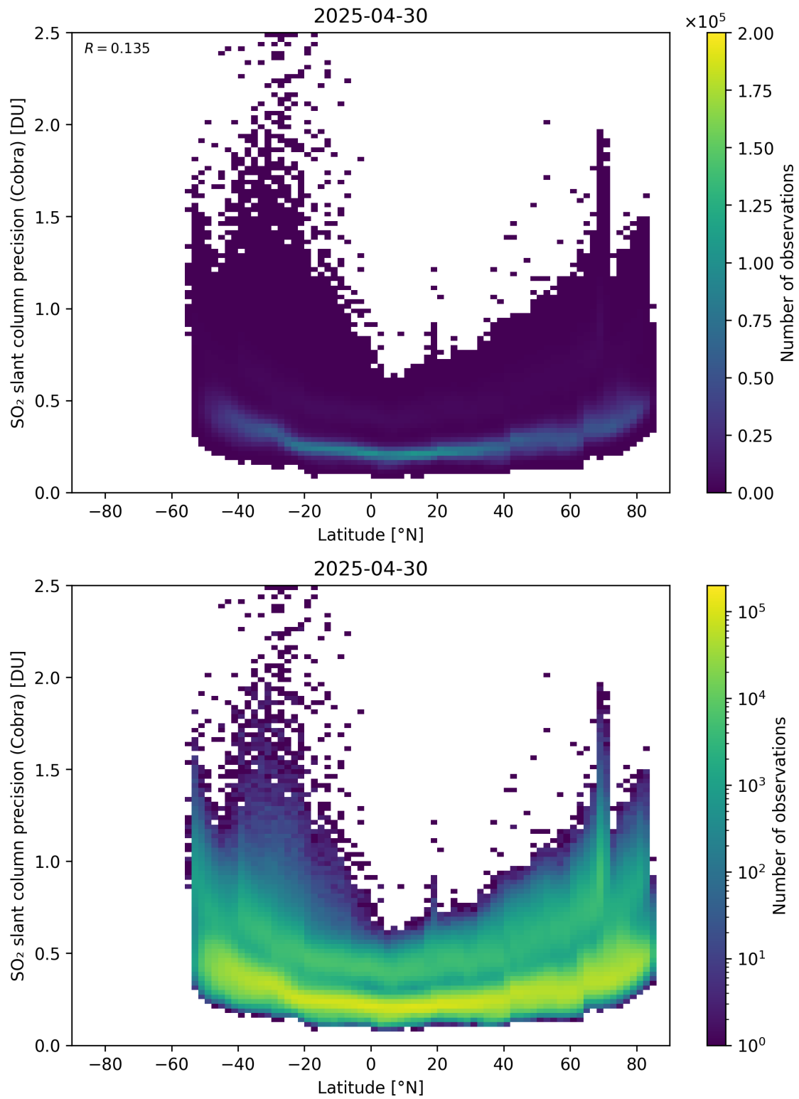
Figure 158: Scatter density plot of “Latitude” against “SO 2 slant column precision (Cobra)” for 2025-04-29 to 2025-05-01.
