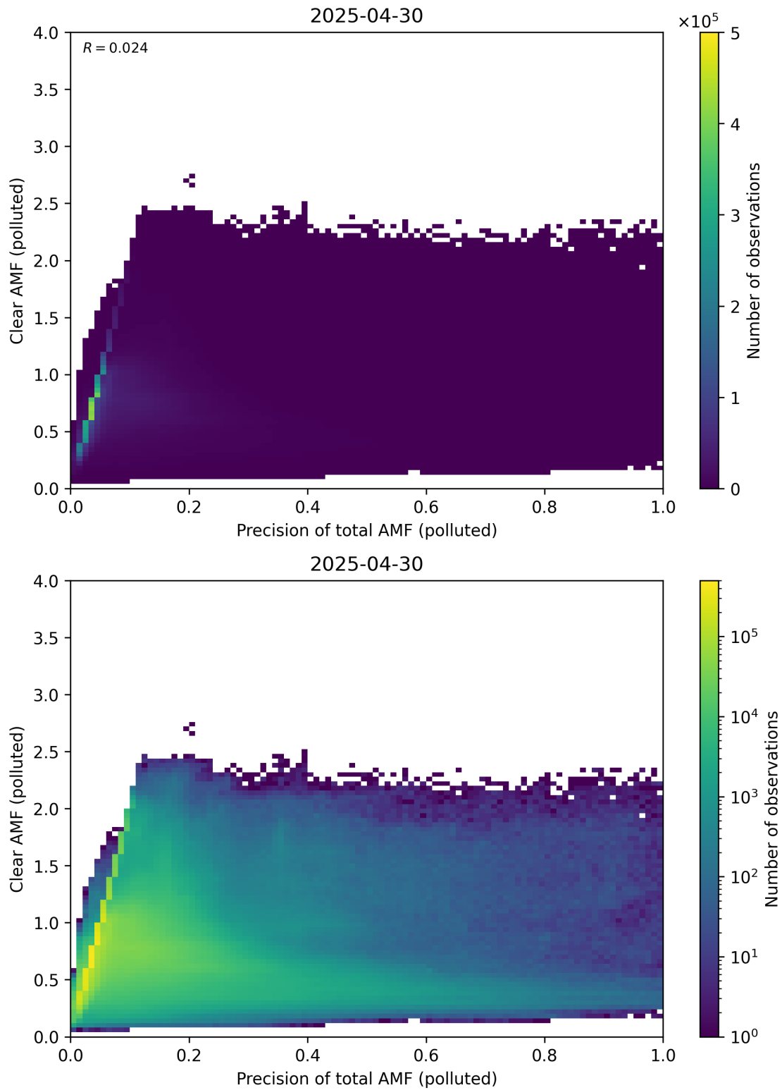
Figure 320: Scatter density plot of “Precision of total AMF (polluted)” against “Clear AMF (polluted)” for 2025-04-29 to 2025-05-01.
