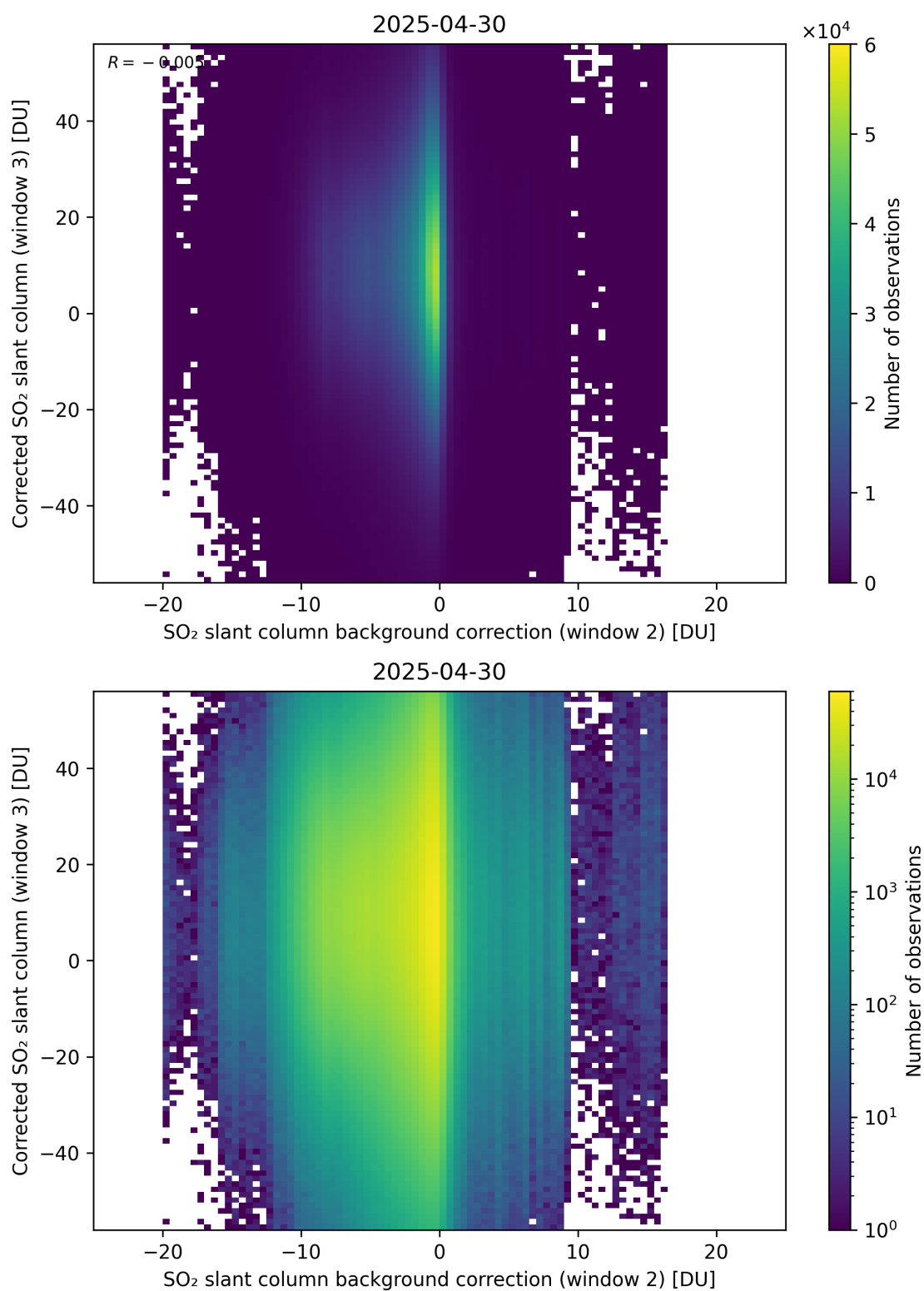
Figure 127: Scatter density plot of “SO 2 slant column background correction (window 2)” against “Corrected SO 2 slant column (window 3)” for 2025-04-29 to 2025-05-01.
