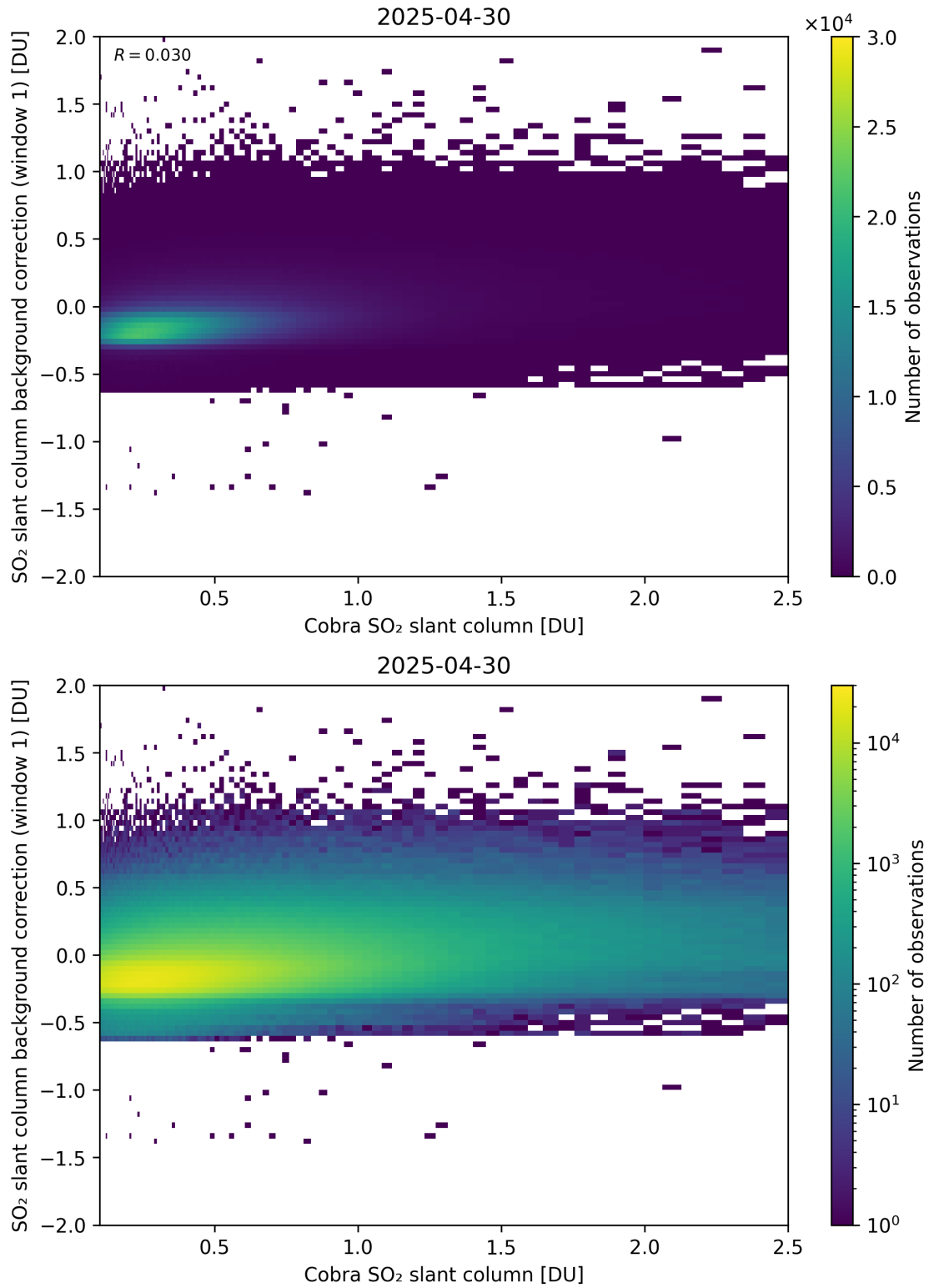
Figure 193: Scatter density plot of “Cobra SO 2 slant column” against “SO 2 slant column background correction (window 1)” for 2025-04-29 to 2025-05-01.
