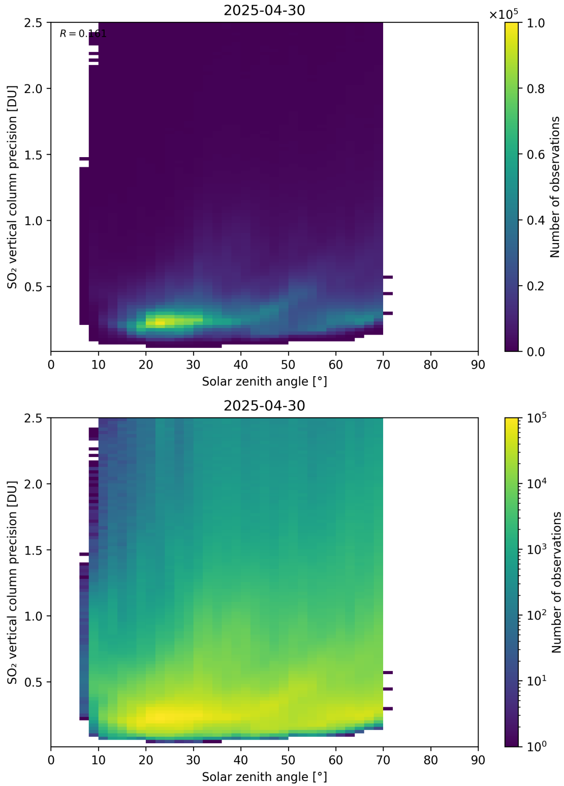
Figure 192: Scatter density plot of “Solar zenith angle” against “SO 2 vertical column precision” for 2025-04-29 to 2025-05-01.
