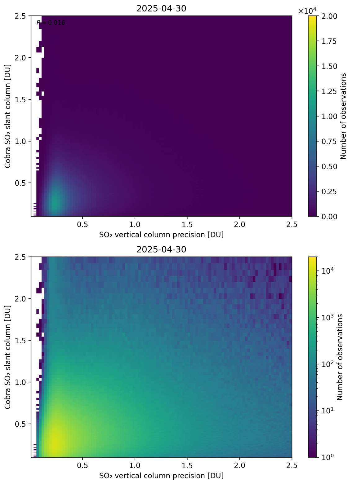
Figure 336: Scatter density plot of “SO 2 vertical column precision” against “Cobra SO 2 slant column” for 2025-04-29 to 2025-05-01.
