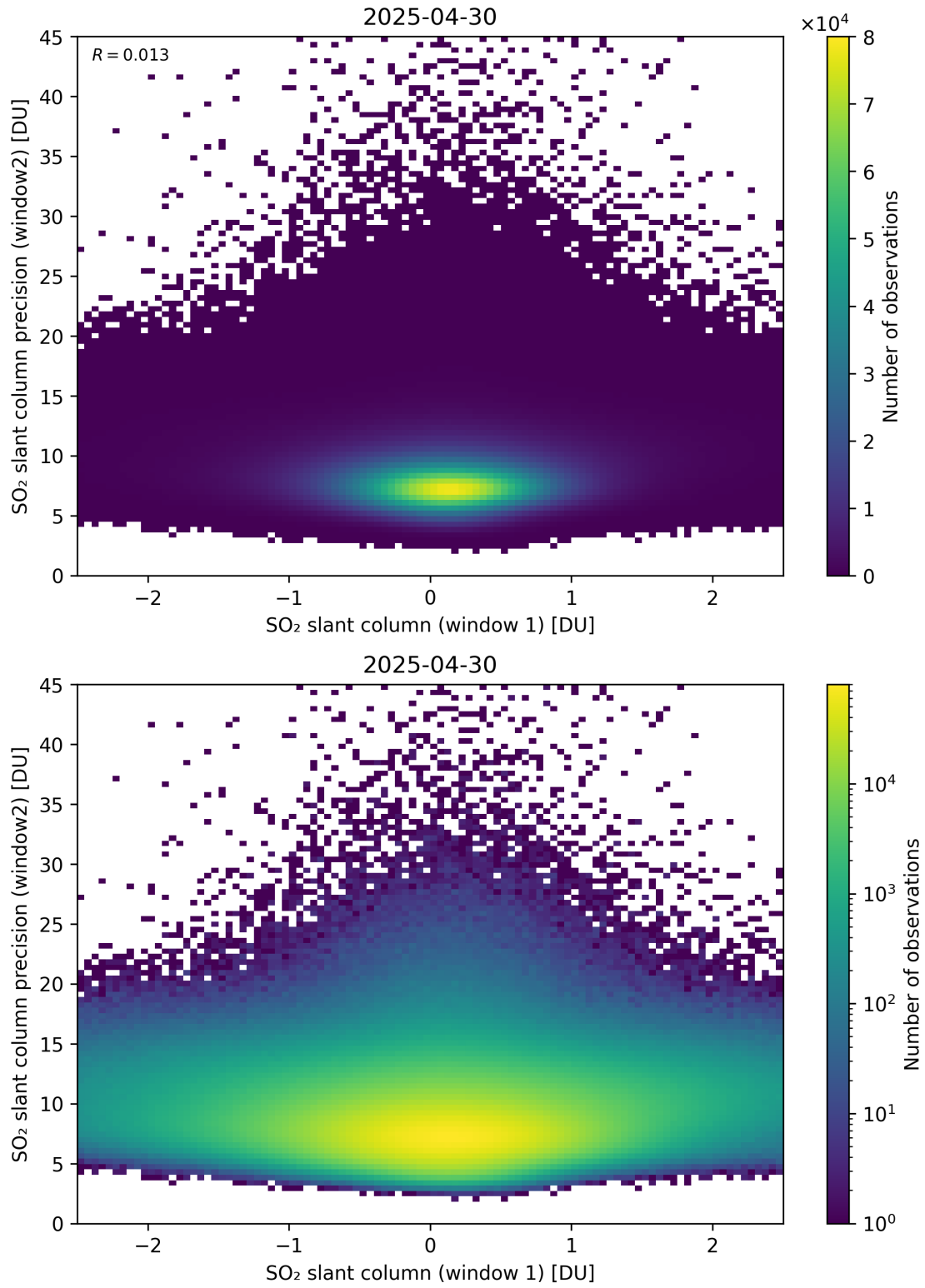
Figure 286: Scatter density plot of “SO 2 slant column (window 1)” against “SO 2 slant column precision (window2)” for 2025-04-29 to 2025-05-01.
