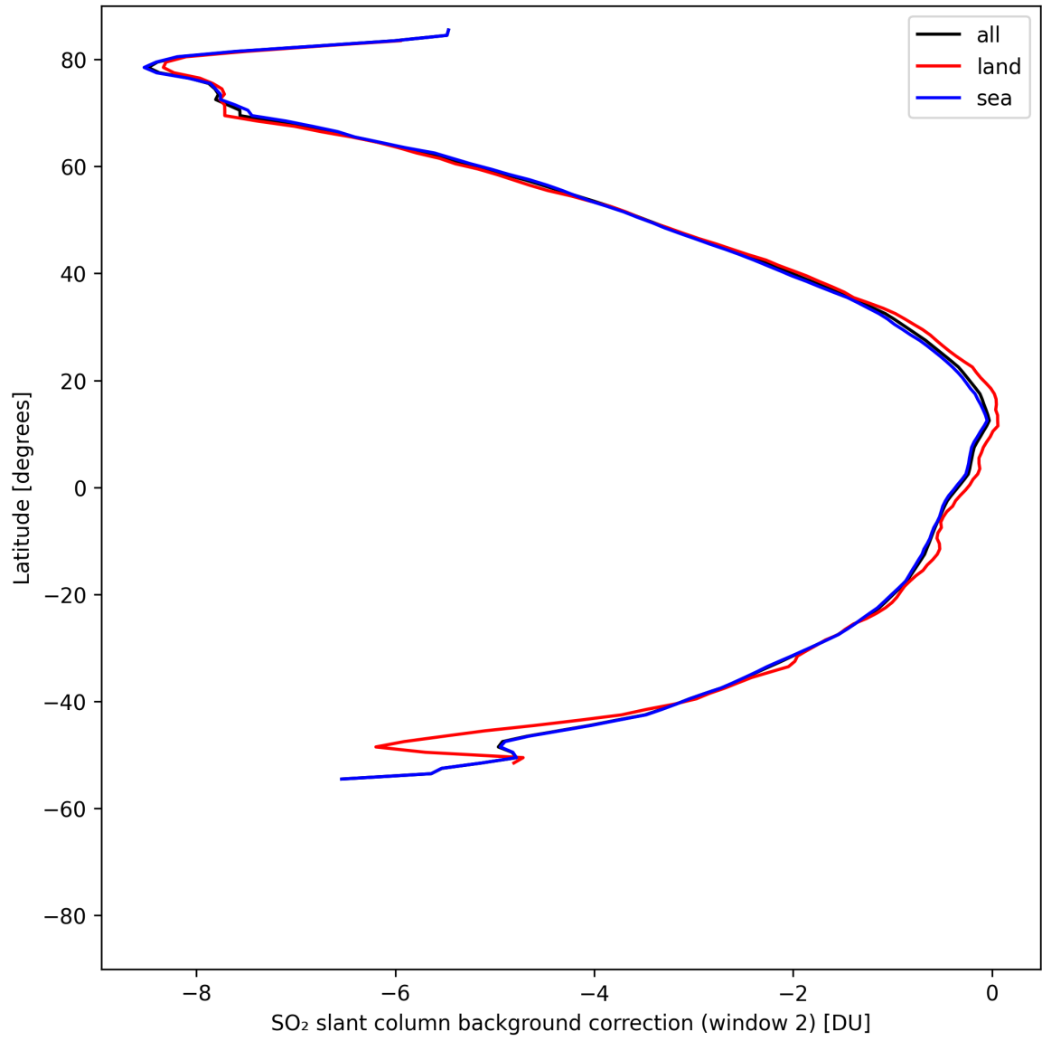
Figure 44: Zonal average of “SO 2 slant column background correction (window 2)” for 2025-04-29 to 2025-05-01.
