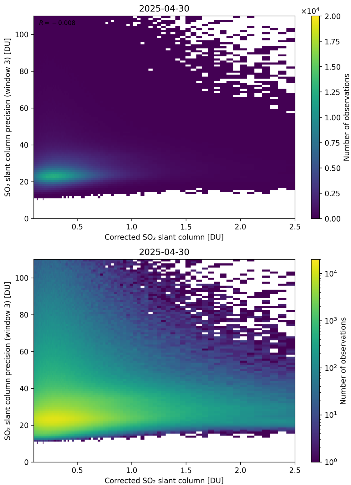
Figure 241: Scatter density plot of “Corrected SO 2 slant column” against “SO 2 slant column precision (window 3)” for 2025-04-29 to 2025-05-01.
