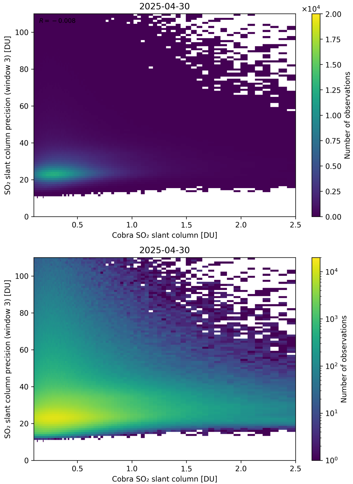
Figure 223: Scatter density plot of “Cobra SO 2 slant column” against “SO 2 slant column precision (window 3)” for 2025-04-29 to 2025-05-01.
