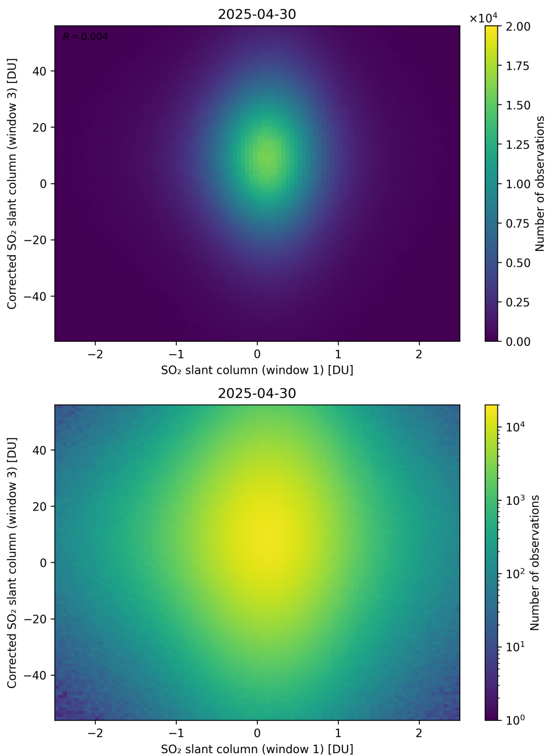
Figure 284: Scatter density plot of “SO 2 slant column (window 1)” against “Corrected SO 2 slant column (window 3)” for 2025-04-29 to 2025-05-01.
