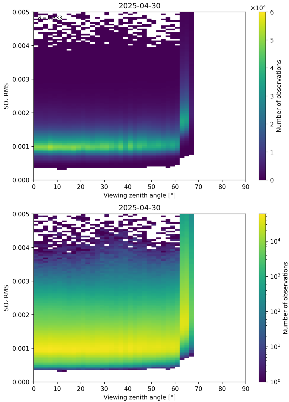
Figure 367: Scatter density plot of “Viewing zenith angle” against “SO 2 RMS” for 2025-04-29 to 2025-05-01.
