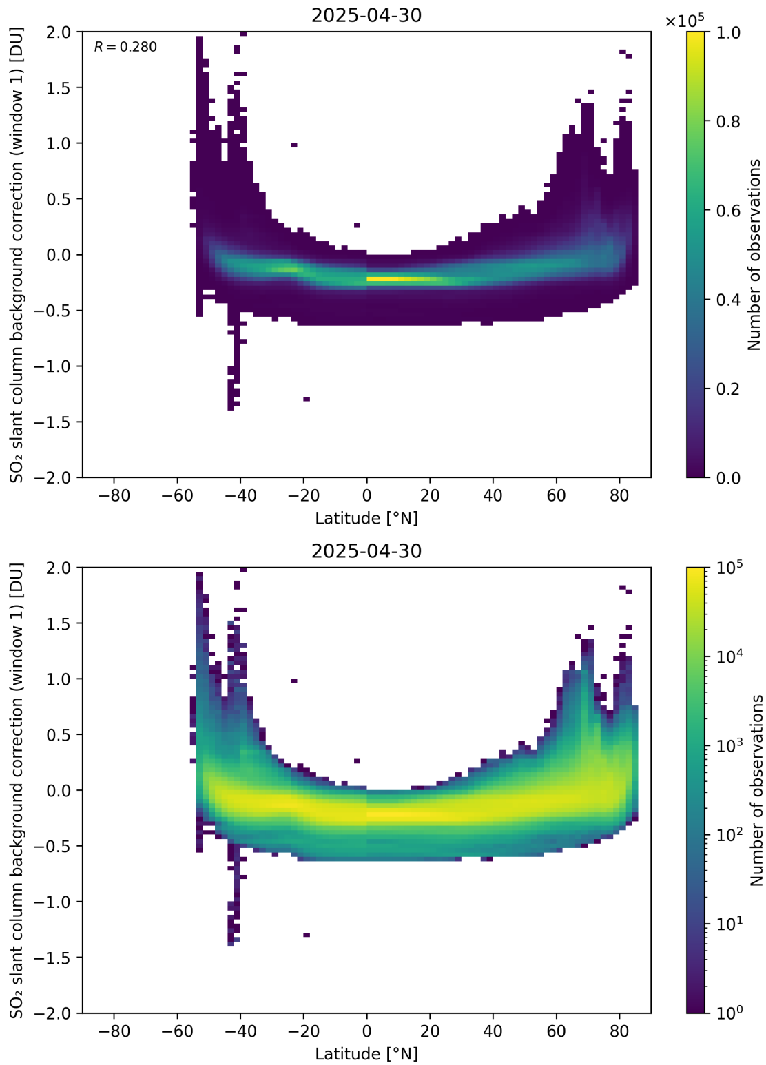
Figure 150: Scatter density plot of “Latitude” against “SO 2 slant column background correction (window 1)” for 2025-04-29 to 2025-05-01.
