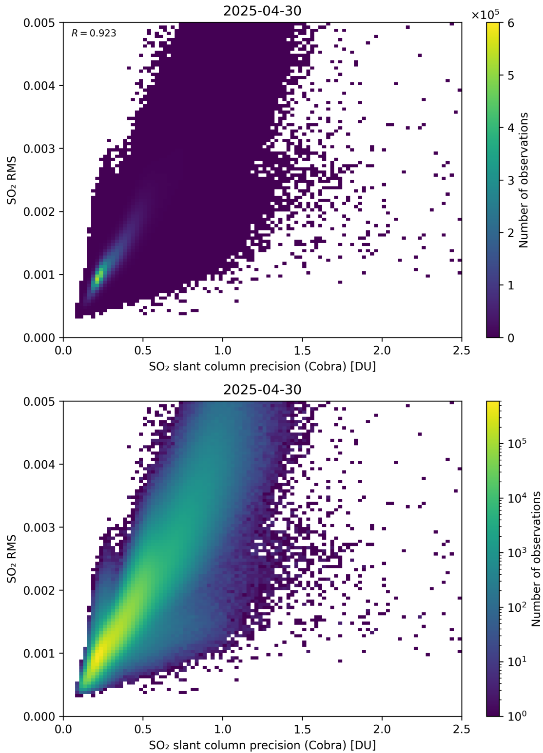
Figure 204: Scatter density plot of “SO 2 slant column precision (Cobra)” against “SO 2 RMS” for 2025-04-29 to 2025-05-01.
