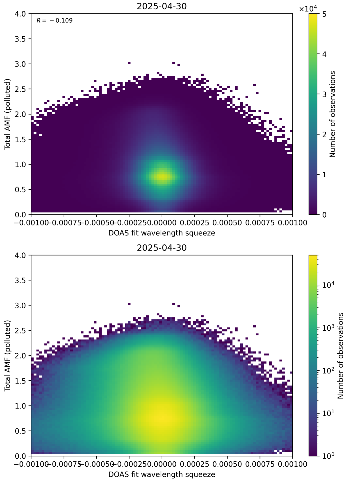
Figure 145: Scatter density plot of “DOAS fit wavelength squeeze” against “Total AMF (polluted)” for 2025-04-29 to 2025-05-01.
