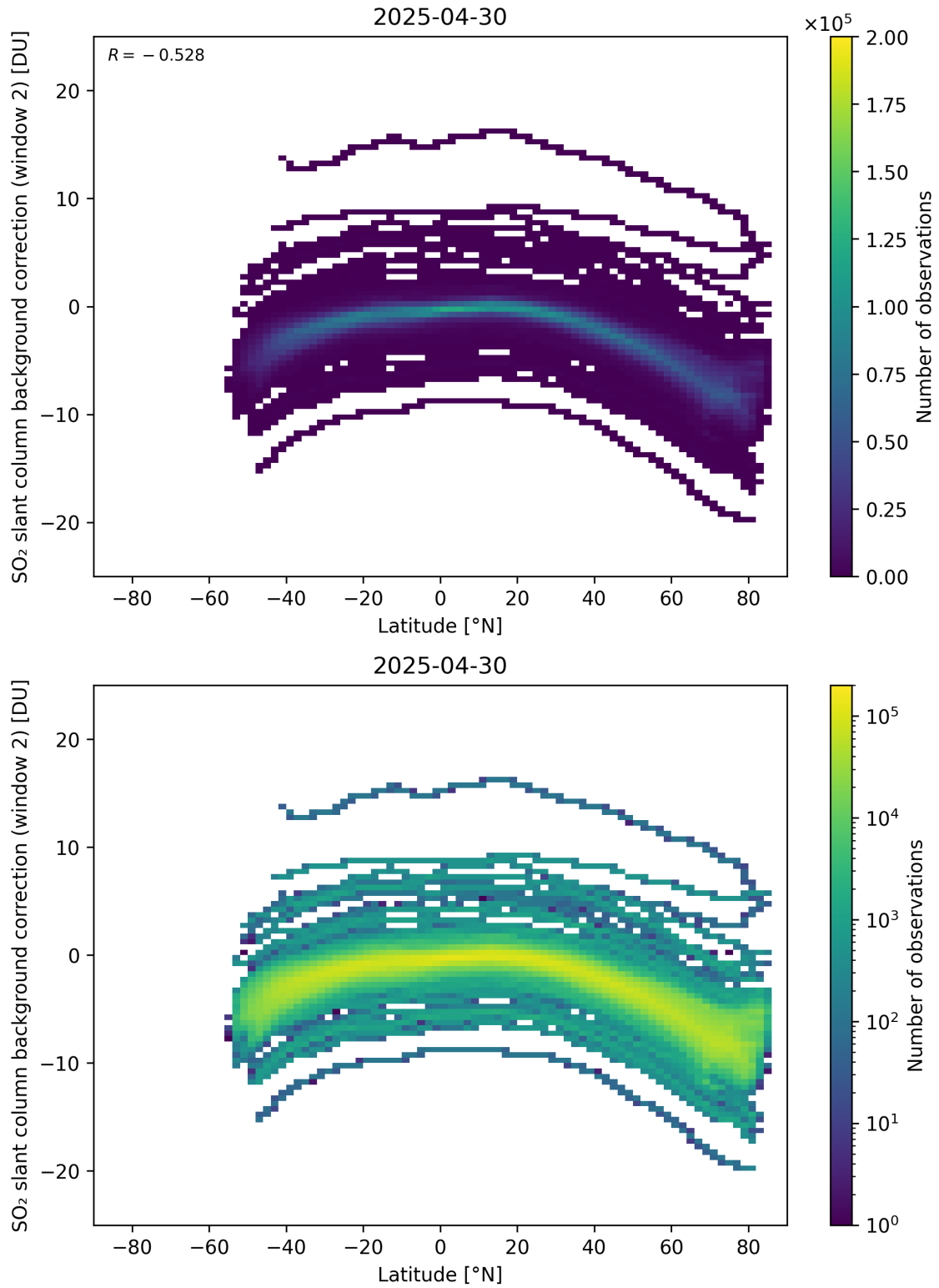
Figure 151: Scatter density plot of “Latitude” against “SO 2 slant column background correction (window 2)” for 2025-04-29 to 2025-05-01.
