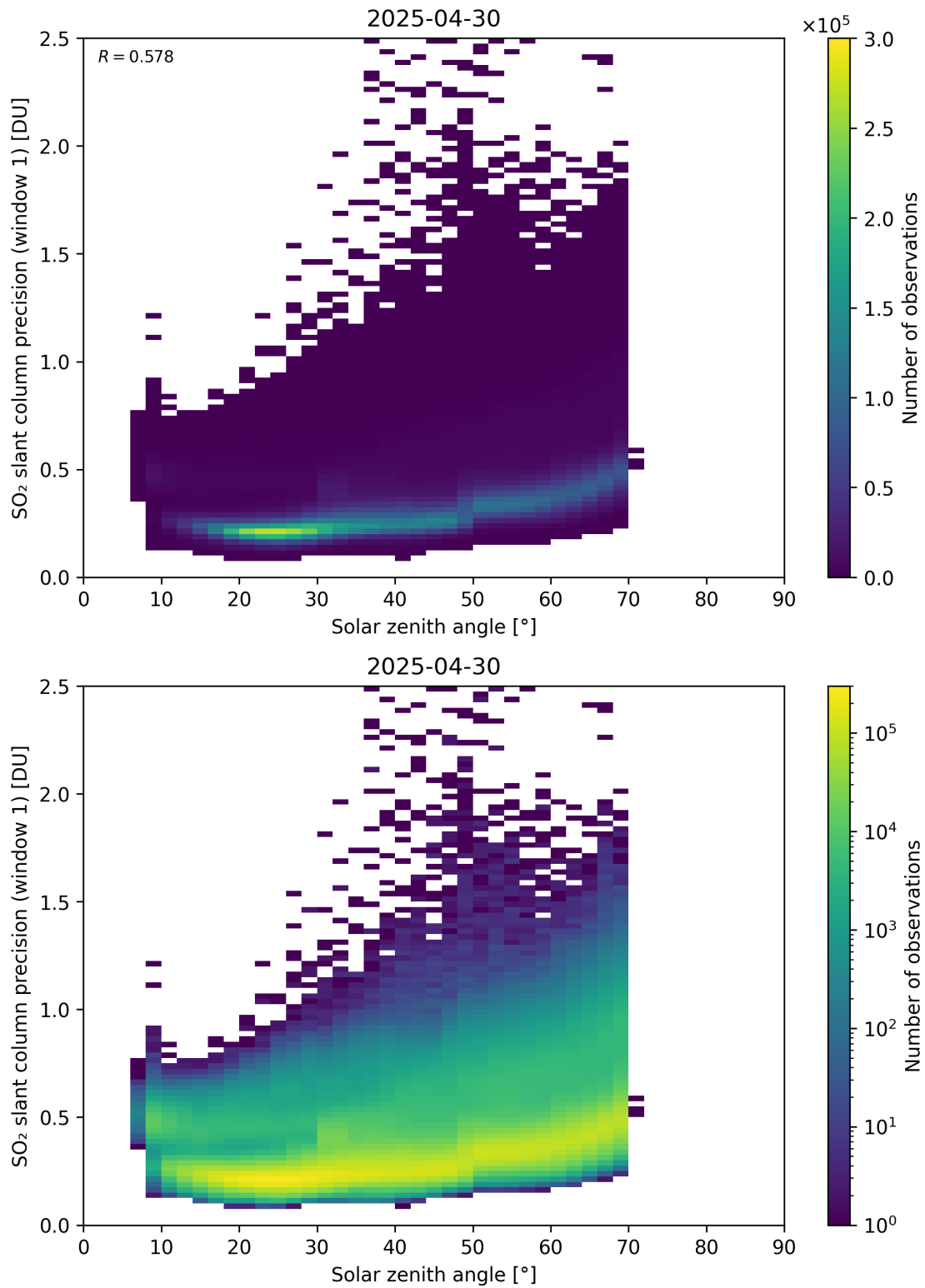
Figure 185: Scatter density plot of “Solar zenith angle” against “SO 2 slant column precision (window 1)” for 2025-04-29 to 2025-05-01.
