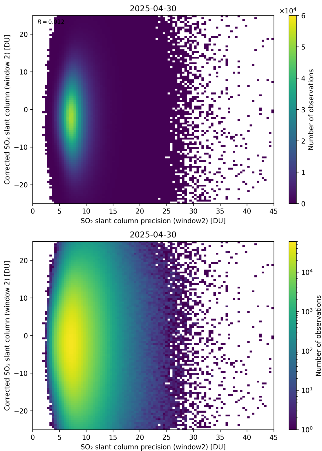
Figure 297: Scatter density plot of “SO 2 slant column precision (window2)” against “Corrected SO 2 slant column (window 2)” for 2025-04-29 to 2025-05-01.
