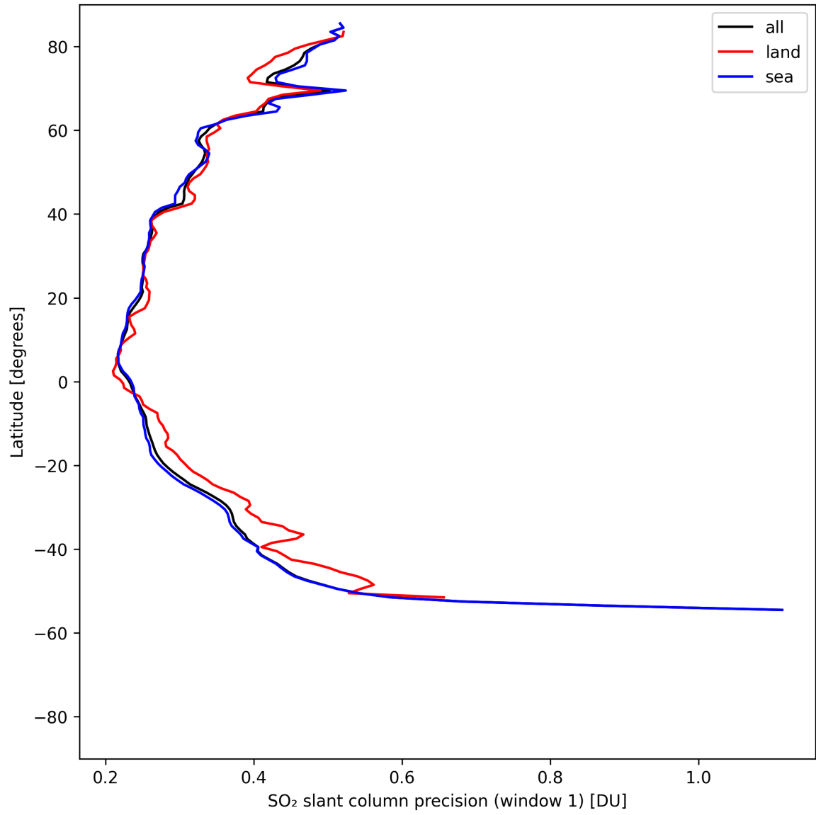
Figure 38: Zonal average of “SO 2 slant column precision (window 1)” for 2025-04-29 to 2025-05-01.
