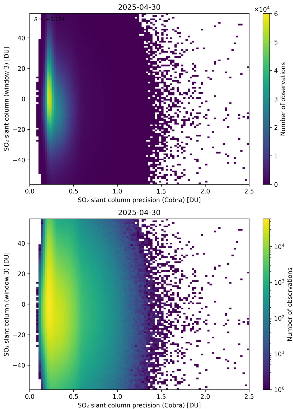
Figure 211: Scatter density plot of “SO 2 slant column precision (Cobra)” against “SO 2 slant column (window 3)” for 2025-04-29 to 2025-05-01.
