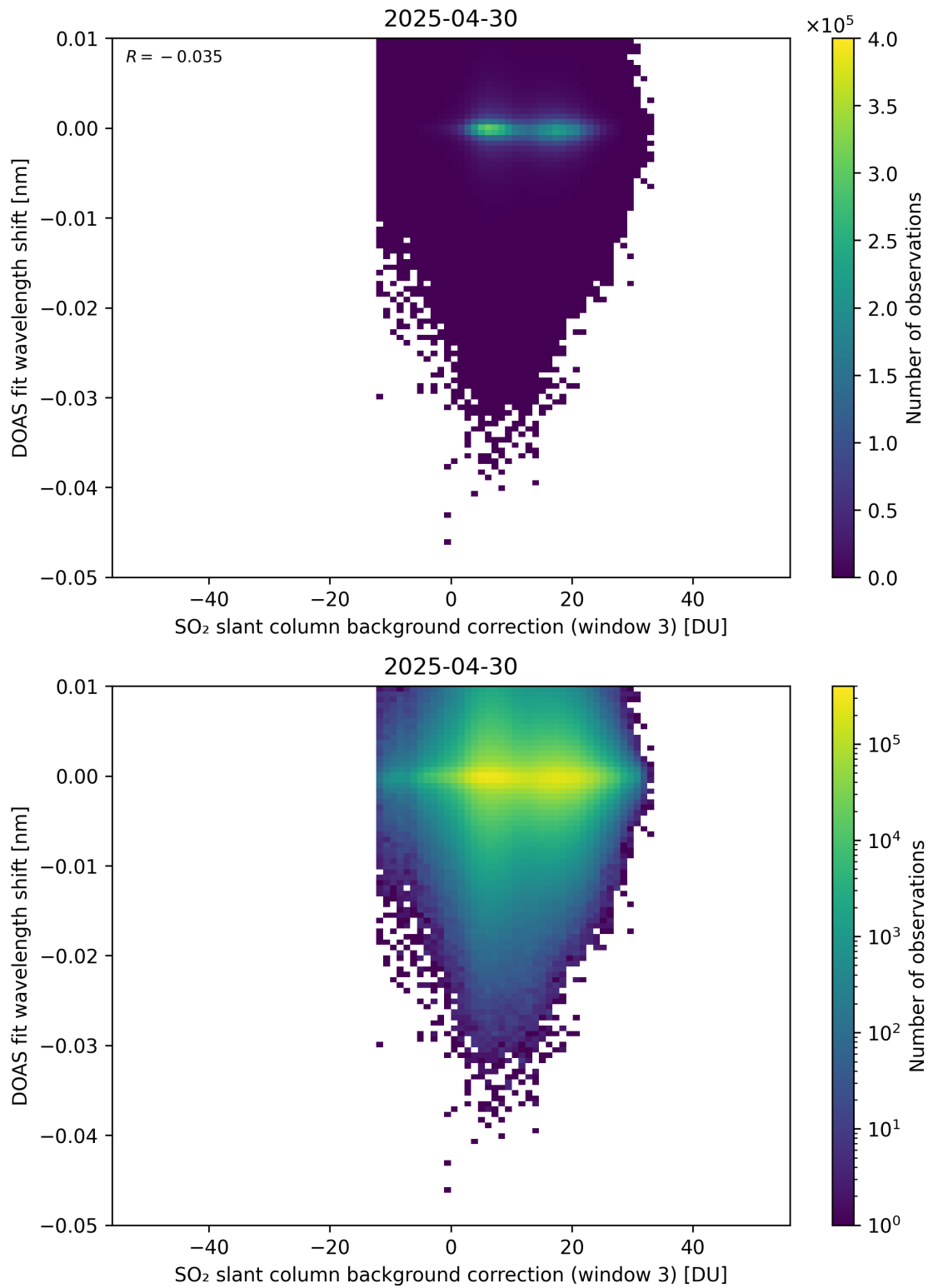
Figure 132: Scatter density plot of “SO 2 slant column background correction (window 3)” against “DOAS fit wavelength shift” for 2025-04-29 to 2025-05-01.
