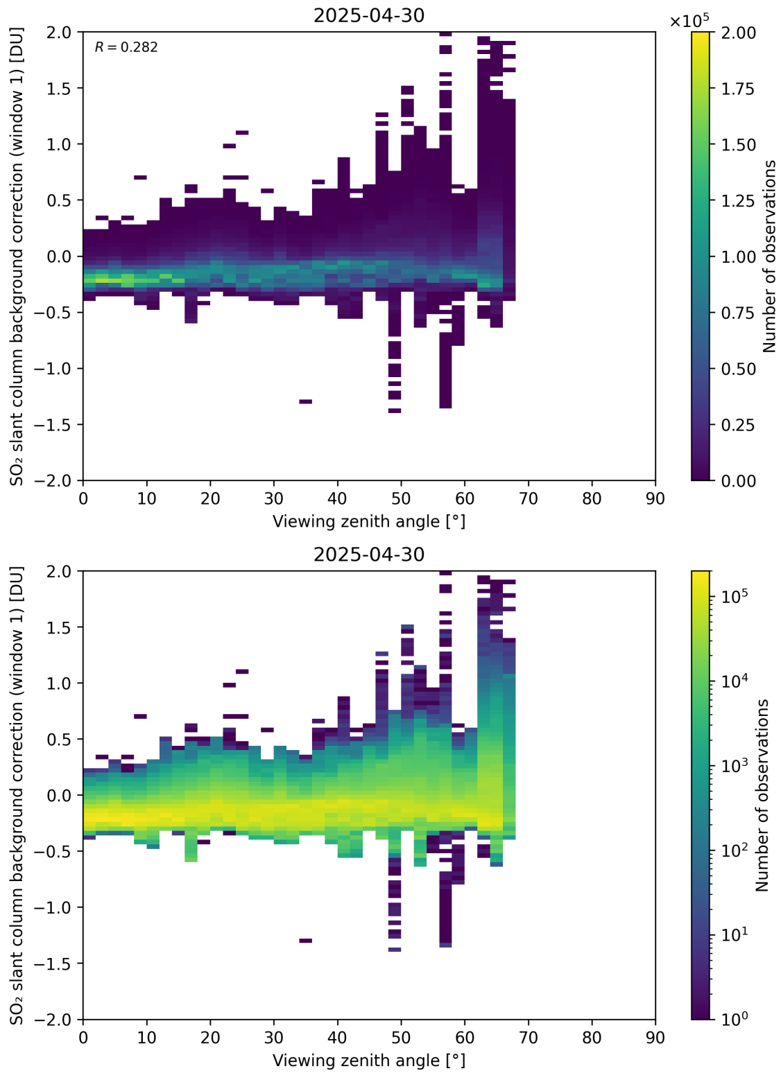
Figure 362: Scatter density plot of “Viewing zenith angle” against “SO 2 slant column background correction (window 1)” for 2025-04-29 to 2025-05-01.
