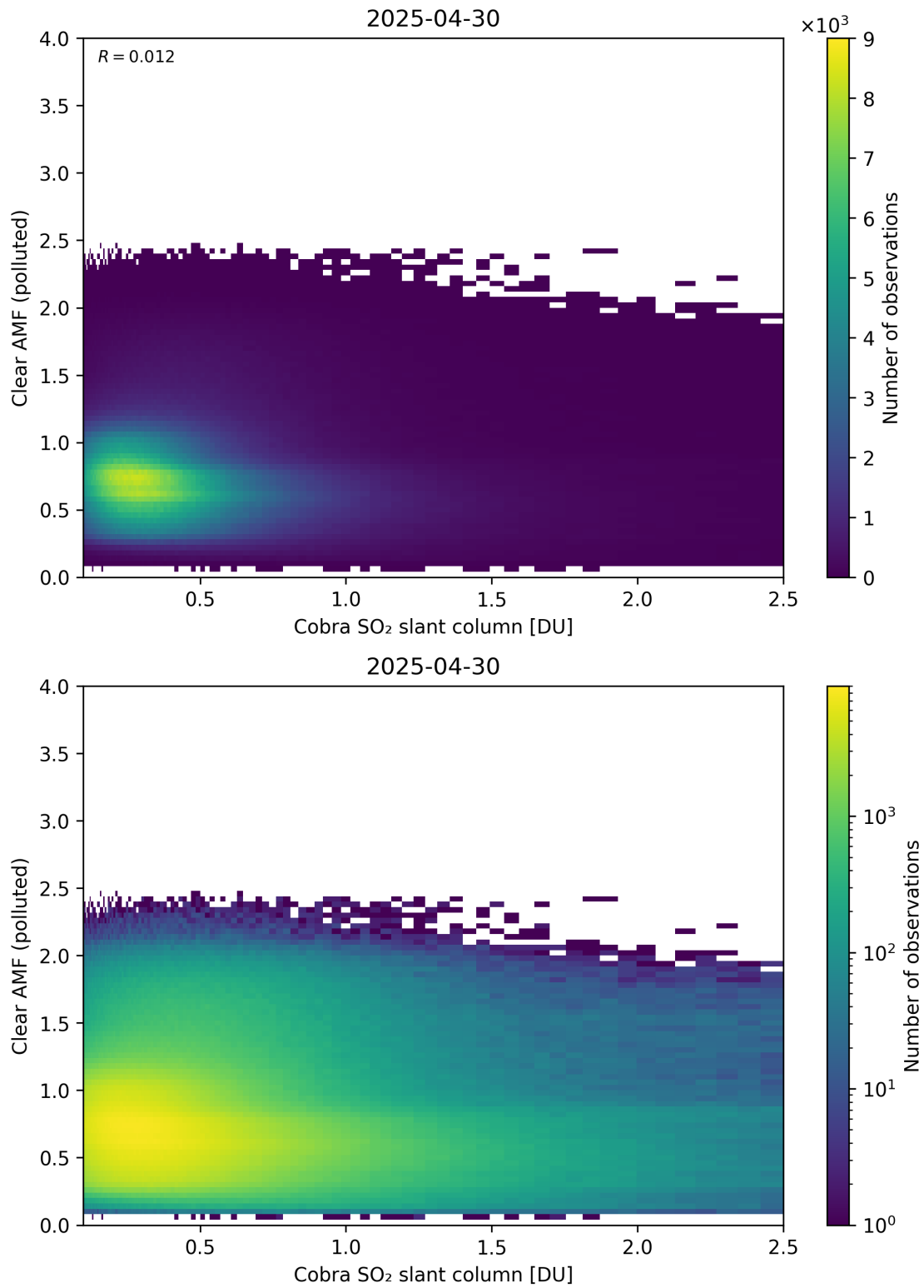
Figure 215: Scatter density plot of “Cobra SO 2 slant column” against “Clear AMF (polluted)” for 2025-04-29 to 2025-05-01.
