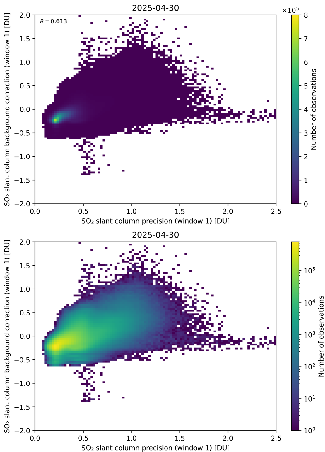
Figure 268: Scatter density plot of “SO 2 slant column precision (window 1)” against “SO 2 slant column background correction (window 1)” for 2025-04-29 to 2025-05-01.
