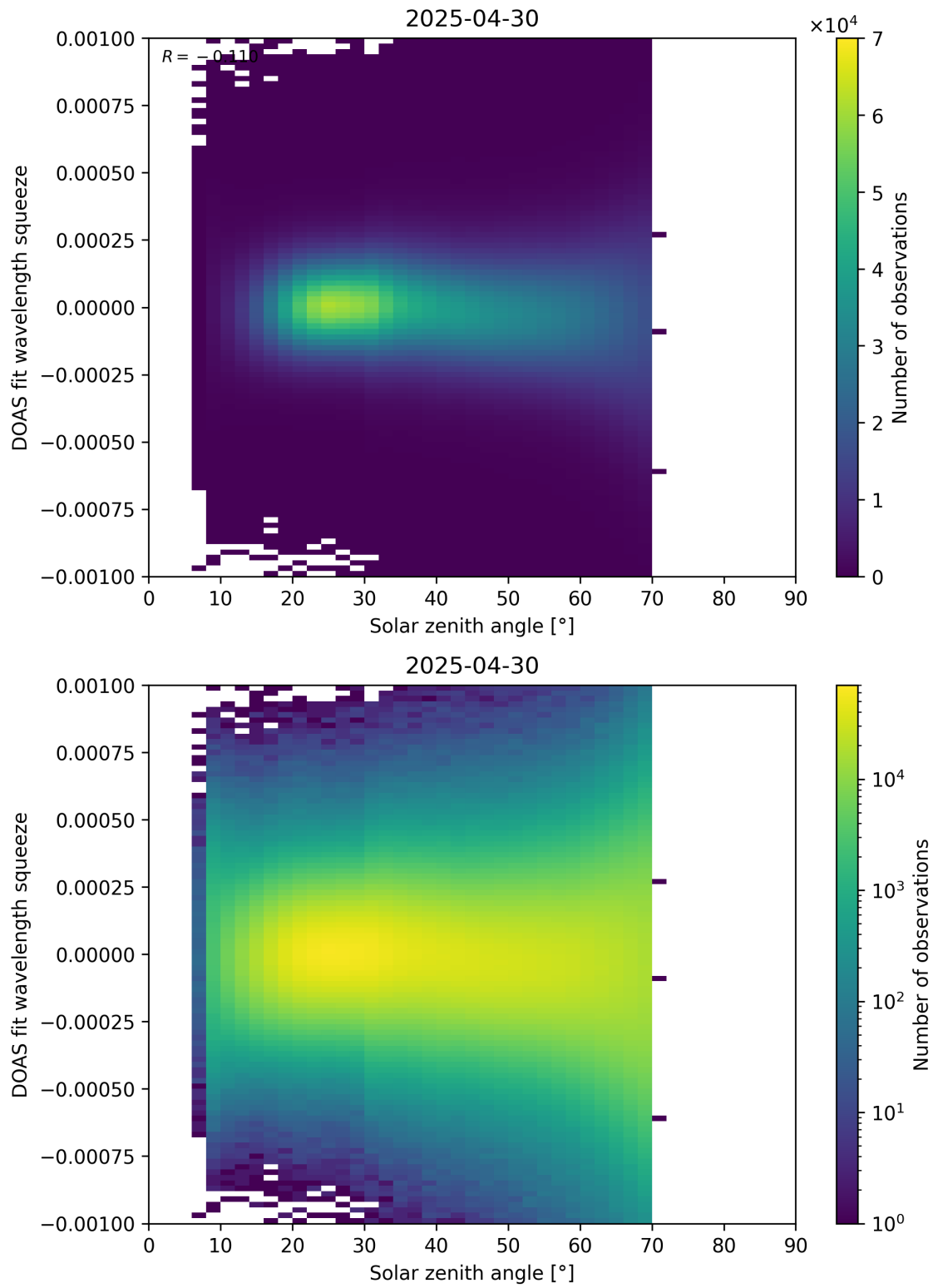
Figure 175: Scatter density plot of “Solar zenith angle” against “DOAS fit wavelength squeeze” for 2025-04-29 to 2025-05-01.
