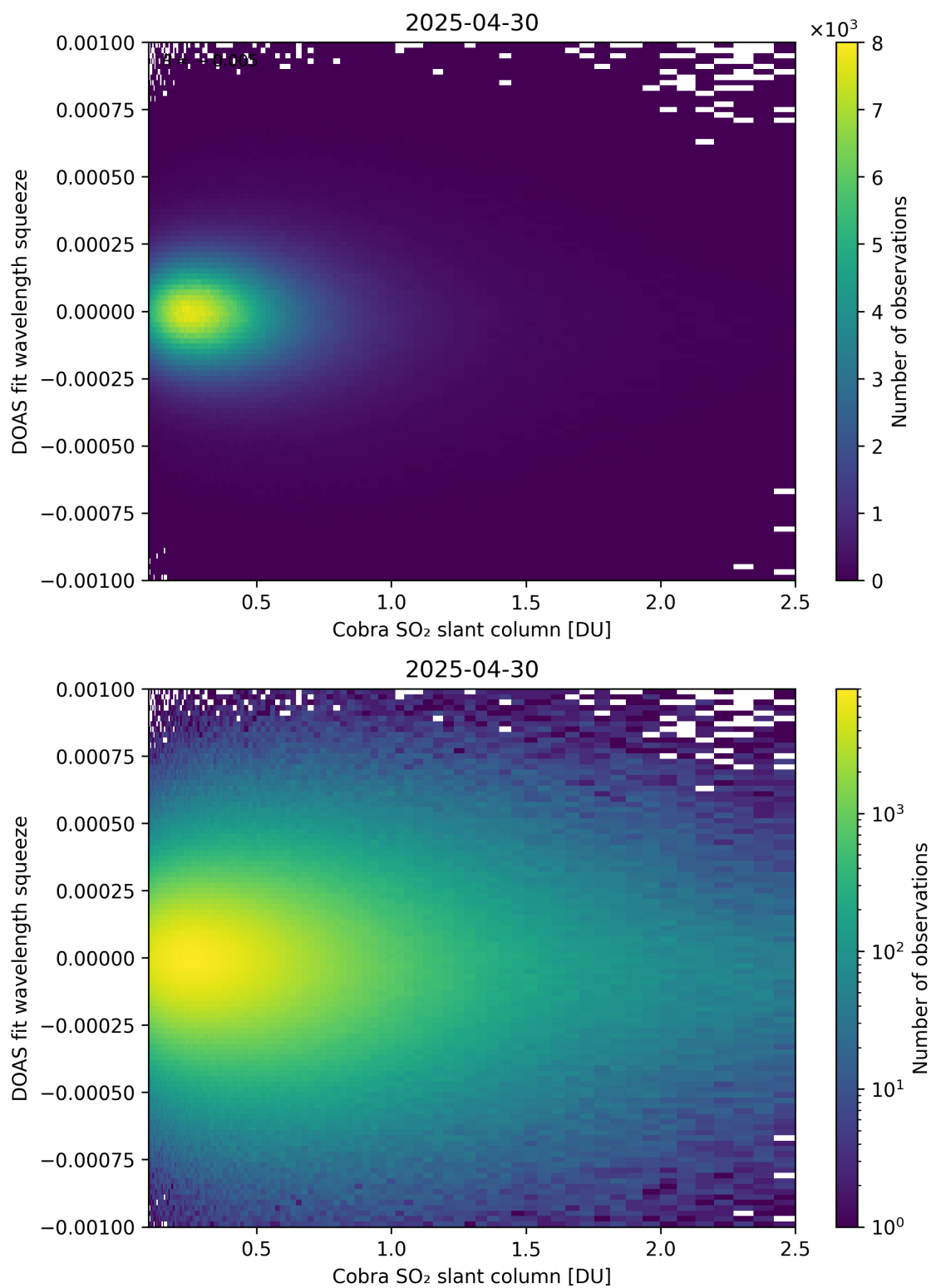
Figure 197: Scatter density plot of “Cobra SO 2 slant column” against “DOAS fit wavelength squeeze” for 2025-04-29 to 2025-05-01.
