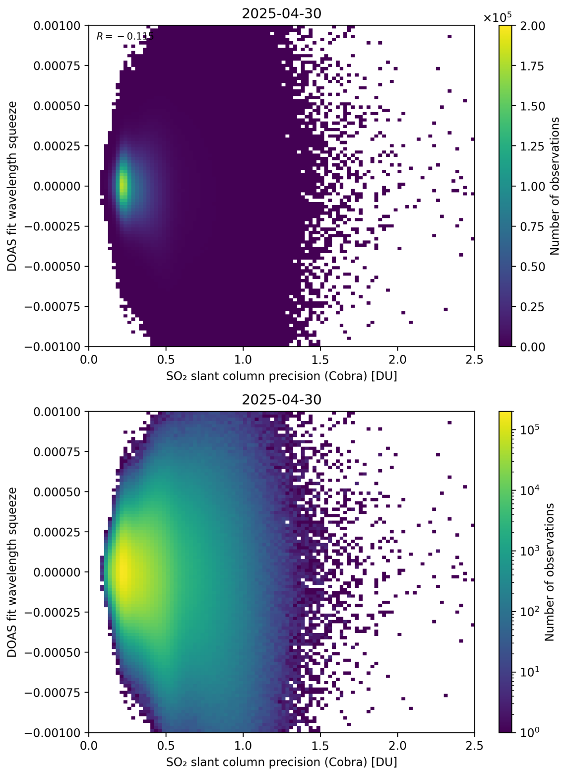
Figure 203: Scatter density plot of “SO 2 slant column precision (Cobra)” against “DOAS fit wavelength squeeze” for 2025-04-29 to 2025-05-01.
