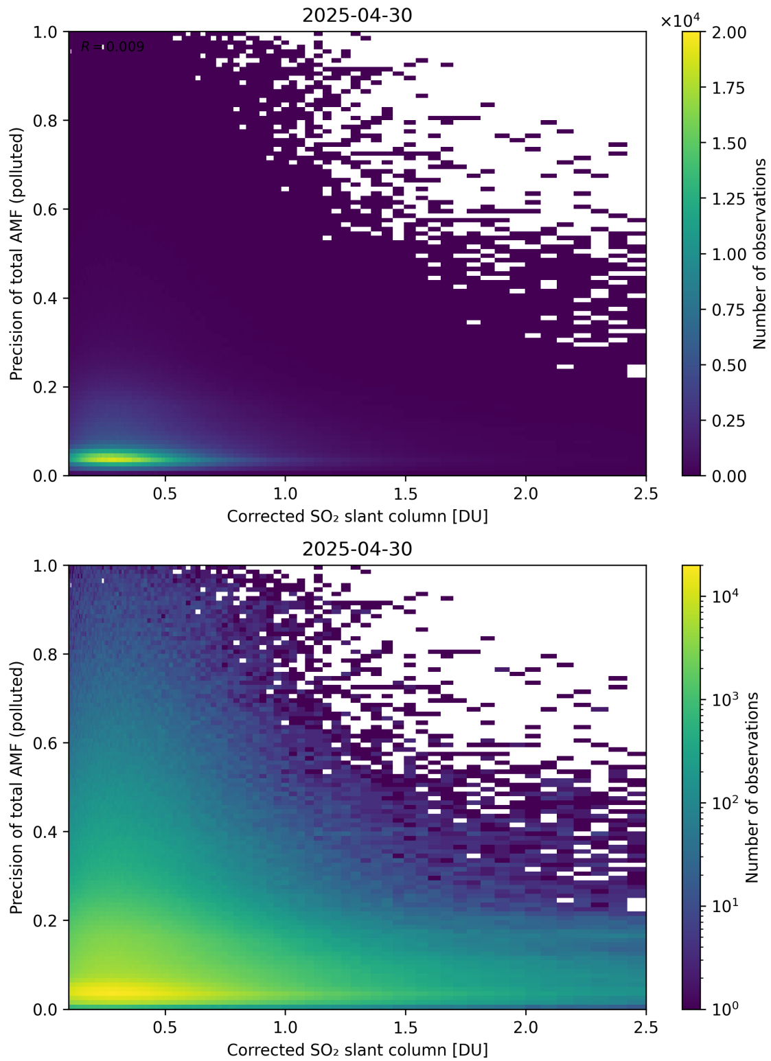
Figure 243: Scatter density plot of “Corrected SO 2 slant column” against “Precision of total AMF (polluted)” for 2025-04-29 to 2025-05-01.
