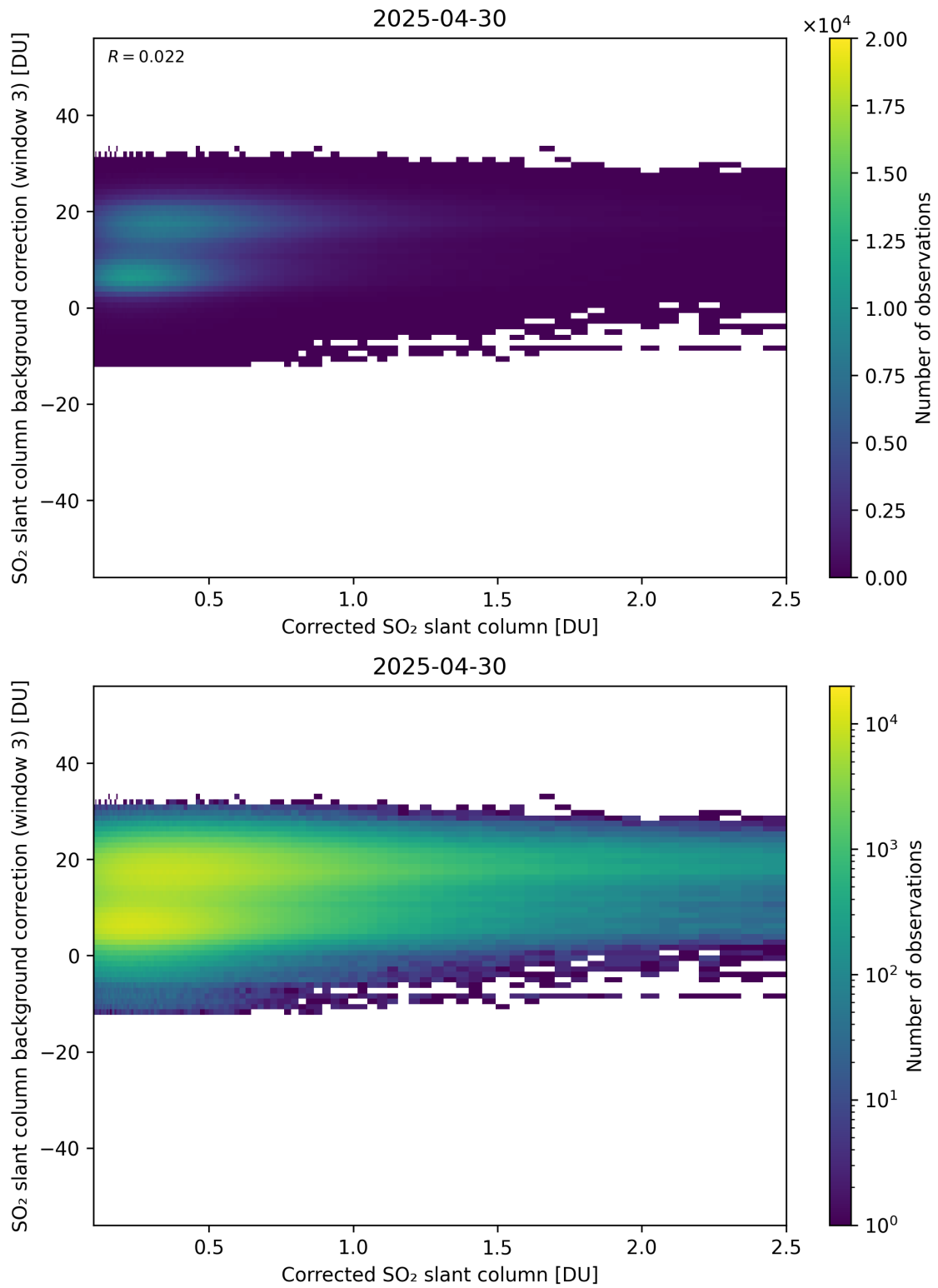
Figure 228: Scatter density plot of “Corrected SO 2 slant column” against “SO 2 slant column background correction (window 3)” for 2025-04-29 to 2025-05-01.
