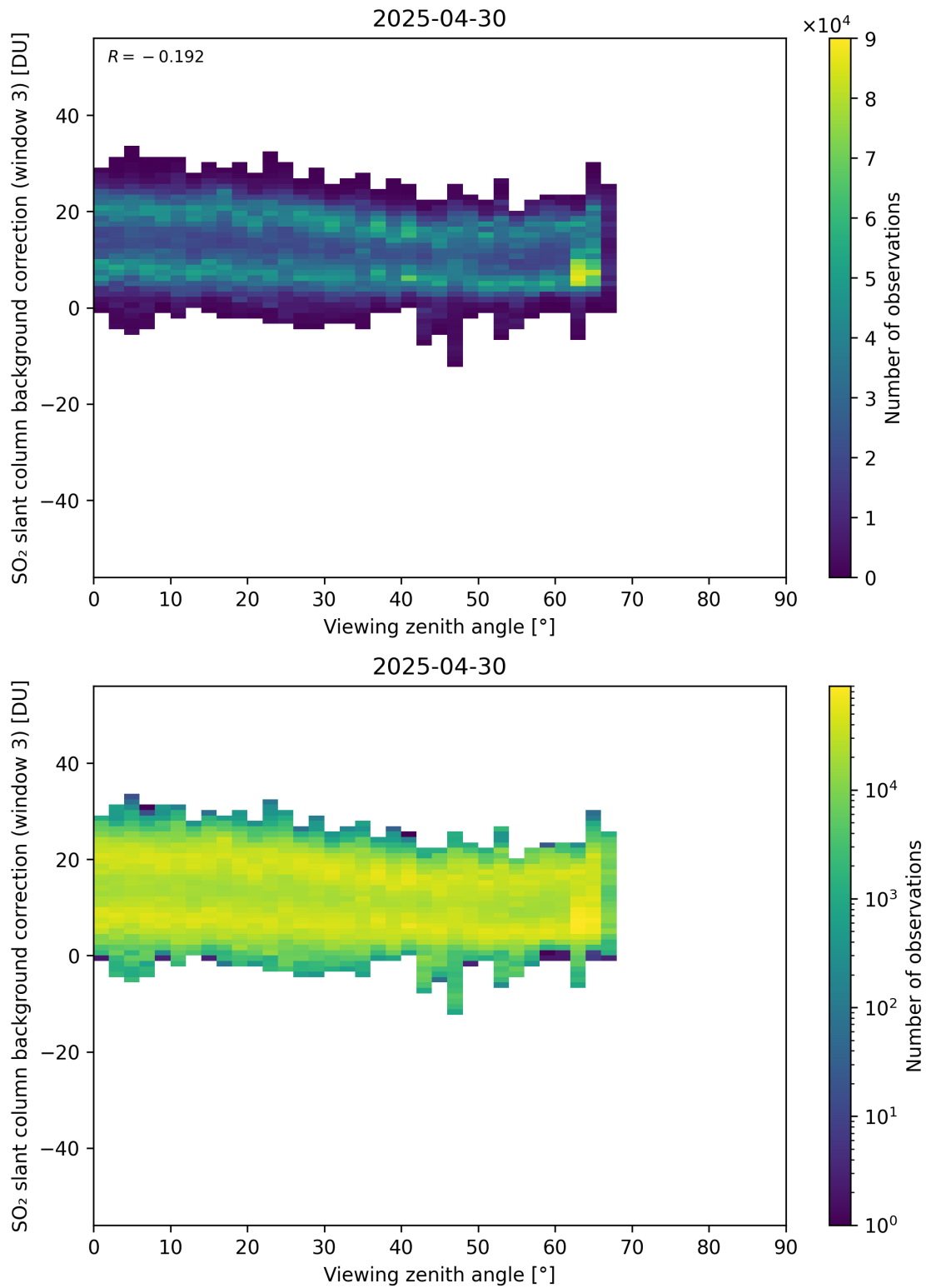
Figure 364: Scatter density plot of “Viewing zenith angle” against “SO 2 slant column background correction (window 3)” for 2025-04-29 to 2025-05-01.
