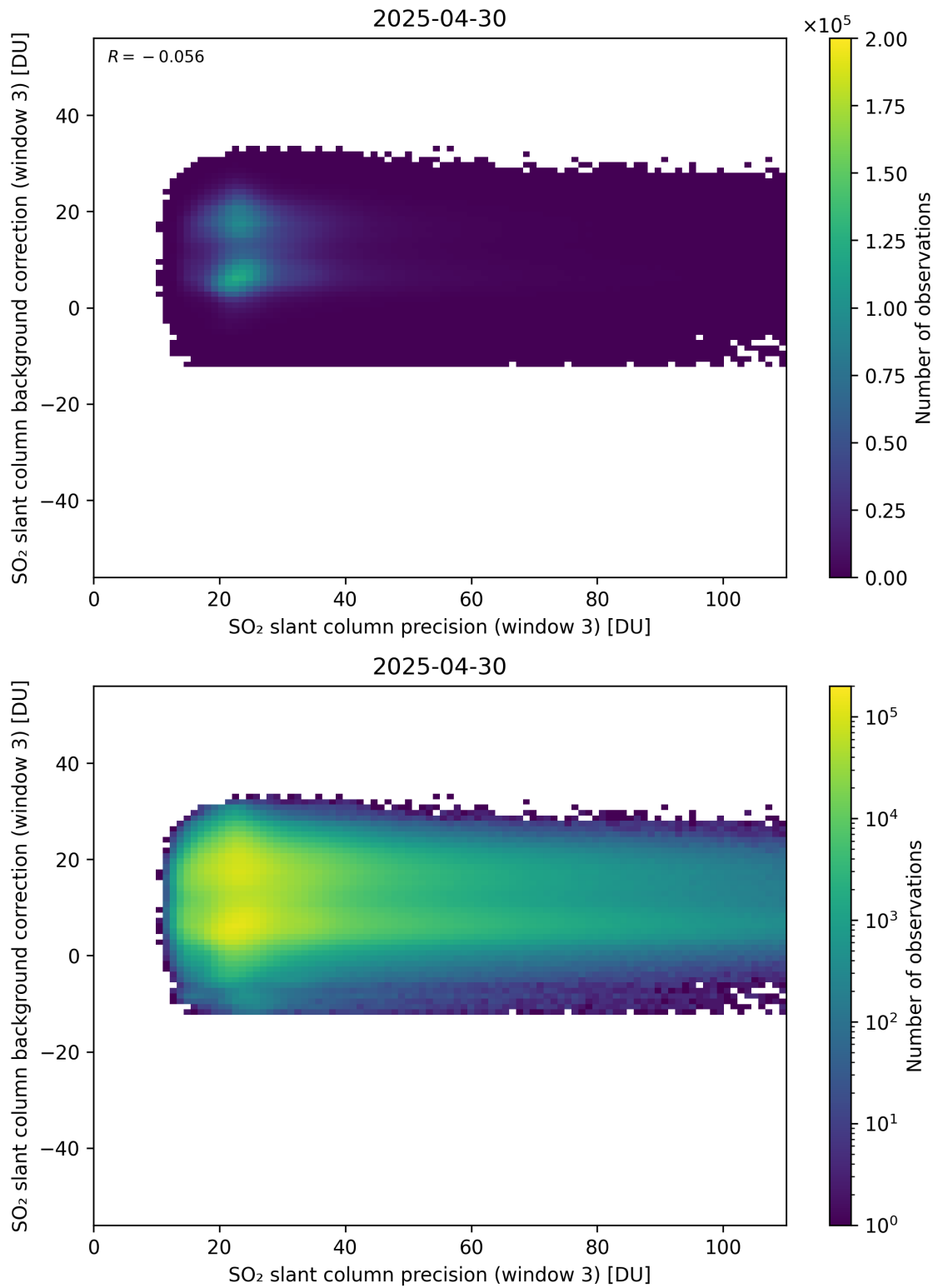
Figure 307: Scatter density plot of “SO 2 slant column precision (window 3)” against “SO 2 slant column background correction (window 3)” for 2025-04-29 to 2025-05-01.
