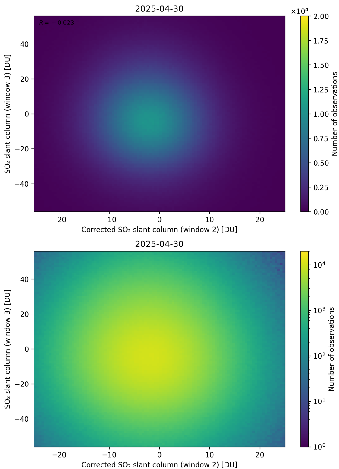
Figure 251: Scatter density plot of “Corrected SO 2 slant column (window 2)” against “SO 2 slant column (window 3)” for 2025-04-29 to 2025-05-01.
