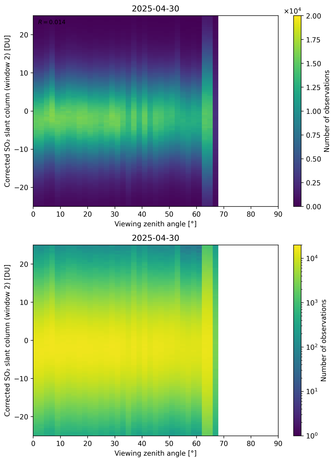
Figure 374: Scatter density plot of “Viewing zenith angle” against “Corrected SO 2 slant column (window 2)” for 2025-04-29 to 2025-05-01.
