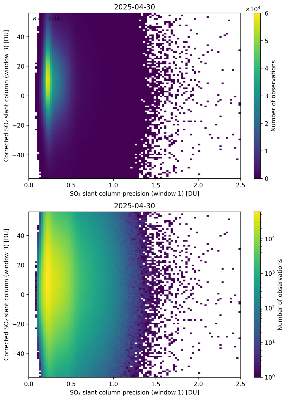
Figure 276: Scatter density plot of “SO 2 slant column precision (window 1)” against “Corrected SO 2 slant column (window 3)” for 2025-04-29 to 2025-05-01.
