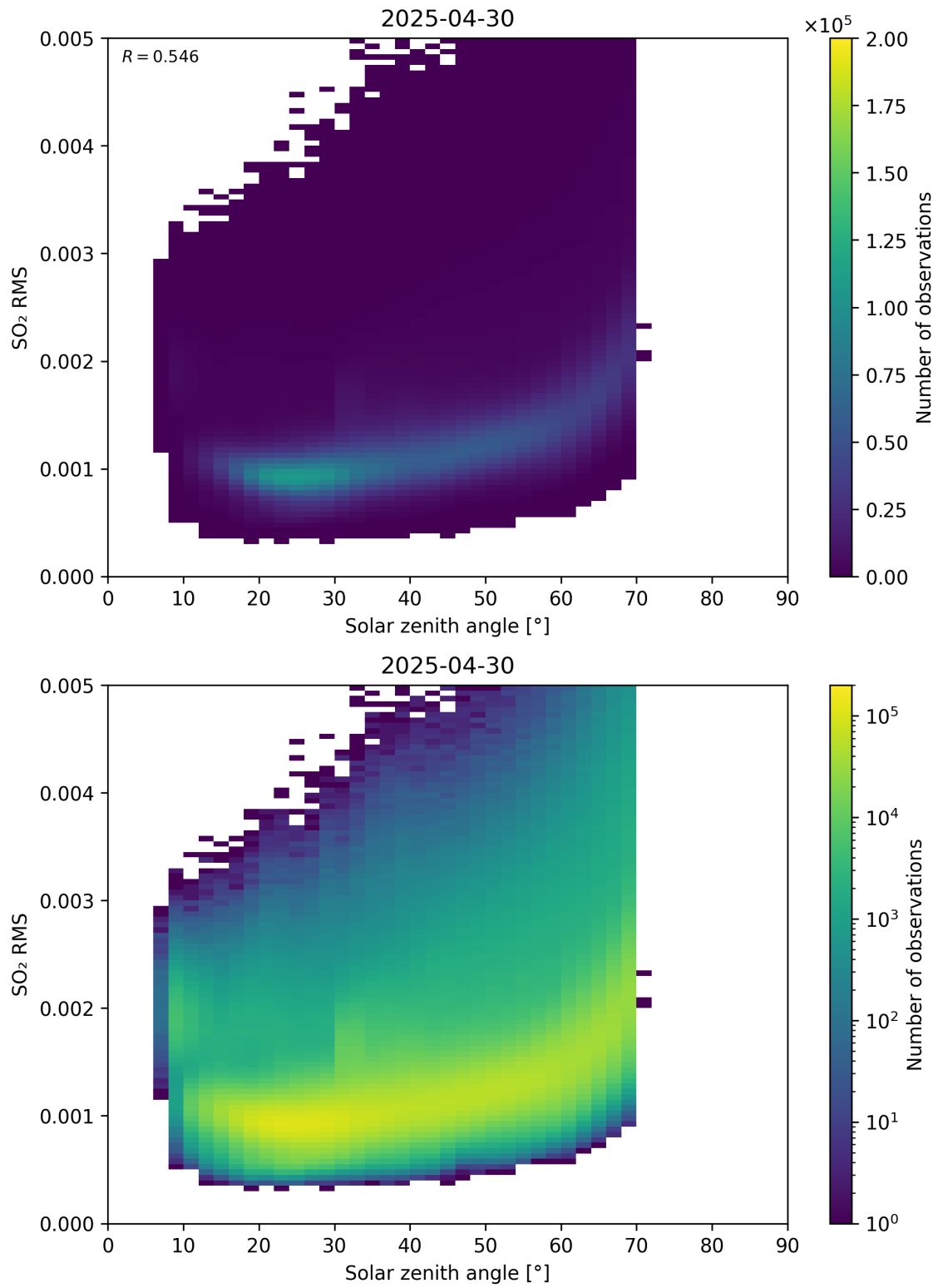
Figure 176: Scatter density plot of “Solar zenith angle” against “SO 2 RMS” for 2025-04-29 to 2025-05-01.
