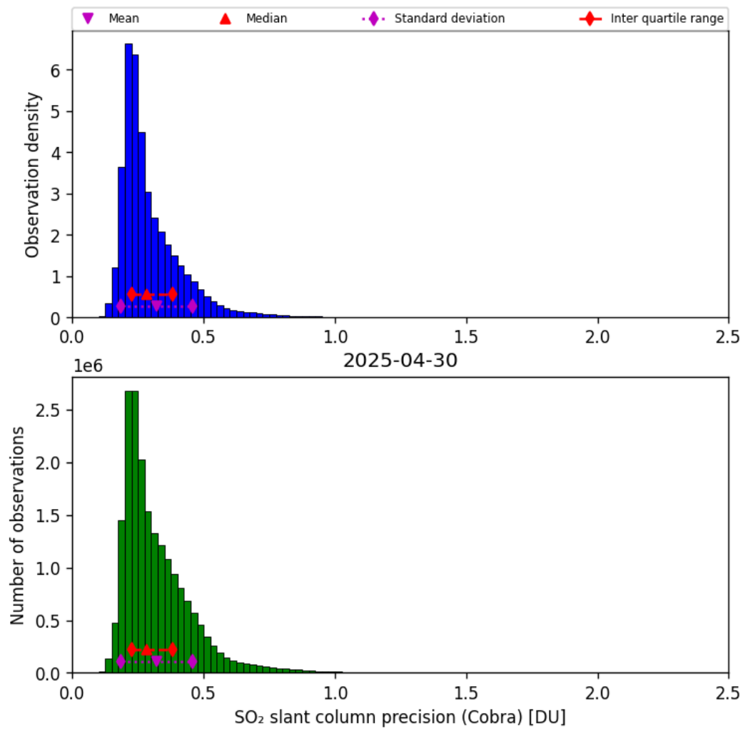
Figure 62: Histogram of “SO 2 slant column precision (Cobra)” for 2025-04-29 to 2025-05-01
