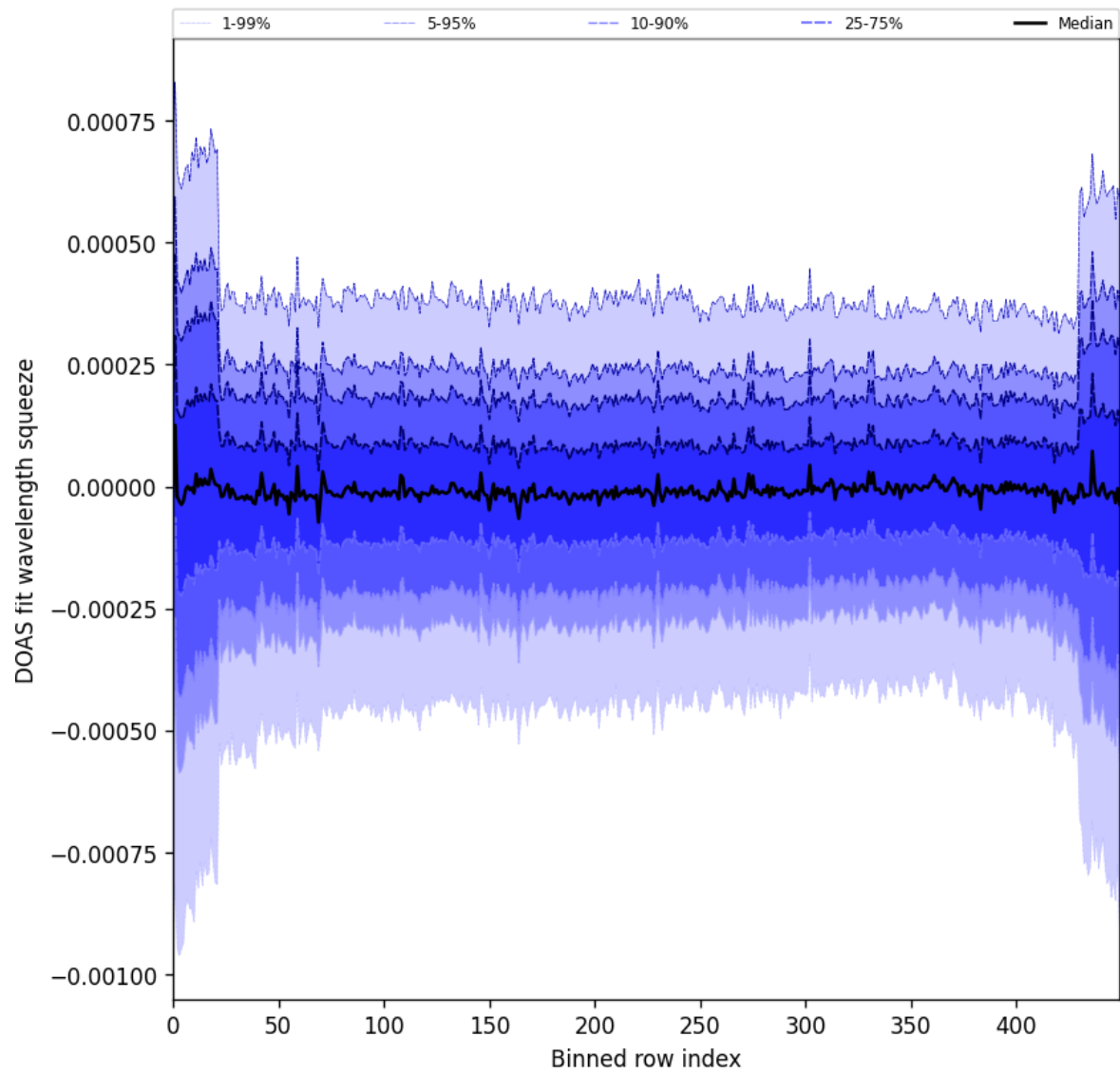
Figure 103: Along track statistics of “DOAS fit wavelength squeeze” for 2025-04-29 to 2025-05-01
