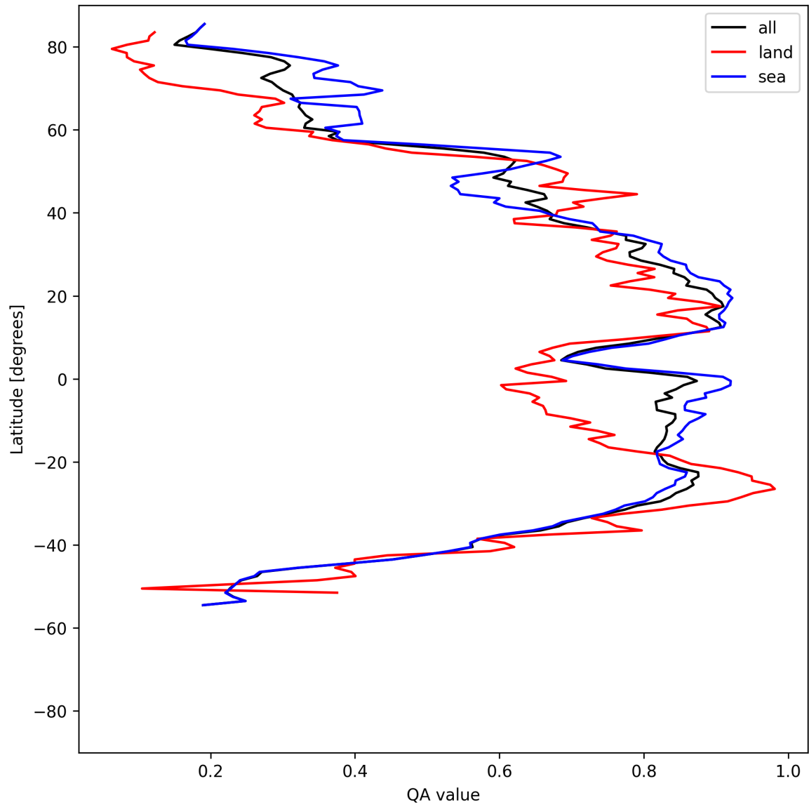
Figure 31: Zonal average of “QA value” for 2025-04-29 to 2025-05-01.
