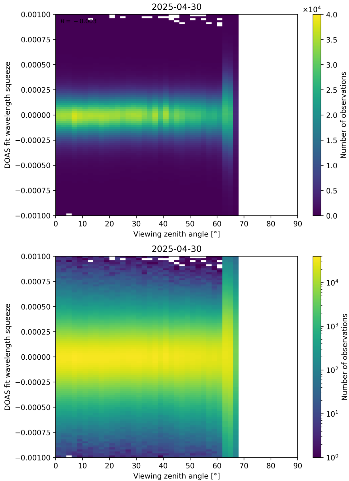
Figure 366: Scatter density plot of “Viewing zenith angle” against “DOAS fit wavelength squeeze” for 2025-04-29 to 2025-05-01.
