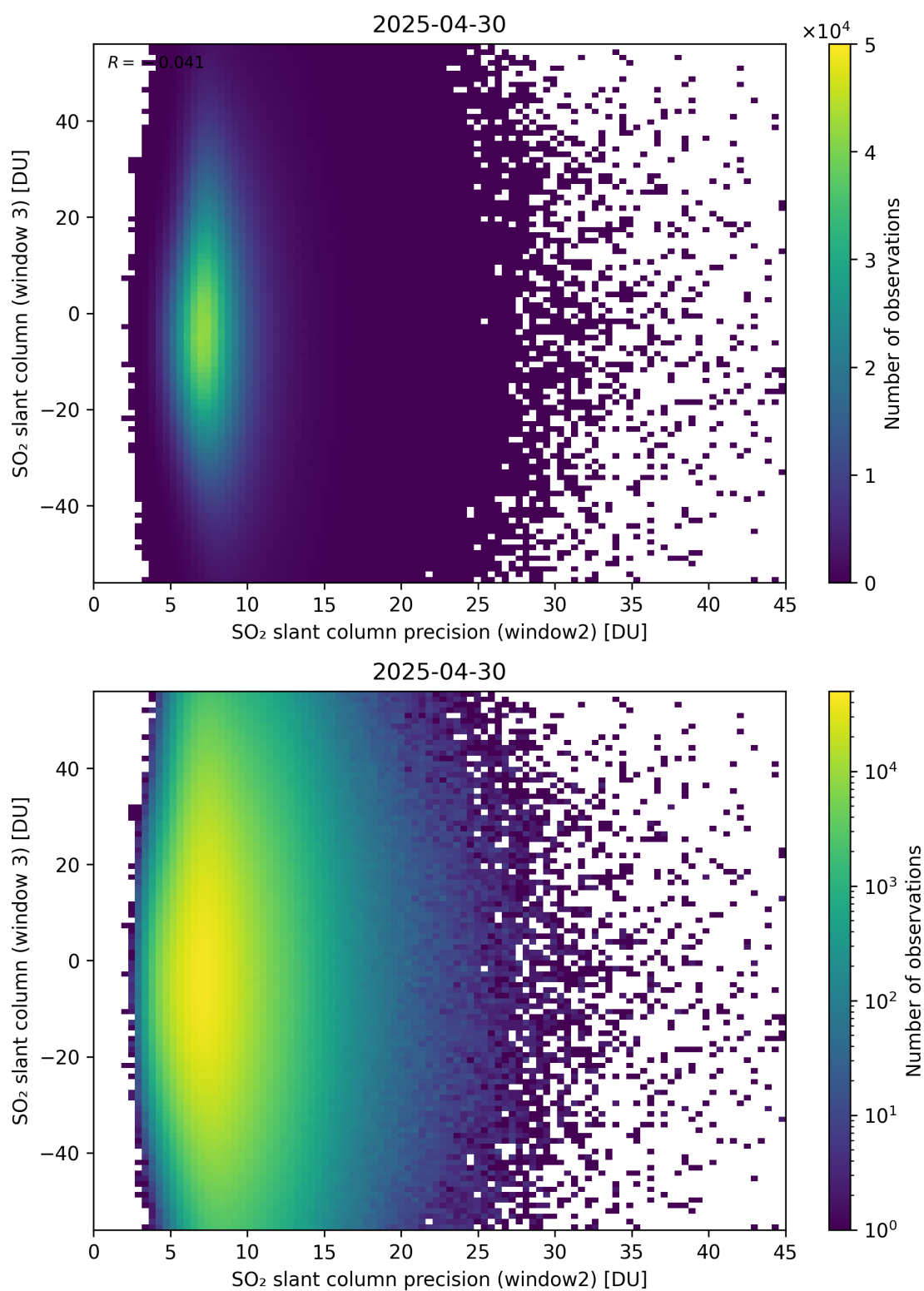
Figure 299: Scatter density plot of “SO 2 slant column precision (window2)” against “SO 2 slant column (window 3)” for 2025-04-29 to 2025-05-01.
