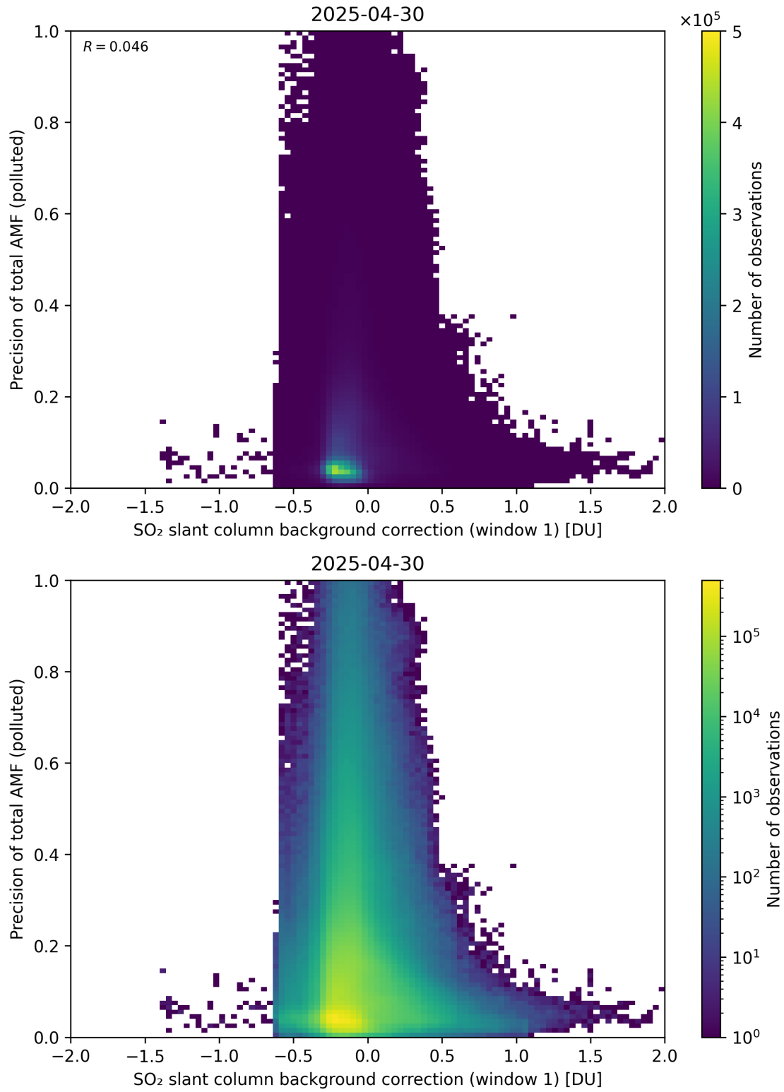
Figure 121: Scatter density plot of “SO 2 slant column background correction (window 1)” against “Precision of total AMF (polluted)” for 2025-04-29 to 2025-05-01.
