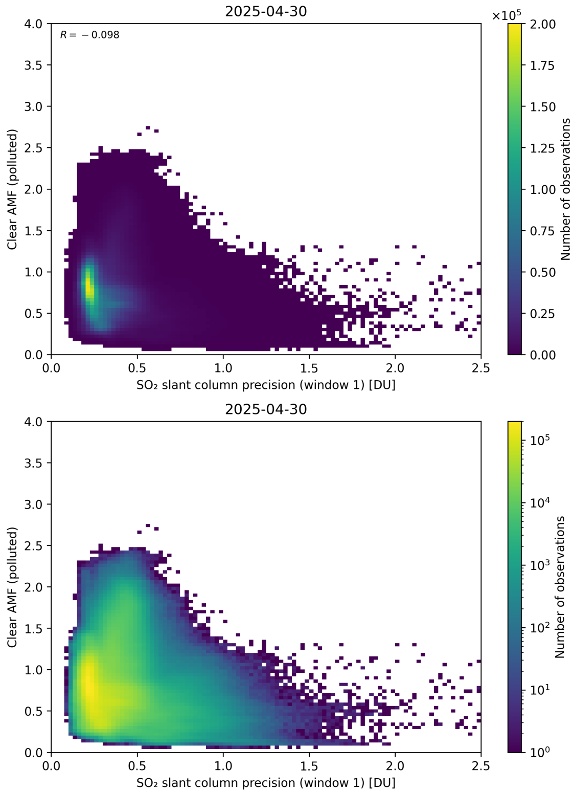
Figure 274: Scatter density plot of “SO 2 slant column precision (window 1)” against “Clear AMF (polluted)” for 2025-04-29 to 2025-05-01.
