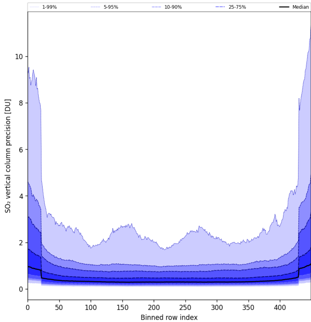
Figure 85: Along track statistics of “SO 2 vertical column precision” for 2025-04-29 to 2025-05-01
