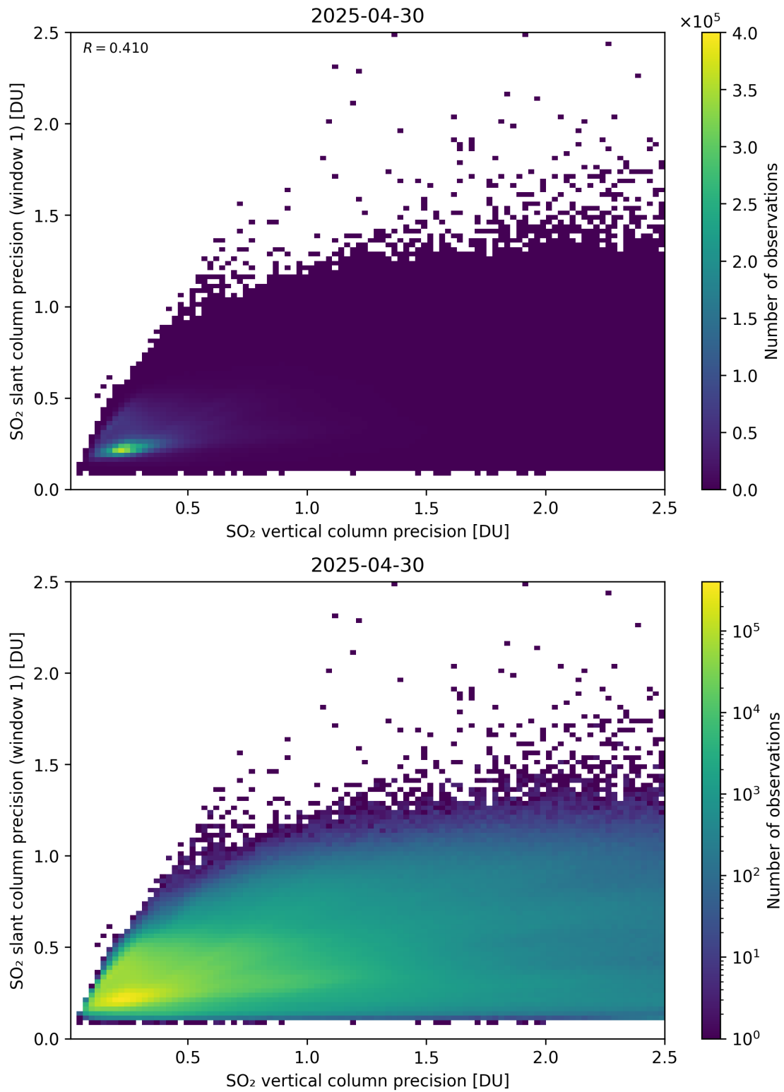
Figure 342: Scatter density plot of “SO 2 vertical column precision” against “SO 2 slant column precision (window 1)” for 2025-04-29 to 2025-05-01.
