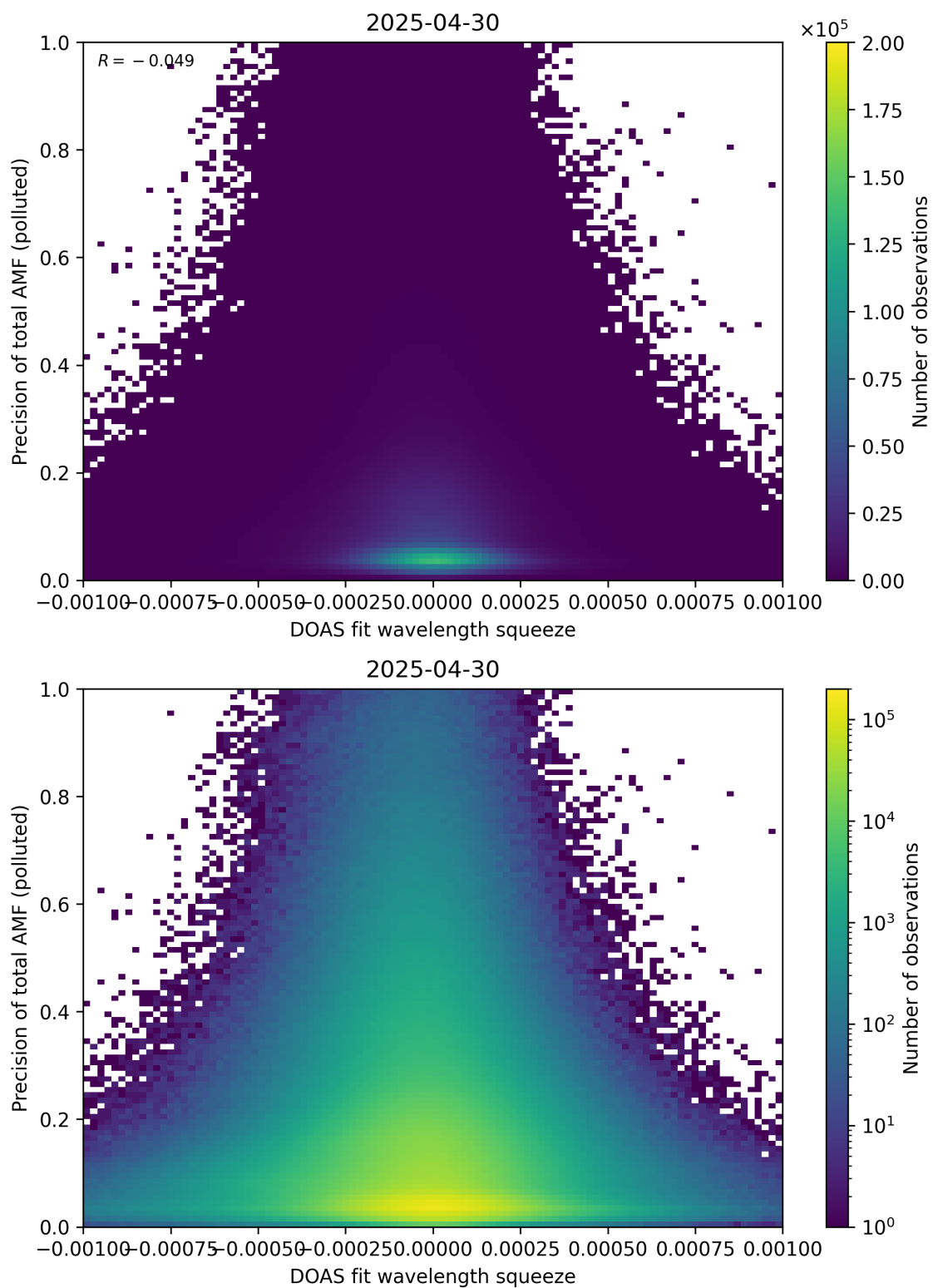
Figure 146: Scatter density plot of “DOAS fit wavelength squeeze” against “Precision of total AMF (polluted)” for 2025-04-29 to 2025-05-01.
