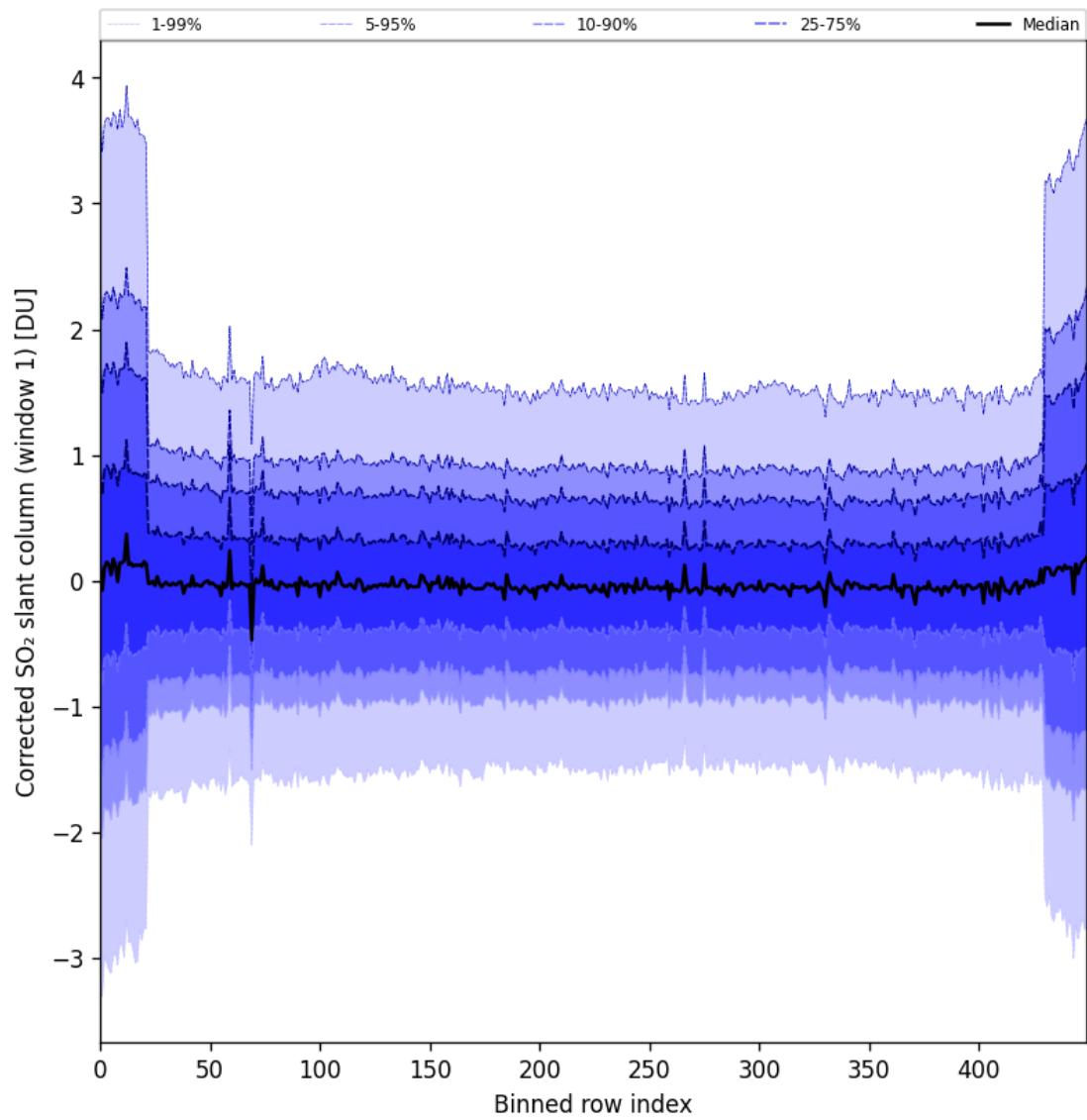
Figure 91: Along track statistics of “Corrected SO 2 slant column (window 1)” for 2025-04-29 to 2025-05-01
