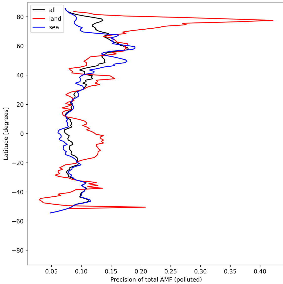
Figure 54: Zonal average of “Precision of total AMF (polluted)” for 2025-04-29 to 2025-05-01.
