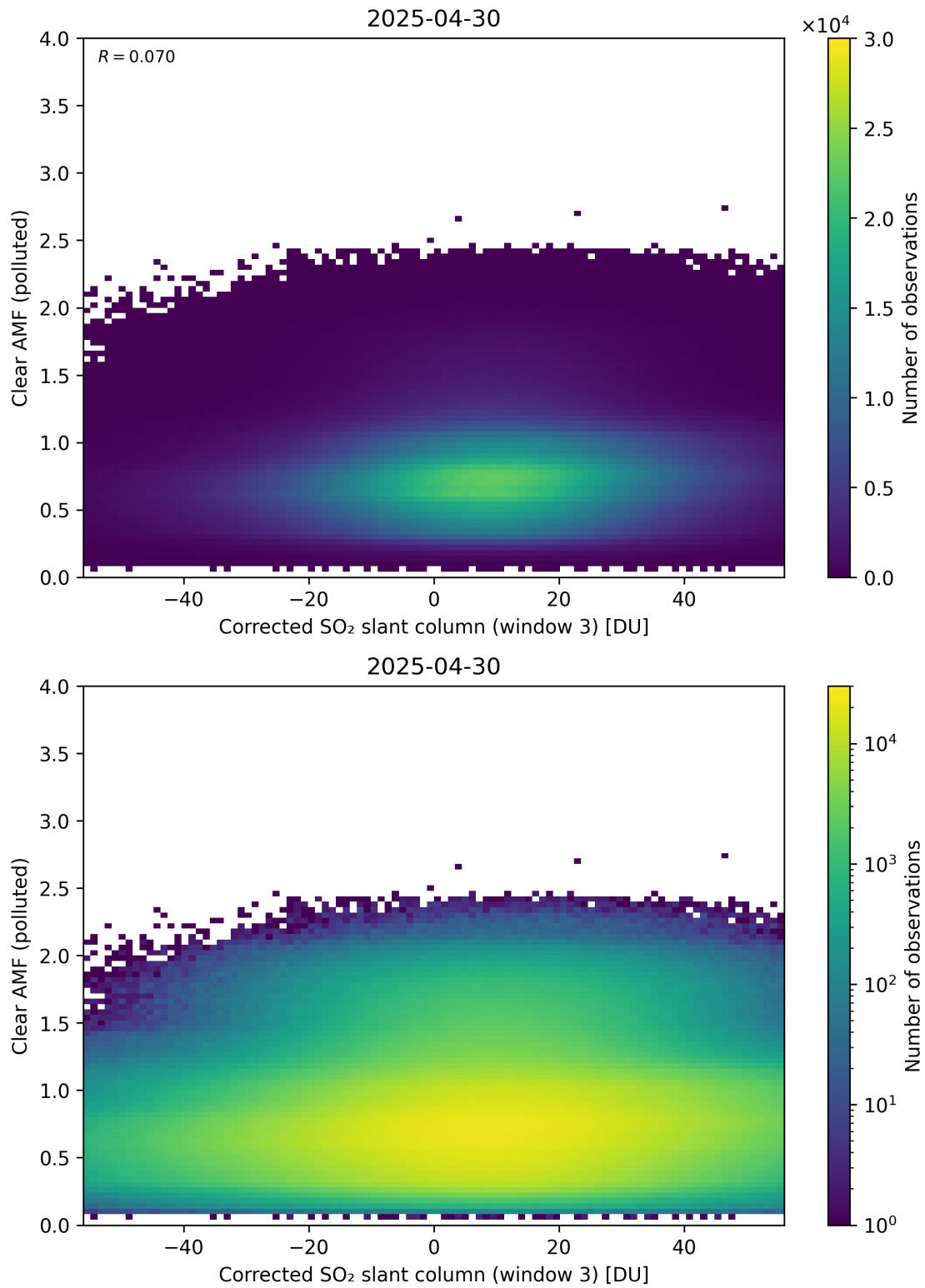
Figure 259: Scatter density plot of “Corrected SO 2 slant column (window 3)” against “Clear AMF (polluted)” for 2025-04-29 to 2025-05-01.
