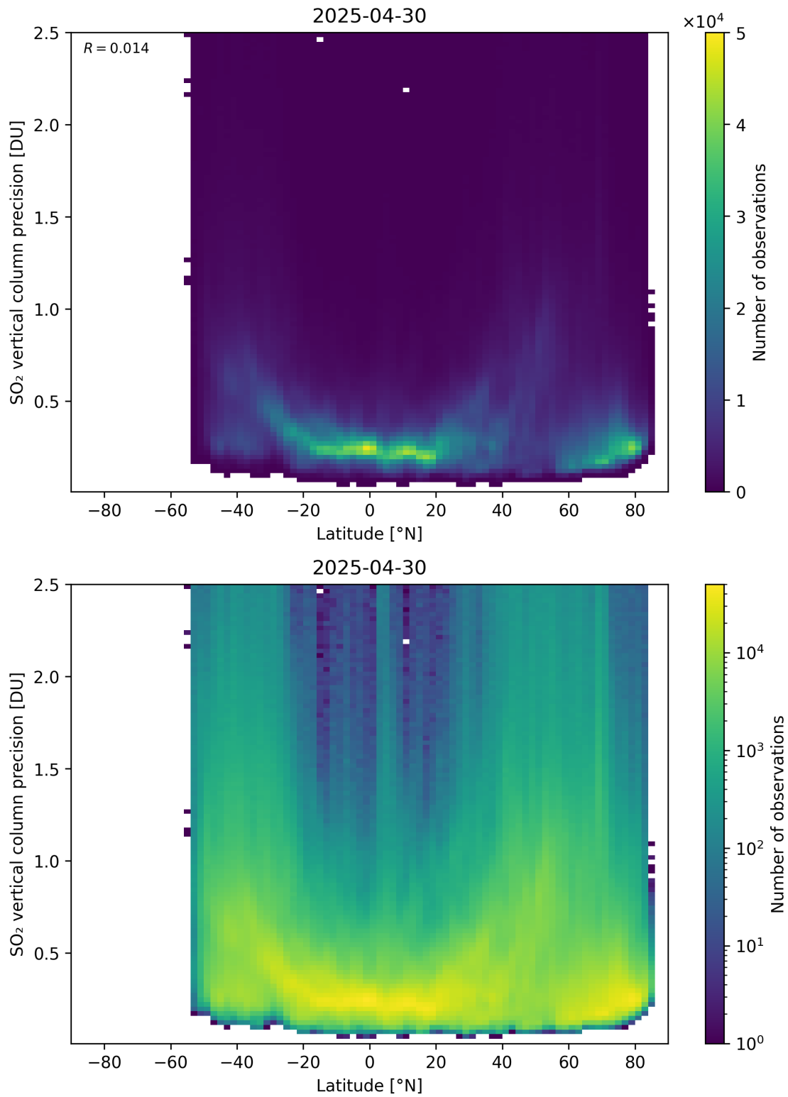
Figure 170: Scatter density plot of “Latitude” against “SO 2 vertical column precision” for 2025-04-29 to 2025-05-01.
