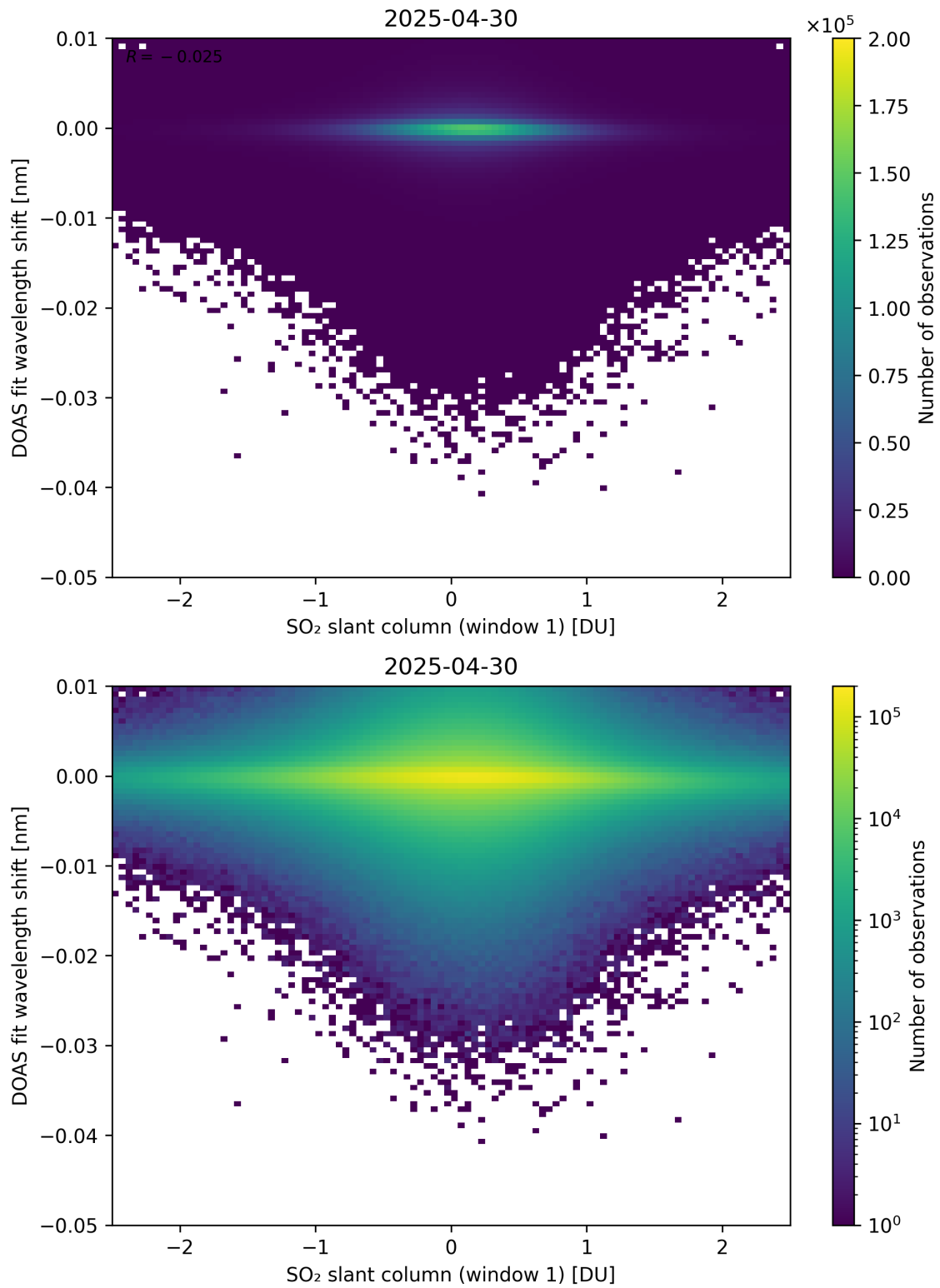
Figure 265: Scatter density plot of “SO 2 slant column (window 1)” against “DOAS fit wavelength shift” for 2025-04-29 to 2025-05-01.
