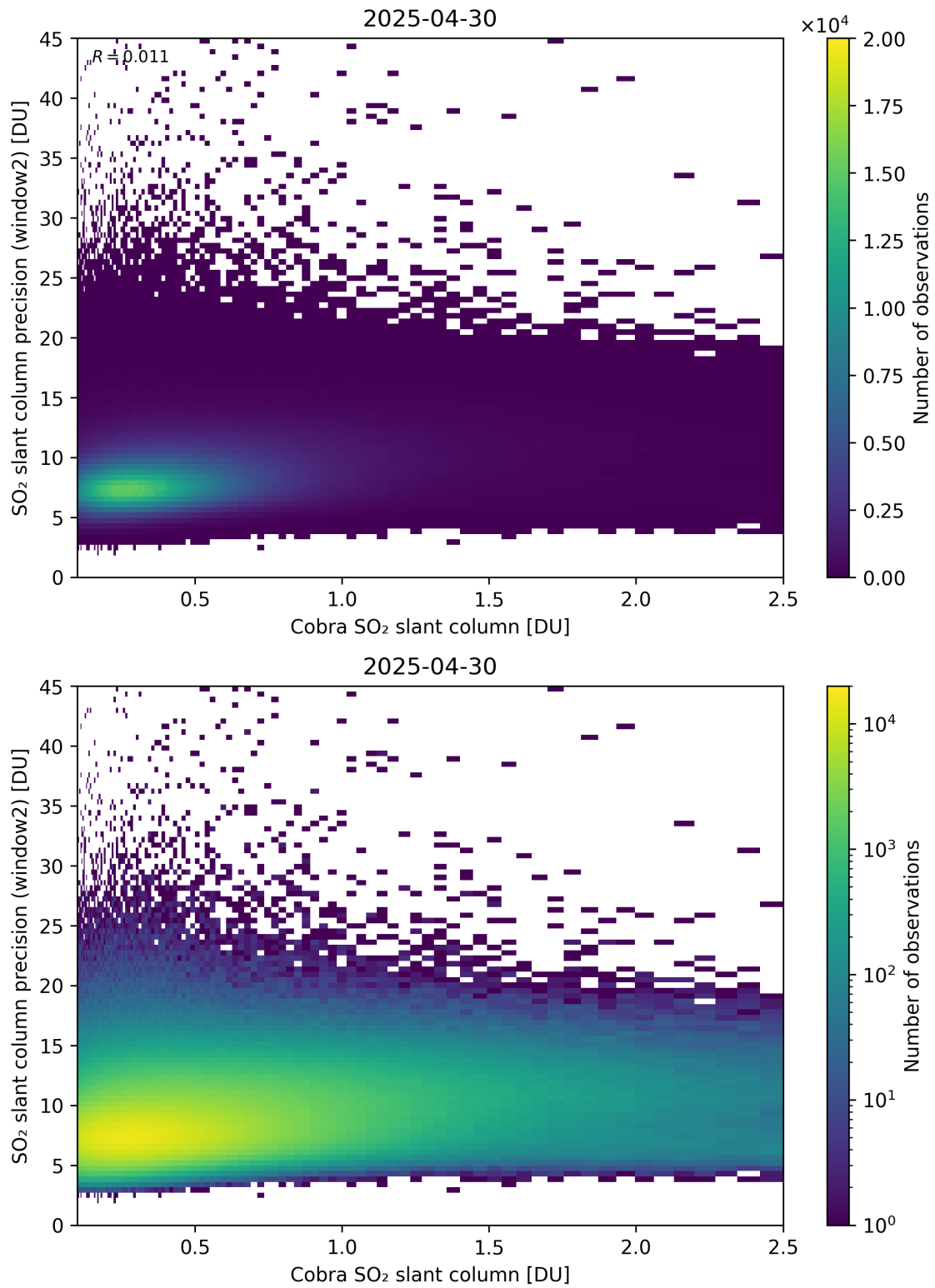
Figure 221: Scatter density plot of “Cobra SO 2 slant column” against “SO 2 slant column precision (window2)” for 2025-04-29 to 2025-05-01.
