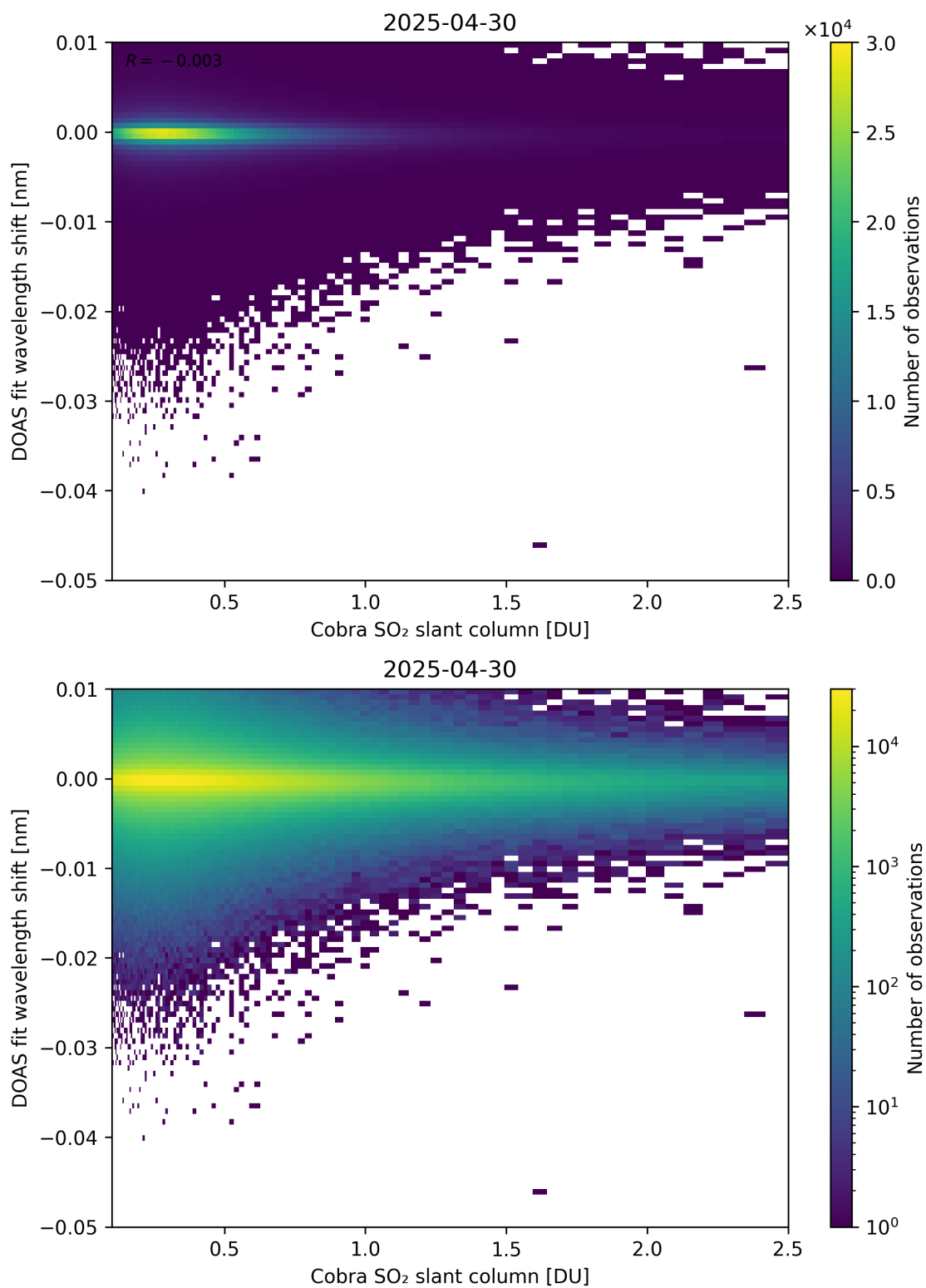
Figure 196: Scatter density plot of “Cobra SO 2 slant column” against “DOAS fit wavelength shift” for 2025-04-29 to 2025-05-01.
