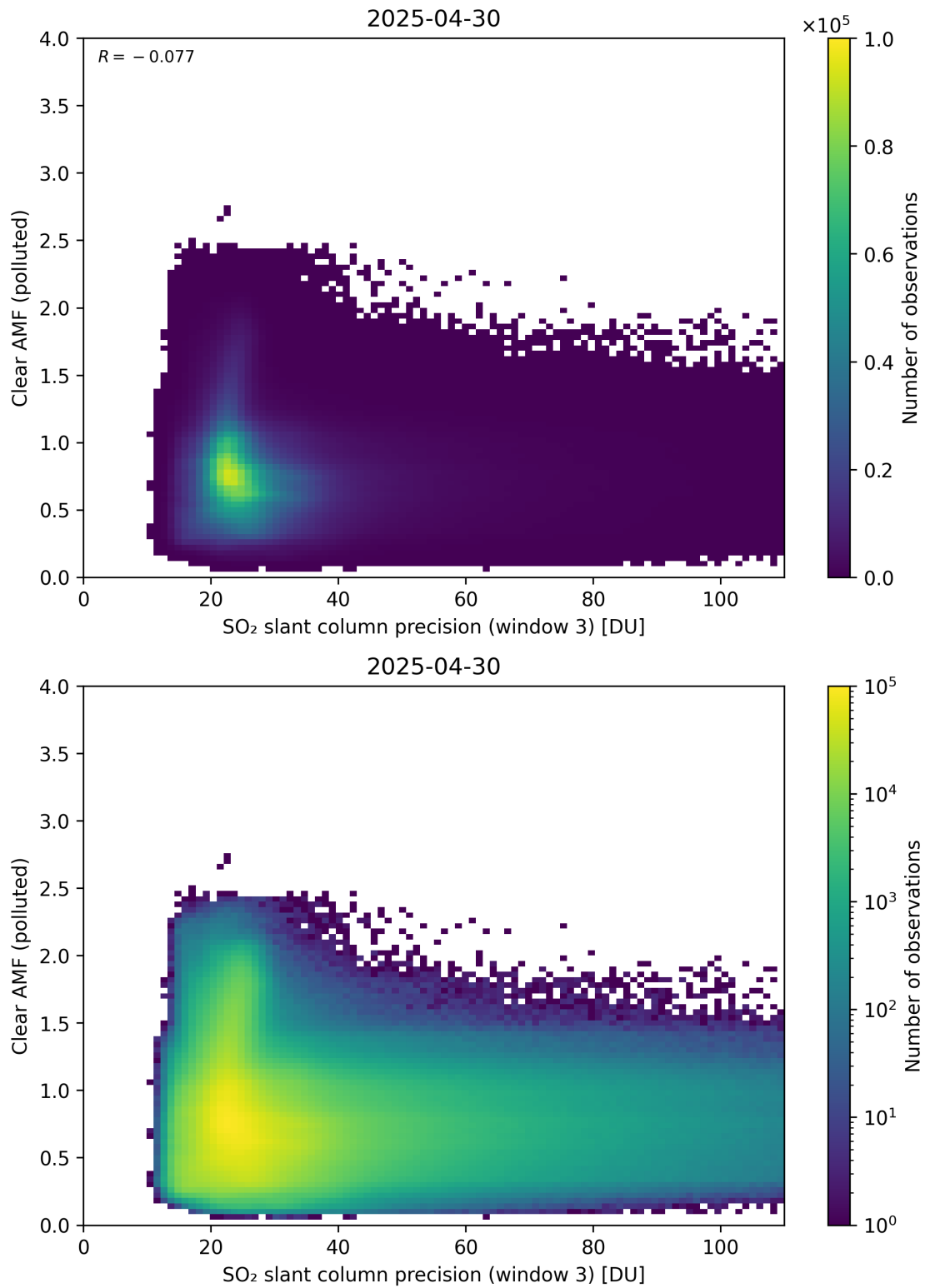
Figure 311: Scatter density plot of “SO 2 slant column precision (window 3)” against “Clear AMF (polluted)” for 2025-04-29 to 2025-05-01.
