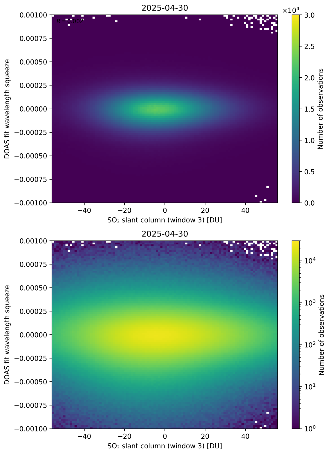
Figure 305: Scatter density plot of “SO 2 slant column (window 3)” against “DOAS fit wavelength squeeze” for 2025-04-29 to 2025-05-01.
