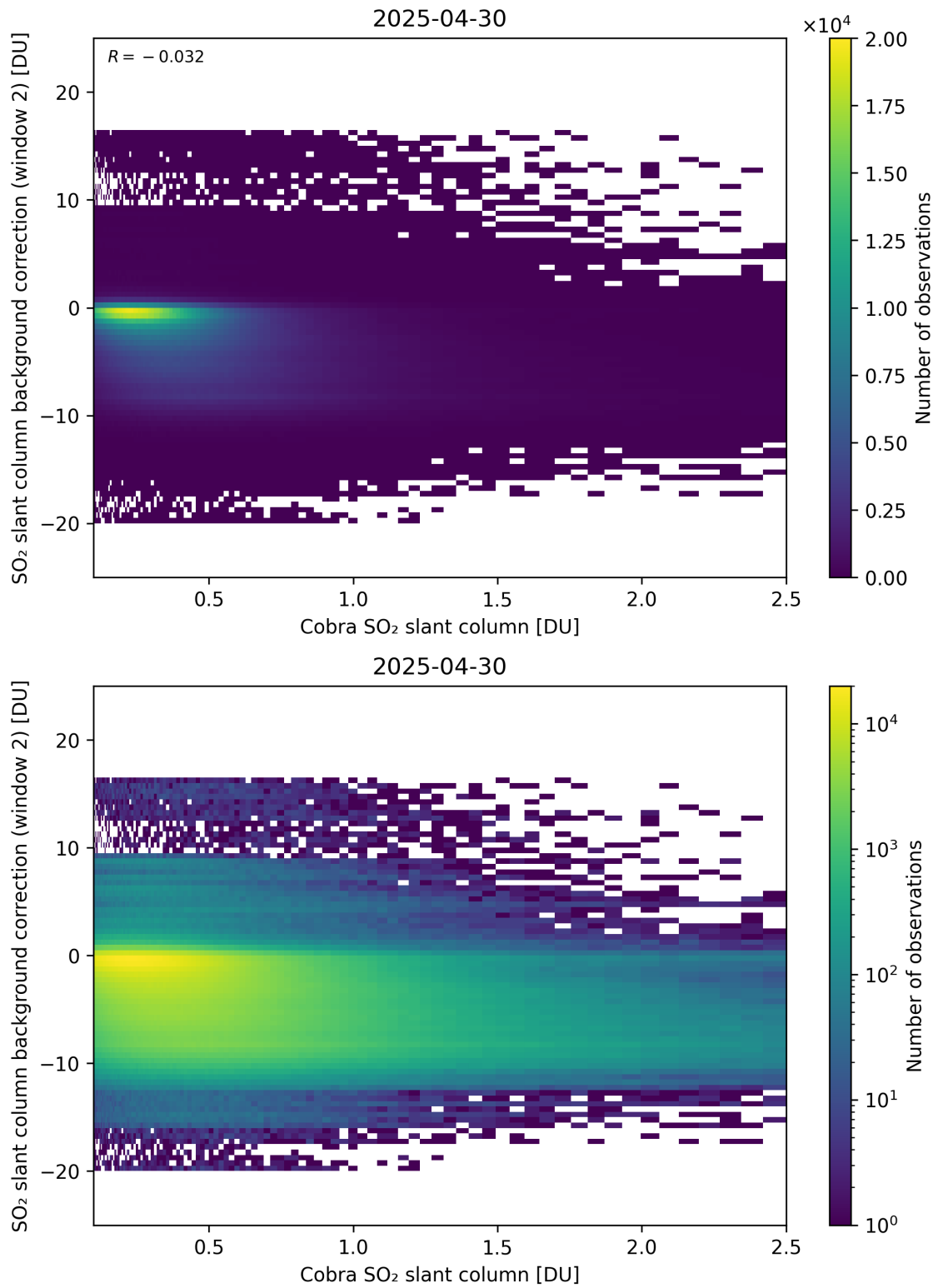
Figure 194: Scatter density plot of “Cobra SO 2 slant column” against “SO 2 slant column background correction (window 2)” for 2025-04-29 to 2025-05-01.
