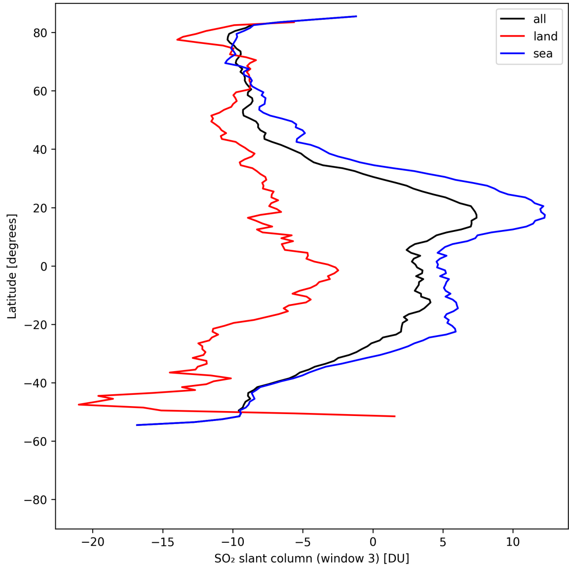
Figure 45: Zonal average of “SO 2 slant column (window 3)” for 2025-04-29 to 2025-05-01.
