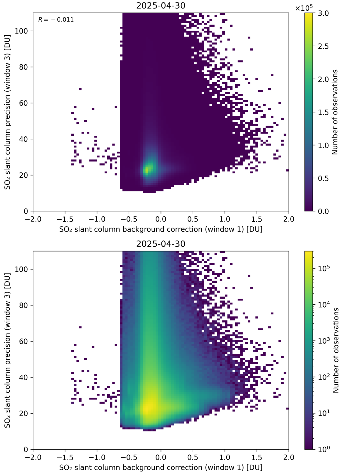
Figure 119: Scatter density plot of “SO 2 slant column background correction (window 1)” against “SO 2 slant column precision (window 3)” for 2025-04-29 to 2025-05-01.
