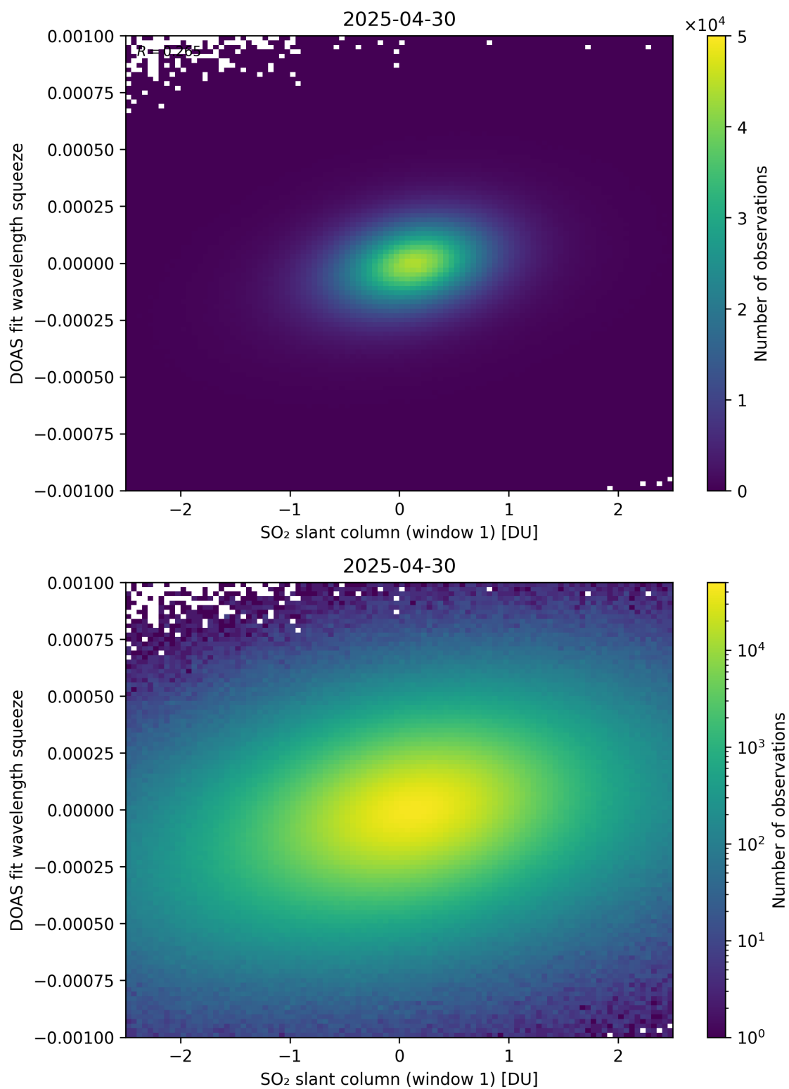
Figure 266: Scatter density plot of “SO 2 slant column (window 1)” against “DOAS fit wavelength squeeze” for 2025-04-29 to 2025-05-01.
