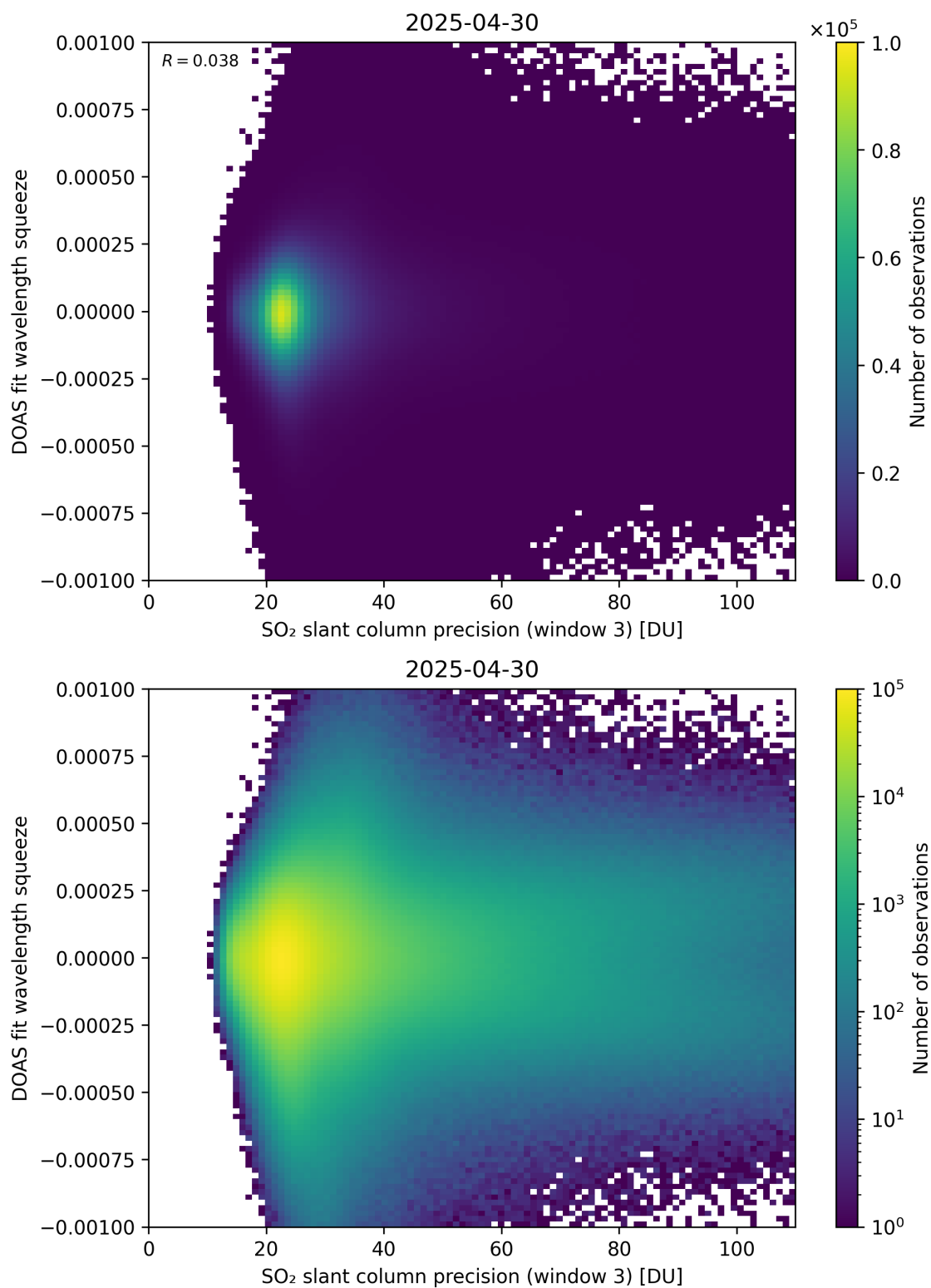
Figure 309: Scatter density plot of “SO 2 slant column precision (window 3)” against “DOAS fit wavelength squeeze” for 2025-04-29 to 2025-05-01.
