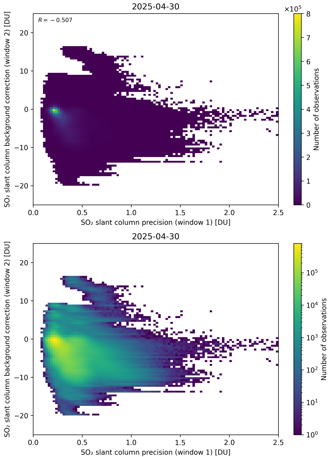
Figure 269: Scatter density plot of “SO 2 slant column precision (window 1)” against “SO 2 slant column background correction (window 2)” for 2025-04-29 to 2025-05-01.
