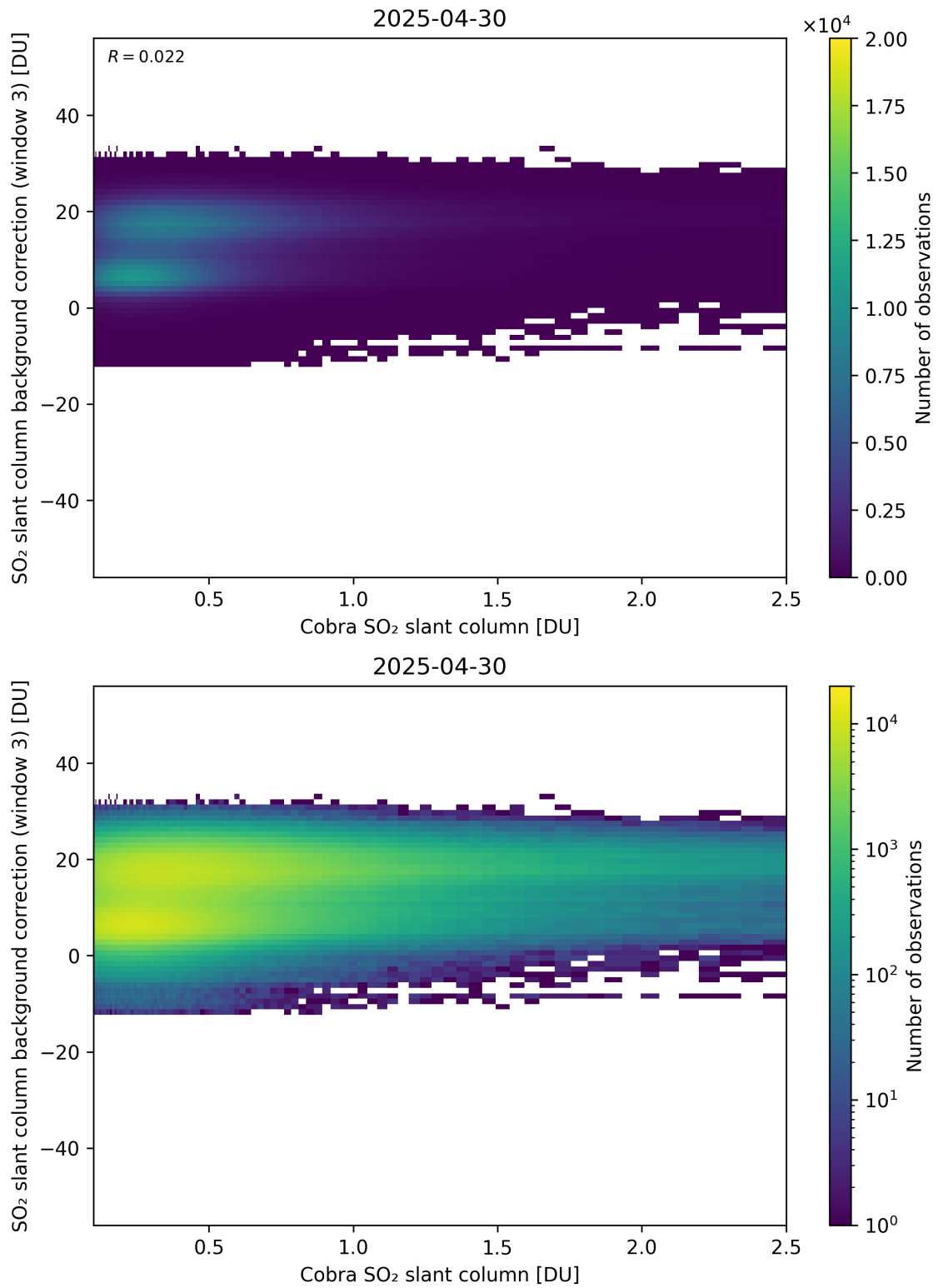
Figure 195: Scatter density plot of “Cobra SO 2 slant column” against “SO 2 slant column background correction (window 3)” for 2025-04-29 to 2025-05-01.
