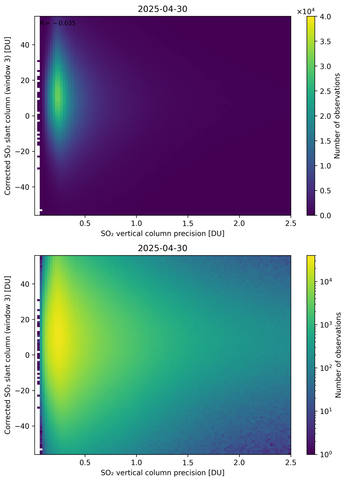
Figure 340: Scatter density plot of “SO 2 vertical column precision” against “Corrected SO 2 slant column (window 3)” for 2025-04-29 to 2025-05-01.
