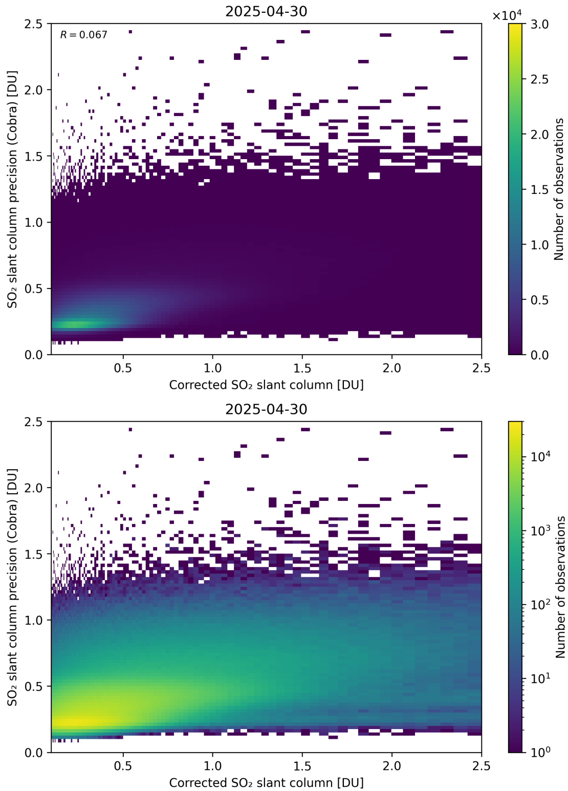
Figure 234: Scatter density plot of “Corrected SO 2 slant column” against “SO 2 slant column precision (Cobra)” for 2025-04-29 to 2025-05-01.
