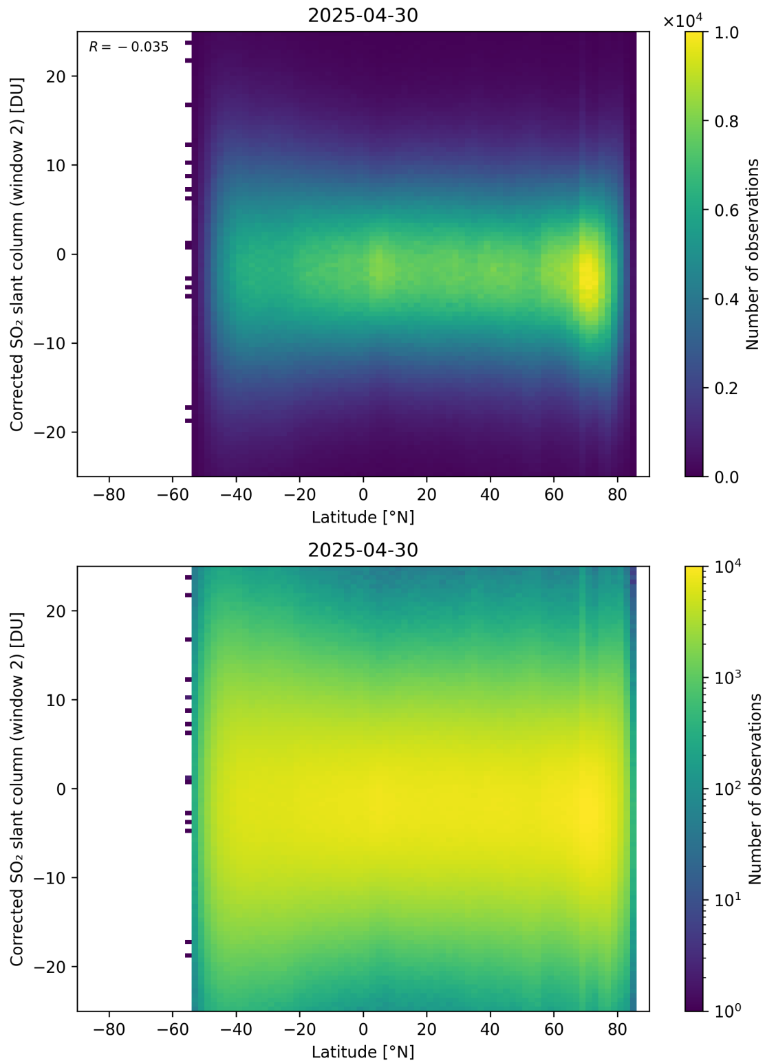
Figure 160: Scatter density plot of “Latitude” against “Corrected SO 2 slant column (window 2)” for 2025-04-29 to 2025-05-01.
