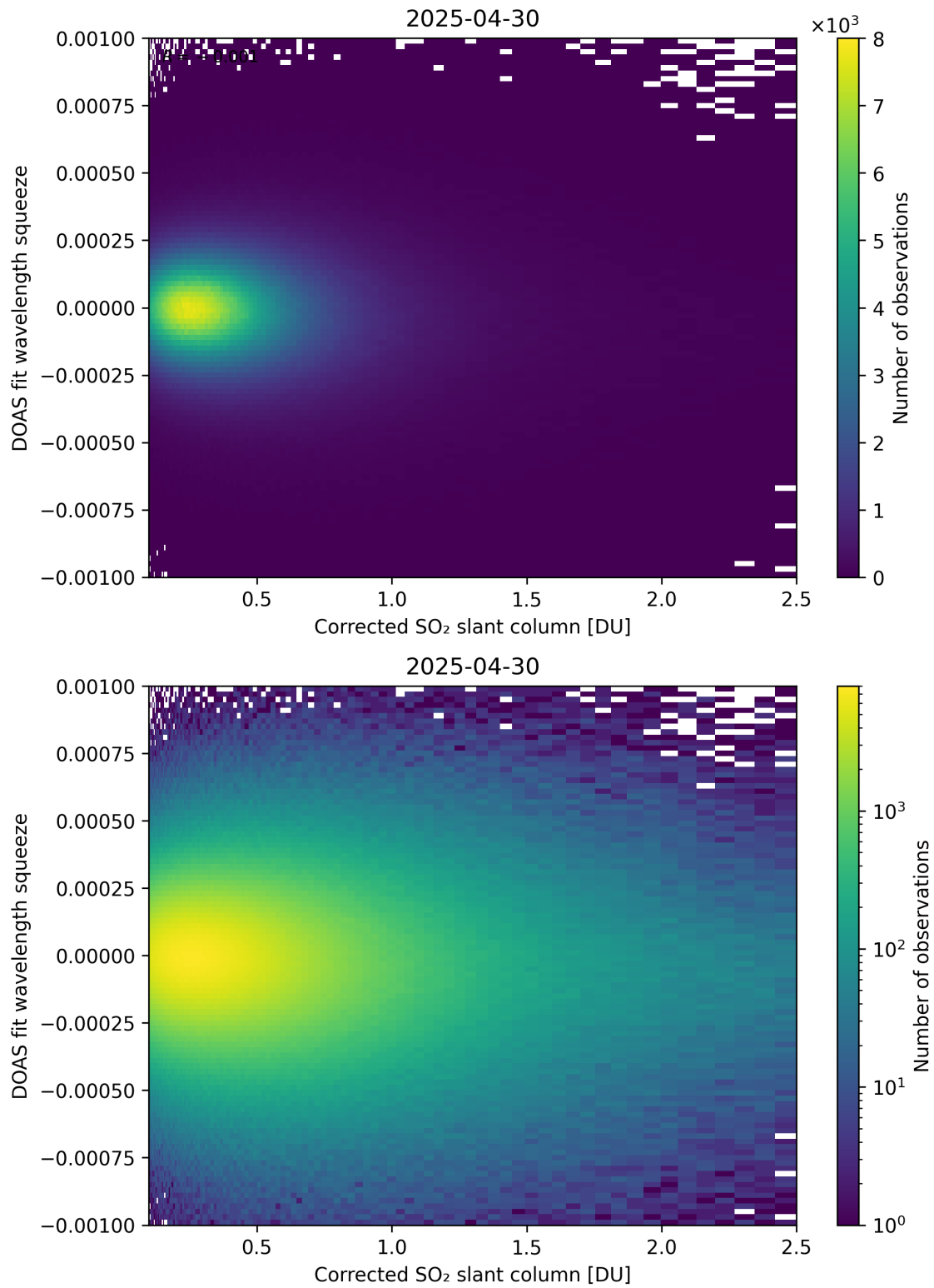
Figure 230: Scatter density plot of "Corrected SO 2 slant column" against "DOAS fit wavelength squeeze" for 2025-04-29 to 2025-05-01.
