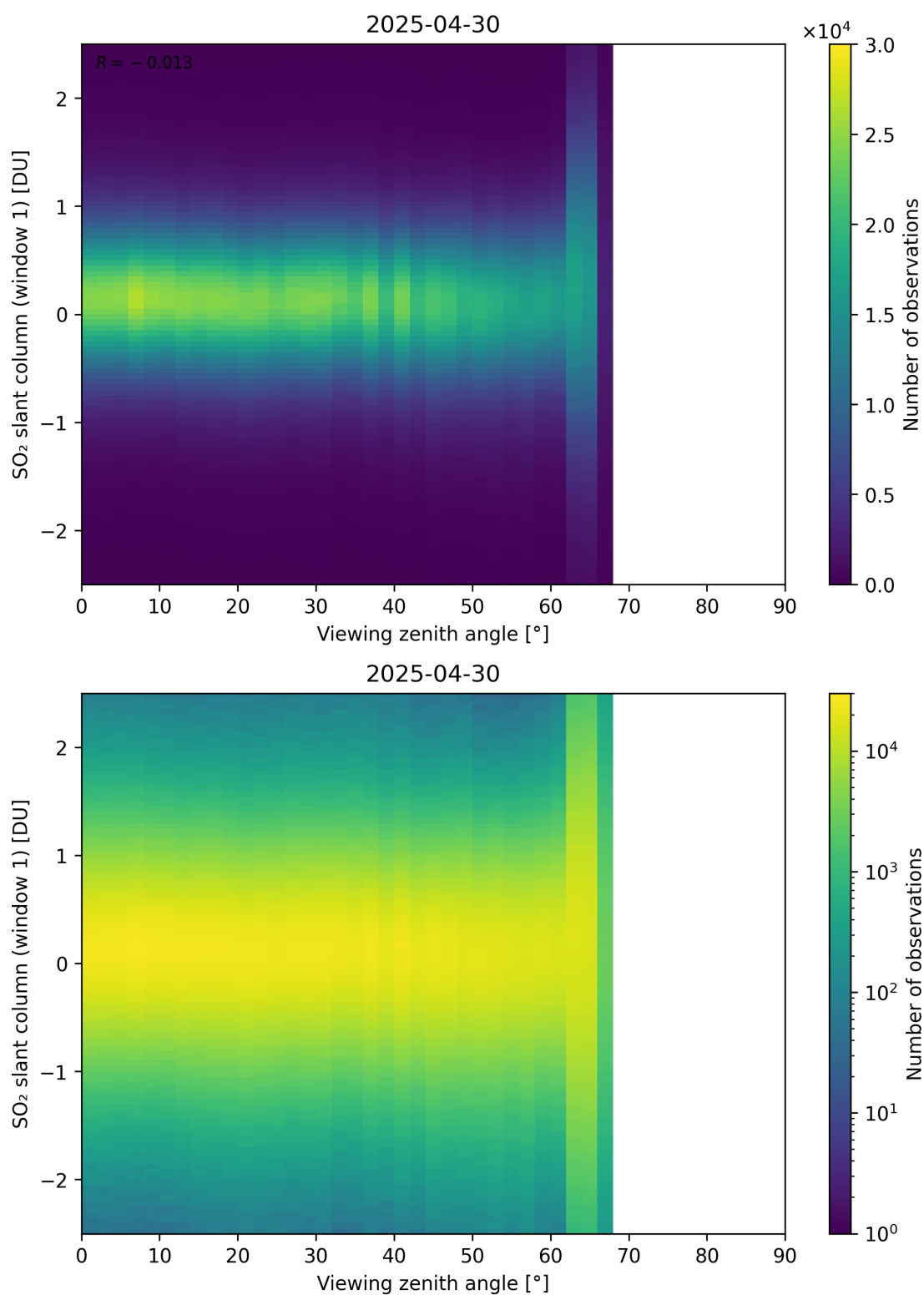
Figure 376: Scatter density plot of “Viewing zenith angle” against “SO 2 slant column (window 1)” for 2025-04-29 to 2025-05-01.
