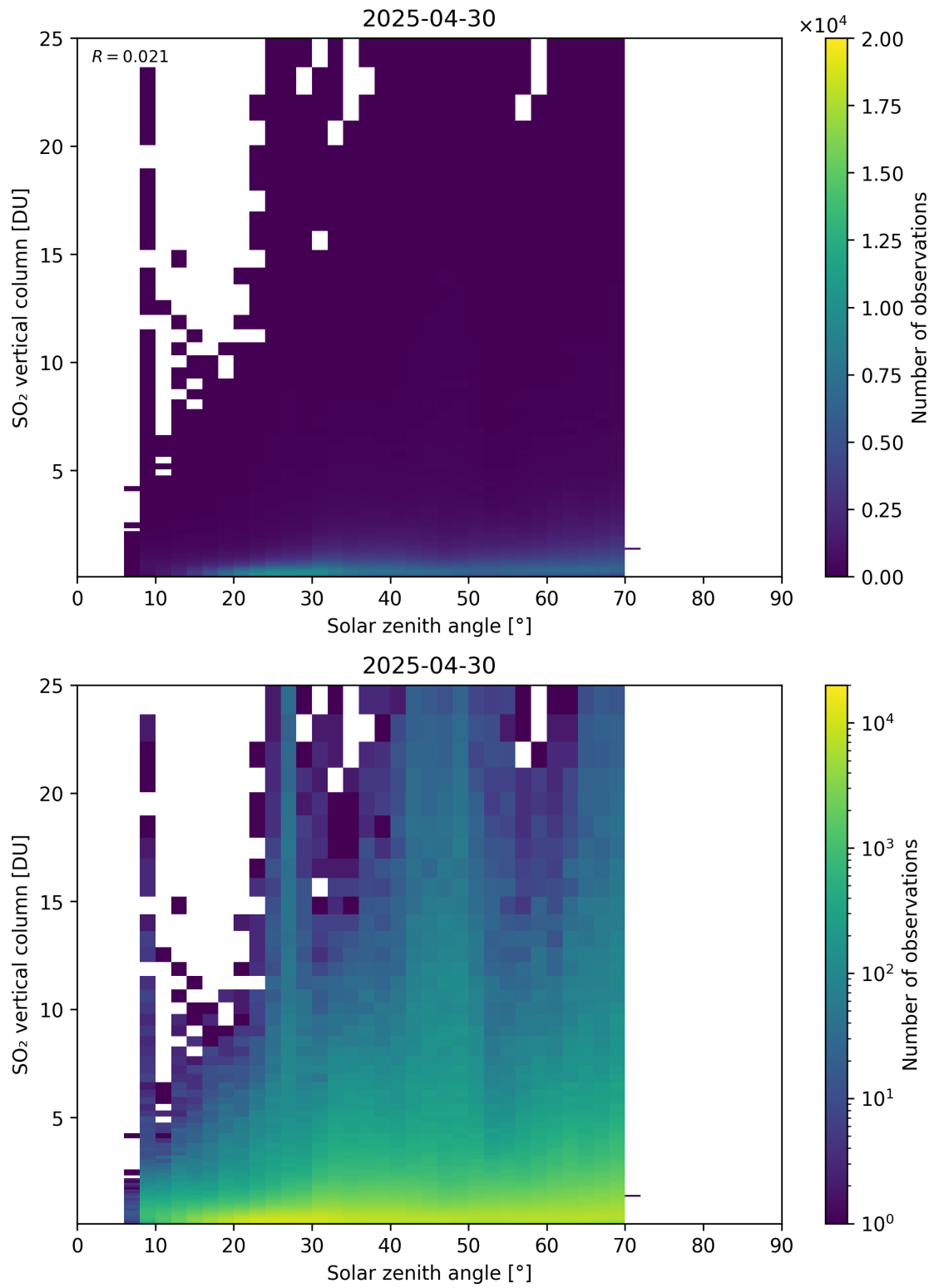
Figure 191: Scatter density plot of “Solar zenith angle” against “SO 2 vertical column” for 2025-04-29 to 2025-05-01.
