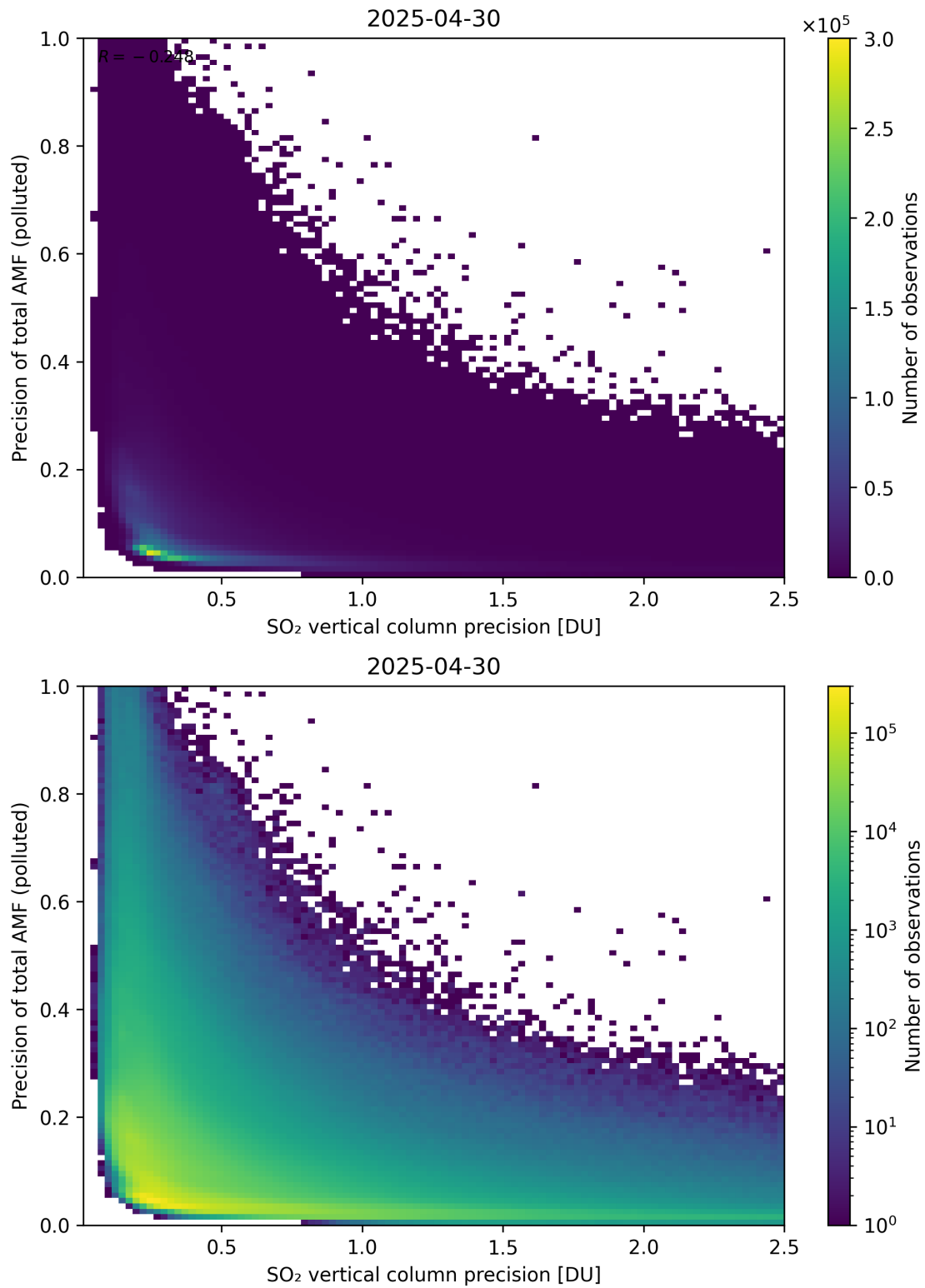
Figure 347: Scatter density plot of “SO 2 vertical column precision” against “Precision of total AMF (polluted)” for 2025-04-29 to 2025-05-01.
