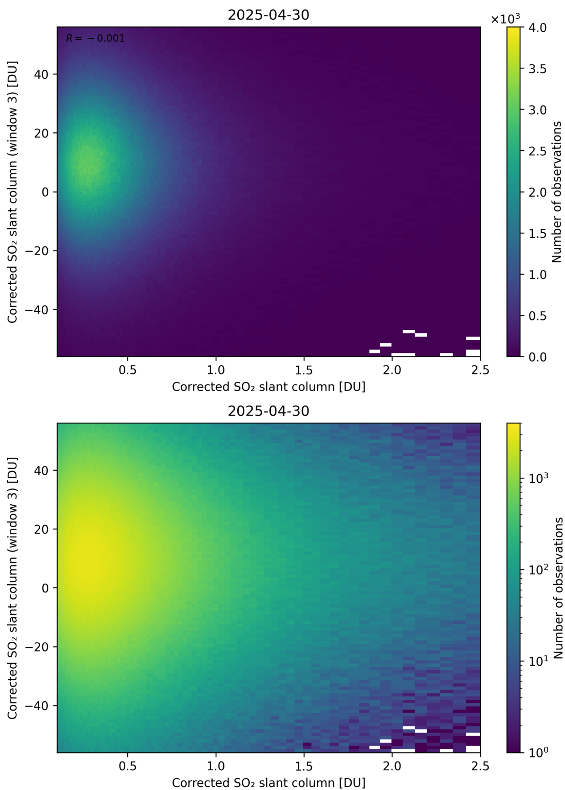
Figure 236: Scatter density plot of “Corrected SO 2 slant column” against “Corrected SO 2 slant column (window 3)” for 2025-04-29 to 2025-05-01.
