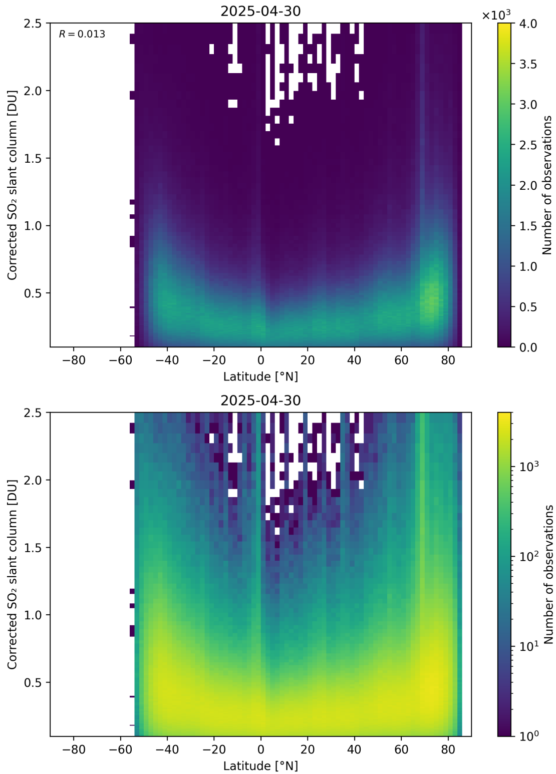
Figure 159: Scatter density plot of “Latitude” against “Corrected SO 2 slant column” for 2025-04-29 to 2025-05-01.
