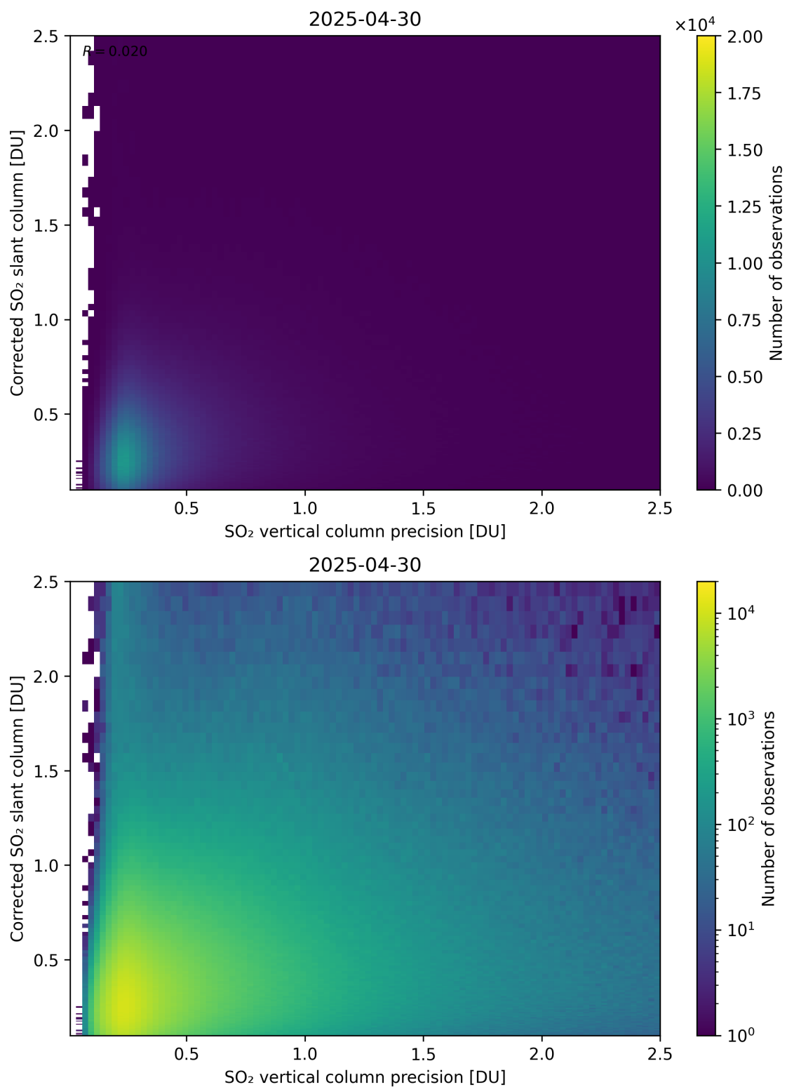
Figure 338: Scatter density plot of “SO 2 vertical column precision” against “Corrected SO 2 slant column” for 2025-04-29 to 2025-05-01.
