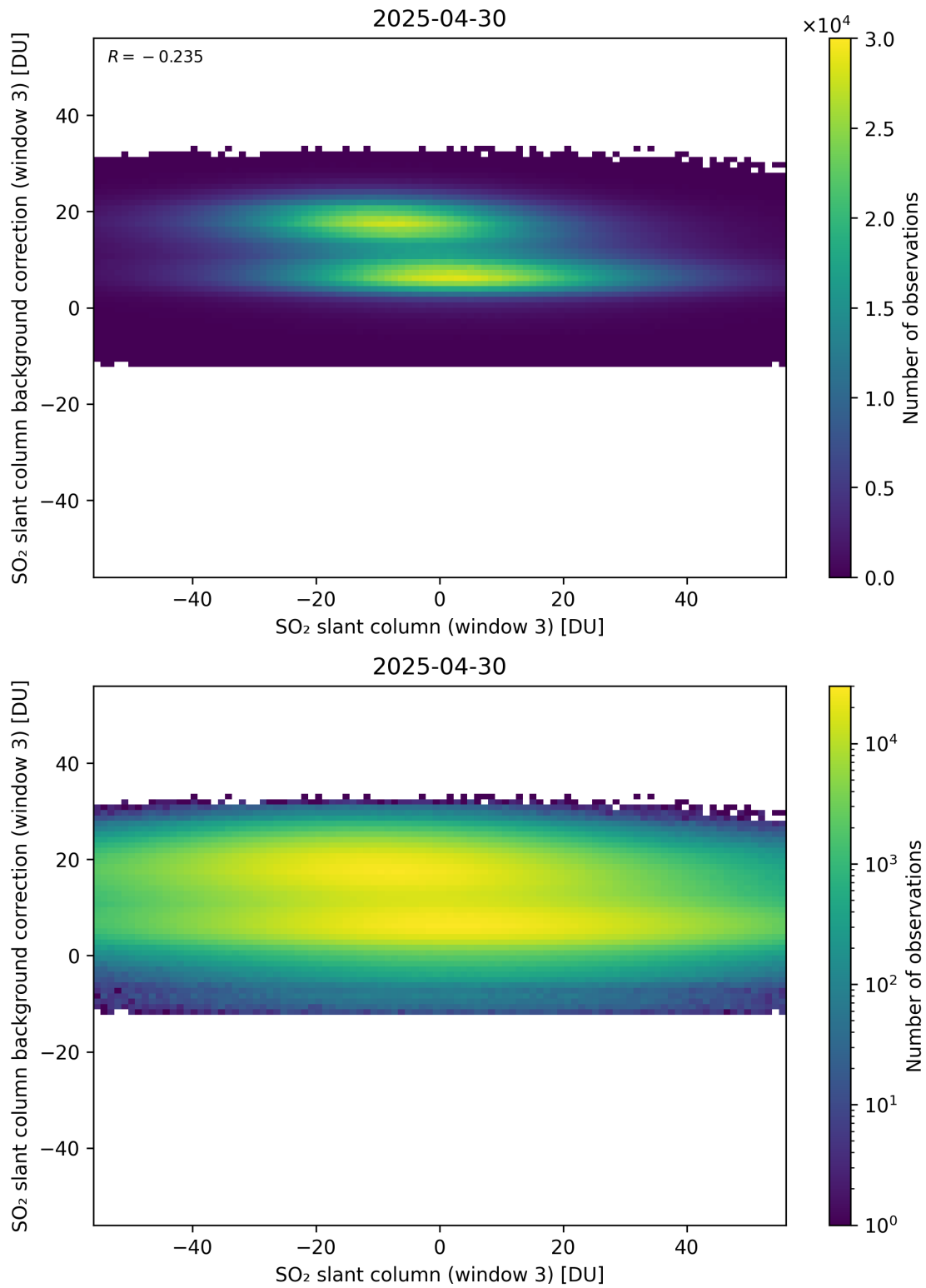
Figure 303: Scatter density plot of “SO 2 slant column (window 3)” against “SO 2 slant column background correction (window 3)” for 2025-04-29 to 2025-05-01.
