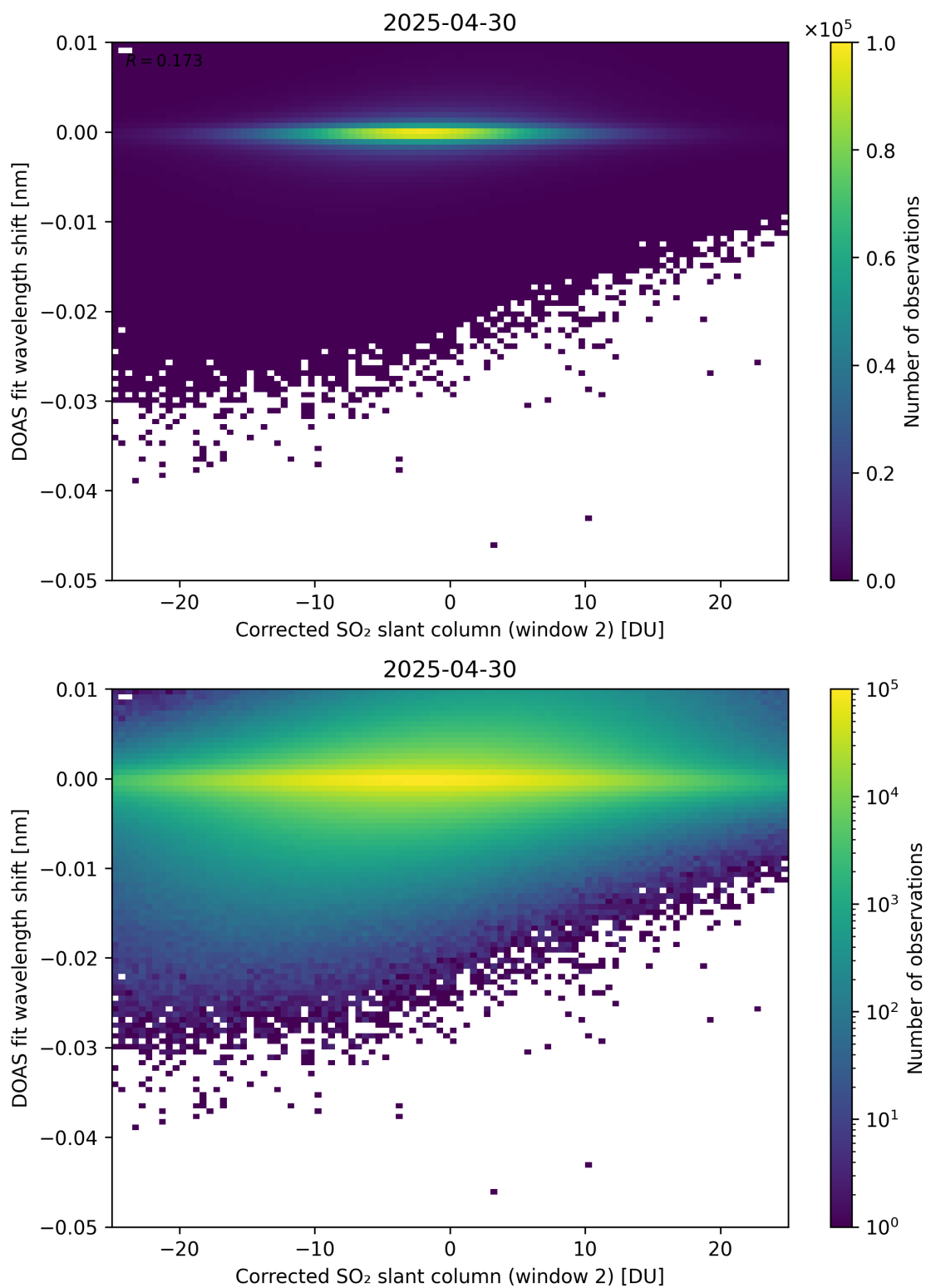
Figure 246: Scatter density plot of “Corrected SO 2 slant column (window 2)” against “DOAS fit wavelength shift” for 2025-04-29 to 2025-05-01.
