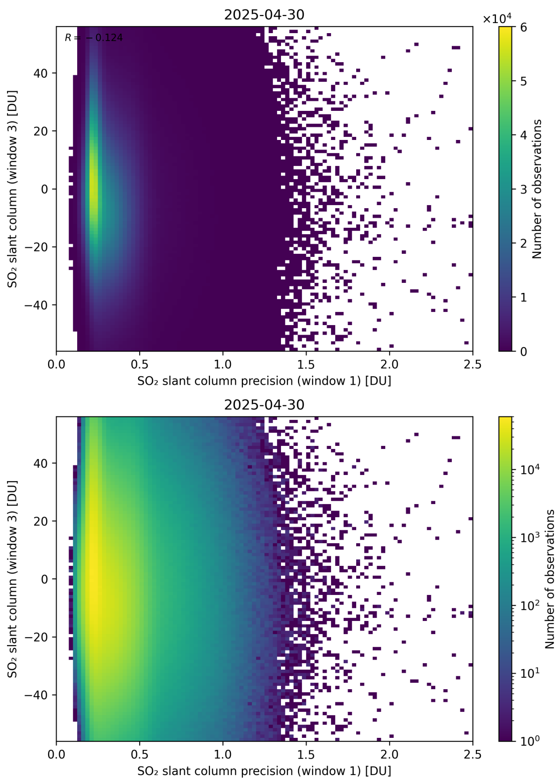
Figure 278: Scatter density plot of “SO 2 slant column precision (window 1)” against “SO 2 slant column (window 3)” for 2025-04-29 to 2025-05-01.
