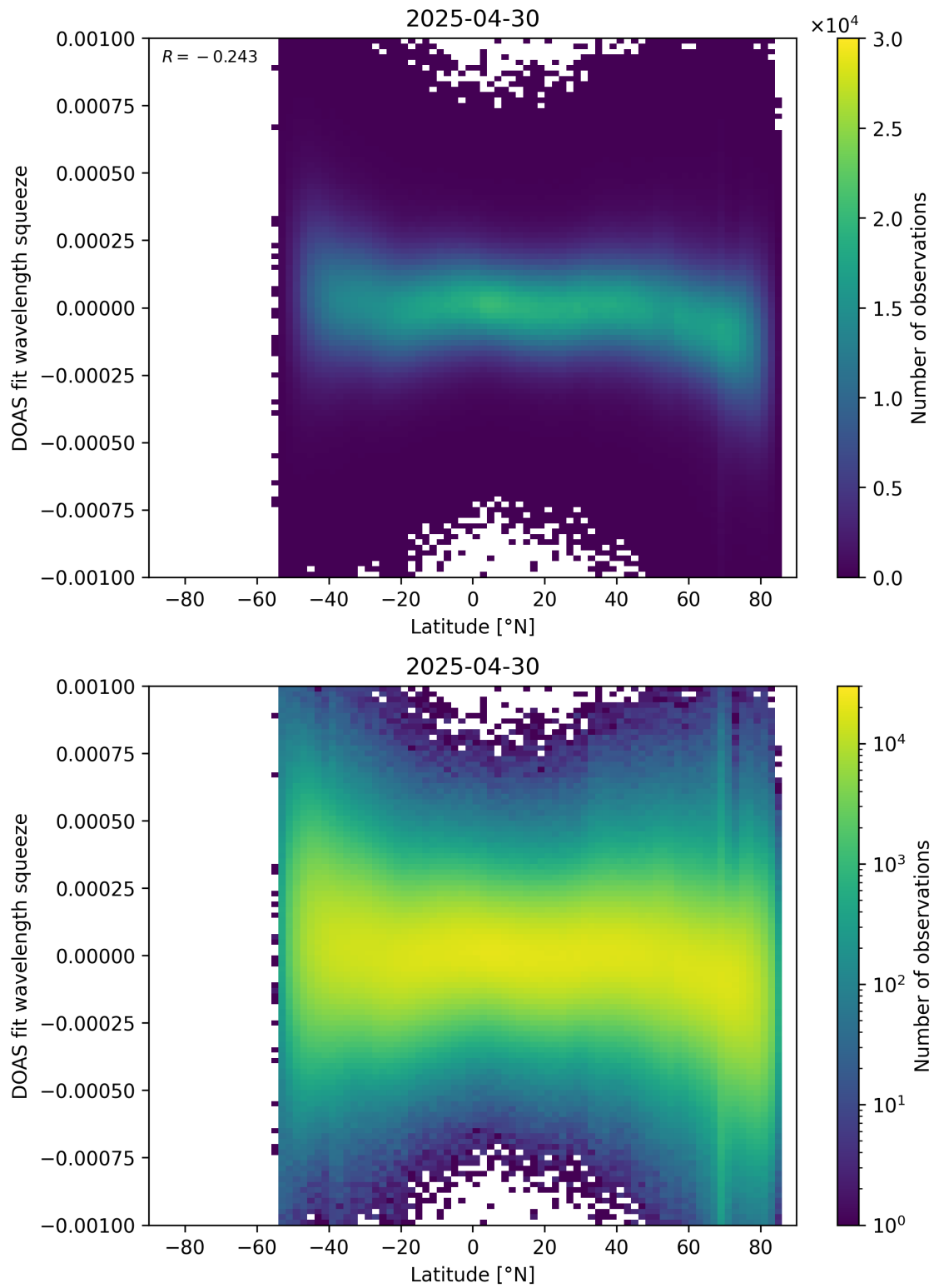
Figure 154: Scatter density plot of “Latitude” against “DOAS fit wavelength squeeze” for 2025-04-29 to 2025-05-01.
