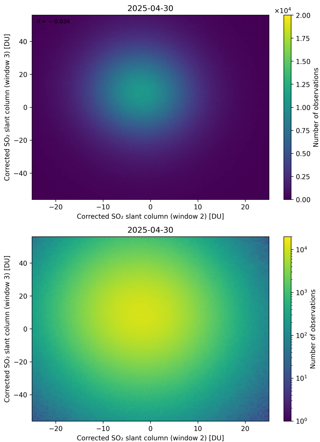
Figure 250: Scatter density plot of “Corrected SO 2 slant column (window 2)” against “Corrected SO 2 slant column (window 3)” for 2025-04-29 to 2025-05-01.
