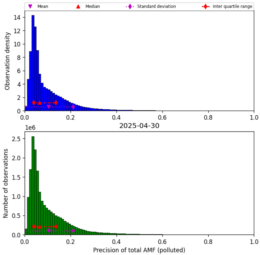
Figure 80: Histogram of “Precision of total AMF (polluted)” for 2025-04-29 to 2025-05-01
