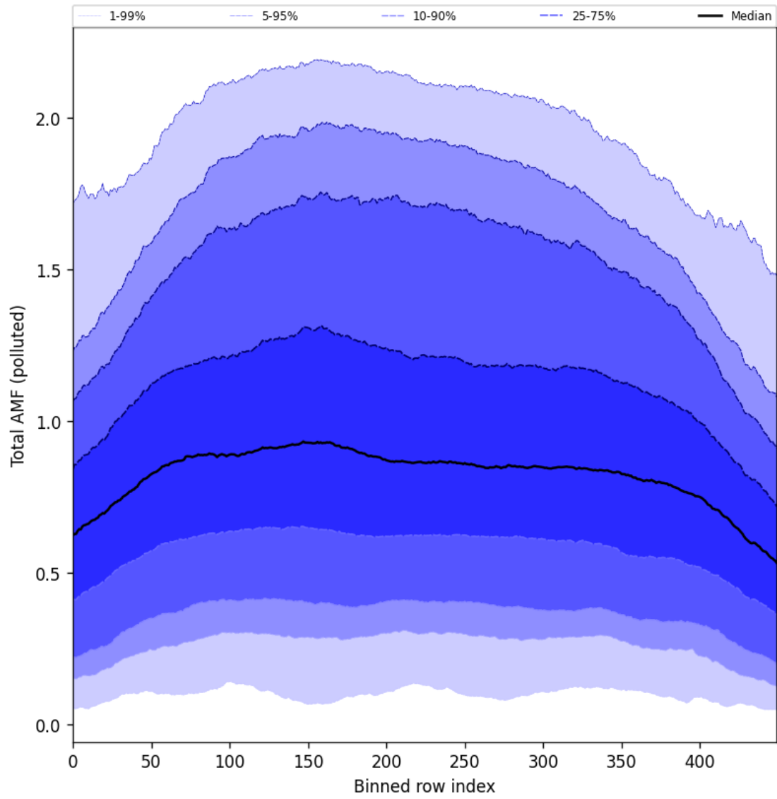
Figure 105: Along track statistics of “Total AMF (polluted)” for 2025-04-29 to 2025-05-01
