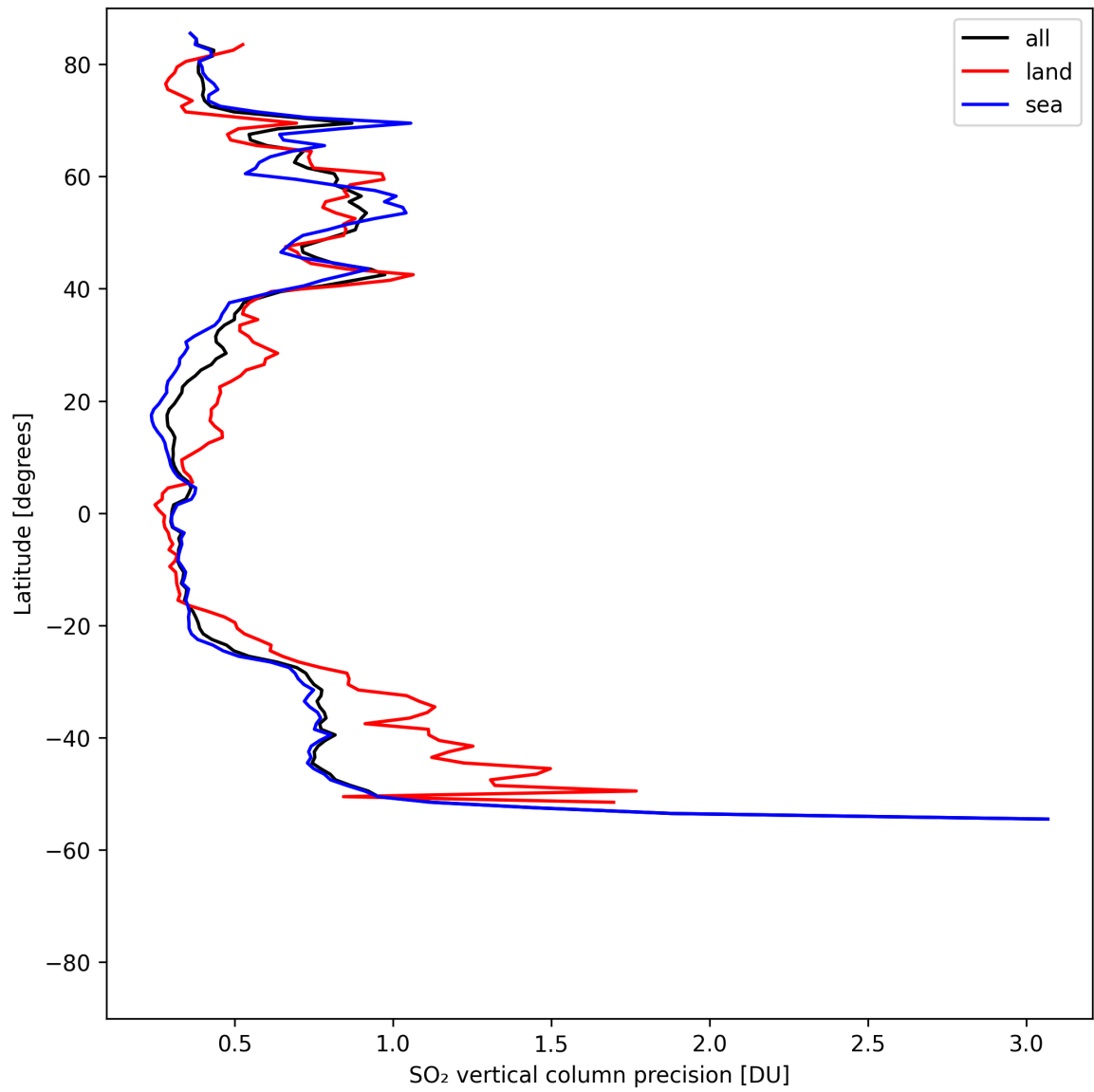
Figure 33: Zonal average of “SO 2 vertical column precision” for 2025-04-29 to 2025-05-01.
