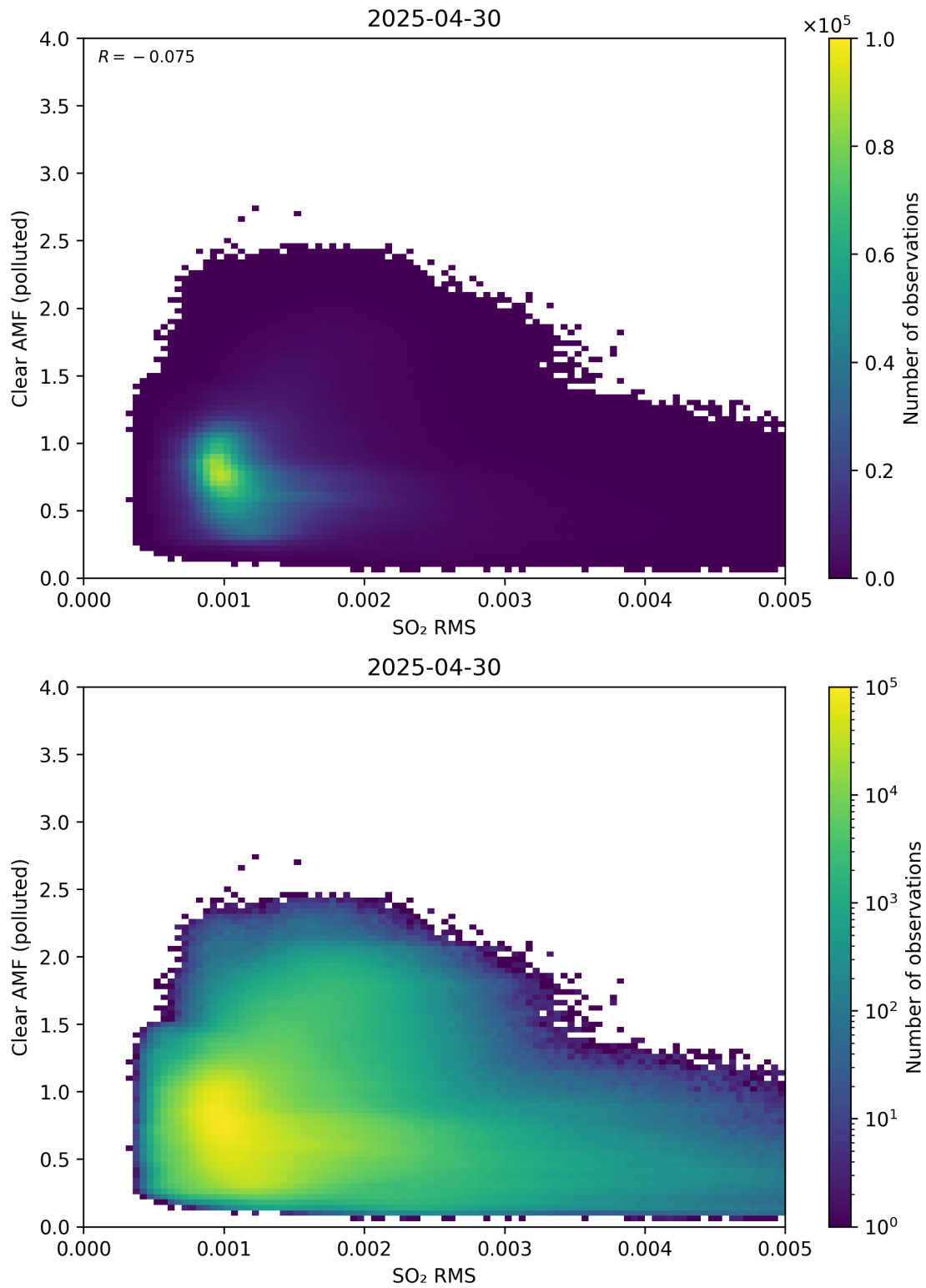
Figure 147: Scatter density plot of “SO 2 RMS” against “Clear AMF (polluted)” for 2025-04-29 to 2025-05-01.
