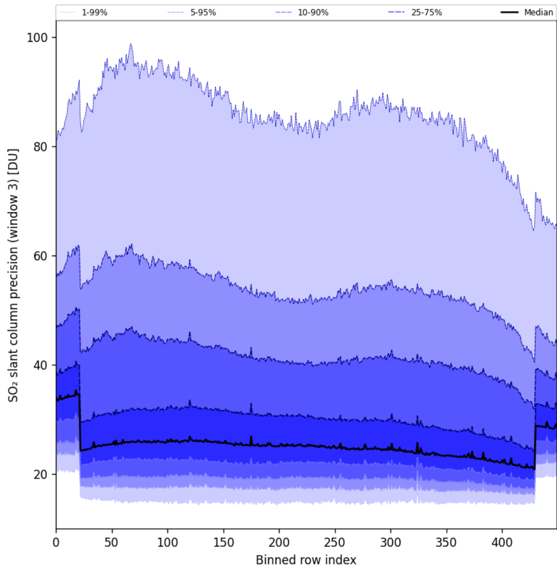
Figure 98: Along track statistics of “SO 2 slant column precision (window 3)” for 2025-04-29 to 2025-05-01
