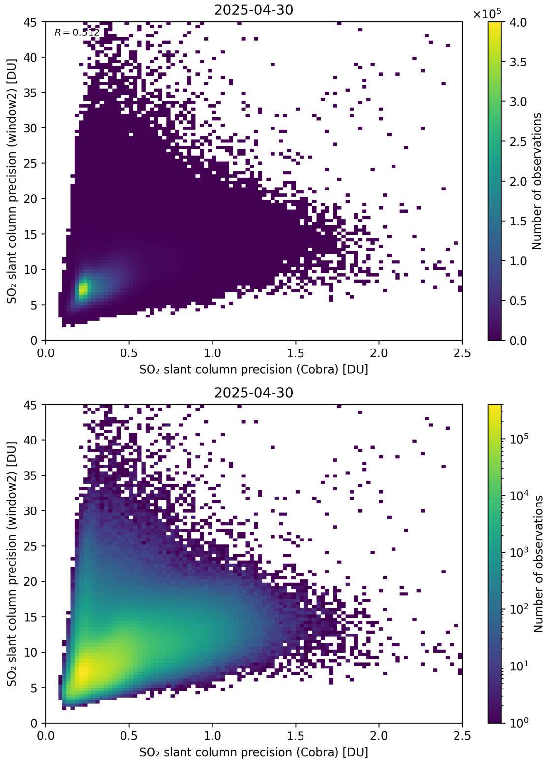
Figure 210: Scatter density plot of “SO 2 slant column precision (Cobra)” against “SO 2 slant column precision (window2)” for 2025-04-29 to 2025-05-01.
