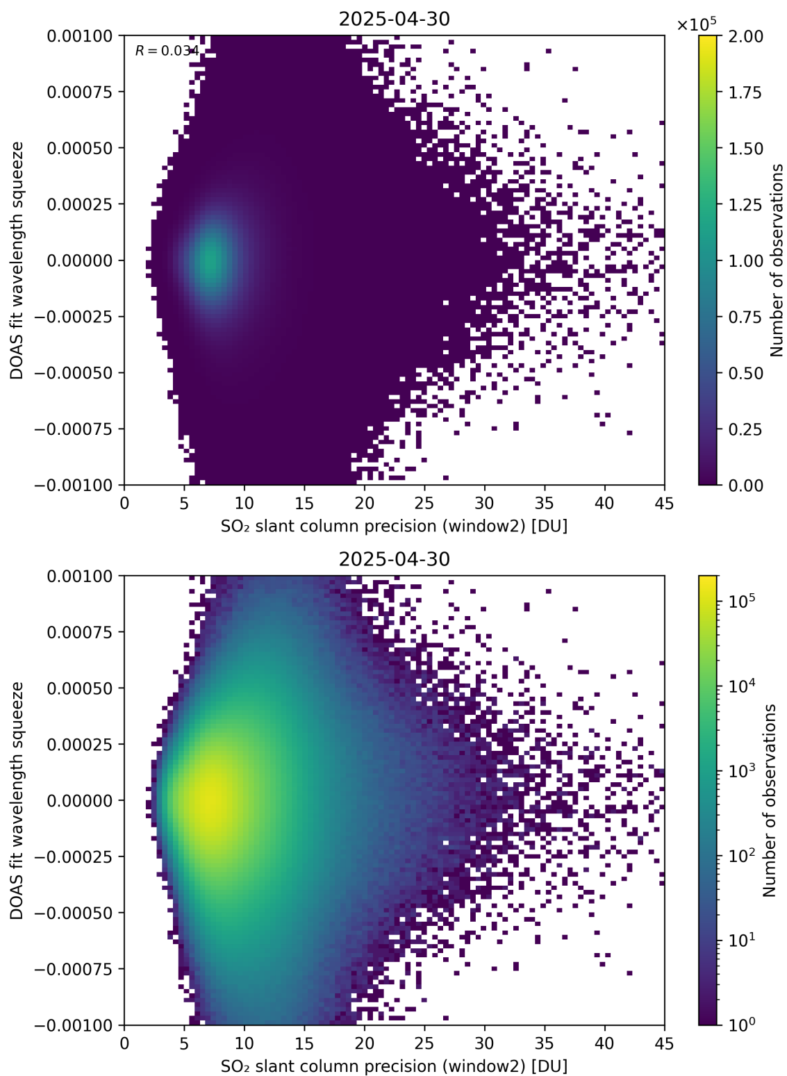
Figure 294: Scatter density plot of “SO 2 slant column precision (window2)” against “DOAS fit wavelength squeeze” for 2025-04-29 to 2025-05-01.
