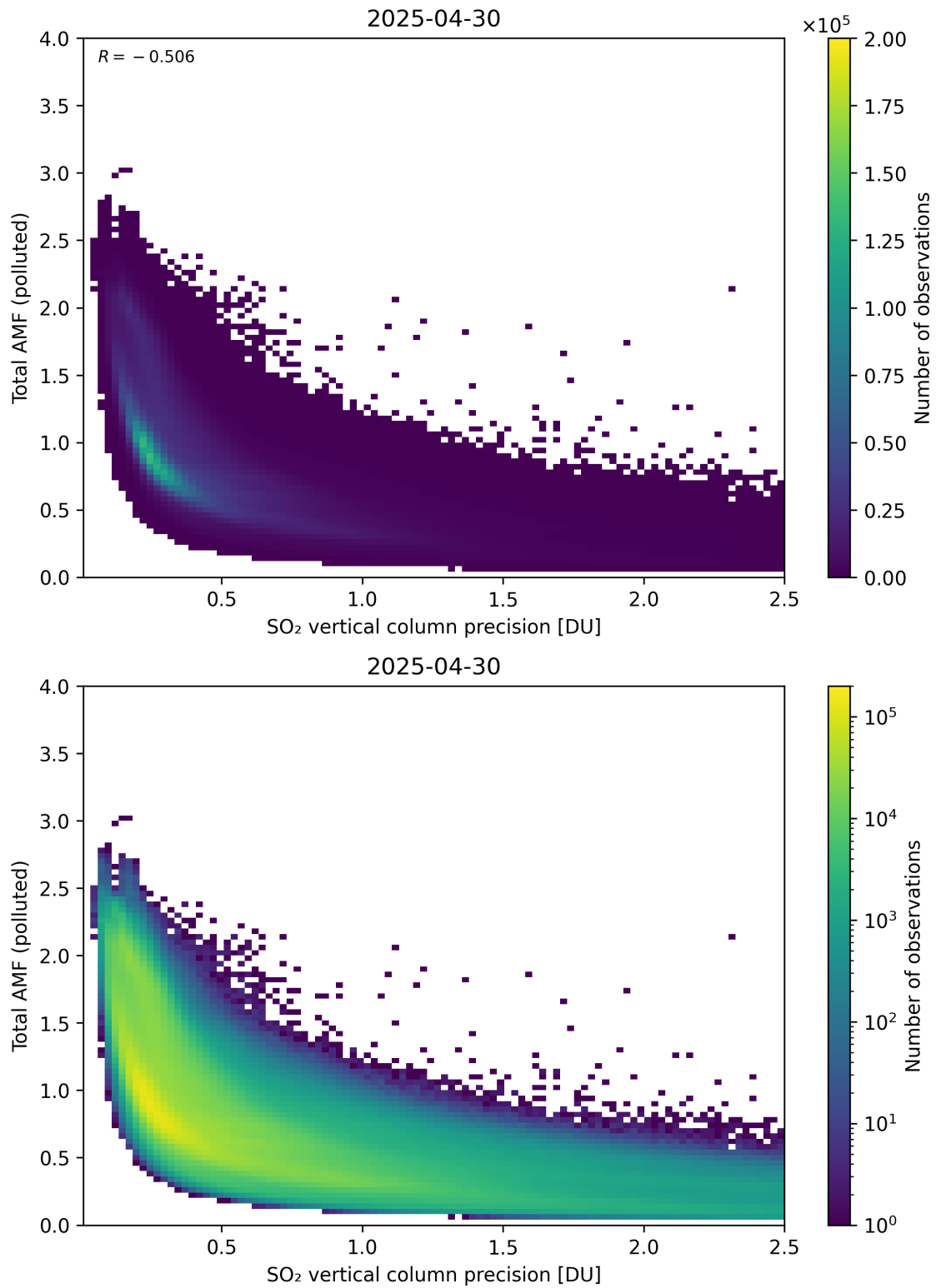
Figure 346: Scatter density plot of “SO 2 vertical column precision” against “Total AMF (polluted)” for 2025-04-29 to 2025-05-01.
