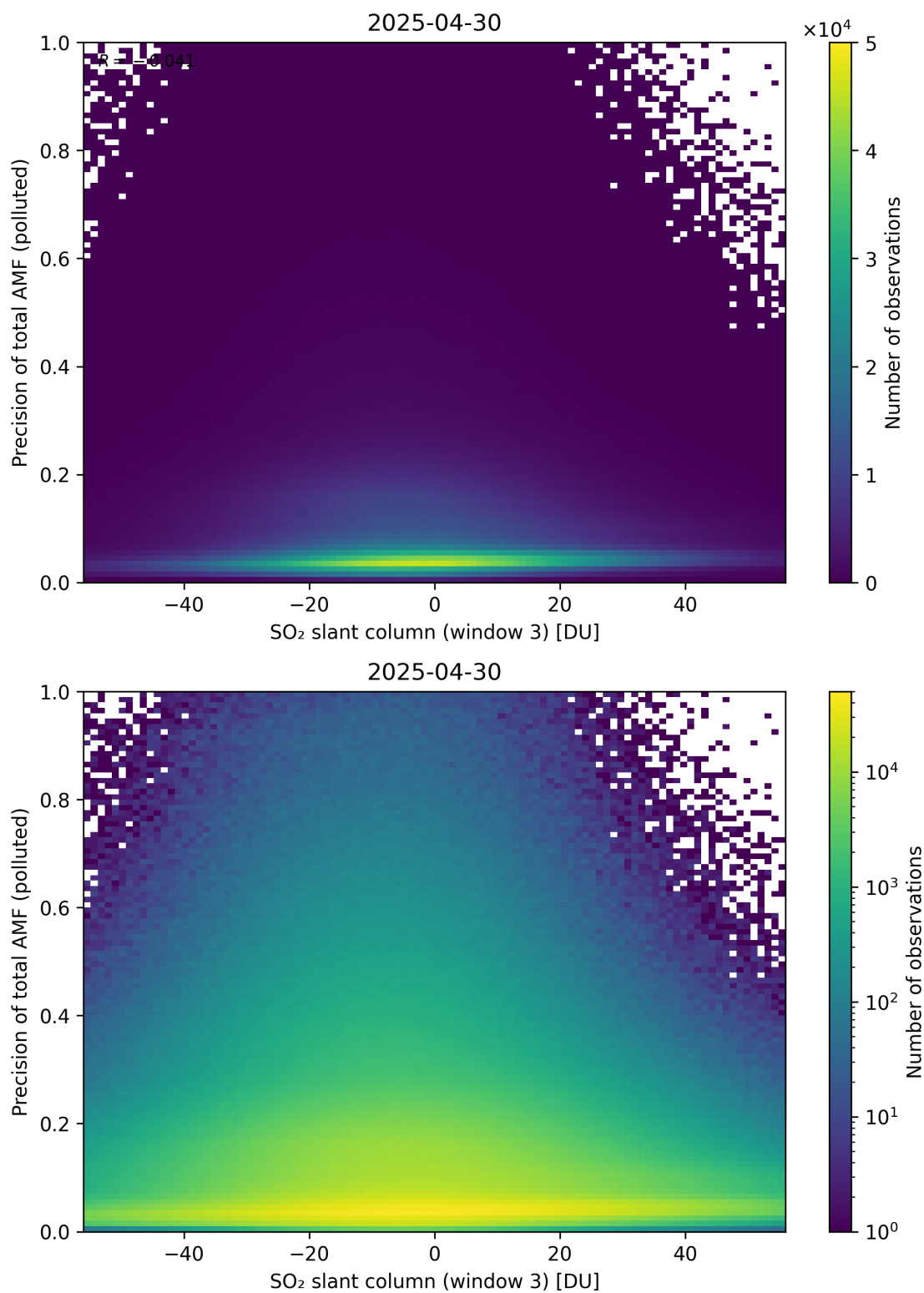
Figure 319: Scatter density plot of “SO 2 slant column (window 3)” against “Precision of total AMF (polluted)” for 2025-04-29 to 2025-05-01.
