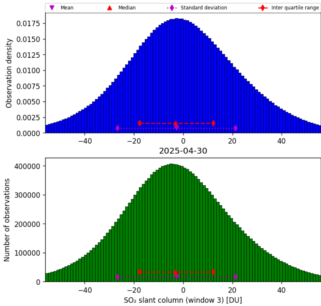
Figure 71: Histogram of “SO 2 slant column (window 3)” for 2025-04-29 to 2025-05-01
