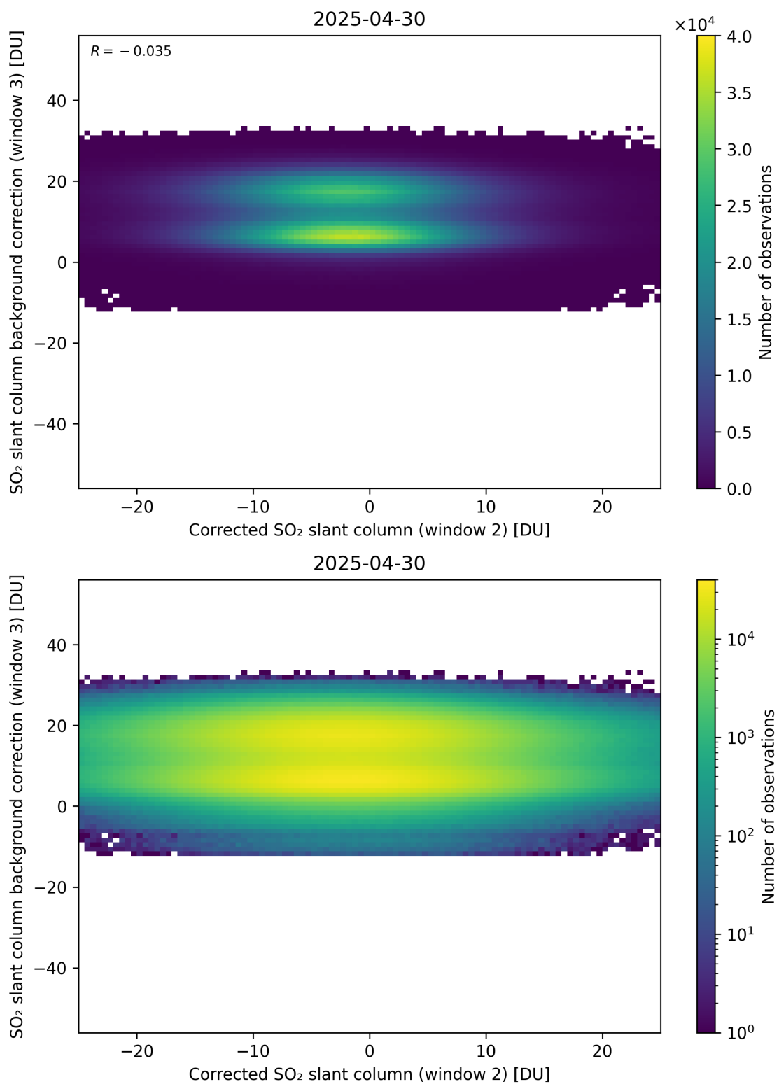
Figure 245: Scatter density plot of “Corrected SO 2 slant column (window 2)” against “SO 2 slant column background correction (window 3)” for 2025-04-29 to 2025-05-01.
