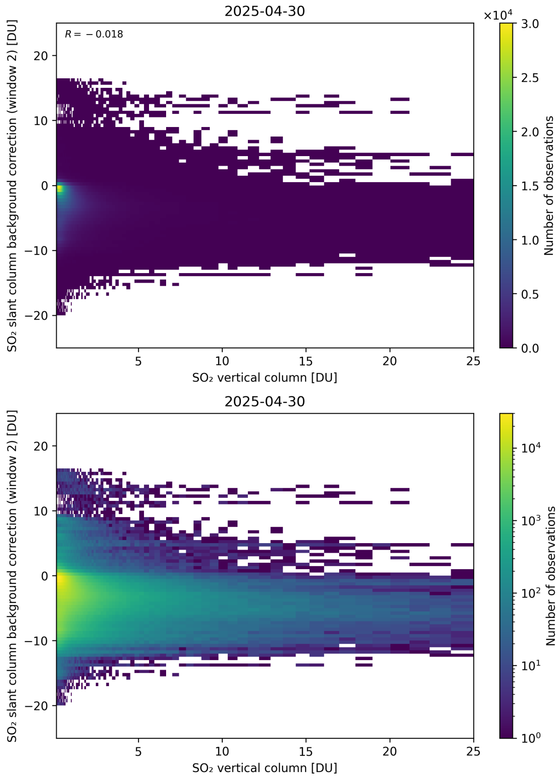
Figure 324: Scatter density plot of “SO 2 vertical column” against “SO 2 slant column background correction (window 2)” for 2025-04-29 to 2025-05-01.
