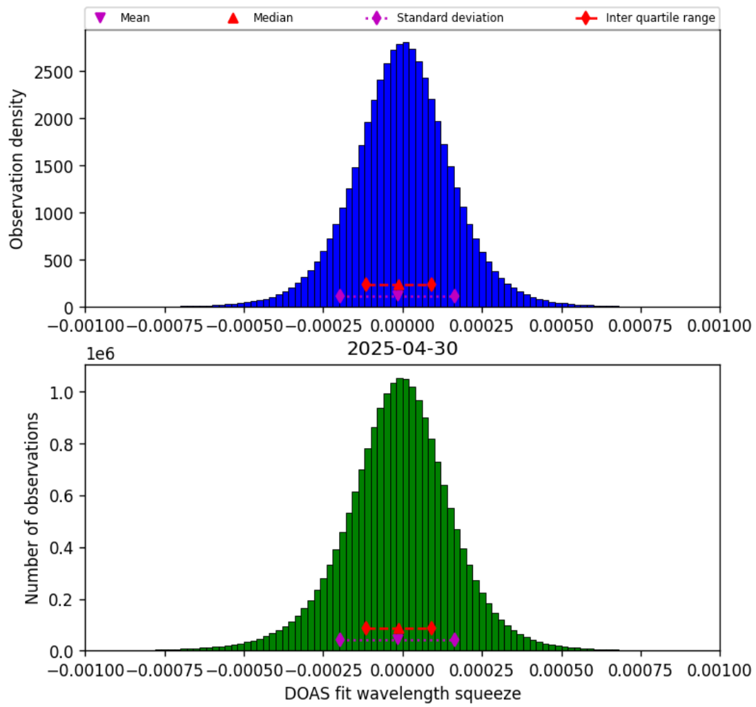
Figure 77: Histogram of “DOAS fit wavelength squeeze” for 2025-04-29 to 2025-05-01
