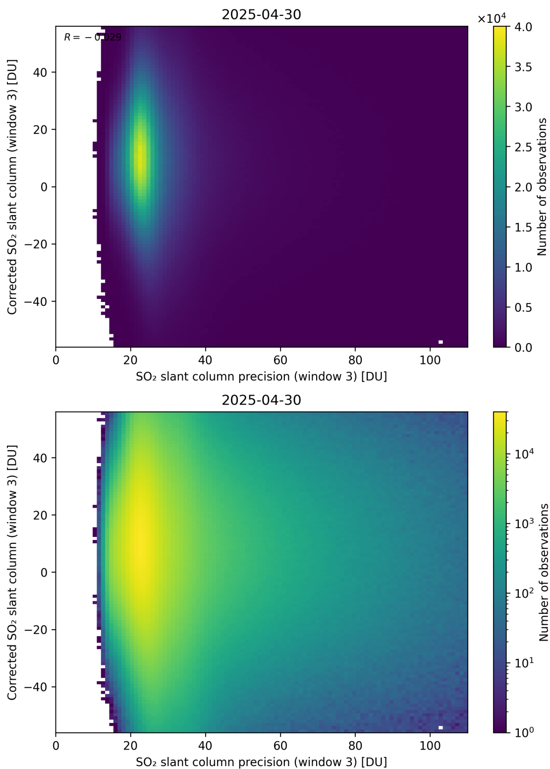
Figure 312: Scatter density plot of “SO 2 slant column precision (window 3)” against “Corrected SO 2 slant column (window 3)” for 2025-04-29 to 2025-05-01.
