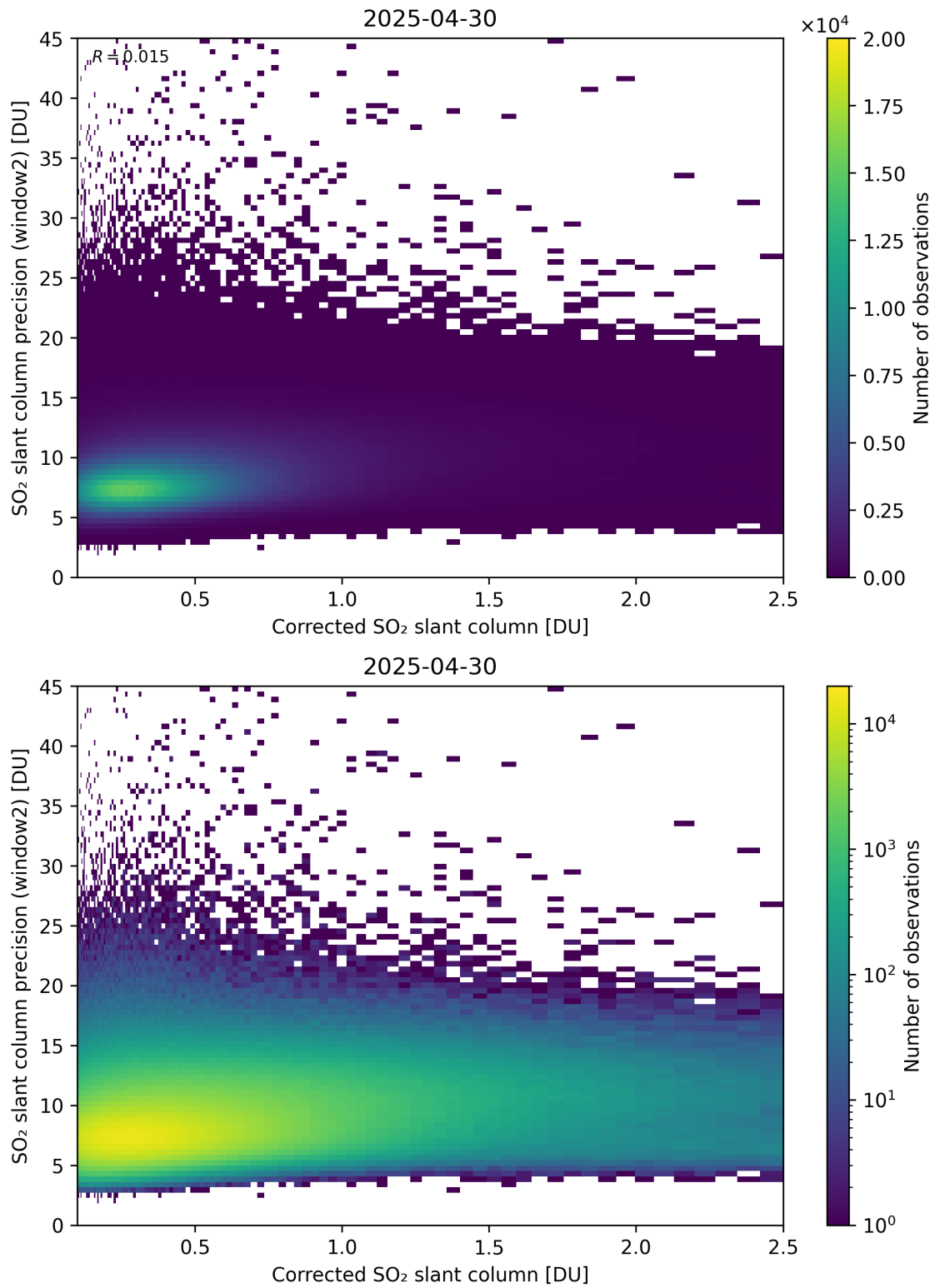
Figure 239: Scatter density plot of “Corrected SO 2 slant column” against “SO 2 slant column precision (window2)” for 2025-04-29 to 2025-05-01.
