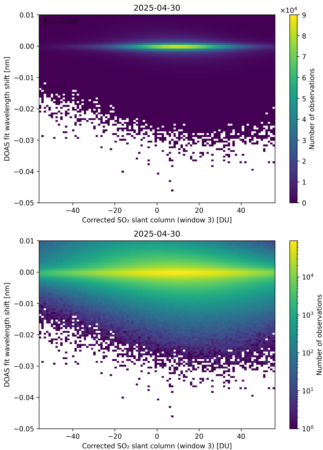
Figure 256: Scatter density plot of “Corrected SO 2 slant column (window 3)” against “DOAS fit wavelength shift” for 2025-04-29 to 2025-05-01.
