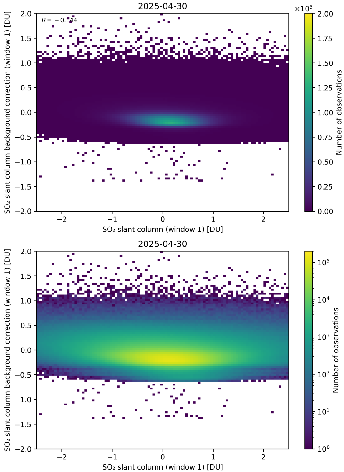
Figure 262: Scatter density plot of “SO 2 slant column (window 1)” against “SO 2 slant column background correction (window 1)” for 2025-04-29 to 2025-05-01.
