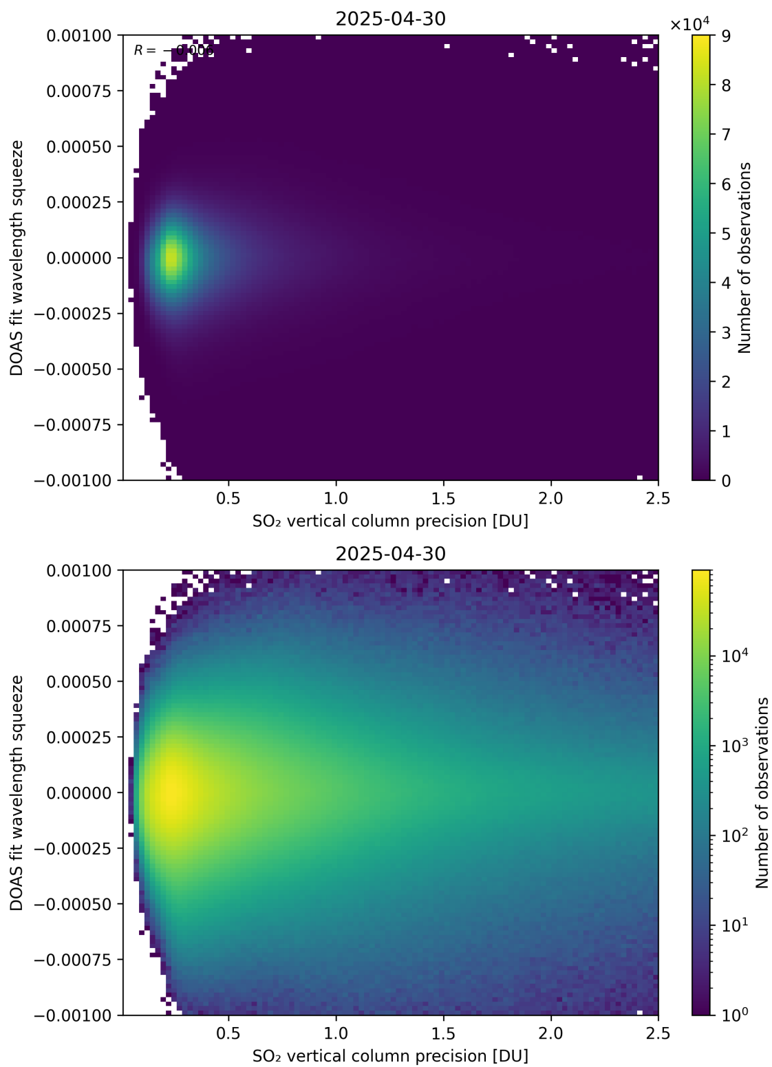
Figure 333: Scatter density plot of “SO 2 vertical column precision” against “DOAS fit wavelength squeeze” for 2025-04-29 to 2025-05-01.
