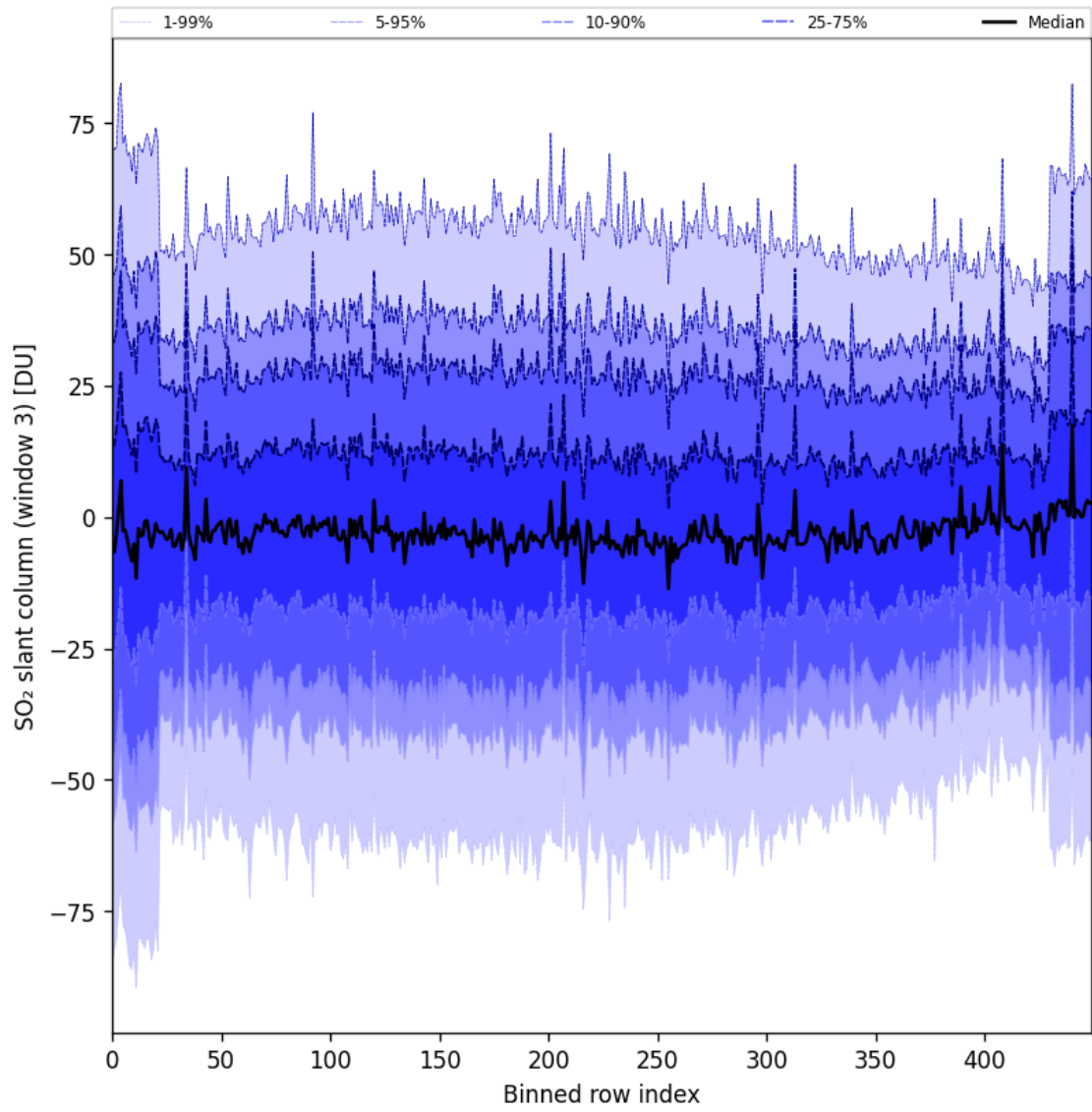
Figure 97: Along track statistics of “SO 2 slant column (window 3)” for 2025-04-29 to 2025-05-01
