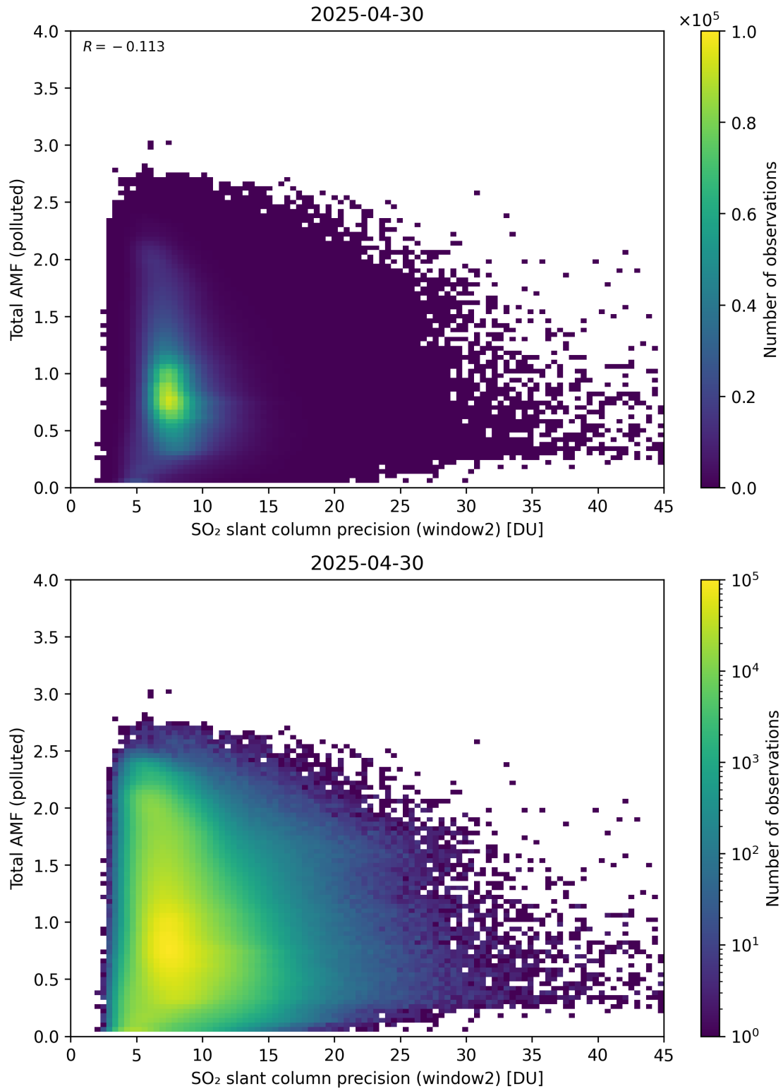
Figure 301: Scatter density plot of “SO 2 slant column precision (window2)” against “Total AMF (polluted)” for 2025-04-29 to 2025-05-01.
