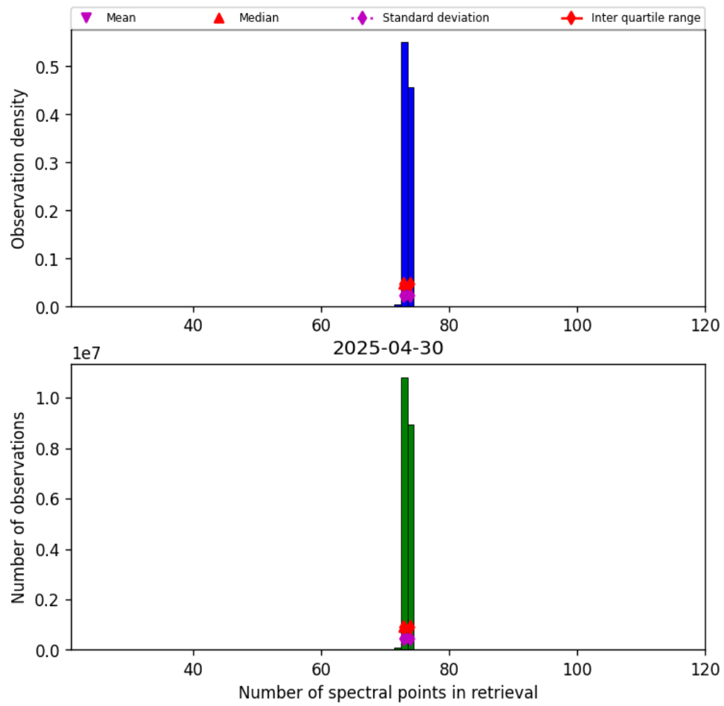
Figure 82: Histogram of “Number of spectral points in retrieval” for 2025-04-29 to 2025-05-01
