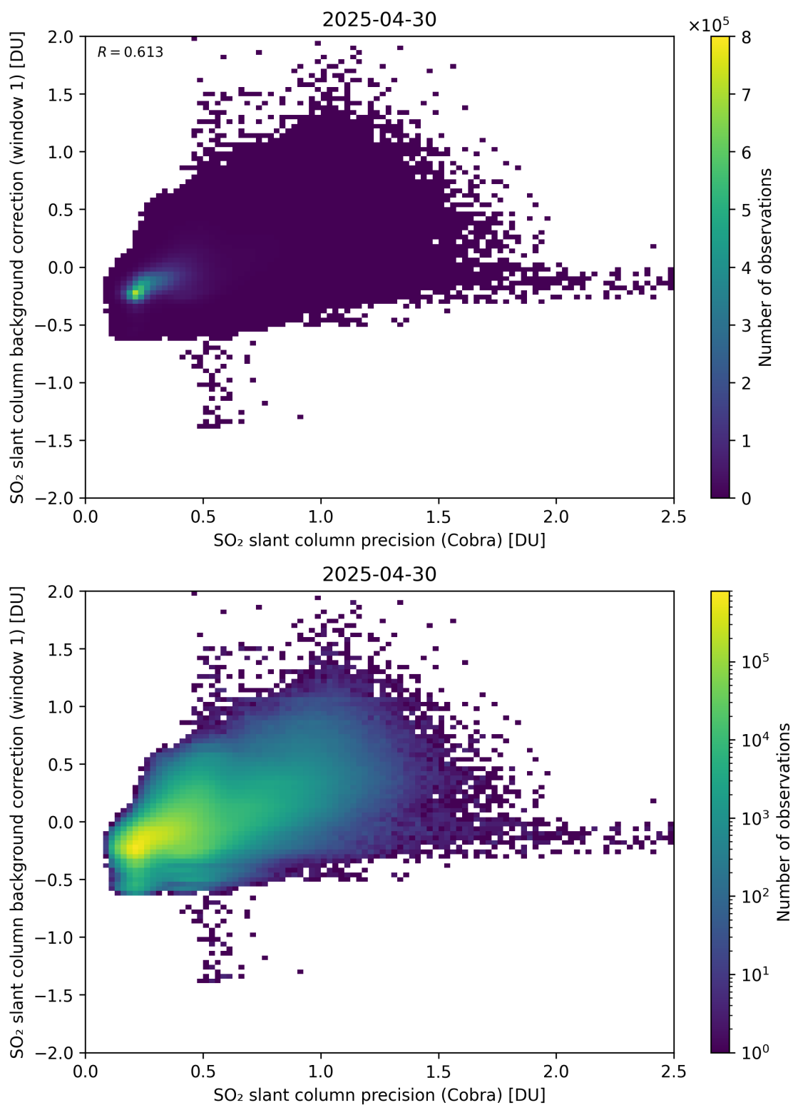
Figure 199: Scatter density plot of “SO 2 slant column precision (Cobra)” against “SO 2 slant column background correction (window 1)” for 2025-04-29 to 2025-05-01.
