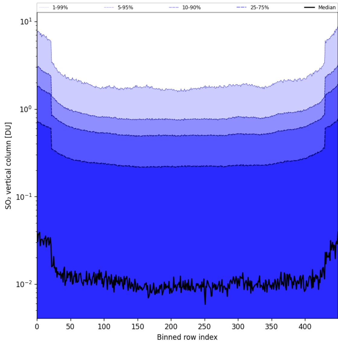
Figure 84: Along track statistics of “SO 2 vertical column” for 2025-04-29 to 2025-05-01
