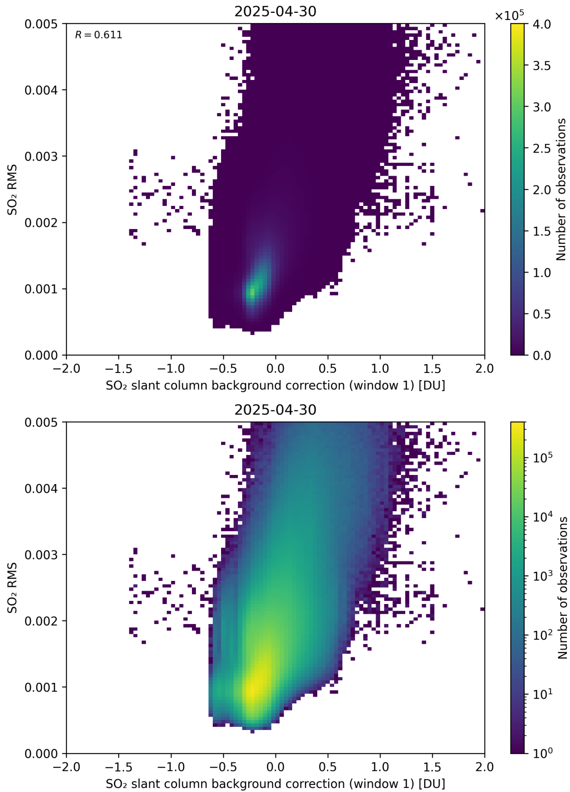
Figure 113: Scatter density plot of “SO 2 slant column background correction (window 1)” against “SO 2 RMS” for 2025-04-29 to 2025-05-01.
