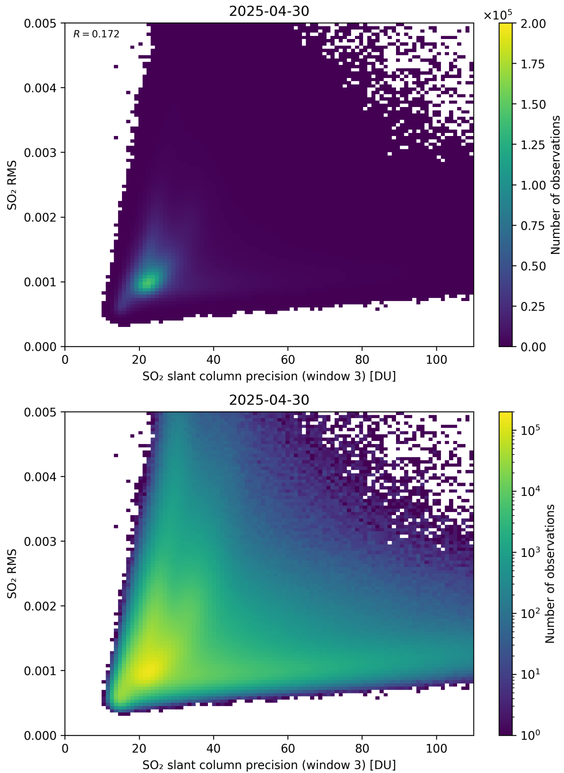
Figure 310: Scatter density plot of “SO 2 slant column precision (window 3)” against “SO 2 RMS” for 2025-04-29 to 2025-05-01.
