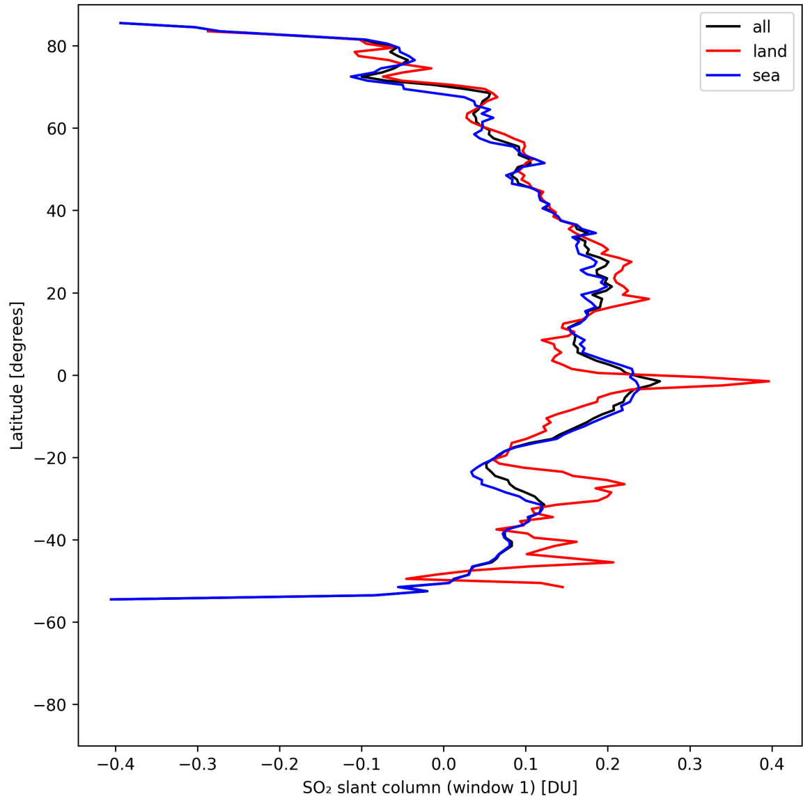
Figure 37: Zonal average of “SO 2 slant column (window 1)” for 2025-04-29 to 2025-05-01.
