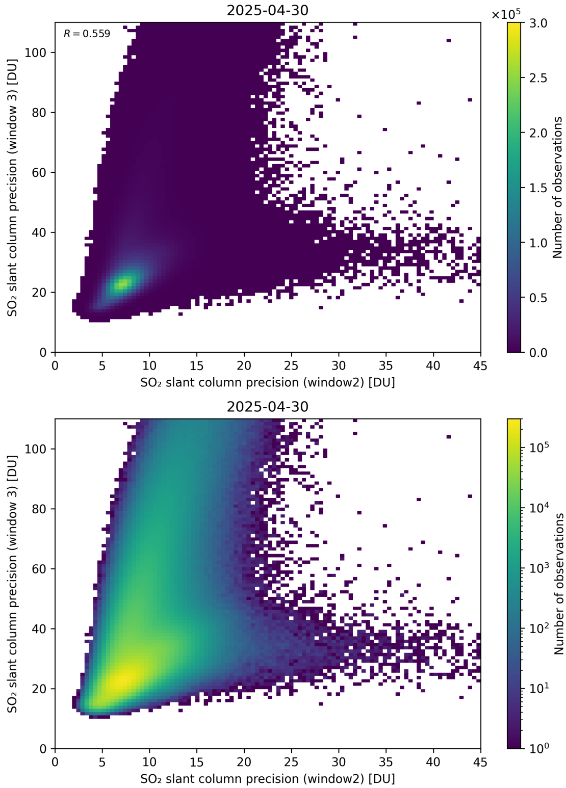
Figure 300: Scatter density plot of “SO 2 slant column precision (window2)” against “SO 2 slant column precision (window 3)” for 2025-04-29 to 2025-05-01.
