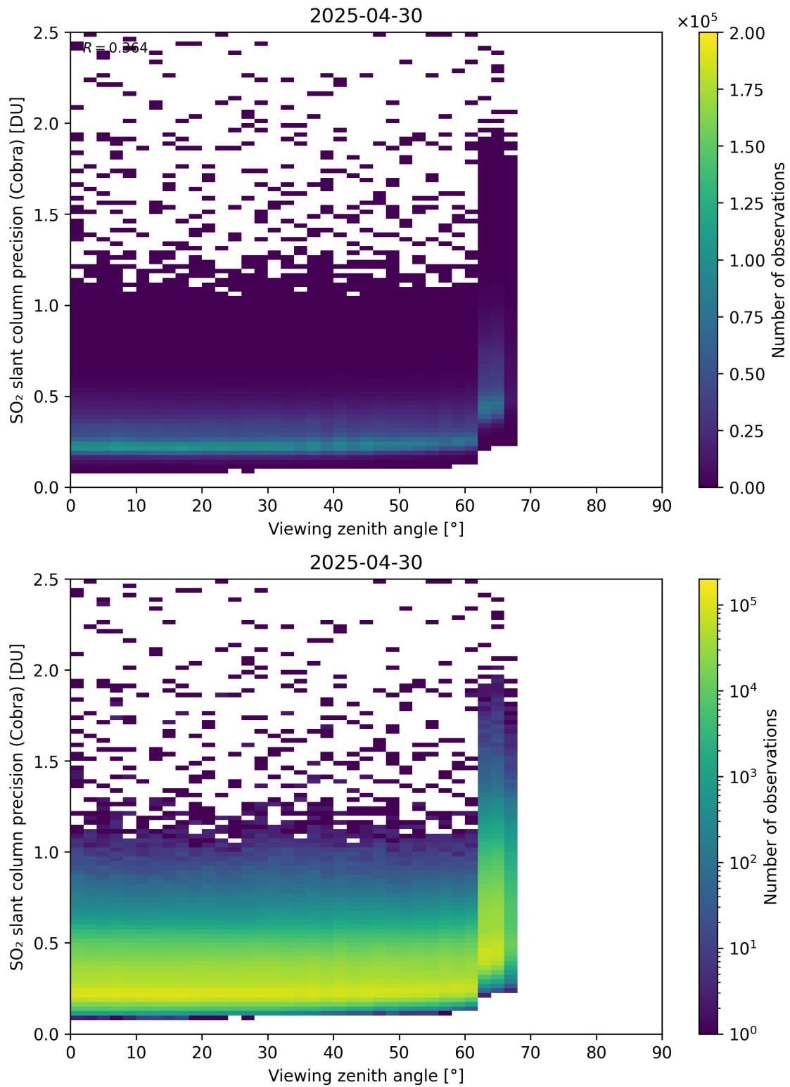
Figure 372: Scatter density plot of “Viewing zenith angle” against “SO 2 slant column precision (Cobra)” for 2025-04-29 to 2025-05-01.
