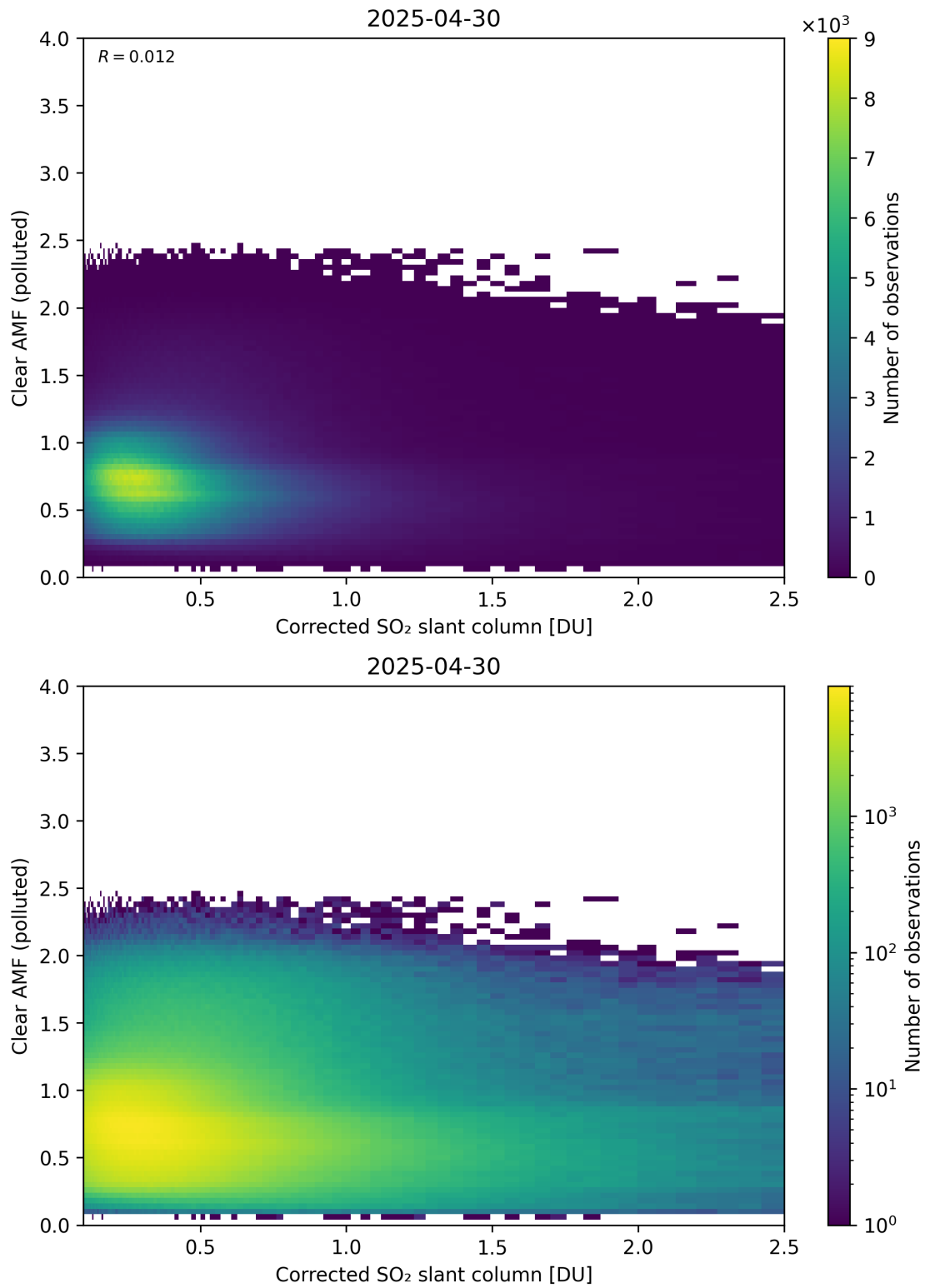
Figure 232: Scatter density plot of “Corrected SO 2 slant column” against “Clear AMF (polluted)” for 2025-04-29 to 2025-05-01.
