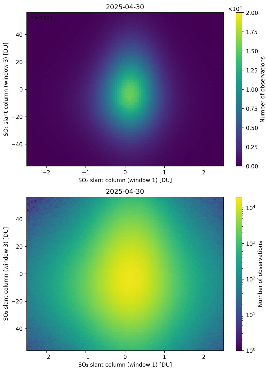
Figure 287: Scatter density plot of “SO 2 slant column (window 1)” against “SO 2 slant column (window 3)” for 2025-04-29 to 2025-05-01.
