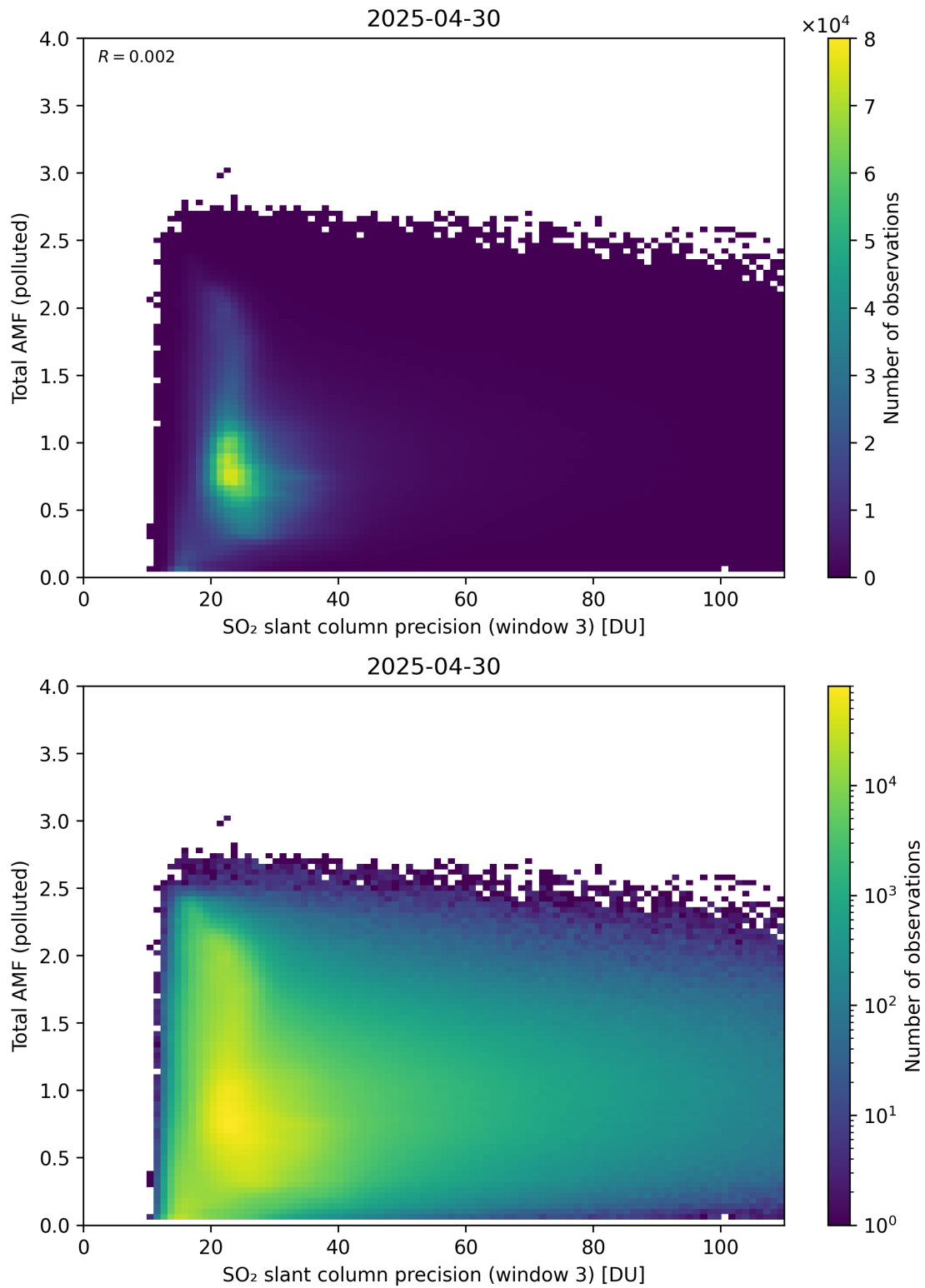
Figure 313: Scatter density plot of “SO 2 slant column precision (window 3)” against “Total AMF (polluted)” for 2025-04-29 to 2025-05-01.
