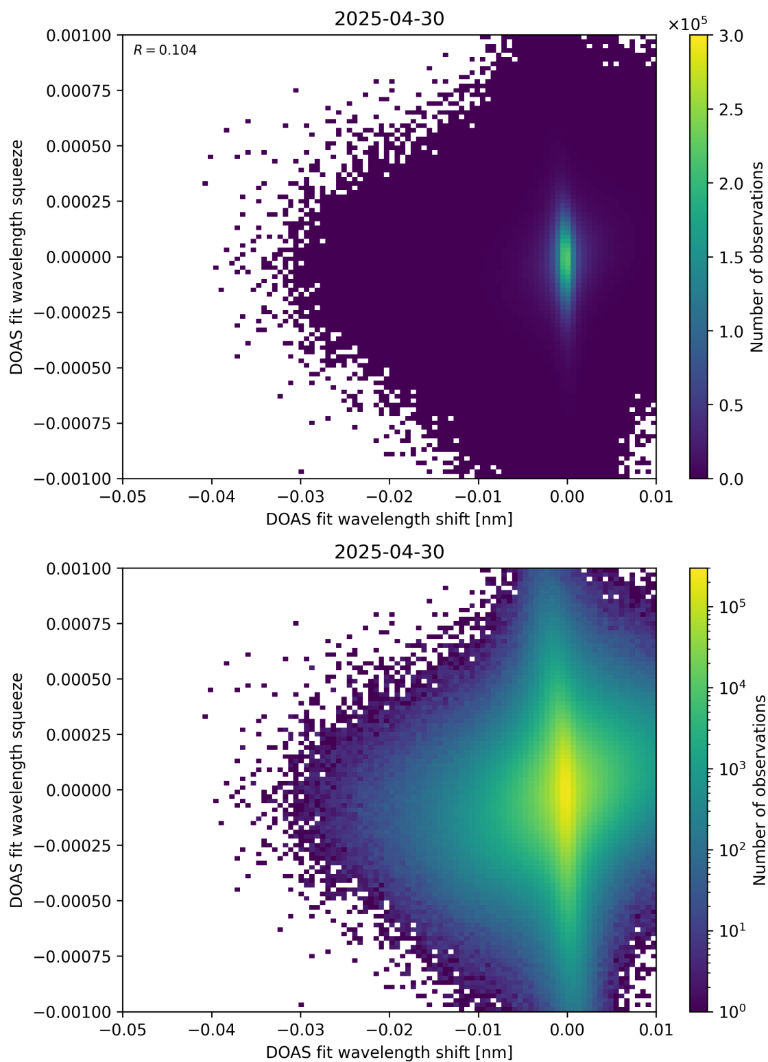
Figure 138: Scatter density plot of “DOAS fit wavelength shift” against “DOAS fit wavelength squeeze” for 2025-04-29 to 2025-05-01.
