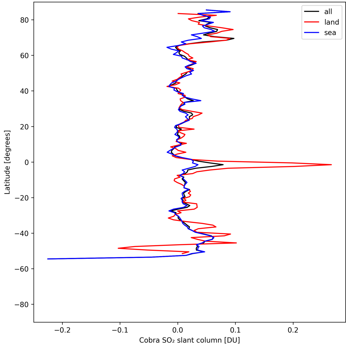
Figure 35: Zonal average of “Cobra SO 2 slant column” for 2025-04-29 to 2025-05-01.
