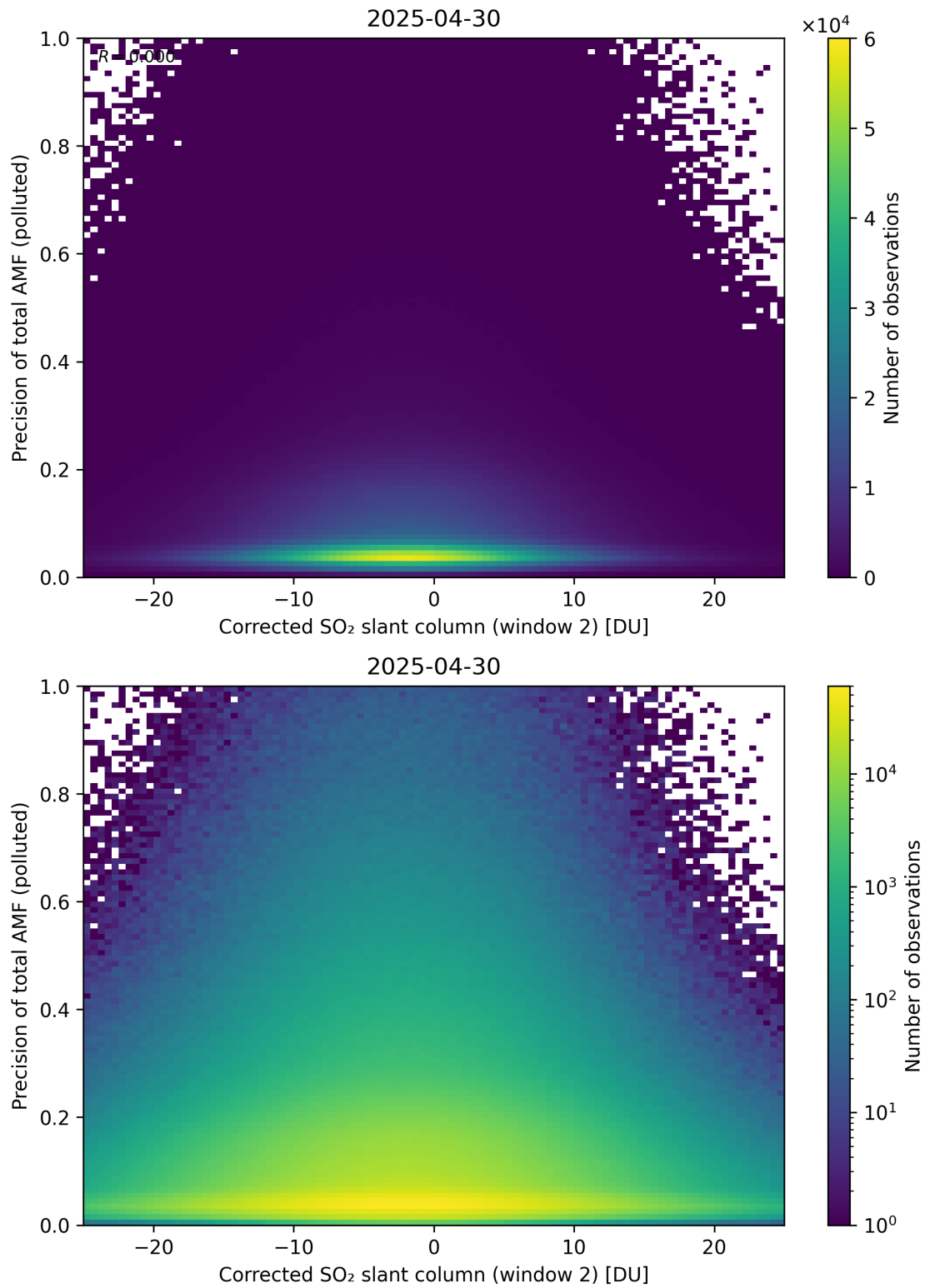
Figure 254: Scatter density plot of “Corrected SO 2 slant column (window 2)” against “Precision of total AMF (polluted)” for 2025-04-29 to 2025-05-01.
