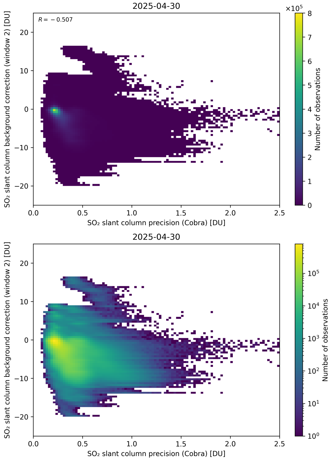
Figure 200: Scatter density plot of “SO 2 slant column precision (Cobra)” against “SO 2 slant column background correction (window 2)” for 2025-04-29 to 2025-05-01.
