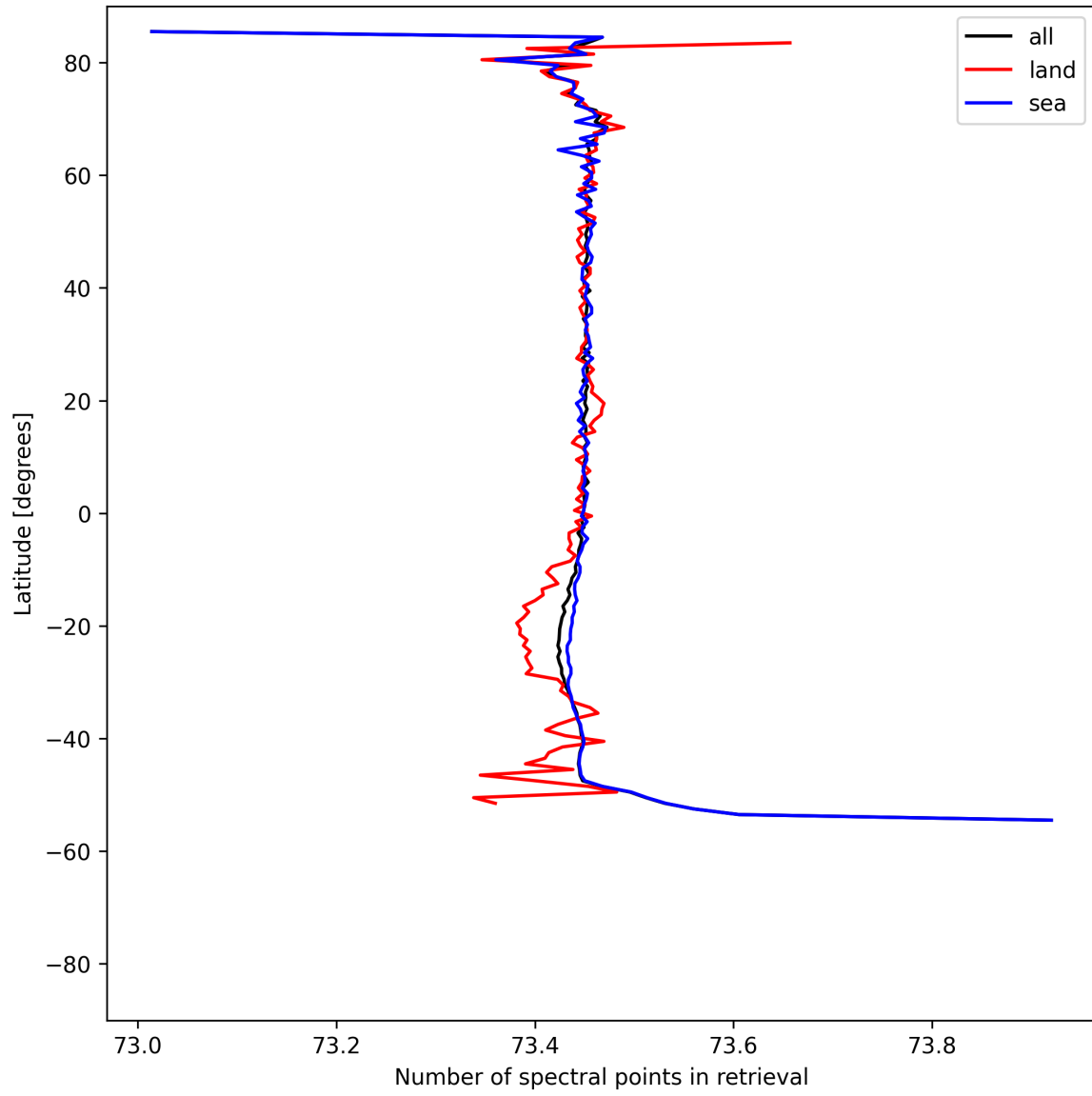
Figure 56: Zonal average of “Number of spectral points in retrieval” for 2025-04-29 to 2025-05-01.
