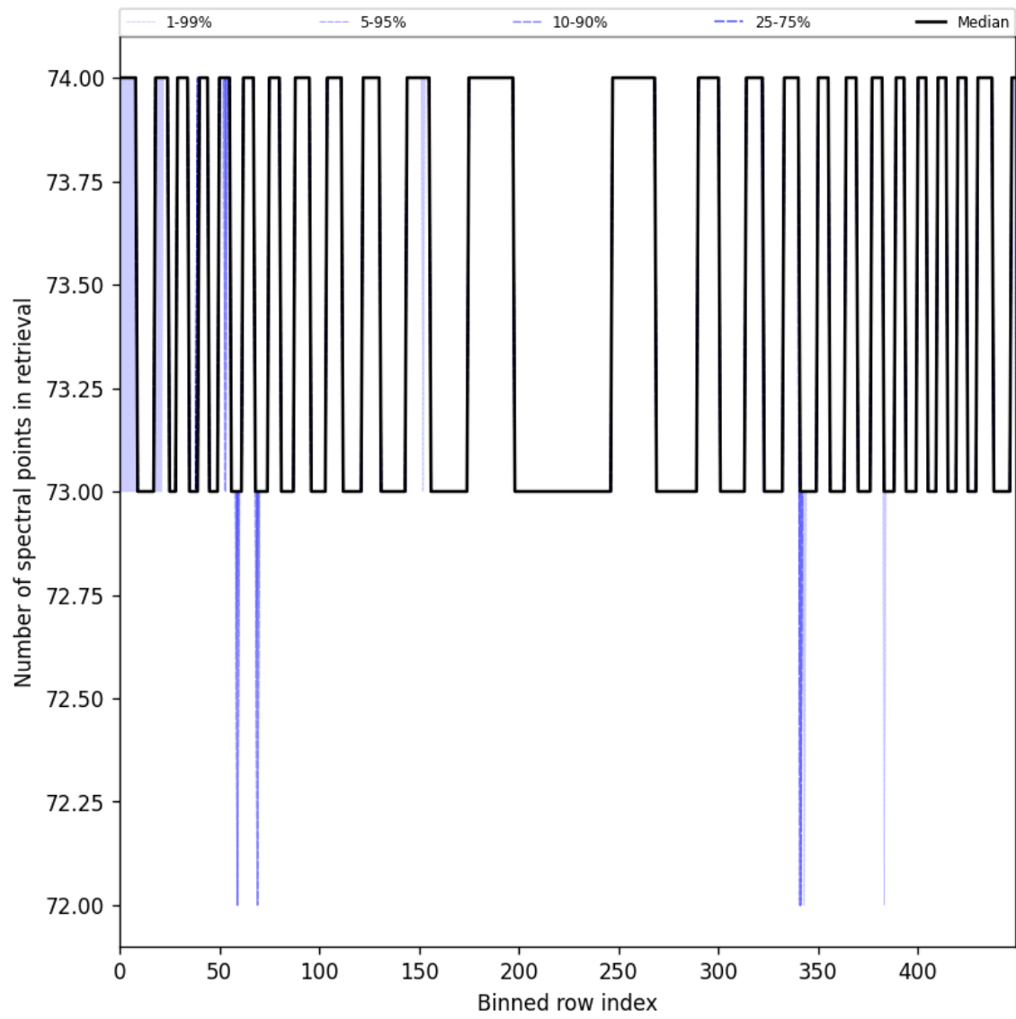
Figure 108: Along track statistics of “Number of spectral points in retrieval” for 2025-04-29 to 2025-05-01
