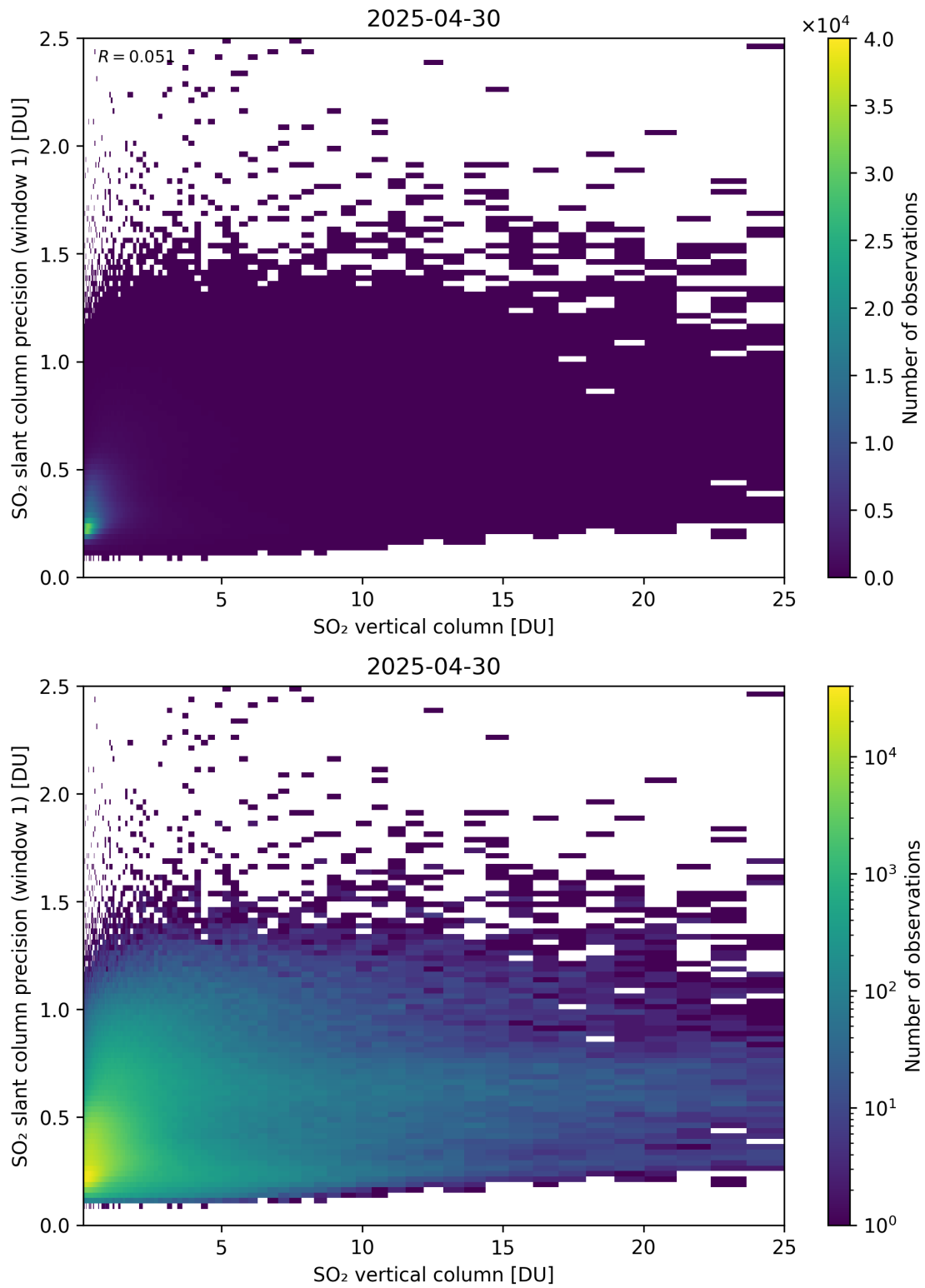
Figure 355: Scatter density plot of “SO 2 vertical column” against “SO 2 slant column precision (window 1)” for 2025-04-29 to 2025-05-01.
