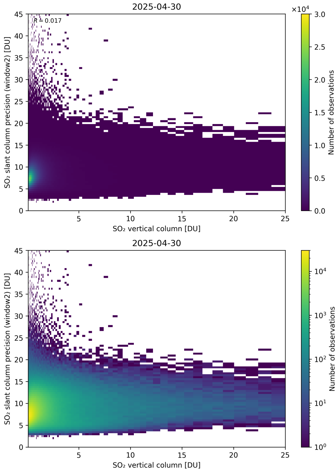
Figure 356: Scatter density plot of “SO 2 vertical column” against “SO 2 slant column precision (window2)” for 2025-04-29 to 2025-05-01.
