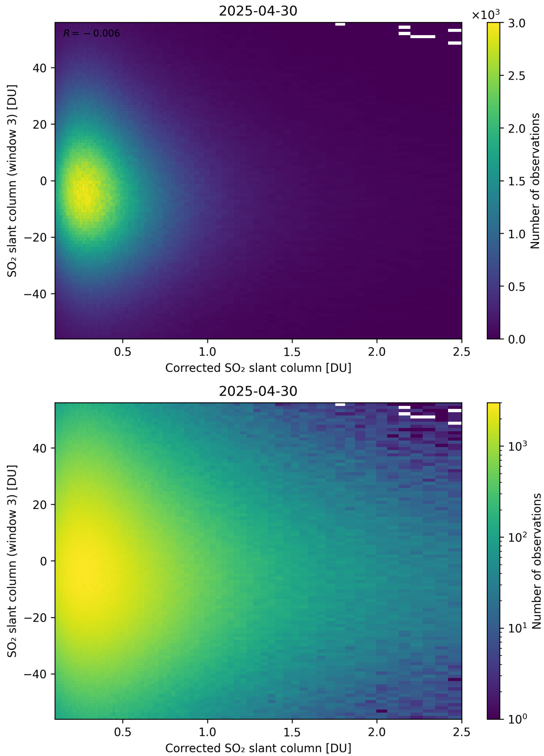
Figure 240: Scatter density plot of “Corrected SO 2 slant column” against “SO 2 slant column (window 3)” for 2025-04-29 to 2025-05-01.
