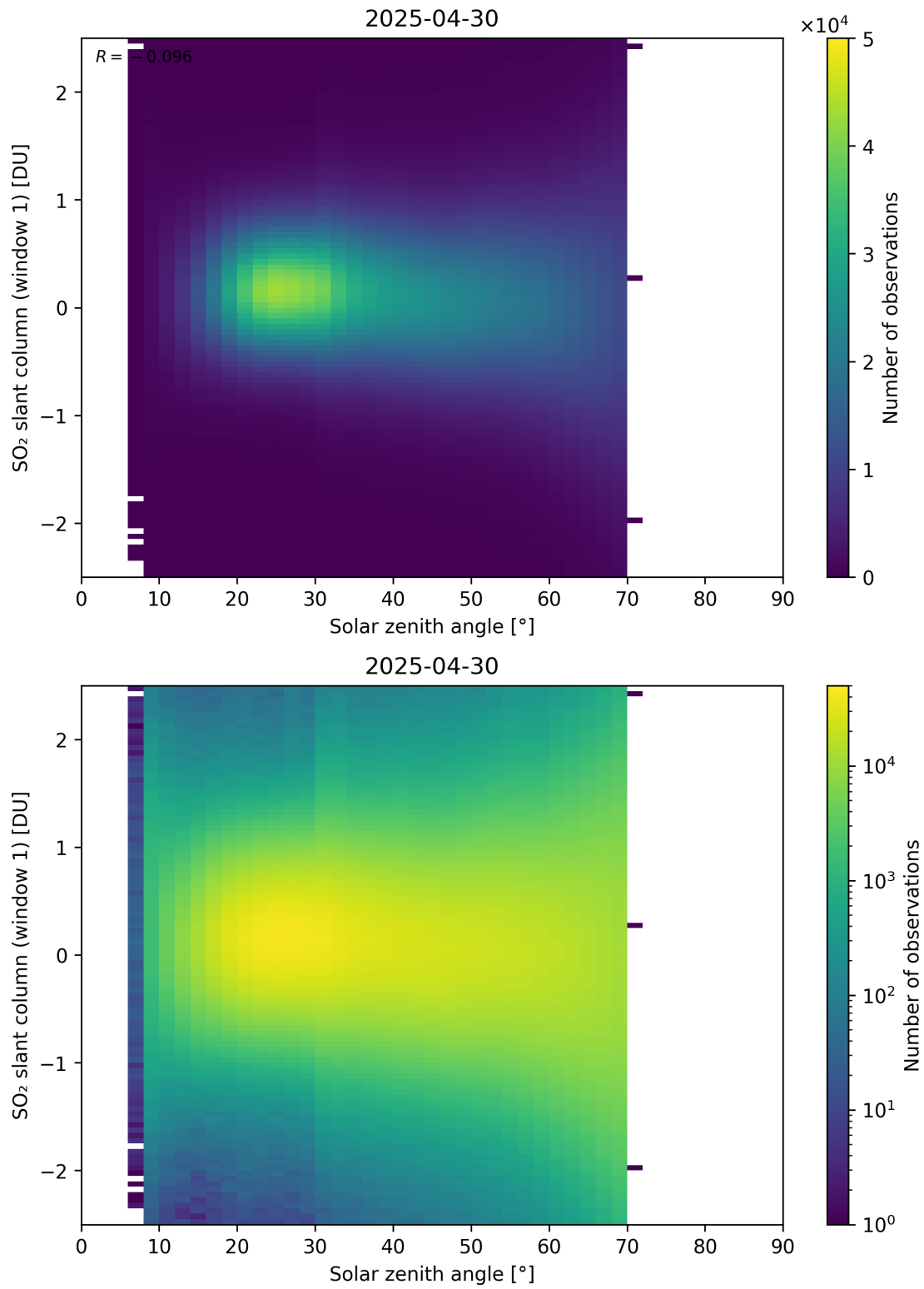
Figure 184: Scatter density plot of “Solar zenith angle” against “SO 2 slant column (window 1)” for 2025-04-29 to 2025-05-01.
