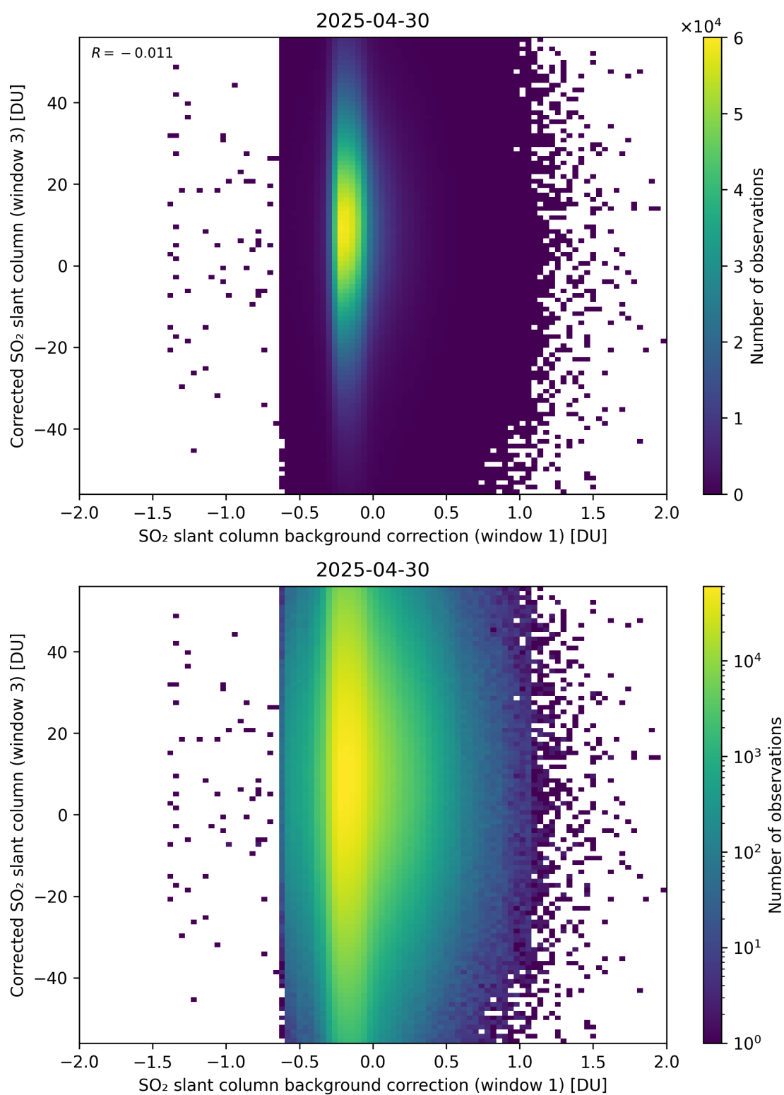
Figure 116: Scatter density plot of “SO 2 slant column background correction (window 1)” against “Corrected SO 2 slant column (window 3)” for 2025-04-29 to 2025-05-01.
