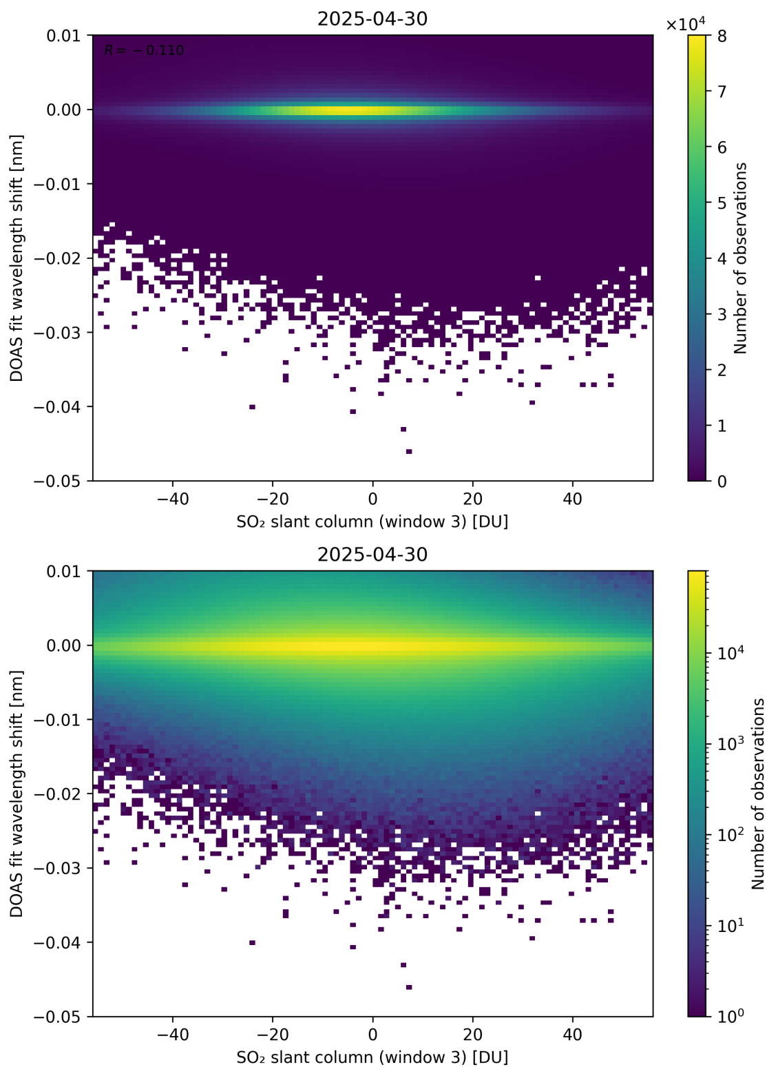
Figure 304: Scatter density plot of “SO 2 slant column (window 3)” against “DOAS fit wavelength shift” for 2025-04-29 to 2025-05-01.
