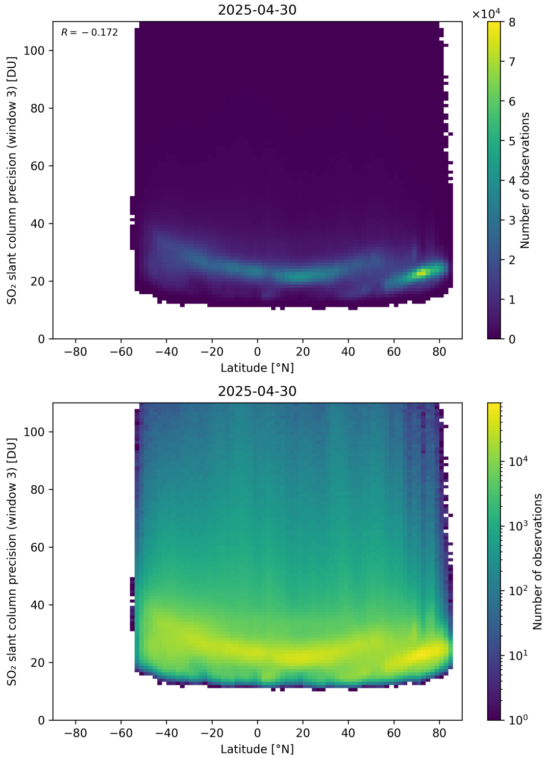
Figure 166: Scatter density plot of “Latitude” against “SO 2 slant column precision (window 3)” for 2025-04-29 to 2025-05-01.
