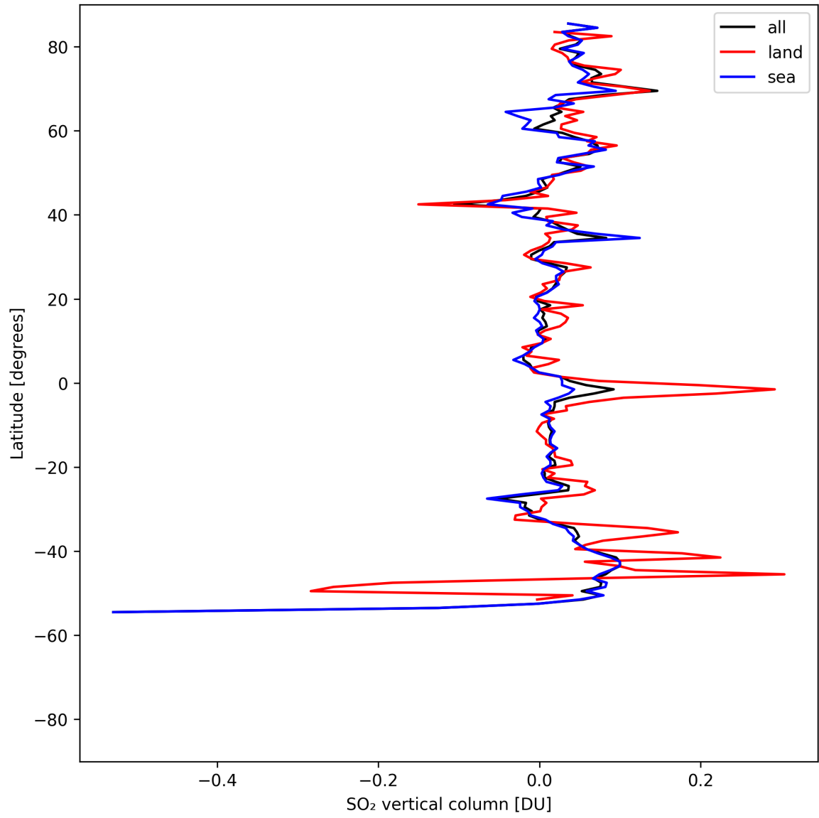
Figure 32: Zonal average of “SO 2 vertical column” for 2025-04-29 to 2025-05-01.
