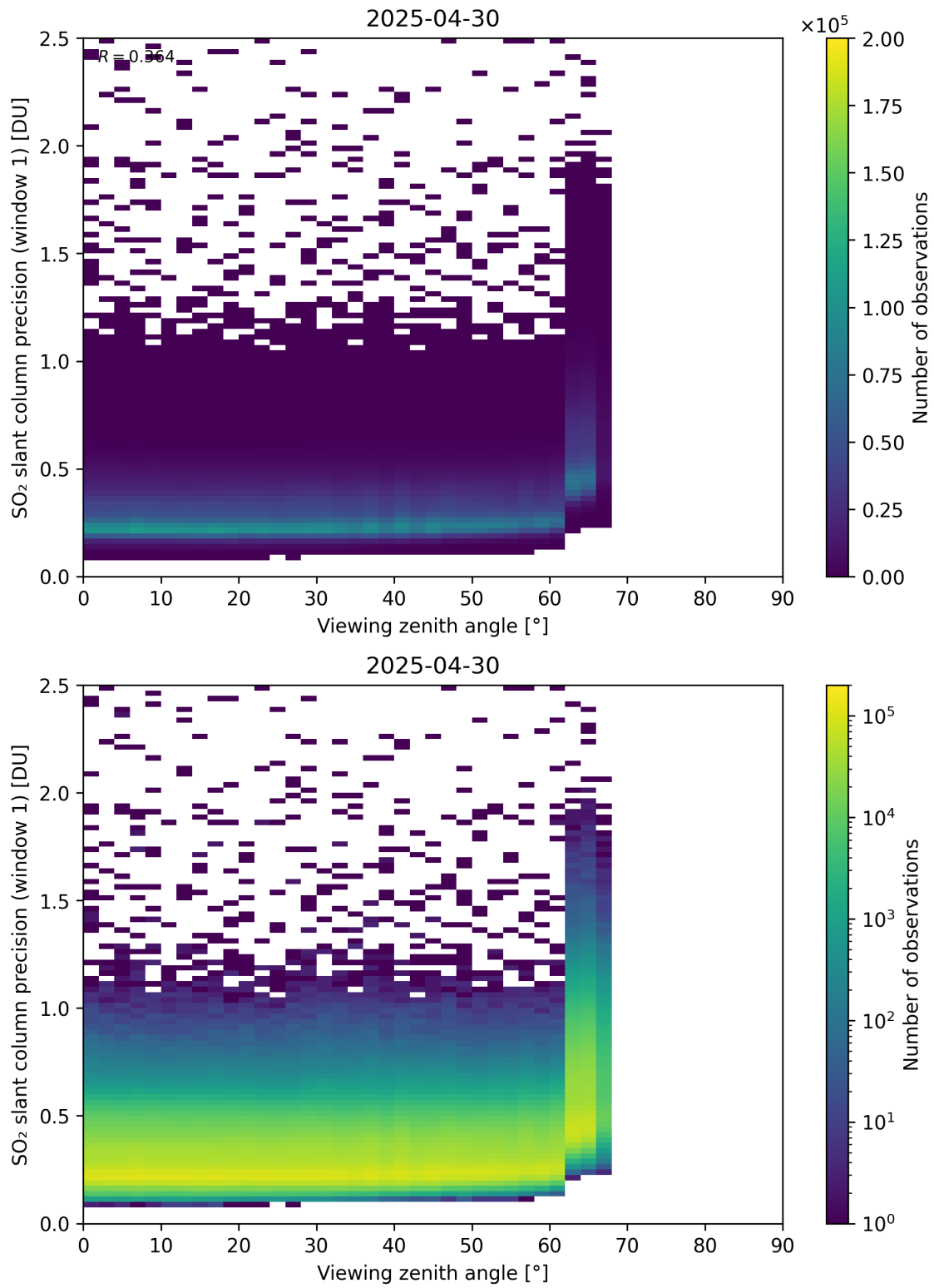
Figure 377: Scatter density plot of “Viewing zenith angle” against “SO 2 slant column precision (window 1)” for 2025-04-29 to 2025-05-01.
