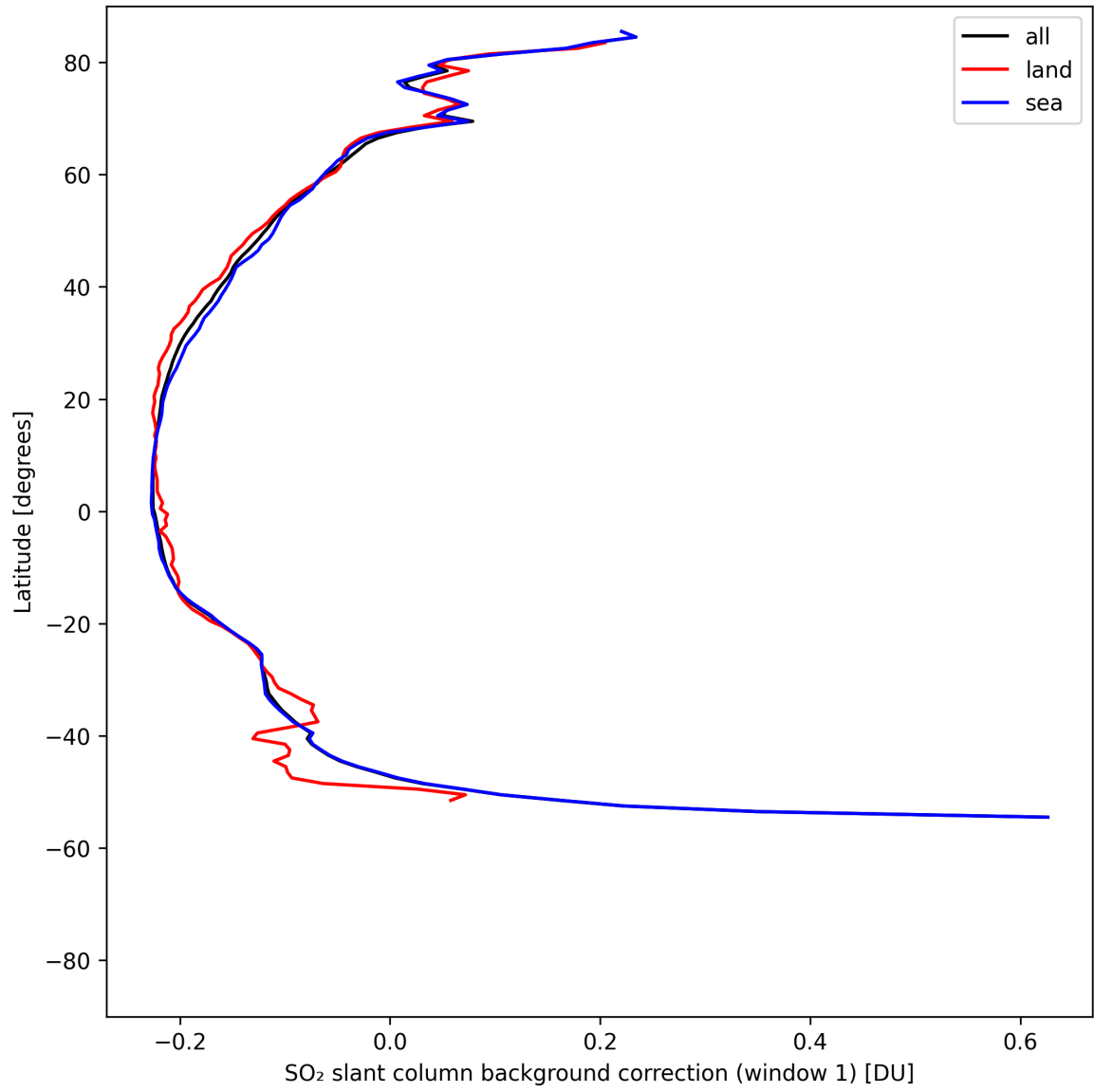
Figure 40: Zonal average of “SO 2 slant column background correction (window 1)” for 2025-04-29 to 2025-05-01.
