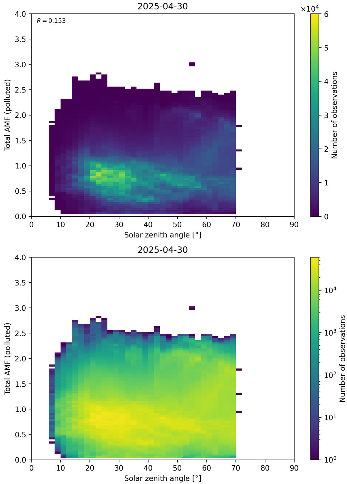
Figure 189: Scatter density plot of “Solar zenith angle” against “Total AMF (polluted)” for 2025-04-29 to 2025-05-01.
