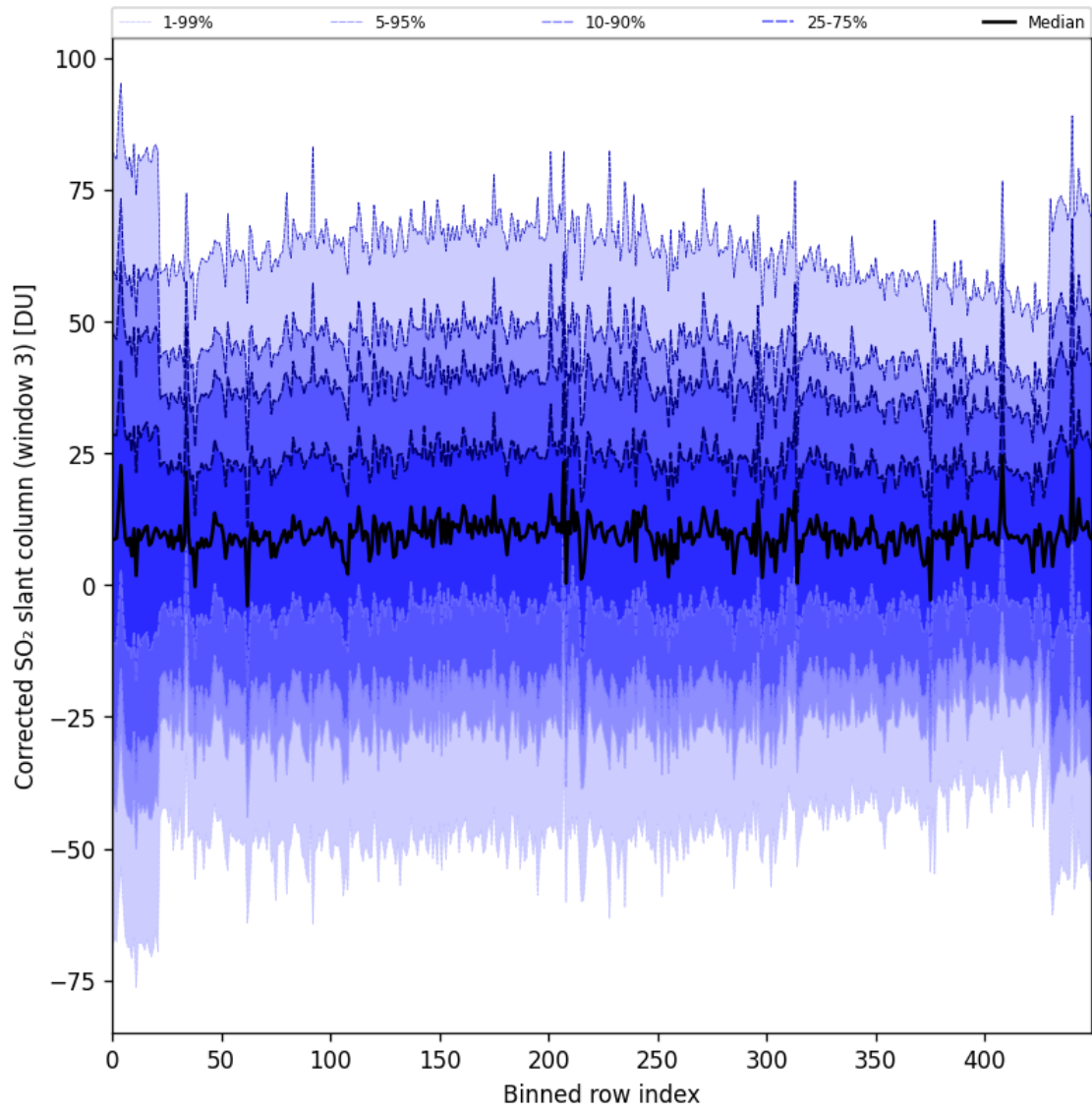
Figure 99: Along track statistics of “Corrected SO 2 slant column (window 3)” for 2025-04-29 to 2025-05-01
