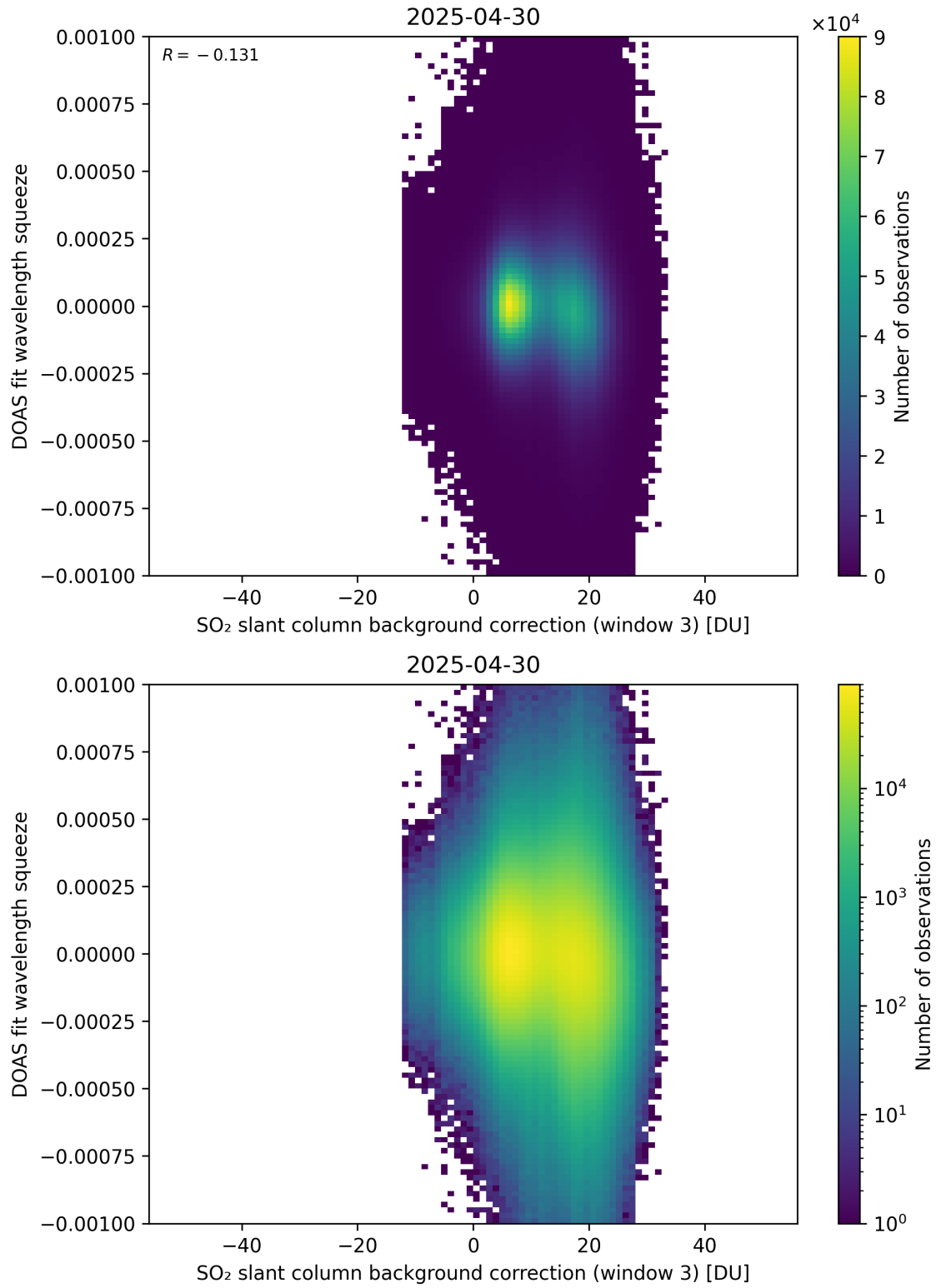
Figure 133: Scatter density plot of “SO 2 slant column background correction (window 3)” against “DOAS fit wavelength squeeze” for 2025-04-29 to 2025-05-01.
