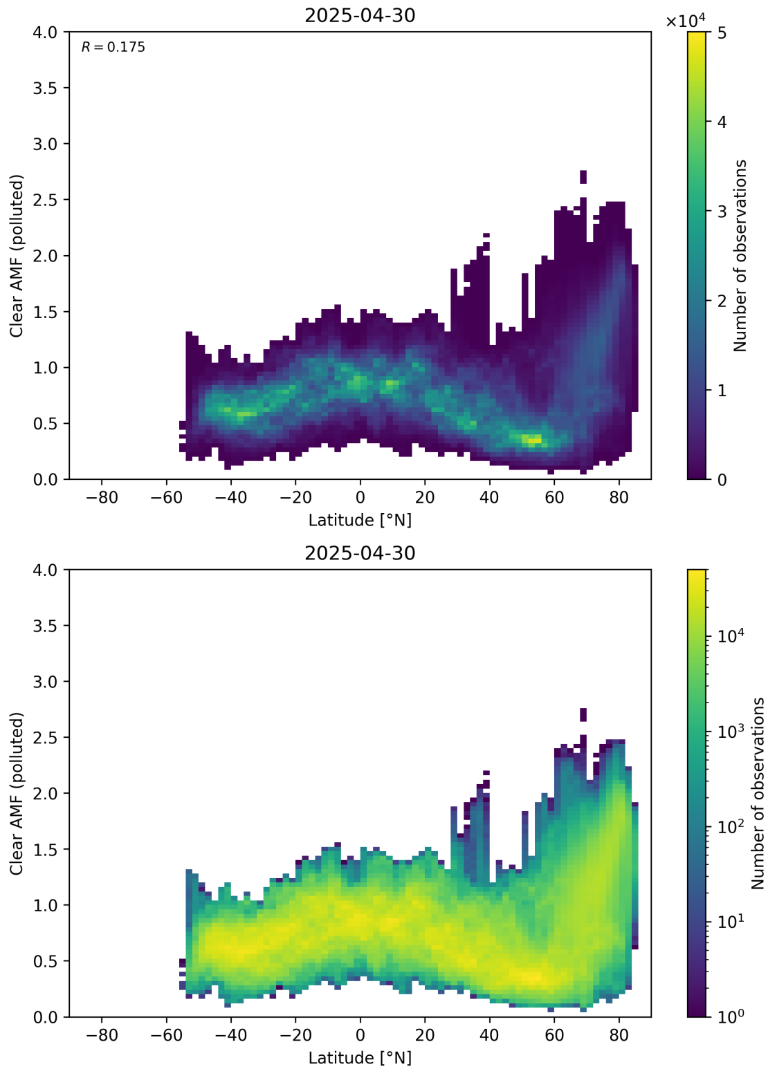
Figure 156: Scatter density plot of “Latitude” against “Clear AMF (polluted)” for 2025-04-29 to 2025-05-01.
