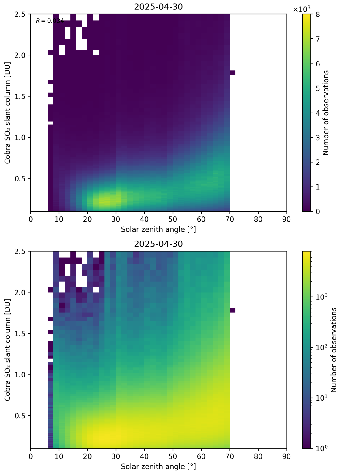
Figure 179: Scatter density plot of “Solar zenith angle” against “Cobra SO 2 slant column” for 2025-04-29 to 2025-05-01.
