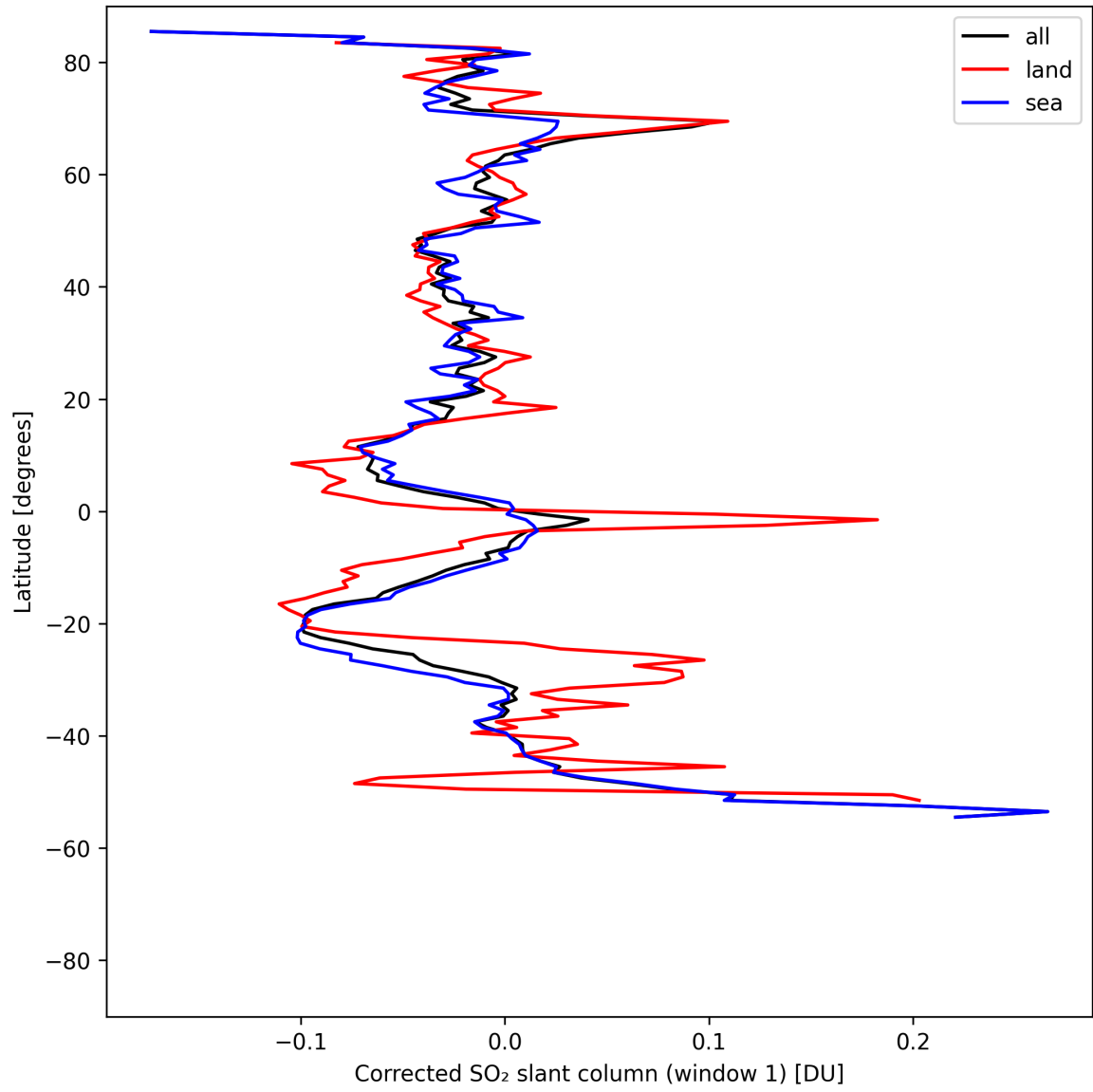
Figure 39: Zonal average of “Corrected SO 2 slant column (window 1)” for 2025-04-29 to 2025-05-01.
