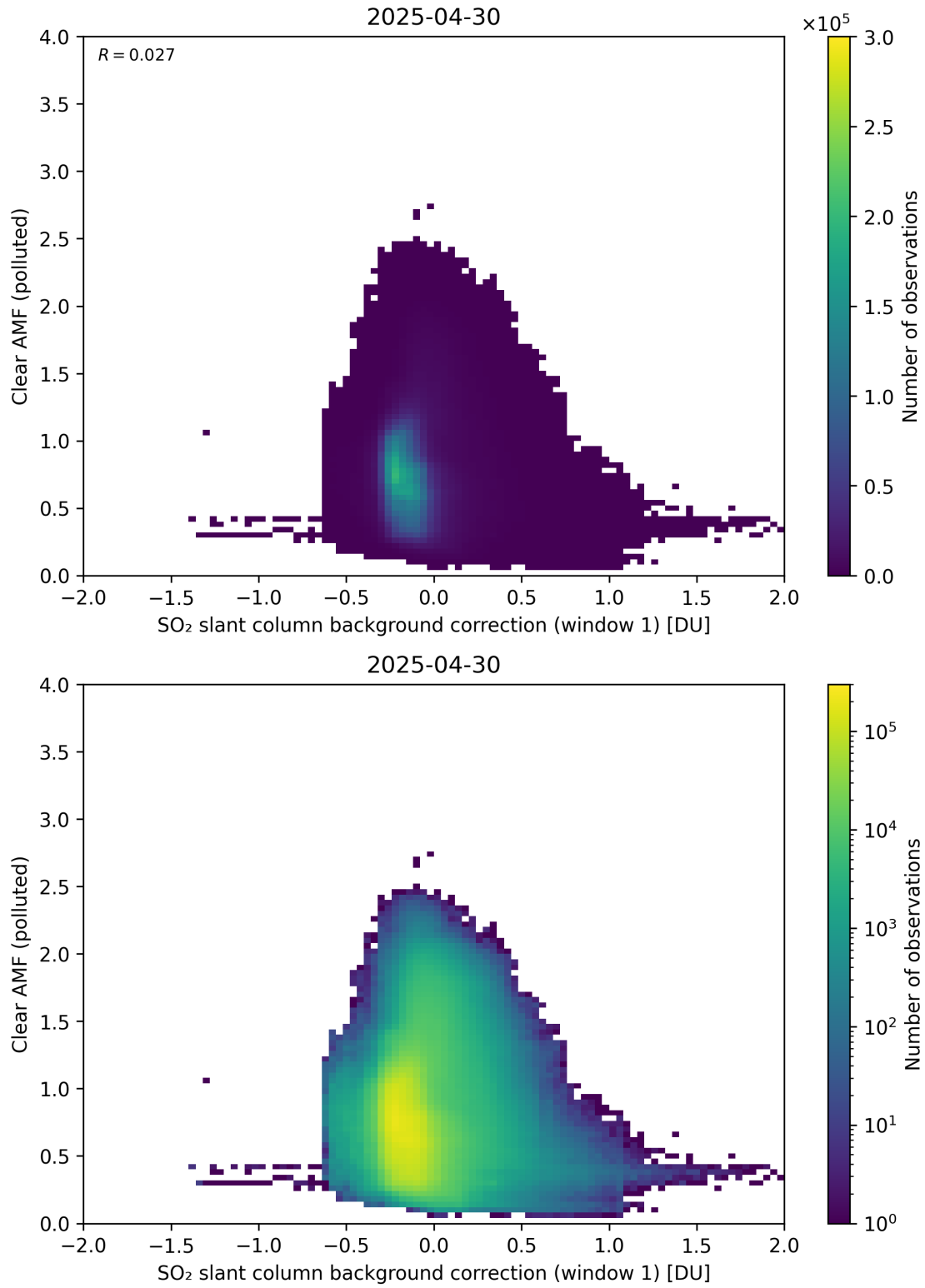
Figure 114: Scatter density plot of “SO 2 slant column background correction (window 1)” against “Clear AMF (polluted)” for 2025-04-29 to 2025-05-01.
