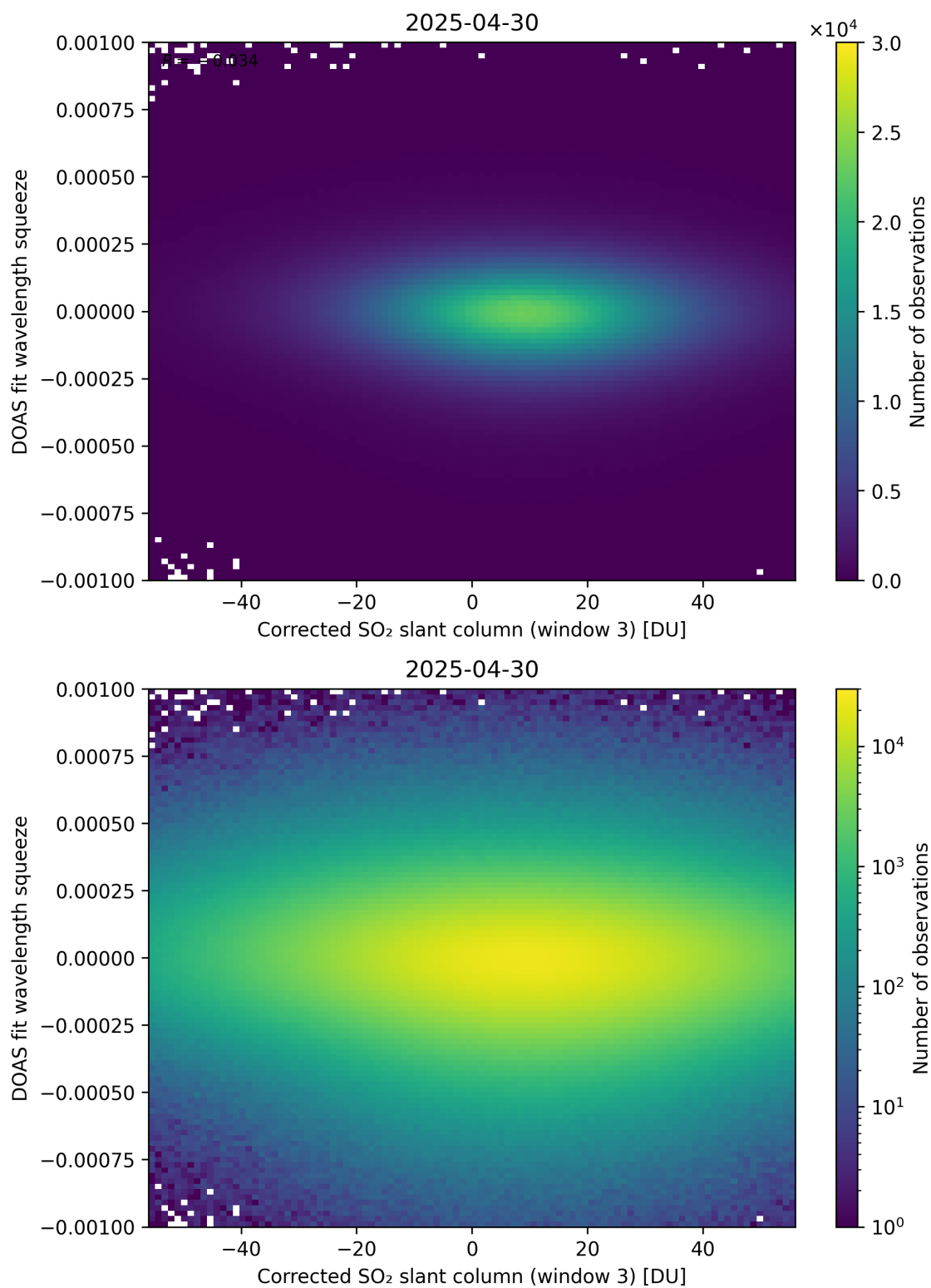
Figure 257: Scatter density plot of “Corrected SO 2 slant column (window 3)” against “DOAS fit wavelength squeeze” for 2025-04-29 to 2025-05-01.
