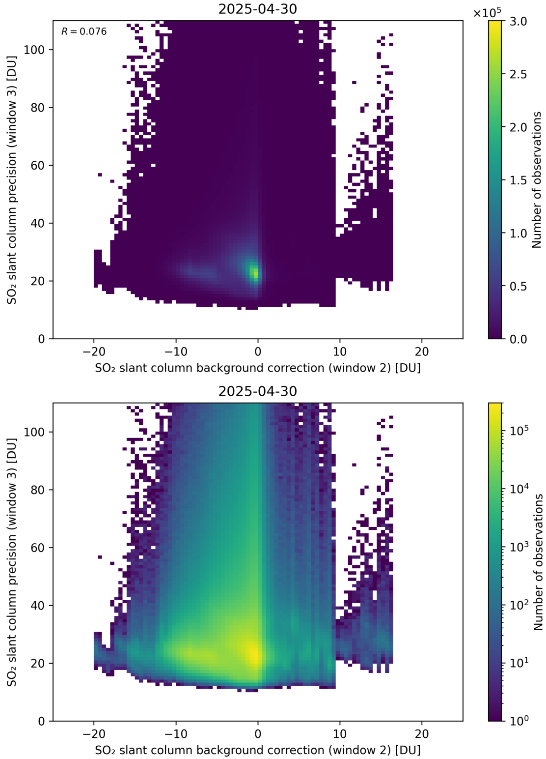
Figure 129: Scatter density plot of “SO 2 slant column background correction (window 2)” against “SO 2 slant column precision (window 3)” for 2025-04-29 to 2025-05-01.
