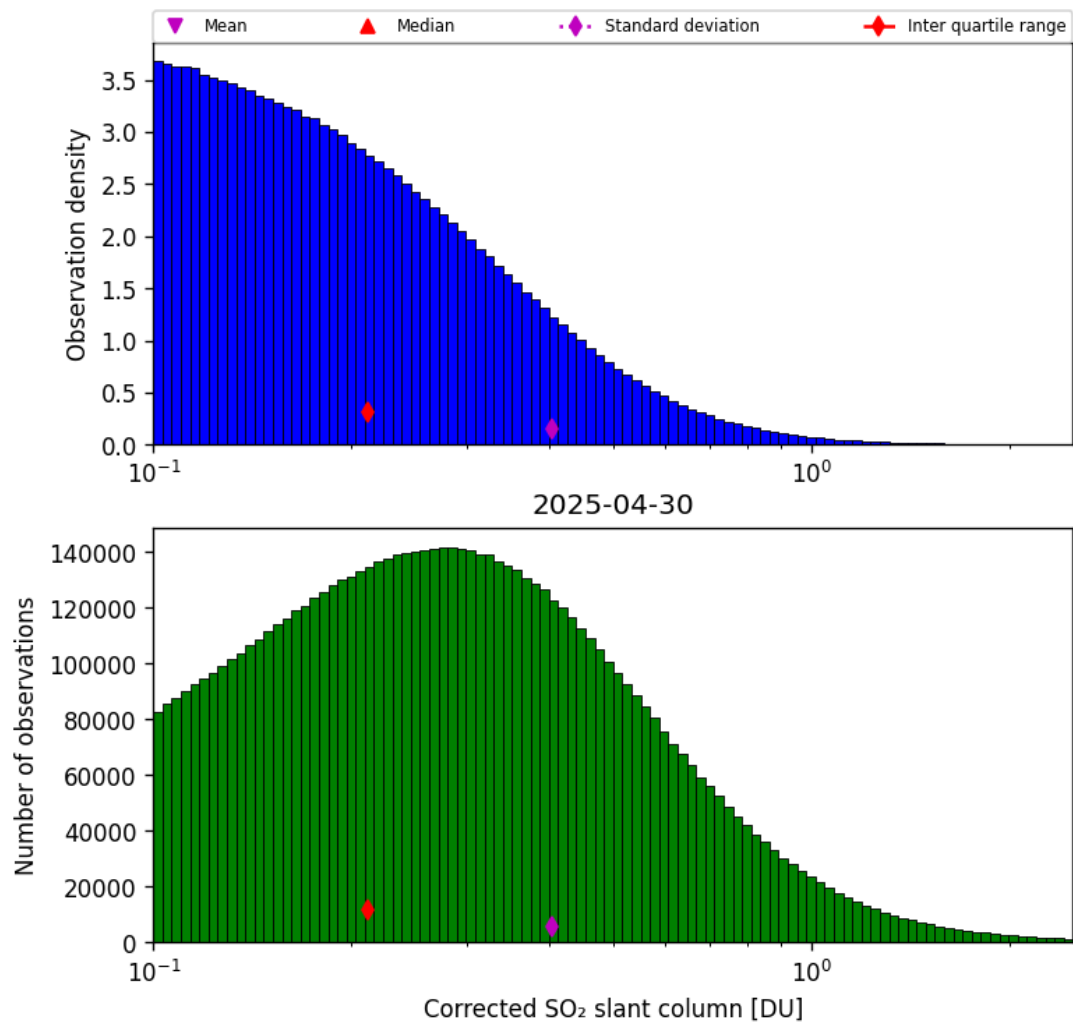
Figure 60: Histogram of "Corrected SO 2 slant column" for 2025-04-29 to 2025-05-01
