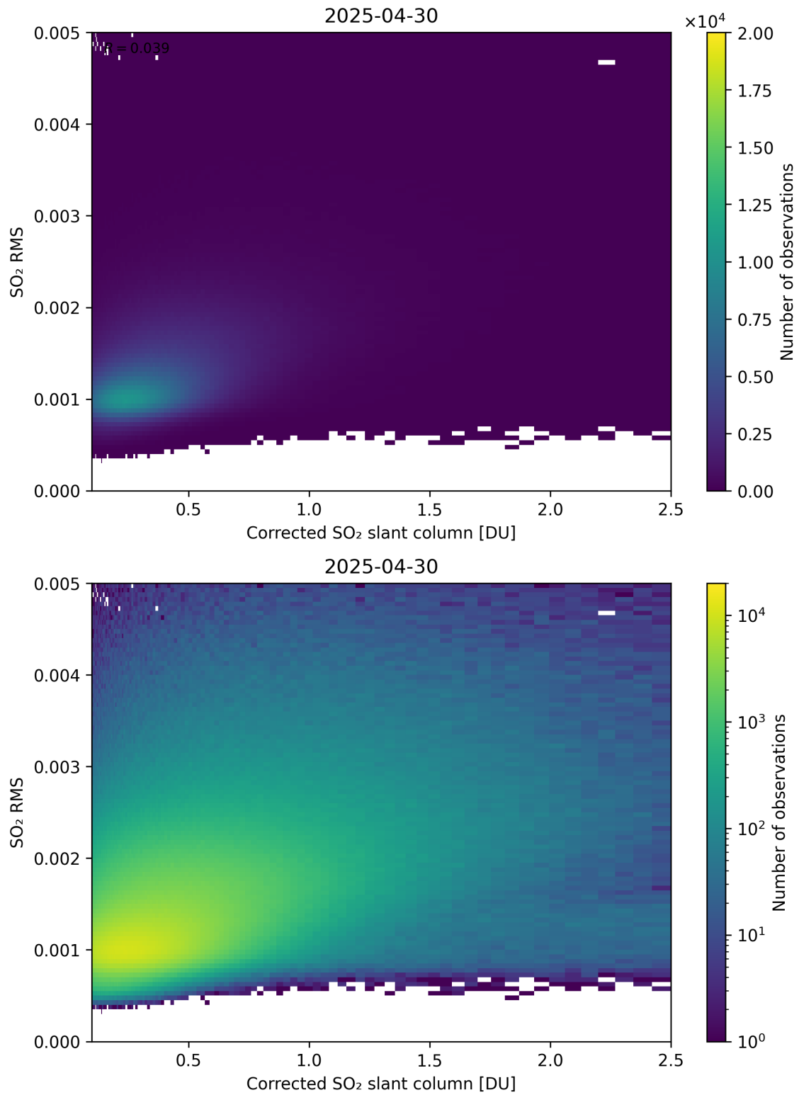
Figure 231: Scatter density plot of “Corrected SO 2 slant column” against “SO 2 RMS” for 2025-04-29 to 2025-05-01.
