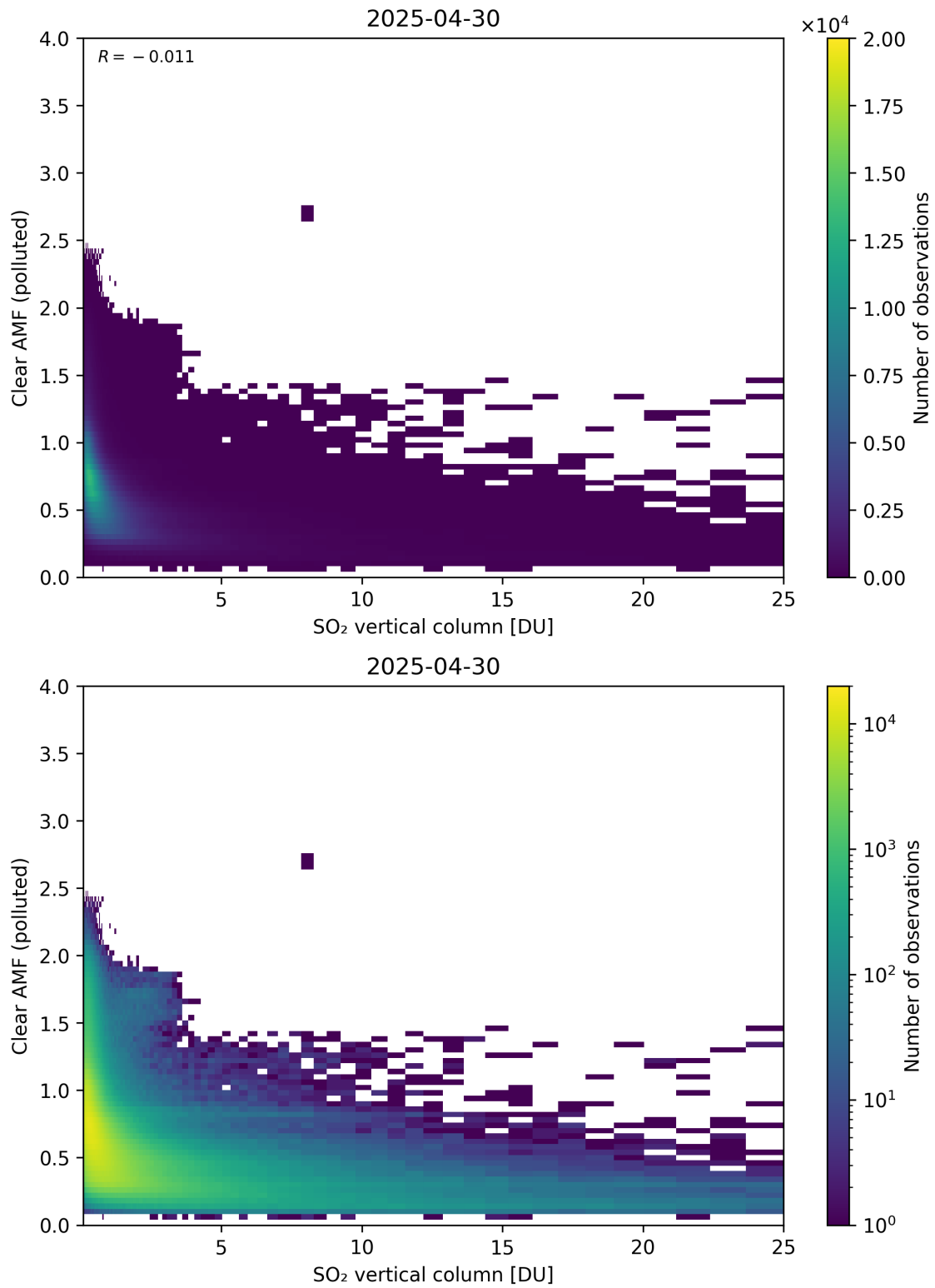
Figure 348: Scatter density plot of “SO 2 vertical column” against “Clear AMF (polluted)” for 2025-04-29 to 2025-05-01.
