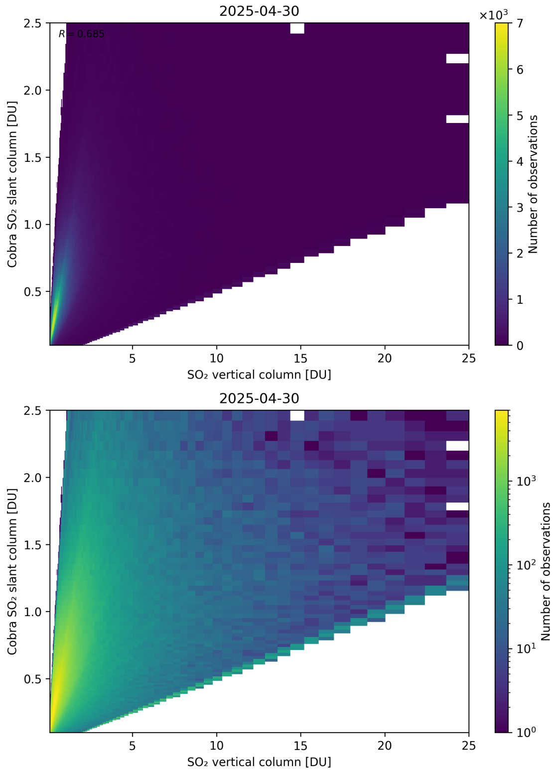
Figure 349: Scatter density plot of “SO 2 vertical column” against “Cobra SO 2 slant column” for 2025-04-29 to 2025-05-01.
