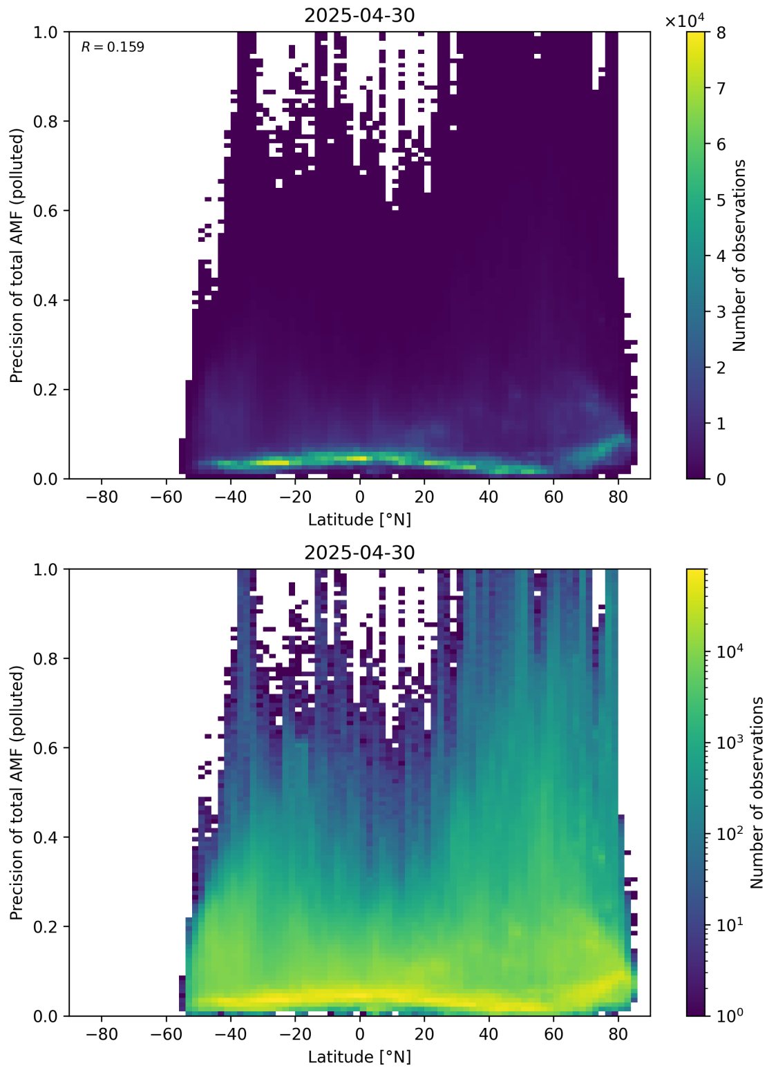
Figure 168: Scatter density plot of “Latitude” against “Precision of total AMF (polluted)” for 2025-04-29 to 2025-05-01.
