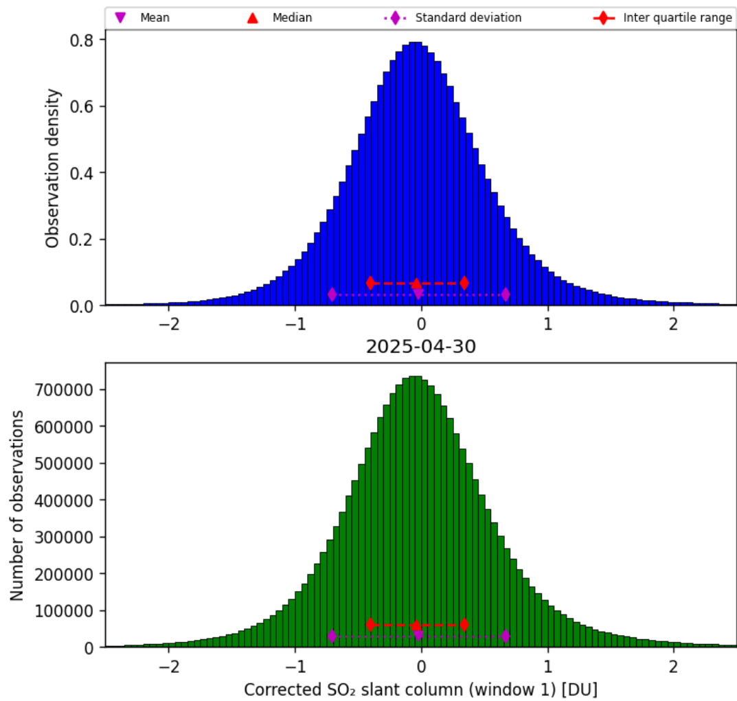
Figure 65: Histogram of “Corrected SO 2 slant column (window 1)” for 2025-04-29 to 2025-05-01
