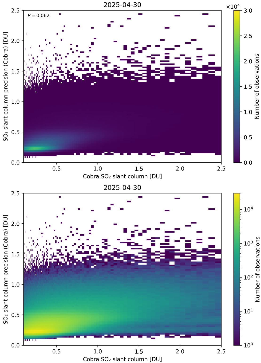
Figure 216: Scatter density plot of “Cobra SO 2 slant column” against “SO 2 slant column precision (Cobra)” for 2025-04-29 to 2025-05-01.
