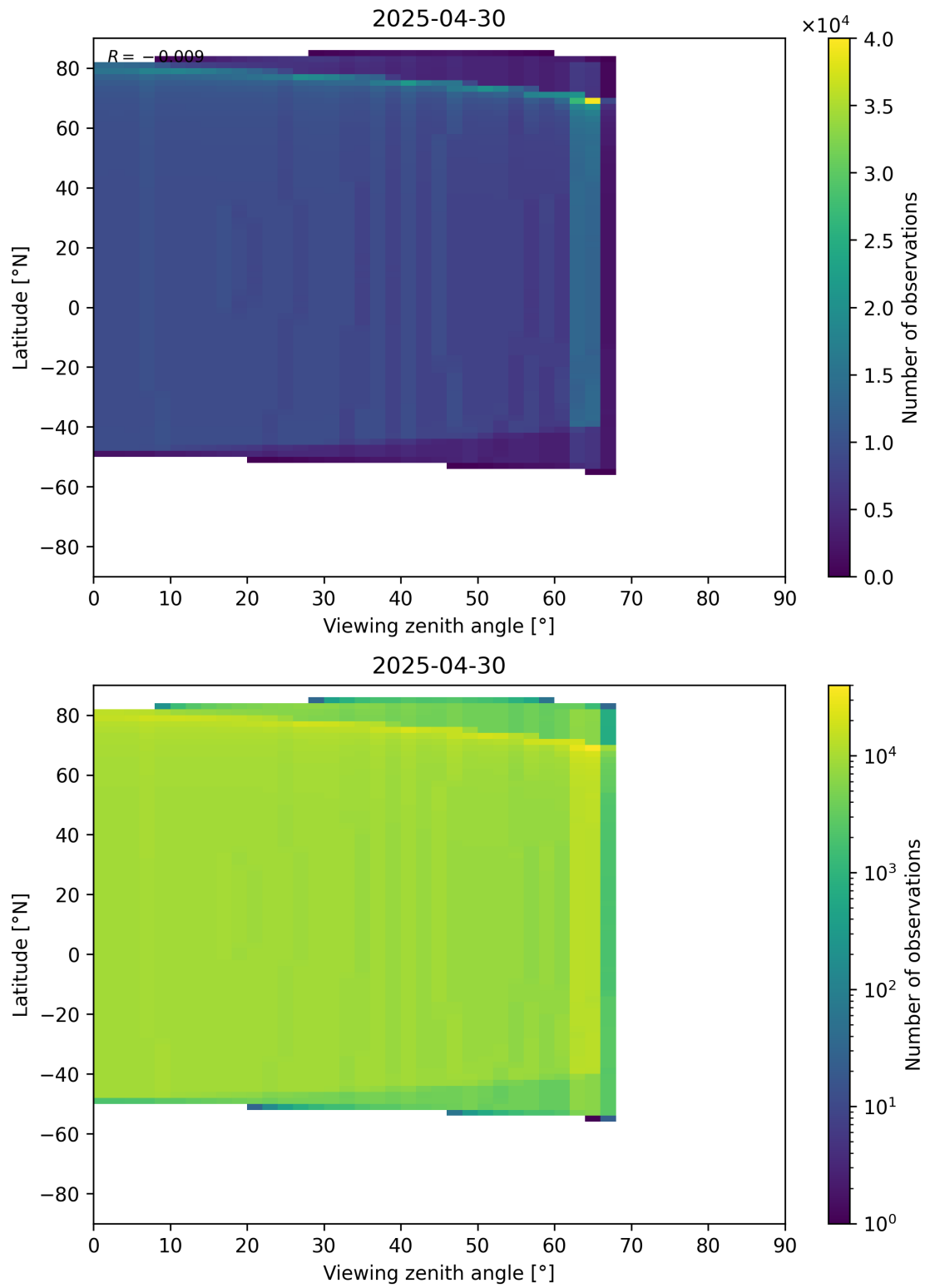
Figure 368: Scatter density plot of “Viewing zenith angle” against “Latitude” for 2025-04-29 to 2025-05-01.
