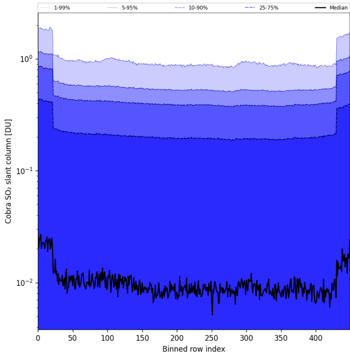
Figure 87: Along track statistics of “Cobra SO 2 slant column” for 2025-04-29 to 2025-05-01
