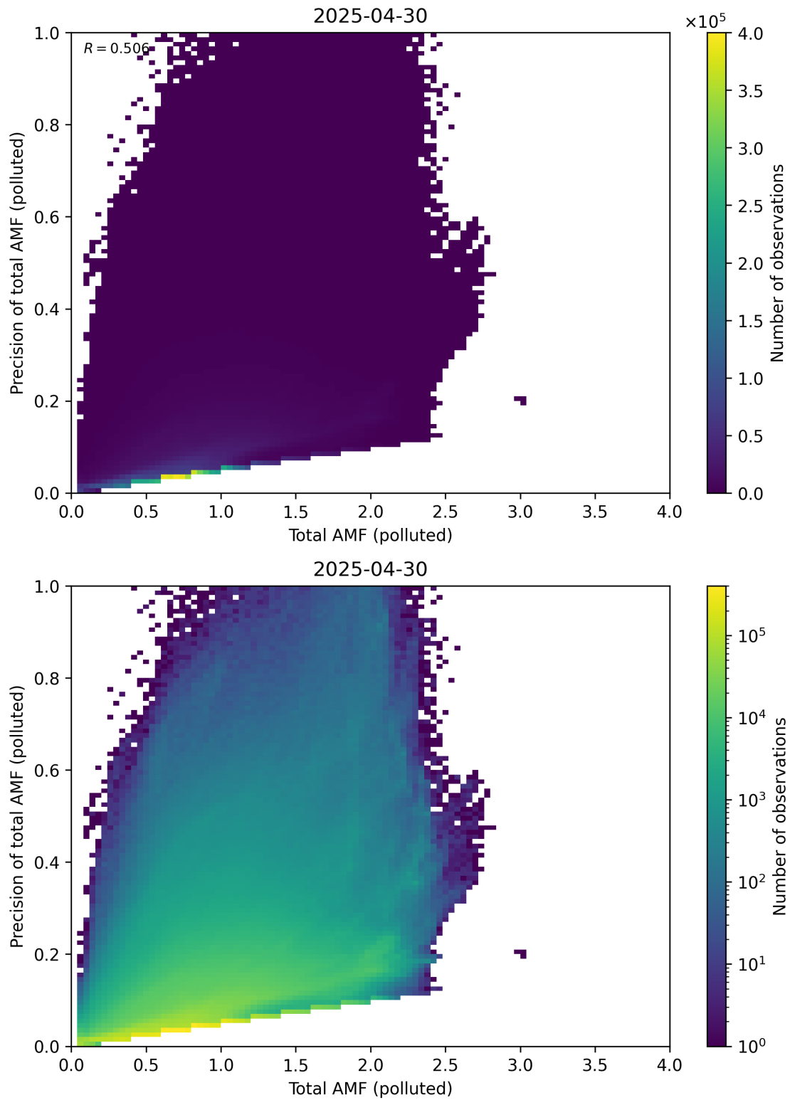
Figure 322: Scatter density plot of “Total AMF (polluted)” against “Precision of total AMF (polluted)” for 2025-04-29 to 2025-05-01.
