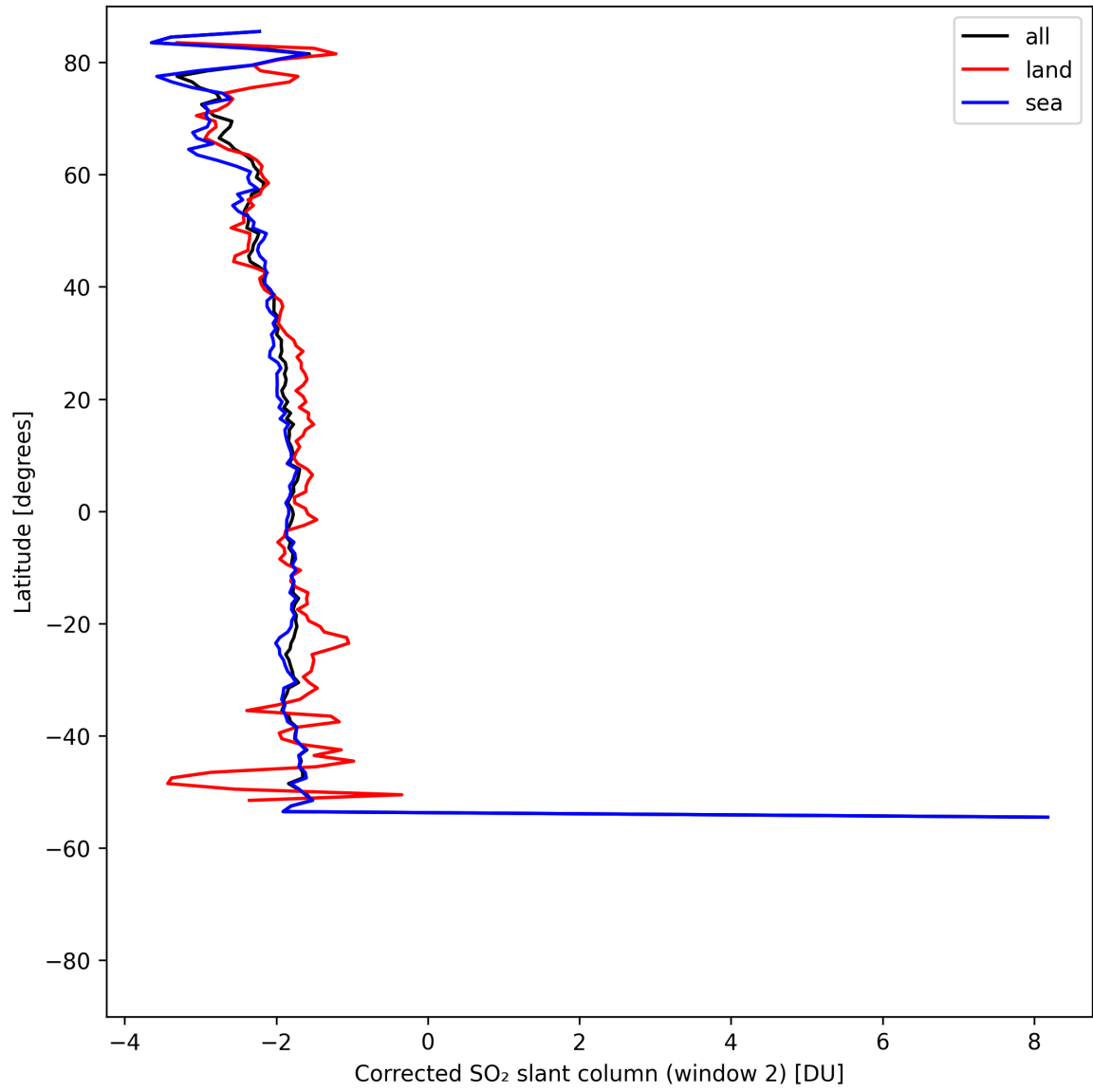
Figure 43: Zonal average of “Corrected SO 2 slant column (window 2)” for 2025-04-29 to 2025-05-01.
