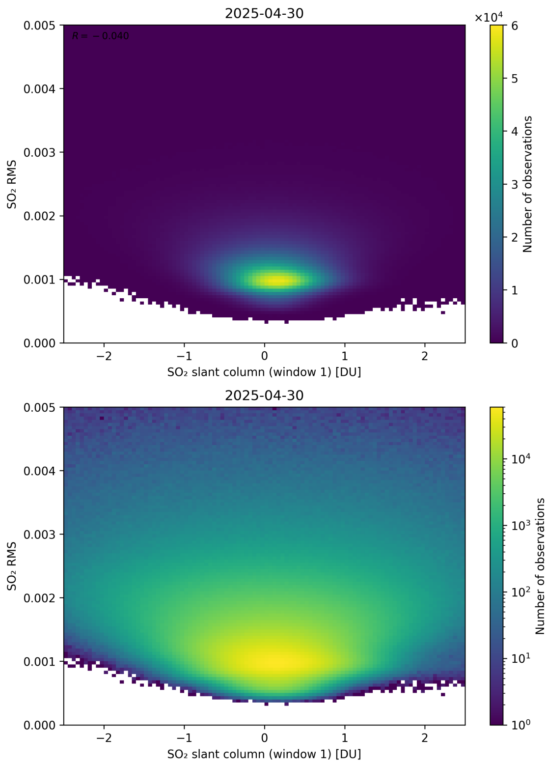
Figure 267: Scatter density plot of “SO 2 slant column (window 1)” against “SO 2 RMS” for 2025-04-29 to 2025-05-01.
