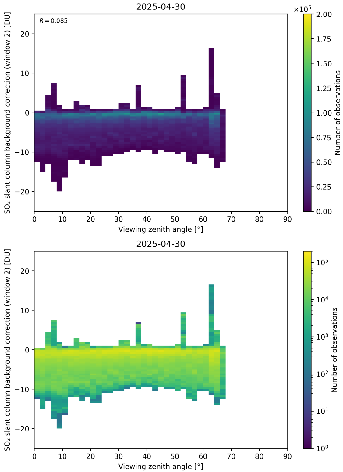
Figure 363: Scatter density plot of “Viewing zenith angle” against “SO 2 slant column background correction (window 2)” for 2025-04-29 to 2025-05-01.
