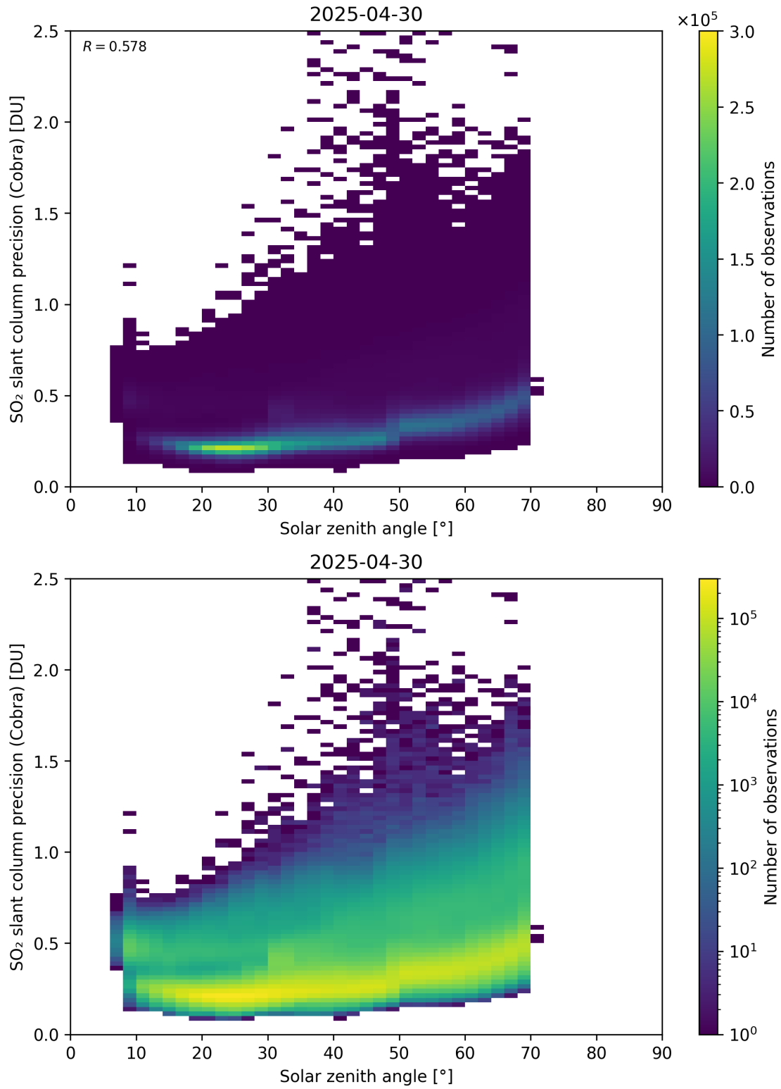
Figure 180: Scatter density plot of “Solar zenith angle” against “SO 2 slant column precision (Cobra)” for 2025-04-29 to 2025-05-01.
