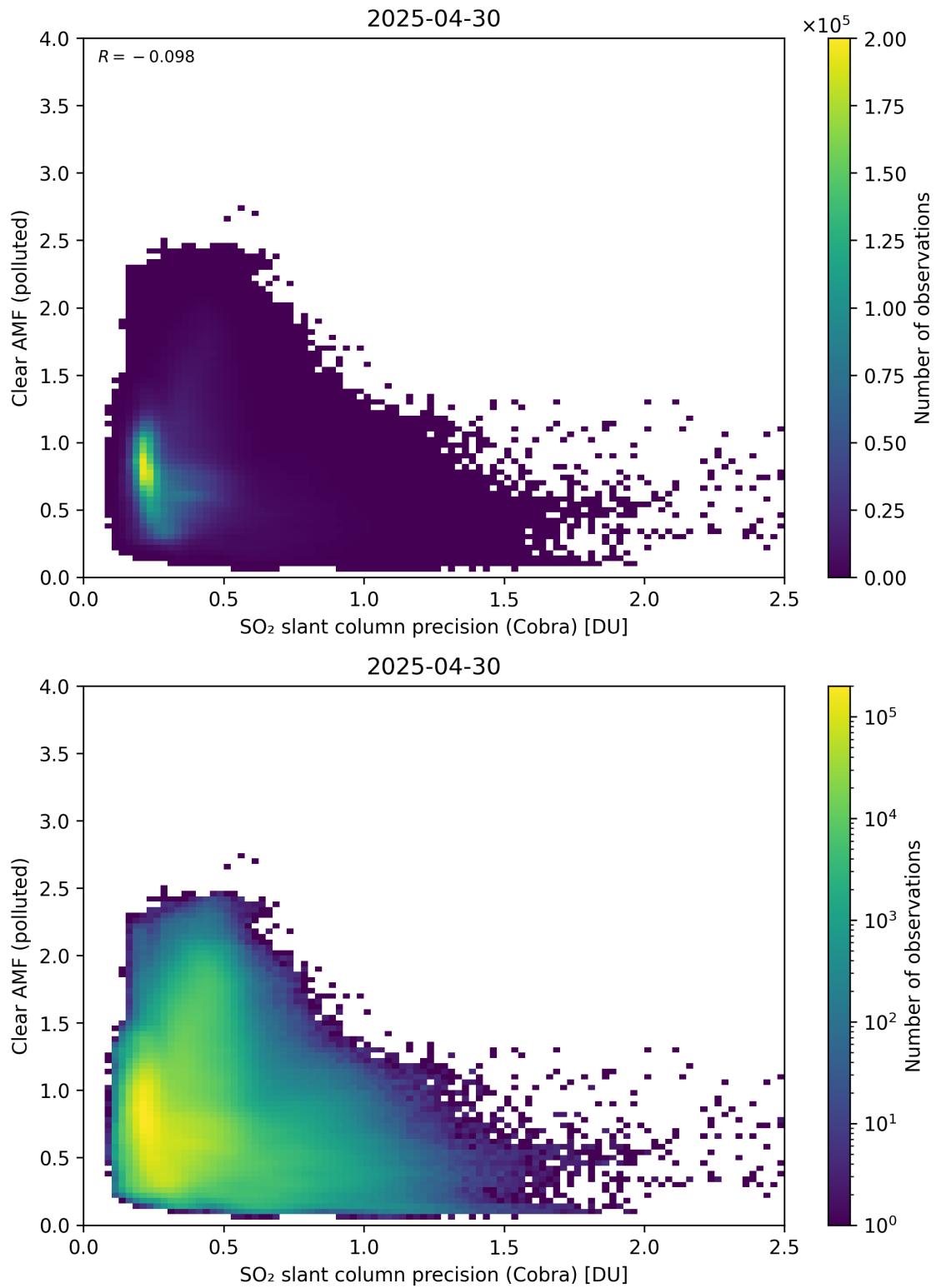
Figure 205: Scatter density plot of “SO 2 slant column precision (Cobra)” against “Clear AMF (polluted)” for 2025-04-29 to 2025-05-01.
