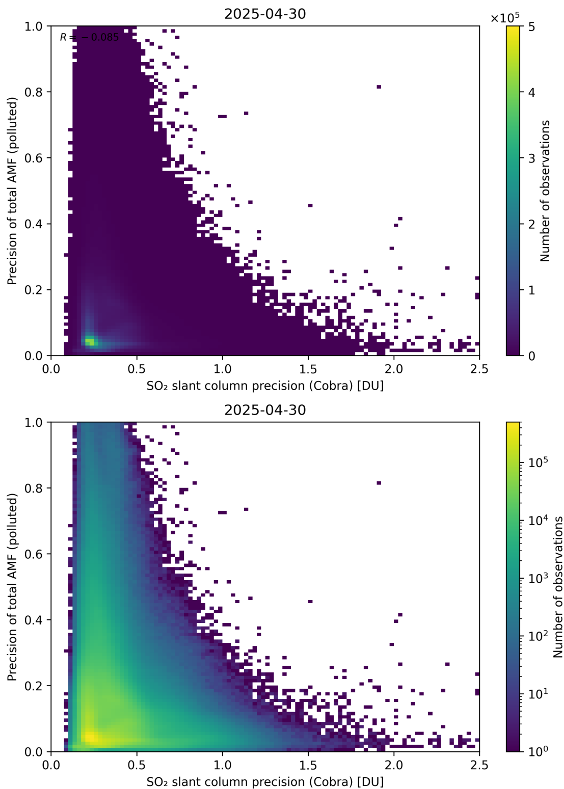
Figure 214: Scatter density plot of “SO 2 slant column precision (Cobra)” against “Precision of total AMF (polluted)” for 2025-04-29 to 2025-05-01.
