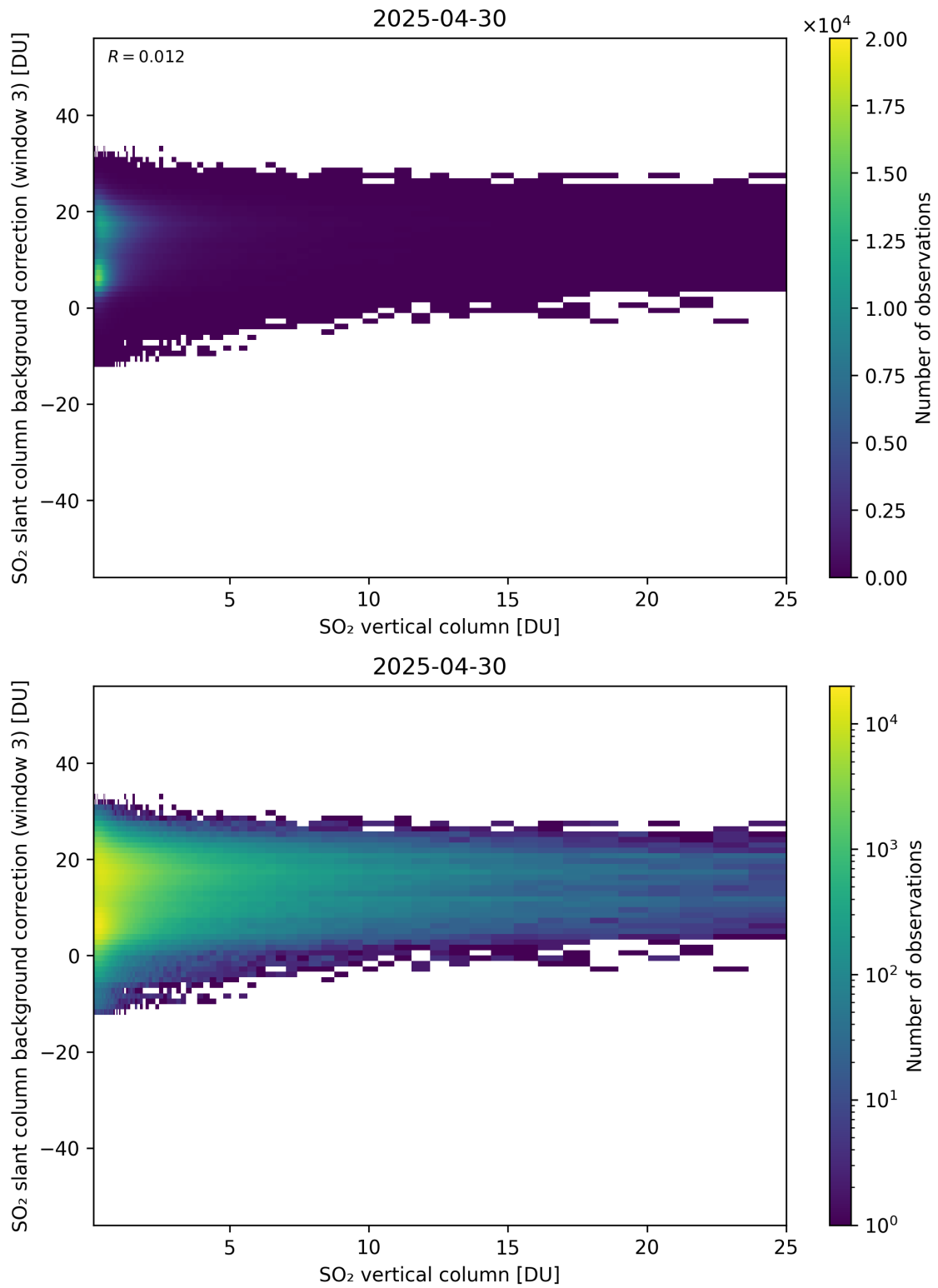
Figure 325: Scatter density plot of “SO 2 vertical column” against “SO 2 slant column background correction (window 3)” for 2025-04-29 to 2025-05-01.
