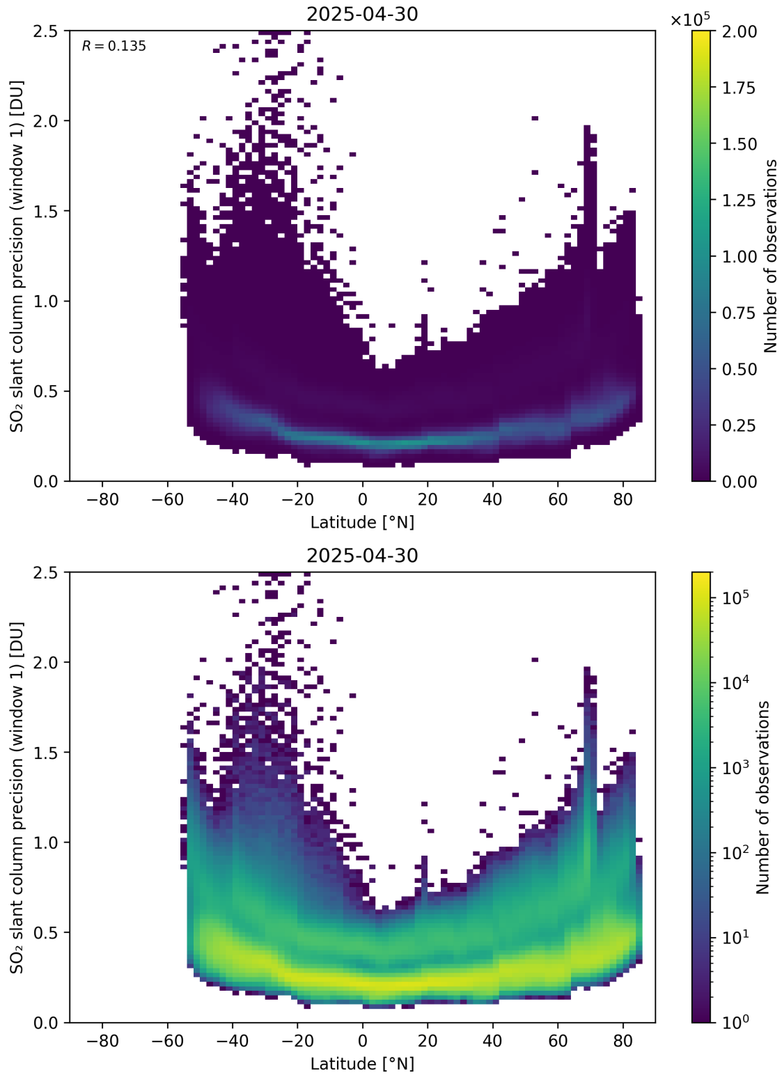
Figure 163: Scatter density plot of “Latitude” against “SO 2 slant column precision (window 1)” for 2025-04-29 to 2025-05-01.
