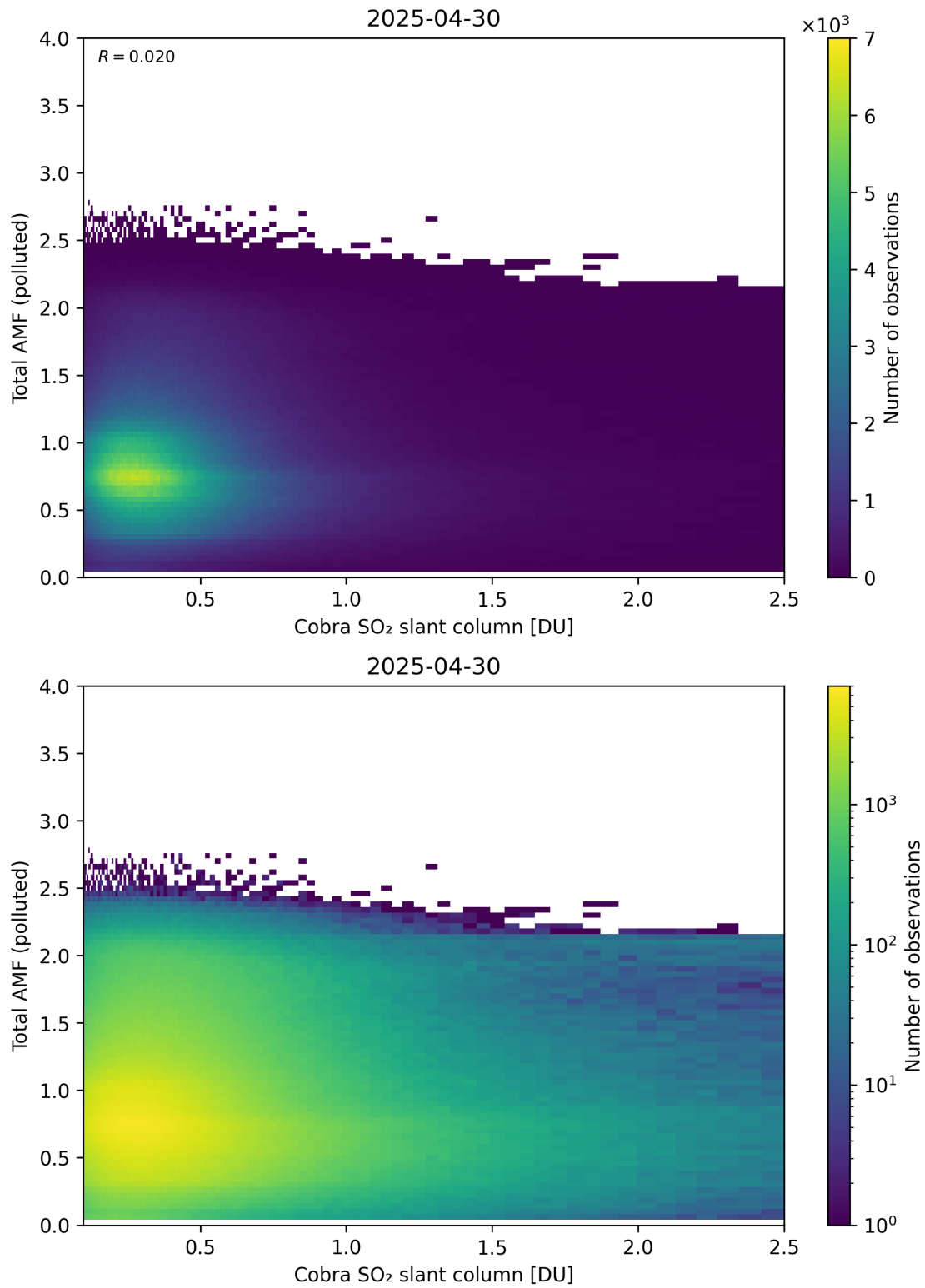
Figure 224: Scatter density plot of “Cobra SO 2 slant column” against “Total AMF (polluted)” for 2025-04-29 to 2025-05-01.
