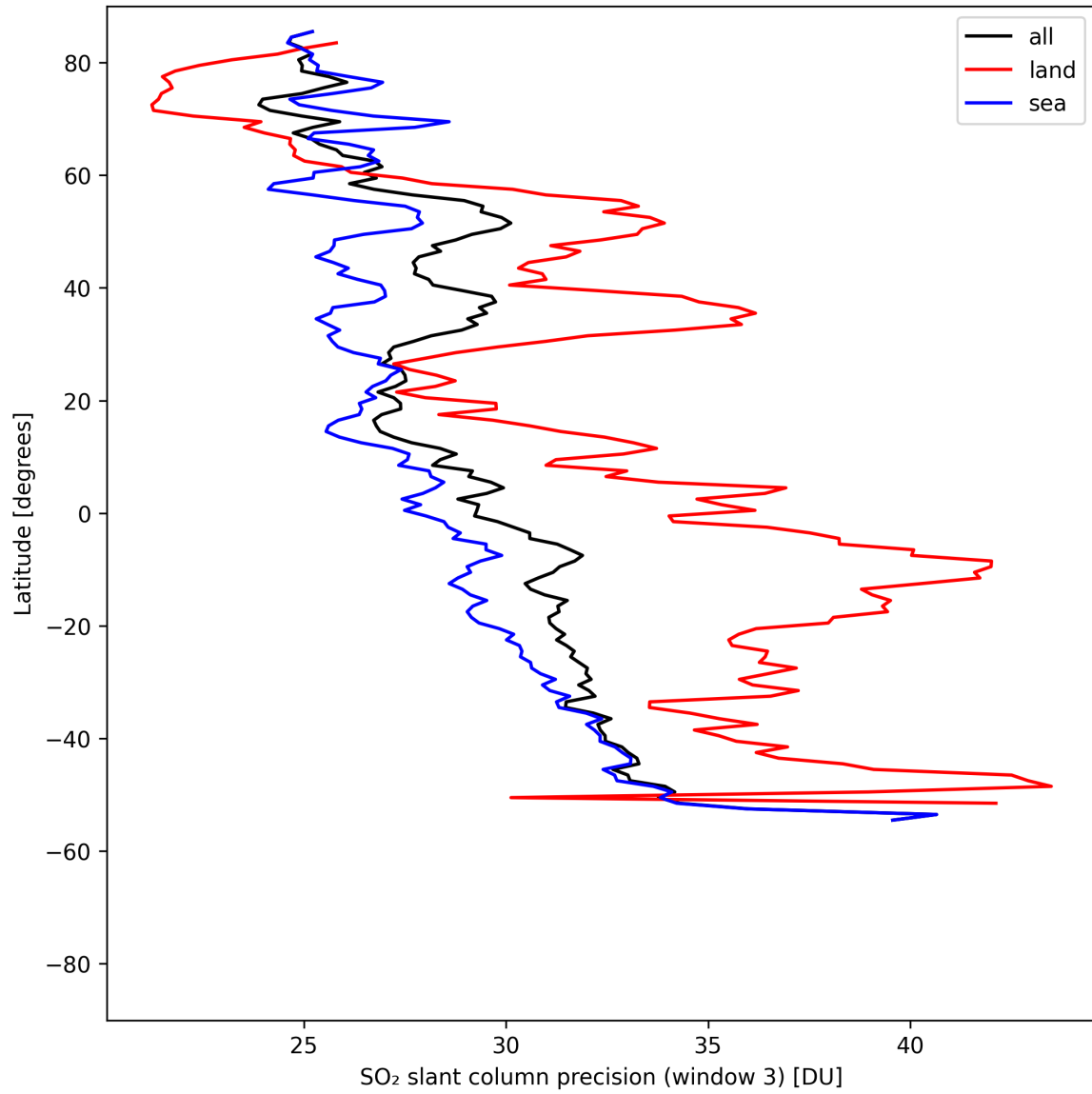
Figure 46: Zonal average of “SO 2 slant column precision (window 3)” for 2025-04-29 to 2025-05-01.
