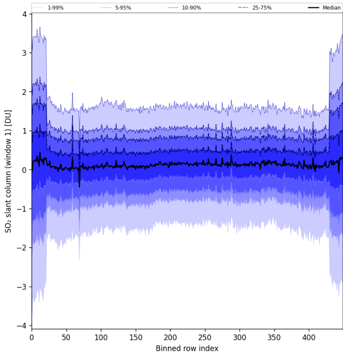
Figure 89: Along track statistics of “SO 2 slant column (window 1)” for 2025-04-29 to 2025-05-01
