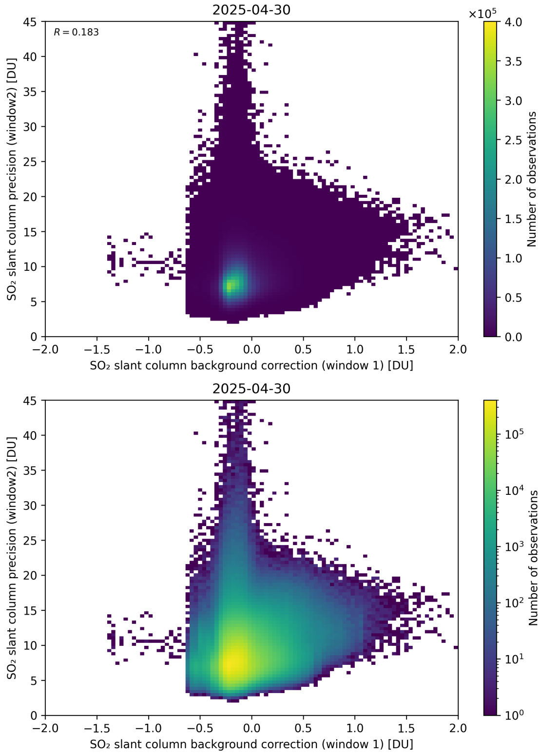
Figure 117: Scatter density plot of “SO 2 slant column background correction (window 1)” against “SO 2 slant column precision (window2)” for 2025-04-29 to 2025-05-01.
