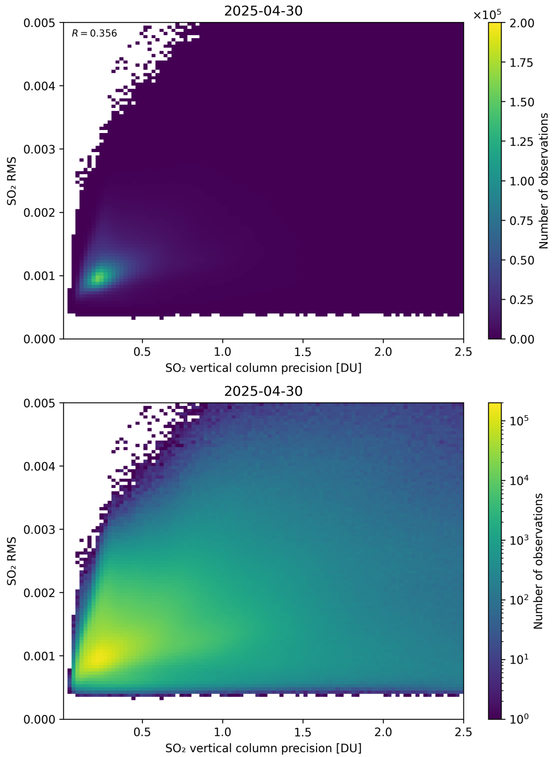
Figure 334: Scatter density plot of “SO 2 vertical column precision” against “SO 2 RMS” for 2025-04-29 to 2025-05-01.
