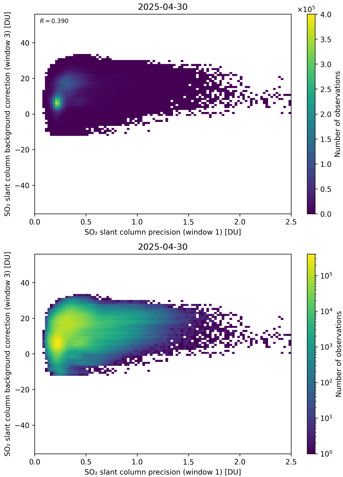
Figure 270: Scatter density plot of “SO 2 slant column precision (window 1)” against “SO 2 slant column background correction (window 3)” for 2025-04-29 to 2025-05-01.
