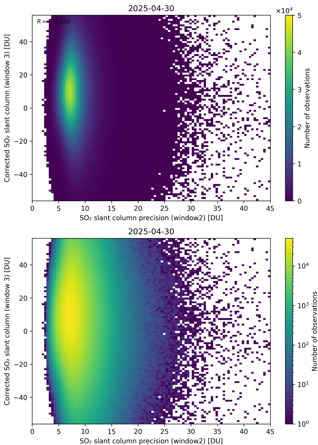
Figure 298: Scatter density plot of “SO 2 slant column precision (window2)” against “Corrected SO 2 slant column (window 3)” for 2025-04-29 to 2025-05-01.
