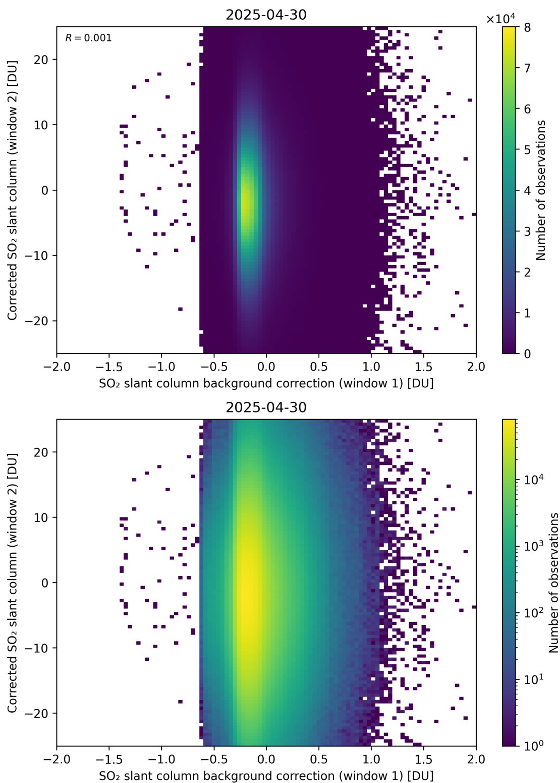
Figure 115: Scatter density plot of “SO 2 slant column background correction (window 1)” against “Corrected SO 2 slant column (window 2)” for 2025-04-29 to 2025-05-01.
