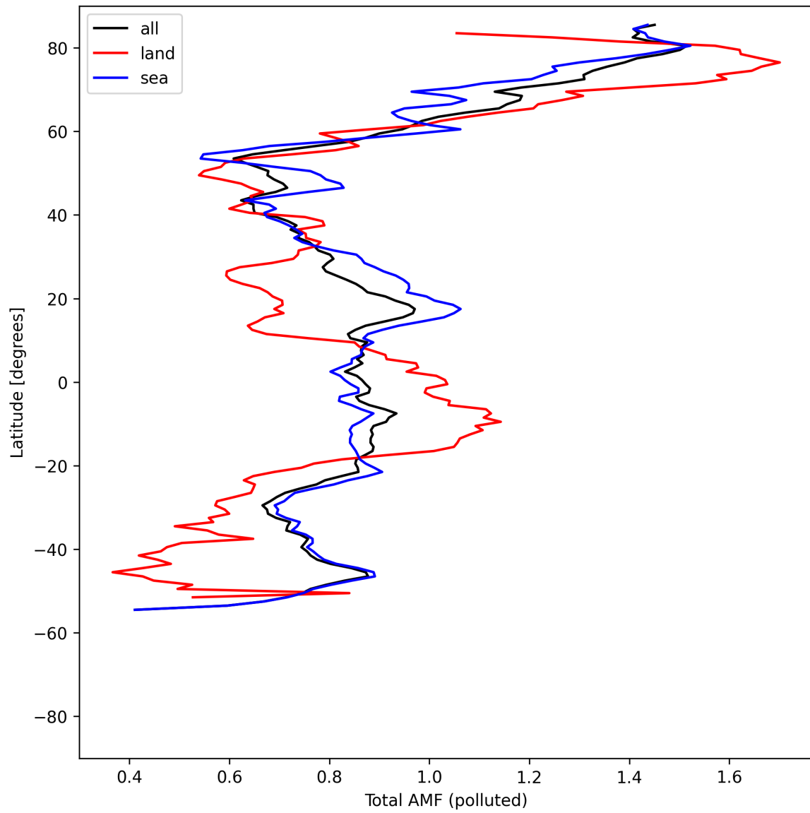
Figure 53: Zonal average of “Total AMF (polluted)” for 2025-04-29 to 2025-05-01.
