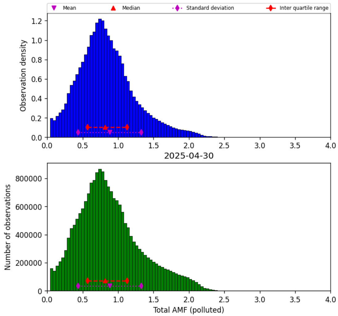
Figure 79: Histogram of “Total AMF (polluted)” for 2025-04-29 to 2025-05-01
