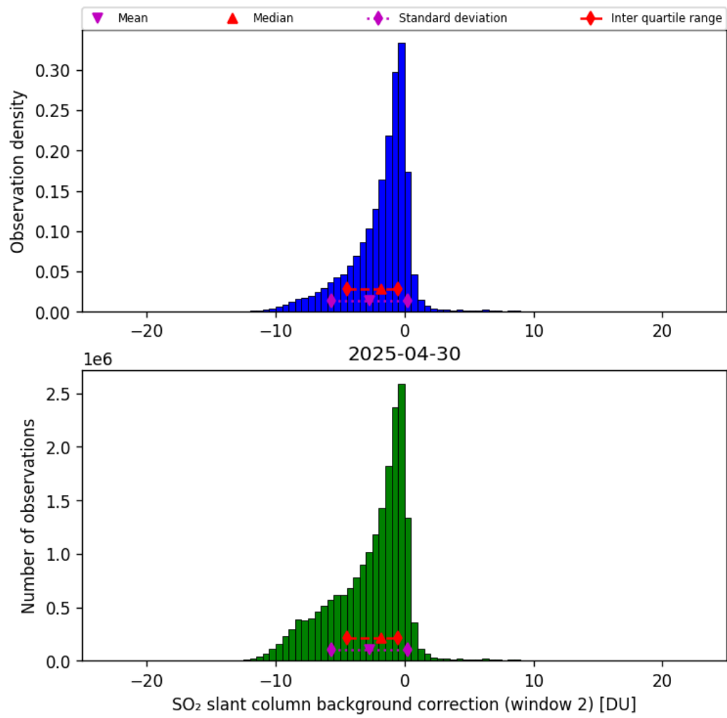
Figure 70: Histogram of “SO 2 slant column background correction (window 2)” for 2025-04-29 to 2025-05-01
