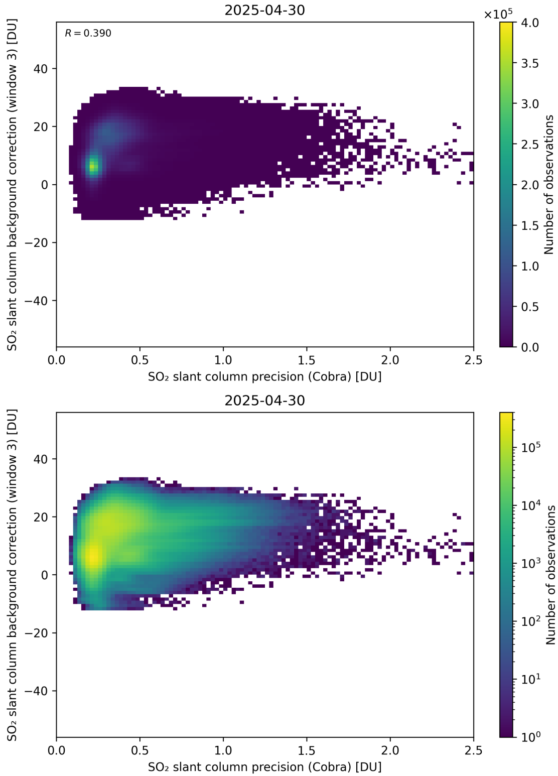
Figure 201: Scatter density plot of “SO 2 slant column precision (Cobra)” against “SO 2 slant column background correction (window 3)” for 2025-04-29 to 2025-05-01.
