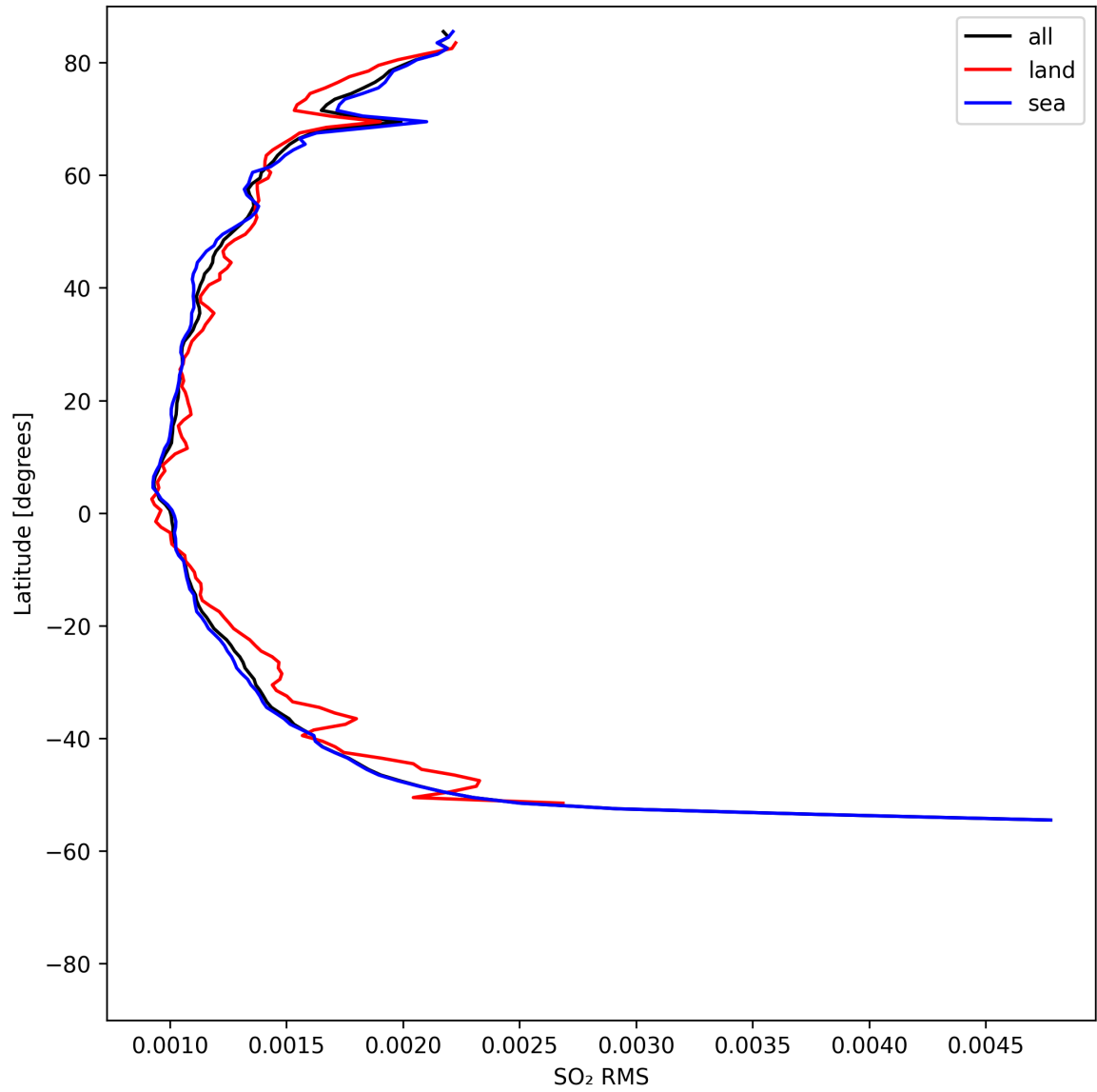
Figure 52: Zonal average of “SO 2 RMS” for 2025-04-29 to 2025-05-01.
