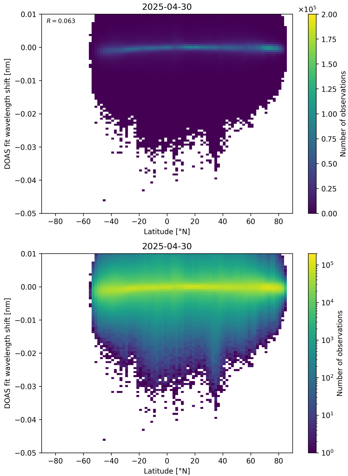
Figure 153: Scatter density plot of “Latitude” against “DOAS fit wavelength shift” for 2025-04-29 to 2025-05-01.
