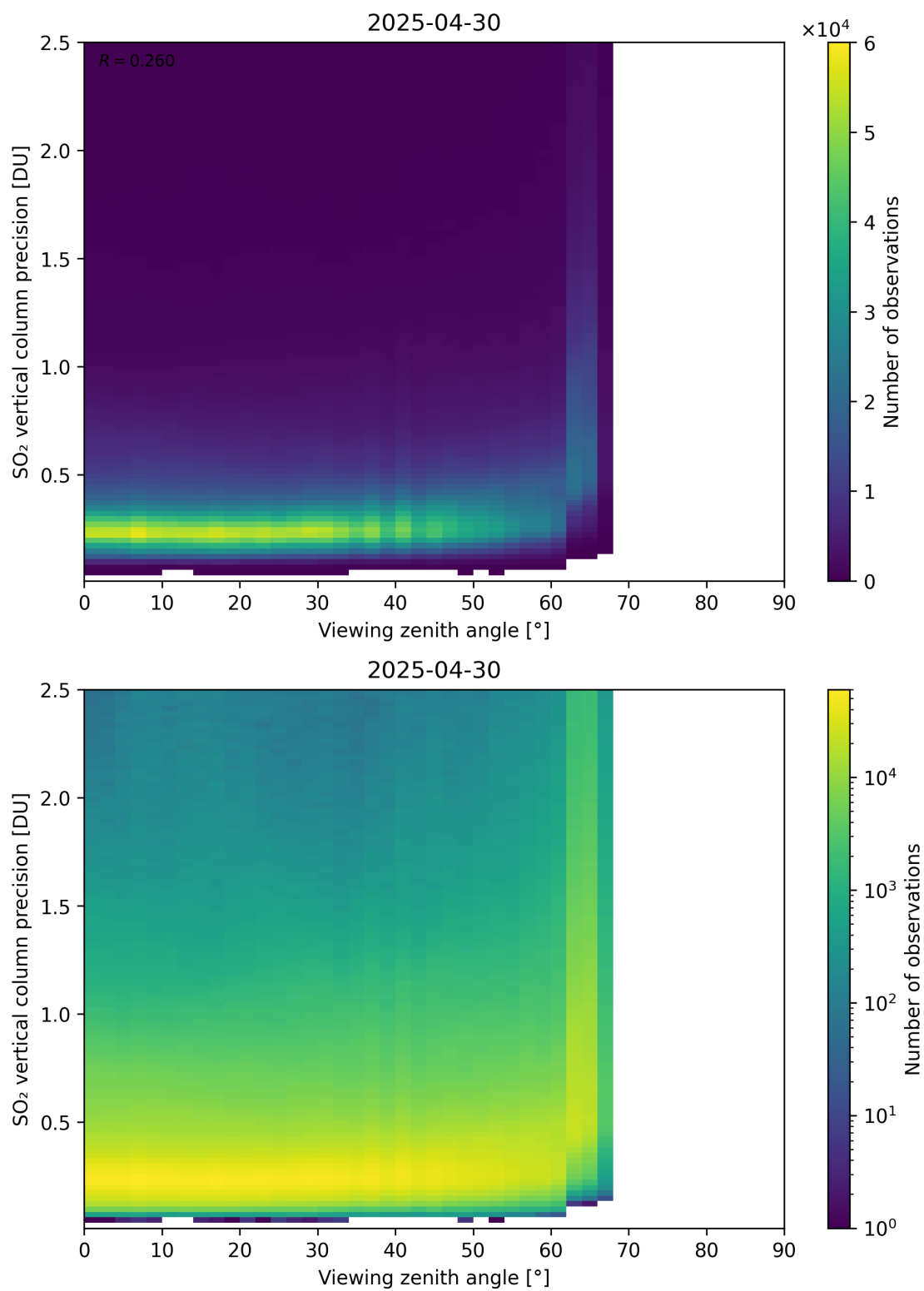
Figure 384: Scatter density plot of “Viewing zenith angle” against “SO 2 vertical column precision” for 2025-04-29 to 2025-05-01.
