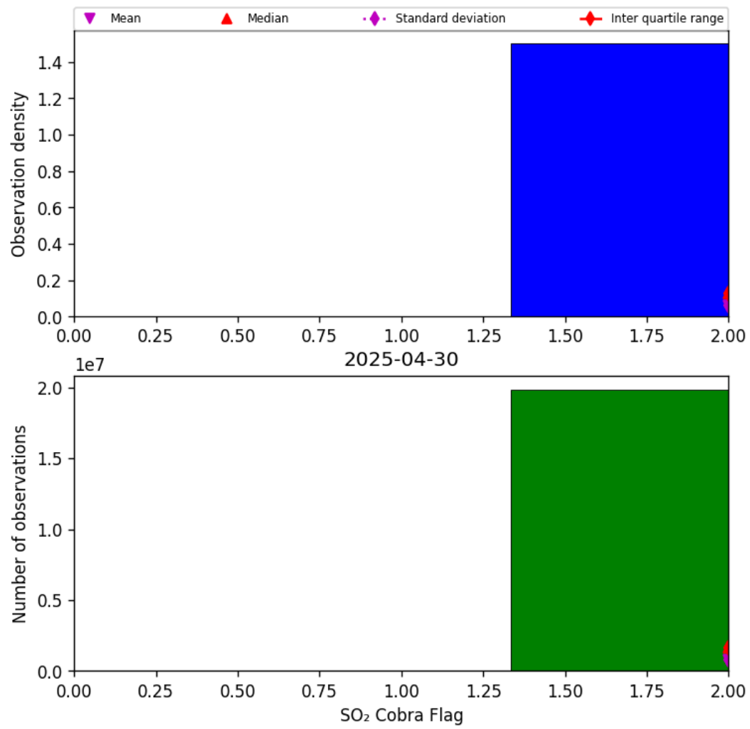
Figure 75: Histogram of “SO 2 Cobra Flag” for 2025-04-29 to 2025-05-01
