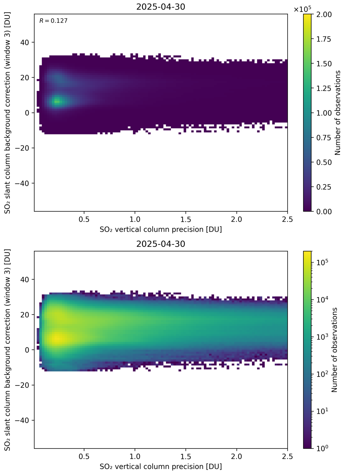
Figure 331: Scatter density plot of “SO 2 vertical column precision” against “SO 2 slant column background correction (window 3)” for 2025-04-29 to 2025-05-01.
