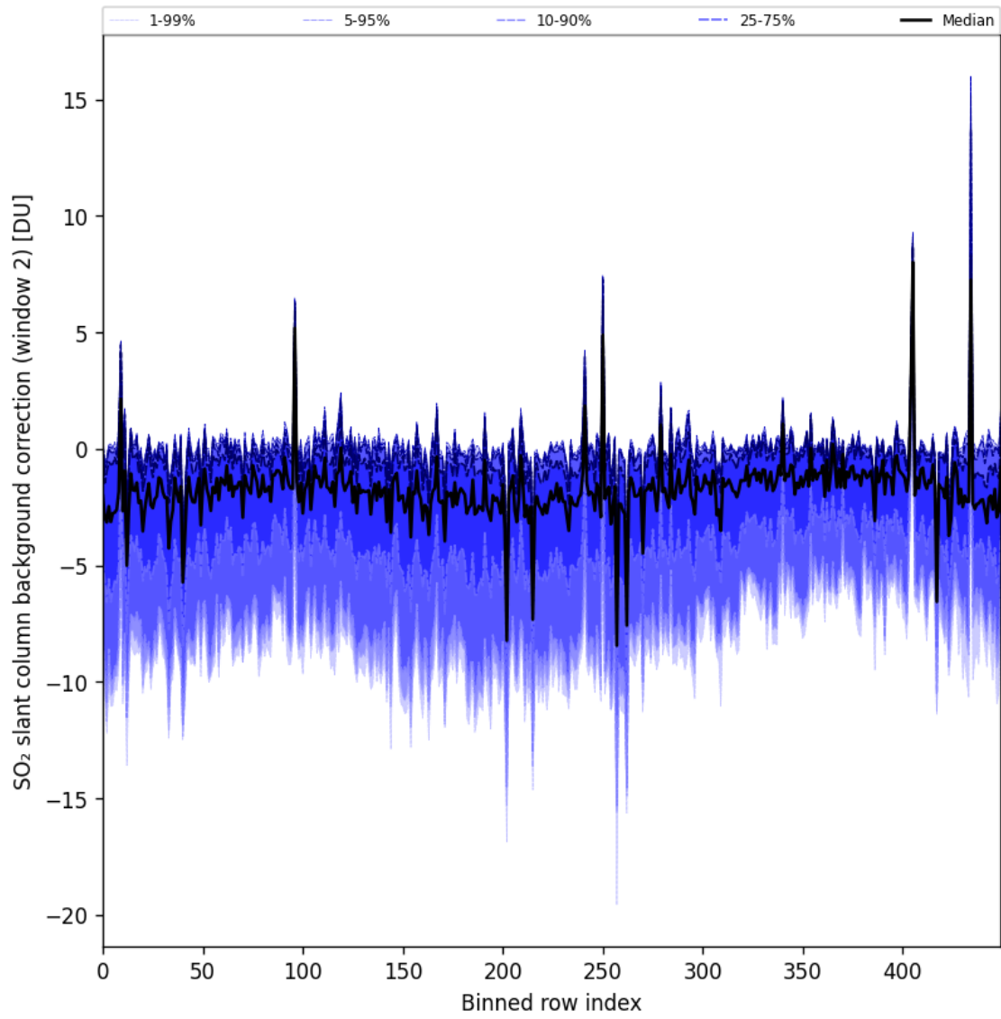
Figure 96: Along track statistics of “SO 2 slant column background correction (window 2)” for 2025-04-29 to 2025-05-01
