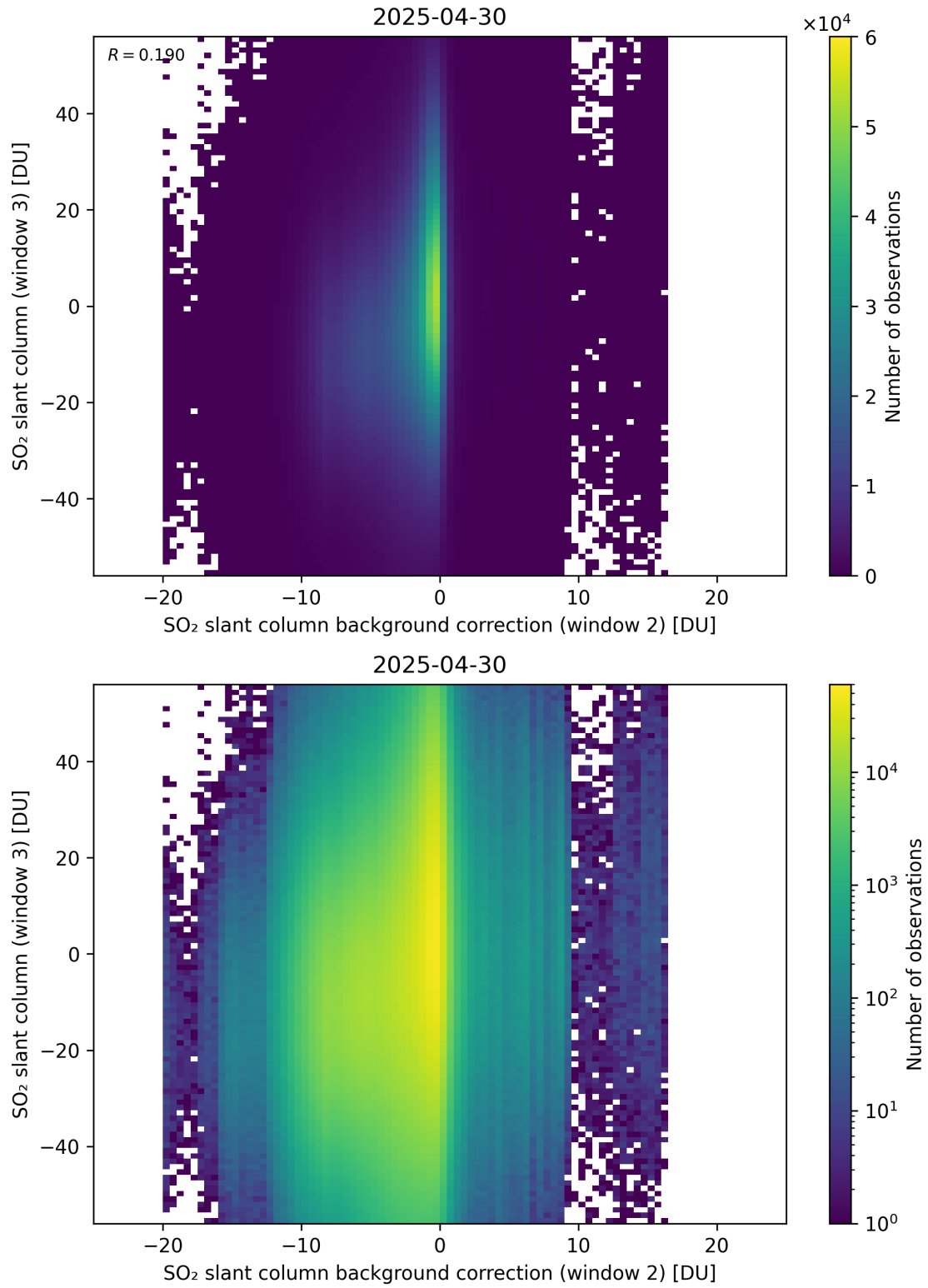
Figure 128: Scatter density plot of “SO 2 slant column background correction (window 2)” against “SO 2 slant column (window 3)” for 2025-04-29 to 2025-05-01.
