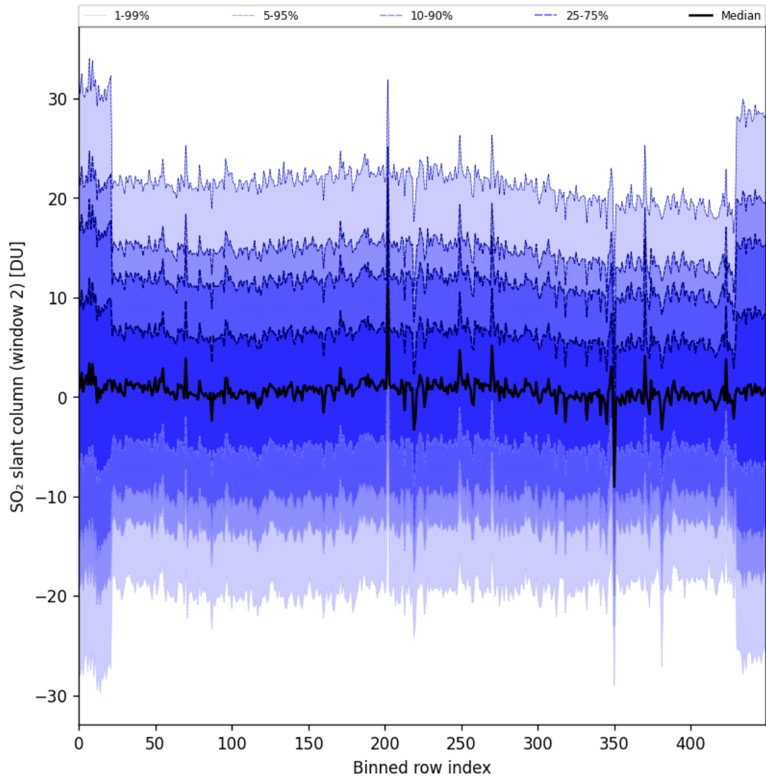
Figure 93: Along track statistics of “SO 2 slant column (window 2)” for 2025-04-29 to 2025-05-01
