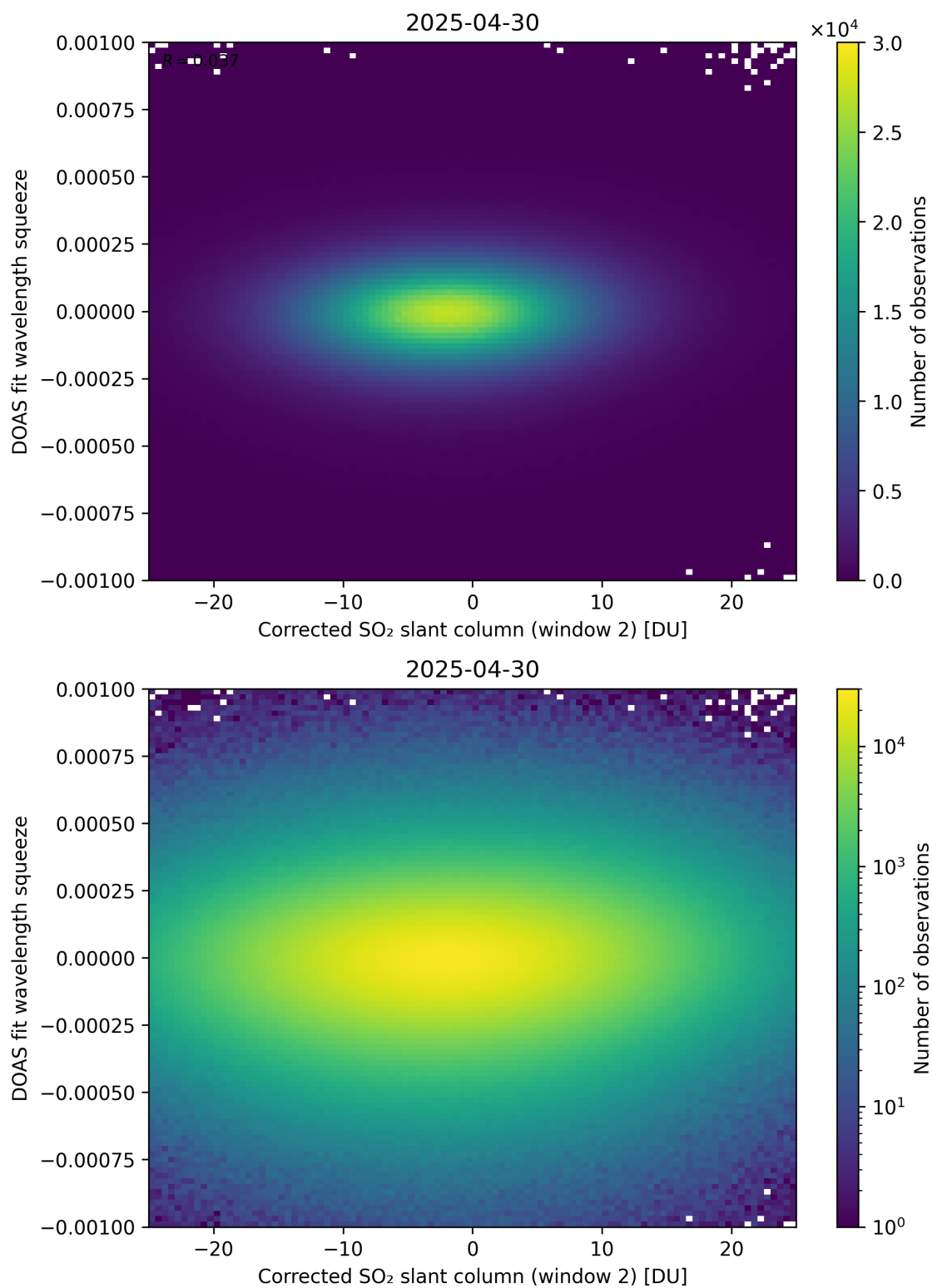
Figure 247: Scatter density plot of “Corrected SO 2 slant column (window 2)” against “DOAS fit wavelength squeeze” for 2025-04-29 to 2025-05-01.
