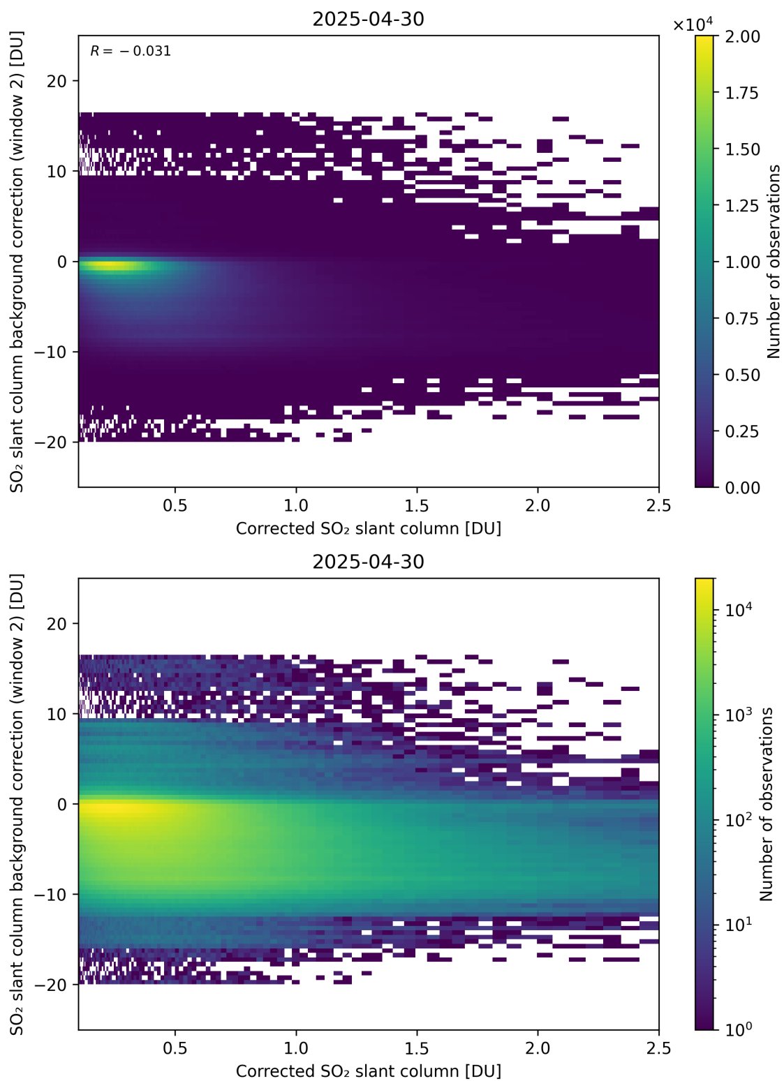
Figure 227: Scatter density plot of “Corrected SO 2 slant column” against “SO 2 slant column background correction (window 2)” for 2025-04-29 to 2025-05-01.
