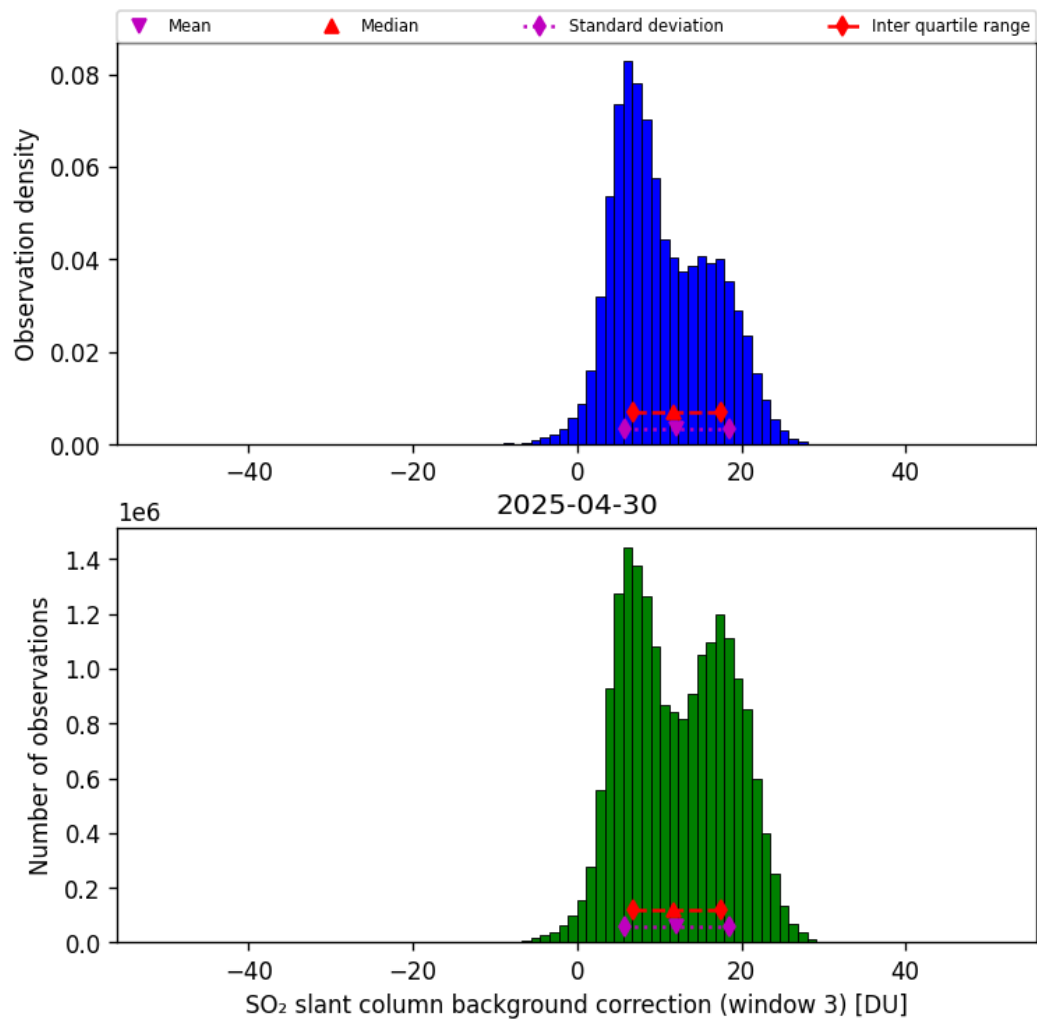
Figure 74: Histogram of “SO 2 slant column background correction (window 3)” for 2025-04-29 to 2025-05-01
