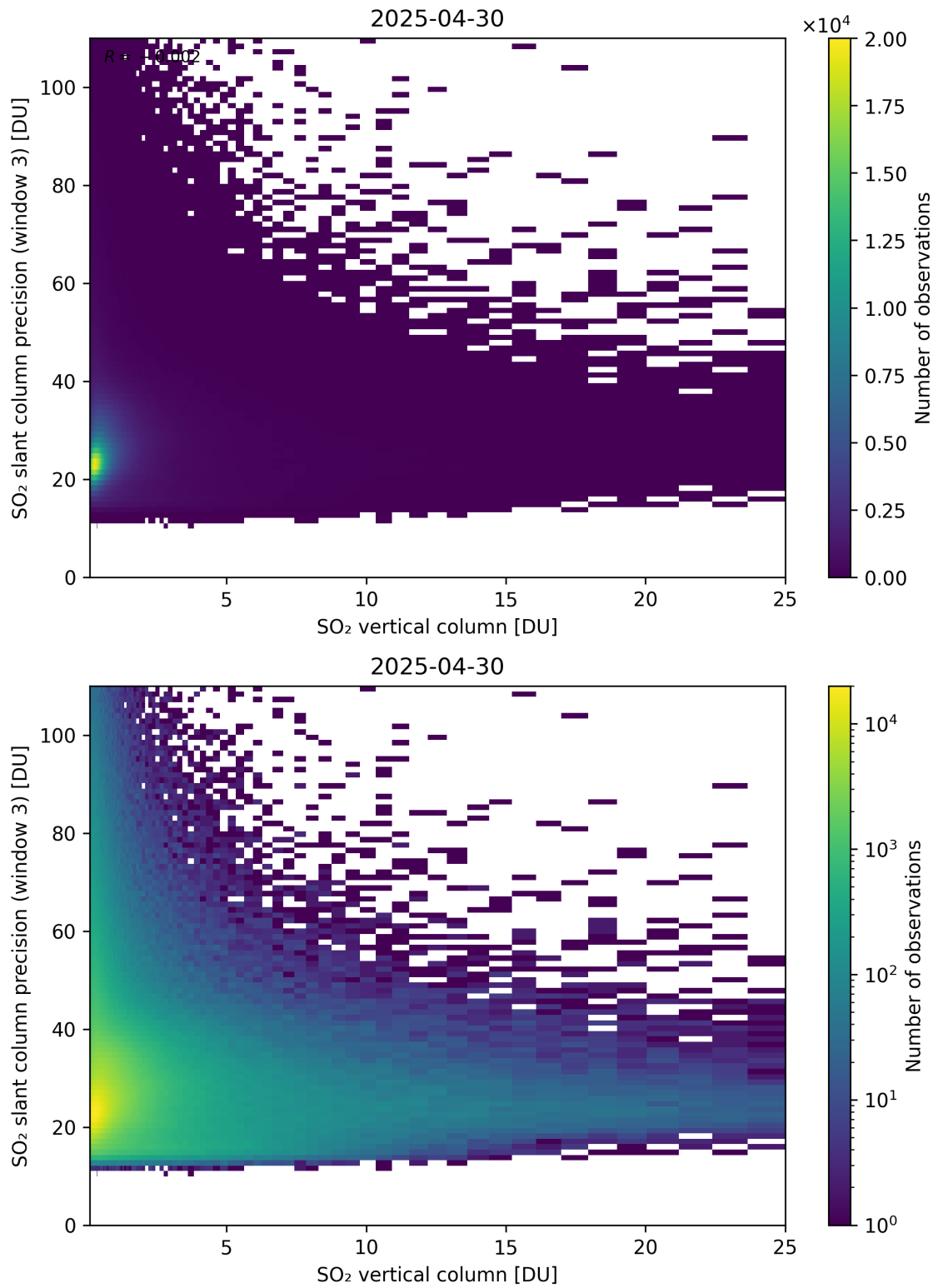
Figure 358: Scatter density plot of “SO 2 vertical column” against “SO 2 slant column precision (window 3)” for 2025-04-29 to 2025-05-01.
