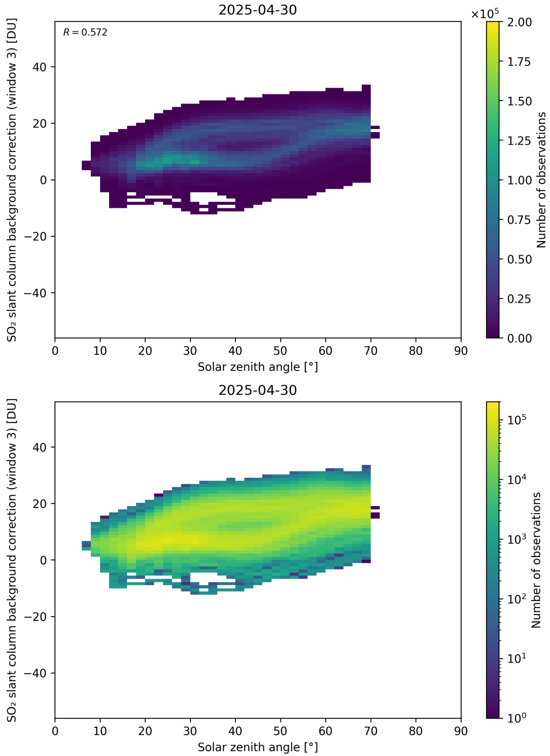
Figure 173: Scatter density plot of “Solar zenith angle” against “SO 2 slant column background correction (window 3)” for 2025-04-29 to 2025-05-01.
