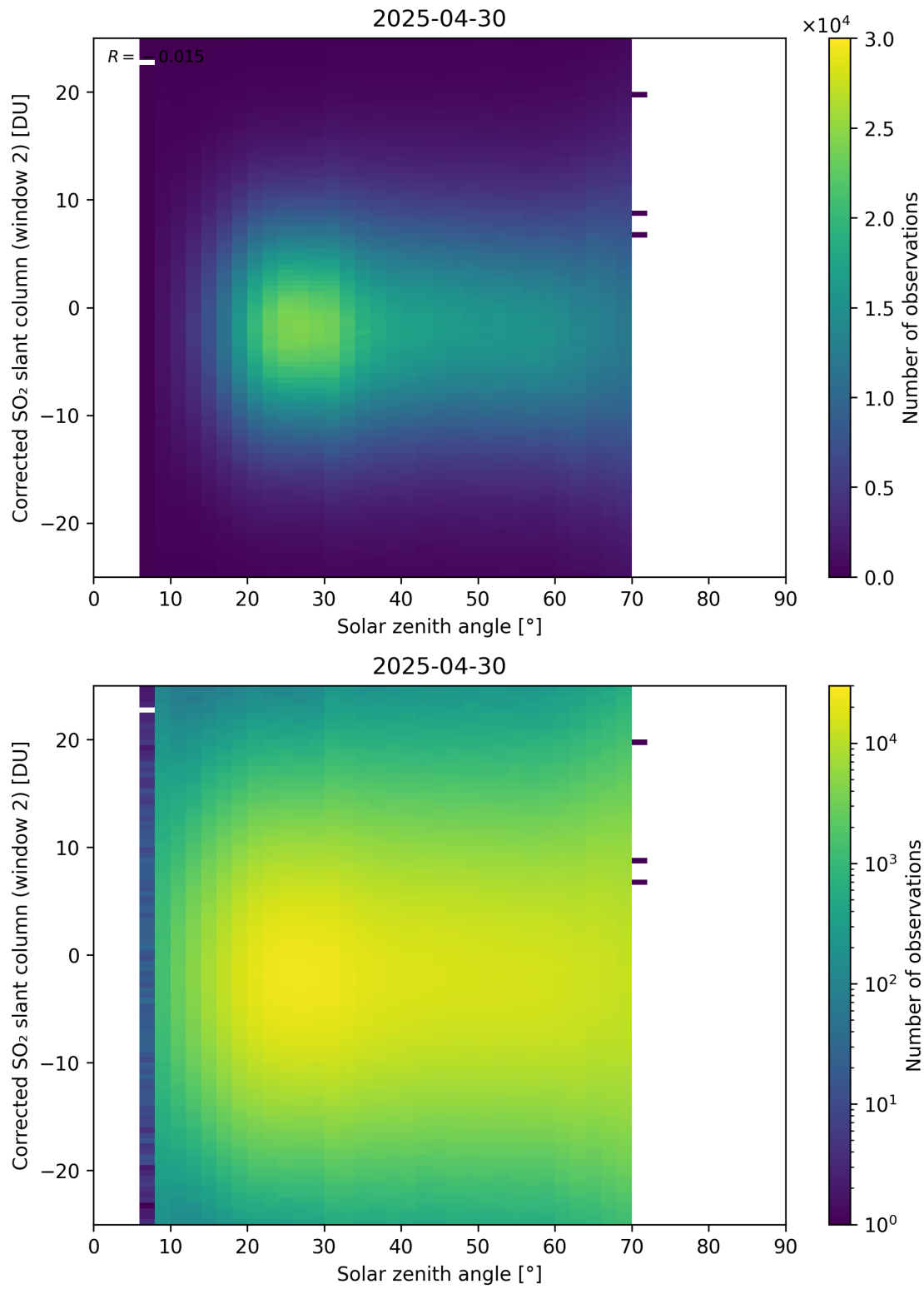
Figure 182: Scatter density plot of “Solar zenith angle” against “Corrected SO 2 slant column (window 2)” for 2025-04-29 to 2025-05-01.
