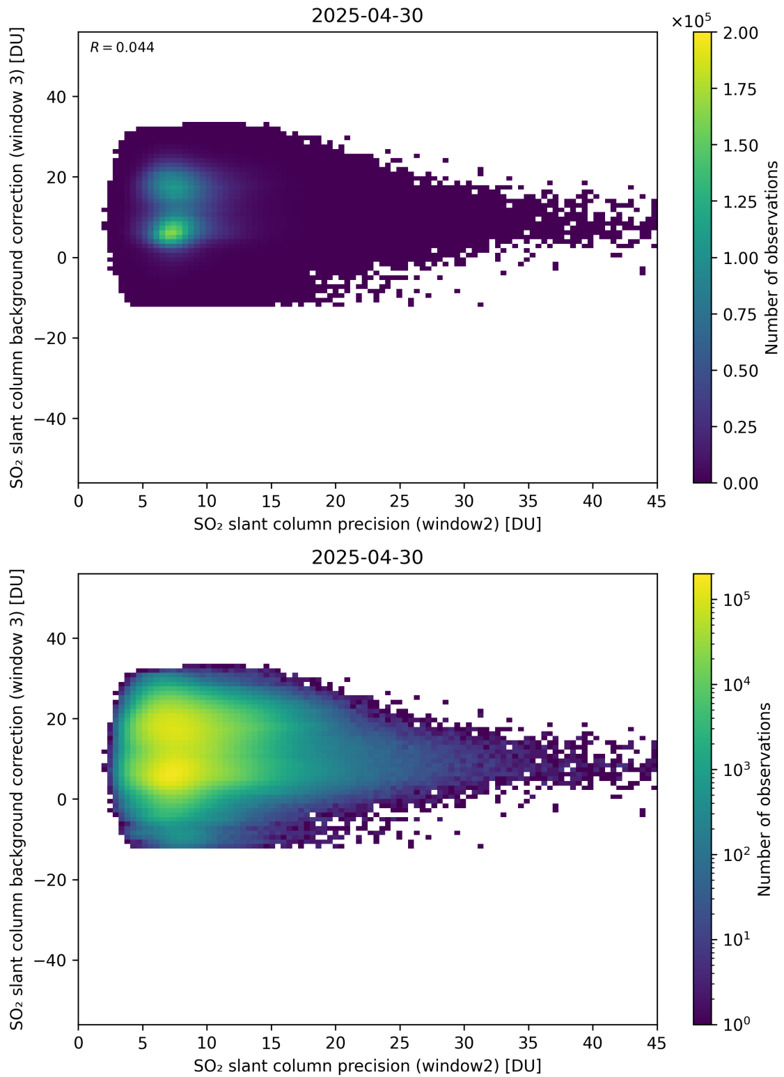
Figure 292: Scatter density plot of “SO 2 slant column precision (window2)” against “SO 2 slant column background correction (window 3)” for 2025-04-29 to 2025-05-01.
