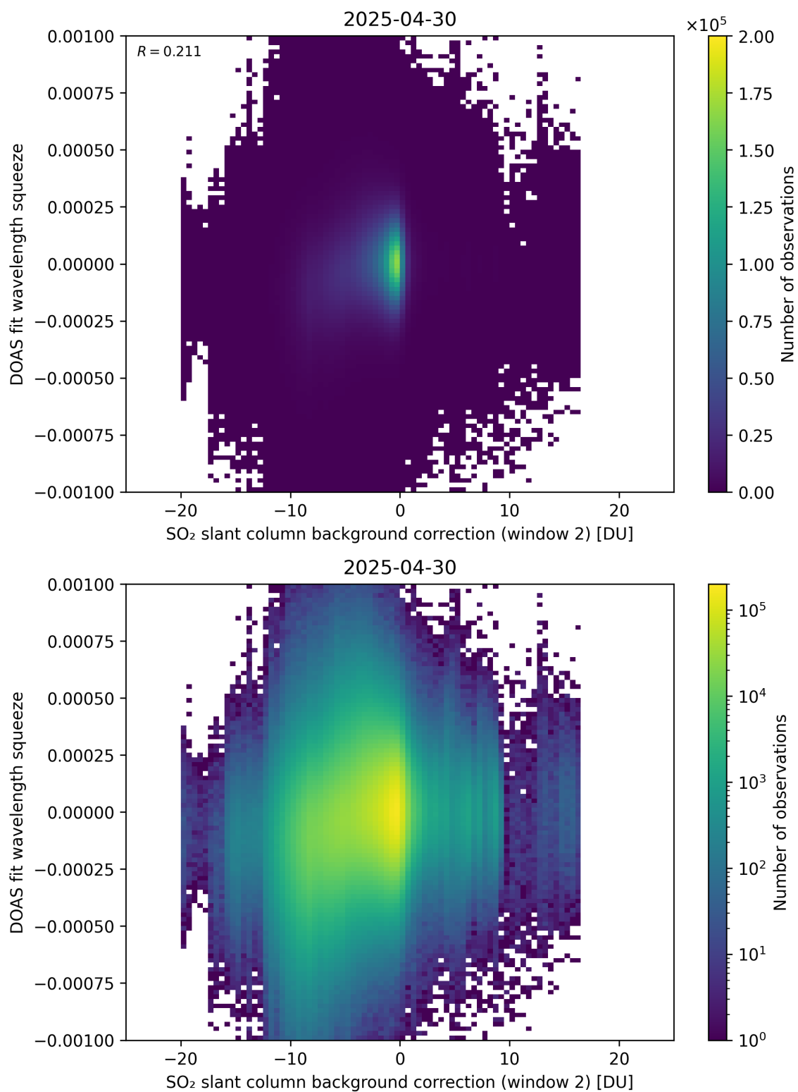
Figure 124: Scatter density plot of “SO 2 slant column background correction (window 2)” against “DOAS fit wavelength squeeze” for 2025-04-29 to 2025-05-01.
