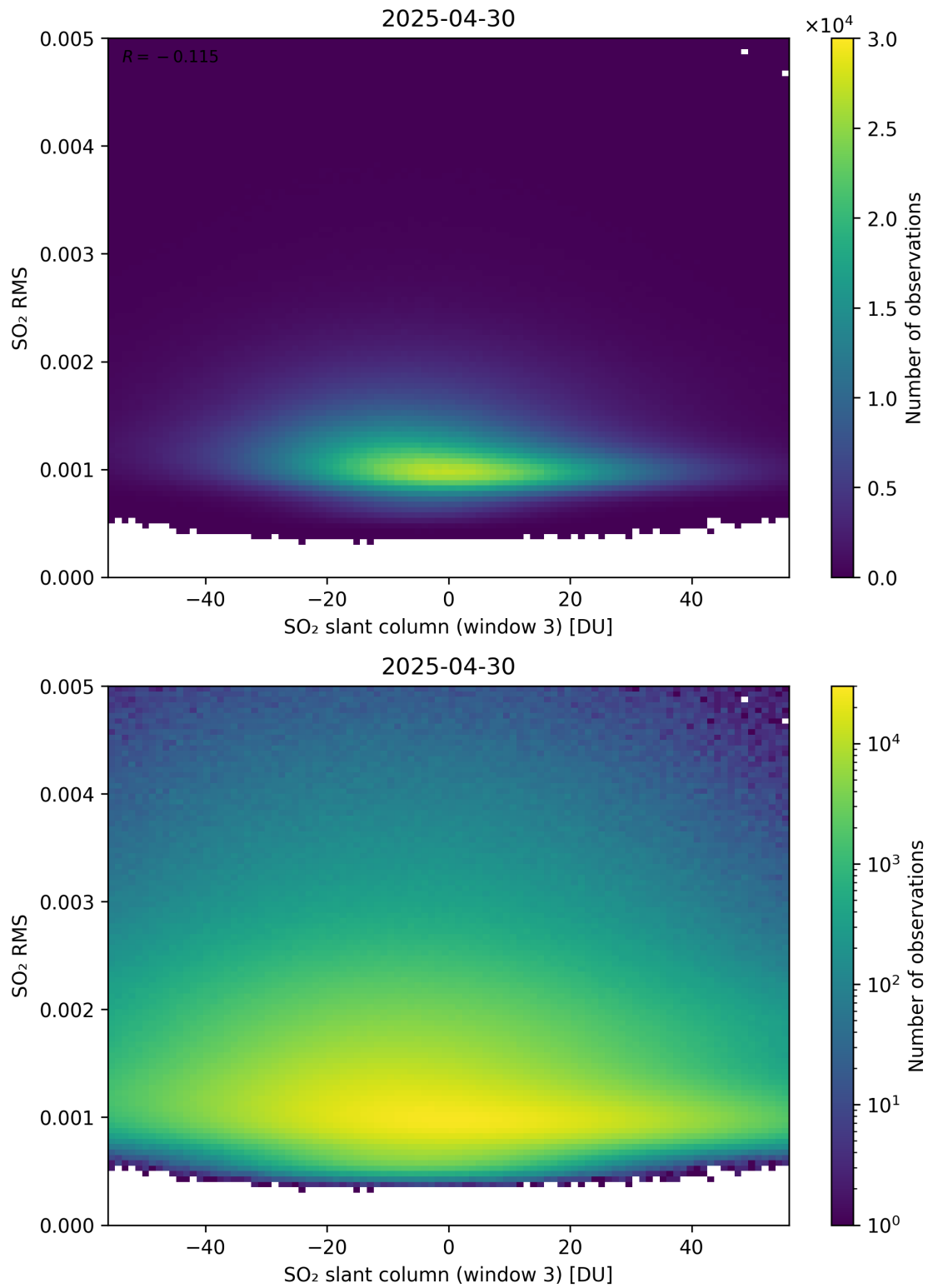
Figure 306: Scatter density plot of “SO 2 slant column (window 3)” against “SO 2 RMS” for 2025-04-29 to 2025-05-01.
