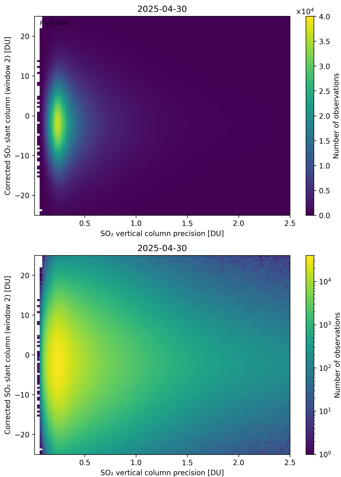
Figure 339: Scatter density plot of “SO 2 vertical column precision” against “Corrected SO 2 slant column (window 2)” for 2025-04-29 to 2025-05-01.
