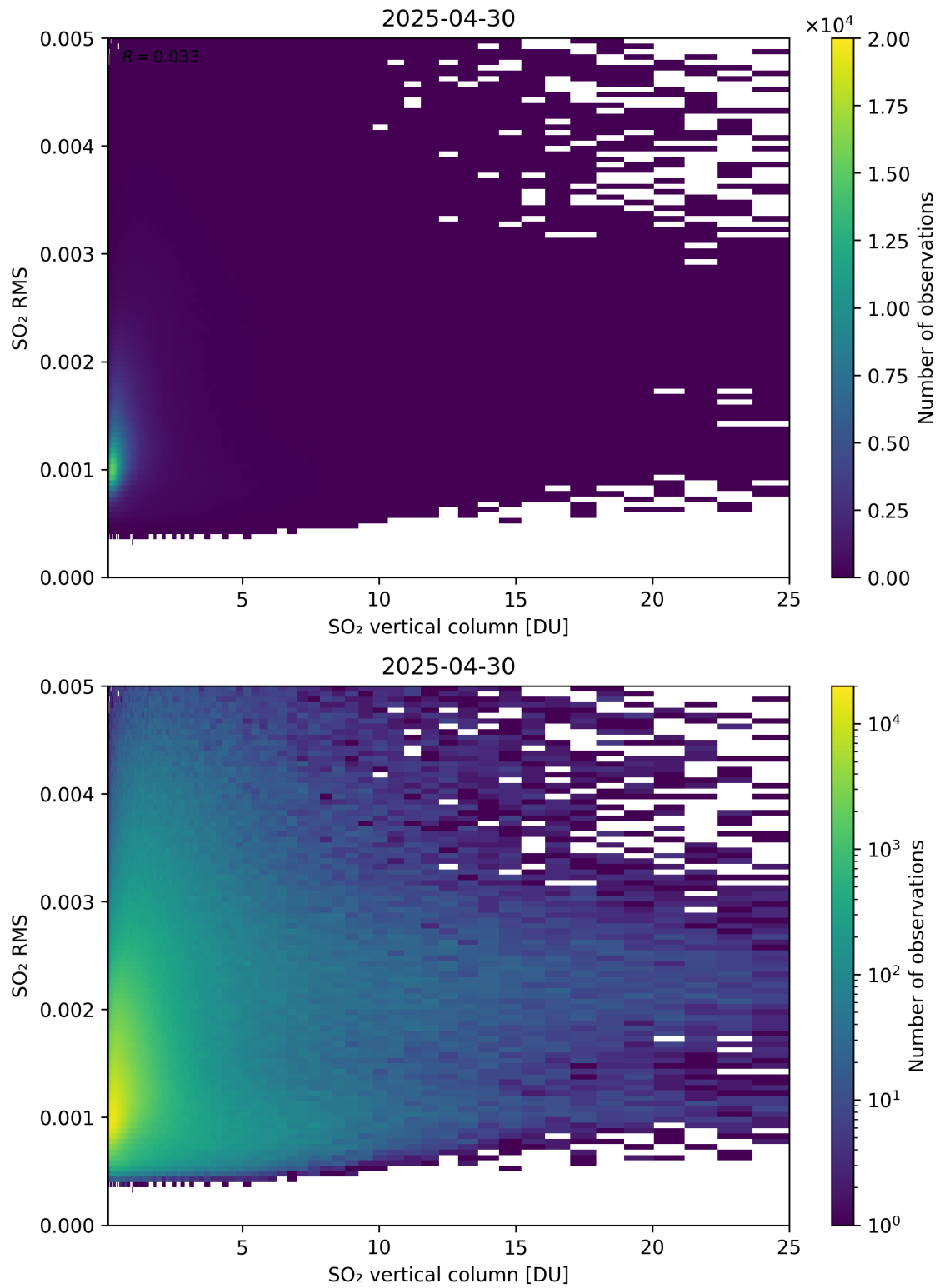
Figure 328: Scatter density plot of “SO 2 vertical column” against “SO 2 RMS” for 2025-04-29 to 2025-05-01.
