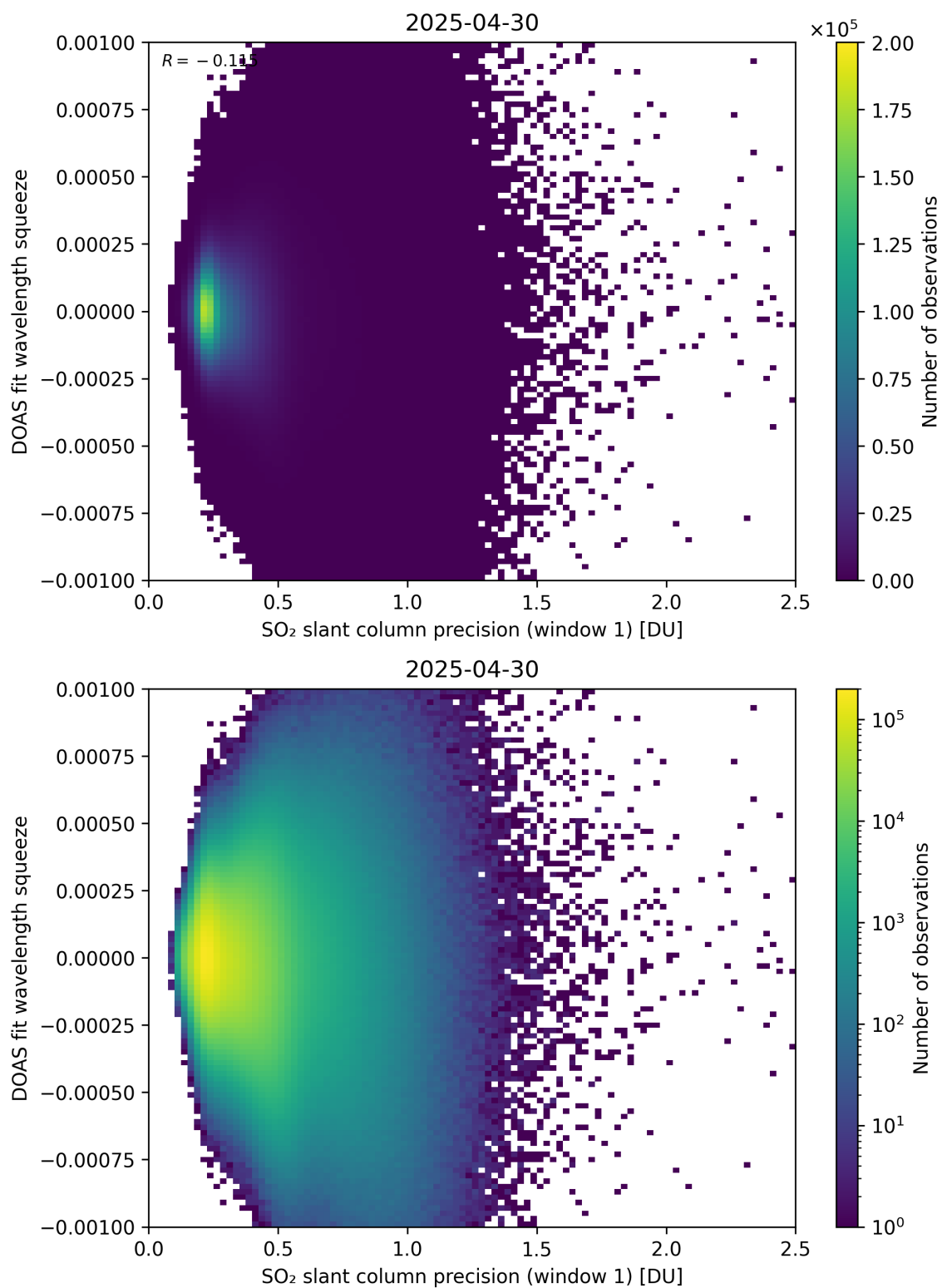
Figure 272: Scatter density plot of “SO 2 slant column precision (window 1)” against “DOAS fit wavelength squeeze” for 2025-04-29 to 2025-05-01.
