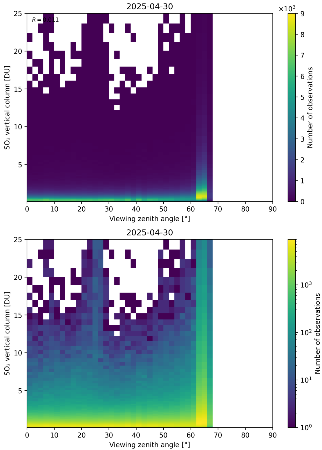
Figure 383: Scatter density plot of “Viewing zenith angle” against “SO 2 vertical column” for 2025-04-29 to 2025-05-01.
