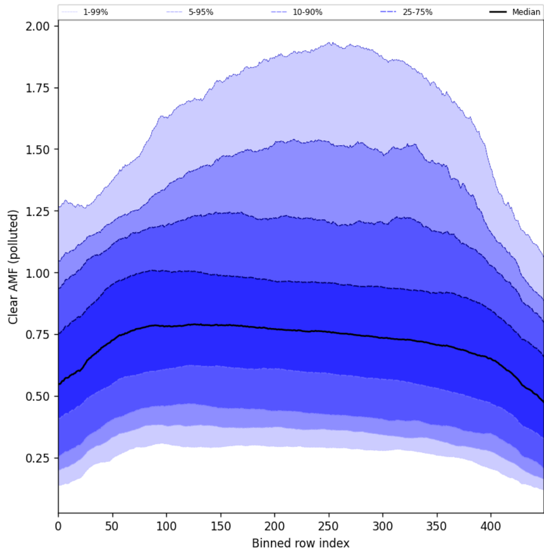
Figure 107: Along track statistics of “Clear AMF (polluted)” for 2025-04-29 to 2025-05-01
