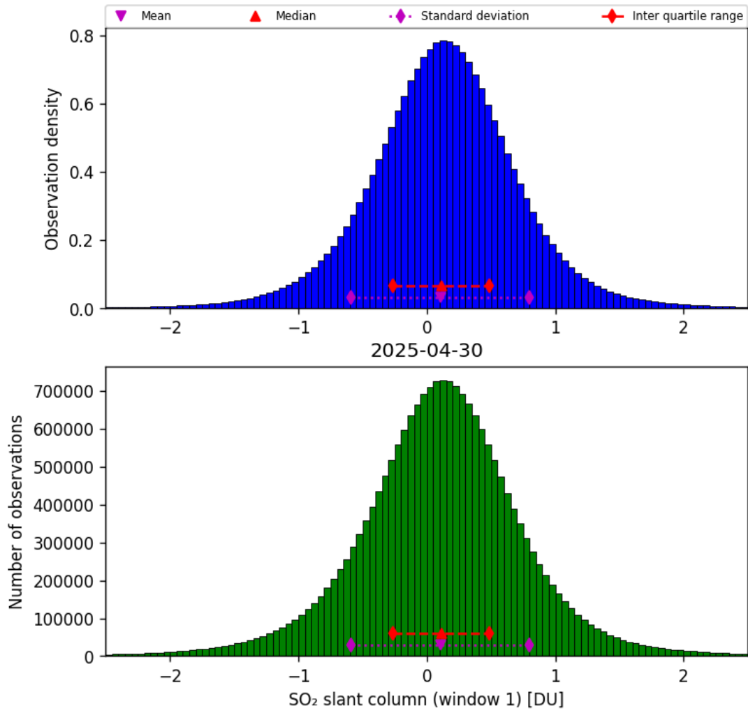
Figure 63: Histogram of “SO 2 slant column (window 1)” for 2025-04-29 to 2025-05-01
