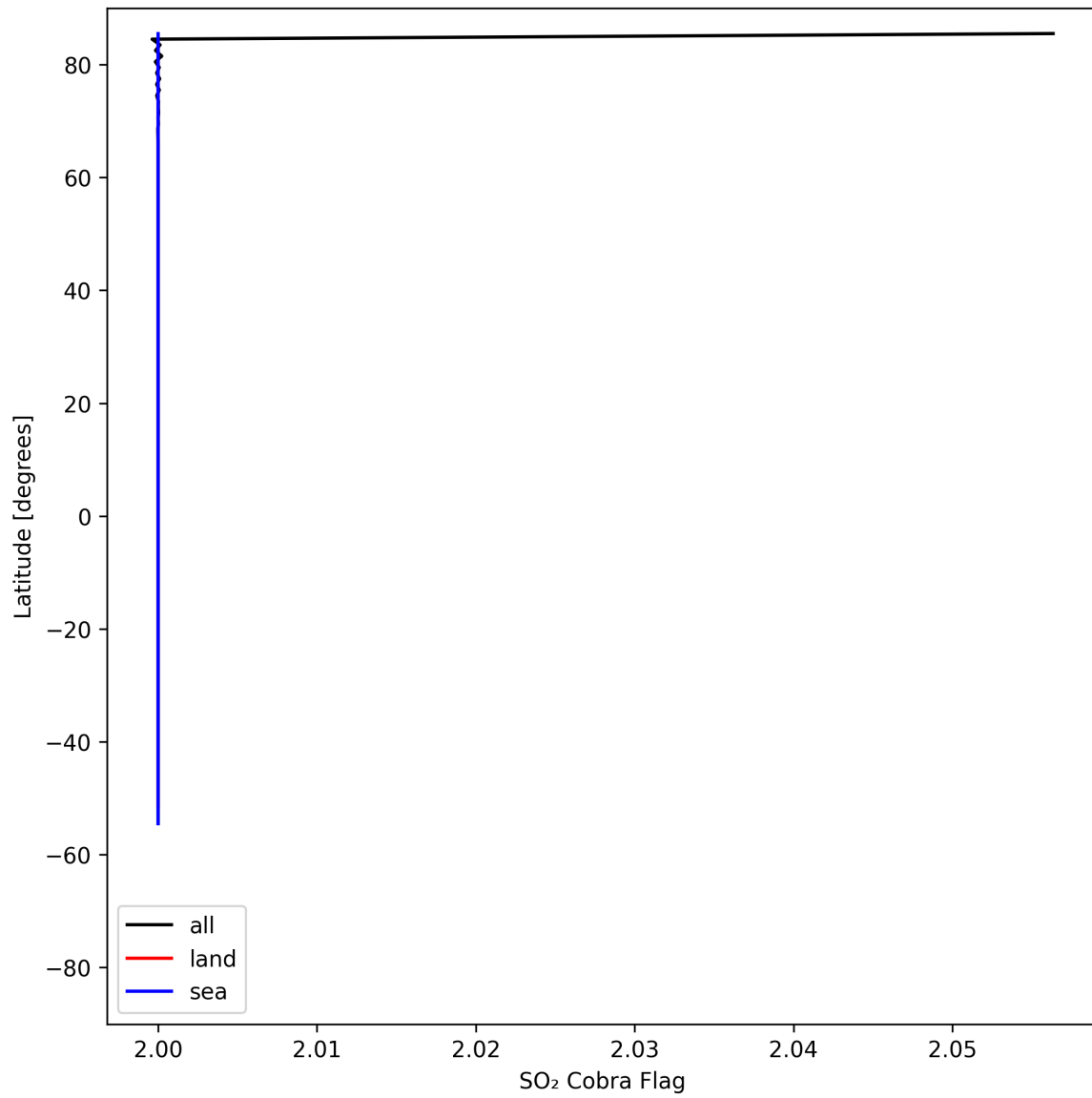
Figure 49: Zonal average of “SO 2 Cobra Flag” for 2025-04-29 to 2025-05-01.
