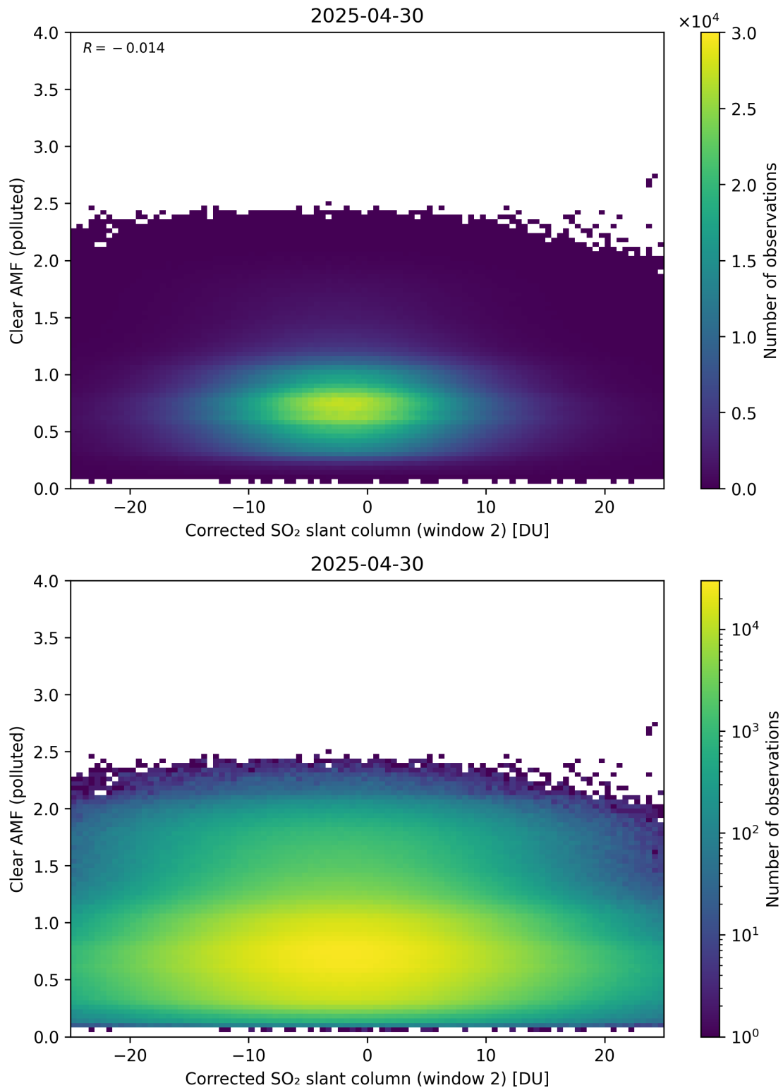
Figure 249: Scatter density plot of “Corrected SO 2 slant column (window 2)” against “Clear AMF (polluted)” for 2025-04-29 to 2025-05-01.
