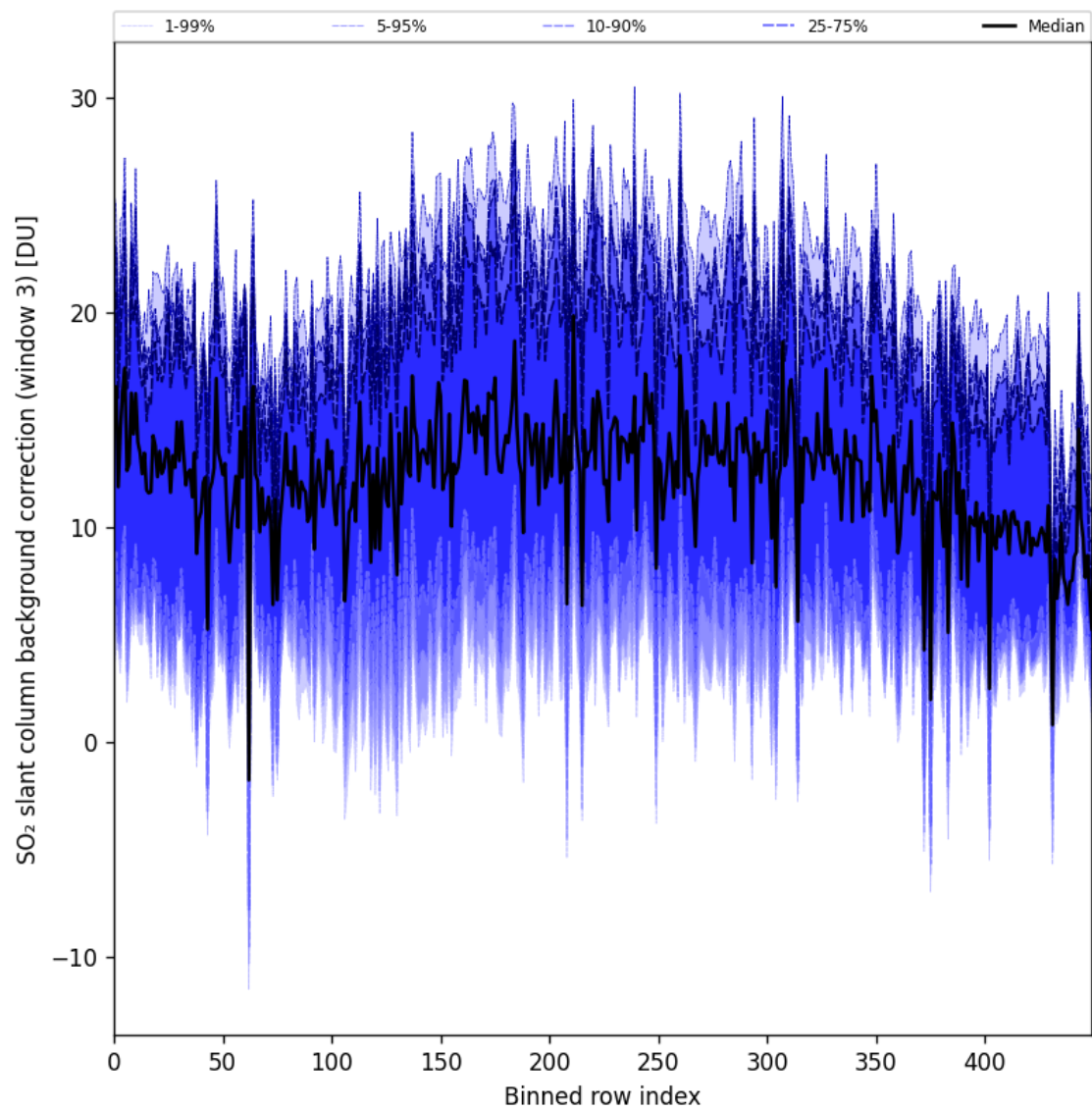
Figure 100: Along track statistics of “SO 2 slant column background correction (window 3)” for 2025-04-29 to 2025-05-01
