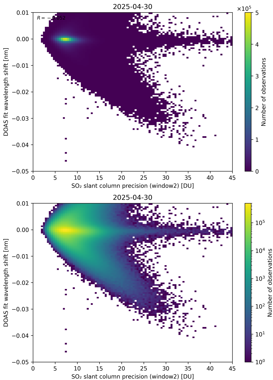
Figure 293: Scatter density plot of “SO 2 slant column precision (window2)” against “DOAS fit wavelength shift” for 2025-04-29 to 2025-05-01.
