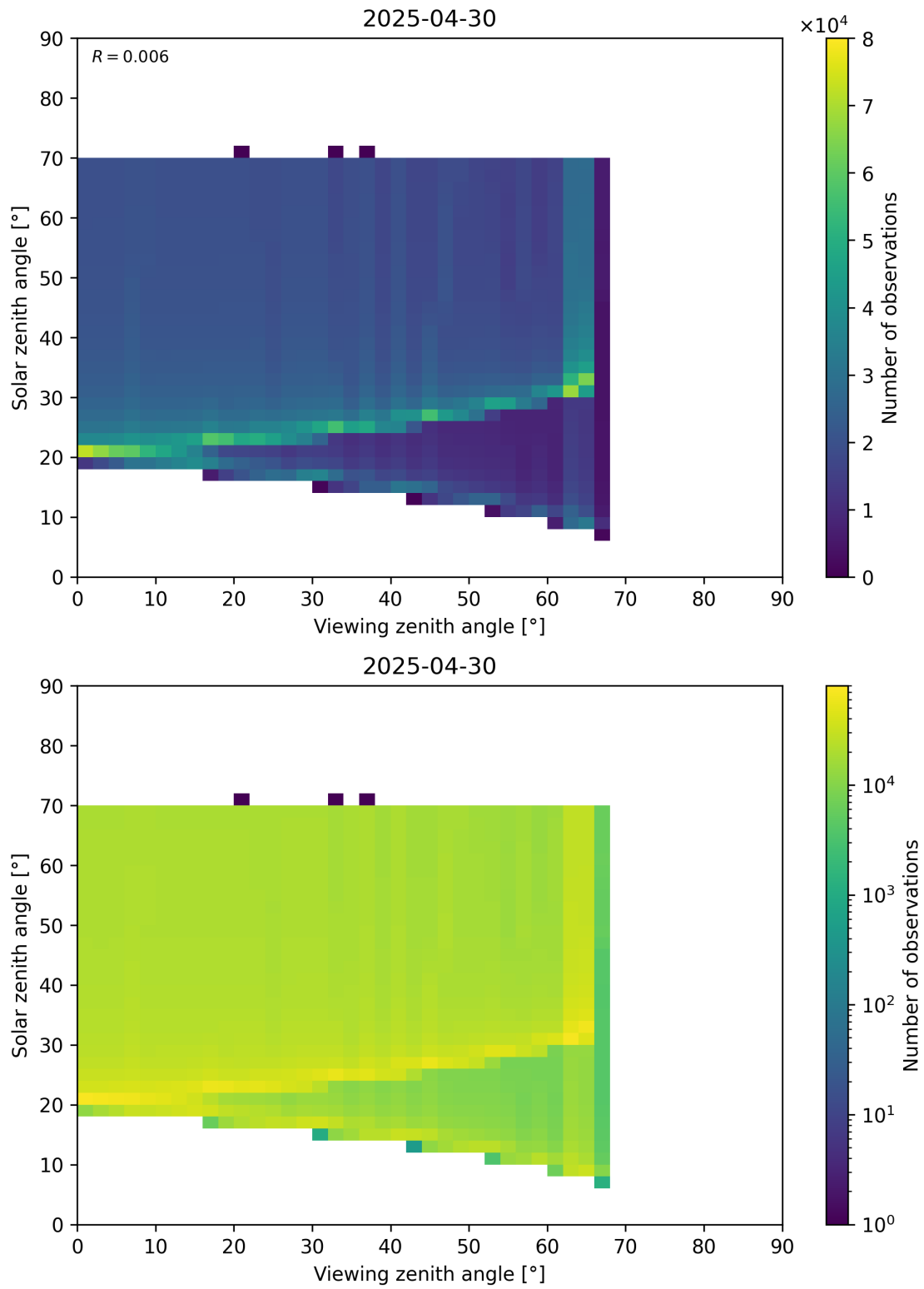
Figure 369: Scatter density plot of “Viewing zenith angle” against “Solar zenith angle” for 2025-04-29 to 2025-05-01.
