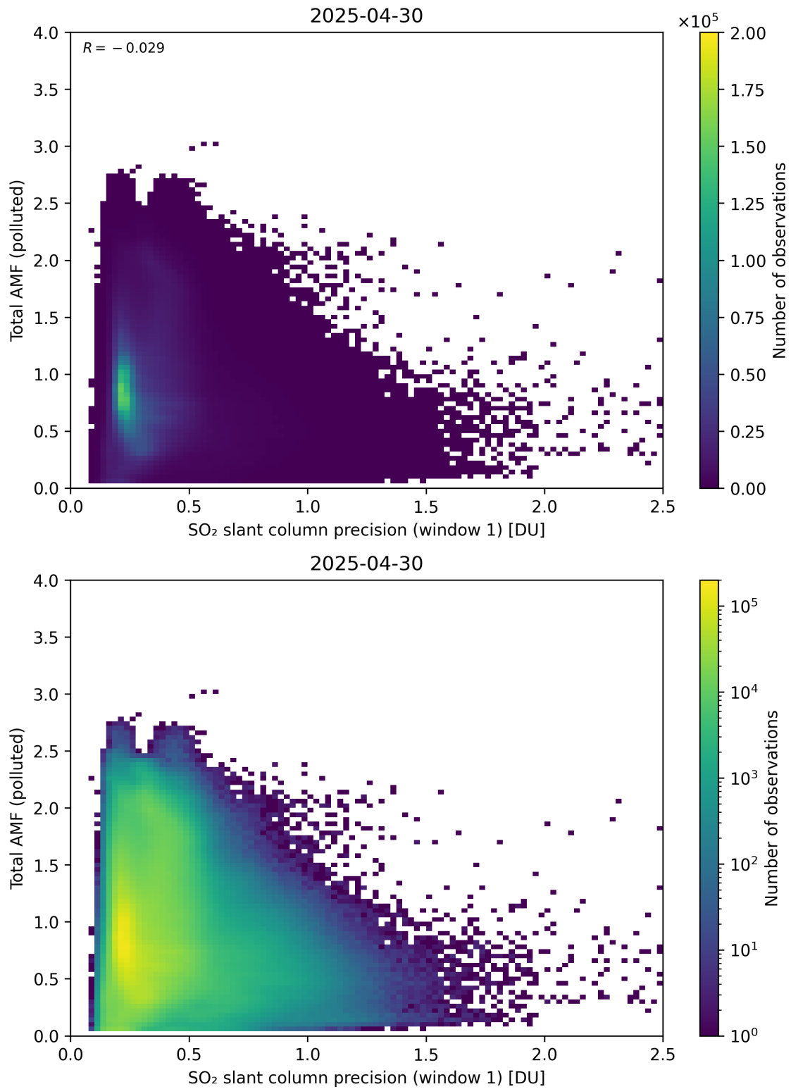
Figure 280: Scatter density plot of “SO 2 slant column precision (window 1)” against “Total AMF (polluted)” for 2025-04-29 to 2025-05-01.
