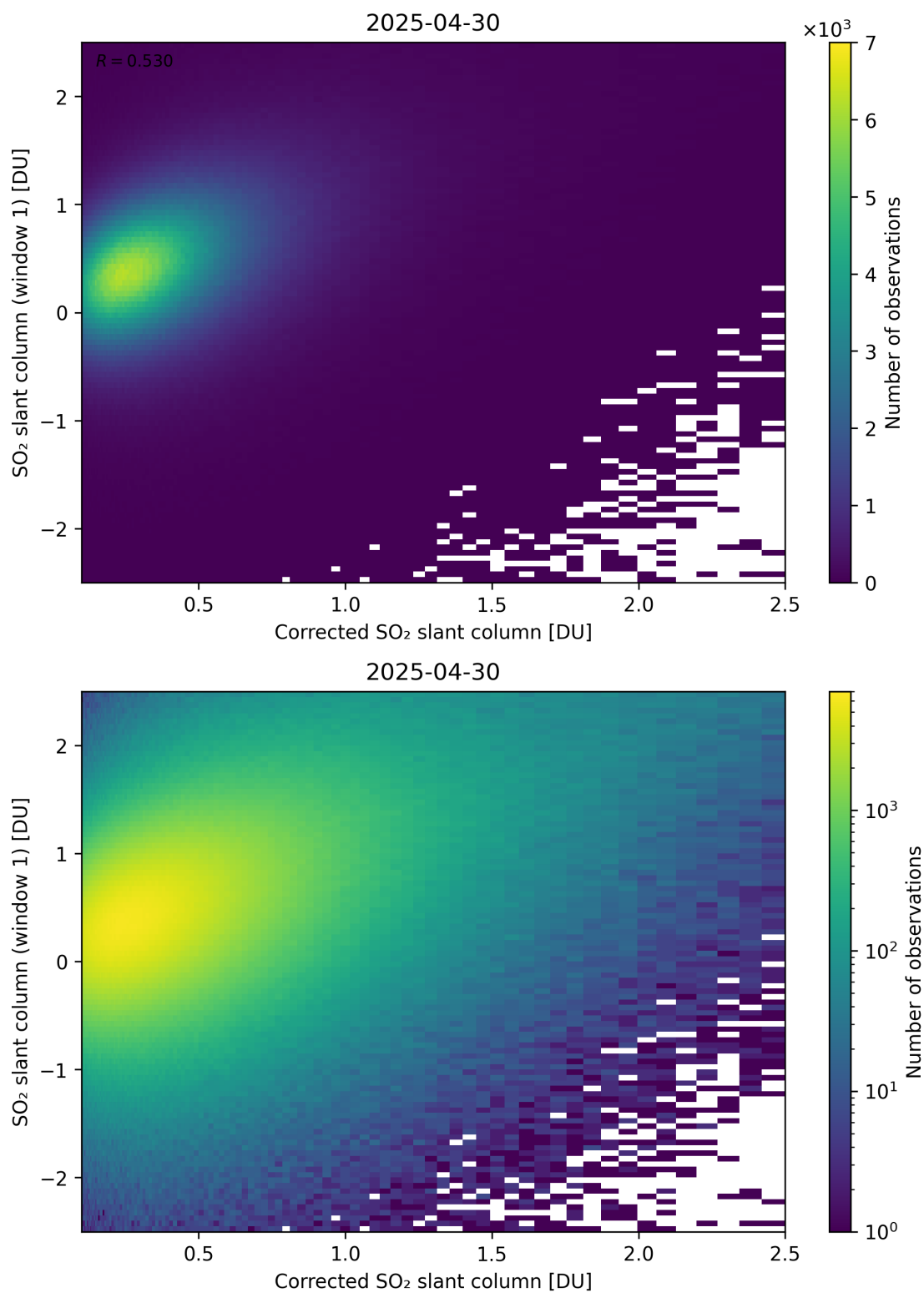
Figure 237: Scatter density plot of “Corrected SO 2 slant column” against “SO 2 slant column (window 1)” for 2025-04-29 to 2025-05-01.
