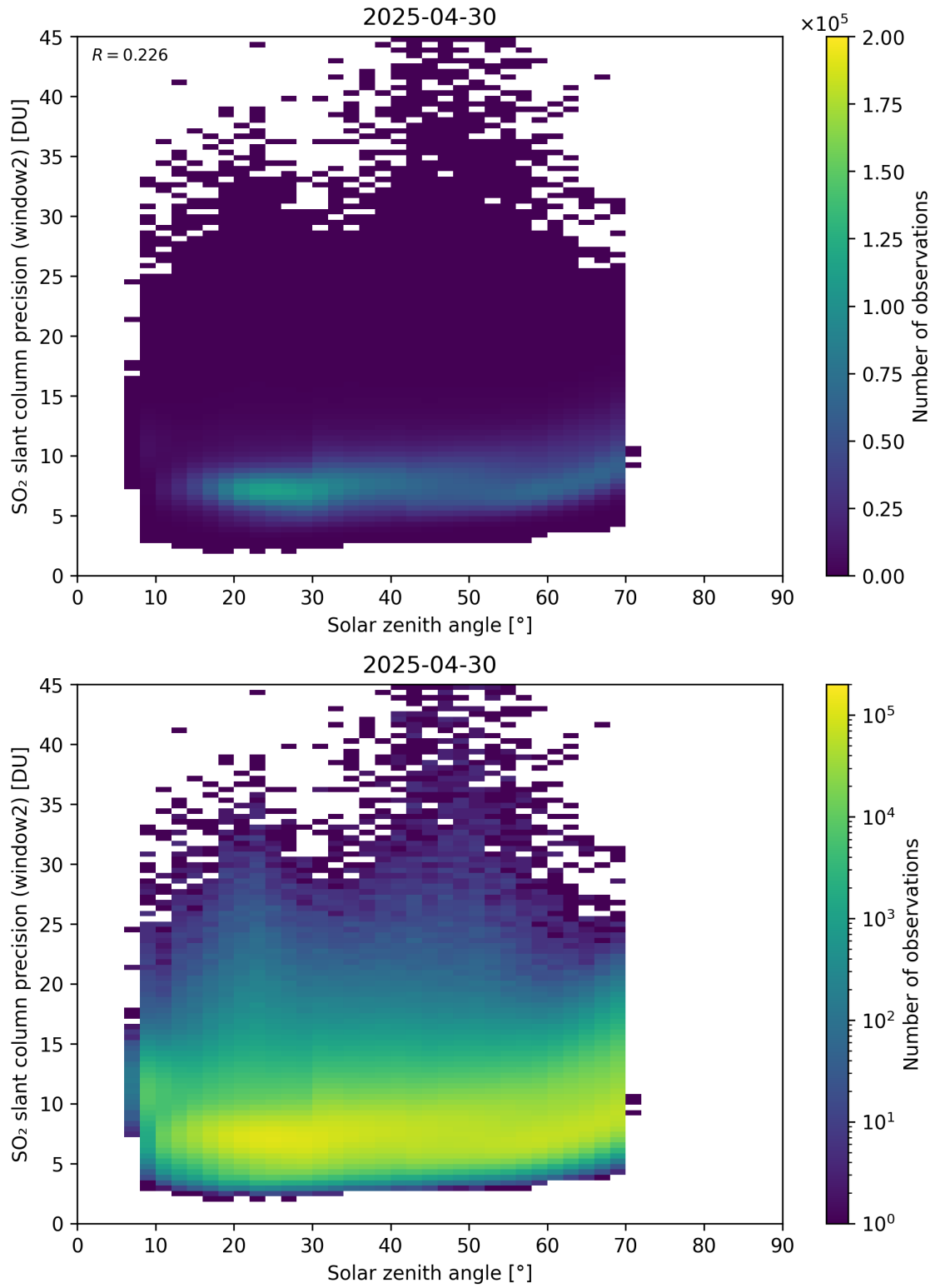
Figure 186: Scatter density plot of “Solar zenith angle” against “SO 2 slant column precision (window2)” for 2025-04-29 to 2025-05-01.
