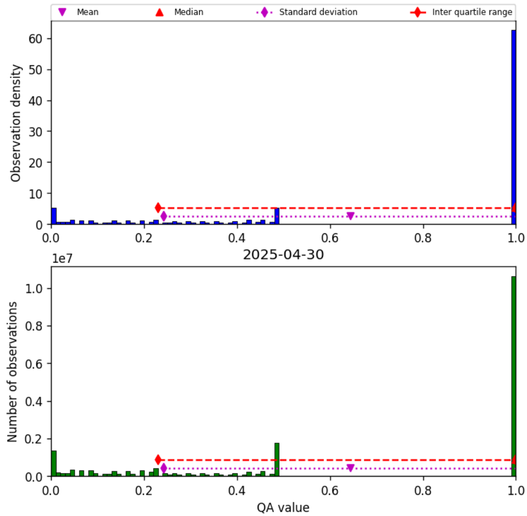
Figure 57: Histogram of “QA value” for 2025-04-29 to 2025-05-01
