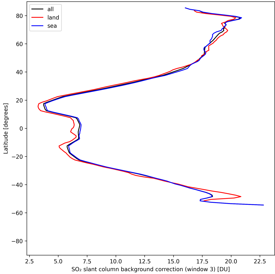
Figure 48: Zonal average of “SO 2 slant column background correction (window 3)” for 2025-04-29 to 2025-05-01.
