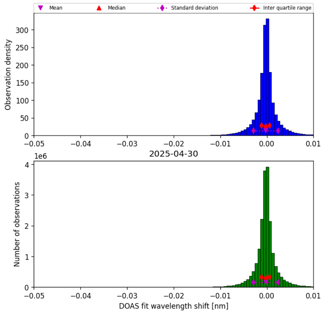
Figure 76: Histogram of “DOAS fit wavelength shift” for 2025-04-29 to 2025-05-01
