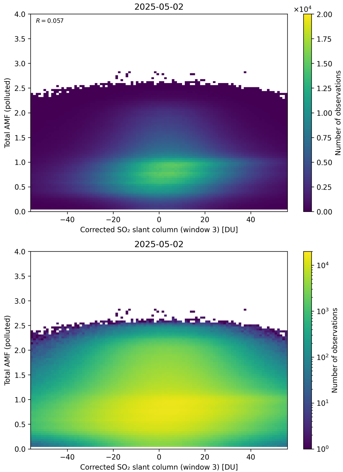
Figure 260: Scatter density plot of “Corrected SO 2 slant column (window 3)” against “Total AMF (polluted)” for 2025-05-01 to 2025-05-03.
