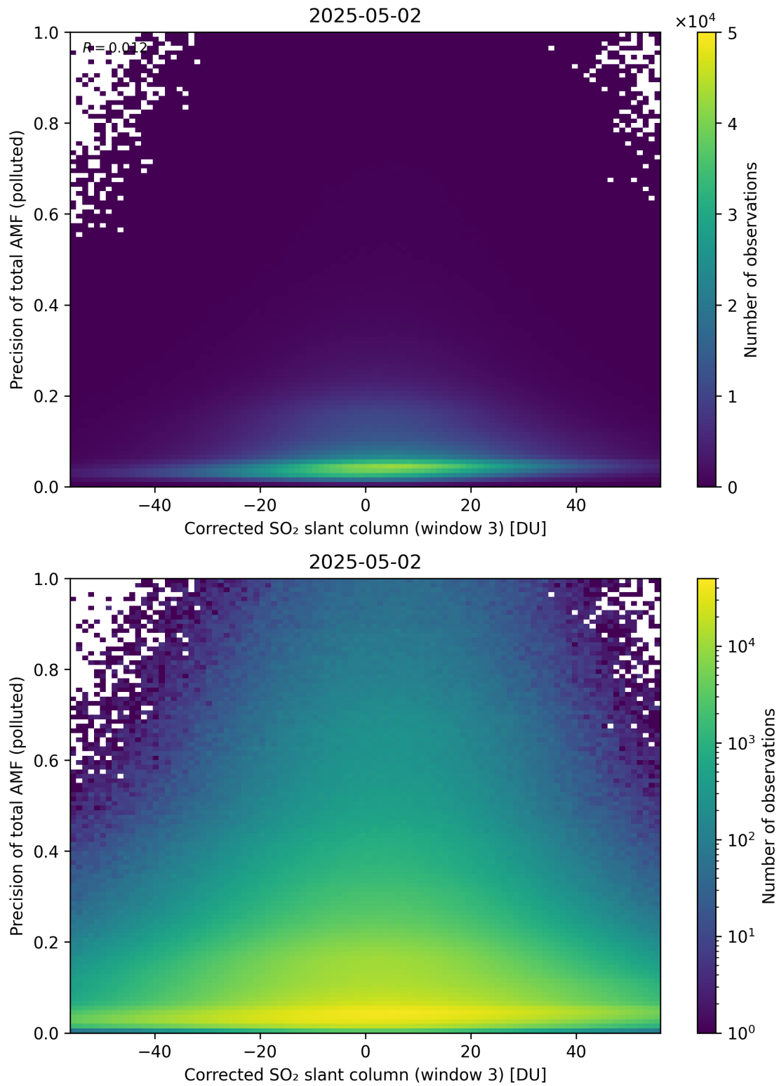
Figure 261: Scatter density plot of “Corrected SO 2 slant column (window 3)” against “Precision of total AMF (polluted)” for 2025-05-01 to 2025-05-03.
