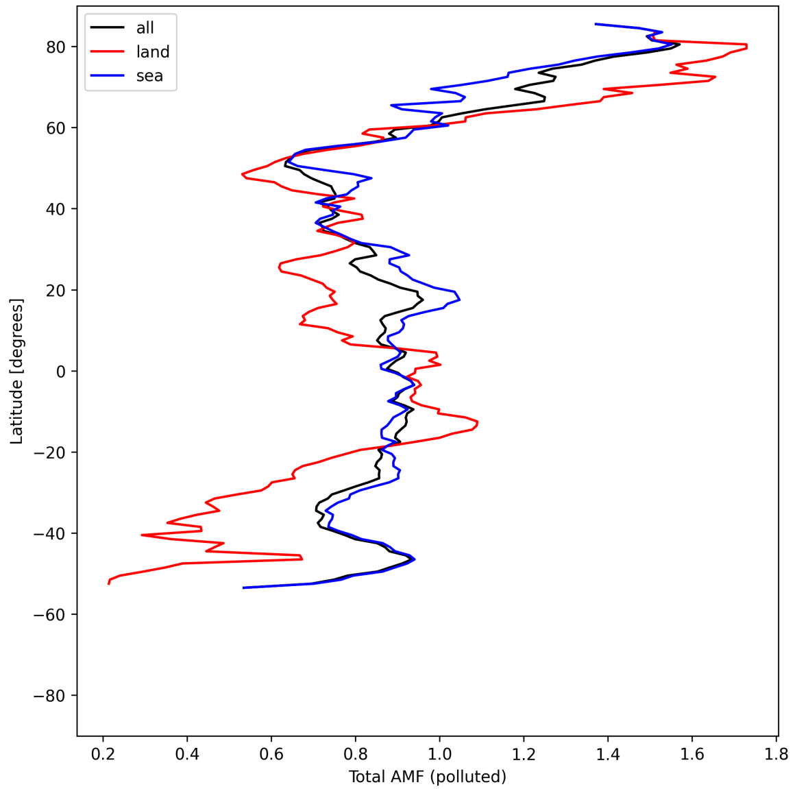
Figure 53: Zonal average of “Total AMF (polluted)” for 2025-05-01 to 2025-05-03.
