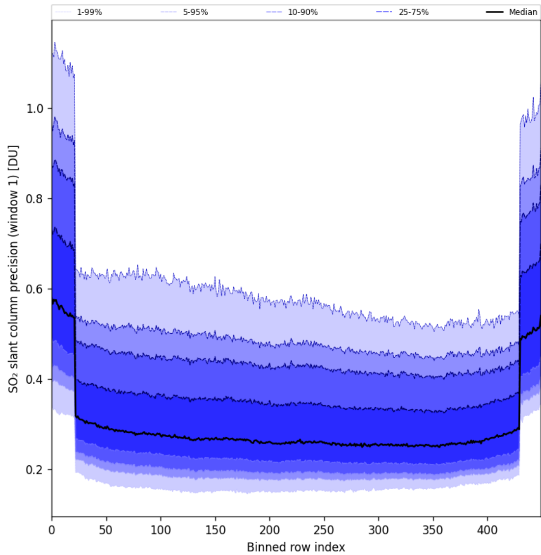
Figure 90: Along track statistics of “SO 2 slant column precision (window 1)” for 2025-05-01 to 2025-05-03
