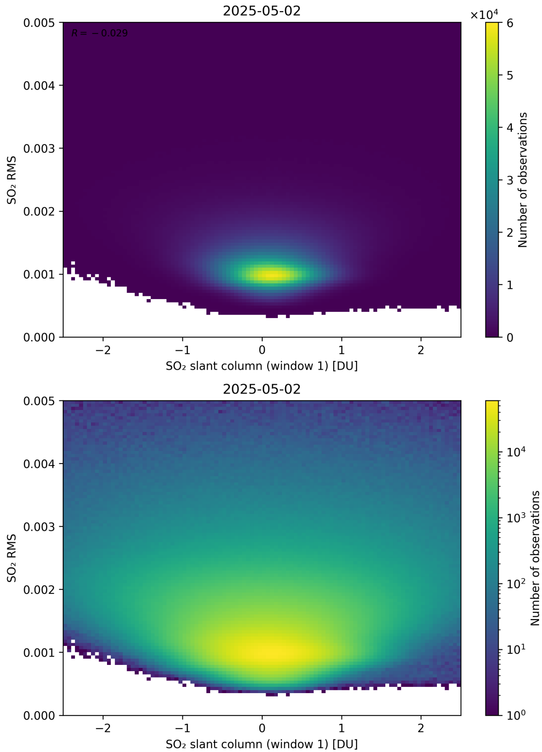
Figure 267: Scatter density plot of “SO 2 slant column (window 1)” against “SO 2 RMS” for 2025-05-01 to 2025-05-03.
