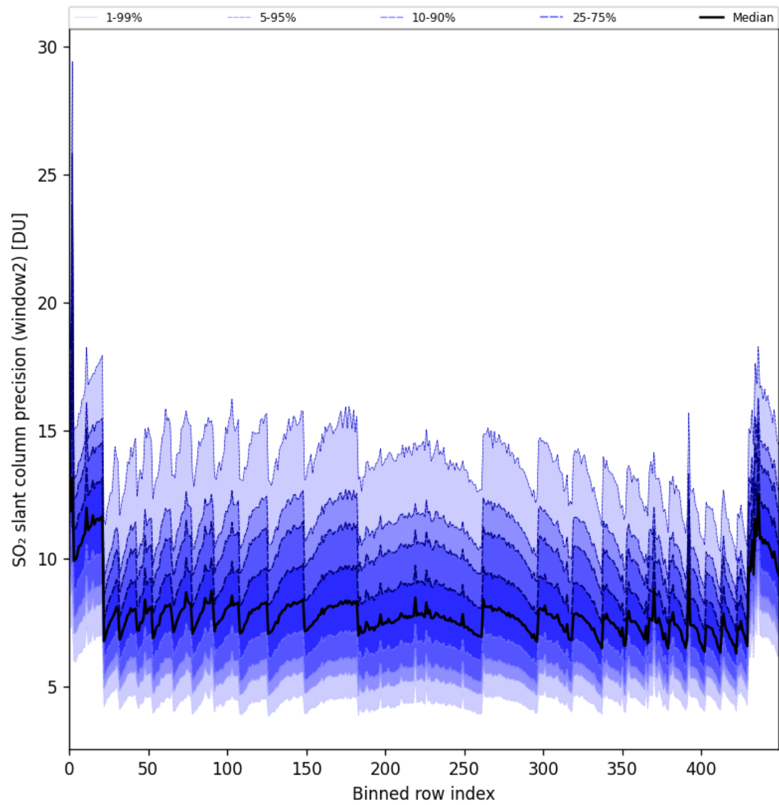
Figure 94: Along track statistics of “SO 2 slant column precision (window2)” for 2025-05-01 to 2025-05-03
