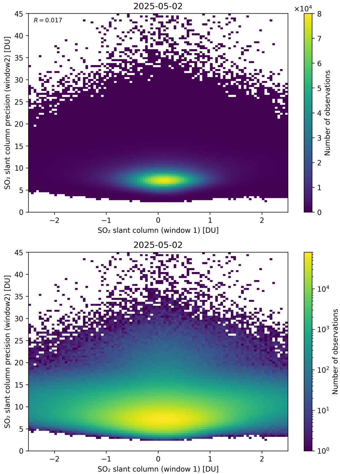
Figure 286: Scatter density plot of “SO 2 slant column (window 1)” against “SO 2 slant column precision (window2)” for 2025-05-01 to 2025-05-03.
