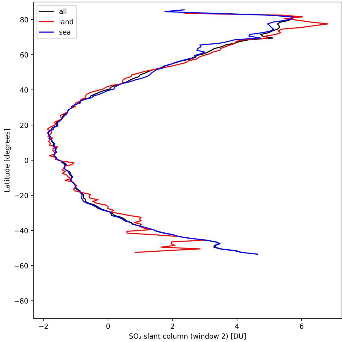
Figure 41: Zonal average of “SO 2 slant column (window 2)” for 2025-05-01 to 2025-05-03.
