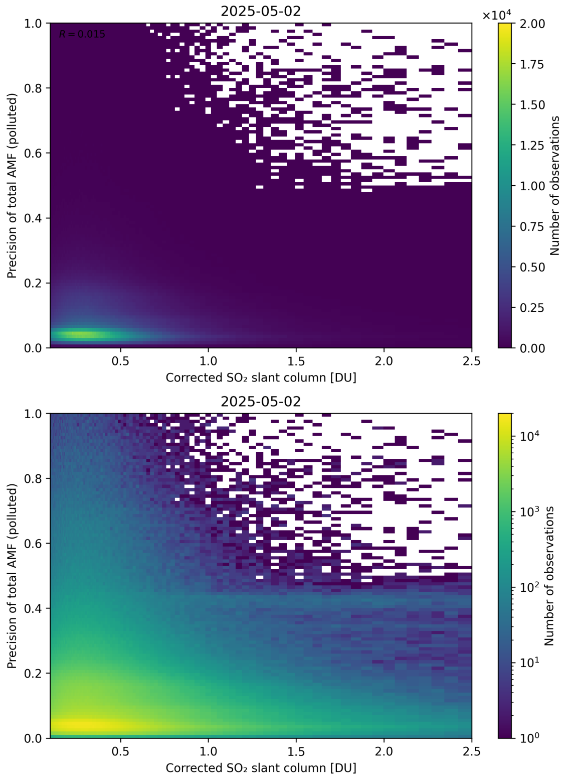
Figure 243: Scatter density plot of “Corrected SO 2 slant column” against “Precision of total AMF (polluted)” for 2025-05-01 to 2025-05-03.
