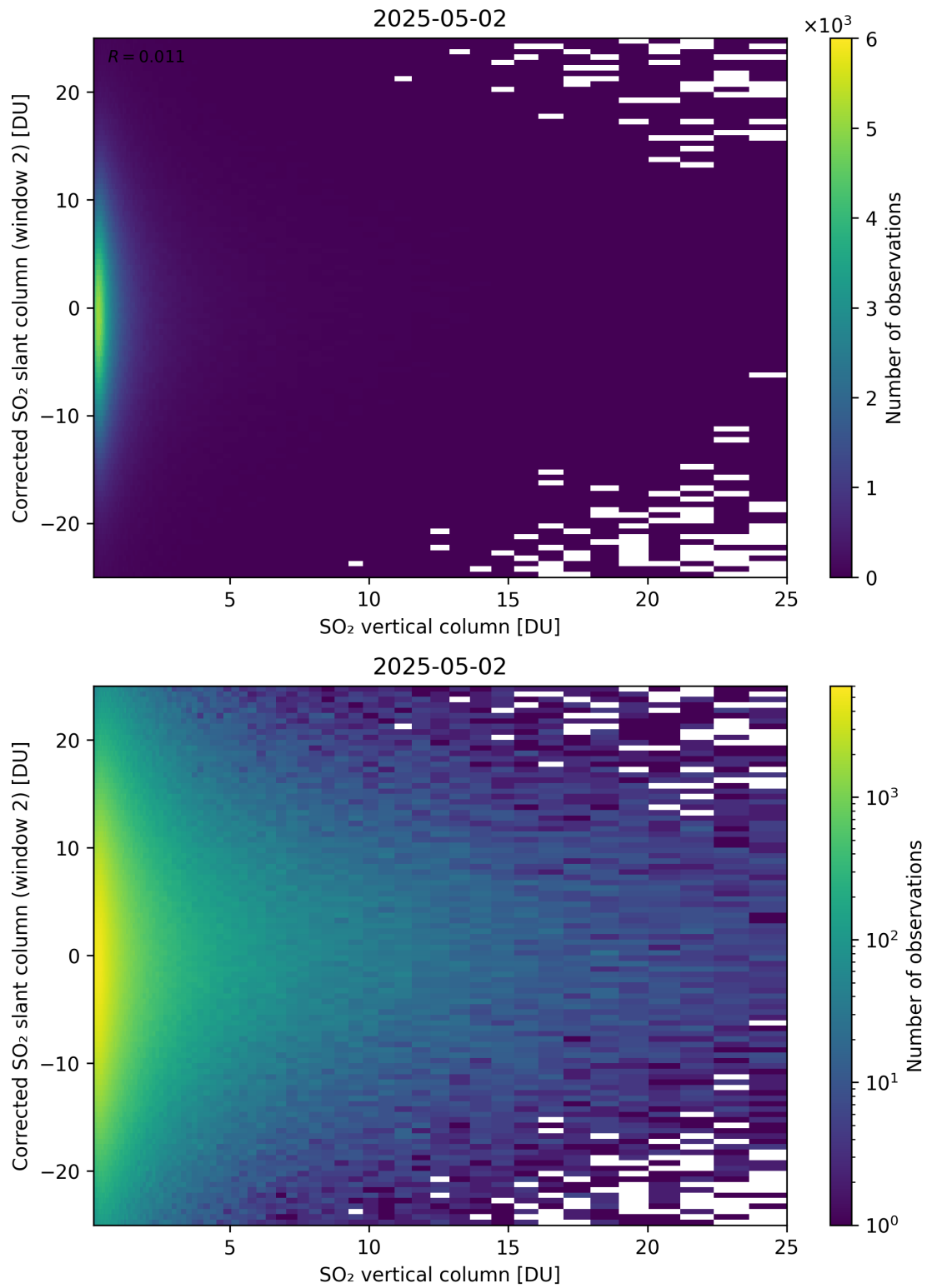
Figure 352: Scatter density plot of “SO 2 vertical column” against “Corrected SO 2 slant column (window 2)” for 2025-05-01 to 2025-05-03.
