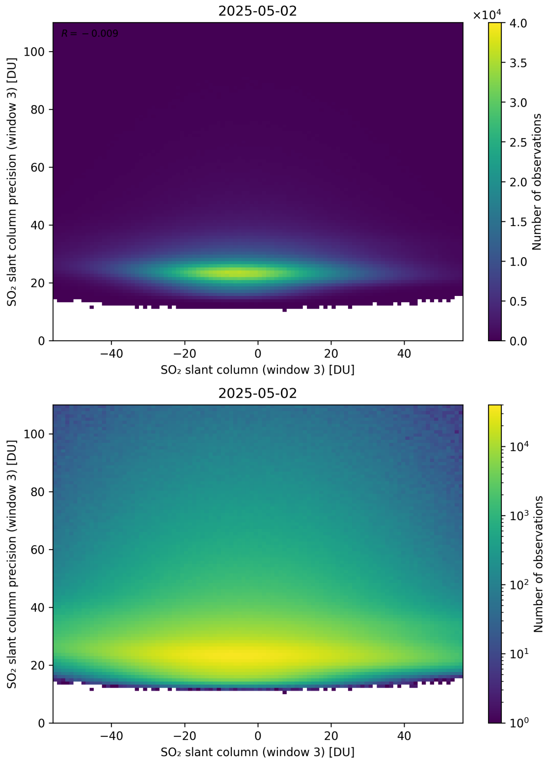
Figure 317: Scatter density plot of “SO 2 slant column (window 3)” against “SO 2 slant column precision (window 3)” for 2025-05-01 to 2025-05-03.
