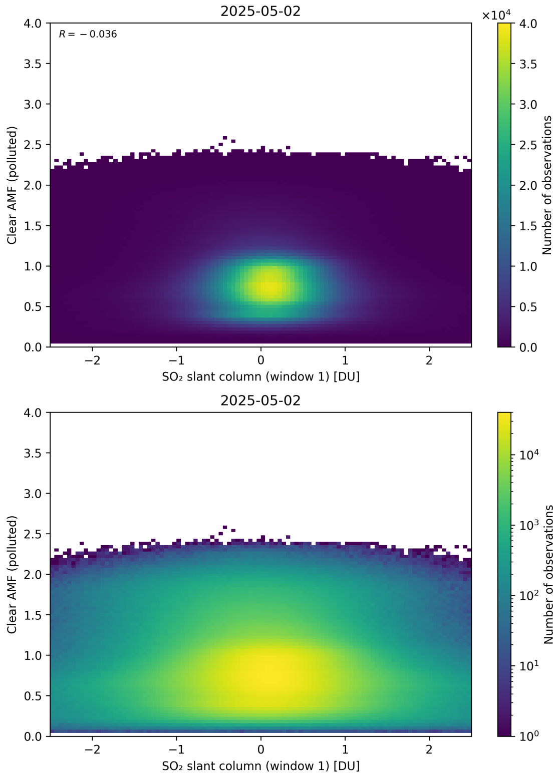
Figure 282: Scatter density plot of “SO 2 slant column (window 1)” against “Clear AMF (polluted)” for 2025-05-01 to 2025-05-03.
