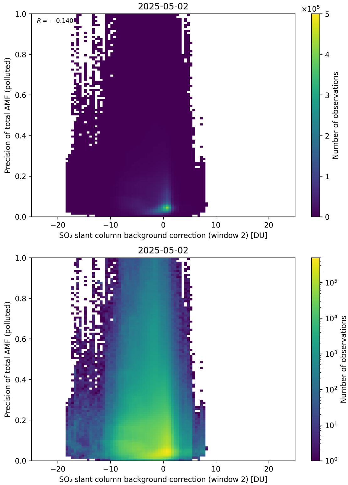
Figure 131: Scatter density plot of “SO 2 slant column background correction (window 2)” against “Precision of total AMF (polluted)” for 2025-05-01 to 2025-05-03.
