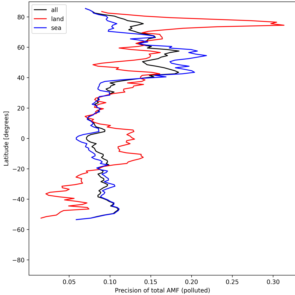
Figure 54: Zonal average of “Precision of total AMF (polluted)” for 2025-05-01 to 2025-05-03.
