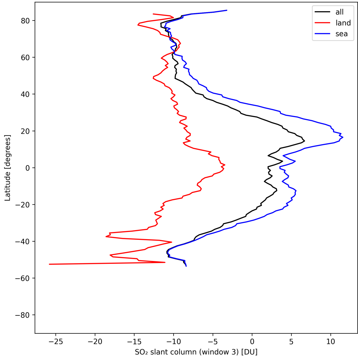
Figure 45: Zonal average of “SO 2 slant column (window 3)” for 2025-05-01 to 2025-05-03.
