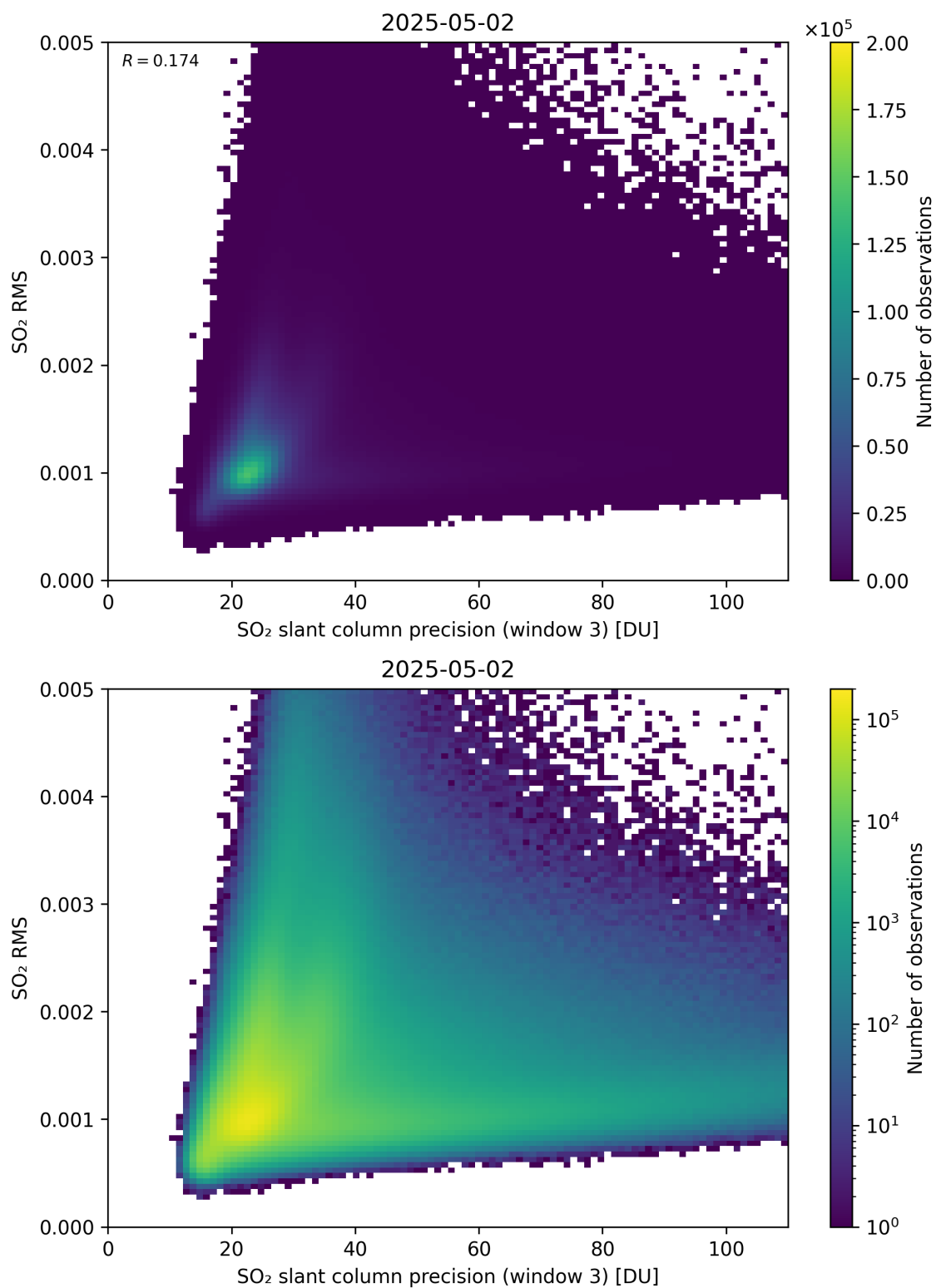
Figure 310: Scatter density plot of “SO 2 slant column precision (window 3)” against “SO 2 RMS” for 2025-05-01 to 2025-05-03.
