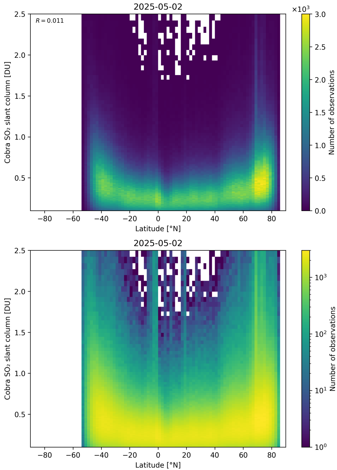
Figure 157: Scatter density plot of “Latitude” against “Cobra SO 2 slant column” for 2025-05-01 to 2025-05-03.
