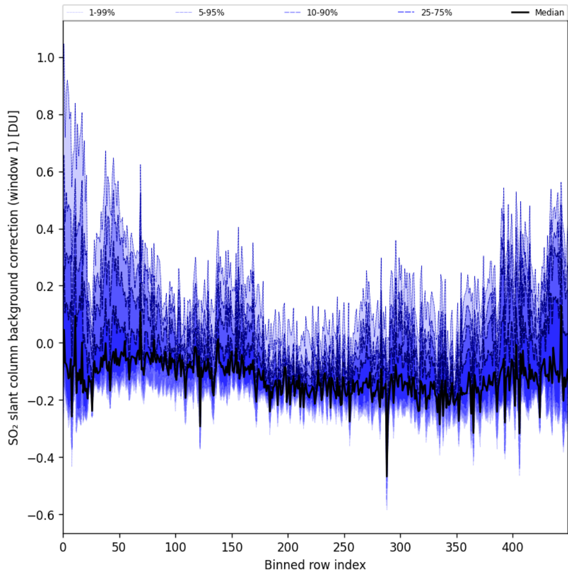
Figure 92: Along track statistics of “SO 2 slant column background correction (window 1)” for 2025-05-01 to 2025-05-03
