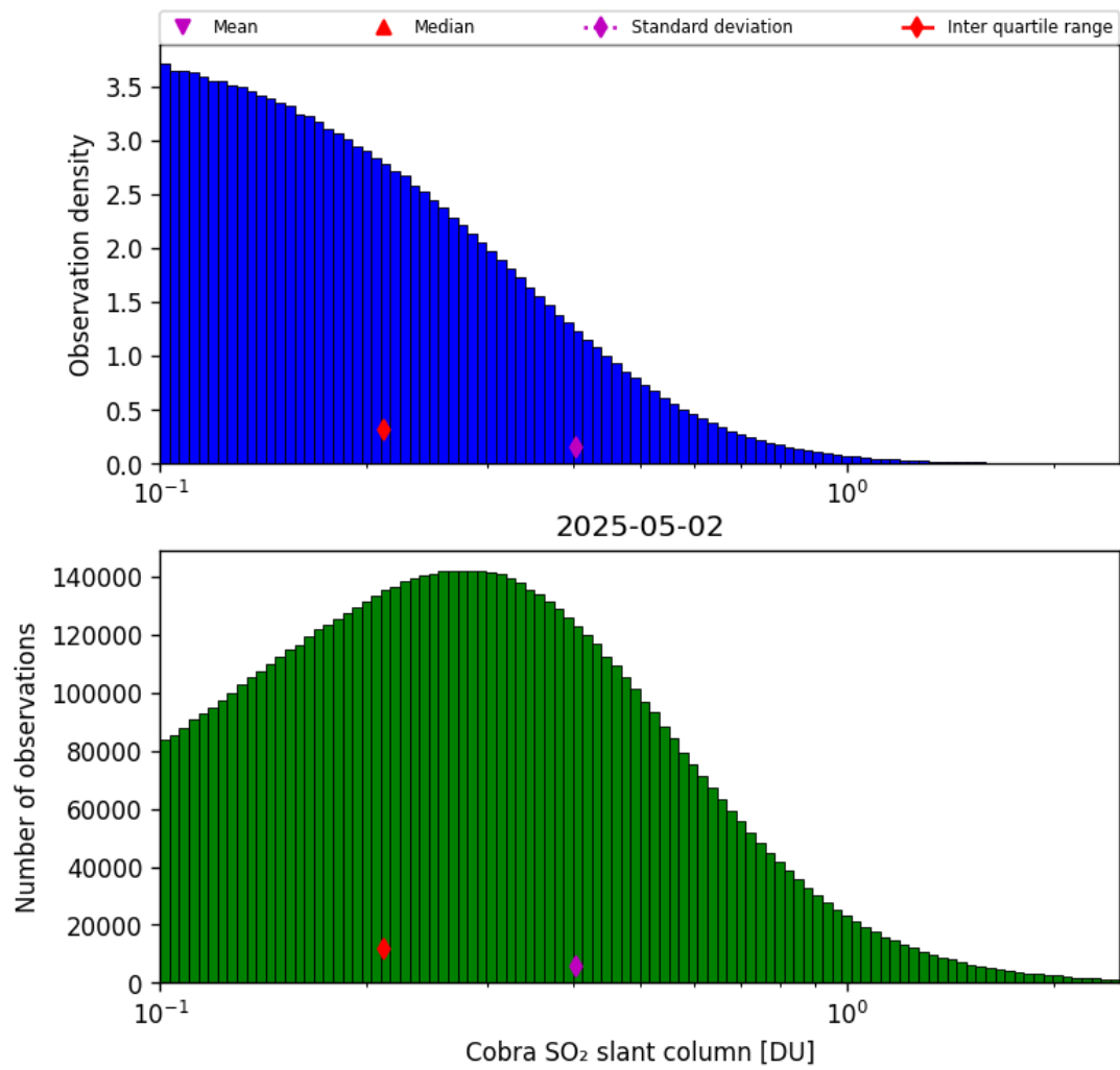
Figure 61: Histogram of “Cobra SO 2 slant column” for 2025-05-01 to 2025-05-03
