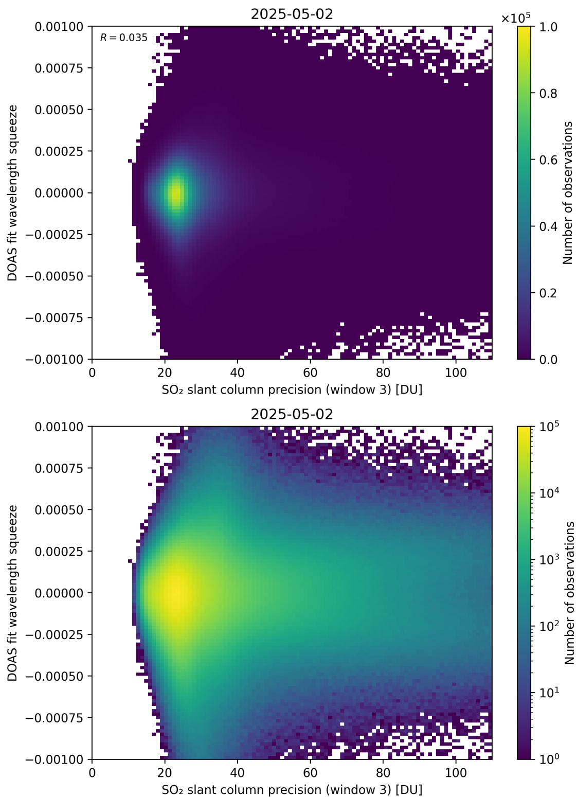
Figure 309: Scatter density plot of “SO 2 slant column precision (window 3)” against “DOAS fit wavelength squeeze” for 2025-05-01 to 2025-05-03.
