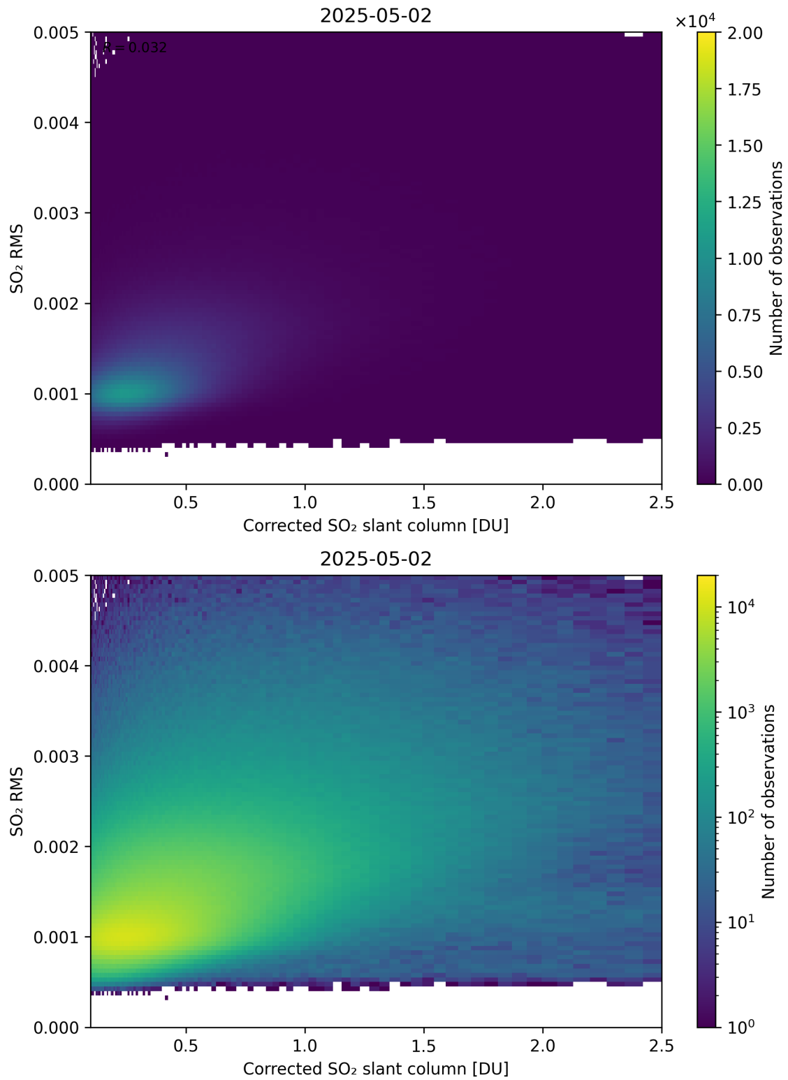
Figure 231: Scatter density plot of “Corrected SO 2 slant column” against “SO 2 RMS” for 2025-05-01 to 2025-05-03.
