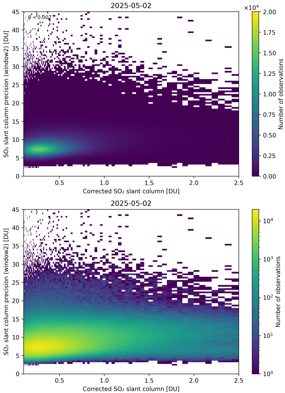
Figure 239: Scatter density plot of “Corrected SO 2 slant column” against “SO 2 slant column precision (window2)” for 2025-05-01 to 2025-05-03.
