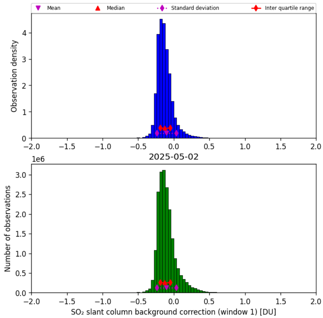
Figure 66: Histogram of “SO 2 slant column background correction (window 1)” for 2025-05-01 to 2025-05-03
