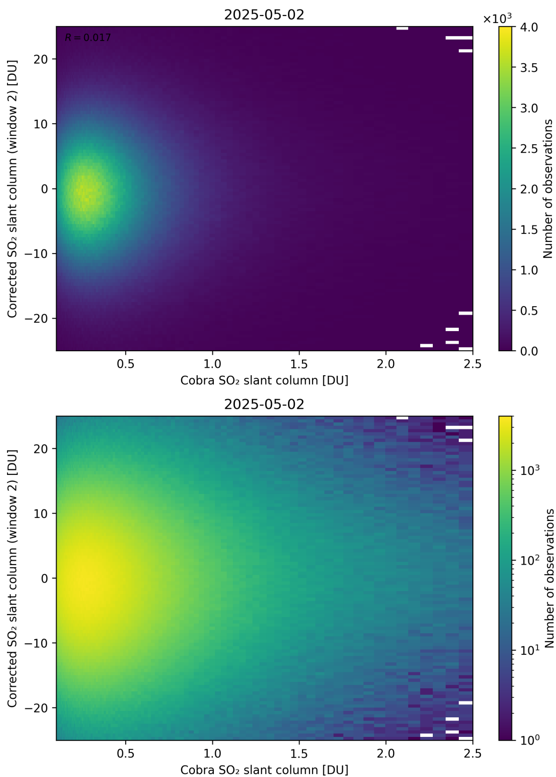
Figure 217: Scatter density plot of “Cobra SO 2 slant column” against “Corrected SO 2 slant column (window 2)” for 2025-05-01 to 2025-05-03.
