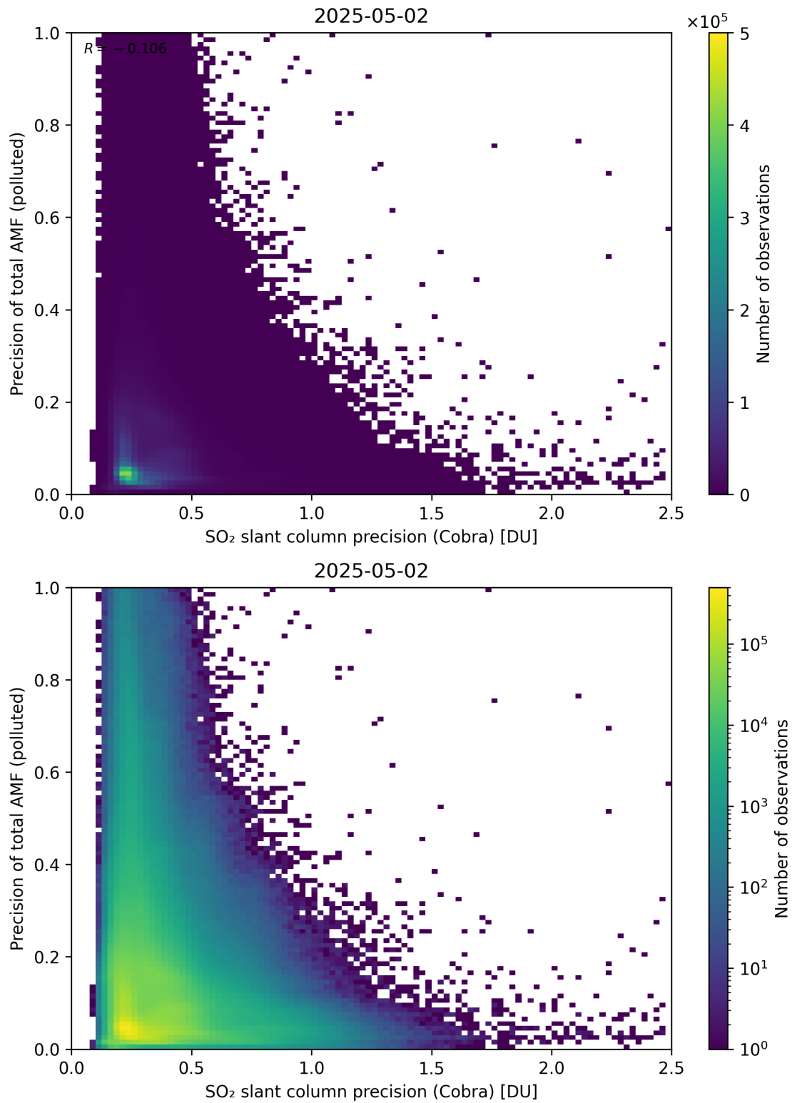
Figure 214: Scatter density plot of “SO 2 slant column precision (Cobra)” against “Precision of total AMF (polluted)” for 2025-05-01 to 2025-05-03.
