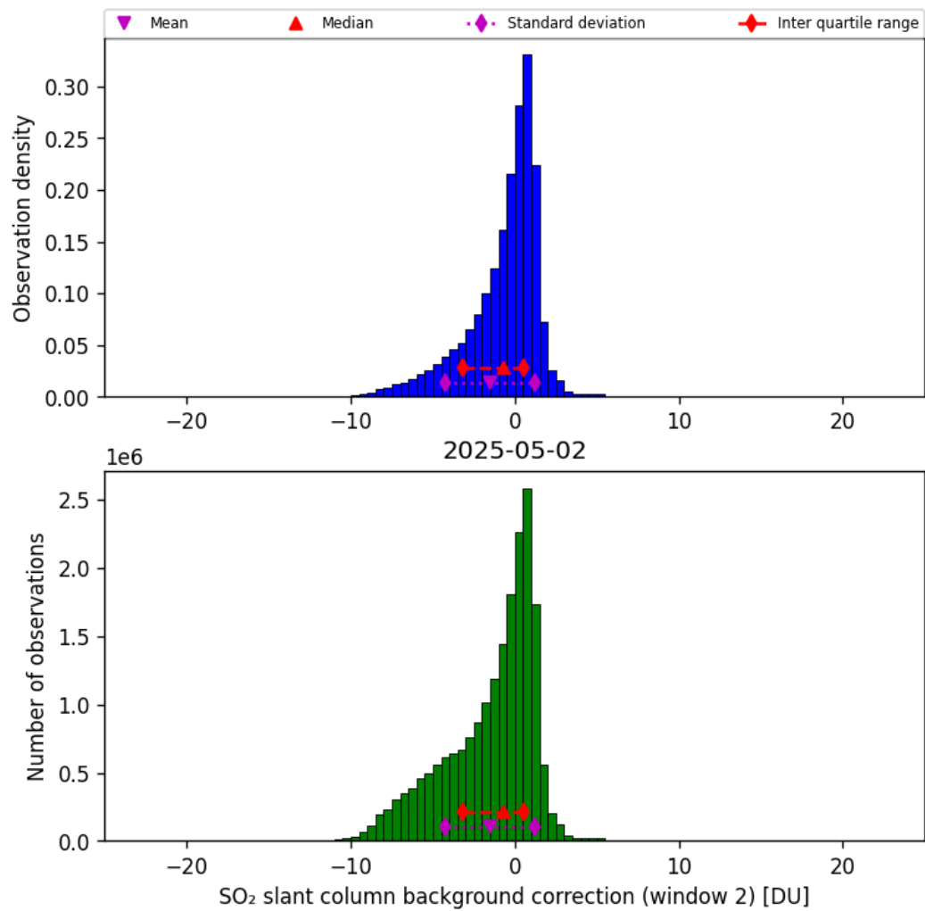
Figure 70: Histogram of “SO 2 slant column background correction (window 2)” for 2025-05-01 to 2025-05-03
