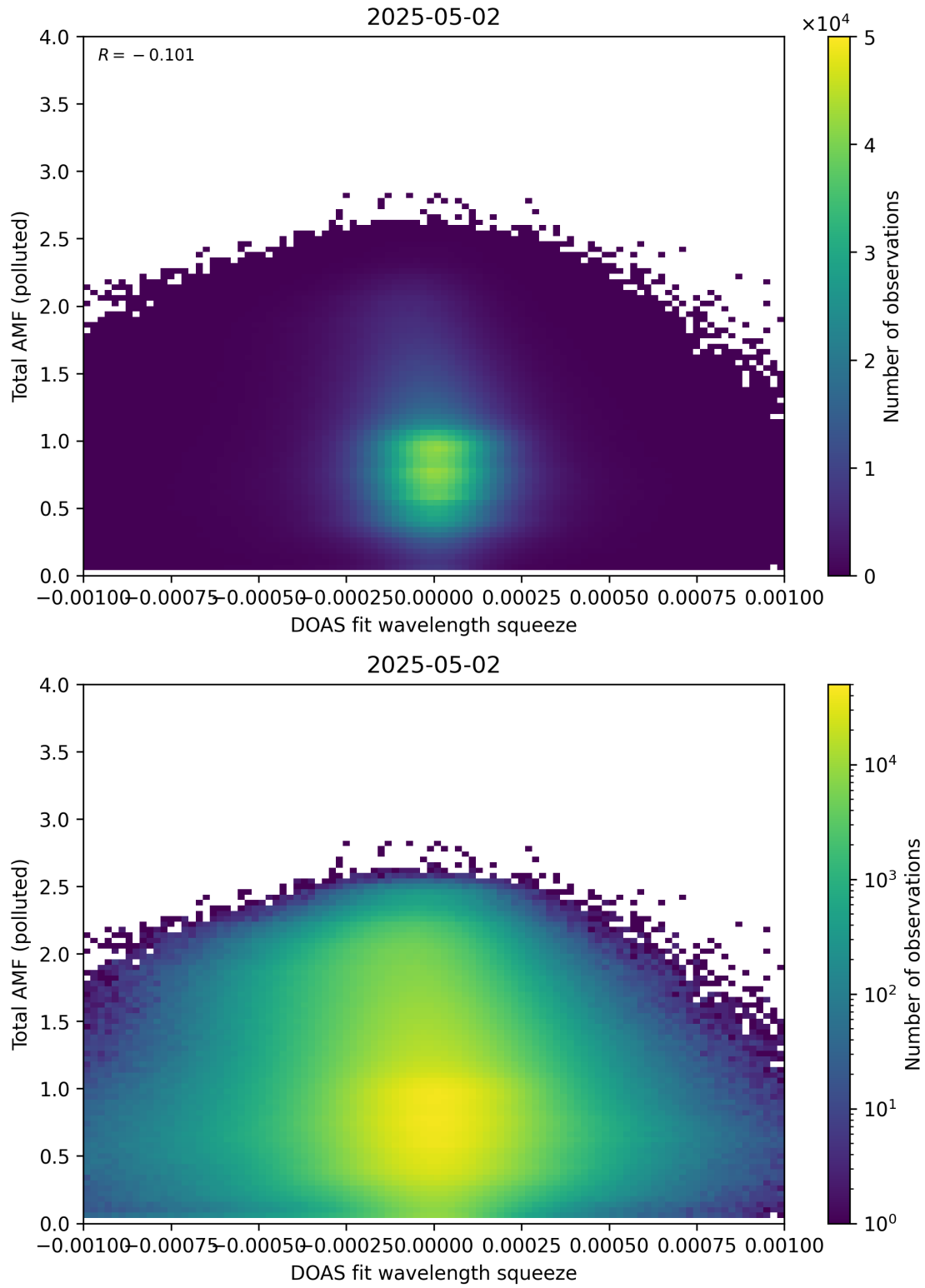
Figure 145: Scatter density plot of “DOAS fit wavelength squeeze” against “Total AMF (polluted)” for 2025-05-01 to 2025-05-03.
