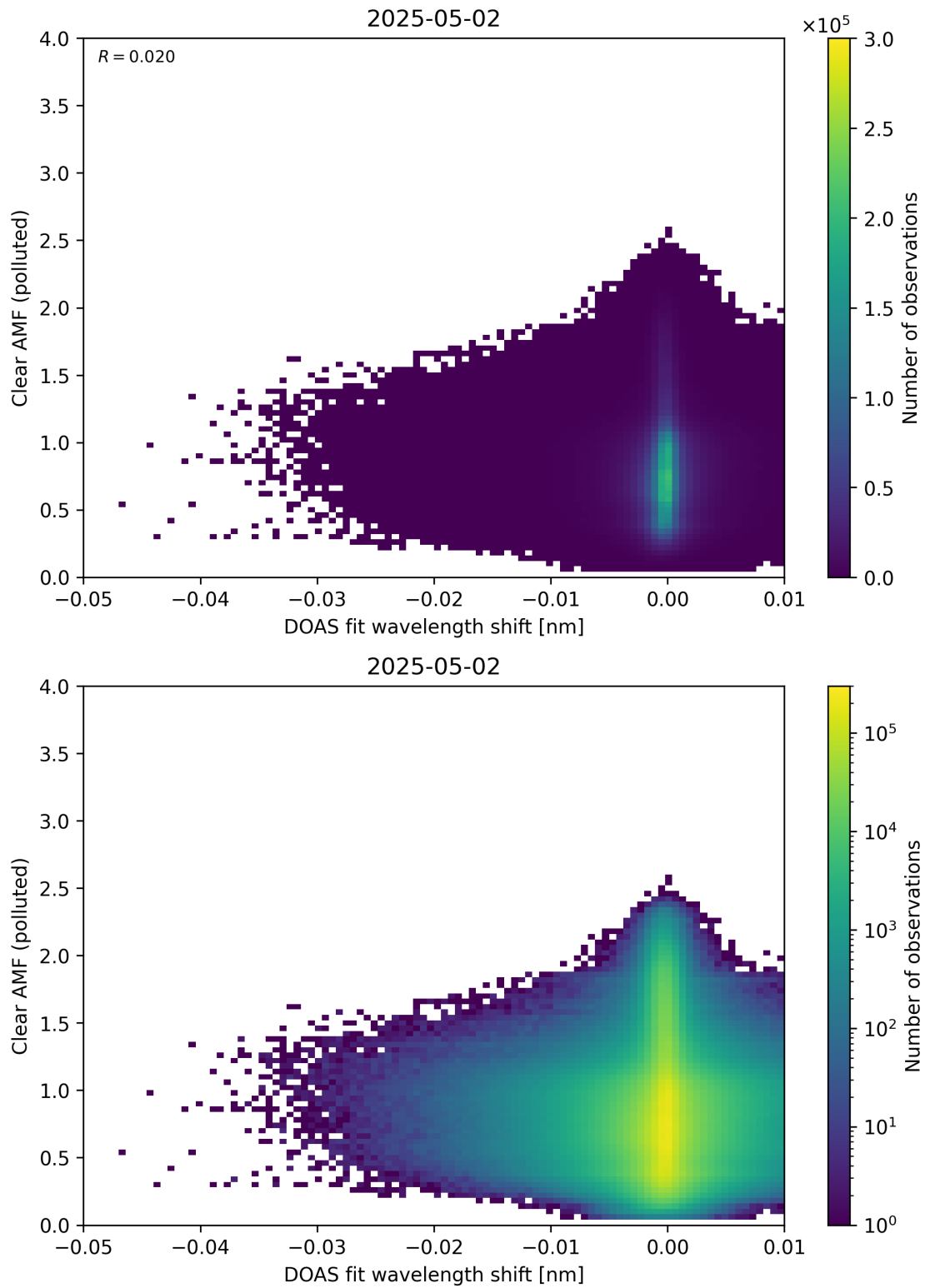
Figure 140: Scatter density plot of “DOAS fit wavelength shift” against “Clear AMF (polluted)” for 2025-05-01 to 2025-05-03.
