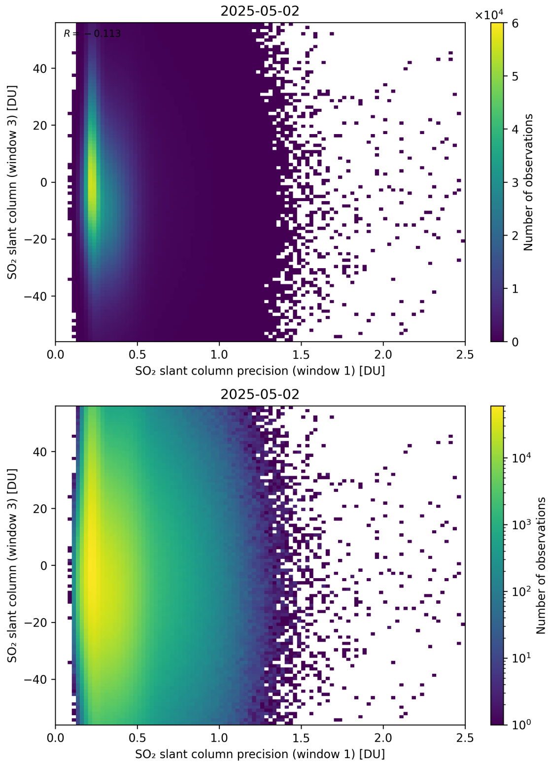
Figure 278: Scatter density plot of “SO 2 slant column precision (window 1)” against “SO 2 slant column (window 3)” for 2025-05-01 to 2025-05-03.
