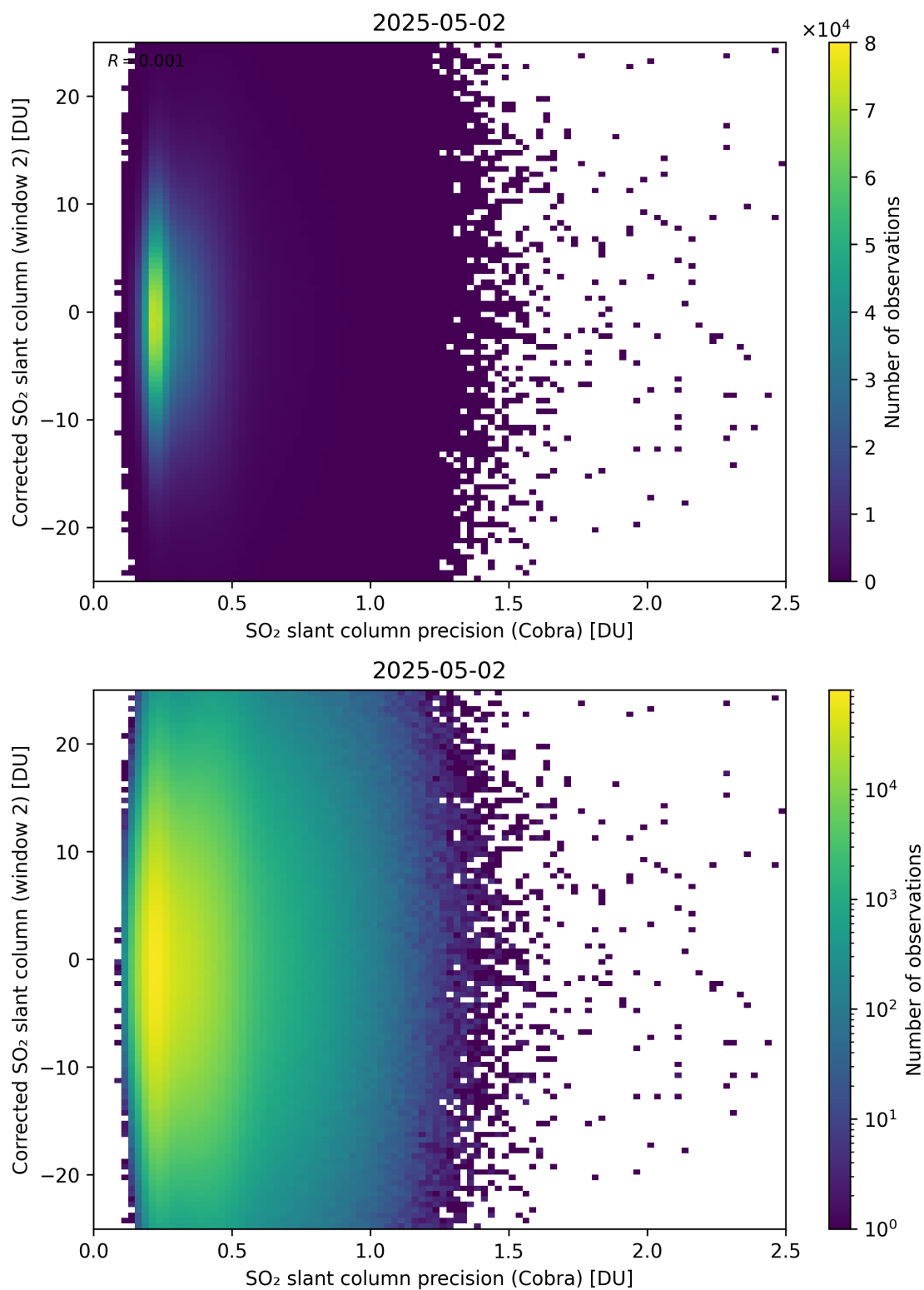
Figure 206: Scatter density plot of “SO 2 slant column precision (Cobra)” against “Corrected SO 2 slant column (window 2)” for 2025-05-01 to 2025-05-03.
