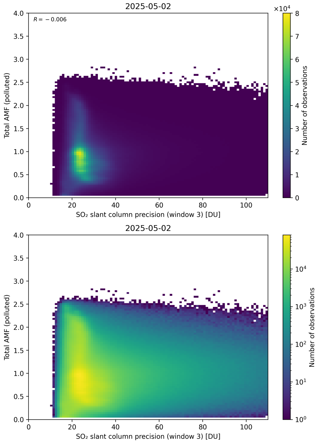
Figure 313: Scatter density plot of “SO 2 slant column precision (window 3)” against “Total AMF (polluted)” for 2025-05-01 to 2025-05-03.
