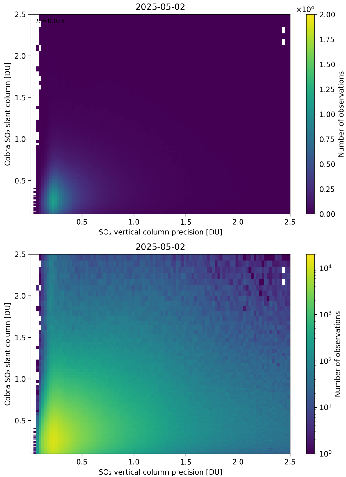
Figure 336: Scatter density plot of “SO 2 vertical column precision” against “Cobra SO 2 slant column” for 2025-05-01 to 2025-05-03.
