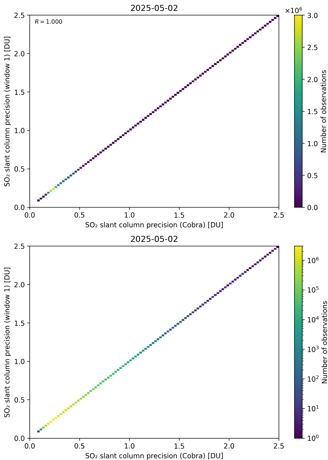
Figure 209: Scatter density plot of “SO 2 slant column precision (Cobra)” against “SO 2 slant column precision (window 1)” for 2025-05-01 to 2025-05-03.
