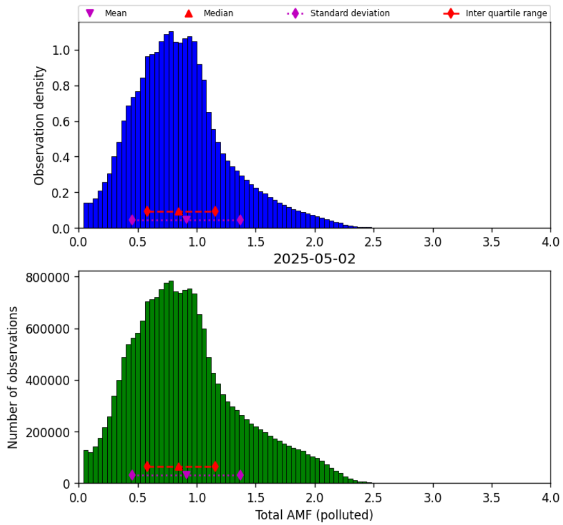
Figure 79: Histogram of “Total AMF (polluted)” for 2025-05-01 to 2025-05-03
