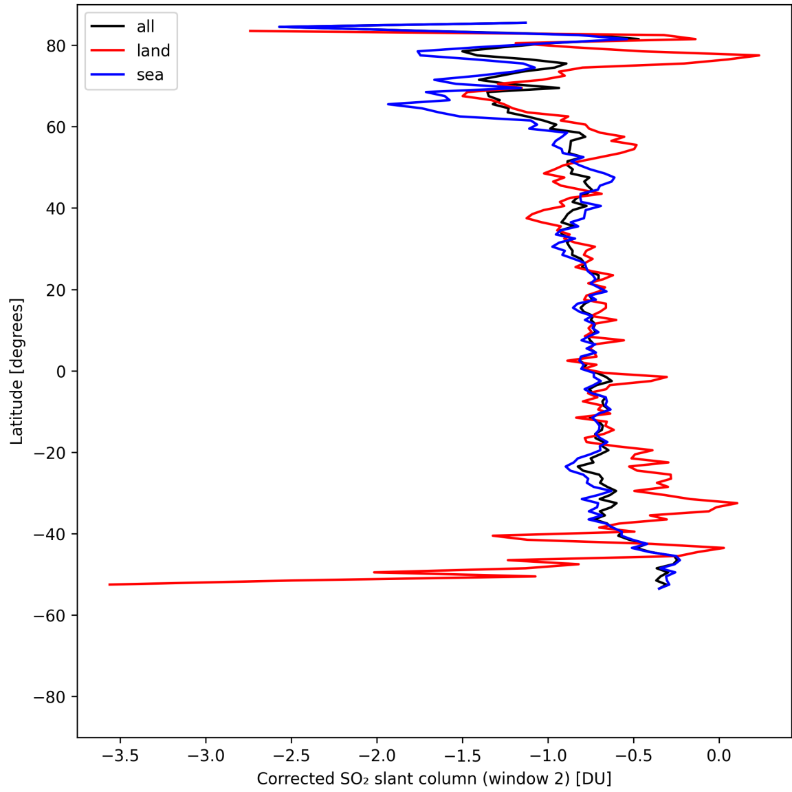
Figure 43: Zonal average of “Corrected SO 2 slant column (window 2)” for 2025-05-01 to 2025-05-03.
