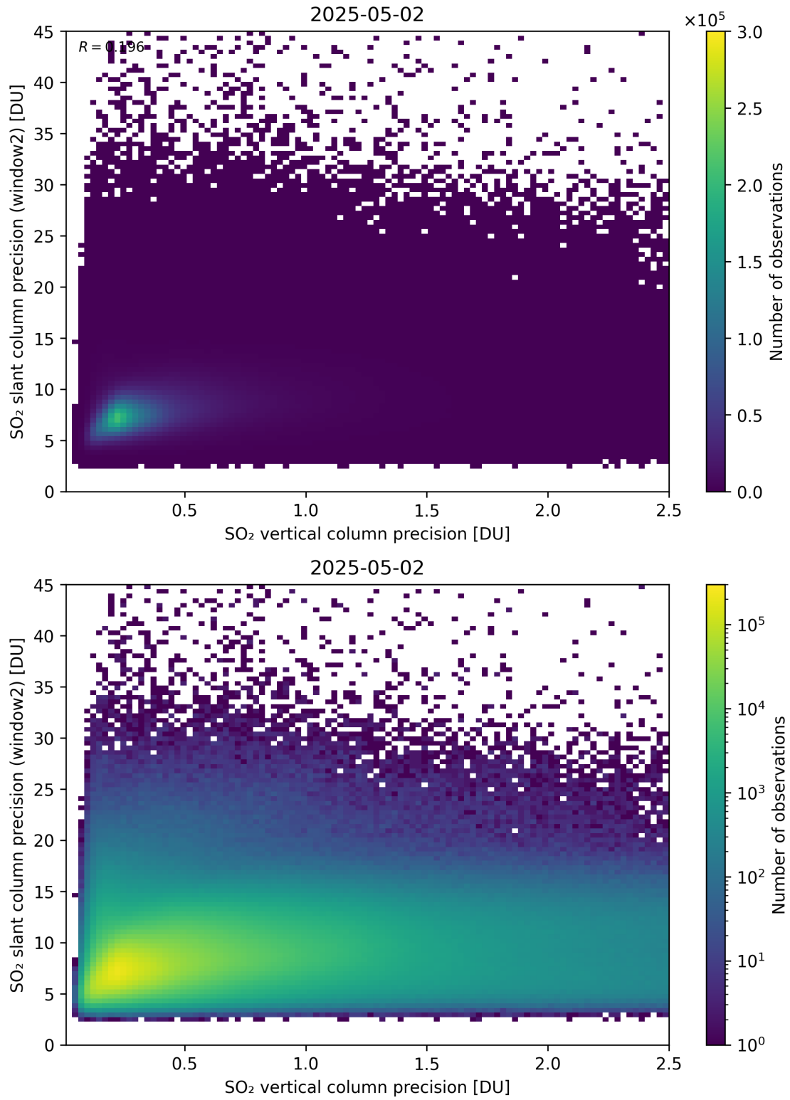
Figure 343: Scatter density plot of “SO 2 vertical column precision” against “SO 2 slant column precision (window2)” for 2025-05-01 to 2025-05-03.
