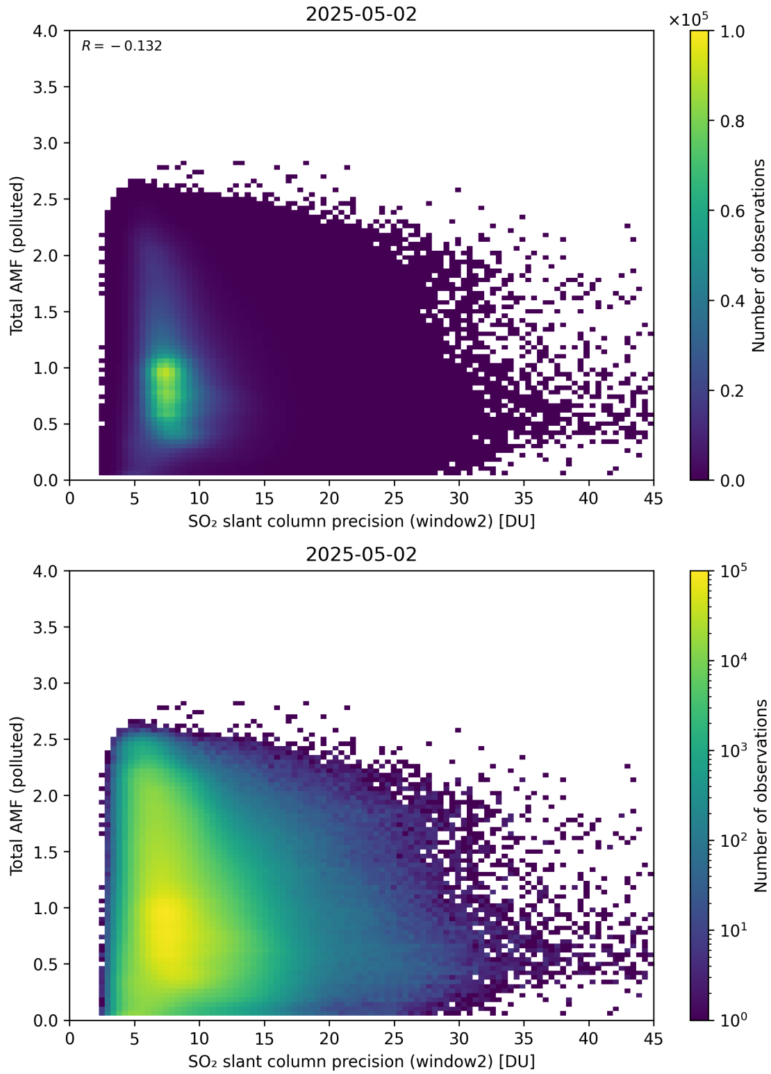
Figure 301: Scatter density plot of “SO 2 slant column precision (window2)” against “Total AMF (polluted)” for 2025-05-01 to 2025-05-03.
