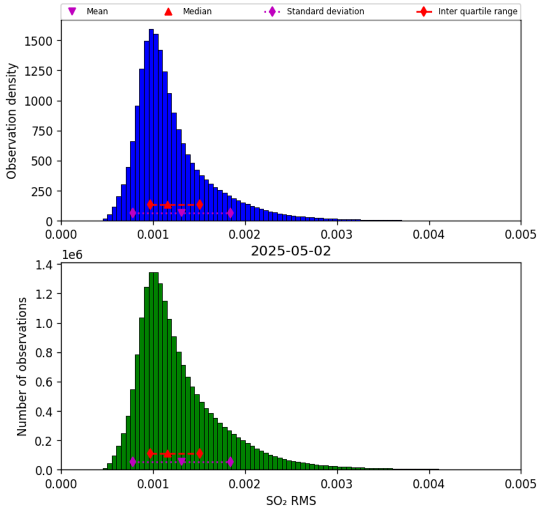
Figure 78: Histogram of “SO 2 RMS” for 2025-05-01 to 2025-05-03
