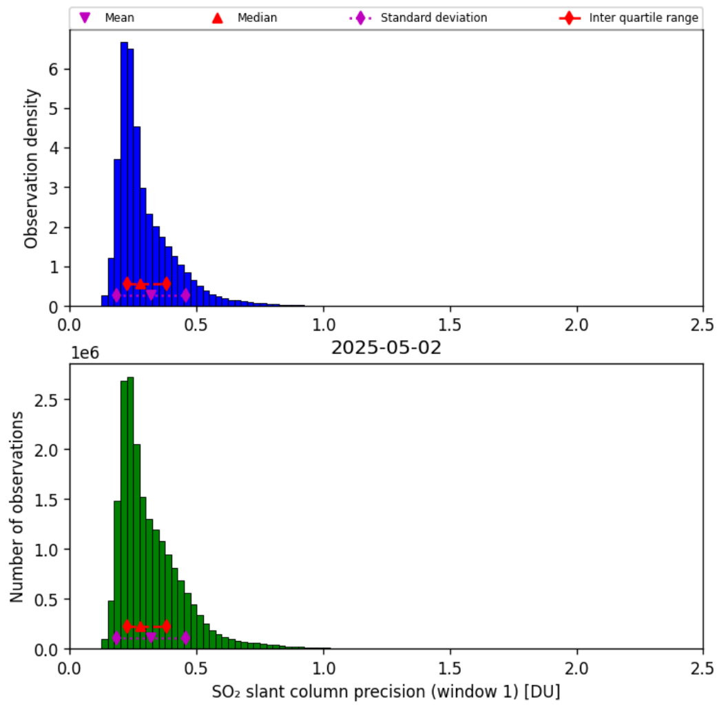
Figure 64: Histogram of “SO 2 slant column precision (window 1)” for 2025-05-01 to 2025-05-03
