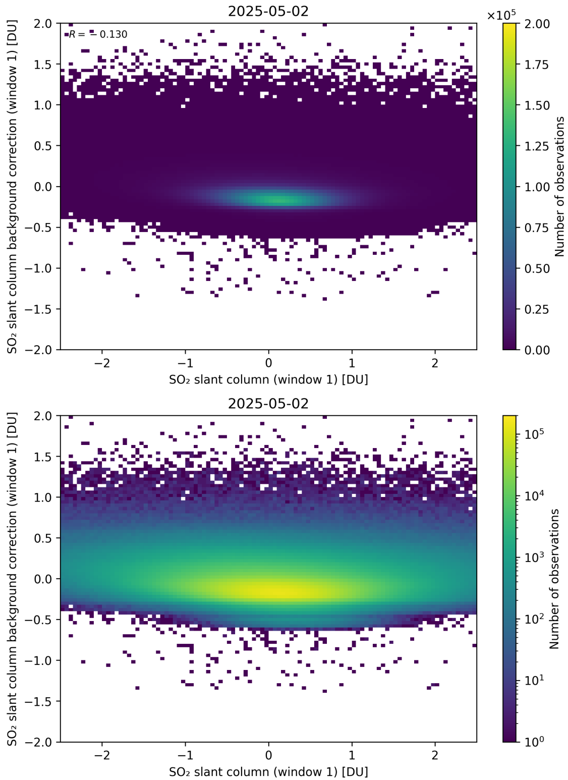
Figure 262: Scatter density plot of “SO 2 slant column (window 1)” against “SO 2 slant column background correction (window 1)” for 2025-05-01 to 2025-05-03.
