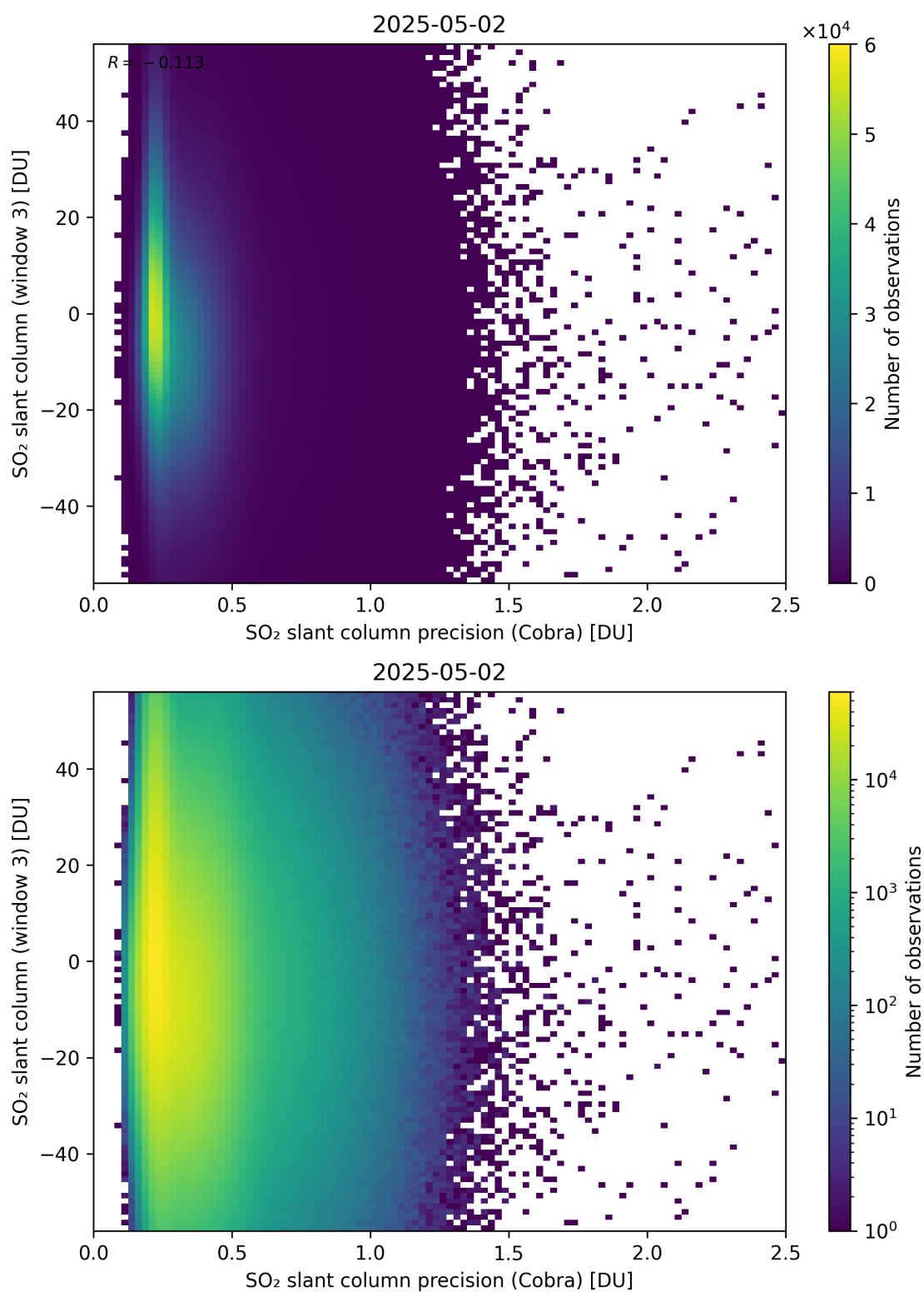
Figure 211: Scatter density plot of “SO 2 slant column precision (Cobra)” against “SO 2 slant column (window 3)” for 2025-05-01 to 2025-05-03.
