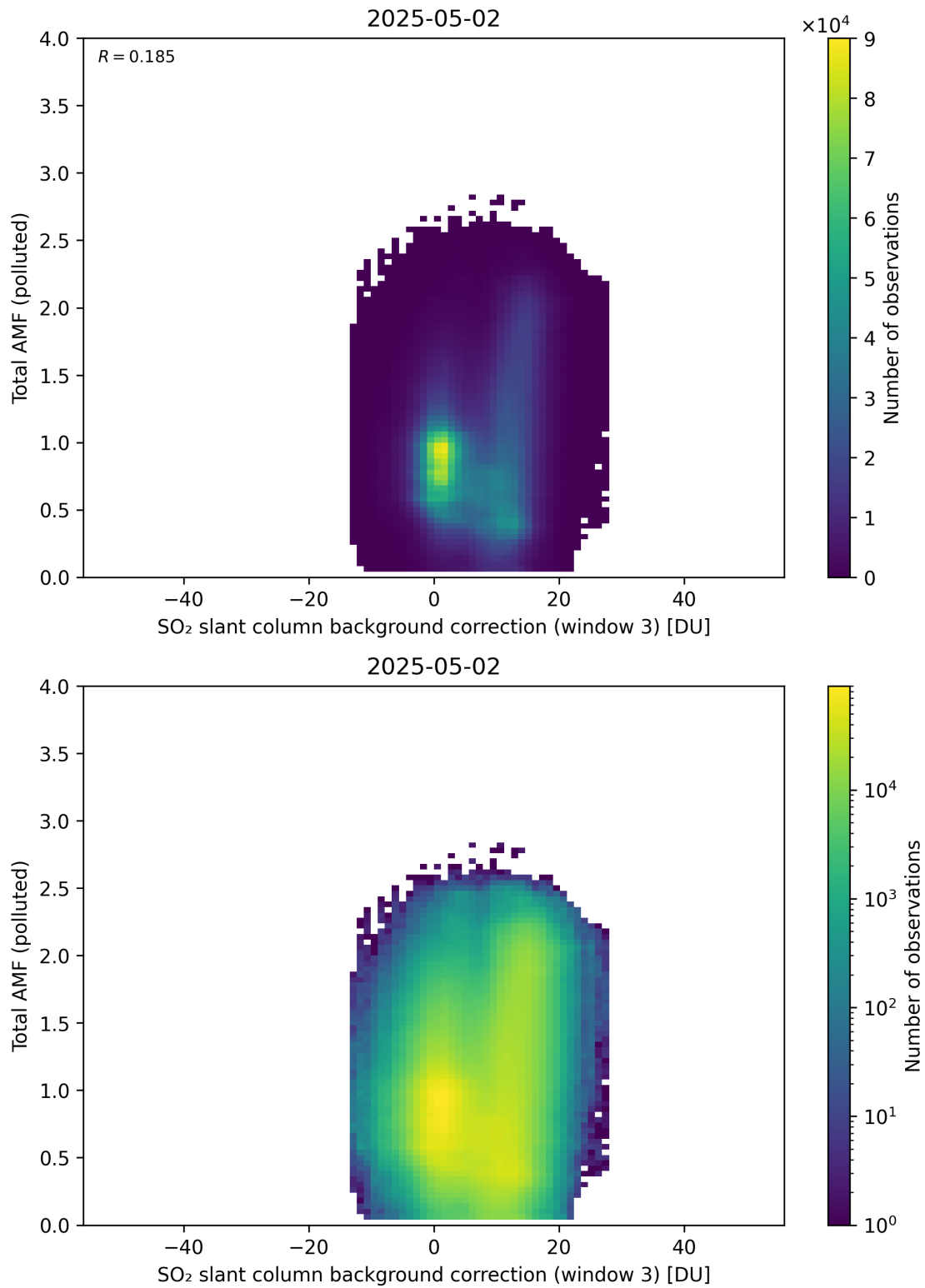
Figure 136: Scatter density plot of “SO 2 slant column background correction (window 3)” against “Total AMF (polluted)” for 2025-05-01 to 2025-05-03.
