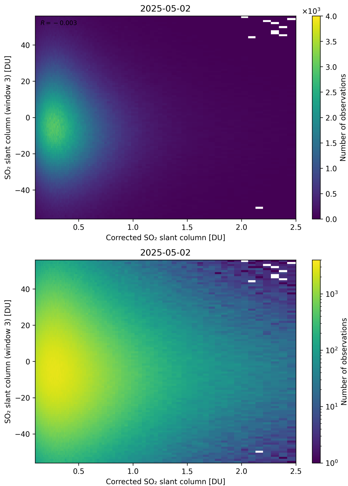
Figure 240: Scatter density plot of “Corrected SO 2 slant column” against “SO 2 slant column (window 3)” for 2025-05-01 to 2025-05-03.
