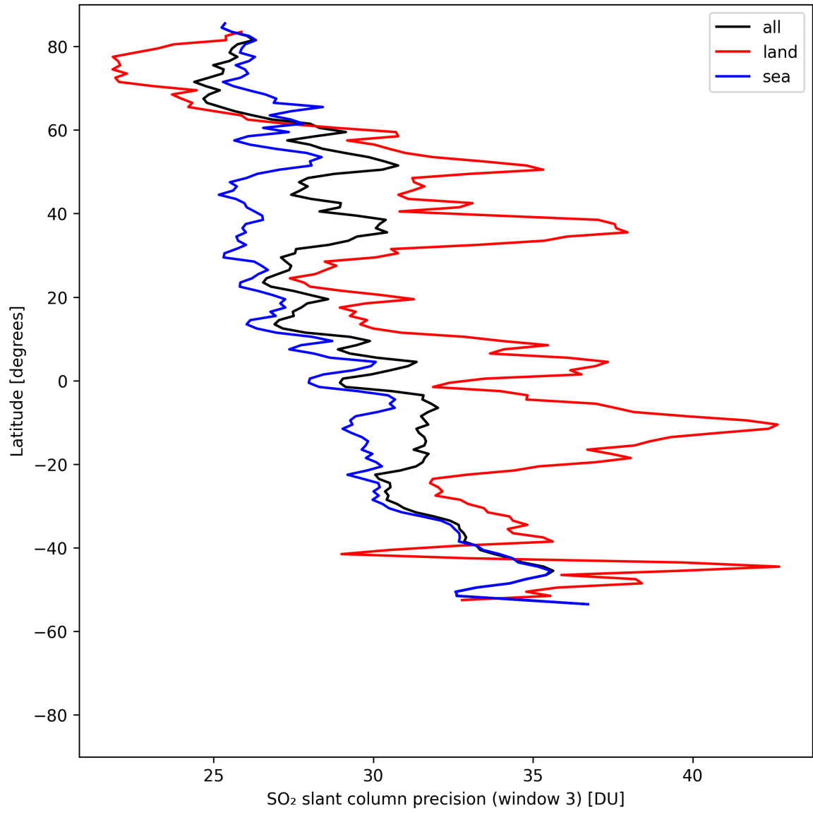
Figure 46: Zonal average of “SO 2 slant column precision (window 3)” for 2025-05-01 to 2025-05-03.
