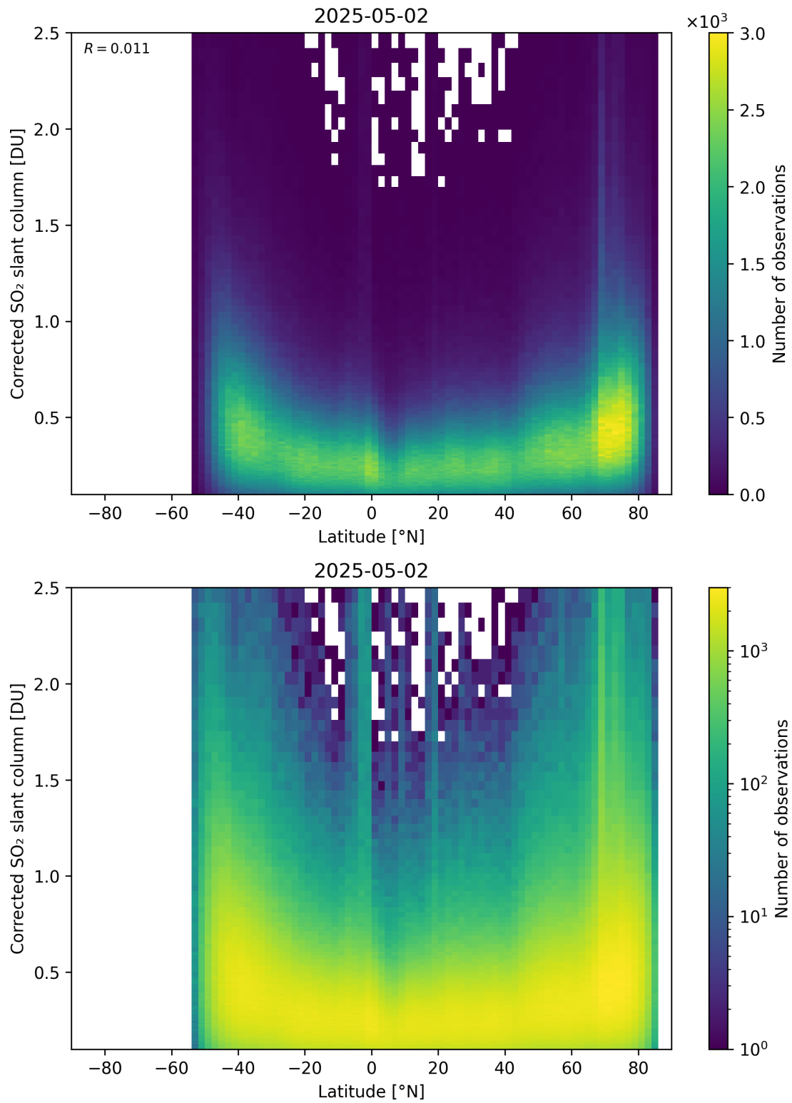
Figure 159: Scatter density plot of “Latitude” against “Corrected SO 2 slant column” for 2025-05-01 to 2025-05-03.
