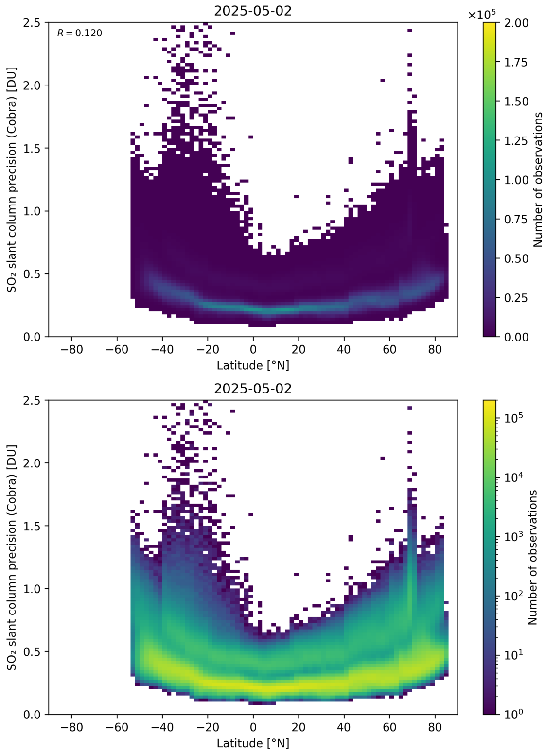
Figure 158: Scatter density plot of “Latitude” against “SO 2 slant column precision (Cobra)” for 2025-05-01 to 2025-05-03.
