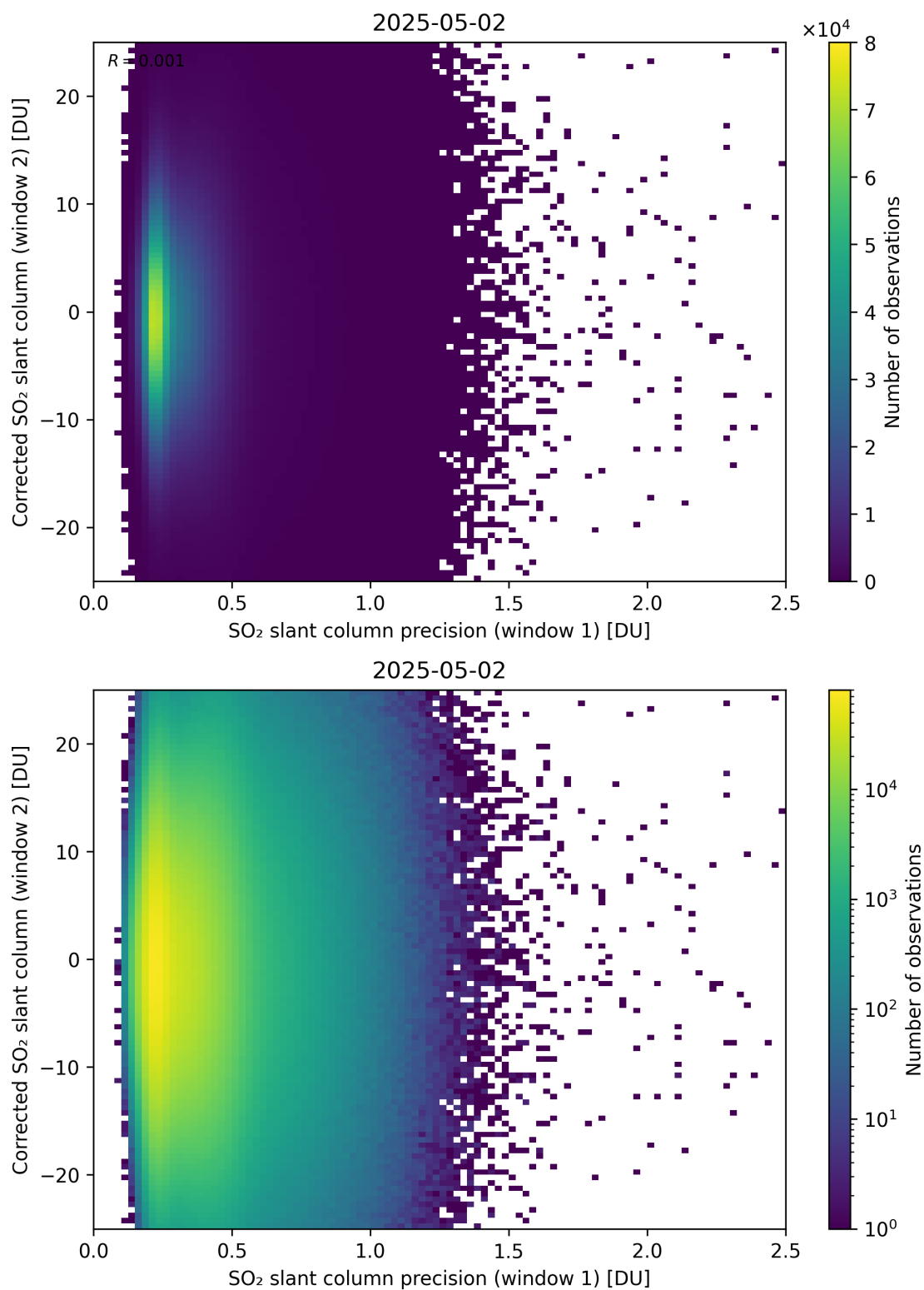
Figure 275: Scatter density plot of “SO 2 slant column precision (window 1)” against “Corrected SO 2 slant column (window 2)” for 2025-05-01 to 2025-05-03.
