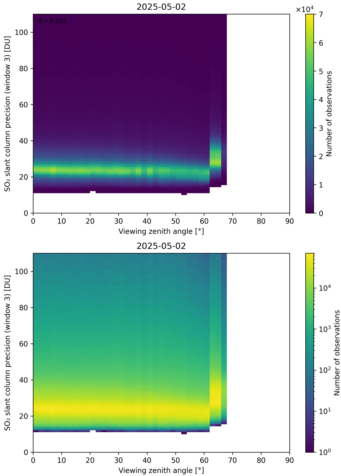
Figure 380: Scatter density plot of “Viewing zenith angle” against “SO 2 slant column precision (window 3)” for 2025-05-01 to 2025-05-03.
