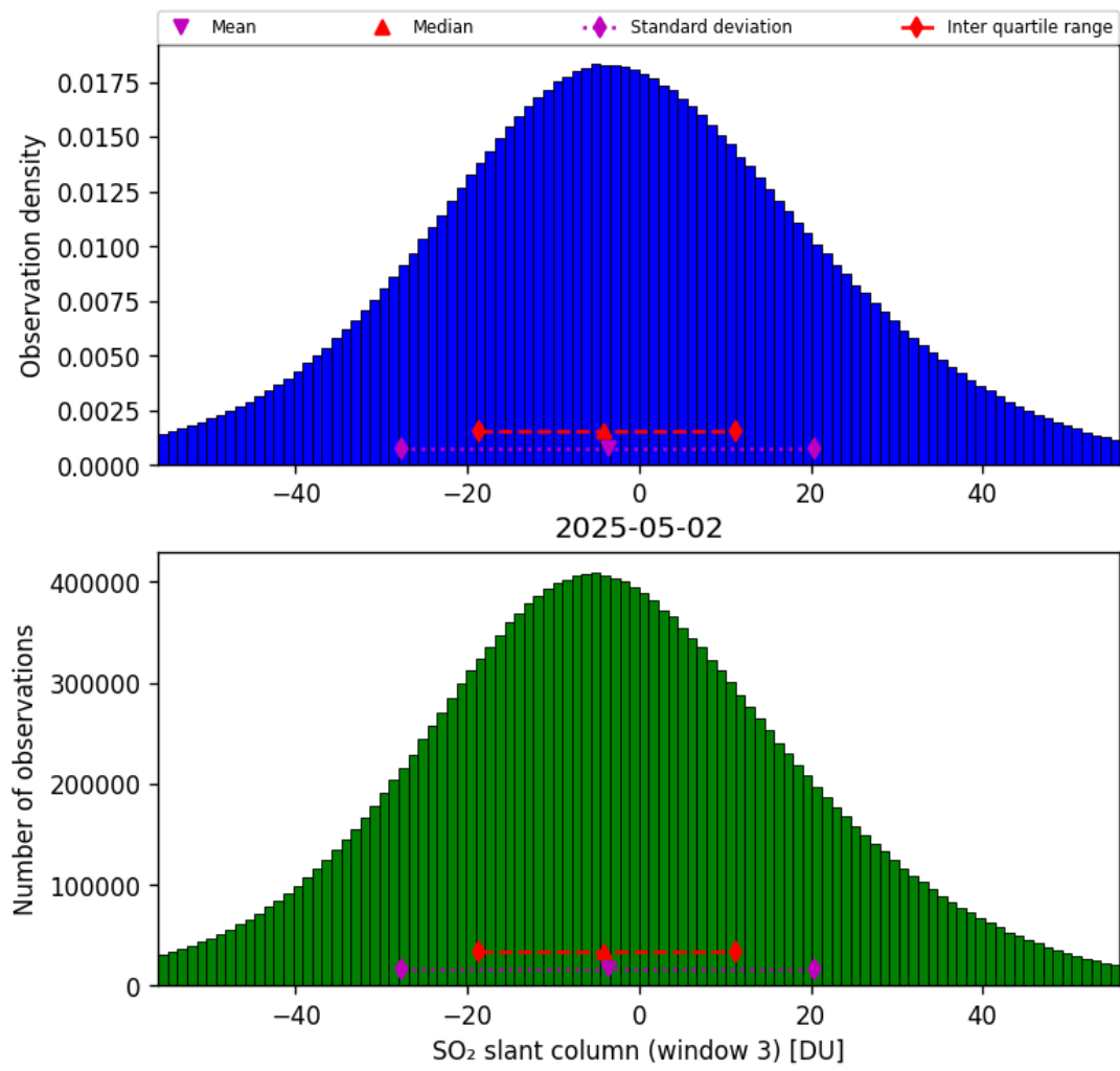
Figure 71: Histogram of “SO 2 slant column (window 3)” for 2025-05-01 to 2025-05-03
