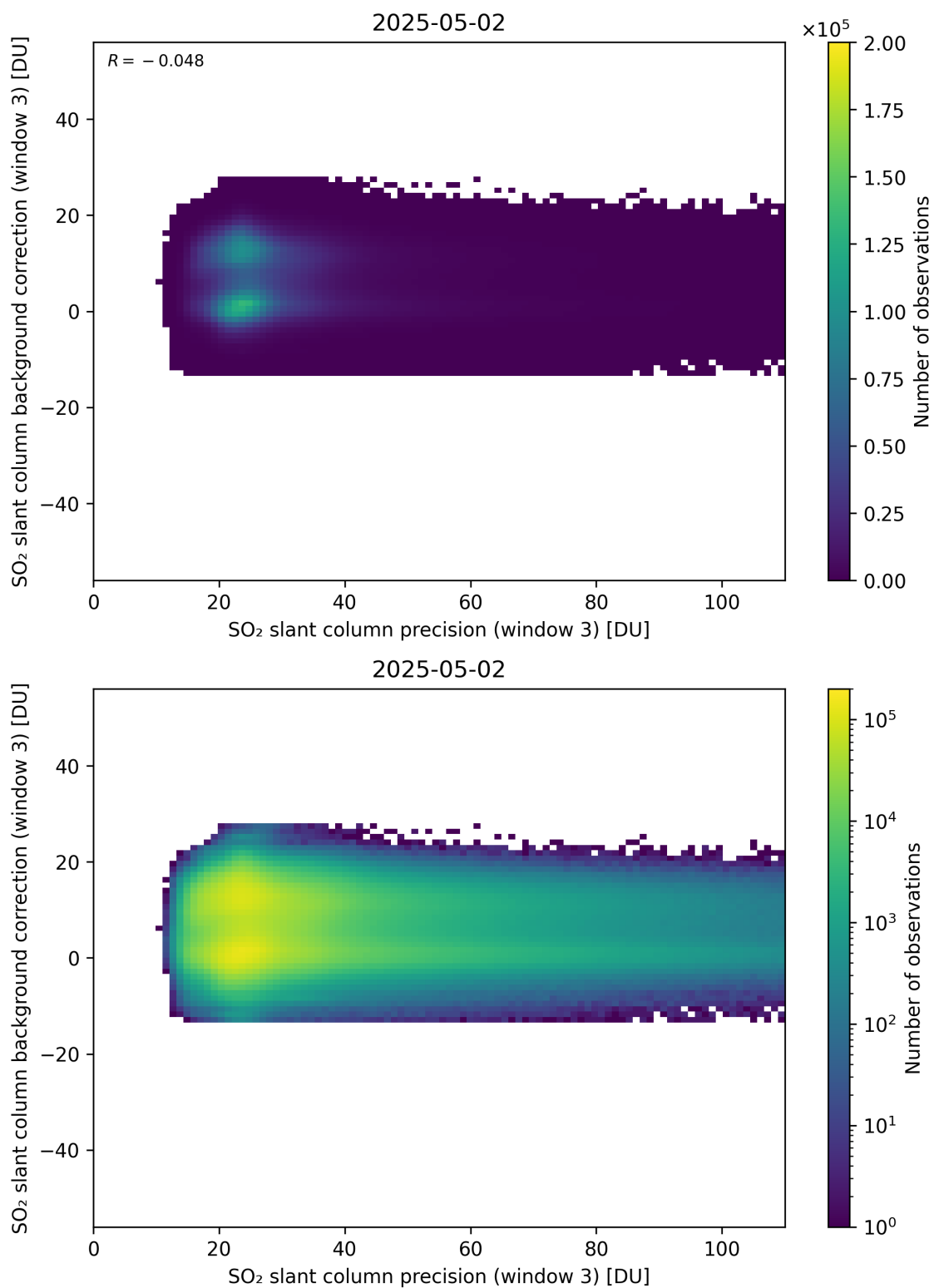
Figure 307: Scatter density plot of “SO 2 slant column precision (window 3)” against “SO 2 slant column background correction (window 3)” for 2025-05-01 to 2025-05-03.
