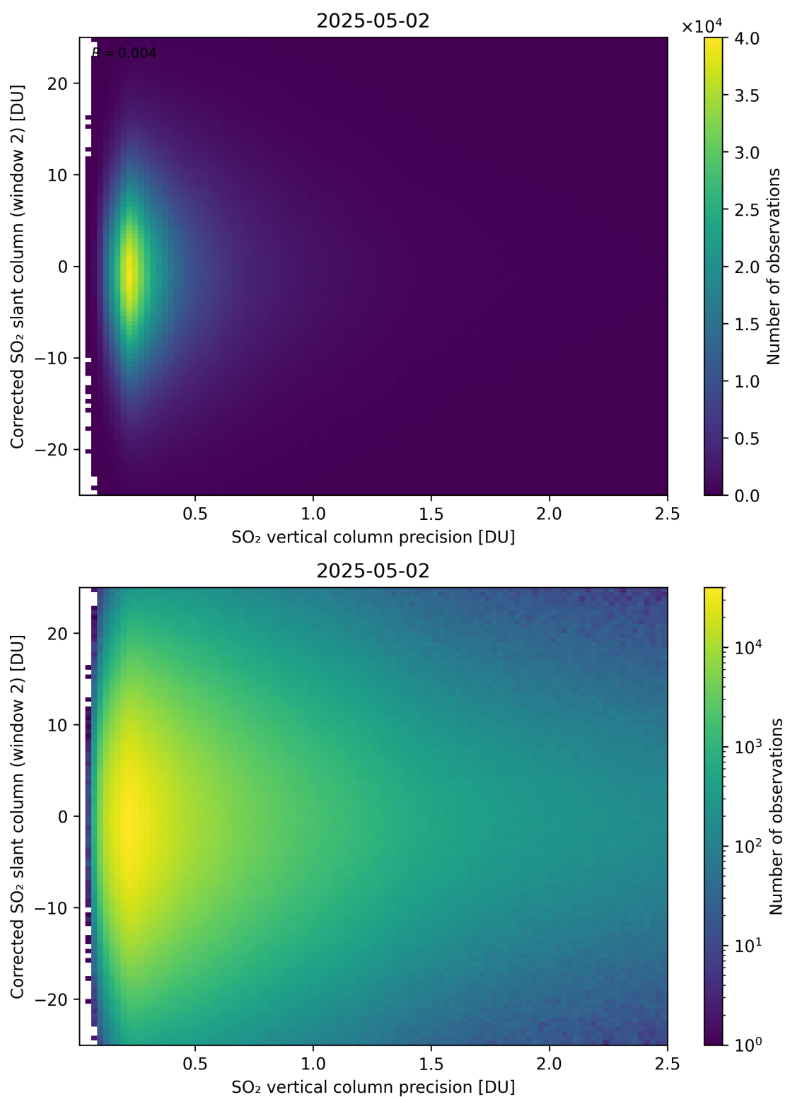
Figure 339: Scatter density plot of “SO 2 vertical column precision” against “Corrected SO 2 slant column (window 2)” for 2025-05-01 to 2025-05-03.
