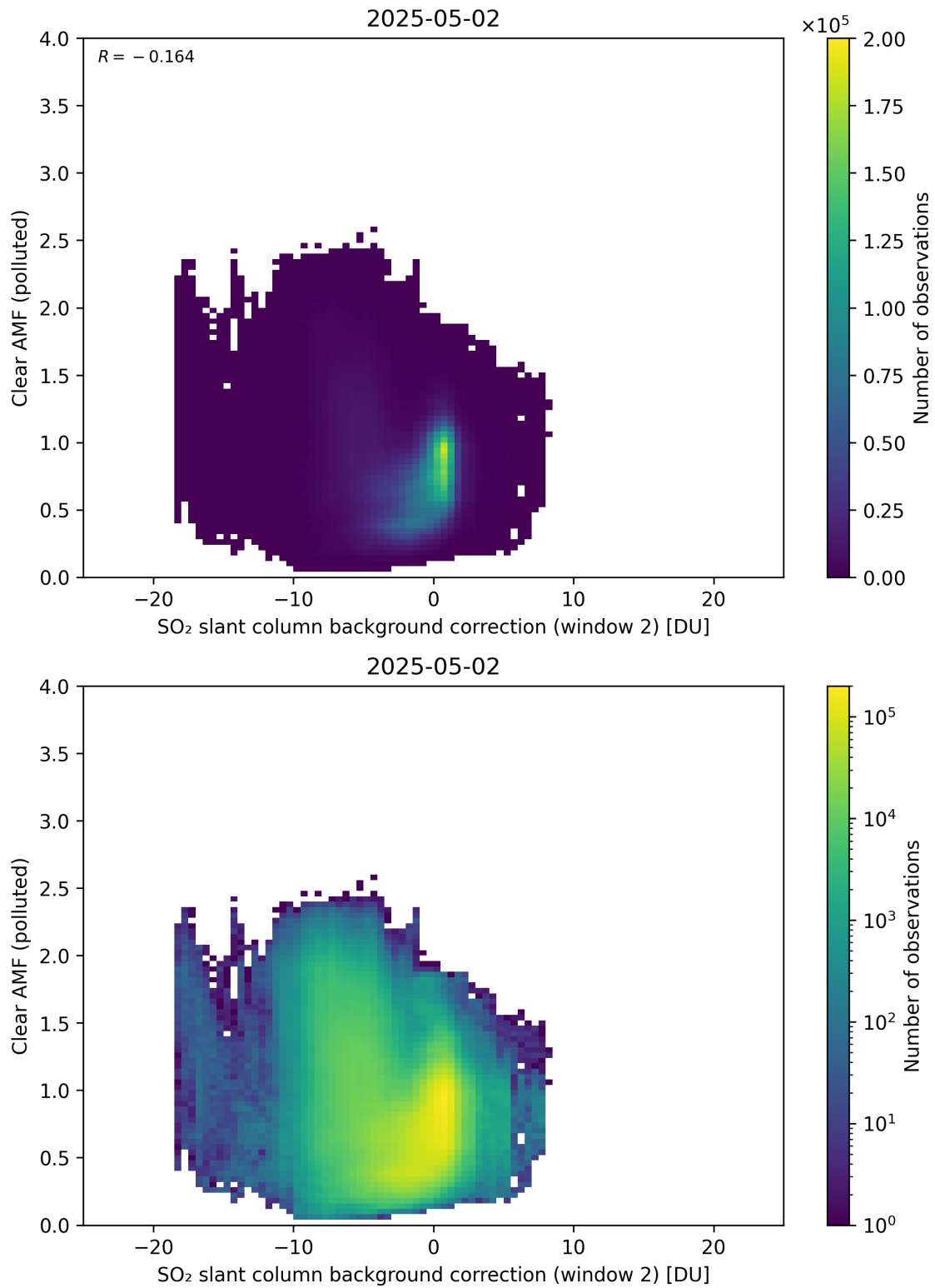
Figure 126: Scatter density plot of “SO 2 slant column background correction (window 2)” against “Clear AMF (polluted)” for 2025-05-01 to 2025-05-03.
