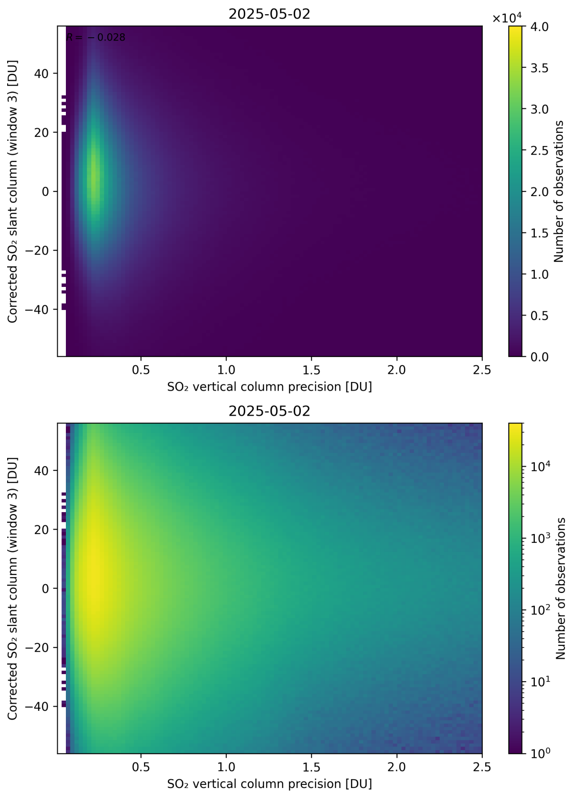
Figure 340: Scatter density plot of “SO 2 vertical column precision” against “Corrected SO 2 slant column (window 3)” for 2025-05-01 to 2025-05-03.
