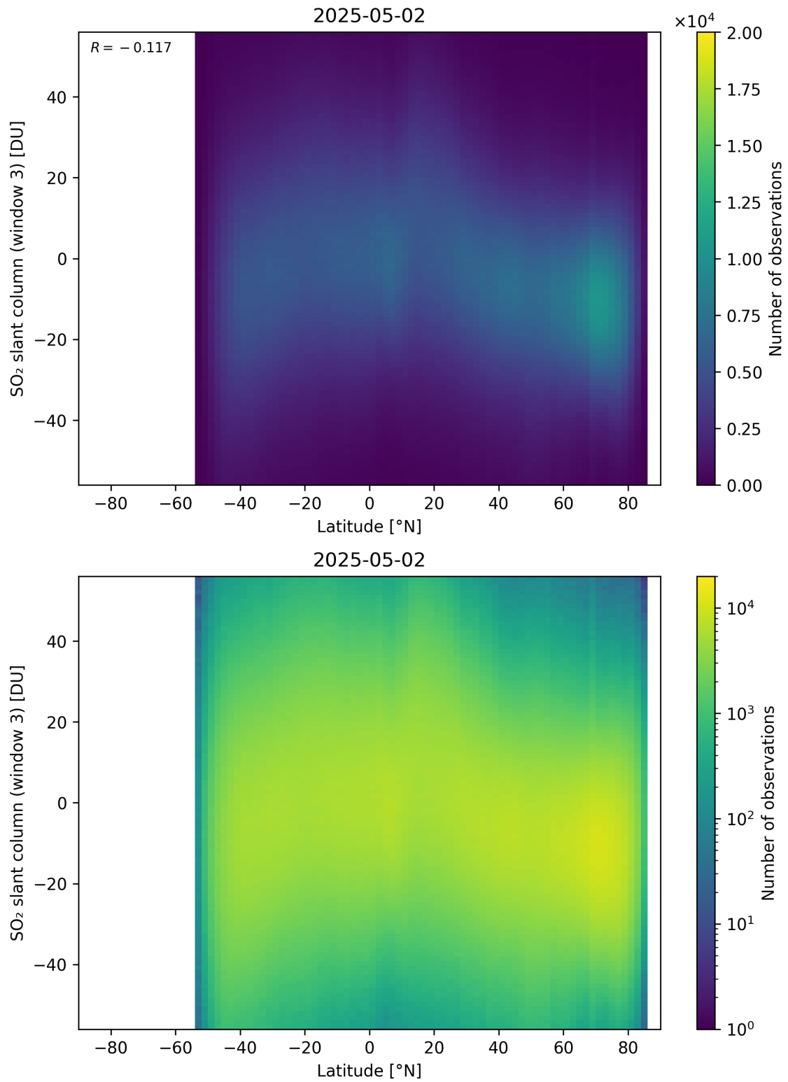
Figure 165: Scatter density plot of “Latitude” against “SO 2 slant column (window 3)” for 2025-05-01 to 2025-05-03.
