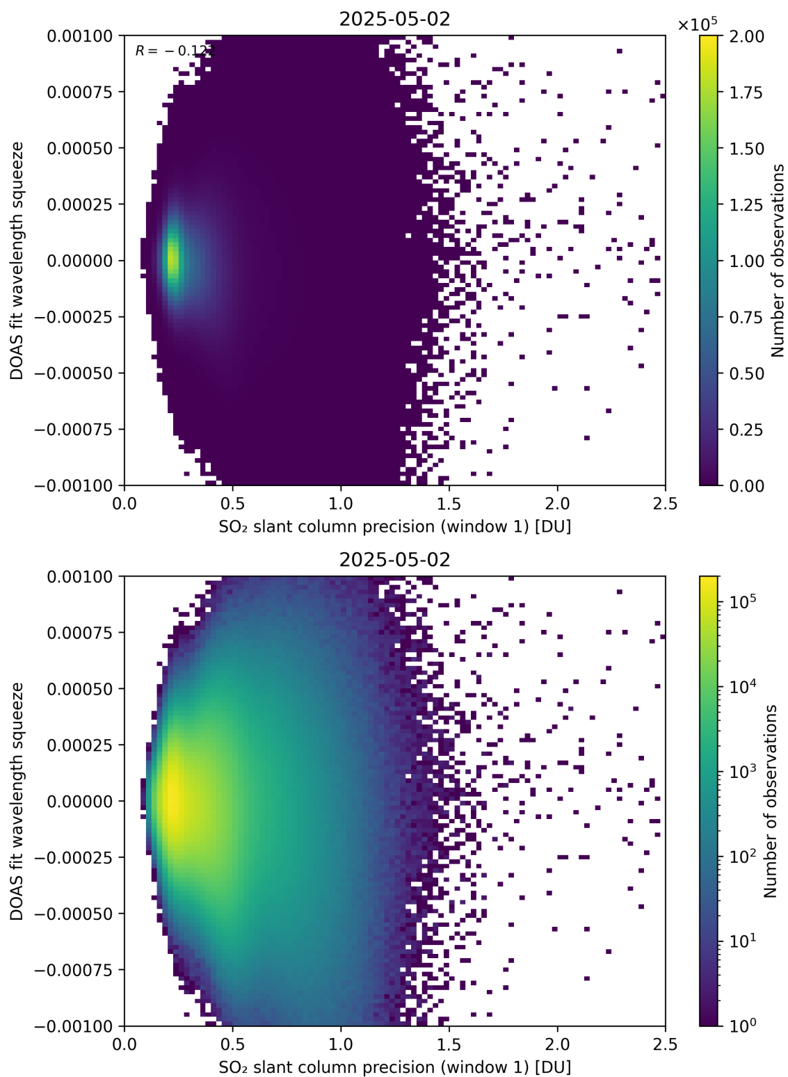
Figure 272: Scatter density plot of “SO 2 slant column precision (window 1)” against “DOAS fit wavelength squeeze” for 2025-05-01 to 2025-05-03.
