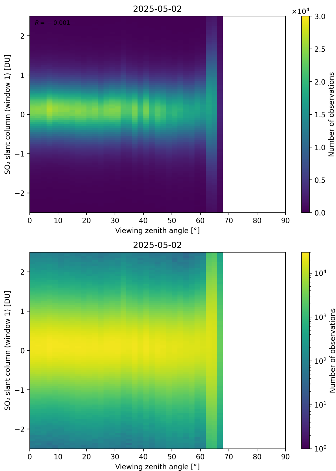
Figure 376: Scatter density plot of “Viewing zenith angle” against “SO 2 slant column (window 1)” for 2025-05-01 to 2025-05-03.
