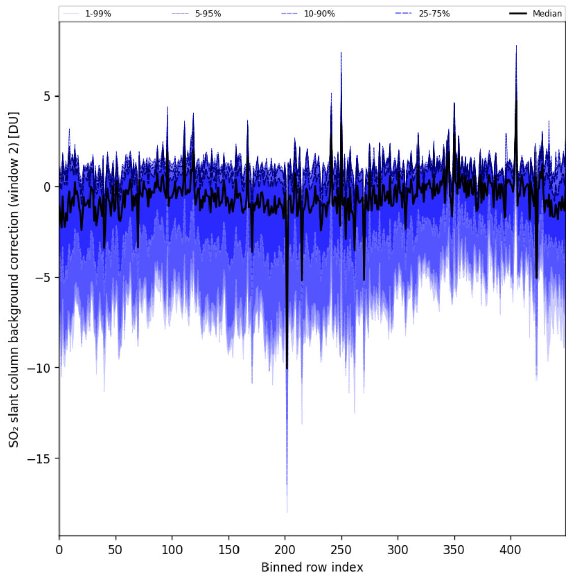
Figure 96: Along track statistics of “SO 2 slant column background correction (window 2)” for 2025-05-01 to 2025-05-03
