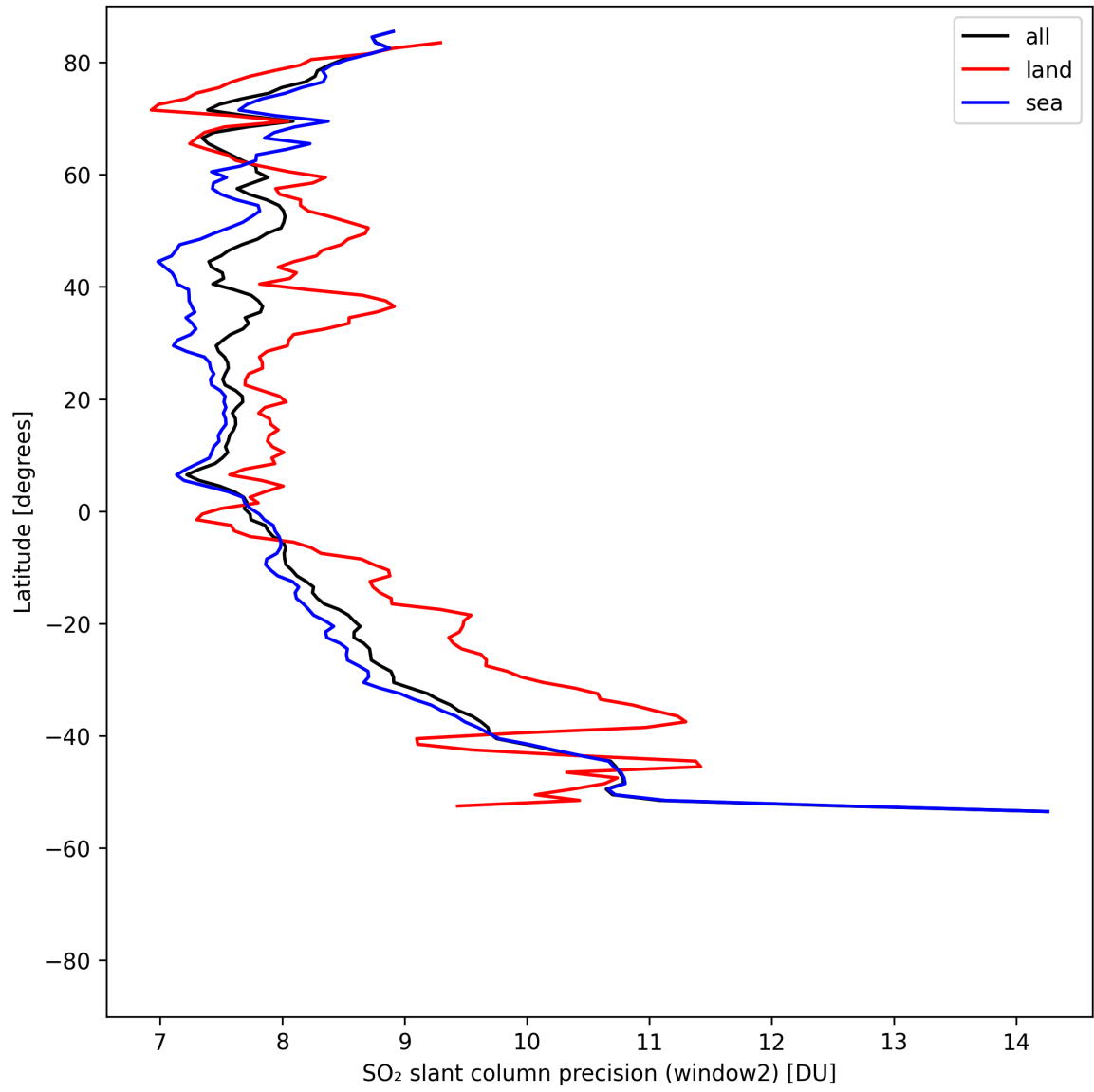
Figure 42: Zonal average of “SO 2 slant column precision (window2)” for 2025-05-01 to 2025-05-03.
