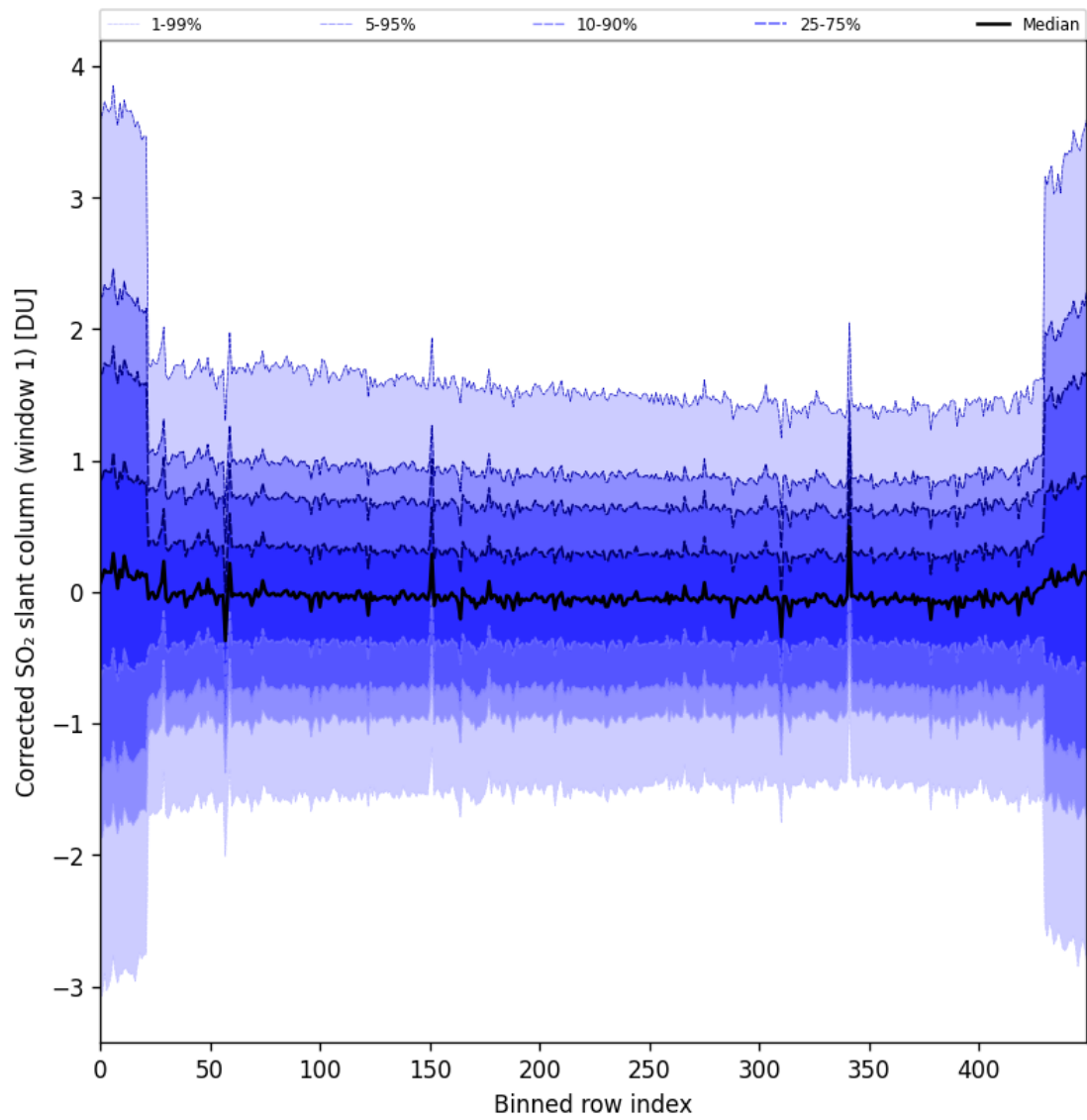
Figure 91: Along track statistics of “Corrected SO 2 slant column (window 1)” for 2025-05-01 to 2025-05-03
