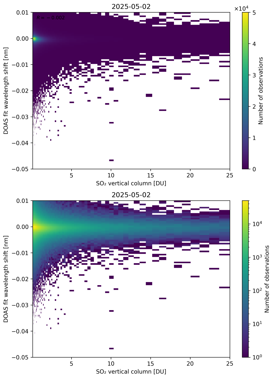
Figure 326: Scatter density plot of “SO 2 vertical column” against “DOAS fit wavelength shift” for 2025-05-01 to 2025-05-03.
