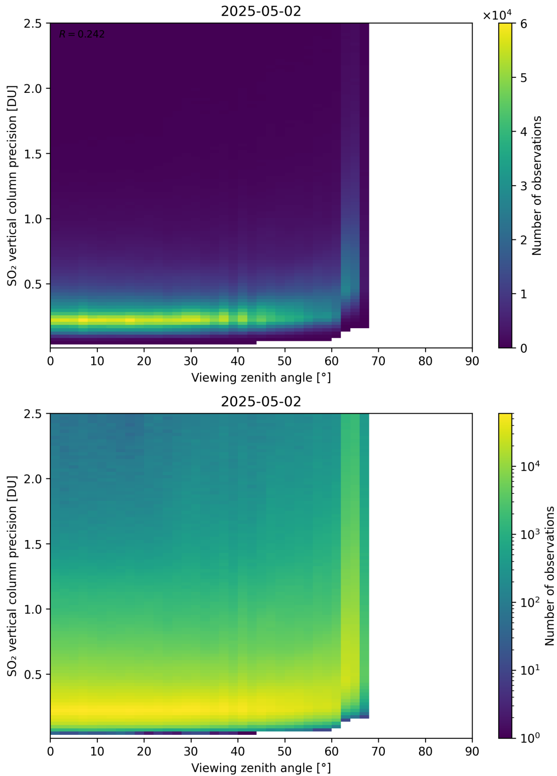
Figure 384: Scatter density plot of “Viewing zenith angle” against “SO 2 vertical column precision” for 2025-05-01 to 2025-05-03.
