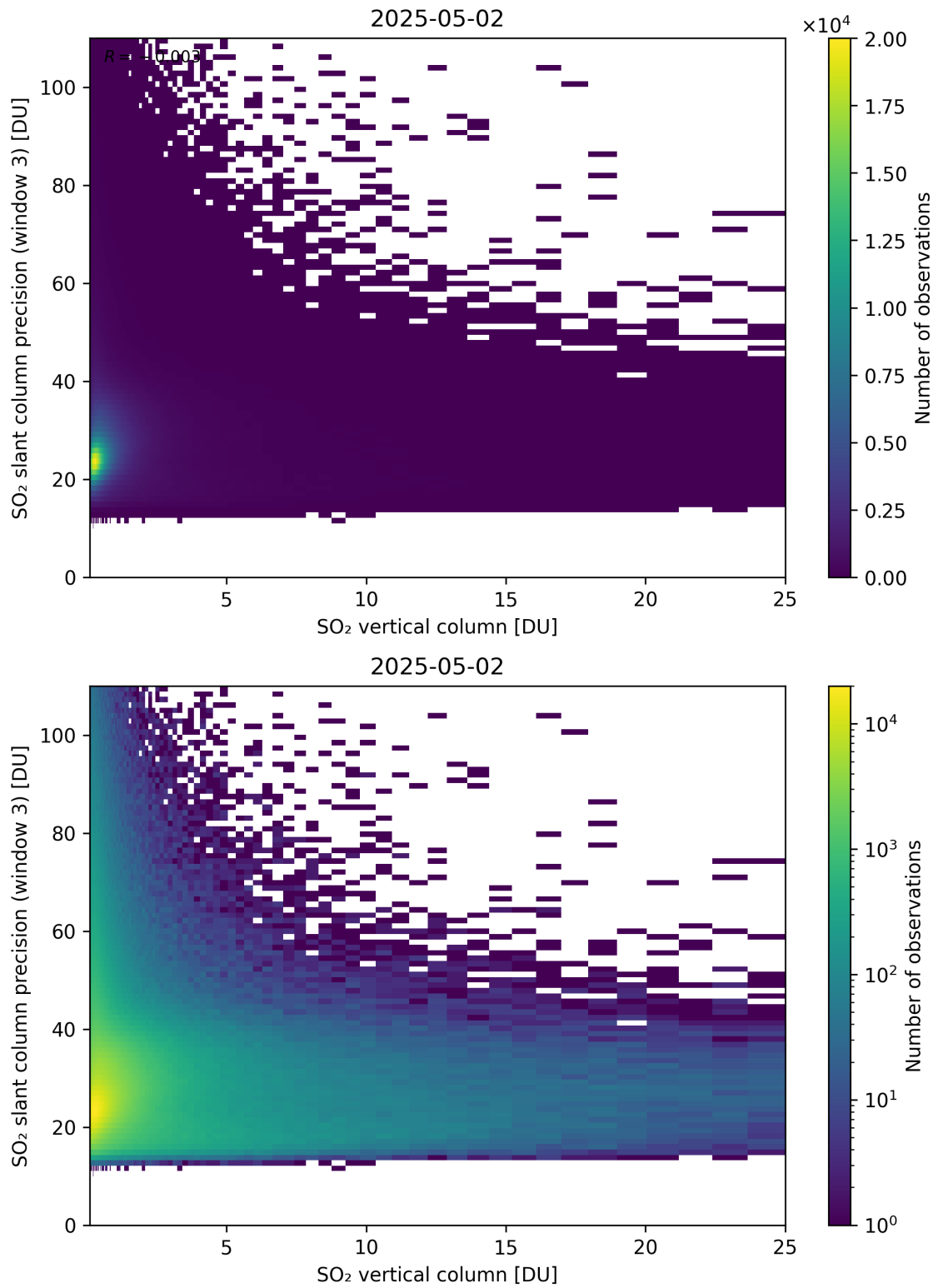
Figure 358: Scatter density plot of “SO 2 vertical column” against “SO 2 slant column precision (window 3)” for 2025-05-01 to 2025-05-03.
