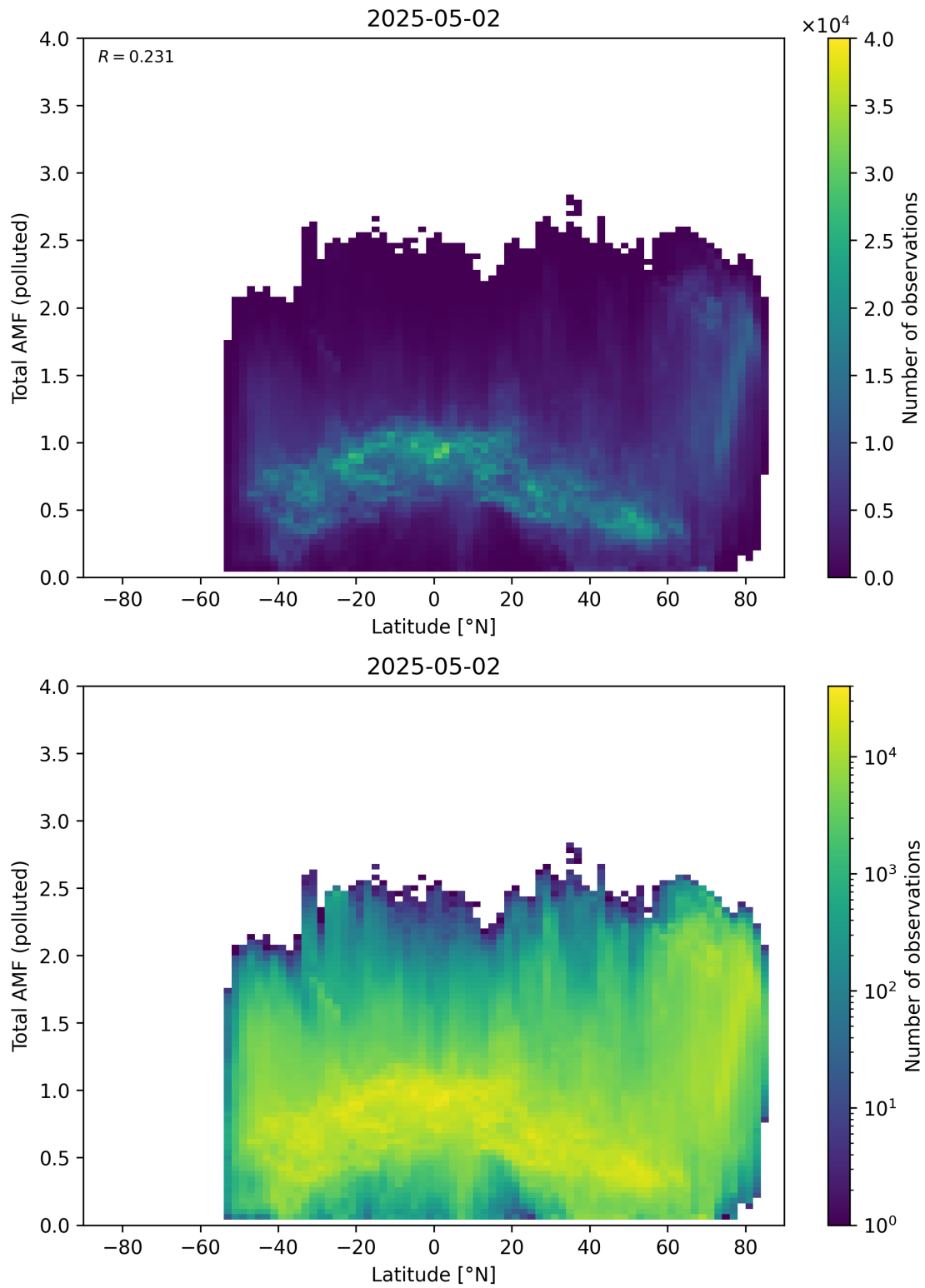
Figure 167: Scatter density plot of “Latitude” against “Total AMF (polluted)” for 2025-05-01 to 2025-05-03.
