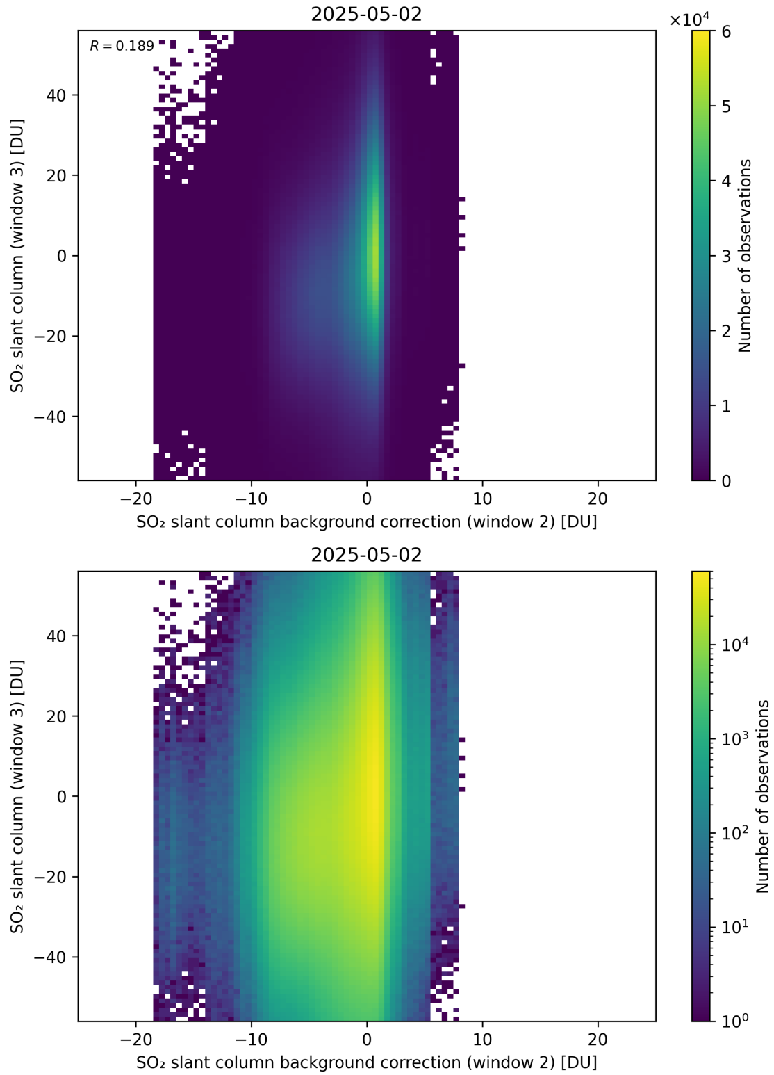
Figure 128: Scatter density plot of “SO 2 slant column background correction (window 2)” against “SO 2 slant column (window 3)” for 2025-05-01 to 2025-05-03.
