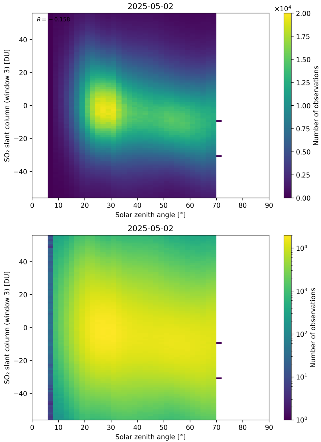
Figure 187: Scatter density plot of “Solar zenith angle” against “SO 2 slant column (window 3)” for 2025-05-01 to 2025-05-03.
