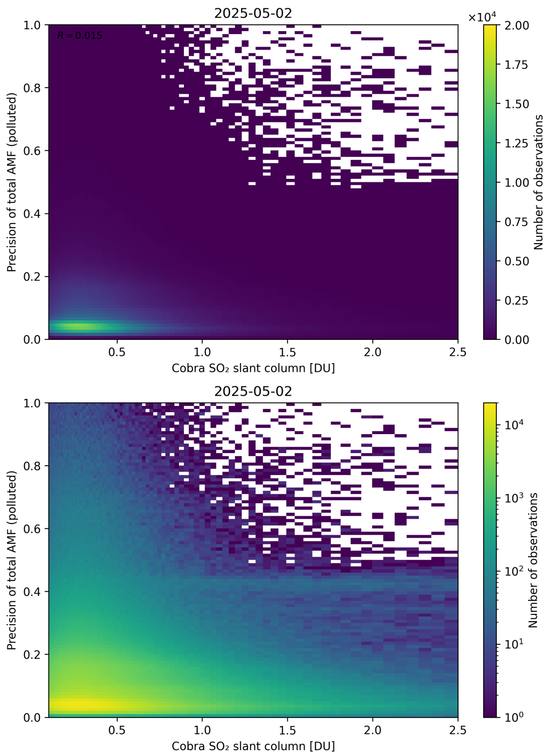
Figure 225: Scatter density plot of “Cobra SO 2 slant column” against “Precision of total AMF (polluted)” for 2025-05-01 to 2025-05-03.
