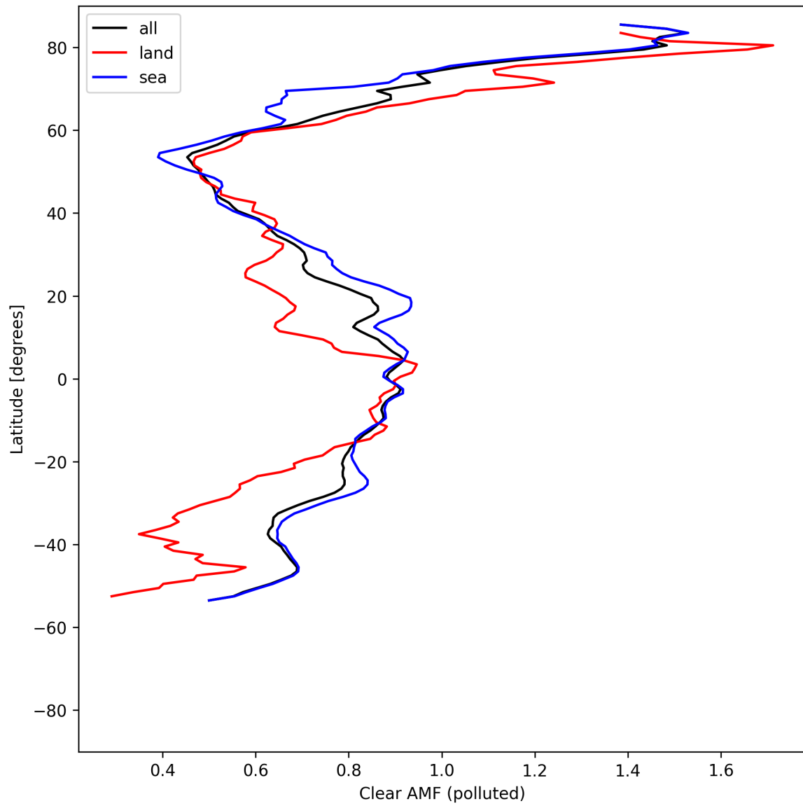
Figure 55: Zonal average of “Clear AMF (polluted)” for 2025-05-01 to 2025-05-03.
