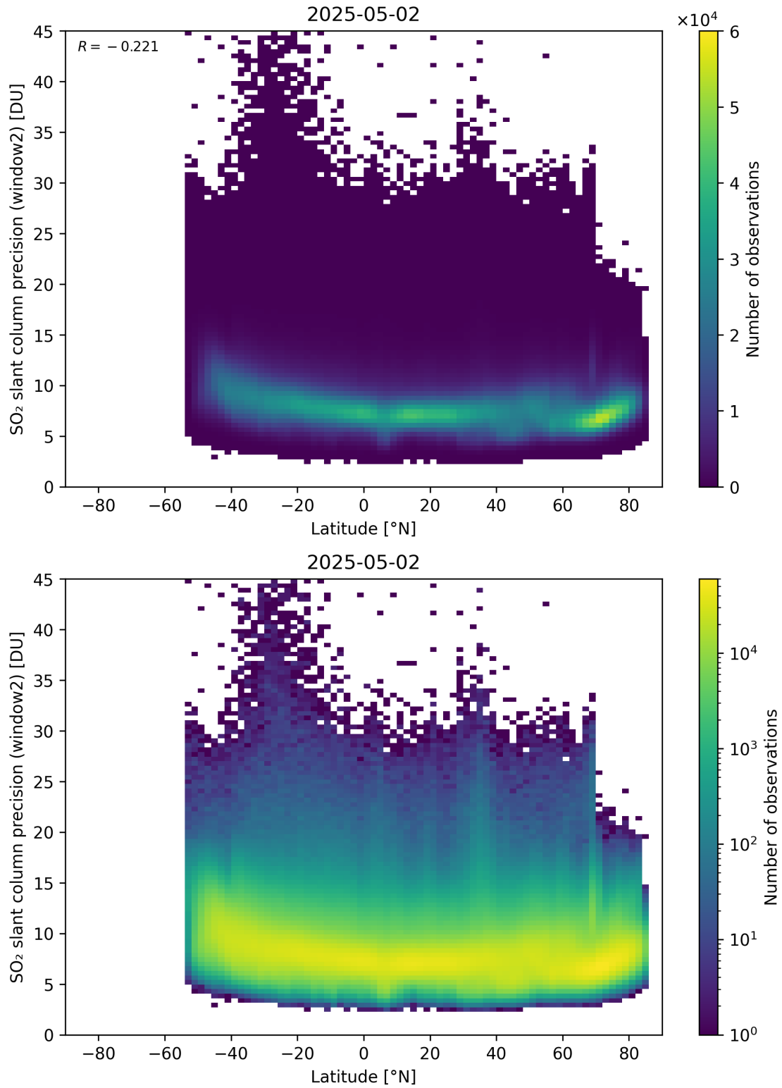
Figure 164: Scatter density plot of “Latitude” against “SO 2 slant column precision (window2)” for 2025-05-01 to 2025-05-03.
