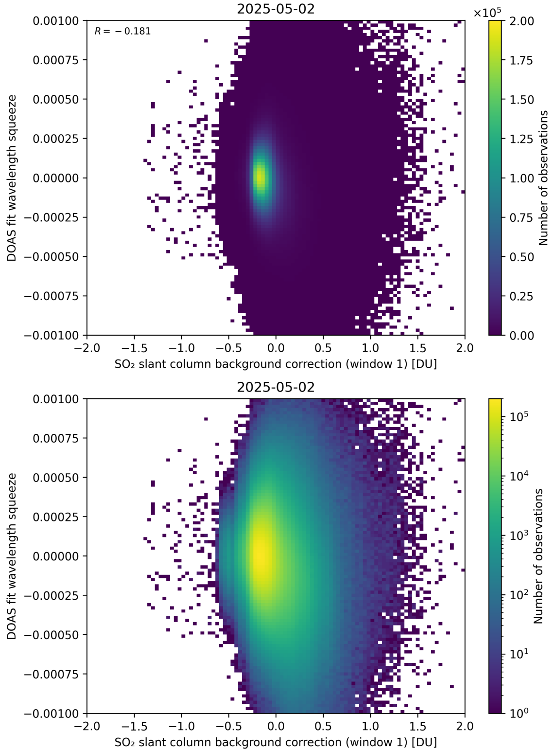
Figure 112: Scatter density plot of “SO 2 slant column background correction (window 1)” against “DOAS fit wavelength squeeze” for 2025-05-01 to 2025-05-03.
