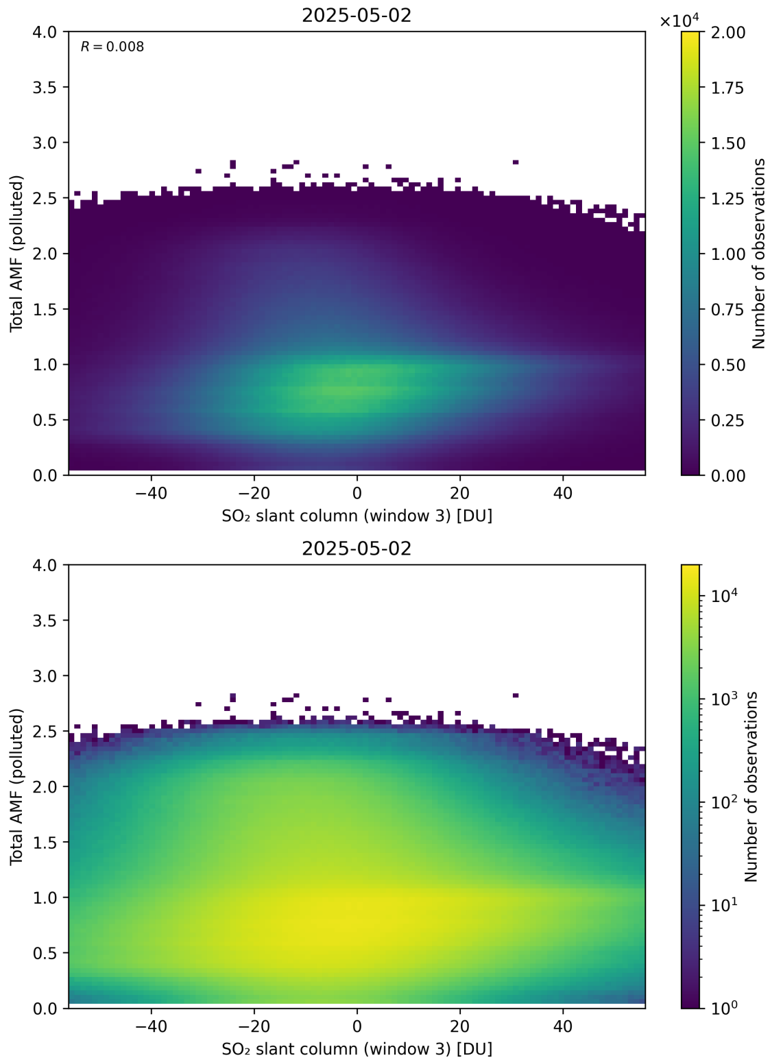
Figure 318: Scatter density plot of “SO 2 slant column (window 3)” against “Total AMF (polluted)” for 2025-05-01 to 2025-05-03.
