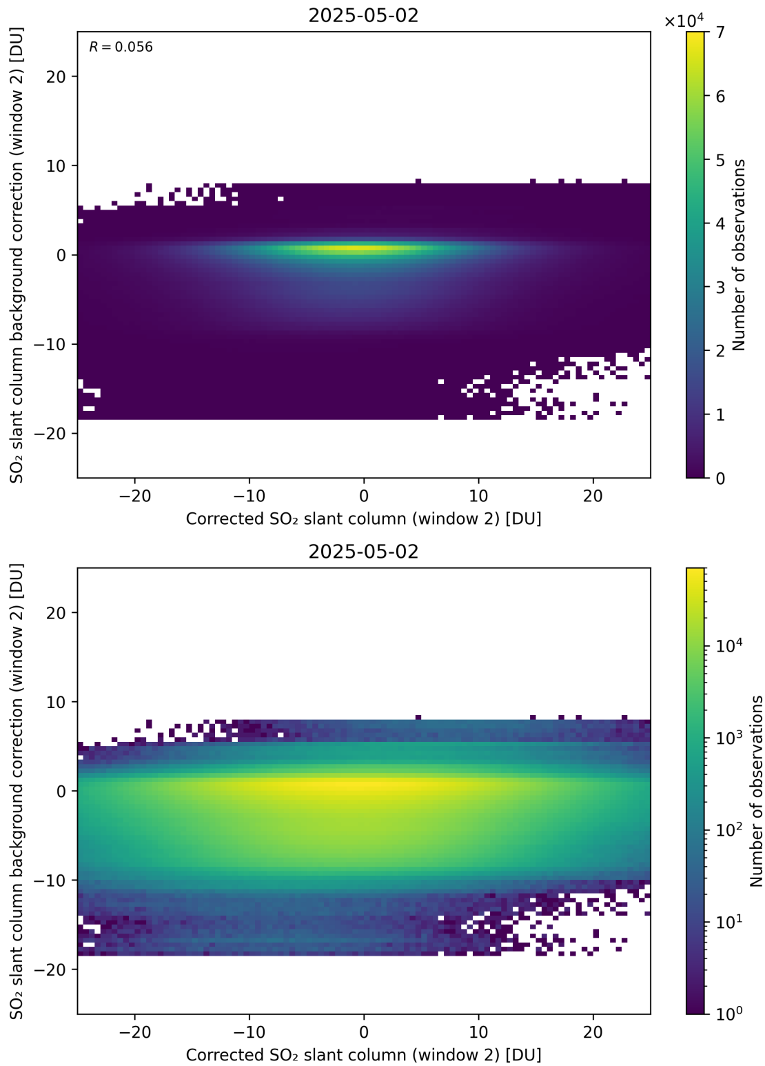
Figure 244: Scatter density plot of “Corrected SO 2 slant column (window 2)” against “SO 2 slant column background correction (window 2)” for 2025-05-01 to 2025-05-03.
