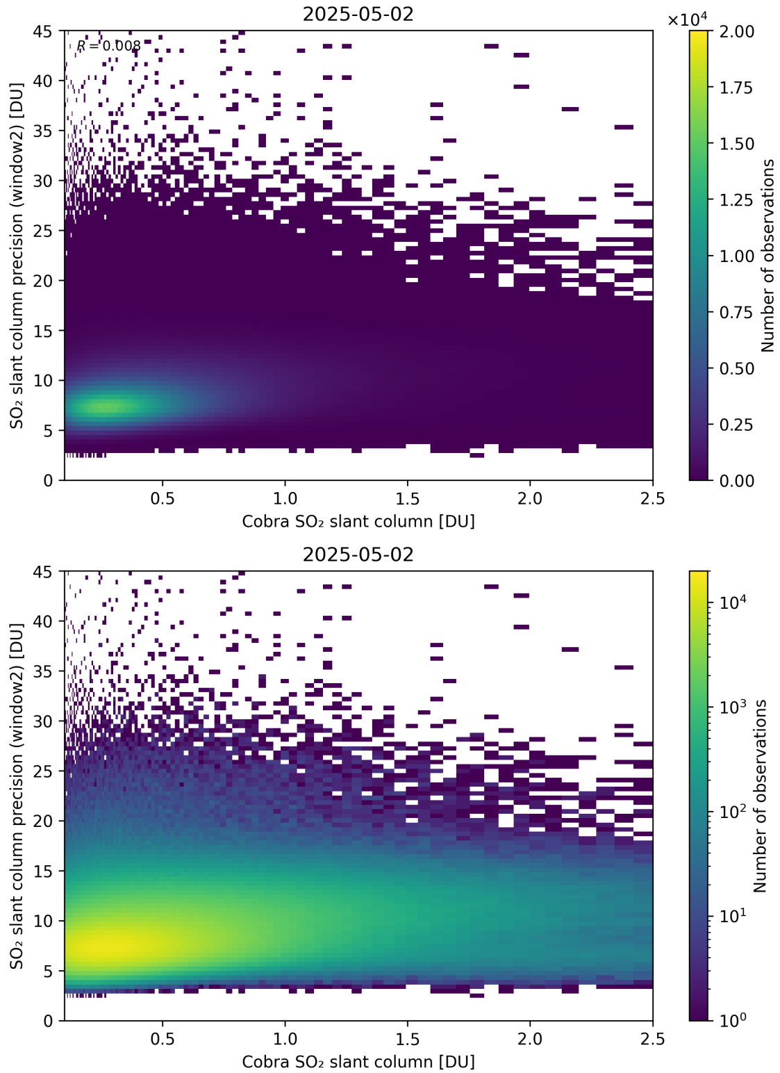
Figure 221: Scatter density plot of “Cobra SO 2 slant column” against “SO 2 slant column precision (window2)” for 2025-05-01 to 2025-05-03.
