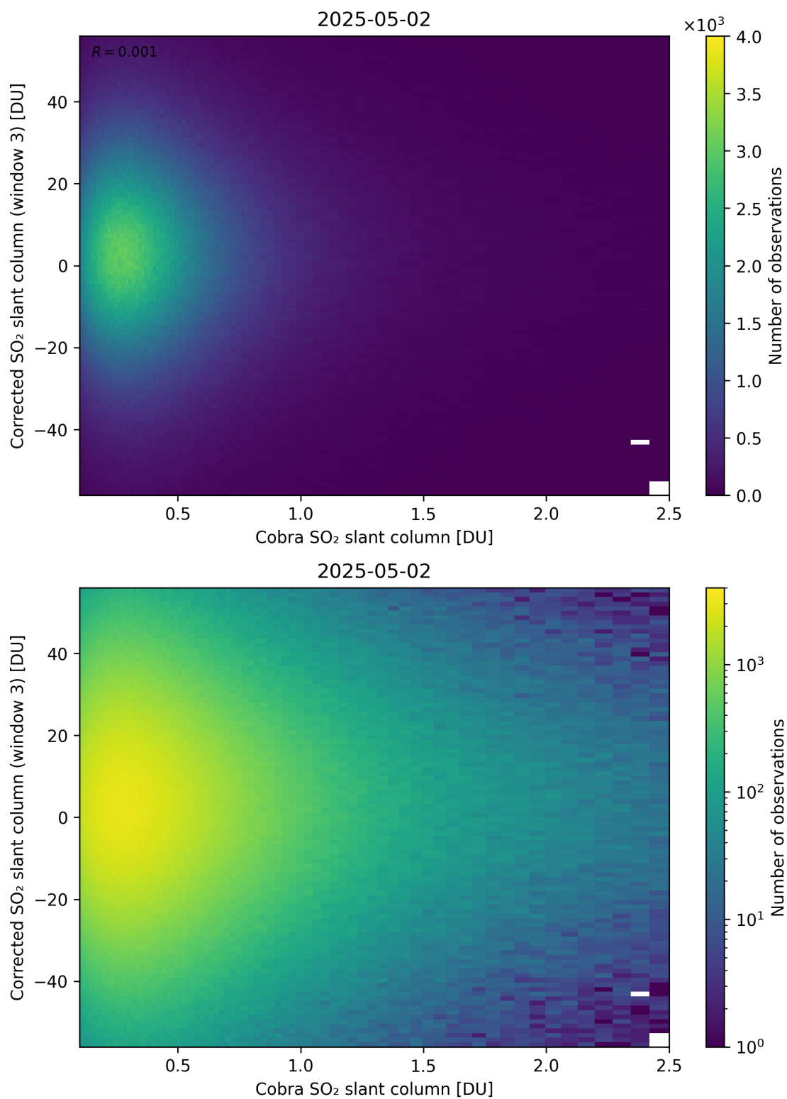
Figure 218: Scatter density plot of “Cobra SO 2 slant column” against “Corrected SO 2 slant column (window 3)” for 2025-05-01 to 2025-05-03.
