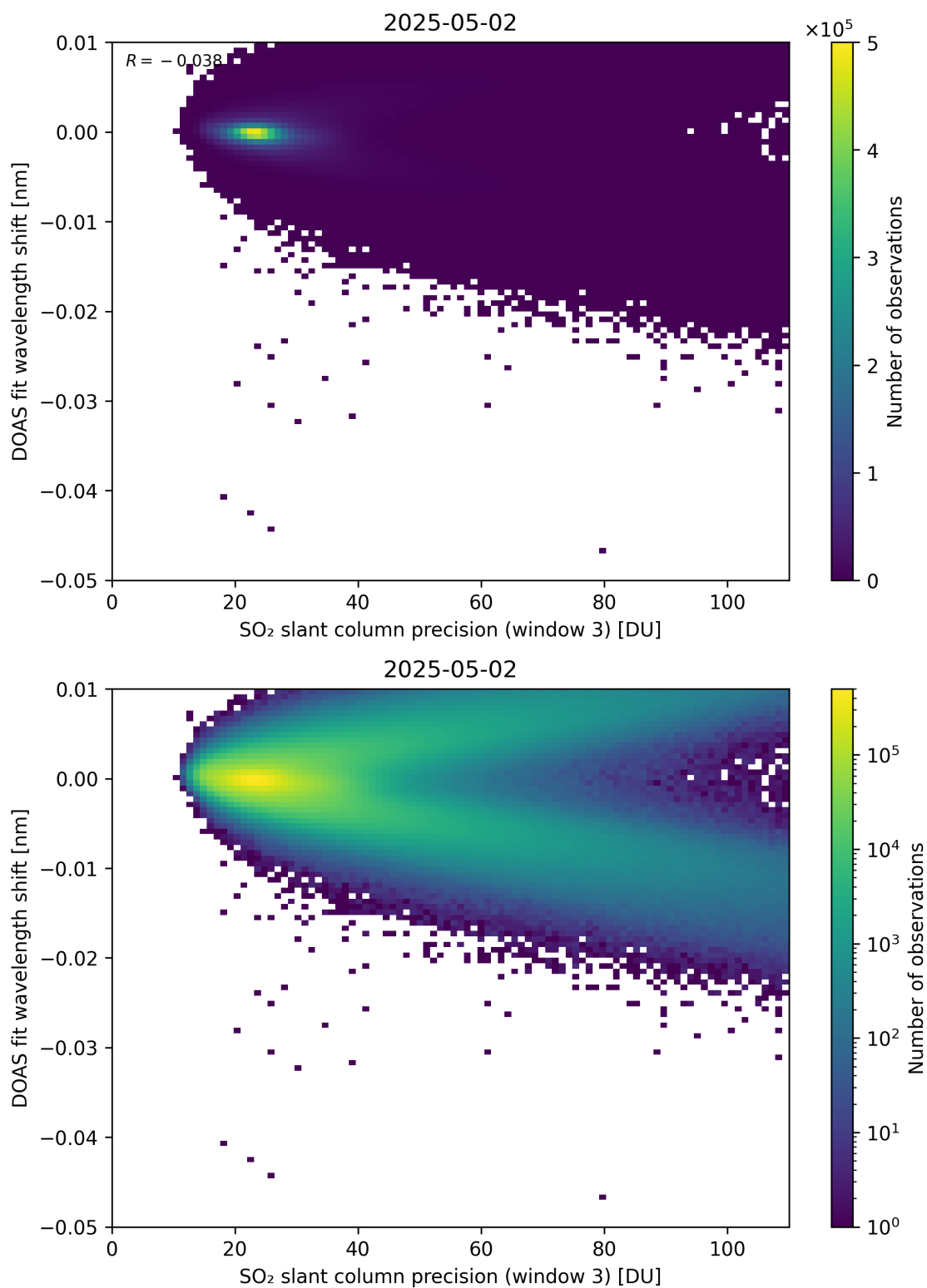
Figure 308: Scatter density plot of “SO 2 slant column precision (window 3)” against “DOAS fit wavelength shift” for 2025-05-01 to 2025-05-03.
