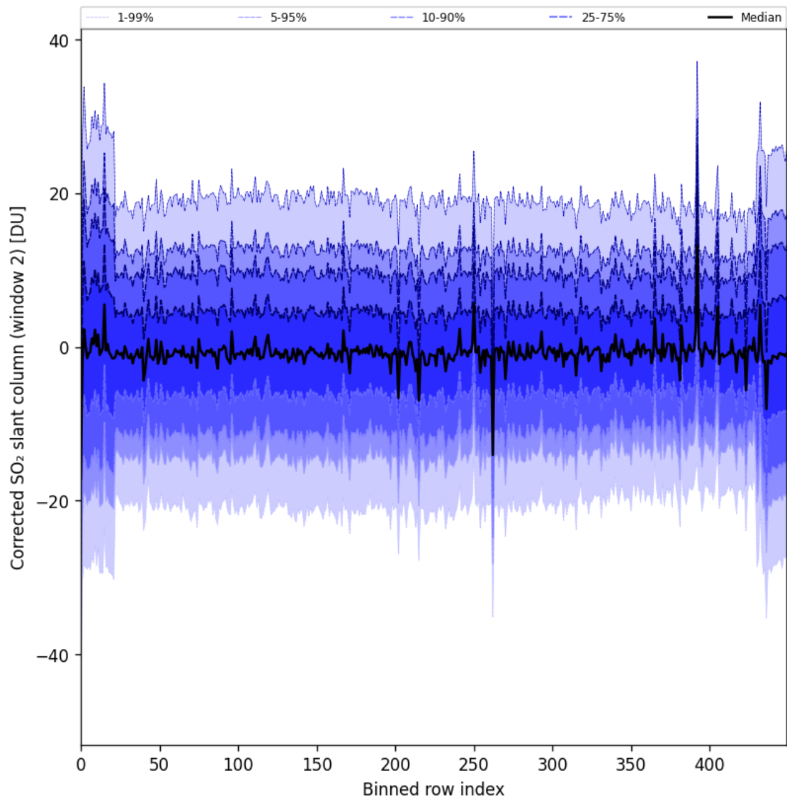
Figure 95: Along track statistics of "Corrected SO 2 slant column (window 2)" for 2025-05-01 to 2025-05-03
