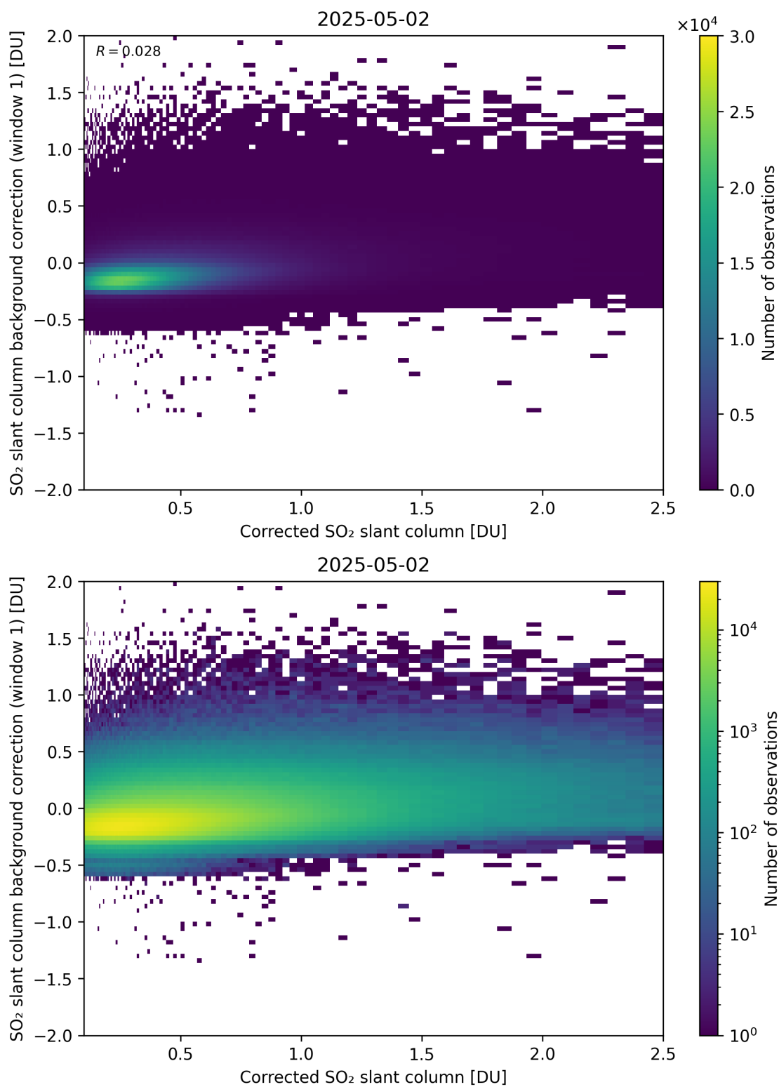
Figure 226: Scatter density plot of “Corrected SO 2 slant column” against “SO 2 slant column background correction (window 1)” for 2025-05-01 to 2025-05-03.
