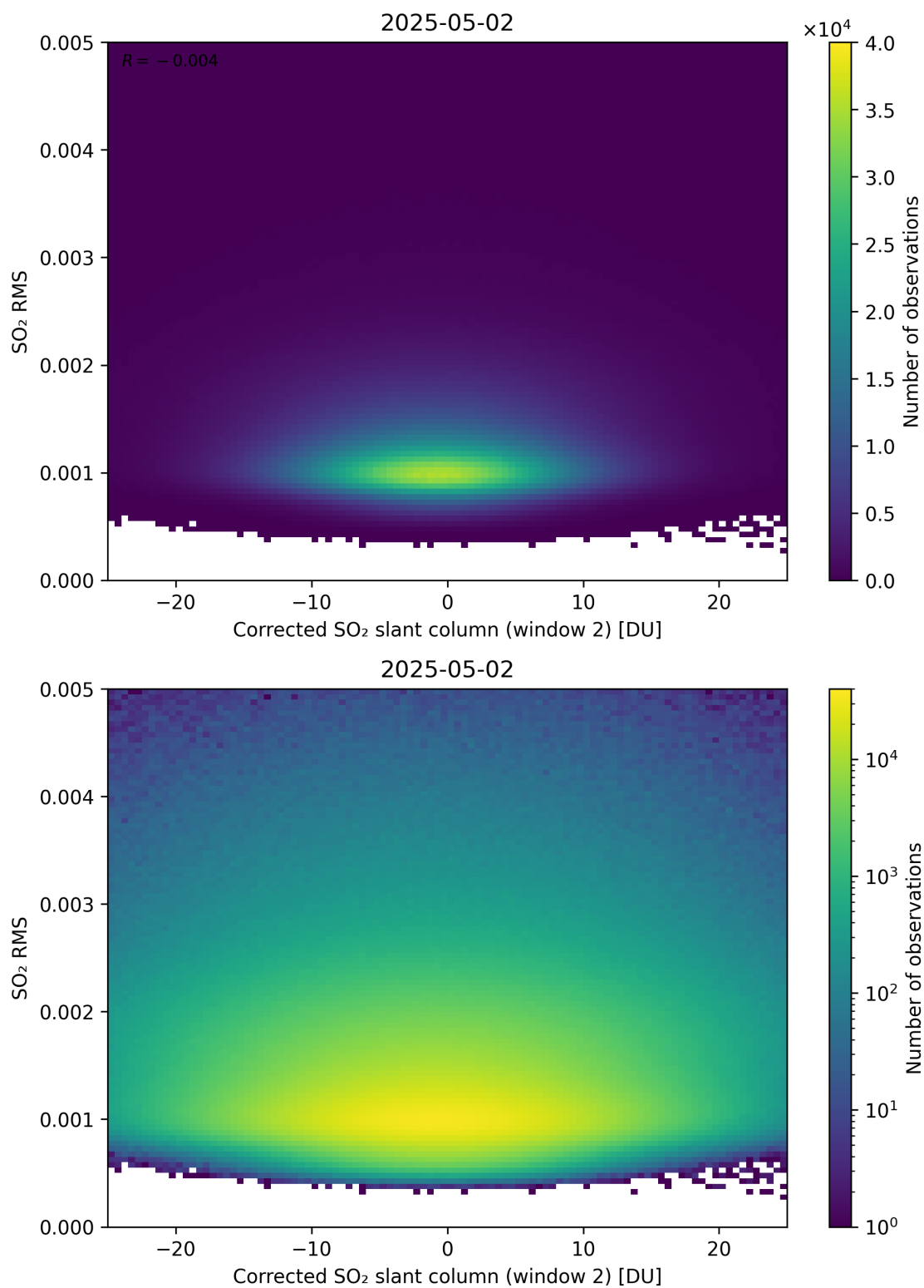
Figure 248: Scatter density plot of “Corrected SO 2 slant column (window 2)” against “SO 2 RMS” for 2025-05-01 to 2025-05-03.
