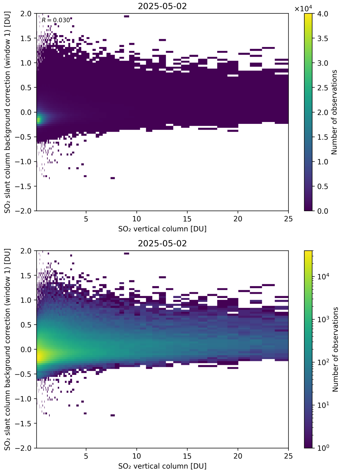
Figure 323: Scatter density plot of “SO 2 vertical column” against “SO 2 slant column background correction (window 1)” for 2025-05-01 to 2025-05-03.
