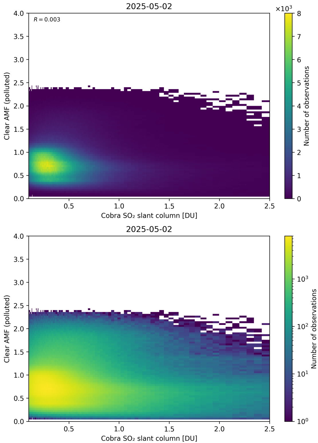
Figure 215: Scatter density plot of “Cobra SO 2 slant column” against “Clear AMF (polluted)” for 2025-05-01 to 2025-05-03.
