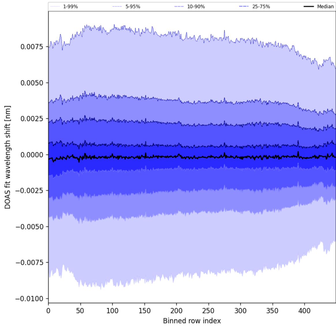
Figure 102: Along track statistics of “DOAS fit wavelength shift” for 2025-05-01 to 2025-05-03
