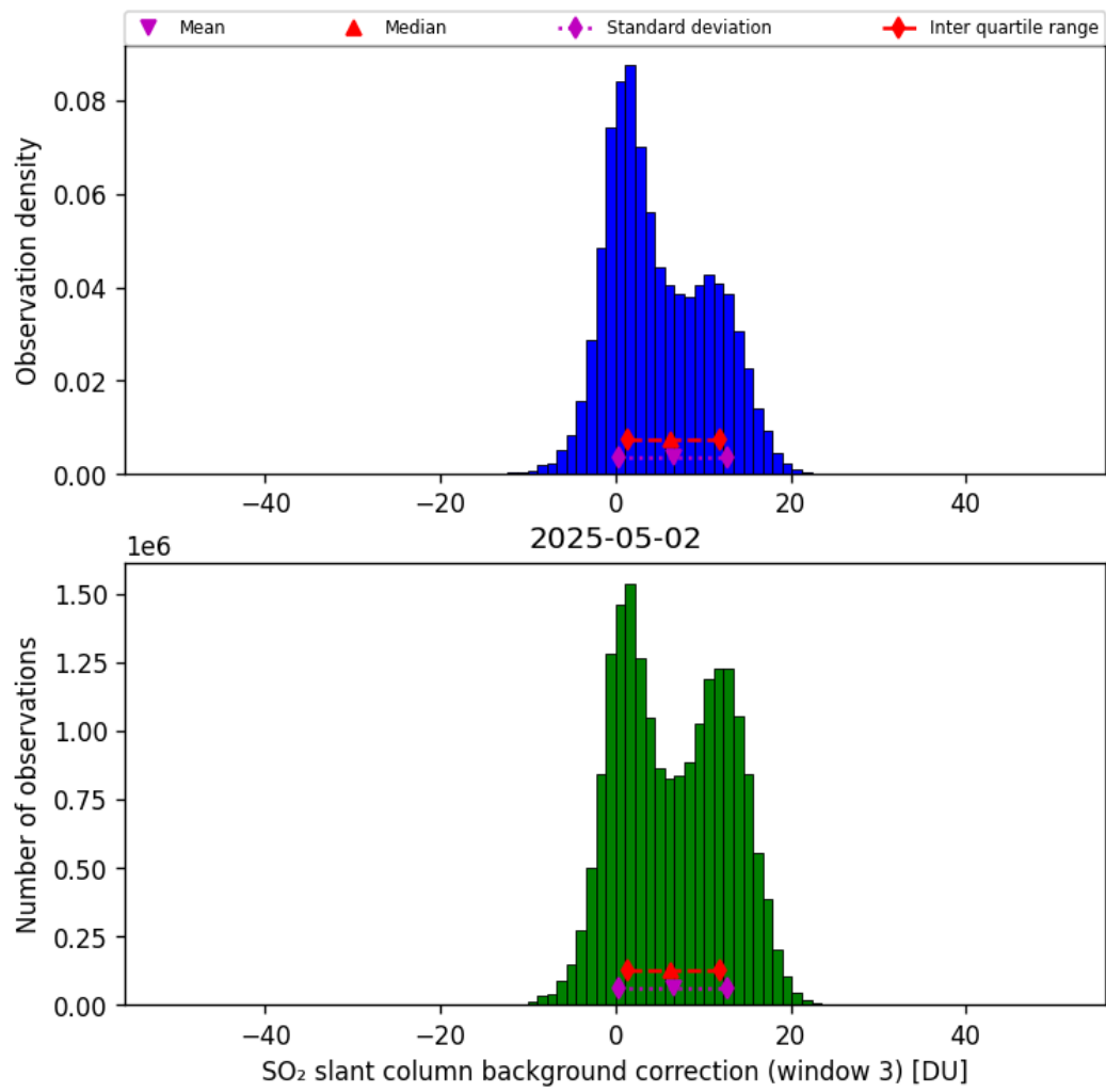
Figure 74: Histogram of “SO 2 slant column background correction (window 3)” for 2025-05-01 to 2025-05-03
