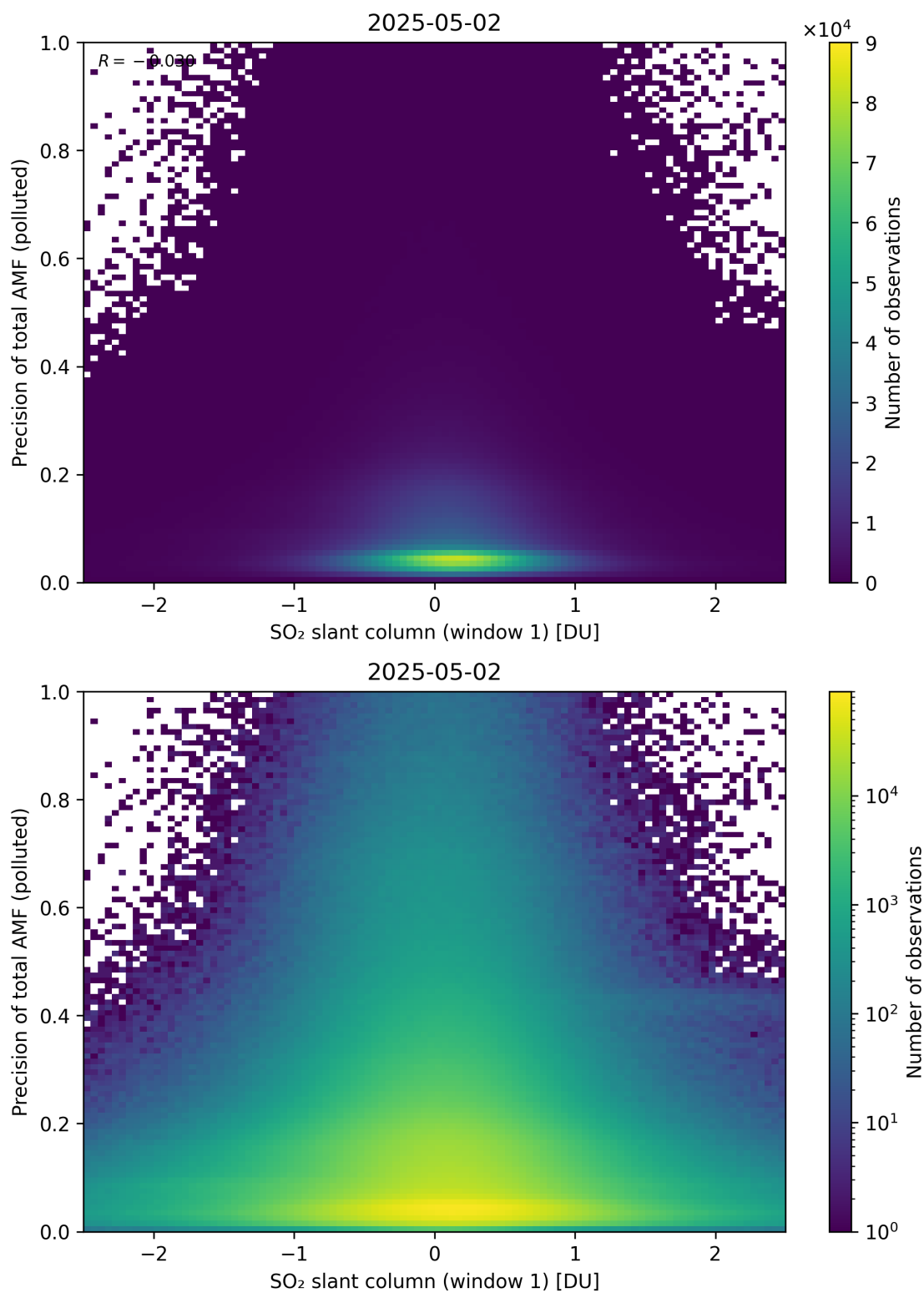
Figure 290: Scatter density plot of “SO 2 slant column (window 1)” against “Precision of total AMF (polluted)” for 2025-05-01 to 2025-05-03.
