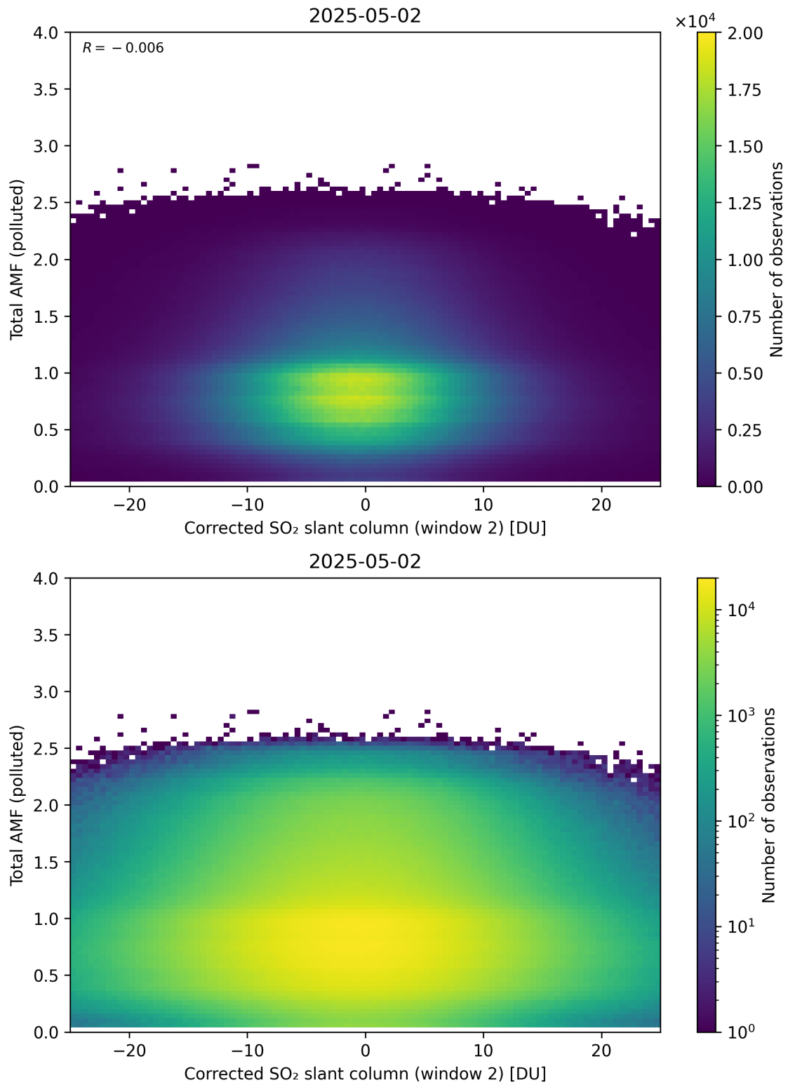
Figure 253: Scatter density plot of “Corrected SO 2 slant column (window 2)” against “Total AMF (polluted)” for 2025-05-01 to 2025-05-03.
