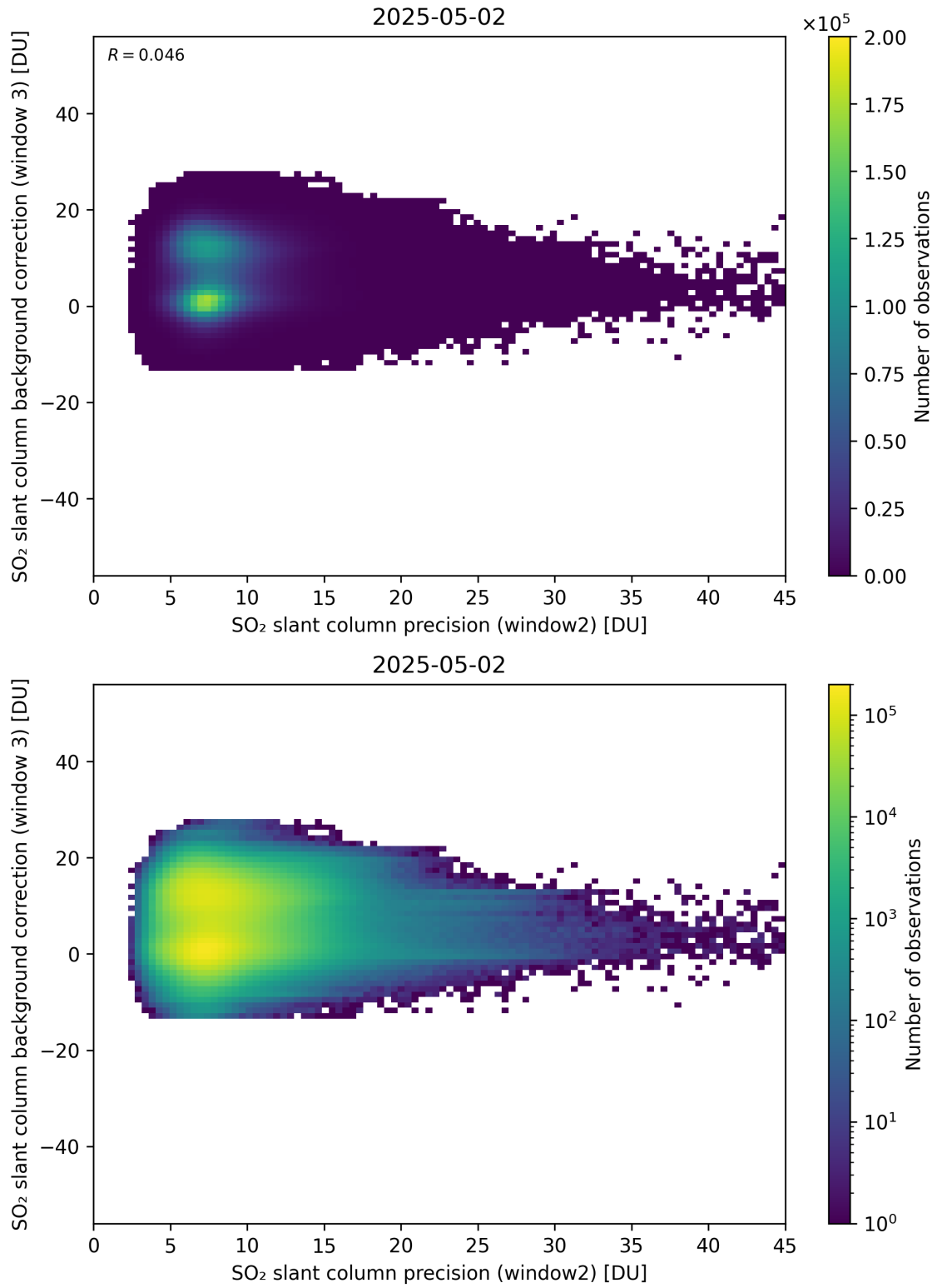
Figure 292: Scatter density plot of “SO 2 slant column precision (window2)” against “SO 2 slant column background correction (window 3)” for 2025-05-01 to 2025-05-03.
