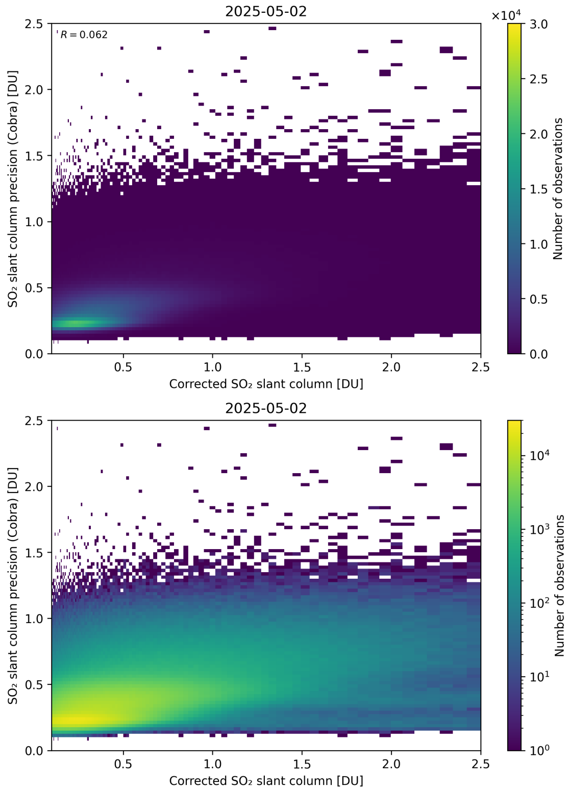
Figure 234: Scatter density plot of “Corrected SO 2 slant column” against “SO 2 slant column precision (Cobra)” for 2025-05-01 to 2025-05-03.
