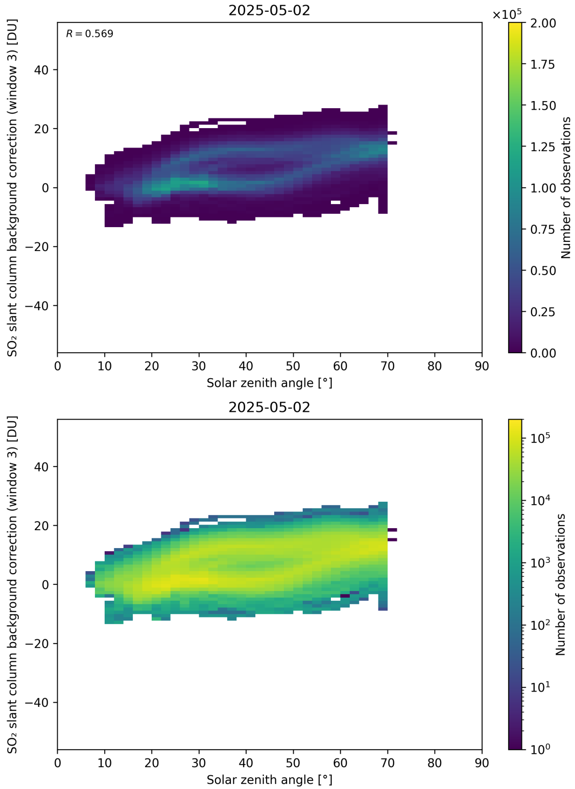
Figure 173: Scatter density plot of “Solar zenith angle” against “SO 2 slant column background correction (window 3)” for 2025-05-01 to 2025-05-03.
