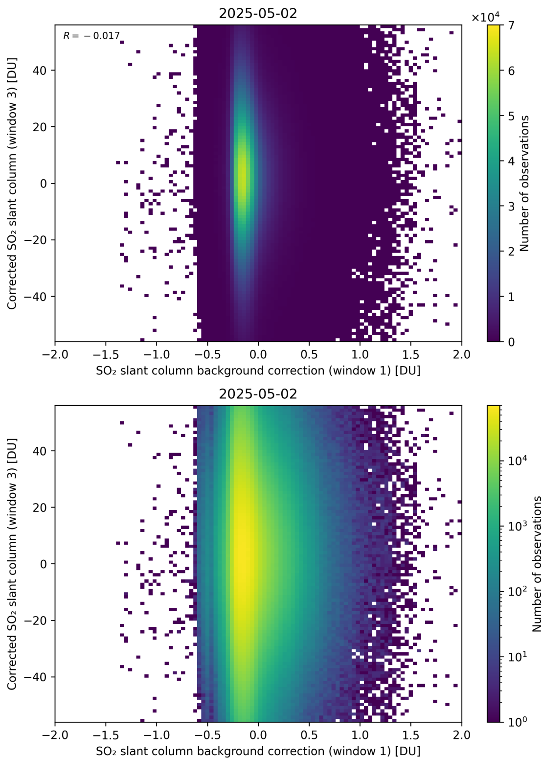
Figure 116: Scatter density plot of “SO 2 slant column background correction (window 1)” against “Corrected SO 2 slant column (window 3)” for 2025-05-01 to 2025-05-03.
