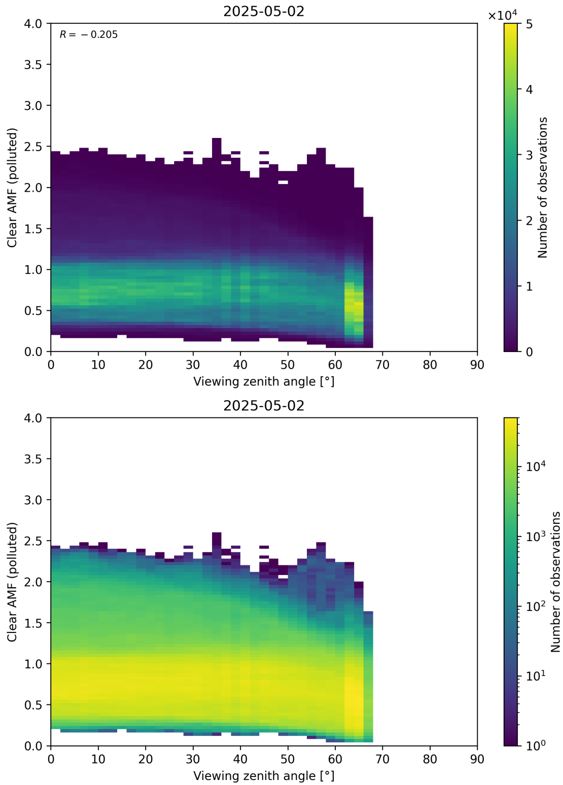
Figure 370: Scatter density plot of “Viewing zenith angle” against “Clear AMF (polluted)” for 2025-05-01 to 2025-05-03.
