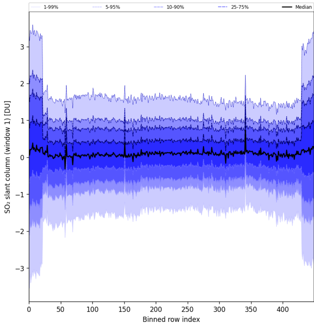
Figure 89: Along track statistics of “SO 2 slant column (window 1)” for 2025-05-01 to 2025-05-03
