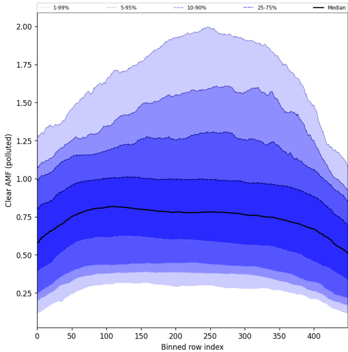
Figure 107: Along track statistics of “Clear AMF (polluted)” for 2025-05-01 to 2025-05-03
