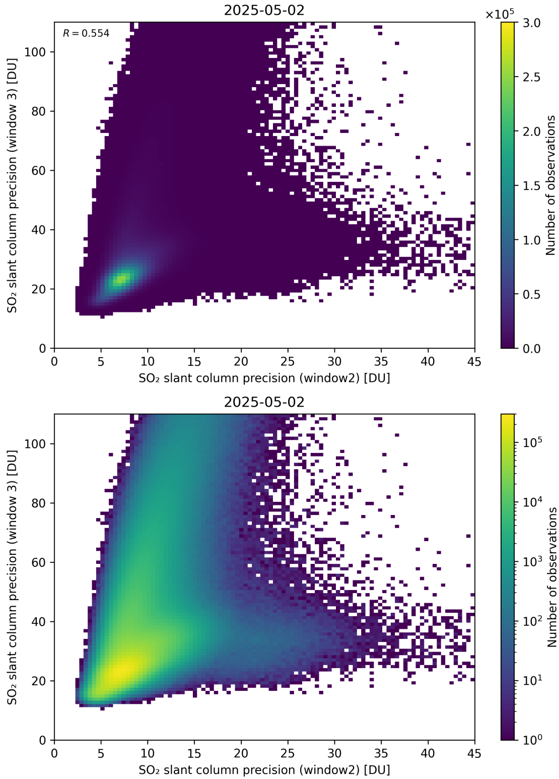
Figure 300: Scatter density plot of “SO 2 slant column precision (window2)” against “SO 2 slant column precision (window 3)” for 2025-05-01 to 2025-05-03.
