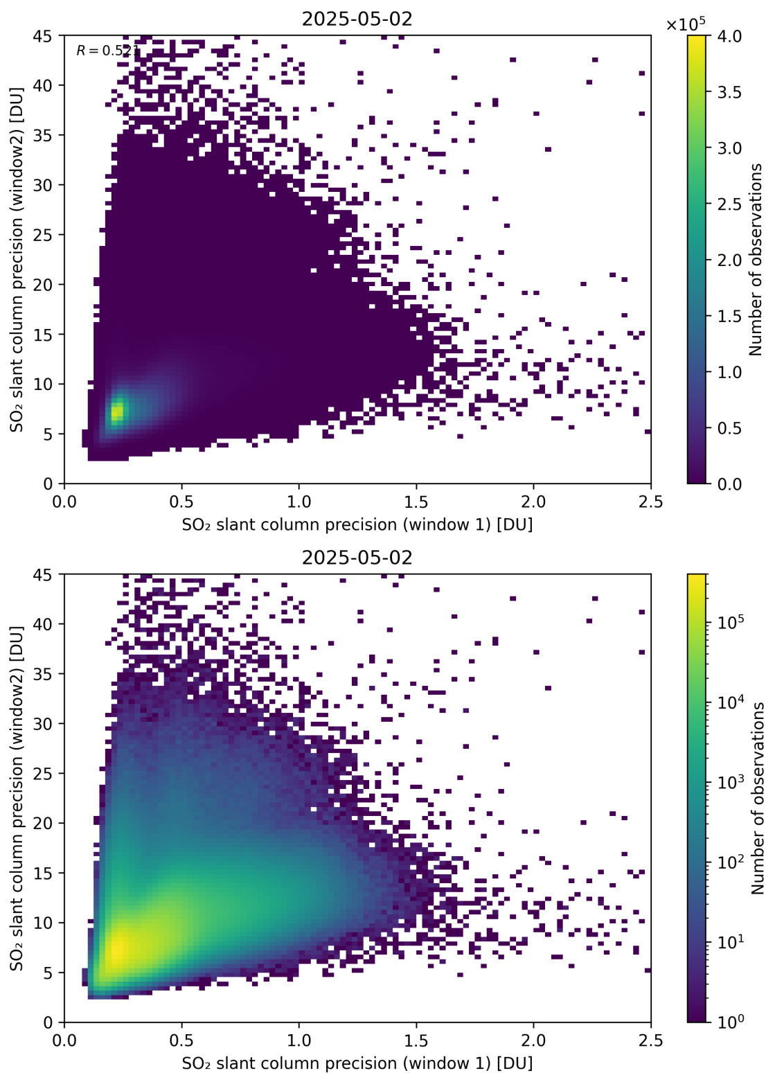
Figure 277: Scatter density plot of “SO 2 slant column precision (window 1)” against “SO 2 slant column precision (window 2)” for 2025-05-01 to 2025-05-03.
