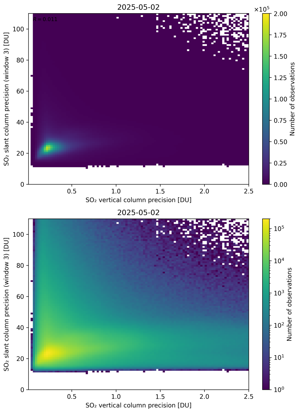
Figure 345: Scatter density plot of “SO 2 vertical column precision” against “SO 2 slant column precision (window 3)” for 2025-05-01 to 2025-05-03.
