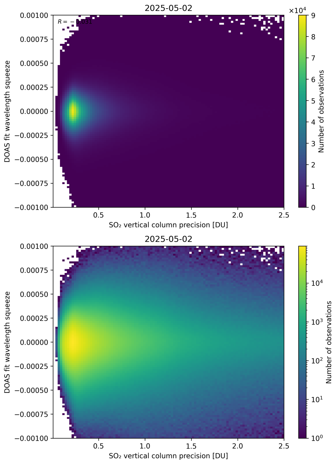
Figure 333: Scatter density plot of “SO 2 vertical column precision” against “DOAS fit wavelength squeeze” for 2025-05-01 to 2025-05-03.
