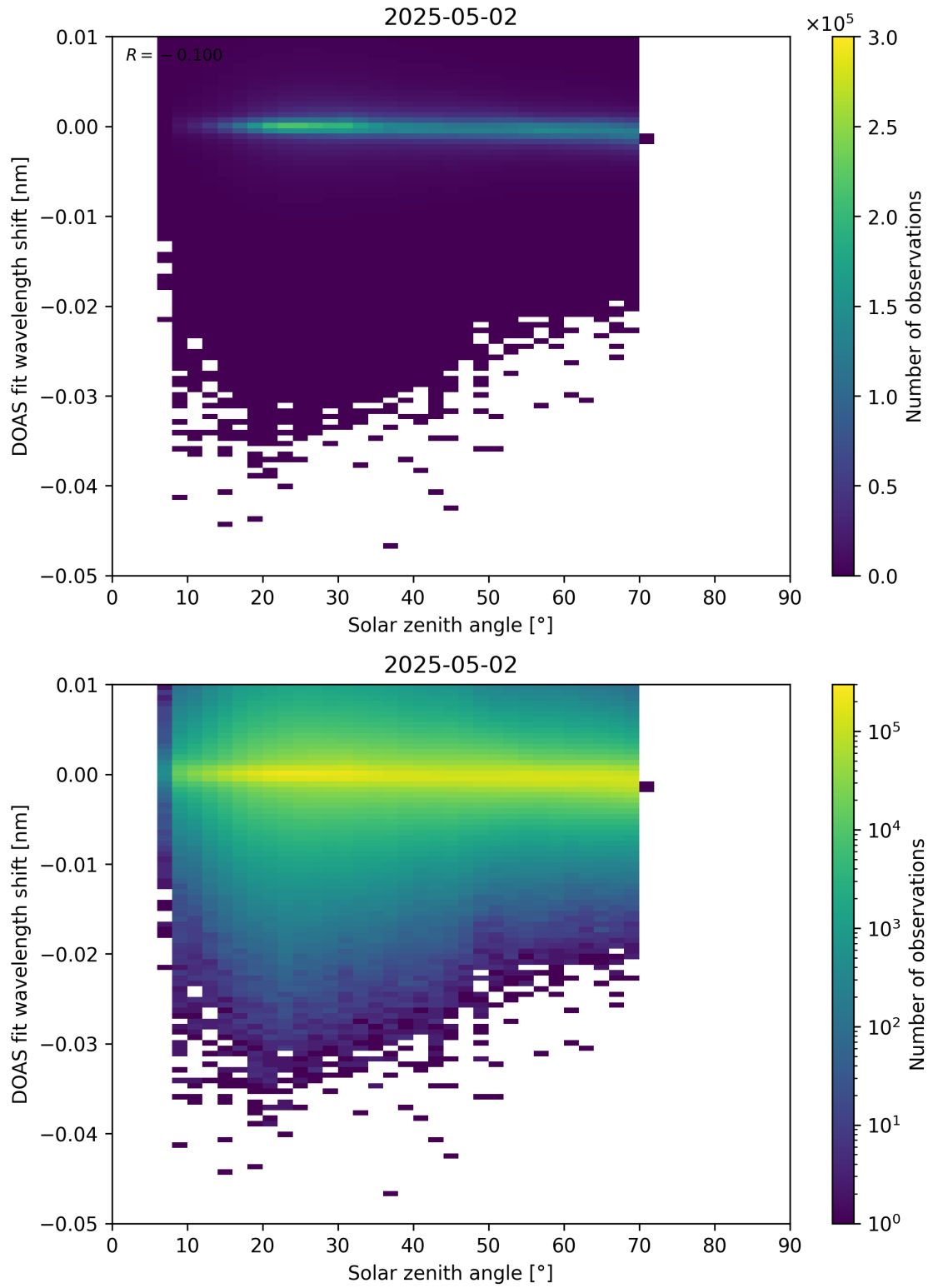
Figure 174: Scatter density plot of “Solar zenith angle” against “DOAS fit wavelength shift” for 2025-05-01 to 2025-05-03.
