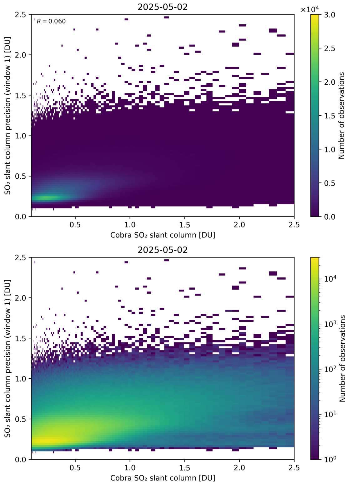
Figure 220: Scatter density plot of “Cobra SO 2 slant column” against “SO 2 slant column precision (window 1)” for 2025-05-01 to 2025-05-03.
