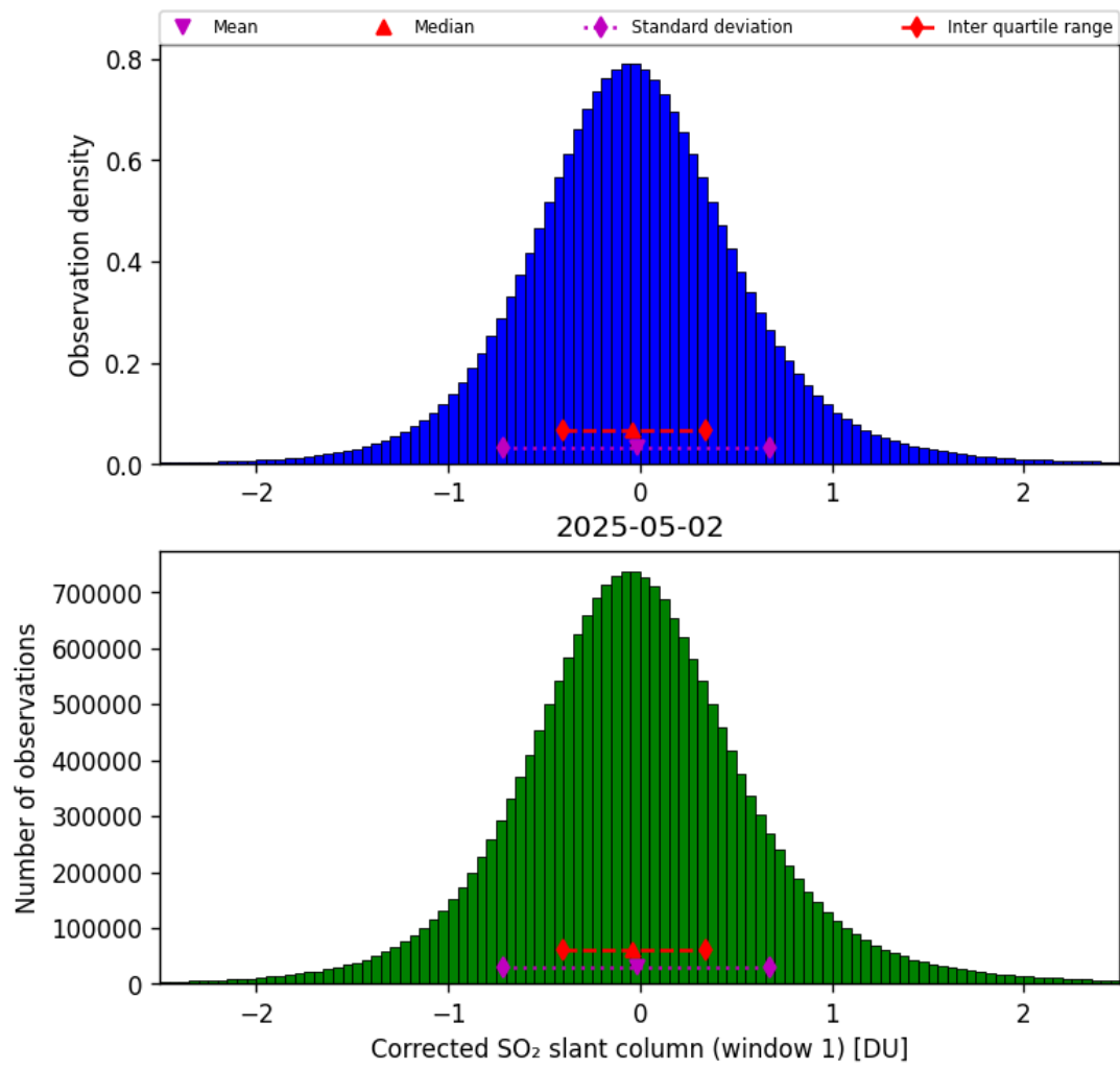
Figure 65: Histogram of “Corrected SO 2 slant column (window 1)” for 2025-05-01 to 2025-05-03
