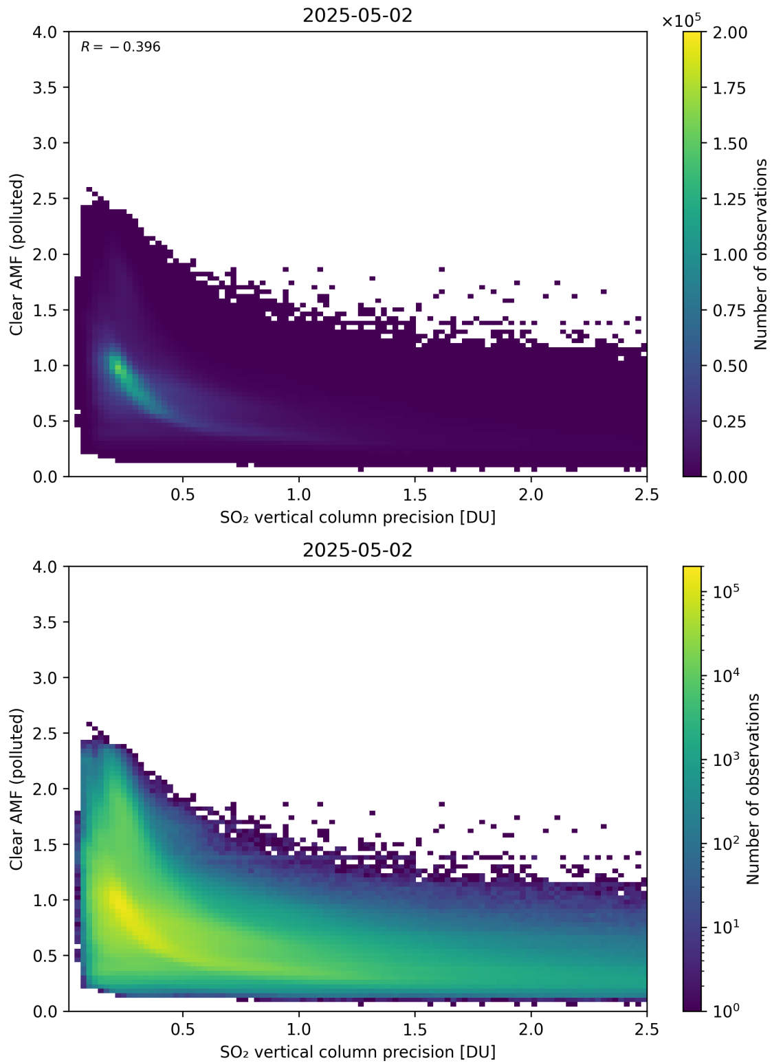
Figure 335: Scatter density plot of “SO 2 vertical column precision” against “Clear AMF (polluted)” for 2025-05-01 to 2025-05-03.
