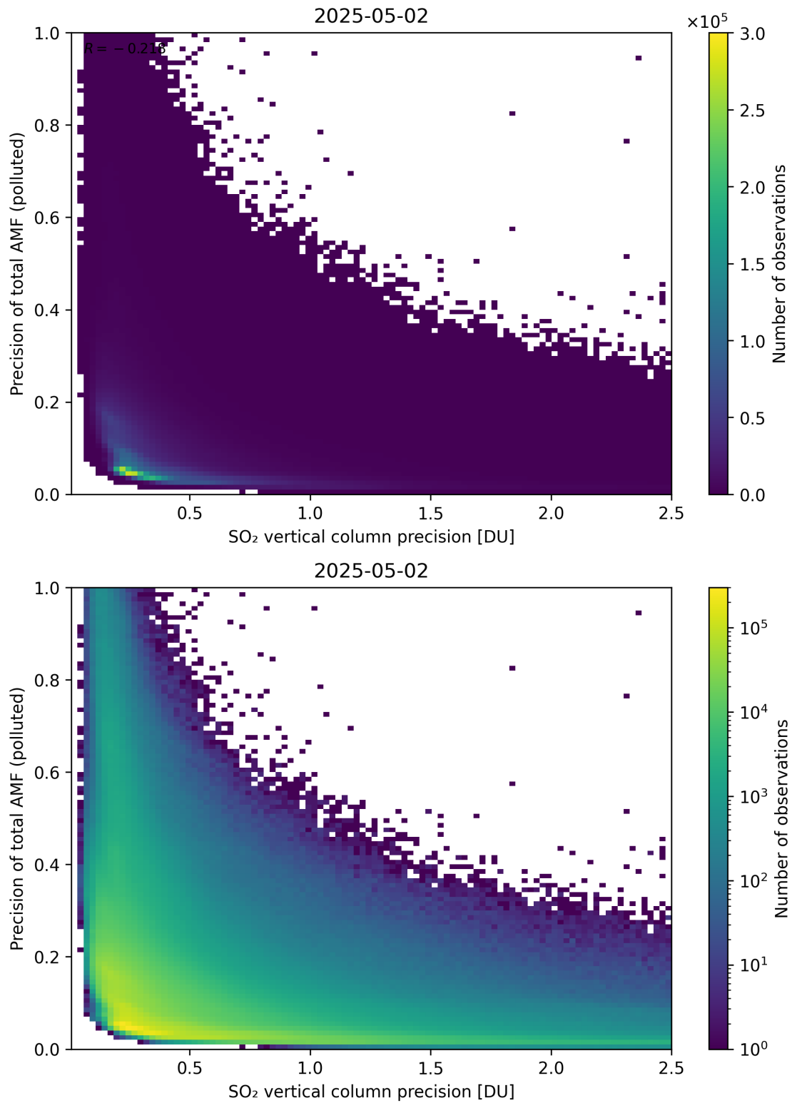
Figure 347: Scatter density plot of “SO 2 vertical column precision” against “Precision of total AMF (polluted)” for 2025-05-01 to 2025-05-03.
