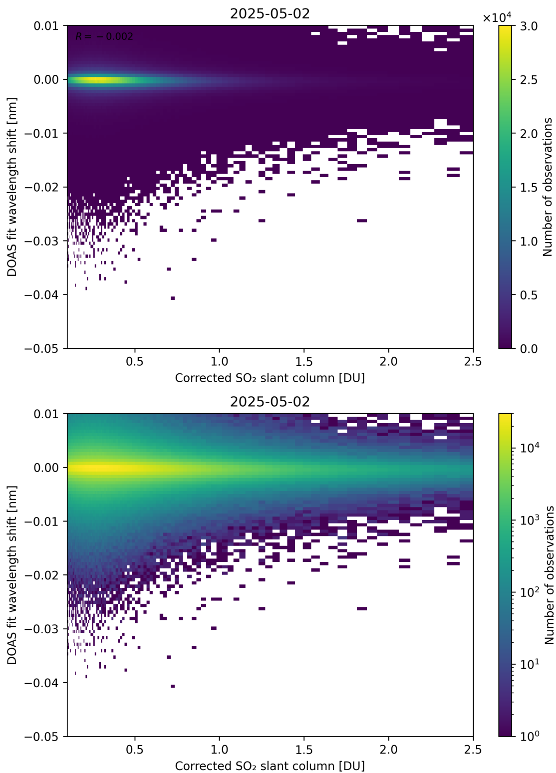
Figure 229: Scatter density plot of “Corrected SO 2 slant column” against “DOAS fit wavelength shift” for 2025-05-01 to 2025-05-03.
