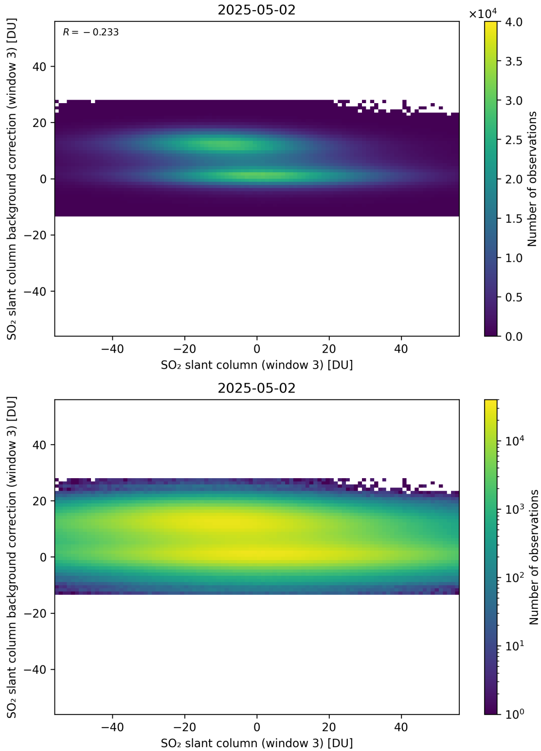
Figure 303: Scatter density plot of “SO 2 slant column (window 3)” against “SO 2 slant column background correction (window 3)” for 2025-05-01 to 2025-05-03.
