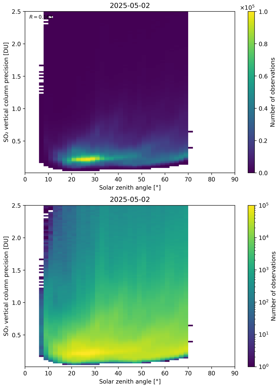
Figure 192: Scatter density plot of “Solar zenith angle” against “SO 2 vertical column precision” for 2025-05-01 to 2025-05-03.
