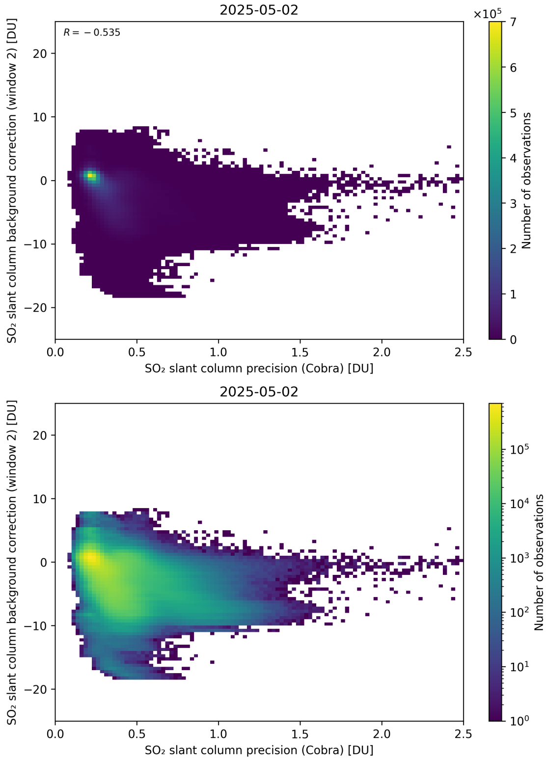
Figure 200: Scatter density plot of “SO 2 slant column precision (Cobra)” against “SO 2 slant column background correction (window 2)” for 2025-05-01 to 2025-05-03.
