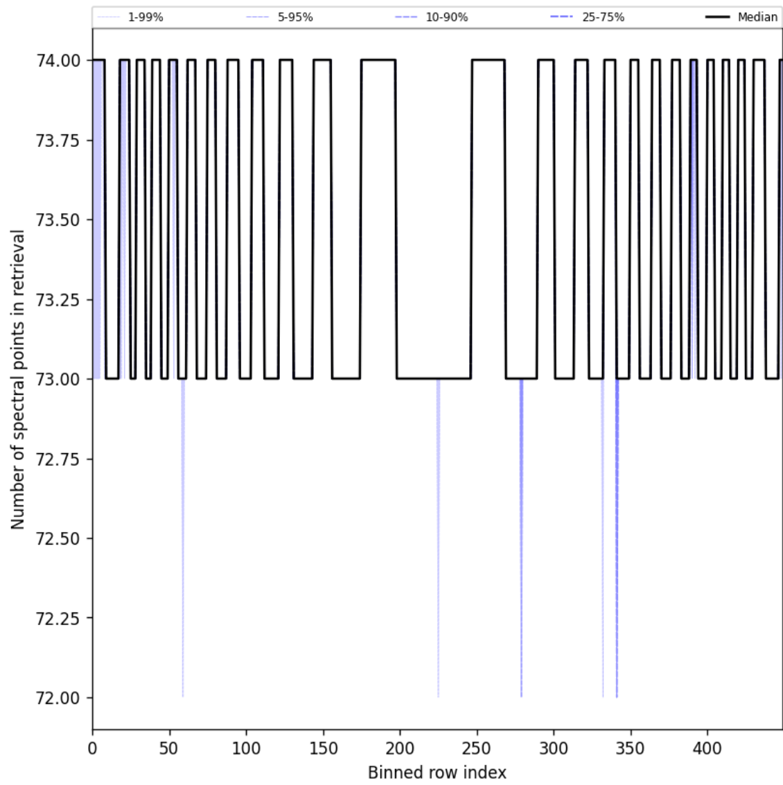
Figure 108: Along track statistics of “Number of spectral points in retrieval” for 2025-05-01 to 2025-05-03
