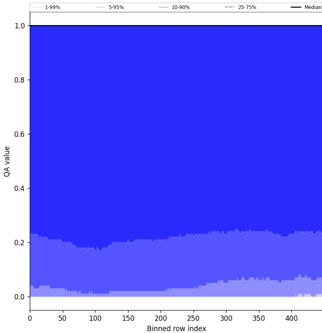
Figure 83: Along track statistics of “QA value” for 2025-05-01 to 2025-05-03
