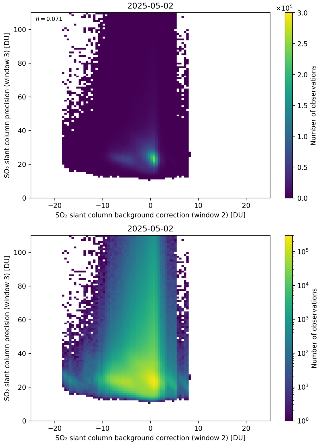
Figure 129: Scatter density plot of “SO 2 slant column background correction (window 2)” against “SO 2 slant column precision (window 3)” for 2025-05-01 to 2025-05-03.
