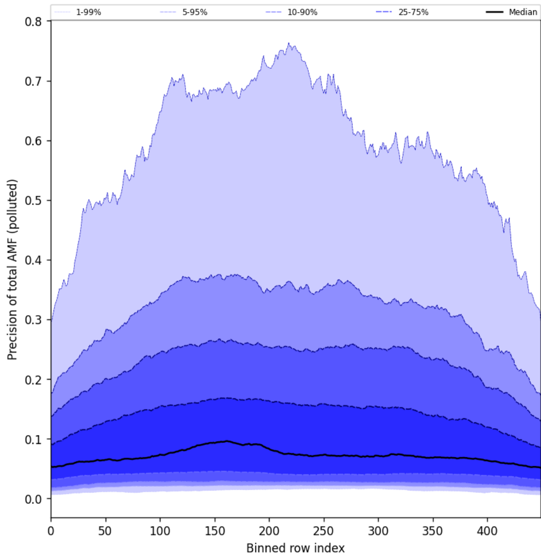
Figure 106: Along track statistics of “Precision of total AMF (polluted)” for 2025-05-01 to 2025-05-03
