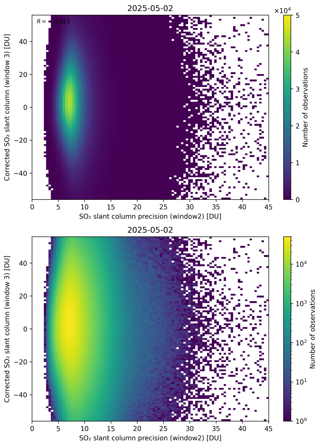
Figure 298: Scatter density plot of “SO 2 slant column precision (window2)” against “Corrected SO 2 slant column (window 3)” for 2025-05-01 to 2025-05-03.
