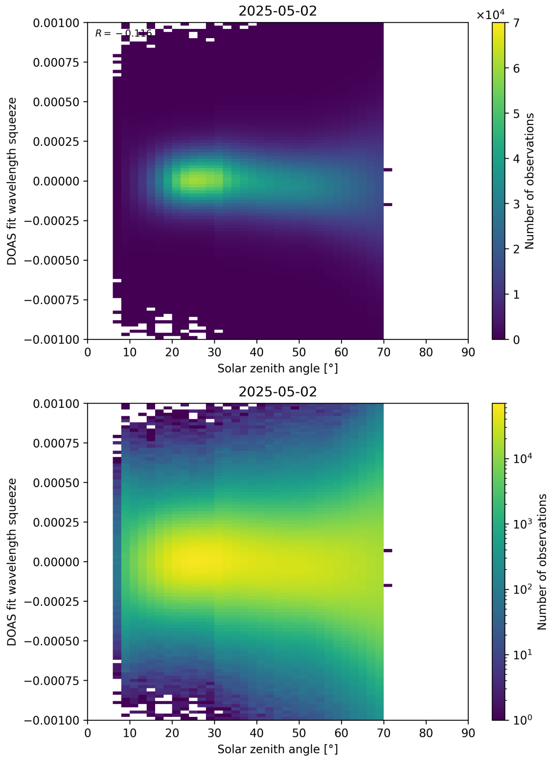
Figure 175: Scatter density plot of “Solar zenith angle” against “DOAS fit wavelength squeeze” for 2025-05-01 to 2025-05-03.
