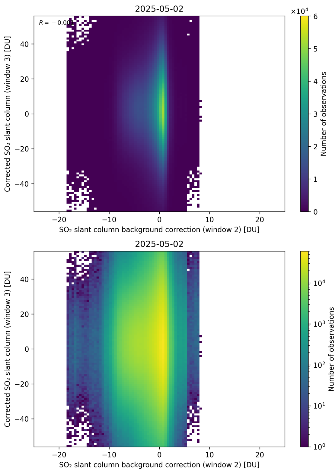
Figure 127: Scatter density plot of “SO 2 slant column background correction (window 2)” against “Corrected SO 2 slant column (window 3)” for 2025-05-01 to 2025-05-03.
