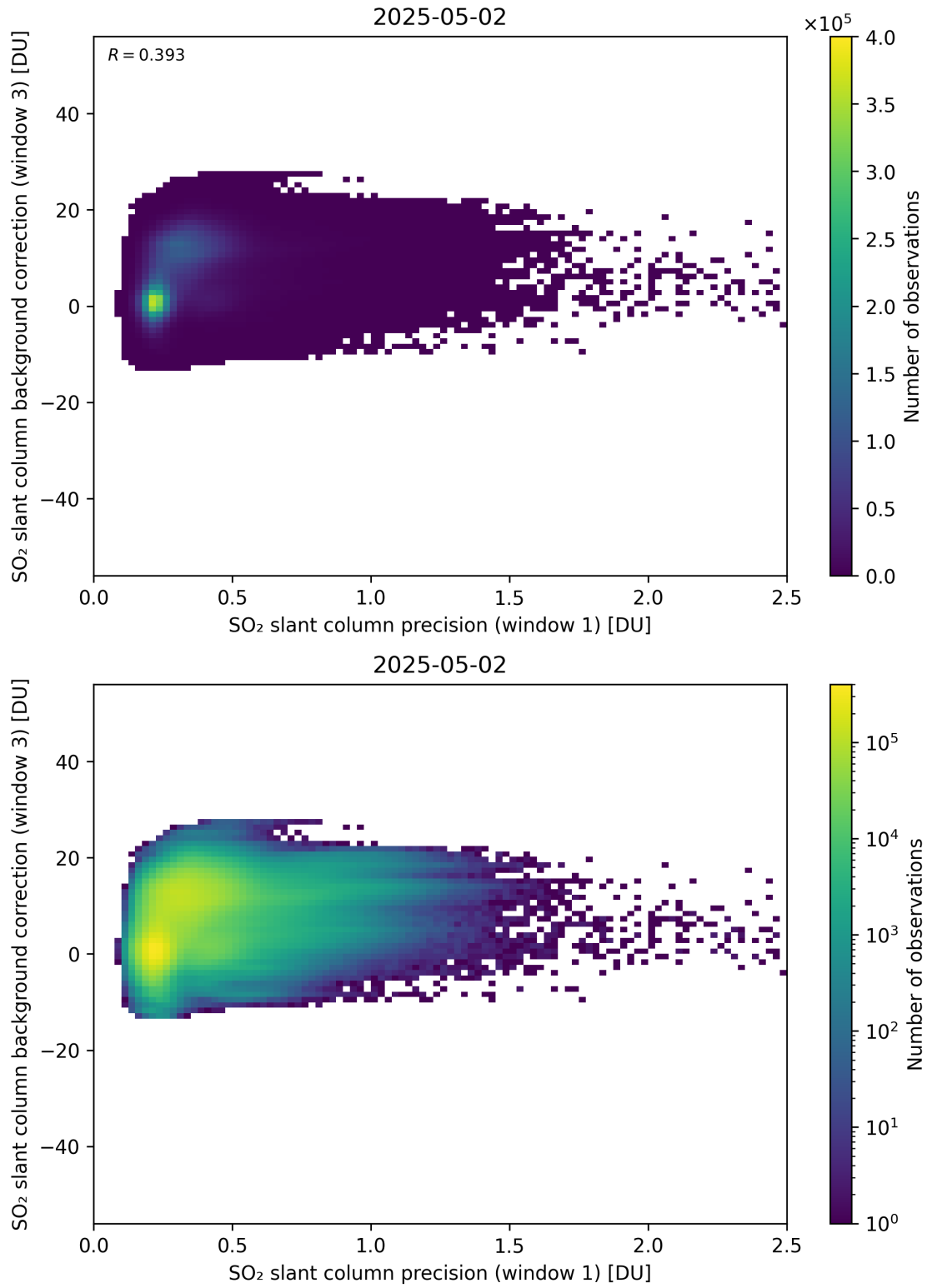
Figure 270: Scatter density plot of “SO 2 slant column precision (window 1)” against “SO 2 slant column background correction (window 3)” for 2025-05-01 to 2025-05-03.
