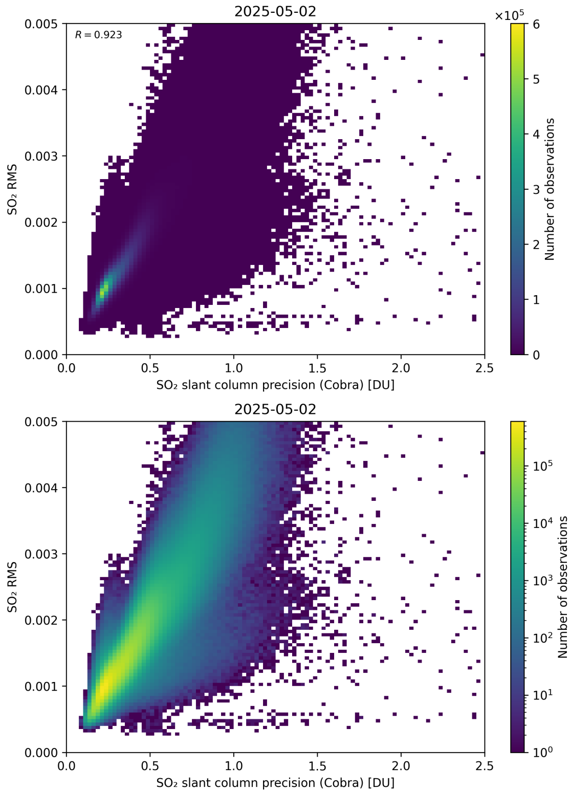
Figure 204: Scatter density plot of “SO 2 slant column precision (Cobra)” against “SO 2 RMS” for 2025-05-01 to 2025-05-03.
