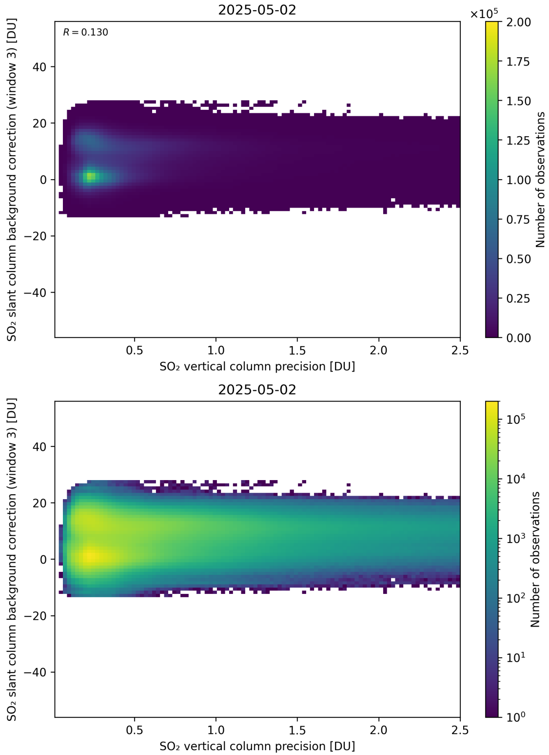
Figure 331: Scatter density plot of “SO 2 vertical column precision” against “SO 2 slant column background correction (window 3)” for 2025-05-01 to 2025-05-03.
