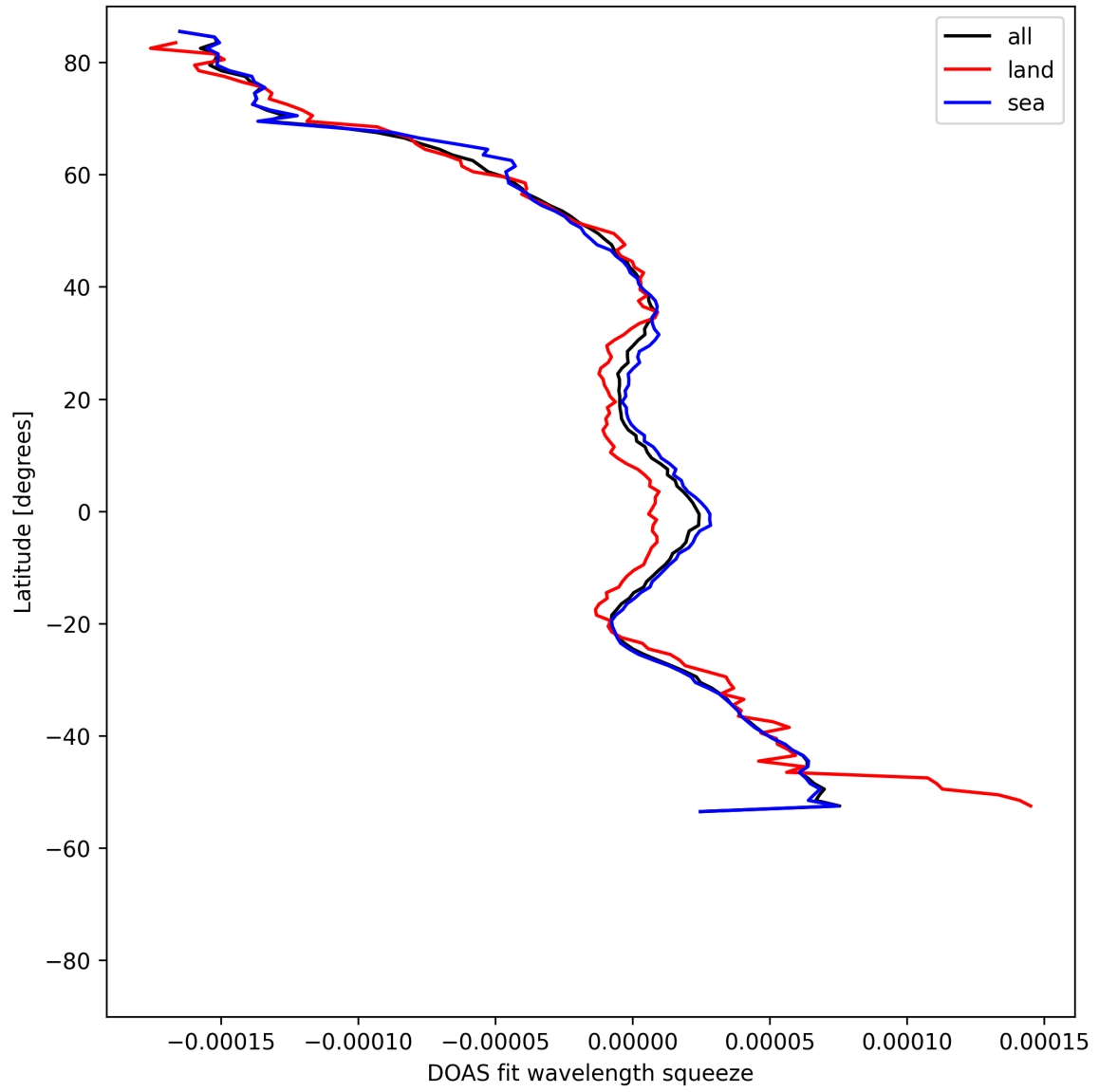
Figure 51: Zonal average of “DOAS fit wavelength squeeze” for 2025-05-01 to 2025-05-03.
