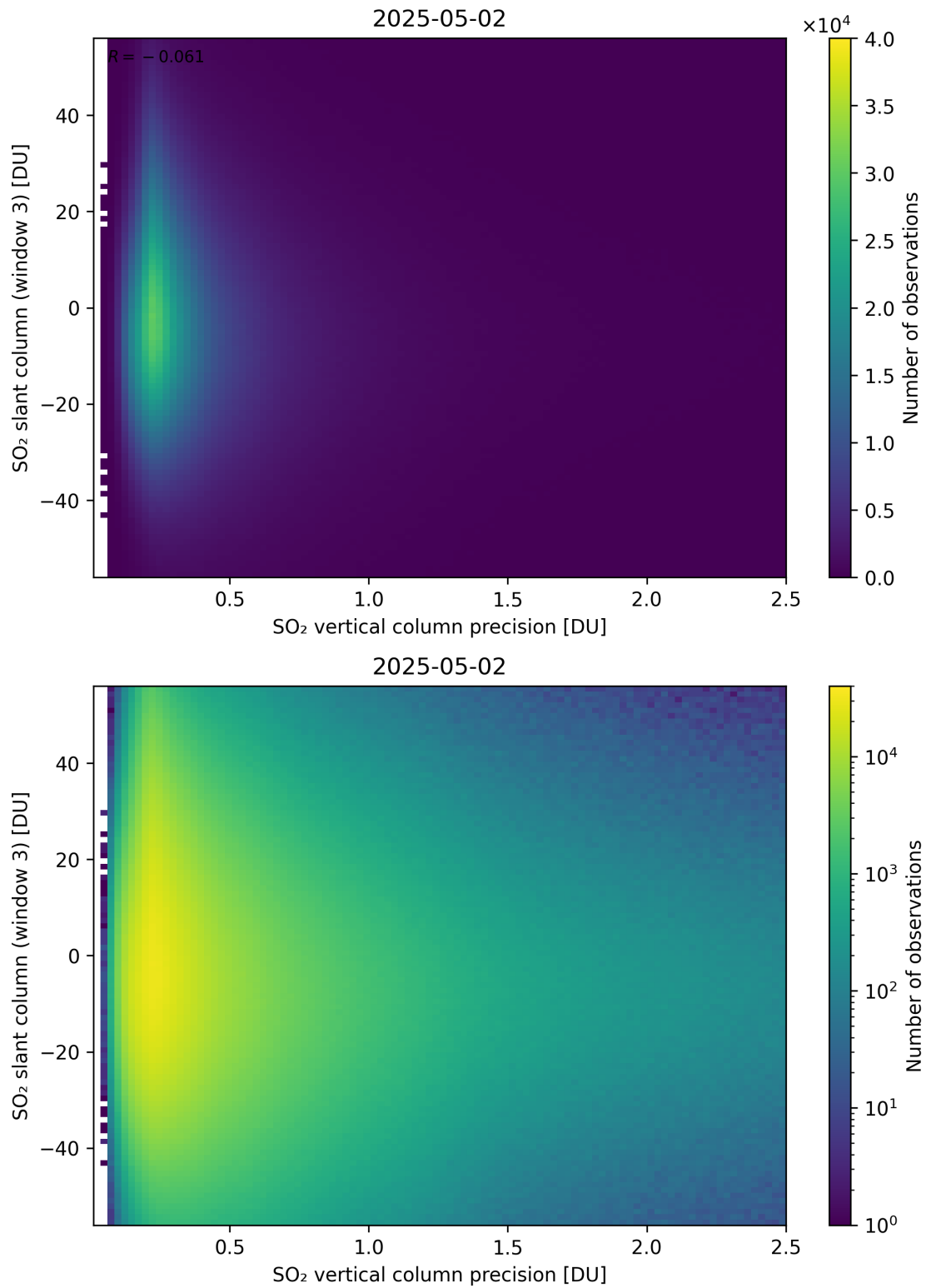
Figure 344: Scatter density plot of “SO 2 vertical column precision” against “SO 2 slant column (window 3)” for 2025-05-01 to 2025-05-03.
