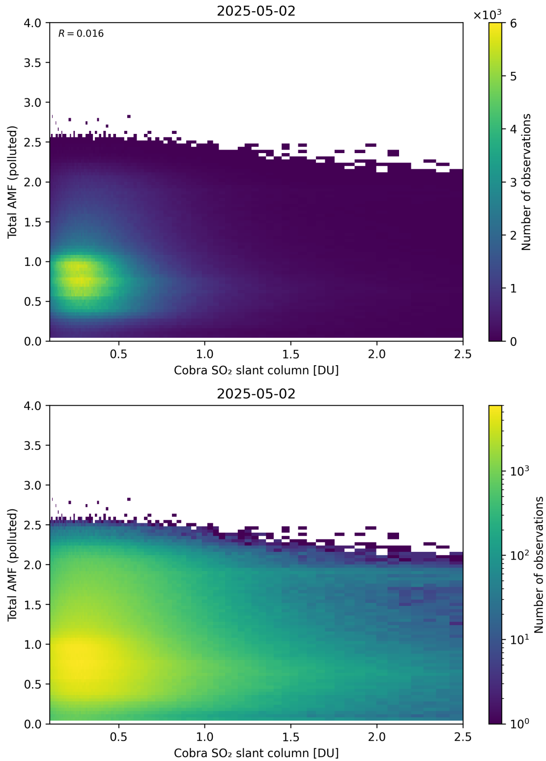
Figure 224: Scatter density plot of “Cobra SO 2 slant column” against “Total AMF (polluted)” for 2025-05-01 to 2025-05-03.
