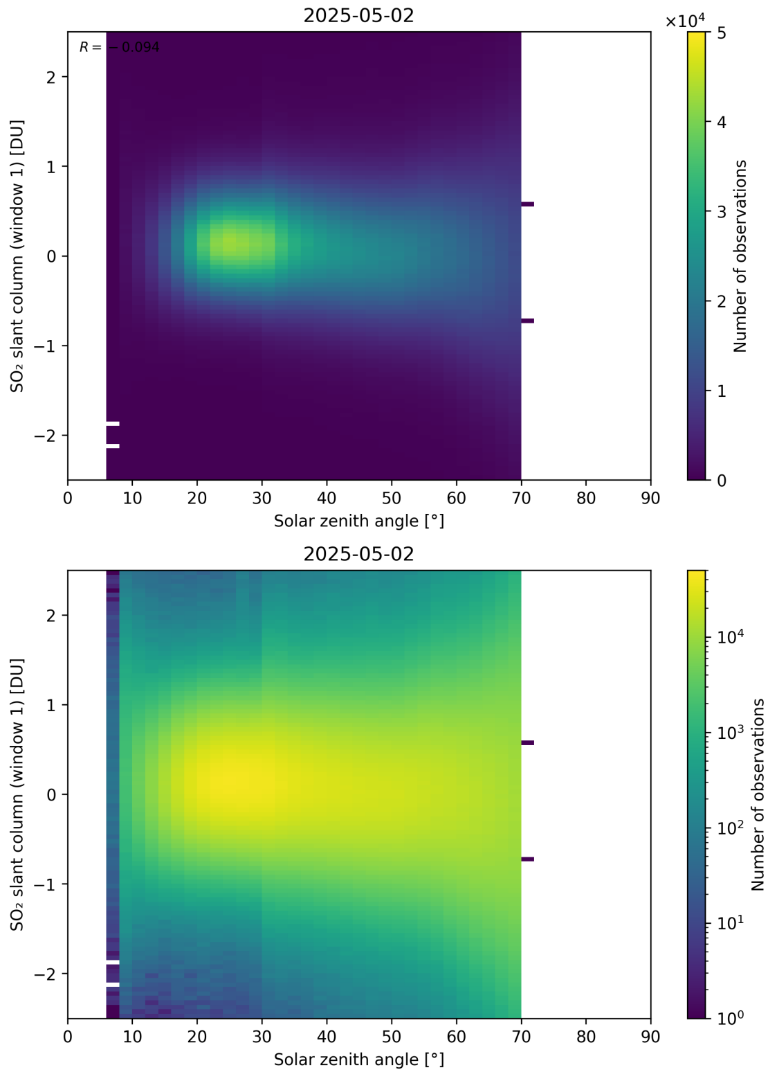
Figure 184: Scatter density plot of “Solar zenith angle” against “SO 2 slant column (window 1)” for 2025-05-01 to 2025-05-03.
