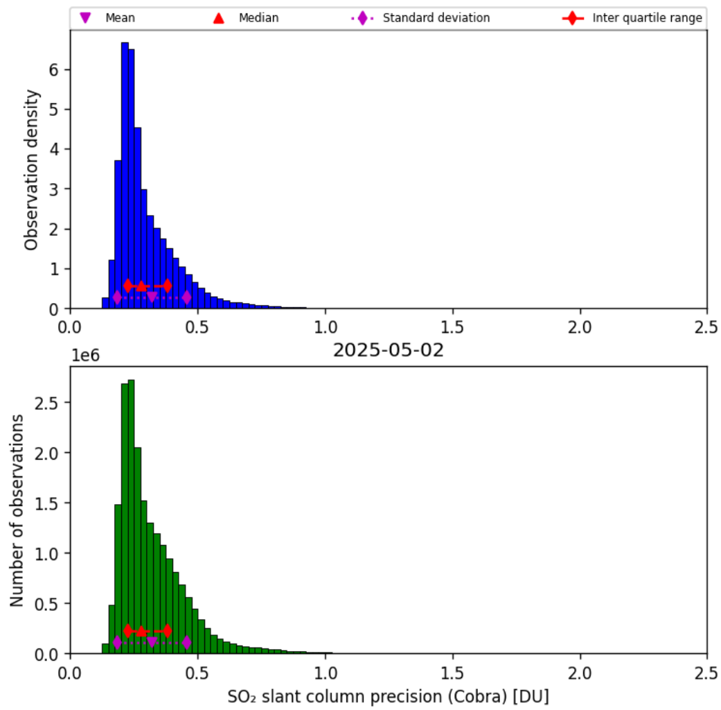
Figure 62: Histogram of “SO 2 slant column precision (Cobra)” for 2025-05-01 to 2025-05-03
