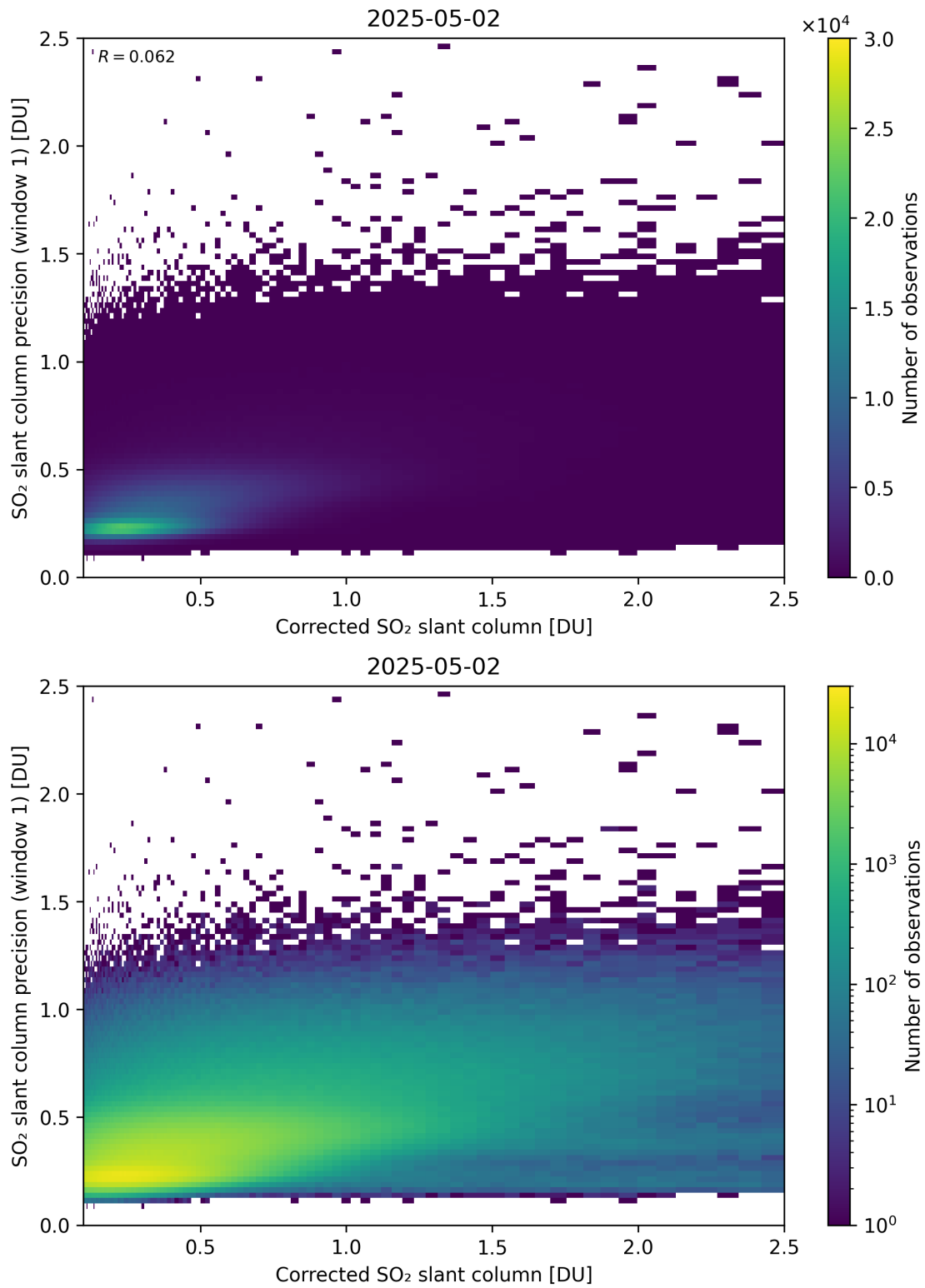
Figure 238: Scatter density plot of “Corrected SO 2 slant column” against “SO 2 slant column precision (window 1)” for 2025-05-01 to 2025-05-03.
