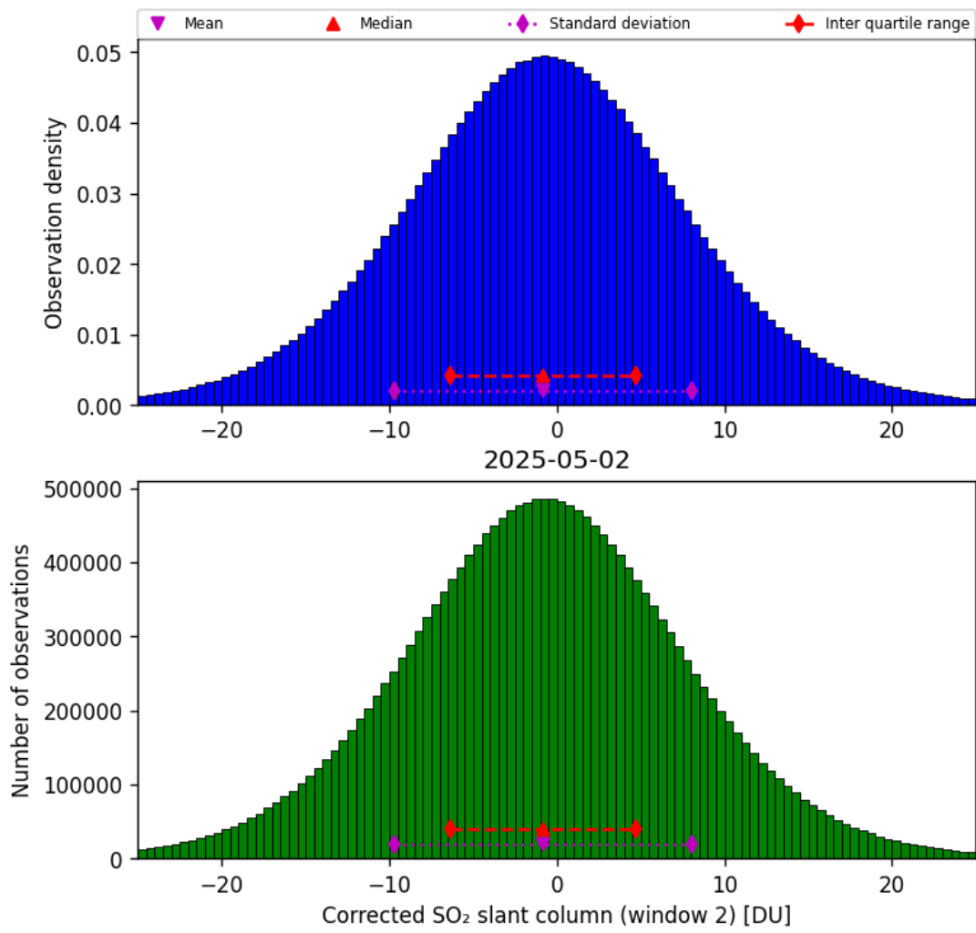
Figure 69: Histogram of “Corrected SO 2 slant column (window 2)” for 2025-05-01 to 2025-05-03
