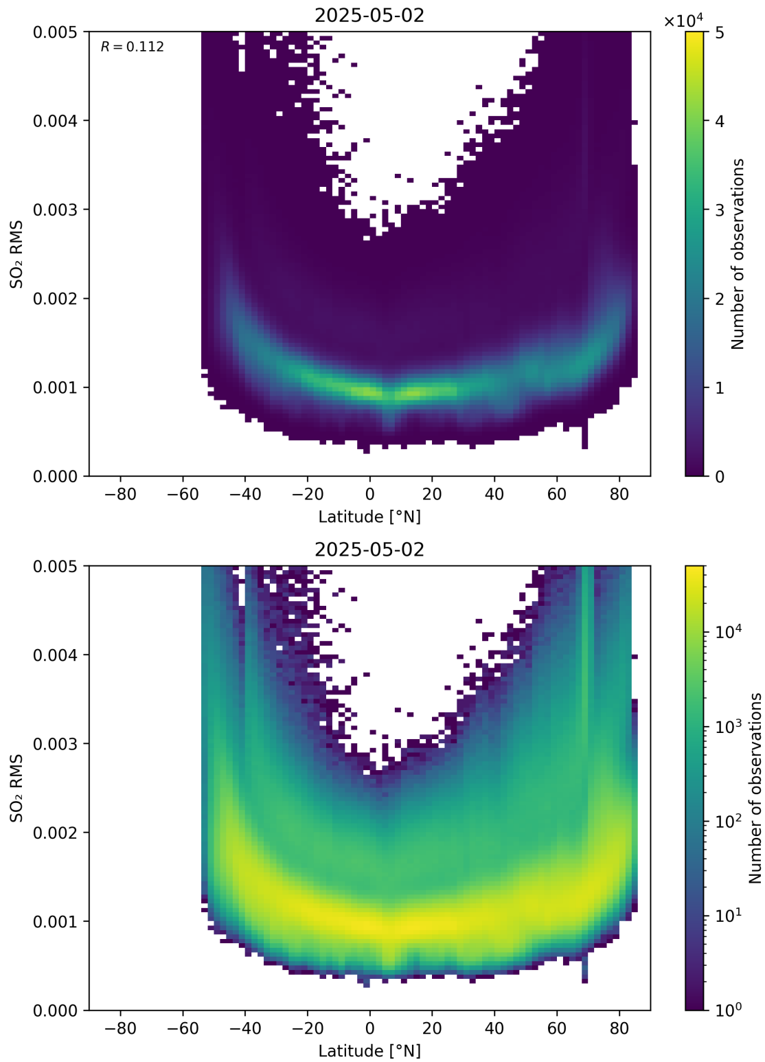
Figure 155: Scatter density plot of “Latitude” against “SO 2 RMS” for 2025-05-01 to 2025-05-03.
