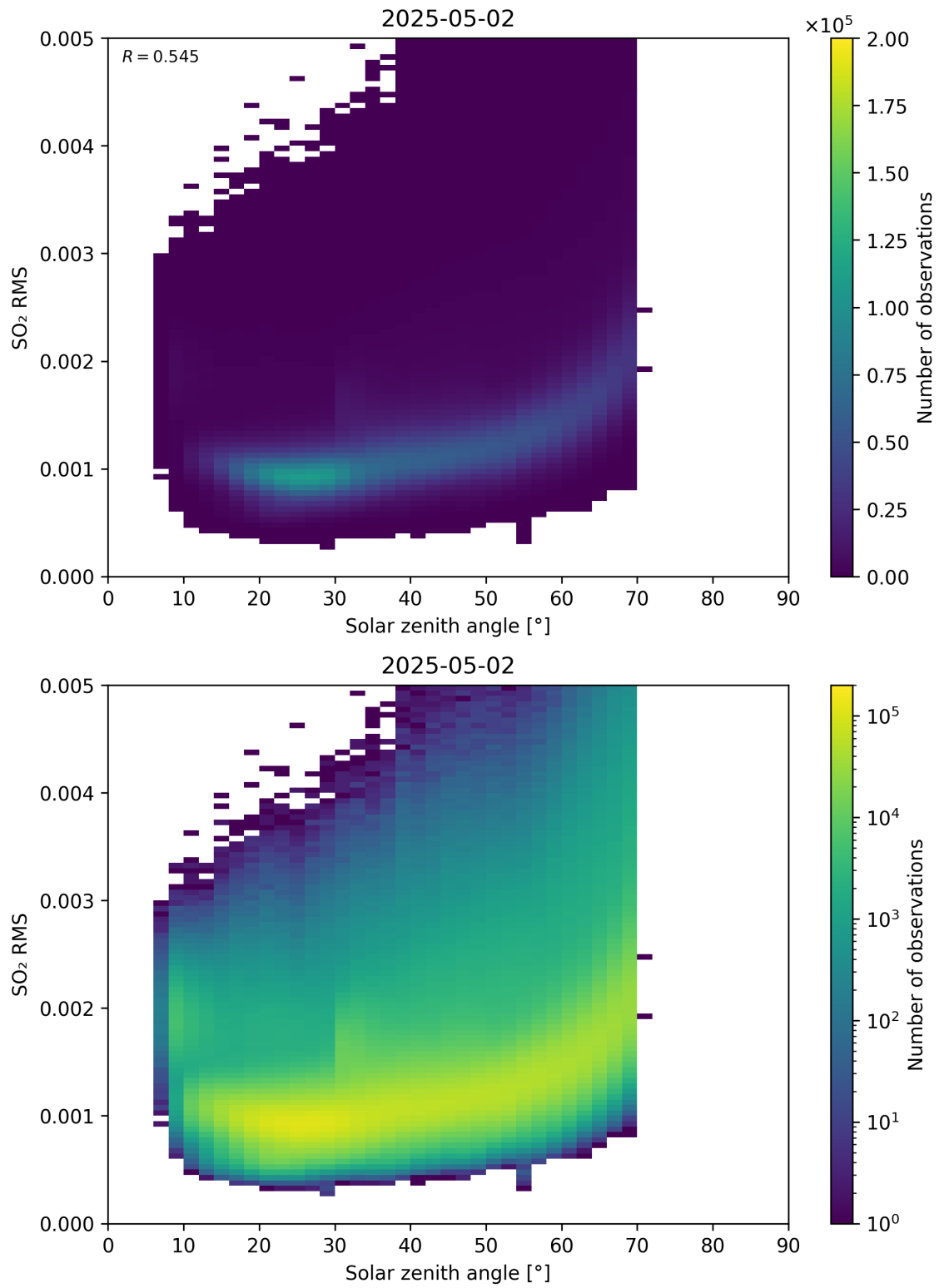
Figure 176: Scatter density plot of “Solar zenith angle” against “SO 2 RMS” for 2025-05-01 to 2025-05-03.
