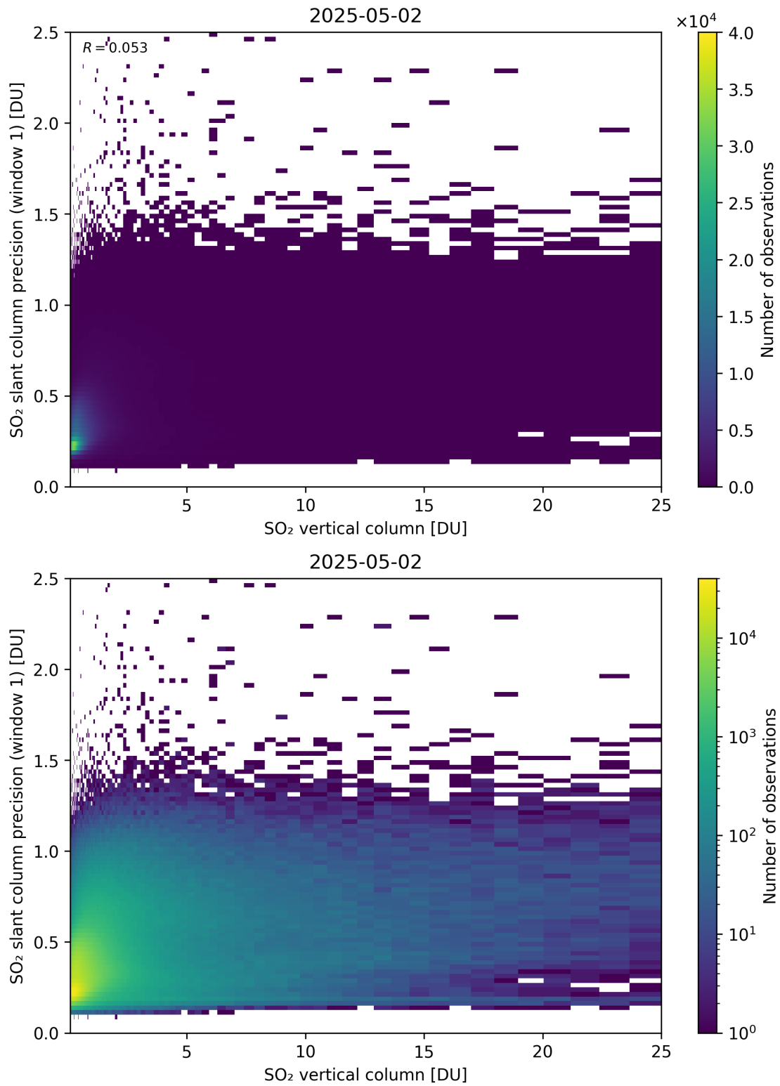
Figure 355: Scatter density plot of “SO 2 vertical column” against “SO 2 slant column precision (window 1)” for 2025-05-01 to 2025-05-03.
