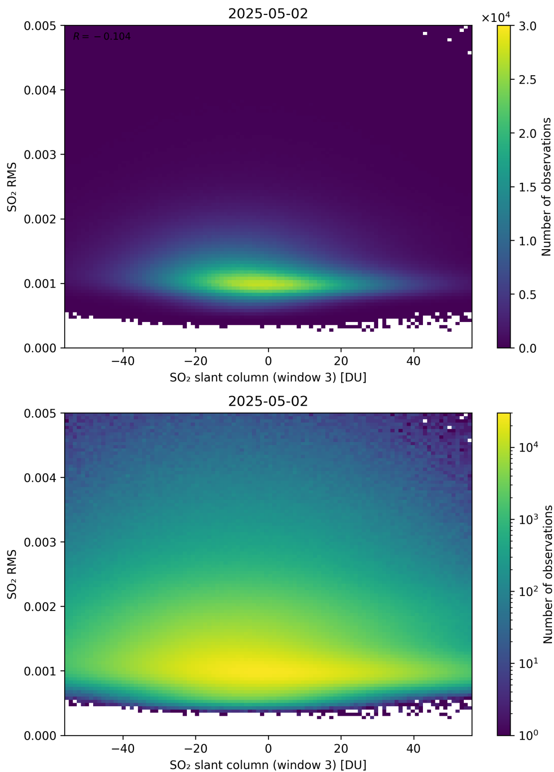
Figure 306: Scatter density plot of “SO 2 slant column (window 3)” against “SO 2 RMS” for 2025-05-01 to 2025-05-03.
