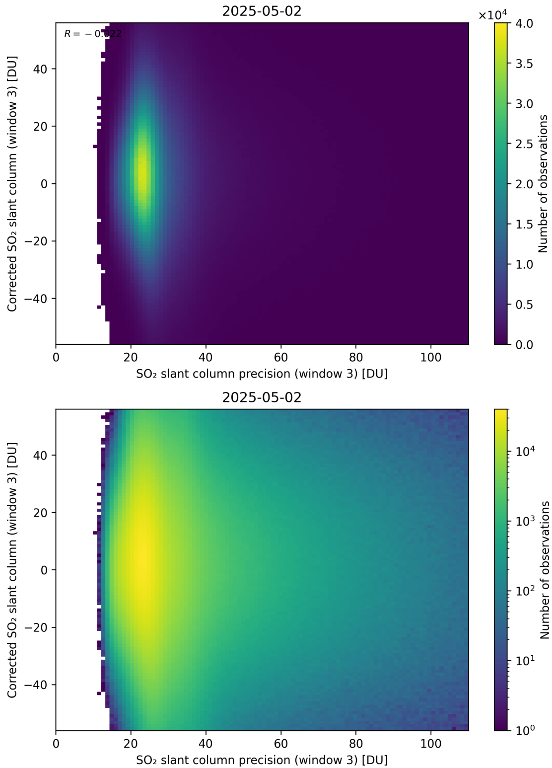
Figure 312: Scatter density plot of “SO 2 slant column precision (window 3)” against “Corrected SO 2 slant column (window 3)” for 2025-05-01 to 2025-05-03.
