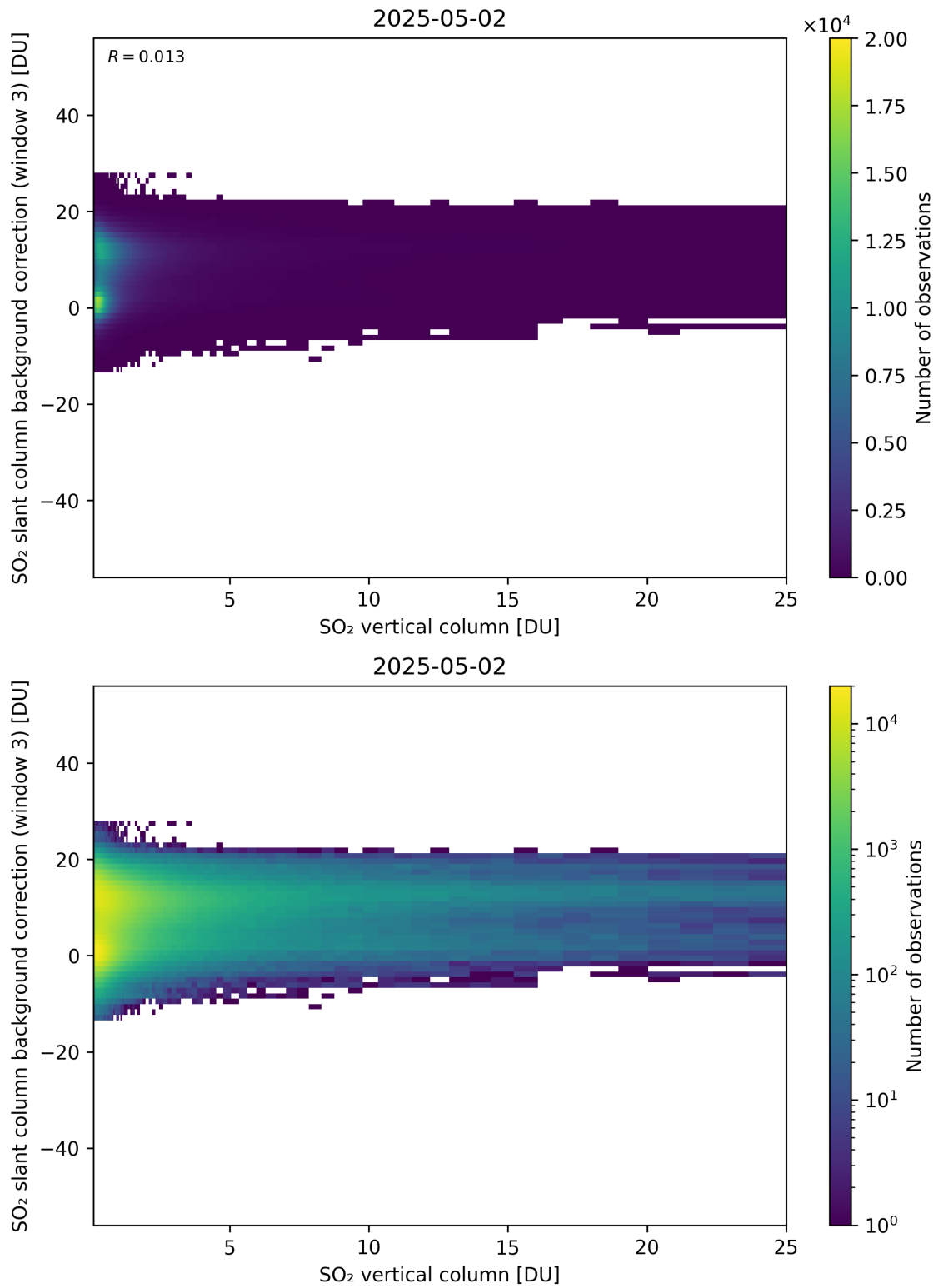
Figure 325: Scatter density plot of “SO 2 vertical column” against “SO 2 slant column background correction (window 3)” for 2025-05-01 to 2025-05-03.
