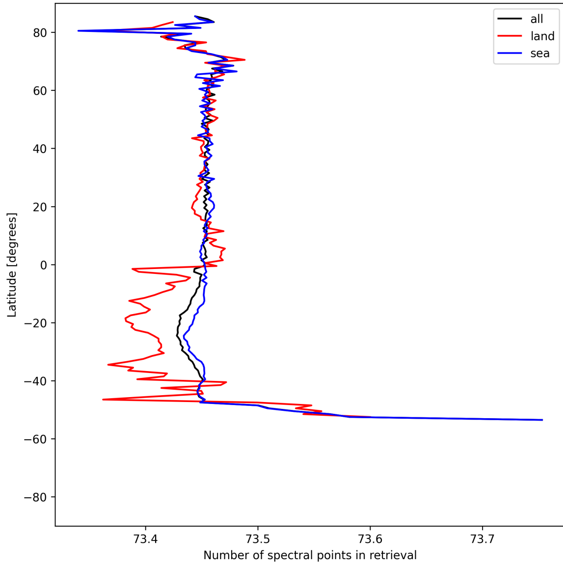
Figure 56: Zonal average of “Number of spectral points in retrieval” for 2025-05-01 to 2025-05-03.
