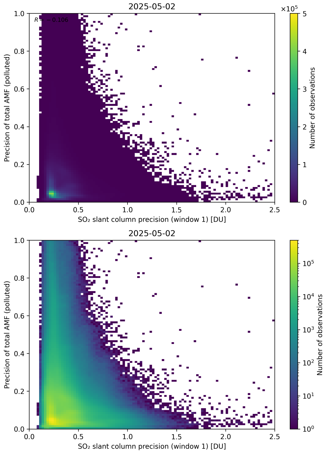
Figure 281: Scatter density plot of “SO 2 slant column precision (window 1)” against “Precision of total AMF (polluted)” for 2025-05-01 to 2025-05-03.
