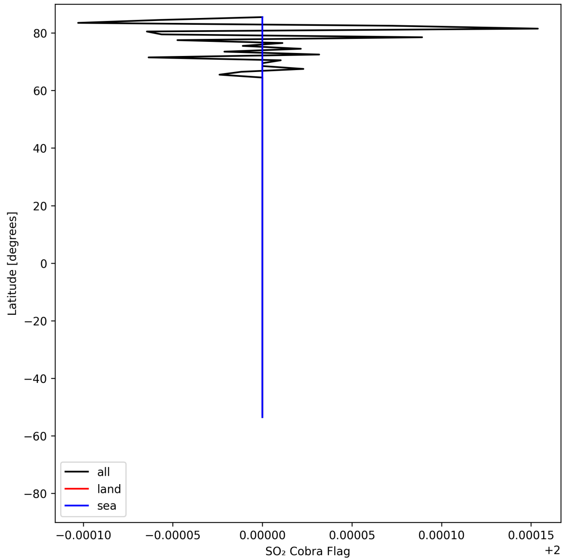
Figure 49: Zonal average of "SO 2 Cobra Flag" for 2025-05-01 to 2025-05-03.
