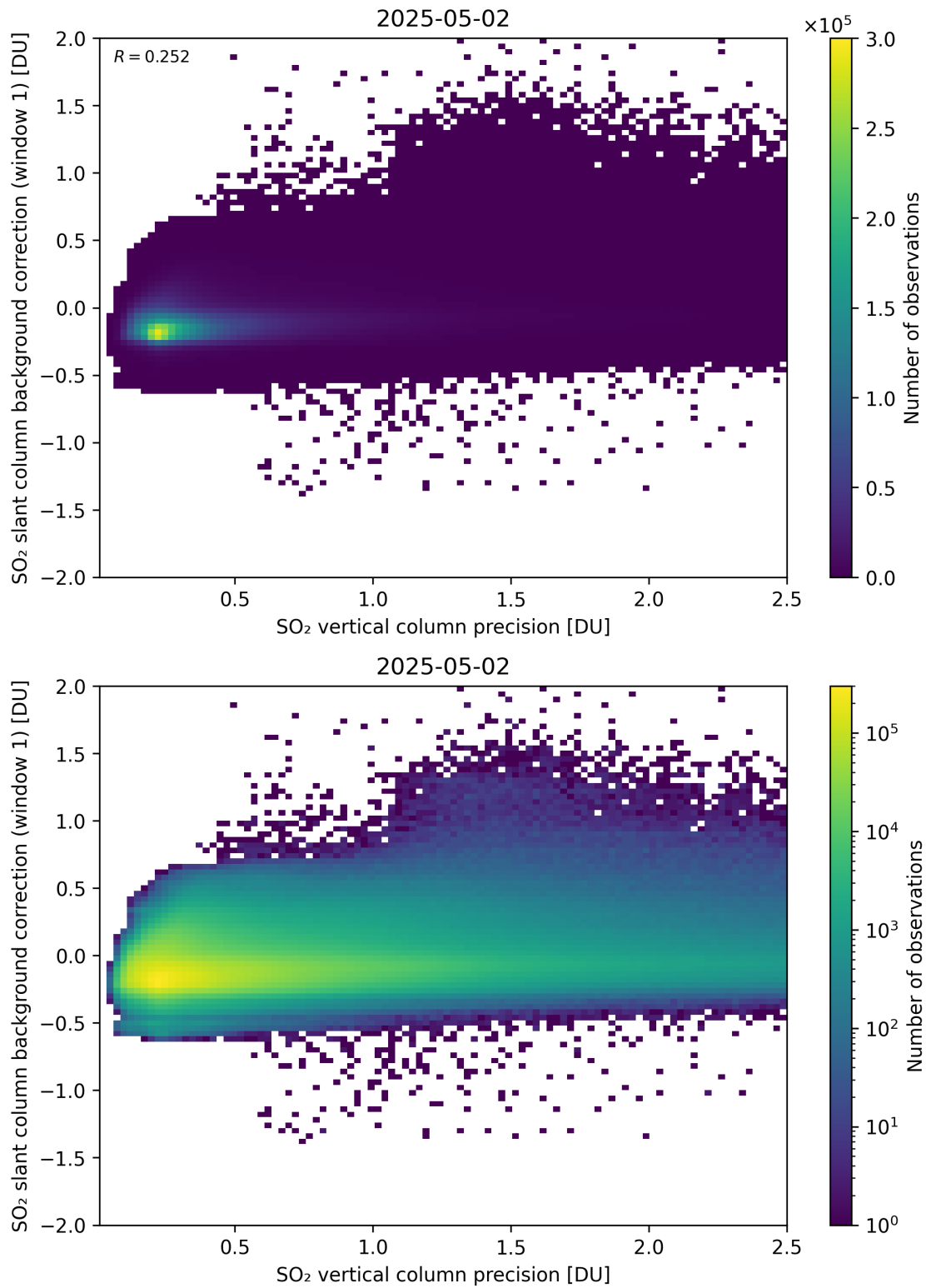
Figure 329: Scatter density plot of “SO 2 vertical column precision” against “SO 2 slant column background correction (window 1)” for 2025-05-01 to 2025-05-03.
