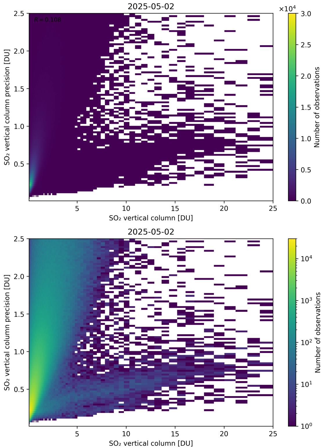
Figure 361: Scatter density plot of “SO 2 vertical column” against “SO 2 vertical column precision” for 2025-05-01 to 2025-05-03.
