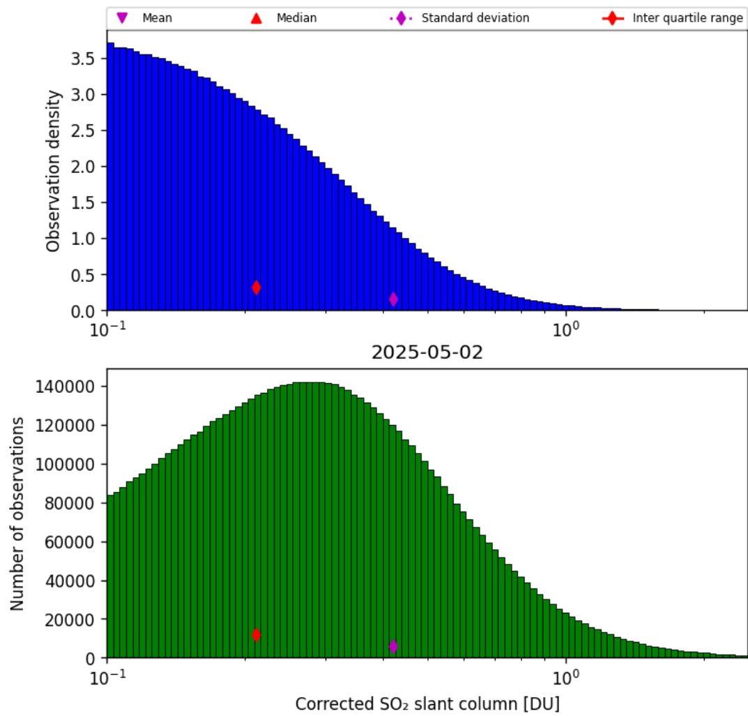
Figure 60: Histogram of "Corrected SO 2 slant column" for 2025-05-01 to 2025-05-03
