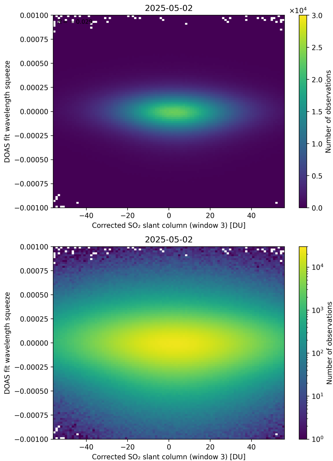
Figure 257: Scatter density plot of “Corrected SO 2 slant column (window 3)” against “DOAS fit wavelength squeeze” for 2025-05-01 to 2025-05-03.
