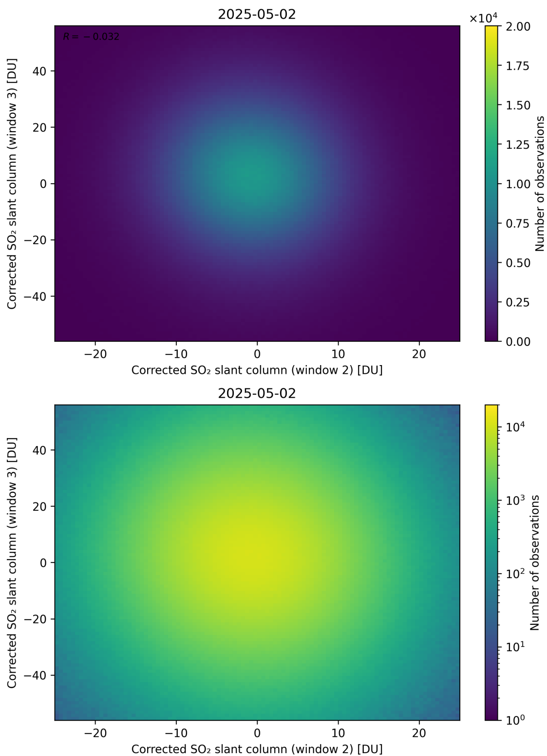
Figure 250: Scatter density plot of “Corrected SO 2 slant column (window 2)” against “Corrected SO 2 slant column (window 3)” for 2025-05-01 to 2025-05-03.
