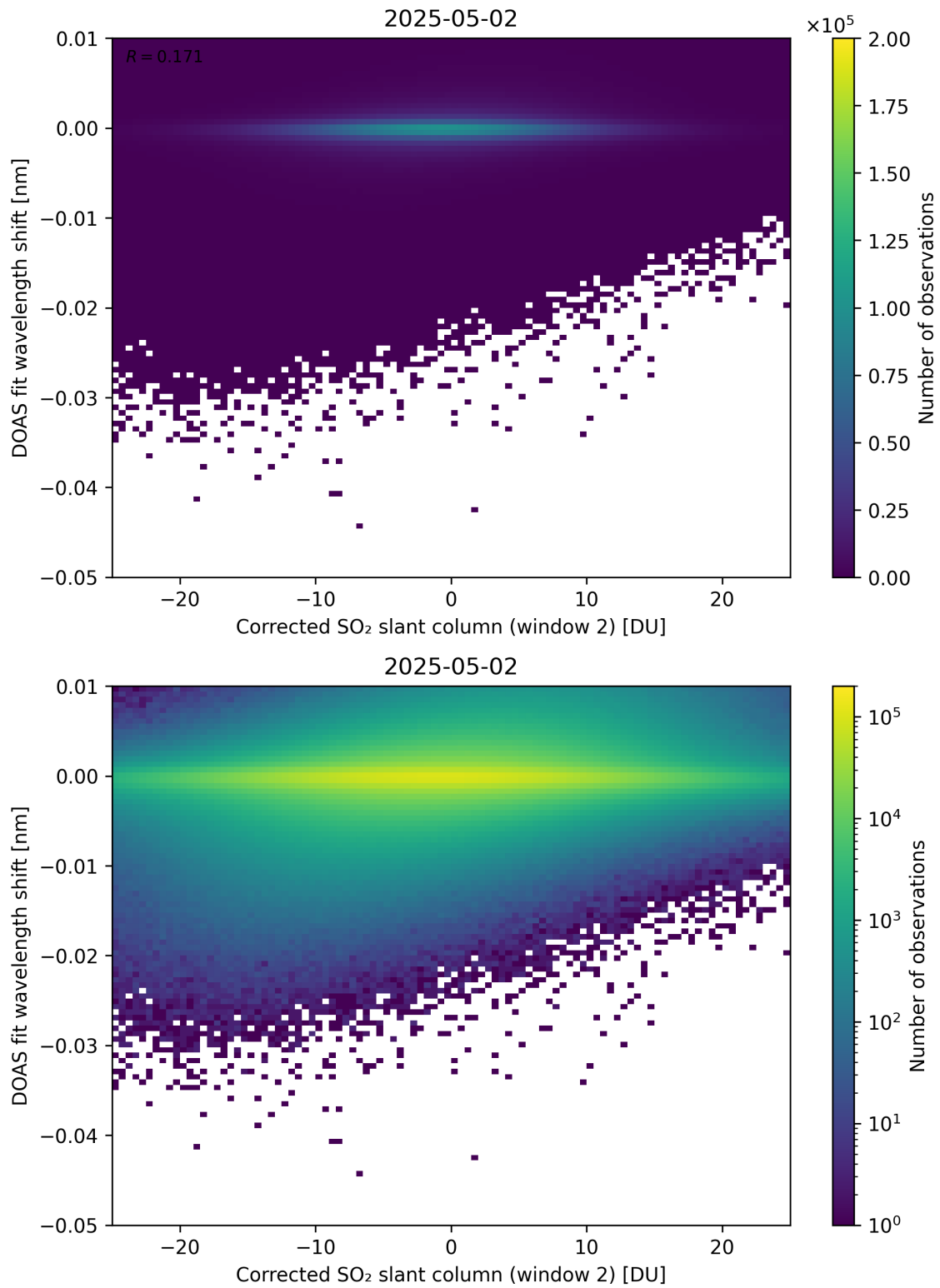
Figure 246: Scatter density plot of “Corrected SO 2 slant column (window 2)” against “DOAS fit wavelength shift” for 2025-05-01 to 2025-05-03.
