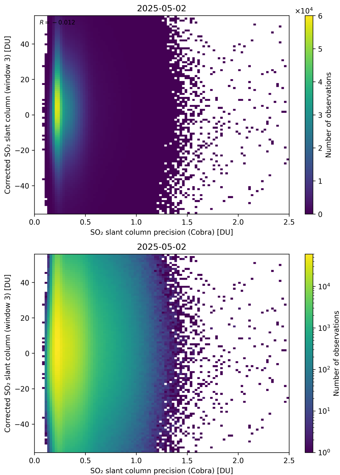
Figure 207: Scatter density plot of “SO 2 slant column precision (Cobra)” against “Corrected SO 2 slant column (window 3)” for 2025-05-01 to 2025-05-03.
