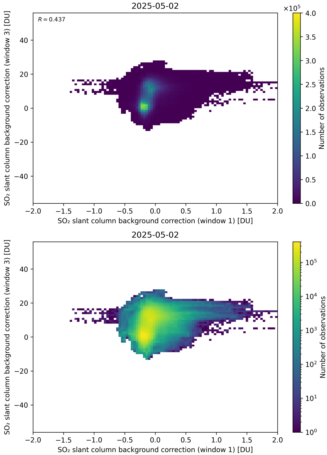
Figure 110: Scatter density plot of “SO 2 slant column background correction (window 1)” against “SO 2 slant column background correction (window 3)” for 2025-05-01 to 2025-05-03.
