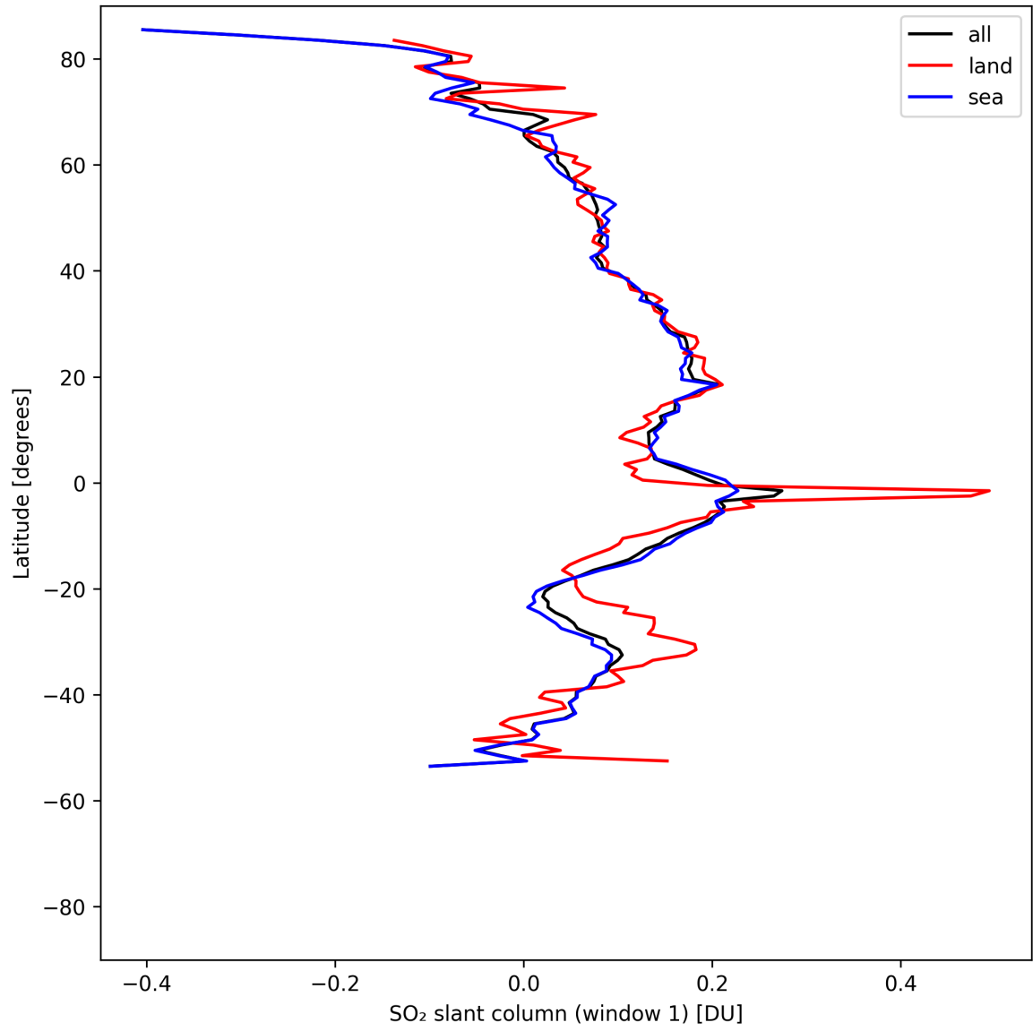
Figure 37: Zonal average of “SO 2 slant column (window 1)” for 2025-05-01 to 2025-05-03.
