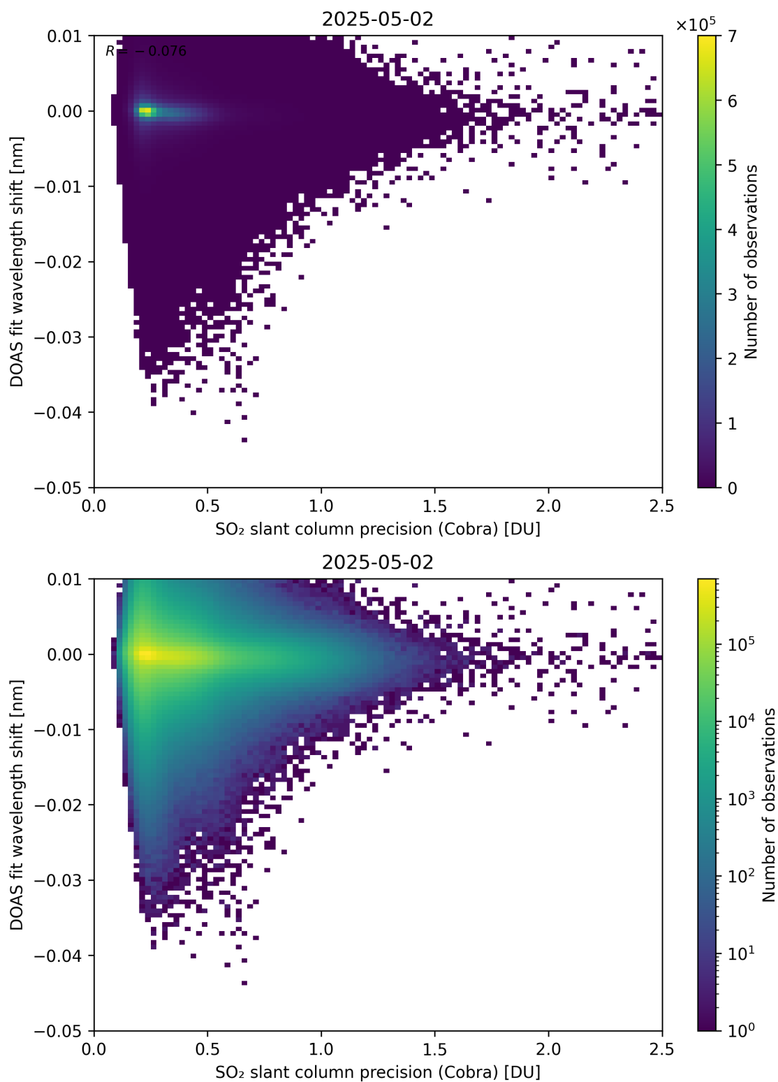
Figure 202: Scatter density plot of “SO 2 slant column precision (Cobra)” against “DOAS fit wavelength shift” for 2025-05-01 to 2025-05-03.
