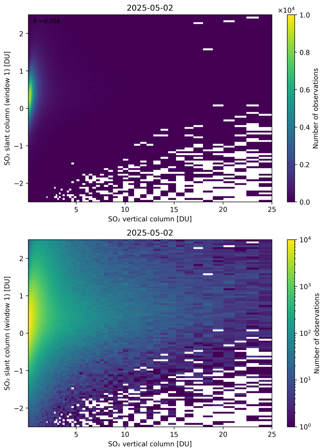
Figure 354: Scatter density plot of “SO 2 vertical column” against “SO 2 slant column (window 1)” for 2025-05-01 to 2025-05-03.
