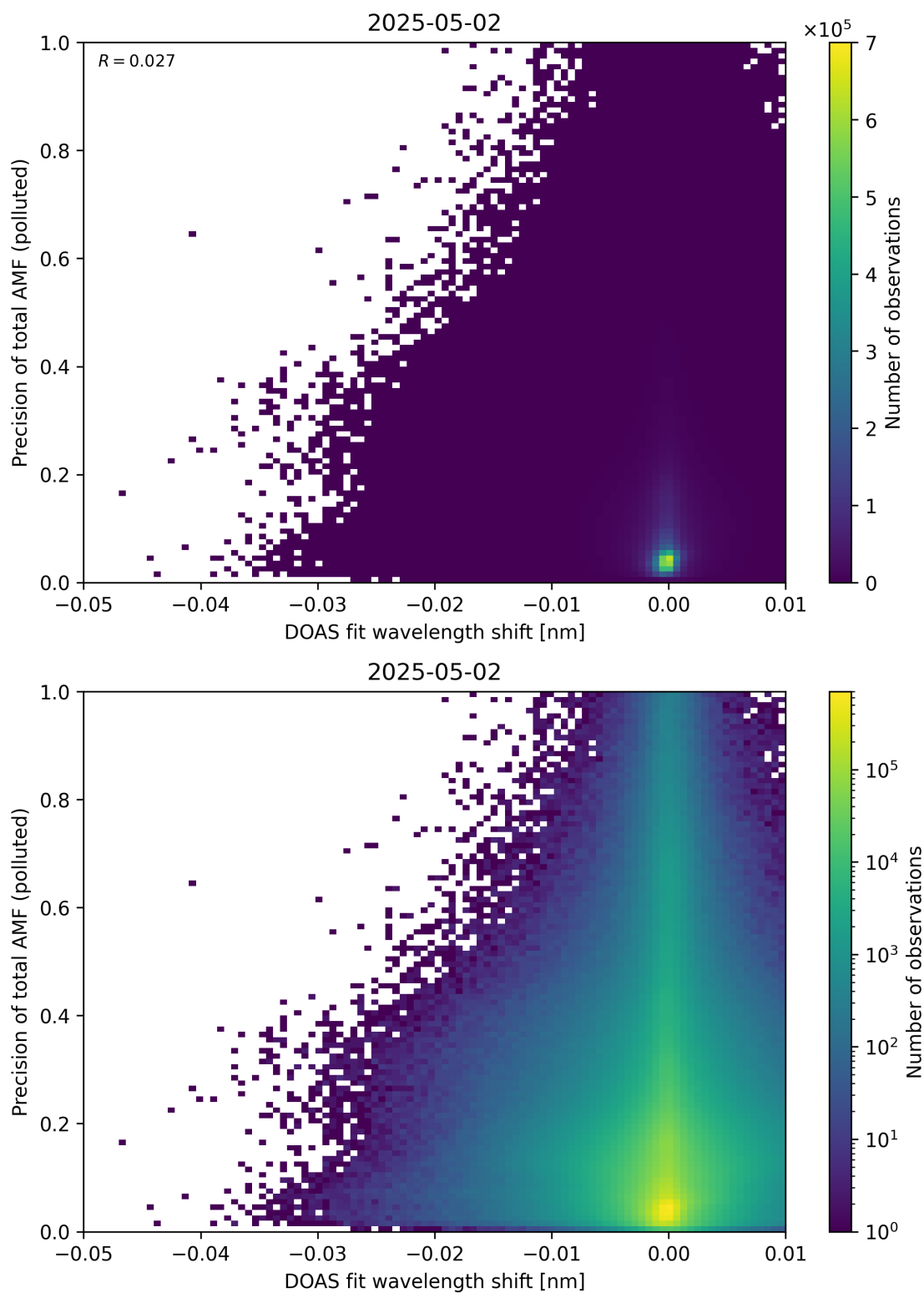
Figure 142: Scatter density plot of “DOAS fit wavelength shift” against “Precision of total AMF (polluted)” for 2025-05-01 to 2025-05-03.
