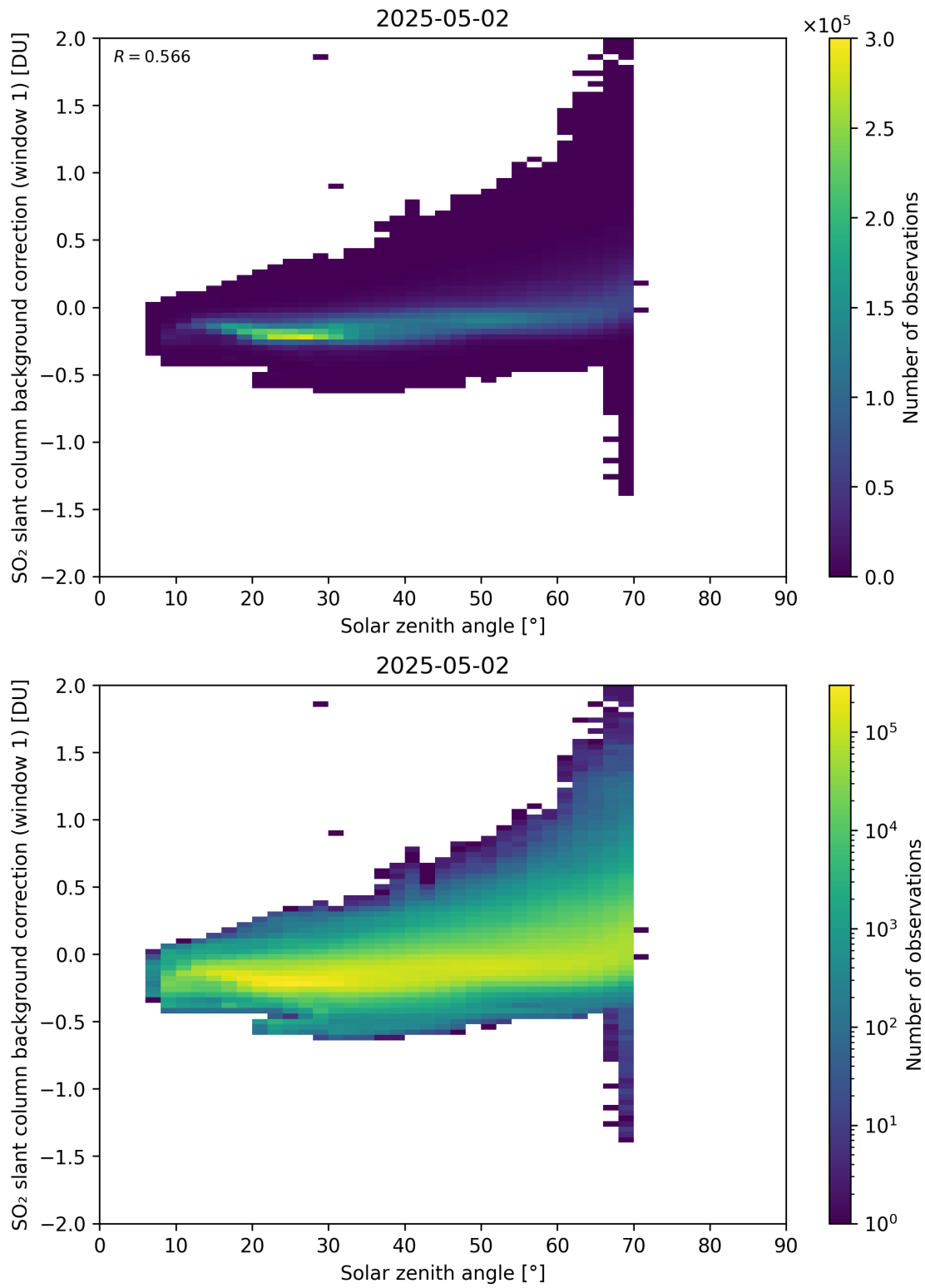
Figure 171: Scatter density plot of “Solar zenith angle” against “SO 2 slant column background correction (window 1)” for 2025-05-01 to 2025-05-03.
