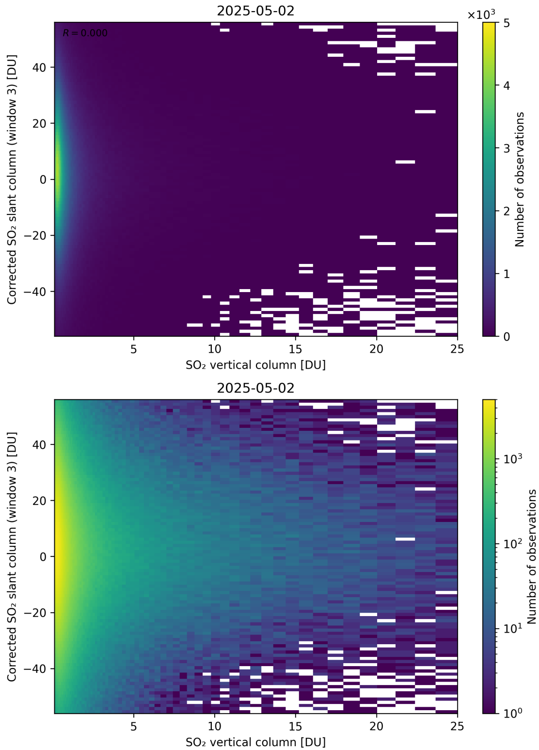
Figure 353: Scatter density plot of “SO 2 vertical column” against “Corrected SO 2 slant column (window 3)” for 2025-05-01 to 2025-05-03.
