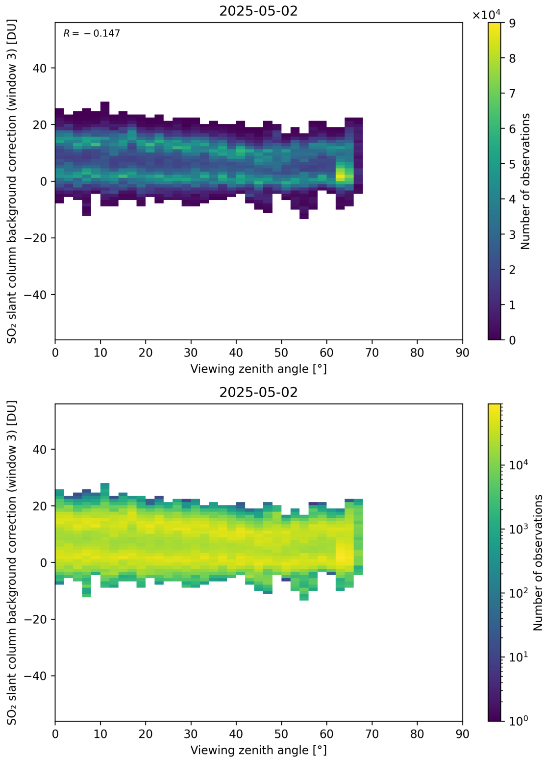
Figure 364: Scatter density plot of “Viewing zenith angle” against “SO 2 slant column background correction (window 3)” for 2025-05-01 to 2025-05-03.
