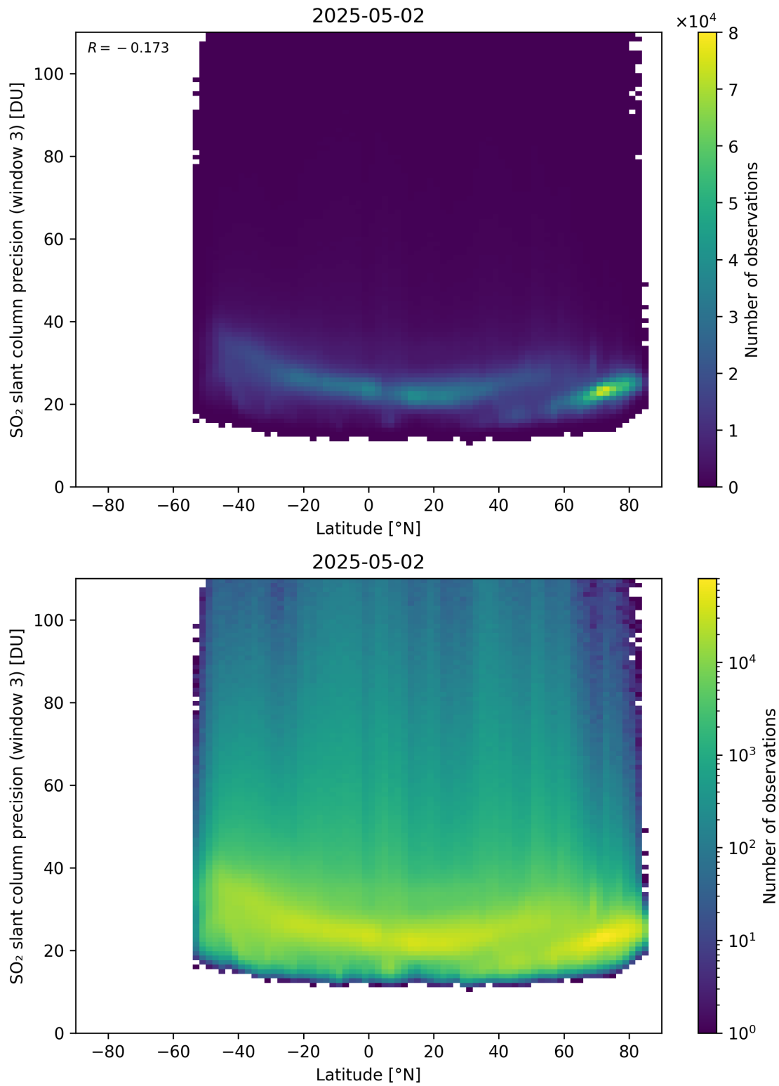
Figure 166: Scatter density plot of “Latitude” against “SO 2 slant column precision (window 3)” for 2025-05-01 to 2025-05-03.
