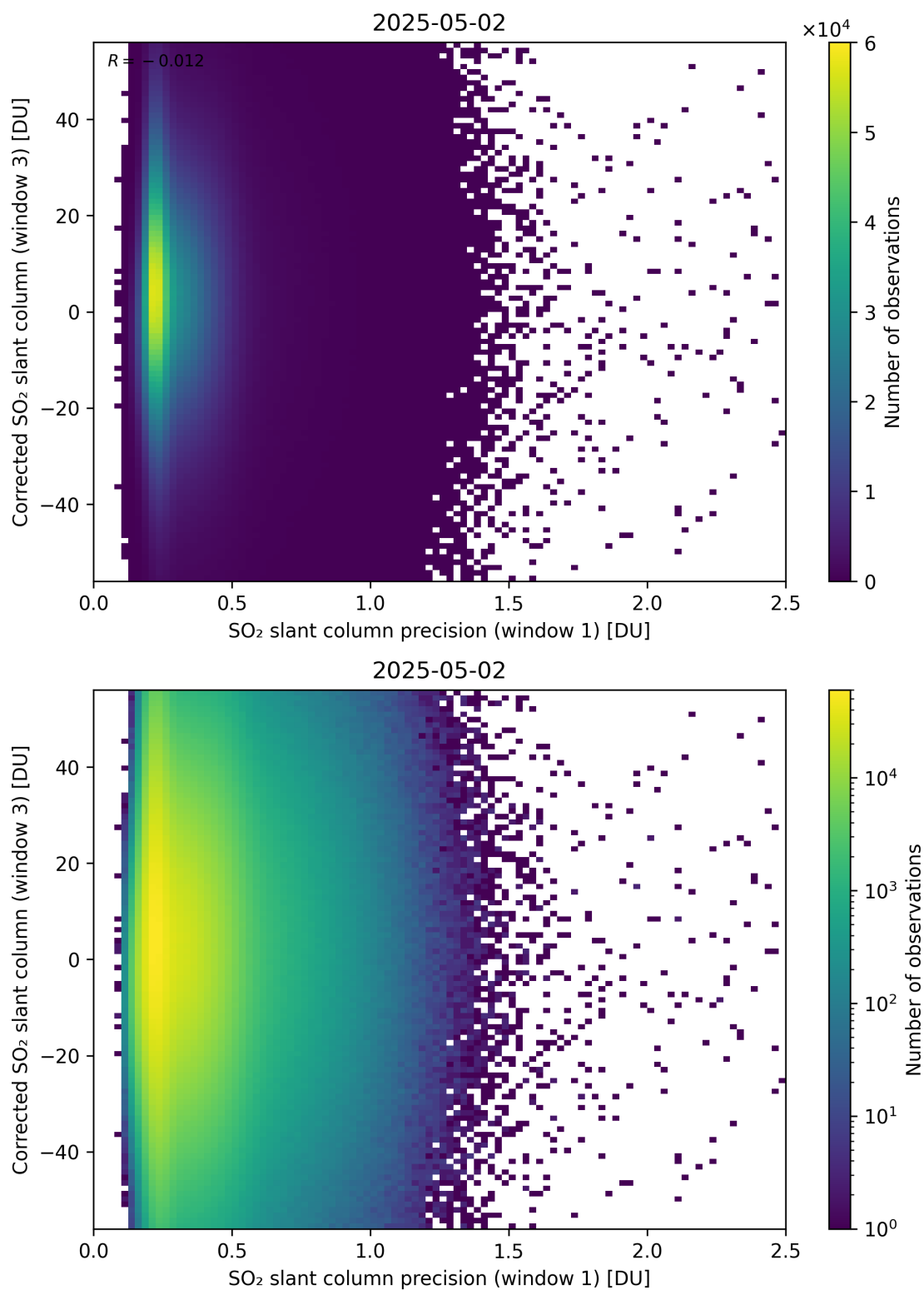
Figure 276: Scatter density plot of “SO 2 slant column precision (window 1)” against “Corrected SO 2 slant column (window 3)” for 2025-05-01 to 2025-05-03.
