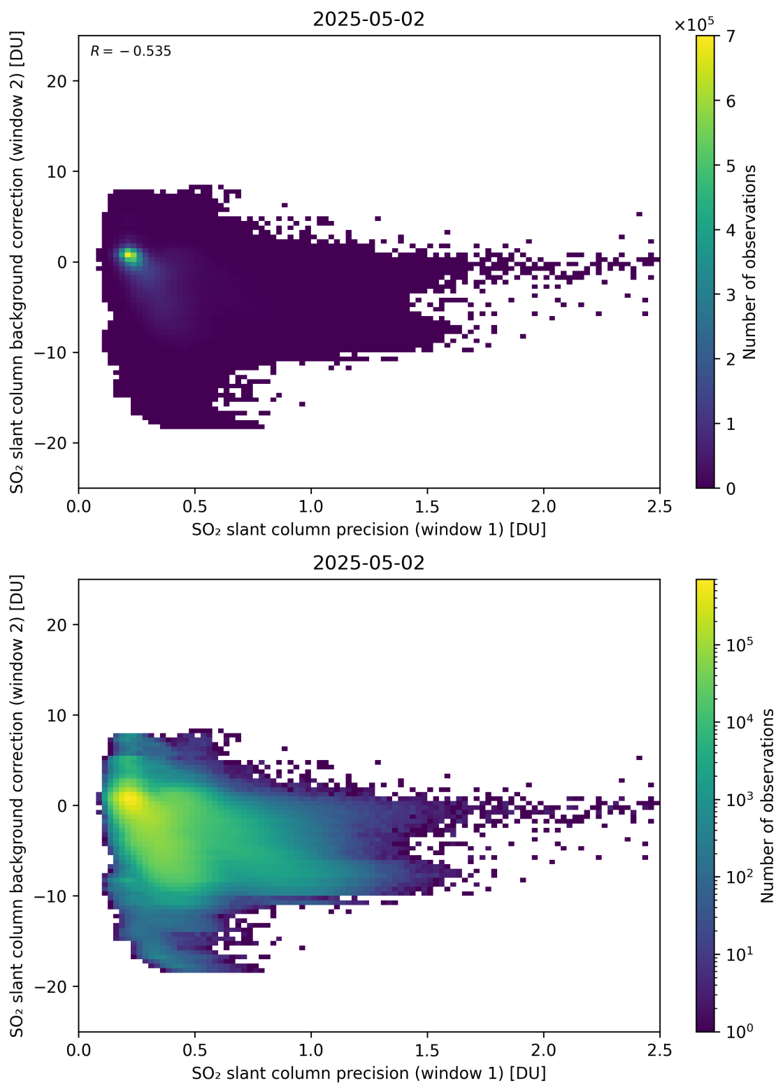
Figure 269: Scatter density plot of “SO 2 slant column precision (window 1)” against “SO 2 slant column background correction (window 2)” for 2025-05-01 to 2025-05-03.
