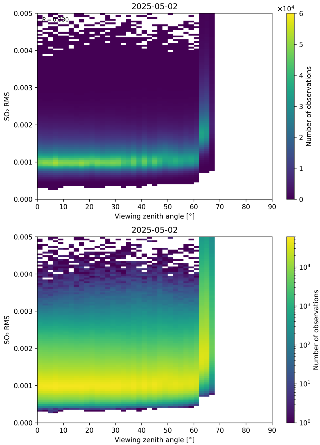
Figure 367: Scatter density plot of “Viewing zenith angle” against “SO 2 RMS” for 2025-05-01 to 2025-05-03.
