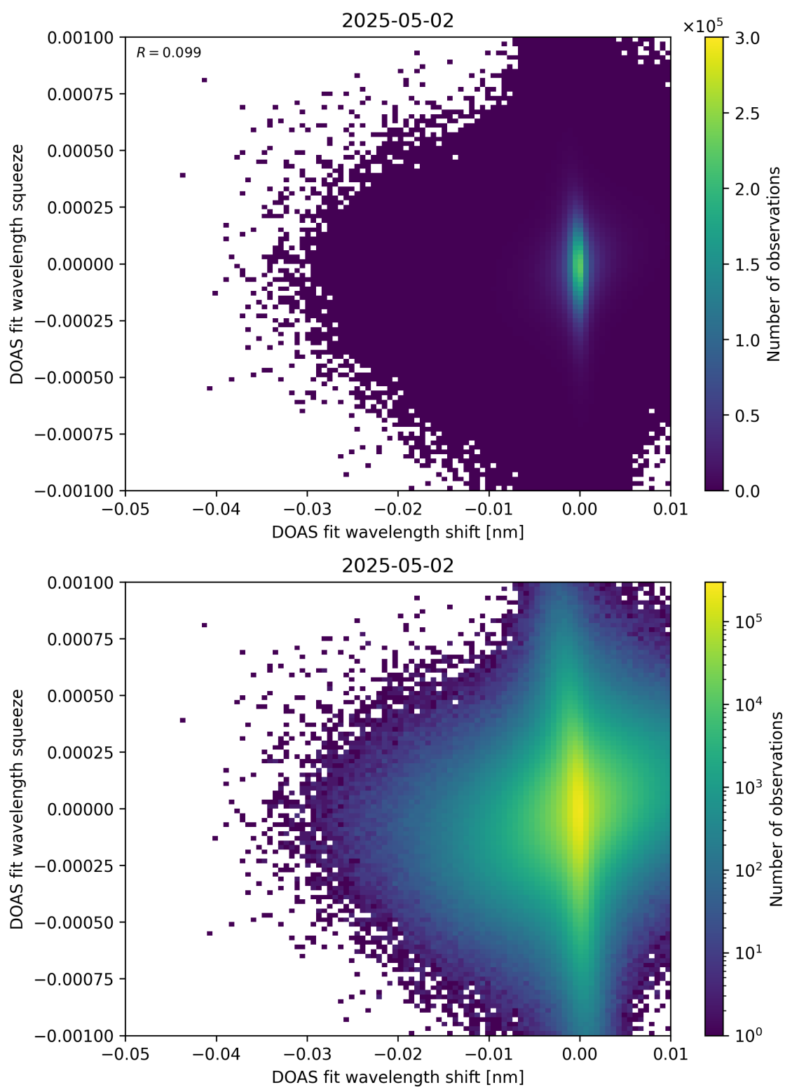
Figure 138: Scatter density plot of “DOAS fit wavelength shift” against “DOAS fit wavelength squeeze” for 2025-05-01 to 2025-05-03.
