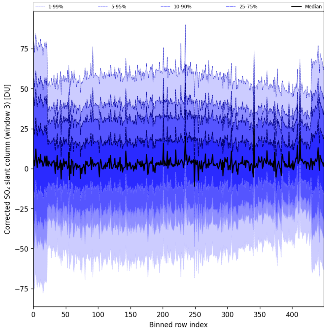
Figure 99: Along track statistics of “Corrected SO 2 slant column (window 3)” for 2025-05-01 to 2025-05-03
