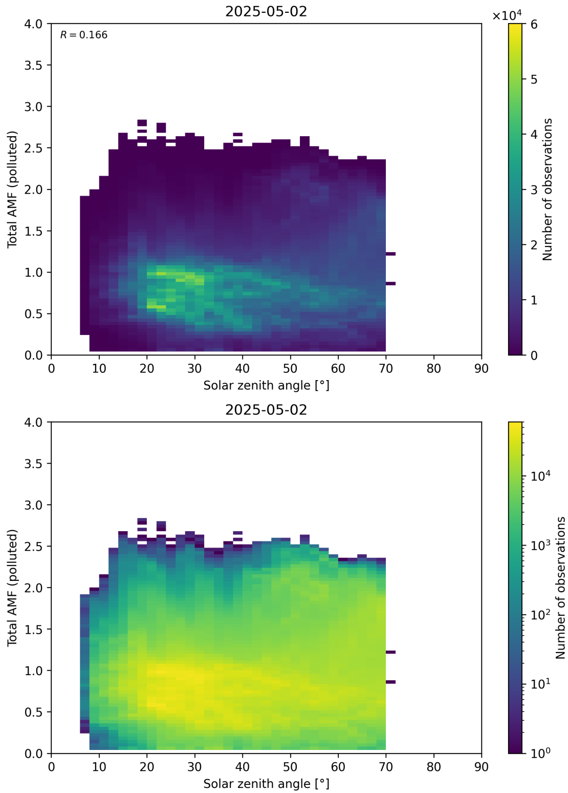
Figure 189: Scatter density plot of “Solar zenith angle” against “Total AMF (polluted)” for 2025-05-01 to 2025-05-03.
