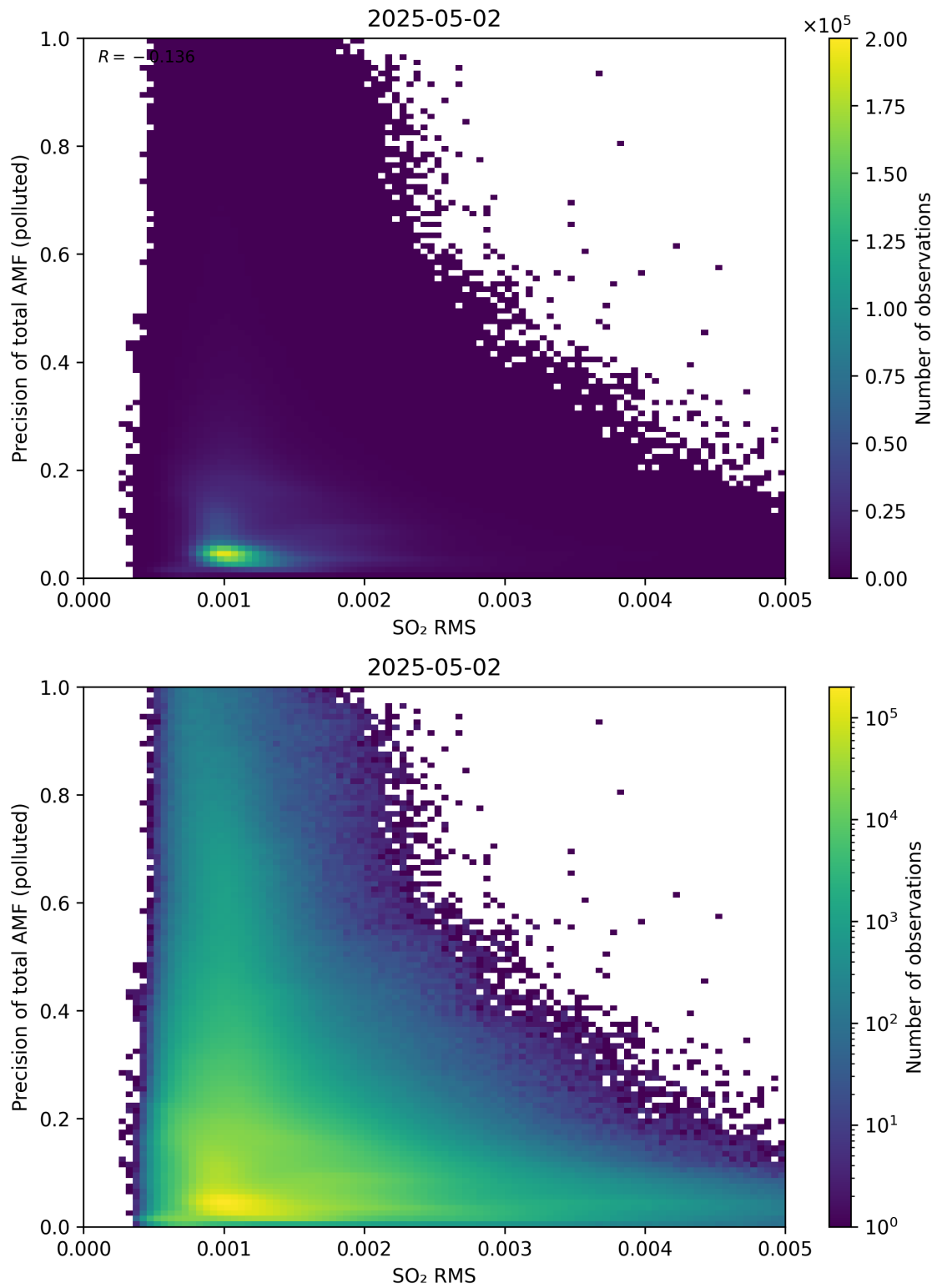
Figure 149: Scatter density plot of “SO 2 RMS” against “Precision of total AMF (polluted)” for 2025-05-01 to 2025-05-03.
