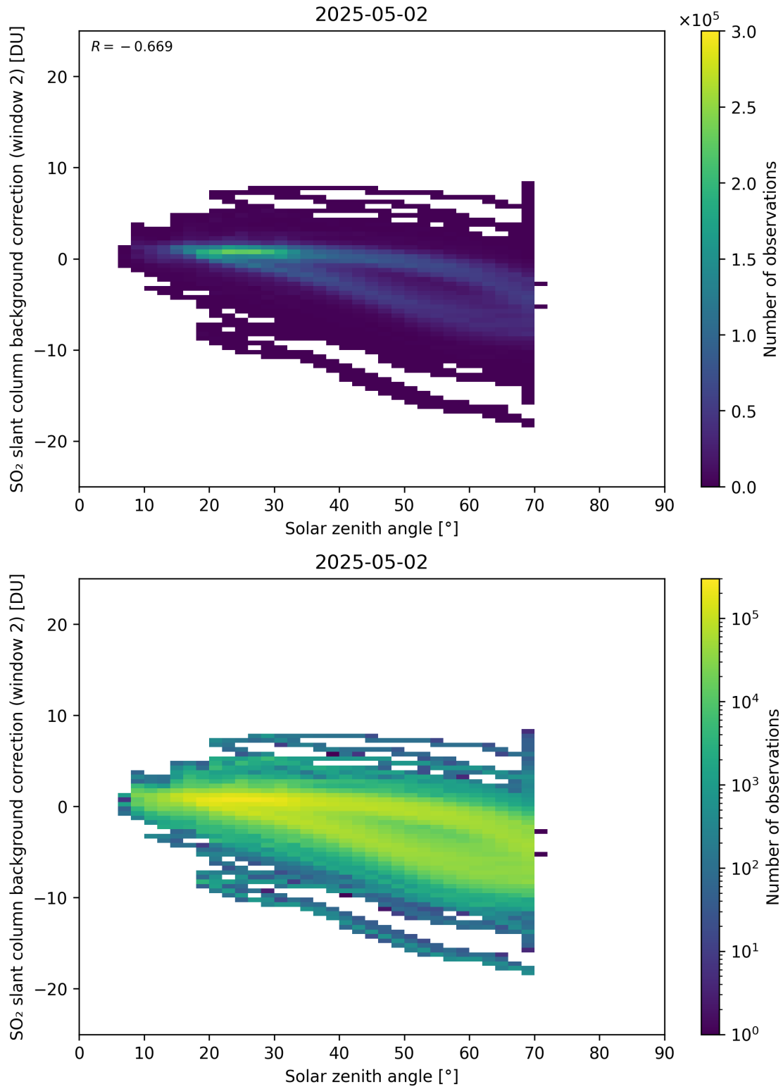
Figure 172: Scatter density plot of “Solar zenith angle” against “SO 2 slant column background correction (window 2)” for 2025-05-01 to 2025-05-03.
