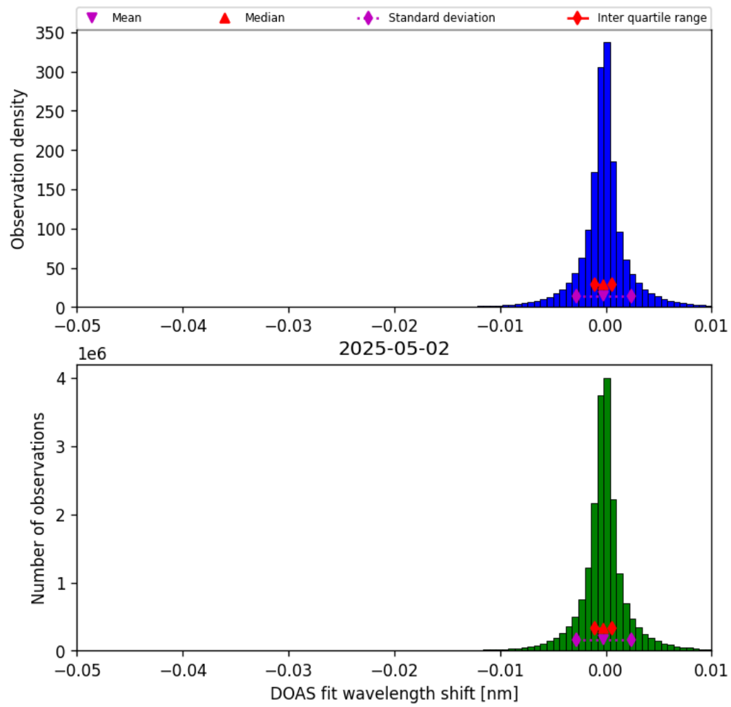
Figure 76: Histogram of “DOAS fit wavelength shift” for 2025-05-01 to 2025-05-03
