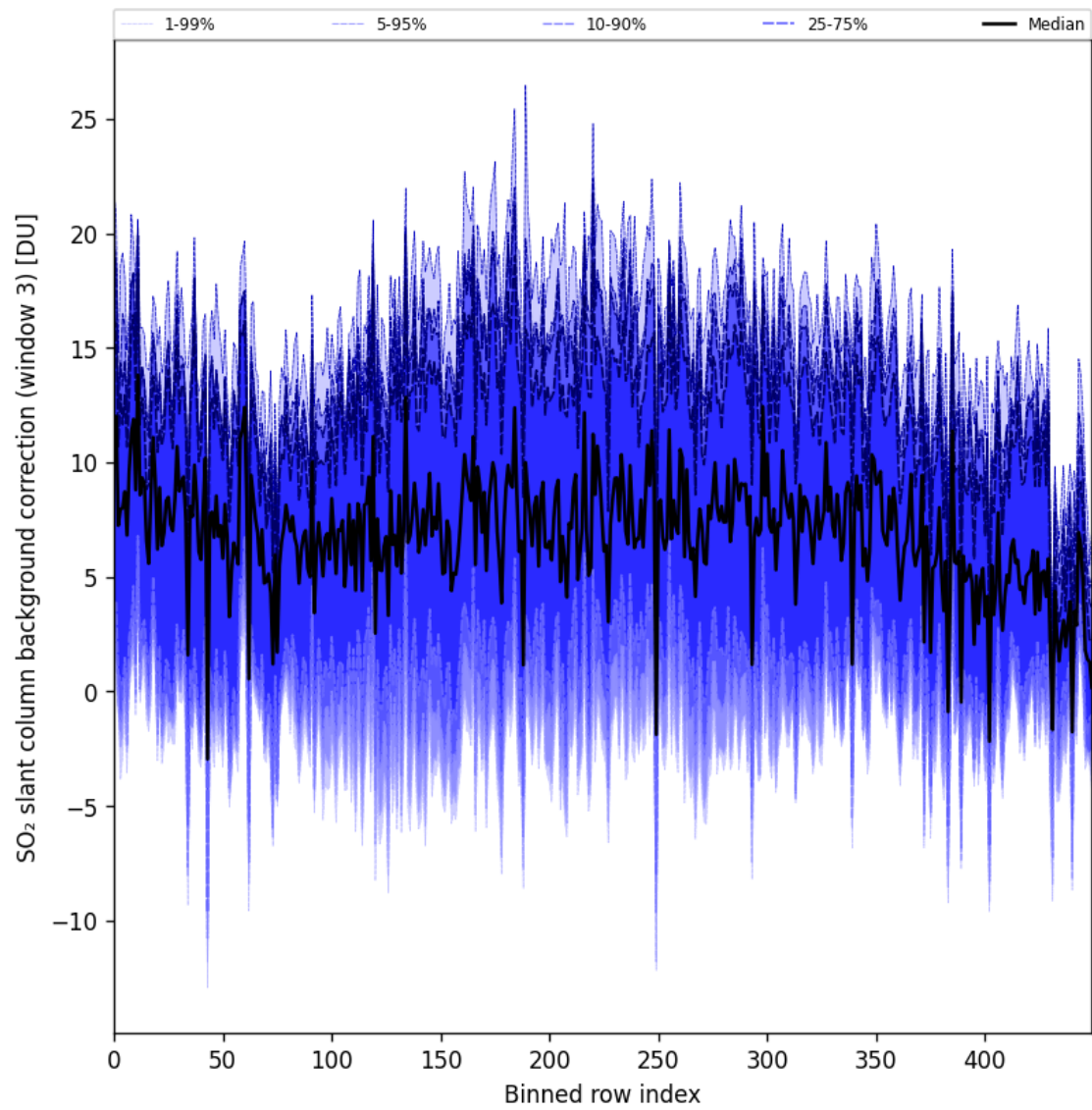
Figure 100: Along track statistics of “SO 2 slant column background correction (window 3)” for 2025-05-01 to 2025-05-03
