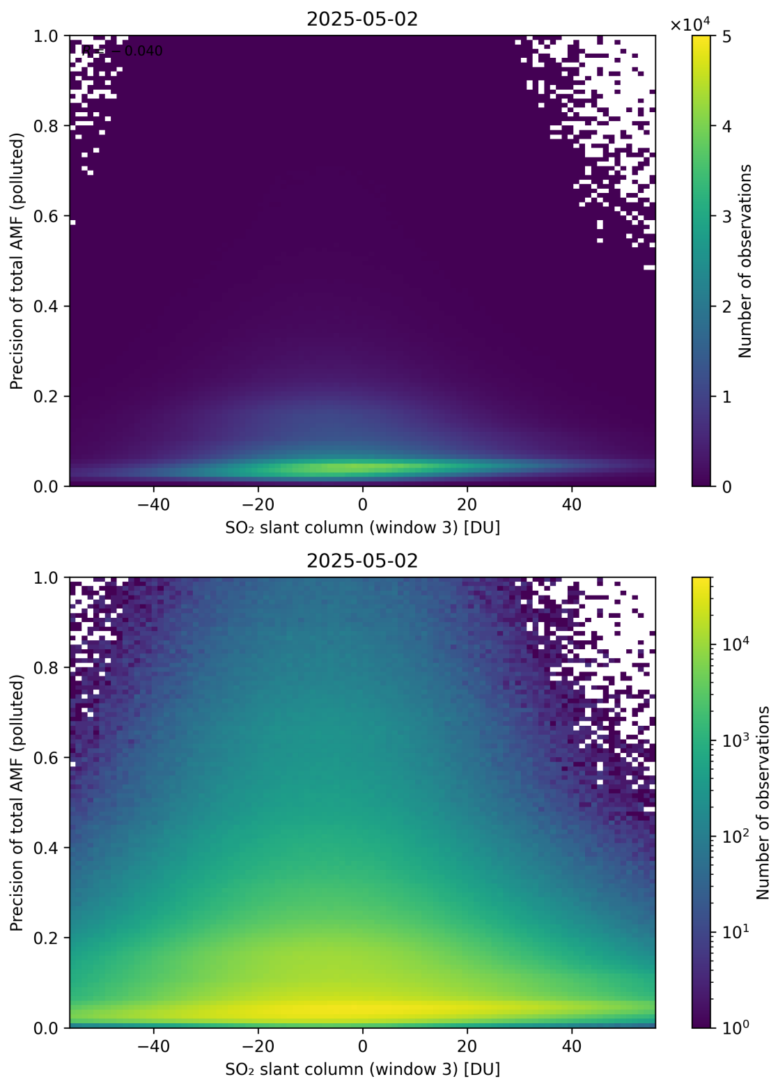
Figure 319: Scatter density plot of “SO 2 slant column (window 3)” against “Precision of total AMF (polluted)” for 2025-05-01 to 2025-05-03.
