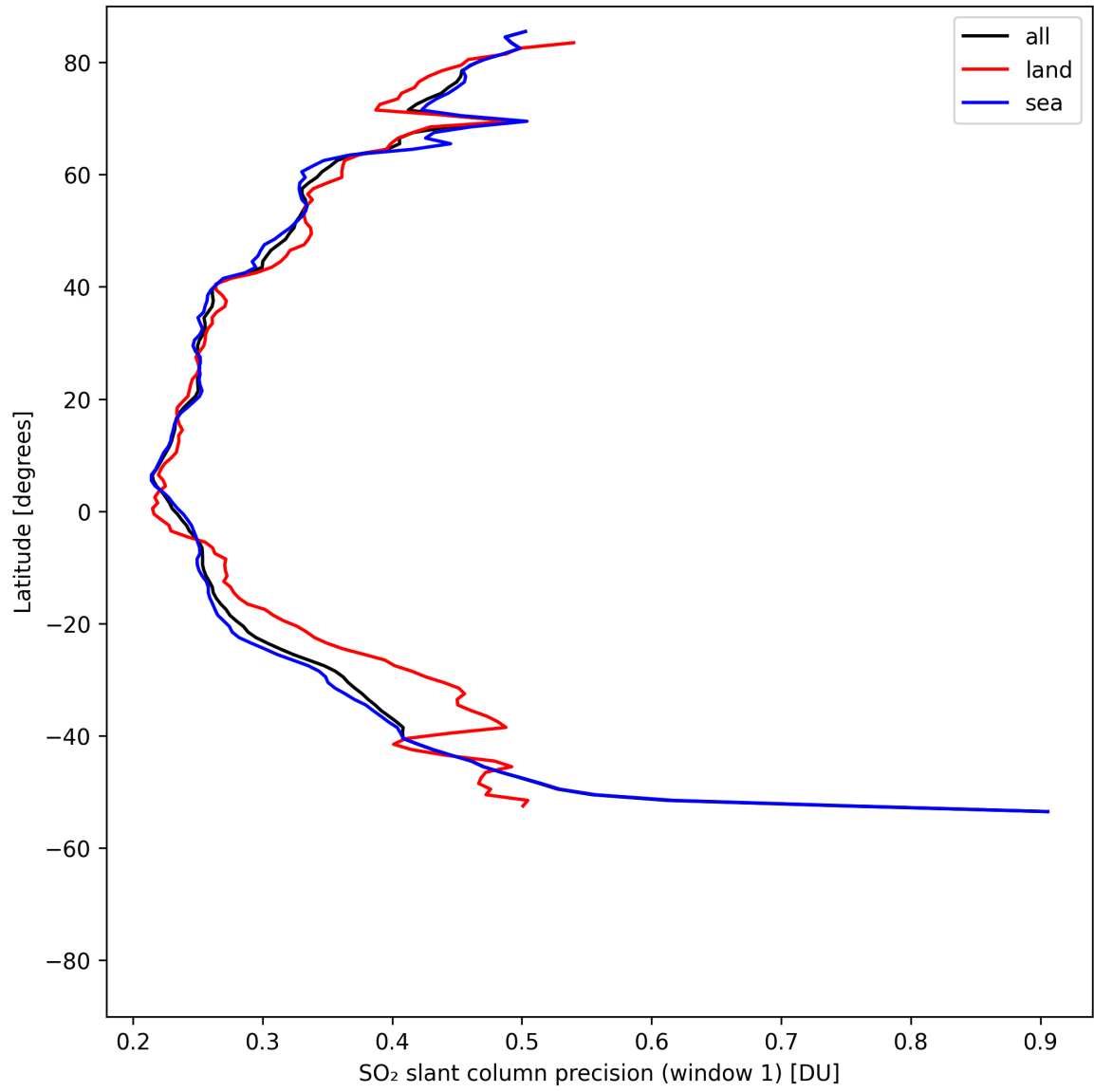
Figure 38: Zonal average of “SO 2 slant column precision (window 1)” for 2025-05-01 to 2025-05-03.
