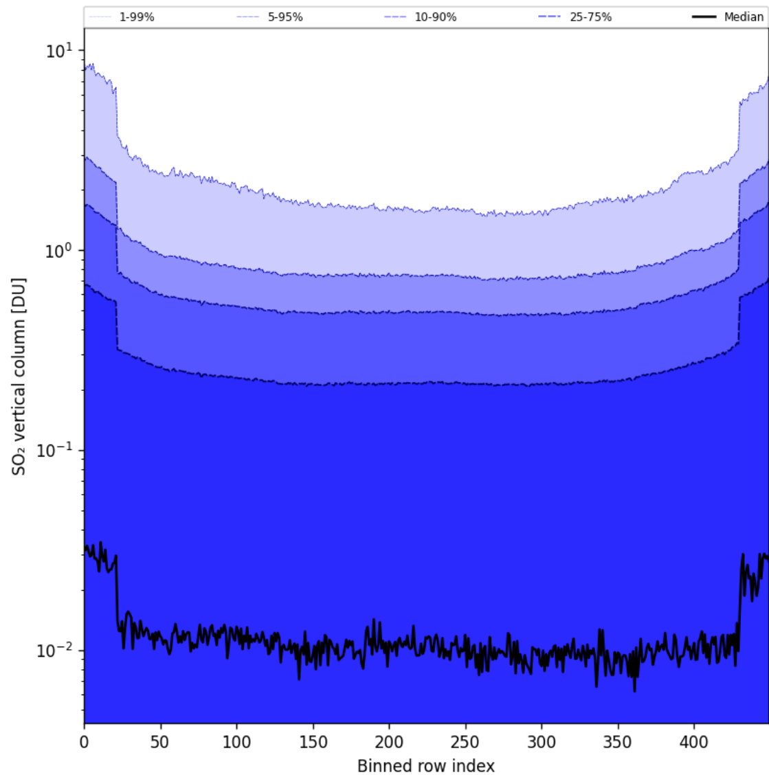
Figure 84: Along track statistics of “SO 2 vertical column” for 2025-05-01 to 2025-05-03
