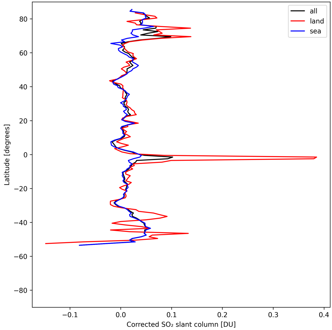
Figure 34: Zonal average of “Corrected SO 2 slant column” for 2025-05-01 to 2025-05-03.
