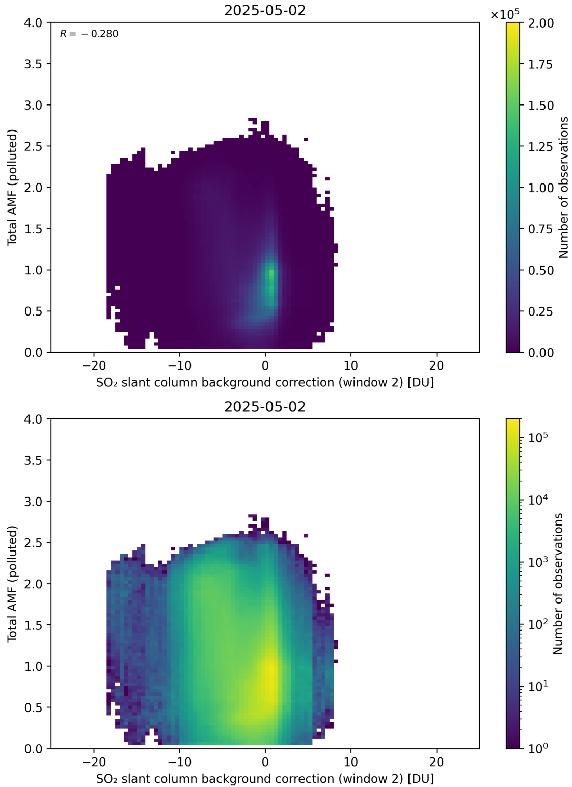
Figure 130: Scatter density plot of “SO 2 slant column background correction (window 2)” against “Total AMF (polluted)” for 2025-05-01 to 2025-05-03.
