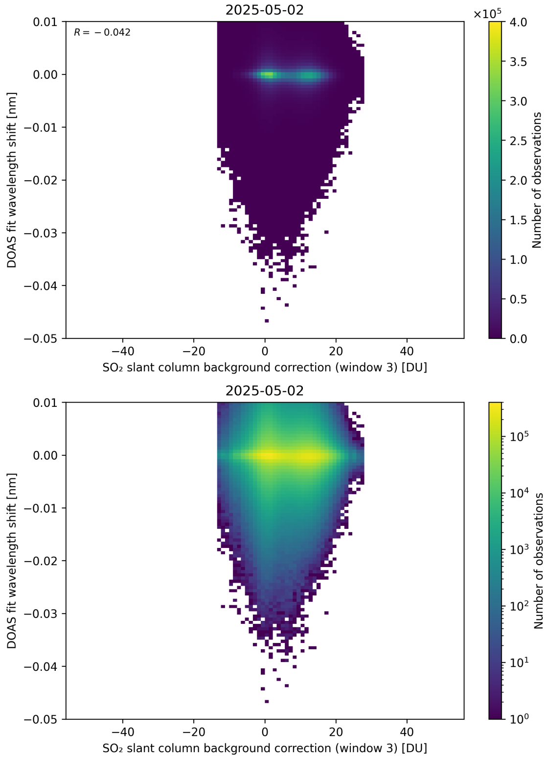
Figure 132: Scatter density plot of “SO 2 slant column background correction (window 3)” against “DOAS fit wavelength shift” for 2025-05-01 to 2025-05-03.
