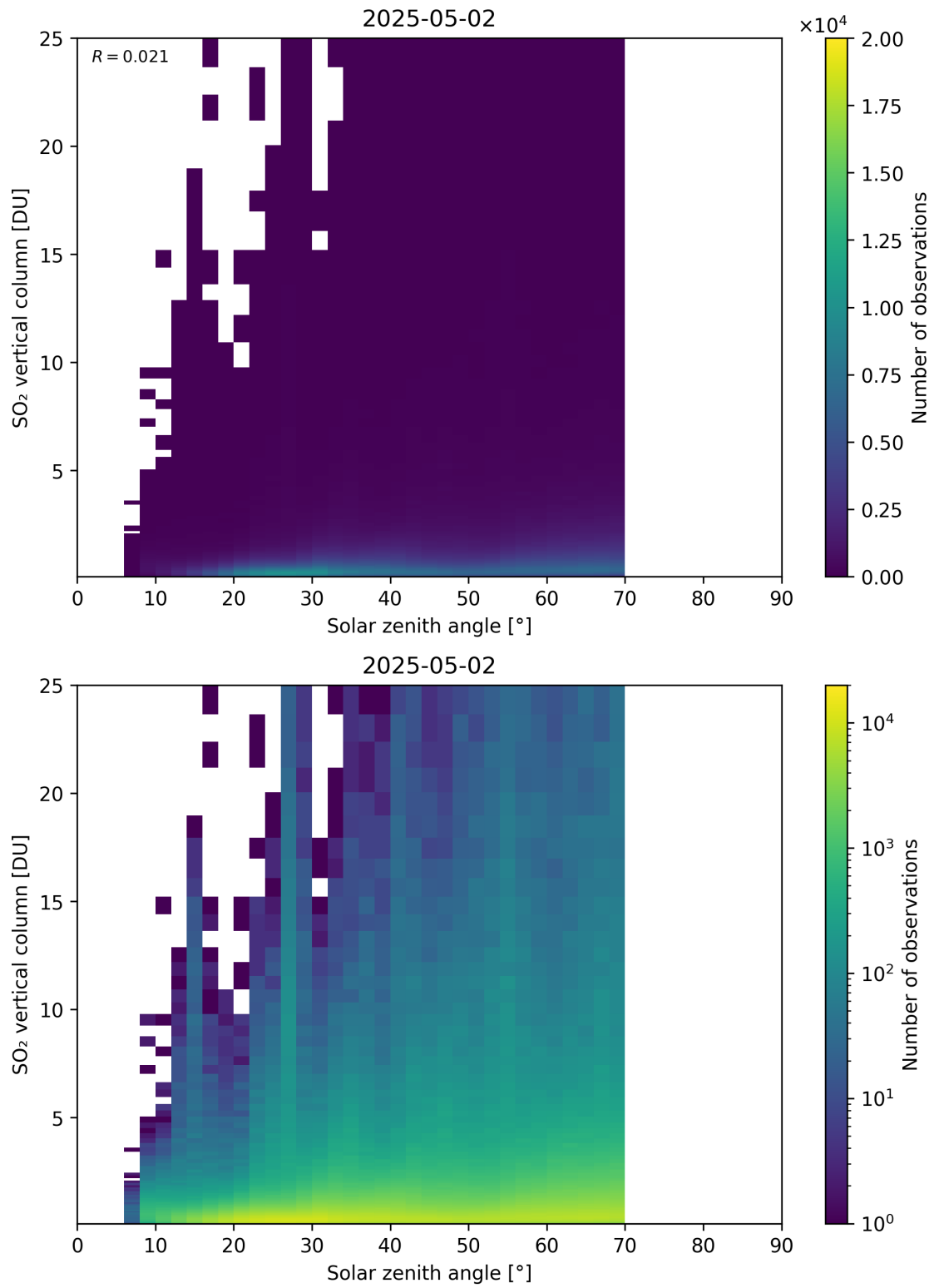
Figure 191: Scatter density plot of “Solar zenith angle” against “SO 2 vertical column” for 2025-05-01 to 2025-05-03.
