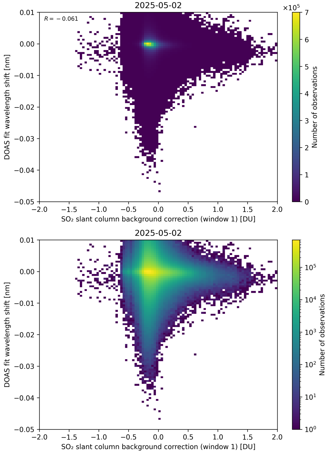
Figure 111: Scatter density plot of “SO 2 slant column background correction (window 1)” against “DOAS fit wavelength shift” for 2025-05-01 to 2025-05-03.
