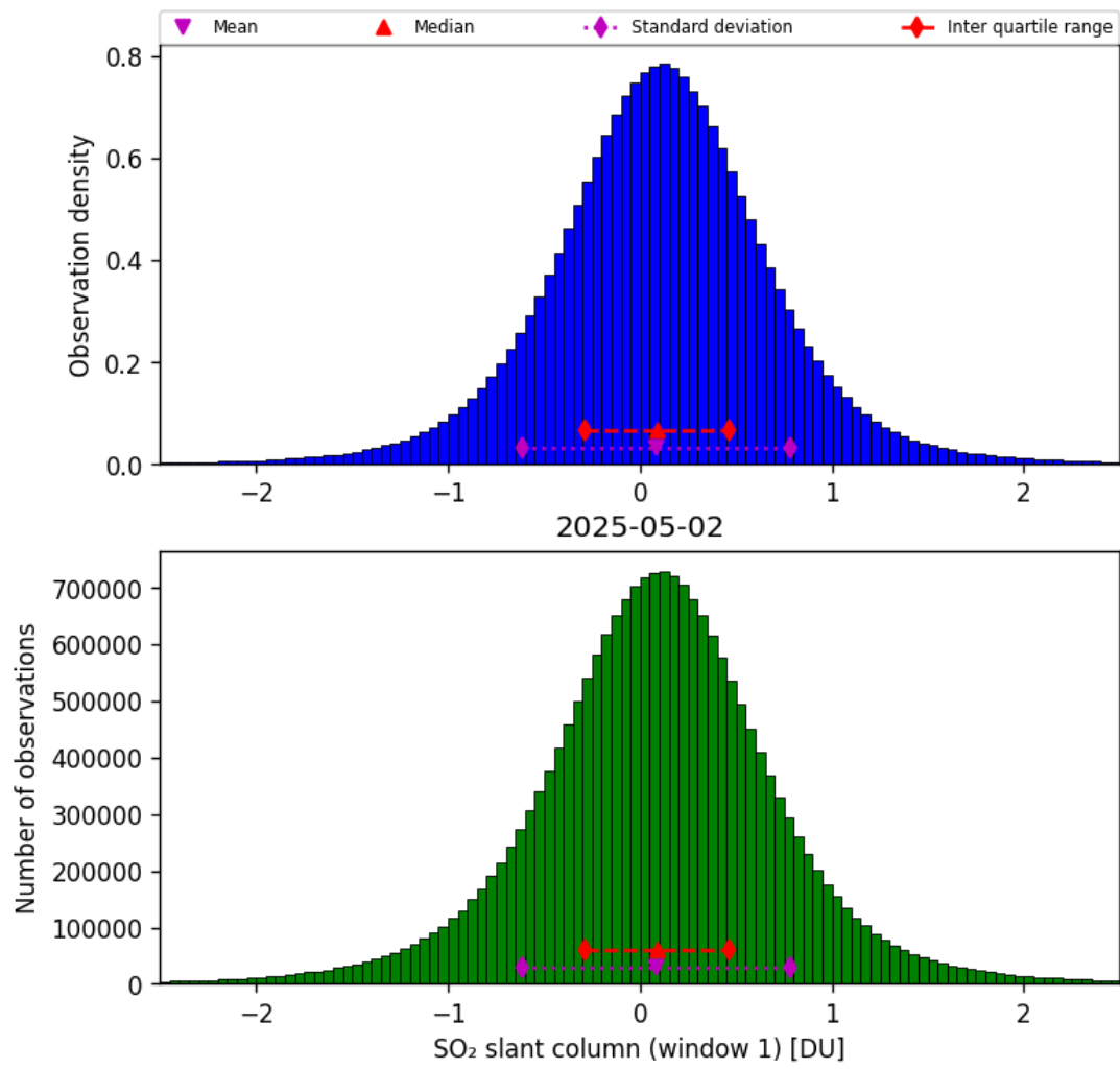
Figure 63: Histogram of “SO 2 slant column (window 1)” for 2025-05-01 to 2025-05-03
