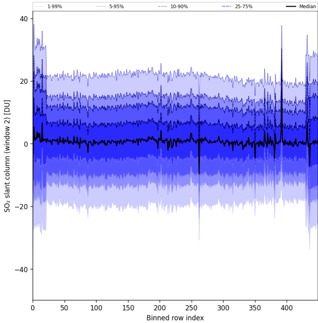
Figure 93: Along track statistics of "SO 2 slant column (window 2)" for 2025-05-01 to 2025-05-03
