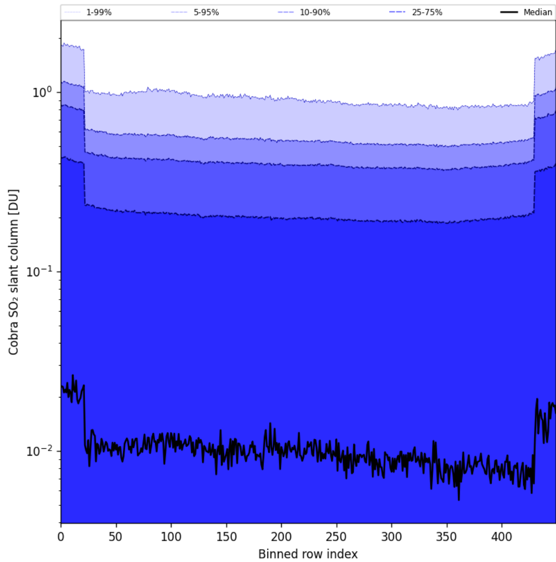
Figure 87: Along track statistics of “Cobra SO 2 slant column” for 2025-05-01 to 2025-05-03
