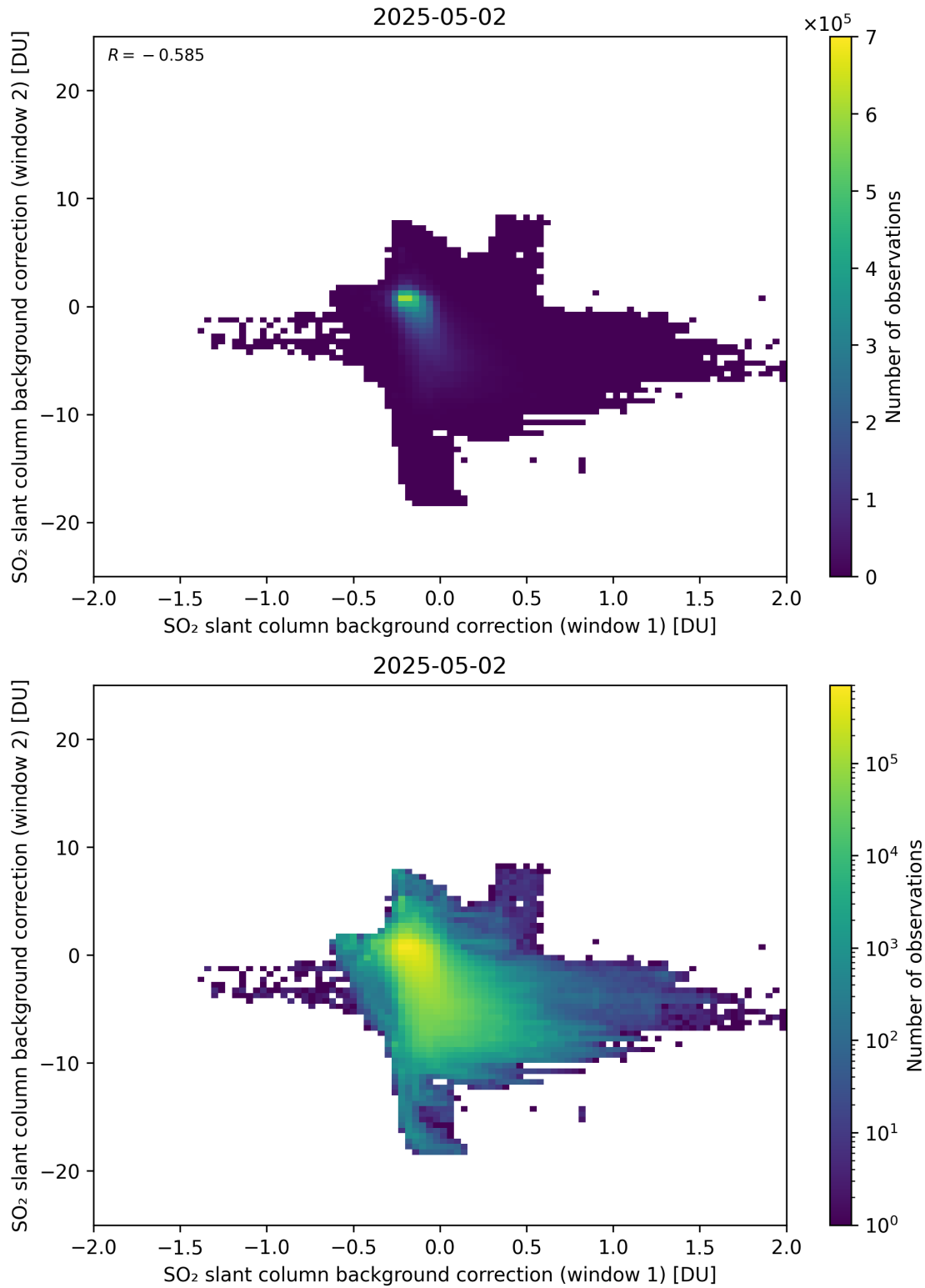
Figure 109: Scatter density plot of “SO 2 slant column background correction (window 1)” against “SO 2 slant column background correction (window 2)” for 2025-05-01 to 2025-05-03.
