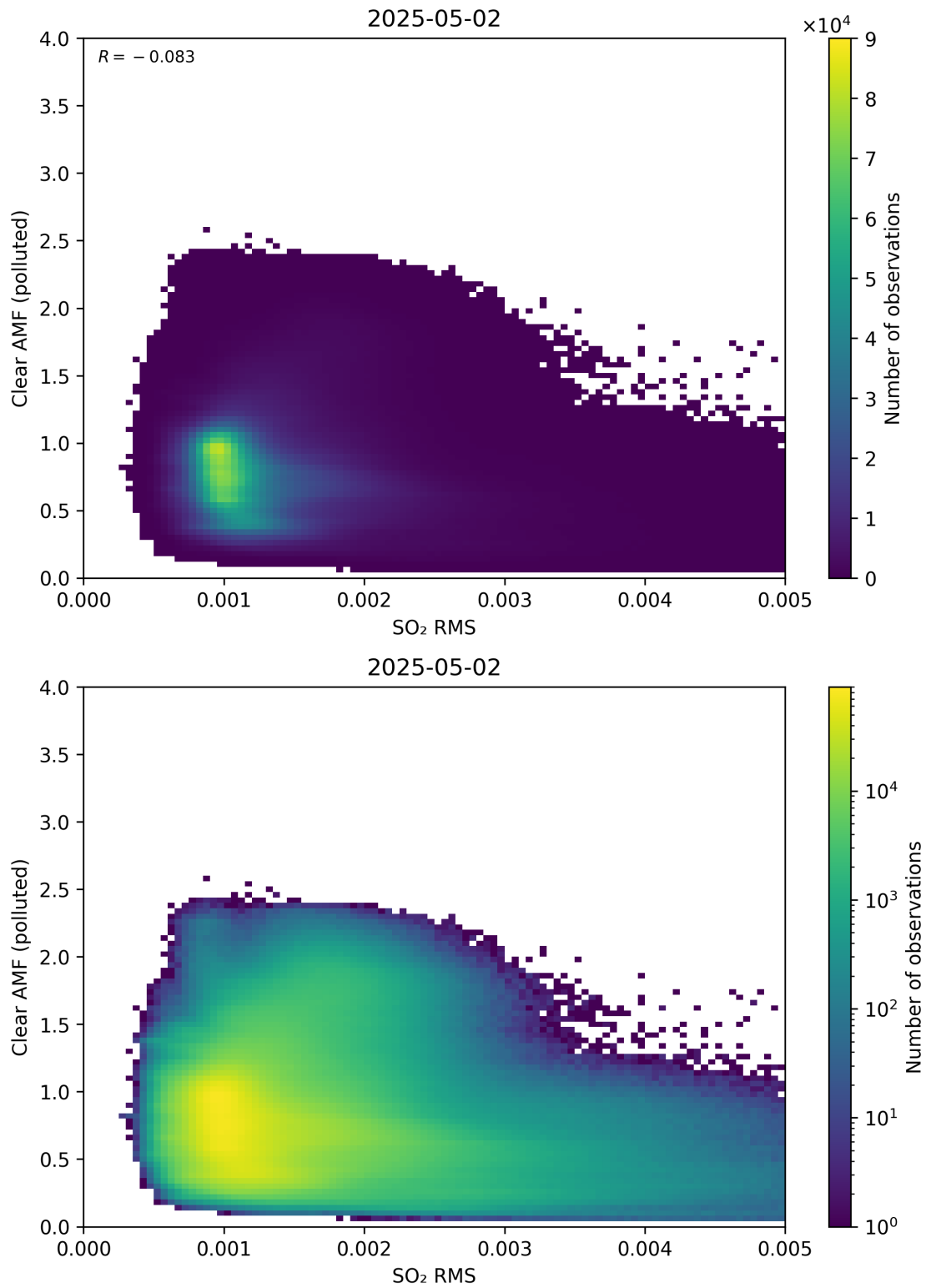
Figure 147: Scatter density plot of “SO 2 RMS” against “Clear AMF (polluted)” for 2025-05-01 to 2025-05-03.
