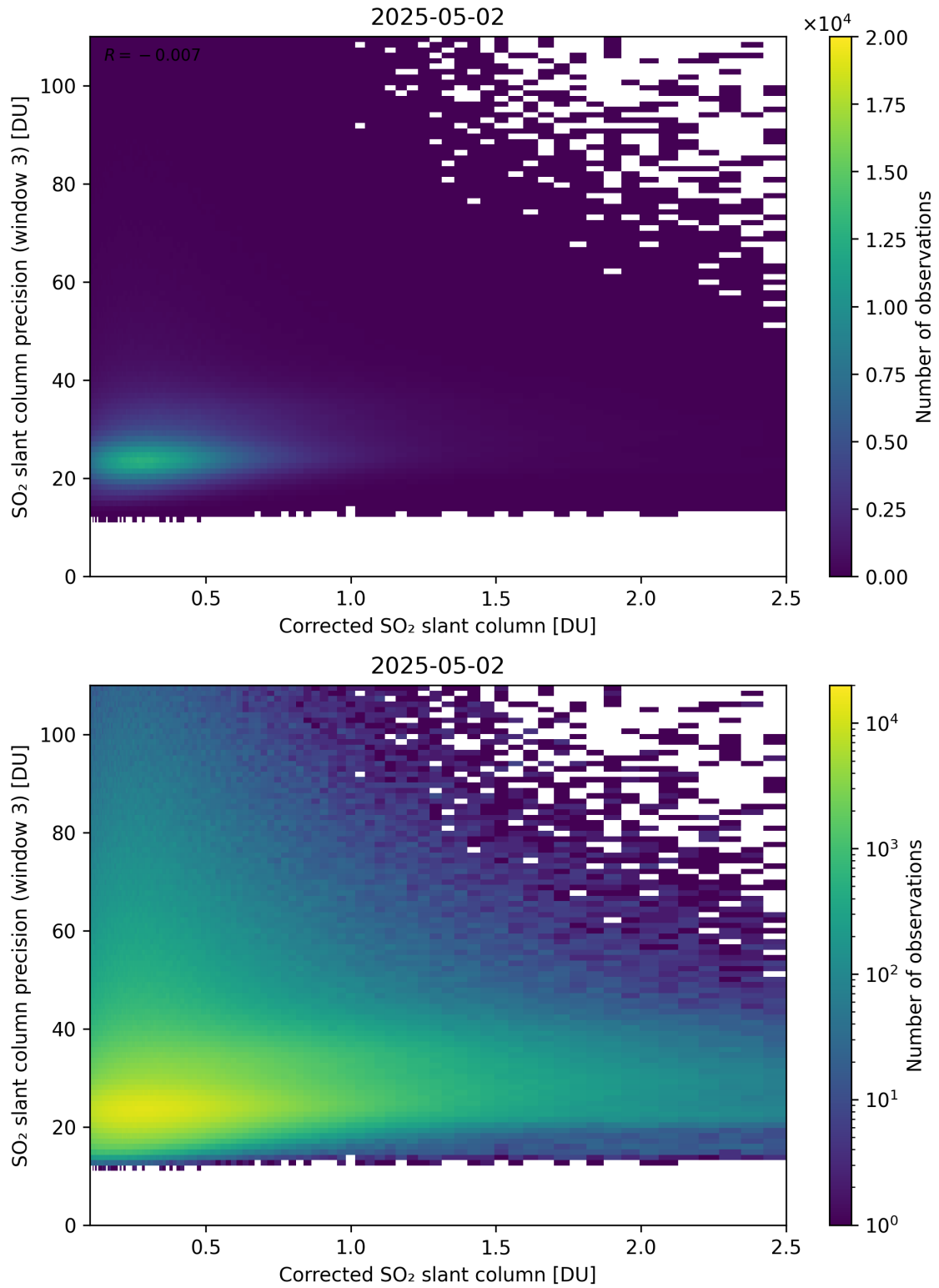
Figure 241: Scatter density plot of “Corrected SO 2 slant column” against “SO 2 slant column precision (window 3)” for 2025-05-01 to 2025-05-03.
