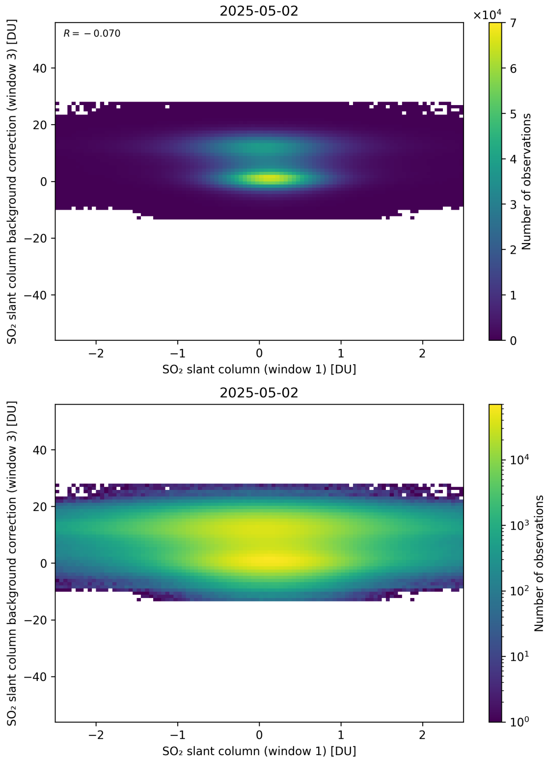
Figure 264: Scatter density plot of “SO 2 slant column (window 1)” against “SO 2 slant column background correction (window 3)” for 2025-05-01 to 2025-05-03.
