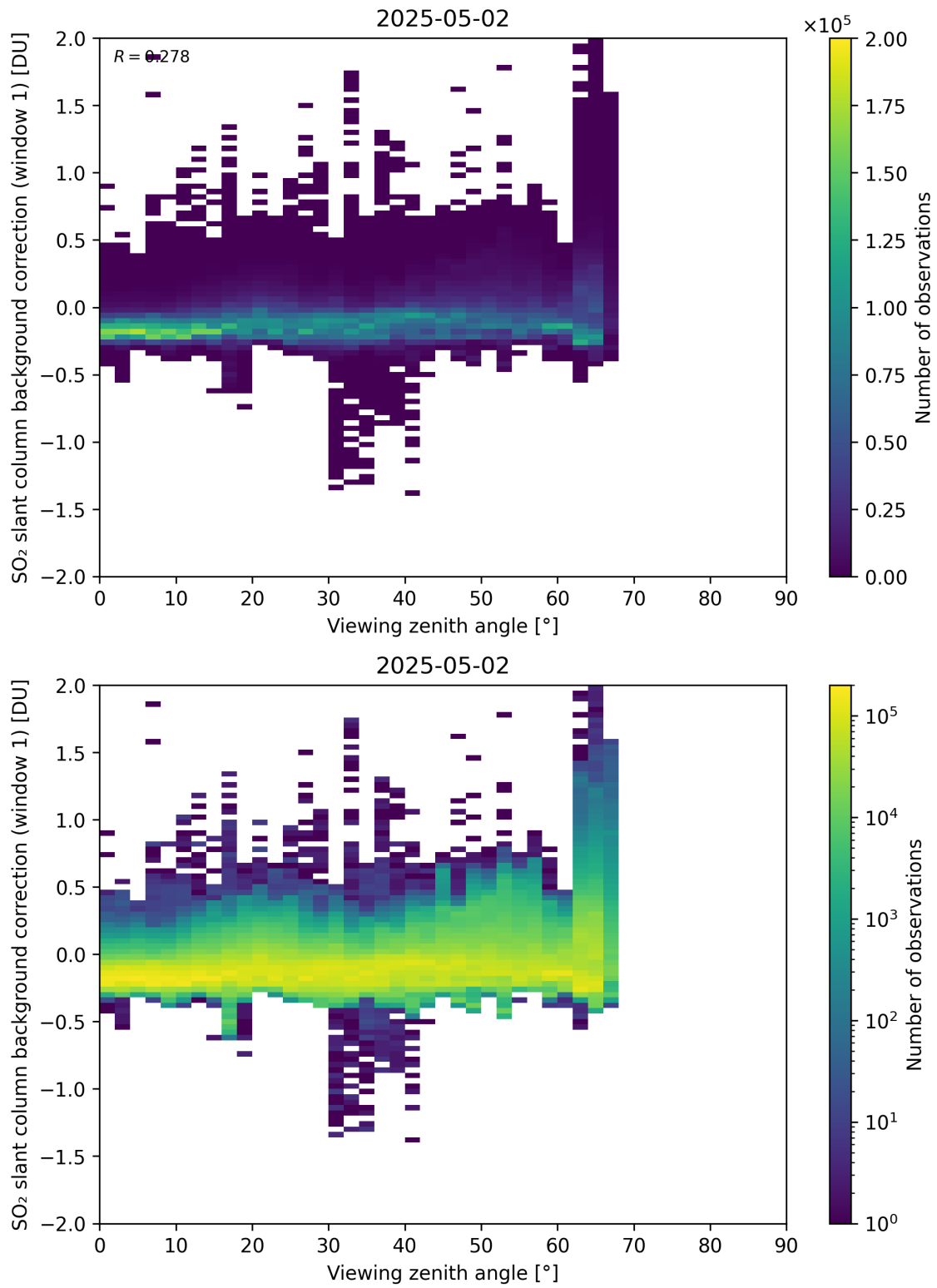
Figure 362: Scatter density plot of “Viewing zenith angle” against “SO 2 slant column background correction (window 1)” for 2025-05-01 to 2025-05-03.
