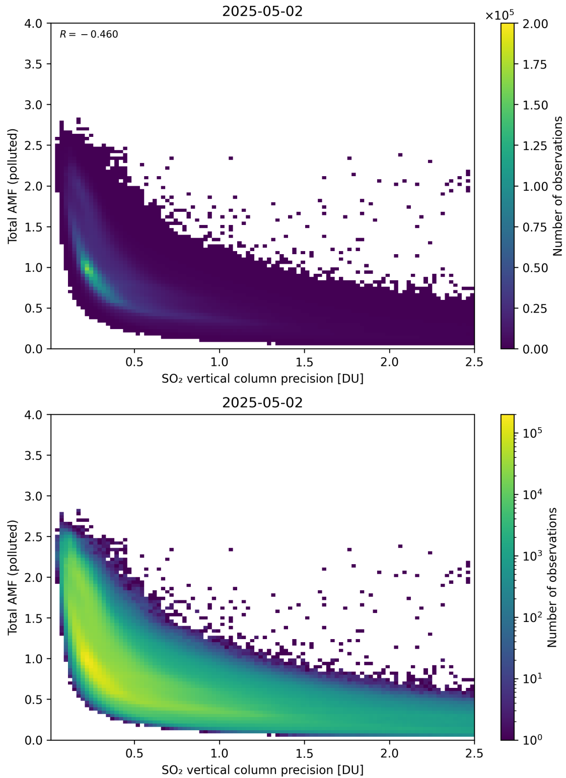
Figure 346: Scatter density plot of “SO 2 vertical column precision” against “Total AMF (polluted)” for 2025-05-01 to 2025-05-03.
