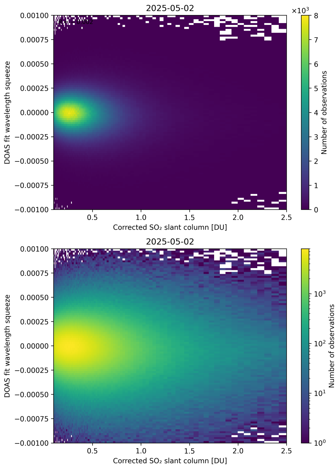
Figure 230: Scatter density plot of “Corrected SO 2 slant column” against “DOAS fit wavelength squeeze” for 2025-05-01 to 2025-05-03.
