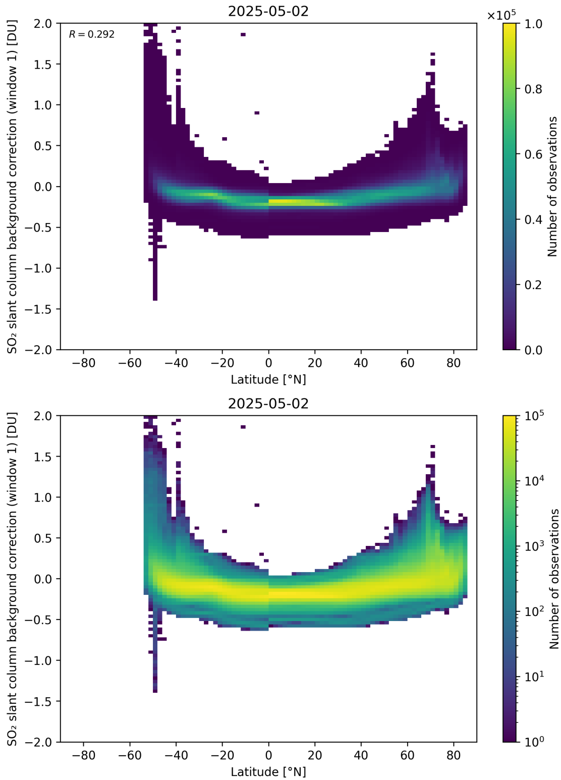
Figure 150: Scatter density plot of “Latitude” against “SO 2 slant column background correction (window 1)” for 2025-05-01 to 2025-05-03.
