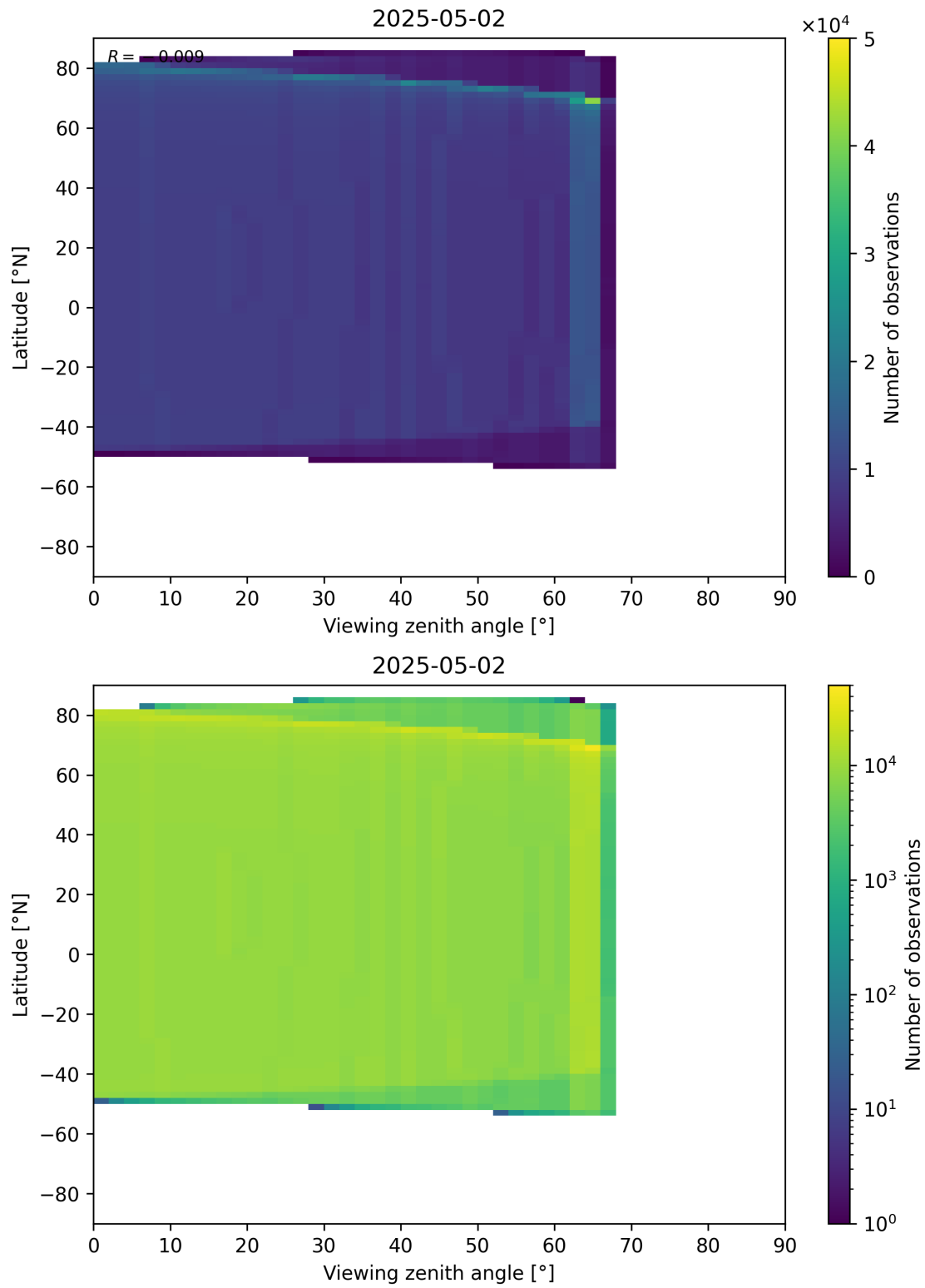
Figure 368: Scatter density plot of “Viewing zenith angle” against “Latitude” for 2025-05-01 to 2025-05-03.
