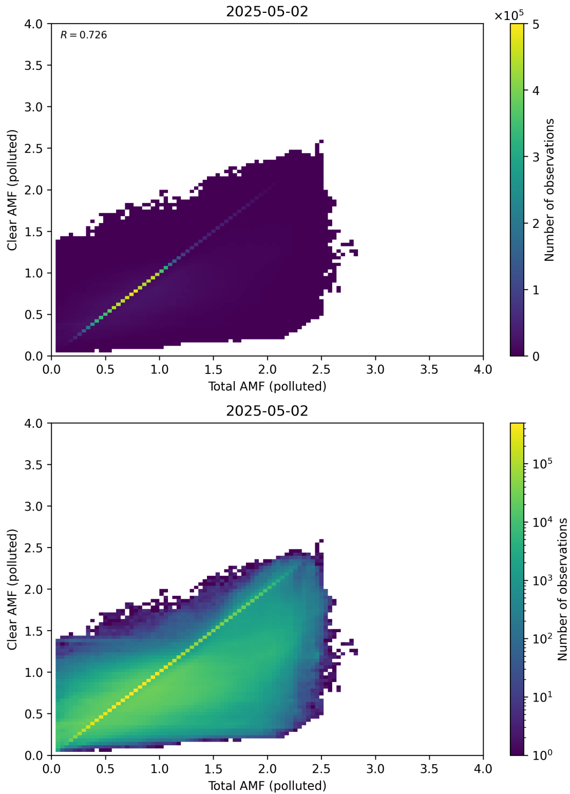
Figure 321: Scatter density plot of “Total AMF (polluted)” against “Clear AMF (polluted)” for 2025-05-01 to 2025-05-03.
