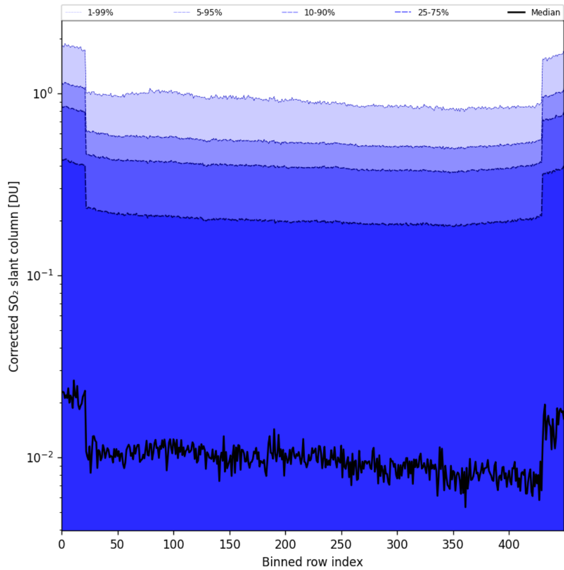
Figure 86: Along track statistics of “Corrected SO 2 slant column” for 2025-05-01 to 2025-05-03
