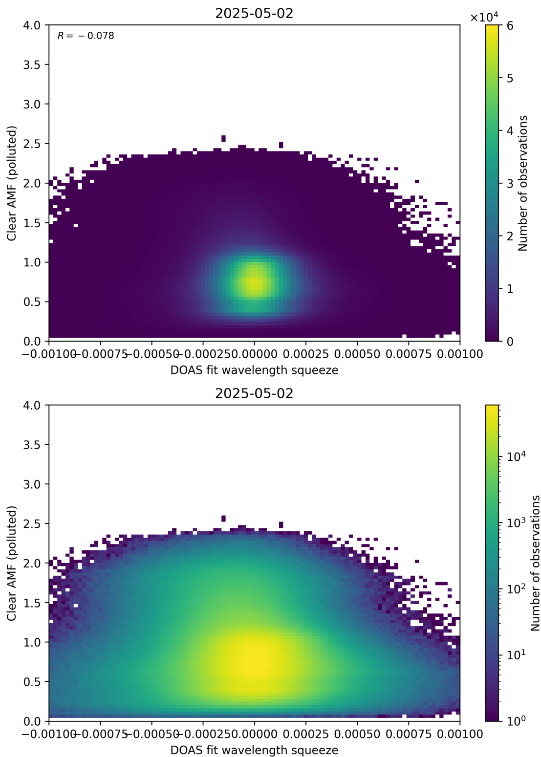
Figure 144: Scatter density plot of “DOAS fit wavelength squeeze” against “Clear AMF (polluted)” for 2025-05-01 to 2025-05-03.
