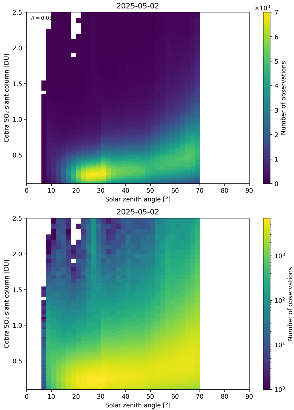
Figure 179: Scatter density plot of “Solar zenith angle” against “Cobra SO 2 slant column” for 2025-05-01 to 2025-05-03.
