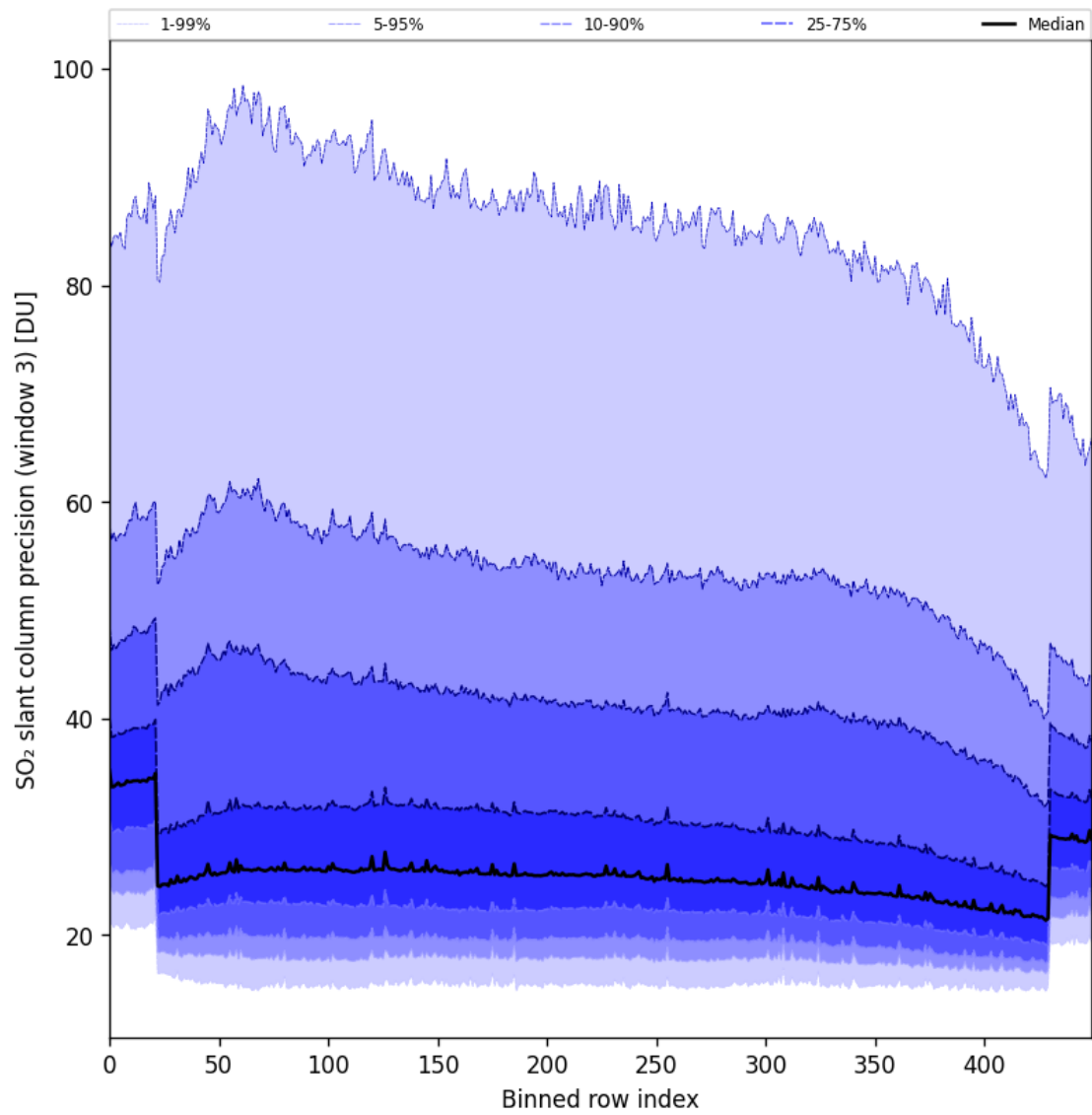
Figure 98: Along track statistics of “SO 2 slant column precision (window 3)” for 2025-05-01 to 2025-05-03
