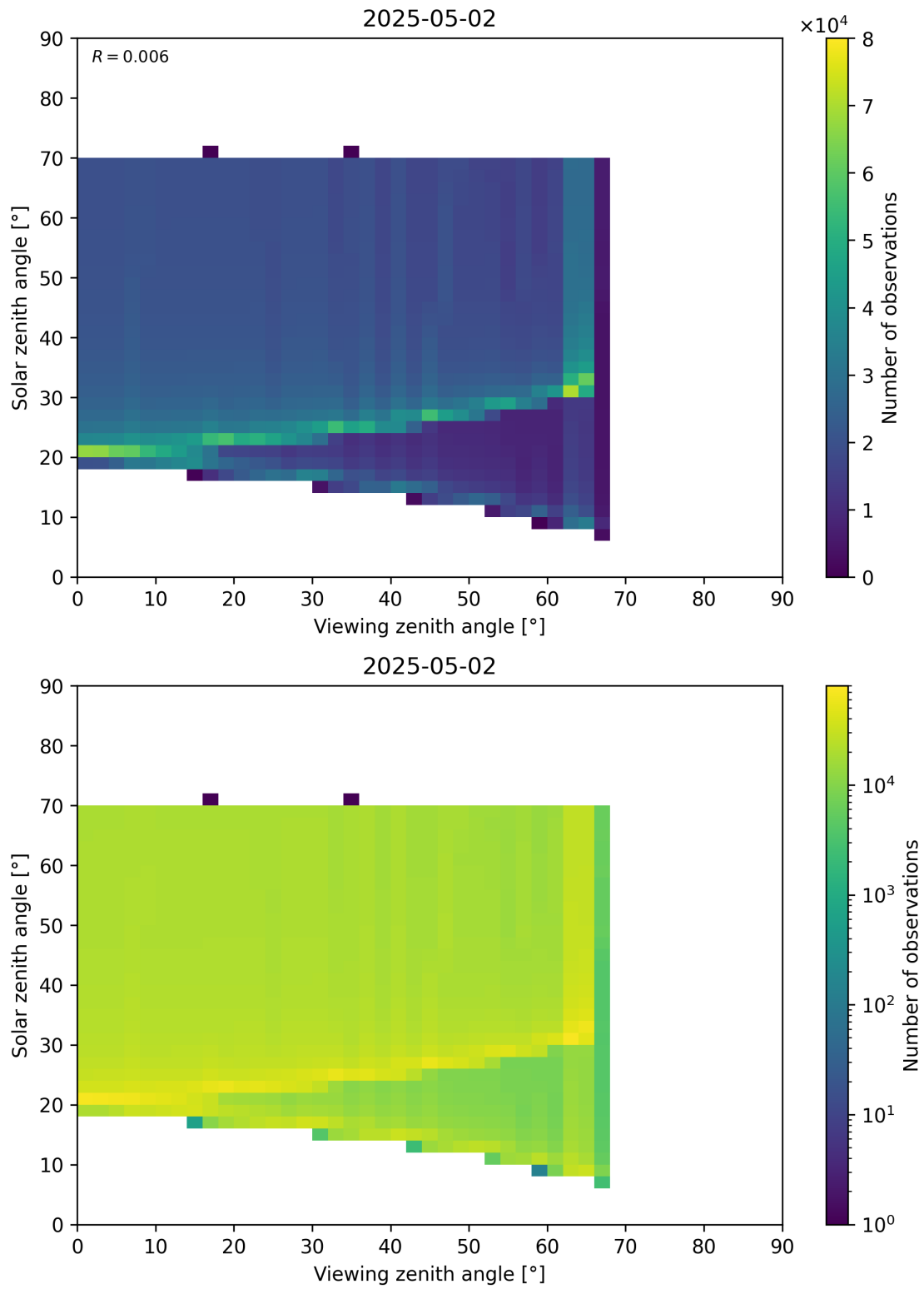
Figure 369: Scatter density plot of “Viewing zenith angle” against “Solar zenith angle” for 2025-05-01 to 2025-05-03.
