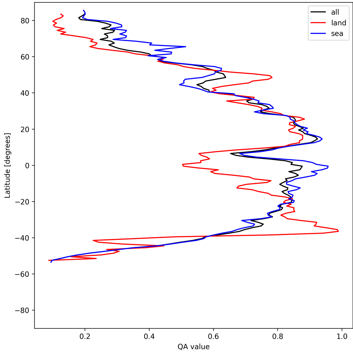
Figure 31: Zonal average of “QA value” for 2025-05-01 to 2025-05-03.
