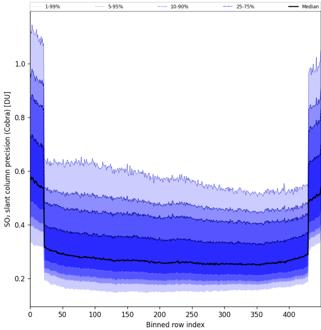
Figure 88: Along track statistics of “SO 2 slant column precision (Cobra)” for 2025-05-01 to 2025-05-03
