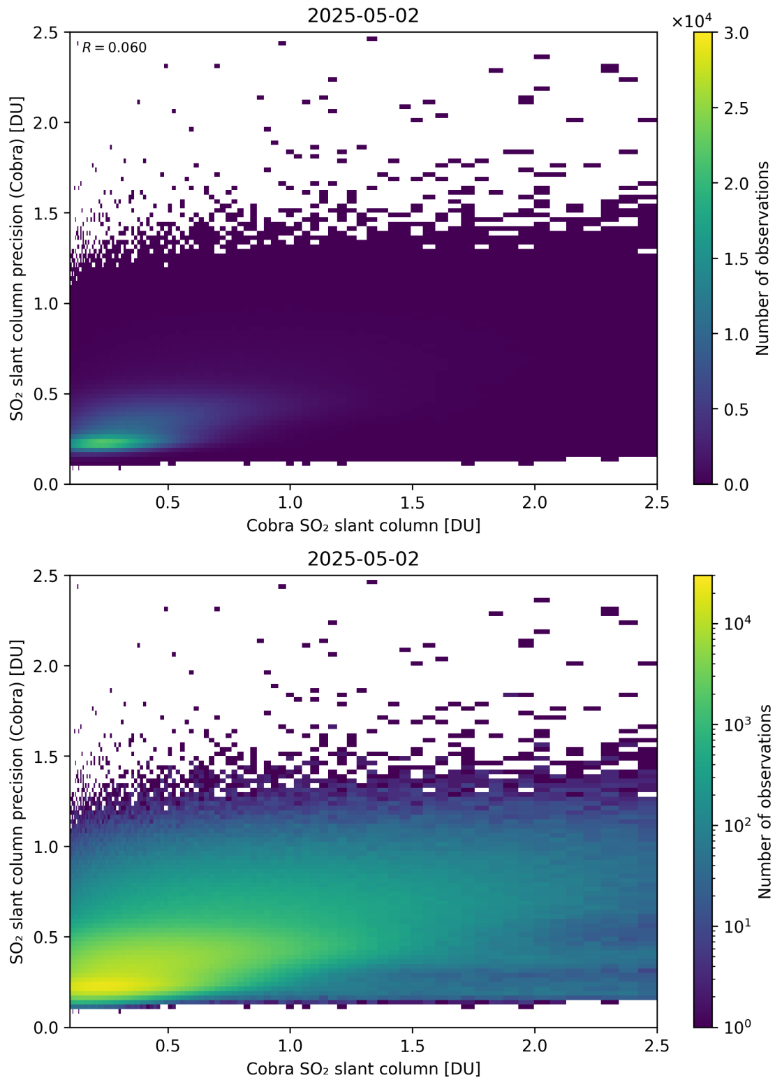
Figure 216: Scatter density plot of “Cobra SO 2 slant column” against “SO 2 slant column precision (Cobra)” for 2025-05-01 to 2025-05-03.
