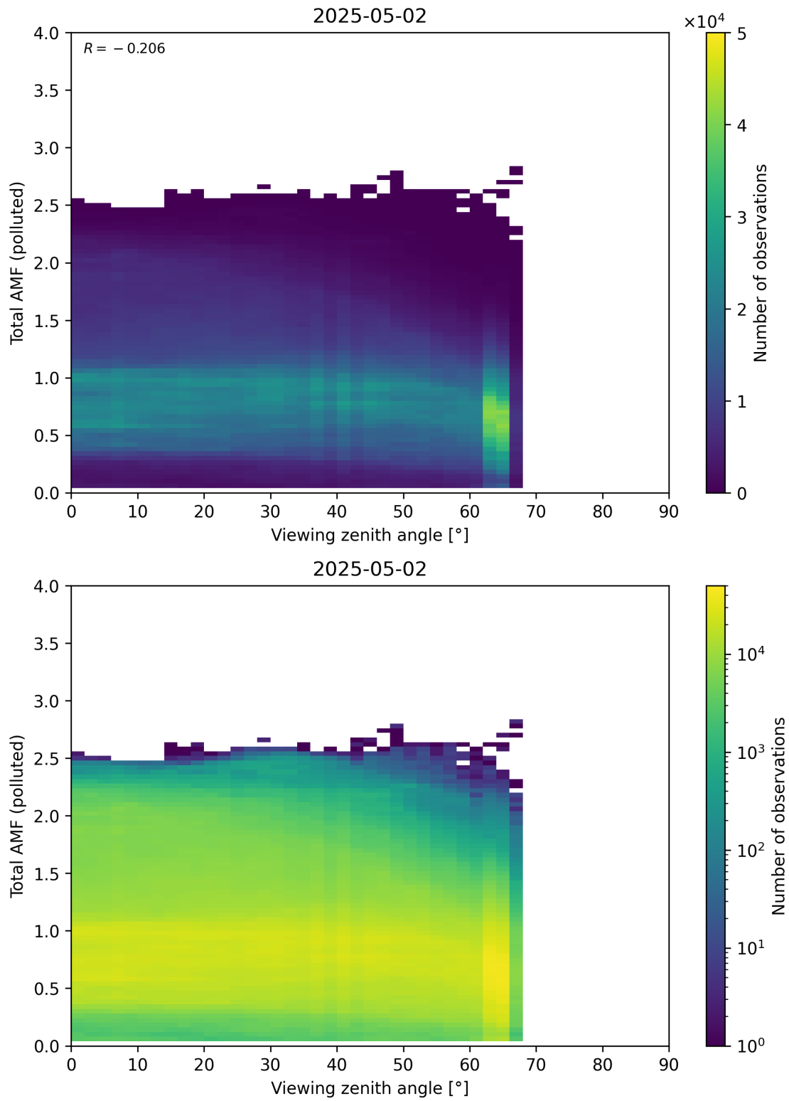
Figure 381: Scatter density plot of “Viewing zenith angle” against “Total AMF (polluted)” for 2025-05-01 to 2025-05-03.
