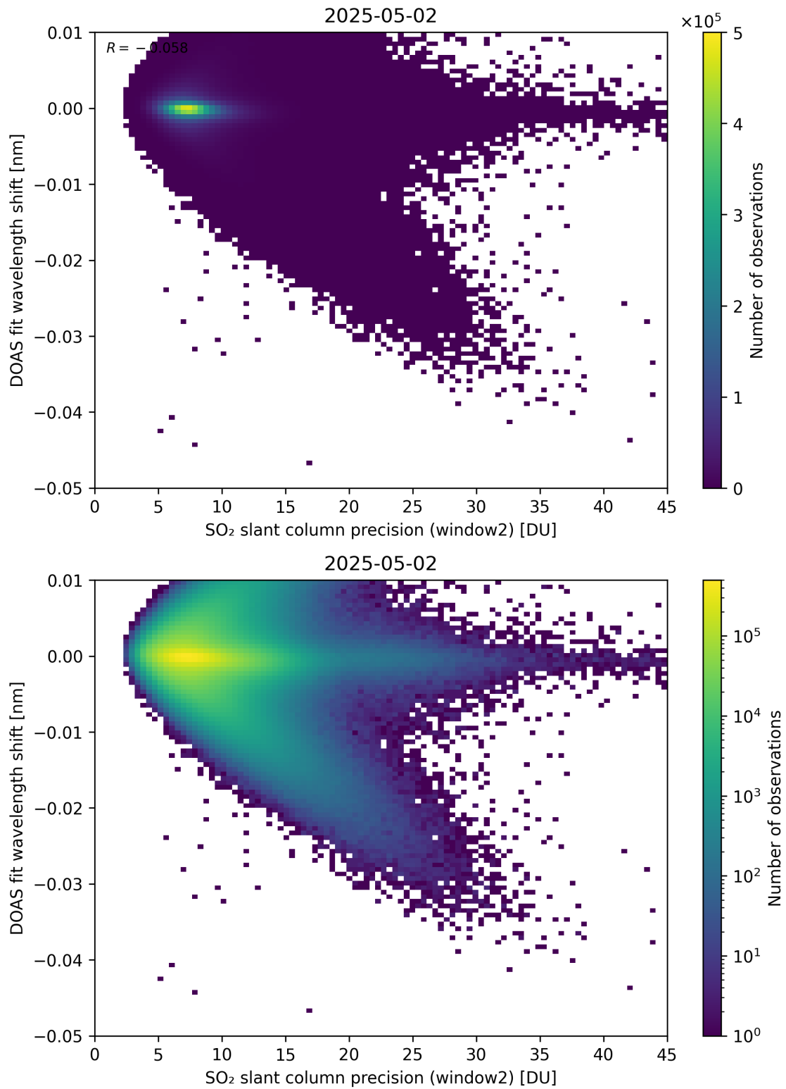
Figure 293: Scatter density plot of “SO 2 slant column precision (window2)” against “DOAS fit wavelength shift” for 2025-05-01 to 2025-05-03.
