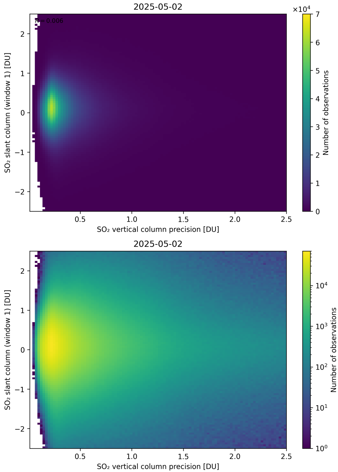
Figure 341: Scatter density plot of “SO 2 vertical column precision” against “SO 2 slant column (window 1)” for 2025-05-01 to 2025-05-03.
