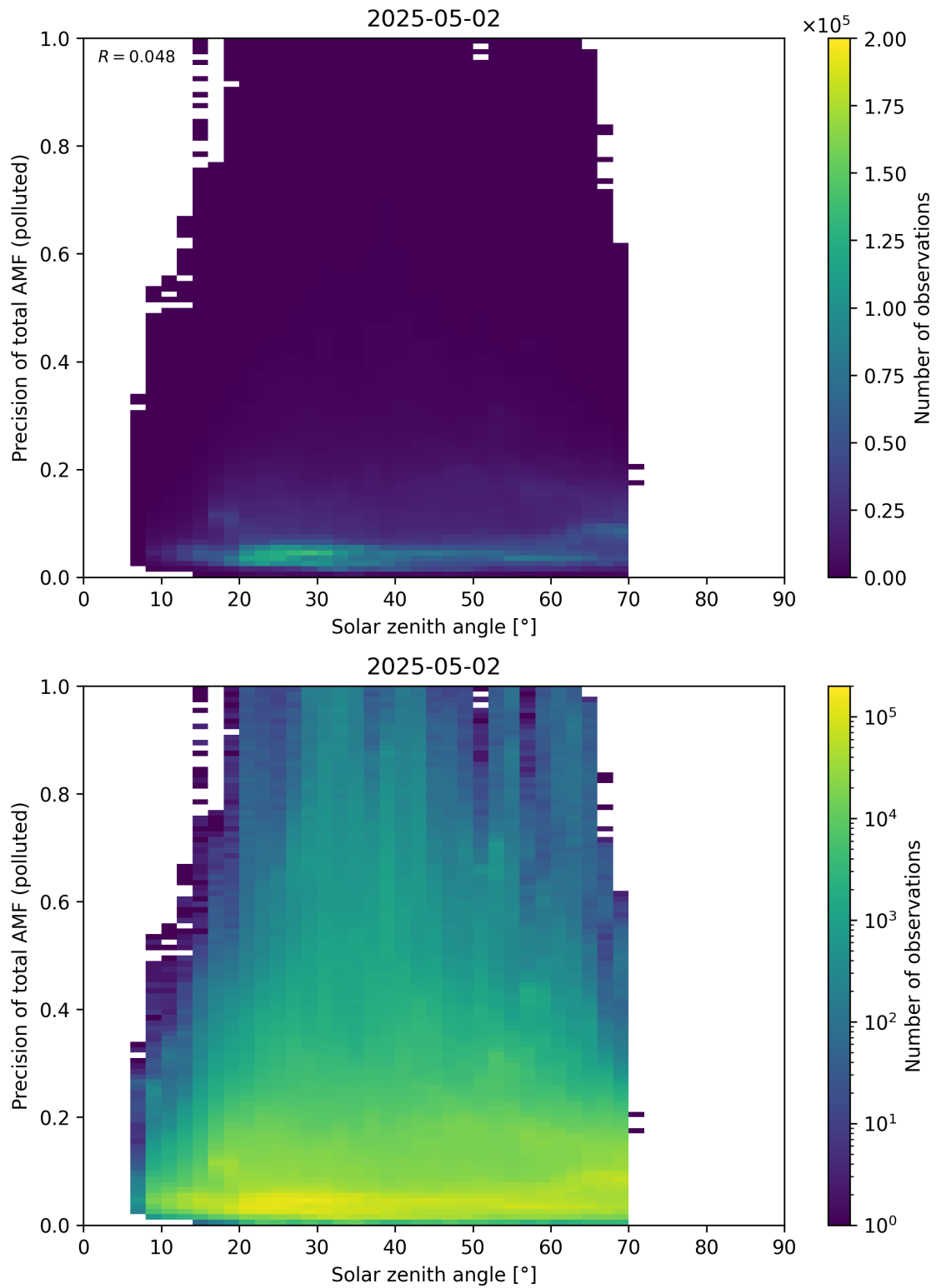
Figure 190: Scatter density plot of “Solar zenith angle” against “Precision of total AMF (polluted)” for 2025-05-01 to 2025-05-03.
