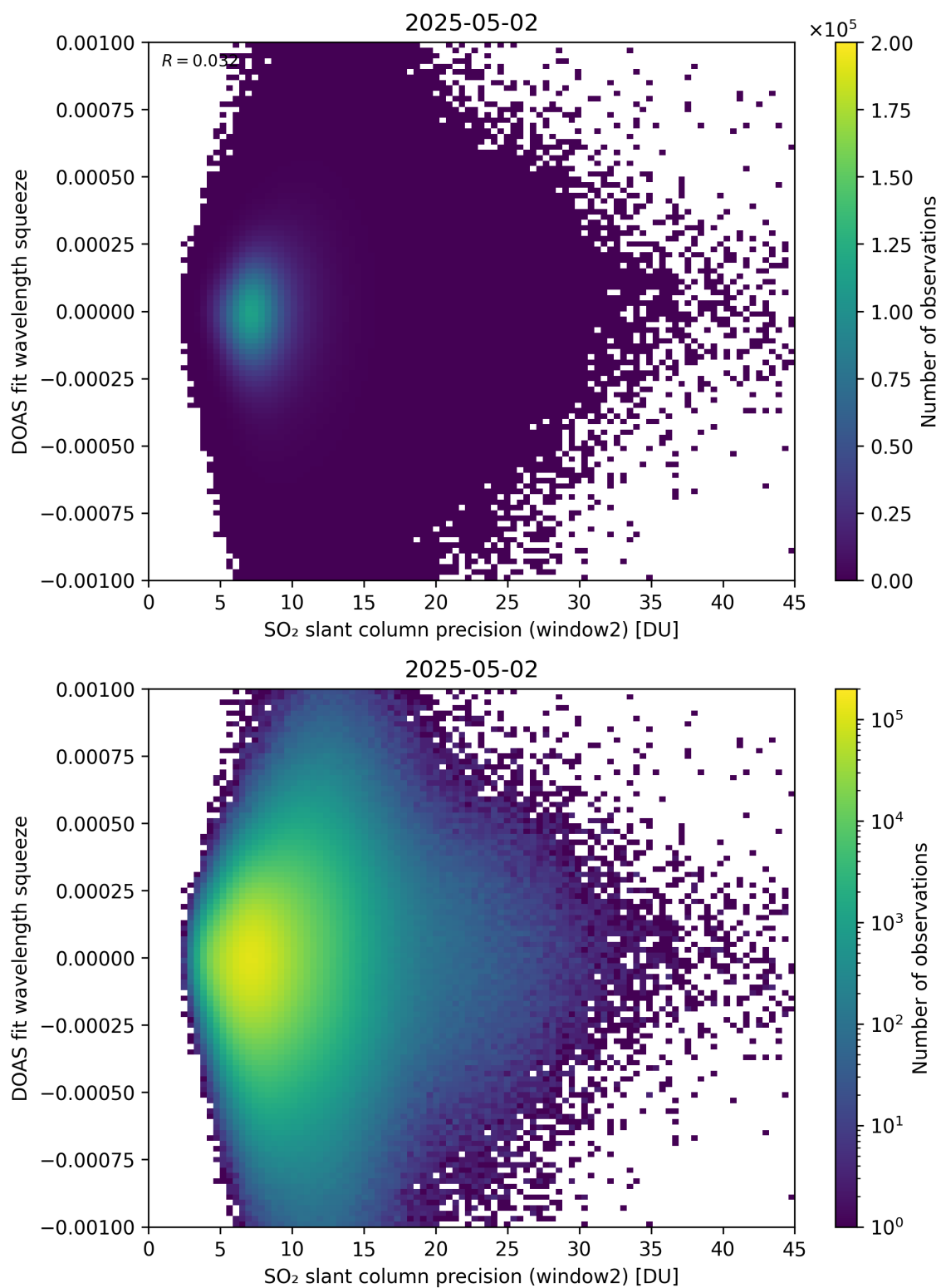
Figure 294: Scatter density plot of “SO 2 slant column precision (window2)” against “DOAS fit wavelength squeeze” for 2025-05-01 to 2025-05-03.
