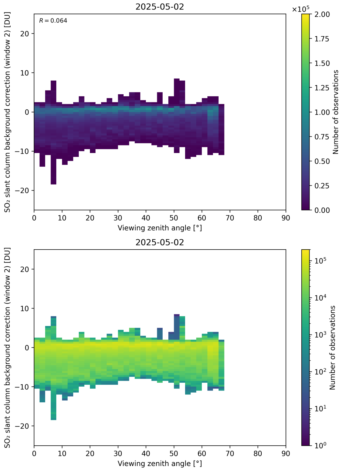
Figure 363: Scatter density plot of “Viewing zenith angle” against “SO 2 slant column background correction (window 2)” for 2025-05-01 to 2025-05-03.
