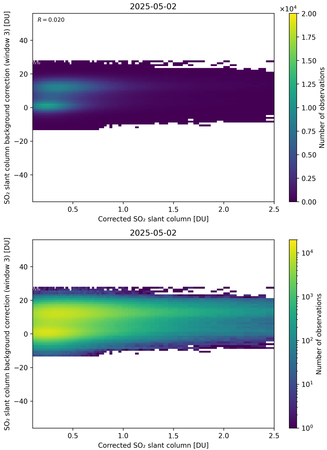
Figure 228: Scatter density plot of “Corrected SO 2 slant column” against “SO 2 slant column background correction (window 3)” for 2025-05-01 to 2025-05-03.
