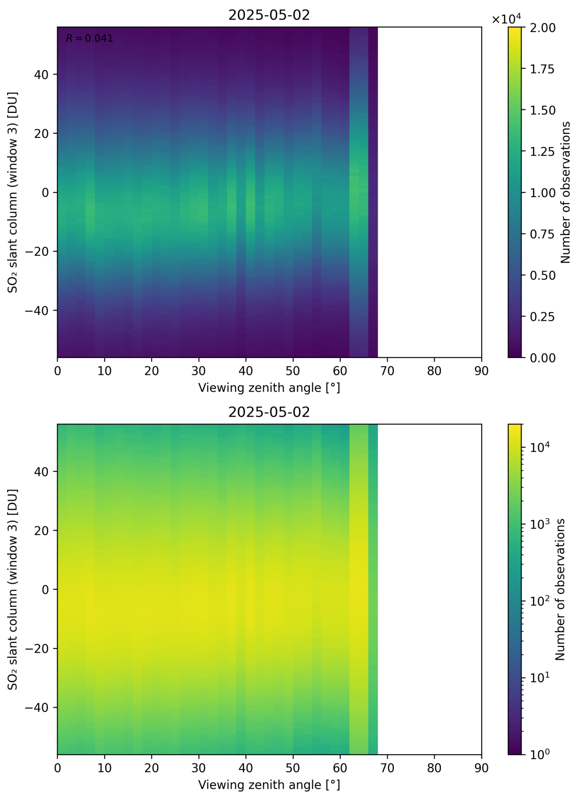
Figure 379: Scatter density plot of “Viewing zenith angle” against “SO 2 slant column (window 3)” for 2025-05-01 to 2025-05-03.
