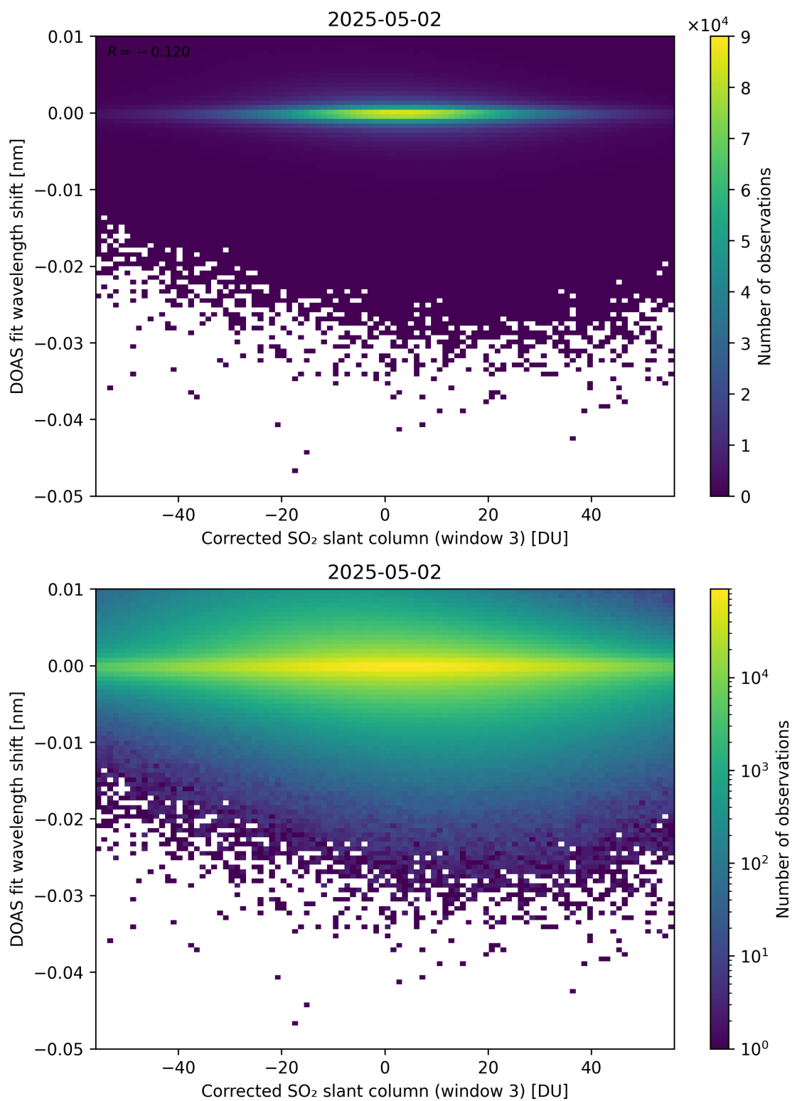
Figure 256: Scatter density plot of “Corrected SO 2 slant column (window 3)” against “DOAS fit wavelength shift” for 2025-05-01 to 2025-05-03.
