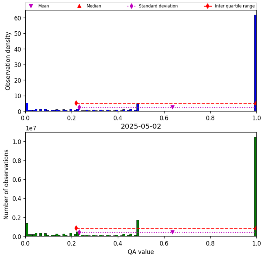
Figure 57: Histogram of “QA value” for 2025-05-01 to 2025-05-03
