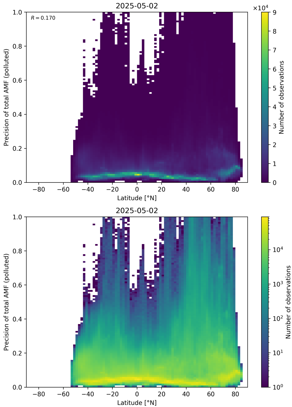
Figure 168: Scatter density plot of “Latitude” against “Precision of total AMF (polluted)” for 2025-05-01 to 2025-05-03.
