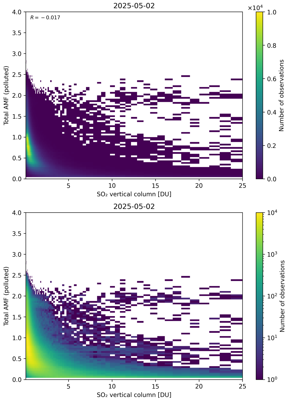
Figure 359: Scatter density plot of “SO 2 vertical column” against “Total AMF (polluted)” for 2025-05-01 to 2025-05-03.
