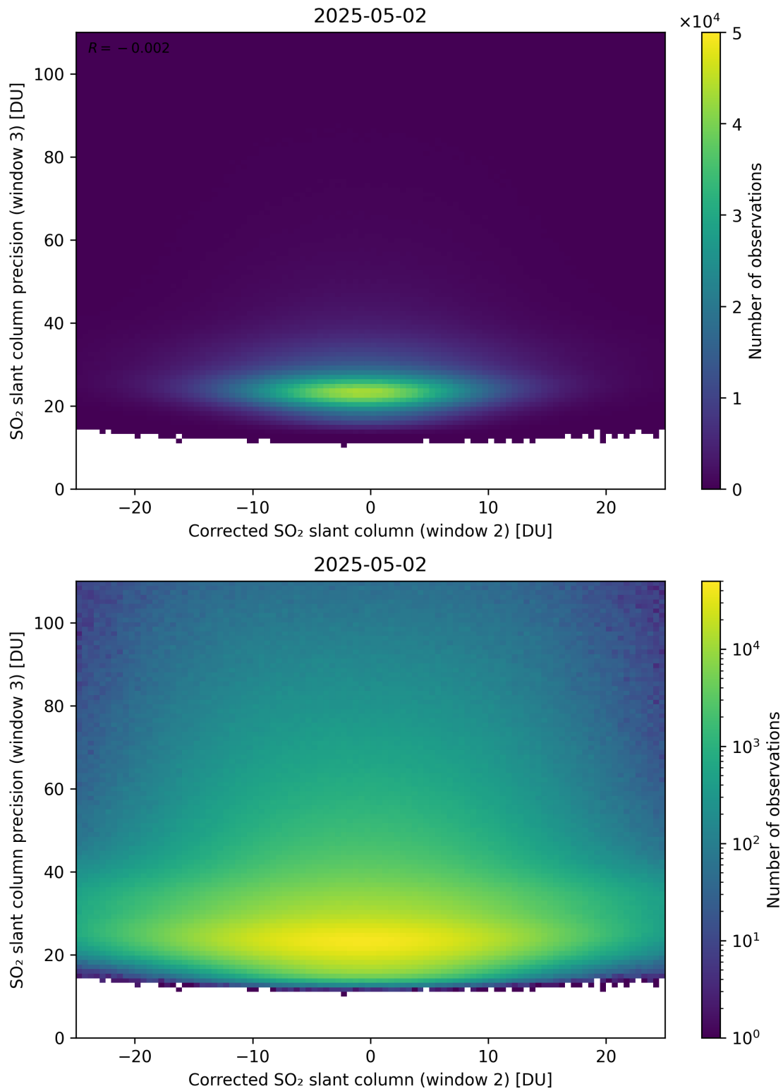
Figure 252: Scatter density plot of “Corrected SO 2 slant column (window 2)” against “SO 2 slant column precision (window 3)” for 2025-05-01 to 2025-05-03.
