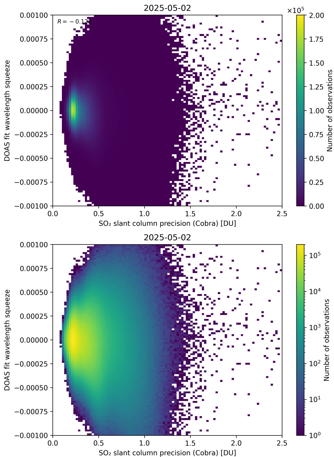
Figure 203: Scatter density plot of “SO 2 slant column precision (Cobra)” against “DOAS fit wavelength squeeze” for 2025-05-01 to 2025-05-03.
