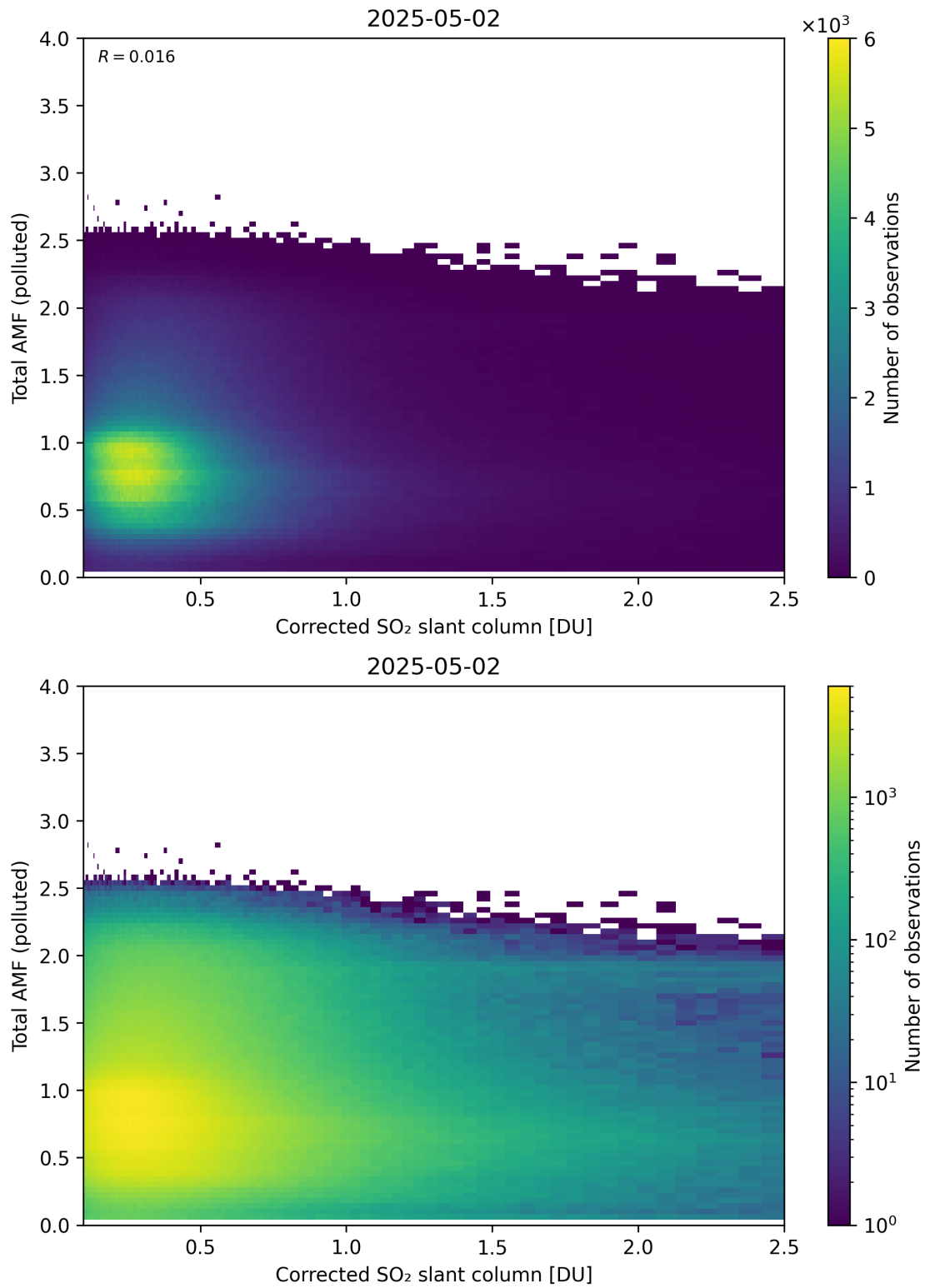
Figure 242: Scatter density plot of “Corrected SO 2 slant column” against “Total AMF (polluted)” for 2025-05-01 to 2025-05-03.
