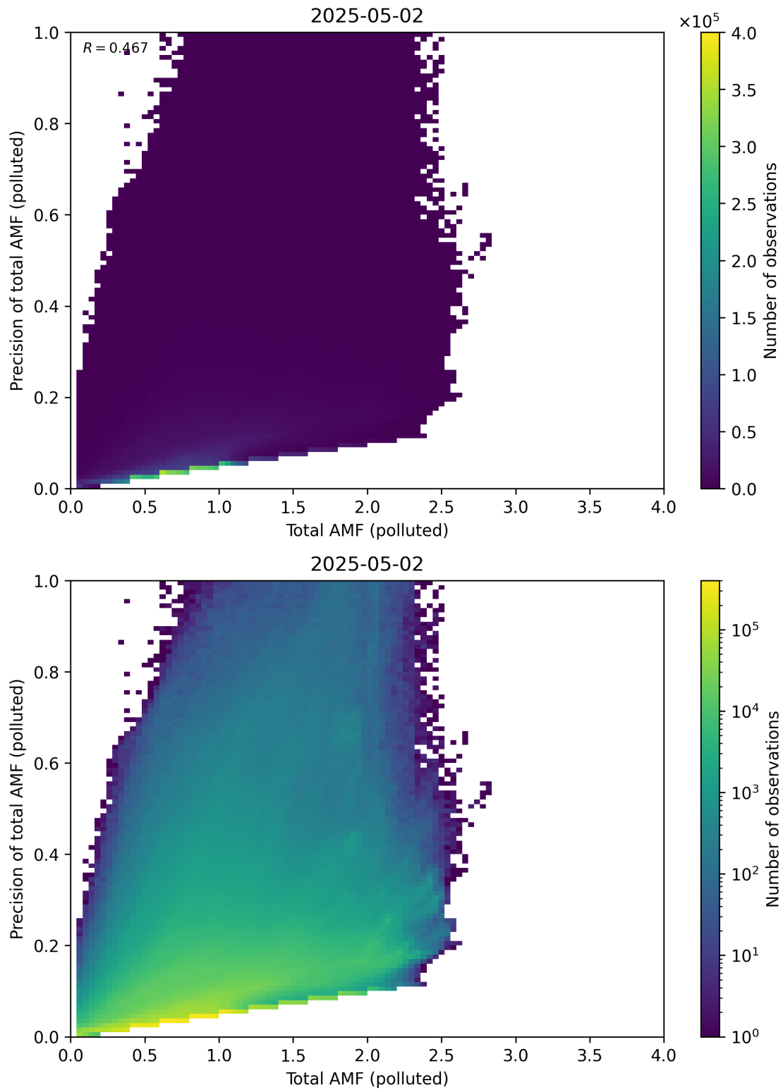
Figure 322: Scatter density plot of “Total AMF (polluted)” against “Precision of total AMF (polluted)” for 2025-05-01 to 2025-05-03.
