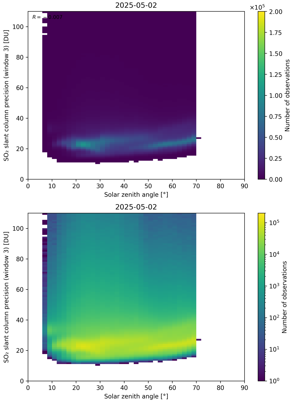
Figure 188: Scatter density plot of “Solar zenith angle” against “SO 2 slant column precision (window 3)” for 2025-05-01 to 2025-05-03.
