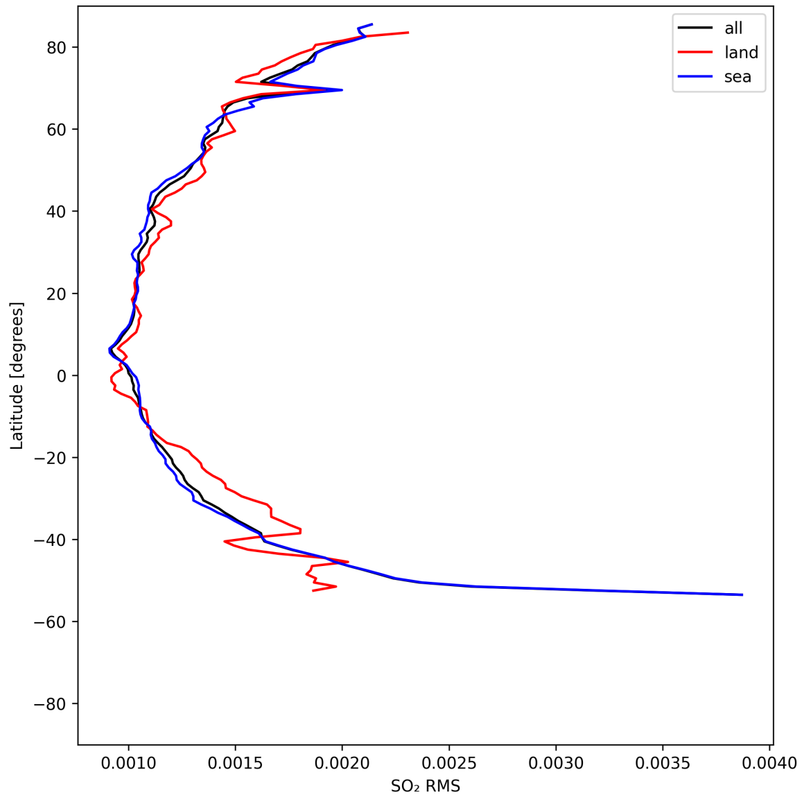
Figure 52: Zonal average of “SO 2 RMS” for 2025-05-01 to 2025-05-03.
