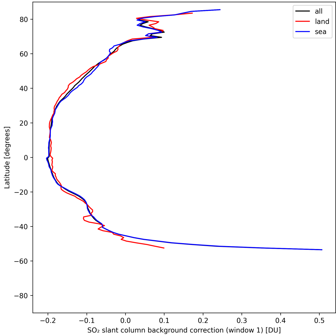
Figure 40: Zonal average of “SO 2 slant column background correction (window 1)” for 2025-05-01 to 2025-05-03.
