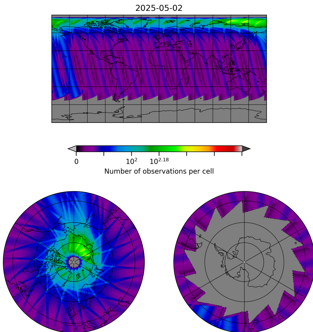
Figure 30: Map of the number of observations for 2025-05-01 to 2025-05-03
