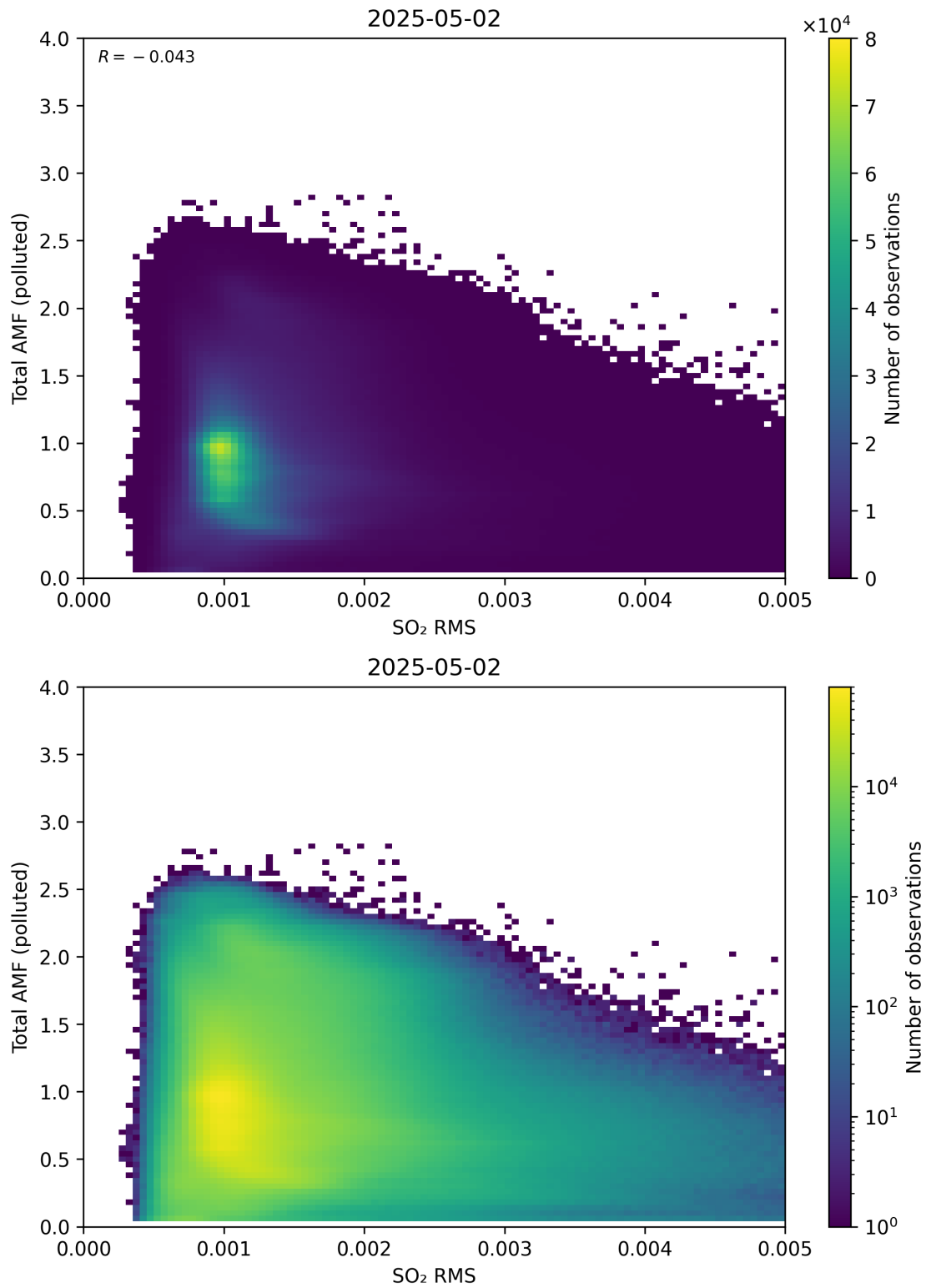
Figure 148: Scatter density plot of “SO 2 RMS” against “Total AMF (polluted)” for 2025-05-01 to 2025-05-03.
