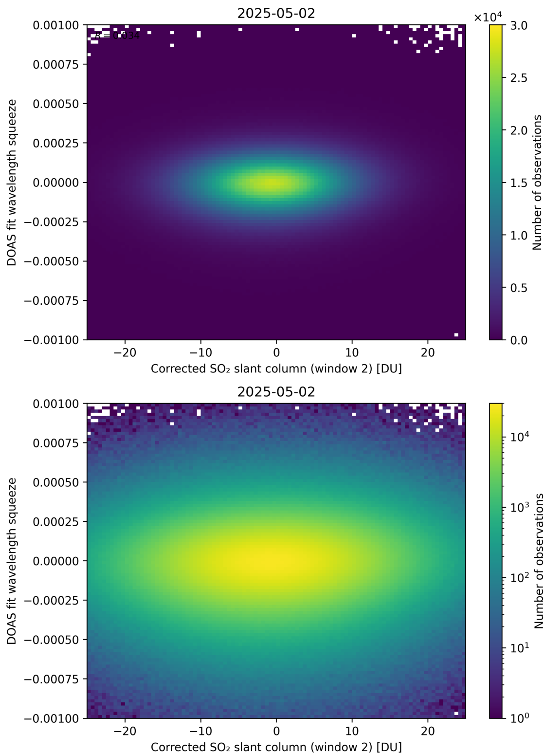
Figure 247: Scatter density plot of “Corrected SO 2 slant column (window 2)” against “DOAS fit wavelength squeeze” for 2025-05-01 to 2025-05-03.
