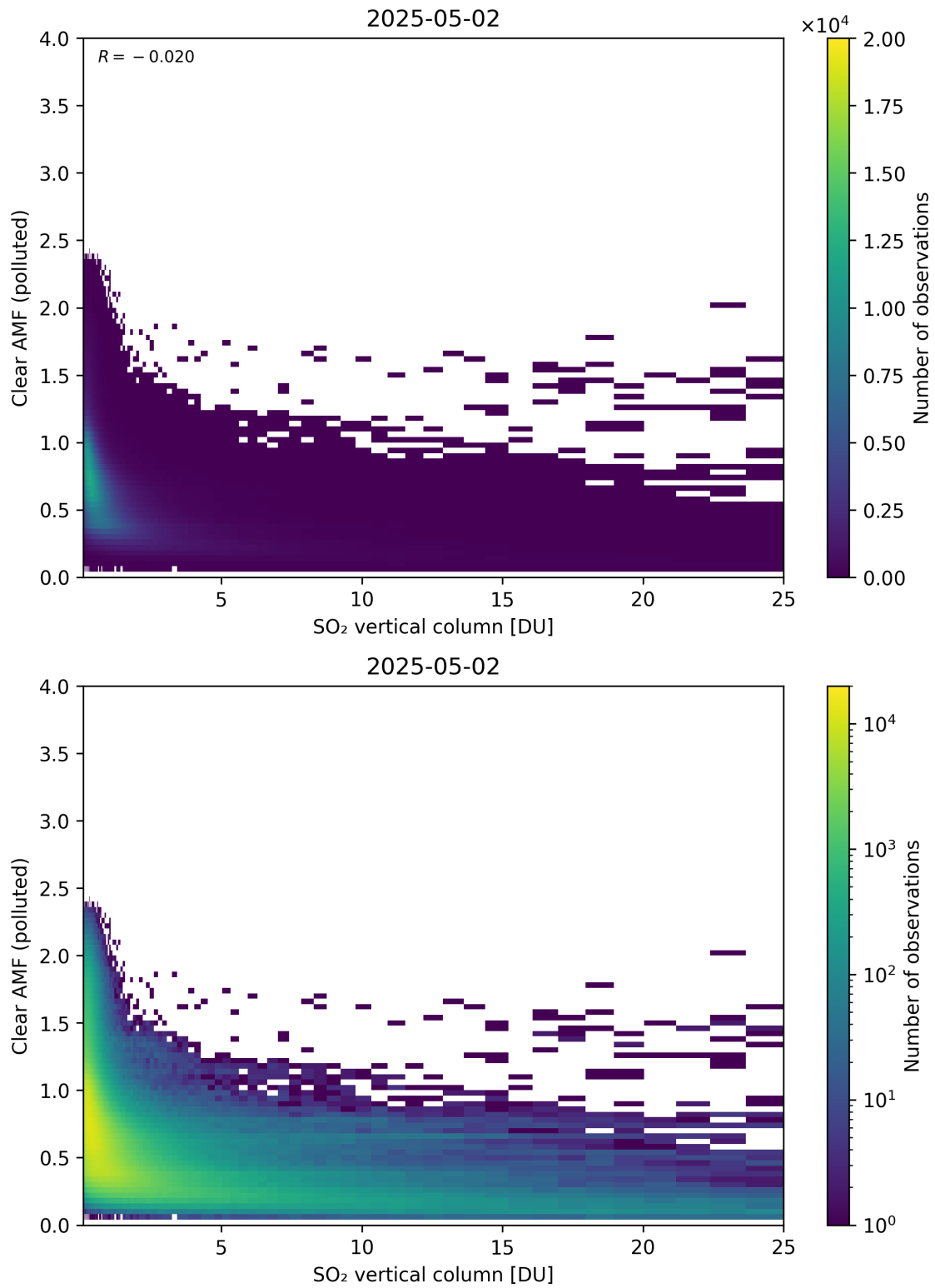
Figure 348: Scatter density plot of “SO 2 vertical column” against “Clear AMF (polluted)” for 2025-05-01 to 2025-05-03.
