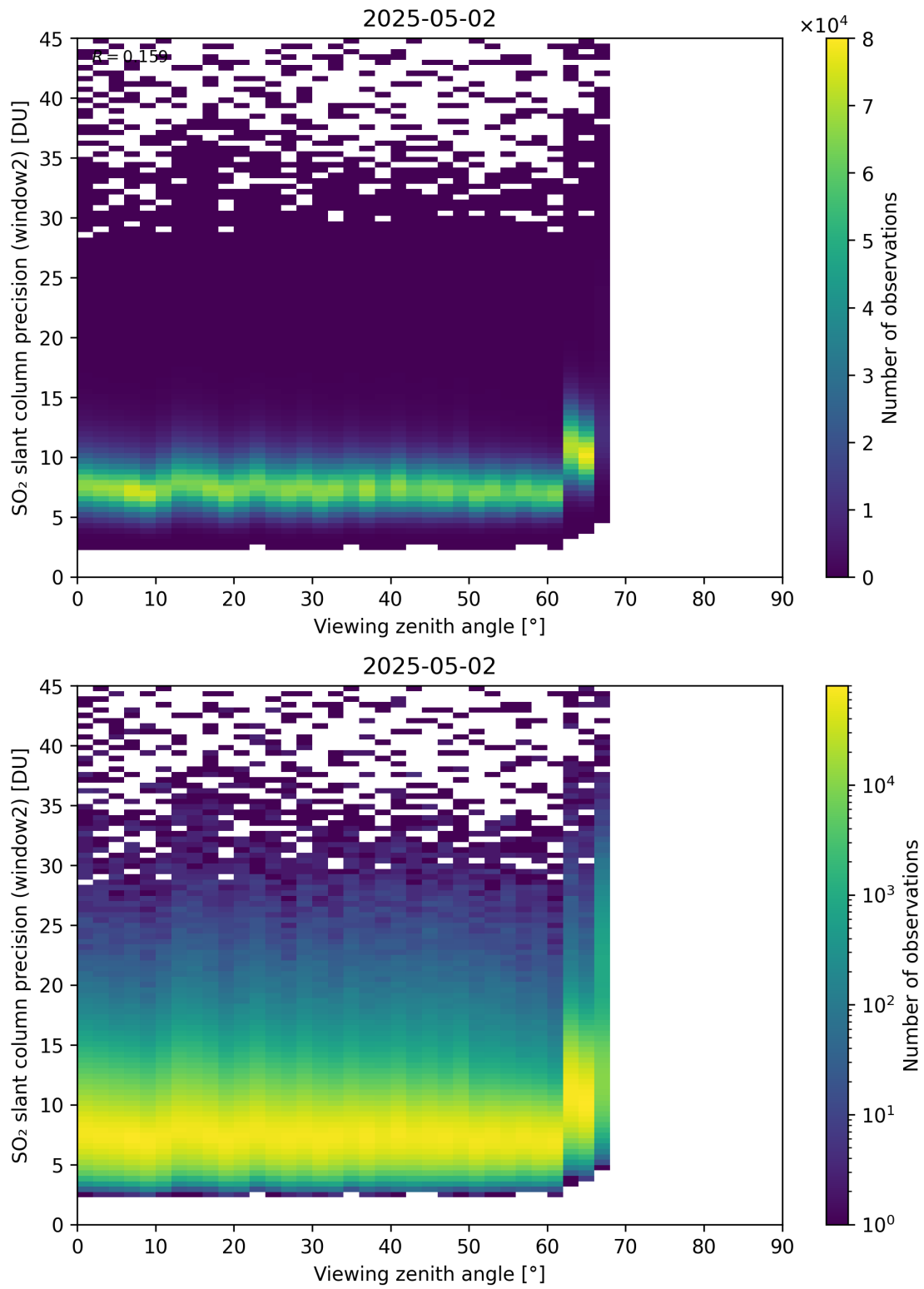
Figure 378: Scatter density plot of “Viewing zenith angle” against “SO 2 slant column precision (window2)” for 2025-05-01 to 2025-05-03.
