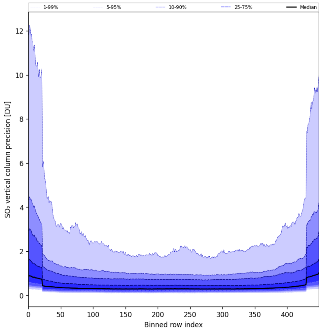
Figure 85: Along track statistics of “SO 2 vertical column precision” for 2025-05-01 to 2025-05-03
