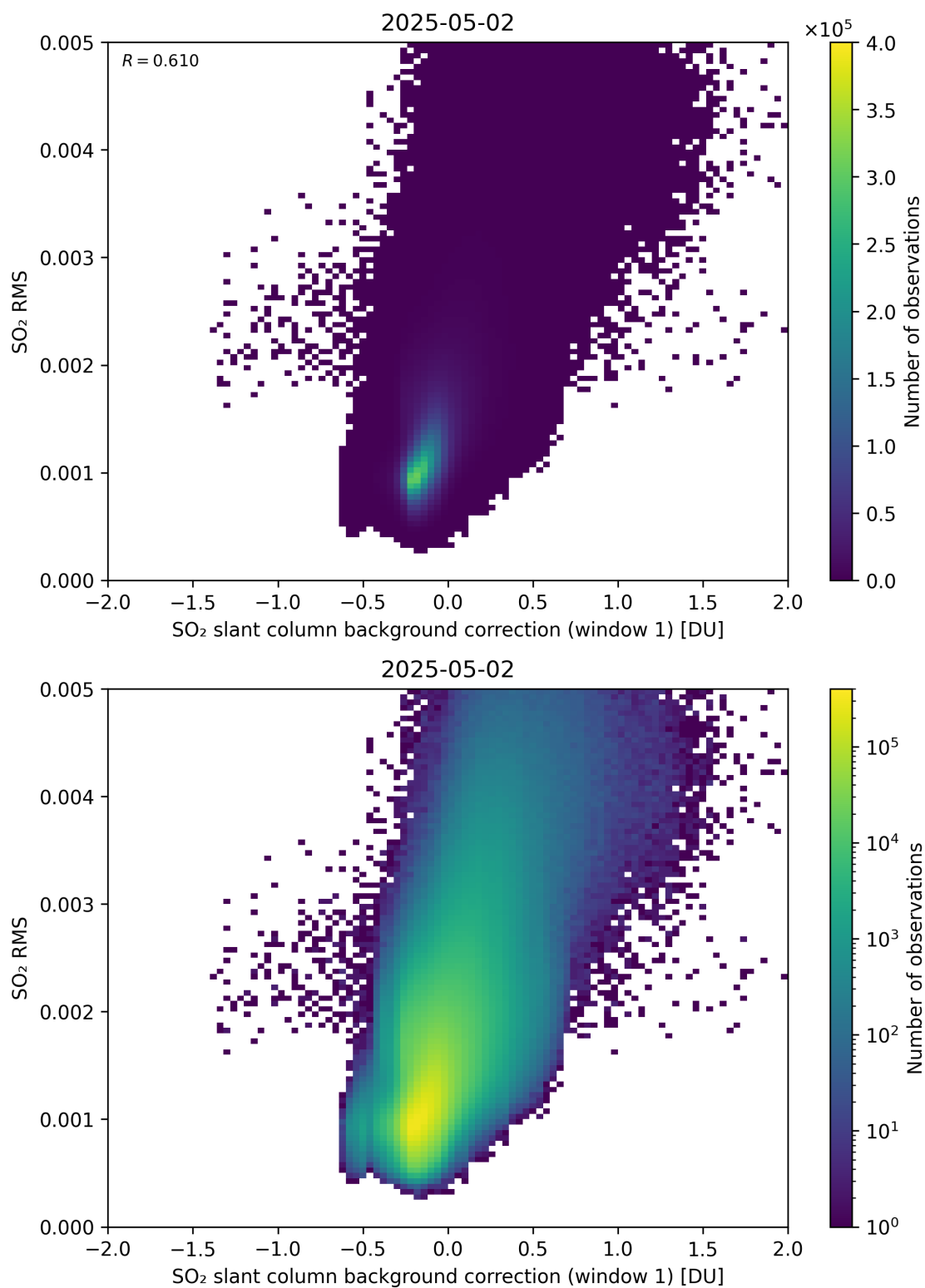
Figure 113: Scatter density plot of “SO 2 slant column background correction (window 1)” against “SO 2 RMS” for 2025-05-01 to 2025-05-03.
