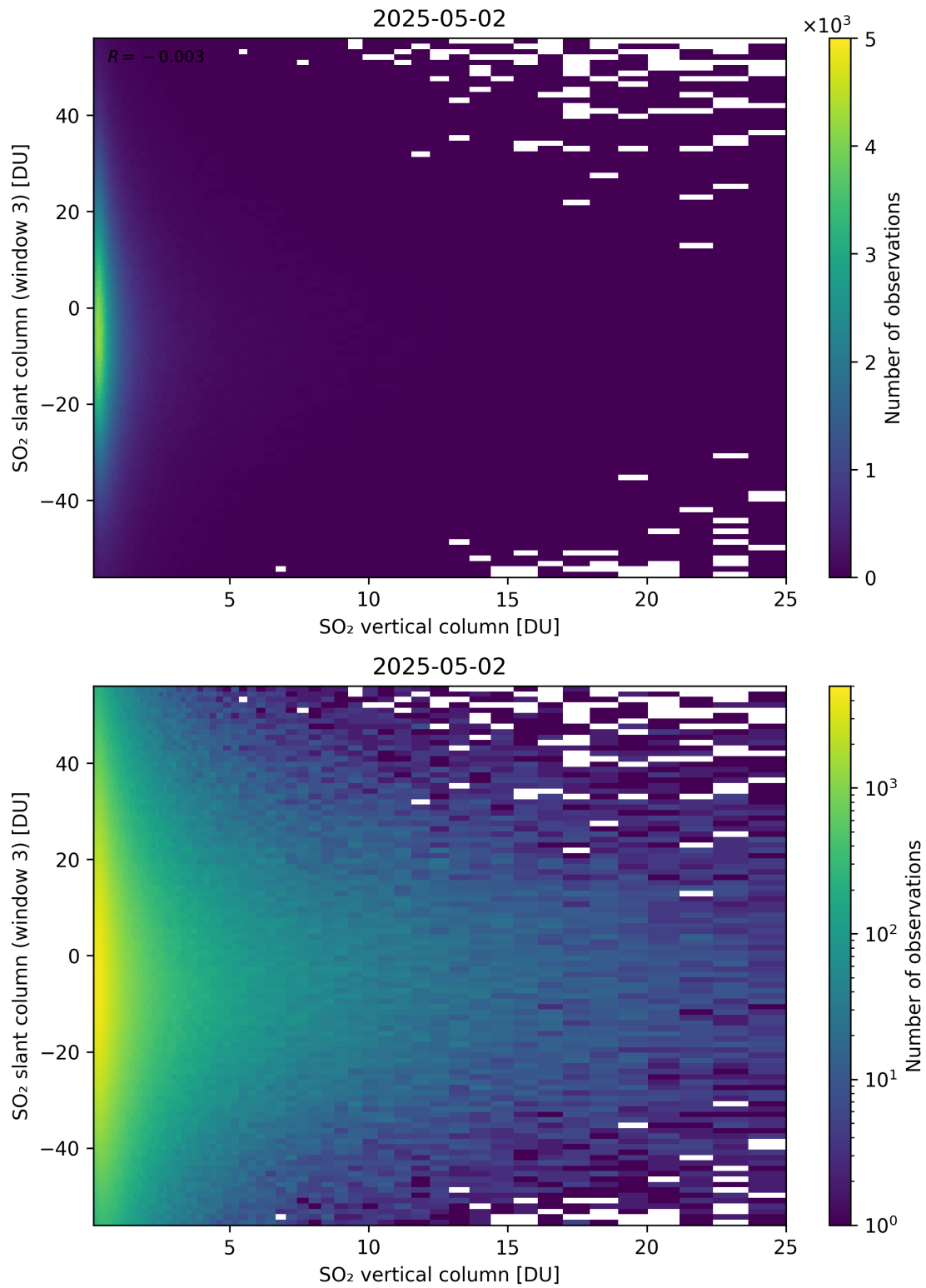
Figure 357: Scatter density plot of “SO 2 vertical column” against “SO 2 slant column (window 3)” for 2025-05-01 to 2025-05-03.
