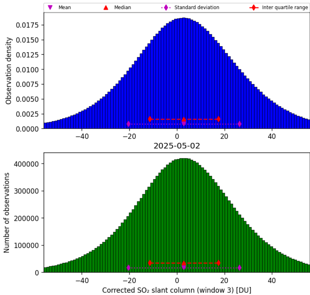
Figure 73: Histogram of “Corrected SO 2 slant column (window 3)” for 2025-05-01 to 2025-05-03
