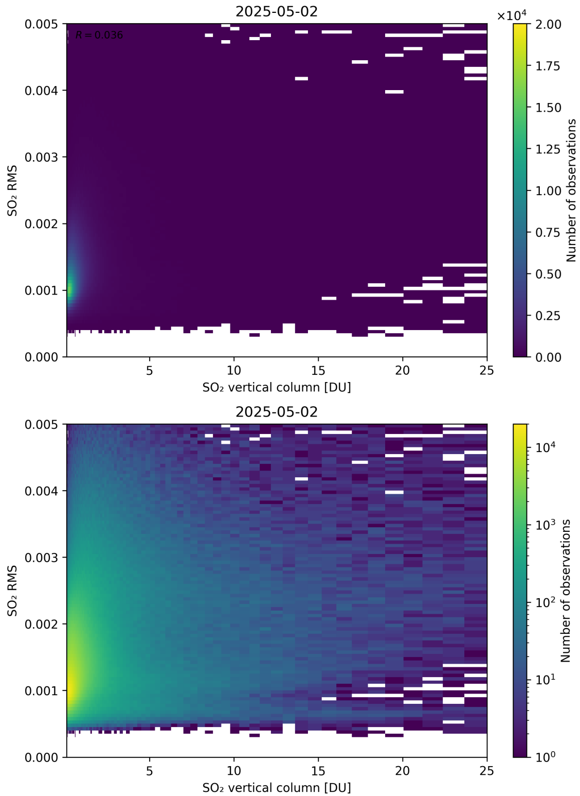
Figure 328: Scatter density plot of “SO 2 vertical column” against “SO 2 RMS” for 2025-05-01 to 2025-05-03.
