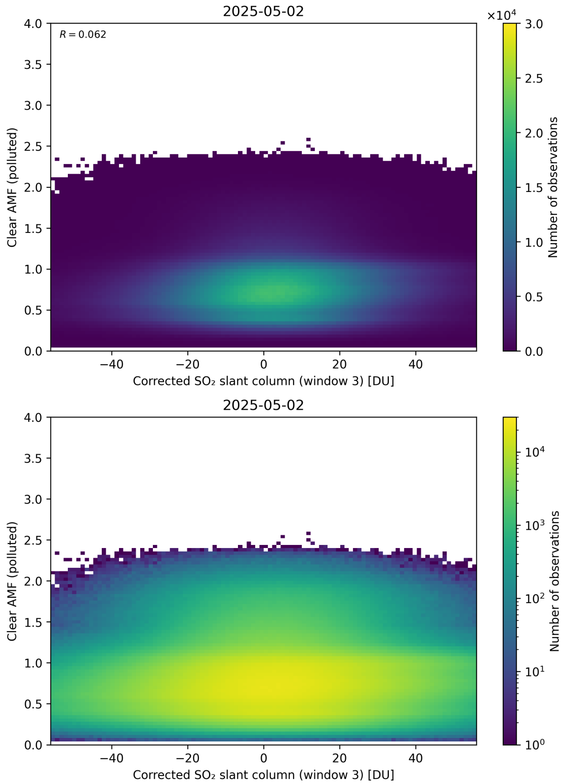
Figure 259: Scatter density plot of “Corrected SO 2 slant column (window 3)” against “Clear AMF (polluted)” for 2025-05-01 to 2025-05-03.
