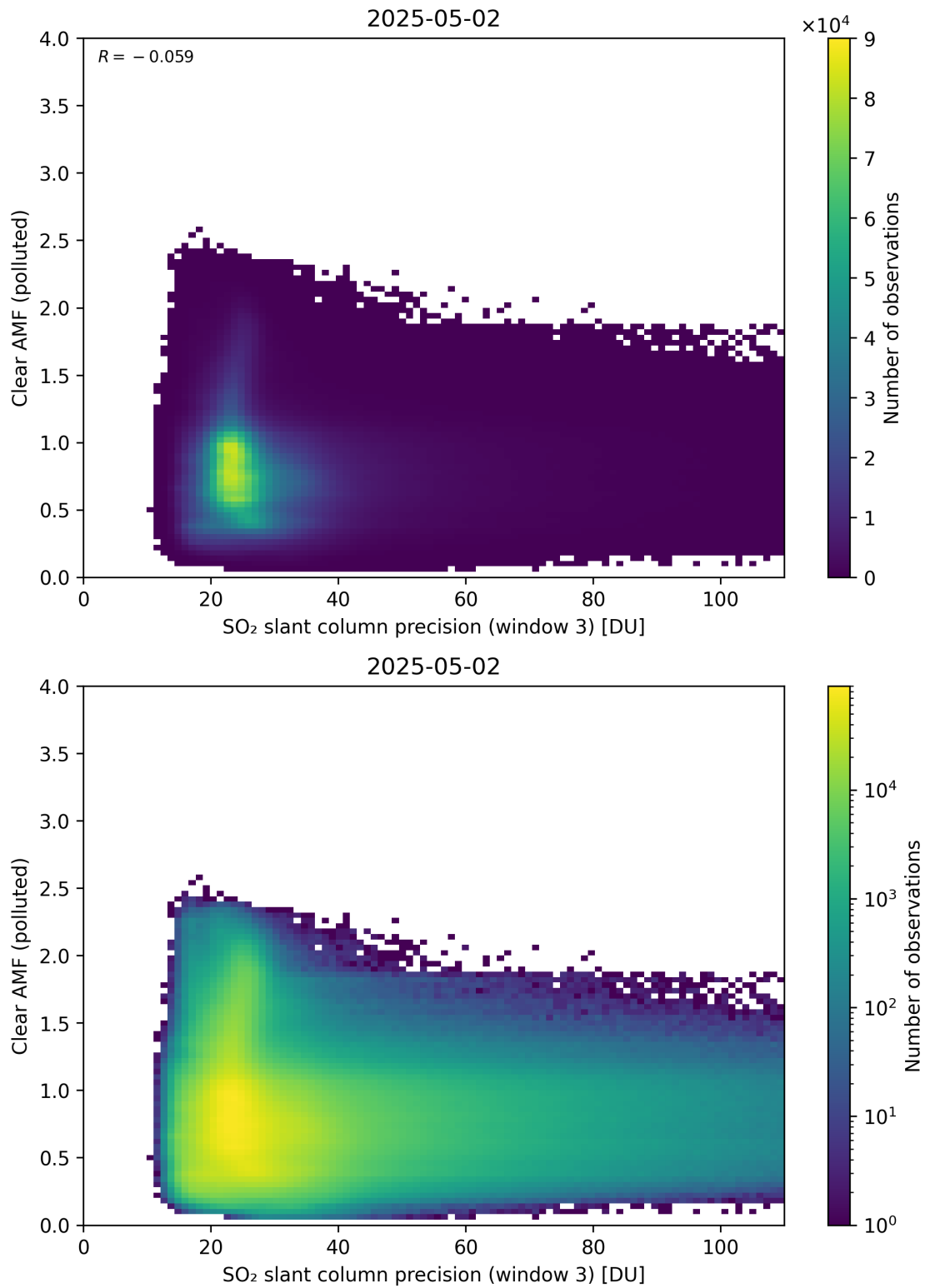
Figure 311: Scatter density plot of “SO 2 slant column precision (window 3)” against “Clear AMF (polluted)” for 2025-05-01 to 2025-05-03.
