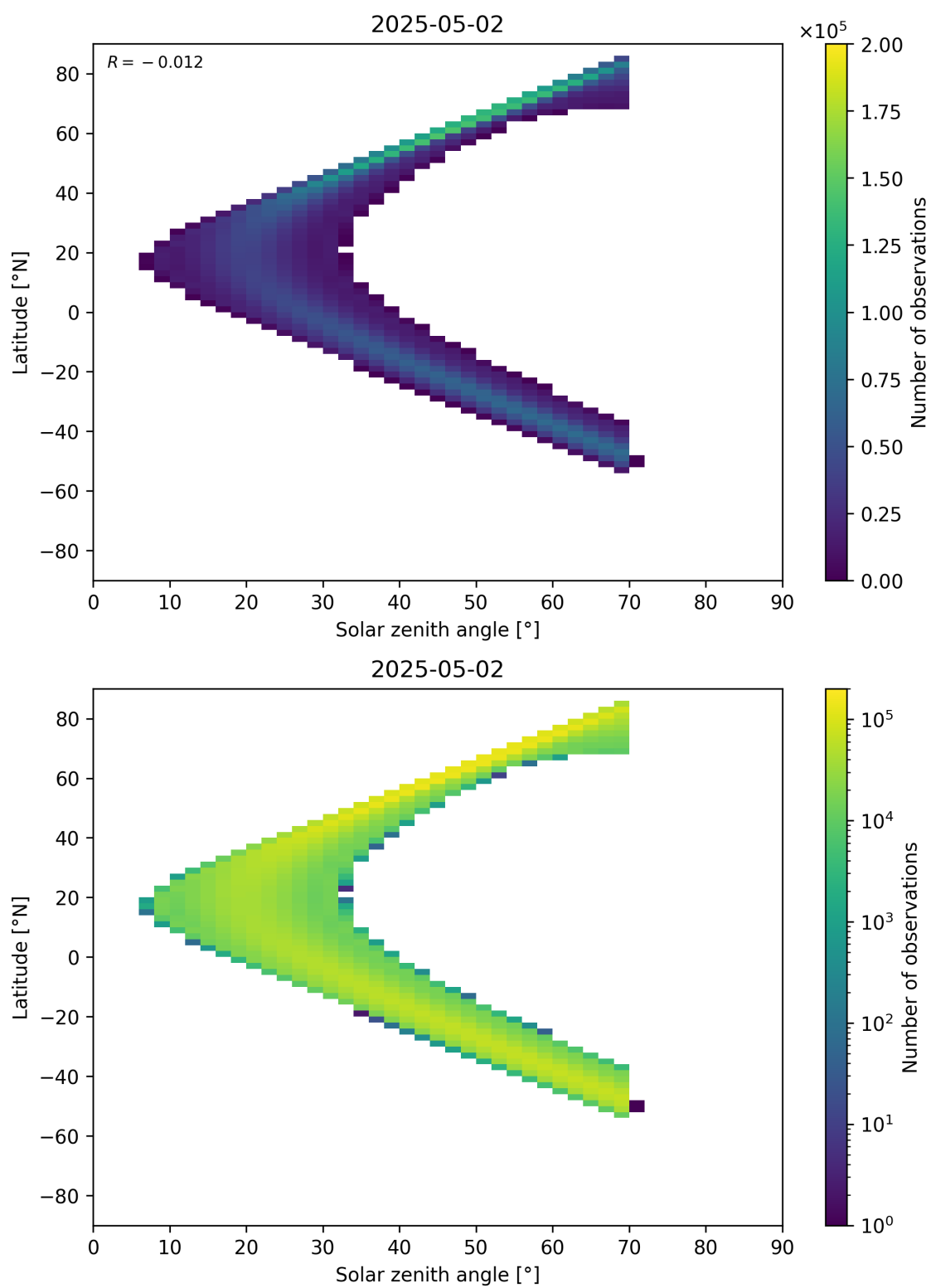
Figure 177: Scatter density plot of “Solar zenith angle” against “Latitude” for 2025-05-01 to 2025-05-03.
