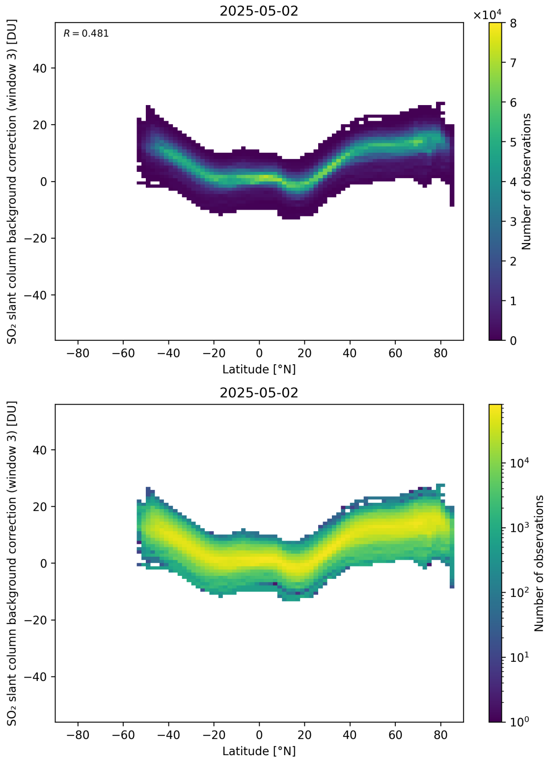
Figure 152: Scatter density plot of “Latitude” against “SO 2 slant column background correction (window 3)” for 2025-05-01 to 2025-05-03.
