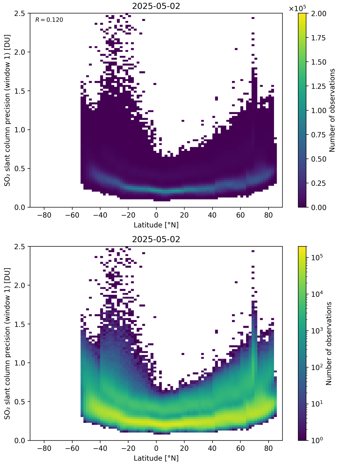
Figure 163: Scatter density plot of “Latitude” against “SO 2 slant column precision (window 1)” for 2025-05-01 to 2025-05-03.
