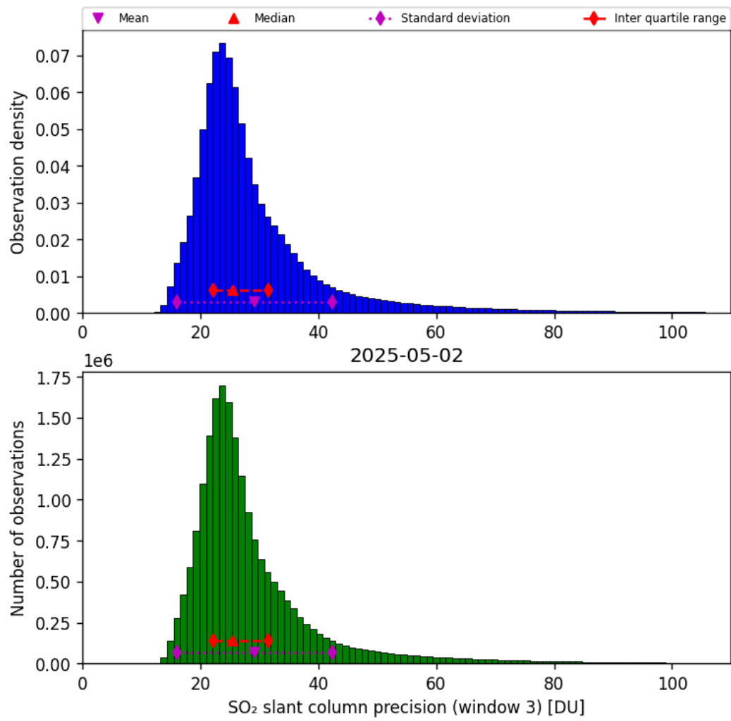
Figure 72: Histogram of “SO 2 slant column precision (window 3)” for 2025-05-01 to 2025-05-03
