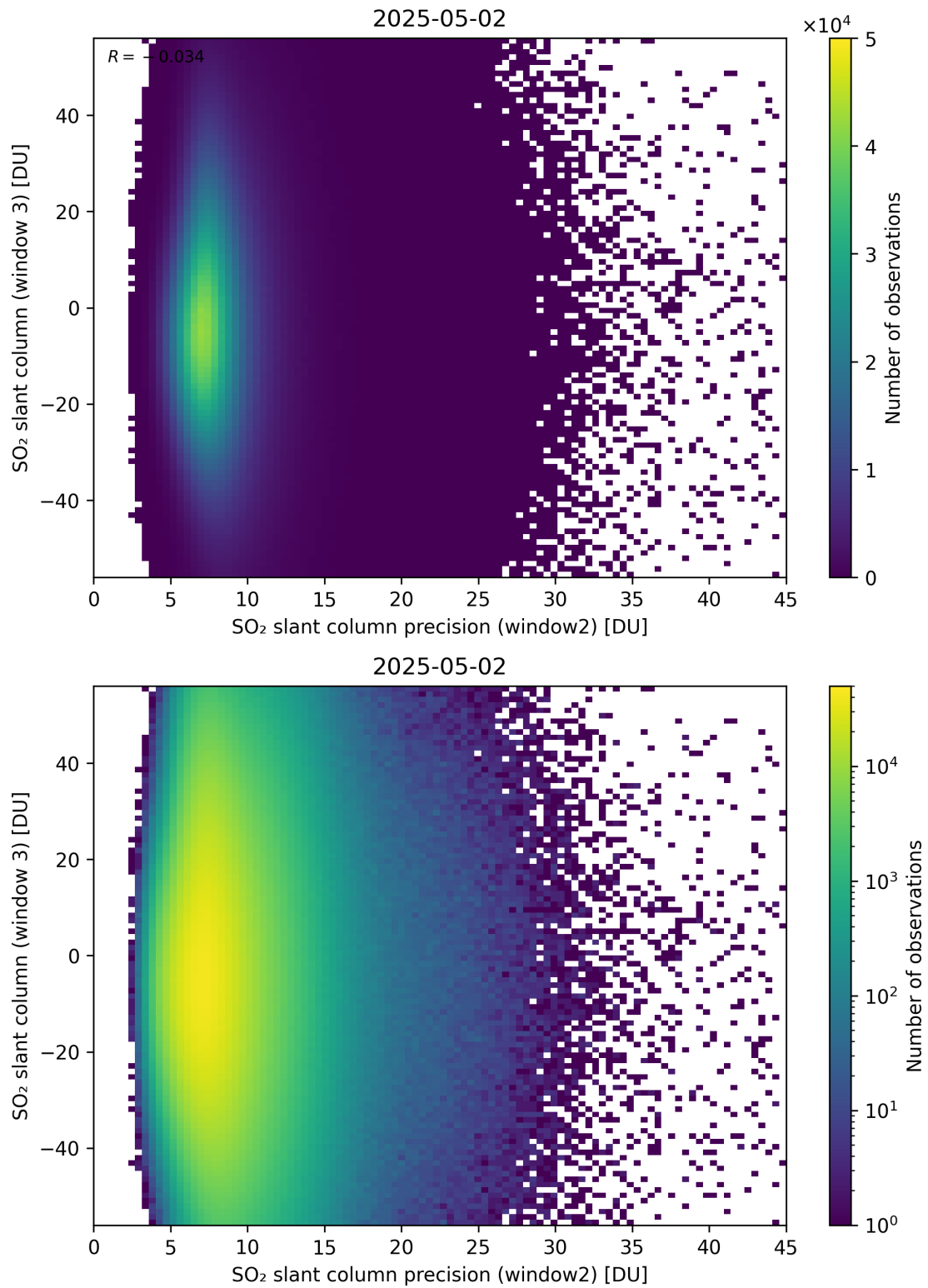
Figure 299: Scatter density plot of “SO 2 slant column precision (window2)” against “SO 2 slant column (window 3)” for 2025-05-01 to 2025-05-03.
