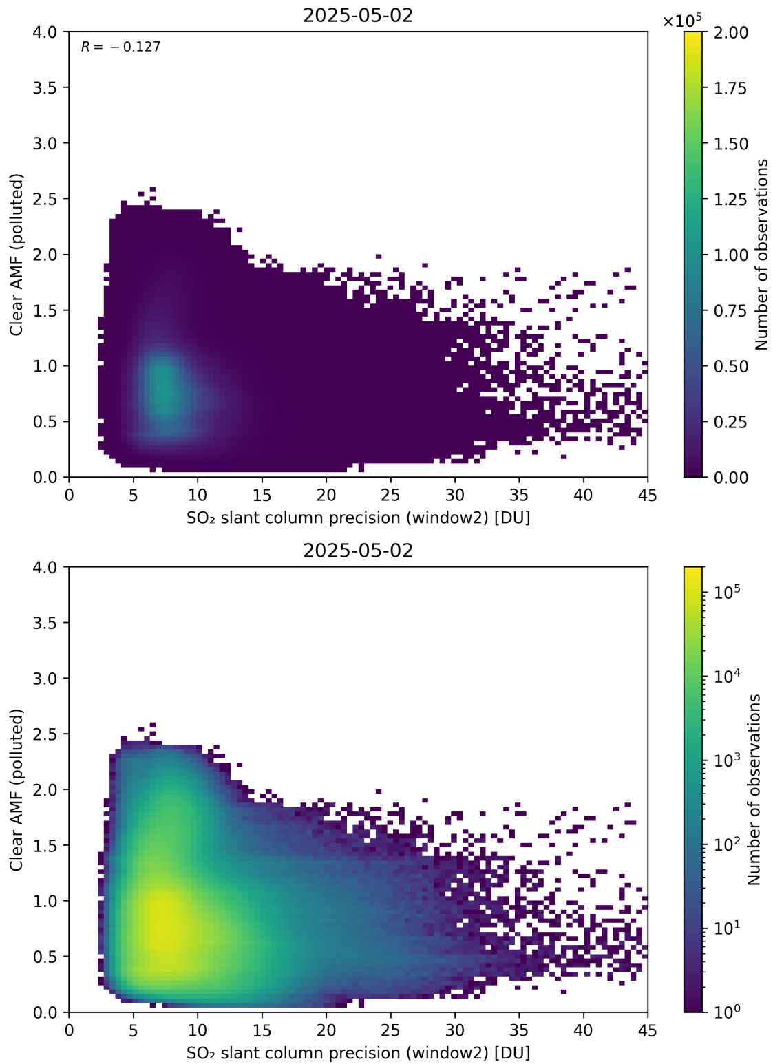
Figure 296: Scatter density plot of “SO 2 slant column precision (window2)” against “Clear AMF (polluted)” for 2025-05-01 to 2025-05-03.
