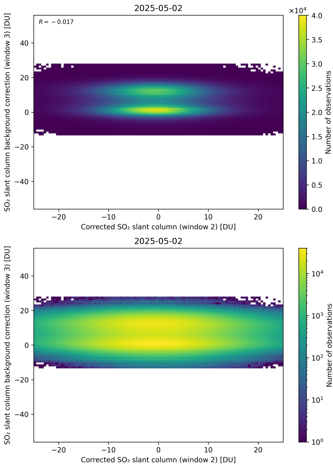
Figure 245: Scatter density plot of “Corrected SO 2 slant column (window 2)” against “SO 2 slant column background correction (window 3)” for 2025-05-01 to 2025-05-03.
