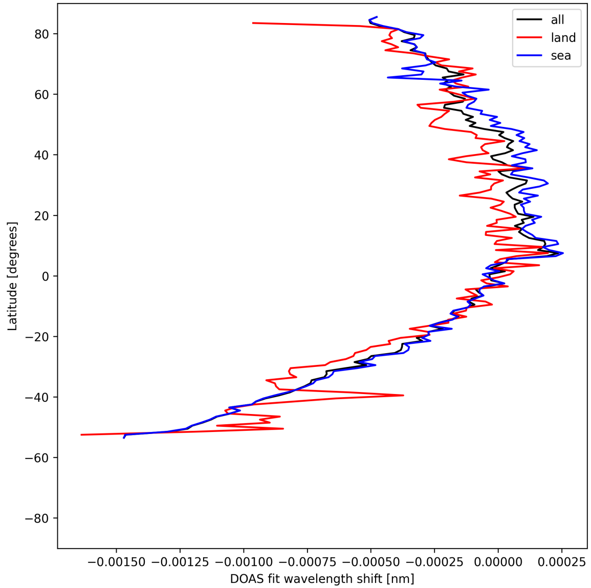
Figure 50: Zonal average of “DOAS fit wavelength shift” for 2025-05-01 to 2025-05-03.
