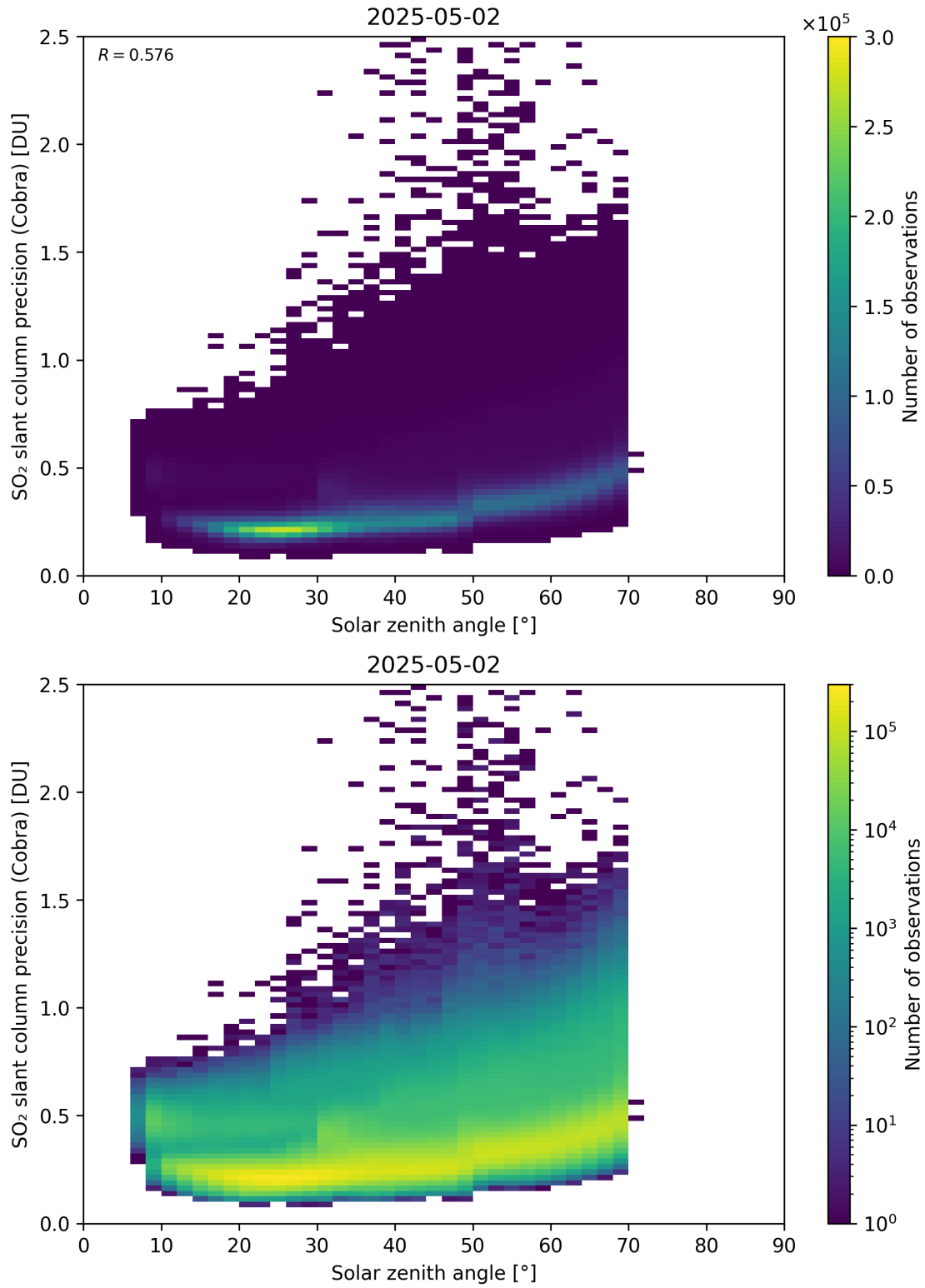
Figure 180: Scatter density plot of “Solar zenith angle” against “SO 2 slant column precision (Cobra)” for 2025-05-01 to 2025-05-03.
