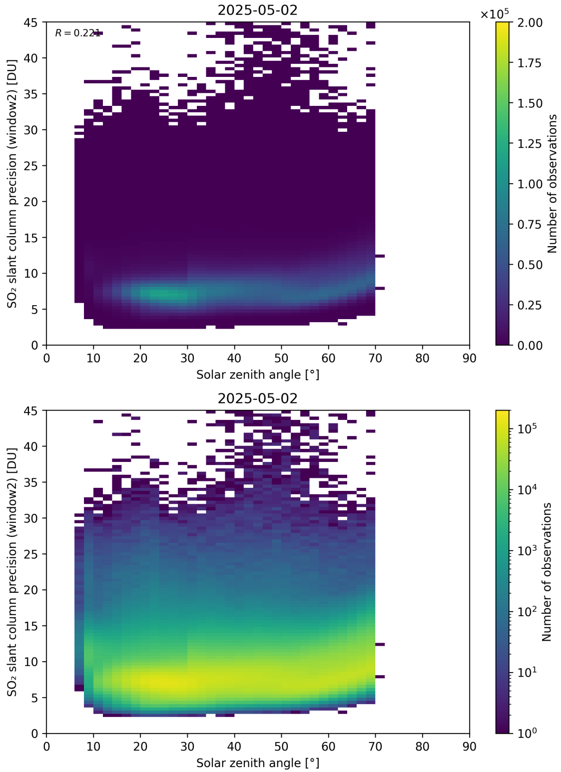
Figure 186: Scatter density plot of “Solar zenith angle” against “SO 2 slant column precision (window2)” for 2025-05-01 to 2025-05-03.
