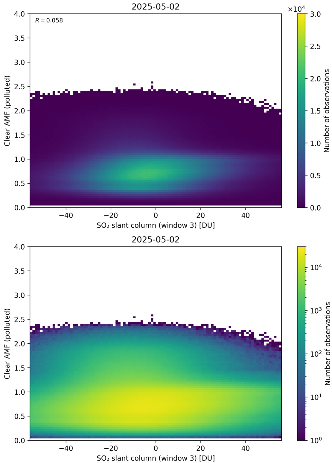
Figure 315: Scatter density plot of “SO 2 slant column (window 3)” against “Clear AMF (polluted)” for 2025-05-01 to 2025-05-03.
