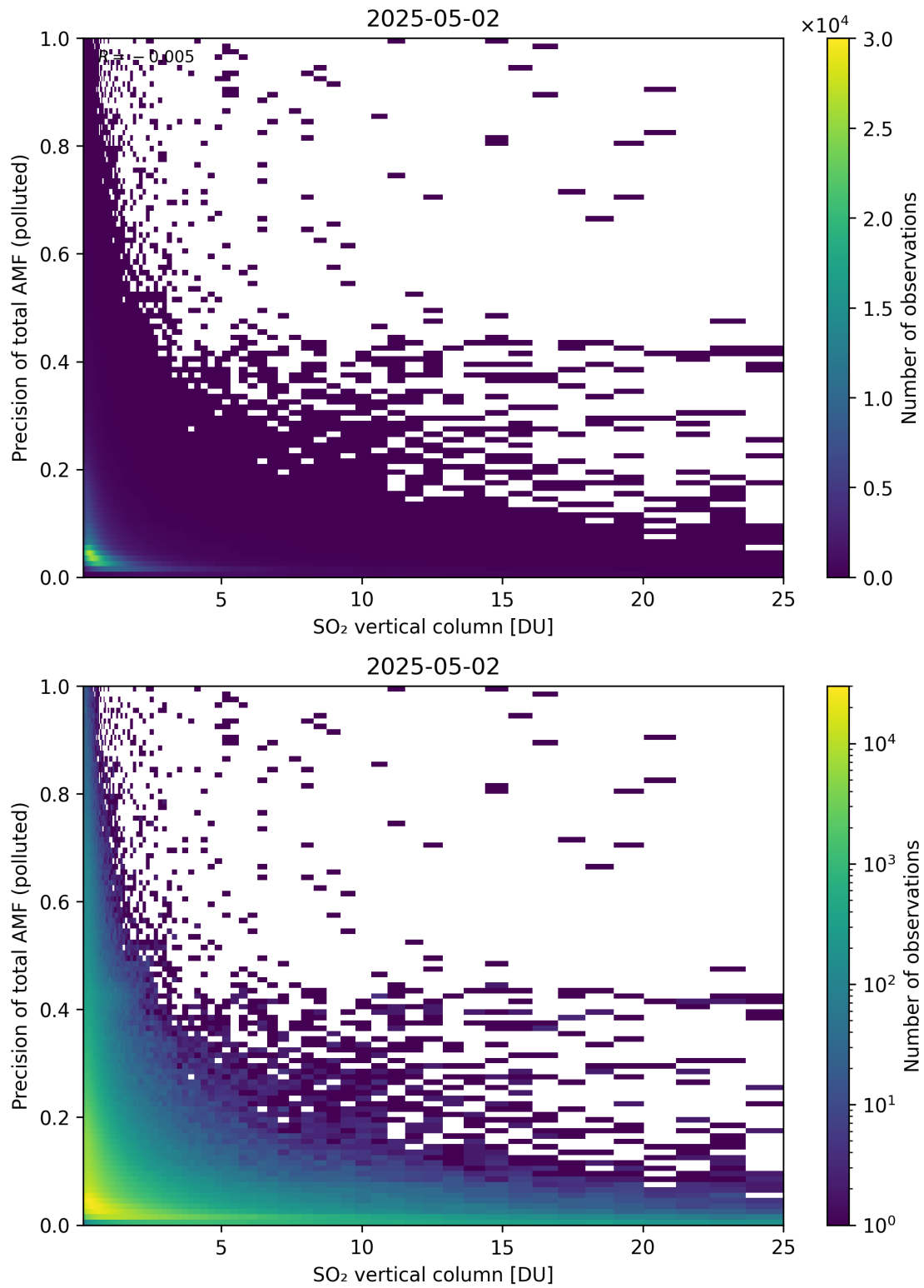
Figure 360: Scatter density plot of “SO 2 vertical column” against “Precision of total AMF (polluted)” for 2025-05-01 to 2025-05-03.
