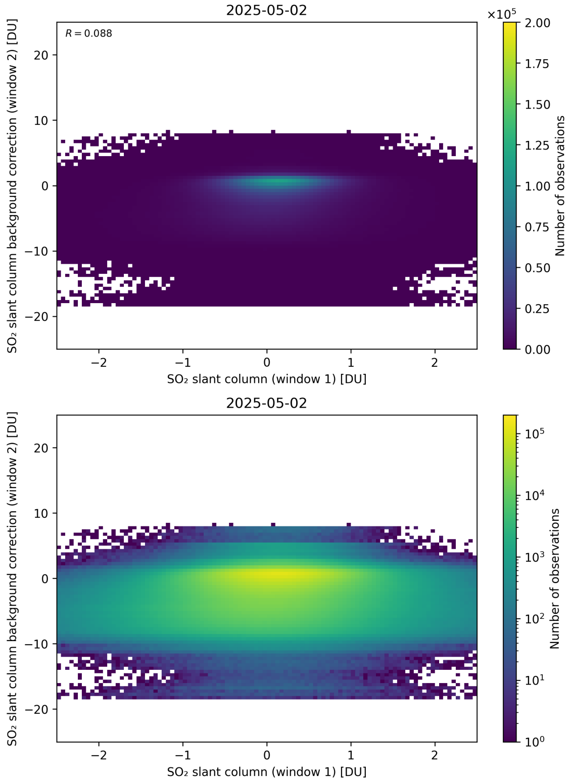
Figure 263: Scatter density plot of “SO 2 slant column (window 1)” against “SO 2 slant column background correction (window 2)” for 2025-05-01 to 2025-05-03.
