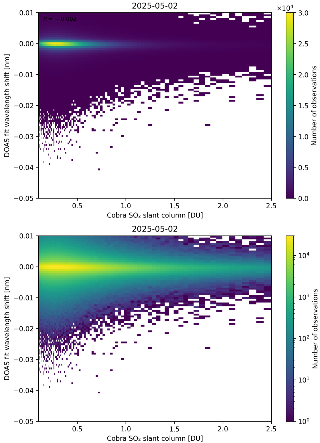
Figure 196: Scatter density plot of “Cobra SO 2 slant column” against “DOAS fit wavelength shift” for 2025-05-01 to 2025-05-03.
