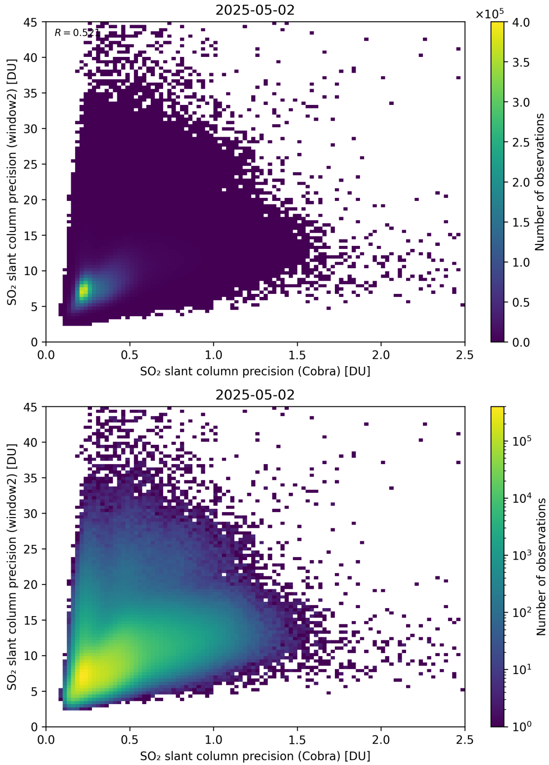
Figure 210: Scatter density plot of “SO 2 slant column precision (Cobra)” against “SO 2 slant column precision (window2)” for 2025-05-01 to 2025-05-03.
