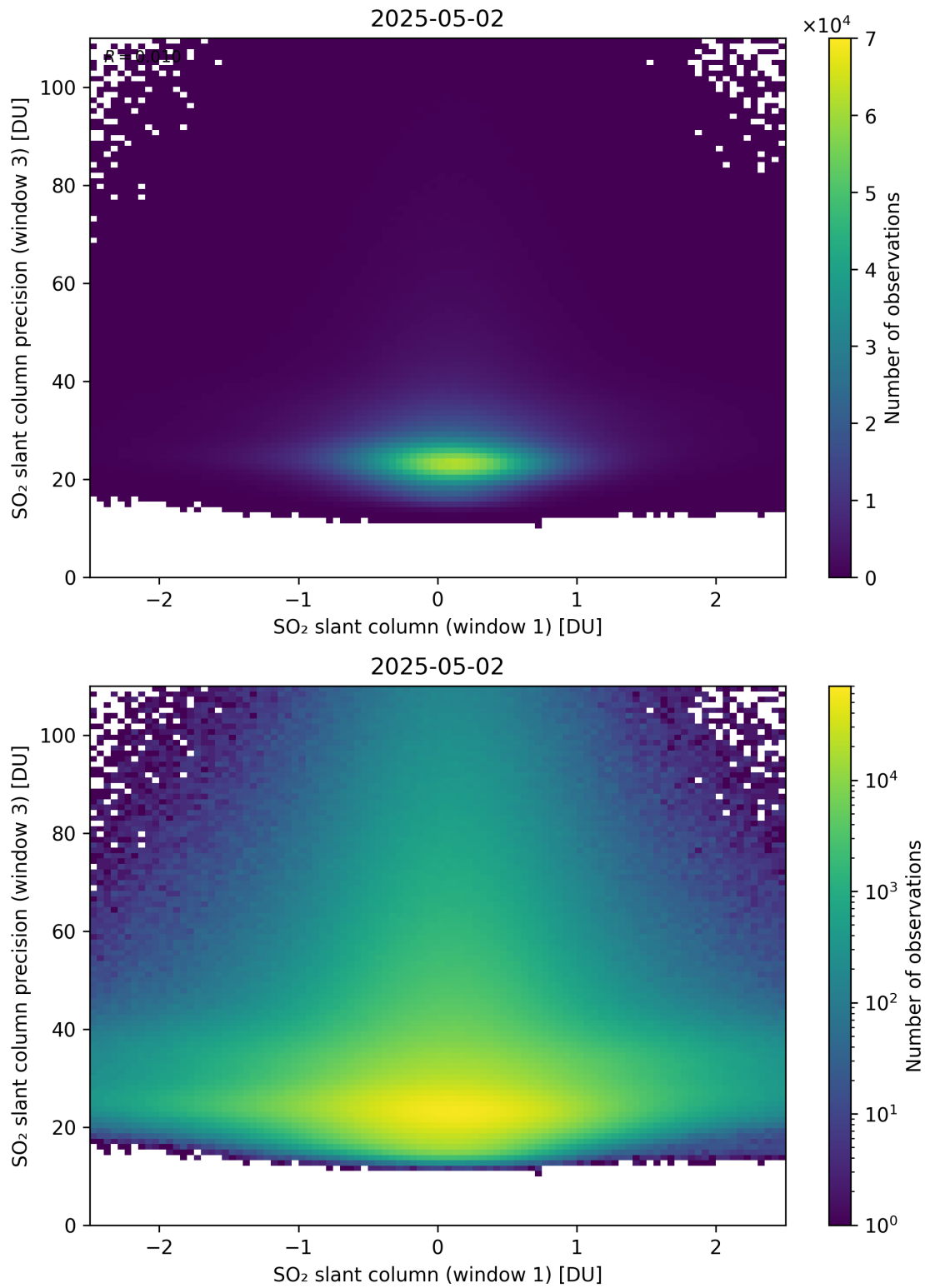
Figure 288: Scatter density plot of “SO 2 slant column (window 1)” against “SO 2 slant column precision (window 3)” for 2025-05-01 to 2025-05-03.
