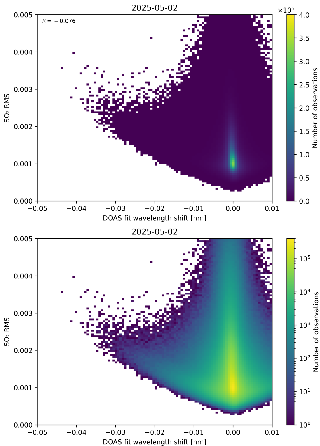
Figure 139: Scatter density plot of “DOAS fit wavelength shift” against “SO 2 RMS” for 2025-05-01 to 2025-05-03.
