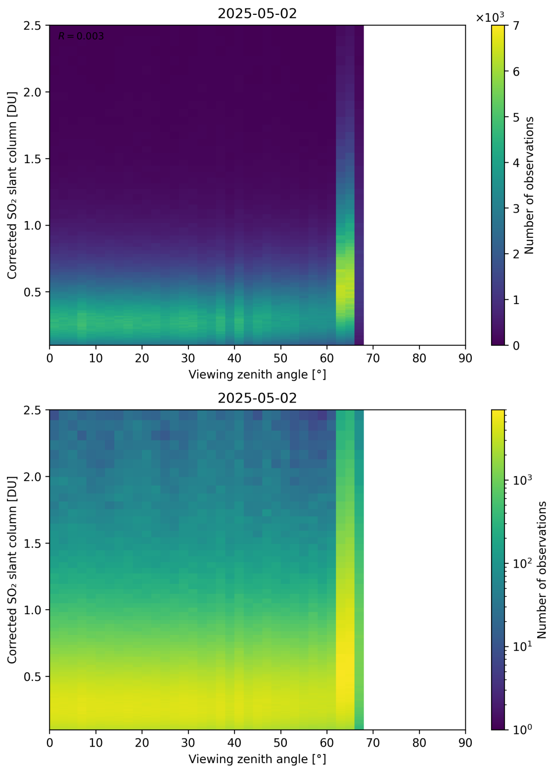
Figure 373: Scatter density plot of “Viewing zenith angle” against “Corrected SO 2 slant column” for 2025-05-01 to 2025-05-03.
