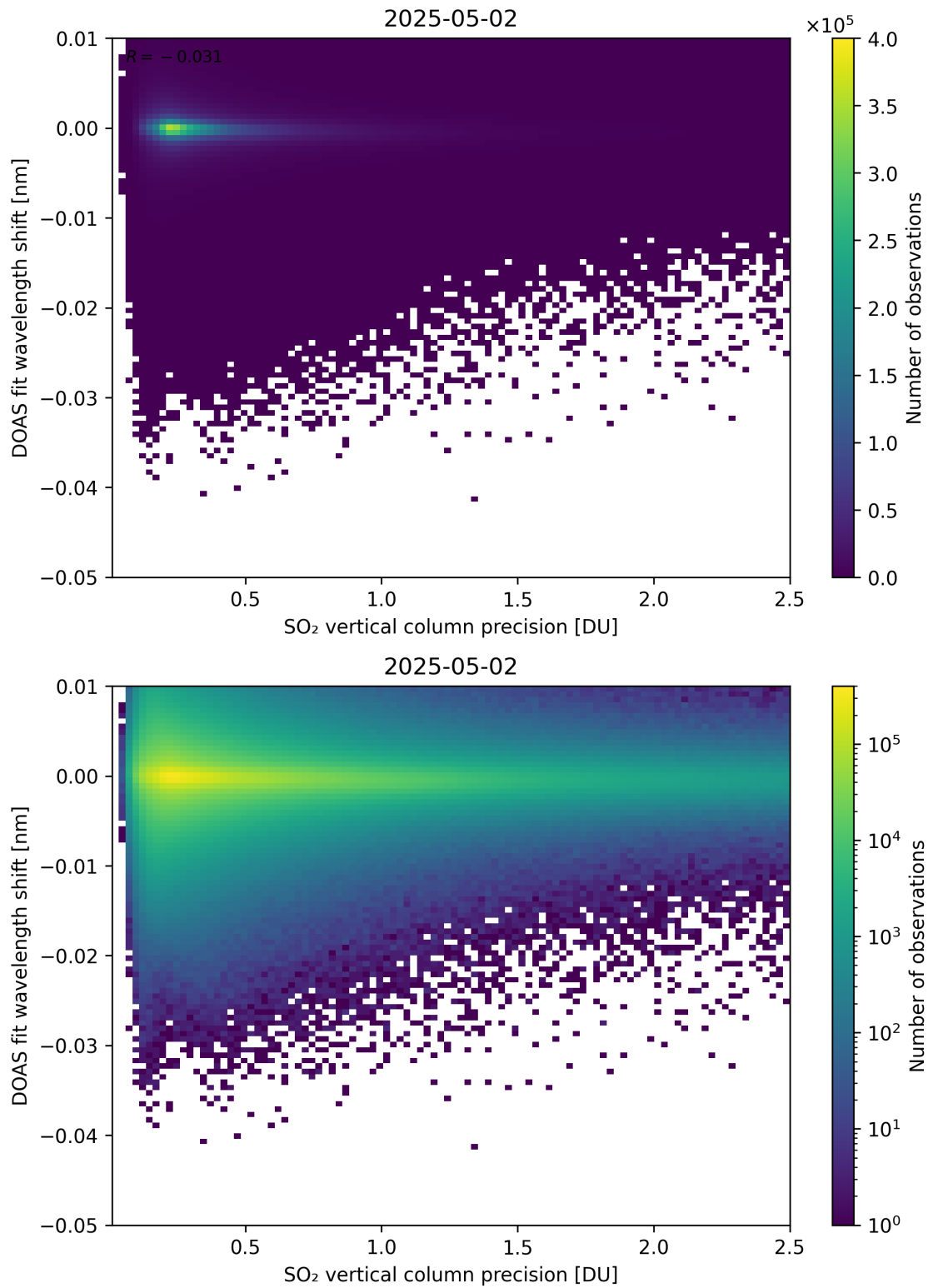
Figure 332: Scatter density plot of “SO 2 vertical column precision” against “DOAS fit wavelength shift” for 2025-05-01 to 2025-05-03.
