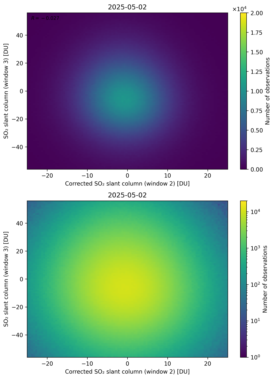
Figure 251: Scatter density plot of “Corrected SO 2 slant column (window 2)” against “SO 2 slant column (window 3)” for 2025-05-01 to 2025-05-03.
