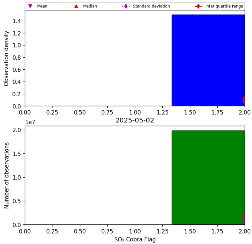
Figure 75: Histogram of “SO 2 Cobra Flag” for 2025-05-01 to 2025-05-03
