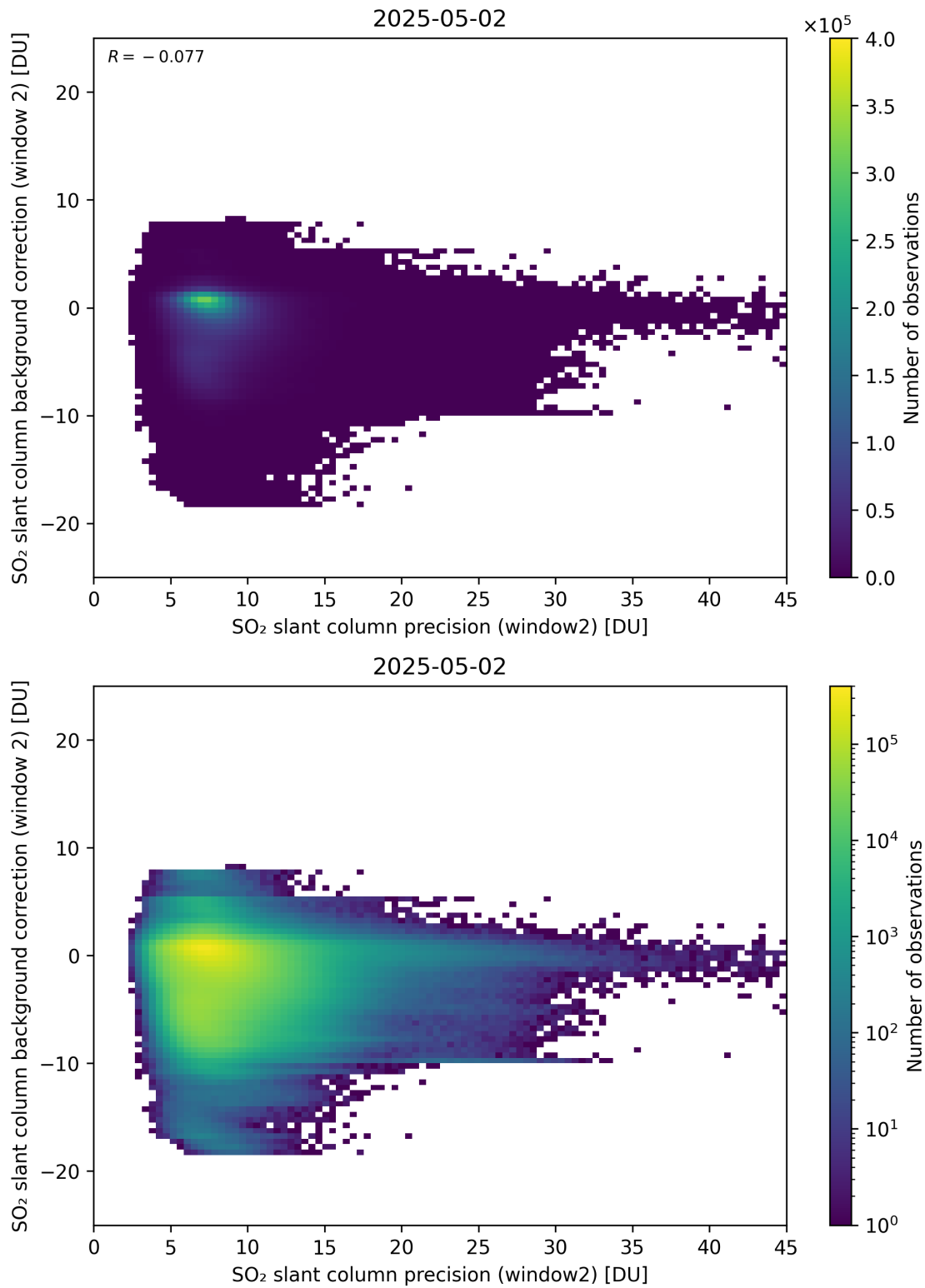
Figure 291: Scatter density plot of “SO 2 slant column precision (window2)” against “SO 2 slant column background correction (window 2)” for 2025-05-01 to 2025-05-03.
