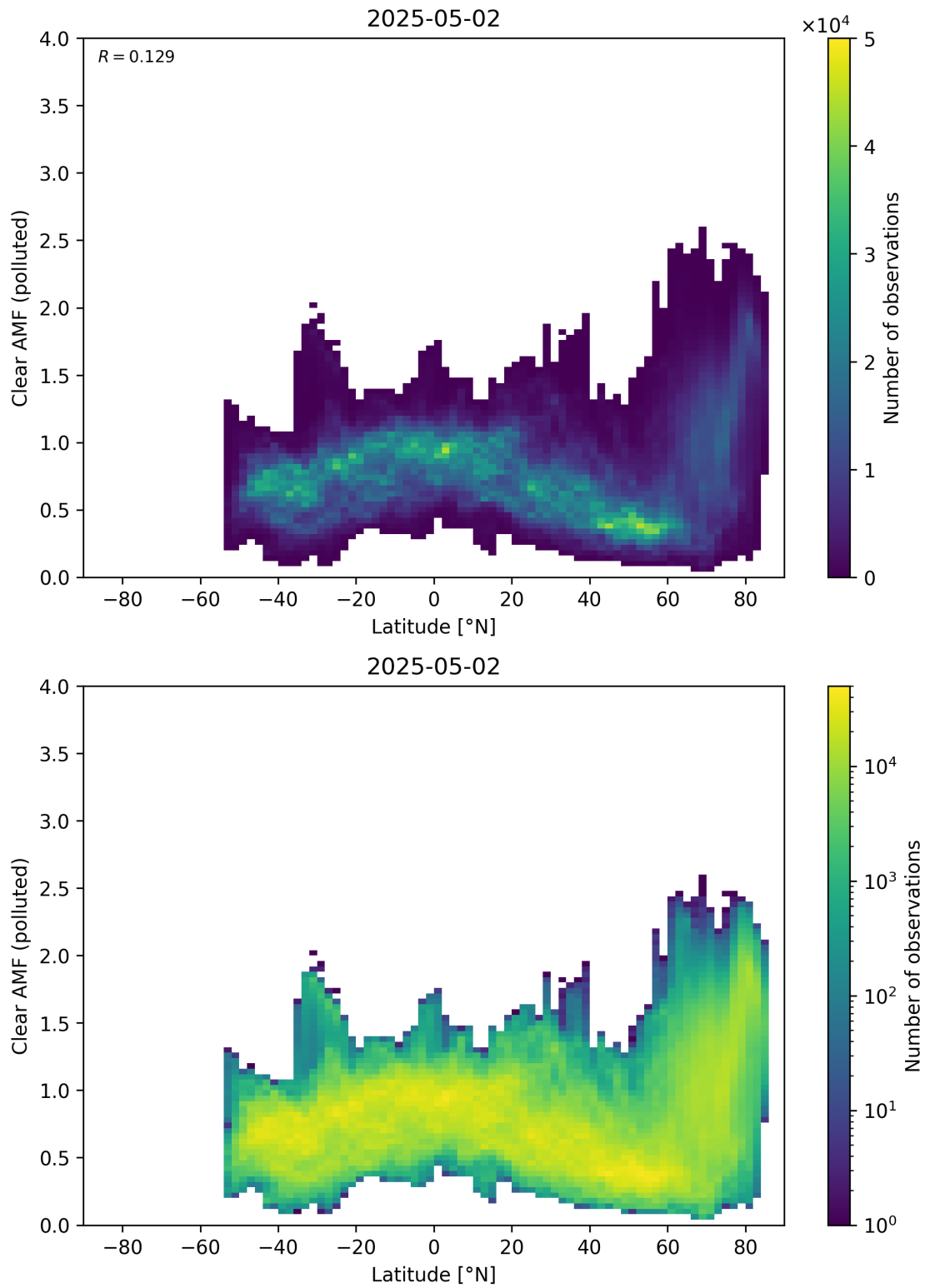
Figure 156: Scatter density plot of “Latitude” against “Clear AMF (polluted)” for 2025-05-01 to 2025-05-03.
