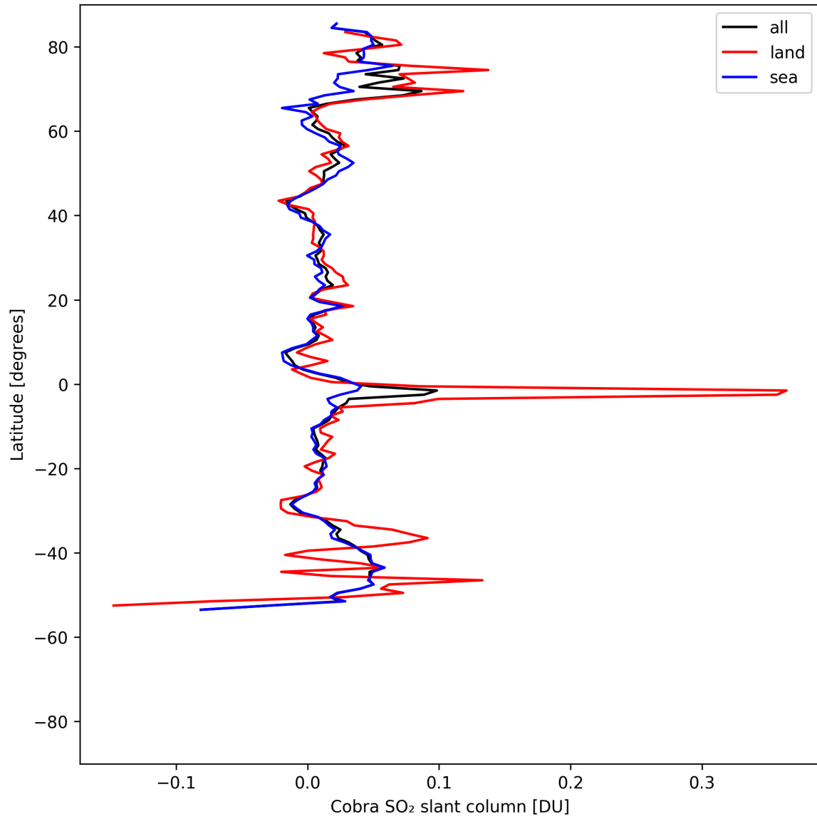
Figure 35: Zonal average of “Cobra SO 2 slant column” for 2025-05-01 to 2025-05-03.
