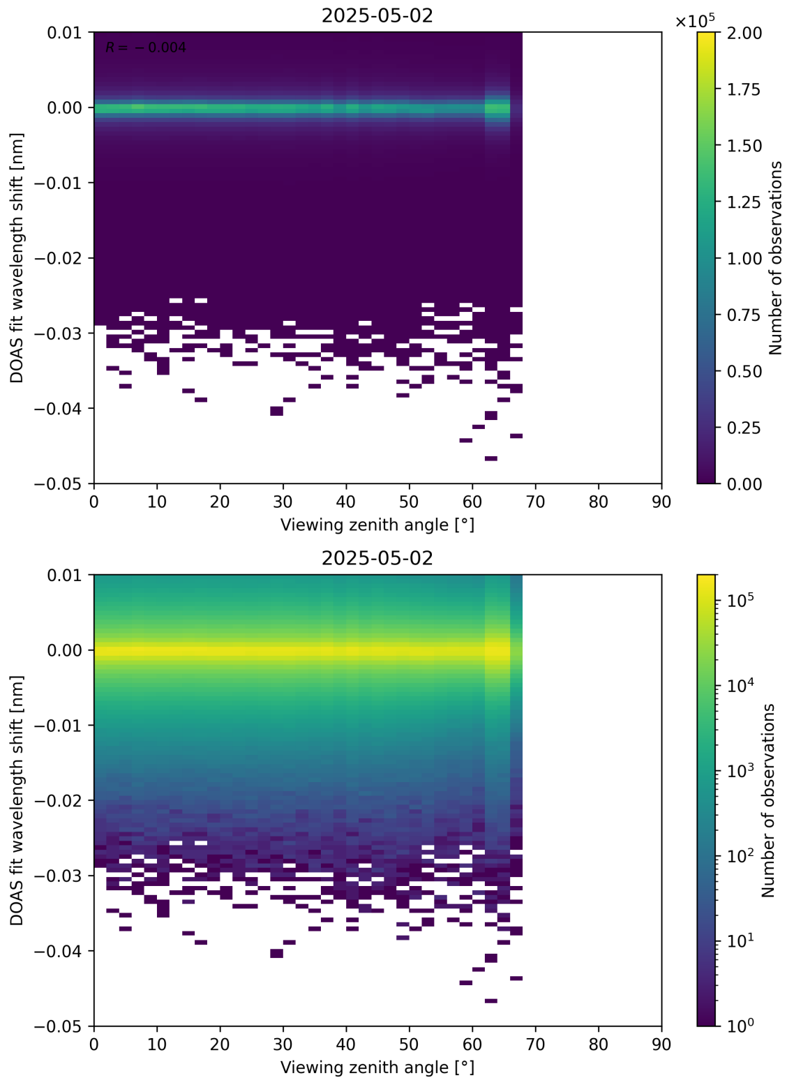
Figure 365: Scatter density plot of “Viewing zenith angle” against “DOAS fit wavelength shift” for 2025-05-01 to 2025-05-03.
