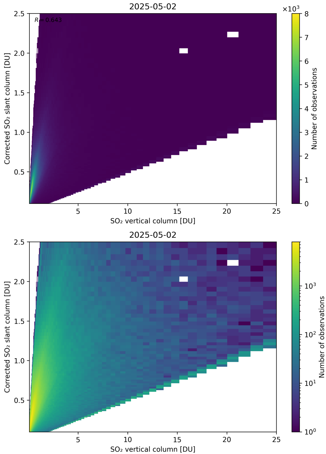
Figure 351: Scatter density plot of “SO 2 vertical column” against “Corrected SO 2 slant column” for 2025-05-01 to 2025-05-03.
