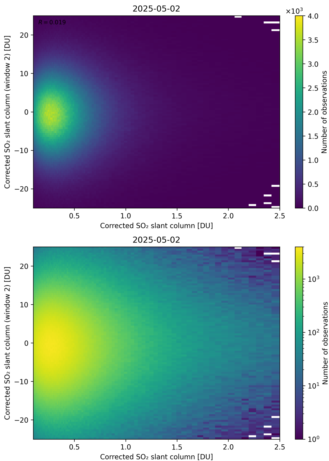
Figure 235: Scatter density plot of “Corrected SO 2 slant column” against “Corrected SO 2 slant column (window 2)” for 2025-05-01 to 2025-05-03.
