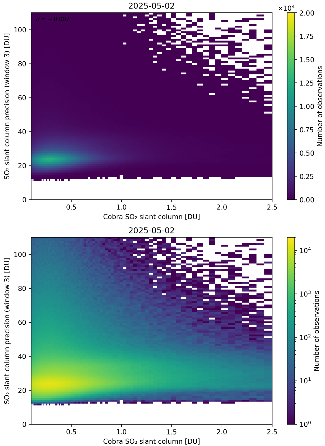
Figure 223: Scatter density plot of “Cobra SO 2 slant column” against “SO 2 slant column precision (window 3)” for 2025-05-01 to 2025-05-03.
