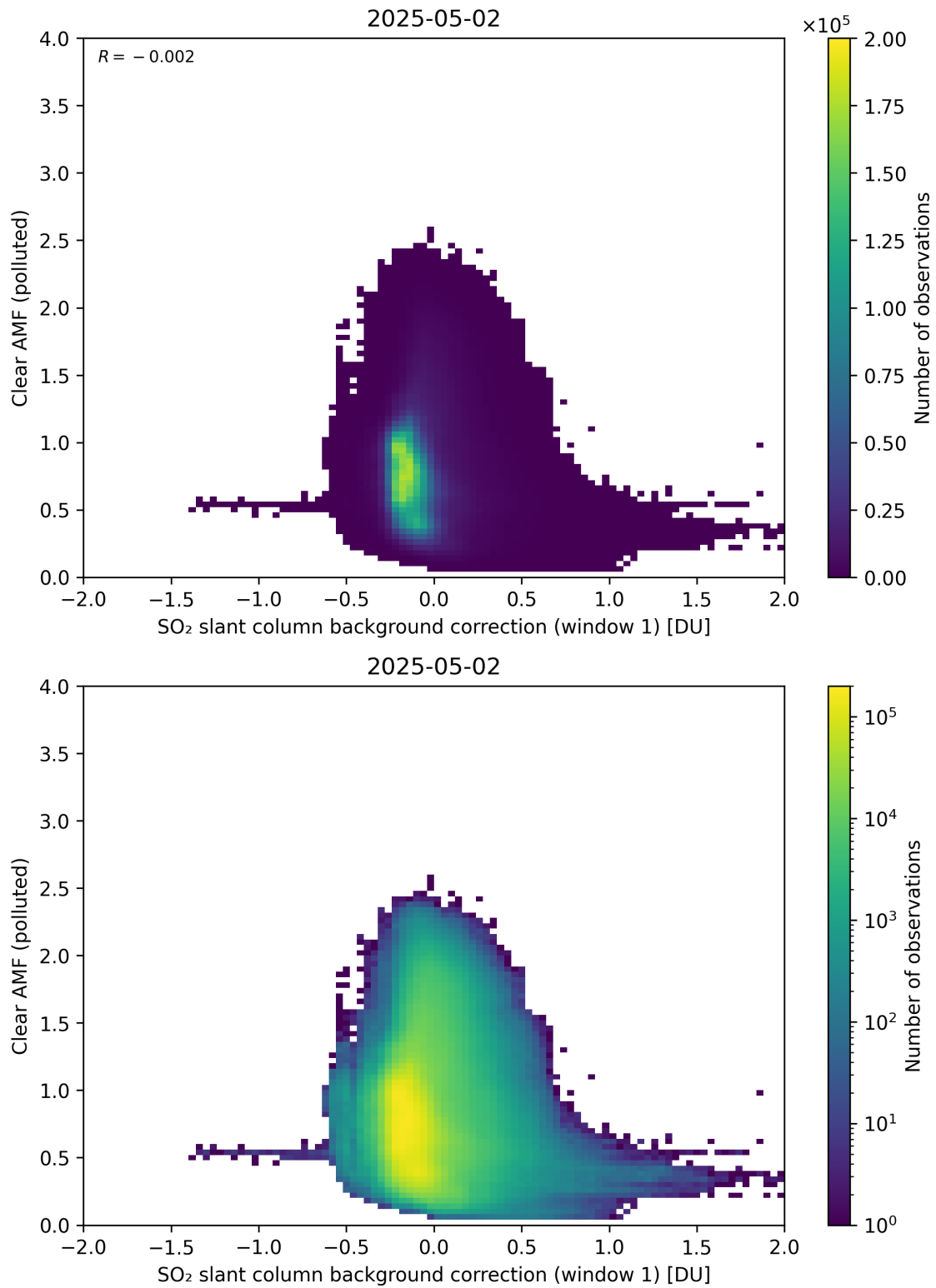
Figure 114: Scatter density plot of “SO 2 slant column background correction (window 1)” against “Clear AMF (polluted)” for 2025-05-01 to 2025-05-03.
