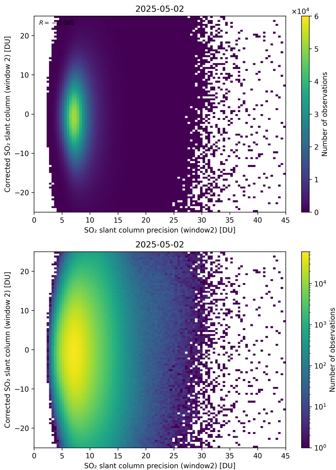
Figure 297: Scatter density plot of “SO 2 slant column precision (window2)” against “Corrected SO 2 slant column (window 2)” for 2025-05-01 to 2025-05-03.
