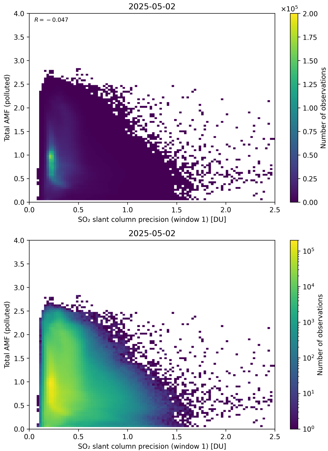
Figure 280: Scatter density plot of “SO 2 slant column precision (window 1)” against “Total AMF (polluted)” for 2025-05-01 to 2025-05-03.
