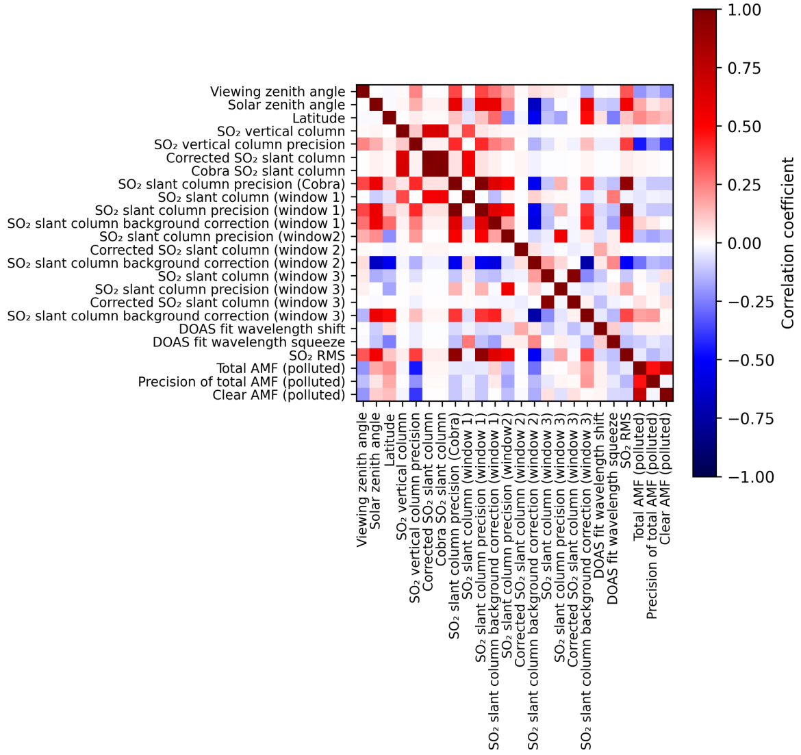
Figure 2: Map of correlation matrix for 2025-05-01 to 2025-05-03.
