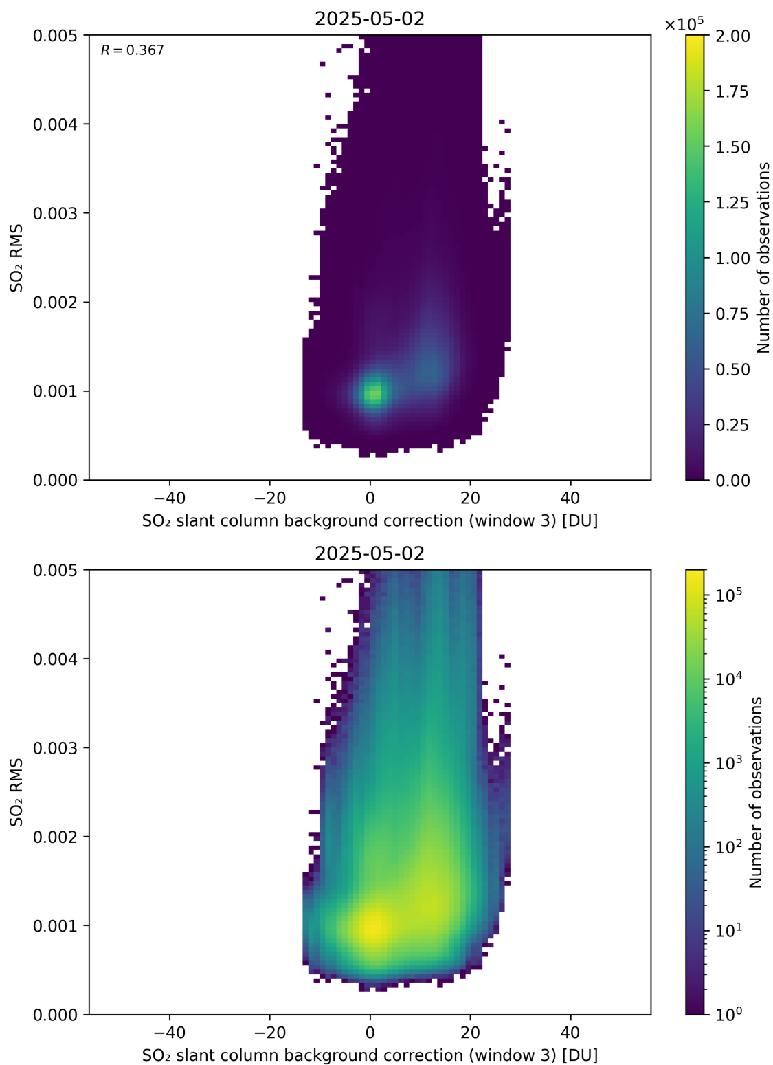
Figure 134: Scatter density plot of “SO 2 slant column background correction (window 3)” against “SO 2 RMS” for 2025-05-01 to 2025-05-03.
