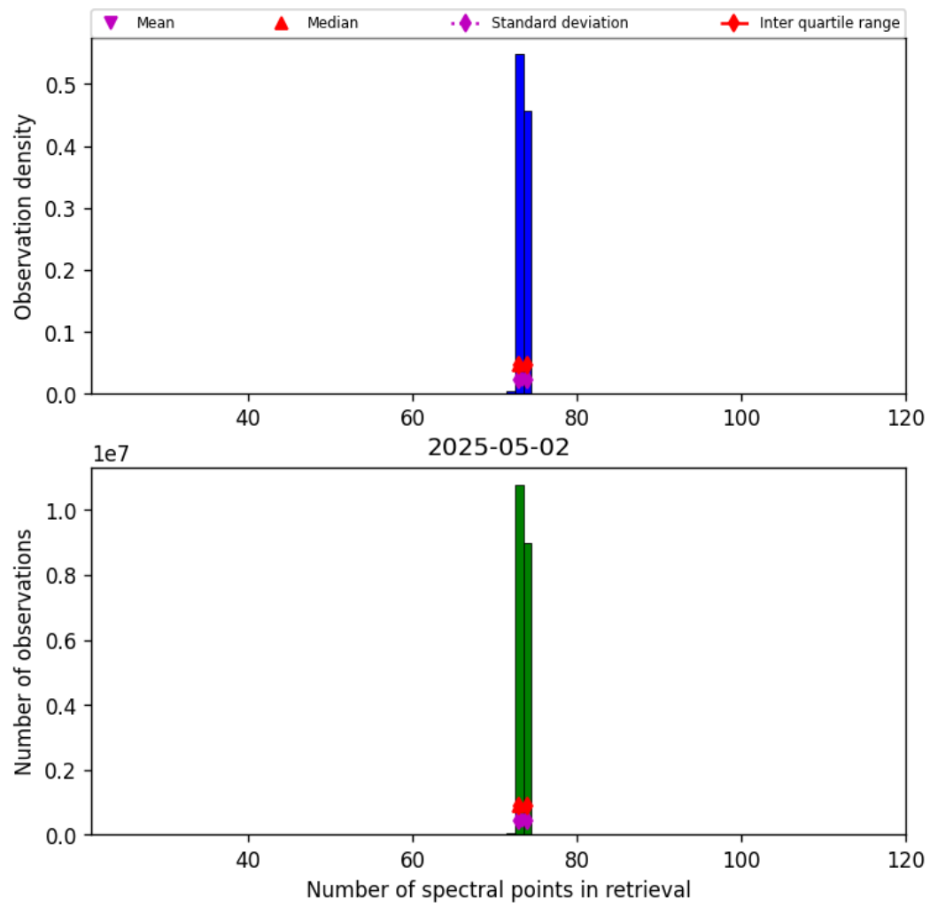
Figure 82: Histogram of “Number of spectral points in retrieval” for 2025-05-01 to 2025-05-03
