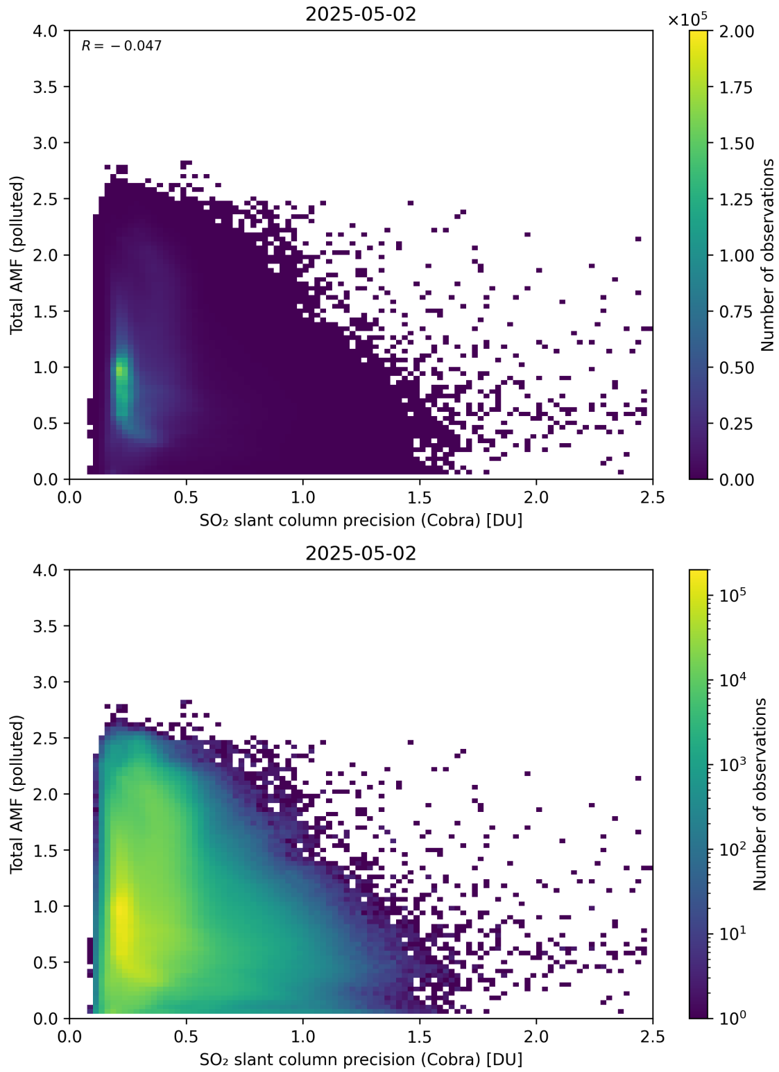
Figure 213: Scatter density plot of “SO 2 slant column precision (Cobra)” against “Total AMF (polluted)” for 2025-05-01 to 2025-05-03.
