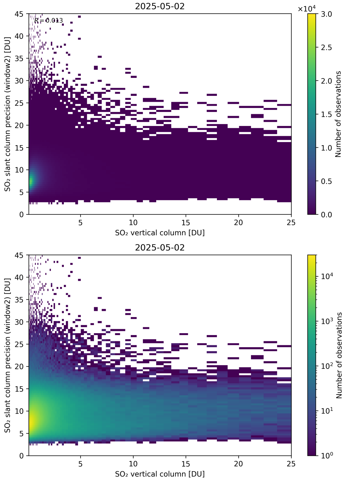
Figure 356: Scatter density plot of “SO 2 vertical column” against “SO 2 slant column precision (window2)” for 2025-05-01 to 2025-05-03.
