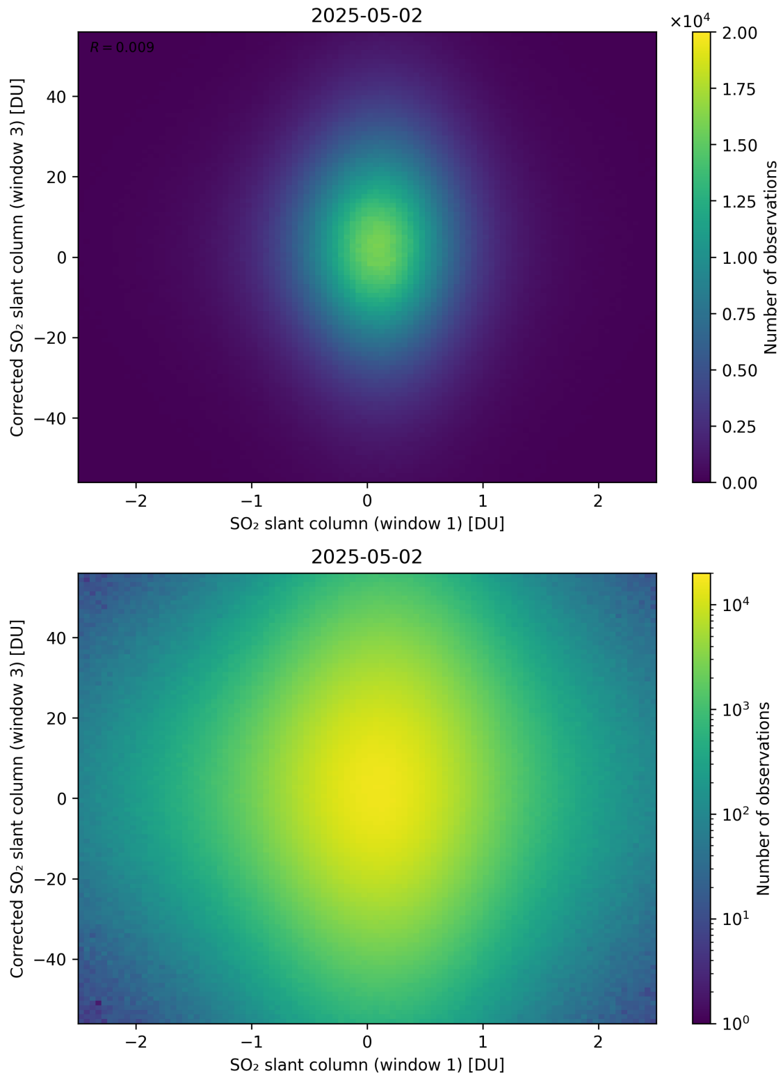
Figure 284: Scatter density plot of “SO 2 slant column (window 1)” against “Corrected SO 2 slant column (window 3)” for 2025-05-01 to 2025-05-03.
