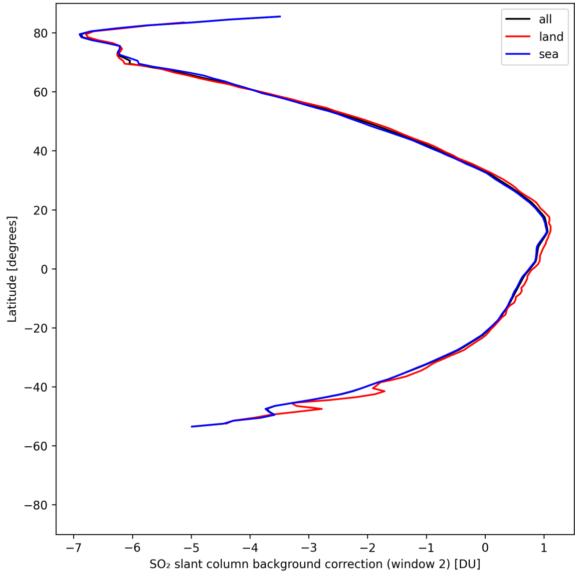
Figure 44: Zonal average of “SO 2 slant column background correction (window 2)” for 2025-05-01 to 2025-05-03.
