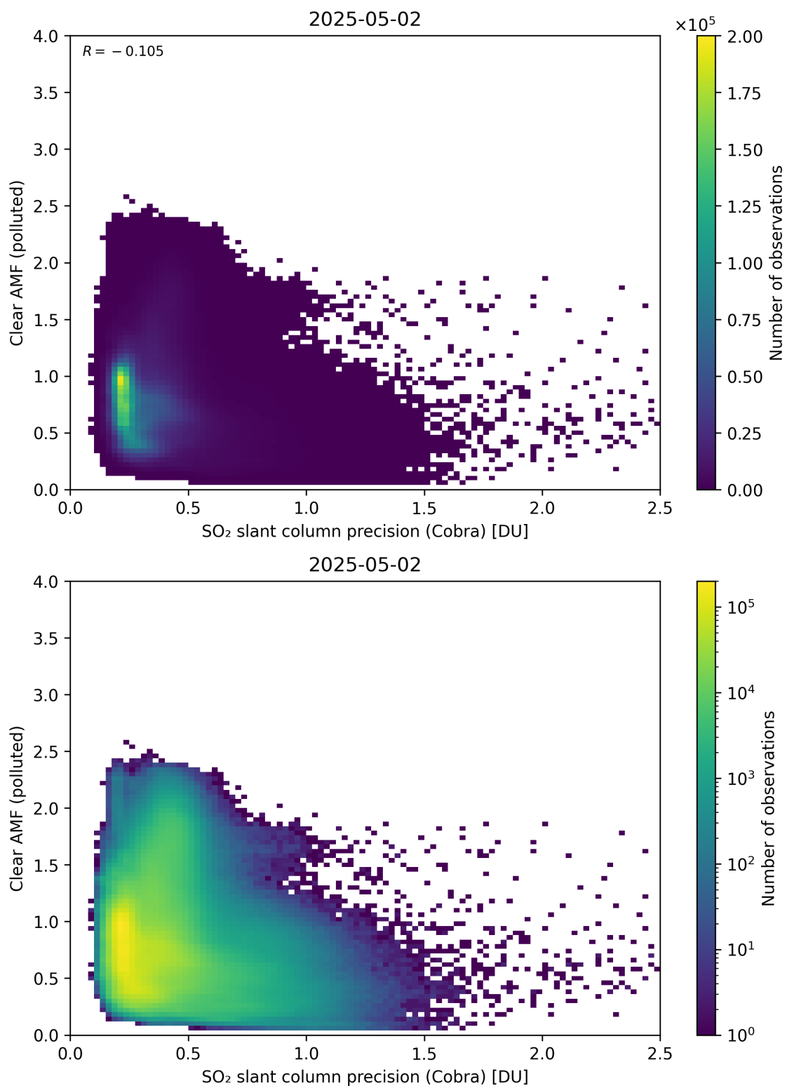
Figure 205: Scatter density plot of “SO 2 slant column precision (Cobra)” against “Clear AMF (polluted)” for 2025-05-01 to 2025-05-03.
