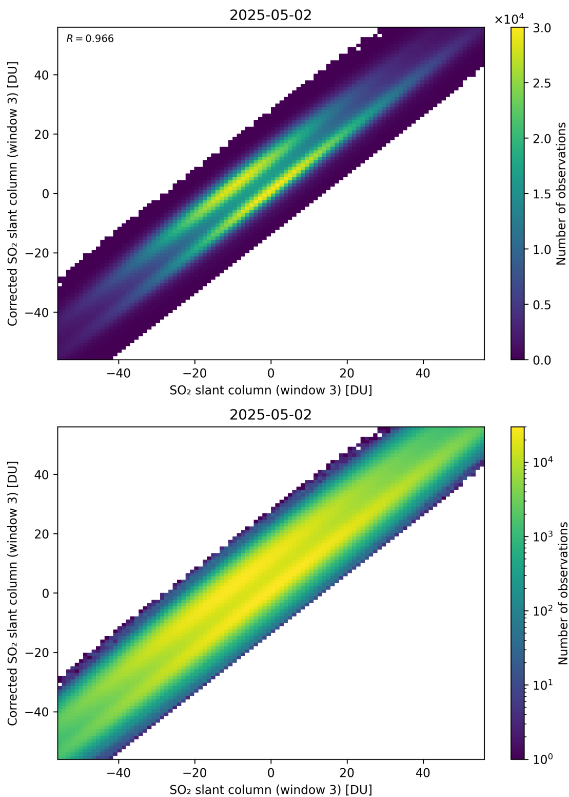
Figure 316: Scatter density plot of “SO 2 slant column (window 3)” against “Corrected SO 2 slant column (window 3)” for 2025-05-01 to 2025-05-03.
