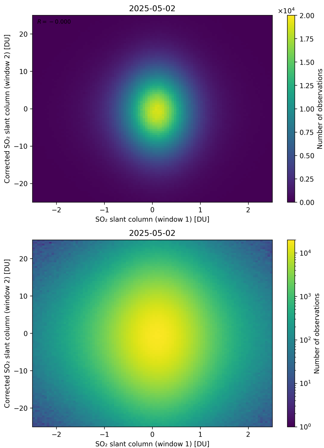
Figure 283: Scatter density plot of “SO 2 slant column (window 1)” against “Corrected SO 2 slant column (window 2)” for 2025-05-01 to 2025-05-03.
