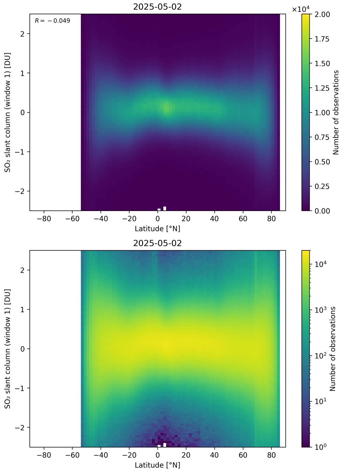
Figure 162: Scatter density plot of “Latitude” against “SO 2 slant column (window 1)” for 2025-05-01 to 2025-05-03.
