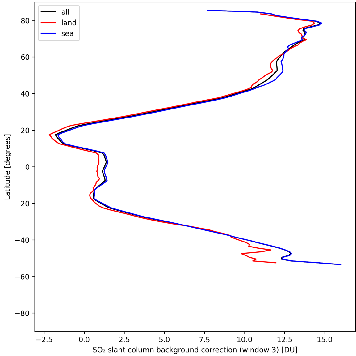
Figure 48: Zonal average of “SO 2 slant column background correction (window 3)” for 2025-05-01 to 2025-05-03.
