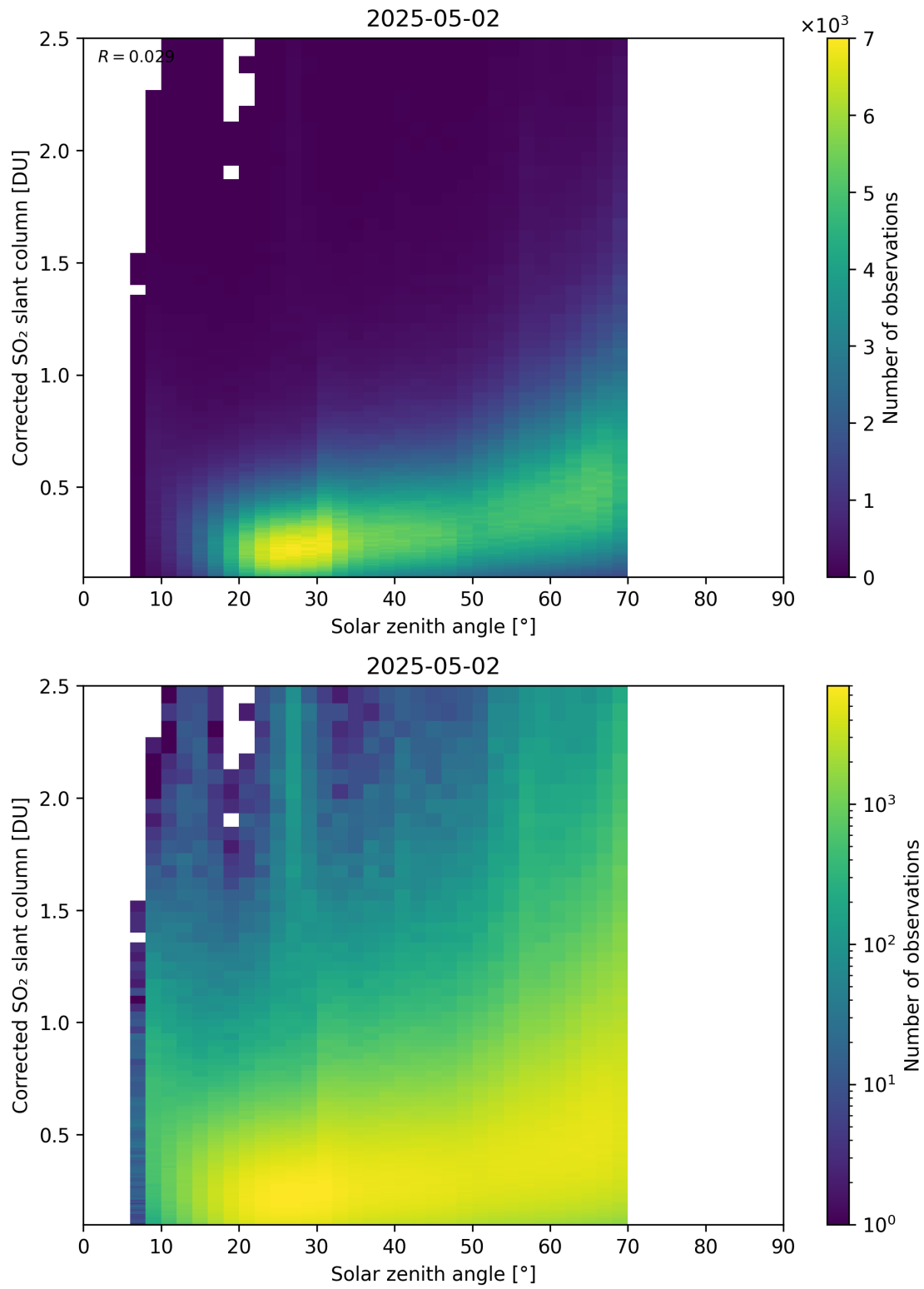
Figure 181: Scatter density plot of “Solar zenith angle” against “Corrected SO 2 slant column” for 2025-05-01 to 2025-05-03.
