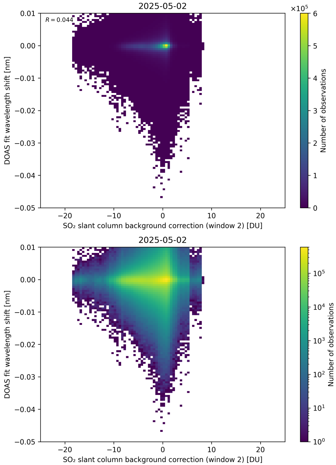
Figure 123: Scatter density plot of “SO 2 slant column background correction (window 2)” against “DOAS fit wavelength shift” for 2025-05-01 to 2025-05-03.
