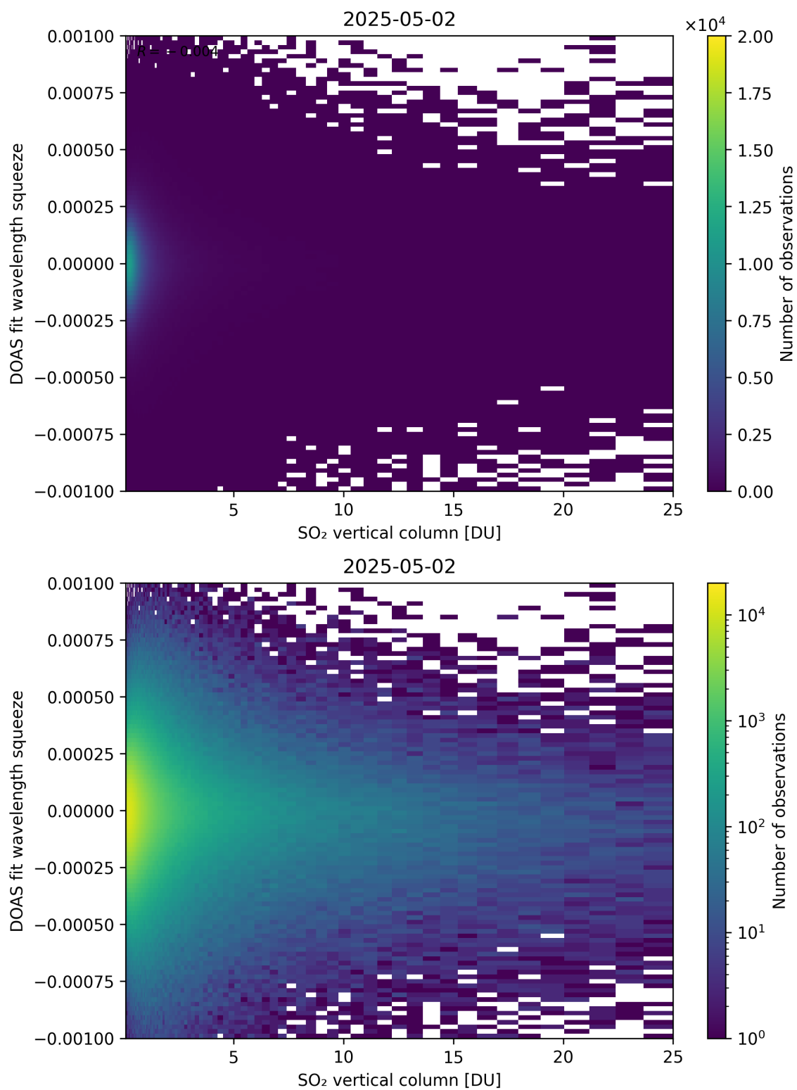
Figure 327: Scatter density plot of “SO 2 vertical column” against “DOAS fit wavelength squeeze” for 2025-05-01 to 2025-05-03.
