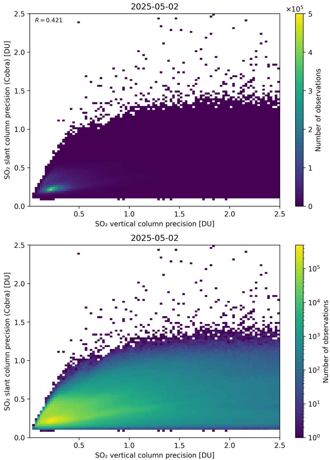
Figure 337: Scatter density plot of “SO 2 vertical column precision” against “SO 2 slant column precision (Cobra)” for 2025-05-01 to 2025-05-03.
