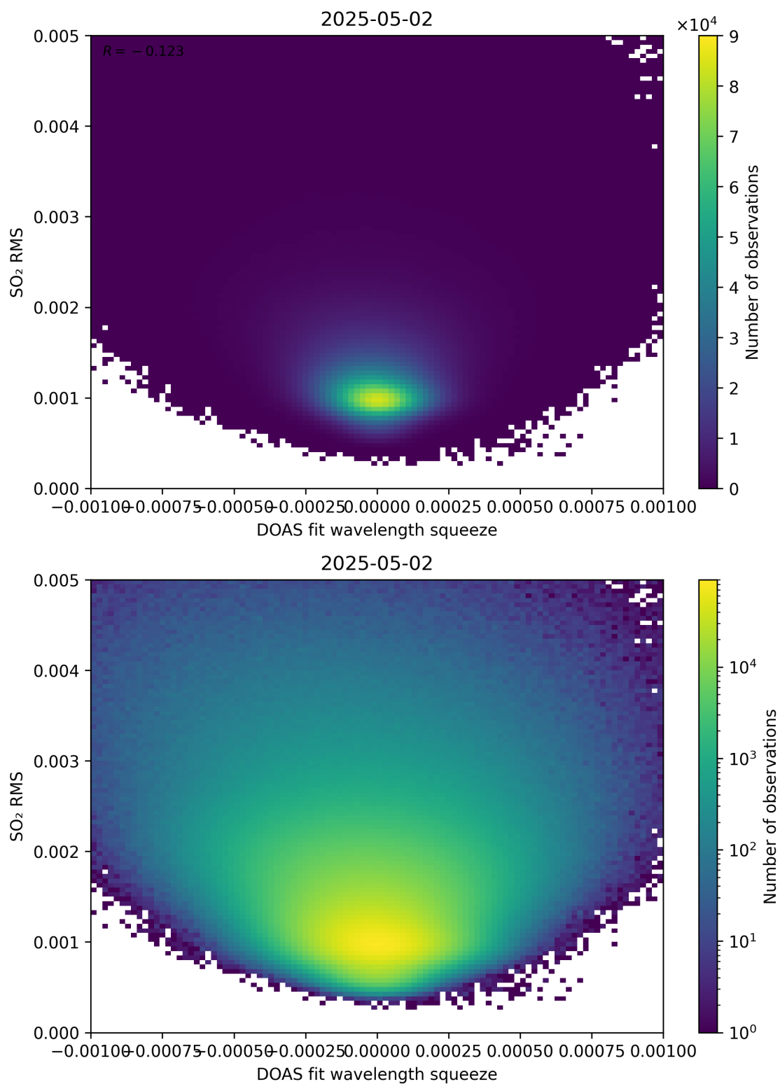
Figure 143: Scatter density plot of “DOAS fit wavelength squeeze” against “SO 2 RMS” for 2025-05-01 to 2025-05-03.
