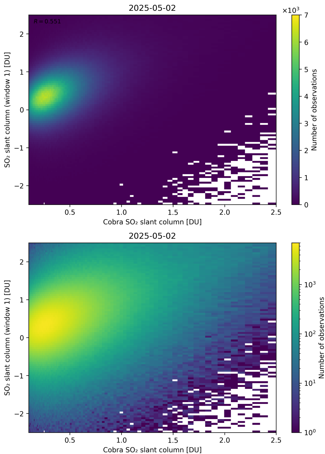
Figure 219: Scatter density plot of “Cobra SO 2 slant column” against “SO 2 slant column (window 1)” for 2025-05-01 to 2025-05-03.
