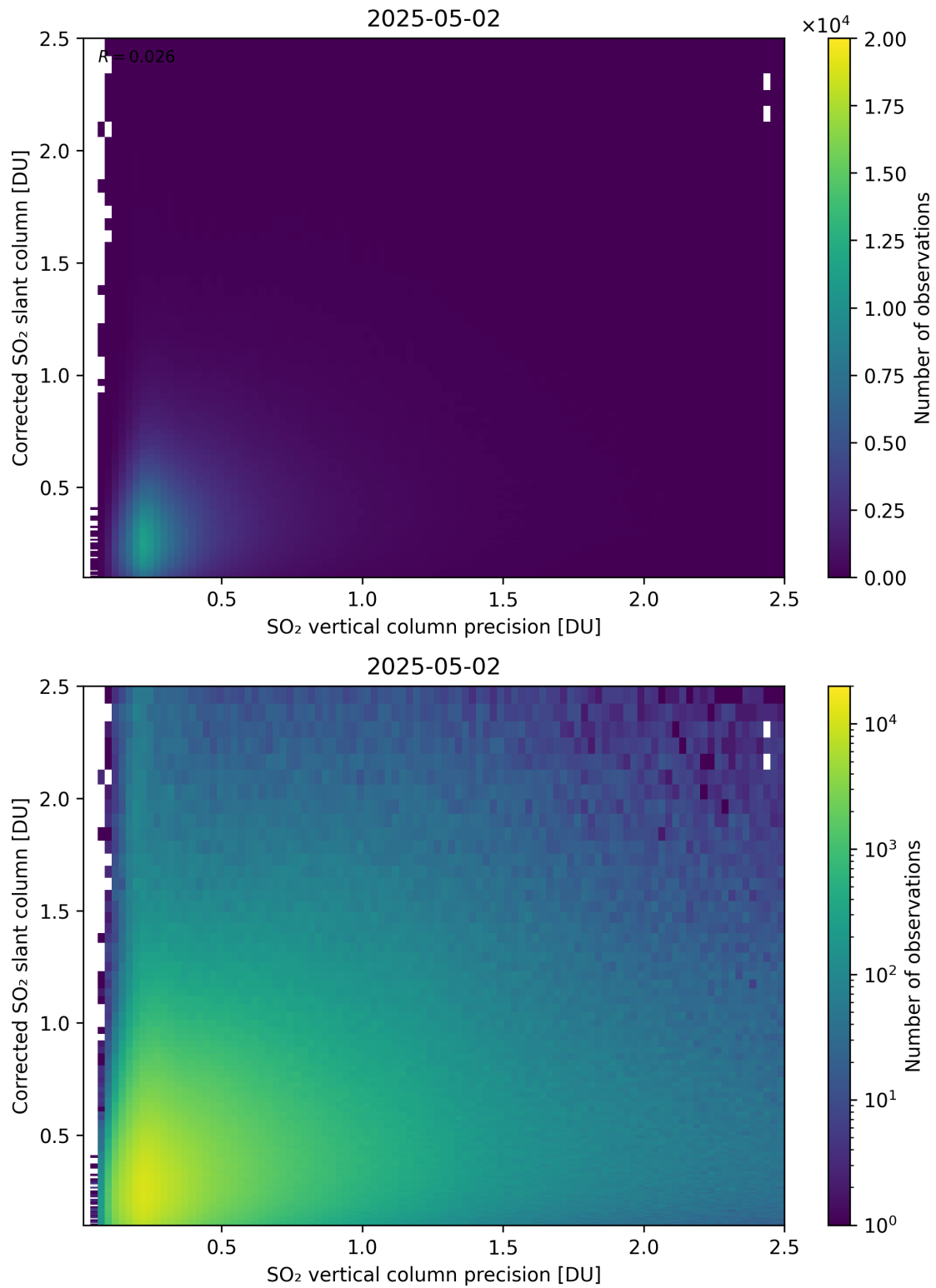
Figure 338: Scatter density plot of “SO 2 vertical column precision” against “Corrected SO 2 slant column” for 2025-05-01 to 2025-05-03.
