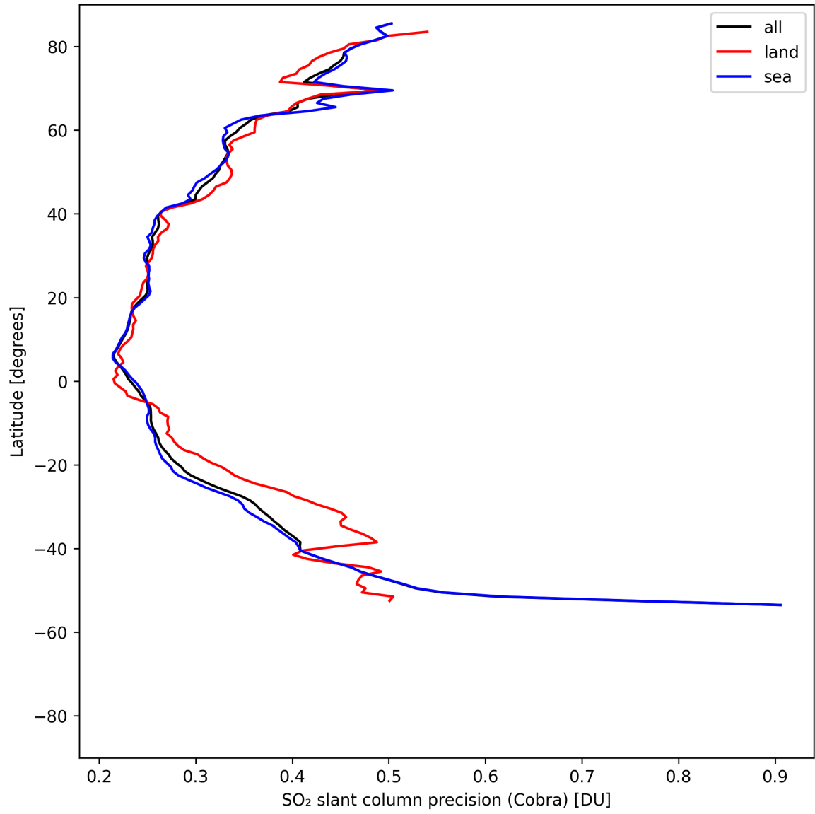
Figure 36: Zonal average of "SO 2 slant column precision (Cobra)" for 2025-05-01 to 2025-05-03.
