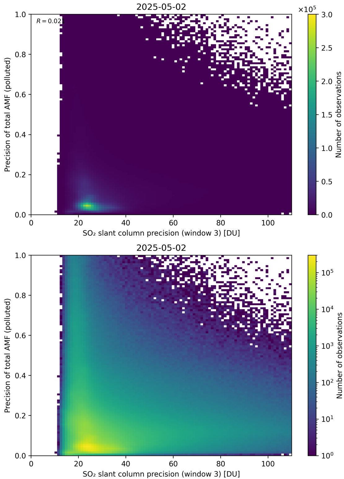
Figure 314: Scatter density plot of “SO 2 slant column precision (window 3)” against “Precision of total AMF (polluted)” for 2025-05-01 to 2025-05-03.
