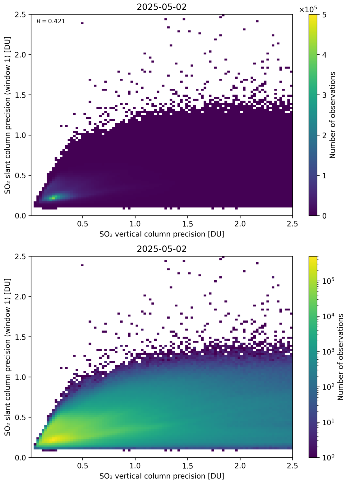
Figure 342: Scatter density plot of “SO 2 vertical column precision” against “SO 2 slant column precision (window 1)” for 2025-05-01 to 2025-05-03.
