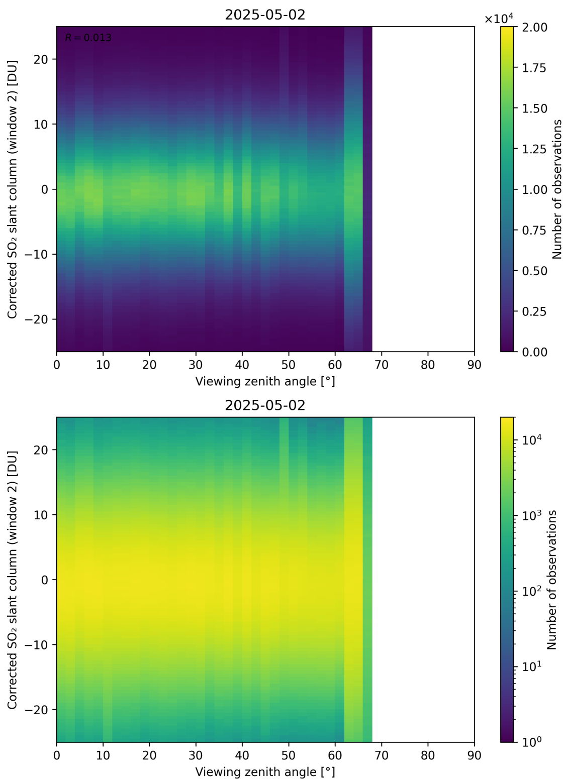
Figure 374: Scatter density plot of “Viewing zenith angle” against “Corrected SO 2 slant column (window 2)” for 2025-05-01 to 2025-05-03.
