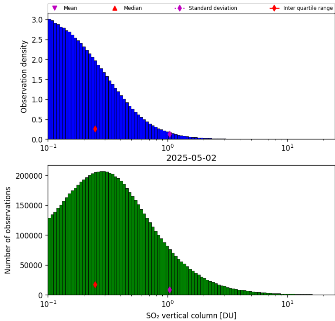
Figure 58: Histogram of “SO 2 vertical column” for 2025-05-01 to 2025-05-03
