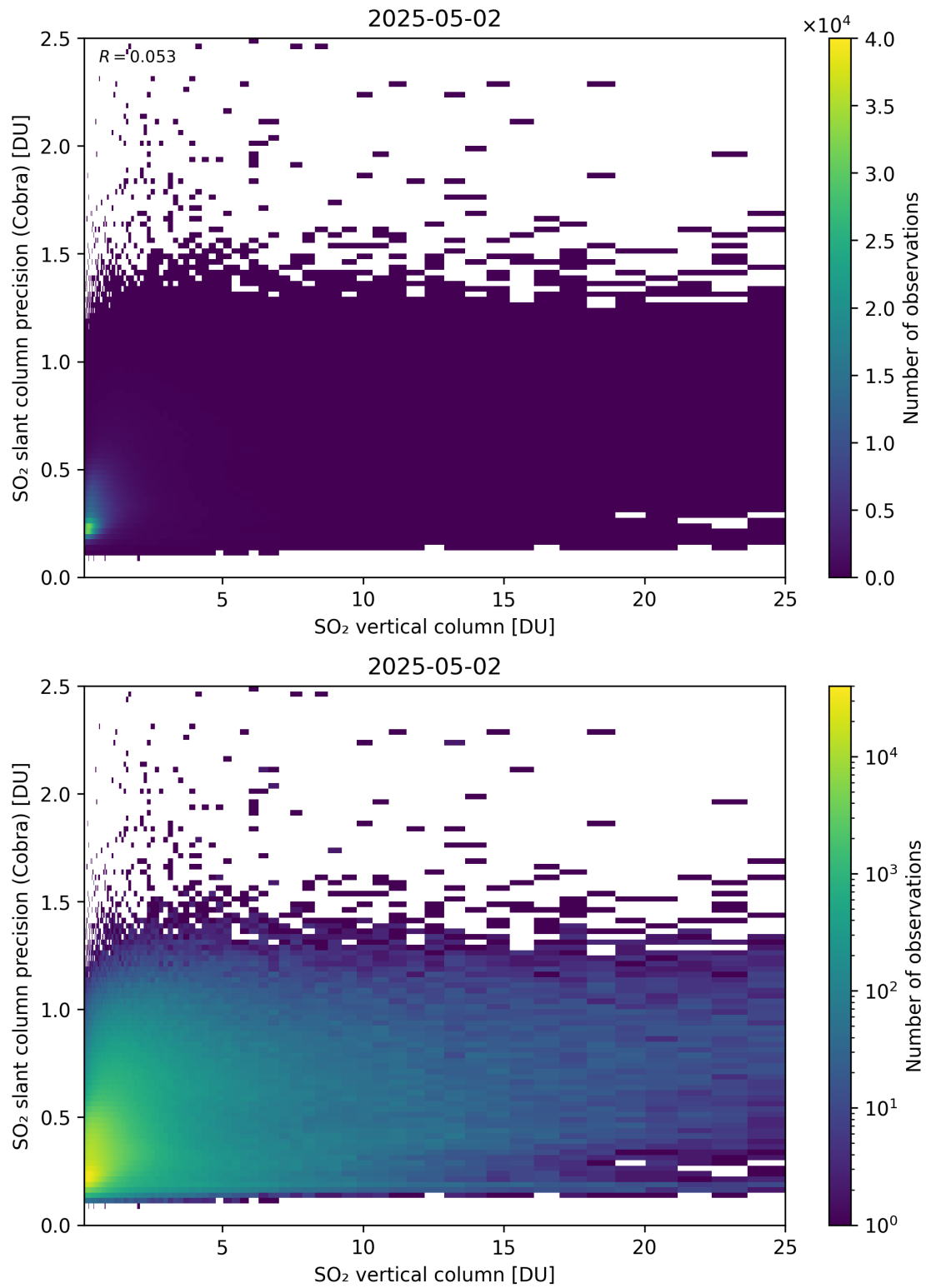
Figure 350: Scatter density plot of “SO 2 vertical column” against “SO 2 slant column precision (Cobra)” for 2025-05-01 to 2025-05-03.
