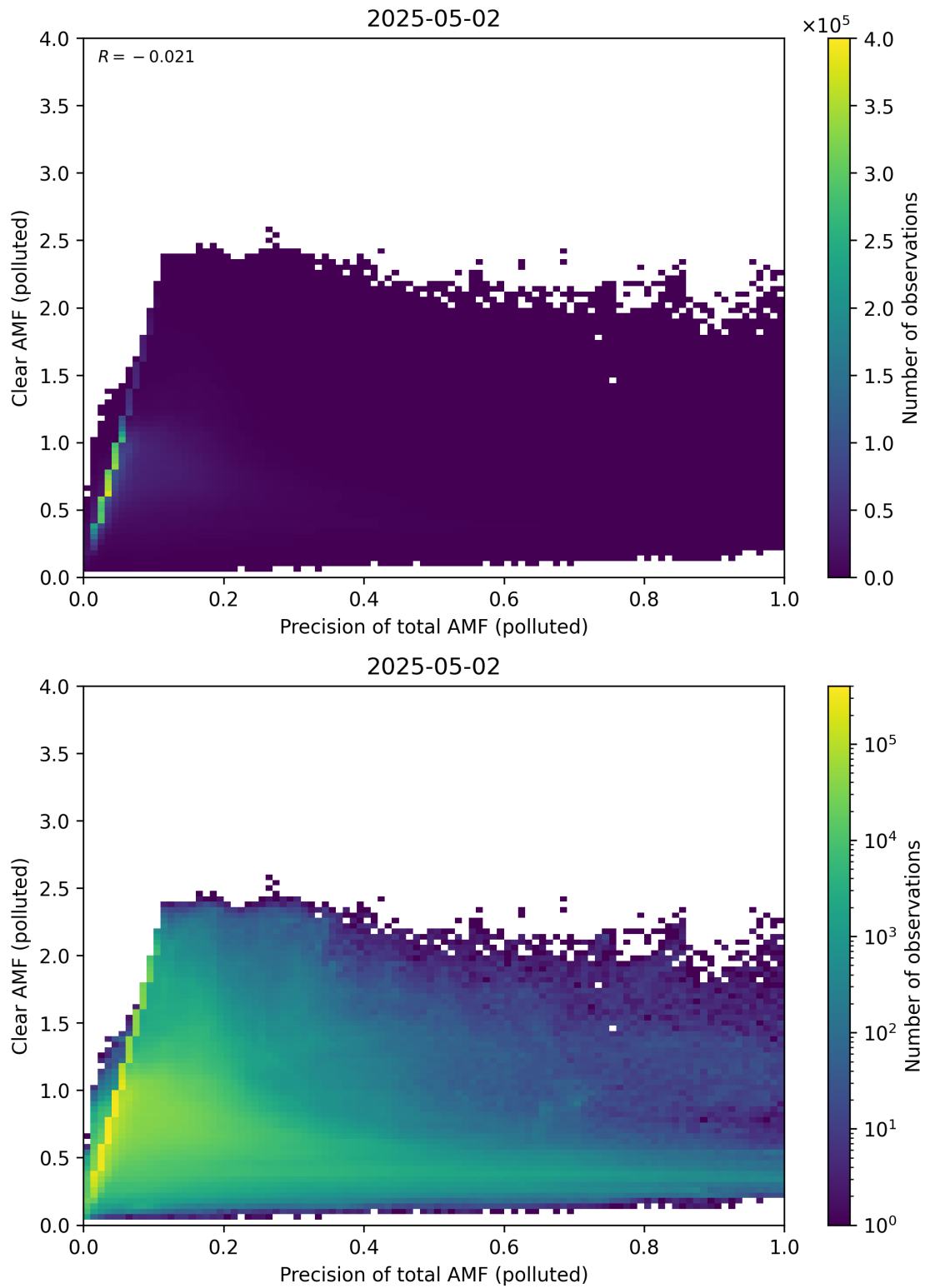
Figure 320: Scatter density plot of “Precision of total AMF (polluted)” against “Clear AMF (polluted)” for 2025-05-01 to 2025-05-03.
