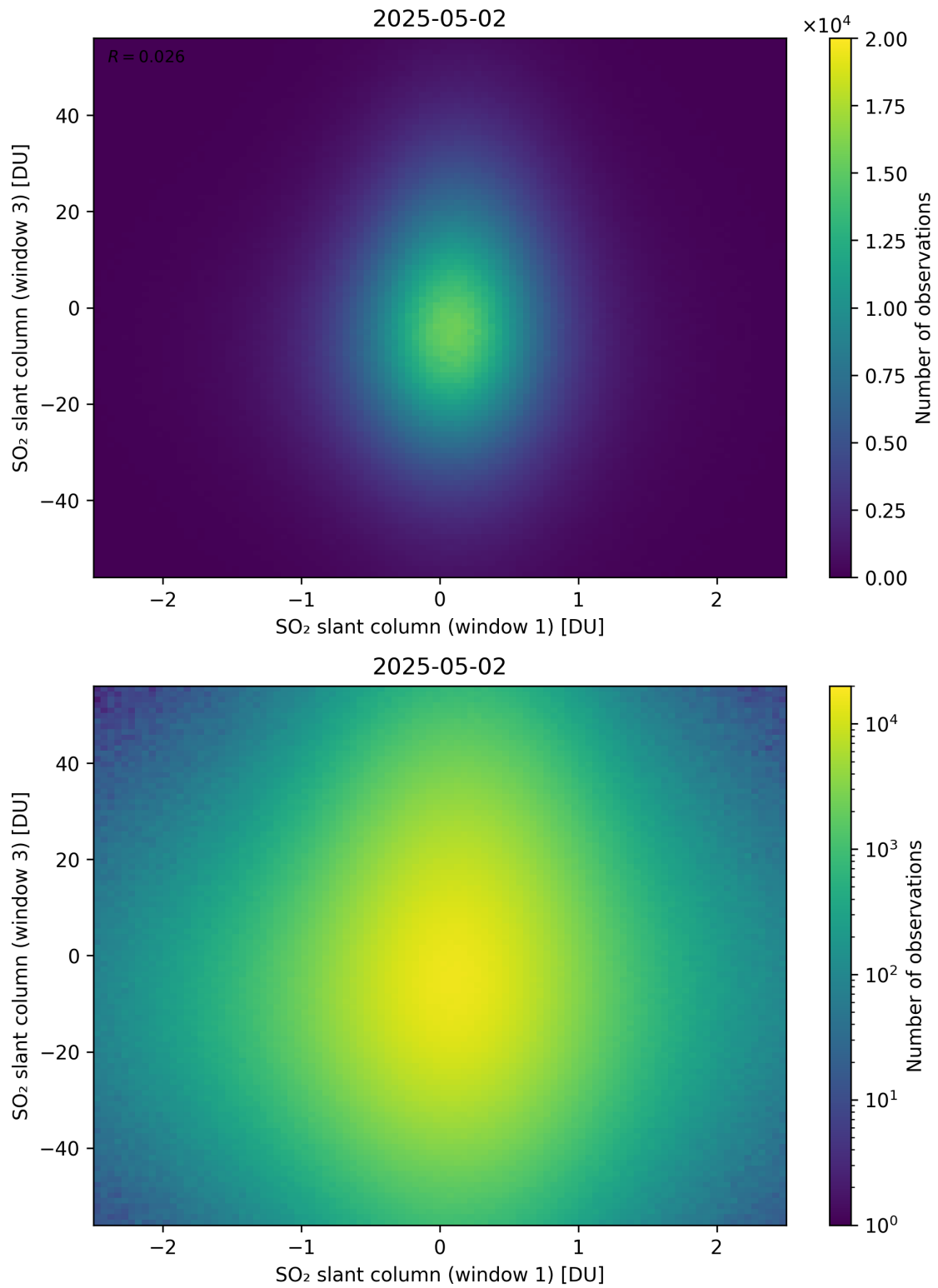
Figure 287: Scatter density plot of “SO 2 slant column (window 1)” against “SO 2 slant column (window 3)” for 2025-05-01 to 2025-05-03.
