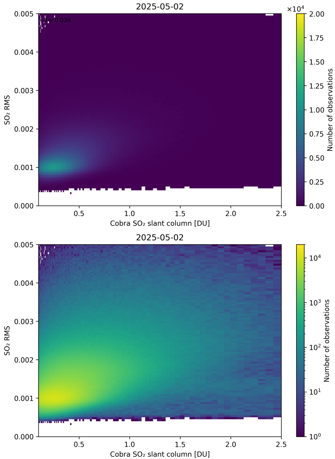
Figure 198: Scatter density plot of “Cobra SO 2 slant column” against “SO 2 RMS” for 2025-05-01 to 2025-05-03.
