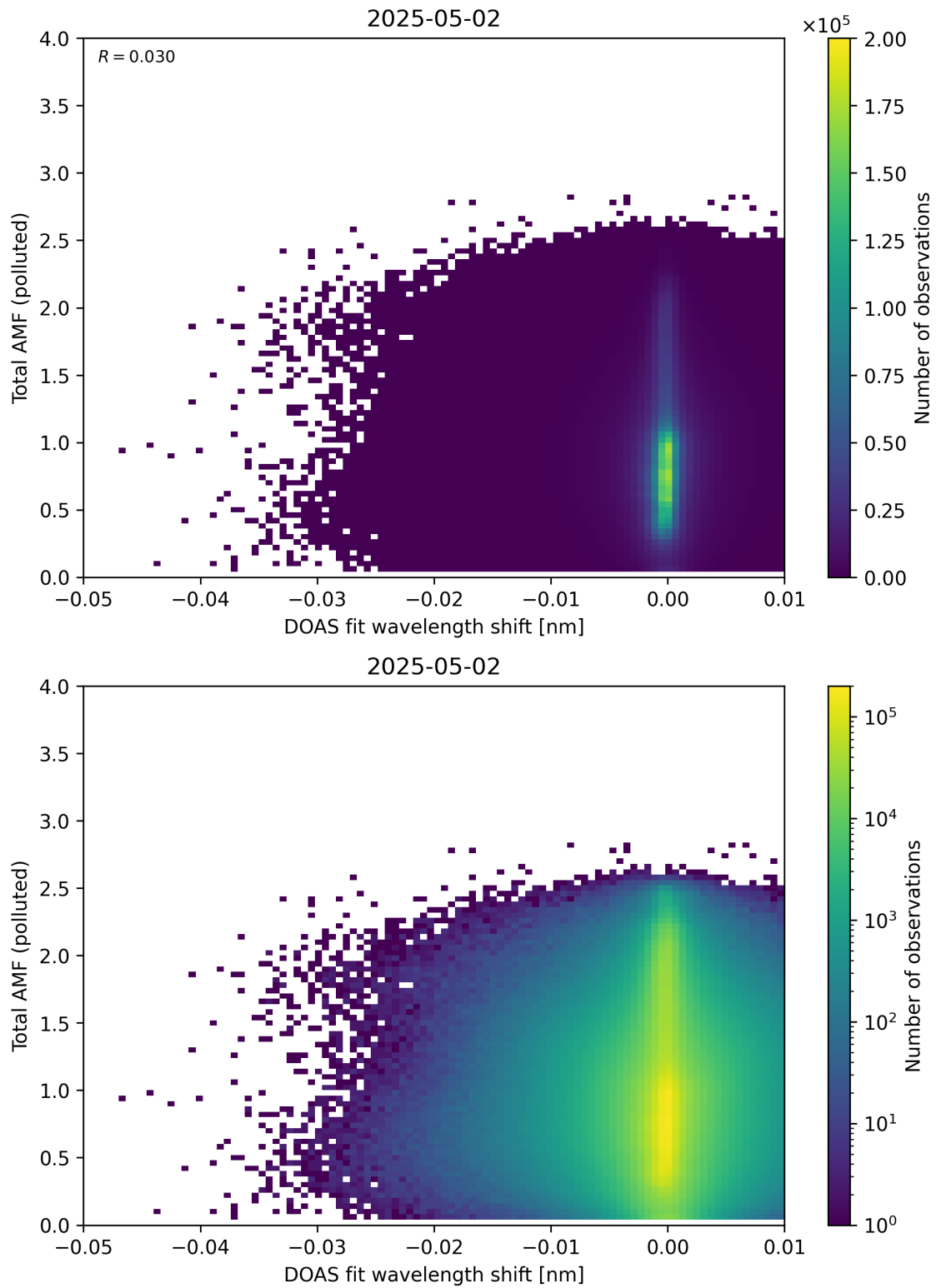
Figure 141: Scatter density plot of “DOAS fit wavelength shift” against “Total AMF (polluted)” for 2025-05-01 to 2025-05-03.
