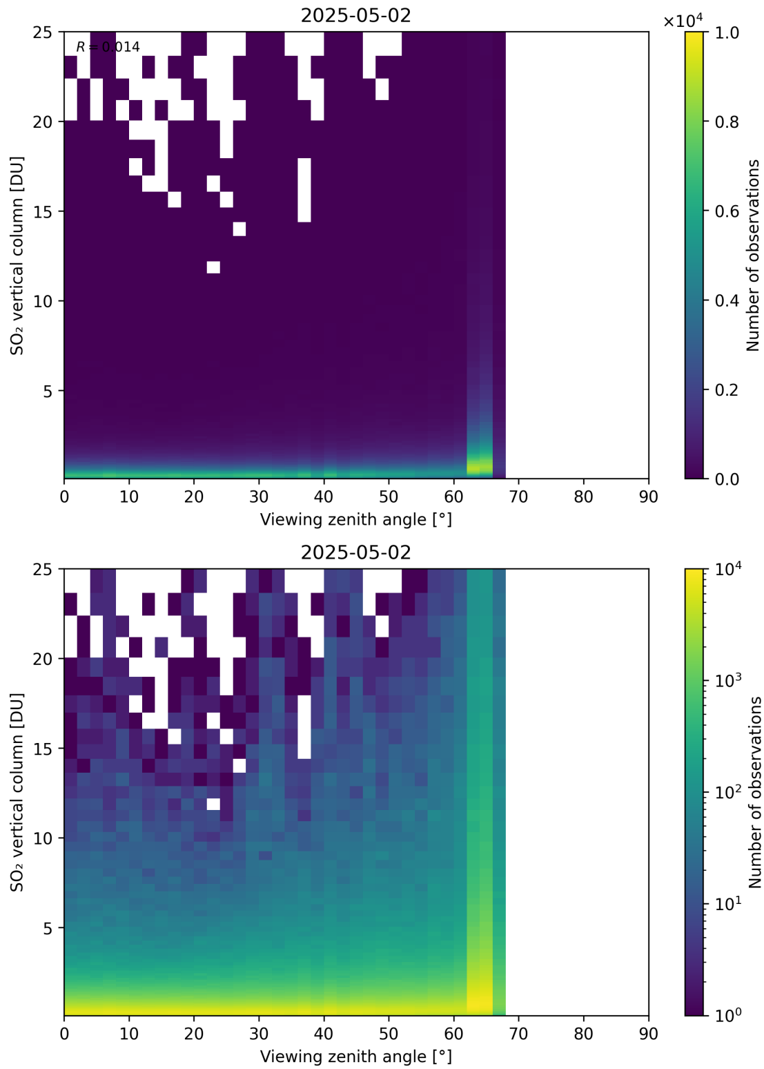
Figure 383: Scatter density plot of “Viewing zenith angle” against “SO 2 vertical column” for 2025-05-01 to 2025-05-03.
