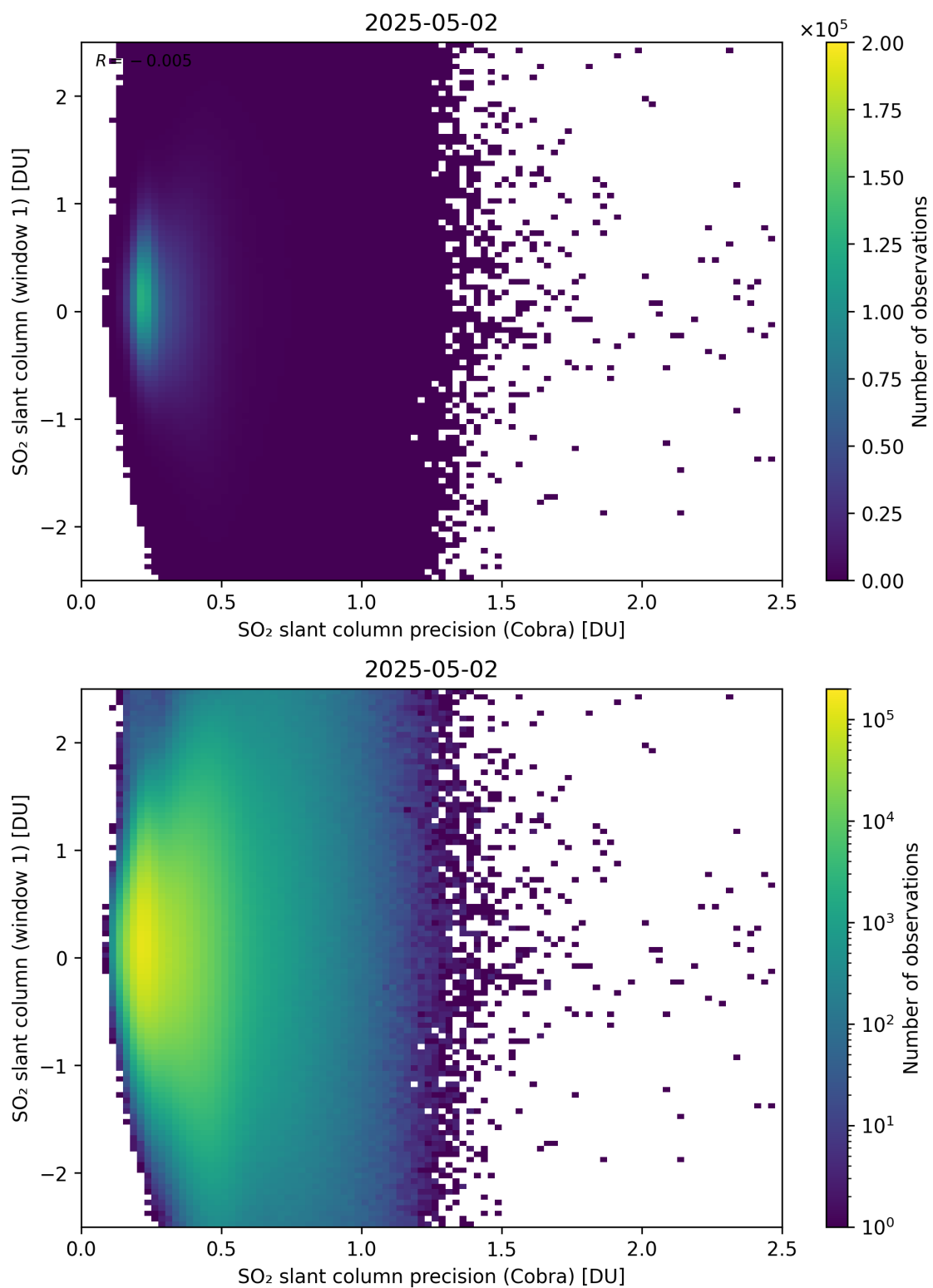
Figure 208: Scatter density plot of “SO 2 slant column precision (Cobra)” against “SO 2 slant column (window 1)” for 2025-05-01 to 2025-05-03.
