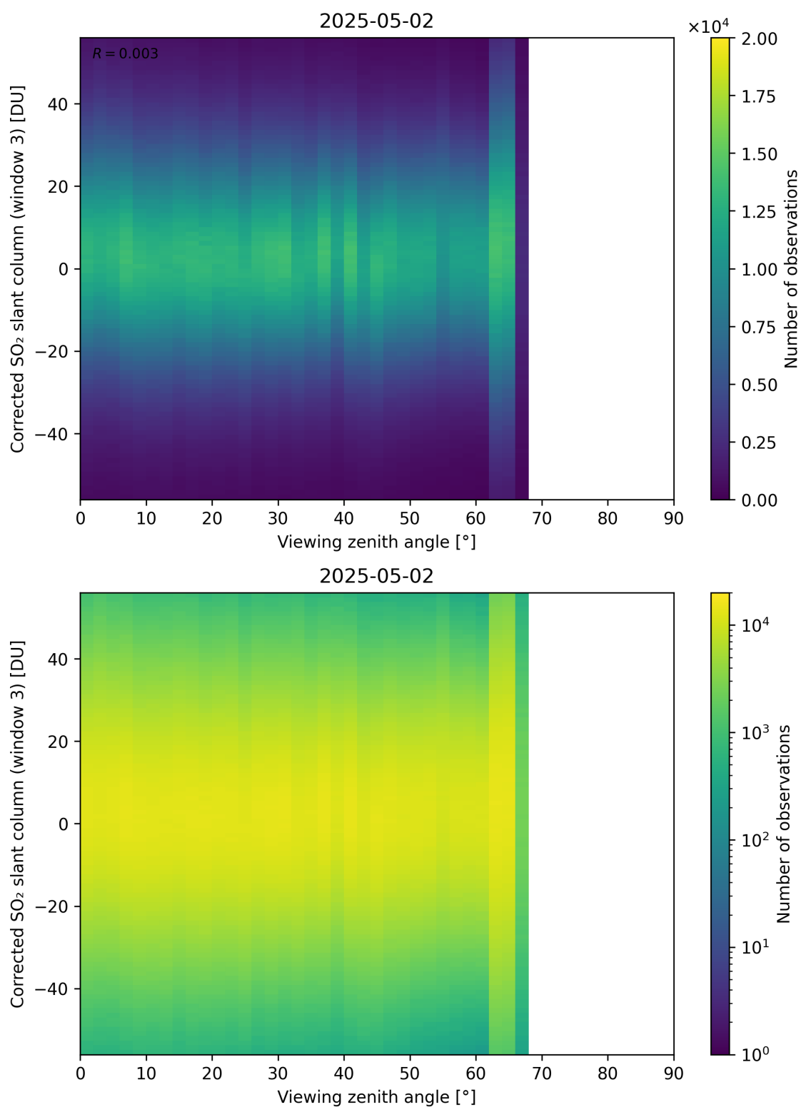
Figure 375: Scatter density plot of “Viewing zenith angle” against “Corrected SO 2 slant column (window 3)” for 2025-05-01 to 2025-05-03.
