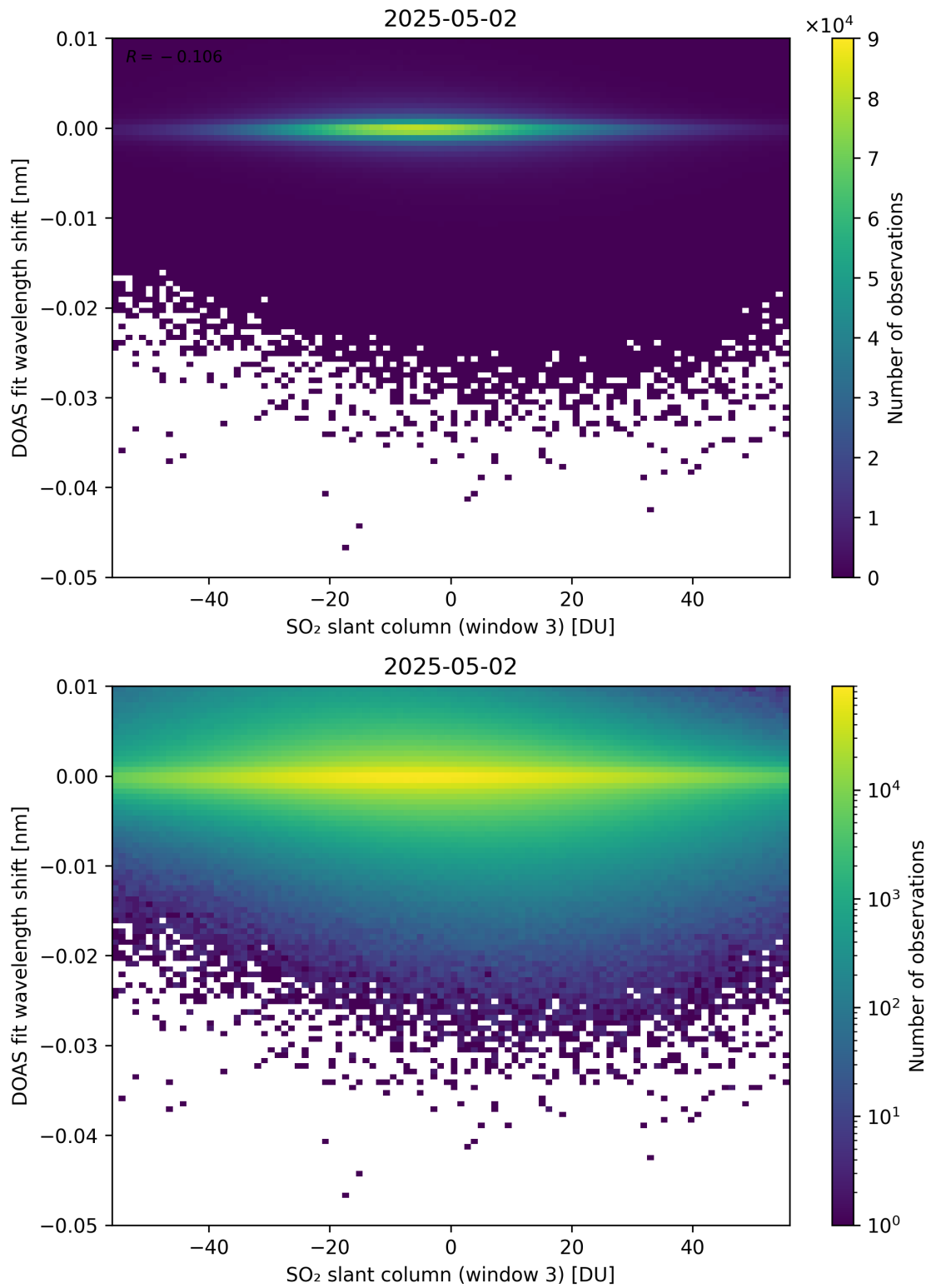
Figure 304: Scatter density plot of “SO 2 slant column (window 3)” against “DOAS fit wavelength shift” for 2025-05-01 to 2025-05-03.
