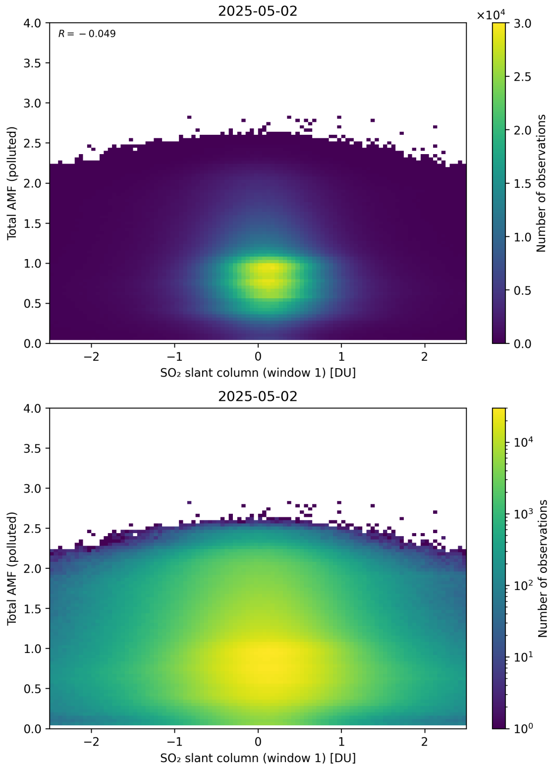
Figure 289: Scatter density plot of “SO 2 slant column (window 1)” against “Total AMF (polluted)” for 2025-05-01 to 2025-05-03.
