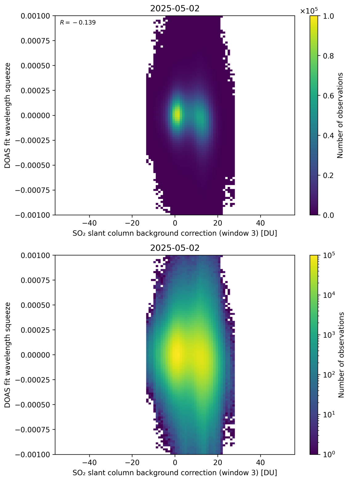
Figure 133: Scatter density plot of “SO 2 slant column background correction (window 3)” against “DOAS fit wavelength squeeze” for 2025-05-01 to 2025-05-03.
