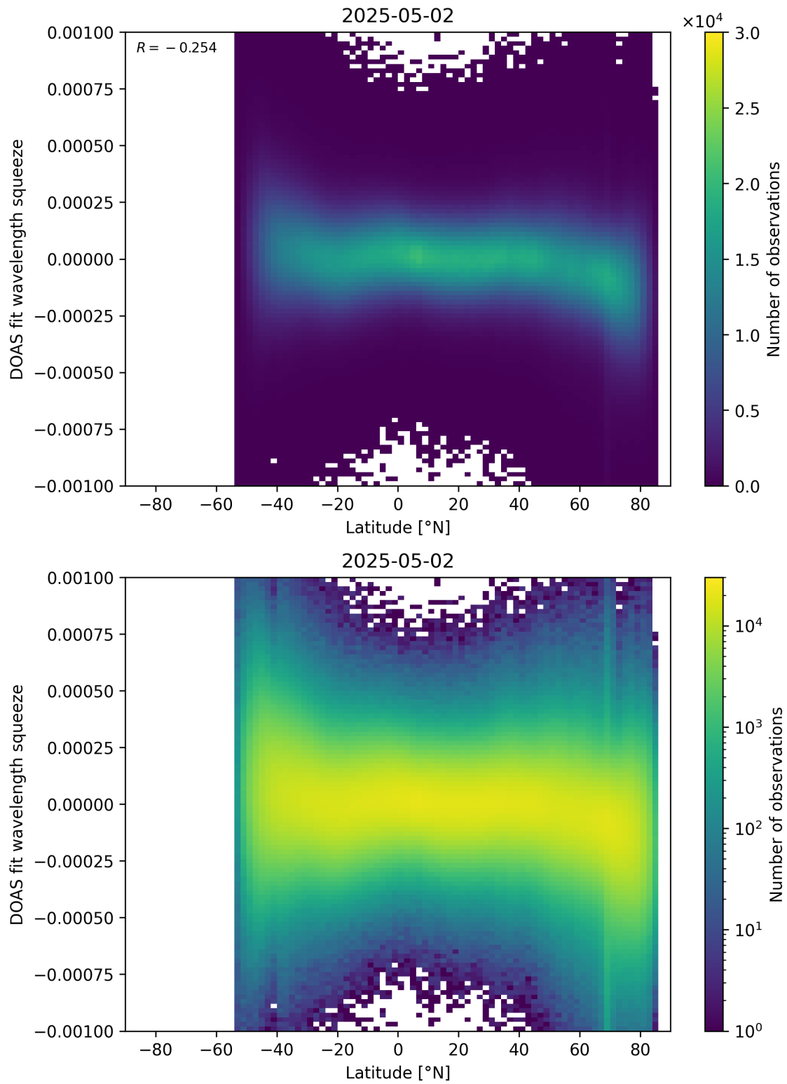
Figure 154: Scatter density plot of “Latitude” against “DOAS fit wavelength squeeze” for 2025-05-01 to 2025-05-03.
