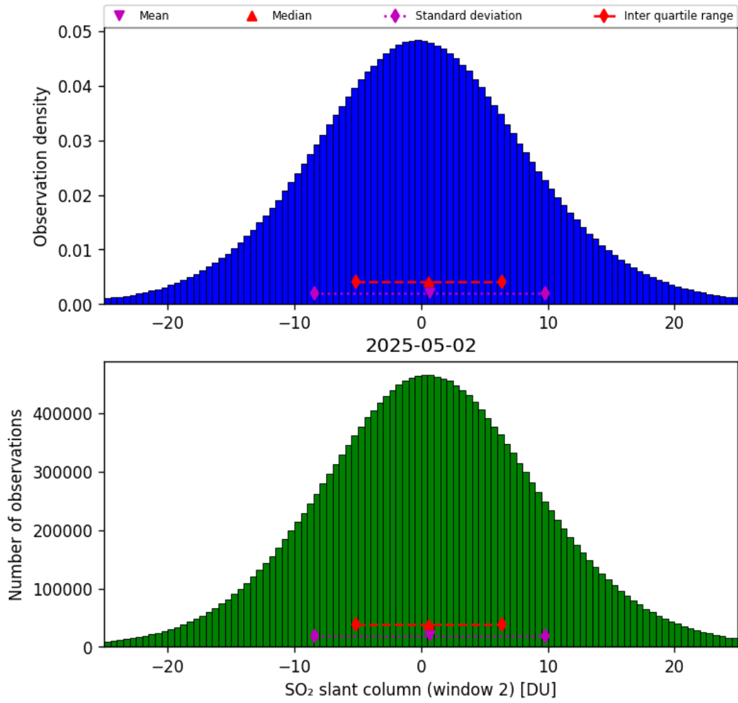
Figure 67: Histogram of “SO 2 slant column (window 2)” for 2025-05-01 to 2025-05-03
