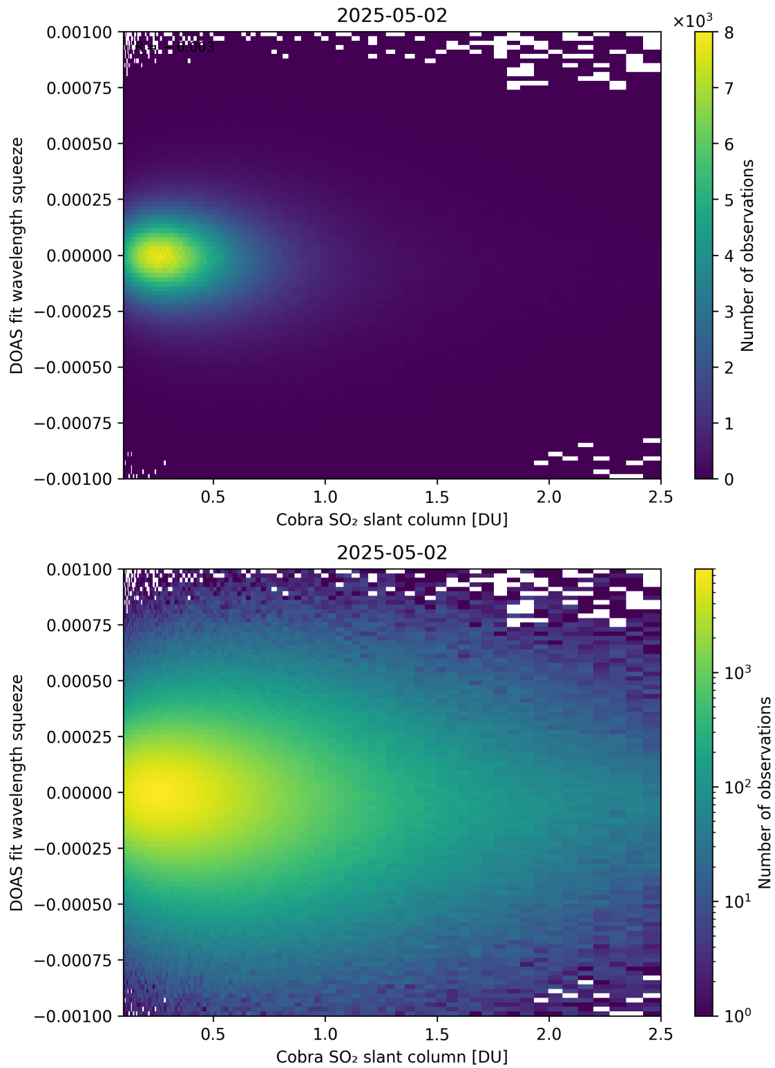
Figure 197: Scatter density plot of “Cobra SO 2 slant column” against “DOAS fit wavelength squeeze” for 2025-05-01 to 2025-05-03.
