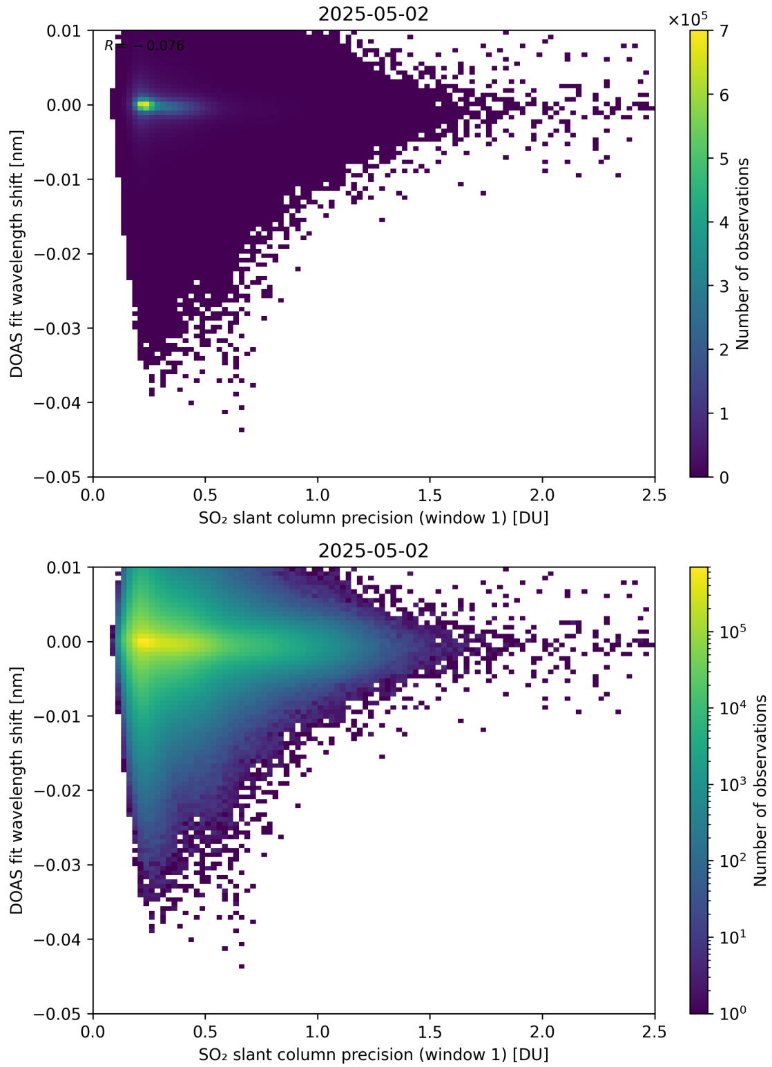
Figure 271: Scatter density plot of “SO 2 slant column precision (window 1)” against “DOAS fit wavelength shift” for 2025-05-01 to 2025-05-03.
