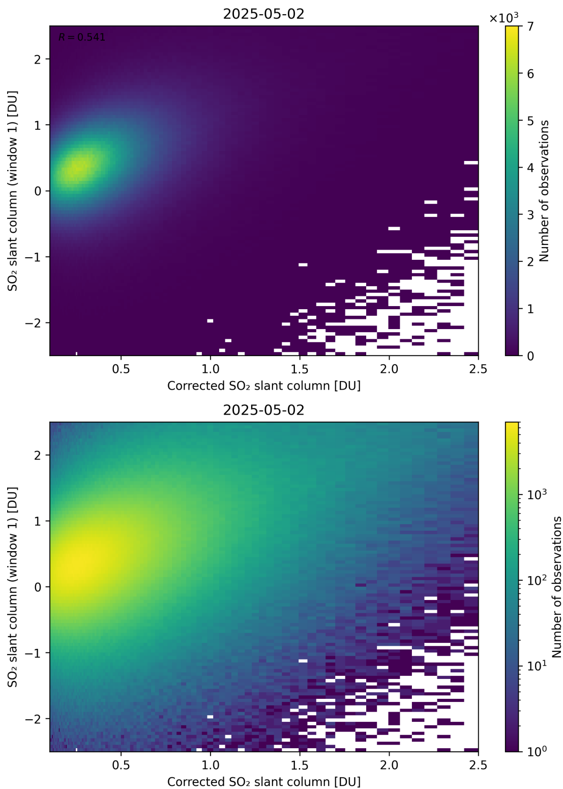
Figure 237: Scatter density plot of “Corrected SO 2 slant column” against “SO 2 slant column (window 1)” for 2025-05-01 to 2025-05-03.
