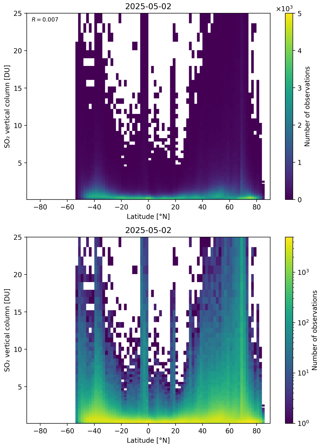
Figure 169: Scatter density plot of “Latitude” against “SO 2 vertical column” for 2025-05-01 to 2025-05-03.
