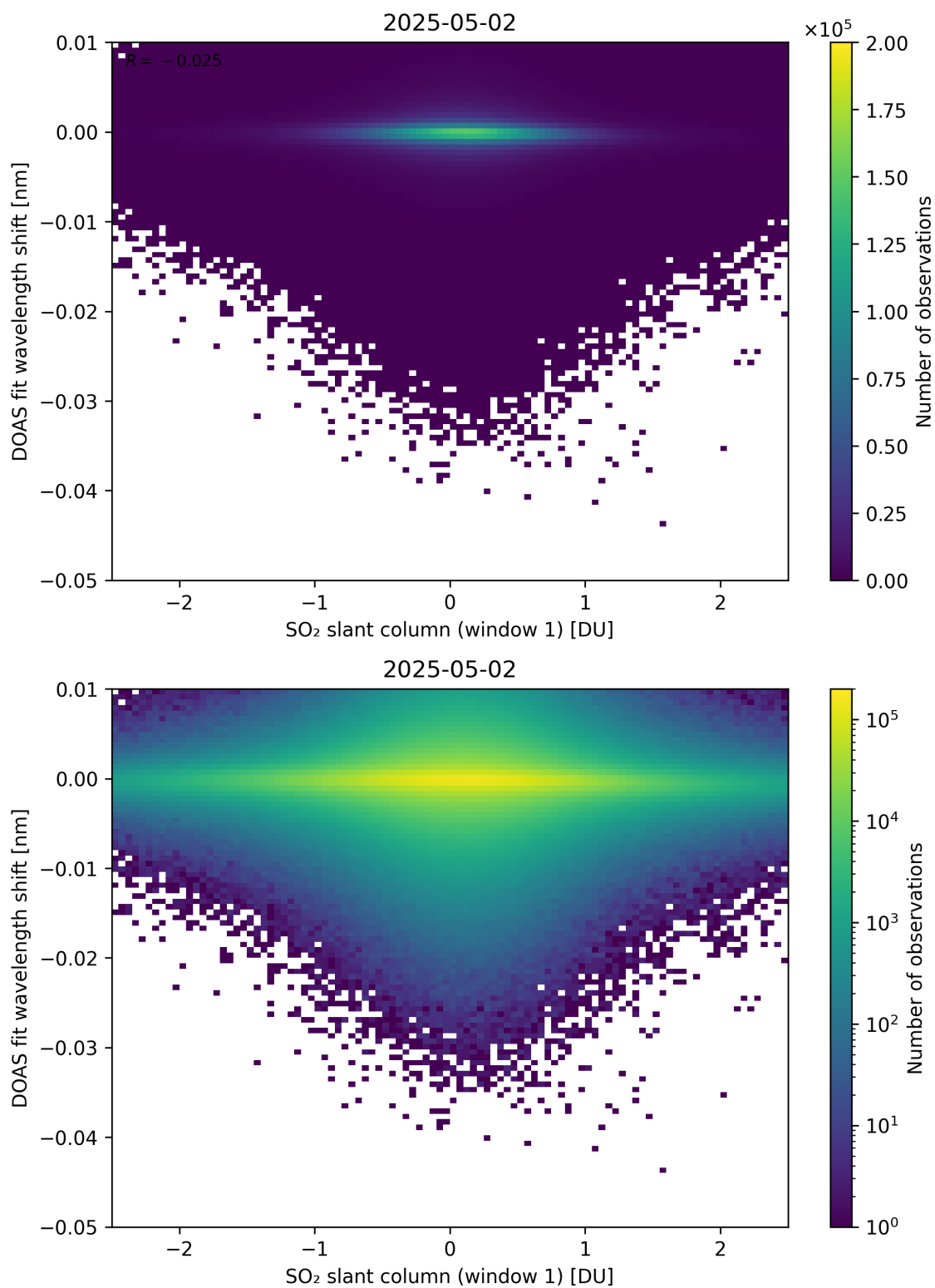
Figure 265: Scatter density plot of “SO 2 slant column (window 1)” against “DOAS fit wavelength shift” for 2025-05-01 to 2025-05-03.
