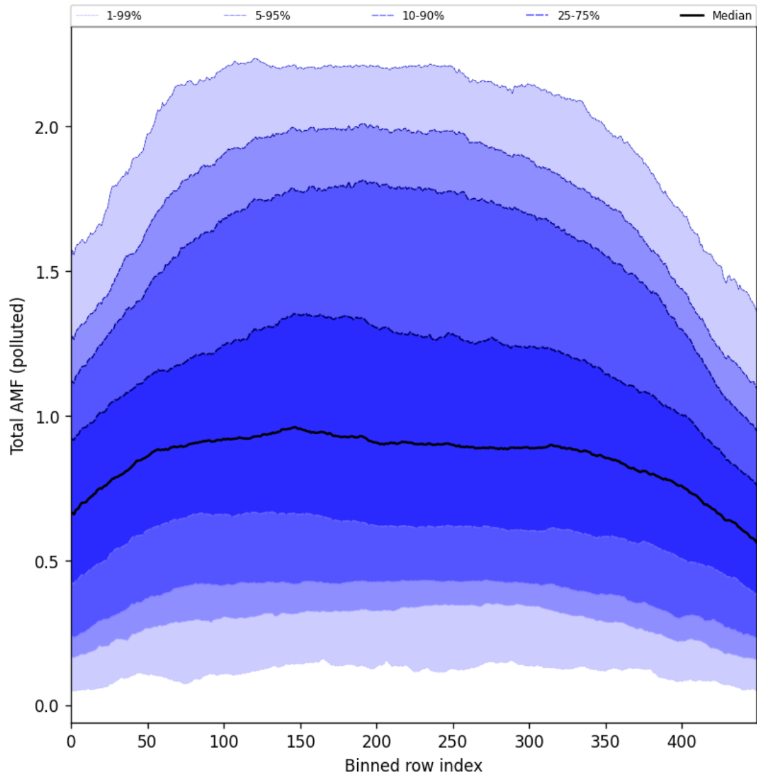
Figure 105: Along track statistics of “Total AMF (polluted)” for 2025-05-01 to 2025-05-03
