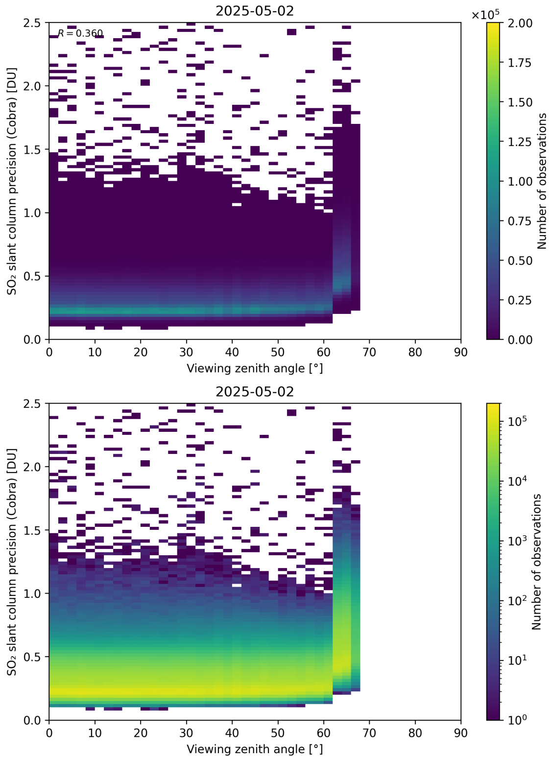
Figure 372: Scatter density plot of “Viewing zenith angle” against “SO 2 slant column precision (Cobra)” for 2025-05-01 to 2025-05-03.
