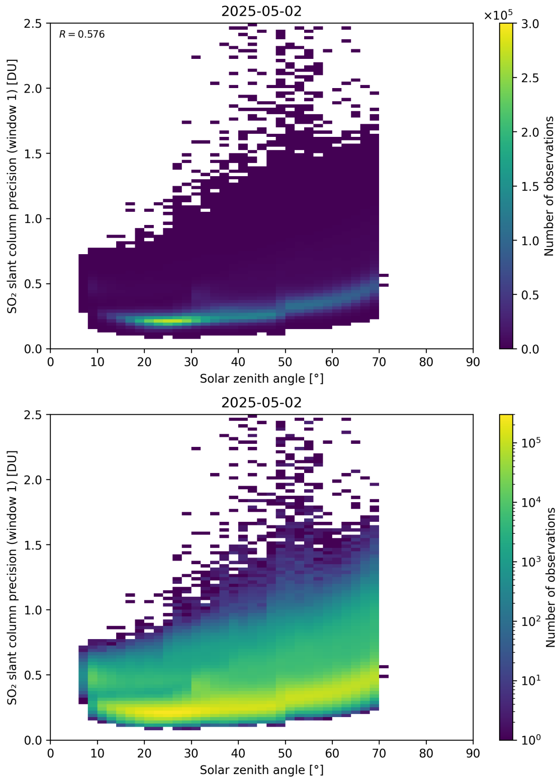
Figure 185: Scatter density plot of “Solar zenith angle” against “SO 2 slant column precision (window 1)” for 2025-05-01 to 2025-05-03.
