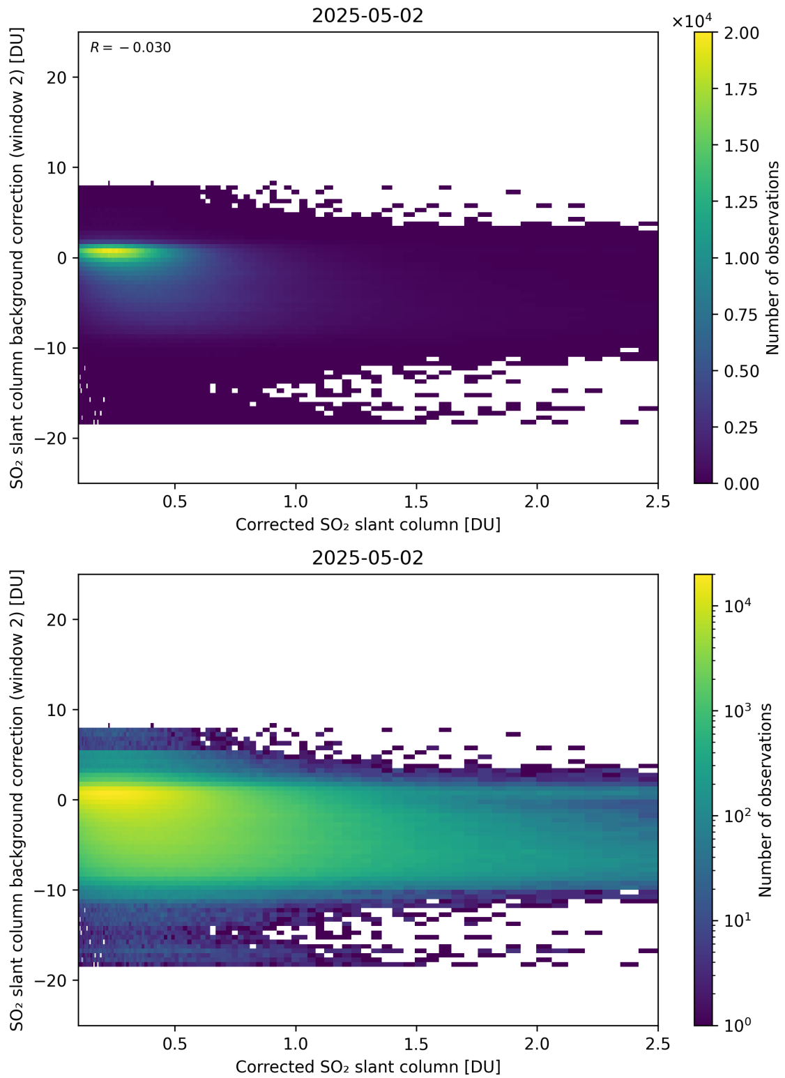
Figure 227: Scatter density plot of “Corrected SO 2 slant column” against “SO 2 slant column background correction (window 2)” for 2025-05-01 to 2025-05-03.
