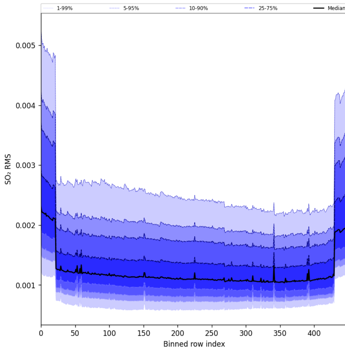
Figure 104: Along track statistics of “SO 2 RMS” for 2025-05-01 to 2025-05-03
