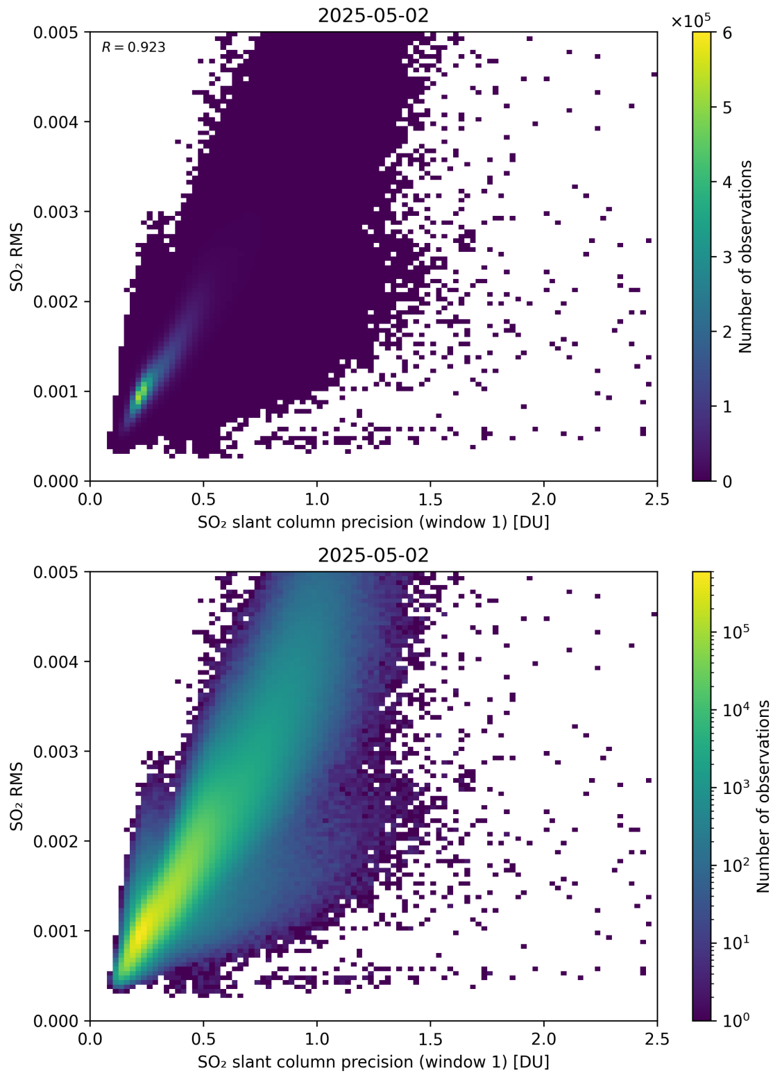
Figure 273: Scatter density plot of “SO 2 slant column precision (window 1)” against “SO 2 RMS” for 2025-05-01 to 2025-05-03.
