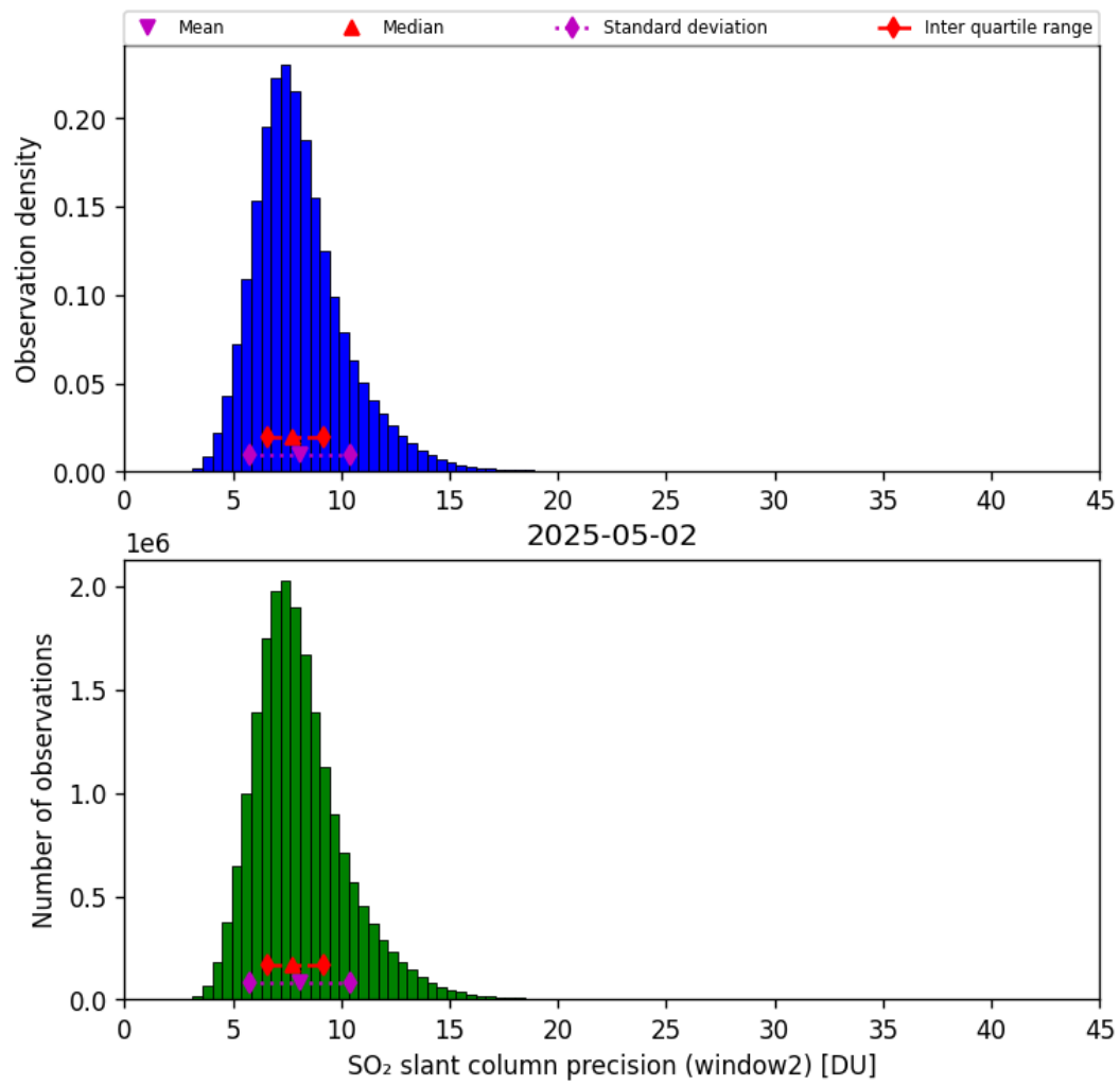
Figure 68: Histogram of “SO 2 slant column precision (window2)” for 2025-05-01 to 2025-05-03
