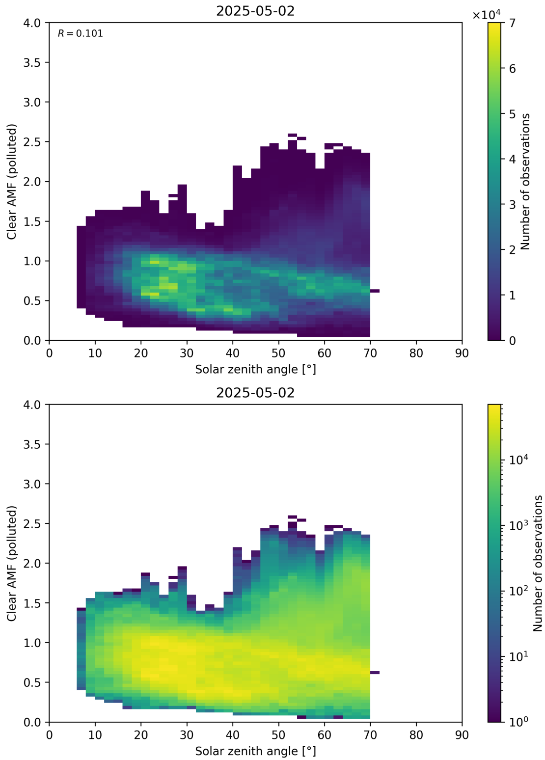
Figure 178: Scatter density plot of “Solar zenith angle” against “Clear AMF (polluted)” for 2025-05-01 to 2025-05-03.
