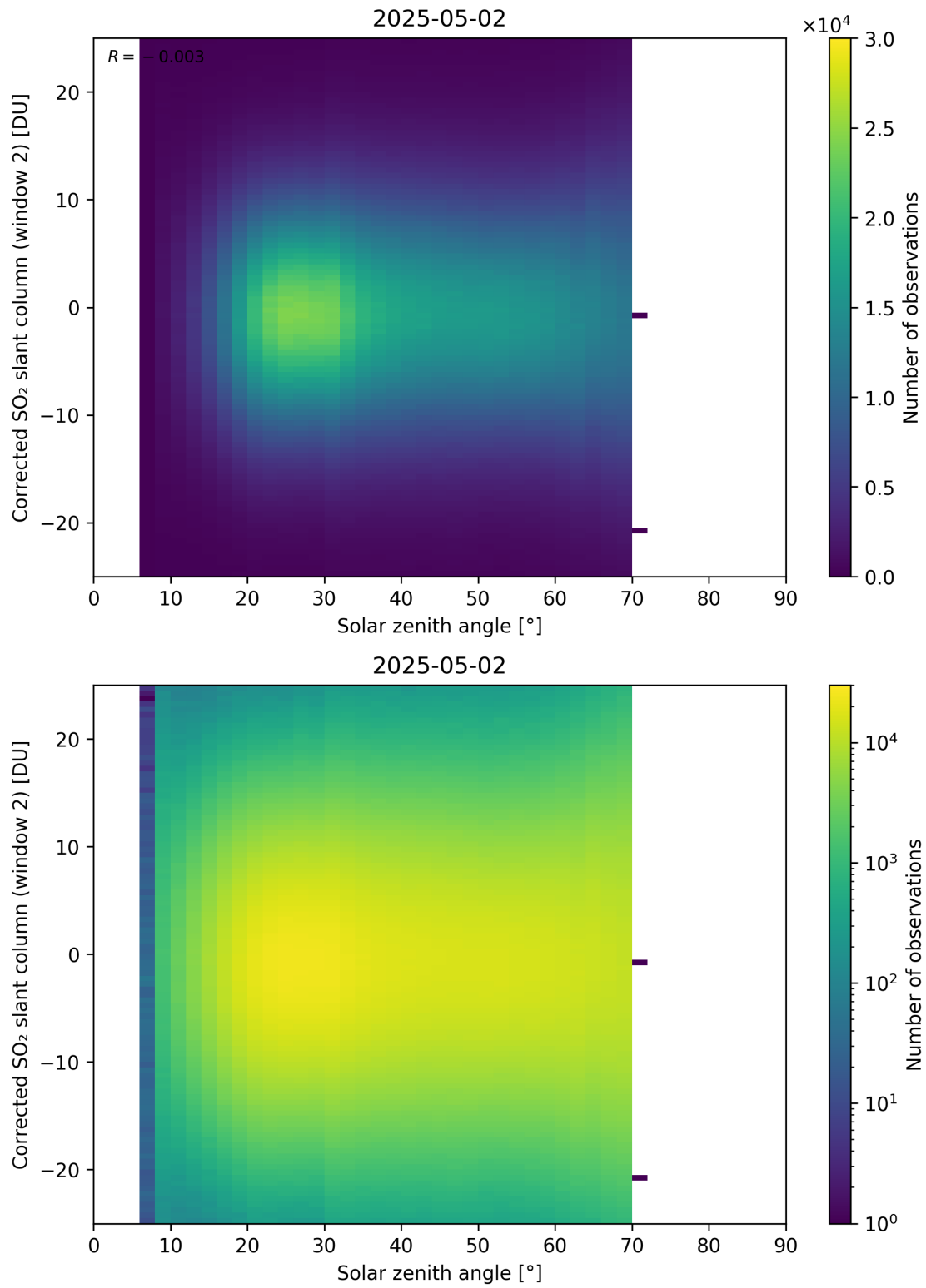
Figure 182: Scatter density plot of “Solar zenith angle” against “Corrected SO 2 slant column (window 2)” for 2025-05-01 to 2025-05-03.
