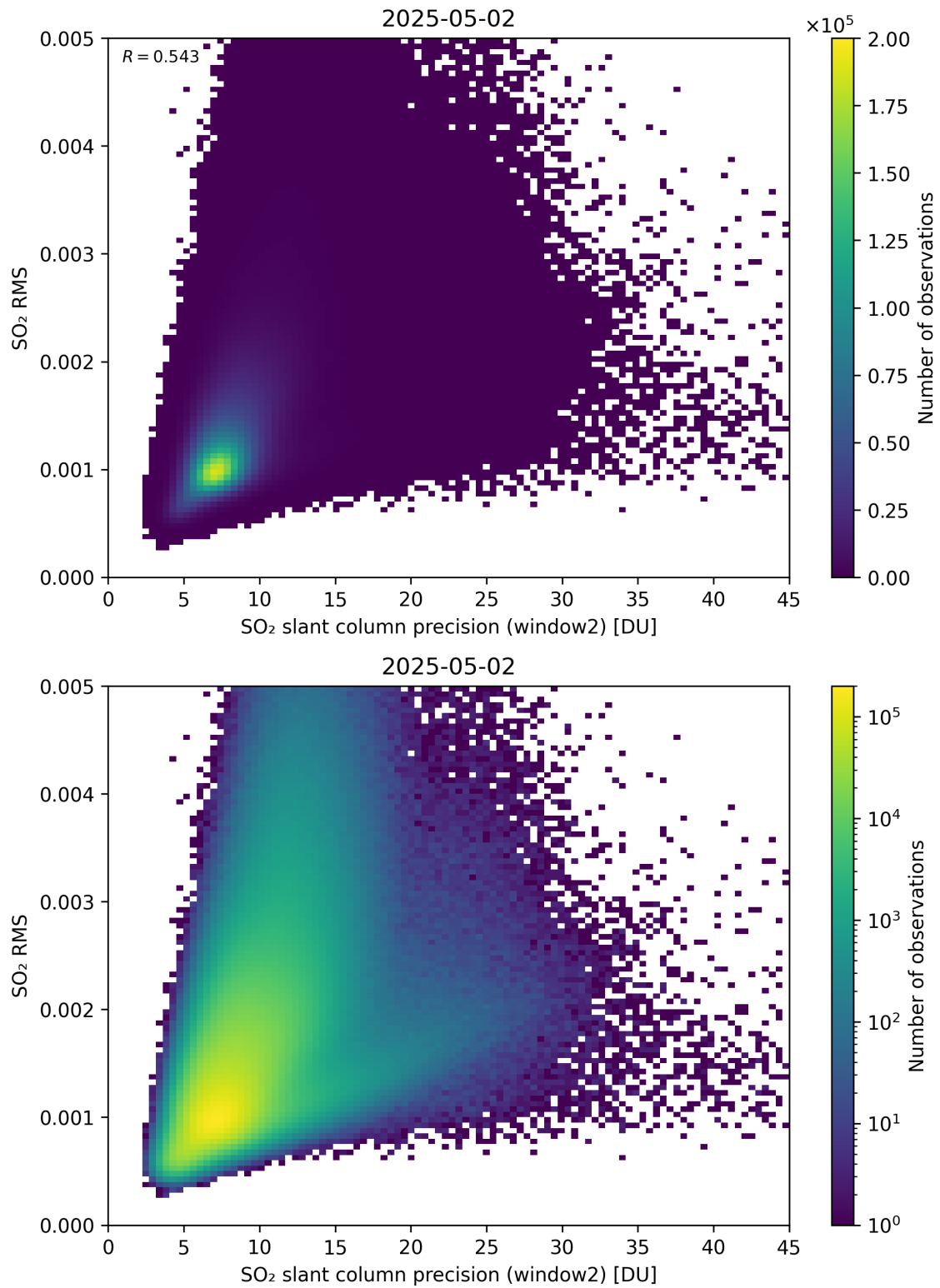
Figure 295: Scatter density plot of “SO 2 slant column precision (window2)” against “SO 2 RMS” for 2025-05-01 to 2025-05-03.
