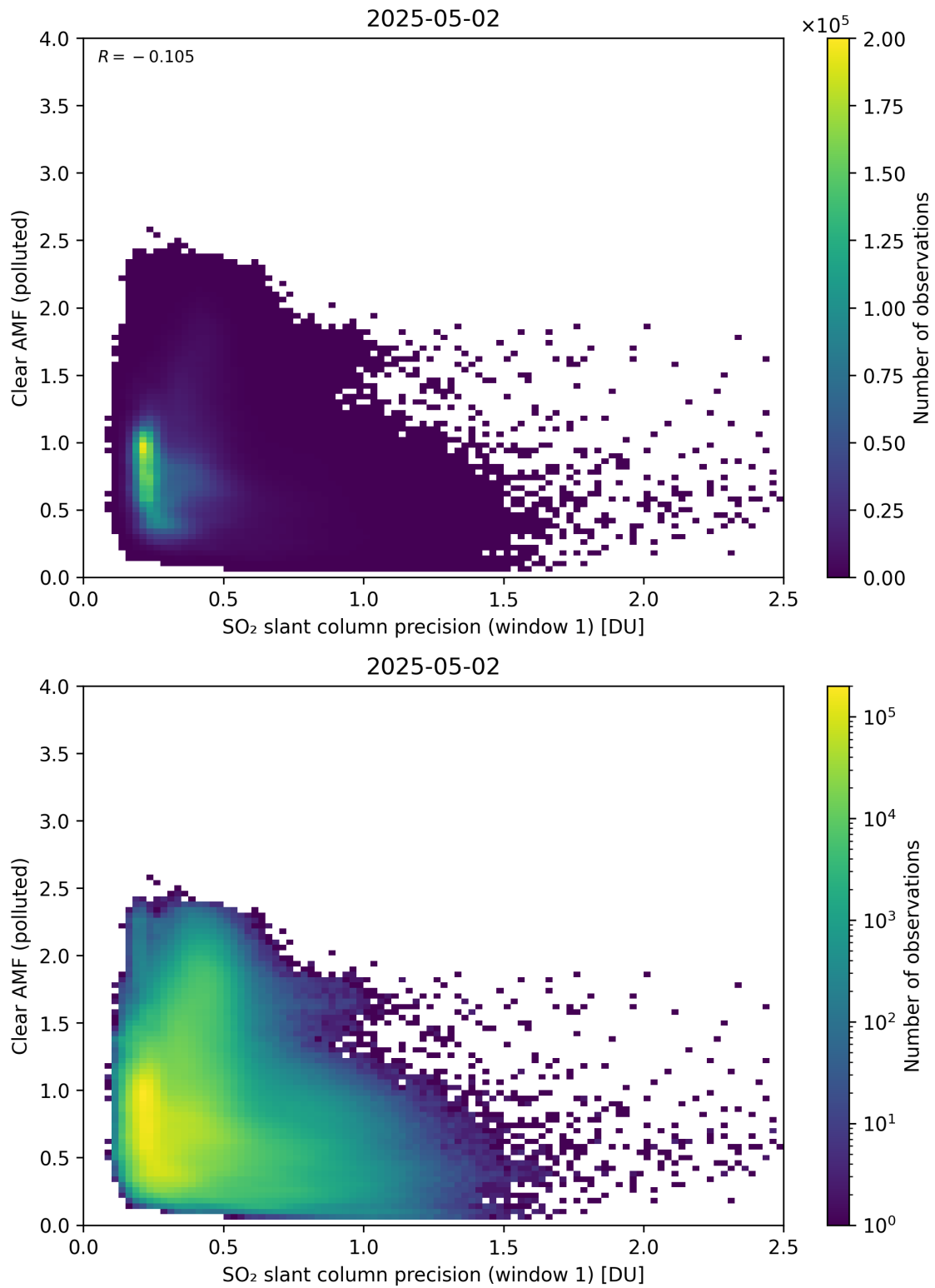
Figure 274: Scatter density plot of “SO 2 slant column precision (window 1)” against “Clear AMF (polluted)” for 2025-05-01 to 2025-05-03.
