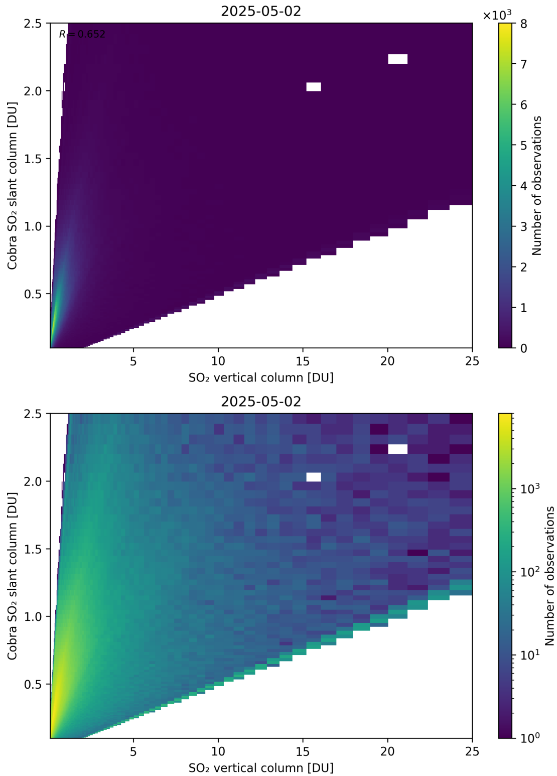
Figure 349: Scatter density plot of “SO 2 vertical column” against “Cobra SO 2 slant column” for 2025-05-01 to 2025-05-03.
