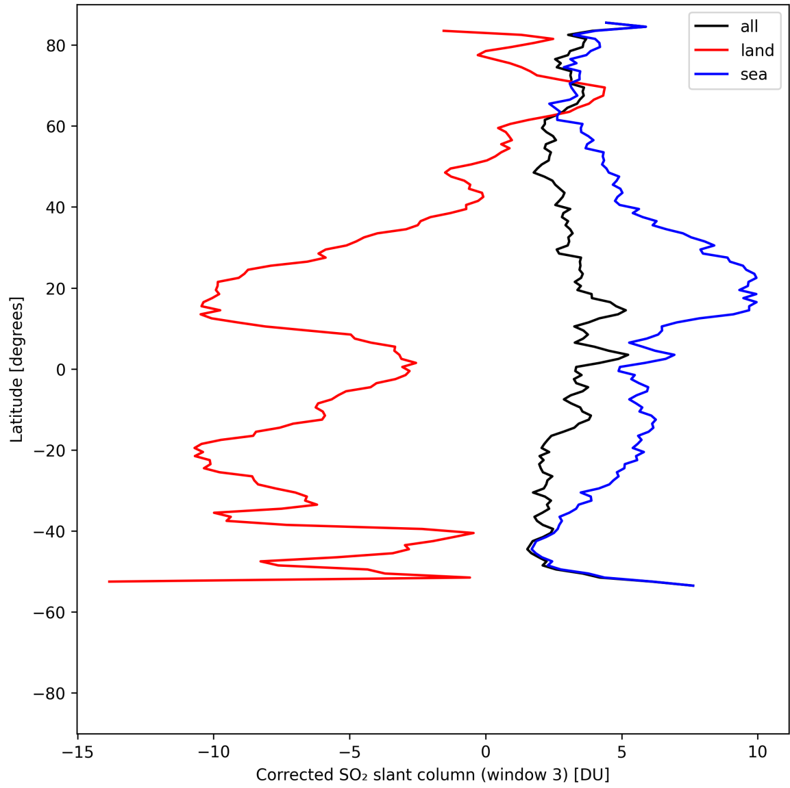
Figure 47: Zonal average of "Corrected SO 2 slant column (window 3)" for 2025-05-01 to 2025-05-03.
