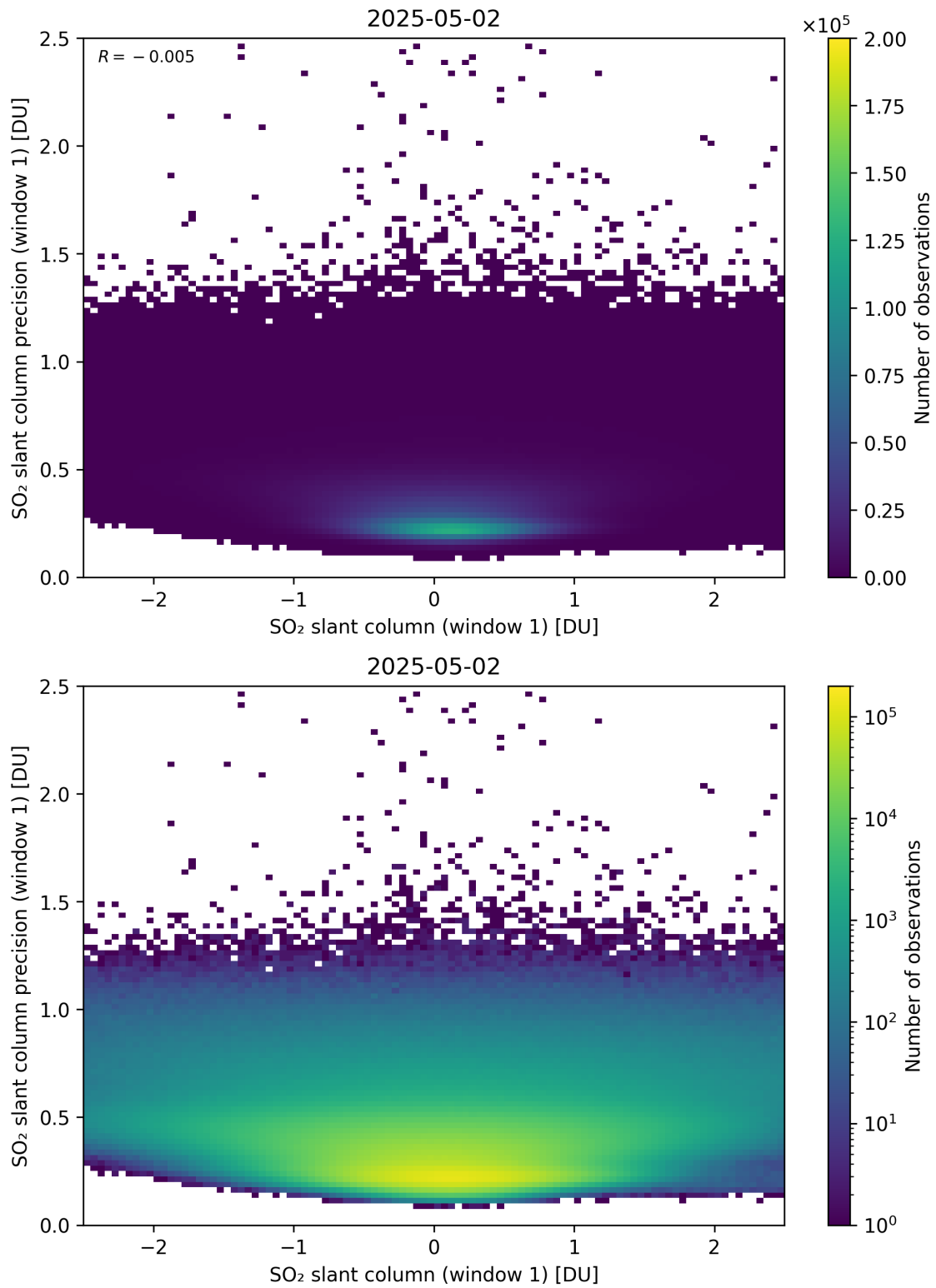
Figure 285: Scatter density plot of “SO 2 slant column (window 1)” against “SO 2 slant column precision (window 1)” for 2025-05-01 to 2025-05-03.
