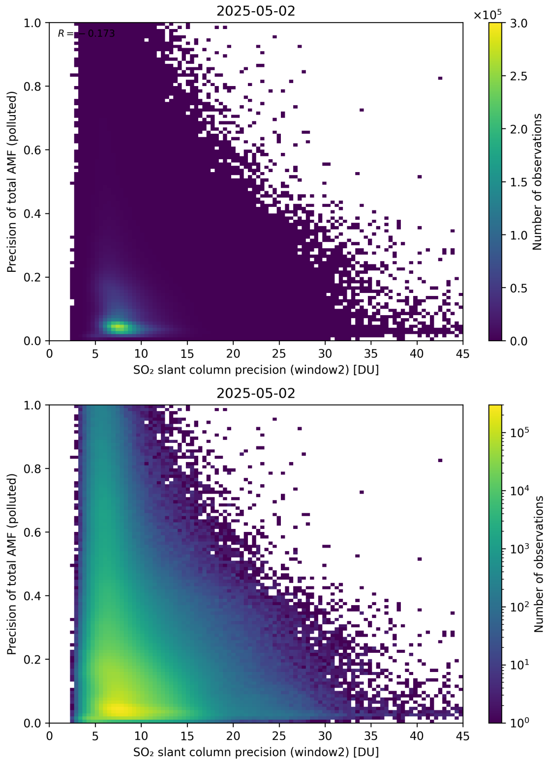
Figure 302: Scatter density plot of “SO 2 slant column precision (window2)” against “Precision of total AMF (polluted)” for 2025-05-01 to 2025-05-03.
