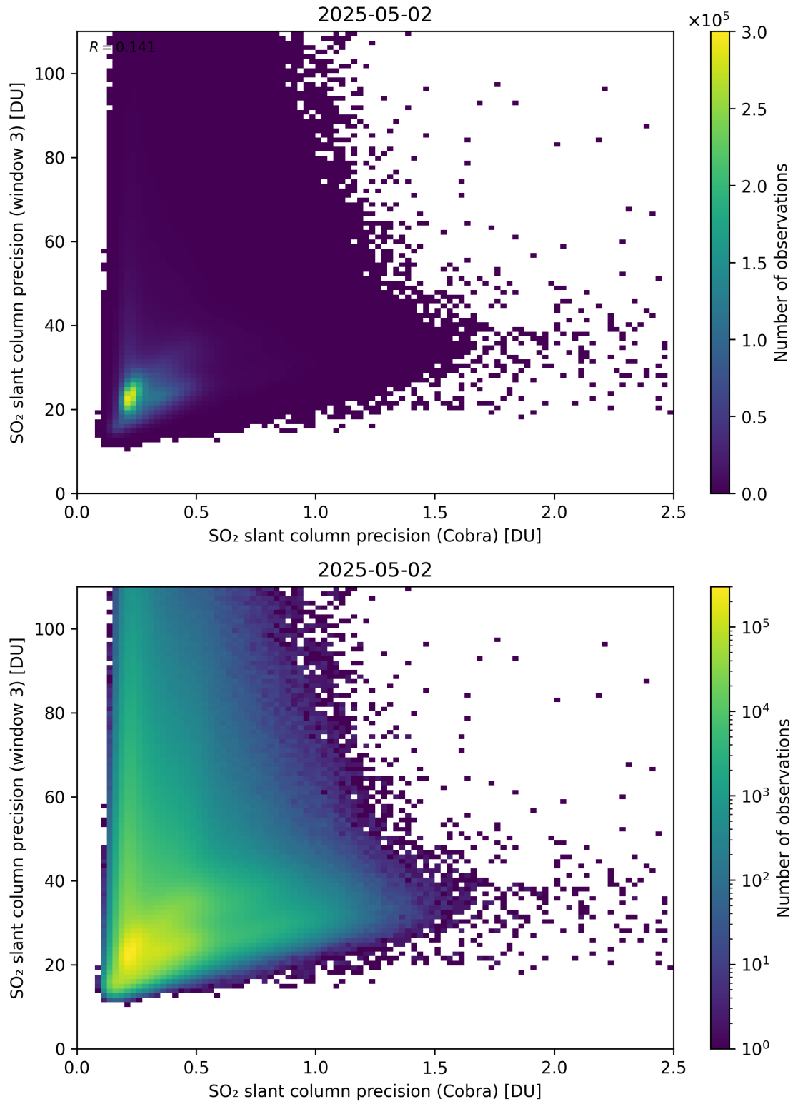
Figure 212: Scatter density plot of “SO 2 slant column precision (Cobra)” against “SO 2 slant column precision (window 3)” for 2025-05-01 to 2025-05-03.
