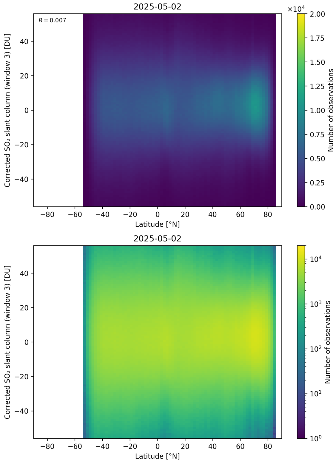
Figure 161: Scatter density plot of “Latitude” against “Corrected SO 2 slant column (window 3)” for 2025-05-01 to 2025-05-03.
