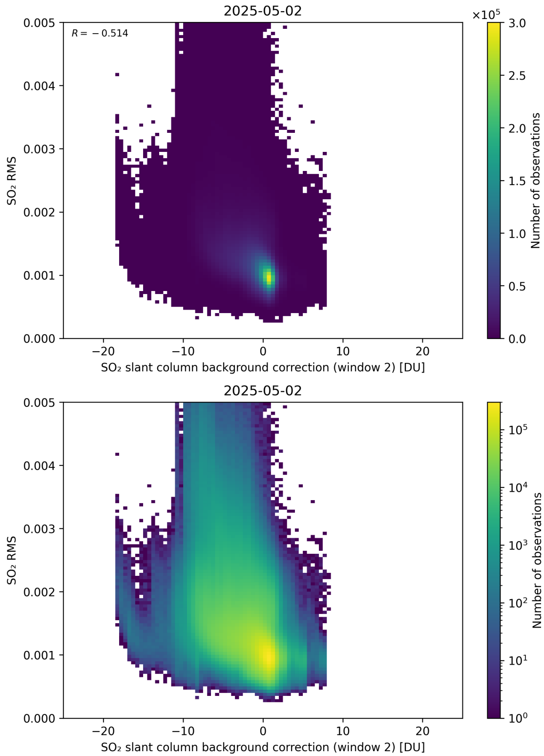
Figure 125: Scatter density plot of “SO 2 slant column background correction (window 2)” against “SO 2 RMS” for 2025-05-01 to 2025-05-03.
