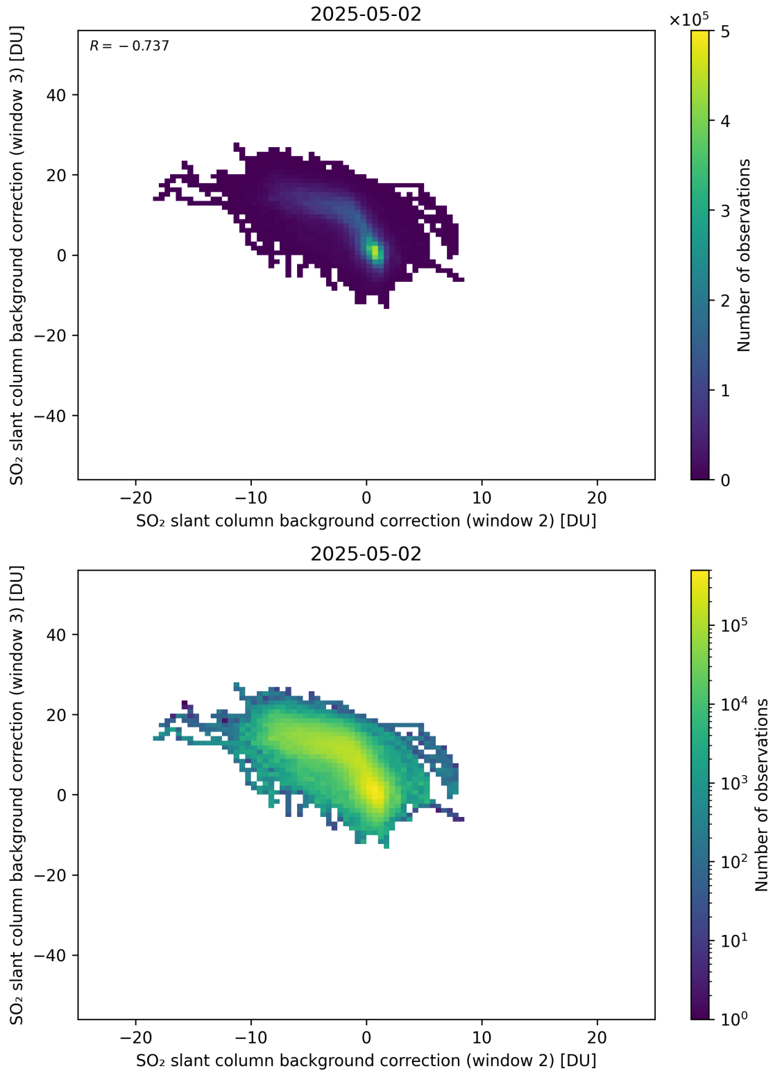
Figure 122: Scatter density plot of “SO 2 slant column background correction (window 2)” against “SO 2 slant column background correction (window 3)” for 2025-05-01 to 2025-05-03.
