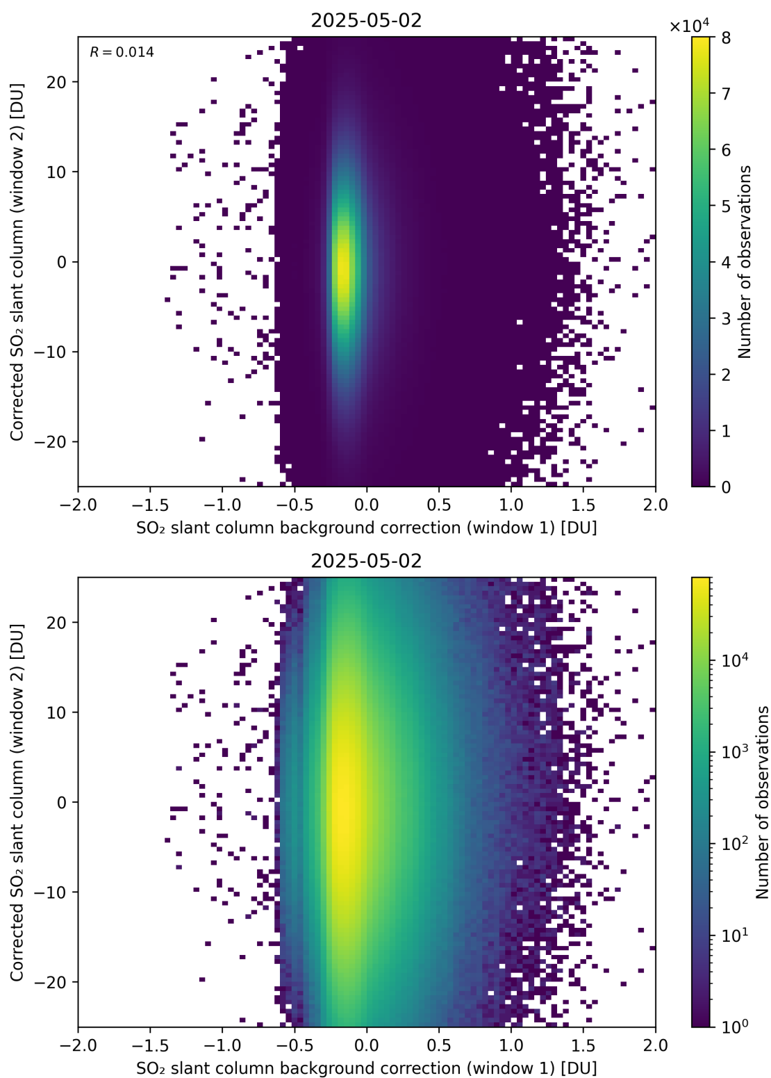
Figure 115: Scatter density plot of “SO 2 slant column background correction (window 1)” against “Corrected SO 2 slant column (window 2)” for 2025-05-01 to 2025-05-03.
