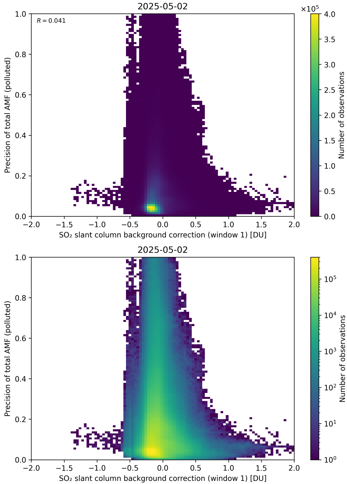
Figure 121: Scatter density plot of “SO 2 slant column background correction (window 1)” against “Precision of total AMF (polluted)” for 2025-05-01 to 2025-05-03.
