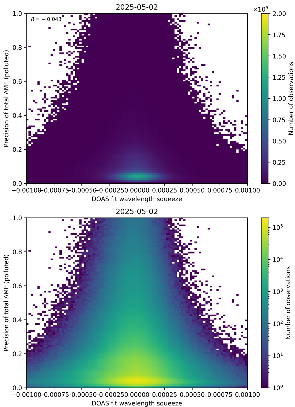
Figure 146: Scatter density plot of “DOAS fit wavelength squeeze” against “Precision of total AMF (polluted)” for 2025-05-01 to 2025-05-03.
