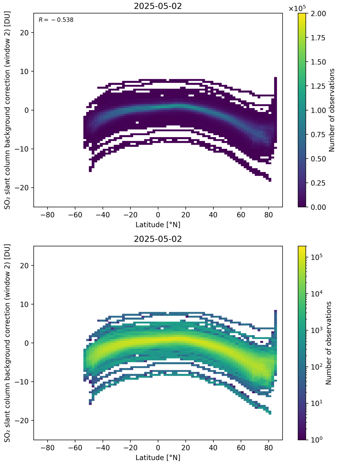
Figure 151: Scatter density plot of “Latitude” against “SO 2 slant column background correction (window 2)” for 2025-05-01 to 2025-05-03.
