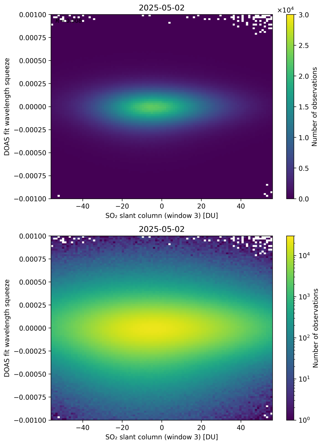
Figure 305: Scatter density plot of “SO 2 slant column (window 3)” against “DOAS fit wavelength squeeze” for 2025-05-01 to 2025-05-03.
