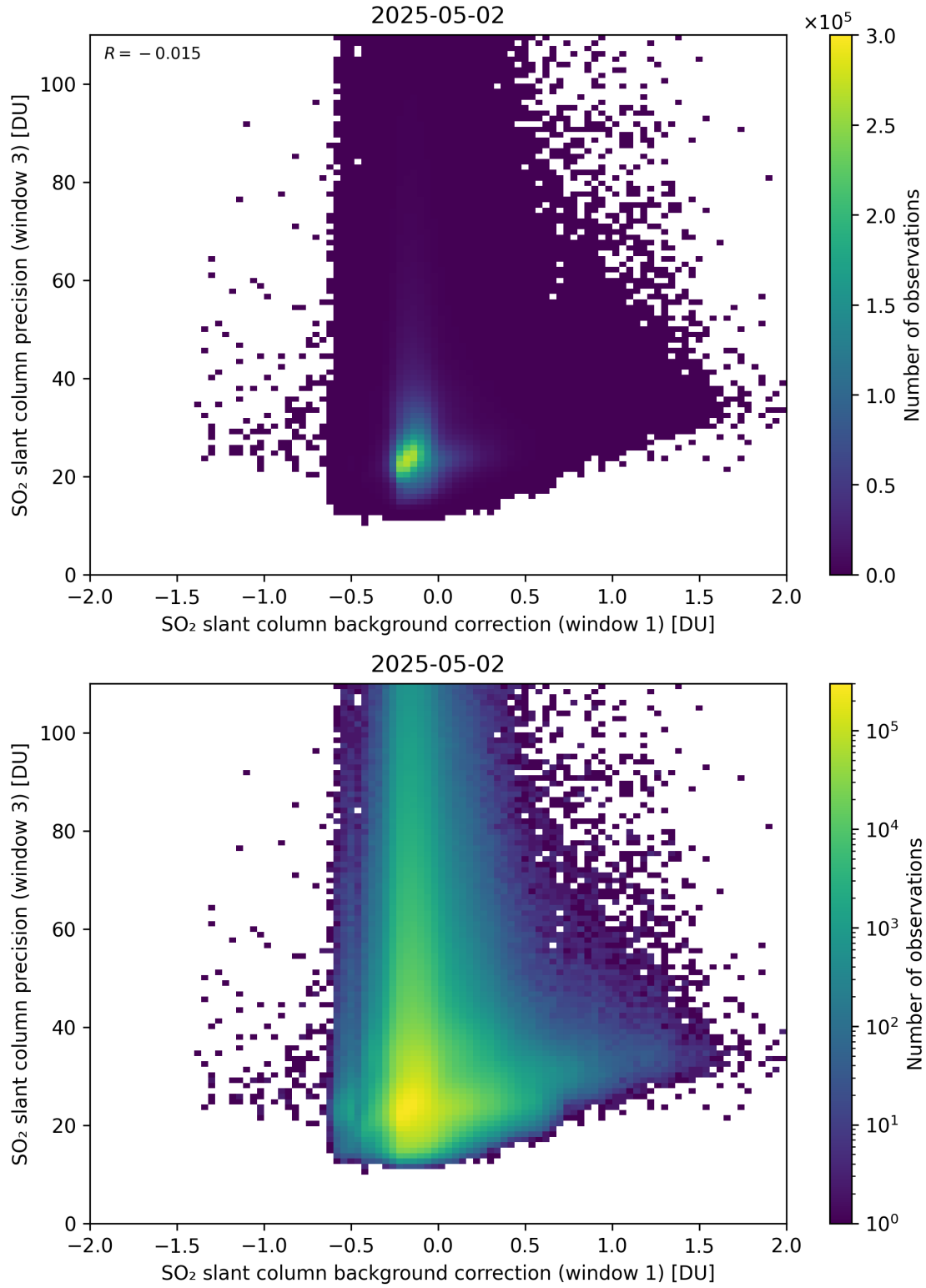
Figure 119: Scatter density plot of “SO 2 slant column background correction (window 1)” against “SO 2 slant column precision (window 3)” for 2025-05-01 to 2025-05-03.
