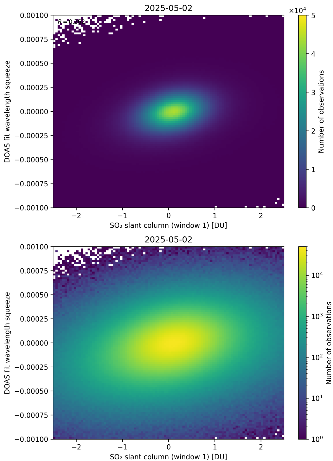
Figure 266: Scatter density plot of “SO 2 slant column (window 1)” against “DOAS fit wavelength squeeze” for 2025-05-01 to 2025-05-03.
