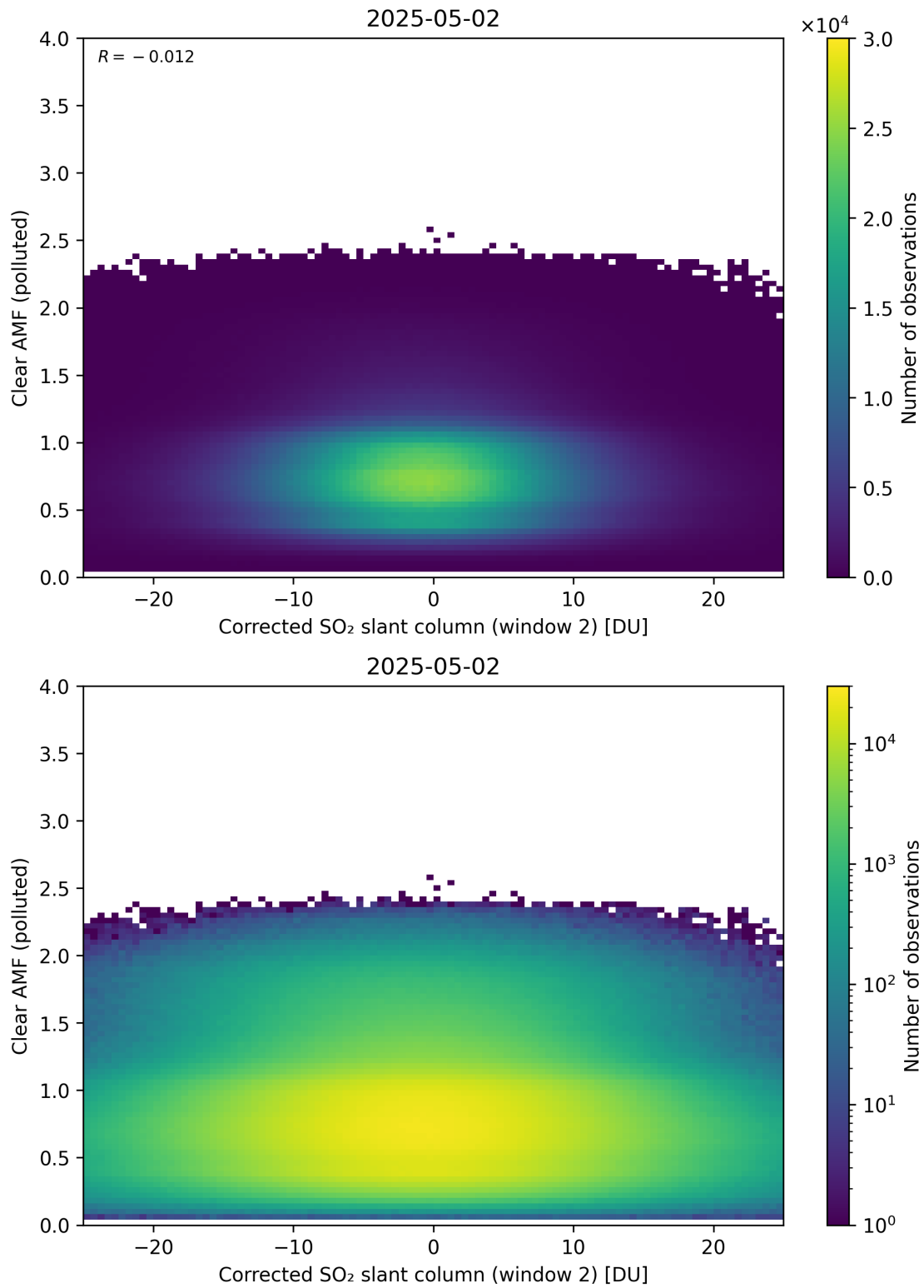
Figure 249: Scatter density plot of “Corrected SO 2 slant column (window 2)” against “Clear AMF (polluted)” for 2025-05-01 to 2025-05-03.
