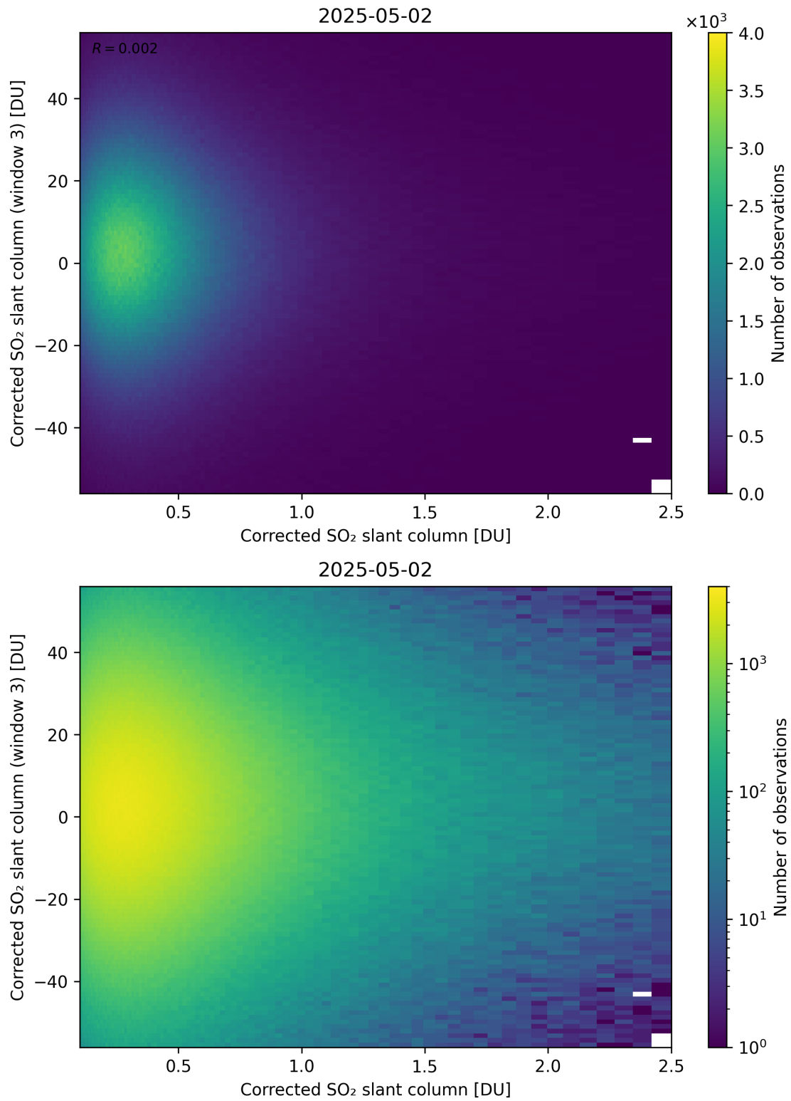
Figure 236: Scatter density plot of “Corrected SO 2 slant column” against “Corrected SO 2 slant column (window 3)” for 2025-05-01 to 2025-05-03.
