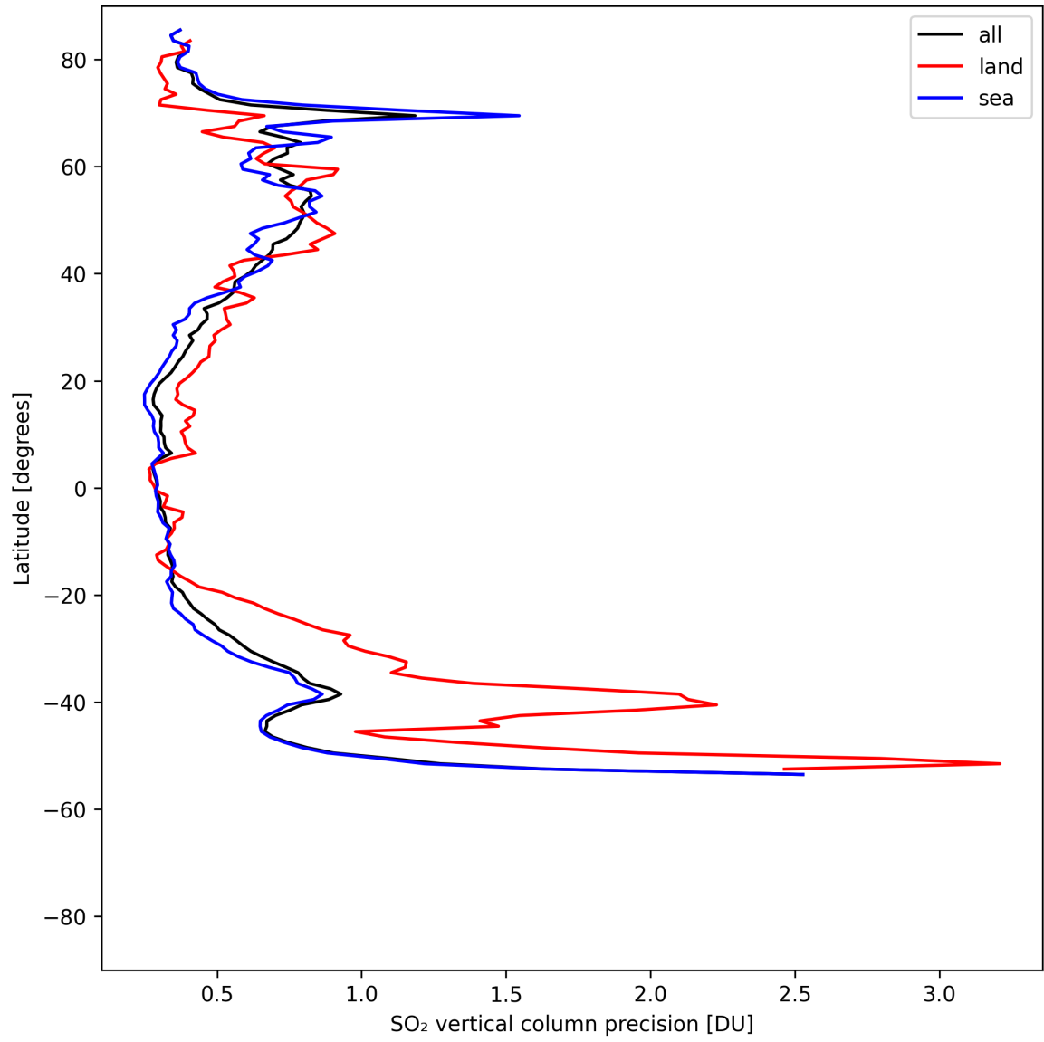
Figure 33: Zonal average of “SO 2 vertical column precision” for 2025-05-01 to 2025-05-03.
