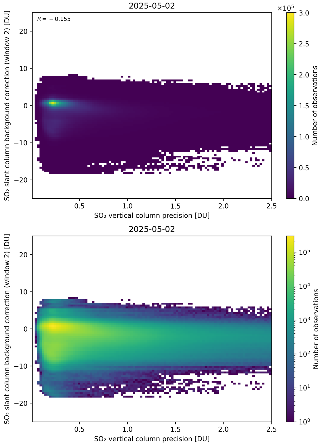
Figure 330: Scatter density plot of “SO 2 vertical column precision” against “SO 2 slant column background correction (window 2)” for 2025-05-01 to 2025-05-03.
