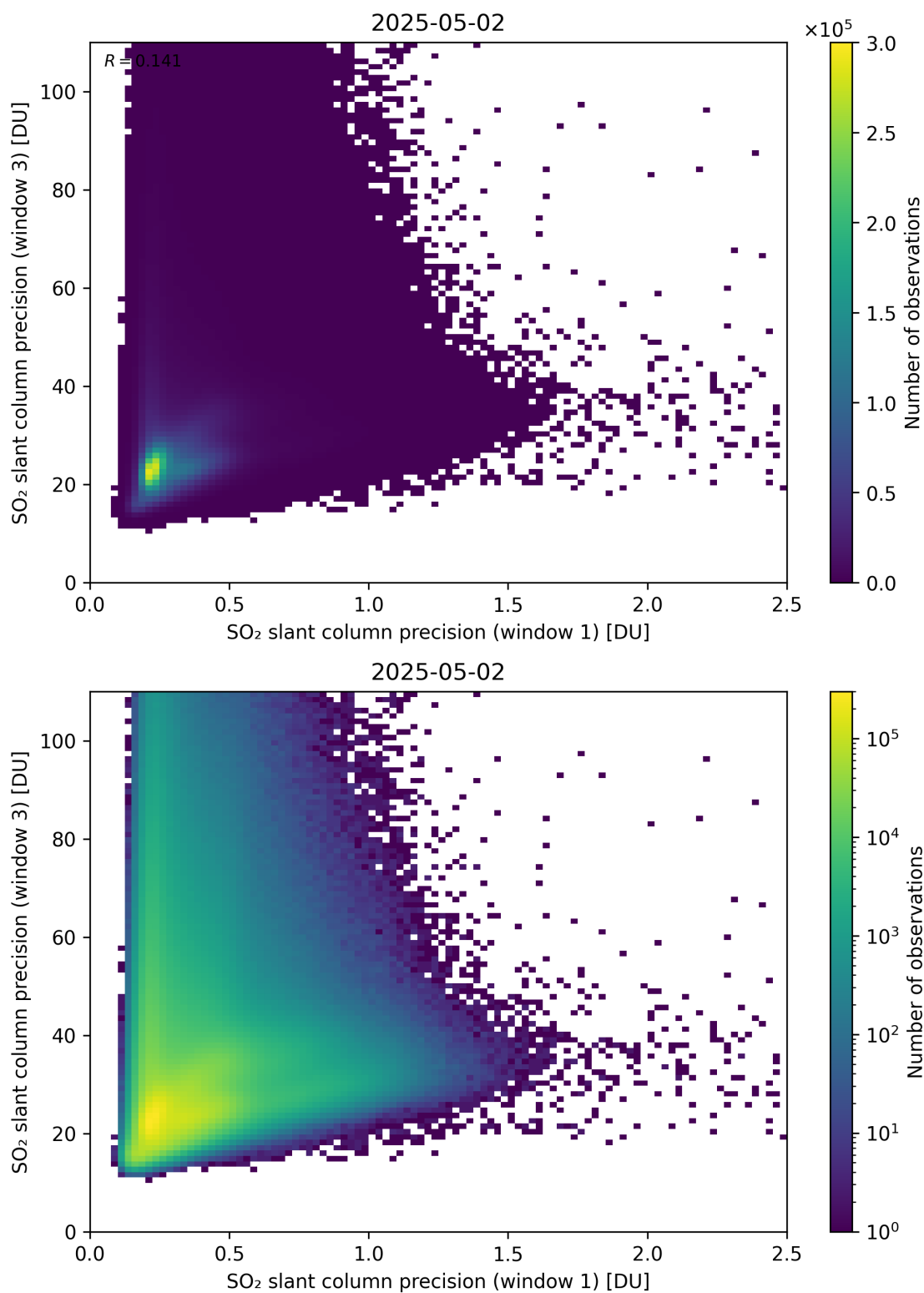
Figure 279: Scatter density plot of “SO 2 slant column precision (window 1)” against “SO 2 slant column precision (window 3)” for 2025-05-01 to 2025-05-03.
