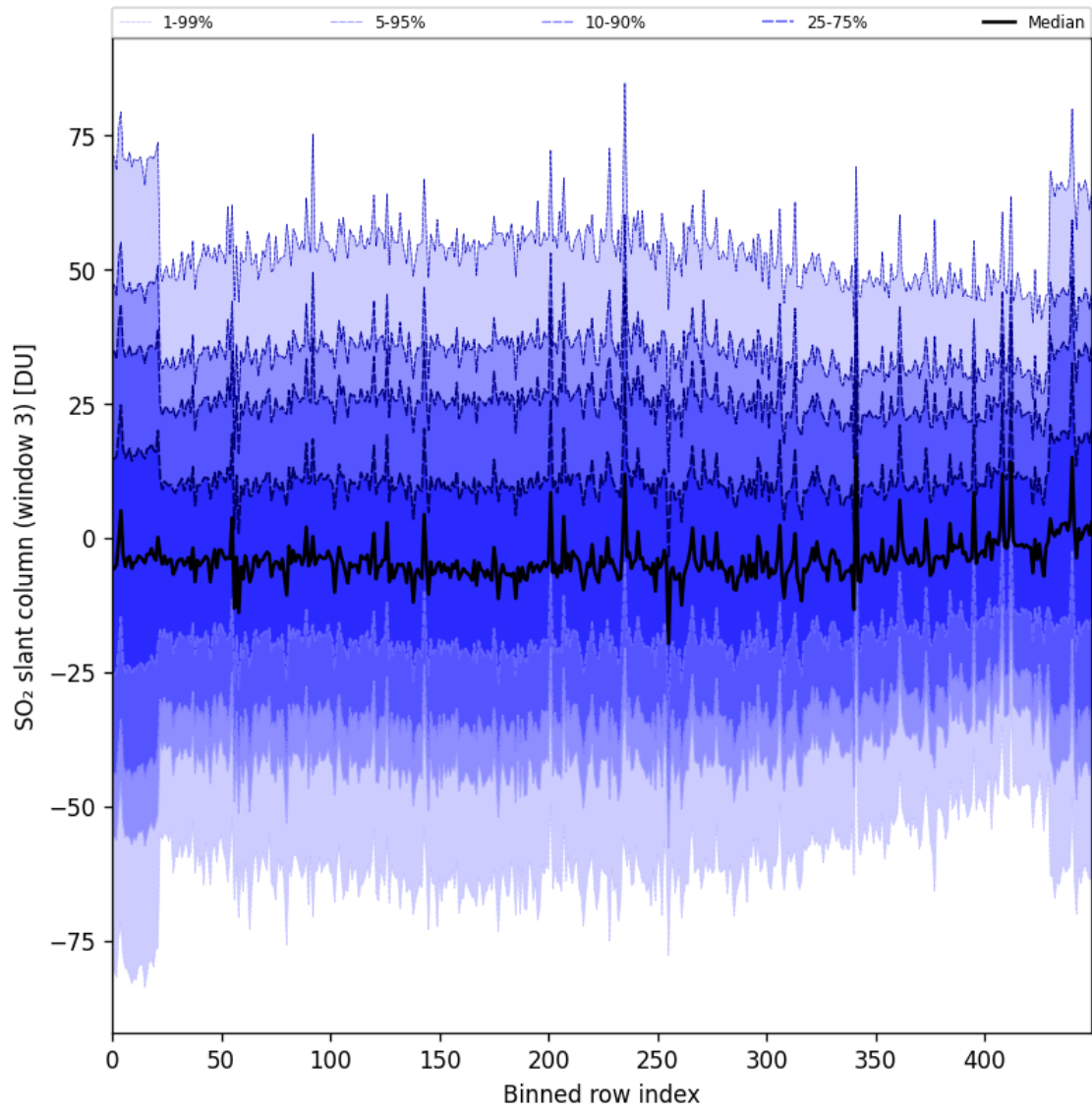
Figure 97: Along track statistics of “SO 2 slant column (window 3)” for 2025-05-01 to 2025-05-03
