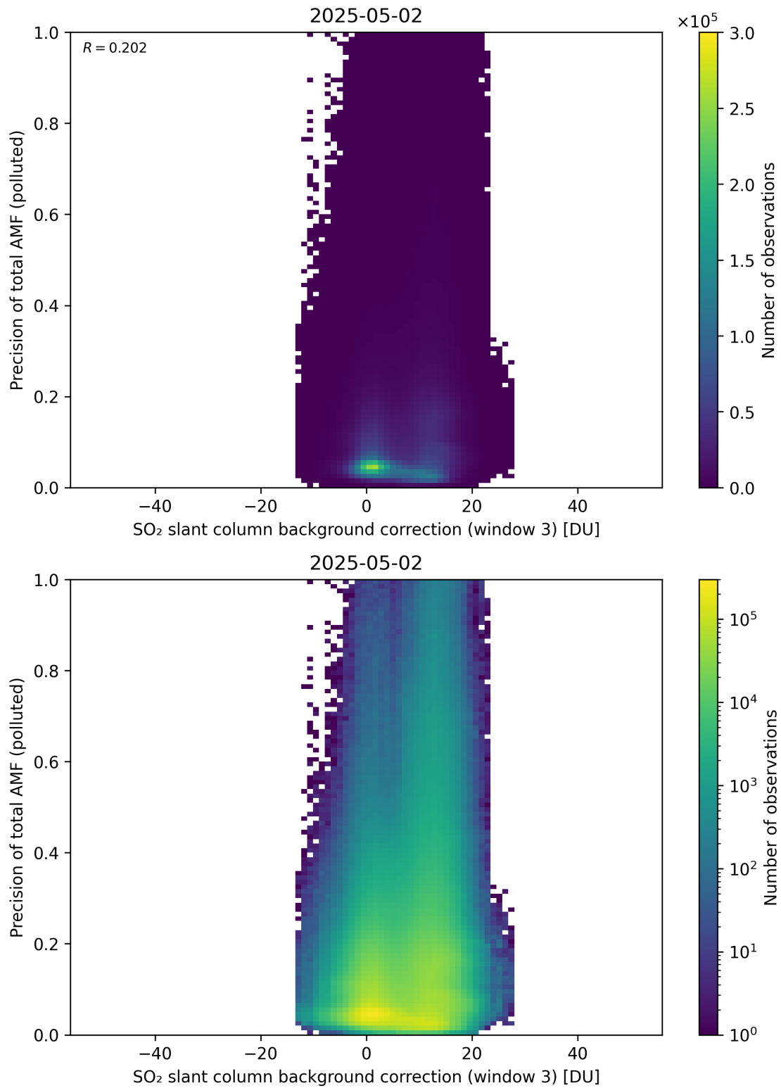
Figure 137: Scatter density plot of “SO 2 slant column background correction (window 3)” against “Precision of total AMF (polluted)” for 2025-05-01 to 2025-05-03.
