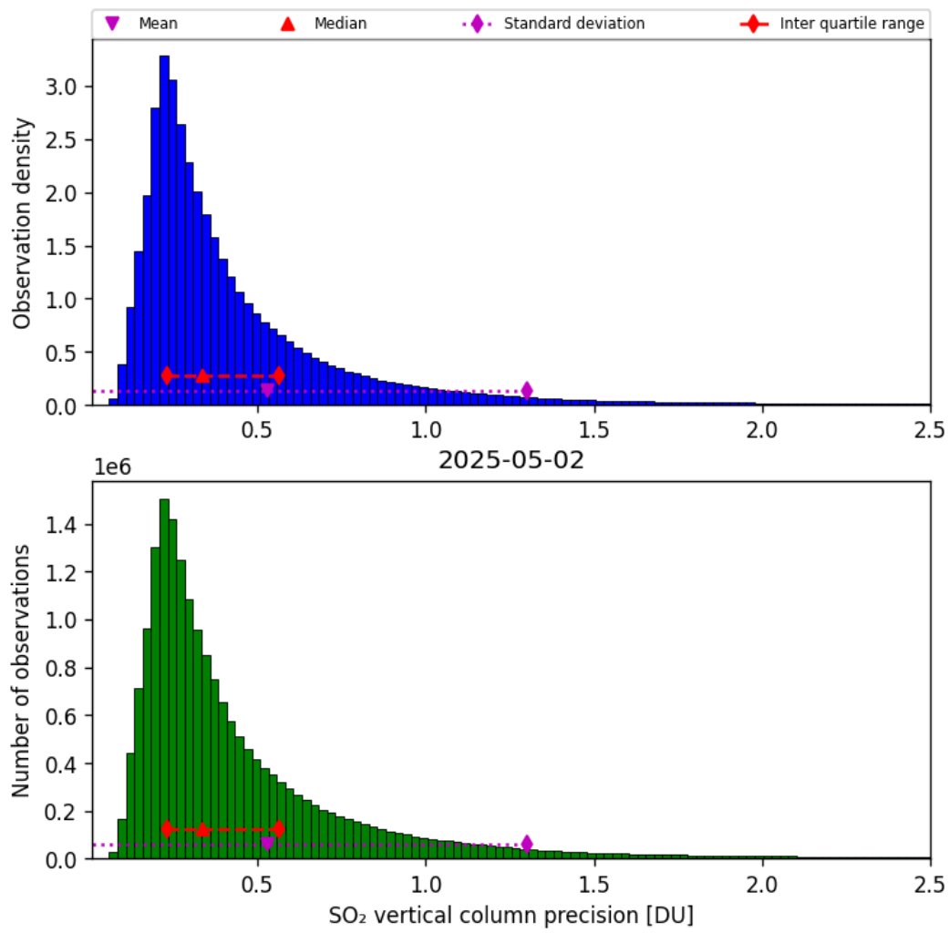
Figure 59: Histogram of “SO 2 vertical column precision” for 2025-05-01 to 2025-05-03
