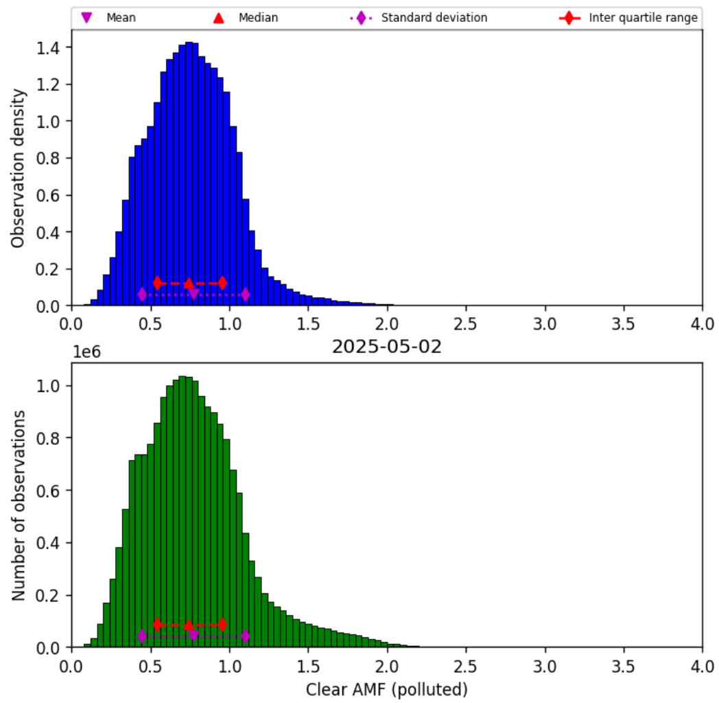
Figure 81: Histogram of “Clear AMF (polluted)” for 2025-05-01 to 2025-05-03
