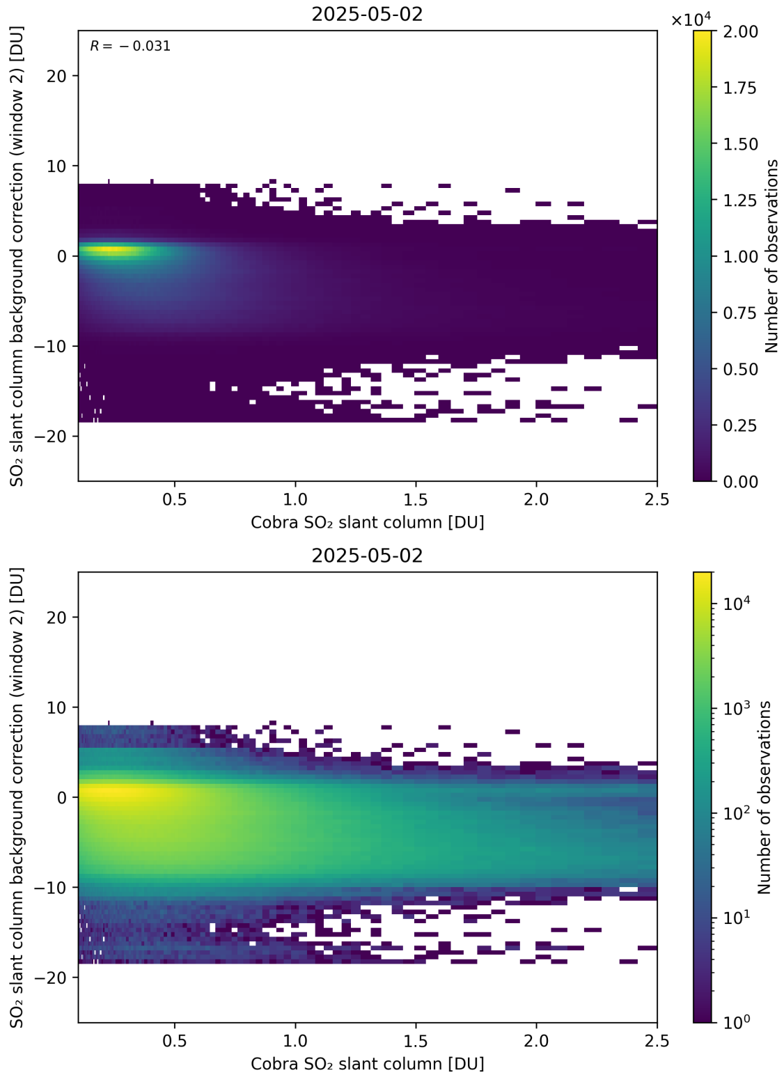
Figure 194: Scatter density plot of “Cobra SO 2 slant column” against “SO 2 slant column background correction (window 2)” for 2025-05-01 to 2025-05-03.
