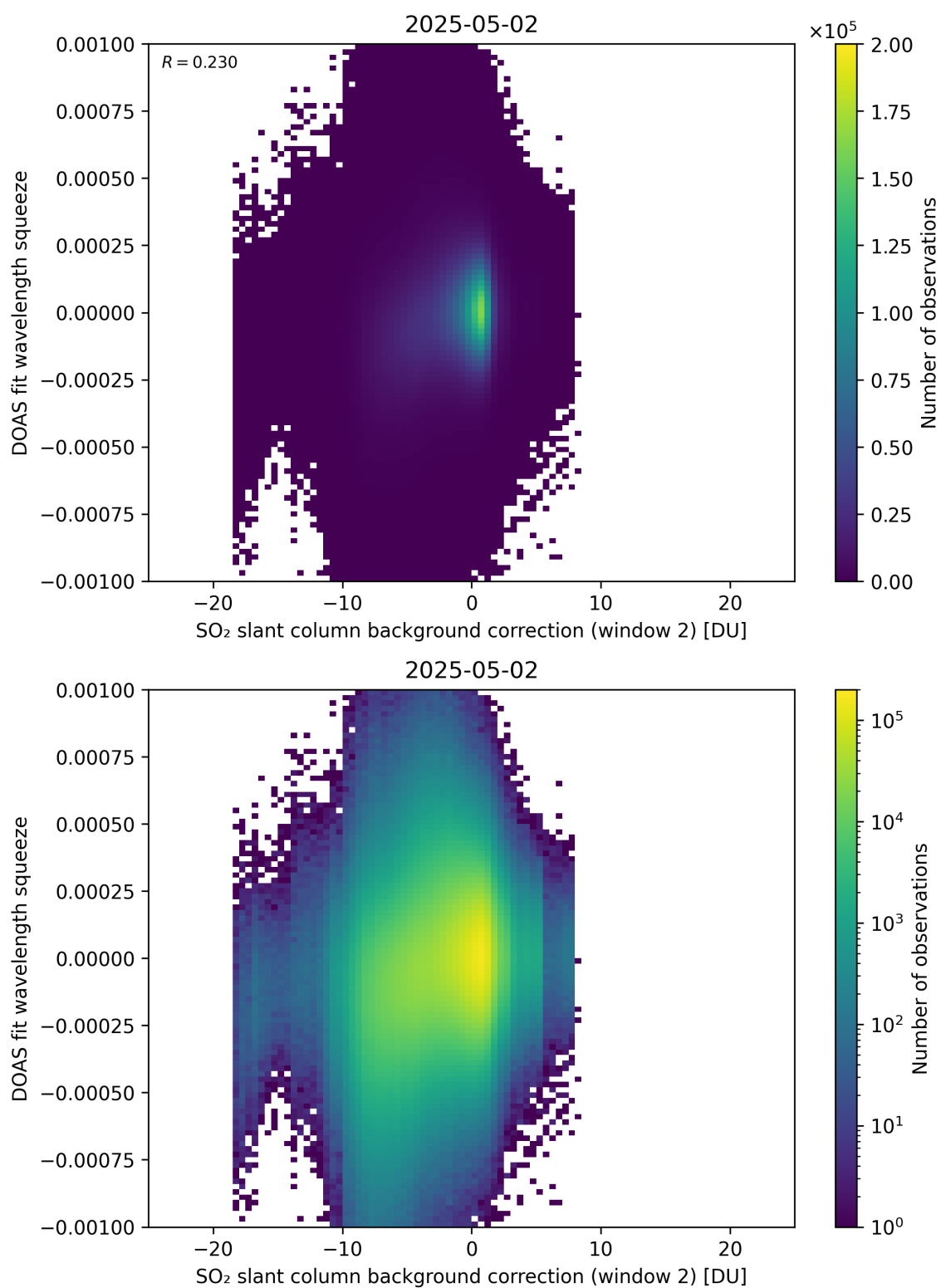
Figure 124: Scatter density plot of “SO 2 slant column background correction (window 2)” against “DOAS fit wavelength squeeze” for 2025-05-01 to 2025-05-03.
