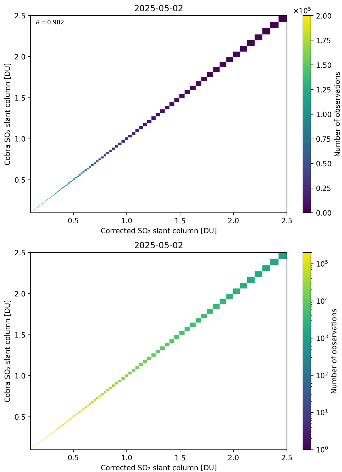
Figure 233: Scatter density plot of “Corrected SO 2 slant column” against “Cobra SO 2 slant column” for 2025-05-01 to 2025-05-03.
