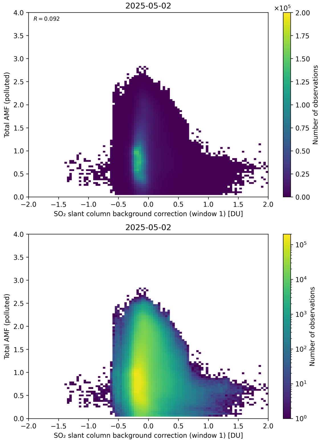
Figure 120: Scatter density plot of “SO 2 slant column background correction (window 1)” against “Total AMF (polluted)” for 2025-05-01 to 2025-05-03.
