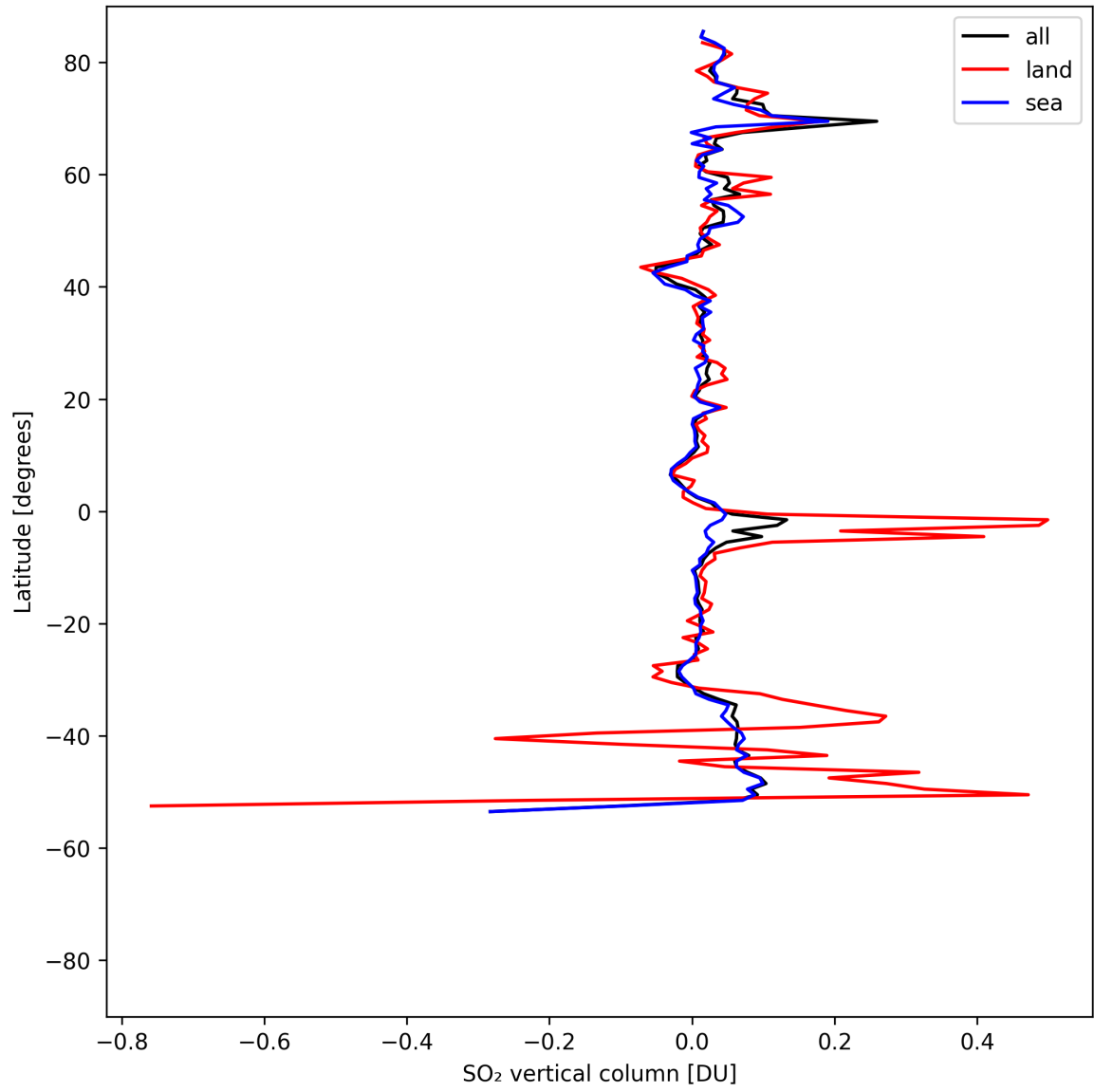
Figure 32: Zonal average of “SO 2 vertical column” for 2025-05-01 to 2025-05-03.
