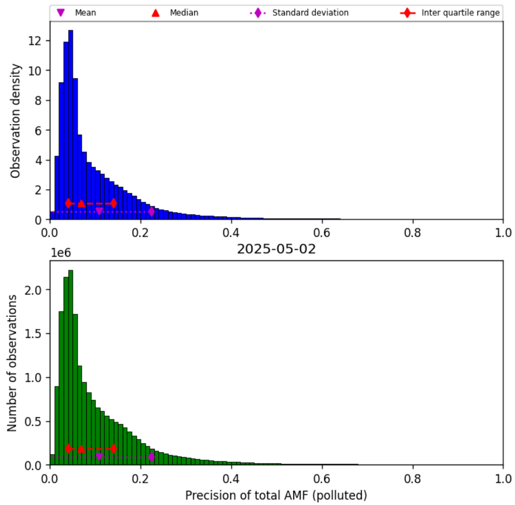
Figure 80: Histogram of “Precision of total AMF (polluted)” for 2025-05-01 to 2025-05-03
