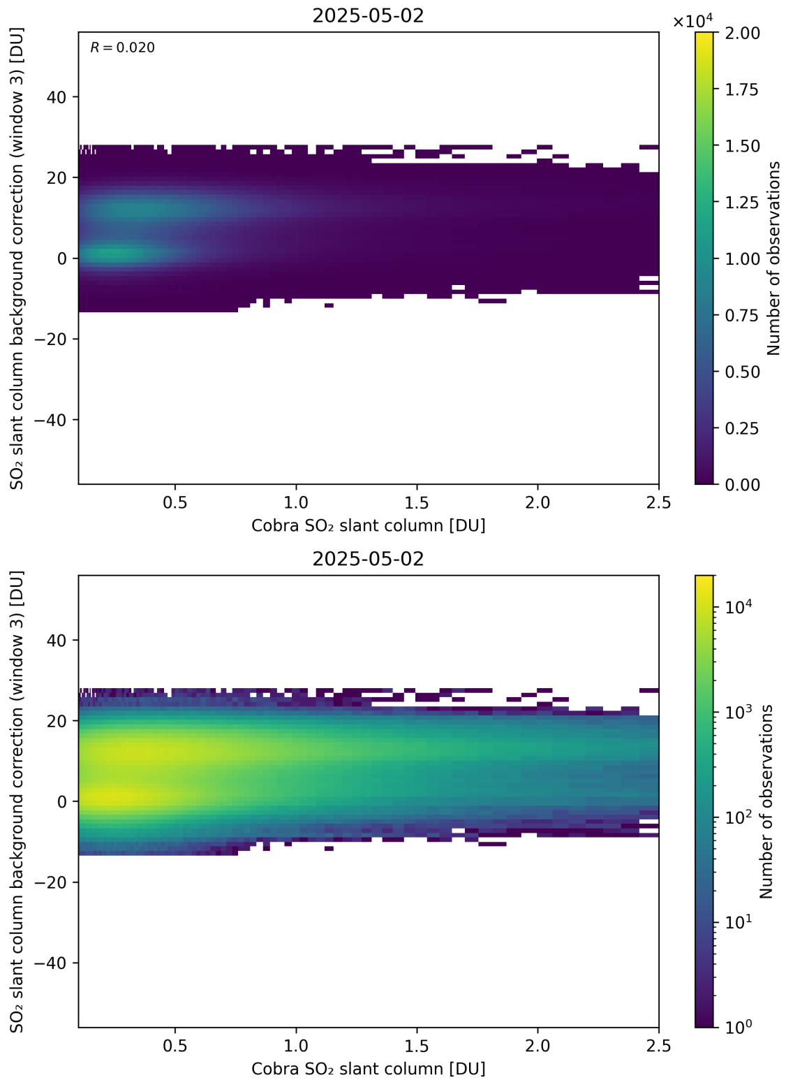
Figure 195: Scatter density plot of “Cobra SO 2 slant column” against “SO 2 slant column background correction (window 3)” for 2025-05-01 to 2025-05-03.
