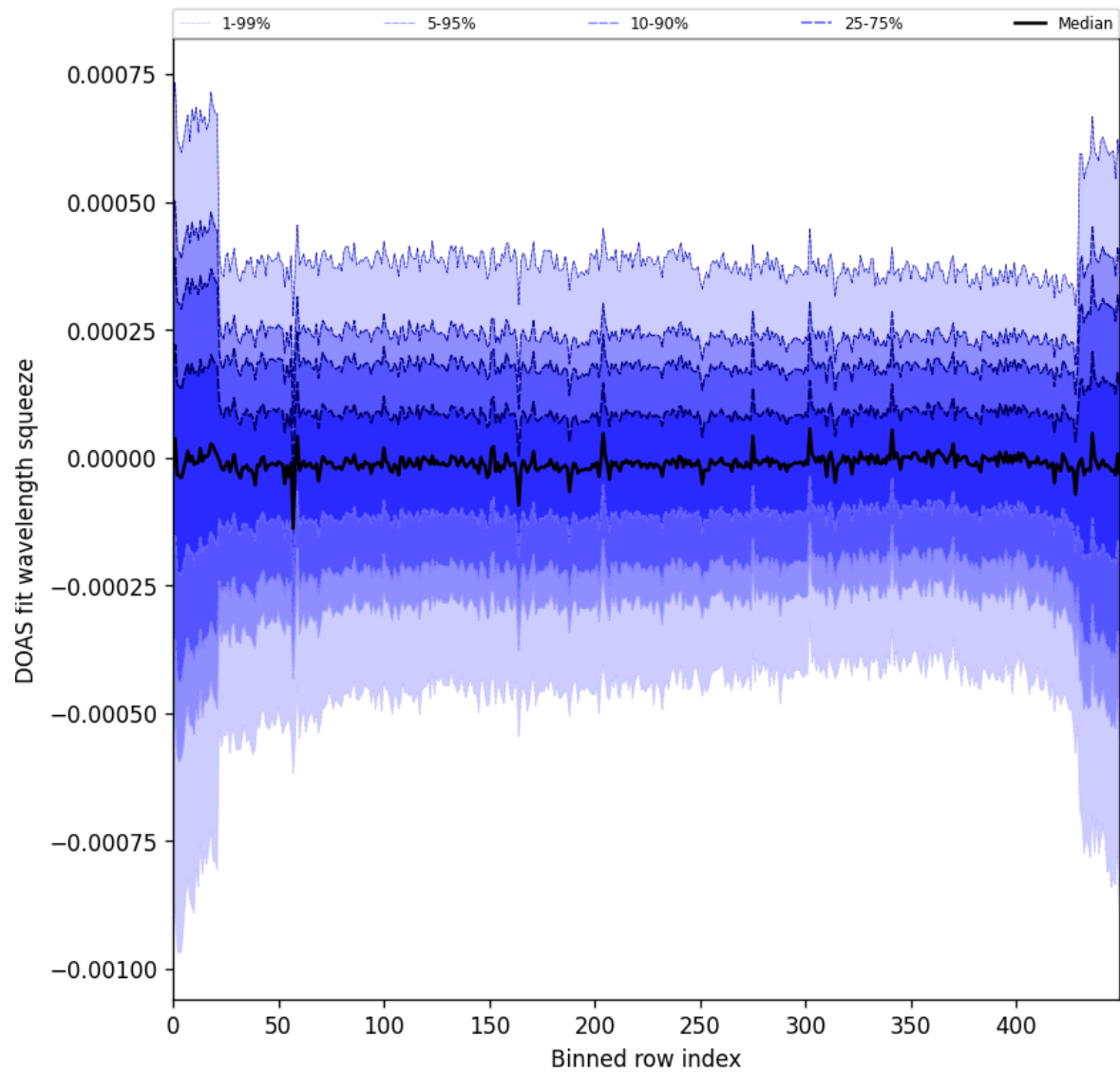
Figure 103: Along track statistics of “DOAS fit wavelength squeeze” for 2025-05-01 to 2025-05-03
