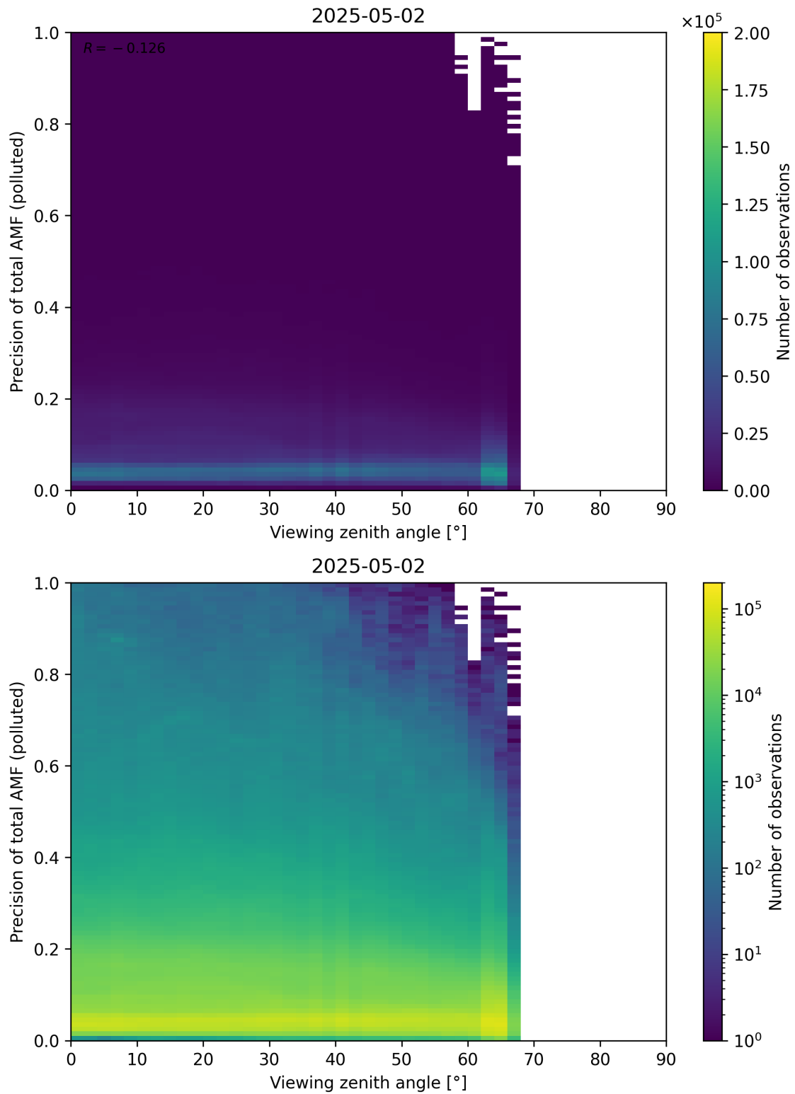
Figure 382: Scatter density plot of “Viewing zenith angle” against “Precision of total AMF (polluted)” for 2025-05-01 to 2025-05-03.
