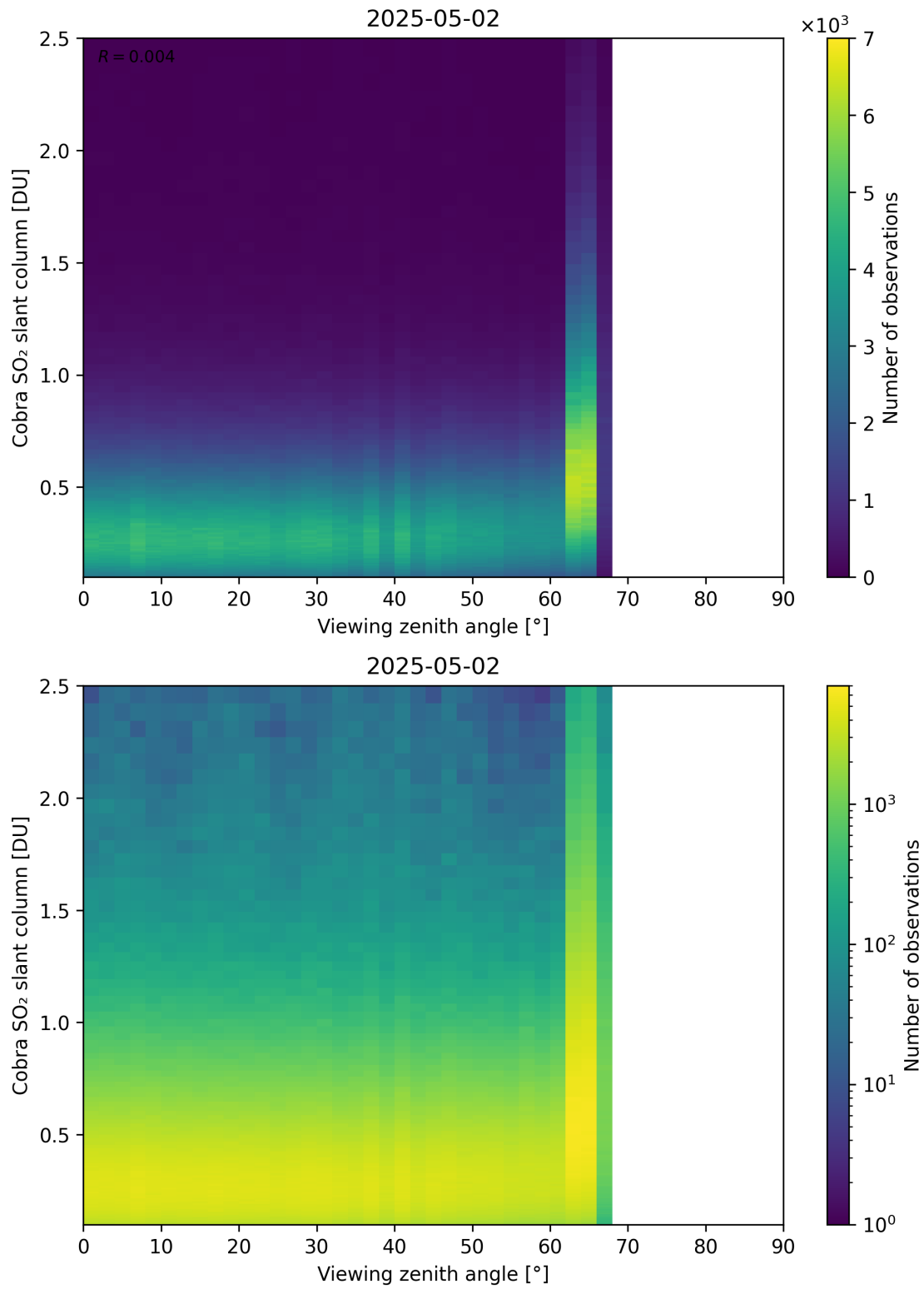
Figure 371: Scatter density plot of “Viewing zenith angle” against “Cobra SO 2 slant column” for 2025-05-01 to 2025-05-03.
