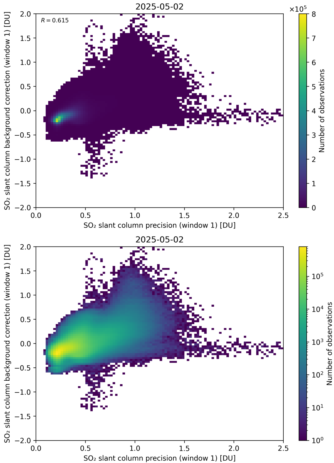
Figure 268: Scatter density plot of “SO 2 slant column precision (window 1)” against “SO 2 slant column background correction (window 1)” for 2025-05-01 to 2025-05-03.
