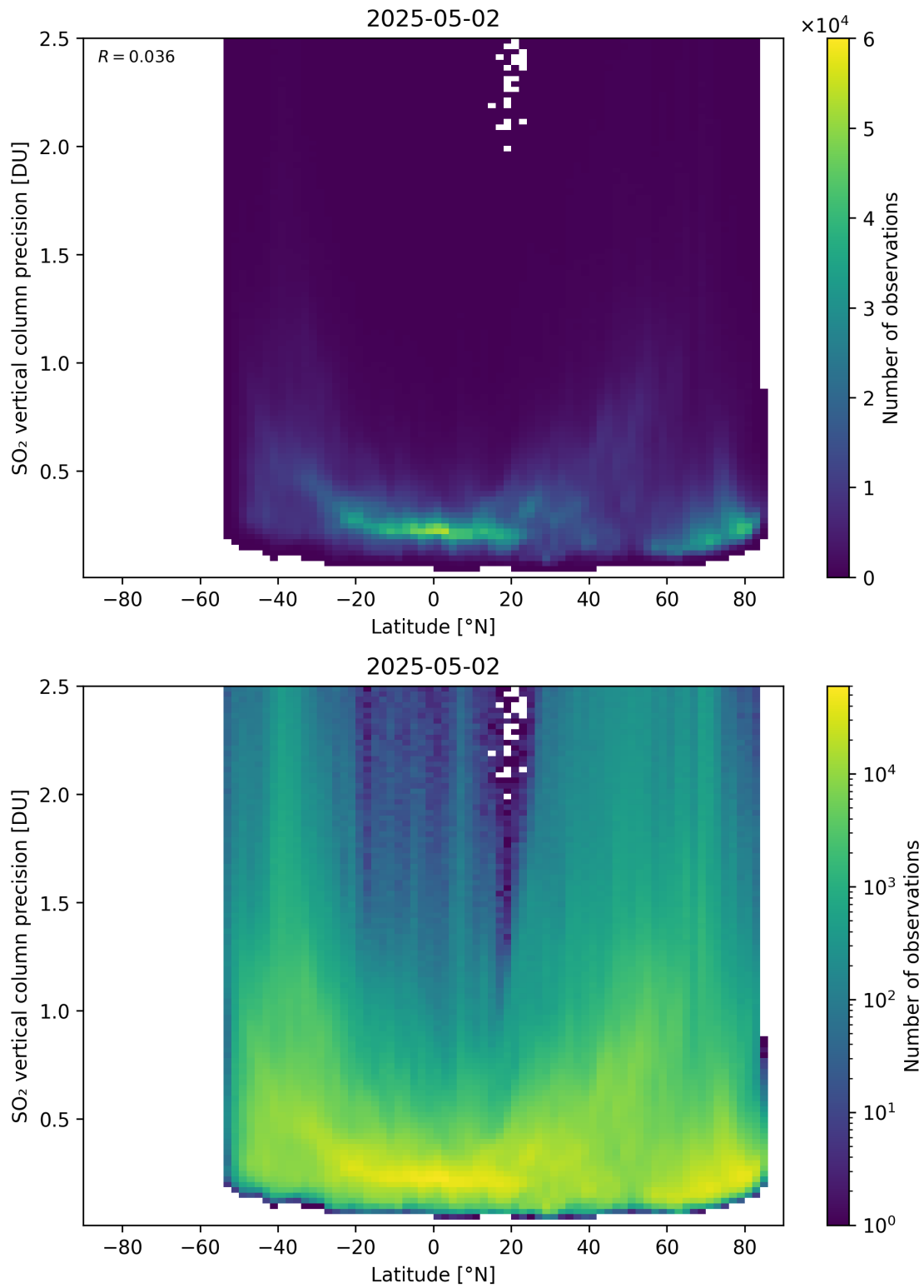
Figure 170: Scatter density plot of “Latitude” against “SO 2 vertical column precision” for 2025-05-01 to 2025-05-03.
