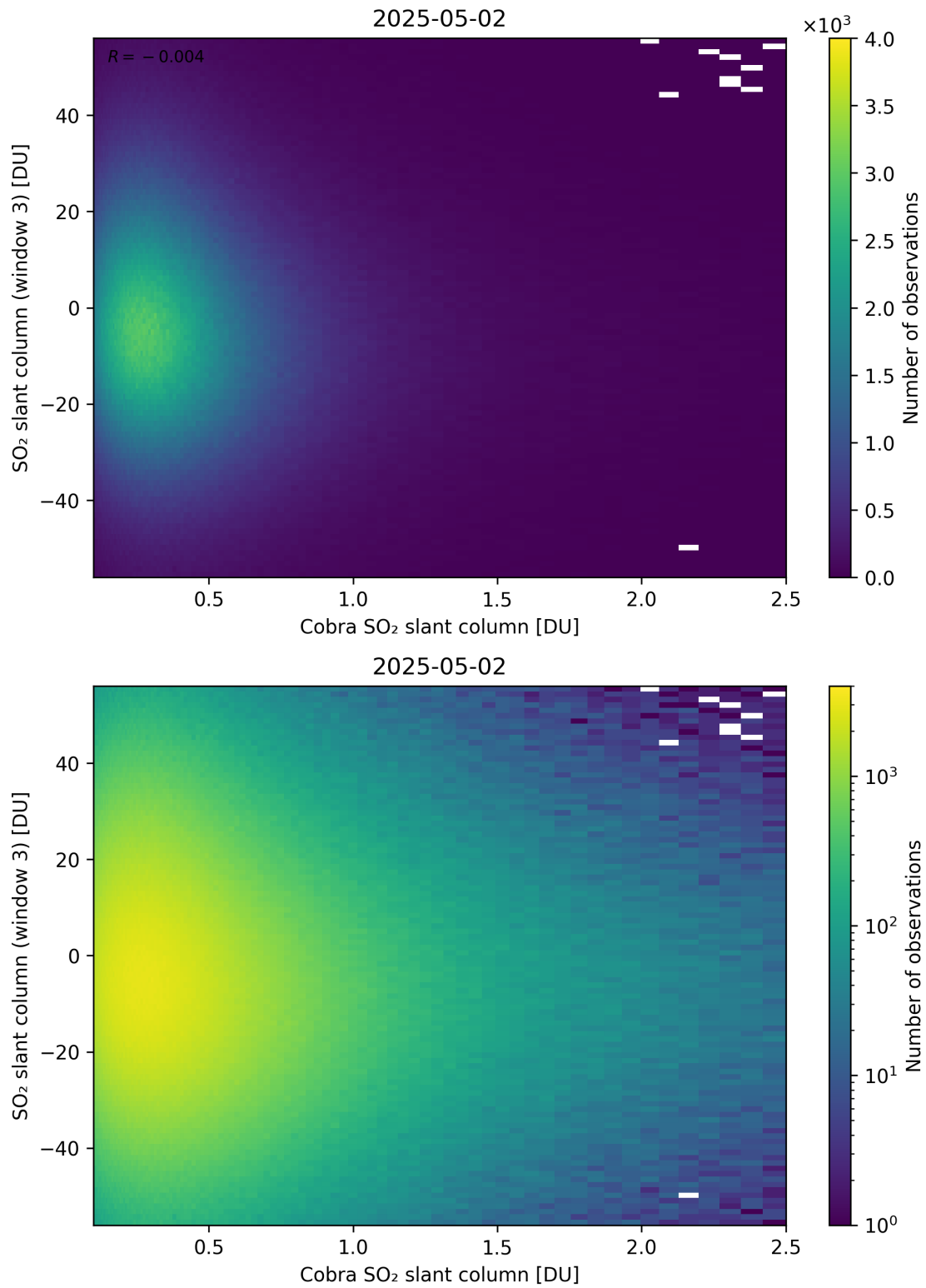
Figure 222: Scatter density plot of “Cobra SO 2 slant column” against “SO 2 slant column (window 3)” for 2025-05-01 to 2025-05-03.
