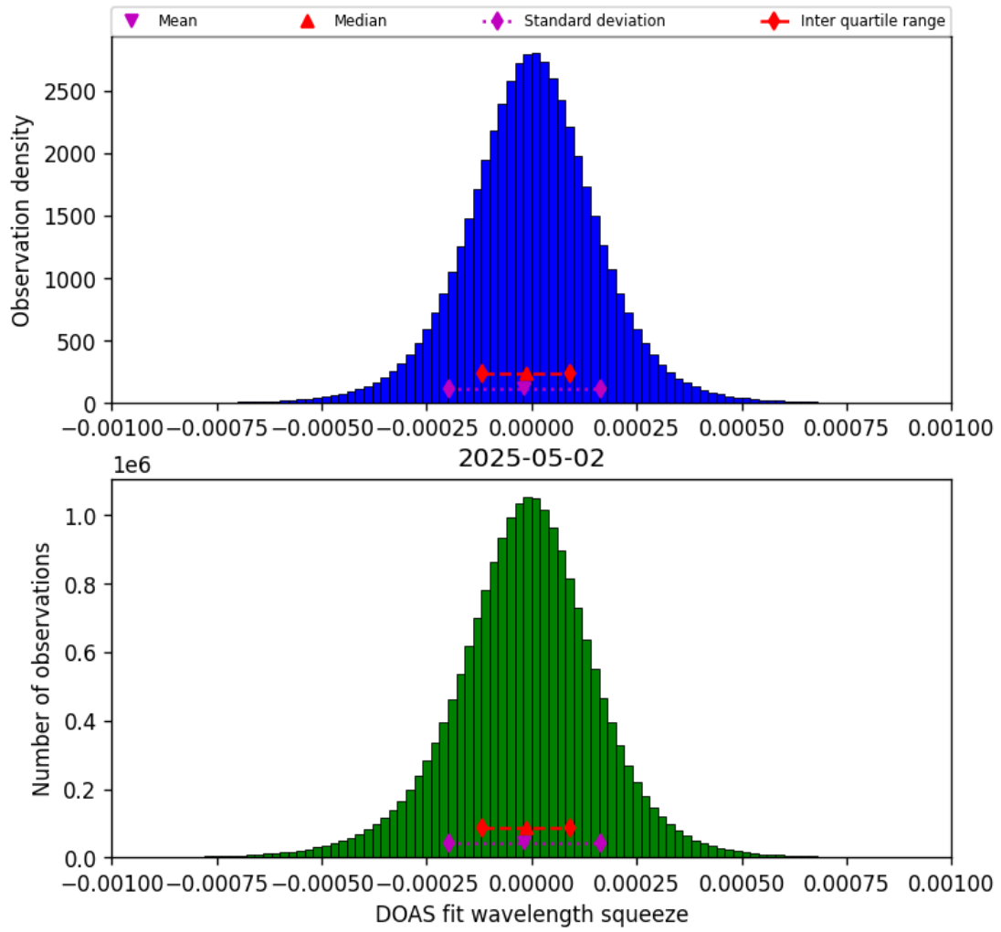
Figure 77: Histogram of “DOAS fit wavelength squeeze” for 2025-05-01 to 2025-05-03
