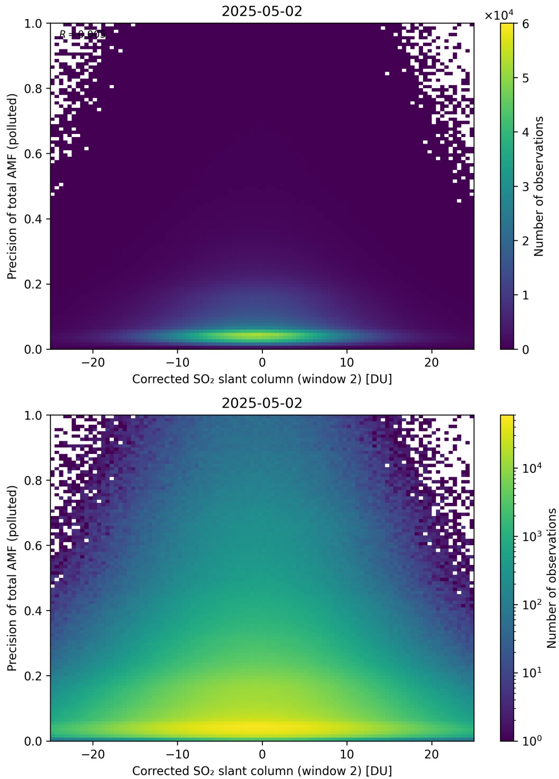
Figure 254: Scatter density plot of “Corrected SO 2 slant column (window 2)” against “Precision of total AMF (polluted)” for 2025-05-01 to 2025-05-03.
