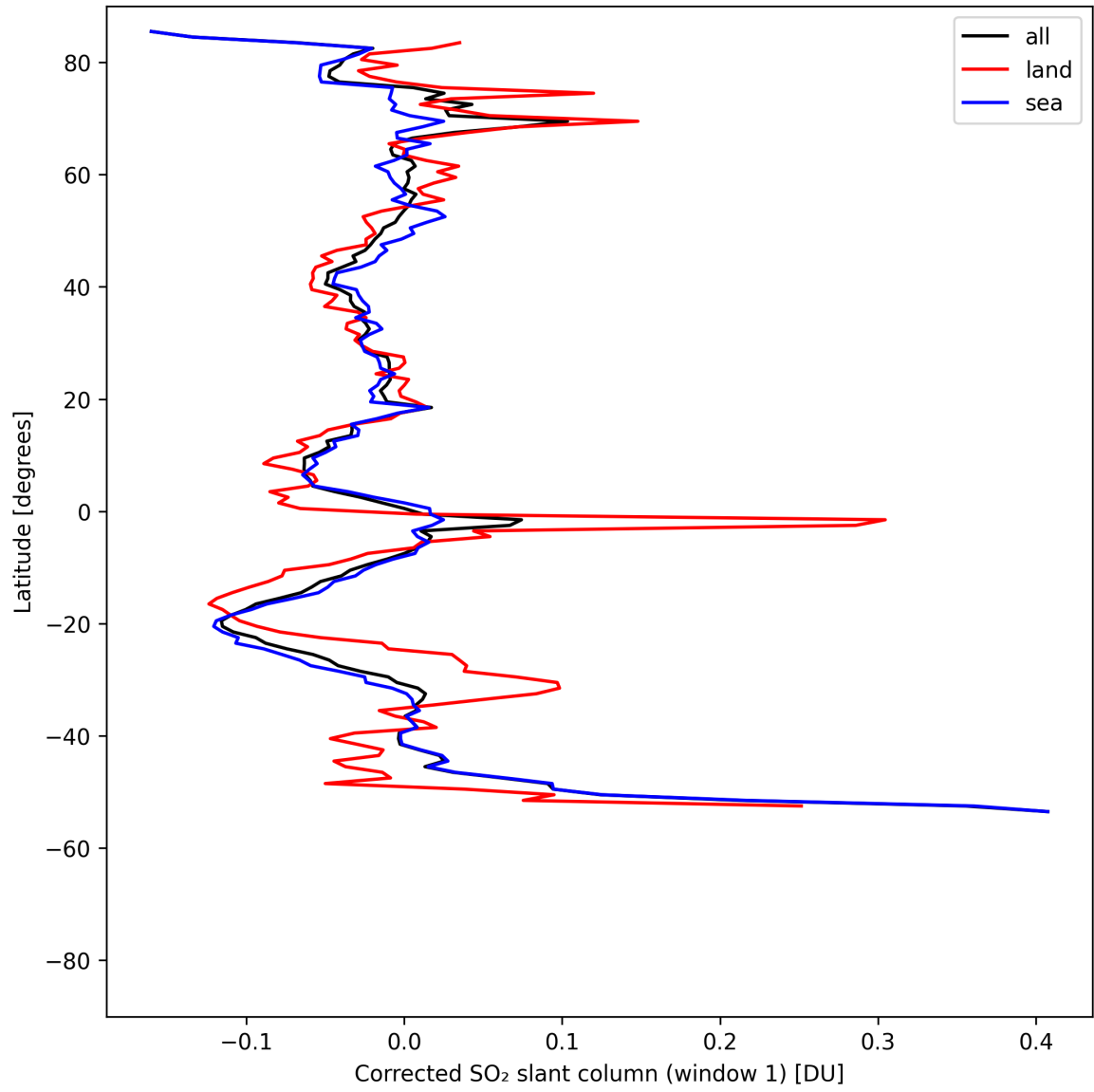
Figure 39: Zonal average of “Corrected SO 2 slant column (window 1)” for 2025-05-01 to 2025-05-03.
