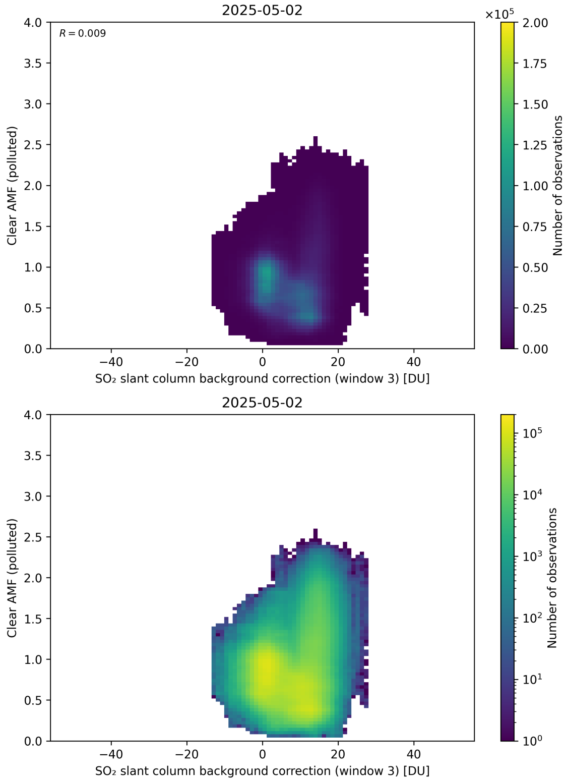
Figure 135: Scatter density plot of “SO 2 slant column background correction (window 3)” against “Clear AMF (polluted)” for 2025-05-01 to 2025-05-03.
