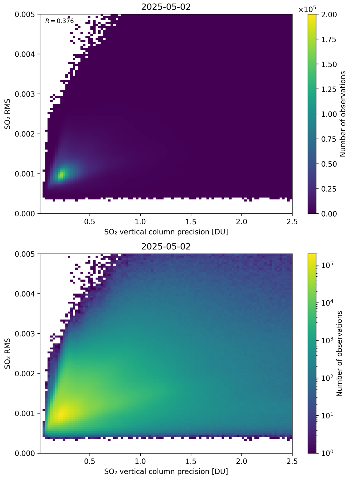
Figure 334: Scatter density plot of “SO 2 vertical column precision” against “SO 2 RMS” for 2025-05-01 to 2025-05-03.
