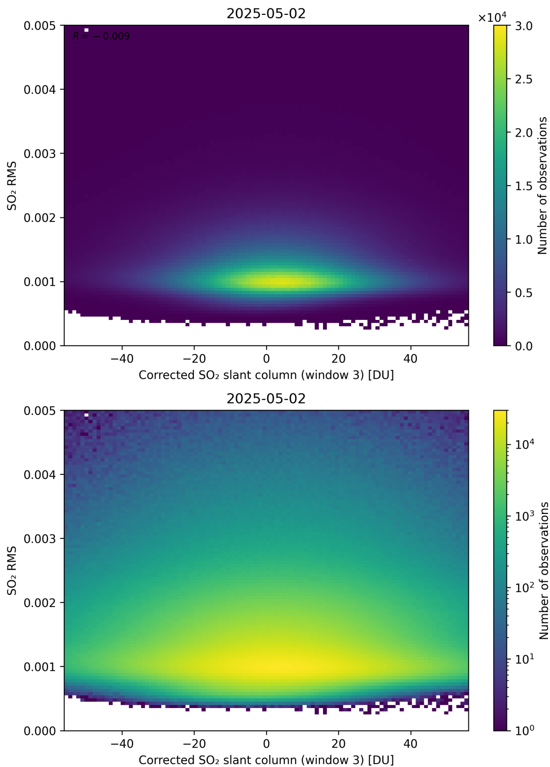
Figure 258: Scatter density plot of “Corrected SO 2 slant column (window 3)” against “SO 2 RMS” for 2025-05-01 to 2025-05-03.
