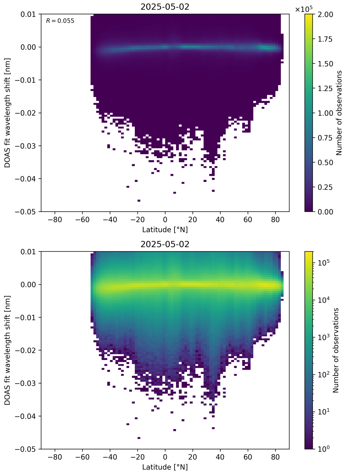
Figure 153: Scatter density plot of “Latitude” against “DOAS fit wavelength shift” for 2025-05-01 to 2025-05-03.
