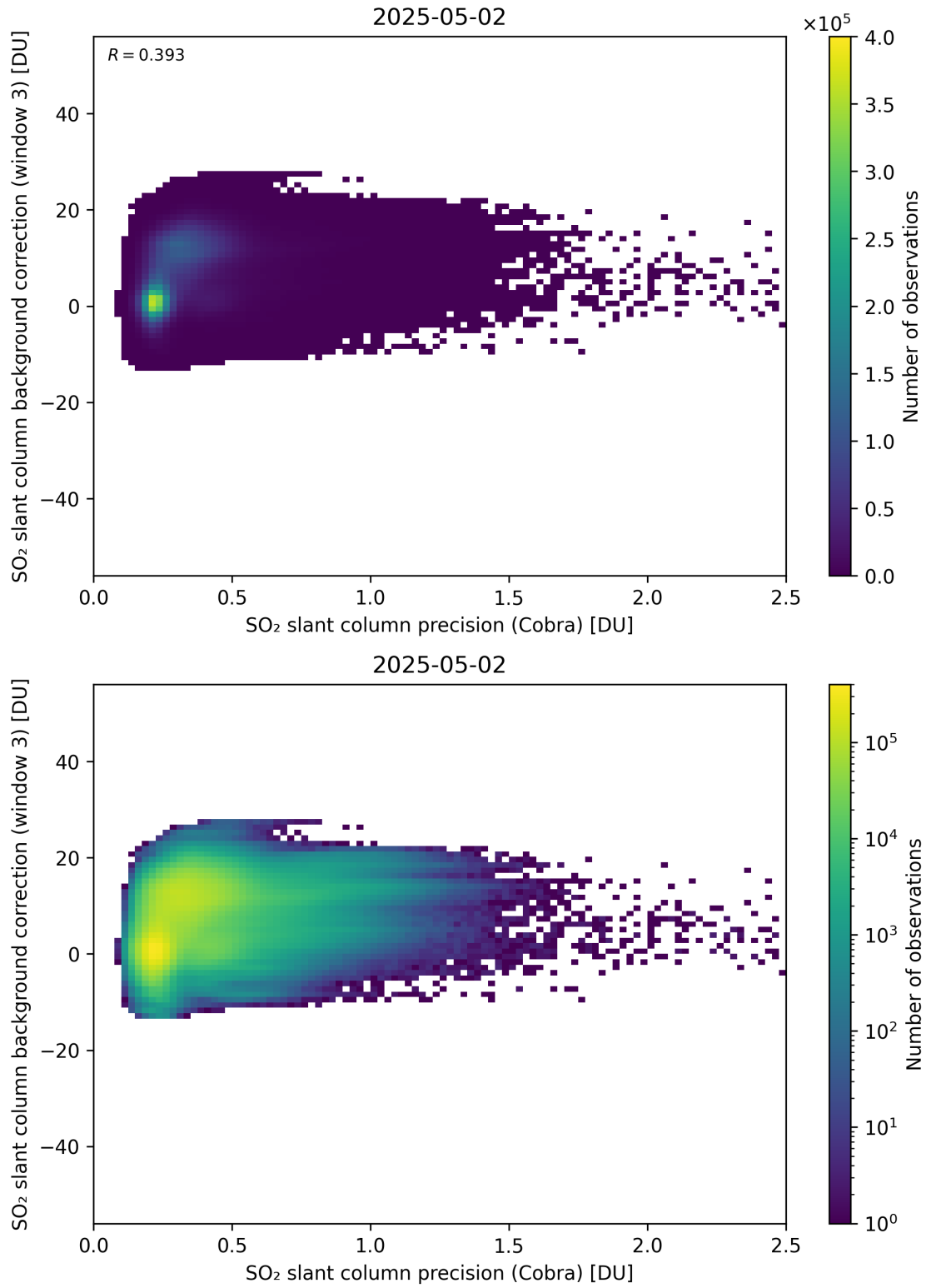
Figure 201: Scatter density plot of “SO 2 slant column precision (Cobra)” against “SO 2 slant column background correction (window 3)” for 2025-05-01 to 2025-05-03.
