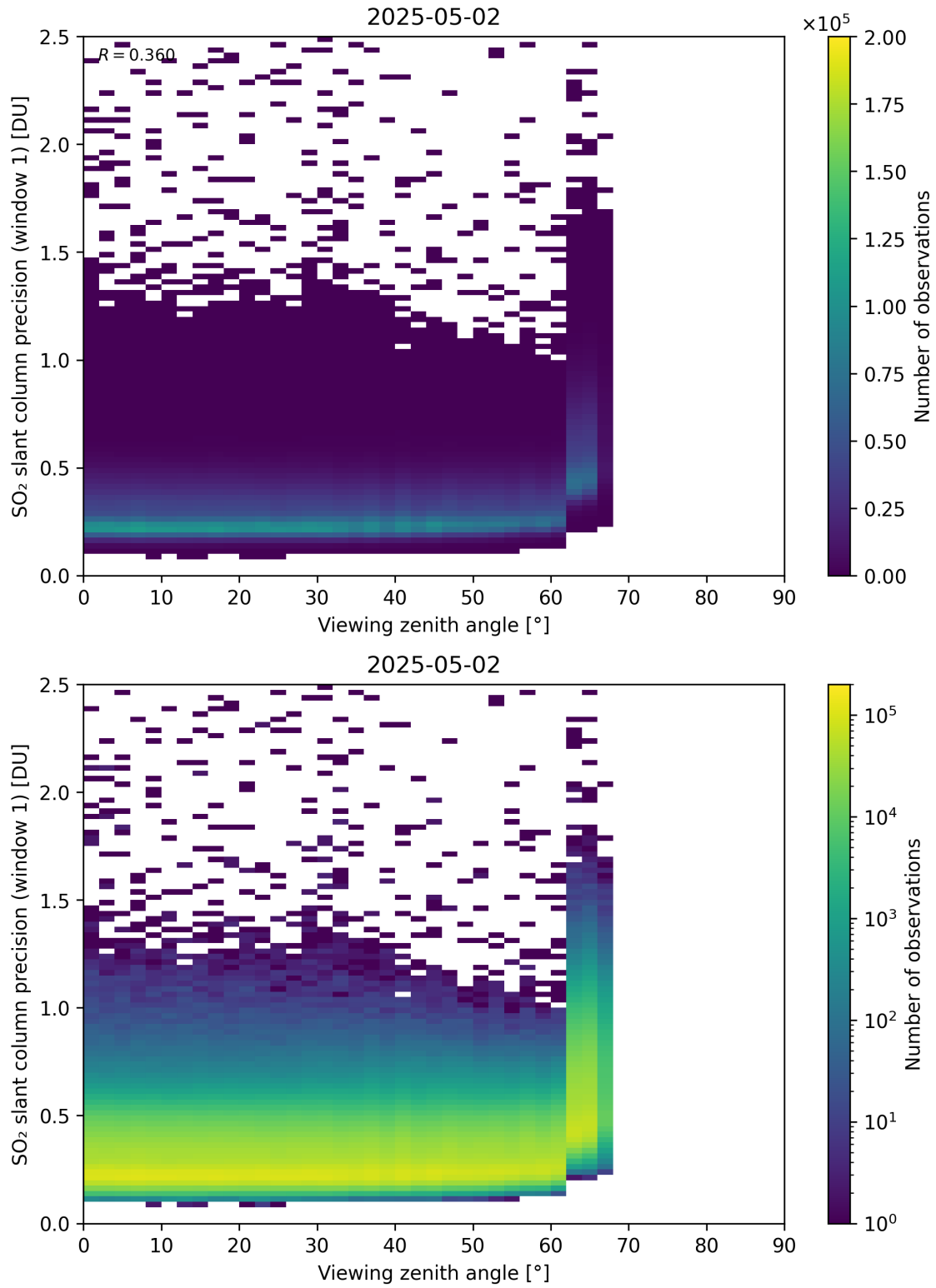
Figure 377: Scatter density plot of “Viewing zenith angle” against “SO 2 slant column precision (window 1)” for 2025-05-01 to 2025-05-03.
