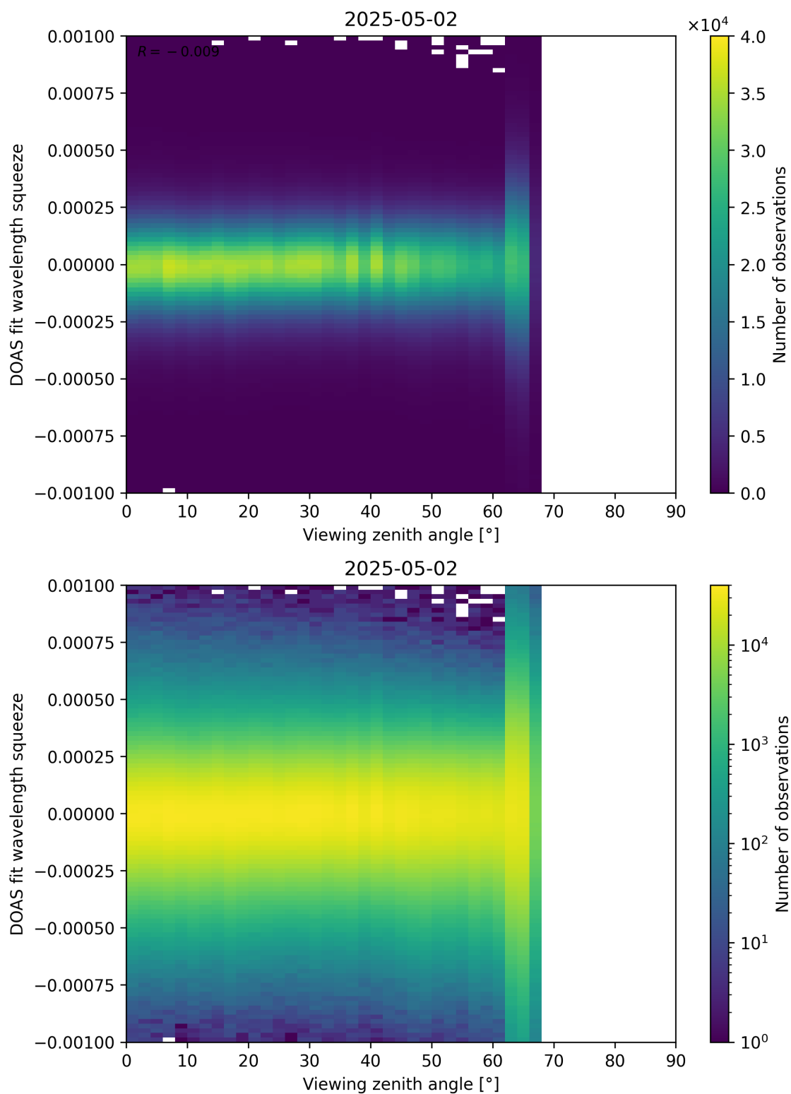
Figure 366: Scatter density plot of “Viewing zenith angle” against “DOAS fit wavelength squeeze” for 2025-05-01 to 2025-05-03.
