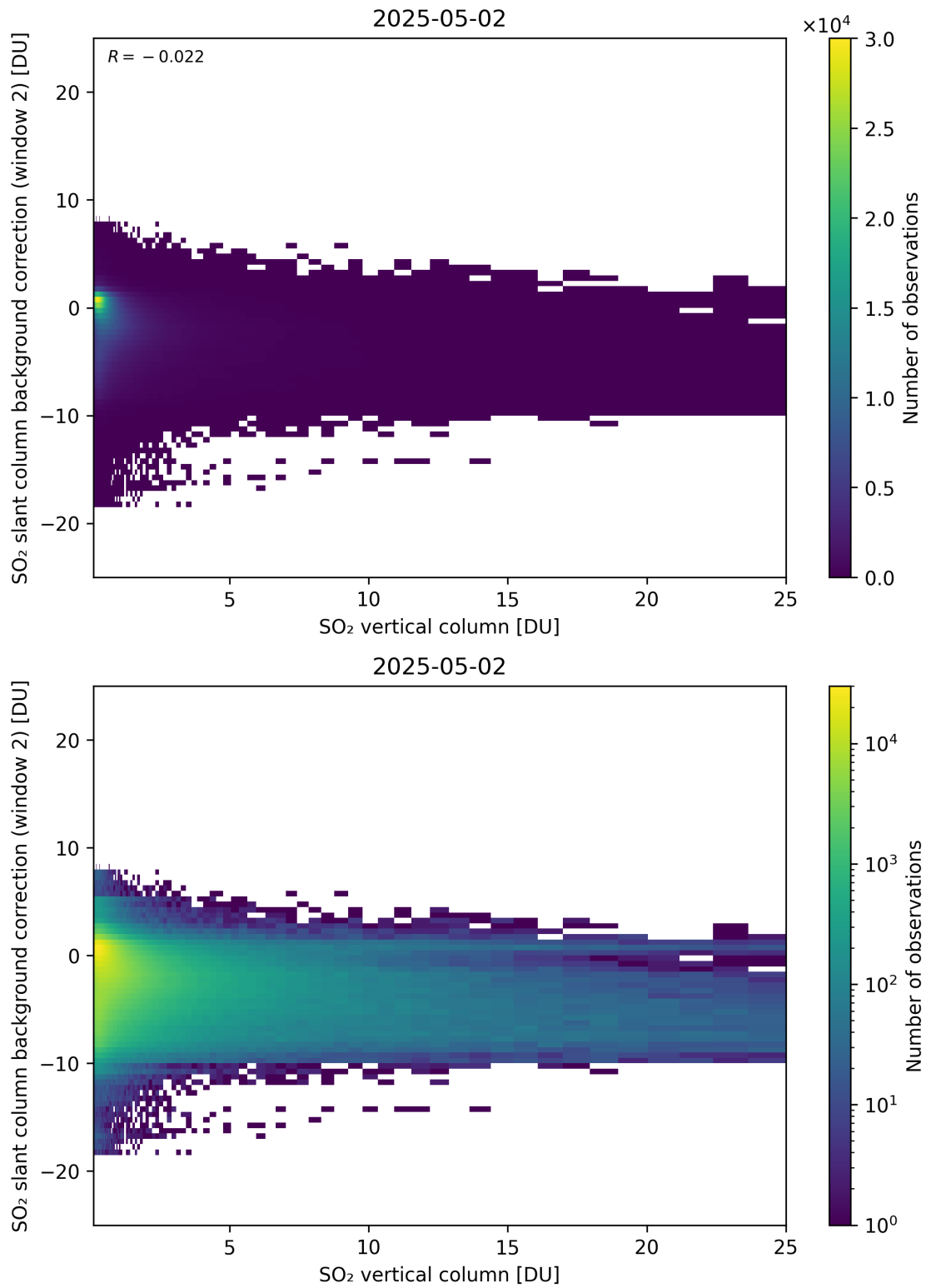
Figure 324: Scatter density plot of “SO 2 vertical column” against “SO 2 slant column background correction (window 2)” for 2025-05-01 to 2025-05-03.
