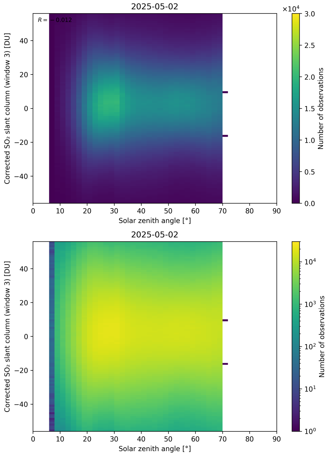
Figure 183: Scatter density plot of “Solar zenith angle” against “Corrected SO 2 slant column (window 3)” for 2025-05-01 to 2025-05-03.
