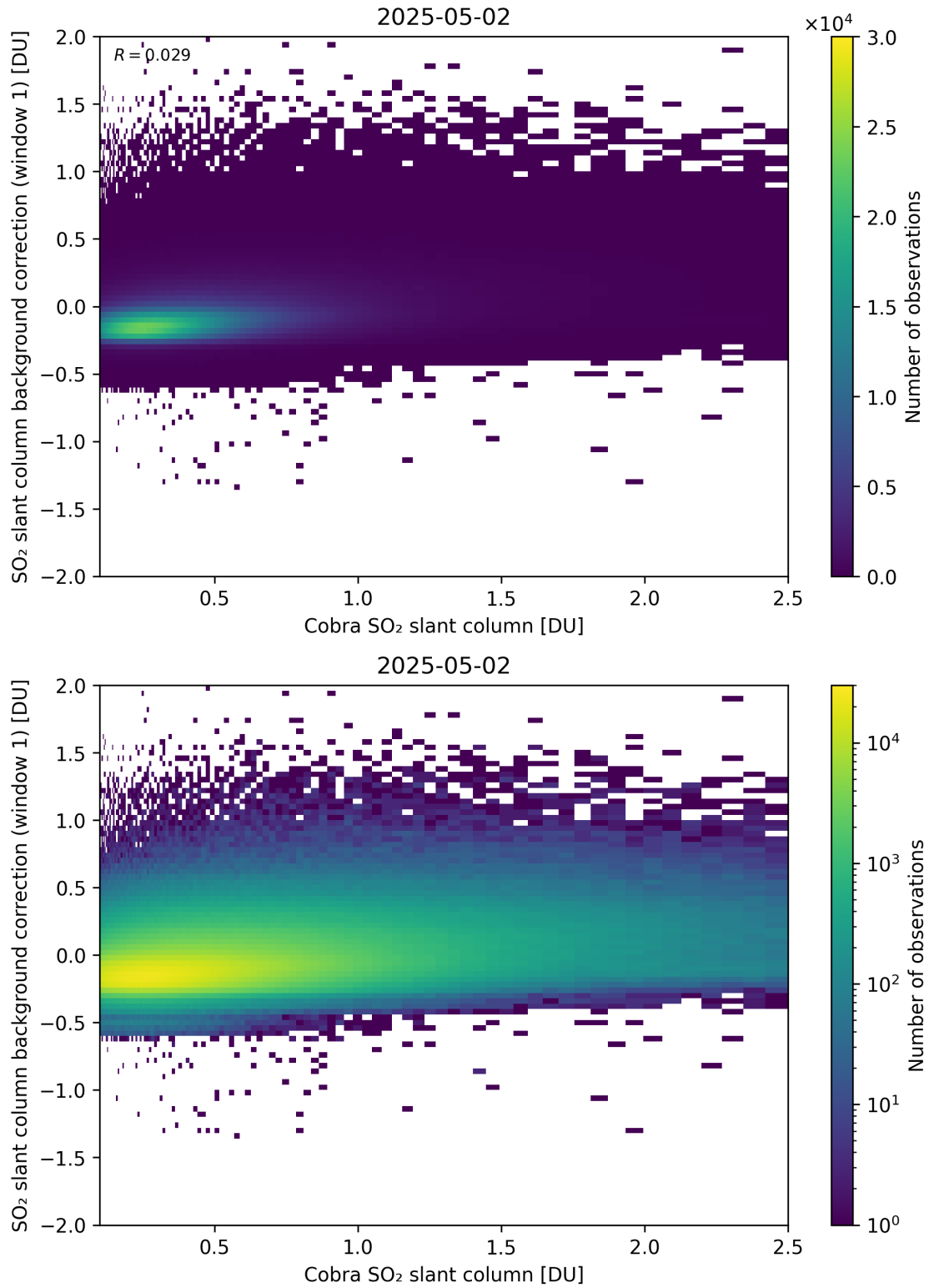
Figure 193: Scatter density plot of “Cobra SO 2 slant column” against “SO 2 slant column background correction (window 1)” for 2025-05-01 to 2025-05-03.
