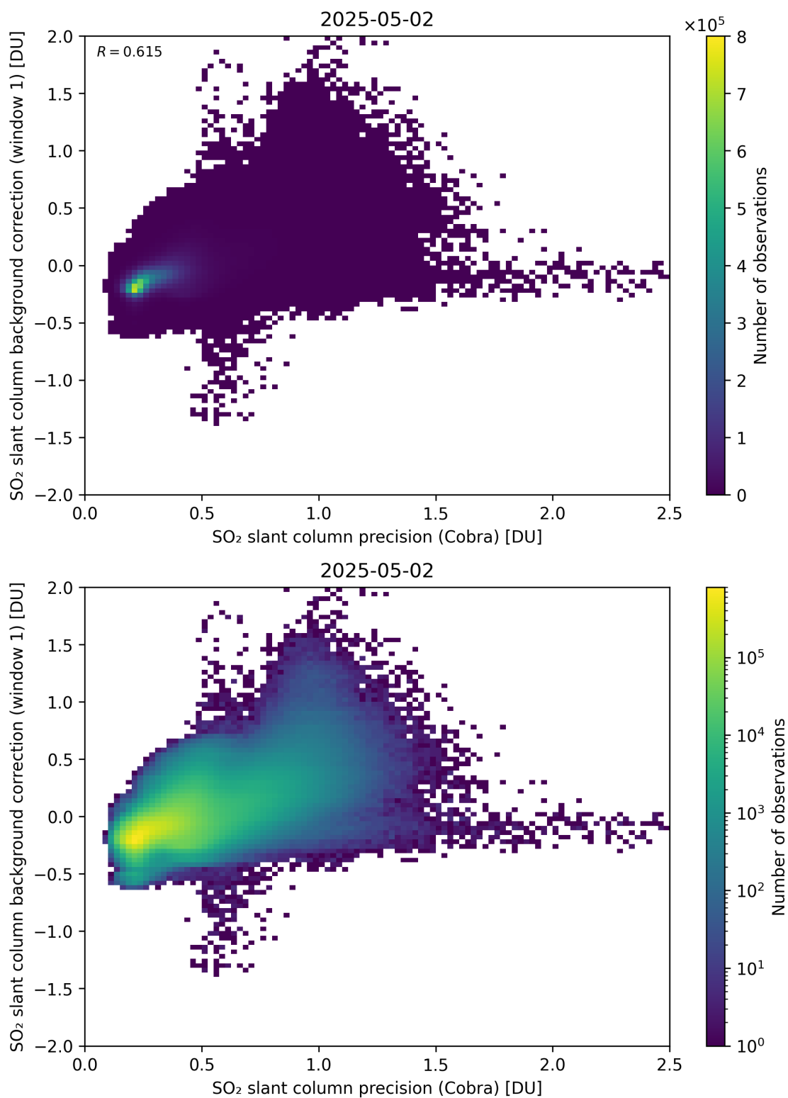
Figure 199: Scatter density plot of “SO 2 slant column precision (Cobra)” against “SO 2 slant column background correction (window 1)” for 2025-05-01 to 2025-05-03.
