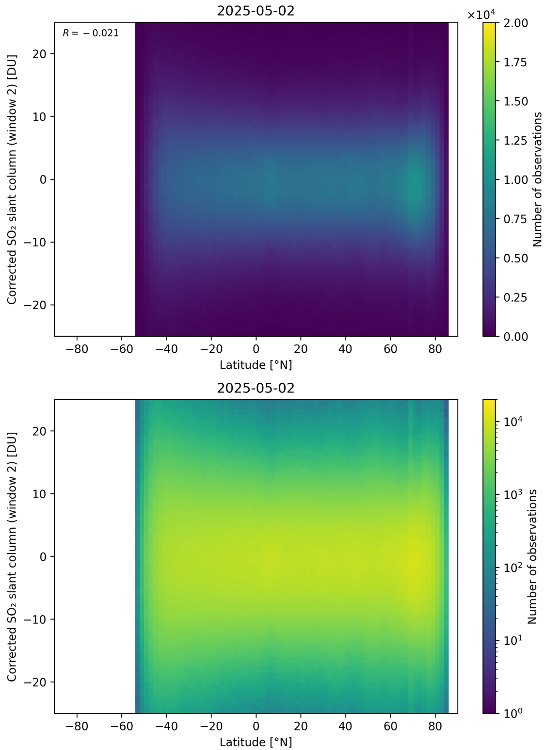
Figure 160: Scatter density plot of “Latitude” against “Corrected SO 2 slant column (window 2)” for 2025-05-01 to 2025-05-03.
