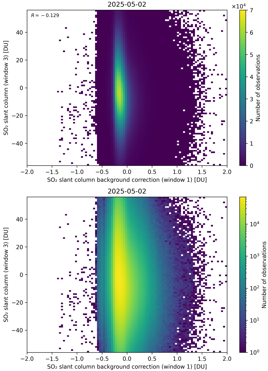
Figure 118: Scatter density plot of “SO 2 slant column background correction (window 1)” against “SO 2 slant column (window 3)” for 2025-05-01 to 2025-05-03.
