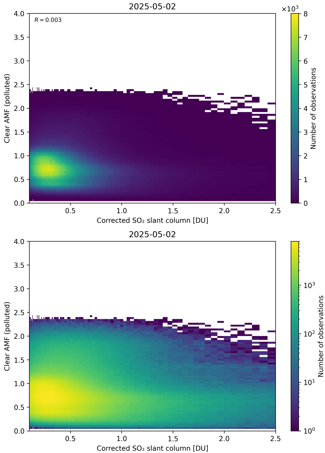
Figure 232: Scatter density plot of “Corrected SO 2 slant column” against “Clear AMF (polluted)” for 2025-05-01 to 2025-05-03.
