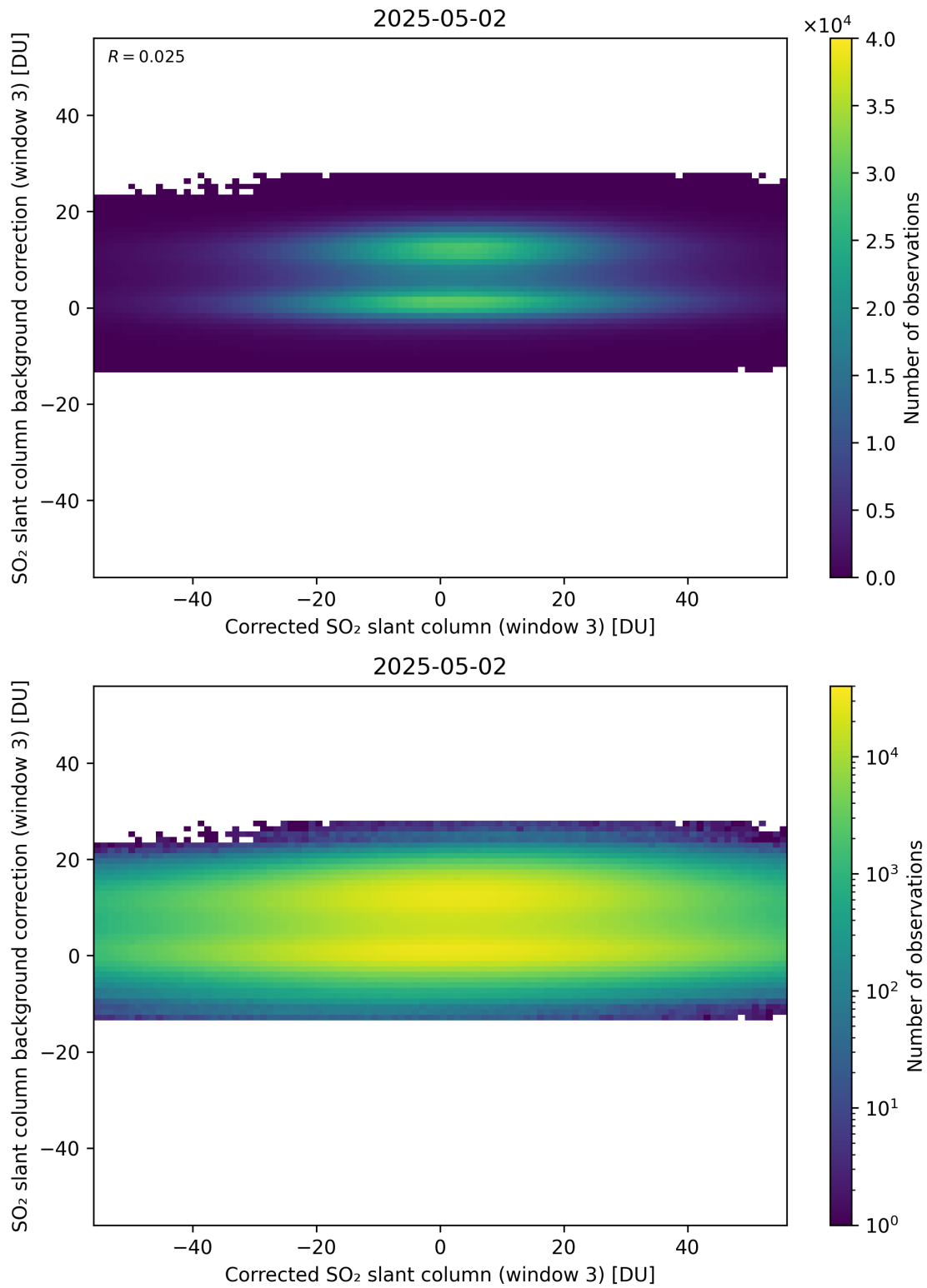
Figure 255: Scatter density plot of “Corrected SO 2 slant column (window 3)” against “SO 2 slant column background correction (window 3)” for 2025-05-01 to 2025-05-03.
