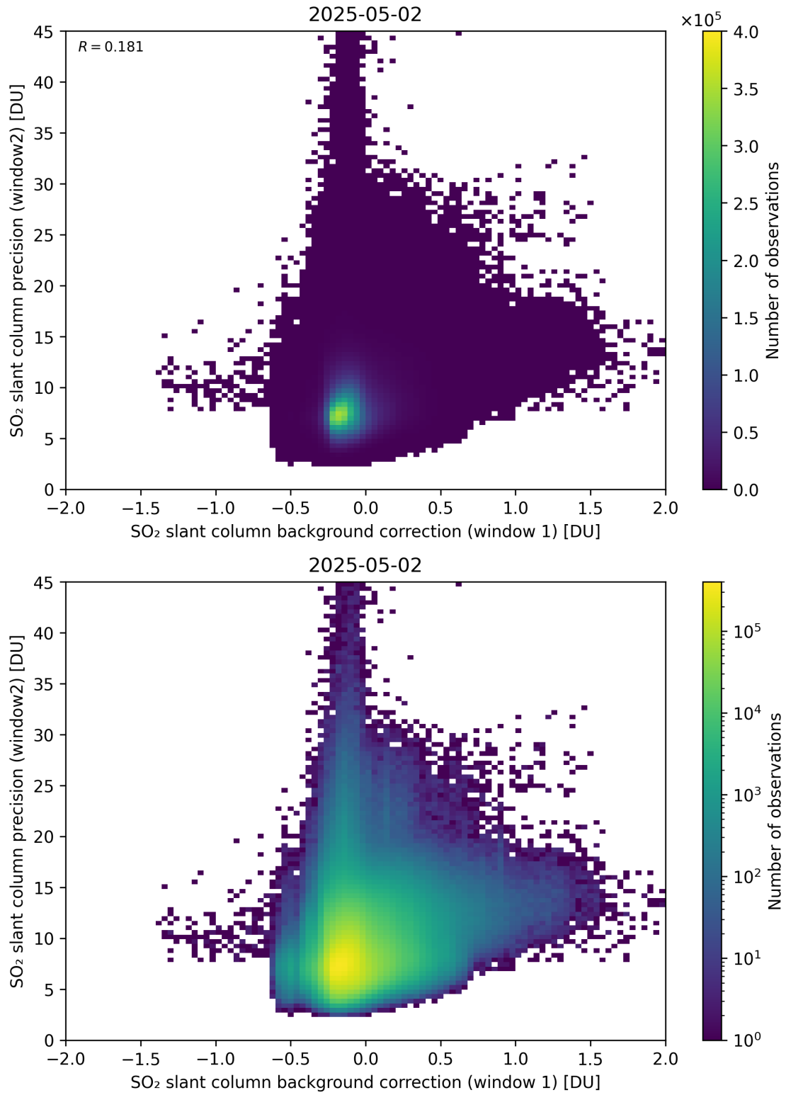
Figure 117: Scatter density plot of “SO 2 slant column background correction (window 1)” against “SO 2 slant column precision (window2)” for 2025-05-01 to 2025-05-03.
