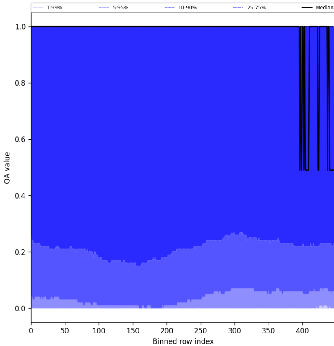
Figure 83: Along track statistics of “QA value” for 2025-05-02 to 2025-05-04
