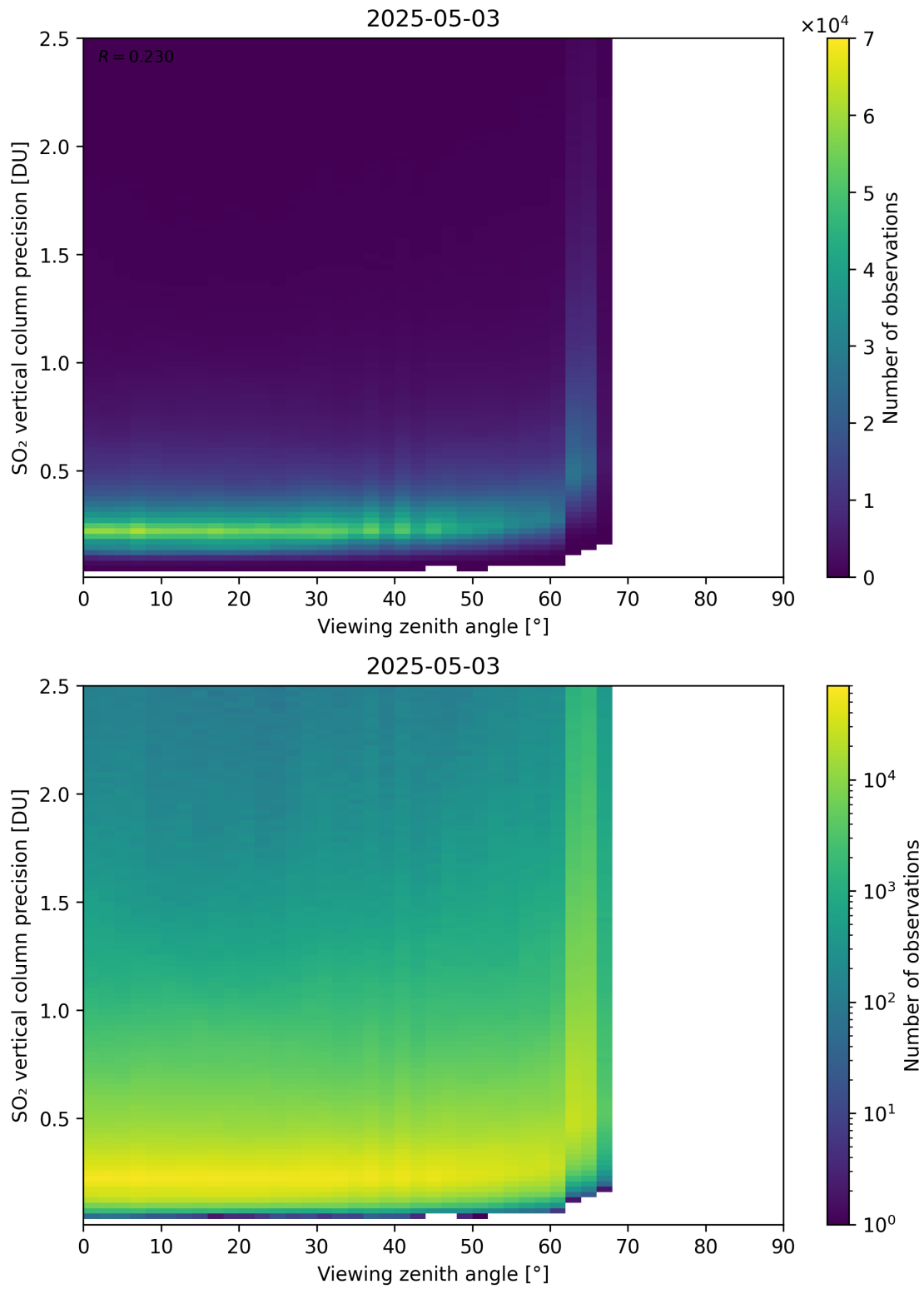
Figure 384: Scatter density plot of “Viewing zenith angle” against “SO 2 vertical column precision” for 2025-05-02 to 2025-05-04.
