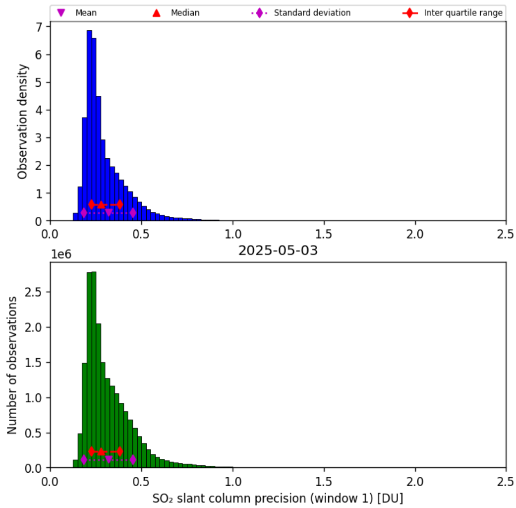
Figure 64: Histogram of “SO 2 slant column precision (window 1)” for 2025-05-02 to 2025-05-04
