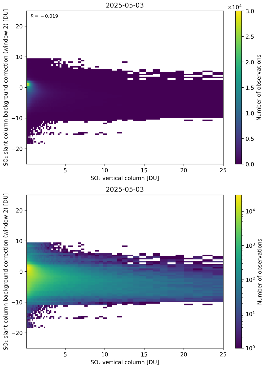
Figure 324: Scatter density plot of “SO 2 vertical column” against “SO 2 slant column background correction (window 2)” for 2025-05-02 to 2025-05-04.
