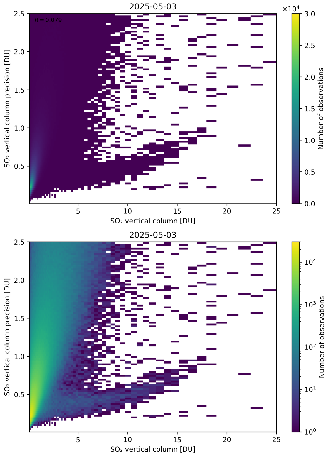
Figure 361: Scatter density plot of “SO 2 vertical column” against “SO 2 vertical column precision” for 2025-05-02 to 2025-05-04.
