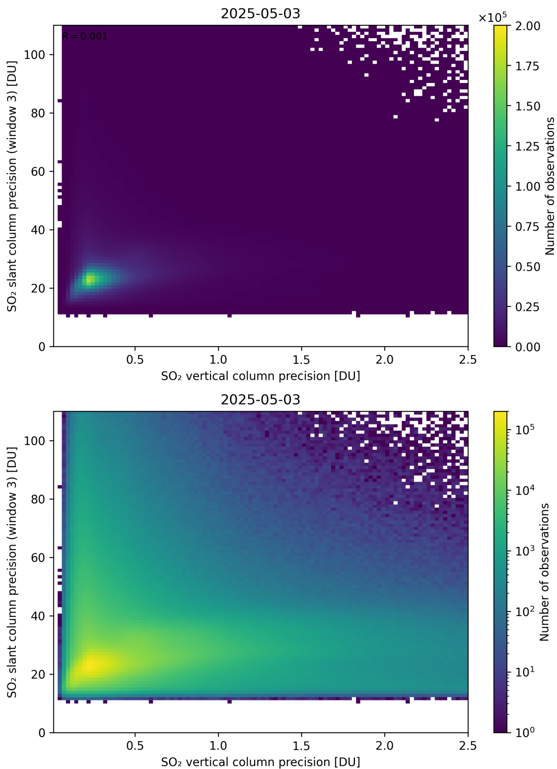
Figure 345: Scatter density plot of “SO 2 vertical column precision” against “SO 2 slant column precision (window 3)” for 2025-05-02 to 2025-05-04.
