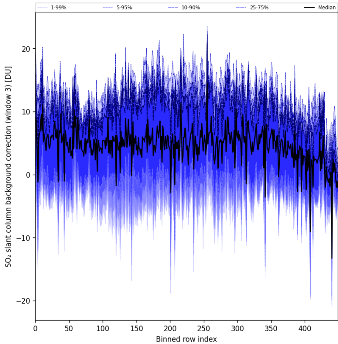
Figure 100: Along track statistics of “SO 2 slant column background correction (window 3)” for 2025-05-02 to 2025-05-04
