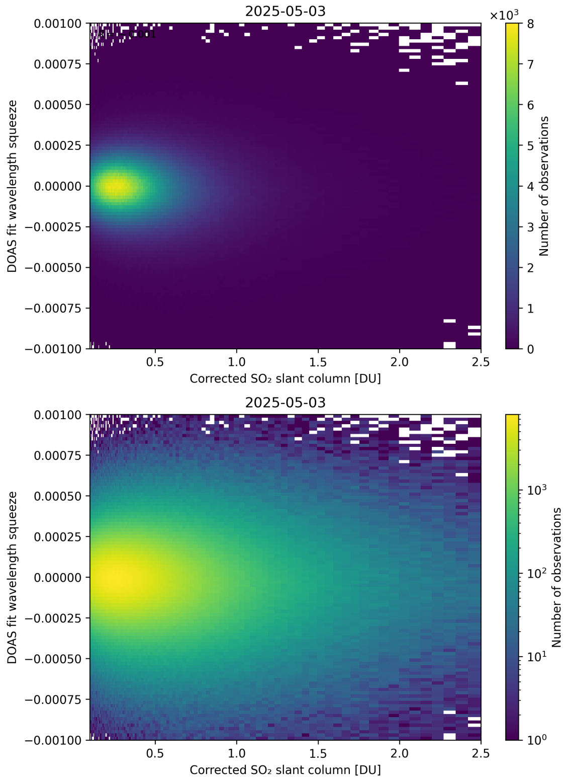
Figure 230: Scatter density plot of “Corrected SO 2 slant column” against “DOAS fit wavelength squeeze” for 2025-05-02 to 2025-05-04.
