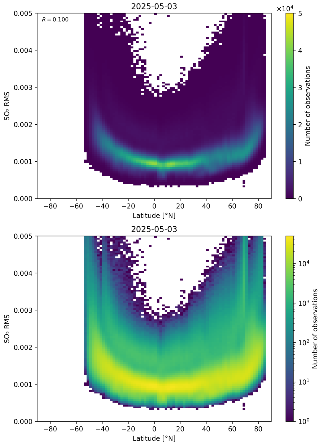
Figure 155: Scatter density plot of “Latitude” against “SO 2 RMS” for 2025-05-02 to 2025-05-04.
