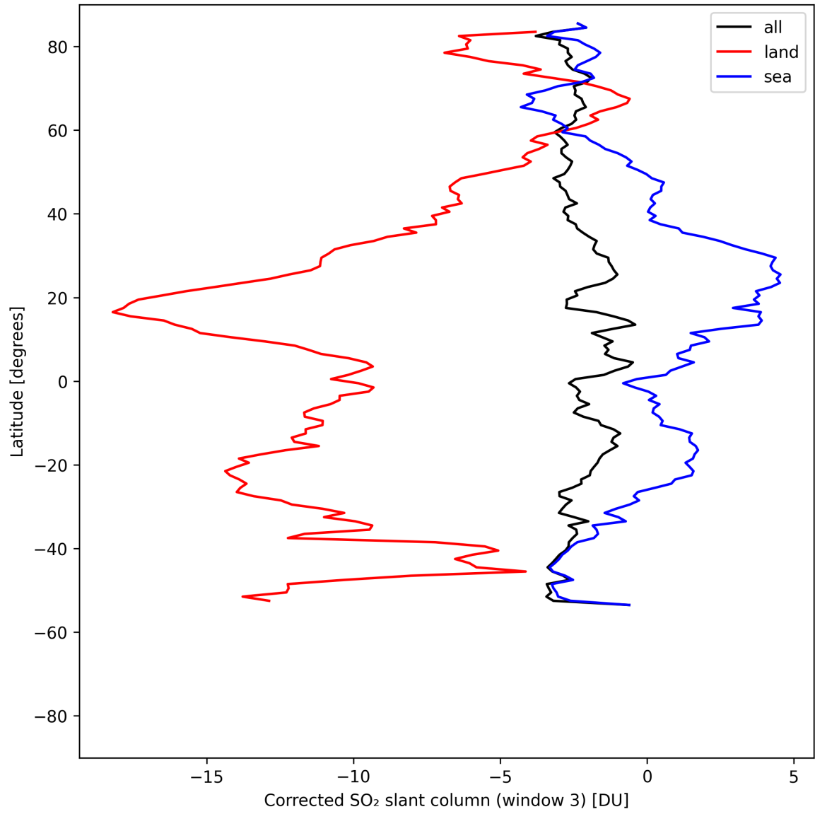
Figure 47: Zonal average of “Corrected SO 2 slant column (window 3)” for 2025-05-02 to 2025-05-04.
