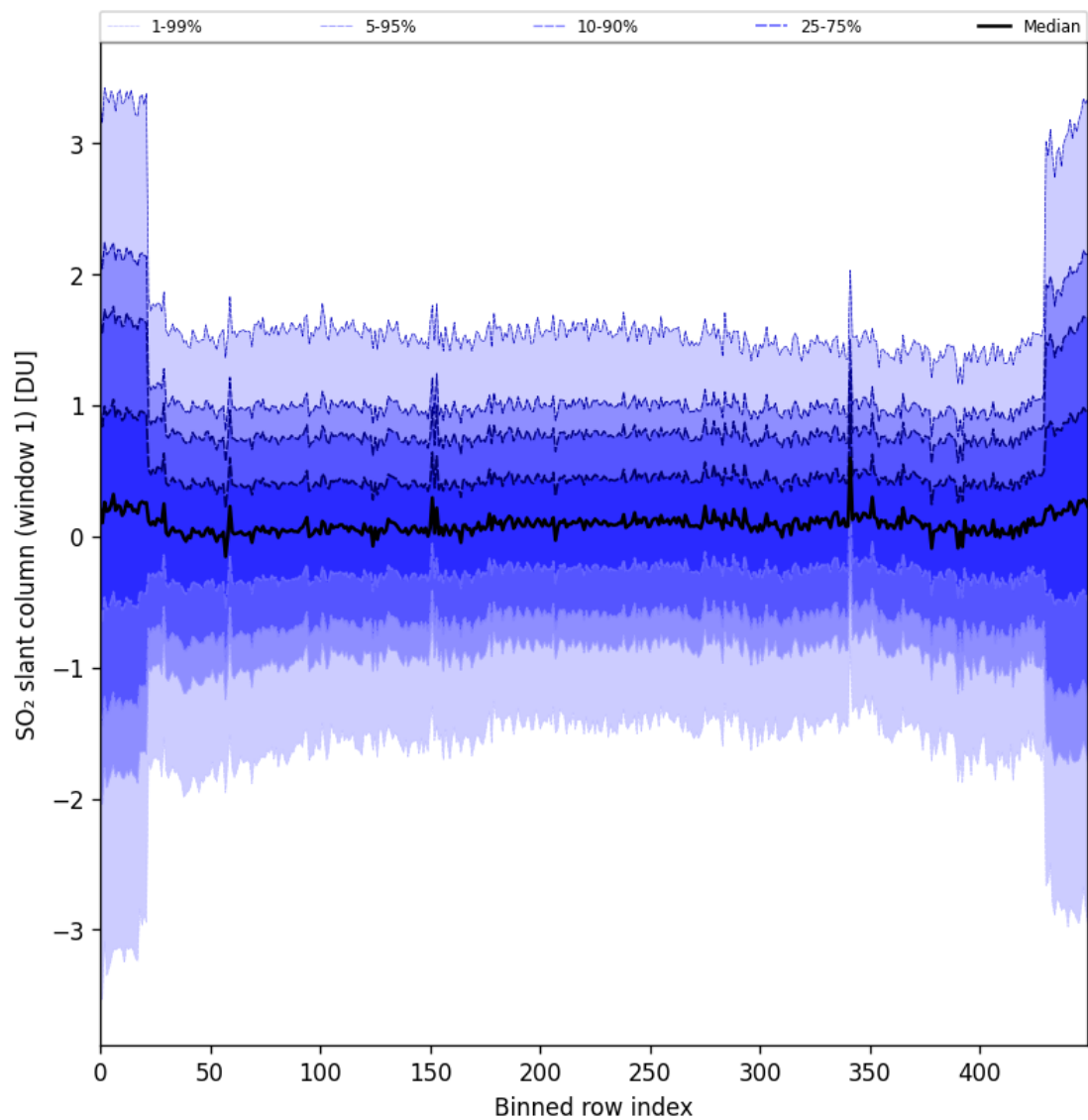
Figure 89: Along track statistics of “SO 2 slant column (window 1)” for 2025-05-02 to 2025-05-04
