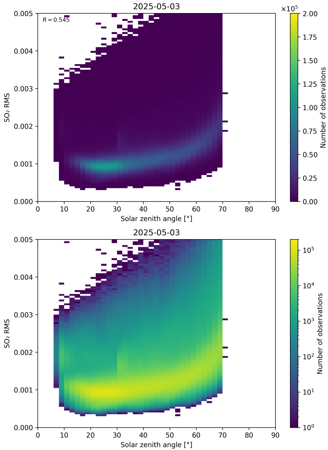
Figure 176: Scatter density plot of “Solar zenith angle” against “SO 2 RMS” for 2025-05-02 to 2025-05-04.
