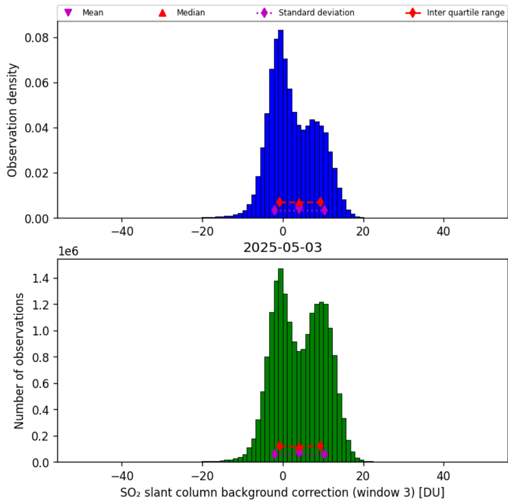
Figure 74: Histogram of “SO 2 slant column background correction (window 3)” for 2025-05-02 to 2025-05-04
