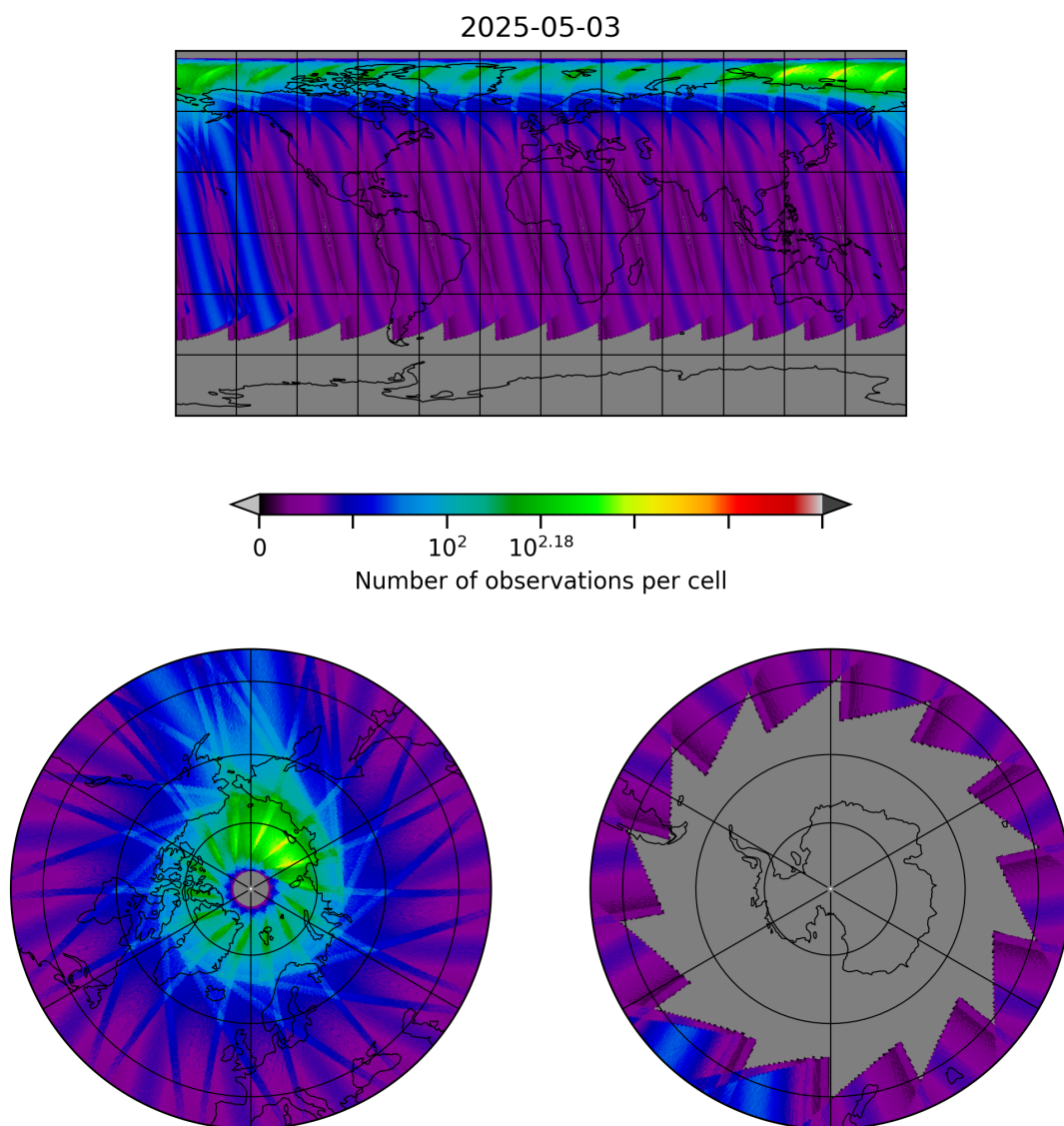
Figure 30: Map of the number of observations for 2025-05-02 to 2025-05-04
