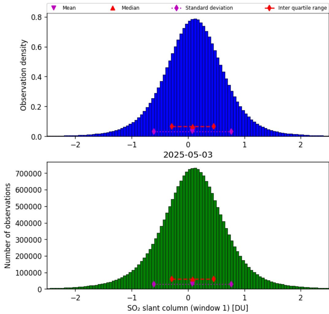
Figure 63: Histogram of “SO 2 slant column (window 1)” for 2025-05-02 to 2025-05-04
