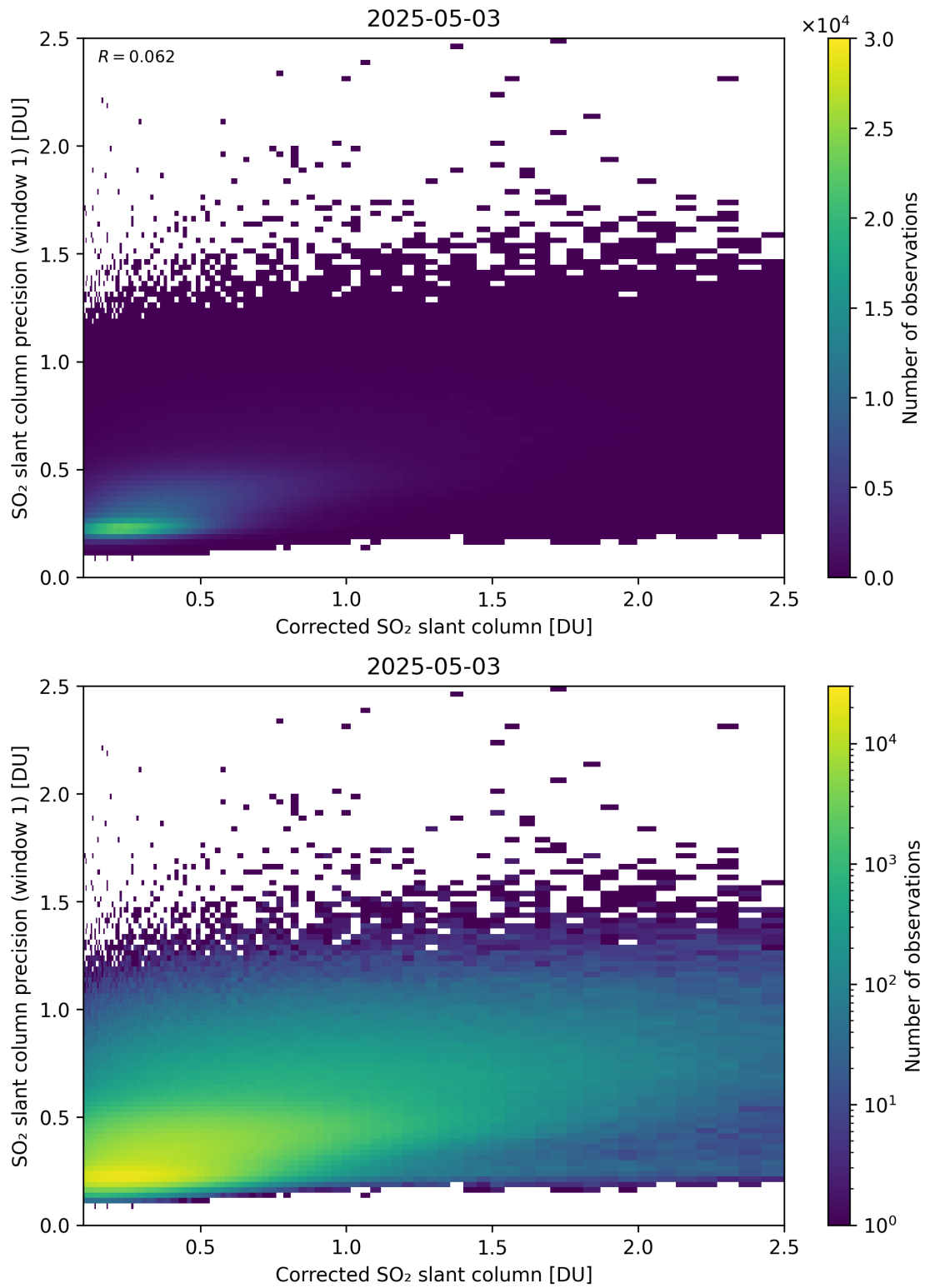
Figure 238: Scatter density plot of “Corrected SO 2 slant column” against “SO 2 slant column precision (window 1)” for 2025-05-02 to 2025-05-04.
