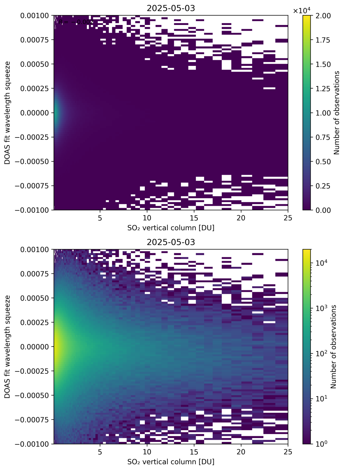
Figure 327: Scatter density plot of “SO 2 vertical column” against “DOAS fit wavelength squeeze” for 2025-05-02 to 2025-05-04.
