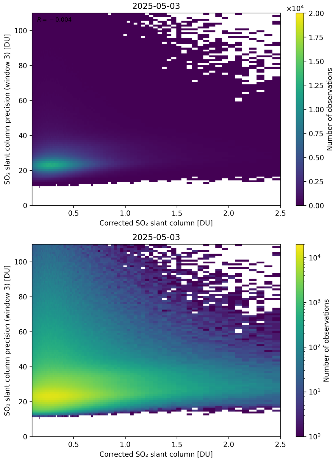
Figure 241: Scatter density plot of “Corrected SO 2 slant column” against “SO 2 slant column precision (window 3)” for 2025-05-02 to 2025-05-04.
