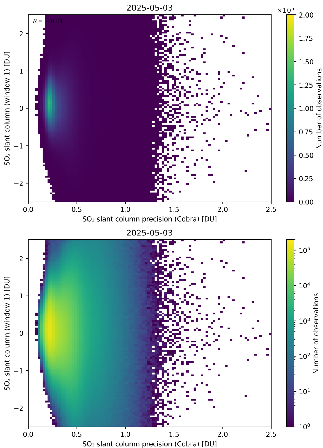
Figure 208: Scatter density plot of “SO 2 slant column precision (Cobra)” against “SO 2 slant column (window 1)” for 2025-05-02 to 2025-05-04.
