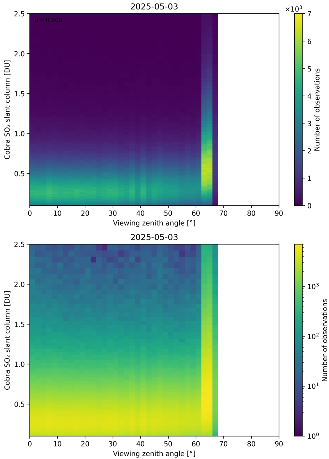
Figure 371: Scatter density plot of “Viewing zenith angle” against “Cobra SO 2 slant column” for 2025-05-02 to 2025-05-04.
