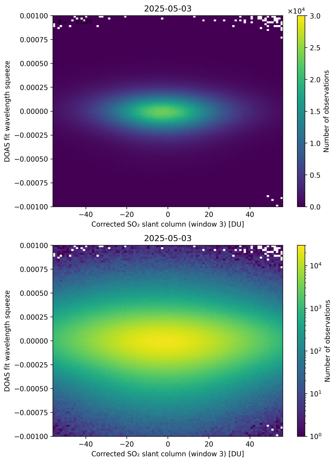
Figure 257: Scatter density plot of “Corrected SO 2 slant column (window 3)” against “DOAS fit wavelength squeeze” for 2025-05-02 to 2025-05-04.
