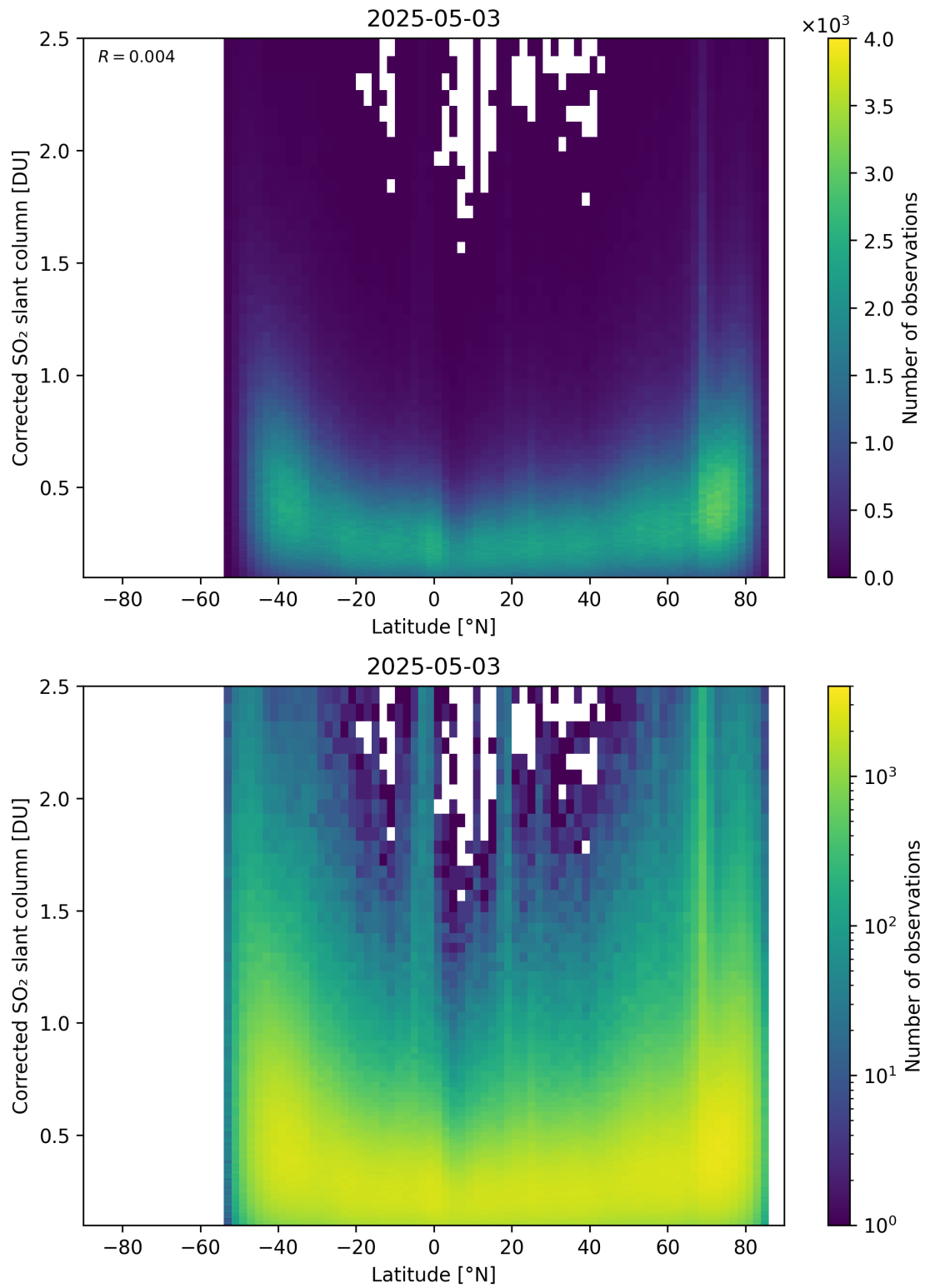
Figure 159: Scatter density plot of “Latitude” against “Corrected SO 2 slant column” for 2025-05-02 to 2025-05-04.
