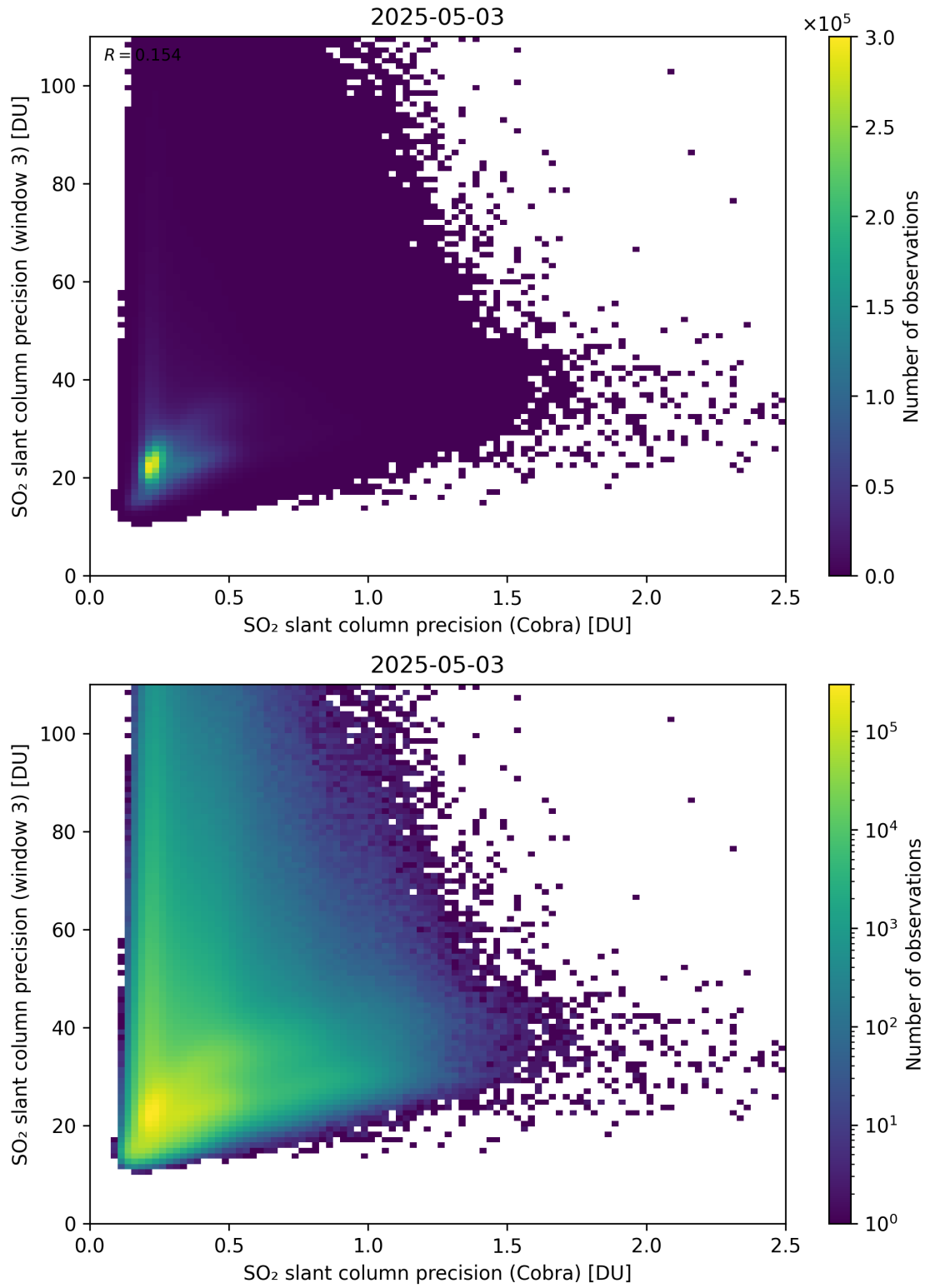
Figure 212: Scatter density plot of “SO 2 slant column precision (Cobra)” against “SO 2 slant column precision (window 3)” for 2025-05-02 to 2025-05-04.
