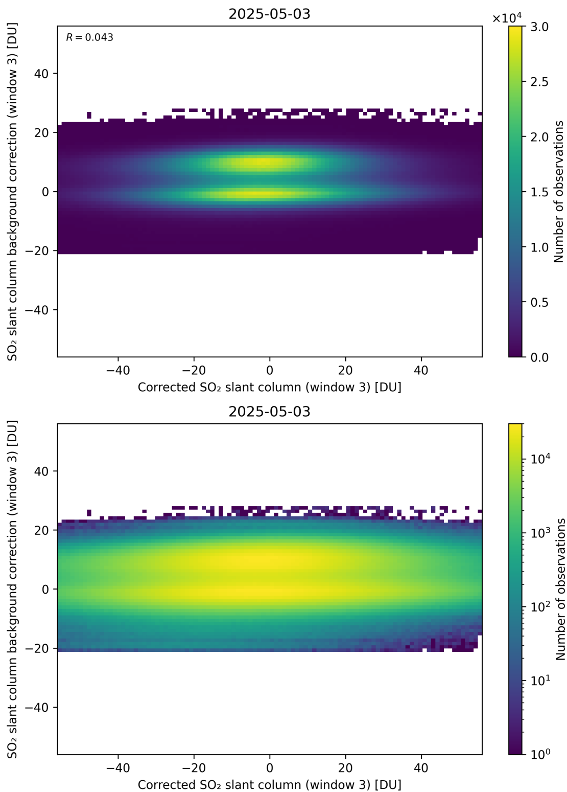
Figure 255: Scatter density plot of “Corrected SO 2 slant column (window 3)” against “SO 2 slant column background correction (window 3)” for 2025-05-02 to 2025-05-04.
