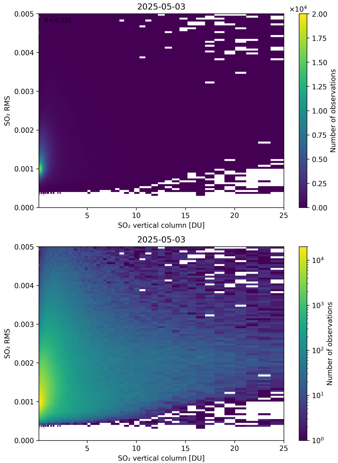
Figure 328: Scatter density plot of “SO 2 vertical column” against “SO 2 RMS” for 2025-05-02 to 2025-05-04.
