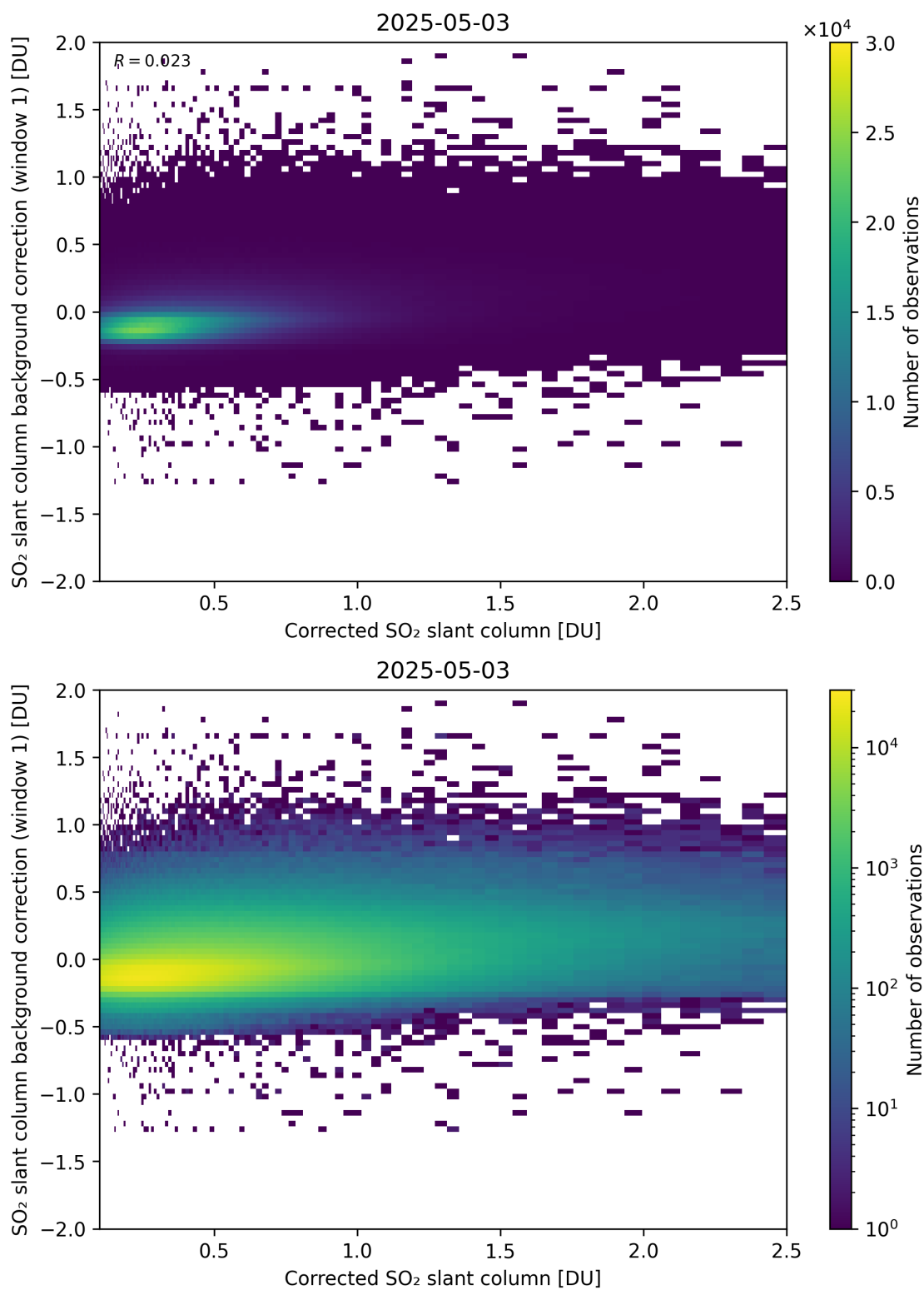
Figure 226: Scatter density plot of “Corrected SO 2 slant column” against “SO 2 slant column background correction (window 1)” for 2025-05-02 to 2025-05-04.
