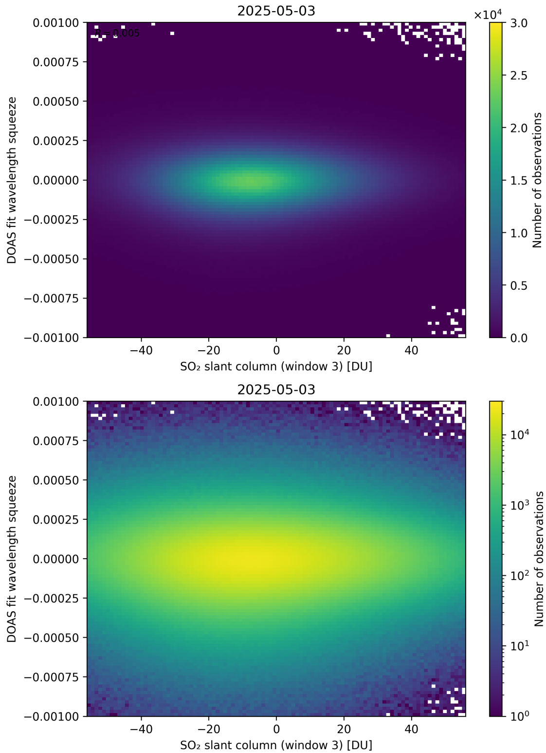
Figure 305: Scatter density plot of “SO 2 slant column (window 3)” against “DOAS fit wavelength squeeze” for 2025-05-02 to 2025-05-04.
