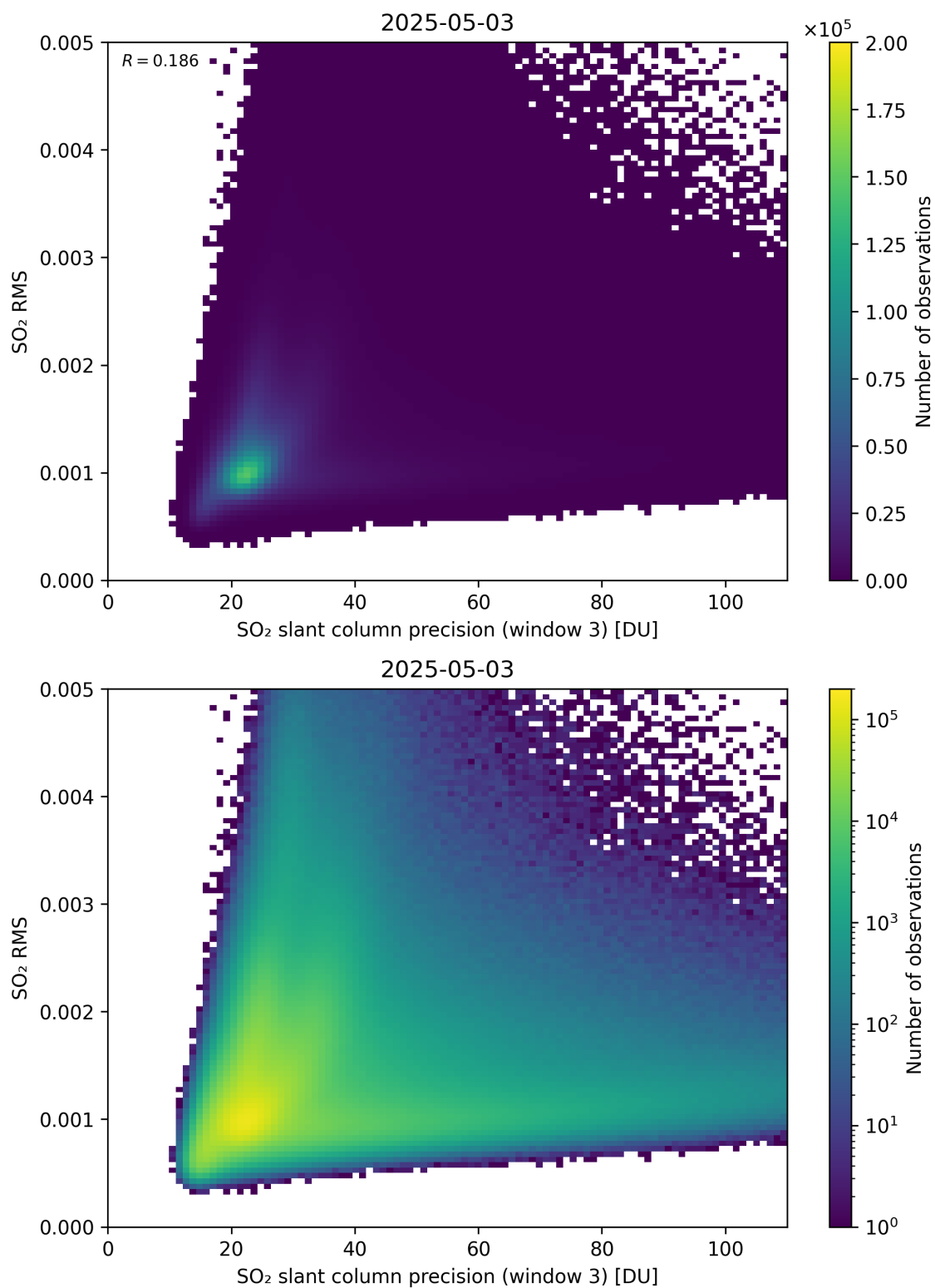
Figure 310: Scatter density plot of “SO 2 slant column precision (window 3)” against “SO 2 RMS” for 2025-05-02 to 2025-05-04.
