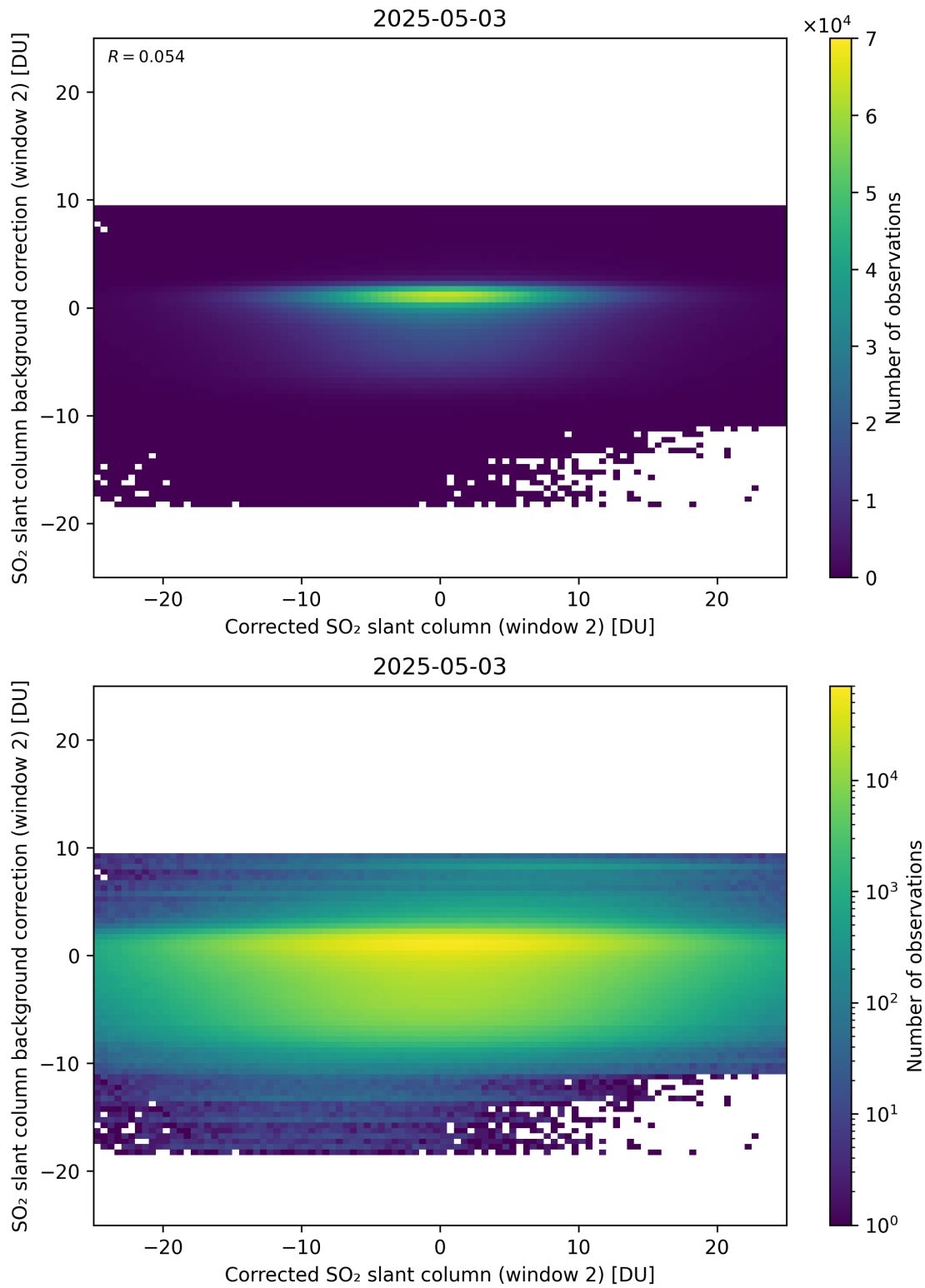
Figure 244: Scatter density plot of “Corrected SO 2 slant column (window 2)” against “SO 2 slant column background correction (window 2)” for 2025-05-02 to 2025-05-04.
