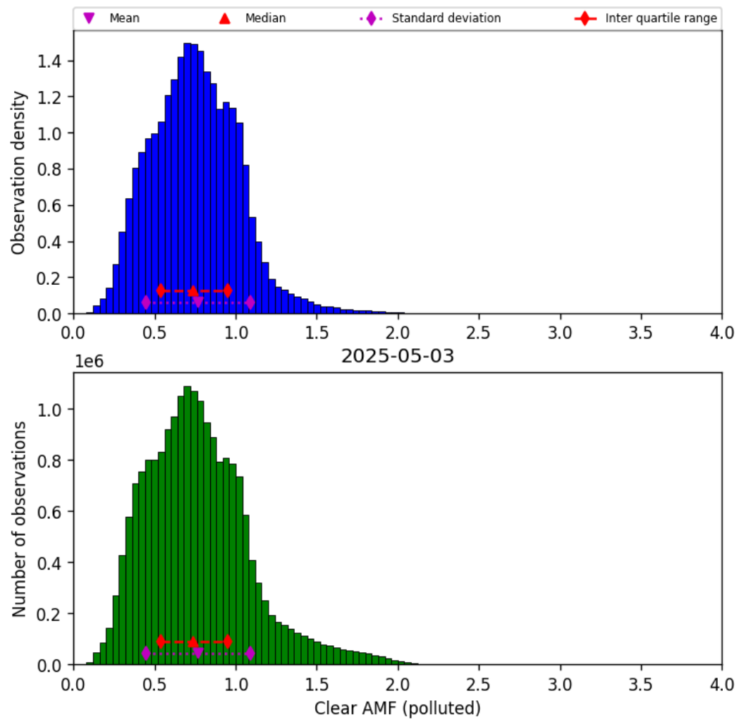
Figure 81: Histogram of “Clear AMF (polluted)” for 2025-05-02 to 2025-05-04
