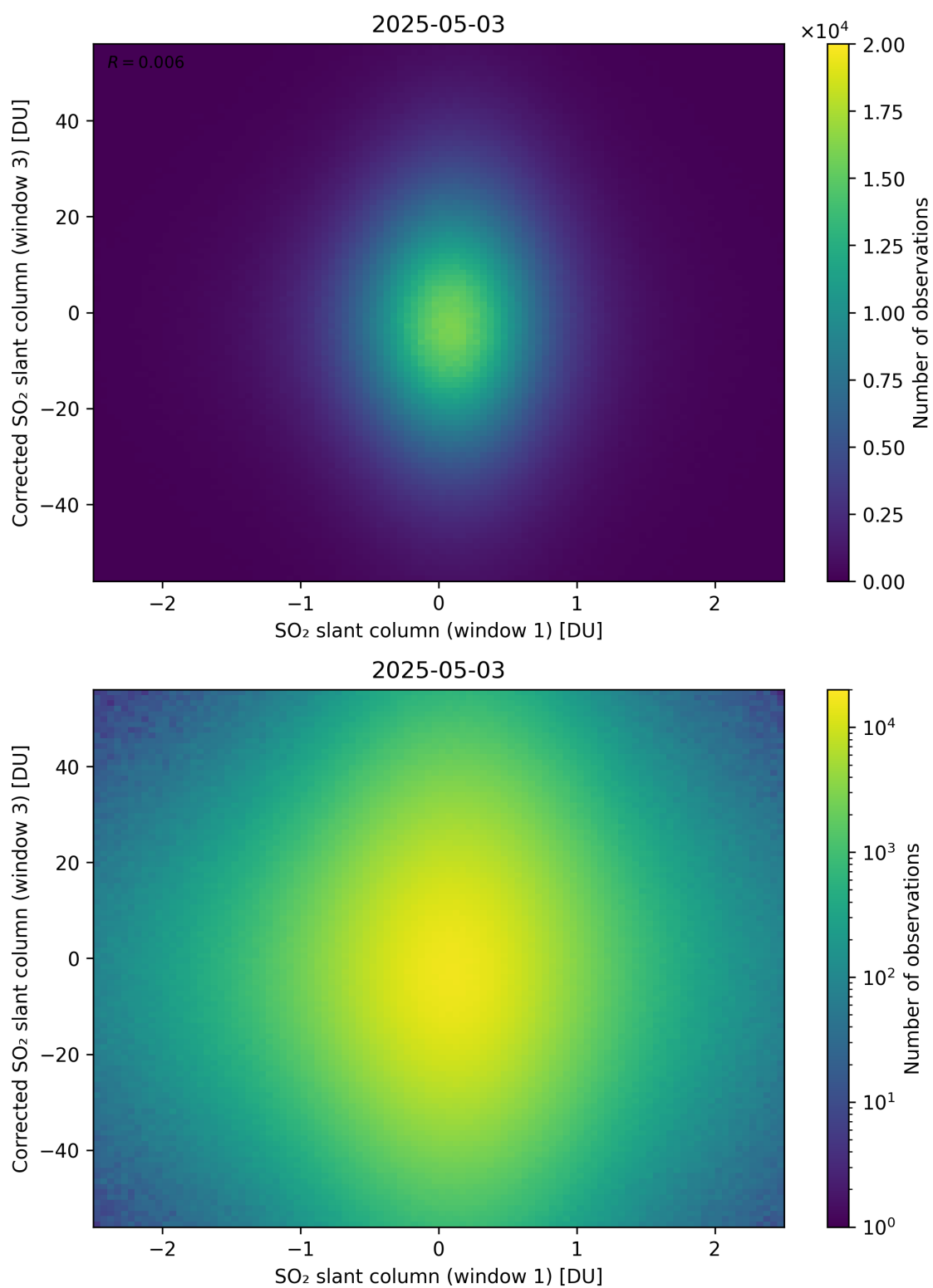
Figure 284: Scatter density plot of “SO 2 slant column (window 1)” against “Corrected SO 2 slant column (window 3)” for 2025-05-02 to 2025-05-04.
