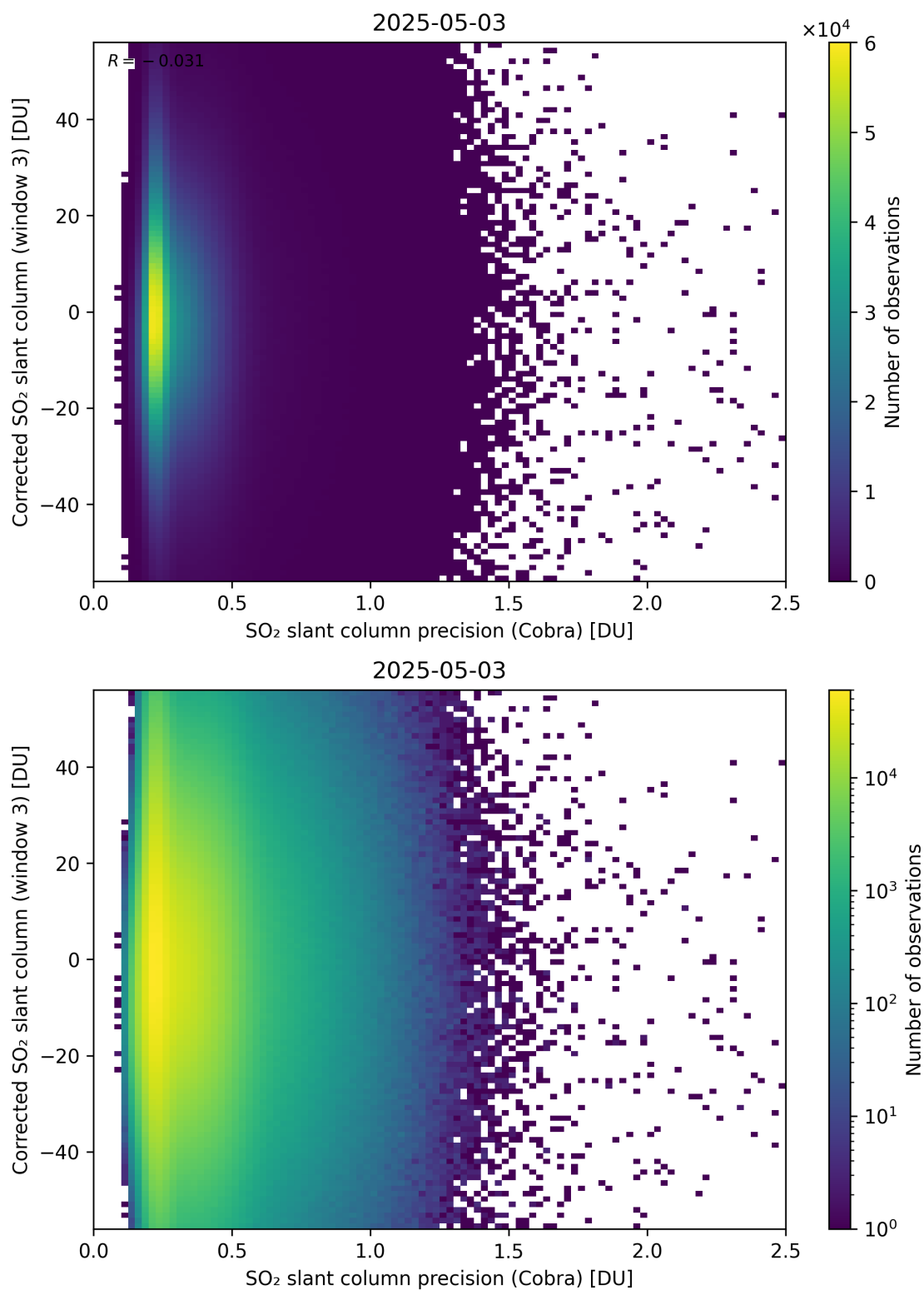
Figure 207: Scatter density plot of “SO 2 slant column precision (Cobra)” against “Corrected SO 2 slant column (window 3)” for 2025-05-02 to 2025-05-04.
