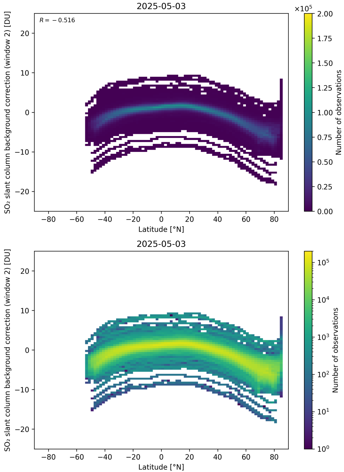
Figure 151: Scatter density plot of “Latitude” against “SO 2 slant column background correction (window 2)” for 2025-05-02 to 2025-05-04.
