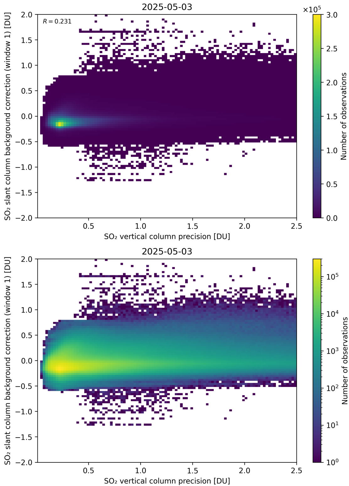
Figure 329: Scatter density plot of “SO 2 vertical column precision” against “SO 2 slant column background correction (window 1)” for 2025-05-02 to 2025-05-04.
