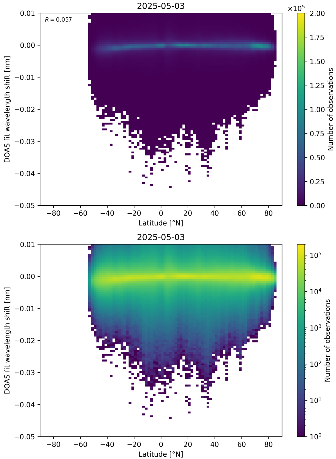
Figure 153: Scatter density plot of “Latitude” against “DOAS fit wavelength shift” for 2025-05-02 to 2025-05-04.
