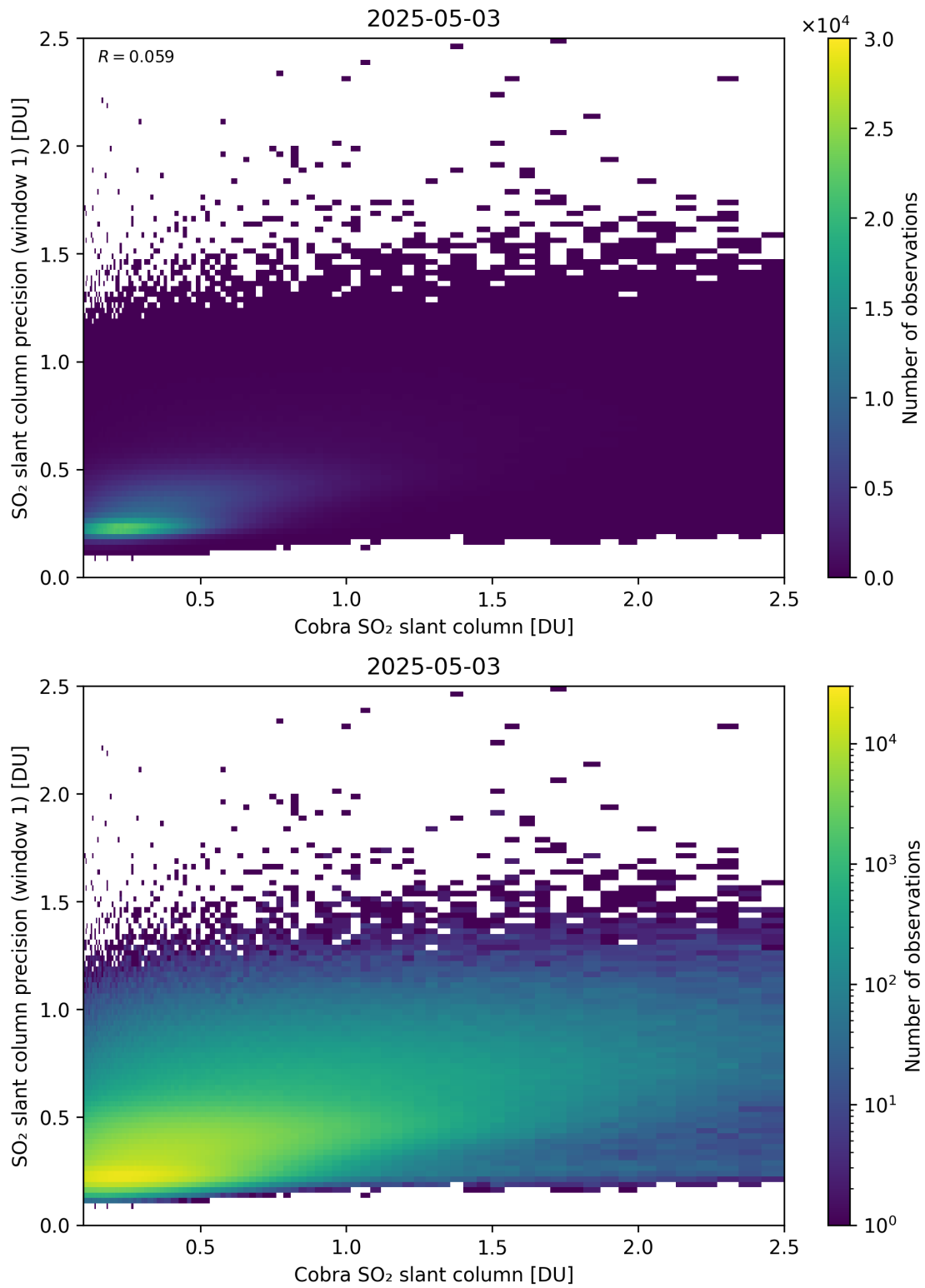
Figure 220: Scatter density plot of “Cobra SO 2 slant column” against “SO 2 slant column precision (window 1)” for 2025-05-02 to 2025-05-04.
