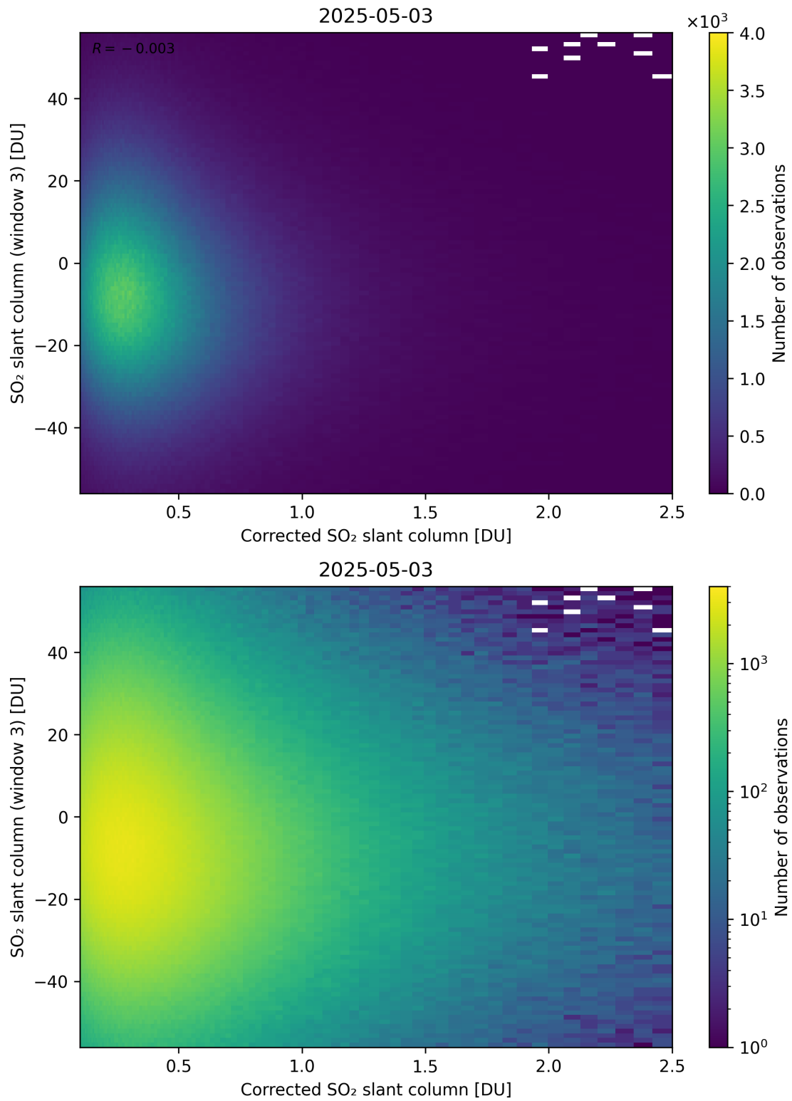
Figure 240: Scatter density plot of “Corrected SO 2 slant column” against “SO 2 slant column (window 3)” for 2025-05-02 to 2025-05-04.
