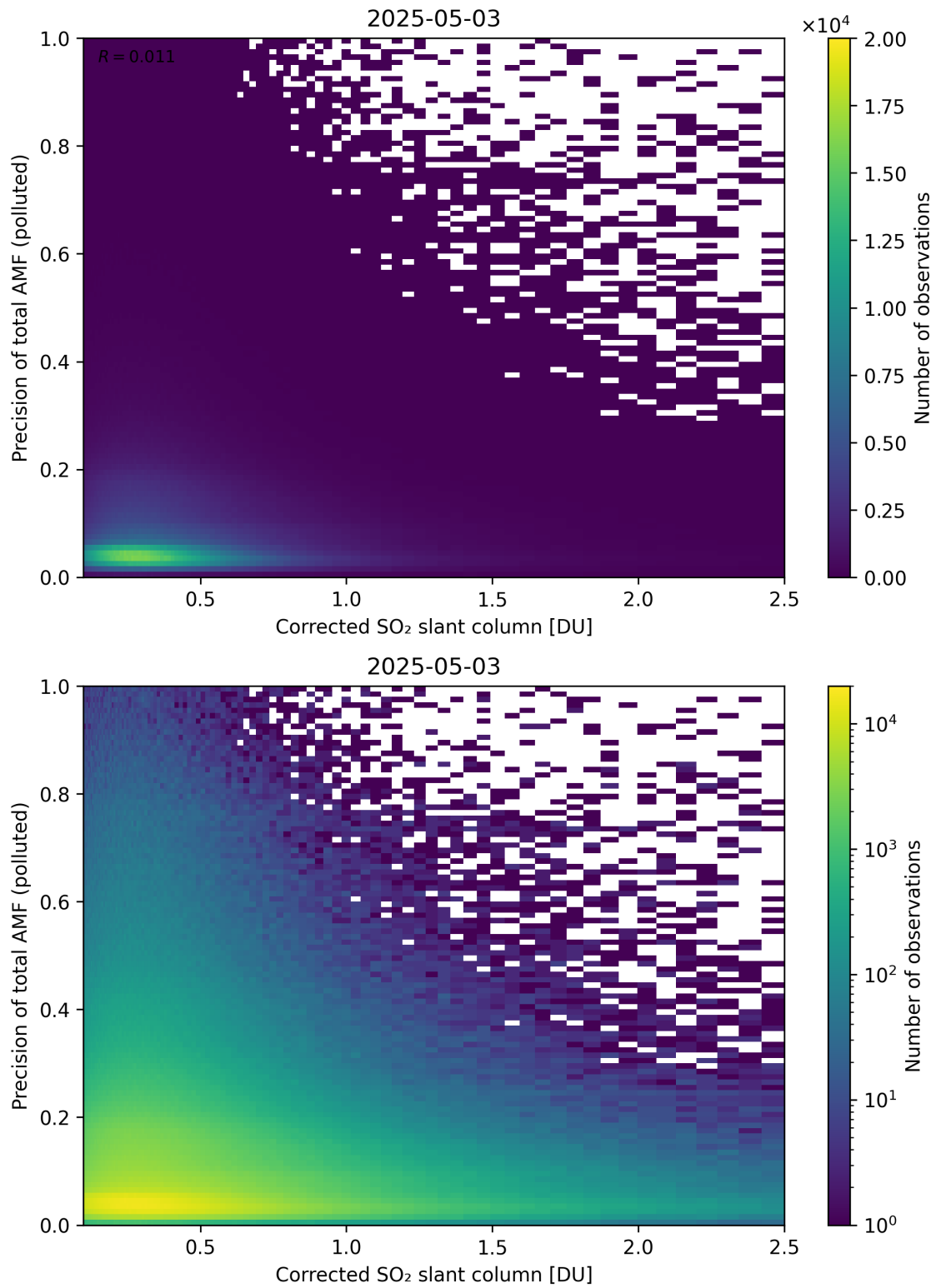
Figure 243: Scatter density plot of “Corrected SO 2 slant column” against “Precision of total AMF (polluted)” for 2025-05-02 to 2025-05-04.
