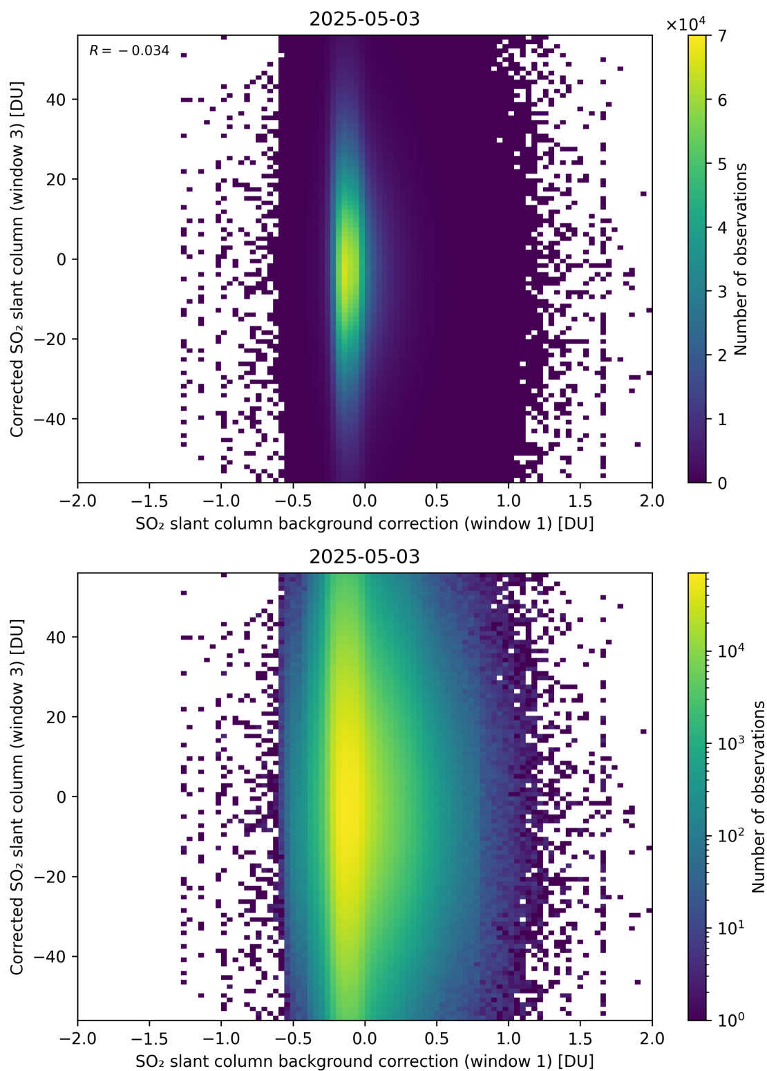
Figure 116: Scatter density plot of “SO 2 slant column background correction (window 1)” against “Corrected SO 2 slant column (window 3)” for 2025-05-02 to 2025-05-04.
