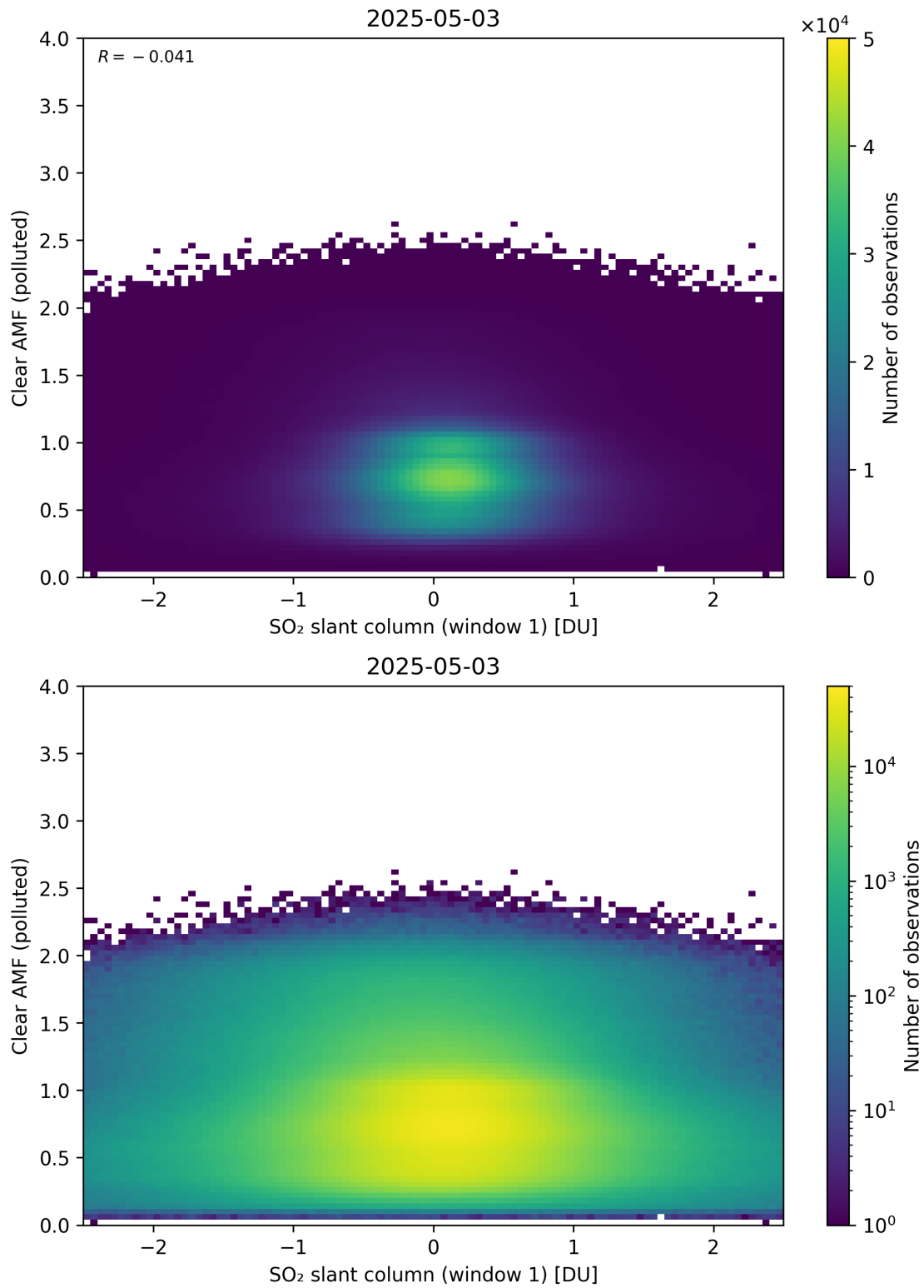
Figure 282: Scatter density plot of “SO 2 slant column (window 1)” against “Clear AMF (polluted)” for 2025-05-02 to 2025-05-04.
