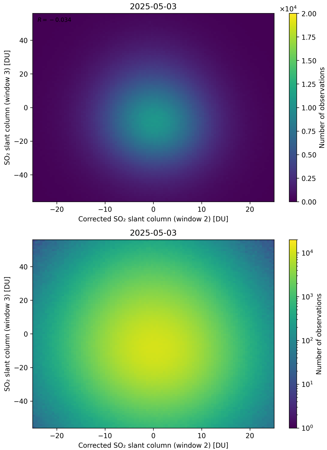
Figure 251: Scatter density plot of “Corrected SO 2 slant column (window 2)” against “SO 2 slant column (window 3)” for 2025-05-02 to 2025-05-04.
