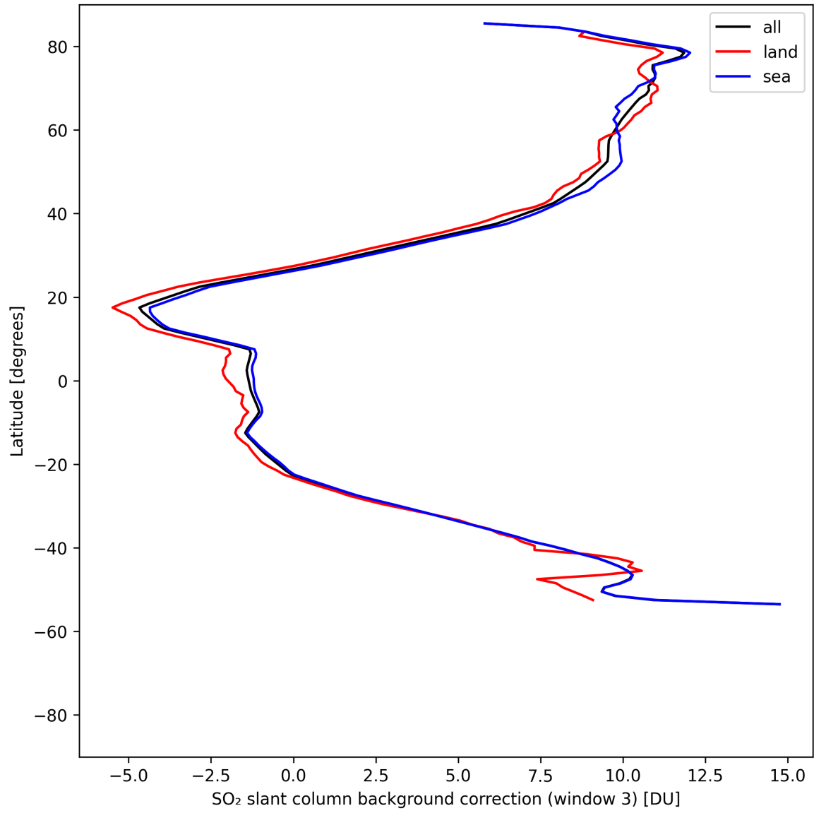
Figure 48: Zonal average of “SO 2 slant column background correction (window 3)” for 2025-05-02 to 2025-05-04.
