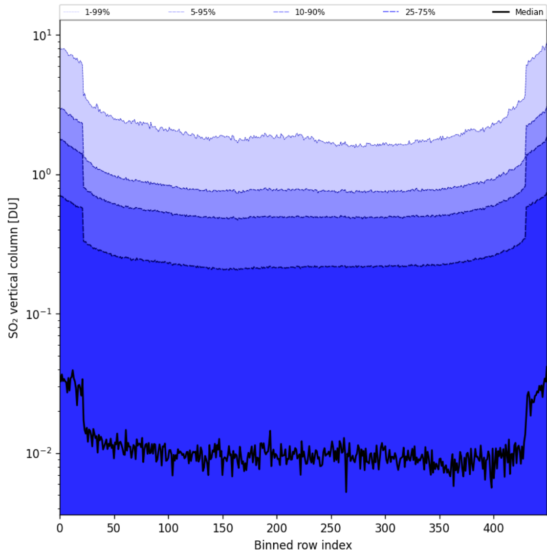
Figure 84: Along track statistics of “SO 2 vertical column” for 2025-05-02 to 2025-05-04
