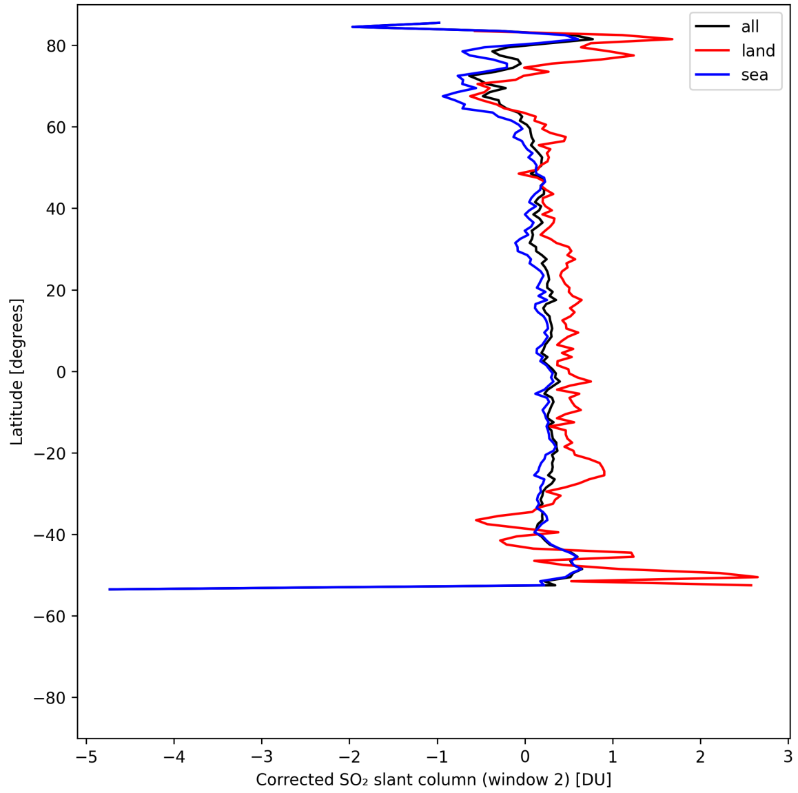
Figure 43: Zonal average of “Corrected SO 2 slant column (window 2)” for 2025-05-02 to 2025-05-04.
