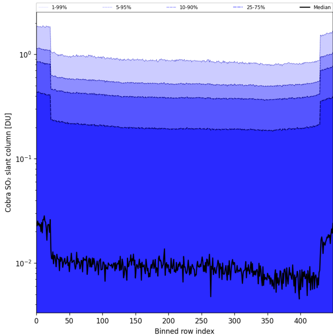
Figure 87: Along track statistics of “Cobra SO 2 slant column” for 2025-05-02 to 2025-05-04
