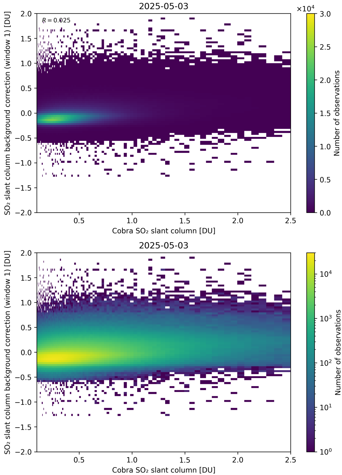
Figure 193: Scatter density plot of “Cobra SO 2 slant column” against “SO 2 slant column background correction (window 1)” for 2025-05-02 to 2025-05-04.
