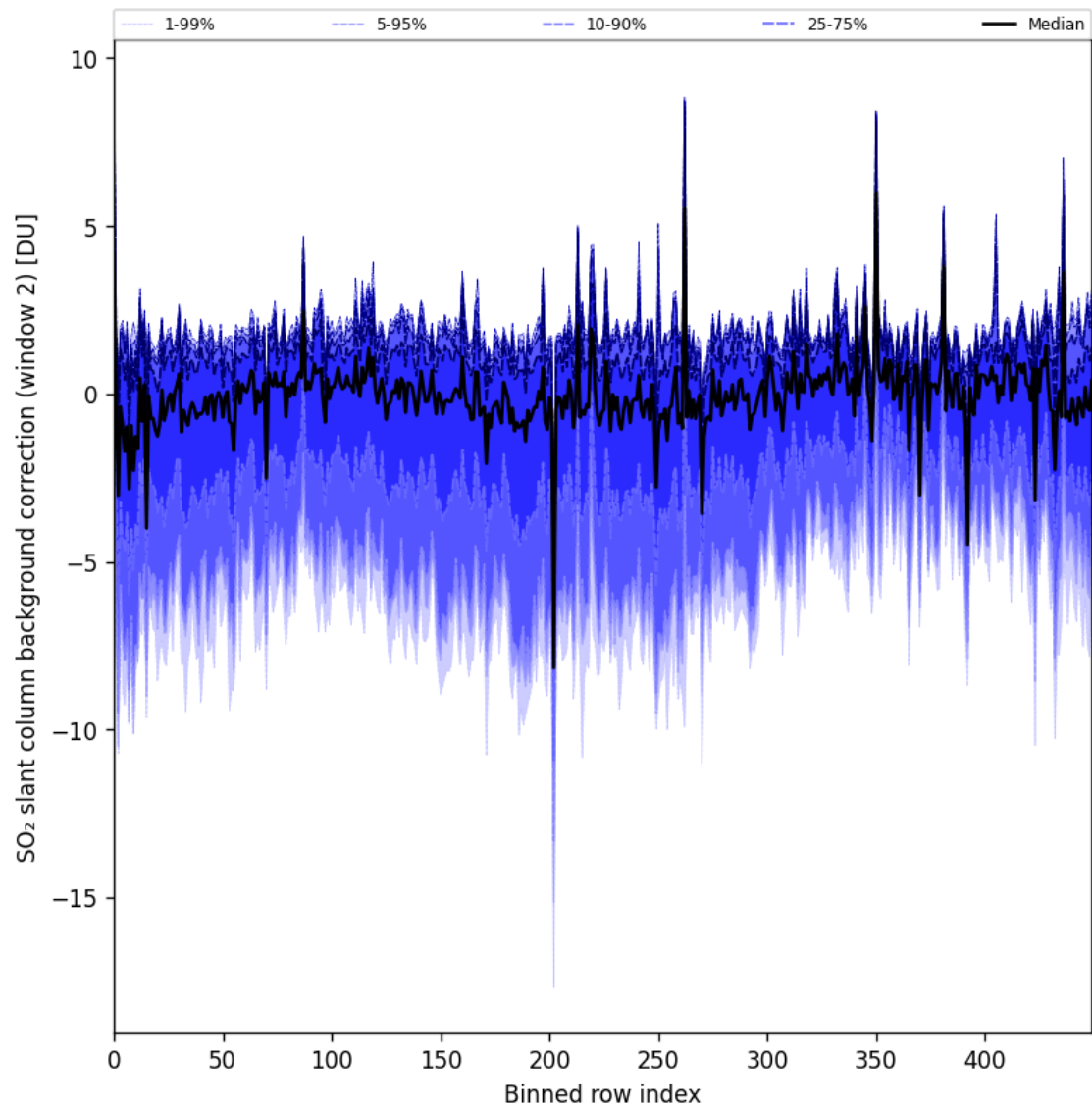
Figure 96: Along track statistics of “SO 2 slant column background correction (window 2)” for 2025-05-02 to 2025-05-04
