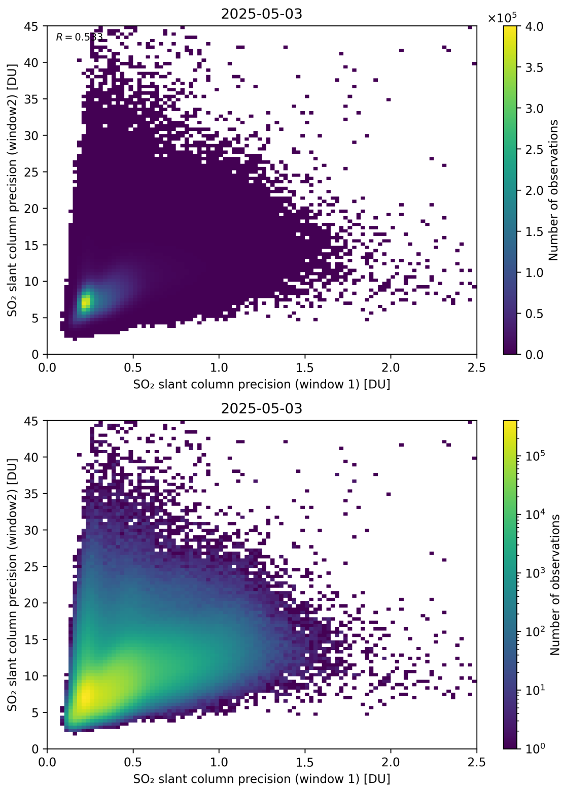
Figure 277: Scatter density plot of “SO 2 slant column precision (window 1)” against “SO 2 slant column precision (window2)” for 2025-05-02 to 2025-05-04.
