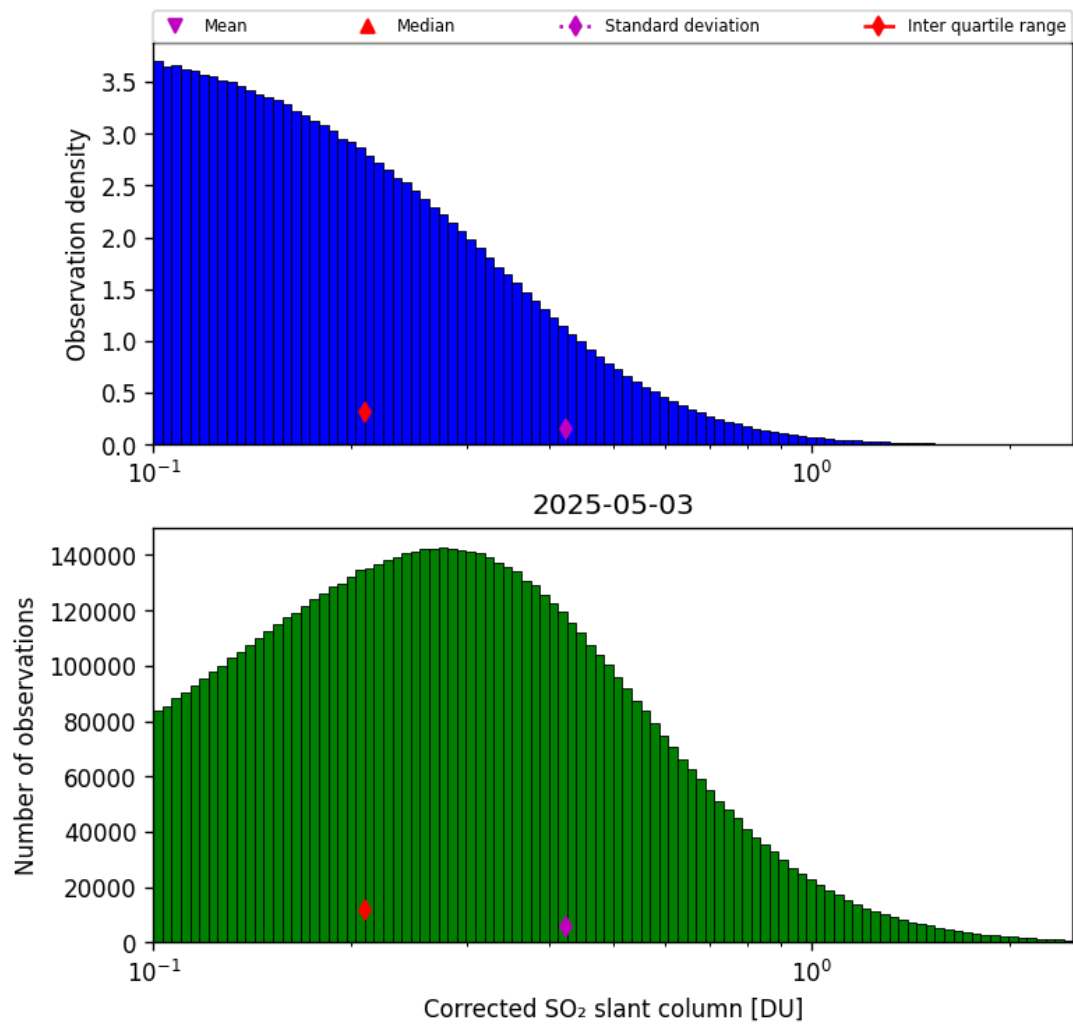
Figure 60: Histogram of "Corrected SO 2 slant column" for 2025-05-02 to 2025-05-04
