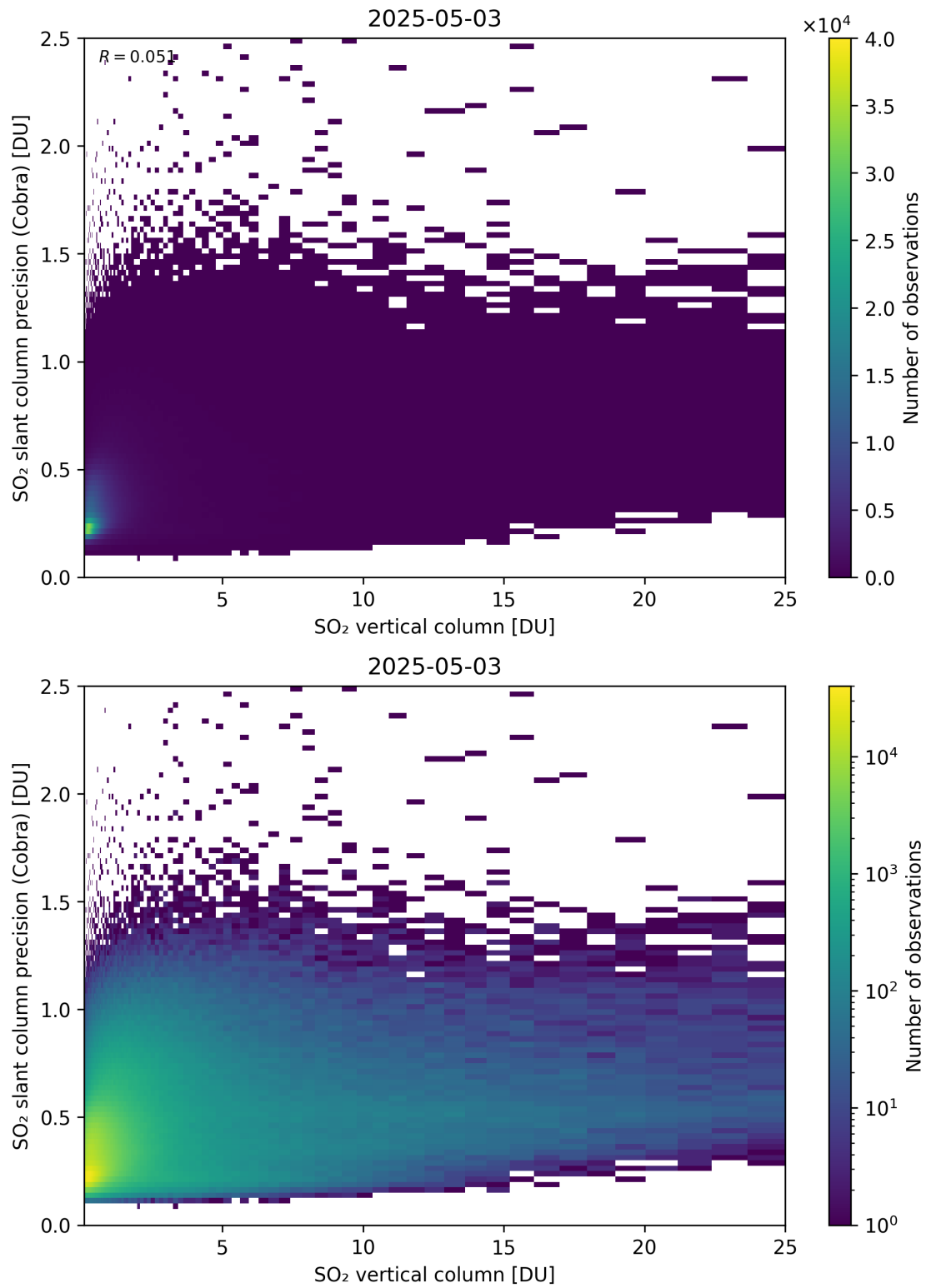
Figure 350: Scatter density plot of “SO 2 vertical column” against “SO 2 slant column precision (Cobra)” for 2025-05-02 to 2025-05-04.
