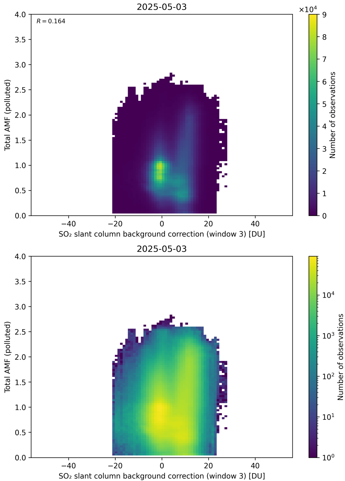
Figure 136: Scatter density plot of “SO 2 slant column background correction (window 3)” against “Total AMF (polluted)” for 2025-05-02 to 2025-05-04.
