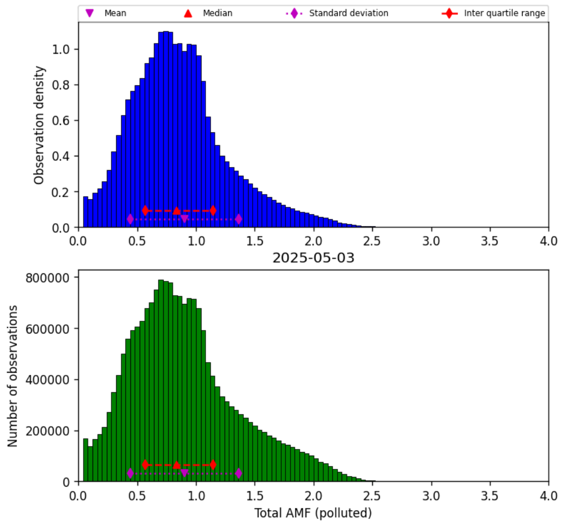
Figure 79: Histogram of “Total AMF (polluted)” for 2025-05-02 to 2025-05-04
