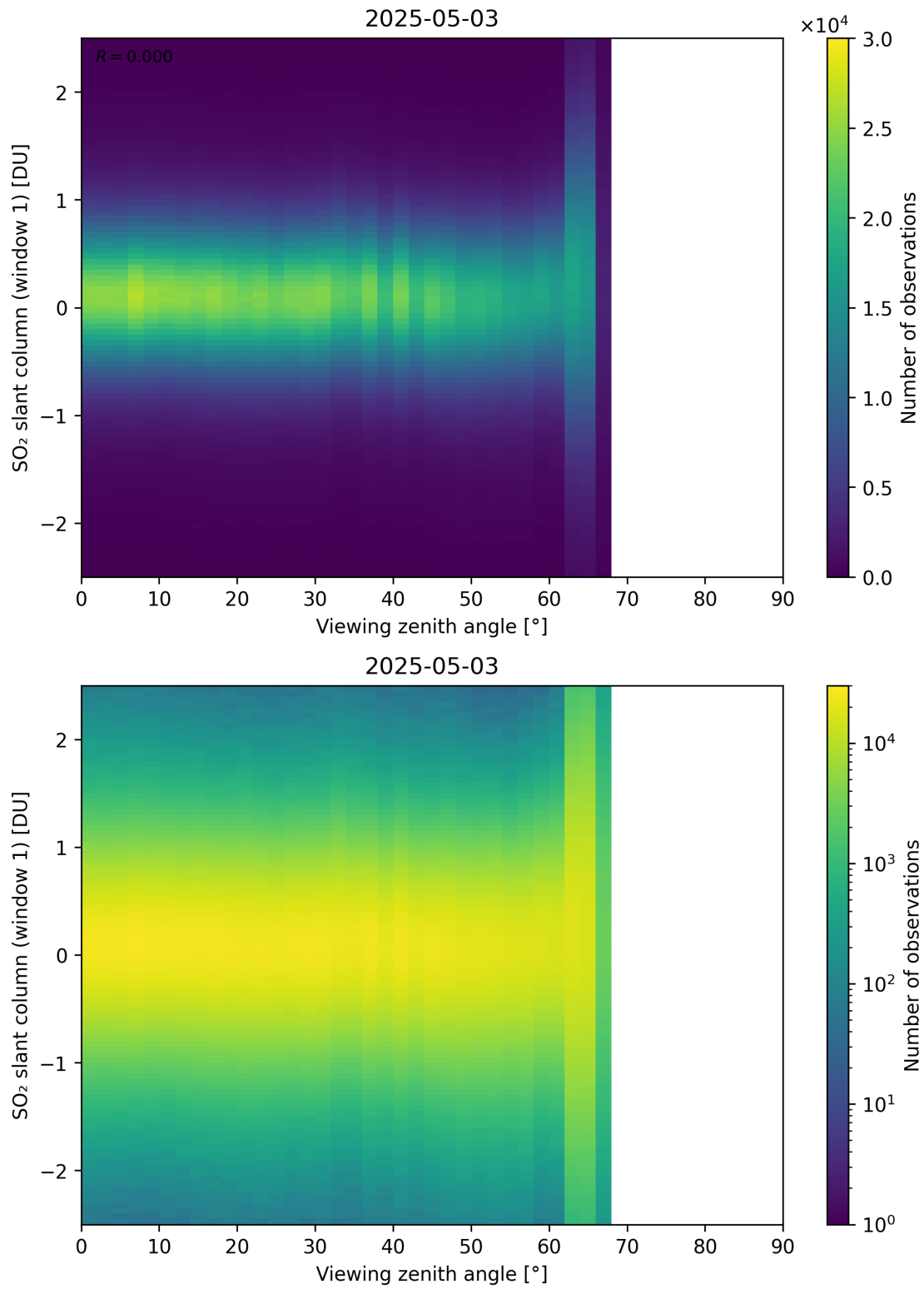
Figure 376: Scatter density plot of “Viewing zenith angle” against “SO 2 slant column (window 1)” for 2025-05-02 to 2025-05-04.
