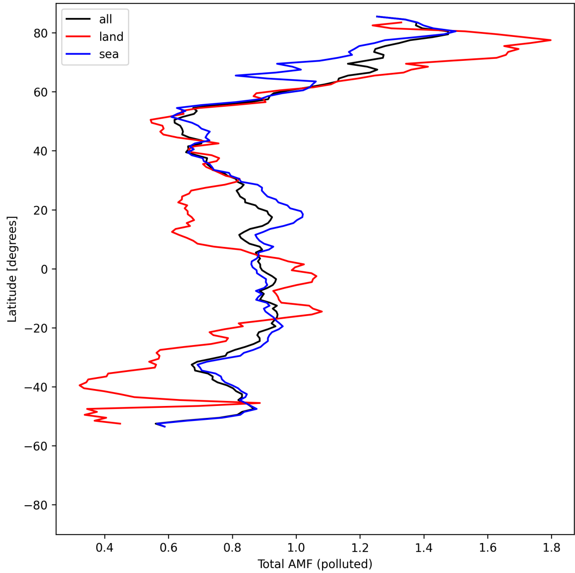
Figure 53: Zonal average of “Total AMF (polluted)” for 2025-05-02 to 2025-05-04.
