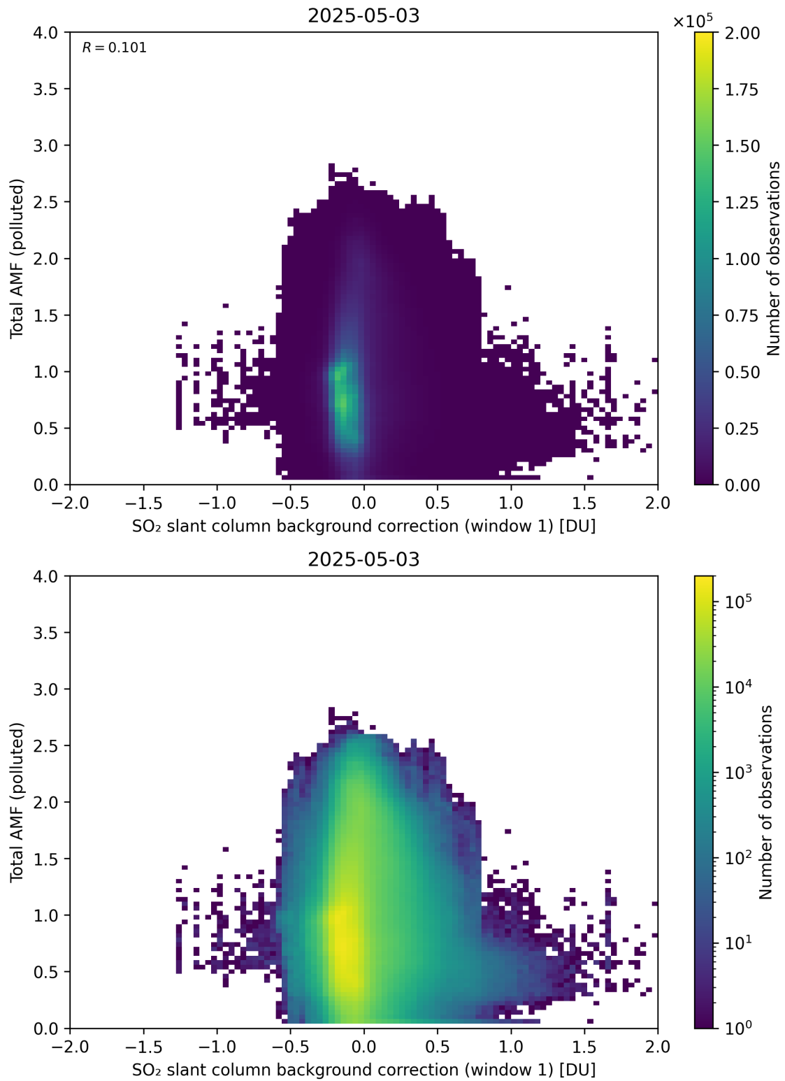
Figure 120: Scatter density plot of “SO 2 slant column background correction (window 1)” against “Total AMF (polluted)” for 2025-05-02 to 2025-05-04.
