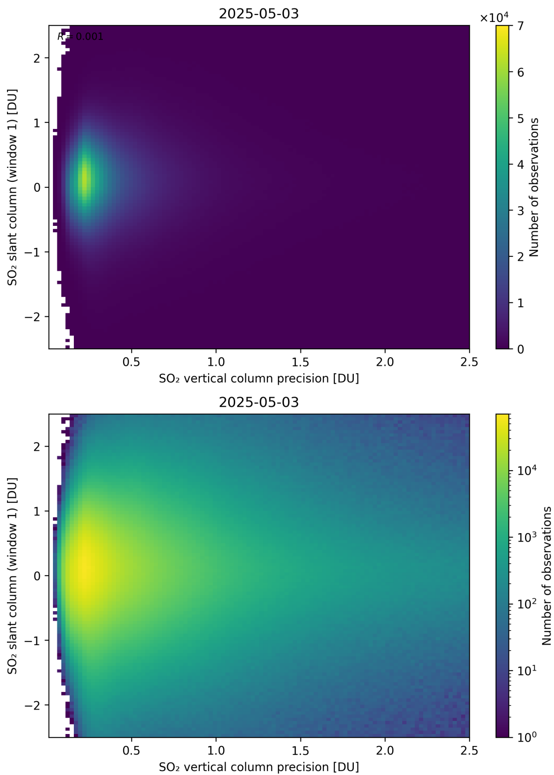
Figure 341: Scatter density plot of “SO 2 vertical column precision” against “SO 2 slant column (window 1)” for 2025-05-02 to 2025-05-04.
