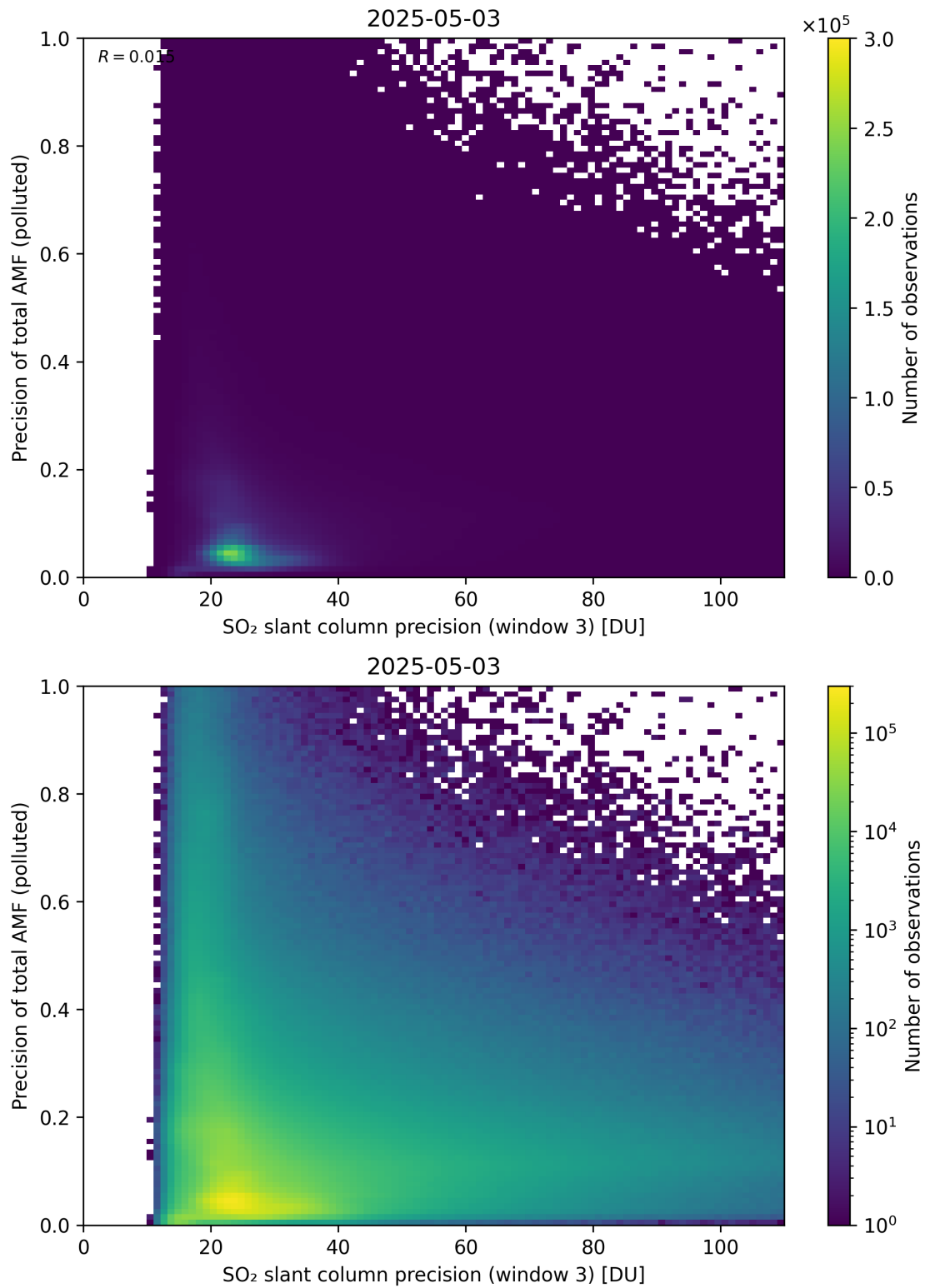
Figure 314: Scatter density plot of “SO 2 slant column precision (window 3)” against “Precision of total AMF (polluted)” for 2025-05-02 to 2025-05-04.
