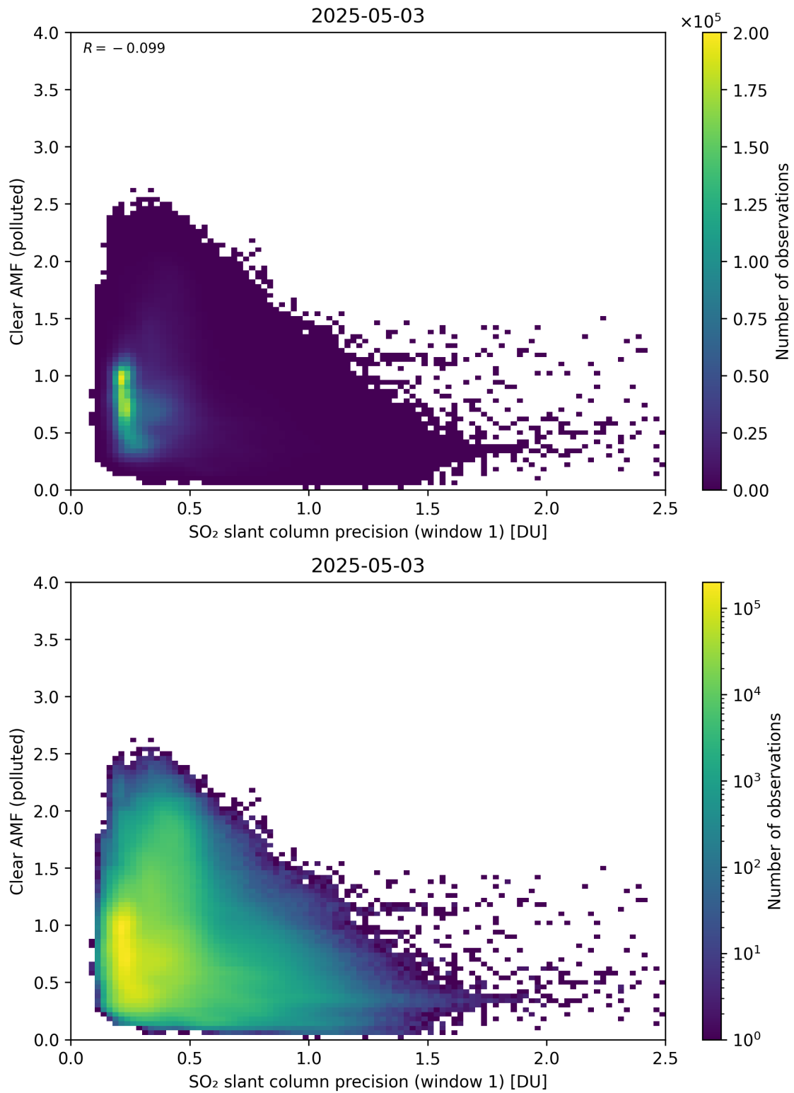
Figure 274: Scatter density plot of “SO 2 slant column precision (window 1)” against “Clear AMF (polluted)” for 2025-05-02 to 2025-05-04.
