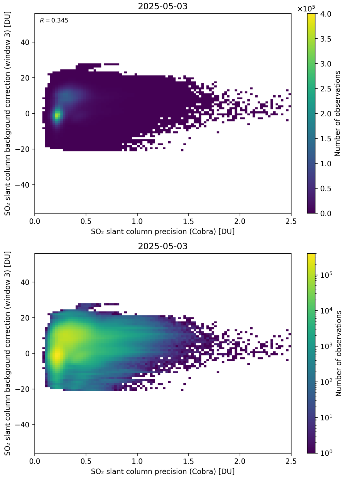
Figure 201: Scatter density plot of “SO 2 slant column precision (Cobra)” against “SO 2 slant column background correction (window 3)” for 2025-05-02 to 2025-05-04.
