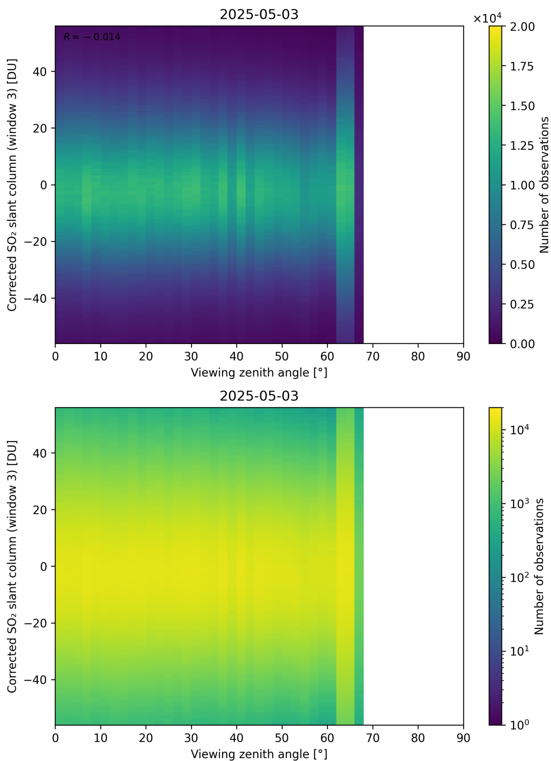
Figure 375: Scatter density plot of “Viewing zenith angle” against “Corrected SO 2 slant column (window 3)” for 2025-05-02 to 2025-05-04.
