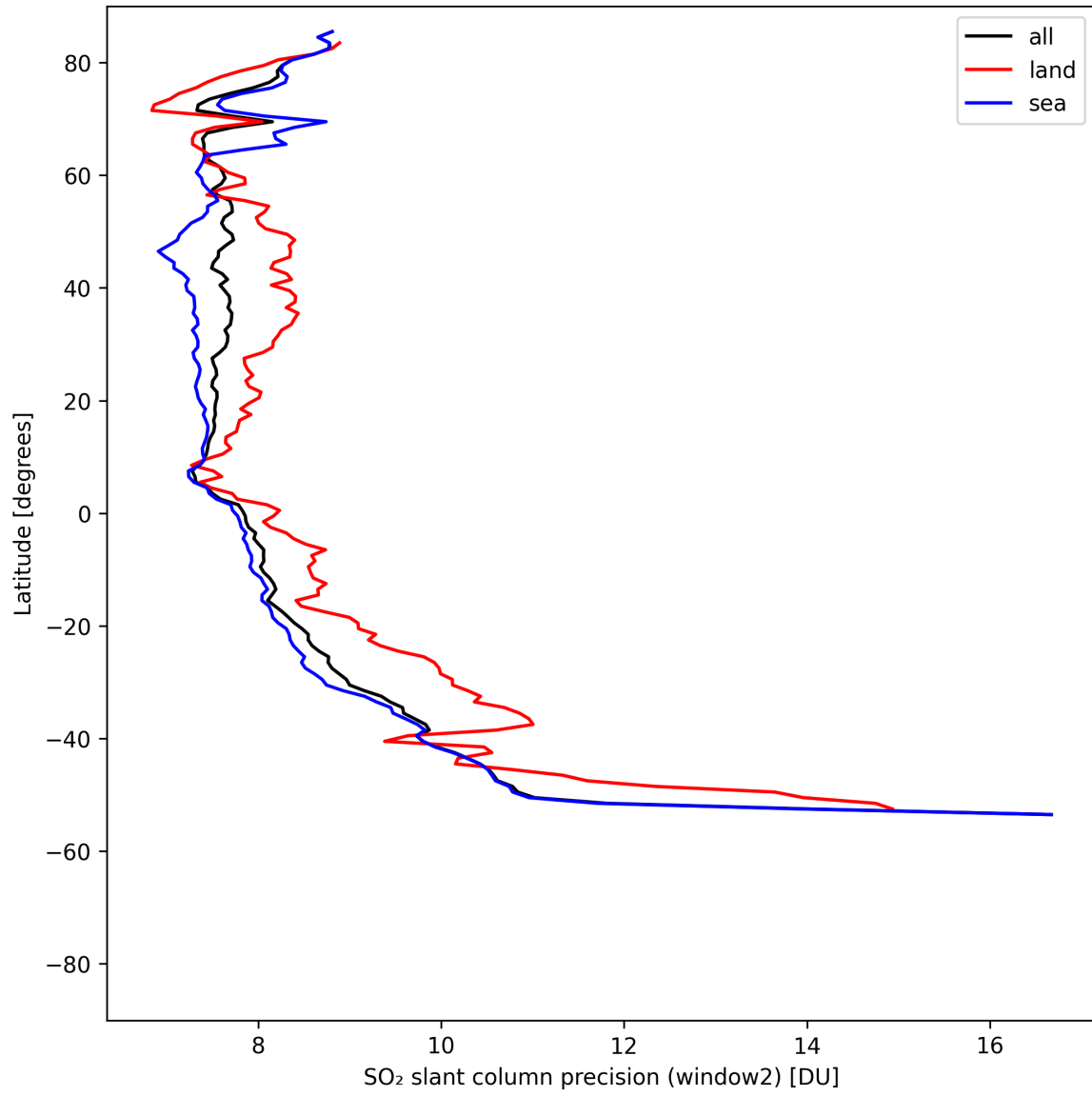
Figure 42: Zonal average of “SO 2 slant column precision (window2)” for 2025-05-02 to 2025-05-04.
