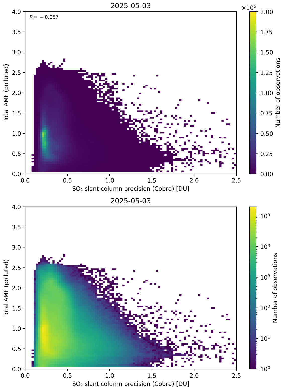
Figure 213: Scatter density plot of “SO 2 slant column precision (Cobra)” against “Total AMF (polluted)” for 2025-05-02 to 2025-05-04.
