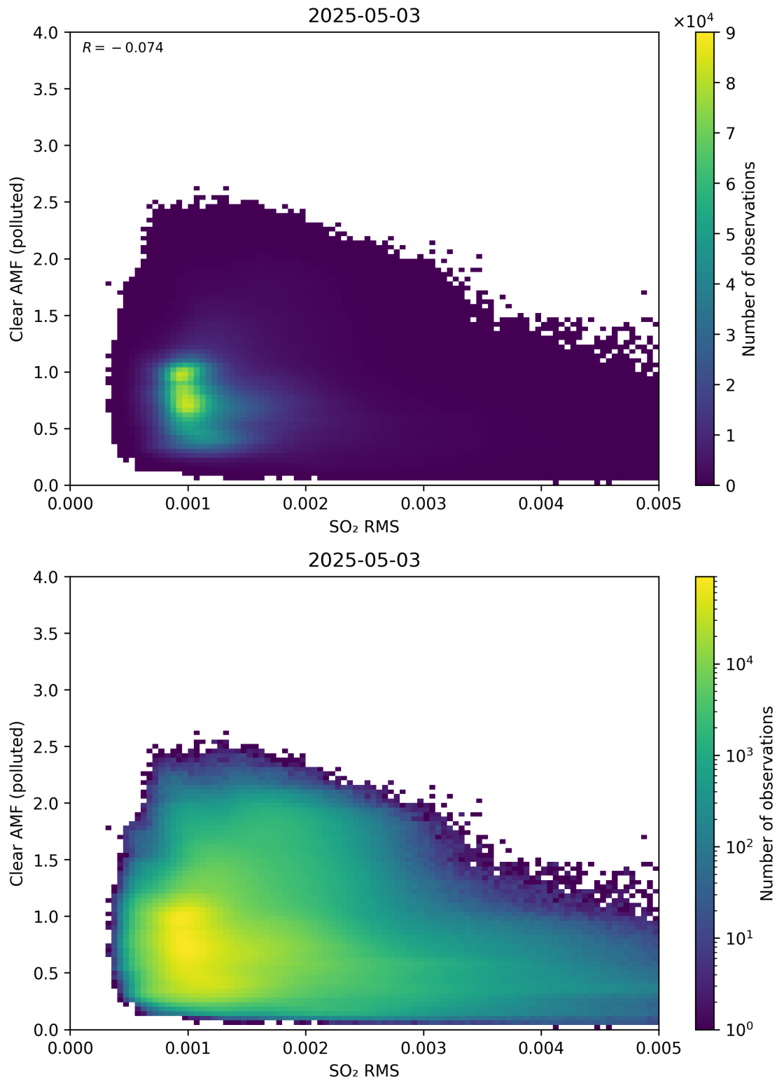
Figure 147: Scatter density plot of “SO 2 RMS” against “Clear AMF (polluted)” for 2025-05-02 to 2025-05-04.
