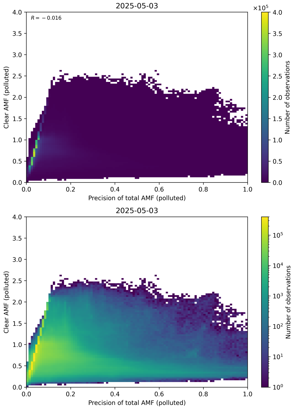
Figure 320: Scatter density plot of “Precision of total AMF (polluted)” against “Clear AMF (polluted)” for 2025-05-02 to 2025-05-04.
