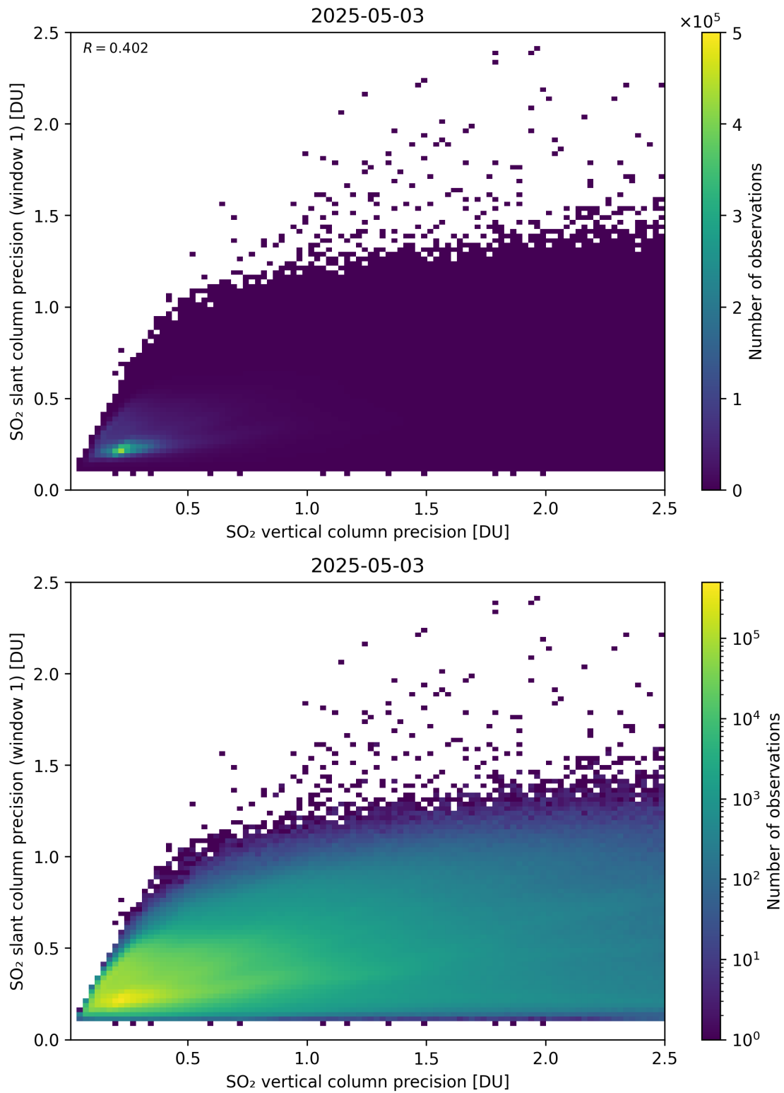
Figure 342: Scatter density plot of “SO 2 vertical column precision” against “SO 2 slant column precision (window 1)” for 2025-05-02 to 2025-05-04.
