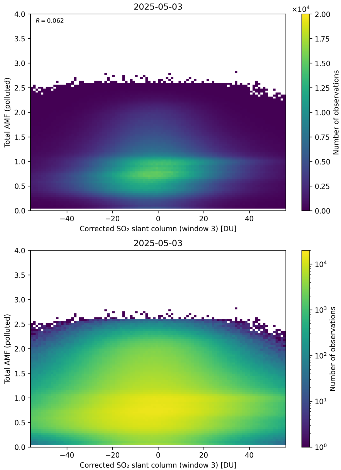
Figure 260: Scatter density plot of “Corrected SO 2 slant column (window 3)” against “Total AMF (polluted)” for 2025-05-02 to 2025-05-04.
