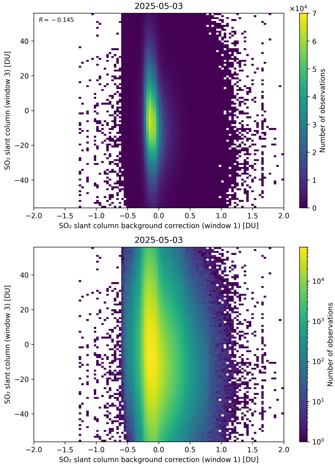
Figure 118: Scatter density plot of “SO 2 slant column background correction (window 1)” against “SO 2 slant column (window 3)” for 2025-05-02 to 2025-05-04.
