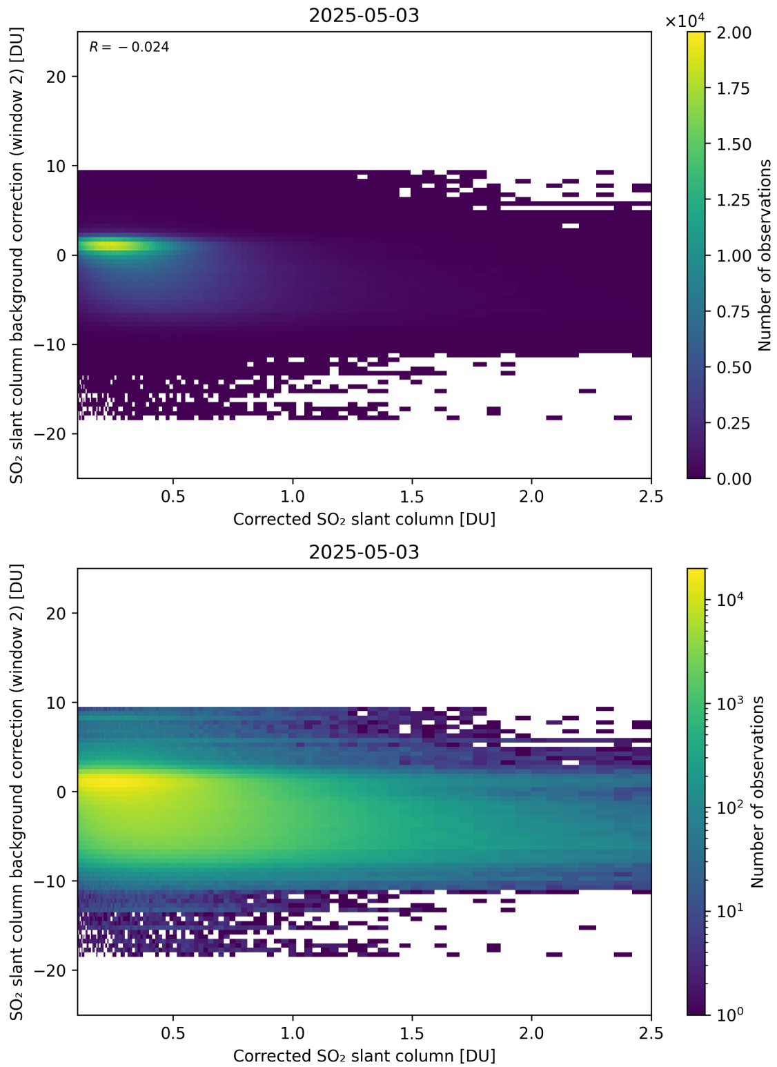
Figure 227: Scatter density plot of “Corrected SO 2 slant column” against “SO 2 slant column background correction (window 2)” for 2025-05-02 to 2025-05-04.
