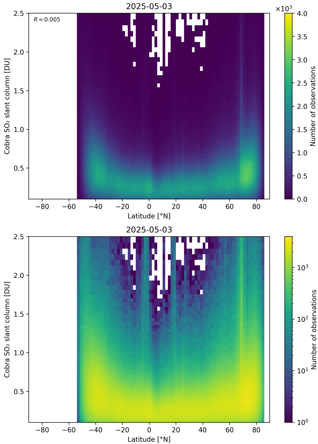
Figure 157: Scatter density plot of “Latitude” against “Cobra SO 2 slant column” for 2025-05-02 to 2025-05-04.
