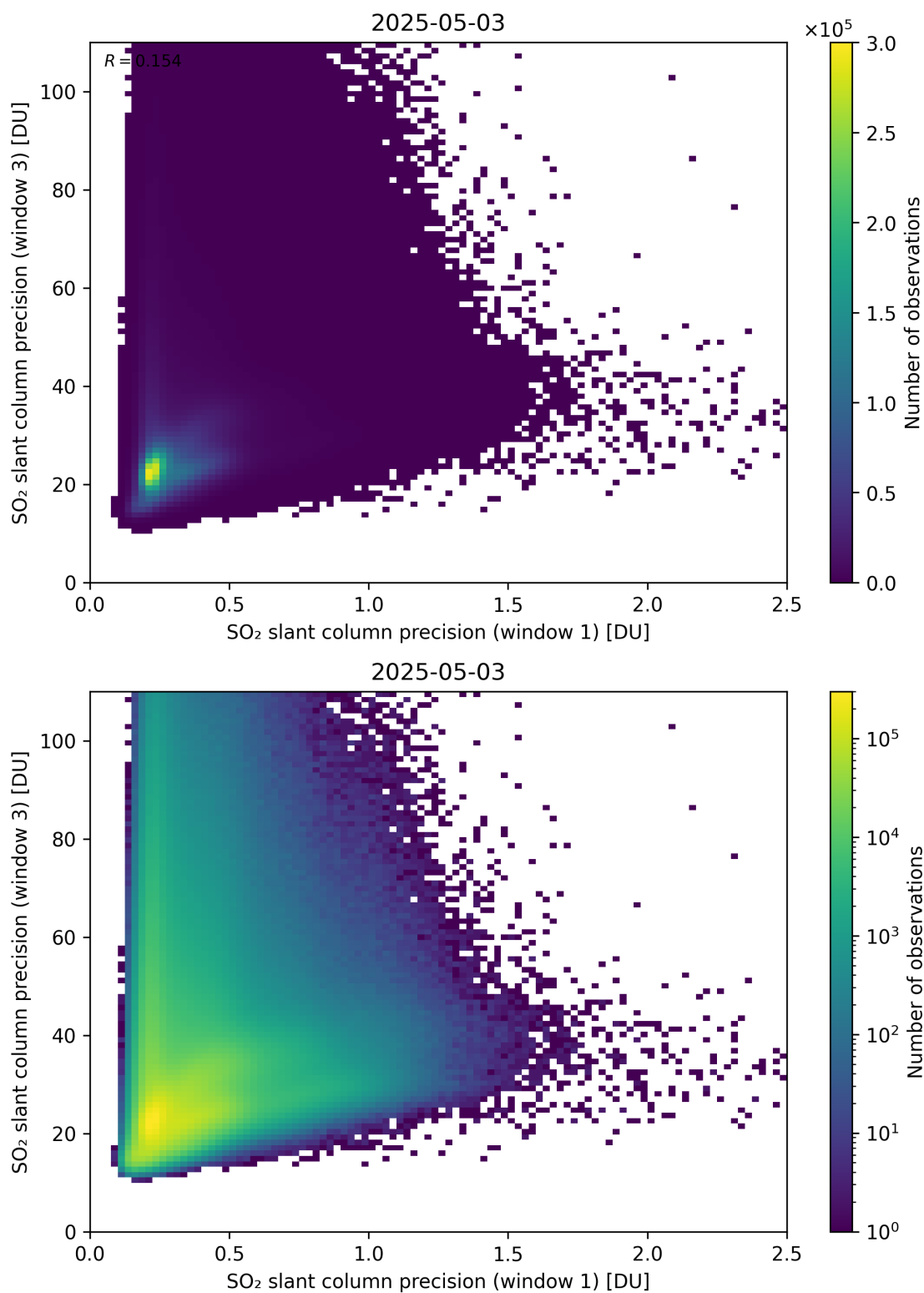
Figure 279: Scatter density plot of “SO 2 slant column precision (window 1)” against “SO 2 slant column precision (window 3)” for 2025-05-02 to 2025-05-04.
