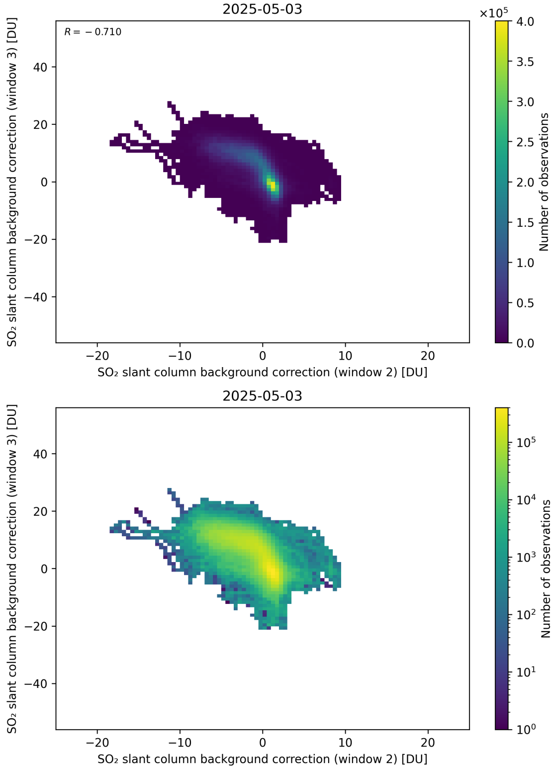
Figure 122: Scatter density plot of “SO 2 slant column background correction (window 2)” against “SO 2 slant column background correction (window 3)” for 2025-05-02 to 2025-05-04.
