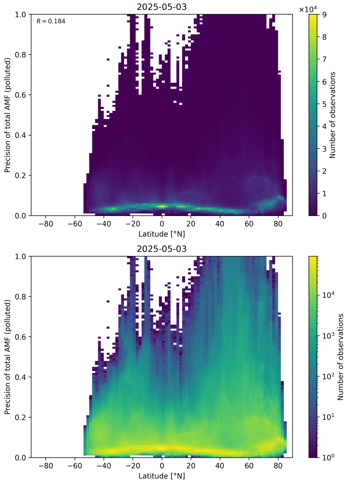
Figure 168: Scatter density plot of “Latitude” against “Precision of total AMF (polluted)” for 2025-05-02 to 2025-05-04.
