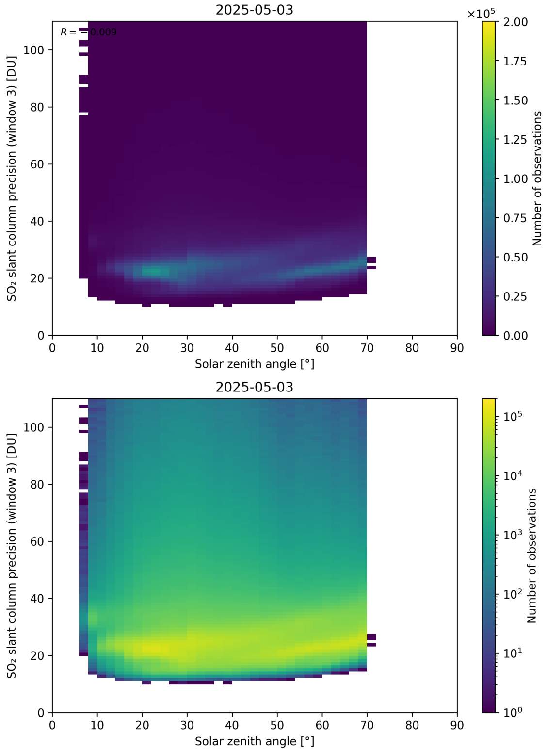
Figure 188: Scatter density plot of “Solar zenith angle” against “SO 2 slant column precision (window 3)” for 2025-05-02 to 2025-05-04.
