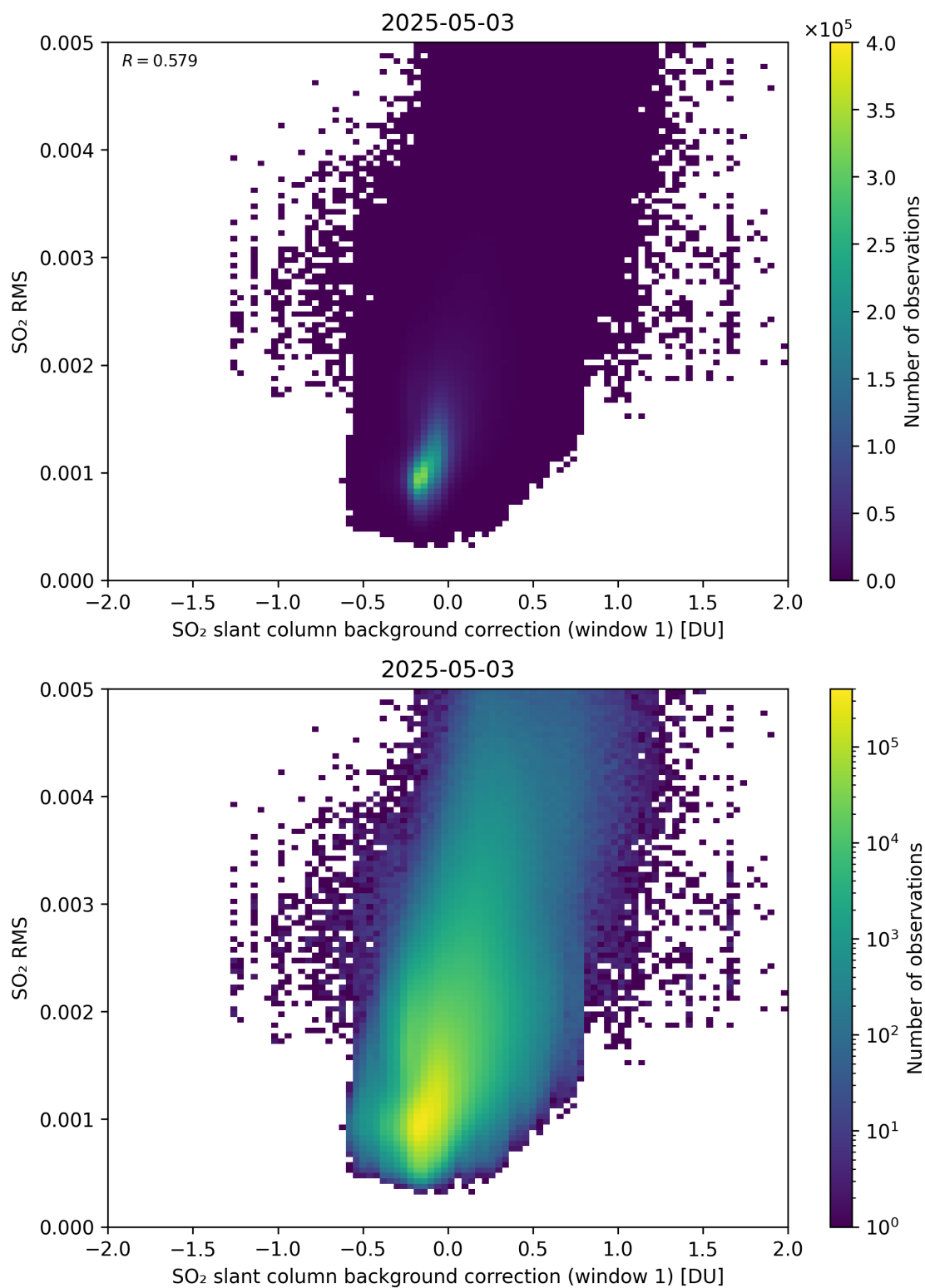
Figure 113: Scatter density plot of “SO 2 slant column background correction (window 1)” against “SO 2 RMS” for 2025-05-02 to 2025-05-04.
