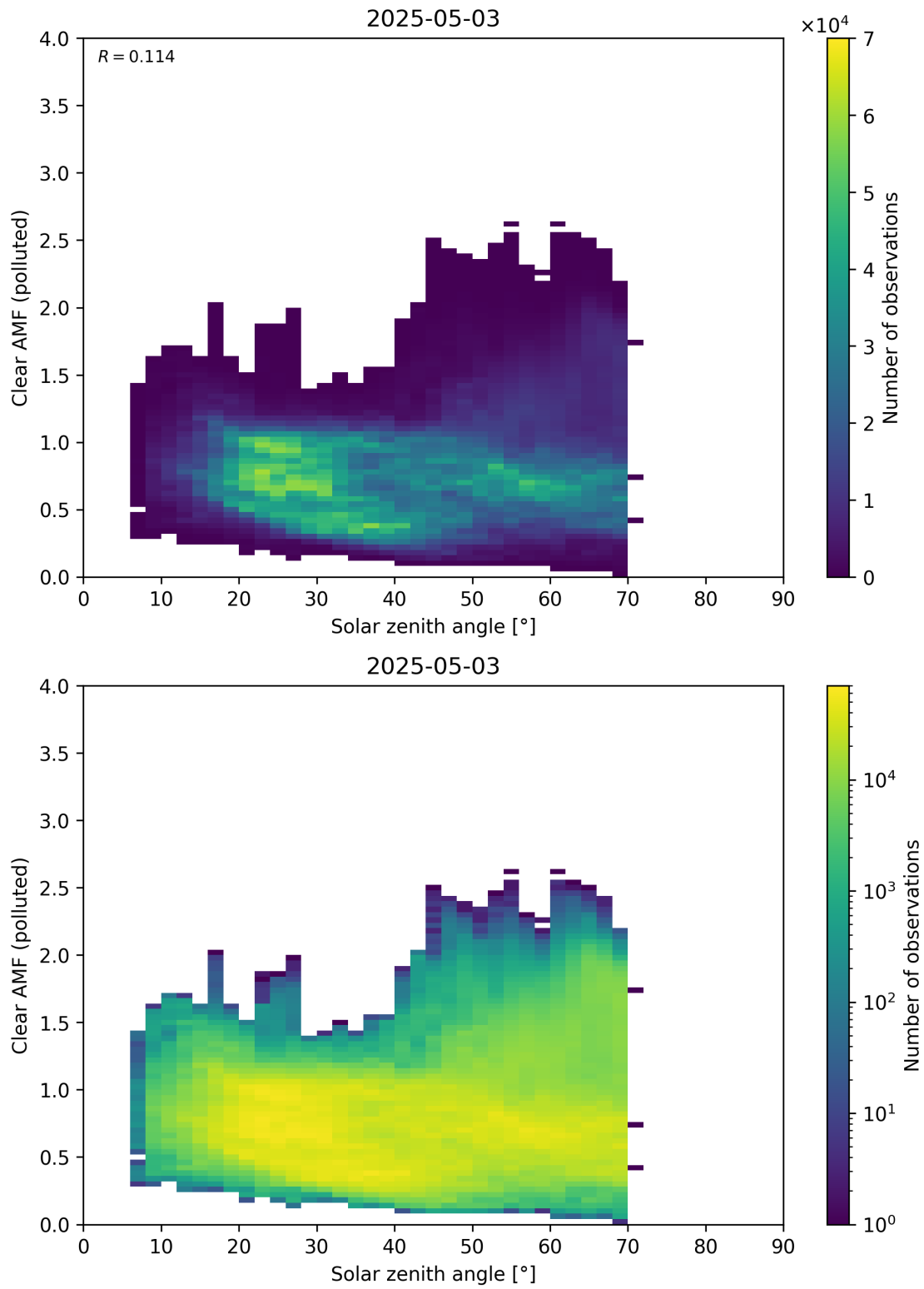
Figure 178: Scatter density plot of “Solar zenith angle” against “Clear AMF (polluted)” for 2025-05-02 to 2025-05-04.
