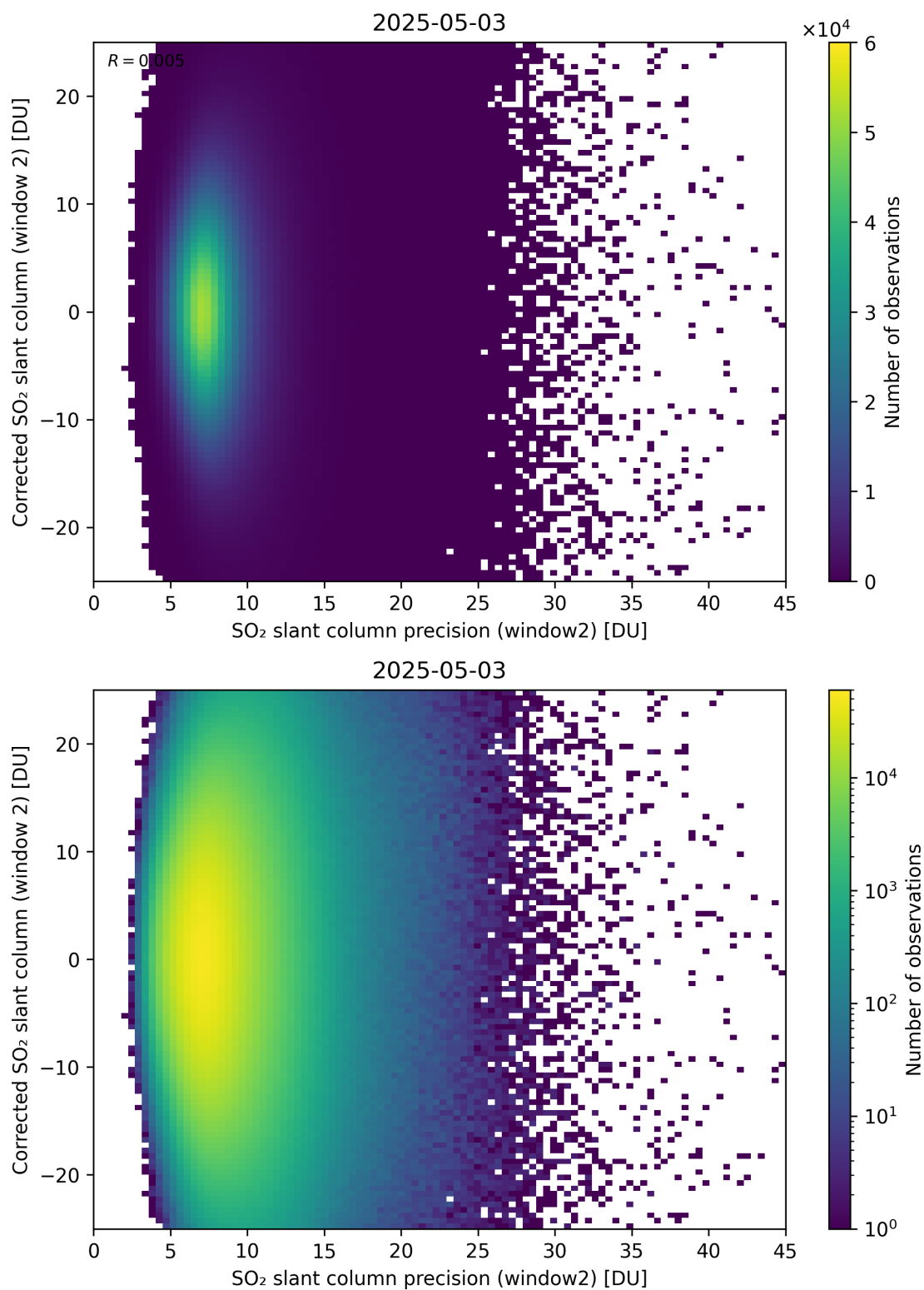
Figure 297: Scatter density plot of “SO 2 slant column precision (window2)” against “Corrected SO 2 slant column (window 2)” for 2025-05-02 to 2025-05-04.
