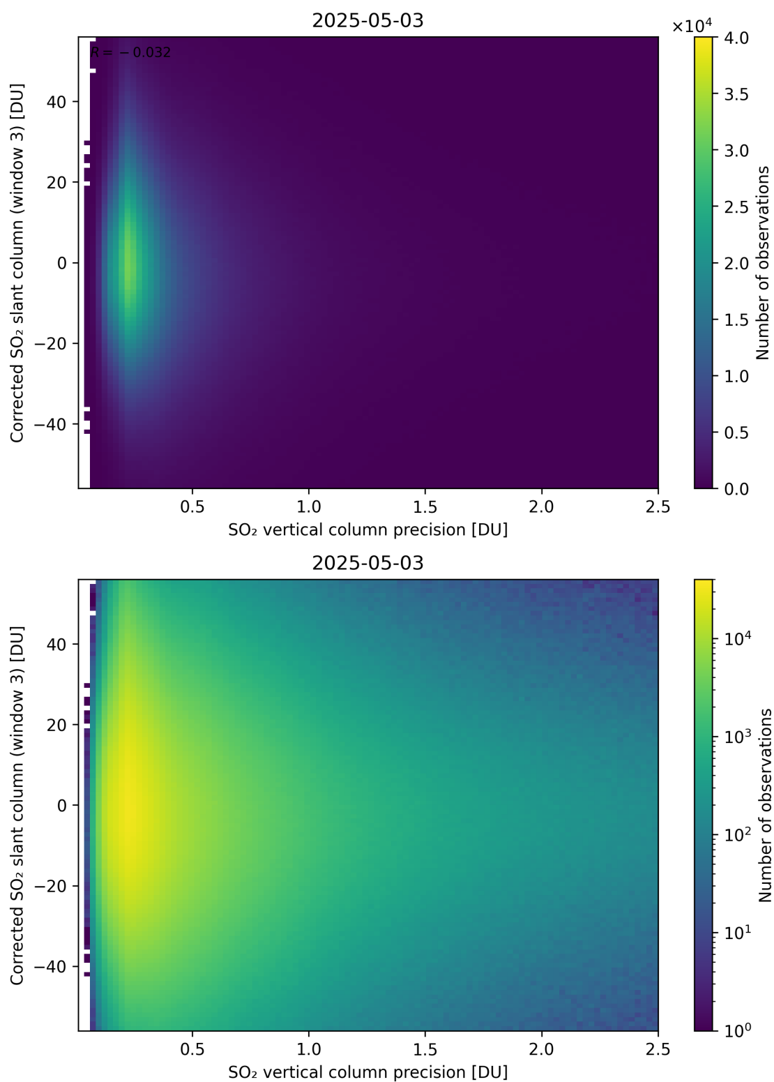
Figure 340: Scatter density plot of “SO 2 vertical column precision” against “Corrected SO 2 slant column (window 3)” for 2025-05-02 to 2025-05-04.
