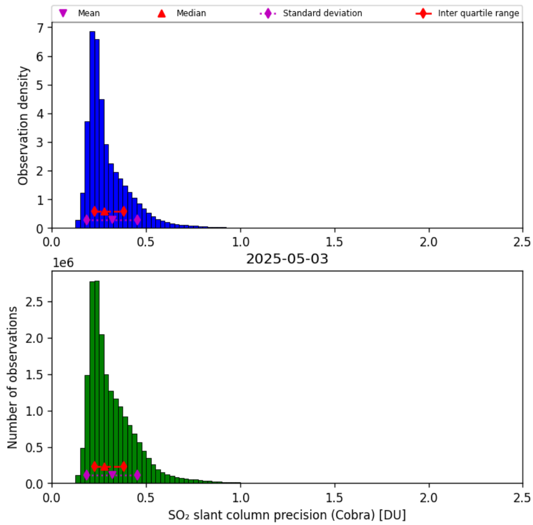
Figure 62: Histogram of “SO 2 slant column precision (Cobra)” for 2025-05-02 to 2025-05-04
