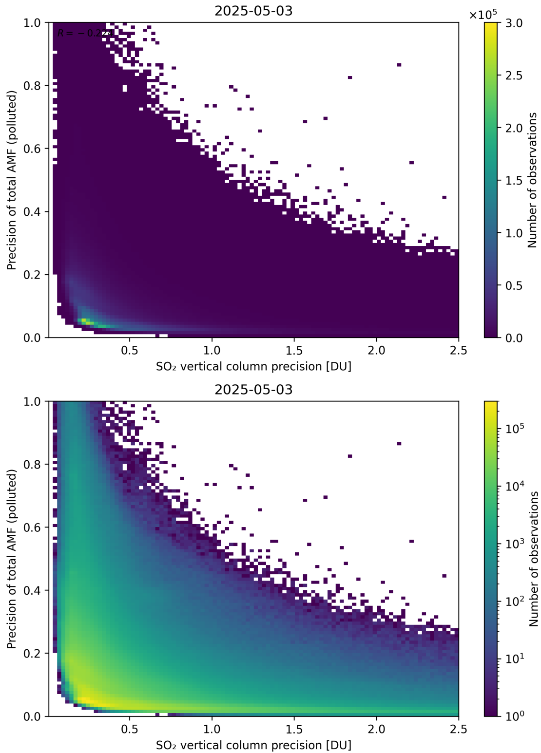
Figure 347: Scatter density plot of “SO 2 vertical column precision” against “Precision of total AMF (polluted)” for 2025-05-02 to 2025-05-04.
