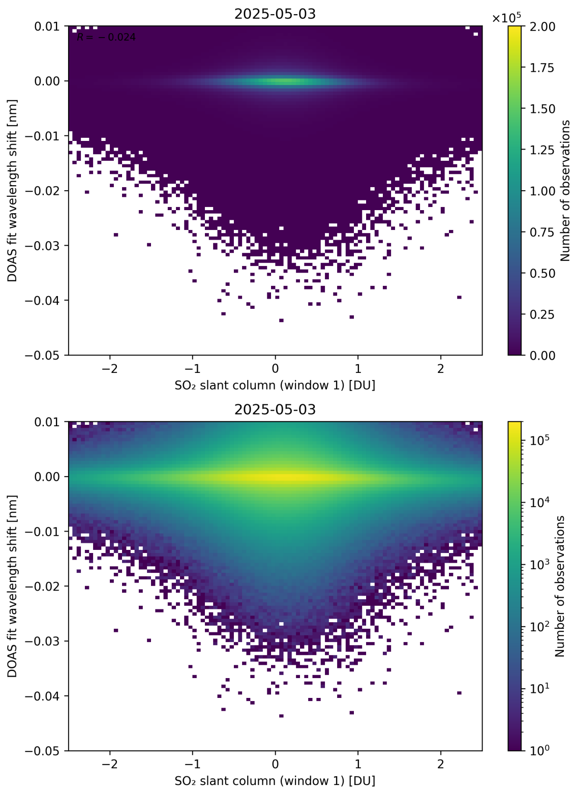
Figure 265: Scatter density plot of “SO 2 slant column (window 1)” against “DOAS fit wavelength shift” for 2025-05-02 to 2025-05-04.
