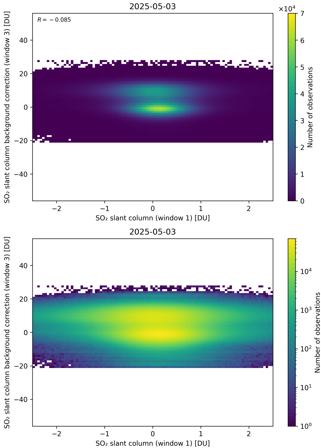
Figure 264: Scatter density plot of “SO 2 slant column (window 1)” against “SO 2 slant column background correction (window 3)” for 2025-05-02 to 2025-05-04.
