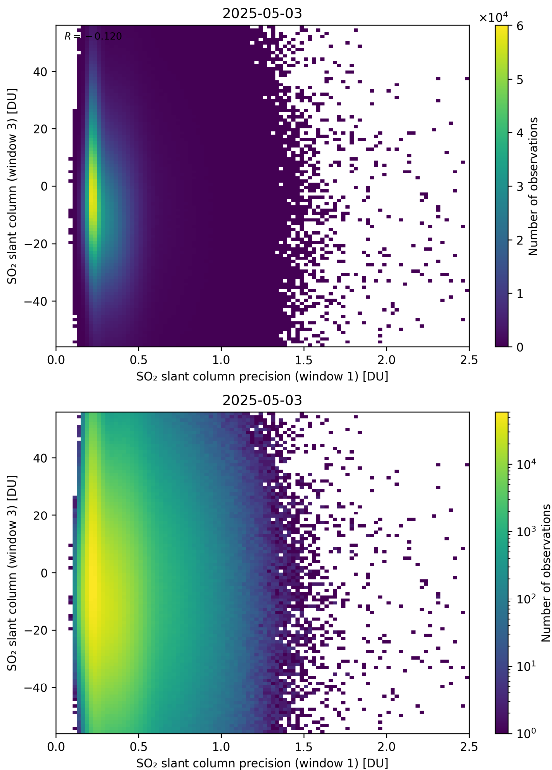
Figure 278: Scatter density plot of “SO 2 slant column precision (window 1)” against “SO 2 slant column (window 3)” for 2025-05-02 to 2025-05-04.
