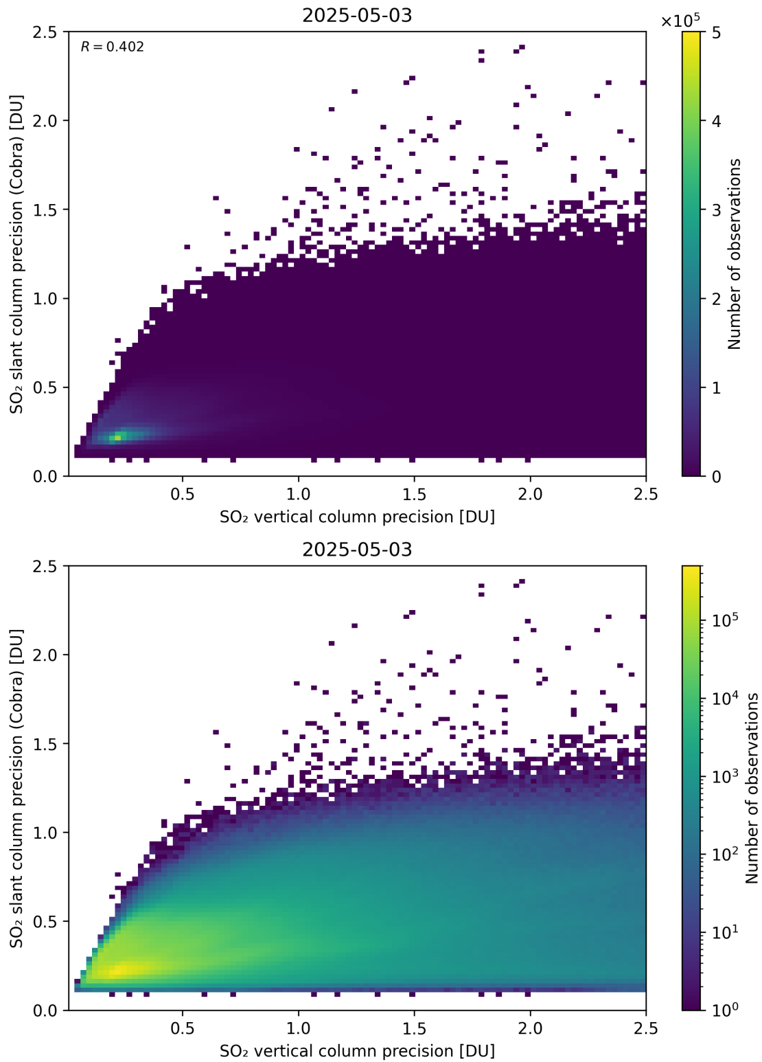
Figure 337: Scatter density plot of “SO 2 vertical column precision” against “SO 2 slant column precision (Cobra)” for 2025-05-02 to 2025-05-04.
