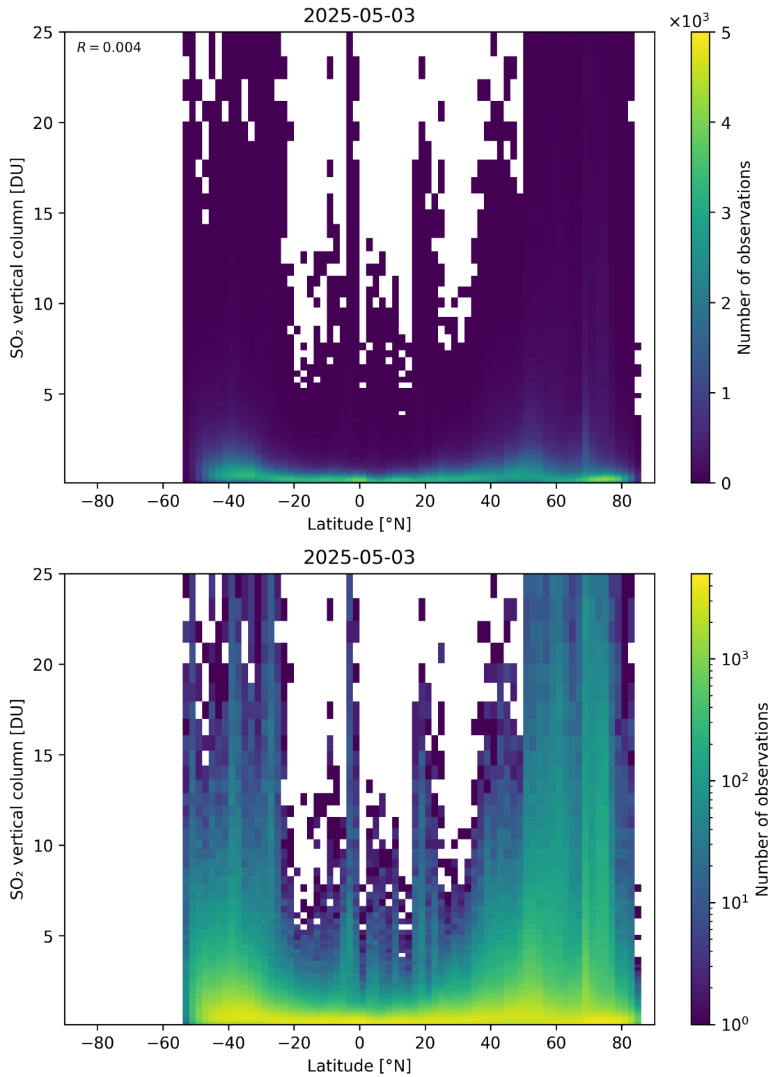
Figure 169: Scatter density plot of “Latitude” against “SO 2 vertical column” for 2025-05-02 to 2025-05-04.
