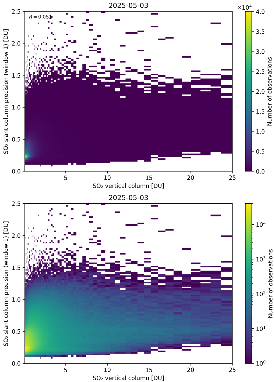
Figure 355: Scatter density plot of “SO 2 vertical column” against “SO 2 slant column precision (window 1)” for 2025-05-02 to 2025-05-04.
