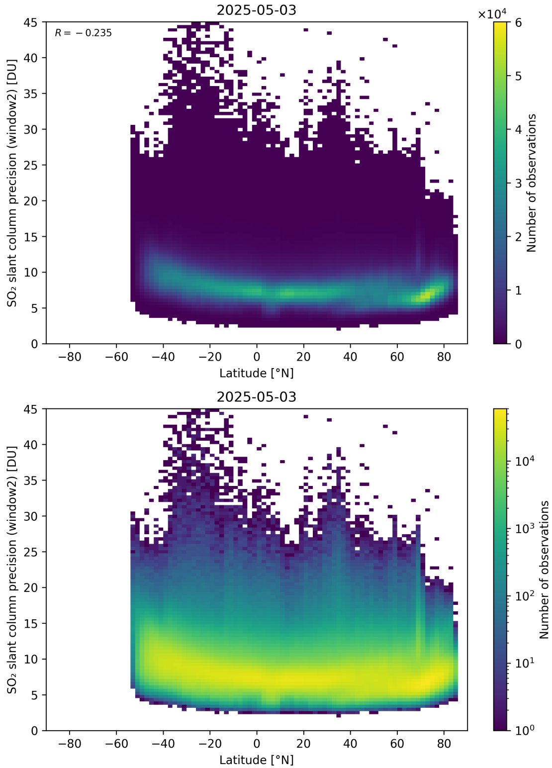
Figure 164: Scatter density plot of “Latitude” against “SO 2 slant column precision (window2)” for 2025-05-02 to 2025-05-04.
