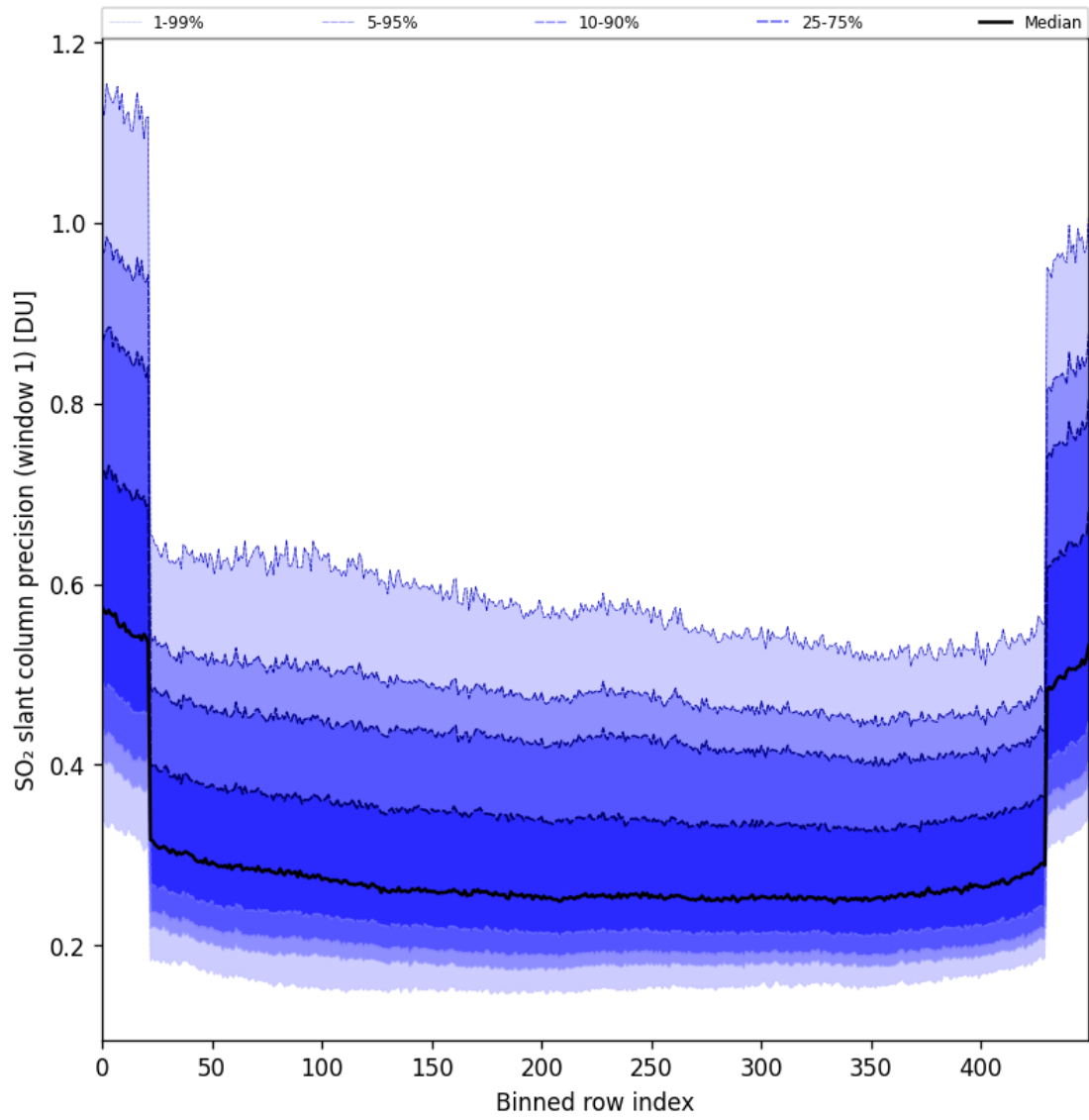
Figure 90: Along track statistics of “SO 2 slant column precision (window 1)” for 2025-05-02 to 2025-05-04
