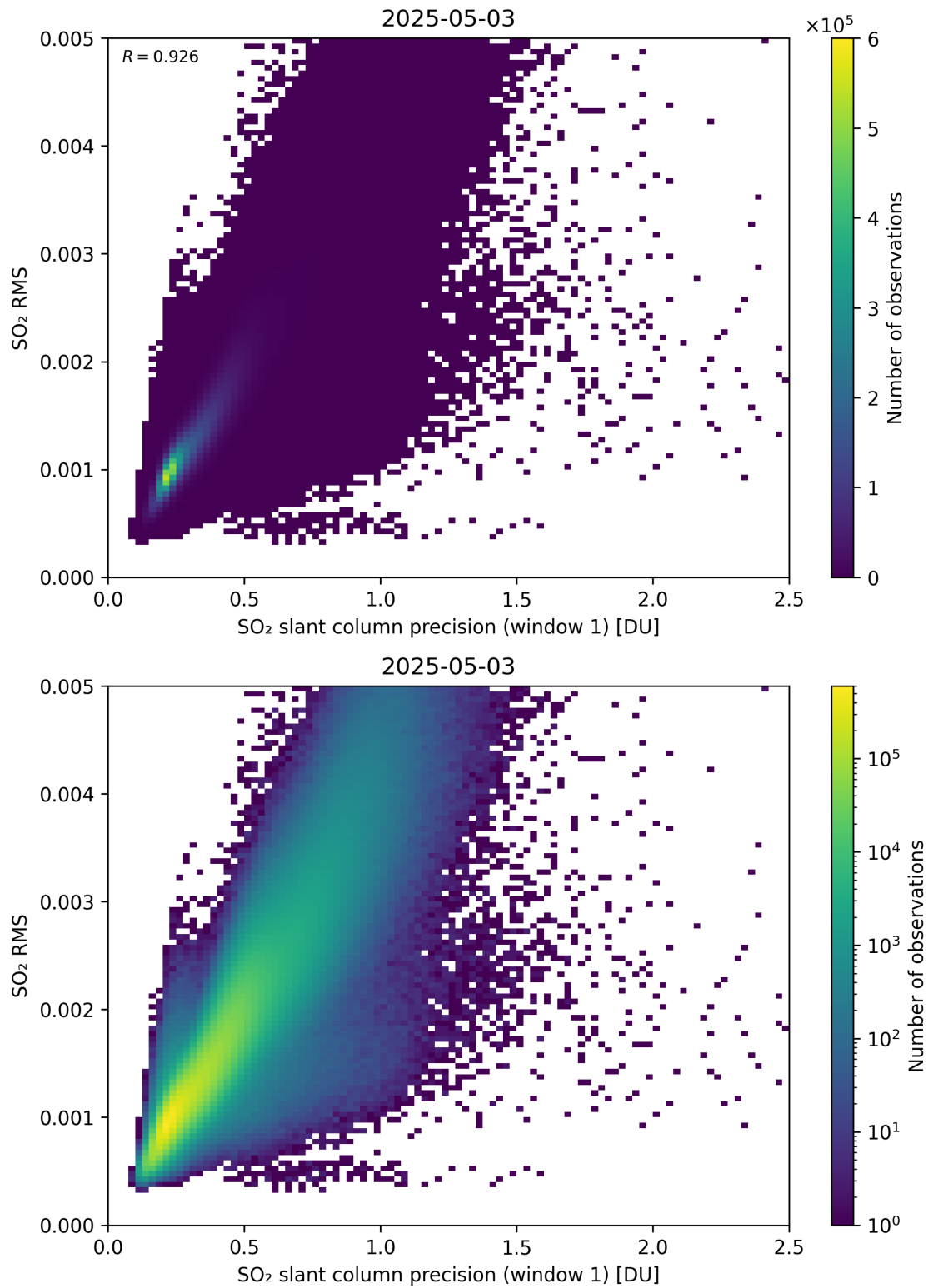
Figure 273: Scatter density plot of “SO 2 slant column precision (window 1)” against “SO 2 RMS” for 2025-05-02 to 2025-05-04.
