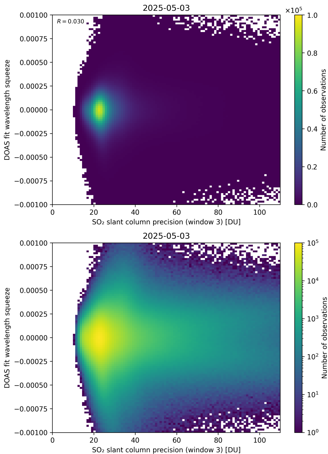
Figure 309: Scatter density plot of “SO 2 slant column precision (window 3)” against “DOAS fit wavelength squeeze” for 2025-05-02 to 2025-05-04.
