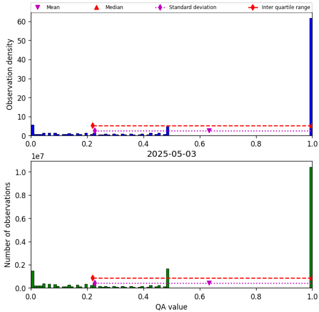
Figure 57: Histogram of “QA value” for 2025-05-02 to 2025-05-04
