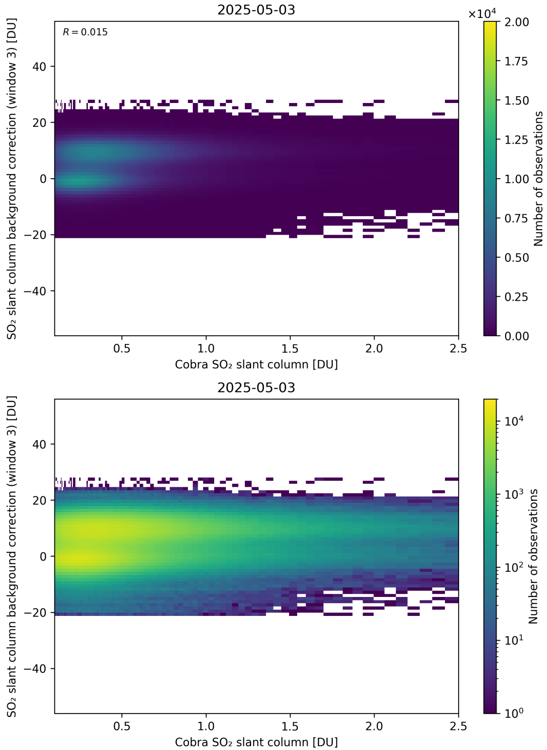
Figure 195: Scatter density plot of “Cobra SO 2 slant column” against “SO 2 slant column background correction (window 3)” for 2025-05-02 to 2025-05-04.
