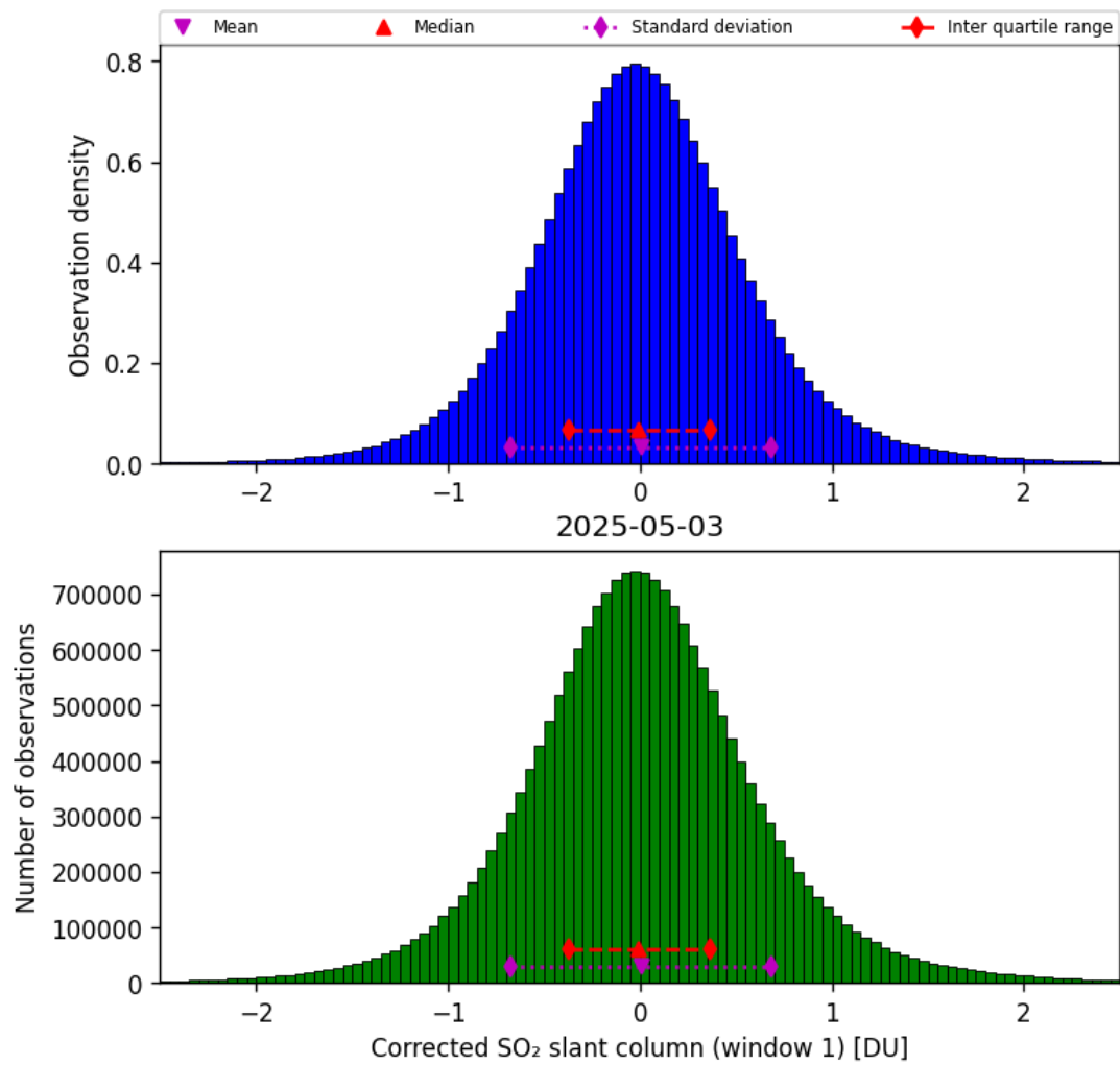
Figure 65: Histogram of “Corrected SO 2 slant column (window 1)” for 2025-05-02 to 2025-05-04
