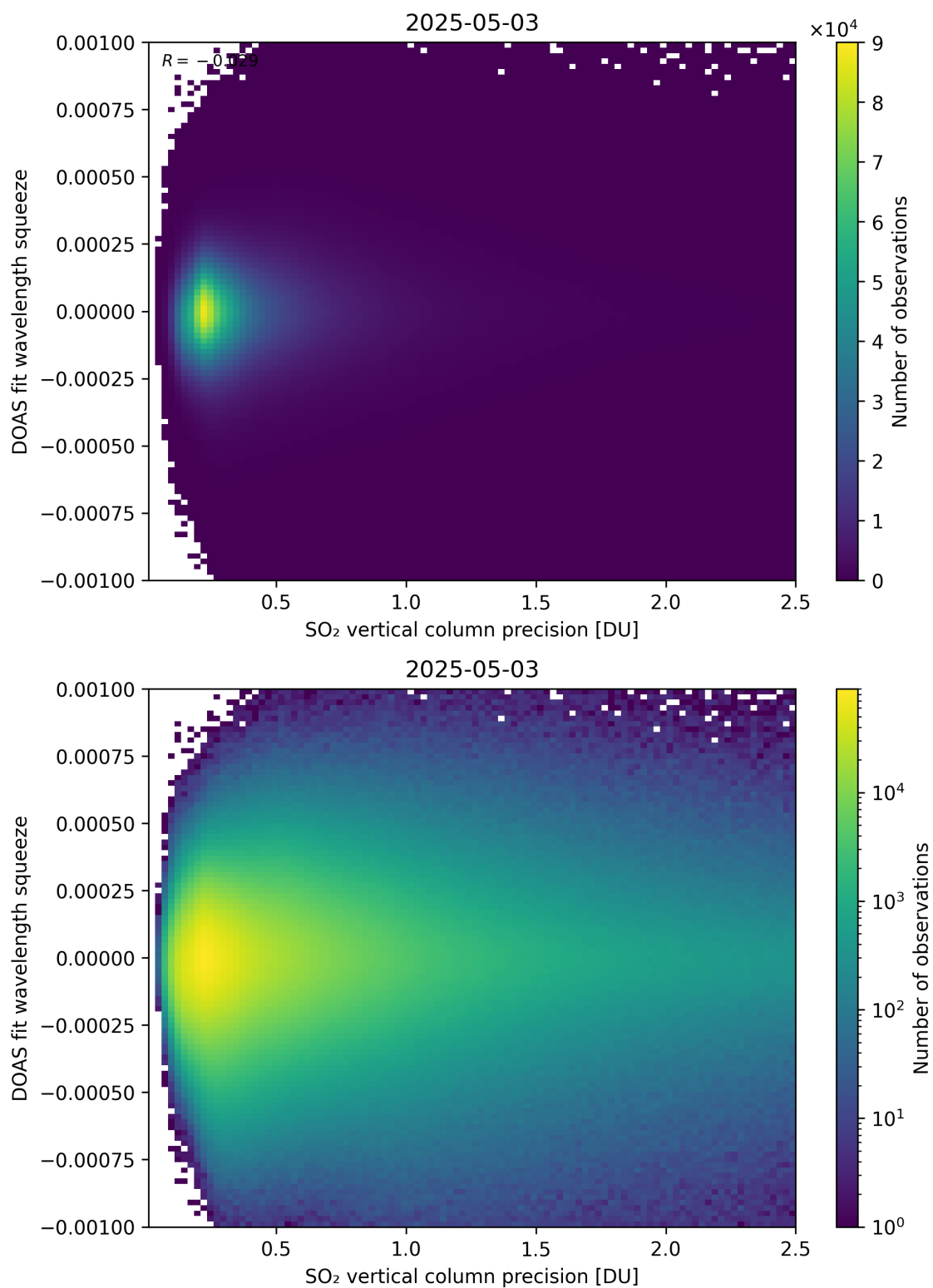
Figure 333: Scatter density plot of “SO 2 vertical column precision” against “DOAS fit wavelength squeeze” for 2025-05-02 to 2025-05-04.
