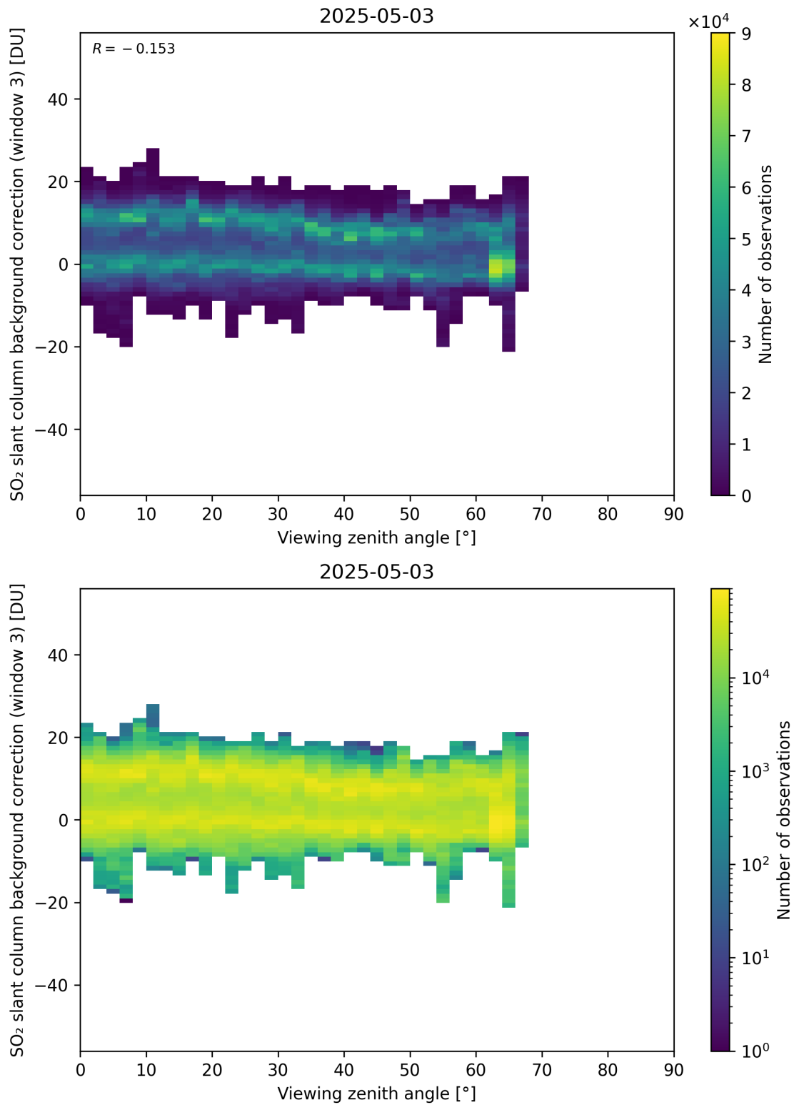
Figure 364: Scatter density plot of “Viewing zenith angle” against “SO 2 slant column background correction (window 3)” for 2025-05-02 to 2025-05-04.
