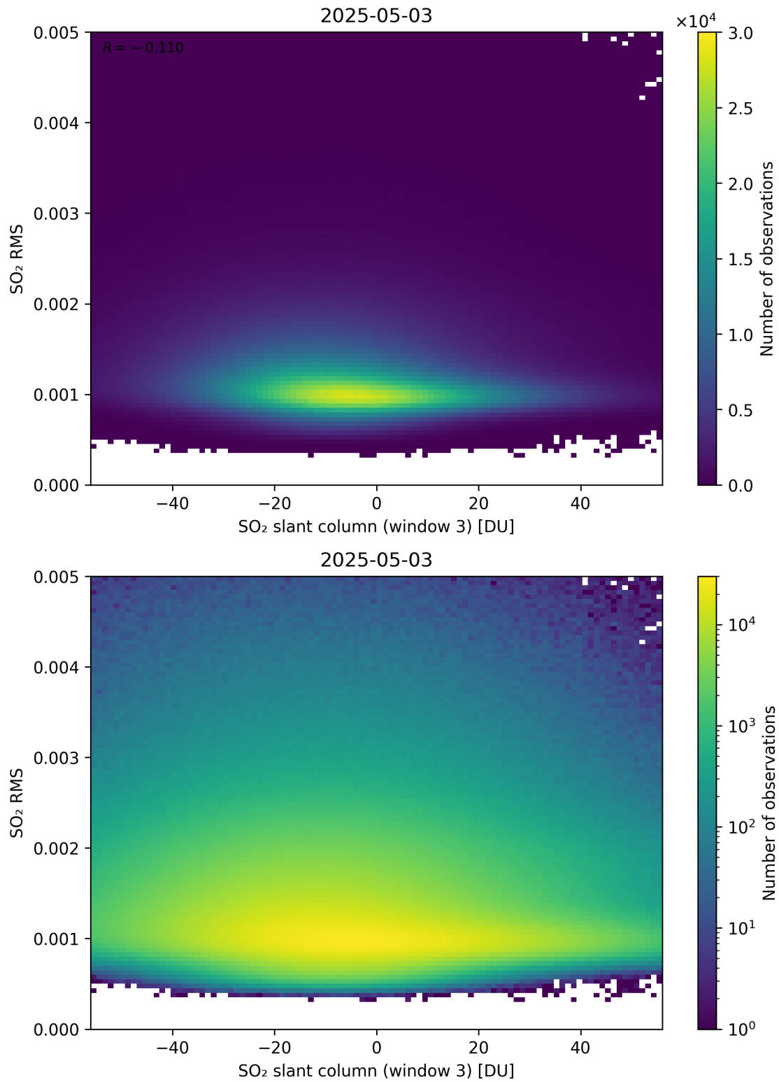
Figure 306: Scatter density plot of “SO 2 slant column (window 3)” against “SO 2 RMS” for 2025-05-02 to 2025-05-04.
