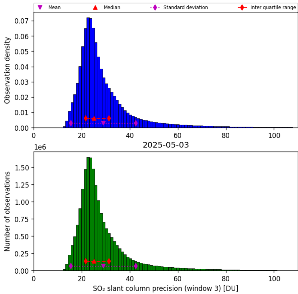
Figure 72: Histogram of “SO 2 slant column precision (window 3)” for 2025-05-02 to 2025-05-04
