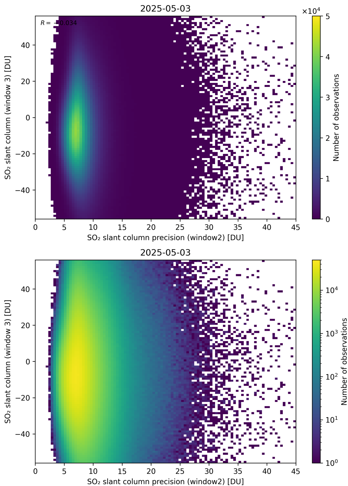
Figure 299: Scatter density plot of “SO 2 slant column precision (window2)” against “SO 2 slant column (window 3)” for 2025-05-02 to 2025-05-04.
