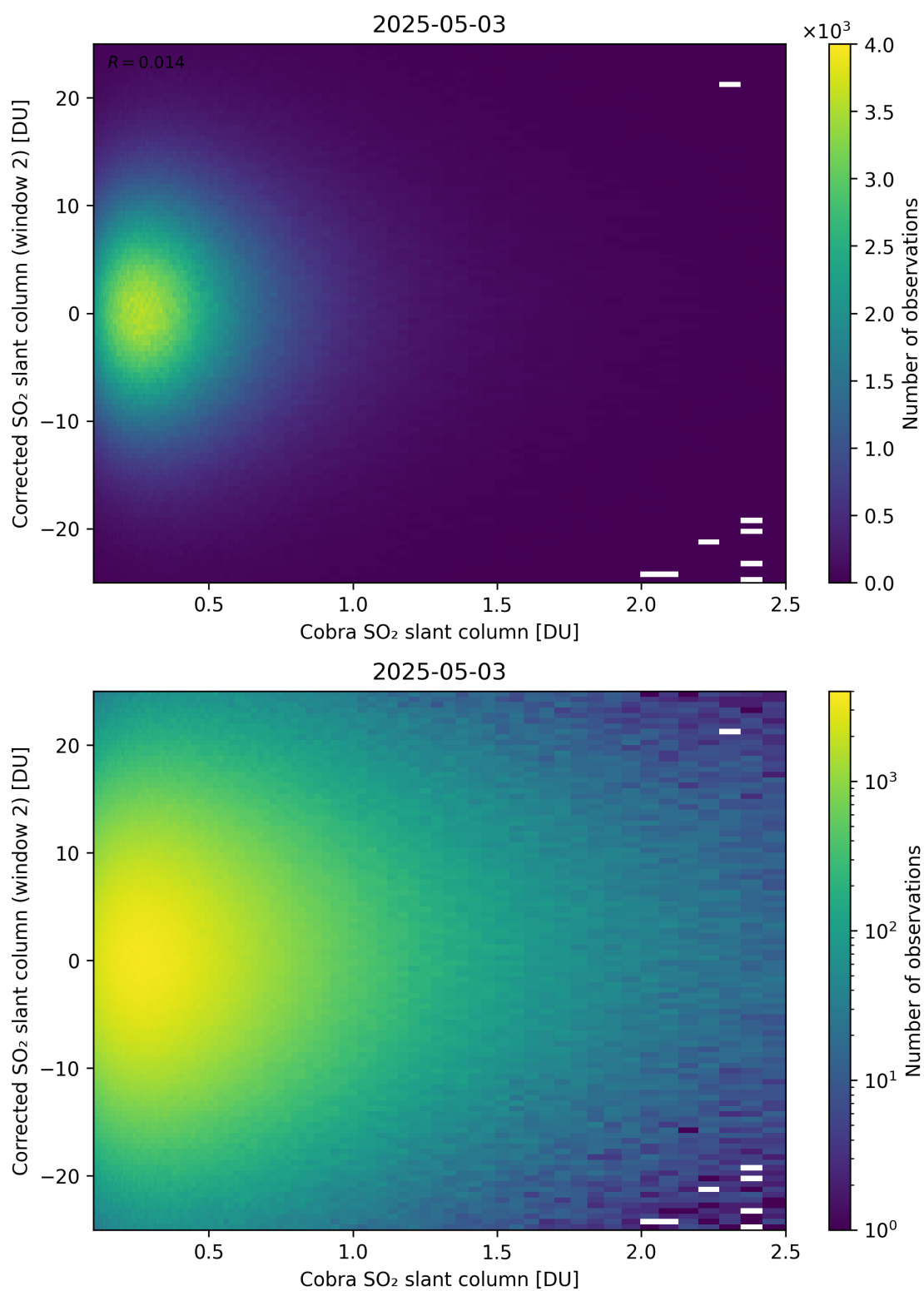
Figure 217: Scatter density plot of “Cobra SO 2 slant column” against “Corrected SO 2 slant column (window 2)” for 2025-05-02 to 2025-05-04.
