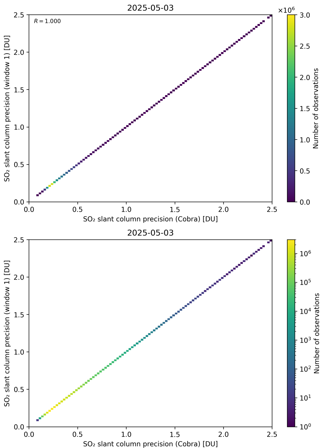
Figure 209: Scatter density plot of “SO 2 slant column precision (Cobra)” against “SO 2 slant column precision (window 1)” for 2025-05-02 to 2025-05-04.
