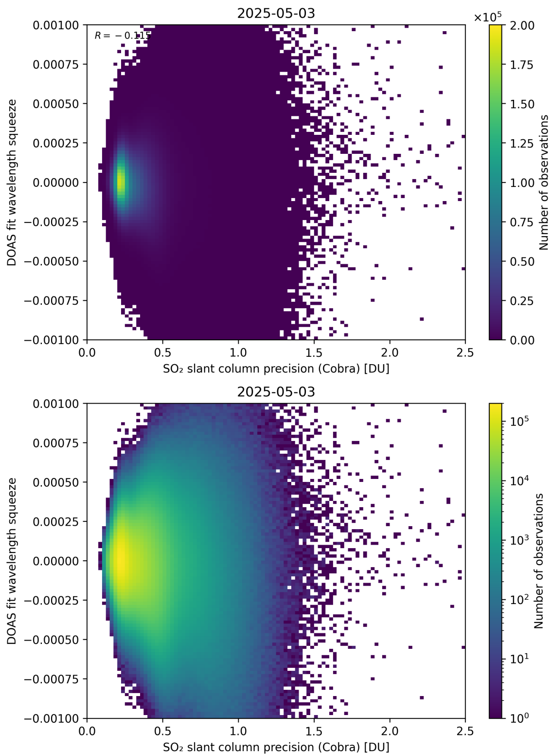
Figure 203: Scatter density plot of “SO 2 slant column precision (Cobra)” against “DOAS fit wavelength squeeze” for 2025-05-02 to 2025-05-04.
