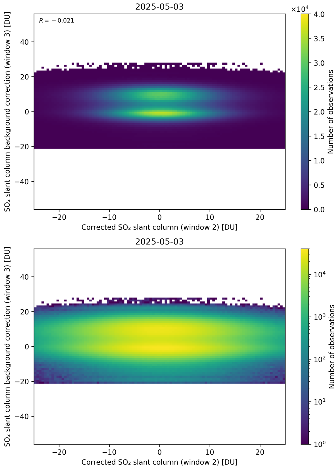
Figure 245: Scatter density plot of “Corrected SO 2 slant column (window 2)” against “SO 2 slant column background correction (window 3)” for 2025-05-02 to 2025-05-04.
