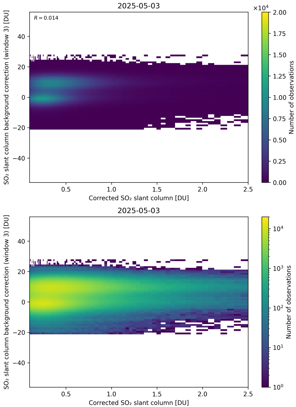
Figure 228: Scatter density plot of “Corrected SO 2 slant column” against “SO 2 slant column background correction (window 3)” for 2025-05-02 to 2025-05-04.
