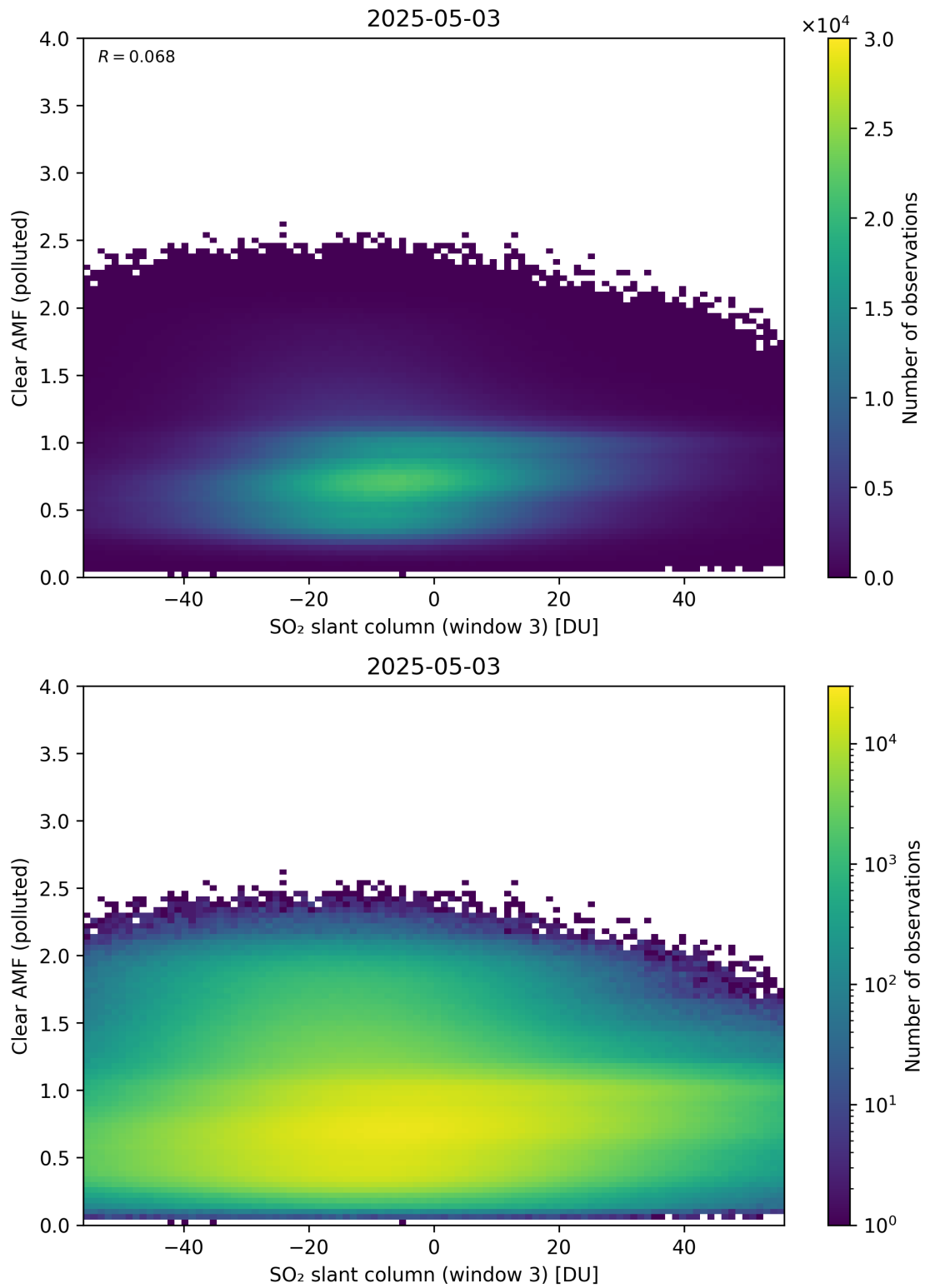
Figure 315: Scatter density plot of “SO 2 slant column (window 3)” against “Clear AMF (polluted)” for 2025-05-02 to 2025-05-04.
