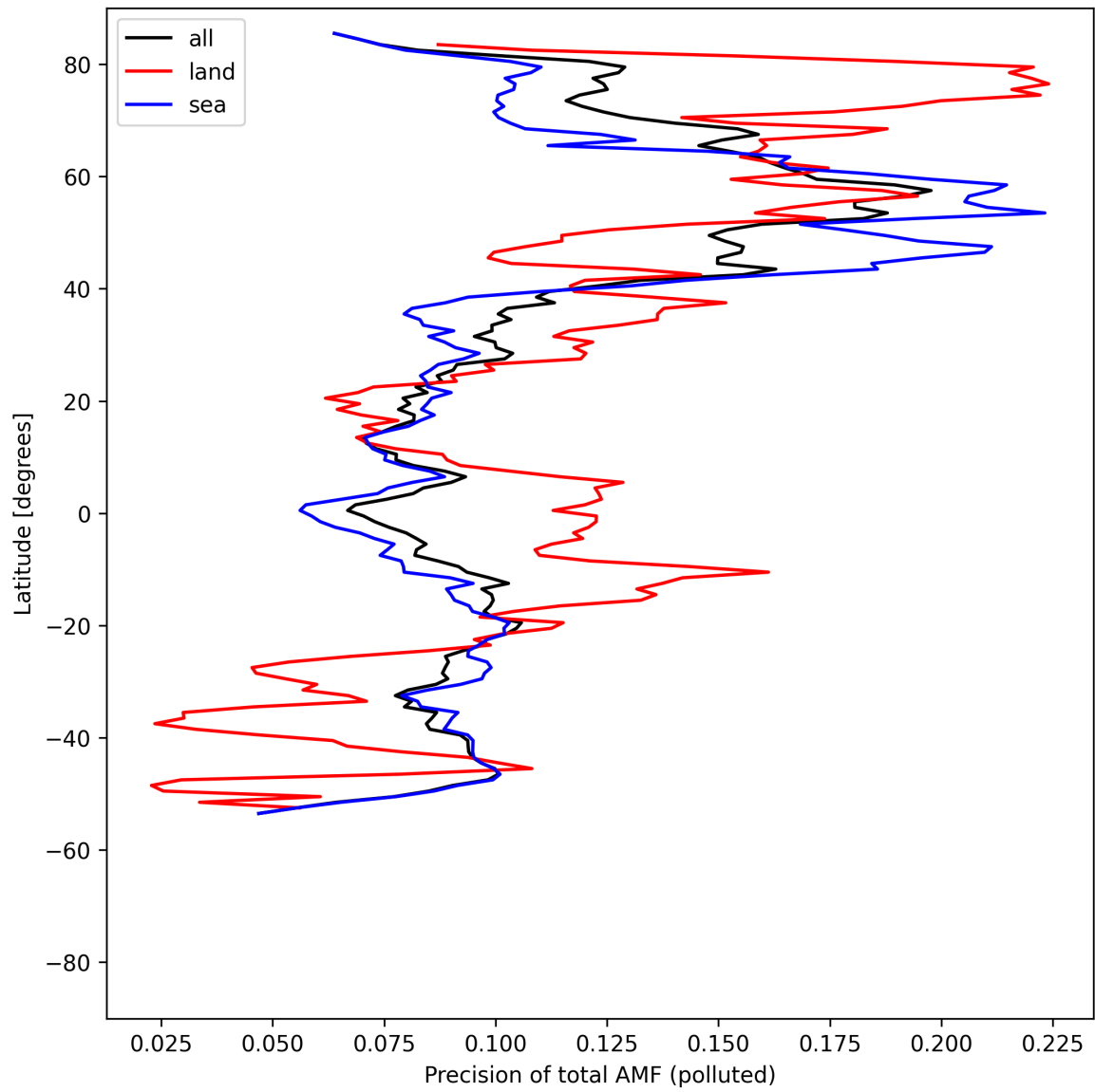
Figure 54: Zonal average of “Precision of total AMF (polluted)” for 2025-05-02 to 2025-05-04.
