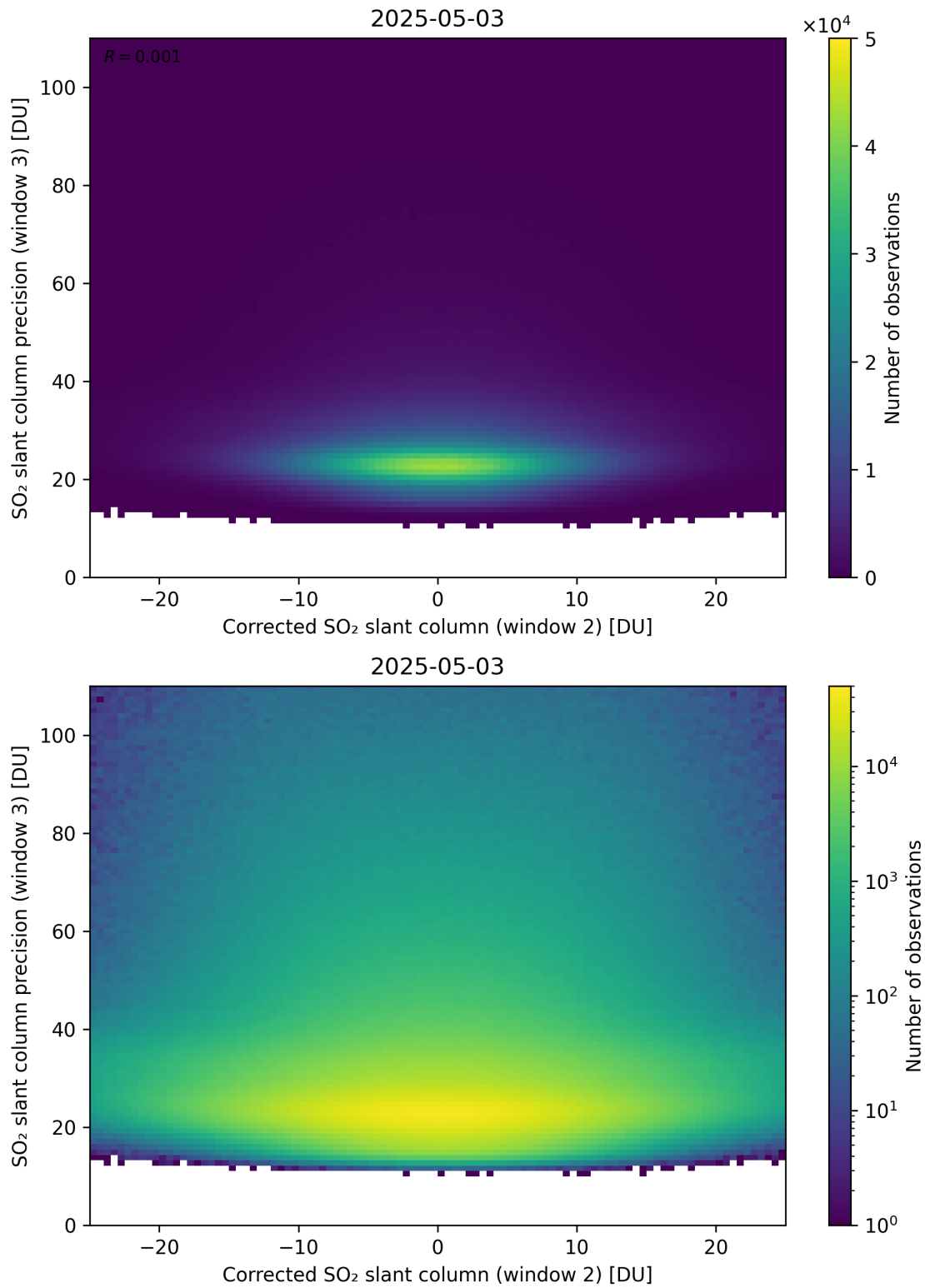
Figure 252: Scatter density plot of “Corrected SO 2 slant column (window 2)” against “SO 2 slant column precision (window 3)” for 2025-05-02 to 2025-05-04.
