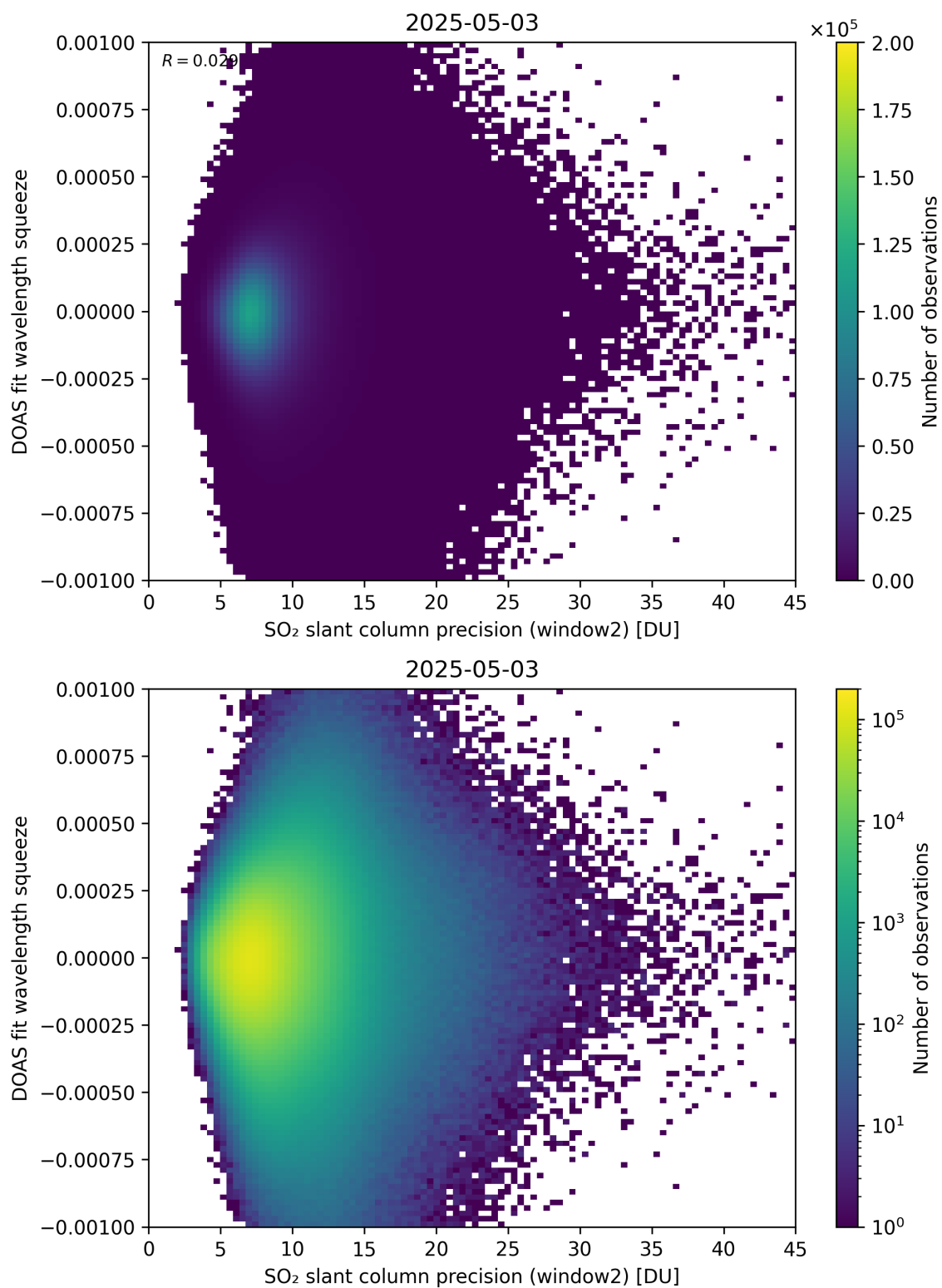
Figure 294: Scatter density plot of “SO 2 slant column precision (window2)” against “DOAS fit wavelength squeeze” for 2025-05-02 to 2025-05-04.
