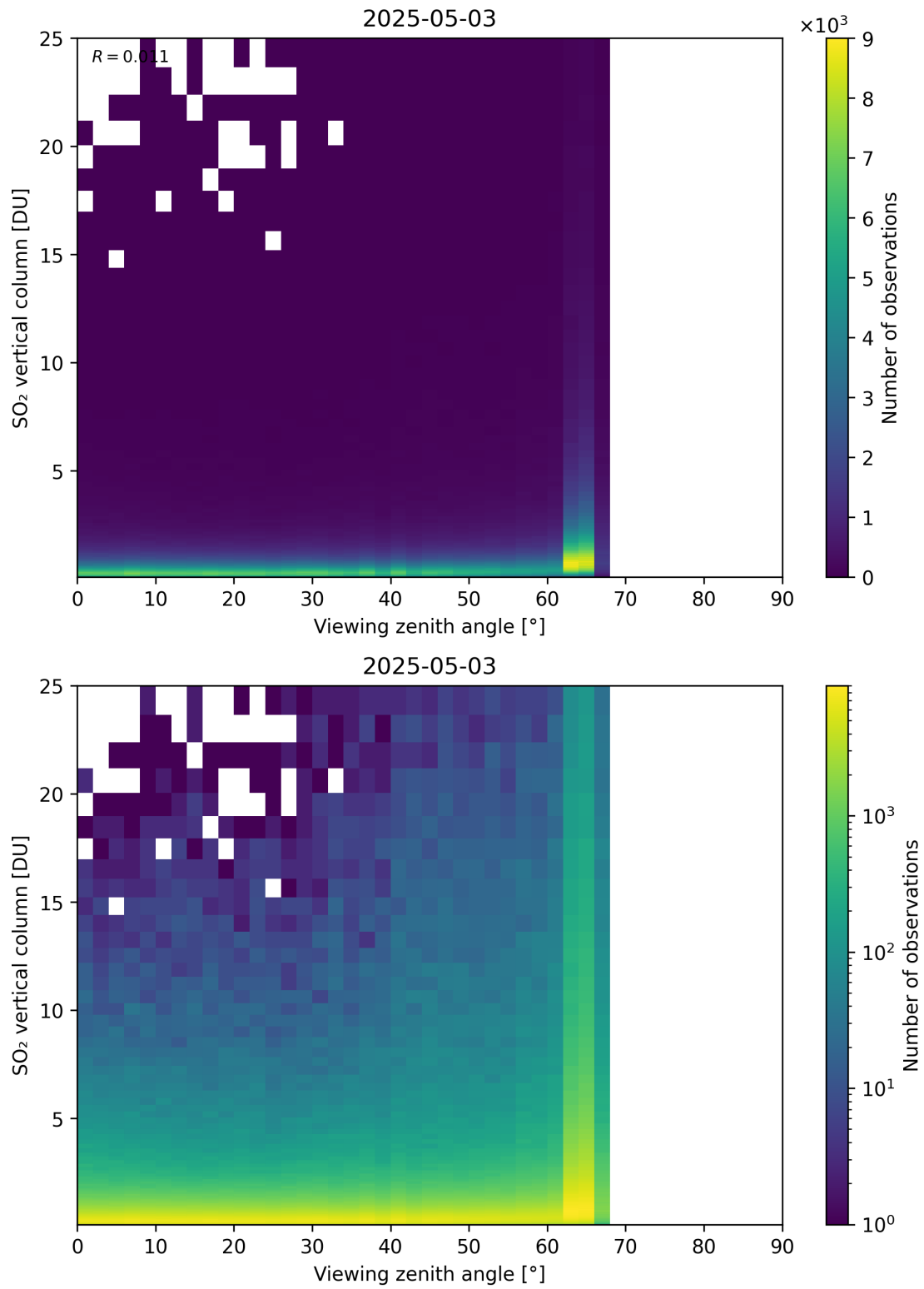
Figure 383: Scatter density plot of “Viewing zenith angle” against “SO 2 vertical column” for 2025-05-02 to 2025-05-04.
