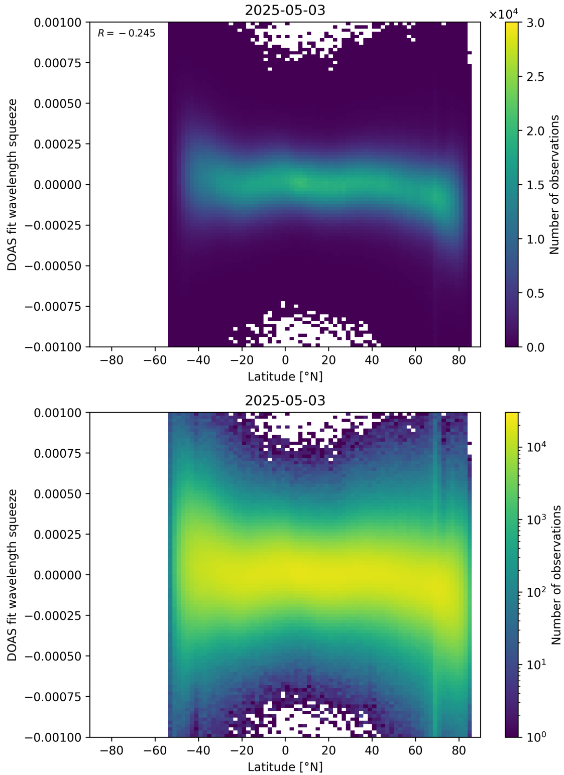
Figure 154: Scatter density plot of “Latitude” against “DOAS fit wavelength squeeze” for 2025-05-02 to 2025-05-04.
