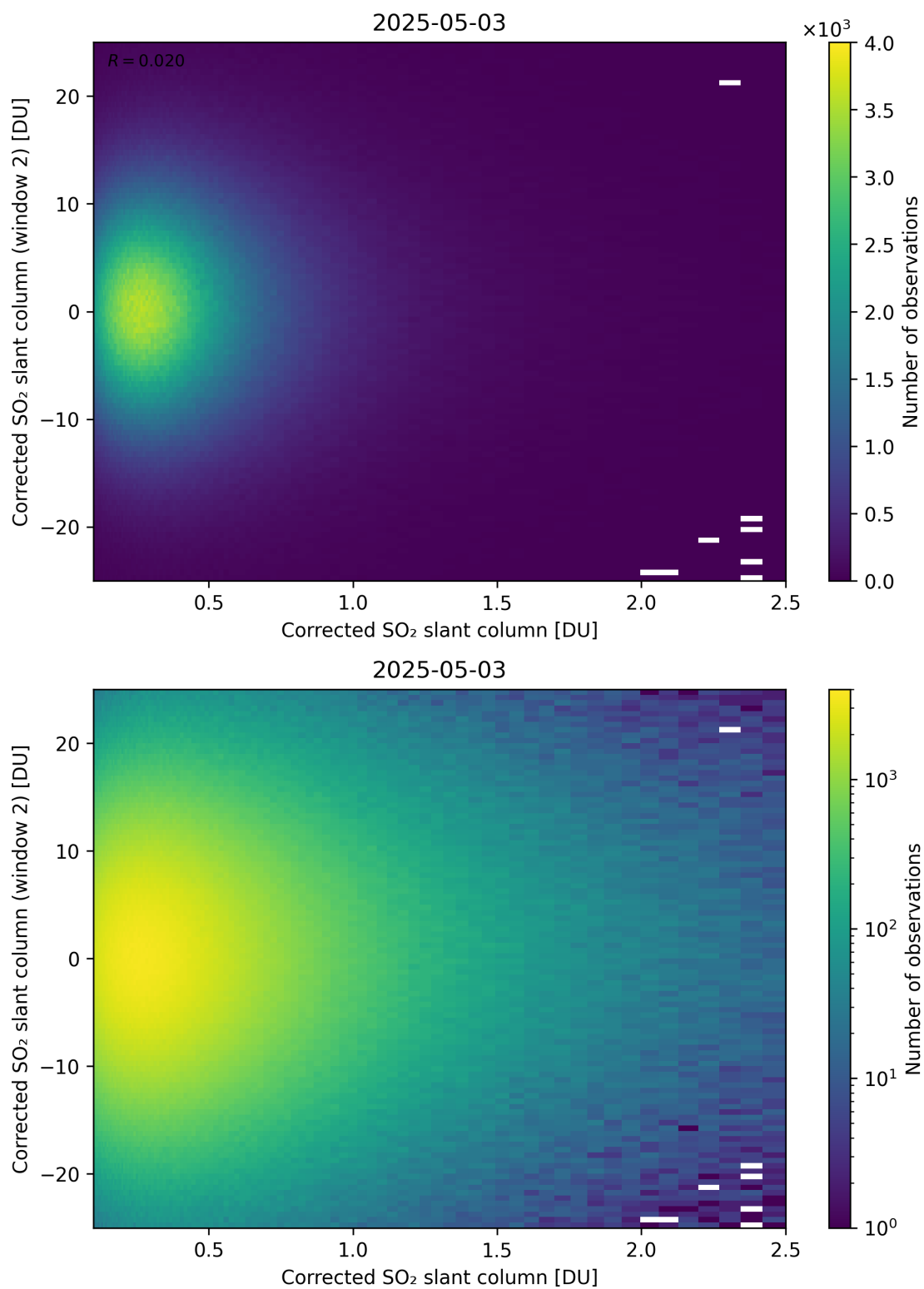
Figure 235: Scatter density plot of “Corrected SO 2 slant column” against “Corrected SO 2 slant column (window 2)” for 2025-05-02 to 2025-05-04.
