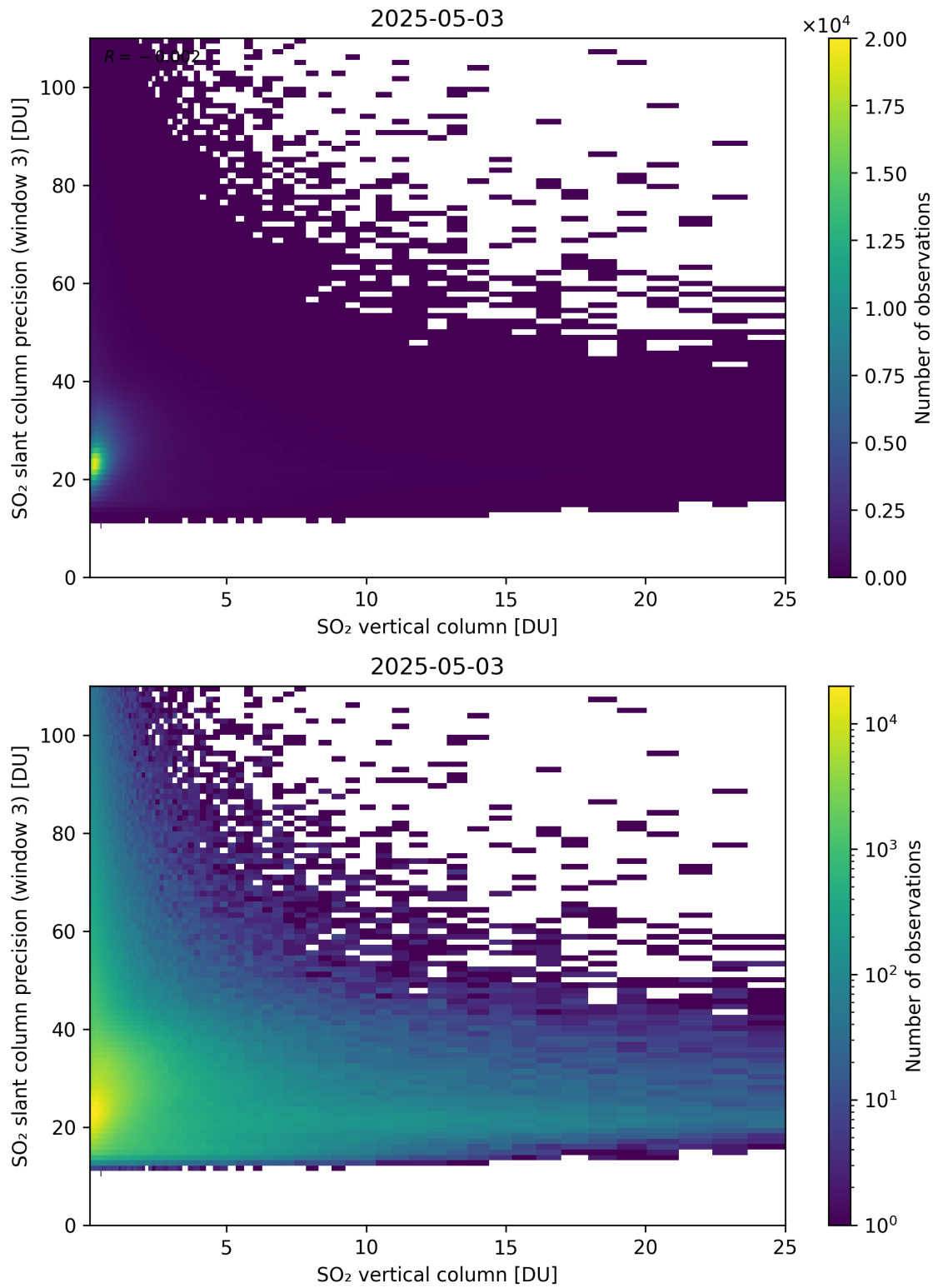
Figure 358: Scatter density plot of “SO 2 vertical column” against “SO 2 slant column precision (window 3)” for 2025-05-02 to 2025-05-04.
