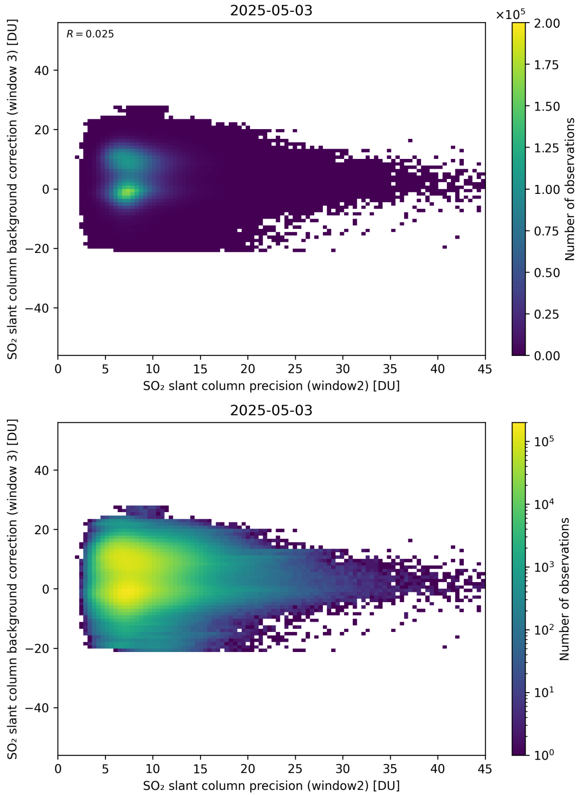
Figure 292: Scatter density plot of “SO 2 slant column precision (window2)” against “SO 2 slant column background correction (window 3)” for 2025-05-02 to 2025-05-04.
