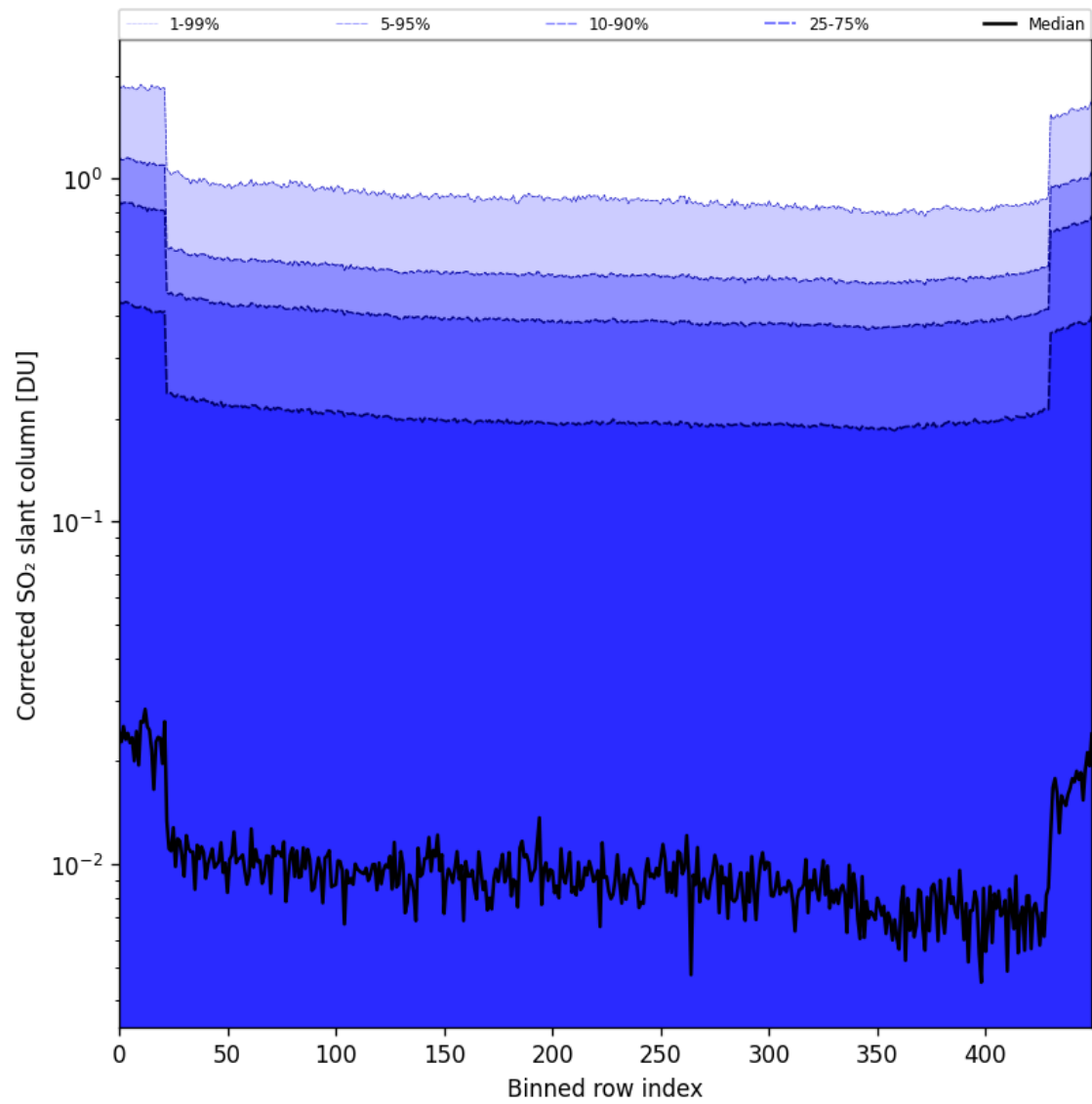
Figure 86: Along track statistics of “Corrected SO 2 slant column” for 2025-05-02 to 2025-05-04
