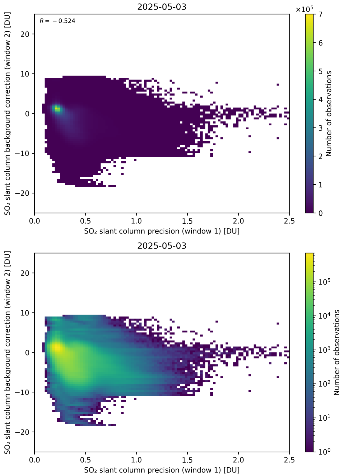
Figure 269: Scatter density plot of “SO 2 slant column precision (window 1)” against “SO 2 slant column background correction (window 2)” for 2025-05-02 to 2025-05-04.
