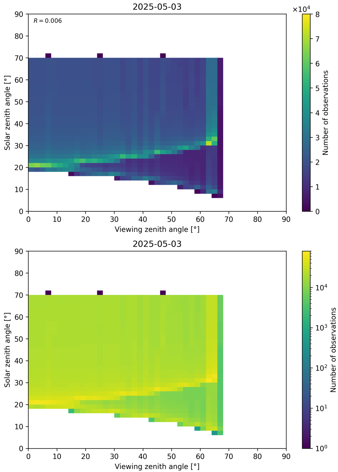
Figure 369: Scatter density plot of “Viewing zenith angle” against “Solar zenith angle” for 2025-05-02 to 2025-05-04.
