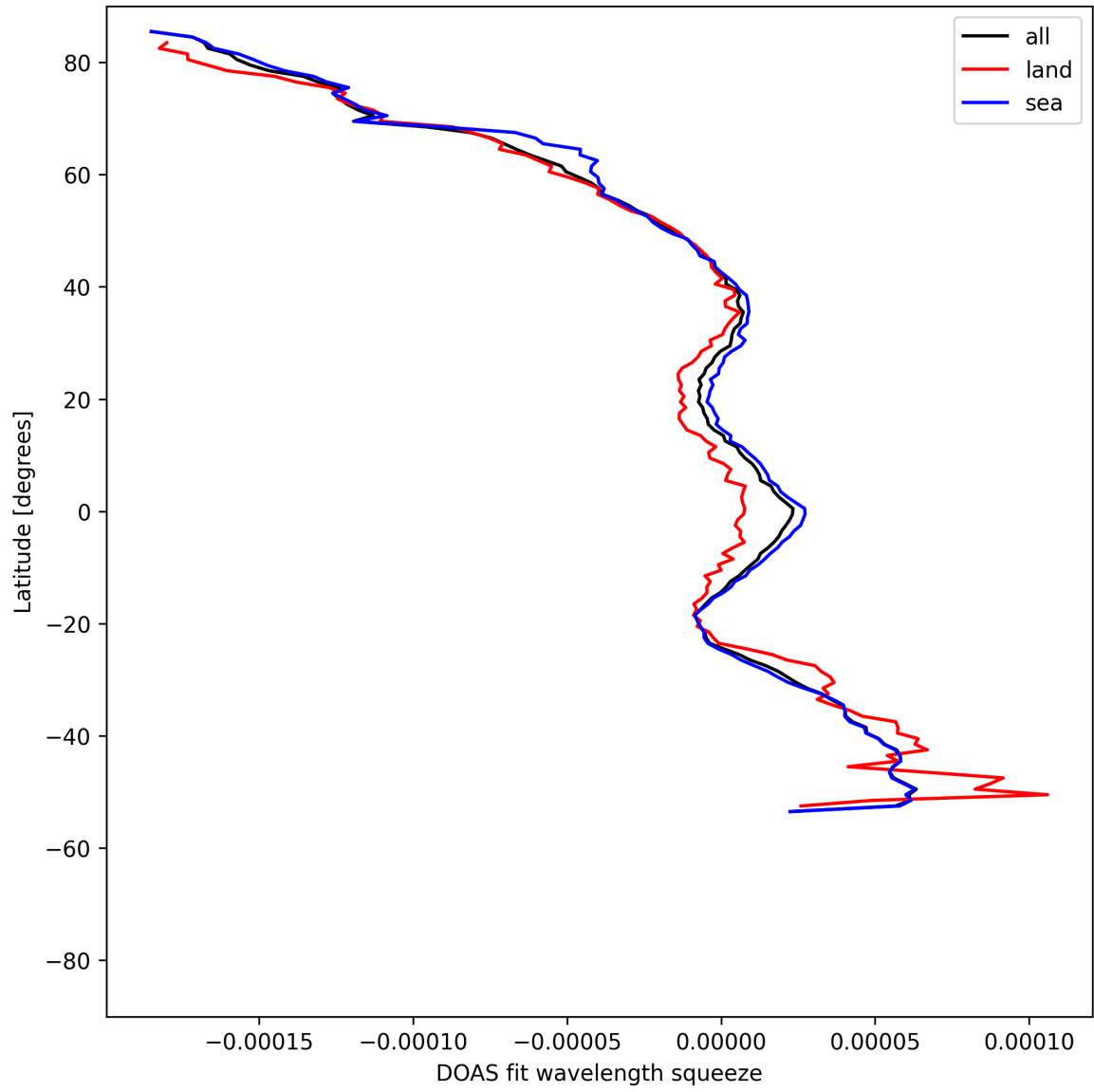
Figure 51: Zonal average of “DOAS fit wavelength squeeze” for 2025-05-02 to 2025-05-04.
