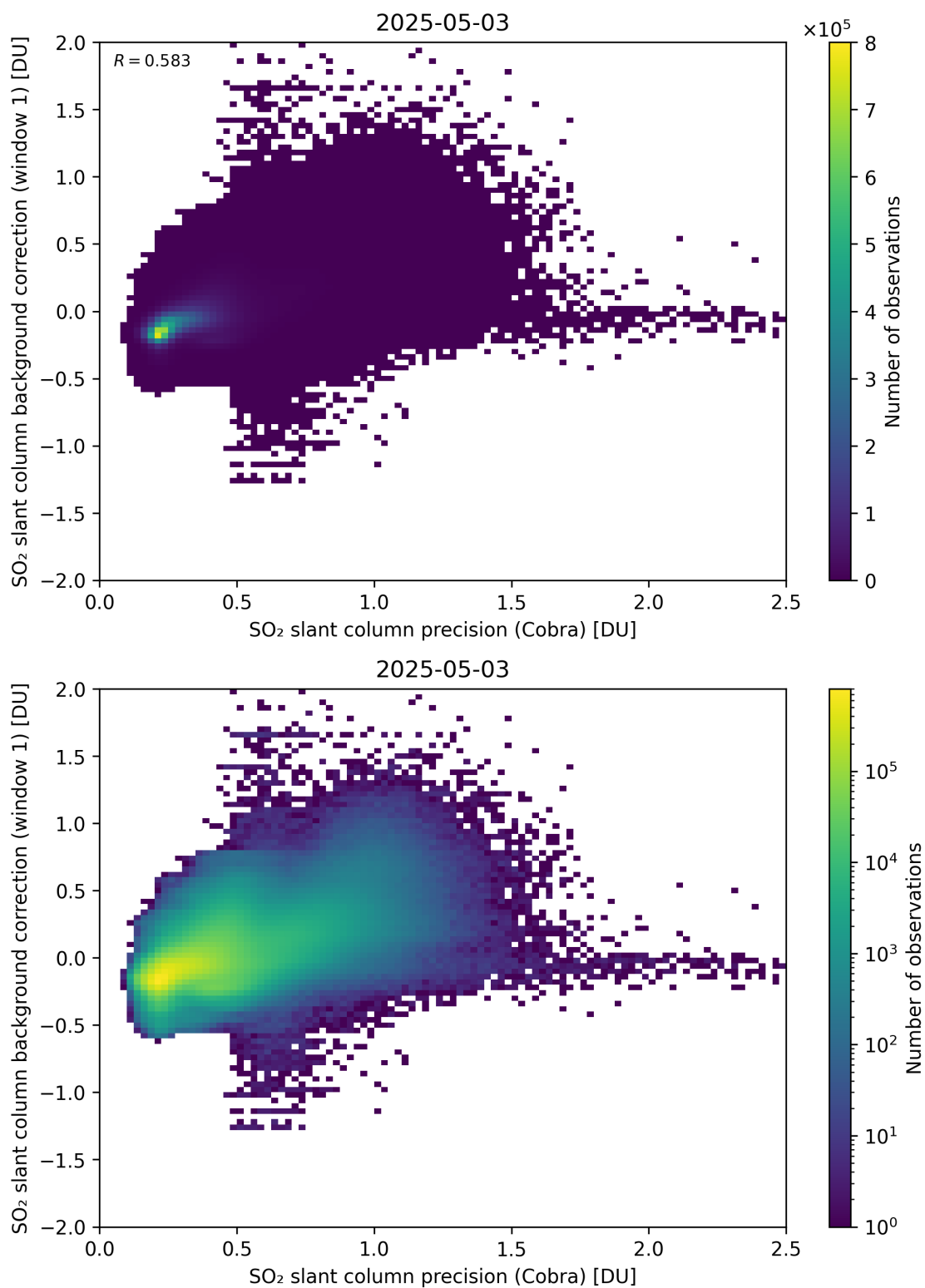
Figure 199: Scatter density plot of “SO 2 slant column precision (Cobra)” against “SO 2 slant column background correction (window 1)” for 2025-05-02 to 2025-05-04.
