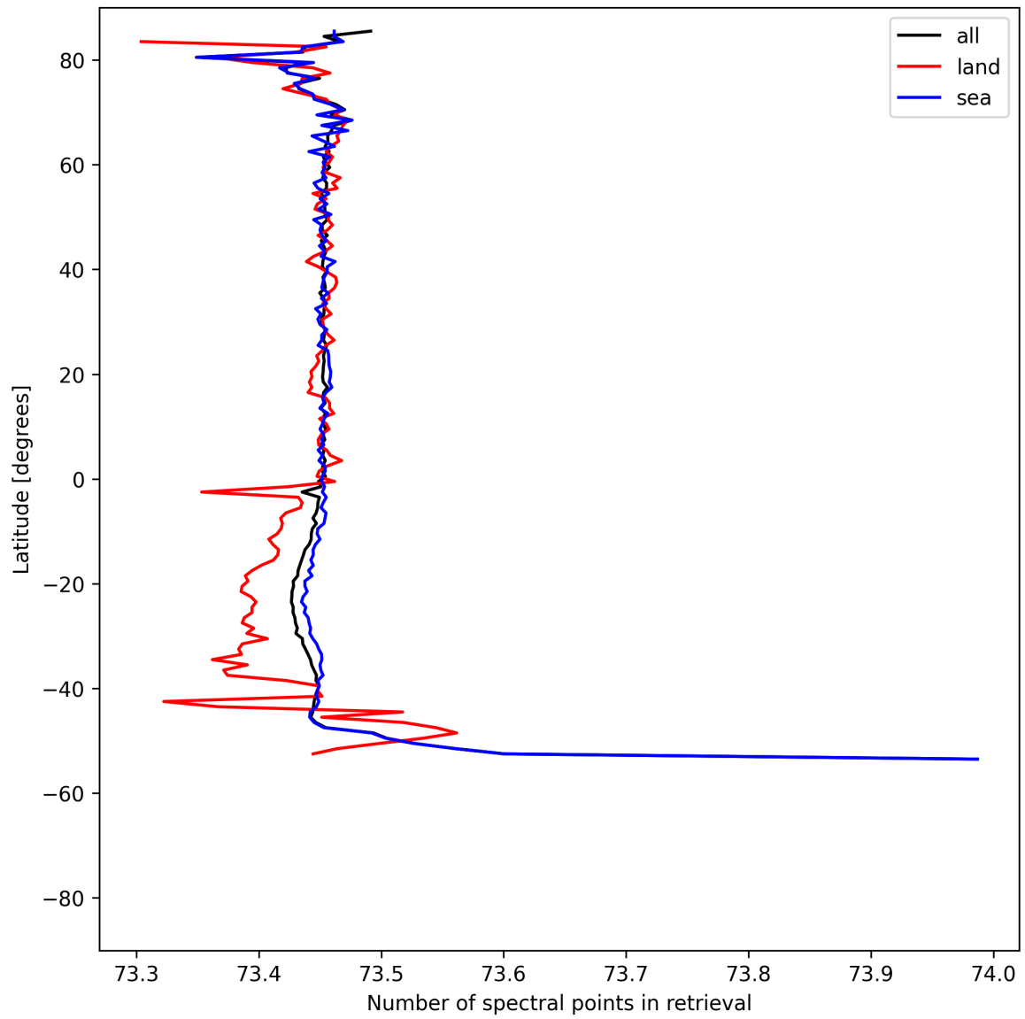
Figure 56: Zonal average of “Number of spectral points in retrieval” for 2025-05-02 to 2025-05-04.
