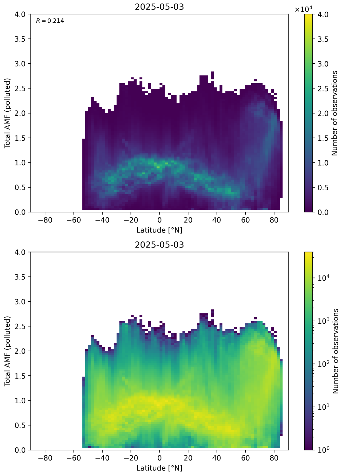
Figure 167: Scatter density plot of “Latitude” against “Total AMF (polluted)” for 2025-05-02 to 2025-05-04.
