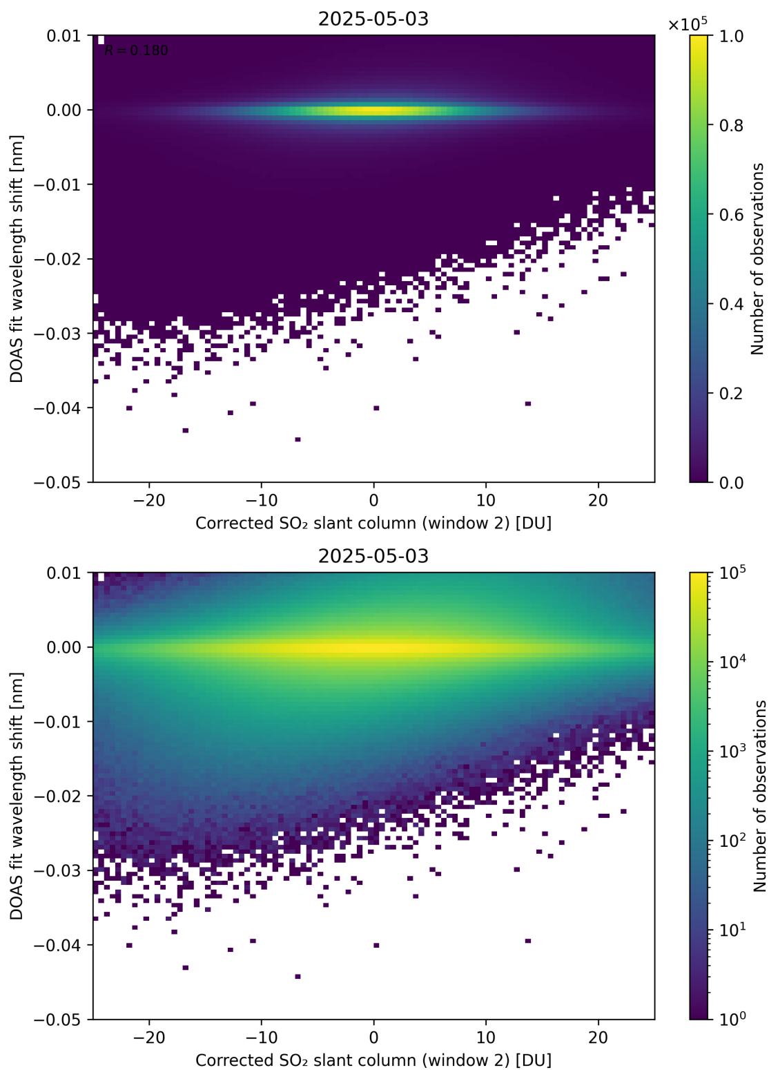
Figure 246: Scatter density plot of “Corrected SO 2 slant column (window 2)” against “DOAS fit wavelength shift” for 2025-05-02 to 2025-05-04.
