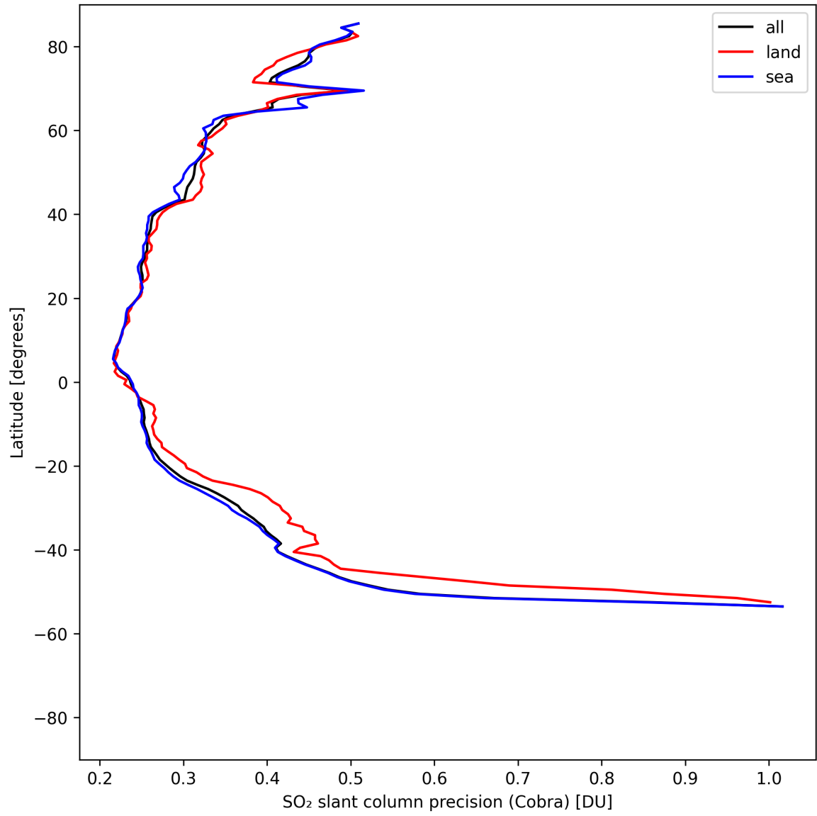
Figure 36: Zonal average of “SO 2 slant column precision (Cobra)” for 2025-05-02 to 2025-05-04.
