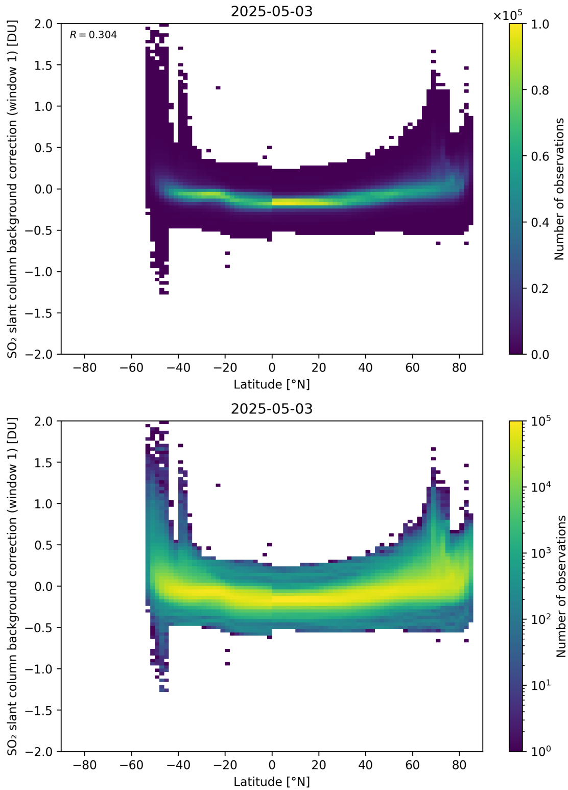
Figure 150: Scatter density plot of “Latitude” against “SO 2 slant column background correction (window 1)” for 2025-05-02 to 2025-05-04.
