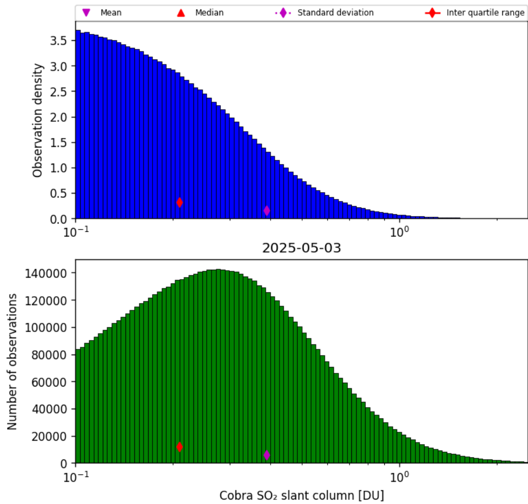
Figure 61: Histogram of “Cobra SO 2 slant column” for 2025-05-02 to 2025-05-04
