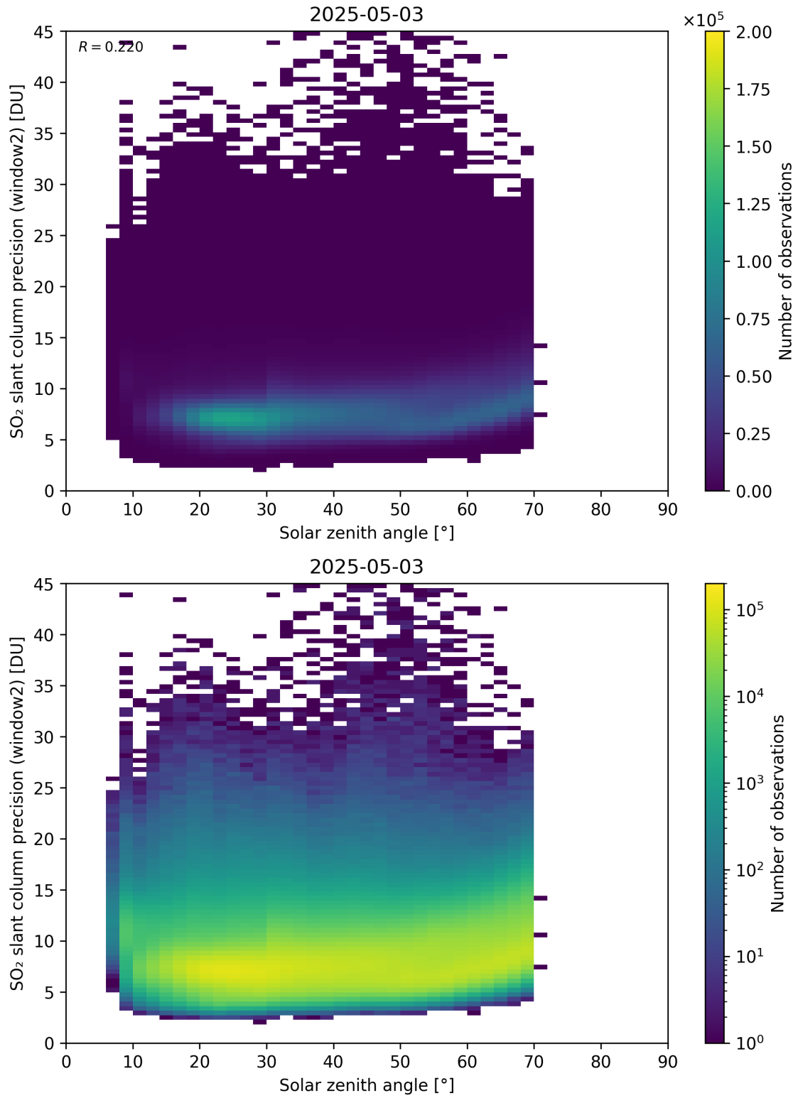
Figure 186: Scatter density plot of “Solar zenith angle” against “SO 2 slant column precision (window2)” for 2025-05-02 to 2025-05-04.
