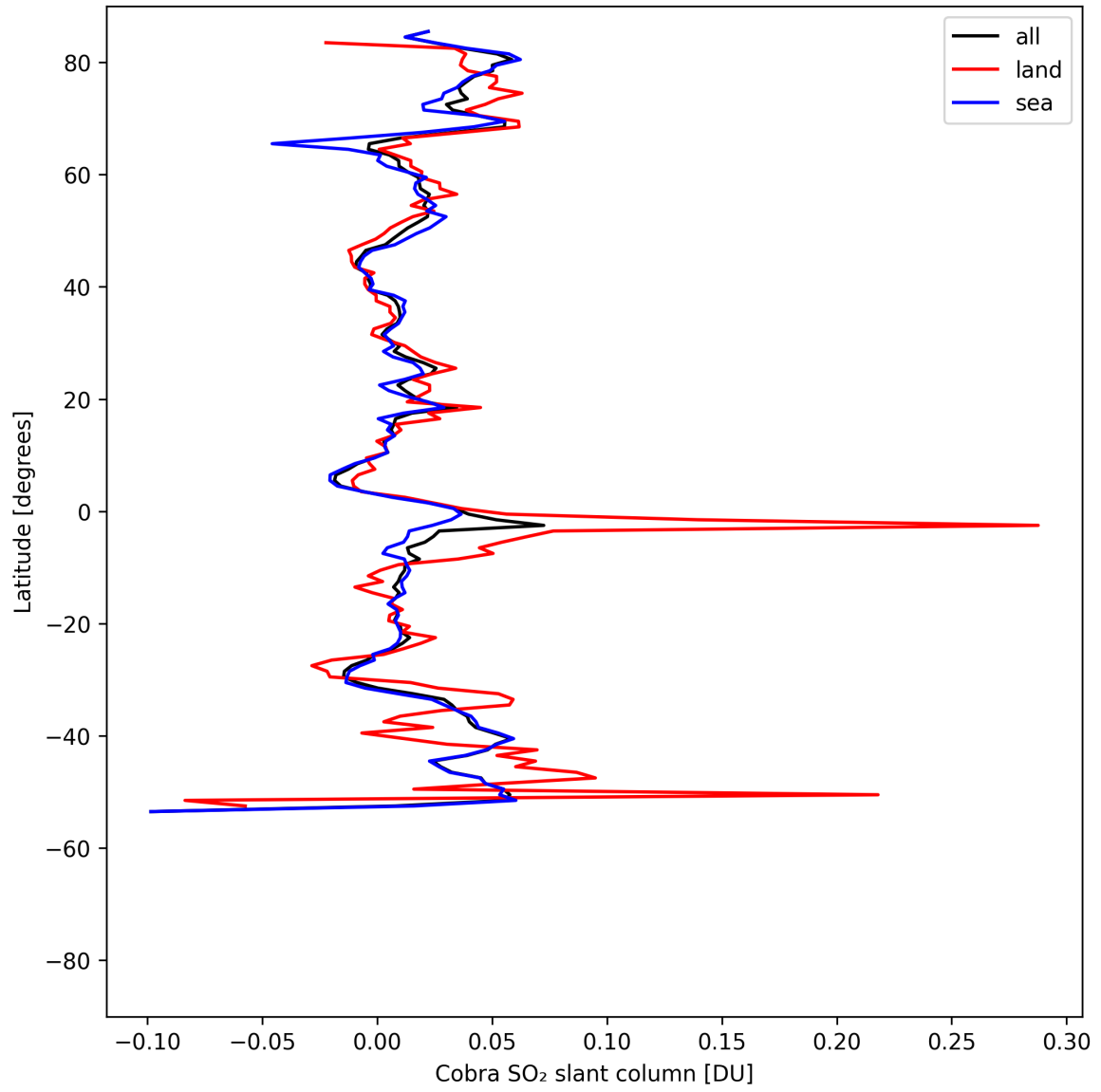
Figure 35: Zonal average of “Cobra SO 2 slant column” for 2025-05-02 to 2025-05-04.
