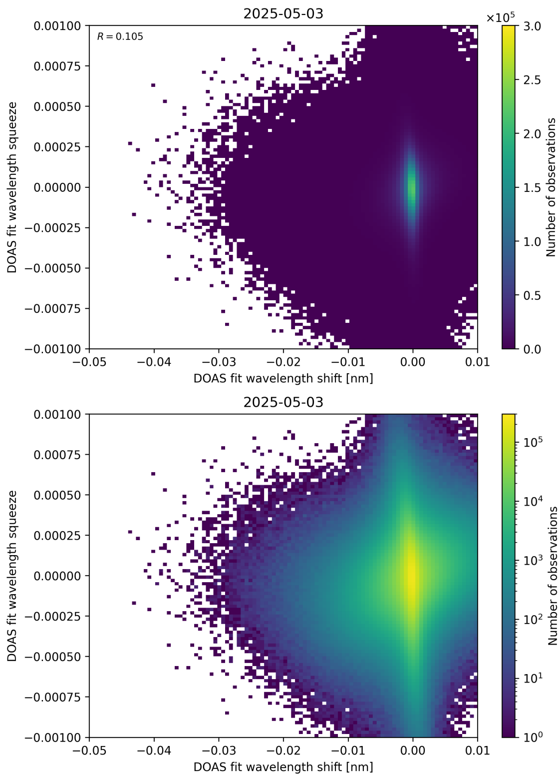
Figure 138: Scatter density plot of “DOAS fit wavelength shift” against “DOAS fit wavelength squeeze” for 2025-05-02 to 2025-05-04.
