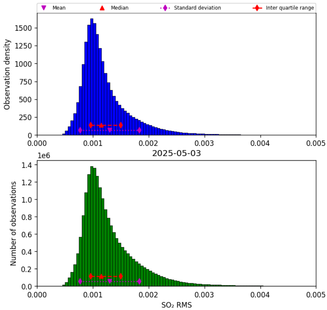
Figure 78: Histogram of “SO 2 RMS” for 2025-05-02 to 2025-05-04
