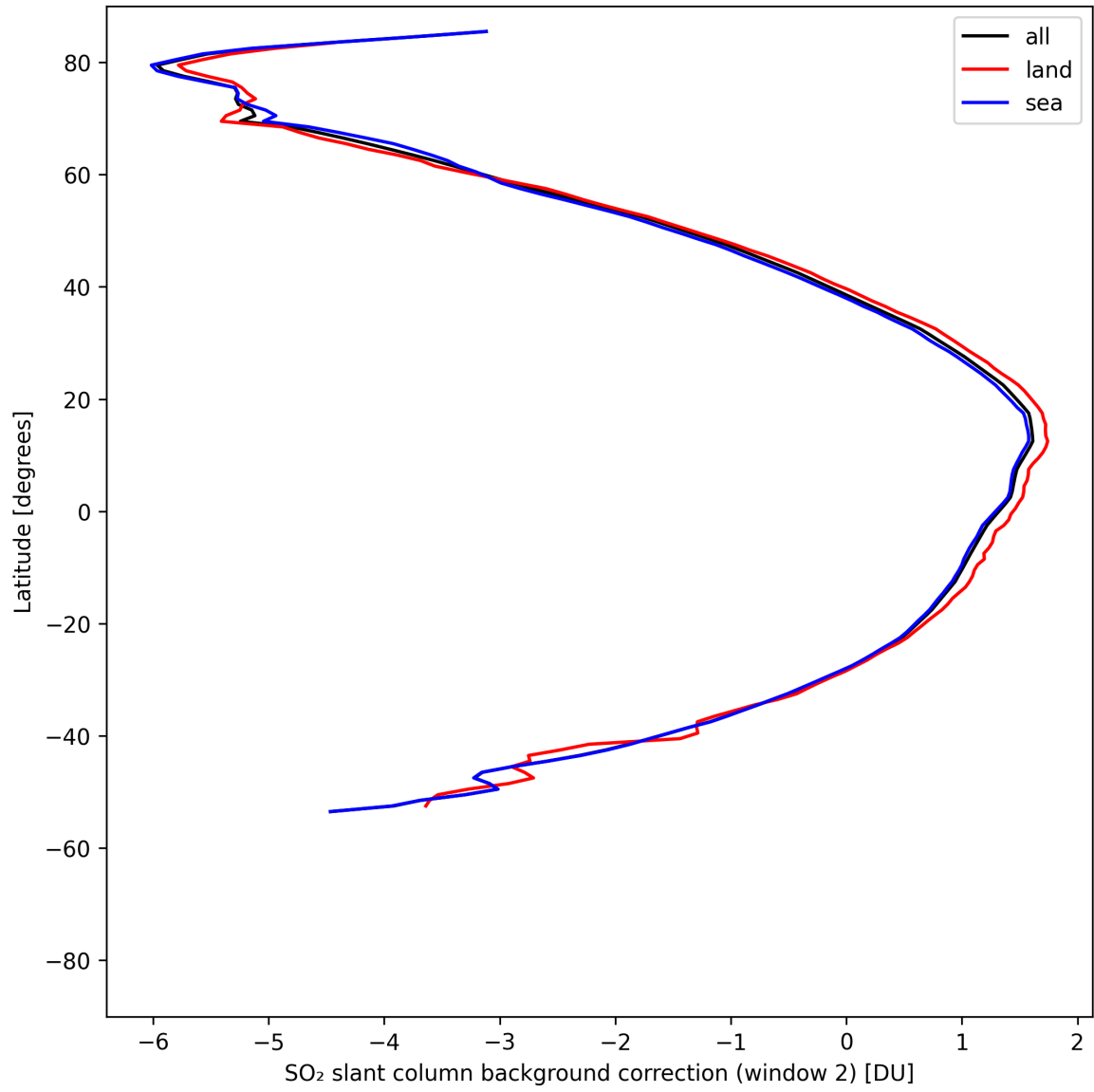
Figure 44: Zonal average of “SO 2 slant column background correction (window 2)” for 2025-05-02 to 2025-05-04.
