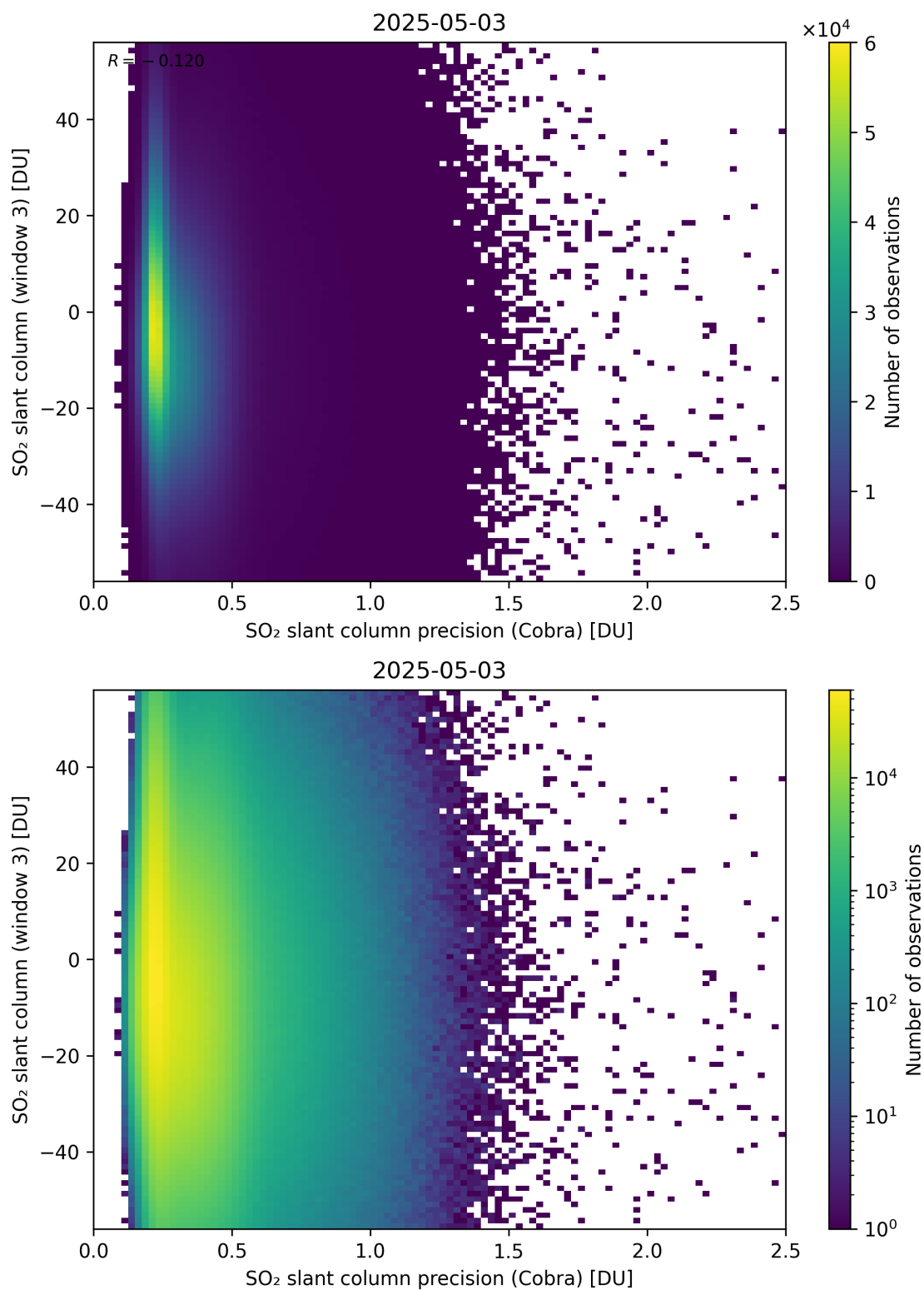
Figure 211: Scatter density plot of “SO 2 slant column precision (Cobra)” against “SO 2 slant column (window 3)” for 2025-05-02 to 2025-05-04.
