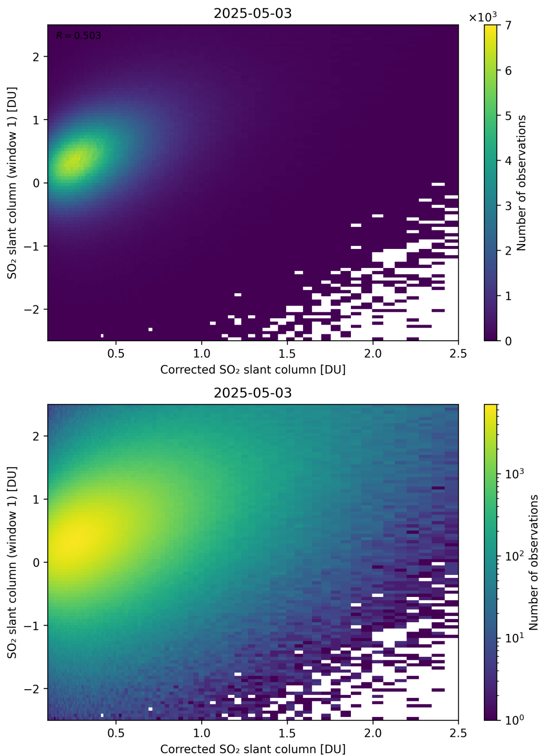
Figure 237: Scatter density plot of “Corrected SO 2 slant column” against “SO 2 slant column (window 1)” for 2025-05-02 to 2025-05-04.
