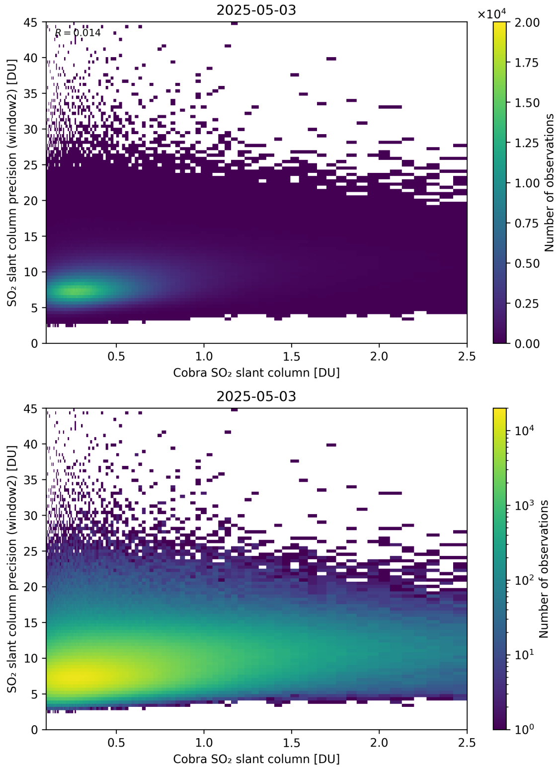
Figure 221: Scatter density plot of “Cobra SO 2 slant column” against “SO 2 slant column precision (window2)” for 2025-05-02 to 2025-05-04.
