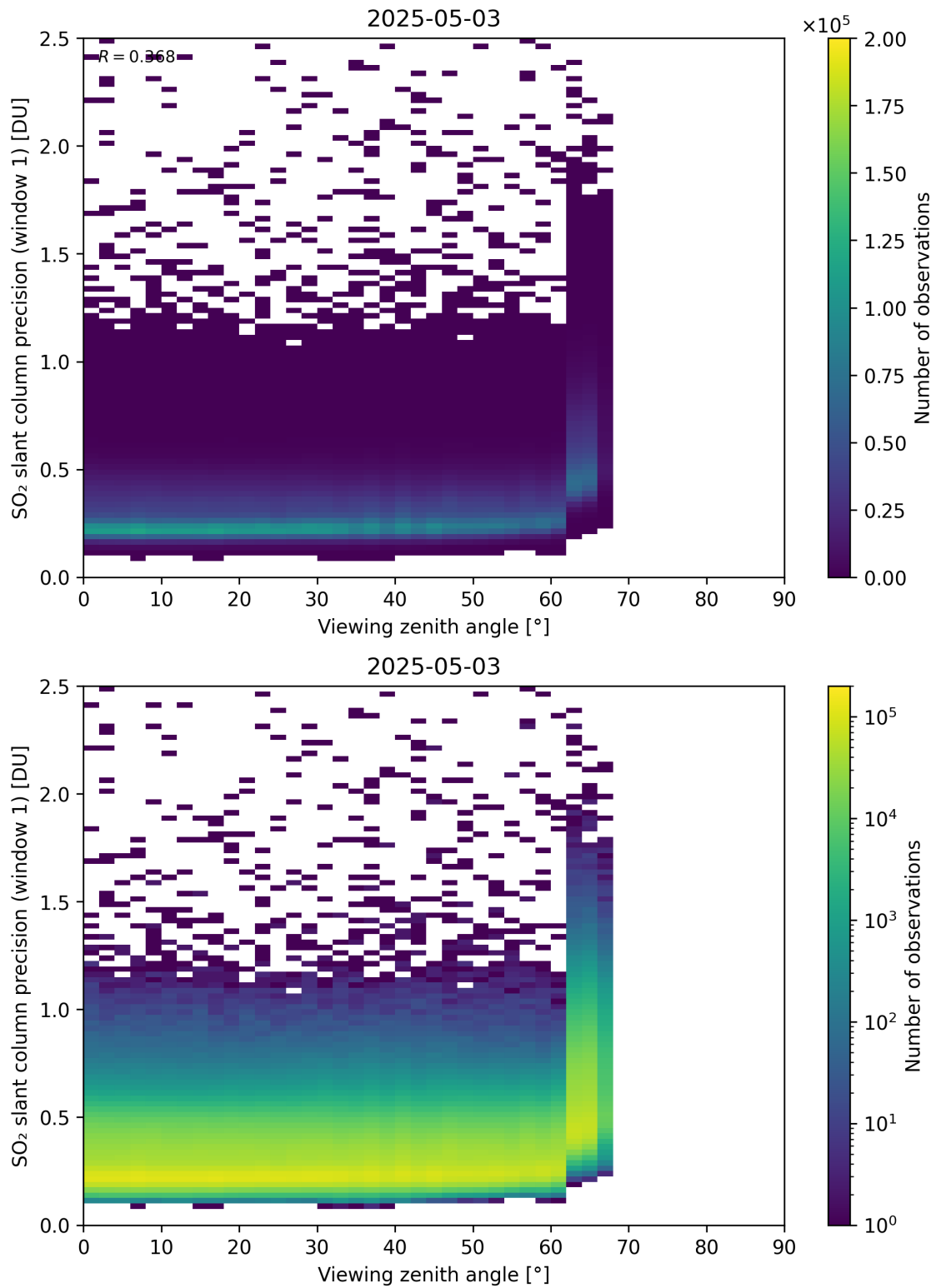
Figure 377: Scatter density plot of “Viewing zenith angle” against “SO 2 slant column precision (window 1)” for 2025-05-02 to 2025-05-04.
