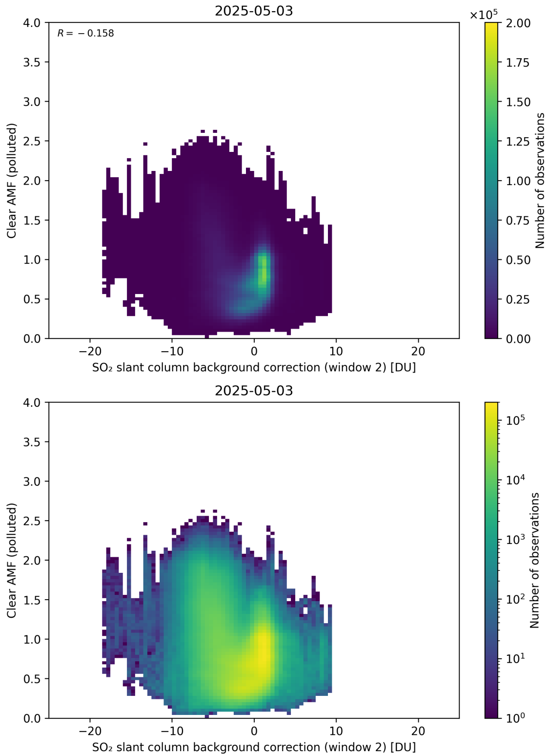
Figure 126: Scatter density plot of “SO 2 slant column background correction (window 2)” against “Clear AMF (polluted)” for 2025-05-02 to 2025-05-04.
