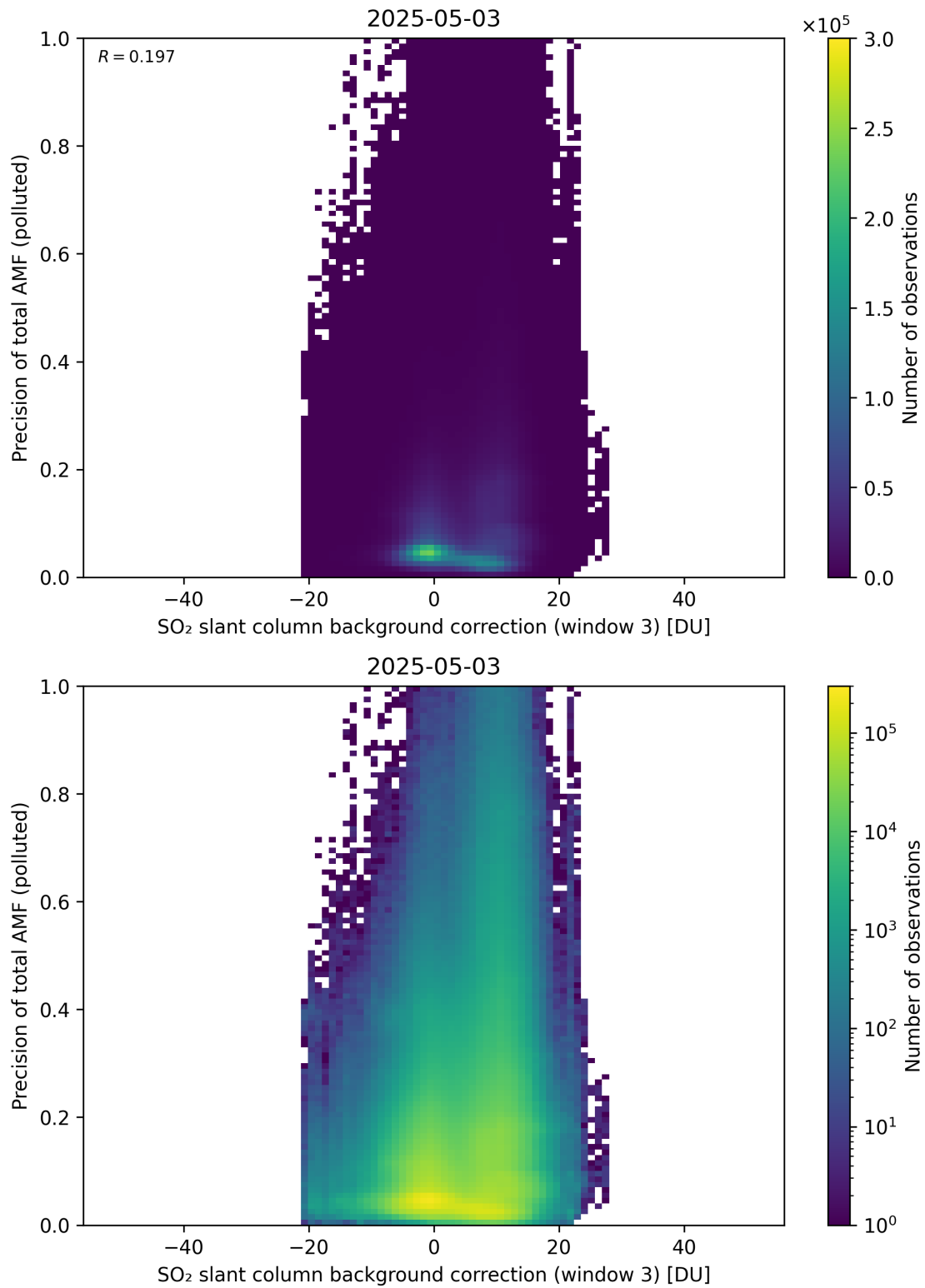
Figure 137: Scatter density plot of “SO 2 slant column background correction (window 3)” against “Precision of total AMF (polluted)” for 2025-05-02 to 2025-05-04.
