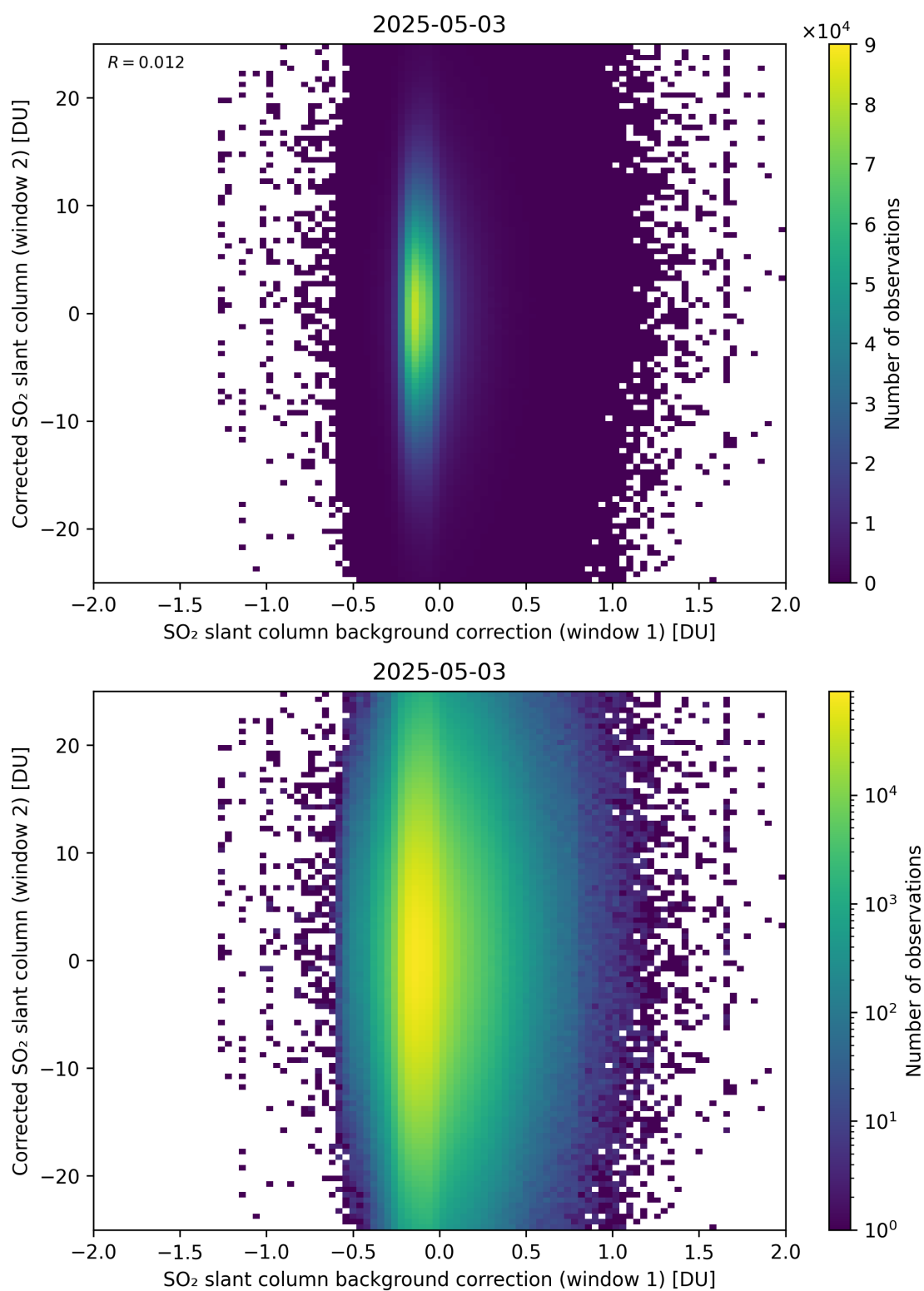
Figure 115: Scatter density plot of “SO 2 slant column background correction (window 1)” against “Corrected SO 2 slant column (window 2)” for 2025-05-02 to 2025-05-04.
