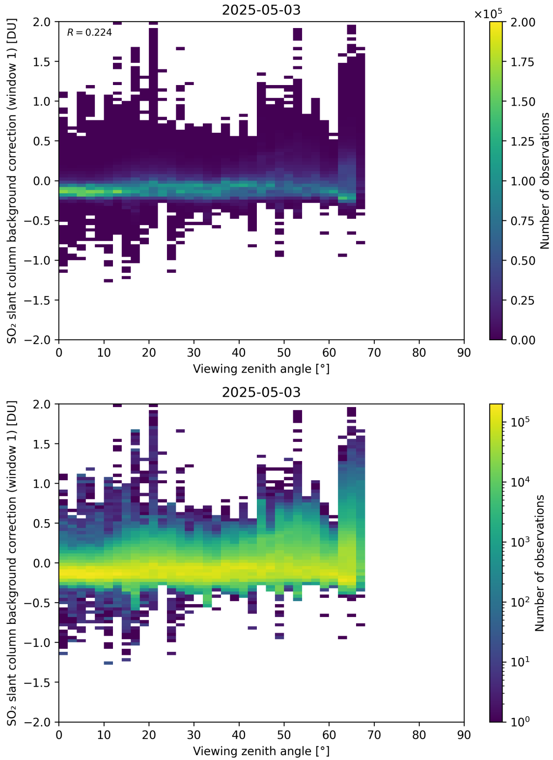
Figure 362: Scatter density plot of “Viewing zenith angle” against “SO 2 slant column background correction (window 1)” for 2025-05-02 to 2025-05-04.
