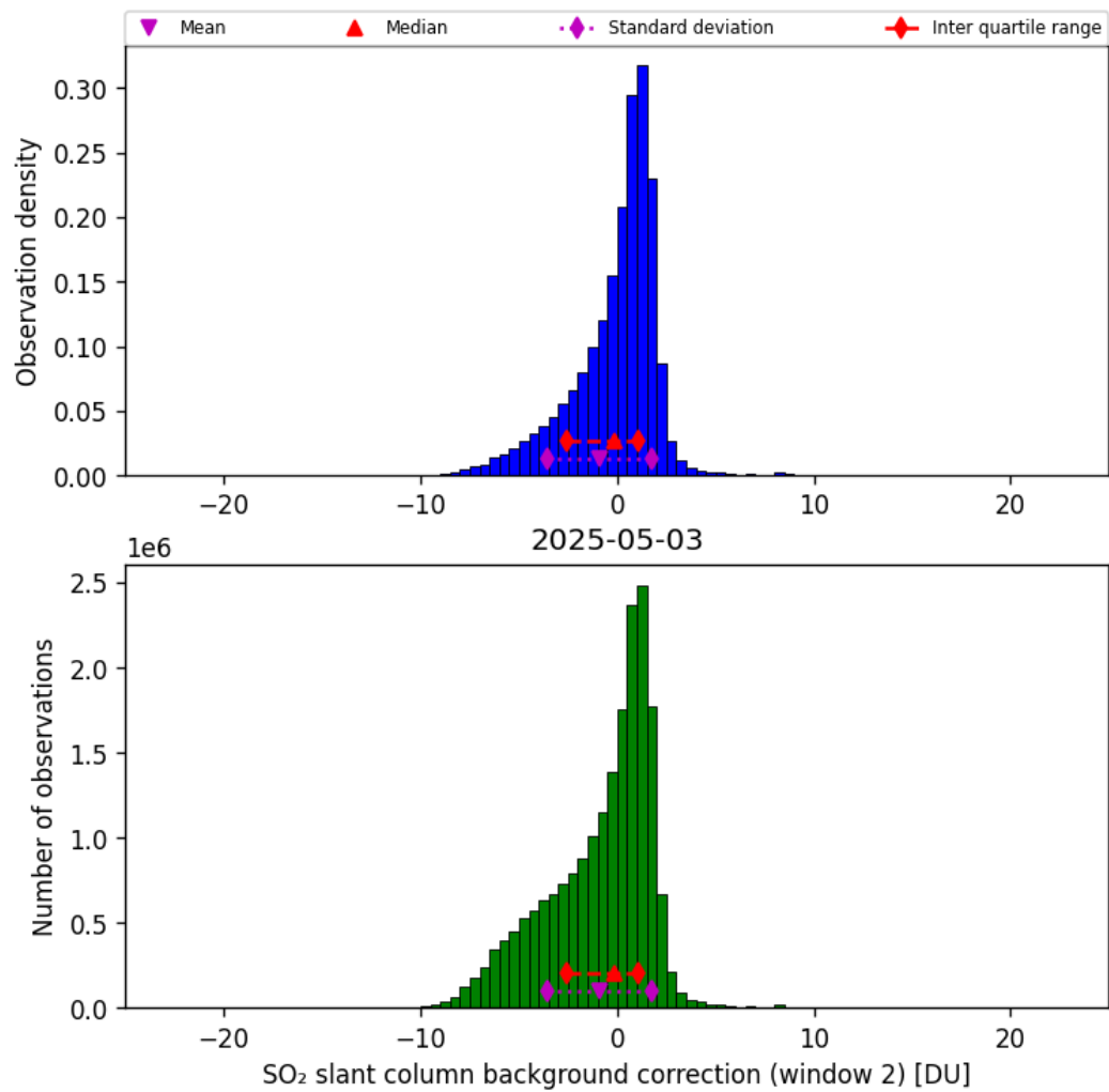
Figure 70: Histogram of “SO 2 slant column background correction (window 2)” for 2025-05-02 to 2025-05-04
