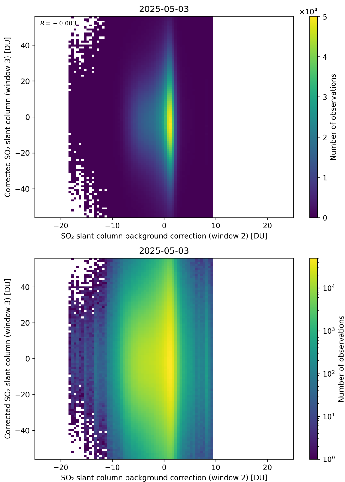
Figure 127: Scatter density plot of “SO 2 slant column background correction (window 2)” against “Corrected SO 2 slant column (window 3)” for 2025-05-02 to 2025-05-04.
