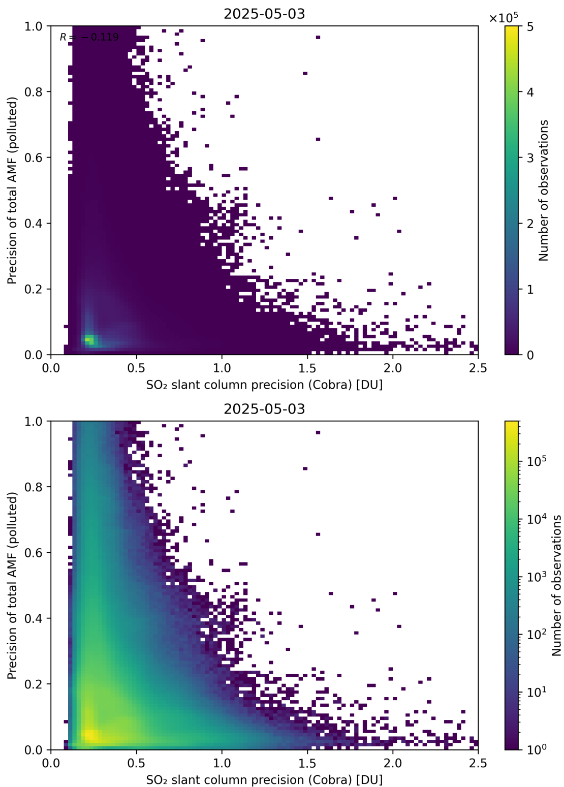
Figure 214: Scatter density plot of “SO 2 slant column precision (Cobra)” against “Precision of total AMF (polluted)” for 2025-05-02 to 2025-05-04.
