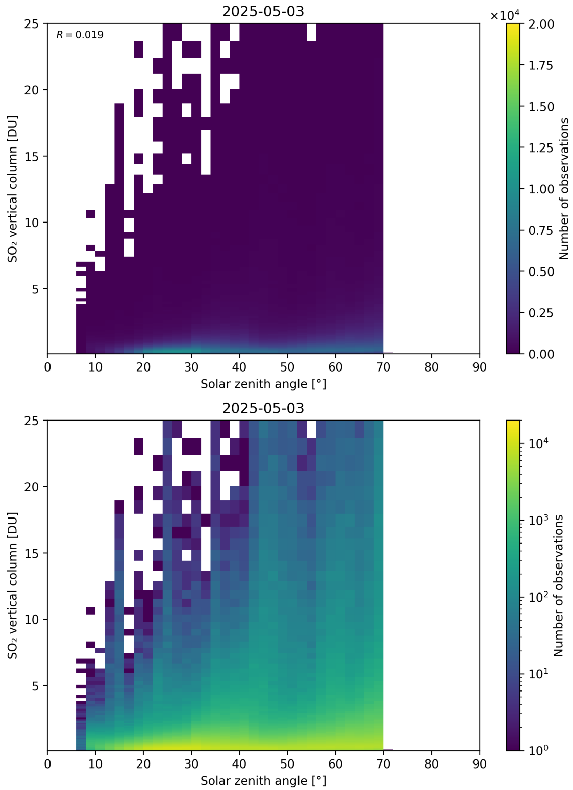
Figure 191: Scatter density plot of “Solar zenith angle” against “SO 2 vertical column” for 2025-05-02 to 2025-05-04.
