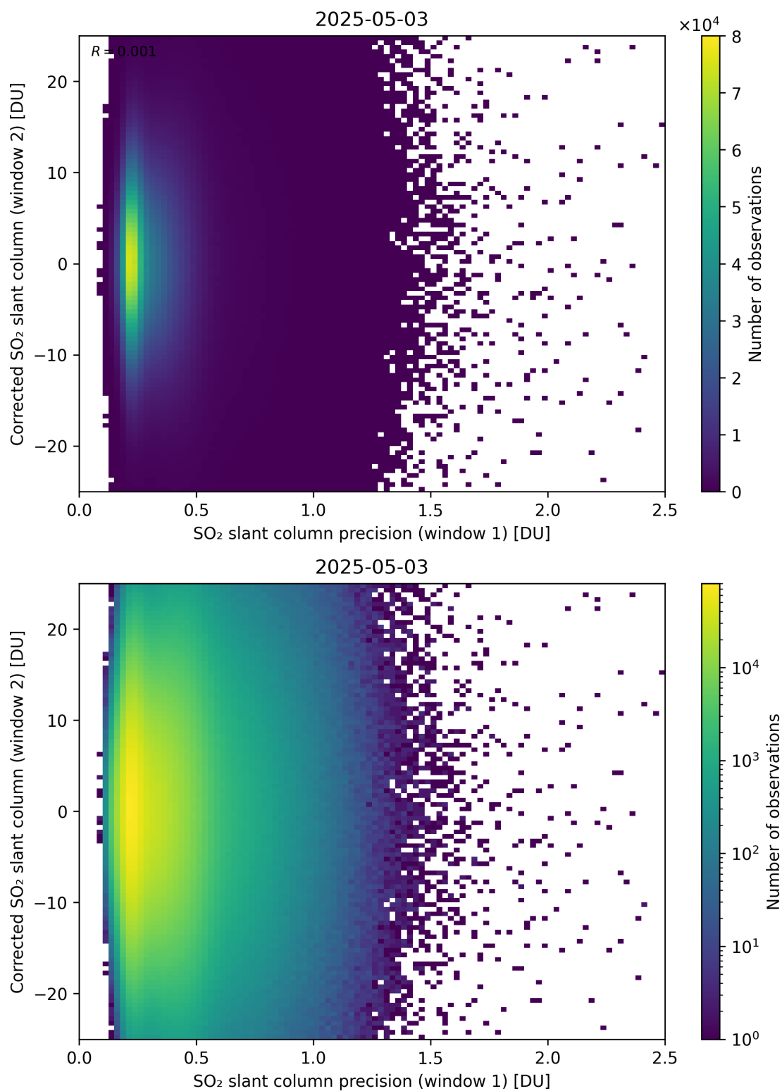
Figure 275: Scatter density plot of “SO 2 slant column precision (window 1)” against “Corrected SO 2 slant column (window 2)” for 2025-05-02 to 2025-05-04.
