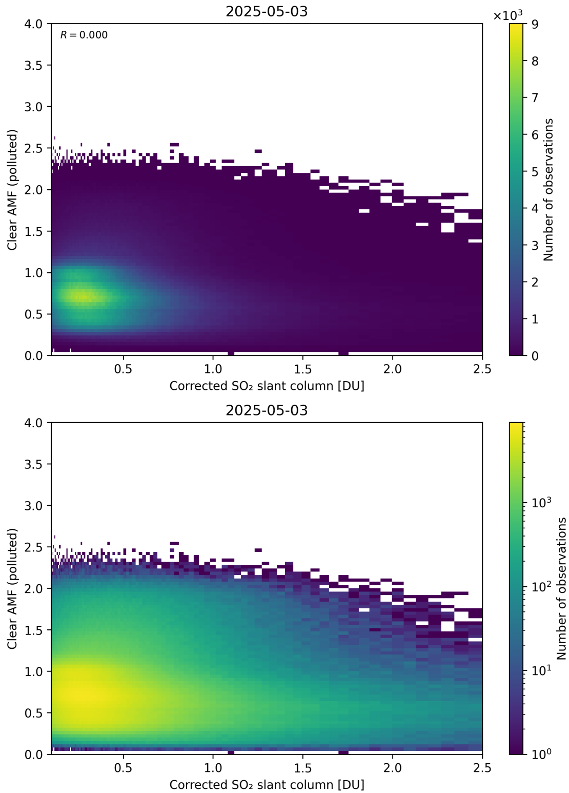
Figure 232: Scatter density plot of “Corrected SO 2 slant column” against “Clear AMF (polluted)” for 2025-05-02 to 2025-05-04.
