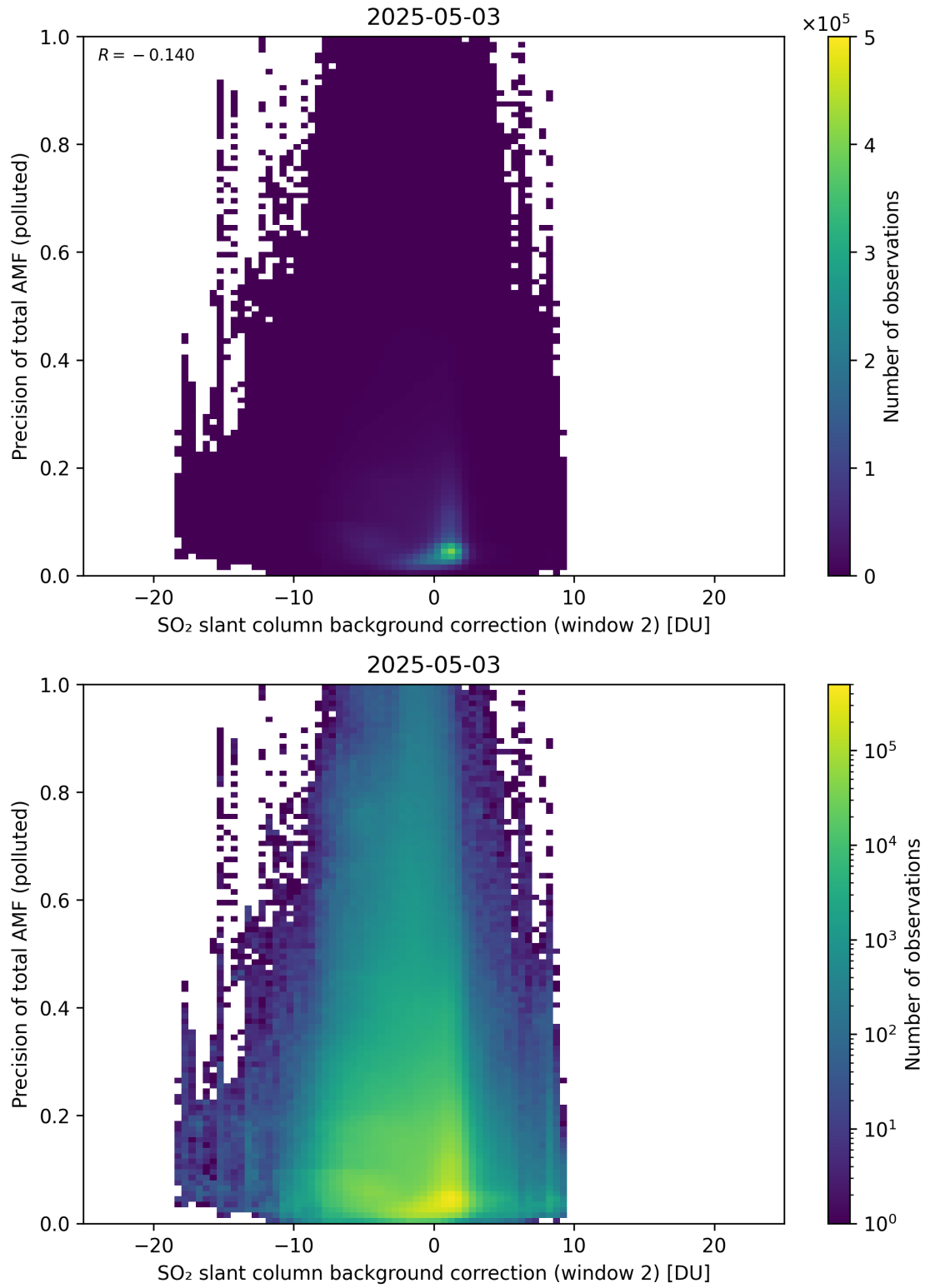
Figure 131: Scatter density plot of “SO 2 slant column background correction (window 2)” against “Precision of total AMF (polluted)” for 2025-05-02 to 2025-05-04.
