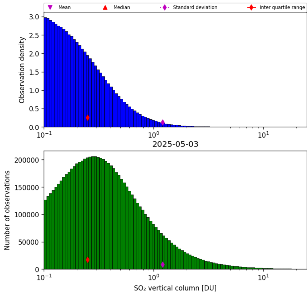
Figure 58: Histogram of “SO 2 vertical column” for 2025-05-02 to 2025-05-04
