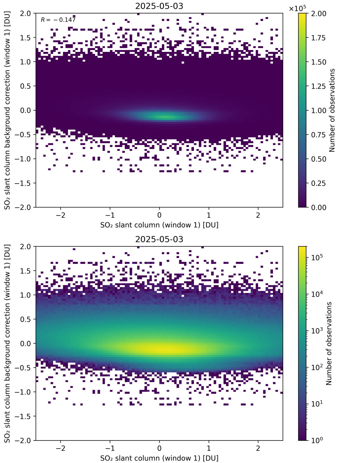
Figure 262: Scatter density plot of “SO 2 slant column (window 1)” against “SO 2 slant column background correction (window 1)” for 2025-05-02 to 2025-05-04.
