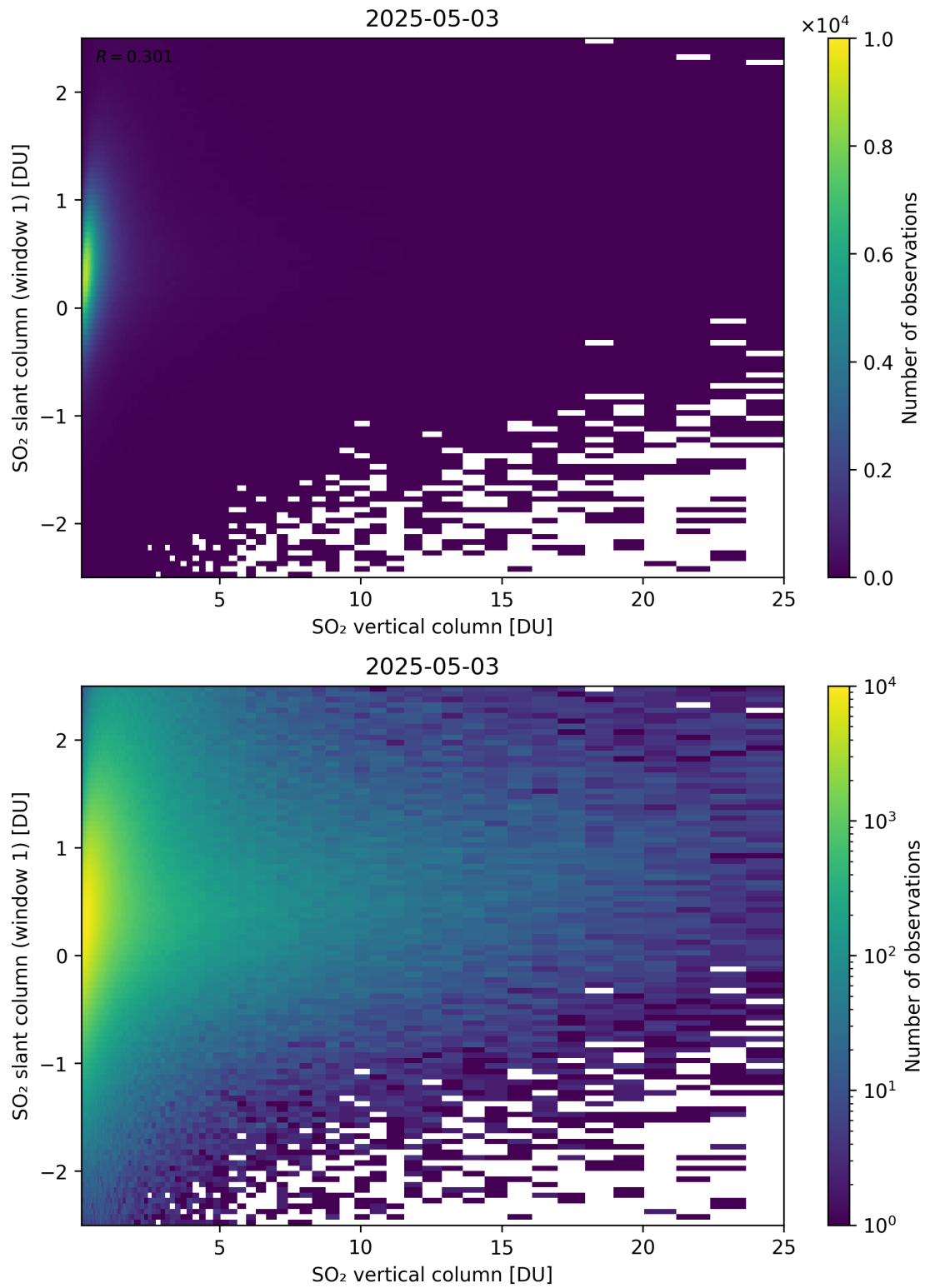
Figure 354: Scatter density plot of “SO 2 vertical column” against “SO 2 slant column (window 1)” for 2025-05-02 to 2025-05-04.
