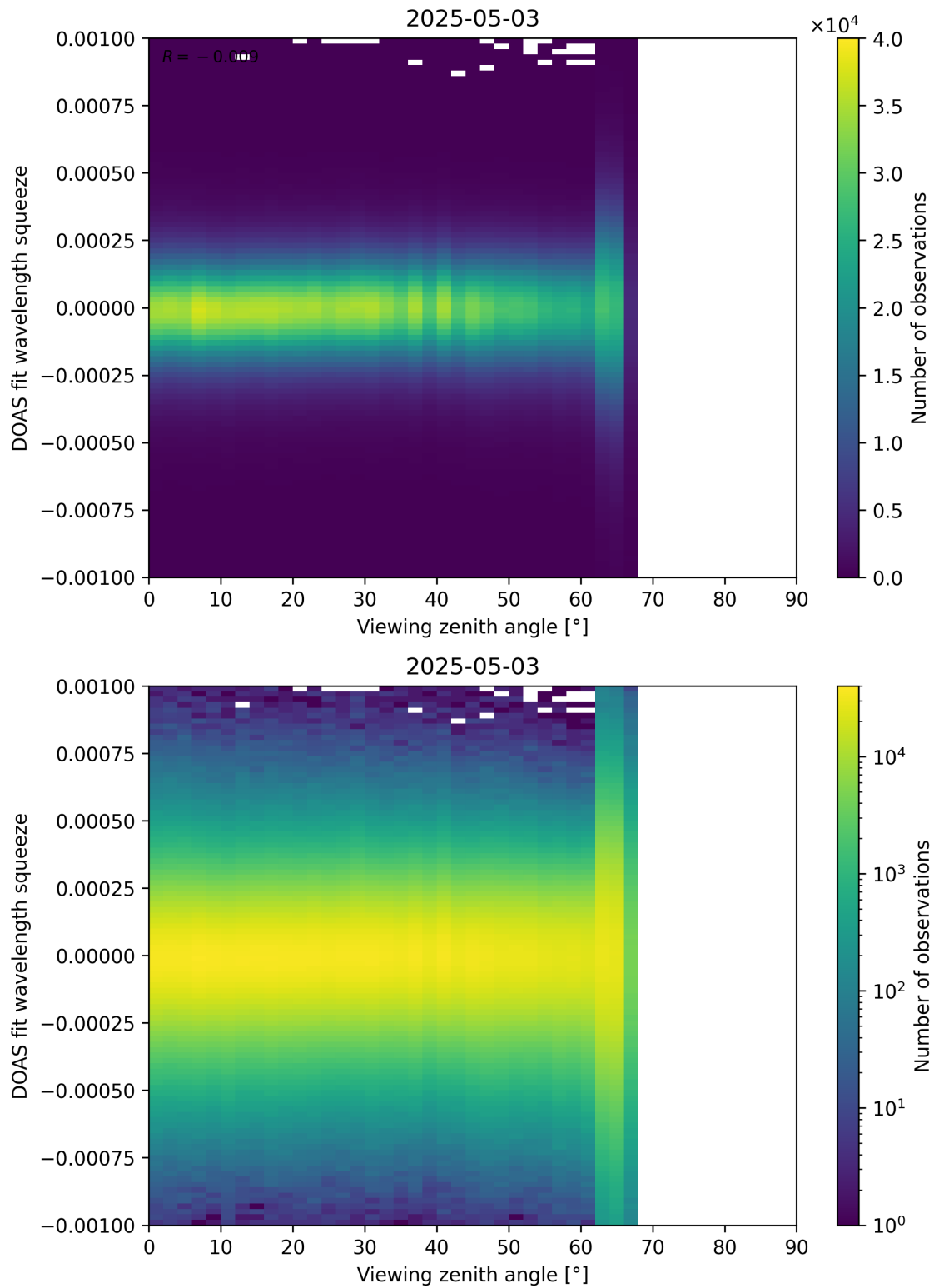
Figure 366: Scatter density plot of “Viewing zenith angle” against “DOAS fit wavelength squeeze” for 2025-05-02 to 2025-05-04.
