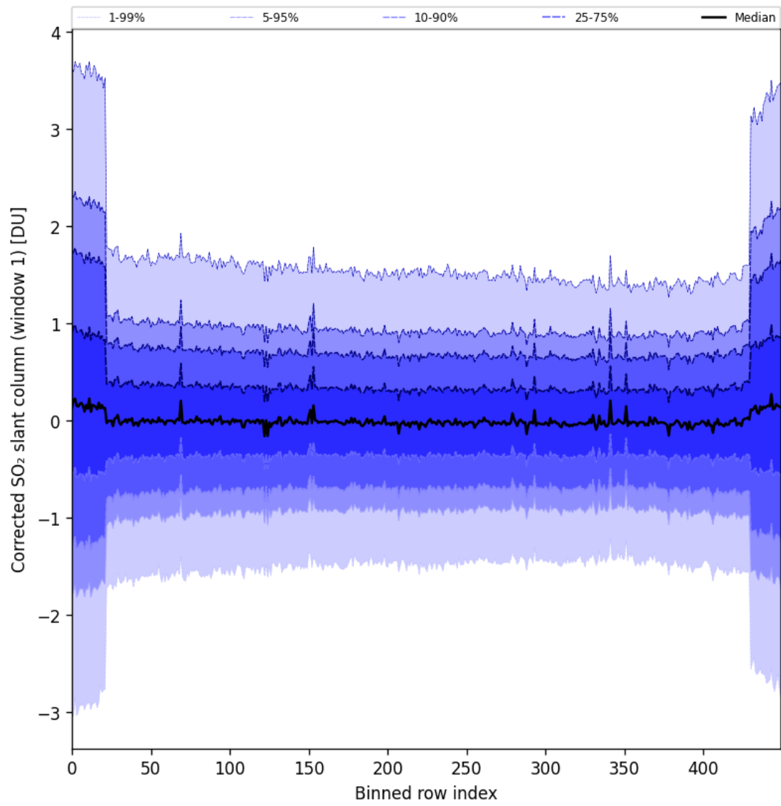
Figure 91: Along track statistics of “Corrected SO 2 slant column (window 1)” for 2025-05-02 to 2025-05-04
