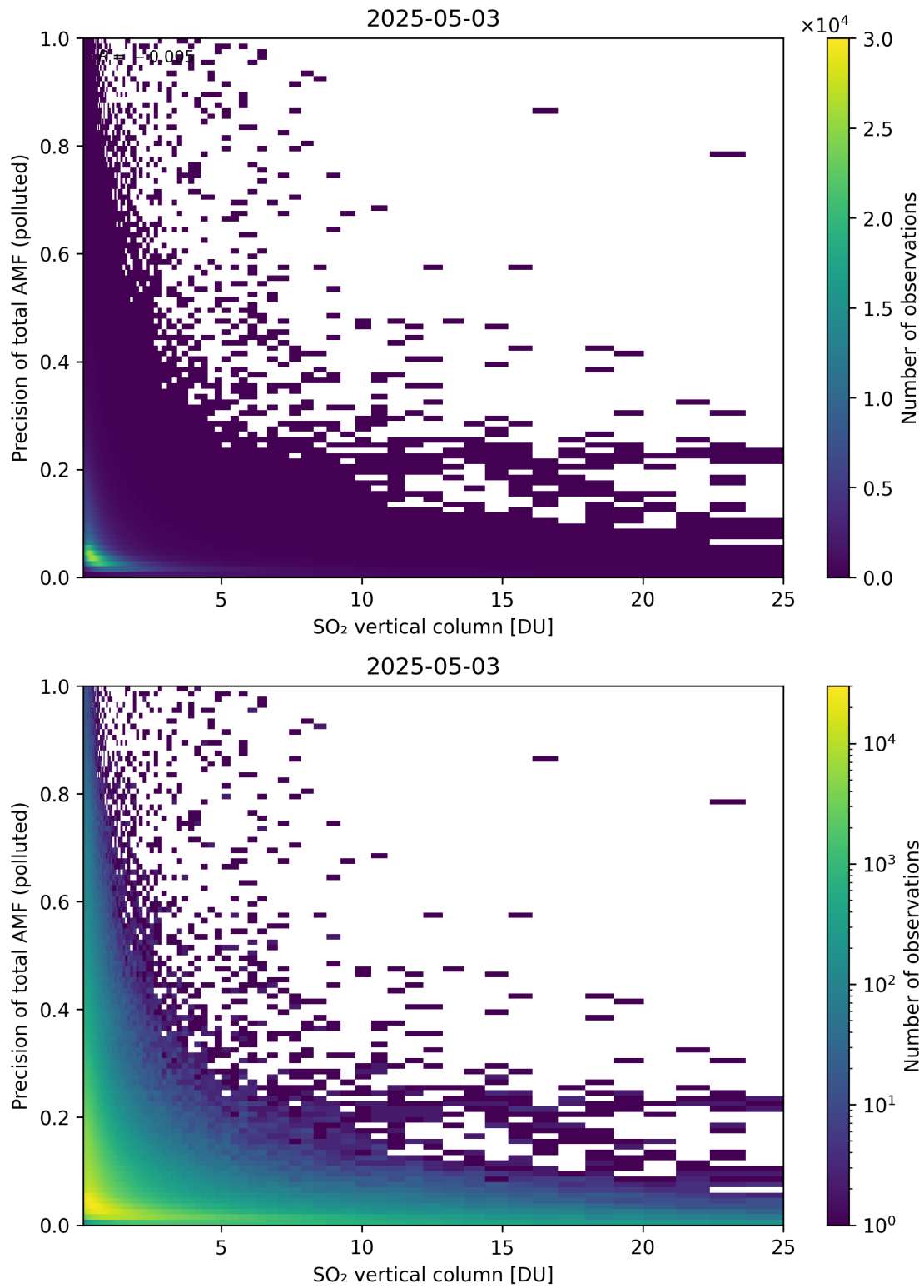
Figure 360: Scatter density plot of “SO 2 vertical column” against “Precision of total AMF (polluted)” for 2025-05-02 to 2025-05-04.
