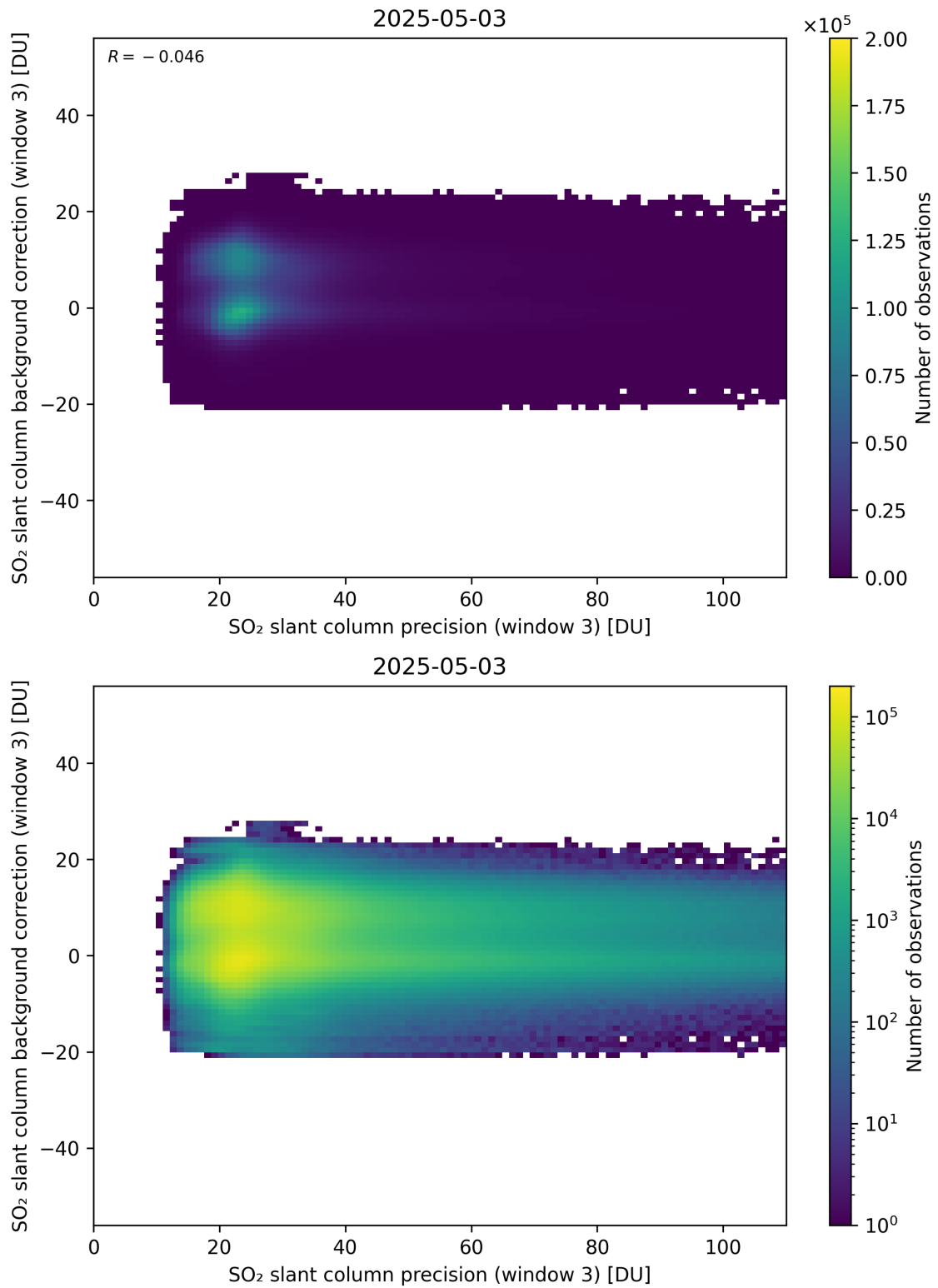
Figure 307: Scatter density plot of “SO 2 slant column precision (window 3)” against “SO 2 slant column background correction (window 3)” for 2025-05-02 to 2025-05-04.
