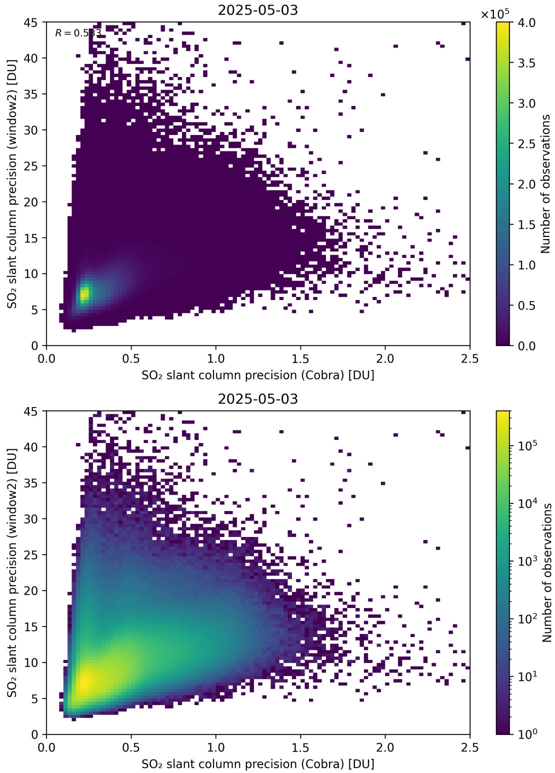
Figure 210: Scatter density plot of “SO 2 slant column precision (Cobra)” against “SO 2 slant column precision (window2)” for 2025-05-02 to 2025-05-04.
