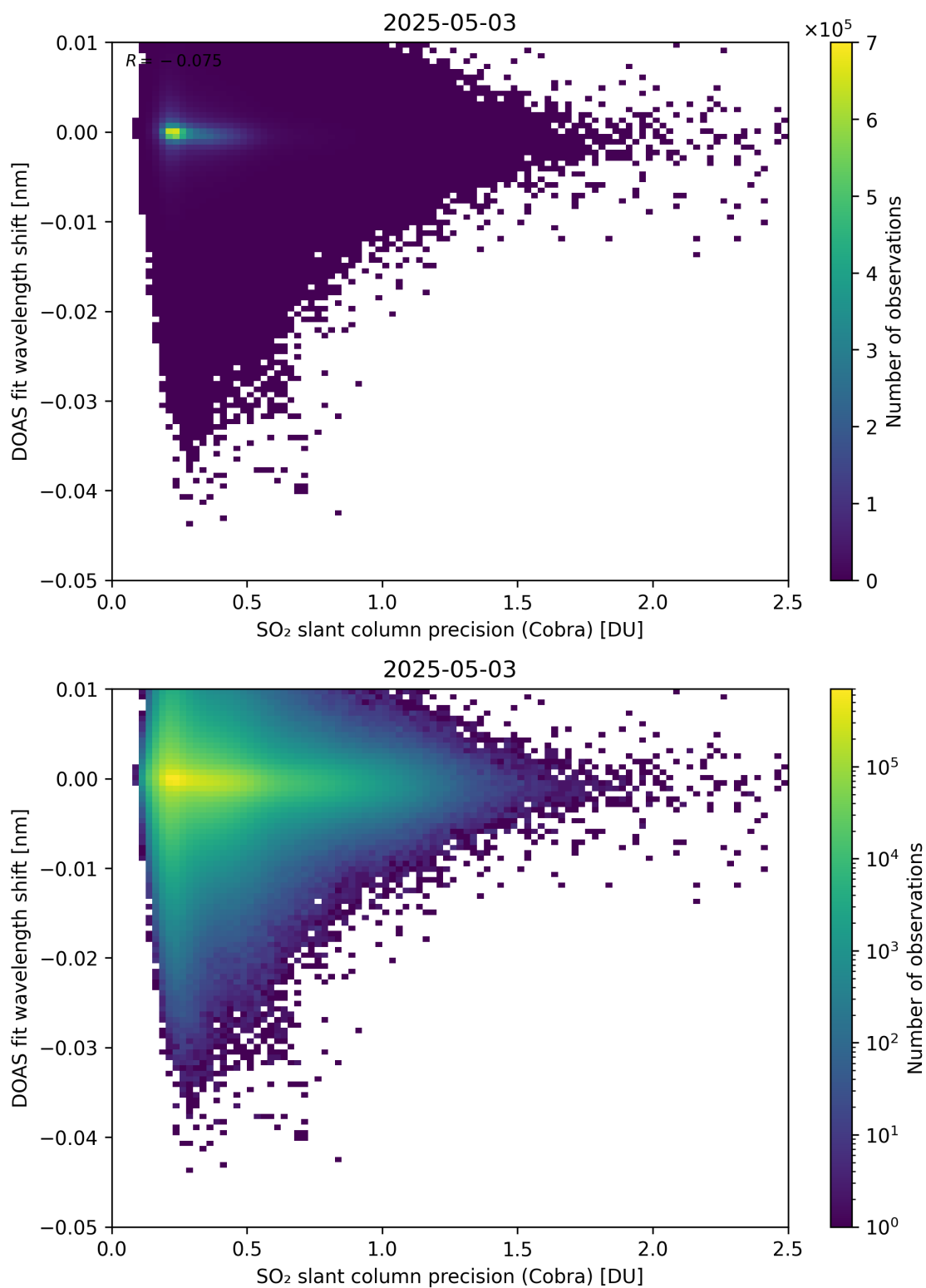
Figure 202: Scatter density plot of “SO 2 slant column precision (Cobra)” against “DOAS fit wavelength shift” for 2025-05-02 to 2025-05-04.
