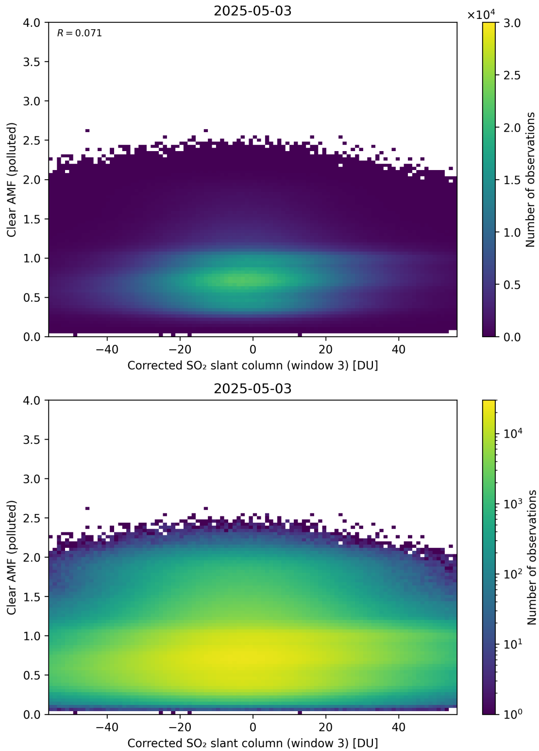
Figure 259: Scatter density plot of “Corrected SO 2 slant column (window 3)” against “Clear AMF (polluted)” for 2025-05-02 to 2025-05-04.
