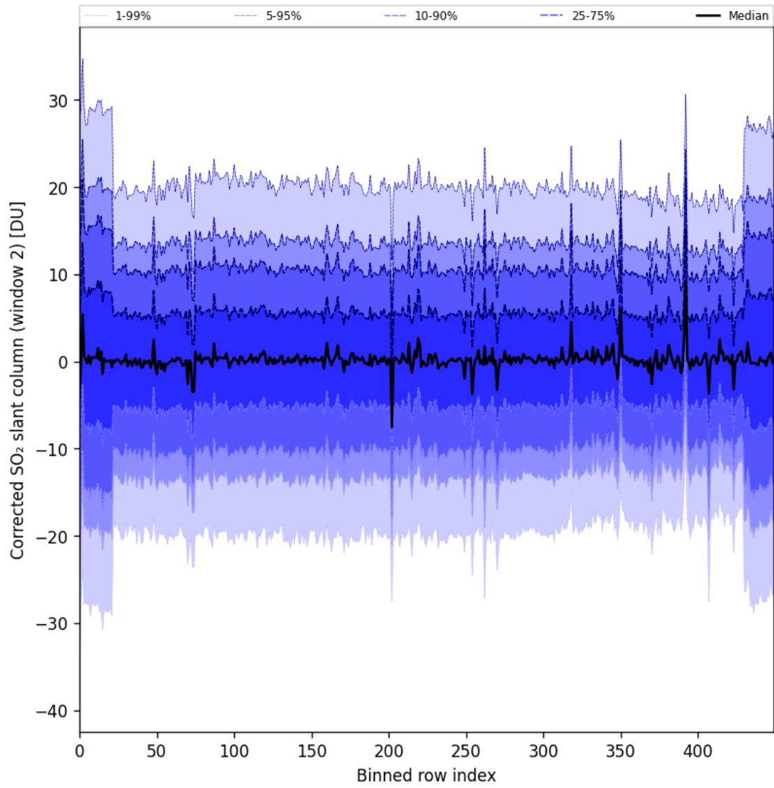
Figure 95: Along track statistics of “Corrected SO 2 slant column (window 2)” for 2025-05-02 to 2025-05-04
