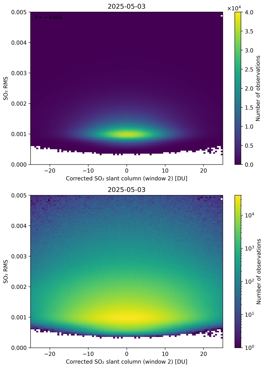
Figure 248: Scatter density plot of “Corrected SO 2 slant column (window 2)” against “SO 2 RMS” for 2025-05-02 to 2025-05-04.
