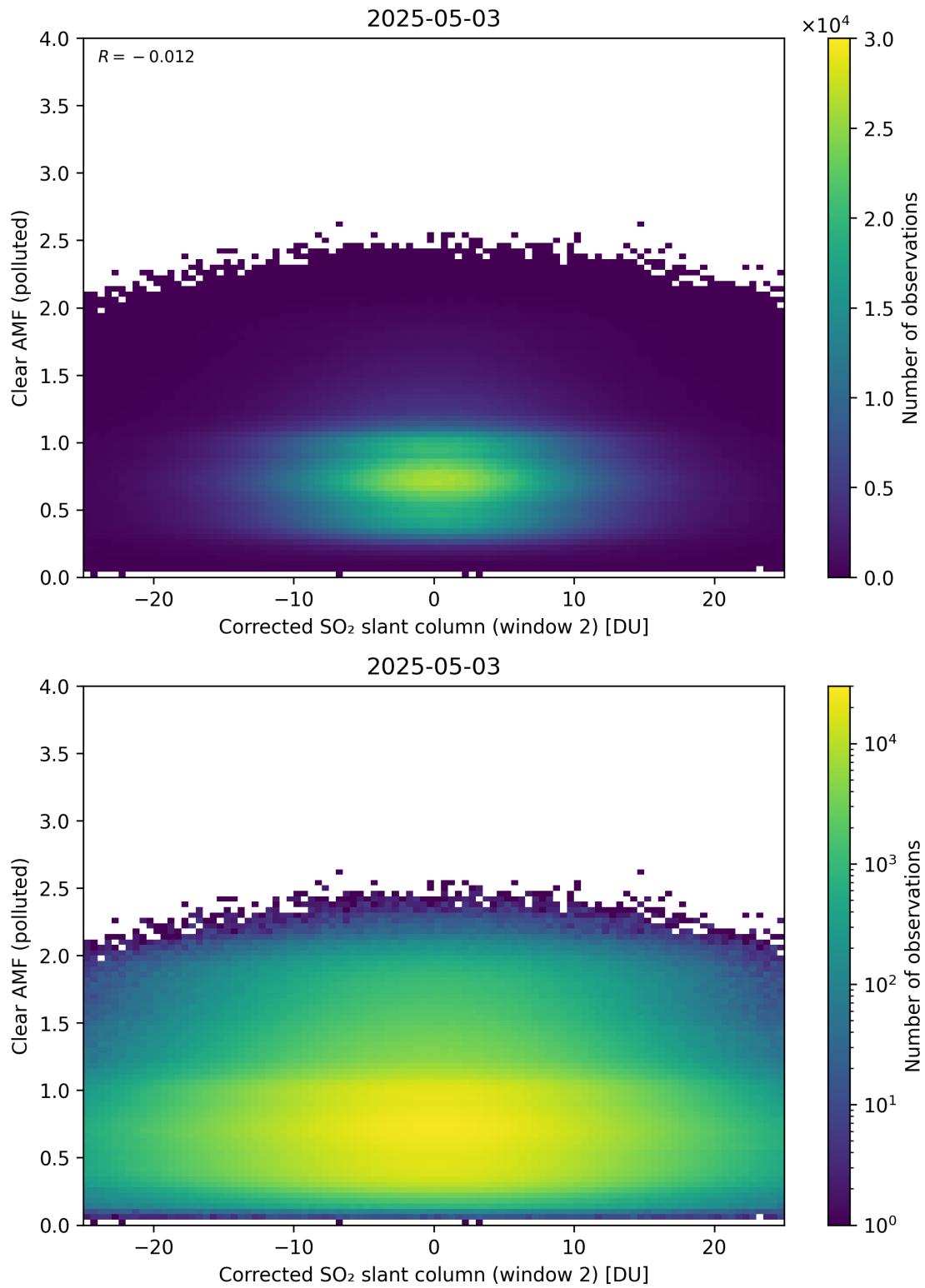
Figure 249: Scatter density plot of “Corrected SO 2 slant column (window 2)” against “Clear AMF (polluted)” for 2025-05-02 to 2025-05-04.
