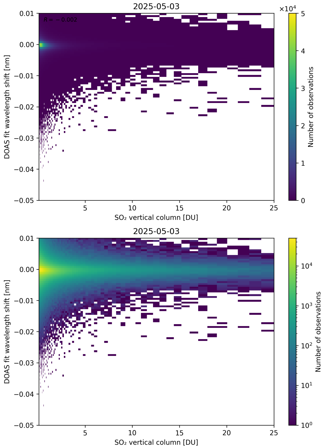
Figure 326: Scatter density plot of “SO 2 vertical column” against “DOAS fit wavelength shift” for 2025-05-02 to 2025-05-04.
