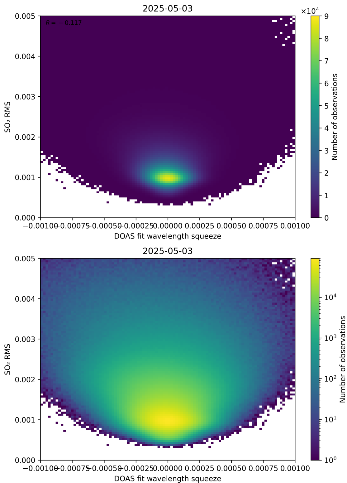
Figure 143: Scatter density plot of “DOAS fit wavelength squeeze” against “SO 2 RMS” for 2025-05-02 to 2025-05-04.
