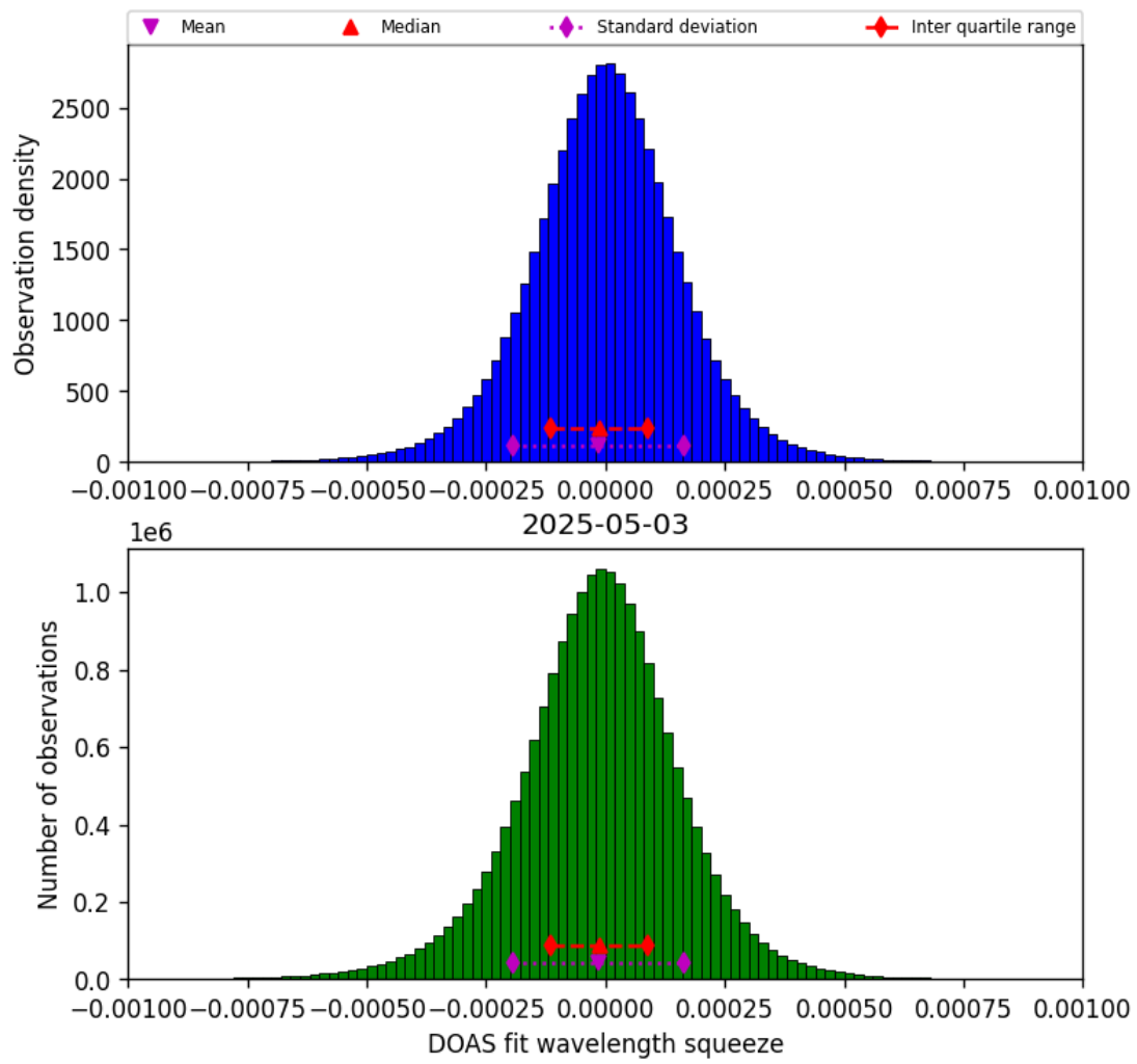
Figure 77: Histogram of “DOAS fit wavelength squeeze” for 2025-05-02 to 2025-05-04
