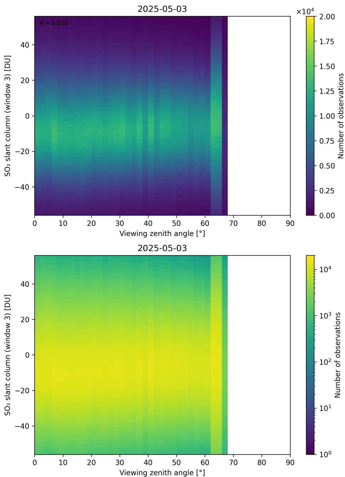
Figure 379: Scatter density plot of “Viewing zenith angle” against “SO 2 slant column (window 3)” for 2025-05-02 to 2025-05-04.
