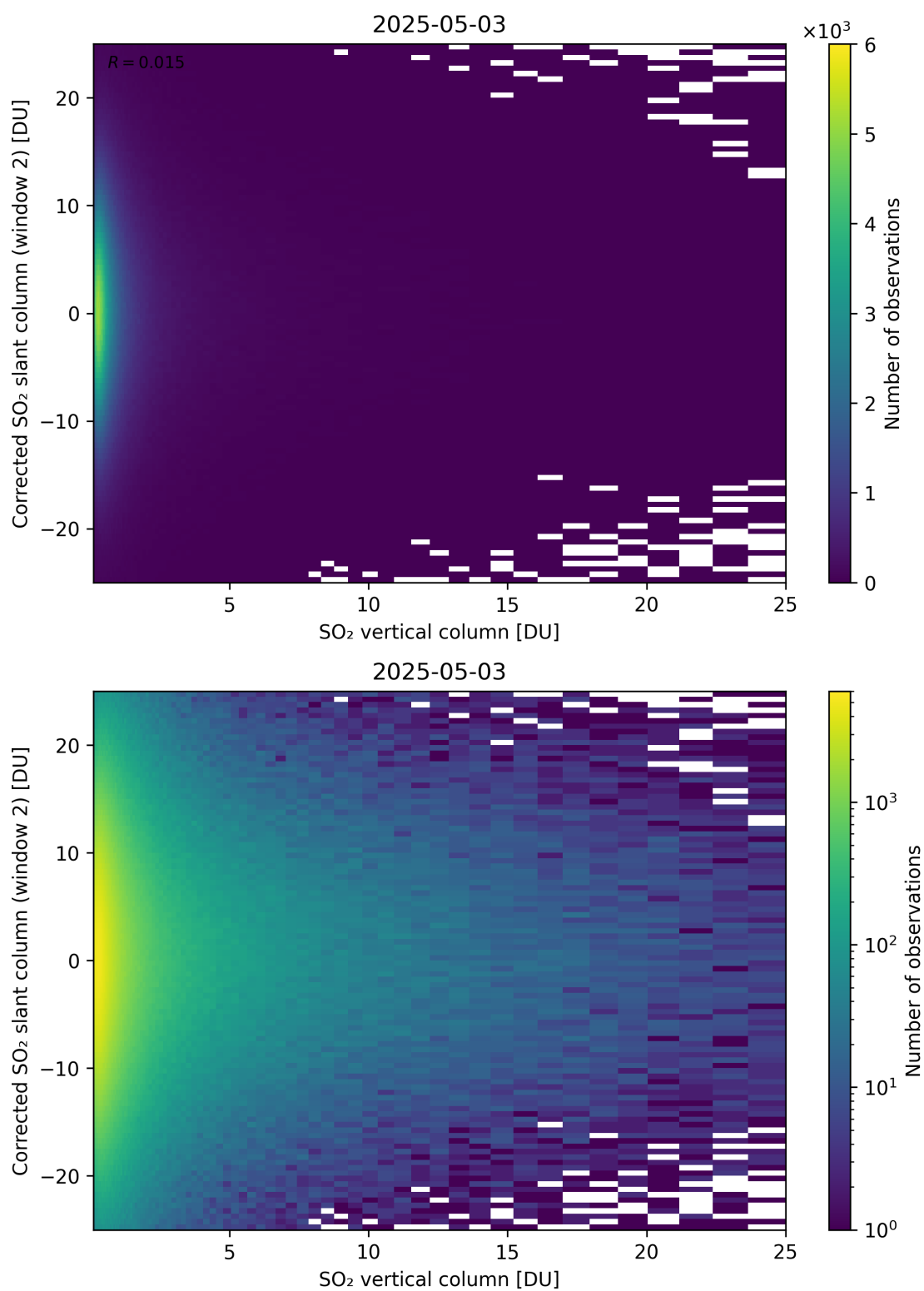
Figure 352: Scatter density plot of “SO 2 vertical column” against “Corrected SO 2 slant column (window 2)” for 2025-05-02 to 2025-05-04.
