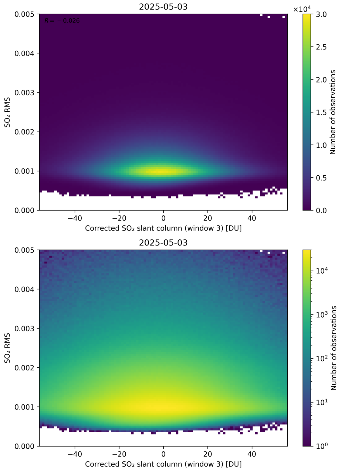
Figure 258: Scatter density plot of “Corrected SO 2 slant column (window 3)” against “SO 2 RMS” for 2025-05-02 to 2025-05-04.
