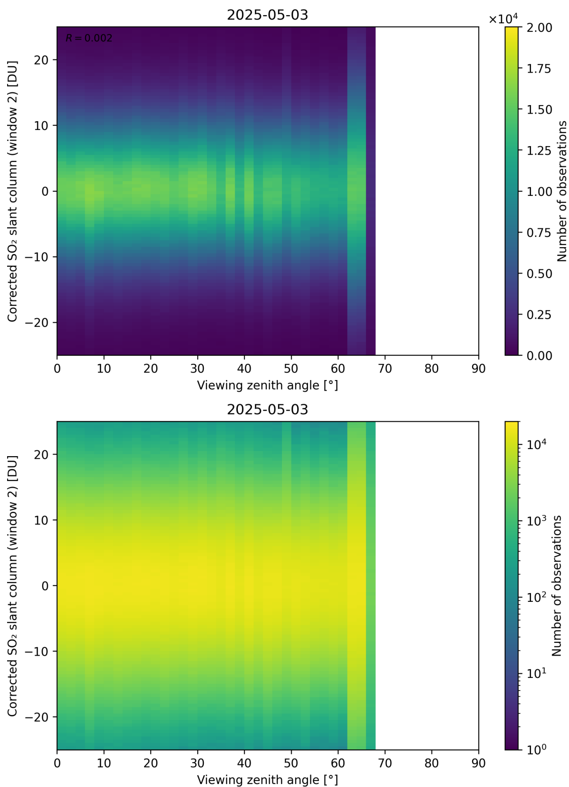
Figure 374: Scatter density plot of “Viewing zenith angle” against “Corrected SO 2 slant column (window 2)” for 2025-05-02 to 2025-05-04.
