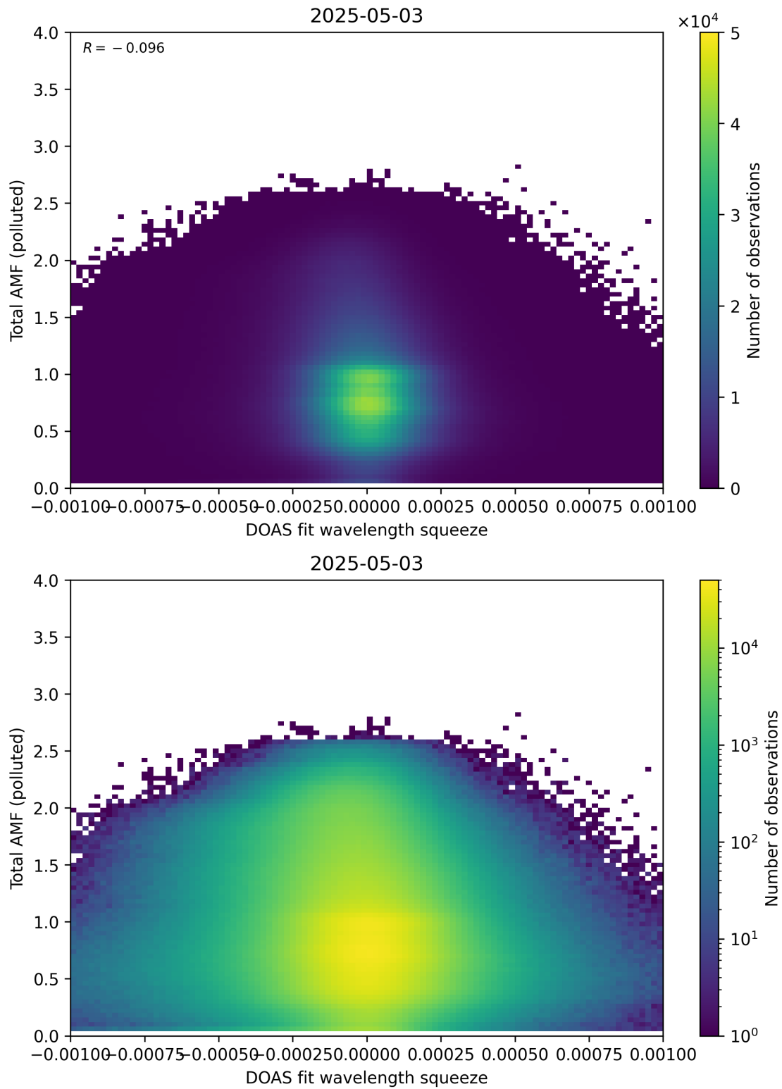
Figure 145: Scatter density plot of “DOAS fit wavelength squeeze” against “Total AMF (polluted)” for 2025-05-02 to 2025-05-04.
