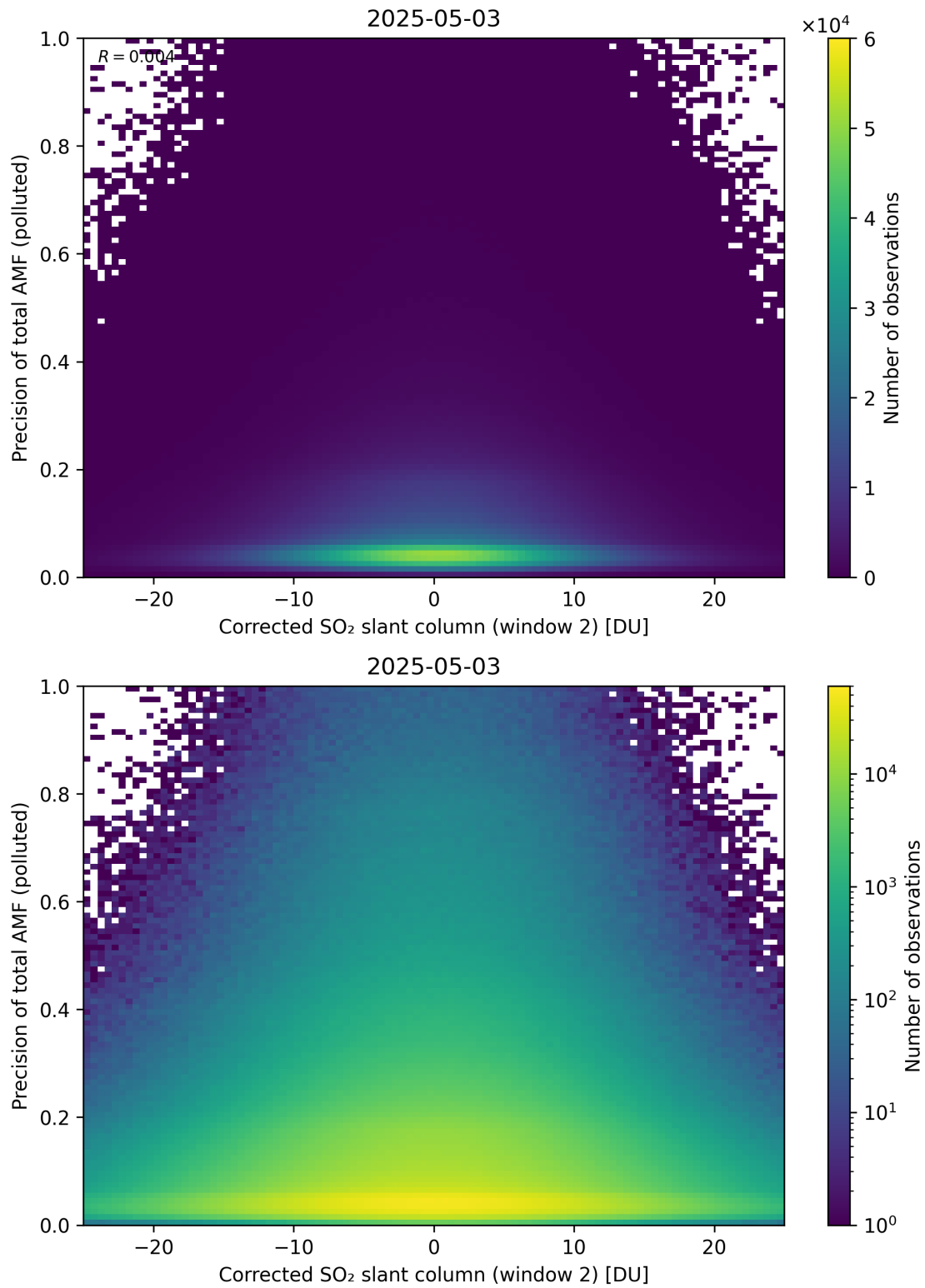
Figure 254: Scatter density plot of “Corrected SO 2 slant column (window 2)” against “Precision of total AMF (polluted)” for 2025-05-02 to 2025-05-04.
