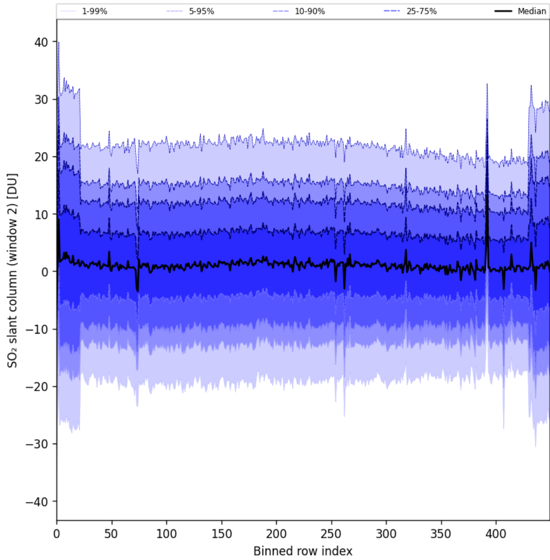
Figure 93: Along track statistics of “SO 2 slant column (window 2)” for 2025-05-02 to 2025-05-04
