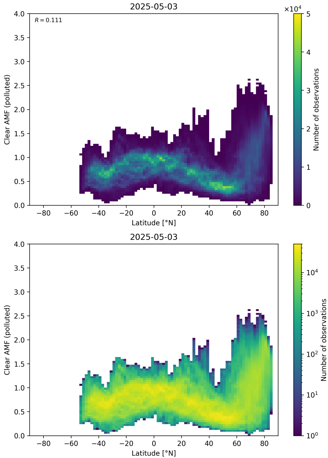
Figure 156: Scatter density plot of “Latitude” against “Clear AMF (polluted)” for 2025-05-02 to 2025-05-04.
