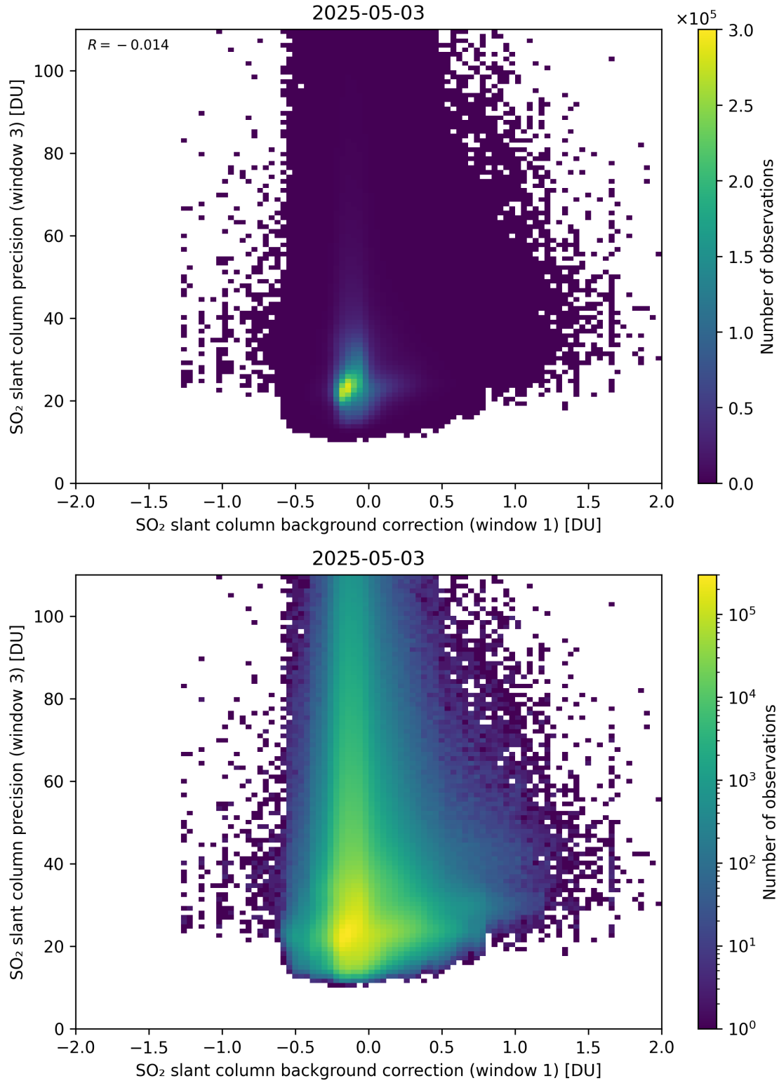
Figure 119: Scatter density plot of “SO 2 slant column background correction (window 1)” against “SO 2 slant column precision (window 3)” for 2025-05-02 to 2025-05-04.
