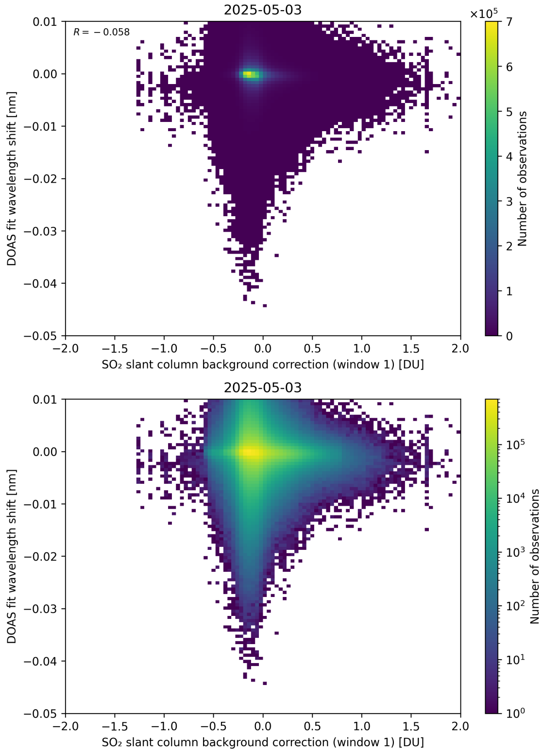
Figure 111: Scatter density plot of “SO 2 slant column background correction (window 1)” against “DOAS fit wavelength shift” for 2025-05-02 to 2025-05-04.
