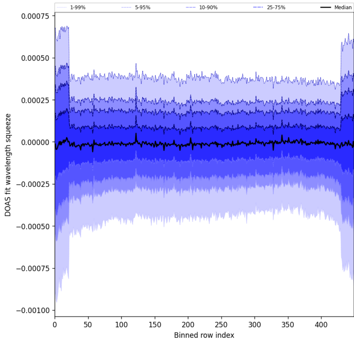
Figure 103: Along track statistics of “DOAS fit wavelength squeeze” for 2025-05-02 to 2025-05-04
