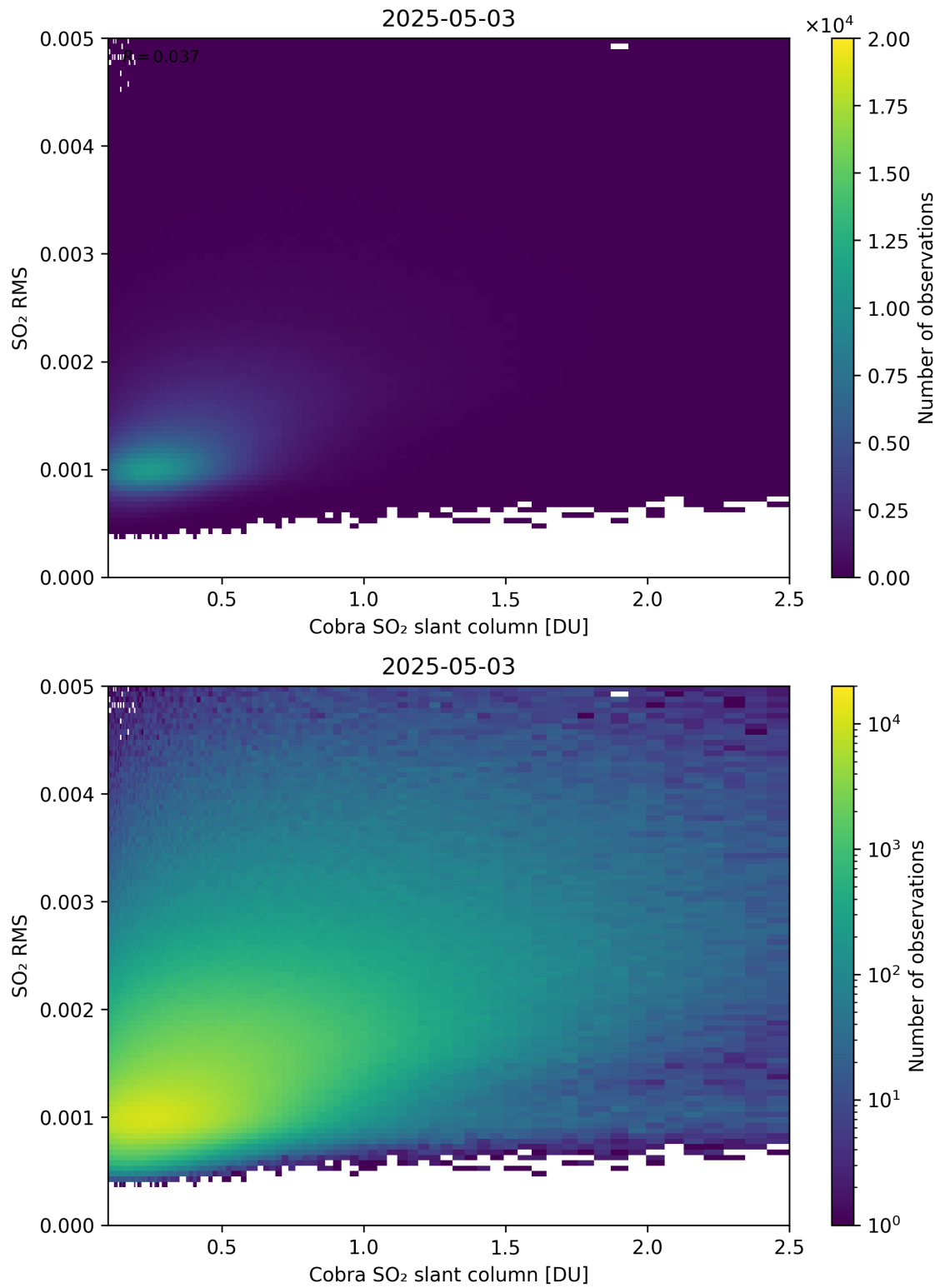
Figure 198: Scatter density plot of “Cobra SO 2 slant column” against “SO 2 RMS” for 2025-05-02 to 2025-05-04.
