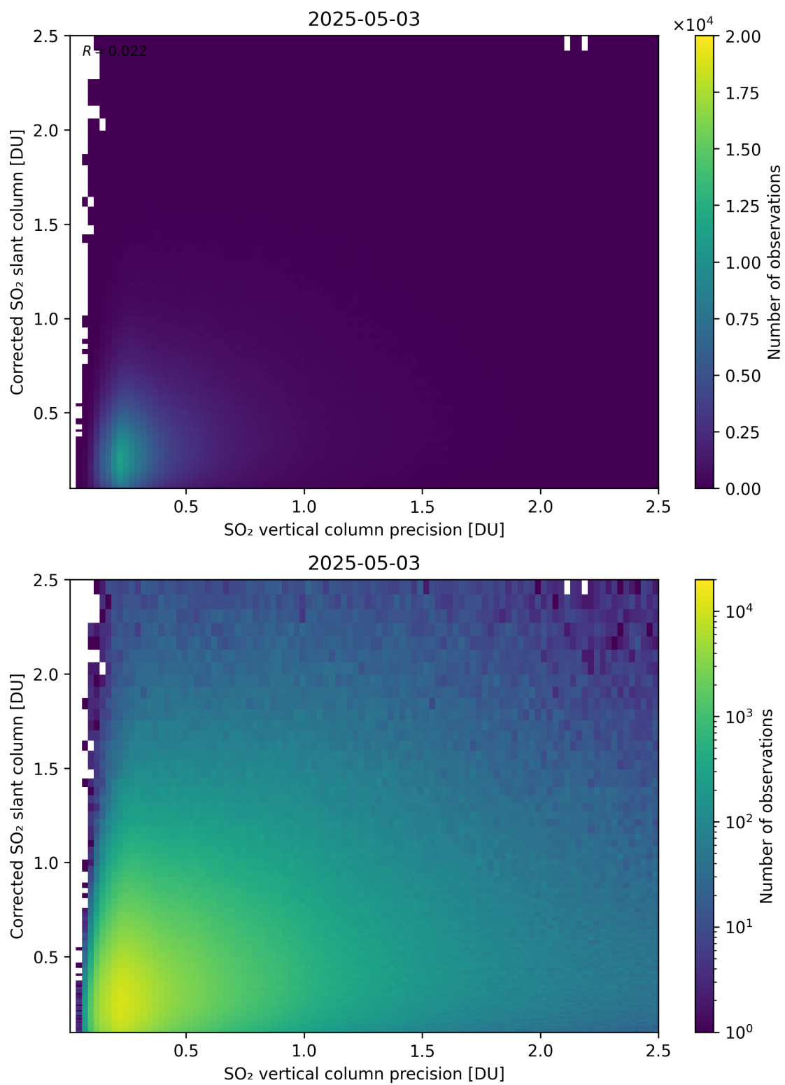
Figure 338: Scatter density plot of “SO 2 vertical column precision” against “Corrected SO 2 slant column” for 2025-05-02 to 2025-05-04.
