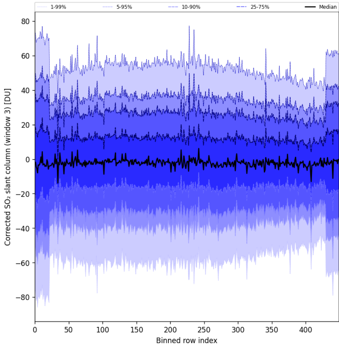
Figure 99: Along track statistics of “Corrected SO 2 slant column (window 3)” for 2025-05-02 to 2025-05-04
