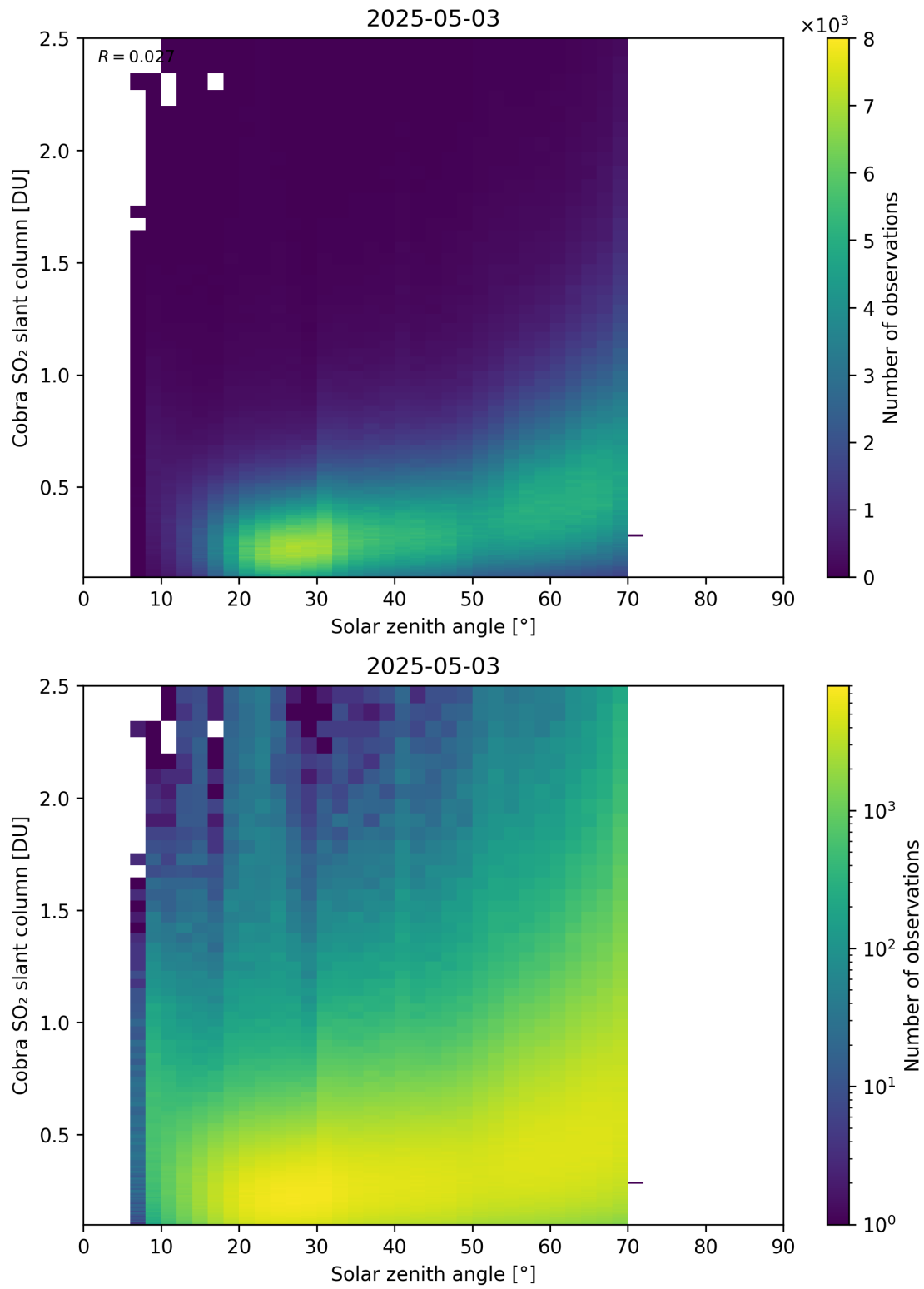
Figure 179: Scatter density plot of “Solar zenith angle” against “Cobra SO 2 slant column” for 2025-05-02 to 2025-05-04.
