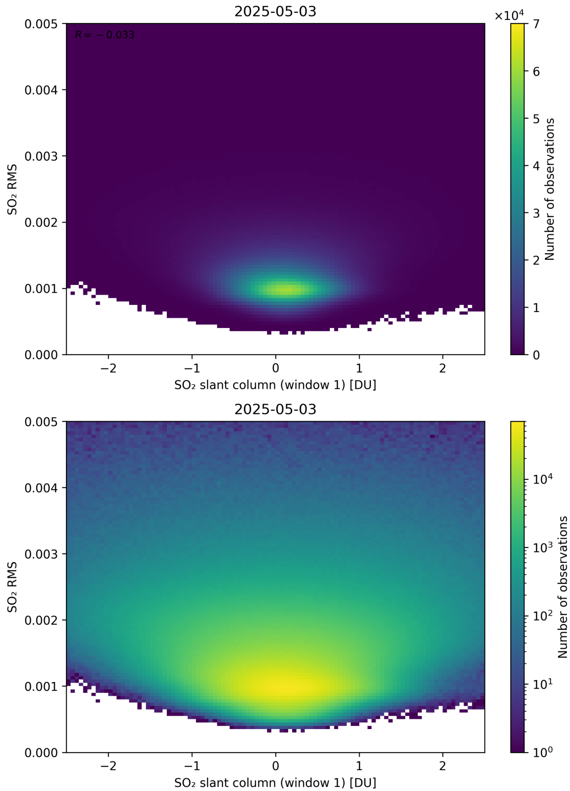
Figure 267: Scatter density plot of “SO 2 slant column (window 1)” against “SO 2 RMS” for 2025-05-02 to 2025-05-04.
