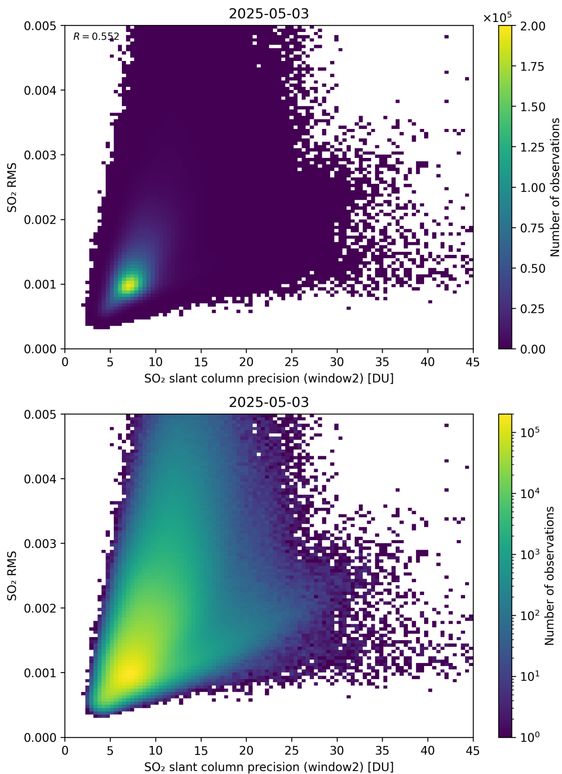
Figure 295: Scatter density plot of “SO 2 slant column precision (window2)” against “SO 2 RMS” for 2025-05-02 to 2025-05-04.
