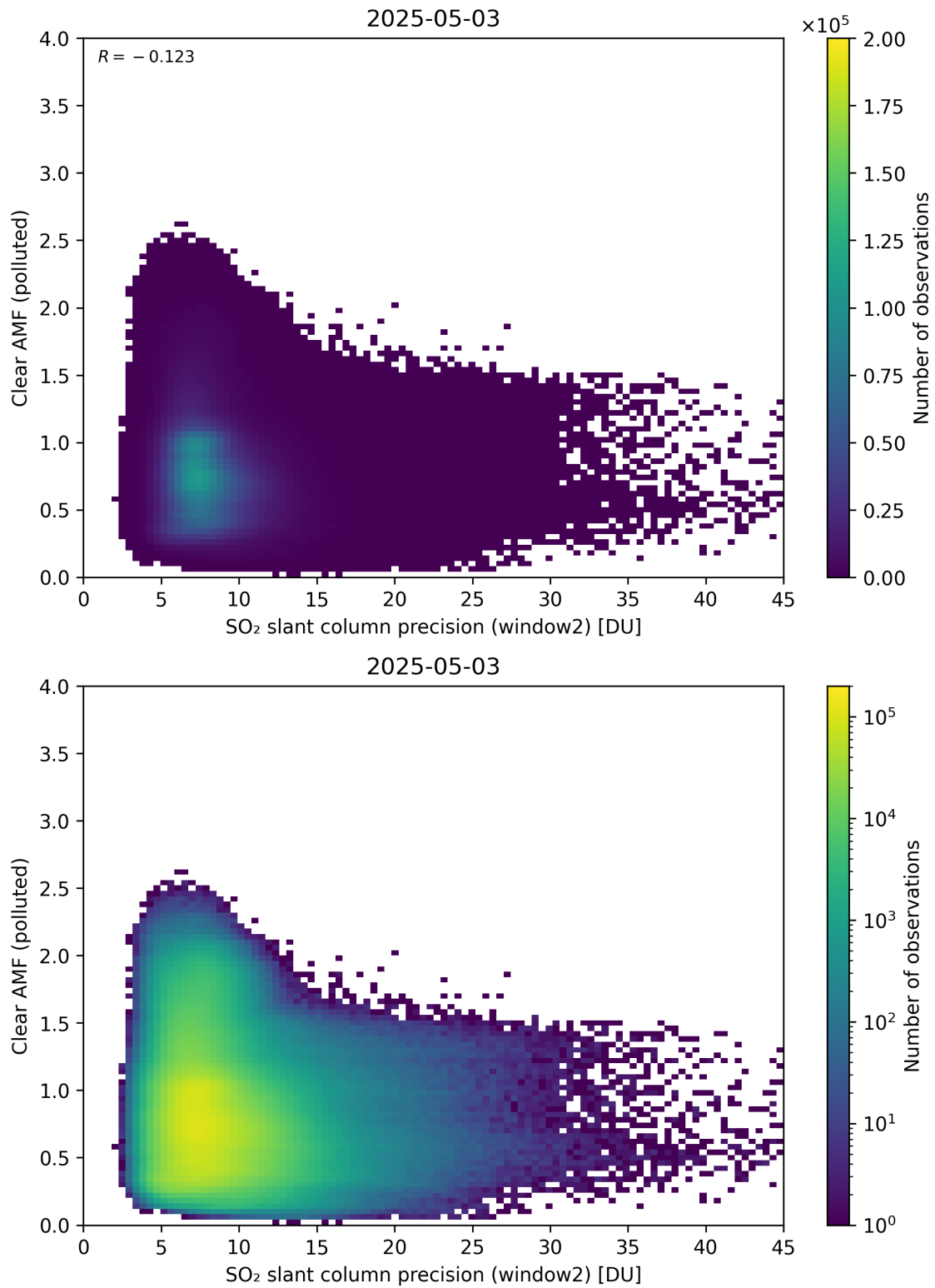
Figure 296: Scatter density plot of “SO 2 slant column precision (window2)” against “Clear AMF (polluted)” for 2025-05-02 to 2025-05-04.
