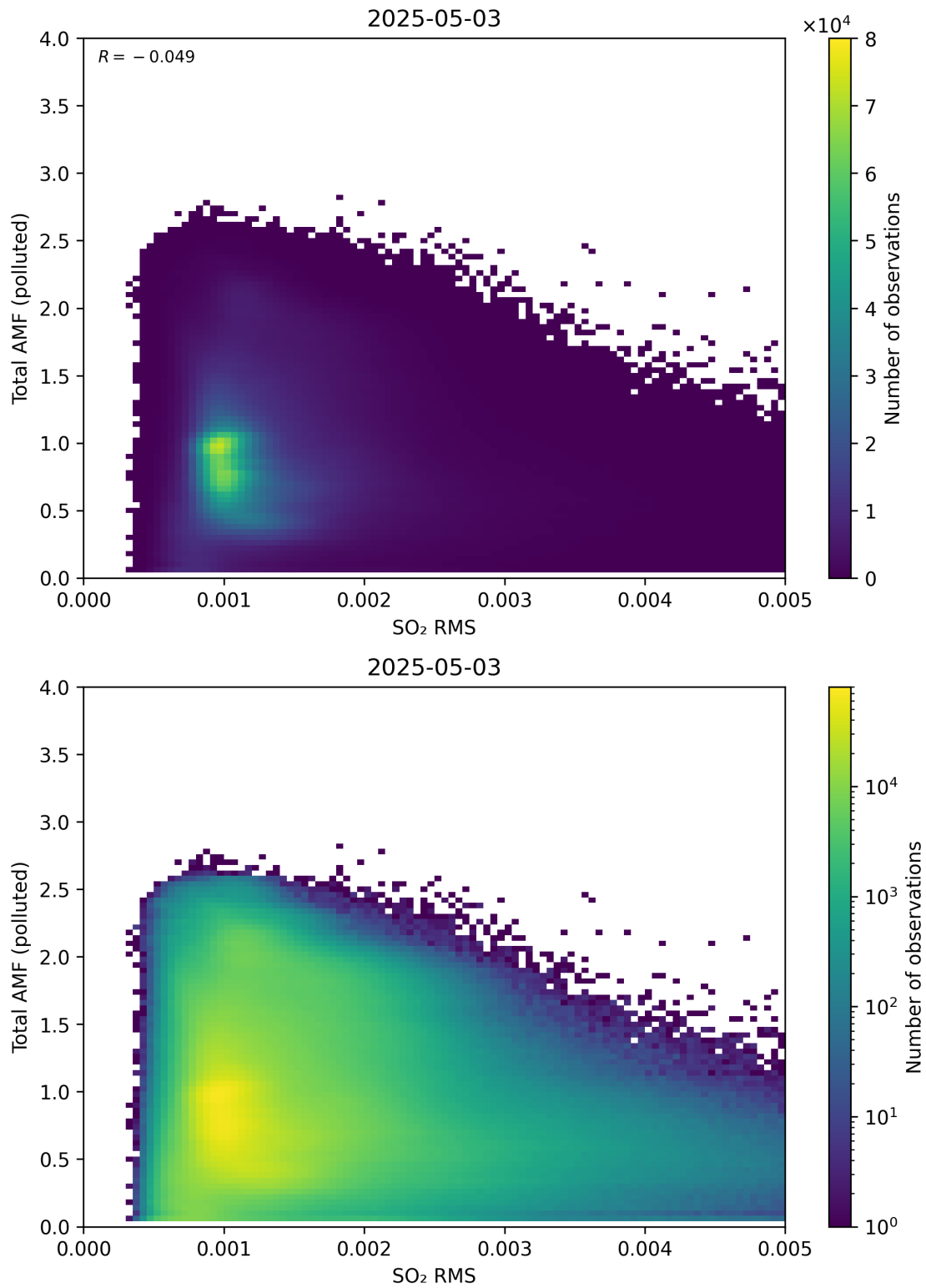
Figure 148: Scatter density plot of “SO 2 RMS” against “Total AMF (polluted)” for 2025-05-02 to 2025-05-04.
