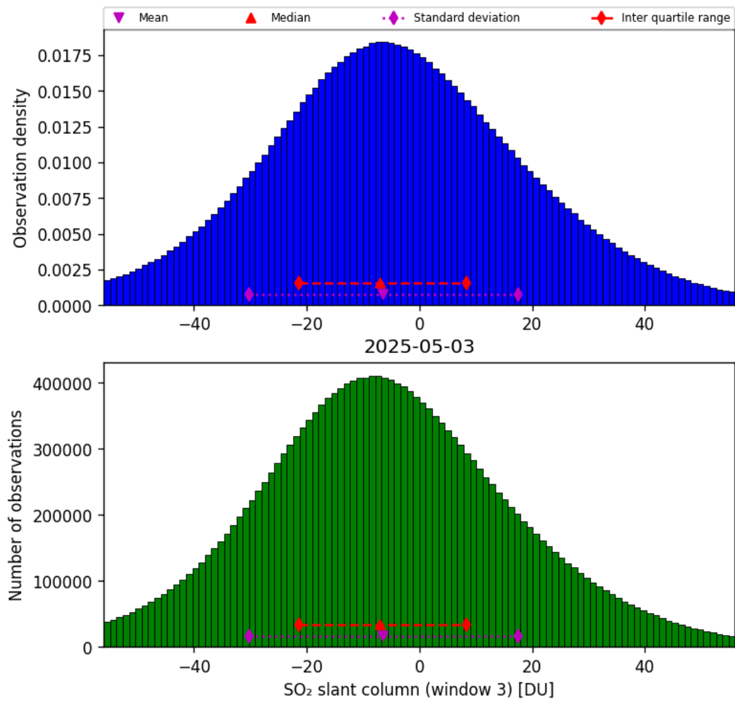
Figure 71: Histogram of “SO 2 slant column (window 3)” for 2025-05-02 to 2025-05-04
