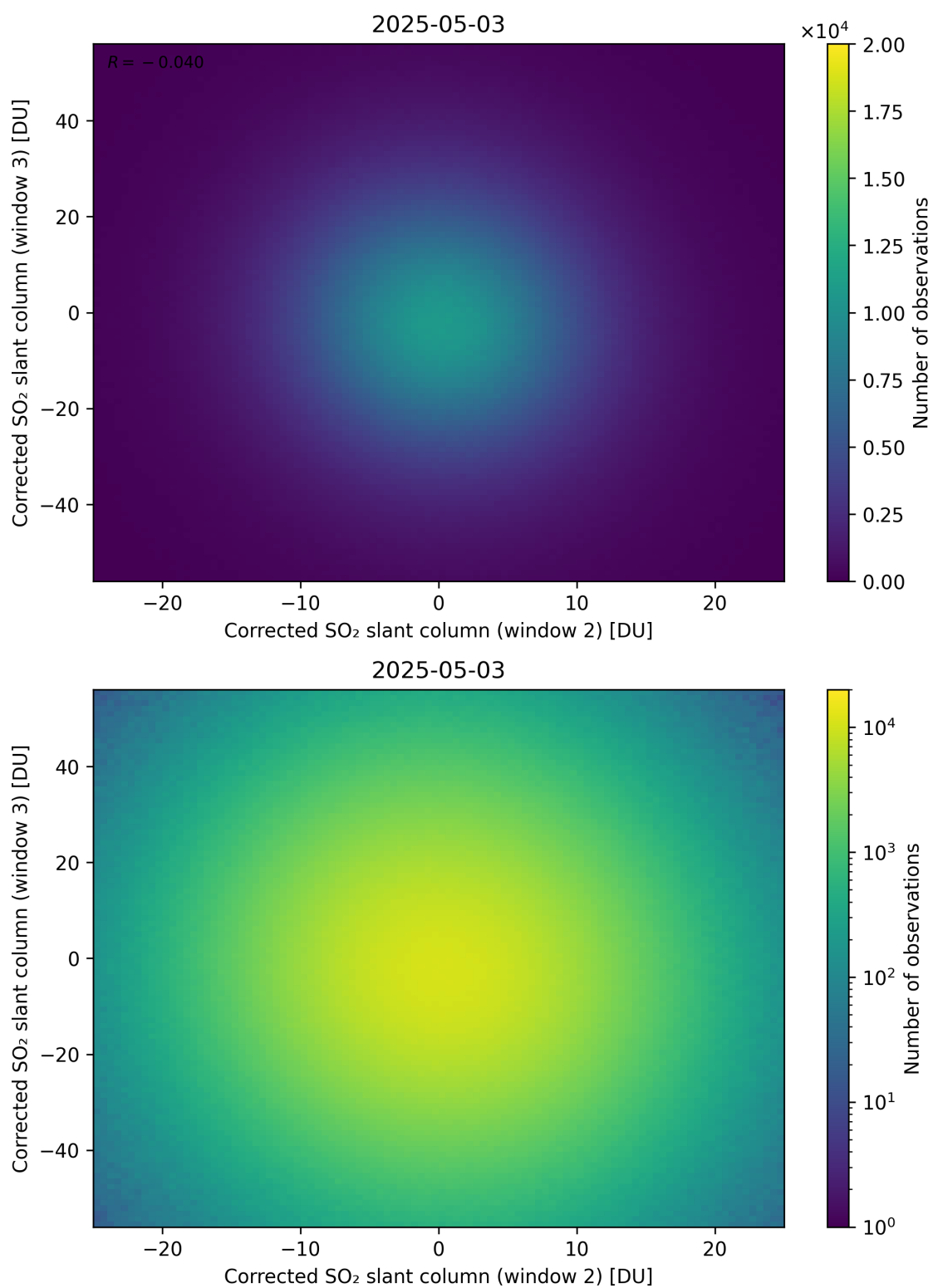
Figure 250: Scatter density plot of “Corrected SO 2 slant column (window 2)” against “Corrected SO 2 slant column (window 3)” for 2025-05-02 to 2025-05-04.
