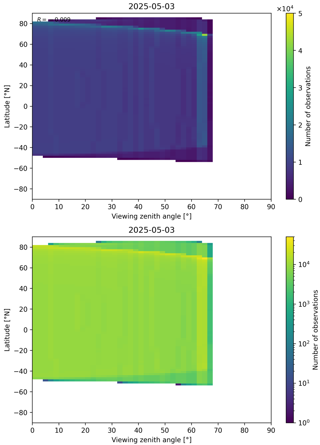
Figure 368: Scatter density plot of “Viewing zenith angle” against “Latitude” for 2025-05-02 to 2025-05-04.
