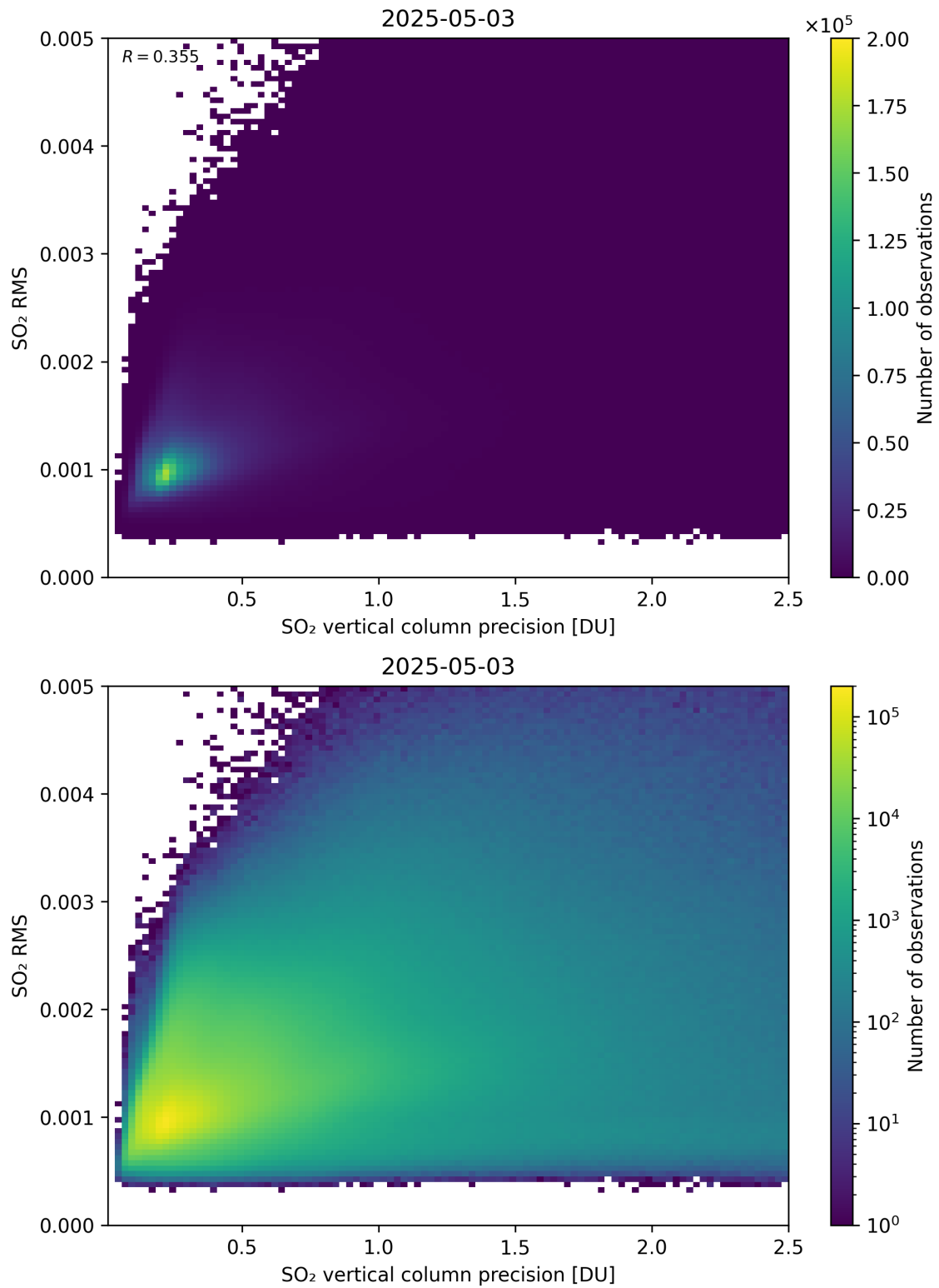
Figure 334: Scatter density plot of “SO 2 vertical column precision” against “SO 2 RMS” for 2025-05-02 to 2025-05-04.
