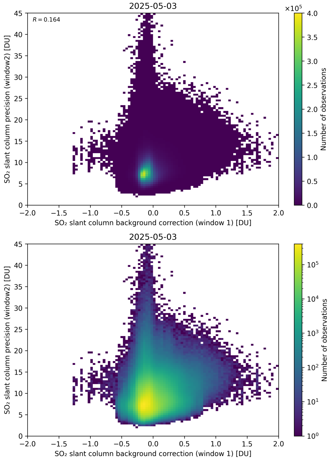
Figure 117: Scatter density plot of “SO 2 slant column background correction (window 1)” against “SO 2 slant column precision (window2)” for 2025-05-02 to 2025-05-04.
