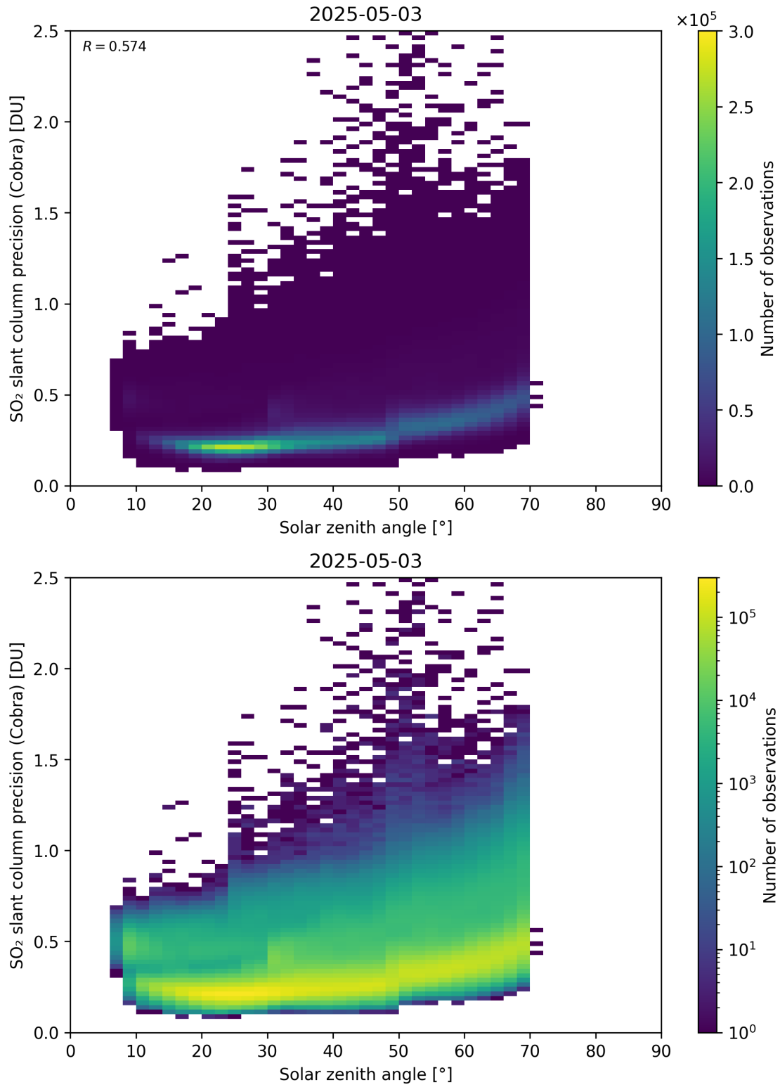
Figure 180: Scatter density plot of “Solar zenith angle” against “SO 2 slant column precision (Cobra)” for 2025-05-02 to 2025-05-04.
