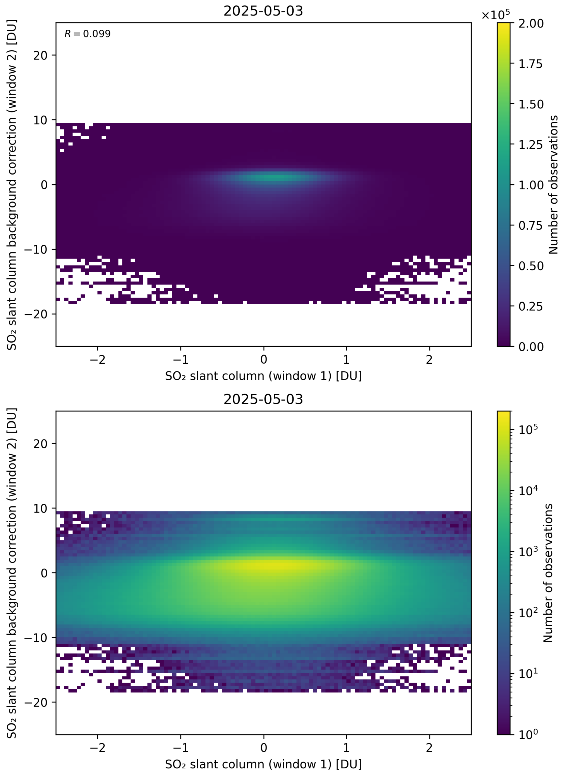
Figure 263: Scatter density plot of “SO 2 slant column (window 1)” against “SO 2 slant column background correction (window 2)” for 2025-05-02 to 2025-05-04.
