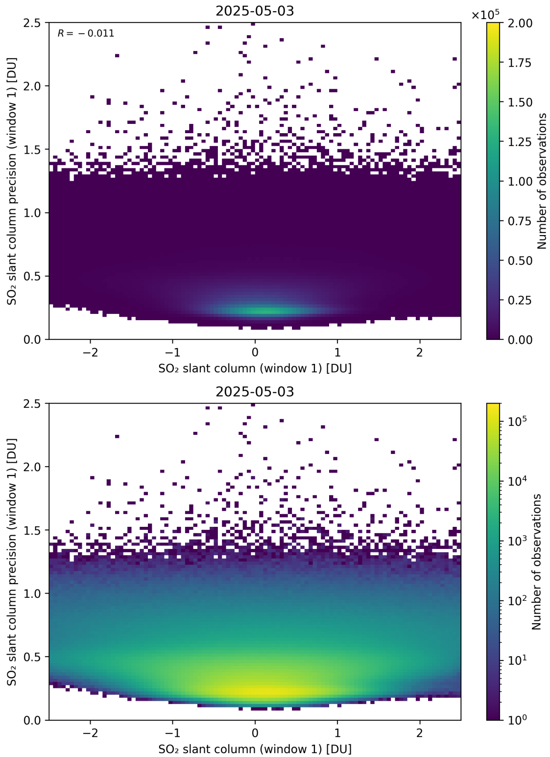
Figure 285: Scatter density plot of “SO 2 slant column (window 1)” against “SO 2 slant column precision (window 1)” for 2025-05-02 to 2025-05-04.
