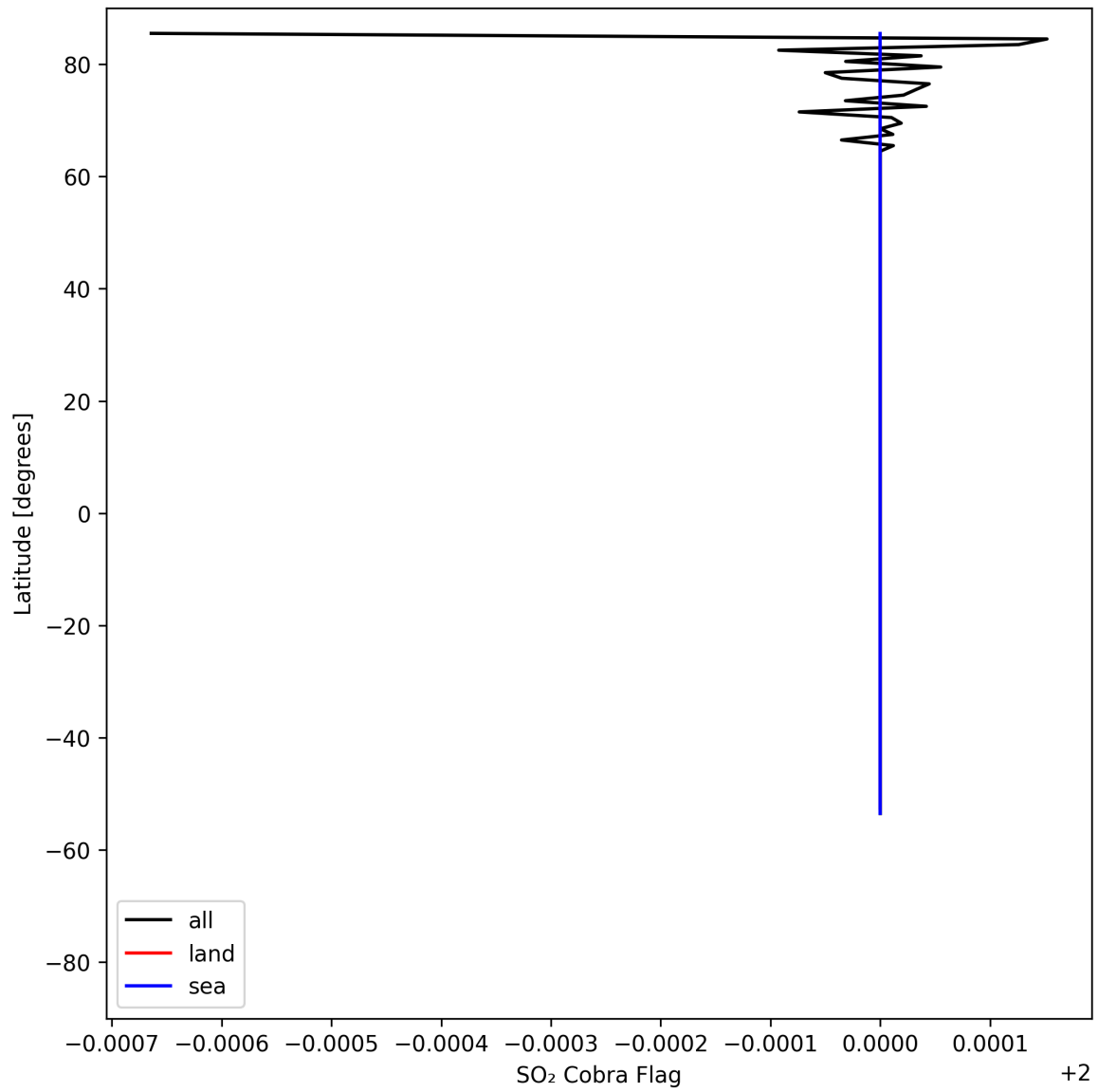
Figure 49: Zonal average of “SO 2 Cobra Flag” for 2025-05-02 to 2025-05-04.
