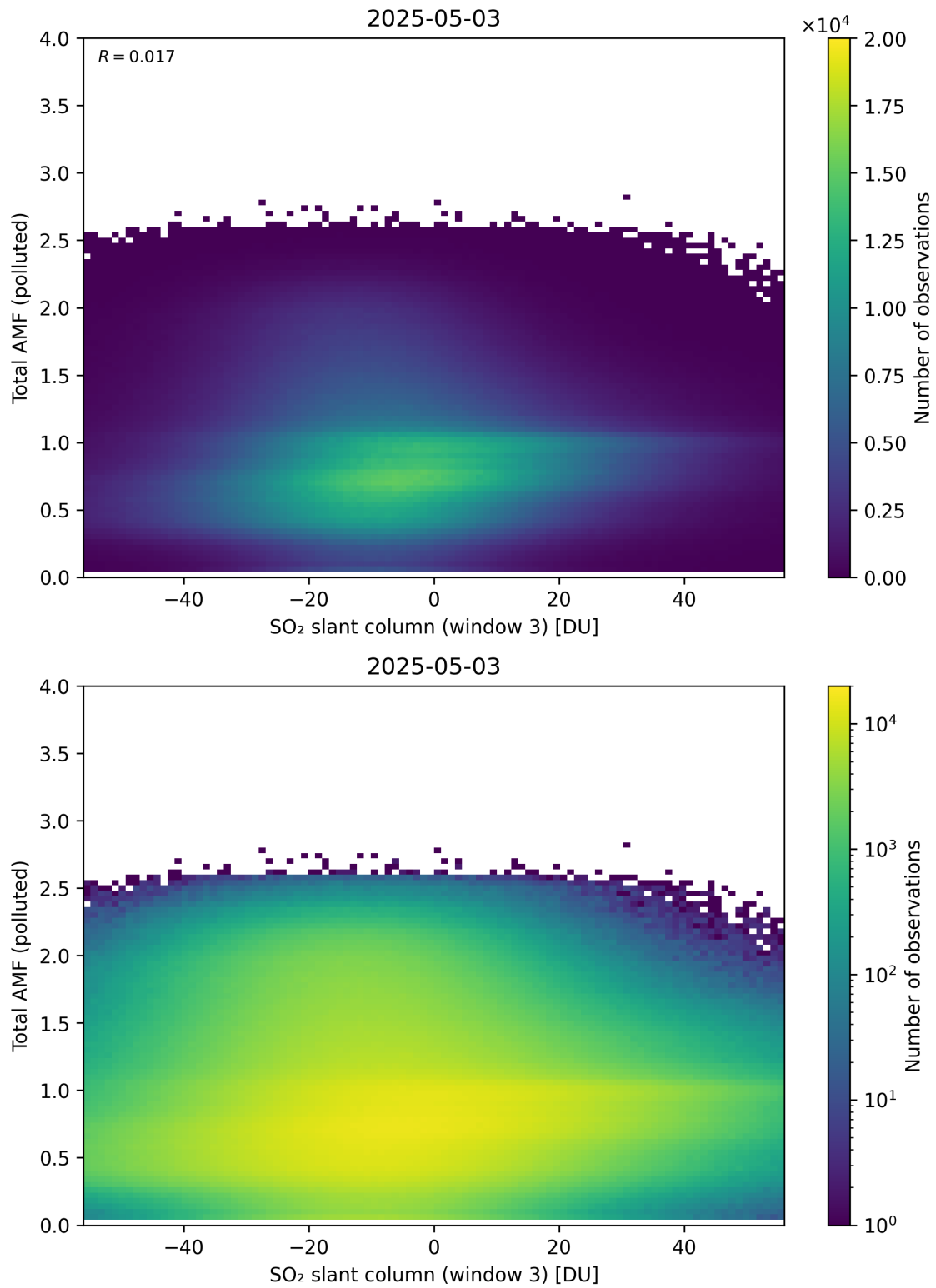
Figure 318: Scatter density plot of “SO 2 slant column (window 3)” against “Total AMF (polluted)” for 2025-05-02 to 2025-05-04.
