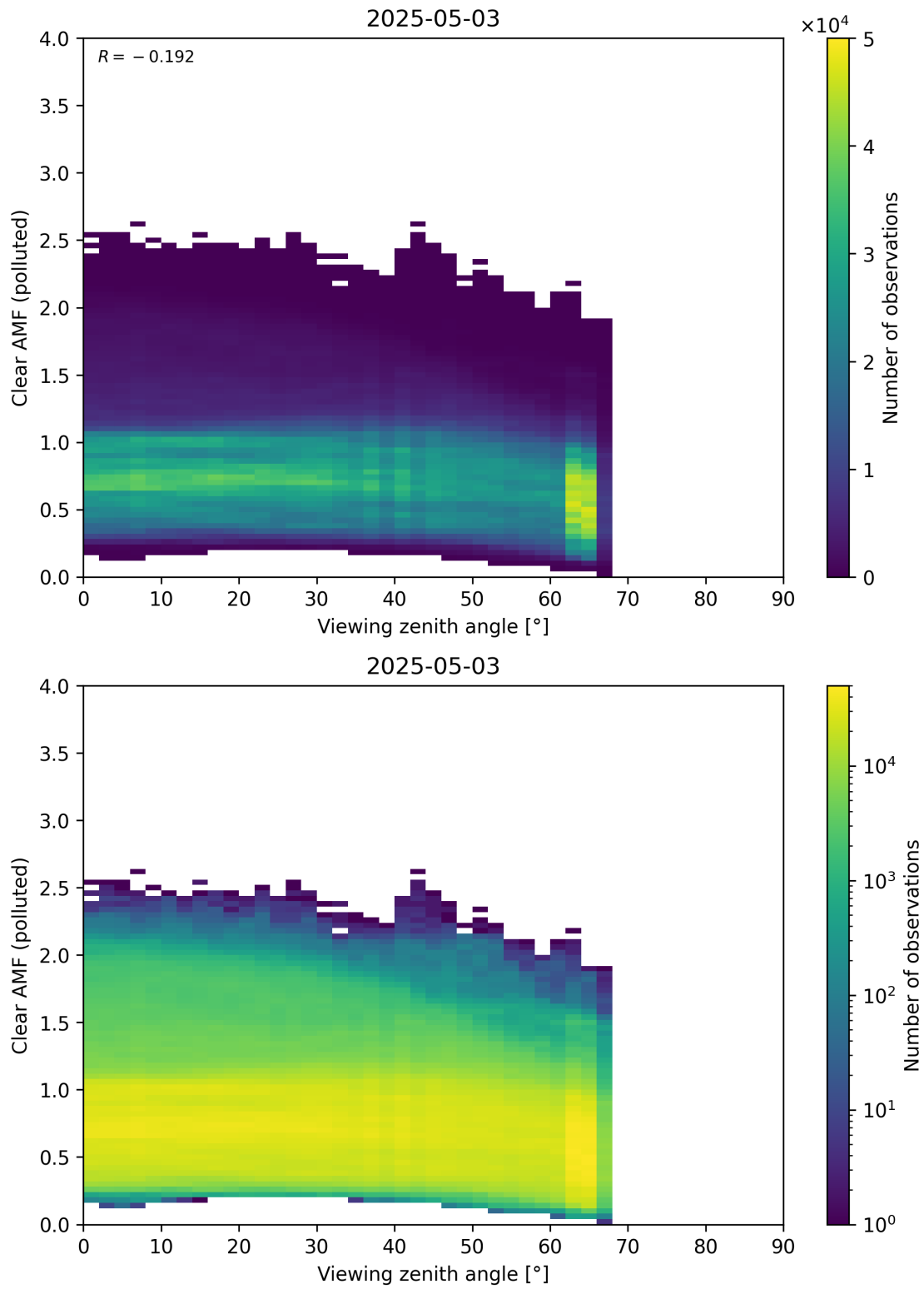
Figure 370: Scatter density plot of “Viewing zenith angle” against “Clear AMF (polluted)” for 2025-05-02 to 2025-05-04.
