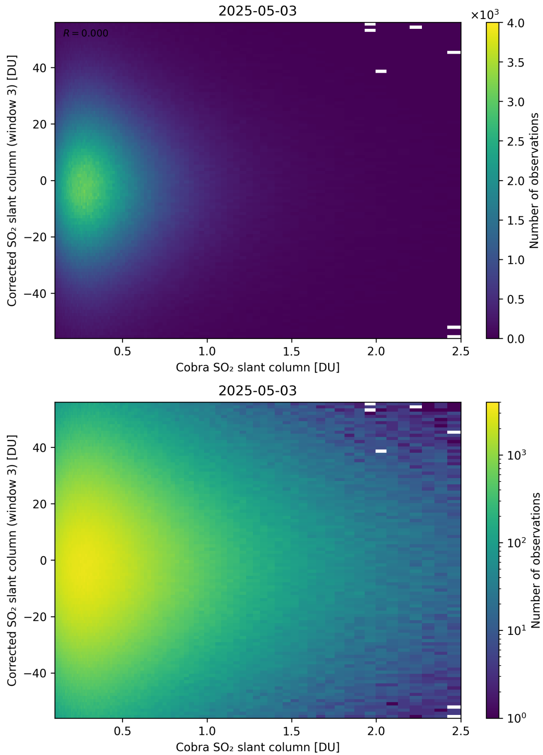
Figure 218: Scatter density plot of “Cobra SO 2 slant column” against “Corrected SO 2 slant column (window 3)” for 2025-05-02 to 2025-05-04.
