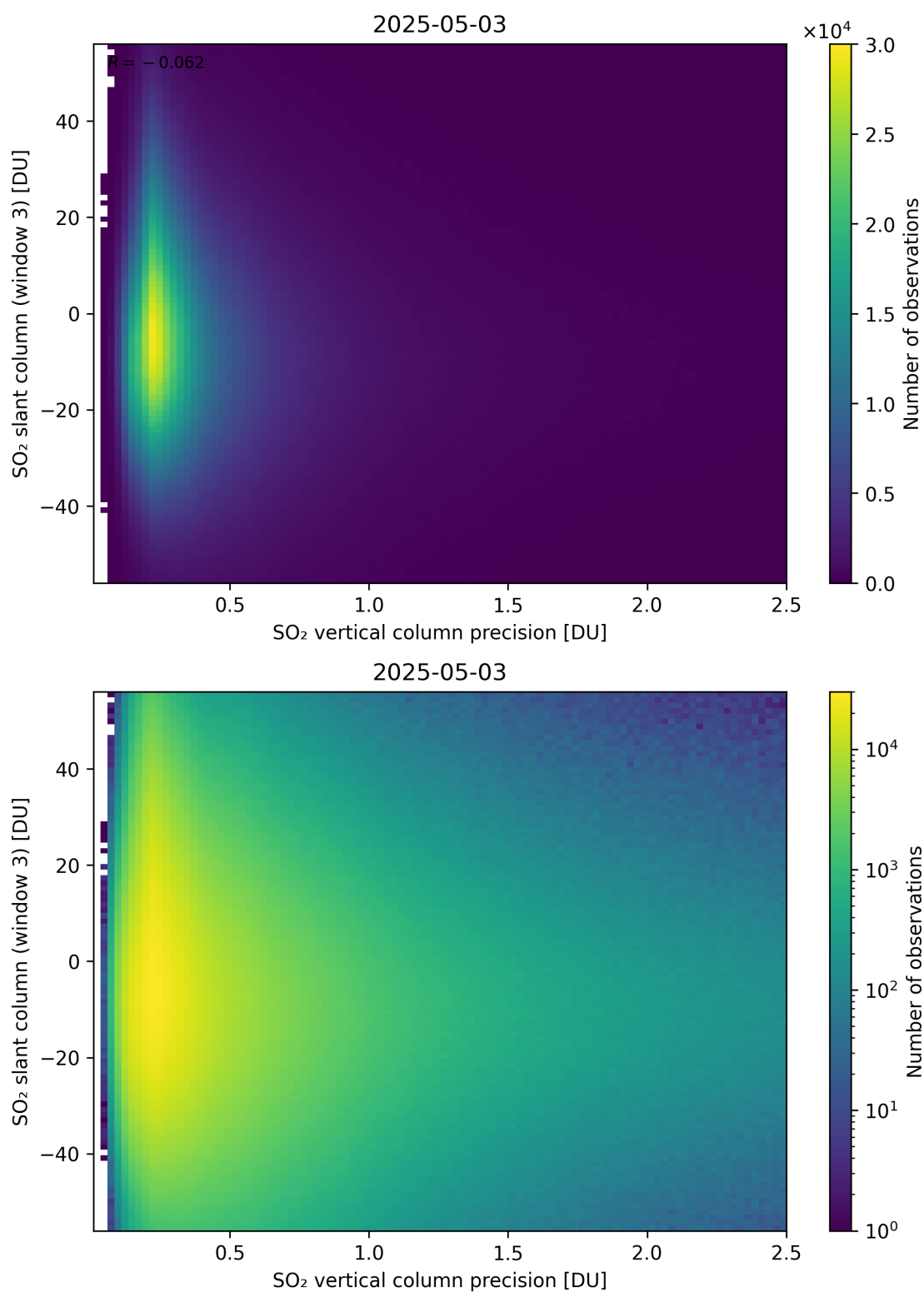
Figure 344: Scatter density plot of “SO 2 vertical column precision” against “SO 2 slant column (window 3)” for 2025-05-02 to 2025-05-04.
