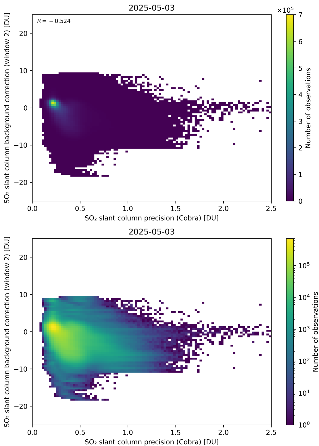
Figure 200: Scatter density plot of “SO 2 slant column precision (Cobra)” against “SO 2 slant column background correction (window 2)” for 2025-05-02 to 2025-05-04.
