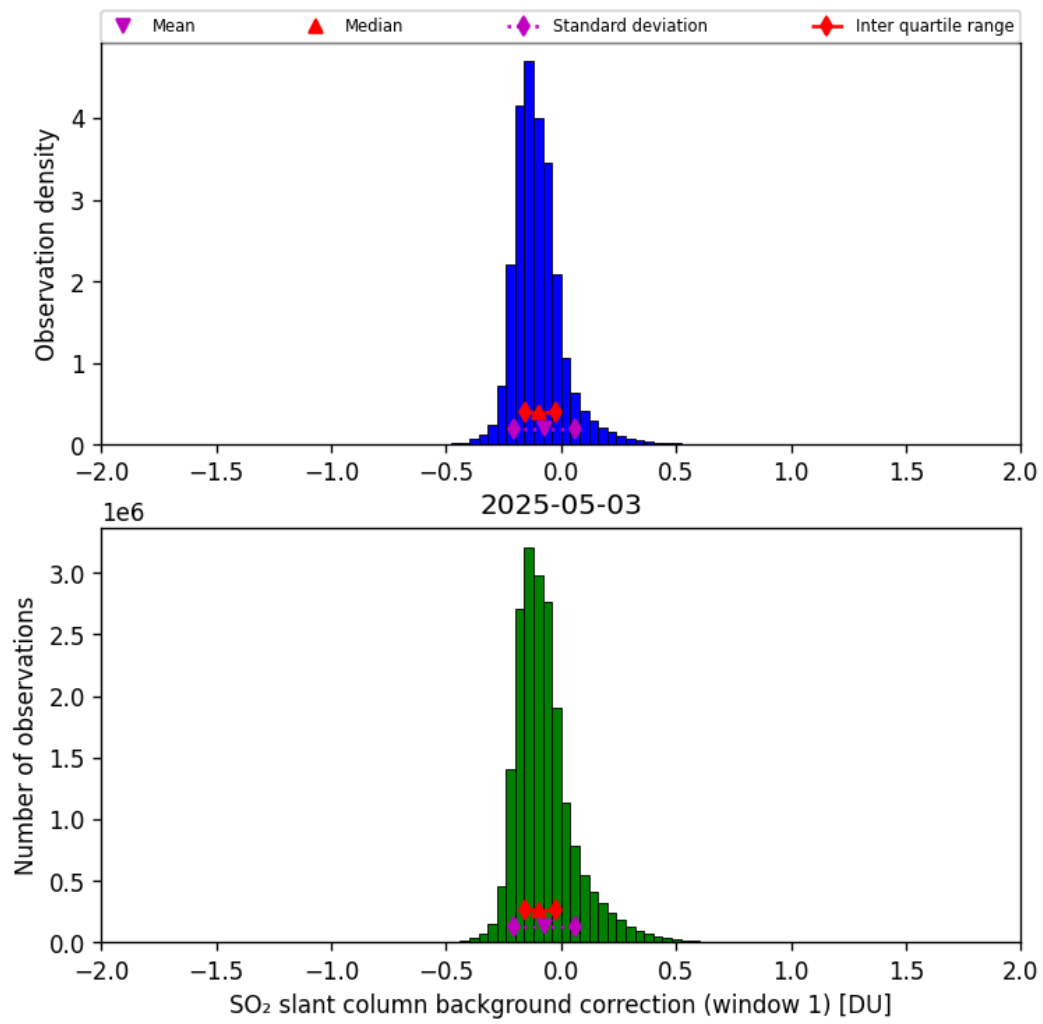
Figure 66: Histogram of “SO 2 slant column background correction (window 1)” for 2025-05-02 to 2025-05-04
