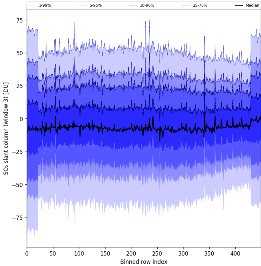
Figure 97: Along track statistics of “SO 2 slant column (window 3)” for 2025-05-02 to 2025-05-04
