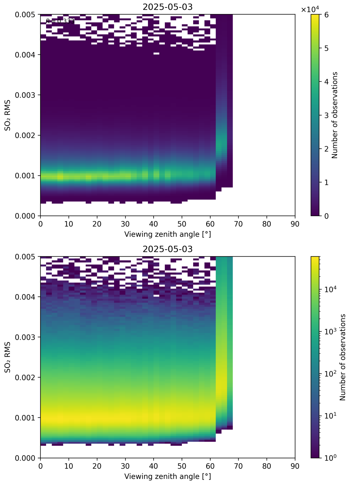
Figure 367: Scatter density plot of “Viewing zenith angle” against “SO 2 RMS” for 2025-05-02 to 2025-05-04.
