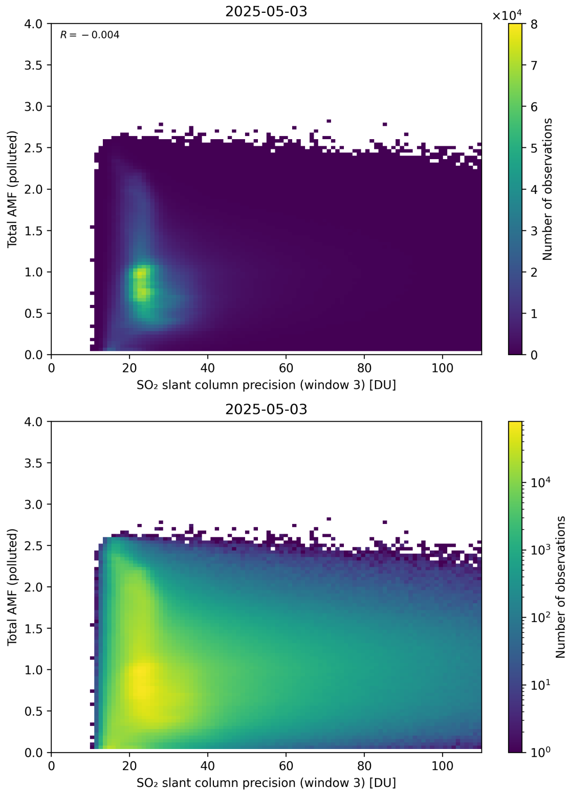
Figure 313: Scatter density plot of “SO 2 slant column precision (window 3)” against “Total AMF (polluted)” for 2025-05-02 to 2025-05-04.
