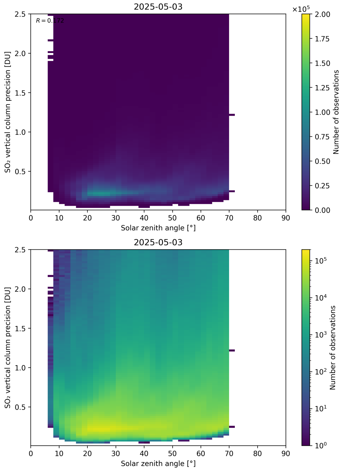
Figure 192: Scatter density plot of “Solar zenith angle” against “SO 2 vertical column precision” for 2025-05-02 to 2025-05-04.
