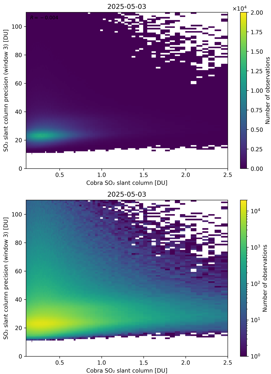
Figure 223: Scatter density plot of “Cobra SO 2 slant column” against “SO 2 slant column precision (window 3)” for 2025-05-02 to 2025-05-04.
