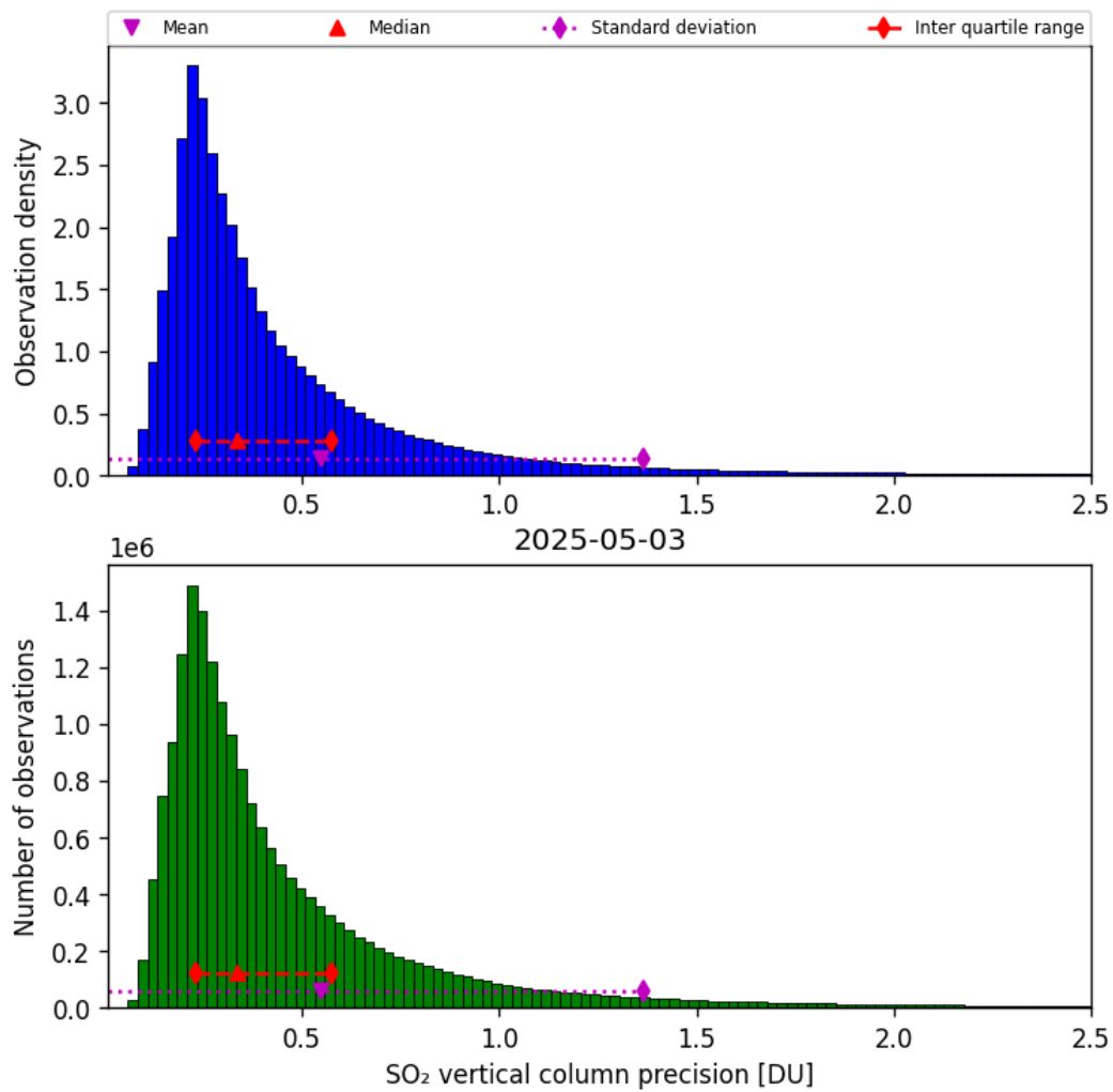
Figure 59: Histogram of “SO 2 vertical column precision” for 2025-05-02 to 2025-05-04
