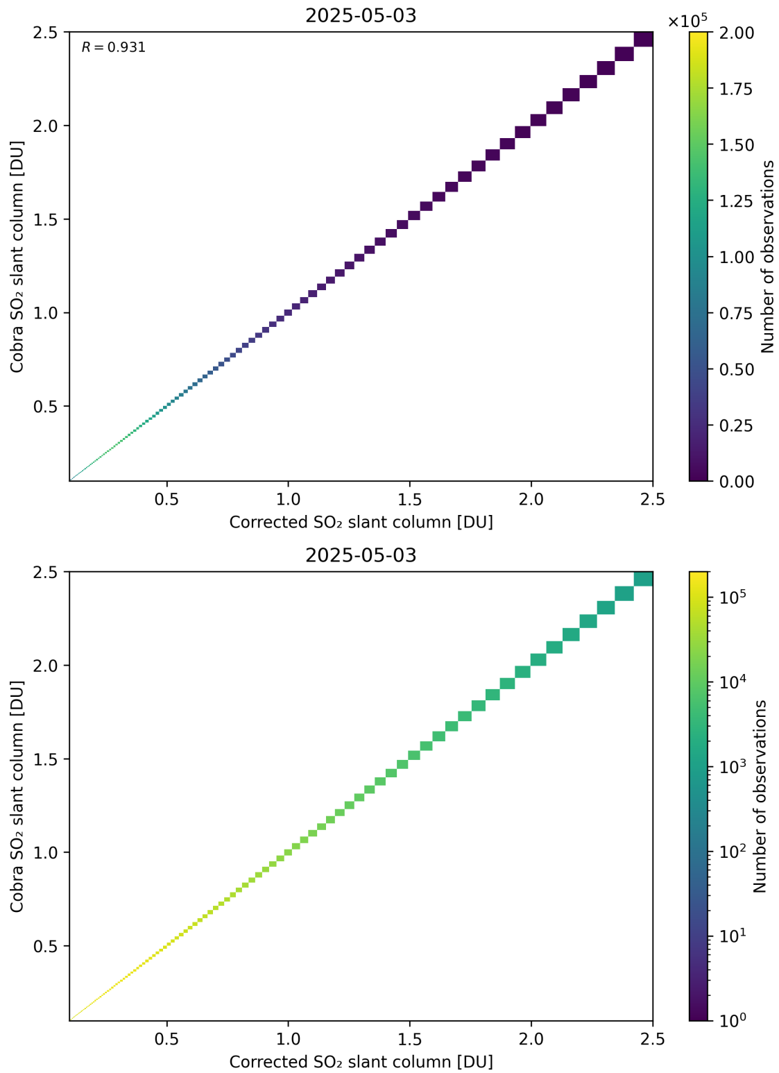
Figure 233: Scatter density plot of “Corrected SO 2 slant column” against “Cobra SO 2 slant column” for 2025-05-02 to 2025-05-04.
