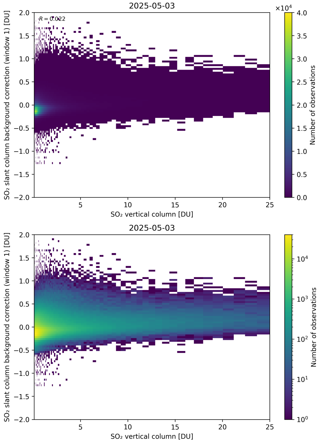
Figure 323: Scatter density plot of “SO 2 vertical column” against “SO 2 slant column background correction (window 1)” for 2025-05-02 to 2025-05-04.
