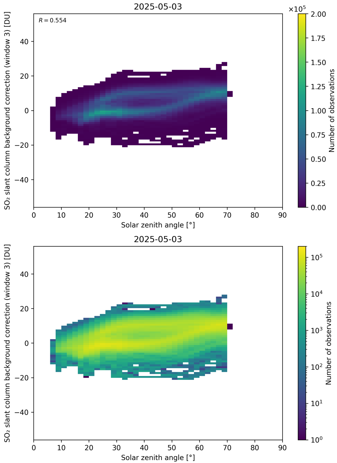
Figure 173: Scatter density plot of “Solar zenith angle” against “SO 2 slant column background correction (window 3)” for 2025-05-02 to 2025-05-04.
