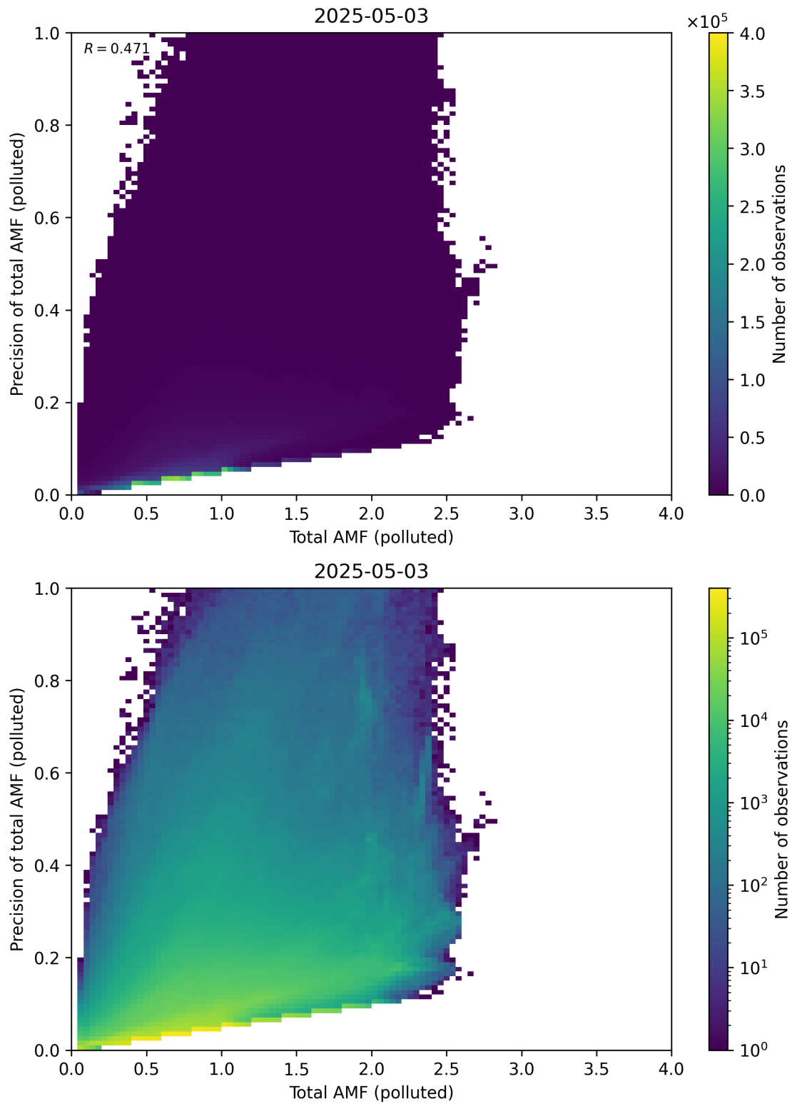
Figure 322: Scatter density plot of “Total AMF (polluted)” against “Precision of total AMF (polluted)” for 2025-05-02 to 2025-05-04.
