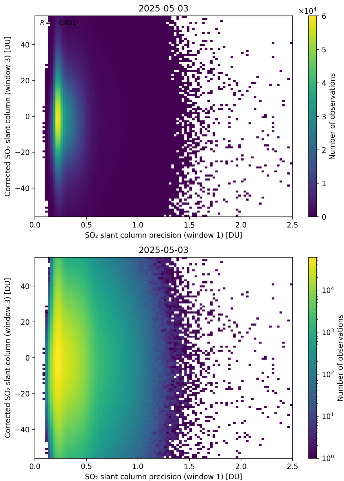
Figure 276: Scatter density plot of “SO 2 slant column precision (window 1)” against “Corrected SO 2 slant column (window 3)” for 2025-05-02 to 2025-05-04.
