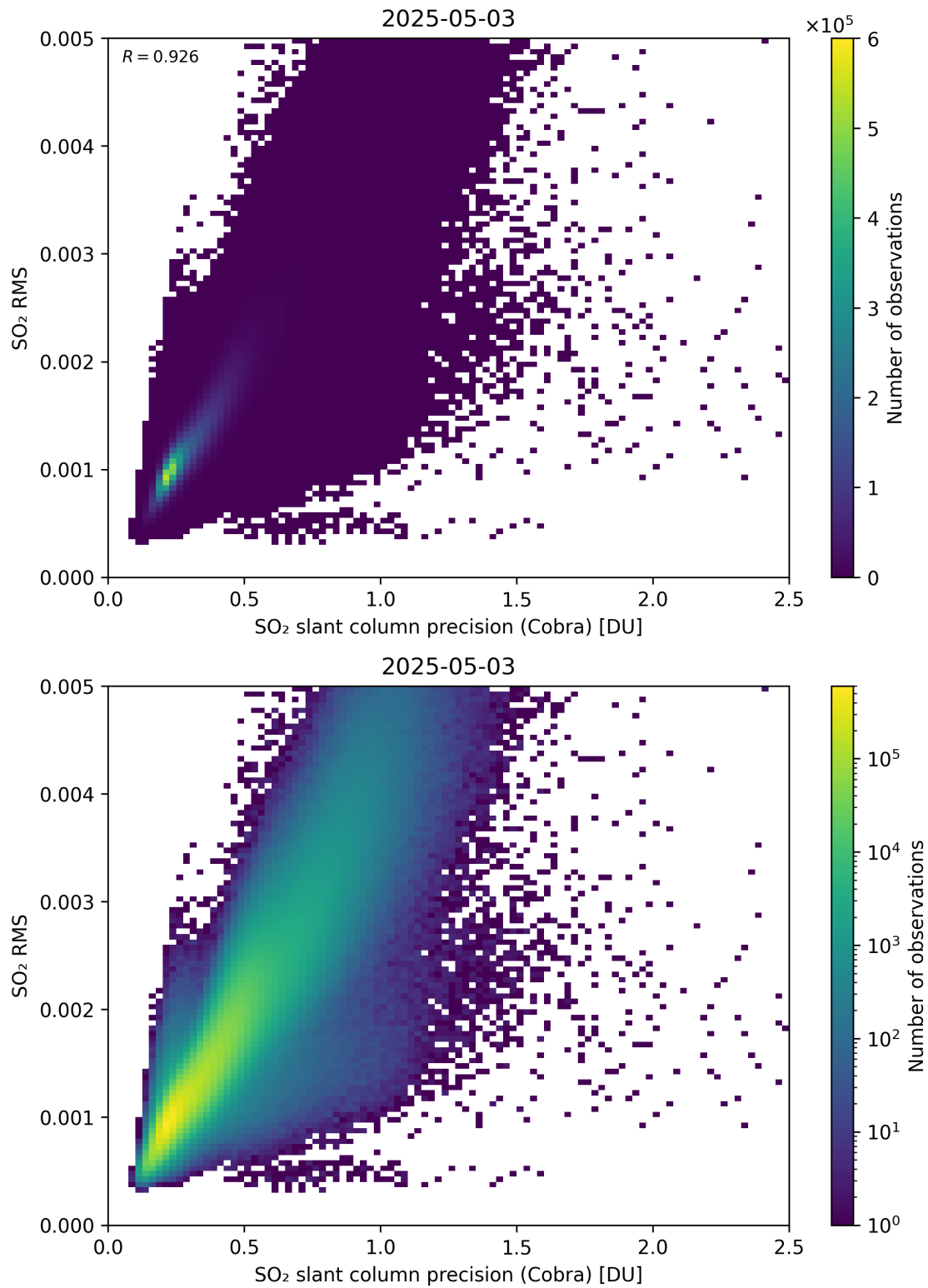
Figure 204: Scatter density plot of “SO 2 slant column precision (Cobra)” against “SO 2 RMS” for 2025-05-02 to 2025-05-04.
