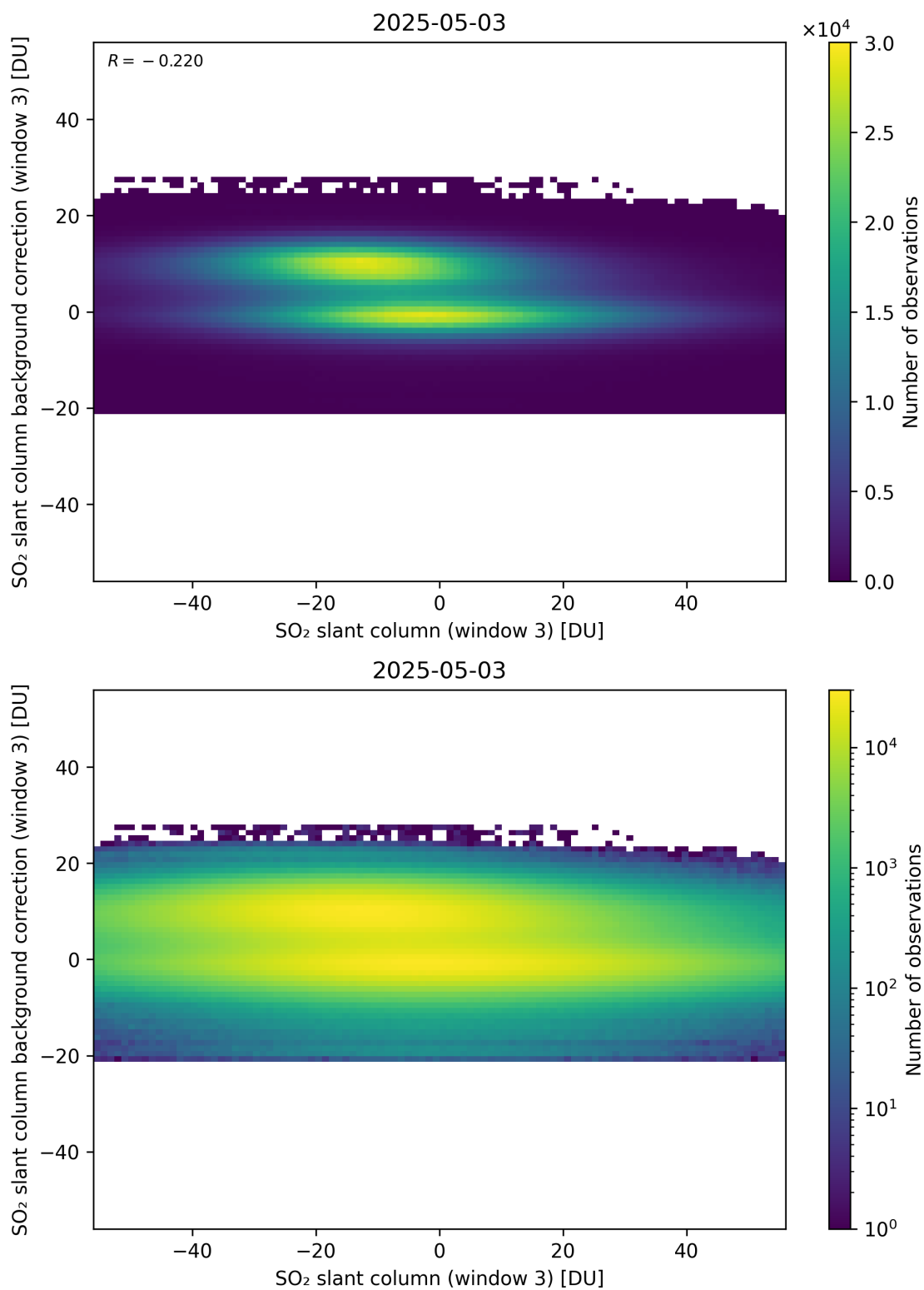
Figure 303: Scatter density plot of “SO 2 slant column (window 3)” against “SO 2 slant column background correction (window 3)” for 2025-05-02 to 2025-05-04.
