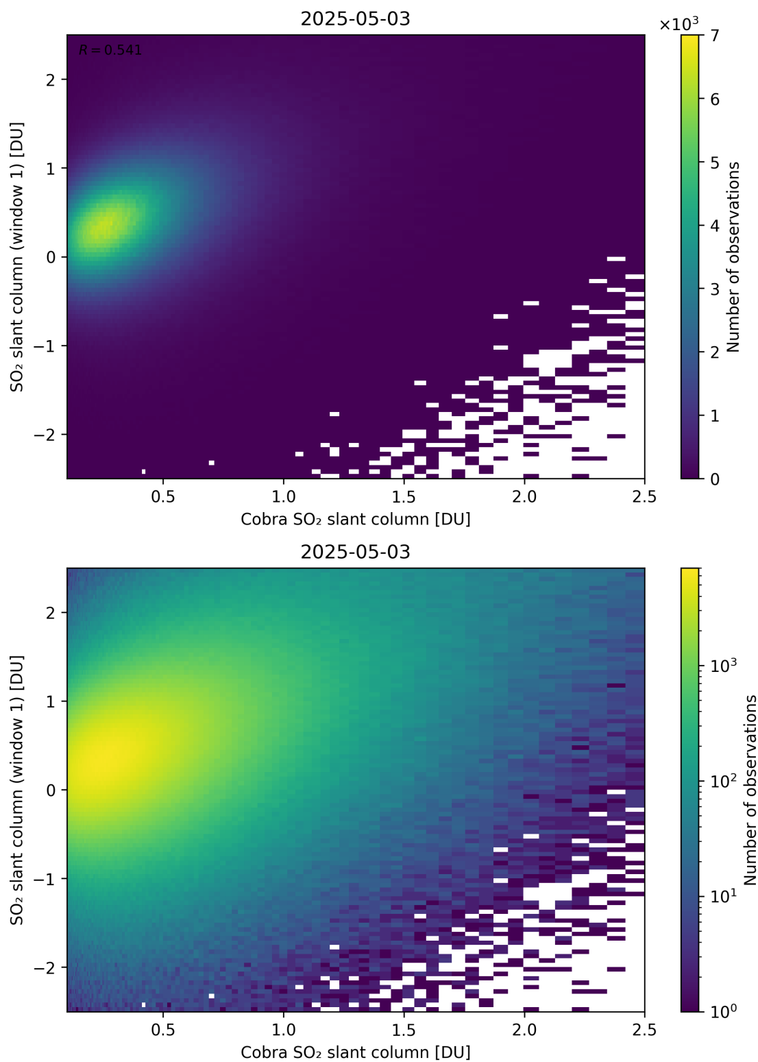
Figure 219: Scatter density plot of “Cobra SO 2 slant column” against “SO 2 slant column (window 1)” for 2025-05-02 to 2025-05-04.
