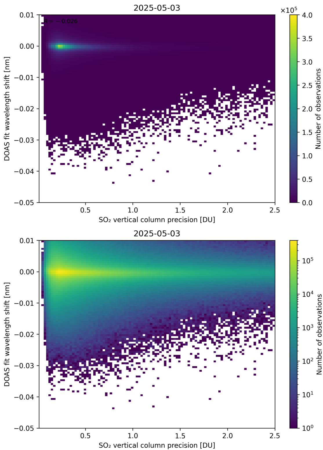
Figure 332: Scatter density plot of “SO 2 vertical column precision” against “DOAS fit wavelength shift” for 2025-05-02 to 2025-05-04.
