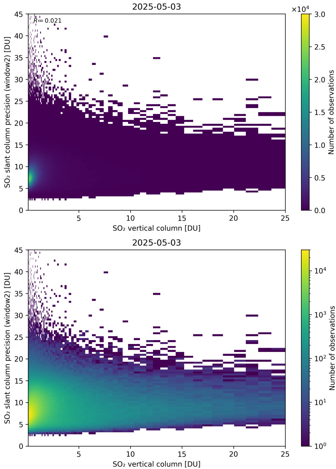
Figure 356: Scatter density plot of “SO 2 vertical column” against “SO 2 slant column precision (window2)” for 2025-05-02 to 2025-05-04.
