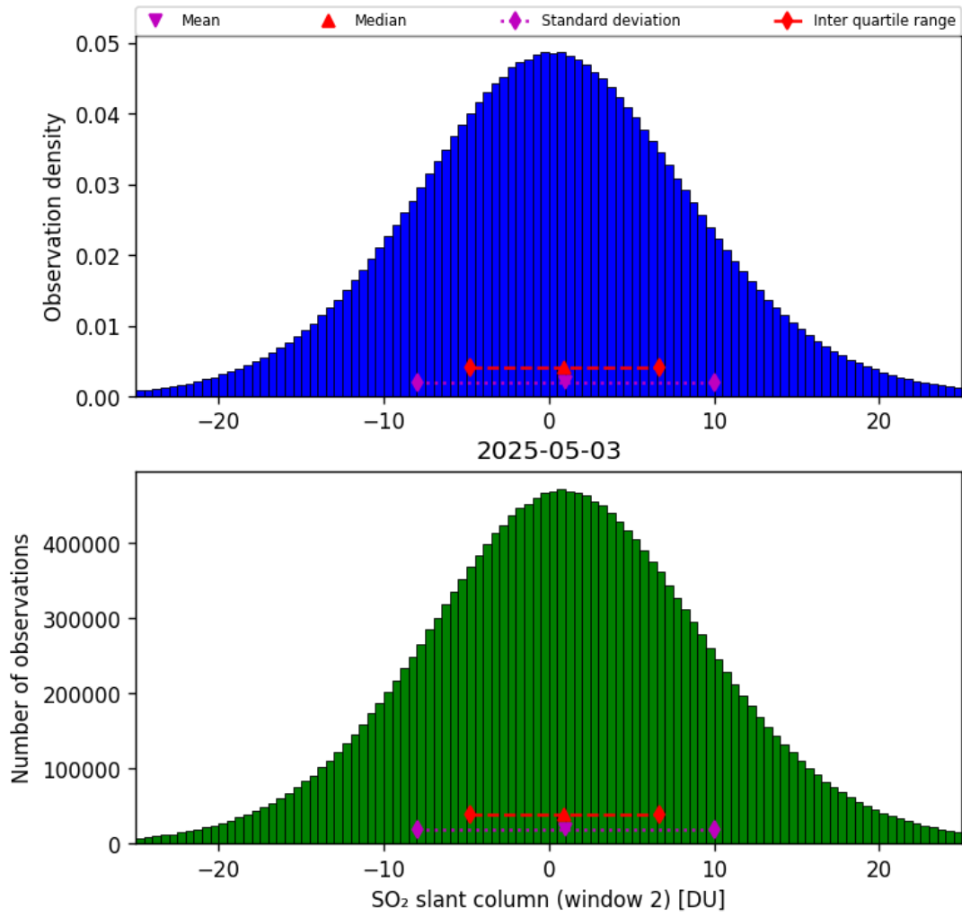
Figure 67: Histogram of “SO 2 slant column (window 2)” for 2025-05-02 to 2025-05-04
