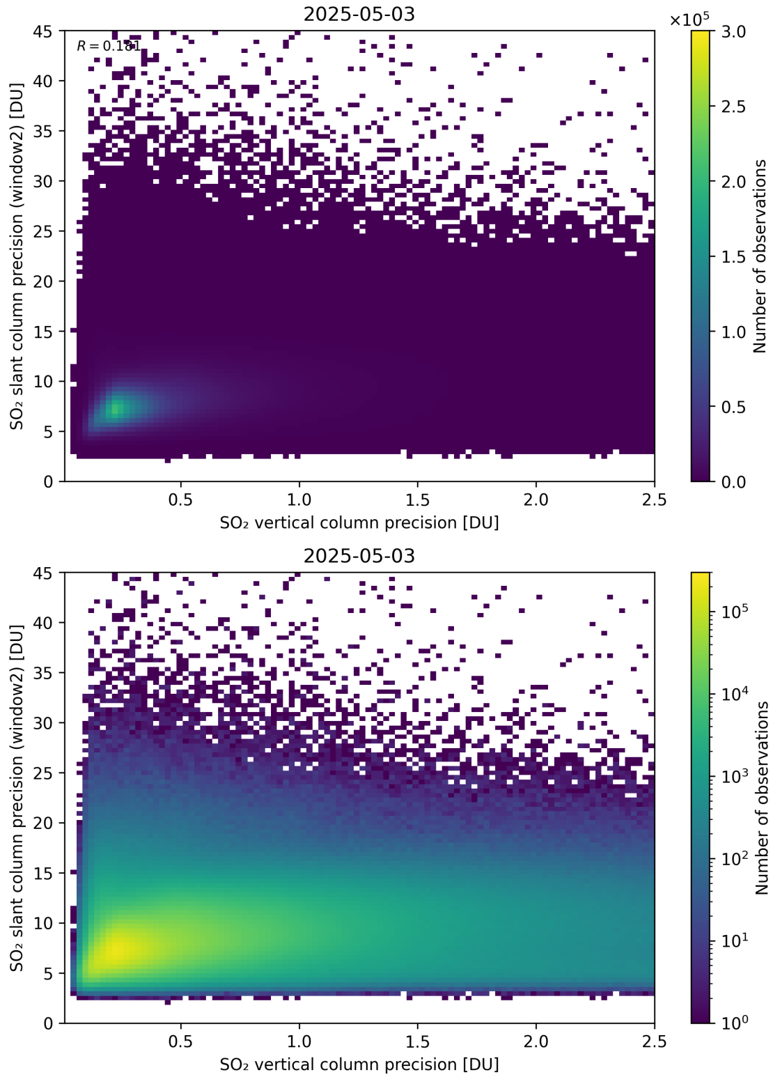
Figure 343: Scatter density plot of “SO 2 vertical column precision” against “SO 2 slant column precision (window2)” for 2025-05-02 to 2025-05-04.
