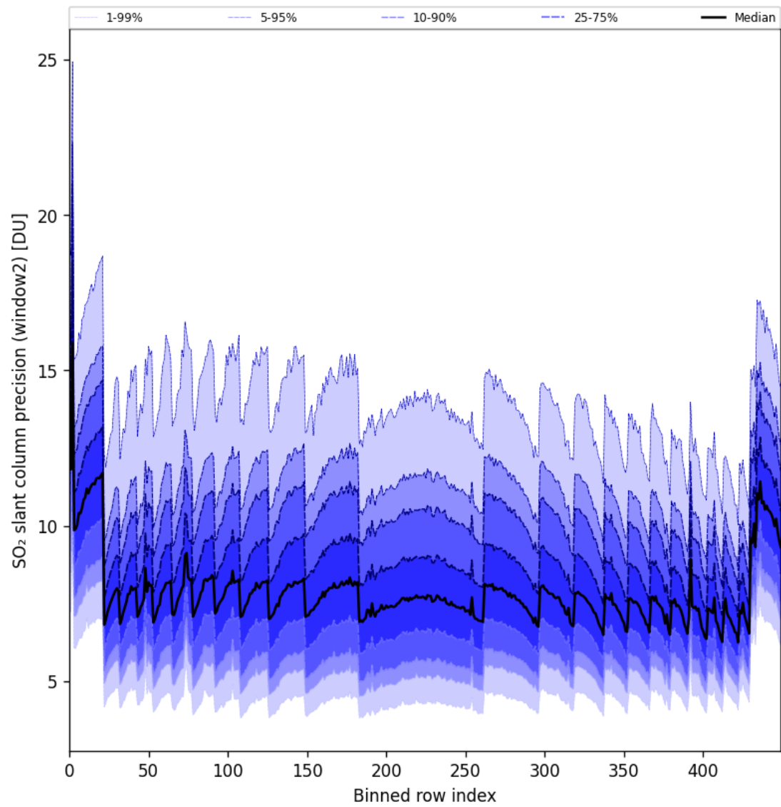
Figure 94: Along track statistics of “SO 2 slant column precision (window2)” for 2025-05-02 to 2025-05-04
