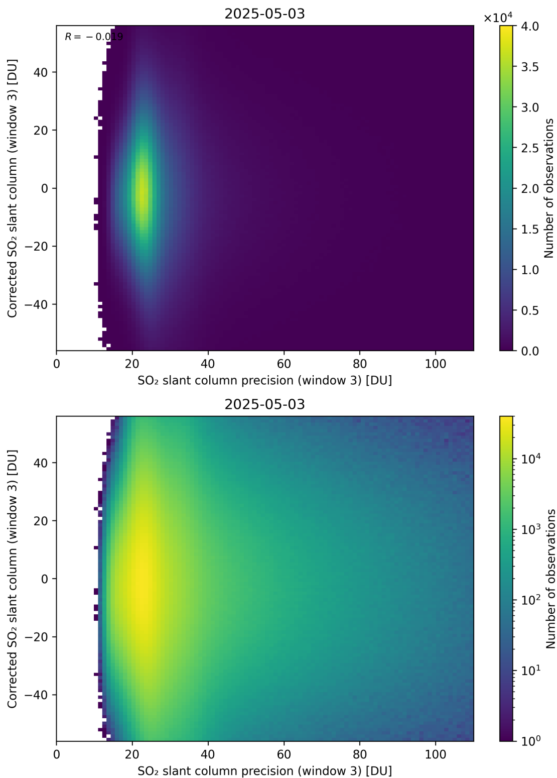
Figure 312: Scatter density plot of “SO 2 slant column precision (window 3)” against “Corrected SO 2 slant column (window 3)” for 2025-05-02 to 2025-05-04.
