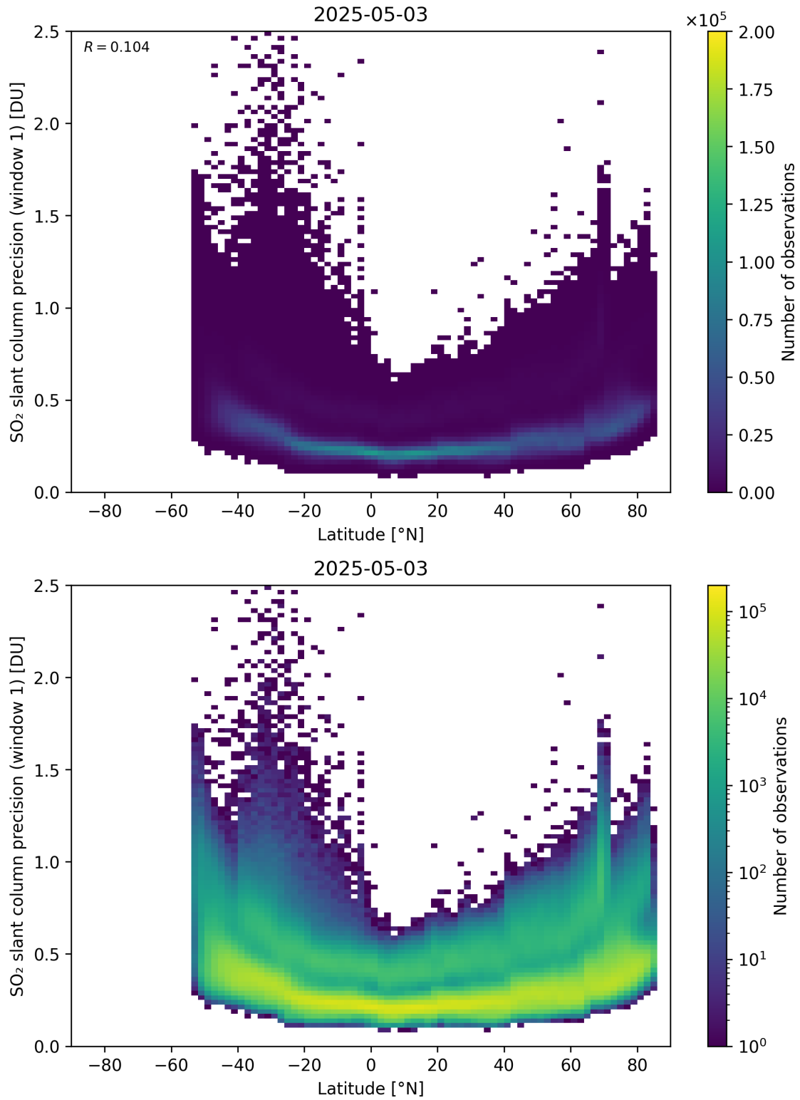
Figure 163: Scatter density plot of “Latitude” against “SO 2 slant column precision (window 1)” for 2025-05-02 to 2025-05-04.
