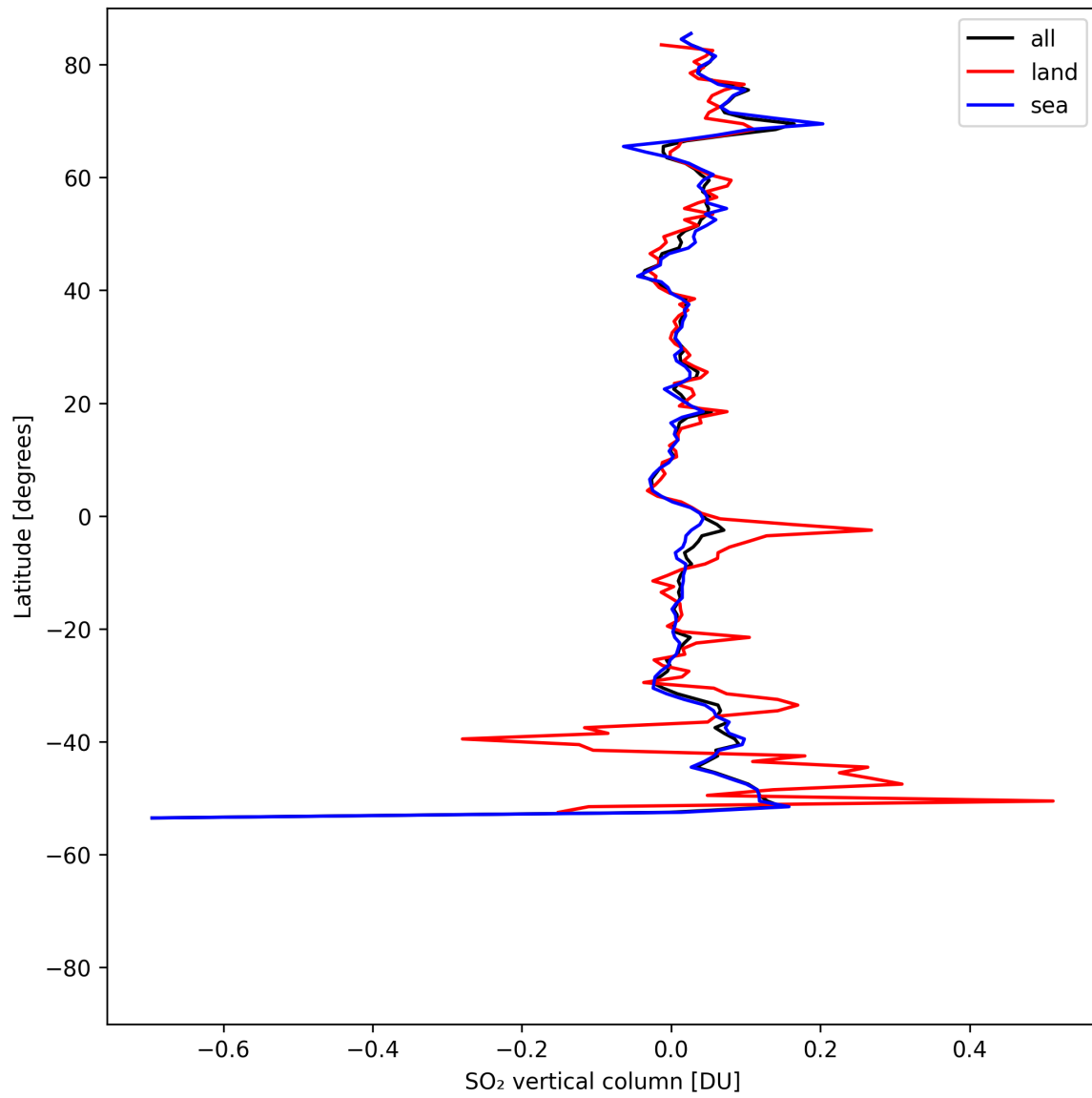
Figure 32: Zonal average of “SO 2 vertical column” for 2025-05-02 to 2025-05-04.
