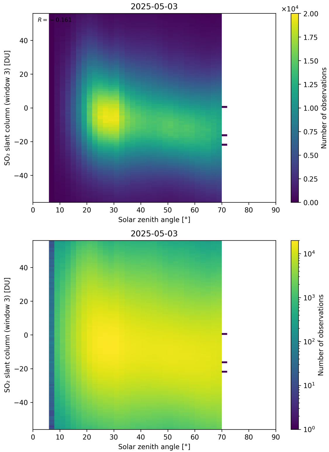
Figure 187: Scatter density plot of “Solar zenith angle” against “SO 2 slant column (window 3)” for 2025-05-02 to 2025-05-04.
