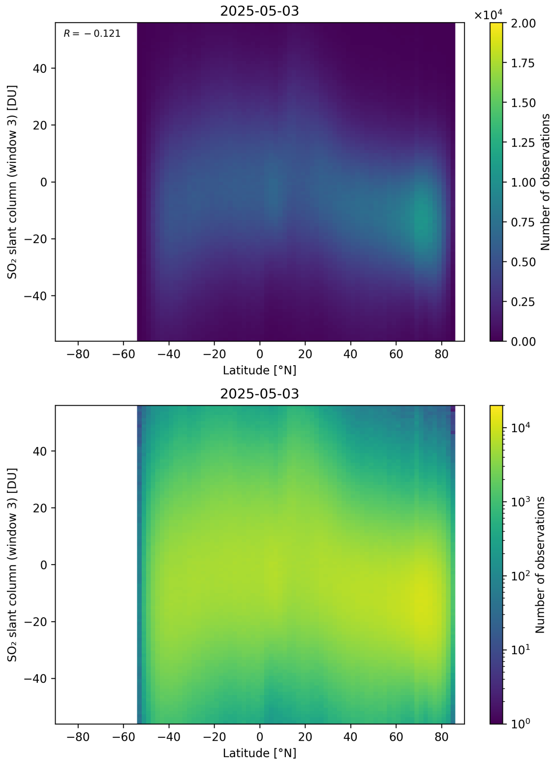
Figure 165: Scatter density plot of “Latitude” against “SO 2 slant column (window 3)” for 2025-05-02 to 2025-05-04.
