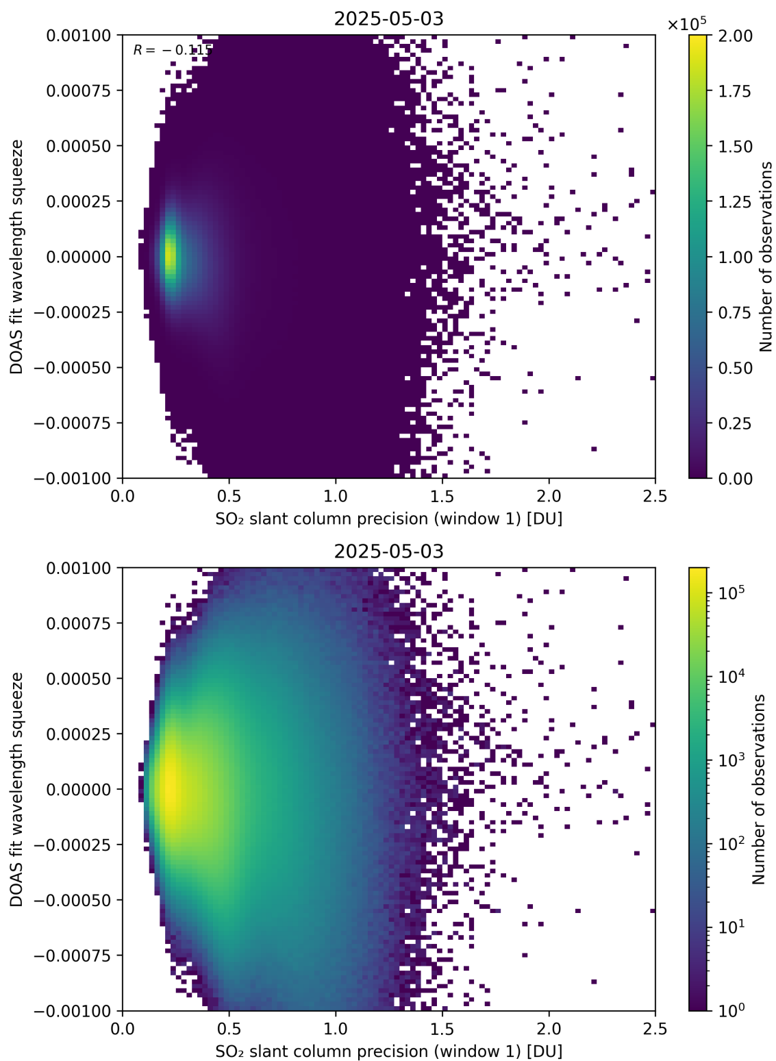
Figure 272: Scatter density plot of “SO 2 slant column precision (window 1)” against “DOAS fit wavelength squeeze” for 2025-05-02 to 2025-05-04.
