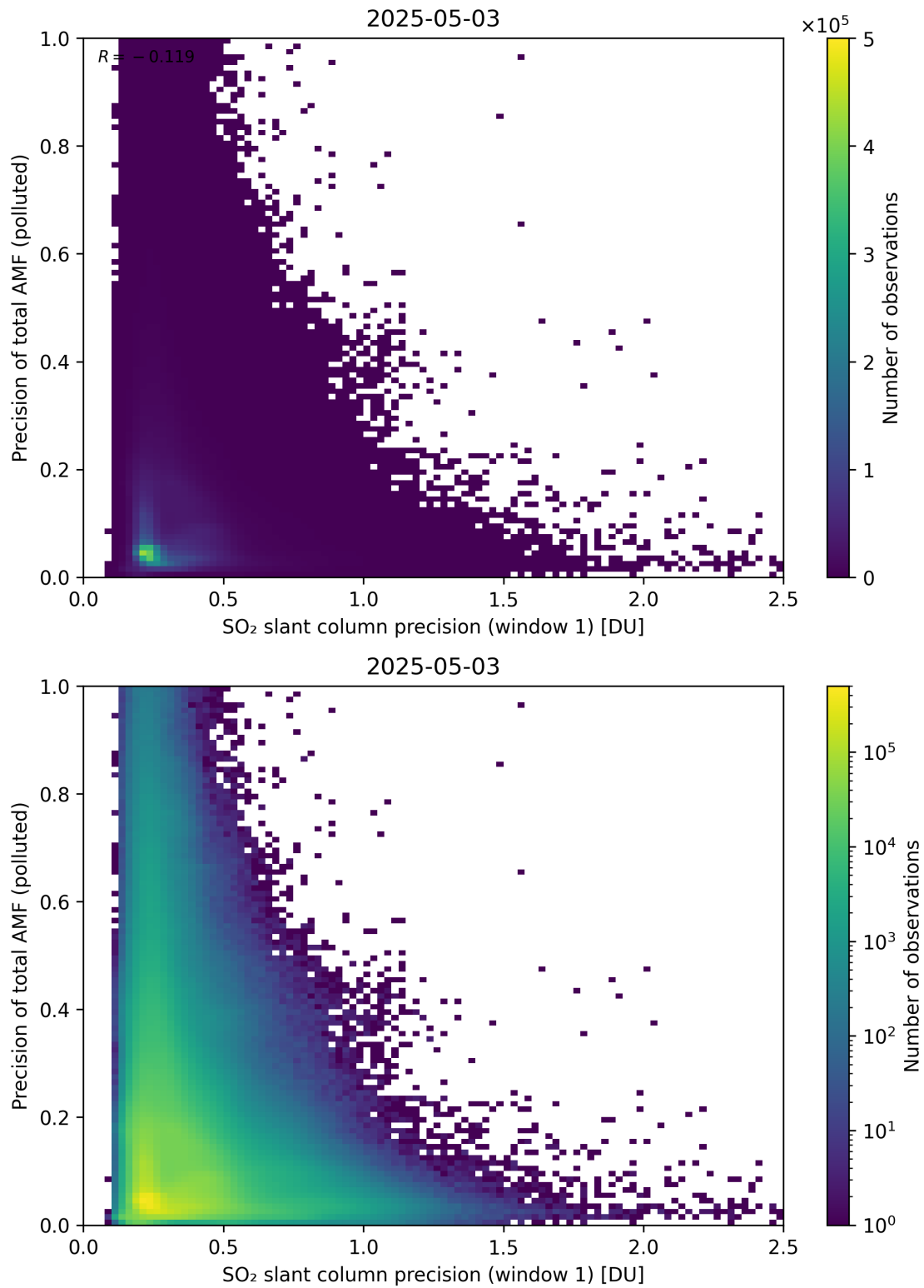
Figure 281: Scatter density plot of “SO 2 slant column precision (window 1)” against “Precision of total AMF (polluted)” for 2025-05-02 to 2025-05-04.
