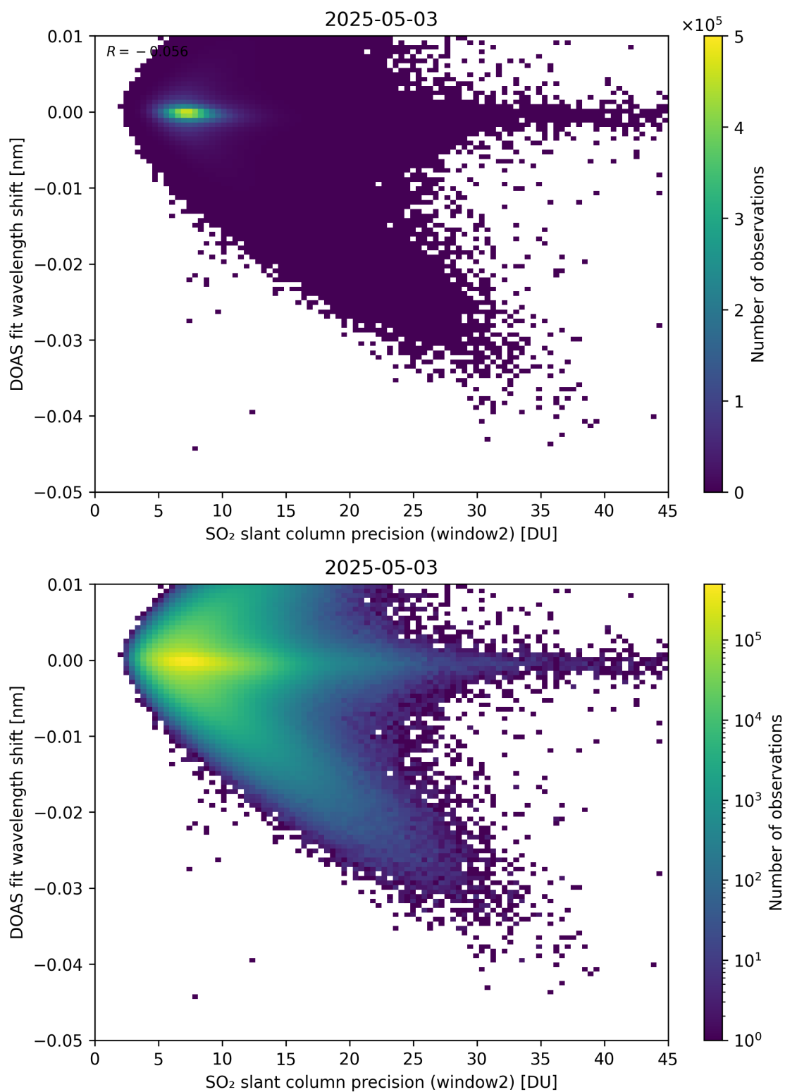
Figure 293: Scatter density plot of “SO 2 slant column precision (window2)” against “DOAS fit wavelength shift” for 2025-05-02 to 2025-05-04.
