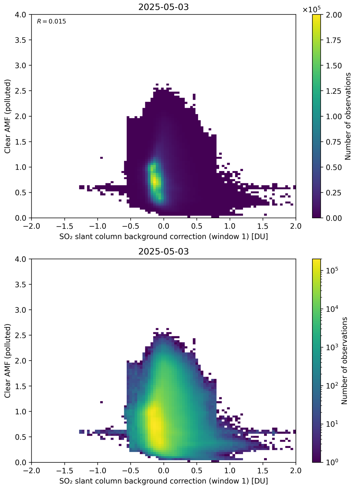
Figure 114: Scatter density plot of “SO 2 slant column background correction (window 1)” against “Clear AMF (polluted)” for 2025-05-02 to 2025-05-04.
