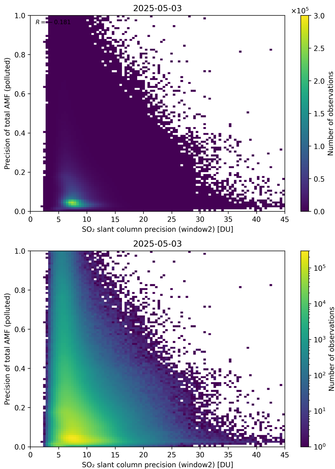
Figure 302: Scatter density plot of “SO 2 slant column precision (window2)” against “Precision of total AMF (polluted)” for 2025-05-02 to 2025-05-04.
