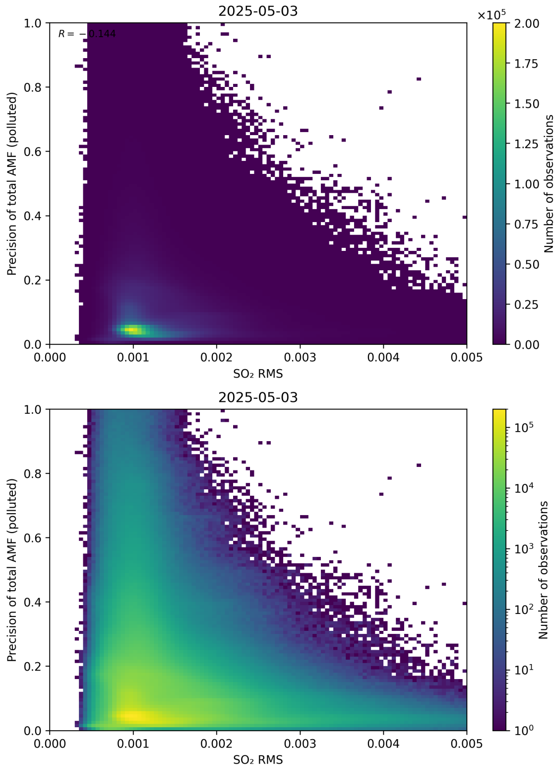
Figure 149: Scatter density plot of “SO 2 RMS” against “Precision of total AMF (polluted)” for 2025-05-02 to 2025-05-04.
