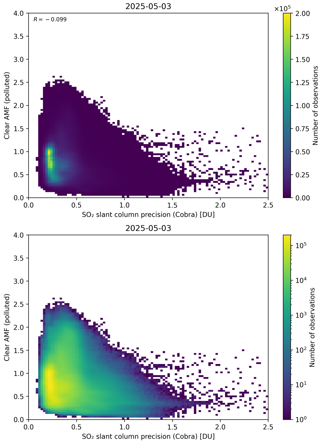
Figure 205: Scatter density plot of “SO 2 slant column precision (Cobra)” against “Clear AMF (polluted)” for 2025-05-02 to 2025-05-04.
