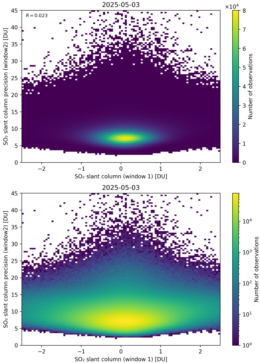
Figure 286: Scatter density plot of “SO 2 slant column (window 1)” against “SO 2 slant column precision (window2)” for 2025-05-02 to 2025-05-04.
