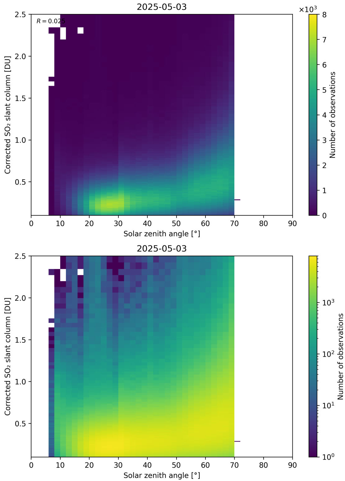
Figure 181: Scatter density plot of “Solar zenith angle” against “Corrected SO 2 slant column” for 2025-05-02 to 2025-05-04.
