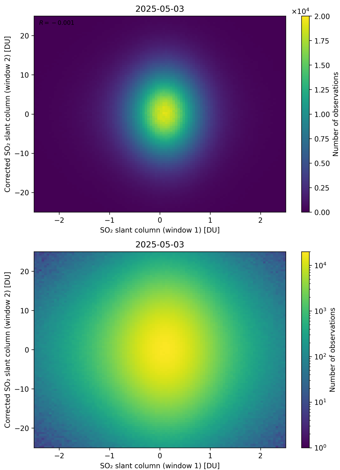
Figure 283: Scatter density plot of “SO 2 slant column (window 1)” against “Corrected SO 2 slant column (window 2)” for 2025-05-02 to 2025-05-04.
