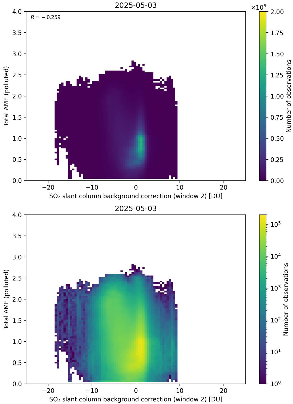
Figure 130: Scatter density plot of “SO 2 slant column background correction (window 2)” against “Total AMF (polluted)” for 2025-05-02 to 2025-05-04.
