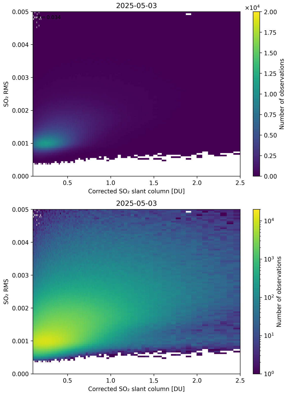
Figure 231: Scatter density plot of “Corrected SO 2 slant column” against “SO 2 RMS” for 2025-05-02 to 2025-05-04.
