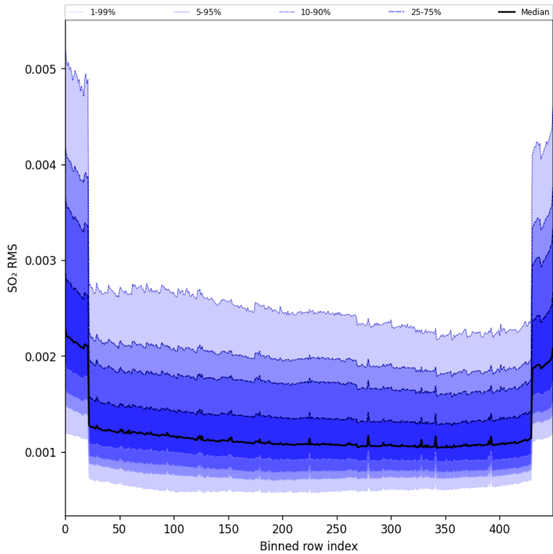
Figure 104: Along track statistics of “SO 2 RMS” for 2025-05-02 to 2025-05-04
