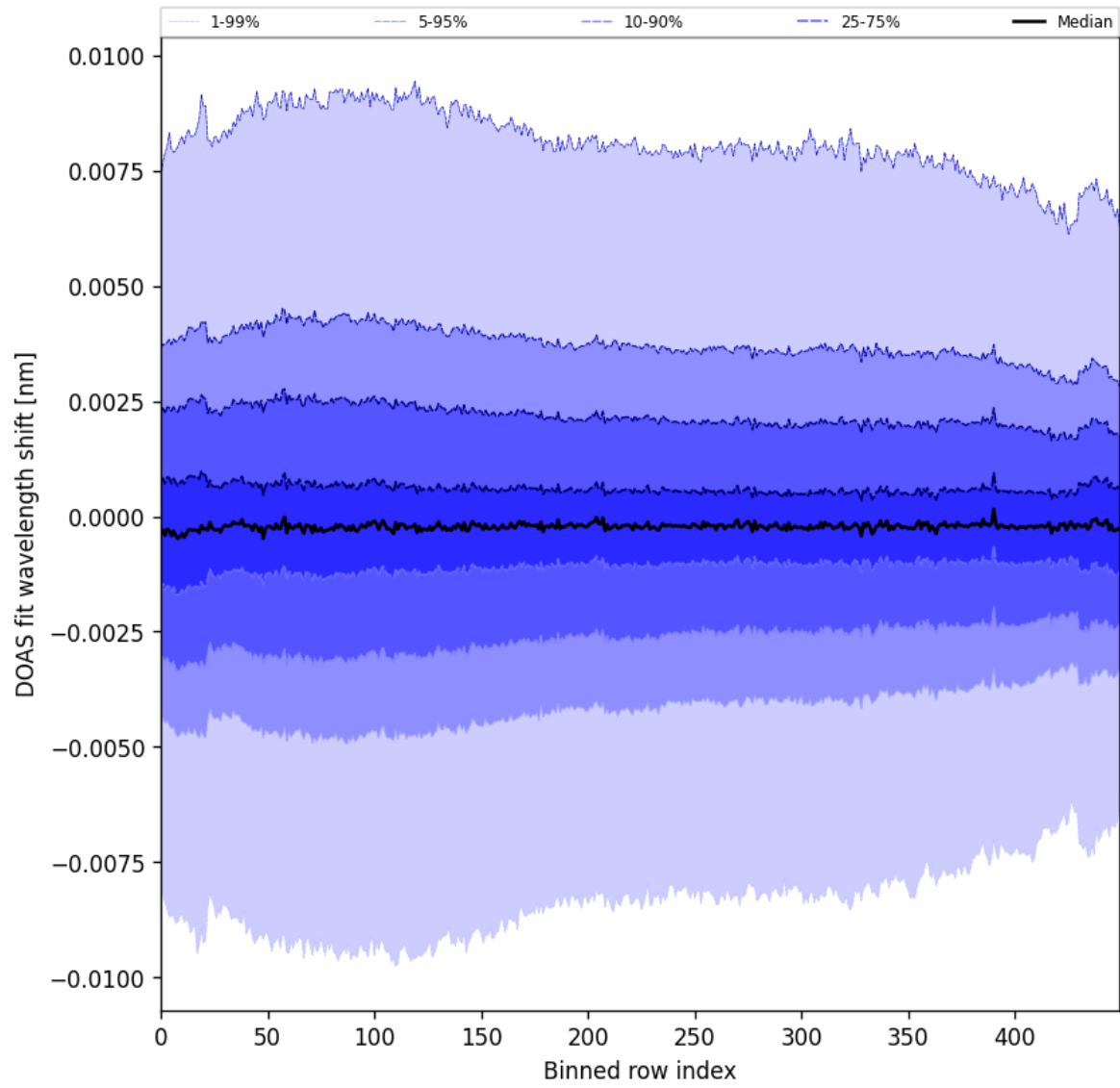
Figure 102: Along track statistics of “DOAS fit wavelength shift” for 2025-05-02 to 2025-05-04
