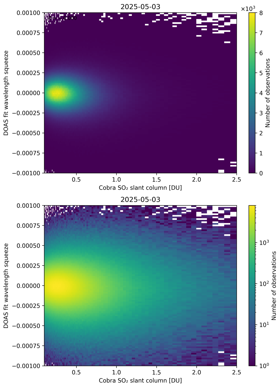
Figure 197: Scatter density plot of “Cobra SO 2 slant column” against “DOAS fit wavelength squeeze” for 2025-05-02 to 2025-05-04.
