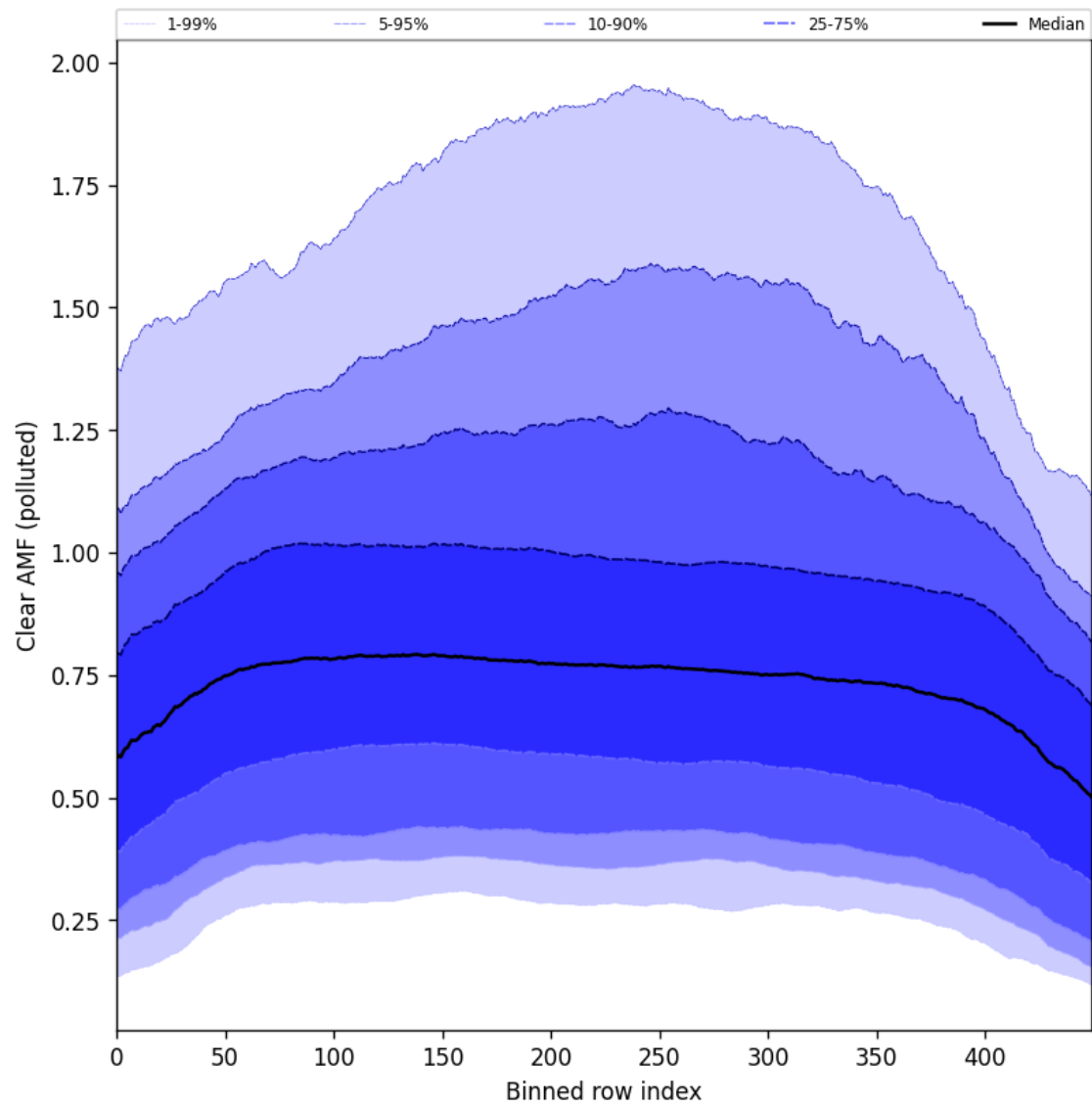
Figure 107: Along track statistics of “Clear AMF (polluted)” for 2025-05-02 to 2025-05-04
