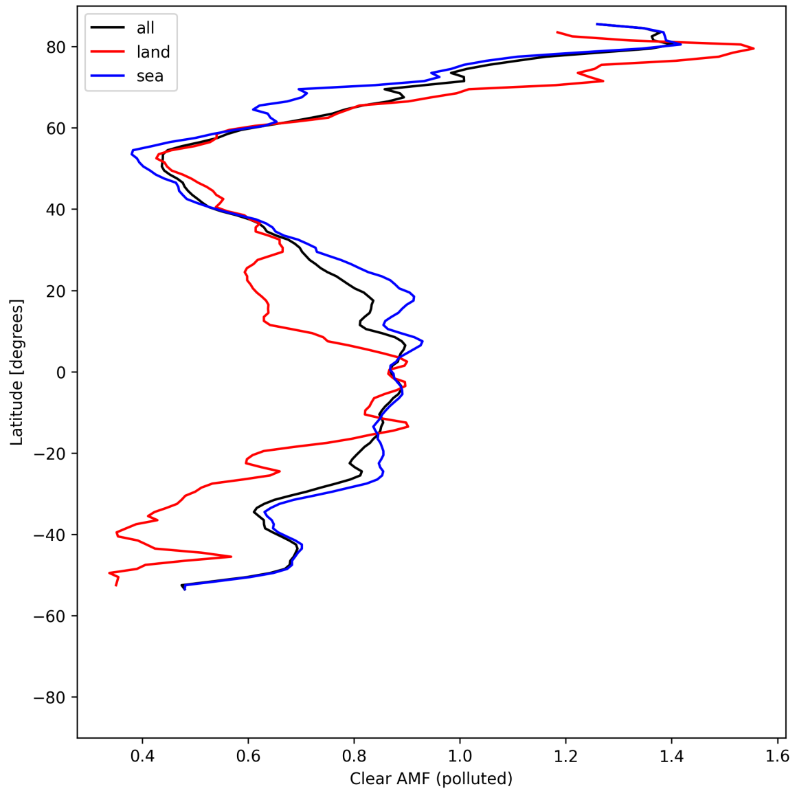
Figure 55: Zonal average of “Clear AMF (polluted)” for 2025-05-02 to 2025-05-04.
