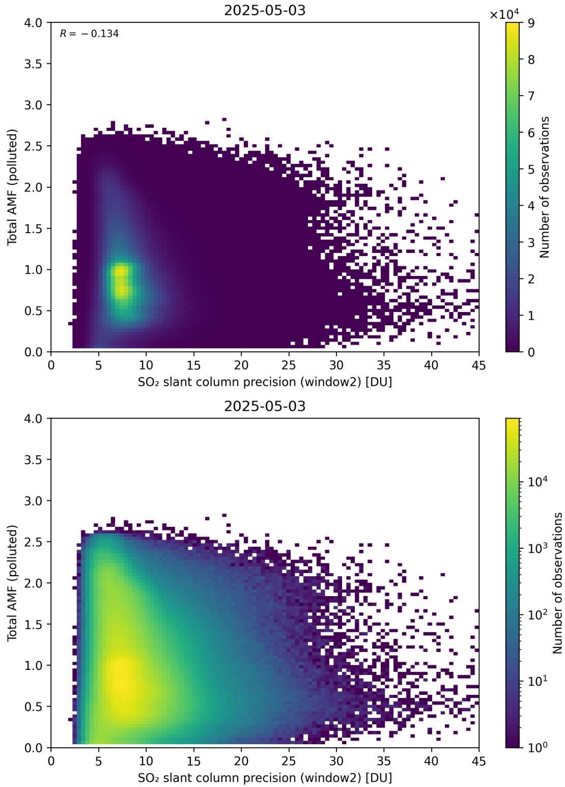
Figure 301: Scatter density plot of “SO 2 slant column precision (window2)” against “Total AMF (polluted)” for 2025-05-02 to 2025-05-04.
