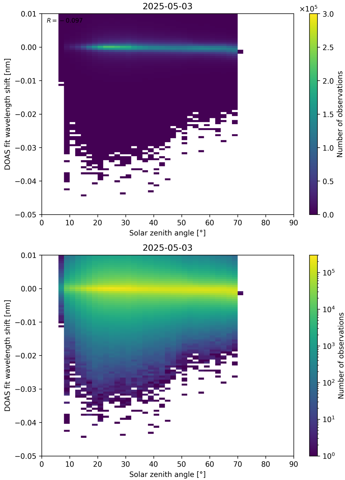
Figure 174: Scatter density plot of “Solar zenith angle” against “DOAS fit wavelength shift” for 2025-05-02 to 2025-05-04.
