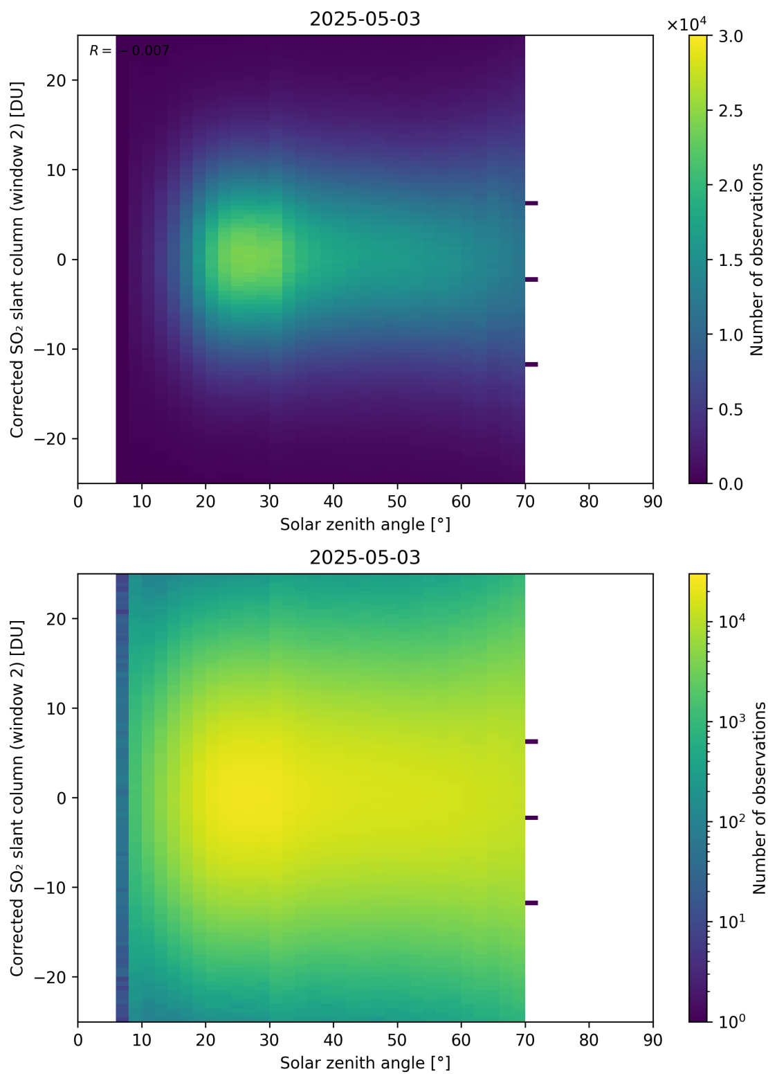
Figure 182: Scatter density plot of “Solar zenith angle” against “Corrected SO 2 slant column (window 2)” for 2025-05-02 to 2025-05-04.
