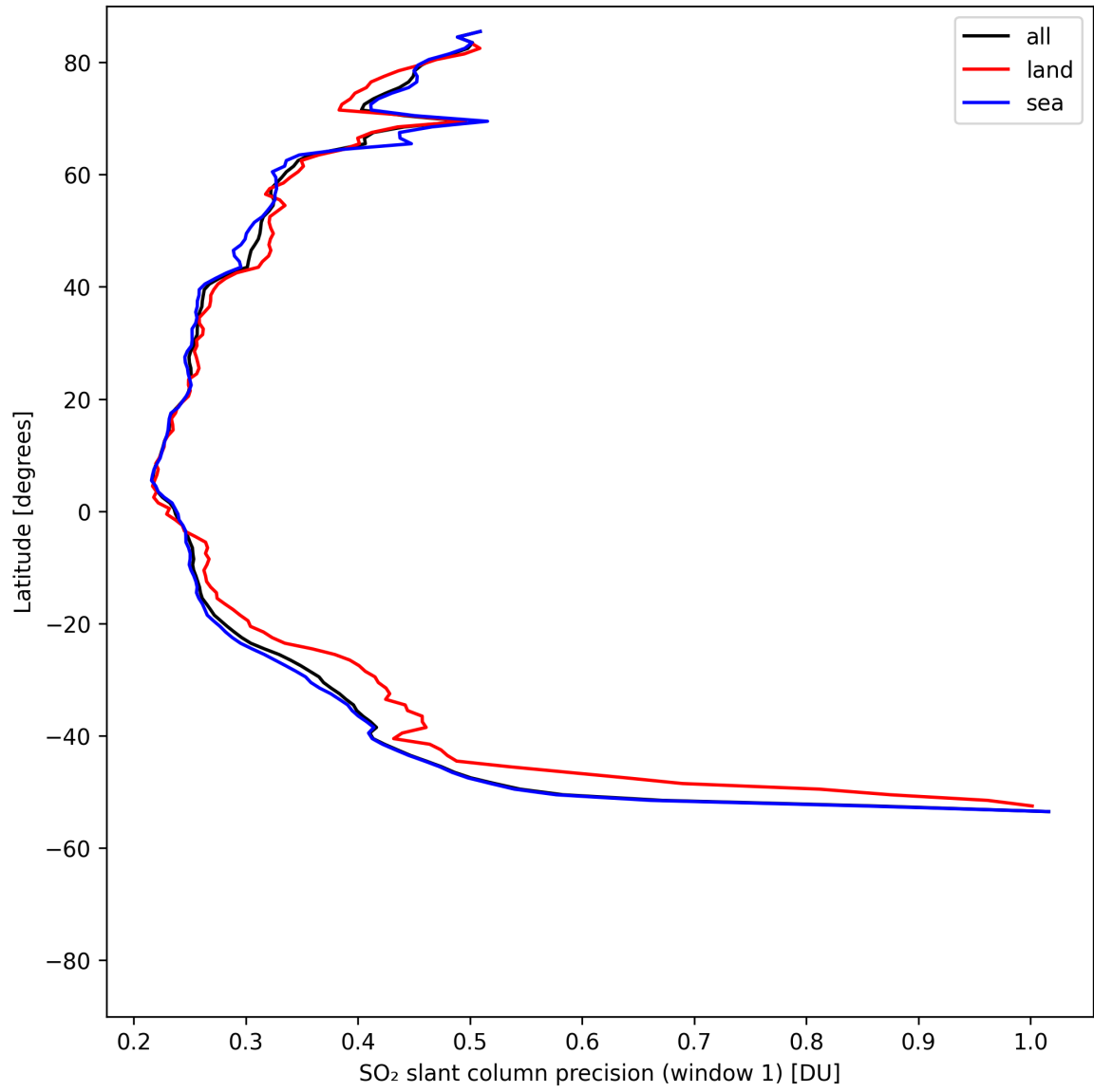
Figure 38: Zonal average of “SO 2 slant column precision (window 1)” for 2025-05-02 to 2025-05-04.
