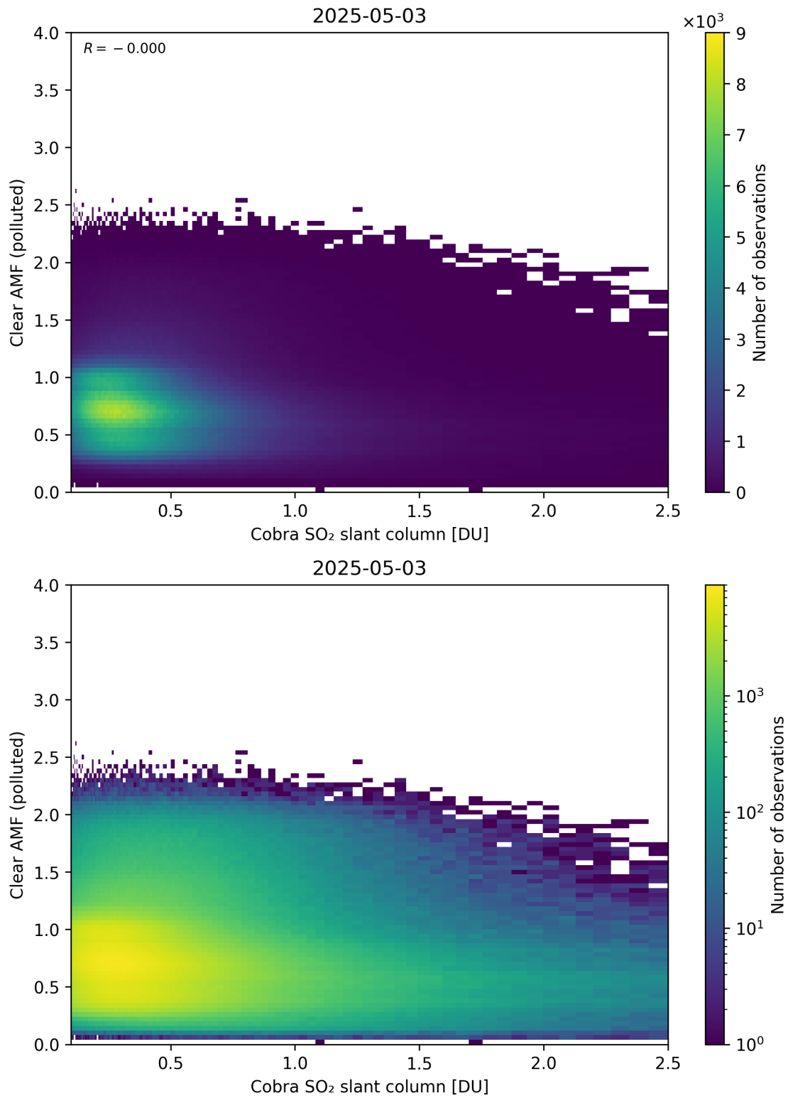
Figure 215: Scatter density plot of “Cobra SO 2 slant column” against “Clear AMF (polluted)” for 2025-05-02 to 2025-05-04.
