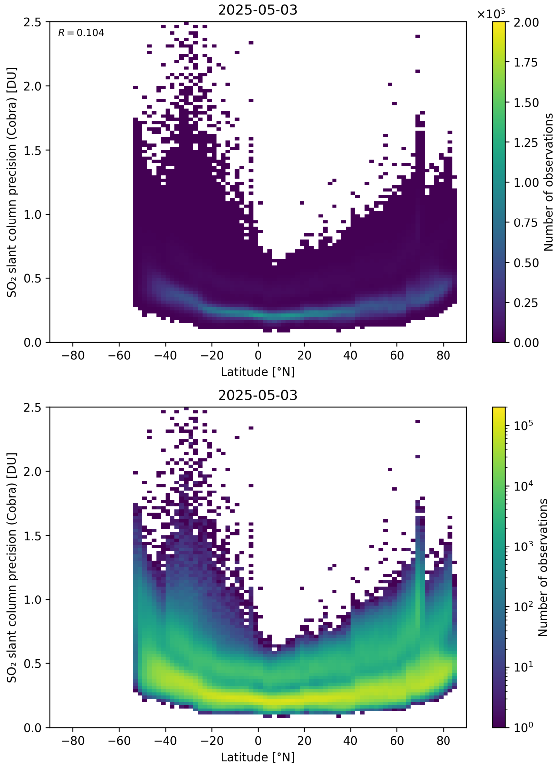
Figure 158: Scatter density plot of “Latitude” against “SO 2 slant column precision (Cobra)” for 2025-05-02 to 2025-05-04.
