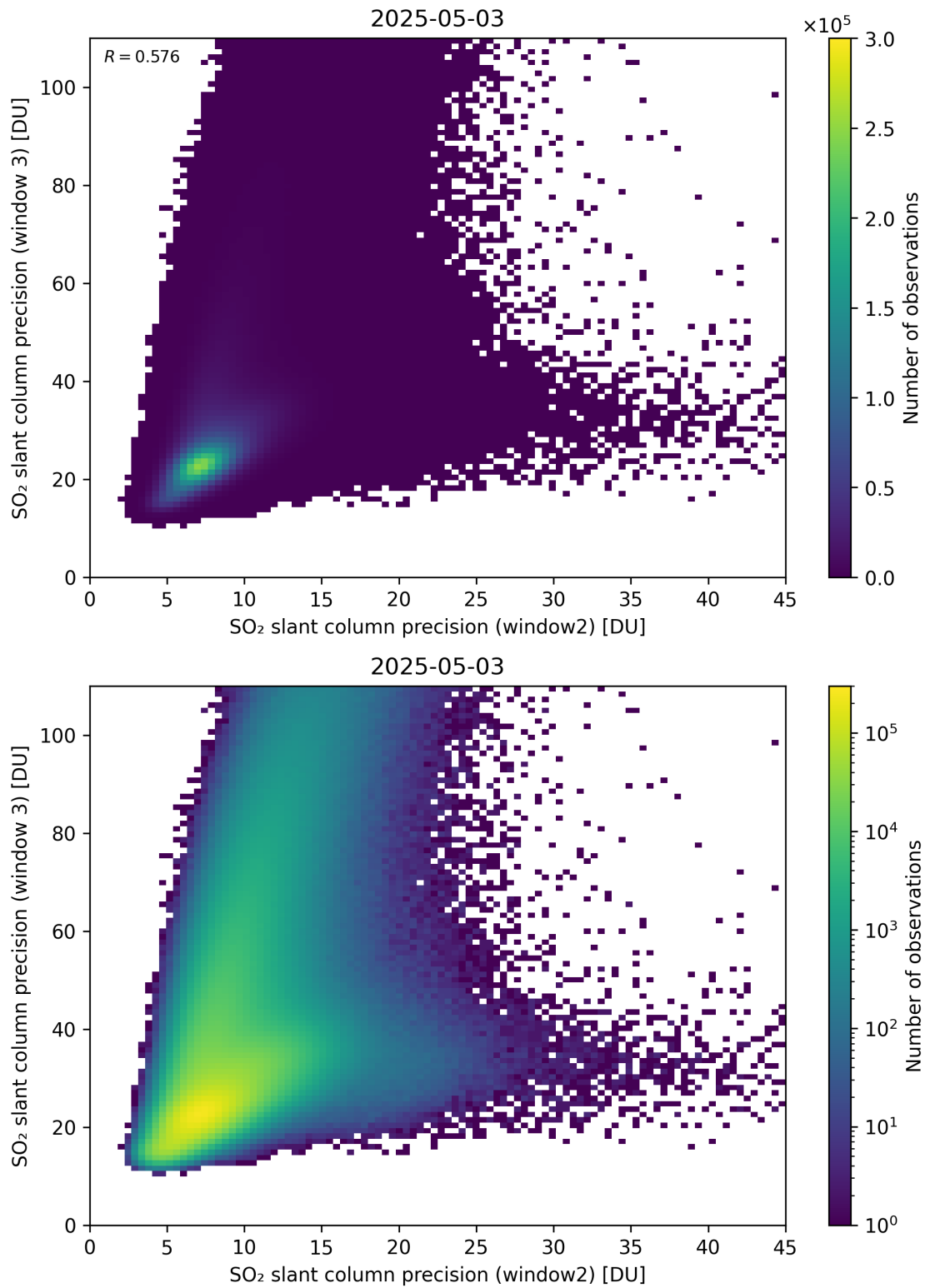
Figure 300: Scatter density plot of “SO 2 slant column precision (window2)” against “SO 2 slant column precision (window 3)” for 2025-05-02 to 2025-05-04.
