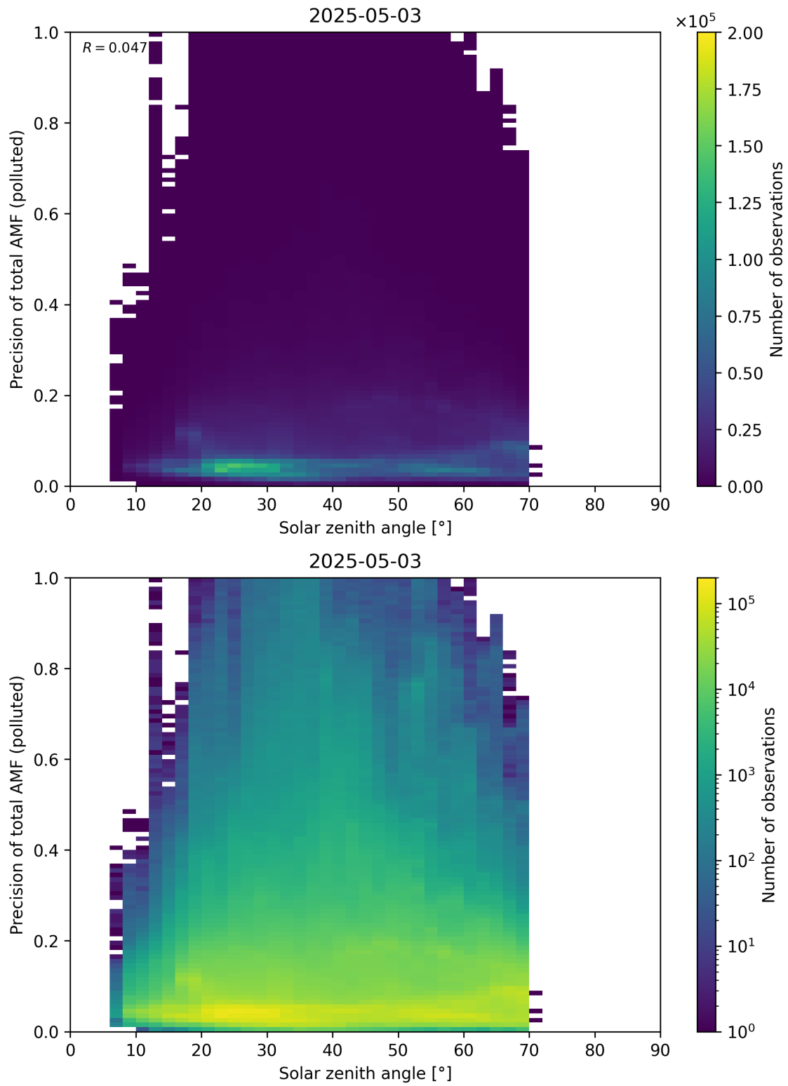
Figure 190: Scatter density plot of “Solar zenith angle” against “Precision of total AMF (polluted)” for 2025-05-02 to 2025-05-04.
