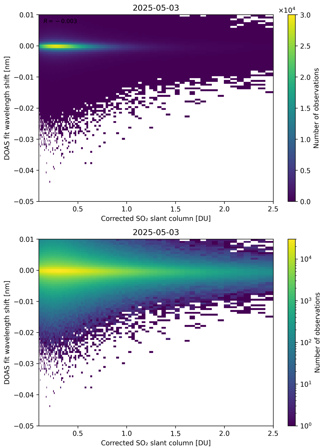
Figure 229: Scatter density plot of “Corrected SO 2 slant column” against “DOAS fit wavelength shift” for 2025-05-02 to 2025-05-04.
