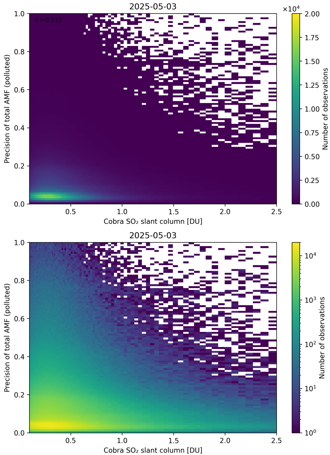
Figure 225: Scatter density plot of “Cobra SO 2 slant column” against “Precision of total AMF (polluted)” for 2025-05-02 to 2025-05-04.
