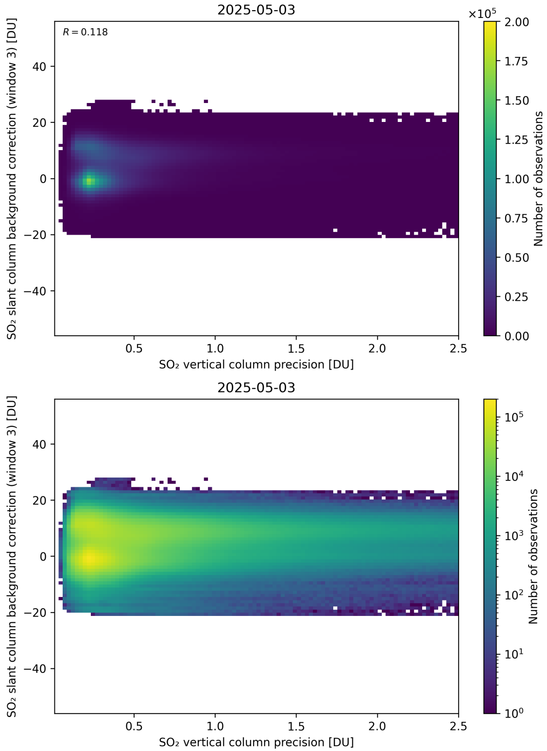
Figure 331: Scatter density plot of “SO 2 vertical column precision” against “SO 2 slant column background correction (window 3)” for 2025-05-02 to 2025-05-04.
