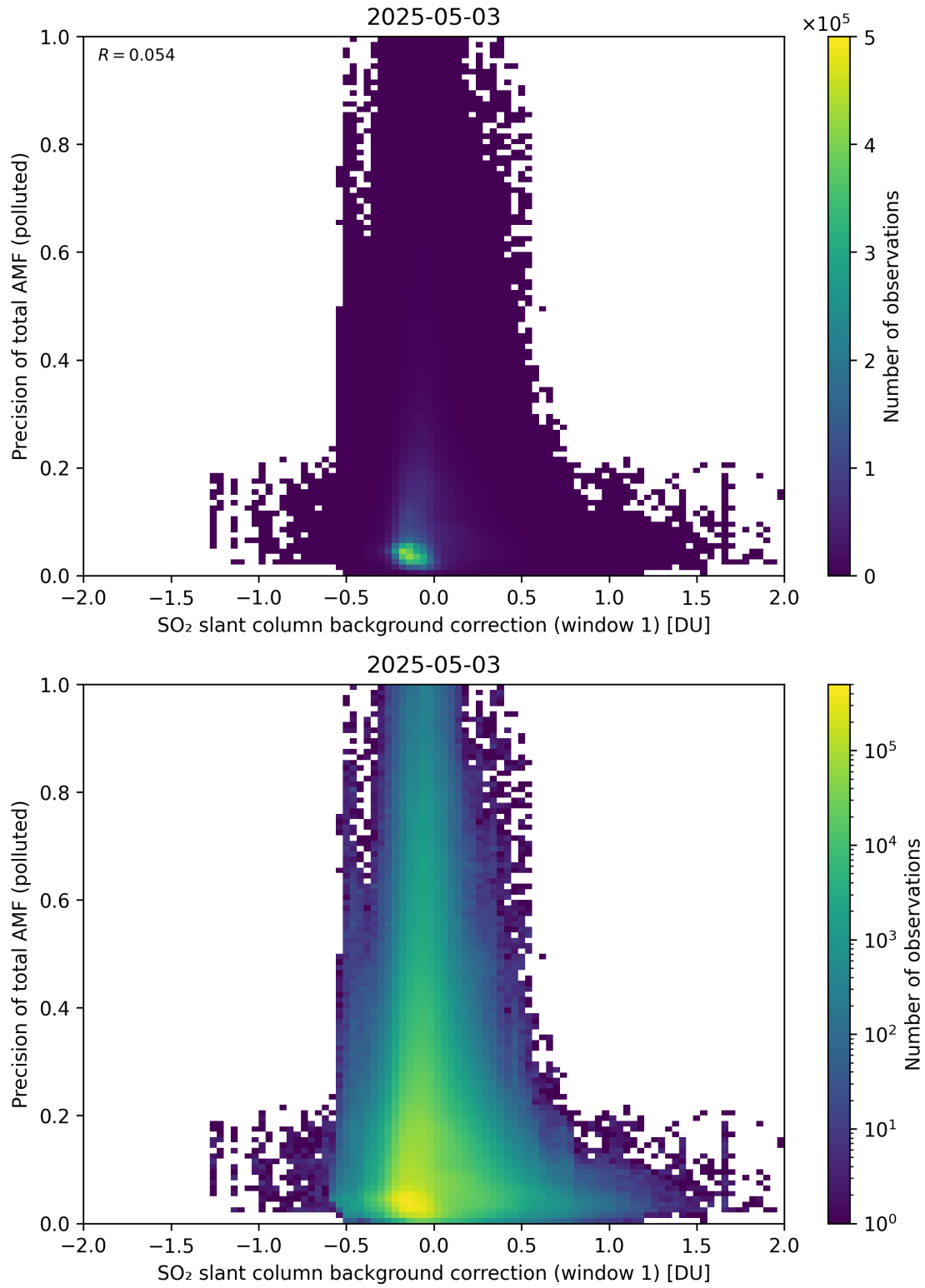
Figure 121: Scatter density plot of “SO 2 slant column background correction (window 1)” against “Precision of total AMF (polluted)” for 2025-05-02 to 2025-05-04.
