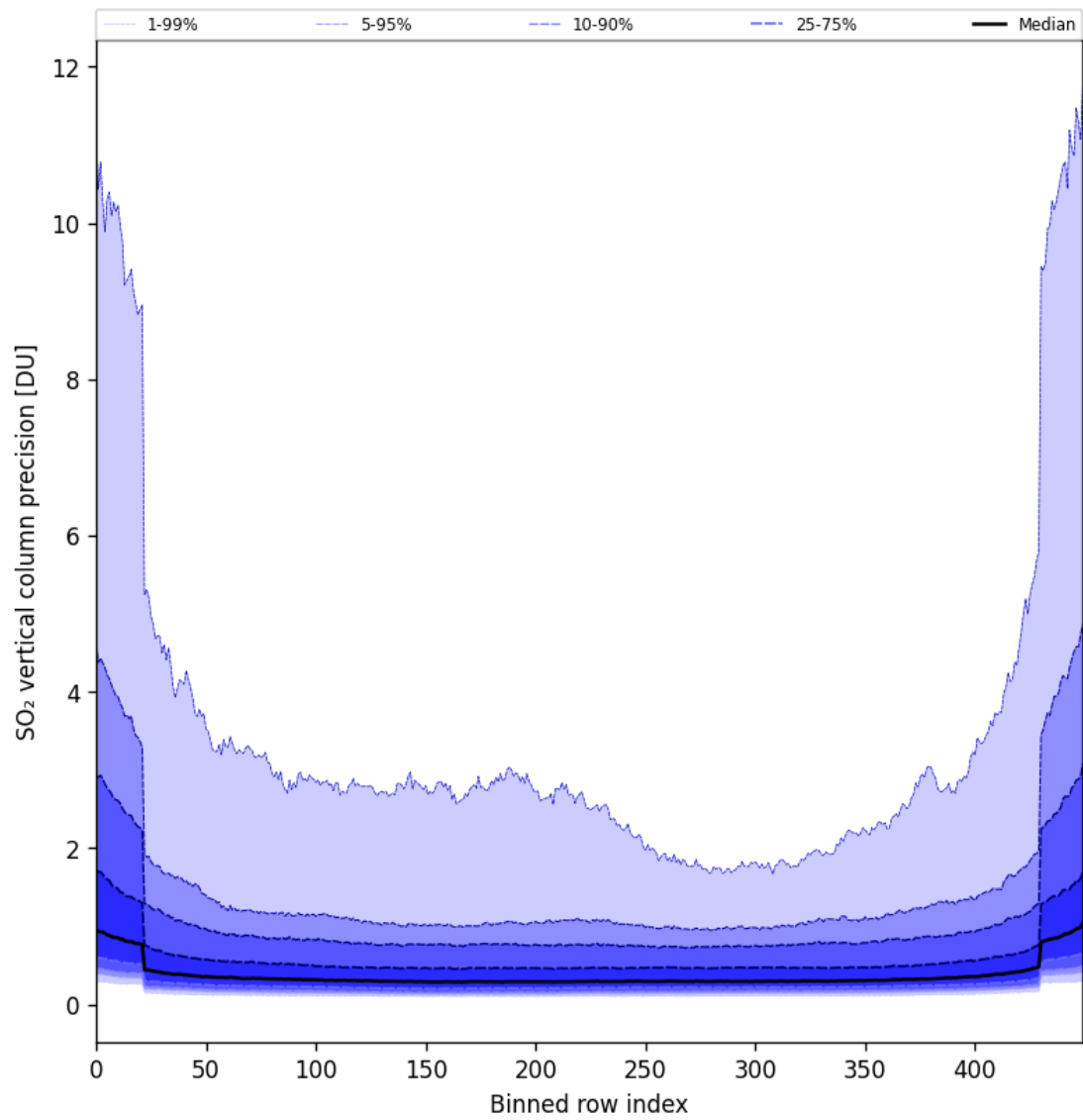
Figure 85: Along track statistics of “SO 2 vertical column precision” for 2025-05-02 to 2025-05-04
