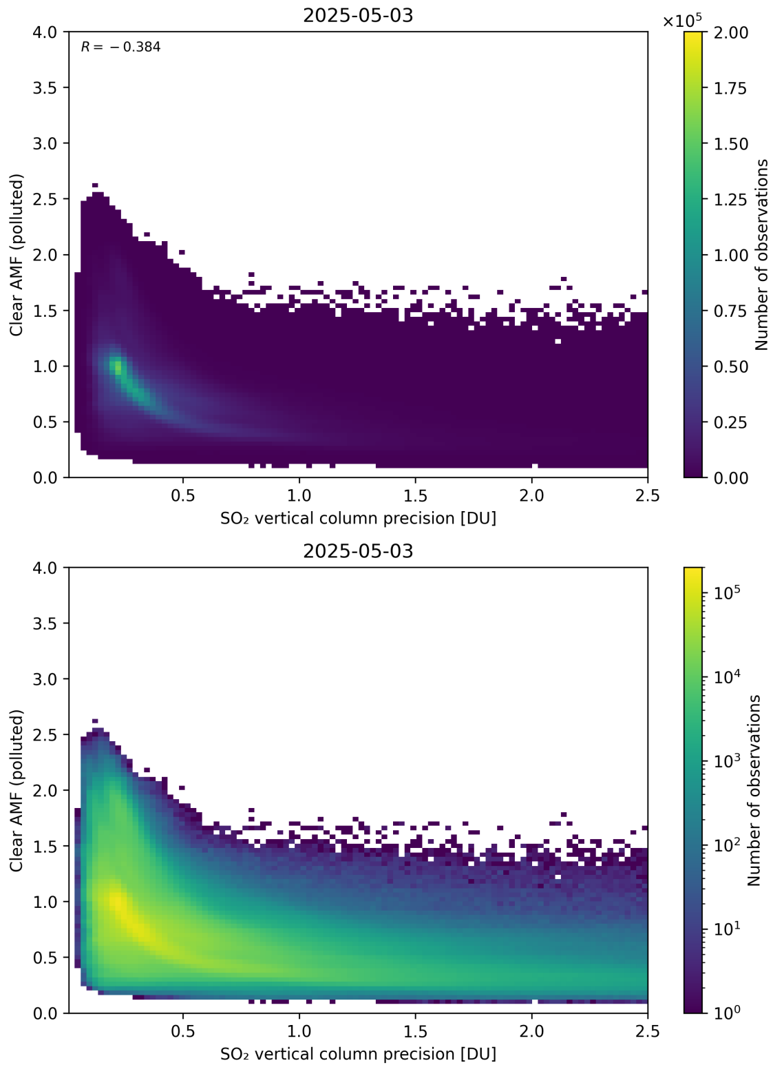
Figure 335: Scatter density plot of “SO 2 vertical column precision” against “Clear AMF (polluted)” for 2025-05-02 to 2025-05-04.
