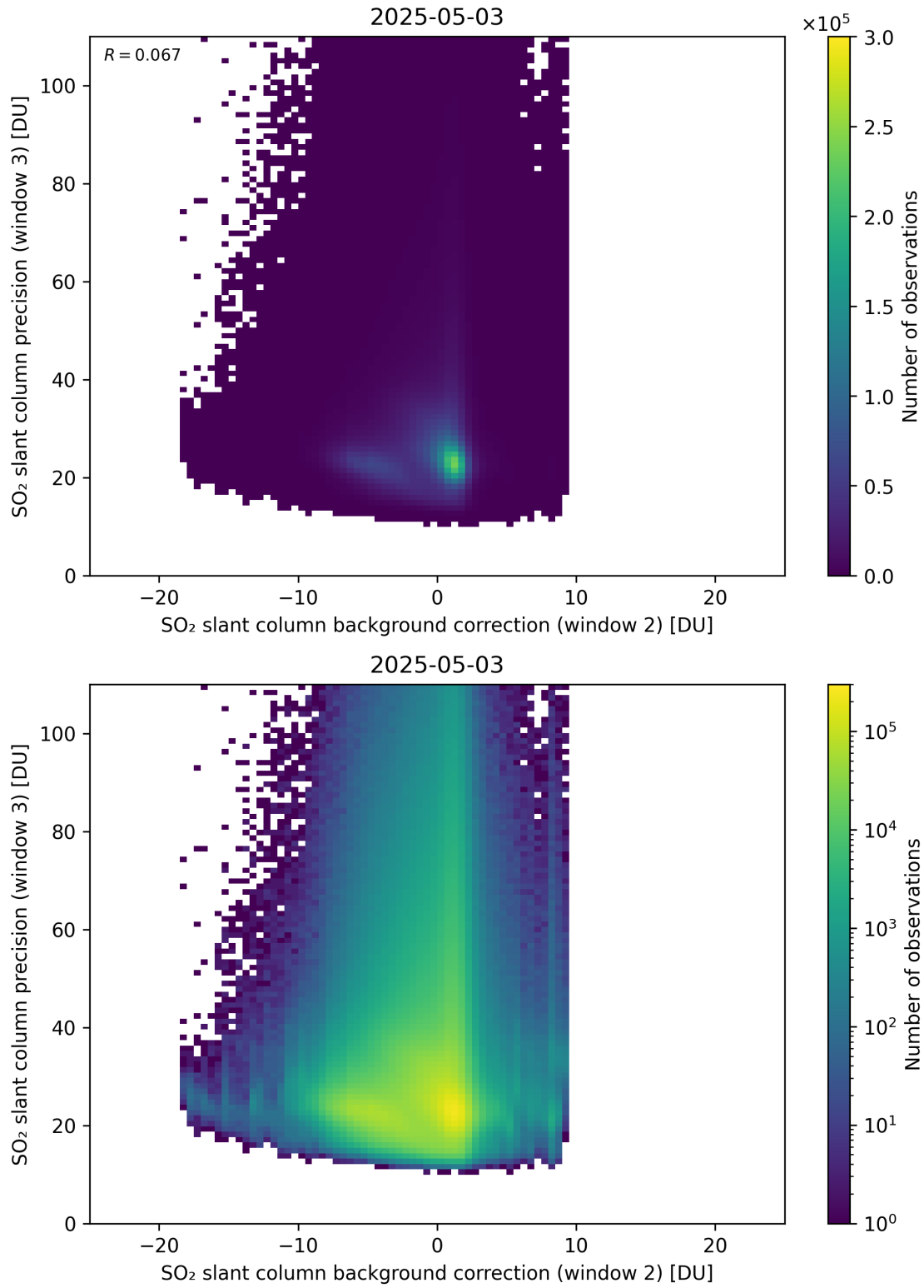
Figure 129: Scatter density plot of “SO 2 slant column background correction (window 2)” against “SO 2 slant column precision (window 3)” for 2025-05-02 to 2025-05-04.
