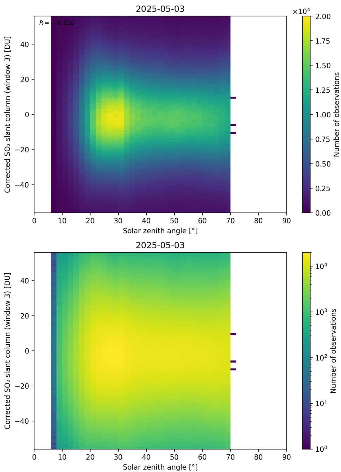
Figure 183: Scatter density plot of “Solar zenith angle” against “Corrected SO 2 slant column (window 3)” for 2025-05-02 to 2025-05-04.
