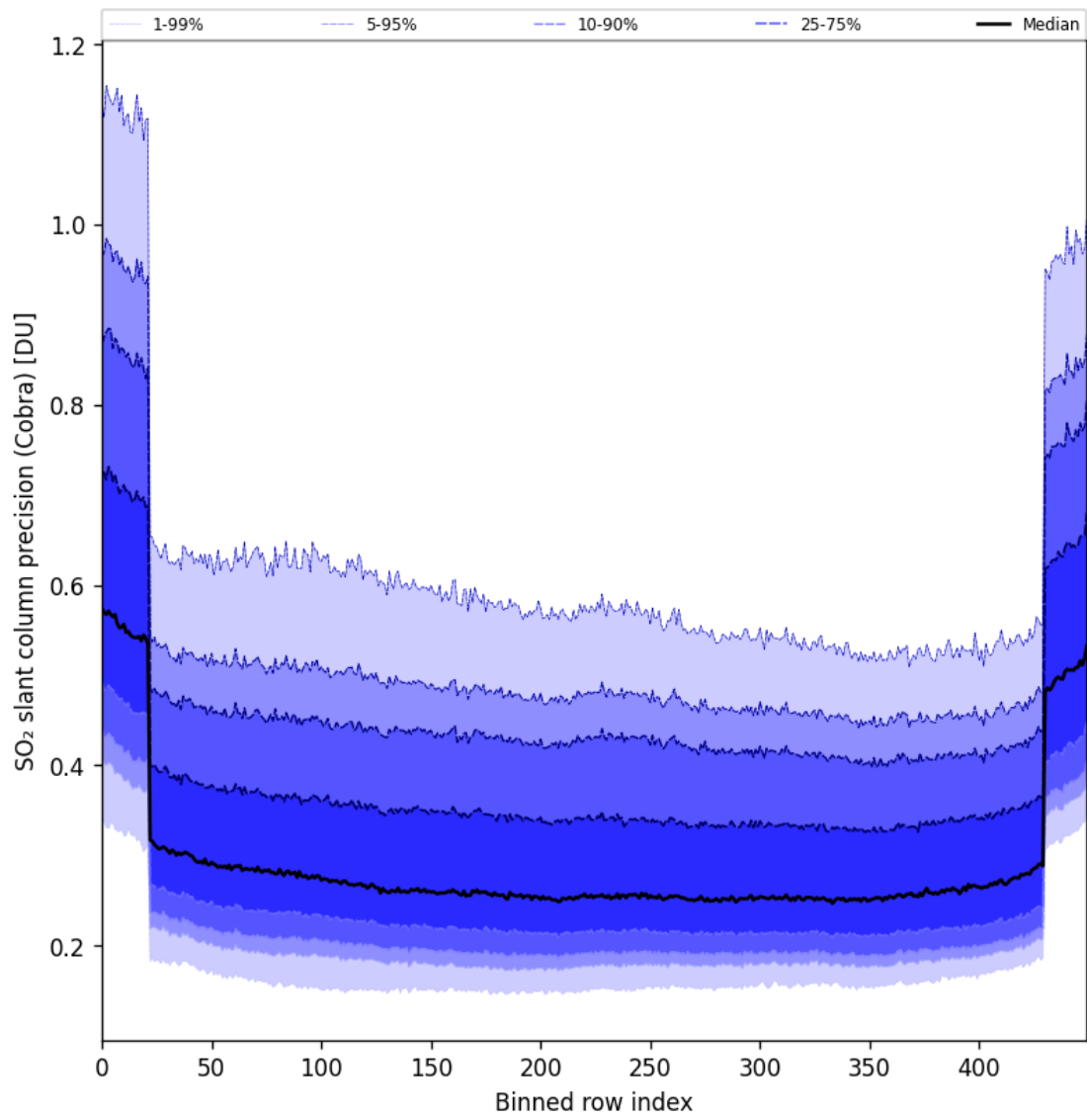
Figure 88: Along track statistics of “SO 2 slant column precision (Cobra)” for 2025-05-02 to 2025-05-04
