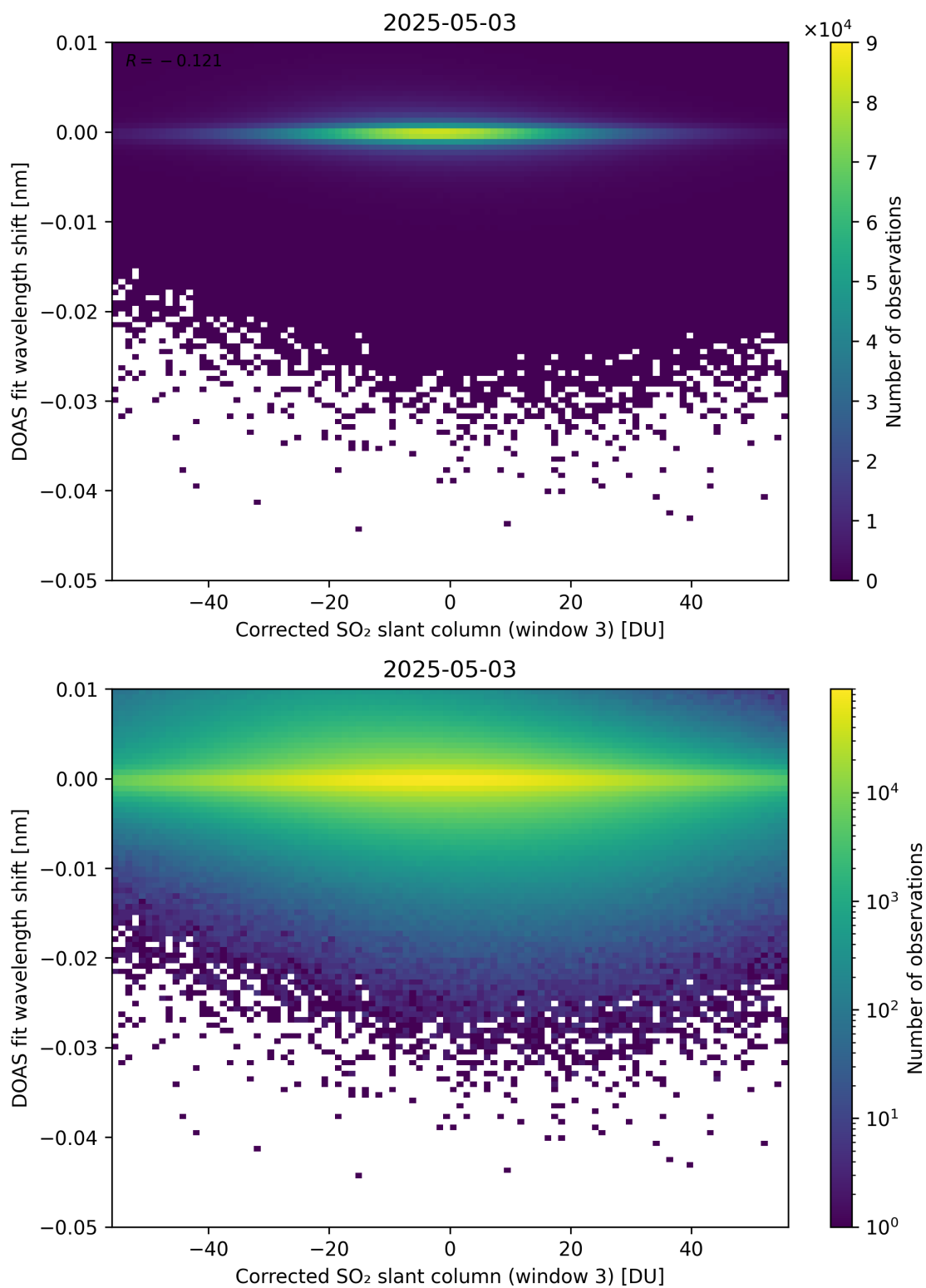
Figure 256: Scatter density plot of “Corrected SO 2 slant column (window 3)” against “DOAS fit wavelength shift” for 2025-05-02 to 2025-05-04.
