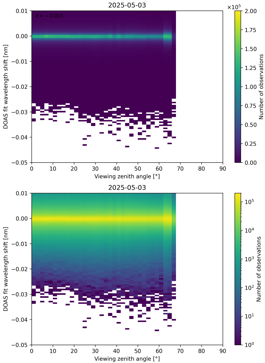
Figure 365: Scatter density plot of “Viewing zenith angle” against “DOAS fit wavelength shift” for 2025-05-02 to 2025-05-04.
