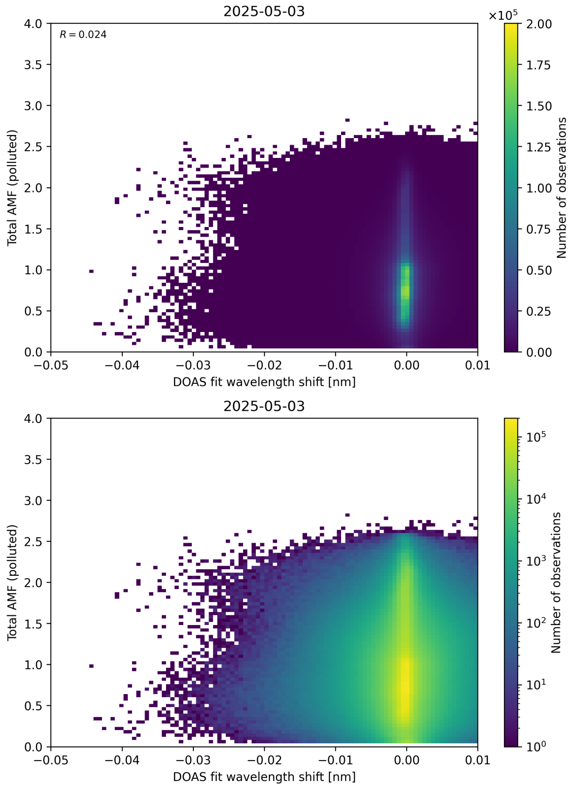
Figure 141: Scatter density plot of “DOAS fit wavelength shift” against “Total AMF (polluted)” for 2025-05-02 to 2025-05-04.
