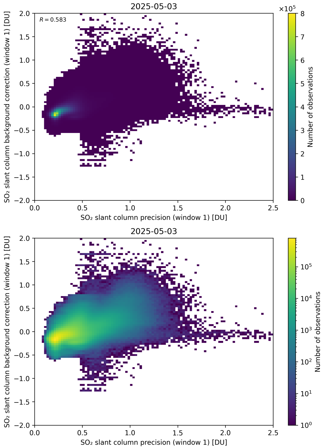
Figure 268: Scatter density plot of “SO 2 slant column precision (window 1)” against “SO 2 slant column background correction (window 1)” for 2025-05-02 to 2025-05-04.
