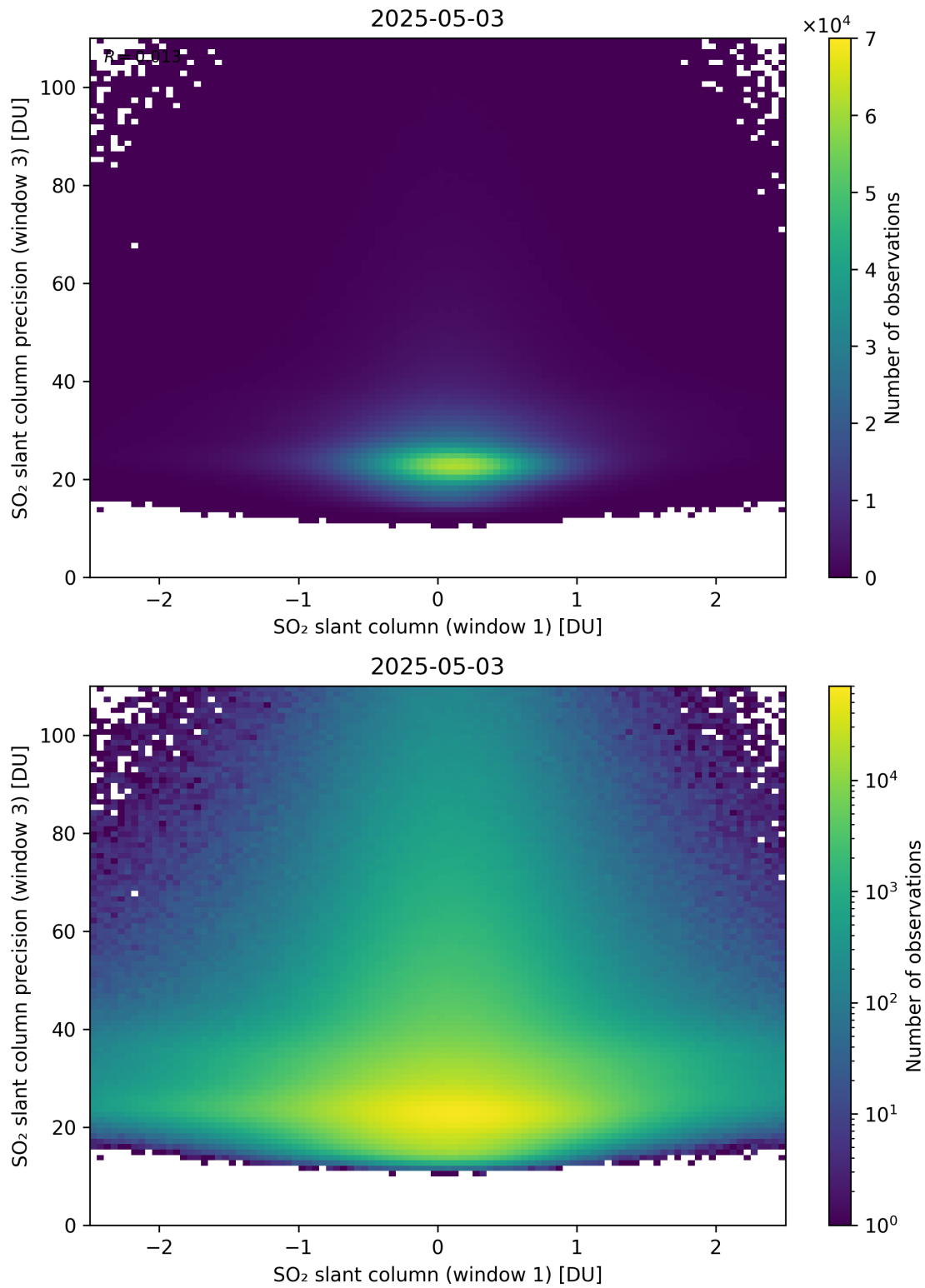
Figure 288: Scatter density plot of “SO 2 slant column (window 1)” against “SO 2 slant column precision (window 3)” for 2025-05-02 to 2025-05-04.
