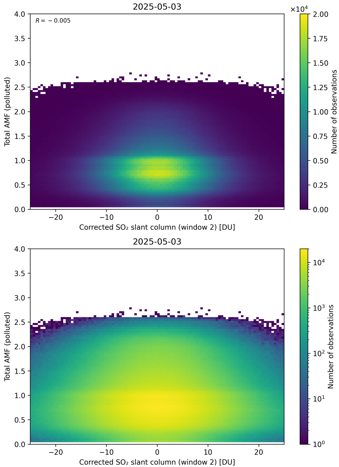
Figure 253: Scatter density plot of “Corrected SO 2 slant column (window 2)” against “Total AMF (polluted)” for 2025-05-02 to 2025-05-04.
