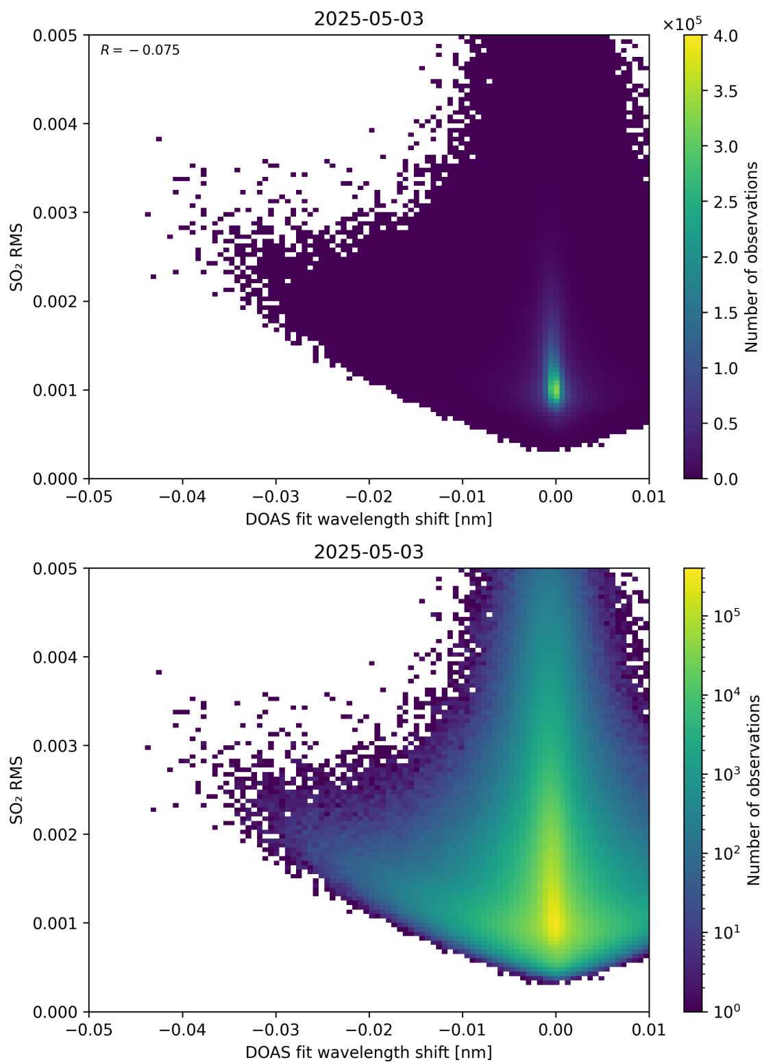
Figure 139: Scatter density plot of “DOAS fit wavelength shift” against “SO 2 RMS” for 2025-05-02 to 2025-05-04.
