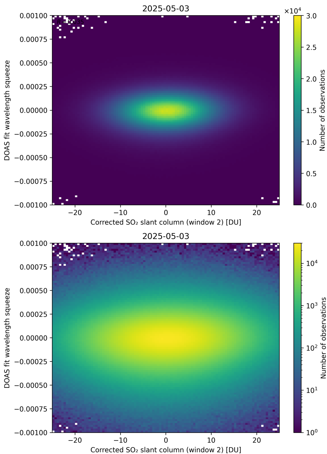
Figure 247: Scatter density plot of “Corrected SO 2 slant column (window 2)” against “DOAS fit wavelength squeeze” for 2025-05-02 to 2025-05-04.
