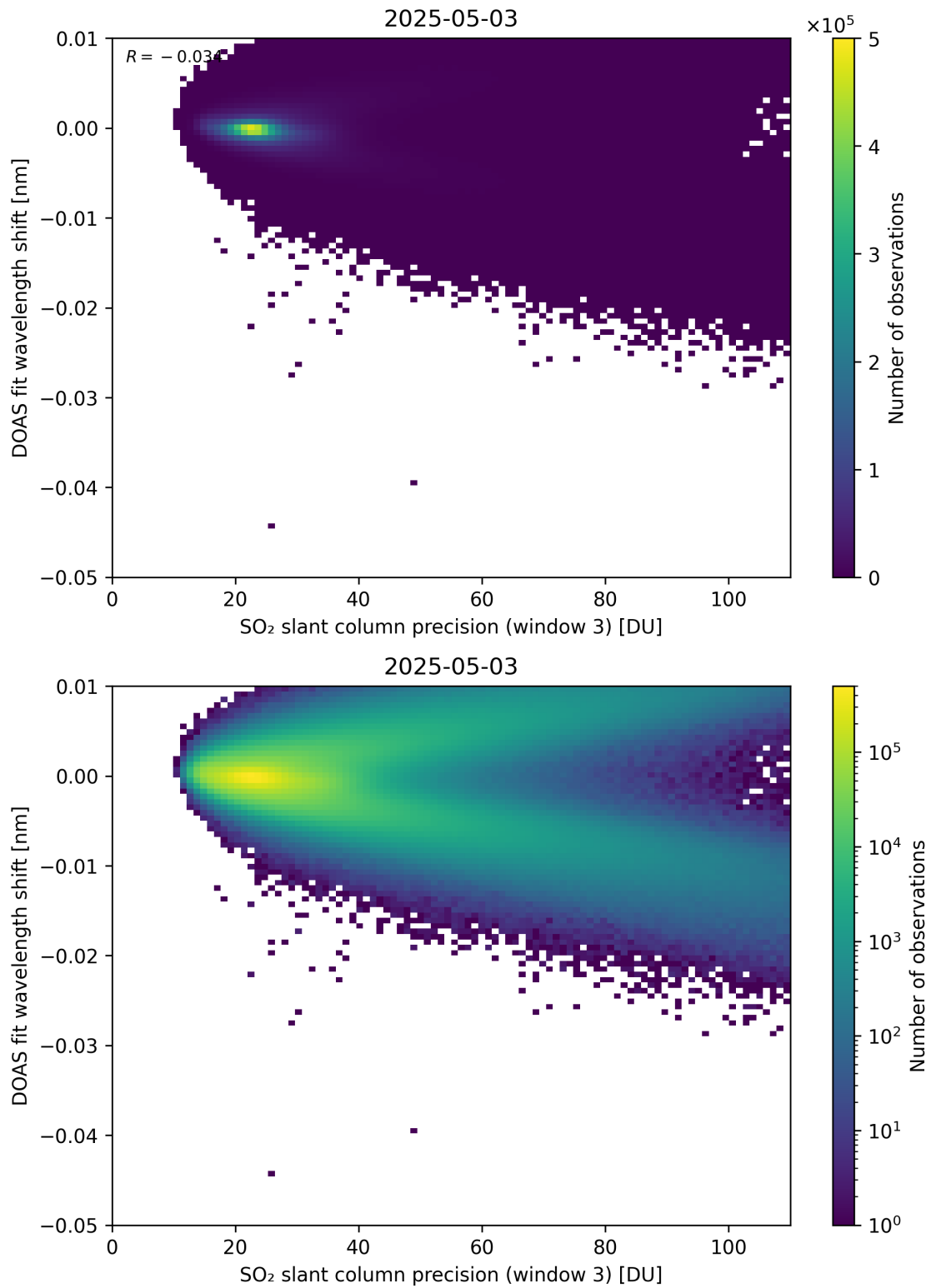
Figure 308: Scatter density plot of “SO 2 slant column precision (window 3)” against “DOAS fit wavelength shift” for 2025-05-02 to 2025-05-04.
