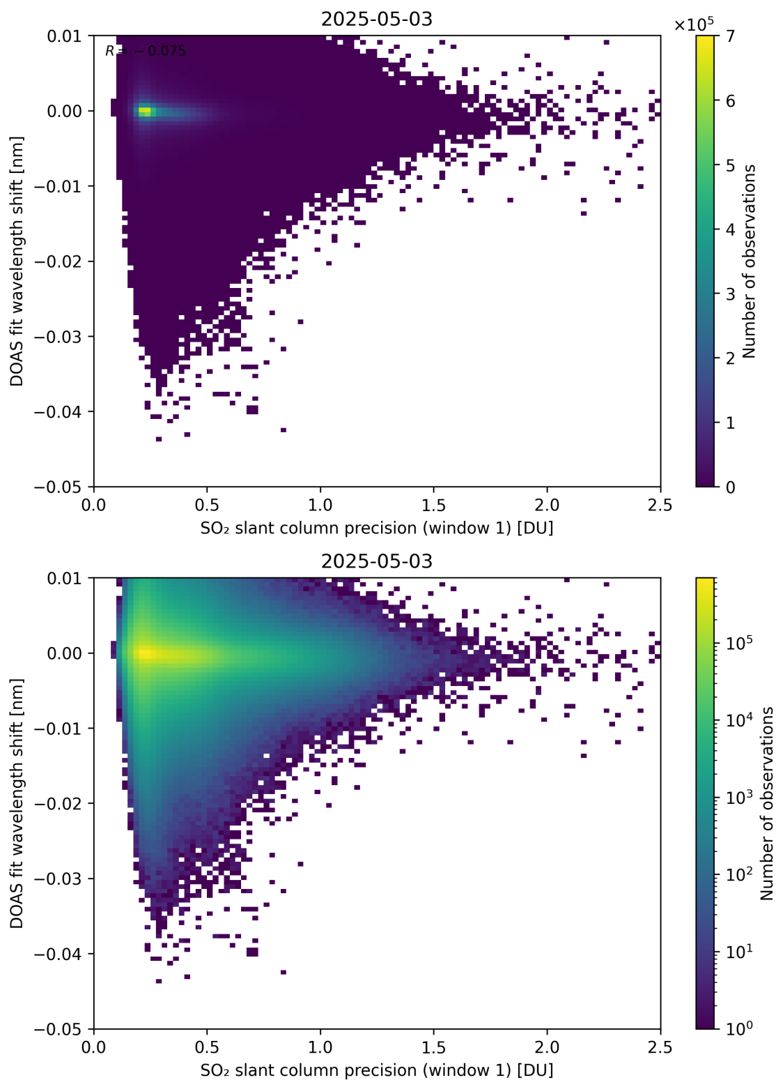
Figure 271: Scatter density plot of “SO 2 slant column precision (window 1)” against “DOAS fit wavelength shift” for 2025-05-02 to 2025-05-04.
