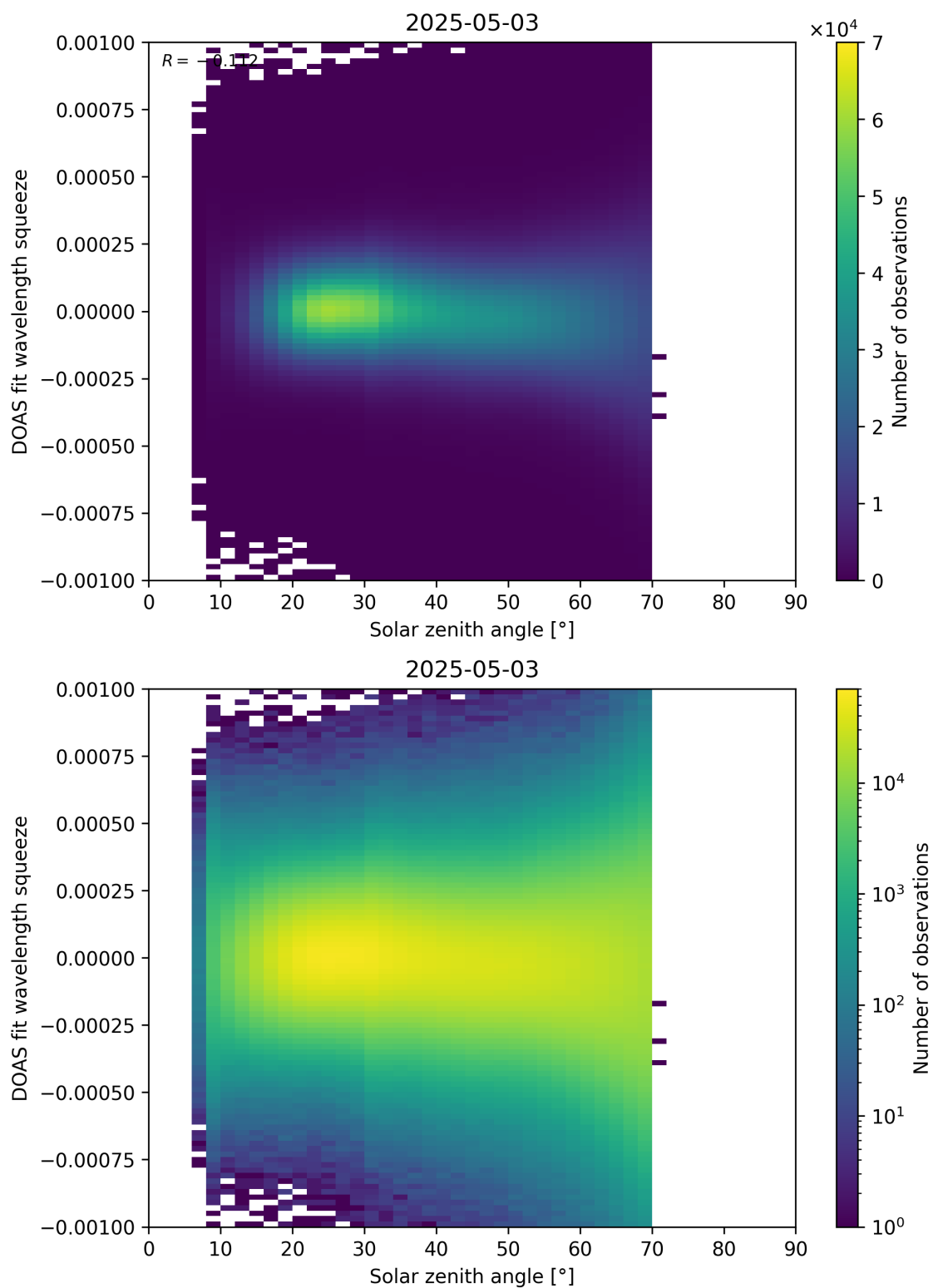
Figure 175: Scatter density plot of “Solar zenith angle” against “DOAS fit wavelength squeeze” for 2025-05-02 to 2025-05-04.
