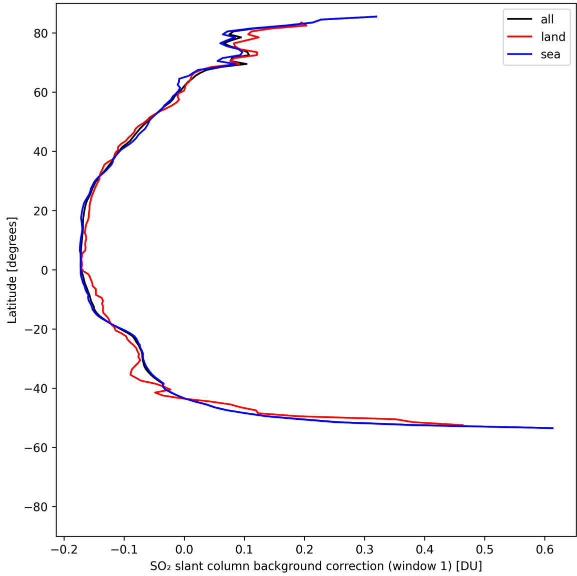
Figure 40: Zonal average of “SO 2 slant column background correction (window 1)” for 2025-05-02 to 2025-05-04.
