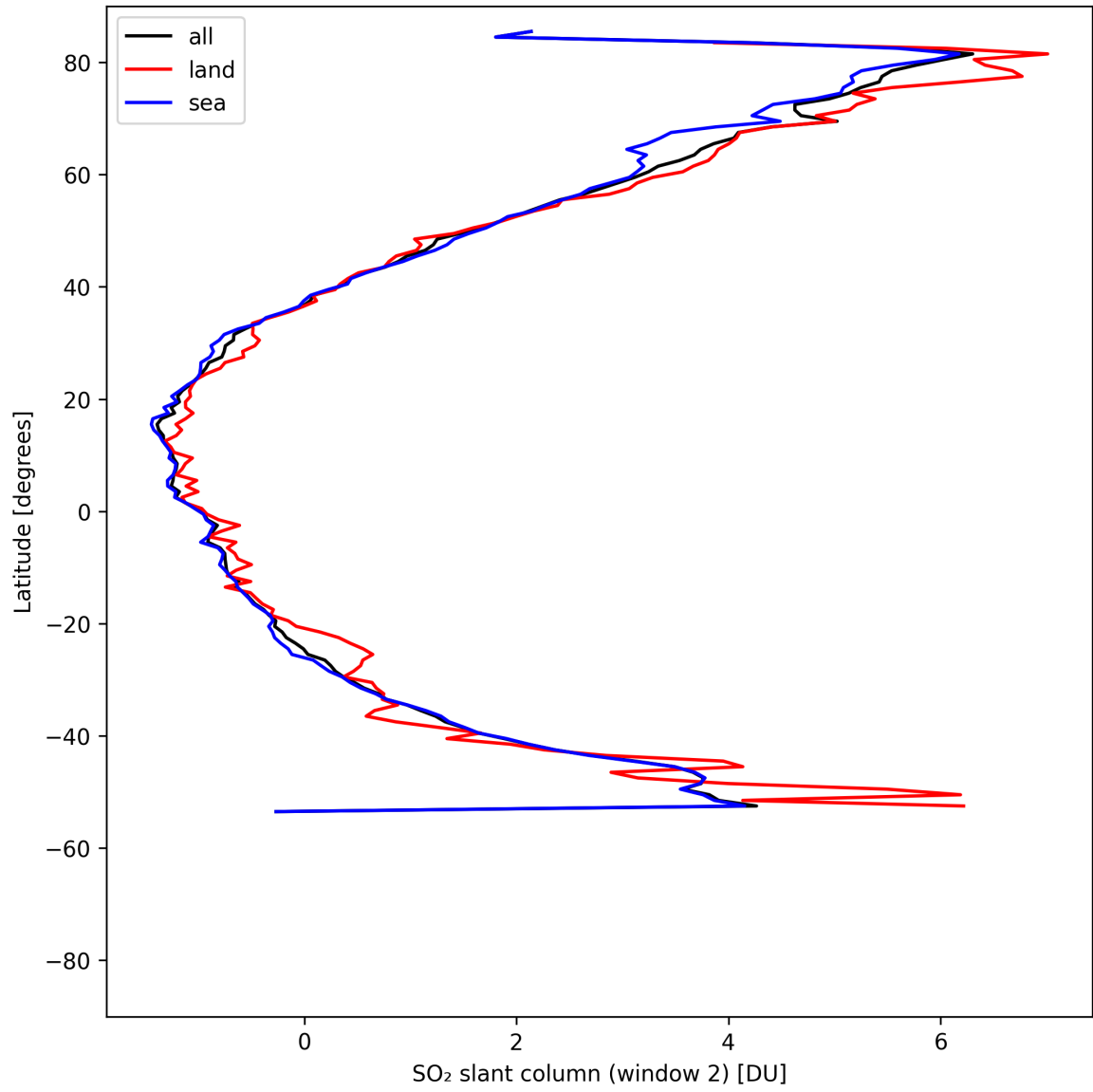
Figure 41: Zonal average of “SO 2 slant column (window 2)” for 2025-05-02 to 2025-05-04.
