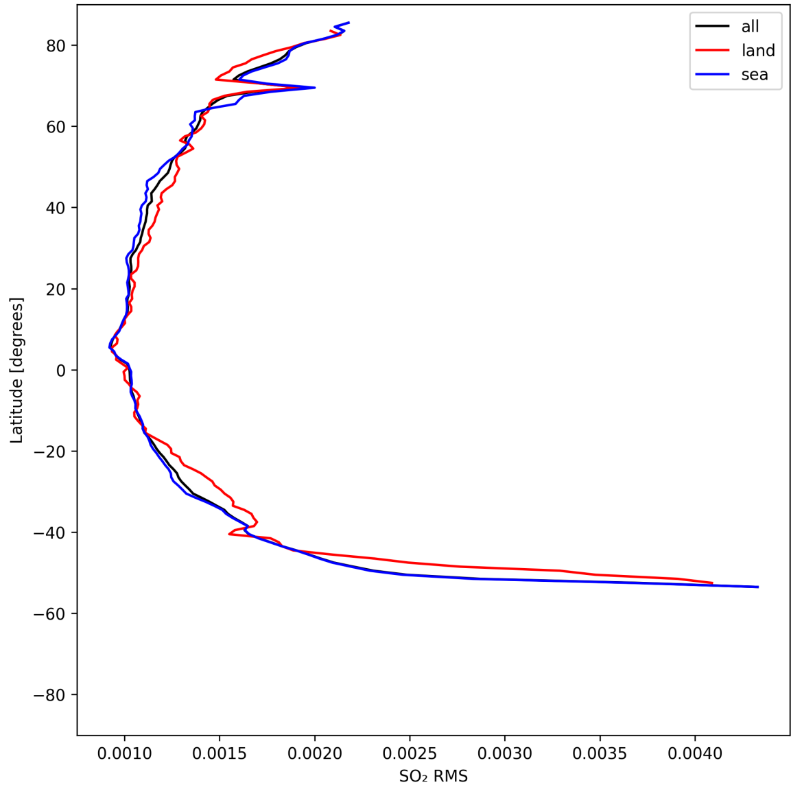
Figure 52: Zonal average of “SO 2 RMS” for 2025-05-02 to 2025-05-04.
