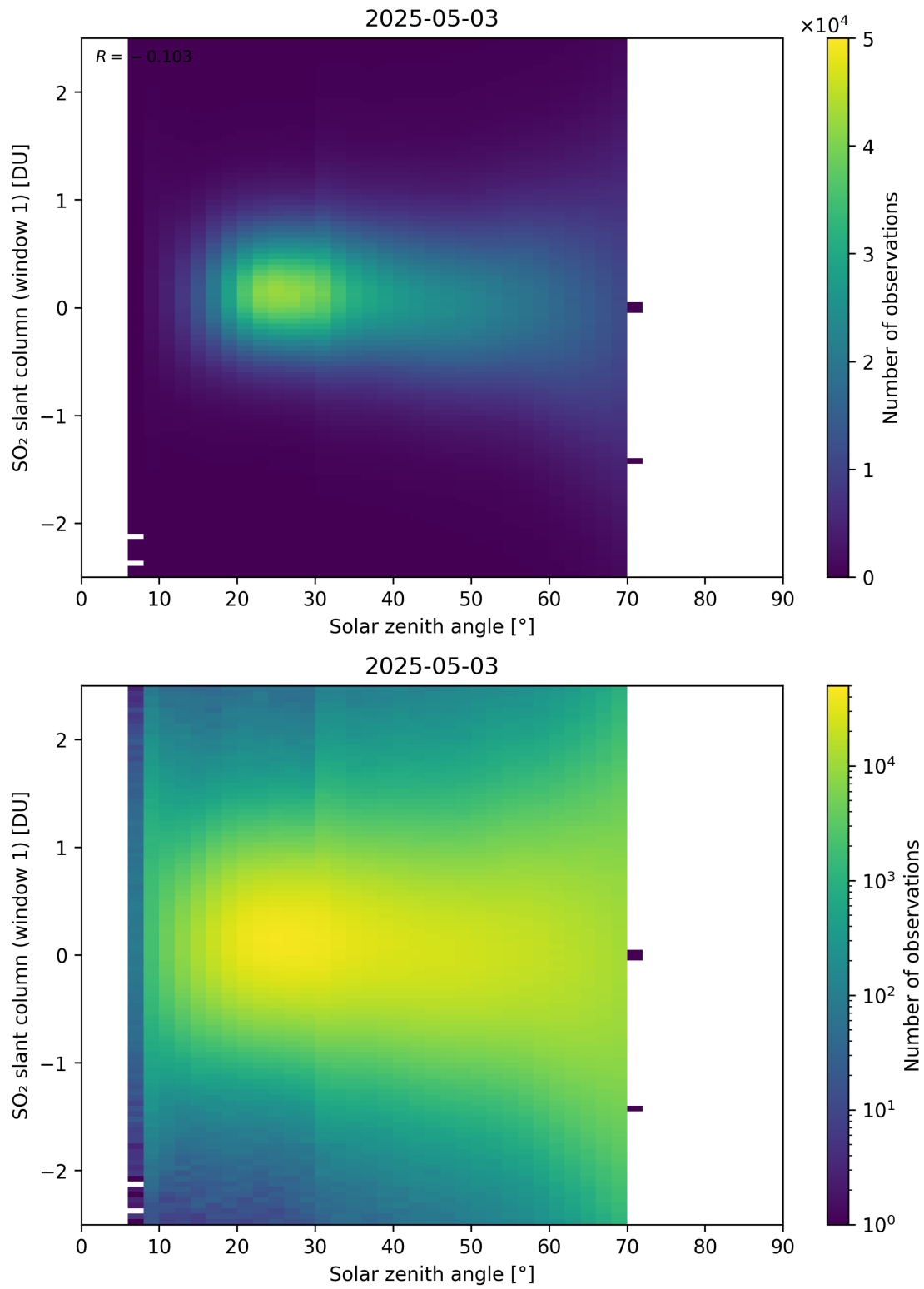
Figure 184: Scatter density plot of “Solar zenith angle” against “SO 2 slant column (window 1)” for 2025-05-02 to 2025-05-04.
