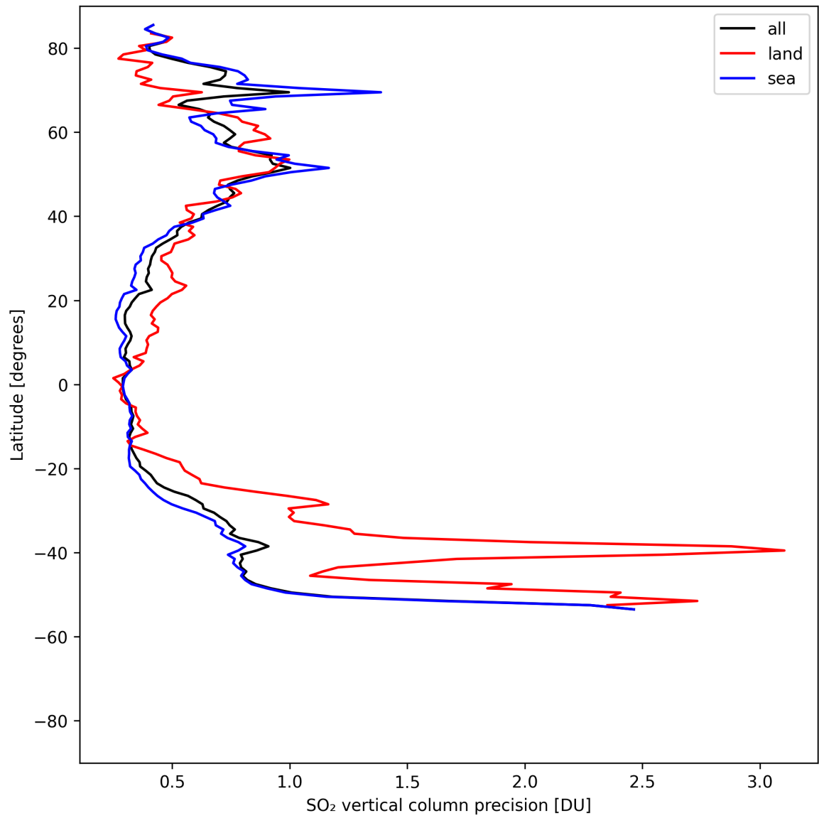
Figure 33: Zonal average of “SO 2 vertical column precision” for 2025-05-02 to 2025-05-04.
