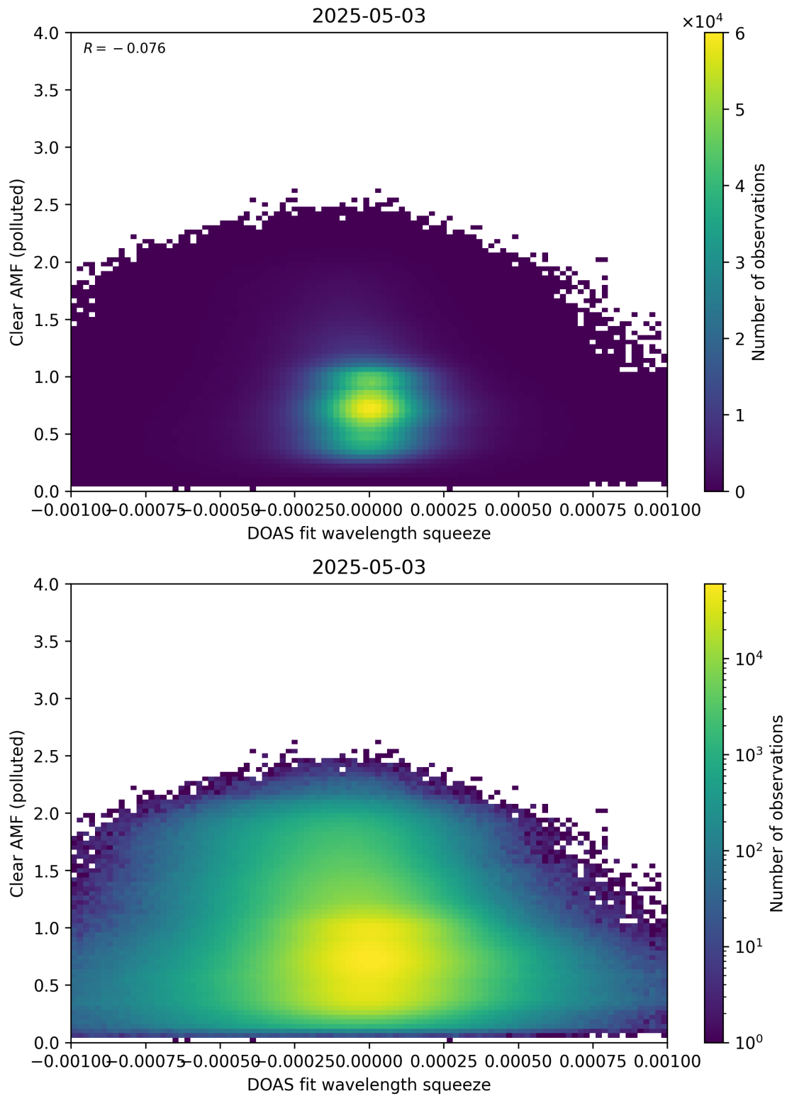
Figure 144: Scatter density plot of “DOAS fit wavelength squeeze” against “Clear AMF (polluted)” for 2025-05-02 to 2025-05-04.
