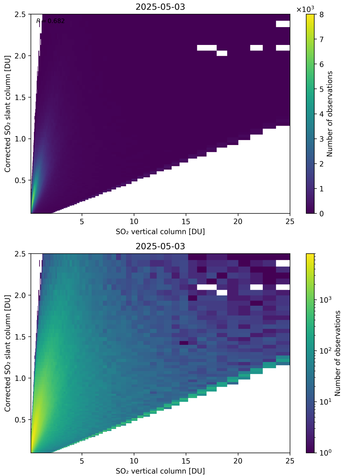
Figure 351: Scatter density plot of “SO 2 vertical column” against “Corrected SO 2 slant column” for 2025-05-02 to 2025-05-04.
