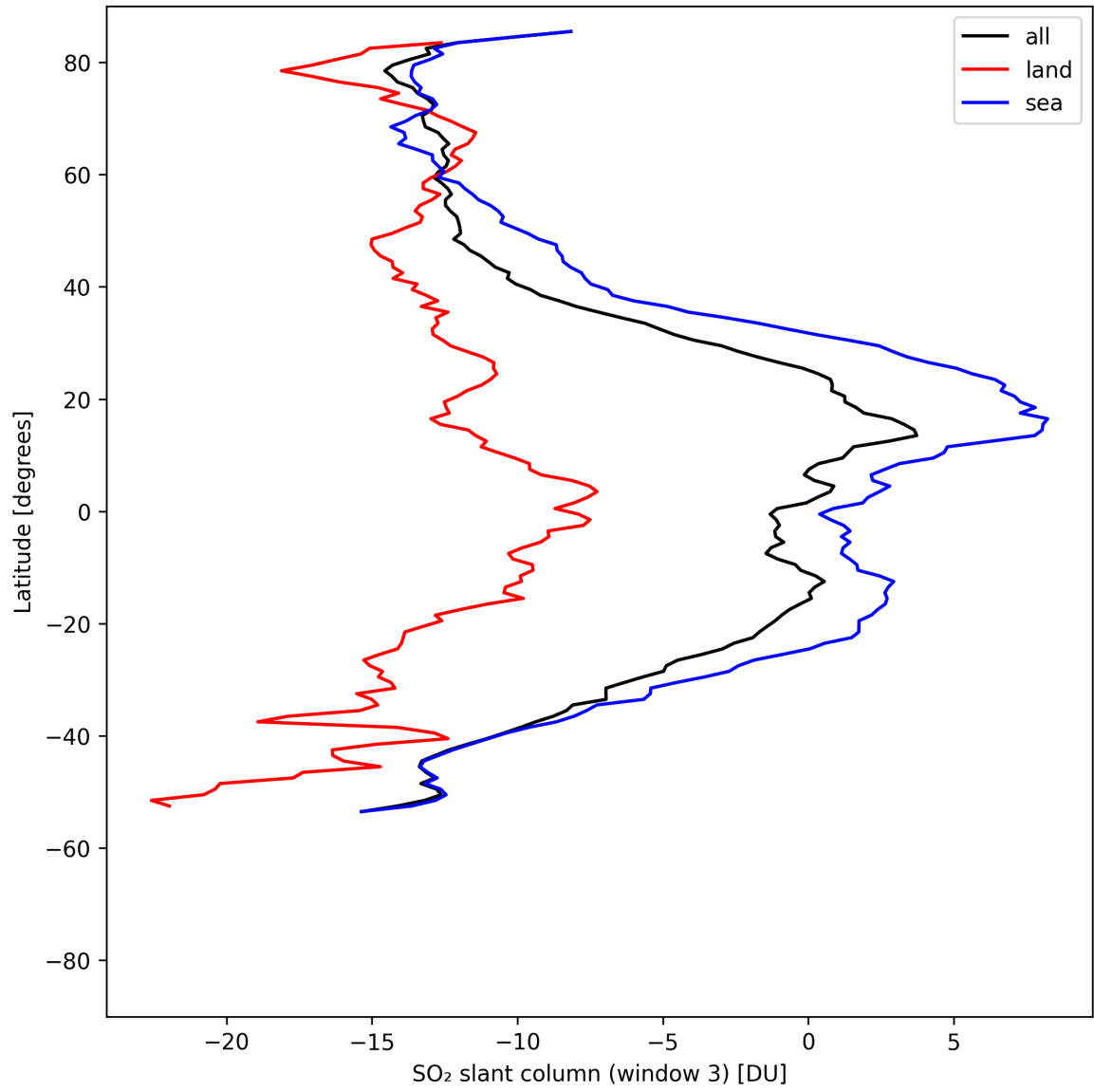
Figure 45: Zonal average of “SO 2 slant column (window 3)” for 2025-05-02 to 2025-05-04.
