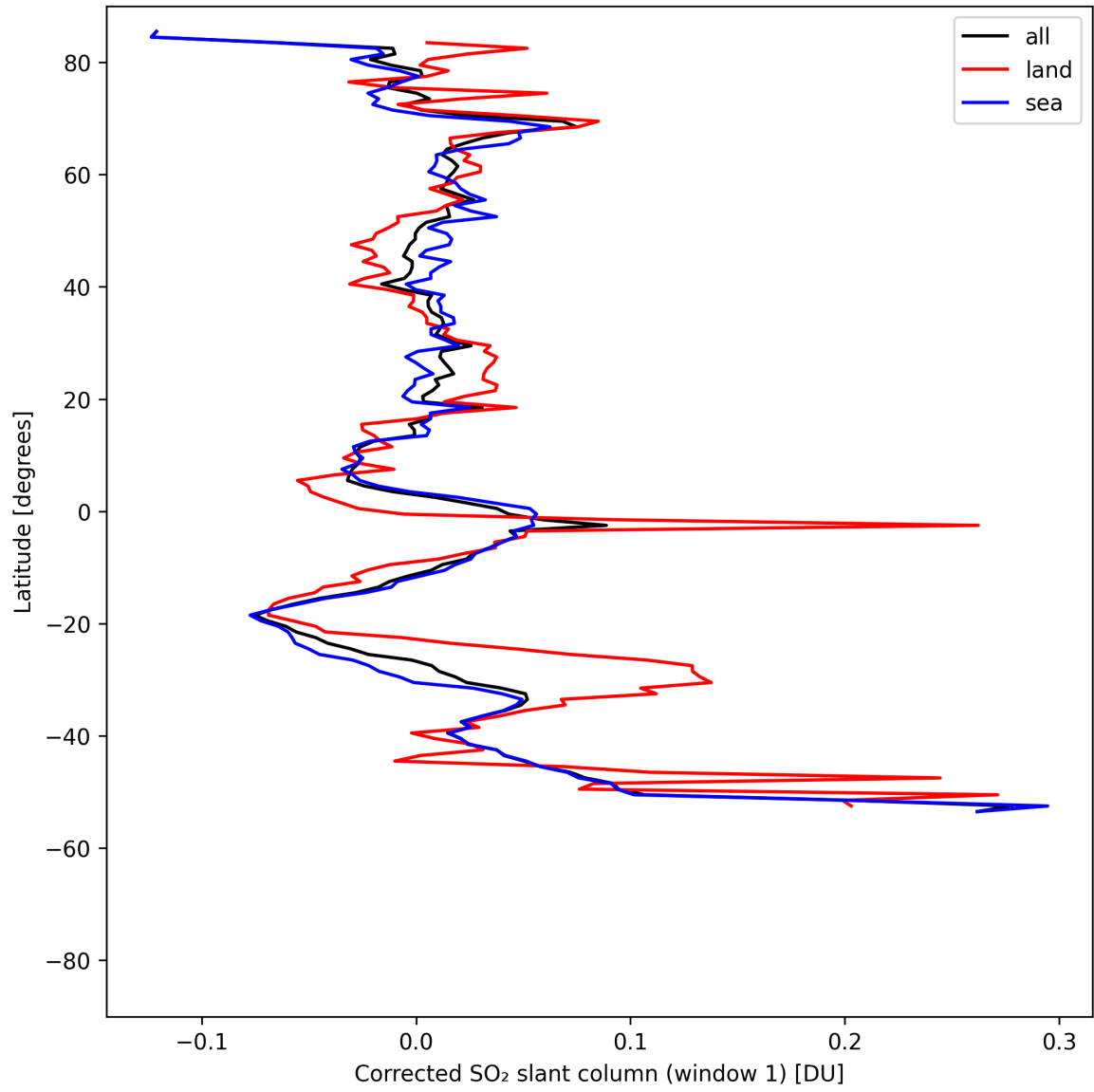
Figure 39: Zonal average of “Corrected SO 2 slant column (window 1)” for 2025-05-02 to 2025-05-04.
