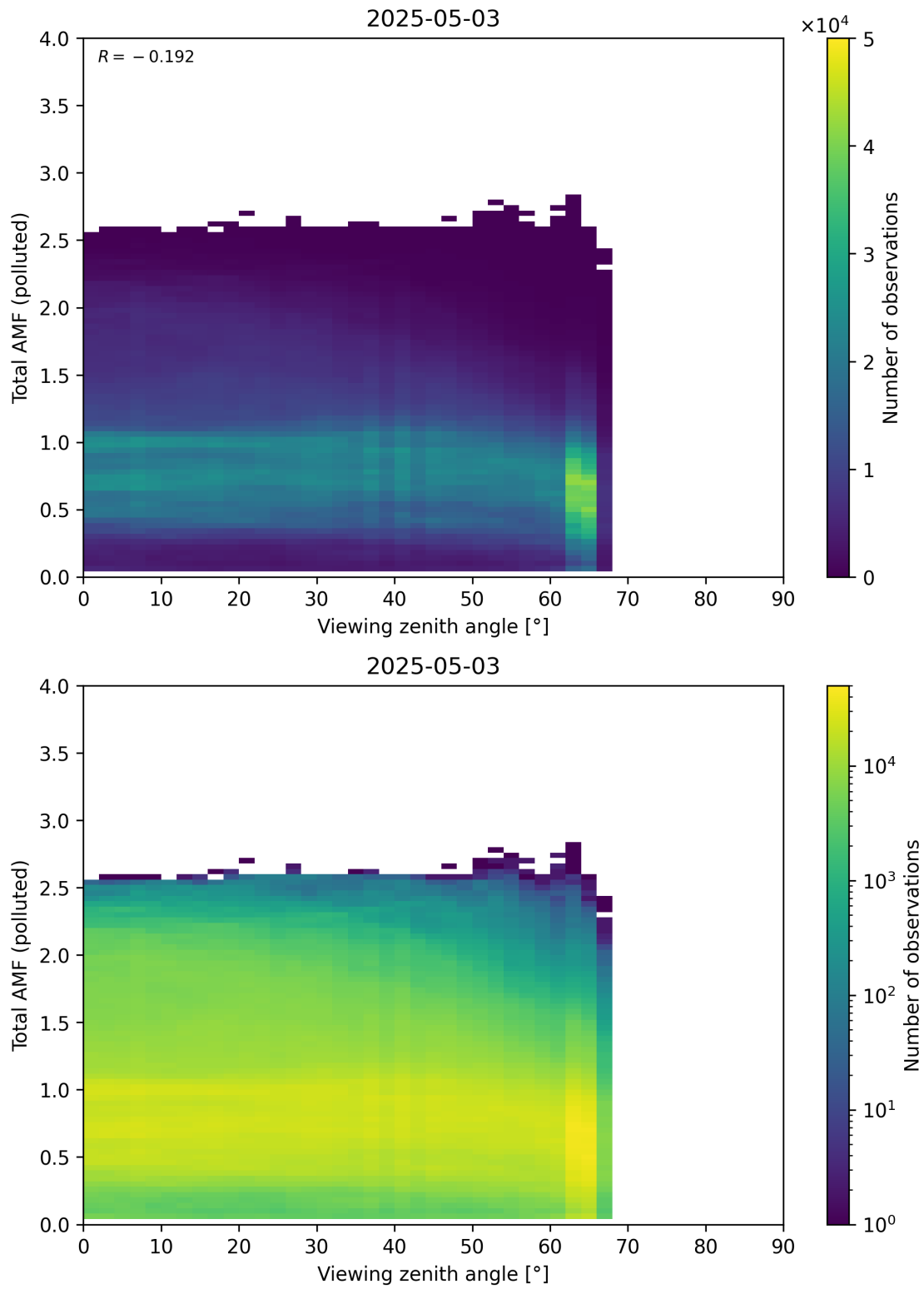
Figure 381: Scatter density plot of “Viewing zenith angle” against “Total AMF (polluted)” for 2025-05-02 to 2025-05-04.
