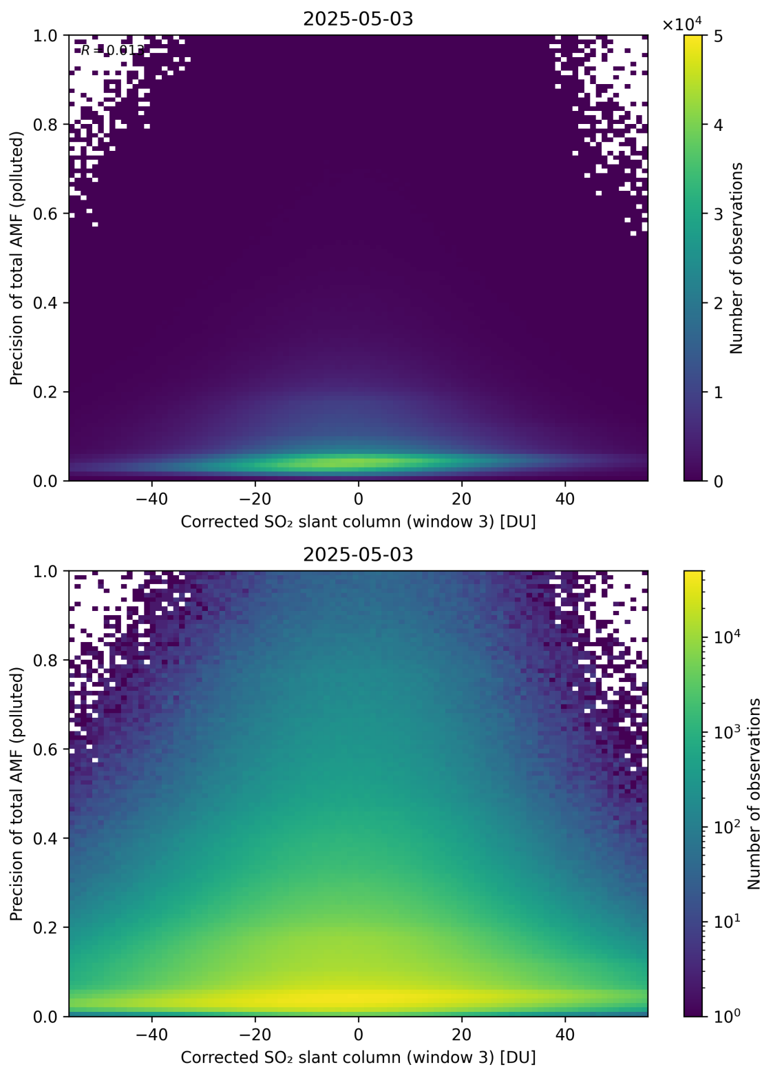
Figure 261: Scatter density plot of “Corrected SO 2 slant column (window 3)” against “Precision of total AMF (polluted)” for 2025-05-02 to 2025-05-04.
