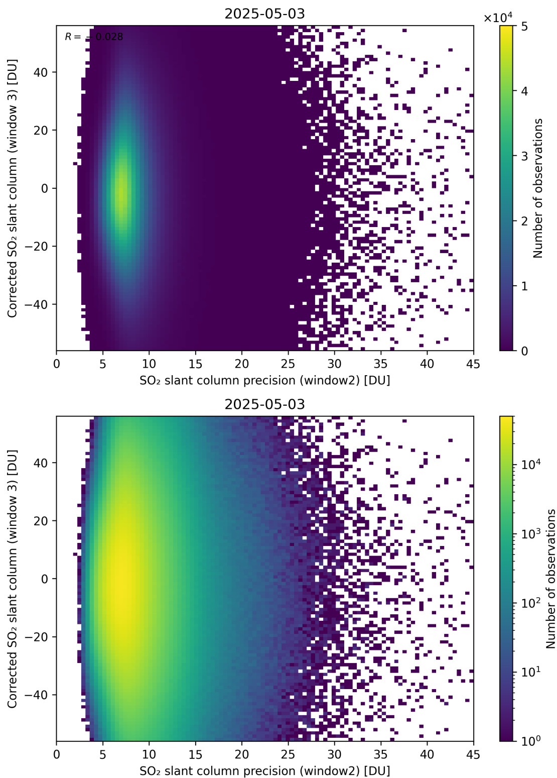
Figure 298: Scatter density plot of “SO 2 slant column precision (window2)” against “Corrected SO 2 slant column (window 3)” for 2025-05-02 to 2025-05-04.
