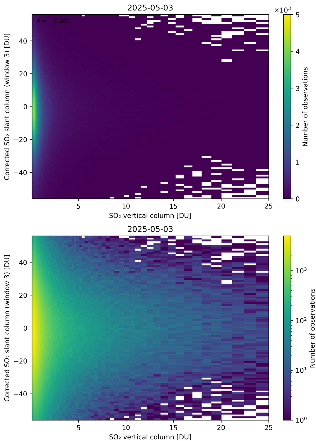
Figure 353: Scatter density plot of “SO 2 vertical column” against “Corrected SO 2 slant column (window 3)” for 2025-05-02 to 2025-05-04.
