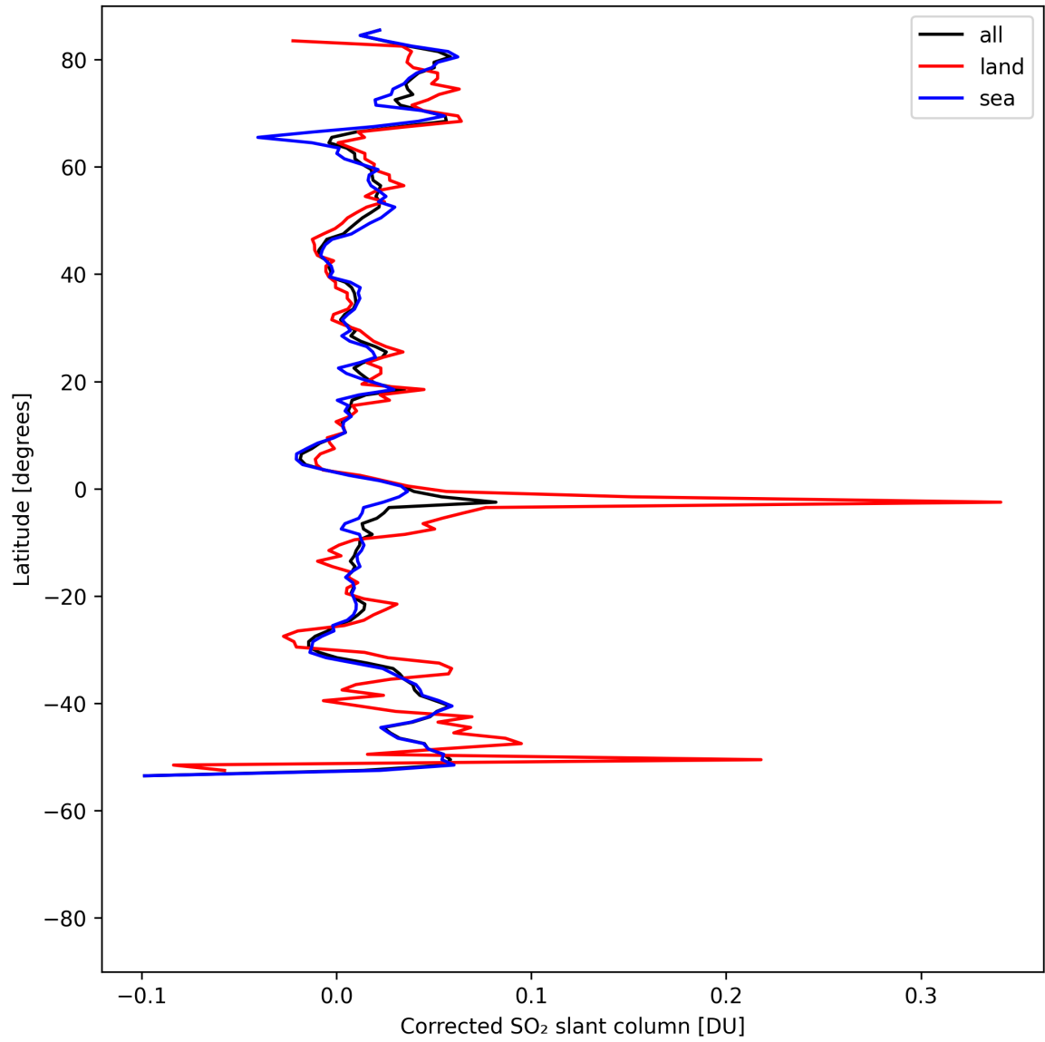
Figure 34: Zonal average of “Corrected SO 2 slant column” for 2025-05-02 to 2025-05-04.
