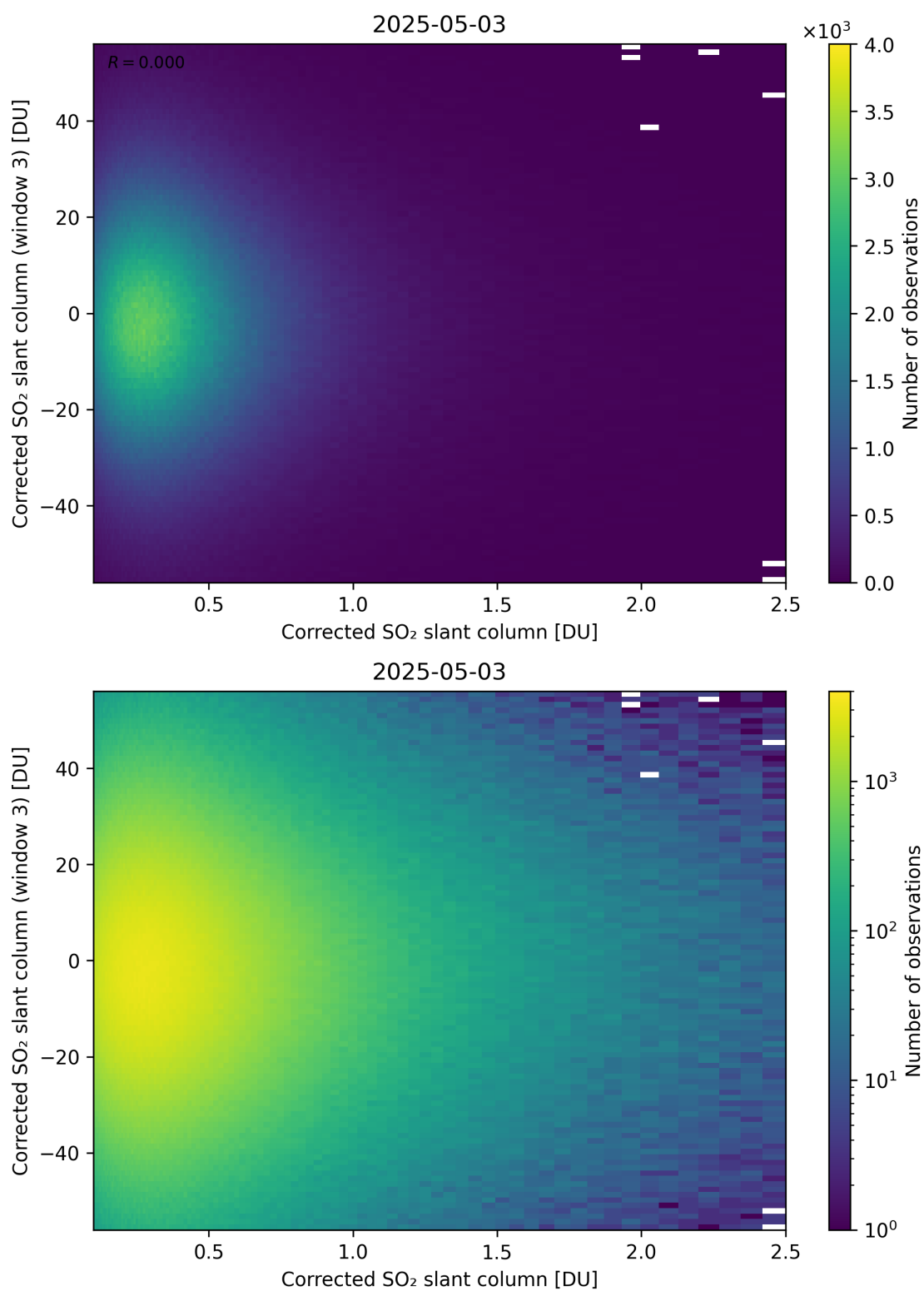
Figure 236: Scatter density plot of “Corrected SO 2 slant column” against “Corrected SO 2 slant column (window 3)” for 2025-05-02 to 2025-05-04.
