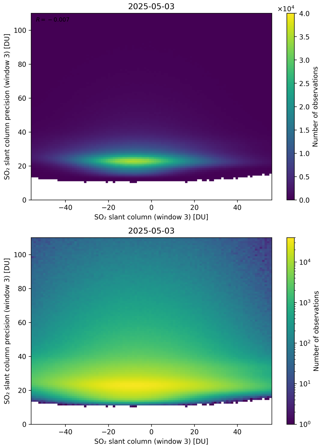
Figure 317: Scatter density plot of “SO 2 slant column (window 3)” against “SO 2 slant column precision (window 3)” for 2025-05-02 to 2025-05-04.
