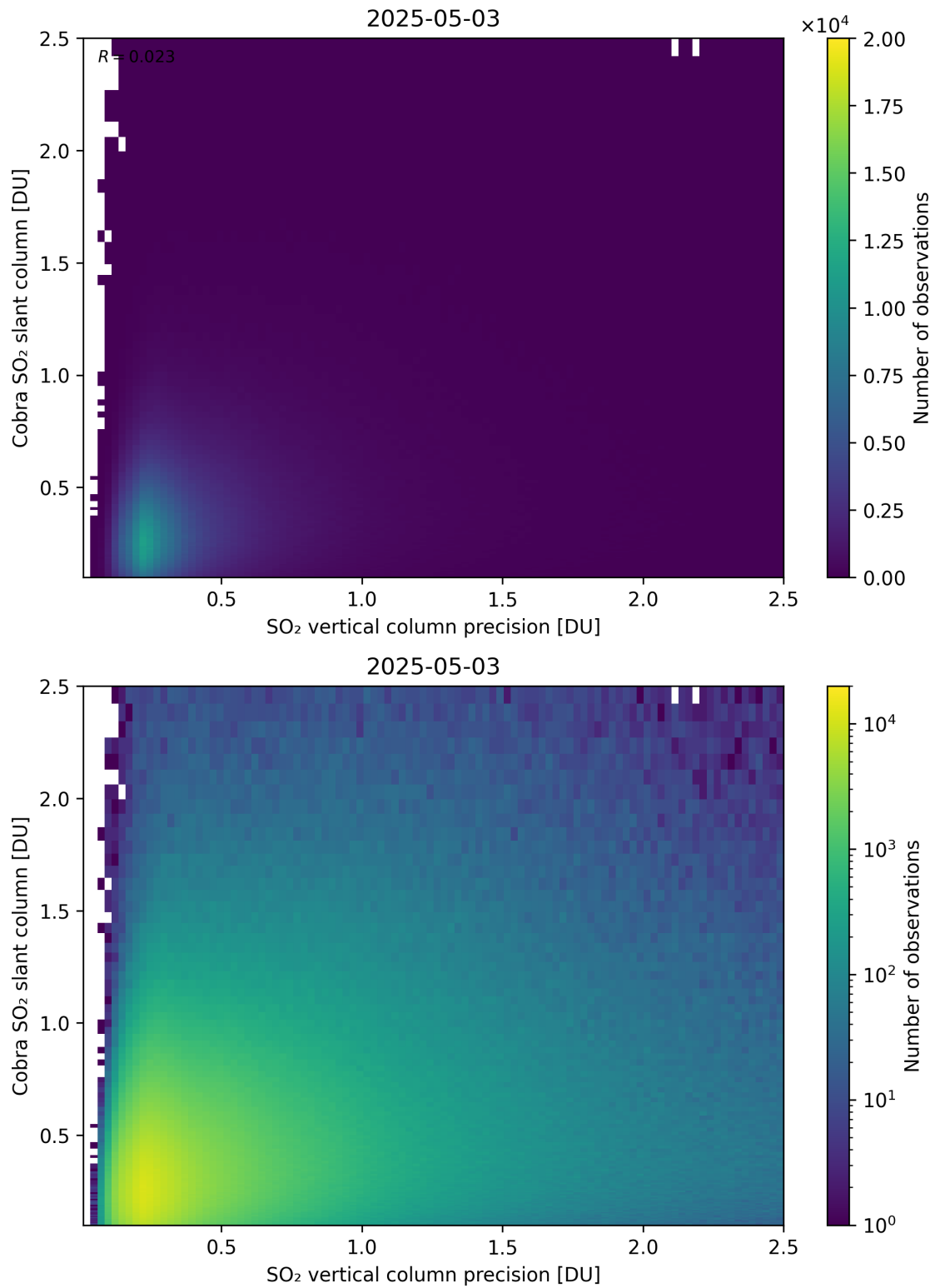
Figure 336: Scatter density plot of “SO 2 vertical column precision” against “Cobra SO 2 slant column” for 2025-05-02 to 2025-05-04.
