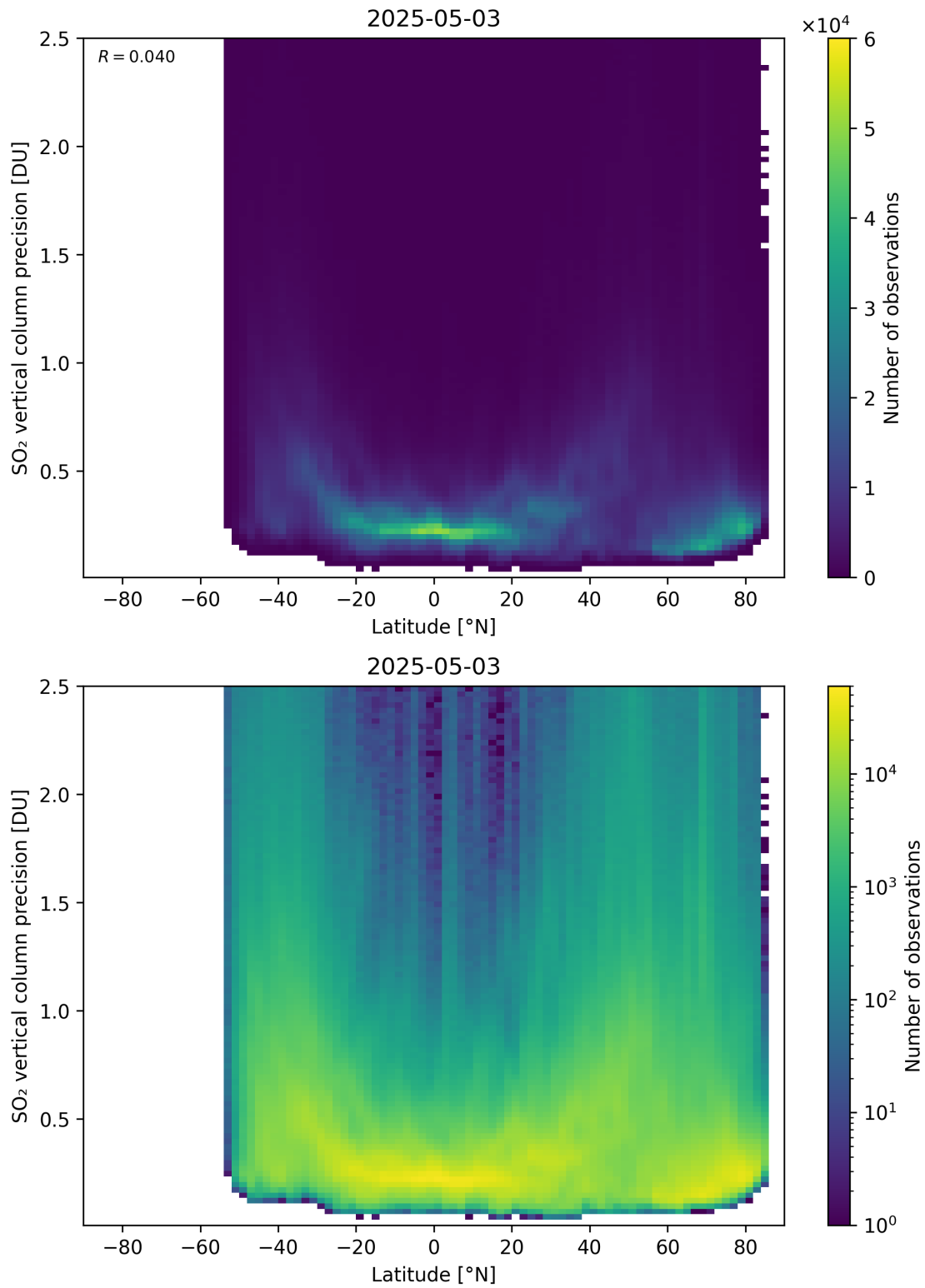
Figure 170: Scatter density plot of “Latitude” against “SO 2 vertical column precision” for 2025-05-02 to 2025-05-04.
