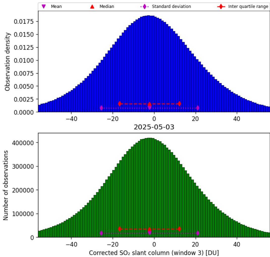
Figure 73: Histogram of “Corrected SO 2 slant column (window 3)” for 2025-05-02 to 2025-05-04
