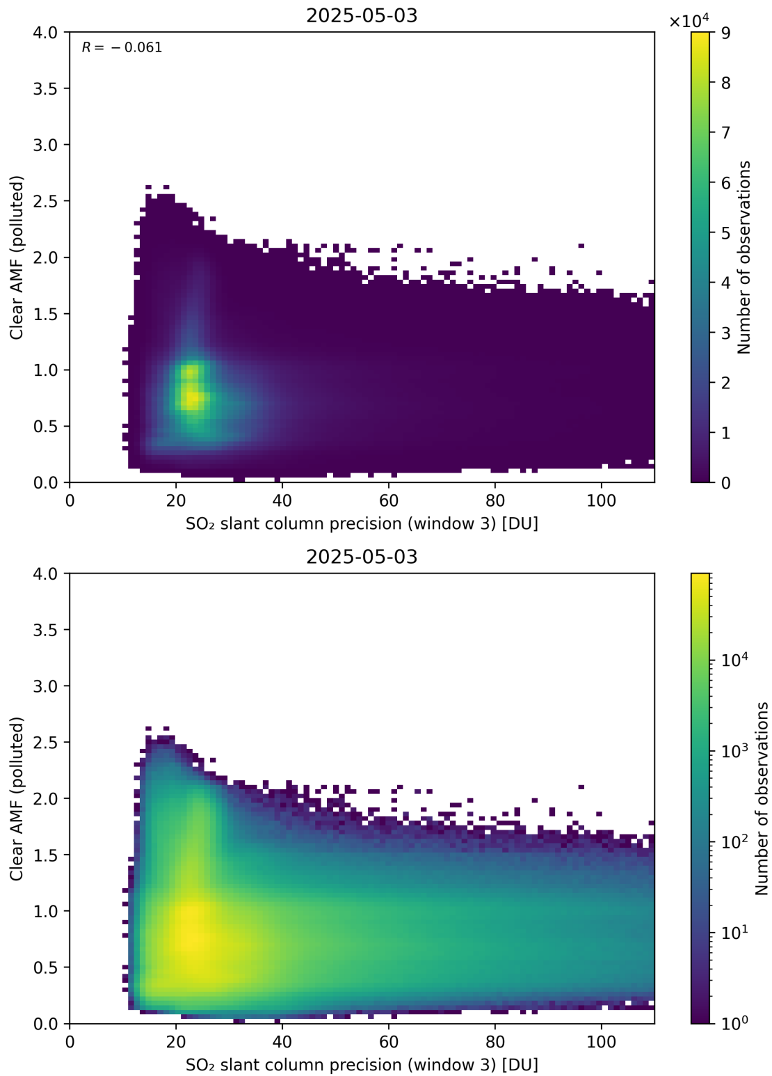
Figure 311: Scatter density plot of “SO 2 slant column precision (window 3)” against “Clear AMF (polluted)” for 2025-05-02 to 2025-05-04.
