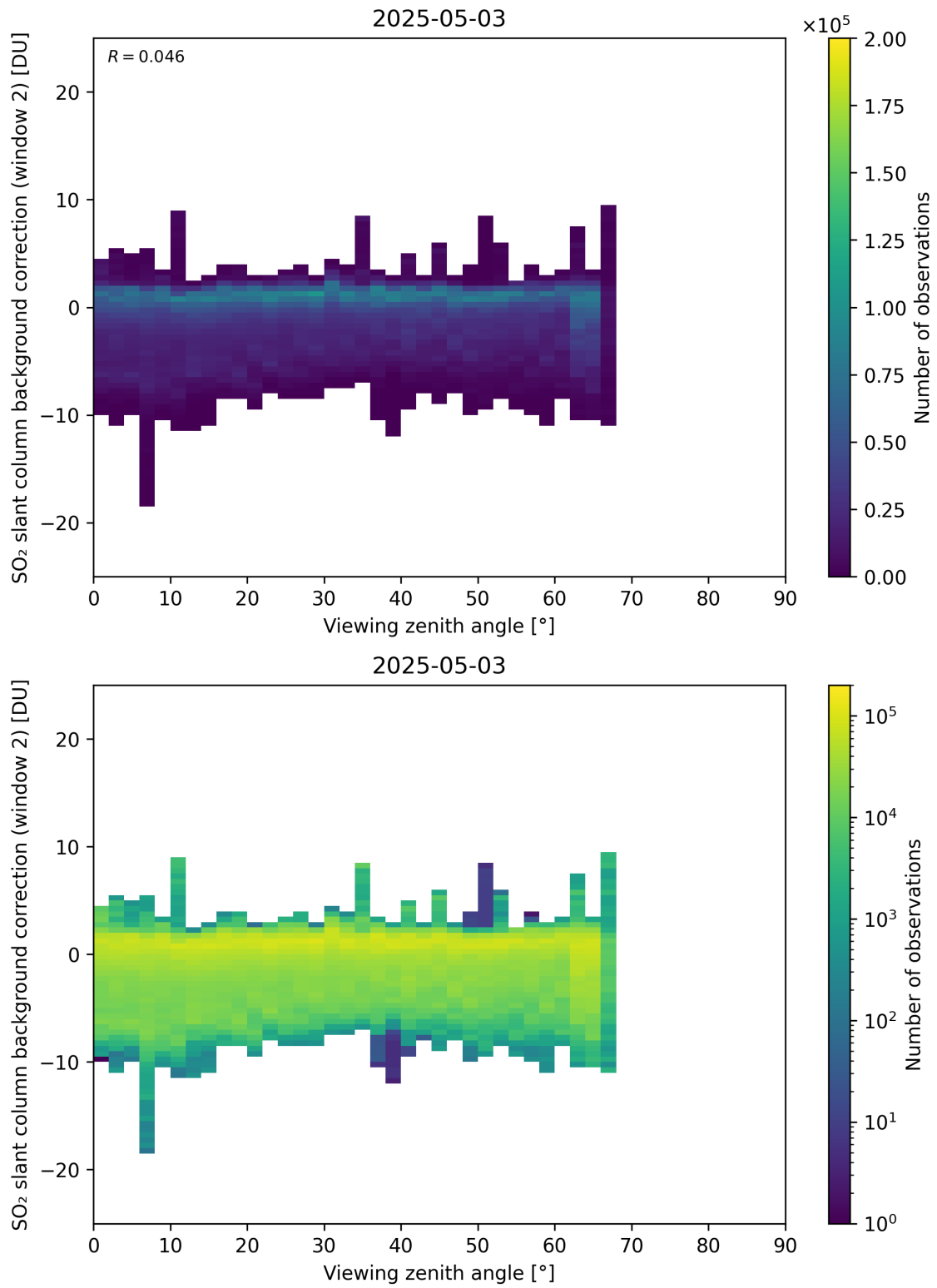
Figure 363: Scatter density plot of “Viewing zenith angle” against “SO 2 slant column background correction (window 2)” for 2025-05-02 to 2025-05-04.
