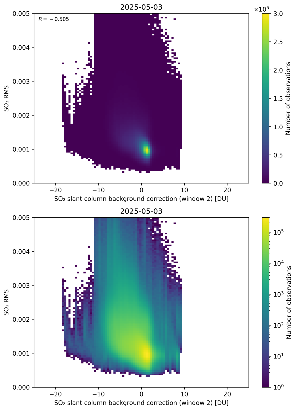
Figure 125: Scatter density plot of “SO 2 slant column background correction (window 2)” against “SO 2 RMS” for 2025-05-02 to 2025-05-04.
