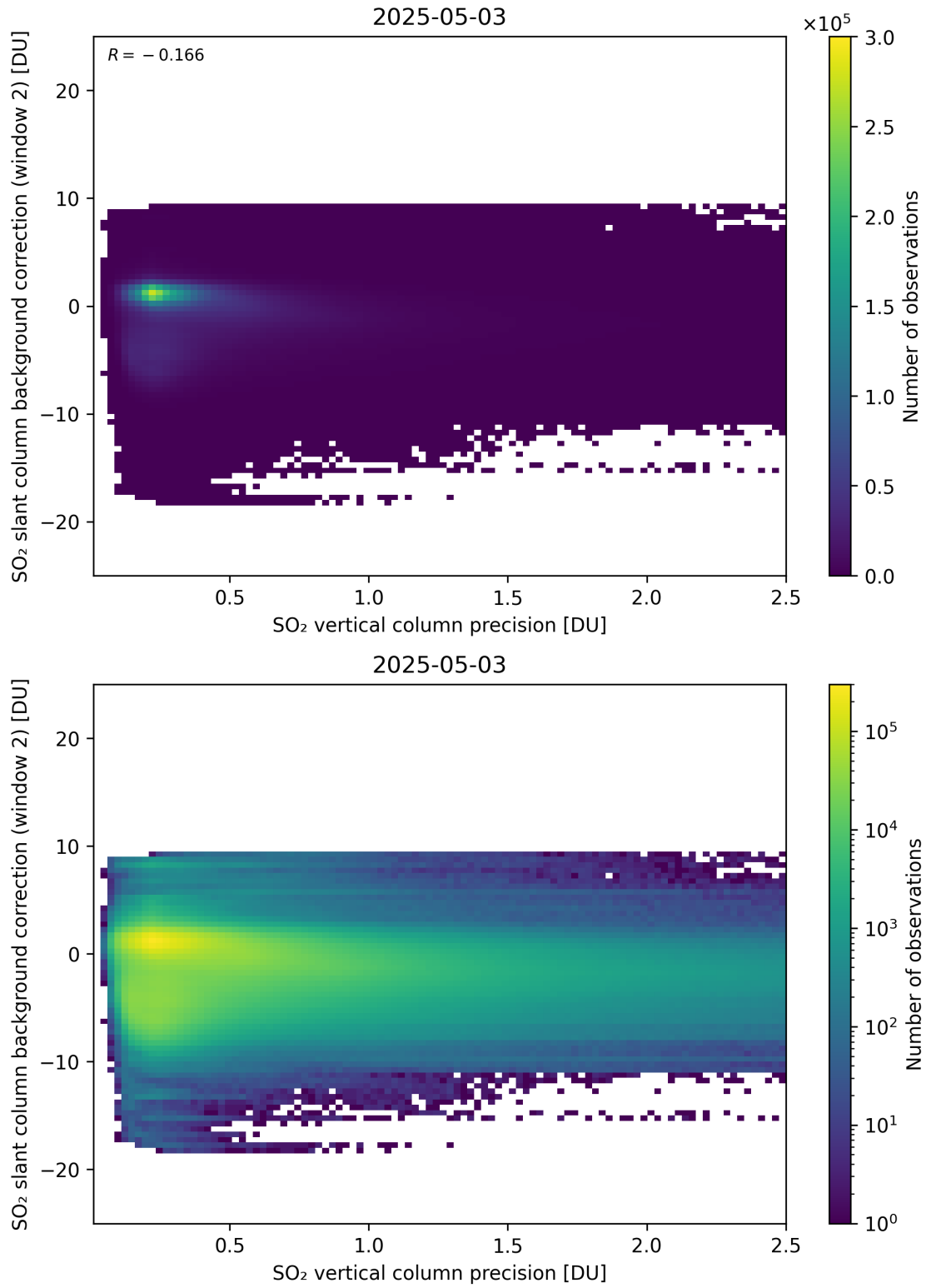
Figure 330: Scatter density plot of “SO 2 vertical column precision” against “SO 2 slant column background correction (window 2)” for 2025-05-02 to 2025-05-04.
