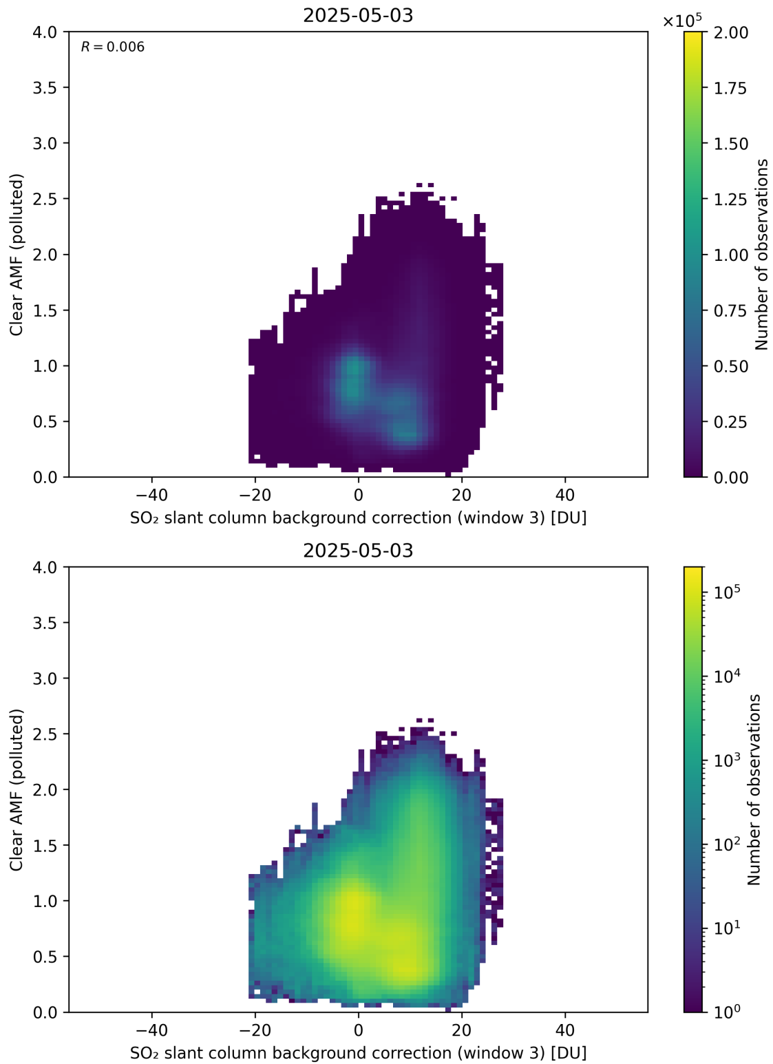
Figure 135: Scatter density plot of “SO 2 slant column background correction (window 3)” against “Clear AMF (polluted)” for 2025-05-02 to 2025-05-04.
