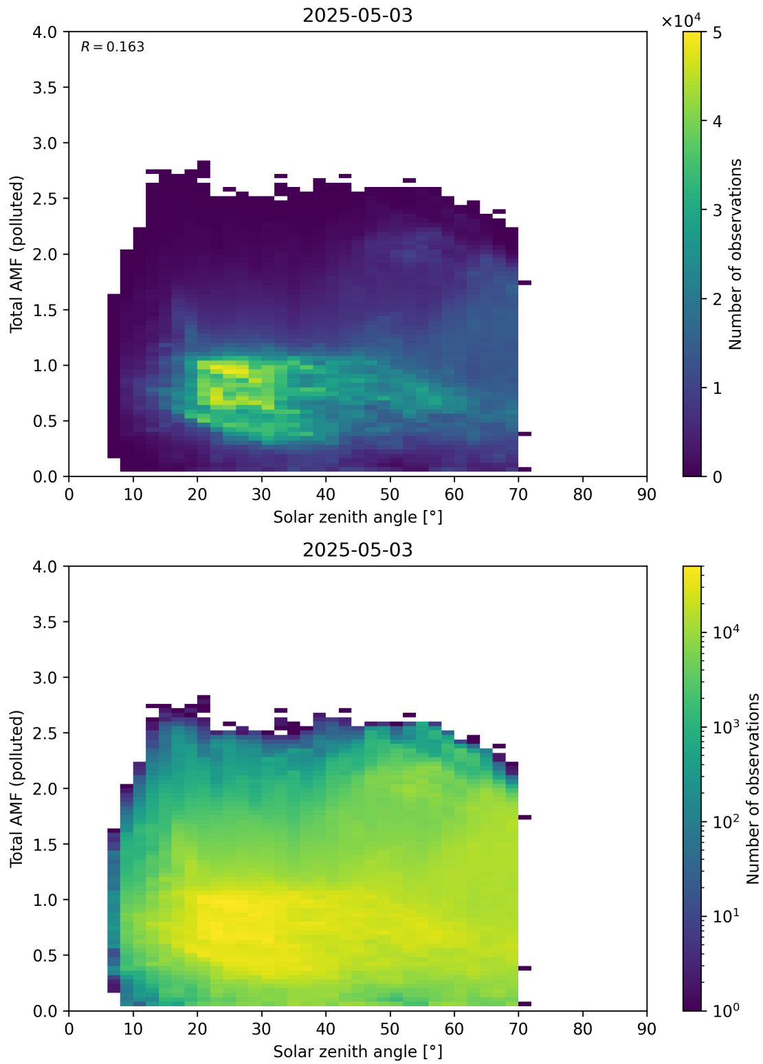
Figure 189: Scatter density plot of “Solar zenith angle” against “Total AMF (polluted)” for 2025-05-02 to 2025-05-04.
