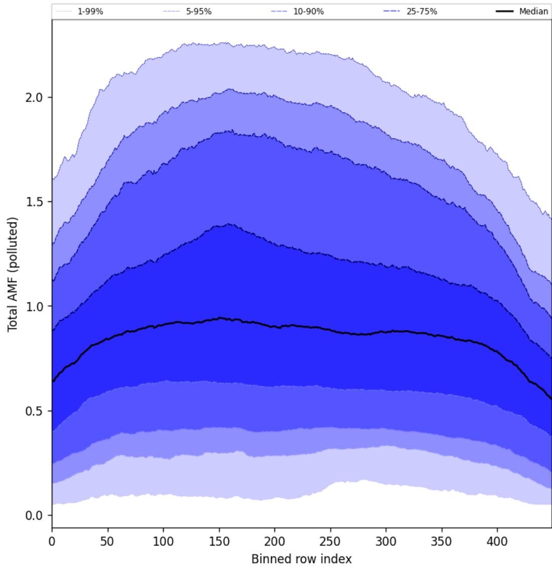
Figure 105: Along track statistics of “Total AMF (polluted)” for 2025-05-02 to 2025-05-04
