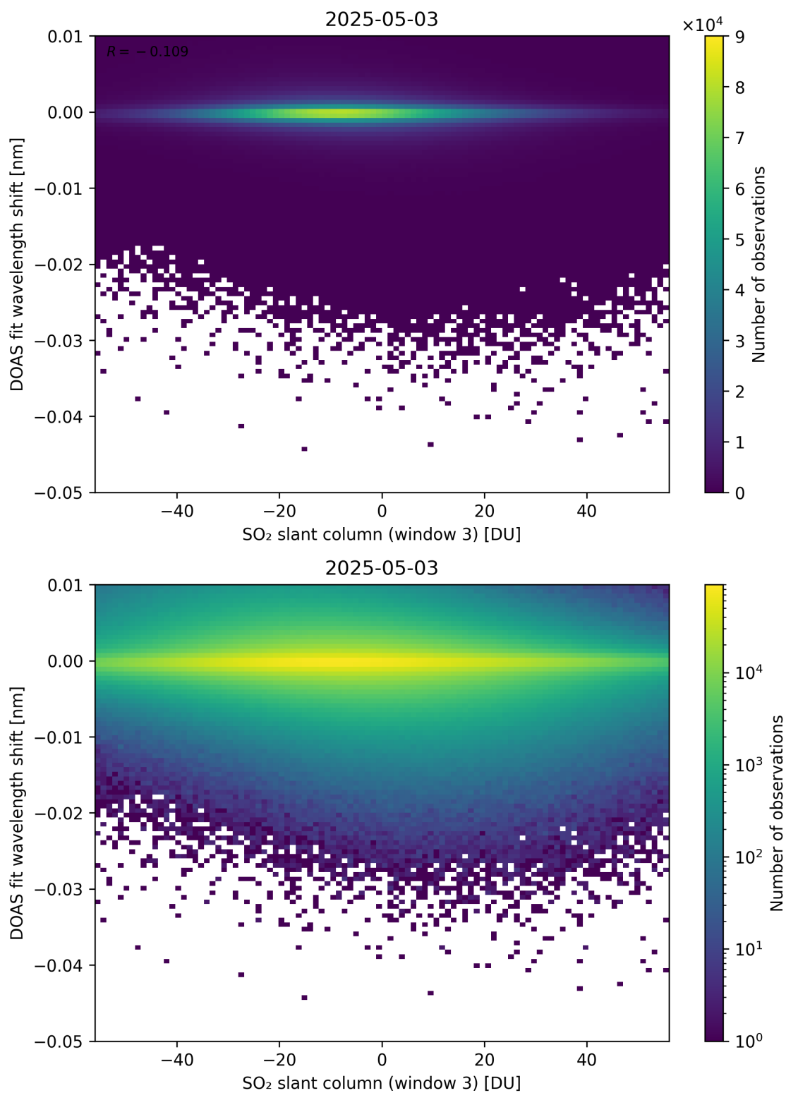
Figure 304: Scatter density plot of “SO 2 slant column (window 3)” against “DOAS fit wavelength shift” for 2025-05-02 to 2025-05-04.
