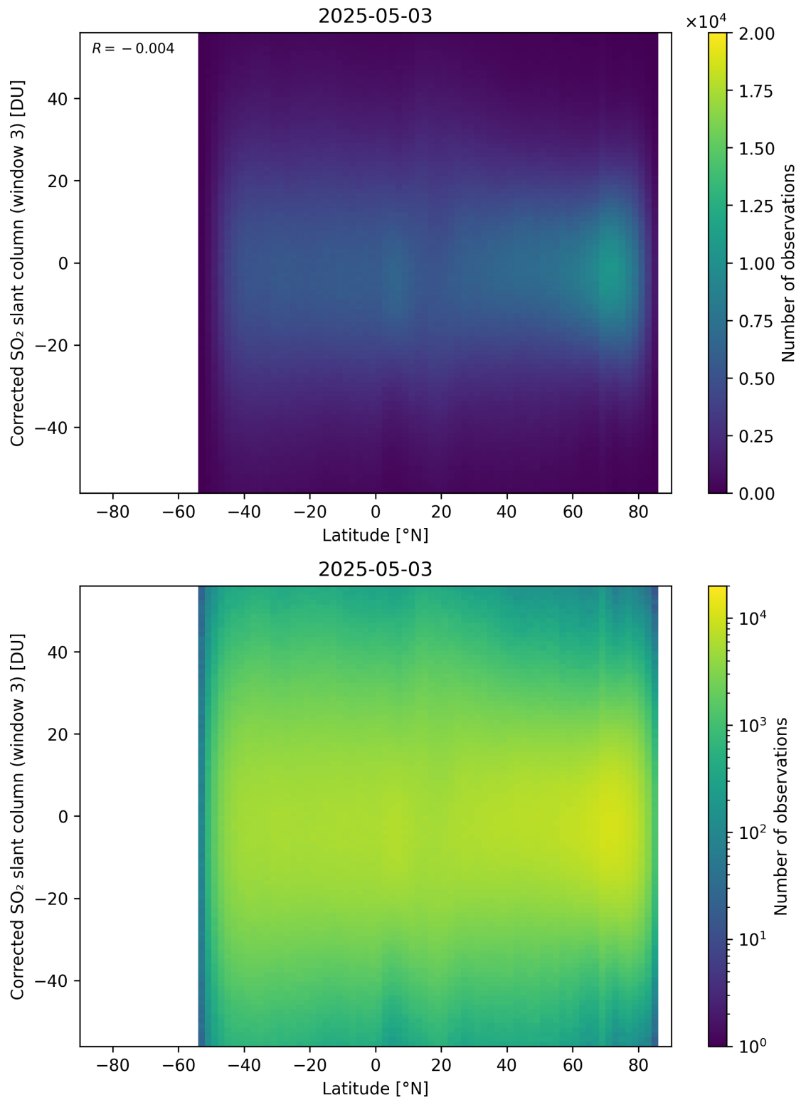
Figure 161: Scatter density plot of “Latitude” against “Corrected SO 2 slant column (window 3)” for 2025-05-02 to 2025-05-04.
