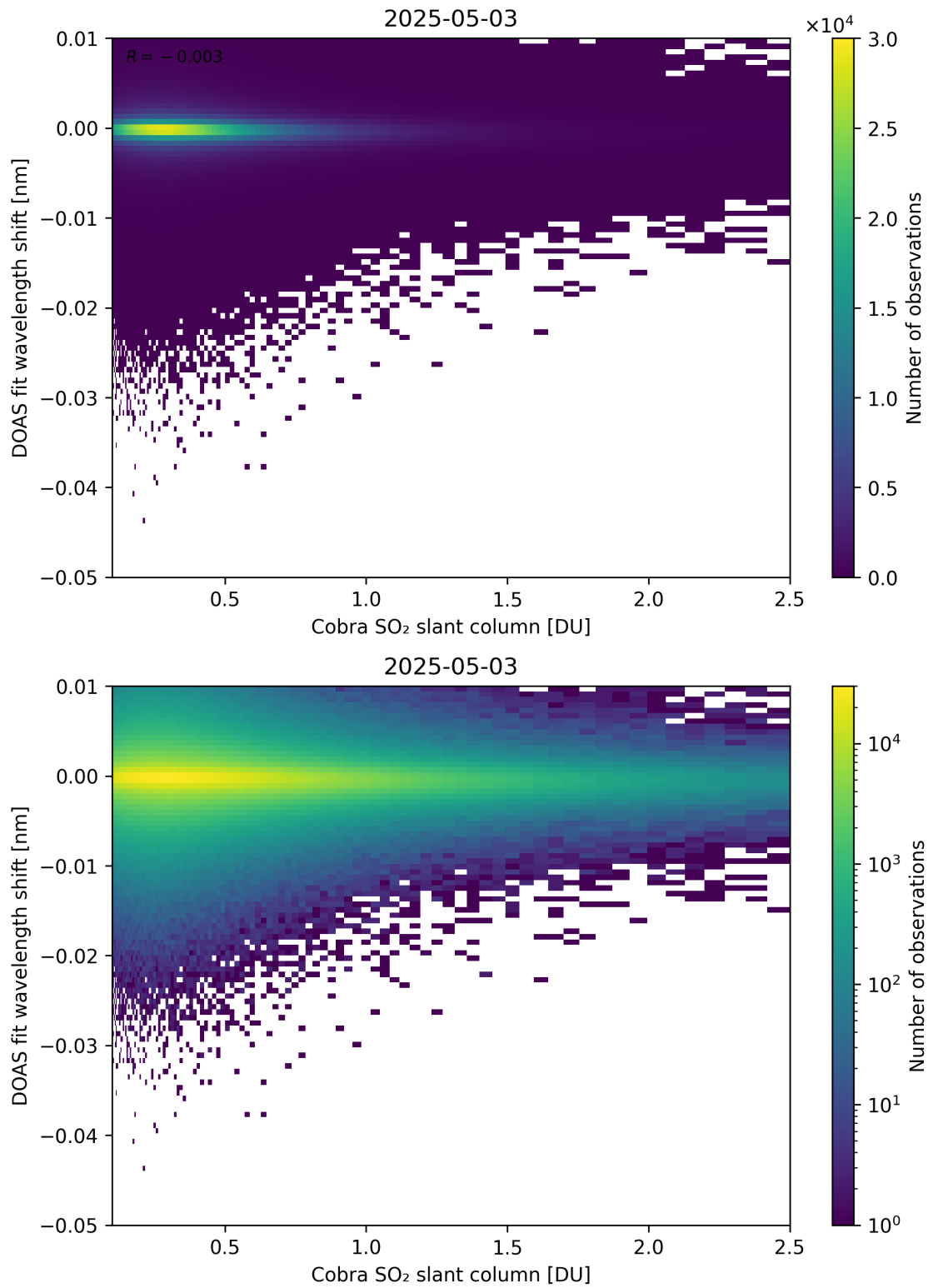
Figure 196: Scatter density plot of “Cobra SO 2 slant column” against “DOAS fit wavelength shift” for 2025-05-02 to 2025-05-04.
