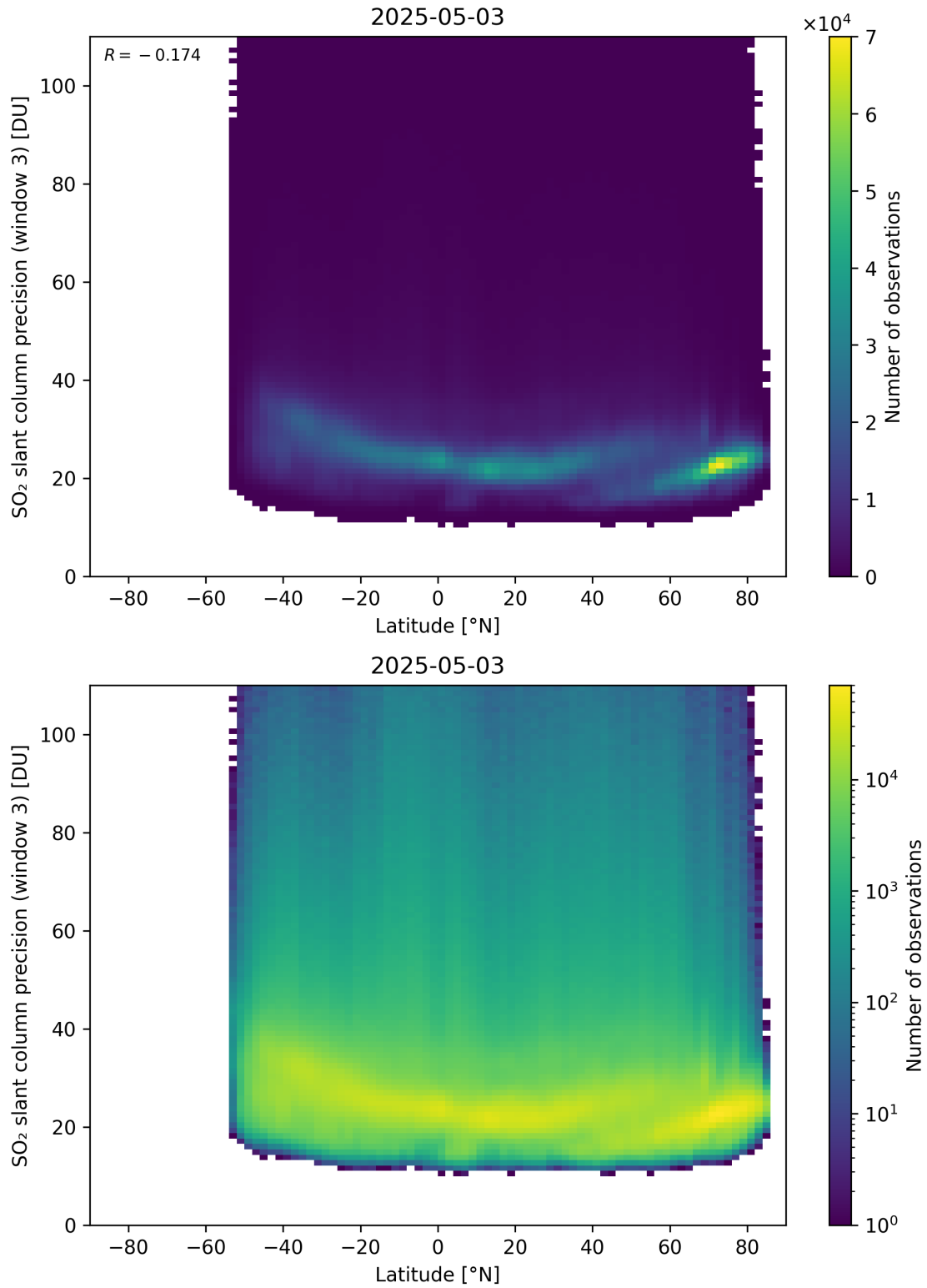
Figure 166: Scatter density plot of “Latitude” against “SO 2 slant column precision (window 3)” for 2025-05-02 to 2025-05-04.
