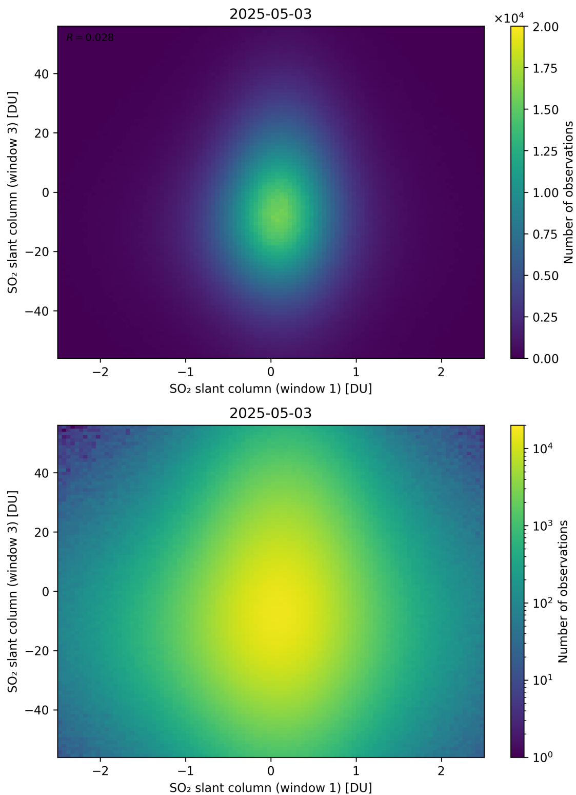
Figure 287: Scatter density plot of “SO 2 slant column (window 1)” against “SO 2 slant column (window 3)” for 2025-05-02 to 2025-05-04.
