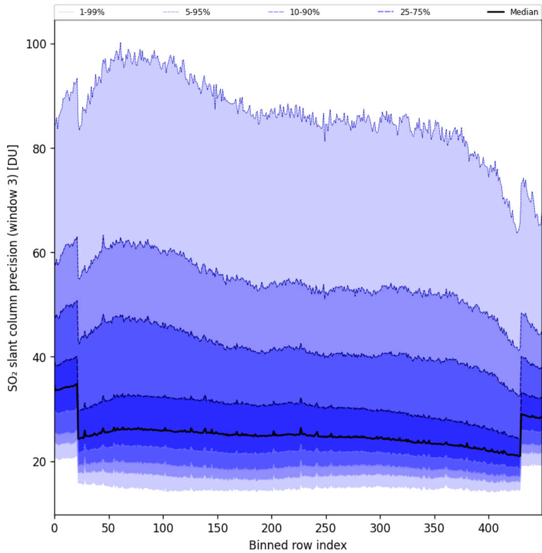
Figure 98: Along track statistics of “SO 2 slant column precision (window 3)” for 2025-05-02 to 2025-05-04
