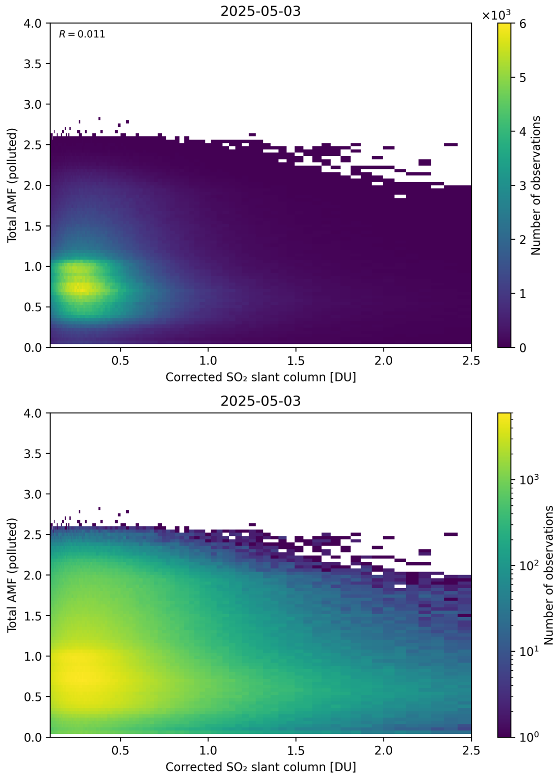
Figure 242: Scatter density plot of “Corrected SO 2 slant column” against “Total AMF (polluted)” for 2025-05-02 to 2025-05-04.
