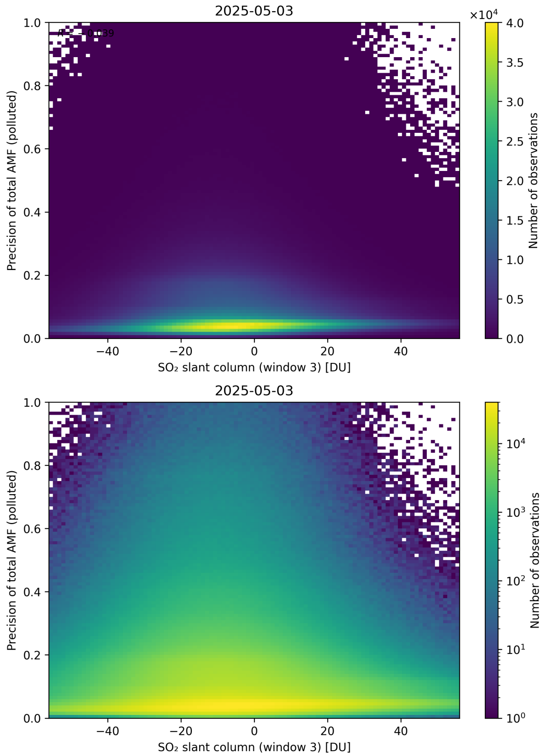
Figure 319: Scatter density plot of “SO 2 slant column (window 3)” against “Precision of total AMF (polluted)” for 2025-05-02 to 2025-05-04.
