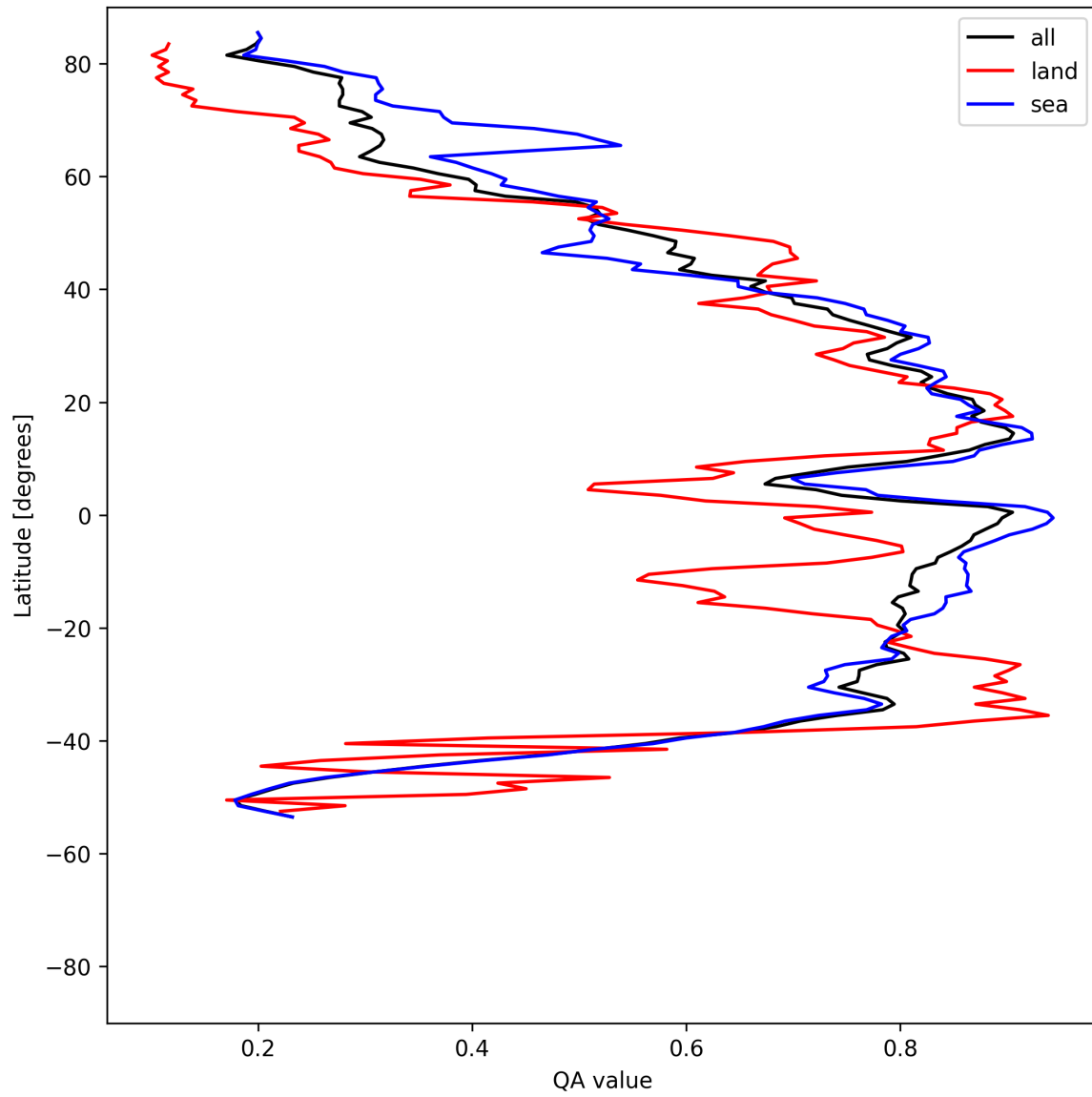
Figure 31: Zonal average of “QA value” for 2025-05-02 to 2025-05-04.
