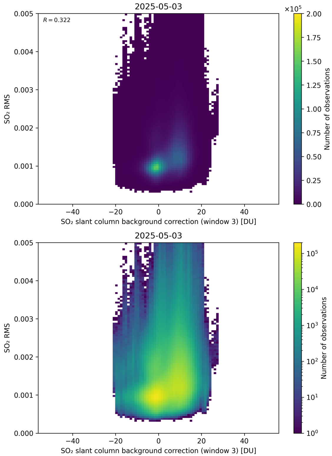
Figure 134: Scatter density plot of “SO 2 slant column background correction (window 3)” against “SO 2 RMS” for 2025-05-02 to 2025-05-04.
