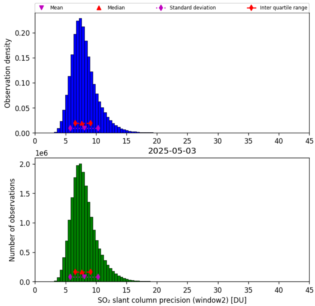
Figure 68: Histogram of “SO 2 slant column precision (window2)” for 2025-05-02 to 2025-05-04
