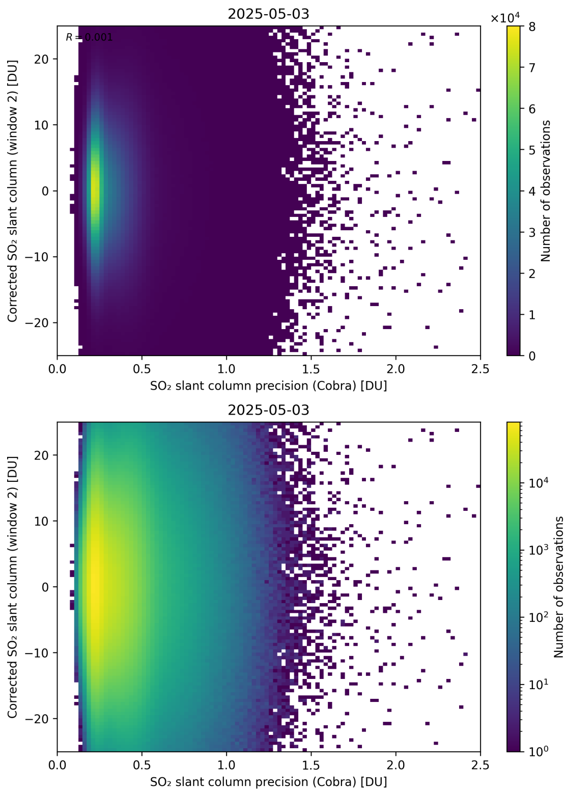
Figure 206: Scatter density plot of “SO 2 slant column precision (Cobra)” against “Corrected SO 2 slant column (window 2)” for 2025-05-02 to 2025-05-04.
