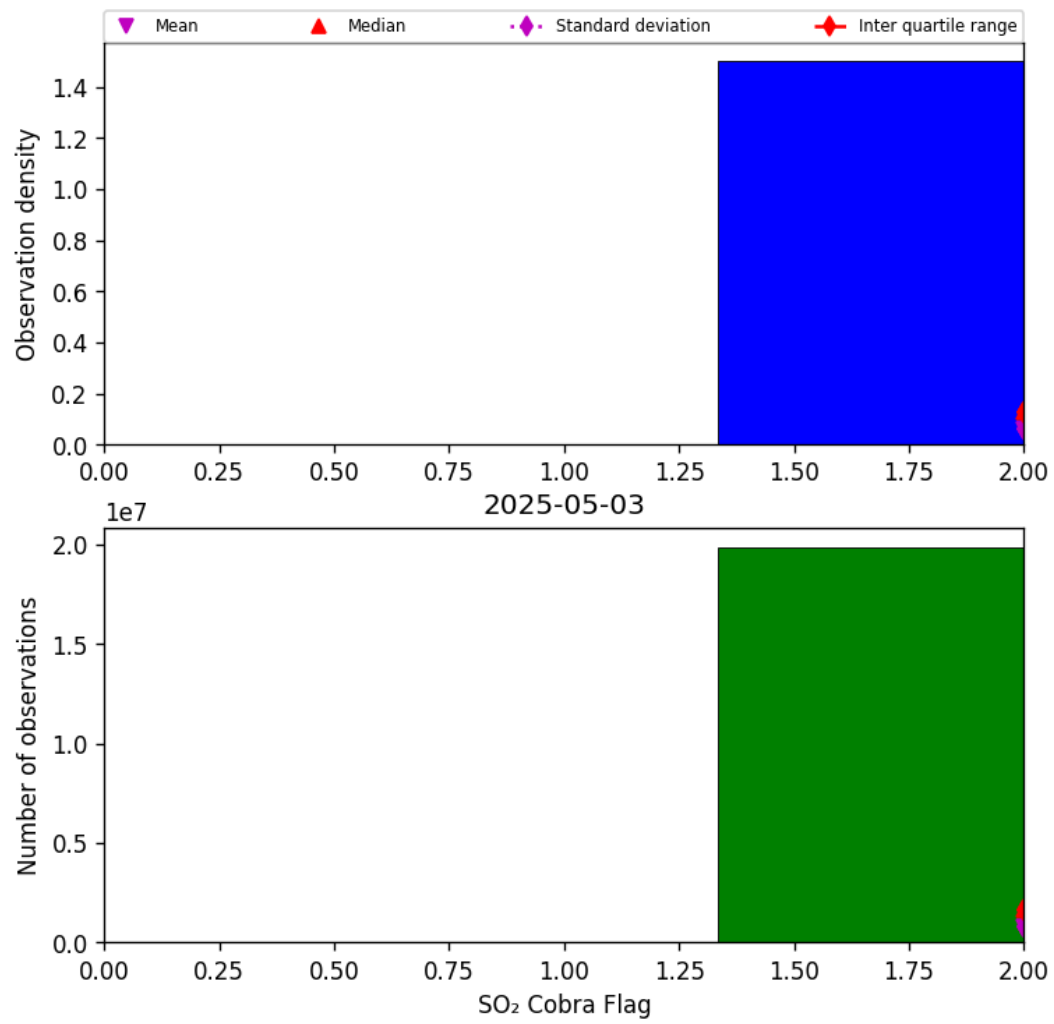
Figure 75: Histogram of “SO 2 Cobra Flag” for 2025-05-02 to 2025-05-04
