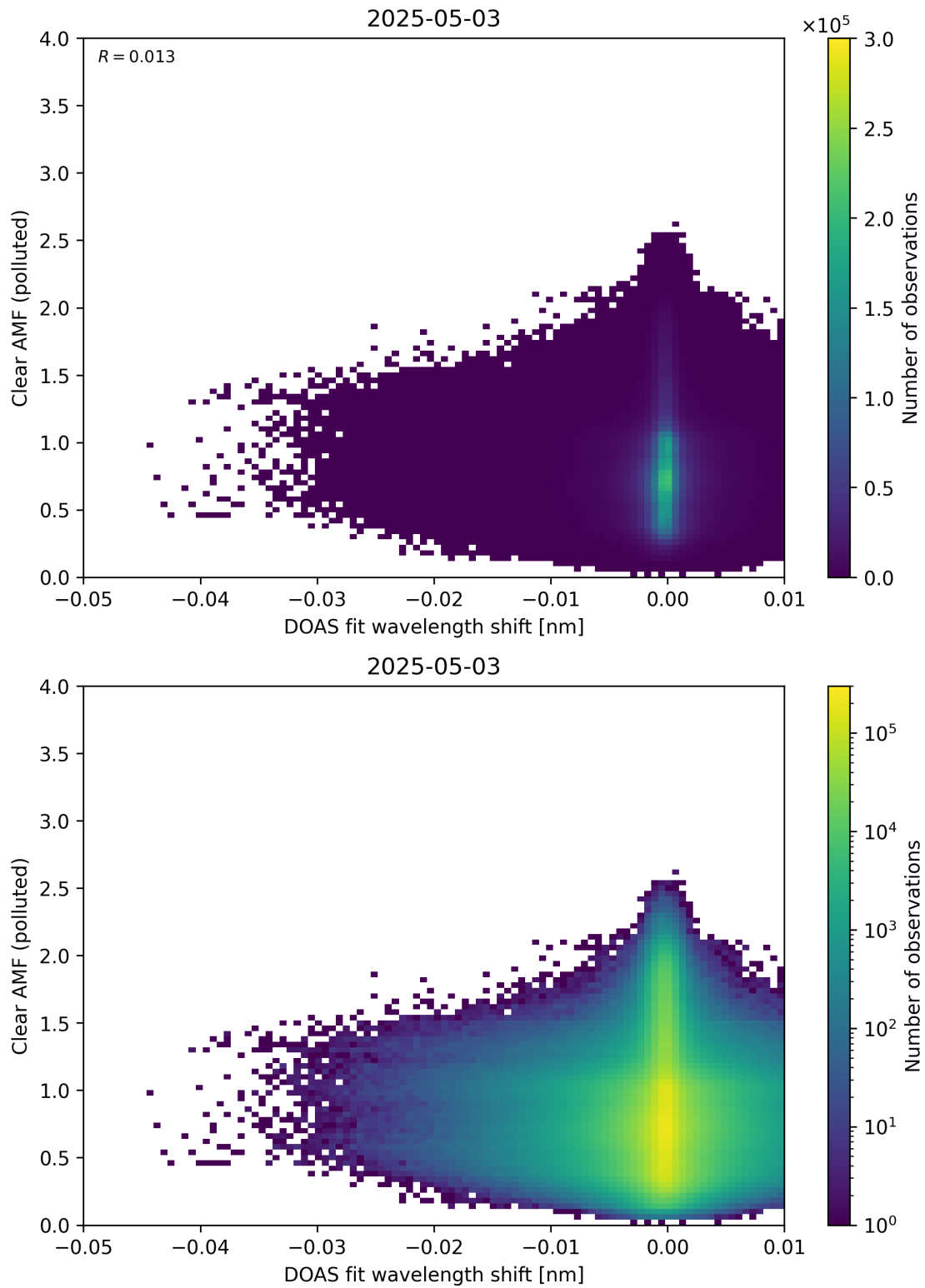
Figure 140: Scatter density plot of “DOAS fit wavelength shift” against “Clear AMF (polluted)” for 2025-05-02 to 2025-05-04.
