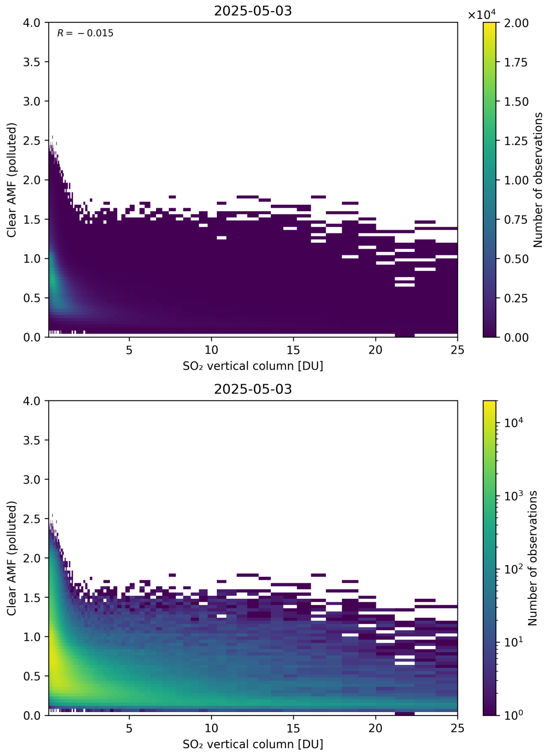
Figure 348: Scatter density plot of “SO 2 vertical column” against “Clear AMF (polluted)” for 2025-05-02 to 2025-05-04.
