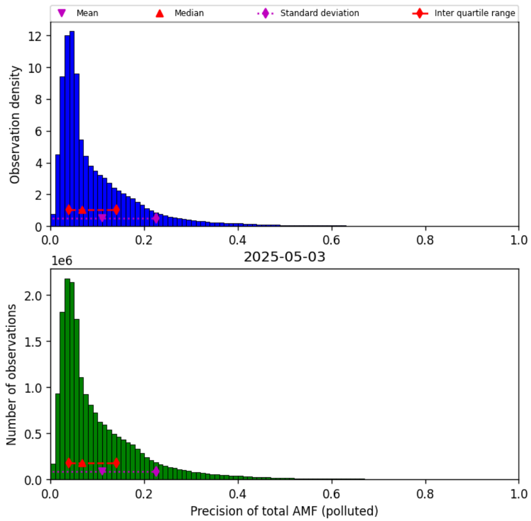
Figure 80: Histogram of “Precision of total AMF (polluted)” for 2025-05-02 to 2025-05-04
