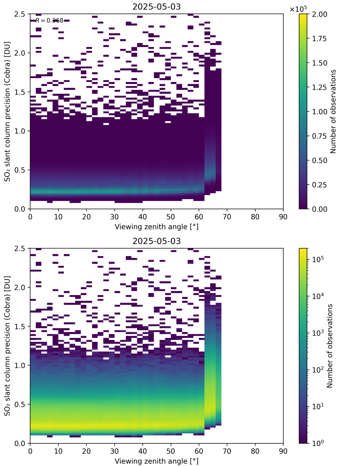
Figure 372: Scatter density plot of “Viewing zenith angle” against “SO 2 slant column precision (Cobra)” for 2025-05-02 to 2025-05-04.
