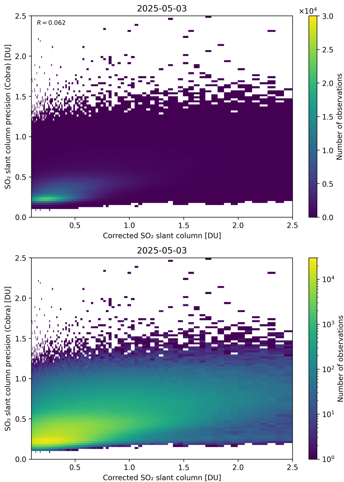
Figure 234: Scatter density plot of “Corrected SO 2 slant column” against “SO 2 slant column precision (Cobra)” for 2025-05-02 to 2025-05-04.
