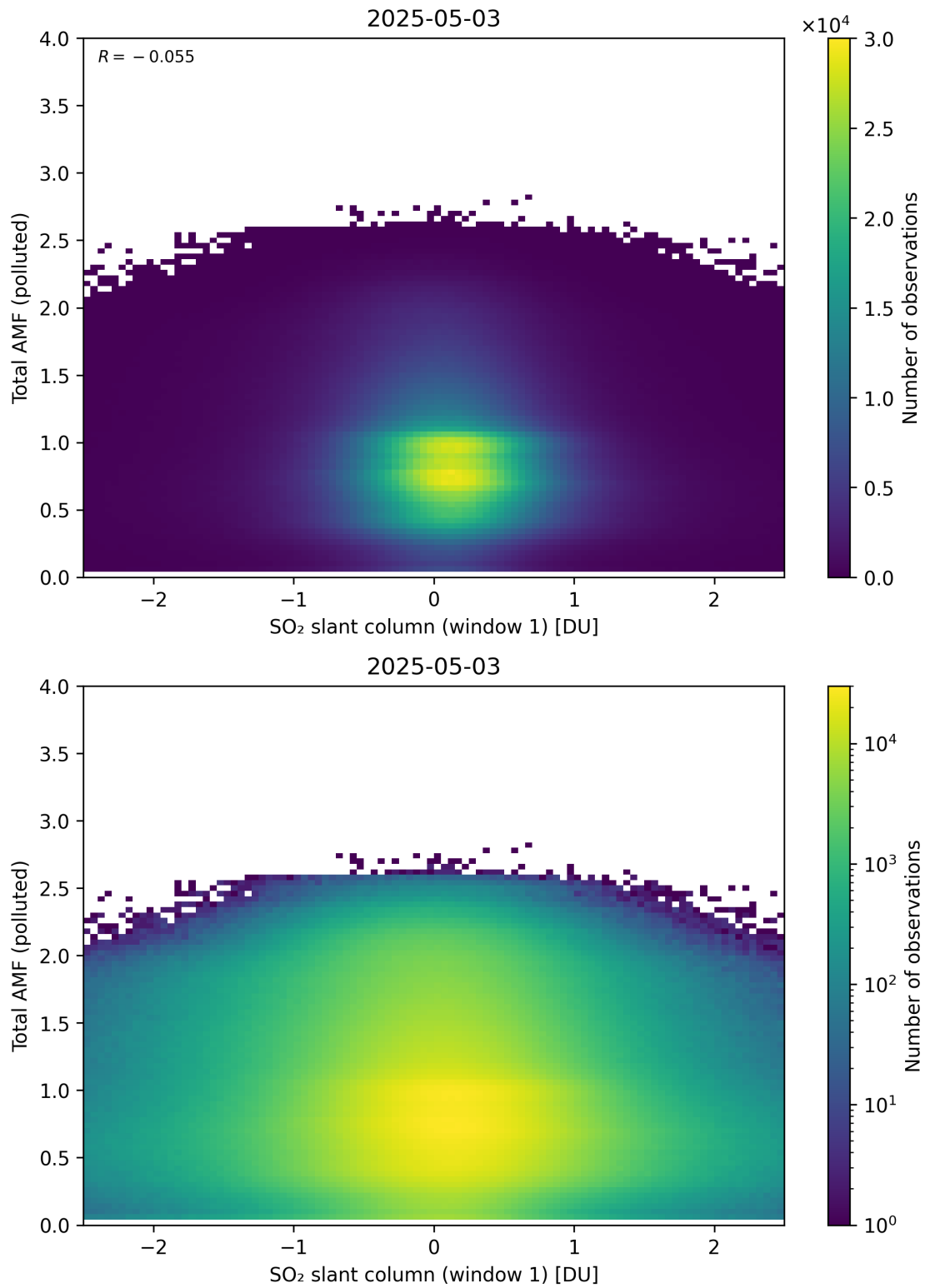
Figure 289: Scatter density plot of “SO 2 slant column (window 1)” against “Total AMF (polluted)” for 2025-05-02 to 2025-05-04.
