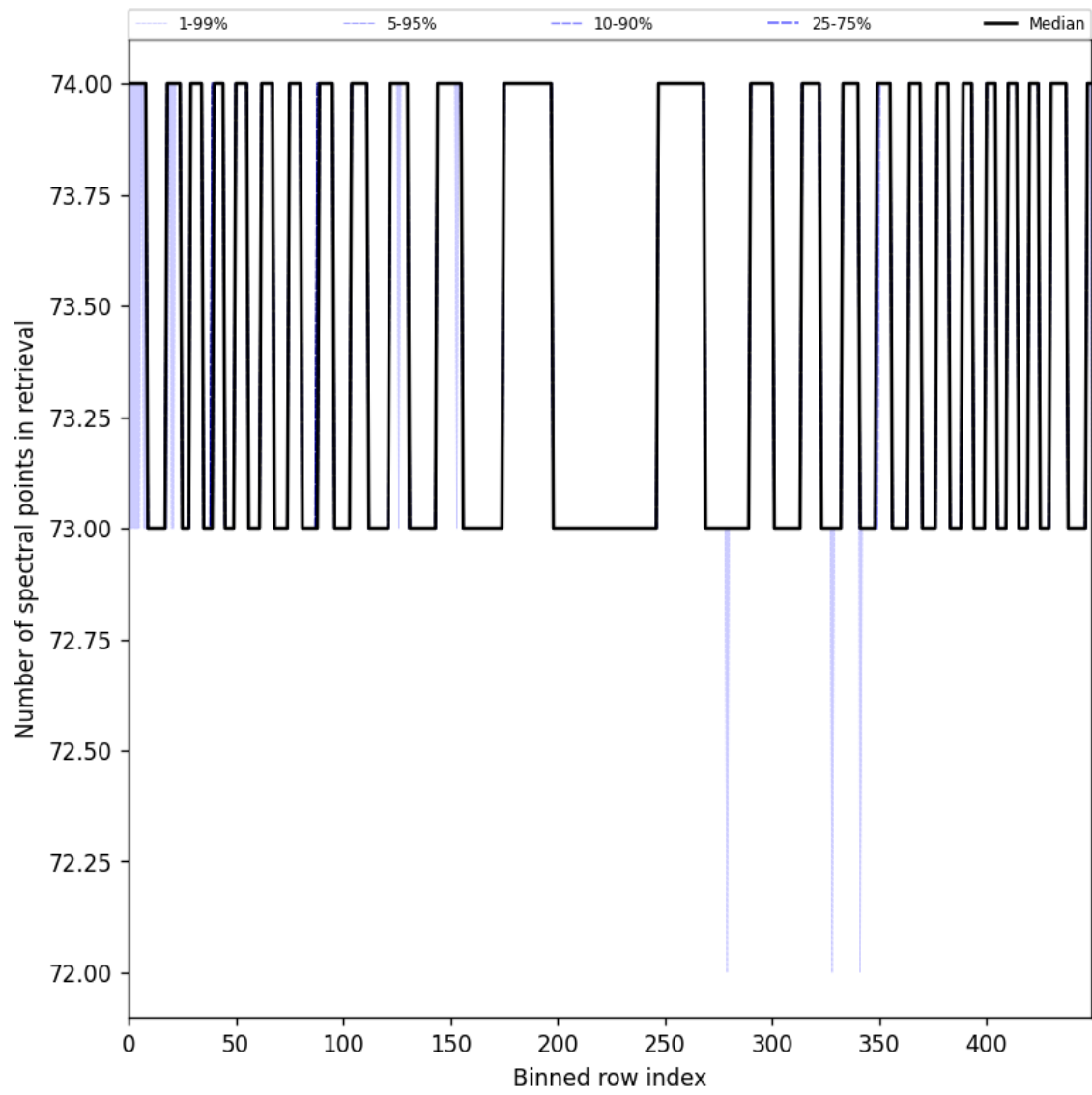
Figure 108: Along track statistics of “Number of spectral points in retrieval” for 2025-05-02 to 2025-05-04
