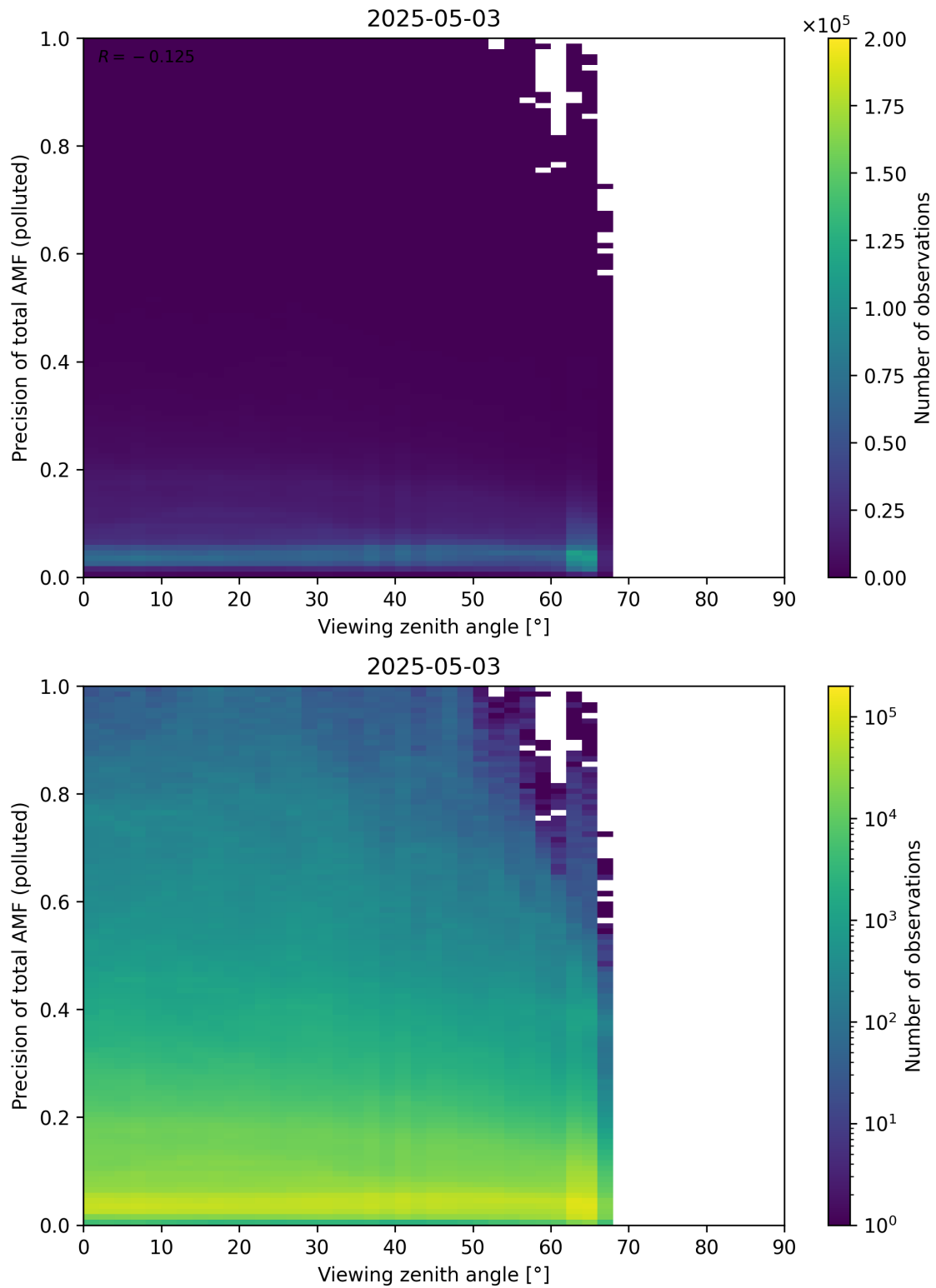
Figure 382: Scatter density plot of “Viewing zenith angle” against “Precision of total AMF (polluted)” for 2025-05-02 to 2025-05-04.
