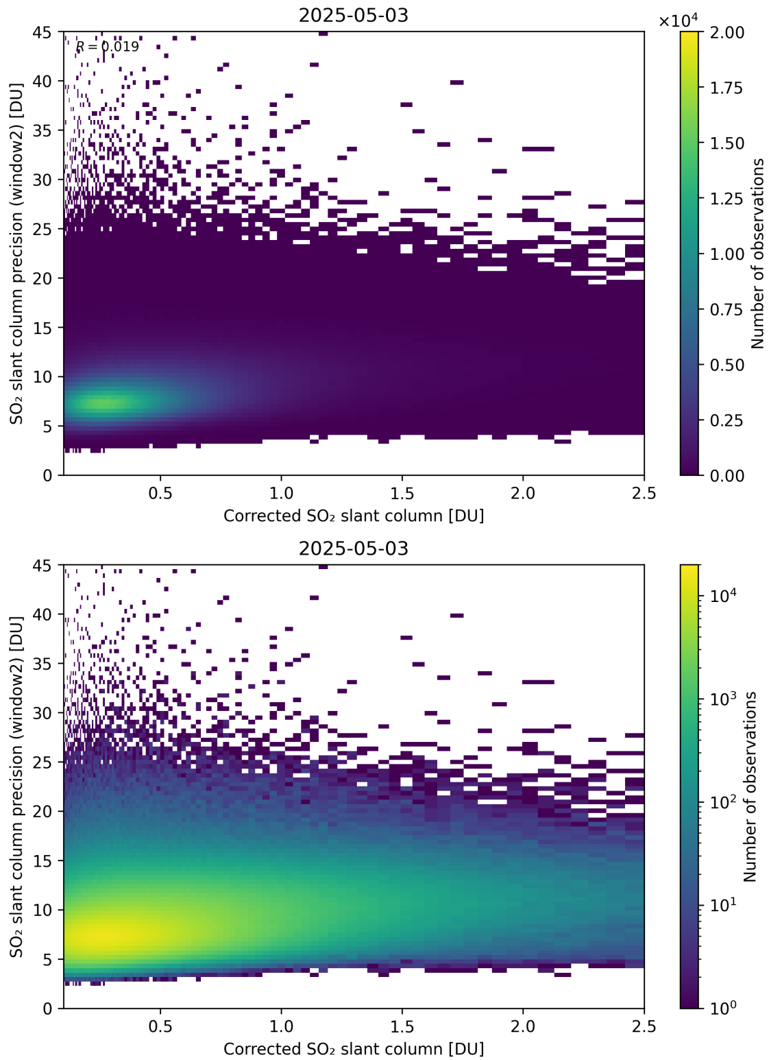
Figure 239: Scatter density plot of “Corrected SO 2 slant column” against “SO 2 slant column precision (window2)” for 2025-05-02 to 2025-05-04.
