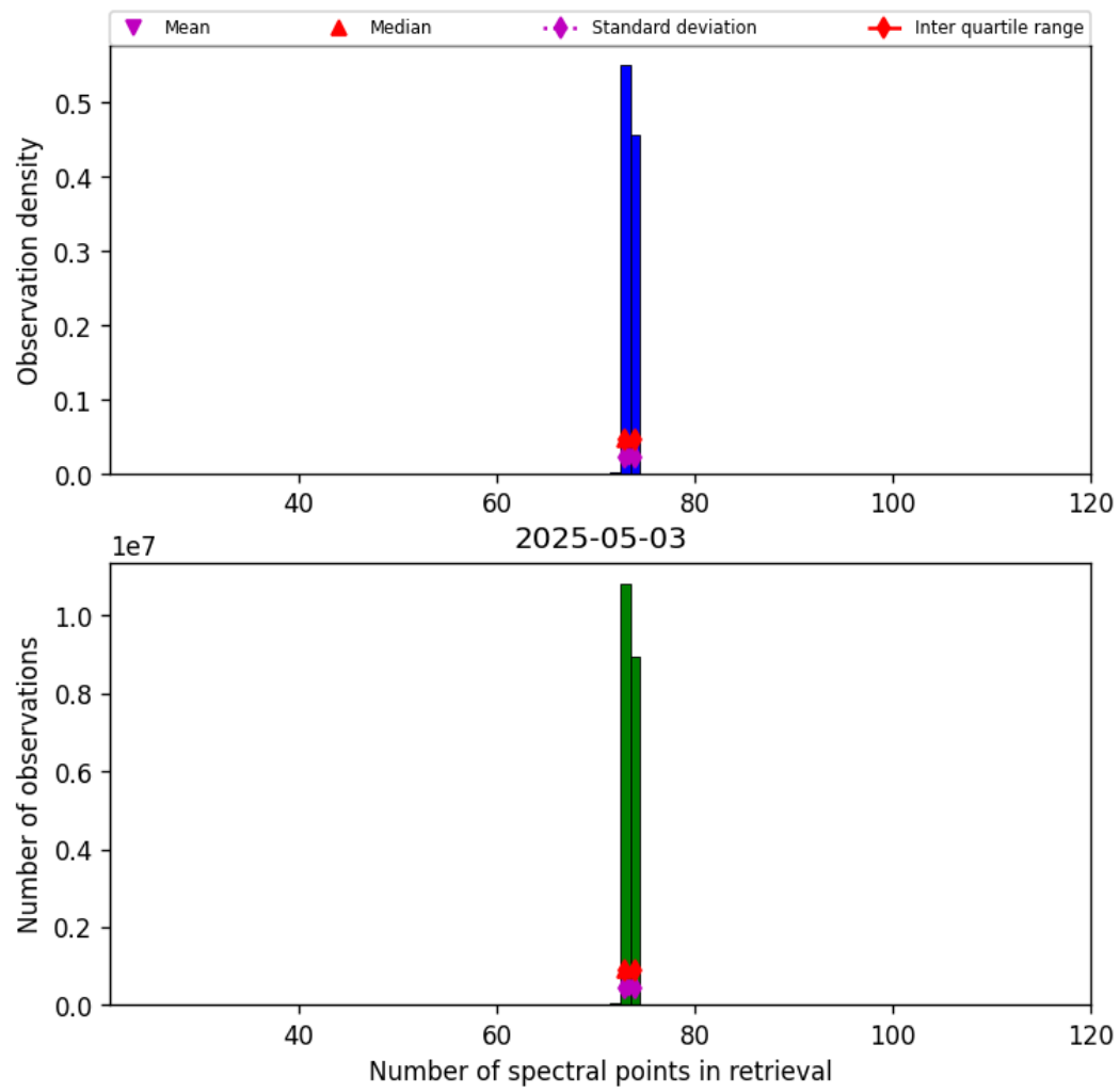
Figure 82: Histogram of “Number of spectral points in retrieval” for 2025-05-02 to 2025-05-04
