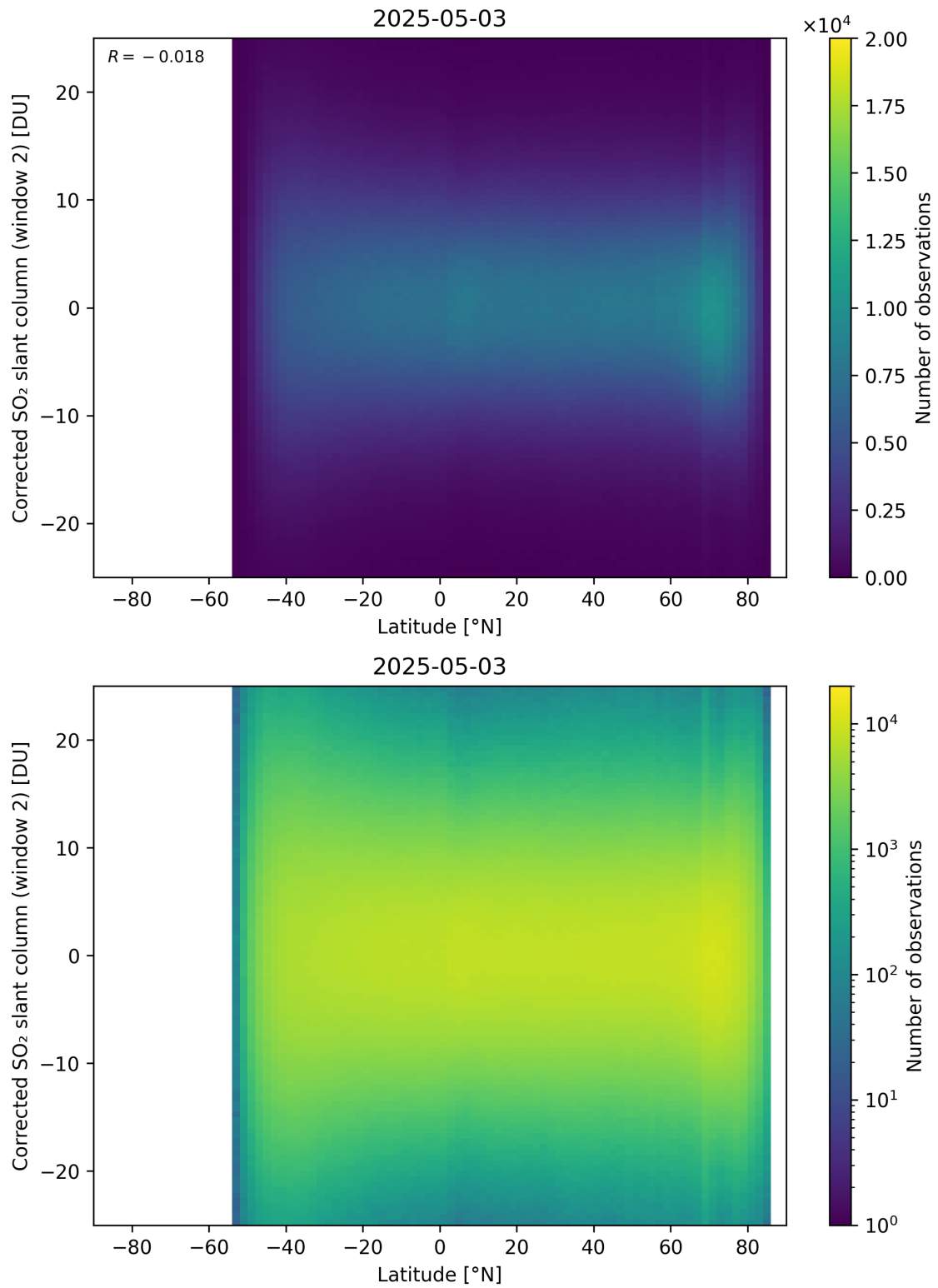
Figure 160: Scatter density plot of “Latitude” against “Corrected SO 2 slant column (window 2)” for 2025-05-02 to 2025-05-04.
