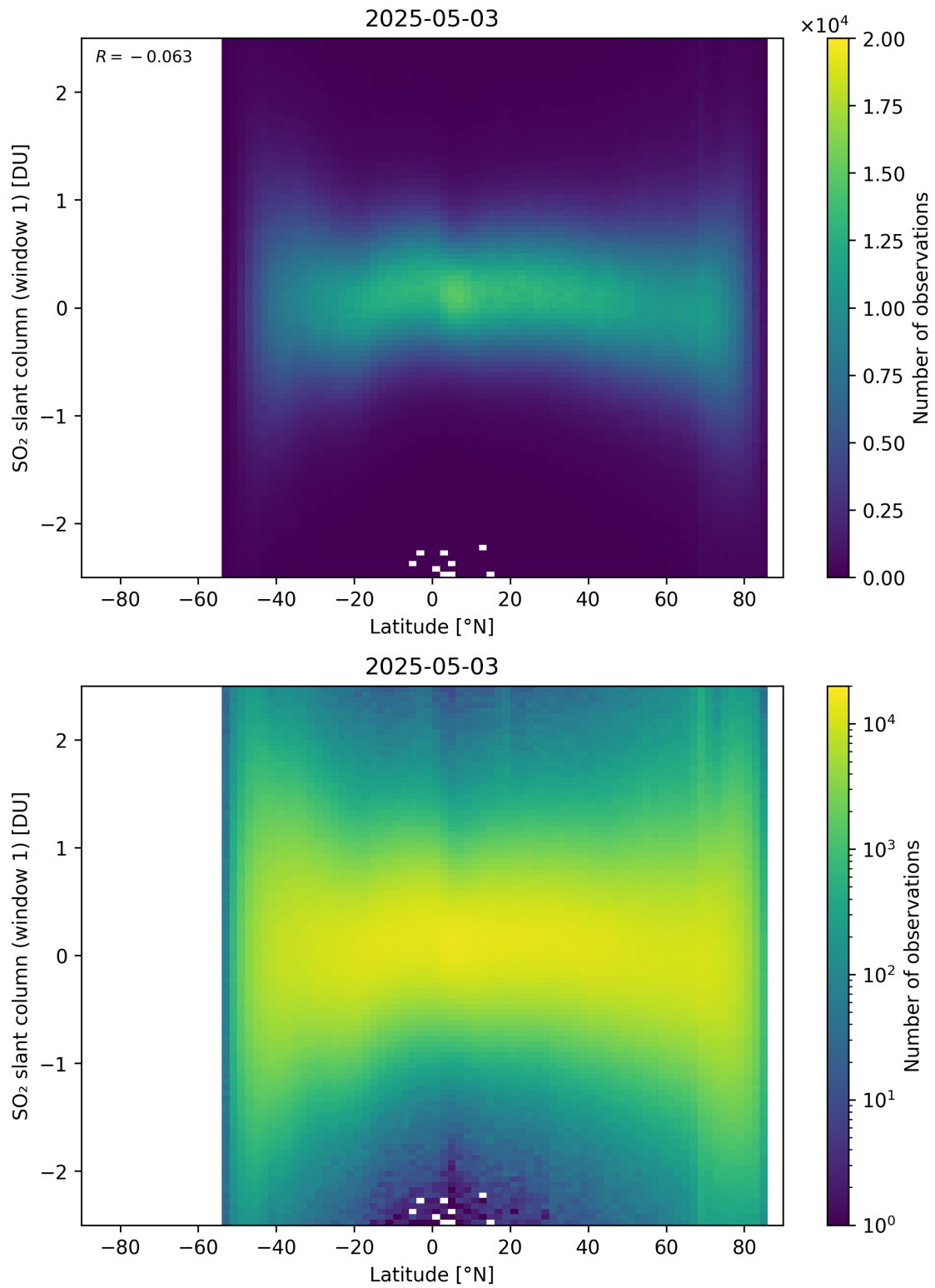
Figure 162: Scatter density plot of “Latitude” against “SO 2 slant column (window 1)” for 2025-05-02 to 2025-05-04.
