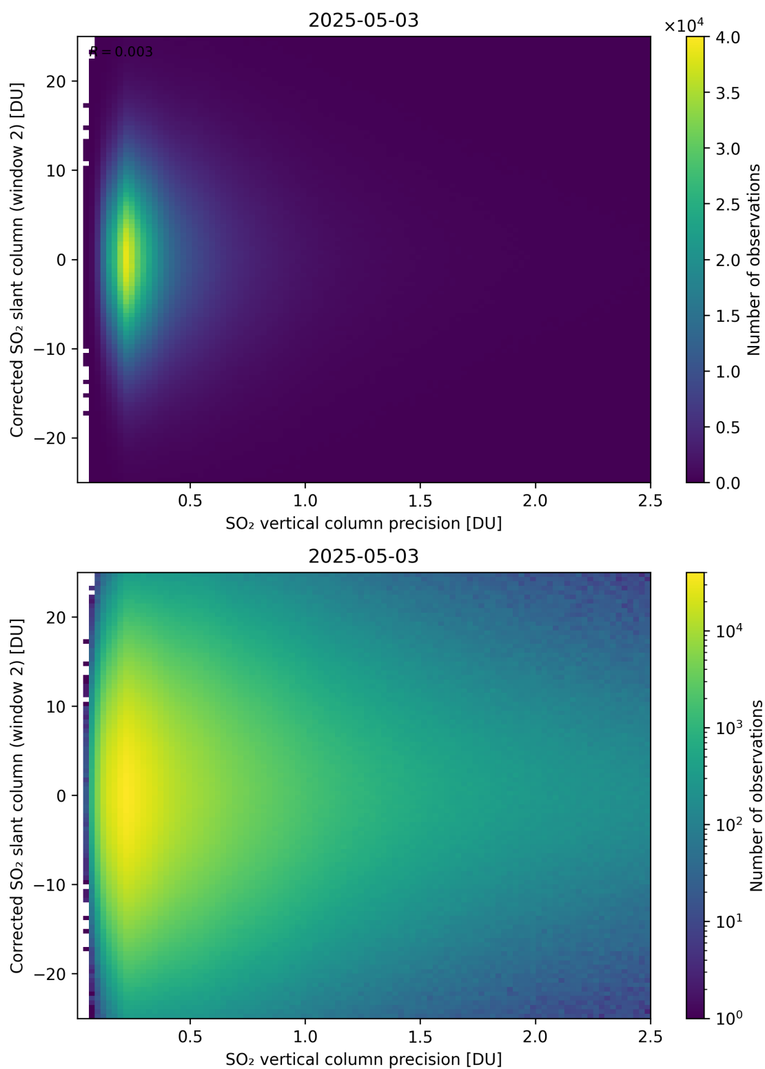
Figure 339: Scatter density plot of “SO 2 vertical column precision” against “Corrected SO 2 slant column (window 2)” for 2025-05-02 to 2025-05-04.
