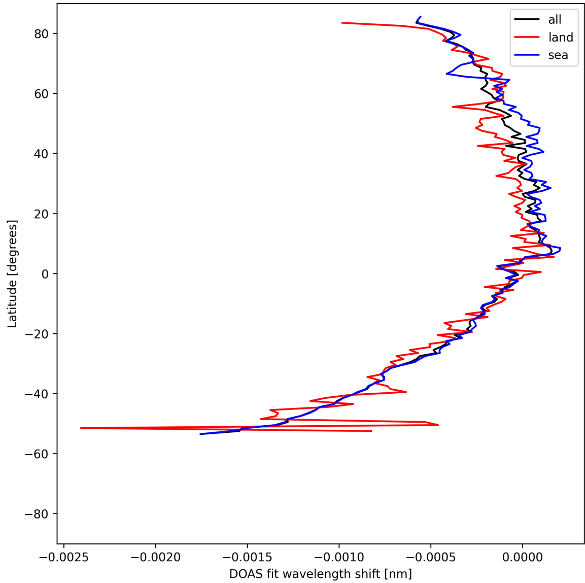
Figure 50: Zonal average of “DOAS fit wavelength shift” for 2025-05-02 to 2025-05-04.
