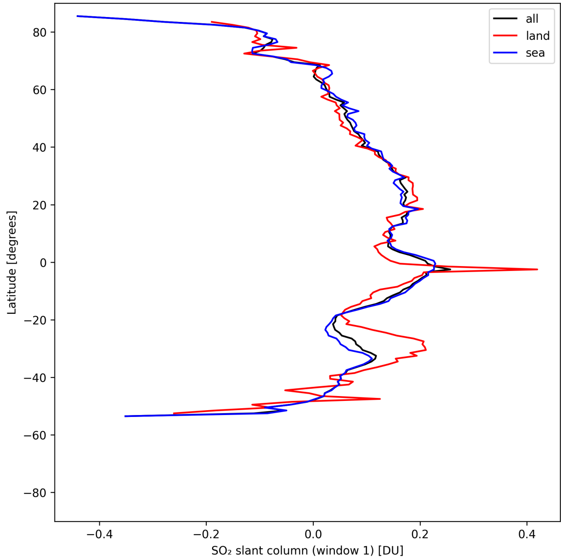
Figure 37: Zonal average of “SO 2 slant column (window 1)” for 2025-05-02 to 2025-05-04.
