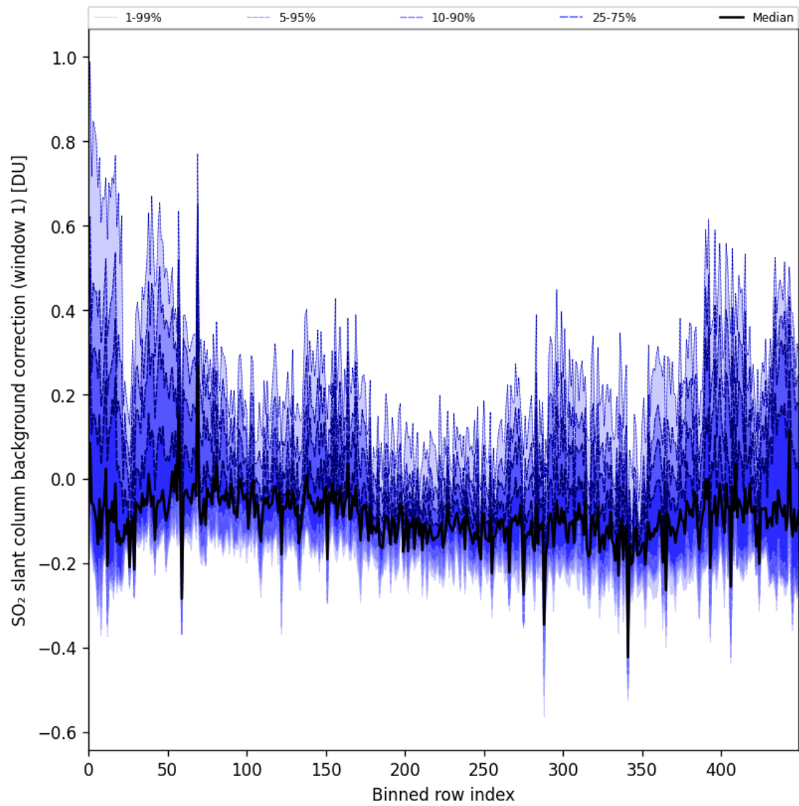
Figure 92: Along track statistics of “SO 2 slant column background correction (window 1)” for 2025-05-02 to 2025-05-04
