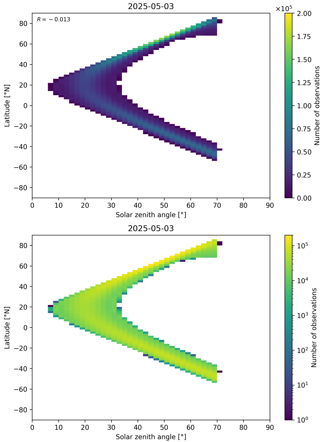
Figure 177: Scatter density plot of “Solar zenith angle” against “Latitude” for 2025-05-02 to 2025-05-04.
