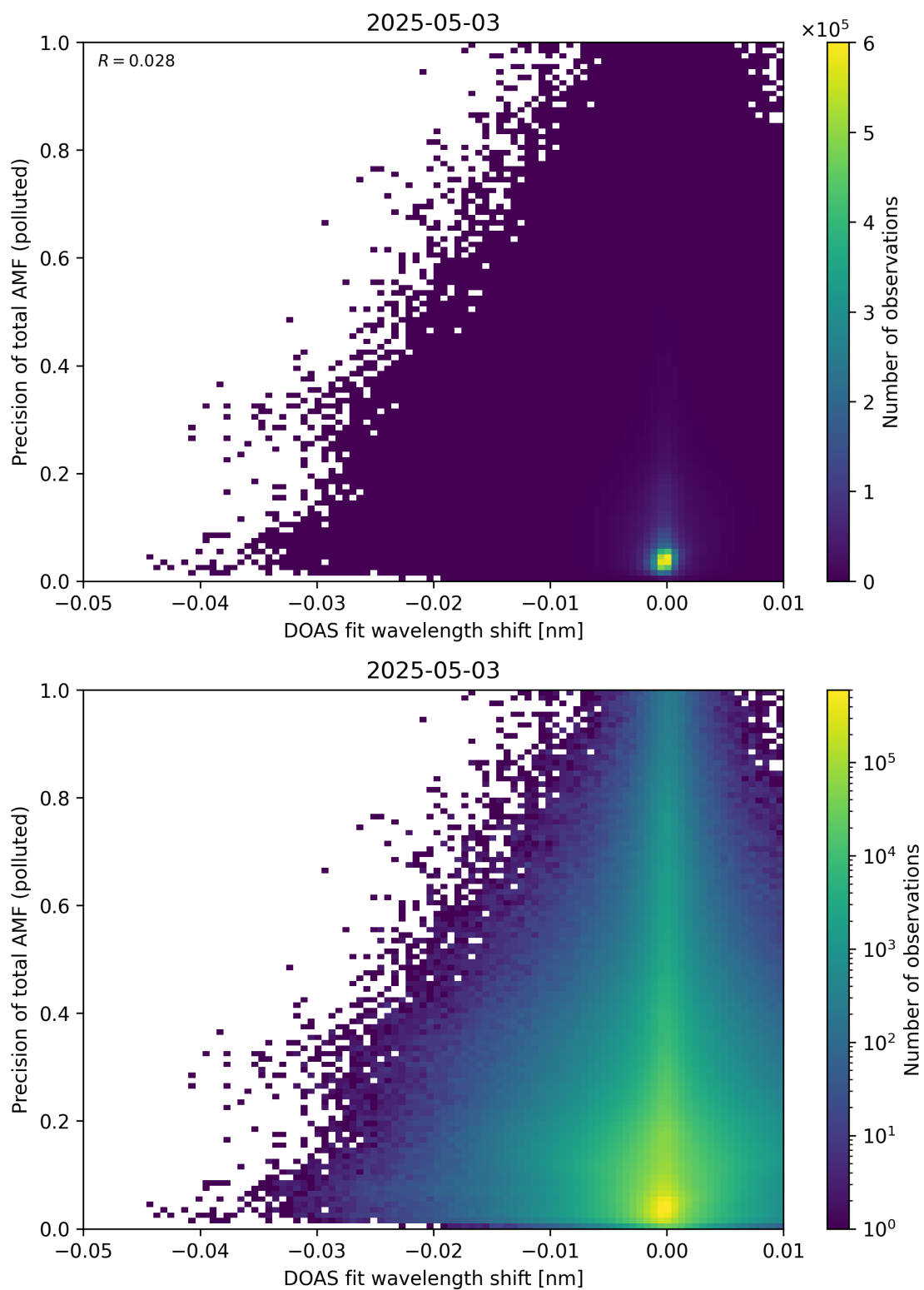
Figure 142: Scatter density plot of “DOAS fit wavelength shift” against “Precision of total AMF (polluted)” for 2025-05-02 to 2025-05-04.
