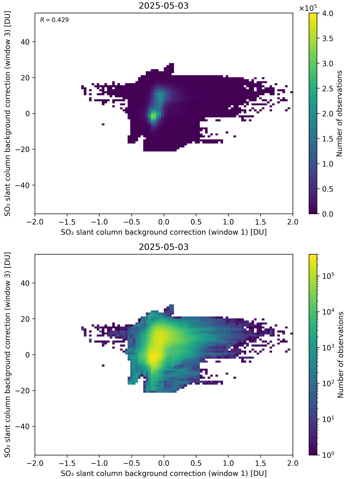
Figure 110: Scatter density plot of “SO 2 slant column background correction (window 1)” against “SO 2 slant column background correction (window 3)” for 2025-05-02 to 2025-05-04.
