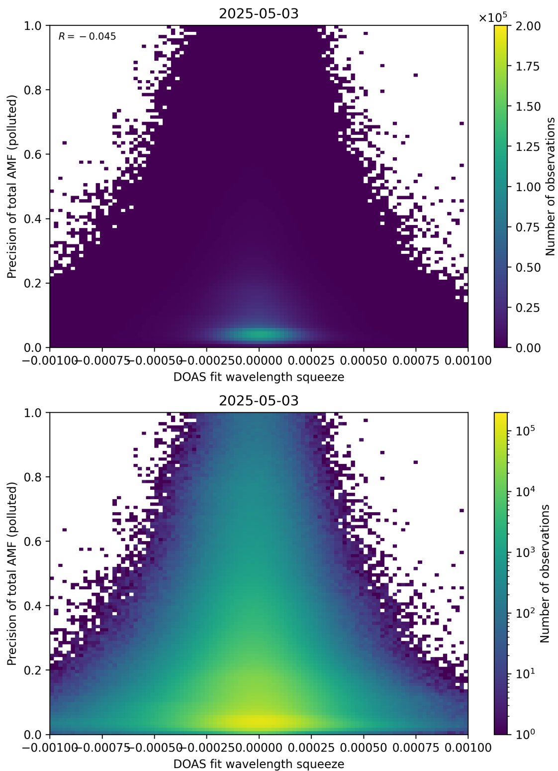
Figure 146: Scatter density plot of “DOAS fit wavelength squeeze” against “Precision of total AMF (polluted)” for 2025-05-02 to 2025-05-04.
