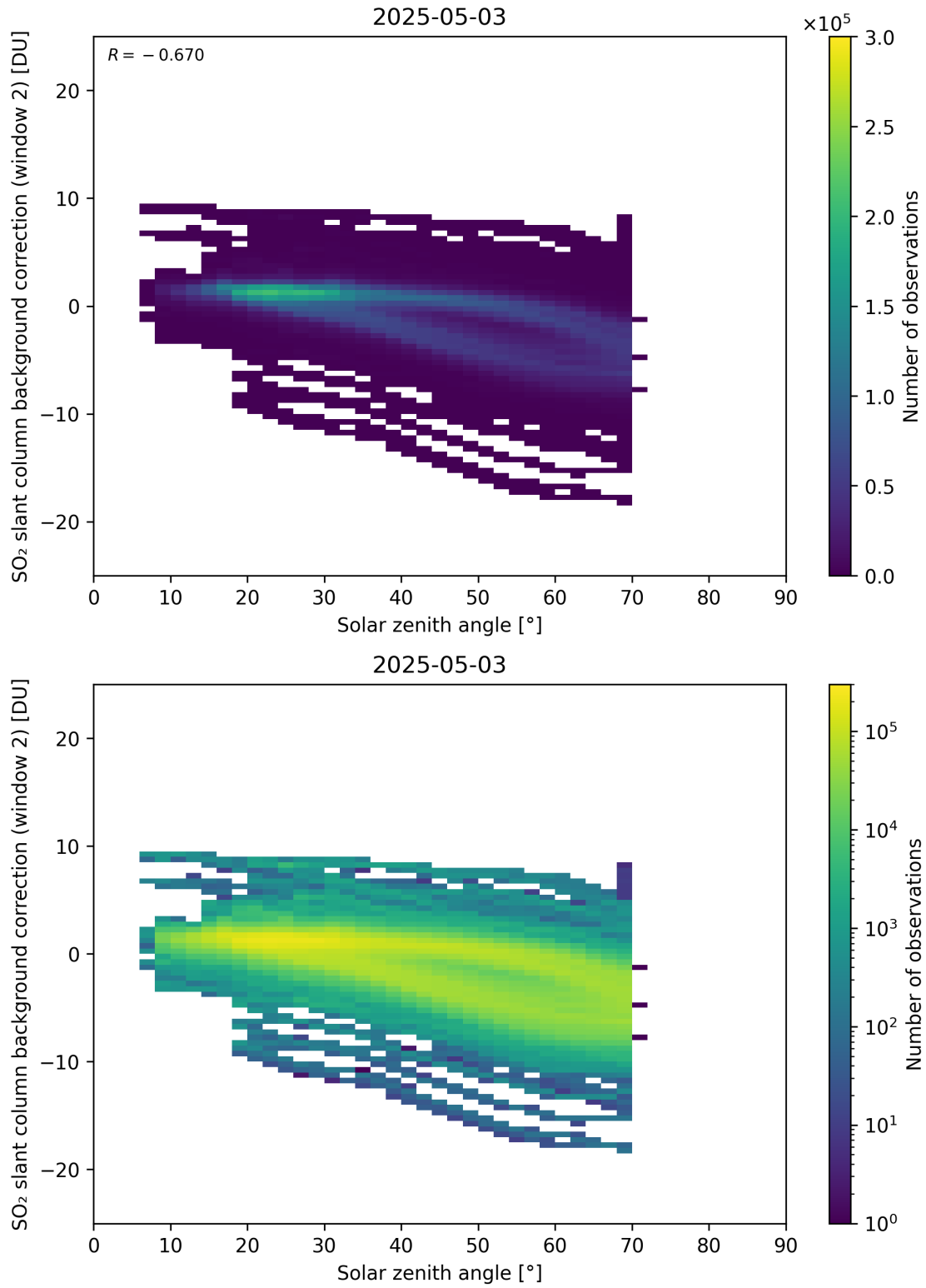
Figure 172: Scatter density plot of “Solar zenith angle” against “SO 2 slant column background correction (window 2)” for 2025-05-02 to 2025-05-04.
