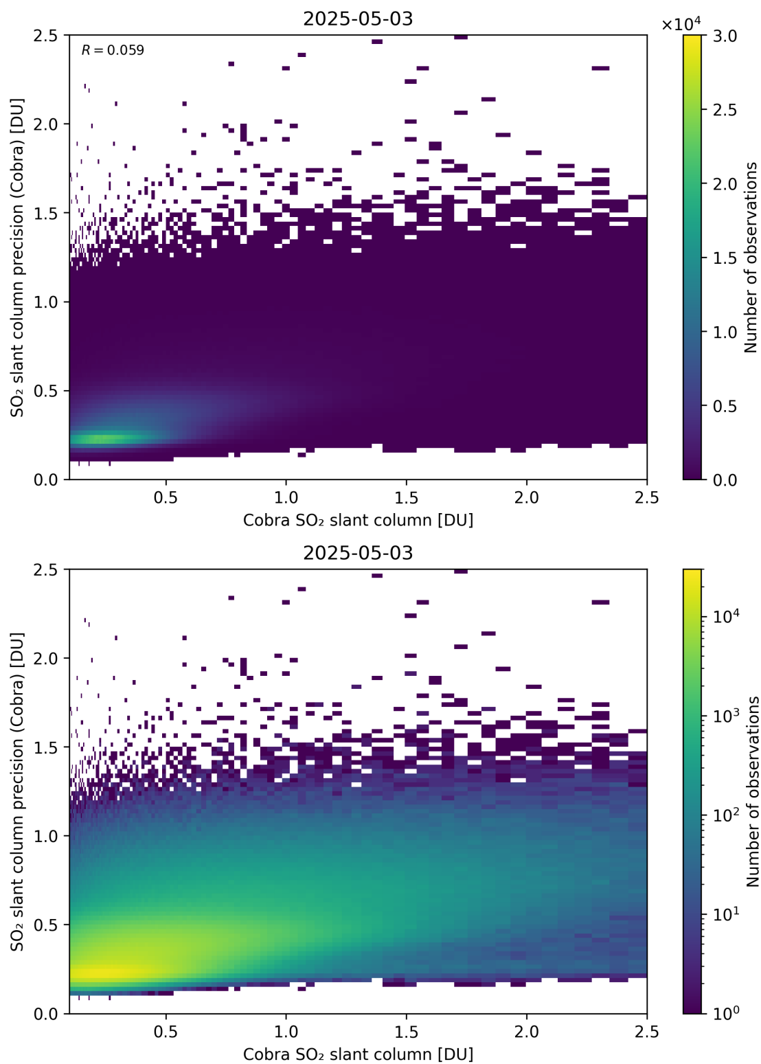
Figure 216: Scatter density plot of “Cobra SO 2 slant column” against “SO 2 slant column precision (Cobra)” for 2025-05-02 to 2025-05-04.
