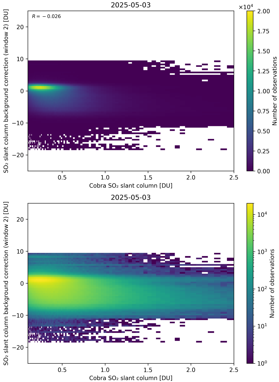
Figure 194: Scatter density plot of “Cobra SO 2 slant column” against “SO 2 slant column background correction (window 2)” for 2025-05-02 to 2025-05-04.
