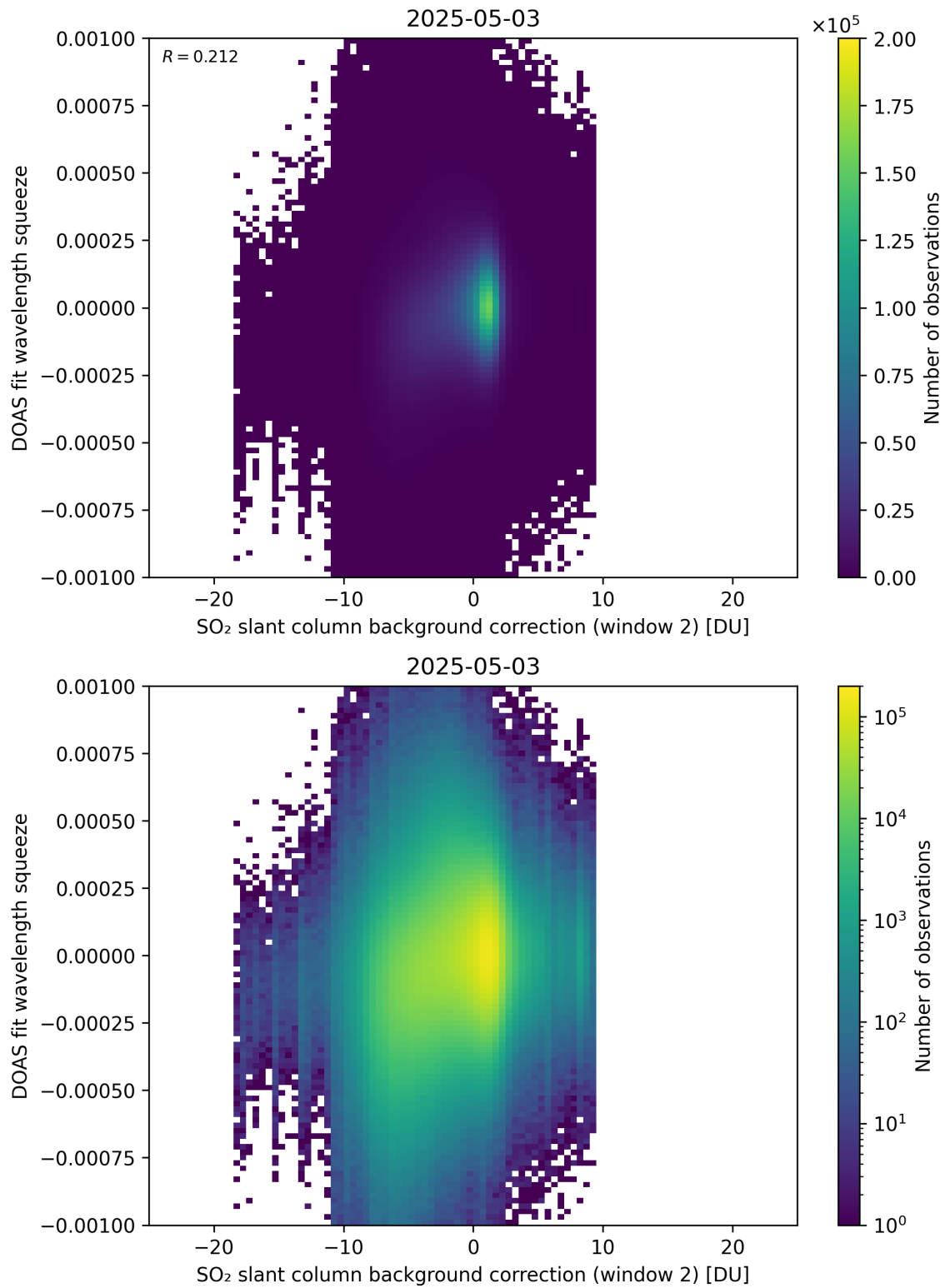
Figure 124: Scatter density plot of “SO 2 slant column background correction (window 2)” against “DOAS fit wavelength squeeze” for 2025-05-02 to 2025-05-04.
