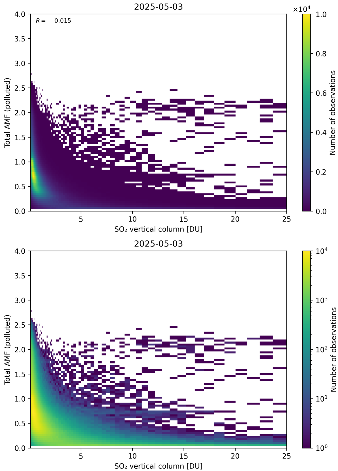
Figure 359: Scatter density plot of “SO 2 vertical column” against “Total AMF (polluted)” for 2025-05-02 to 2025-05-04.
