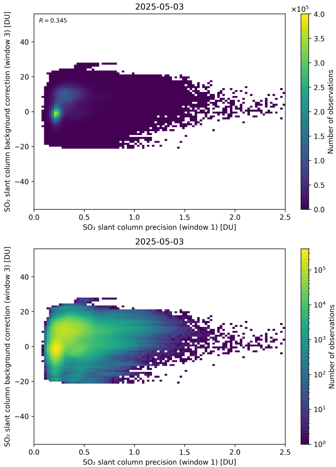
Figure 270: Scatter density plot of “SO 2 slant column precision (window 1)” against “SO 2 slant column background correction (window 3)” for 2025-05-02 to 2025-05-04.
