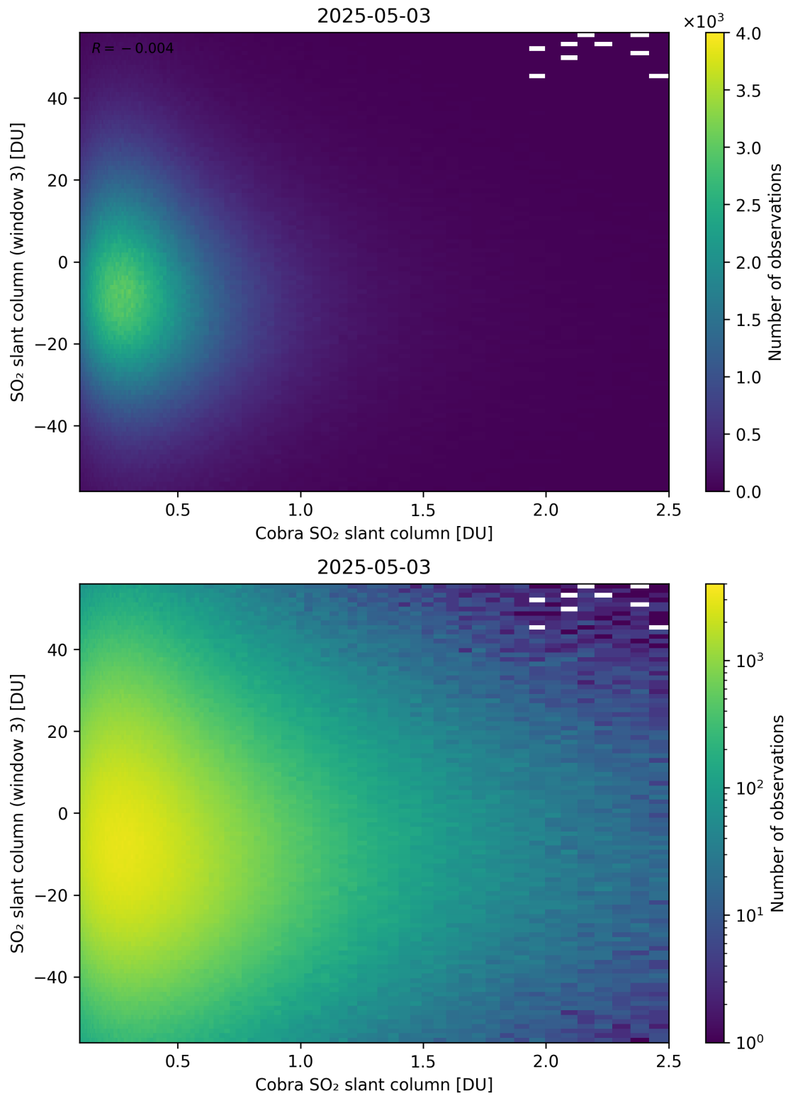
Figure 222: Scatter density plot of “Cobra SO 2 slant column” against “SO 2 slant column (window 3)” for 2025-05-02 to 2025-05-04.
