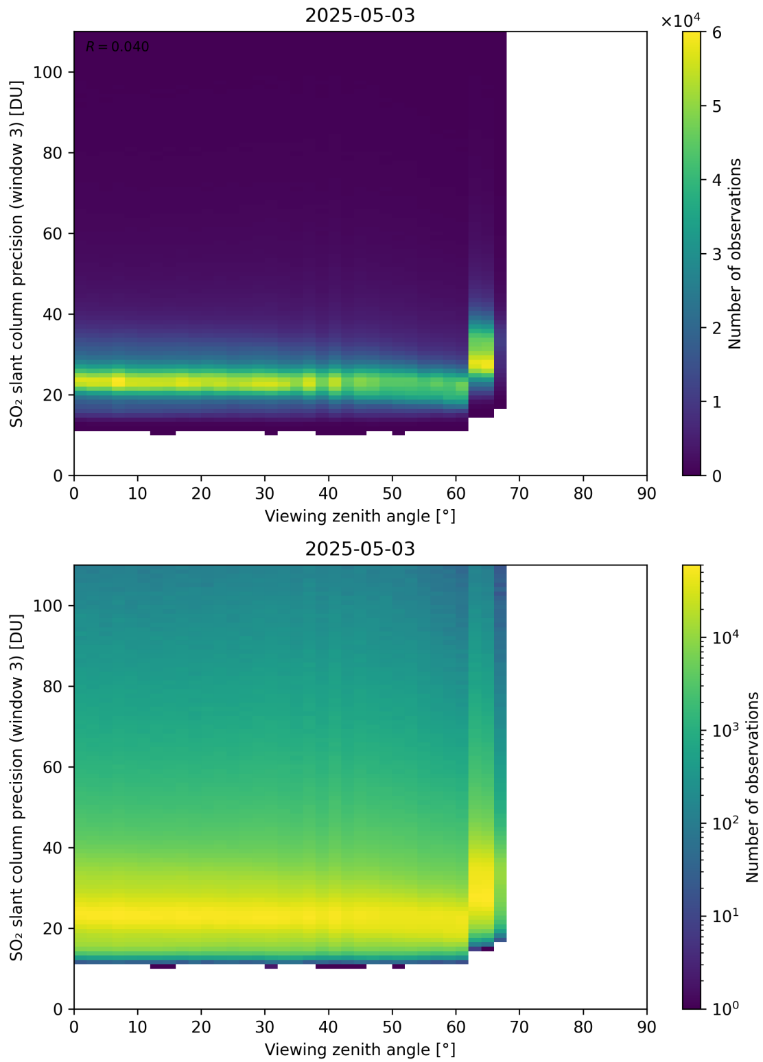
Figure 380: Scatter density plot of “Viewing zenith angle” against “SO 2 slant column precision (window 3)” for 2025-05-02 to 2025-05-04.
