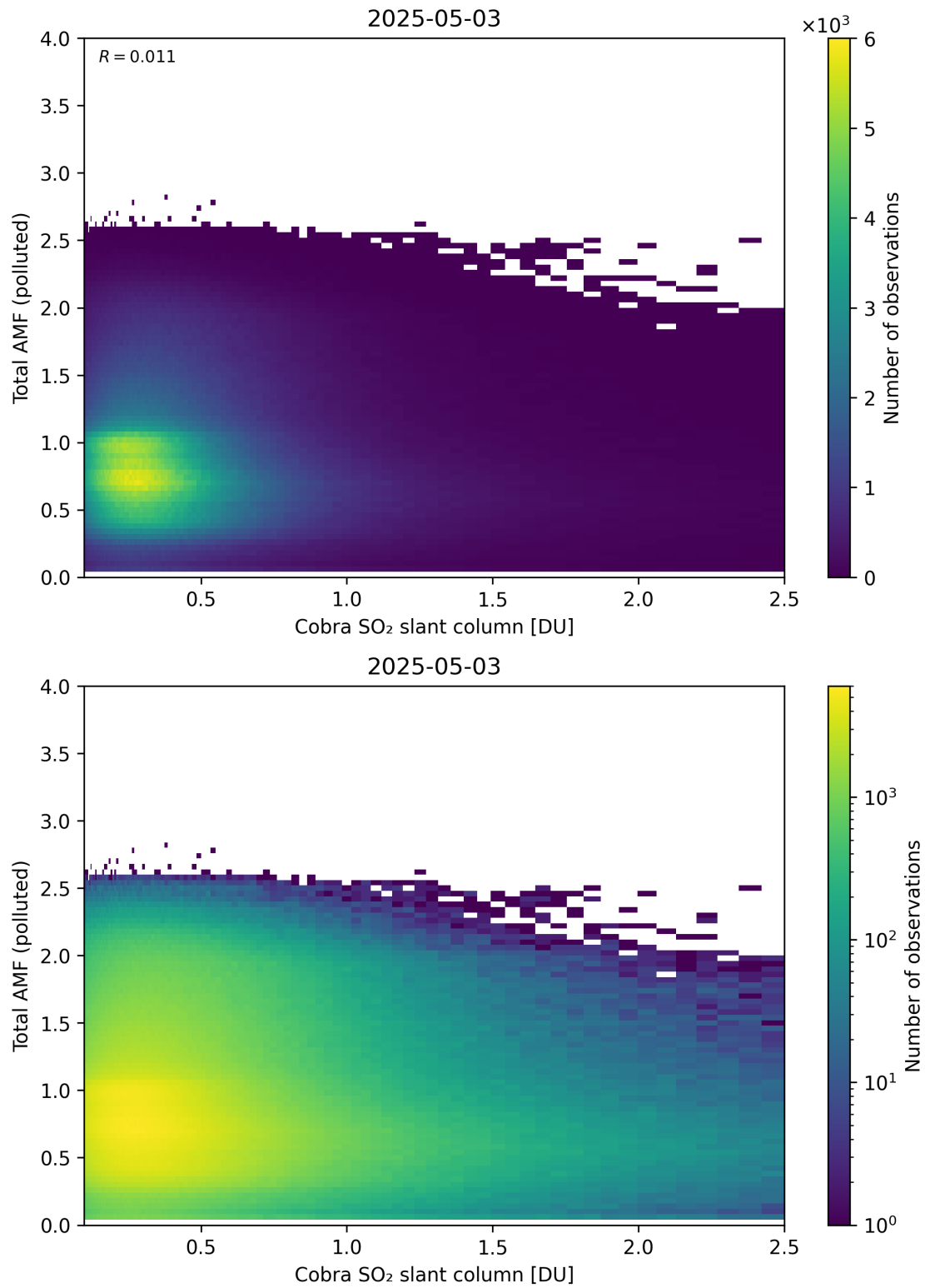
Figure 224: Scatter density plot of “Cobra SO 2 slant column” against “Total AMF (polluted)” for 2025-05-02 to 2025-05-04.
