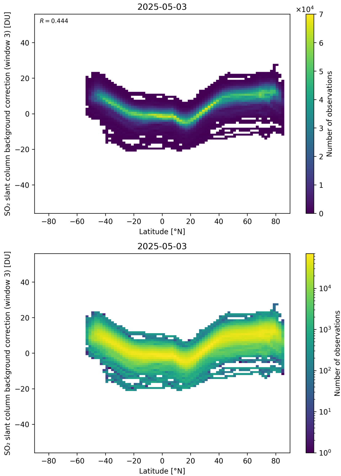
Figure 152: Scatter density plot of “Latitude” against “SO 2 slant column background correction (window 3)” for 2025-05-02 to 2025-05-04.
