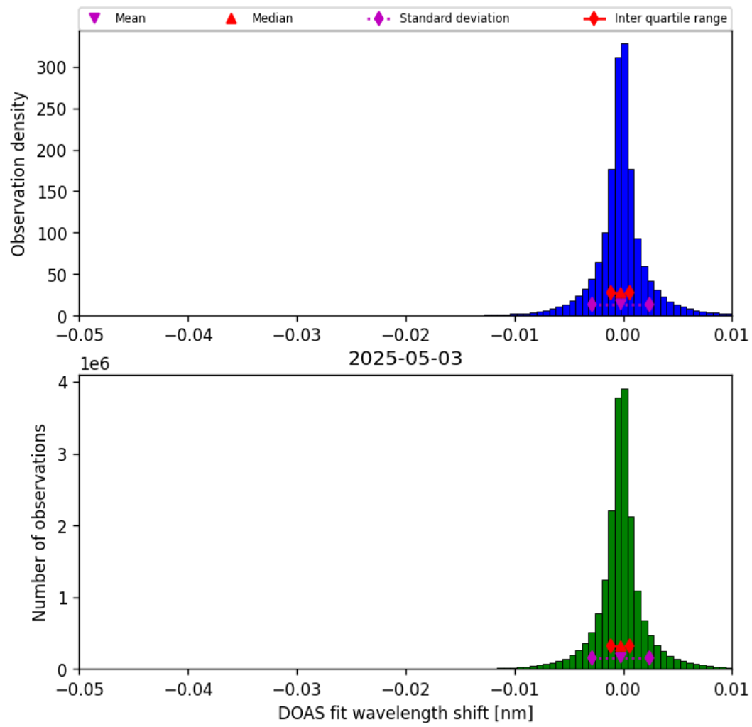
Figure 76: Histogram of “DOAS fit wavelength shift” for 2025-05-02 to 2025-05-04
