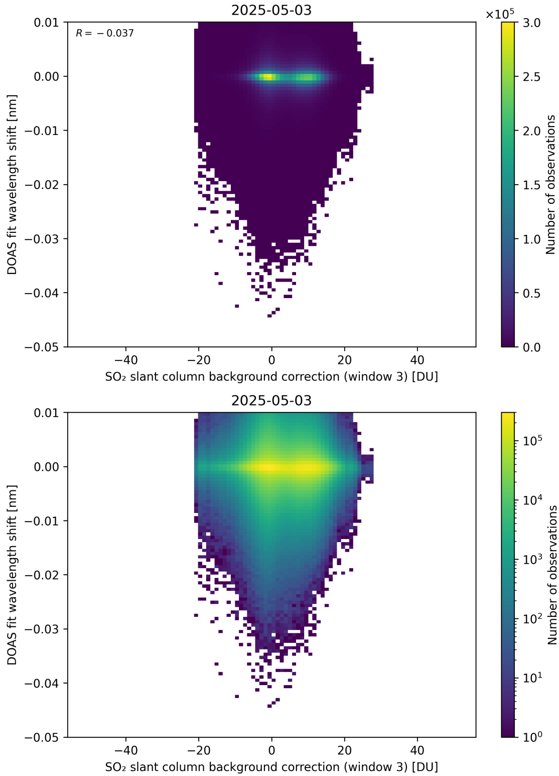
Figure 132: Scatter density plot of “SO 2 slant column background correction (window 3)” against “DOAS fit wavelength shift” for 2025-05-02 to 2025-05-04.
