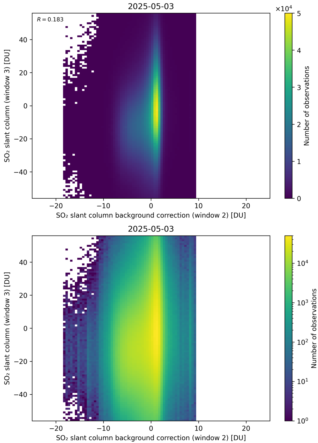
Figure 128: Scatter density plot of “SO 2 slant column background correction (window 2)” against “SO 2 slant column (window 3)” for 2025-05-02 to 2025-05-04.
