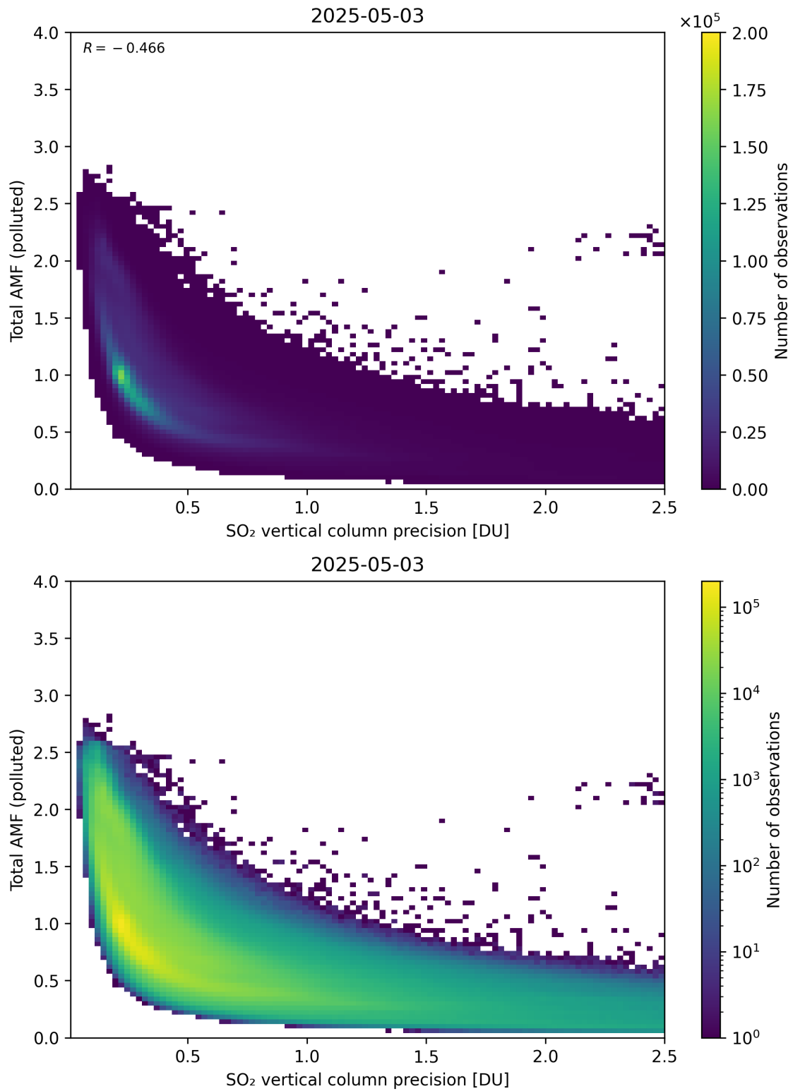
Figure 346: Scatter density plot of “SO 2 vertical column precision” against “Total AMF (polluted)” for 2025-05-02 to 2025-05-04.
