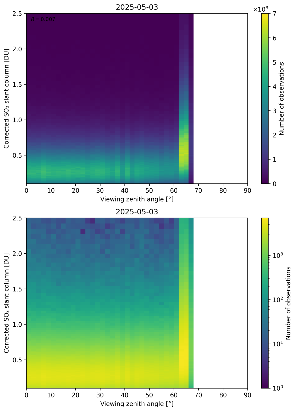
Figure 373: Scatter density plot of “Viewing zenith angle” against “Corrected SO 2 slant column” for 2025-05-02 to 2025-05-04.
