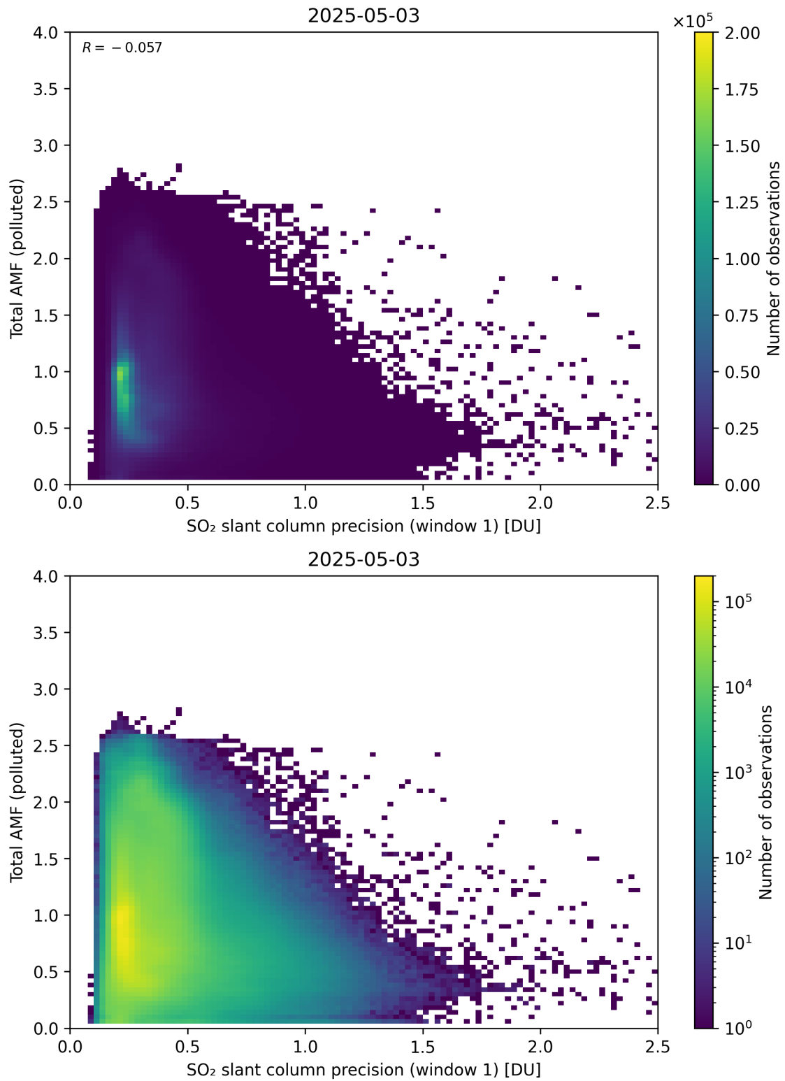
Figure 280: Scatter density plot of “SO 2 slant column precision (window 1)” against “Total AMF (polluted)” for 2025-05-02 to 2025-05-04.
