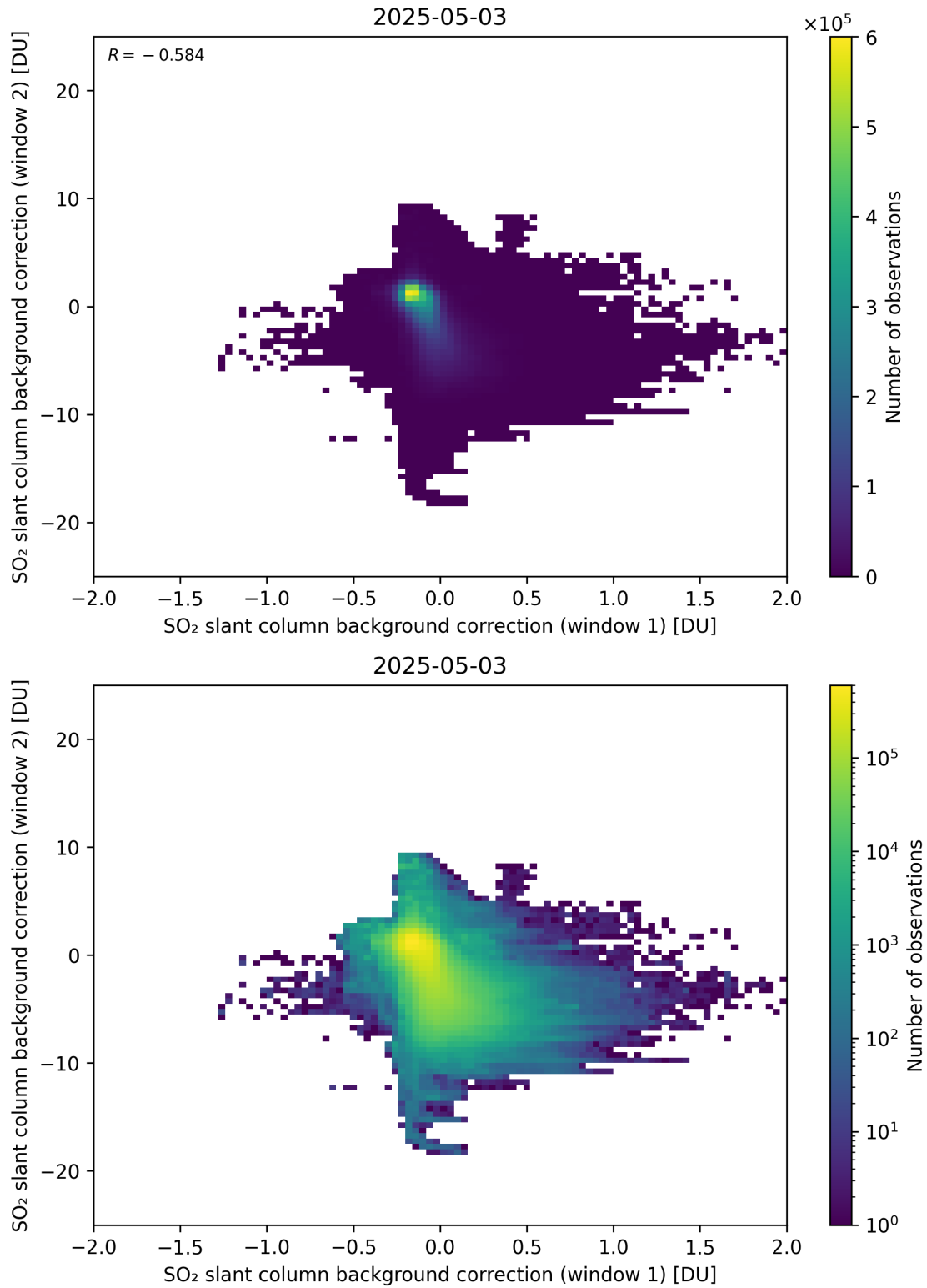
Figure 109: Scatter density plot of “SO 2 slant column background correction (window 1)” against “SO 2 slant column background correction (window 2)” for 2025-05-02 to 2025-05-04.
