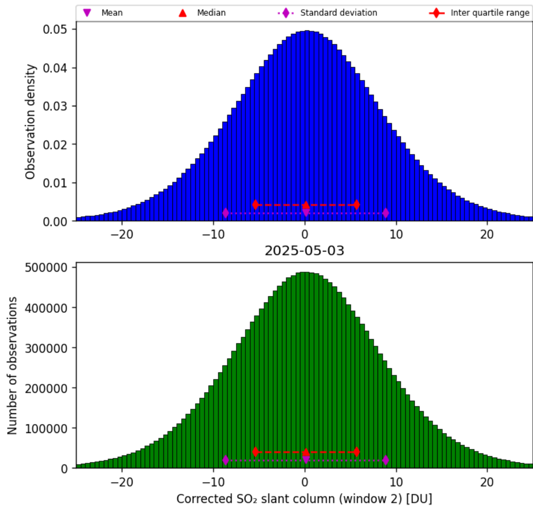
Figure 69: Histogram of “Corrected SO 2 slant column (window 2)” for 2025-05-02 to 2025-05-04
