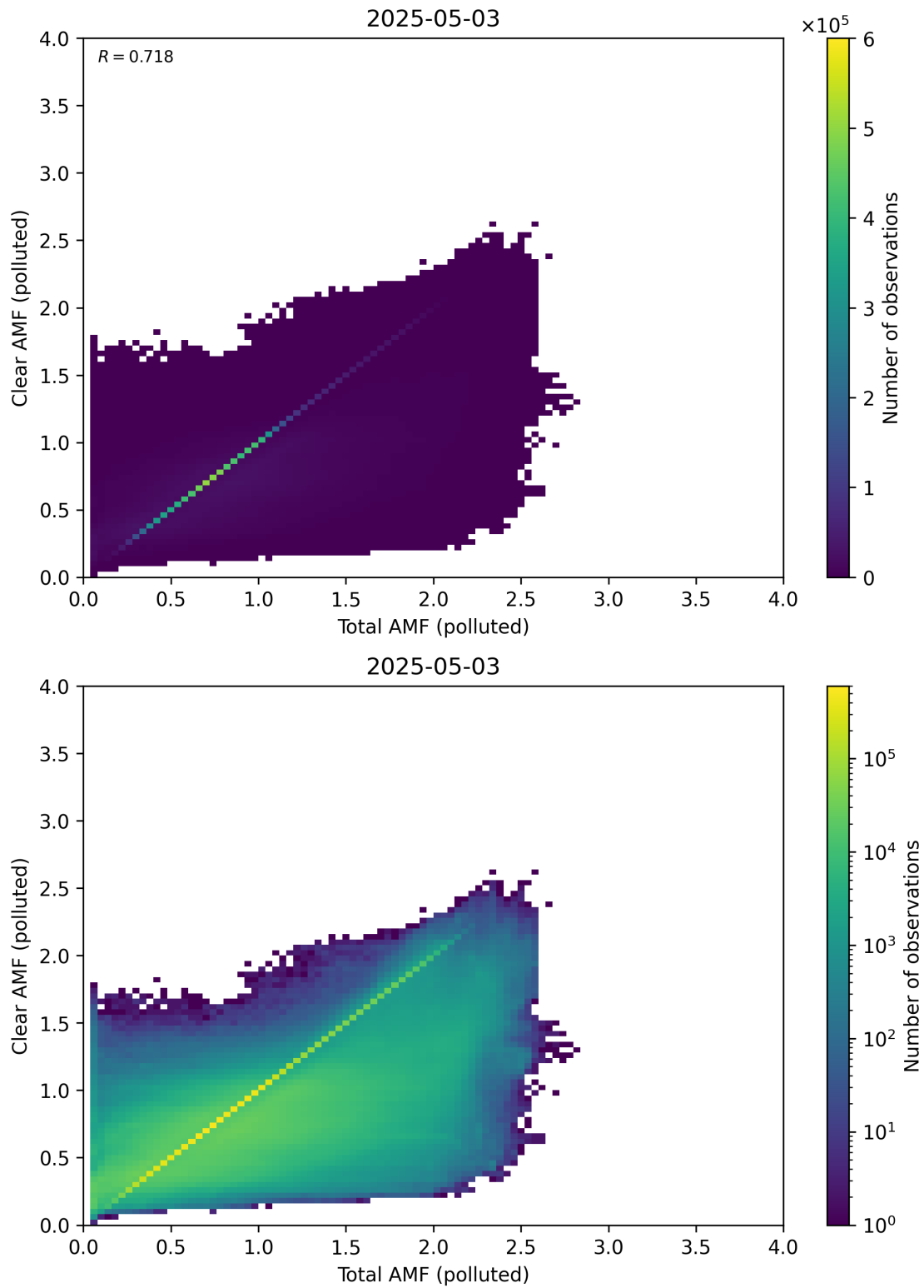
Figure 321: Scatter density plot of “Total AMF (polluted)” against “Clear AMF (polluted)” for 2025-05-02 to 2025-05-04.
