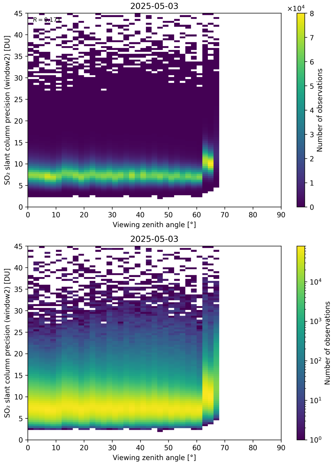
Figure 378: Scatter density plot of “Viewing zenith angle” against “SO 2 slant column precision (window2)” for 2025-05-02 to 2025-05-04.
