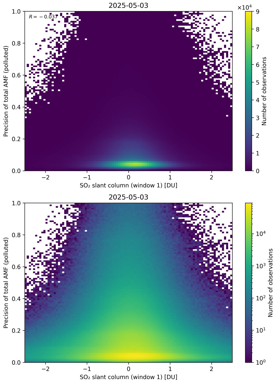
Figure 290: Scatter density plot of “SO 2 slant column (window 1)” against “Precision of total AMF (polluted)” for 2025-05-02 to 2025-05-04.
