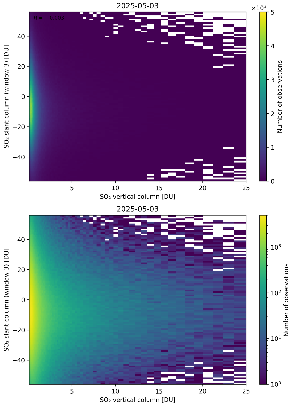
Figure 357: Scatter density plot of “SO 2 vertical column” against “SO 2 slant column (window 3)” for 2025-05-02 to 2025-05-04.
