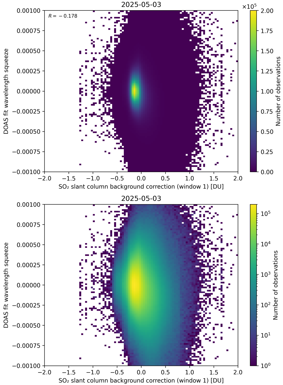
Figure 112: Scatter density plot of “SO 2 slant column background correction (window 1)” against “DOAS fit wavelength squeeze” for 2025-05-02 to 2025-05-04.
