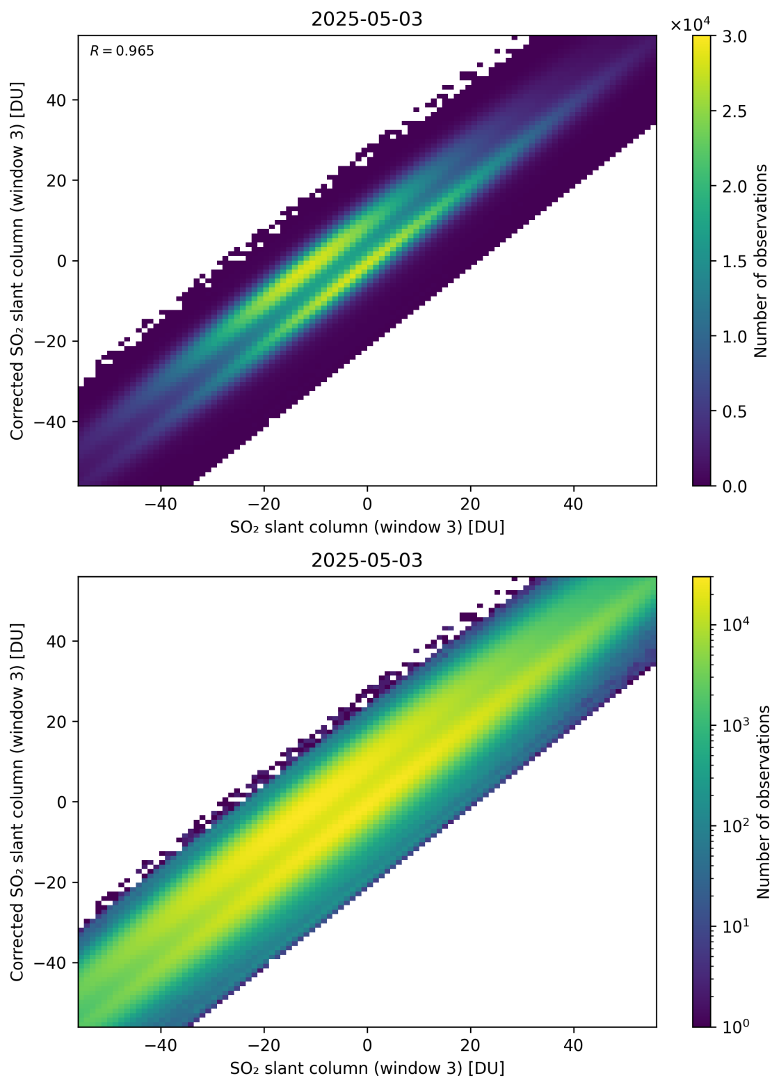
Figure 316: Scatter density plot of “SO 2 slant column (window 3)” against “Corrected SO 2 slant column (window 3)” for 2025-05-02 to 2025-05-04.
