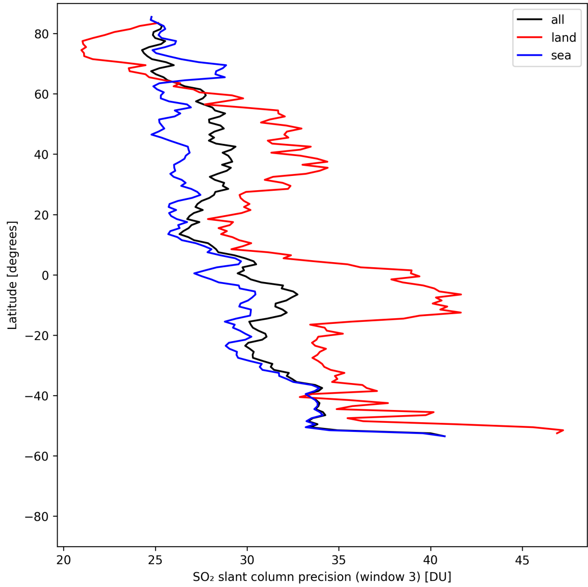
Figure 46: Zonal average of “SO 2 slant column precision (window 3)” for 2025-05-02 to 2025-05-04.
