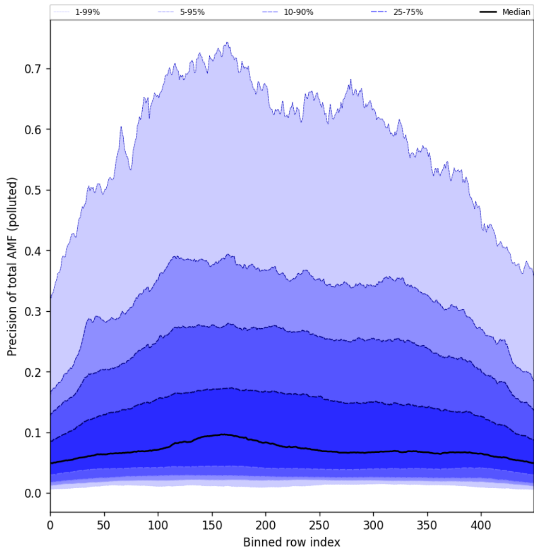
Figure 106: Along track statistics of “Precision of total AMF (polluted)” for 2025-05-02 to 2025-05-04
