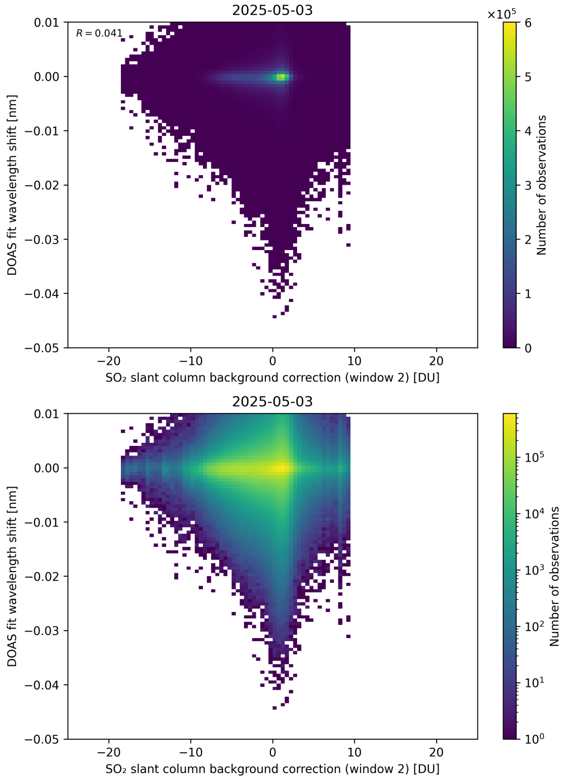
Figure 123: Scatter density plot of “SO 2 slant column background correction (window 2)” against “DOAS fit wavelength shift” for 2025-05-02 to 2025-05-04.
