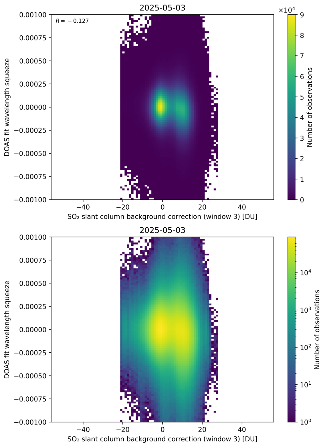
Figure 133: Scatter density plot of “SO 2 slant column background correction (window 3)” against “DOAS fit wavelength squeeze” for 2025-05-02 to 2025-05-04.
