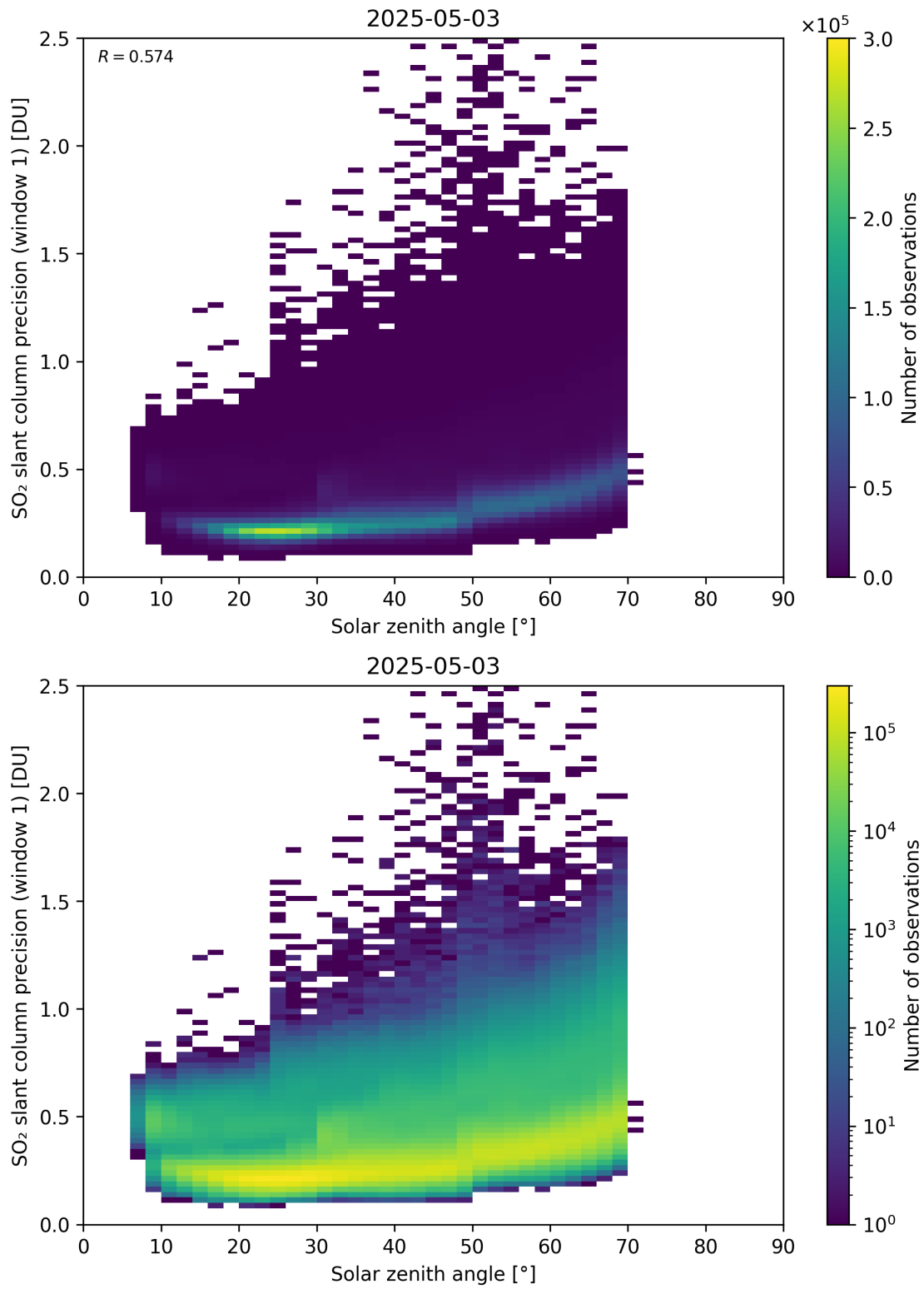
Figure 185: Scatter density plot of “Solar zenith angle” against “SO 2 slant column precision (window 1)” for 2025-05-02 to 2025-05-04.
