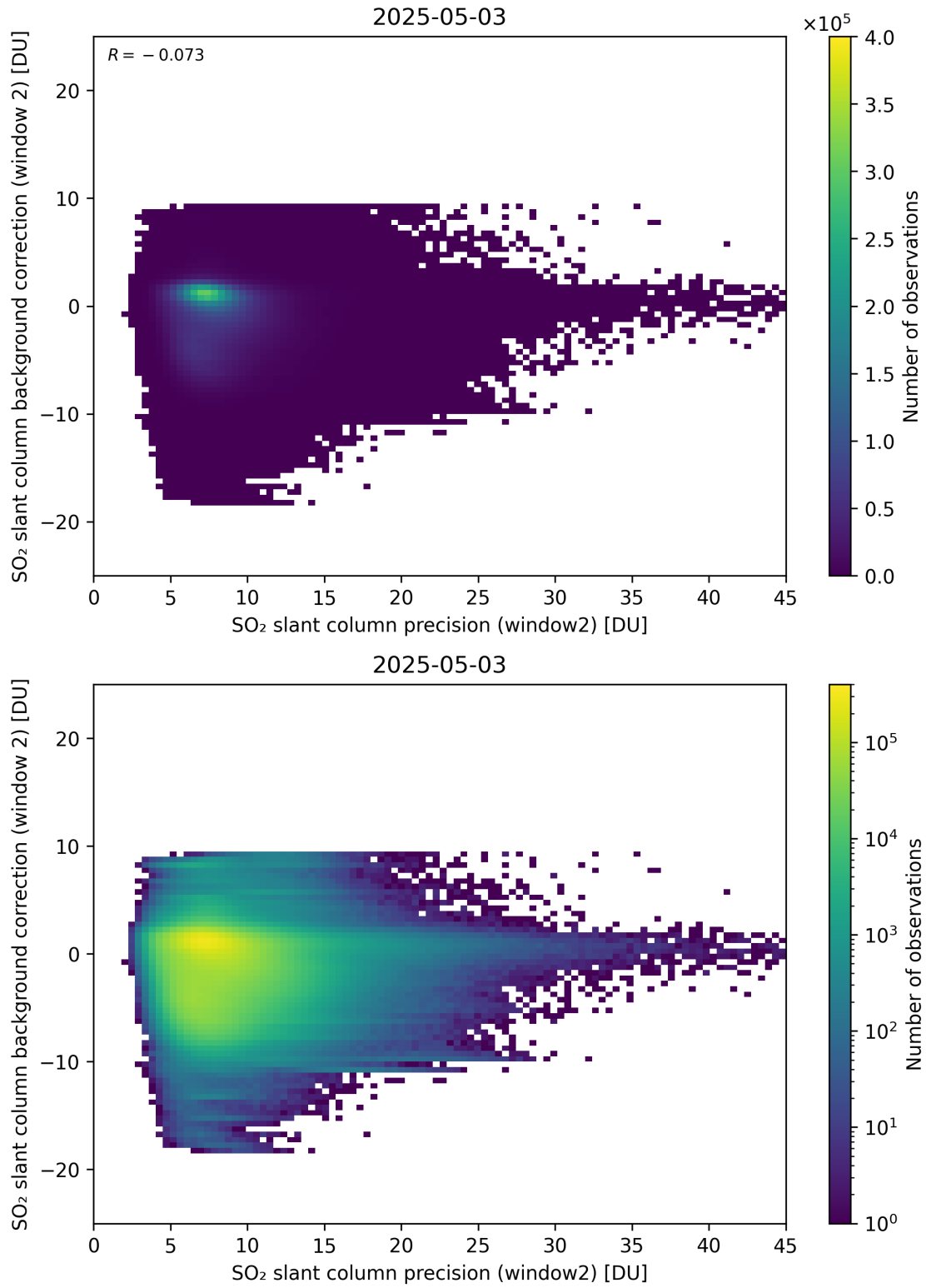
Figure 291: Scatter density plot of “SO 2 slant column precision (window2)” against “SO 2 slant column background correction (window 2)” for 2025-05-02 to 2025-05-04.
