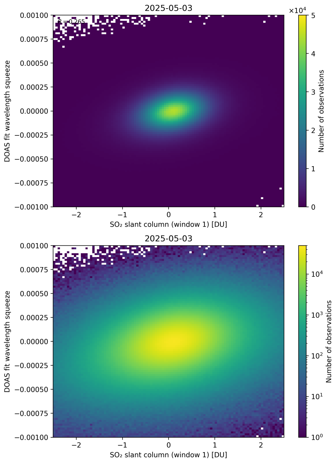
Figure 266: Scatter density plot of “SO 2 slant column (window 1)” against “DOAS fit wavelength squeeze” for 2025-05-02 to 2025-05-04.
