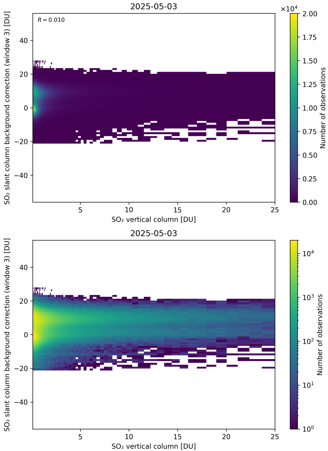
Figure 325: Scatter density plot of “SO 2 vertical column” against “SO 2 slant column background correction (window 3)” for 2025-05-02 to 2025-05-04.
