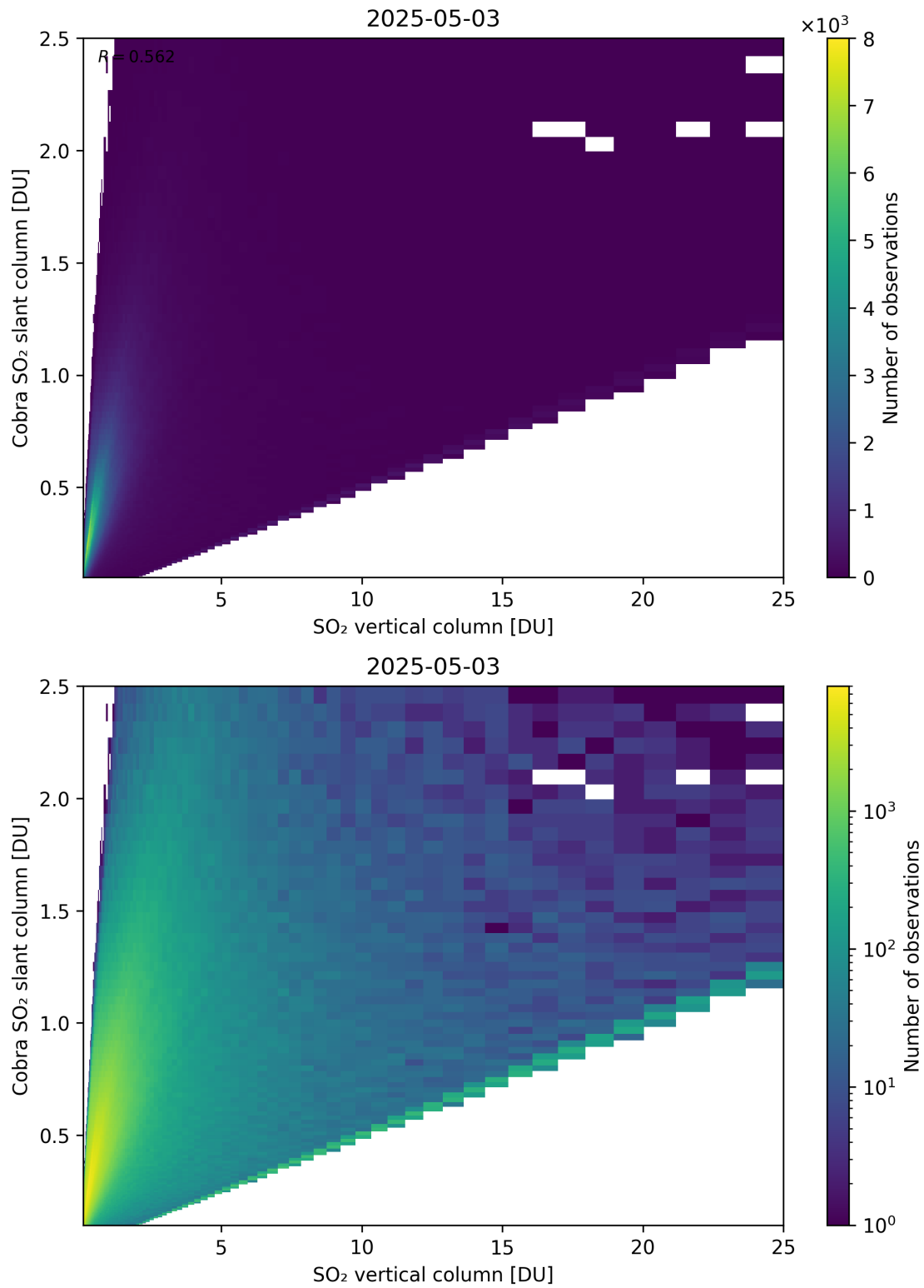
Figure 349: Scatter density plot of “SO 2 vertical column” against “Cobra SO 2 slant column” for 2025-05-02 to 2025-05-04.
