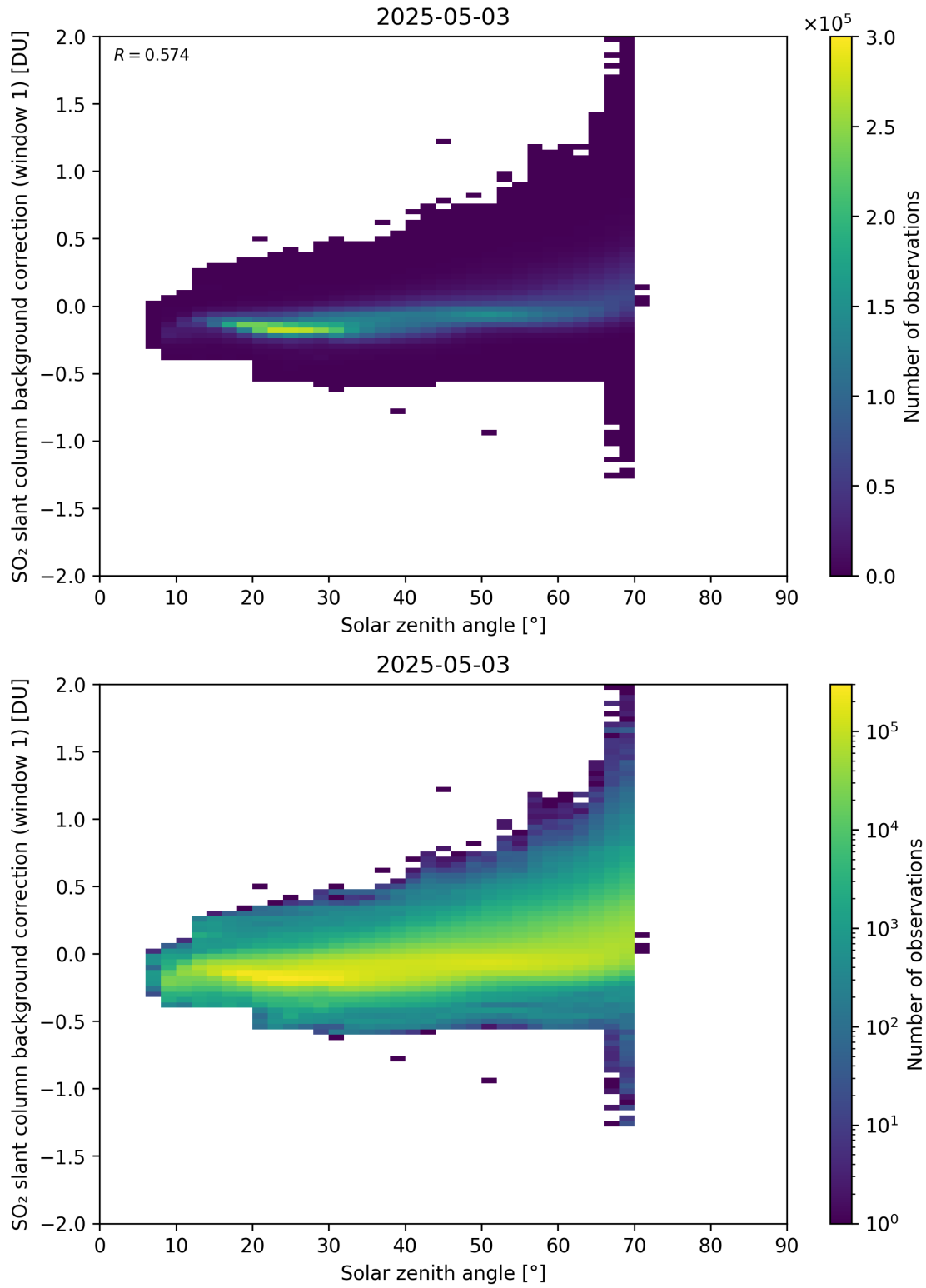
Figure 171: Scatter density plot of “Solar zenith angle” against “SO 2 slant column background correction (window 1)” for 2025-05-02 to 2025-05-04.
