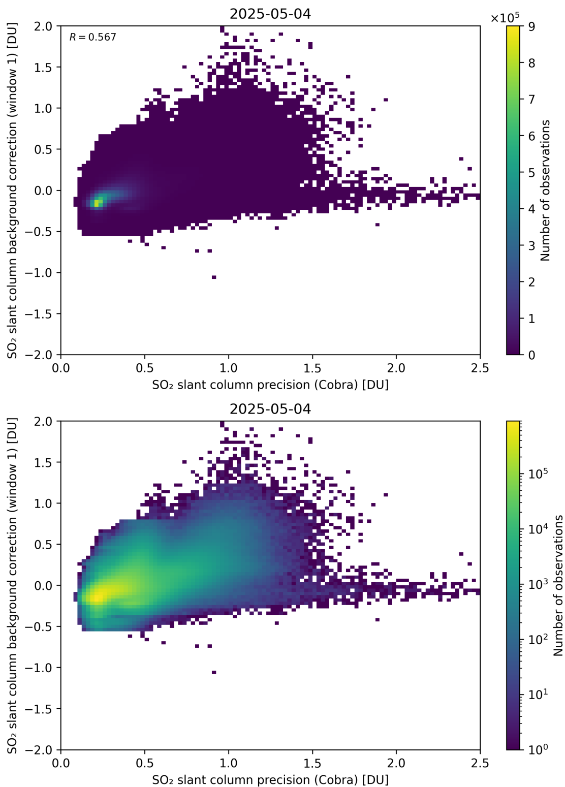
Figure 199: Scatter density plot of “SO 2 slant column precision (Cobra)” against “SO 2 slant column background correction (window 1)” for 2025-05-03 to 2025-05-05.
