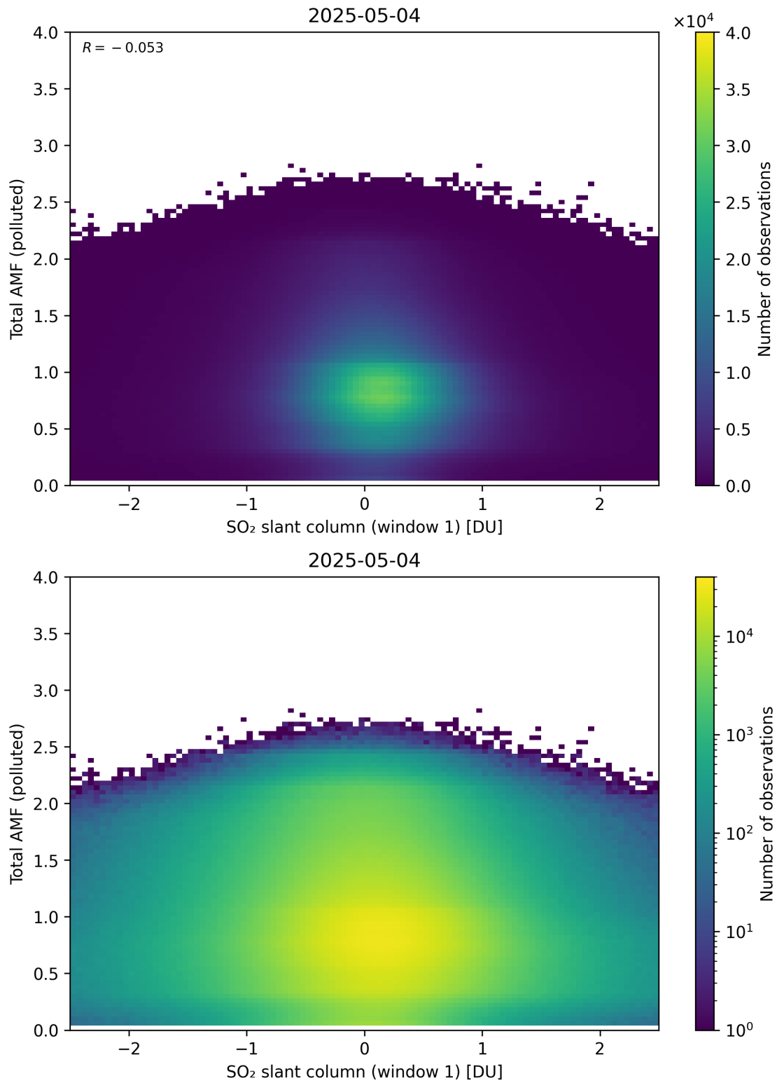
Figure 289: Scatter density plot of “SO 2 slant column (window 1)” against “Total AMF (polluted)” for 2025-05-03 to 2025-05-05.
