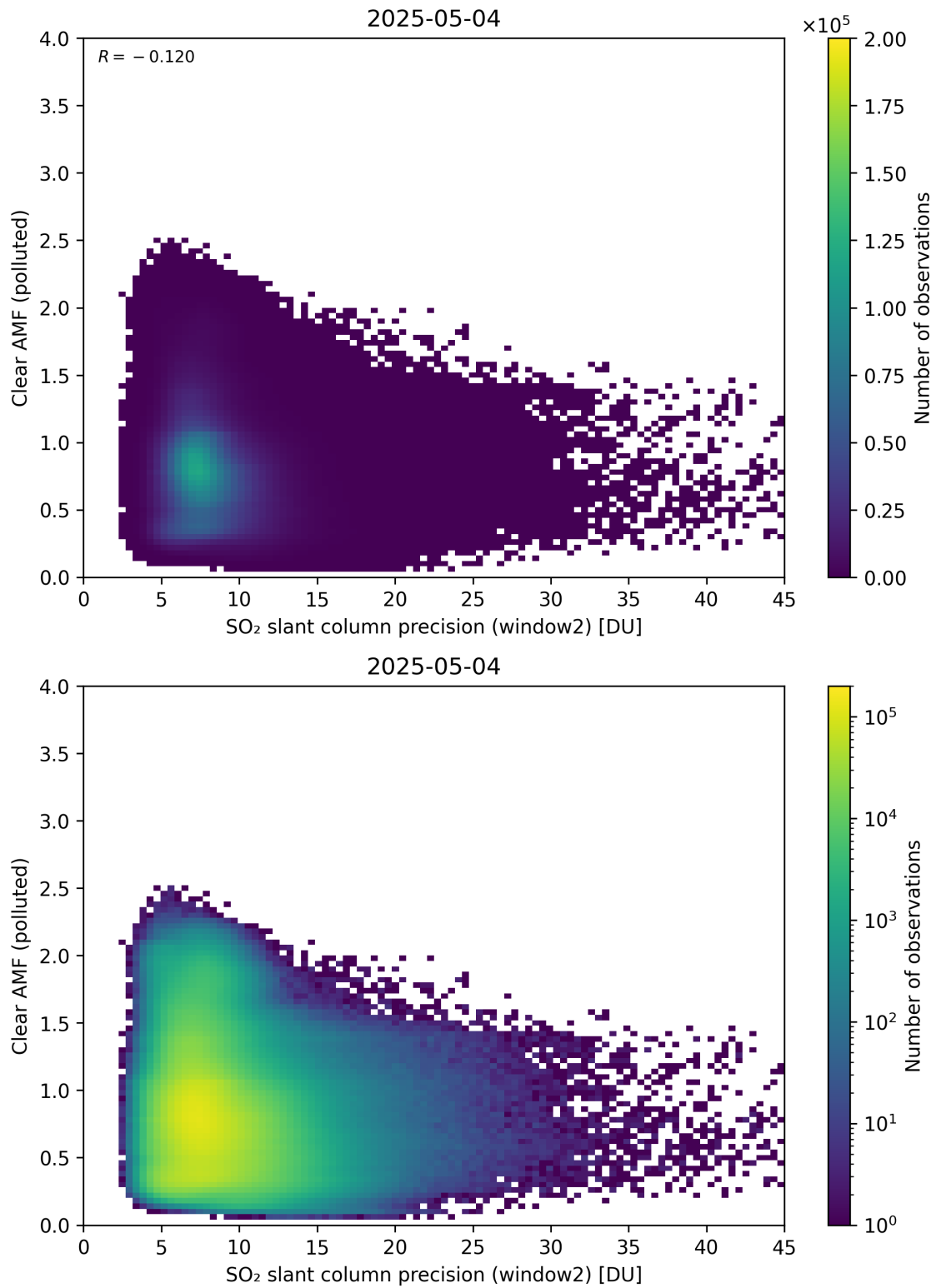
Figure 296: Scatter density plot of “SO 2 slant column precision (window2)” against “Clear AMF (polluted)” for 2025-05-03 to 2025-05-05.
