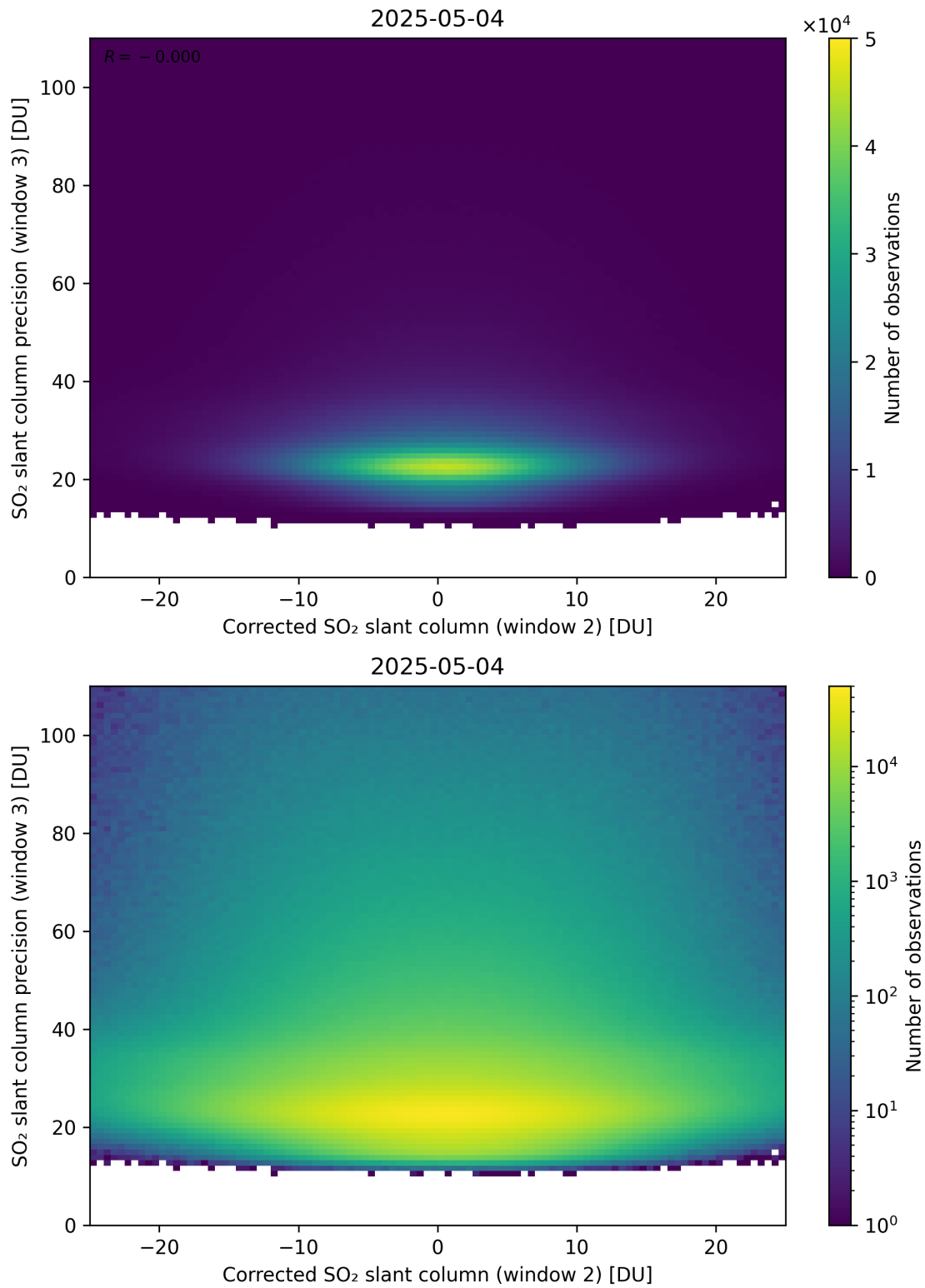
Figure 252: Scatter density plot of “Corrected SO 2 slant column (window 2)” against “SO 2 slant column precision (window 3)” for 2025-05-03 to 2025-05-05.
