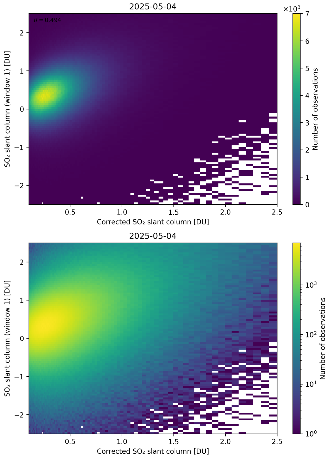
Figure 237: Scatter density plot of “Corrected SO 2 slant column” against “SO 2 slant column (window 1)” for 2025-05-03 to 2025-05-05.
