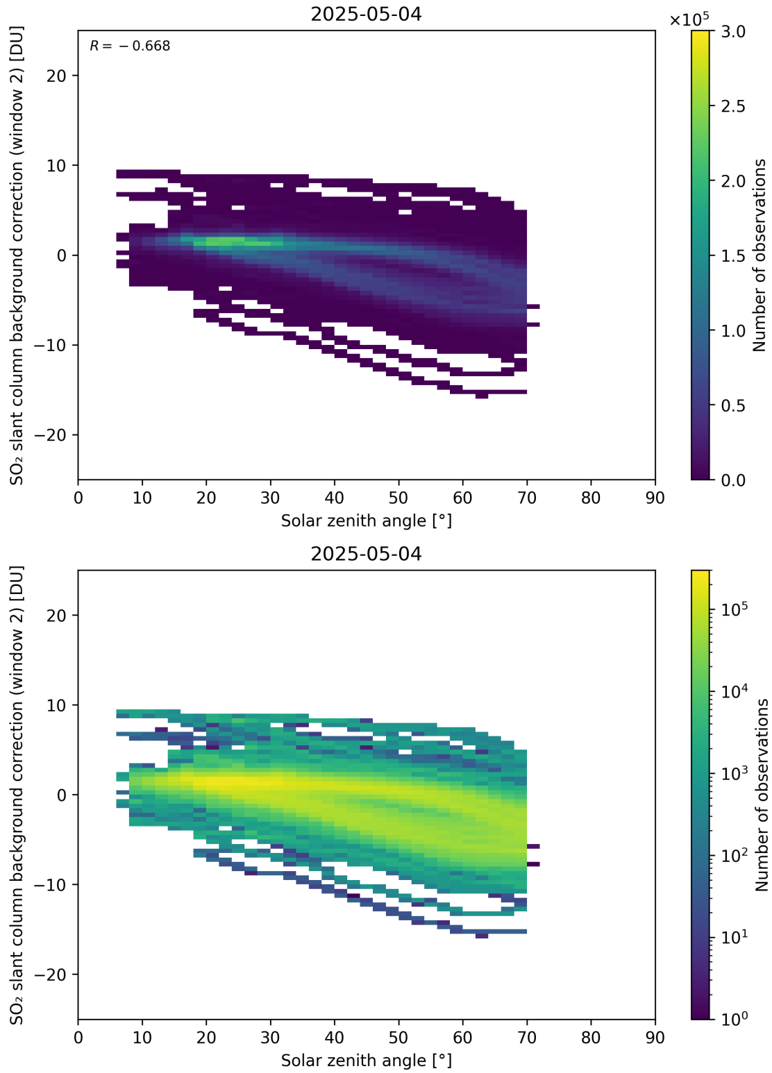
Figure 172: Scatter density plot of “Solar zenith angle” against “SO 2 slant column background correction (window 2)” for 2025-05-03 to 2025-05-05.
