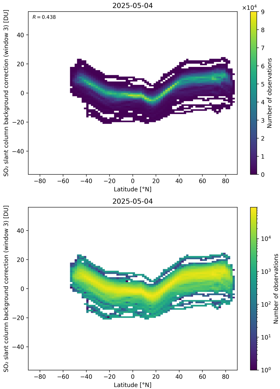
Figure 152: Scatter density plot of “Latitude” against “SO 2 slant column background correction (window 3)” for 2025-05-03 to 2025-05-05.
