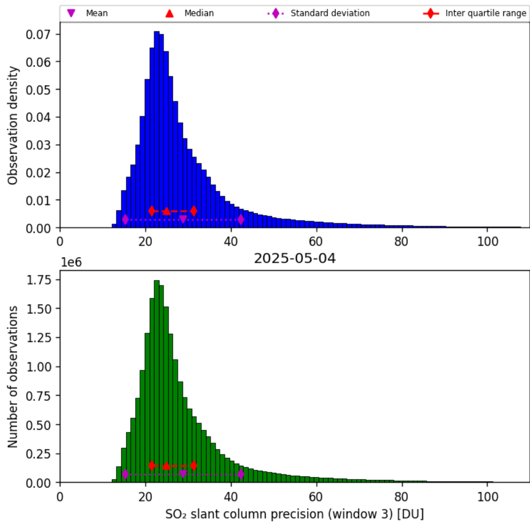
Figure 72: Histogram of “SO 2 slant column precision (window 3)” for 2025-05-03 to 2025-05-05
