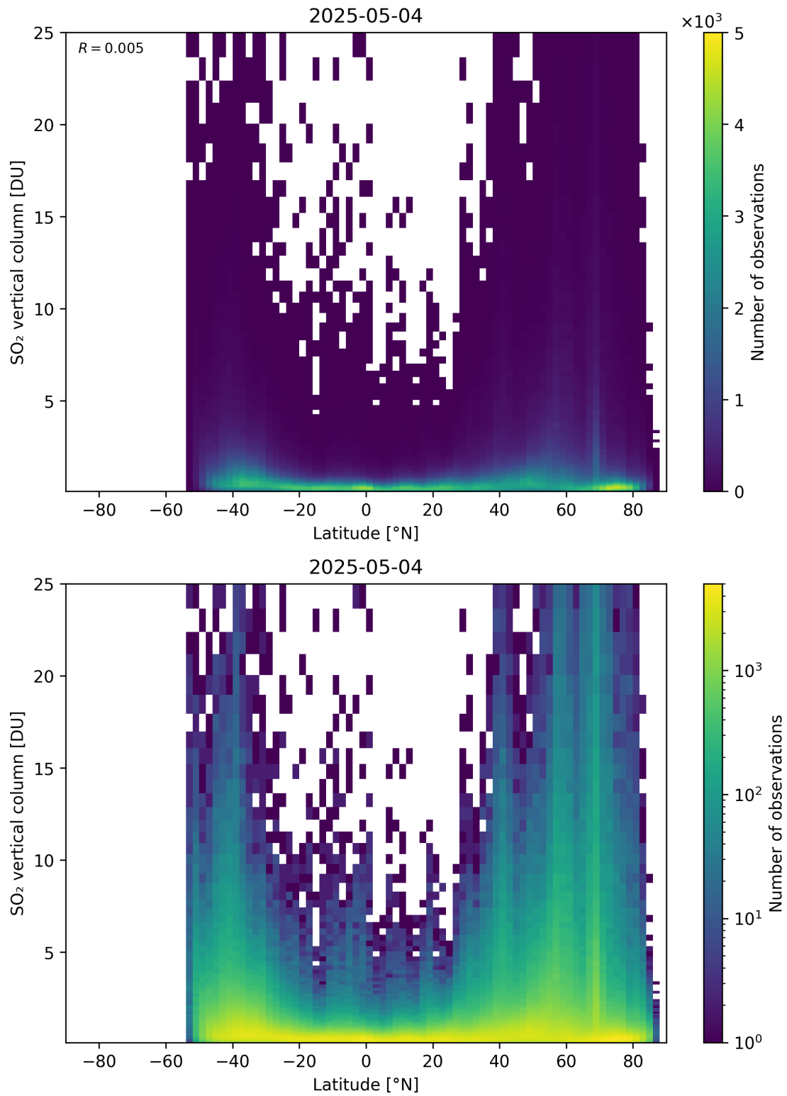
Figure 169: Scatter density plot of “Latitude” against “SO 2 vertical column” for 2025-05-03 to 2025-05-05.
