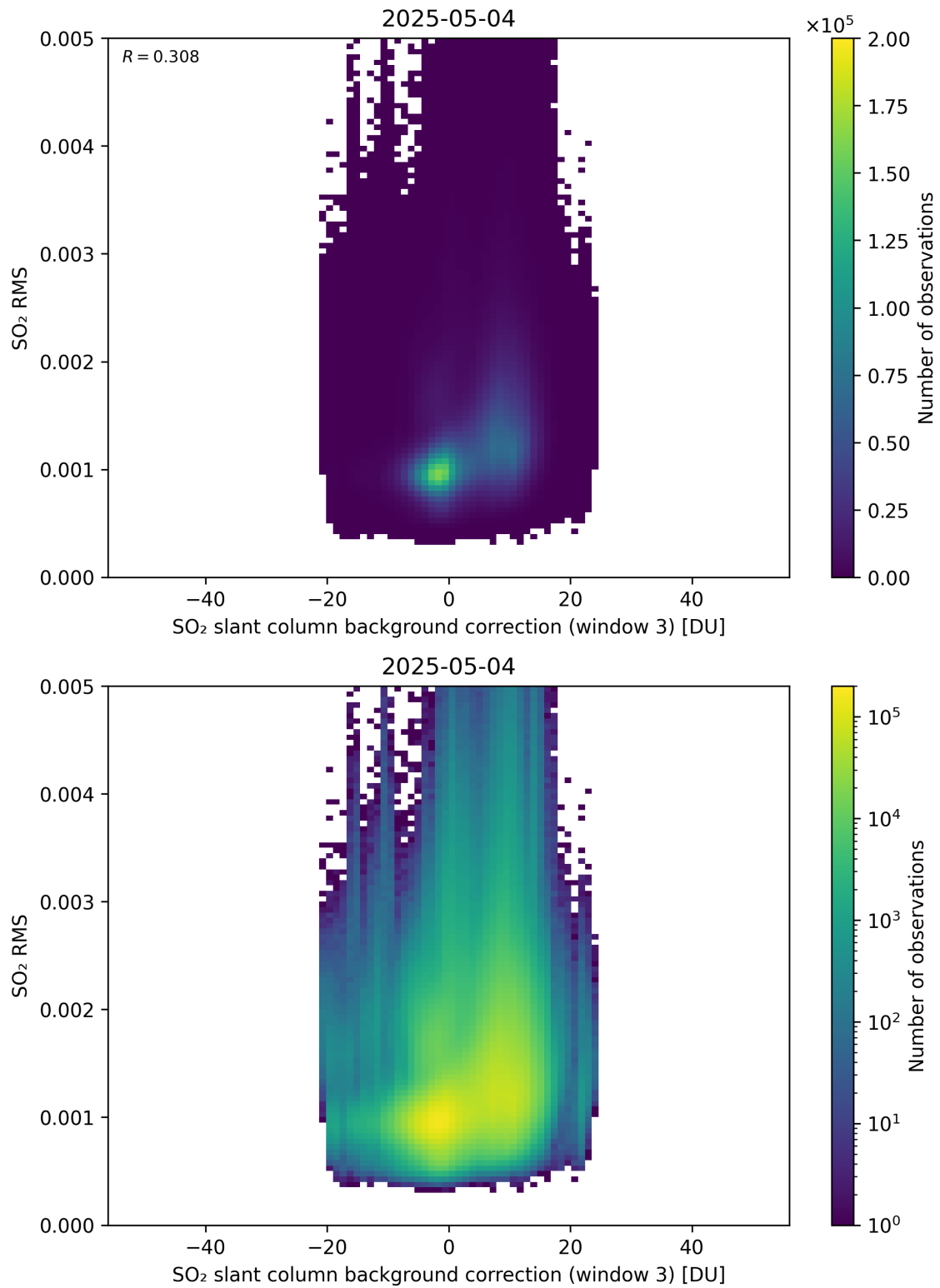
Figure 134: Scatter density plot of “SO 2 slant column background correction (window 3)” against “SO 2 RMS” for 2025-05-03 to 2025-05-05.
