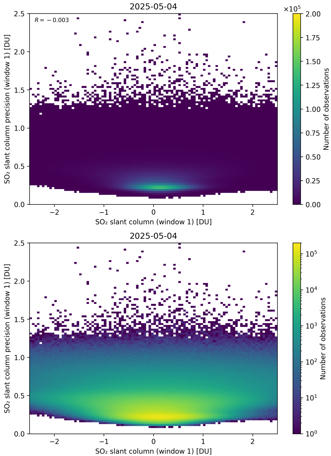
Figure 285: Scatter density plot of “SO 2 slant column (window 1)” against “SO 2 slant column precision (window 1)” for 2025-05-03 to 2025-05-05.
