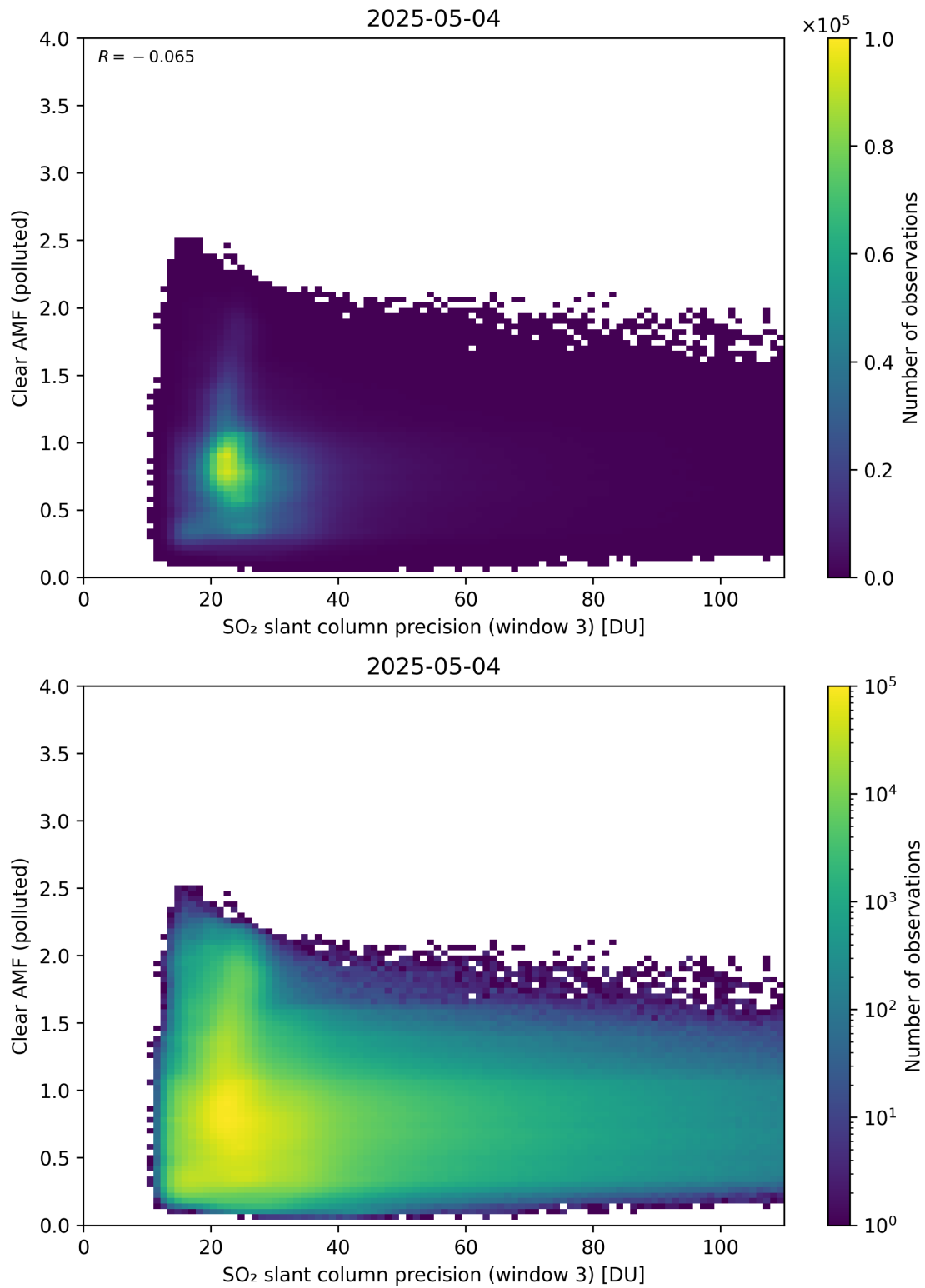
Figure 311: Scatter density plot of “SO 2 slant column precision (window 3)” against “Clear AMF (polluted)” for 2025-05-03 to 2025-05-05.
