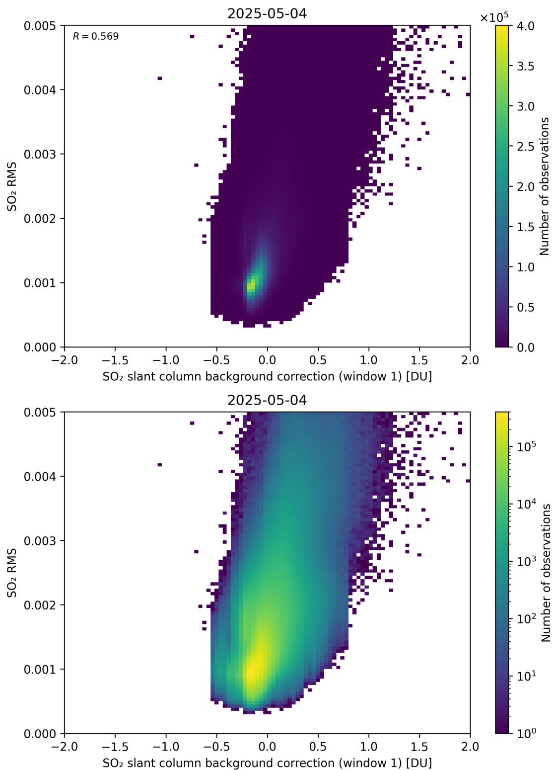
Figure 113: Scatter density plot of “SO 2 slant column background correction (window 1)” against “SO 2 RMS” for 2025-05-03 to 2025-05-05.
