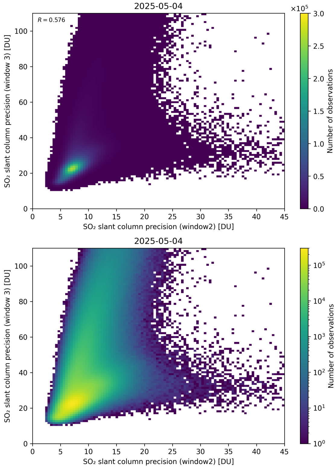
Figure 300: Scatter density plot of “SO 2 slant column precision (window2)” against “SO 2 slant column precision (window 3)” for 2025-05-03 to 2025-05-05.
