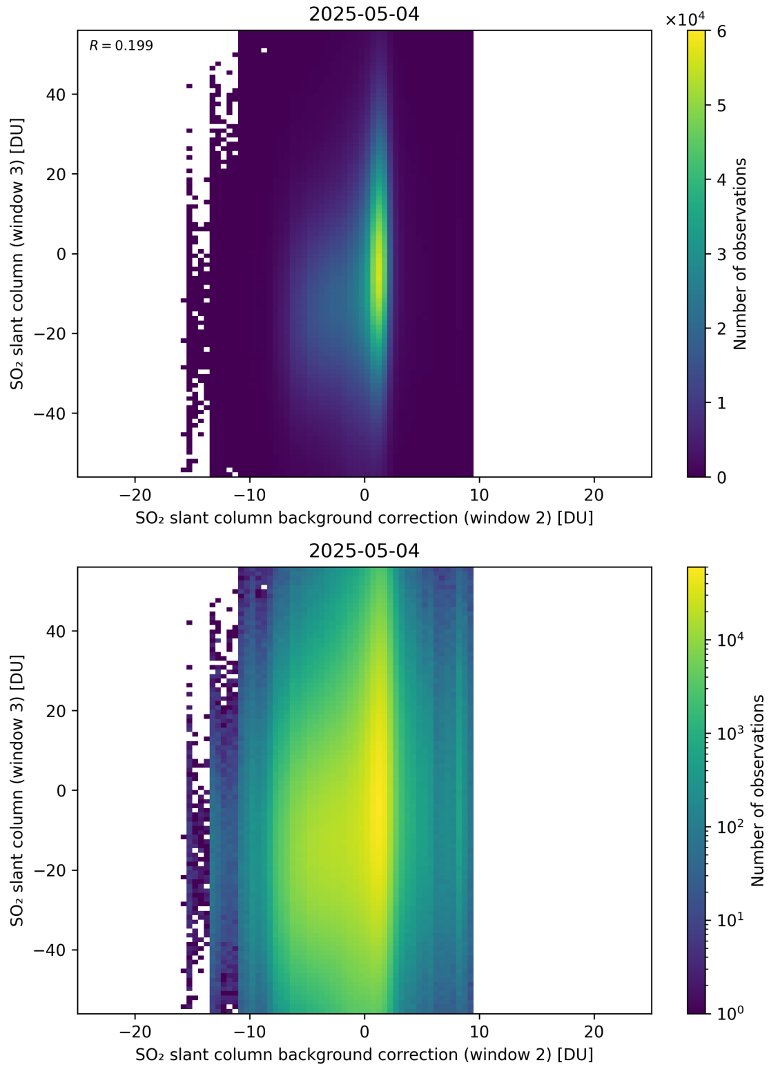
Figure 128: Scatter density plot of “SO 2 slant column background correction (window 2)” against “SO 2 slant column (window 3)” for 2025-05-03 to 2025-05-05.
