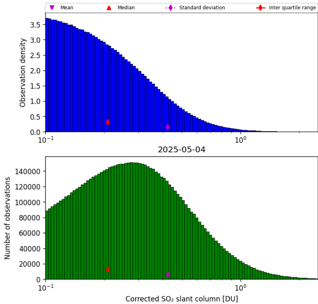
Figure 60: Histogram of “Corrected SO 2 slant column” for 2025-05-03 to 2025-05-05
