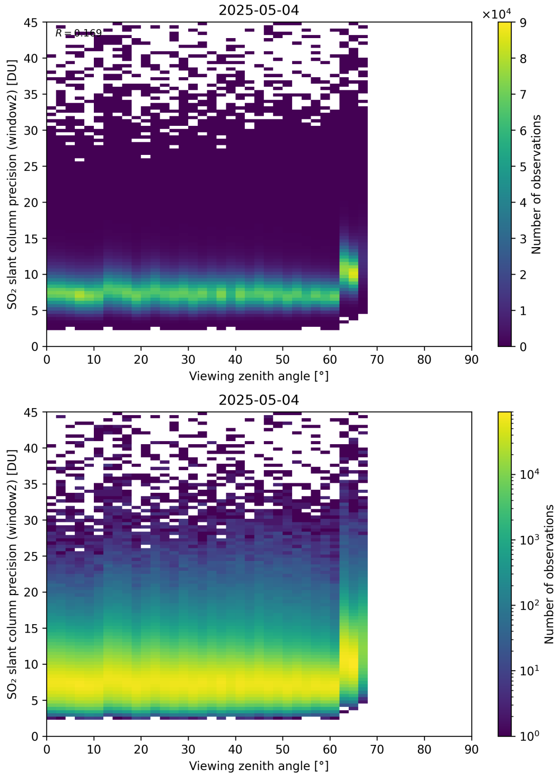
Figure 378: Scatter density plot of “Viewing zenith angle” against “SO 2 slant column precision (window2)” for 2025-05-03 to 2025-05-05.
