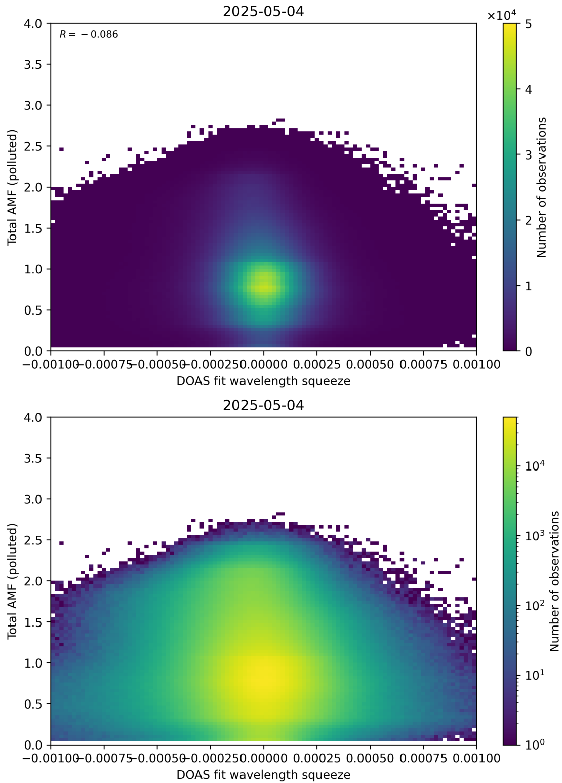
Figure 145: Scatter density plot of “DOAS fit wavelength squeeze” against “Total AMF (polluted)” for 2025-05-03 to 2025-05-05.
