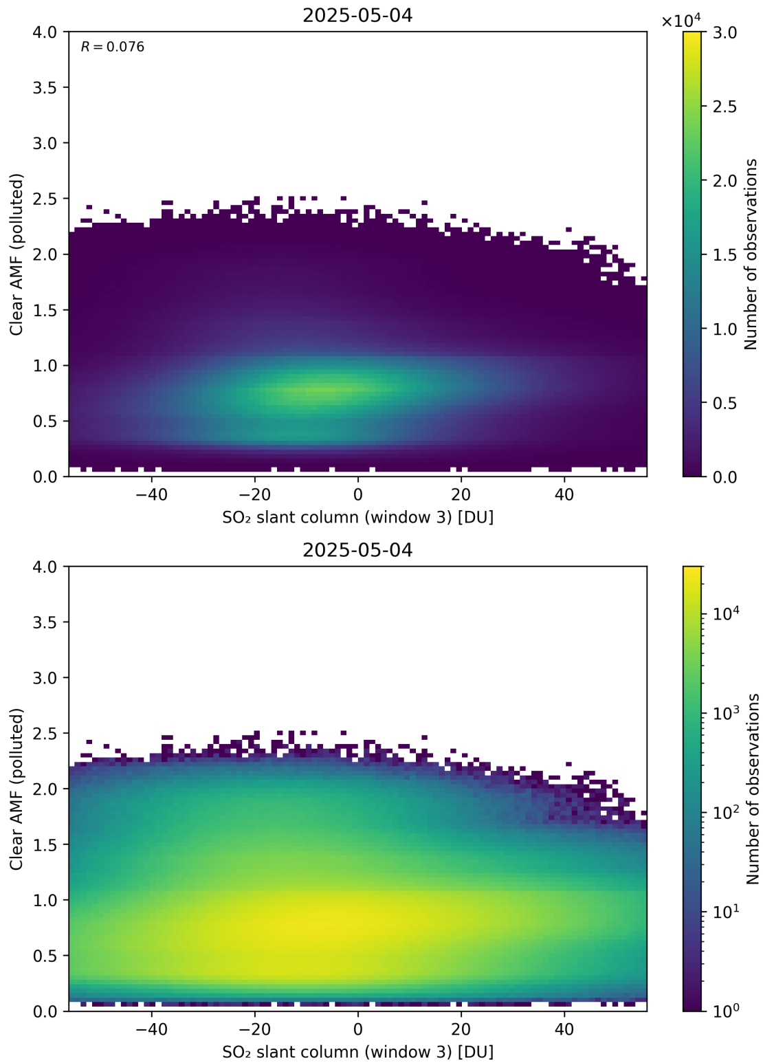
Figure 315: Scatter density plot of “SO 2 slant column (window 3)” against “Clear AMF (polluted)” for 2025-05-03 to 2025-05-05.
