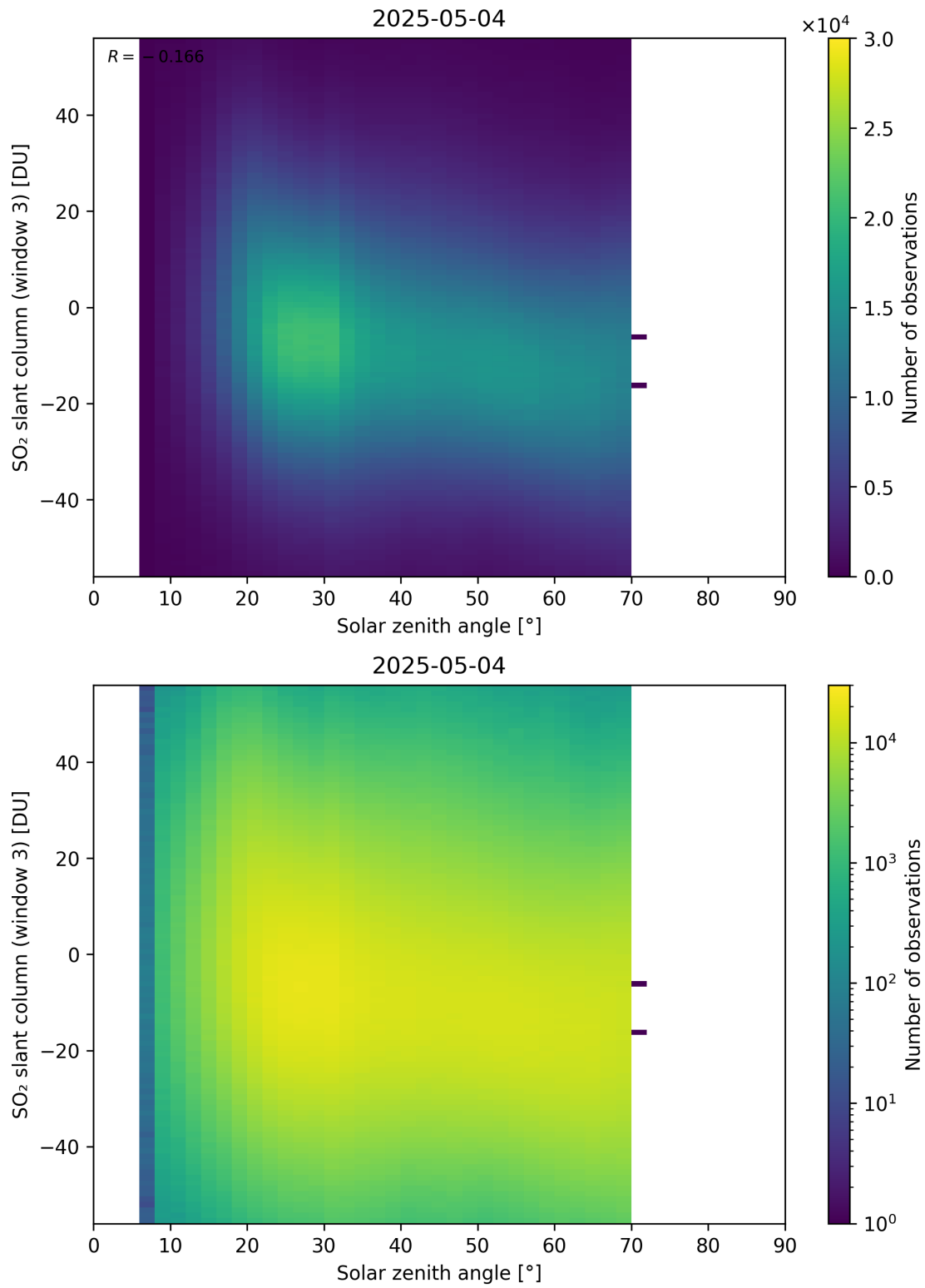
Figure 187: Scatter density plot of “Solar zenith angle” against “SO 2 slant column (window 3)” for 2025-05-03 to 2025-05-05.
