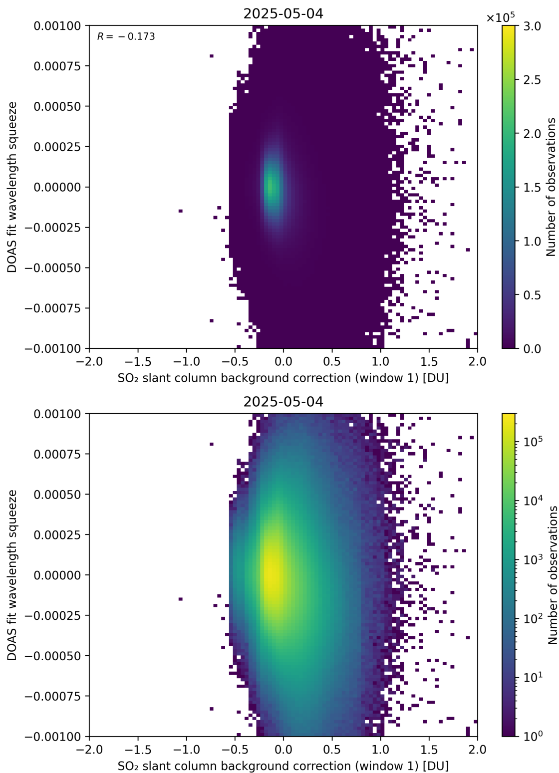
Figure 112: Scatter density plot of “SO 2 slant column background correction (window 1)” against “DOAS fit wavelength squeeze” for 2025-05-03 to 2025-05-05.
