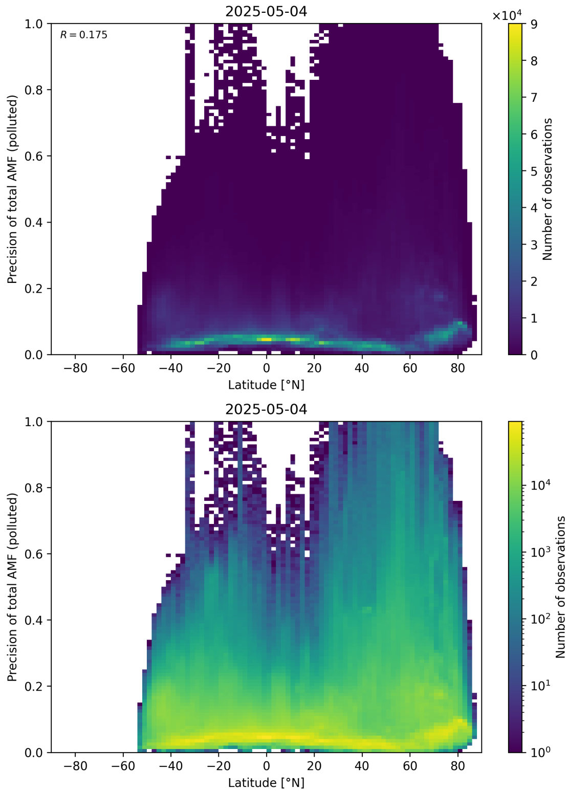
Figure 168: Scatter density plot of “Latitude” against “Precision of total AMF (polluted)” for 2025-05-03 to 2025-05-05.
