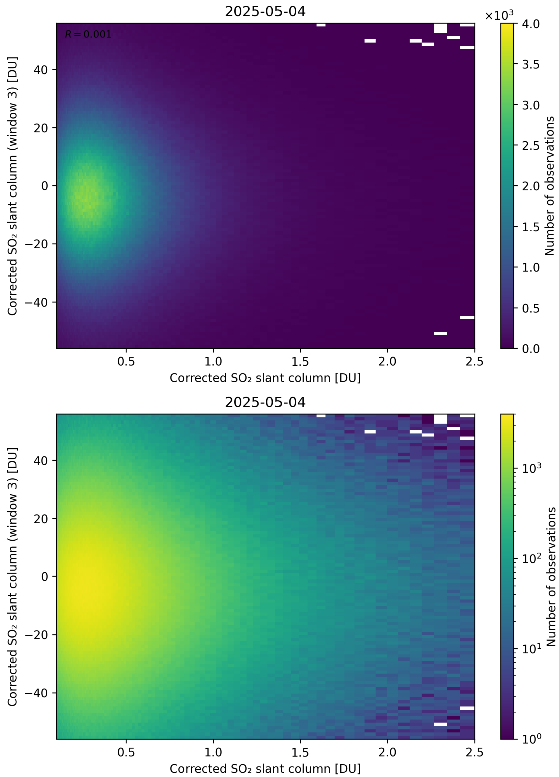
Figure 236: Scatter density plot of “Corrected SO 2 slant column” against “Corrected SO 2 slant column (window 3)” for 2025-05-03 to 2025-05-05.
