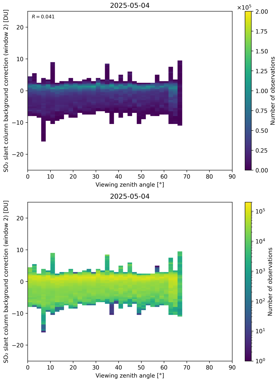
Figure 363: Scatter density plot of “Viewing zenith angle” against “SO 2 slant column background correction (window 2)” for 2025-05-03 to 2025-05-05.
