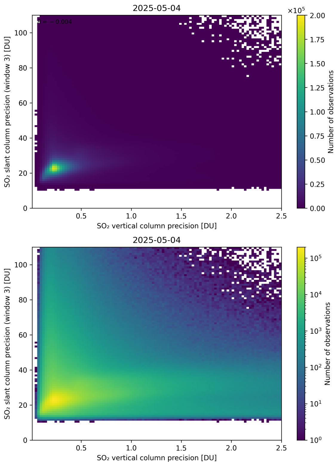
Figure 345: Scatter density plot of “SO 2 vertical column precision” against “SO 2 slant column precision (window 3)” for 2025-05-03 to 2025-05-05.
