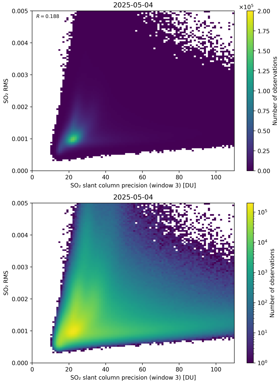
Figure 310: Scatter density plot of “SO 2 slant column precision (window 3)” against “SO 2 RMS” for 2025-05-03 to 2025-05-05.
