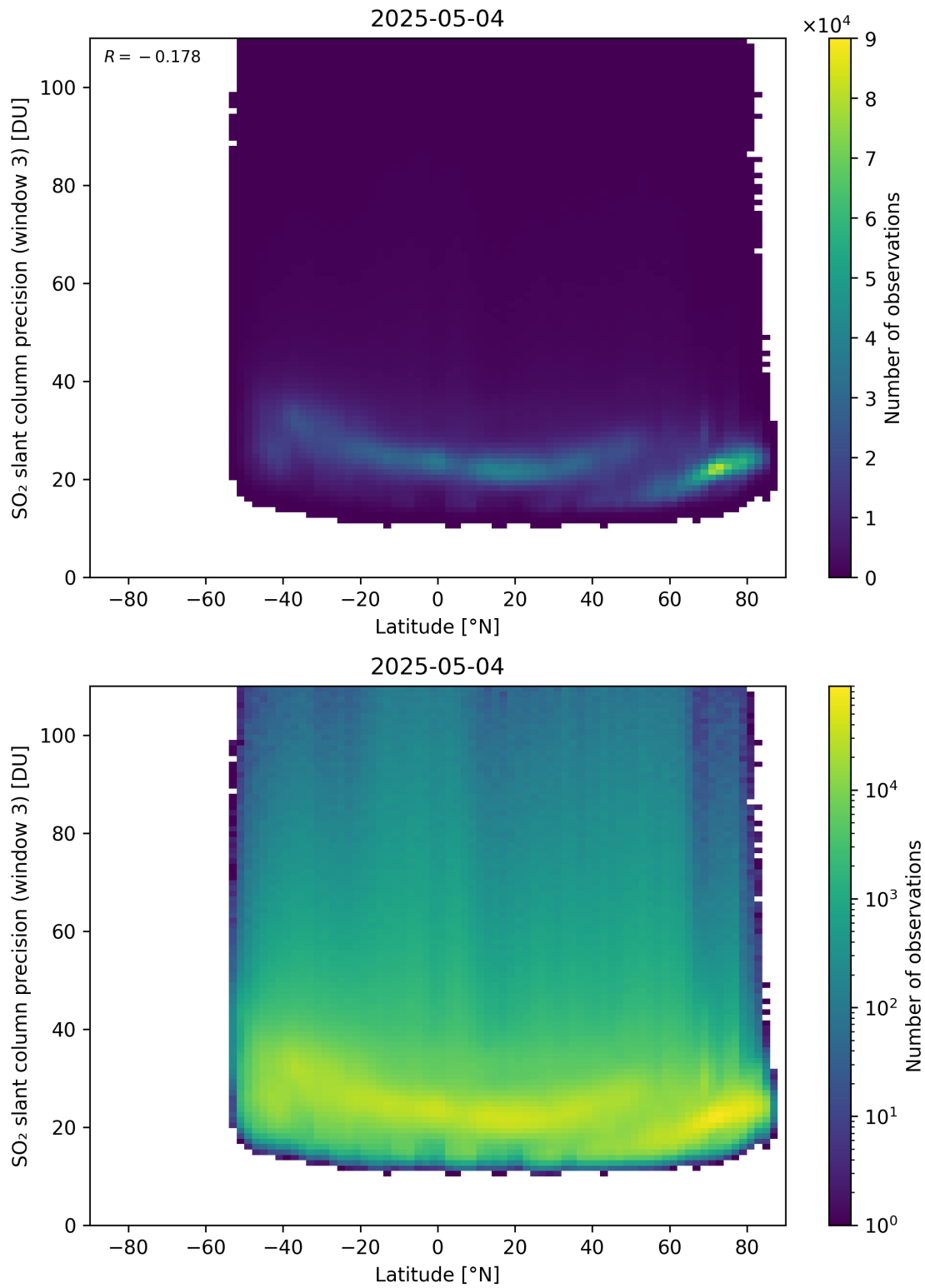
Figure 166: Scatter density plot of “Latitude” against “SO 2 slant column precision (window 3)” for 2025-05-03 to 2025-05-05.
