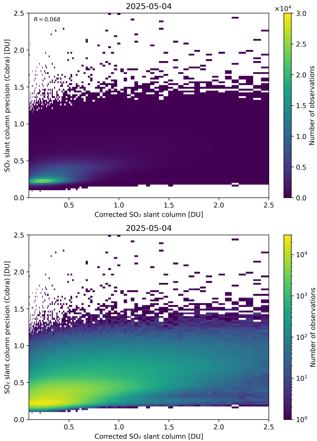
Figure 234: Scatter density plot of “Corrected SO 2 slant column” against “SO 2 slant column precision (Cobra)” for 2025-05-03 to 2025-05-05.
