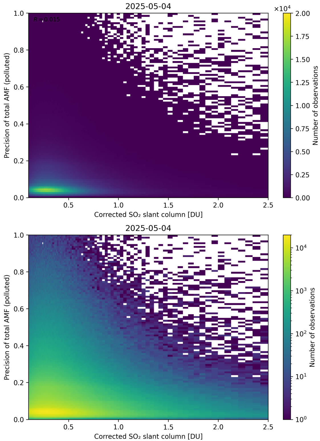
Figure 243: Scatter density plot of “Corrected SO 2 slant column” against “Precision of total AMF (polluted)” for 2025-05-03 to 2025-05-05.
