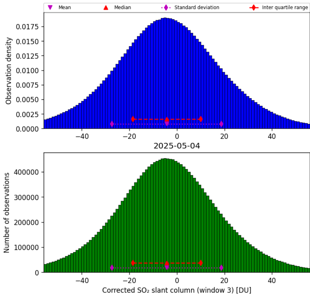
Figure 73: Histogram of “Corrected SO 2 slant column (window 3)” for 2025-05-03 to 2025-05-05
