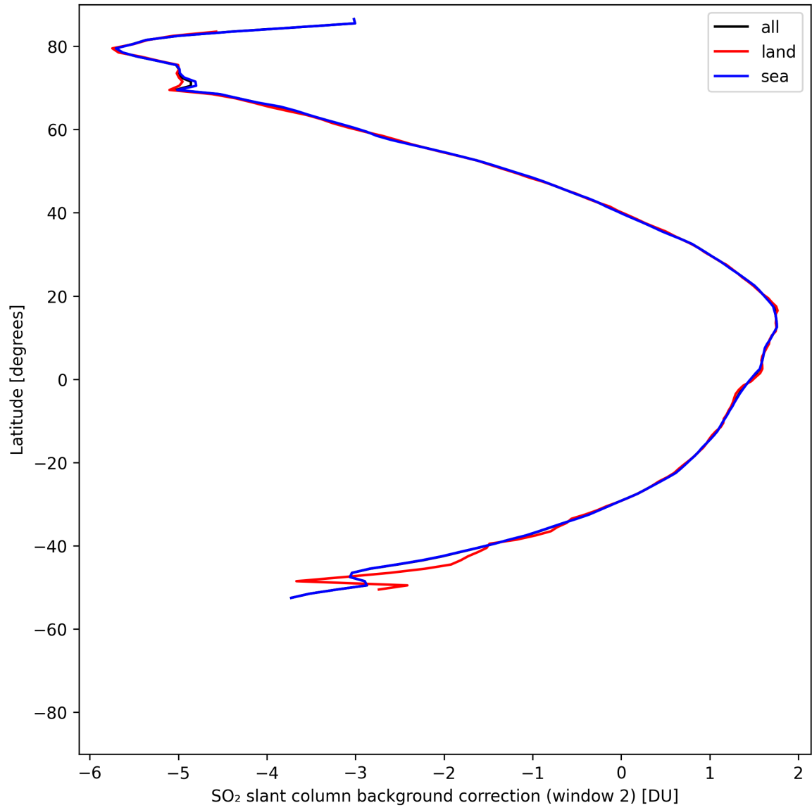
Figure 44: Zonal average of “SO 2 slant column background correction (window 2)” for 2025-05-03 to 2025-05-05.
