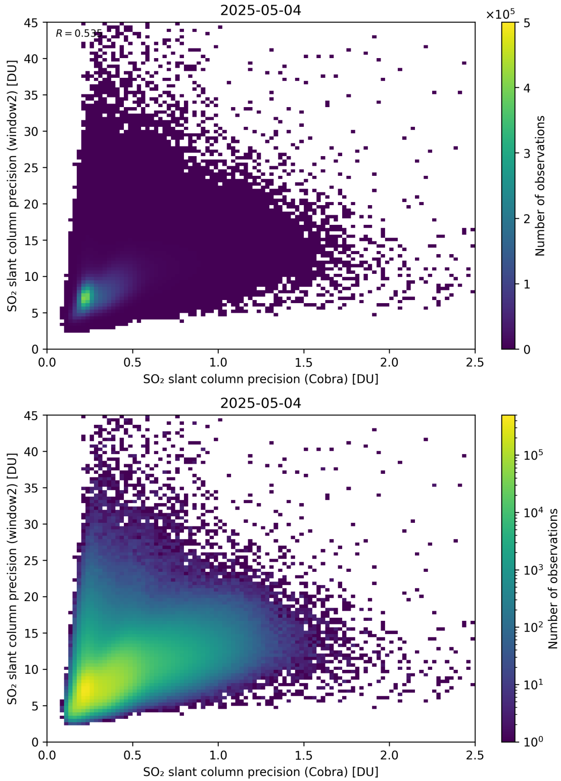
Figure 210: Scatter density plot of “SO 2 slant column precision (Cobra)” against “SO 2 slant column precision (window2)” for 2025-05-03 to 2025-05-05.
