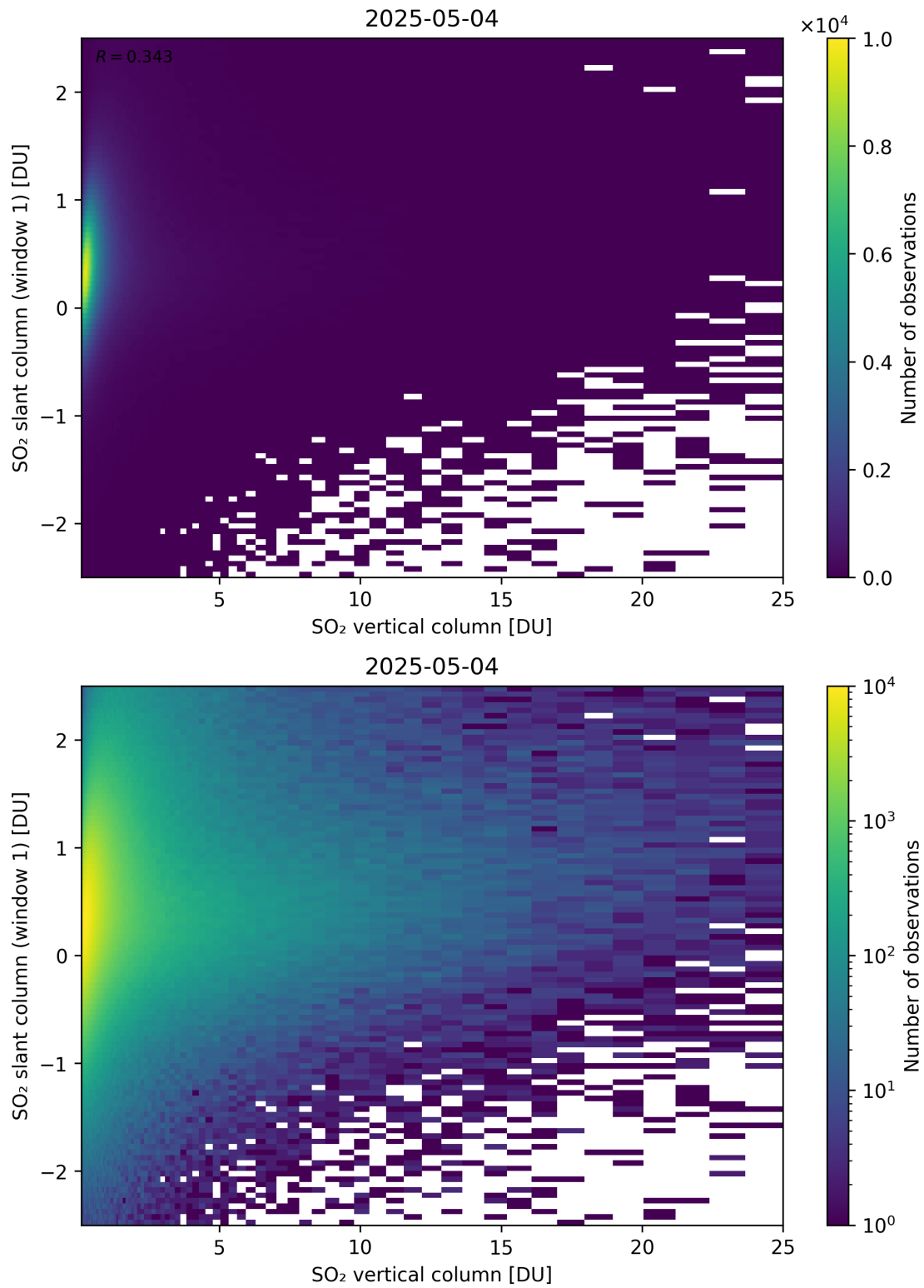
Figure 354: Scatter density plot of “SO 2 vertical column” against “SO 2 slant column (window 1)” for 2025-05-03 to 2025-05-05.
