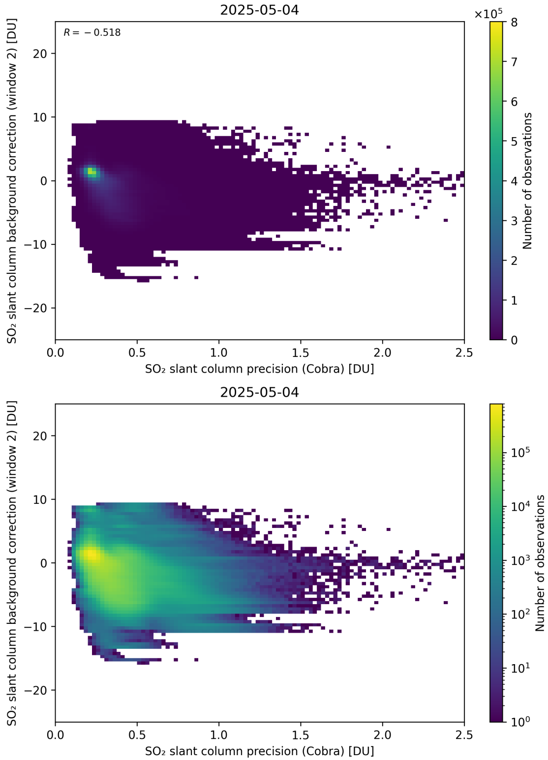
Figure 200: Scatter density plot of “SO 2 slant column precision (Cobra)” against “SO 2 slant column background correction (window 2)” for 2025-05-03 to 2025-05-05.
