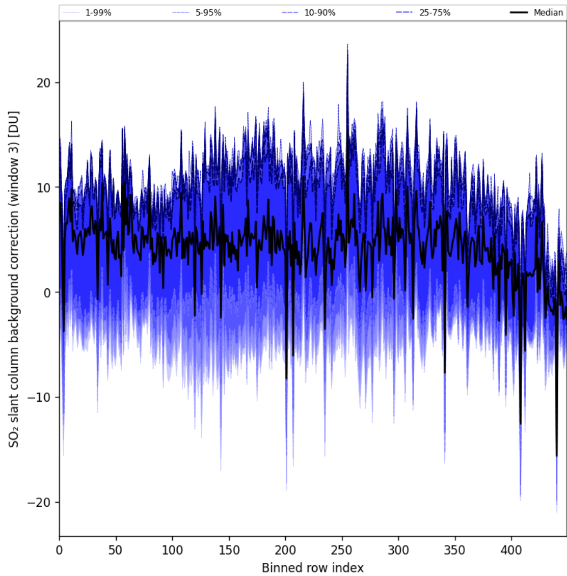
Figure 100: Along track statistics of “SO 2 slant column background correction (window 3)” for 2025-05-03 to 2025-05-05
