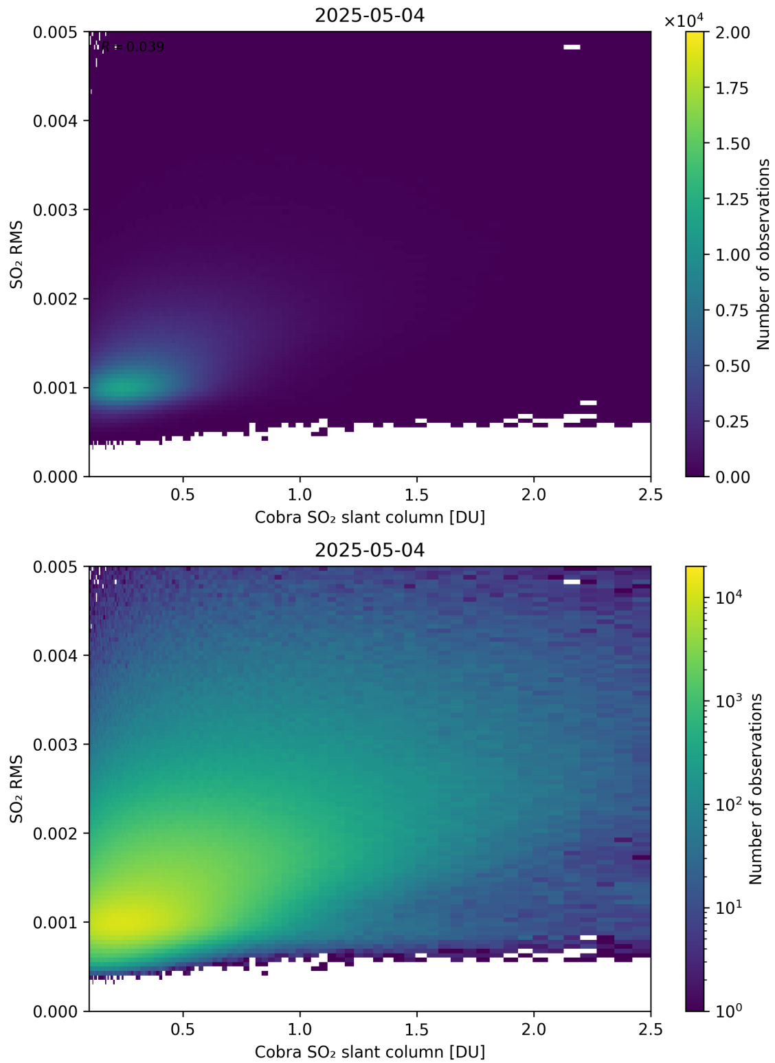
Figure 198: Scatter density plot of “Cobra SO 2 slant column” against “SO 2 RMS” for 2025-05-03 to 2025-05-05.
