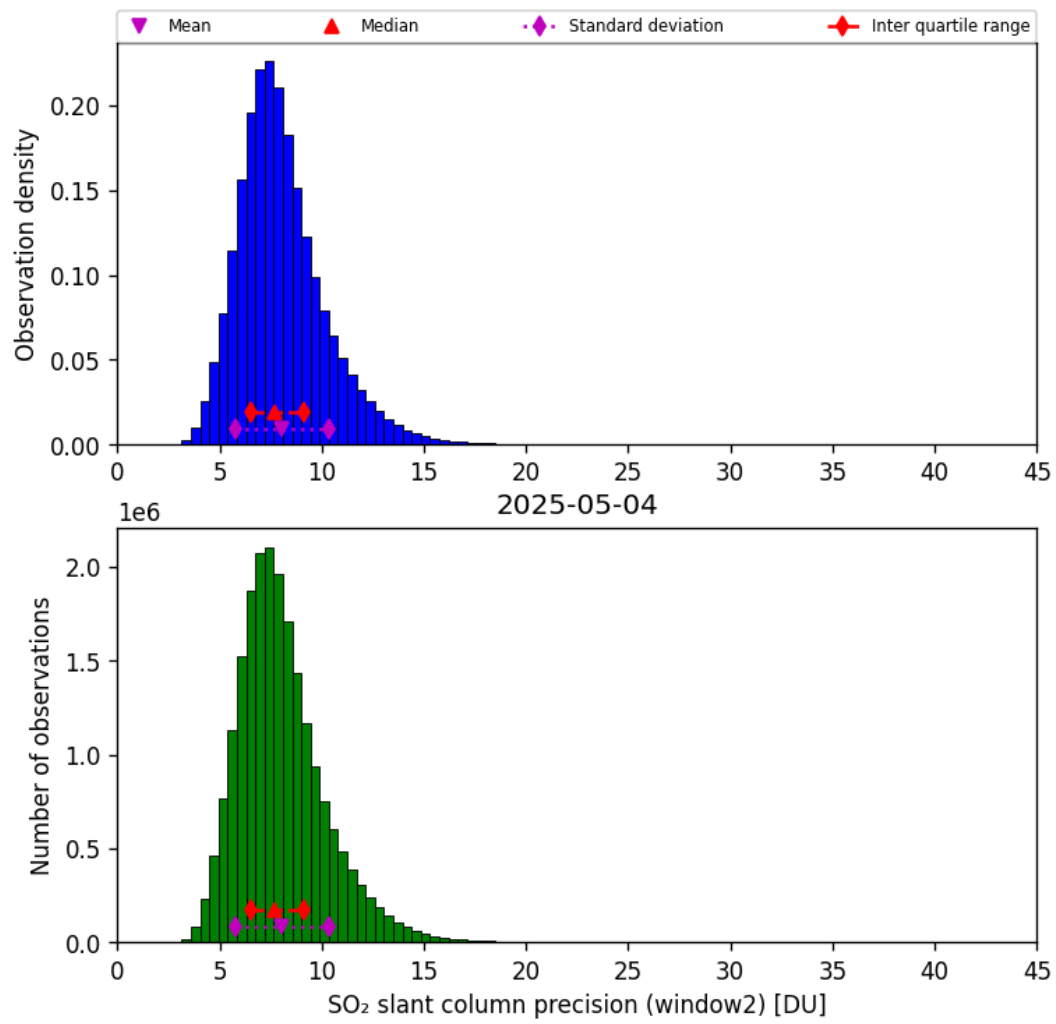
Figure 68: Histogram of “SO 2 slant column precision (window2)” for 2025-05-03 to 2025-05-05
