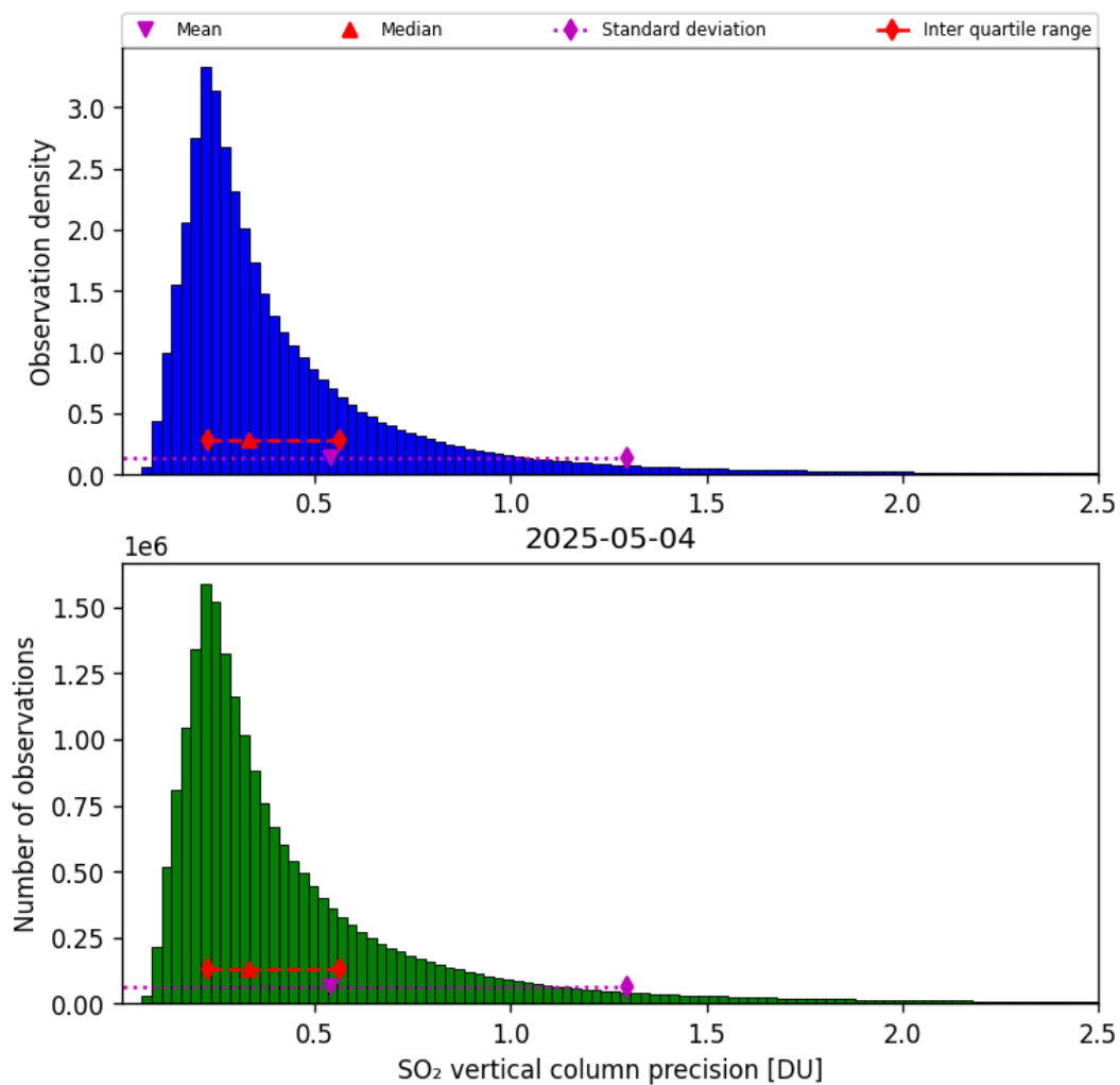
Figure 59: Histogram of “SO 2 vertical column precision” for 2025-05-03 to 2025-05-05
