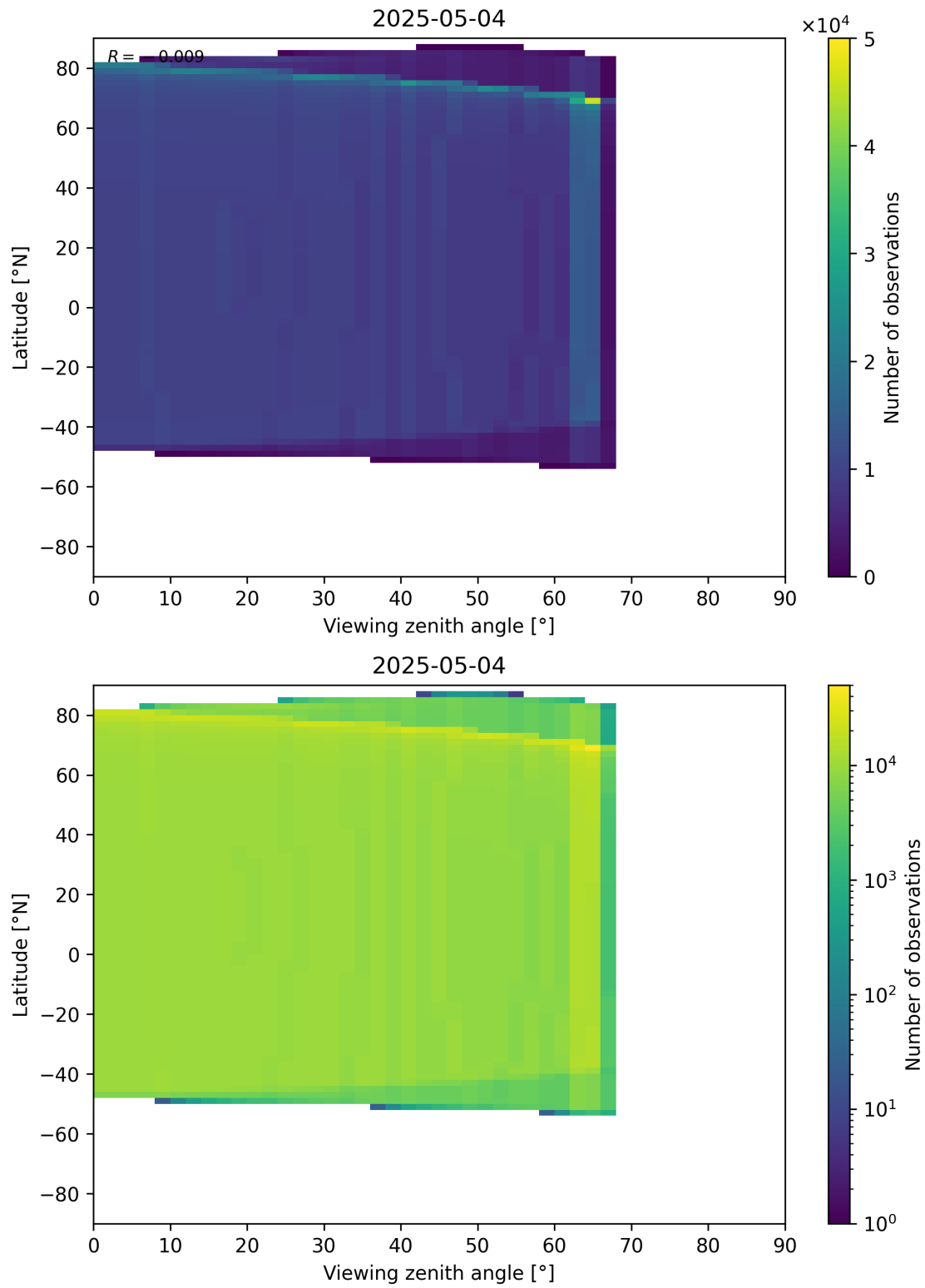
Figure 368: Scatter density plot of “Viewing zenith angle” against “Latitude” for 2025-05-03 to 2025-05-05.
