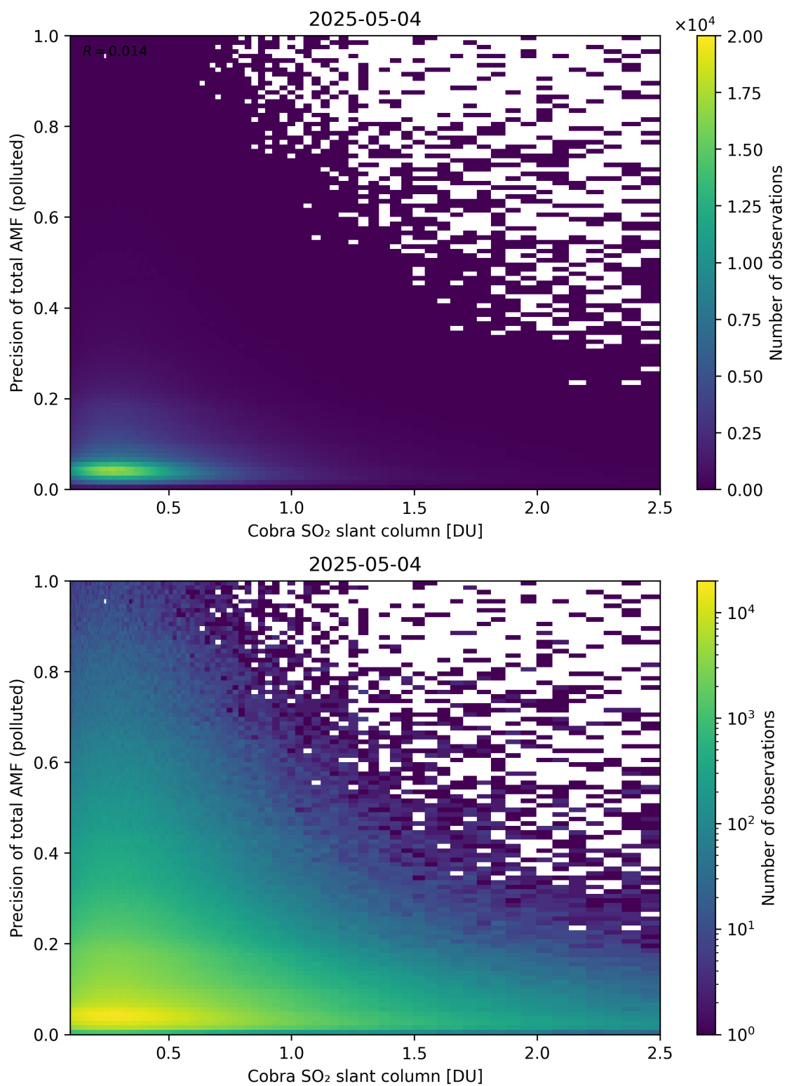
Figure 225: Scatter density plot of “Cobra SO 2 slant column” against “Precision of total AMF (polluted)” for 2025-05-03 to 2025-05-05.
