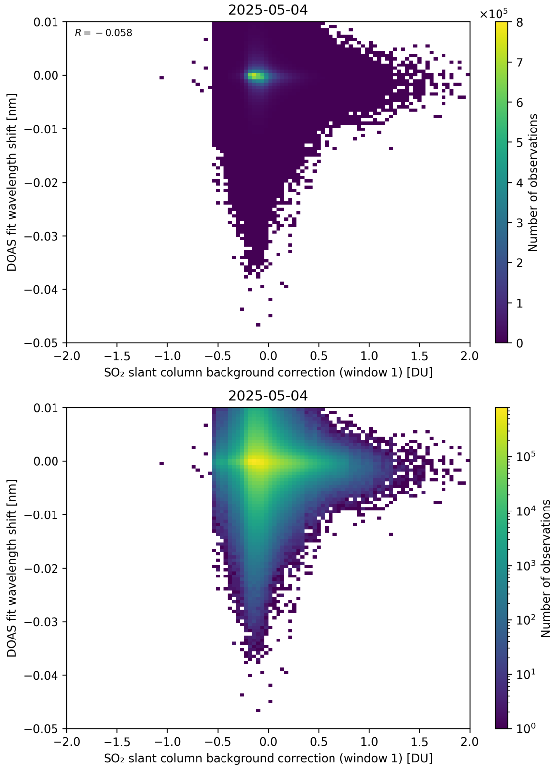
Figure 111: Scatter density plot of “SO 2 slant column background correction (window 1)” against “DOAS fit wavelength shift” for 2025-05-03 to 2025-05-05.
