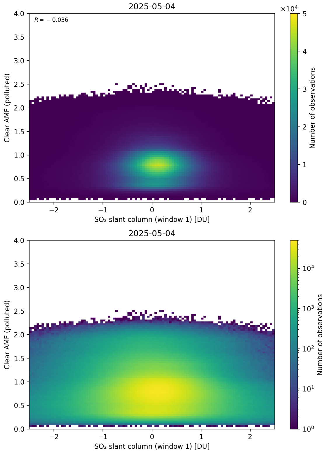
Figure 282: Scatter density plot of “SO 2 slant column (window 1)” against “Clear AMF (polluted)” for 2025-05-03 to 2025-05-05.
