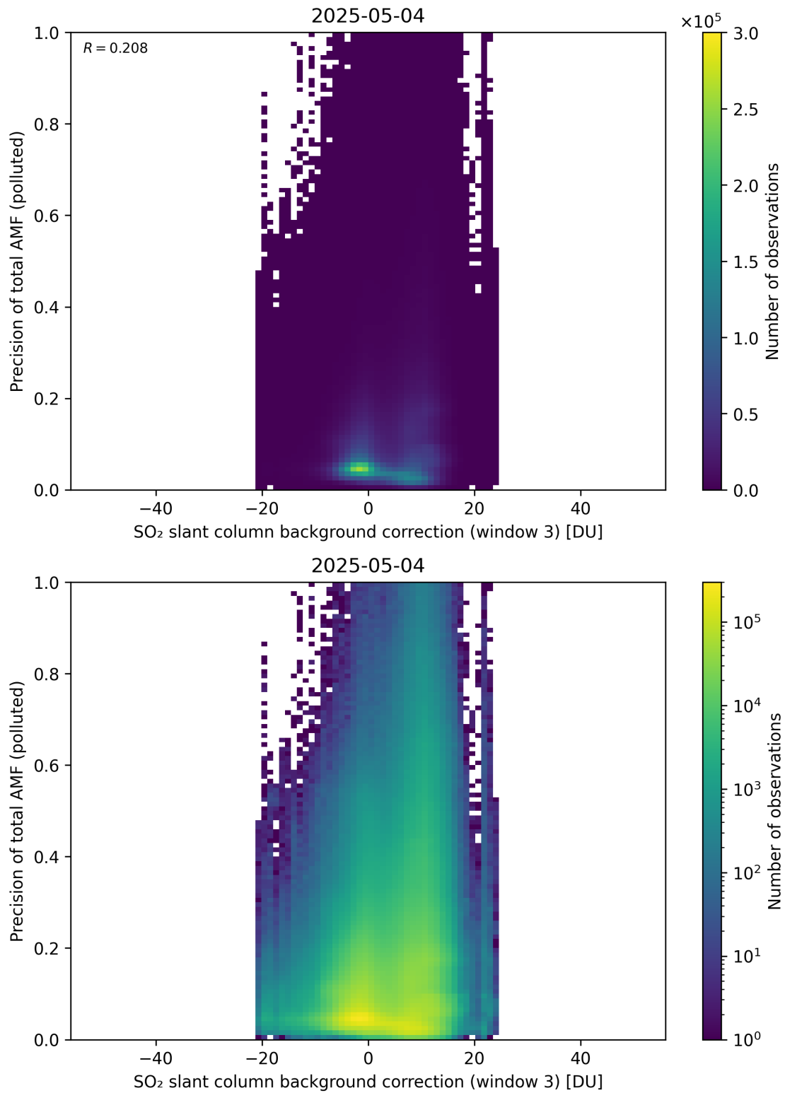
Figure 137: Scatter density plot of “SO 2 slant column background correction (window 3)” against “Precision of total AMF (polluted)” for 2025-05-03 to 2025-05-05.
