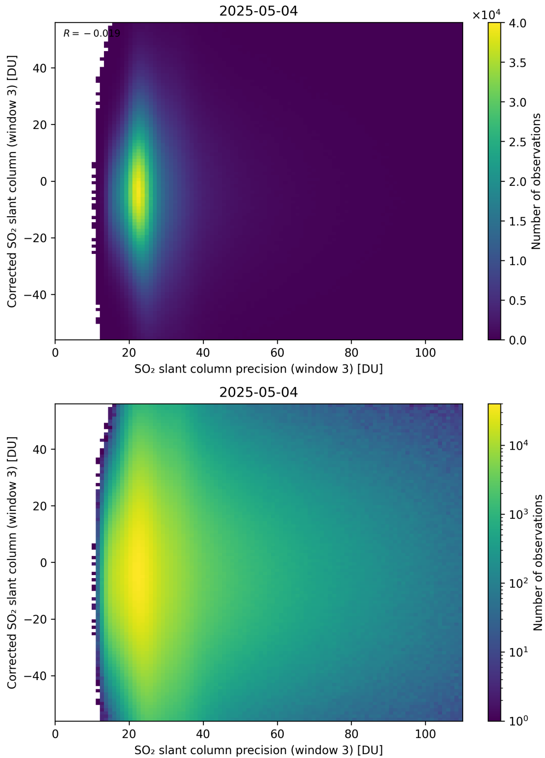
Figure 312: Scatter density plot of “SO 2 slant column precision (window 3)” against “Corrected SO 2 slant column (window 3)” for 2025-05-03 to 2025-05-05.
