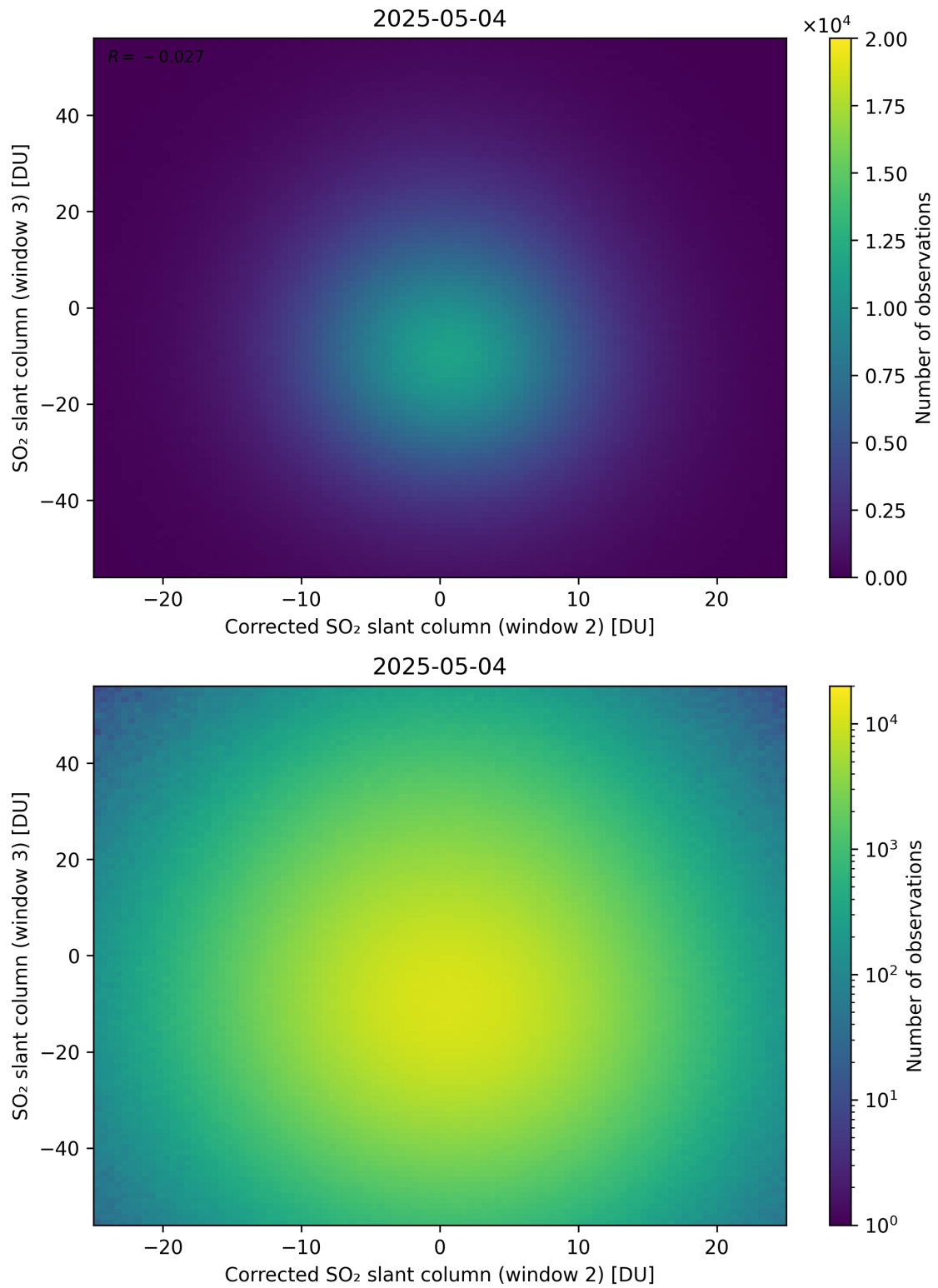
Figure 251: Scatter density plot of “Corrected SO 2 slant column (window 2)” against “SO 2 slant column (window 3)” for 2025-05-03 to 2025-05-05.
