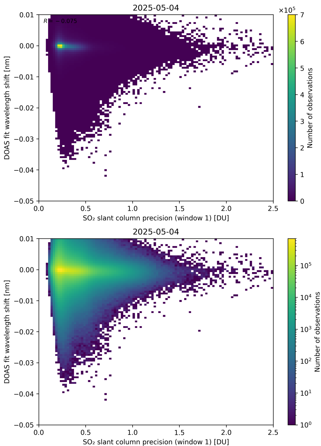
Figure 271: Scatter density plot of “SO 2 slant column precision (window 1)” against “DOAS fit wavelength shift” for 2025-05-03 to 2025-05-05.
