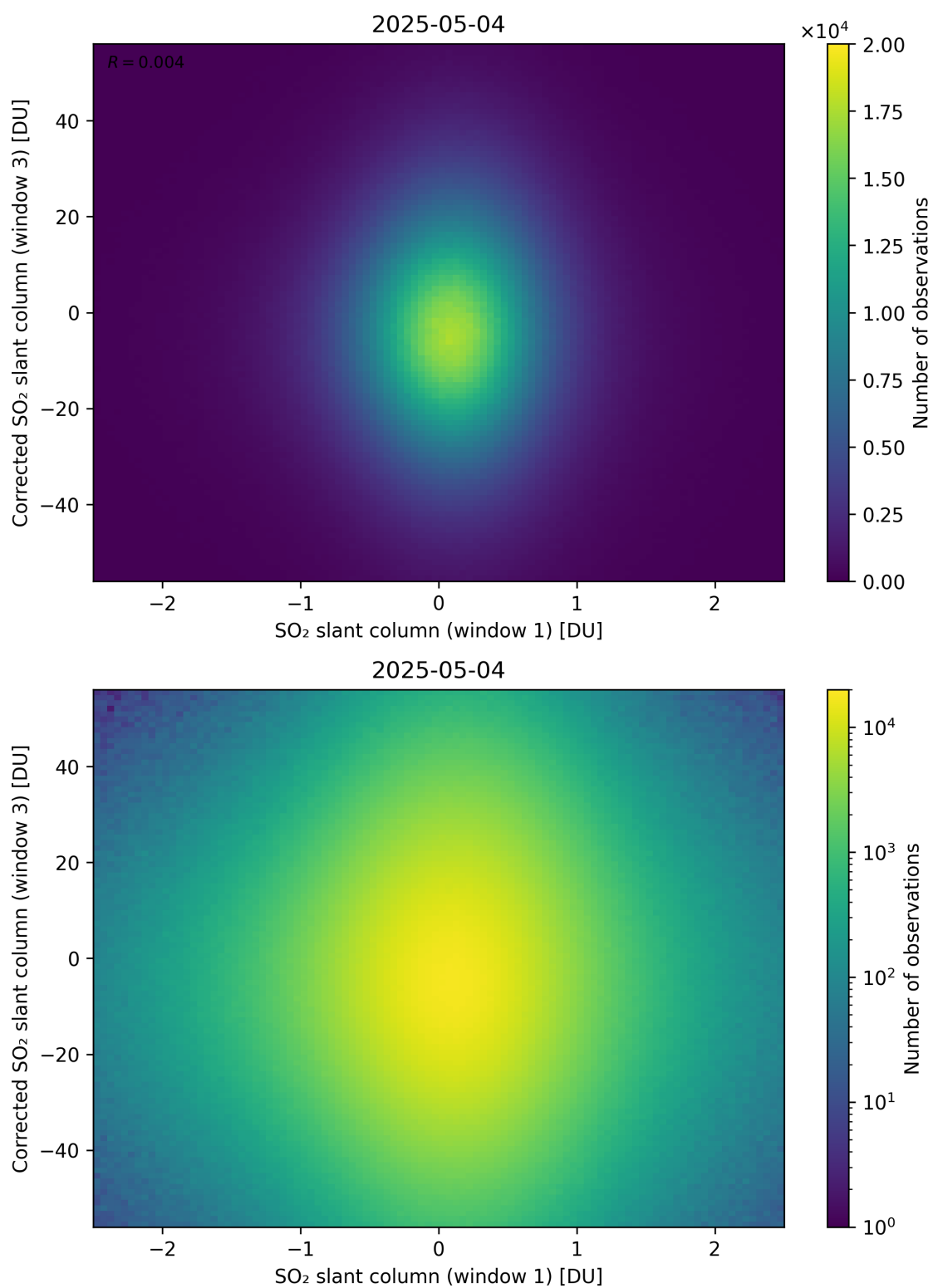
Figure 284: Scatter density plot of “SO 2 slant column (window 1)” against “Corrected SO 2 slant column (window 3)” for 2025-05-03 to 2025-05-05.
