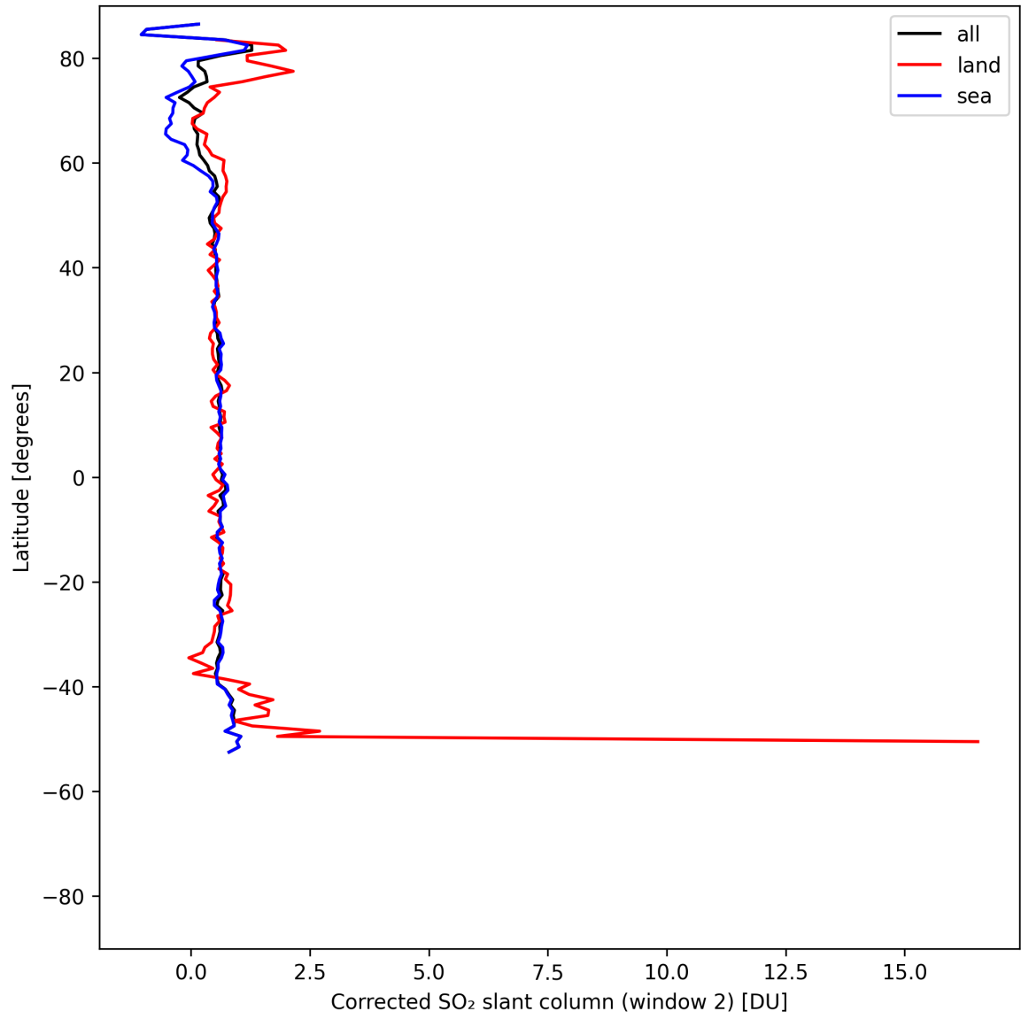
Figure 43: Zonal average of “Corrected SO 2 slant column (window 2)” for 2025-05-03 to 2025-05-05.
