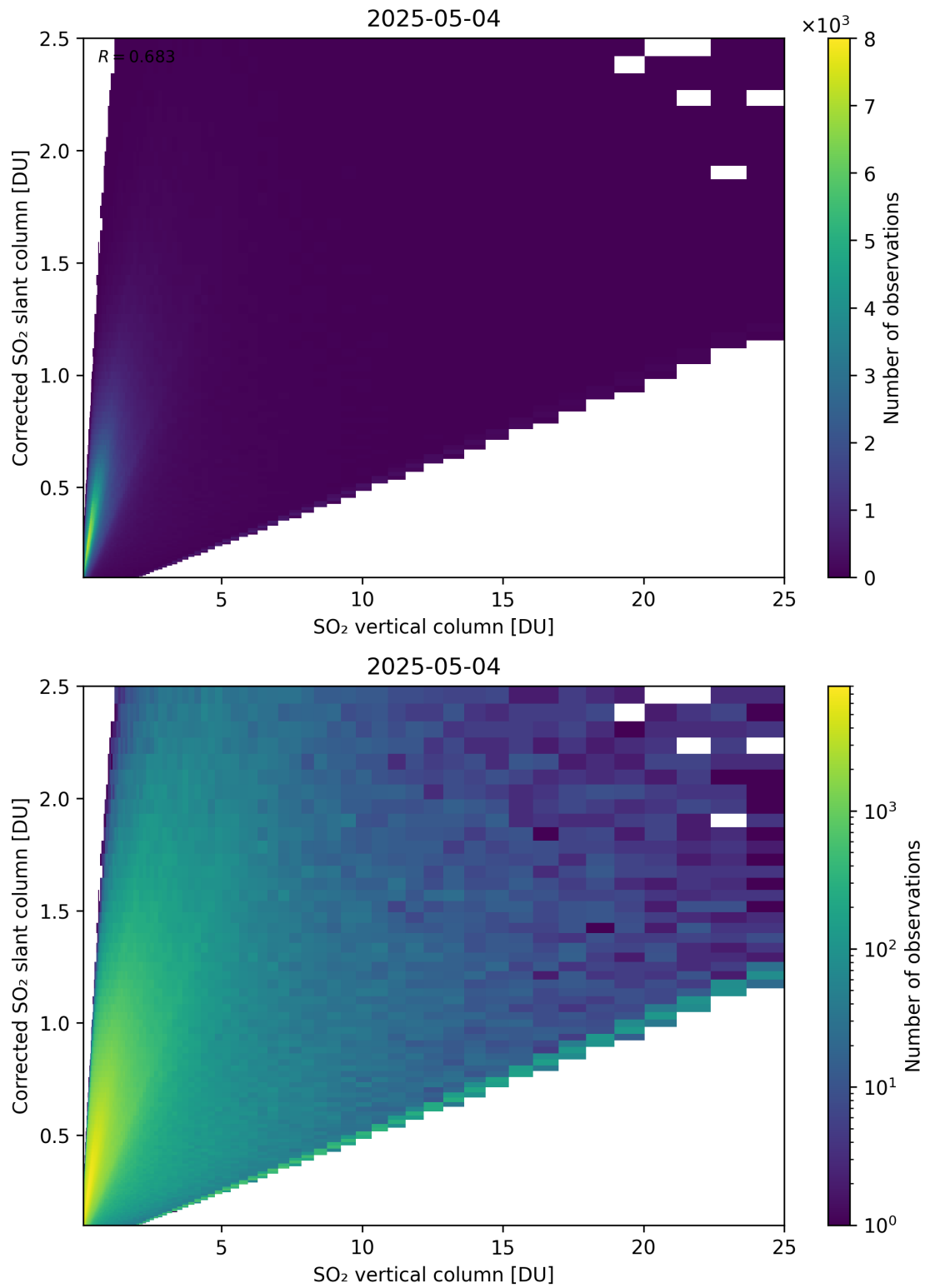
Figure 351: Scatter density plot of “SO 2 vertical column” against “Corrected SO 2 slant column” for 2025-05-03 to 2025-05-05.
