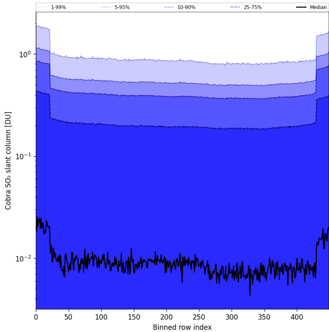
Figure 87: Along track statistics of “Cobra SO 2 slant column” for 2025-05-03 to 2025-05-05
