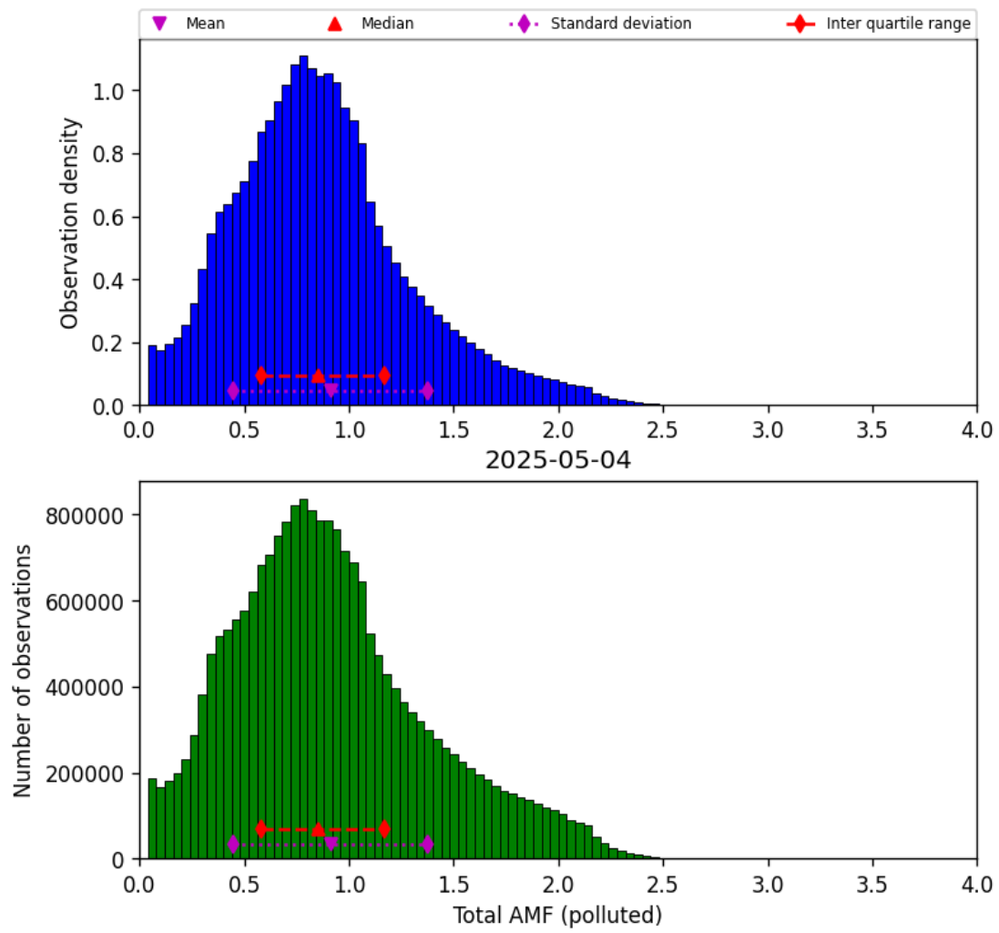
Figure 79: Histogram of “Total AMF (polluted)” for 2025-05-03 to 2025-05-05
