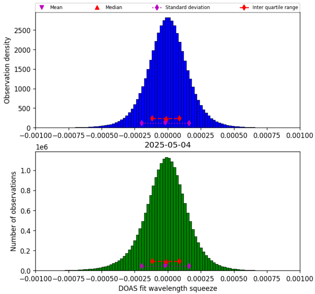
Figure 77: Histogram of “DOAS fit wavelength squeeze” for 2025-05-03 to 2025-05-05
