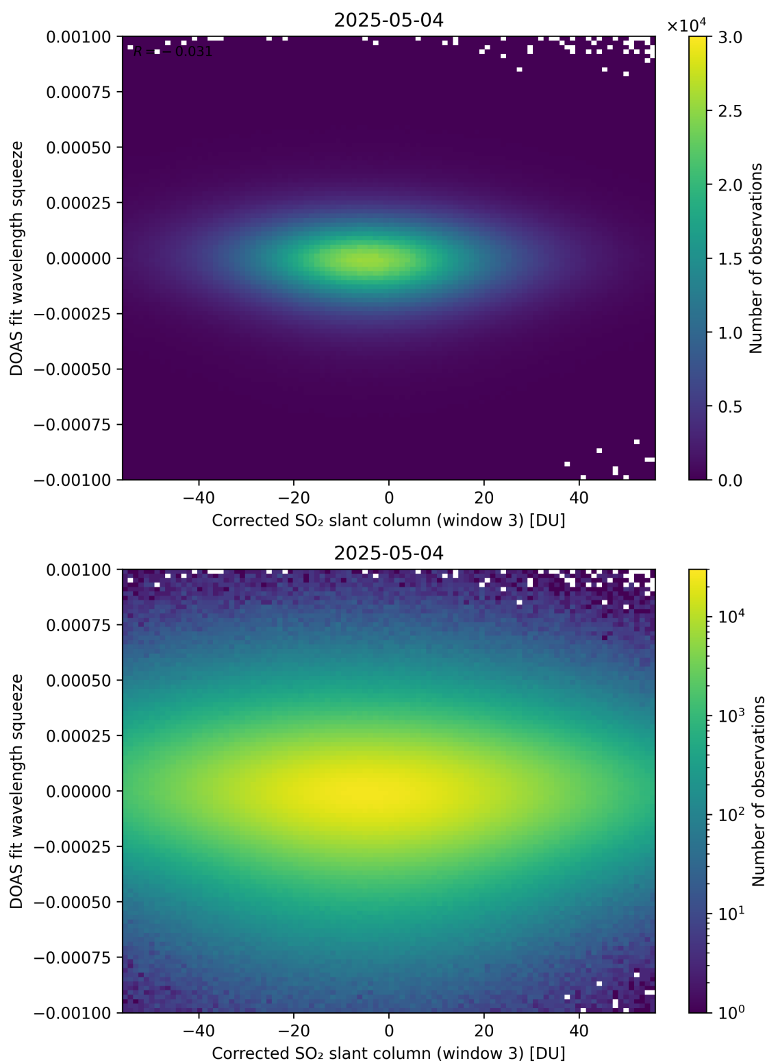
Figure 257: Scatter density plot of “Corrected SO 2 slant column (window 3)” against “DOAS fit wavelength squeeze” for 2025-05-03 to 2025-05-05.
