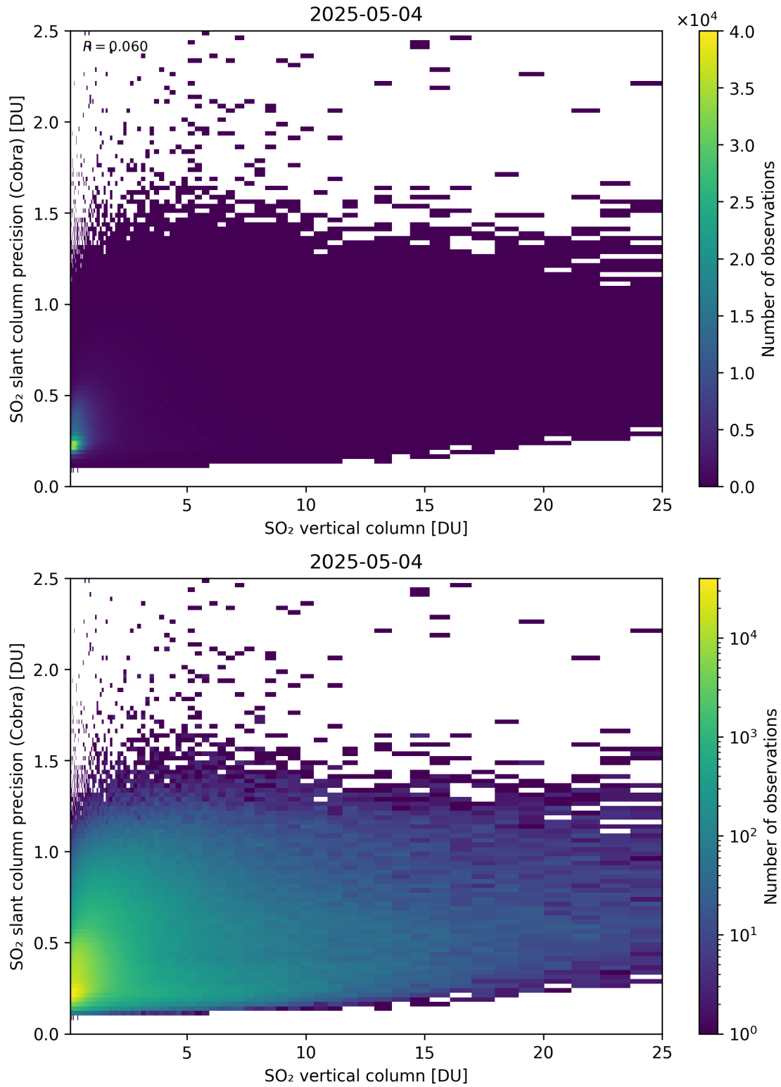
Figure 350: Scatter density plot of “SO 2 vertical column” against “SO 2 slant column precision (Cobra)” for 2025-05-03 to 2025-05-05.
