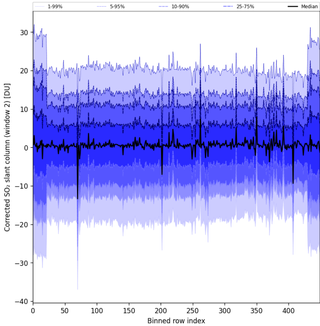
Figure 95: Along track statistics of “Corrected SO 2 slant column (window 2)” for 2025-05-03 to 2025-05-05
