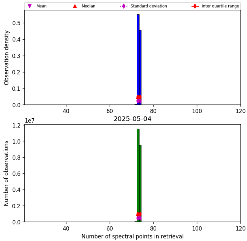
Figure 82: Histogram of “Number of spectral points in retrieval” for 2025-05-03 to 2025-05-05
