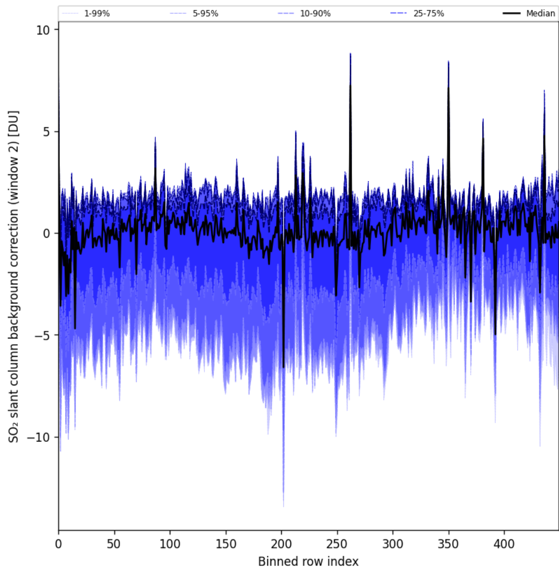
Figure 96: Along track statistics of “SO 2 slant column background correction (window 2)” for 2025-05-03 to 2025-05-05
