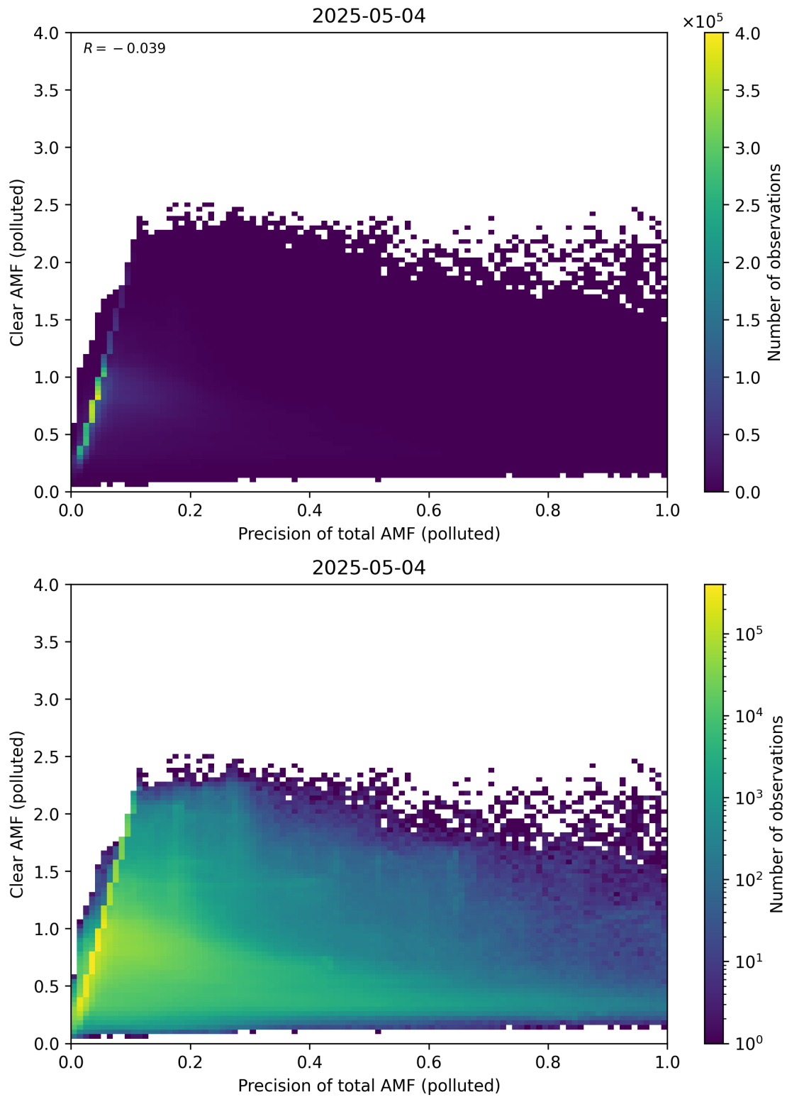
Figure 320: Scatter density plot of “Precision of total AMF (polluted)” against “Clear AMF (polluted)” for 2025-05-03 to 2025-05-05.
