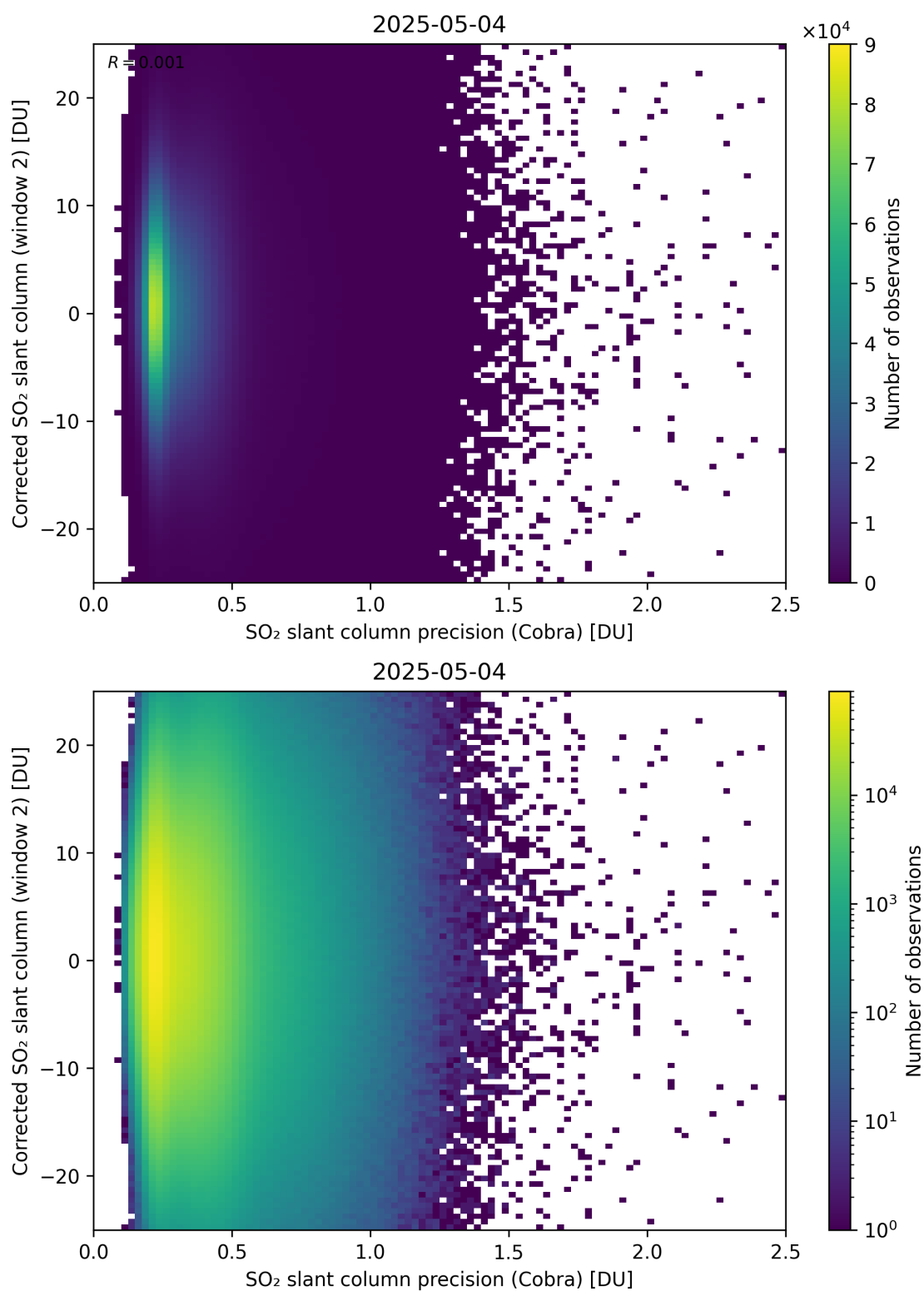
Figure 206: Scatter density plot of “SO 2 slant column precision (Cobra)” against “Corrected SO 2 slant column (window 2)” for 2025-05-03 to 2025-05-05.
