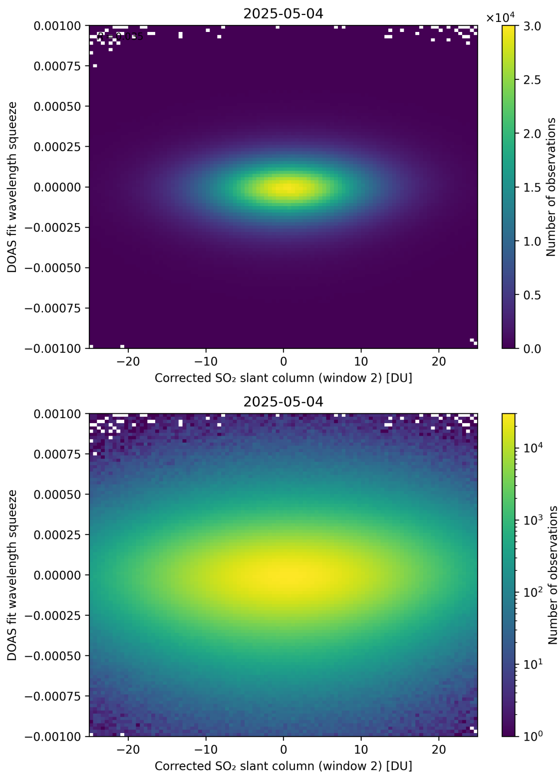
Figure 247: Scatter density plot of “Corrected SO 2 slant column (window 2)” against “DOAS fit wavelength squeeze” for 2025-05-03 to 2025-05-05.
