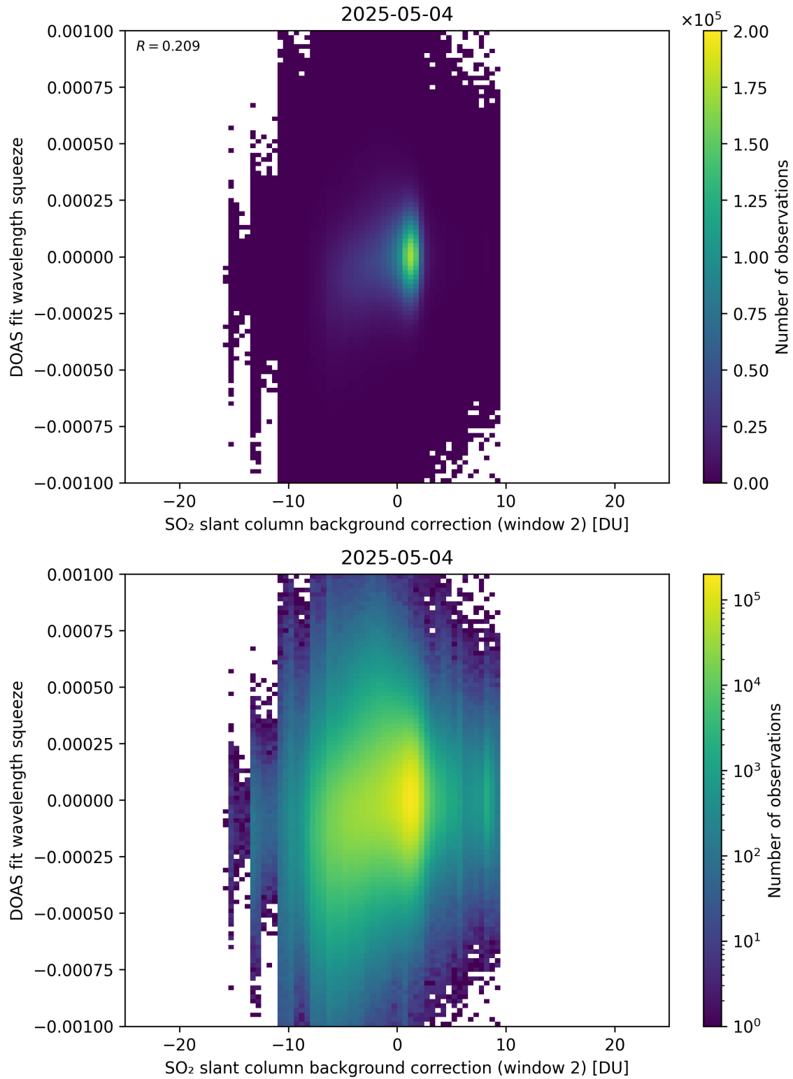
Figure 124: Scatter density plot of “SO 2 slant column background correction (window 2)” against “DOAS fit wavelength squeeze” for 2025-05-03 to 2025-05-05.
