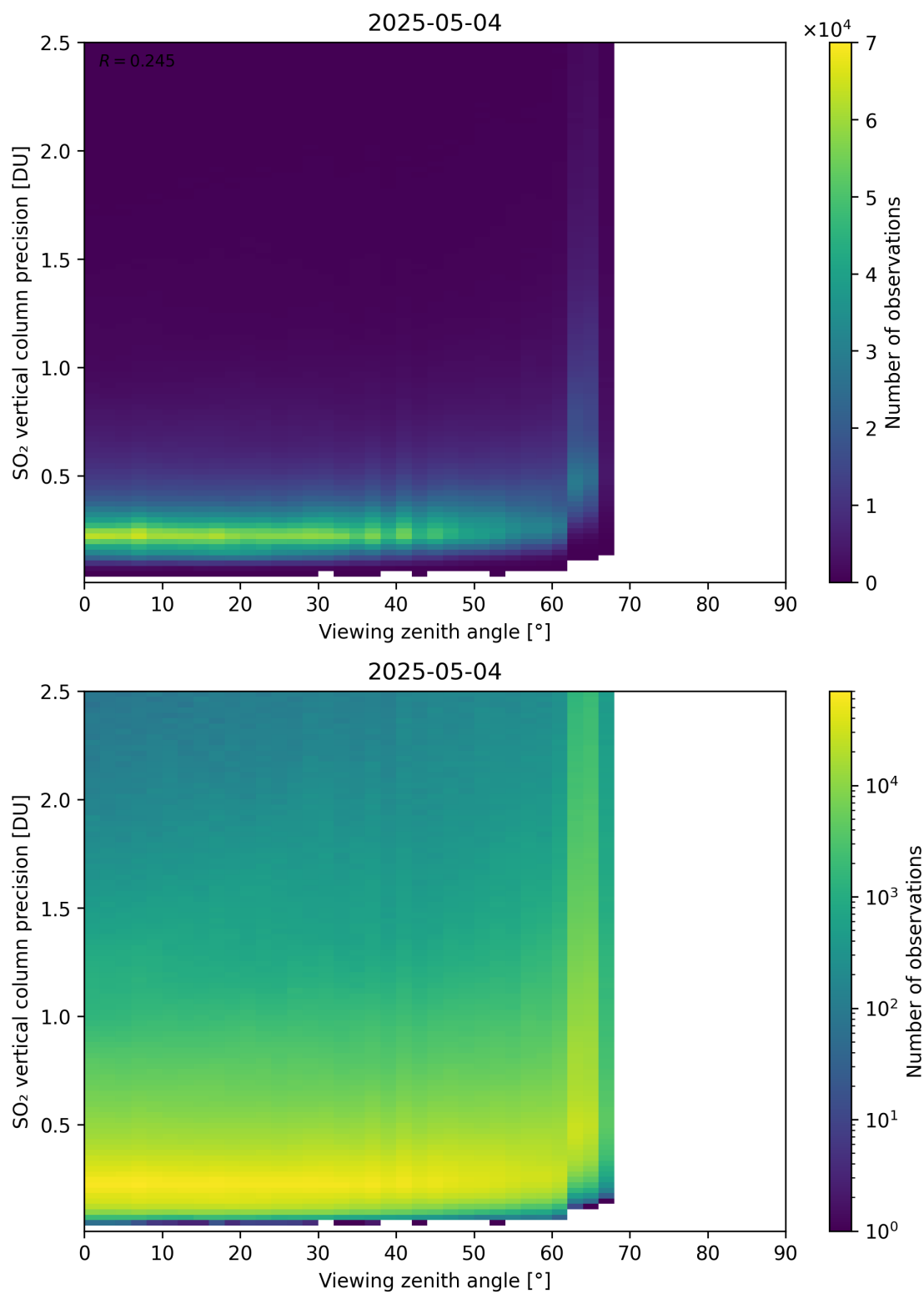
Figure 384: Scatter density plot of “Viewing zenith angle” against “SO 2 vertical column precision” for 2025-05-03 to 2025-05-05.
