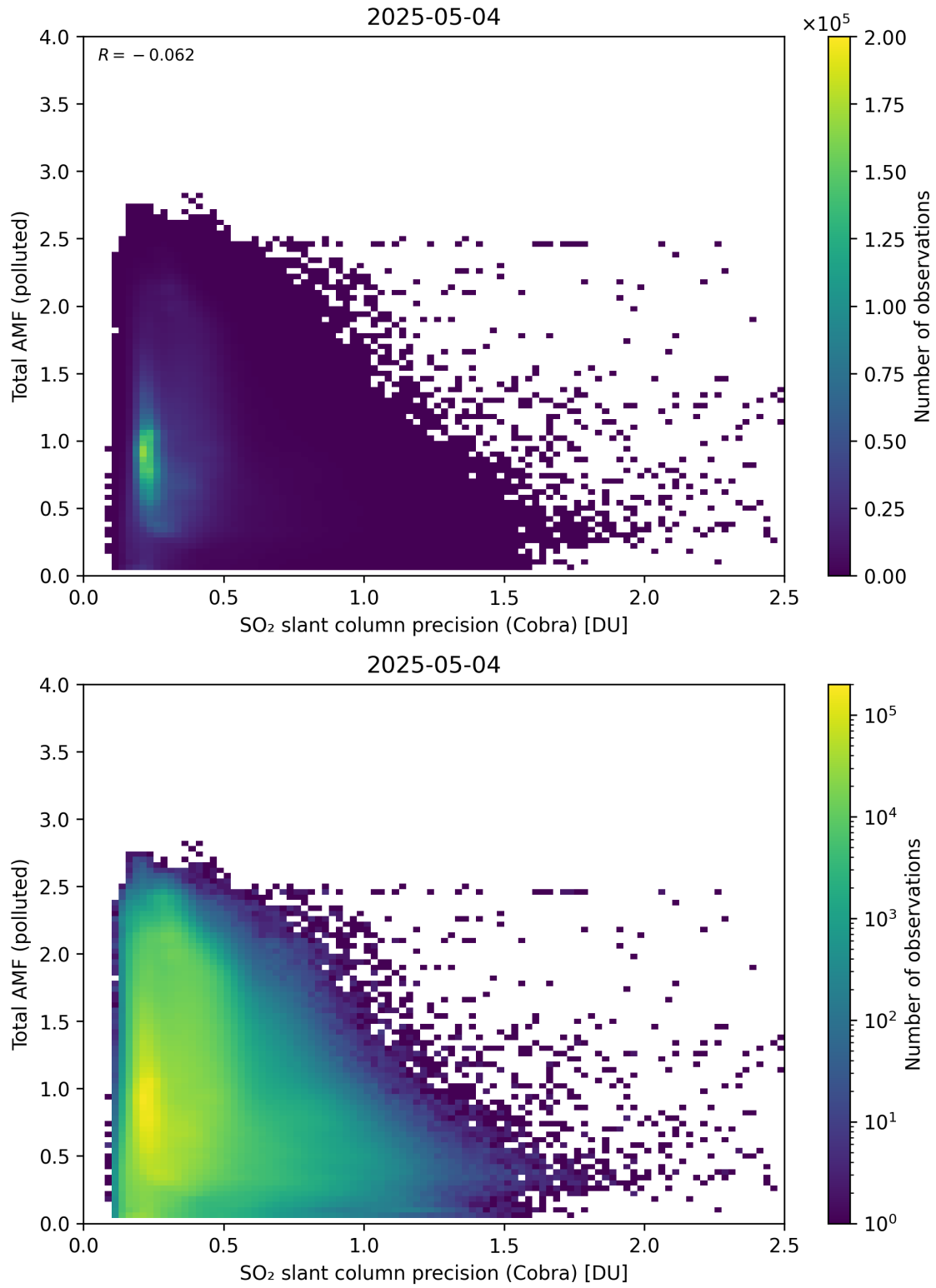
Figure 213: Scatter density plot of “SO 2 slant column precision (Cobra)” against “Total AMF (polluted)” for 2025-05-03 to 2025-05-05.
