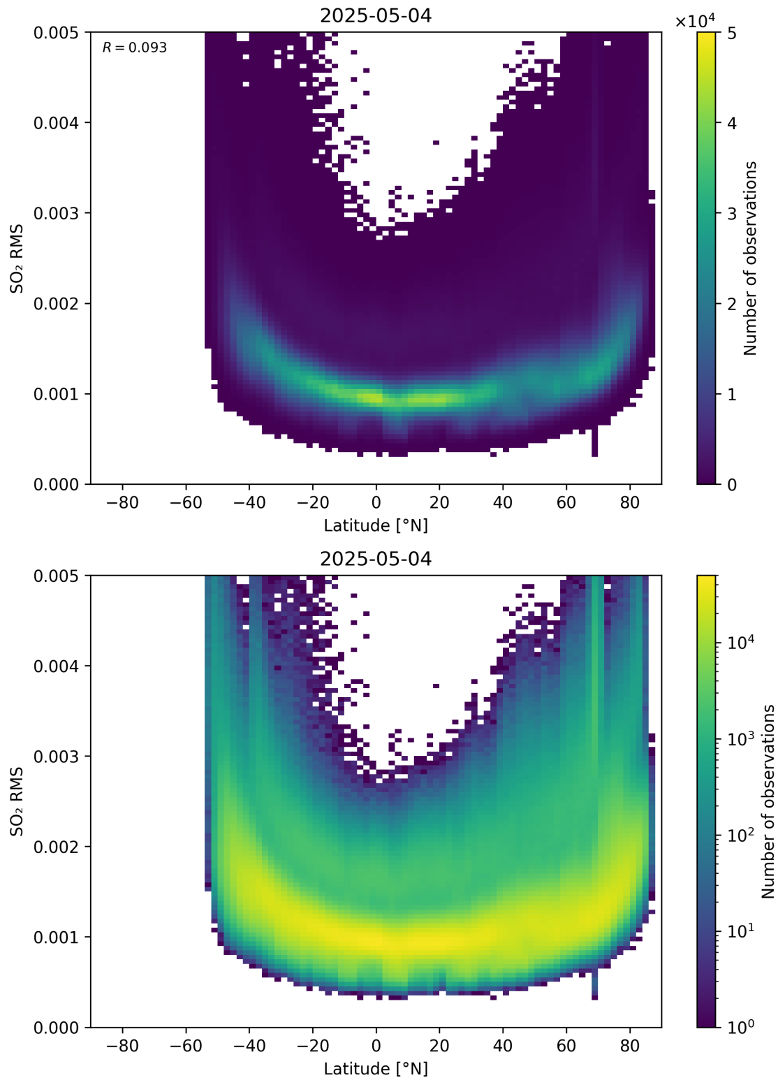
Figure 155: Scatter density plot of “Latitude” against “SO 2 RMS” for 2025-05-03 to 2025-05-05.
