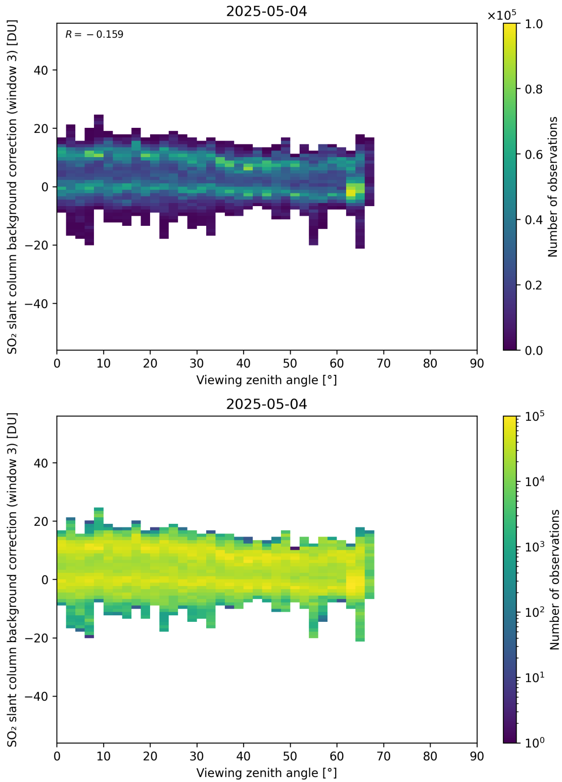
Figure 364: Scatter density plot of “Viewing zenith angle” against “SO 2 slant column background correction (window 3)” for 2025-05-03 to 2025-05-05.
