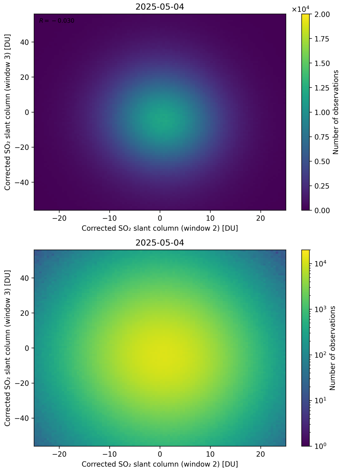
Figure 250: Scatter density plot of “Corrected SO 2 slant column (window 2)” against “Corrected SO 2 slant column (window 3)” for 2025-05-03 to 2025-05-05.
