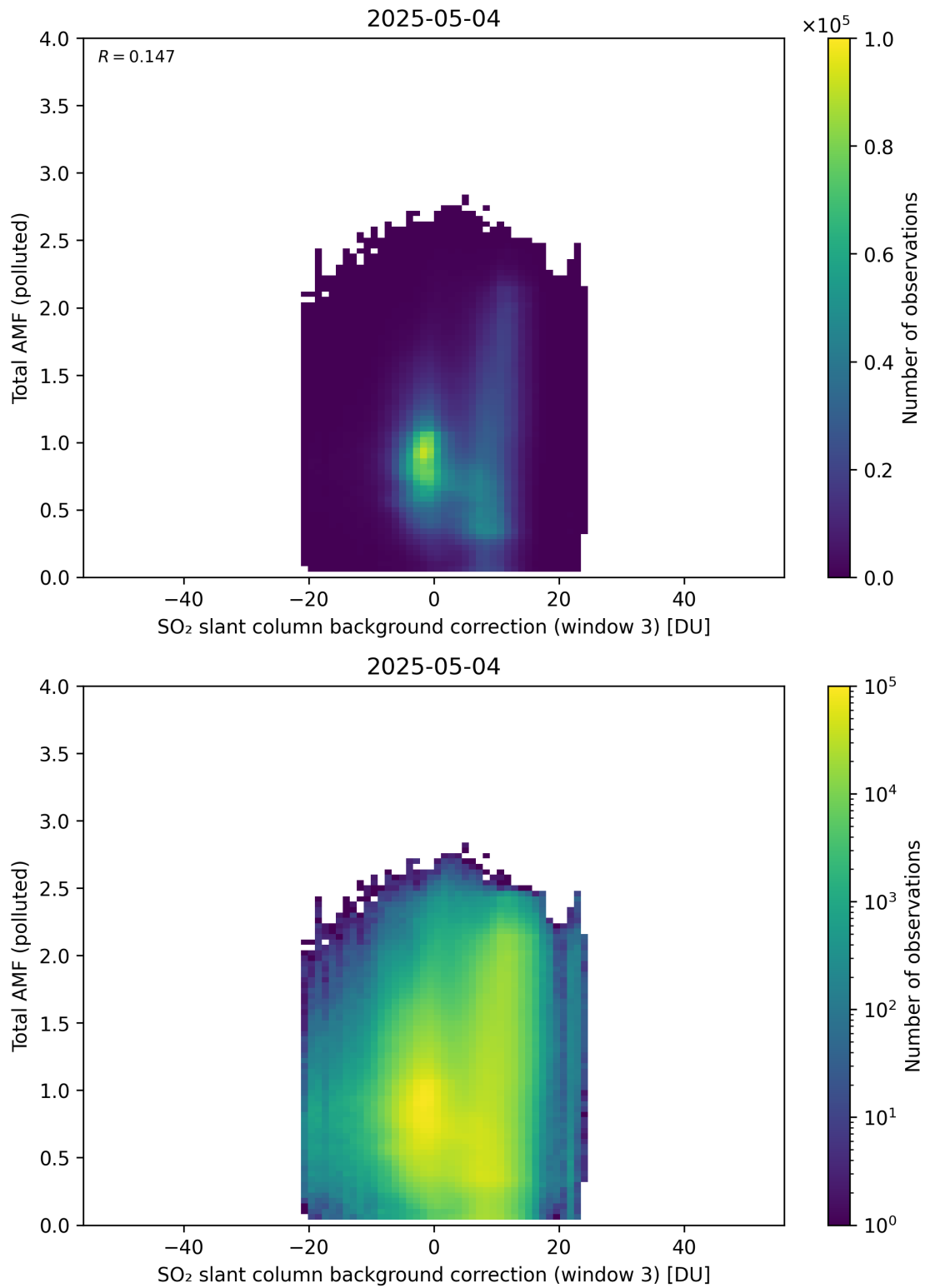
Figure 136: Scatter density plot of “SO 2 slant column background correction (window 3)” against “Total AMF (polluted)” for 2025-05-03 to 2025-05-05.
