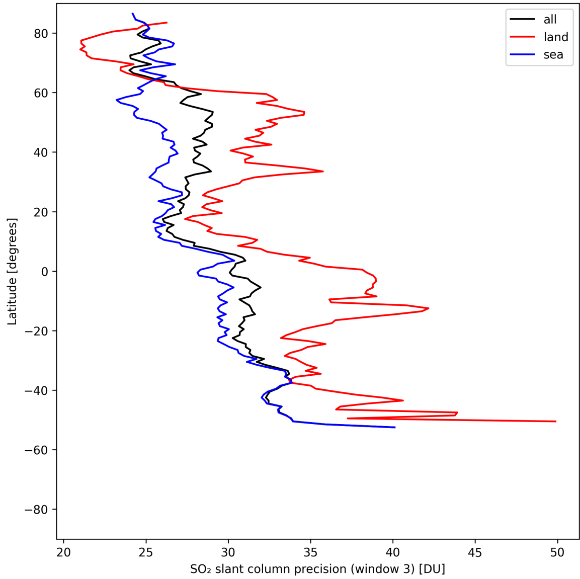
Figure 46: Zonal average of “SO 2 slant column precision (window 3)” for 2025-05-03 to 2025-05-05.
