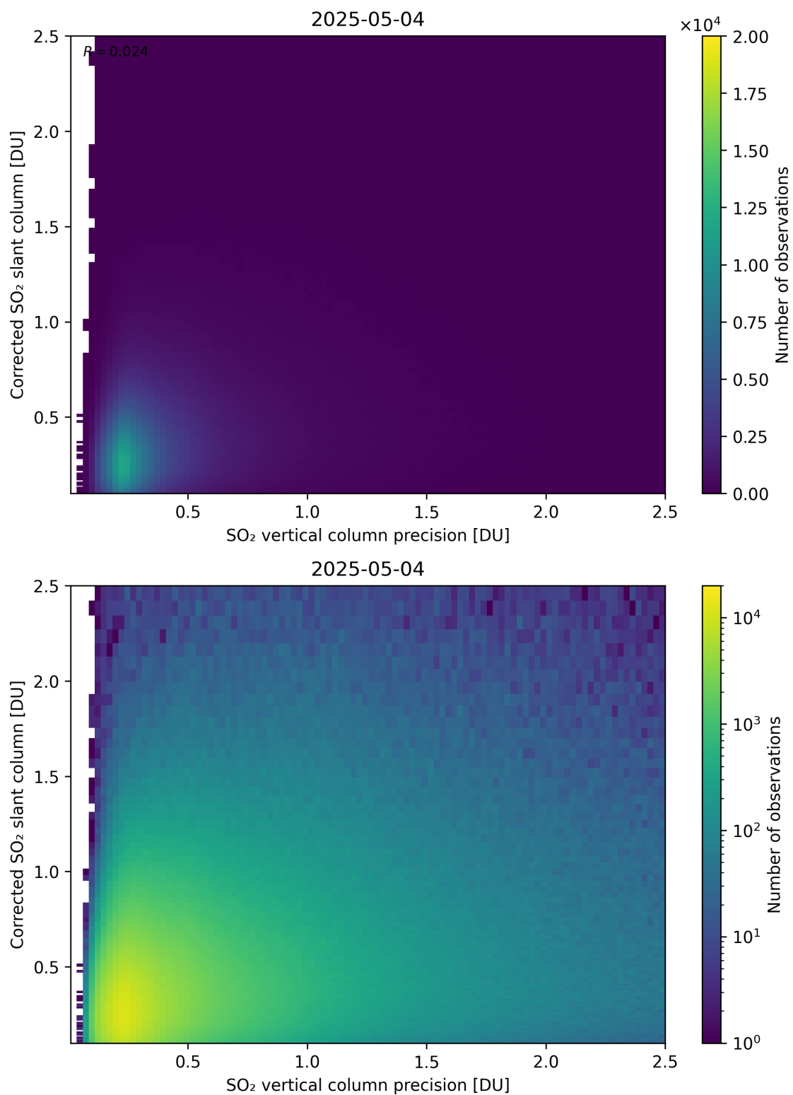
Figure 338: Scatter density plot of “SO 2 vertical column precision” against “Corrected SO 2 slant column” for 2025-05-03 to 2025-05-05.
