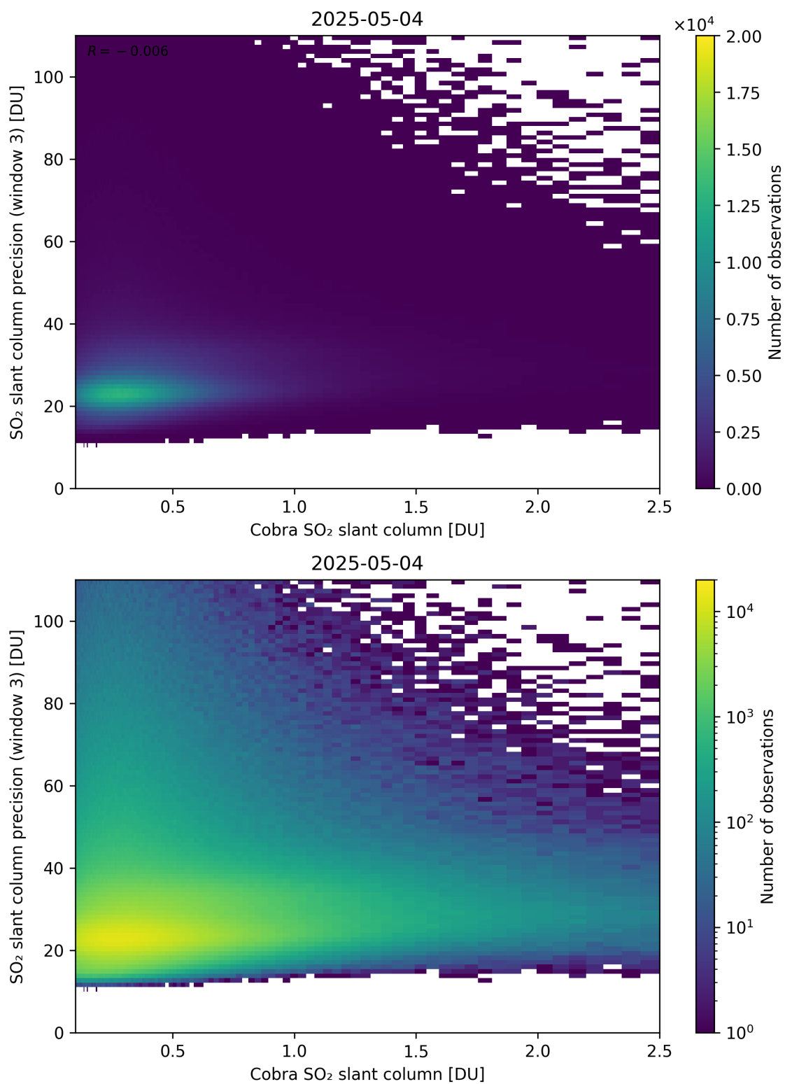
Figure 223: Scatter density plot of “Cobra SO 2 slant column” against “SO 2 slant column precision (window 3)” for 2025-05-03 to 2025-05-05.
