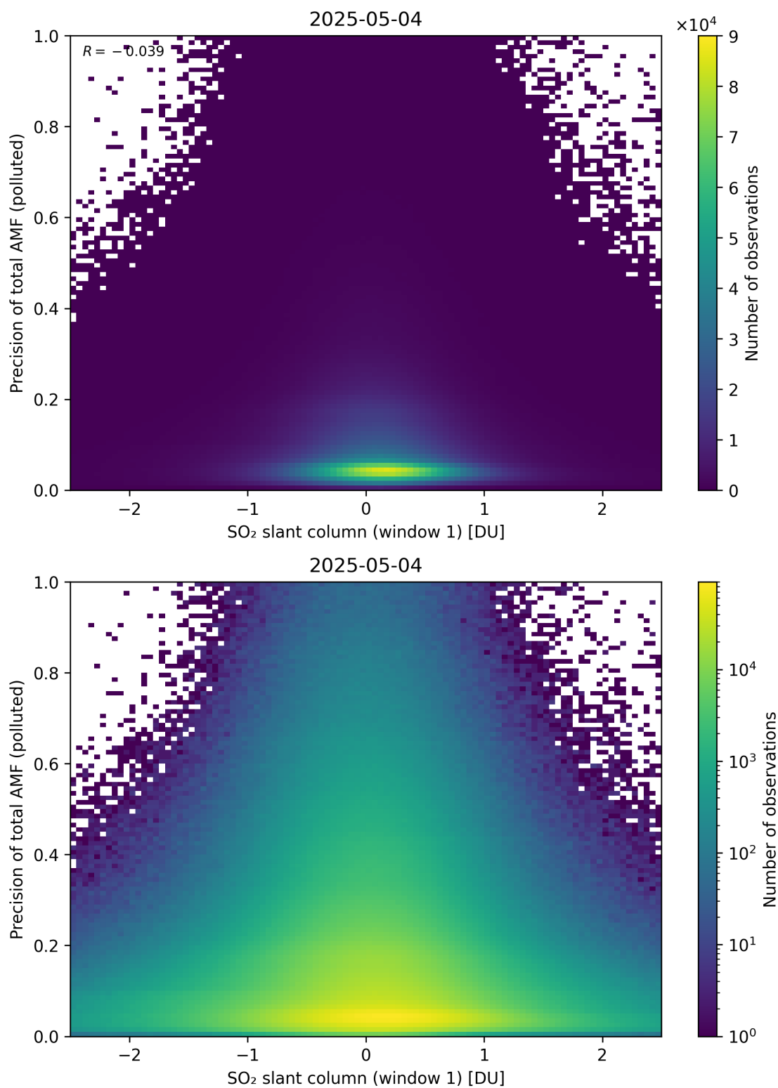
Figure 290: Scatter density plot of “SO 2 slant column (window 1)” against “Precision of total AMF (polluted)” for 2025-05-03 to 2025-05-05.
