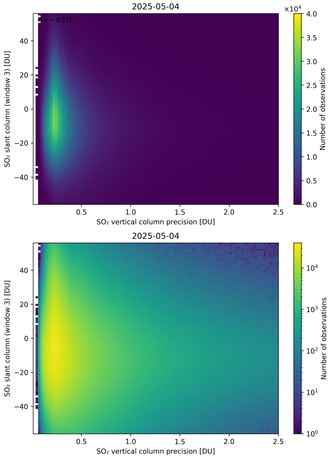
Figure 344: Scatter density plot of “SO 2 vertical column precision” against “SO 2 slant column (window 3)” for 2025-05-03 to 2025-05-05.
