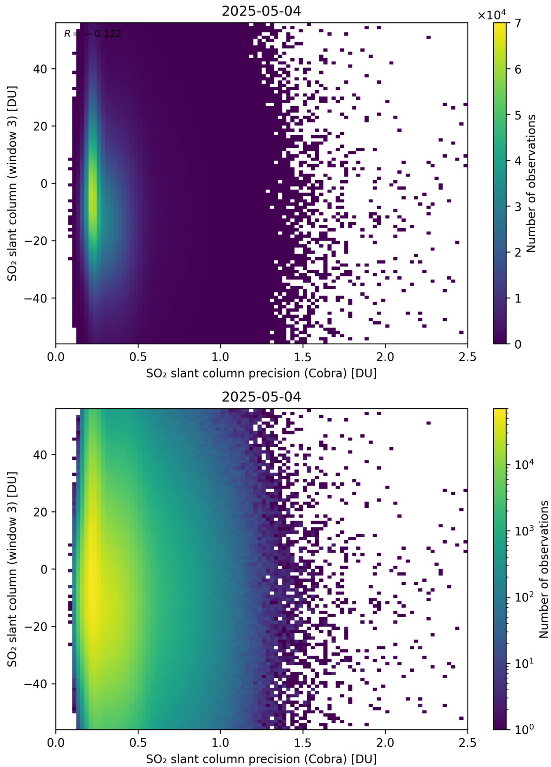
Figure 211: Scatter density plot of “SO 2 slant column precision (Cobra)” against “SO 2 slant column (window 3)” for 2025-05-03 to 2025-05-05.
