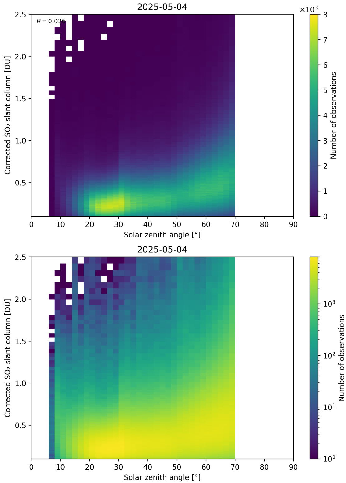
Figure 181: Scatter density plot of “Solar zenith angle” against “Corrected SO 2 slant column” for 2025-05-03 to 2025-05-05.
