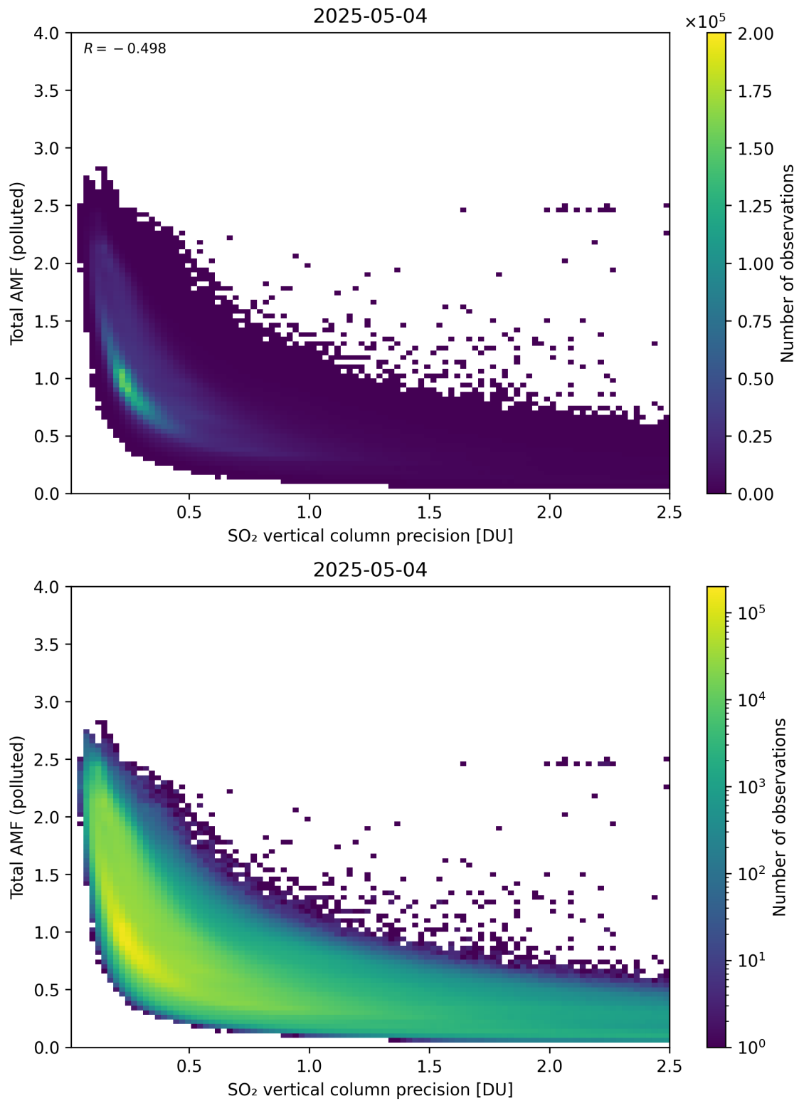
Figure 346: Scatter density plot of “SO 2 vertical column precision” against “Total AMF (polluted)” for 2025-05-03 to 2025-05-05.
