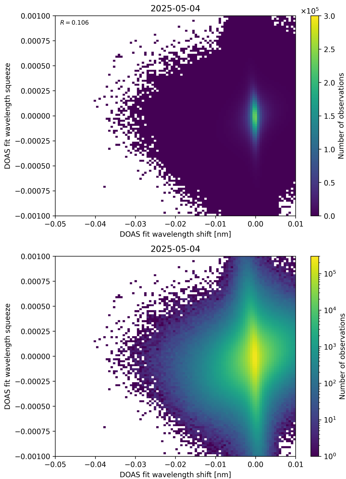
Figure 138: Scatter density plot of “DOAS fit wavelength shift” against “DOAS fit wavelength squeeze” for 2025-05-03 to 2025-05-05.
