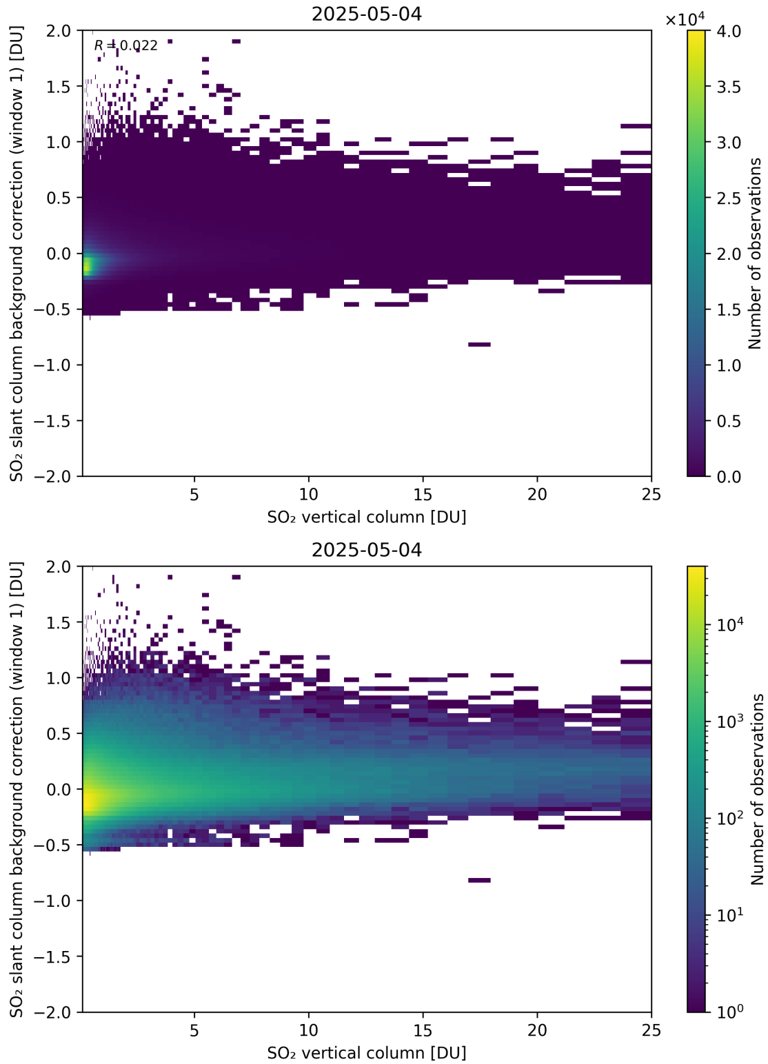
Figure 323: Scatter density plot of “SO 2 vertical column” against “SO 2 slant column background correction (window 1)” for 2025-05-03 to 2025-05-05.
