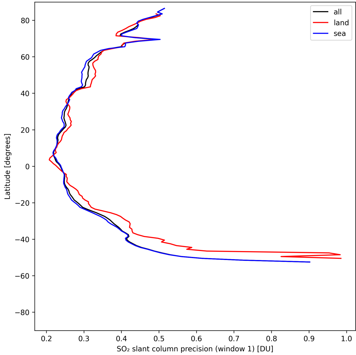
Figure 38: Zonal average of “SO 2 slant column precision (window 1)” for 2025-05-03 to 2025-05-05.
