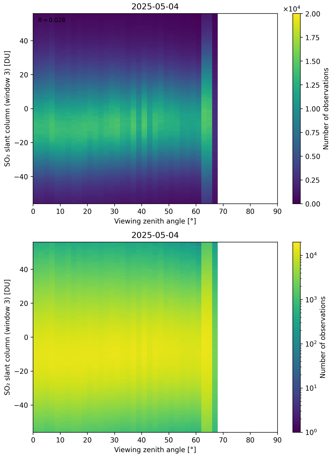
Figure 379: Scatter density plot of “Viewing zenith angle” against “SO 2 slant column (window 3)” for 2025-05-03 to 2025-05-05.
