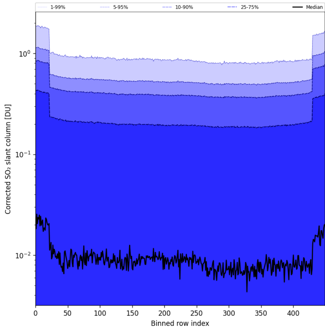
Figure 86: Along track statistics of “Corrected SO 2 slant column” for 2025-05-03 to 2025-05-05
