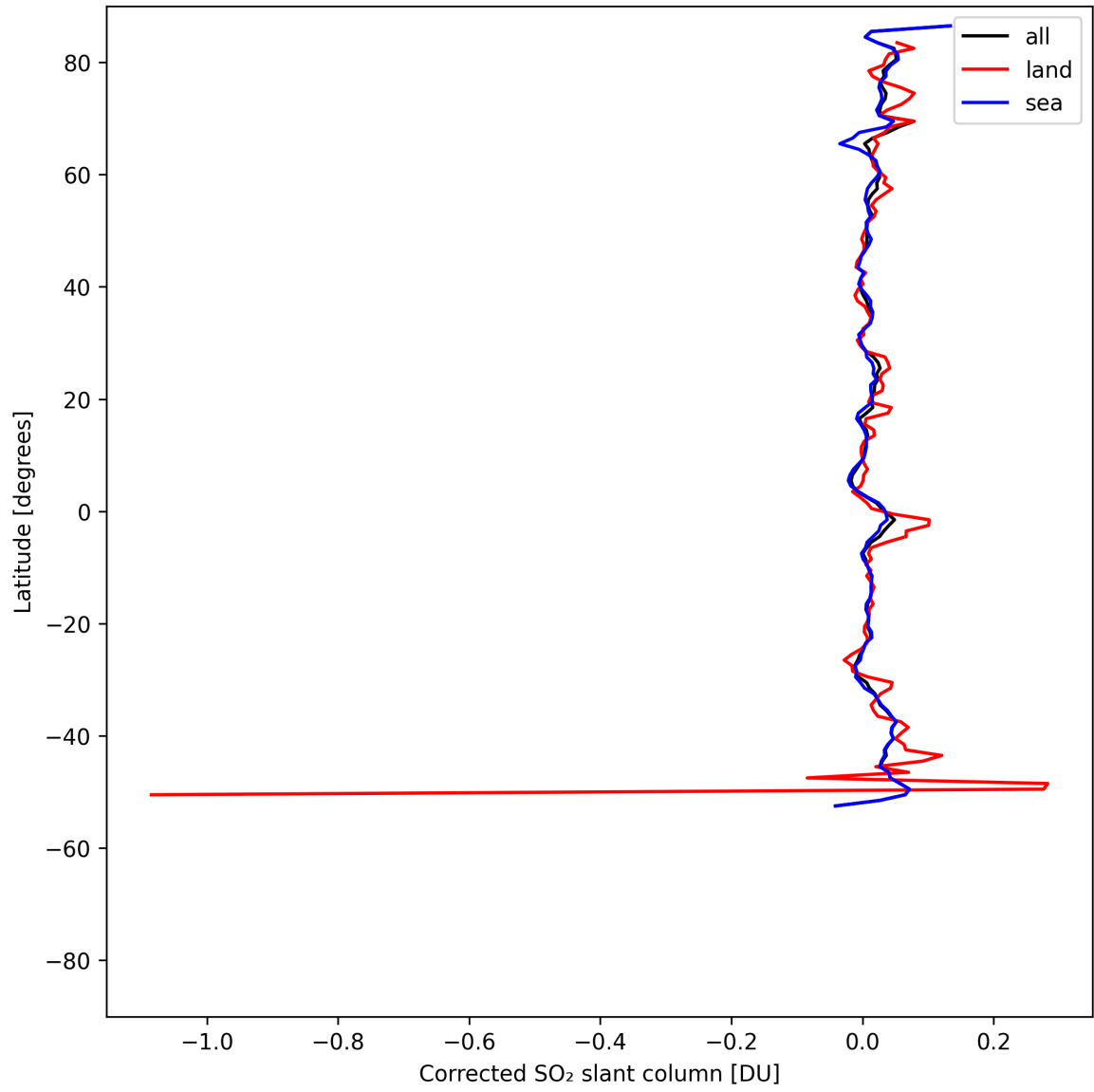
Figure 34: Zonal average of “Corrected SO 2 slant column” for 2025-05-03 to 2025-05-05.
