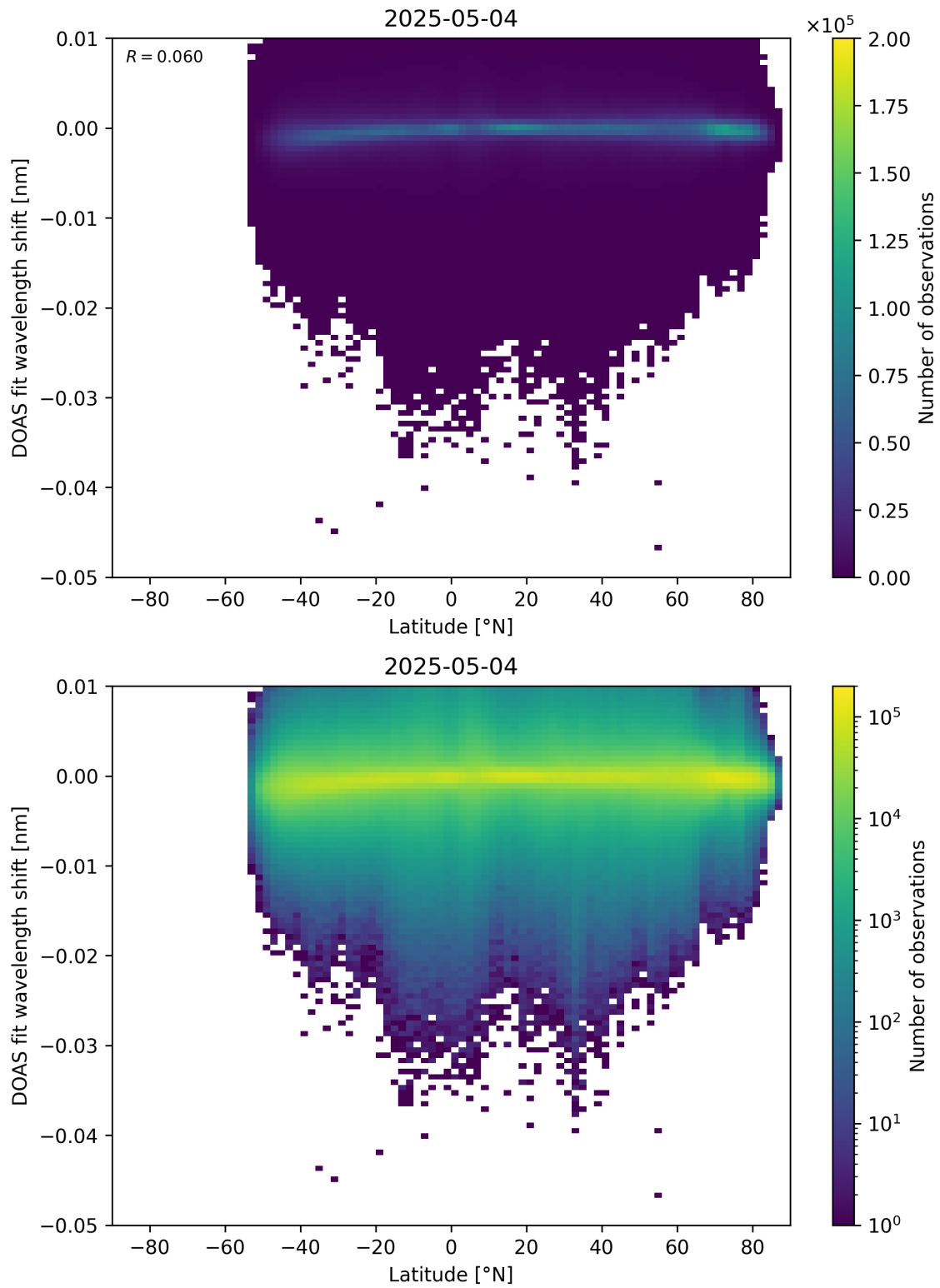
Figure 153: Scatter density plot of “Latitude” against “DOAS fit wavelength shift” for 2025-05-03 to 2025-05-05.
