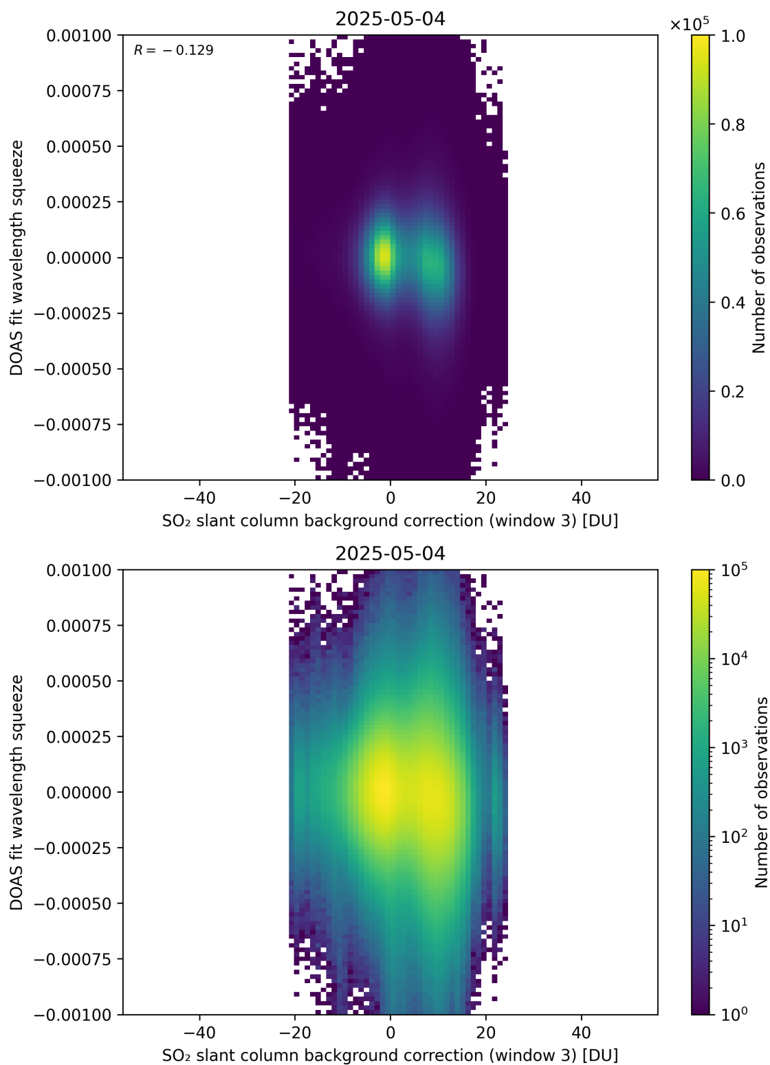
Figure 133: Scatter density plot of “SO 2 slant column background correction (window 3)” against “DOAS fit wavelength squeeze” for 2025-05-03 to 2025-05-05.
