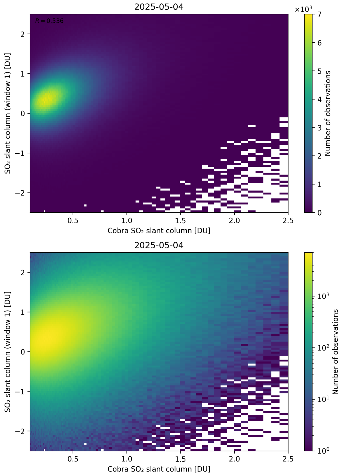
Figure 219: Scatter density plot of “Cobra SO 2 slant column” against “SO 2 slant column (window 1)” for 2025-05-03 to 2025-05-05.
