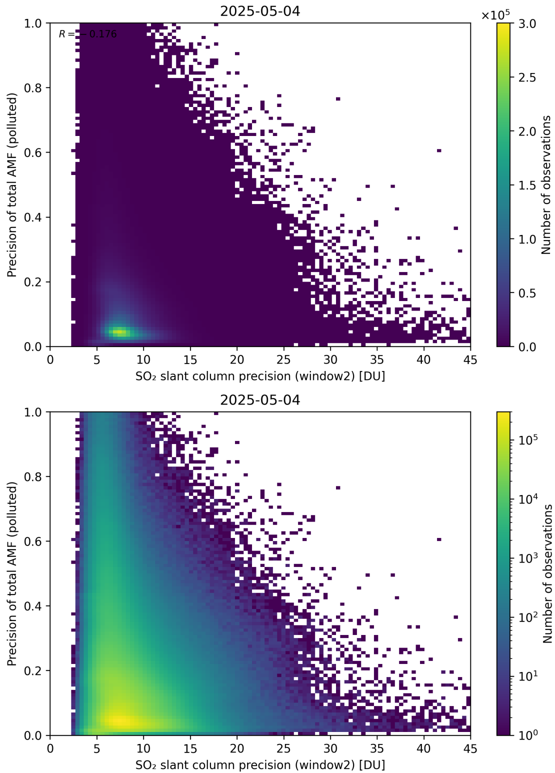
Figure 302: Scatter density plot of “SO 2 slant column precision (window2)” against “Precision of total AMF (polluted)” for 2025-05-03 to 2025-05-05.
