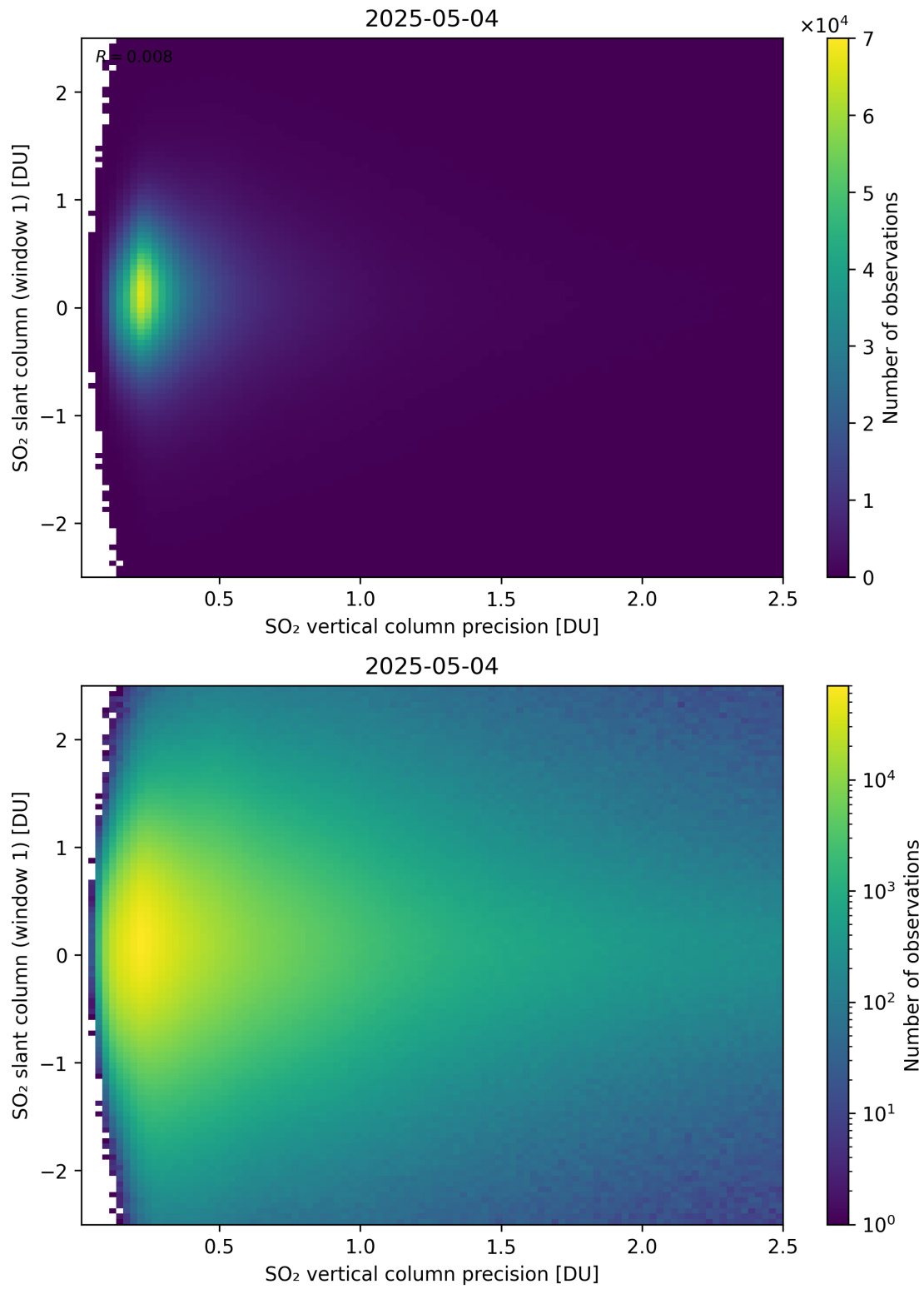
Figure 341: Scatter density plot of “SO 2 vertical column precision” against “SO 2 slant column (window 1)” for 2025-05-03 to 2025-05-05.
