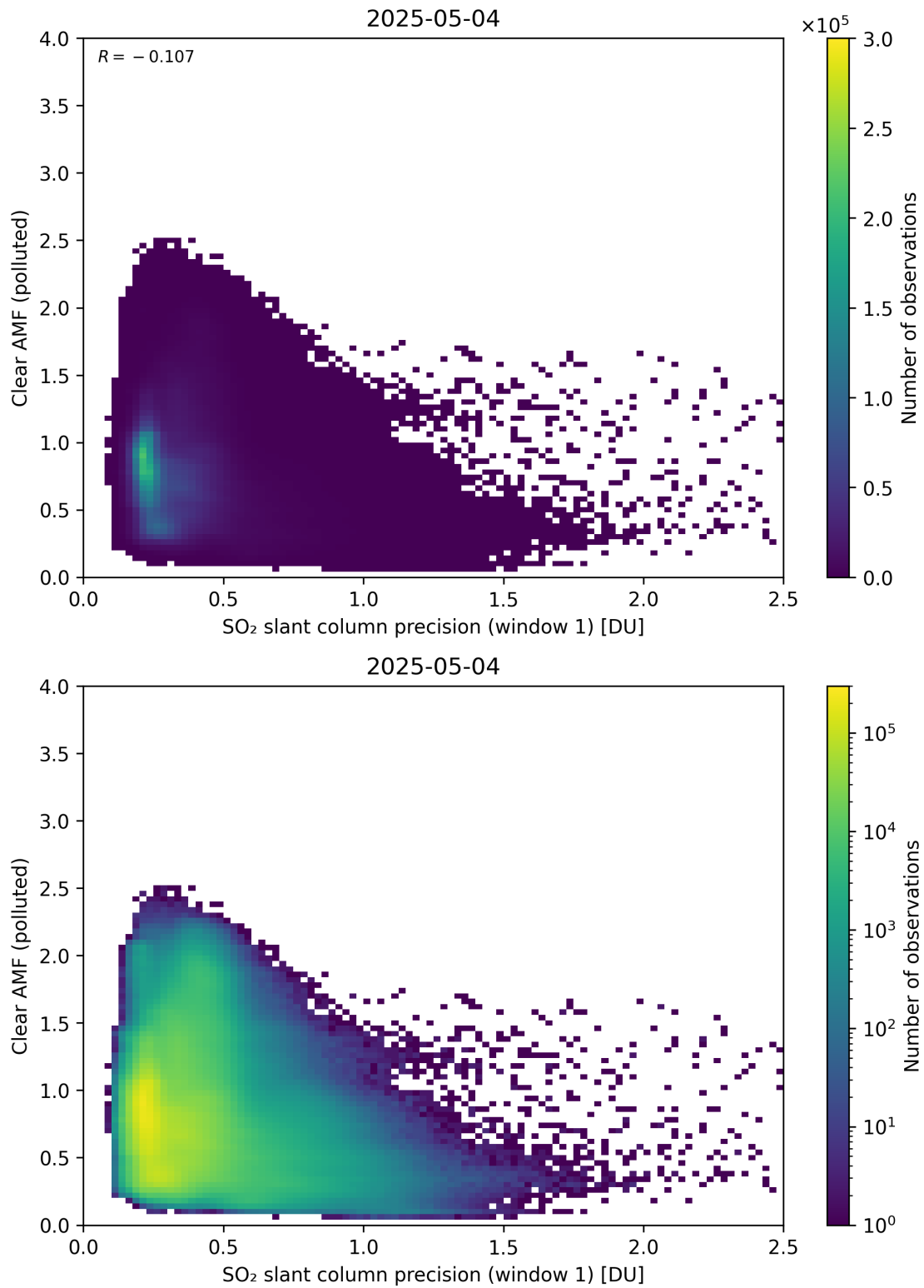
Figure 274: Scatter density plot of “SO 2 slant column precision (window 1)” against “Clear AMF (polluted)” for 2025-05-03 to 2025-05-05.
