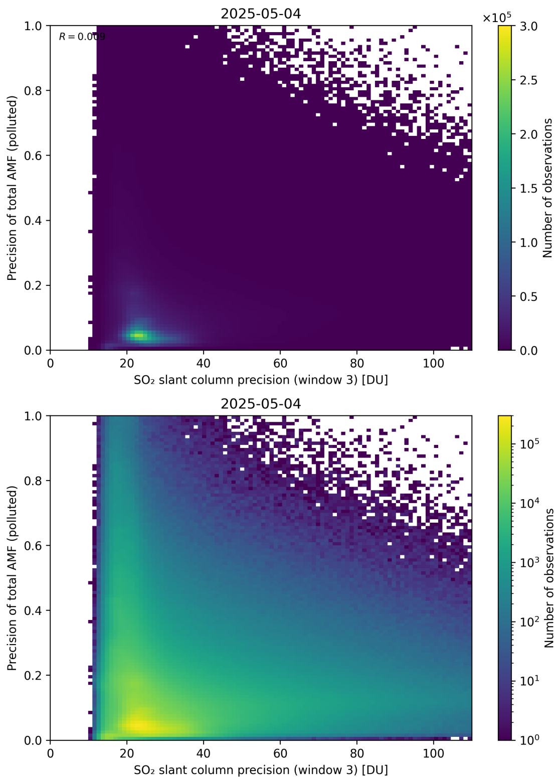
Figure 314: Scatter density plot of “SO 2 slant column precision (window 3)” against “Precision of total AMF (polluted)” for 2025-05-03 to 2025-05-05.
