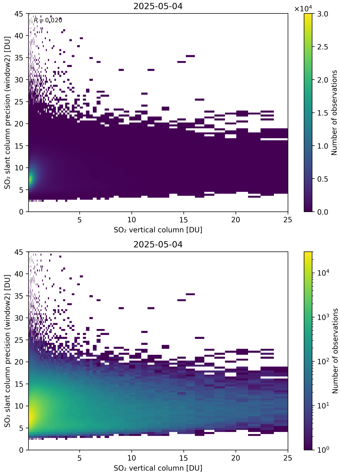
Figure 356: Scatter density plot of “SO 2 vertical column” against “SO 2 slant column precision (window2)” for 2025-05-03 to 2025-05-05.
