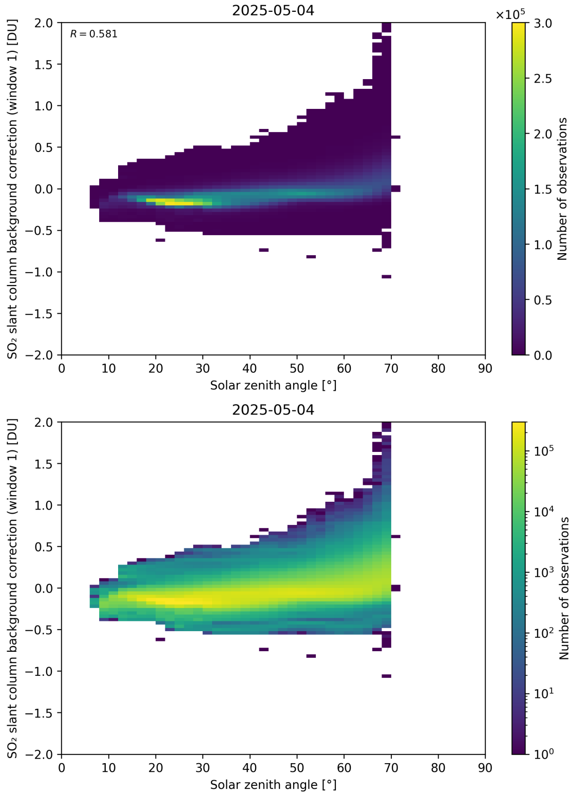
Figure 171: Scatter density plot of “Solar zenith angle” against “SO 2 slant column background correction (window 1)” for 2025-05-03 to 2025-05-05.
