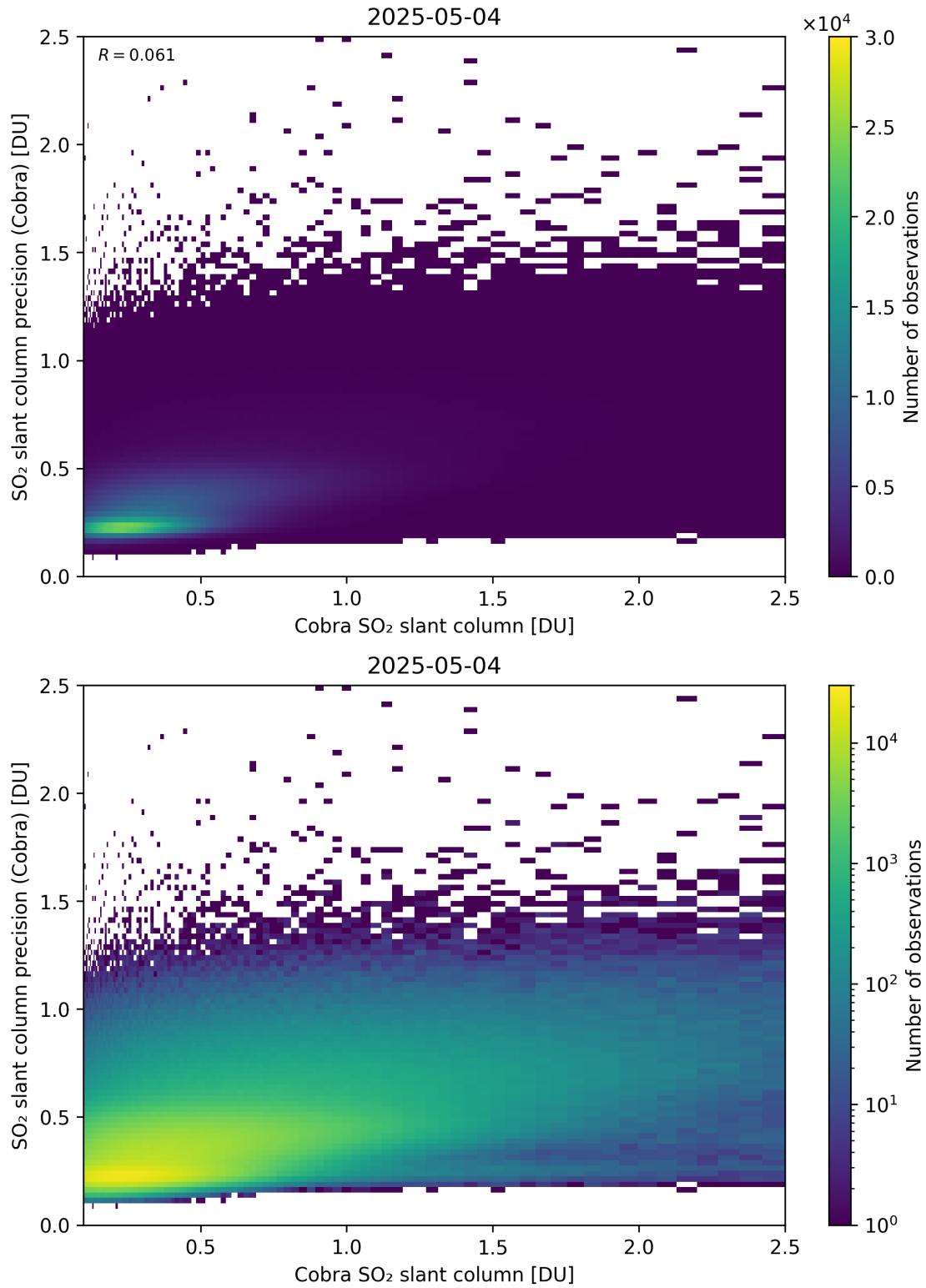
Figure 216: Scatter density plot of “Cobra SO 2 slant column” against “SO 2 slant column precision (Cobra)” for 2025-05-03 to 2025-05-05.
