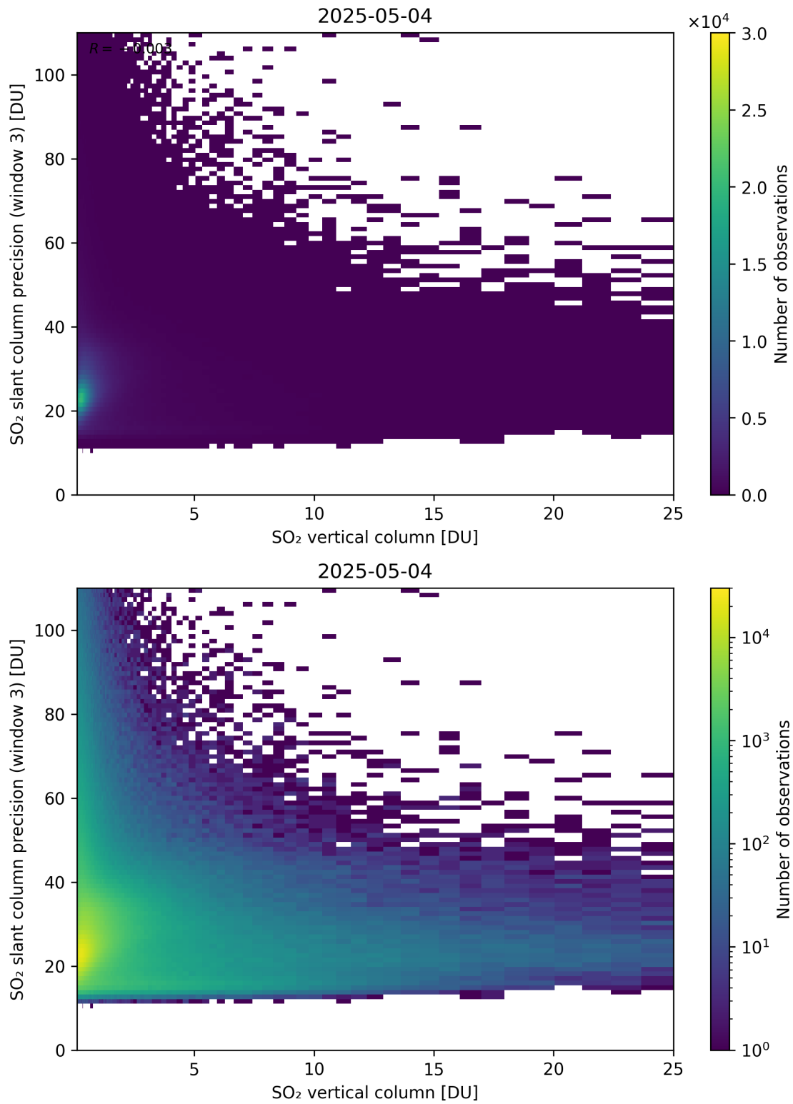
Figure 358: Scatter density plot of “SO 2 vertical column” against “SO 2 slant column precision (window 3)” for 2025-05-03 to 2025-05-05.
