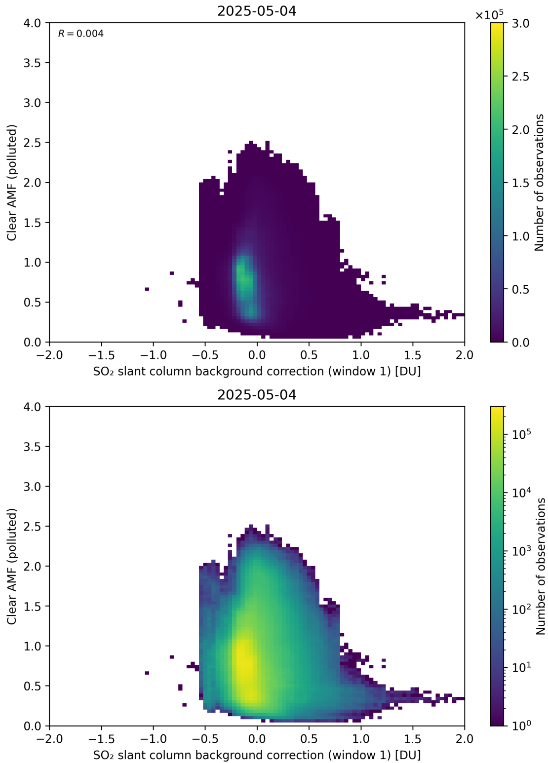
Figure 114: Scatter density plot of “SO 2 slant column background correction (window 1)” against “Clear AMF (polluted)” for 2025-05-03 to 2025-05-05.
