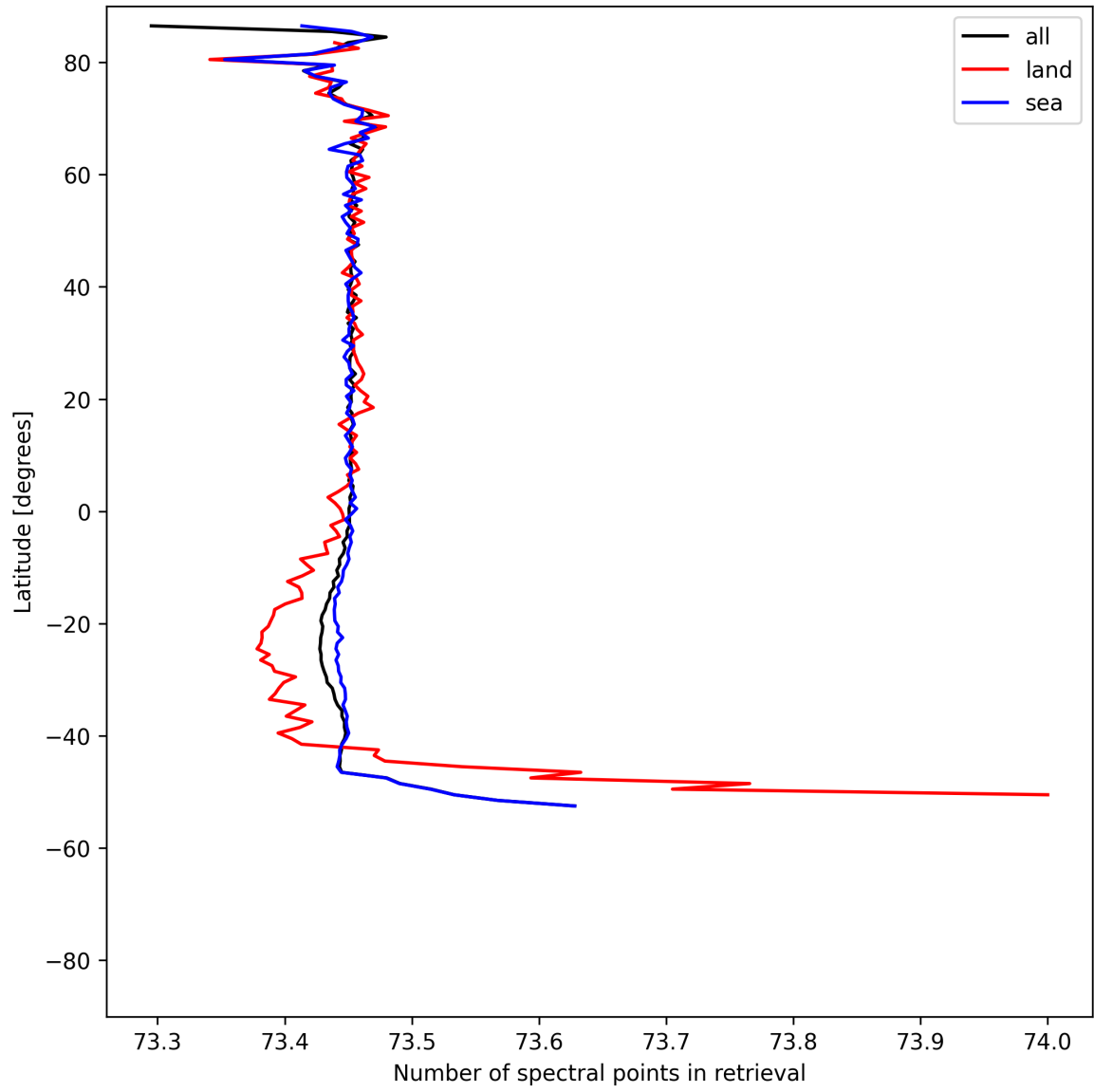
Figure 56: Zonal average of “Number of spectral points in retrieval” for 2025-05-03 to 2025-05-05.
