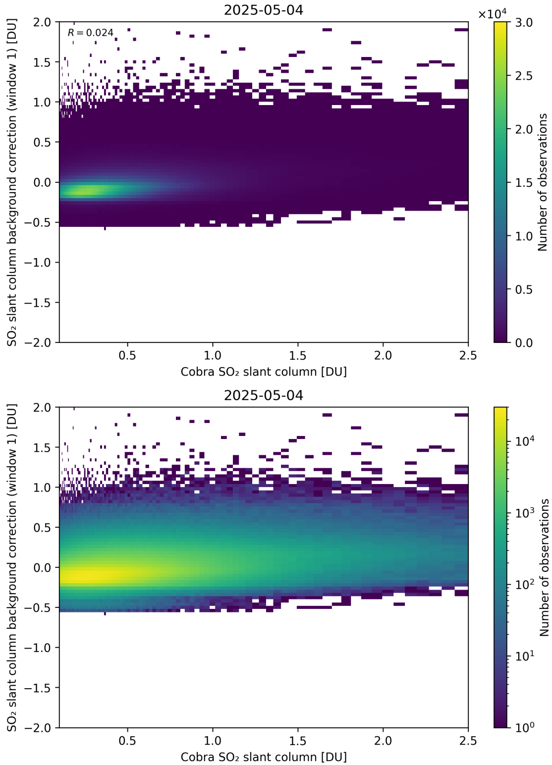
Figure 193: Scatter density plot of “Cobra SO 2 slant column” against “SO 2 slant column background correction (window 1)” for 2025-05-03 to 2025-05-05.
