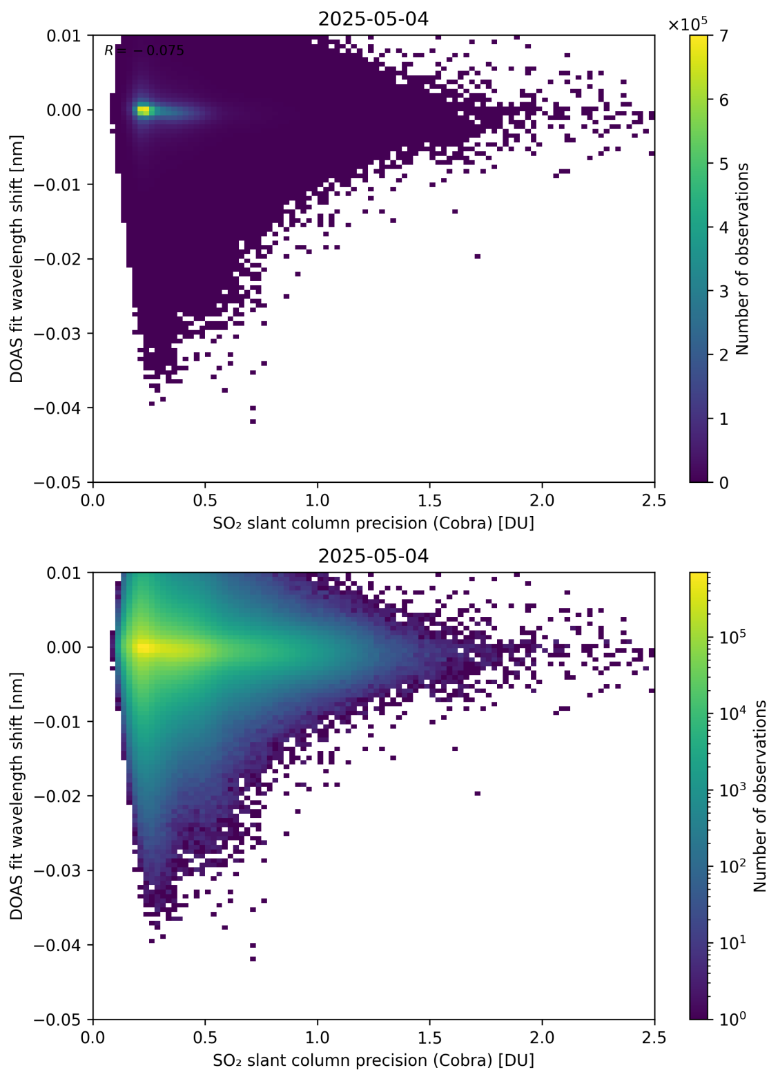
Figure 202: Scatter density plot of “SO 2 slant column precision (Cobra)” against “DOAS fit wavelength shift” for 2025-05-03 to 2025-05-05.
