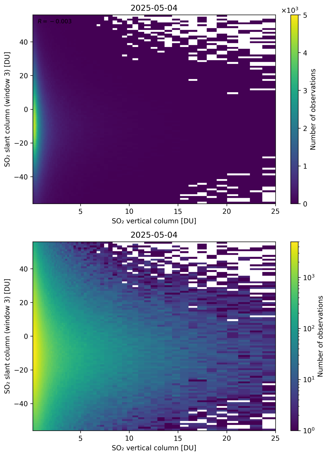
Figure 357: Scatter density plot of “SO 2 vertical column” against “SO 2 slant column (window 3)” for 2025-05-03 to 2025-05-05.
