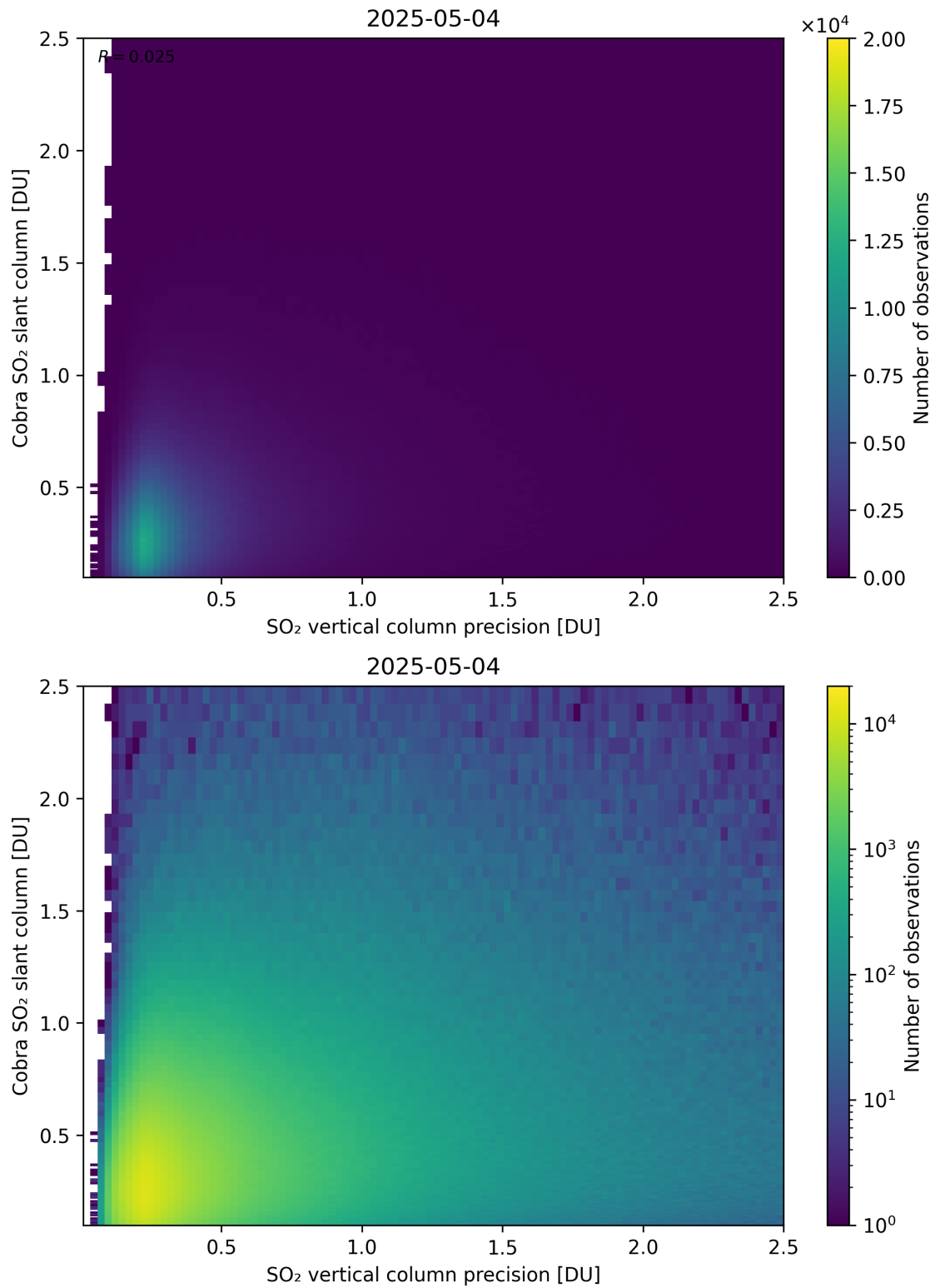
Figure 336: Scatter density plot of “SO 2 vertical column precision” against “Cobra SO 2 slant column” for 2025-05-03 to 2025-05-05.
