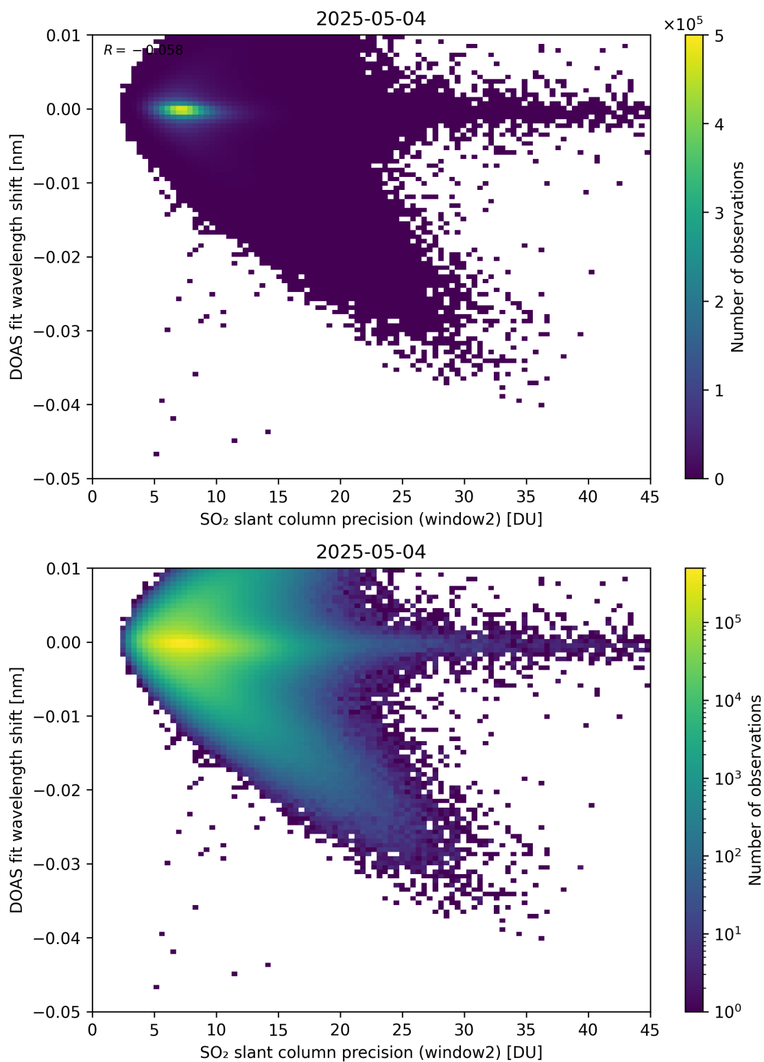
Figure 293: Scatter density plot of “SO 2 slant column precision (window2)” against “DOAS fit wavelength shift” for 2025-05-03 to 2025-05-05.
