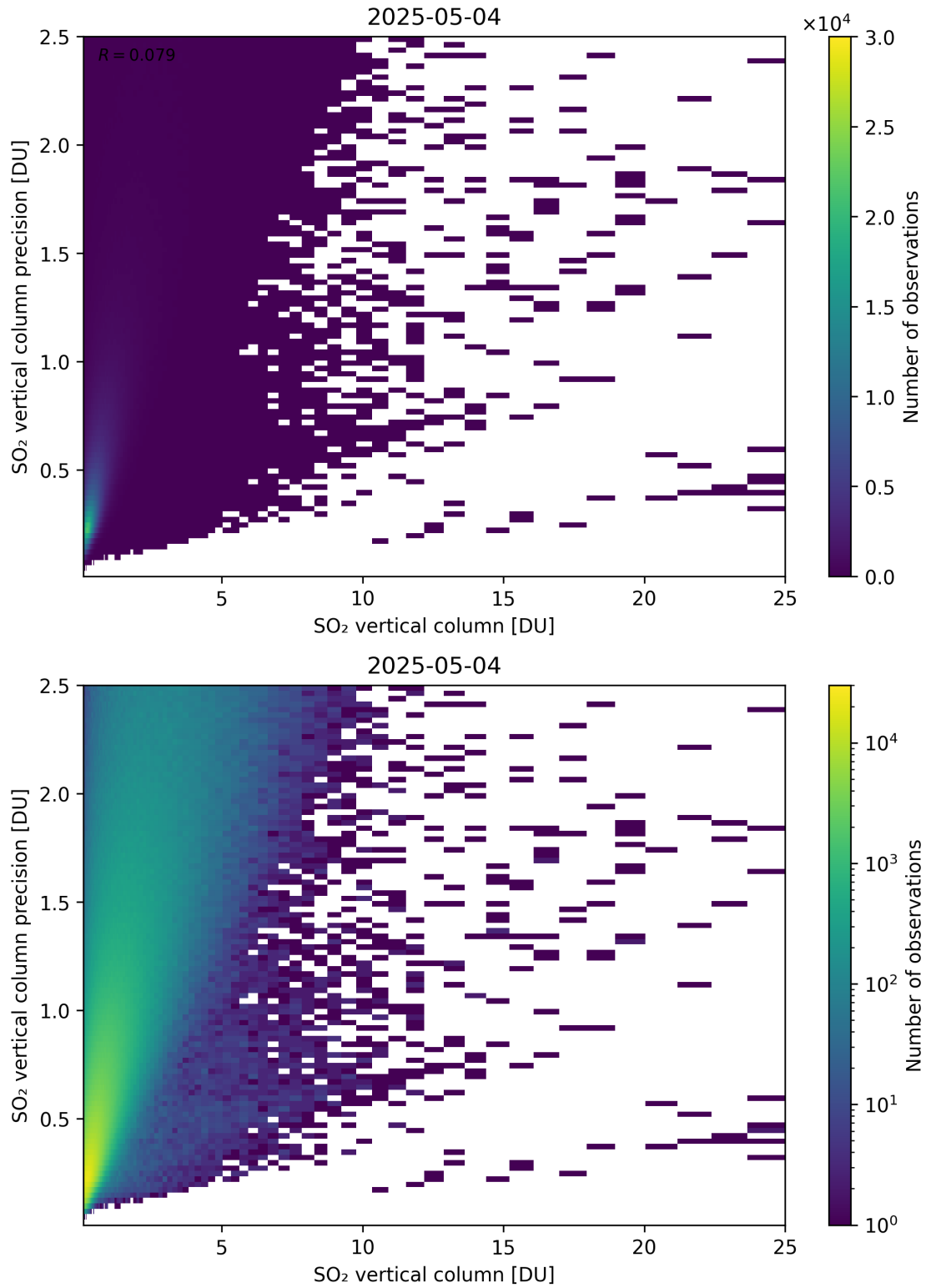
Figure 361: Scatter density plot of “SO 2 vertical column” against “SO 2 vertical column precision” for 2025-05-03 to 2025-05-05.
