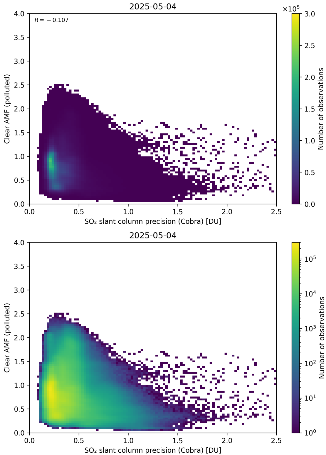
Figure 205: Scatter density plot of “SO 2 slant column precision (Cobra)” against “Clear AMF (polluted)” for 2025-05-03 to 2025-05-05.
