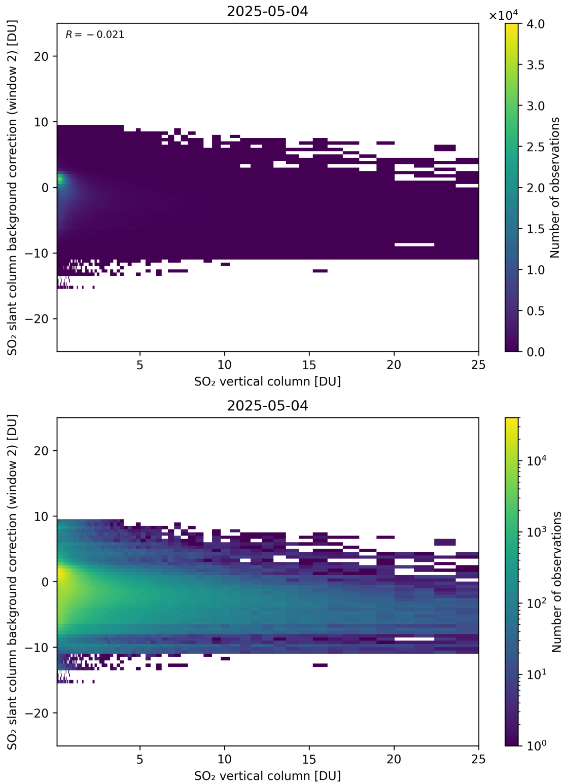
Figure 324: Scatter density plot of “SO 2 vertical column” against “SO 2 slant column background correction (window 2)” for 2025-05-03 to 2025-05-05.
