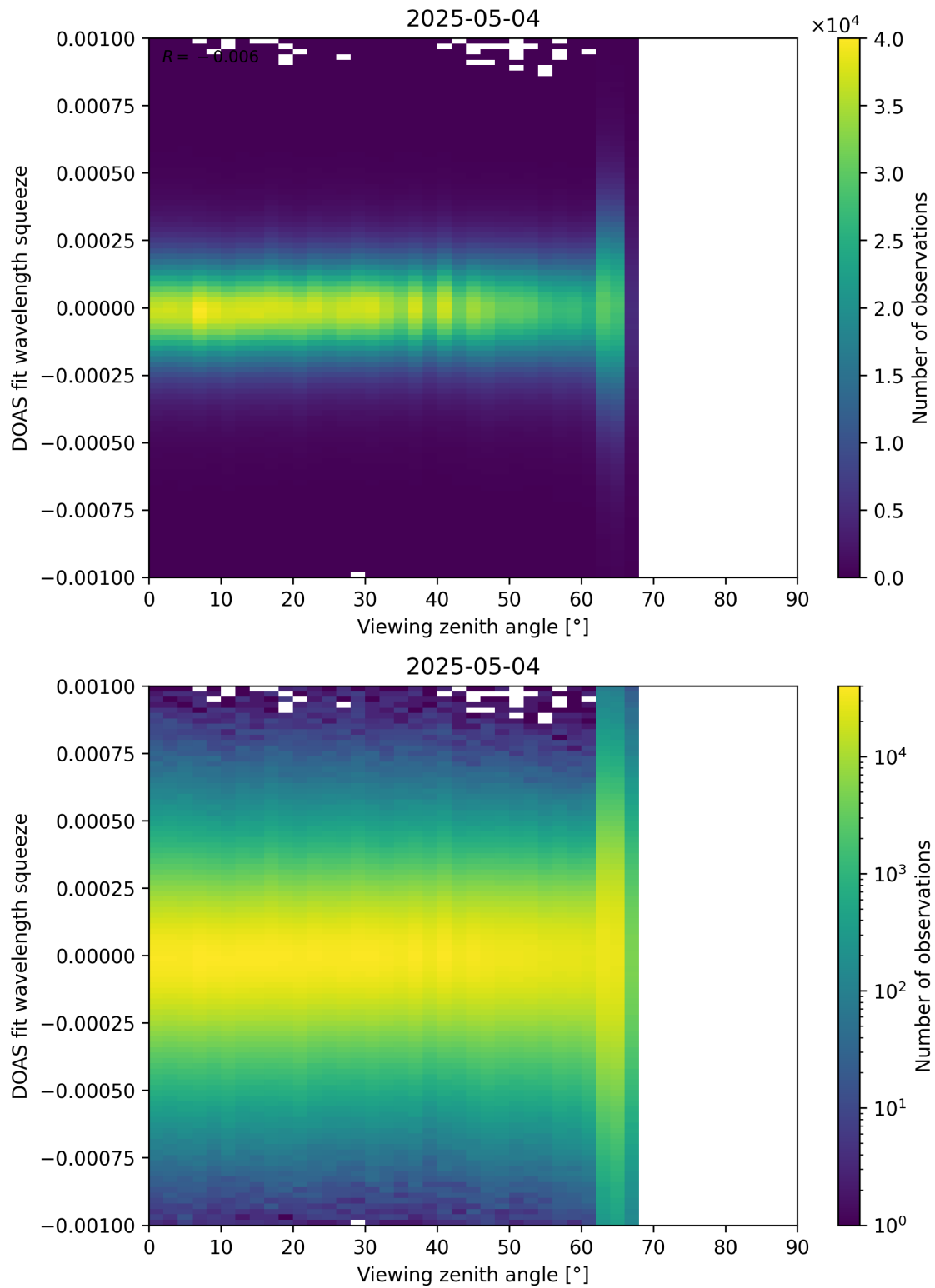
Figure 366: Scatter density plot of “Viewing zenith angle” against “DOAS fit wavelength squeeze” for 2025-05-03 to 2025-05-05.
