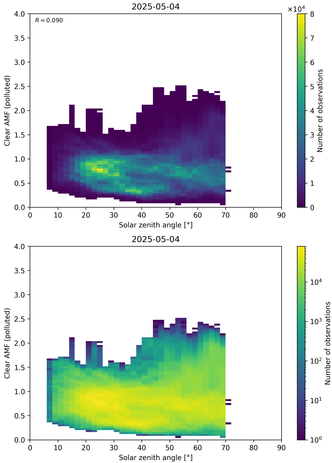
Figure 178: Scatter density plot of “Solar zenith angle” against “Clear AMF (polluted)” for 2025-05-03 to 2025-05-05.
