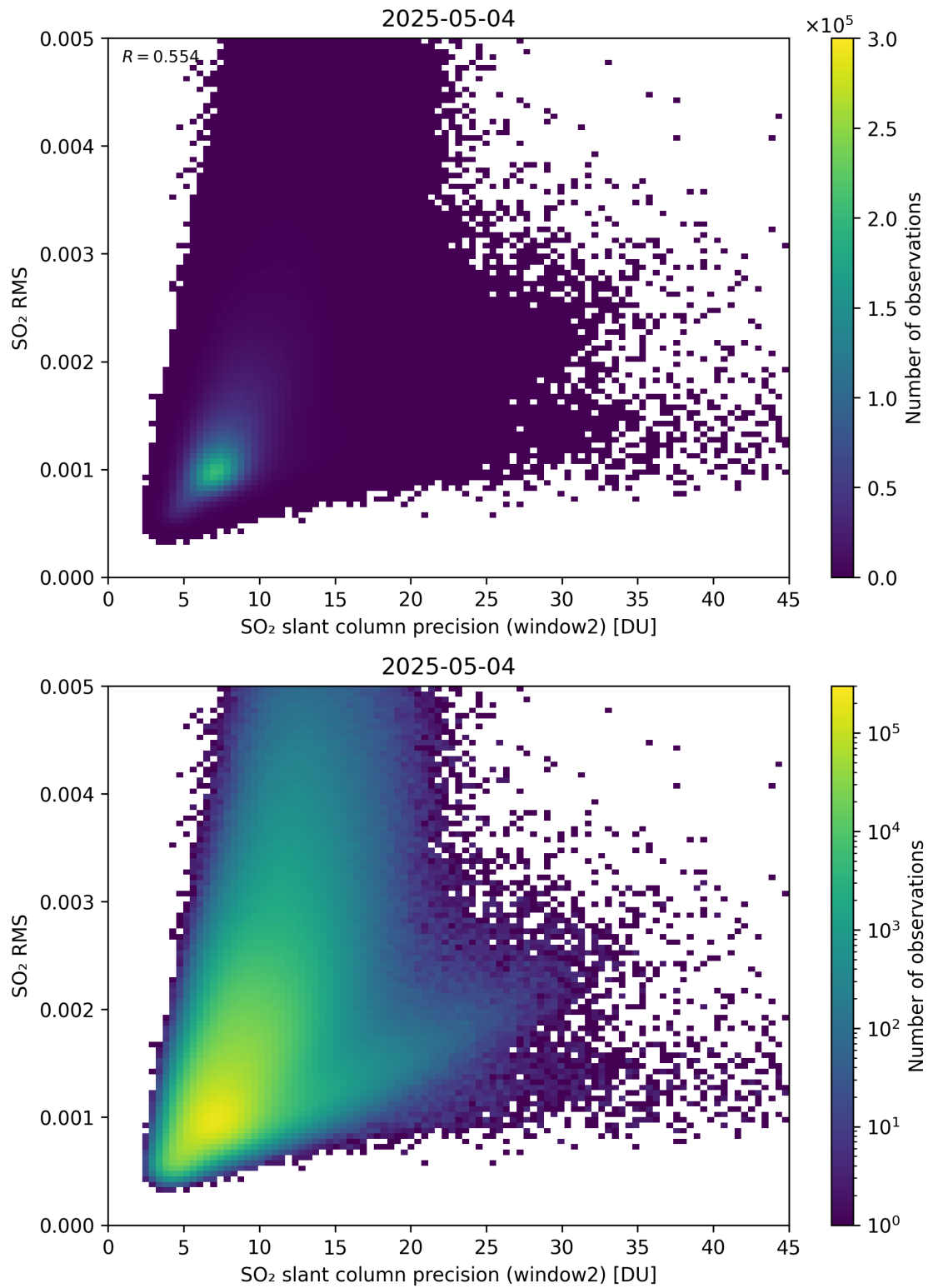
Figure 295: Scatter density plot of “SO 2 slant column precision (window2)” against “SO 2 RMS” for 2025-05-03 to 2025-05-05.
