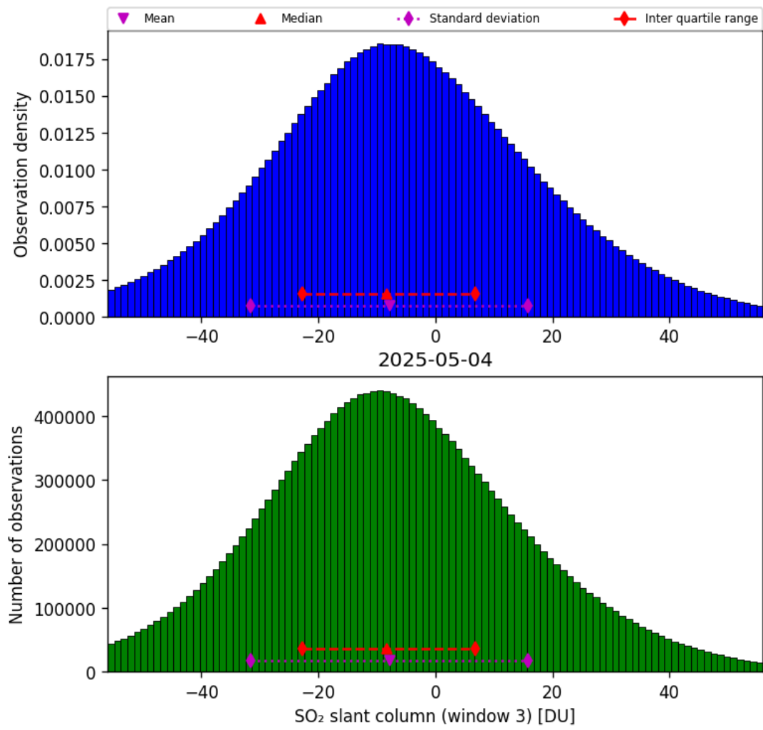
Figure 71: Histogram of “SO 2 slant column (window 3)” for 2025-05-03 to 2025-05-05
