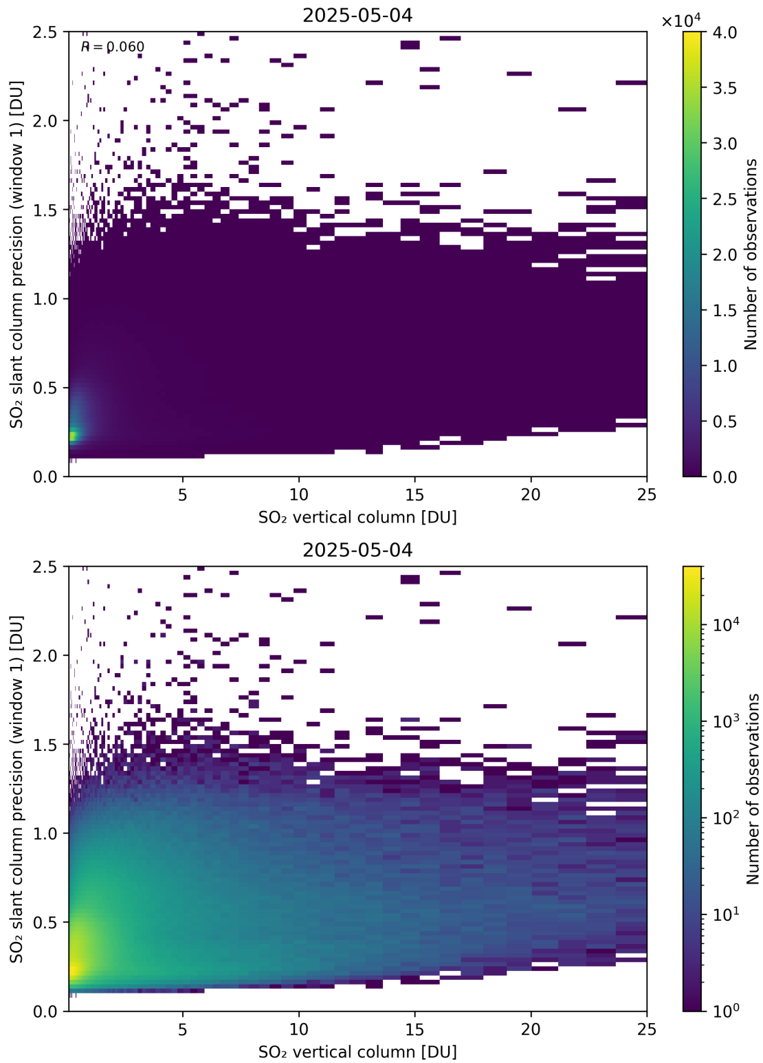
Figure 355: Scatter density plot of “SO 2 vertical column” against “SO 2 slant column precision (window 1)” for 2025-05-03 to 2025-05-05.
