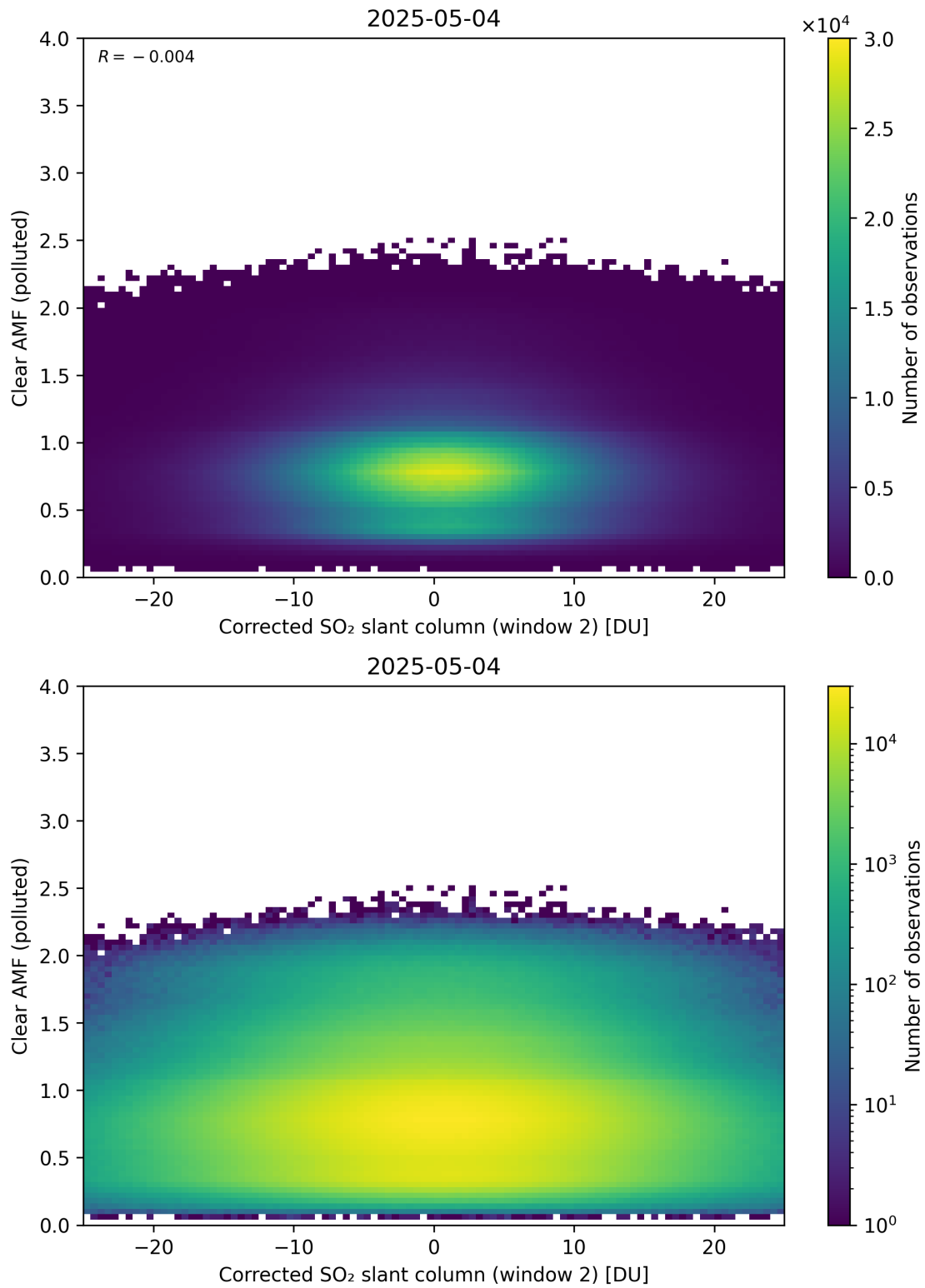
Figure 249: Scatter density plot of “Corrected SO 2 slant column (window 2)” against “Clear AMF (polluted)” for 2025-05-03 to 2025-05-05.
