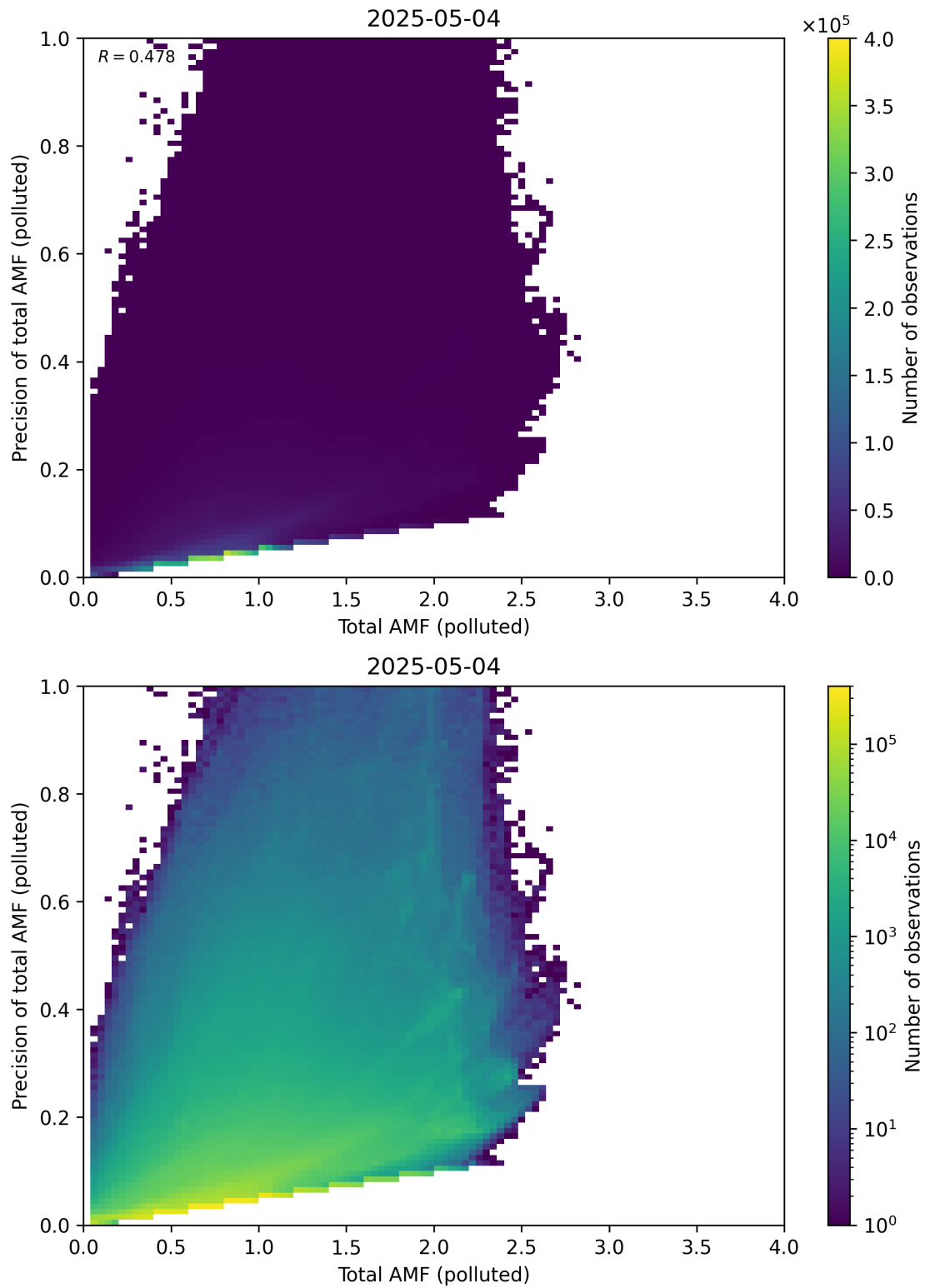
Figure 322: Scatter density plot of “Total AMF (polluted)” against “Precision of total AMF (polluted)” for 2025-05-03 to 2025-05-05.
