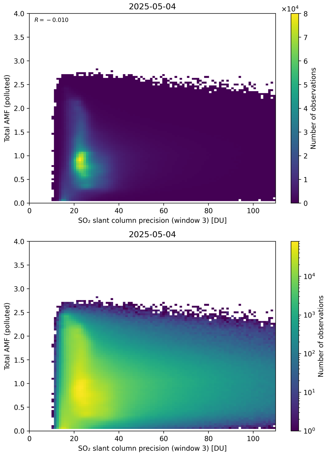
Figure 313: Scatter density plot of “SO 2 slant column precision (window 3)” against “Total AMF (polluted)” for 2025-05-03 to 2025-05-05.
