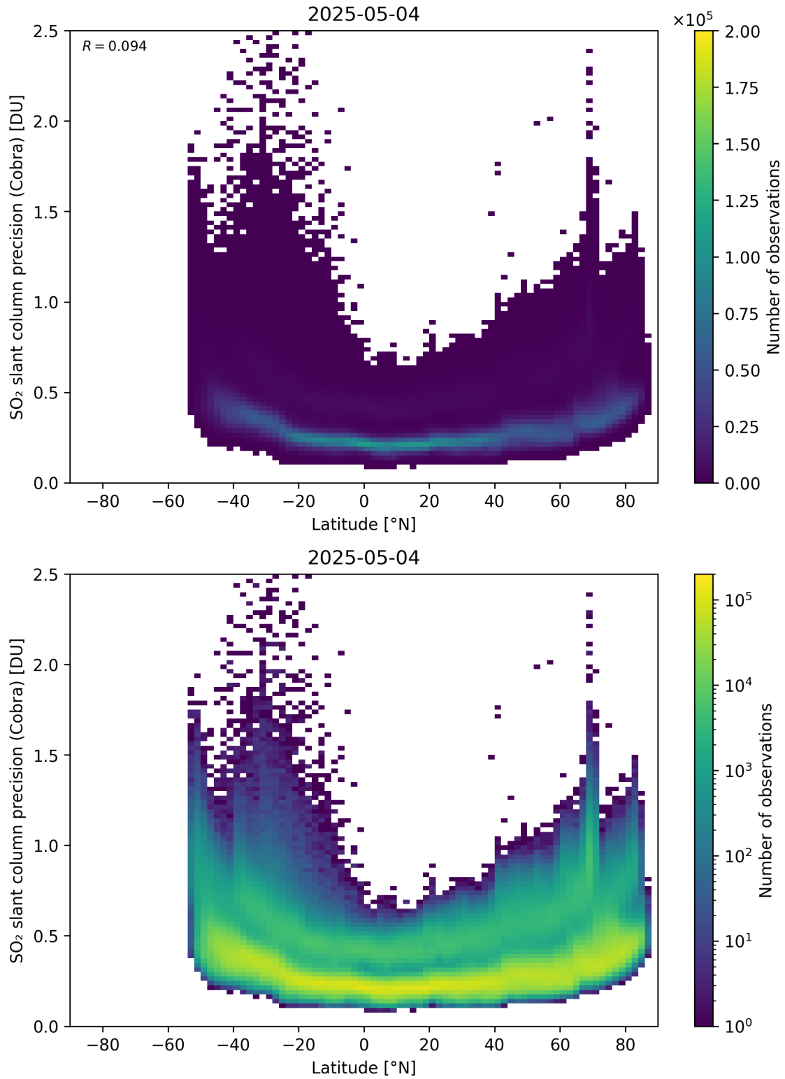
Figure 158: Scatter density plot of “Latitude” against “SO 2 slant column precision (Cobra)” for 2025-05-03 to 2025-05-05.
