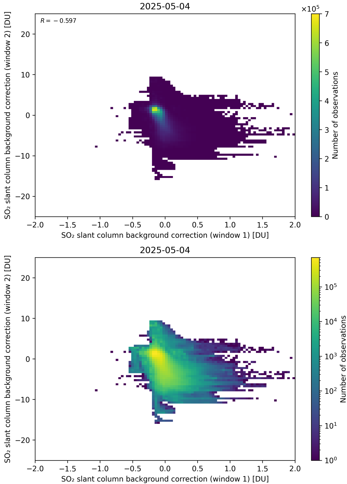
Figure 109: Scatter density plot of “SO 2 slant column background correction (window 1)” against “SO 2 slant column background correction (window 2)” for 2025-05-03 to 2025-05-05.
