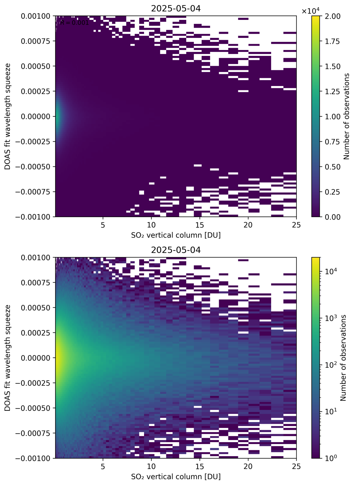
Figure 327: Scatter density plot of “SO 2 vertical column” against “DOAS fit wavelength squeeze” for 2025-05-03 to 2025-05-05.
