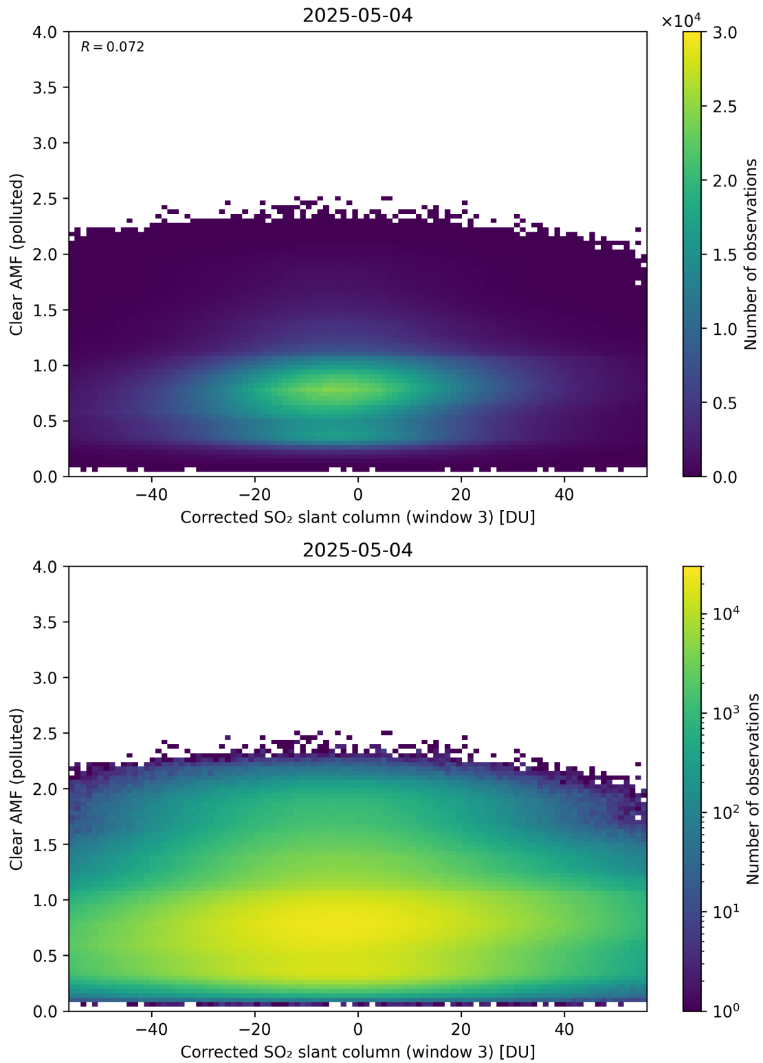
Figure 259: Scatter density plot of “Corrected SO 2 slant column (window 3)” against “Clear AMF (polluted)” for 2025-05-03 to 2025-05-05.
