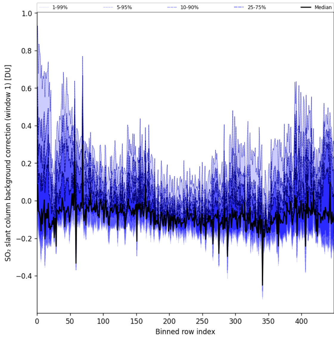
Figure 92: Along track statistics of “SO 2 slant column background correction (window 1)” for 2025-05-03 to 2025-05-05
