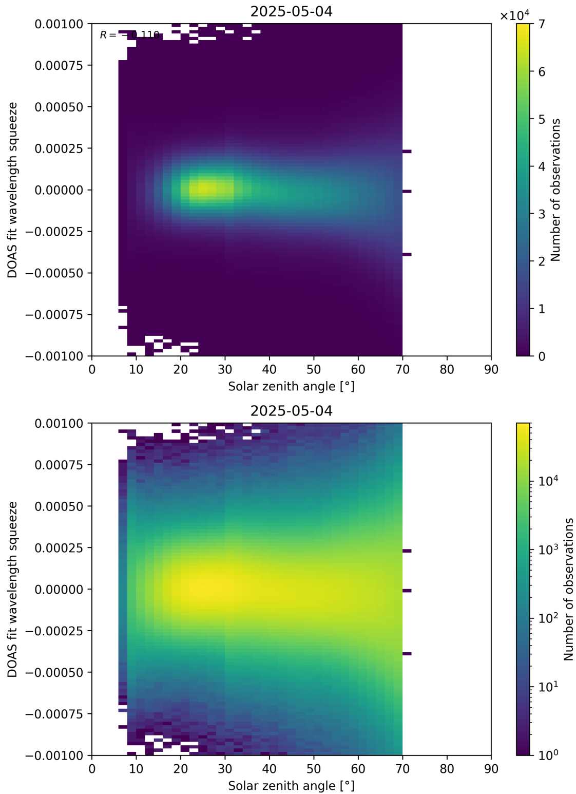
Figure 175: Scatter density plot of “Solar zenith angle” against “DOAS fit wavelength squeeze” for 2025-05-03 to 2025-05-05.
