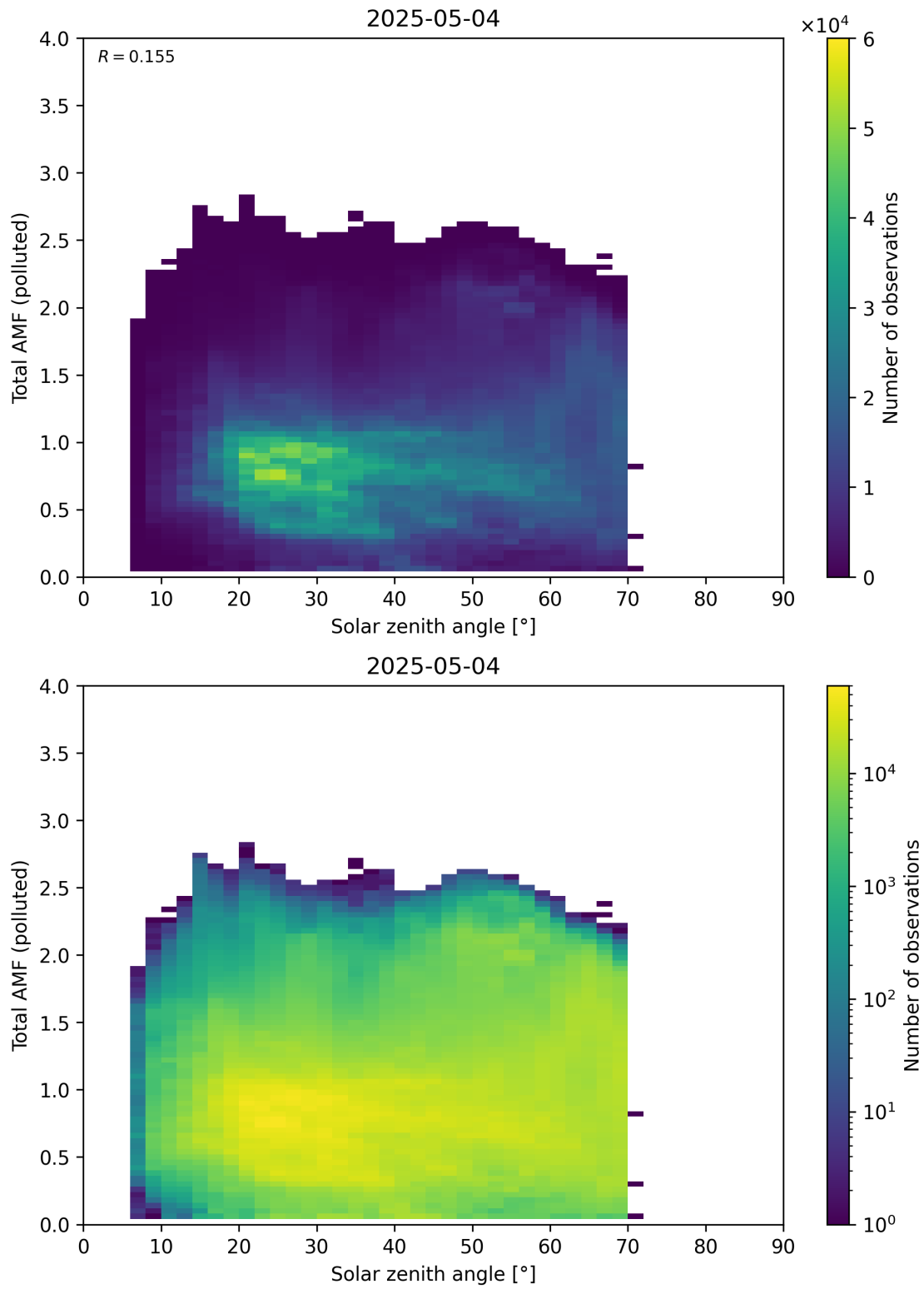
Figure 189: Scatter density plot of “Solar zenith angle” against “Total AMF (polluted)” for 2025-05-03 to 2025-05-05.
