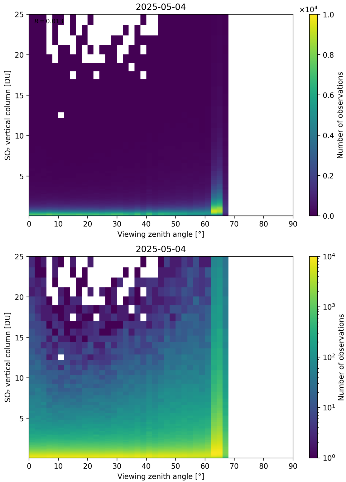
Figure 383: Scatter density plot of “Viewing zenith angle” against “SO 2 vertical column” for 2025-05-03 to 2025-05-05.
