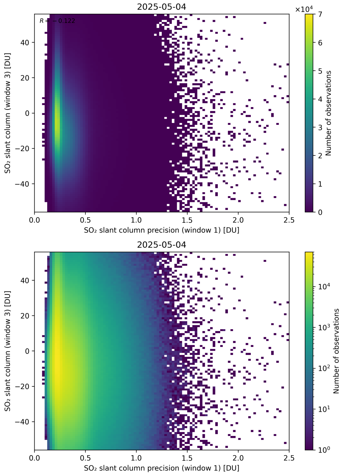
Figure 278: Scatter density plot of “SO 2 slant column precision (window 1)” against “SO 2 slant column (window 3)” for 2025-05-03 to 2025-05-05.
