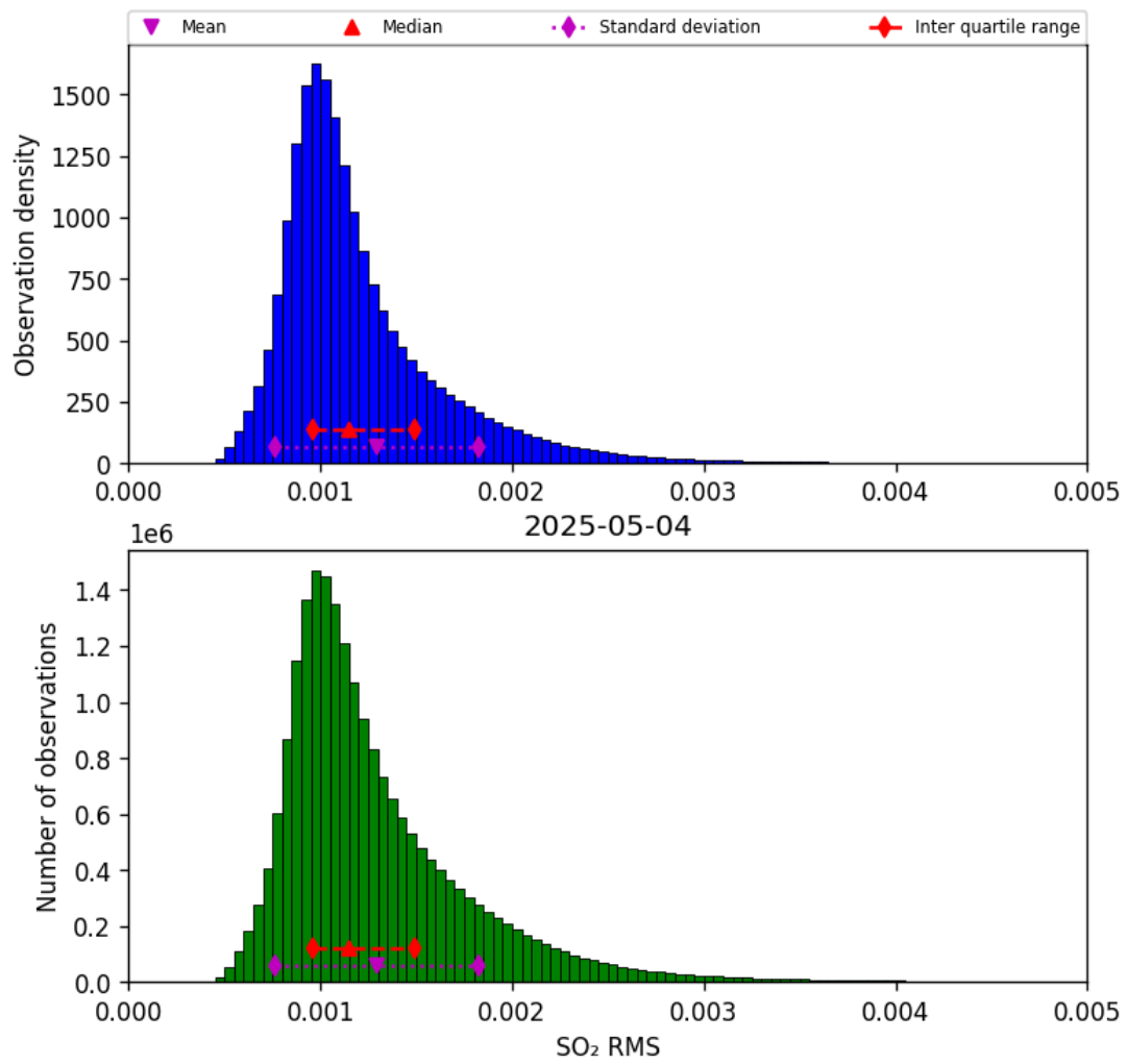
Figure 78: Histogram of “SO 2 RMS” for 2025-05-03 to 2025-05-05
