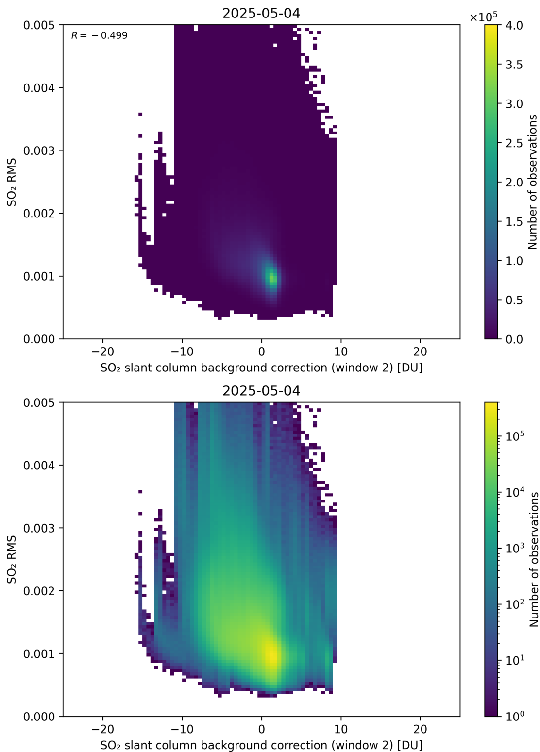
Figure 125: Scatter density plot of “SO 2 slant column background correction (window 2)” against “SO 2 RMS” for 2025-05-03 to 2025-05-05.
