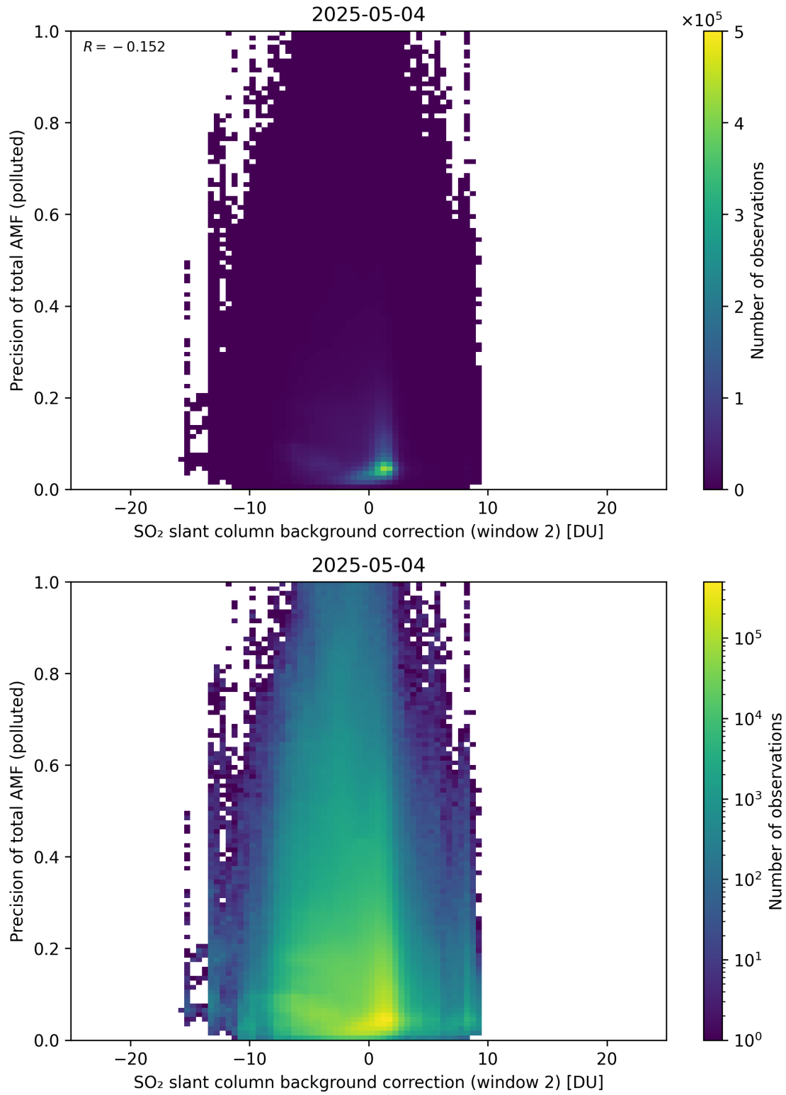
Figure 131: Scatter density plot of “SO 2 slant column background correction (window 2)” against “Precision of total AMF (polluted)” for 2025-05-03 to 2025-05-05.
