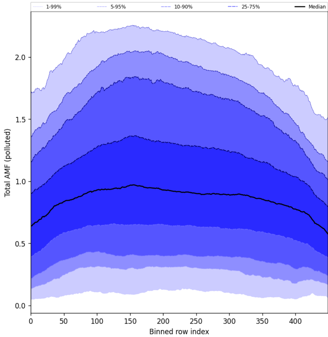
Figure 105: Along track statistics of “Total AMF (polluted)” for 2025-05-03 to 2025-05-05
