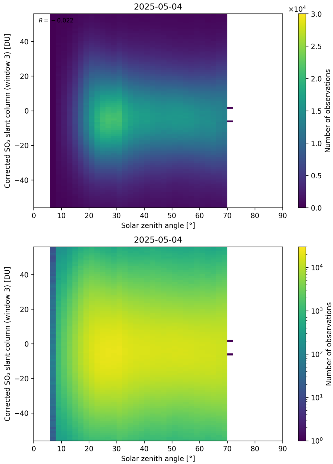
Figure 183: Scatter density plot of “Solar zenith angle” against “Corrected SO 2 slant column (window 3)” for 2025-05-03 to 2025-05-05.
