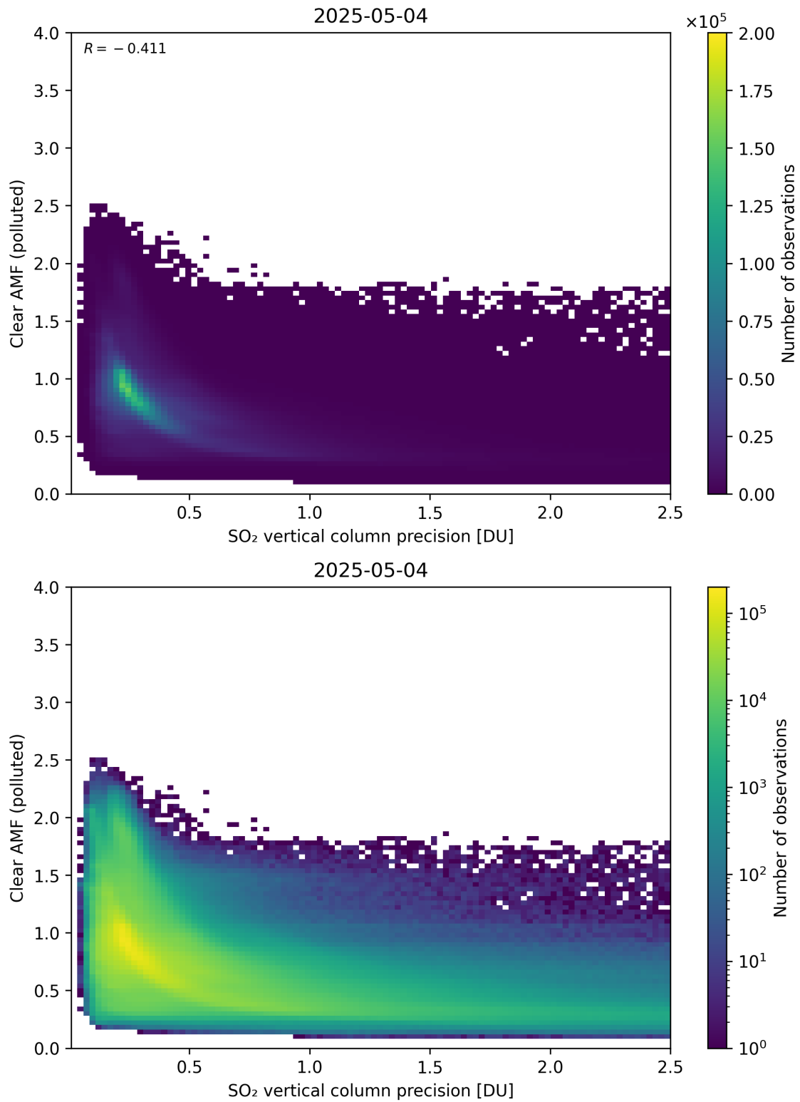
Figure 335: Scatter density plot of “SO 2 vertical column precision” against “Clear AMF (polluted)” for 2025-05-03 to 2025-05-05.
