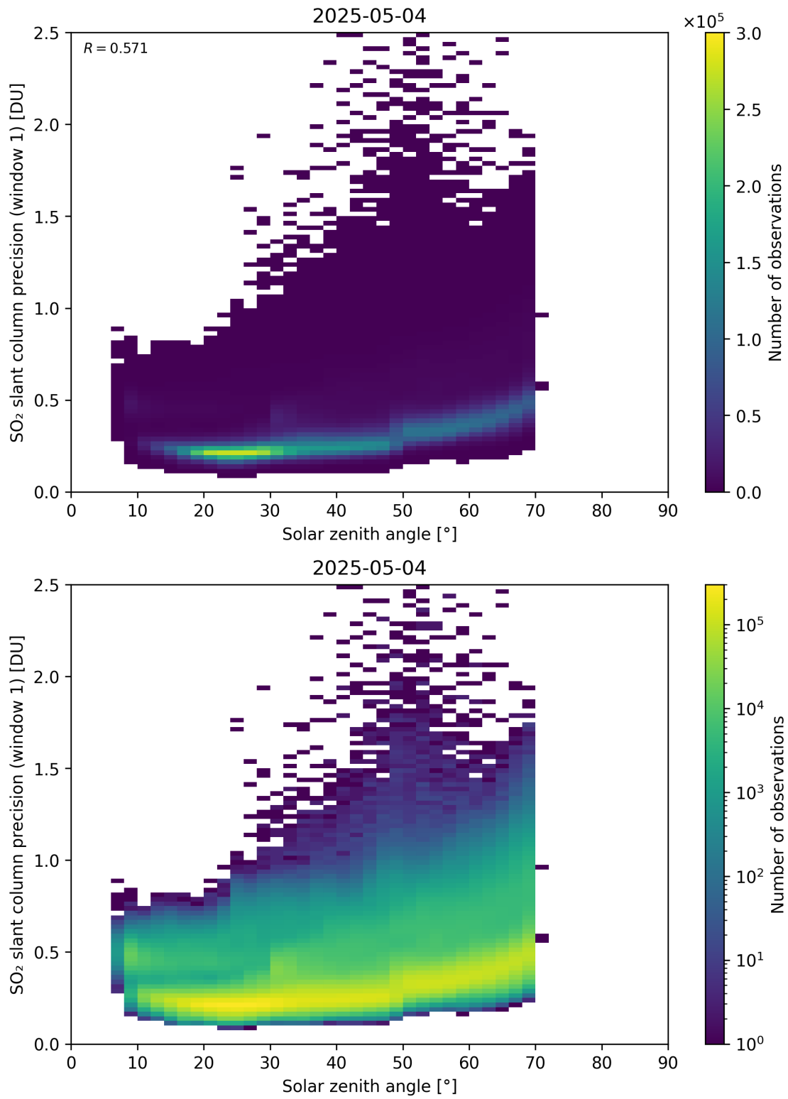
Figure 185: Scatter density plot of “Solar zenith angle” against “SO 2 slant column precision (window 1)” for 2025-05-03 to 2025-05-05.
