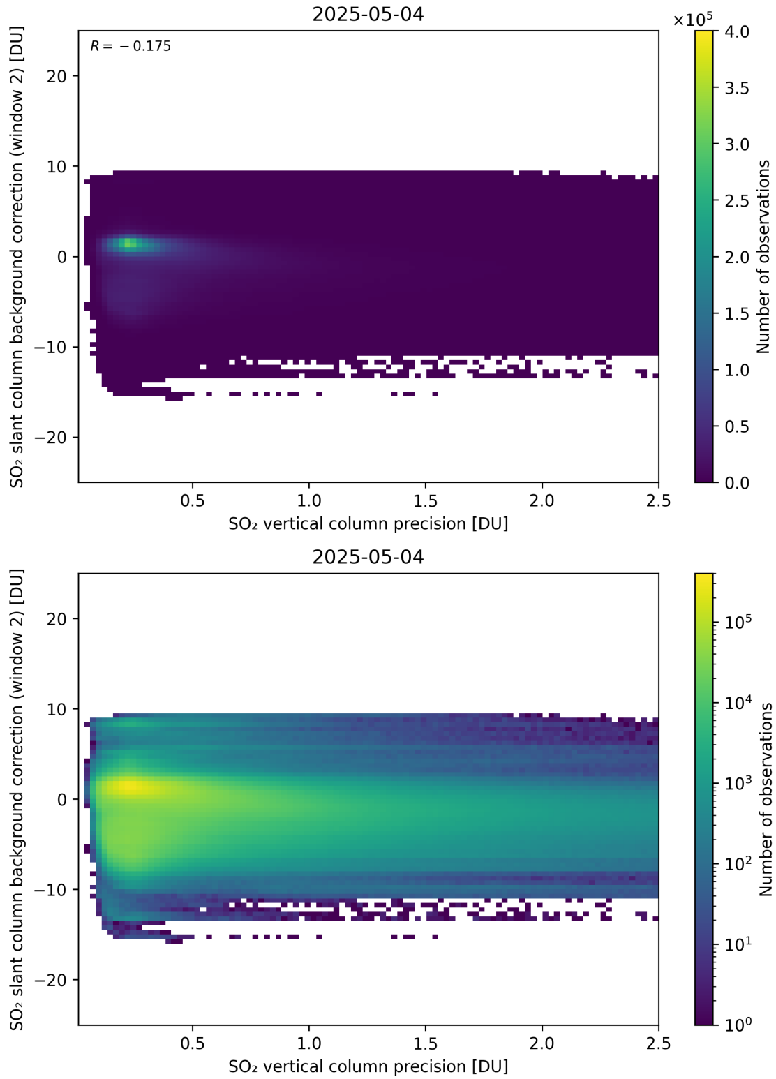
Figure 330: Scatter density plot of “SO 2 vertical column precision” against “SO 2 slant column background correction (window 2)” for 2025-05-03 to 2025-05-05.
