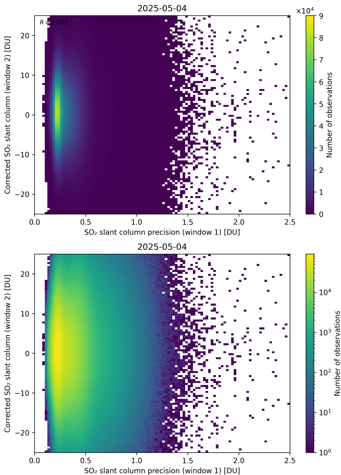
Figure 275: Scatter density plot of “SO 2 slant column precision (window 1)” against “Corrected SO 2 slant column (window 2)” for 2025-05-03 to 2025-05-05.
