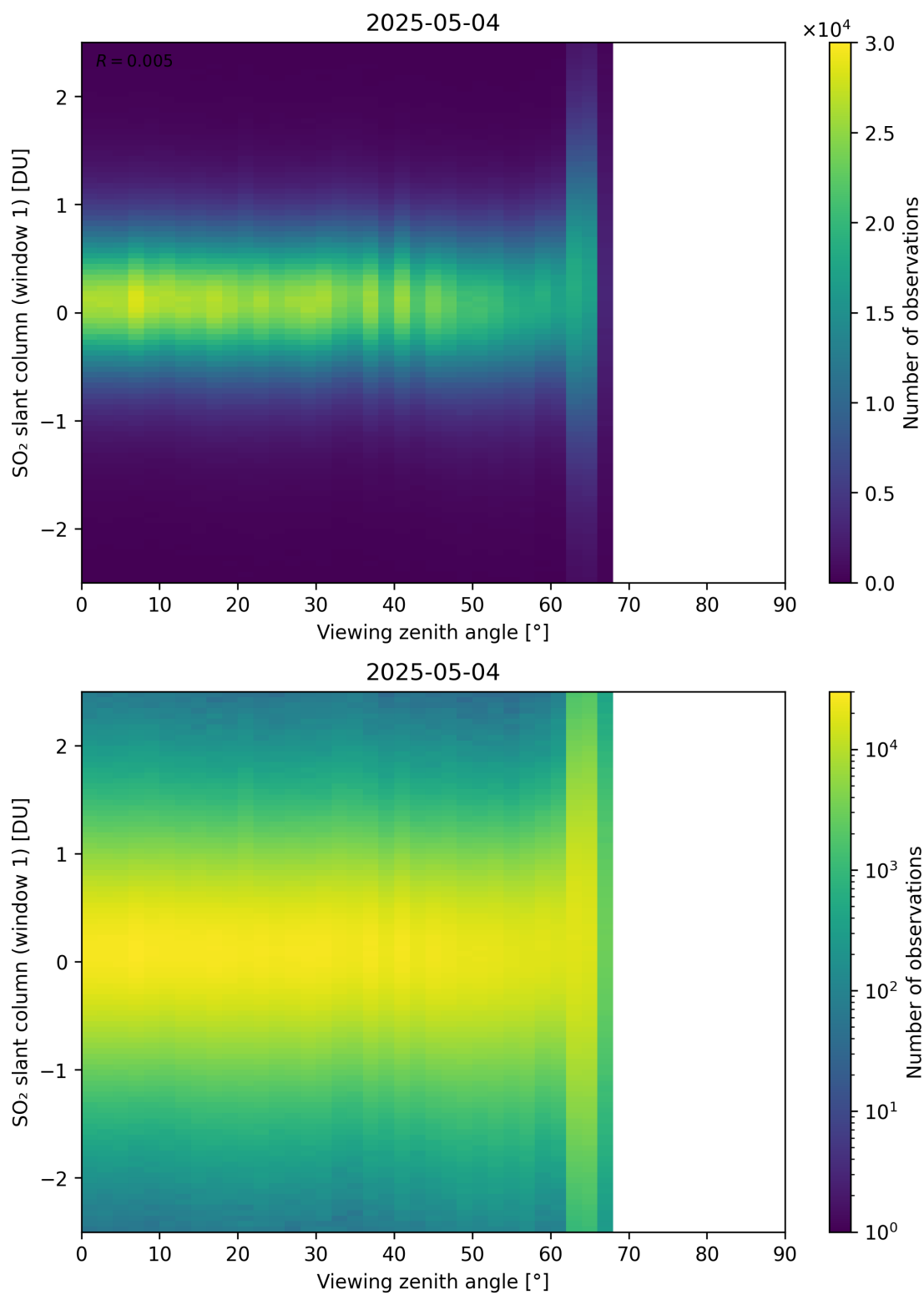
Figure 376: Scatter density plot of “Viewing zenith angle” against “SO 2 slant column (window 1)” for 2025-05-03 to 2025-05-05.
