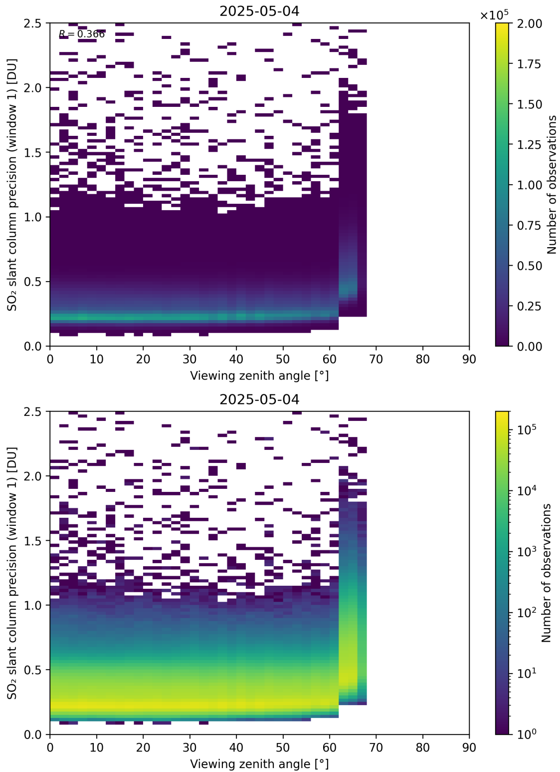
Figure 377: Scatter density plot of “Viewing zenith angle” against “SO 2 slant column precision (window 1)” for 2025-05-03 to 2025-05-05.
