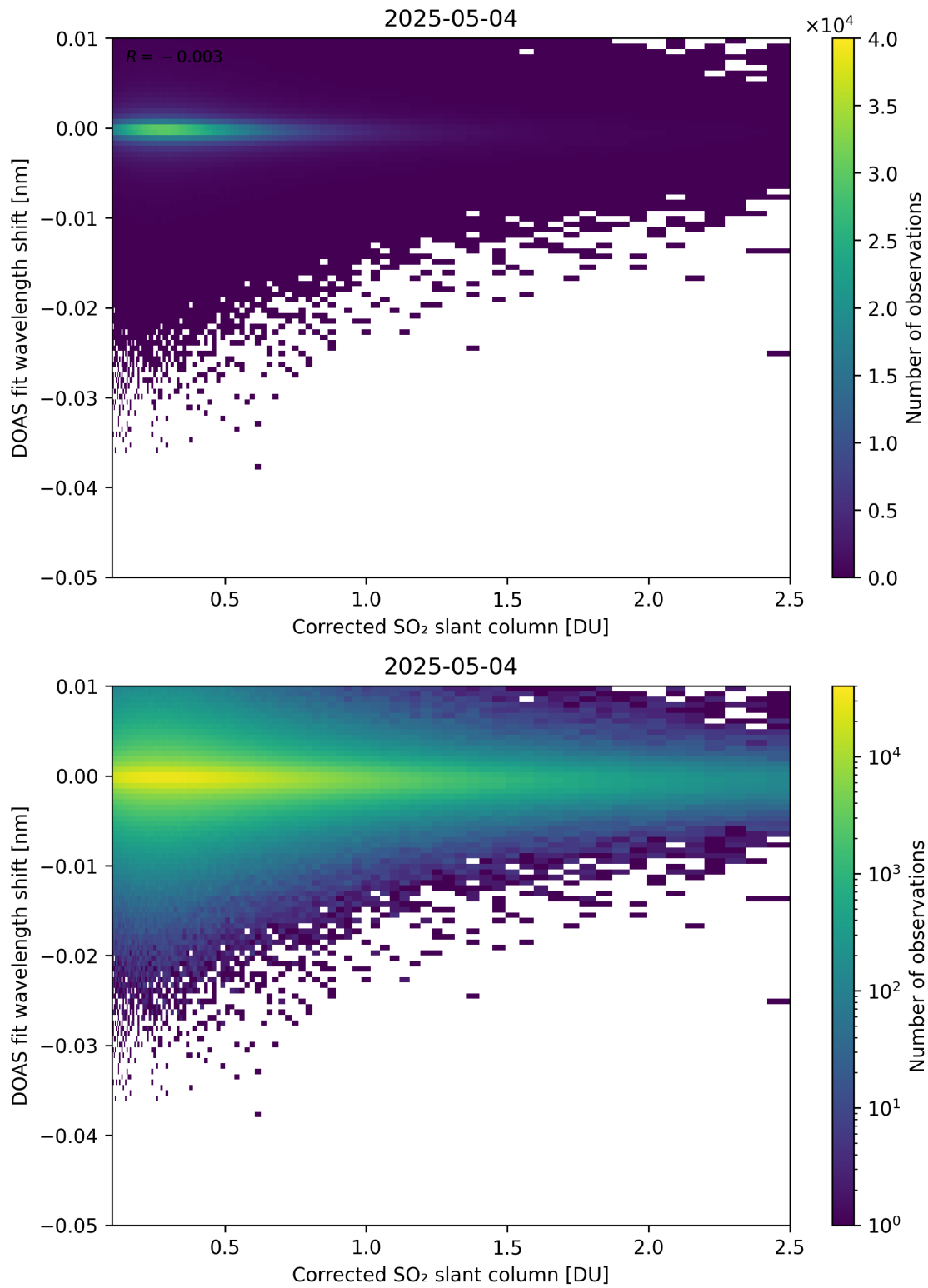
Figure 229: Scatter density plot of “Corrected SO 2 slant column” against “DOAS fit wavelength shift” for 2025-05-03 to 2025-05-05.
