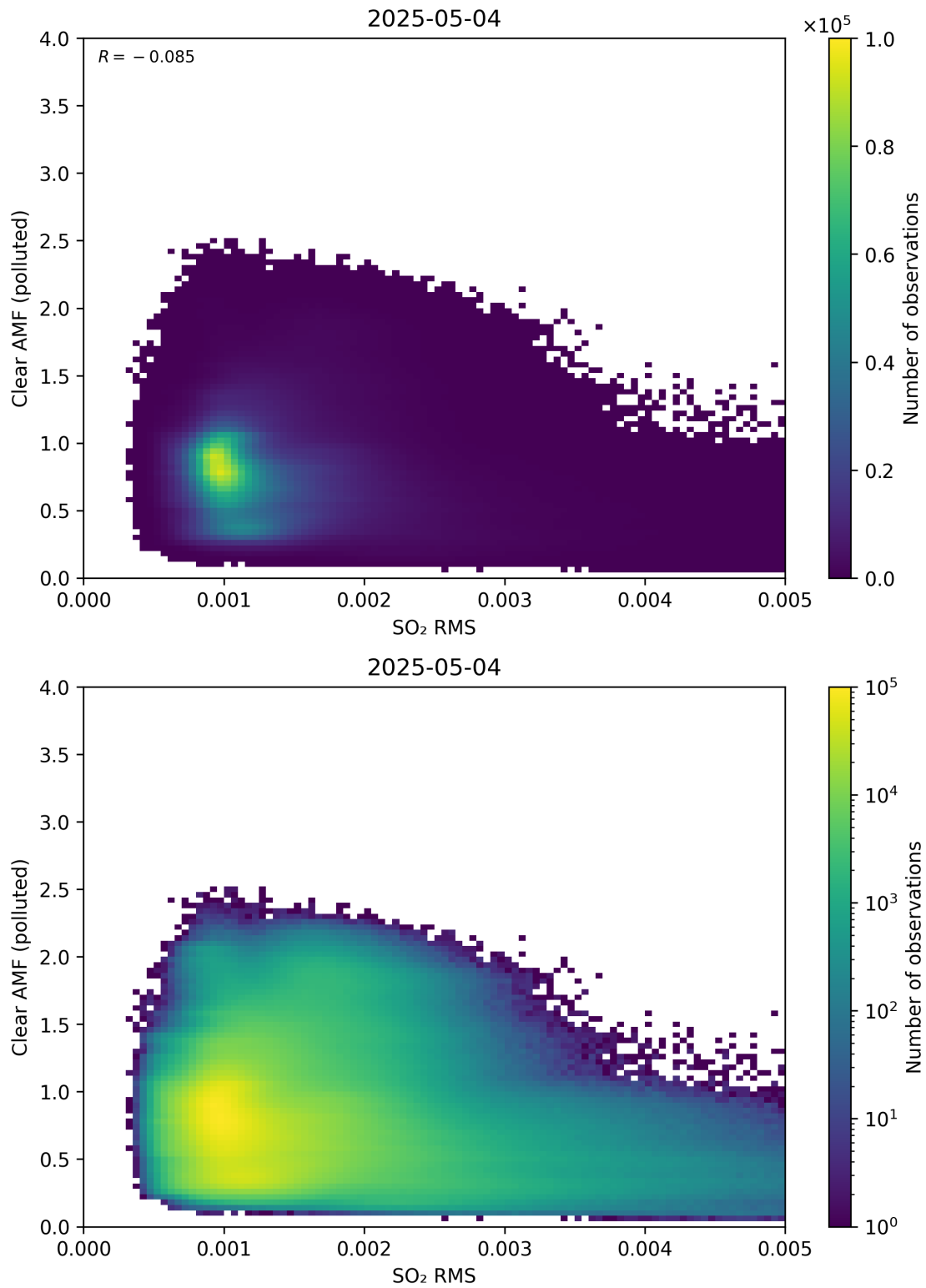
Figure 147: Scatter density plot of “SO 2 RMS” against “Clear AMF (polluted)” for 2025-05-03 to 2025-05-05.
