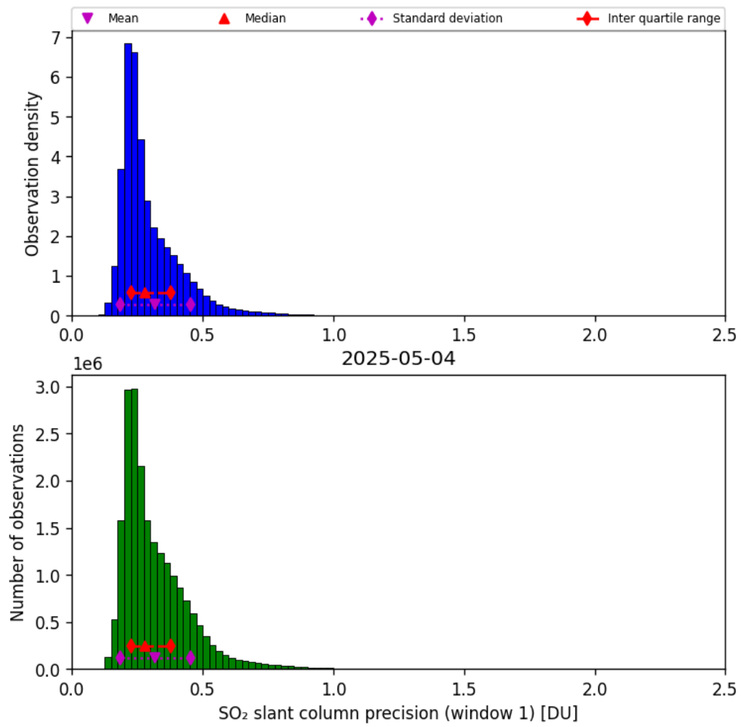
Figure 64: Histogram of “SO 2 slant column precision (window 1)” for 2025-05-03 to 2025-05-05
