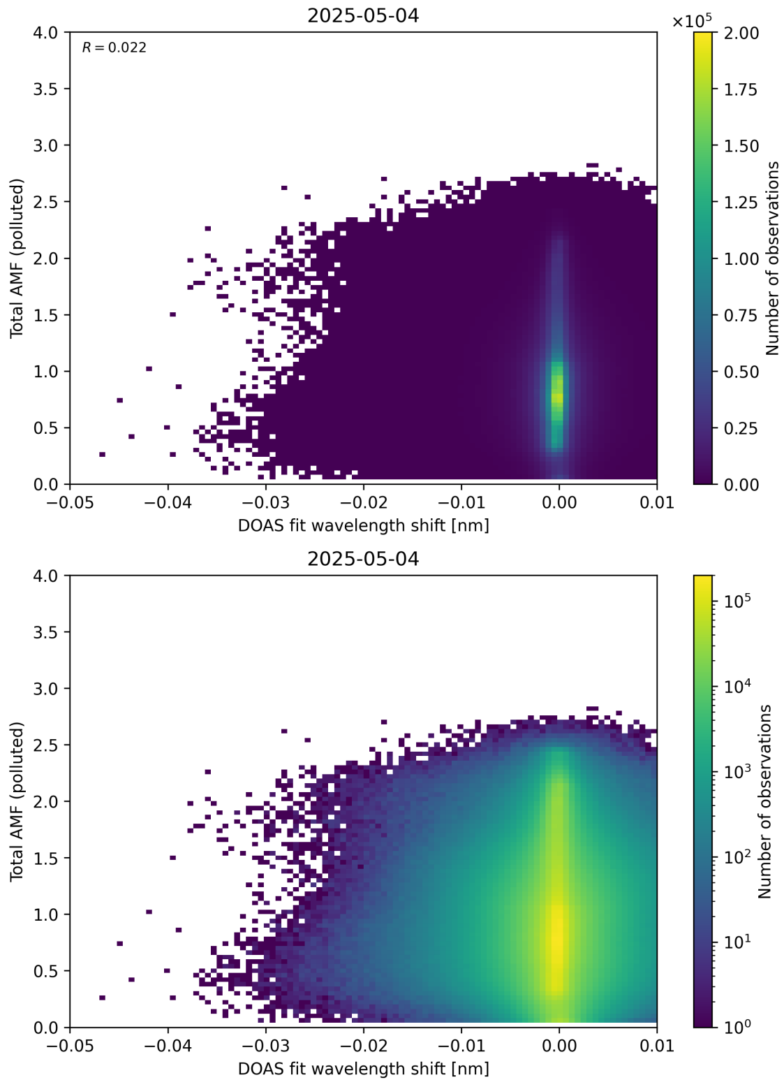
Figure 141: Scatter density plot of “DOAS fit wavelength shift” against “Total AMF (polluted)” for 2025-05-03 to 2025-05-05.
