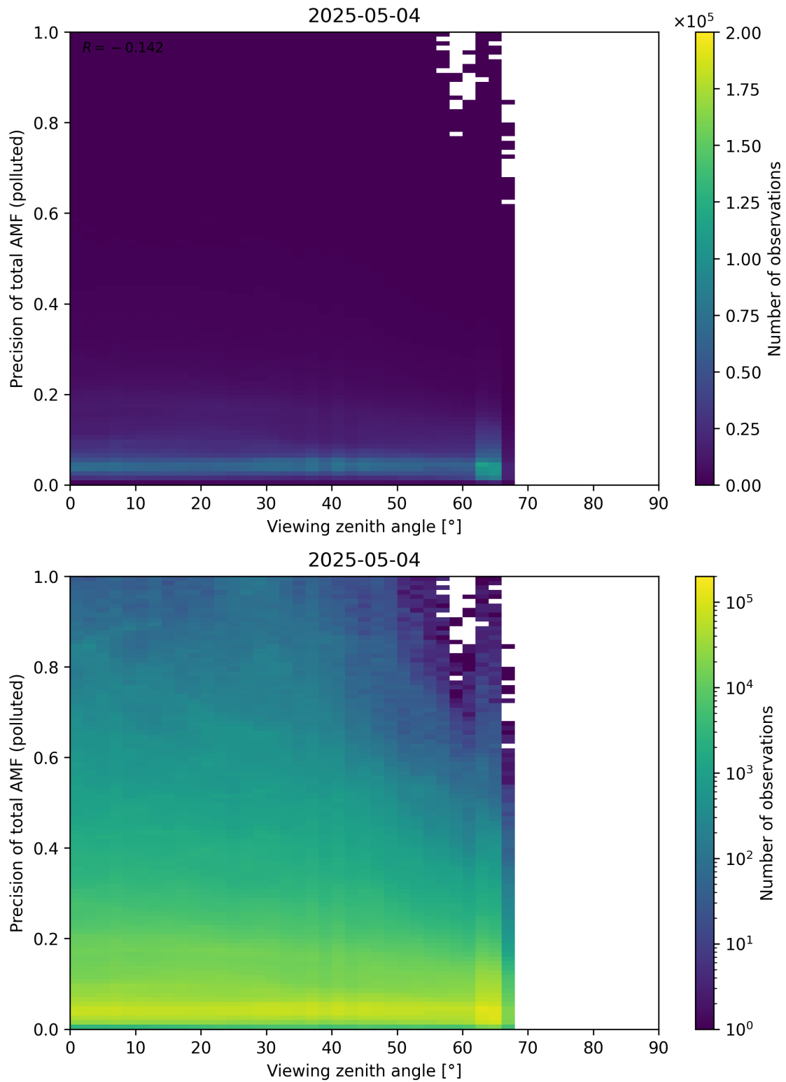
Figure 382: Scatter density plot of “Viewing zenith angle” against “Precision of total AMF (polluted)” for 2025-05-03 to 2025-05-05.
