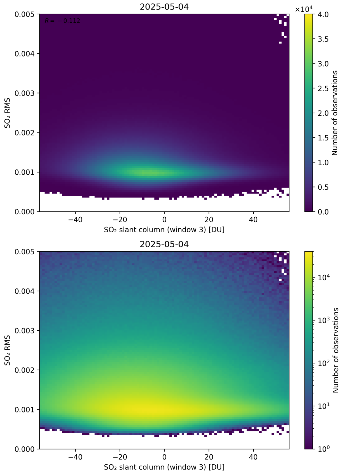
Figure 306: Scatter density plot of “SO 2 slant column (window 3)” against “SO 2 RMS” for 2025-05-03 to 2025-05-05.
