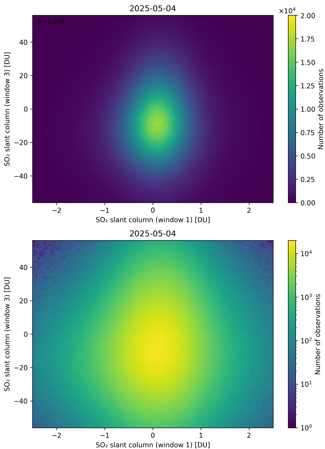
Figure 287: Scatter density plot of “SO 2 slant column (window 1)” against “SO 2 slant column (window 3)” for 2025-05-03 to 2025-05-05.
