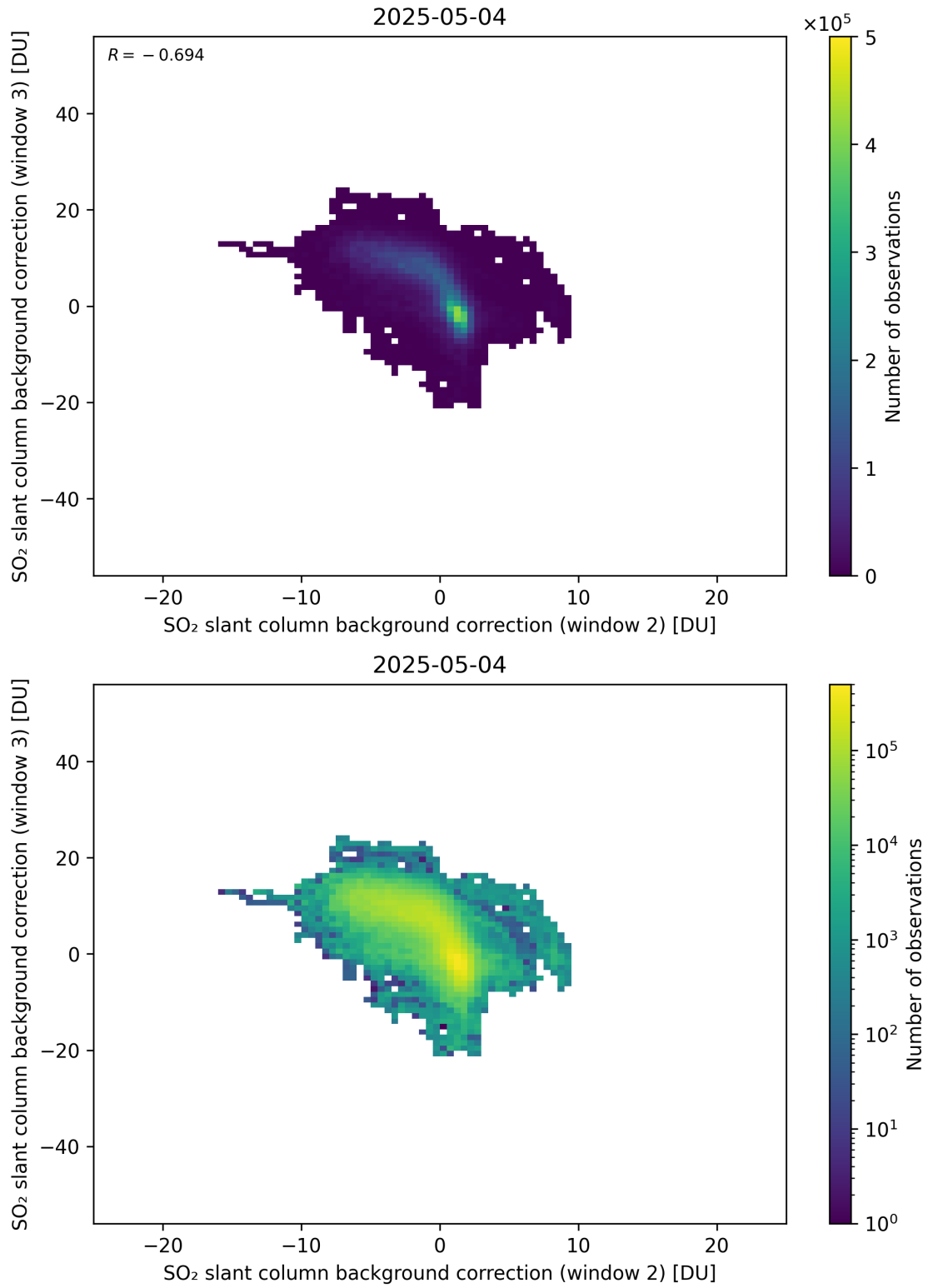
Figure 122: Scatter density plot of “SO 2 slant column background correction (window 2)” against “SO 2 slant column background correction (window 3)” for 2025-05-03 to 2025-05-05.
