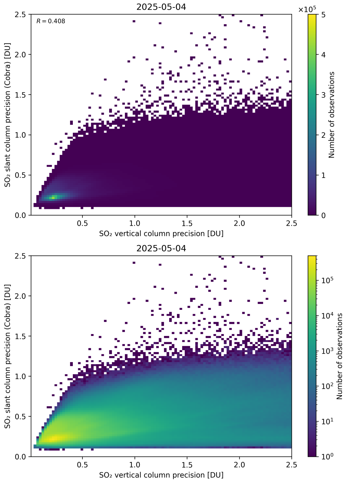
Figure 337: Scatter density plot of “SO 2 vertical column precision” against “SO 2 slant column precision (Cobra)” for 2025-05-03 to 2025-05-05.
