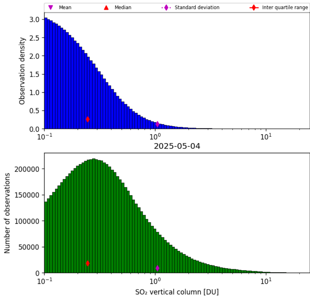
Figure 58: Histogram of “SO 2 vertical column” for 2025-05-03 to 2025-05-05
