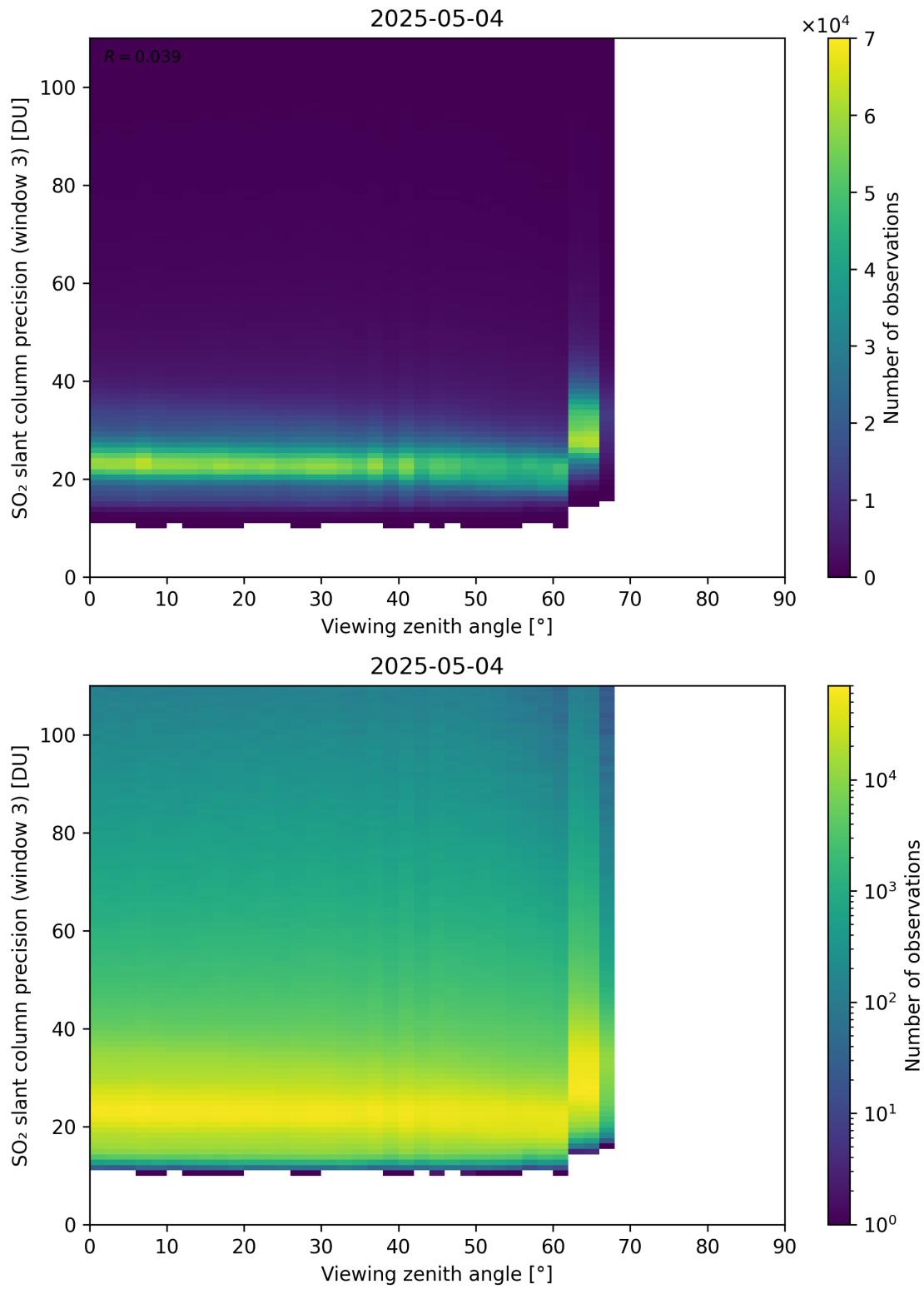
Figure 380: Scatter density plot of “Viewing zenith angle” against “SO 2 slant column precision (window 3)” for 2025-05-03 to 2025-05-05.
