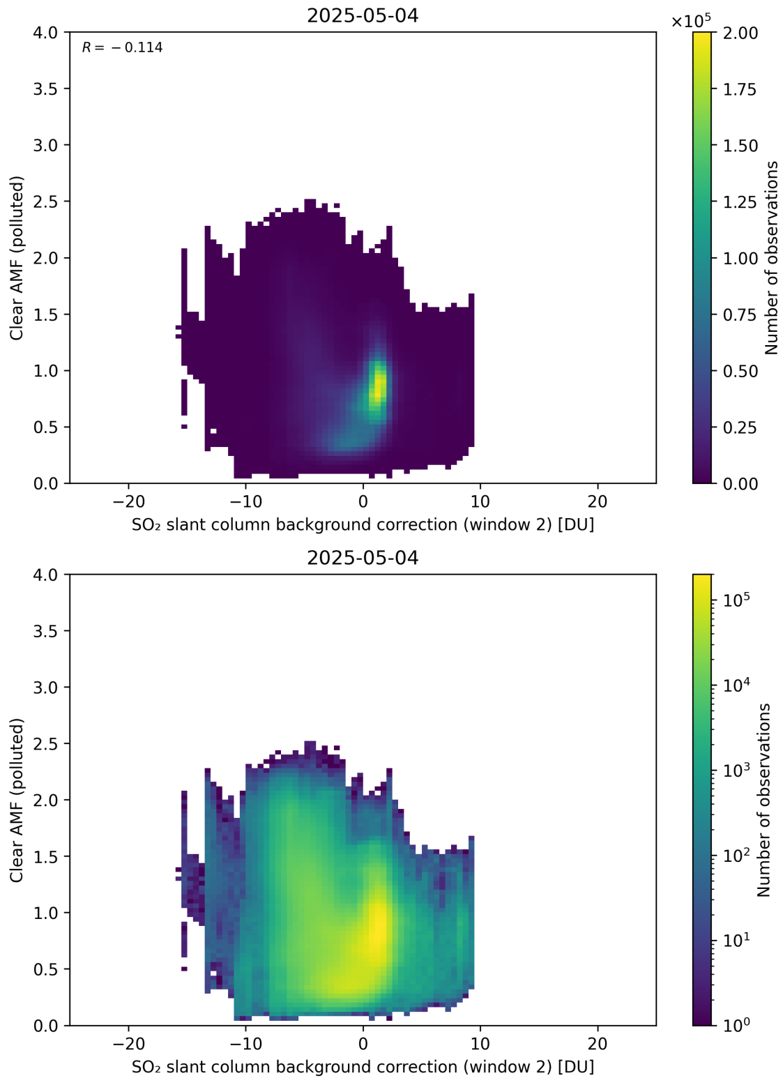
Figure 126: Scatter density plot of “SO 2 slant column background correction (window 2)” against “Clear AMF (polluted)” for 2025-05-03 to 2025-05-05.
