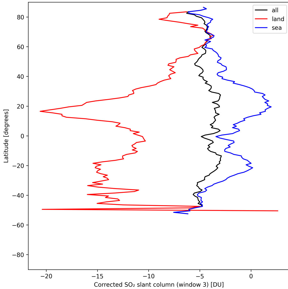
Figure 47: Zonal average of “Corrected SO 2 slant column (window 3)” for 2025-05-03 to 2025-05-05.
