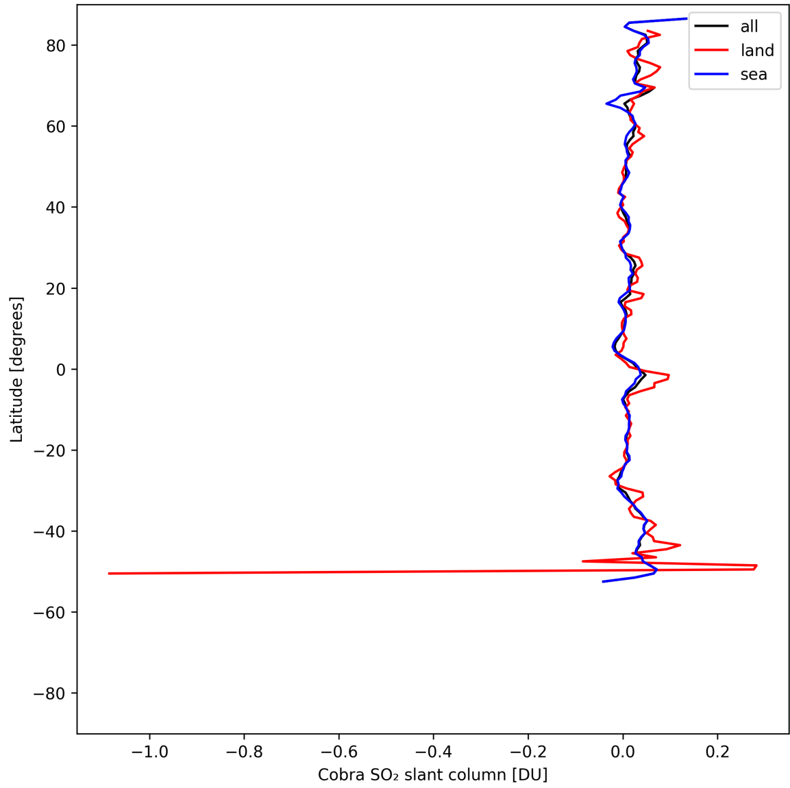
Figure 35: Zonal average of “Cobra SO 2 slant column” for 2025-05-03 to 2025-05-05.
