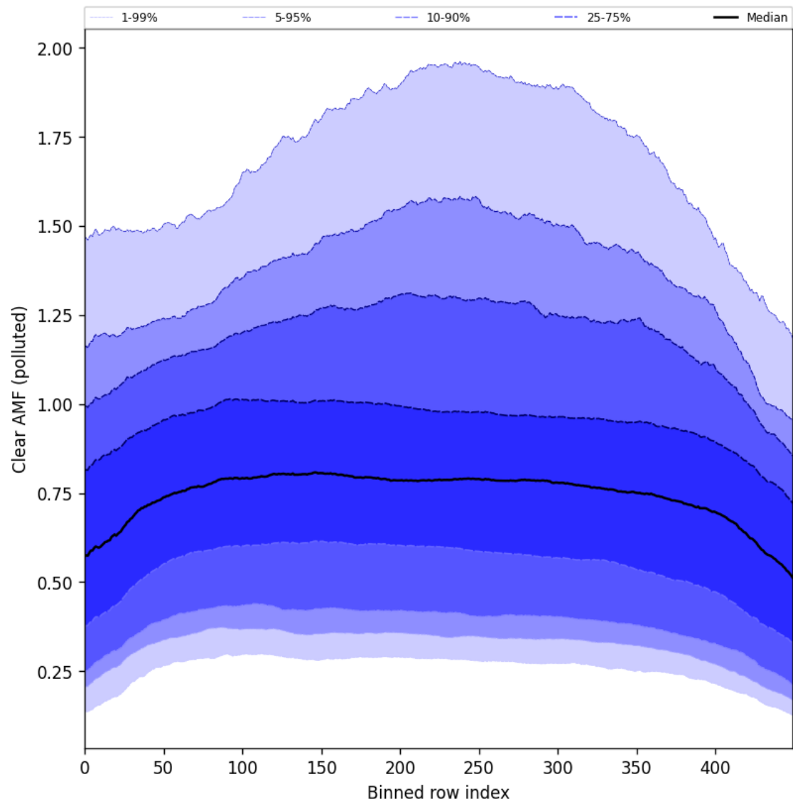
Figure 107: Along track statistics of “Clear AMF (polluted)” for 2025-05-03 to 2025-05-05
