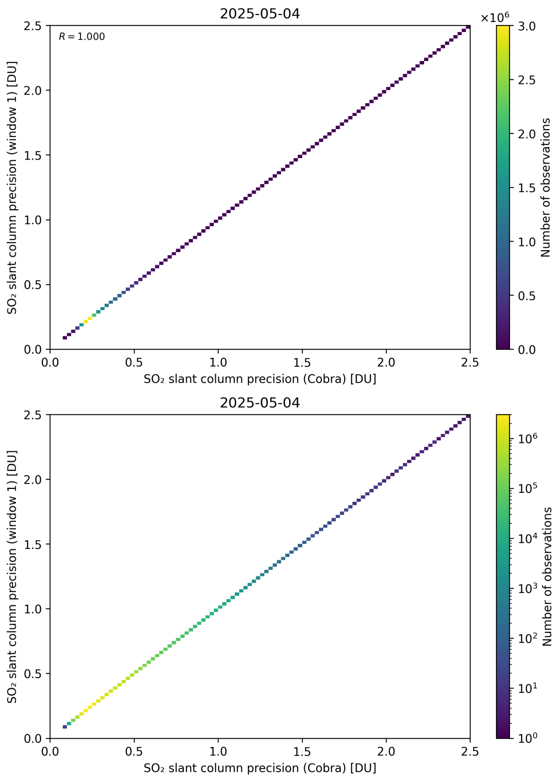
Figure 209: Scatter density plot of “SO 2 slant column precision (Cobra)” against “SO 2 slant column precision (window 1)” for 2025-05-03 to 2025-05-05.
