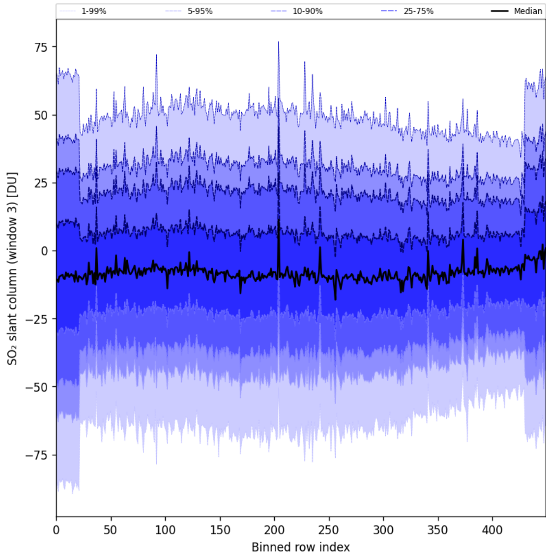
Figure 97: Along track statistics of "SO 2 slant column (window 3)" for 2025-05-03 to 2025-05-05
