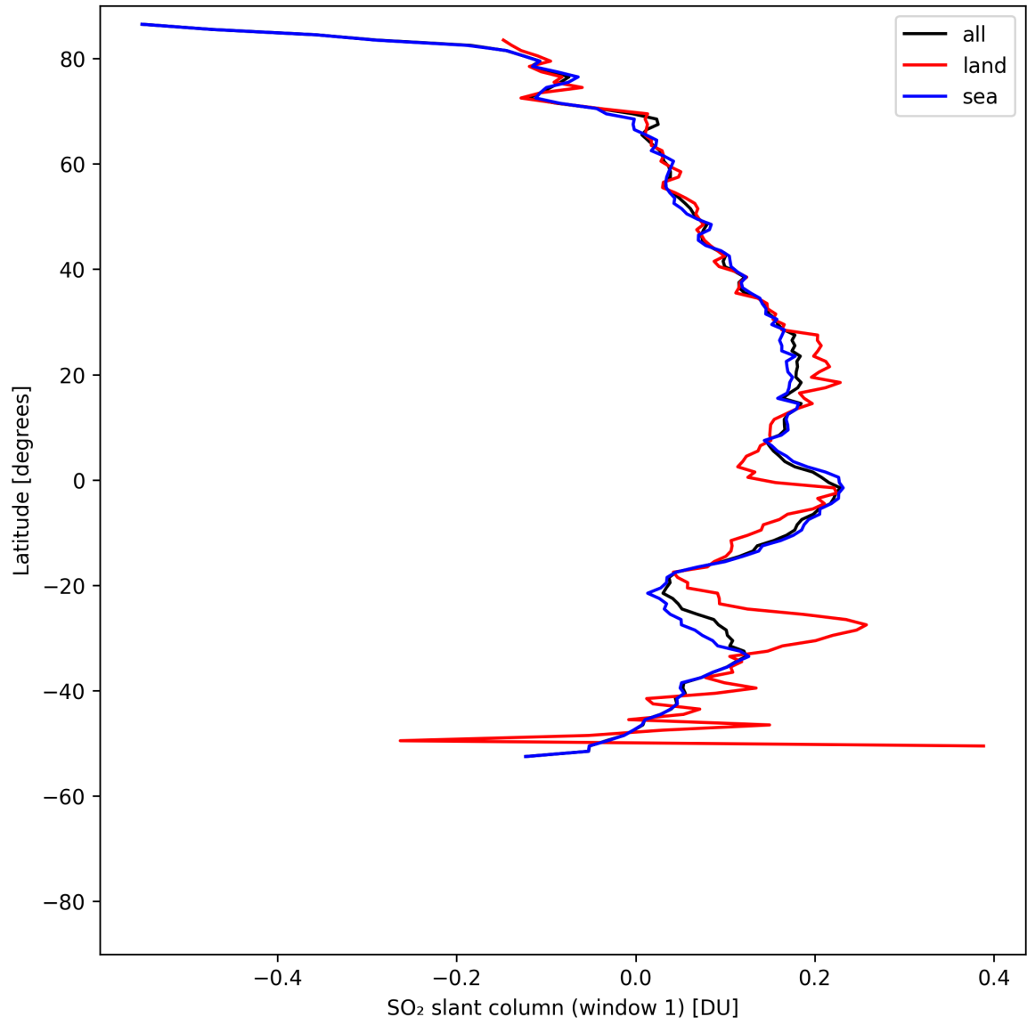
Figure 37: Zonal average of “SO 2 slant column (window 1)” for 2025-05-03 to 2025-05-05.
