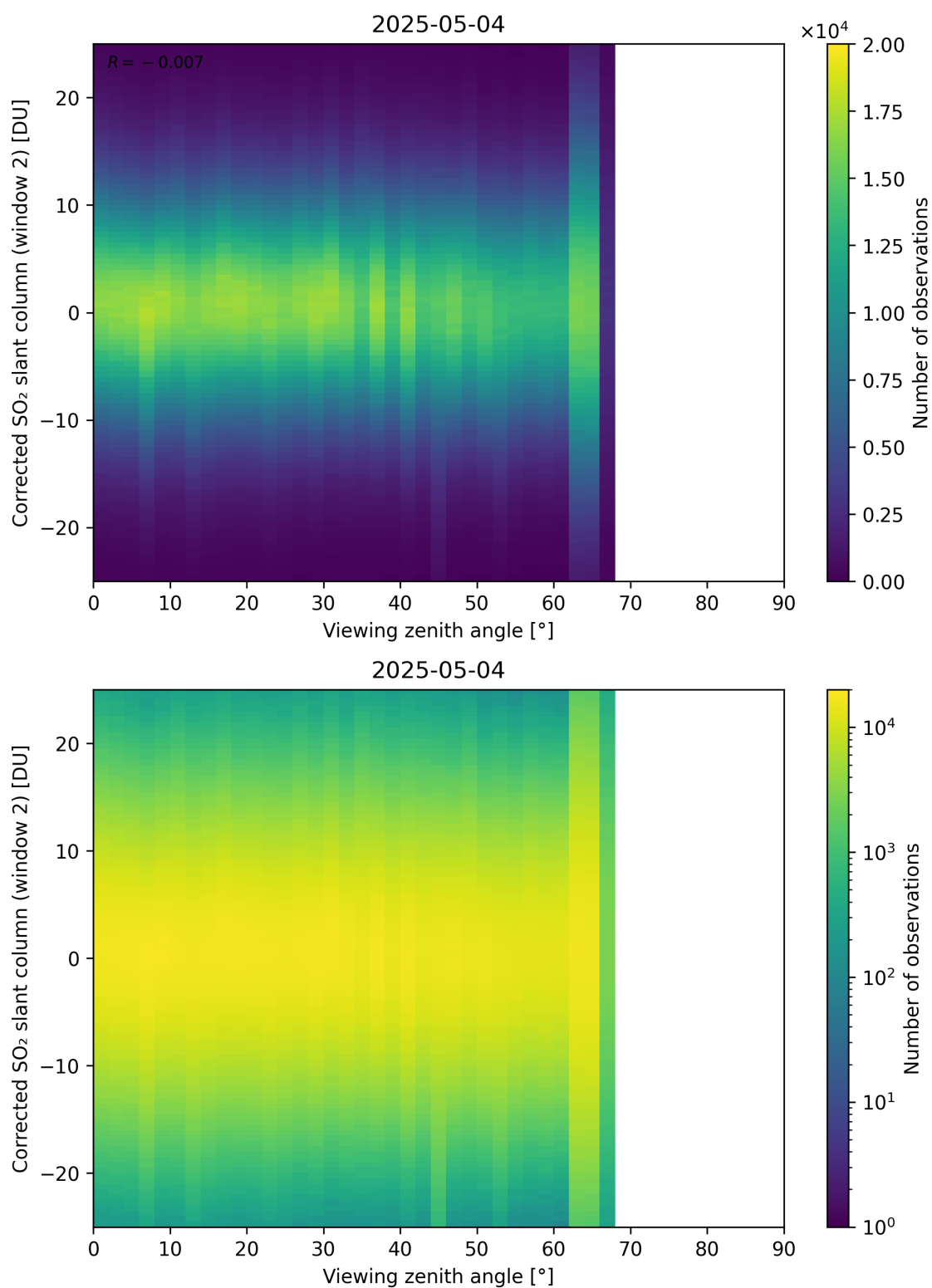
Figure 374: Scatter density plot of “Viewing zenith angle” against “Corrected SO 2 slant column (window 2)” for 2025-05-03 to 2025-05-05.
