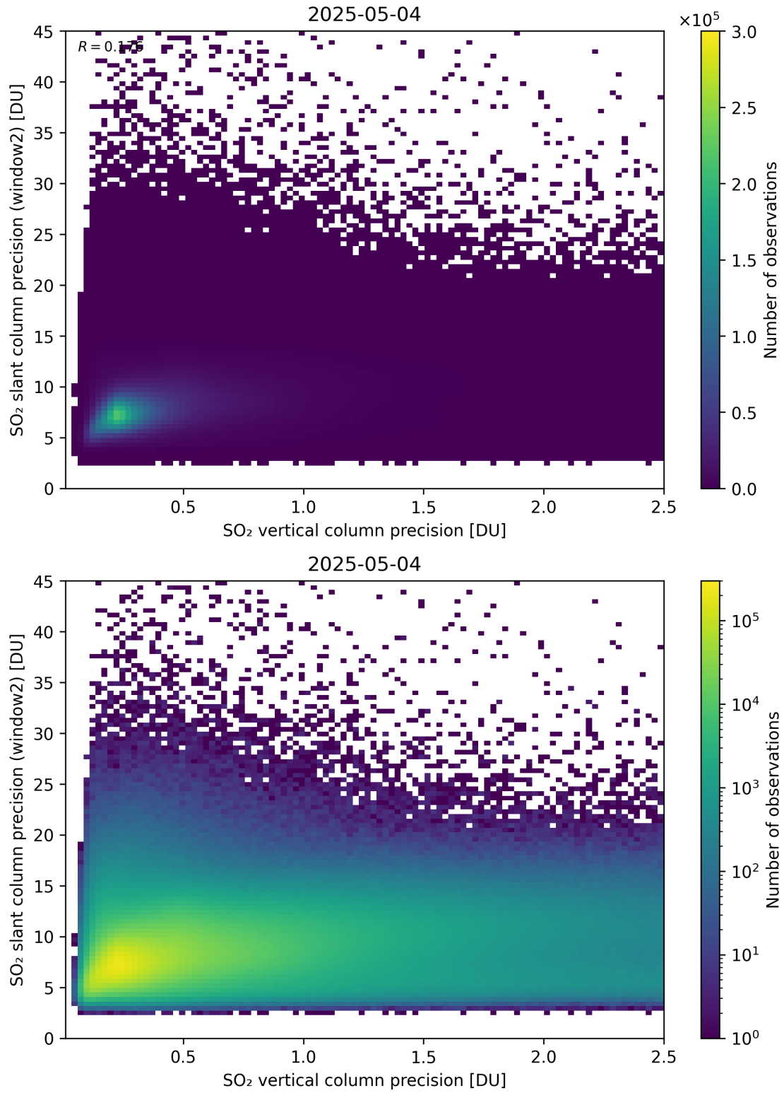
Figure 343: Scatter density plot of “SO 2 vertical column precision” against “SO 2 slant column precision (window2)” for 2025-05-03 to 2025-05-05.
