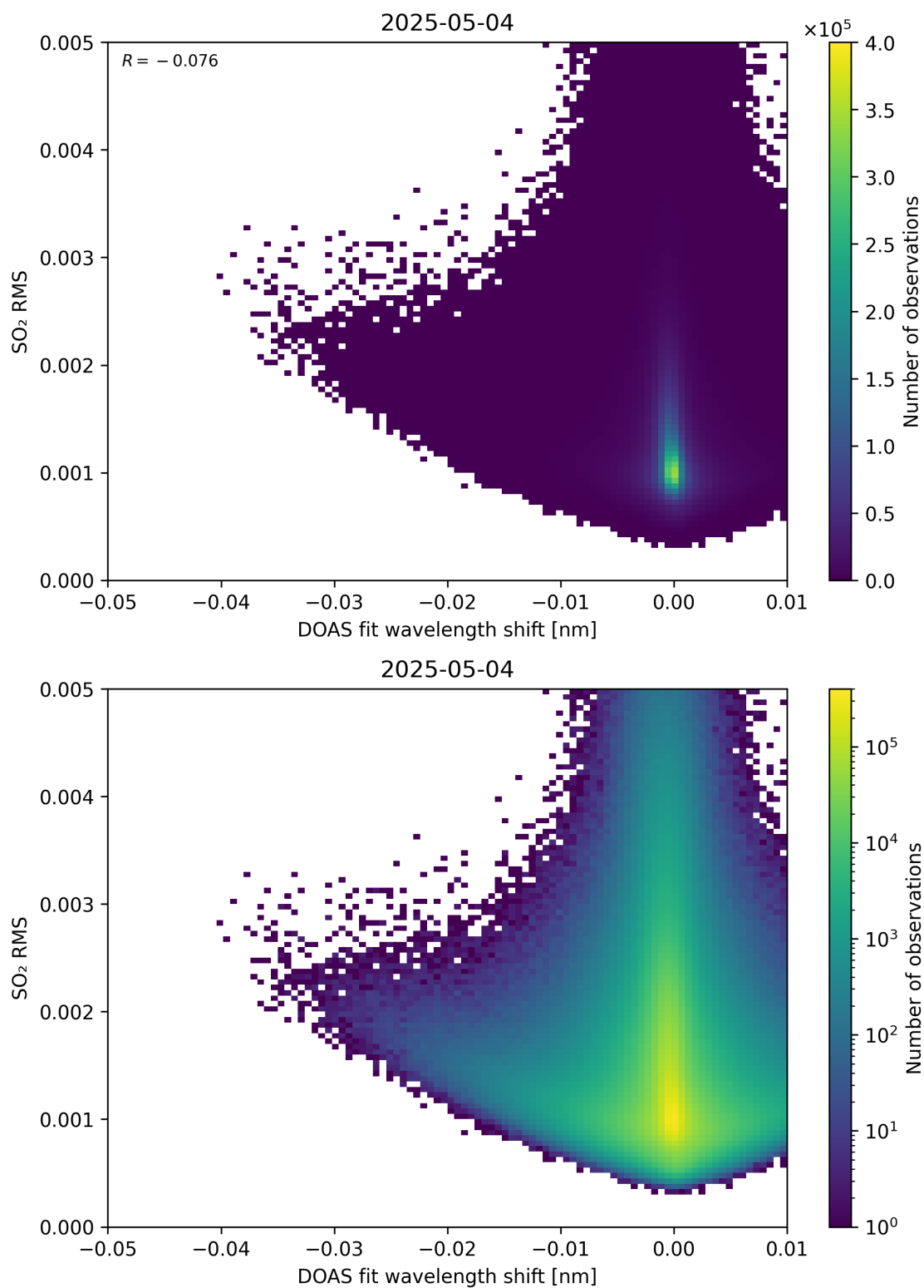
Figure 139: Scatter density plot of “DOAS fit wavelength shift” against “SO 2 RMS” for 2025-05-03 to 2025-05-05.
