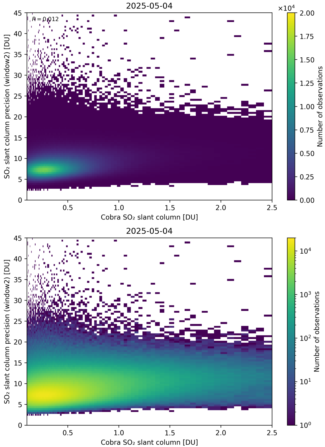
Figure 221: Scatter density plot of “Cobra SO 2 slant column” against “SO 2 slant column precision (window2)” for 2025-05-03 to 2025-05-05.
