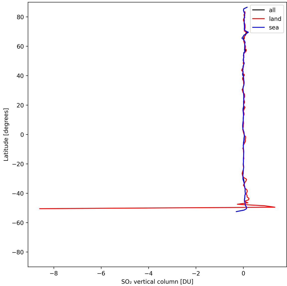
Figure 32: Zonal average of “SO 2 vertical column” for 2025-05-03 to 2025-05-05.
