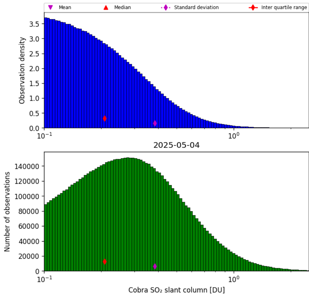
Figure 61: Histogram of “Cobra SO 2 slant column” for 2025-05-03 to 2025-05-05
