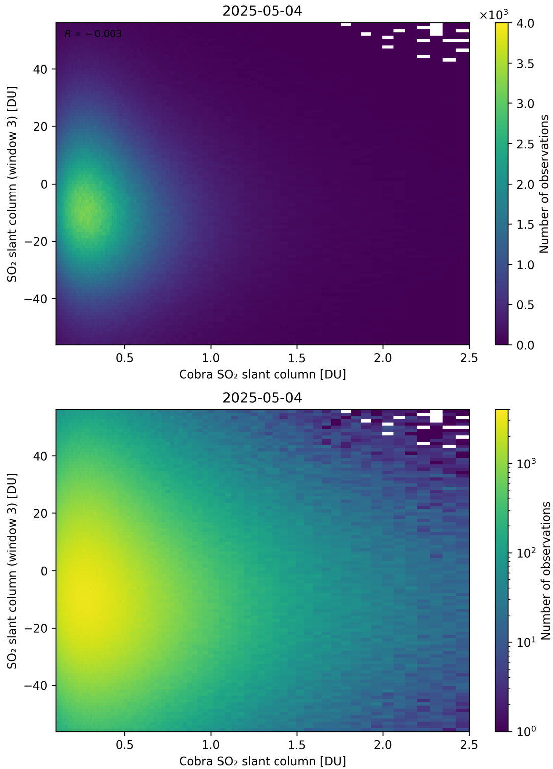
Figure 222: Scatter density plot of “Cobra SO 2 slant column” against “SO 2 slant column (window 3)” for 2025-05-03 to 2025-05-05.
