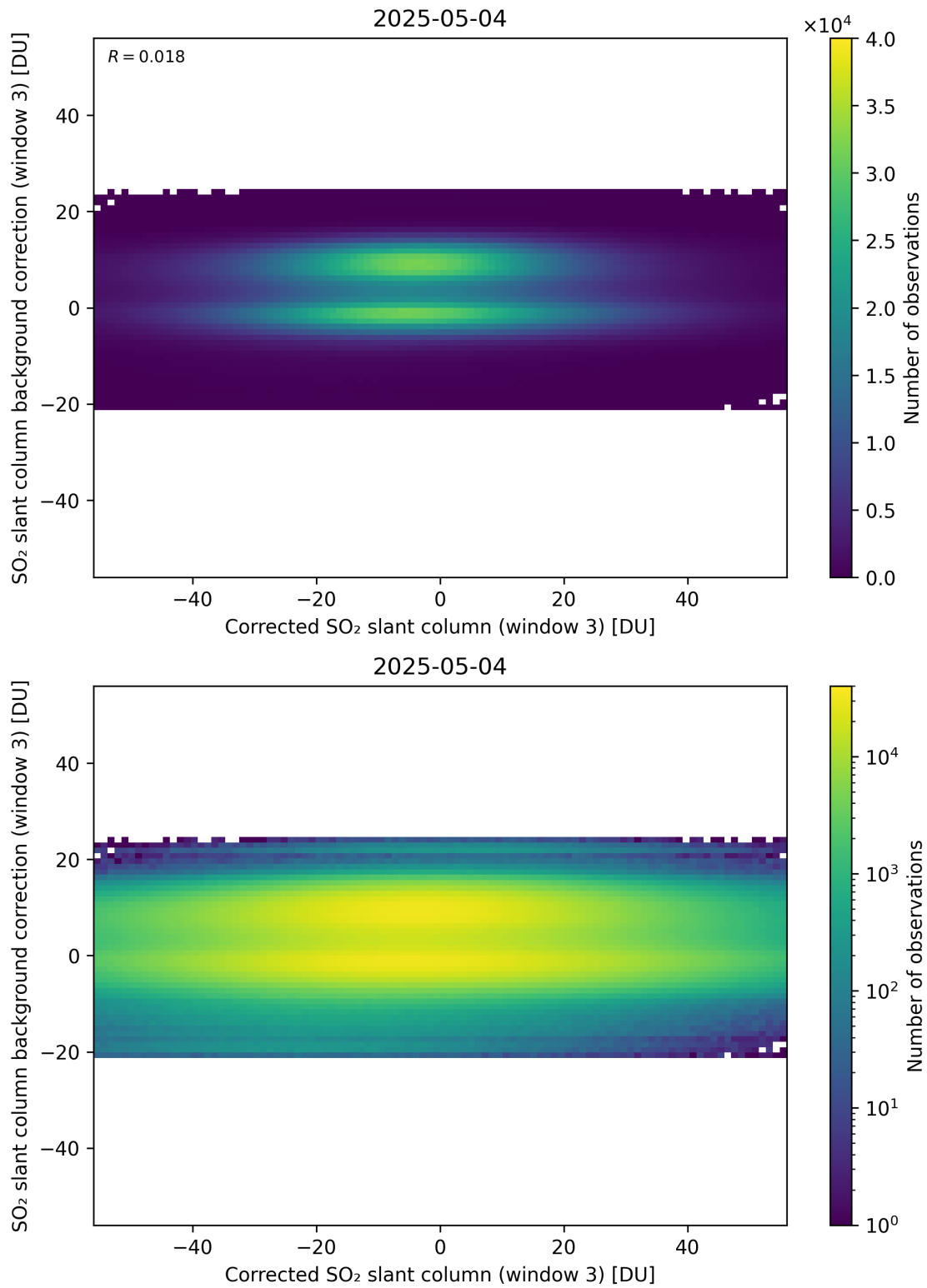
Figure 255: Scatter density plot of “Corrected SO 2 slant column (window 3)” against “SO 2 slant column background correction (window 3)” for 2025-05-03 to 2025-05-05.
