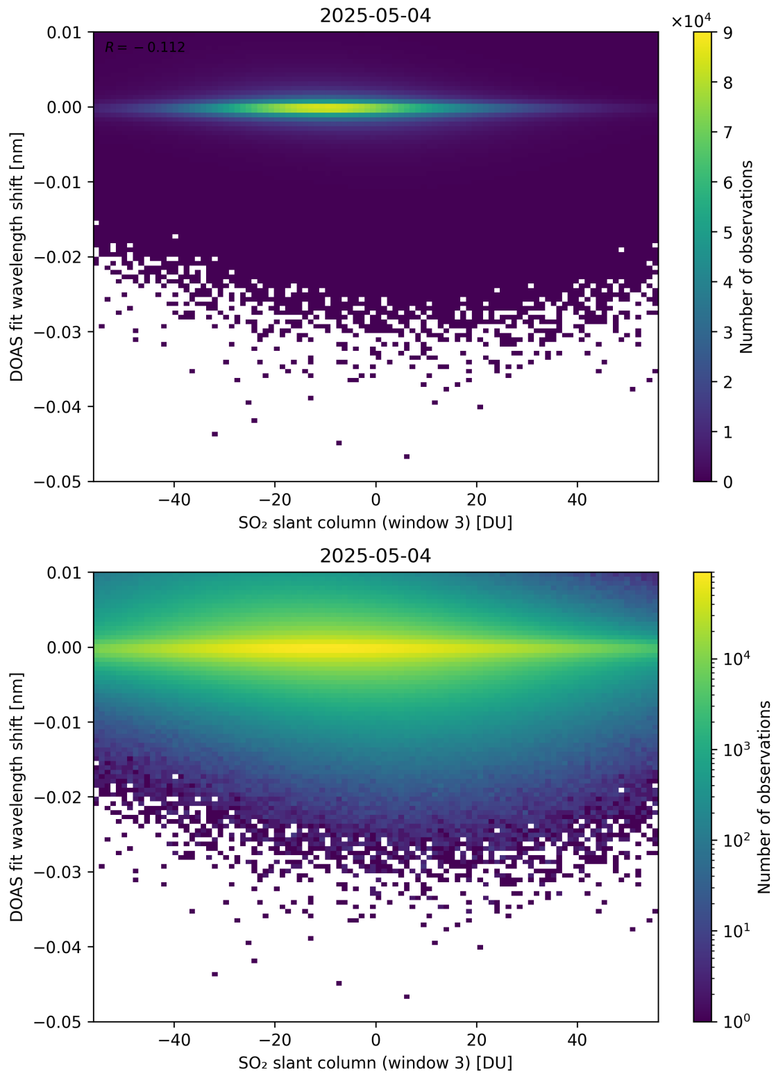
Figure 304: Scatter density plot of “SO 2 slant column (window 3)” against “DOAS fit wavelength shift” for 2025-05-03 to 2025-05-05.
