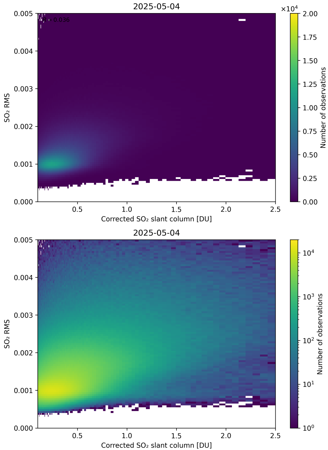
Figure 231: Scatter density plot of “Corrected SO 2 slant column” against “SO 2 RMS” for 2025-05-03 to 2025-05-05.
