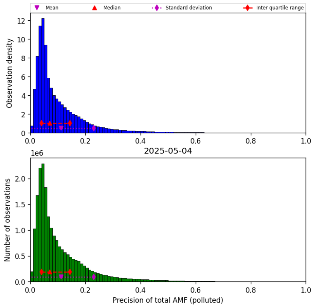
Figure 80: Histogram of “Precision of total AMF (polluted)” for 2025-05-03 to 2025-05-05
