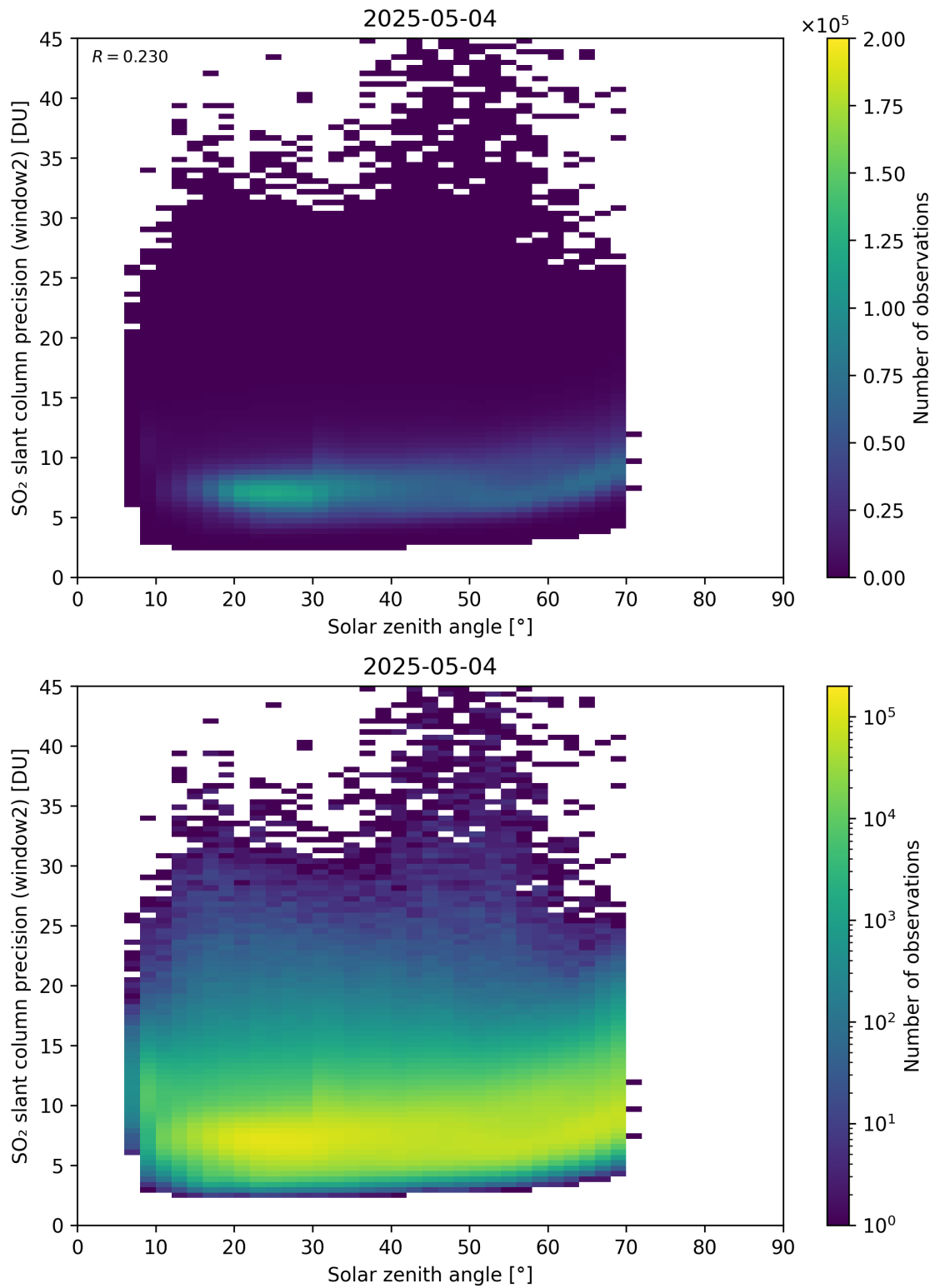
Figure 186: Scatter density plot of “Solar zenith angle” against “SO 2 slant column precision (window2)” for 2025-05-03 to 2025-05-05.
