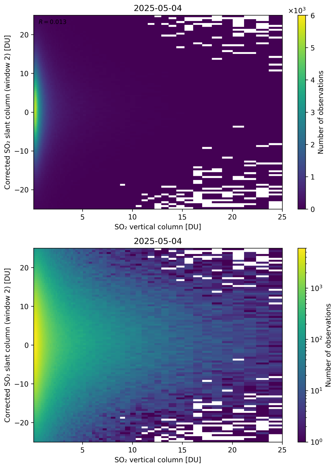
Figure 352: Scatter density plot of “SO 2 vertical column” against “Corrected SO 2 slant column (window 2)” for 2025-05-03 to 2025-05-05.
