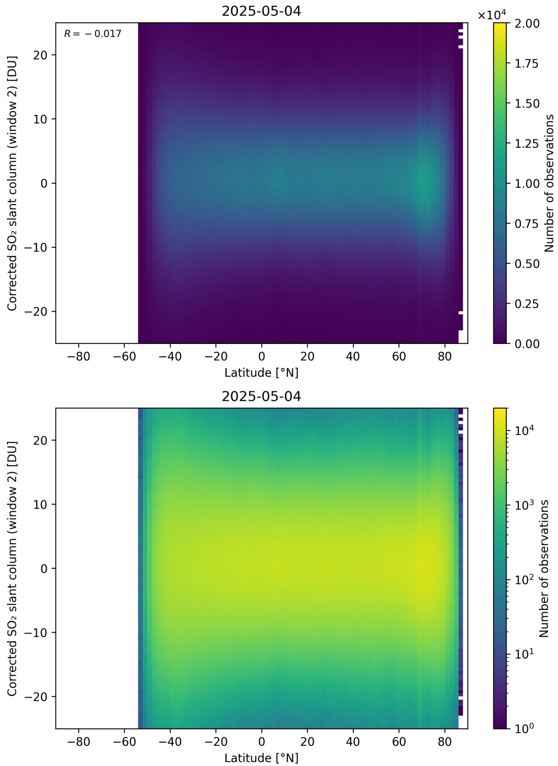
Figure 160: Scatter density plot of “Latitude” against “Corrected SO 2 slant column (window 2)” for 2025-05-03 to 2025-05-05.
