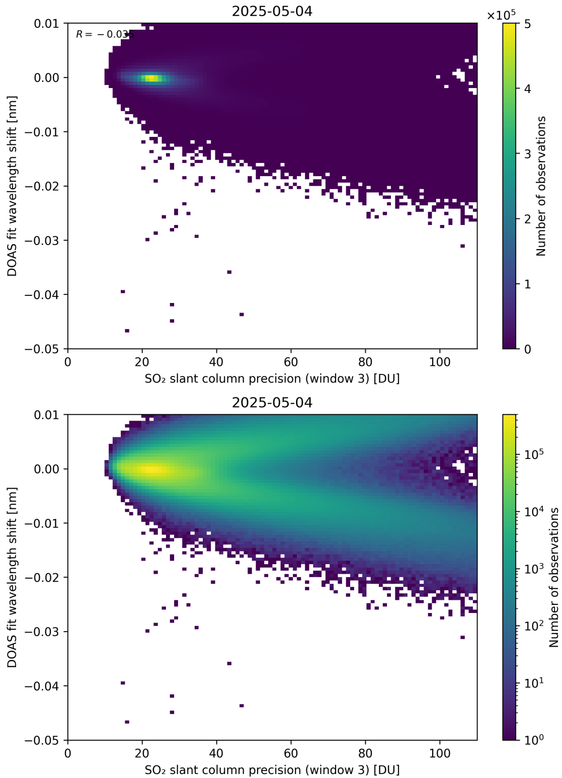
Figure 308: Scatter density plot of “SO 2 slant column precision (window 3)” against “DOAS fit wavelength shift” for 2025-05-03 to 2025-05-05.
