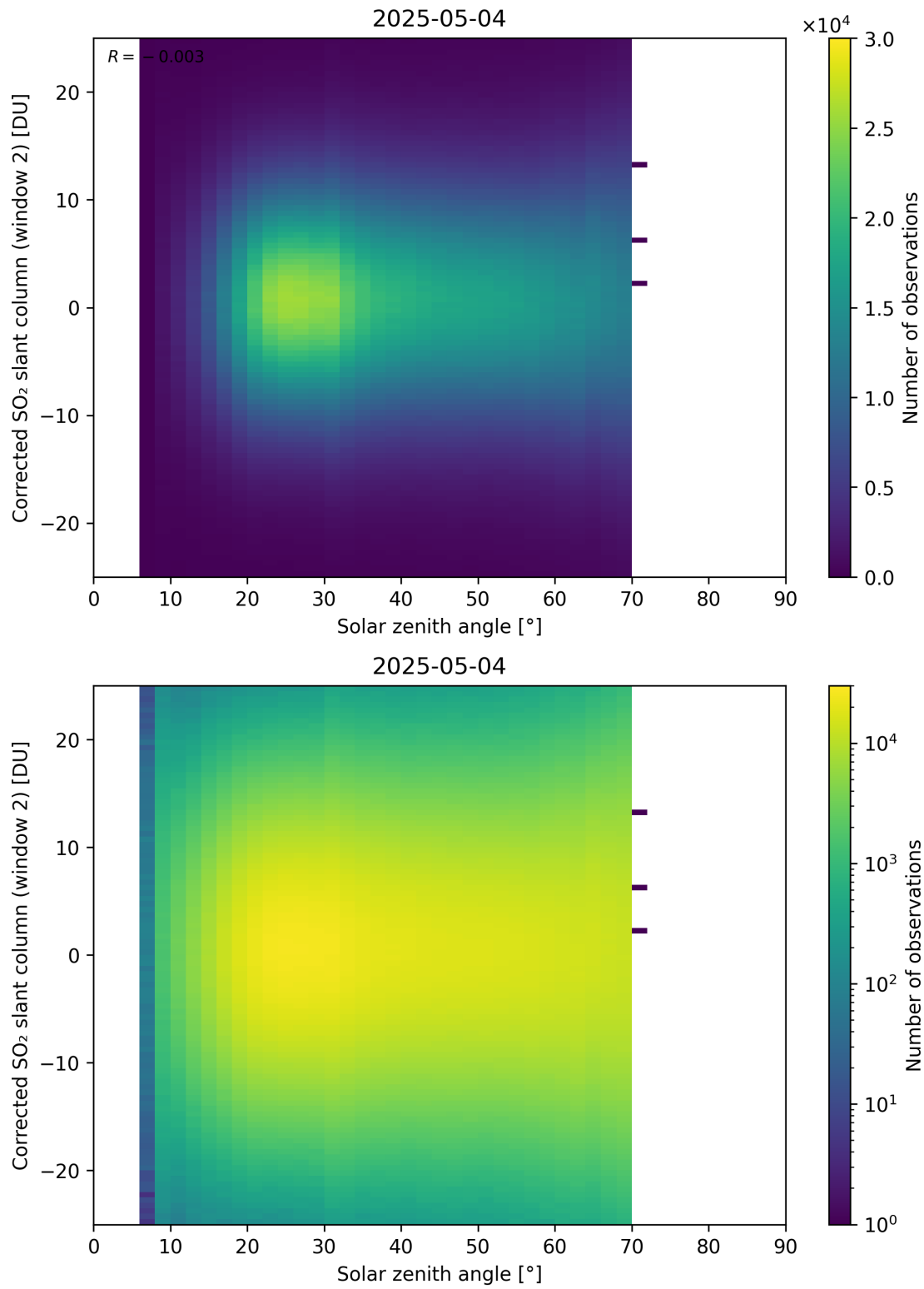
Figure 182: Scatter density plot of “Solar zenith angle” against “Corrected SO 2 slant column (window 2)” for 2025-05-03 to 2025-05-05.
