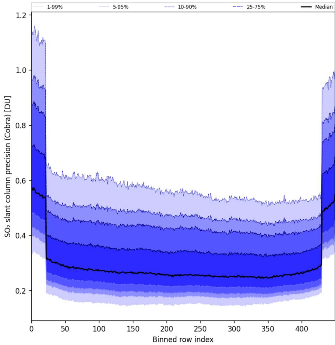
Figure 88: Along track statistics of “SO 2 slant column precision (Cobra)” for 2025-05-03 to 2025-05-05
