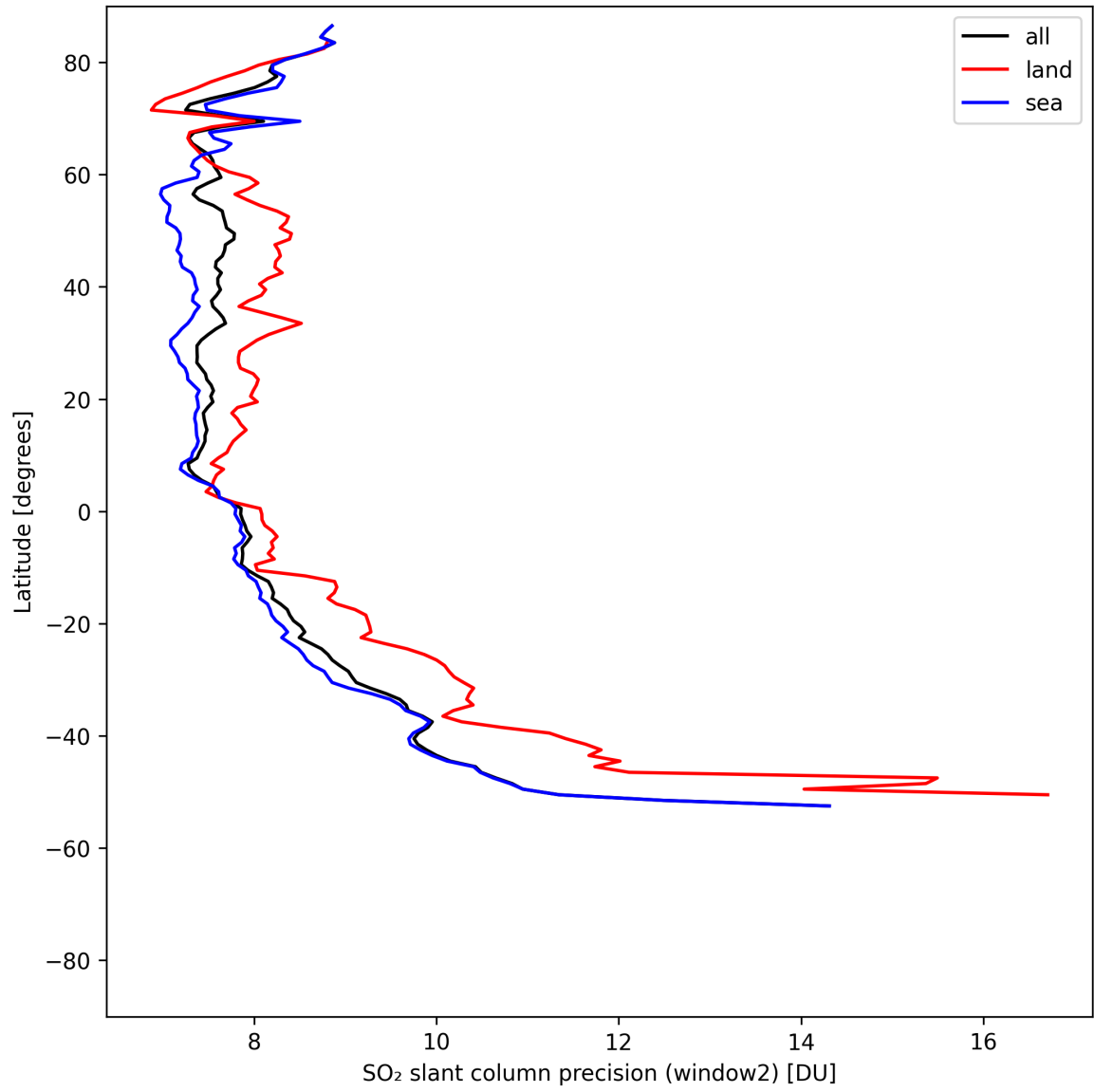
Figure 42: Zonal average of “SO 2 slant column precision (window2)” for 2025-05-03 to 2025-05-05.
