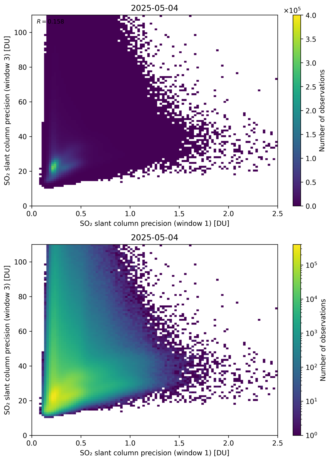
Figure 279: Scatter density plot of “SO 2 slant column precision (window 1)” against “SO 2 slant column precision (window 3)” for 2025-05-03 to 2025-05-05.
