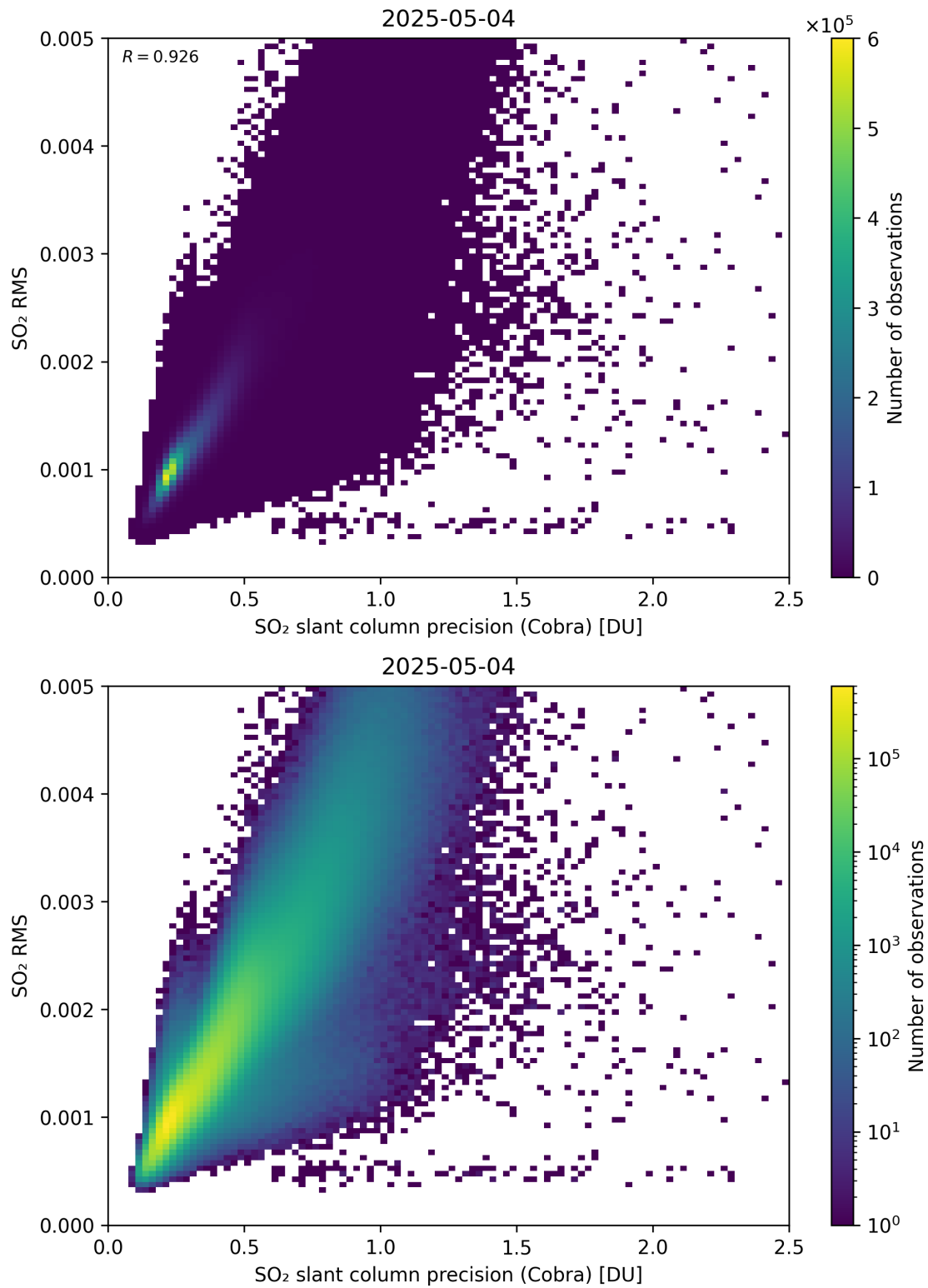
Figure 204: Scatter density plot of “SO 2 slant column precision (Cobra)” against “SO 2 RMS” for 2025-05-03 to 2025-05-05.
