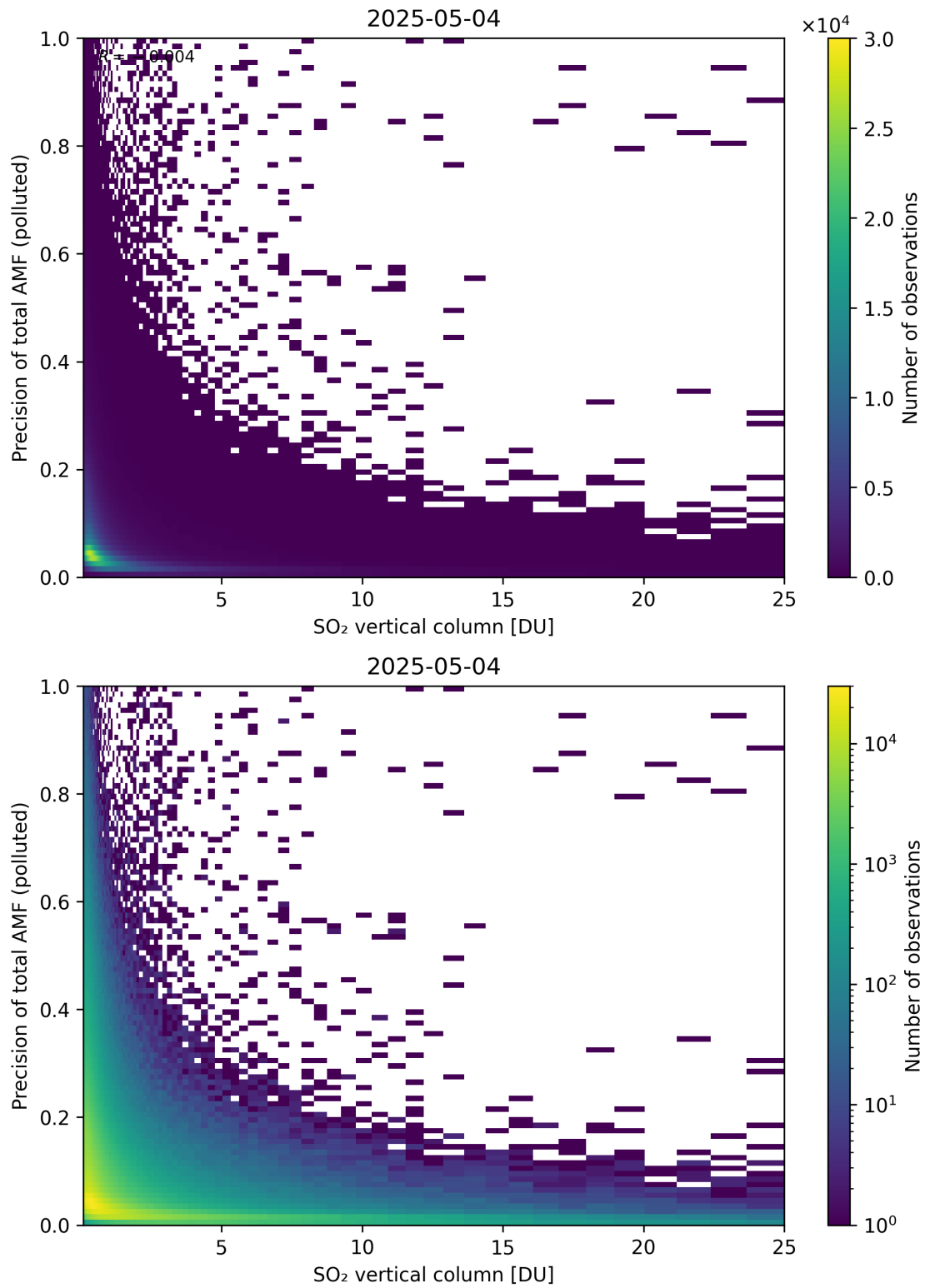
Figure 360: Scatter density plot of “SO 2 vertical column” against “Precision of total AMF (polluted)” for 2025-05-03 to 2025-05-05.
