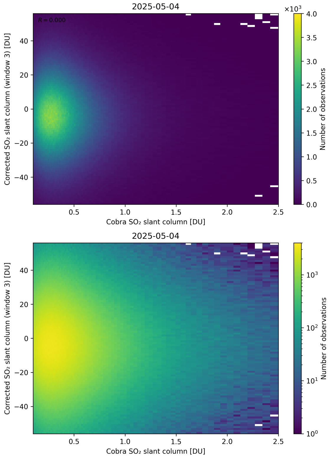
Figure 218: Scatter density plot of “Cobra SO 2 slant column” against “Corrected SO 2 slant column (window 3)” for 2025-05-03 to 2025-05-05.
