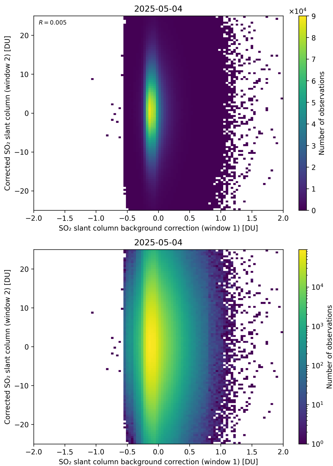
Figure 115: Scatter density plot of “SO 2 slant column background correction (window 1)” against “Corrected SO 2 slant column (window 2)” for 2025-05-03 to 2025-05-05.
