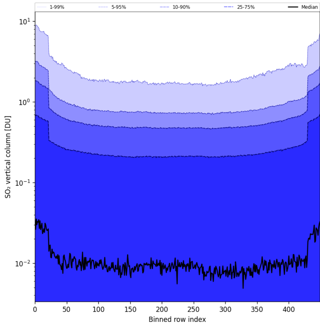
Figure 84: Along track statistics of “SO 2 vertical column” for 2025-05-03 to 2025-05-05
