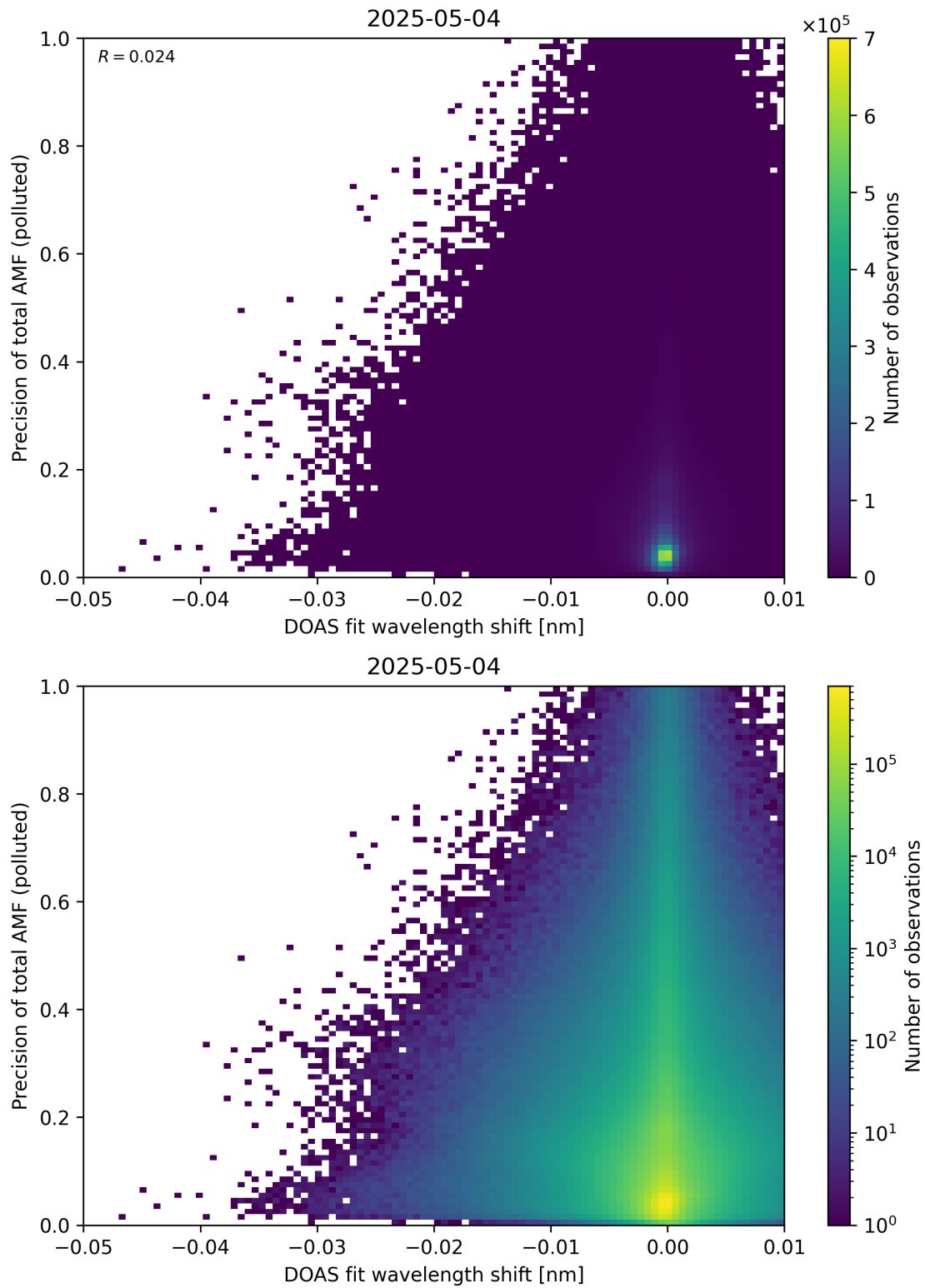
Figure 142: Scatter density plot of “DOAS fit wavelength shift” against “Precision of total AMF (polluted)” for 2025-05-03 to 2025-05-05.
