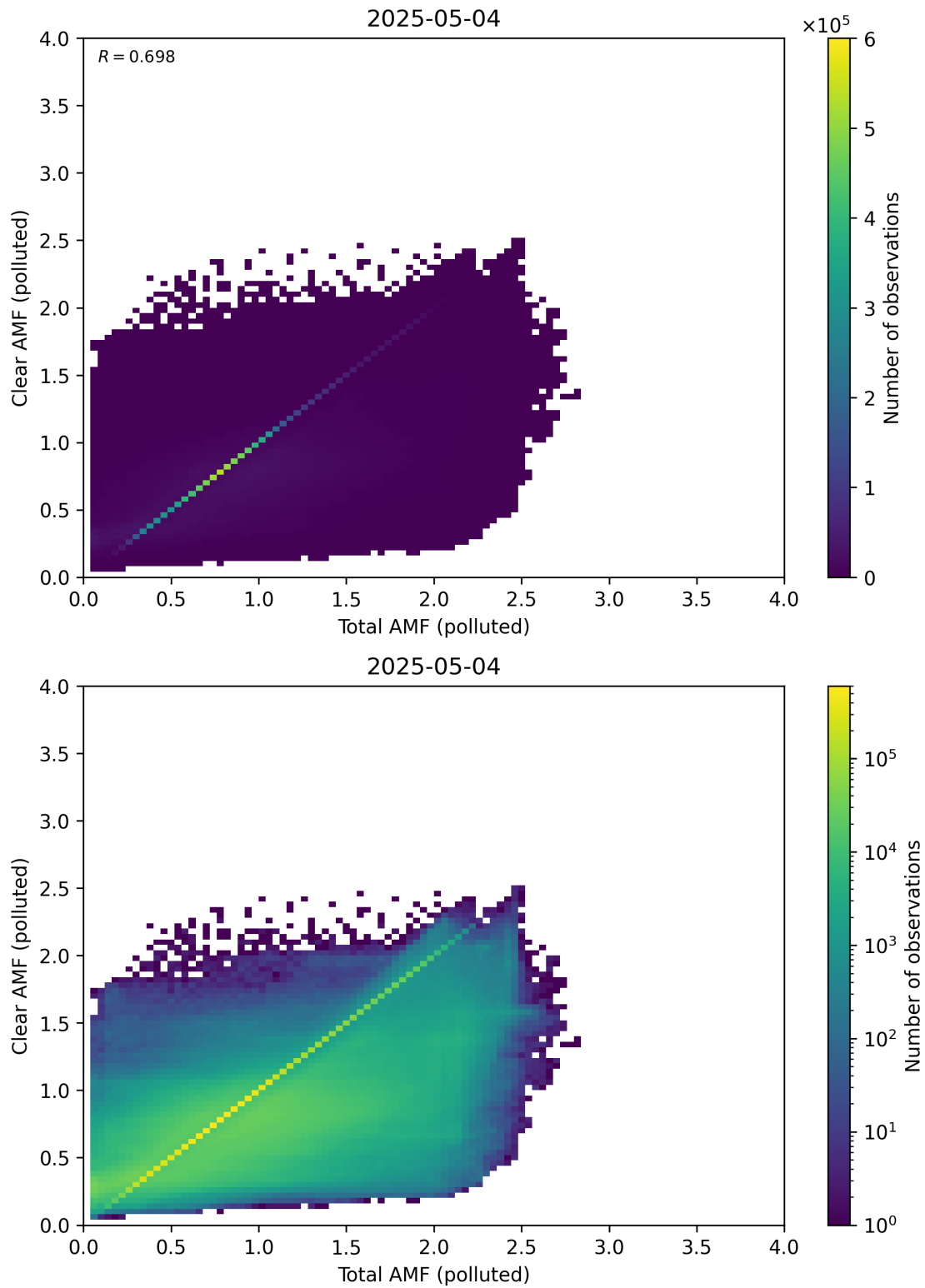
Figure 321: Scatter density plot of “Total AMF (polluted)” against “Clear AMF (polluted)” for 2025-05-03 to 2025-05-05.
