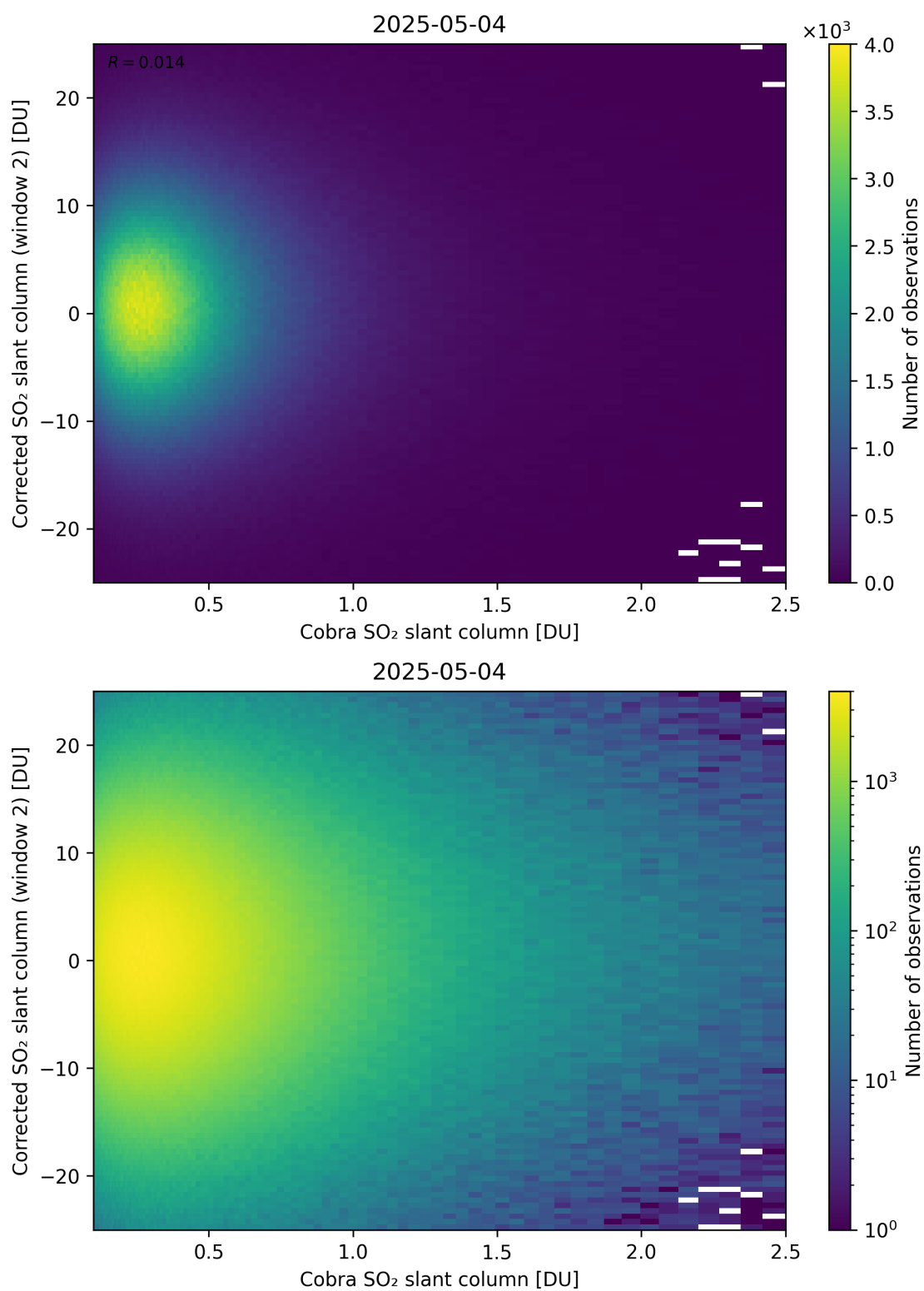
Figure 217: Scatter density plot of “Cobra SO 2 slant column” against “Corrected SO 2 slant column (window 2)” for 2025-05-03 to 2025-05-05.
