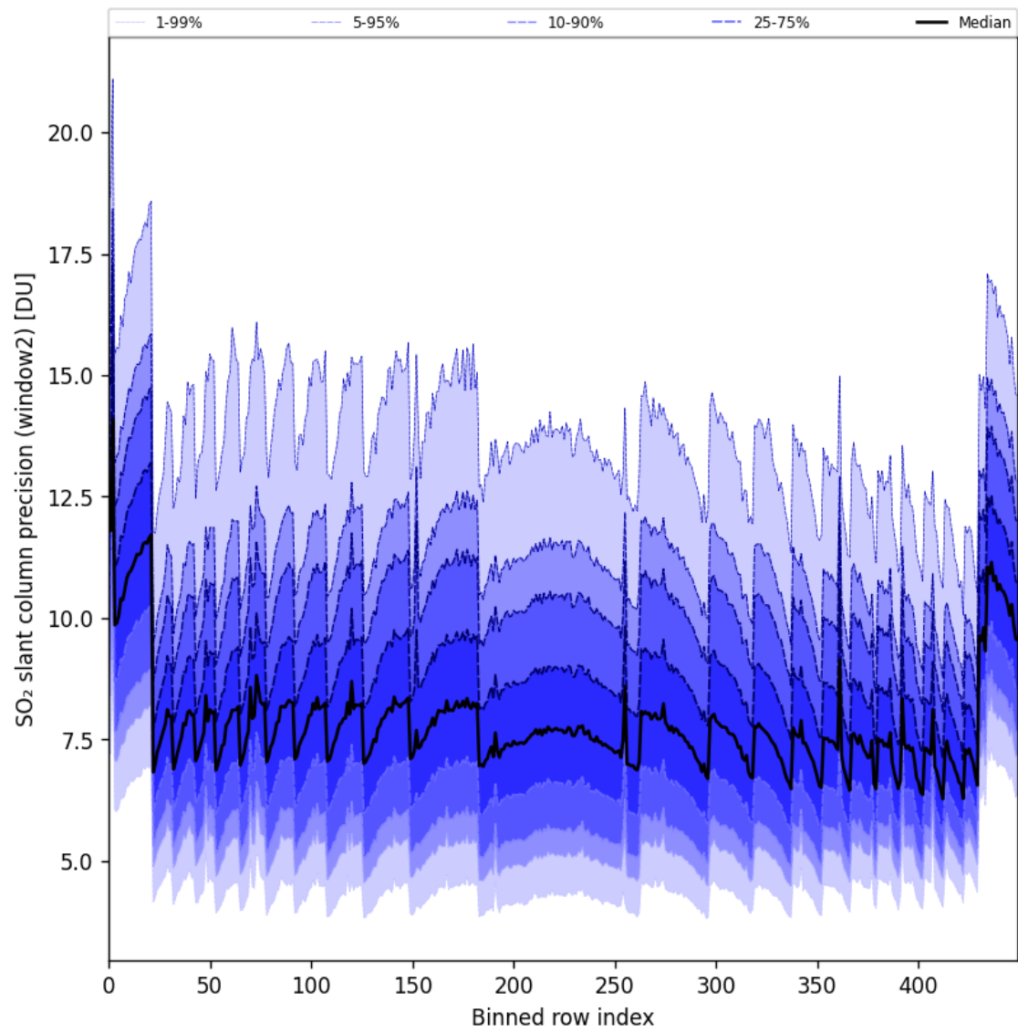
Figure 94: Along track statistics of “SO 2 slant column precision (window2)” for 2025-05-03 to 2025-05-05
