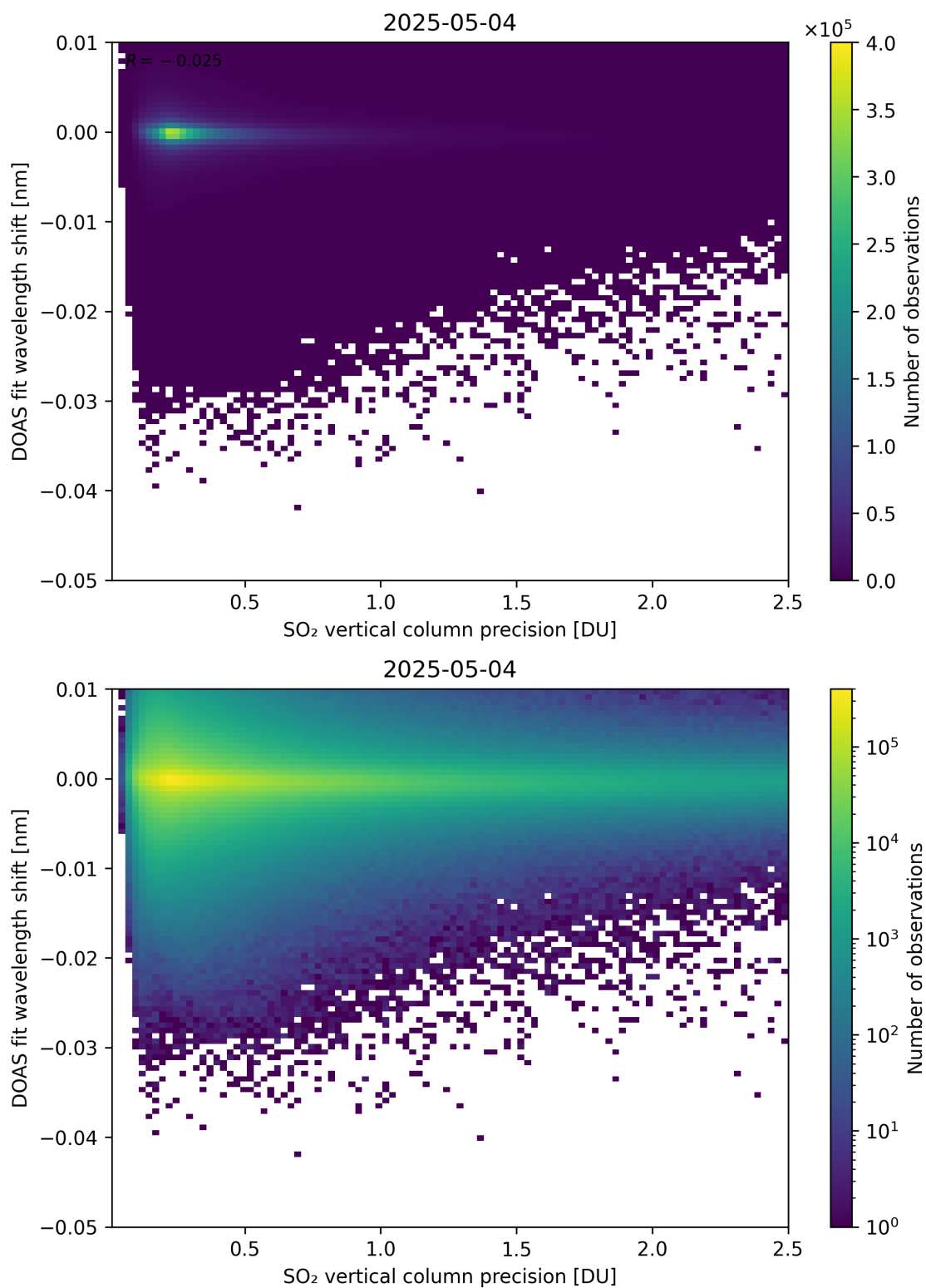
Figure 332: Scatter density plot of “SO 2 vertical column precision” against “DOAS fit wavelength shift” for 2025-05-03 to 2025-05-05.
