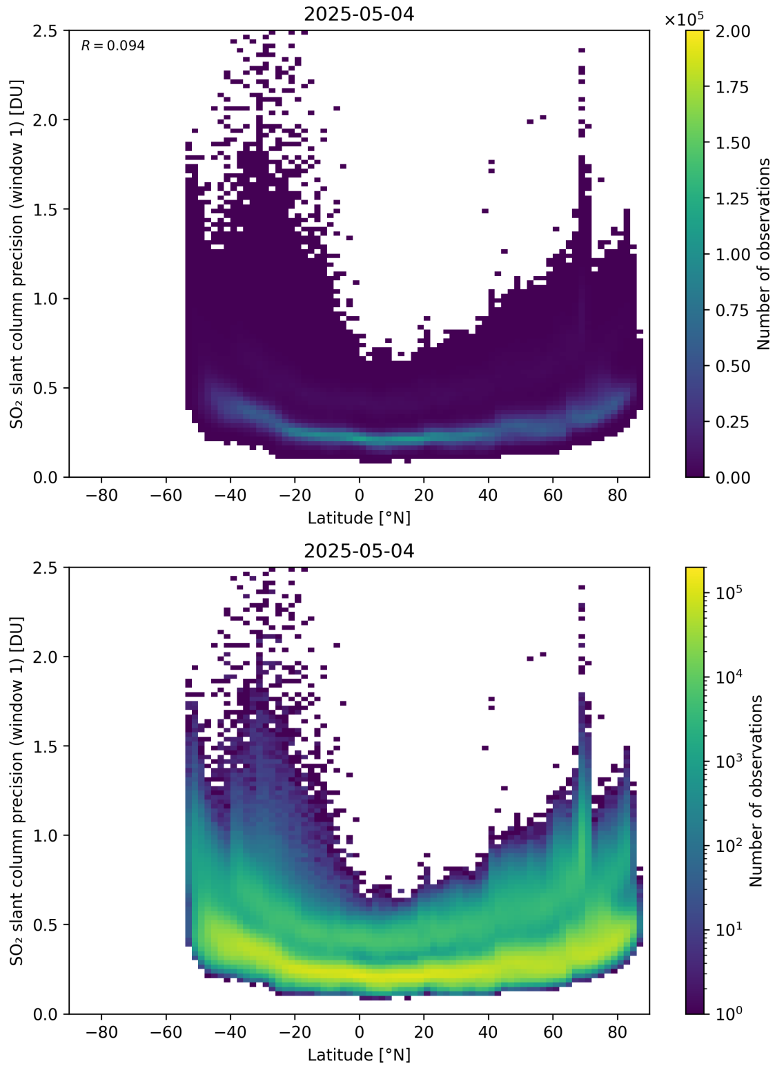
Figure 163: Scatter density plot of “Latitude” against “SO 2 slant column precision (window 1)” for 2025-05-03 to 2025-05-05.
