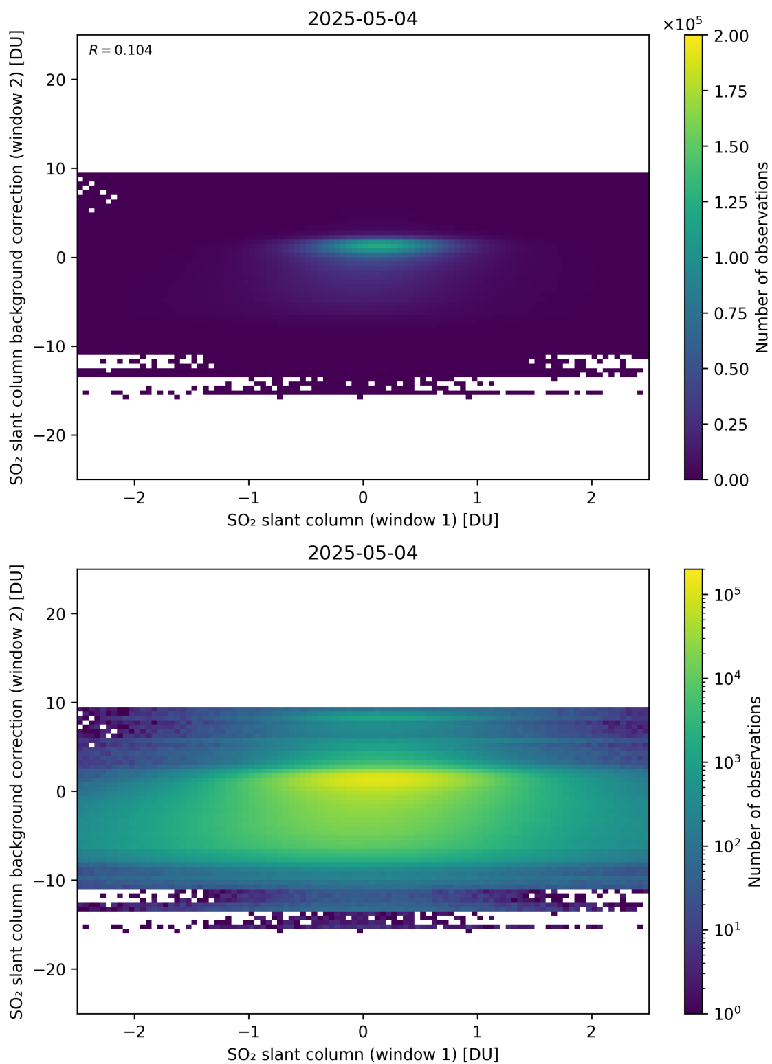
Figure 263: Scatter density plot of “SO 2 slant column (window 1)” against “SO 2 slant column background correction (window 2)” for 2025-05-03 to 2025-05-05.
