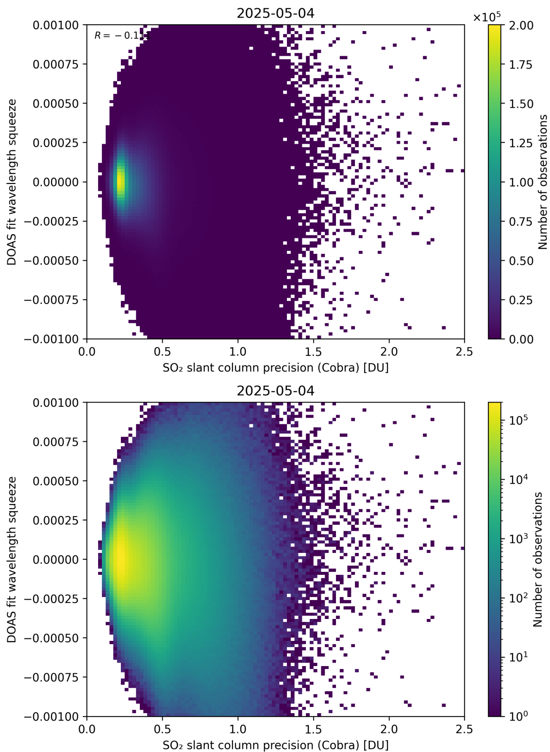
Figure 203: Scatter density plot of “SO 2 slant column precision (Cobra)” against “DOAS fit wavelength squeeze” for 2025-05-03 to 2025-05-05.
