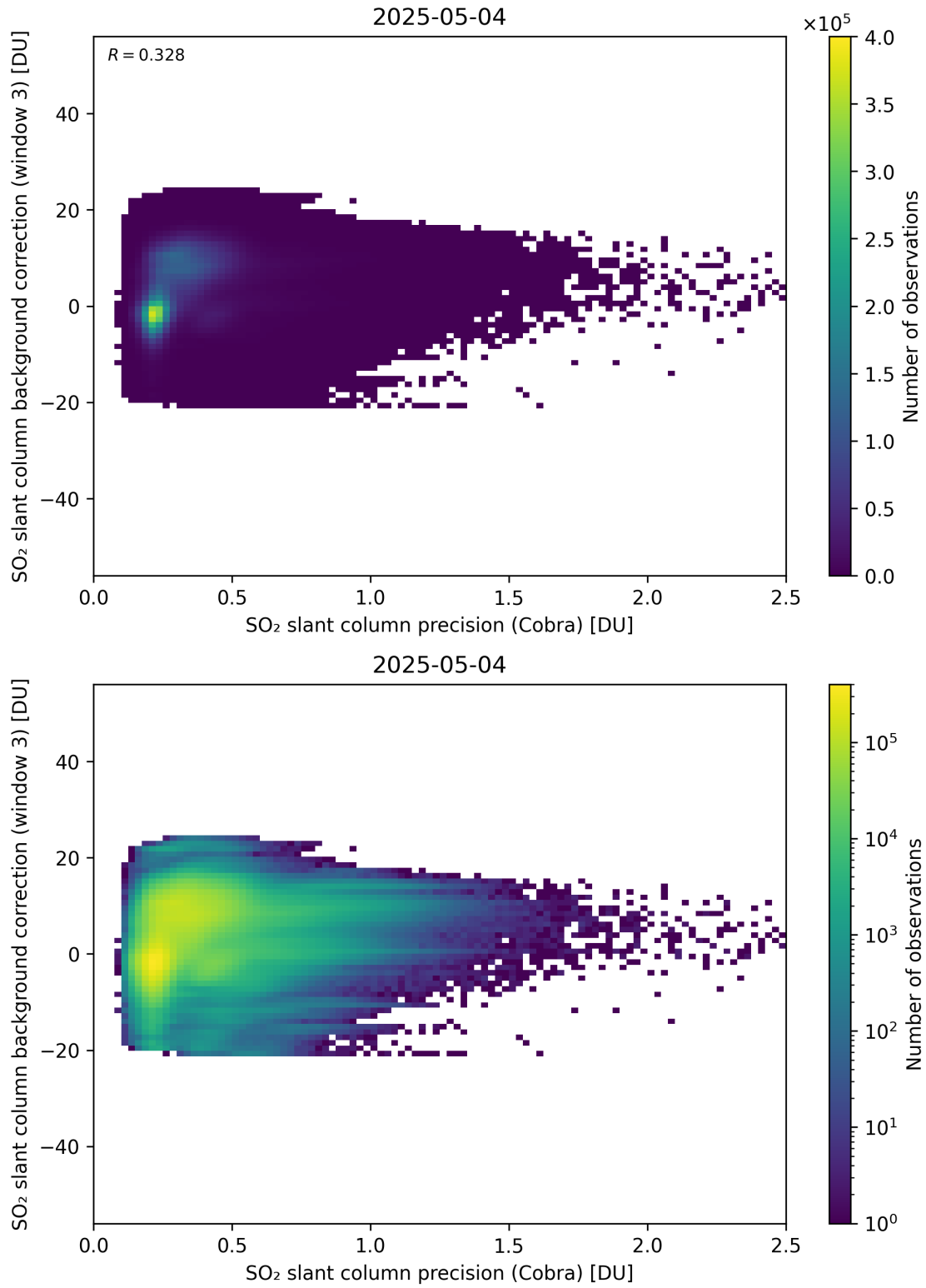
Figure 201: Scatter density plot of “SO 2 slant column precision (Cobra)” against “SO 2 slant column background correction (window 3)” for 2025-05-03 to 2025-05-05.
