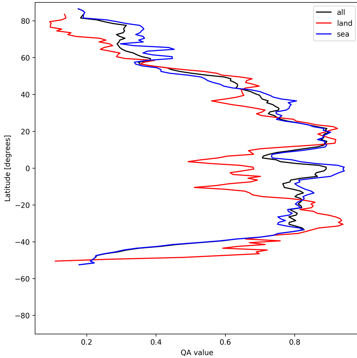
Figure 31: Zonal average of “QA value” for 2025-05-03 to 2025-05-05.
