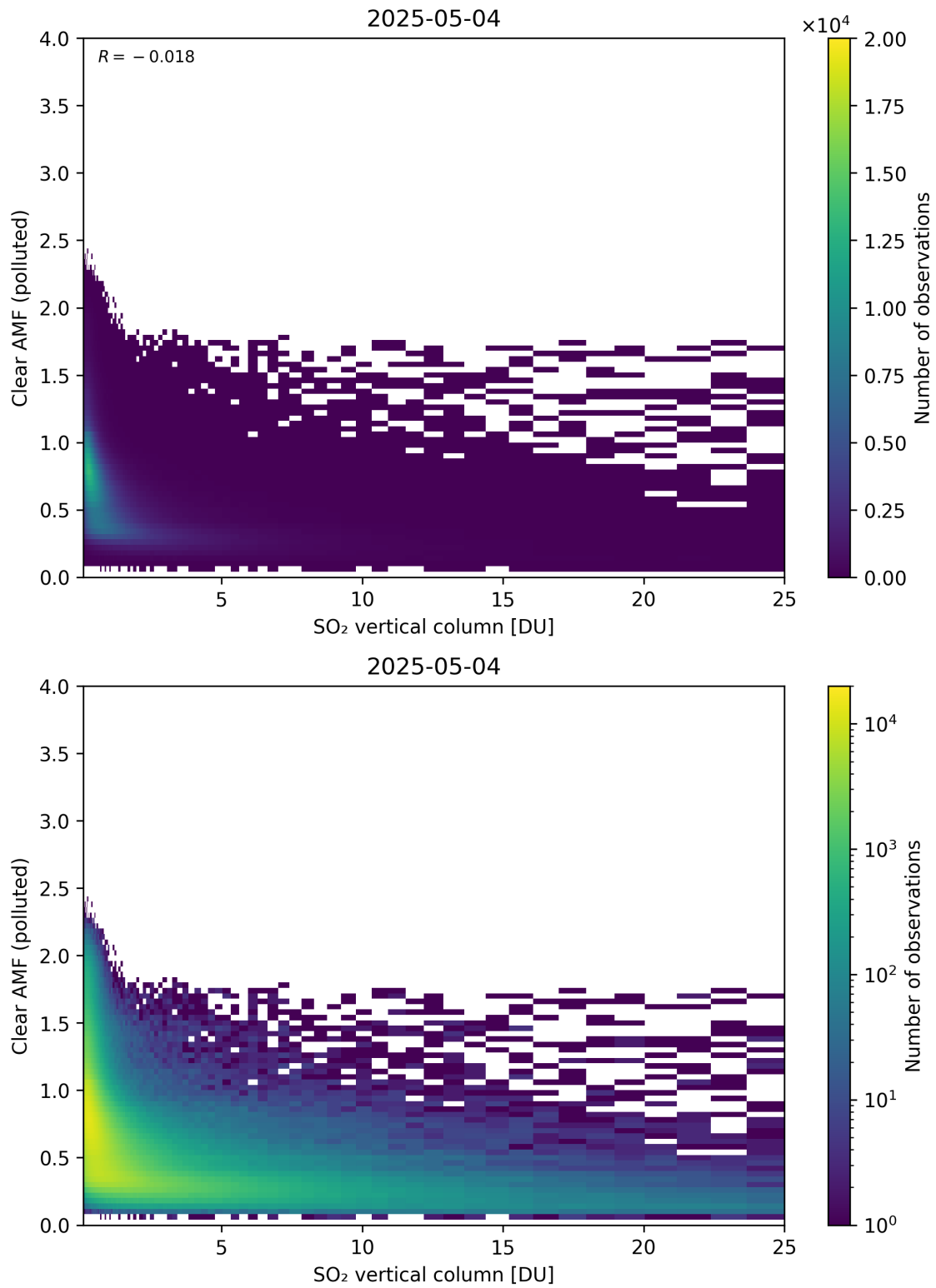
Figure 348: Scatter density plot of “SO 2 vertical column” against “Clear AMF (polluted)” for 2025-05-03 to 2025-05-05.
