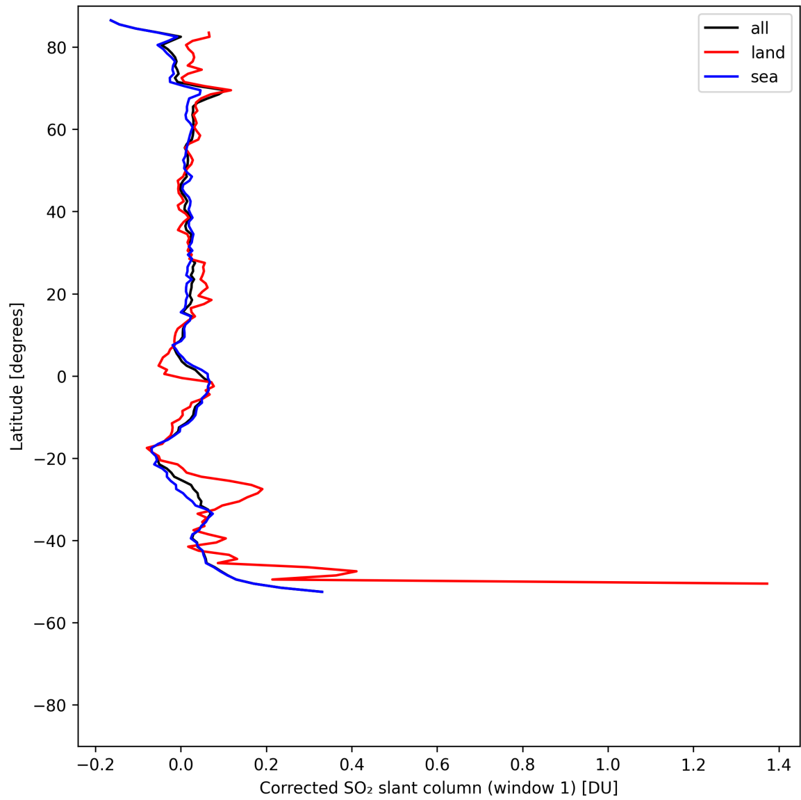
Figure 39: Zonal average of “Corrected SO 2 slant column (window 1)” for 2025-05-03 to 2025-05-05.
