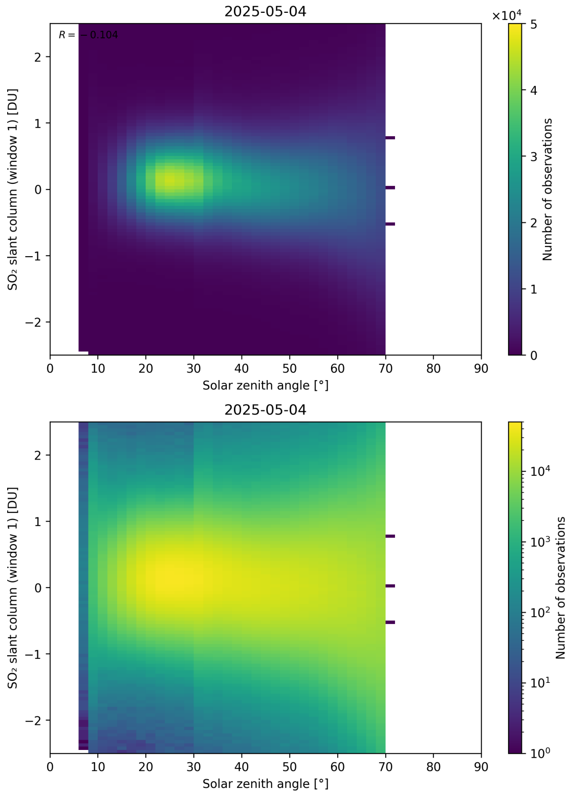
Figure 184: Scatter density plot of “Solar zenith angle” against “SO 2 slant column (window 1)” for 2025-05-03 to 2025-05-05.
