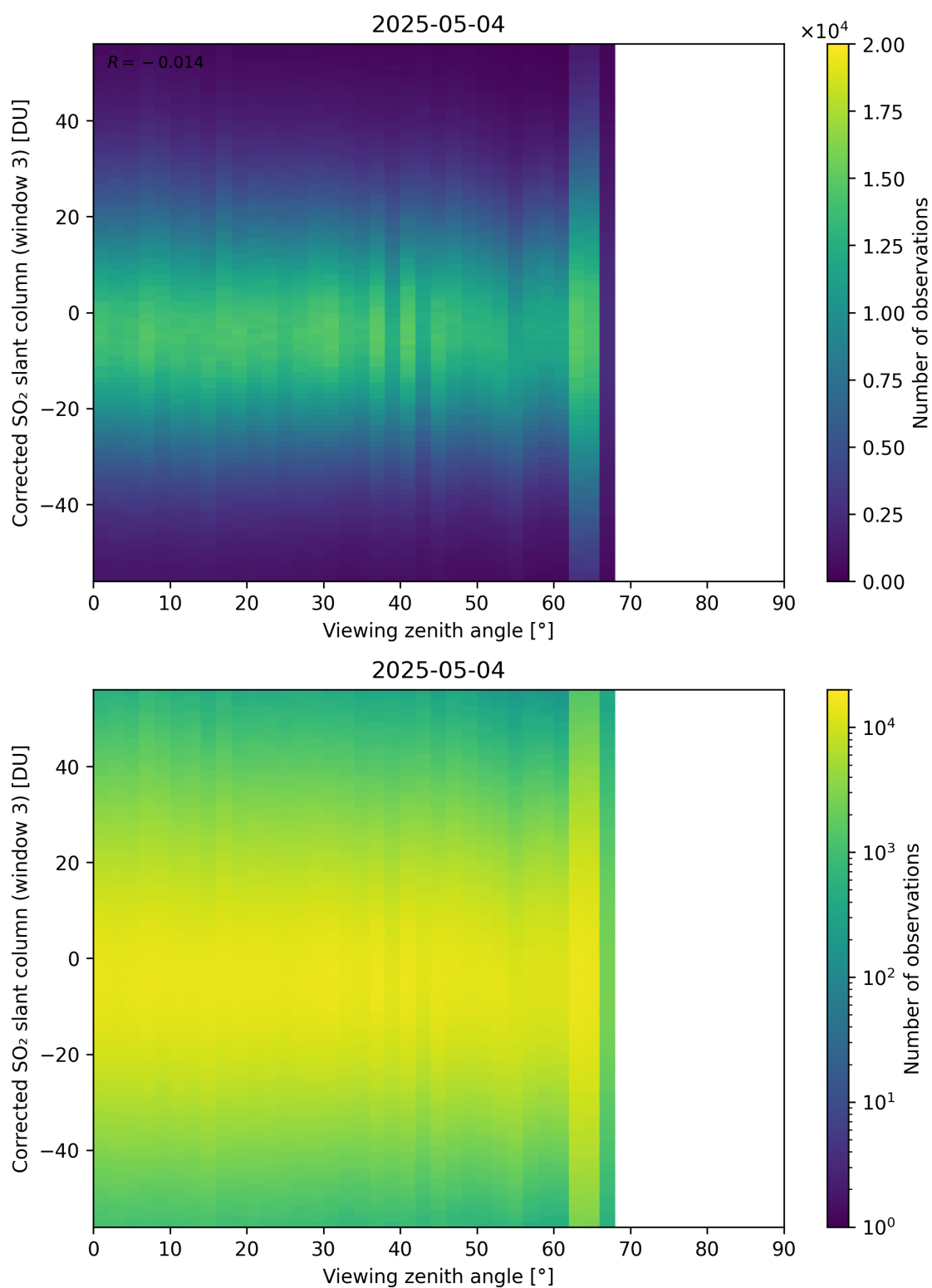
Figure 375: Scatter density plot of “Viewing zenith angle” against “Corrected SO 2 slant column (window 3)” for 2025-05-03 to 2025-05-05.
