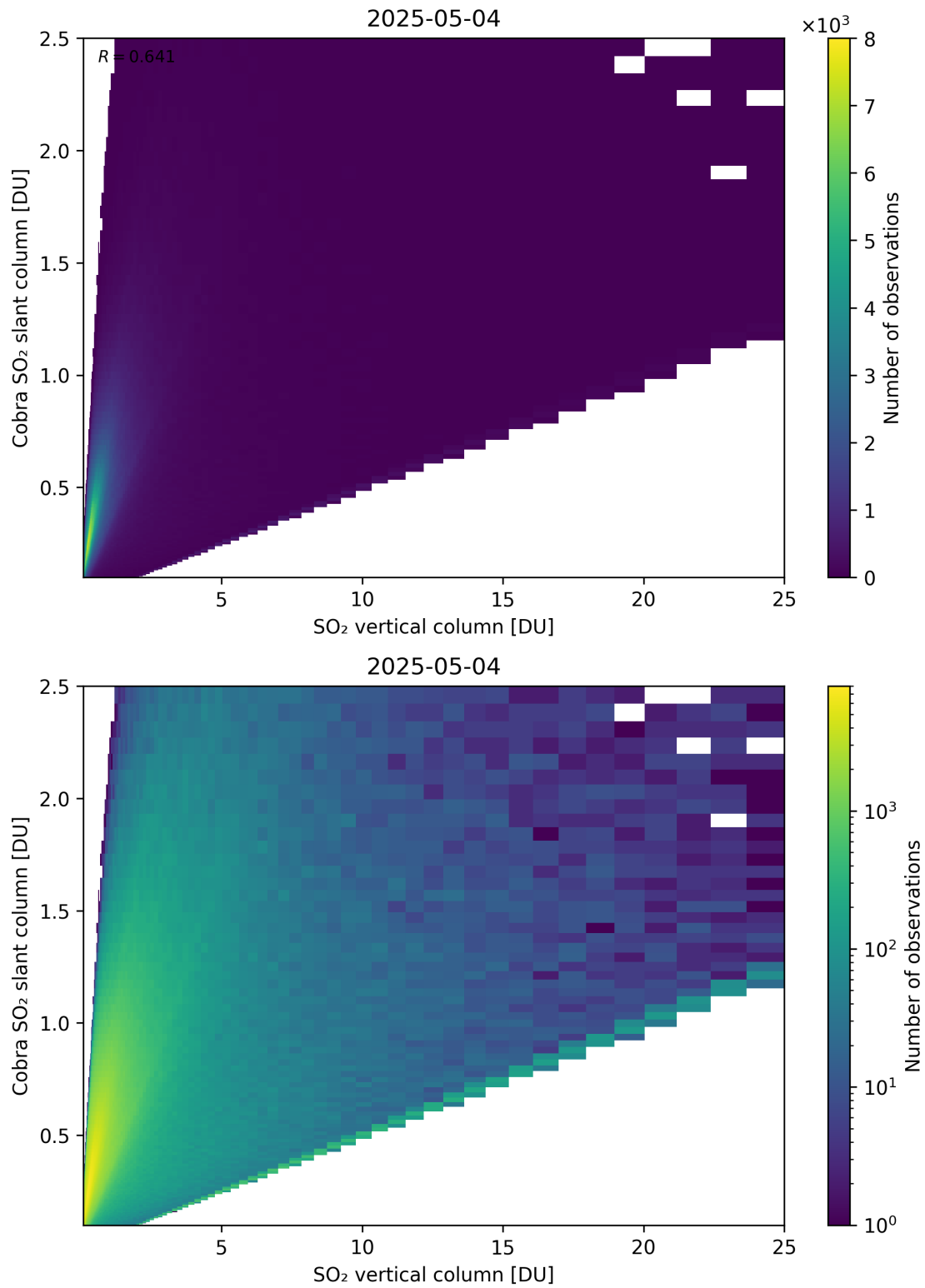
Figure 349: Scatter density plot of “SO 2 vertical column” against “Cobra SO 2 slant column” for 2025-05-03 to 2025-05-05.
