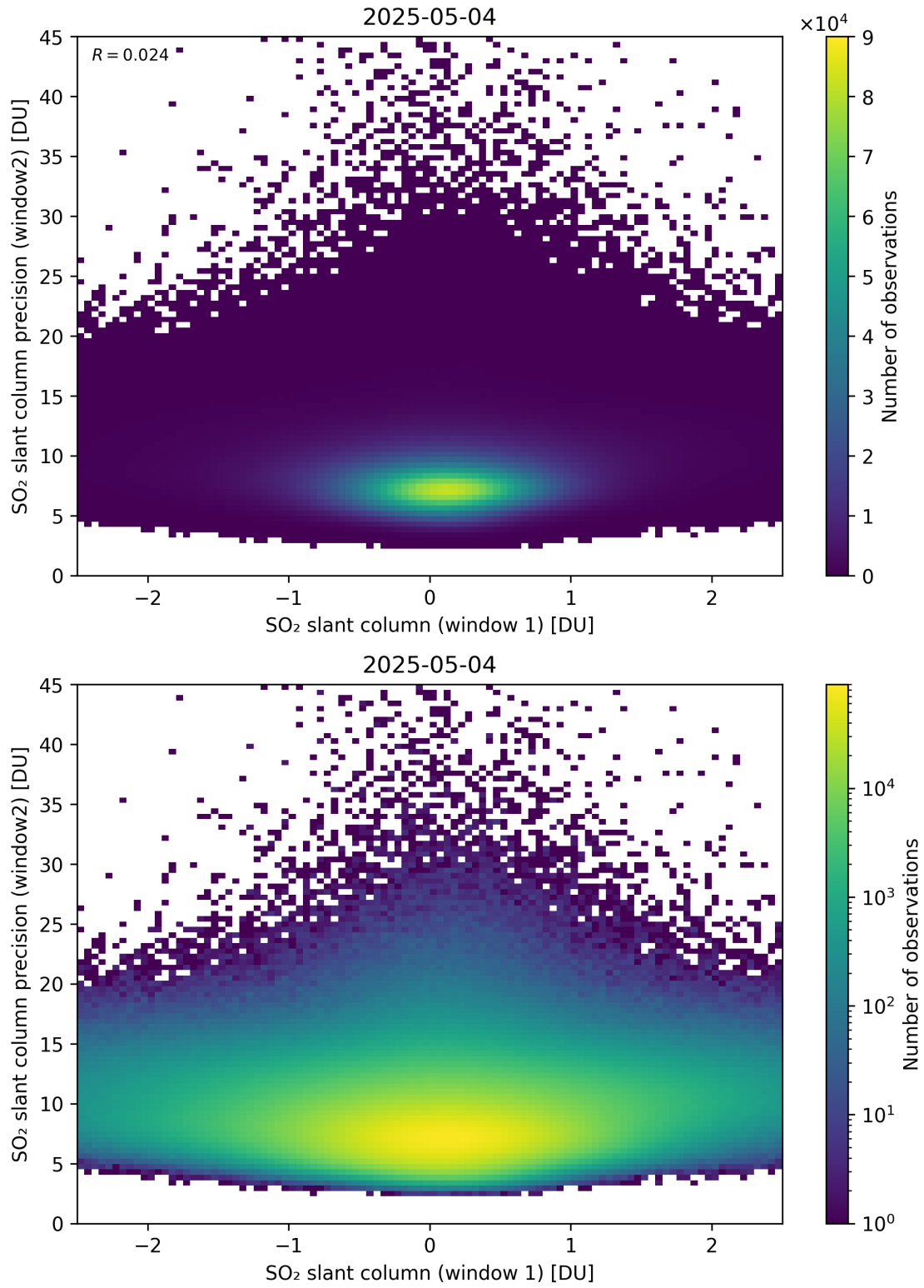
Figure 286: Scatter density plot of “SO 2 slant column (window 1)” against “SO 2 slant column precision (window2)” for 2025-05-03 to 2025-05-05.
