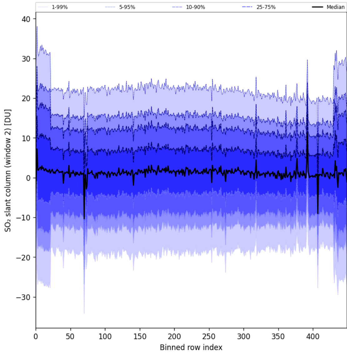
Figure 93: Along track statistics of “SO 2 slant column (window 2)” for 2025-05-03 to 2025-05-05
