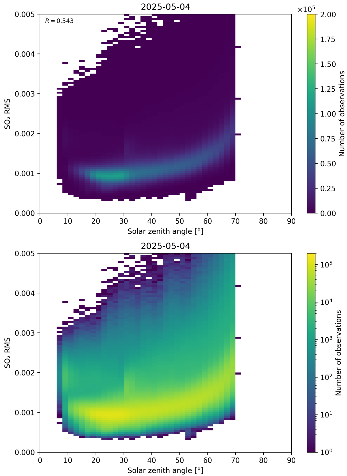
Figure 176: Scatter density plot of “Solar zenith angle” against “SO 2 RMS” for 2025-05-03 to 2025-05-05.
