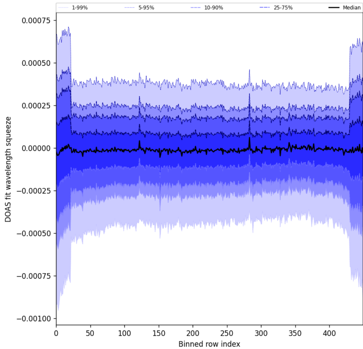
Figure 103: Along track statistics of “DOAS fit wavelength squeeze” for 2025-05-03 to 2025-05-05
