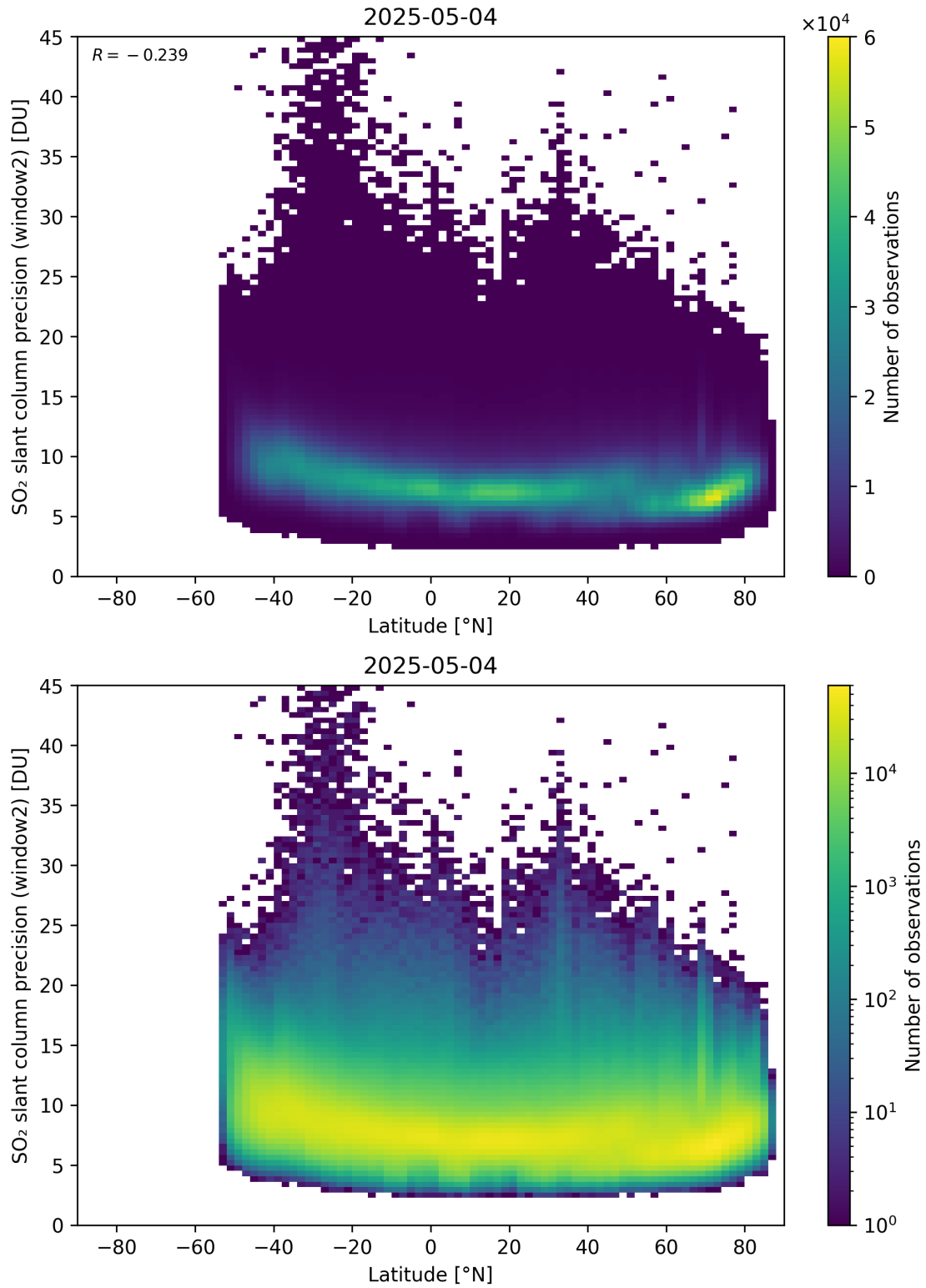
Figure 164: Scatter density plot of “Latitude” against “SO 2 slant column precision (window2)” for 2025-05-03 to 2025-05-05.
