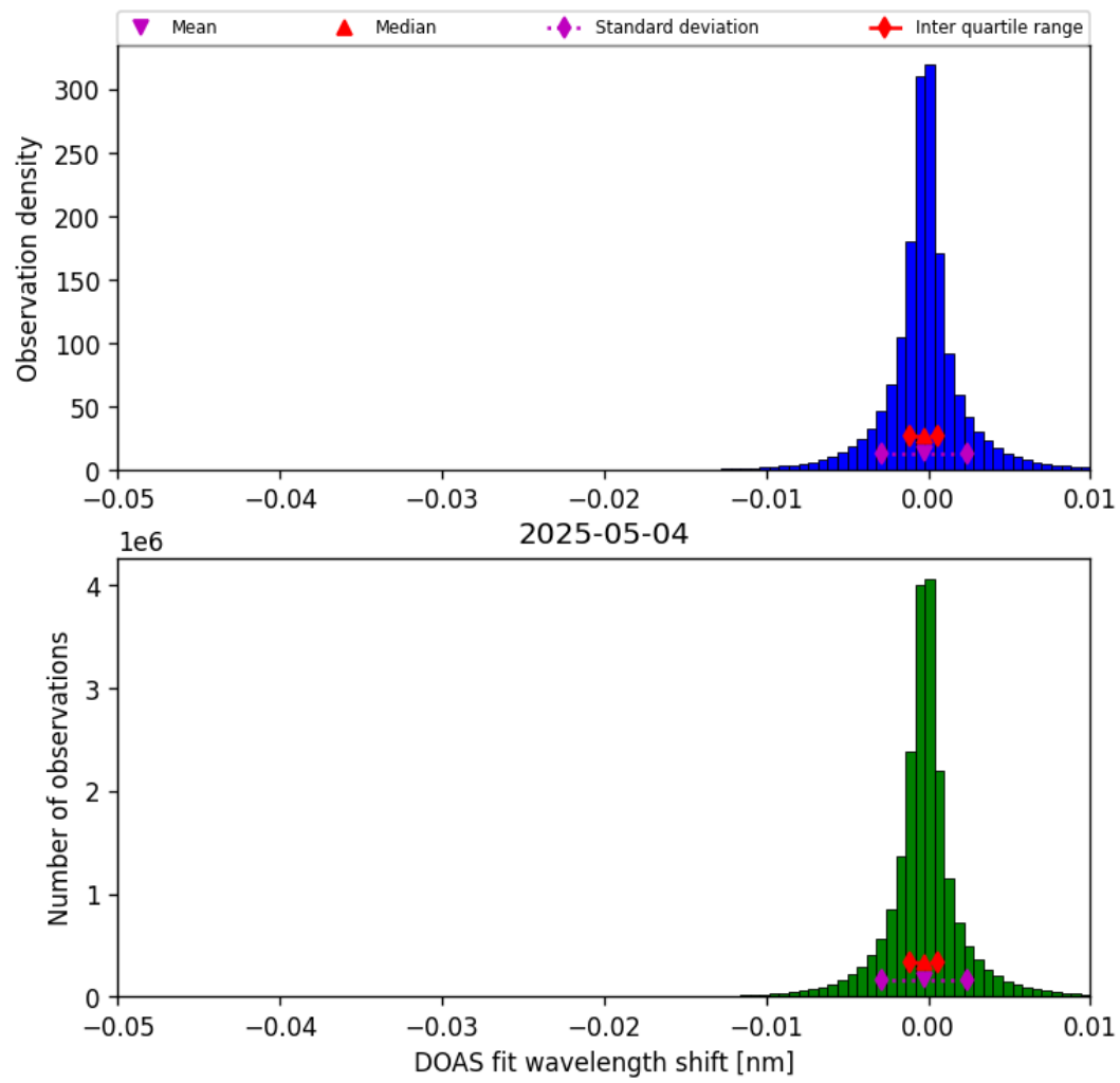
Figure 76: Histogram of “DOAS fit wavelength shift” for 2025-05-03 to 2025-05-05
