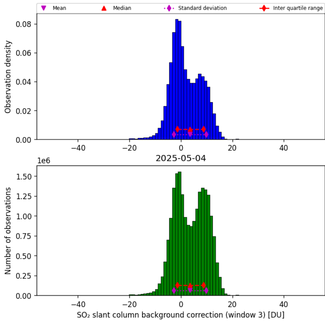
Figure 74: Histogram of “SO 2 slant column background correction (window 3)” for 2025-05-03 to 2025-05-05
