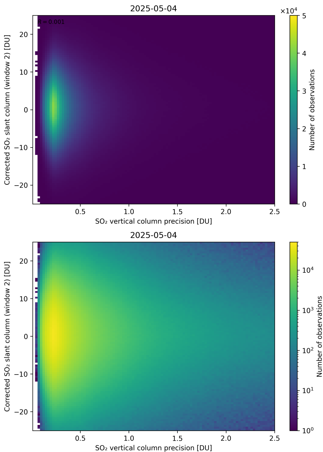
Figure 339: Scatter density plot of “SO 2 vertical column precision” against “Corrected SO 2 slant column (window 2)” for 2025-05-03 to 2025-05-05.
