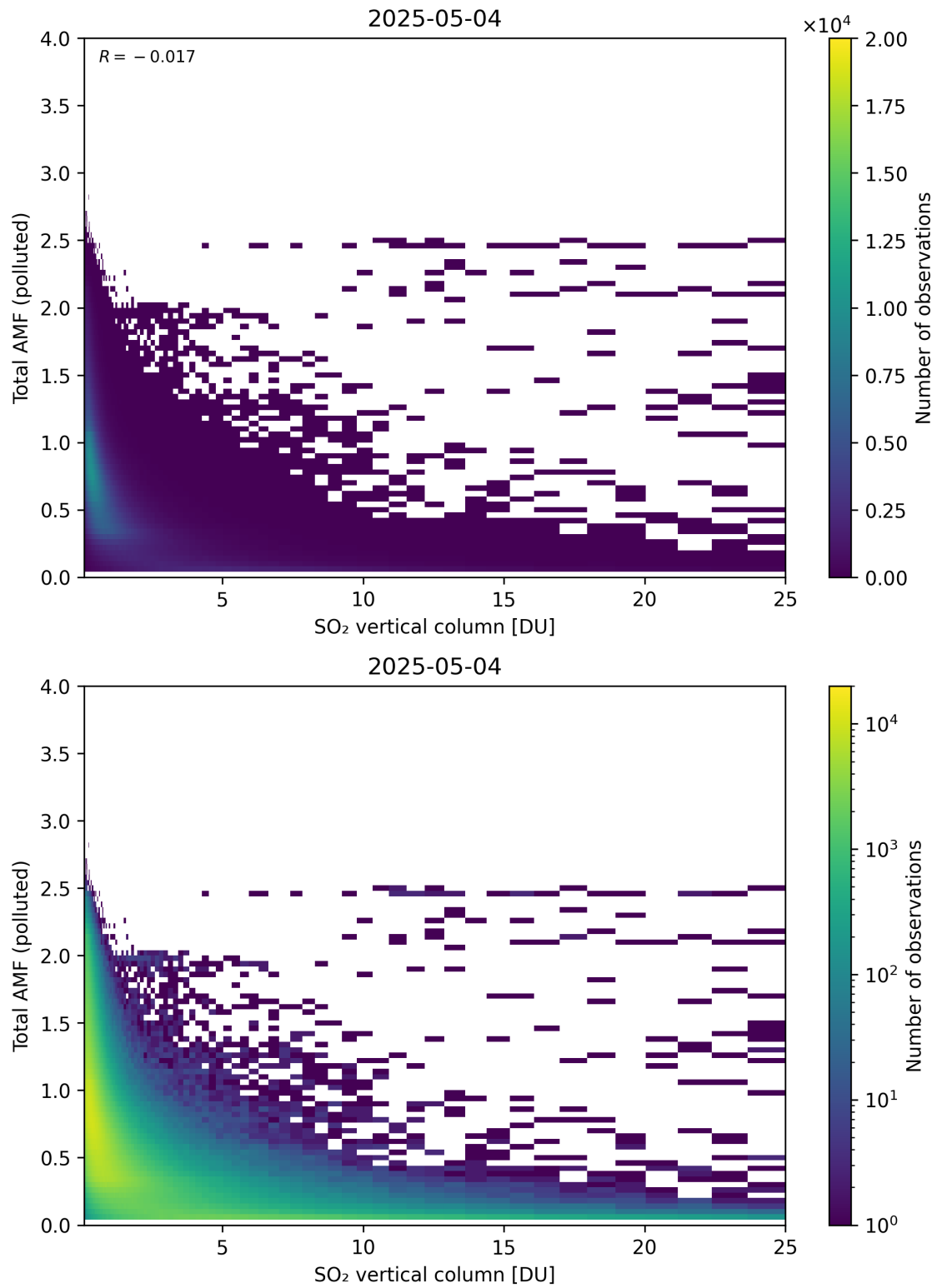
Figure 359: Scatter density plot of “SO 2 vertical column” against “Total AMF (polluted)” for 2025-05-03 to 2025-05-05.
