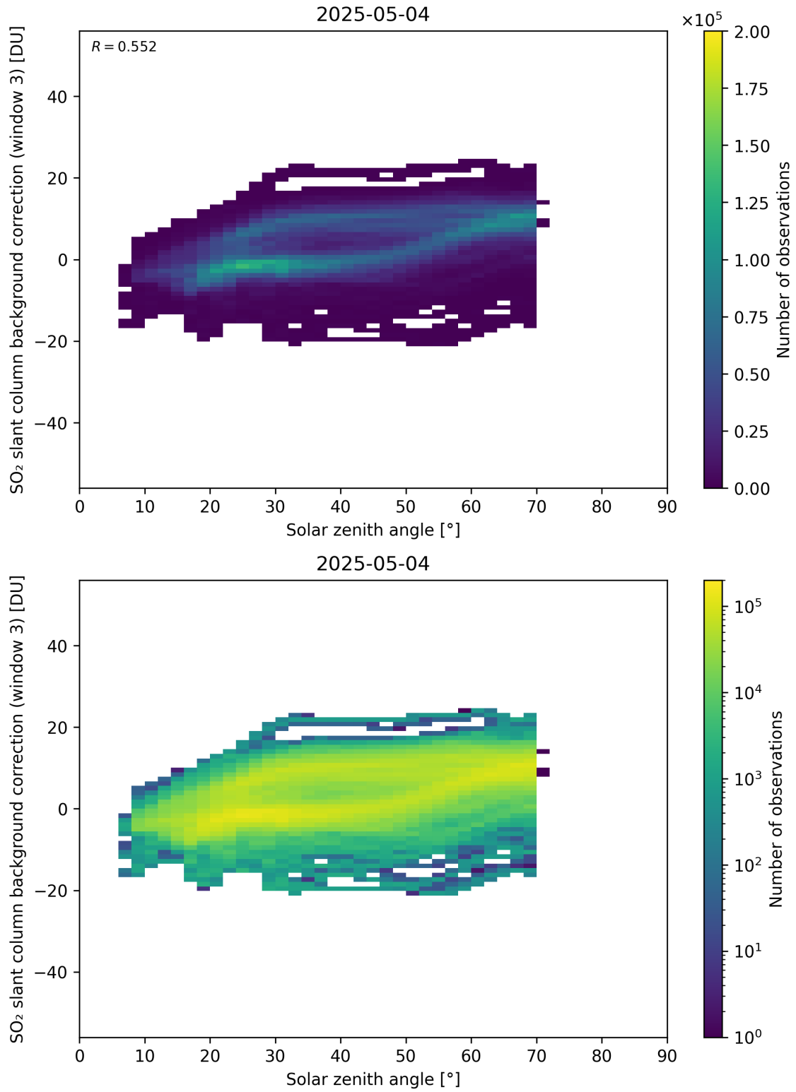
Figure 173: Scatter density plot of “Solar zenith angle” against “SO 2 slant column background correction (window 3)” for 2025-05-03 to 2025-05-05.
