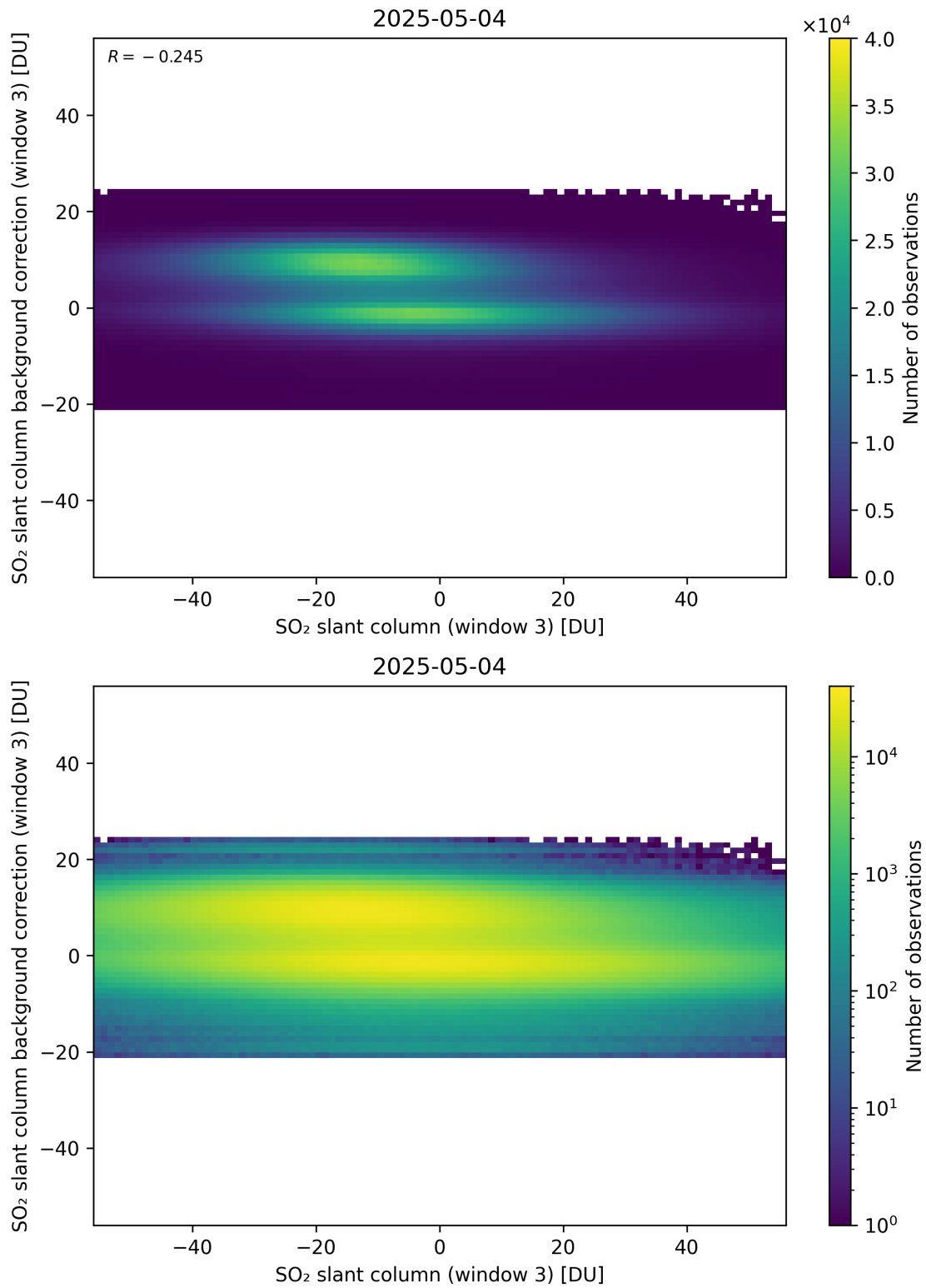
Figure 303: Scatter density plot of “SO 2 slant column (window 3)” against “SO 2 slant column background correction (window 3)” for 2025-05-03 to 2025-05-05.
