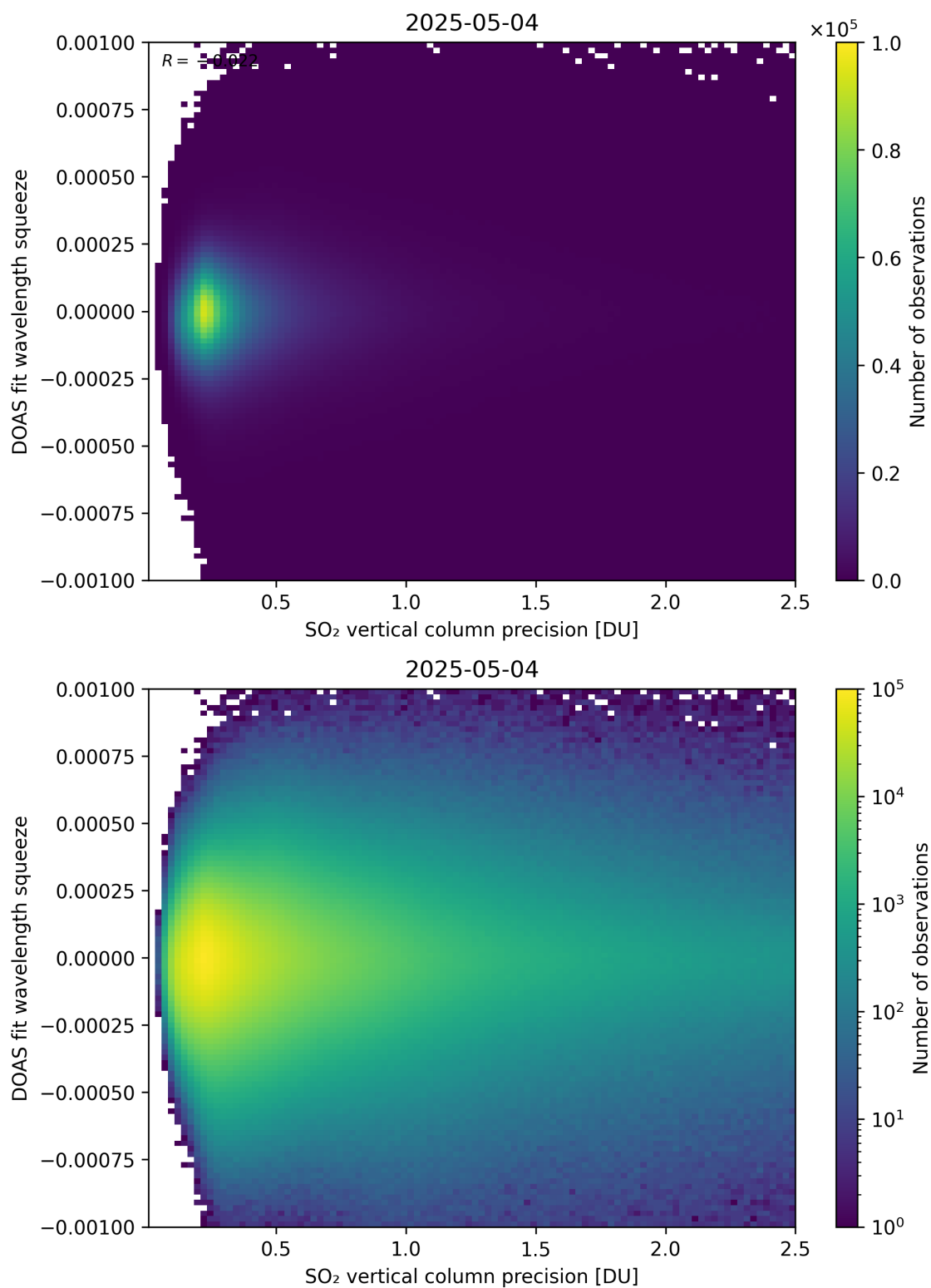
Figure 333: Scatter density plot of “SO 2 vertical column precision” against “DOAS fit wavelength squeeze” for 2025-05-03 to 2025-05-05.
