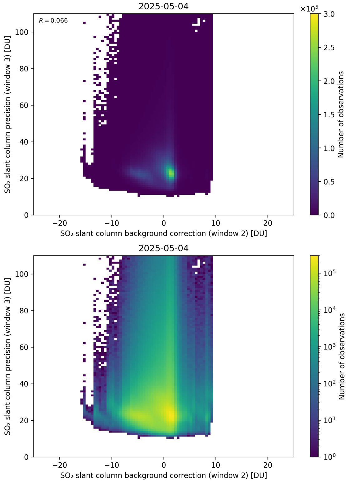
Figure 129: Scatter density plot of “SO 2 slant column background correction (window 2)” against “SO 2 slant column precision (window 3)” for 2025-05-03 to 2025-05-05.
