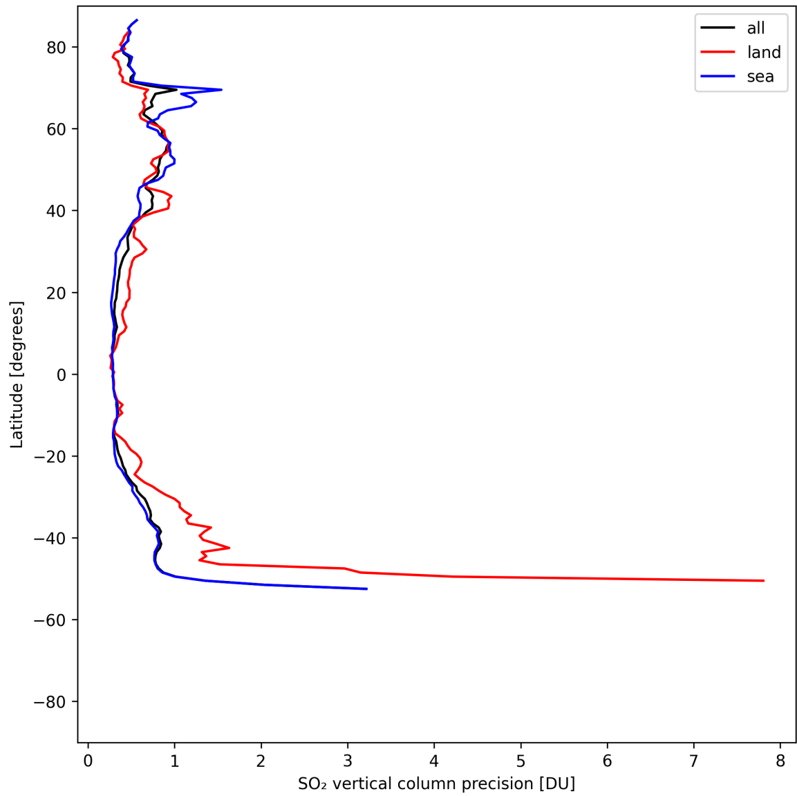
Figure 33: Zonal average of “SO 2 vertical column precision” for 2025-05-03 to 2025-05-05.
