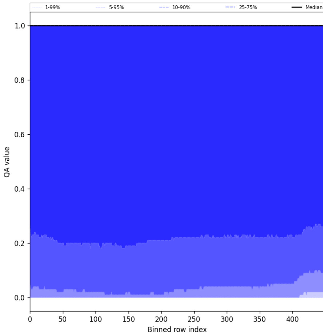
Figure 83: Along track statistics of “QA value” for 2025-05-03 to 2025-05-05
