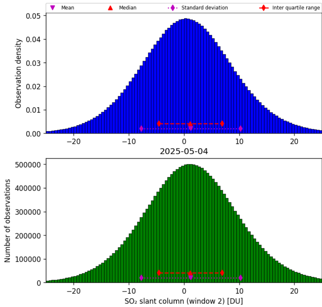
Figure 67: Histogram of “SO 2 slant column (window 2)” for 2025-05-03 to 2025-05-05
