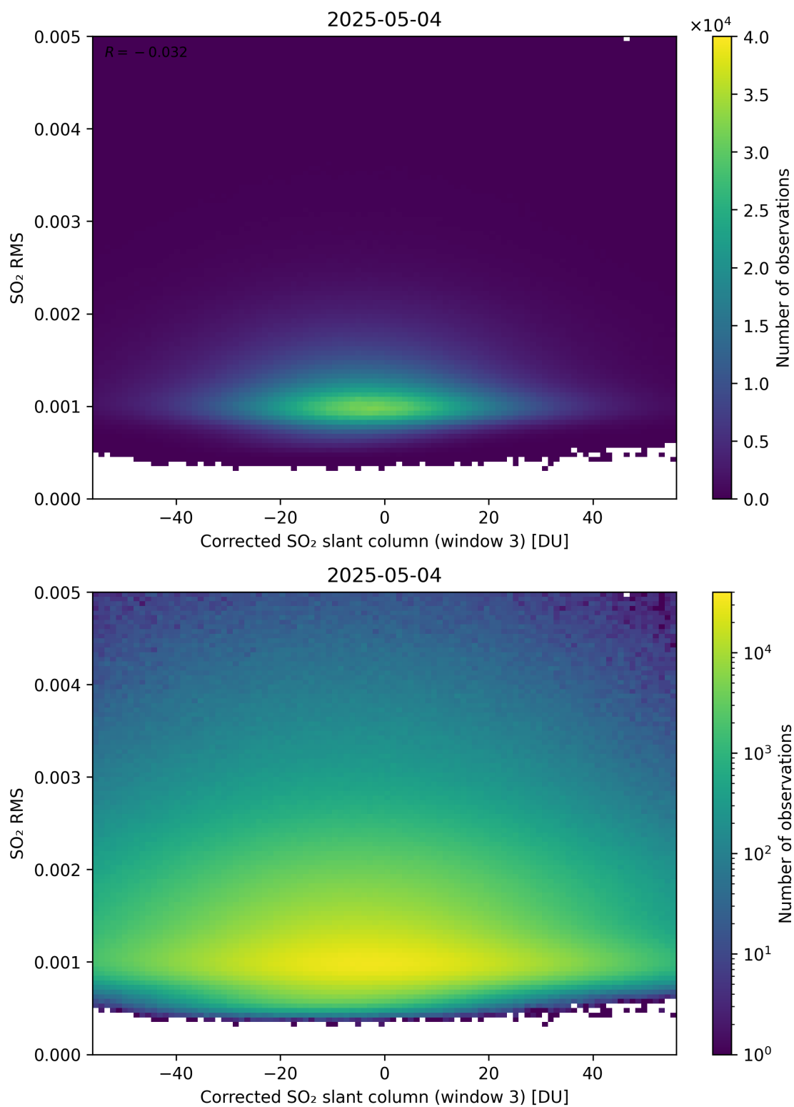
Figure 258: Scatter density plot of “Corrected SO 2 slant column (window 3)” against “SO 2 RMS” for 2025-05-03 to 2025-05-05.
