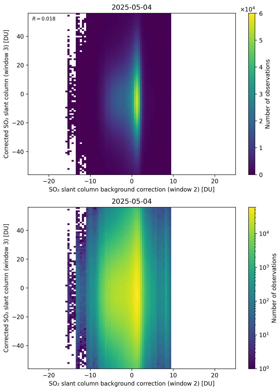
Figure 127: Scatter density plot of “SO 2 slant column background correction (window 2)” against “Corrected SO 2 slant column (window 3)” for 2025-05-03 to 2025-05-05.
