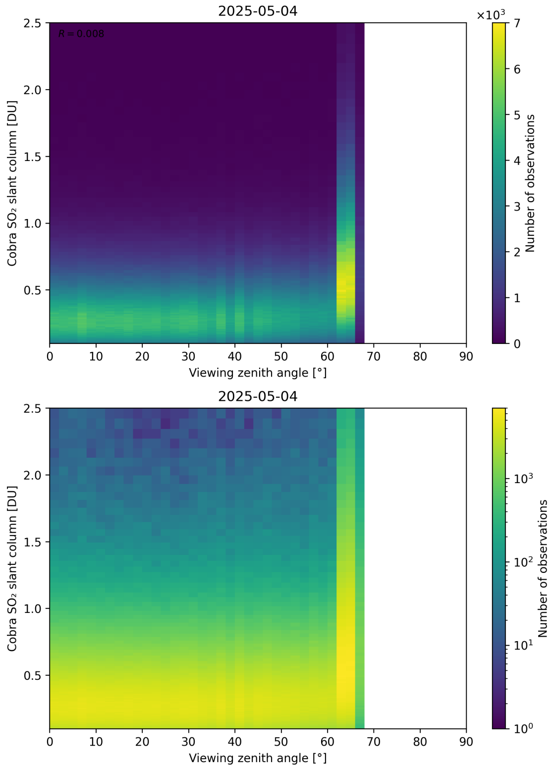
Figure 371: Scatter density plot of “Viewing zenith angle” against “Cobra SO 2 slant column” for 2025-05-03 to 2025-05-05.
