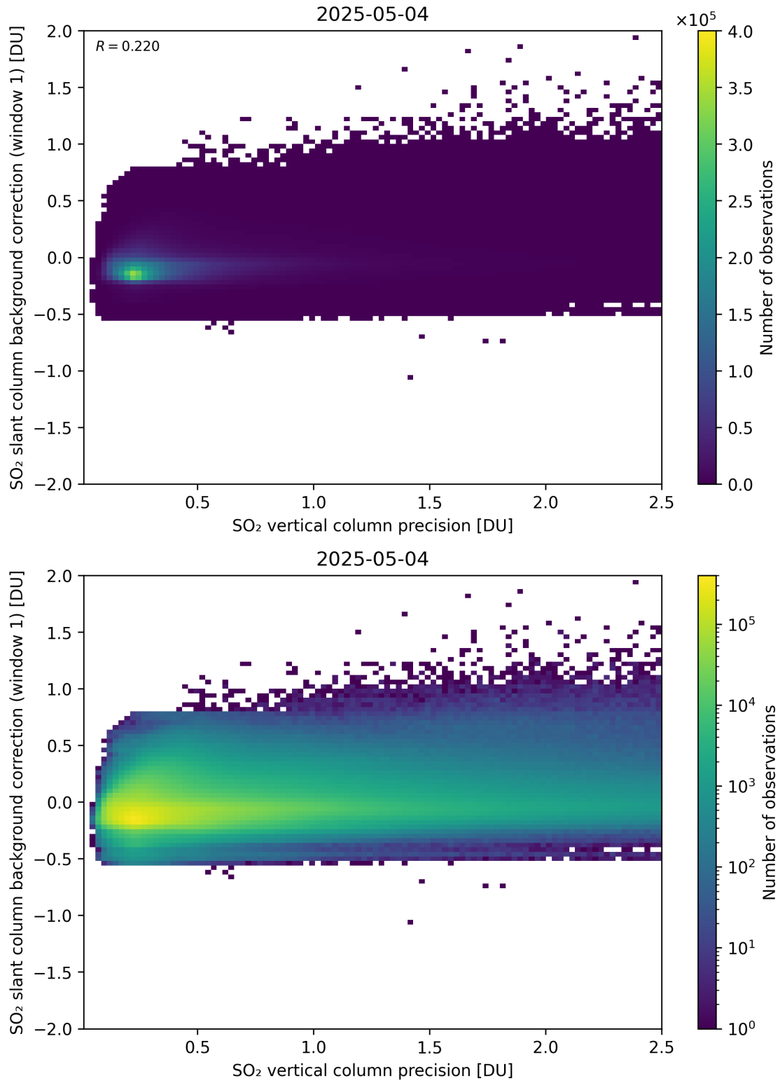
Figure 329: Scatter density plot of “SO 2 vertical column precision” against “SO 2 slant column background correction (window 1)” for 2025-05-03 to 2025-05-05.
