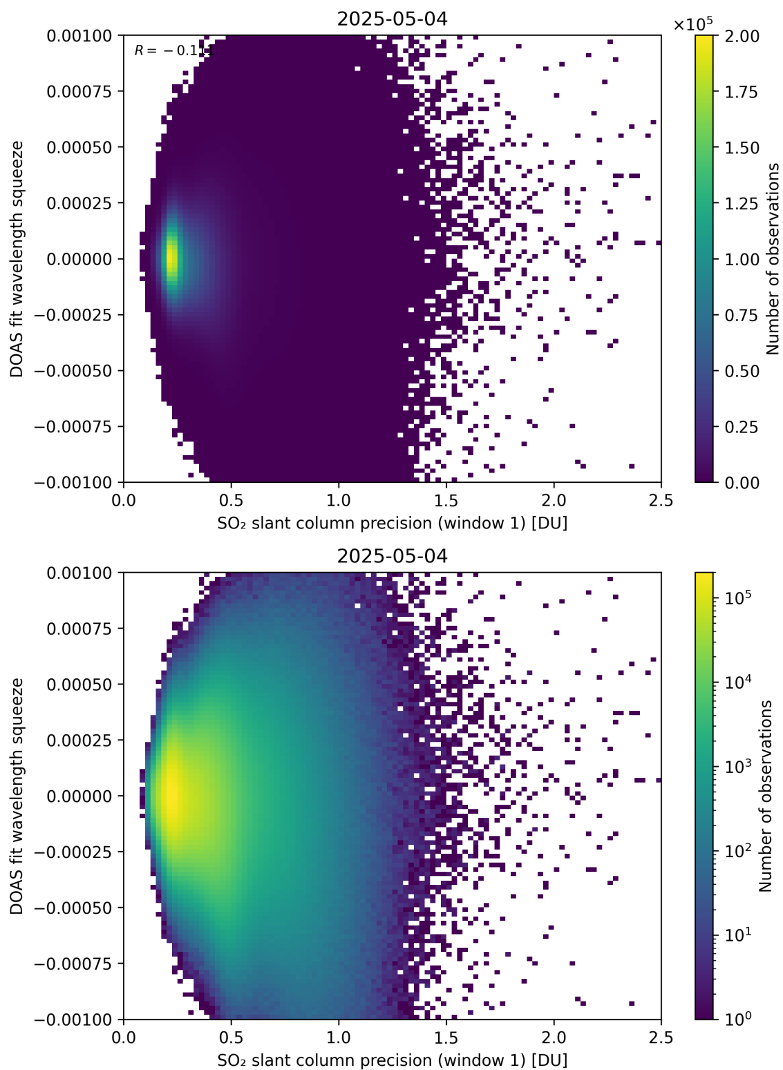
Figure 272: Scatter density plot of “SO 2 slant column precision (window 1)” against “DOAS fit wavelength squeeze” for 2025-05-03 to 2025-05-05.
