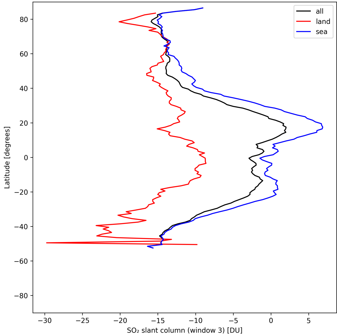
Figure 45: Zonal average of “SO 2 slant column (window 3)” for 2025-05-03 to 2025-05-05.
