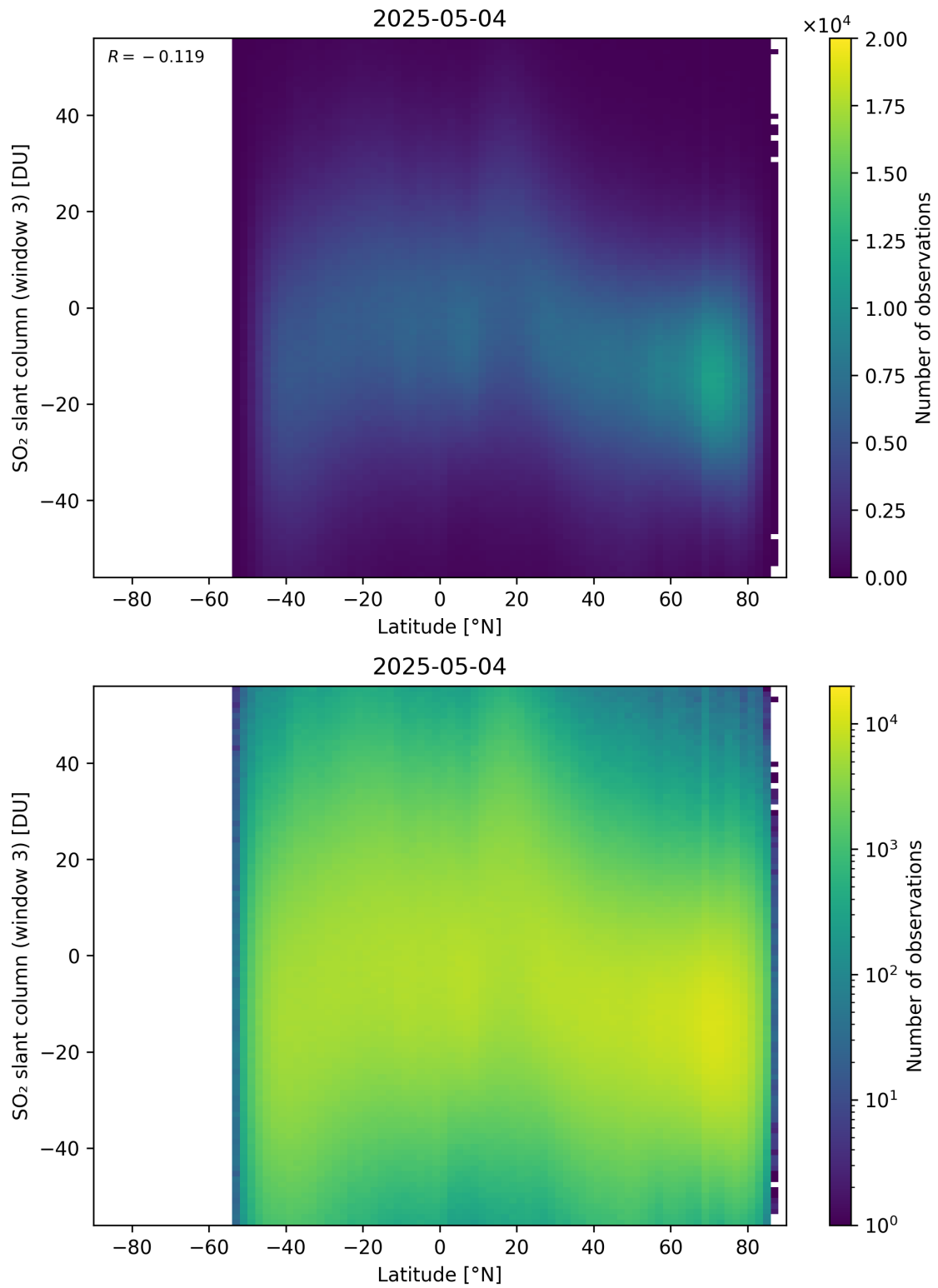
Figure 165: Scatter density plot of “Latitude” against “SO 2 slant column (window 3)” for 2025-05-03 to 2025-05-05.
