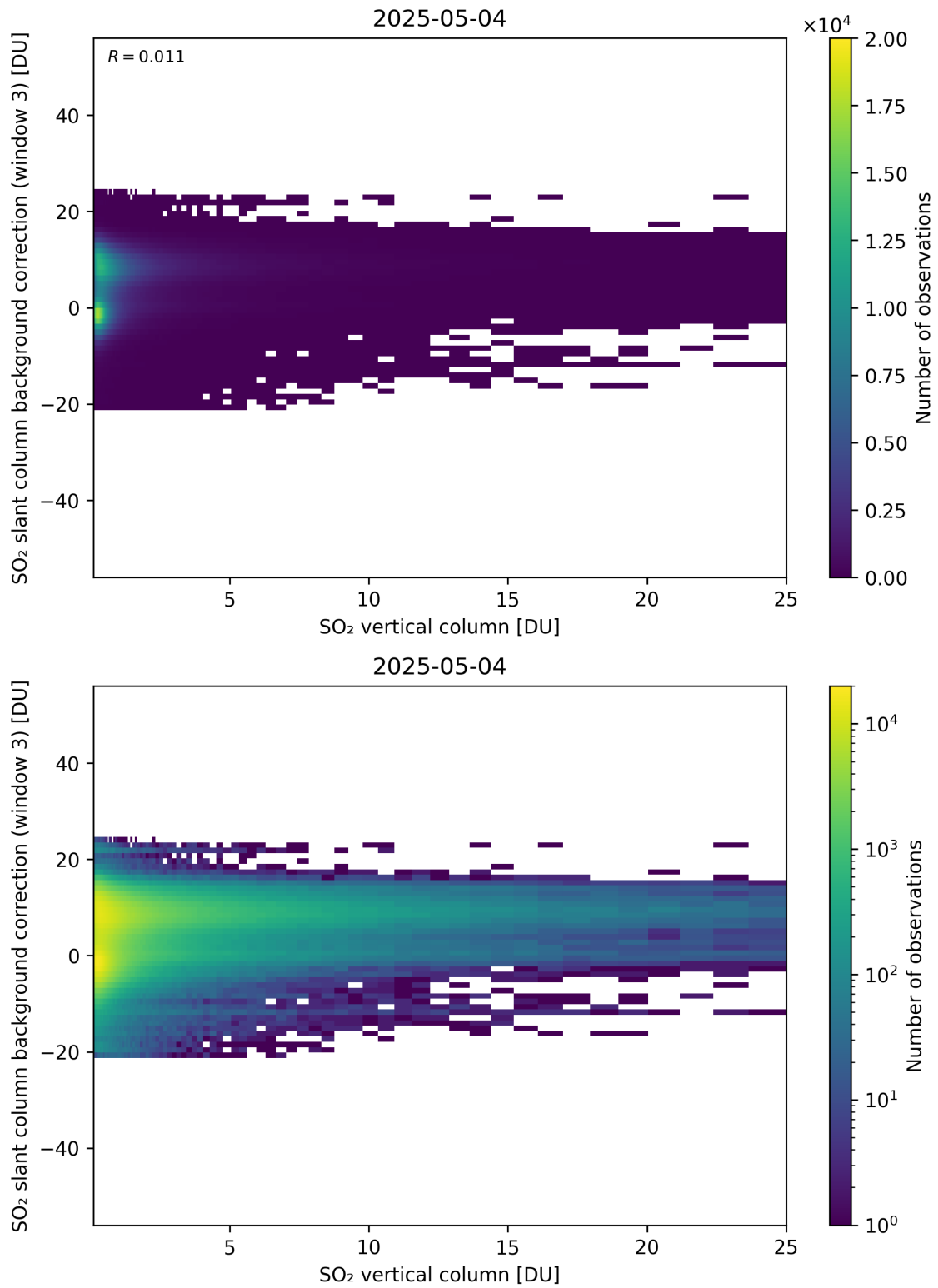
Figure 325: Scatter density plot of “SO 2 vertical column” against “SO 2 slant column background correction (window 3)” for 2025-05-03 to 2025-05-05.
