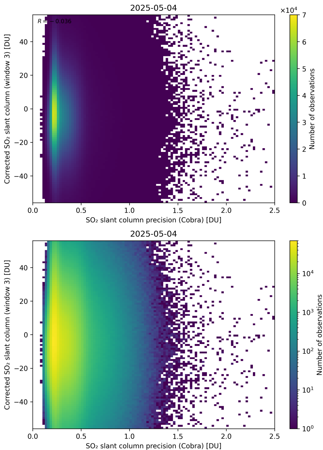
Figure 207: Scatter density plot of “SO 2 slant column precision (Cobra)” against “Corrected SO 2 slant column (window 3)” for 2025-05-03 to 2025-05-05.
