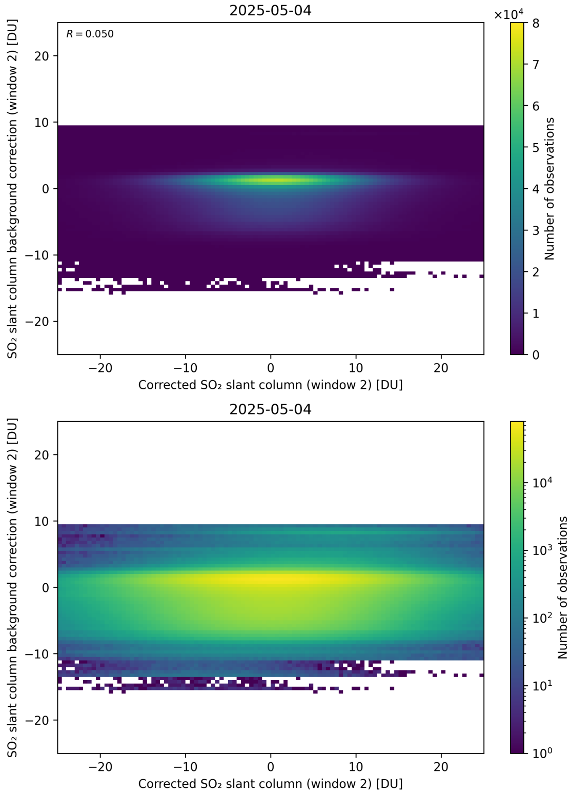
Figure 244: Scatter density plot of “Corrected SO 2 slant column (window 2)” against “SO 2 slant column background correction (window 2)” for 2025-05-03 to 2025-05-05.
