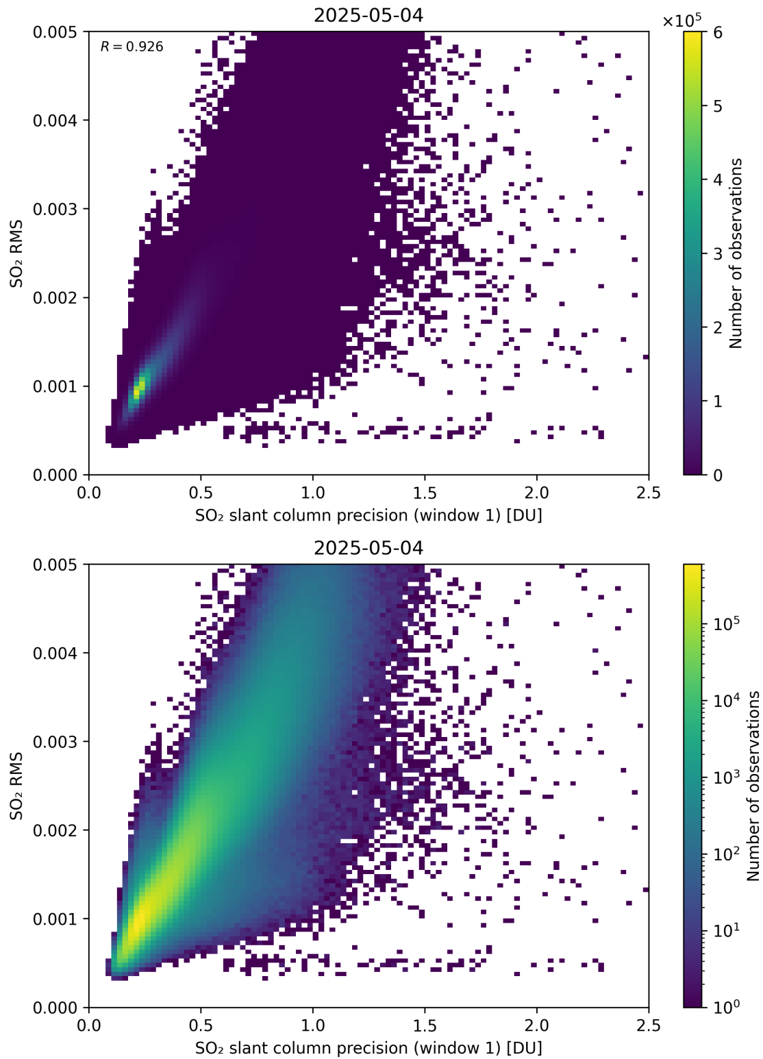
Figure 273: Scatter density plot of “SO 2 slant column precision (window 1)” against “SO 2 RMS” for 2025-05-03 to 2025-05-05.
