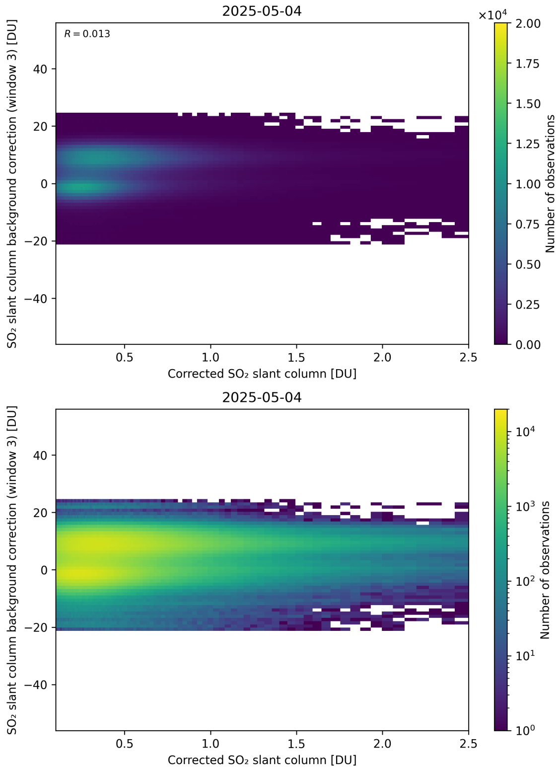
Figure 228: Scatter density plot of “Corrected SO 2 slant column” against “SO 2 slant column background correction (window 3)” for 2025-05-03 to 2025-05-05.
