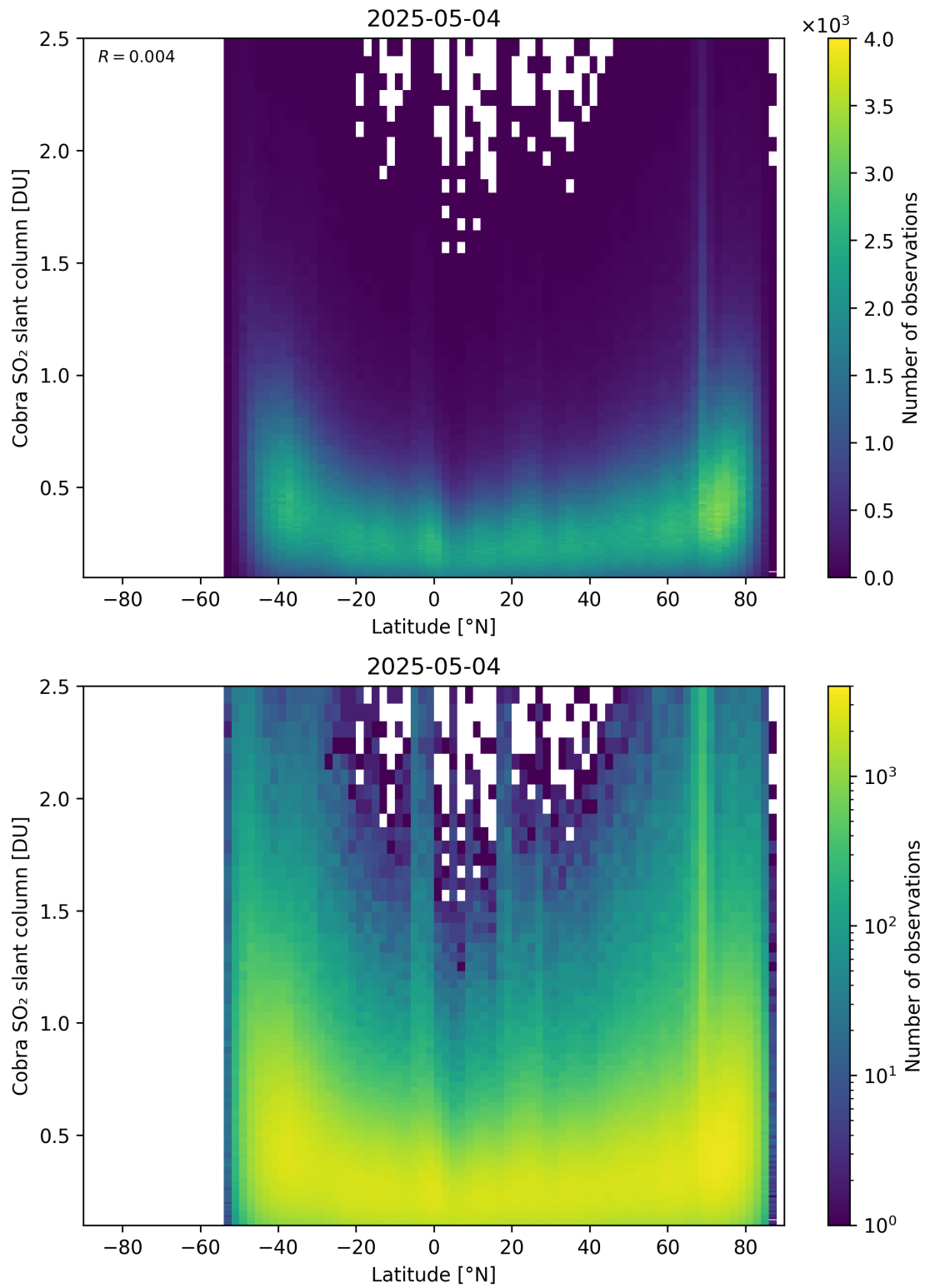
Figure 157: Scatter density plot of “Latitude” against “Cobra SO 2 slant column” for 2025-05-03 to 2025-05-05.
