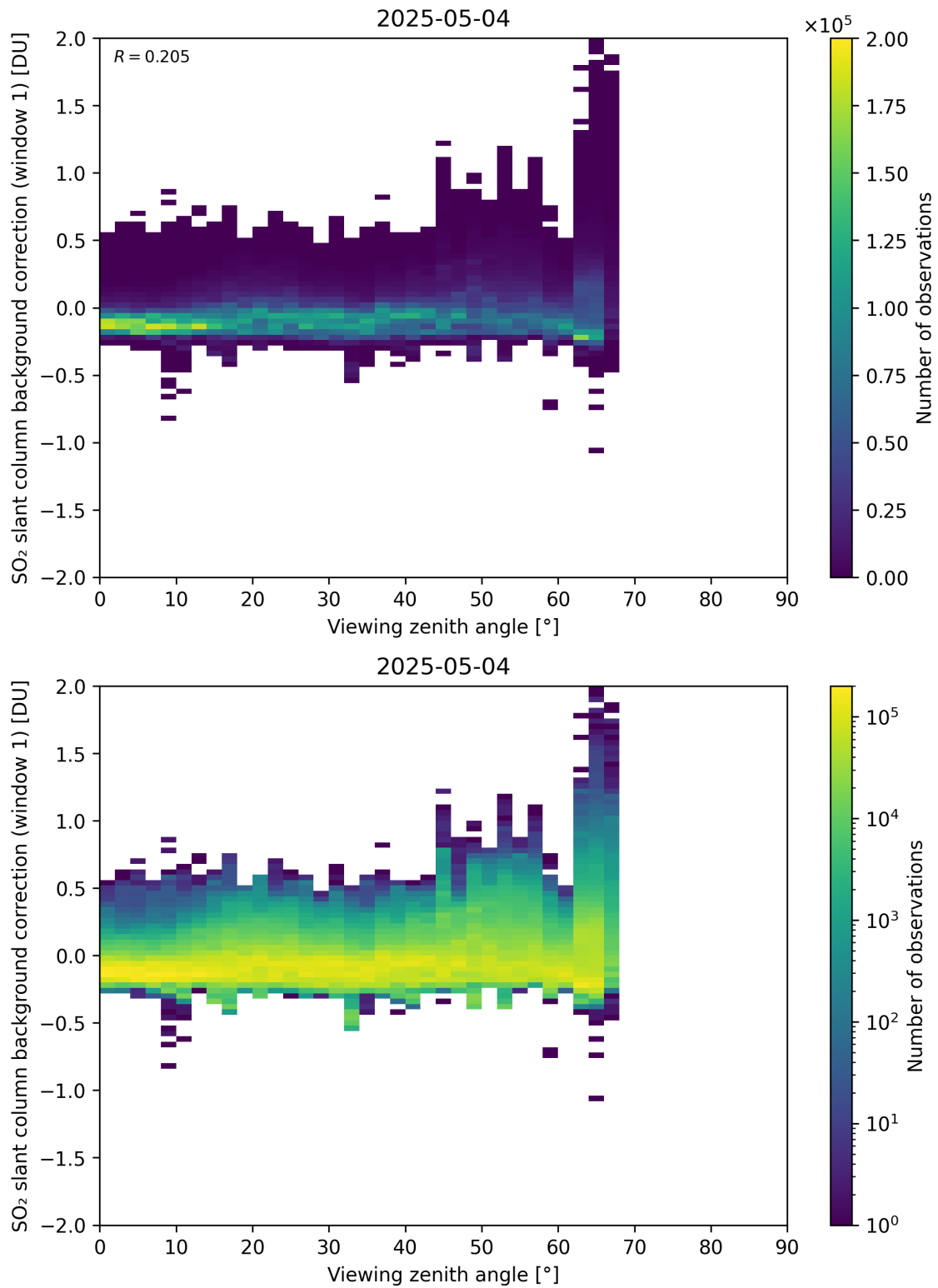
Figure 362: Scatter density plot of “Viewing zenith angle” against “SO 2 slant column background correction (window 1)” for 2025-05-03 to 2025-05-05.
