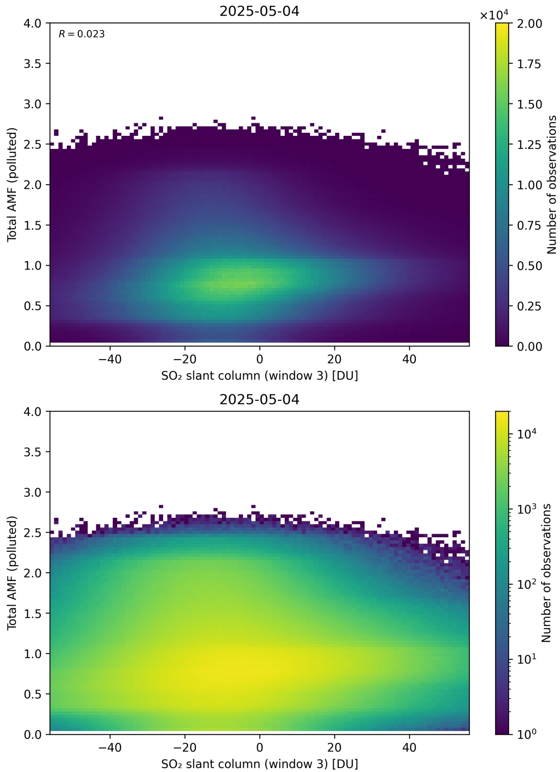
Figure 318: Scatter density plot of “SO 2 slant column (window 3)” against “Total AMF (polluted)” for 2025-05-03 to 2025-05-05.
