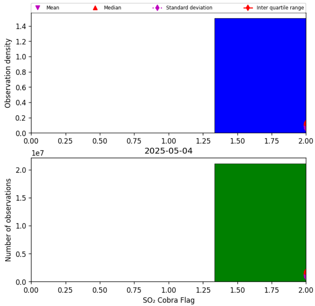
Figure 75: Histogram of “SO 2 Cobra Flag” for 2025-05-03 to 2025-05-05
