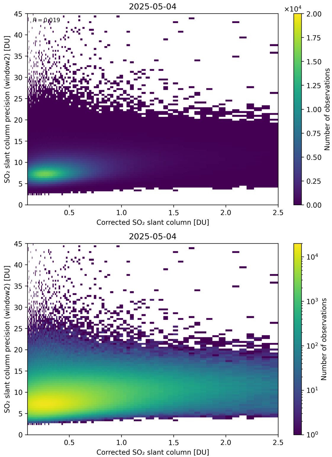
Figure 239: Scatter density plot of “Corrected SO 2 slant column” against “SO 2 slant column precision (window2)” for 2025-05-03 to 2025-05-05.
