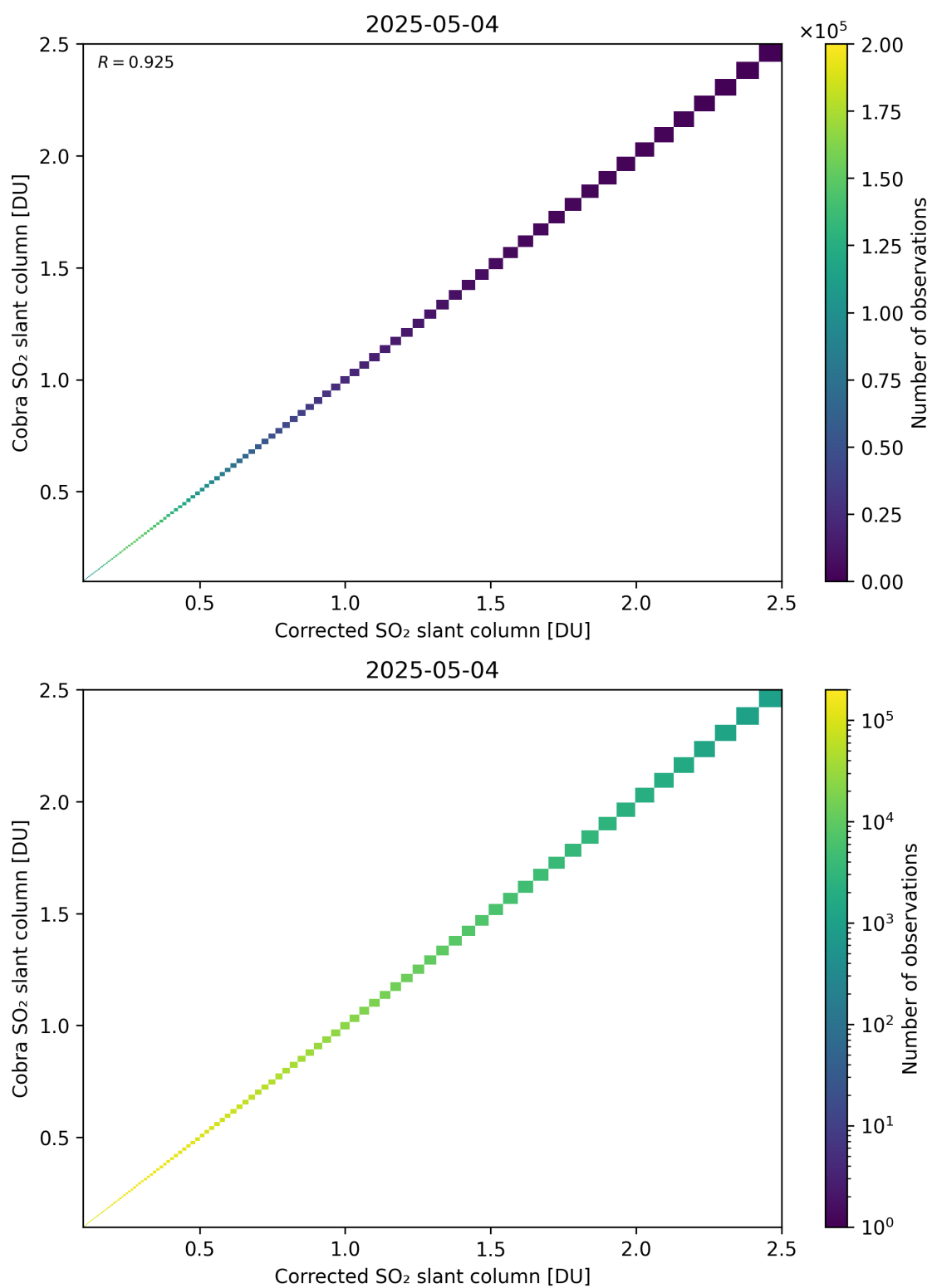
Figure 233: Scatter density plot of “Corrected SO 2 slant column” against “Cobra SO 2 slant column” for 2025-05-03 to 2025-05-05.
