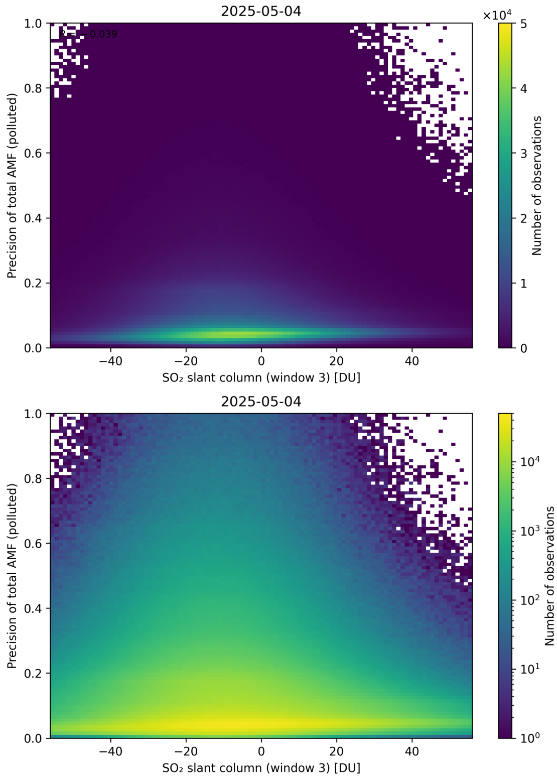
Figure 319: Scatter density plot of “SO 2 slant column (window 3)” against “Precision of total AMF (polluted)” for 2025-05-03 to 2025-05-05.
