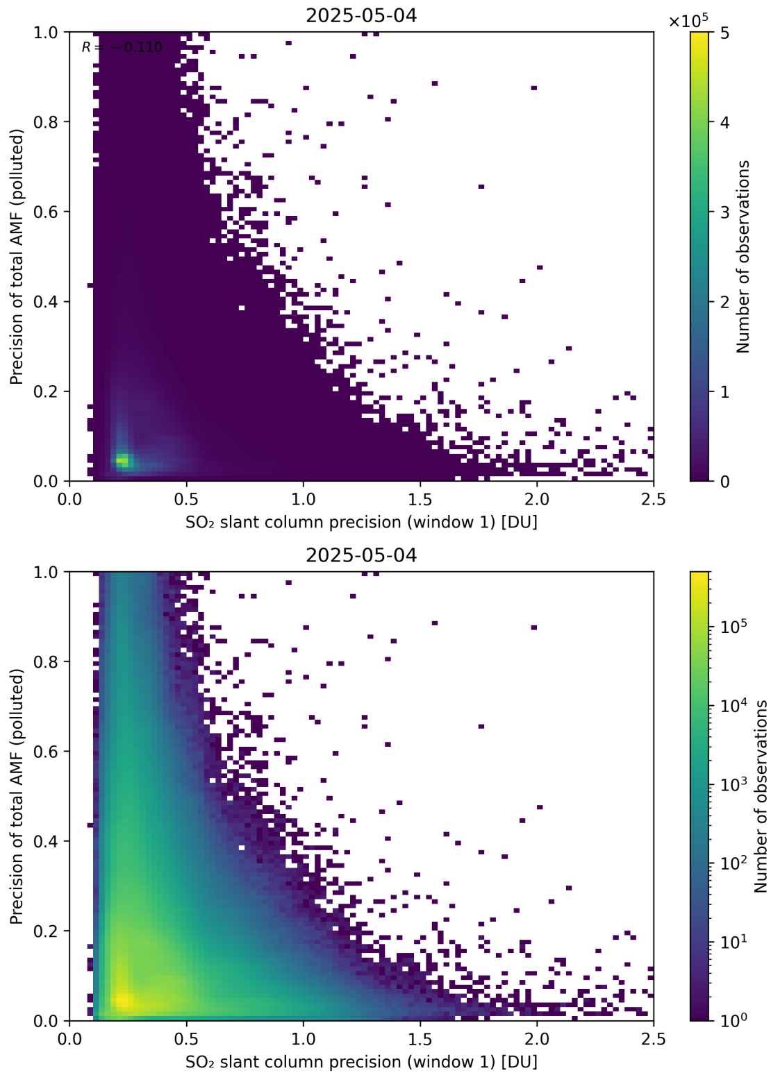
Figure 281: Scatter density plot of “SO 2 slant column precision (window 1)” against “Precision of total AMF (polluted)” for 2025-05-03 to 2025-05-05.
