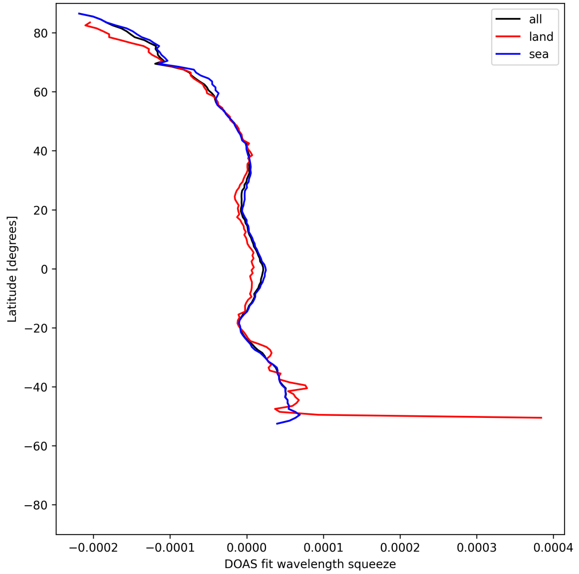
Figure 51: Zonal average of “DOAS fit wavelength squeeze” for 2025-05-03 to 2025-05-05.
