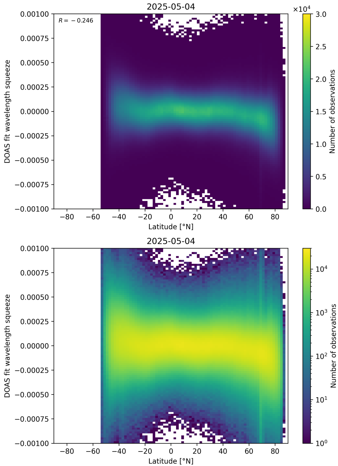
Figure 154: Scatter density plot of “Latitude” against “DOAS fit wavelength squeeze” for 2025-05-03 to 2025-05-05.
