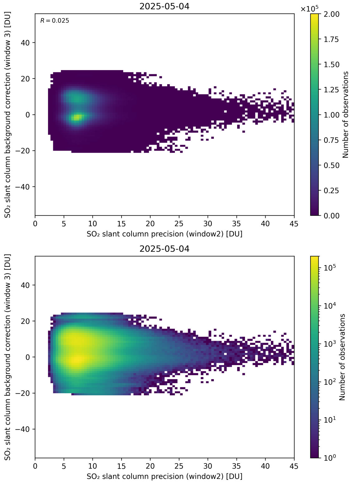
Figure 292: Scatter density plot of “SO 2 slant column precision (window2)” against “SO 2 slant column background correction (window 3)” for 2025-05-03 to 2025-05-05.
