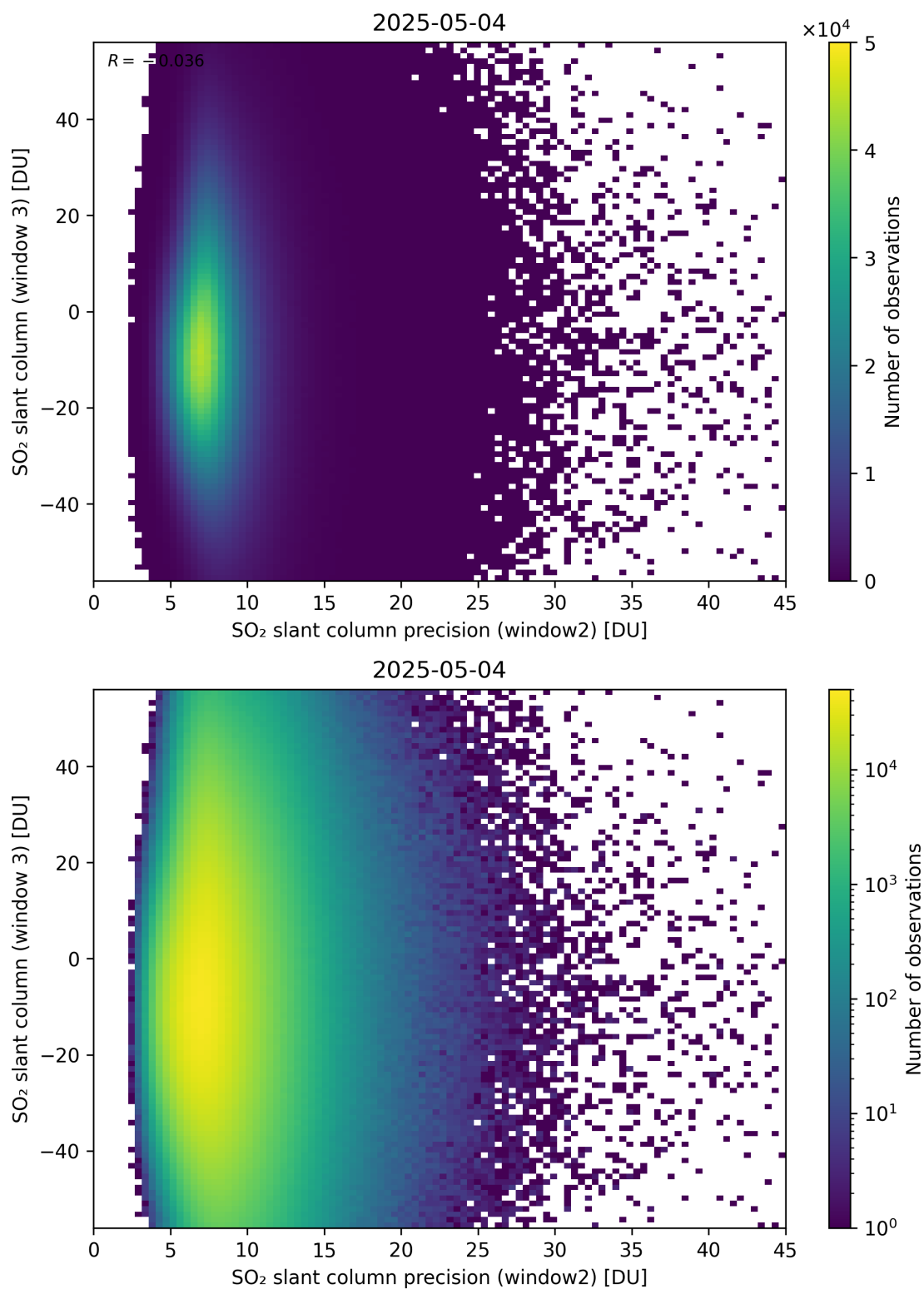
Figure 299: Scatter density plot of “SO 2 slant column precision (window2)” against “SO 2 slant column (window 3)” for 2025-05-03 to 2025-05-05.
