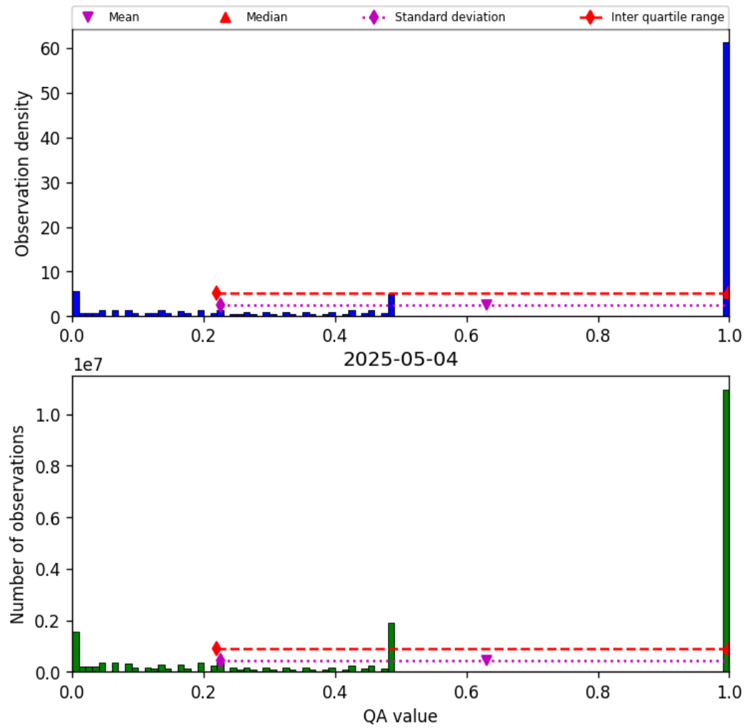
Figure 57: Histogram of “QA value” for 2025-05-03 to 2025-05-05
