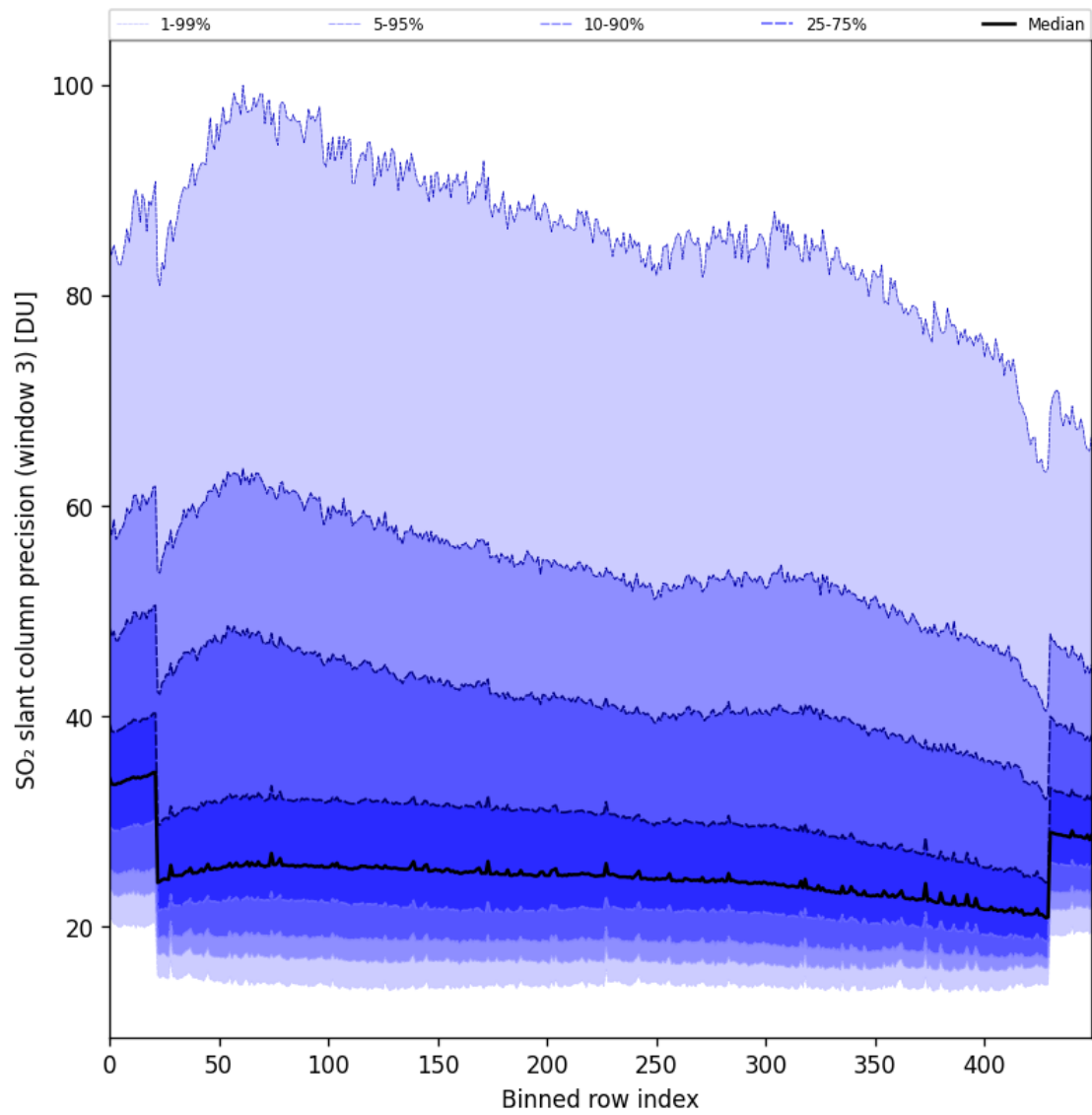
Figure 98: Along track statistics of “SO 2 slant column precision (window 3)” for 2025-05-03 to 2025-05-05
