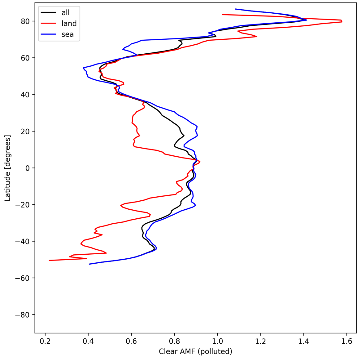
Figure 55: Zonal average of “Clear AMF (polluted)” for 2025-05-03 to 2025-05-05.
