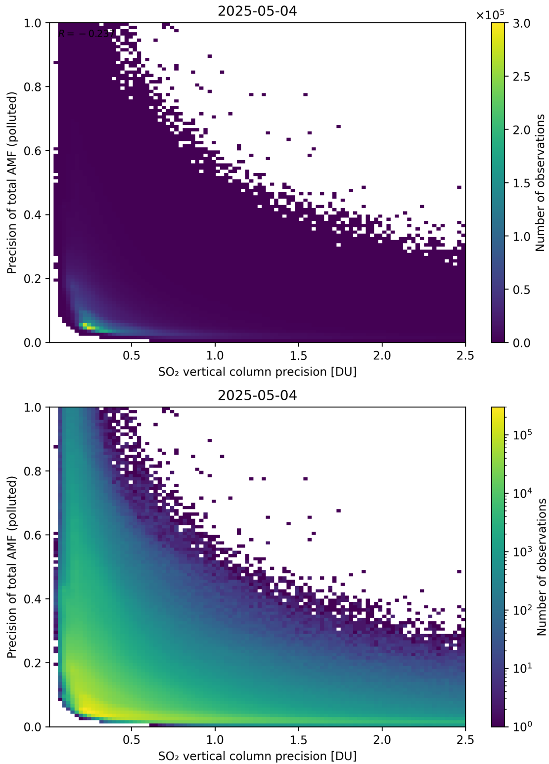
Figure 347: Scatter density plot of “SO 2 vertical column precision” against “Precision of total AMF (polluted)” for 2025-05-03 to 2025-05-05.
