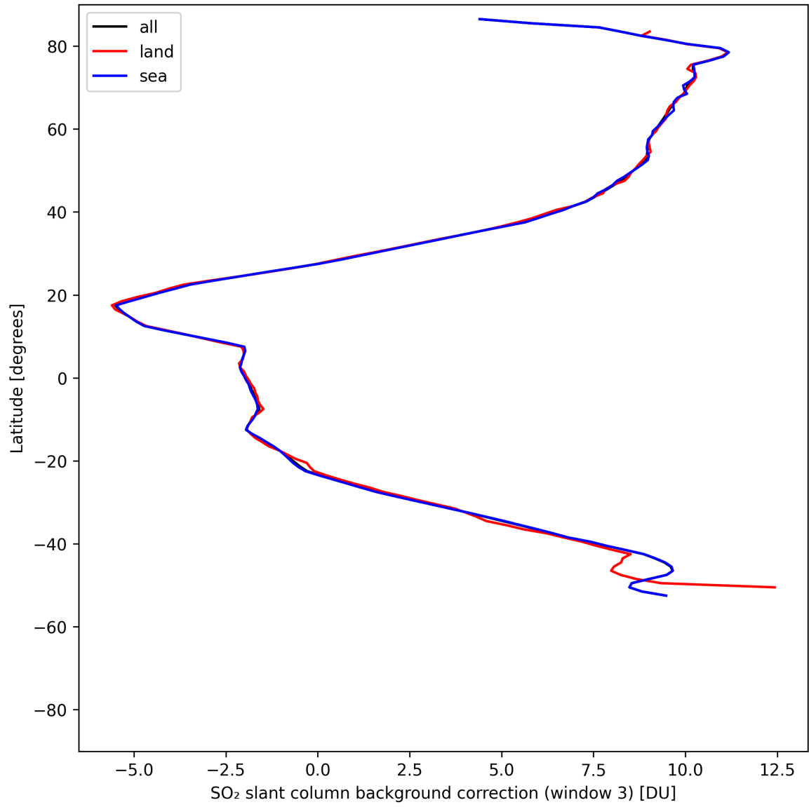
Figure 48: Zonal average of "SO 2 slant column background correction (window 3)" for 2025-05-03 to 2025-05-05.
