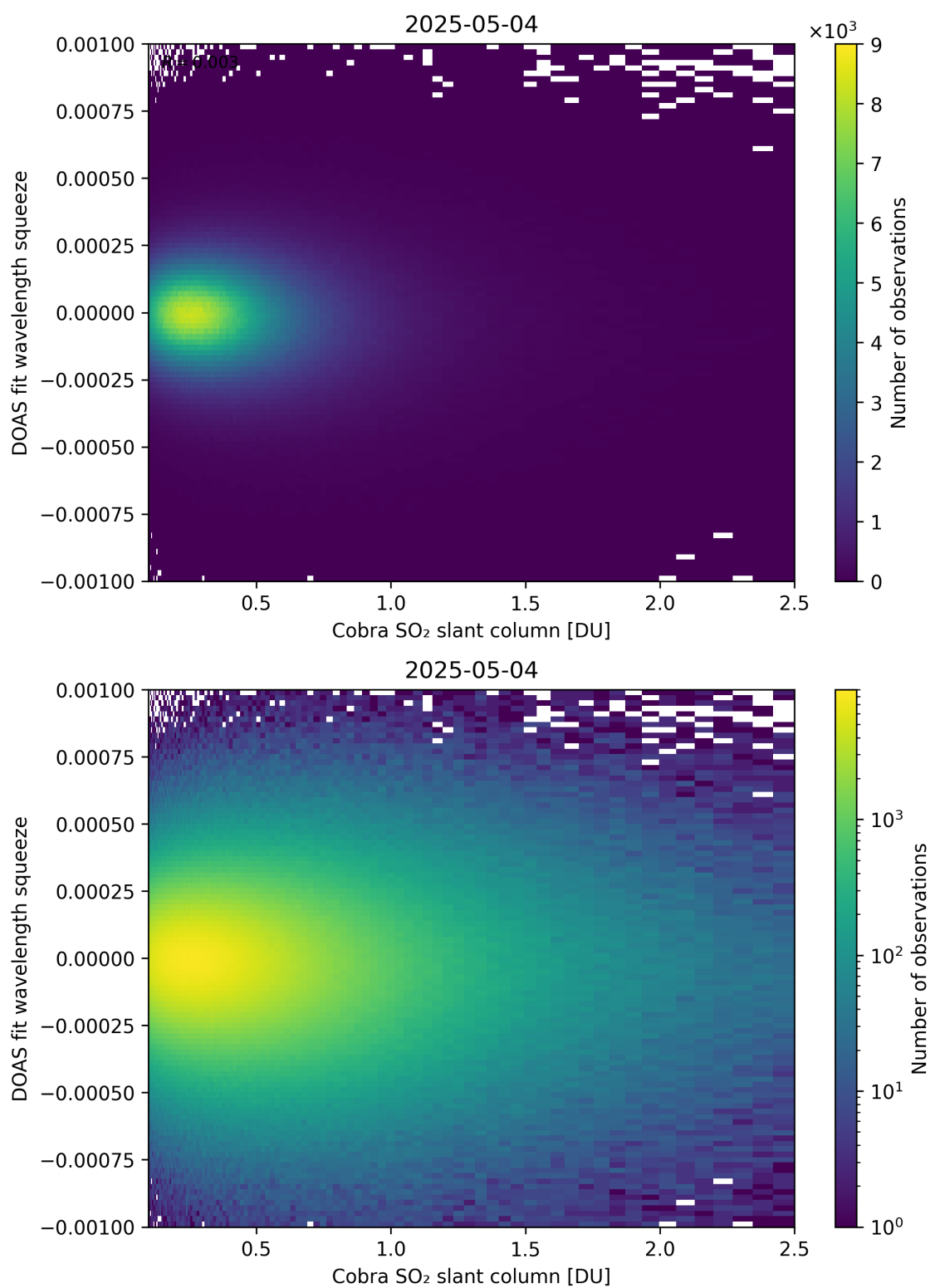
Figure 197: Scatter density plot of “Cobra SO 2 slant column” against “DOAS fit wavelength squeeze” for 2025-05-03 to 2025-05-05.
