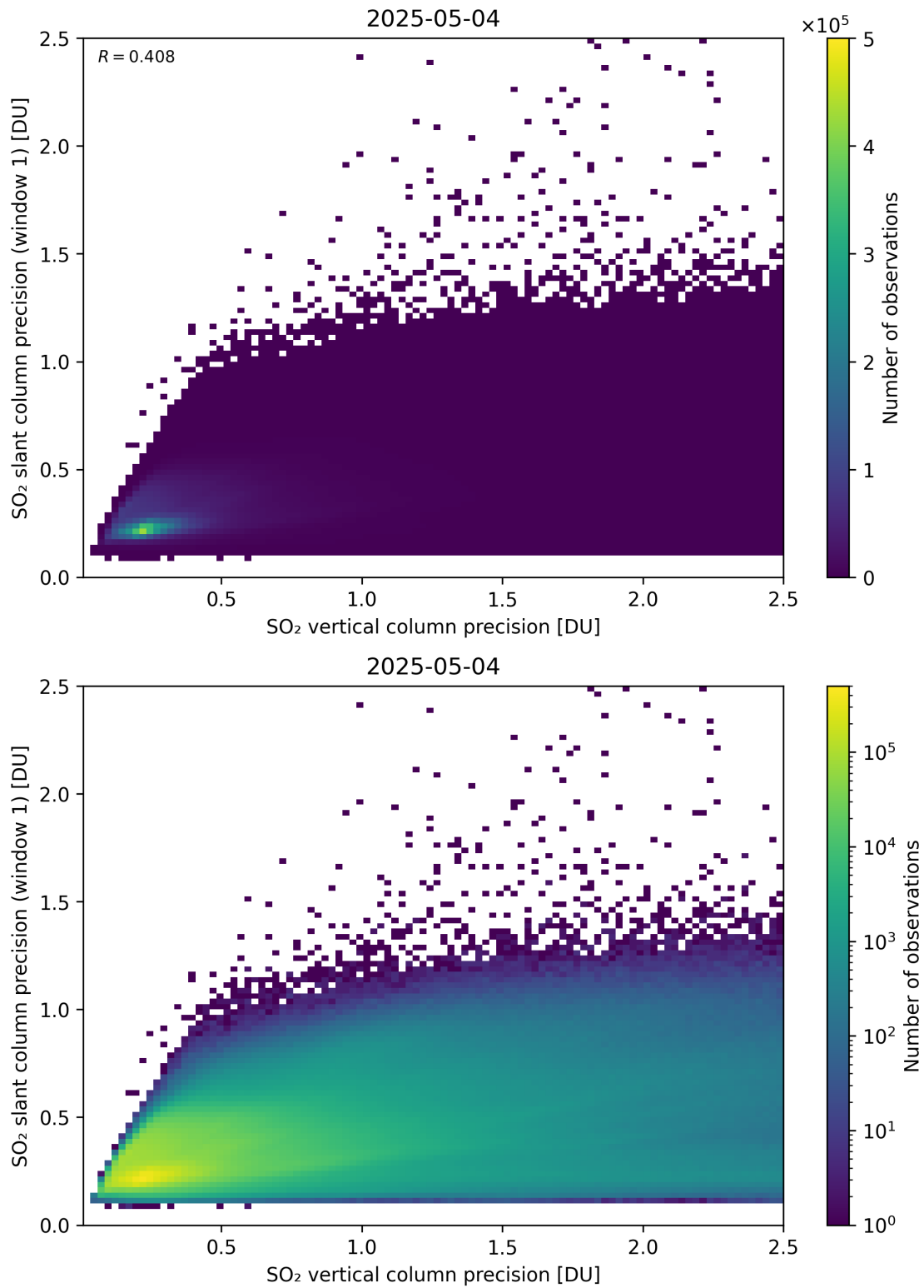
Figure 342: Scatter density plot of “SO 2 vertical column precision” against “SO 2 slant column precision (window 1)” for 2025-05-03 to 2025-05-05.
