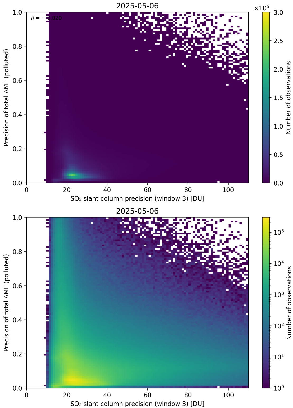
Figure 314: Scatter density plot of “SO 2 slant column precision (window 3)” against “Precision of total AMF (polluted)” for 2025-05-05 to 2025-05-07.
