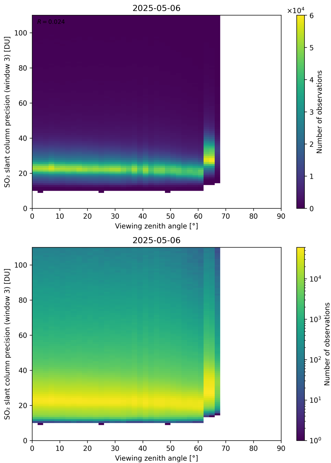
Figure 380: Scatter density plot of “Viewing zenith angle” against “SO 2 slant column precision (window 3)” for 2025-05-05 to 2025-05-07.
