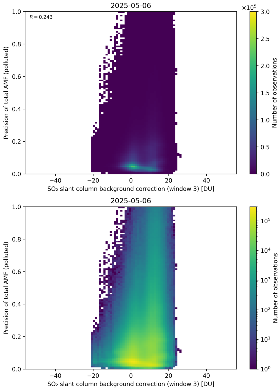
Figure 137: Scatter density plot of “SO 2 slant column background correction (window 3)” against “Precision of total AMF (polluted)” for 2025-05-05 to 2025-05-07.
