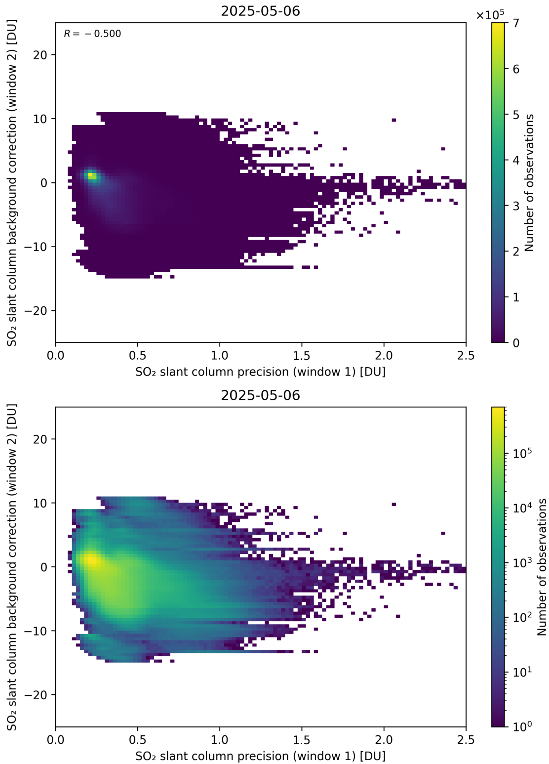
Figure 269: Scatter density plot of “SO 2 slant column precision (window 1)” against “SO 2 slant column background correction (window 2)” for 2025-05-05 to 2025-05-07.
