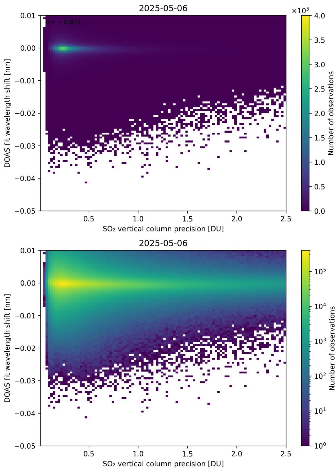
Figure 332: Scatter density plot of “SO 2 vertical column precision” against “DOAS fit wavelength shift” for 2025-05-05 to 2025-05-07.
