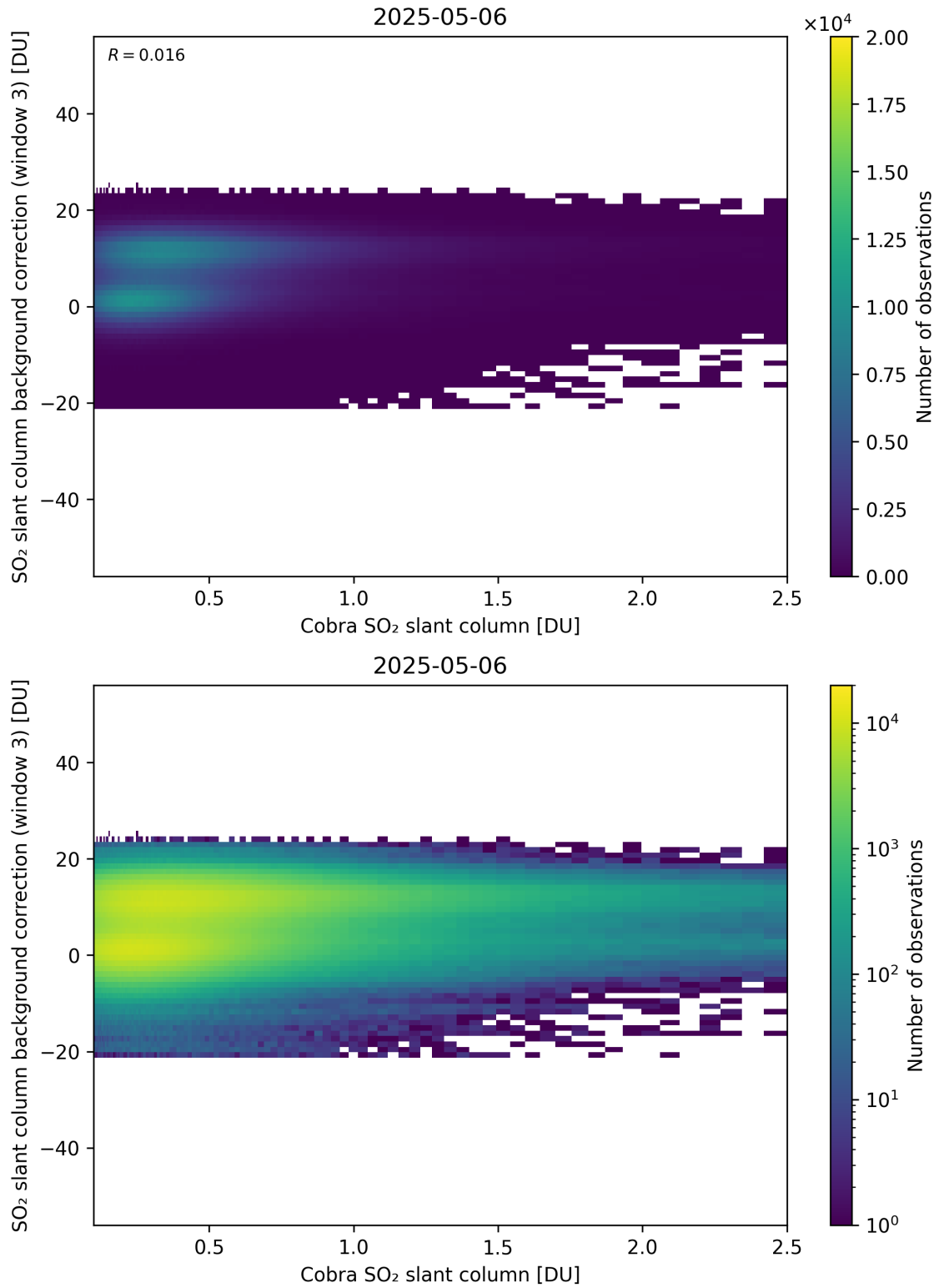
Figure 195: Scatter density plot of “Cobra SO 2 slant column” against “SO 2 slant column background correction (window 3)” for 2025-05-05 to 2025-05-07.
