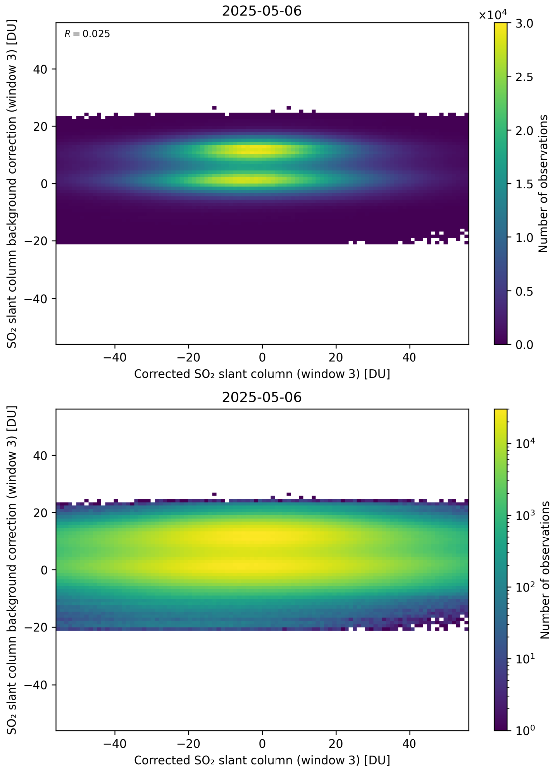
Figure 255: Scatter density plot of “Corrected SO 2 slant column (window 3)” against “SO 2 slant column background correction (window 3)” for 2025-05-05 to 2025-05-07.
