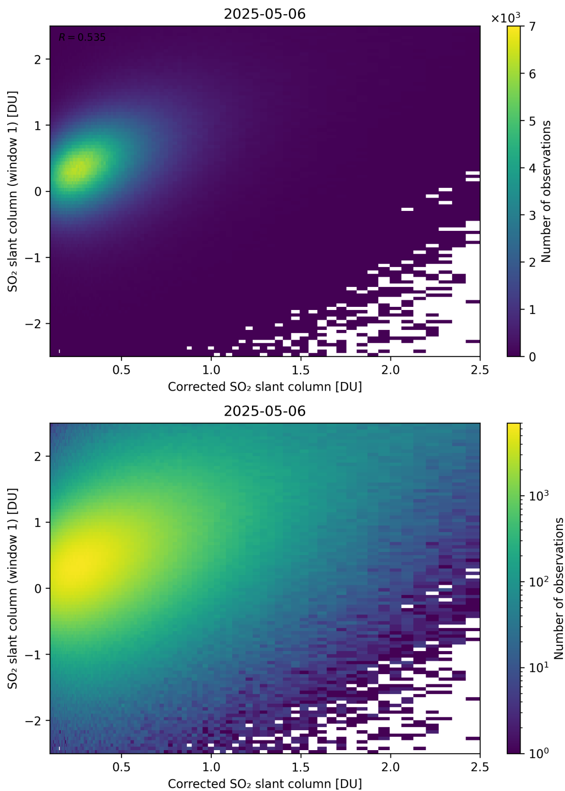
Figure 237: Scatter density plot of “Corrected SO 2 slant column” against “SO 2 slant column (window 1)” for 2025-05-05 to 2025-05-07.
