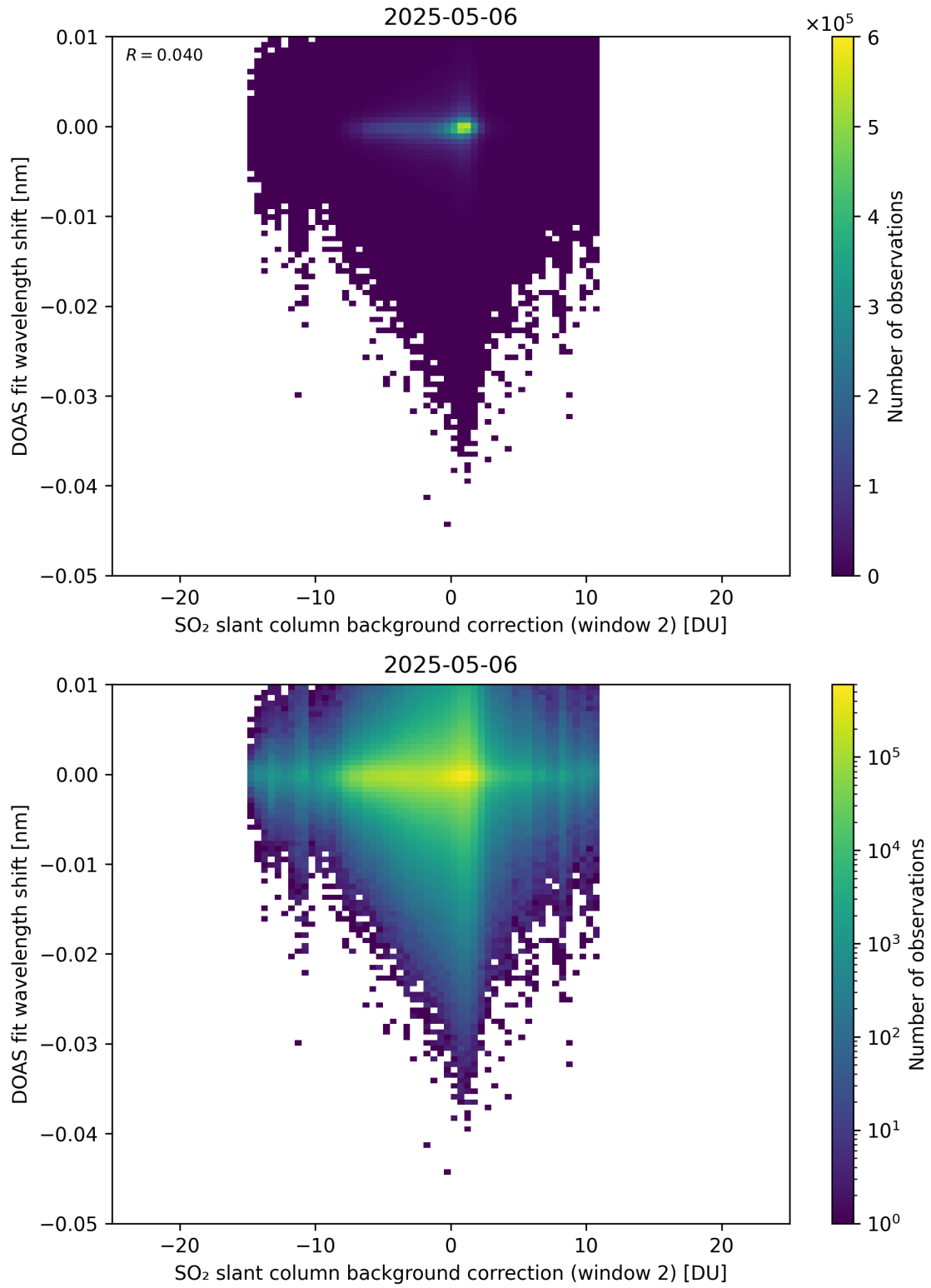
Figure 123: Scatter density plot of “SO 2 slant column background correction (window 2)” against “DOAS fit wavelength shift” for 2025-05-05 to 2025-05-07.
