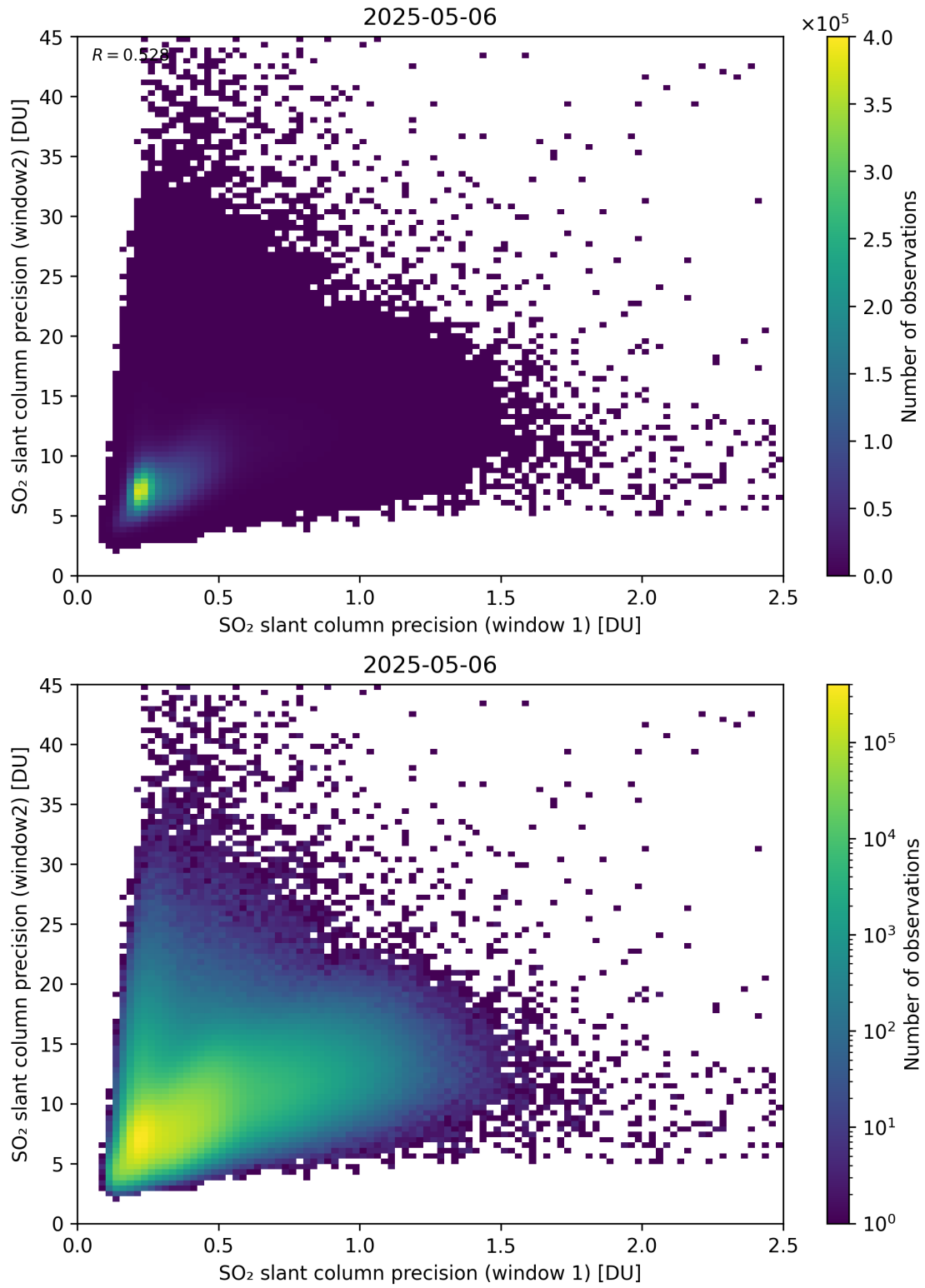
Figure 277: Scatter density plot of “SO 2 slant column precision (window 1)” against “SO 2 slant column precision (window2)” for 2025-05-05 to 2025-05-07.
