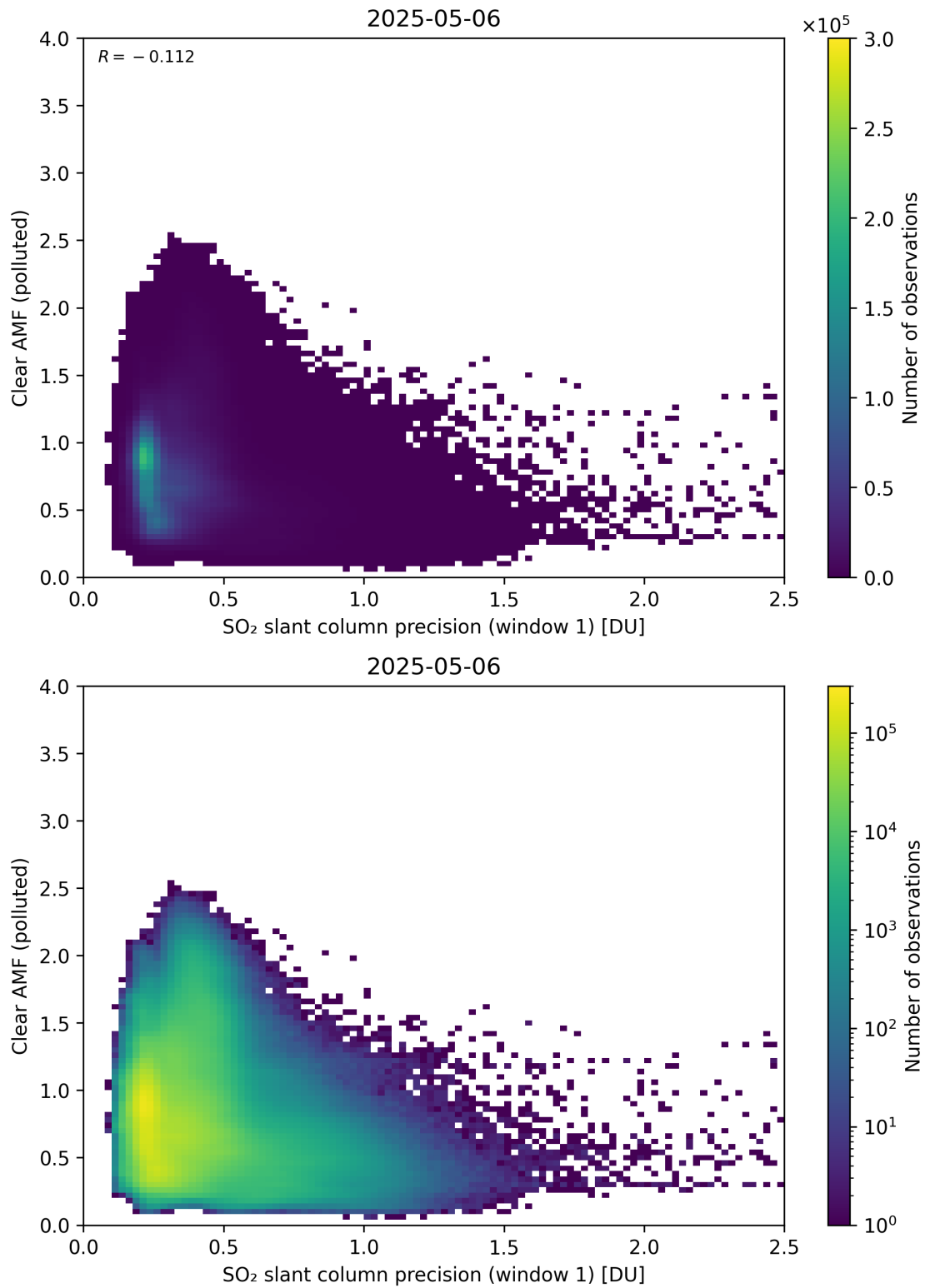
Figure 274: Scatter density plot of “SO 2 slant column precision (window 1)” against “Clear AMF (polluted)” for 2025-05-05 to 2025-05-07.
