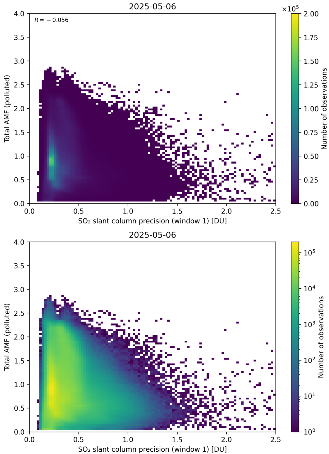
Figure 280: Scatter density plot of “SO 2 slant column precision (window 1)” against “Total AMF (polluted)” for 2025-05-05 to 2025-05-07.
