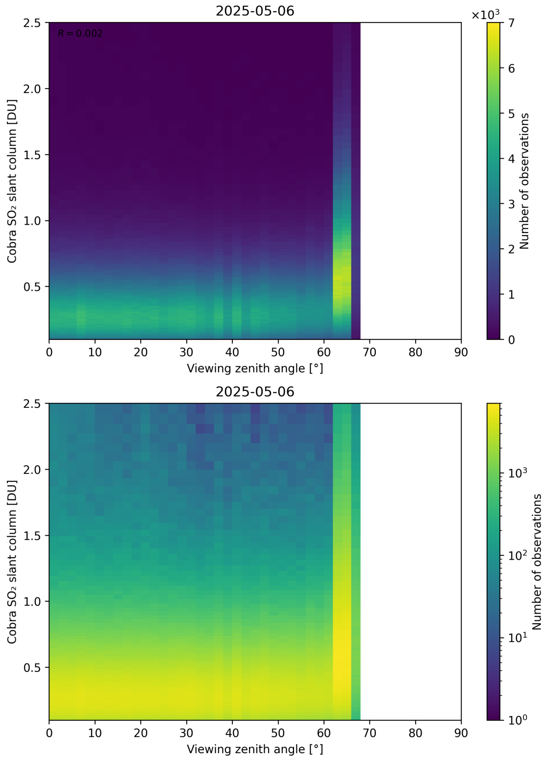
Figure 371: Scatter density plot of “Viewing zenith angle” against “Cobra SO 2 slant column” for 2025-05-05 to 2025-05-07.
