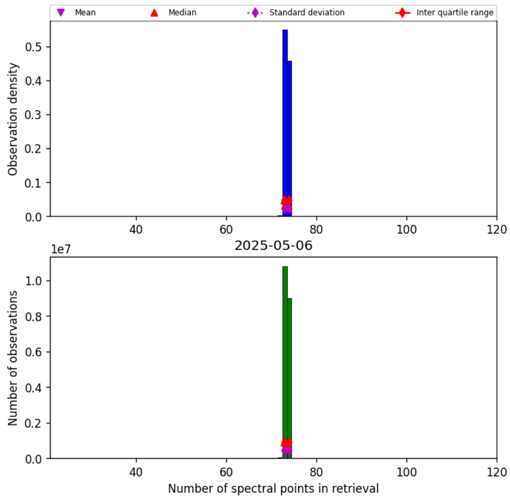
Figure 82: Histogram of “Number of spectral points in retrieval” for 2025-05-05 to 2025-05-07
