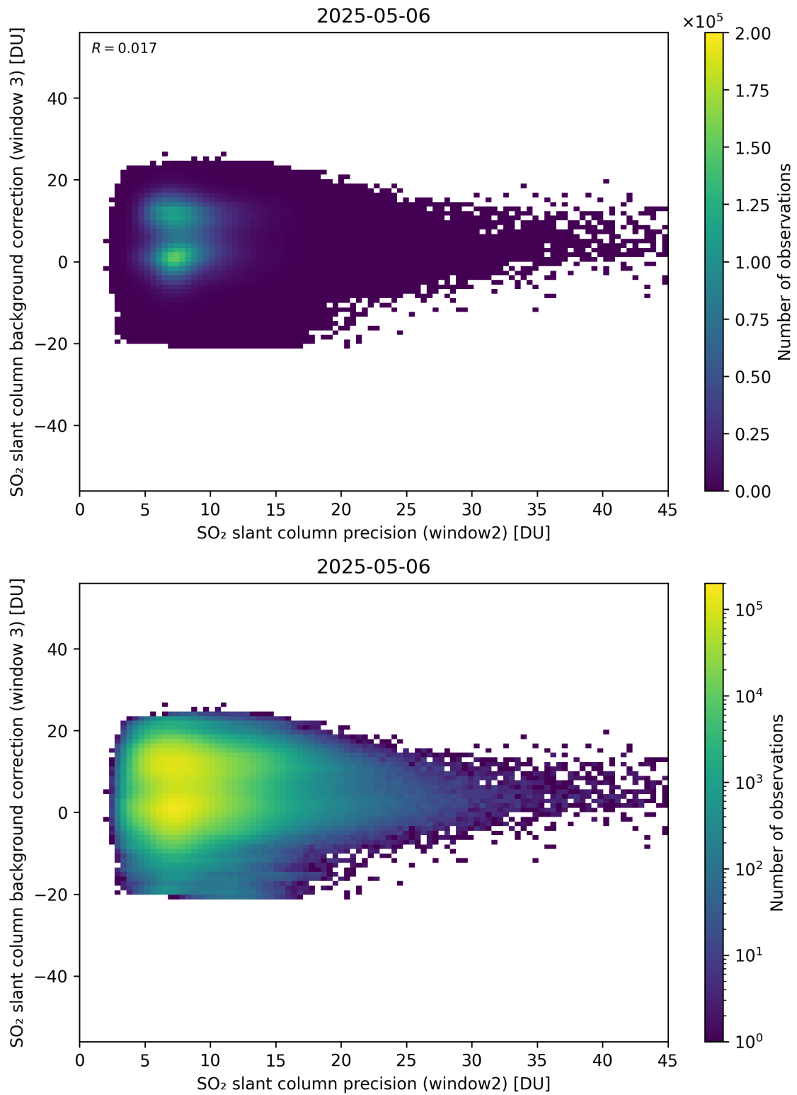
Figure 292: Scatter density plot of “SO 2 slant column precision (window2)” against “SO 2 slant column background correction (window 3)” for 2025-05-05 to 2025-05-07.
