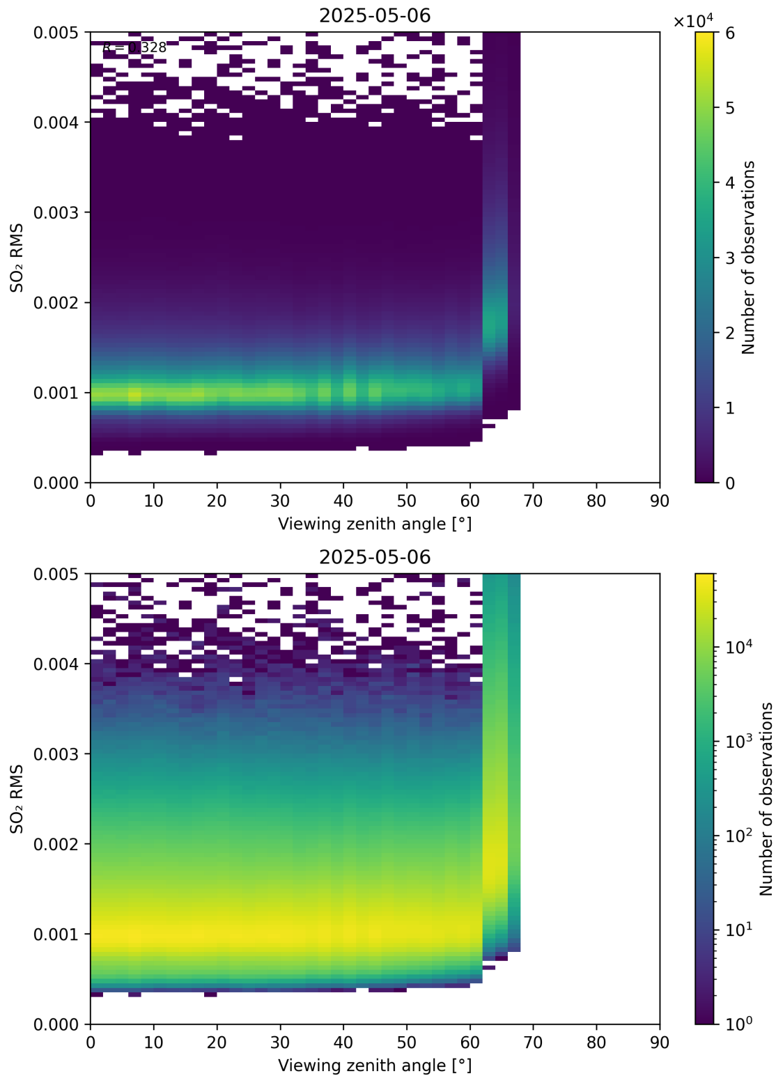
Figure 367: Scatter density plot of “Viewing zenith angle” against “SO 2 RMS” for 2025-05-05 to 2025-05-07.
