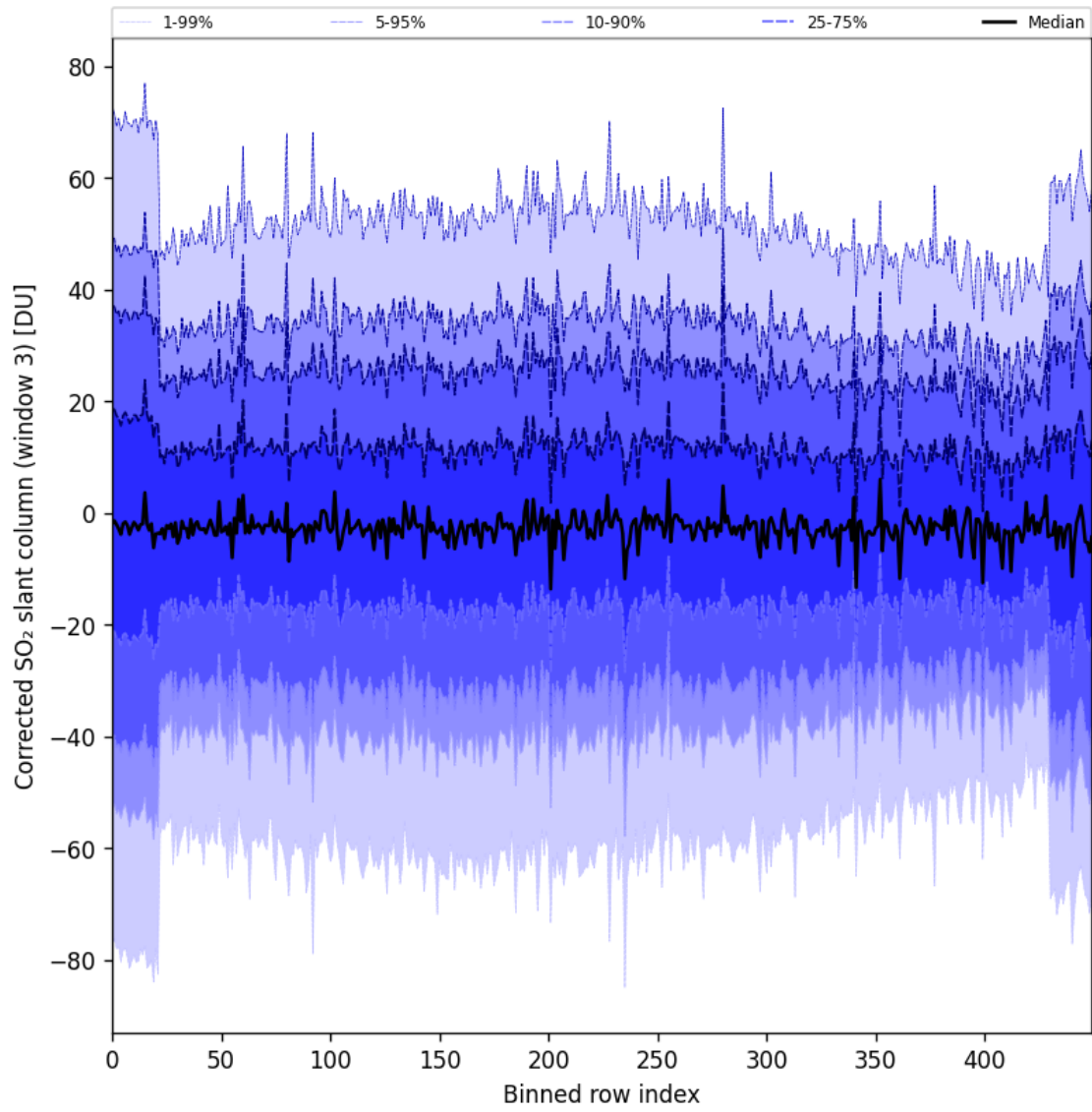
Figure 99: Along track statistics of “Corrected SO 2 slant column (window 3)” for 2025-05-05 to 2025-05-07
