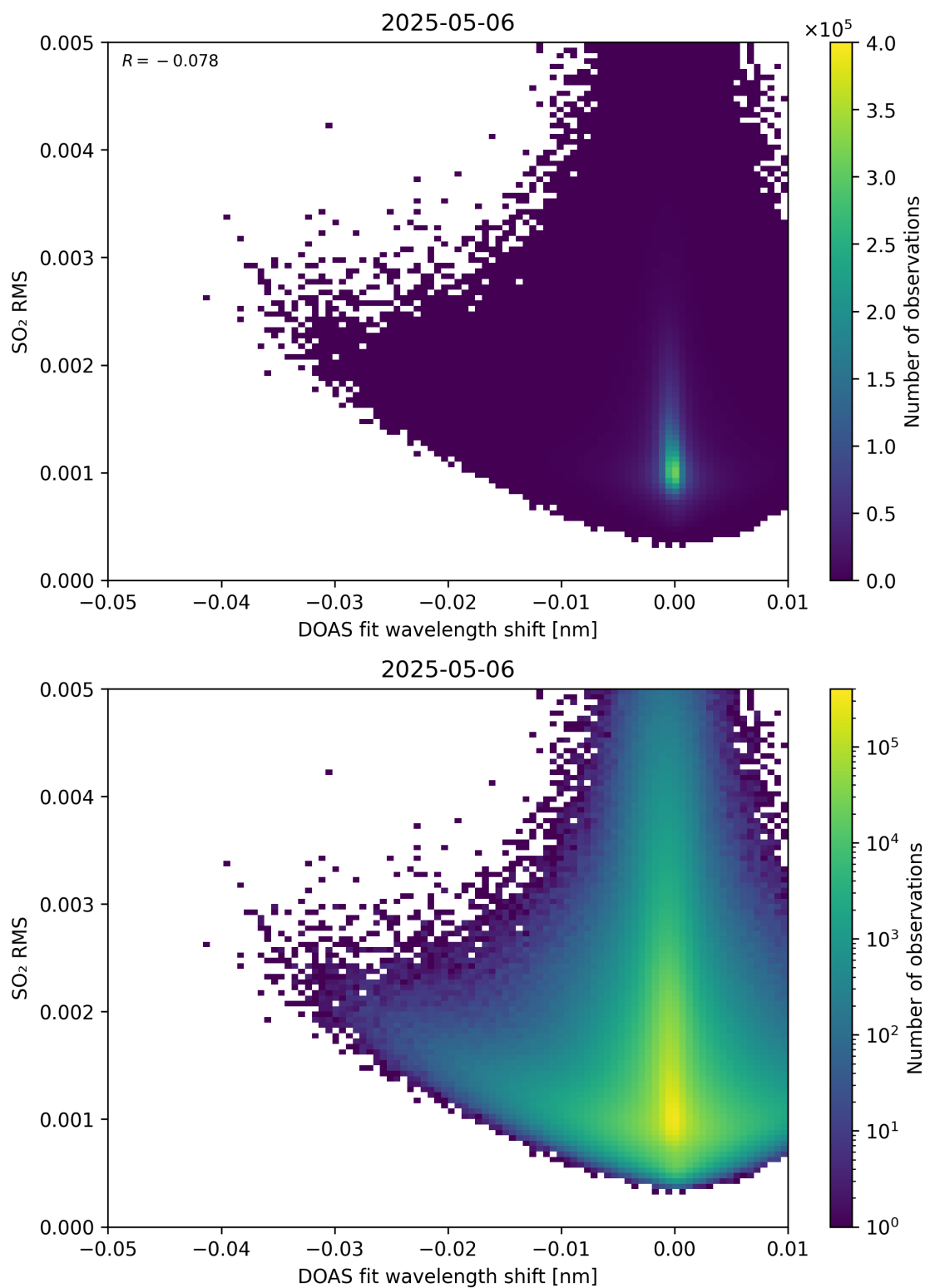
Figure 139: Scatter density plot of “DOAS fit wavelength shift” against “SO 2 RMS” for 2025-05-05 to 2025-05-07.
