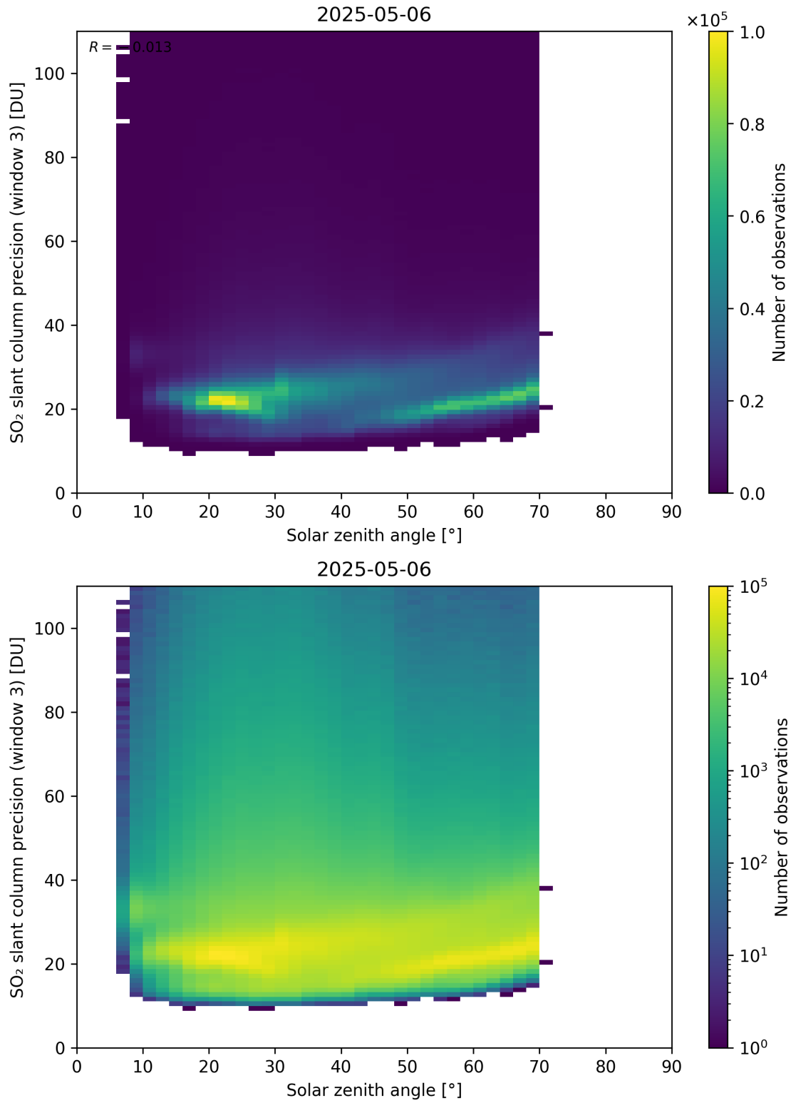
Figure 188: Scatter density plot of “Solar zenith angle” against “SO 2 slant column precision (window 3)” for 2025-05-05 to 2025-05-07.
