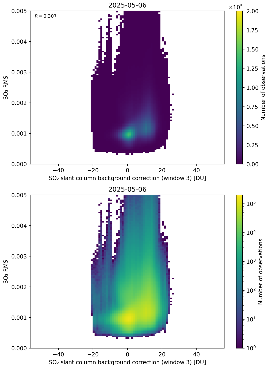
Figure 134: Scatter density plot of “SO 2 slant column background correction (window 3)” against “SO 2 RMS” for 2025-05-05 to 2025-05-07.
