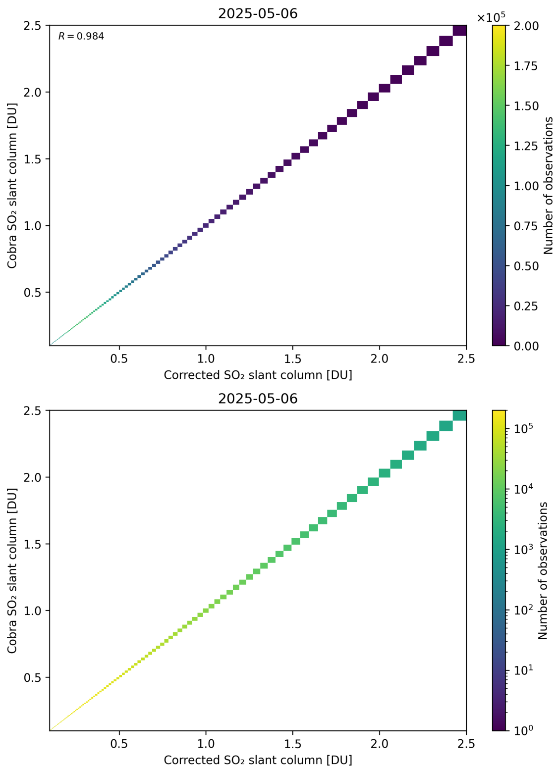
Figure 233: Scatter density plot of “Corrected SO 2 slant column” against “Cobra SO 2 slant column” for 2025-05-05 to 2025-05-07.
