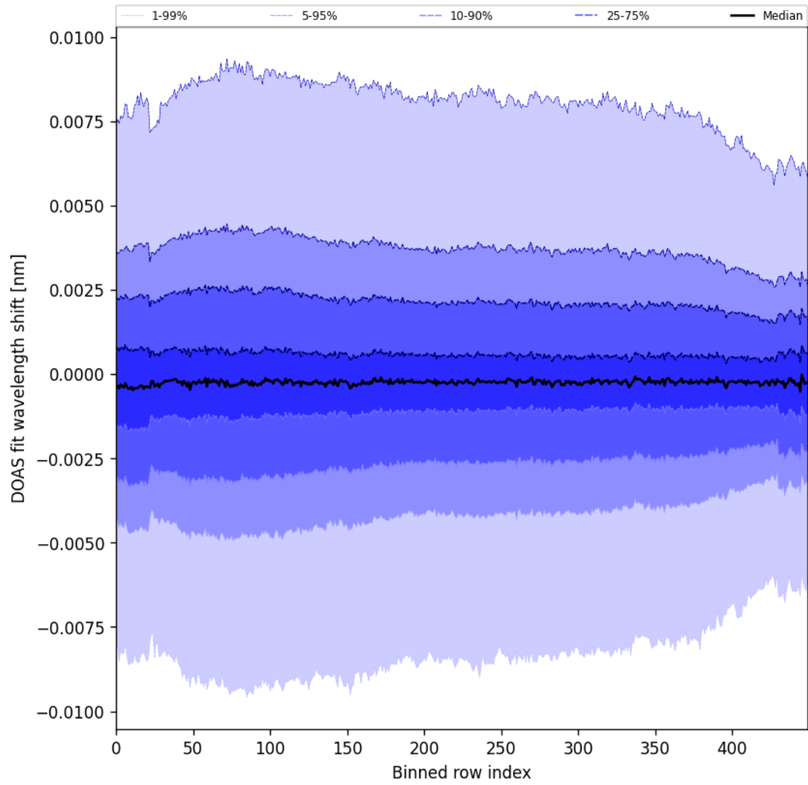
Figure 102: Along track statistics of “DOAS fit wavelength shift” for 2025-05-05 to 2025-05-07
