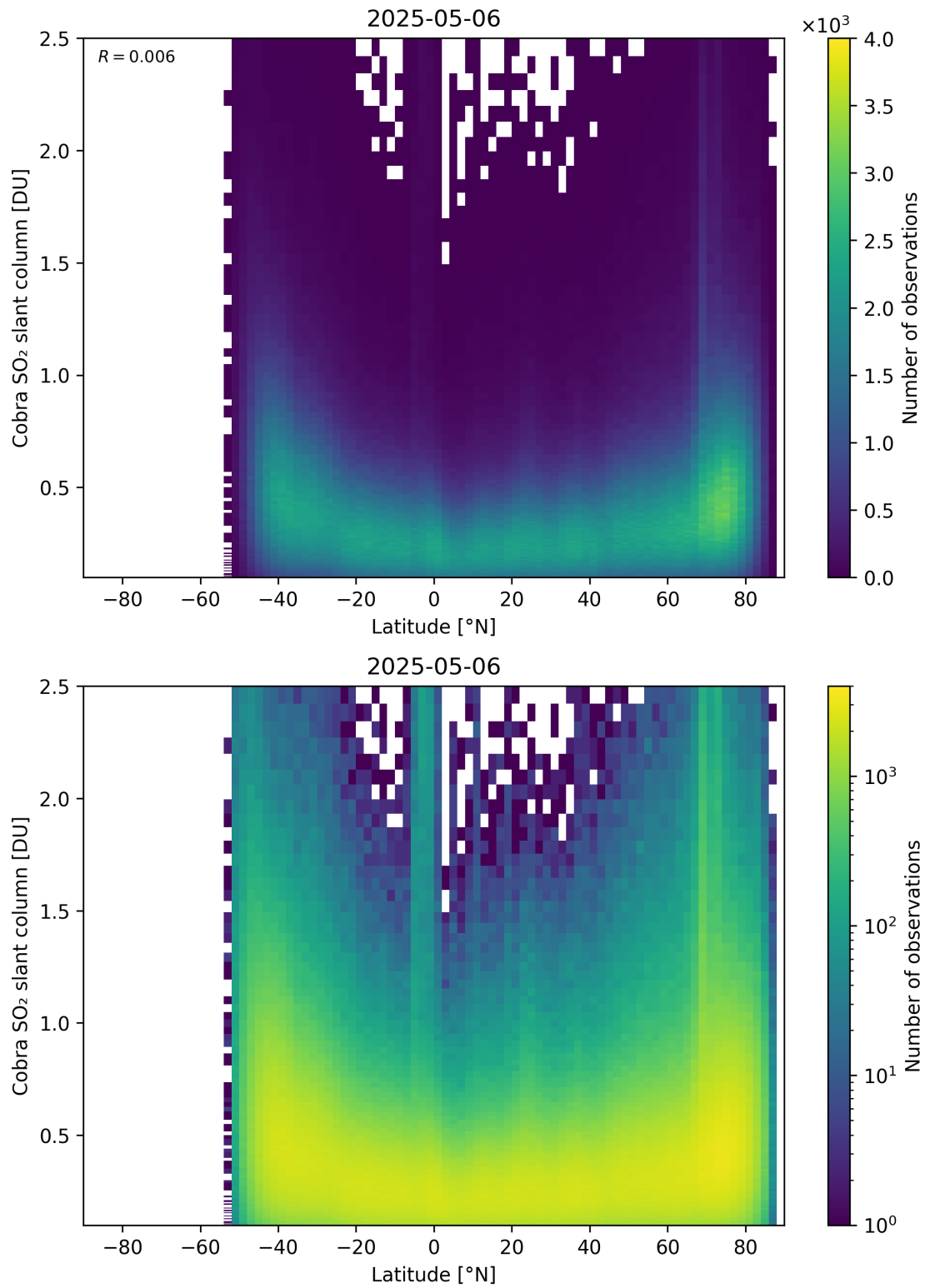
Figure 157: Scatter density plot of “Latitude” against “Cobra SO 2 slant column” for 2025-05-05 to 2025-05-07.
