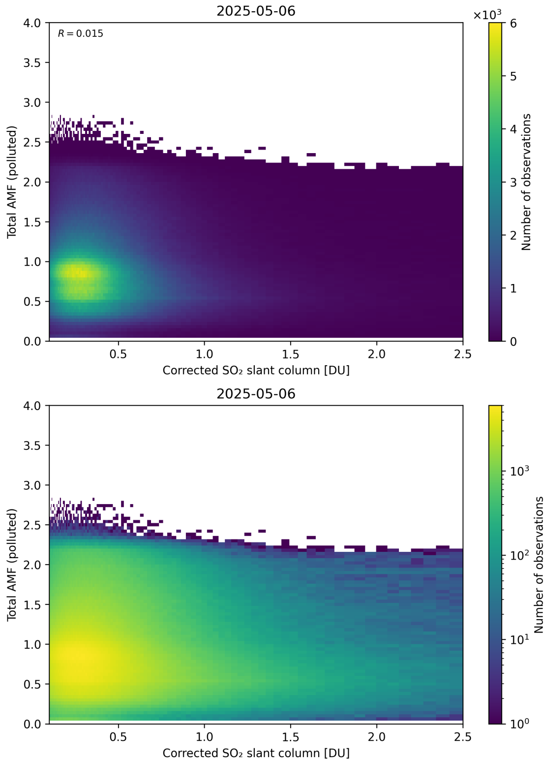
Figure 242: Scatter density plot of “Corrected SO 2 slant column” against “Total AMF (polluted)” for 2025-05-05 to 2025-05-07.
