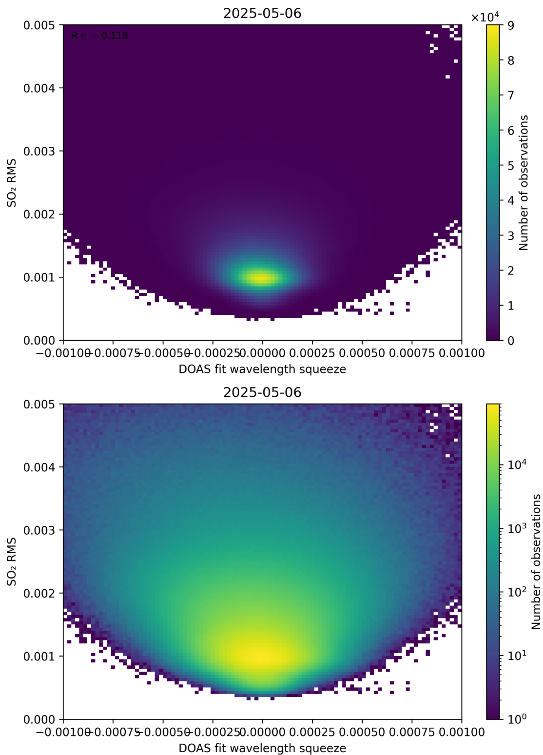
Figure 143: Scatter density plot of “DOAS fit wavelength squeeze” against “SO 2 RMS” for 2025-05-05 to 2025-05-07.
