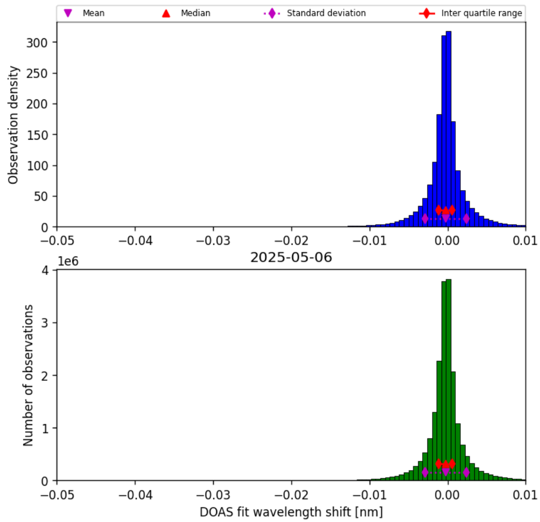
Figure 76: Histogram of “DOAS fit wavelength shift” for 2025-05-05 to 2025-05-07
