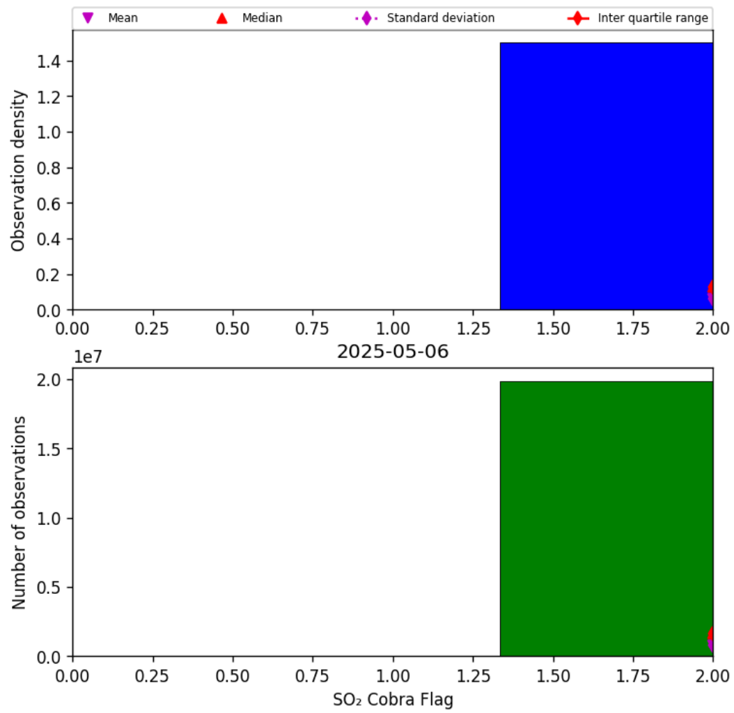
Figure 75: Histogram of “SO 2 Cobra Flag” for 2025-05-05 to 2025-05-07
