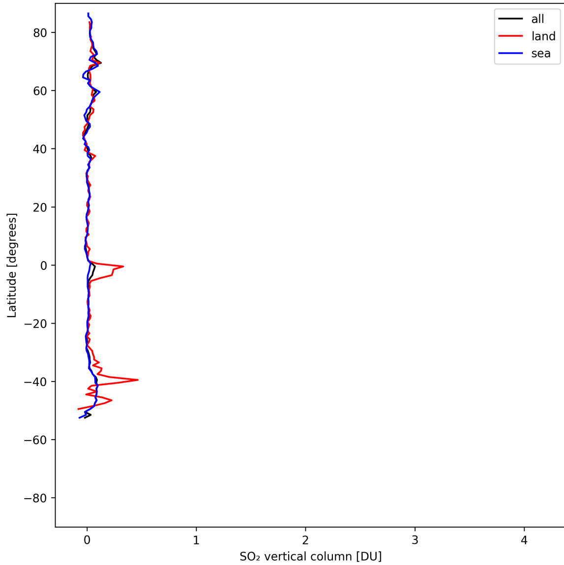
Figure 32: Zonal average of “SO 2 vertical column” for 2025-05-05 to 2025-05-07.
