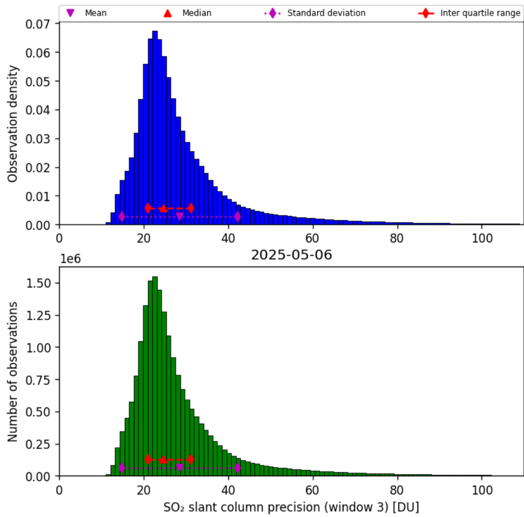
Figure 72: Histogram of “SO 2 slant column precision (window 3)” for 2025-05-05 to 2025-05-07
