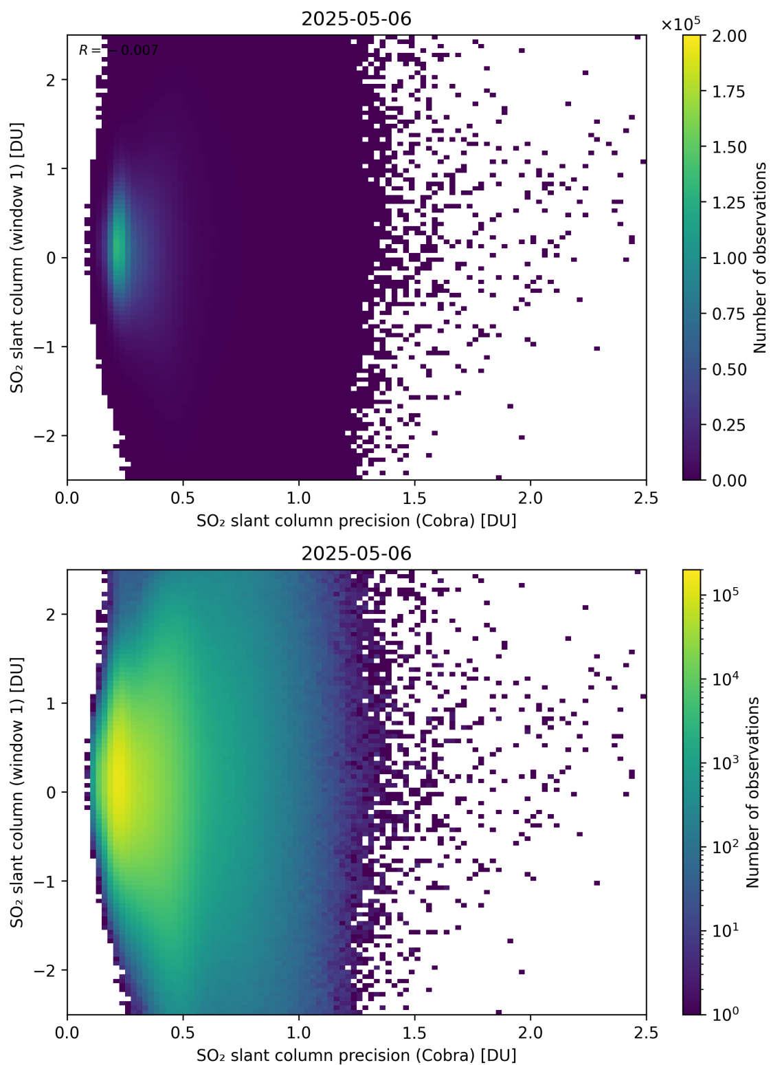
Figure 208: Scatter density plot of “SO 2 slant column precision (Cobra)” against “SO 2 slant column (window 1)” for 2025-05-05 to 2025-05-07.
