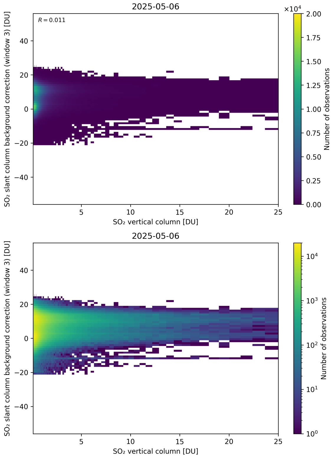
Figure 325: Scatter density plot of “SO 2 vertical column” against “SO 2 slant column background correction (window 3)” for 2025-05-05 to 2025-05-07.
