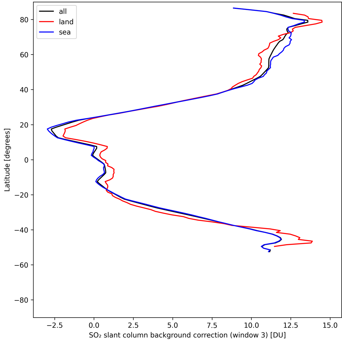
Figure 48: Zonal average of “SO 2 slant column background correction (window 3)” for 2025-05-05 to 2025-05-07.
