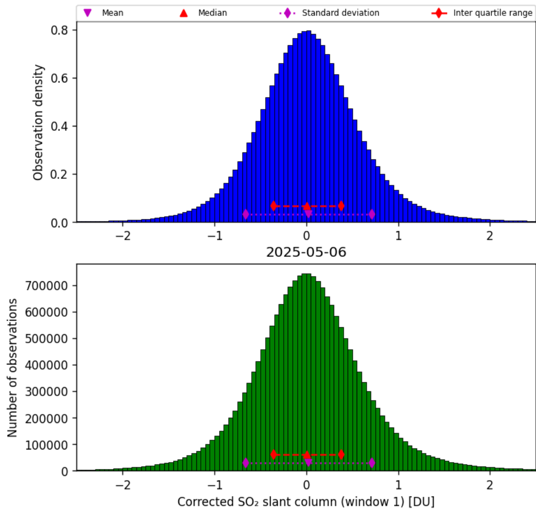
Figure 65: Histogram of “Corrected SO 2 slant column (window 1)” for 2025-05-05 to 2025-05-07
