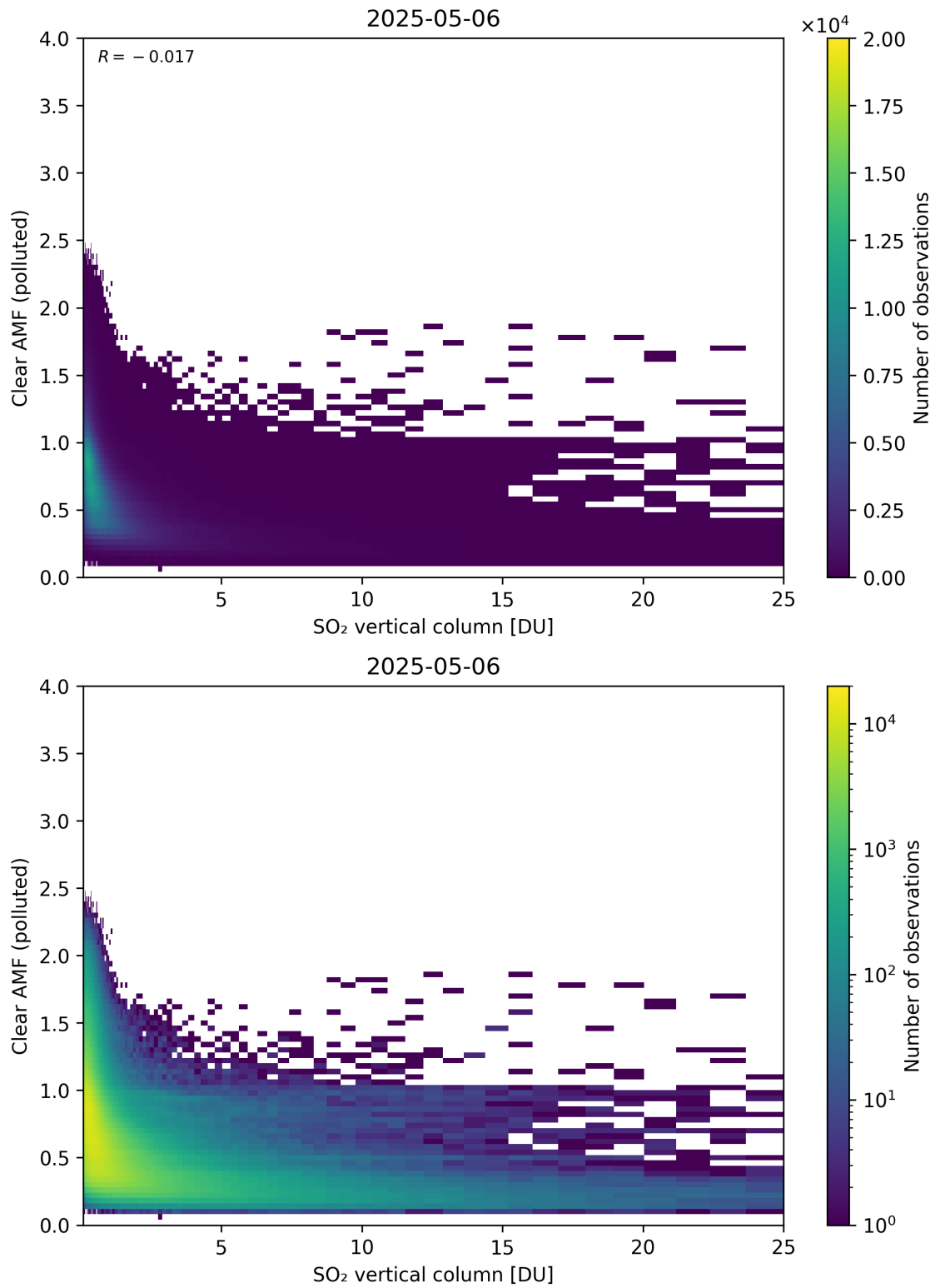
Figure 348: Scatter density plot of “SO 2 vertical column” against “Clear AMF (polluted)” for 2025-05-05 to 2025-05-07.
