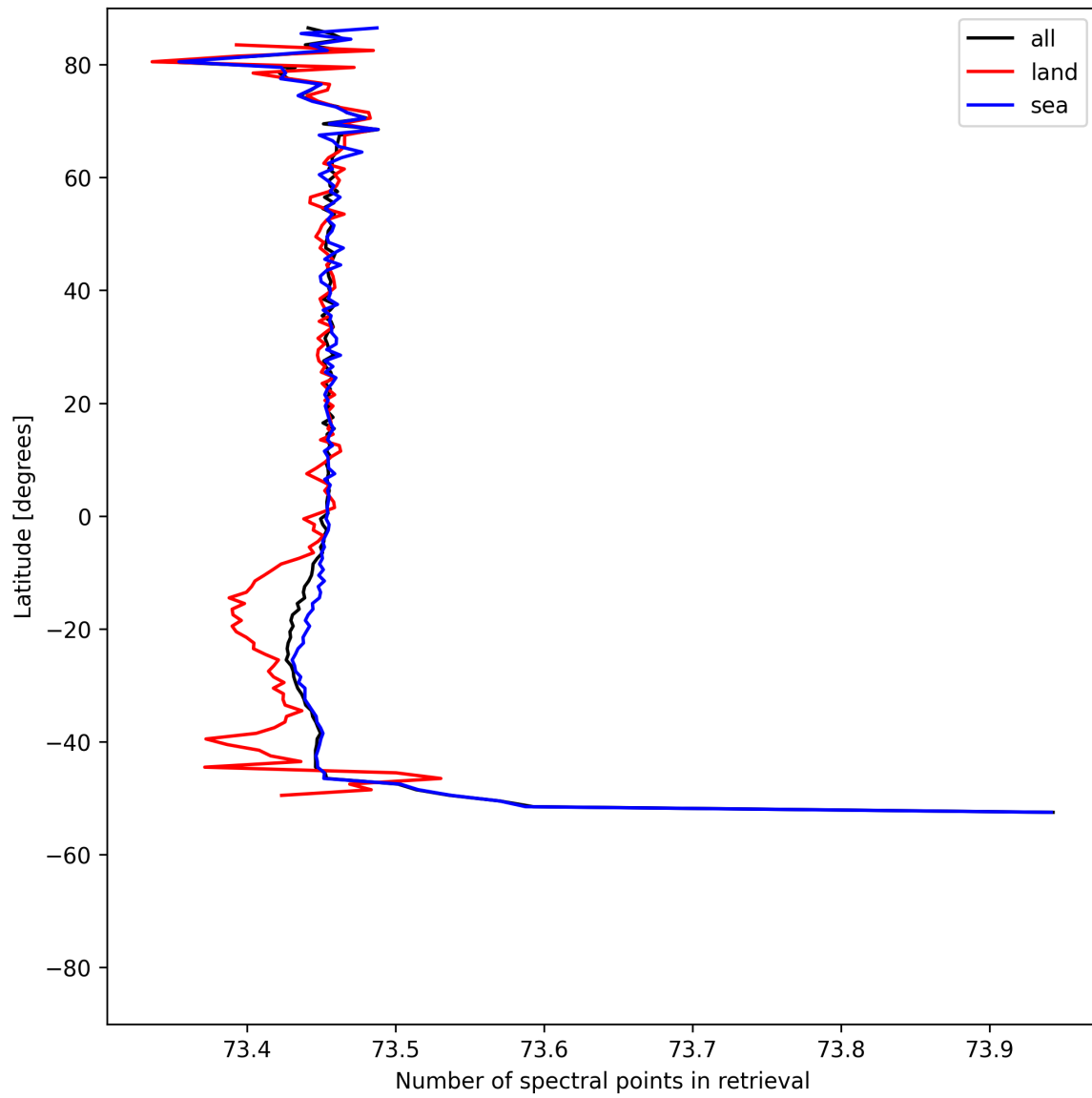
Figure 56: Zonal average of “Number of spectral points in retrieval” for 2025-05-05 to 2025-05-07.
