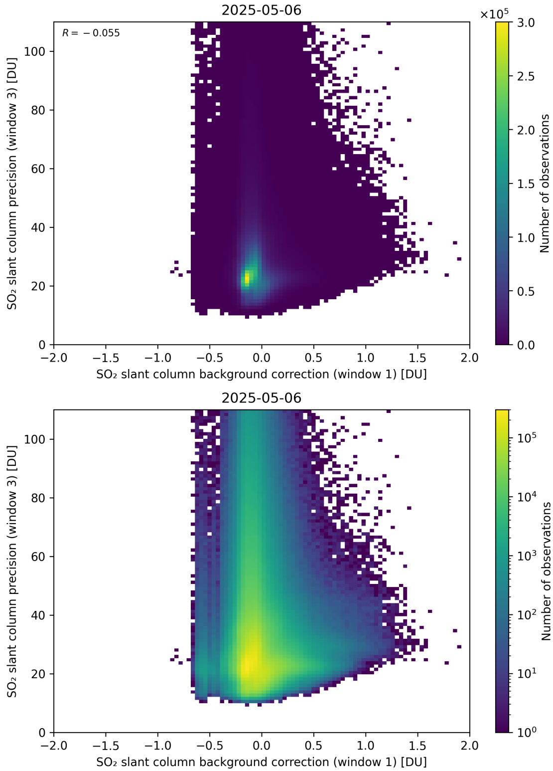
Figure 119: Scatter density plot of “SO 2 slant column background correction (window 1)” against “SO 2 slant column precision (window 3)” for 2025-05-05 to 2025-05-07.
