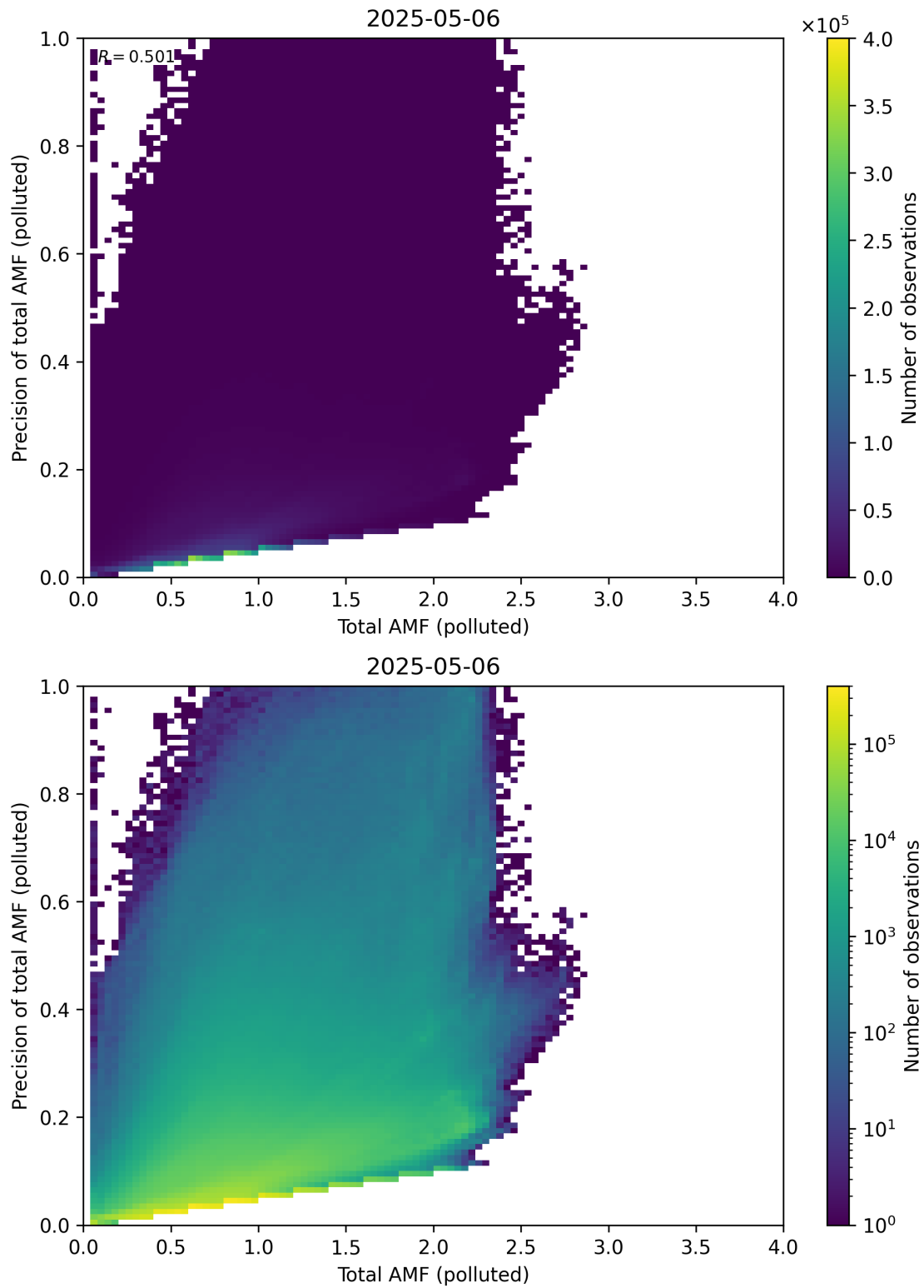
Figure 322: Scatter density plot of “Total AMF (polluted)” against “Precision of total AMF (polluted)” for 2025-05-05 to 2025-05-07.
