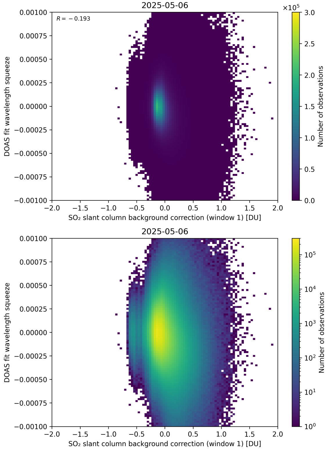
Figure 112: Scatter density plot of “SO 2 slant column background correction (window 1)” against “DOAS fit wavelength squeeze” for 2025-05-05 to 2025-05-07.
