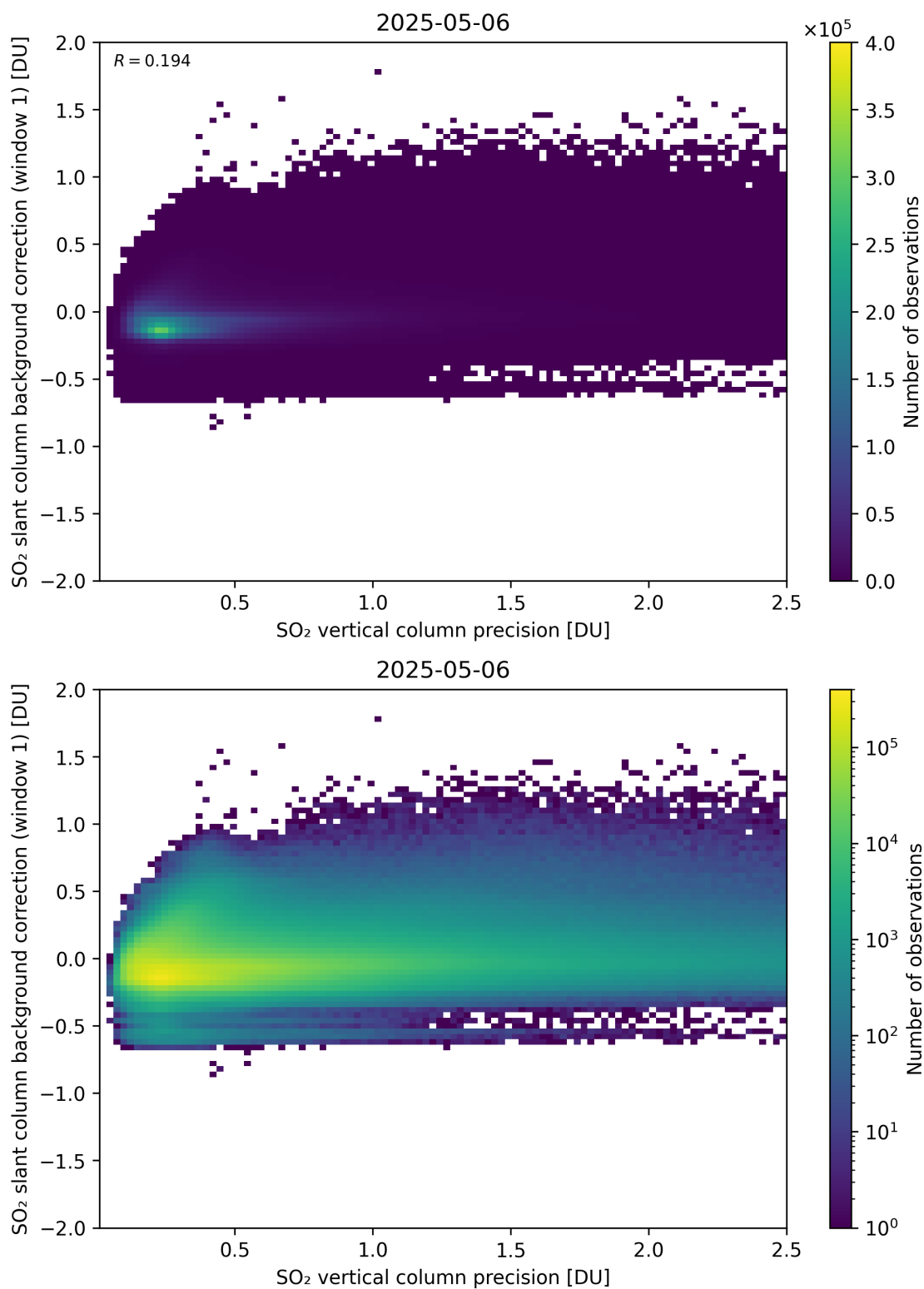
Figure 329: Scatter density plot of “SO 2 vertical column precision” against “SO 2 slant column background correction (window 1)” for 2025-05-05 to 2025-05-07.
