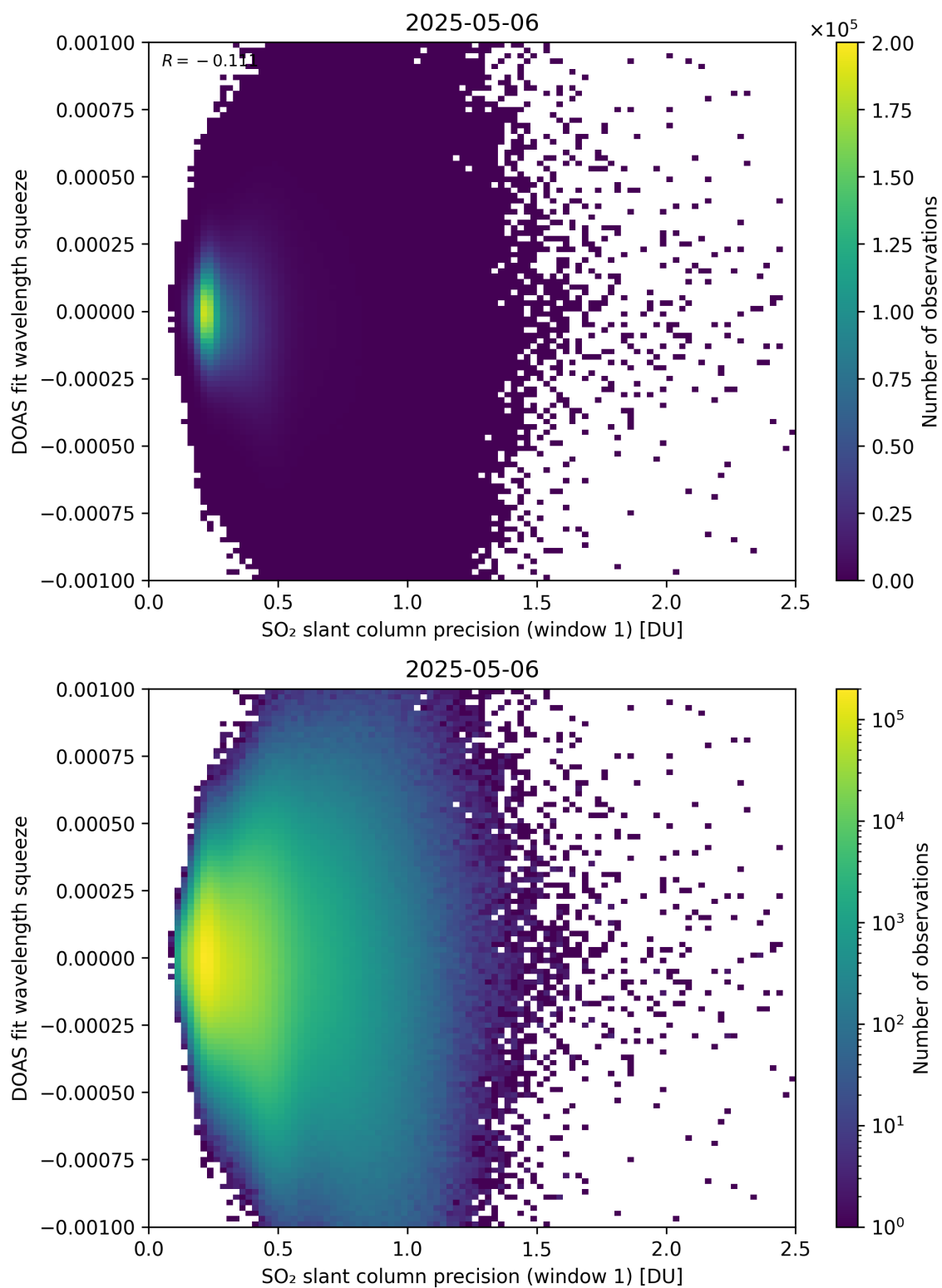
Figure 272: Scatter density plot of “SO 2 slant column precision (window 1)” against “DOAS fit wavelength squeeze” for 2025-05-05 to 2025-05-07.
