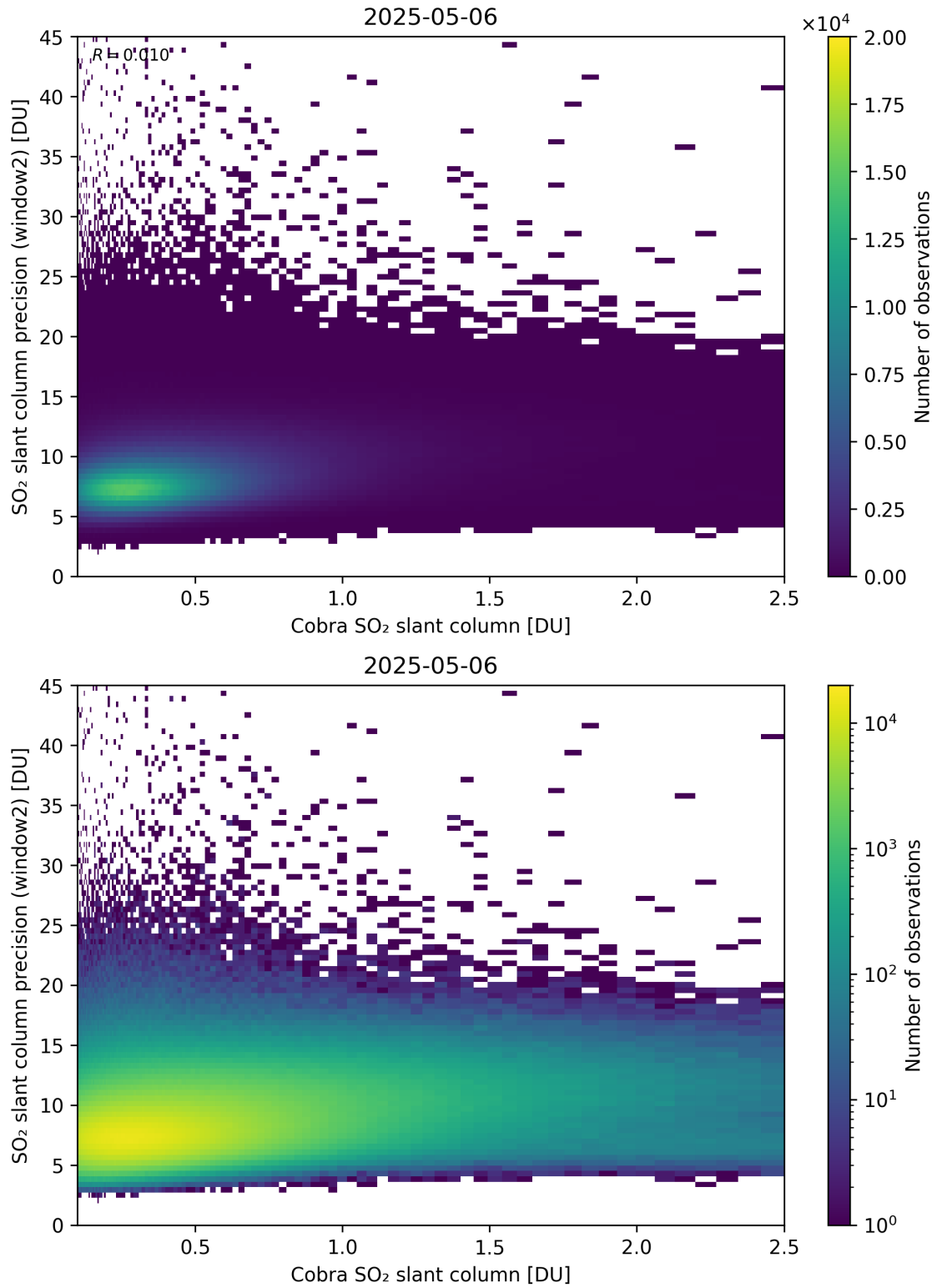
Figure 221: Scatter density plot of “Cobra SO 2 slant column” against “SO 2 slant column precision (window2)” for 2025-05-05 to 2025-05-07.
