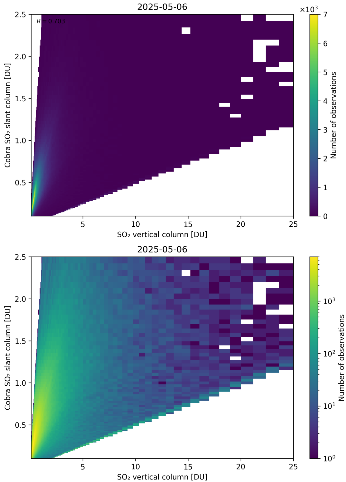
Figure 349: Scatter density plot of “SO 2 vertical column” against “Cobra SO 2 slant column” for 2025-05-05 to 2025-05-07.
