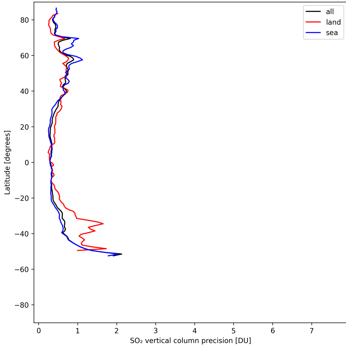
Figure 33: Zonal average of “SO 2 vertical column precision” for 2025-05-05 to 2025-05-07.
