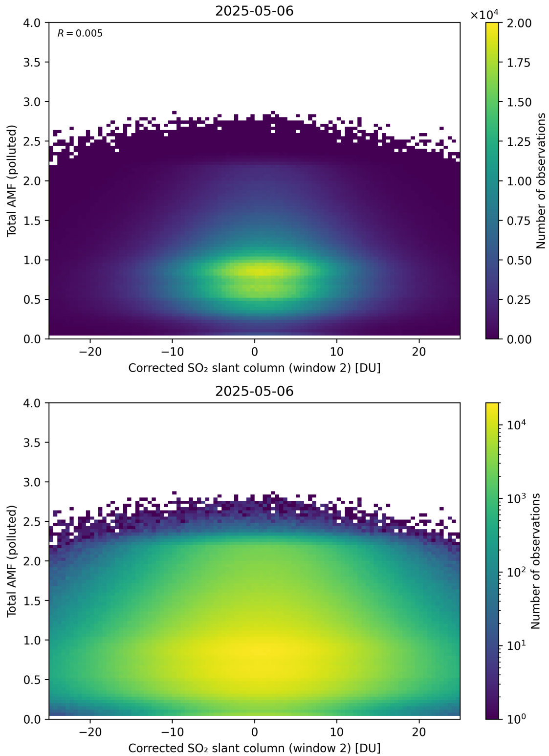
Figure 253: Scatter density plot of “Corrected SO 2 slant column (window 2)” against “Total AMF (polluted)” for 2025-05-05 to 2025-05-07.
