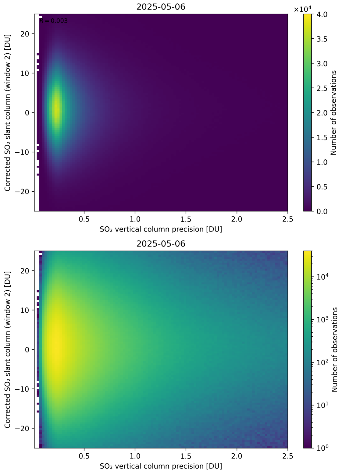
Figure 339: Scatter density plot of “SO 2 vertical column precision” against “Corrected SO 2 slant column (window 2)” for 2025-05-05 to 2025-05-07.
