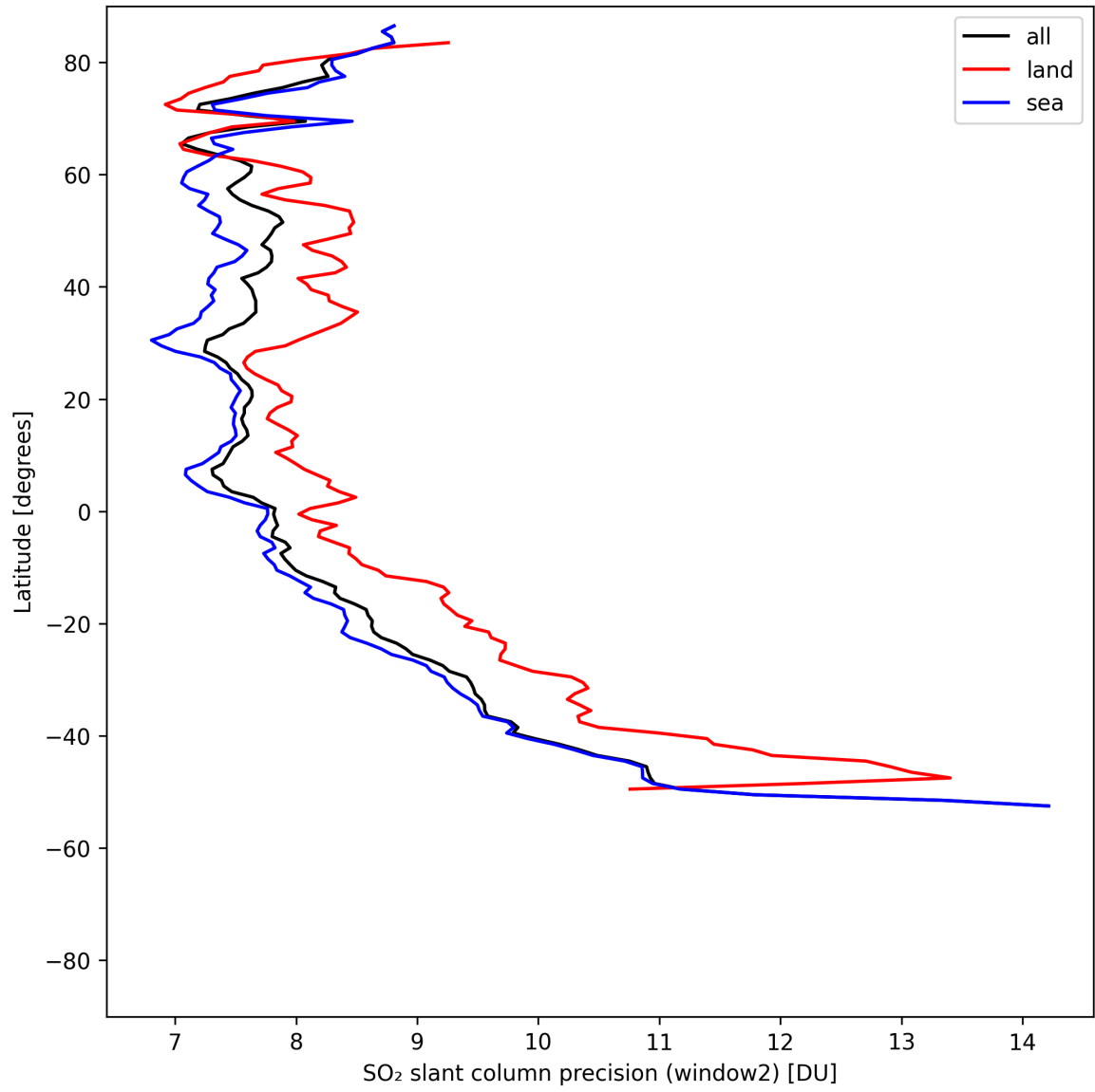
Figure 42: Zonal average of “SO 2 slant column precision (window2)” for 2025-05-05 to 2025-05-07.
