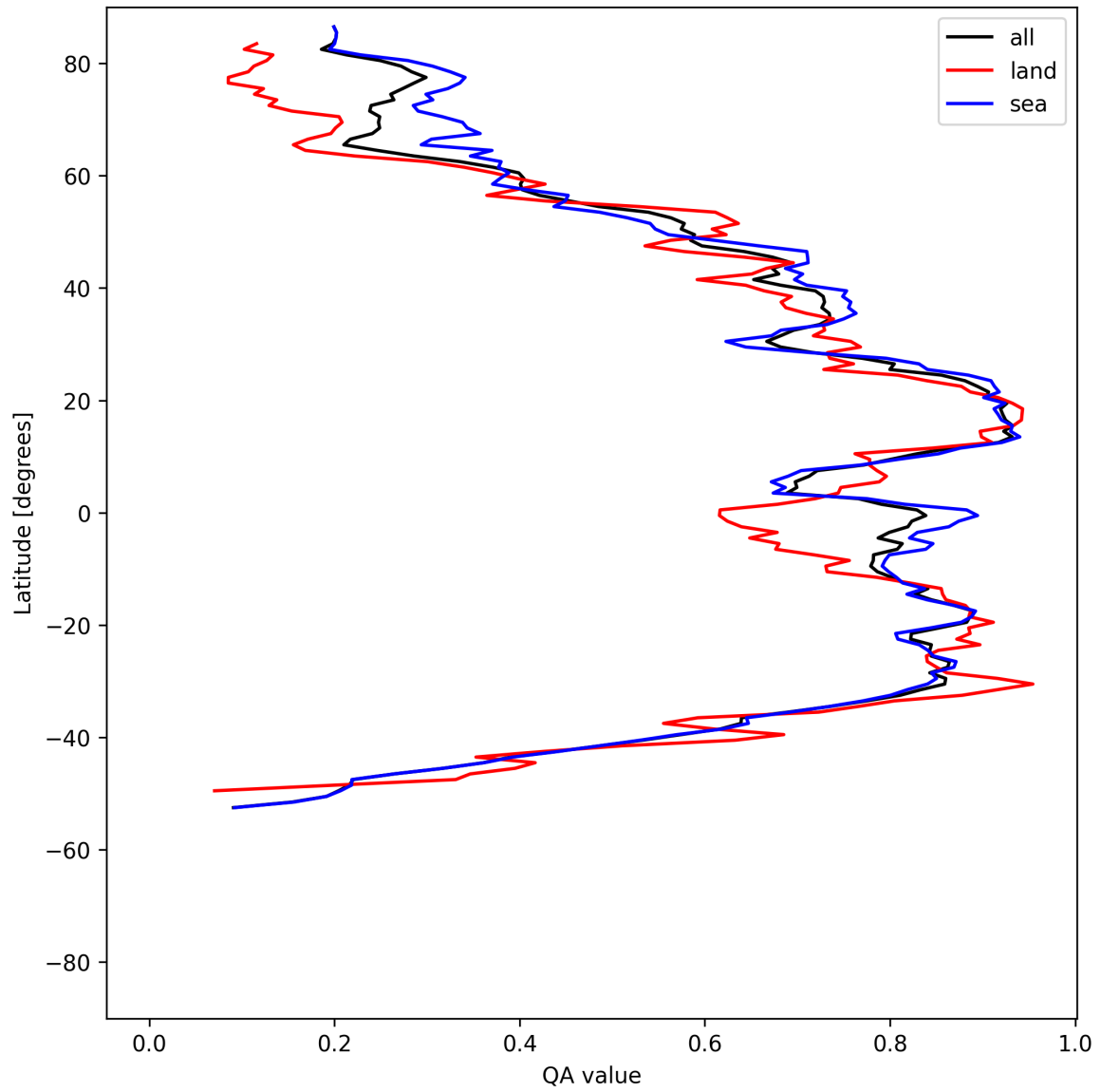
Figure 31: Zonal average of “QA value” for 2025-05-05 to 2025-05-07.
