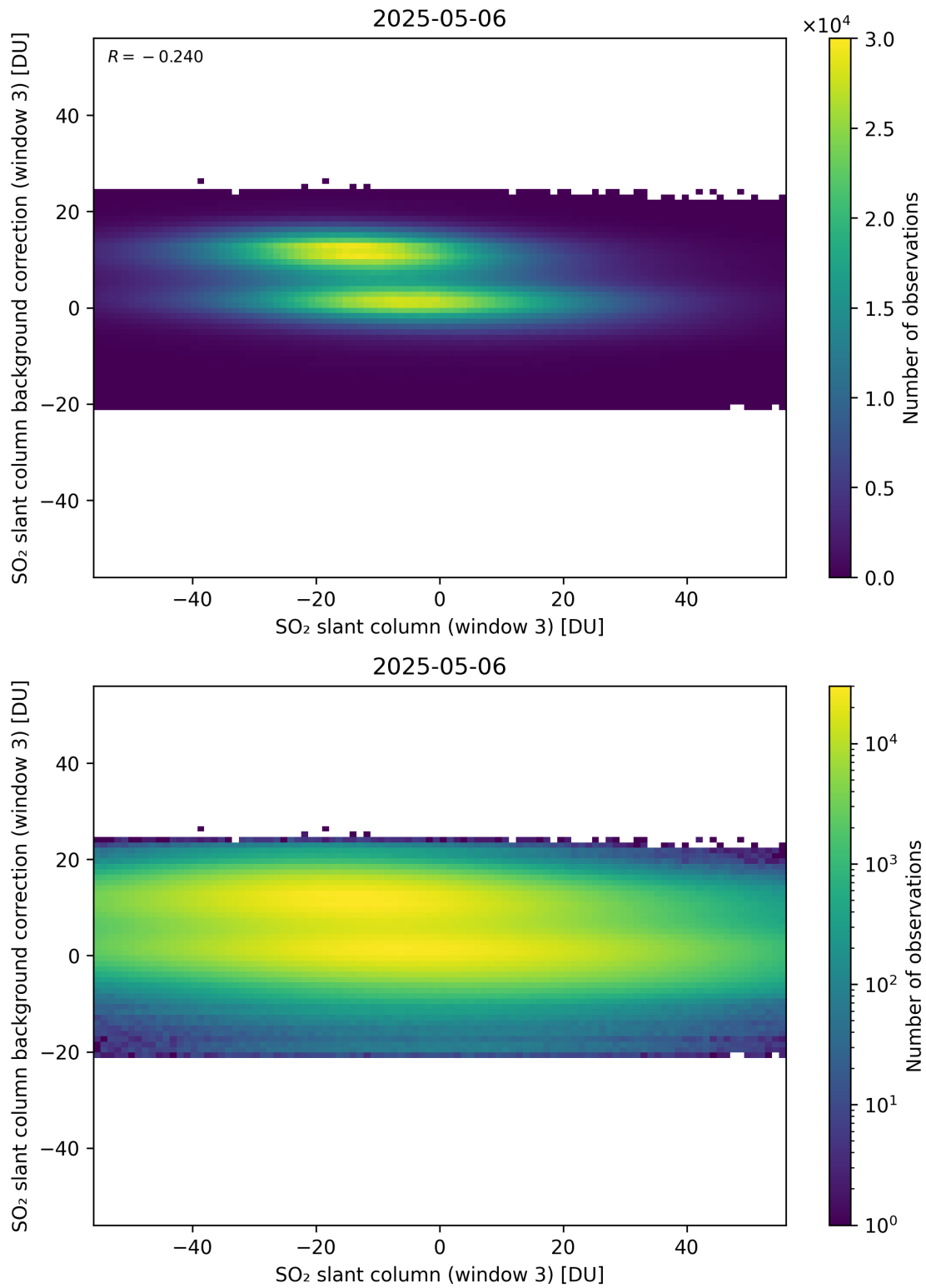
Figure 303: Scatter density plot of “SO 2 slant column (window 3)” against “SO 2 slant column background correction (window 3)” for 2025-05-05 to 2025-05-07.
