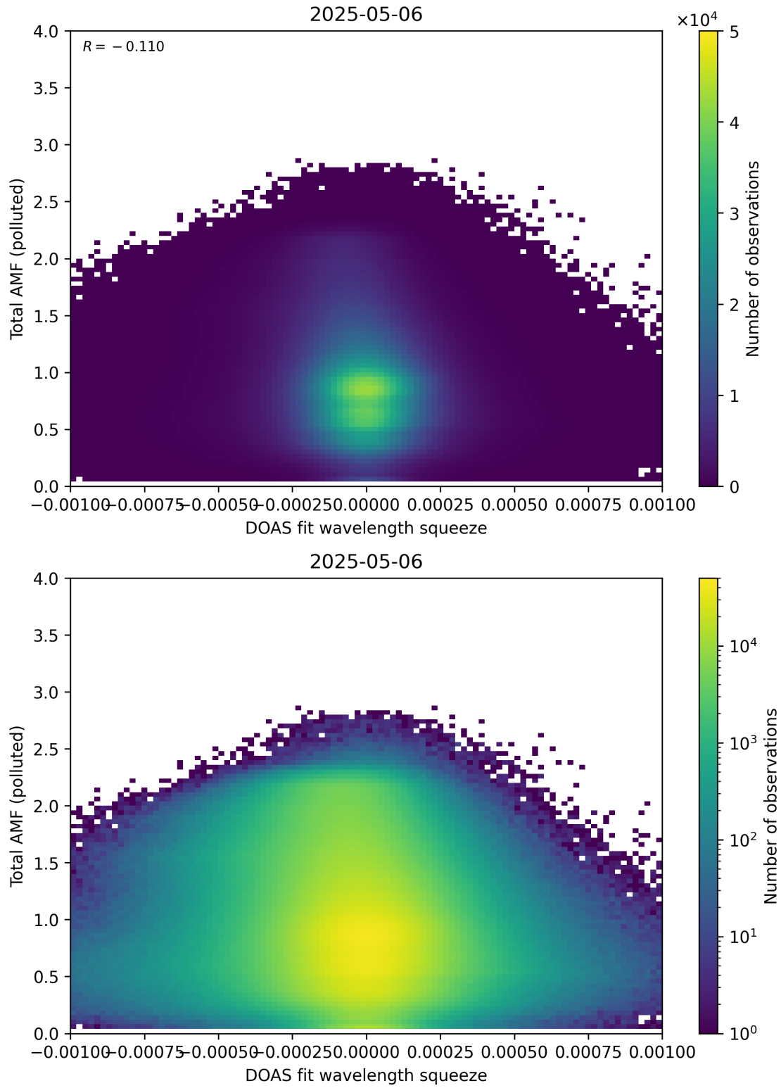
Figure 145: Scatter density plot of “DOAS fit wavelength squeeze” against “Total AMF (polluted)” for 2025-05-05 to 2025-05-07.
