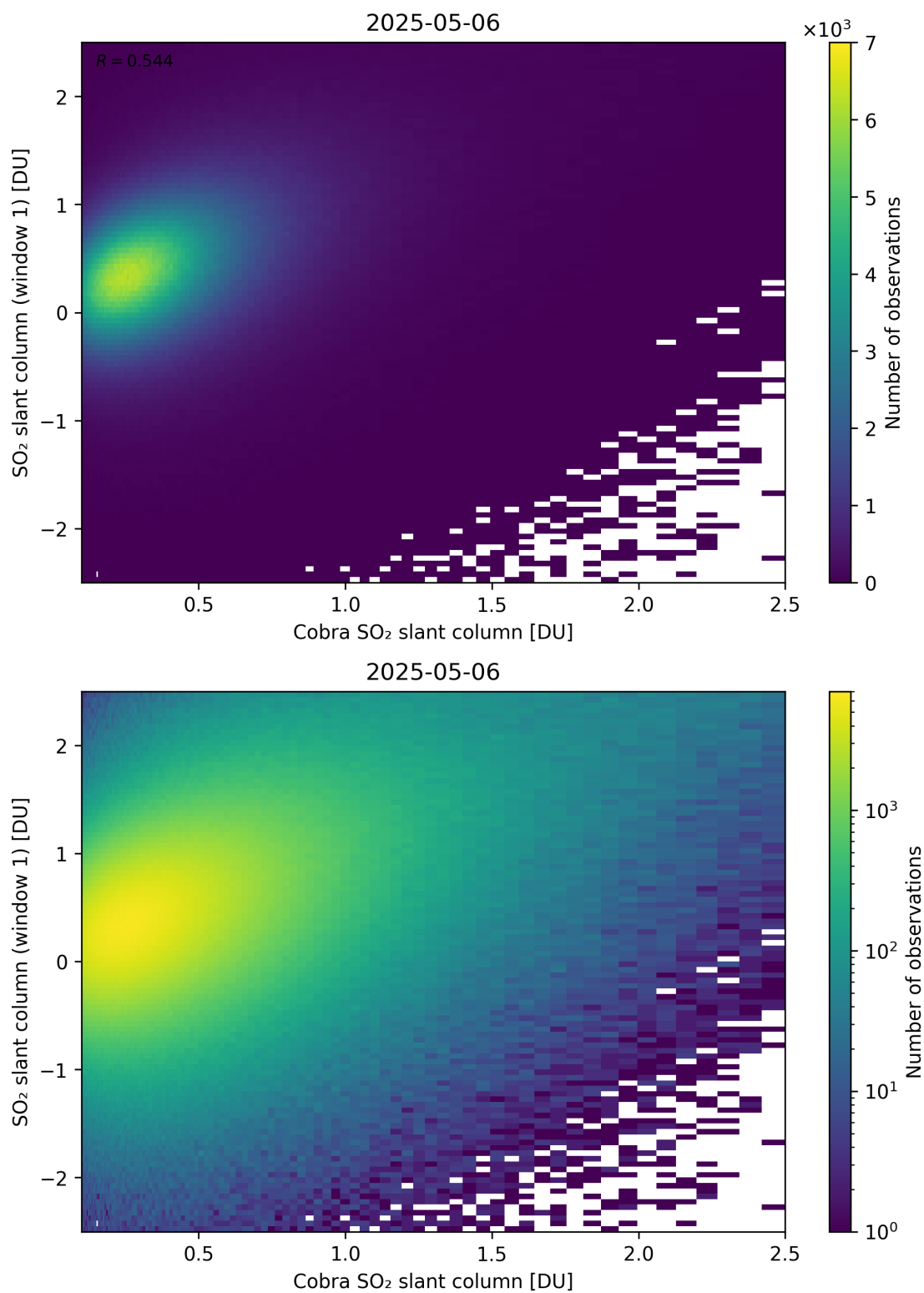
Figure 219: Scatter density plot of “Cobra SO 2 slant column” against “SO 2 slant column (window 1)” for 2025-05-05 to 2025-05-07.
