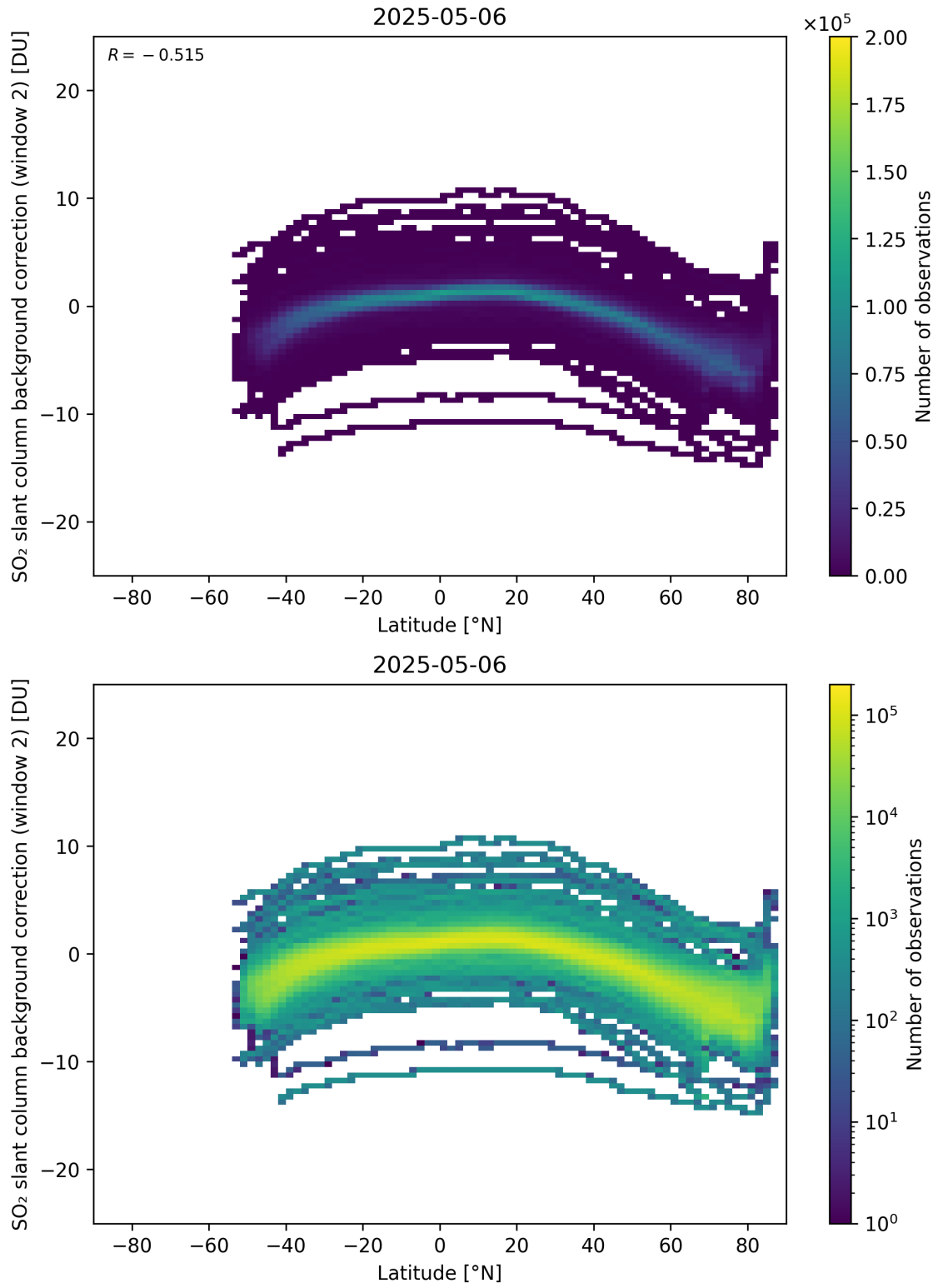
Figure 151: Scatter density plot of “Latitude” against “SO 2 slant column background correction (window 2)” for 2025-05-05 to 2025-05-07.
