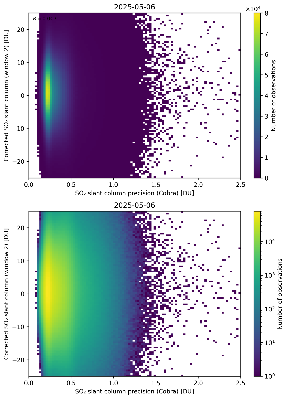
Figure 206: Scatter density plot of “SO 2 slant column precision (Cobra)” against “Corrected SO 2 slant column (window 2)” for 2025-05-05 to 2025-05-07.
