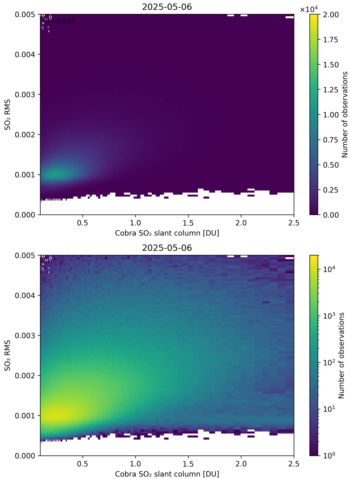
Figure 198: Scatter density plot of “Cobra SO 2 slant column” against “SO 2 RMS” for 2025-05-05 to 2025-05-07.
