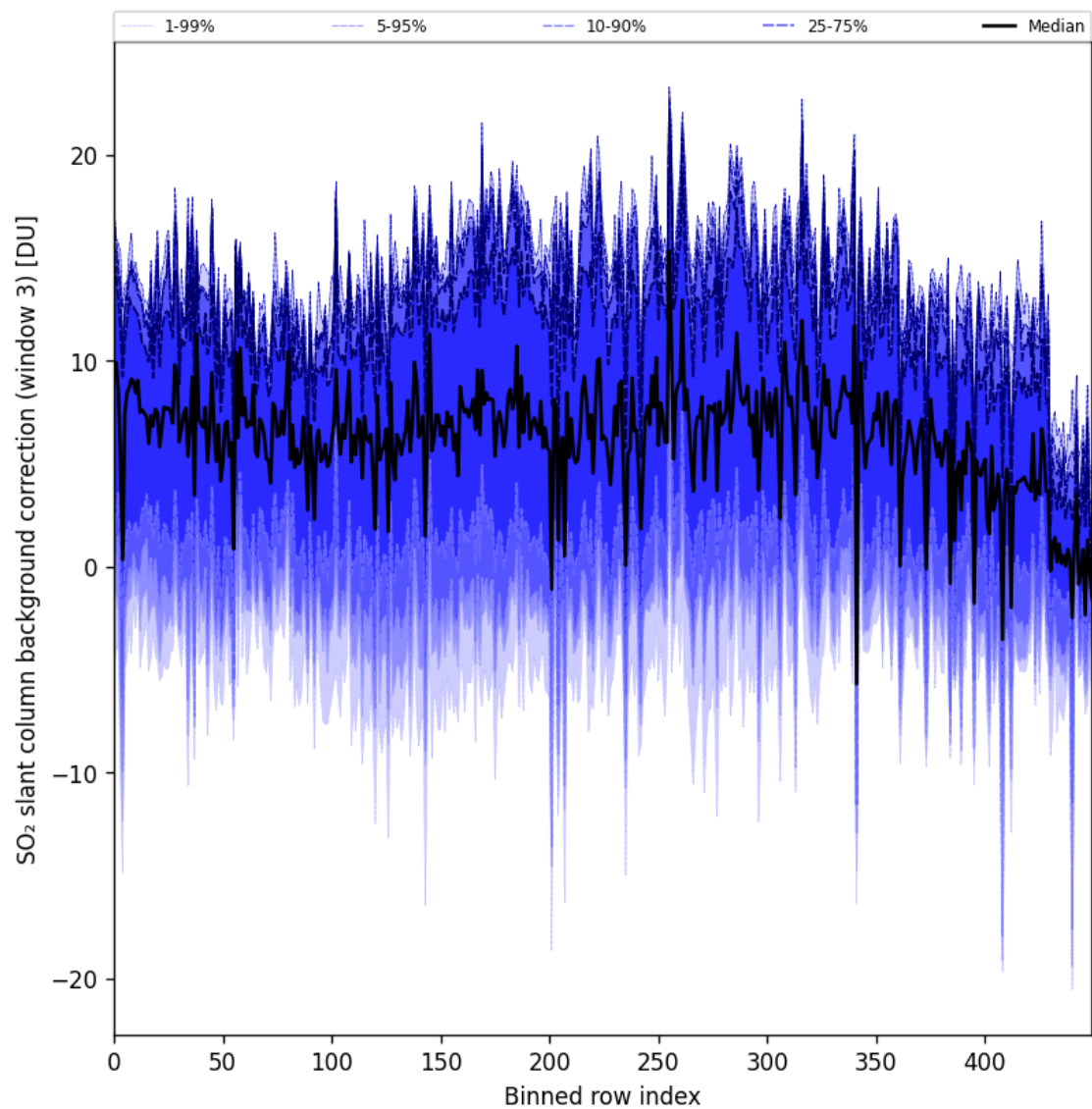
Figure 100: Along track statistics of “SO 2 slant column background correction (window 3)” for 2025-05-05 to 2025-05-07
