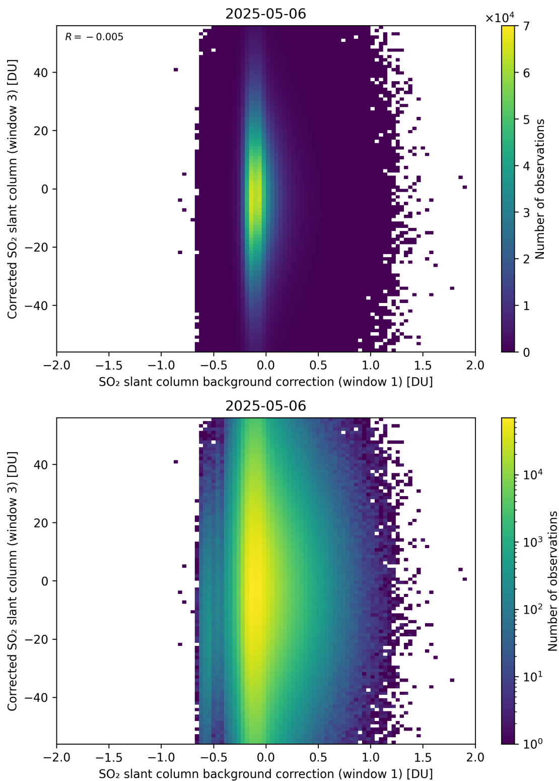
Figure 116: Scatter density plot of “SO 2 slant column background correction (window 1)” against “Corrected SO 2 slant column (window 3)” for 2025-05-05 to 2025-05-07.
