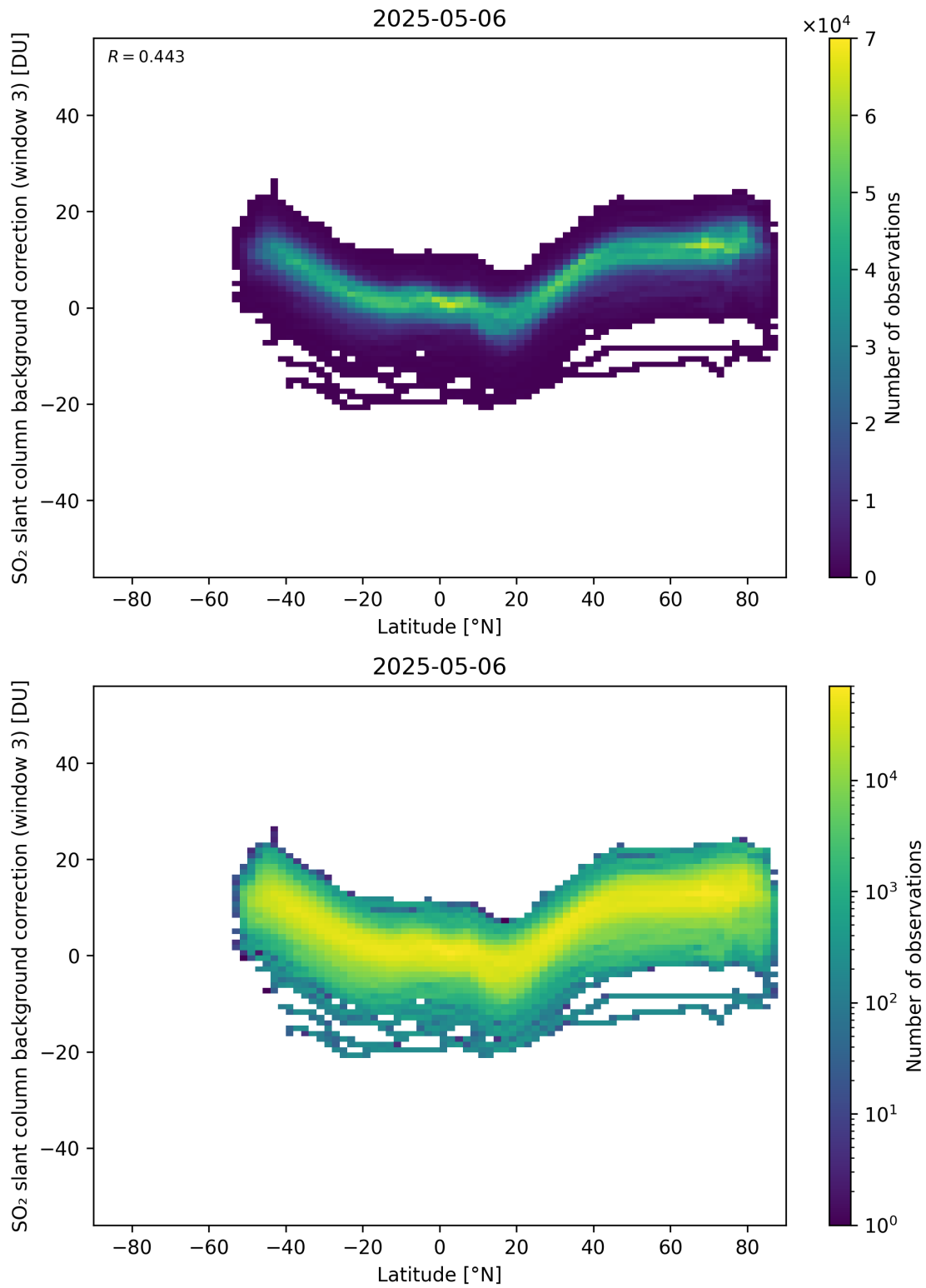
Figure 152: Scatter density plot of “Latitude” against “SO 2 slant column background correction (window 3)” for 2025-05-05 to 2025-05-07.
