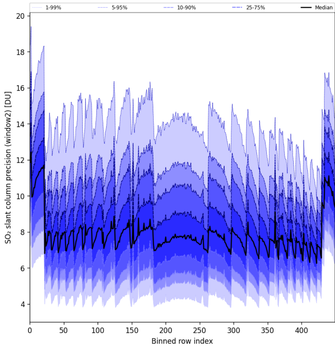
Figure 94: Along track statistics of “SO 2 slant column precision (window2)” for 2025-05-05 to 2025-05-07
