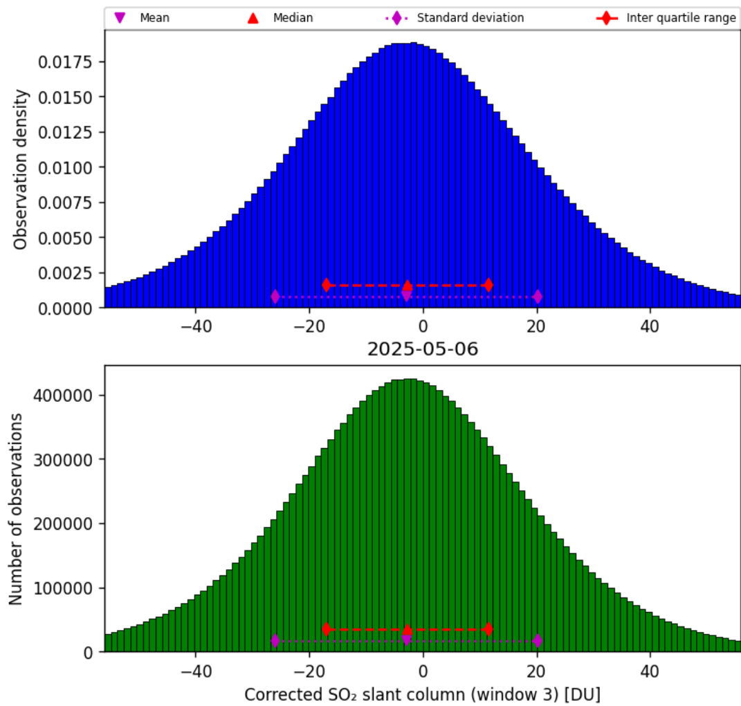
Figure 73: Histogram of “Corrected SO 2 slant column (window 3)” for 2025-05-05 to 2025-05-07
