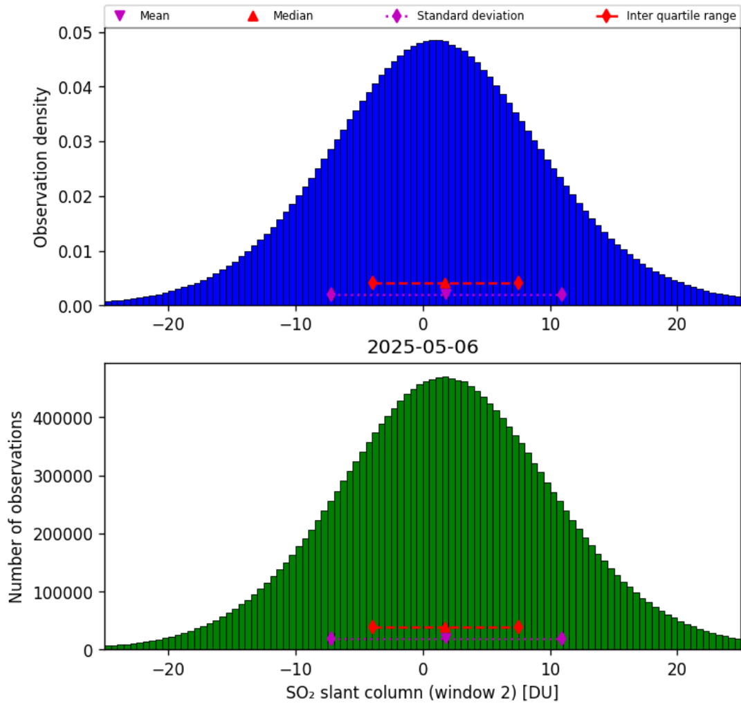
Figure 67: Histogram of “SO 2 slant column (window 2)” for 2025-05-05 to 2025-05-07
