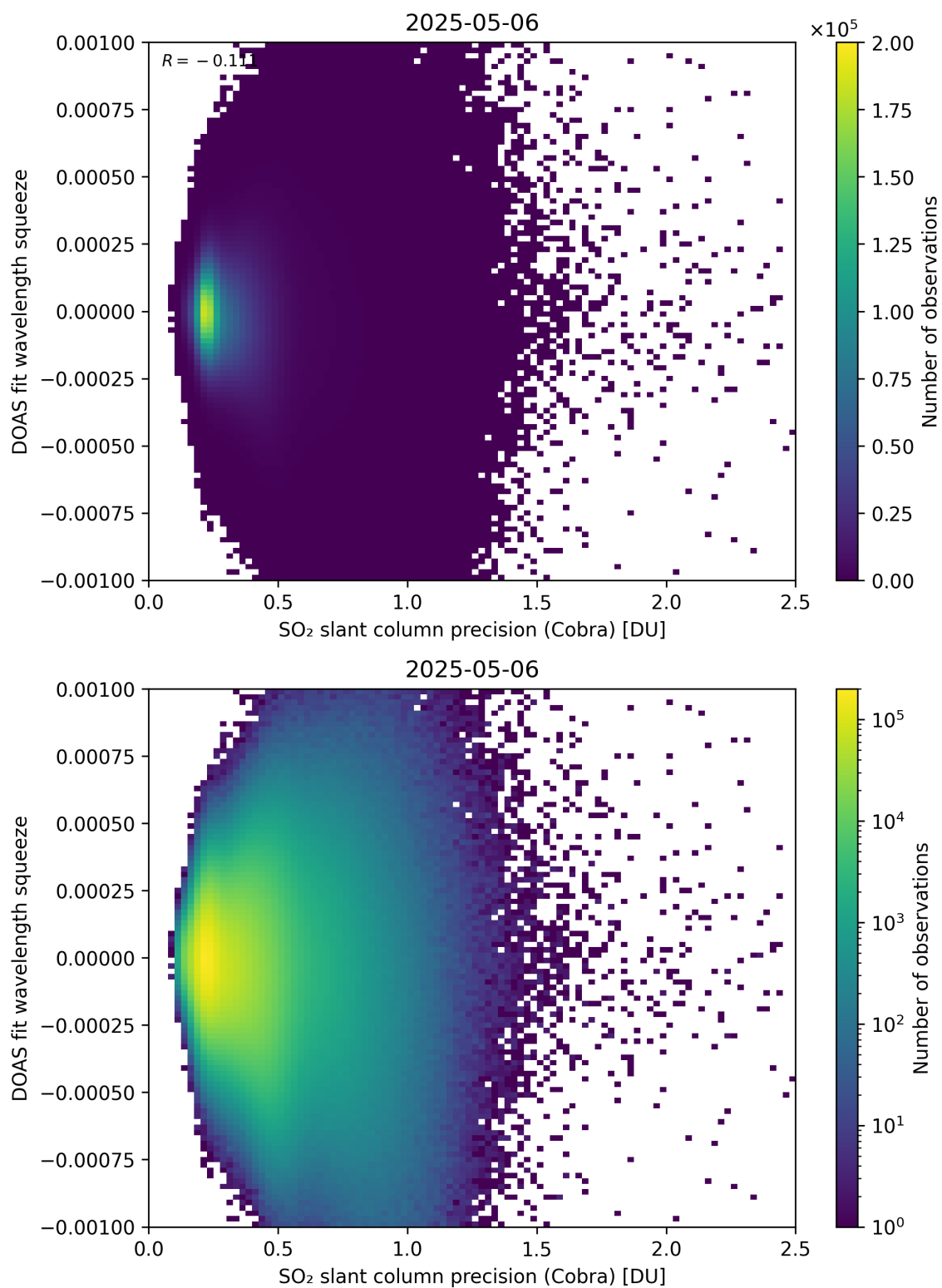
Figure 203: Scatter density plot of “SO 2 slant column precision (Cobra)” against “DOAS fit wavelength squeeze” for 2025-05-05 to 2025-05-07.
