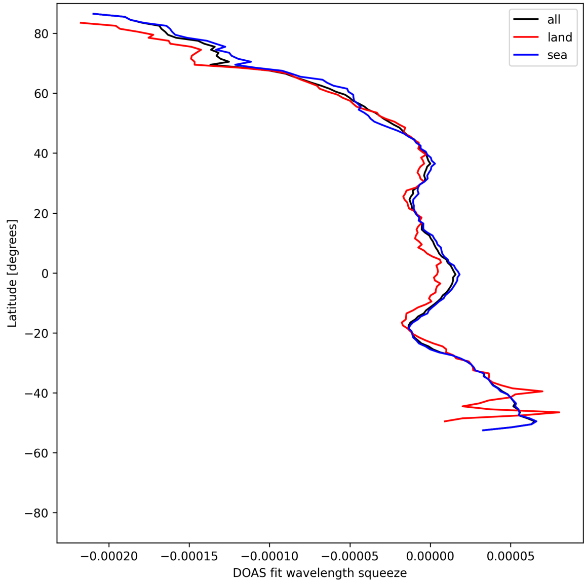
Figure 51: Zonal average of “DOAS fit wavelength squeeze” for 2025-05-05 to 2025-05-07.
