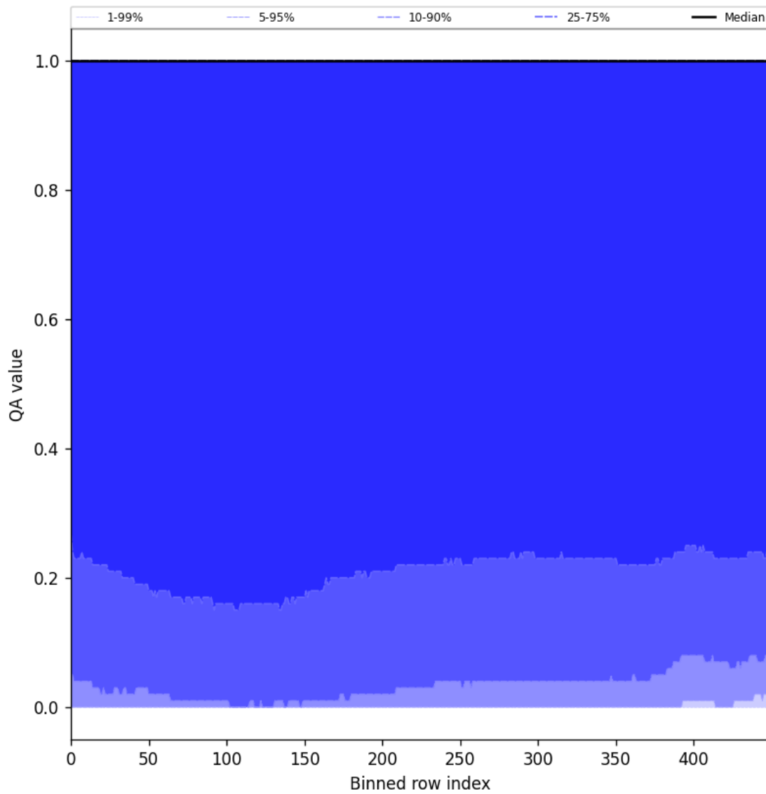
Figure 83: Along track statistics of “QA value” for 2025-05-05 to 2025-05-07
