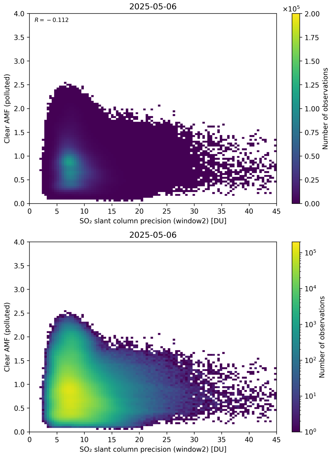
Figure 296: Scatter density plot of “SO 2 slant column precision (window2)” against “Clear AMF (polluted)” for 2025-05-05 to 2025-05-07.
