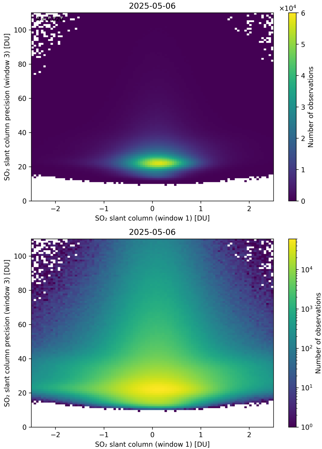
Figure 288: Scatter density plot of “SO 2 slant column (window 1)” against “SO 2 slant column precision (window 3)” for 2025-05-05 to 2025-05-07.
