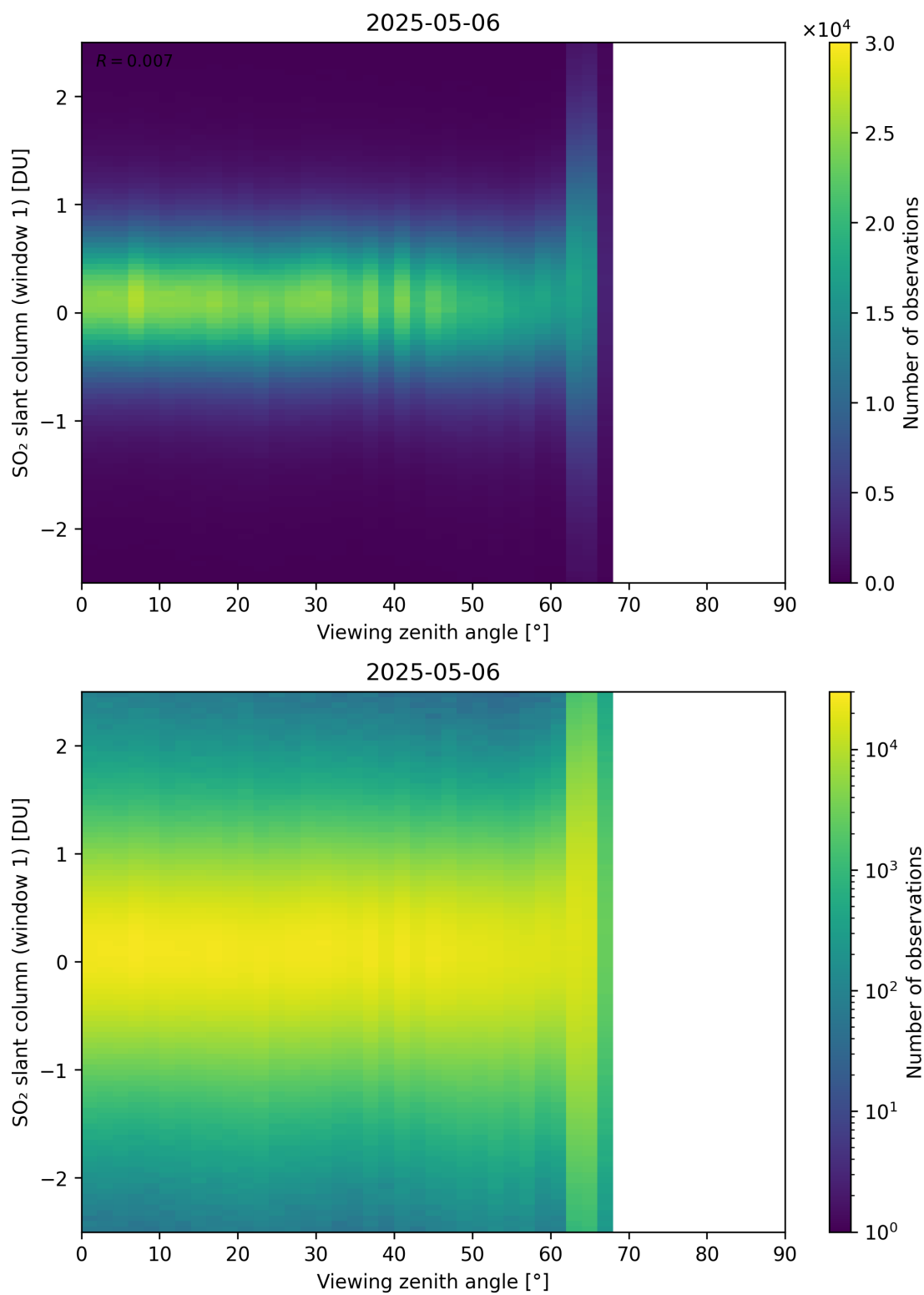
Figure 376: Scatter density plot of “Viewing zenith angle” against “SO 2 slant column (window 1)” for 2025-05-05 to 2025-05-07.
