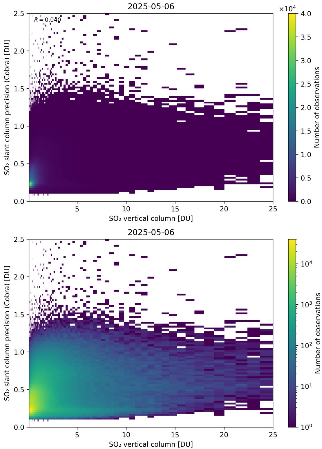
Figure 350: Scatter density plot of “SO 2 vertical column” against “SO 2 slant column precision (Cobra)” for 2025-05-05 to 2025-05-07.
