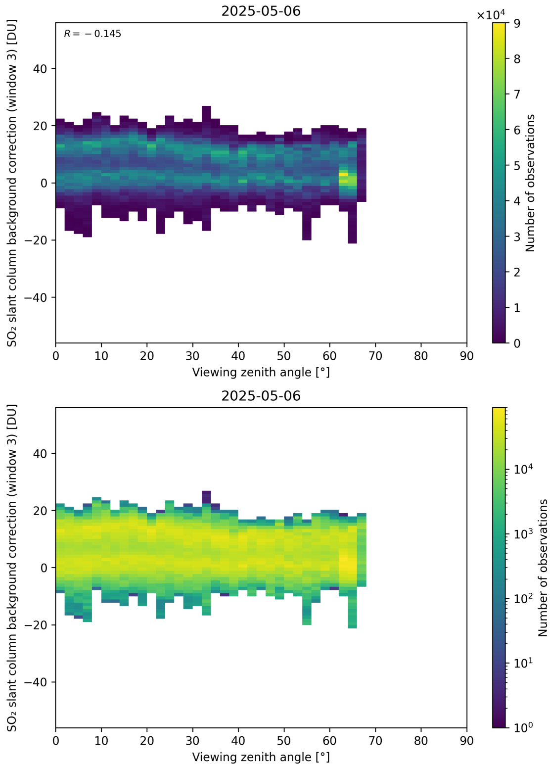
Figure 364: Scatter density plot of “Viewing zenith angle” against “SO 2 slant column background correction (window 3)” for 2025-05-05 to 2025-05-07.
