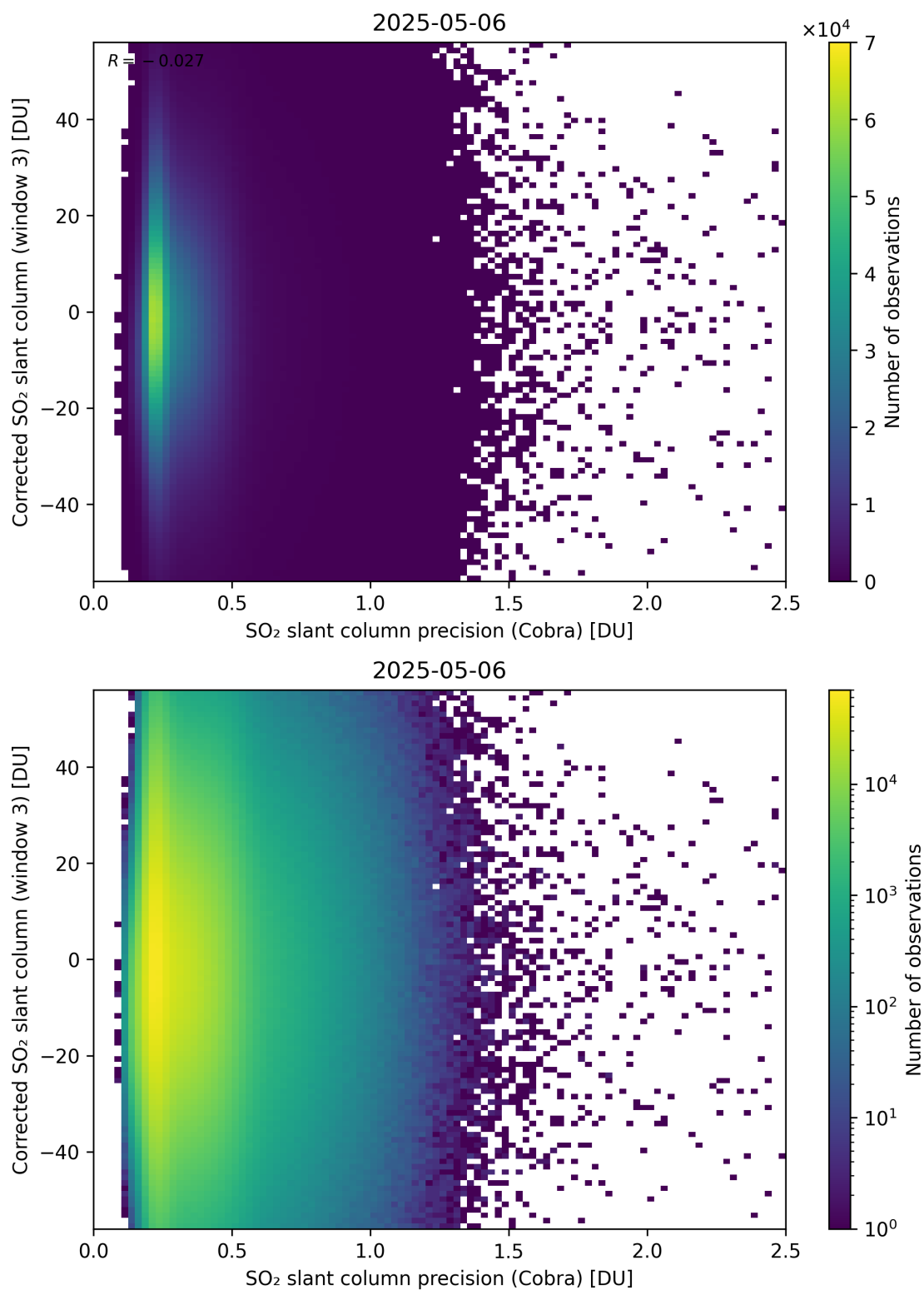
Figure 207: Scatter density plot of “SO 2 slant column precision (Cobra)” against “Corrected SO 2 slant column (window 3)” for 2025-05-05 to 2025-05-07.
