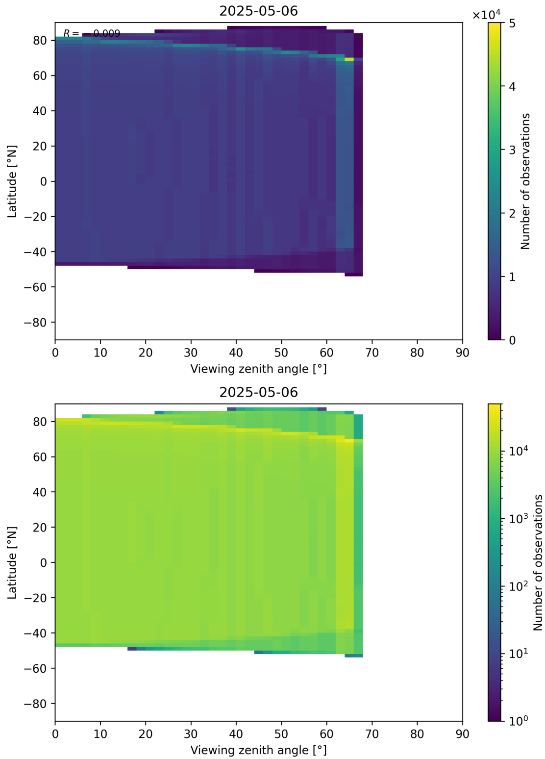
Figure 368: Scatter density plot of “Viewing zenith angle” against “Latitude” for 2025-05-05 to 2025-05-07.
