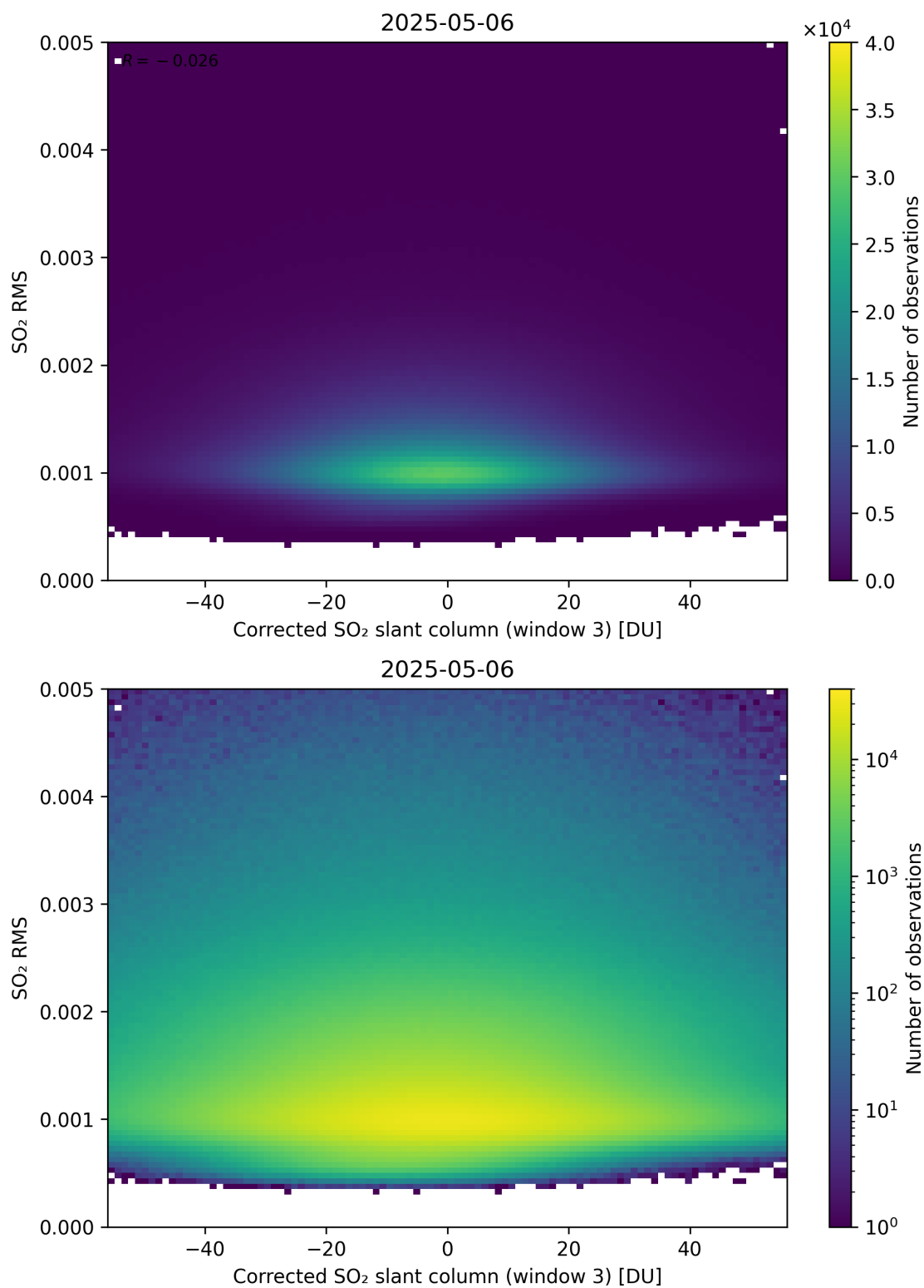
Figure 258: Scatter density plot of “Corrected SO 2 slant column (window 3)” against “SO 2 RMS” for 2025-05-05 to 2025-05-07.
