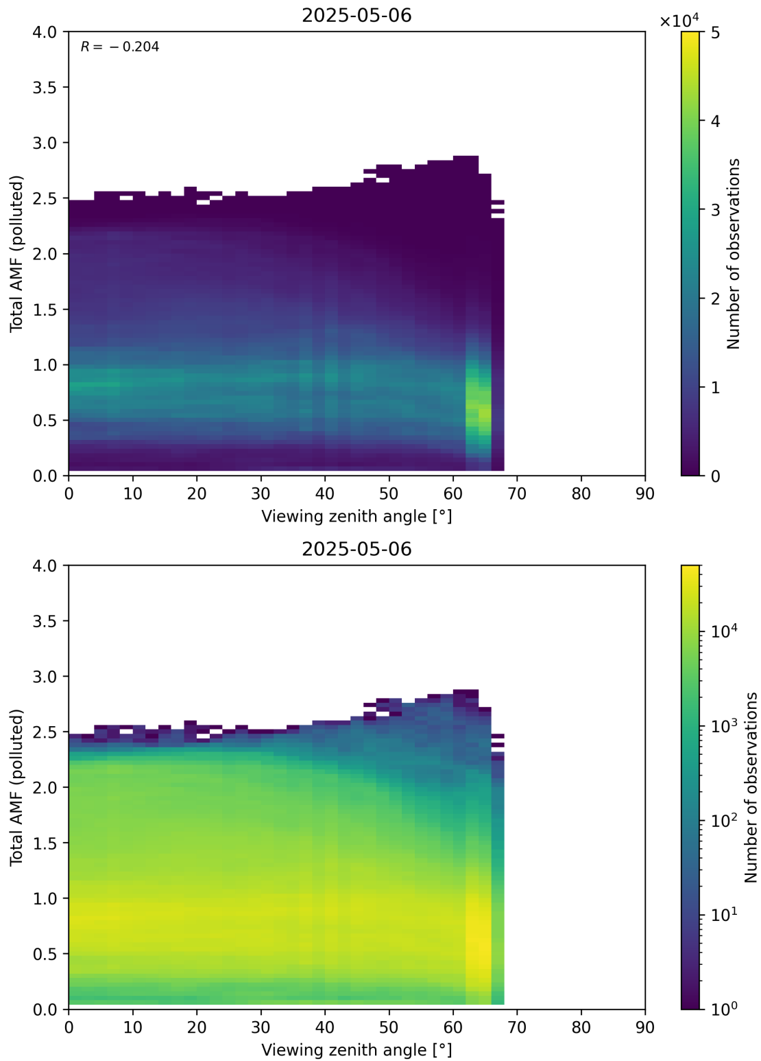
Figure 381: Scatter density plot of “Viewing zenith angle” against “Total AMF (polluted)” for 2025-05-05 to 2025-05-07.
