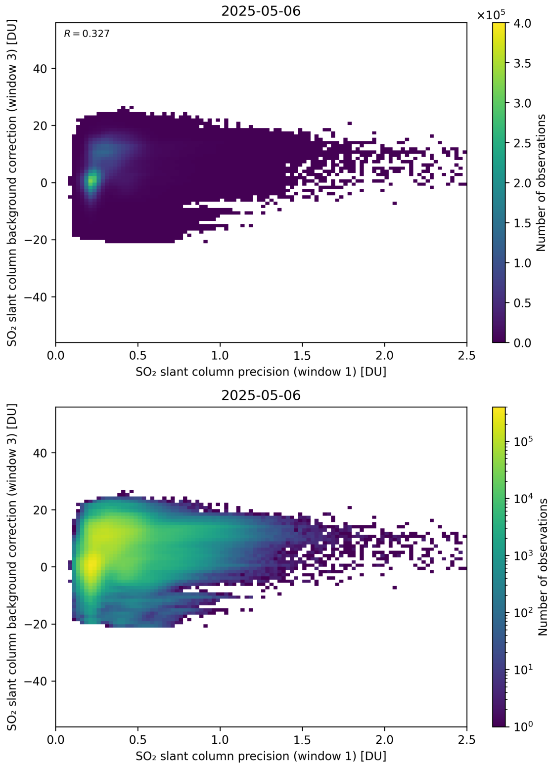
Figure 270: Scatter density plot of “SO 2 slant column precision (window 1)” against “SO 2 slant column background correction (window 3)” for 2025-05-05 to 2025-05-07.
