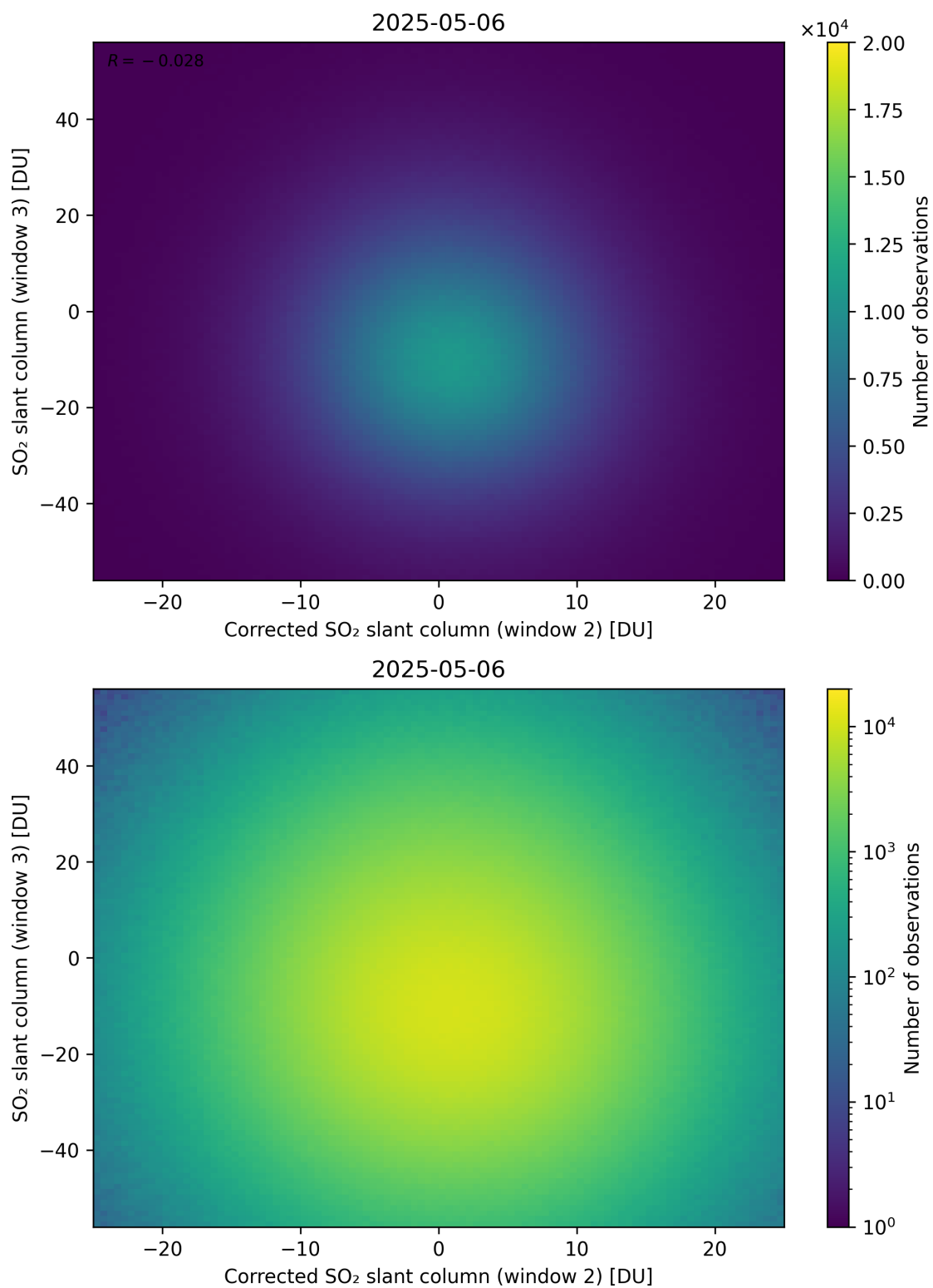
Figure 251: Scatter density plot of “Corrected SO 2 slant column (window 2)” against “SO 2 slant column (window 3)” for 2025-05-05 to 2025-05-07.
