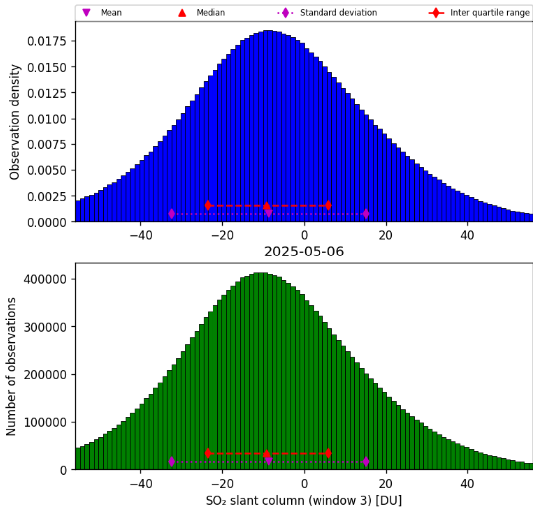
Figure 71: Histogram of “SO 2 slant column (window 3)” for 2025-05-05 to 2025-05-07
