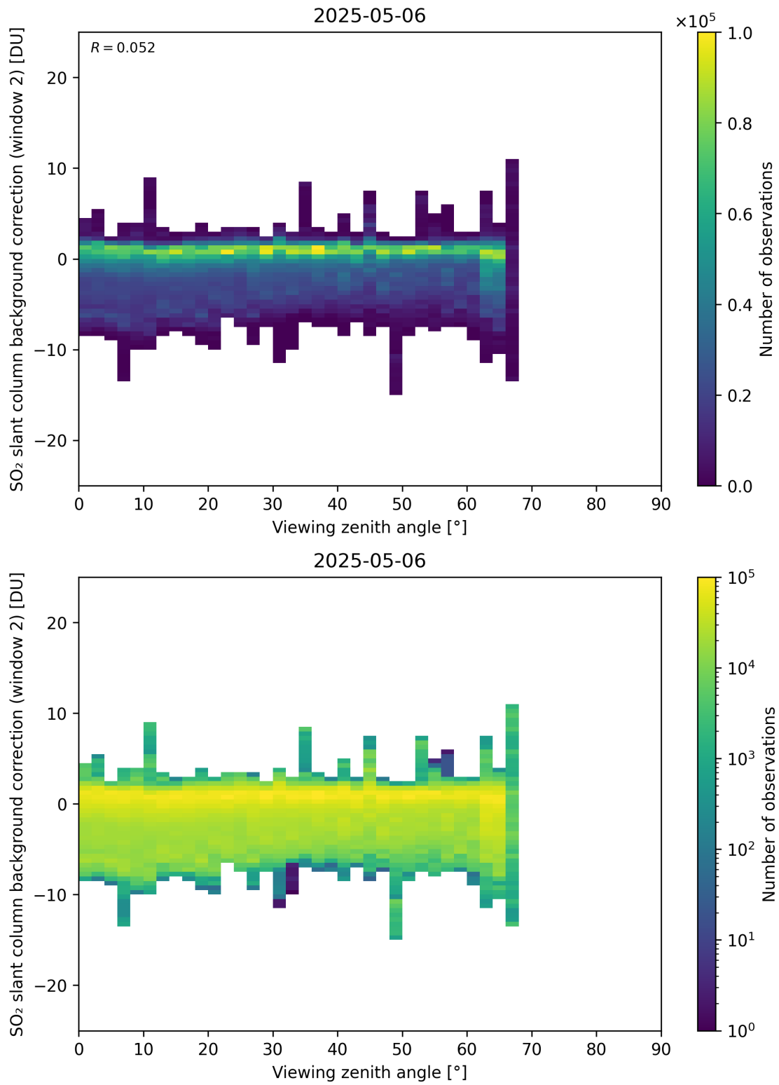
Figure 363: Scatter density plot of “Viewing zenith angle” against “SO 2 slant column background correction (window 2)” for 2025-05-05 to 2025-05-07.
