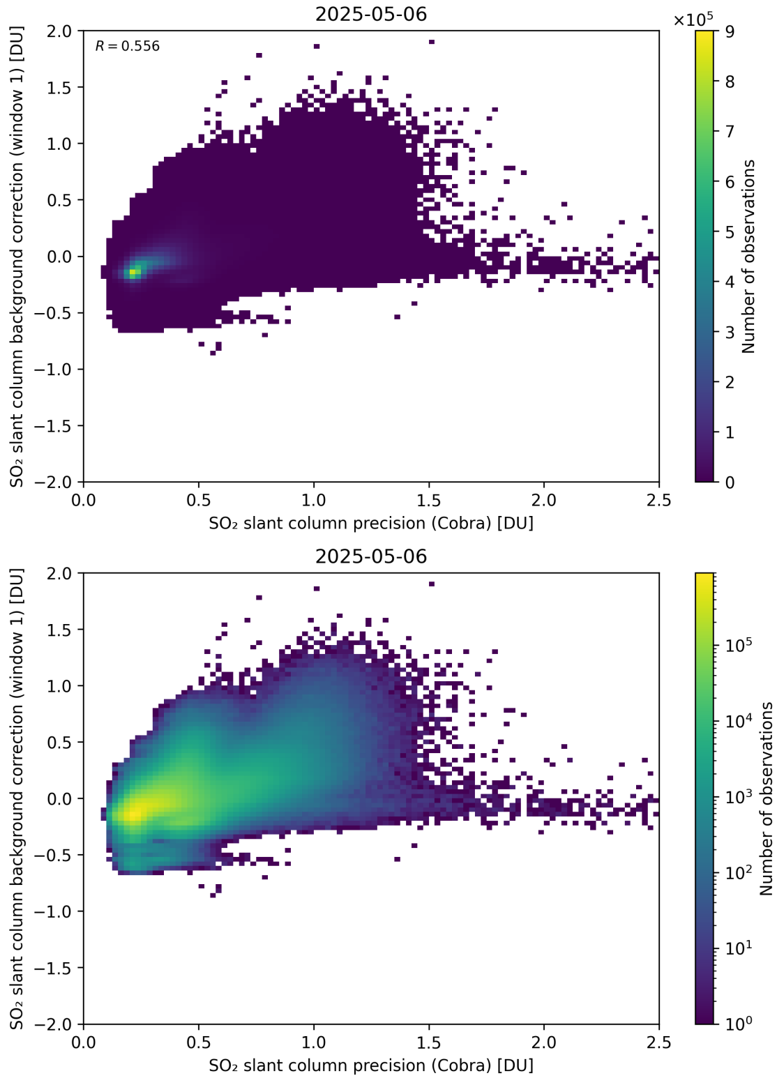
Figure 199: Scatter density plot of “SO 2 slant column precision (Cobra)” against “SO 2 slant column background correction (window 1)” for 2025-05-05 to 2025-05-07.
