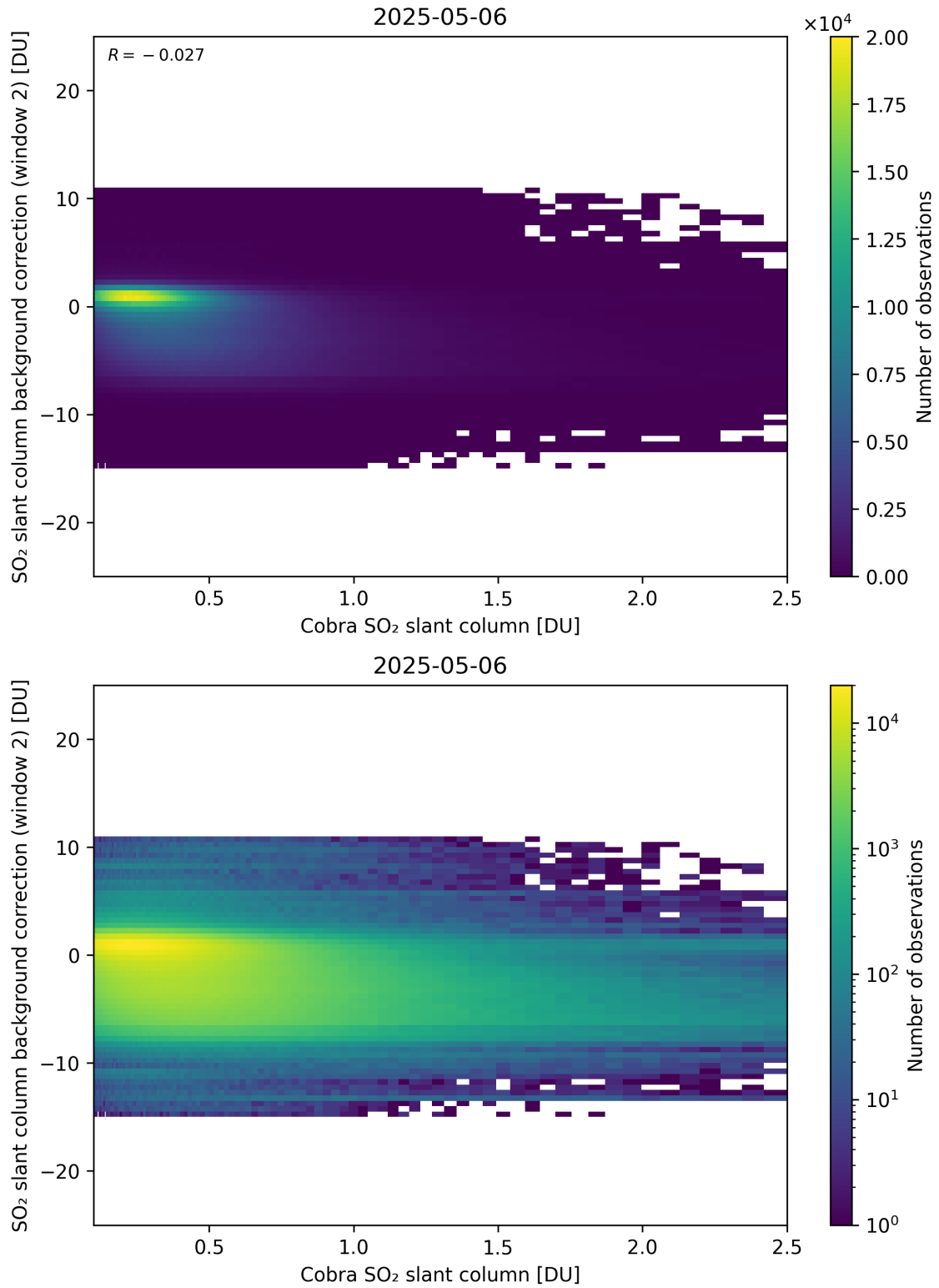
Figure 194: Scatter density plot of “Cobra SO 2 slant column” against “SO 2 slant column background correction (window 2)” for 2025-05-05 to 2025-05-07.
