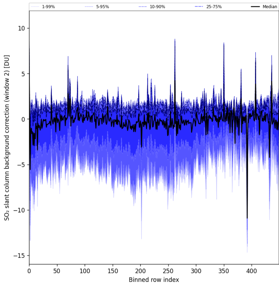
Figure 96: Along track statistics of “SO 2 slant column background correction (window 2)” for 2025-05-05 to 2025-05-07
