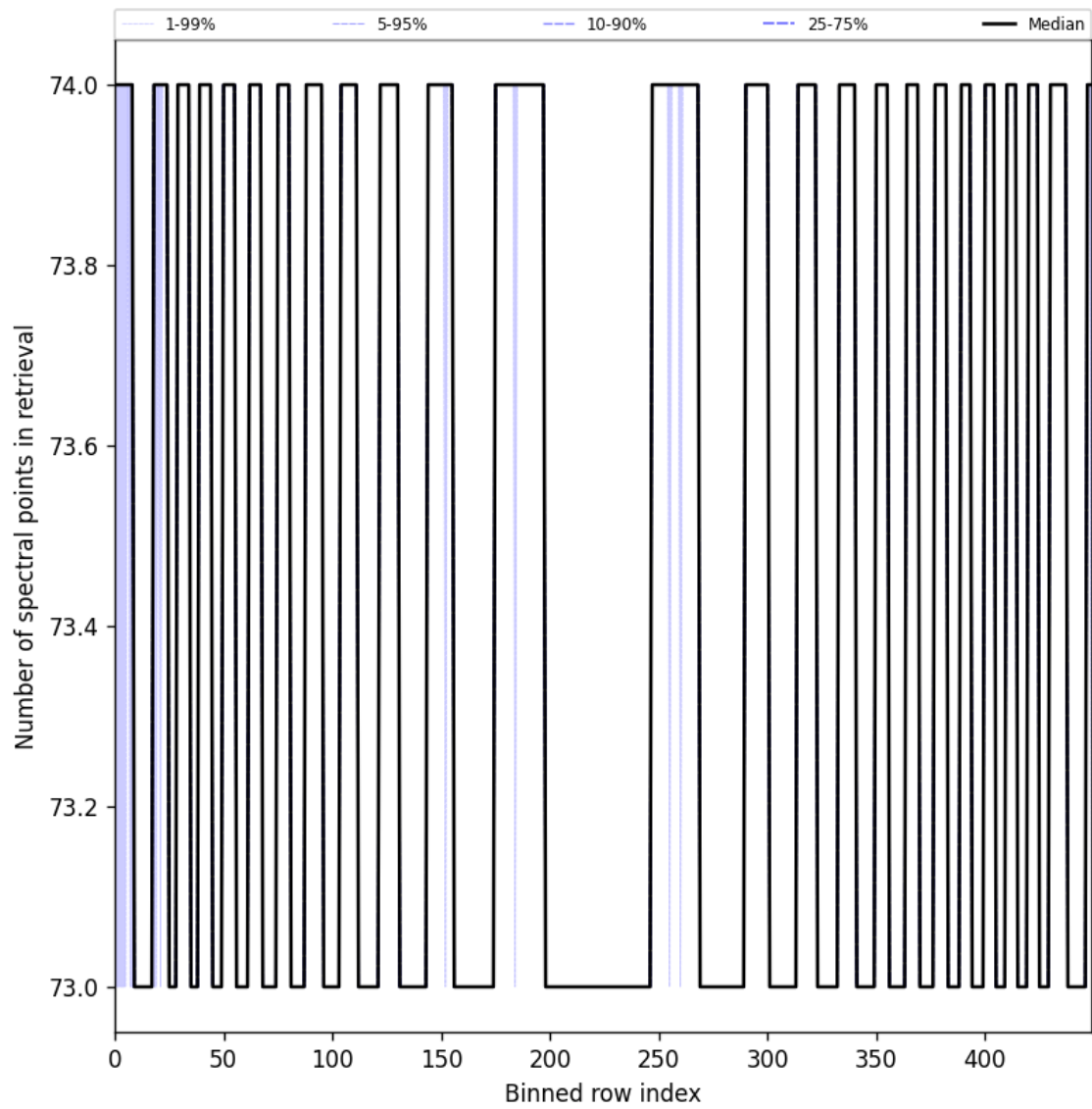
Figure 108: Along track statistics of “Number of spectral points in retrieval” for 2025-05-05 to 2025-05-07
