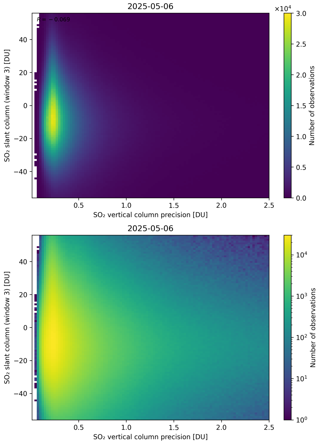
Figure 344: Scatter density plot of “SO 2 vertical column precision” against “SO 2 slant column (window 3)” for 2025-05-05 to 2025-05-07.
