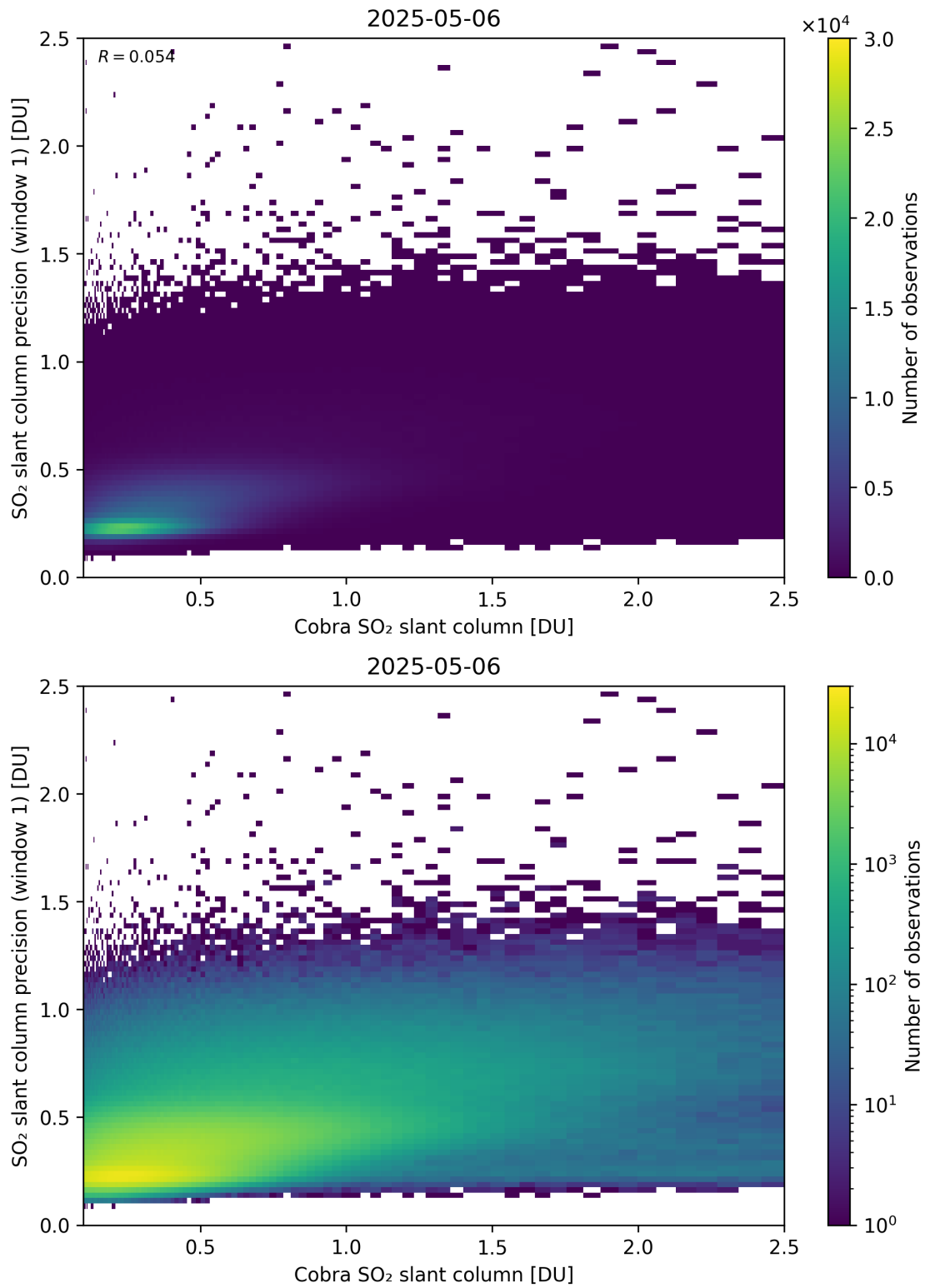
Figure 220: Scatter density plot of “Cobra SO 2 slant column” against “SO 2 slant column precision (window 1)” for 2025-05-05 to 2025-05-07.
