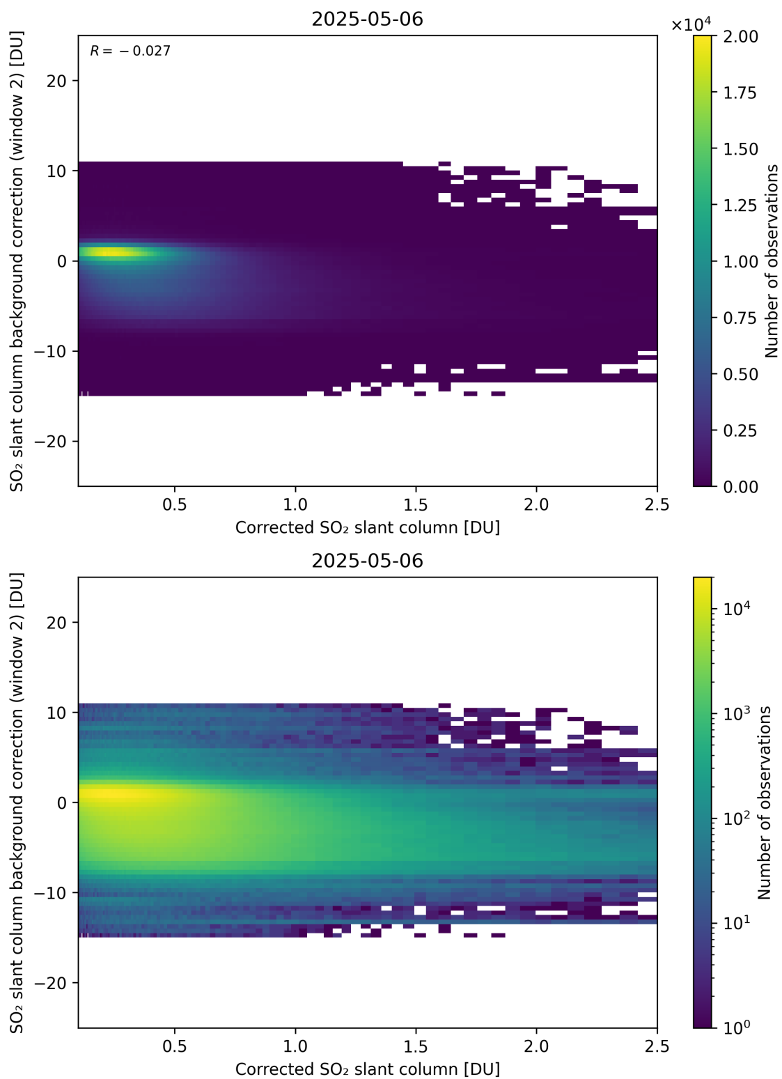
Figure 227: Scatter density plot of “Corrected SO 2 slant column” against “SO 2 slant column background correction (window 2)” for 2025-05-05 to 2025-05-07.
