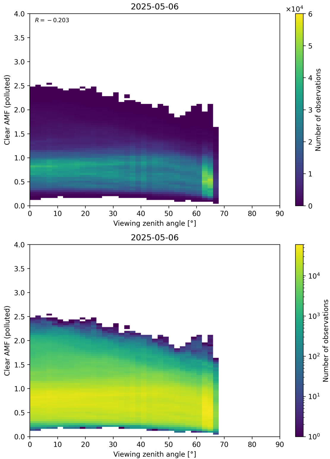
Figure 370: Scatter density plot of “Viewing zenith angle” against “Clear AMF (polluted)” for 2025-05-05 to 2025-05-07.
