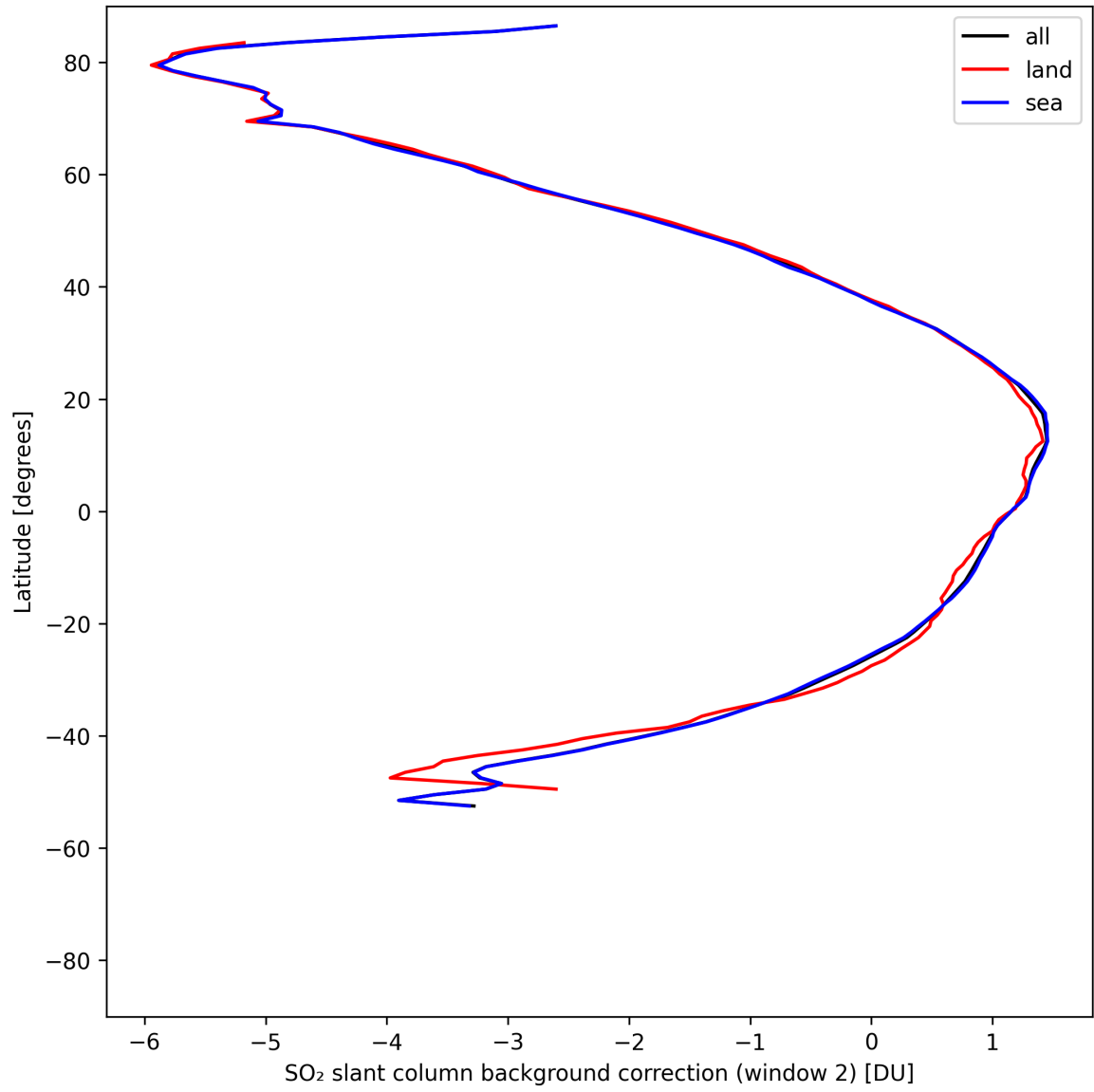
Figure 44: Zonal average of “SO 2 slant column background correction (window 2)” for 2025-05-05 to 2025-05-07.
