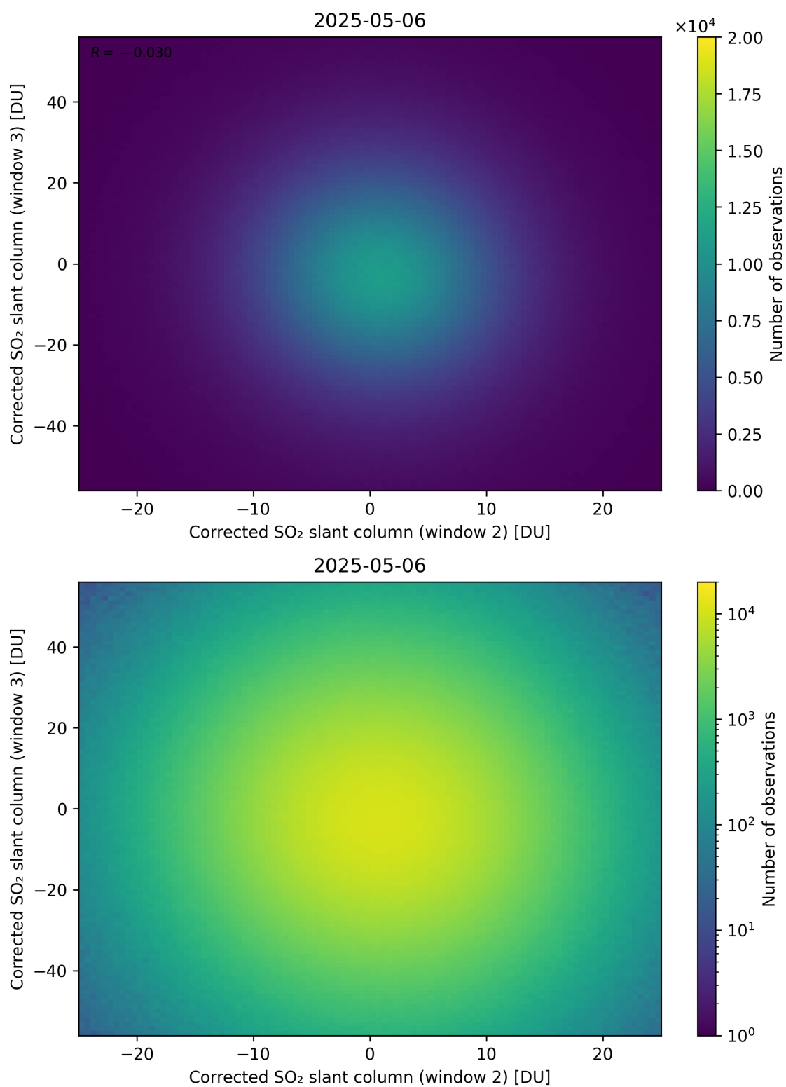
Figure 250: Scatter density plot of “Corrected SO 2 slant column (window 2)” against “Corrected SO 2 slant column (window 3)” for 2025-05-05 to 2025-05-07.
