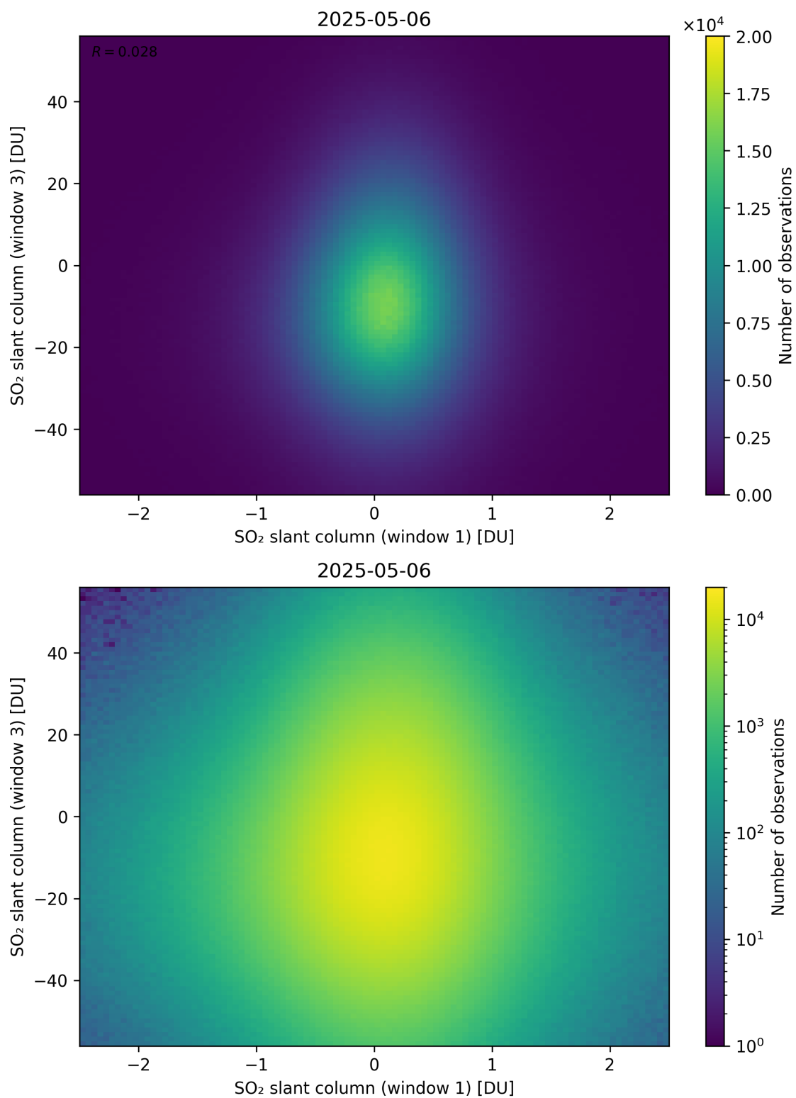
Figure 287: Scatter density plot of “SO 2 slant column (window 1)” against “SO 2 slant column (window 3)” for 2025-05-05 to 2025-05-07.
