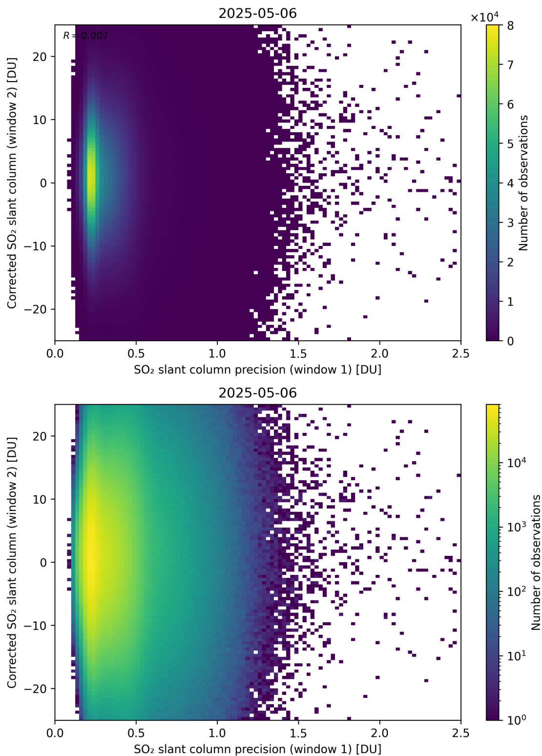
Figure 275: Scatter density plot of “SO 2 slant column precision (window 1)” against “Corrected SO 2 slant column (window 2)” for 2025-05-05 to 2025-05-07.
