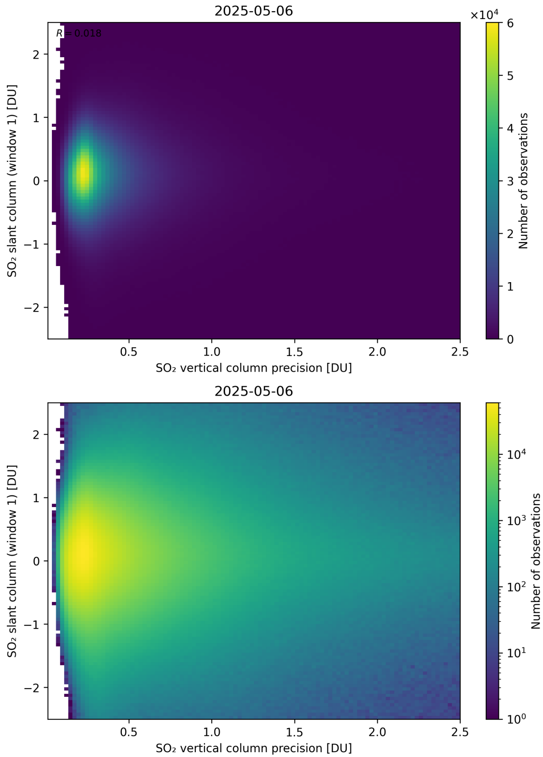
Figure 341: Scatter density plot of “SO 2 vertical column precision” against “SO 2 slant column (window 1)” for 2025-05-05 to 2025-05-07.
