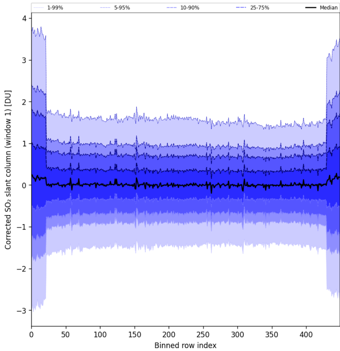
Figure 91: Along track statistics of “Corrected SO 2 slant column (window 1)” for 2025-05-05 to 2025-05-07
