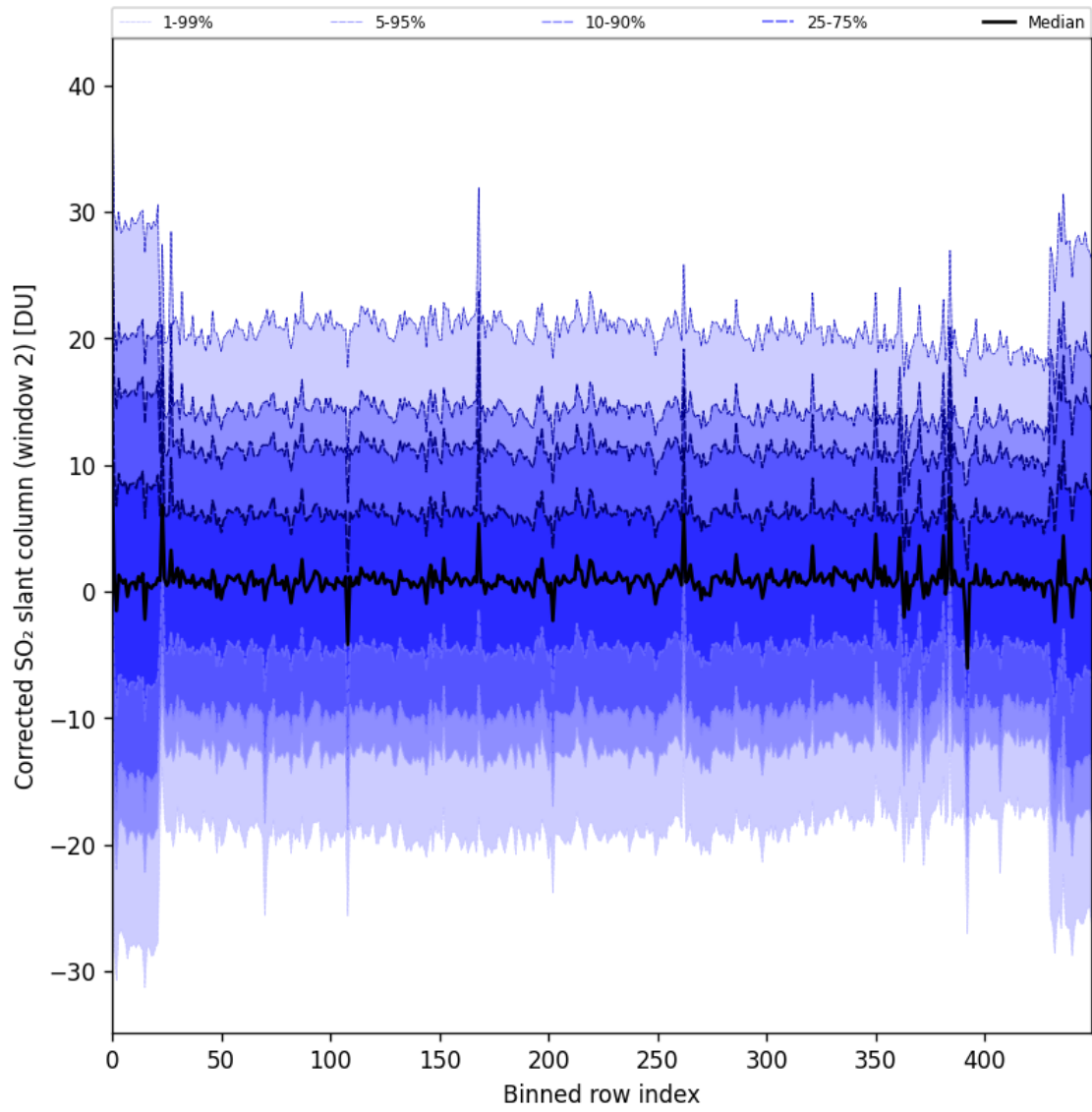
Figure 95: Along track statistics of “Corrected SO 2 slant column (window 2)” for 2025-05-05 to 2025-05-07
