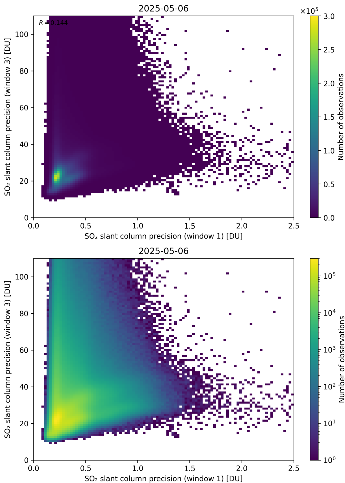
Figure 279: Scatter density plot of “SO 2 slant column precision (window 1)” against “SO 2 slant column precision (window 3)” for 2025-05-05 to 2025-05-07.
