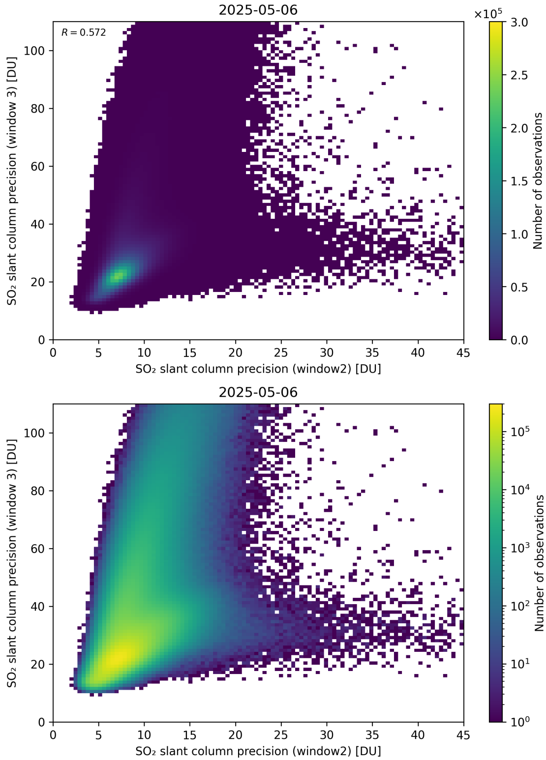
Figure 300: Scatter density plot of “SO 2 slant column precision (window2)” against “SO 2 slant column precision (window 3)” for 2025-05-05 to 2025-05-07.
