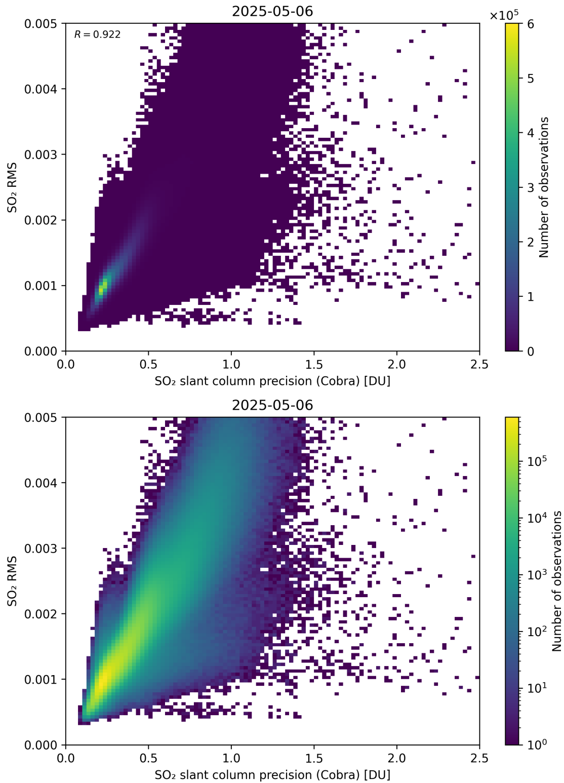
Figure 204: Scatter density plot of “SO 2 slant column precision (Cobra)” against “SO 2 RMS” for 2025-05-05 to 2025-05-07.
