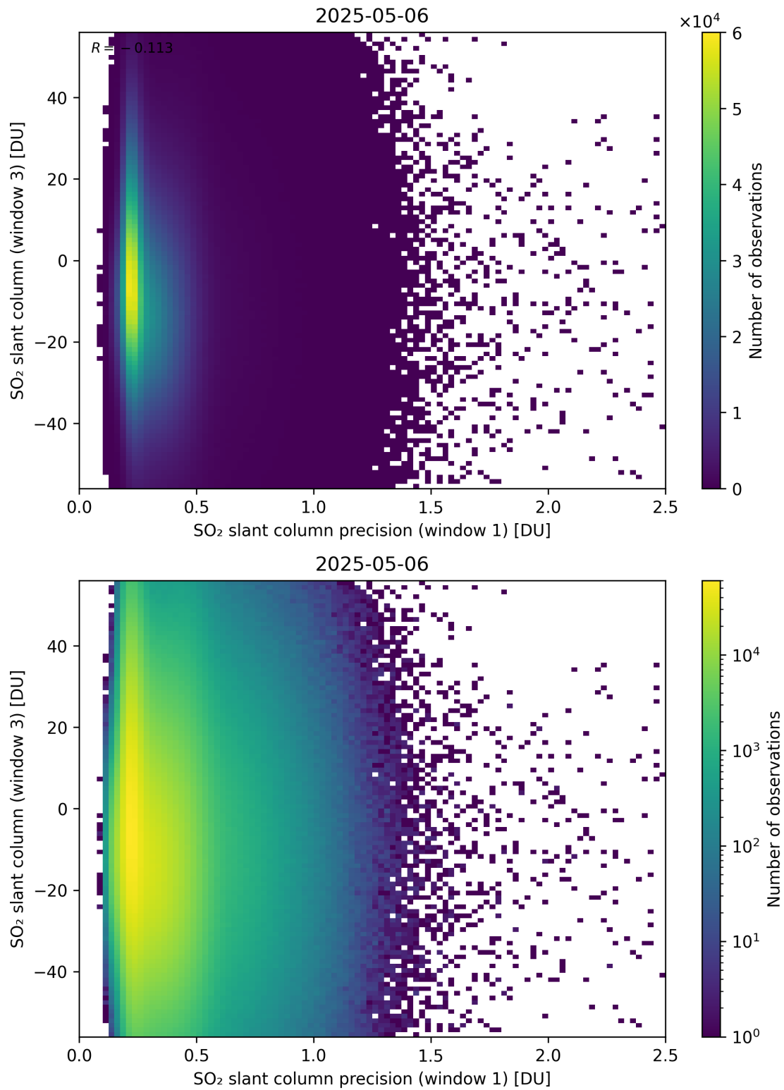
Figure 278: Scatter density plot of “SO 2 slant column precision (window 1)” against “SO 2 slant column (window 3)” for 2025-05-05 to 2025-05-07.
