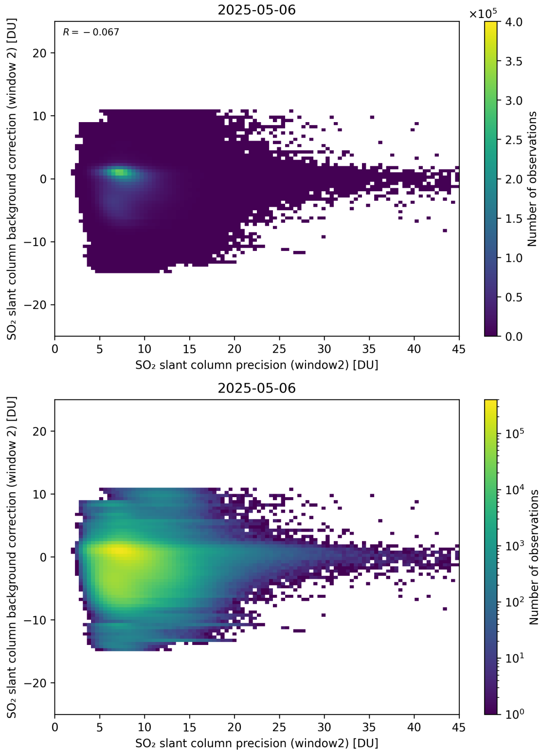
Figure 291: Scatter density plot of “SO 2 slant column precision (window2)” against “SO 2 slant column background correction (window 2)” for 2025-05-05 to 2025-05-07.
