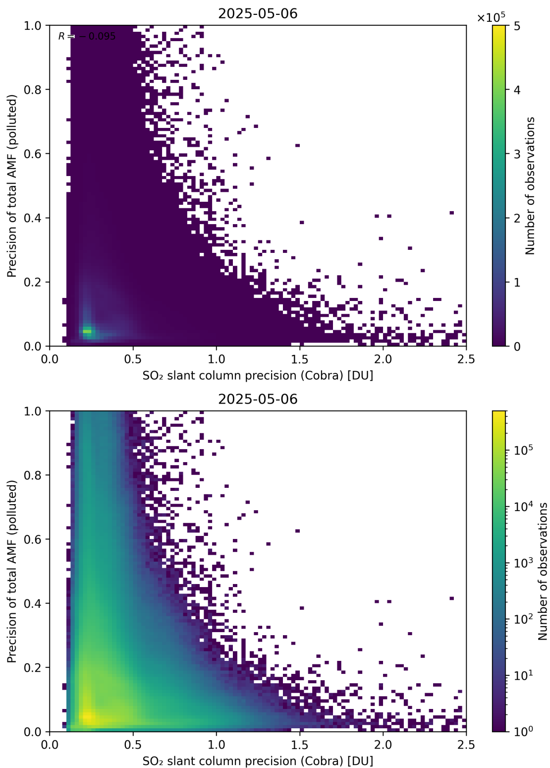
Figure 214: Scatter density plot of “SO 2 slant column precision (Cobra)” against “Precision of total AMF (polluted)” for 2025-05-05 to 2025-05-07.
