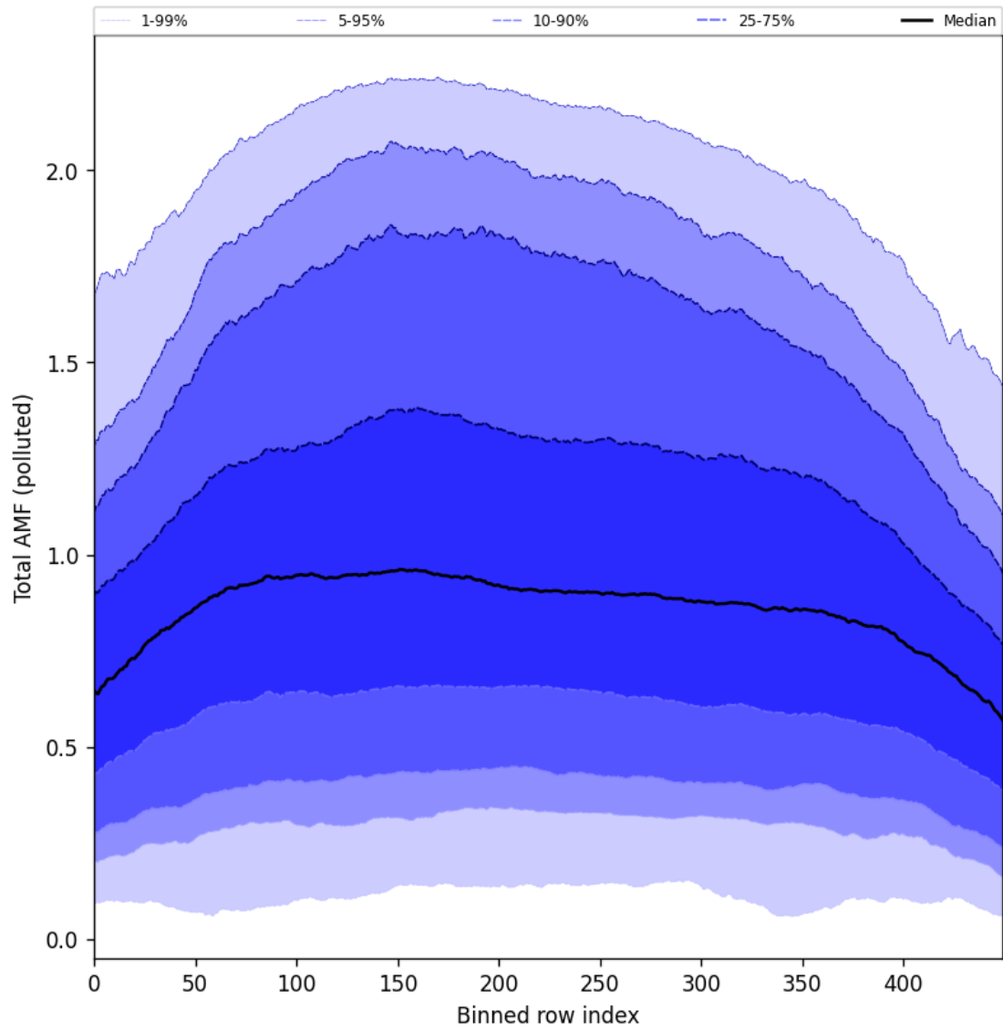
Figure 105: Along track statistics of “Total AMF (polluted)” for 2025-05-05 to 2025-05-07
