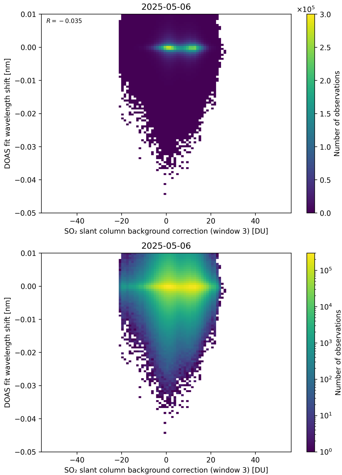
Figure 132: Scatter density plot of “SO 2 slant column background correction (window 3)” against “DOAS fit wavelength shift” for 2025-05-05 to 2025-05-07.
