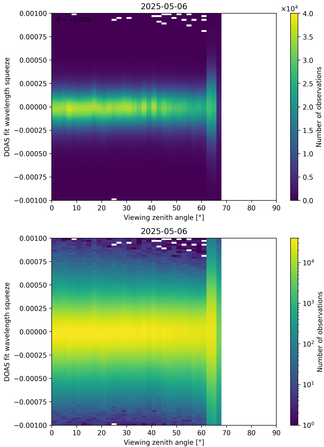
Figure 366: Scatter density plot of “Viewing zenith angle” against “DOAS fit wavelength squeeze” for 2025-05-05 to 2025-05-07.
