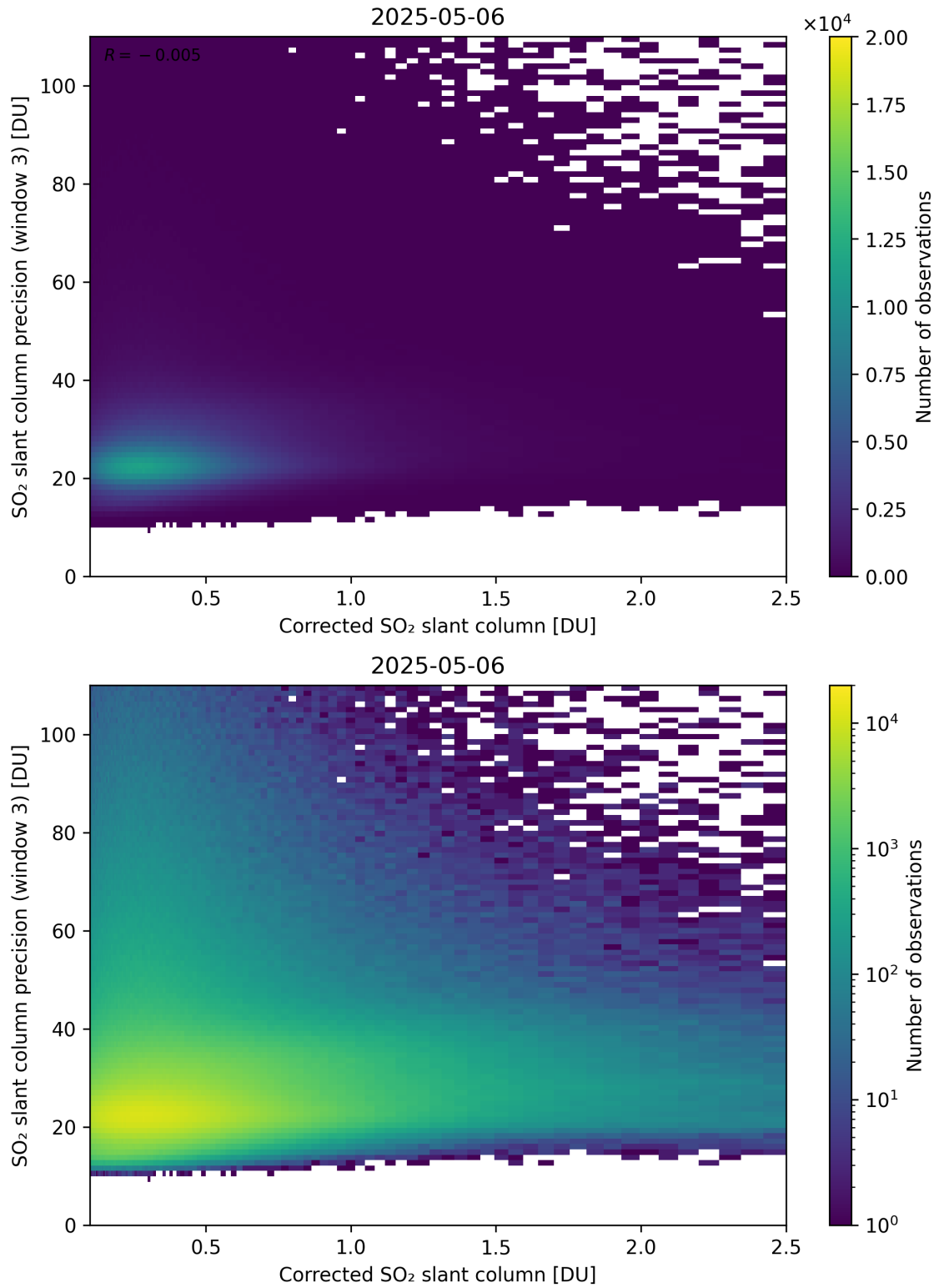
Figure 241: Scatter density plot of “Corrected SO 2 slant column” against “SO 2 slant column precision (window 3)” for 2025-05-05 to 2025-05-07.
