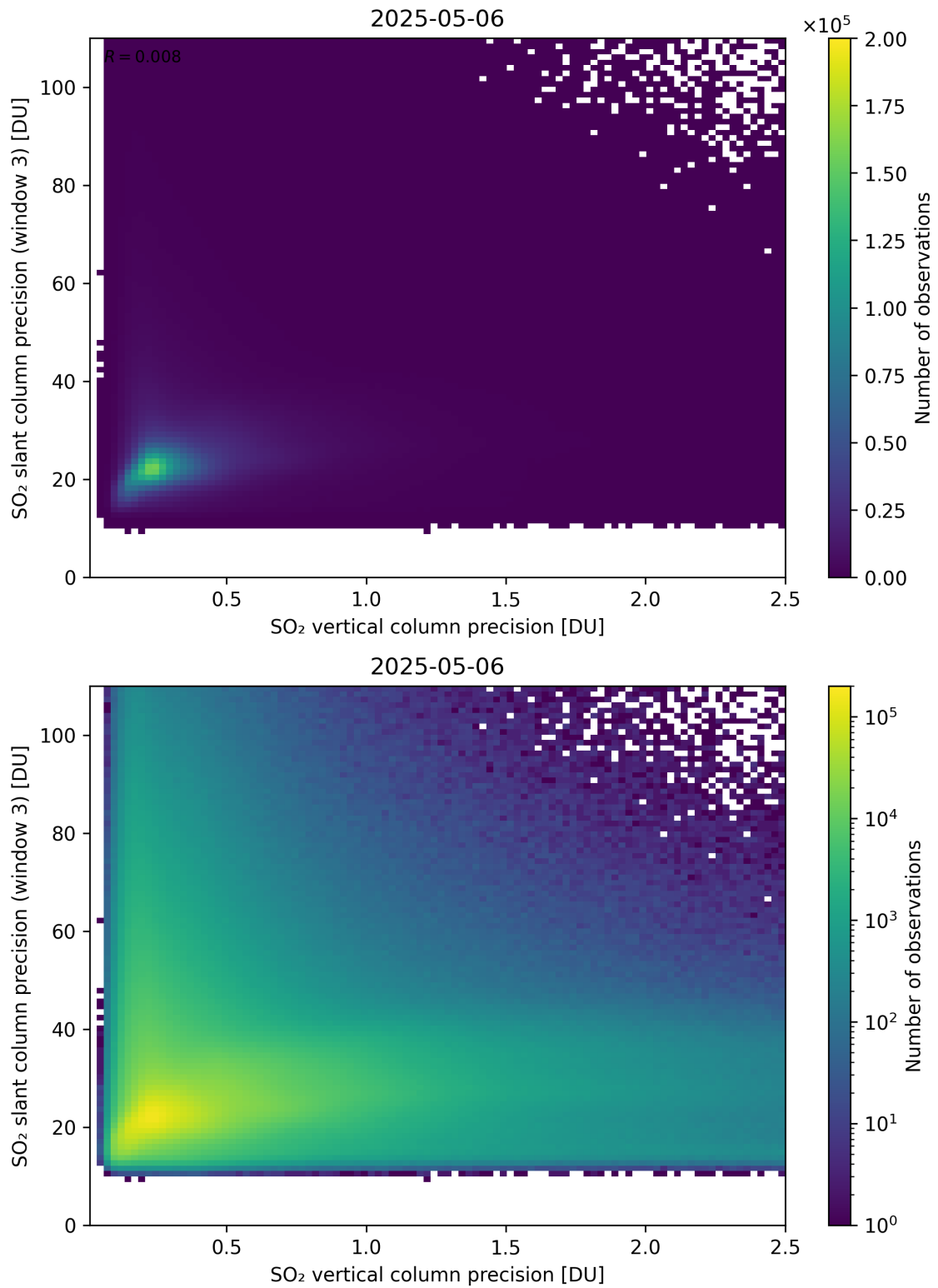
Figure 345: Scatter density plot of “SO 2 vertical column precision” against “SO 2 slant column precision (window 3)” for 2025-05-05 to 2025-05-07.
