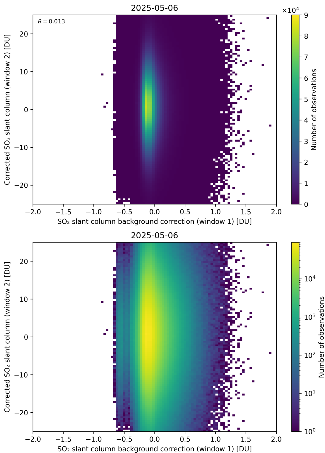
Figure 115: Scatter density plot of “SO 2 slant column background correction (window 1)” against “Corrected SO 2 slant column (window 2)” for 2025-05-05 to 2025-05-07.
