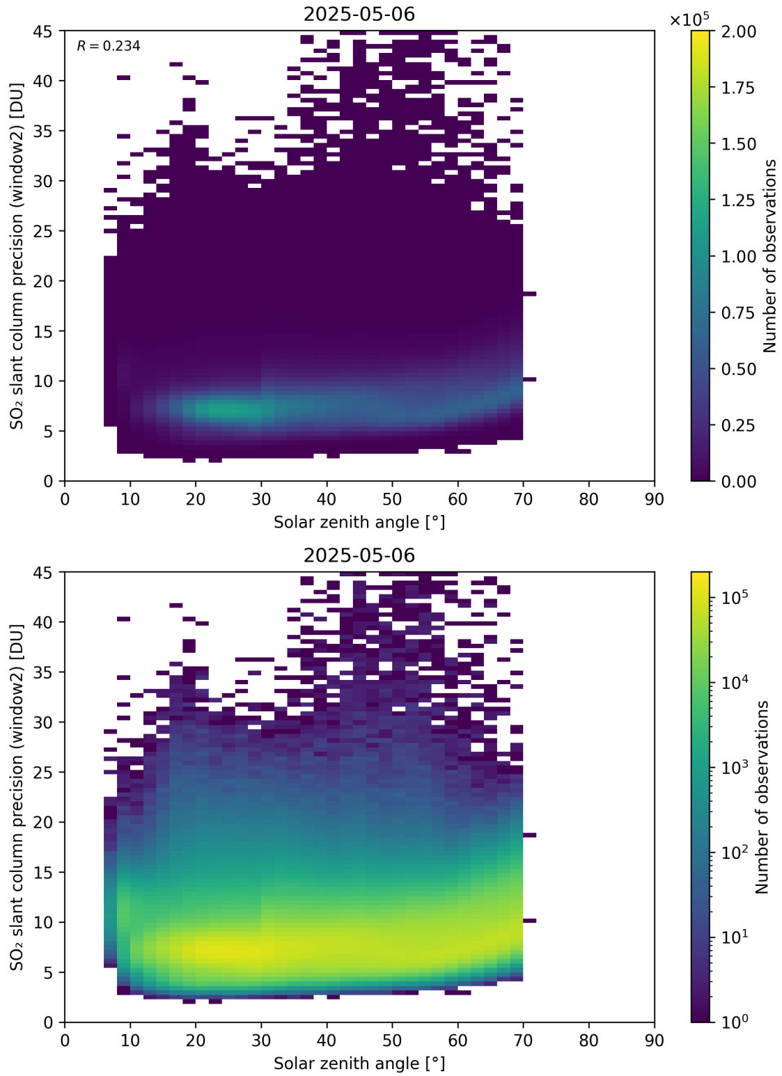
Figure 186: Scatter density plot of “Solar zenith angle” against “SO 2 slant column precision (window2)” for 2025-05-05 to 2025-05-07.
