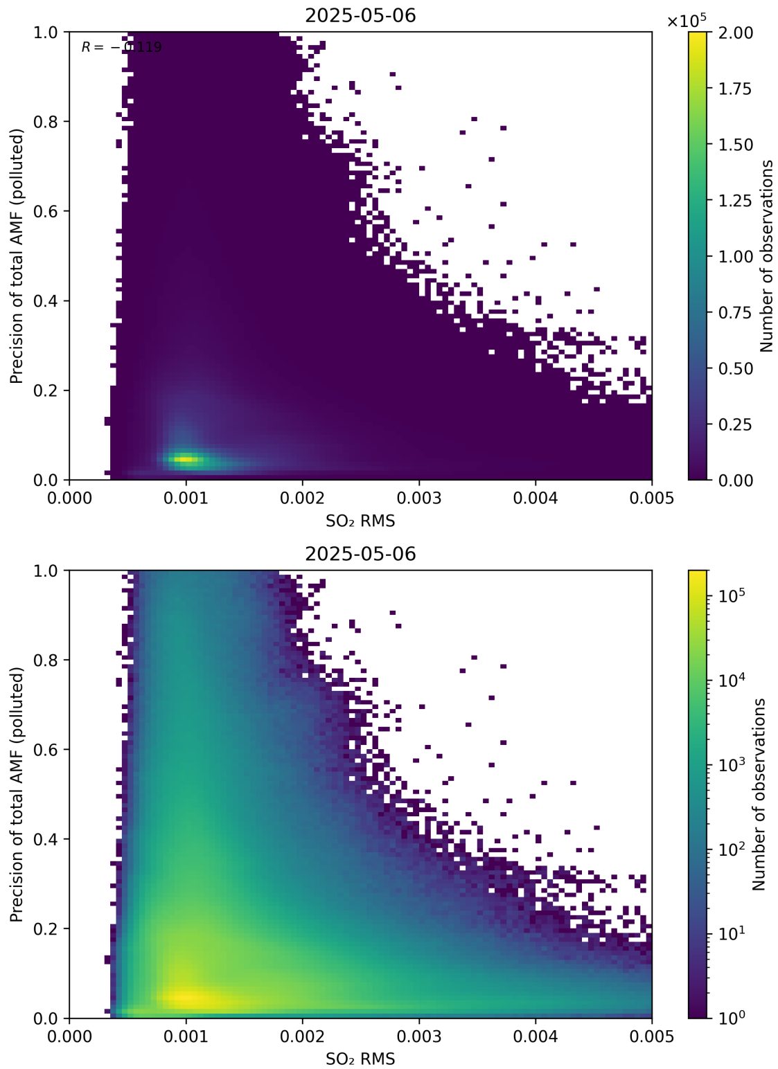
Figure 149: Scatter density plot of “SO 2 RMS” against “Precision of total AMF (polluted)” for 2025-05-05 to 2025-05-07.
