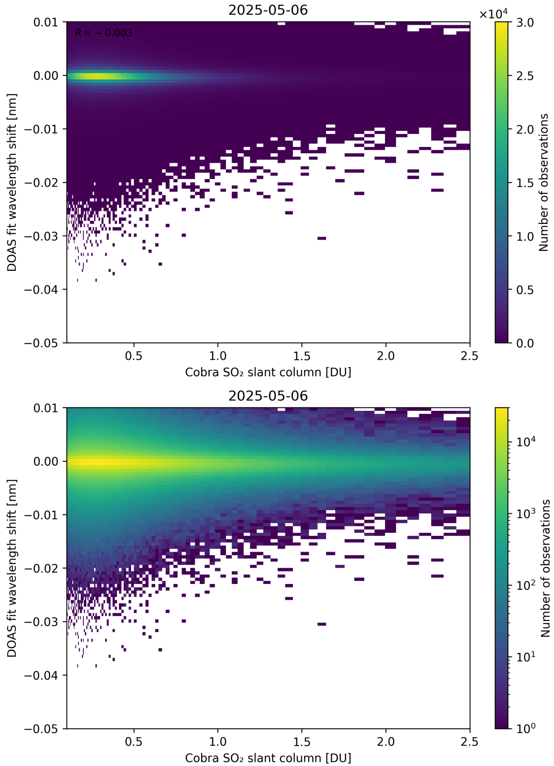
Figure 196: Scatter density plot of “Cobra SO 2 slant column” against “DOAS fit wavelength shift” for 2025-05-05 to 2025-05-07.
