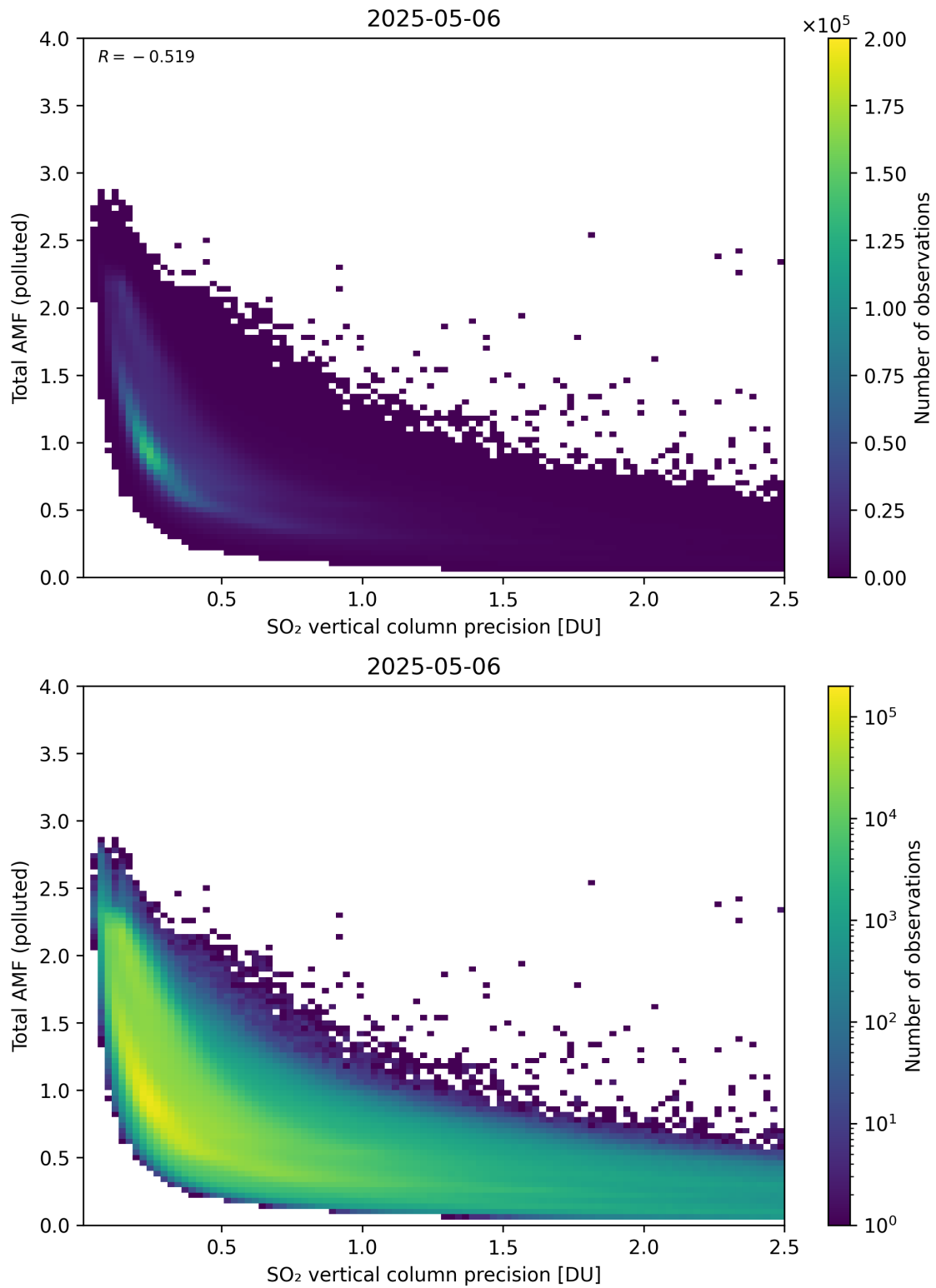
Figure 346: Scatter density plot of “SO 2 vertical column precision” against “Total AMF (polluted)” for 2025-05-05 to 2025-05-07.
