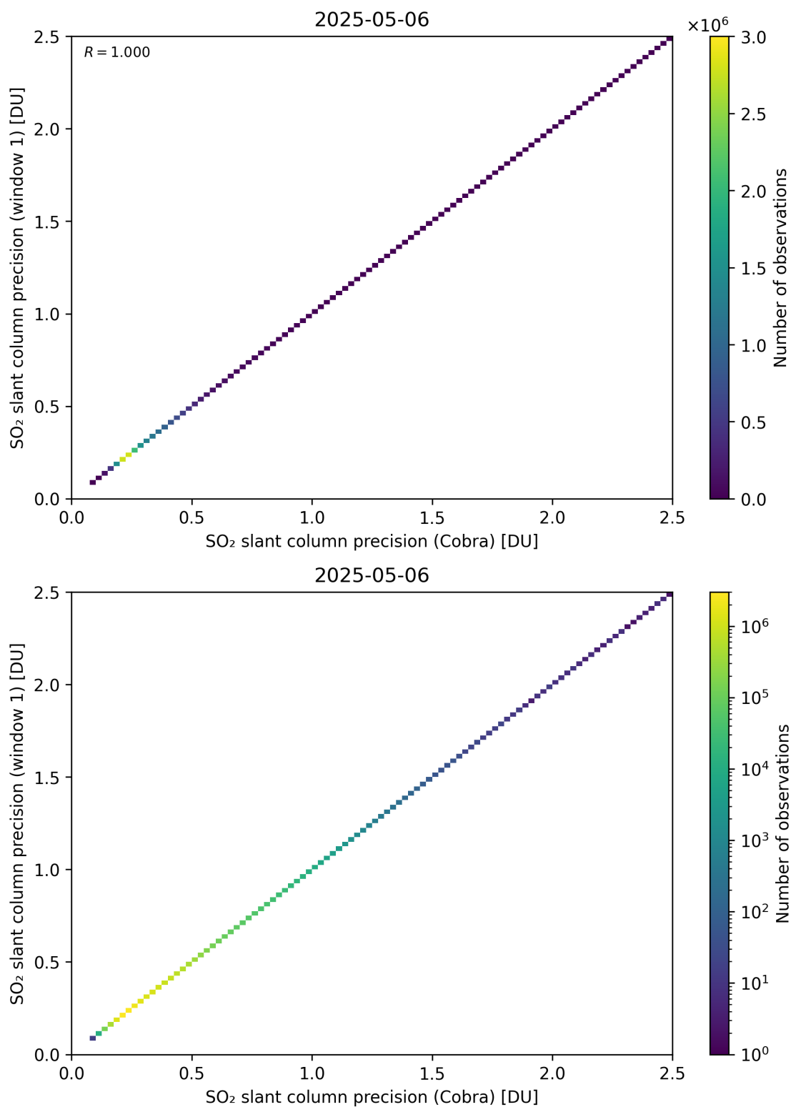
Figure 209: Scatter density plot of “SO 2 slant column precision (Cobra)” against “SO 2 slant column precision (window 1)” for 2025-05-05 to 2025-05-07.
