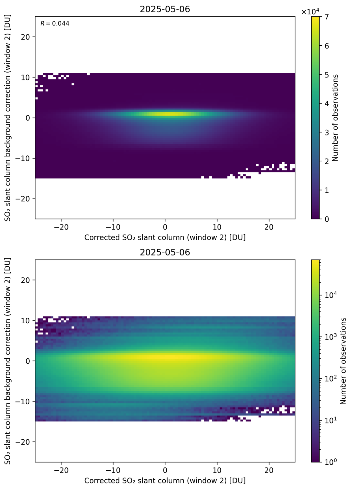
Figure 244: Scatter density plot of “Corrected SO 2 slant column (window 2)” against “SO 2 slant column background correction (window 2)” for 2025-05-05 to 2025-05-07.
