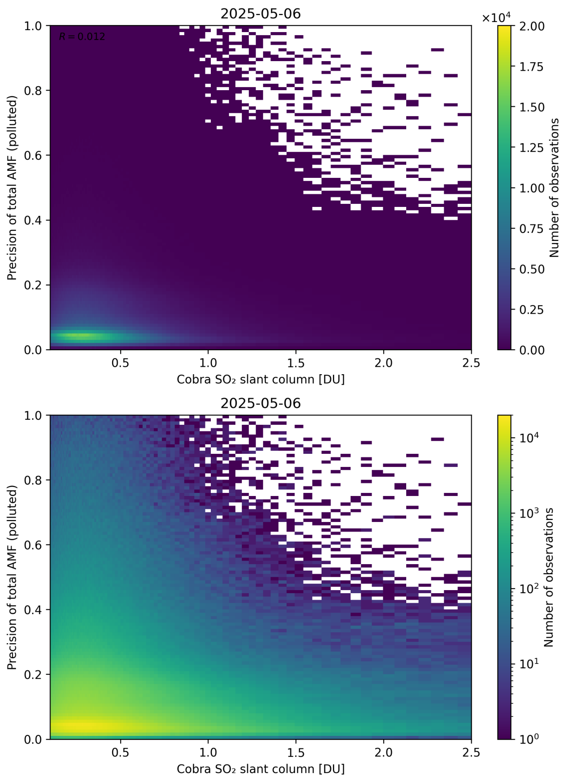
Figure 225: Scatter density plot of “Cobra SO 2 slant column” against “Precision of total AMF (polluted)” for 2025-05-05 to 2025-05-07.
