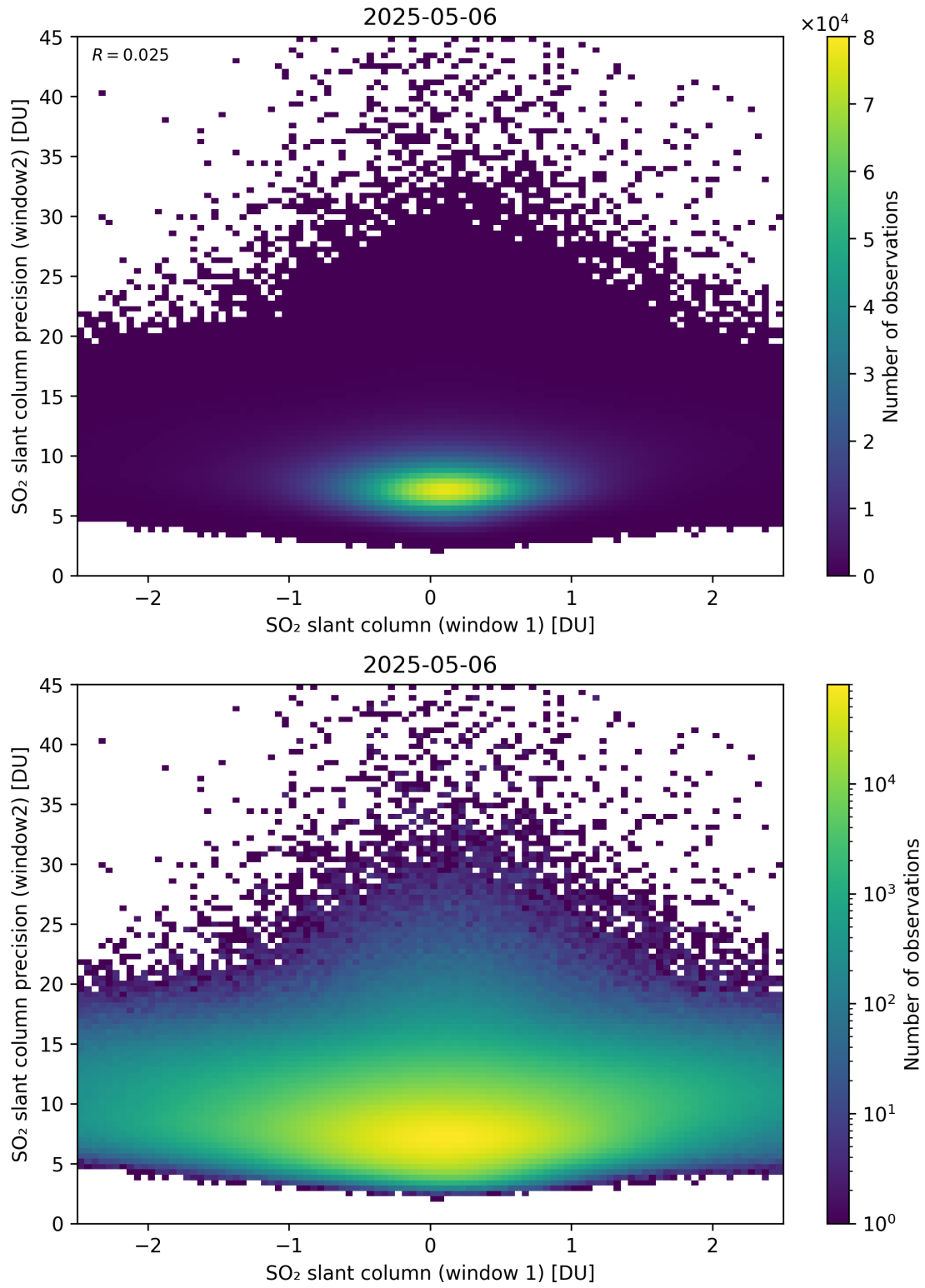
Figure 286: Scatter density plot of “SO 2 slant column (window 1)” against “SO 2 slant column precision (window2)” for 2025-05-05 to 2025-05-07.
