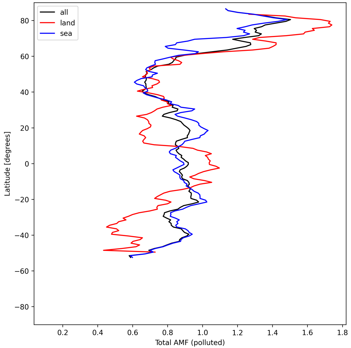
Figure 53: Zonal average of “Total AMF (polluted)” for 2025-05-05 to 2025-05-07.
