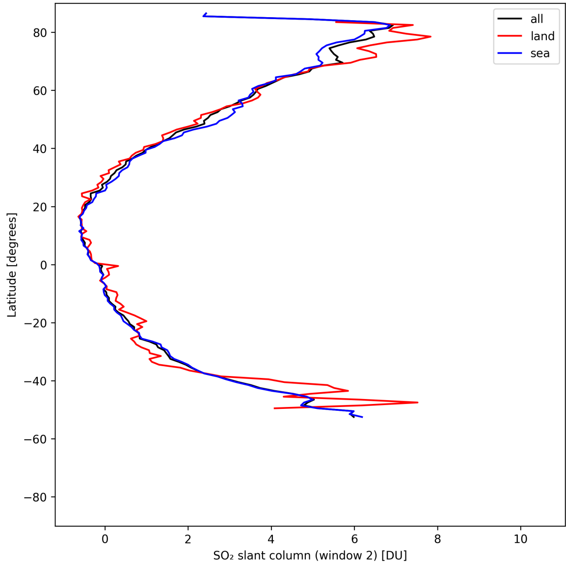
Figure 41: Zonal average of “SO 2 slant column (window 2)” for 2025-05-05 to 2025-05-07.
