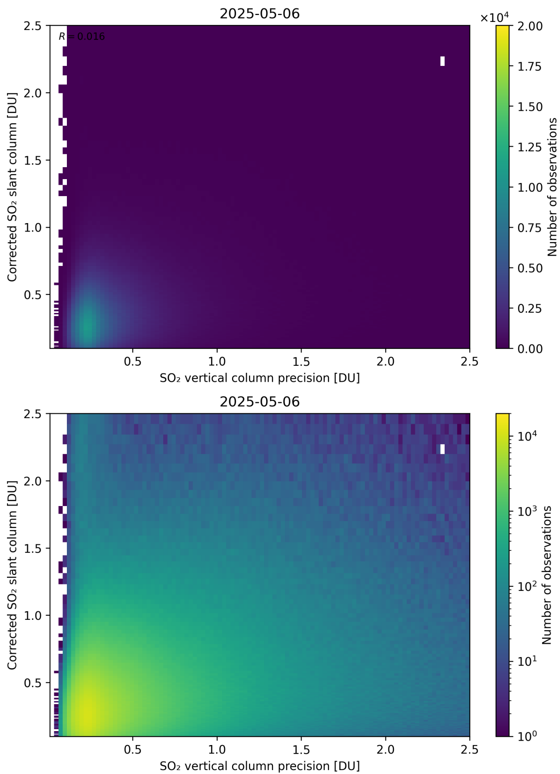
Figure 338: Scatter density plot of “SO 2 vertical column precision” against “Corrected SO 2 slant column” for 2025-05-05 to 2025-05-07.
