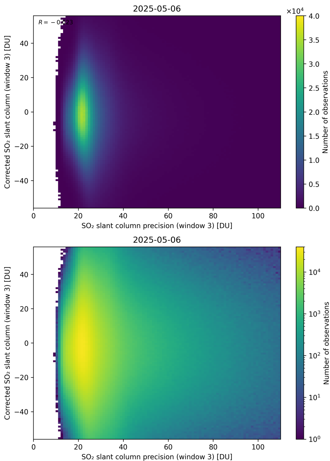
Figure 312: Scatter density plot of “SO 2 slant column precision (window 3)” against “Corrected SO 2 slant column (window 3)” for 2025-05-05 to 2025-05-07.
