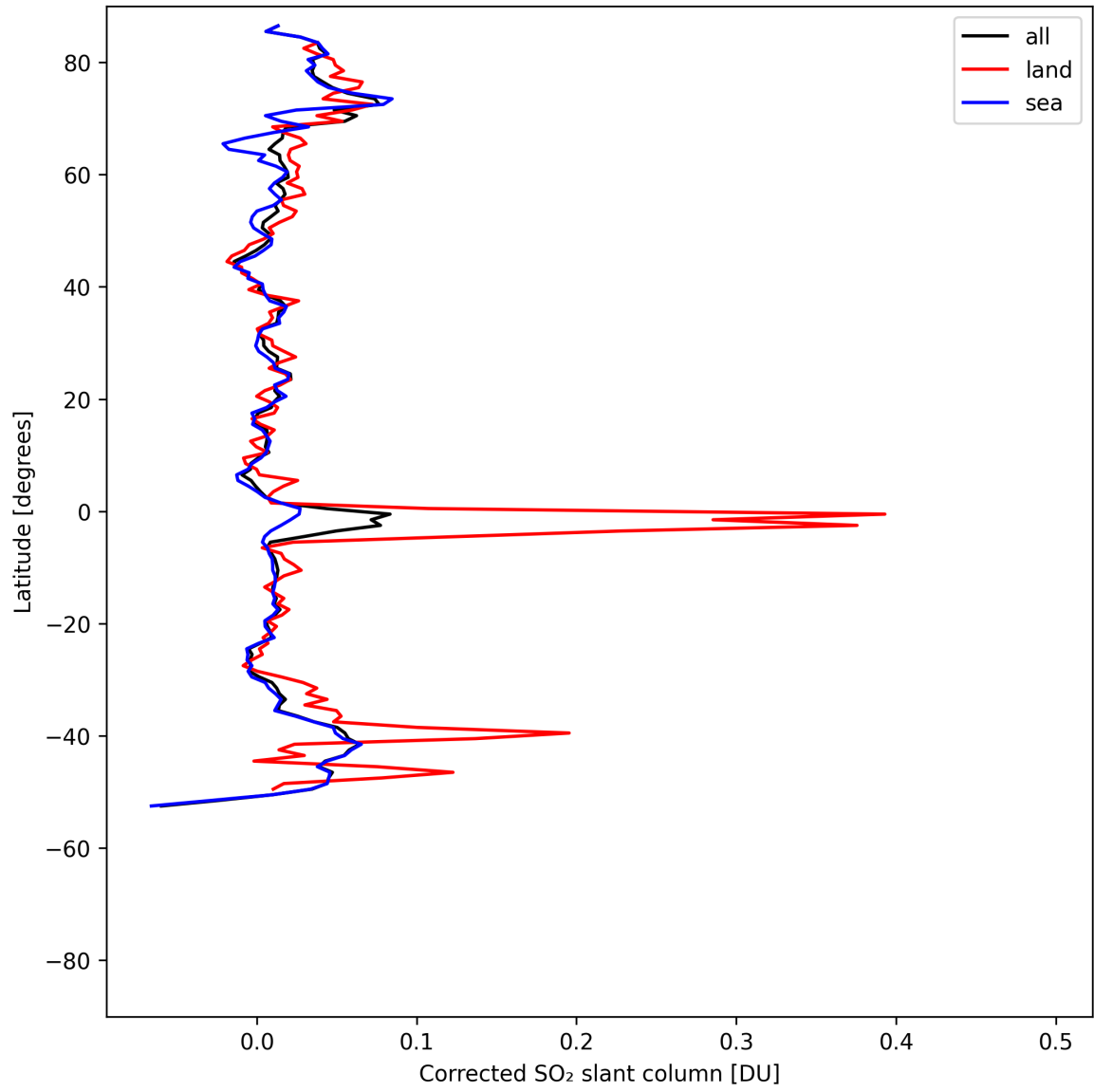
Figure 34: Zonal average of “Corrected SO 2 slant column” for 2025-05-05 to 2025-05-07.
