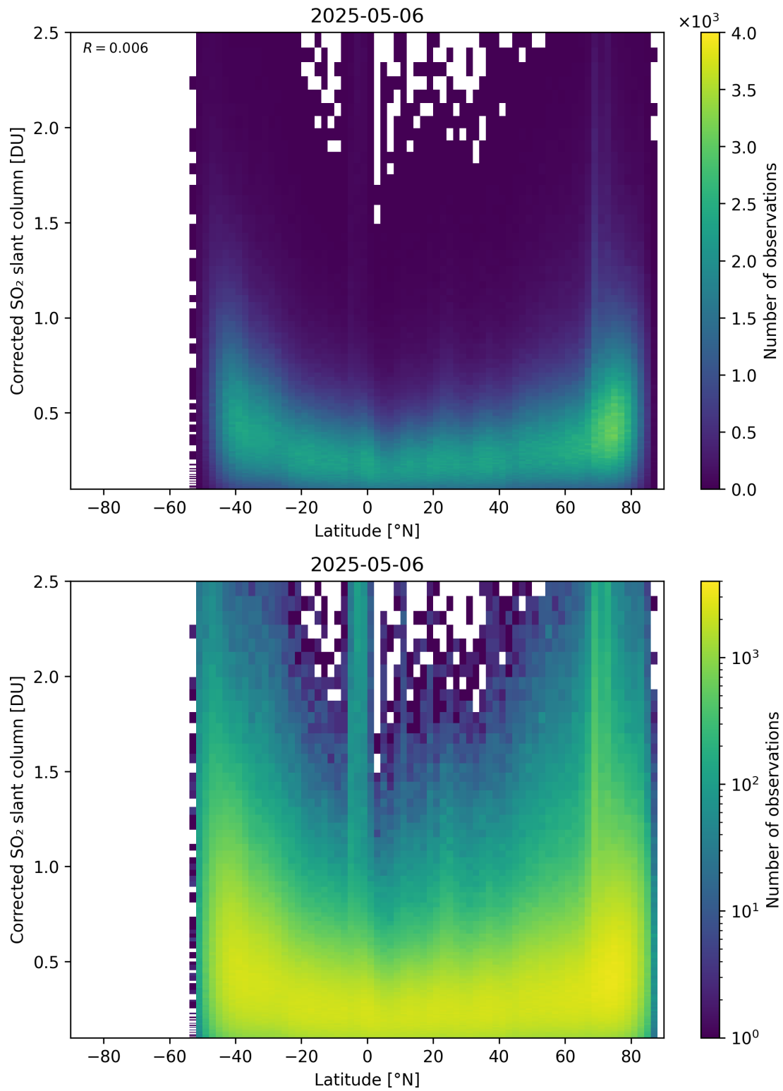
Figure 159: Scatter density plot of “Latitude” against “Corrected SO 2 slant column” for 2025-05-05 to 2025-05-07.
