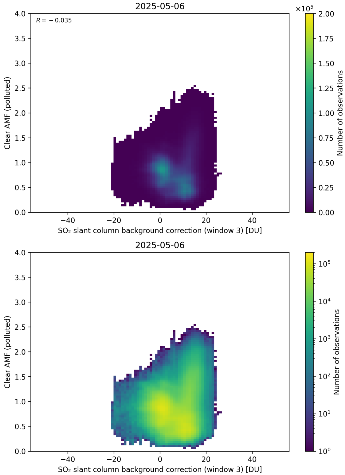
Figure 135: Scatter density plot of “SO 2 slant column background correction (window 3)” against “Clear AMF (polluted)” for 2025-05-05 to 2025-05-07.
