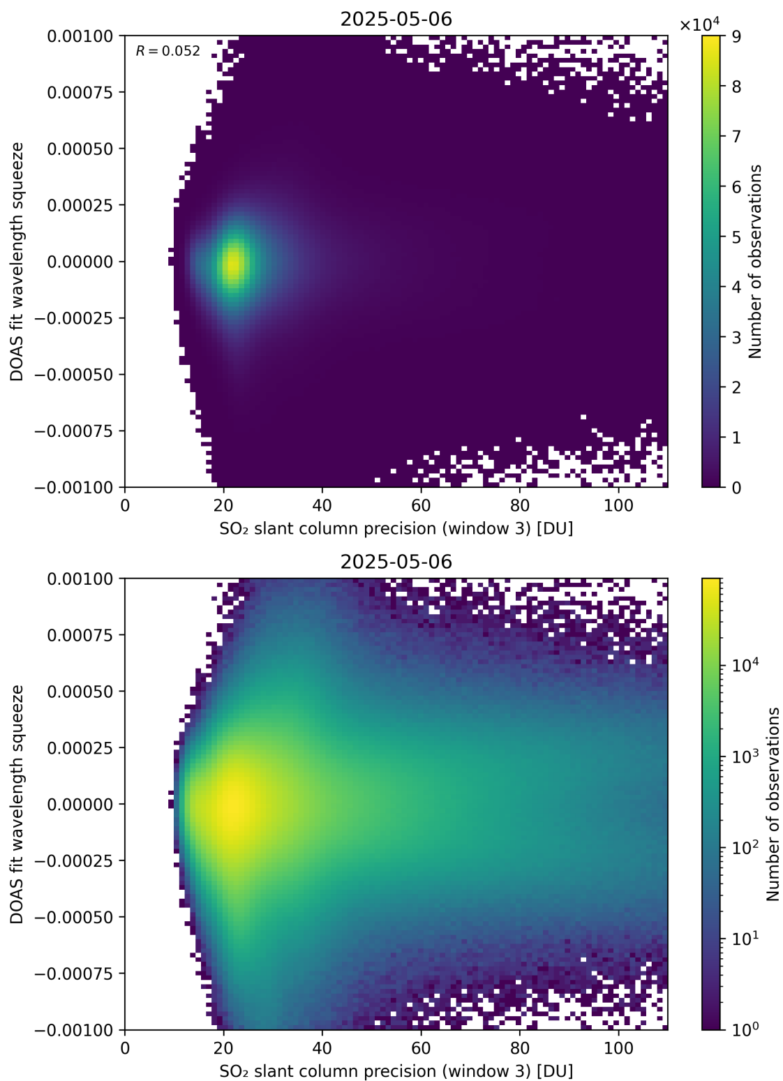
Figure 309: Scatter density plot of “SO 2 slant column precision (window 3)” against “DOAS fit wavelength squeeze” for 2025-05-05 to 2025-05-07.
