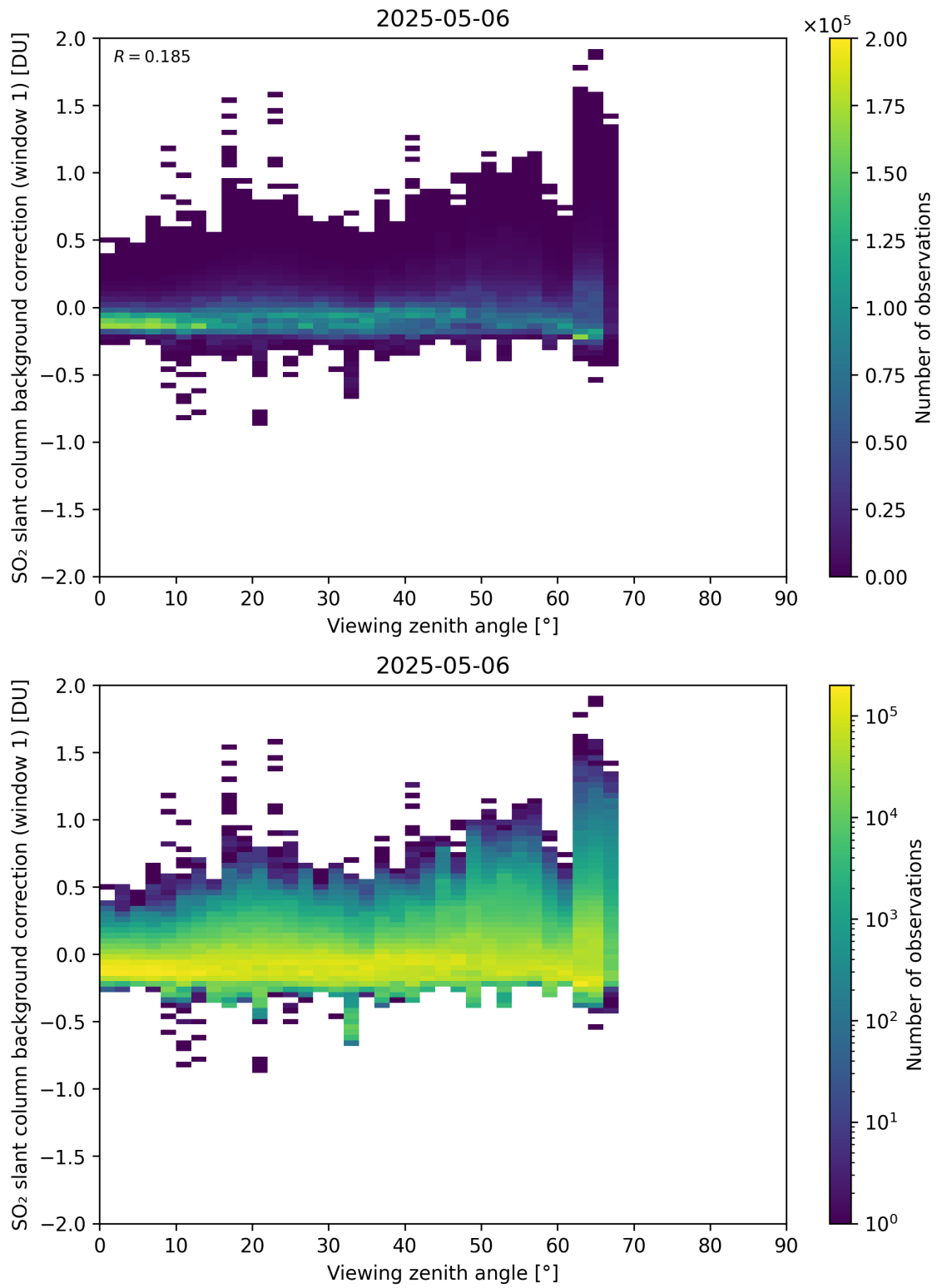
Figure 362: Scatter density plot of “Viewing zenith angle” against “SO 2 slant column background correction (window 1)” for 2025-05-05 to 2025-05-07.
