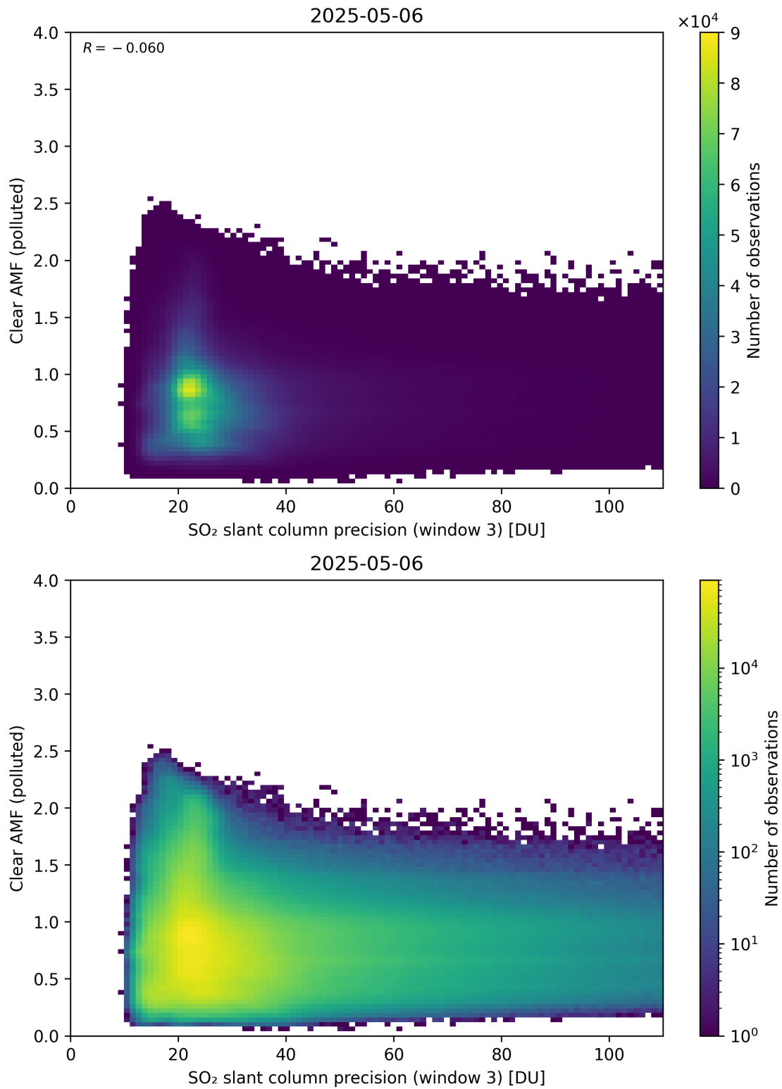
Figure 311: Scatter density plot of “SO 2 slant column precision (window 3)” against “Clear AMF (polluted)” for 2025-05-05 to 2025-05-07.
