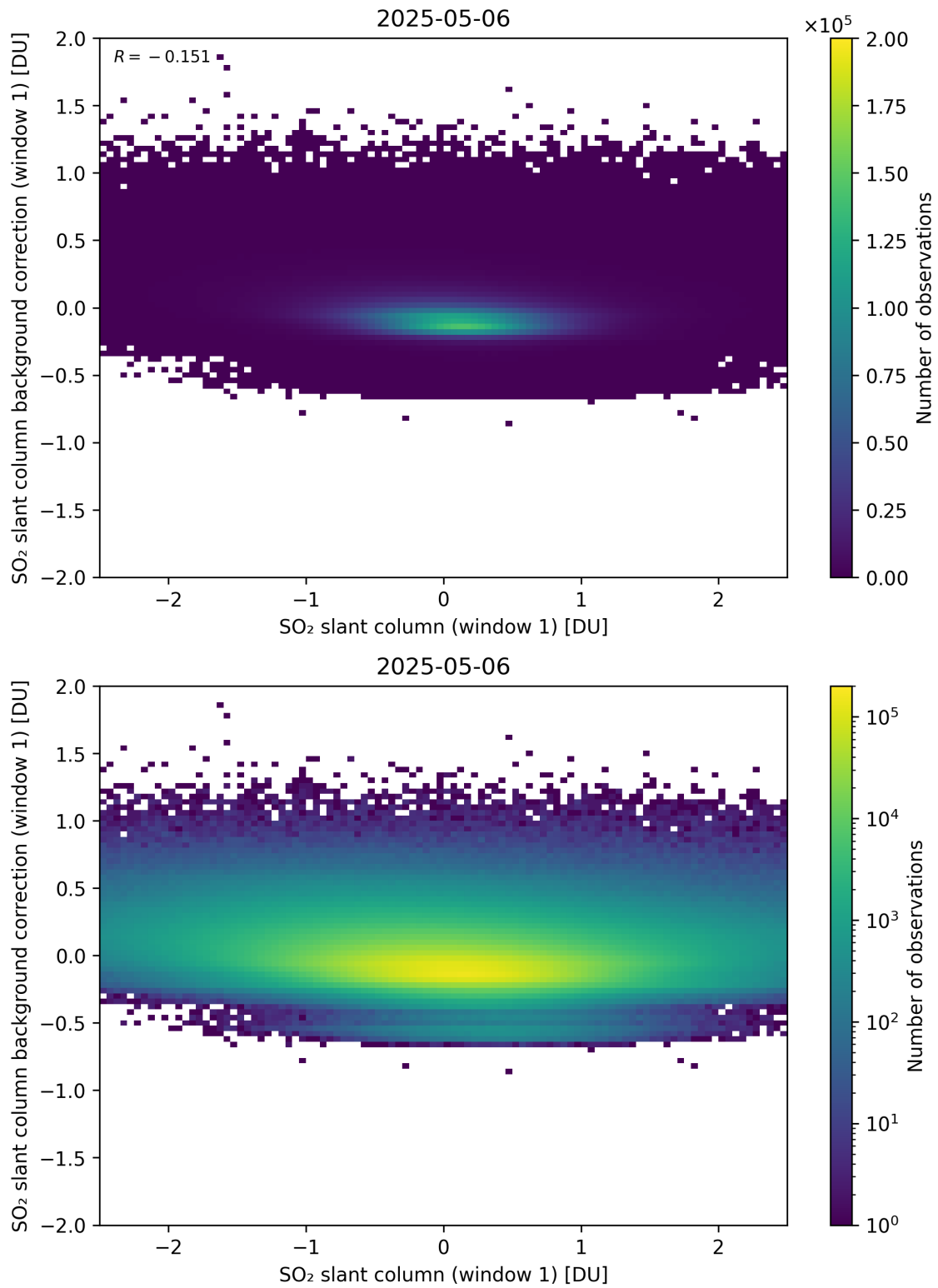
Figure 262: Scatter density plot of “SO 2 slant column (window 1)” against “SO 2 slant column background correction (window 1)” for 2025-05-05 to 2025-05-07.
