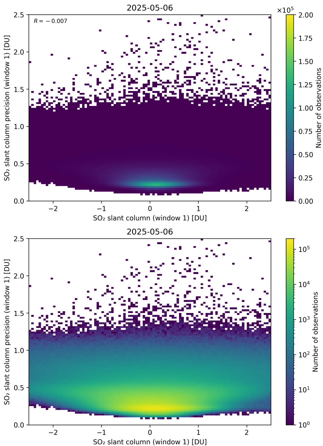
Figure 285: Scatter density plot of “SO 2 slant column (window 1)” against “SO 2 slant column precision (window 1)” for 2025-05-05 to 2025-05-07.
