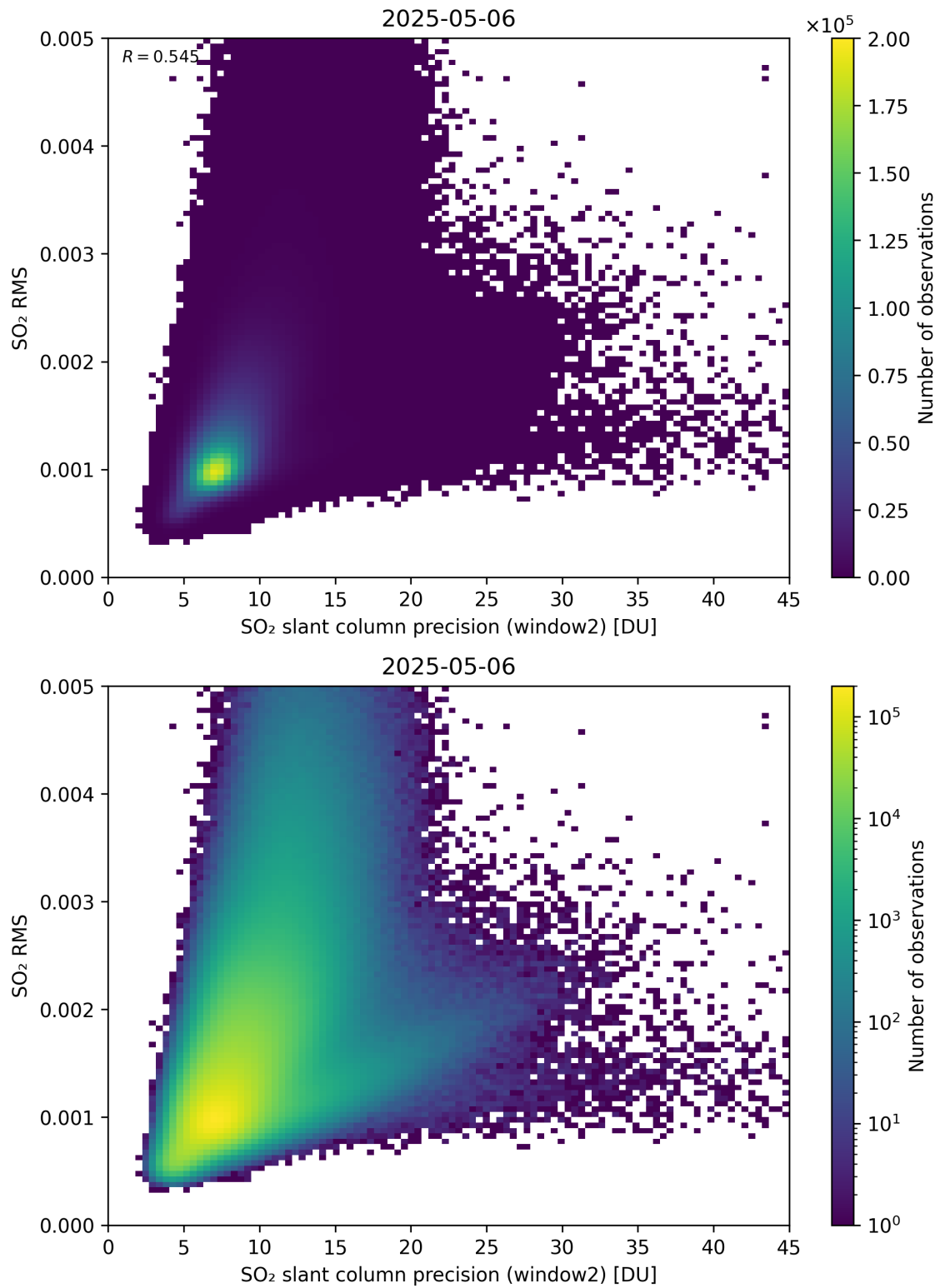
Figure 295: Scatter density plot of “SO 2 slant column precision (window2)” against “SO 2 RMS” for 2025-05-05 to 2025-05-07.
