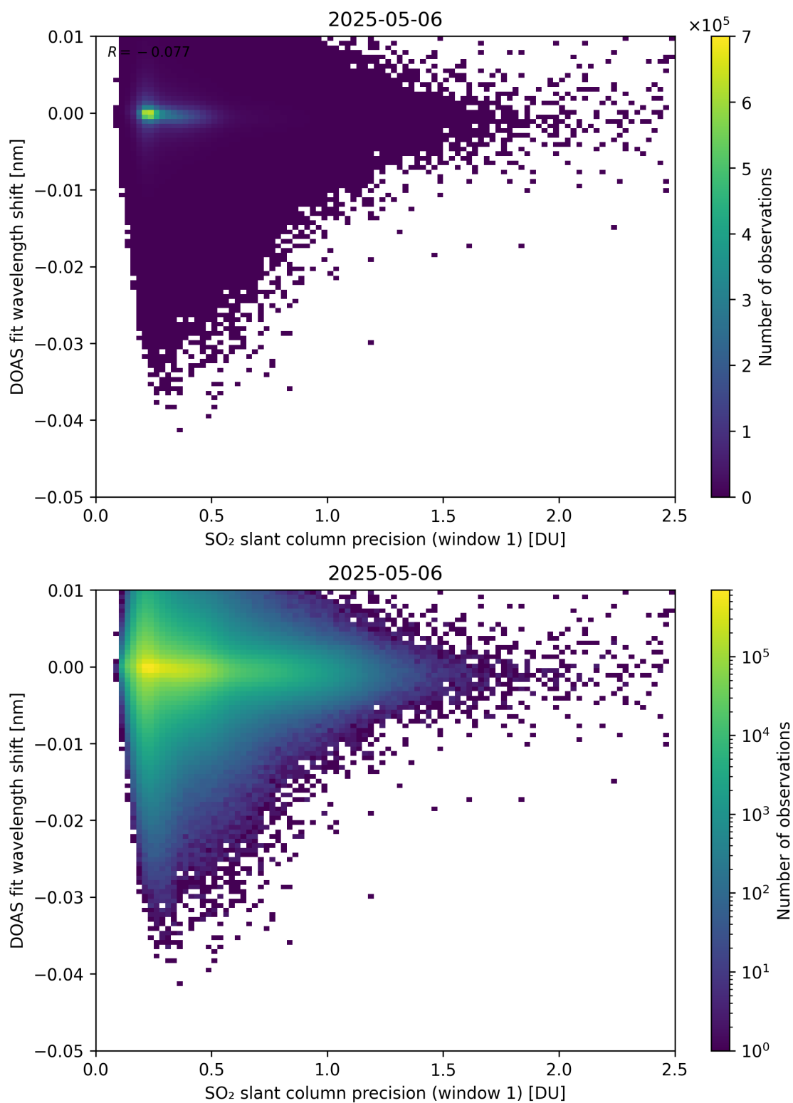
Figure 271: Scatter density plot of “SO 2 slant column precision (window 1)” against “DOAS fit wavelength shift” for 2025-05-05 to 2025-05-07.
