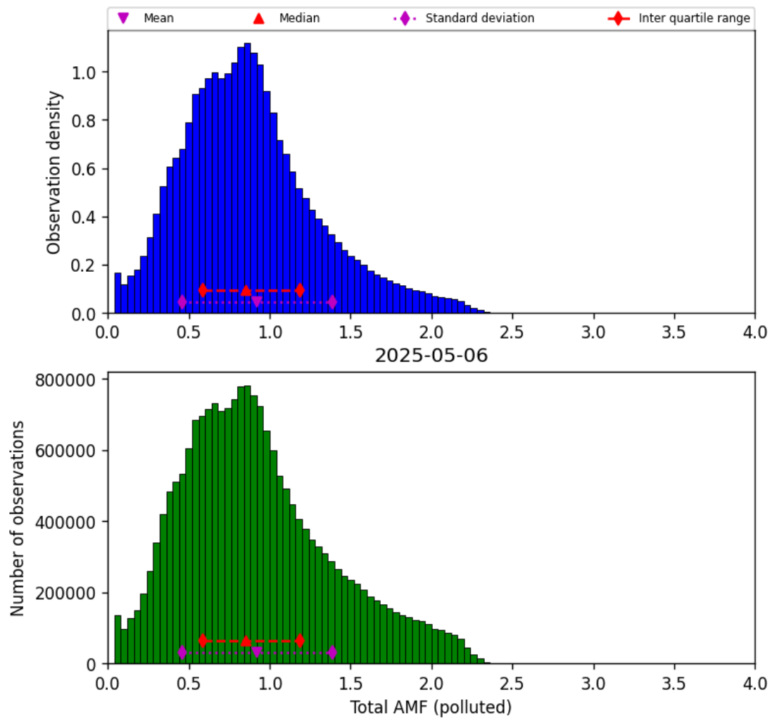
Figure 79: Histogram of “Total AMF (polluted)” for 2025-05-05 to 2025-05-07
