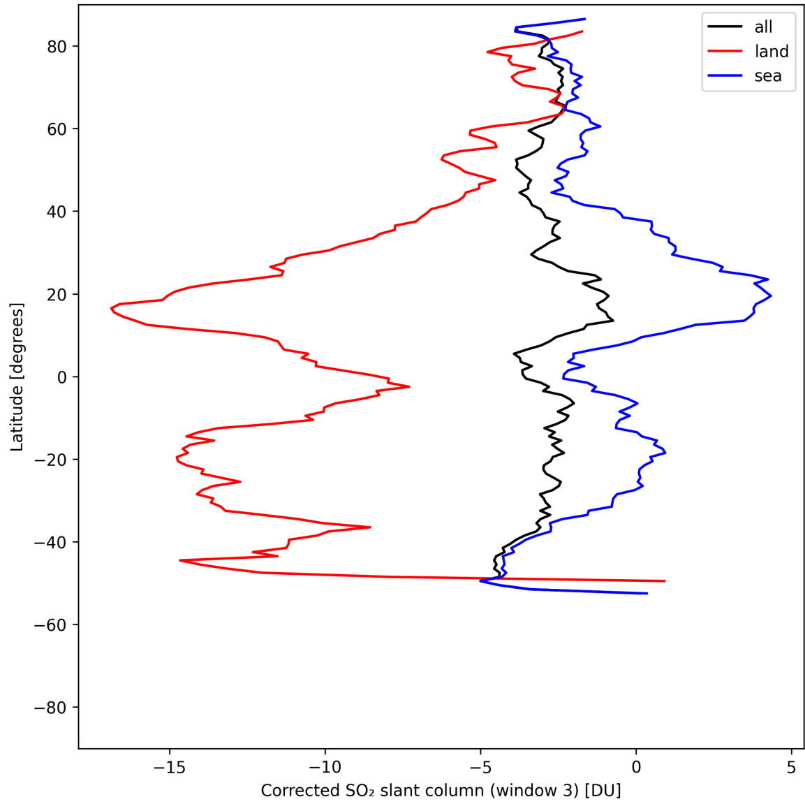
Figure 47: Zonal average of “Corrected SO 2 slant column (window 3)” for 2025-05-05 to 2025-05-07.
