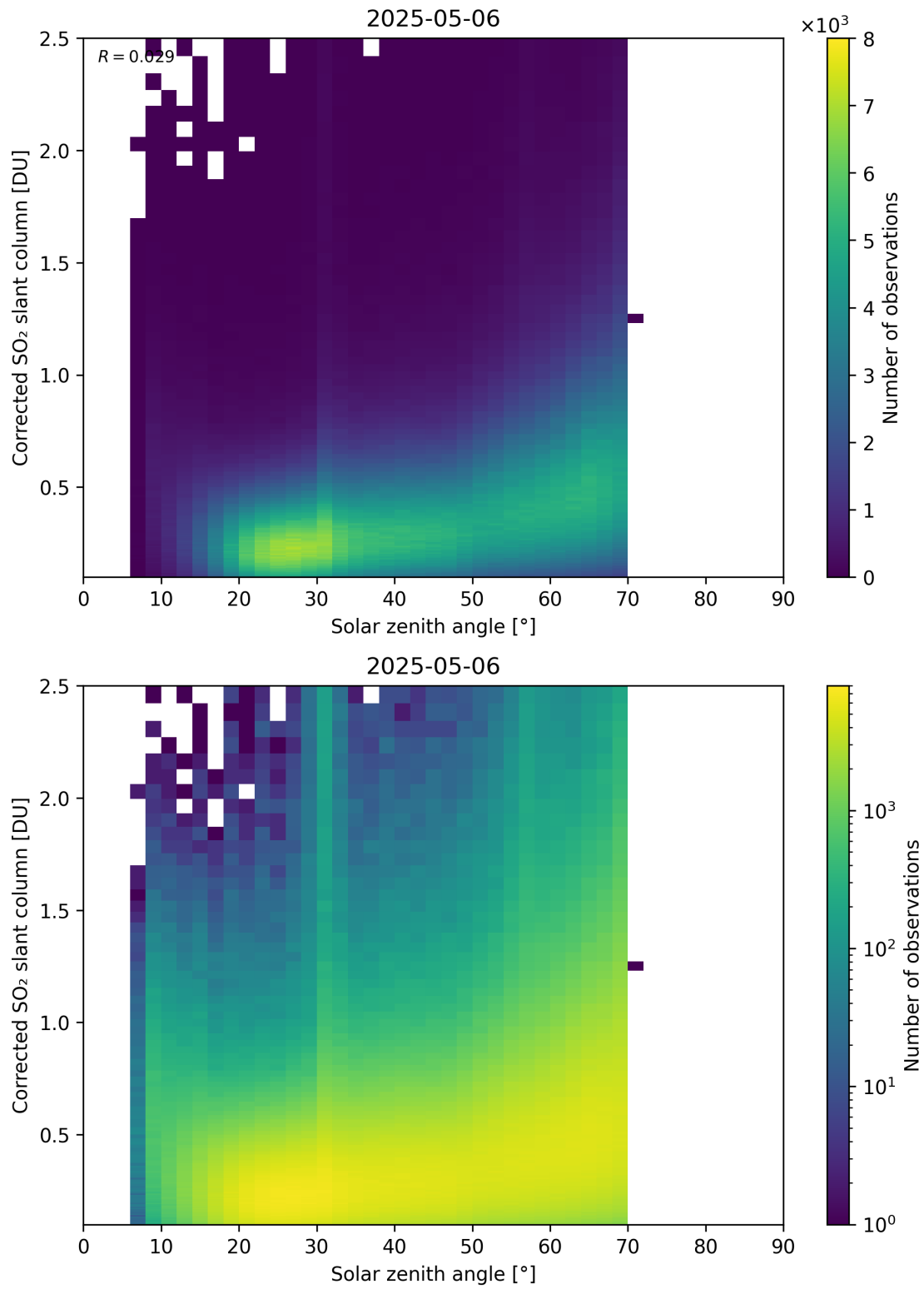
Figure 181: Scatter density plot of “Solar zenith angle” against “Corrected SO 2 slant column” for 2025-05-05 to 2025-05-07.
