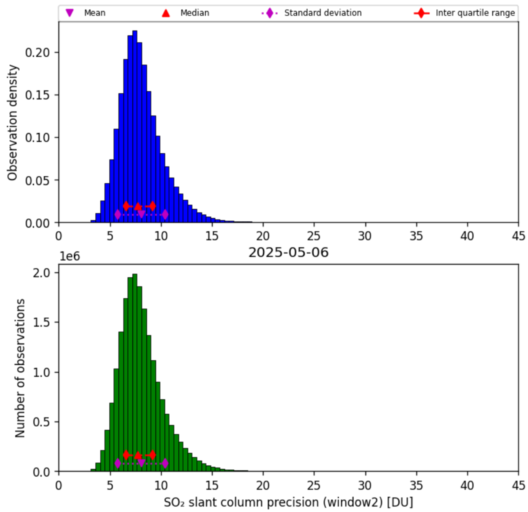
Figure 68: Histogram of “SO 2 slant column precision (window2)” for 2025-05-05 to 2025-05-07
