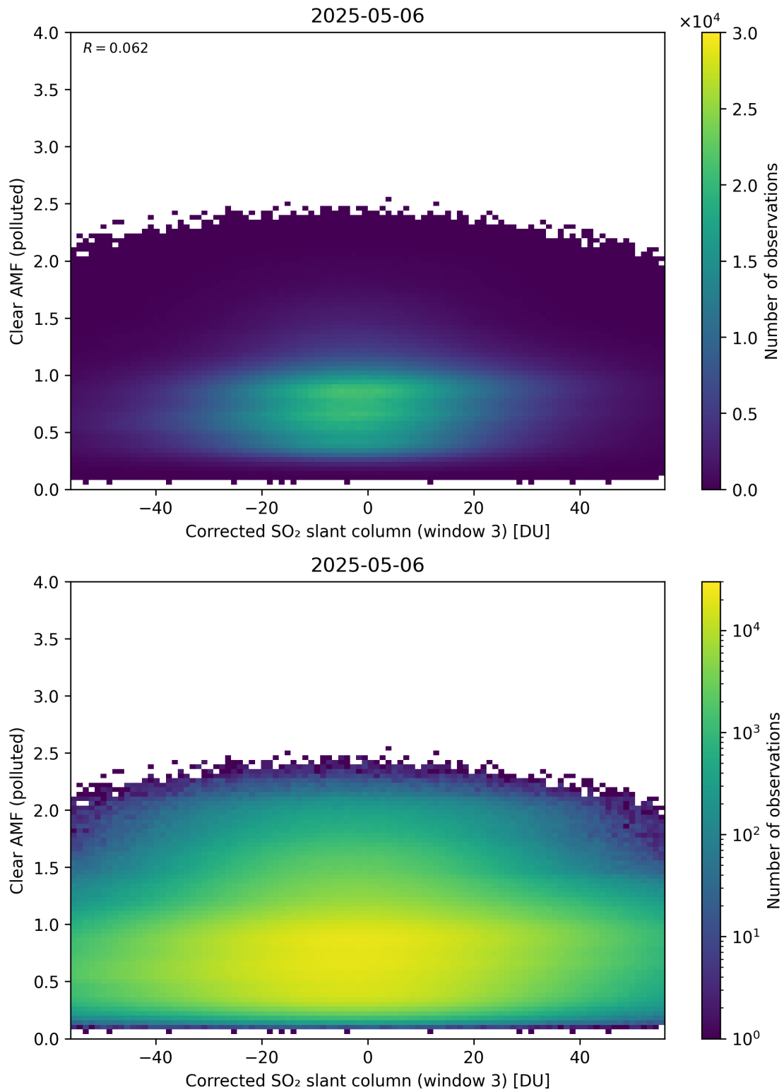
Figure 259: Scatter density plot of “Corrected SO 2 slant column (window 3)” against “Clear AMF (polluted)” for 2025-05-05 to 2025-05-07.
