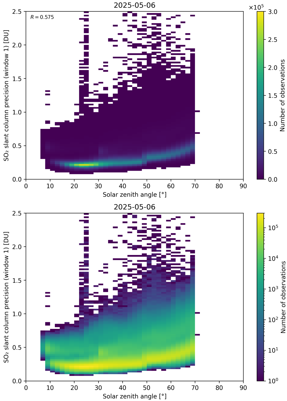
Figure 185: Scatter density plot of “Solar zenith angle” against “SO 2 slant column precision (window 1)” for 2025-05-05 to 2025-05-07.
