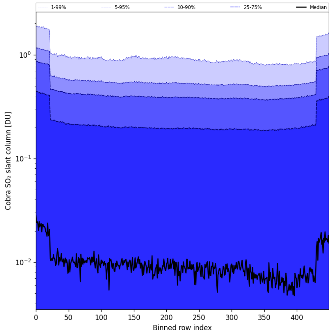
Figure 87: Along track statistics of "Cobra SO 2 slant column" for 2025-05-05 to 2025-05-07
