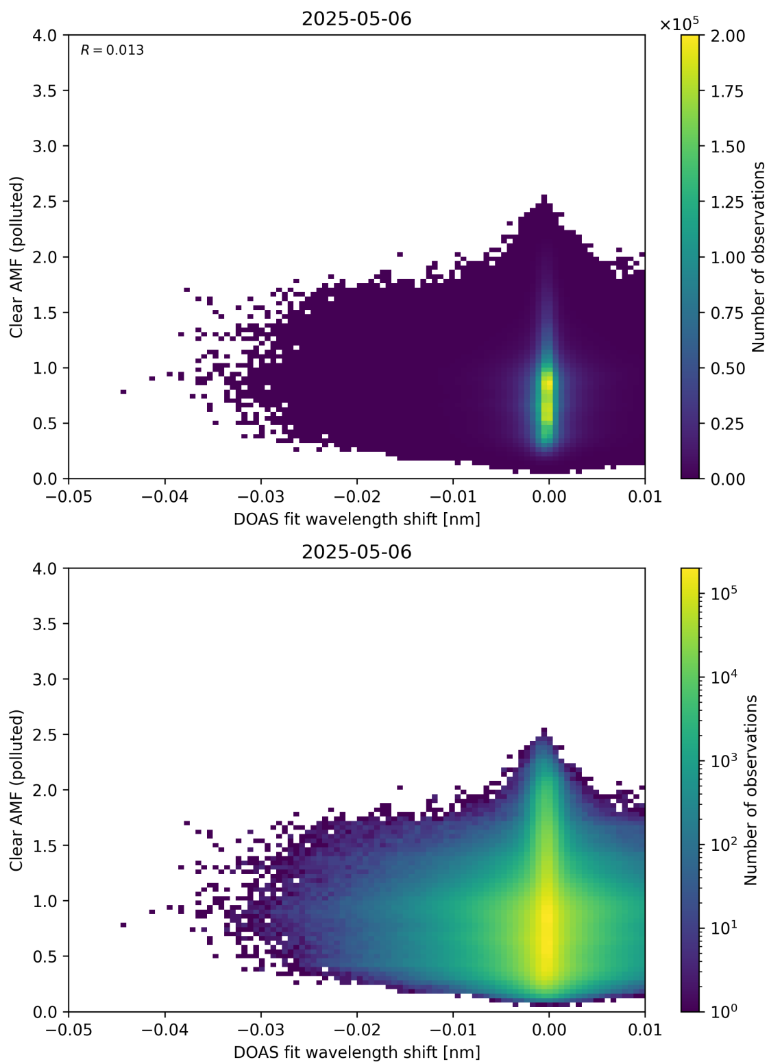
Figure 140: Scatter density plot of “DOAS fit wavelength shift” against “Clear AMF (polluted)” for 2025-05-05 to 2025-05-07.
