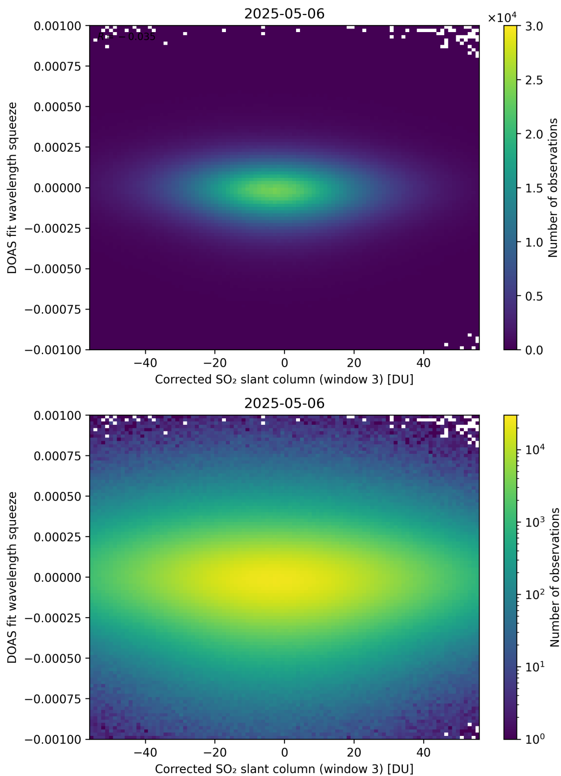
Figure 257: Scatter density plot of “Corrected SO 2 slant column (window 3)” against “DOAS fit wavelength squeeze” for 2025-05-05 to 2025-05-07.
