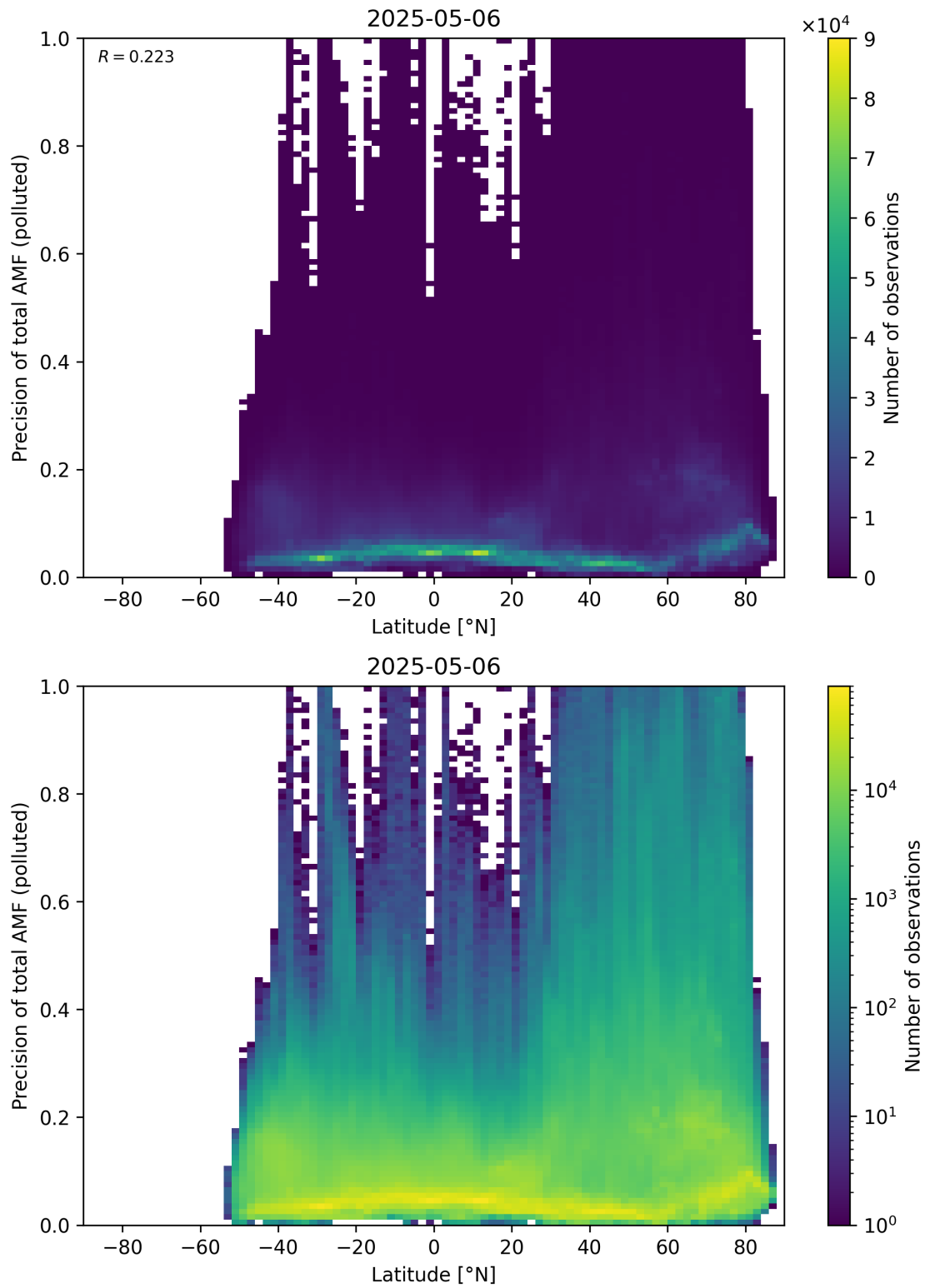
Figure 168: Scatter density plot of “Latitude” against “Precision of total AMF (polluted)” for 2025-05-05 to 2025-05-07.
