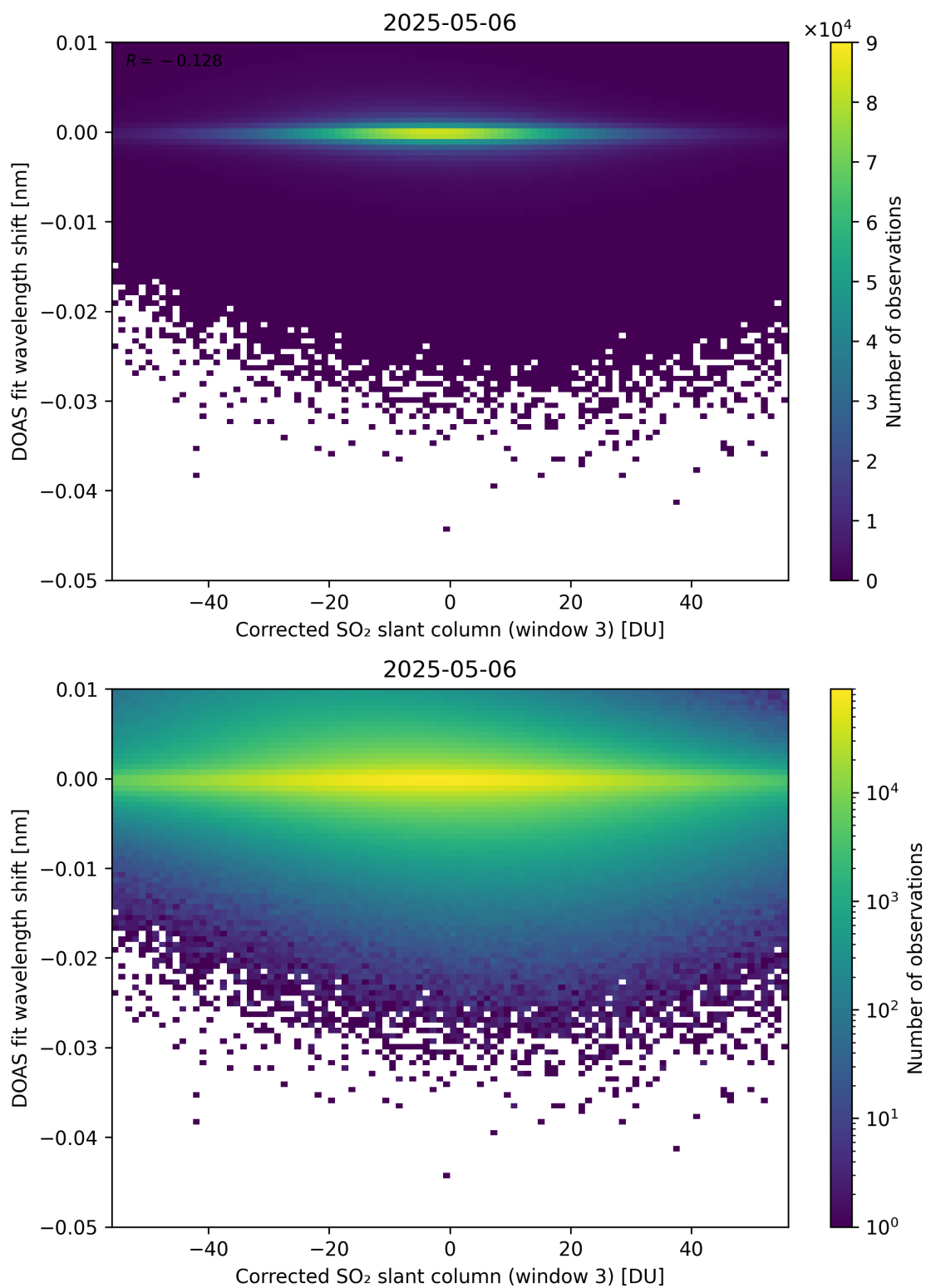
Figure 256: Scatter density plot of “Corrected SO 2 slant column (window 3)” against “DOAS fit wavelength shift” for 2025-05-05 to 2025-05-07.
