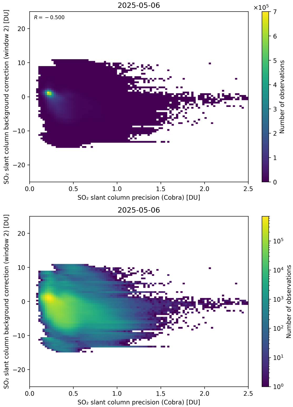
Figure 200: Scatter density plot of “SO 2 slant column precision (Cobra)” against “SO 2 slant column background correction (window 2)” for 2025-05-05 to 2025-05-07.
