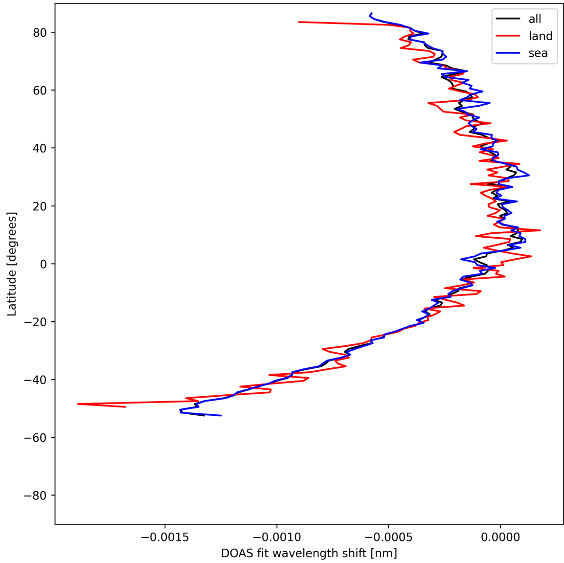
Figure 50: Zonal average of "DOAS fit wavelength shift" for 2025-05-05 to 2025-05-07.
