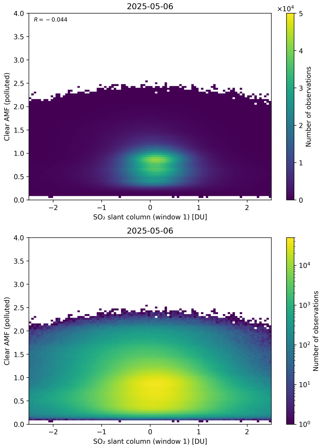
Figure 282: Scatter density plot of “SO 2 slant column (window 1)” against “Clear AMF (polluted)” for 2025-05-05 to 2025-05-07.
