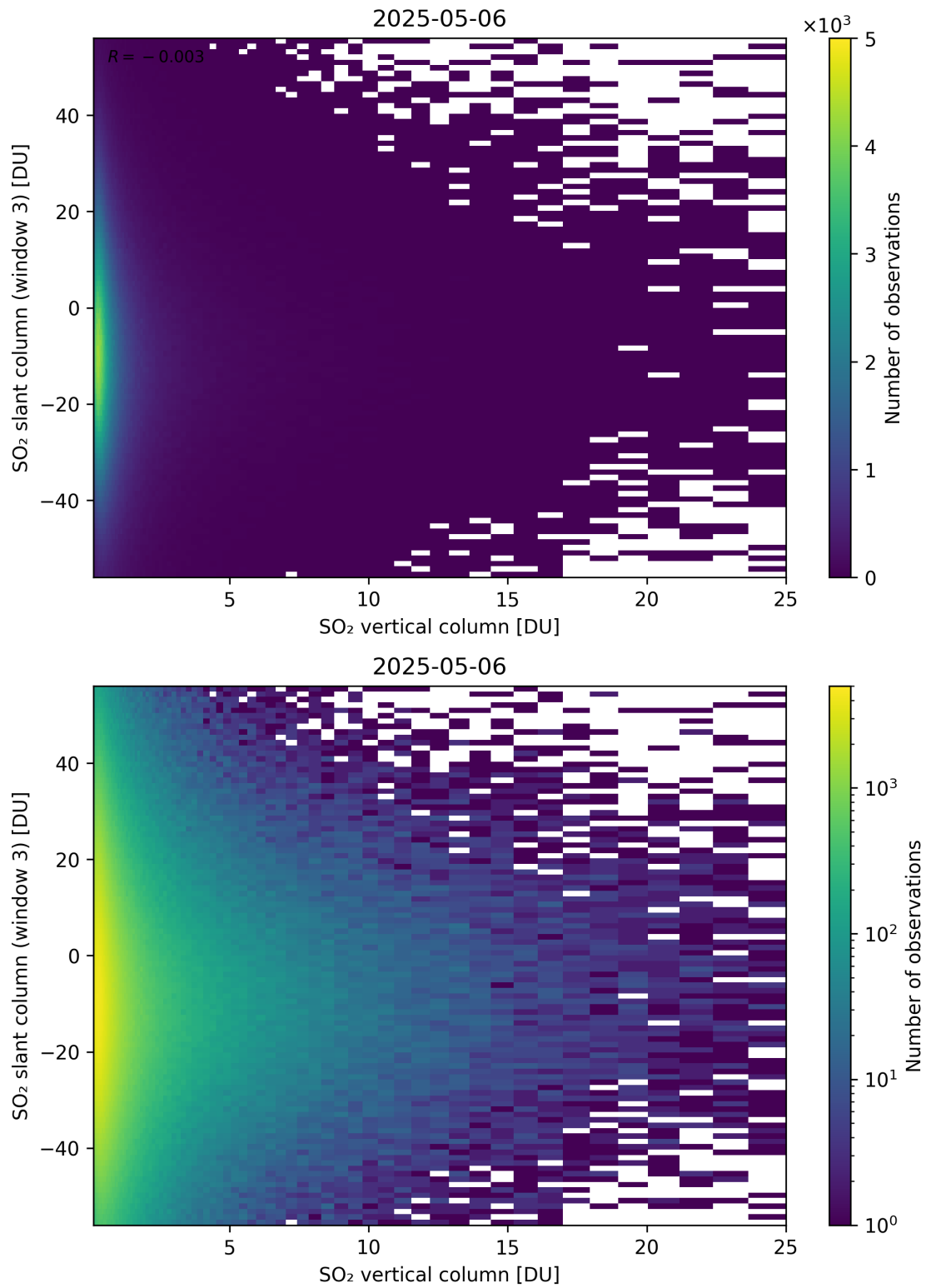
Figure 357: Scatter density plot of “SO 2 vertical column” against “SO 2 slant column (window 3)” for 2025-05-05 to 2025-05-07.
