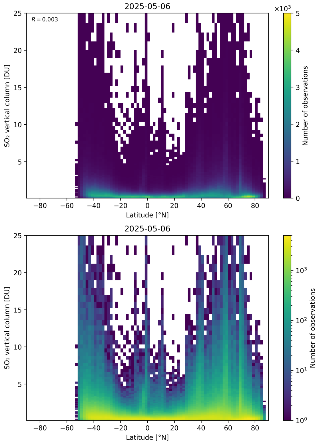
Figure 169: Scatter density plot of “Latitude” against “SO 2 vertical column” for 2025-05-05 to 2025-05-07.
