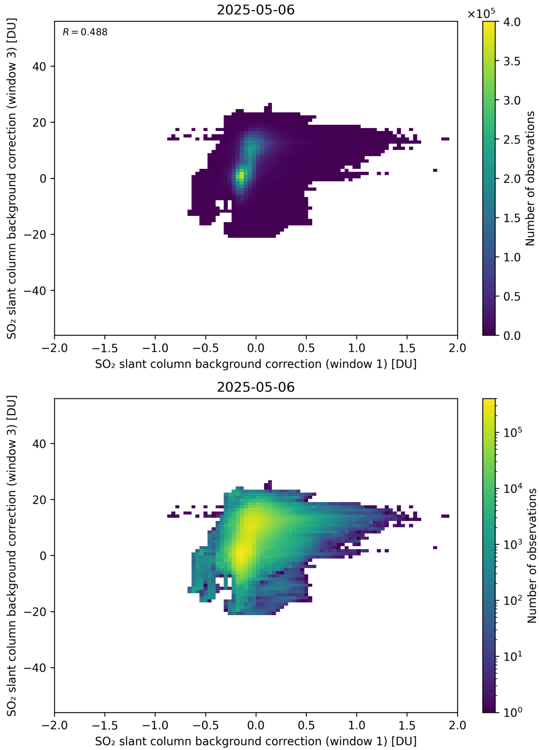
Figure 110: Scatter density plot of “SO 2 slant column background correction (window 1)” against “SO 2 slant column background correction (window 3)” for 2025-05-05 to 2025-05-07.
