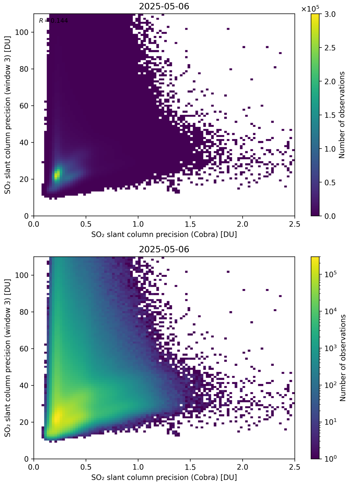
Figure 212: Scatter density plot of “SO 2 slant column precision (Cobra)” against “SO 2 slant column precision (window 3)” for 2025-05-05 to 2025-05-07.
