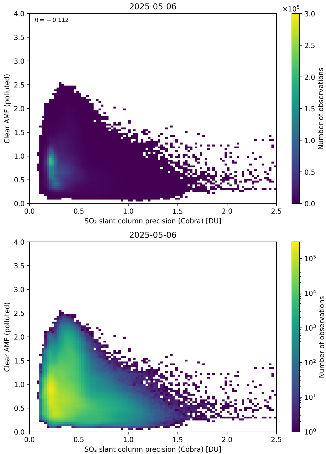
Figure 205: Scatter density plot of “SO 2 slant column precision (Cobra)” against “Clear AMF (polluted)” for 2025-05-05 to 2025-05-07.
