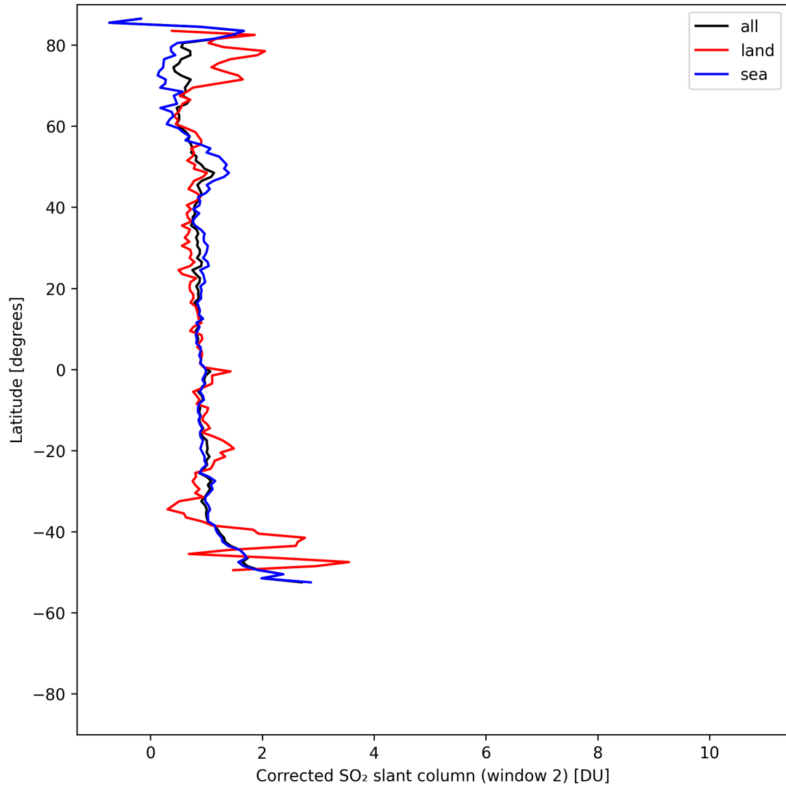
Figure 43: Zonal average of “Corrected SO 2 slant column (window 2)” for 2025-05-05 to 2025-05-07.
