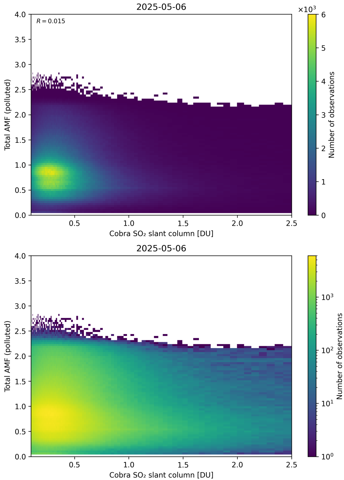
Figure 224: Scatter density plot of “Cobra SO 2 slant column” against “Total AMF (polluted)” for 2025-05-05 to 2025-05-07.
