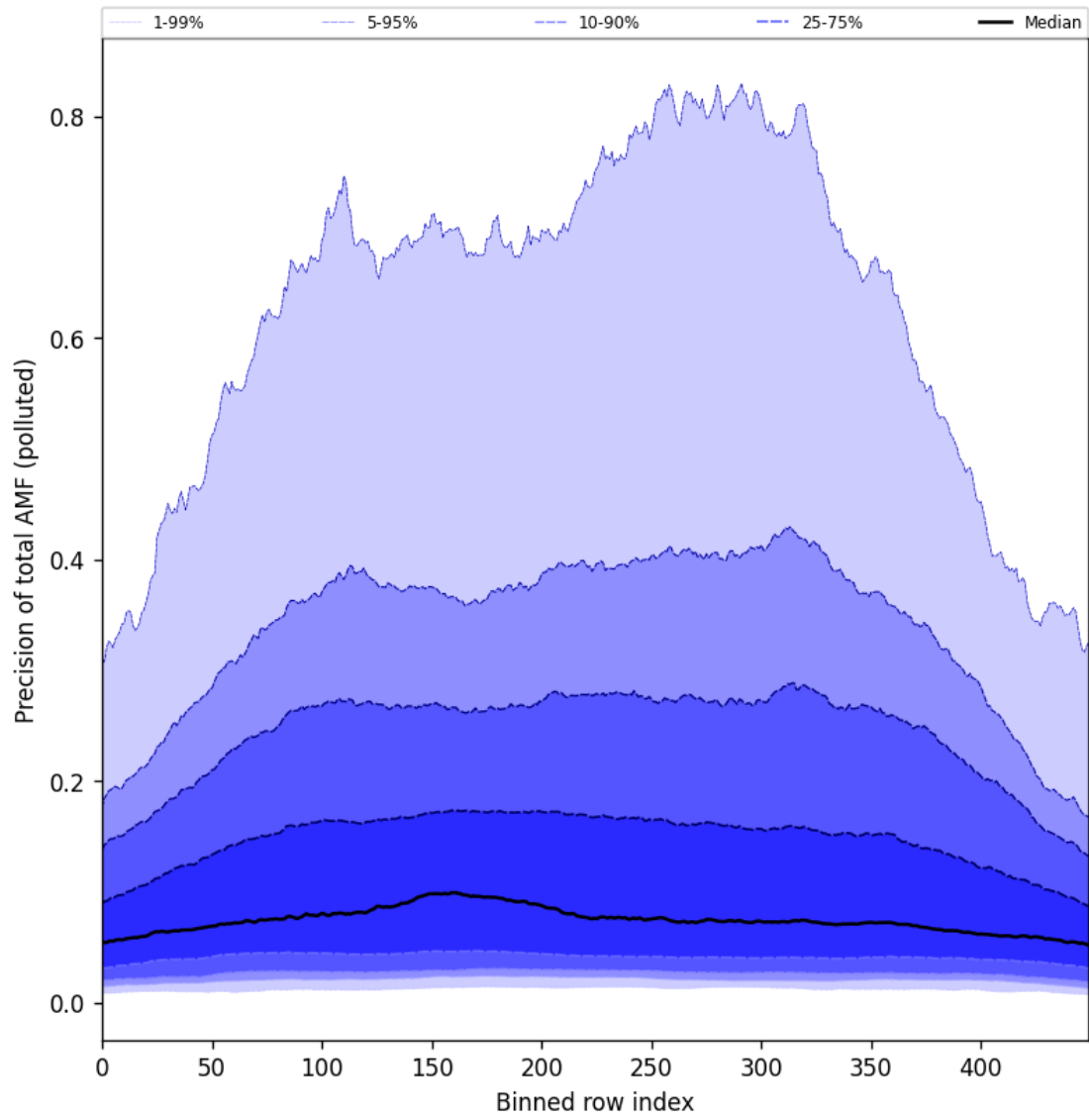
Figure 106: Along track statistics of “Precision of total AMF (polluted)” for 2025-05-05 to 2025-05-07
