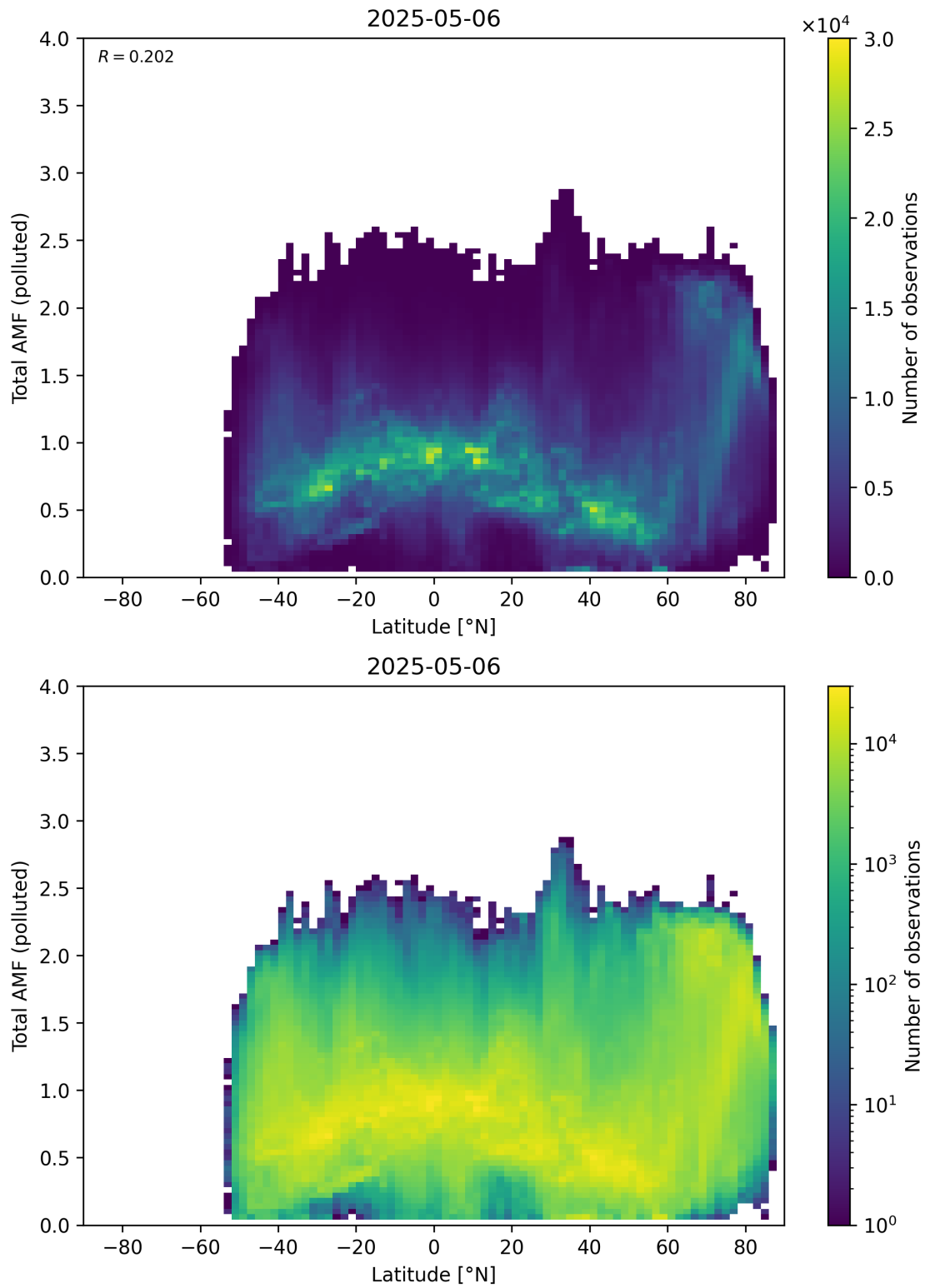
Figure 167: Scatter density plot of “Latitude” against “Total AMF (polluted)” for 2025-05-05 to 2025-05-07.
