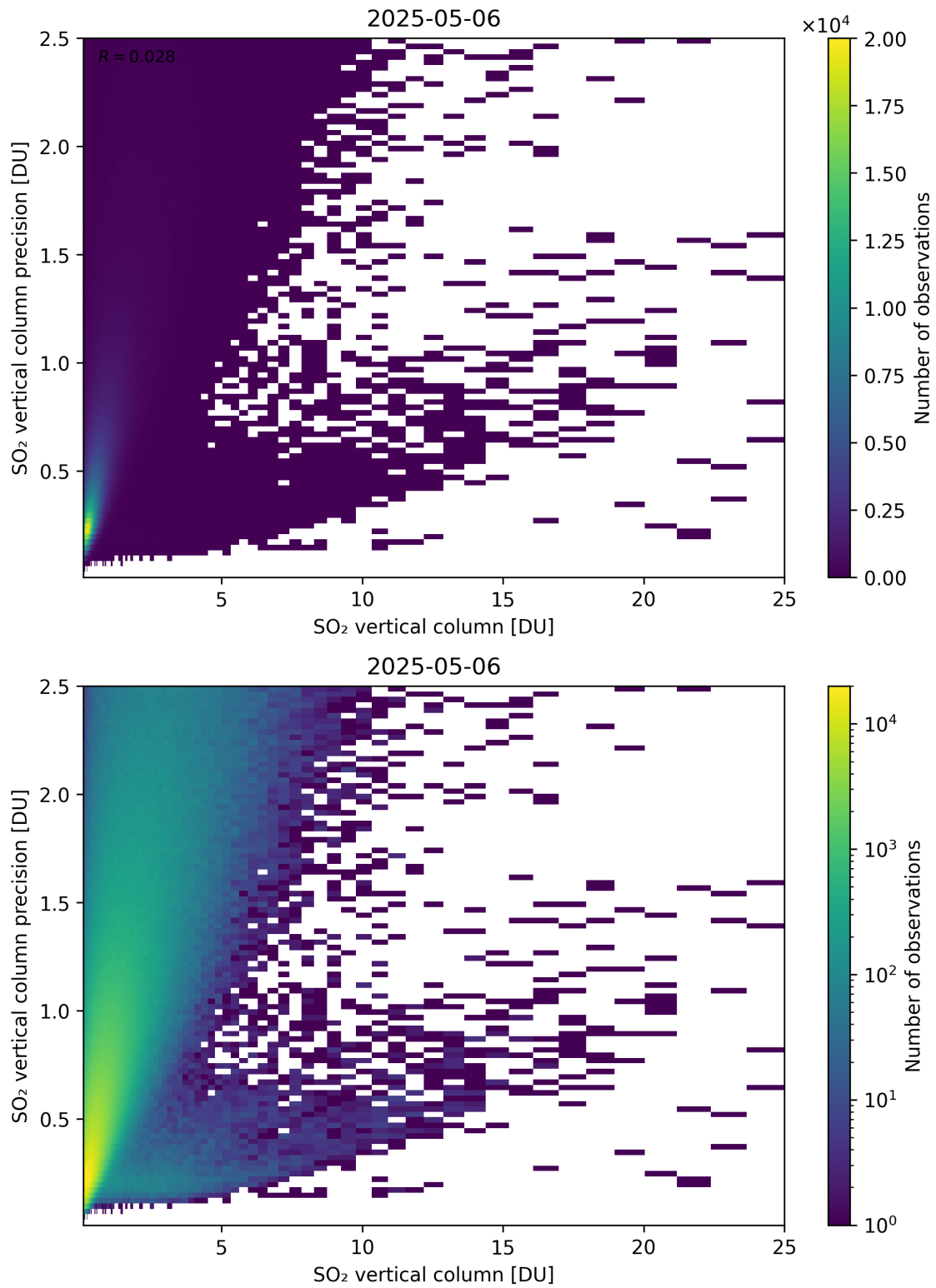
Figure 361: Scatter density plot of “SO 2 vertical column” against “SO 2 vertical column precision” for 2025-05-05 to 2025-05-07.
