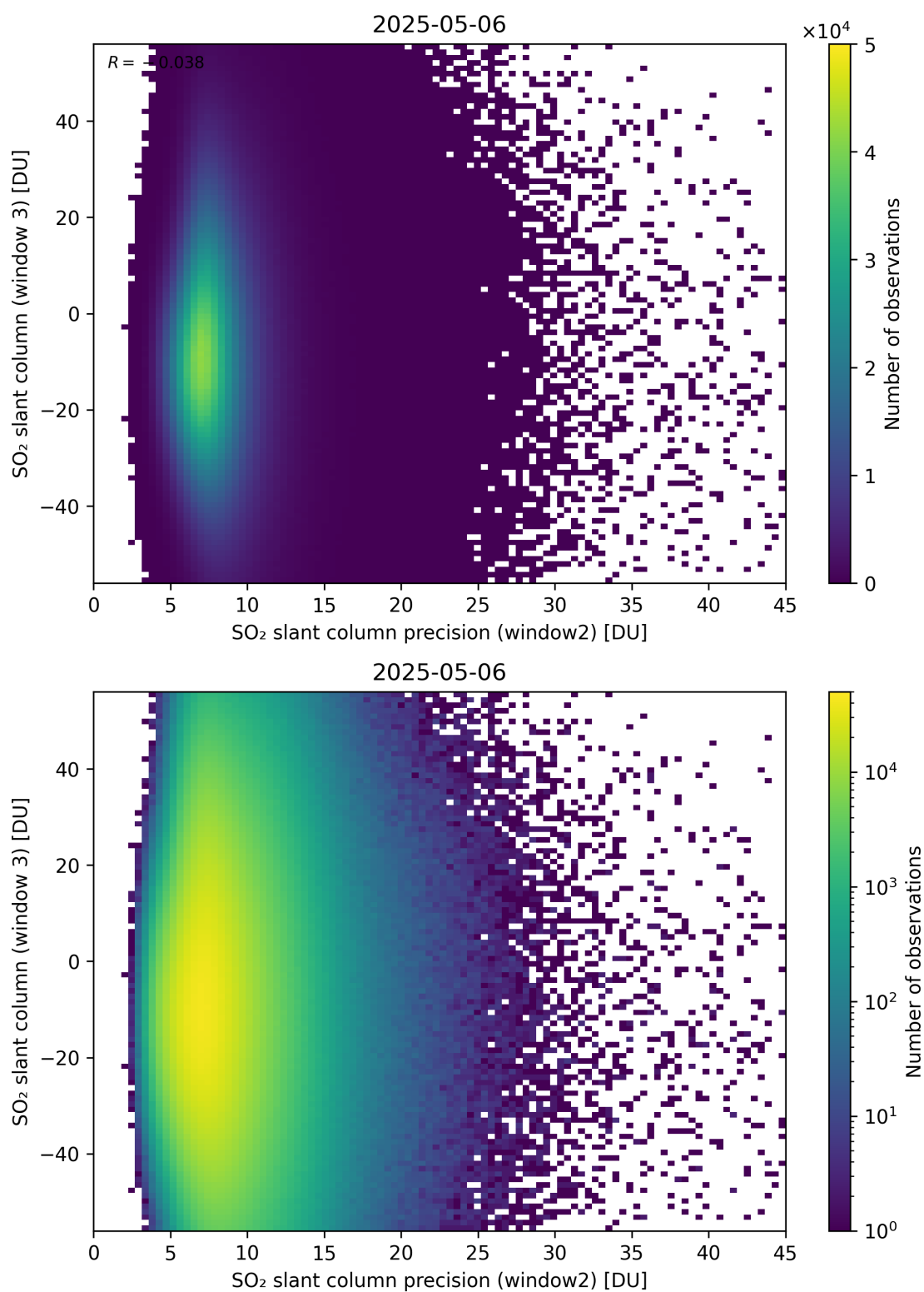
Figure 299: Scatter density plot of “SO 2 slant column precision (window2)” against “SO 2 slant column (window 3)” for 2025-05-05 to 2025-05-07.
