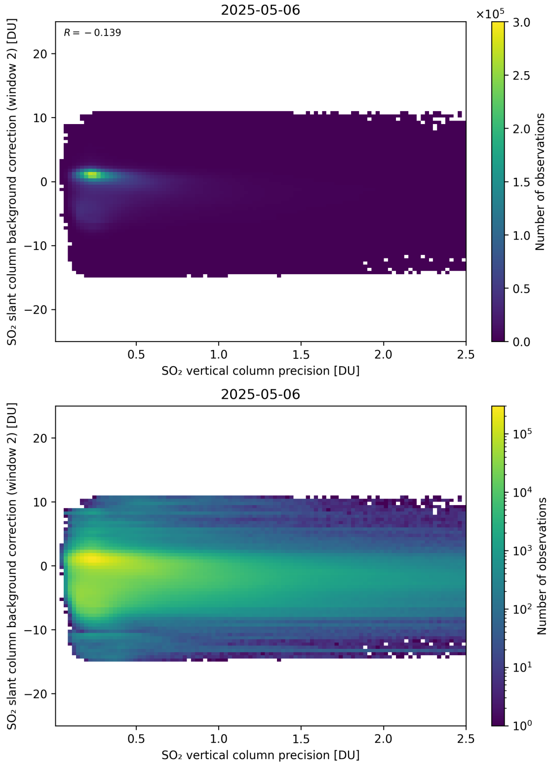
Figure 330: Scatter density plot of “SO 2 vertical column precision” against “SO 2 slant column background correction (window 2)” for 2025-05-05 to 2025-05-07.
