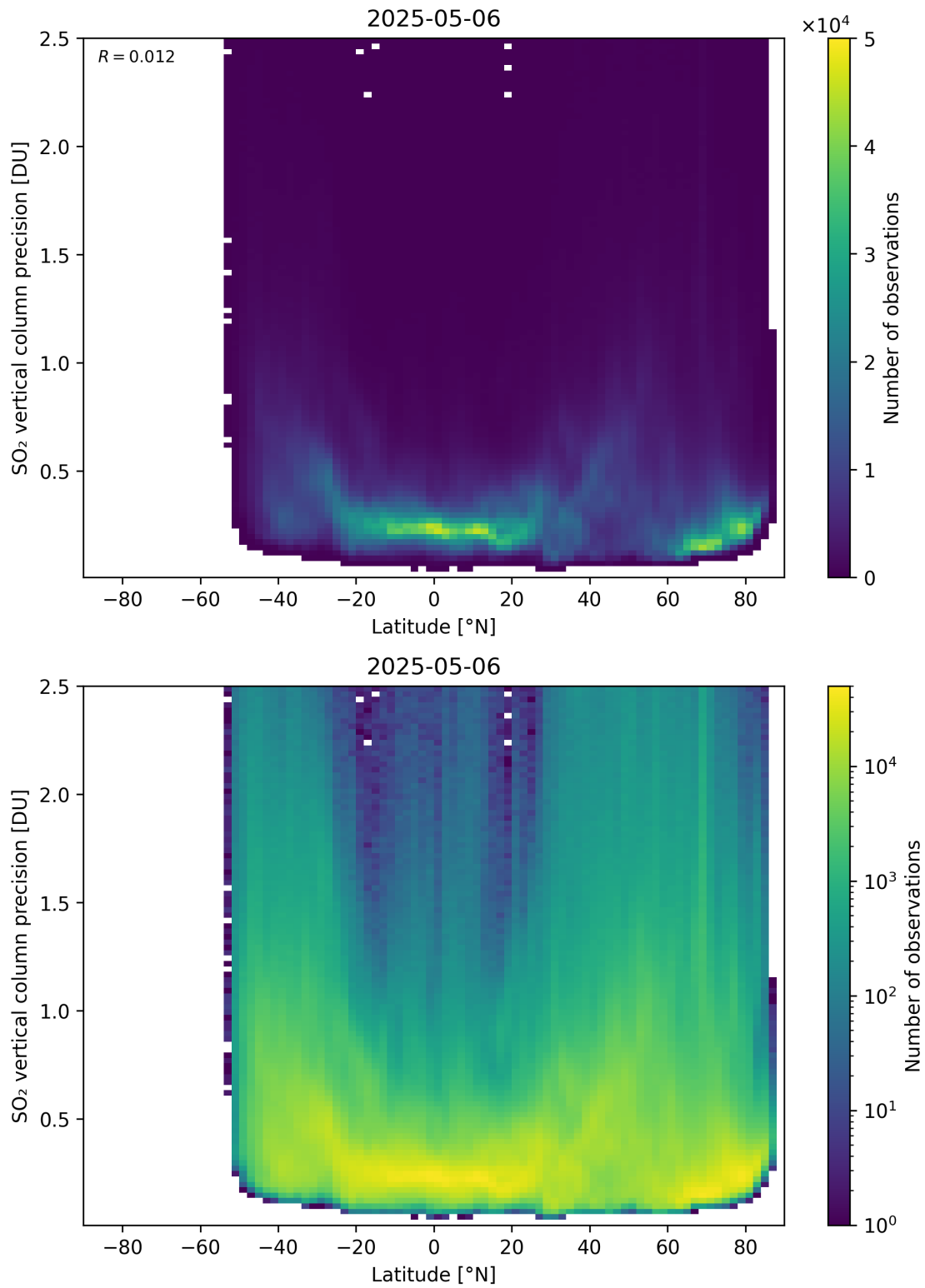
Figure 170: Scatter density plot of “Latitude” against “SO 2 vertical column precision” for 2025-05-05 to 2025-05-07.
