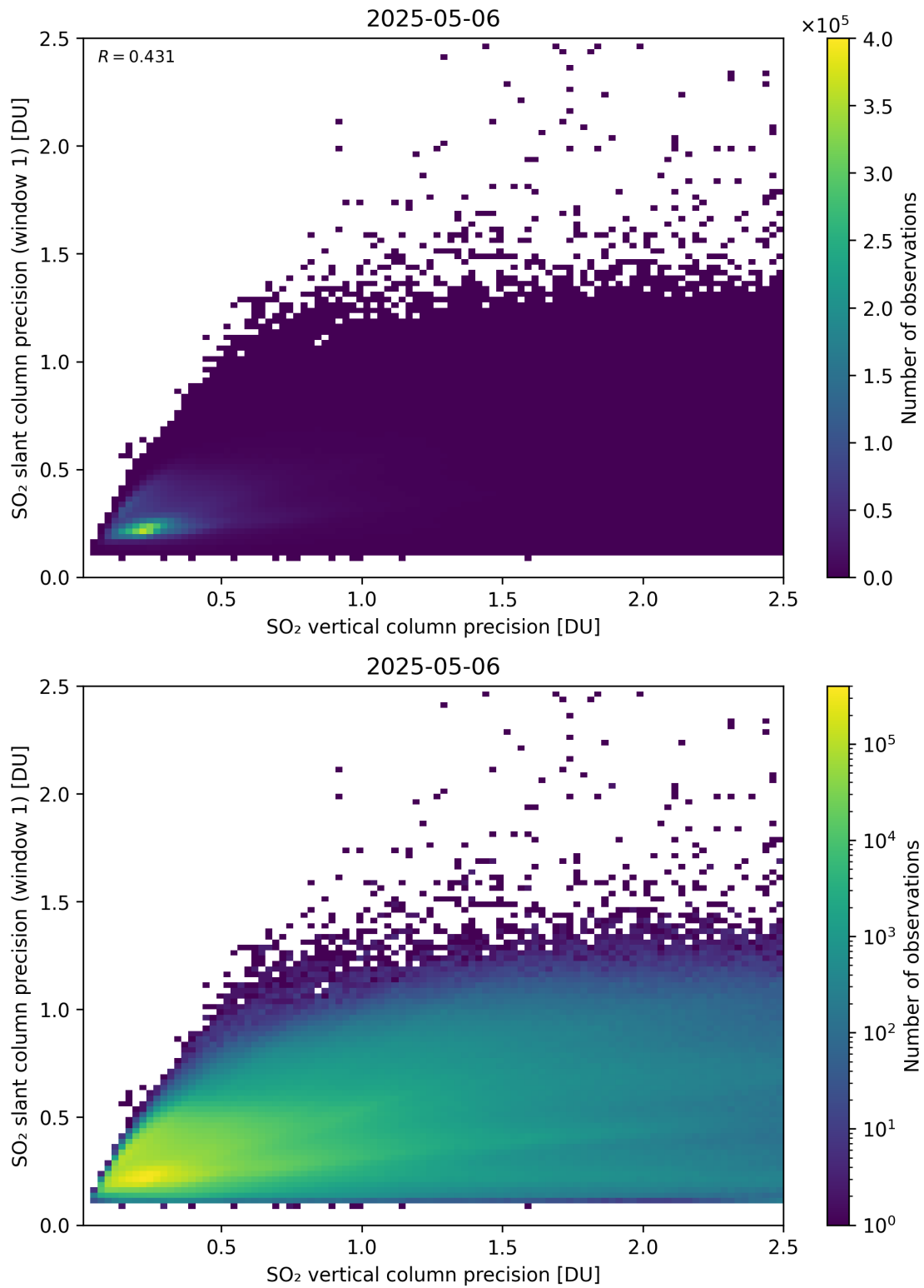
Figure 342: Scatter density plot of “SO 2 vertical column precision” against “SO 2 slant column precision (window 1)” for 2025-05-05 to 2025-05-07.
