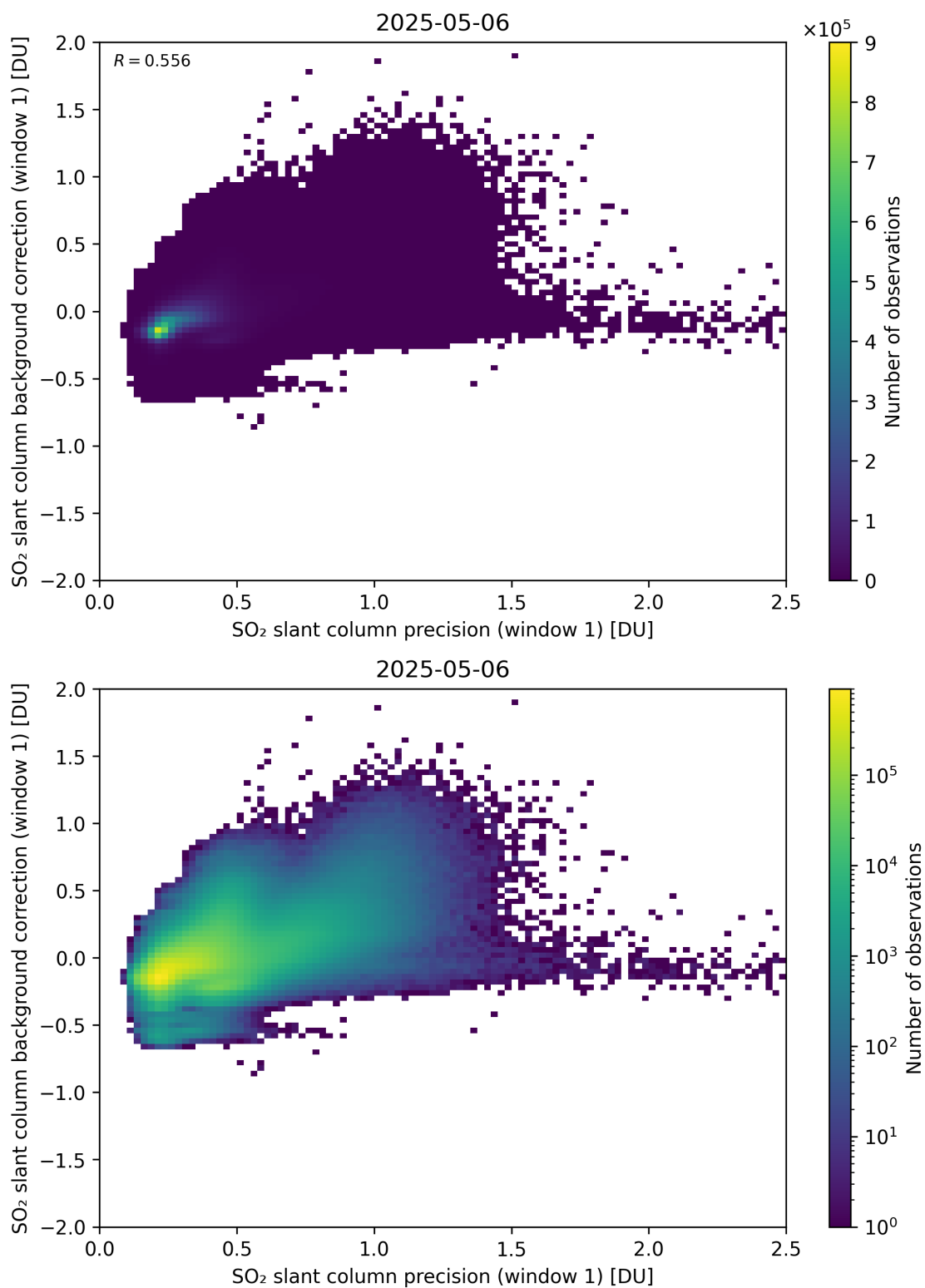
Figure 268: Scatter density plot of “SO 2 slant column precision (window 1)” against “SO 2 slant column background correction (window 1)” for 2025-05-05 to 2025-05-07.
