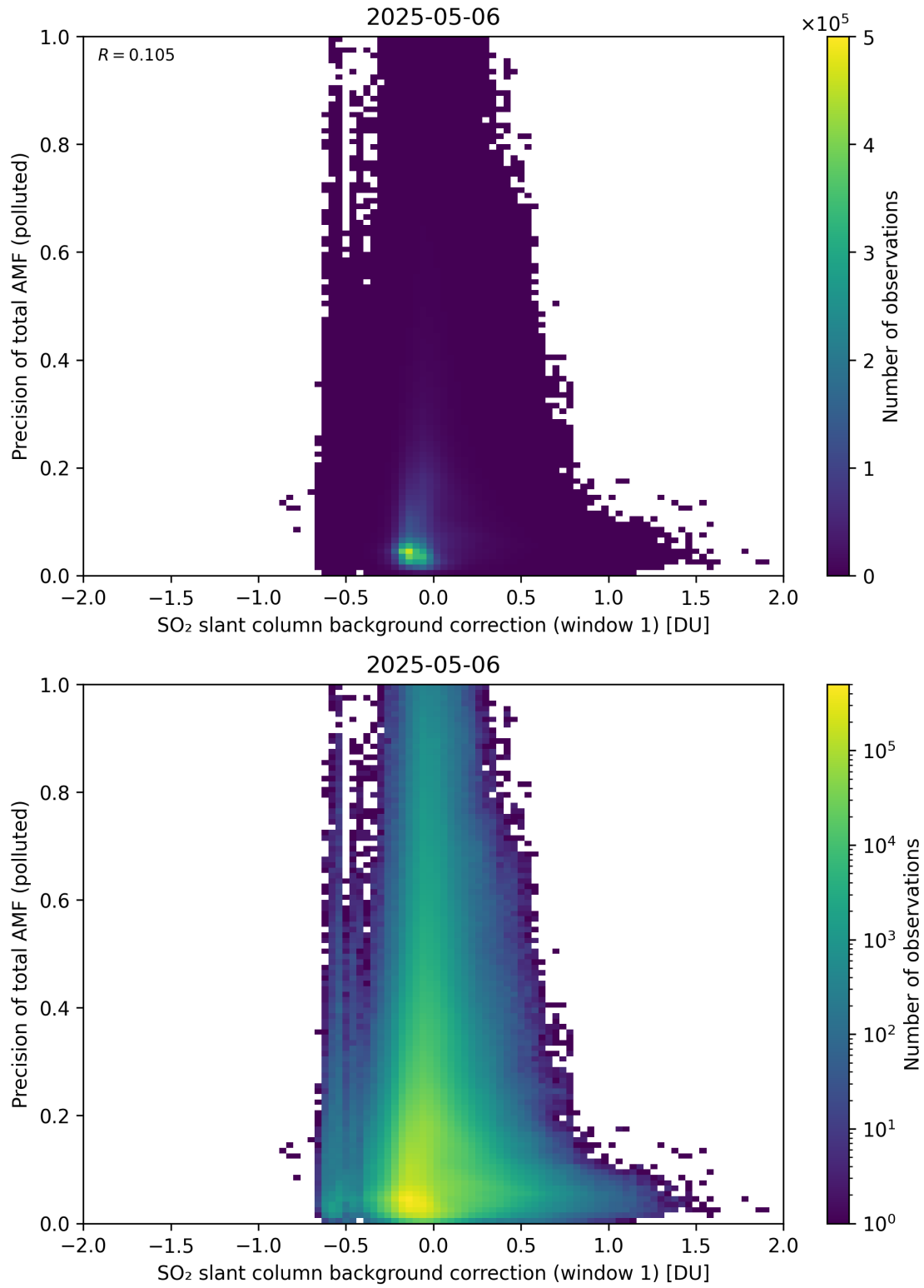
Figure 121: Scatter density plot of “SO 2 slant column background correction (window 1)” against “Precision of total AMF (polluted)” for 2025-05-05 to 2025-05-07.
