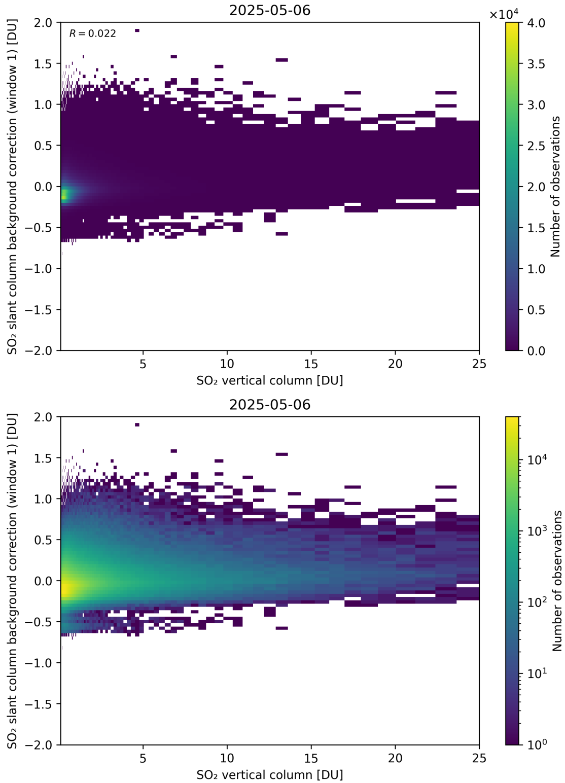
Figure 323: Scatter density plot of “SO 2 vertical column” against “SO 2 slant column background correction (window 1)” for 2025-05-05 to 2025-05-07.
