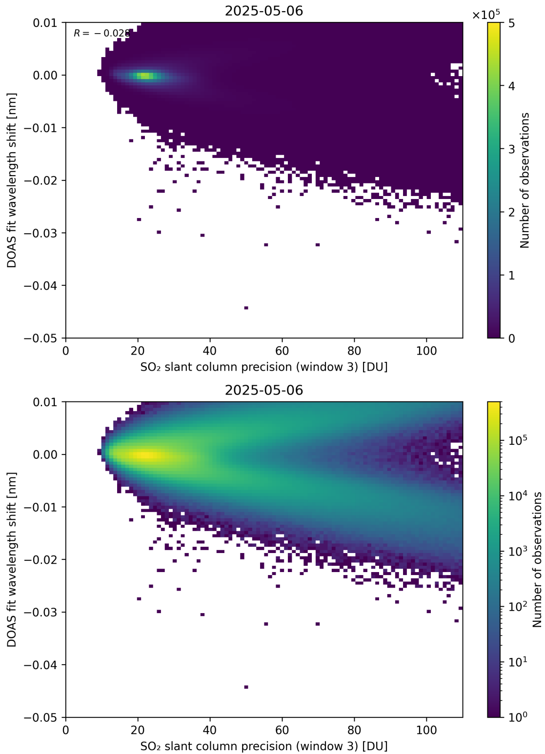
Figure 308: Scatter density plot of “SO 2 slant column precision (window 3)” against “DOAS fit wavelength shift” for 2025-05-05 to 2025-05-07.
