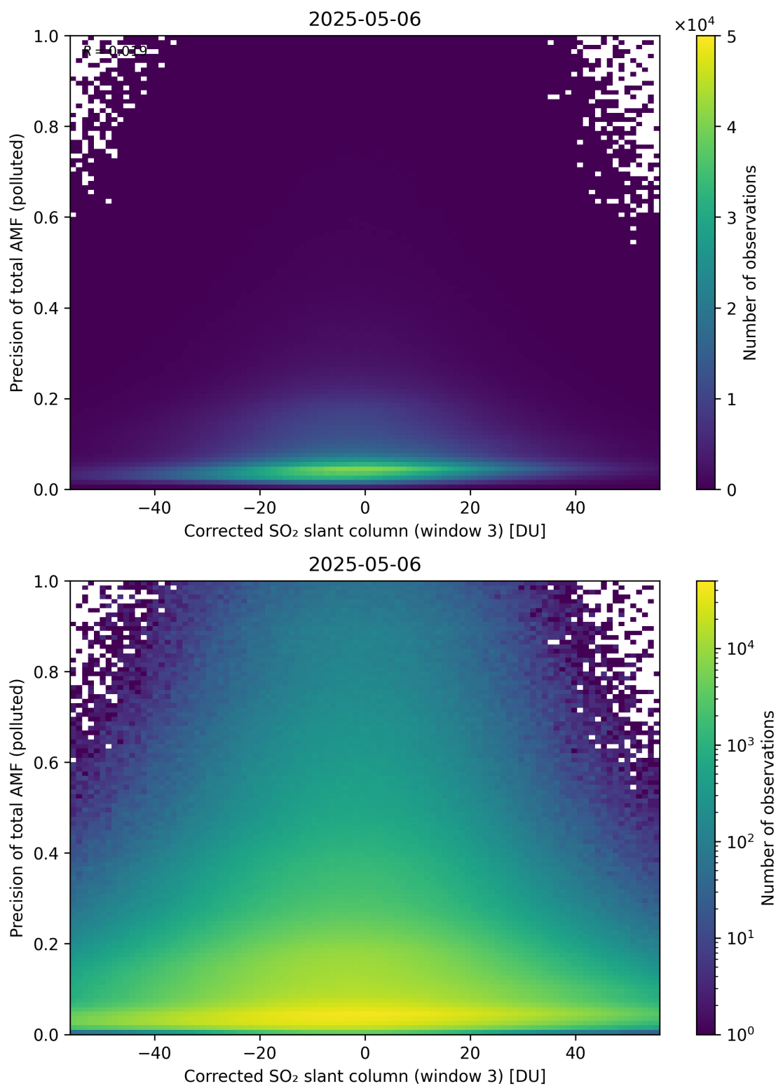
Figure 261: Scatter density plot of “Corrected SO 2 slant column (window 3)” against “Precision of total AMF (polluted)” for 2025-05-05 to 2025-05-07.
