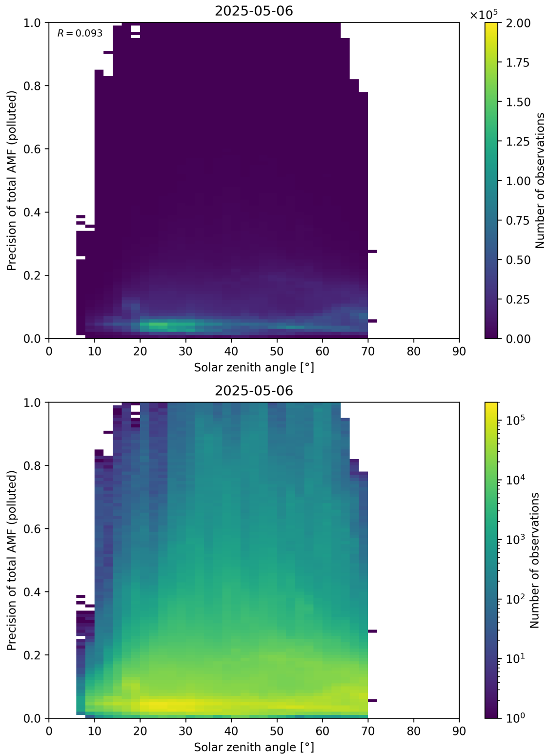
Figure 190: Scatter density plot of “Solar zenith angle” against “Precision of total AMF (polluted)” for 2025-05-05 to 2025-05-07.
