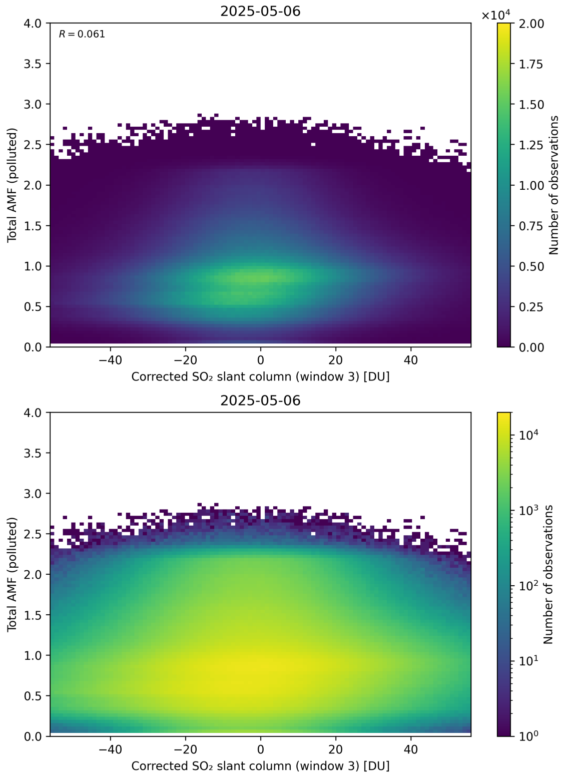
Figure 260: Scatter density plot of “Corrected SO 2 slant column (window 3)” against “Total AMF (polluted)” for 2025-05-05 to 2025-05-07.
