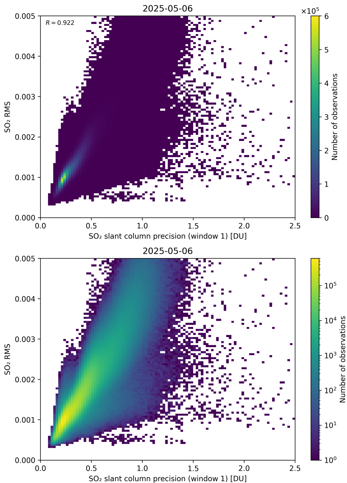
Figure 273: Scatter density plot of “SO 2 slant column precision (window 1)” against “SO 2 RMS” for 2025-05-05 to 2025-05-07.
