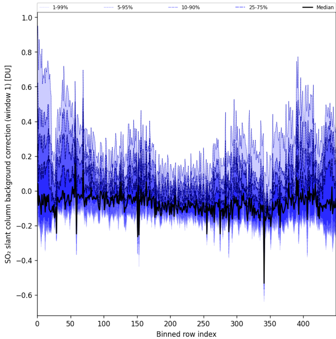
Figure 92: Along track statistics of “SO 2 slant column background correction (window 1)” for 2025-05-05 to 2025-05-07
