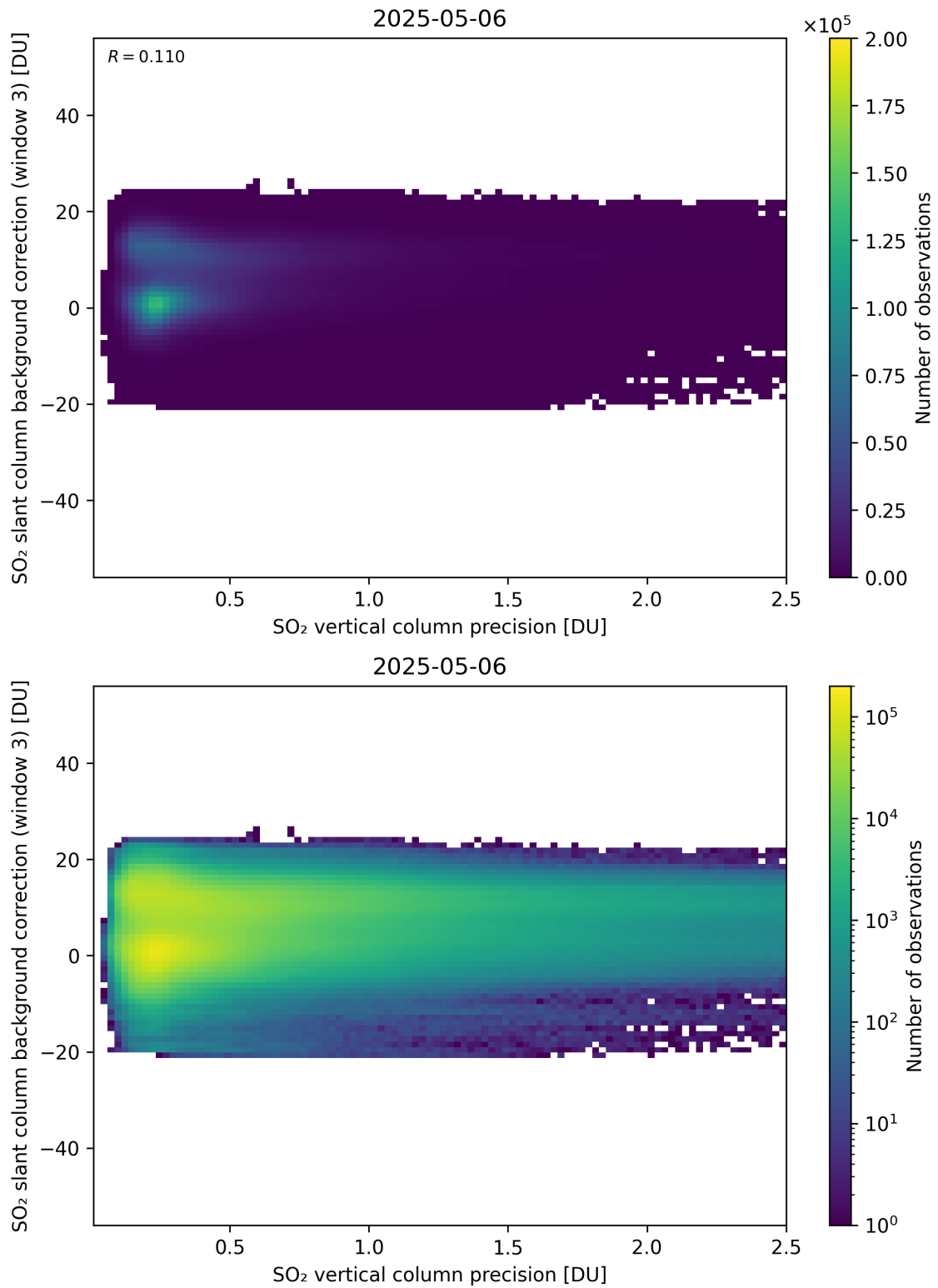
Figure 331: Scatter density plot of “SO 2 vertical column precision” against “SO 2 slant column background correction (window 3)” for 2025-05-05 to 2025-05-07.
