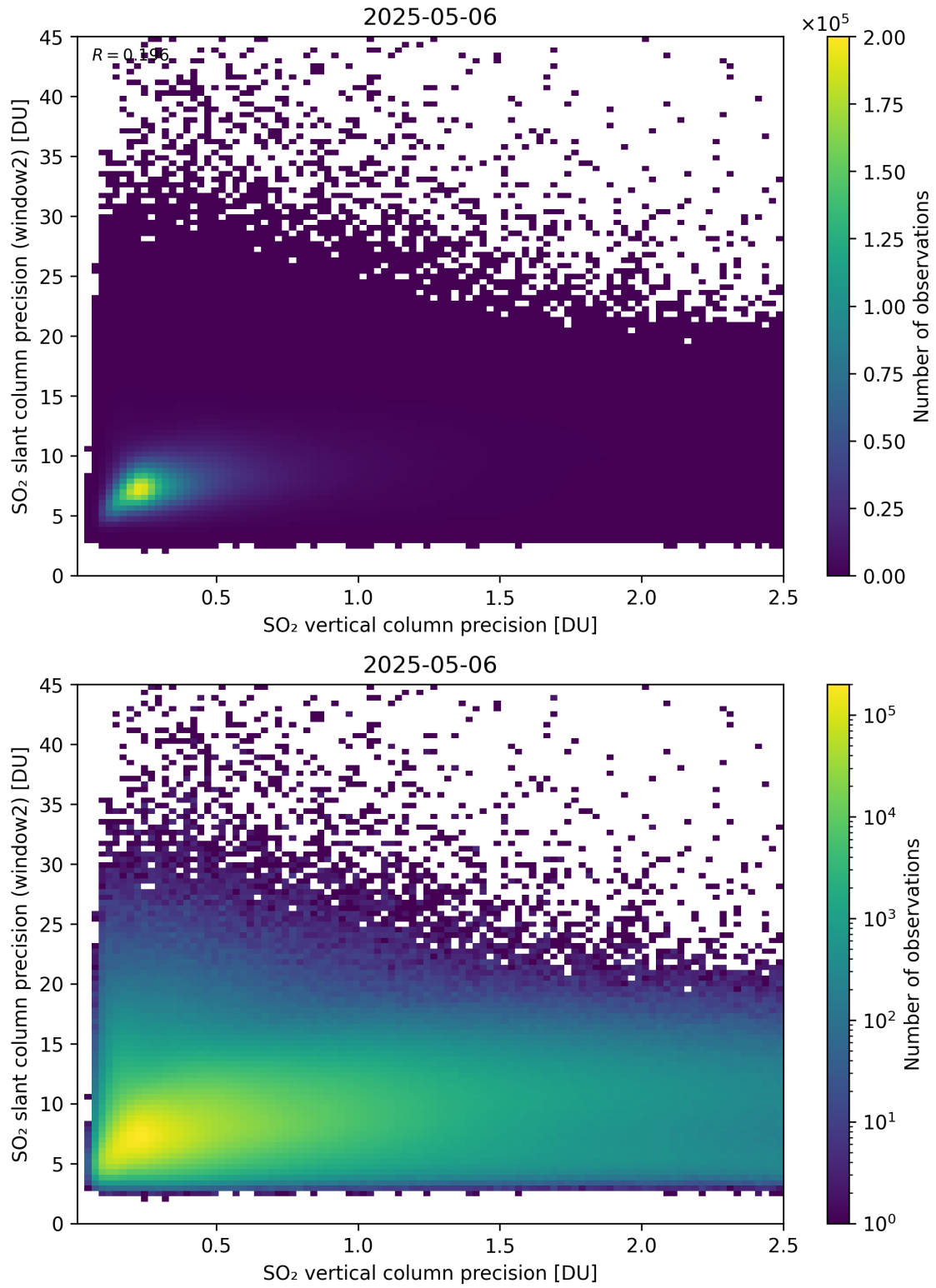
Figure 343: Scatter density plot of “SO 2 vertical column precision” against “SO 2 slant column precision (window2)” for 2025-05-05 to 2025-05-07.
