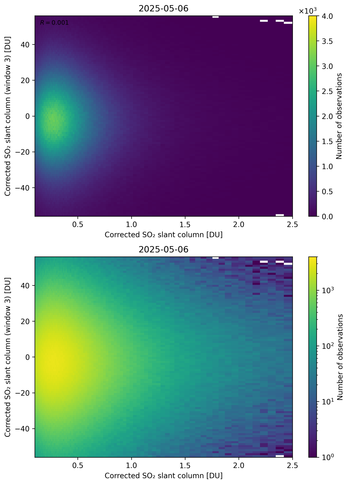
Figure 236: Scatter density plot of “Corrected SO 2 slant column” against “Corrected SO 2 slant column (window 3)” for 2025-05-05 to 2025-05-07.
