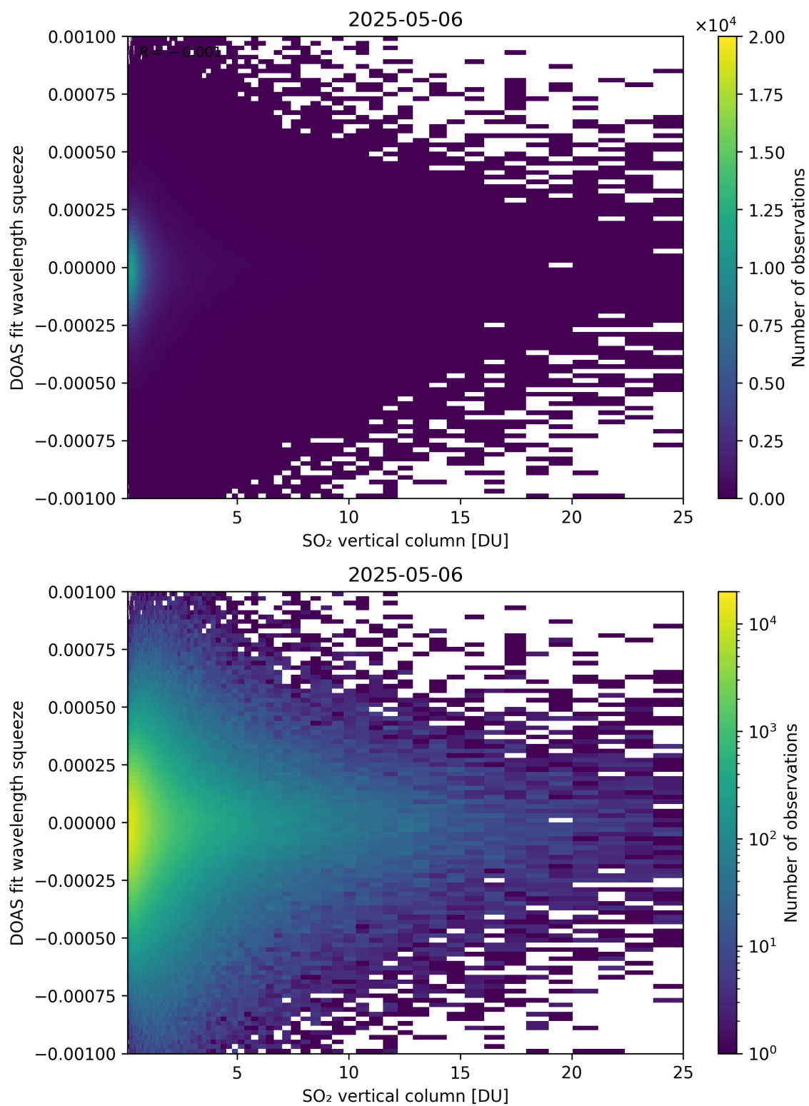
Figure 327: Scatter density plot of “SO 2 vertical column” against “DOAS fit wavelength squeeze” for 2025-05-05 to 2025-05-07.
