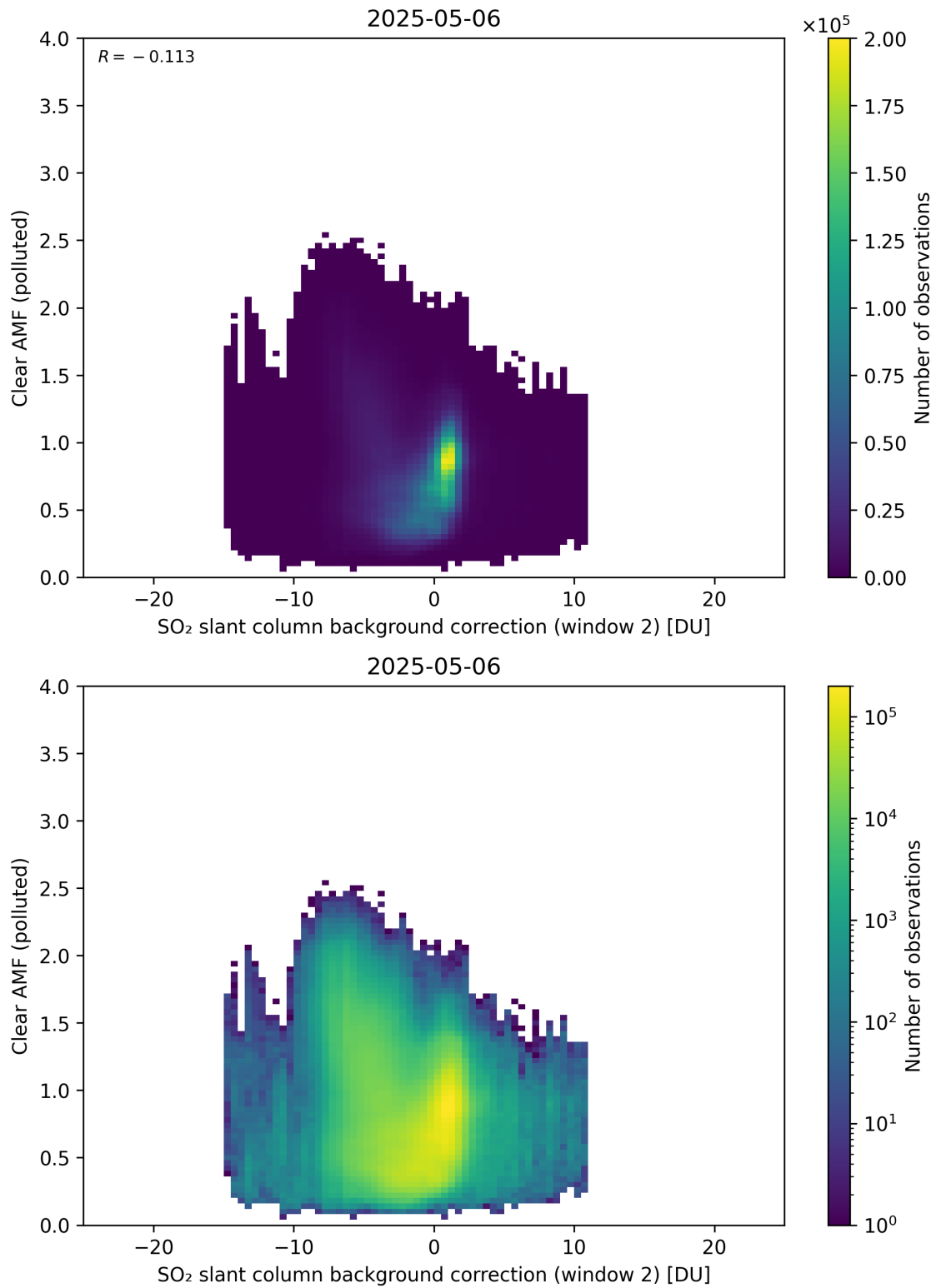
Figure 126: Scatter density plot of “SO 2 slant column background correction (window 2)” against “Clear AMF (polluted)” for 2025-05-05 to 2025-05-07.
