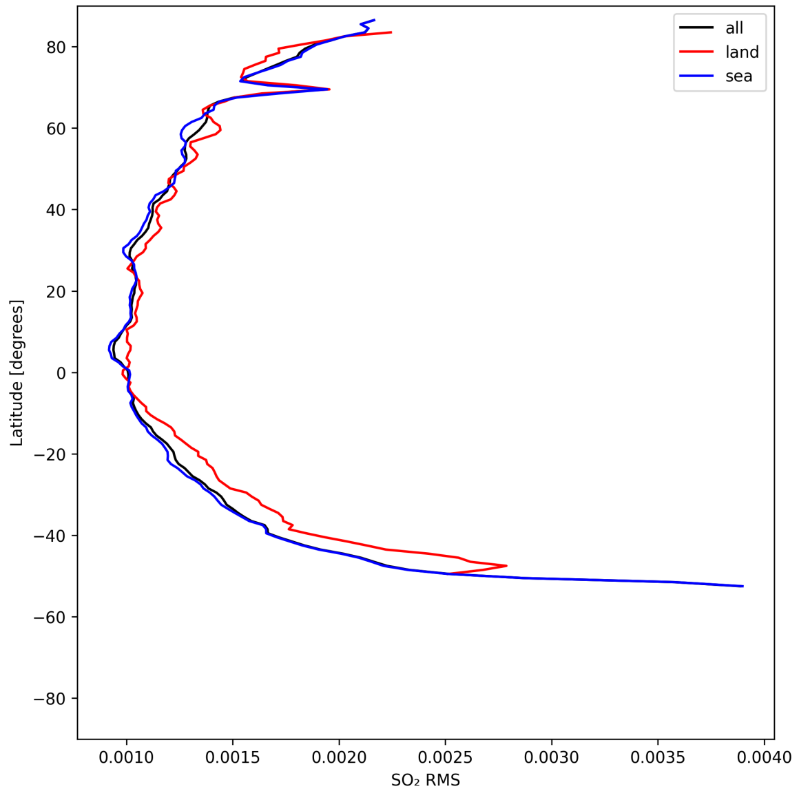
Figure 52: Zonal average of “SO 2 RMS” for 2025-05-05 to 2025-05-07.
