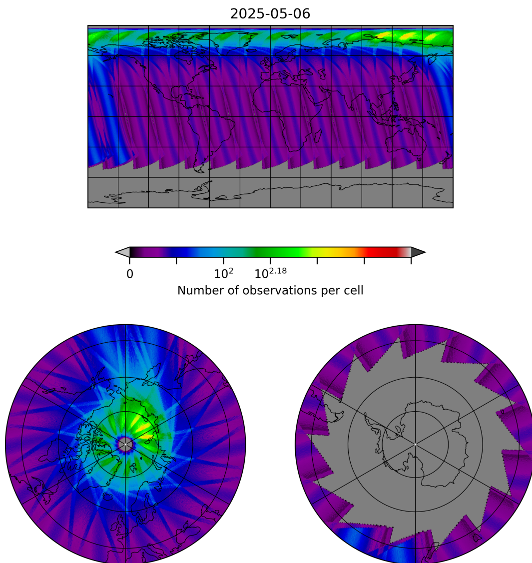
Figure 30: Map of the number of observations for 2025-05-05 to 2025-05-07
