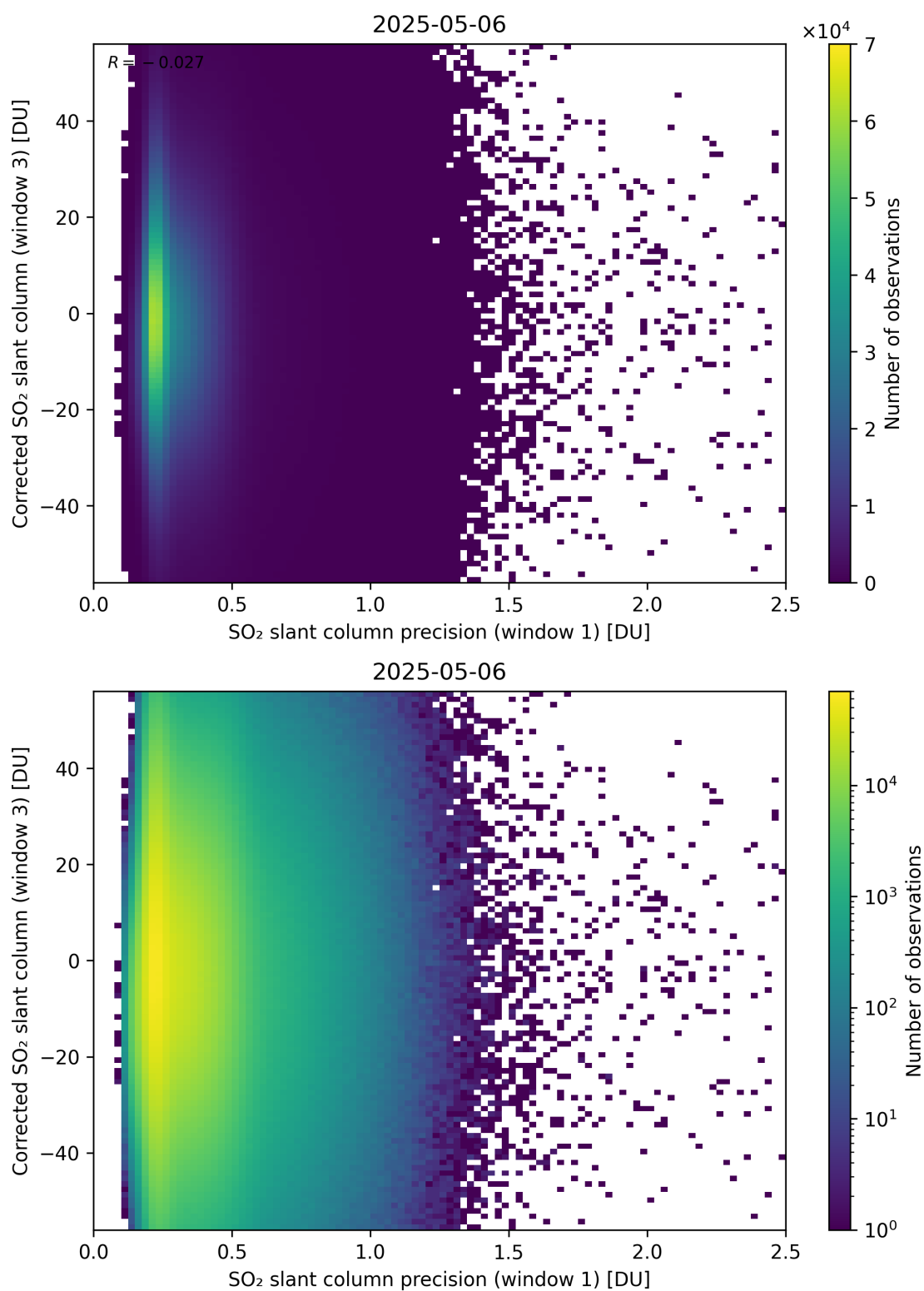
Figure 276: Scatter density plot of “SO 2 slant column precision (window 1)” against “Corrected SO 2 slant column (window 3)” for 2025-05-05 to 2025-05-07.
