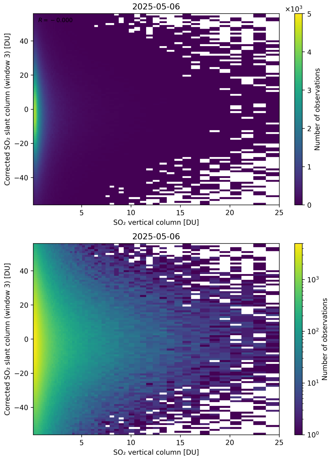
Figure 353: Scatter density plot of “SO 2 vertical column” against “Corrected SO 2 slant column (window 3)” for 2025-05-05 to 2025-05-07.
