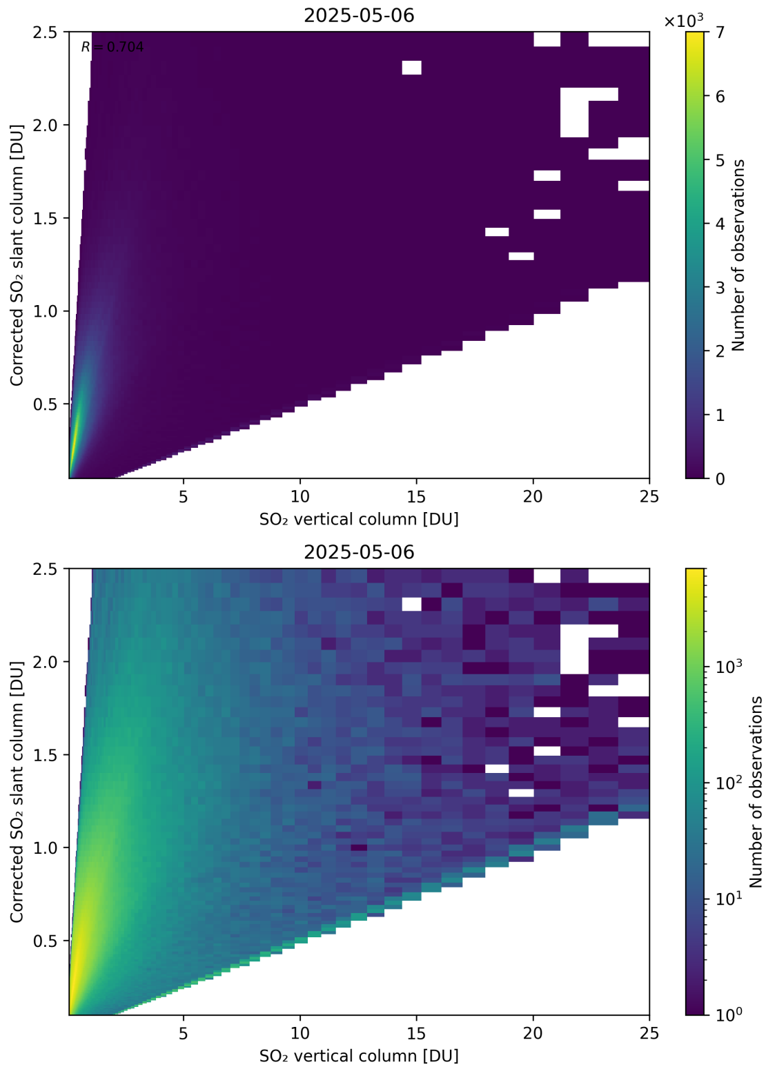
Figure 351: Scatter density plot of “SO 2 vertical column” against “Corrected SO 2 slant column” for 2025-05-05 to 2025-05-07.
