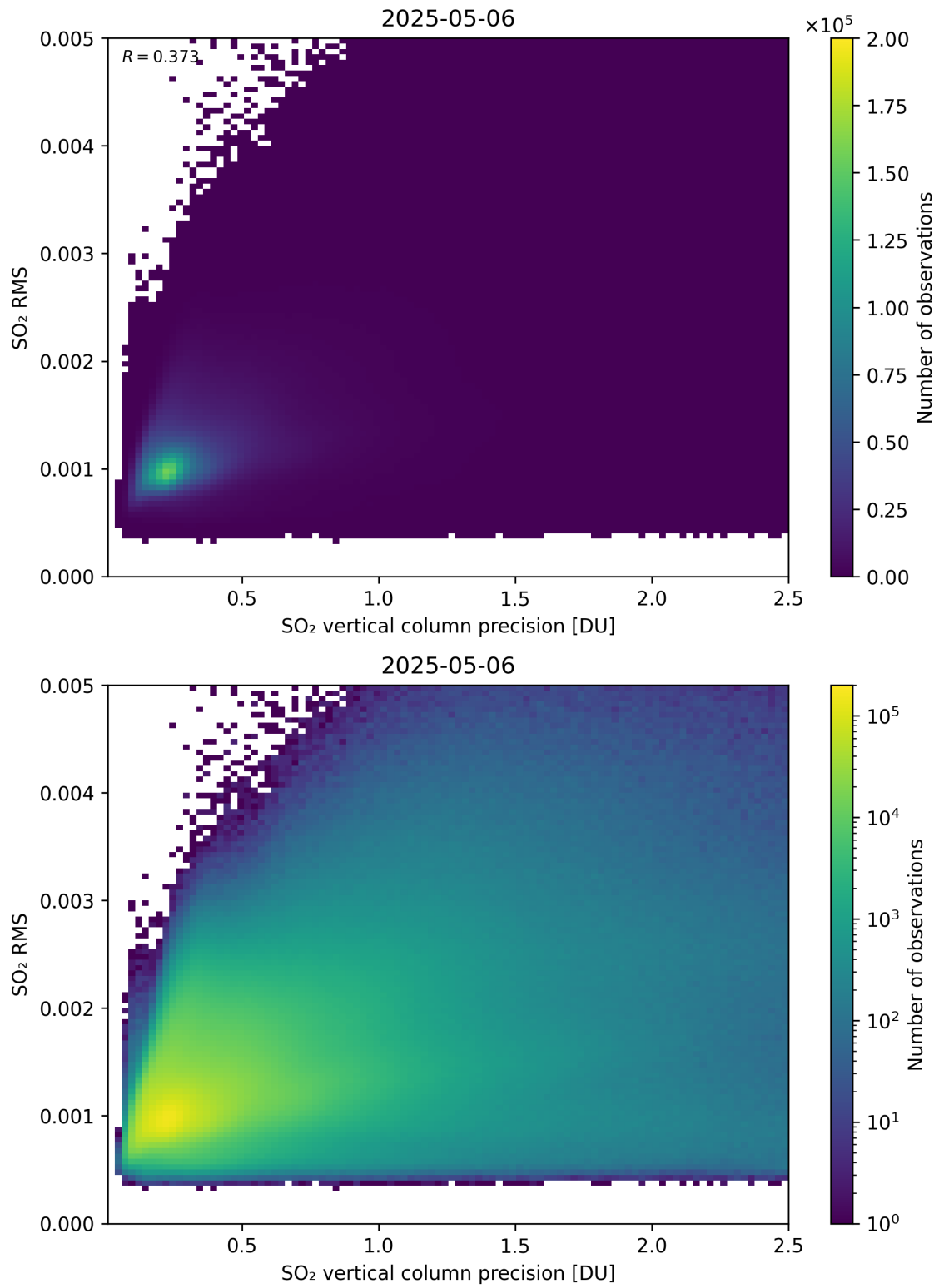
Figure 334: Scatter density plot of “SO 2 vertical column precision” against “SO 2 RMS” for 2025-05-05 to 2025-05-07.
