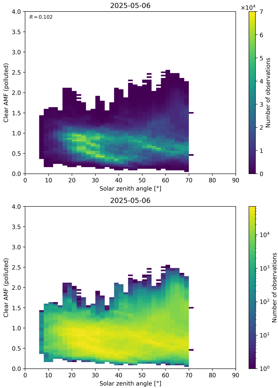
Figure 178: Scatter density plot of “Solar zenith angle” against “Clear AMF (polluted)” for 2025-05-05 to 2025-05-07.
