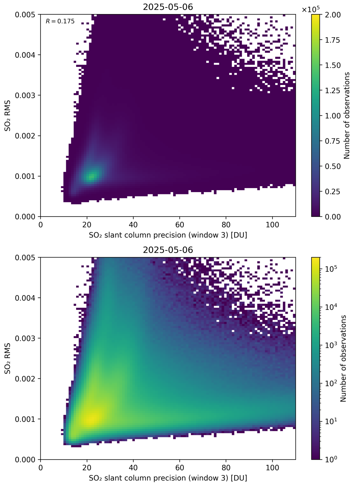
Figure 310: Scatter density plot of “SO 2 slant column precision (window 3)” against “SO 2 RMS” for 2025-05-05 to 2025-05-07.
