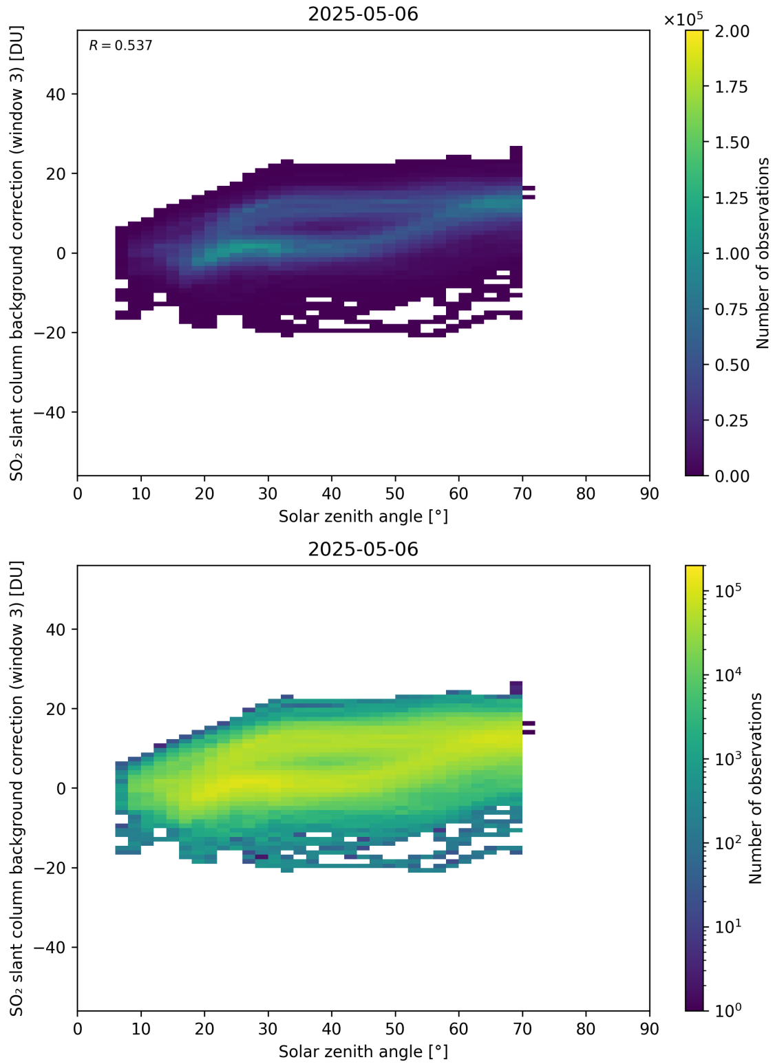
Figure 173: Scatter density plot of “Solar zenith angle” against “SO 2 slant column background correction (window 3)” for 2025-05-05 to 2025-05-07.
