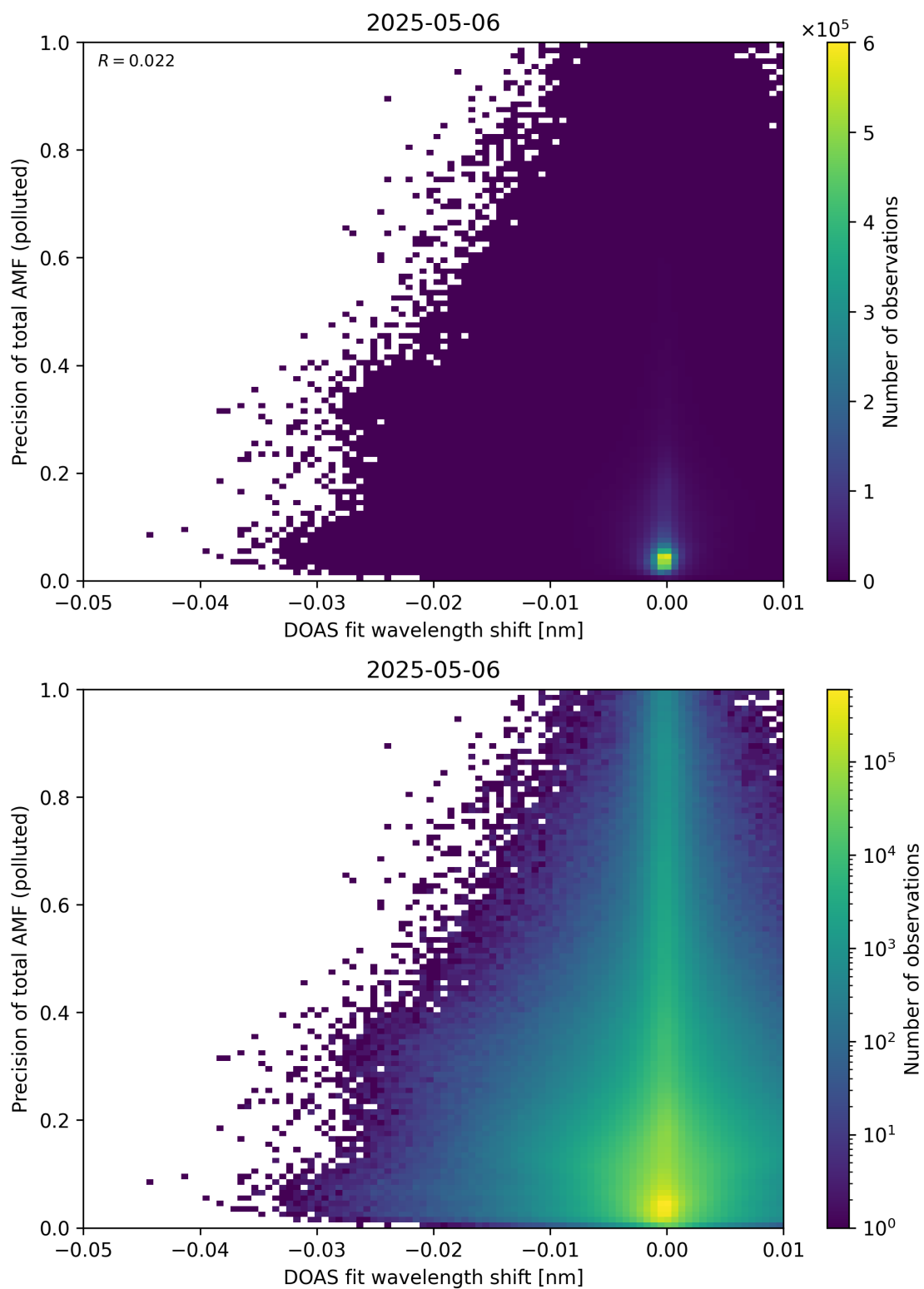
Figure 142: Scatter density plot of “DOAS fit wavelength shift” against “Precision of total AMF (polluted)” for 2025-05-05 to 2025-05-07.
