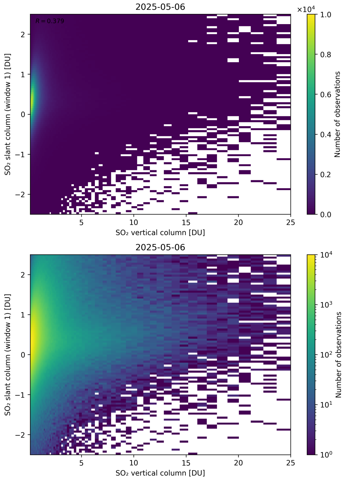
Figure 354: Scatter density plot of “SO 2 vertical column” against “SO 2 slant column (window 1)” for 2025-05-05 to 2025-05-07.
