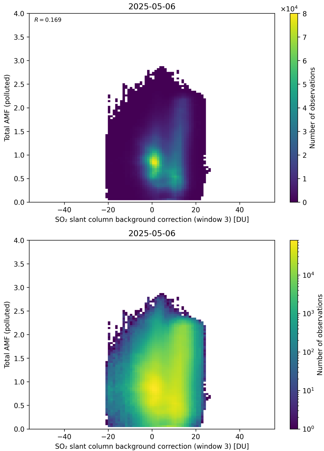
Figure 136: Scatter density plot of “SO 2 slant column background correction (window 3)” against “Total AMF (polluted)” for 2025-05-05 to 2025-05-07.
