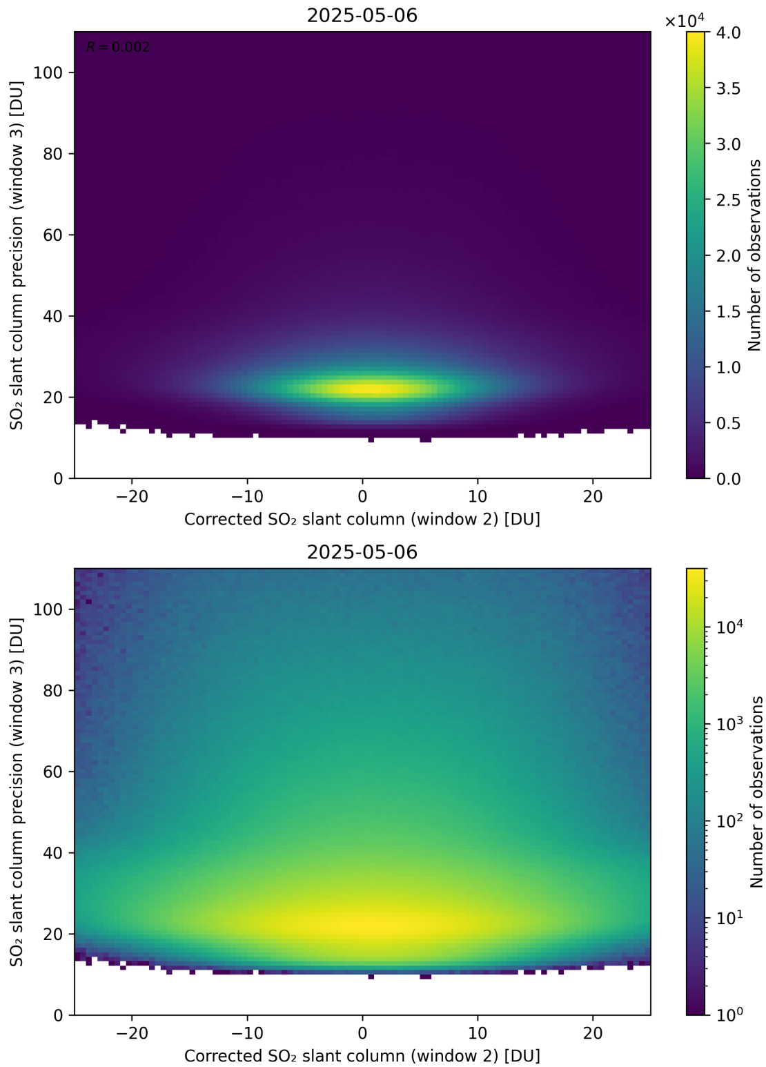
Figure 252: Scatter density plot of “Corrected SO 2 slant column (window 2)” against “SO 2 slant column precision (window 3)” for 2025-05-05 to 2025-05-07.
