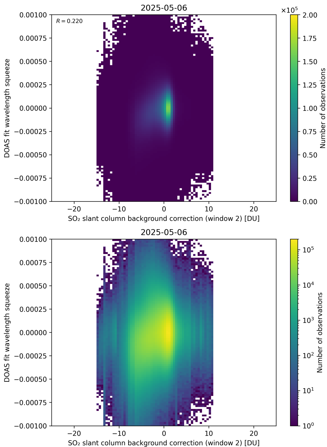
Figure 124: Scatter density plot of “SO 2 slant column background correction (window 2)” against “DOAS fit wavelength squeeze” for 2025-05-05 to 2025-05-07.
