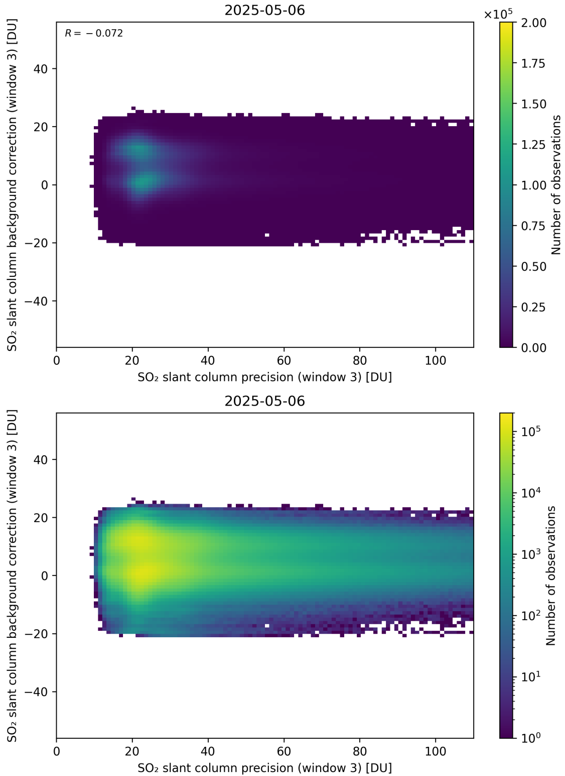
Figure 307: Scatter density plot of “SO 2 slant column precision (window 3)” against “SO 2 slant column background correction (window 3)” for 2025-05-05 to 2025-05-07.
