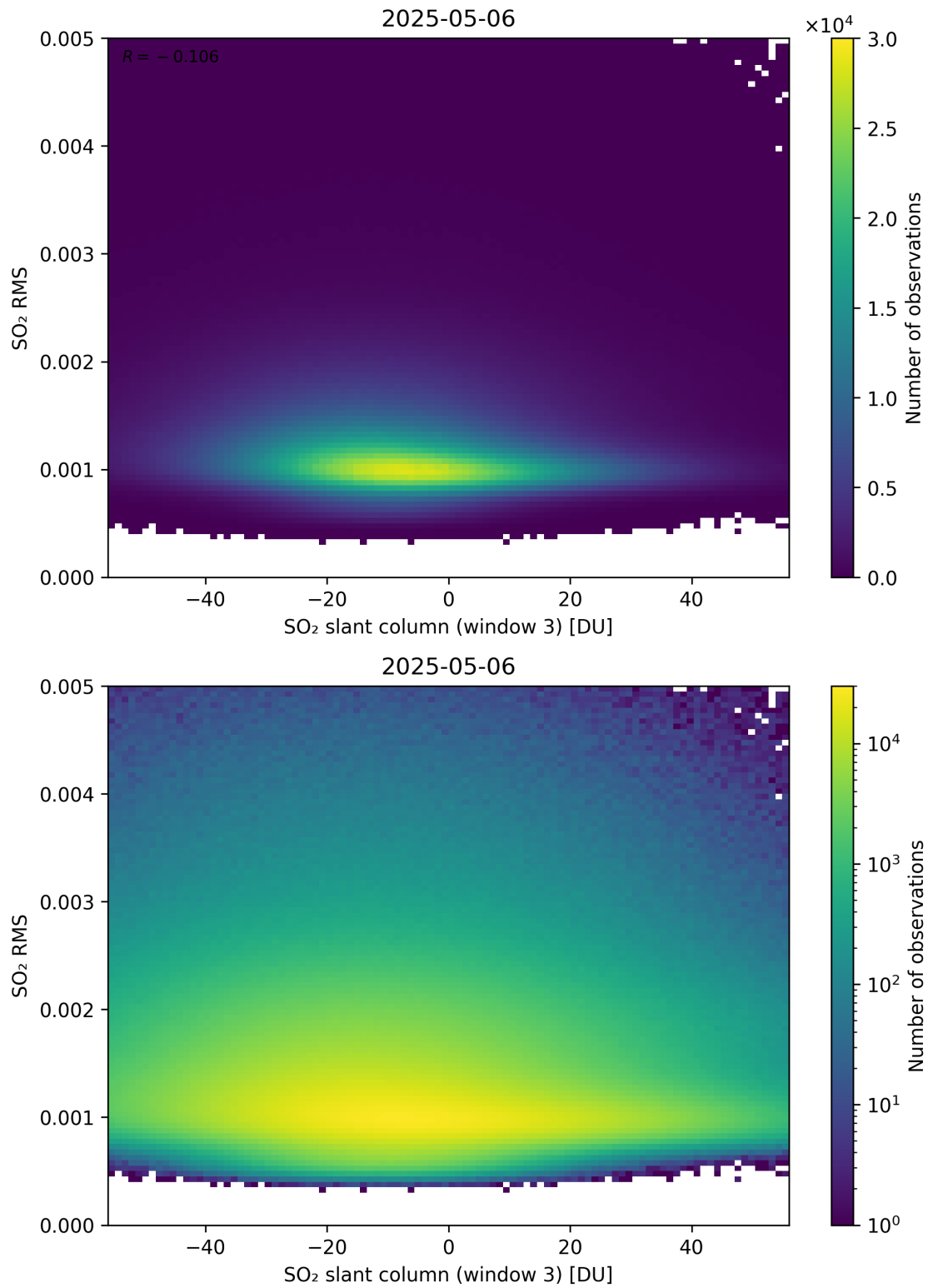
Figure 306: Scatter density plot of “SO 2 slant column (window 3)” against “SO 2 RMS” for 2025-05-05 to 2025-05-07.
