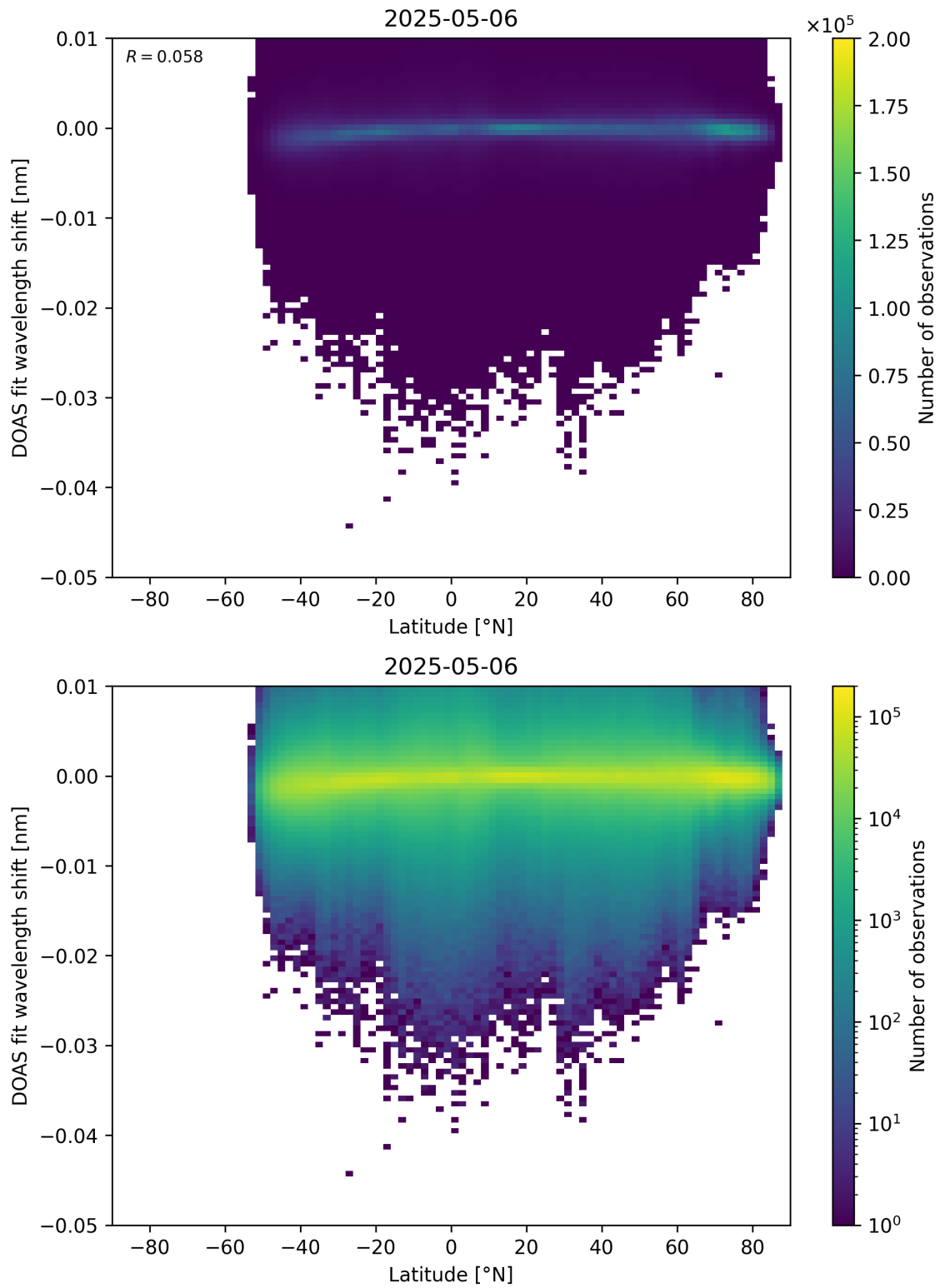
Figure 153: Scatter density plot of “Latitude” against “DOAS fit wavelength shift” for 2025-05-05 to 2025-05-07.
