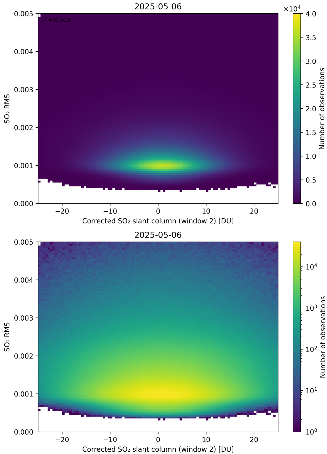
Figure 248: Scatter density plot of “Corrected SO 2 slant column (window 2)” against “SO 2 RMS” for 2025-05-05 to 2025-05-07.
