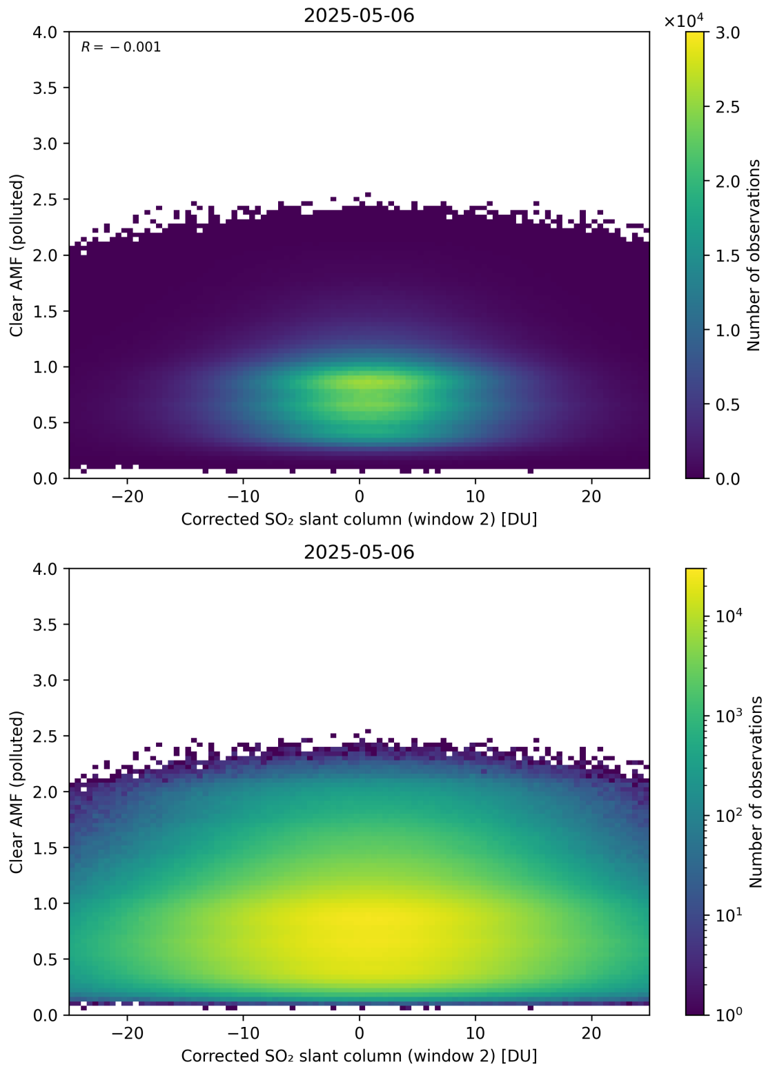
Figure 249: Scatter density plot of “Corrected SO 2 slant column (window 2)” against “Clear AMF (polluted)” for 2025-05-05 to 2025-05-07.
