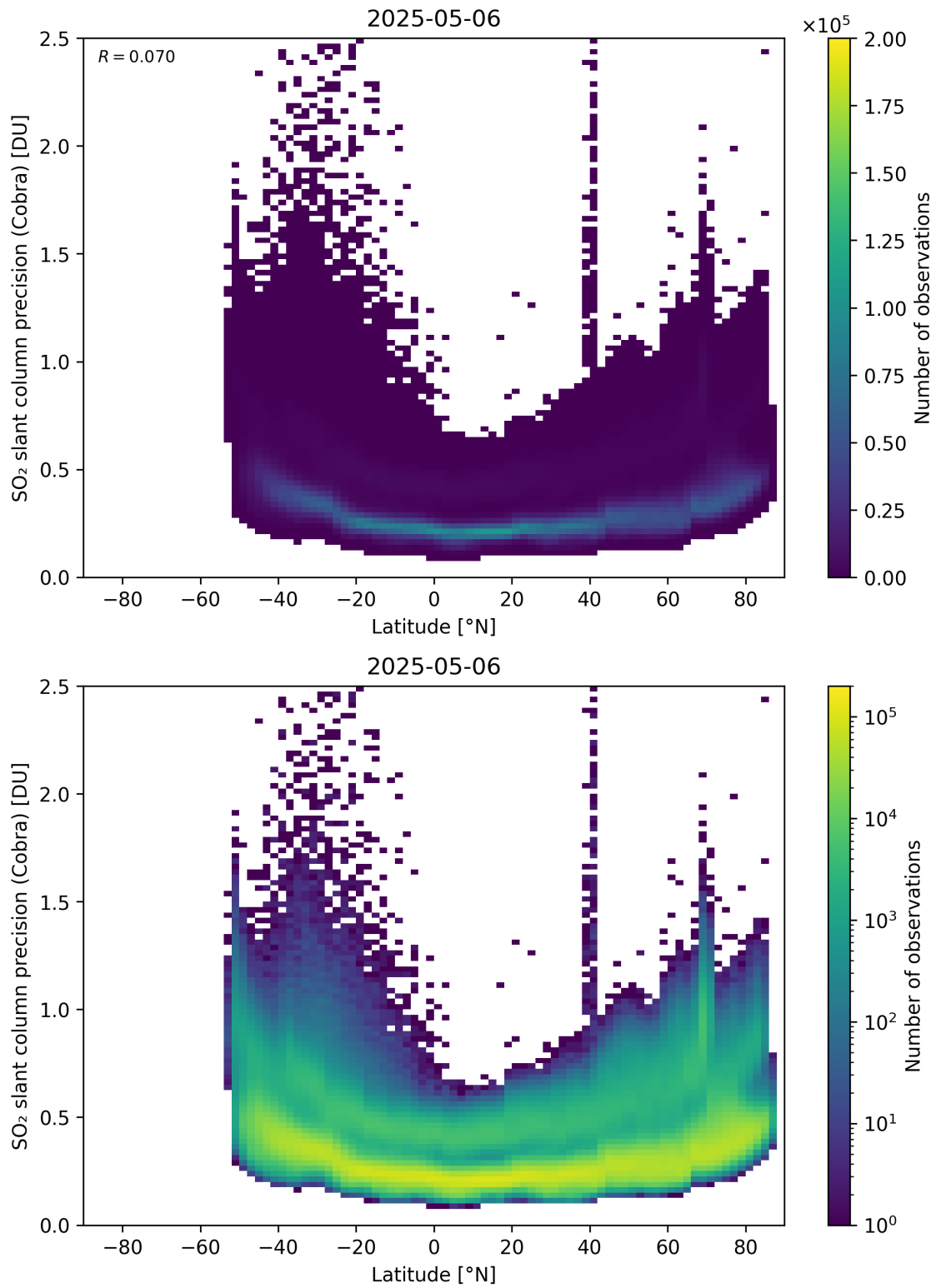
Figure 158: Scatter density plot of “Latitude” against “SO 2 slant column precision (Cobra)” for 2025-05-05 to 2025-05-07.
