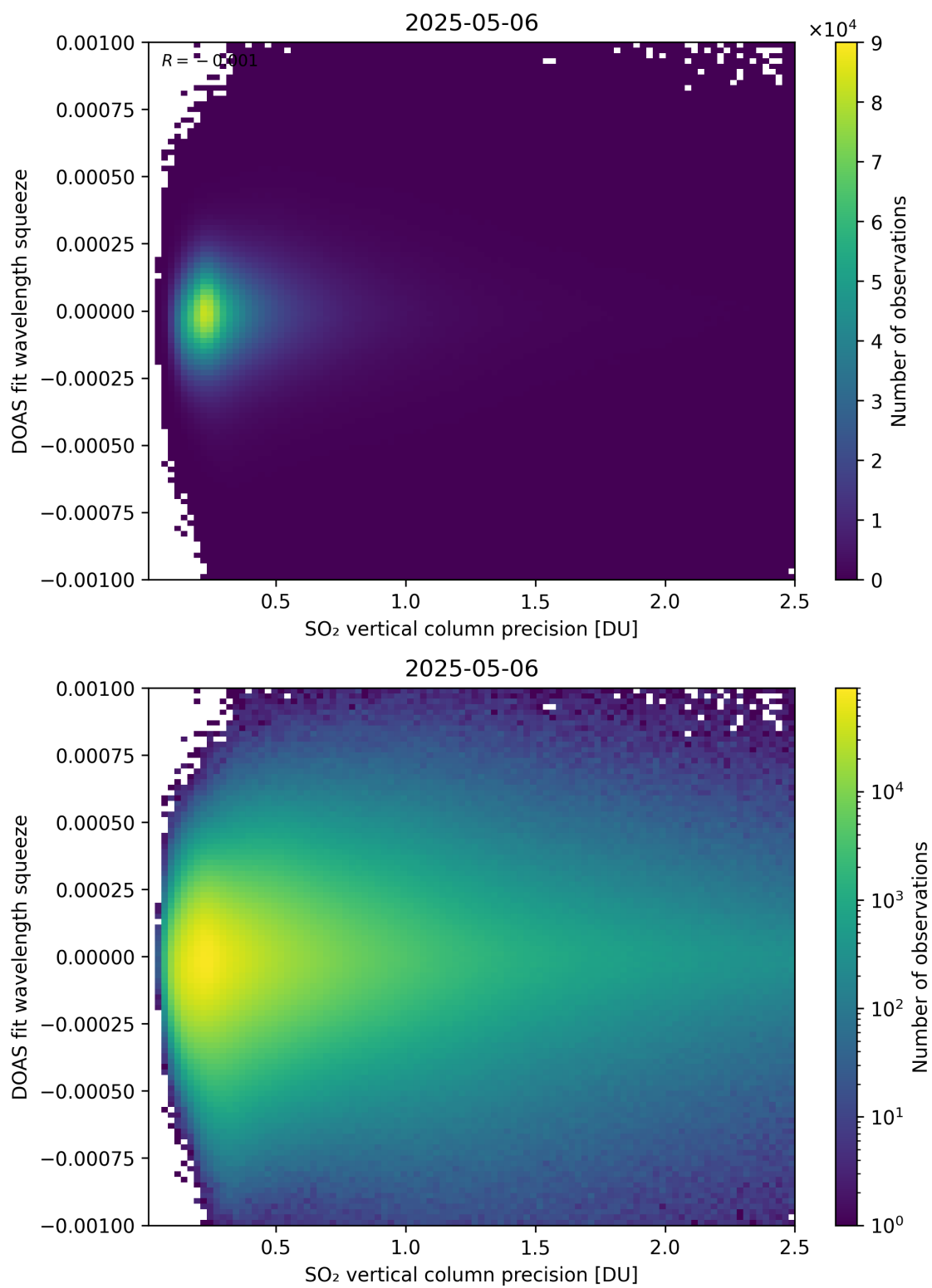
Figure 333: Scatter density plot of “SO 2 vertical column precision” against “DOAS fit wavelength squeeze” for 2025-05-05 to 2025-05-07.
