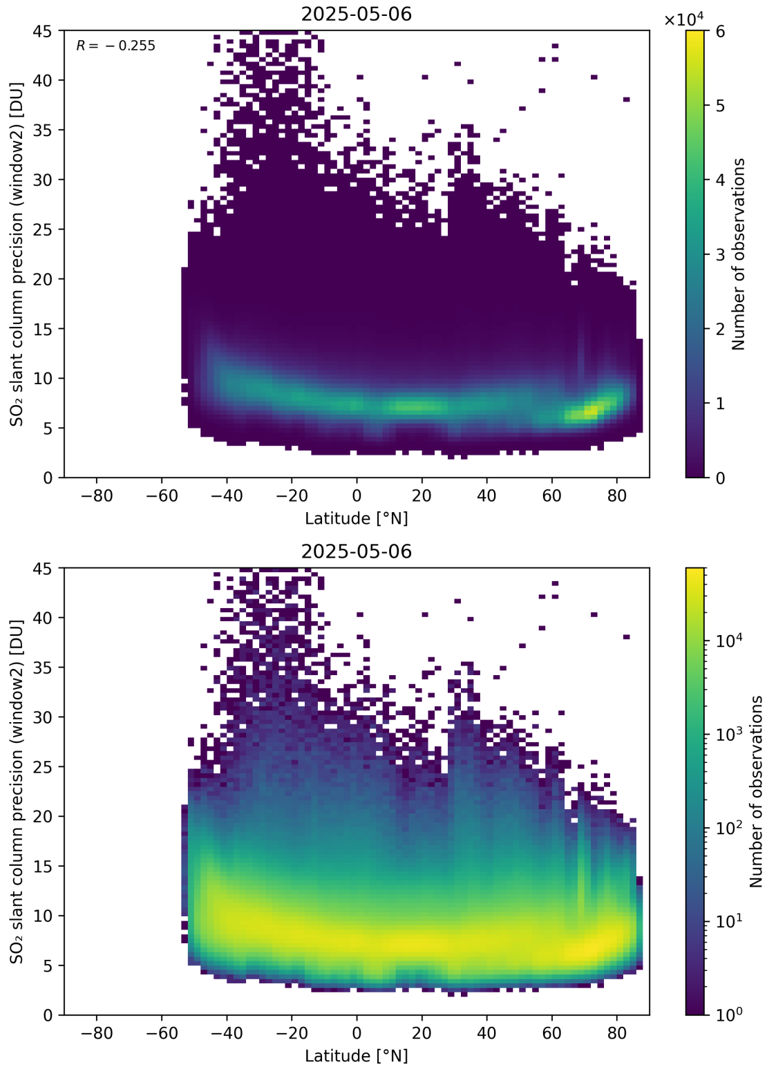
Figure 164: Scatter density plot of “Latitude” against “SO 2 slant column precision (window2)” for 2025-05-05 to 2025-05-07.
