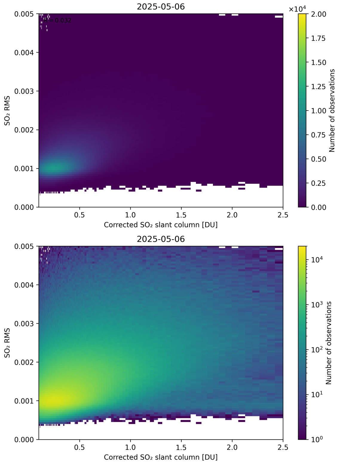
Figure 231: Scatter density plot of “Corrected SO 2 slant column” against “SO 2 RMS” for 2025-05-05 to 2025-05-07.
