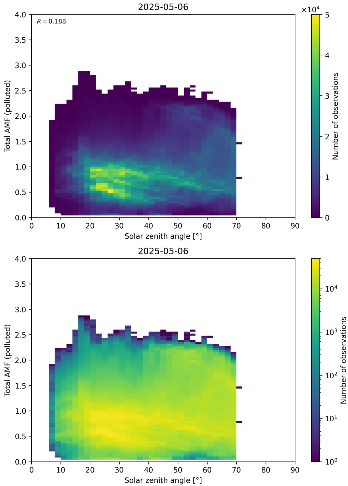
Figure 189: Scatter density plot of “Solar zenith angle” against “Total AMF (polluted)” for 2025-05-05 to 2025-05-07.
