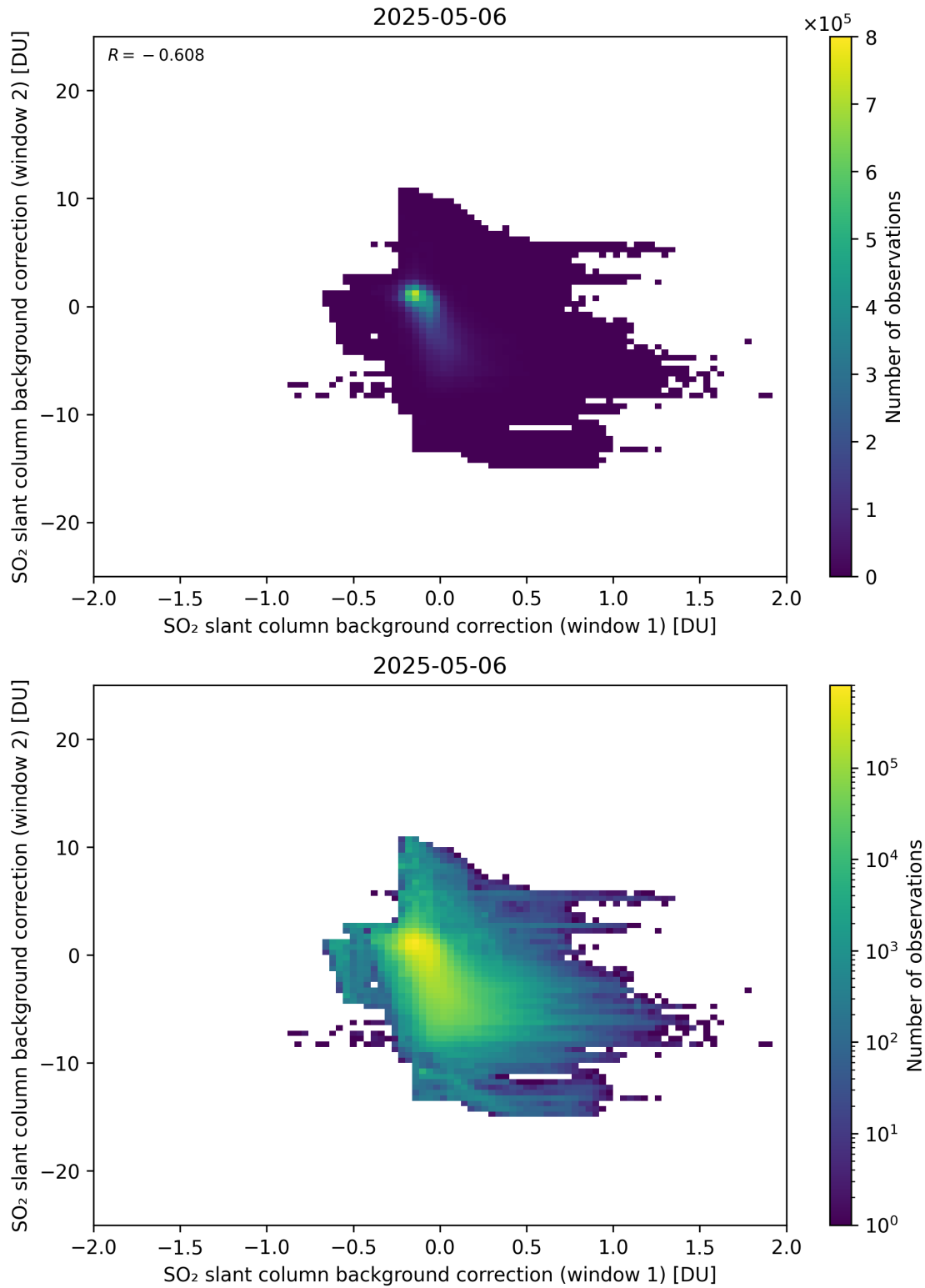
Figure 109: Scatter density plot of “SO 2 slant column background correction (window 1)” against “SO 2 slant column background correction (window 2)” for 2025-05-05 to 2025-05-07.
