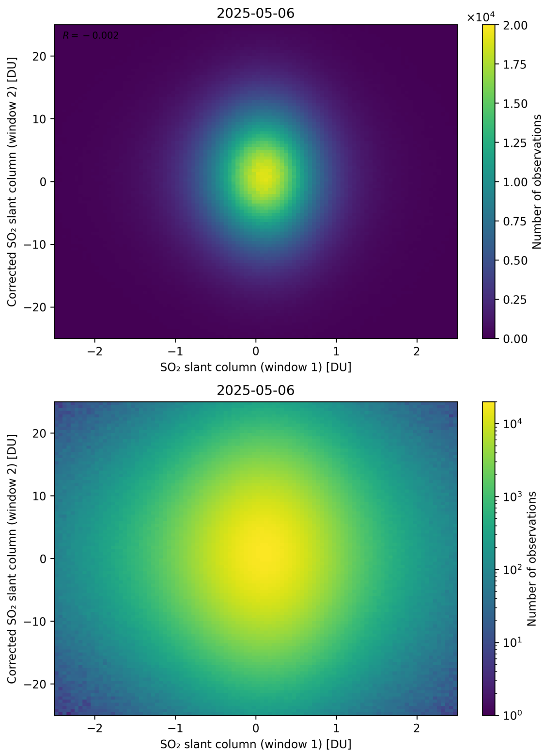
Figure 283: Scatter density plot of “SO 2 slant column (window 1)” against “Corrected SO 2 slant column (window 2)” for 2025-05-05 to 2025-05-07.
