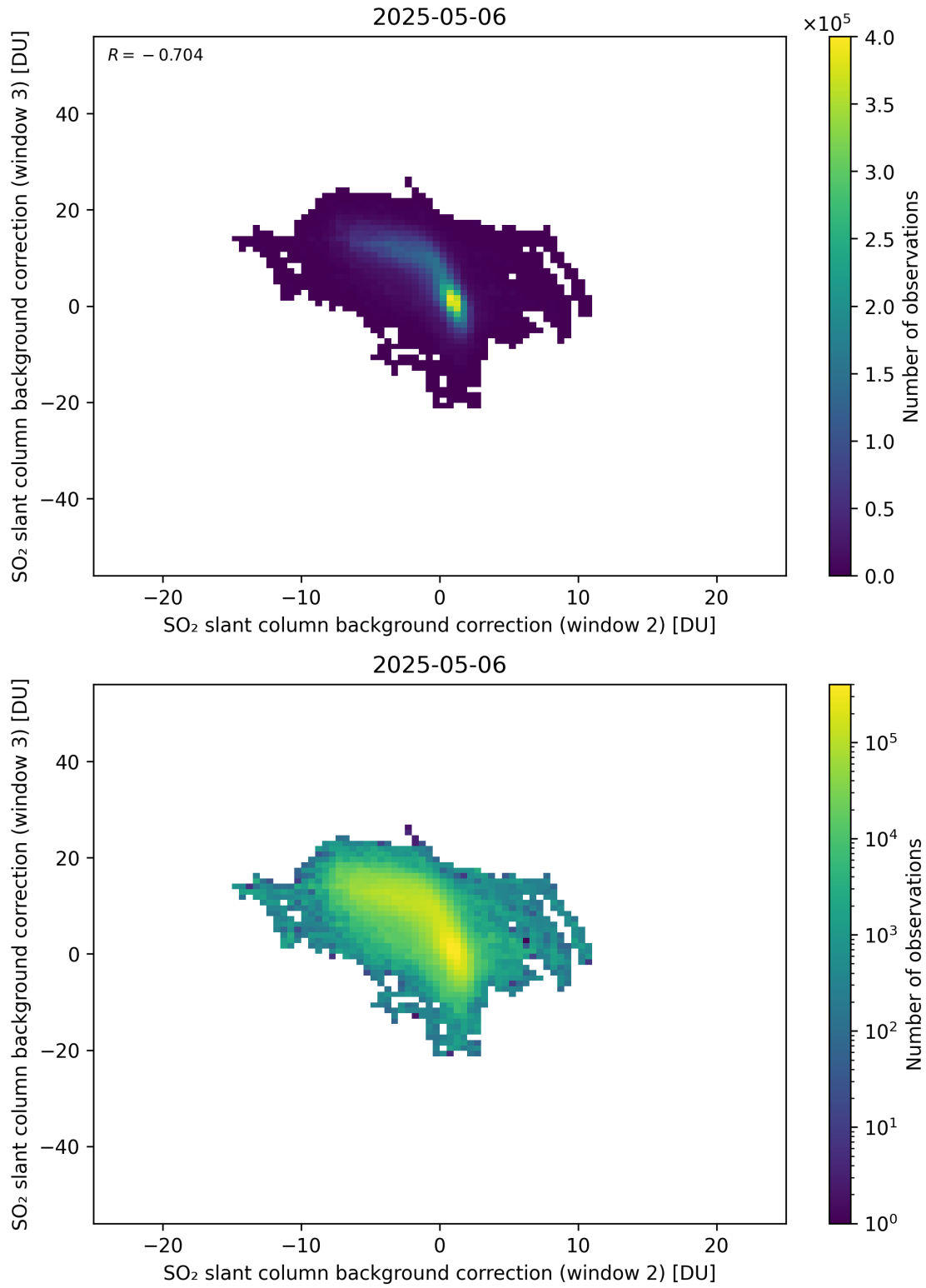
Figure 122: Scatter density plot of “SO 2 slant column background correction (window 2)” against “SO 2 slant column background correction (window 3)” for 2025-05-05 to 2025-05-07.
