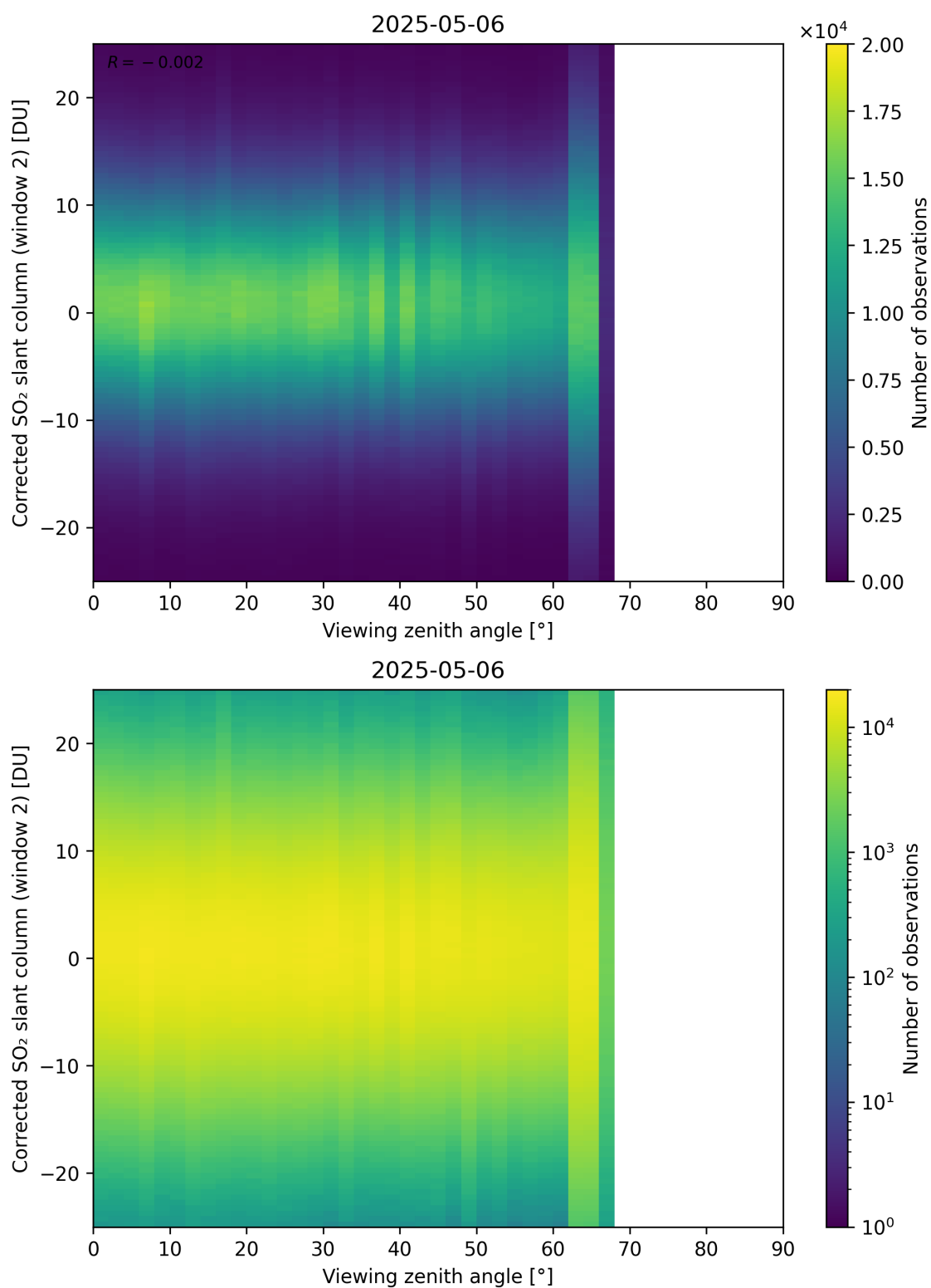
Figure 374: Scatter density plot of “Viewing zenith angle” against “Corrected SO 2 slant column (window 2)” for 2025-05-05 to 2025-05-07.
