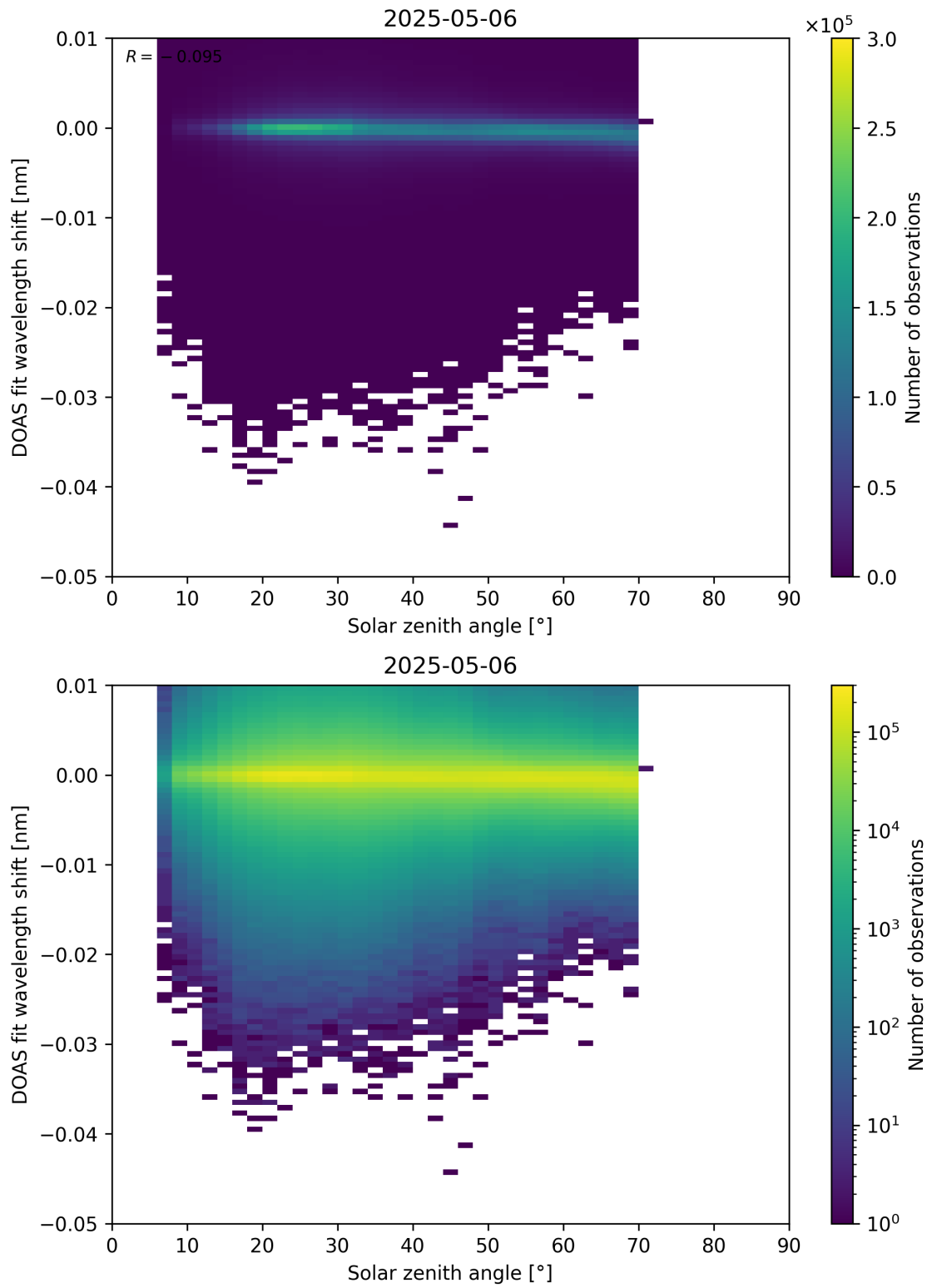
Figure 174: Scatter density plot of “Solar zenith angle” against “DOAS fit wavelength shift” for 2025-05-05 to 2025-05-07.
