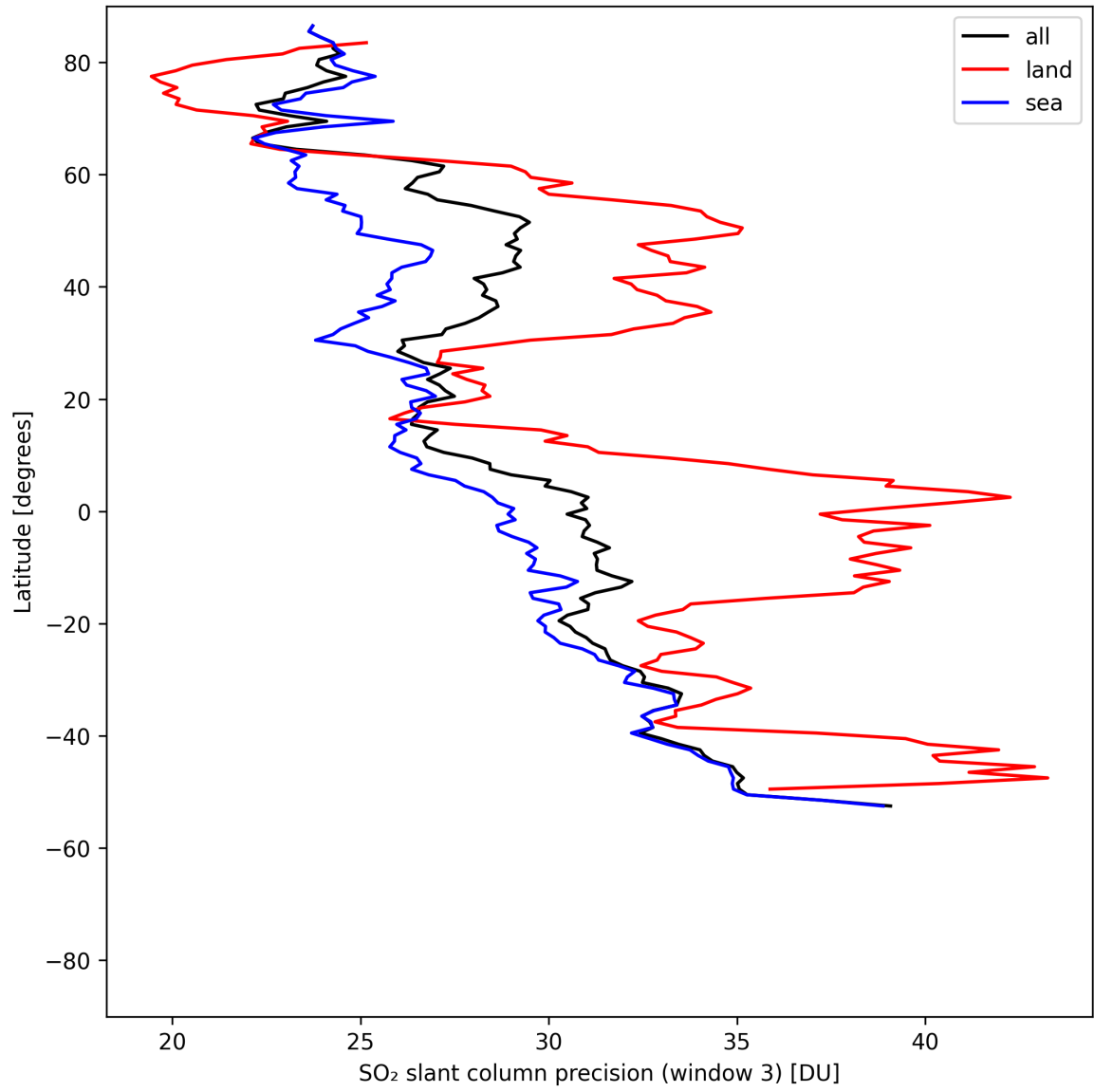
Figure 46: Zonal average of “SO 2 slant column precision (window 3)” for 2025-05-05 to 2025-05-07.
