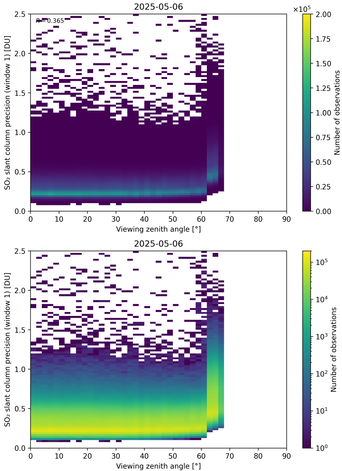
Figure 377: Scatter density plot of “Viewing zenith angle” against “SO 2 slant column precision (window 1)” for 2025-05-05 to 2025-05-07.
