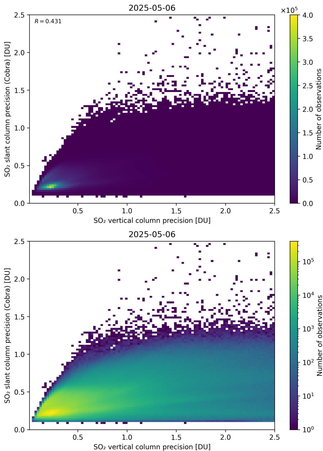
Figure 337: Scatter density plot of “SO 2 vertical column precision” against “SO 2 slant column precision (Cobra)” for 2025-05-05 to 2025-05-07.
