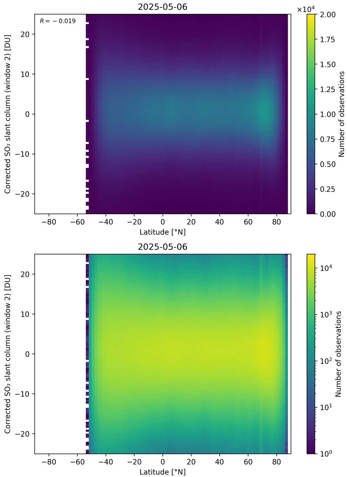
Figure 160: Scatter density plot of “Latitude” against “Corrected SO 2 slant column (window 2)” for 2025-05-05 to 2025-05-07.
