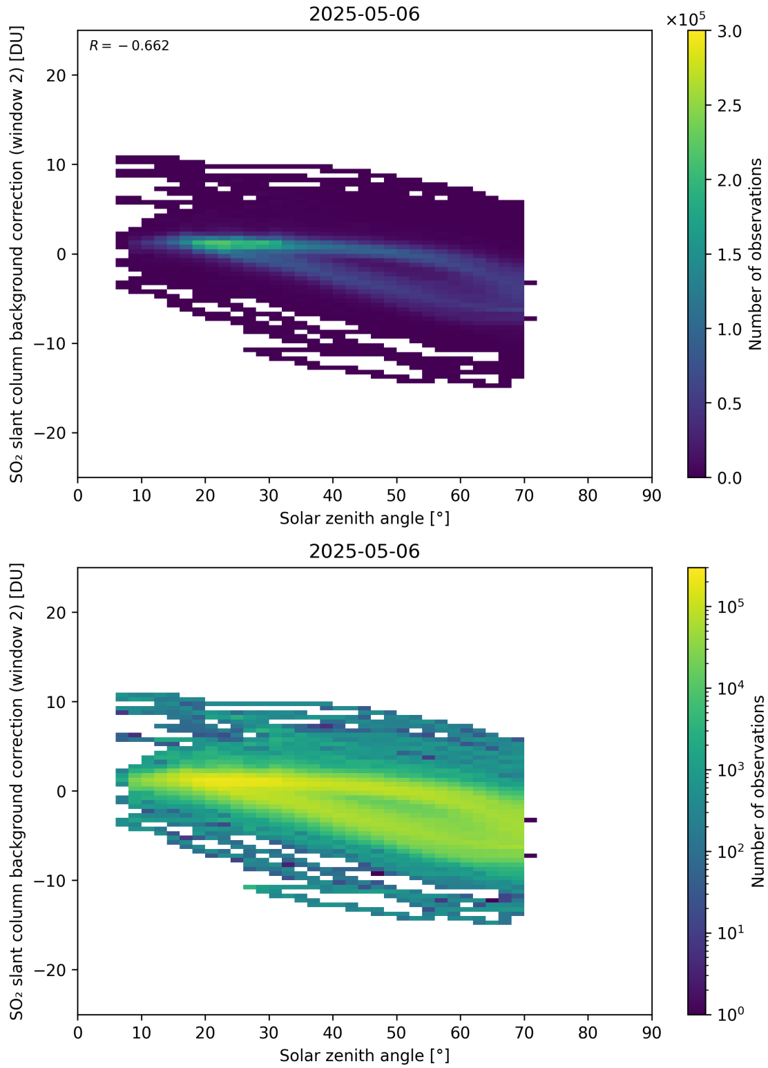
Figure 172: Scatter density plot of “Solar zenith angle” against “SO 2 slant column background correction (window 2)” for 2025-05-05 to 2025-05-07.
