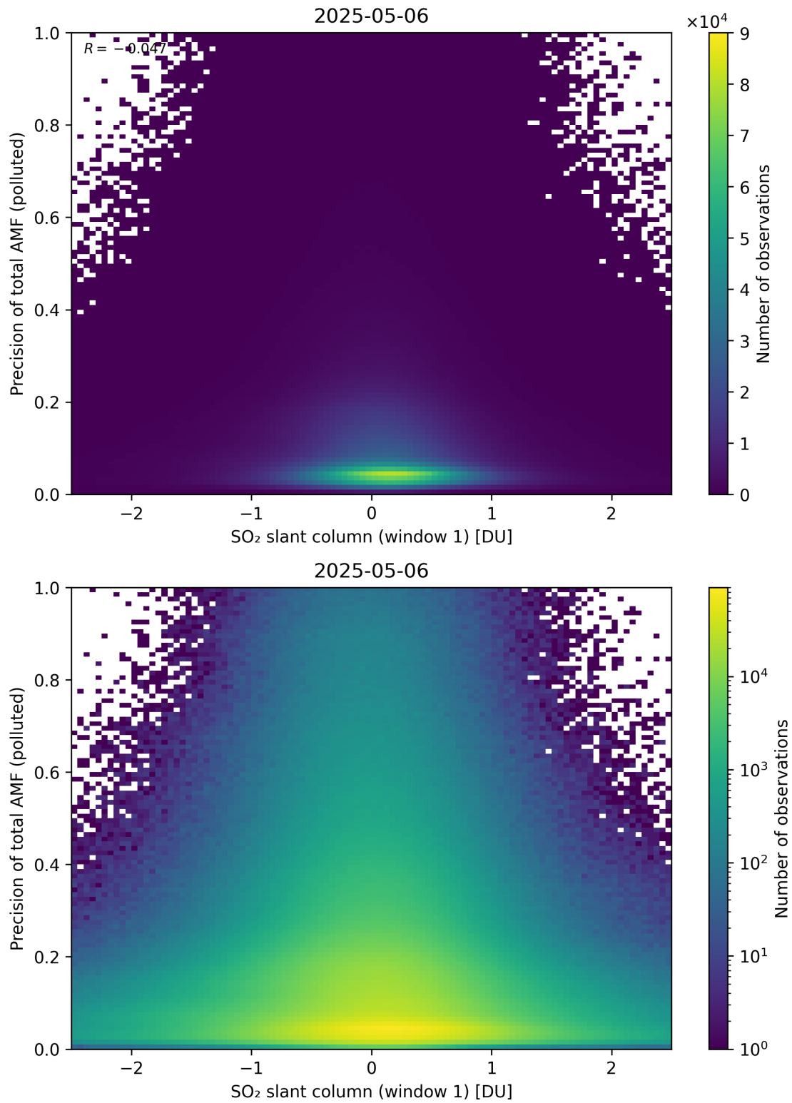
Figure 290: Scatter density plot of “SO 2 slant column (window 1)” against “Precision of total AMF (polluted)” for 2025-05-05 to 2025-05-07.
