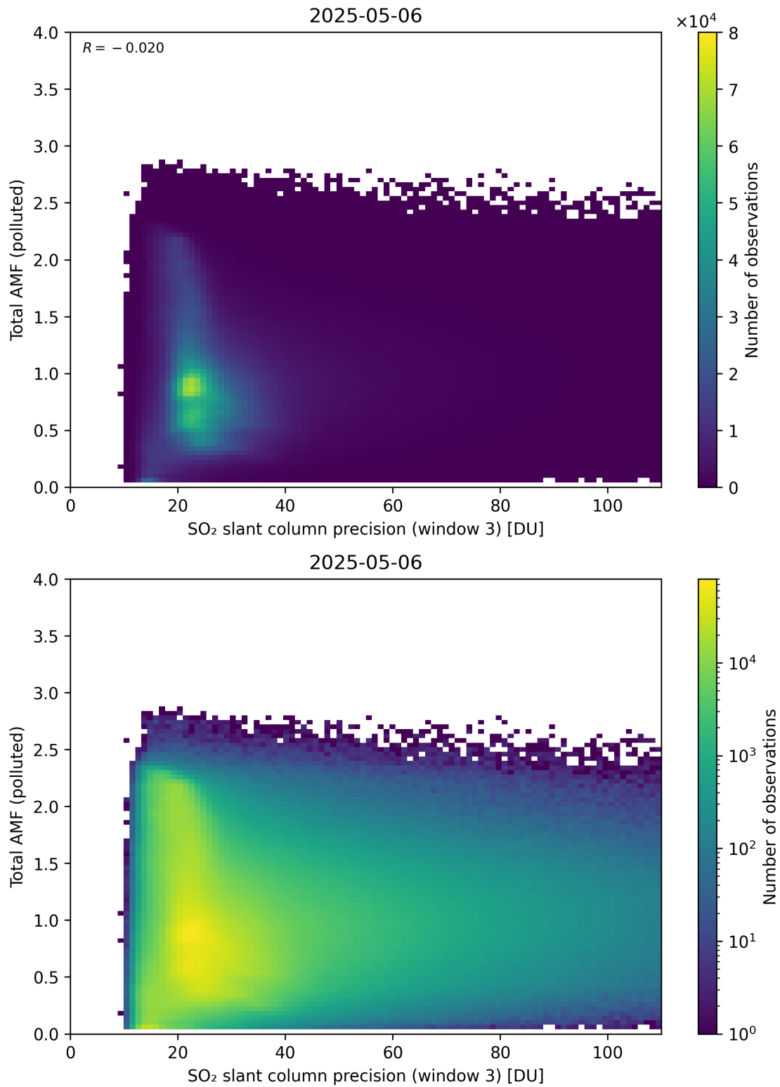
Figure 313: Scatter density plot of “SO 2 slant column precision (window 3)” against “Total AMF (polluted)” for 2025-05-05 to 2025-05-07.
