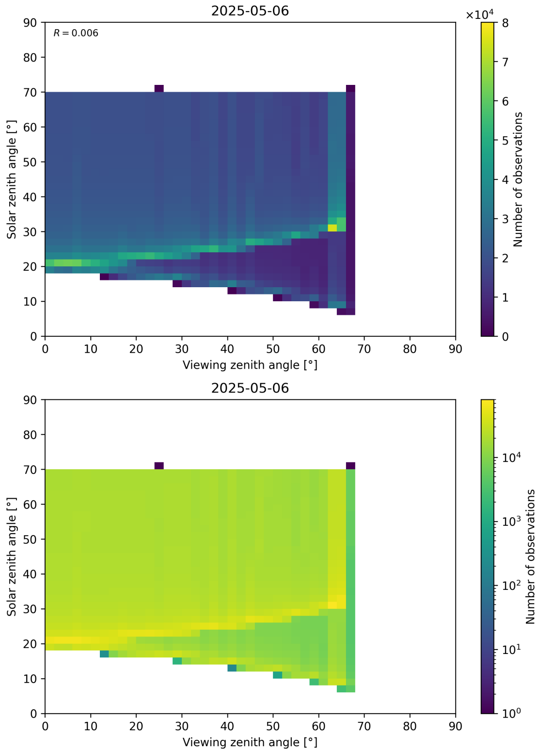
Figure 369: Scatter density plot of “Viewing zenith angle” against “Solar zenith angle” for 2025-05-05 to 2025-05-07.
