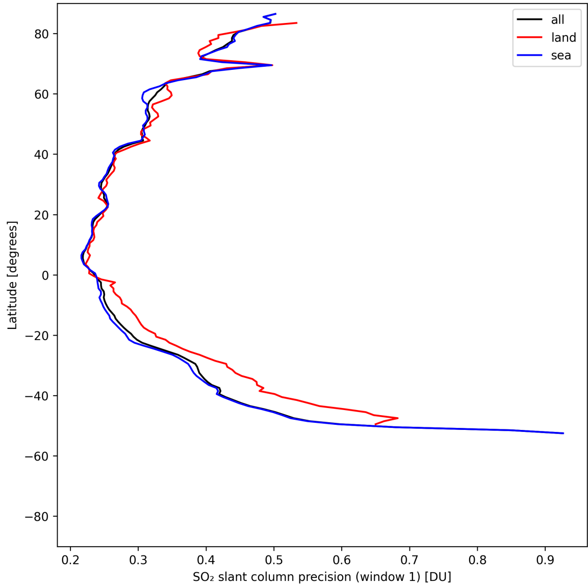
Figure 38: Zonal average of “SO 2 slant column precision (window 1)” for 2025-05-05 to 2025-05-07.
