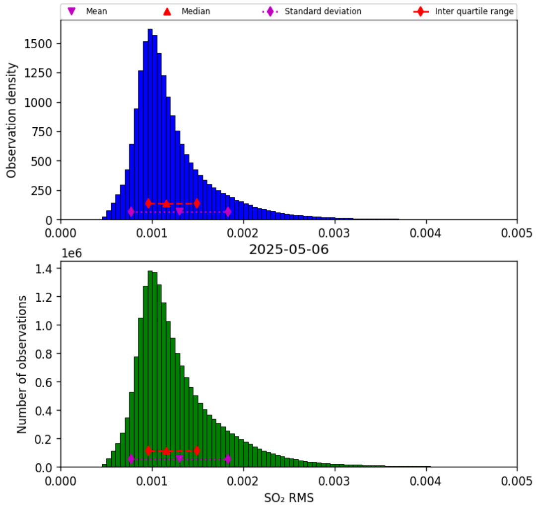
Figure 78: Histogram of “SO 2 RMS” for 2025-05-05 to 2025-05-07
