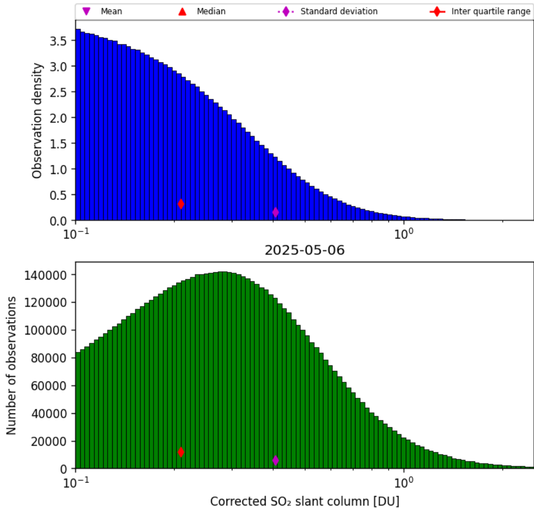
Figure 60: Histogram of “Corrected SO 2 slant column” for 2025-05-05 to 2025-05-07
