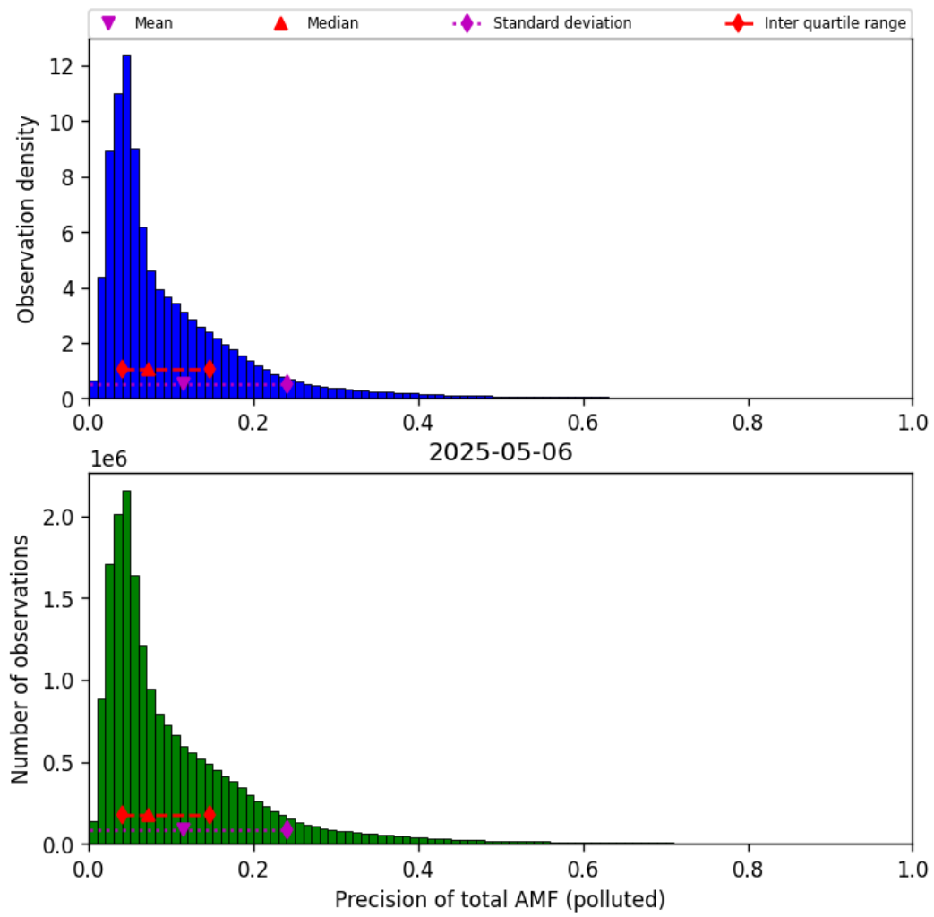
Figure 80: Histogram of “Precision of total AMF (polluted)” for 2025-05-05 to 2025-05-07
