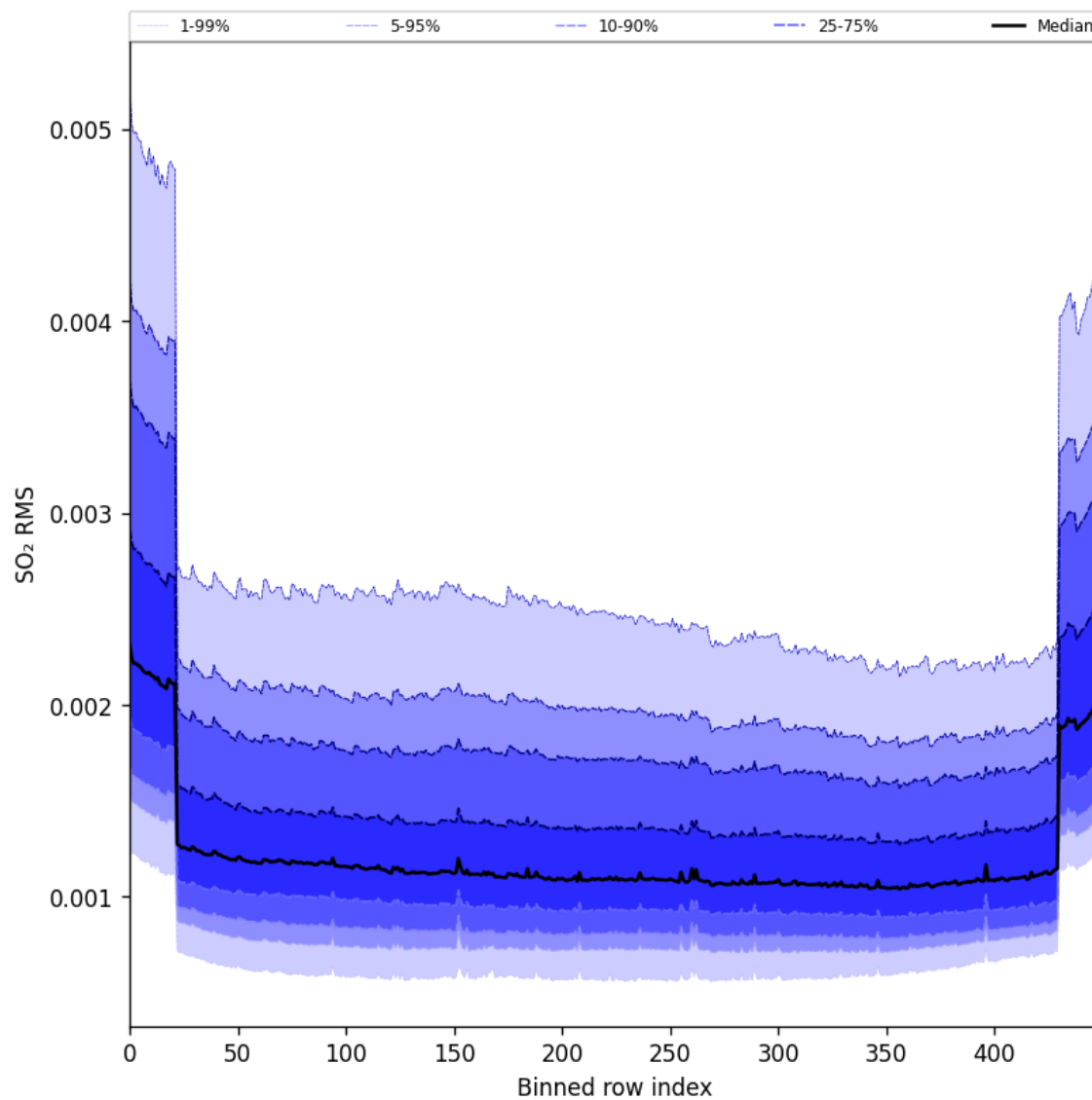
Figure 104: Along track statistics of “SO 2 RMS” for 2025-05-05 to 2025-05-07
