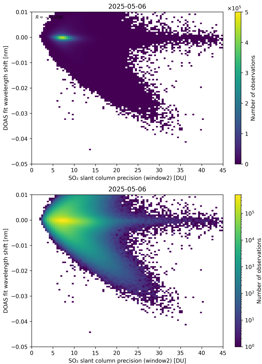
Figure 293: Scatter density plot of “SO 2 slant column precision (window2)” against “DOAS fit wavelength shift” for 2025-05-05 to 2025-05-07.
