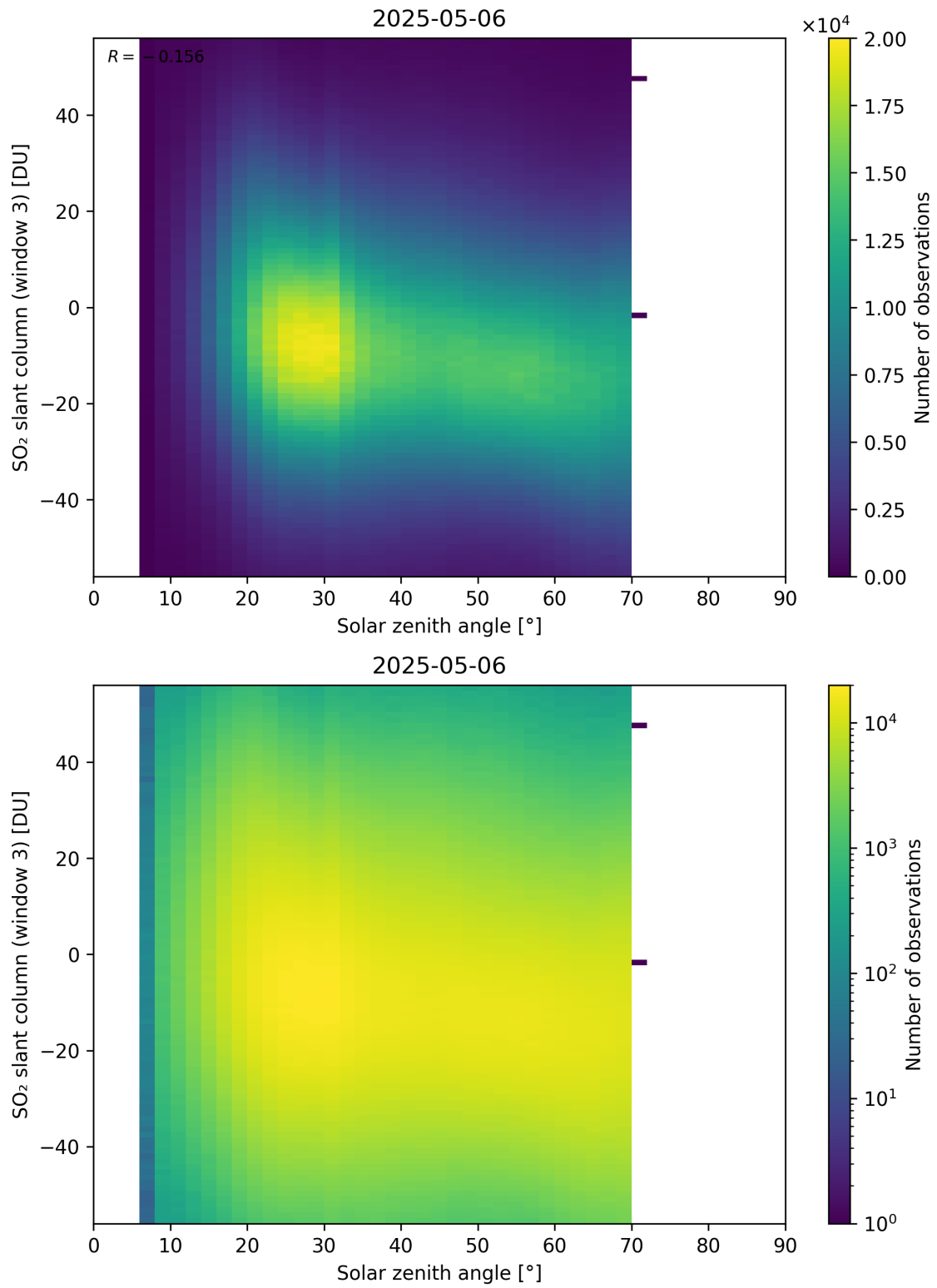
Figure 187: Scatter density plot of “Solar zenith angle” against “SO 2 slant column (window 3)” for 2025-05-05 to 2025-05-07.
