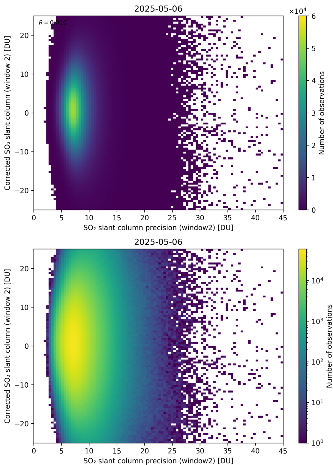
Figure 297: Scatter density plot of “SO 2 slant column precision (window2)” against “Corrected SO 2 slant column (window 2)” for 2025-05-05 to 2025-05-07.
