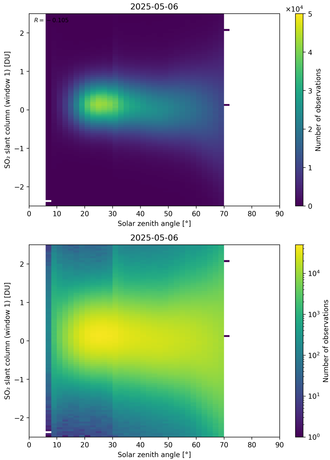
Figure 184: Scatter density plot of “Solar zenith angle” against “SO 2 slant column (window 1)” for 2025-05-05 to 2025-05-07.
