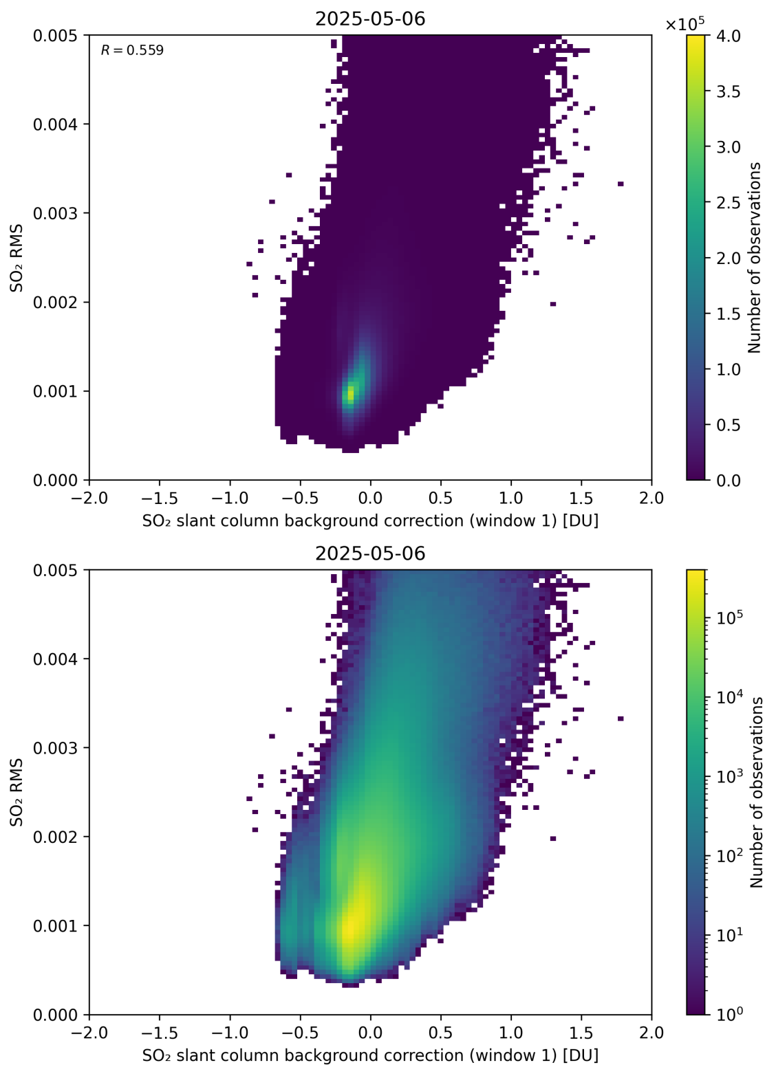
Figure 113: Scatter density plot of “SO 2 slant column background correction (window 1)” against “SO 2 RMS” for 2025-05-05 to 2025-05-07.
