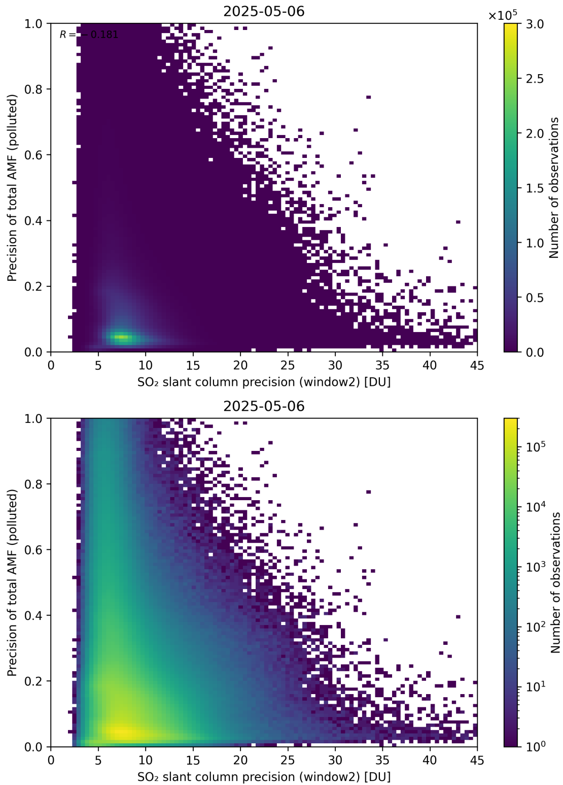
Figure 302: Scatter density plot of “SO 2 slant column precision (window2)” against “Precision of total AMF (polluted)” for 2025-05-05 to 2025-05-07.
