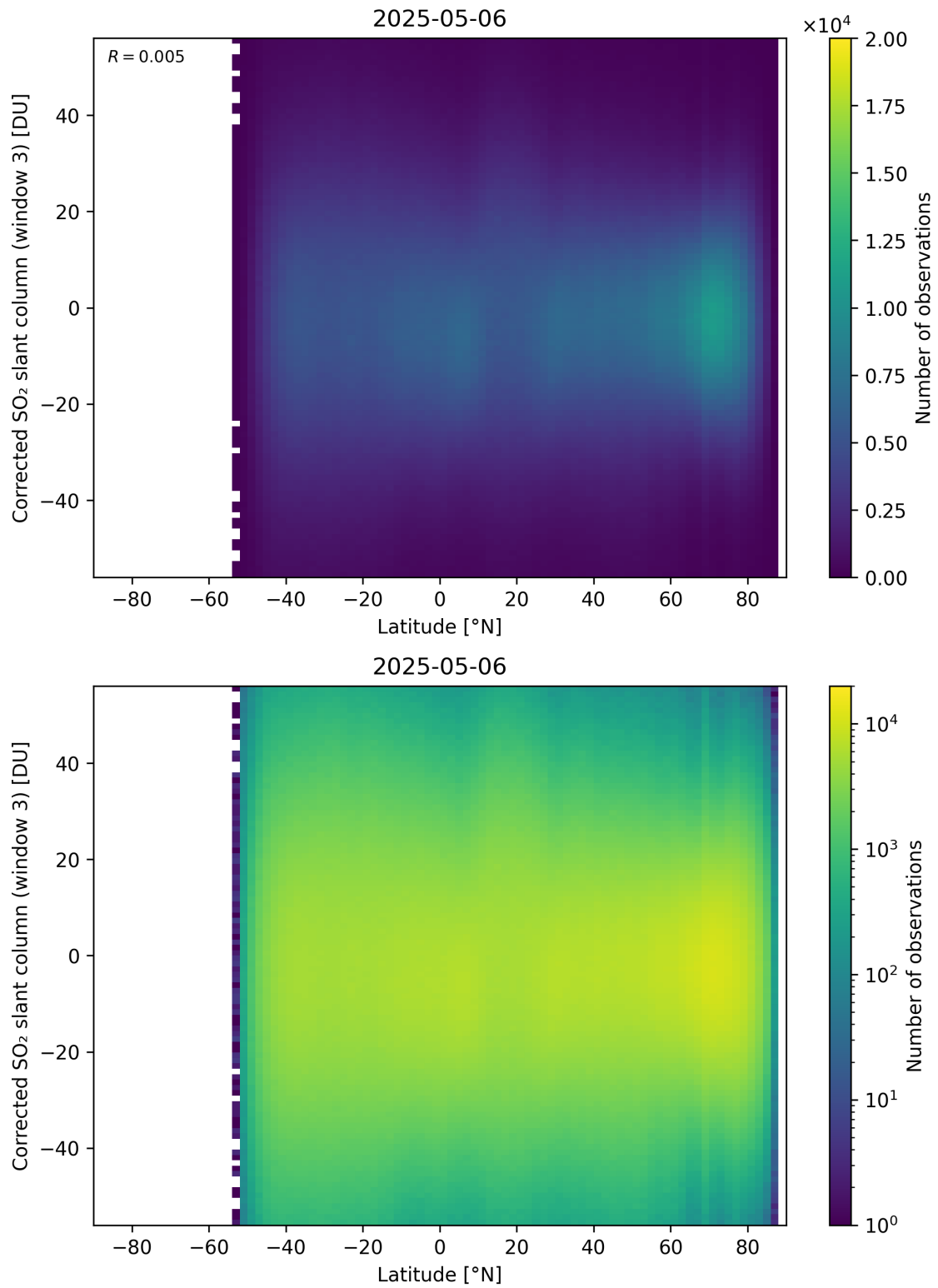
Figure 161: Scatter density plot of “Latitude” against “Corrected SO 2 slant column (window 3)” for 2025-05-05 to 2025-05-07.
