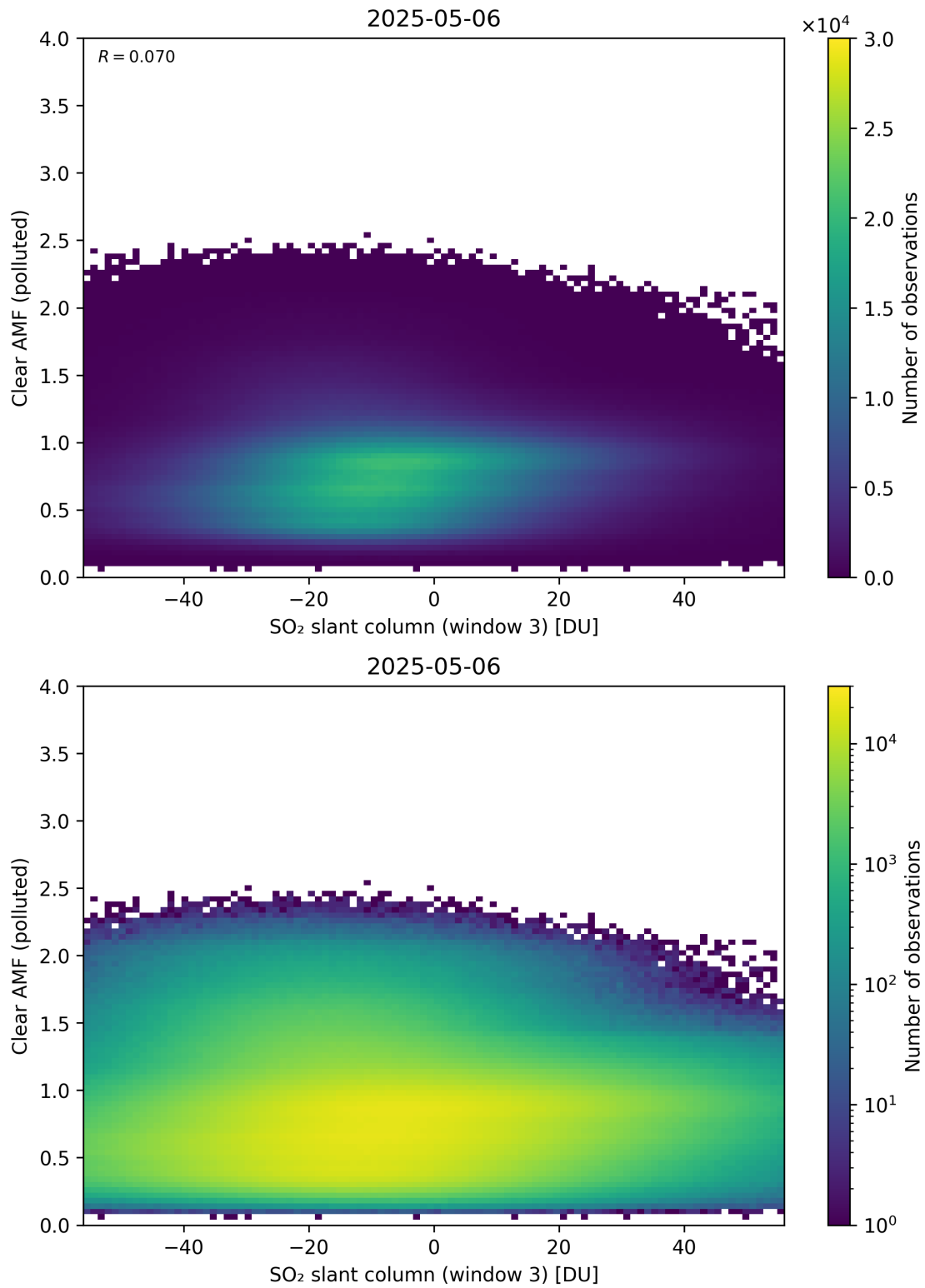
Figure 315: Scatter density plot of “SO 2 slant column (window 3)” against “Clear AMF (polluted)” for 2025-05-05 to 2025-05-07.
