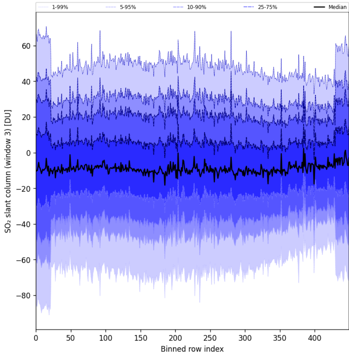
Figure 97: Along track statistics of “SO 2 slant column (window 3)” for 2025-05-05 to 2025-05-07
