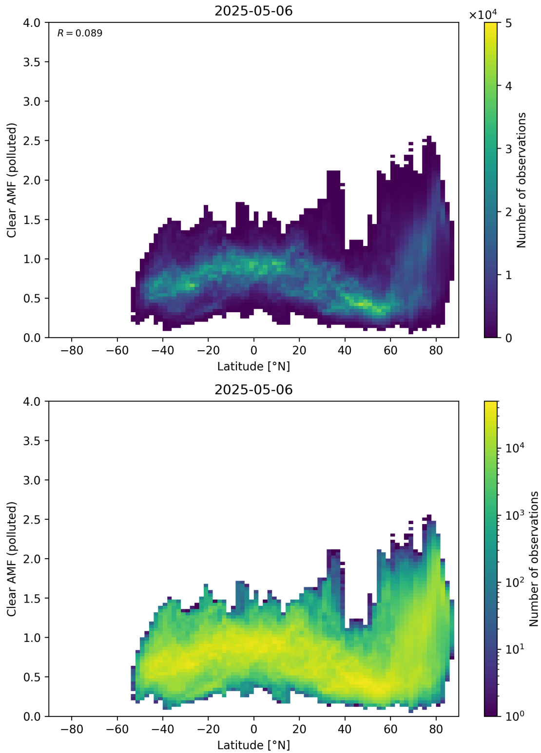
Figure 156: Scatter density plot of “Latitude” against “Clear AMF (polluted)” for 2025-05-05 to 2025-05-07.
