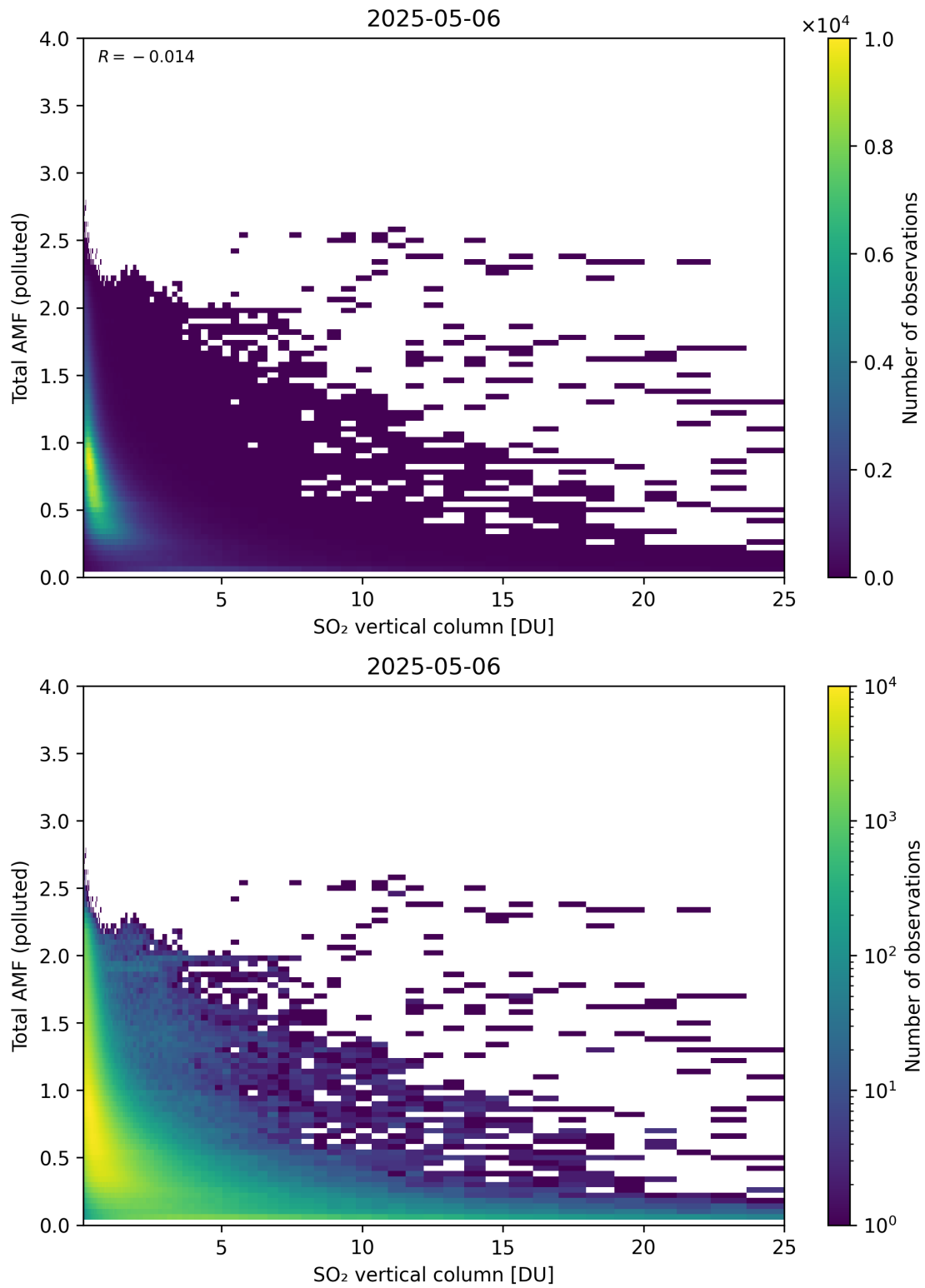
Figure 359: Scatter density plot of “SO 2 vertical column” against “Total AMF (polluted)” for 2025-05-05 to 2025-05-07.
