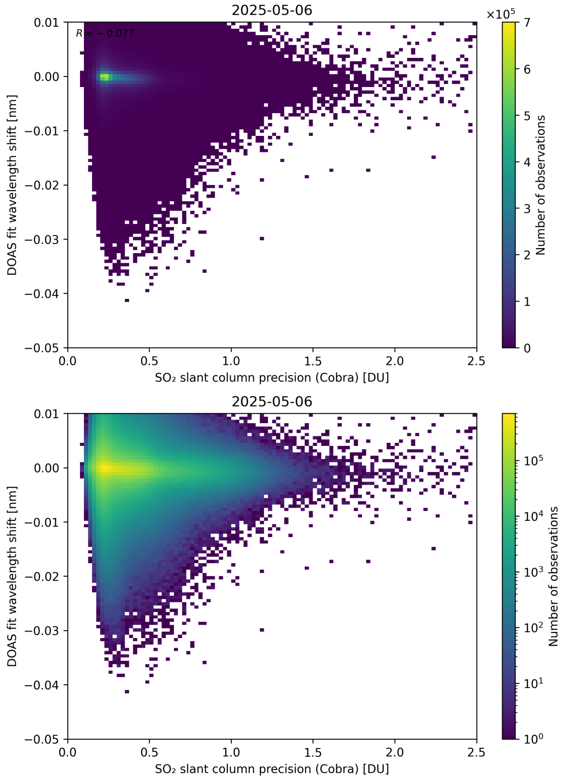
Figure 202: Scatter density plot of “SO 2 slant column precision (Cobra)” against “DOAS fit wavelength shift” for 2025-05-05 to 2025-05-07.
