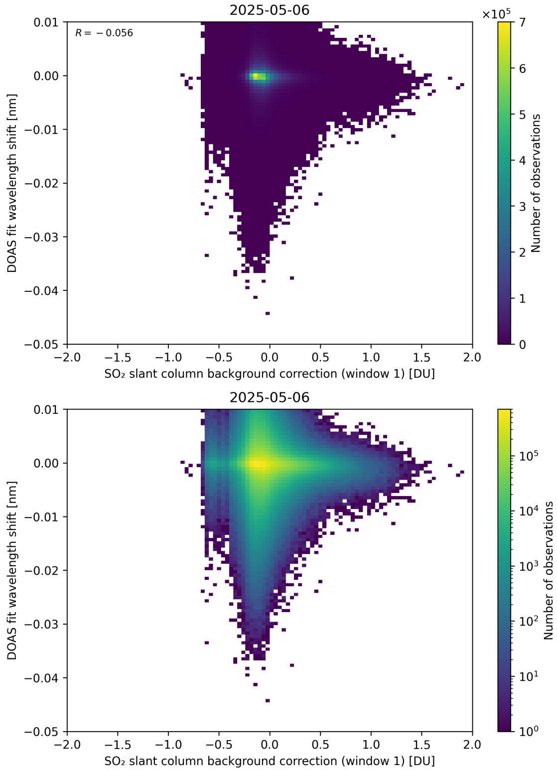
Figure 111: Scatter density plot of “SO 2 slant column background correction (window 1)” against “DOAS fit wavelength shift” for 2025-05-05 to 2025-05-07.
