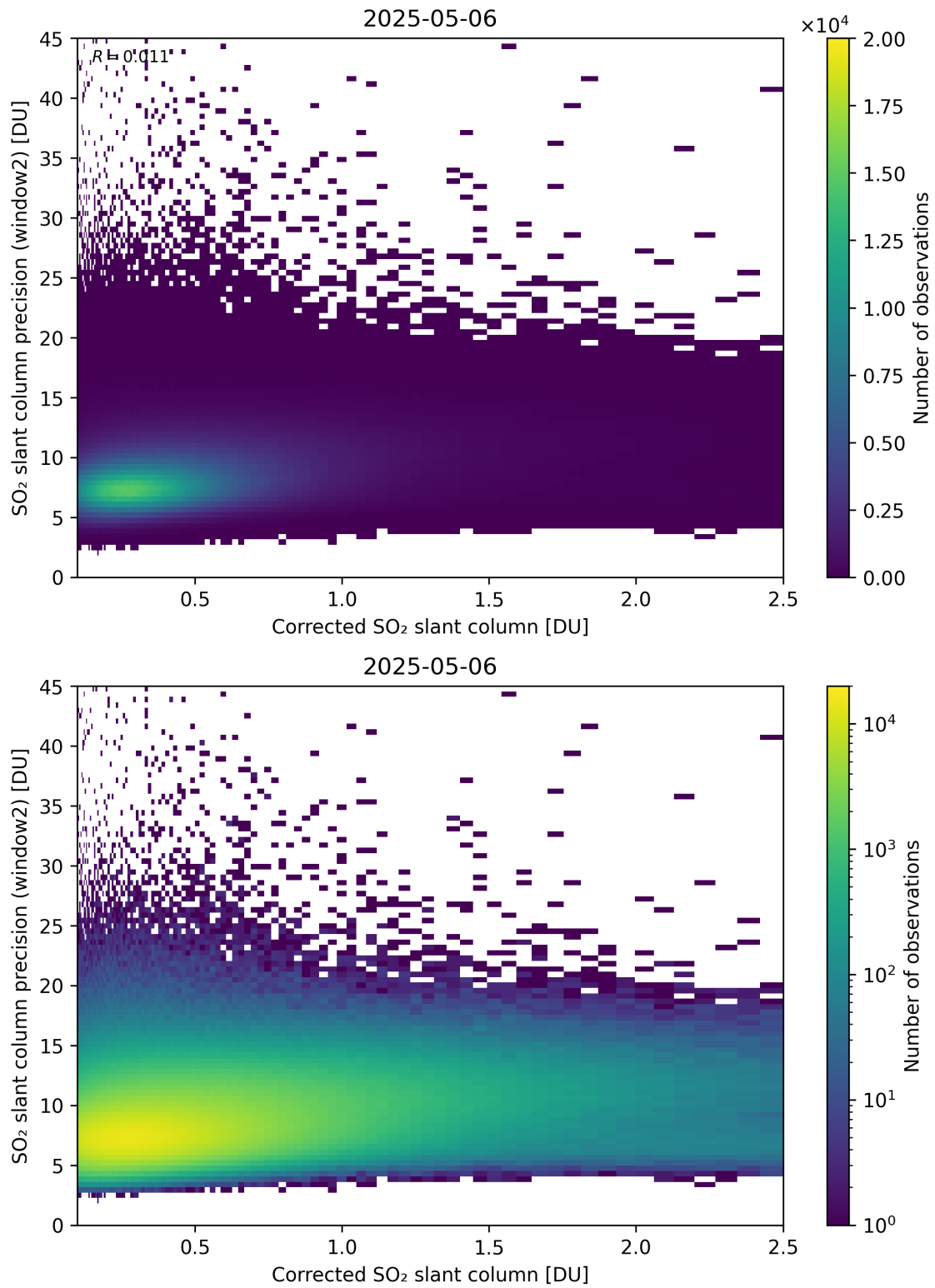
Figure 239: Scatter density plot of “Corrected SO 2 slant column” against “SO 2 slant column precision (window2)” for 2025-05-05 to 2025-05-07.
