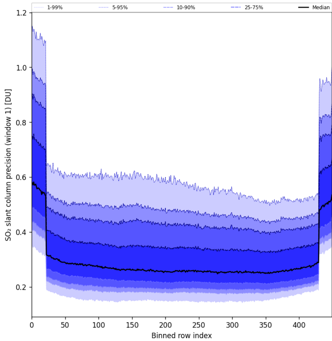
Figure 90: Along track statistics of “SO 2 slant column precision (window 1)” for 2025-05-05 to 2025-05-07
