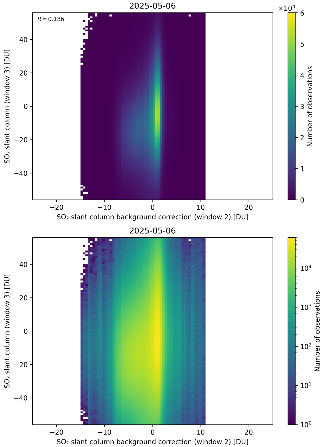
Figure 128: Scatter density plot of “SO 2 slant column background correction (window 2)” against “SO 2 slant column (window 3)” for 2025-05-05 to 2025-05-07.
