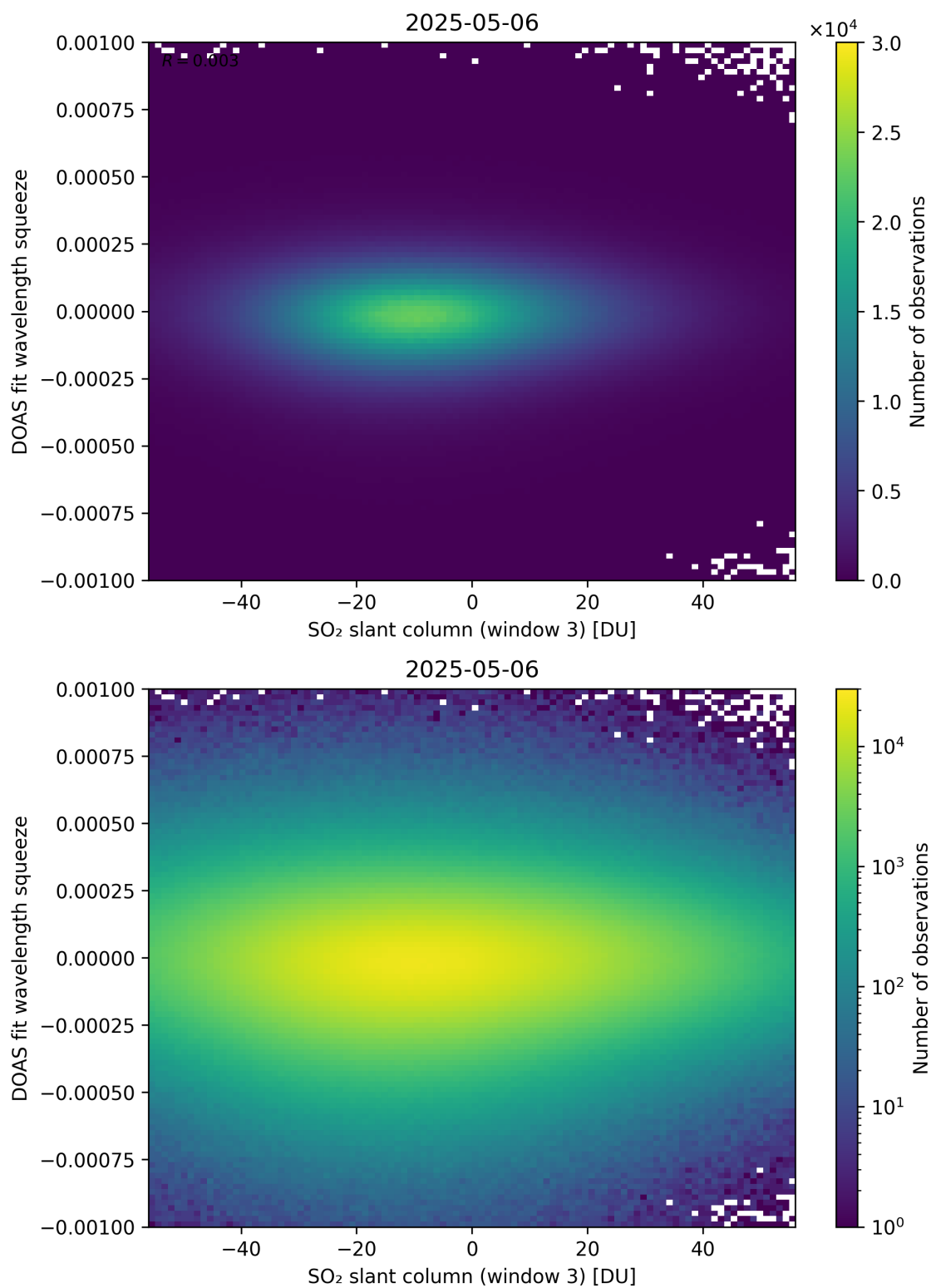
Figure 305: Scatter density plot of “SO 2 slant column (window 3)” against “DOAS fit wavelength squeeze” for 2025-05-05 to 2025-05-07.
