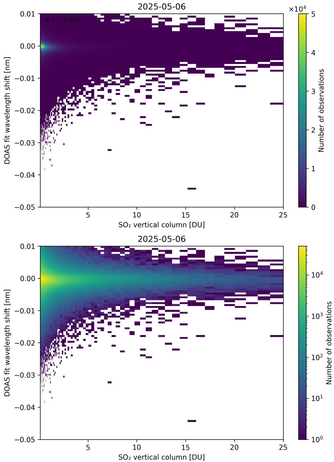
Figure 326: Scatter density plot of “SO 2 vertical column” against “DOAS fit wavelength shift” for 2025-05-05 to 2025-05-07.
