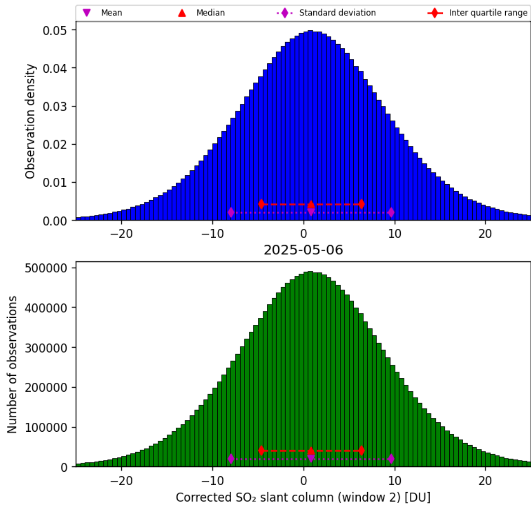
Figure 69: Histogram of “Corrected SO 2 slant column (window 2)” for 2025-05-05 to 2025-05-07
