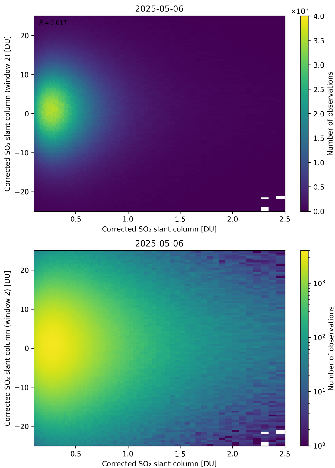
Figure 235: Scatter density plot of “Corrected SO 2 slant column” against “Corrected SO 2 slant column (window 2)” for 2025-05-05 to 2025-05-07.
