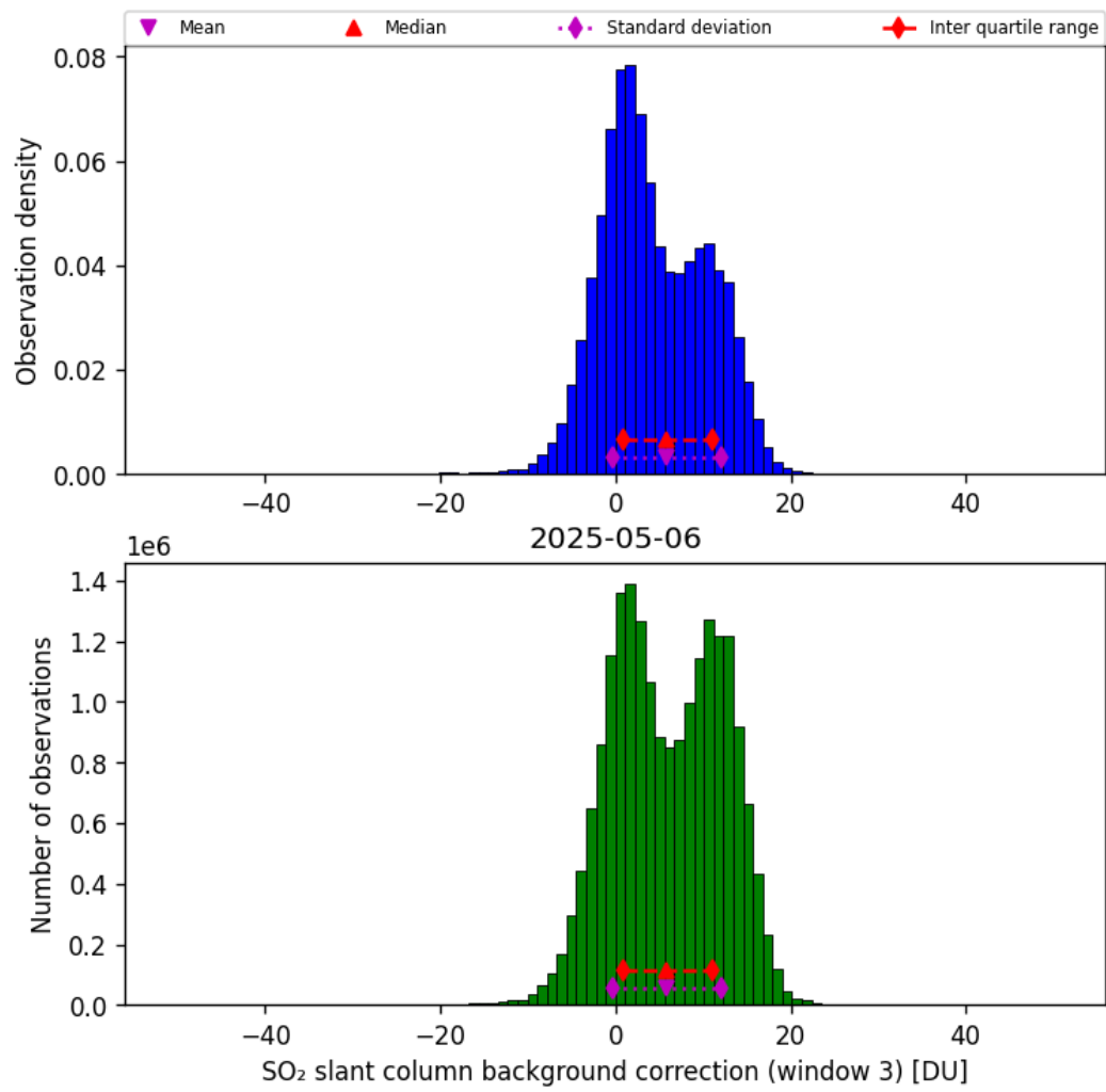
Figure 74: Histogram of “SO 2 slant column background correction (window 3)” for 2025-05-05 to 2025-05-07
