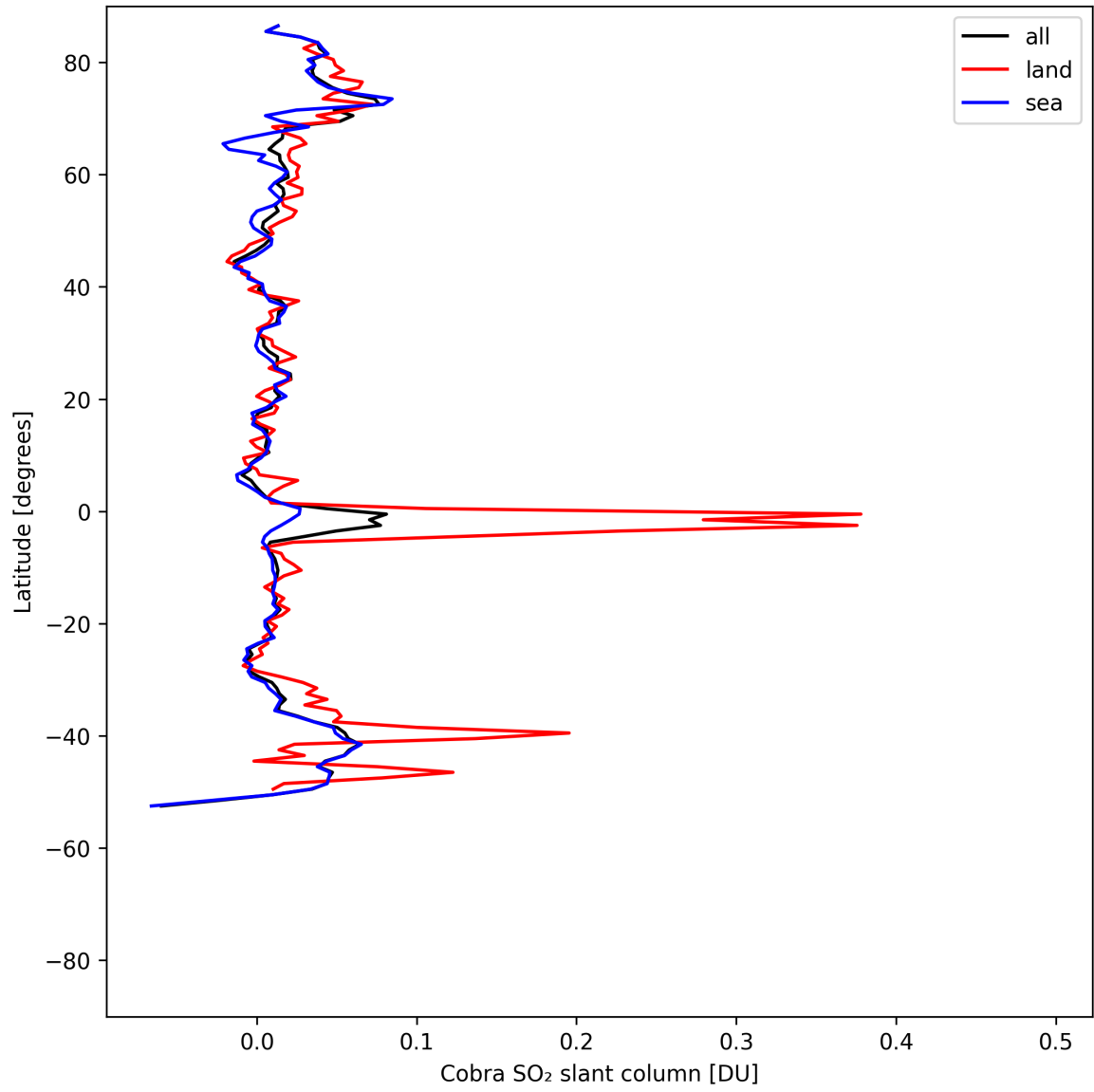
Figure 35: Zonal average of “Cobra SO 2 slant column” for 2025-05-05 to 2025-05-07.
