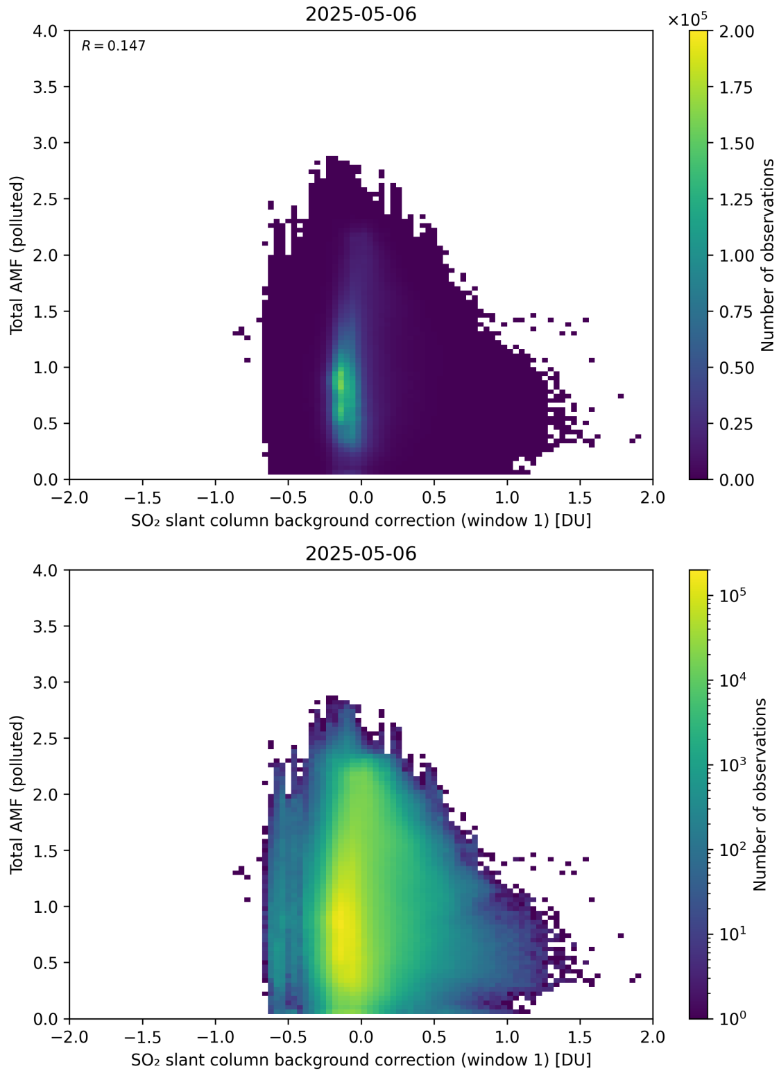
Figure 120: Scatter density plot of “SO 2 slant column background correction (window 1)” against “Total AMF (polluted)” for 2025-05-05 to 2025-05-07.
