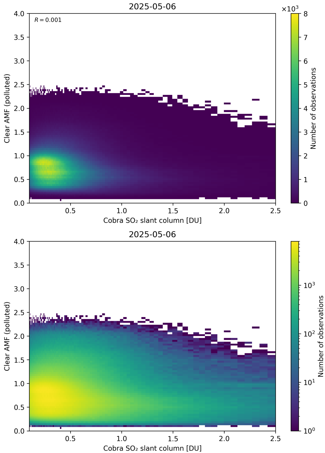
Figure 215: Scatter density plot of “Cobra SO 2 slant column” against “Clear AMF (polluted)” for 2025-05-05 to 2025-05-07.
