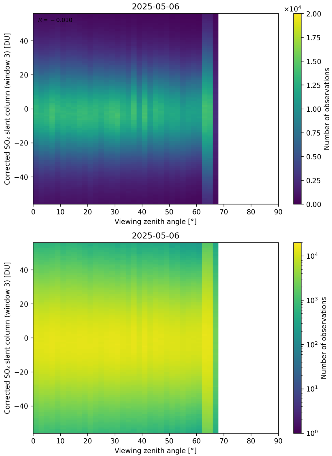
Figure 375: Scatter density plot of “Viewing zenith angle” against “Corrected SO 2 slant column (window 3)” for 2025-05-05 to 2025-05-07.
