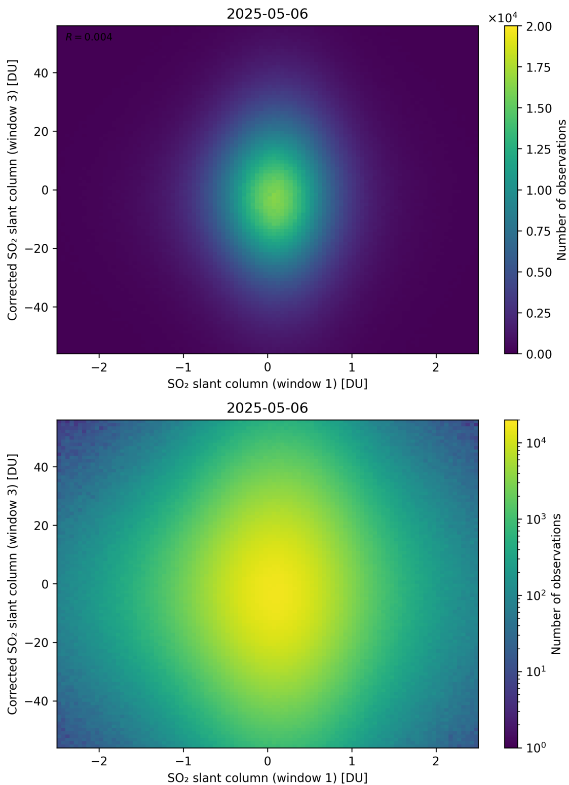
Figure 284: Scatter density plot of “SO 2 slant column (window 1)” against “Corrected SO 2 slant column (window 3)” for 2025-05-05 to 2025-05-07.
