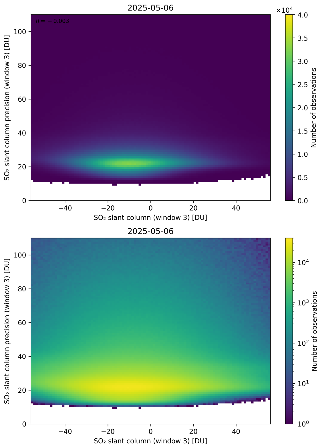
Figure 317: Scatter density plot of “SO 2 slant column (window 3)” against “SO 2 slant column precision (window 3)” for 2025-05-05 to 2025-05-07.
