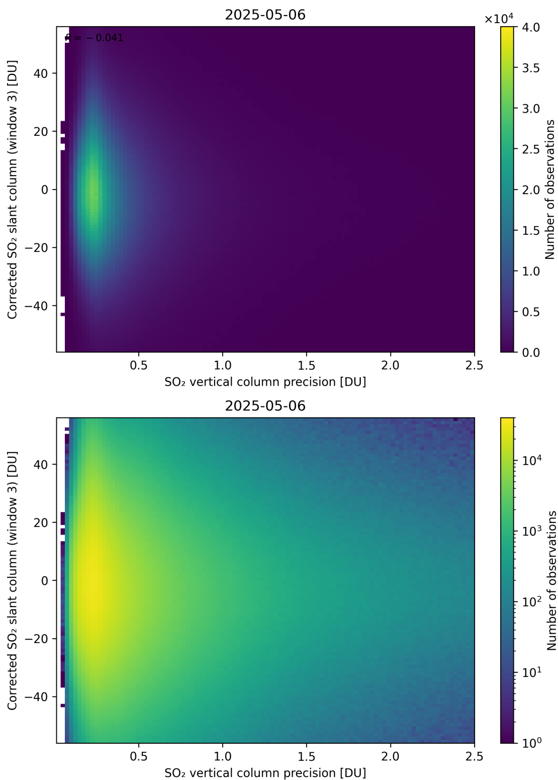
Figure 340: Scatter density plot of “SO 2 vertical column precision” against “Corrected SO 2 slant column (window 3)” for 2025-05-05 to 2025-05-07.
