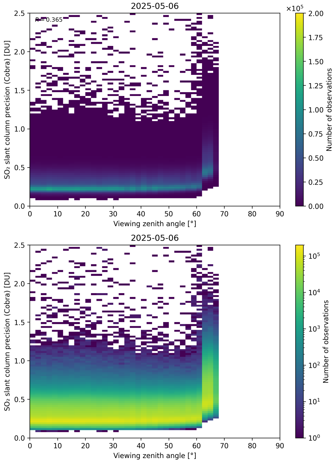
Figure 372: Scatter density plot of “Viewing zenith angle” against “SO 2 slant column precision (Cobra)” for 2025-05-05 to 2025-05-07.
