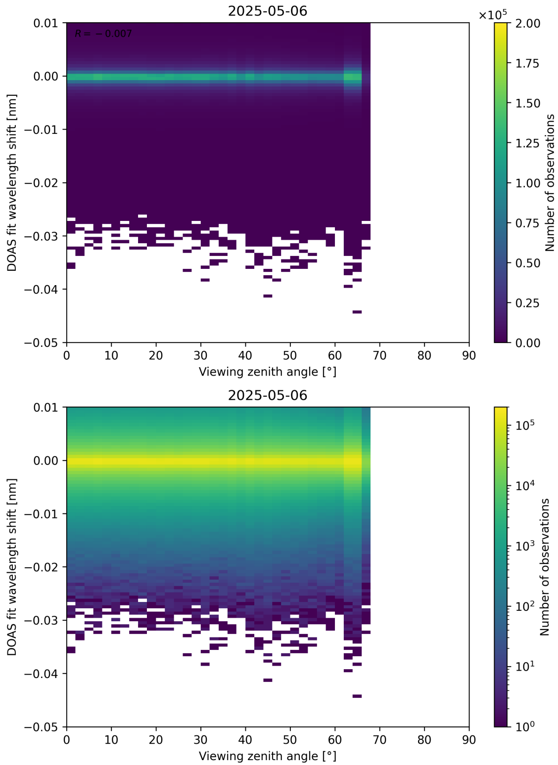
Figure 365: Scatter density plot of “Viewing zenith angle” against “DOAS fit wavelength shift” for 2025-05-05 to 2025-05-07.
