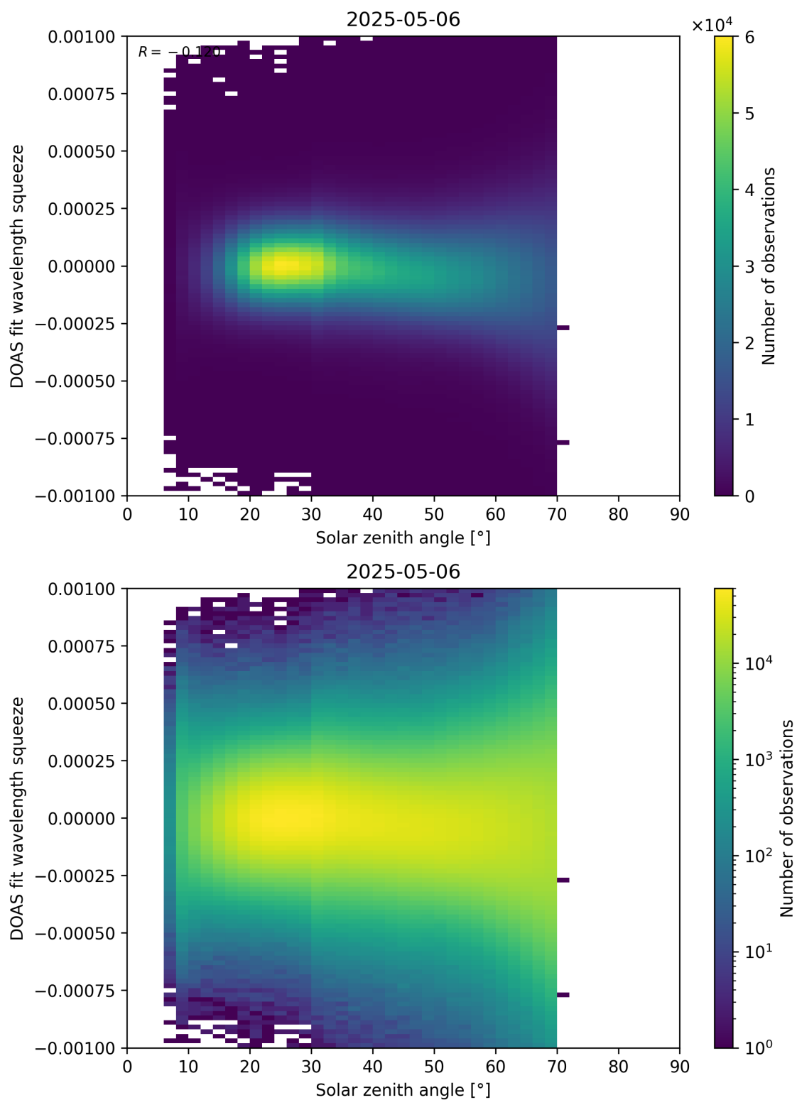
Figure 175: Scatter density plot of “Solar zenith angle” against “DOAS fit wavelength squeeze” for 2025-05-05 to 2025-05-07.
