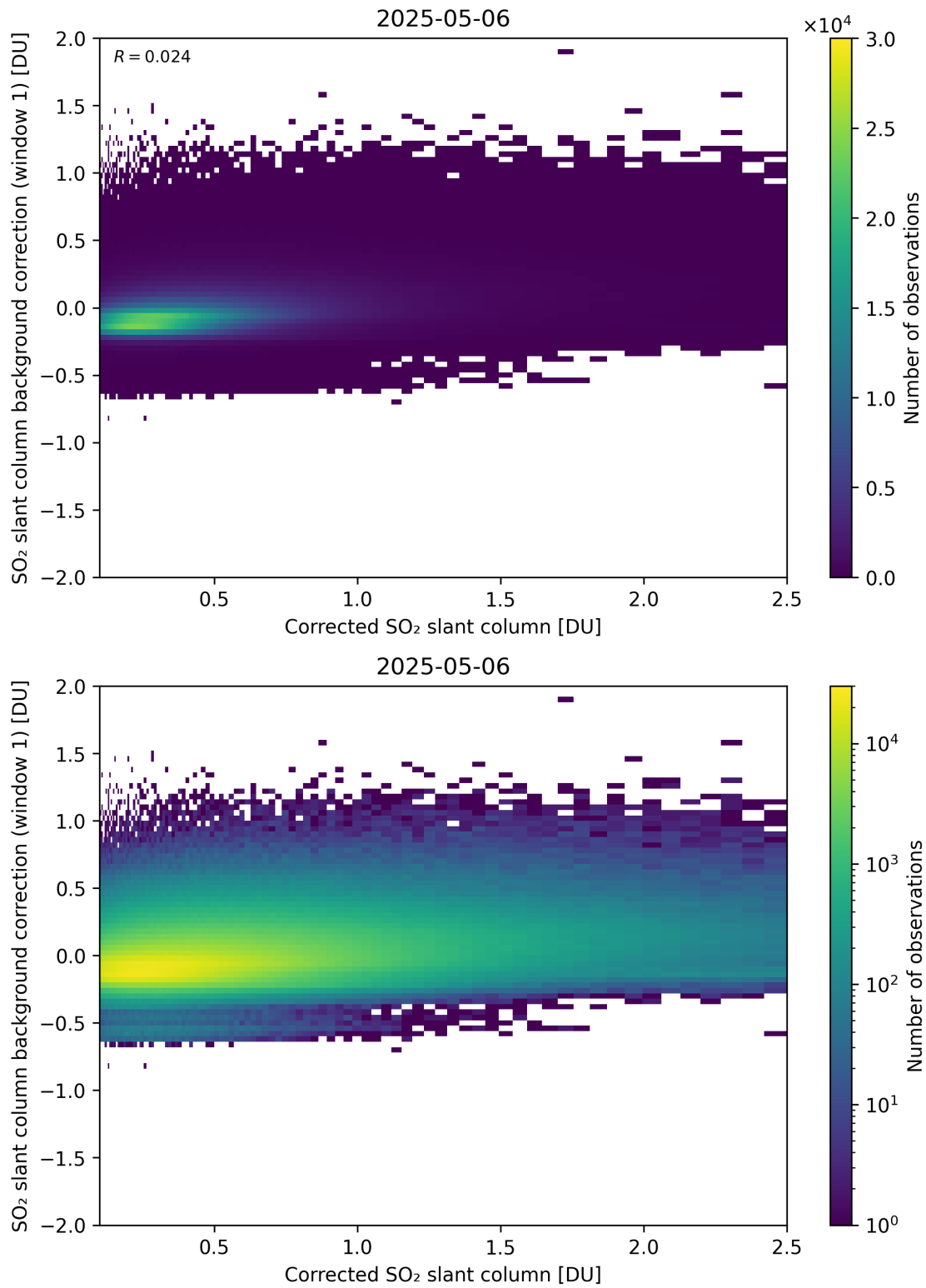
Figure 226: Scatter density plot of “Corrected SO 2 slant column” against “SO 2 slant column background correction (window 1)” for 2025-05-05 to 2025-05-07.
