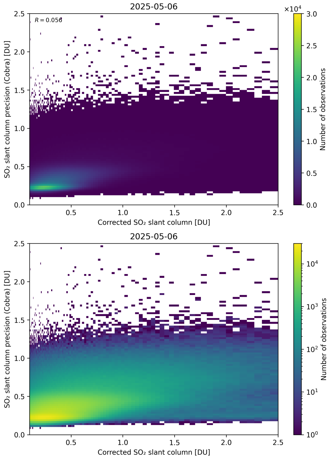
Figure 234: Scatter density plot of “Corrected SO 2 slant column” against “SO 2 slant column precision (Cobra)” for 2025-05-05 to 2025-05-07.
