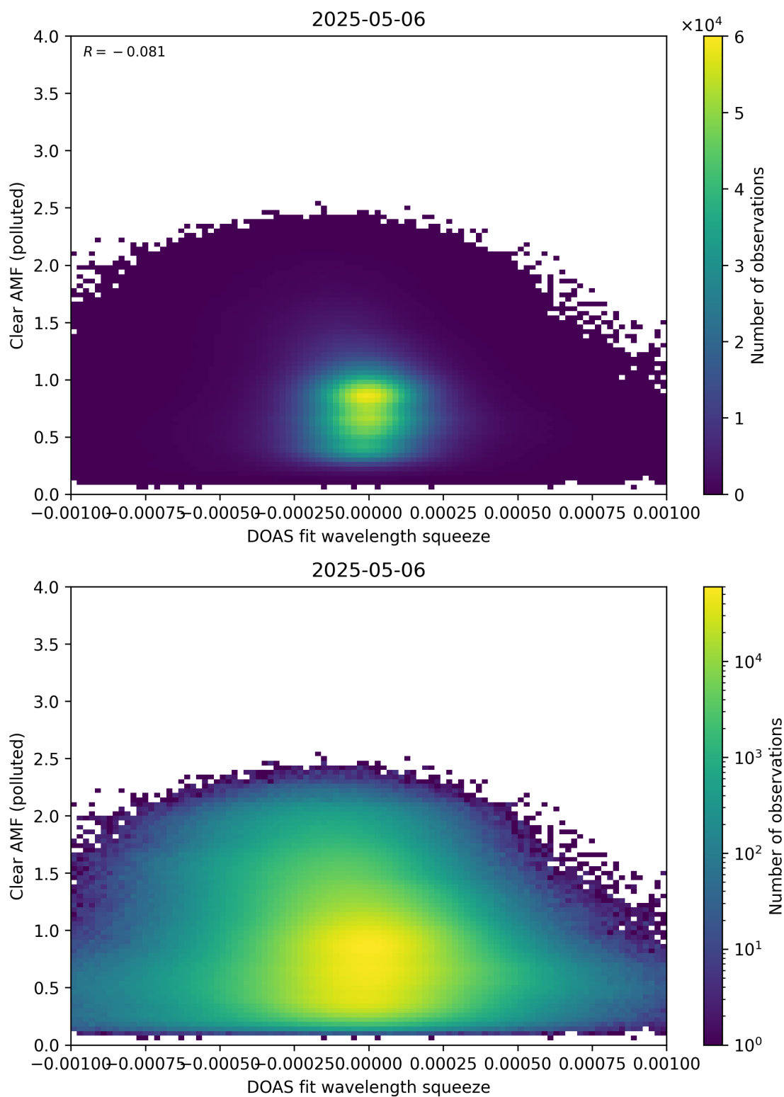
Figure 144: Scatter density plot of “DOAS fit wavelength squeeze” against “Clear AMF (polluted)” for 2025-05-05 to 2025-05-07.
