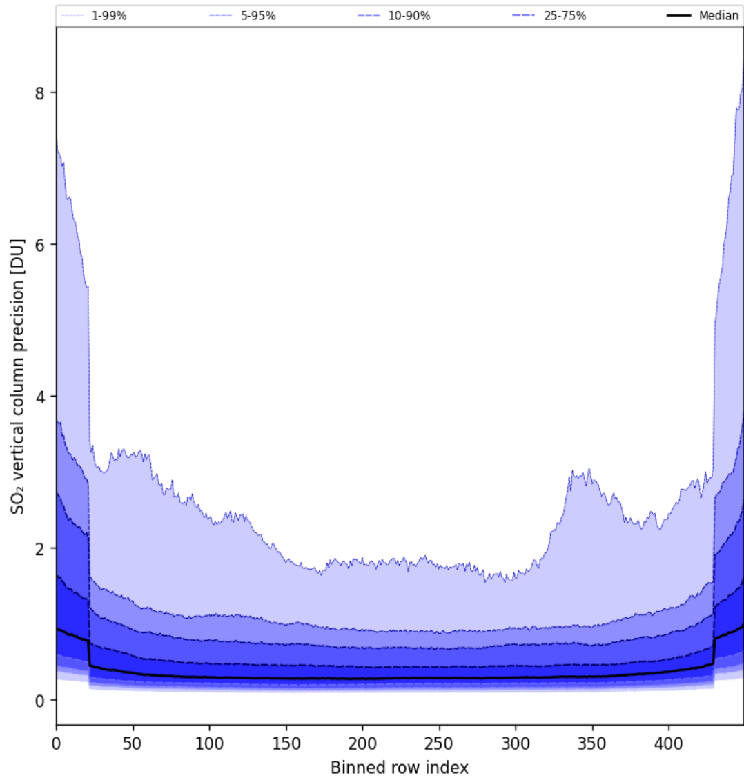
Figure 85: Along track statistics of “SO 2 vertical column precision” for 2025-05-05 to 2025-05-07
