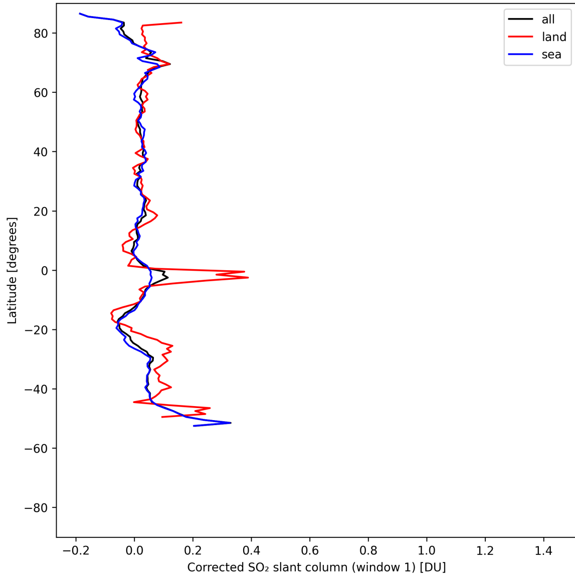
Figure 39: Zonal average of “Corrected SO 2 slant column (window 1)” for 2025-05-05 to 2025-05-07.
