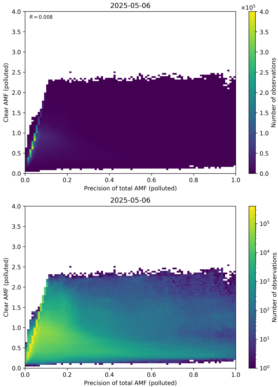
Figure 320: Scatter density plot of “Precision of total AMF (polluted)” against “Clear AMF (polluted)” for 2025-05-05 to 2025-05-07.
