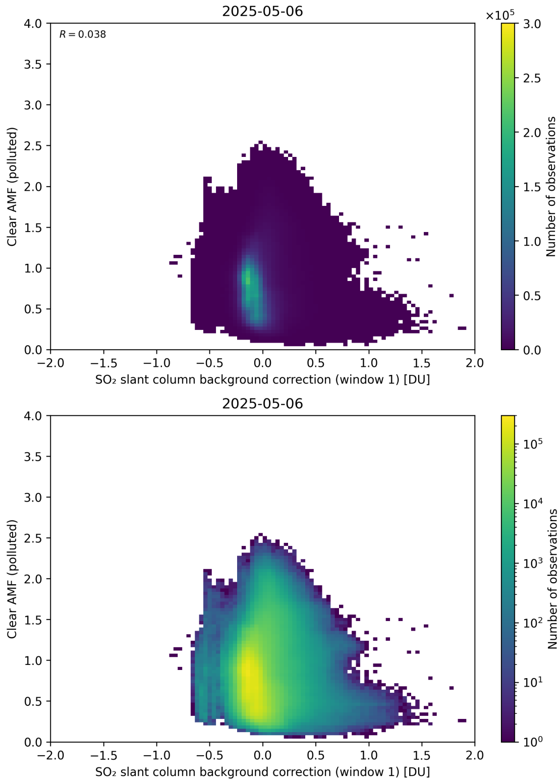
Figure 114: Scatter density plot of “SO 2 slant column background correction (window 1)” against “Clear AMF (polluted)” for 2025-05-05 to 2025-05-07.
