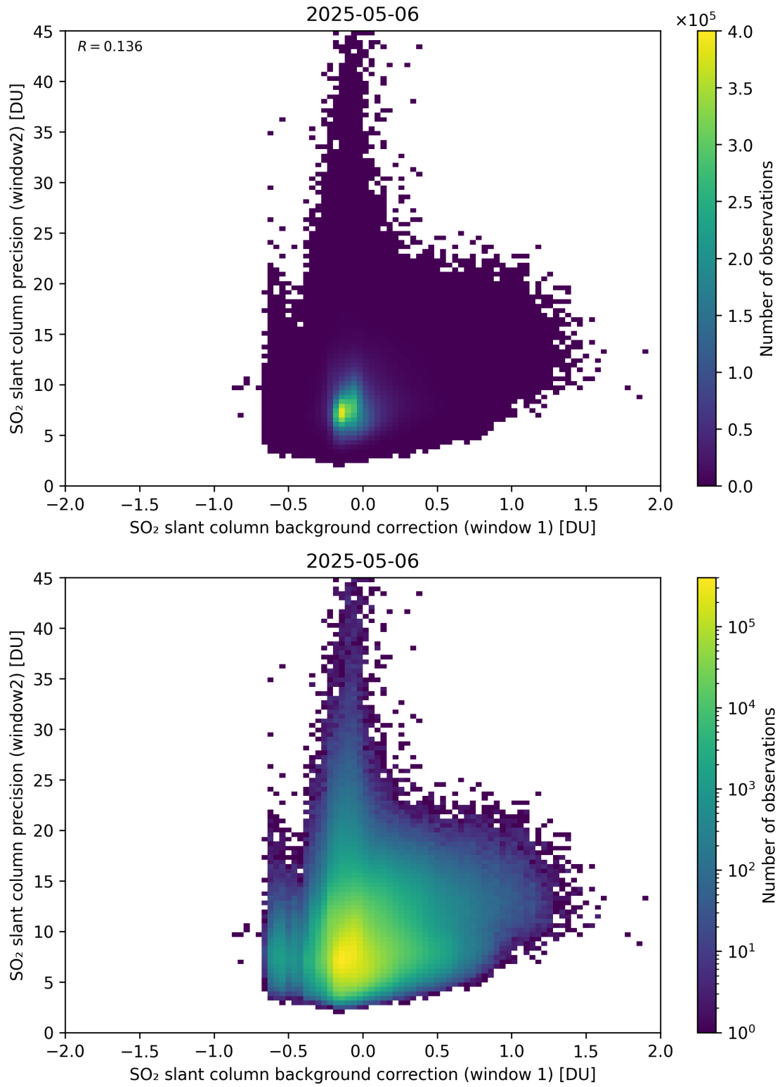
Figure 117: Scatter density plot of “SO 2 slant column background correction (window 1)” against “SO 2 slant column precision (window2)” for 2025-05-05 to 2025-05-07.
