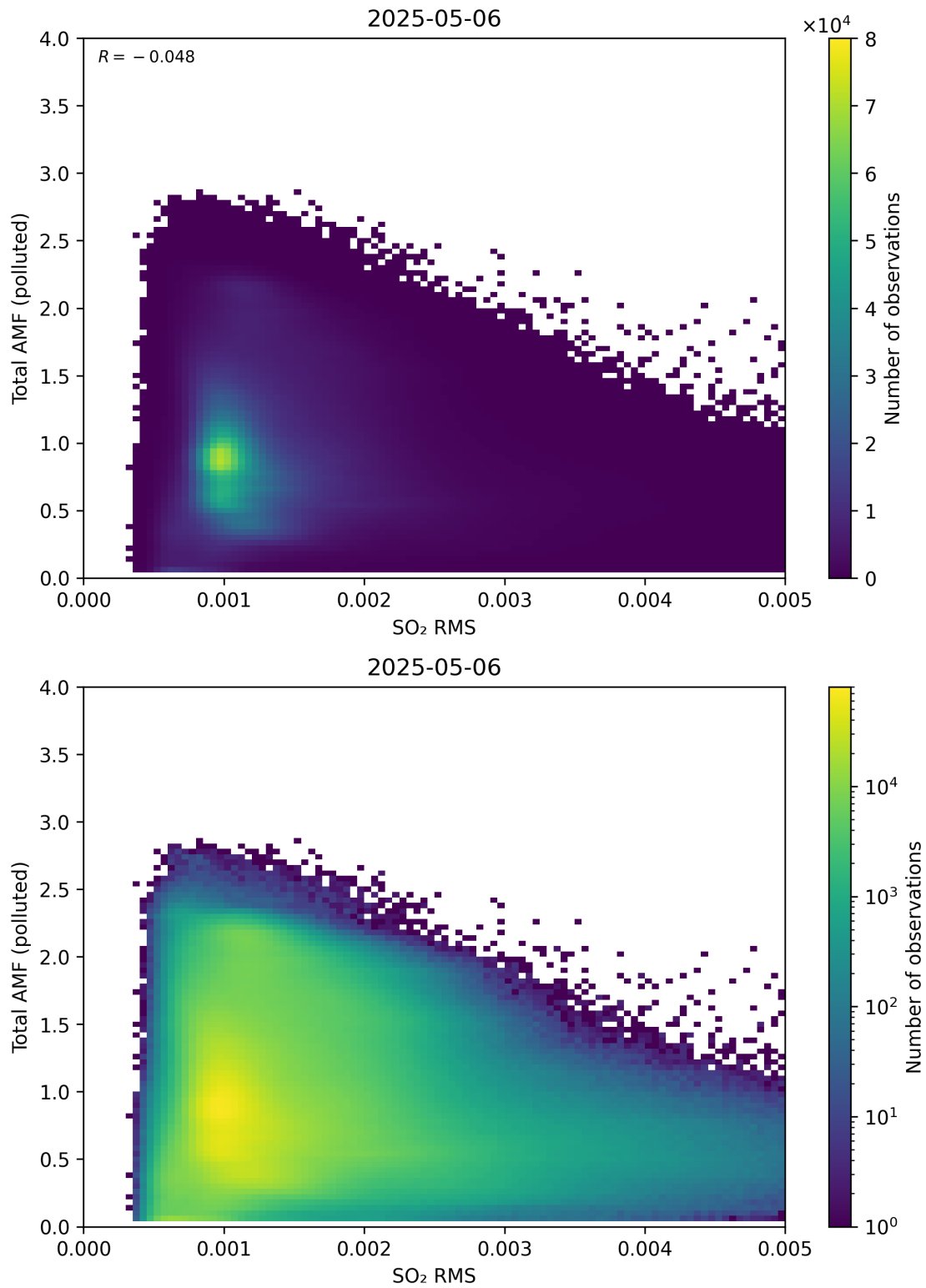
Figure 148: Scatter density plot of “SO 2 RMS” against “Total AMF (polluted)” for 2025-05-05 to 2025-05-07.
