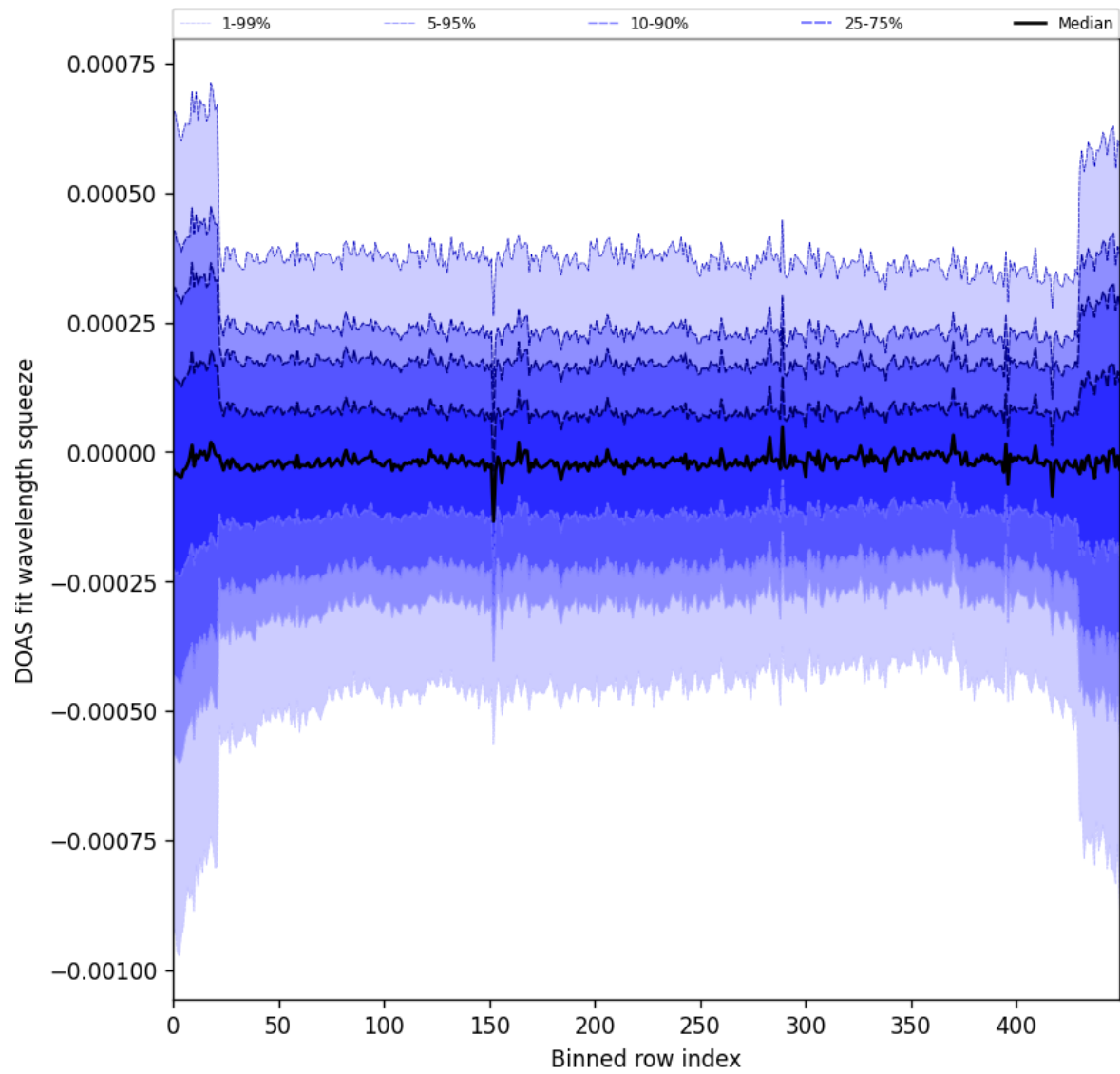
Figure 103: Along track statistics of “DOAS fit wavelength squeeze” for 2025-05-05 to 2025-05-07
