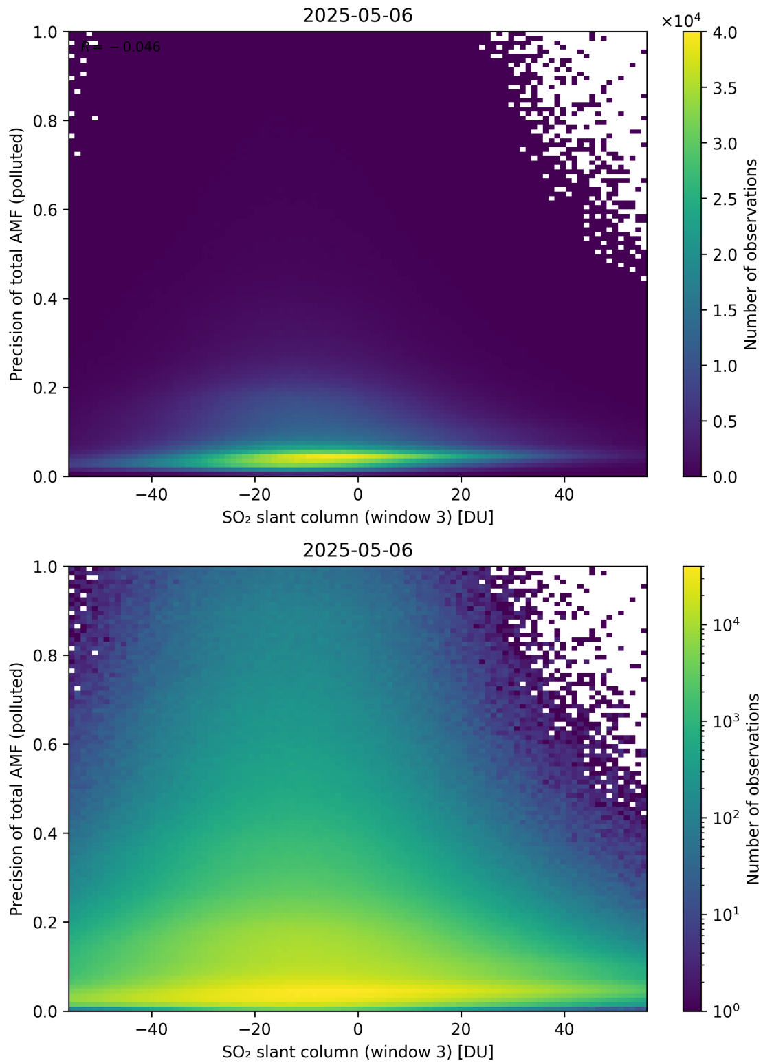
Figure 319: Scatter density plot of “SO 2 slant column (window 3)” against “Precision of total AMF (polluted)” for 2025-05-05 to 2025-05-07.
