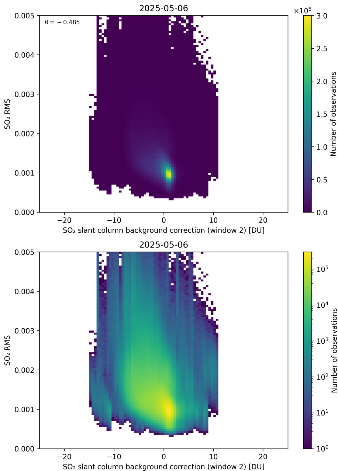
Figure 125: Scatter density plot of “SO 2 slant column background correction (window 2)” against “SO 2 RMS” for 2025-05-05 to 2025-05-07.
