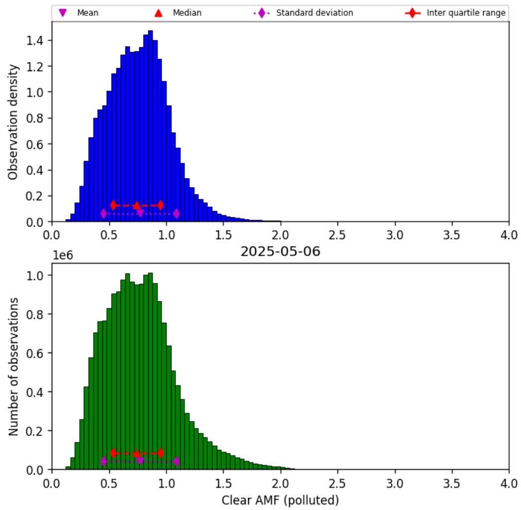
Figure 81: Histogram of “Clear AMF (polluted)” for 2025-05-05 to 2025-05-07
