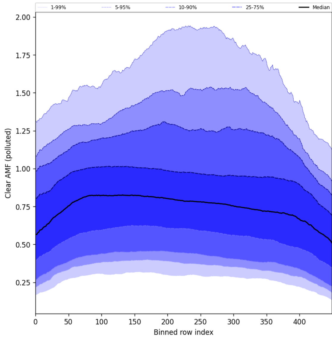
Figure 107: Along track statistics of “Clear AMF (polluted)” for 2025-05-05 to 2025-05-07
