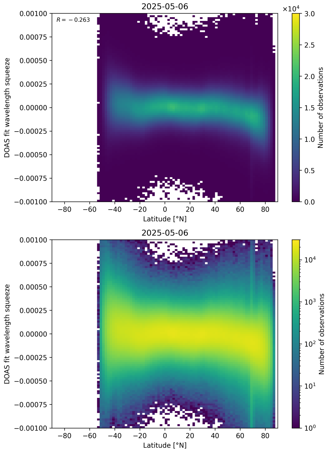
Figure 154: Scatter density plot of “Latitude” against “DOAS fit wavelength squeeze” for 2025-05-05 to 2025-05-07.
