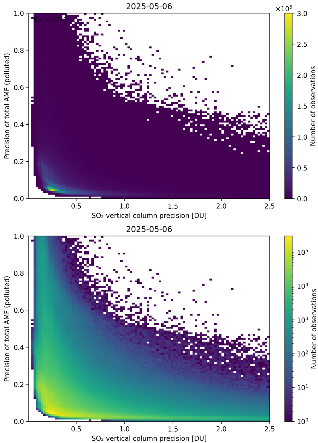
Figure 347: Scatter density plot of “SO 2 vertical column precision” against “Precision of total AMF (polluted)” for 2025-05-05 to 2025-05-07.
