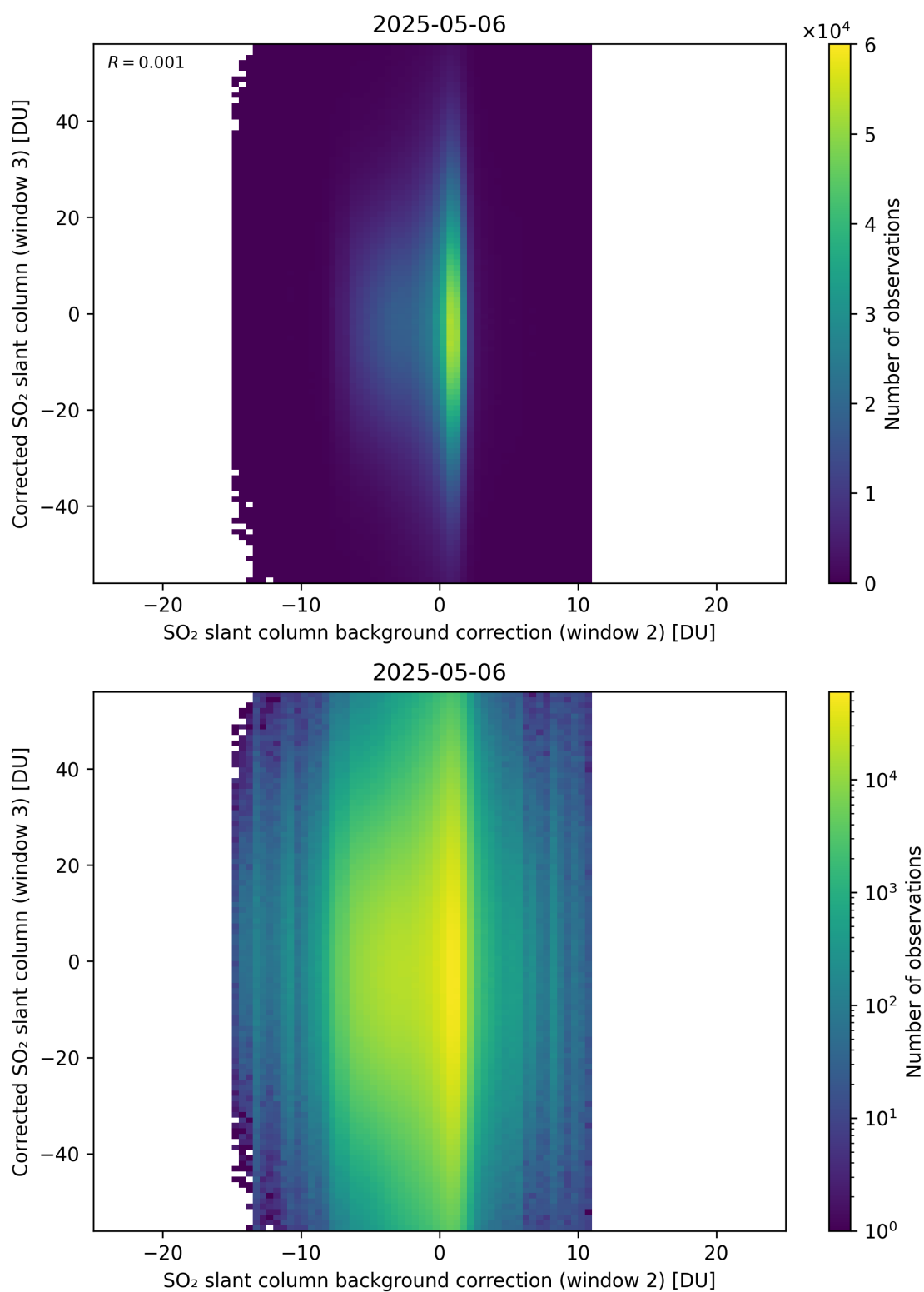
Figure 127: Scatter density plot of “SO 2 slant column background correction (window 2)” against “Corrected SO 2 slant column (window 3)” for 2025-05-05 to 2025-05-07.
