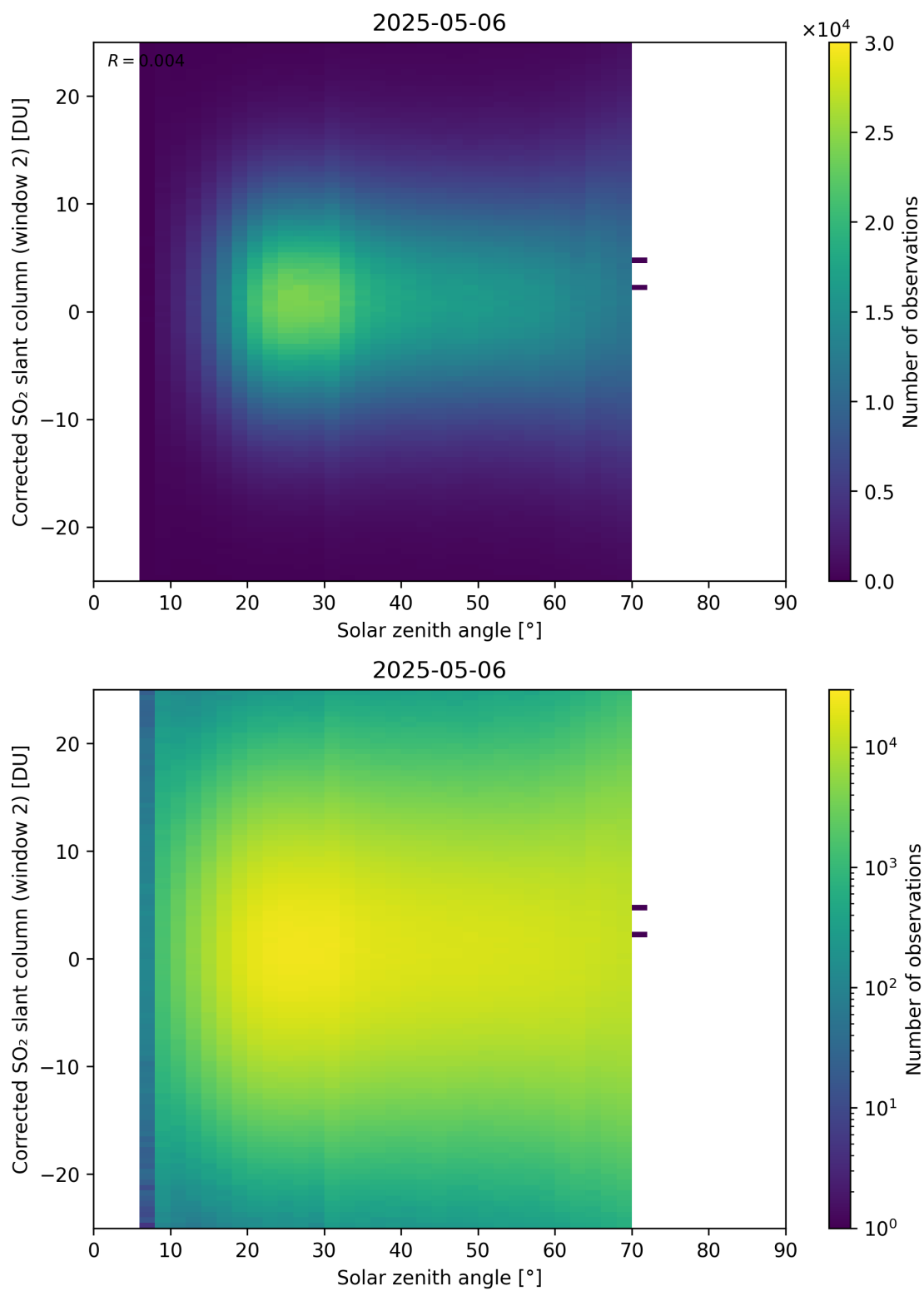
Figure 182: Scatter density plot of “Solar zenith angle” against “Corrected SO 2 slant column (window 2)” for 2025-05-05 to 2025-05-07.
