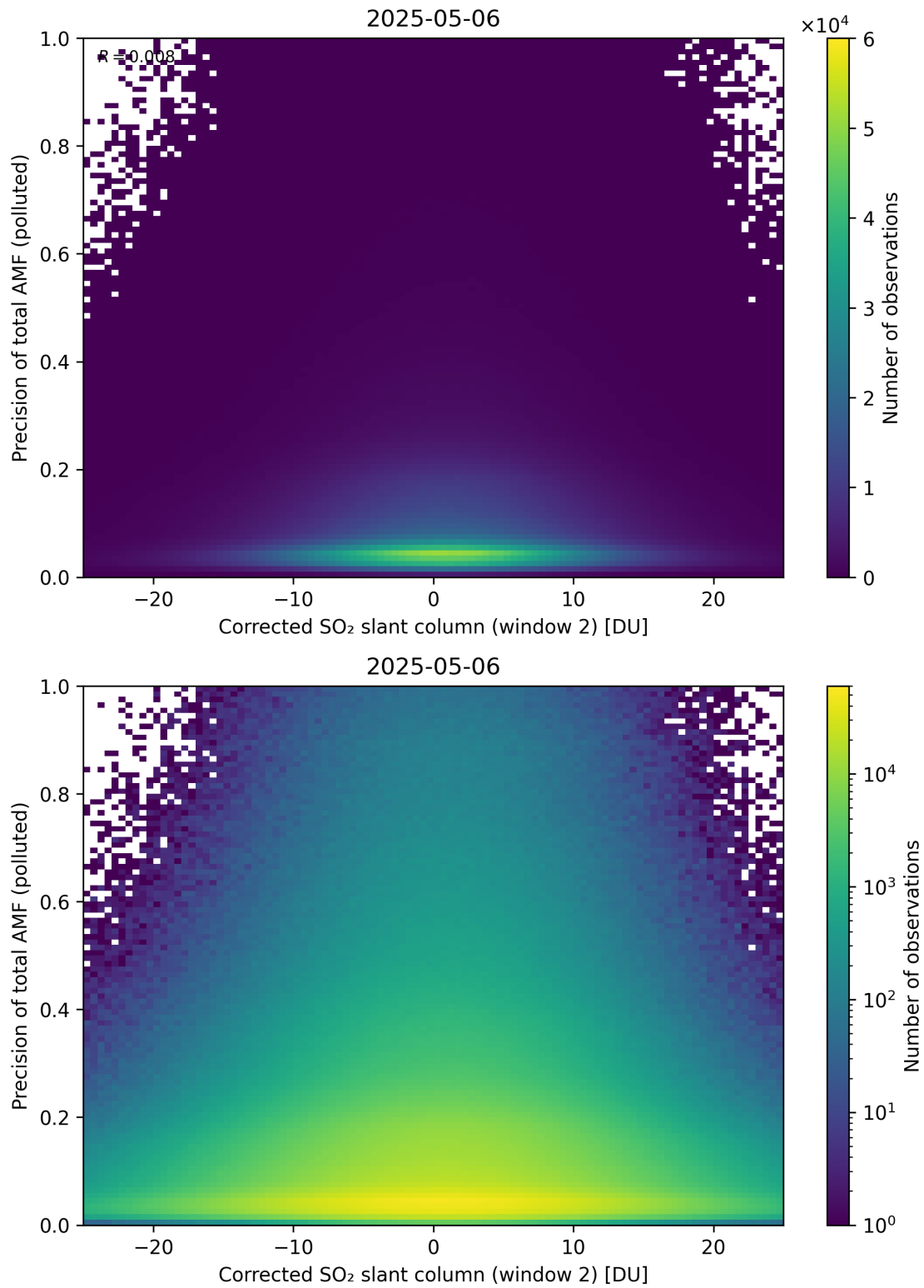
Figure 254: Scatter density plot of “Corrected SO 2 slant column (window 2)” against “Precision of total AMF (polluted)” for 2025-05-05 to 2025-05-07.
