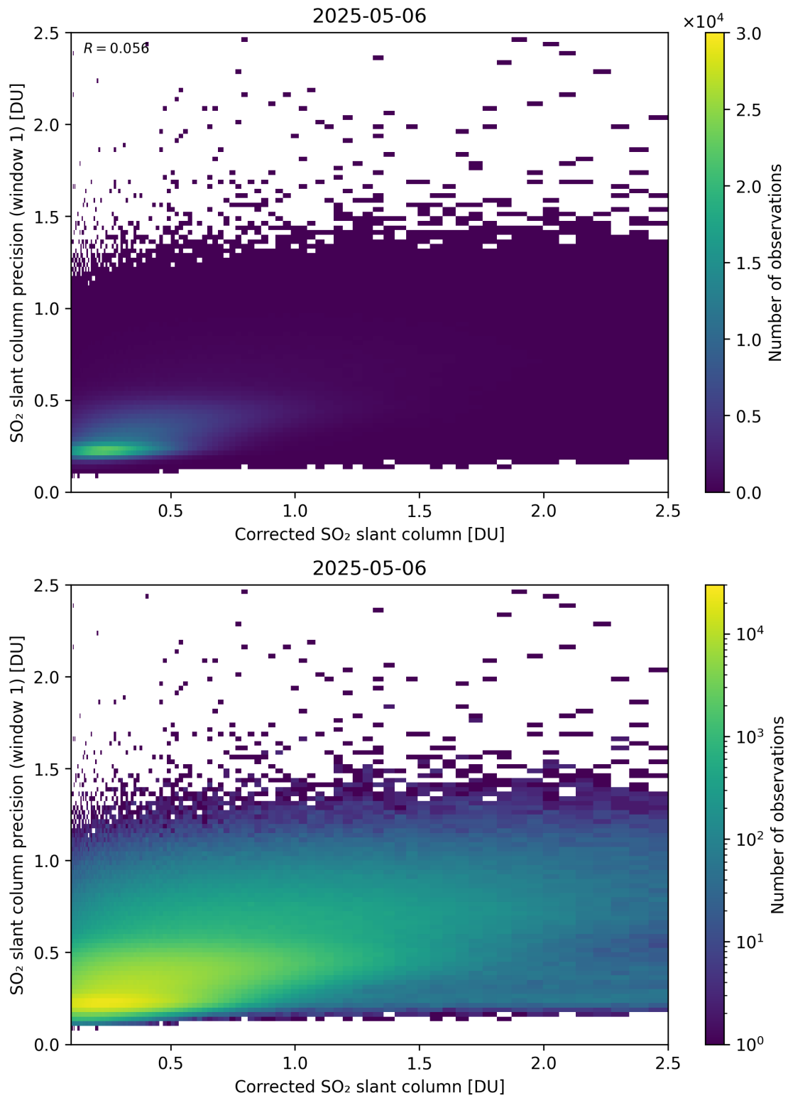
Figure 238: Scatter density plot of “Corrected SO 2 slant column” against “SO 2 slant column precision (window 1)” for 2025-05-05 to 2025-05-07.
