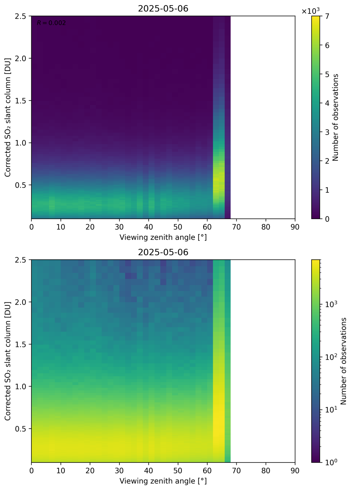
Figure 373: Scatter density plot of “Viewing zenith angle” against “Corrected SO 2 slant column” for 2025-05-05 to 2025-05-07.
