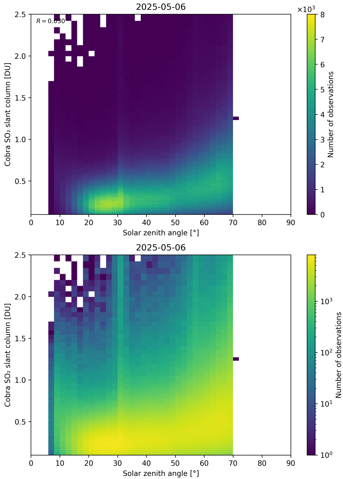
Figure 179: Scatter density plot of “Solar zenith angle” against “Cobra SO 2 slant column” for 2025-05-05 to 2025-05-07.
