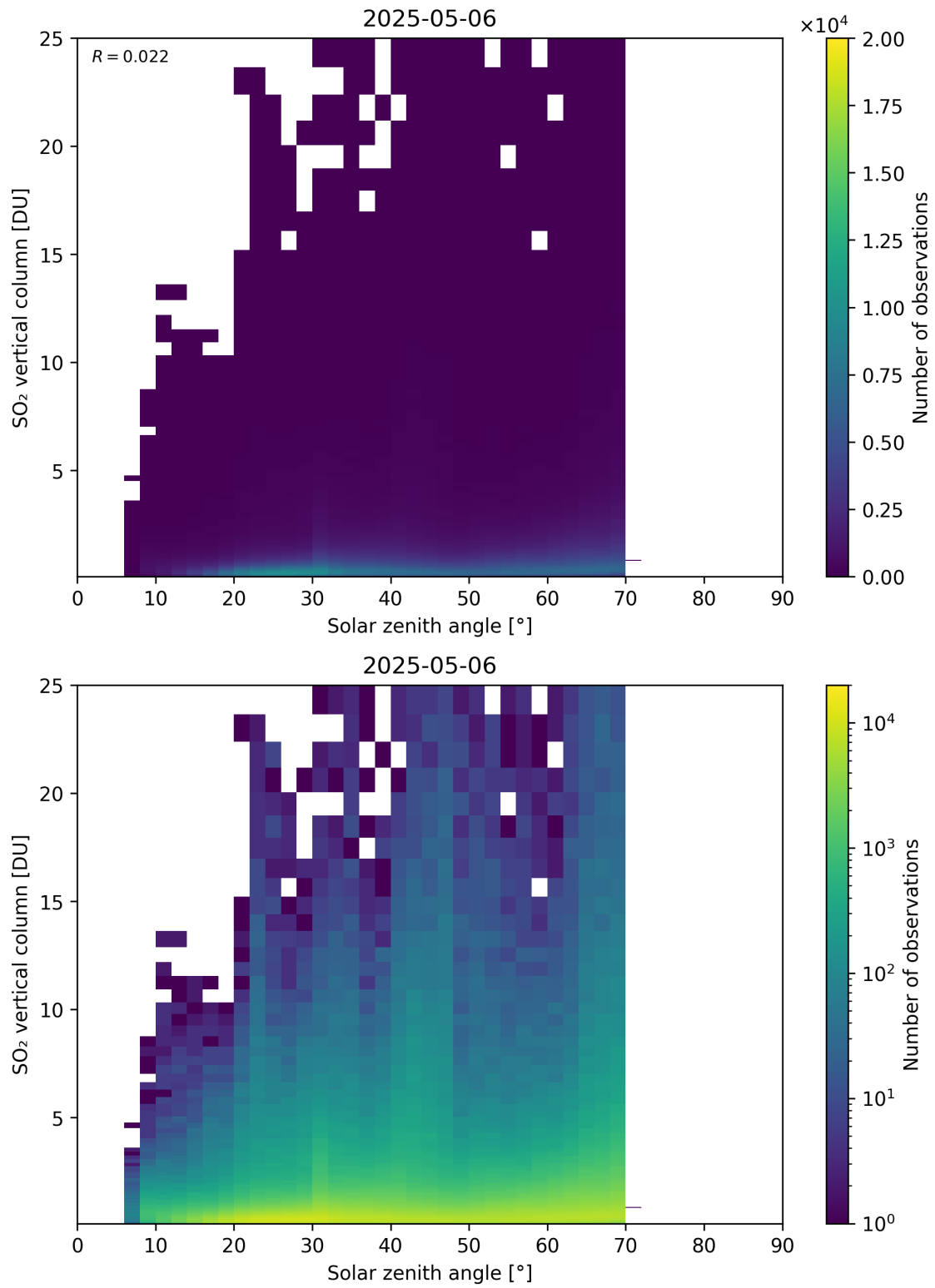
Figure 191: Scatter density plot of “Solar zenith angle” against “SO 2 vertical column” for 2025-05-05 to 2025-05-07.
