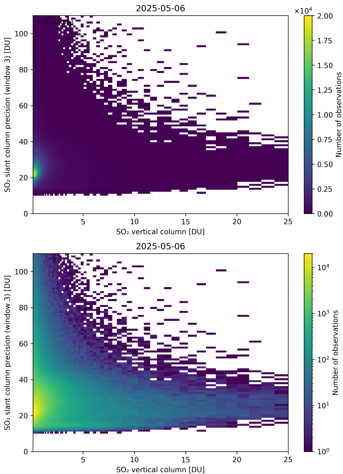
Figure 358: Scatter density plot of “SO 2 vertical column” against “SO 2 slant column precision (window 3)” for 2025-05-05 to 2025-05-07.
