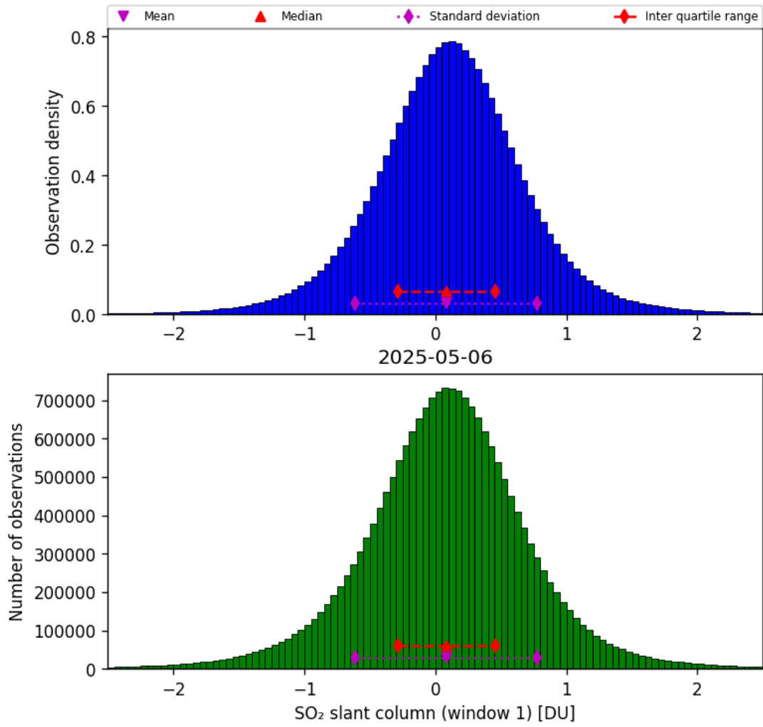
Figure 63: Histogram of “SO 2 slant column (window 1)” for 2025-05-05 to 2025-05-07
