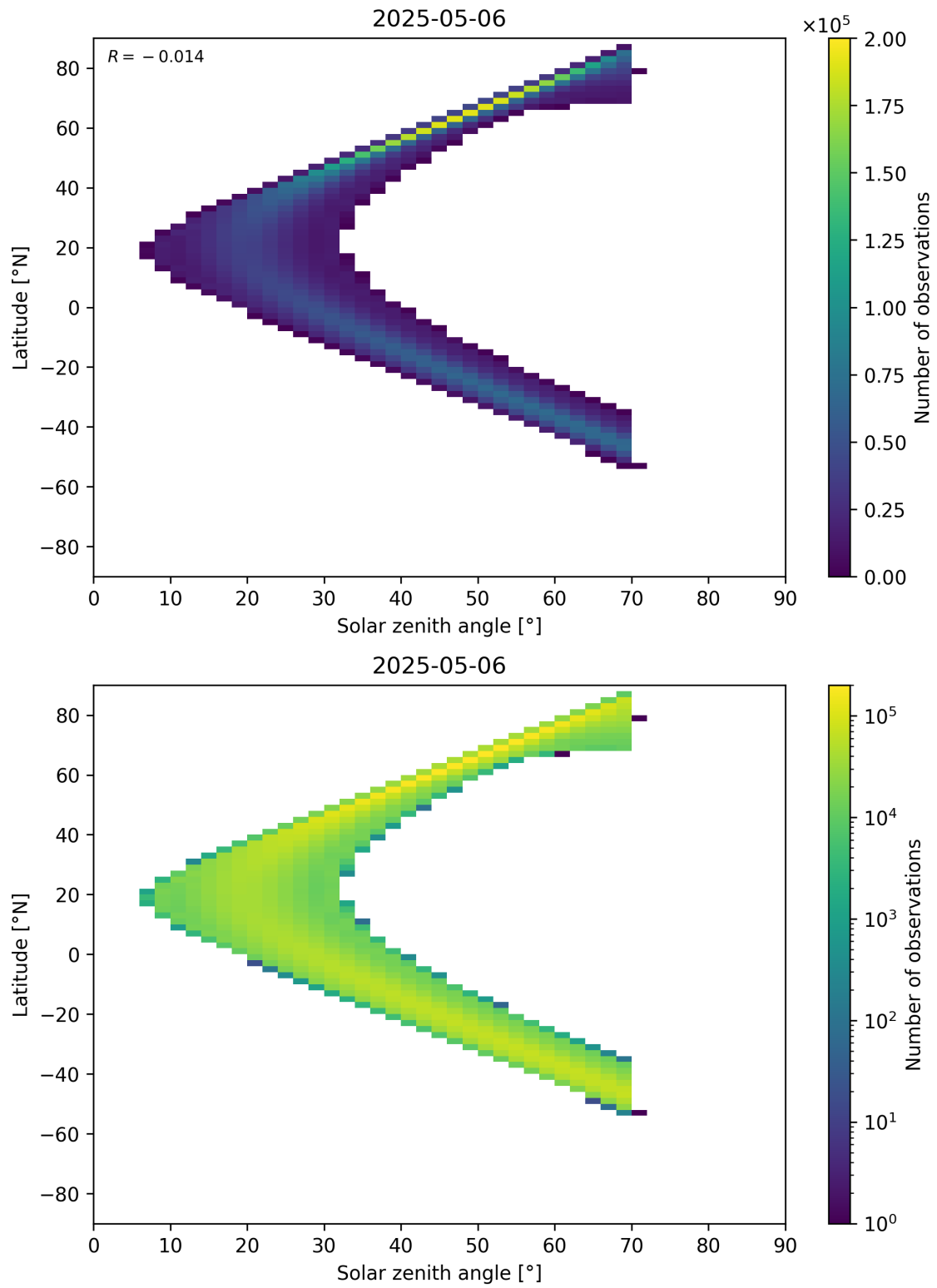
Figure 177: Scatter density plot of “Solar zenith angle” against “Latitude” for 2025-05-05 to 2025-05-07.
