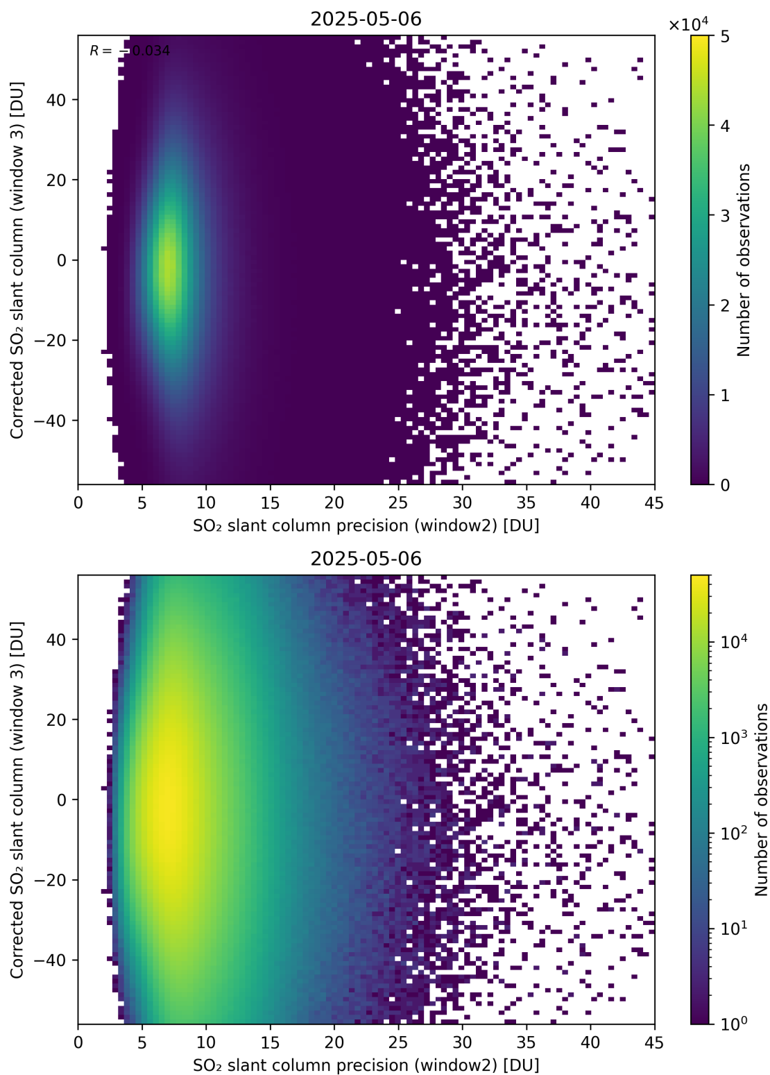
Figure 298: Scatter density plot of “SO 2 slant column precision (window2)” against “Corrected SO 2 slant column (window 3)” for 2025-05-05 to 2025-05-07.
