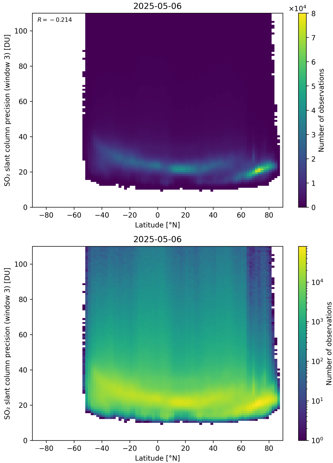
Figure 166: Scatter density plot of “Latitude” against “SO 2 slant column precision (window 3)” for 2025-05-05 to 2025-05-07.
