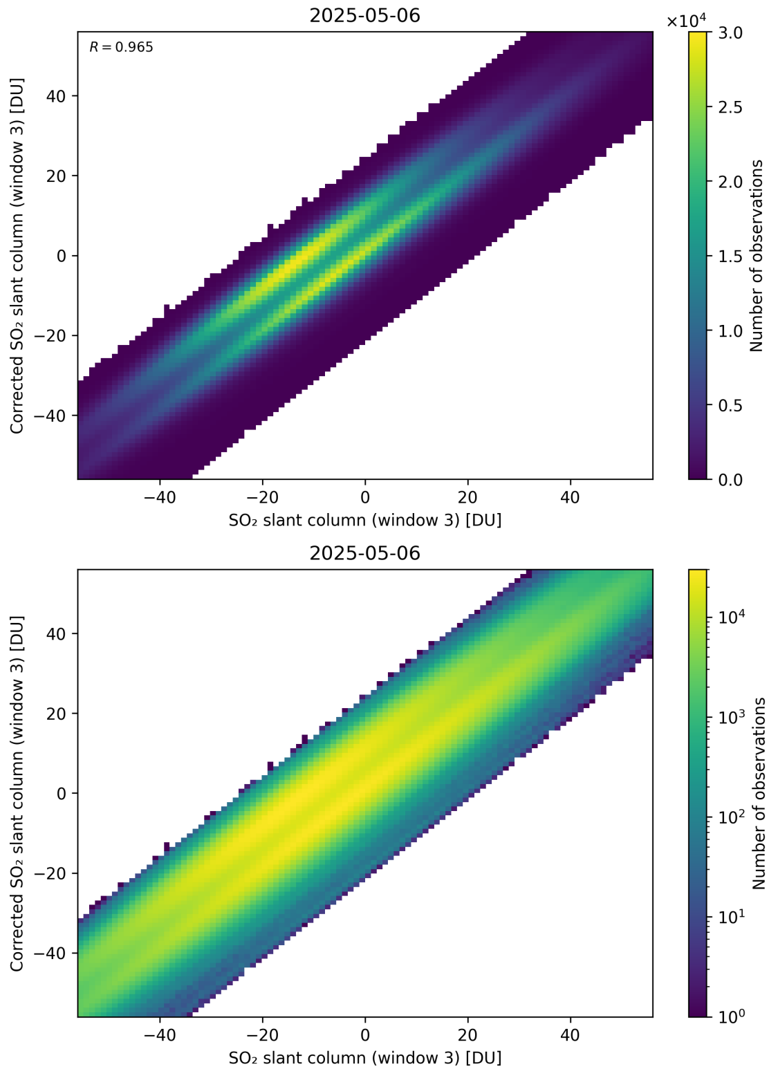
Figure 316: Scatter density plot of “SO 2 slant column (window 3)” against “Corrected SO 2 slant column (window 3)” for 2025-05-05 to 2025-05-07.
