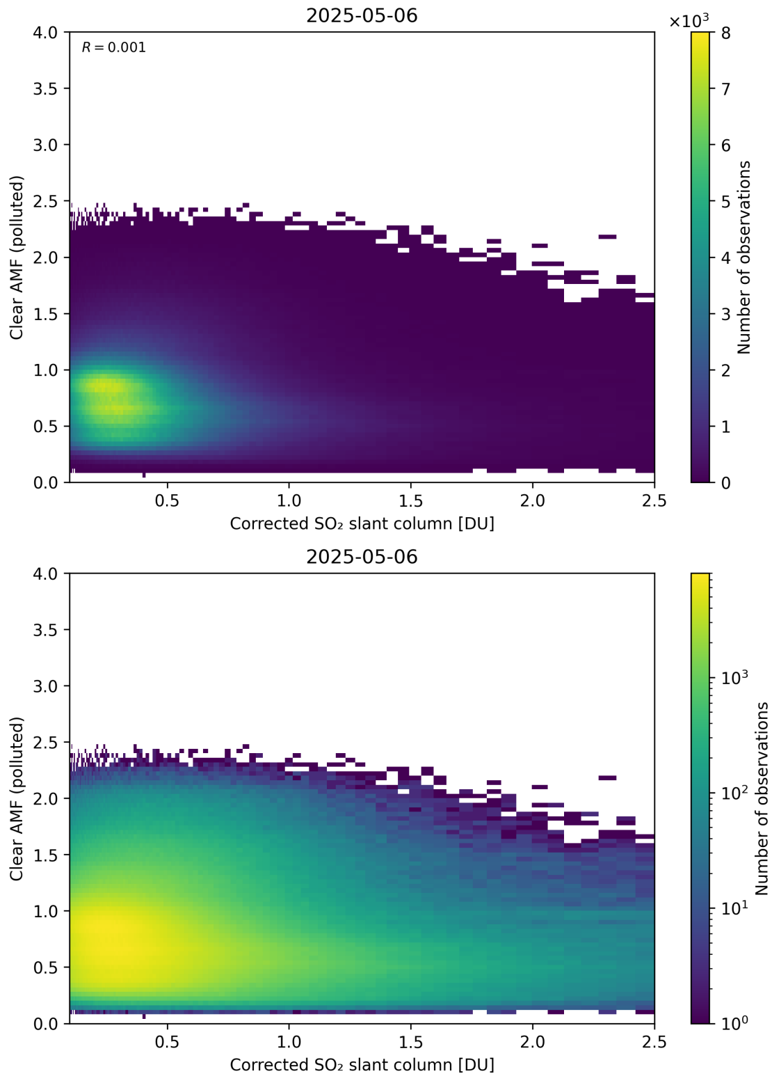
Figure 232: Scatter density plot of “Corrected SO 2 slant column” against “Clear AMF (polluted)” for 2025-05-05 to 2025-05-07.
