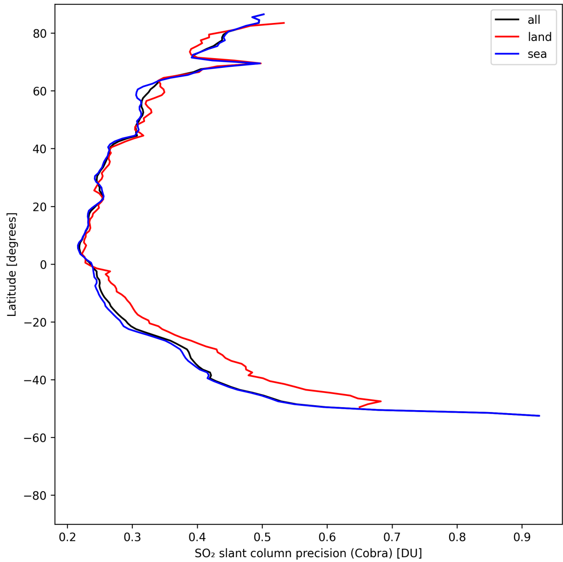
Figure 36: Zonal average of “SO 2 slant column precision (Cobra)” for 2025-05-05 to 2025-05-07.
