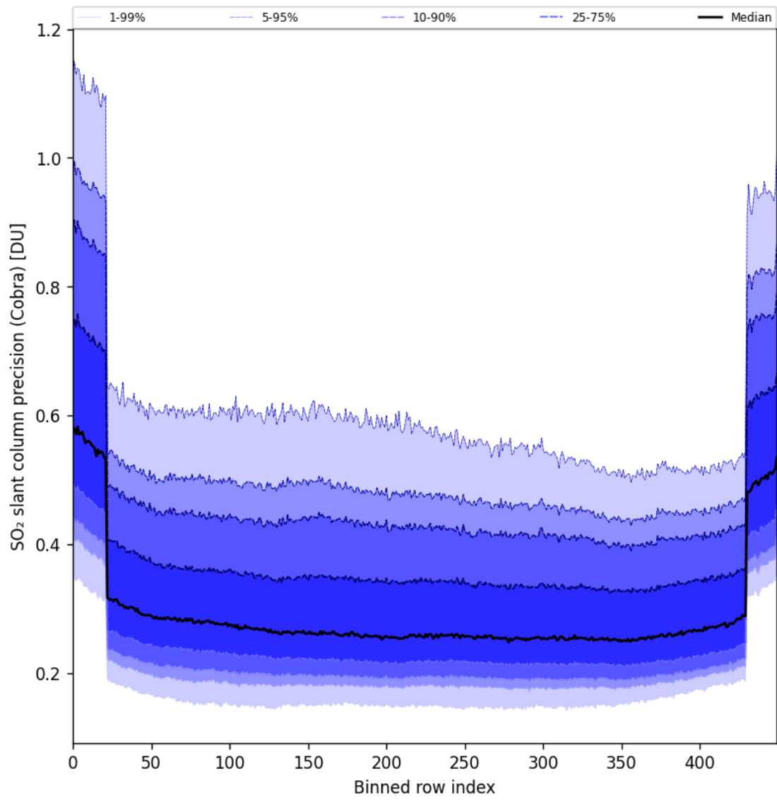
Figure 88: Along track statistics of “SO 2 slant column precision (Cobra)” for 2025-05-05 to 2025-05-07
