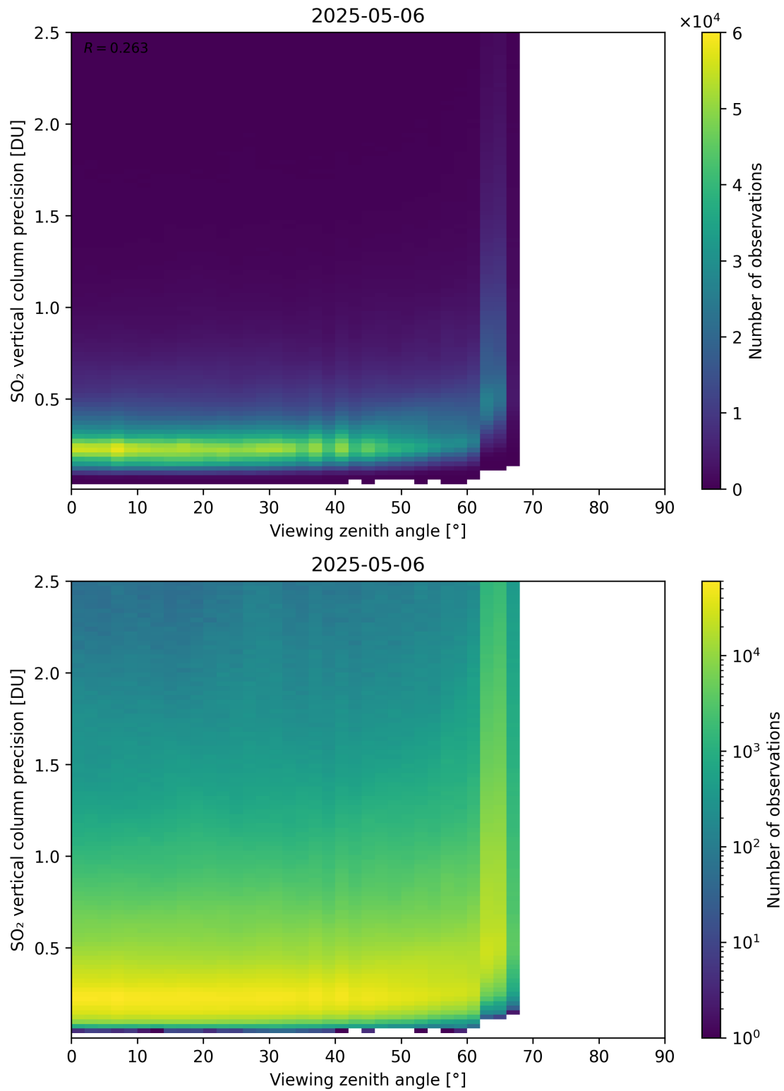
Figure 384: Scatter density plot of “Viewing zenith angle” against “SO 2 vertical column precision” for 2025-05-05 to 2025-05-07.
