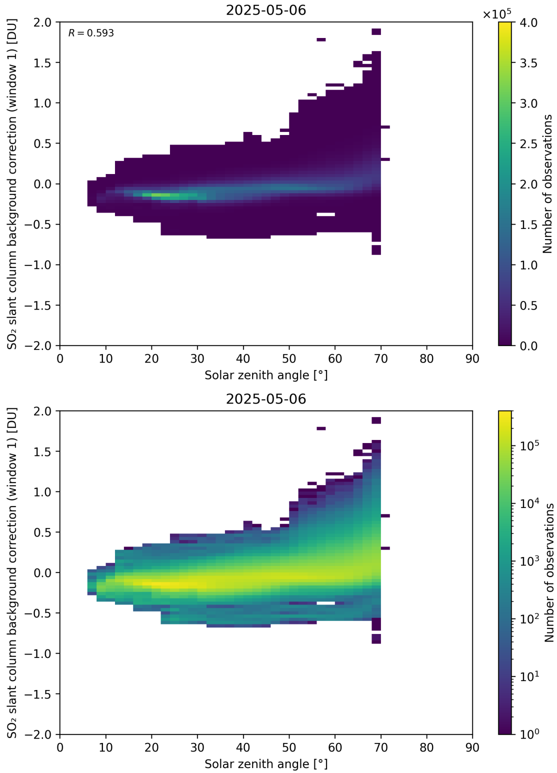
Figure 171: Scatter density plot of “Solar zenith angle” against “SO 2 slant column background correction (window 1)” for 2025-05-05 to 2025-05-07.
