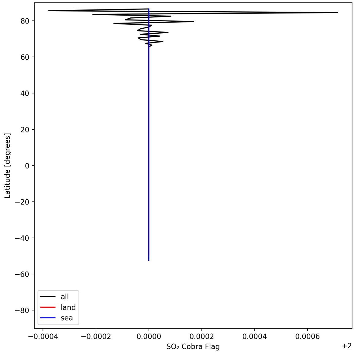
Figure 49: Zonal average of “SO 2 Cobra Flag” for 2025-05-05 to 2025-05-07.
