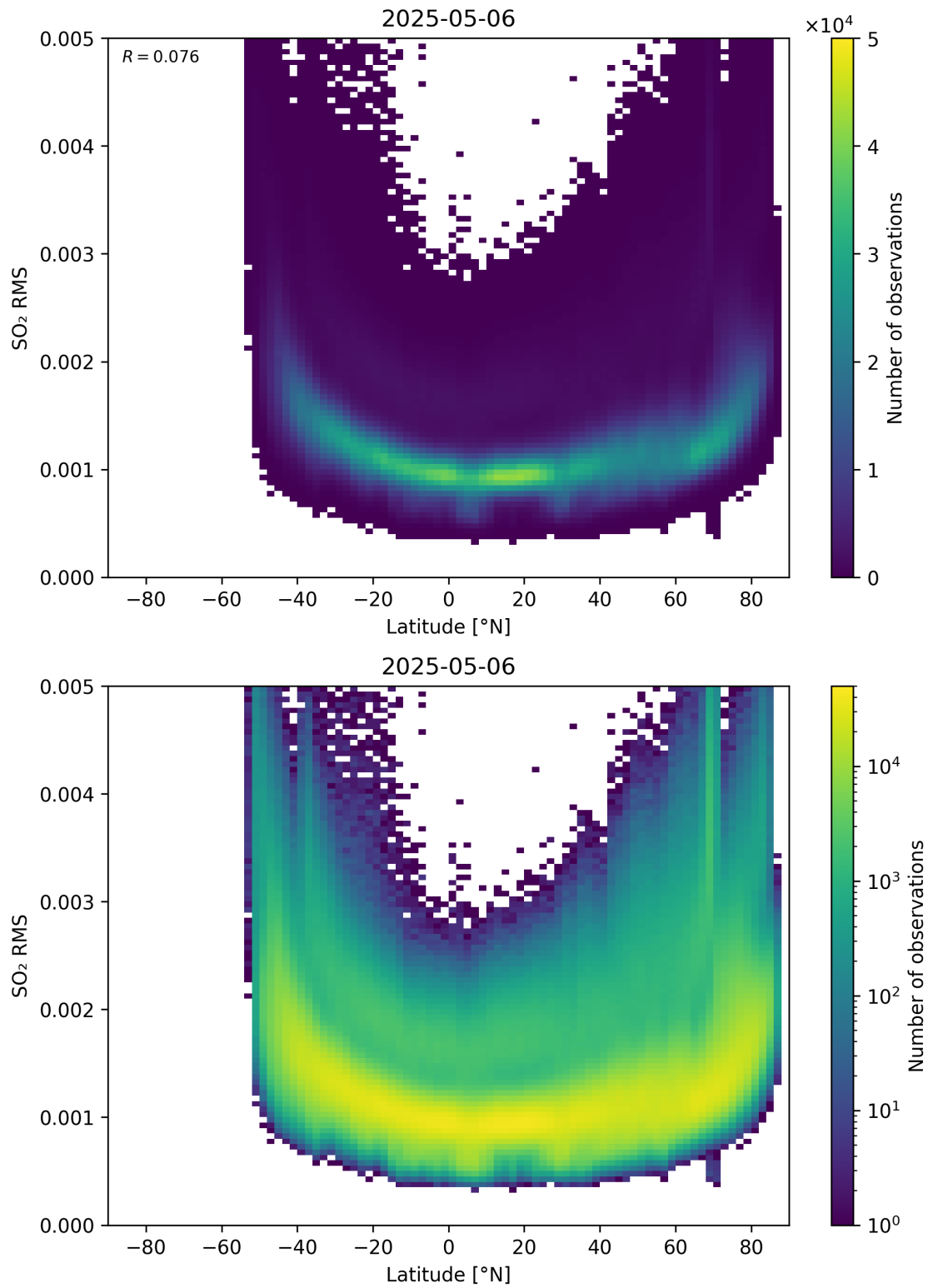
Figure 155: Scatter density plot of “Latitude” against “SO 2 RMS” for 2025-05-05 to 2025-05-07.
