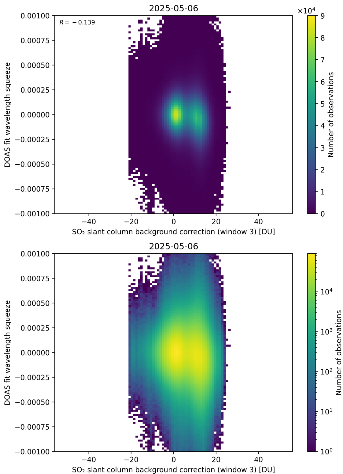
Figure 133: Scatter density plot of “SO 2 slant column background correction (window 3)” against “DOAS fit wavelength squeeze” for 2025-05-05 to 2025-05-07.
