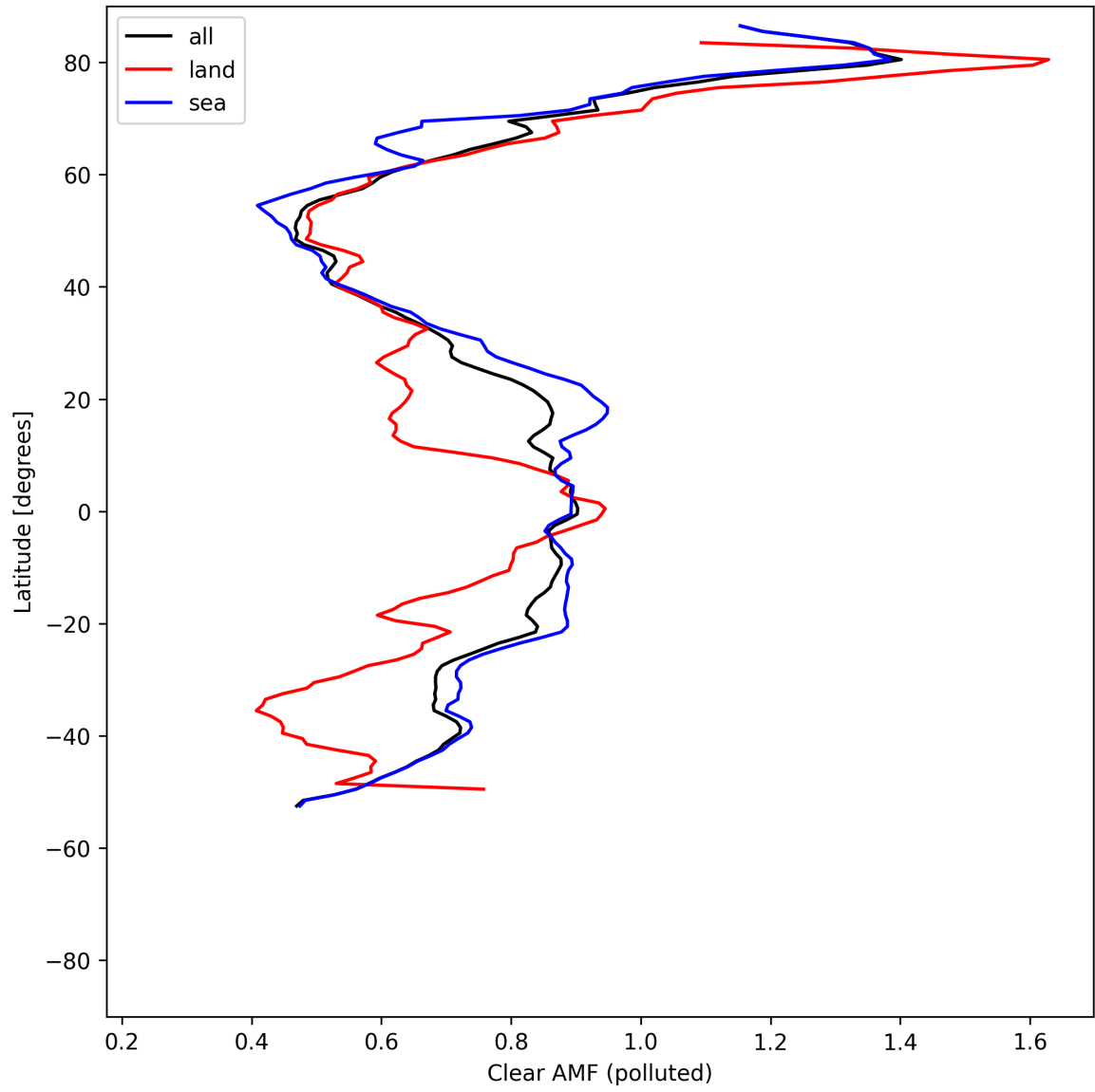
Figure 55: Zonal average of “Clear AMF (polluted)” for 2025-05-05 to 2025-05-07.
