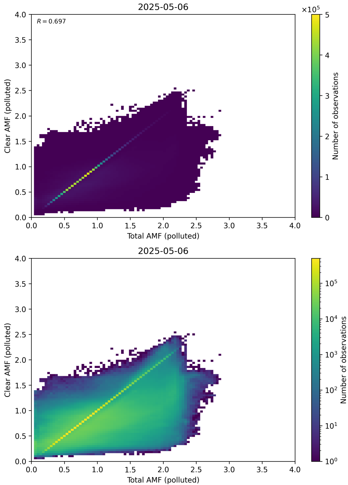
Figure 321: Scatter density plot of “Total AMF (polluted)” against “Clear AMF (polluted)” for 2025-05-05 to 2025-05-07.
