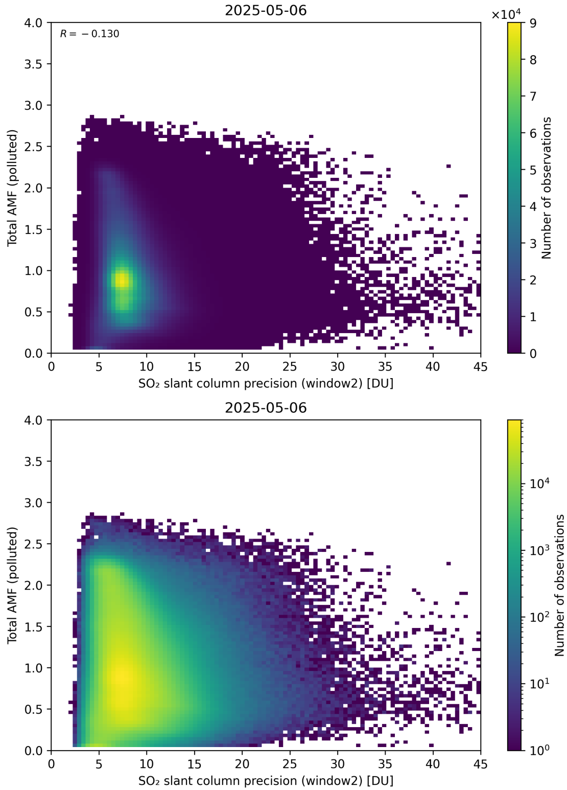
Figure 301: Scatter density plot of “SO 2 slant column precision (window2)” against “Total AMF (polluted)” for 2025-05-05 to 2025-05-07.
