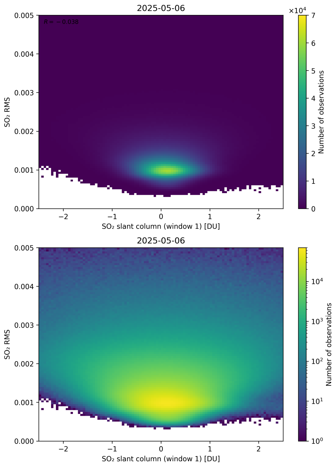
Figure 267: Scatter density plot of “SO 2 slant column (window 1)” against “SO 2 RMS” for 2025-05-05 to 2025-05-07.
