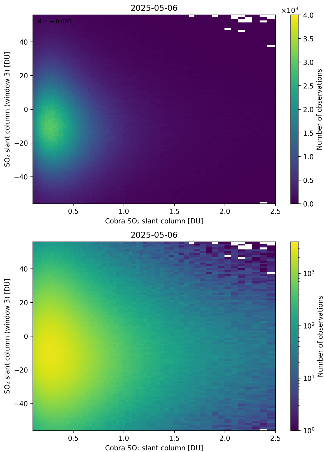
Figure 222: Scatter density plot of “Cobra SO 2 slant column” against “SO 2 slant column (window 3)” for 2025-05-05 to 2025-05-07.
