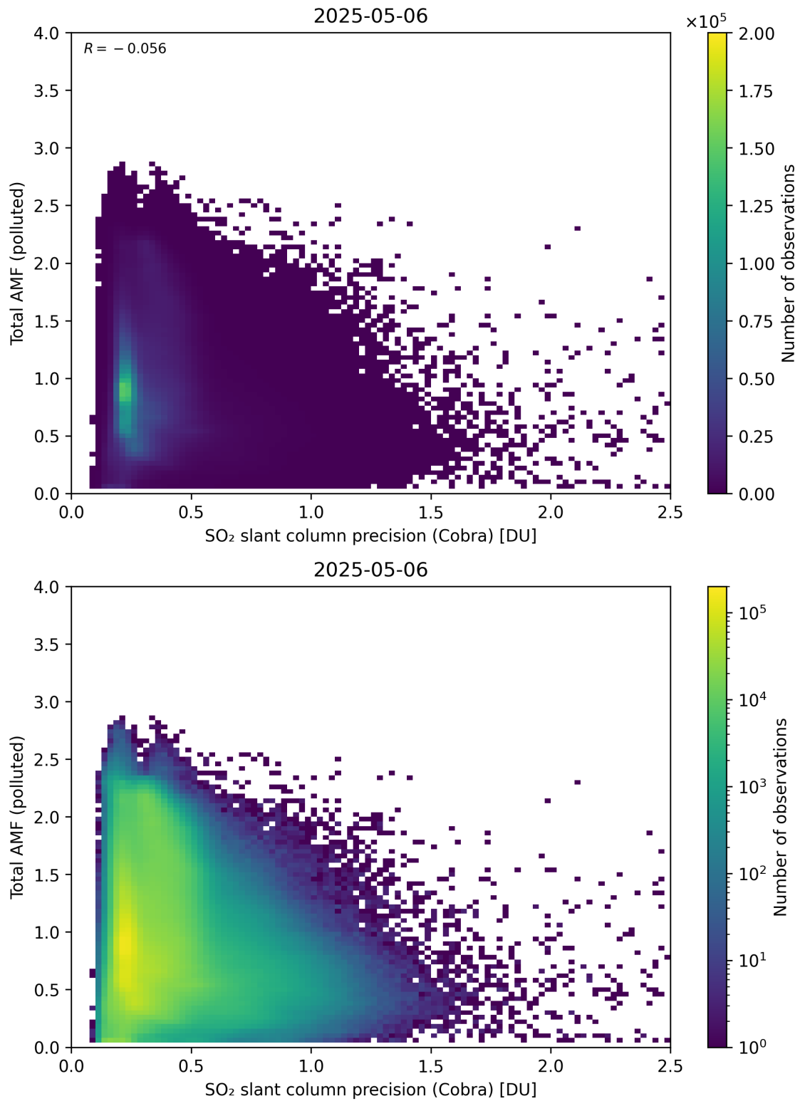
Figure 213: Scatter density plot of “SO 2 slant column precision (Cobra)” against “Total AMF (polluted)” for 2025-05-05 to 2025-05-07.
