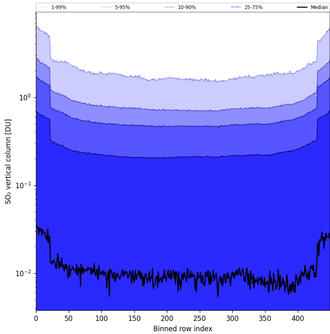
Figure 84: Along track statistics of “SO 2 vertical column” for 2025-05-05 to 2025-05-07
