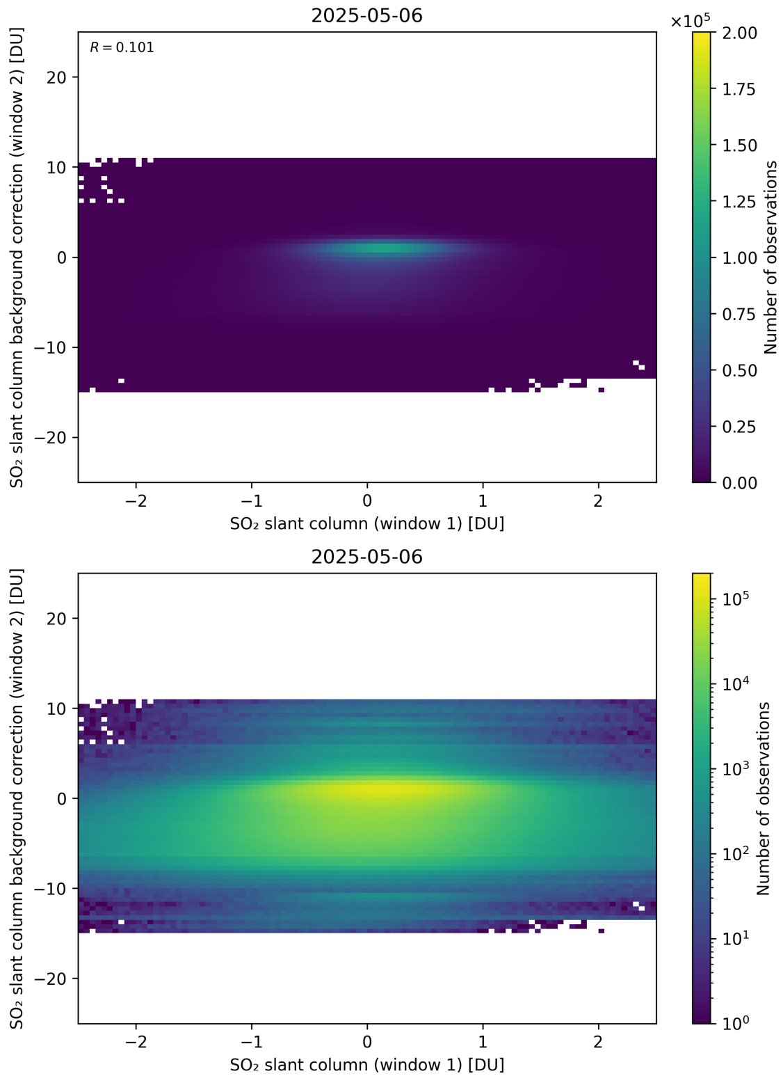
Figure 263: Scatter density plot of “SO 2 slant column (window 1)” against “SO 2 slant column background correction (window 2)” for 2025-05-05 to 2025-05-07.
