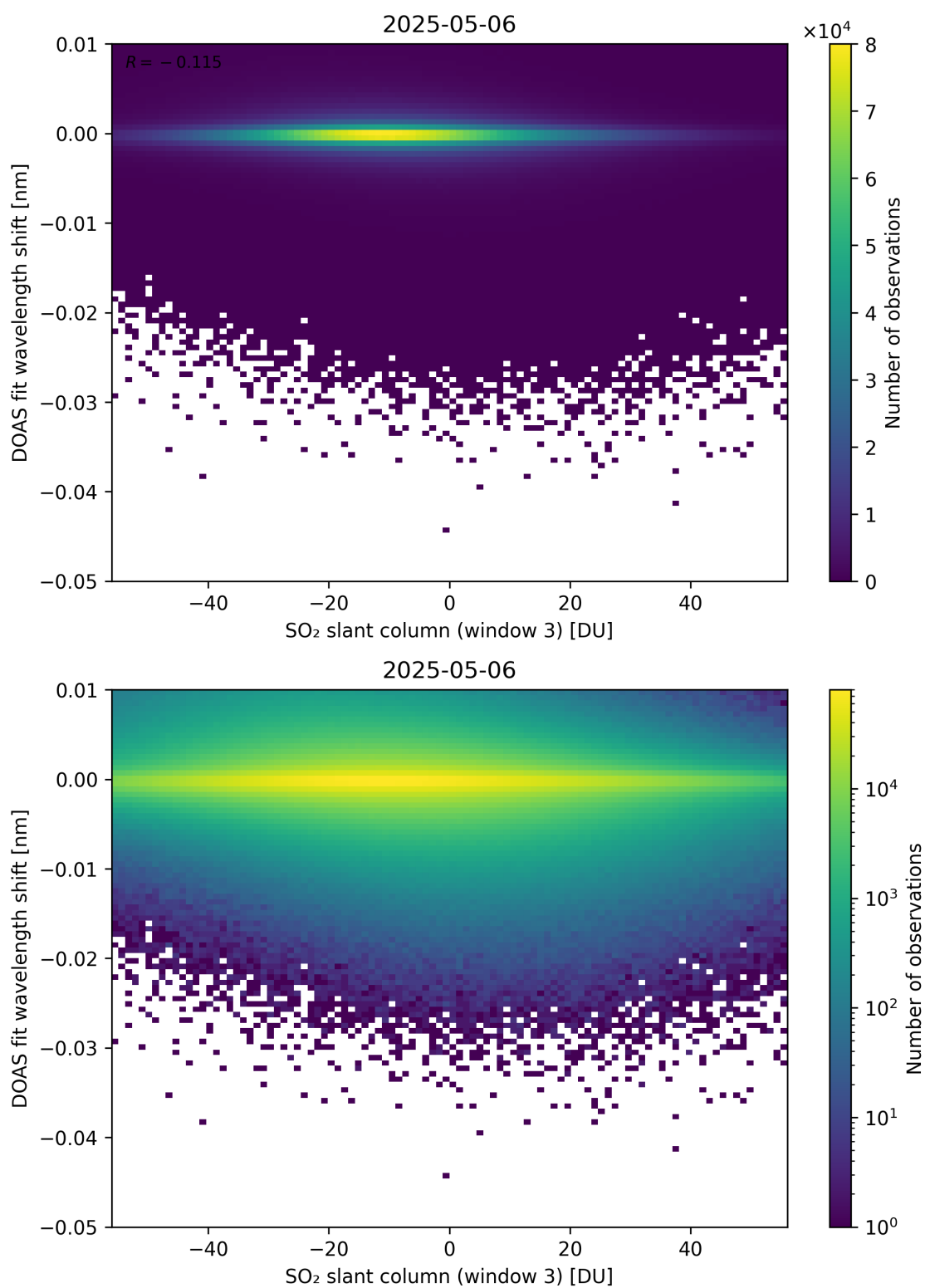
Figure 304: Scatter density plot of “SO 2 slant column (window 3)” against “DOAS fit wavelength shift” for 2025-05-05 to 2025-05-07.
