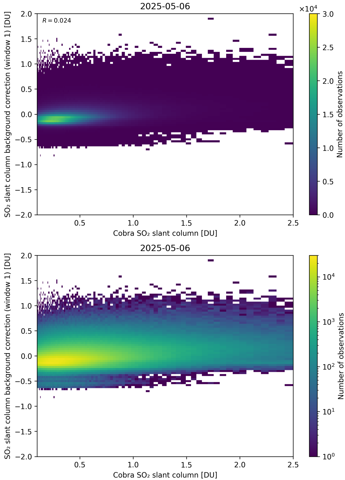
Figure 193: Scatter density plot of “Cobra SO 2 slant column” against “SO 2 slant column background correction (window 1)” for 2025-05-05 to 2025-05-07.
