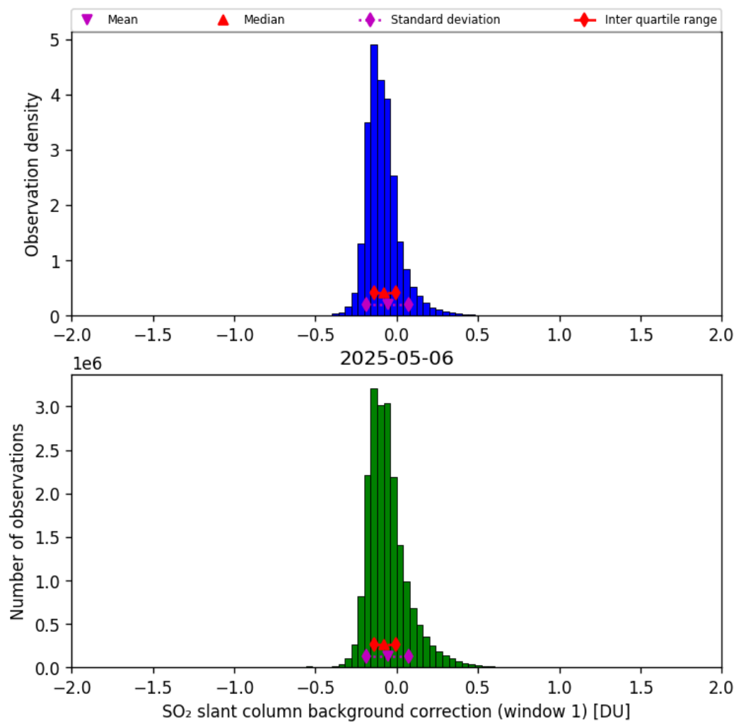
Figure 66: Histogram of “SO 2 slant column background correction (window 1)” for 2025-05-05 to 2025-05-07
