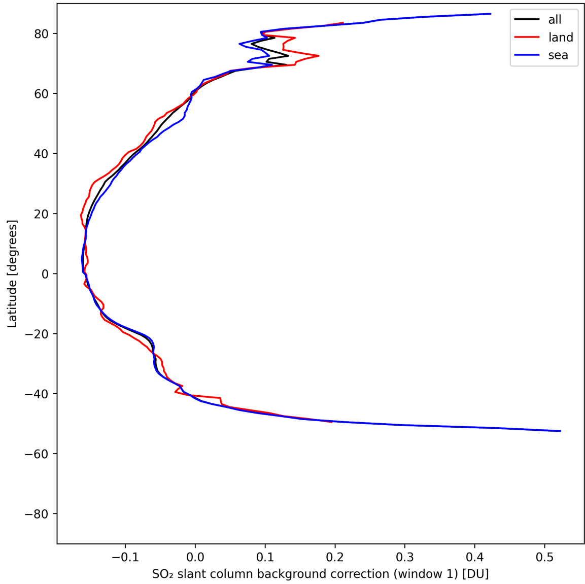
Figure 40: Zonal average of “SO 2 slant column background correction (window 1)” for 2025-05-05 to 2025-05-07.
