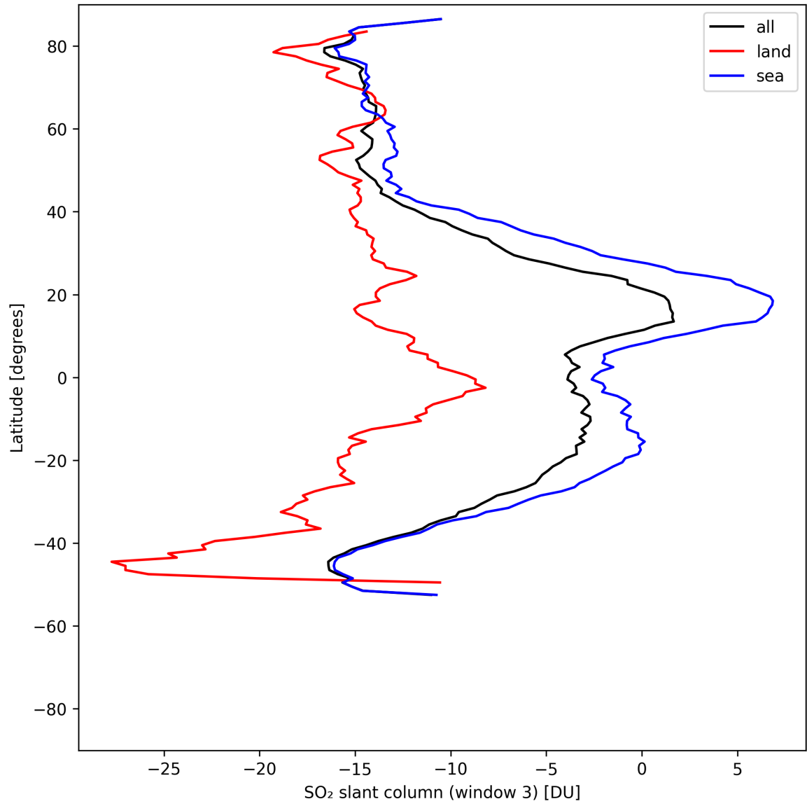
Figure 45: Zonal average of “SO 2 slant column (window 3)” for 2025-05-05 to 2025-05-07.
