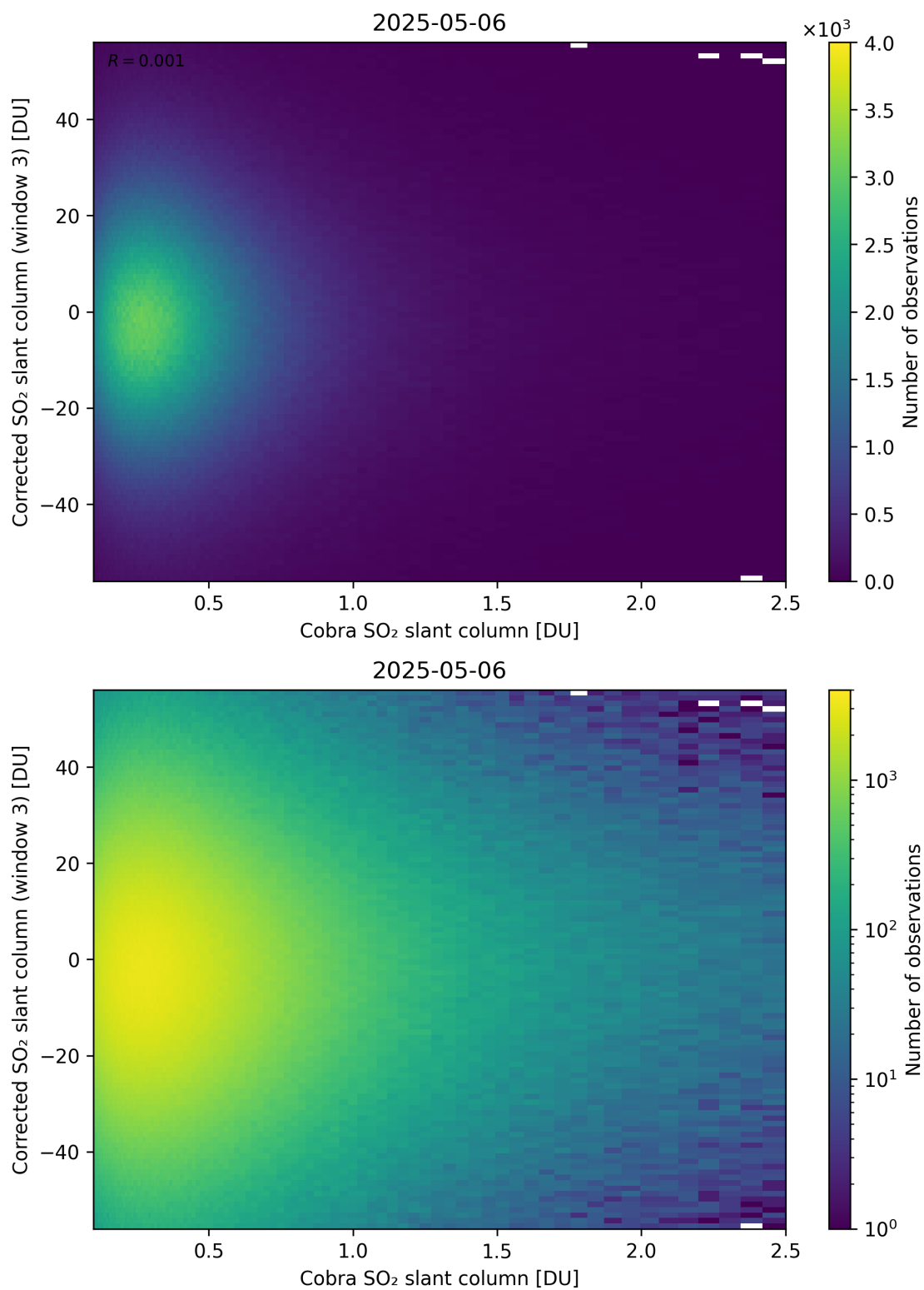
Figure 218: Scatter density plot of “Cobra SO 2 slant column” against “Corrected SO 2 slant column (window 3)” for 2025-05-05 to 2025-05-07.
