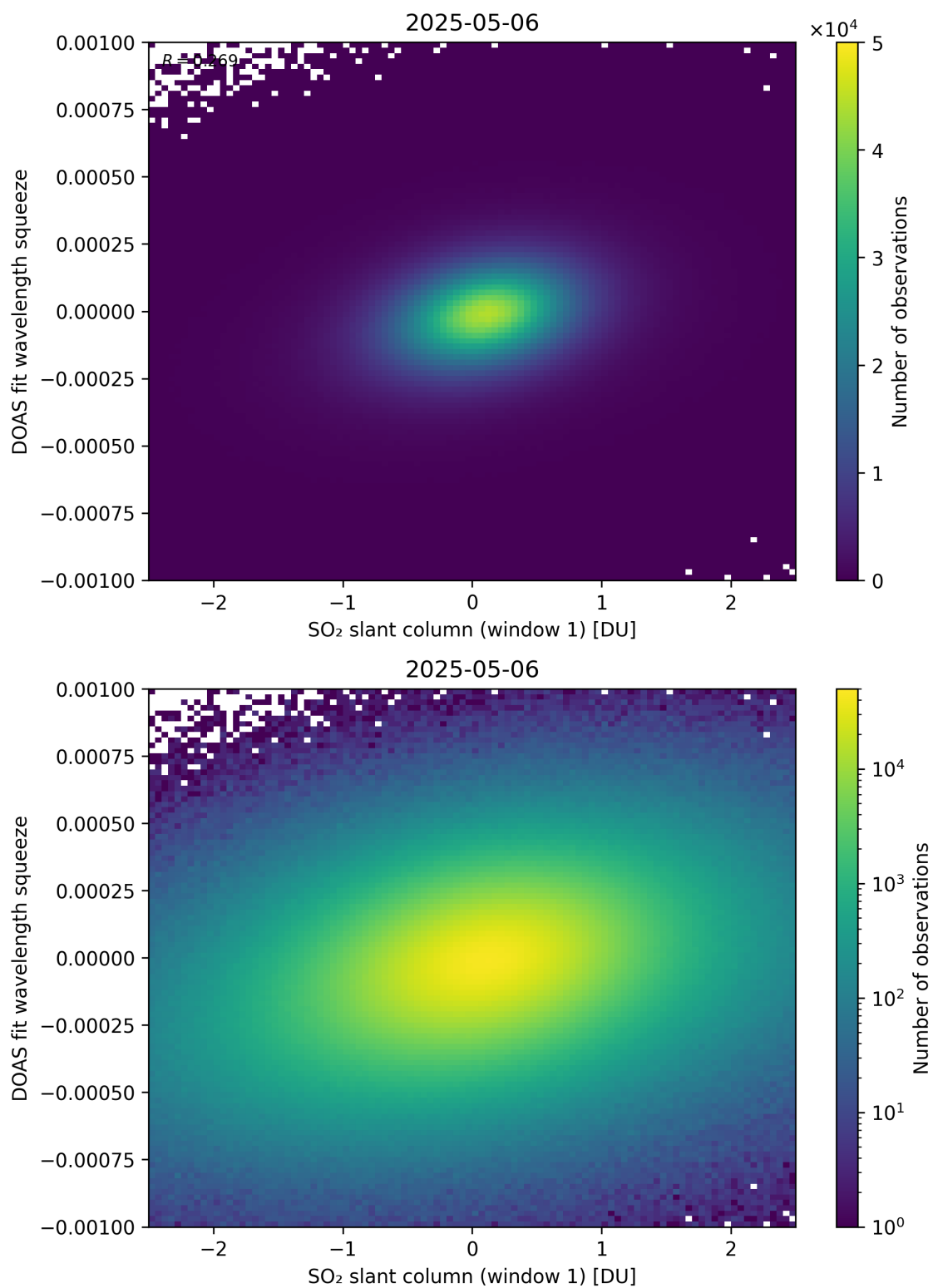
Figure 266: Scatter density plot of “SO 2 slant column (window 1)” against “DOAS fit wavelength squeeze” for 2025-05-05 to 2025-05-07.
