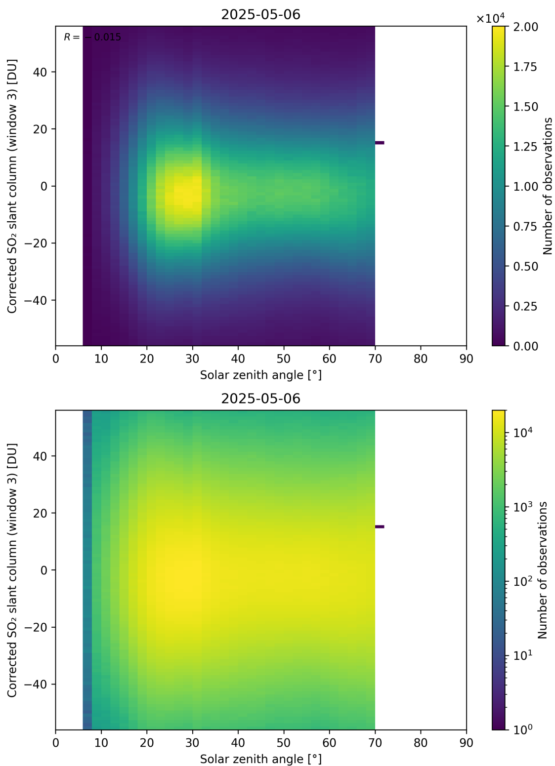
Figure 183: Scatter density plot of “Solar zenith angle” against “Corrected SO 2 slant column (window 3)” for 2025-05-05 to 2025-05-07.
