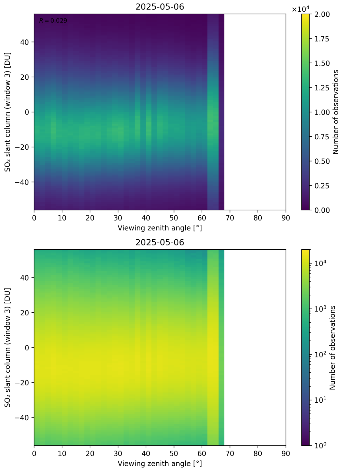
Figure 379: Scatter density plot of “Viewing zenith angle” against “SO 2 slant column (window 3)” for 2025-05-05 to 2025-05-07.
