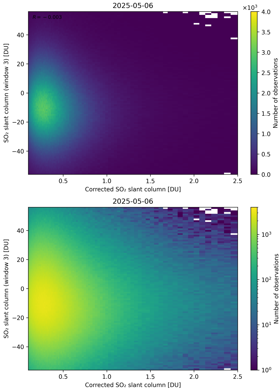
Figure 240: Scatter density plot of “Corrected SO 2 slant column” against “SO 2 slant column (window 3)” for 2025-05-05 to 2025-05-07.
