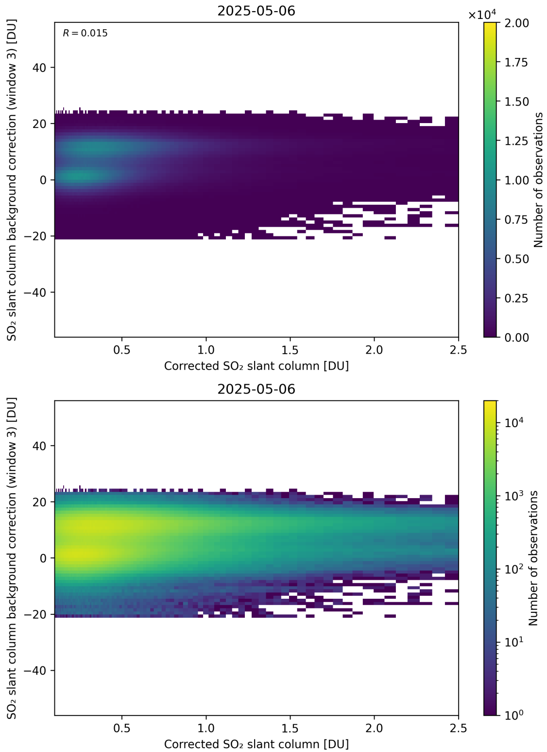
Figure 228: Scatter density plot of “Corrected SO 2 slant column” against “SO 2 slant column background correction (window 3)” for 2025-05-05 to 2025-05-07.
