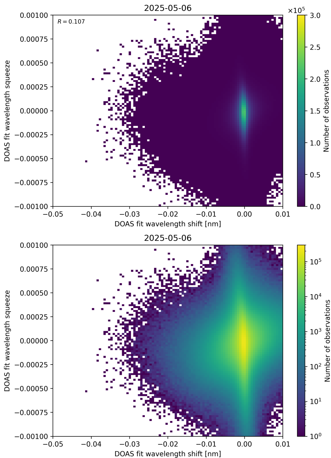
Figure 138: Scatter density plot of “DOAS fit wavelength shift” against “DOAS fit wavelength squeeze” for 2025-05-05 to 2025-05-07.
