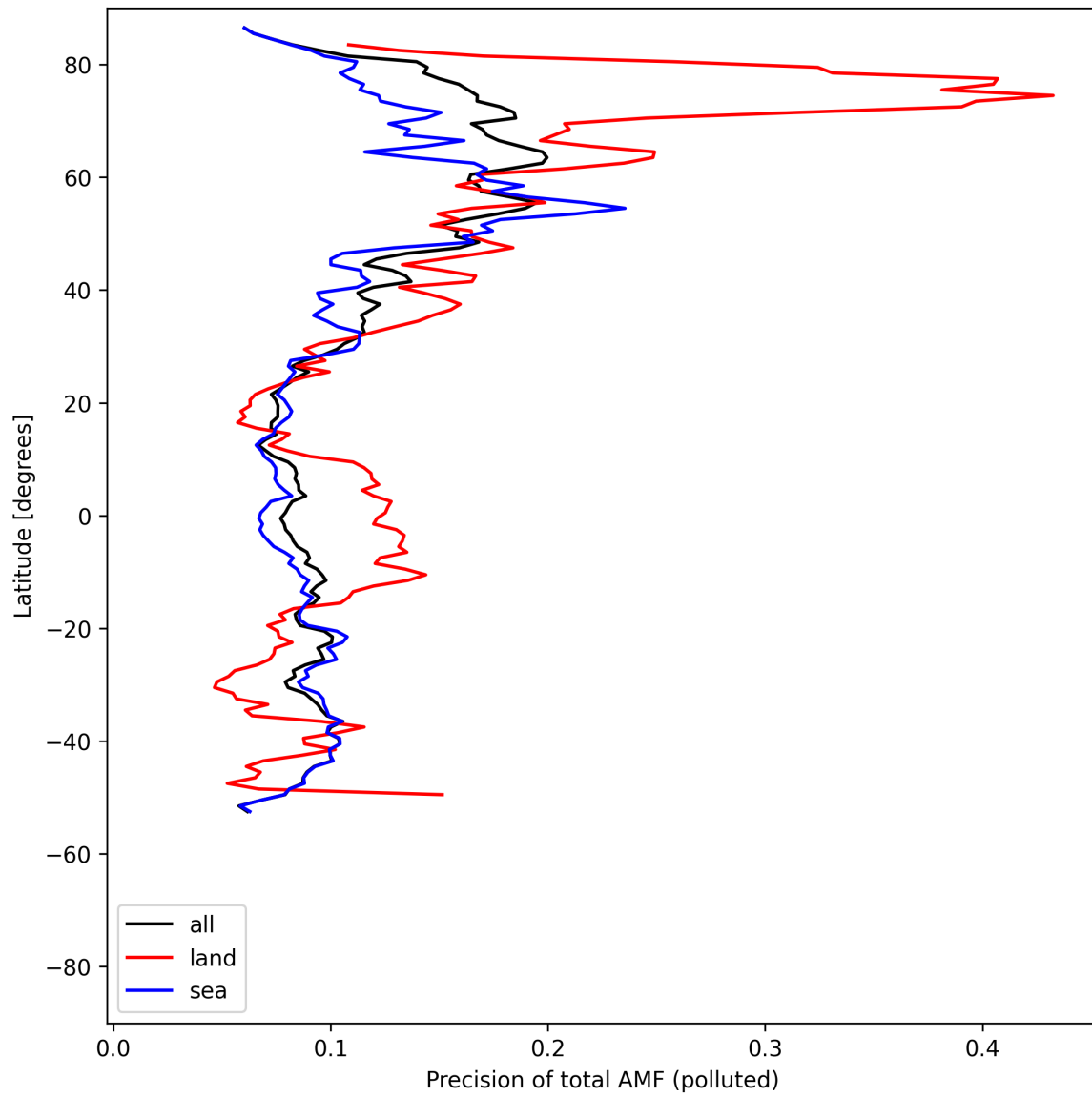
Figure 54: Zonal average of “Precision of total AMF (polluted)” for 2025-05-05 to 2025-05-07.
