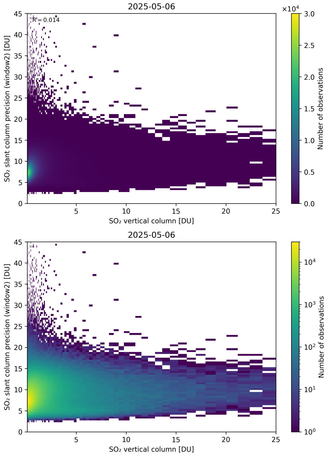
Figure 356: Scatter density plot of “SO 2 vertical column” against “SO 2 slant column precision (window2)” for 2025-05-05 to 2025-05-07.
