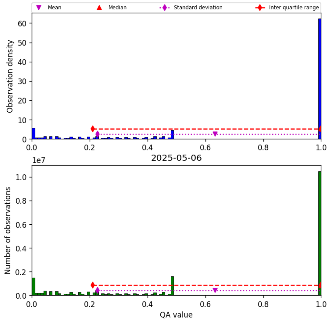
Figure 57: Histogram of “QA value” for 2025-05-05 to 2025-05-07
