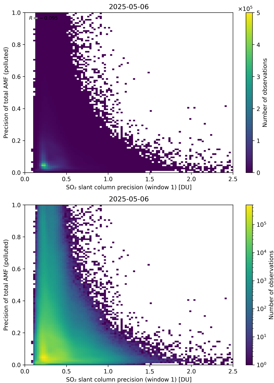
Figure 281: Scatter density plot of “SO 2 slant column precision (window 1)” against “Precision of total AMF (polluted)” for 2025-05-05 to 2025-05-07.
