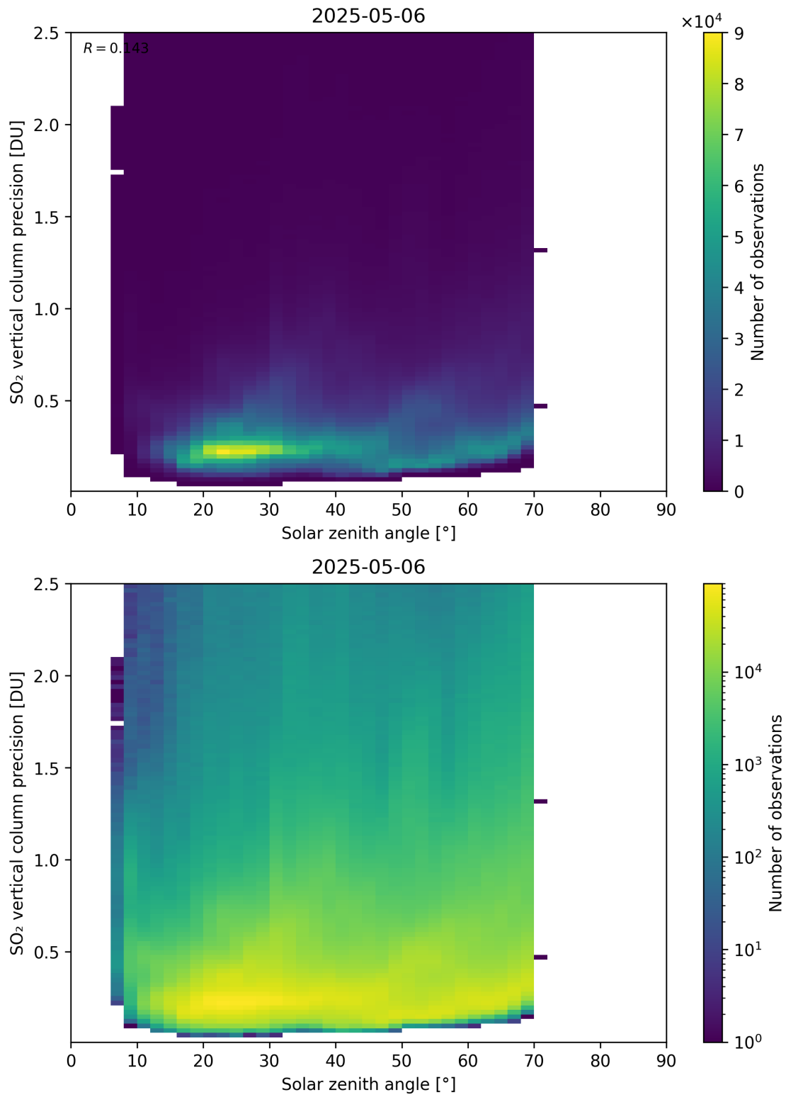
Figure 192: Scatter density plot of “Solar zenith angle” against “SO 2 vertical column precision” for 2025-05-05 to 2025-05-07.
