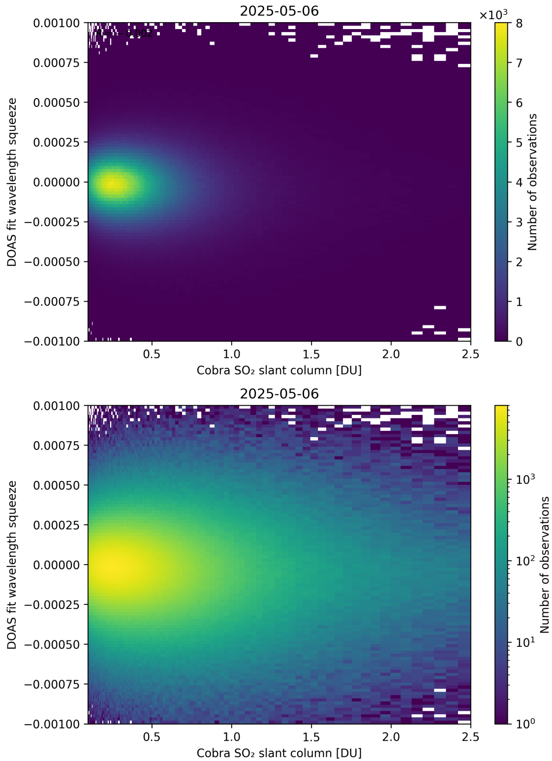
Figure 197: Scatter density plot of “Cobra SO 2 slant column” against “DOAS fit wavelength squeeze” for 2025-05-05 to 2025-05-07.
