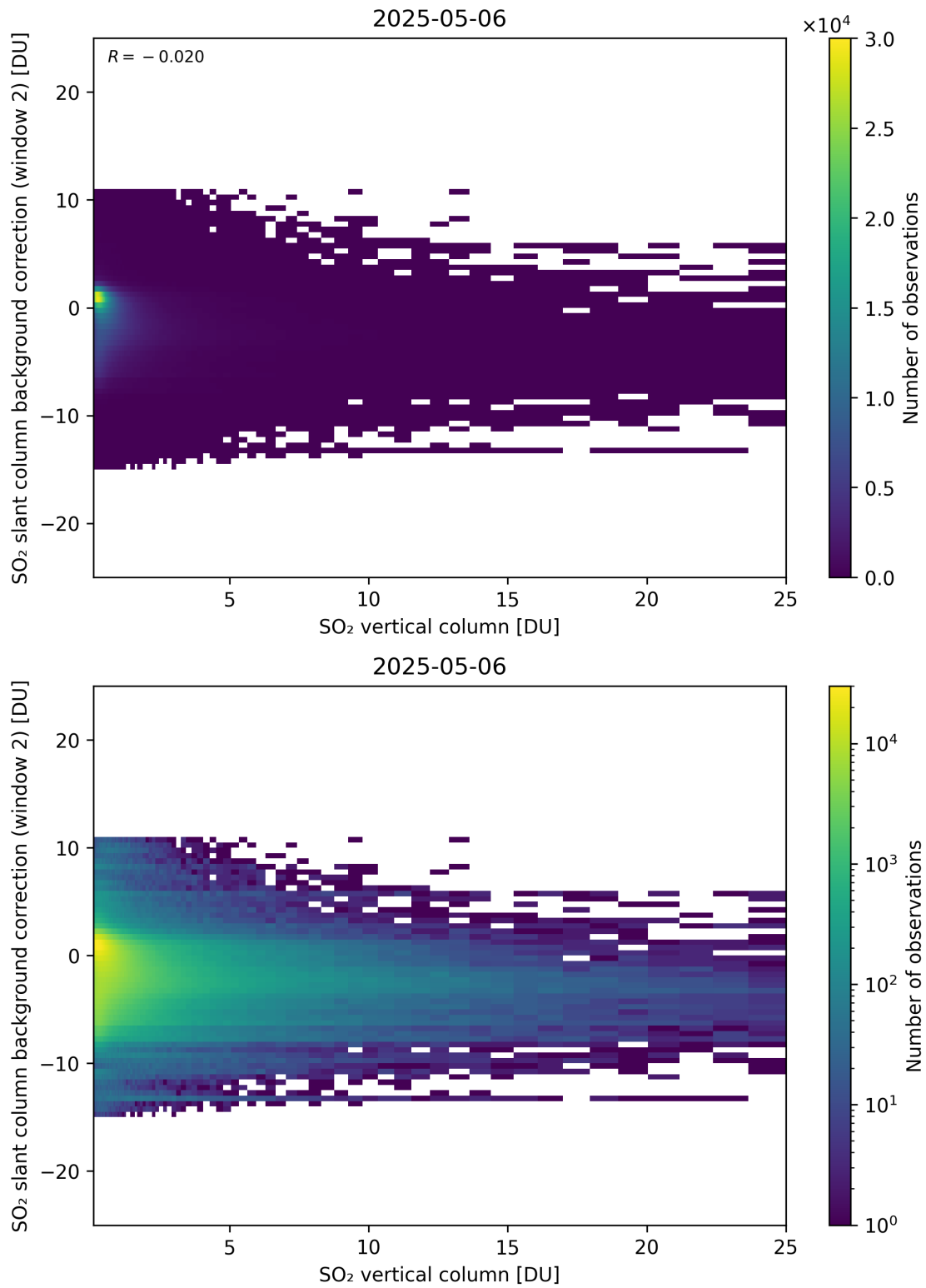
Figure 324: Scatter density plot of “SO 2 vertical column” against “SO 2 slant column background correction (window 2)” for 2025-05-05 to 2025-05-07.
