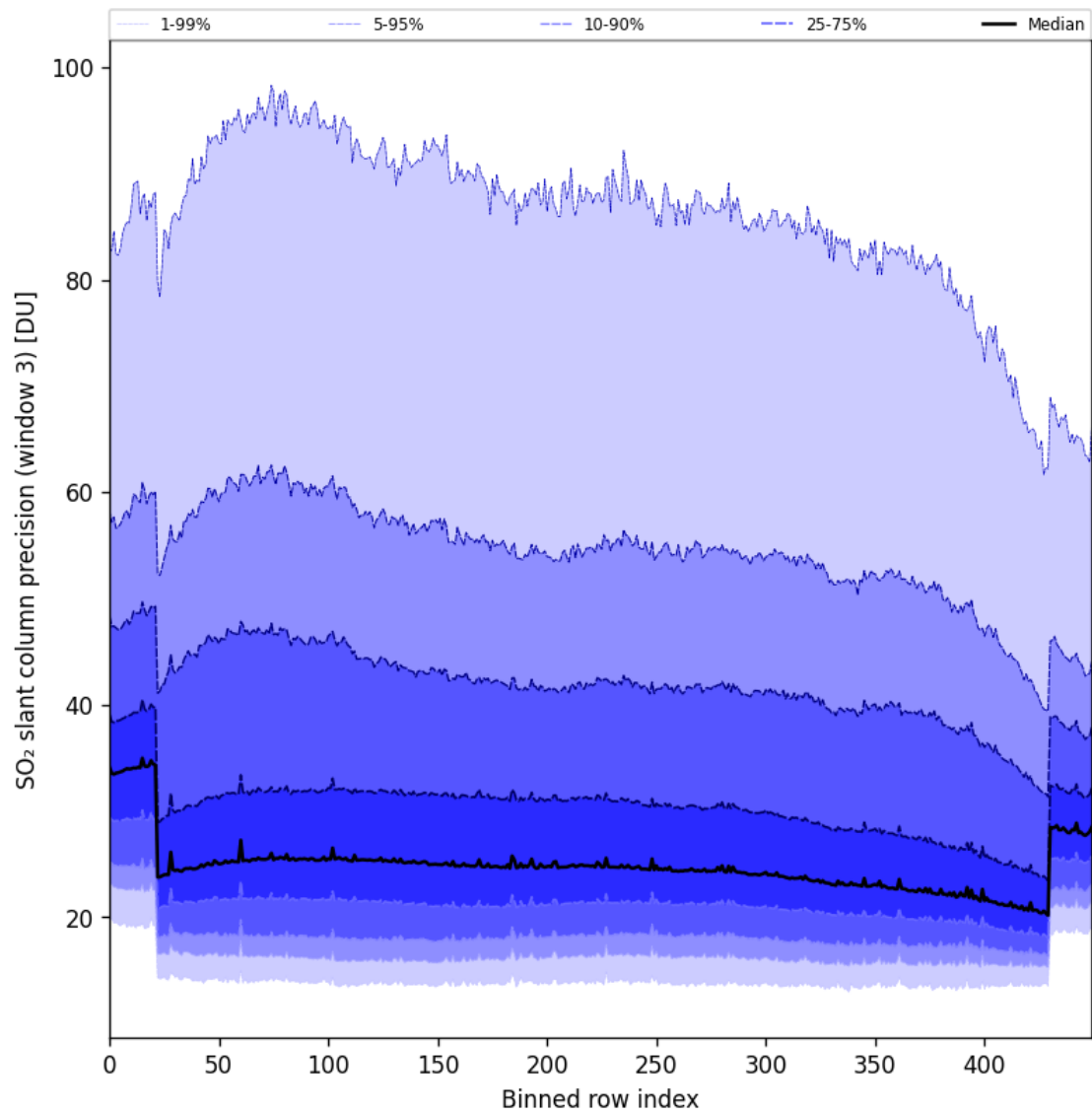
Figure 98: Along track statistics of “SO 2 slant column precision (window 3)” for 2025-05-05 to 2025-05-07
