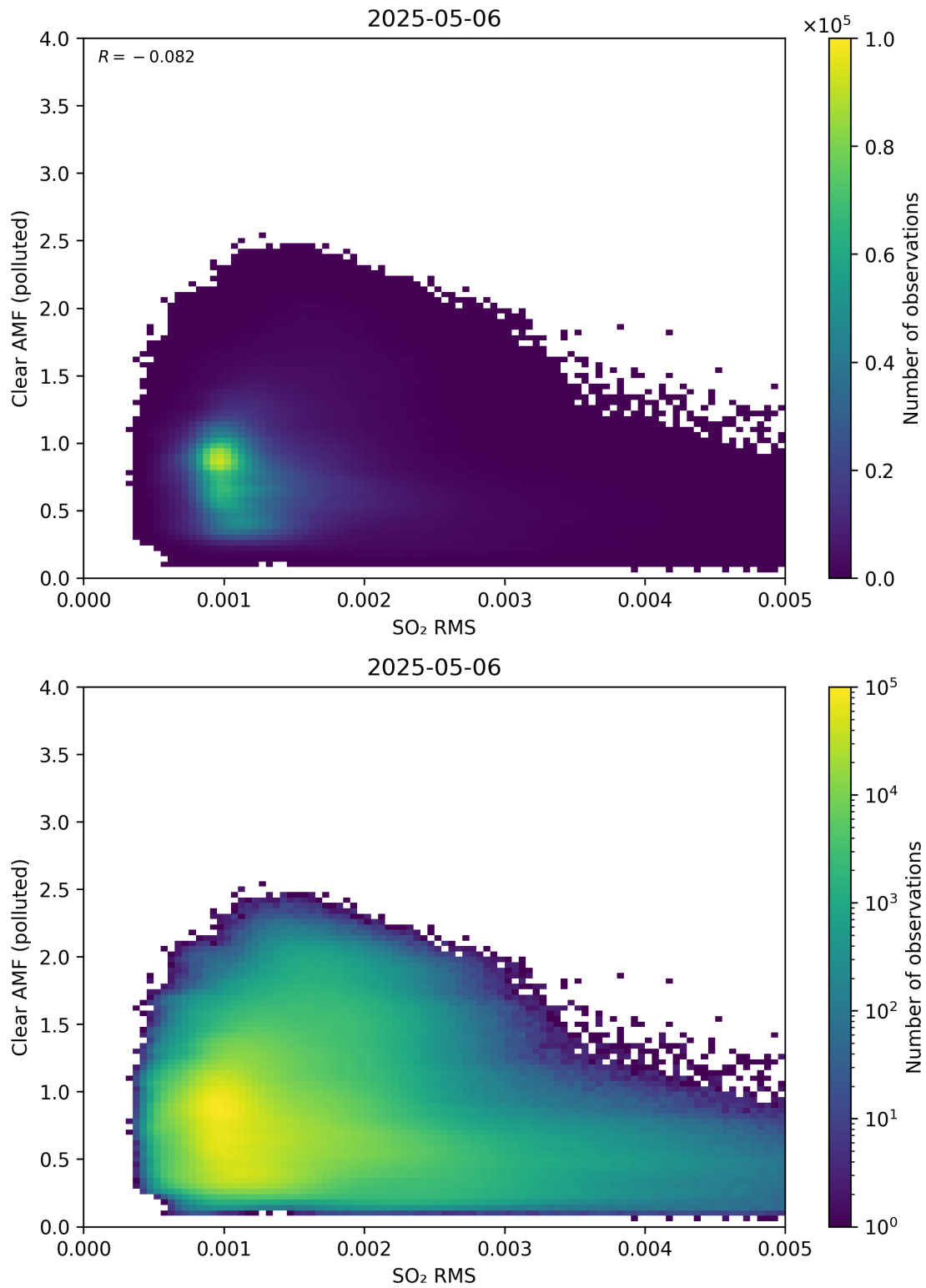
Figure 147: Scatter density plot of “SO 2 RMS” against “Clear AMF (polluted)” for 2025-05-05 to 2025-05-07.
