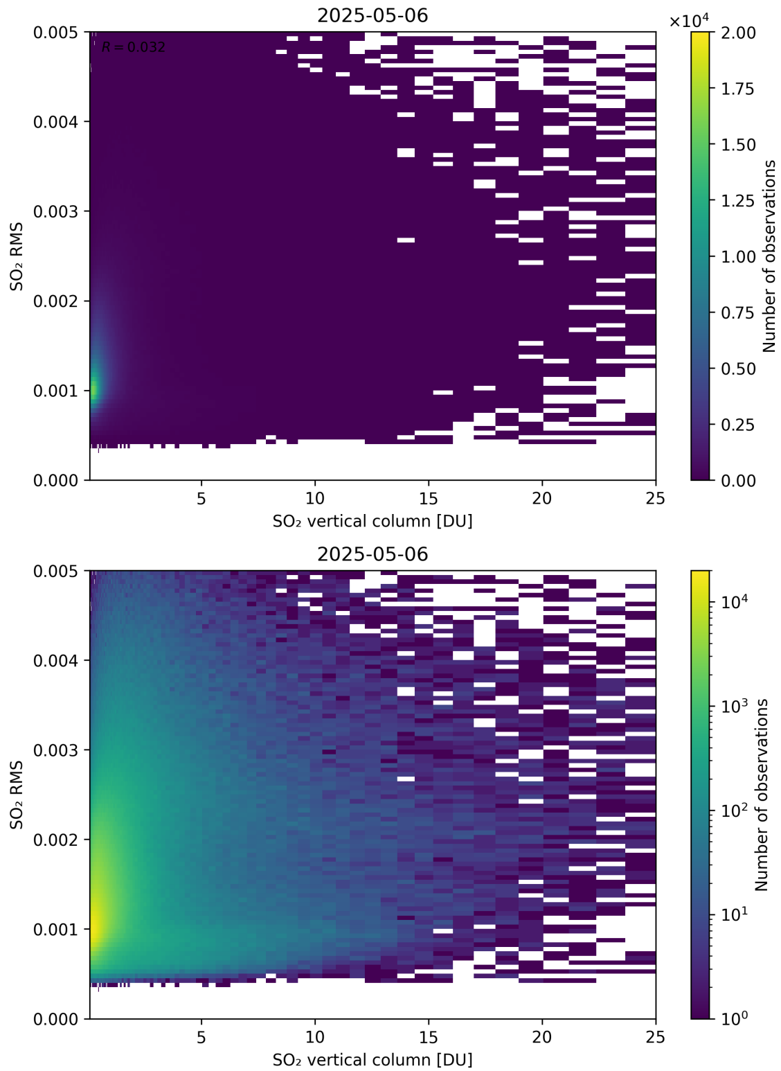
Figure 328: Scatter density plot of “SO 2 vertical column” against “SO 2 RMS” for 2025-05-05 to 2025-05-07.
