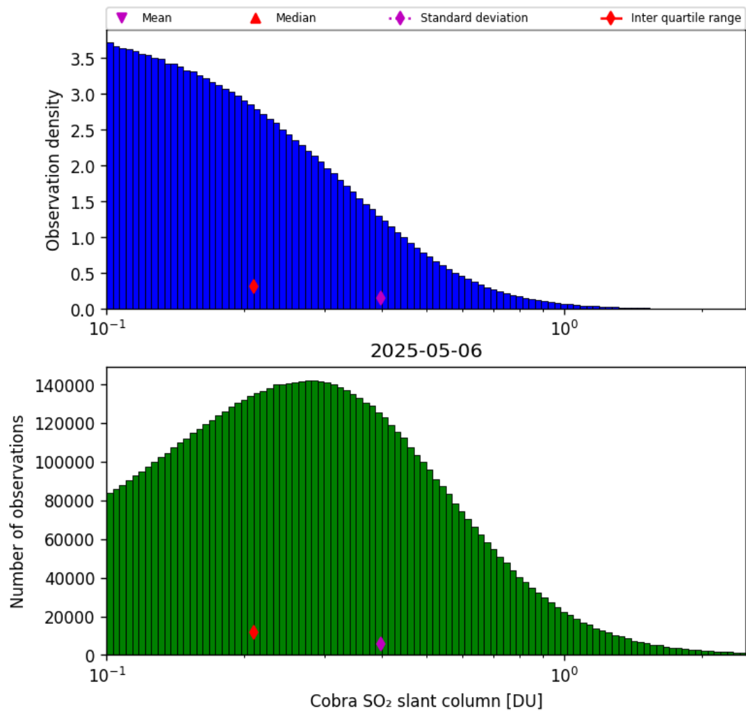
Figure 61: Histogram of “Cobra SO 2 slant column” for 2025-05-05 to 2025-05-07
