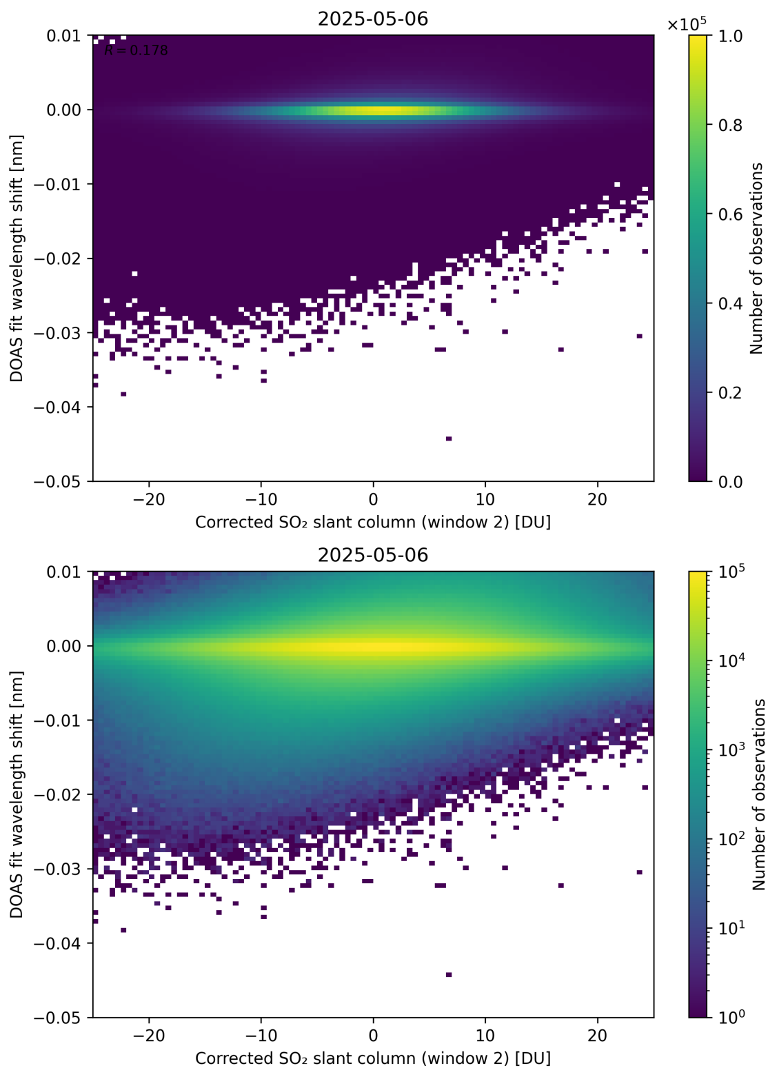
Figure 246: Scatter density plot of “Corrected SO 2 slant column (window 2)” against “DOAS fit wavelength shift” for 2025-05-05 to 2025-05-07.
