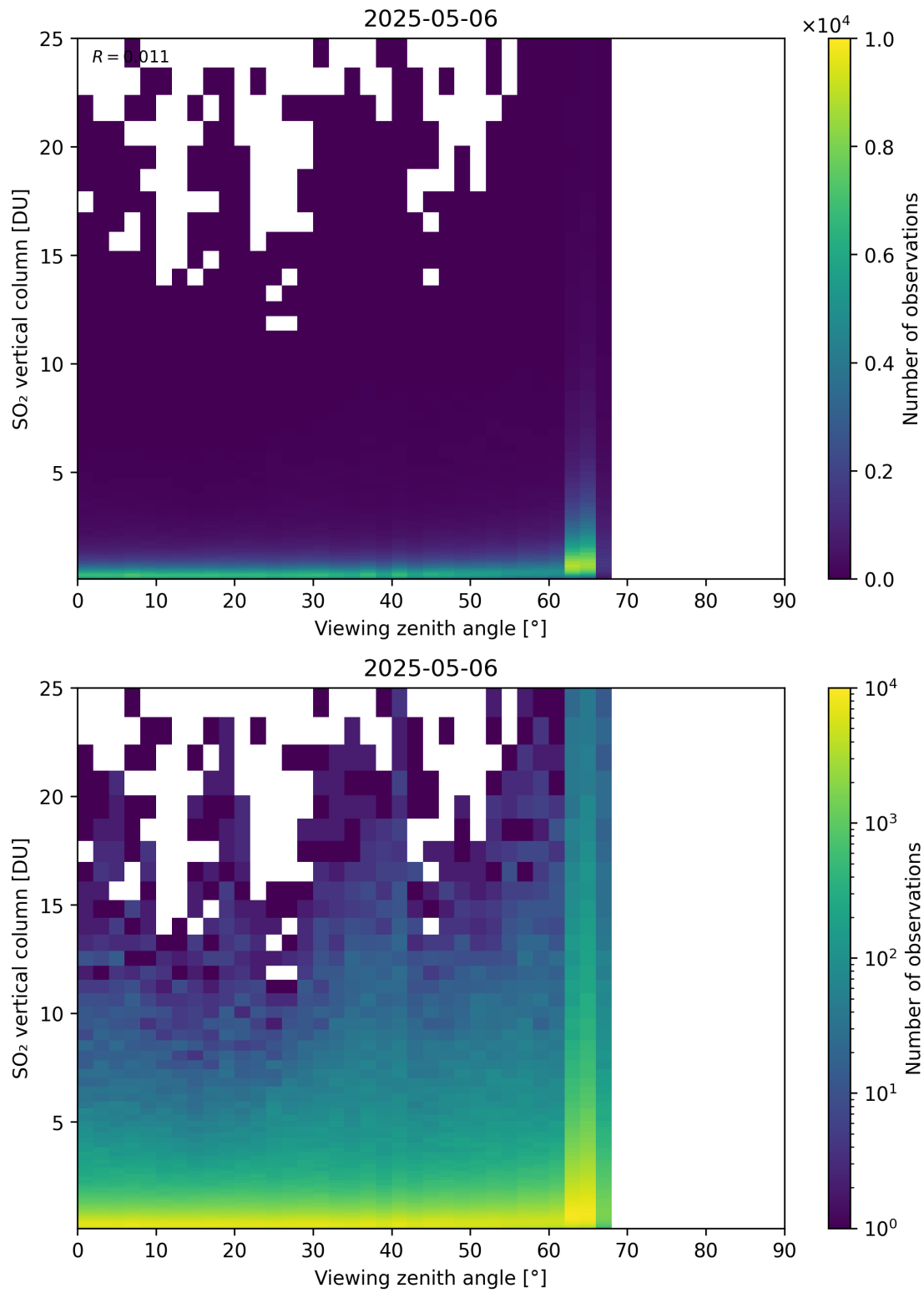
Figure 383: Scatter density plot of “Viewing zenith angle” against “SO 2 vertical column” for 2025-05-05 to 2025-05-07.
