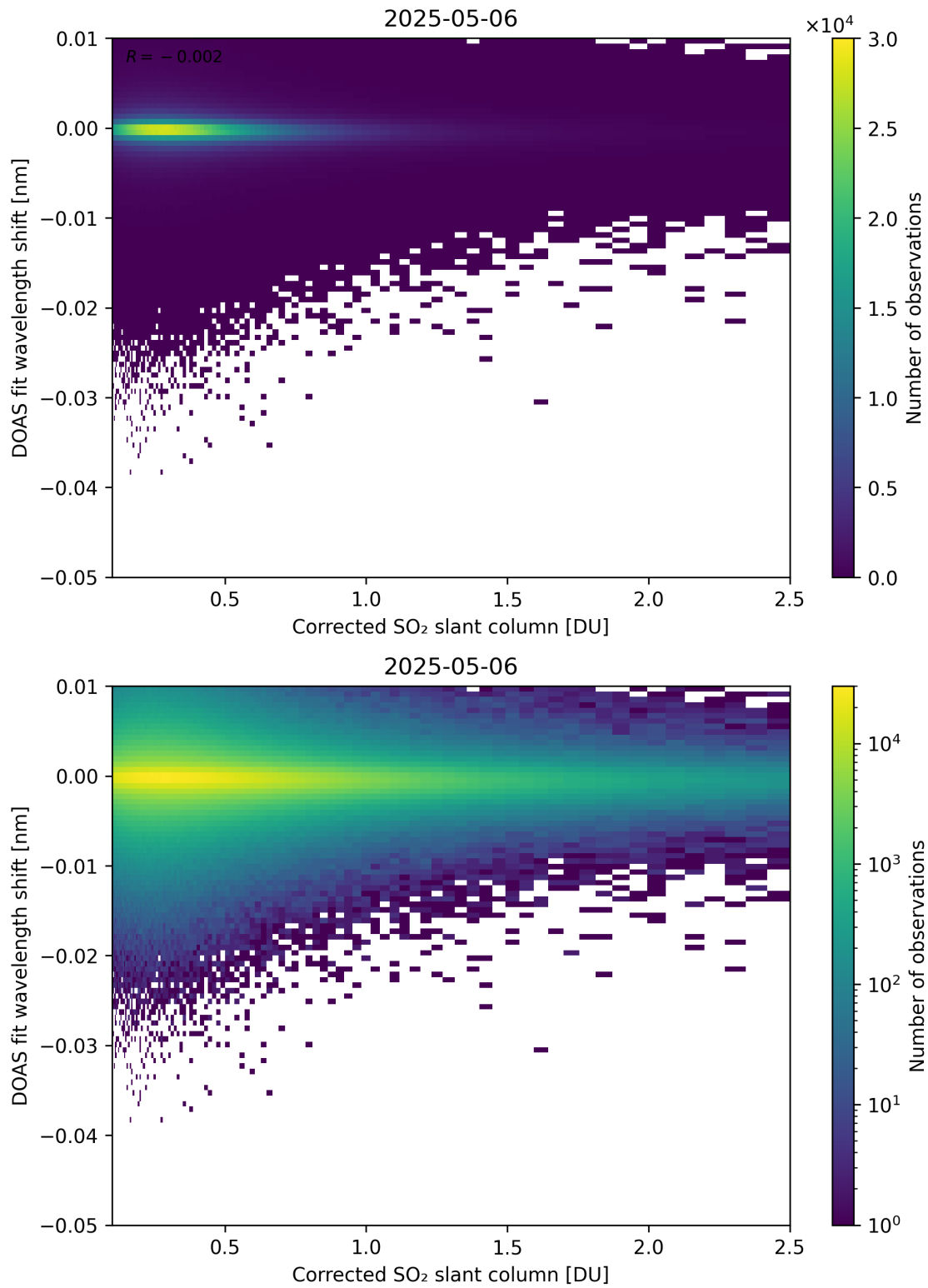
Figure 229: Scatter density plot of “Corrected SO 2 slant column” against “DOAS fit wavelength shift” for 2025-05-05 to 2025-05-07.
