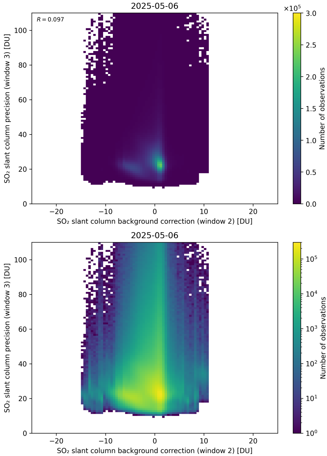
Figure 129: Scatter density plot of “SO 2 slant column background correction (window 2)” against “SO 2 slant column precision (window 3)” for 2025-05-05 to 2025-05-07.
