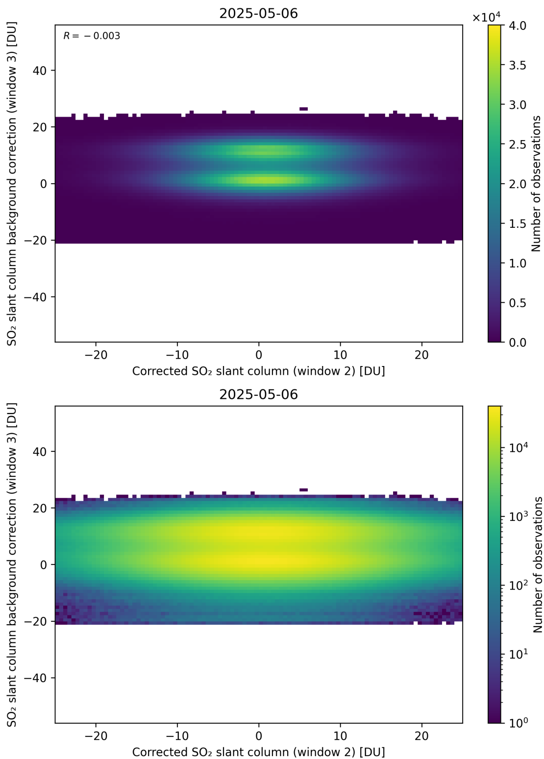
Figure 245: Scatter density plot of “Corrected SO 2 slant column (window 2)” against “SO 2 slant column background correction (window 3)” for 2025-05-05 to 2025-05-07.
