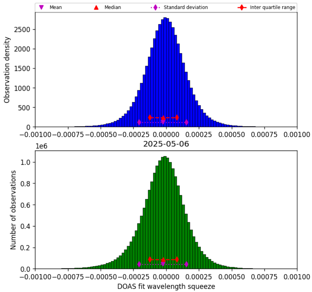
Figure 77: Histogram of “DOAS fit wavelength squeeze” for 2025-05-05 to 2025-05-07
