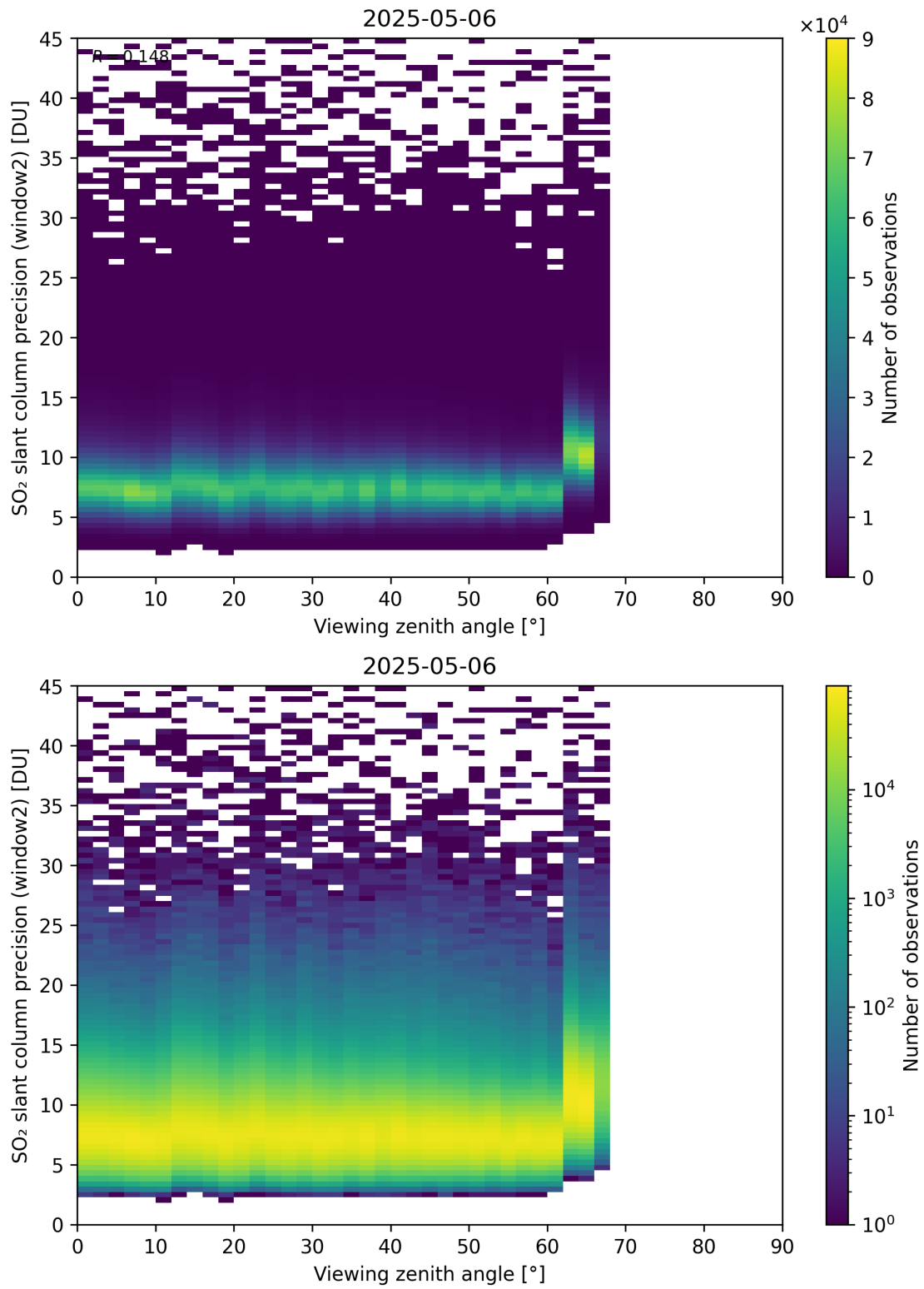
Figure 378: Scatter density plot of “Viewing zenith angle” against “SO 2 slant column precision (window2)” for 2025-05-05 to 2025-05-07.
