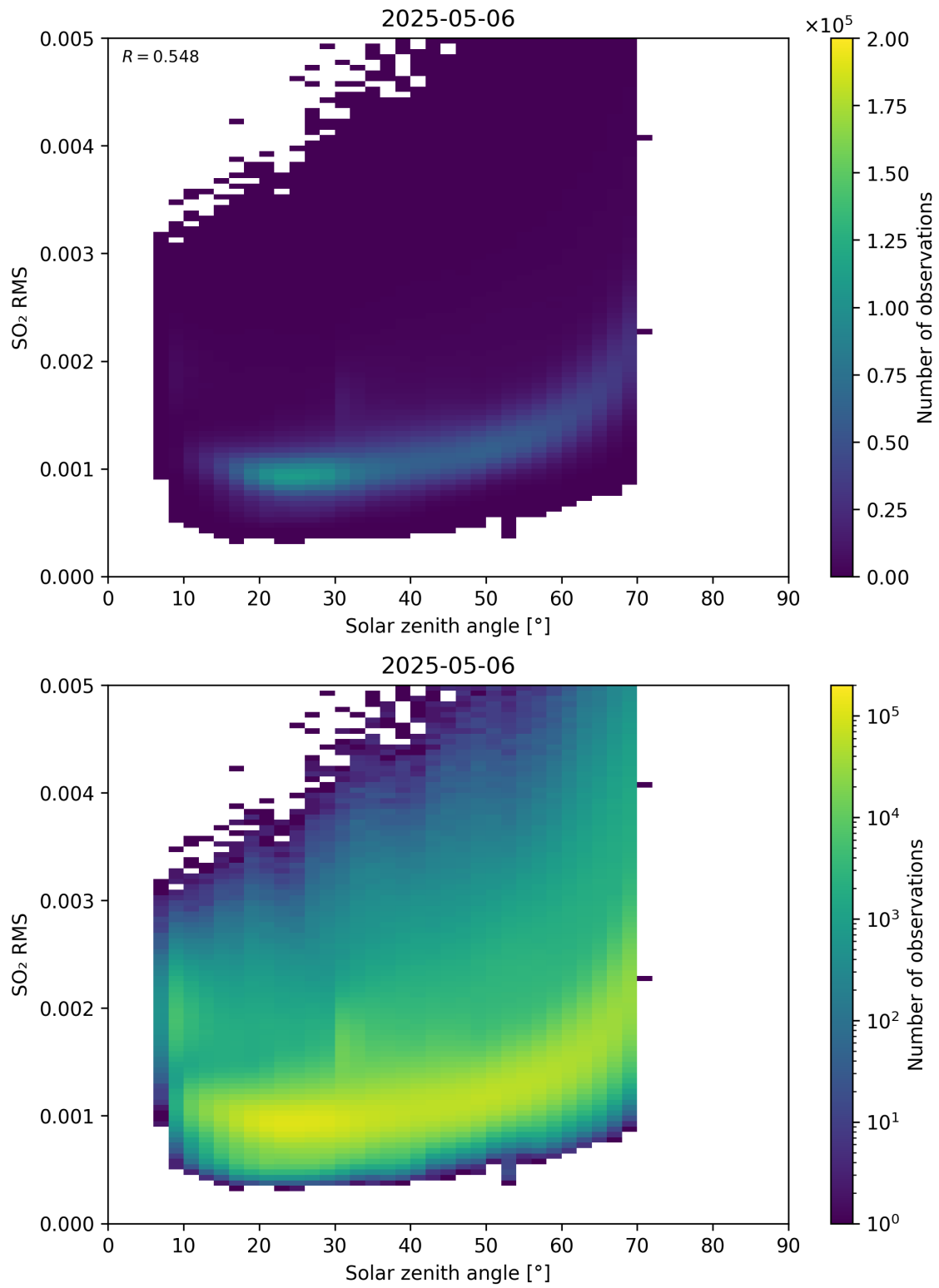
Figure 176: Scatter density plot of “Solar zenith angle” against “SO 2 RMS” for 2025-05-05 to 2025-05-07.
