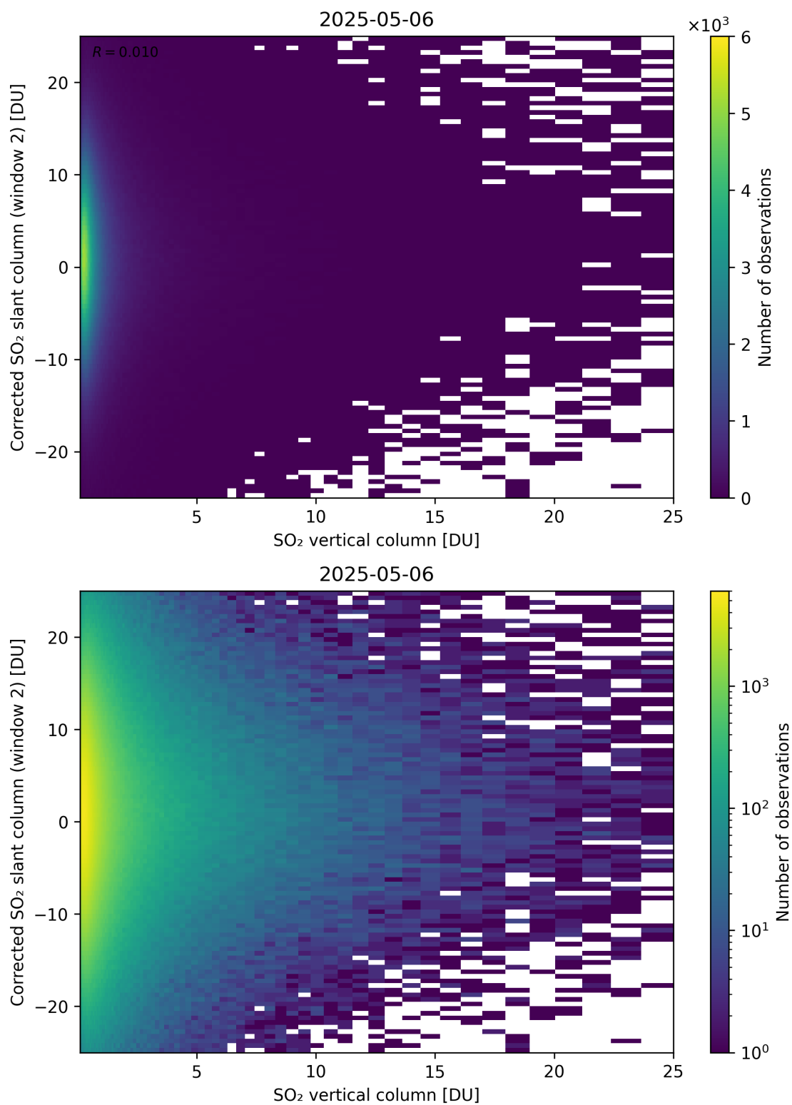
Figure 352: Scatter density plot of “SO 2 vertical column” against “Corrected SO 2 slant column (window 2)” for 2025-05-05 to 2025-05-07.
