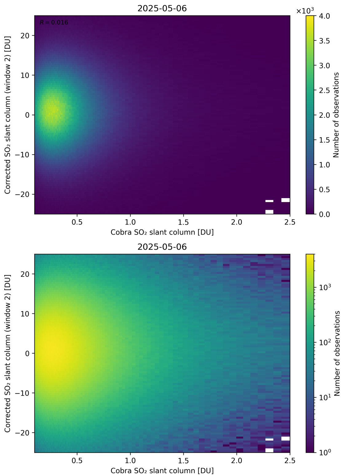
Figure 217: Scatter density plot of “Cobra SO 2 slant column” against “Corrected SO 2 slant column (window 2)” for 2025-05-05 to 2025-05-07.
