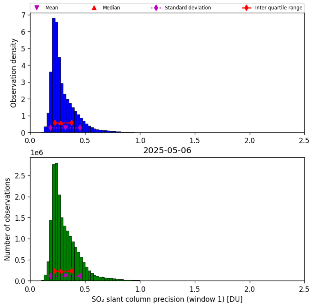
Figure 64: Histogram of “SO 2 slant column precision (window 1)” for 2025-05-05 to 2025-05-07
