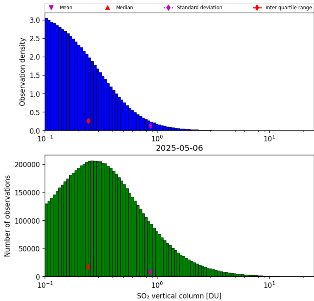
Figure 58: Histogram of “SO 2 vertical column” for 2025-05-05 to 2025-05-07
