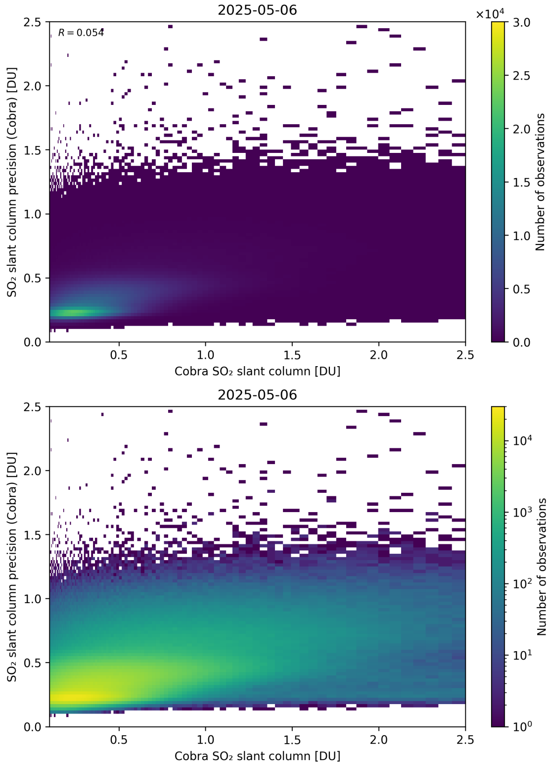
Figure 216: Scatter density plot of “Cobra SO 2 slant column” against “SO 2 slant column precision (Cobra)” for 2025-05-05 to 2025-05-07.
