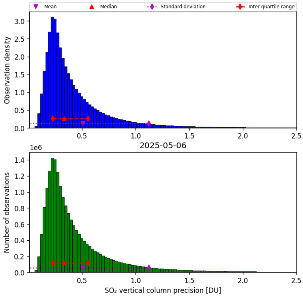
Figure 59: Histogram of "SO 2 vertical column precision" for 2025-05-05 to 2025-05-07
