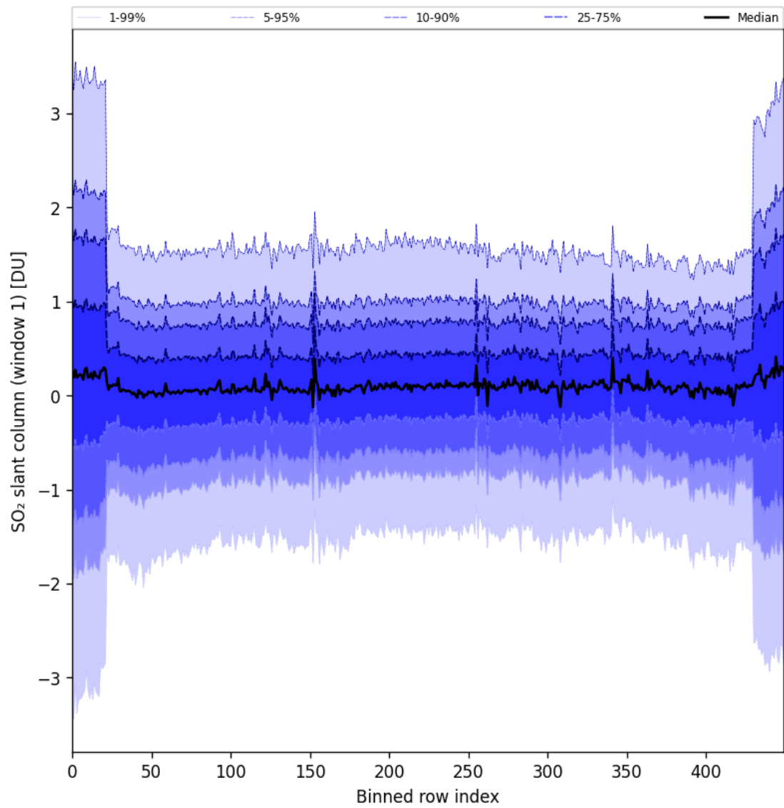
Figure 89: Along track statistics of “SO 2 slant column (window 1)” for 2025-05-05 to 2025-05-07
