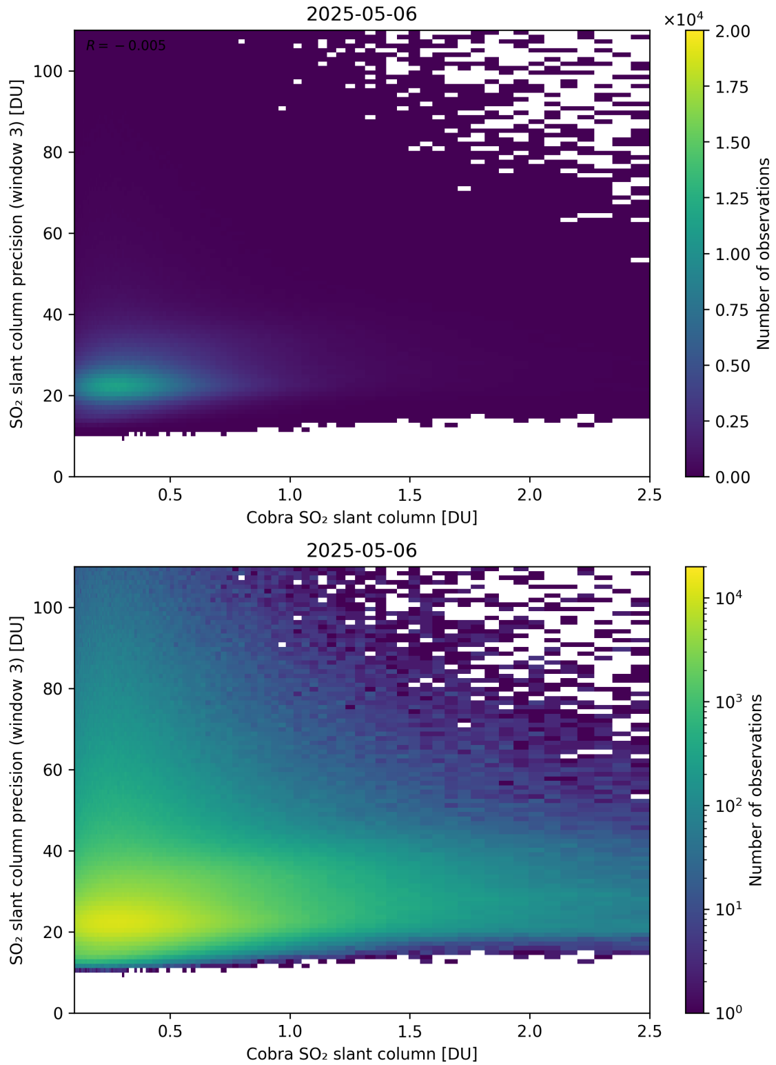
Figure 223: Scatter density plot of “Cobra SO 2 slant column” against “SO 2 slant column precision (window 3)” for 2025-05-05 to 2025-05-07.
