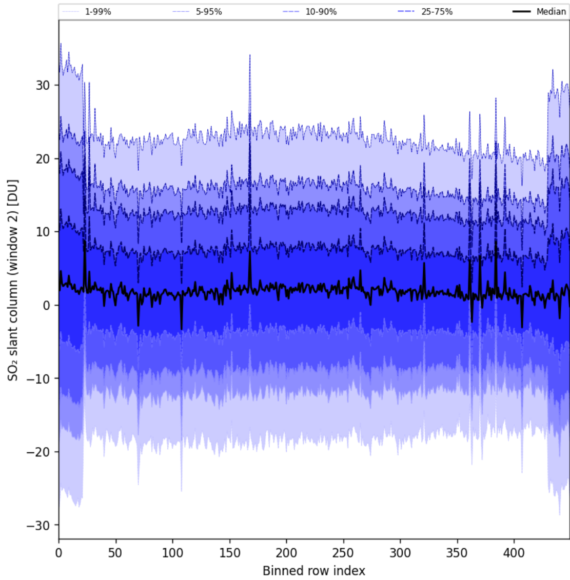
Figure 93: Along track statistics of “SO 2 slant column (window 2)” for 2025-05-05 to 2025-05-07
