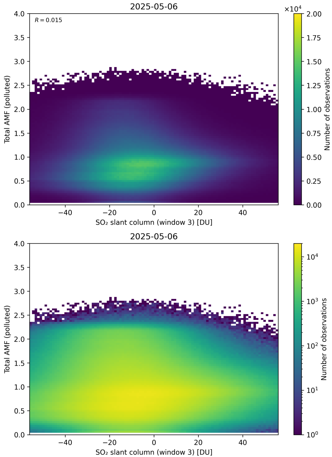
Figure 318: Scatter density plot of “SO 2 slant column (window 3)” against “Total AMF (polluted)” for 2025-05-05 to 2025-05-07.
