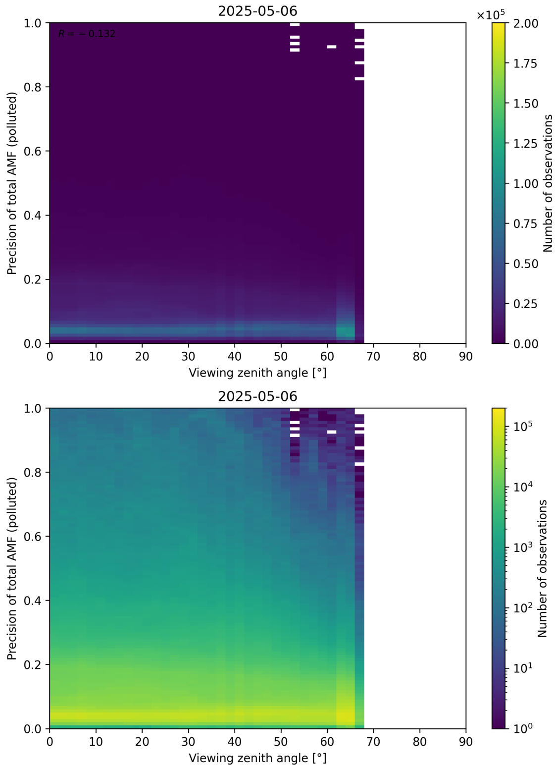
Figure 382: Scatter density plot of “Viewing zenith angle” against “Precision of total AMF (polluted)” for 2025-05-05 to 2025-05-07.
