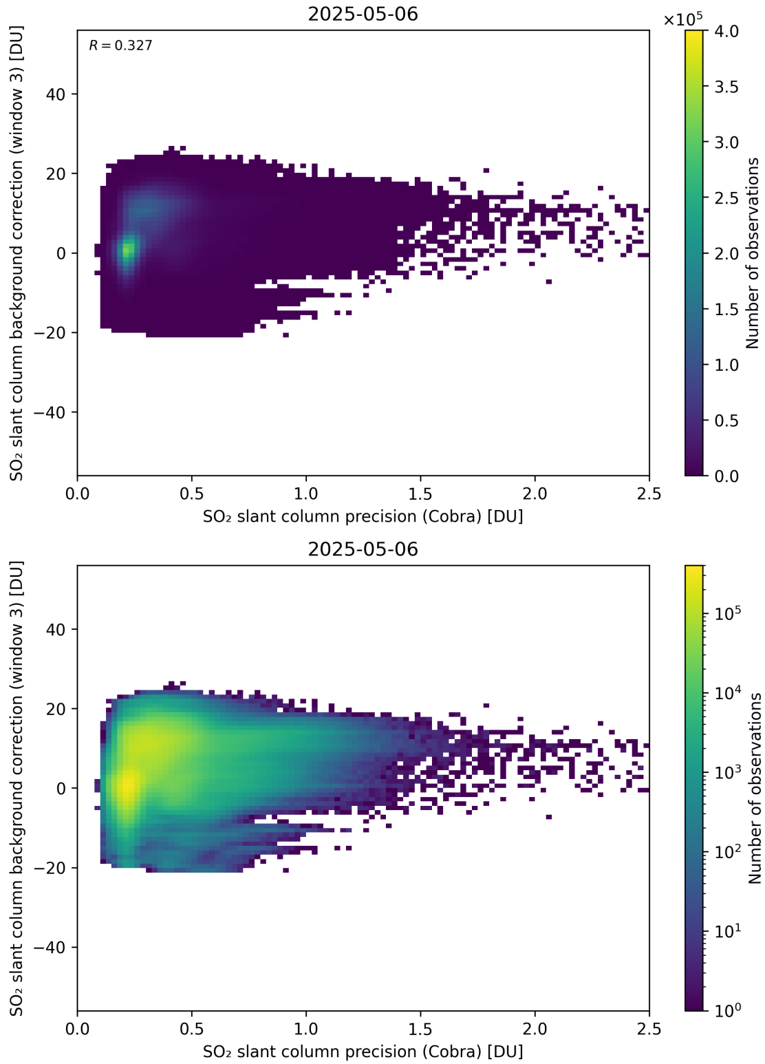
Figure 201: Scatter density plot of “SO 2 slant column precision (Cobra)” against “SO 2 slant column background correction (window 3)” for 2025-05-05 to 2025-05-07.
