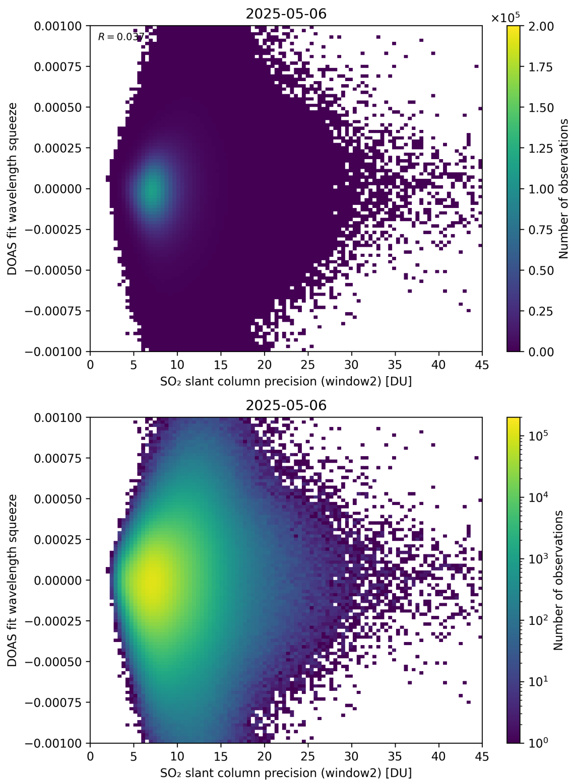
Figure 294: Scatter density plot of “SO 2 slant column precision (window2)” against “DOAS fit wavelength squeeze” for 2025-05-05 to 2025-05-07.
