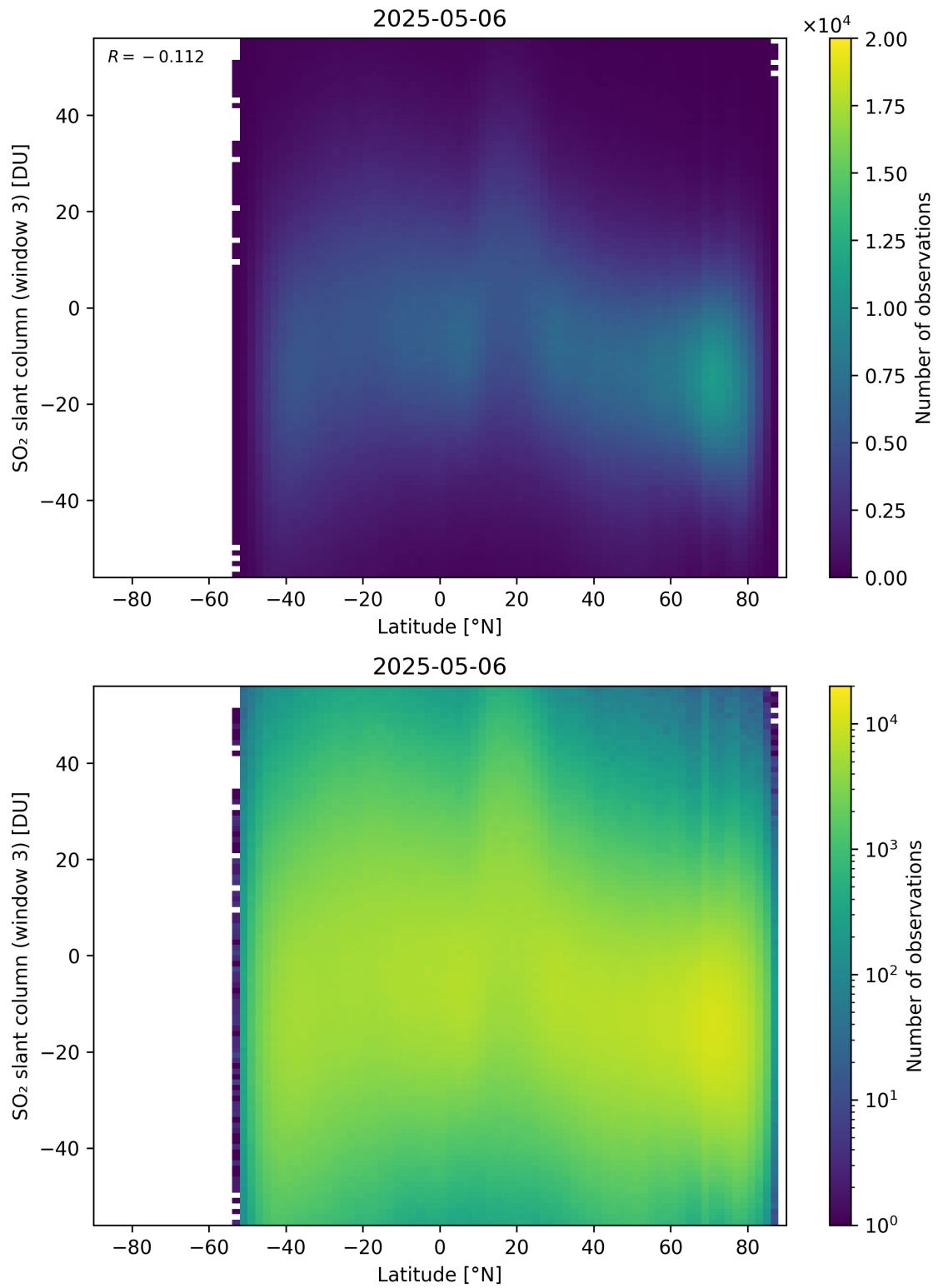
Figure 165: Scatter density plot of “Latitude” against “SO 2 slant column (window 3)” for 2025-05-05 to 2025-05-07.
