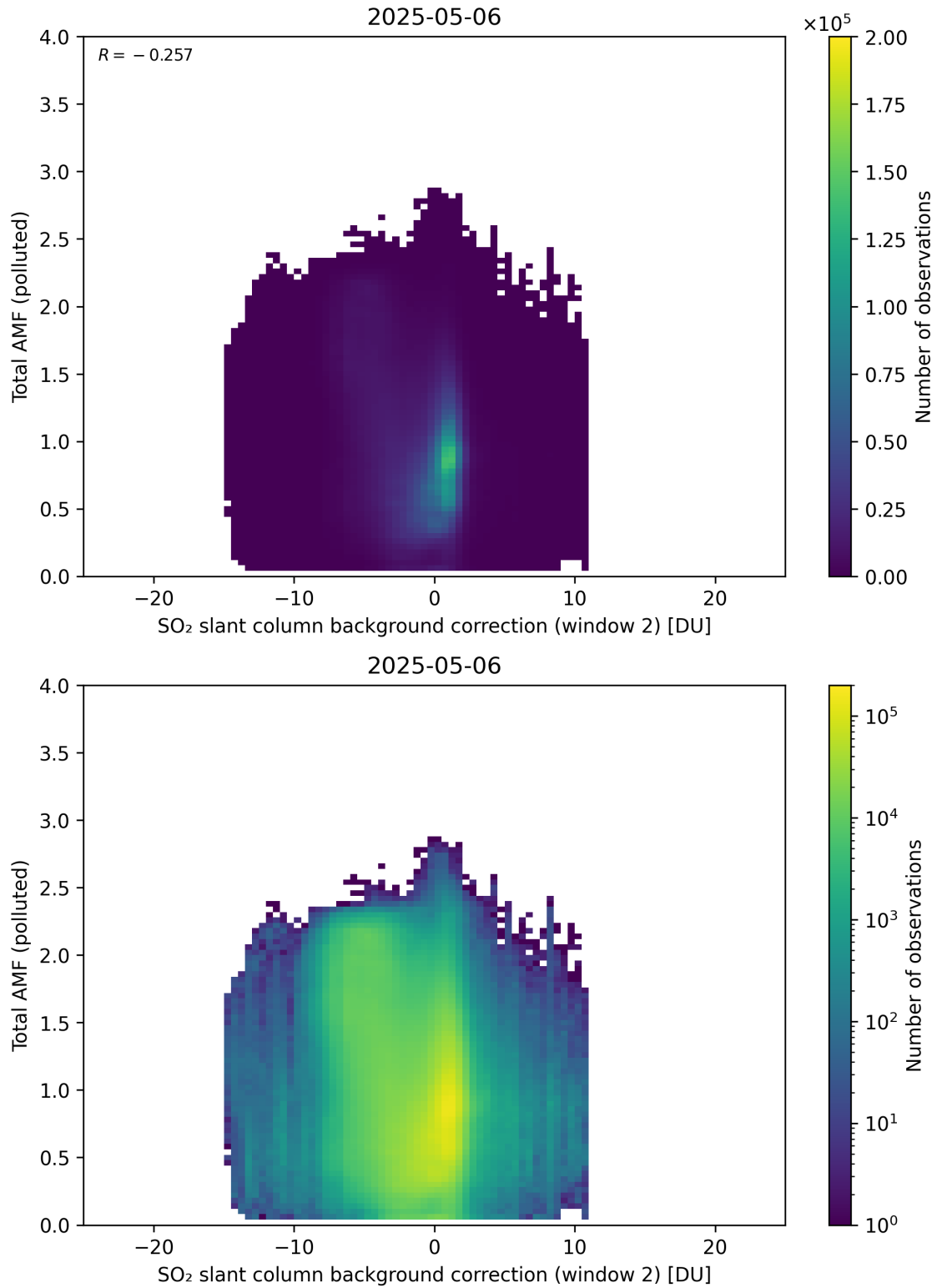
Figure 130: Scatter density plot of “SO 2 slant column background correction (window 2)” against “Total AMF (polluted)” for 2025-05-05 to 2025-05-07.
