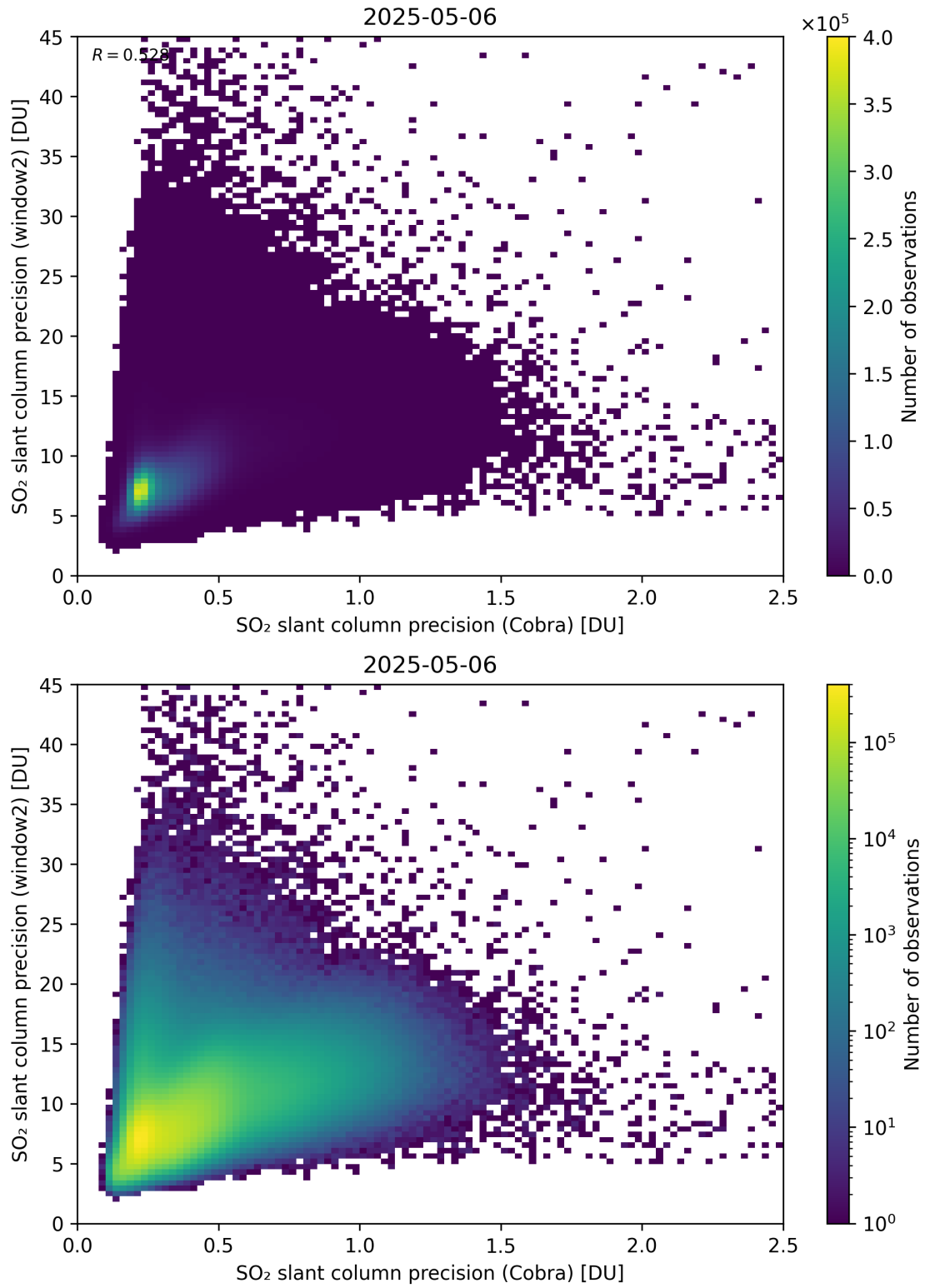
Figure 210: Scatter density plot of “SO 2 slant column precision (Cobra)” against “SO 2 slant column precision (window2)” for 2025-05-05 to 2025-05-07.
