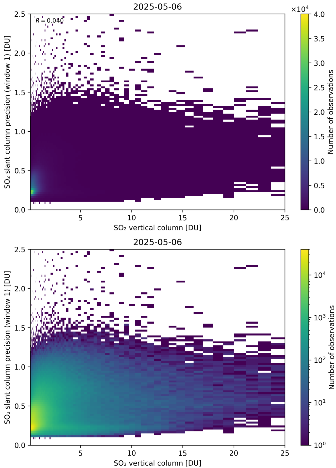
Figure 355: Scatter density plot of “SO 2 vertical column” against “SO 2 slant column precision (window 1)” for 2025-05-05 to 2025-05-07.
