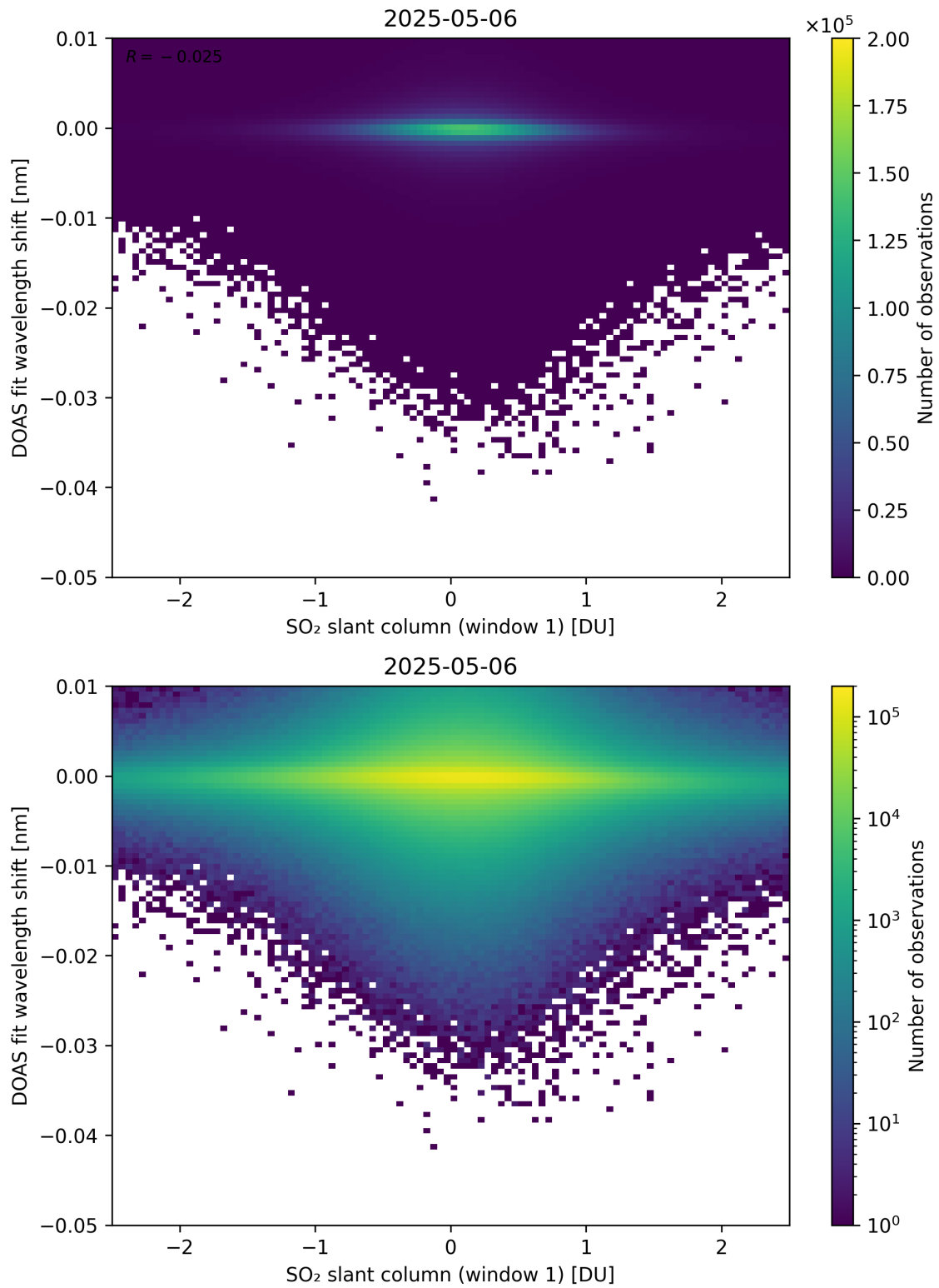
Figure 265: Scatter density plot of “SO 2 slant column (window 1)” against “DOAS fit wavelength shift” for 2025-05-05 to 2025-05-07.
