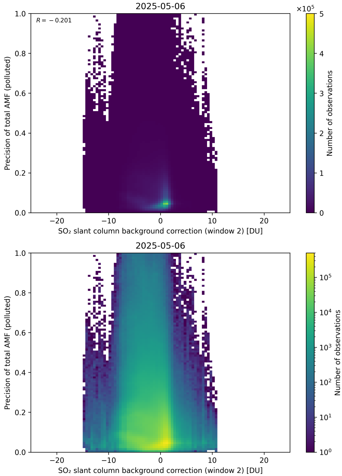
Figure 131: Scatter density plot of “SO 2 slant column background correction (window 2)” against “Precision of total AMF (polluted)” for 2025-05-05 to 2025-05-07.
