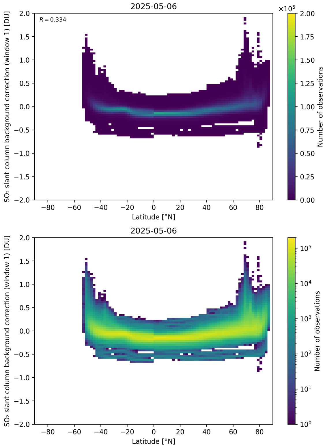
Figure 150: Scatter density plot of “Latitude” against “SO 2 slant column background correction (window 1)” for 2025-05-05 to 2025-05-07.
