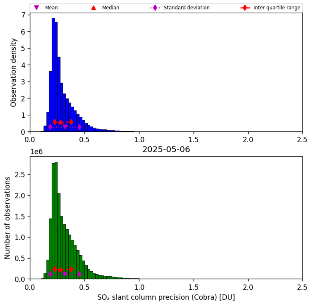
Figure 62: Histogram of “SO 2 slant column precision (Cobra)” for 2025-05-05 to 2025-05-07
