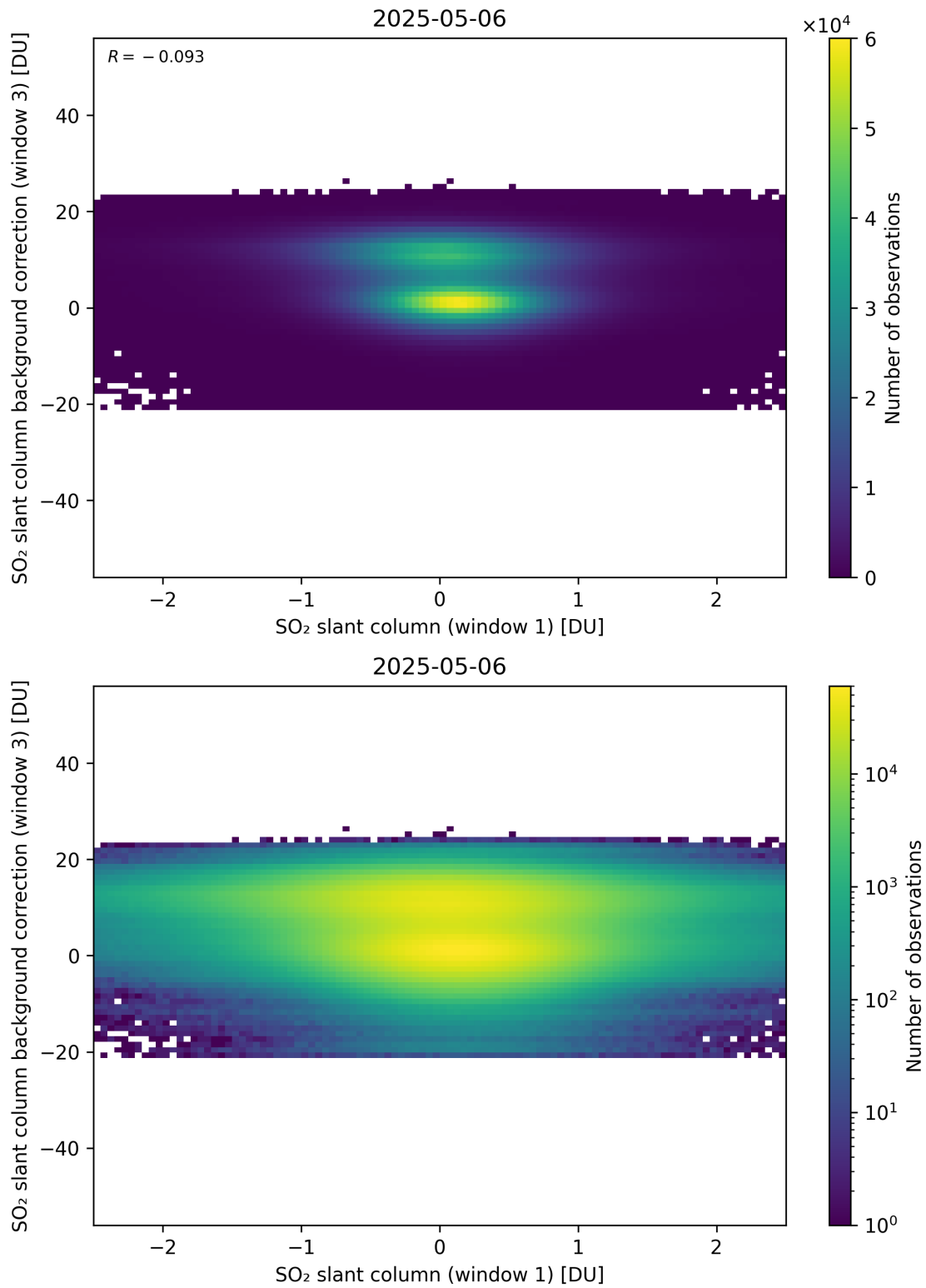
Figure 264: Scatter density plot of “SO 2 slant column (window 1)” against “SO 2 slant column background correction (window 3)” for 2025-05-05 to 2025-05-07.
