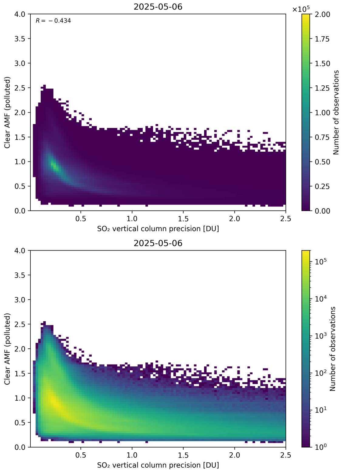
Figure 335: Scatter density plot of “SO 2 vertical column precision” against “Clear AMF (polluted)” for 2025-05-05 to 2025-05-07.
