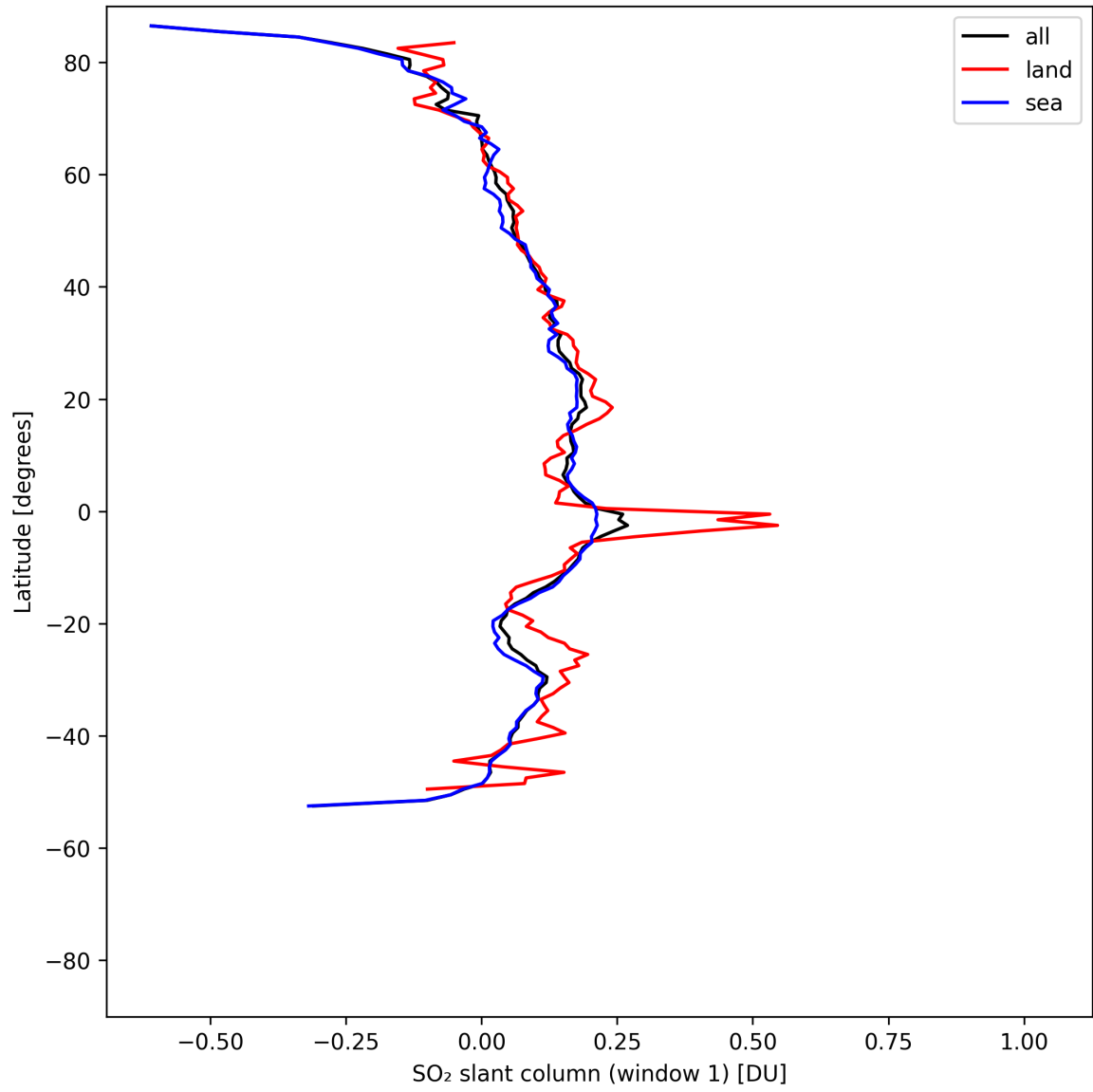
Figure 37: Zonal average of “SO 2 slant column (window 1)” for 2025-05-05 to 2025-05-07.
