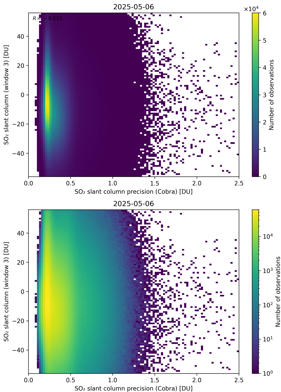
Figure 211: Scatter density plot of “SO 2 slant column precision (Cobra)” against “SO 2 slant column (window 3)” for 2025-05-05 to 2025-05-07.
