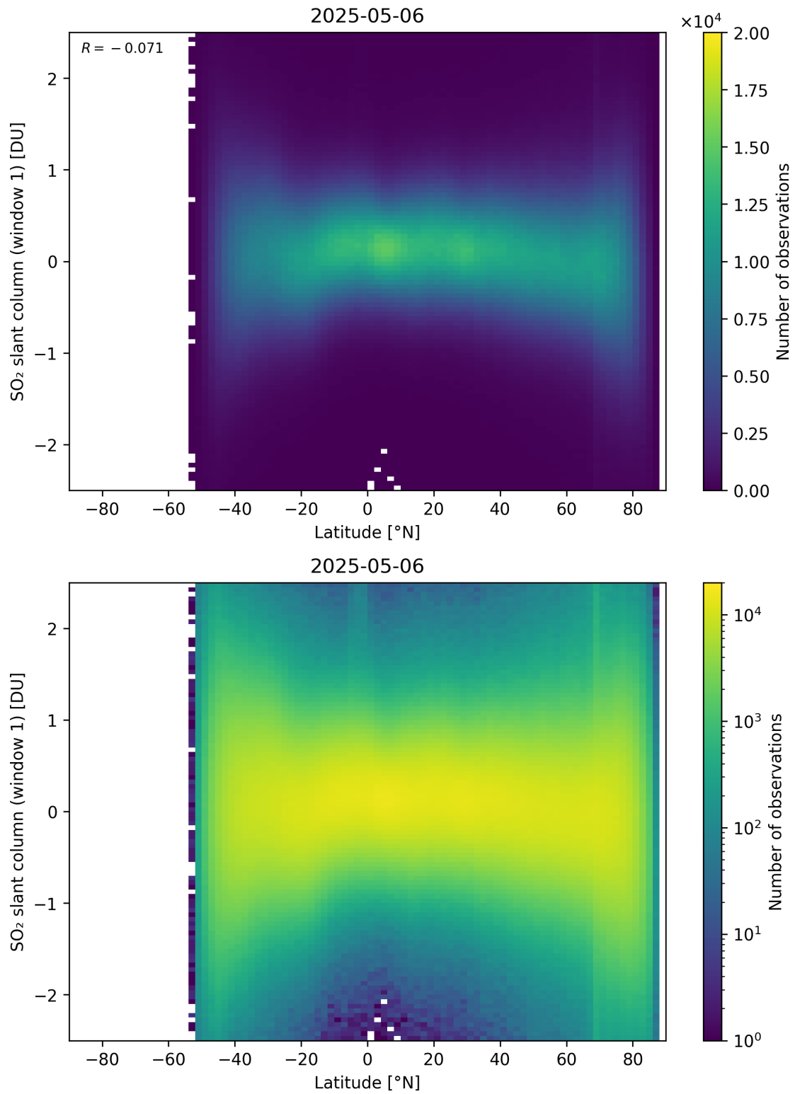
Figure 162: Scatter density plot of “Latitude” against “SO 2 slant column (window 1)” for 2025-05-05 to 2025-05-07.
