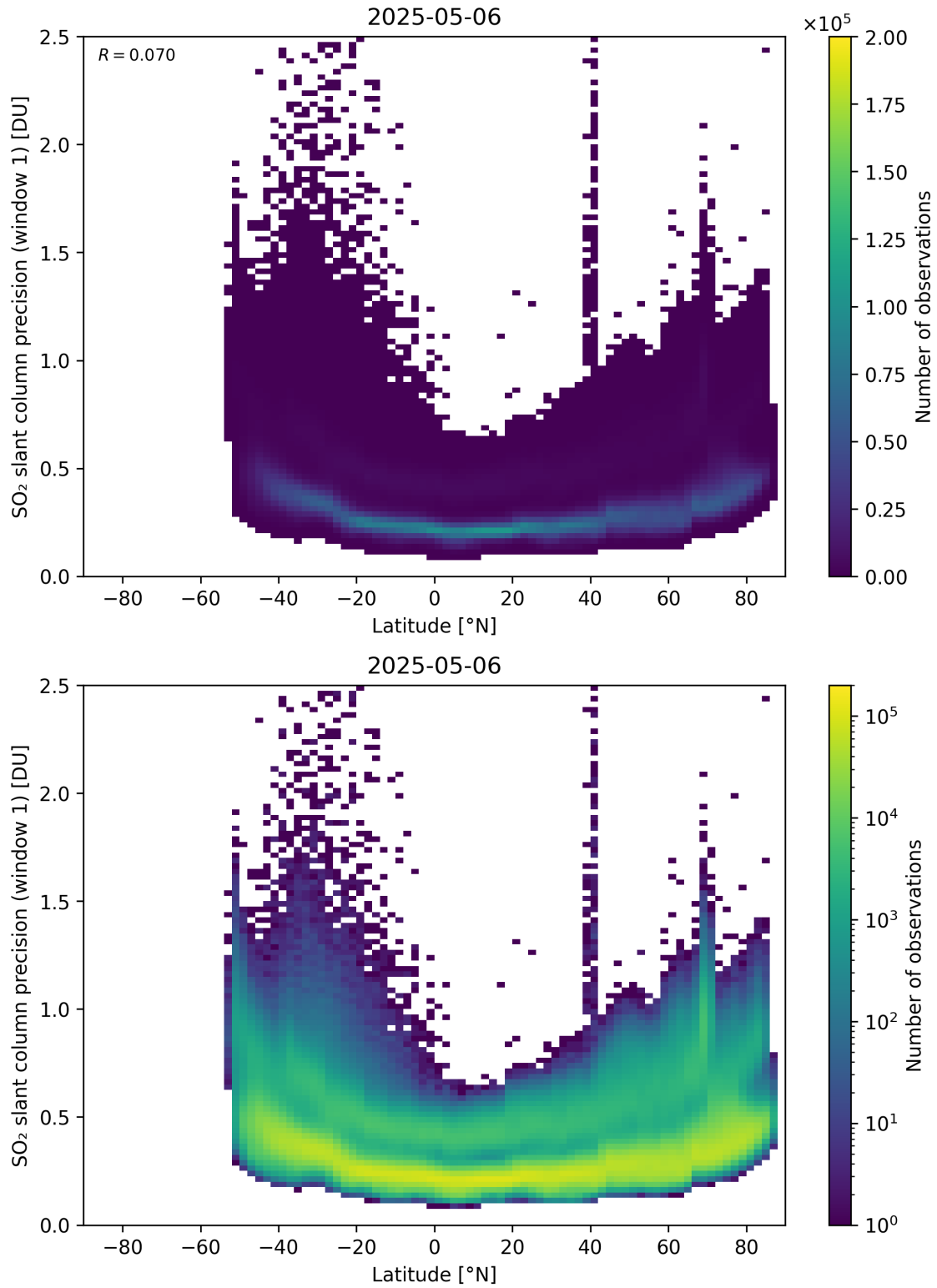
Figure 163: Scatter density plot of “Latitude” against “SO 2 slant column precision (window 1)” for 2025-05-05 to 2025-05-07.
