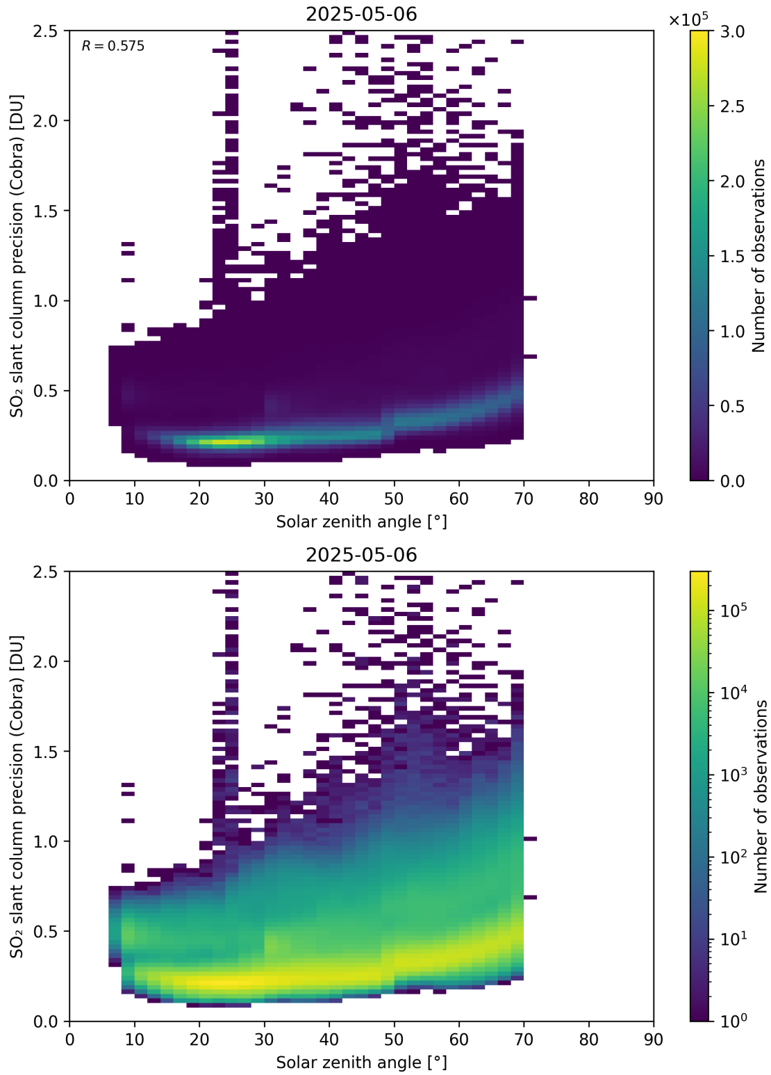
Figure 180: Scatter density plot of “Solar zenith angle” against “SO 2 slant column precision (Cobra)” for 2025-05-05 to 2025-05-07.
