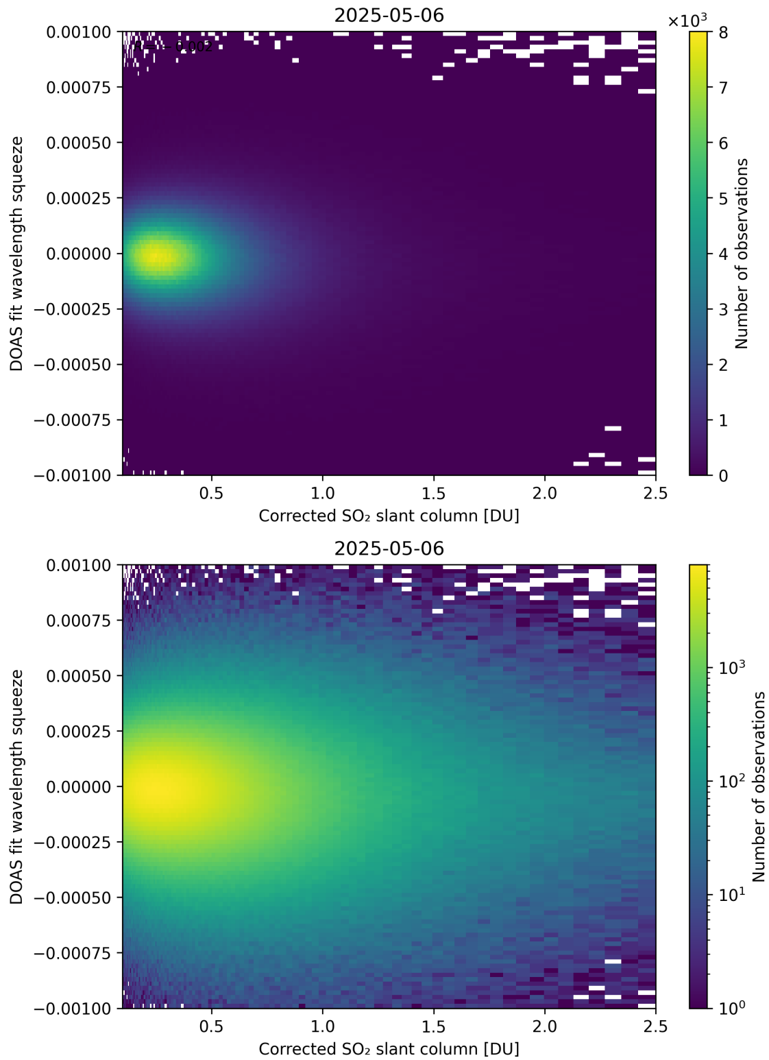
Figure 230: Scatter density plot of “Corrected SO 2 slant column” against “DOAS fit wavelength squeeze” for 2025-05-05 to 2025-05-07.
