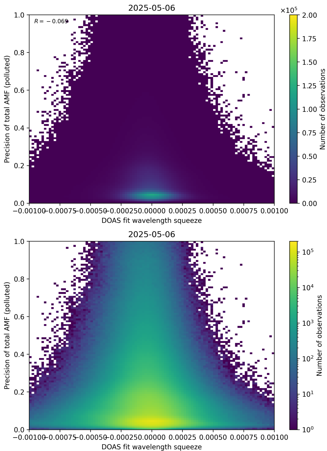
Figure 146: Scatter density plot of “DOAS fit wavelength squeeze” against “Precision of total AMF (polluted)” for 2025-05-05 to 2025-05-07.
