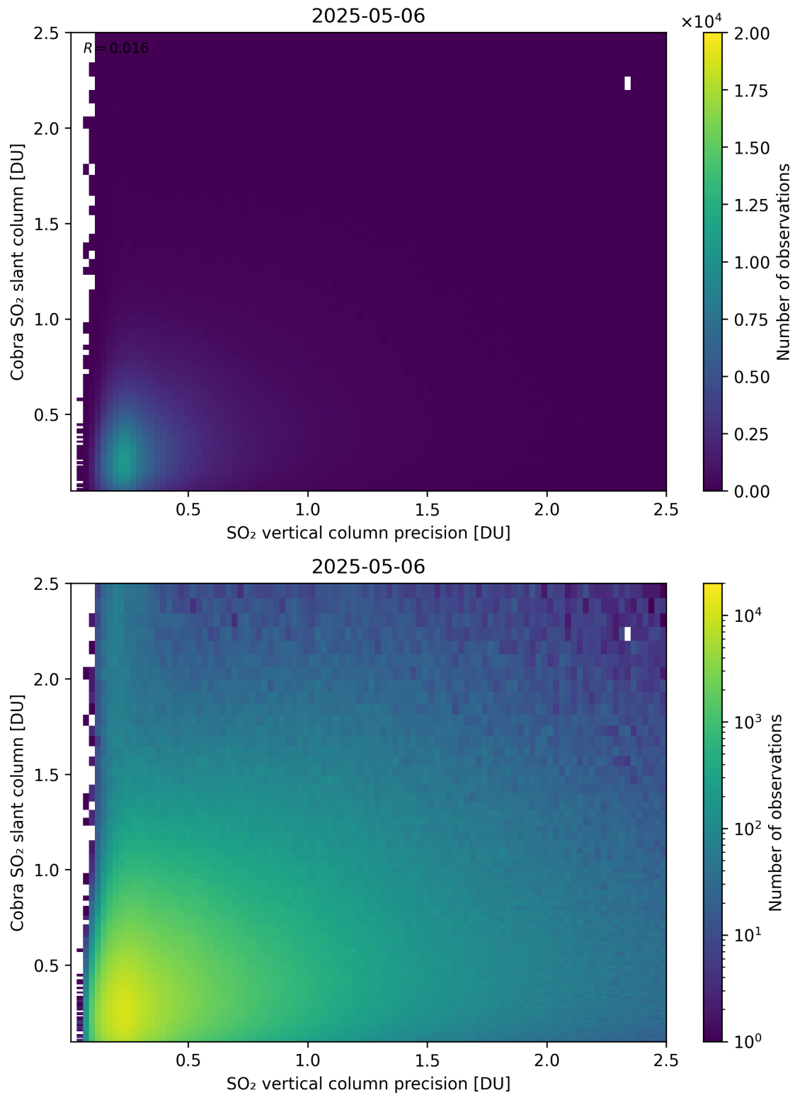
Figure 336: Scatter density plot of “SO 2 vertical column precision” against “Cobra SO 2 slant column” for 2025-05-05 to 2025-05-07.
