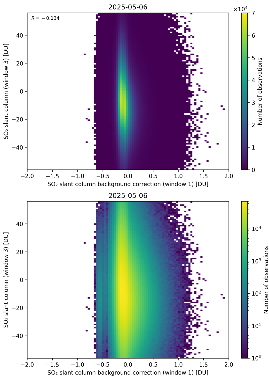
Figure 118: Scatter density plot of “SO 2 slant column background correction (window 1)” against “SO 2 slant column (window 3)” for 2025-05-05 to 2025-05-07.
