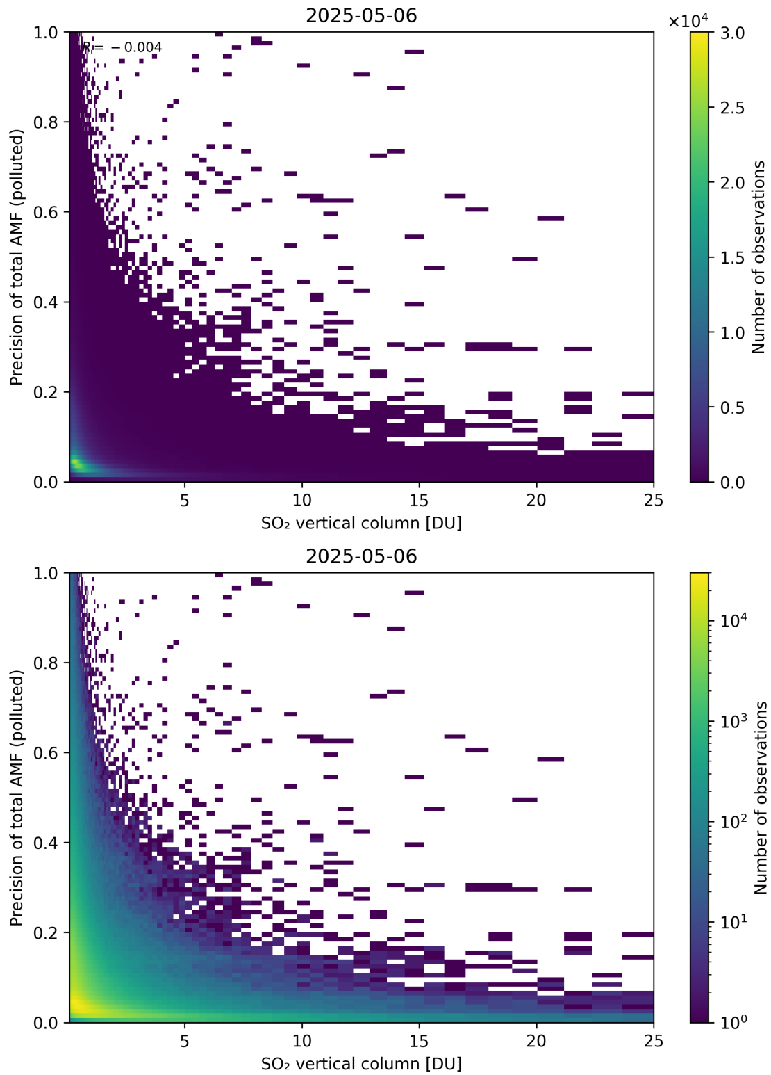
Figure 360: Scatter density plot of “SO 2 vertical column” against “Precision of total AMF (polluted)” for 2025-05-05 to 2025-05-07.
