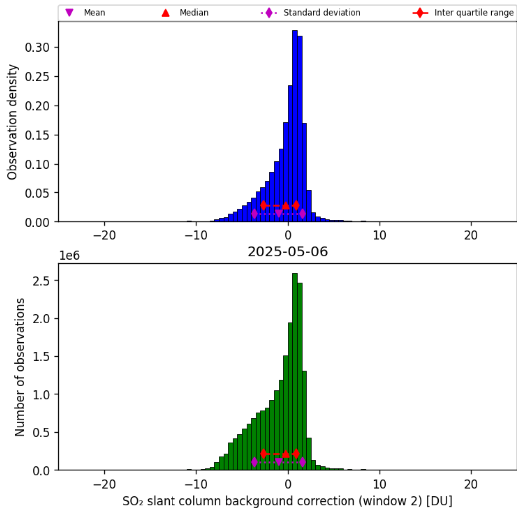
Figure 70: Histogram of “SO 2 slant column background correction (window 2)” for 2025-05-05 to 2025-05-07
