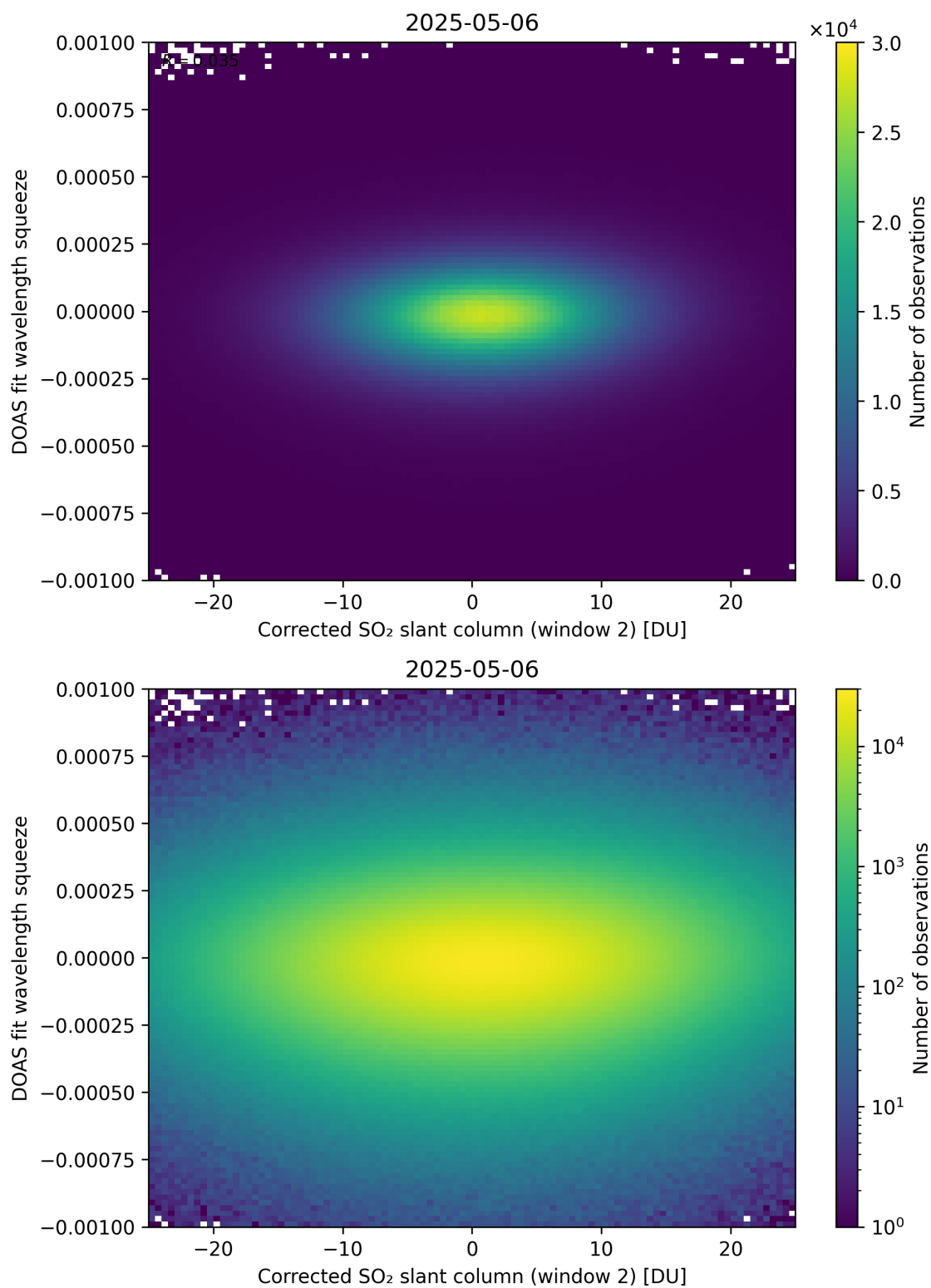
Figure 247: Scatter density plot of “Corrected SO 2 slant column (window 2)” against “DOAS fit wavelength squeeze” for 2025-05-05 to 2025-05-07.
