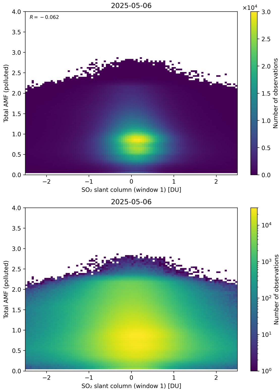
Figure 289: Scatter density plot of “SO 2 slant column (window 1)” against “Total AMF (polluted)” for 2025-05-05 to 2025-05-07.
