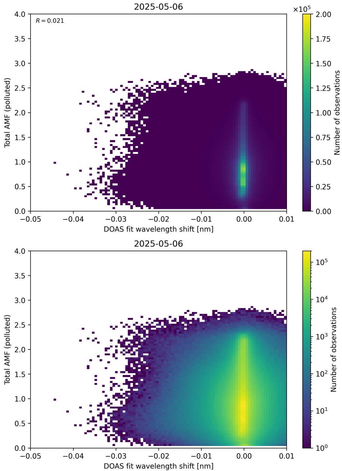
Figure 141: Scatter density plot of “DOAS fit wavelength shift” against “Total AMF (polluted)” for 2025-05-05 to 2025-05-07.
