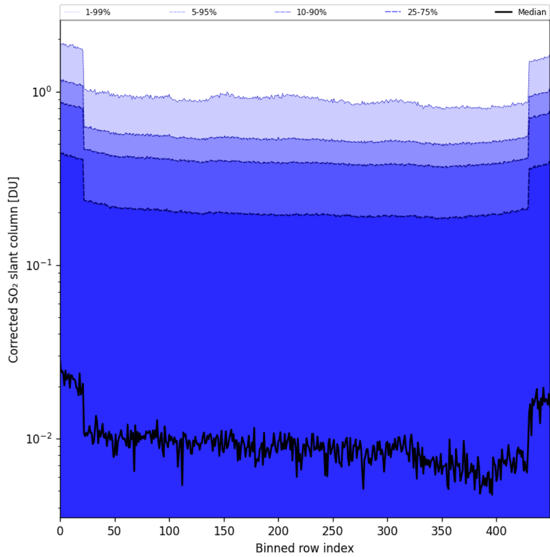
Figure 86: Along track statistics of “Corrected SO 2 slant column” for 2025-05-05 to 2025-05-07
