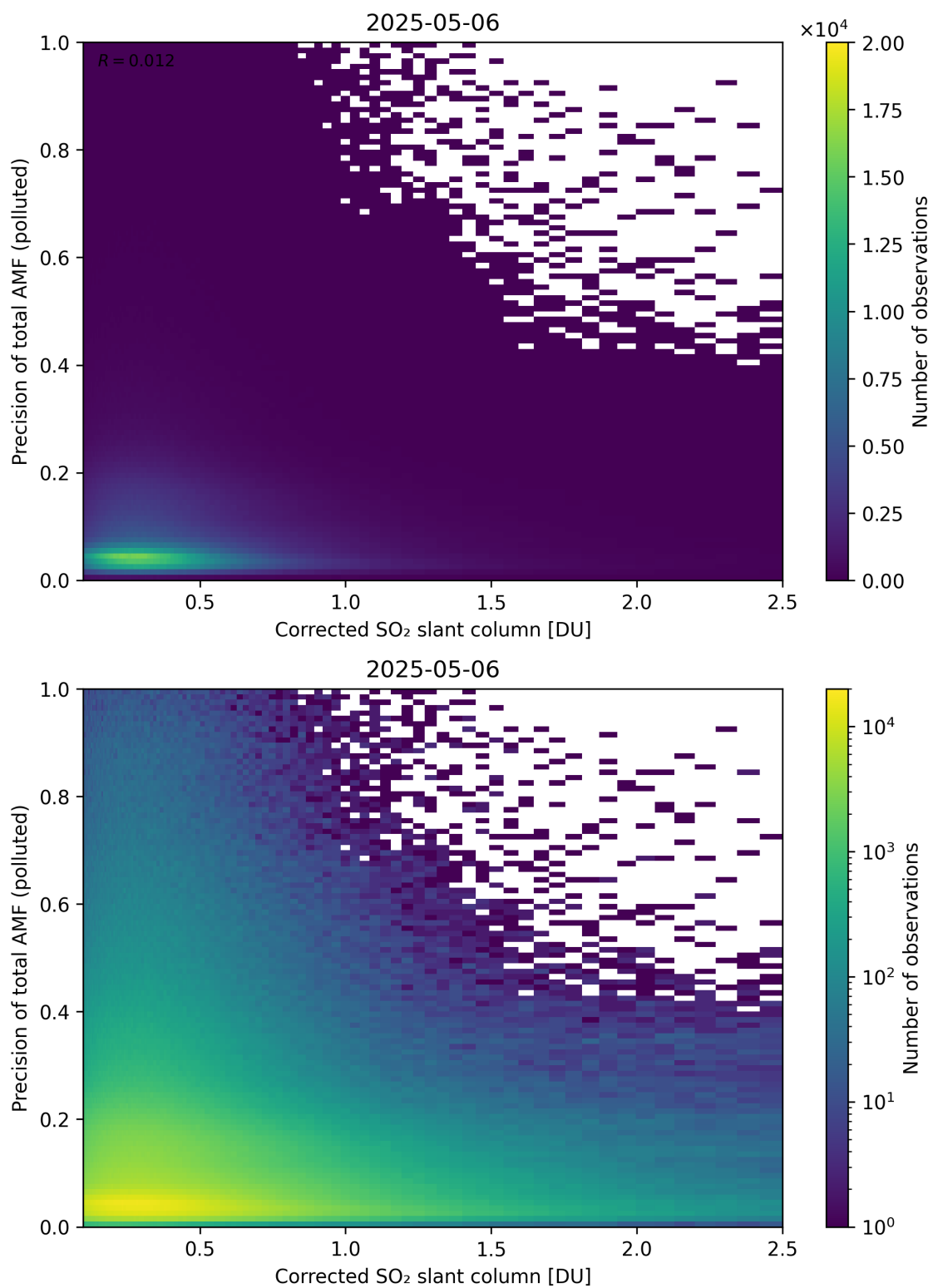
Figure 243: Scatter density plot of “Corrected SO 2 slant column” against “Precision of total AMF (polluted)” for 2025-05-05 to 2025-05-07.
