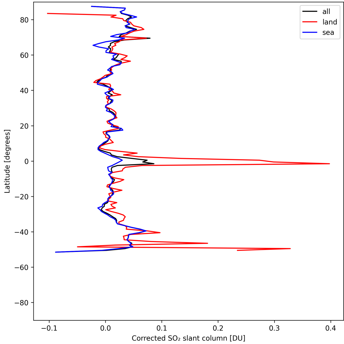
Figure 34: Zonal average of “Corrected SO 2 slant column” for 2025-05-06 to 2025-05-08.
