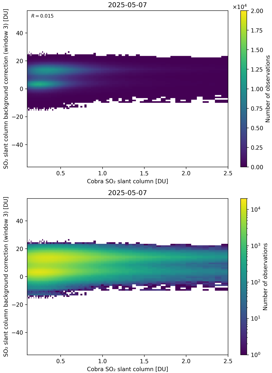
Figure 195: Scatter density plot of “Cobra SO 2 slant column” against “SO 2 slant column background correction (window 3)” for 2025-05-06 to 2025-05-08.
