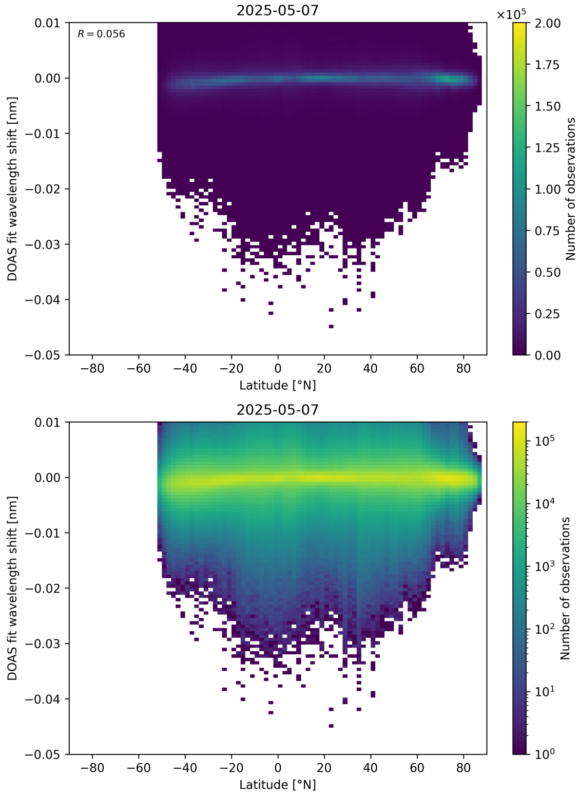
Figure 153: Scatter density plot of “Latitude” against “DOAS fit wavelength shift” for 2025-05-06 to 2025-05-08.
