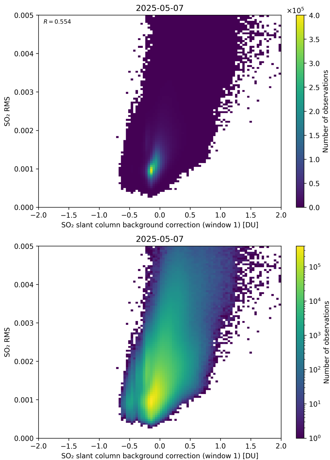
Figure 113: Scatter density plot of “SO 2 slant column background correction (window 1)” against “SO 2 RMS” for 2025-05-06 to 2025-05-08.
