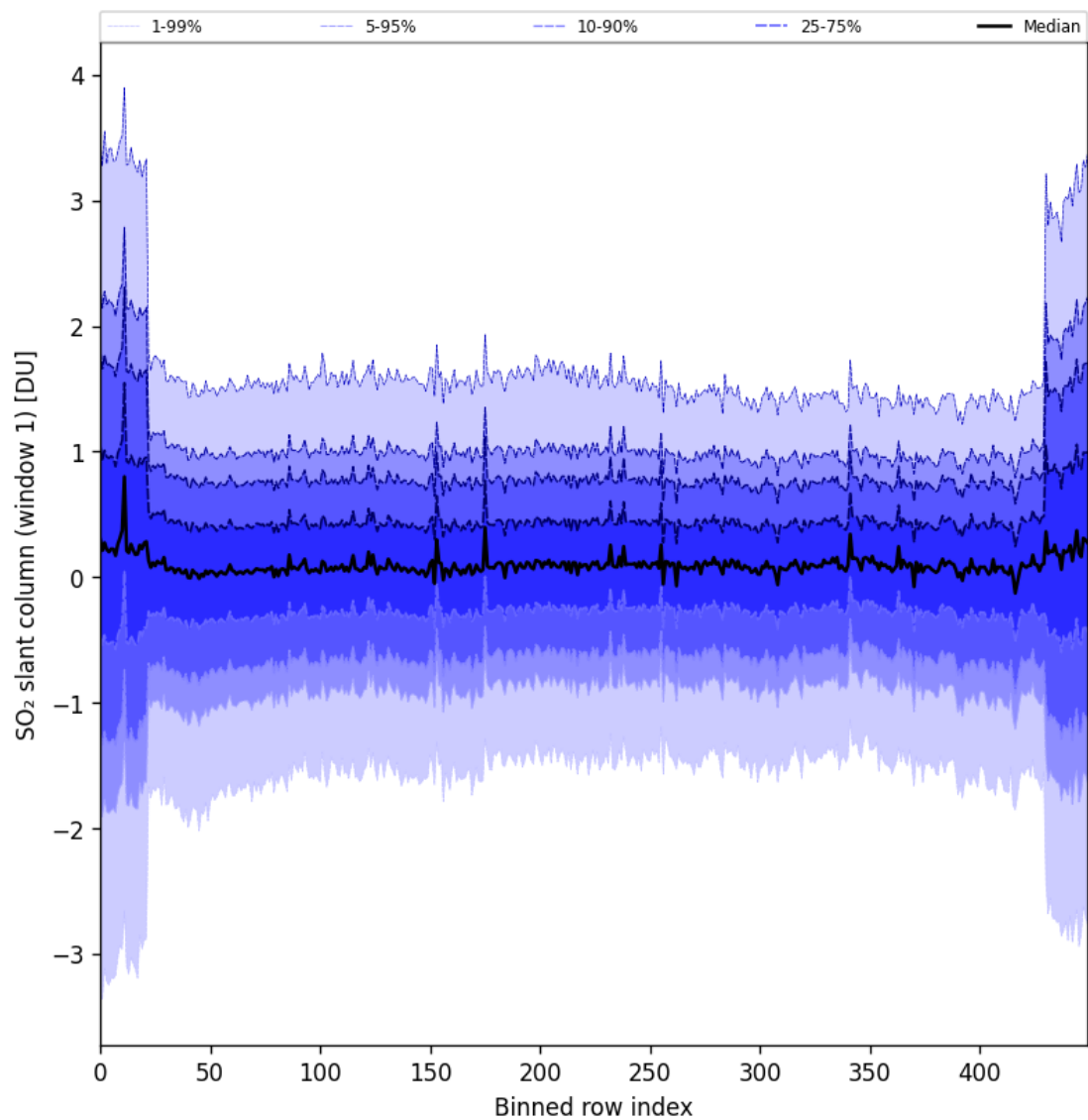
Figure 89: Along track statistics of “SO 2 slant column (window 1)” for 2025-05-06 to 2025-05-08
