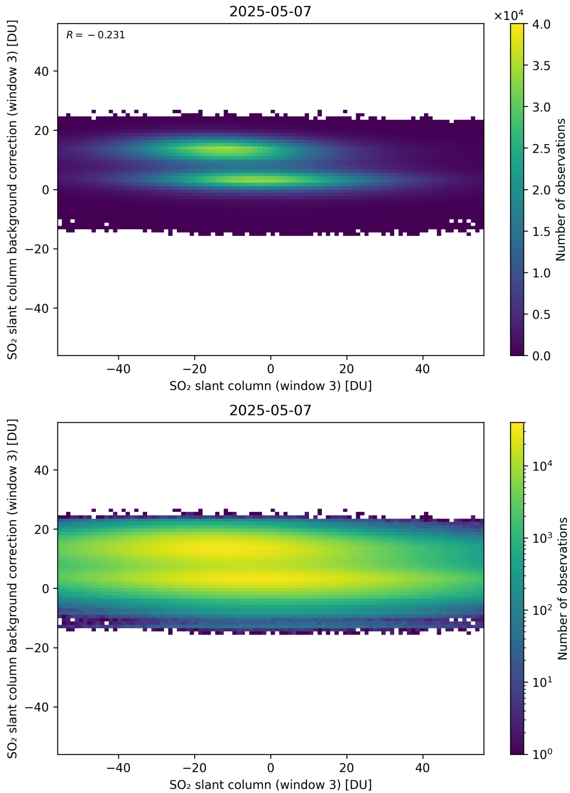
Figure 303: Scatter density plot of “SO 2 slant column (window 3)” against “SO 2 slant column background correction (window 3)” for 2025-05-06 to 2025-05-08.
