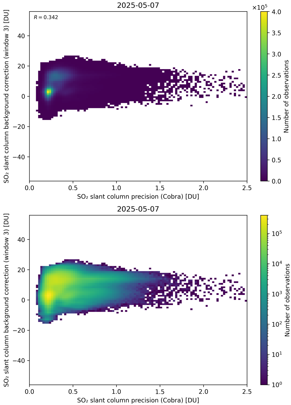
Figure 201: Scatter density plot of “SO 2 slant column precision (Cobra)” against “SO 2 slant column background correction (window 3)” for 2025-05-06 to 2025-05-08.
