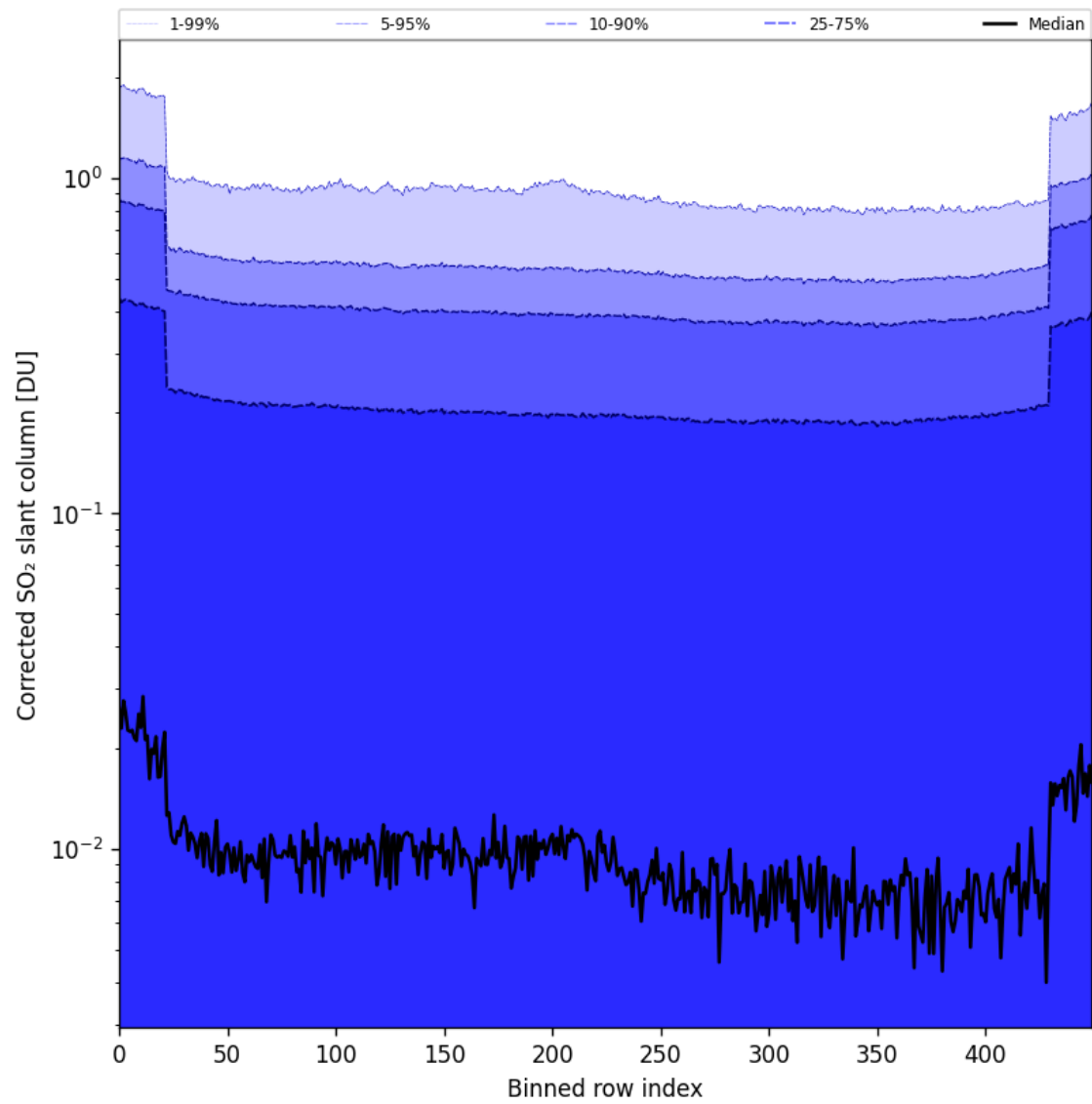
Figure 86: Along track statistics of “Corrected SO 2 slant column” for 2025-05-06 to 2025-05-08
