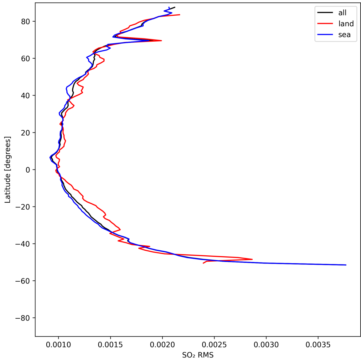
Figure 52: Zonal average of “SO 2 RMS” for 2025-05-06 to 2025-05-08.
