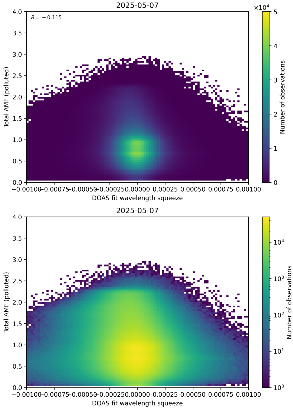
Figure 145: Scatter density plot of “DOAS fit wavelength squeeze” against “Total AMF (polluted)” for 2025-05-06 to 2025-05-08.
