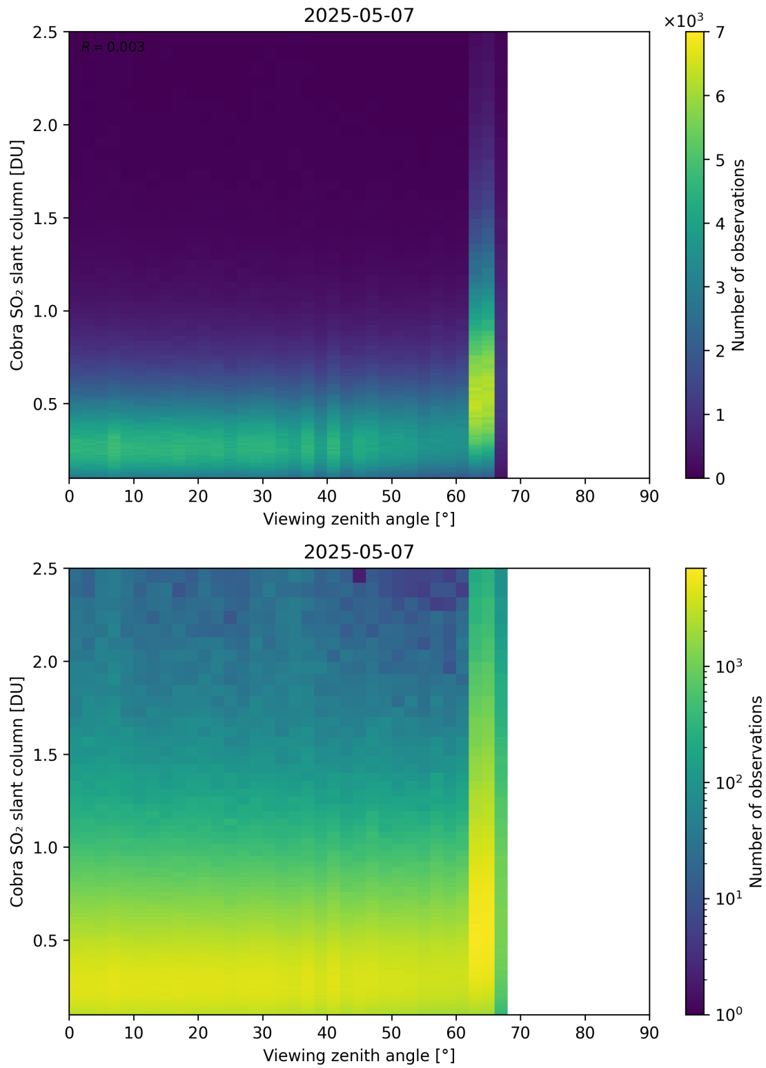
Figure 371: Scatter density plot of “Viewing zenith angle” against “Cobra SO 2 slant column” for 2025-05-06 to 2025-05-08.
