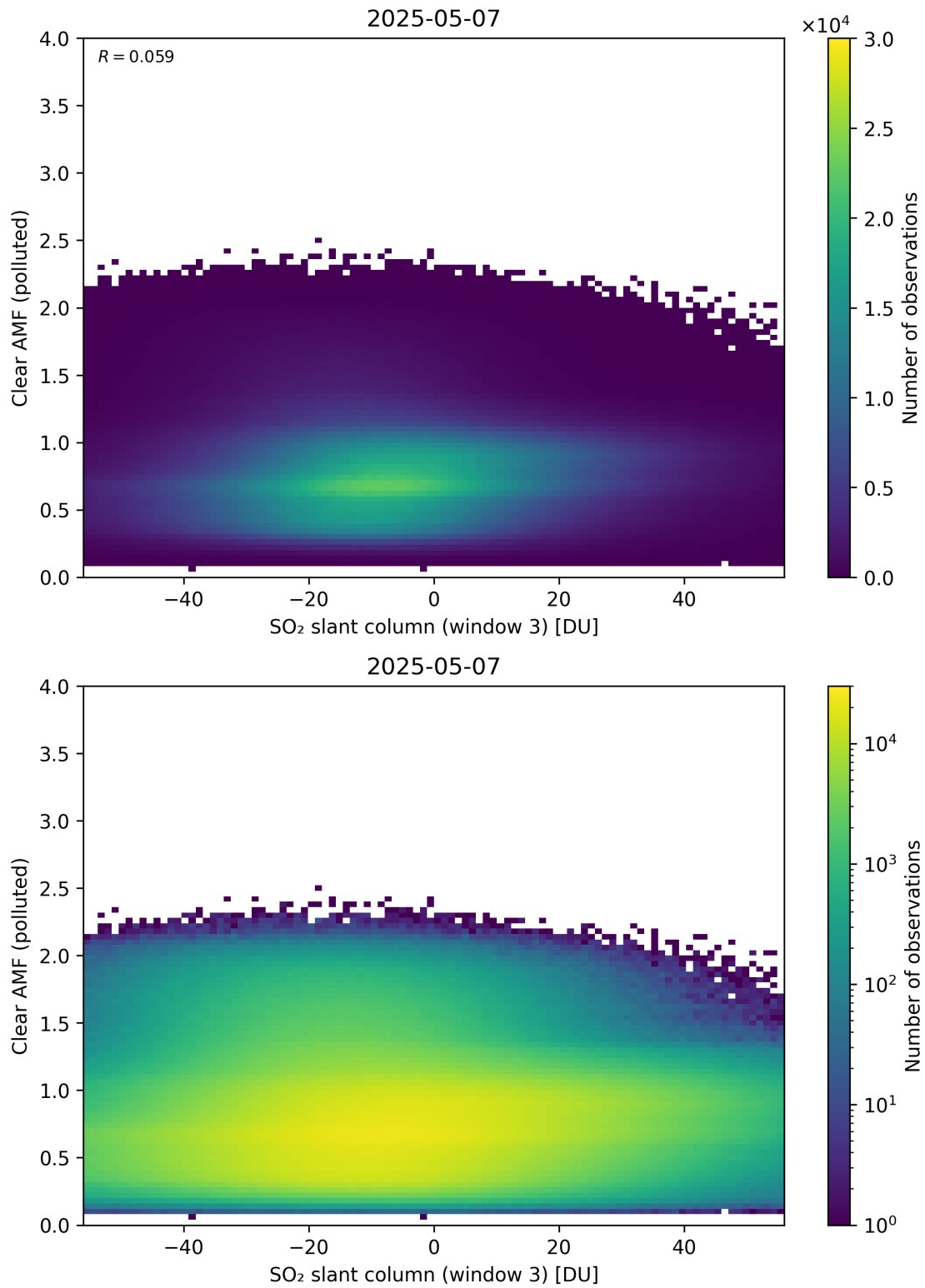
Figure 315: Scatter density plot of “SO 2 slant column (window 3)” against “Clear AMF (polluted)” for 2025-05-06 to 2025-05-08.
