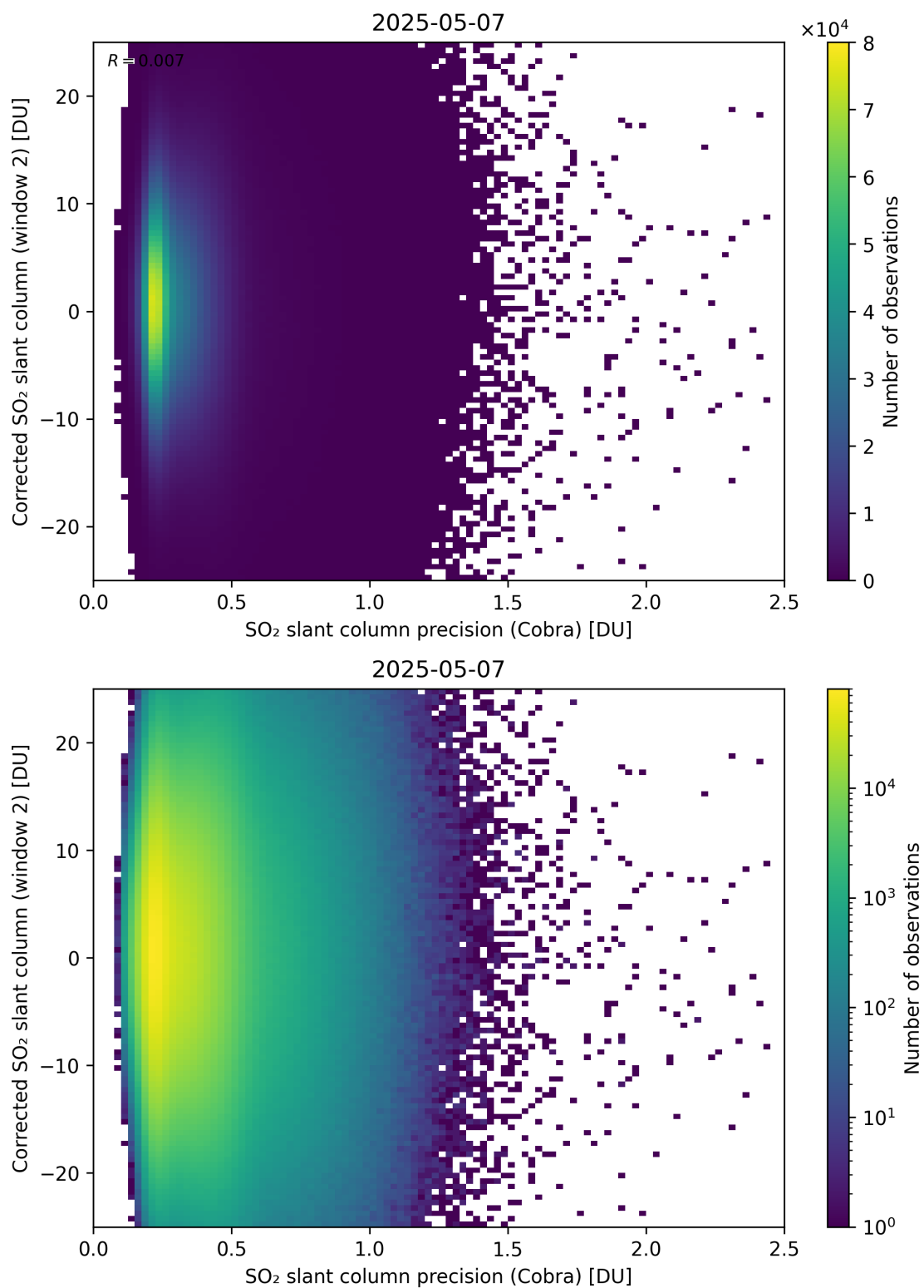
Figure 206: Scatter density plot of “SO 2 slant column precision (Cobra)” against “Corrected SO 2 slant column (window 2)” for 2025-05-06 to 2025-05-08.
