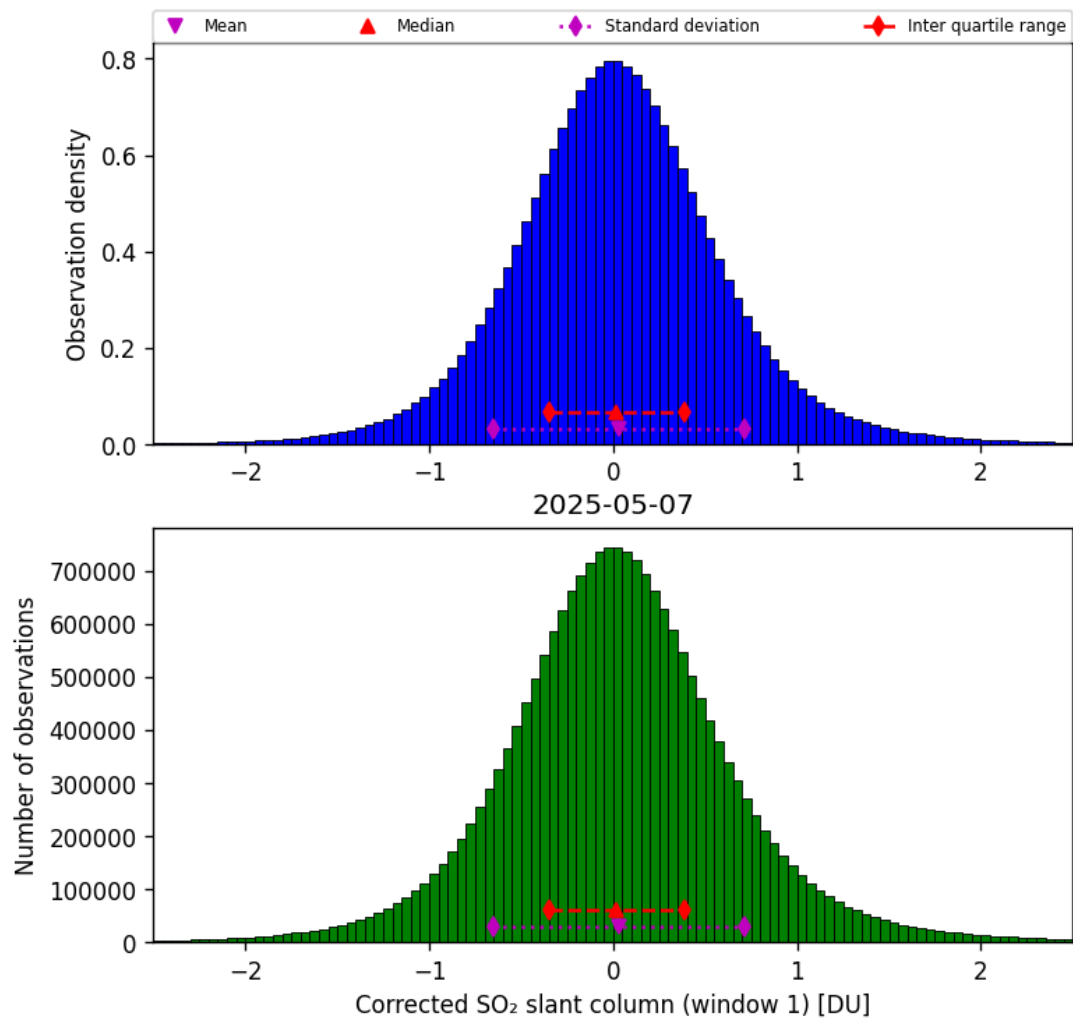
Figure 65: Histogram of “Corrected SO 2 slant column (window 1)” for 2025-05-06 to 2025-05-08
