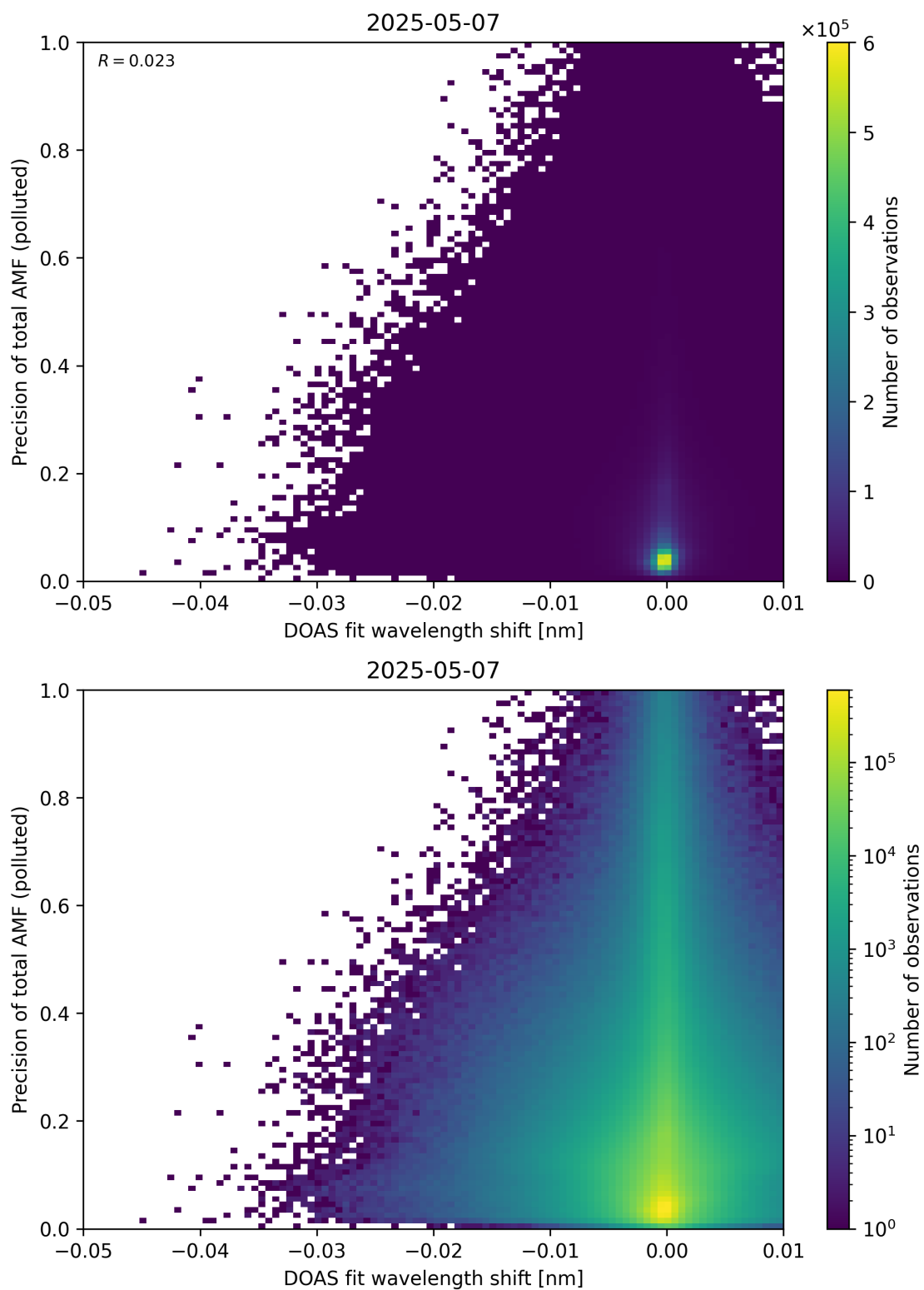
Figure 142: Scatter density plot of “DOAS fit wavelength shift” against “Precision of total AMF (polluted)” for 2025-05-06 to 2025-05-08.
