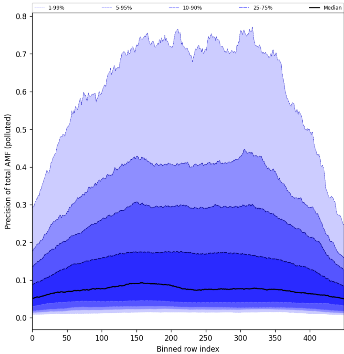
Figure 106: Along track statistics of “Precision of total AMF (polluted)” for 2025-05-06 to 2025-05-08
