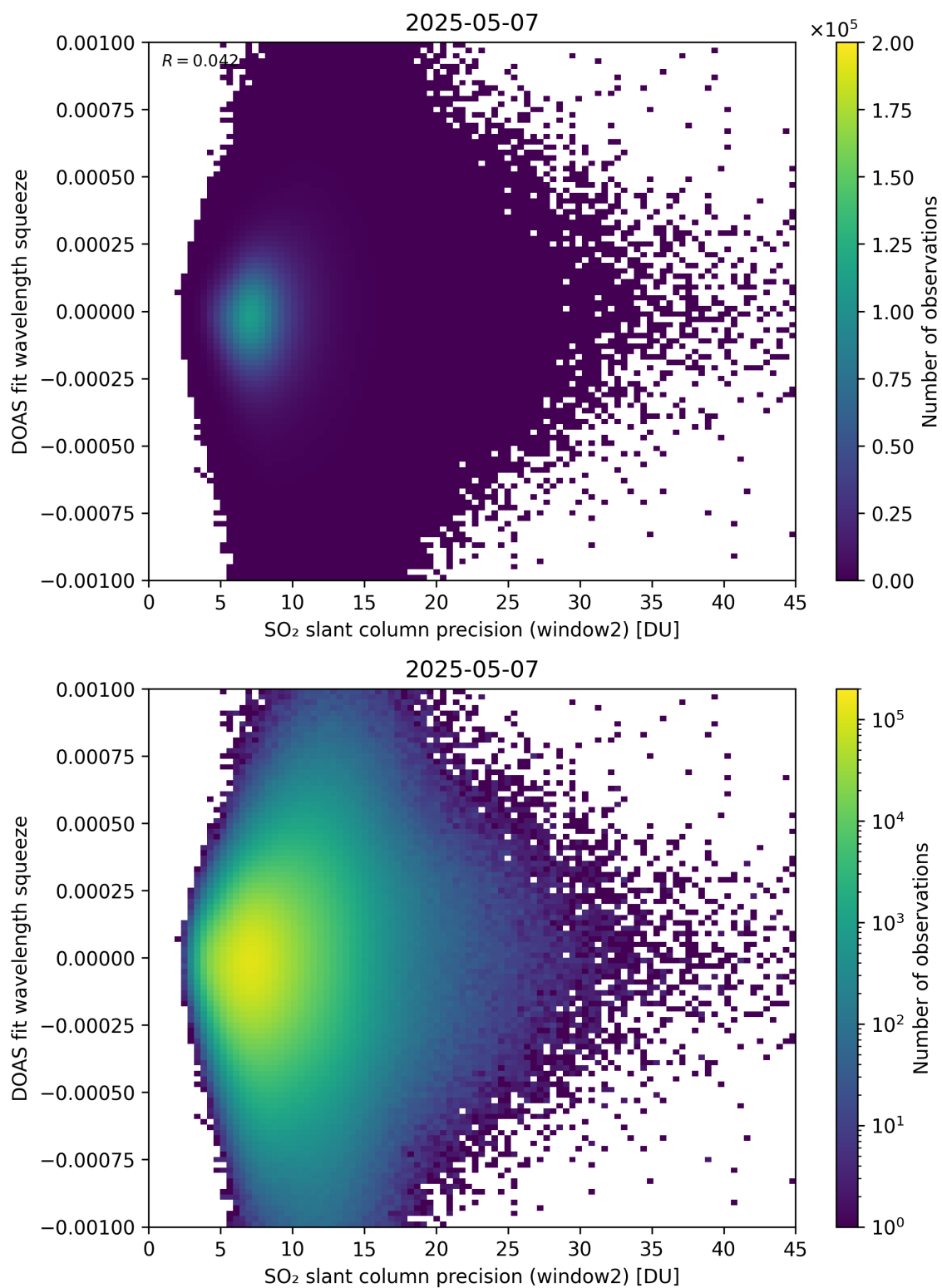
Figure 294: Scatter density plot of “SO 2 slant column precision (window2)” against “DOAS fit wavelength squeeze” for 2025-05-06 to 2025-05-08.
