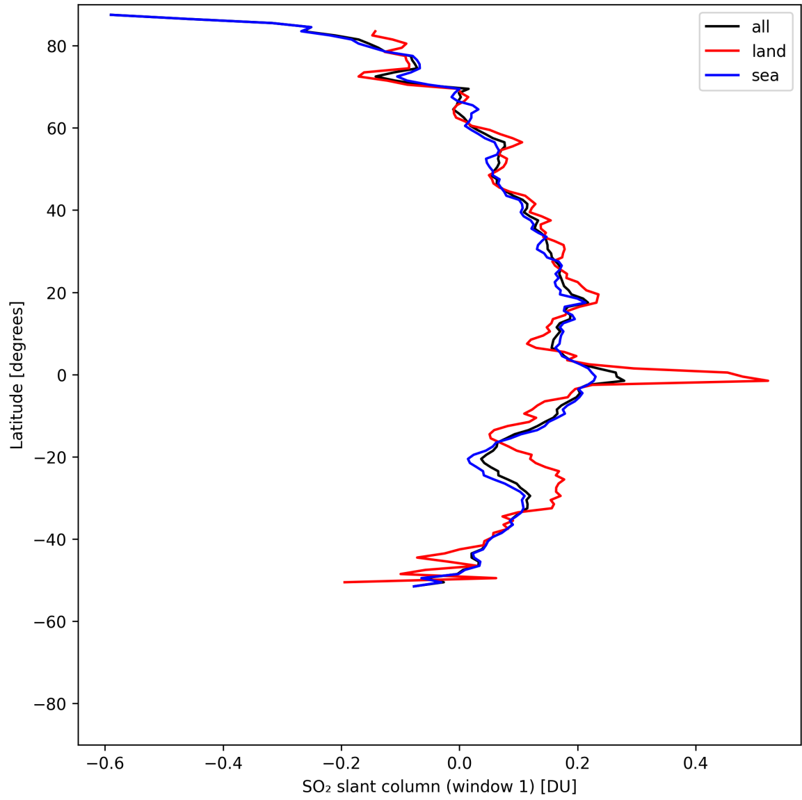
Figure 37: Zonal average of “SO 2 slant column (window 1)” for 2025-05-06 to 2025-05-08.
