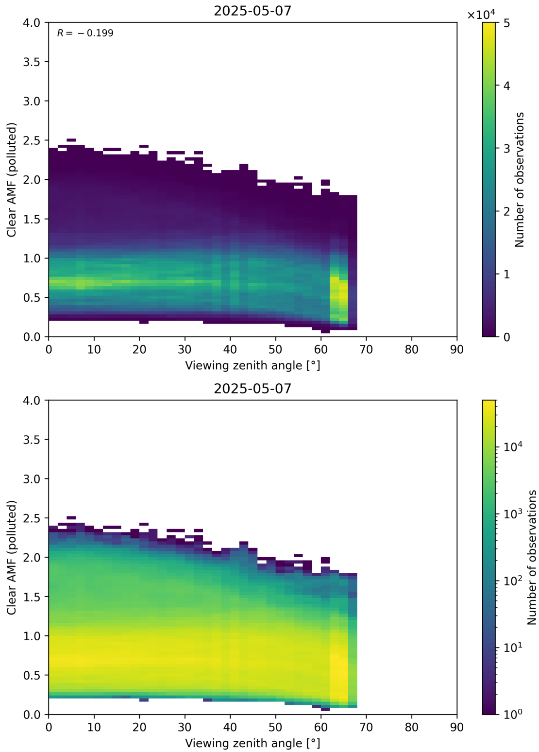
Figure 370: Scatter density plot of “Viewing zenith angle” against “Clear AMF (polluted)” for 2025-05-06 to 2025-05-08.
