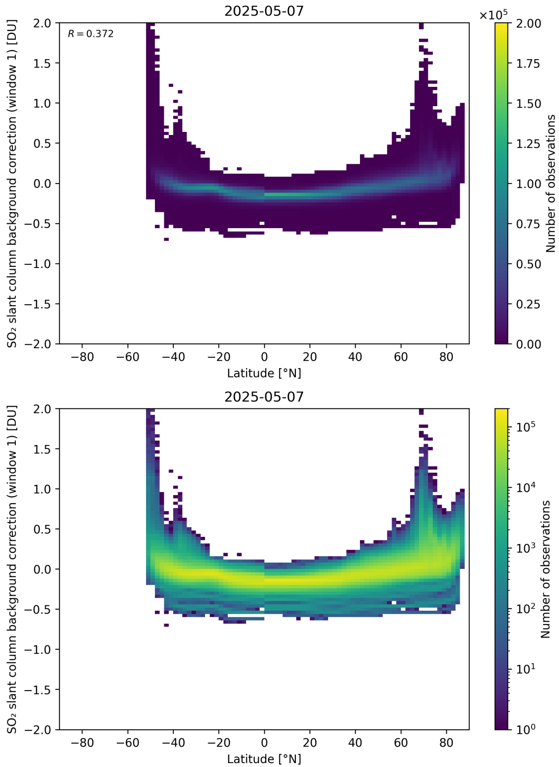
Figure 150: Scatter density plot of “Latitude” against “SO 2 slant column background correction (window 1)” for 2025-05-06 to 2025-05-08.
