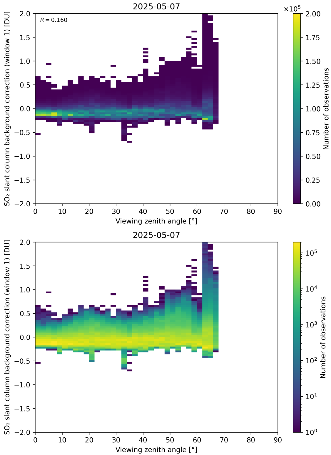
Figure 362: Scatter density plot of “Viewing zenith angle” against “SO 2 slant column background correction (window 1)” for 2025-05-06 to 2025-05-08.
