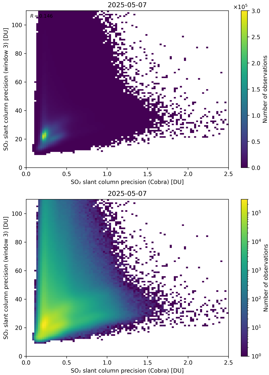
Figure 212: Scatter density plot of “SO 2 slant column precision (Cobra)” against “SO 2 slant column precision (window 3)” for 2025-05-06 to 2025-05-08.
