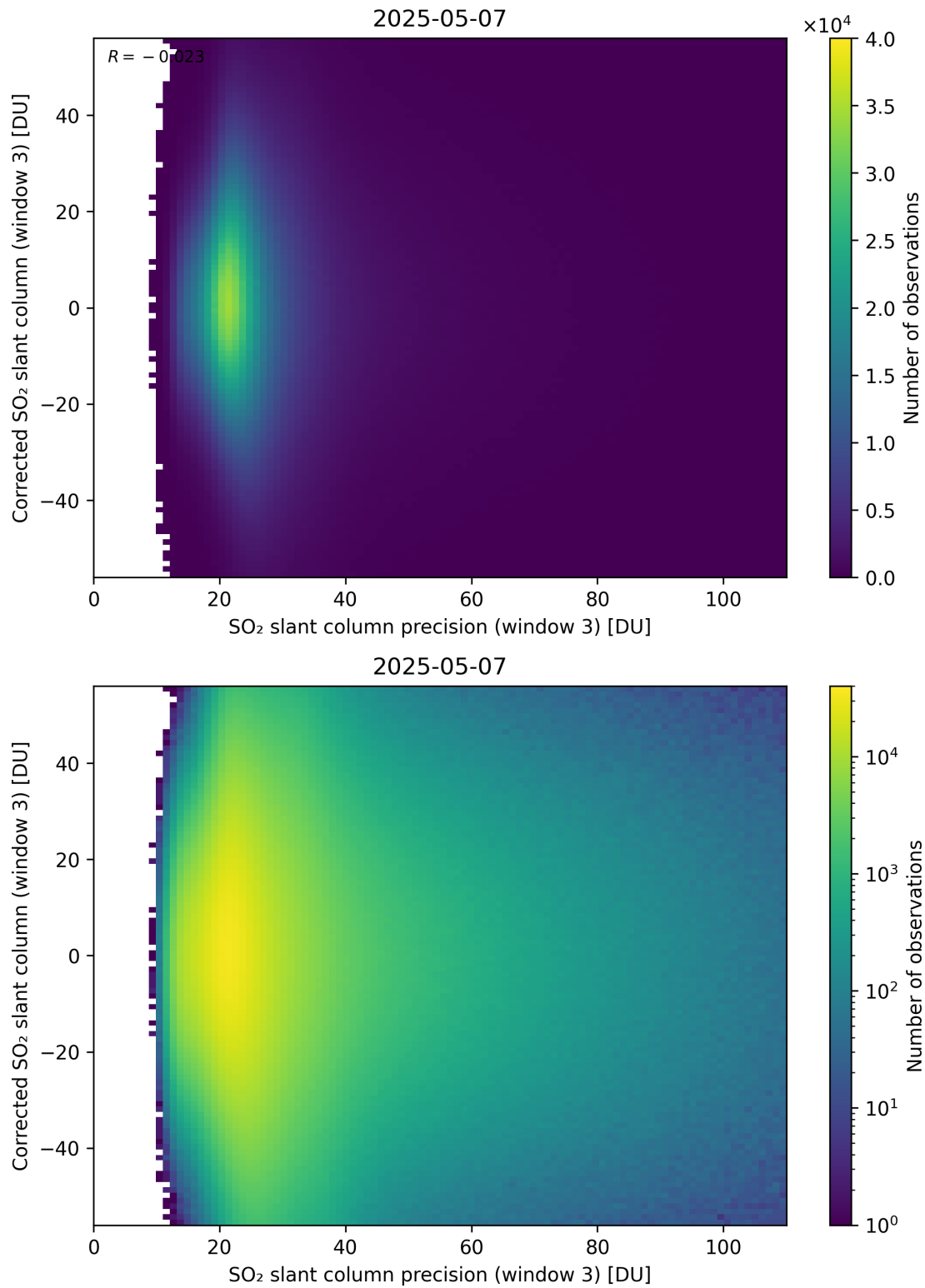
Figure 312: Scatter density plot of “SO 2 slant column precision (window 3)” against “Corrected SO 2 slant column (window 3)” for 2025-05-06 to 2025-05-08.
