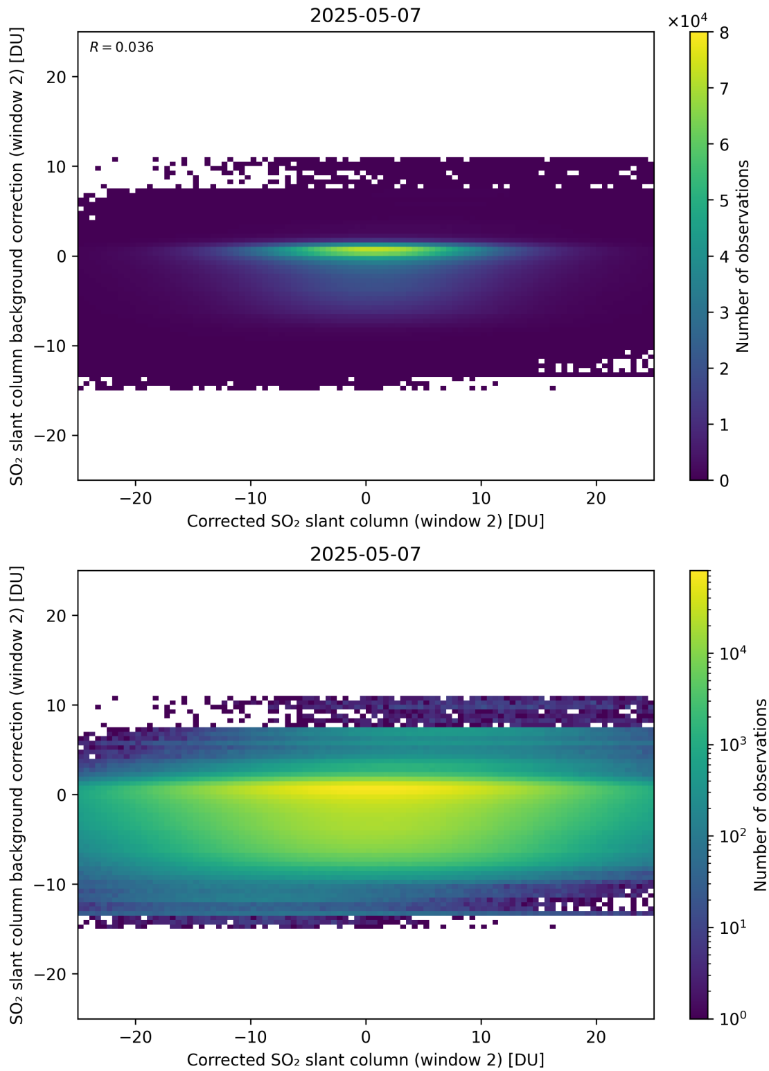
Figure 244: Scatter density plot of “Corrected SO 2 slant column (window 2)” against “SO 2 slant column background correction (window 2)” for 2025-05-06 to 2025-05-08.
