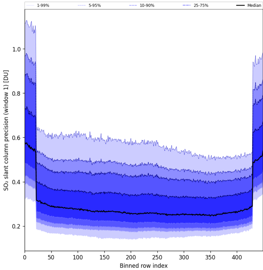
Figure 90: Along track statistics of “SO 2 slant column precision (window 1)” for 2025-05-06 to 2025-05-08
