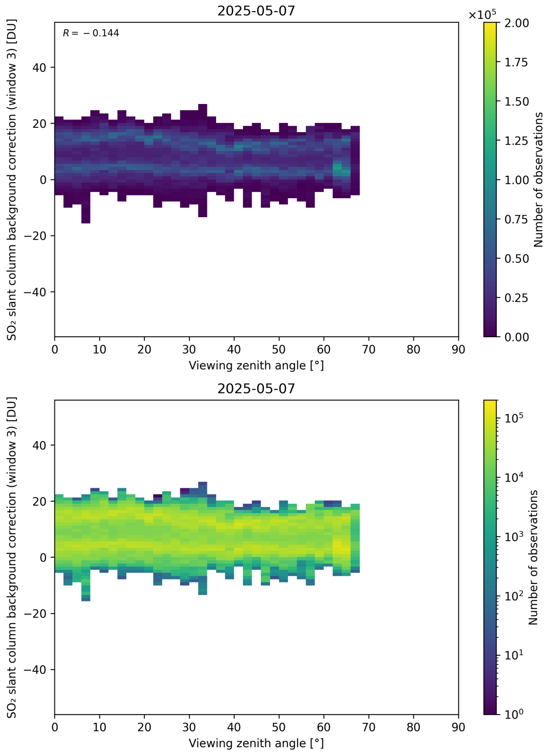
Figure 364: Scatter density plot of “Viewing zenith angle” against “SO 2 slant column background correction (window 3)” for 2025-05-06 to 2025-05-08.
