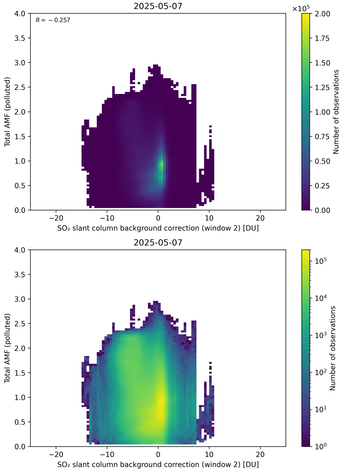
Figure 130: Scatter density plot of “SO 2 slant column background correction (window 2)” against “Total AMF (polluted)” for 2025-05-06 to 2025-05-08.
