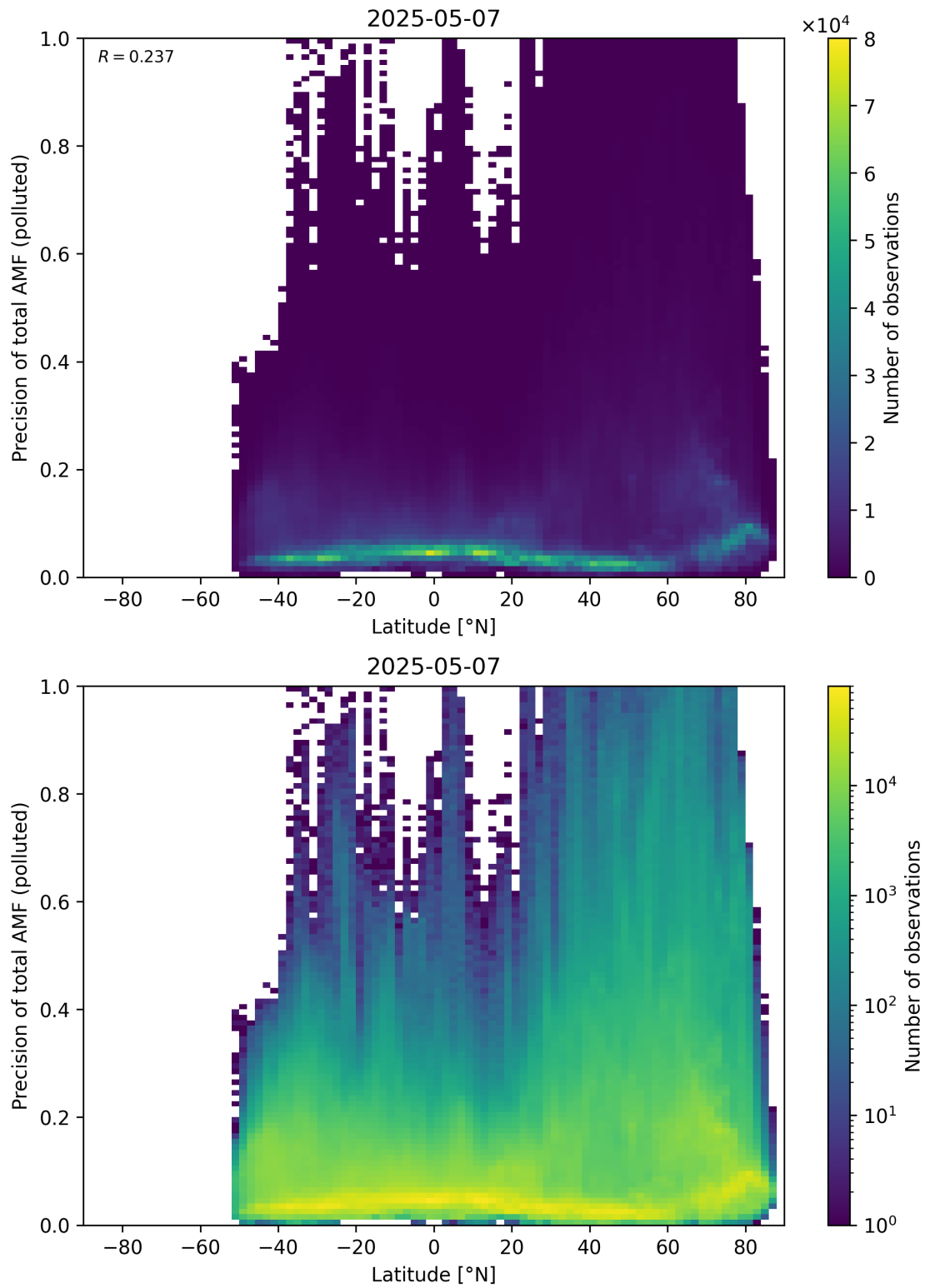
Figure 168: Scatter density plot of “Latitude” against “Precision of total AMF (polluted)” for 2025-05-06 to 2025-05-08.
