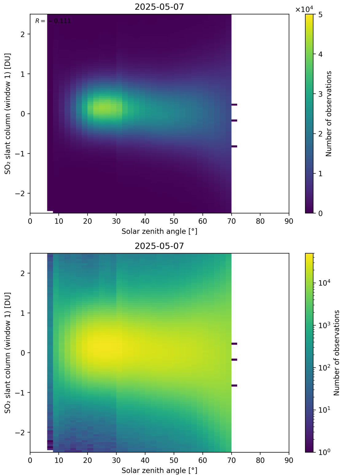
Figure 184: Scatter density plot of “Solar zenith angle” against “SO 2 slant column (window 1)” for 2025-05-06 to 2025-05-08.
