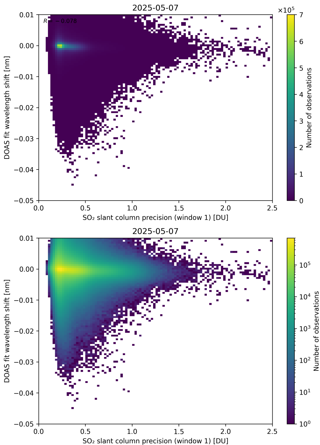
Figure 271: Scatter density plot of “SO 2 slant column precision (window 1)” against “DOAS fit wavelength shift” for 2025-05-06 to 2025-05-08.
