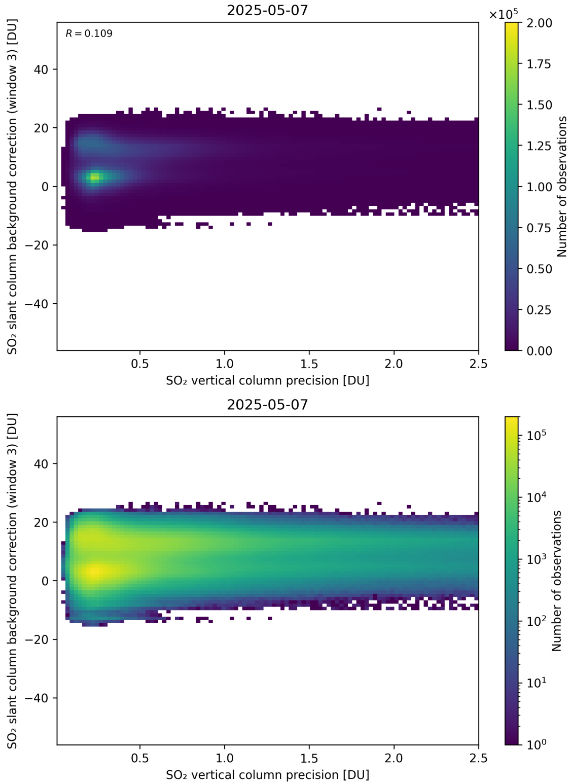
Figure 331: Scatter density plot of “SO 2 vertical column precision” against “SO 2 slant column background correction (window 3)” for 2025-05-06 to 2025-05-08.
