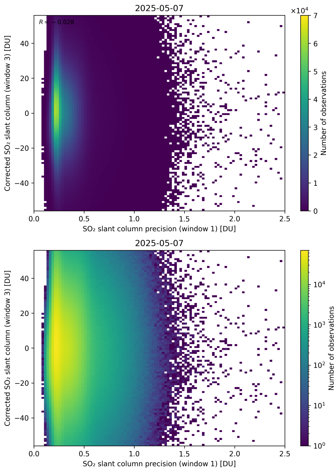
Figure 276: Scatter density plot of “SO 2 slant column precision (window 1)” against “Corrected SO 2 slant column (window 3)” for 2025-05-06 to 2025-05-08.
