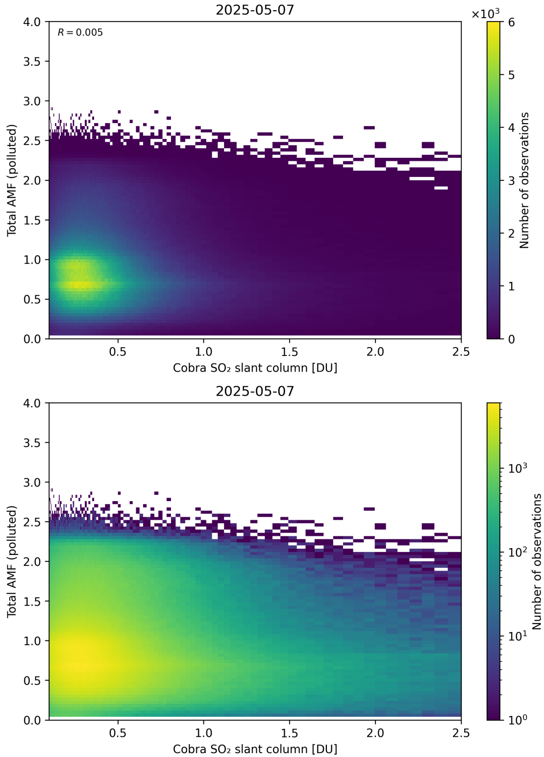
Figure 224: Scatter density plot of “Cobra SO 2 slant column” against “Total AMF (polluted)” for 2025-05-06 to 2025-05-08.
