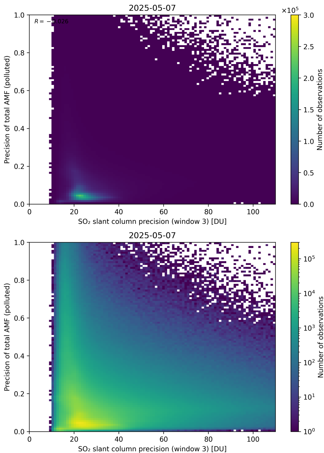
Figure 314: Scatter density plot of “SO 2 slant column precision (window 3)” against “Precision of total AMF (polluted)” for 2025-05-06 to 2025-05-08.
