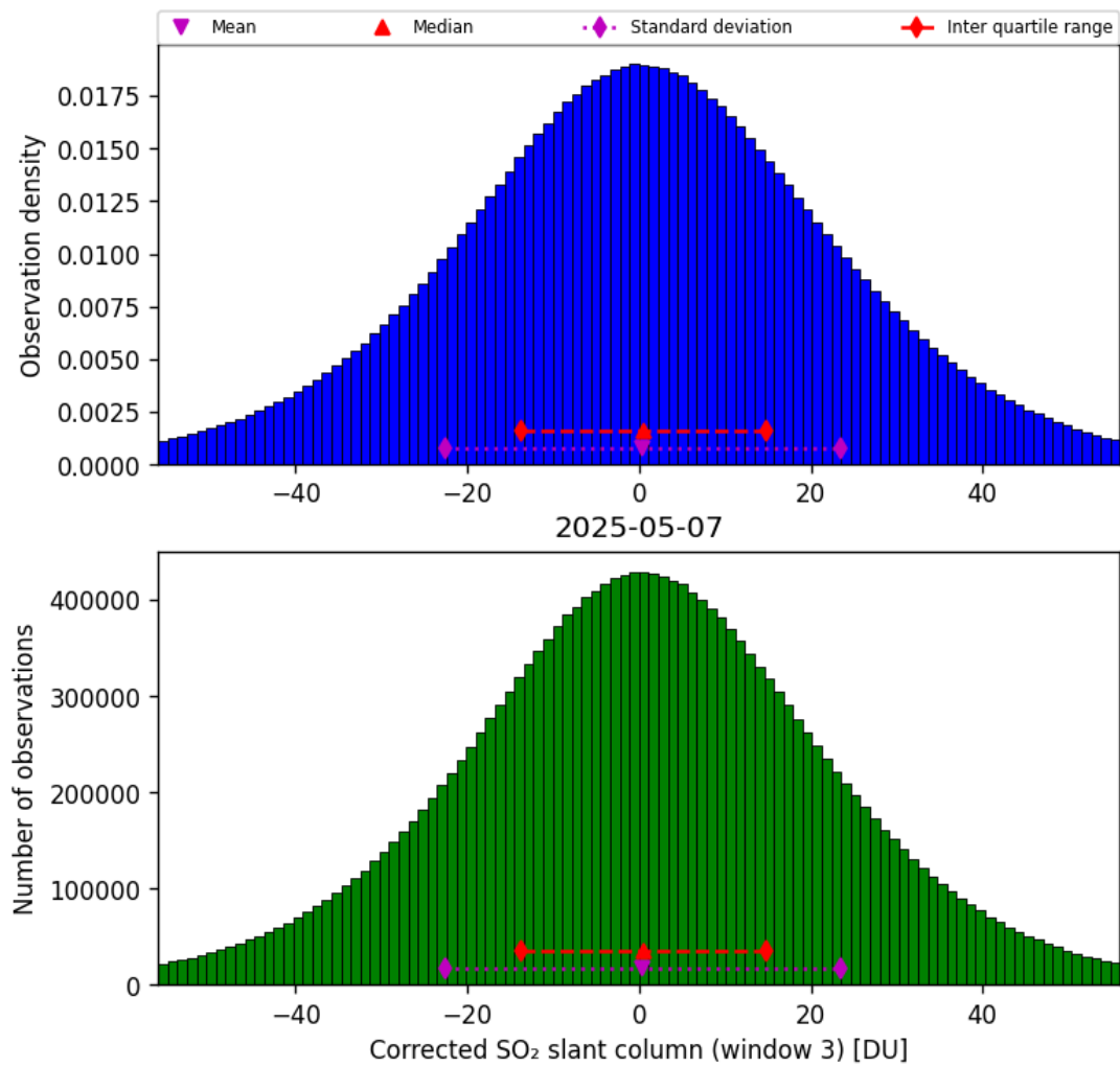
Figure 73: Histogram of “Corrected SO 2 slant column (window 3)” for 2025-05-06 to 2025-05-08
