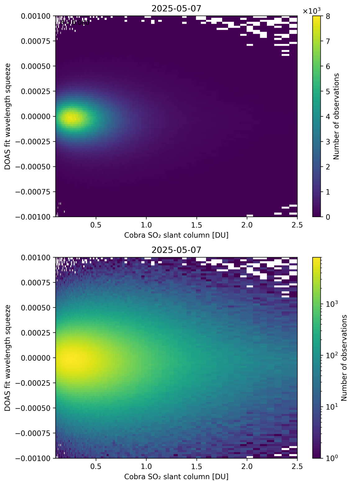
Figure 197: Scatter density plot of “Cobra SO 2 slant column” against “DOAS fit wavelength squeeze” for 2025-05-06 to 2025-05-08.
