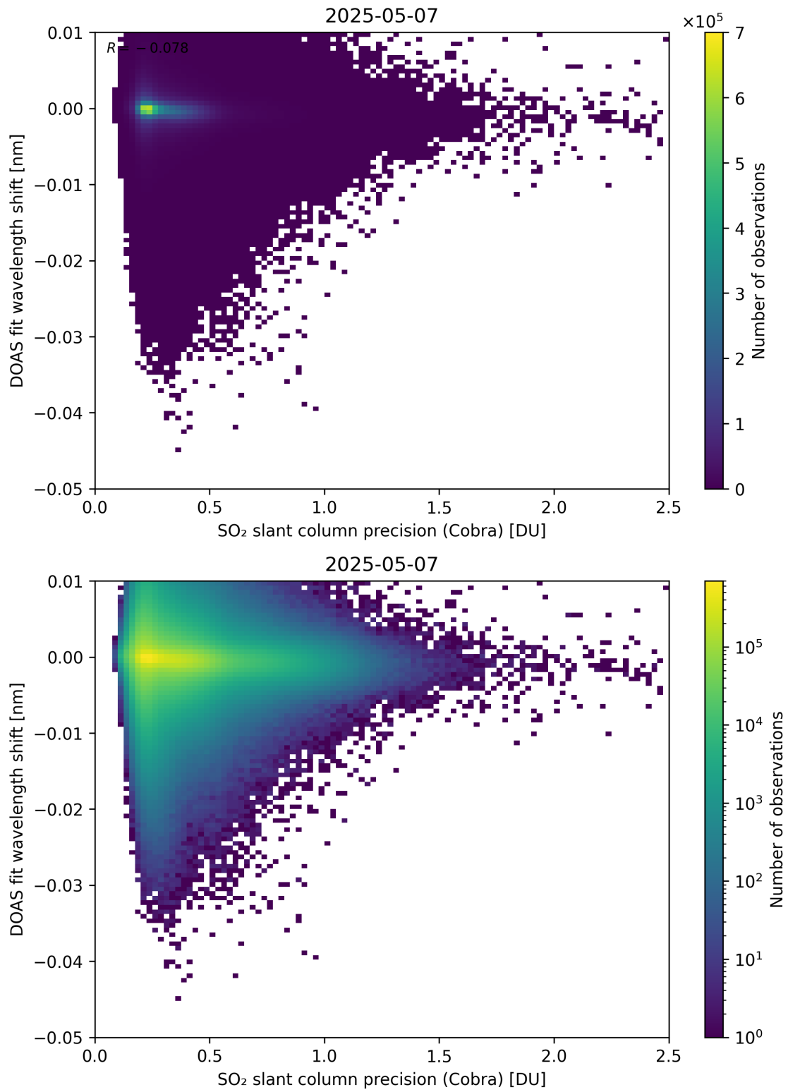
Figure 202: Scatter density plot of “SO 2 slant column precision (Cobra)” against “DOAS fit wavelength shift” for 2025-05-06 to 2025-05-08.
