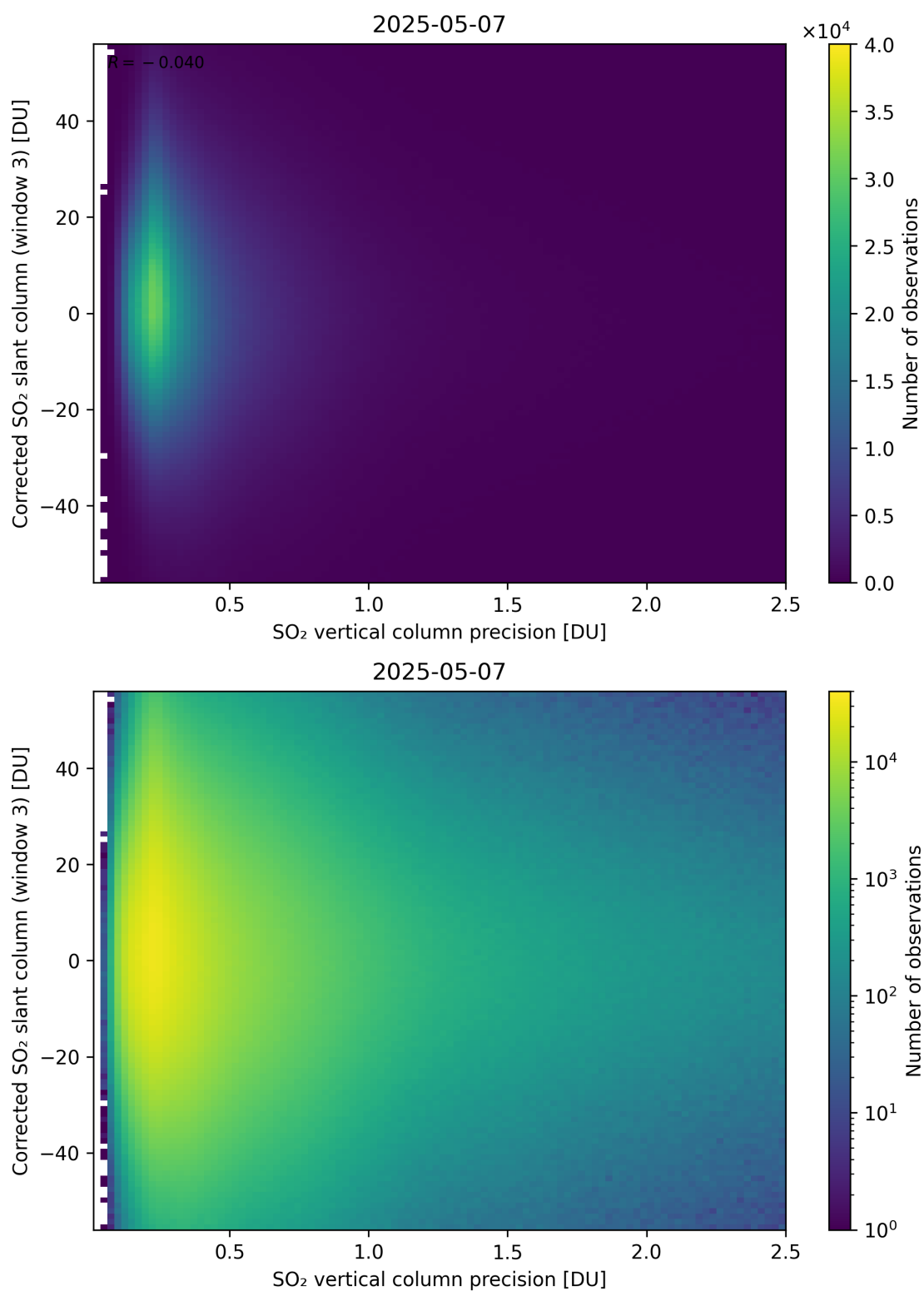
Figure 340: Scatter density plot of “SO 2 vertical column precision” against “Corrected SO 2 slant column (window 3)” for 2025-05-06 to 2025-05-08.
