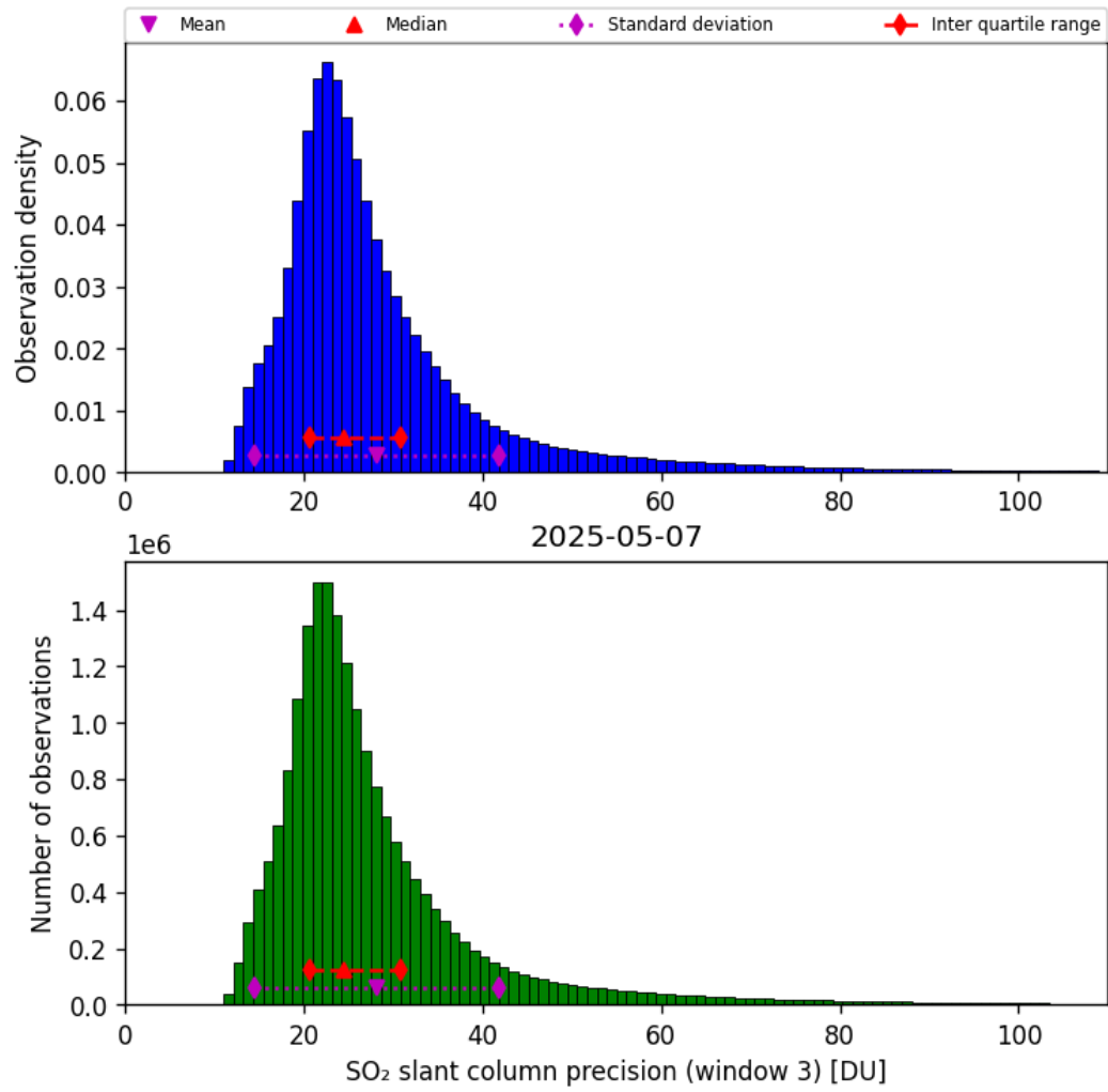
Figure 72: Histogram of “SO 2 slant column precision (window 3)” for 2025-05-06 to 2025-05-08
