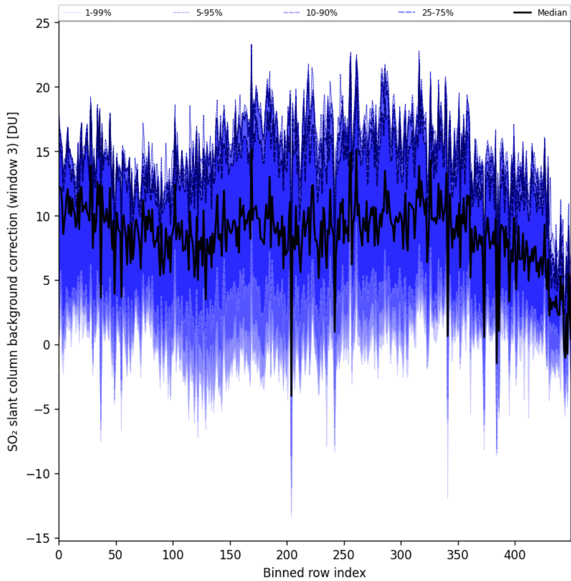
Figure 100: Along track statistics of “SO 2 slant column background correction (window 3)” for 2025-05-06 to 2025-05-08
