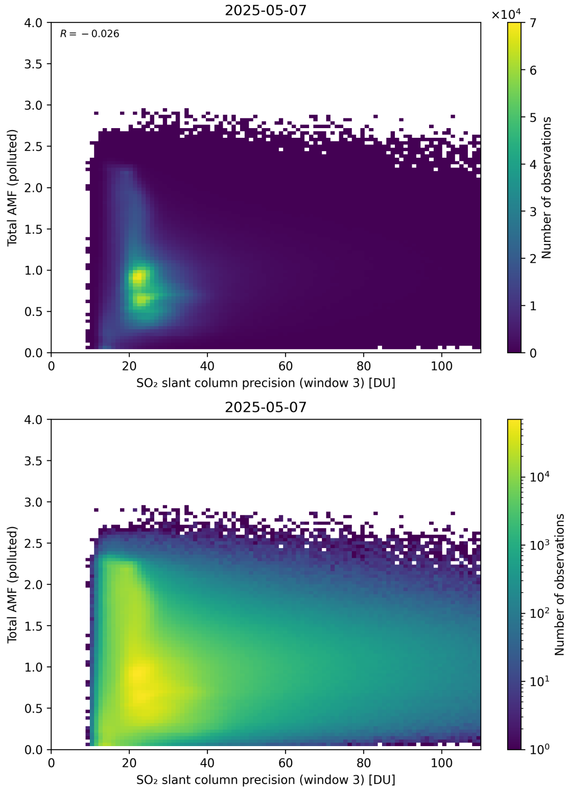
Figure 313: Scatter density plot of “SO 2 slant column precision (window 3)” against “Total AMF (polluted)” for 2025-05-06 to 2025-05-08.
