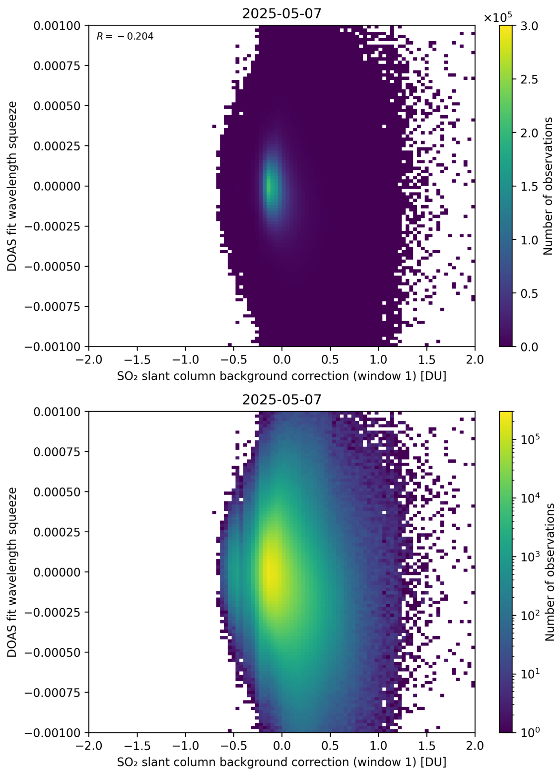
Figure 112: Scatter density plot of “SO 2 slant column background correction (window 1)” against “DOAS fit wavelength squeeze” for 2025-05-06 to 2025-05-08.
