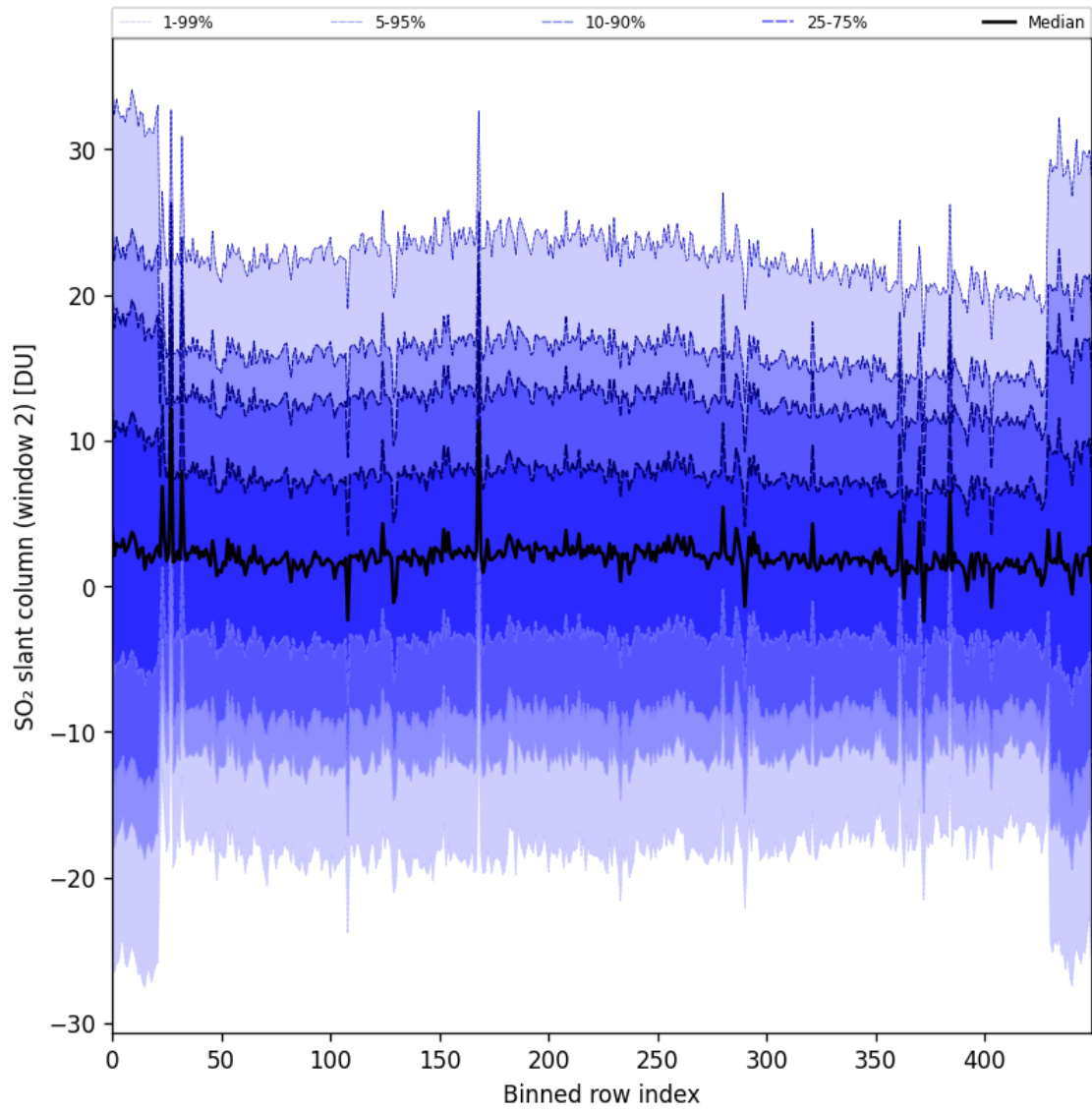
Figure 93: Along track statistics of “SO 2 slant column (window 2)” for 2025-05-06 to 2025-05-08
