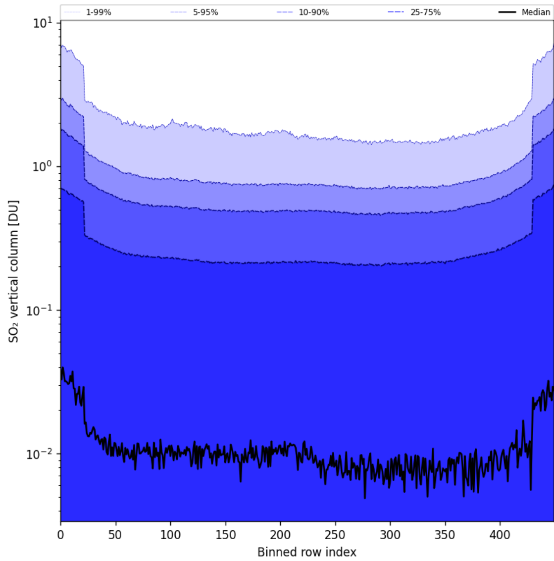
Figure 84: Along track statistics of “SO 2 vertical column” for 2025-05-06 to 2025-05-08
