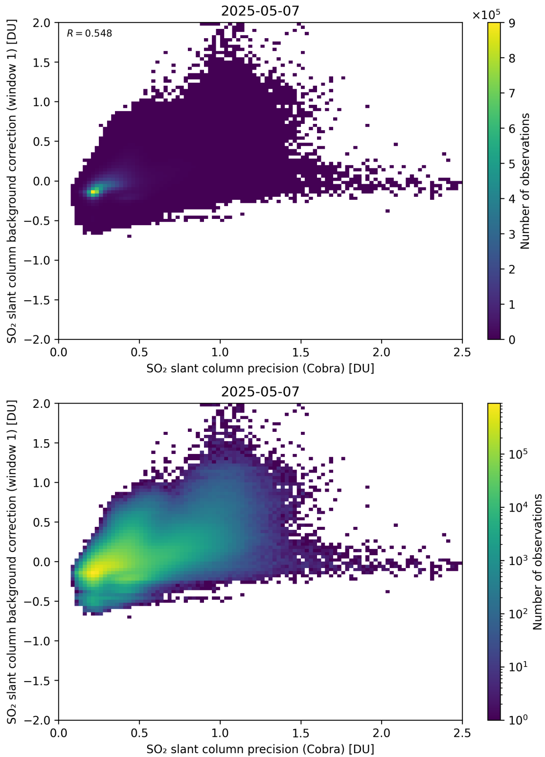
Figure 199: Scatter density plot of “SO 2 slant column precision (Cobra)” against “SO 2 slant column background correction (window 1)” for 2025-05-06 to 2025-05-08.
