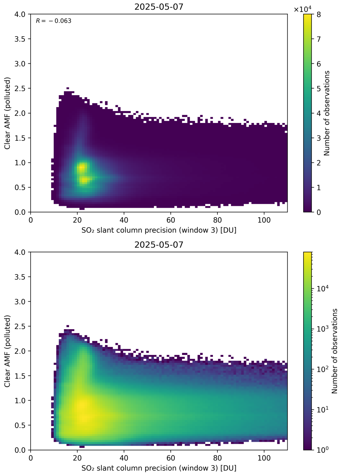
Figure 311: Scatter density plot of “SO 2 slant column precision (window 3)” against “Clear AMF (polluted)” for 2025-05-06 to 2025-05-08.
