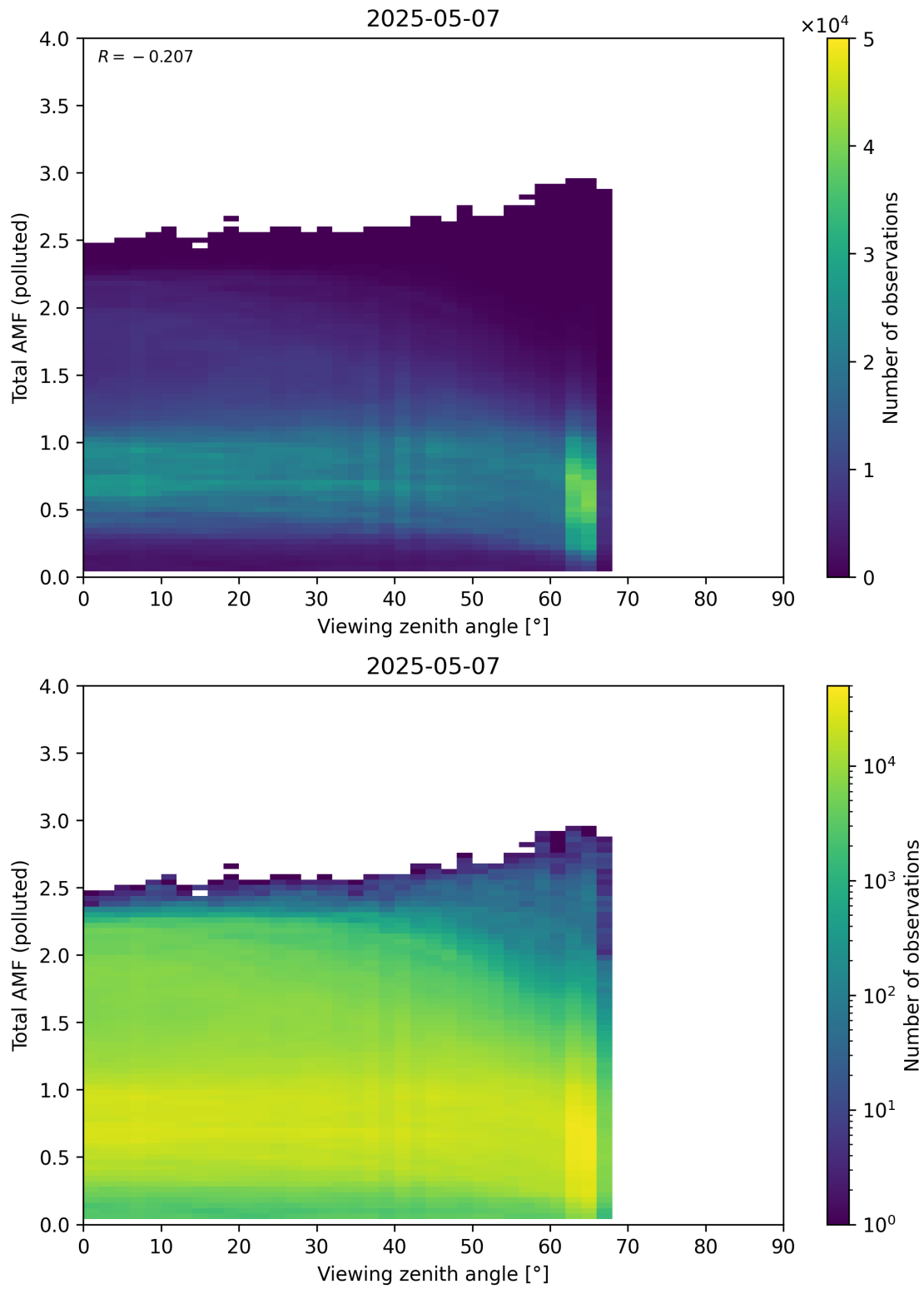
Figure 381: Scatter density plot of “Viewing zenith angle” against “Total AMF (polluted)” for 2025-05-06 to 2025-05-08.
