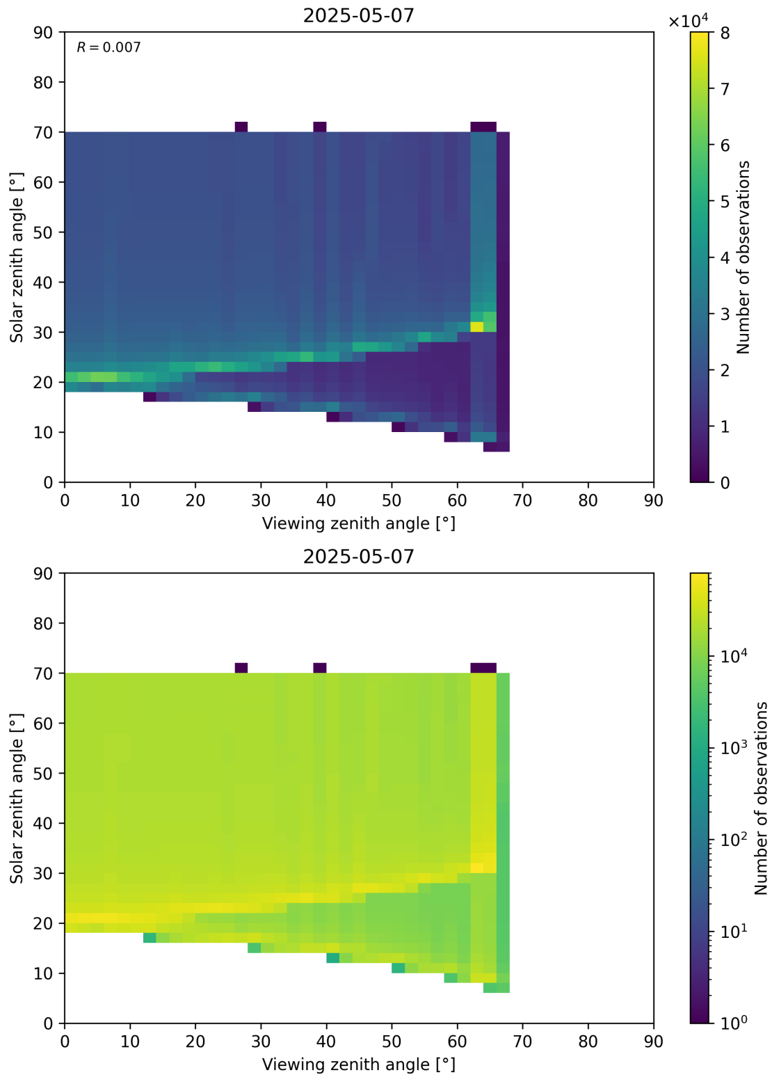
Figure 369: Scatter density plot of “Viewing zenith angle” against “Solar zenith angle” for 2025-05-06 to 2025-05-08.
