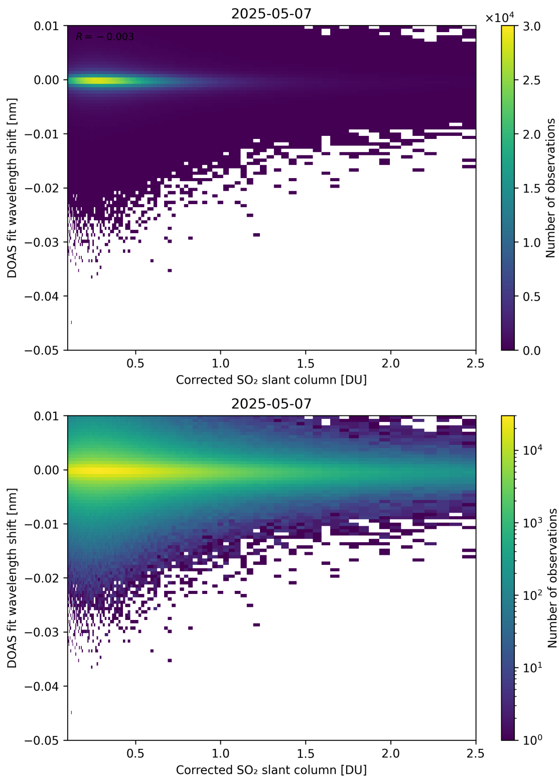
Figure 229: Scatter density plot of “Corrected SO 2 slant column” against “DOAS fit wavelength shift” for 2025-05-06 to 2025-05-08.
