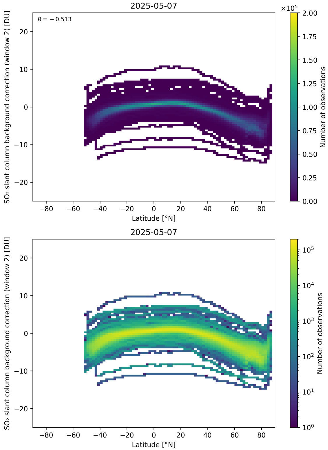
Figure 151: Scatter density plot of “Latitude” against “SO 2 slant column background correction (window 2)” for 2025-05-06 to 2025-05-08.
