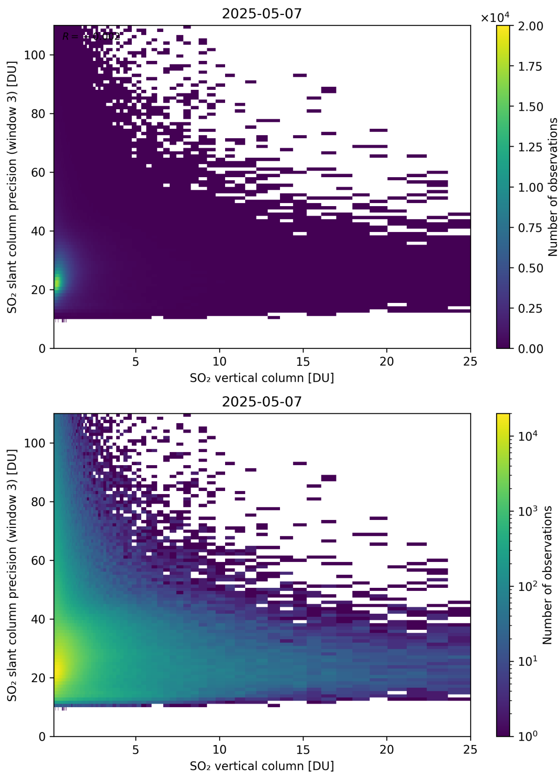
Figure 358: Scatter density plot of “SO 2 vertical column” against “SO 2 slant column precision (window 3)” for 2025-05-06 to 2025-05-08.
