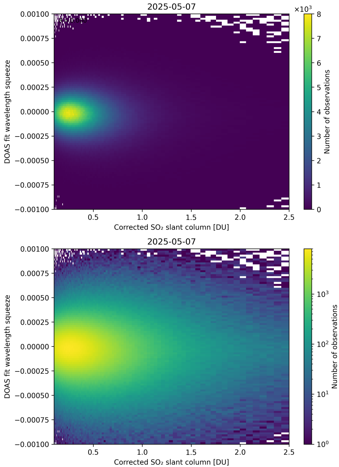
Figure 230: Scatter density plot of “Corrected SO 2 slant column” against “DOAS fit wavelength squeeze” for 2025-05-06 to 2025-05-08.
