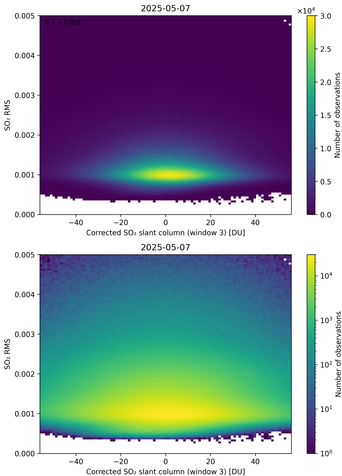
Figure 258: Scatter density plot of “Corrected SO 2 slant column (window 3)” against “SO 2 RMS” for 2025-05-06 to 2025-05-08.
