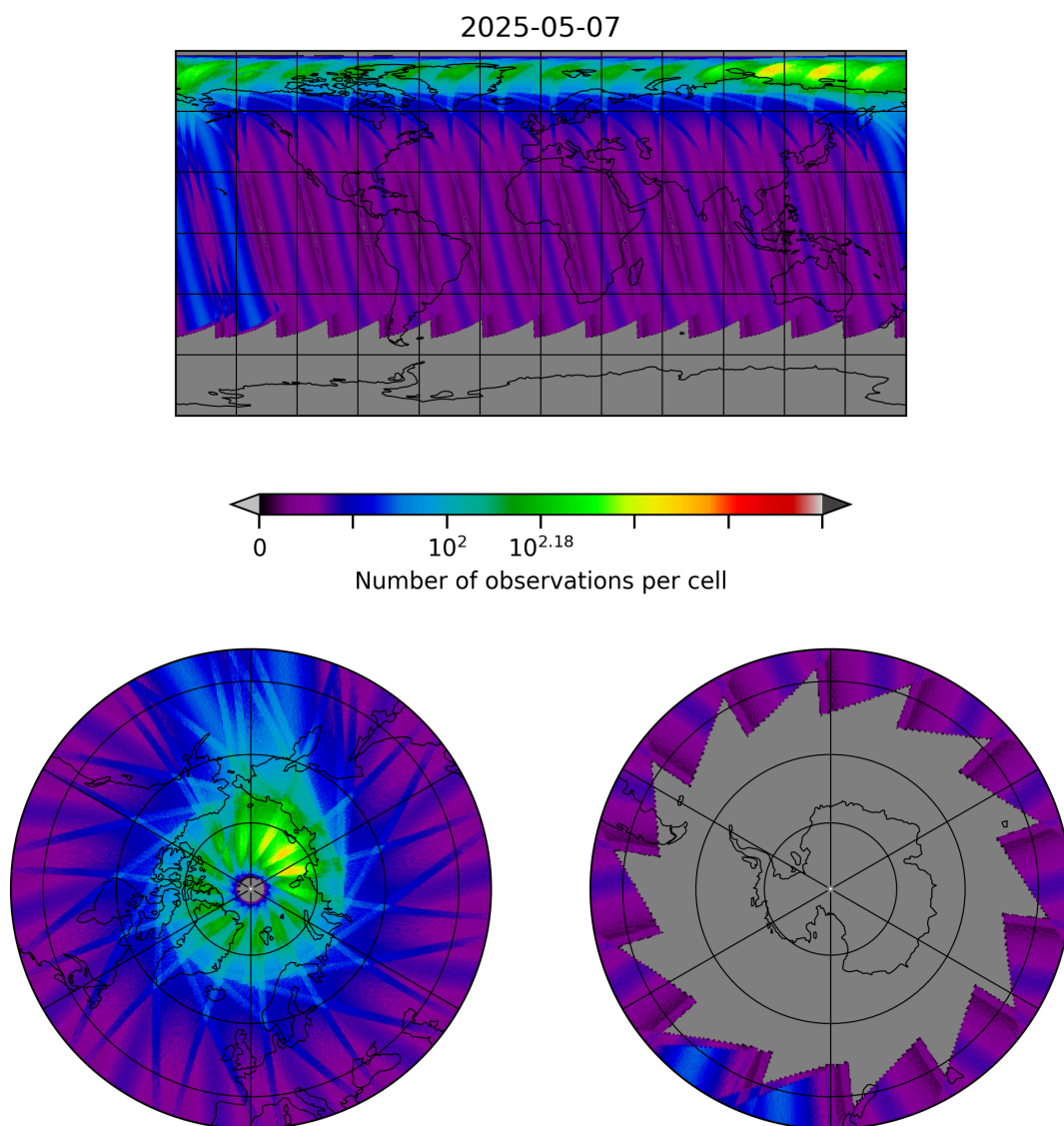
Figure 30: Map of the number of observations for 2025-05-06 to 2025-05-08
