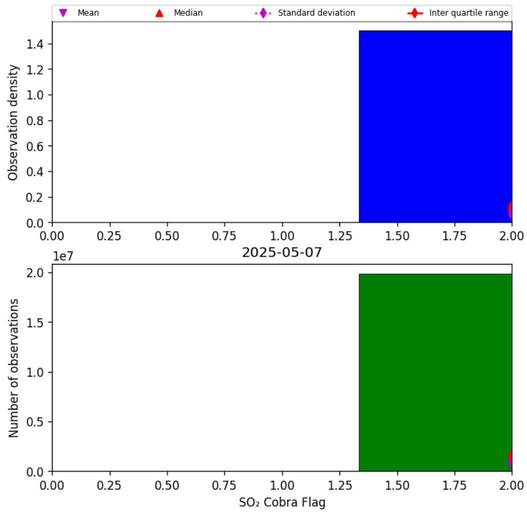
Figure 75: Histogram of “SO 2 Cobra Flag” for 2025-05-06 to 2025-05-08
