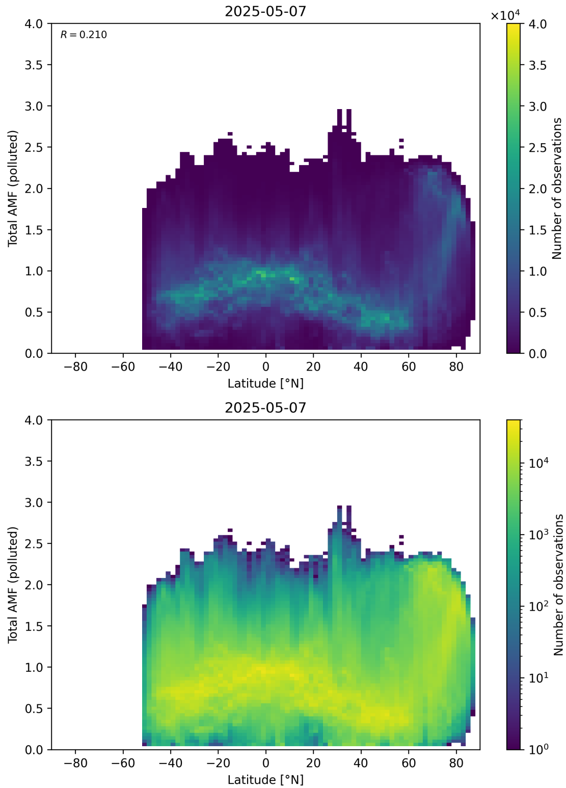
Figure 167: Scatter density plot of “Latitude” against “Total AMF (polluted)” for 2025-05-06 to 2025-05-08.
