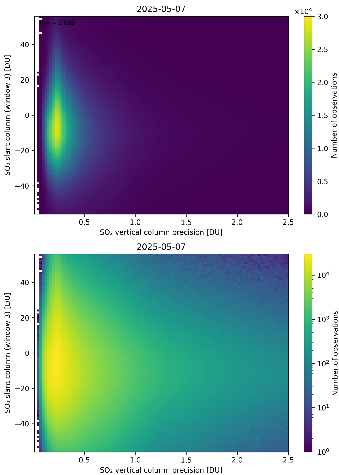
Figure 344: Scatter density plot of “SO 2 vertical column precision” against “SO 2 slant column (window 3)” for 2025-05-06 to 2025-05-08.
