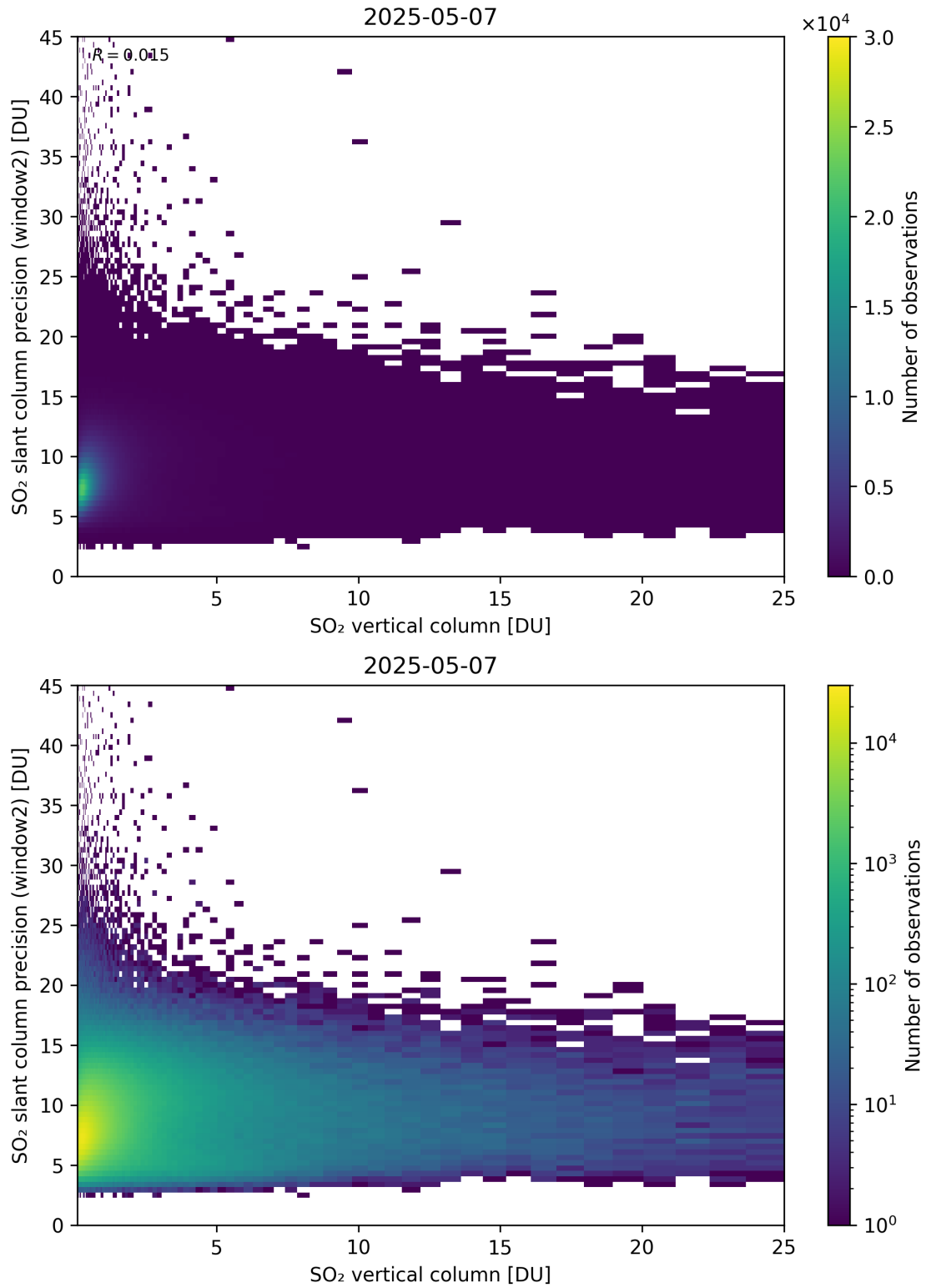
Figure 356: Scatter density plot of “SO 2 vertical column” against “SO 2 slant column precision (window2)” for 2025-05-06 to 2025-05-08.
