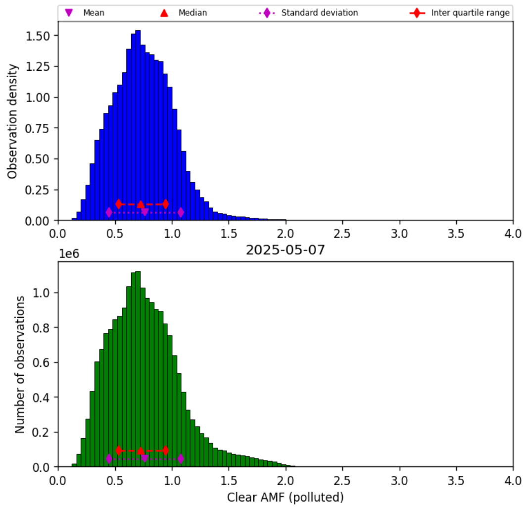
Figure 81: Histogram of “Clear AMF (polluted)” for 2025-05-06 to 2025-05-08
