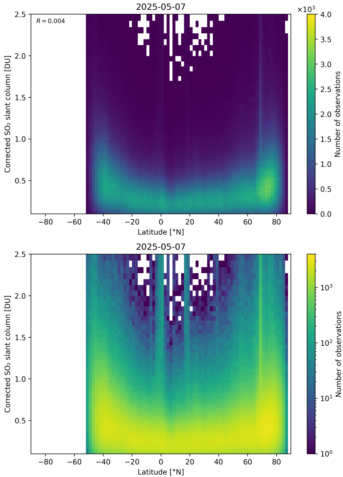
Figure 159: Scatter density plot of “Latitude” against “Corrected SO 2 slant column” for 2025-05-06 to 2025-05-08.
