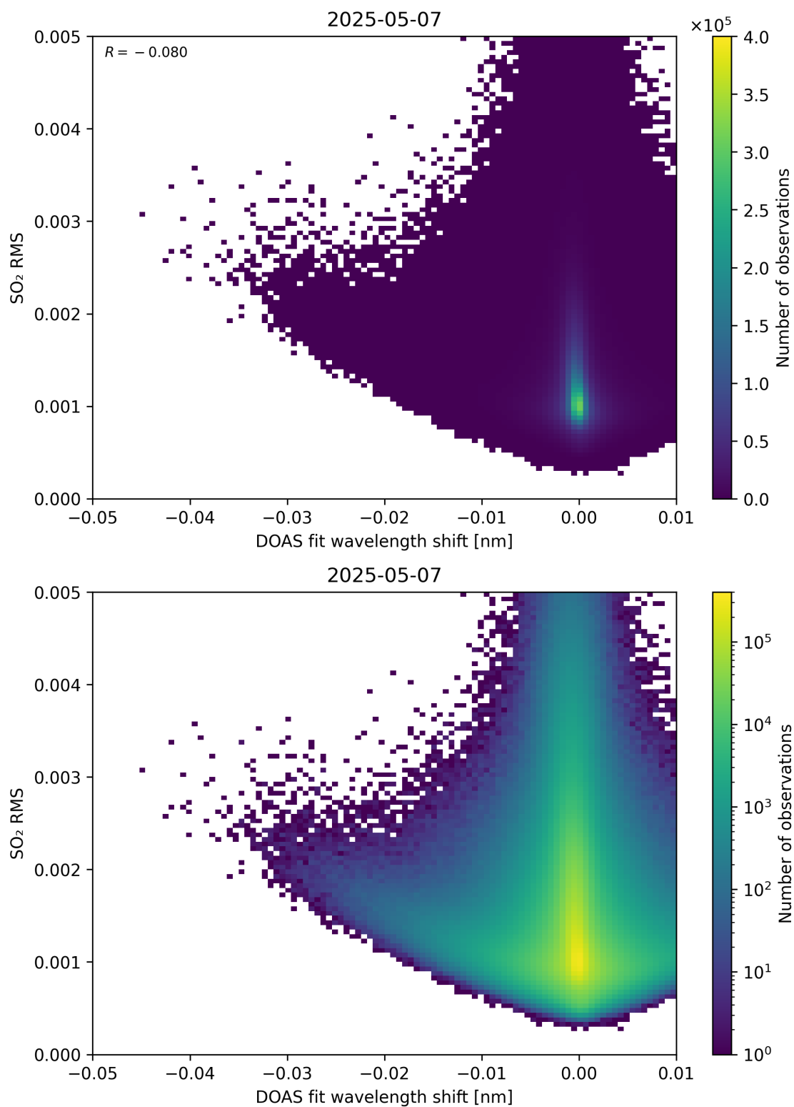
Figure 139: Scatter density plot of “DOAS fit wavelength shift” against “SO 2 RMS” for 2025-05-06 to 2025-05-08.
