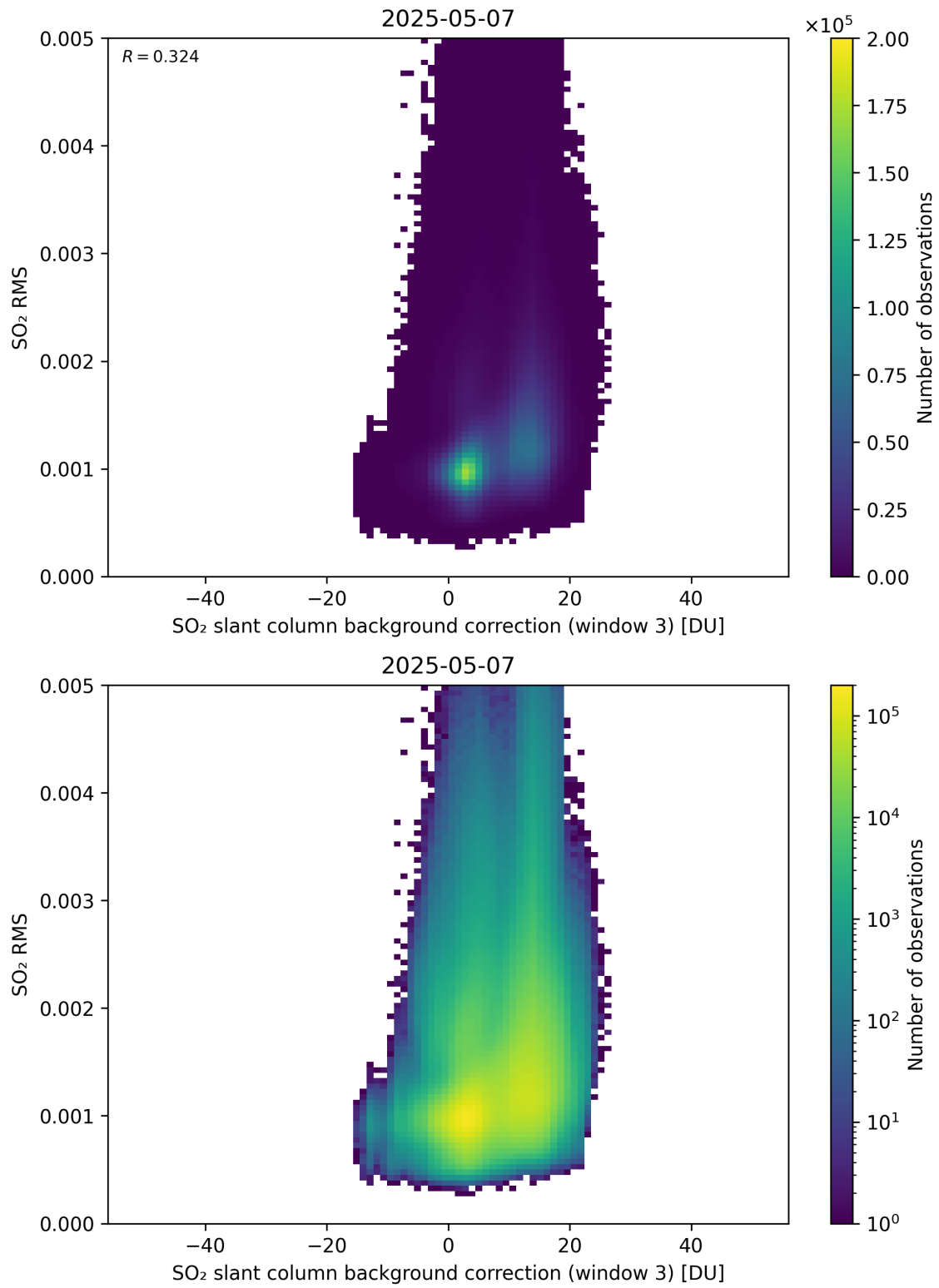
Figure 134: Scatter density plot of “SO 2 slant column background correction (window 3)” against “SO 2 RMS” for 2025-05-06 to 2025-05-08.
