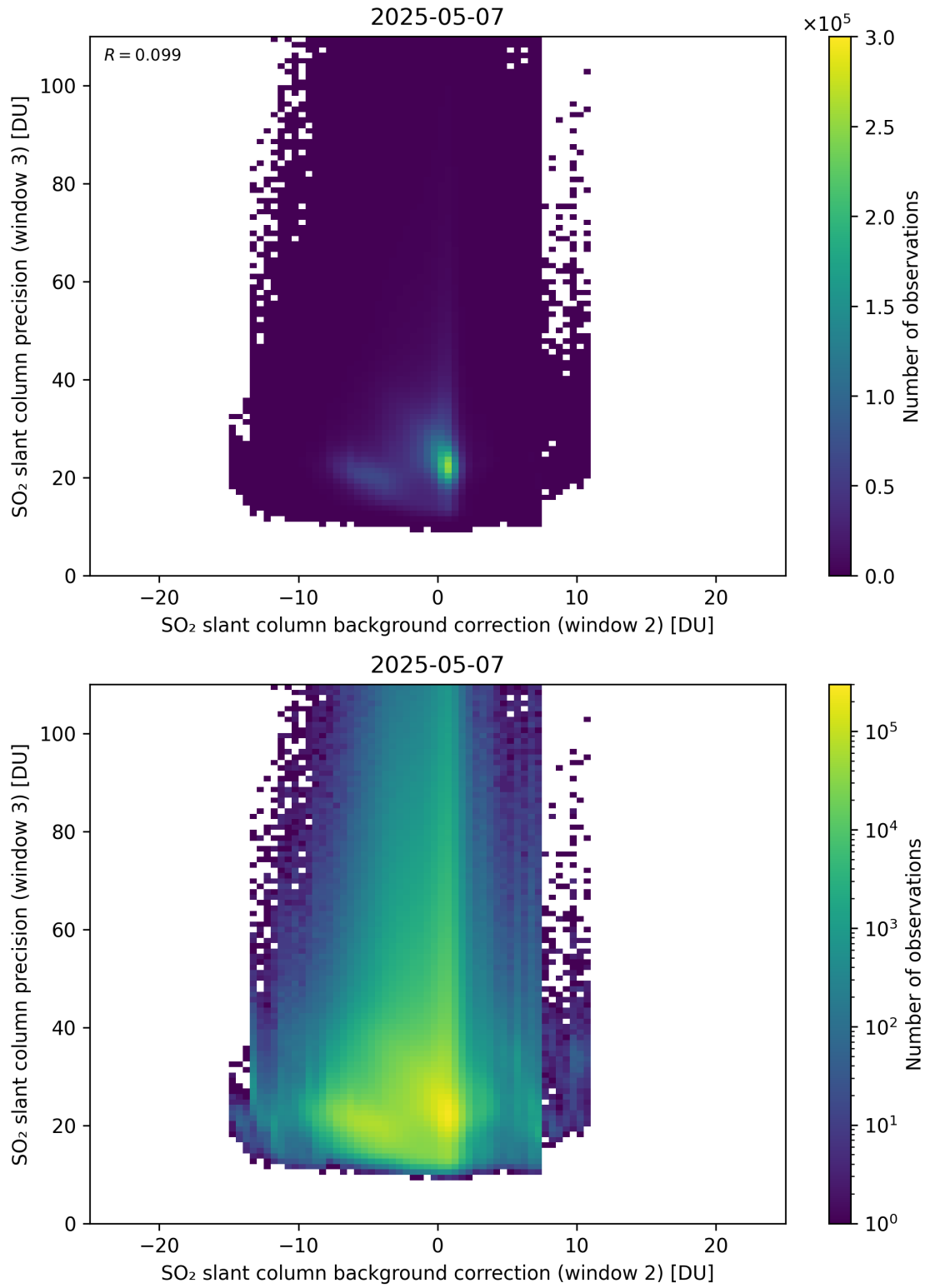
Figure 129: Scatter density plot of “SO 2 slant column background correction (window 2)” against “SO 2 slant column precision (window 3)” for 2025-05-06 to 2025-05-08.
