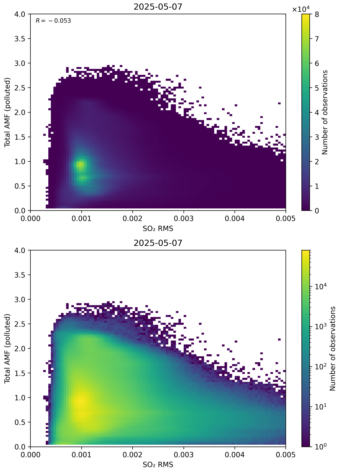
Figure 148: Scatter density plot of “SO 2 RMS” against “Total AMF (polluted)” for 2025-05-06 to 2025-05-08.
