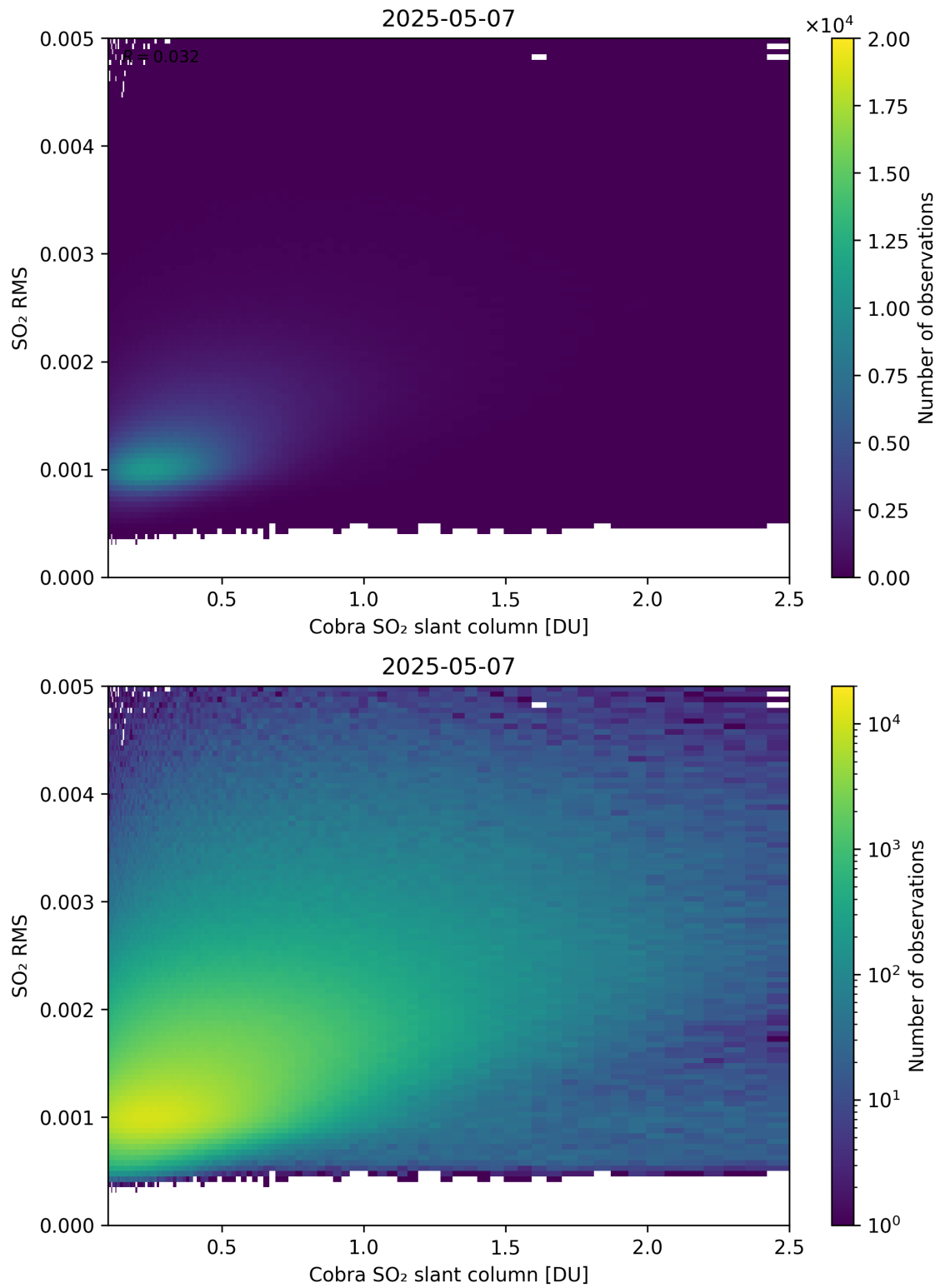
Figure 198: Scatter density plot of “Cobra SO 2 slant column” against “SO 2 RMS” for 2025-05-06 to 2025-05-08.
