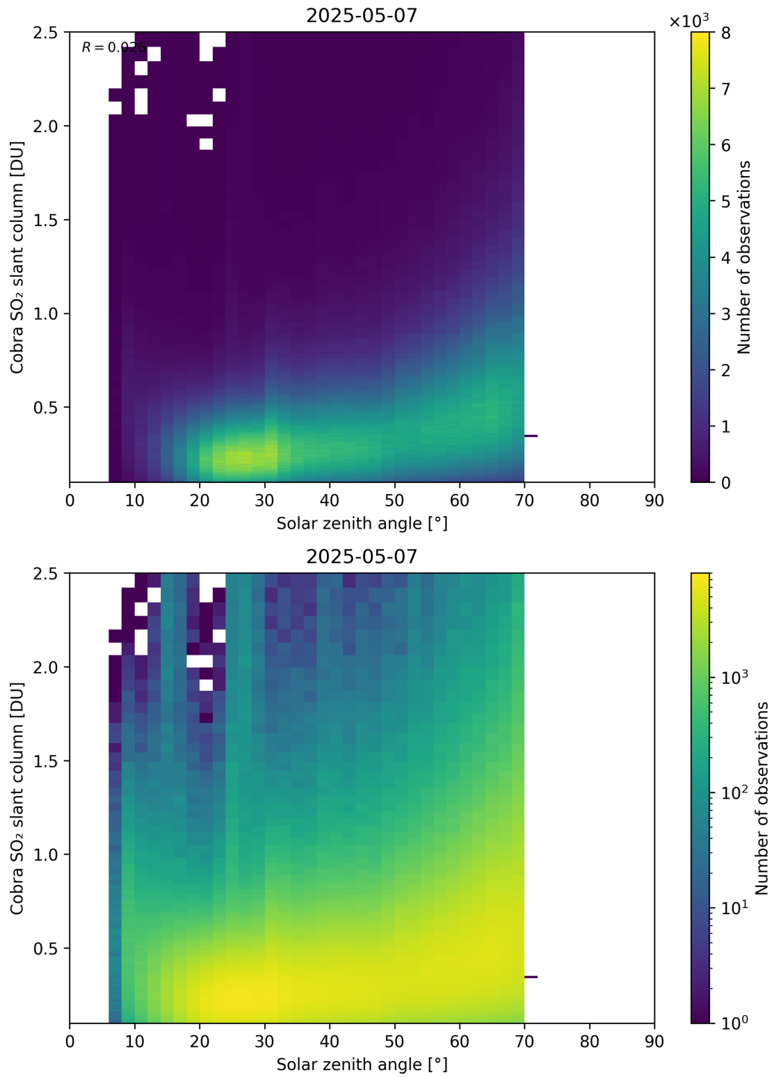
Figure 179: Scatter density plot of “Solar zenith angle” against “Cobra SO 2 slant column” for 2025-05-06 to 2025-05-08.
