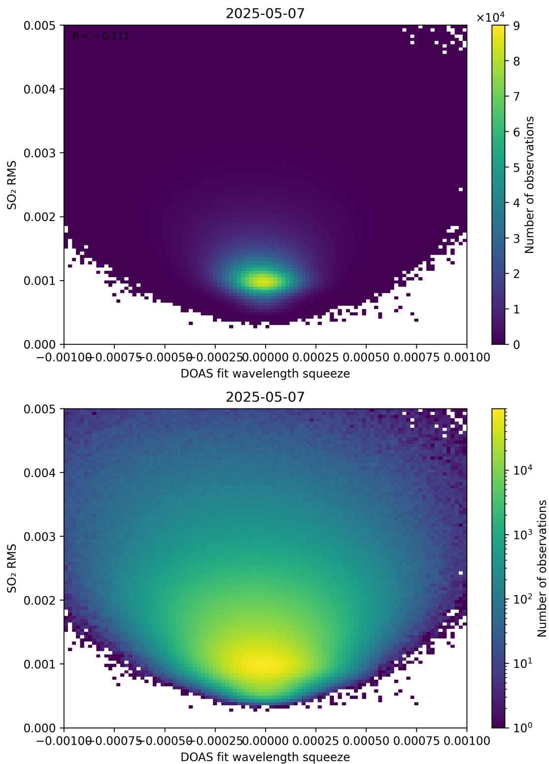
Figure 143: Scatter density plot of “DOAS fit wavelength squeeze” against “SO 2 RMS” for 2025-05-06 to 2025-05-08.
