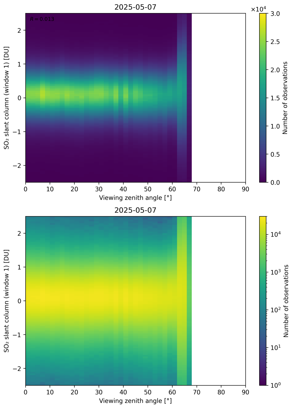
Figure 376: Scatter density plot of “Viewing zenith angle” against “SO 2 slant column (window 1)” for 2025-05-06 to 2025-05-08.
