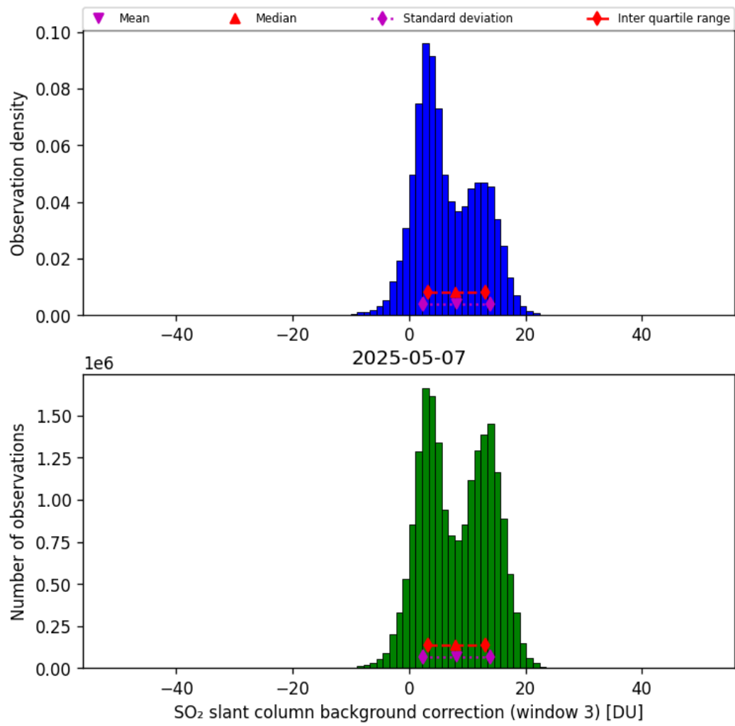
Figure 74: Histogram of “SO 2 slant column background correction (window 3)” for 2025-05-06 to 2025-05-08
