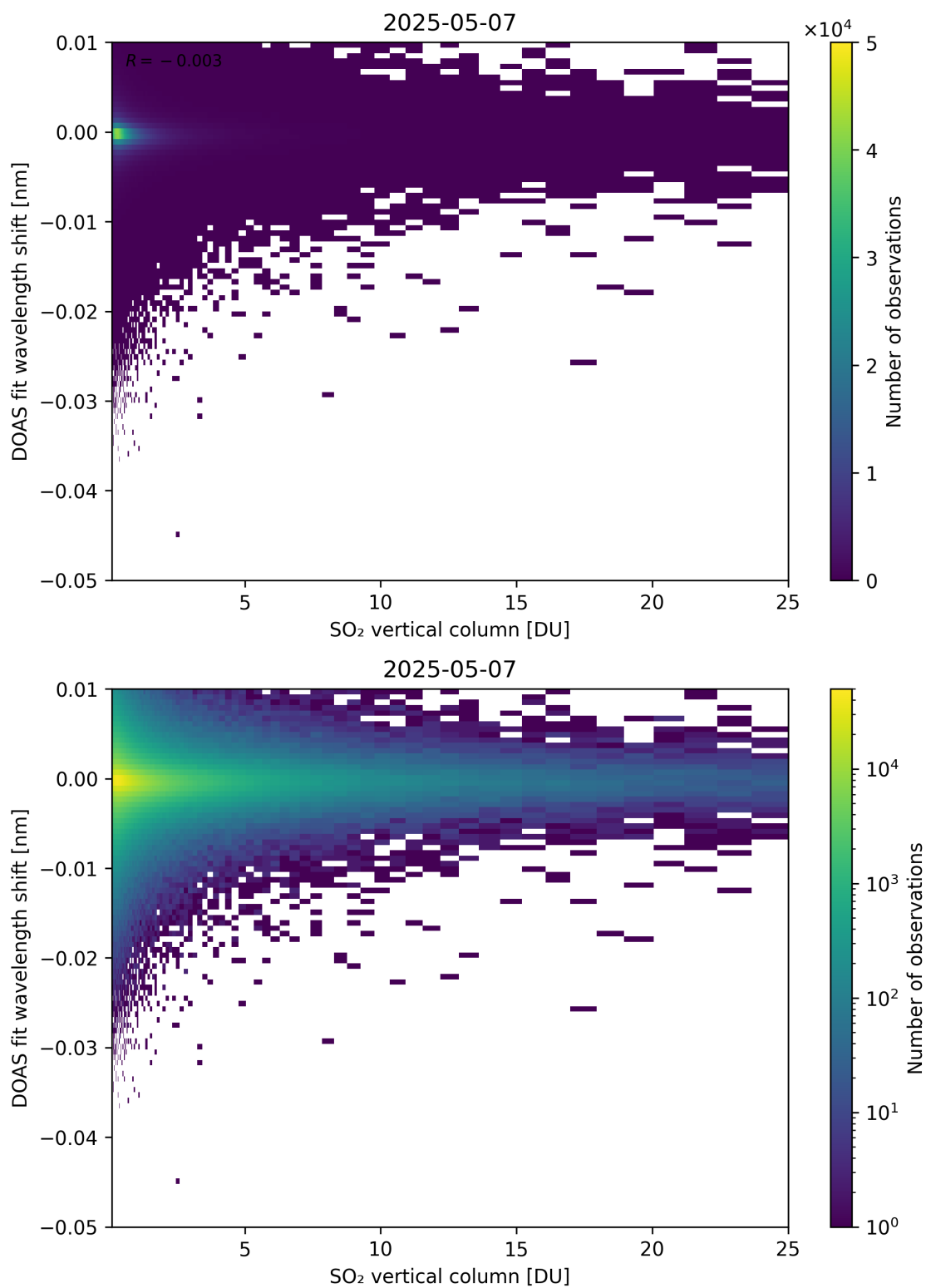
Figure 326: Scatter density plot of “SO 2 vertical column” against “DOAS fit wavelength shift” for 2025-05-06 to 2025-05-08.
