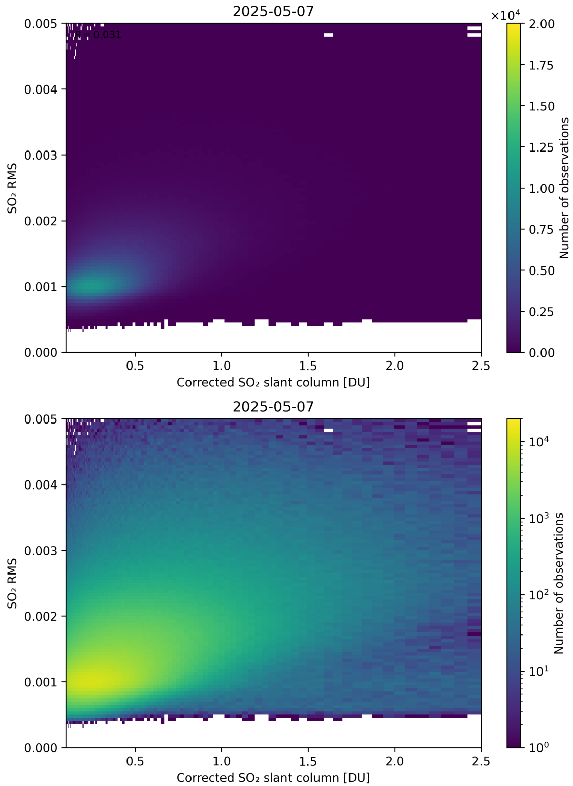
Figure 231: Scatter density plot of “Corrected SO 2 slant column” against “SO 2 RMS” for 2025-05-06 to 2025-05-08.
