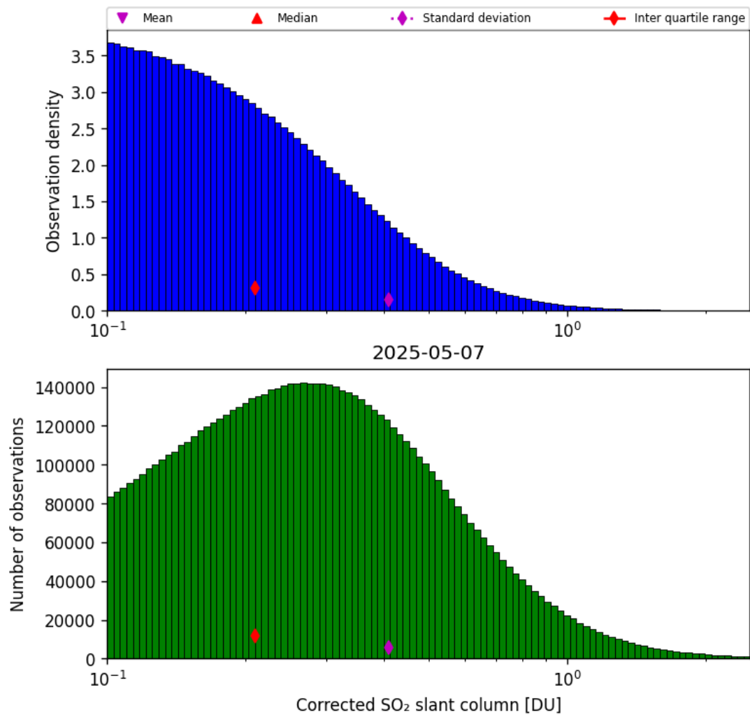
Figure 60: Histogram of "Corrected SO 2 slant column" for 2025-05-06 to 2025-05-08
