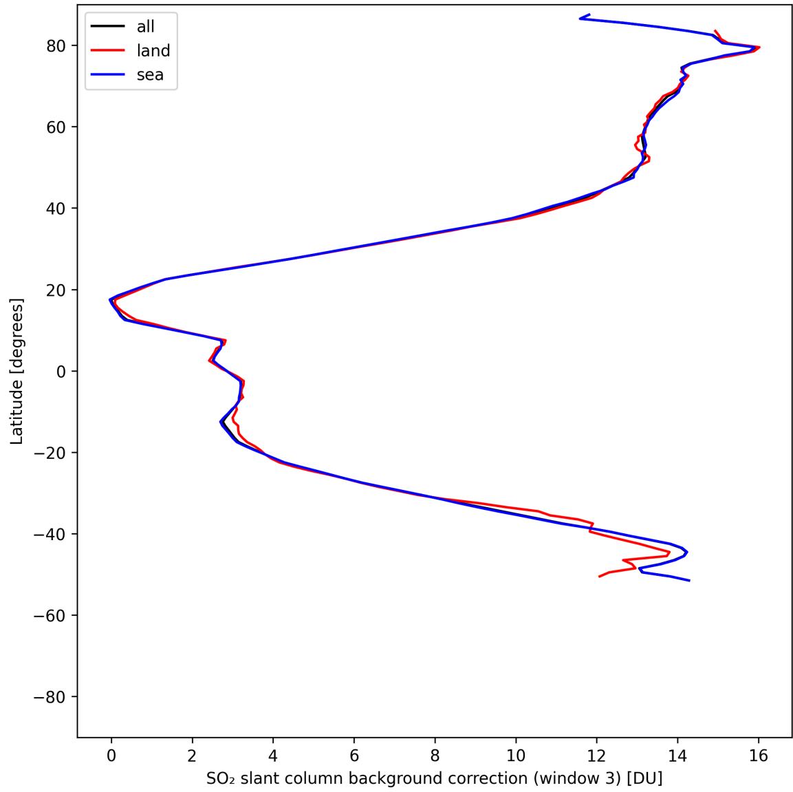
Figure 48: Zonal average of “SO 2 slant column background correction (window 3)” for 2025-05-06 to 2025-05-08.
