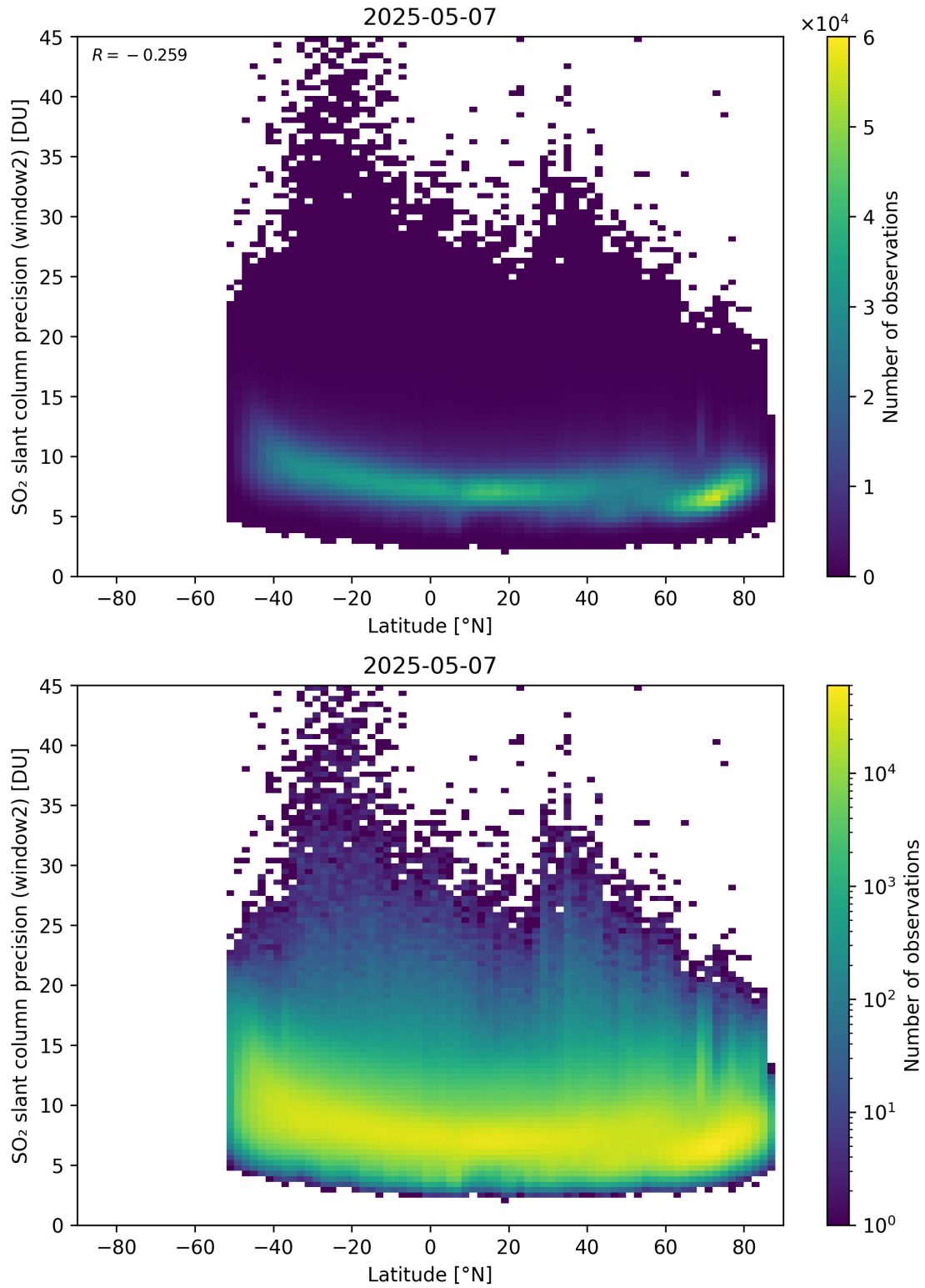
Figure 164: Scatter density plot of “Latitude” against “SO 2 slant column precision (window2)” for 2025-05-06 to 2025-05-08.
