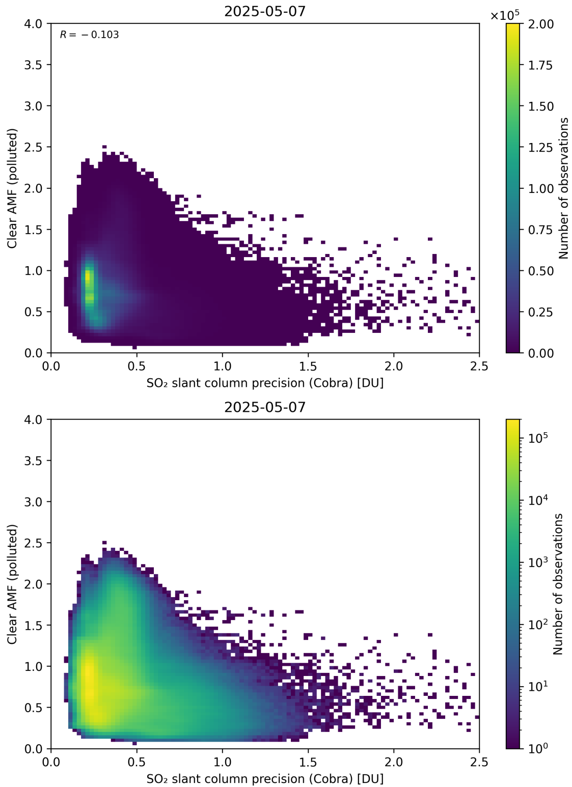
Figure 205: Scatter density plot of “SO 2 slant column precision (Cobra)” against “Clear AMF (polluted)” for 2025-05-06 to 2025-05-08.
