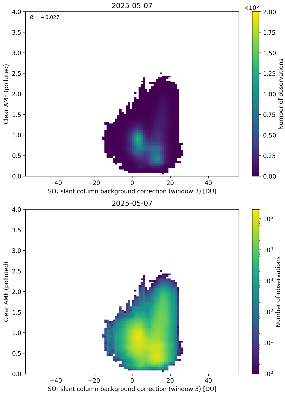
Figure 135: Scatter density plot of “SO 2 slant column background correction (window 3)” against “Clear AMF (polluted)” for 2025-05-06 to 2025-05-08.
