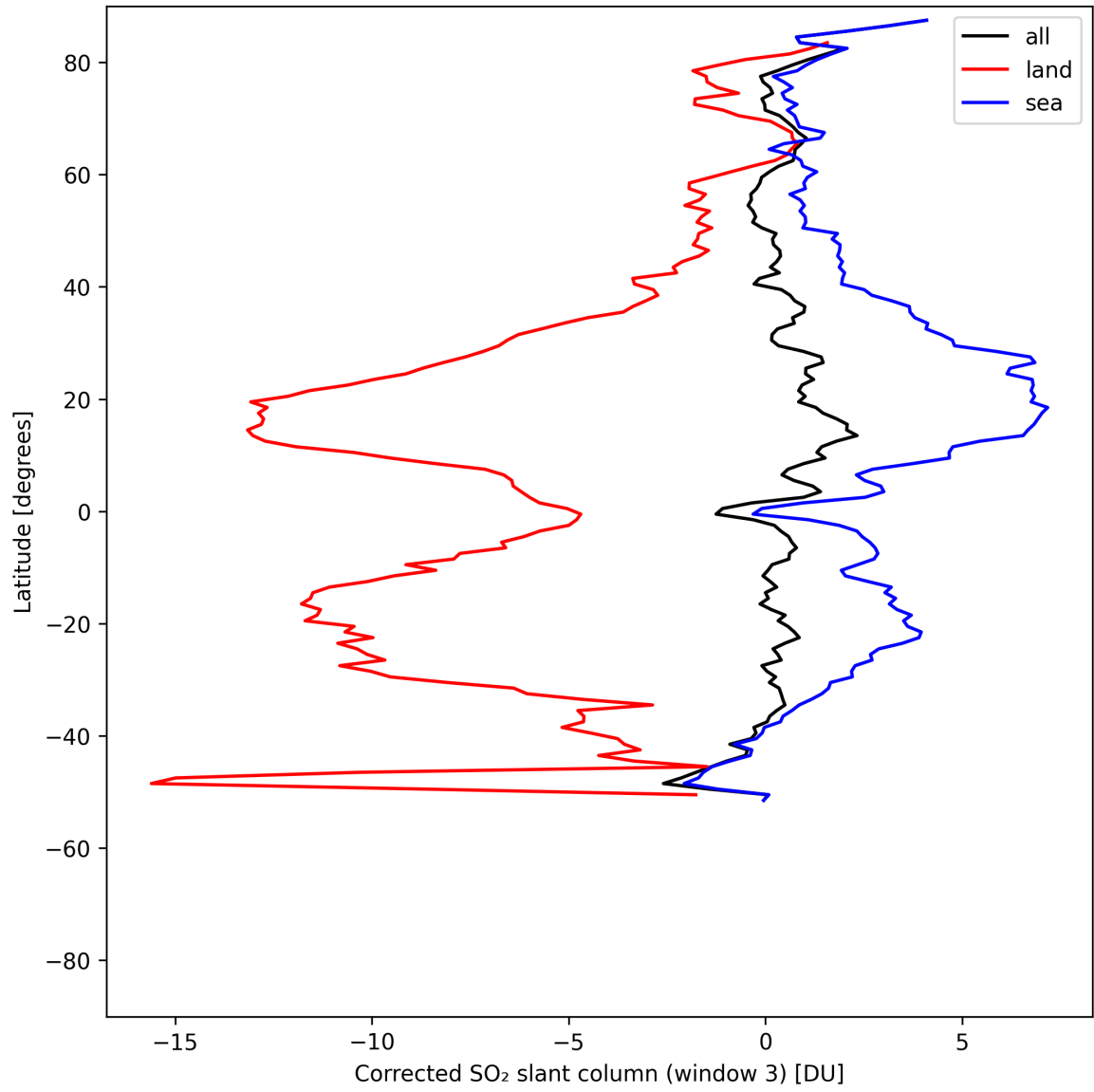
Figure 47: Zonal average of “Corrected SO 2 slant column (window 3)” for 2025-05-06 to 2025-05-08.
