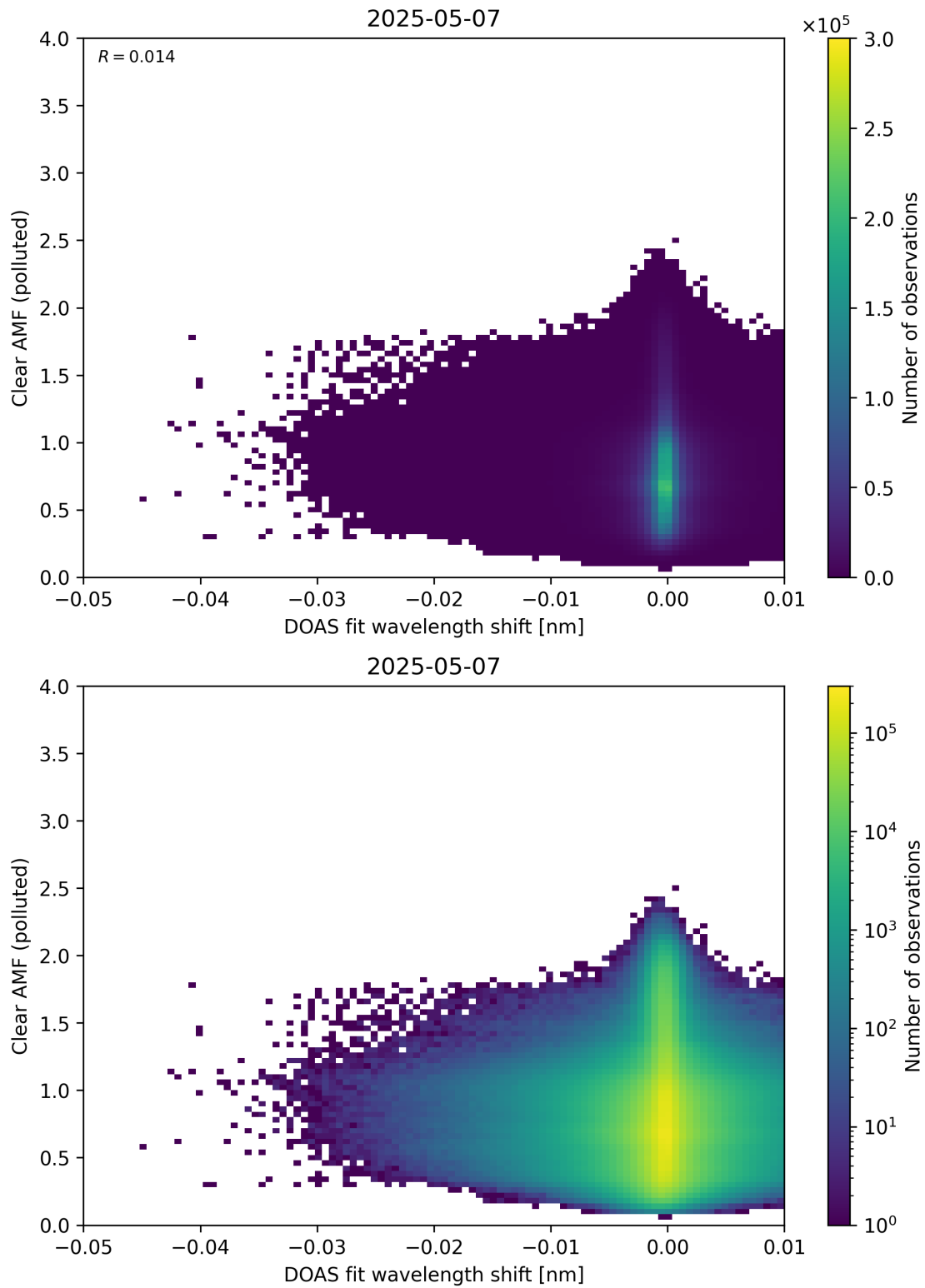
Figure 140: Scatter density plot of “DOAS fit wavelength shift” against “Clear AMF (polluted)” for 2025-05-06 to 2025-05-08.
