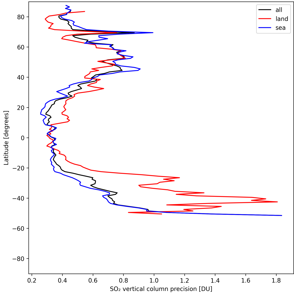
Figure 33: Zonal average of “SO 2 vertical column precision” for 2025-05-06 to 2025-05-08.
