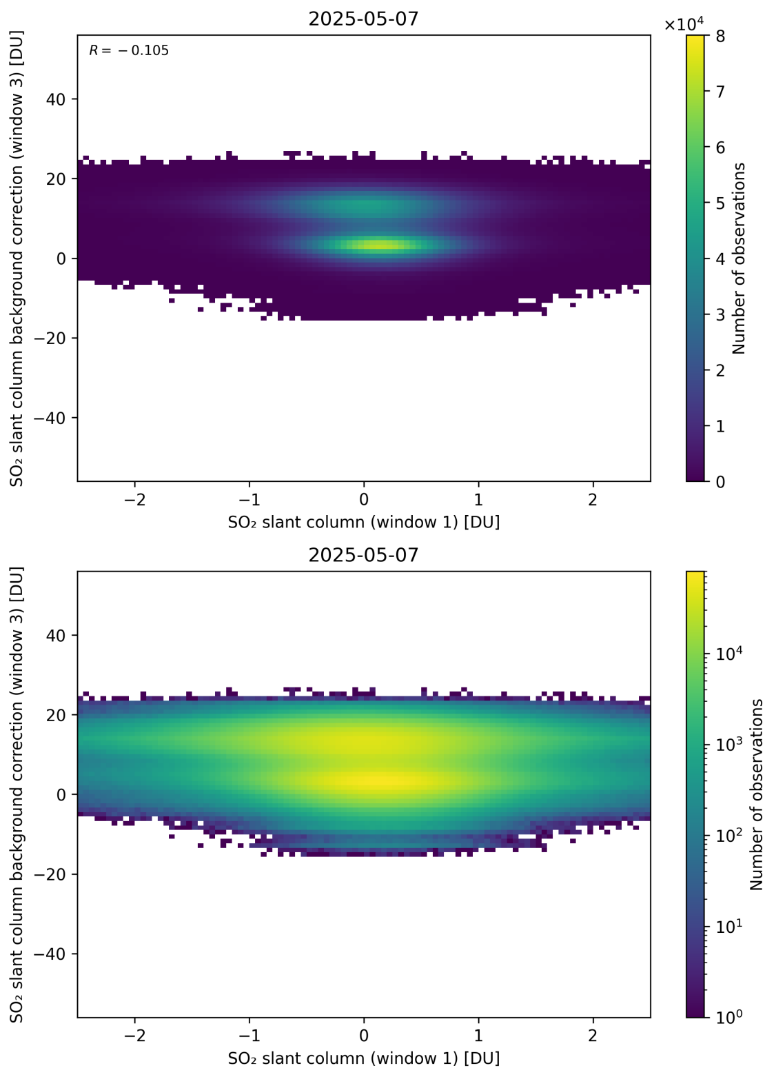
Figure 264: Scatter density plot of “SO 2 slant column (window 1)” against “SO 2 slant column background correction (window 3)” for 2025-05-06 to 2025-05-08.
