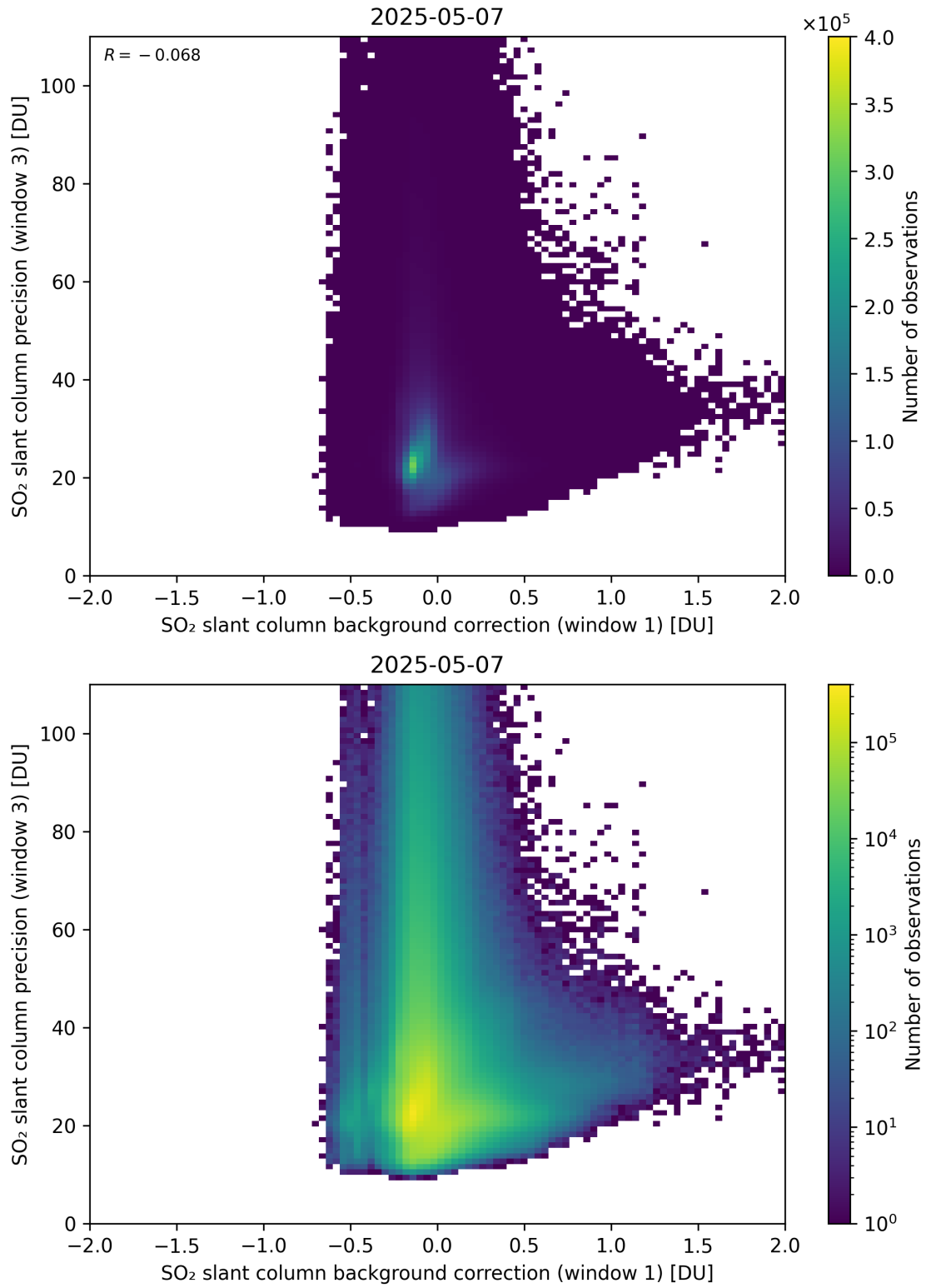
Figure 119: Scatter density plot of “SO 2 slant column background correction (window 1)” against “SO 2 slant column precision (window 3)” for 2025-05-06 to 2025-05-08.
