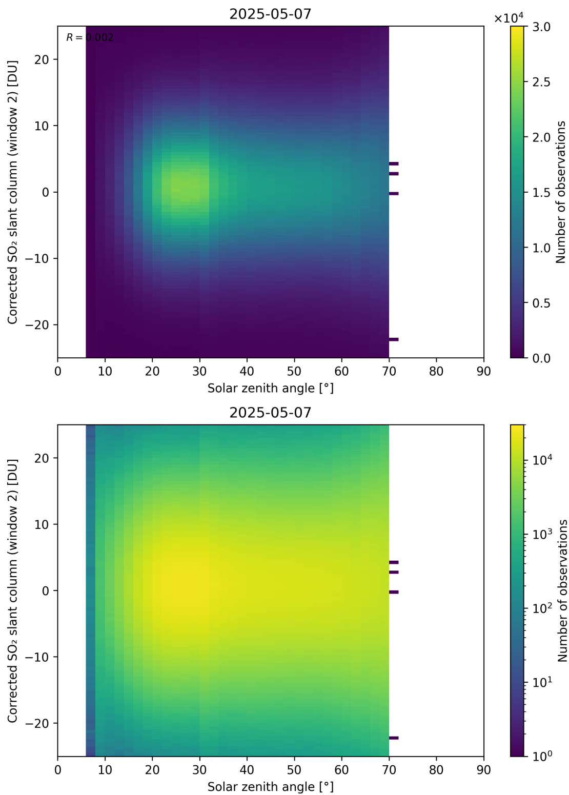
Figure 182: Scatter density plot of “Solar zenith angle” against “Corrected SO 2 slant column (window 2)” for 2025-05-06 to 2025-05-08.
