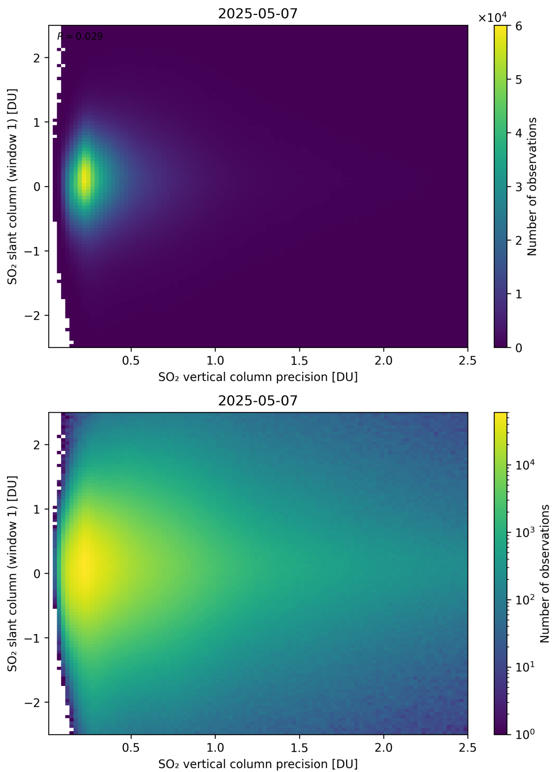
Figure 341: Scatter density plot of “SO 2 vertical column precision” against “SO 2 slant column (window 1)” for 2025-05-06 to 2025-05-08.
