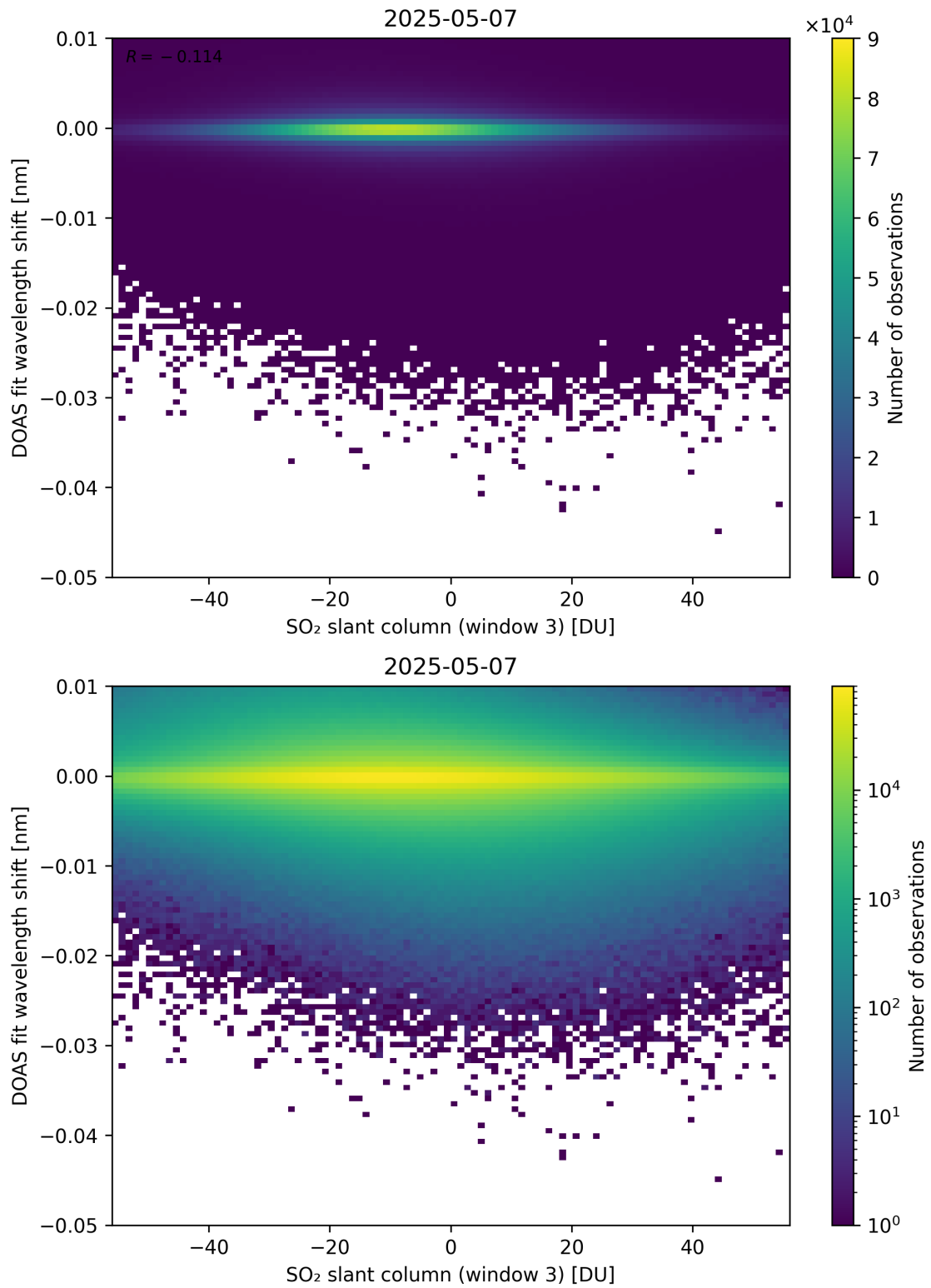
Figure 304: Scatter density plot of “SO 2 slant column (window 3)” against “DOAS fit wavelength shift” for 2025-05-06 to 2025-05-08.
