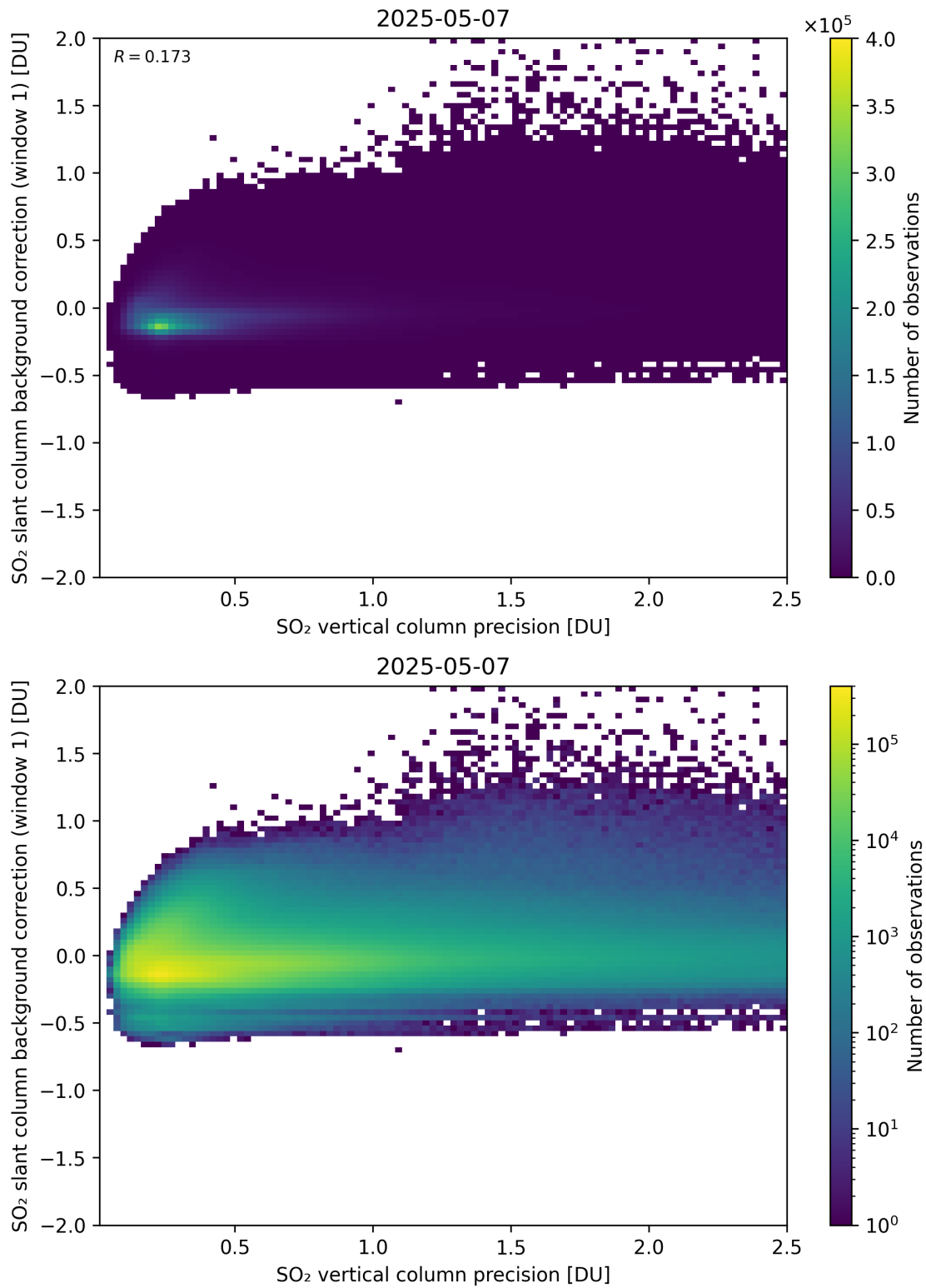
Figure 329: Scatter density plot of “SO 2 vertical column precision” against “SO 2 slant column background correction (window 1)” for 2025-05-06 to 2025-05-08.
