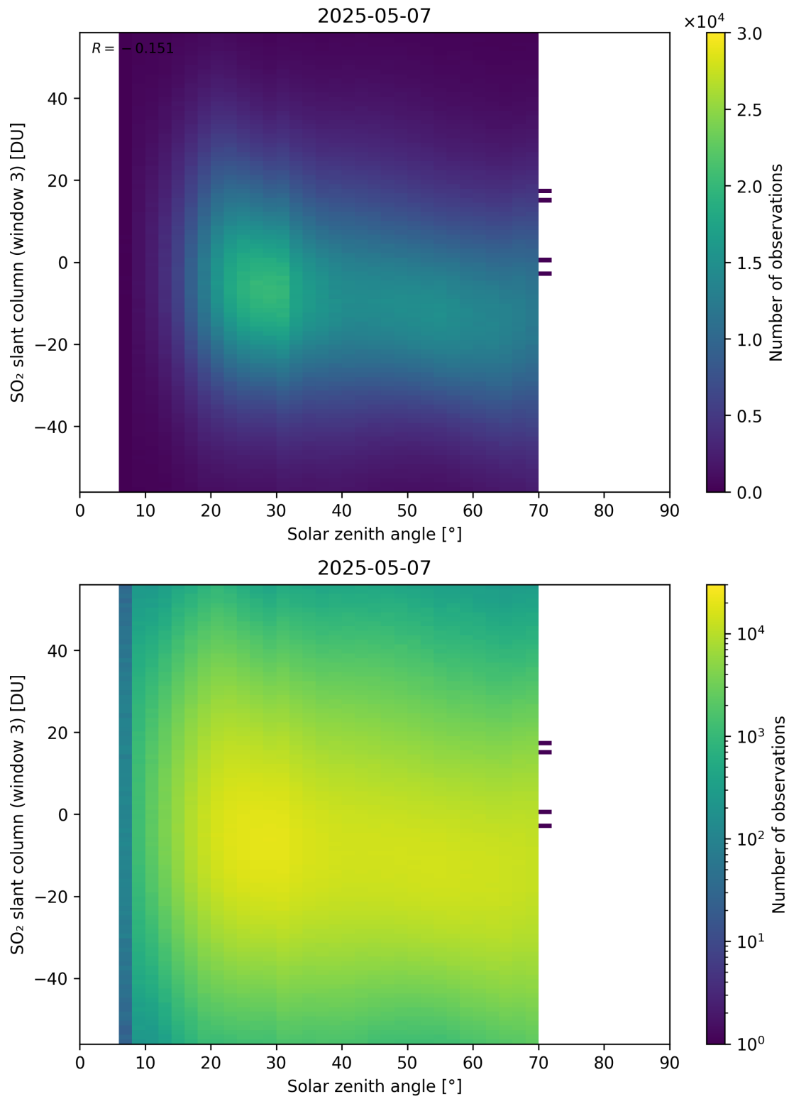
Figure 187: Scatter density plot of “Solar zenith angle” against “SO 2 slant column (window 3)” for 2025-05-06 to 2025-05-08.
