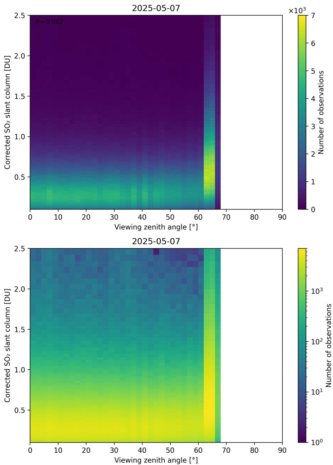
Figure 373: Scatter density plot of “Viewing zenith angle” against “Corrected SO 2 slant column” for 2025-05-06 to 2025-05-08.
