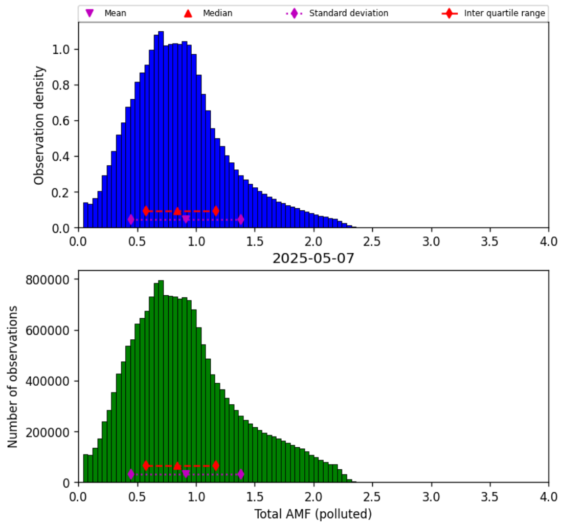
Figure 79: Histogram of “Total AMF (polluted)” for 2025-05-06 to 2025-05-08
