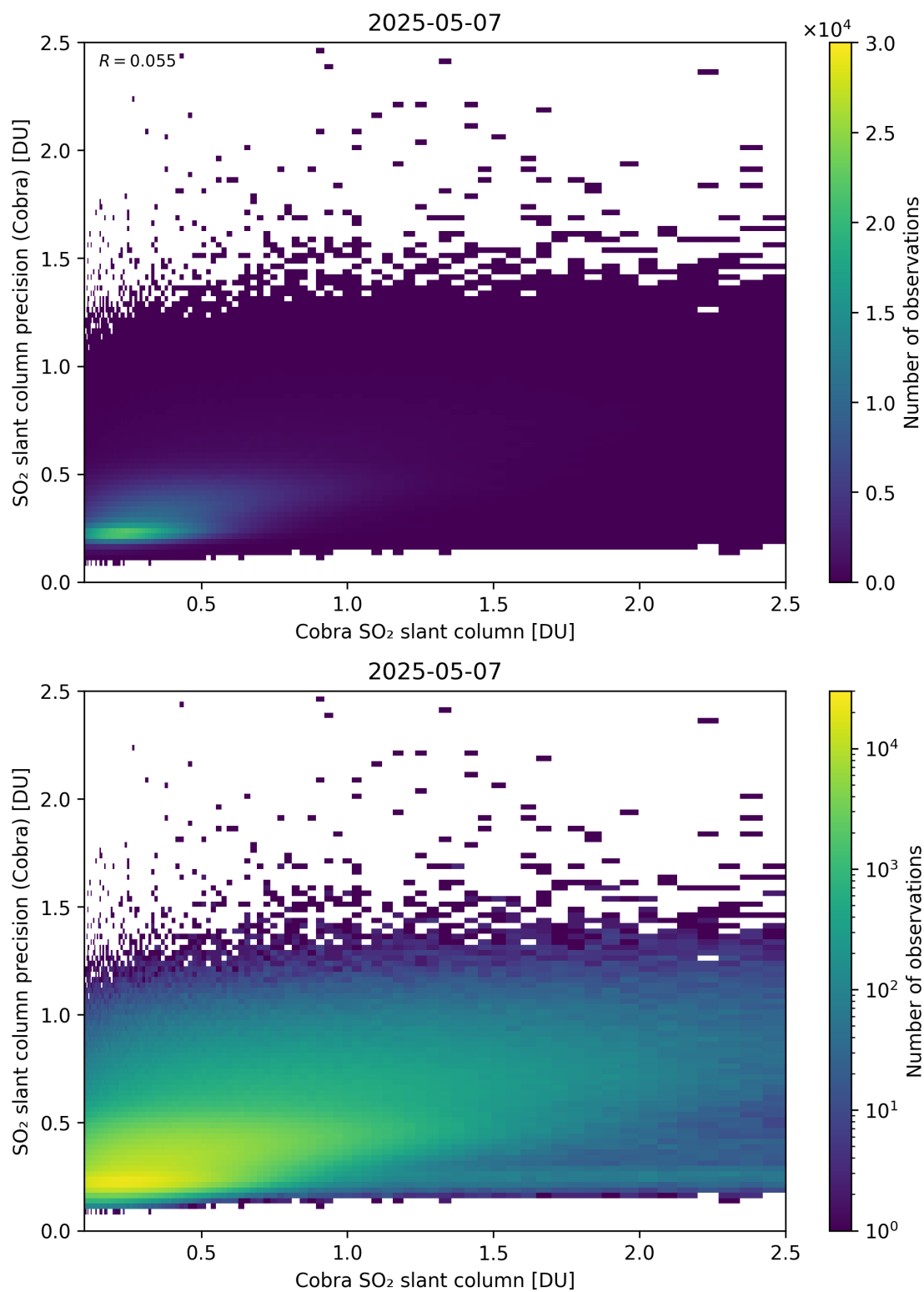
Figure 216: Scatter density plot of “Cobra SO 2 slant column” against “SO 2 slant column precision (Cobra)” for 2025-05-06 to 2025-05-08.
