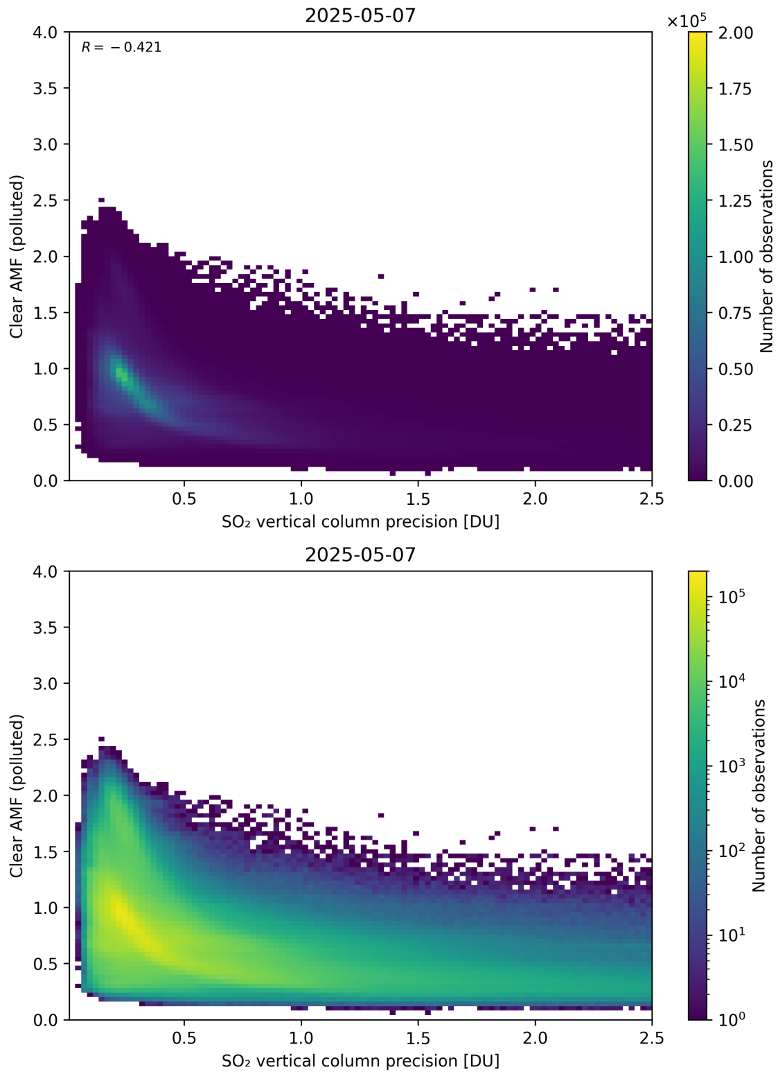
Figure 335: Scatter density plot of “SO 2 vertical column precision” against “Clear AMF (polluted)” for 2025-05-06 to 2025-05-08.
