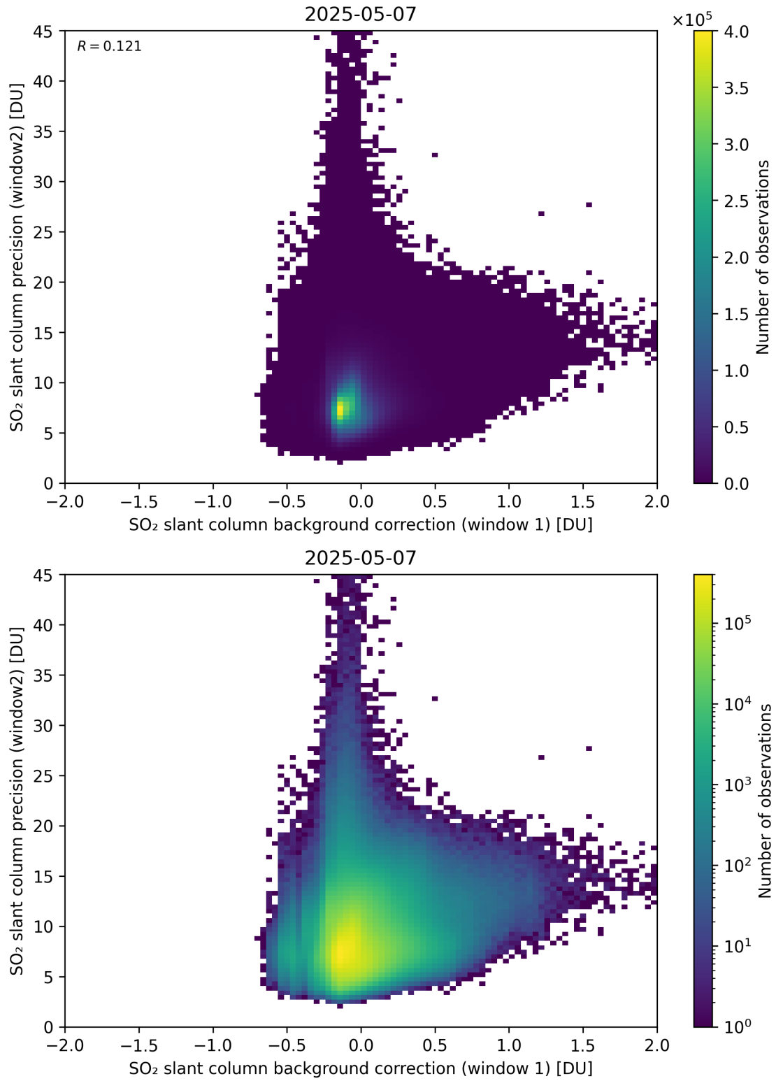
Figure 117: Scatter density plot of “SO 2 slant column background correction (window 1)” against “SO 2 slant column precision (window2)” for 2025-05-06 to 2025-05-08.
