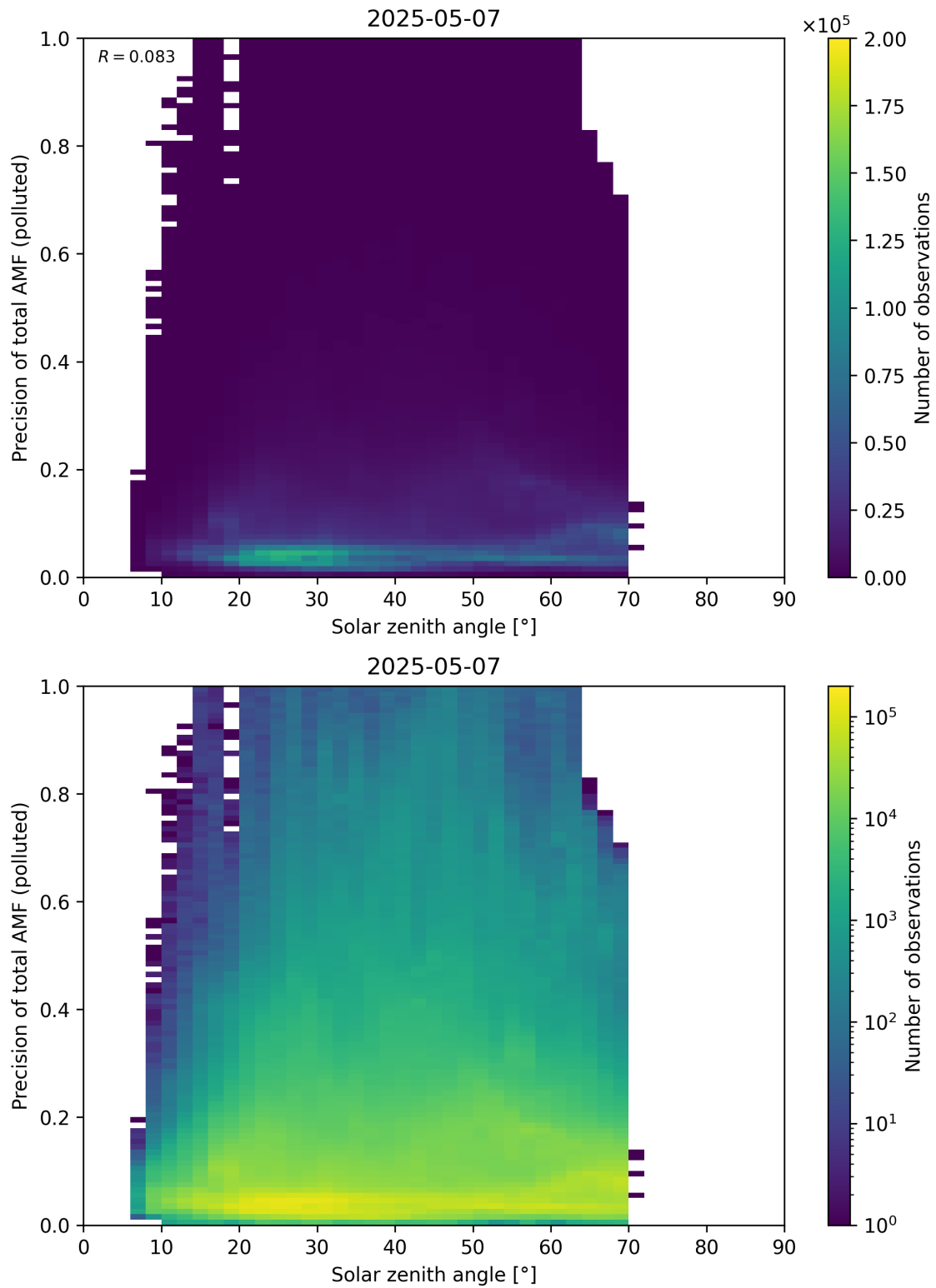
Figure 190: Scatter density plot of “Solar zenith angle” against “Precision of total AMF (polluted)” for 2025-05-06 to 2025-05-08.
