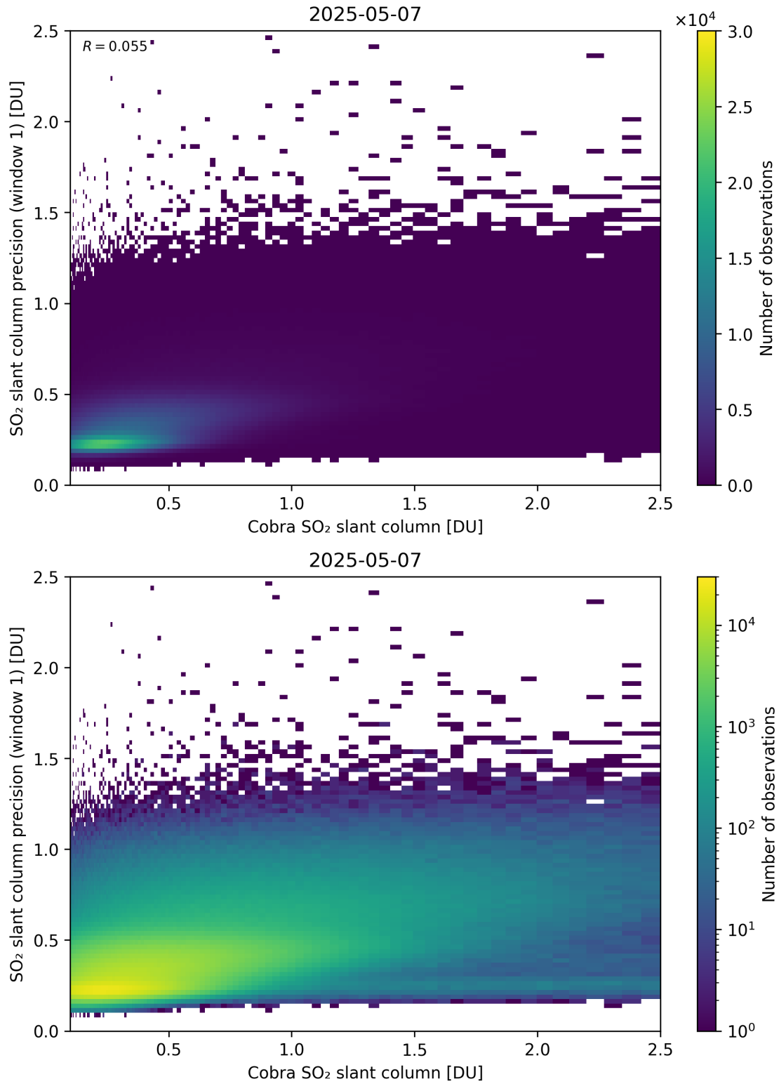
Figure 220: Scatter density plot of “Cobra SO 2 slant column” against “SO 2 slant column precision (window 1)” for 2025-05-06 to 2025-05-08.
