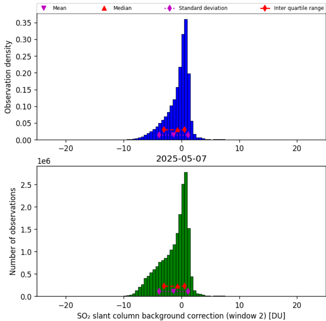
Figure 70: Histogram of “SO 2 slant column background correction (window 2)” for 2025-05-06 to 2025-05-08
