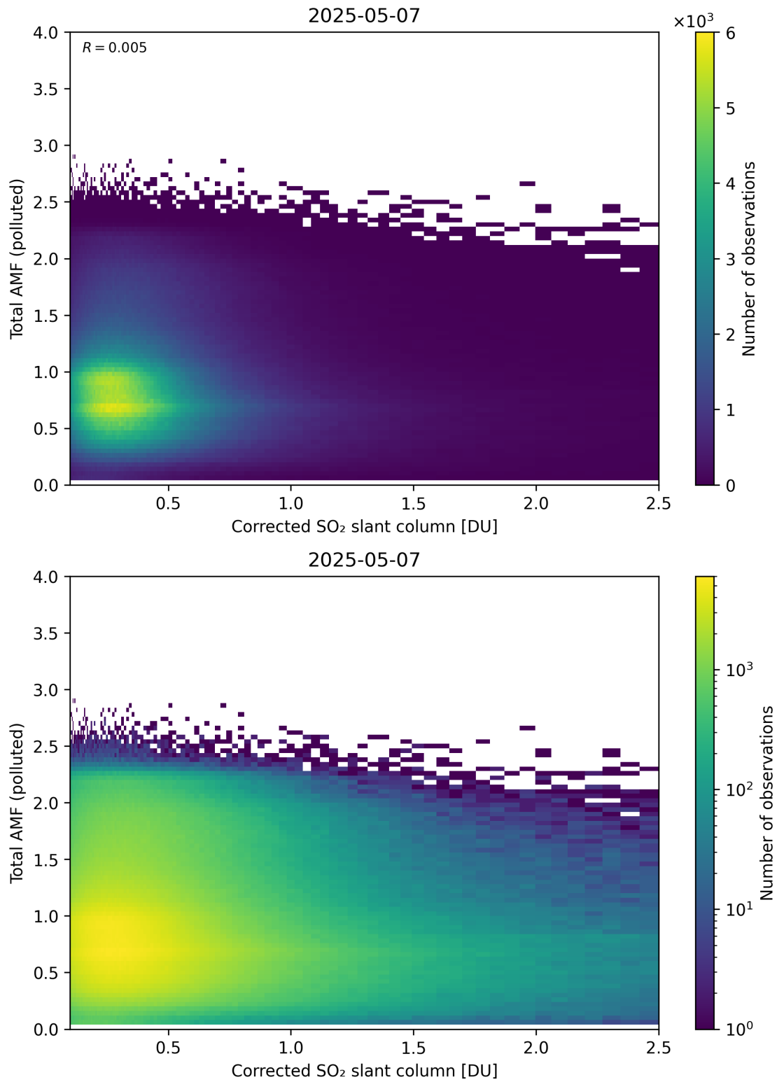
Figure 242: Scatter density plot of “Corrected SO 2 slant column” against “Total AMF (polluted)” for 2025-05-06 to 2025-05-08.
