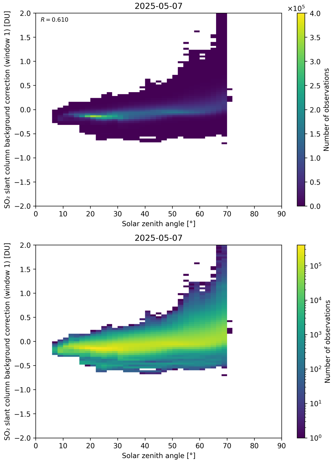
Figure 171: Scatter density plot of “Solar zenith angle” against “SO 2 slant column background correction (window 1)” for 2025-05-06 to 2025-05-08.
