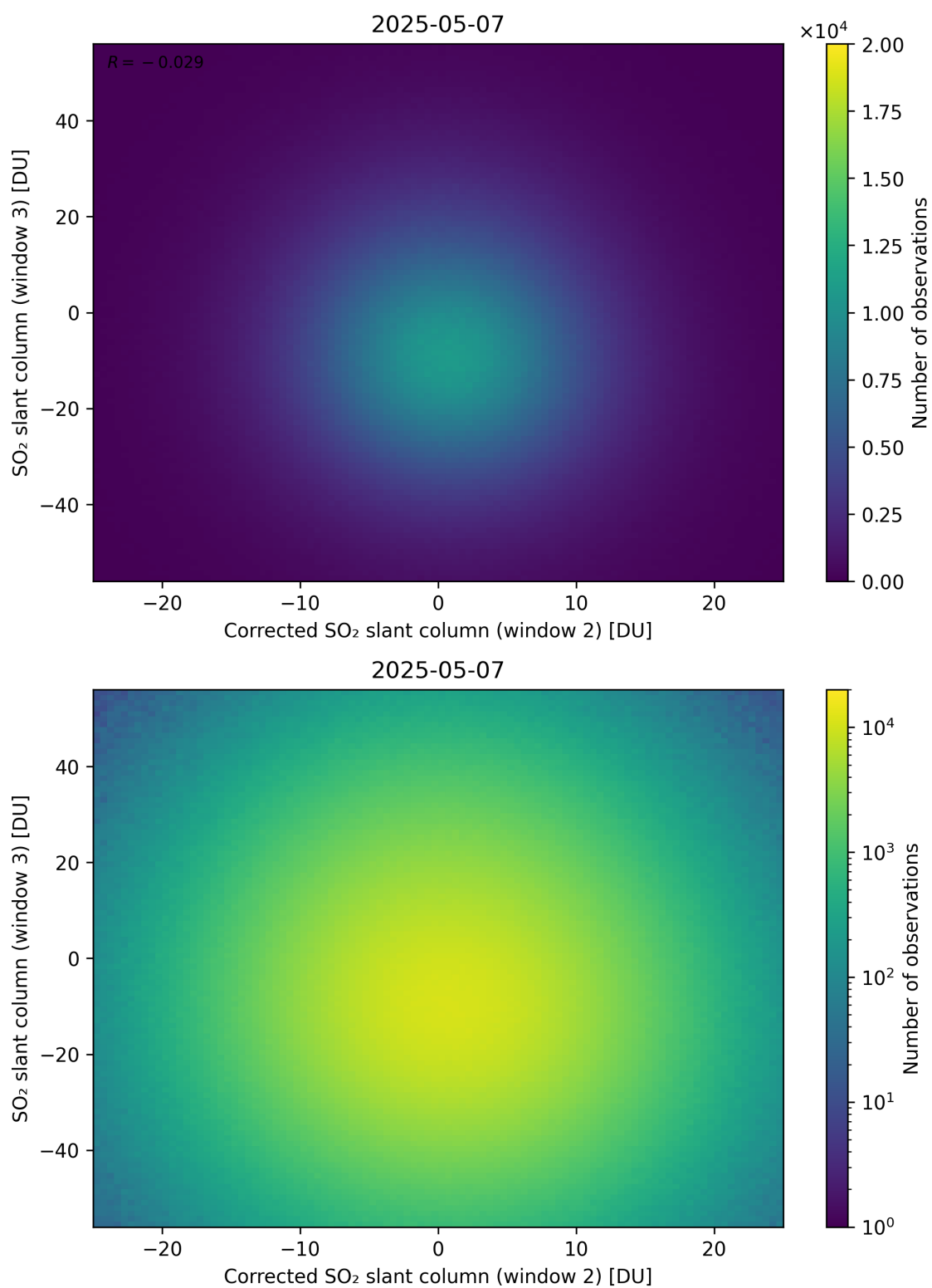
Figure 251: Scatter density plot of “Corrected SO 2 slant column (window 2)” against “SO 2 slant column (window 3)” for 2025-05-06 to 2025-05-08.
