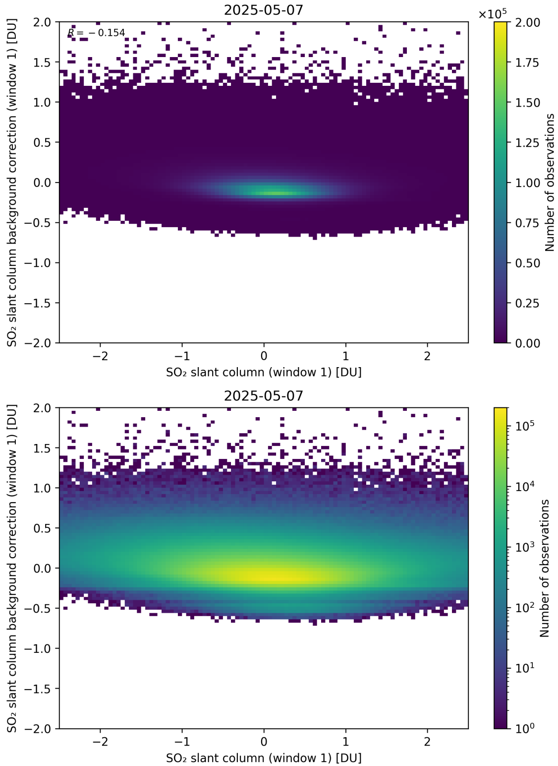
Figure 262: Scatter density plot of “SO 2 slant column (window 1)” against “SO 2 slant column background correction (window 1)” for 2025-05-06 to 2025-05-08.
