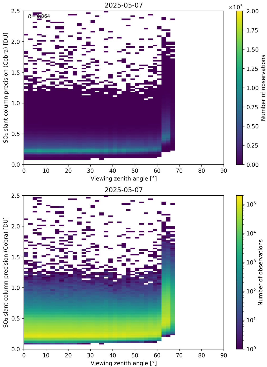
Figure 372: Scatter density plot of “Viewing zenith angle” against “SO 2 slant column precision (Cobra)” for 2025-05-06 to 2025-05-08.
