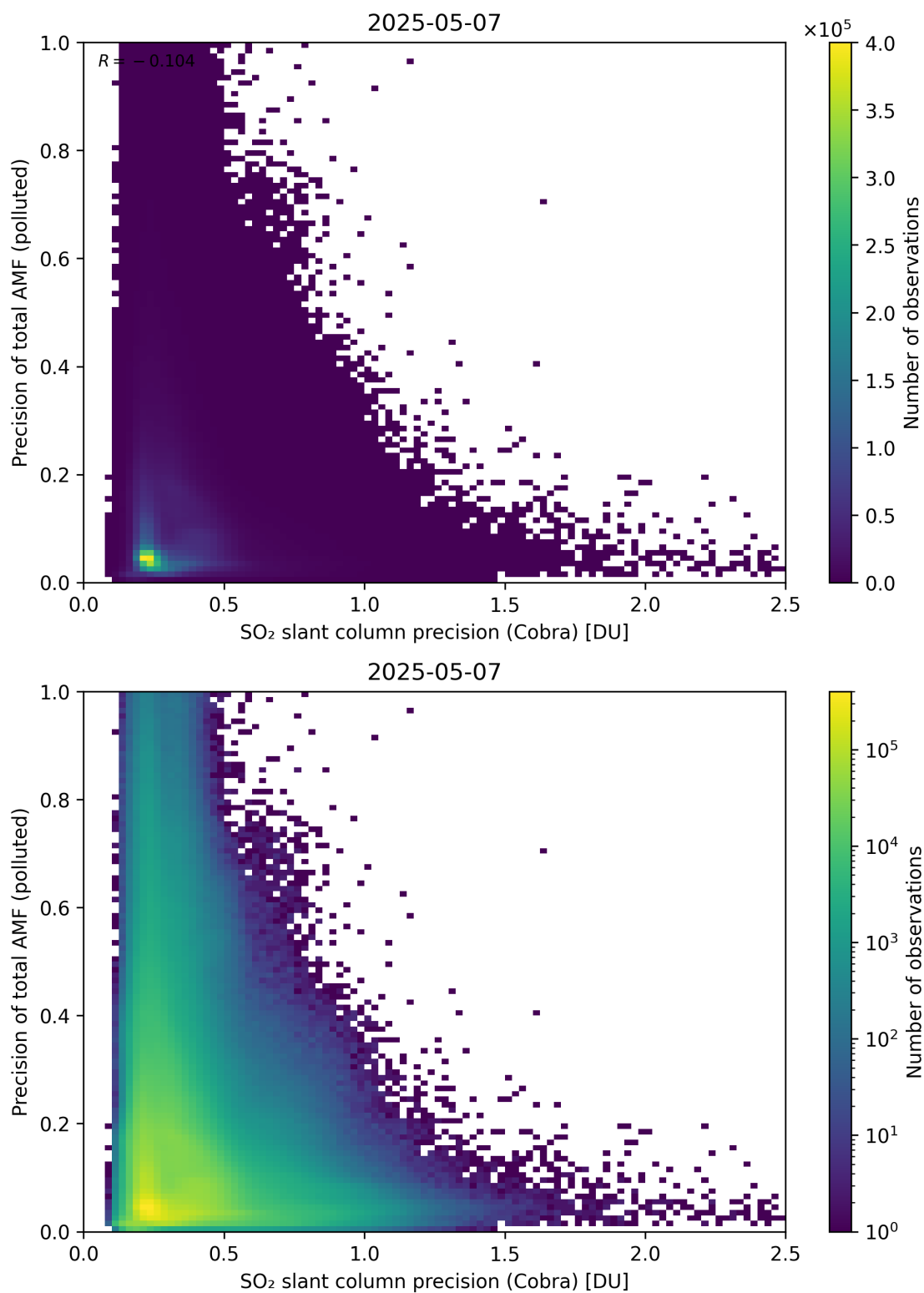
Figure 214: Scatter density plot of “SO 2 slant column precision (Cobra)” against “Precision of total AMF (polluted)” for 2025-05-06 to 2025-05-08.
