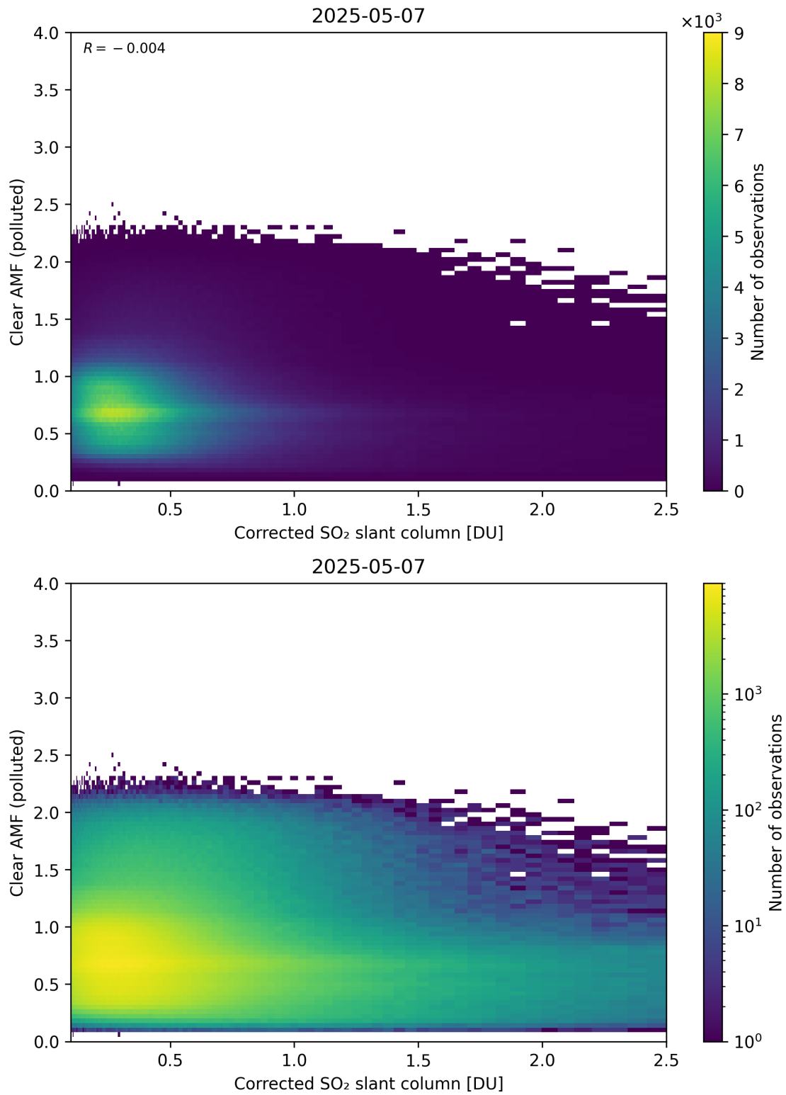
Figure 232: Scatter density plot of “Corrected SO 2 slant column” against “Clear AMF (polluted)” for 2025-05-06 to 2025-05-08.
