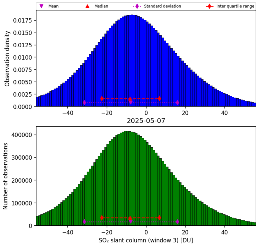
Figure 71: Histogram of “SO 2 slant column (window 3)” for 2025-05-06 to 2025-05-08
