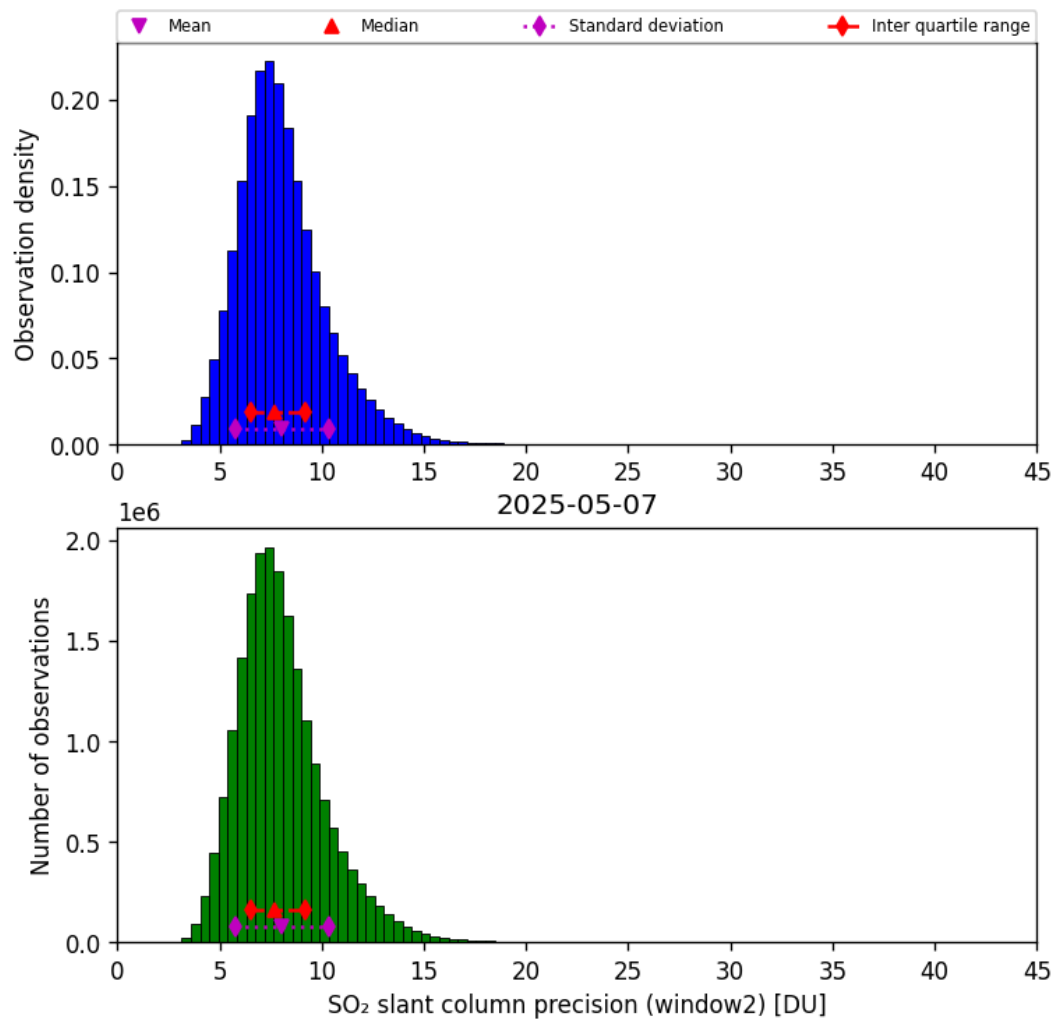
Figure 68: Histogram of “SO 2 slant column precision (window2)” for 2025-05-06 to 2025-05-08
