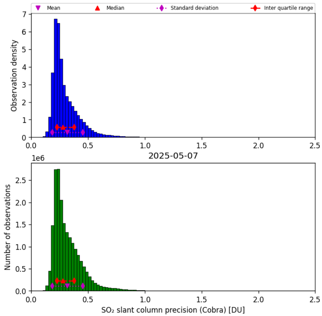
Figure 62: Histogram of “SO 2 slant column precision (Cobra)” for 2025-05-06 to 2025-05-08
