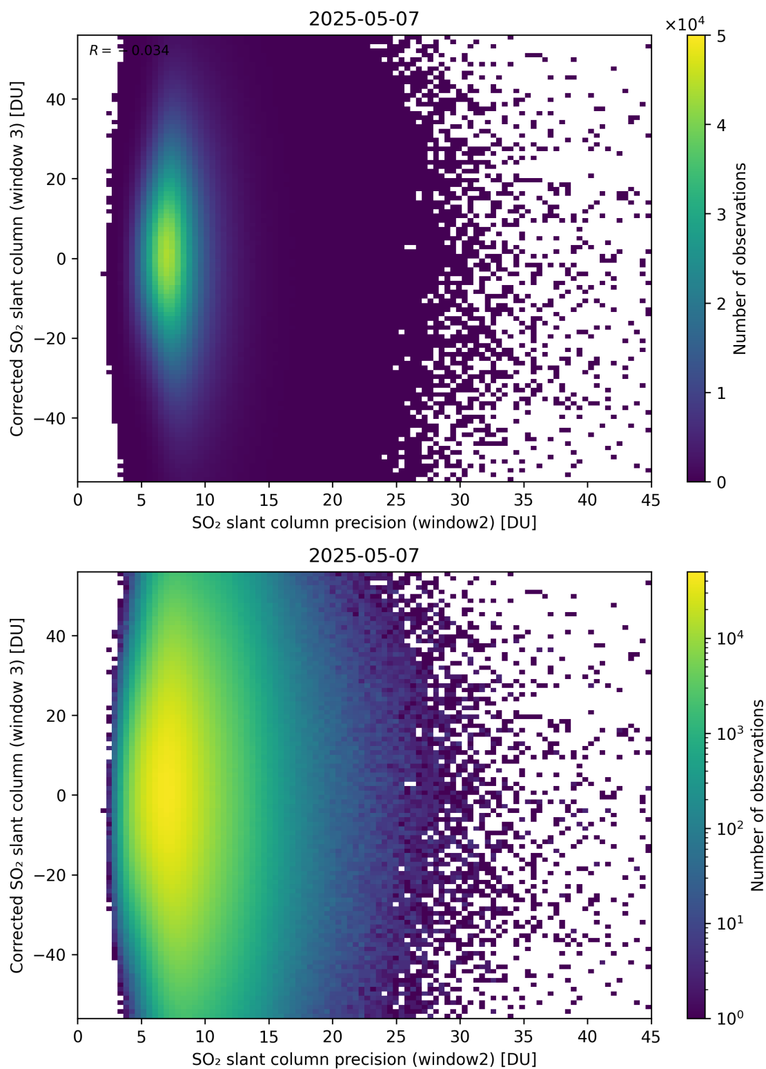
Figure 298: Scatter density plot of “SO 2 slant column precision (window2)” against “Corrected SO 2 slant column (window 3)” for 2025-05-06 to 2025-05-08.
