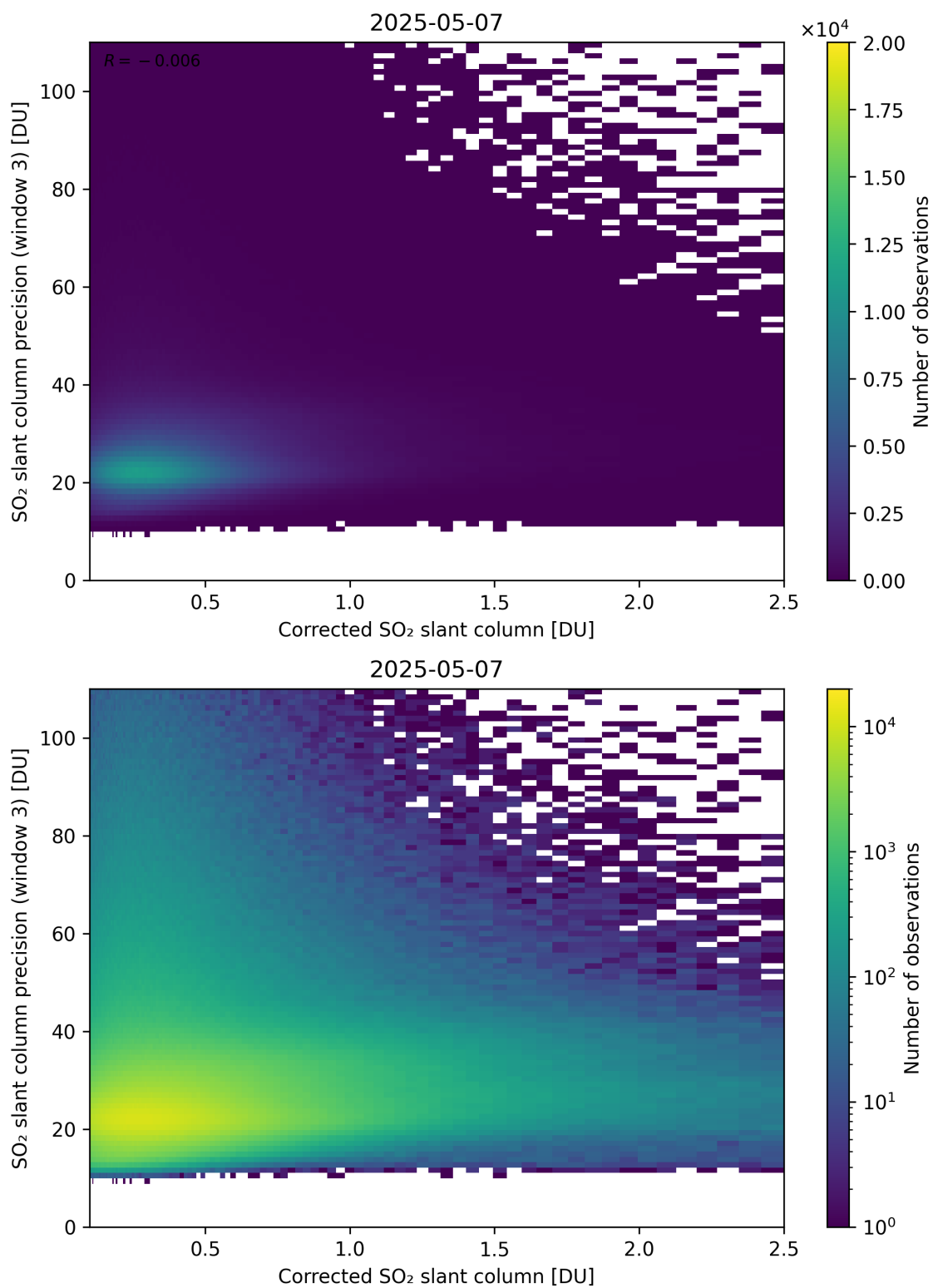
Figure 241: Scatter density plot of “Corrected SO 2 slant column” against “SO 2 slant column precision (window 3)” for 2025-05-06 to 2025-05-08.
