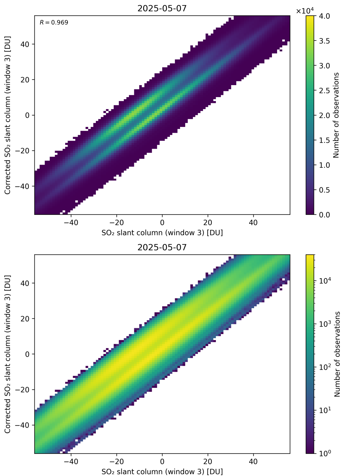
Figure 316: Scatter density plot of “SO 2 slant column (window 3)” against “Corrected SO 2 slant column (window 3)” for 2025-05-06 to 2025-05-08.
