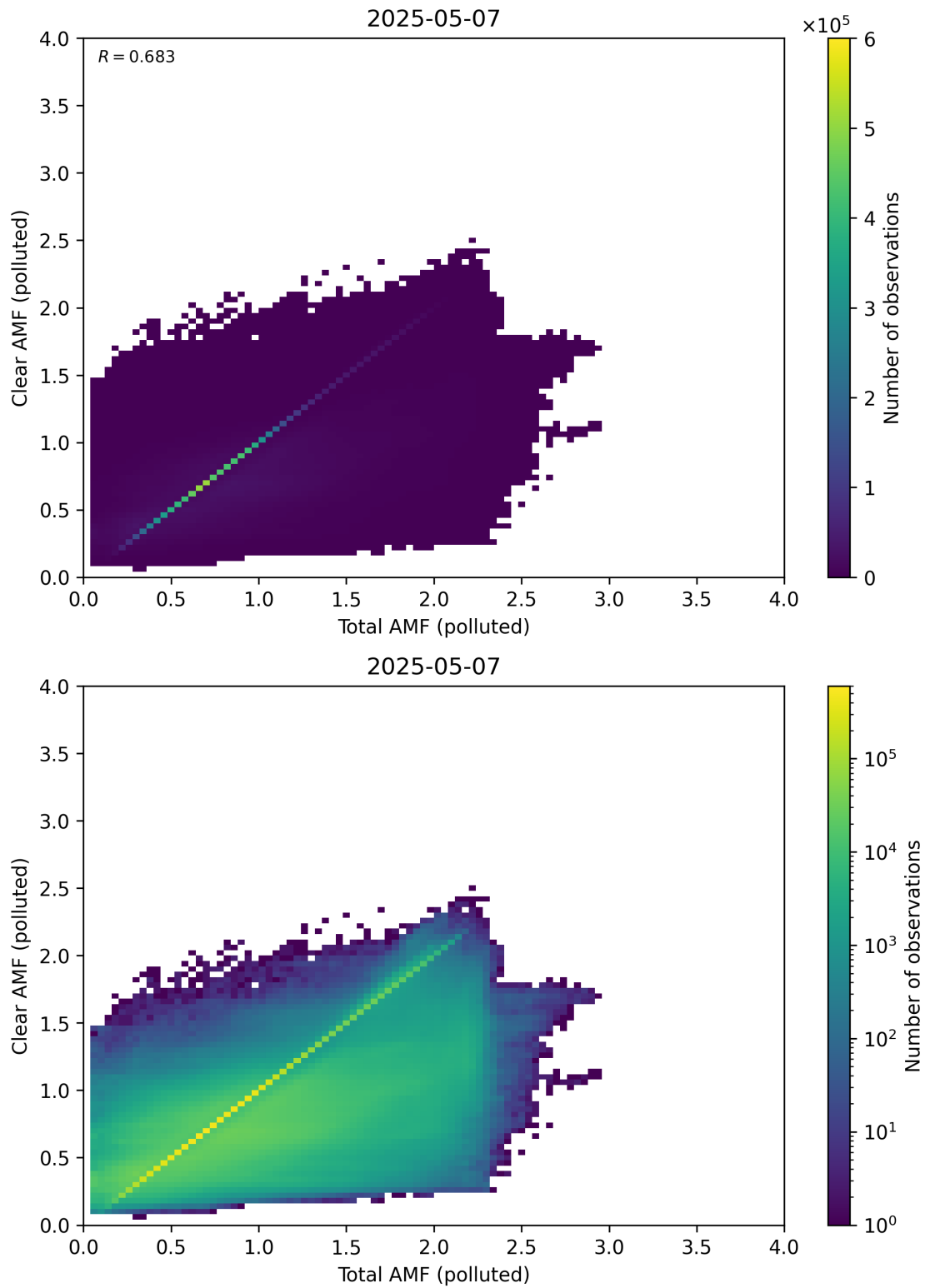
Figure 321: Scatter density plot of “Total AMF (polluted)” against “Clear AMF (polluted)” for 2025-05-06 to 2025-05-08.
