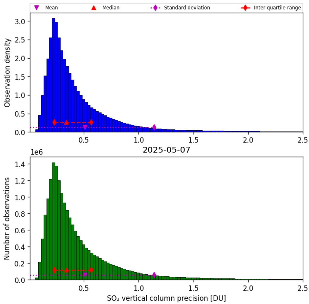
Figure 59: Histogram of “SO 2 vertical column precision” for 2025-05-06 to 2025-05-08
