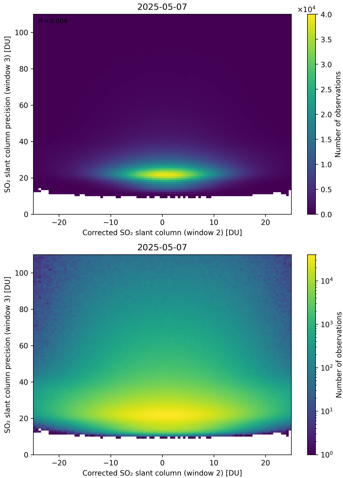
Figure 252: Scatter density plot of “Corrected SO 2 slant column (window 2)” against “SO 2 slant column precision (window 3)” for 2025-05-06 to 2025-05-08.
