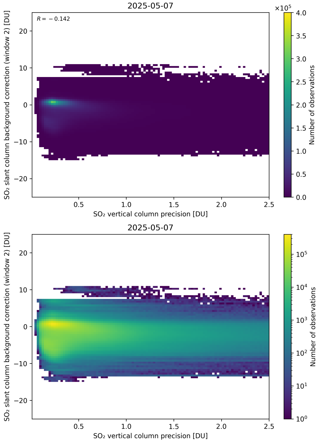
Figure 330: Scatter density plot of “SO 2 vertical column precision” against “SO 2 slant column background correction (window 2)” for 2025-05-06 to 2025-05-08.
