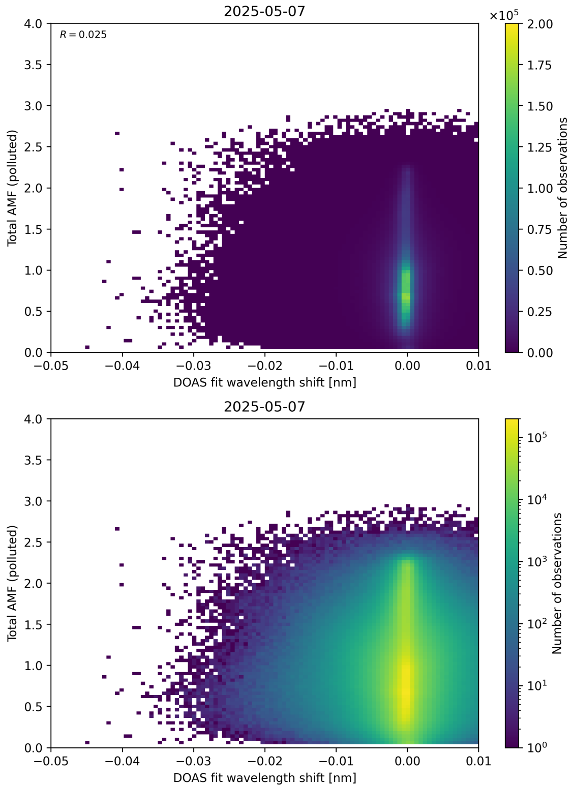
Figure 141: Scatter density plot of “DOAS fit wavelength shift” against “Total AMF (polluted)” for 2025-05-06 to 2025-05-08.
