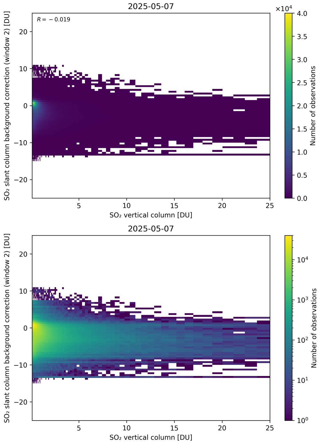
Figure 324: Scatter density plot of “SO 2 vertical column” against “SO 2 slant column background correction (window 2)” for 2025-05-06 to 2025-05-08.
