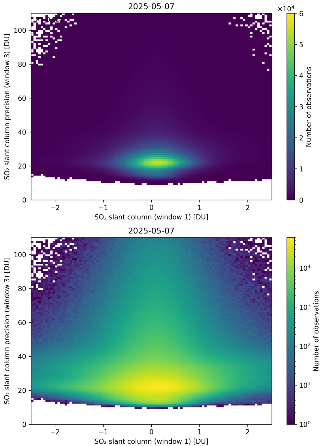
Figure 288: Scatter density plot of “SO 2 slant column (window 1)” against “SO 2 slant column precision (window 3)” for 2025-05-06 to 2025-05-08.
