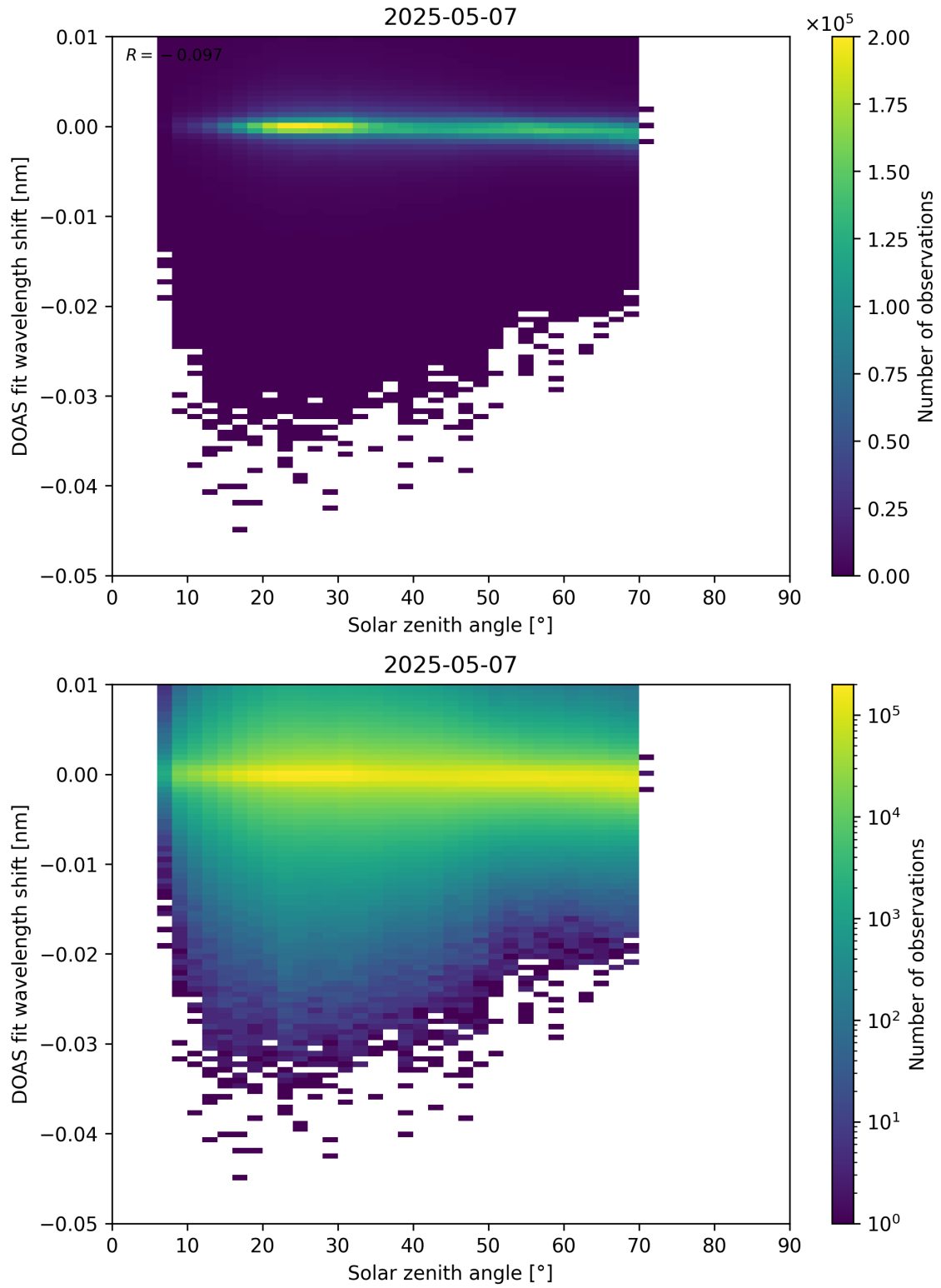
Figure 174: Scatter density plot of “Solar zenith angle” against “DOAS fit wavelength shift” for 2025-05-06 to 2025-05-08.
