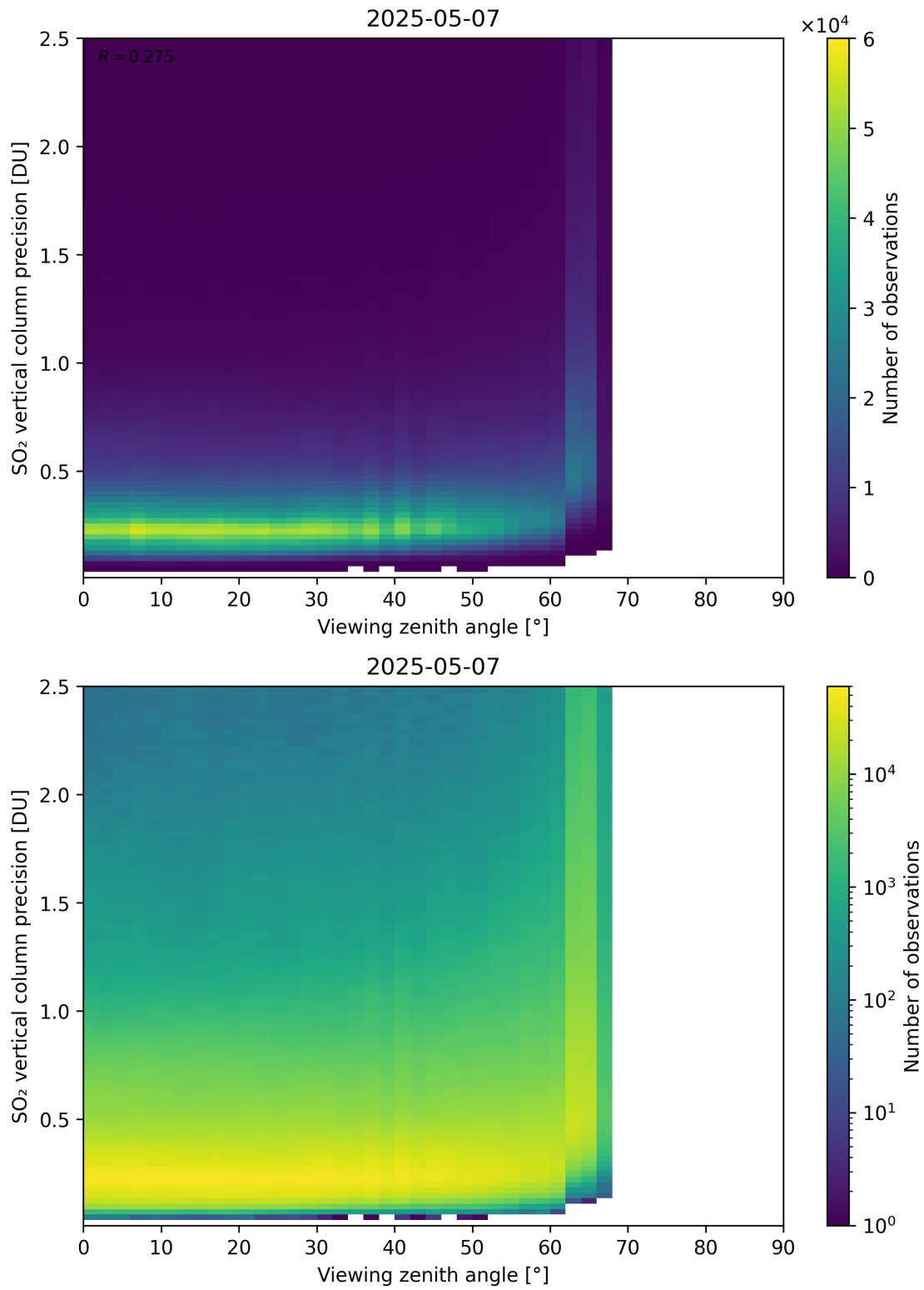
Figure 384: Scatter density plot of “Viewing zenith angle” against “SO 2 vertical column precision” for 2025-05-06 to 2025-05-08.
