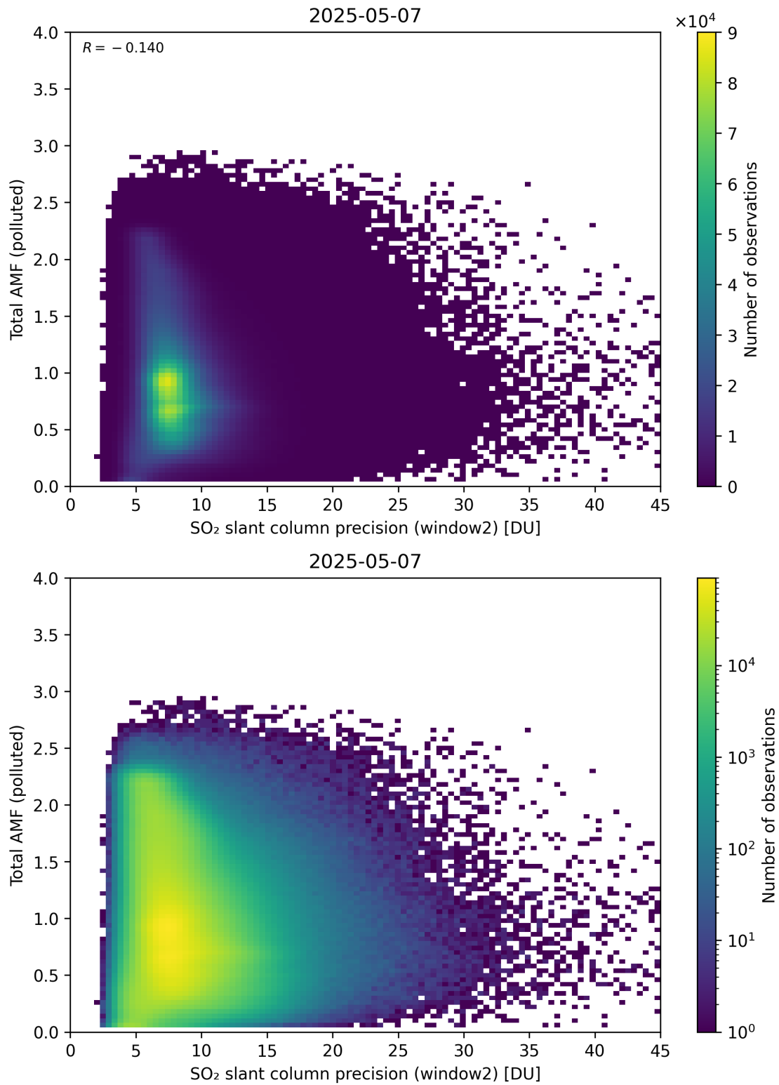
Figure 301: Scatter density plot of “SO 2 slant column precision (window2)” against “Total AMF (polluted)” for 2025-05-06 to 2025-05-08.
