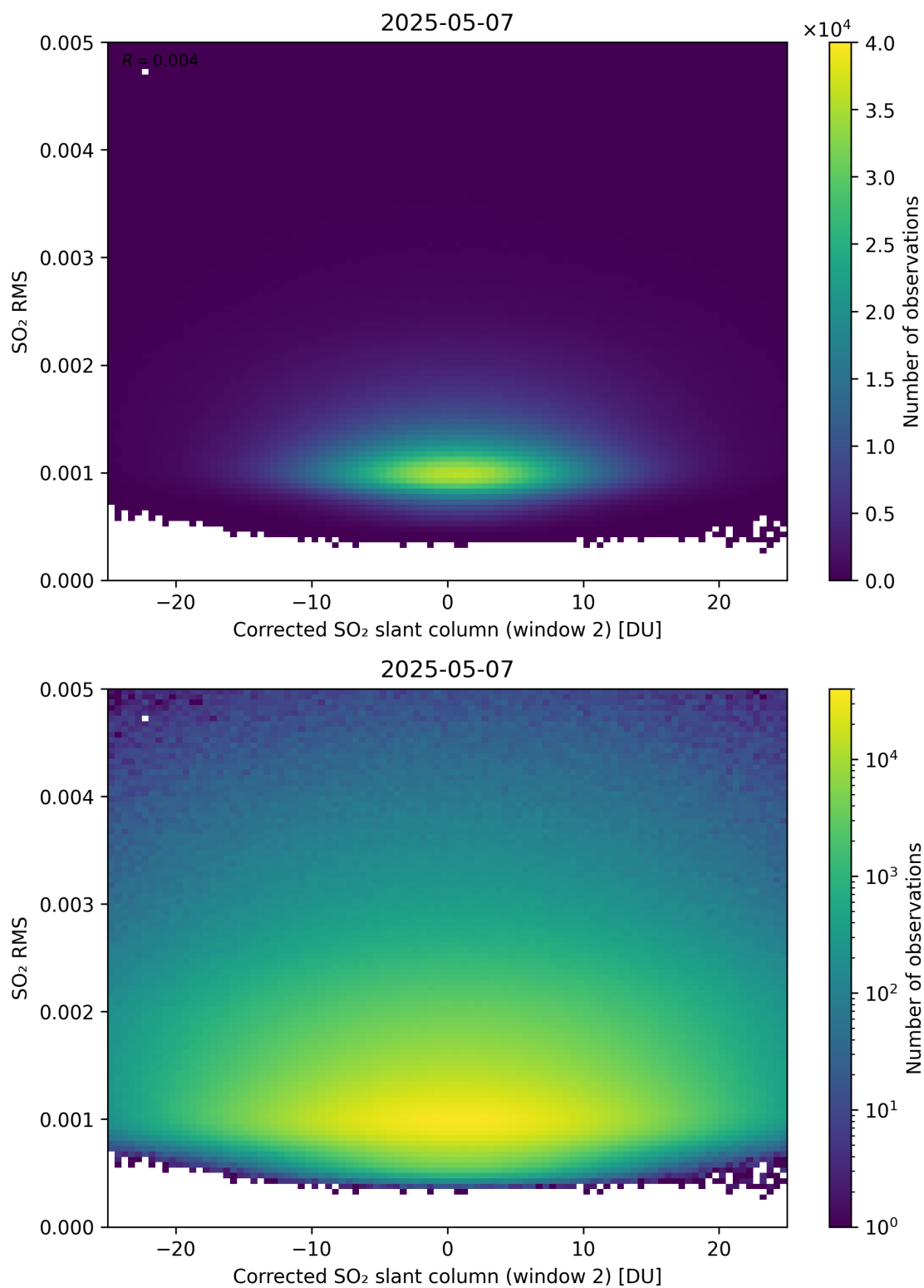
Figure 248: Scatter density plot of “Corrected SO 2 slant column (window 2)” against “SO 2 RMS” for 2025-05-06 to 2025-05-08.
