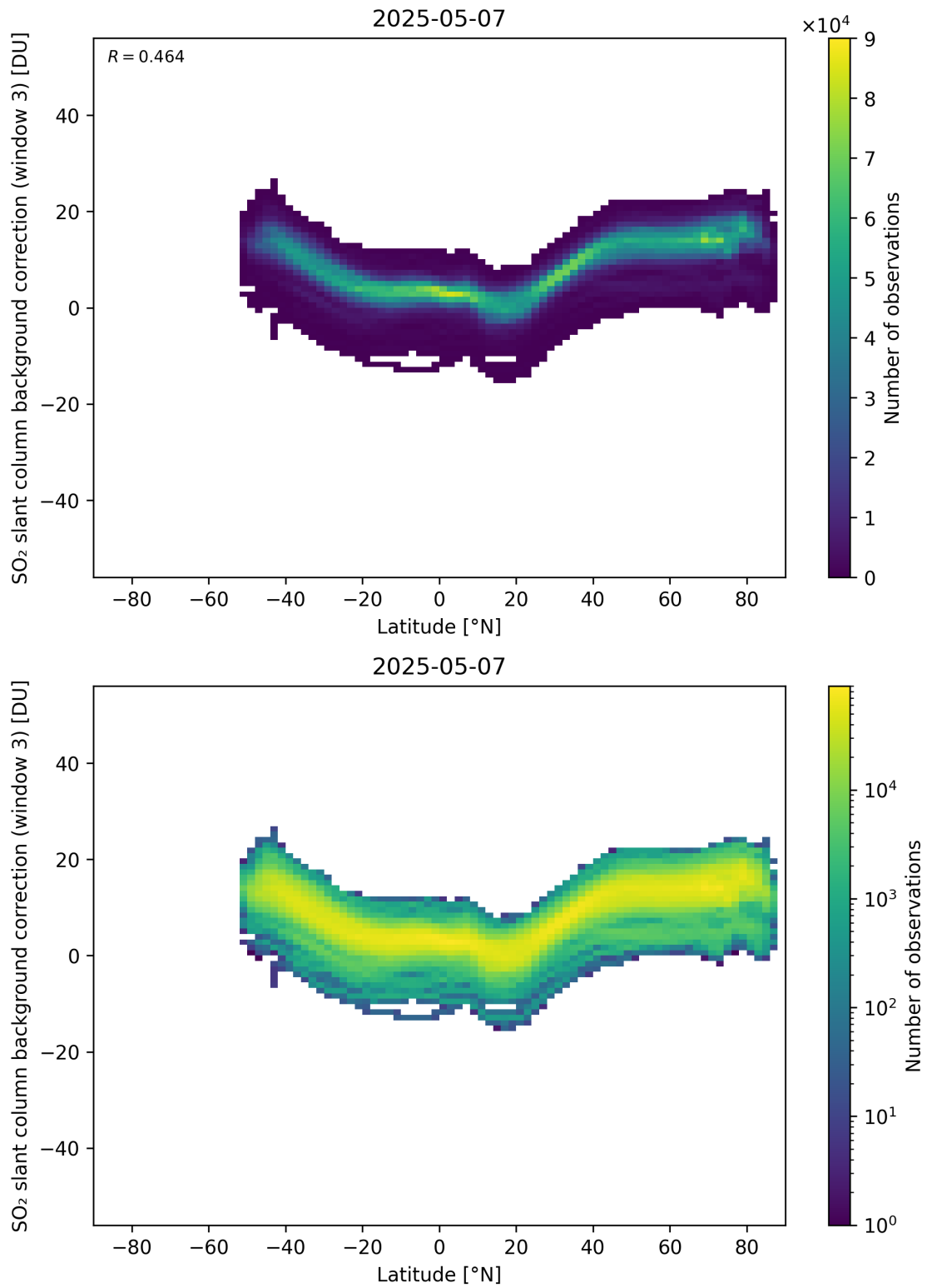
Figure 152: Scatter density plot of “Latitude” against “SO 2 slant column background correction (window 3)” for 2025-05-06 to 2025-05-08.
