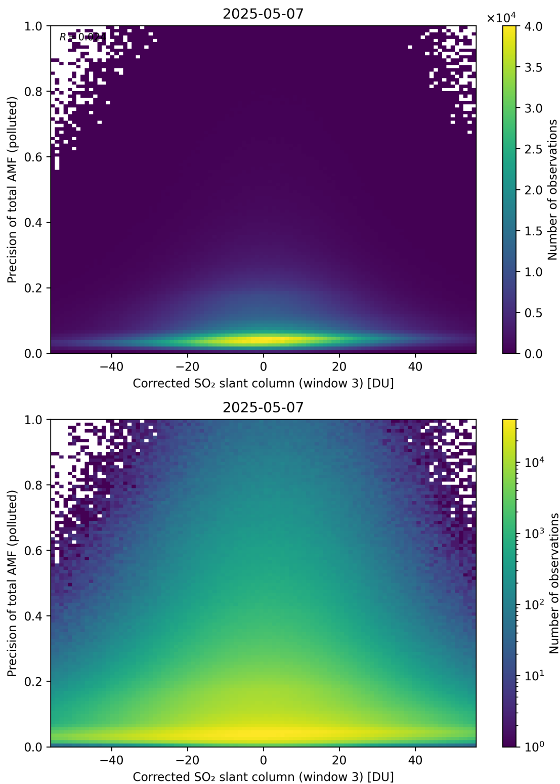
Figure 261: Scatter density plot of “Corrected SO 2 slant column (window 3)” against “Precision of total AMF (polluted)” for 2025-05-06 to 2025-05-08.
