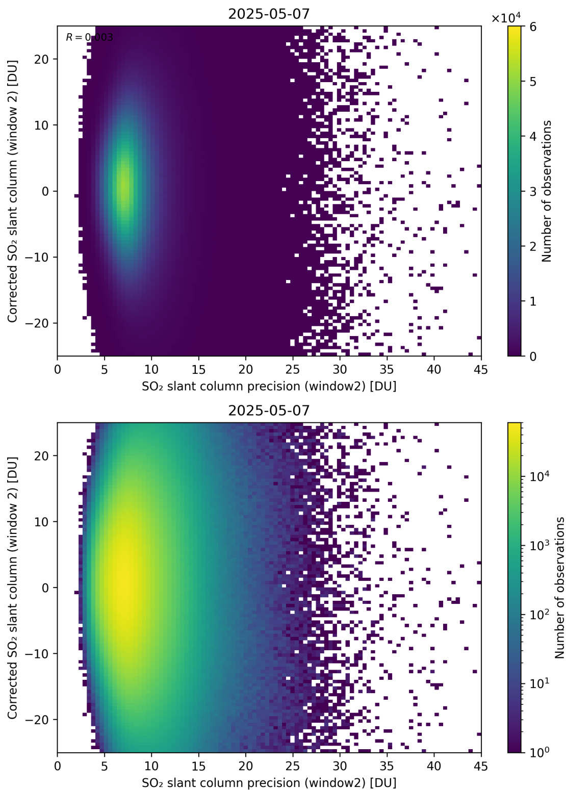
Figure 297: Scatter density plot of “SO 2 slant column precision (window2)” against “Corrected SO 2 slant column (window 2)” for 2025-05-06 to 2025-05-08.
