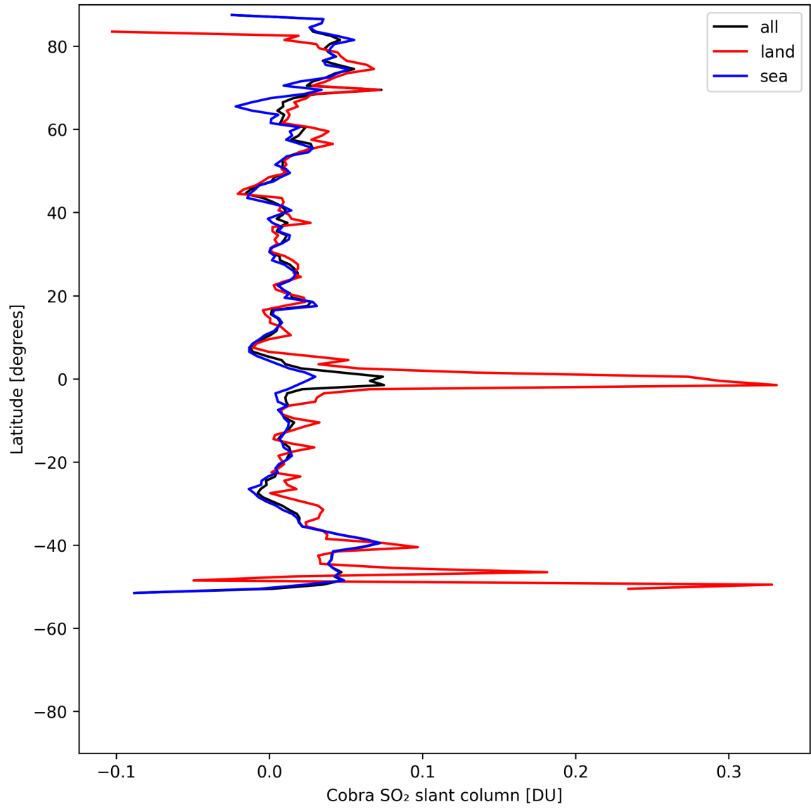
Figure 35: Zonal average of “Cobra SO 2 slant column” for 2025-05-06 to 2025-05-08.
