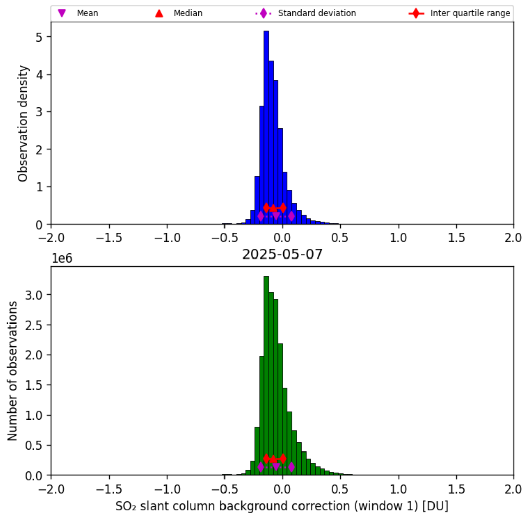
Figure 66: Histogram of “SO 2 slant column background correction (window 1)” for 2025-05-06 to 2025-05-08
