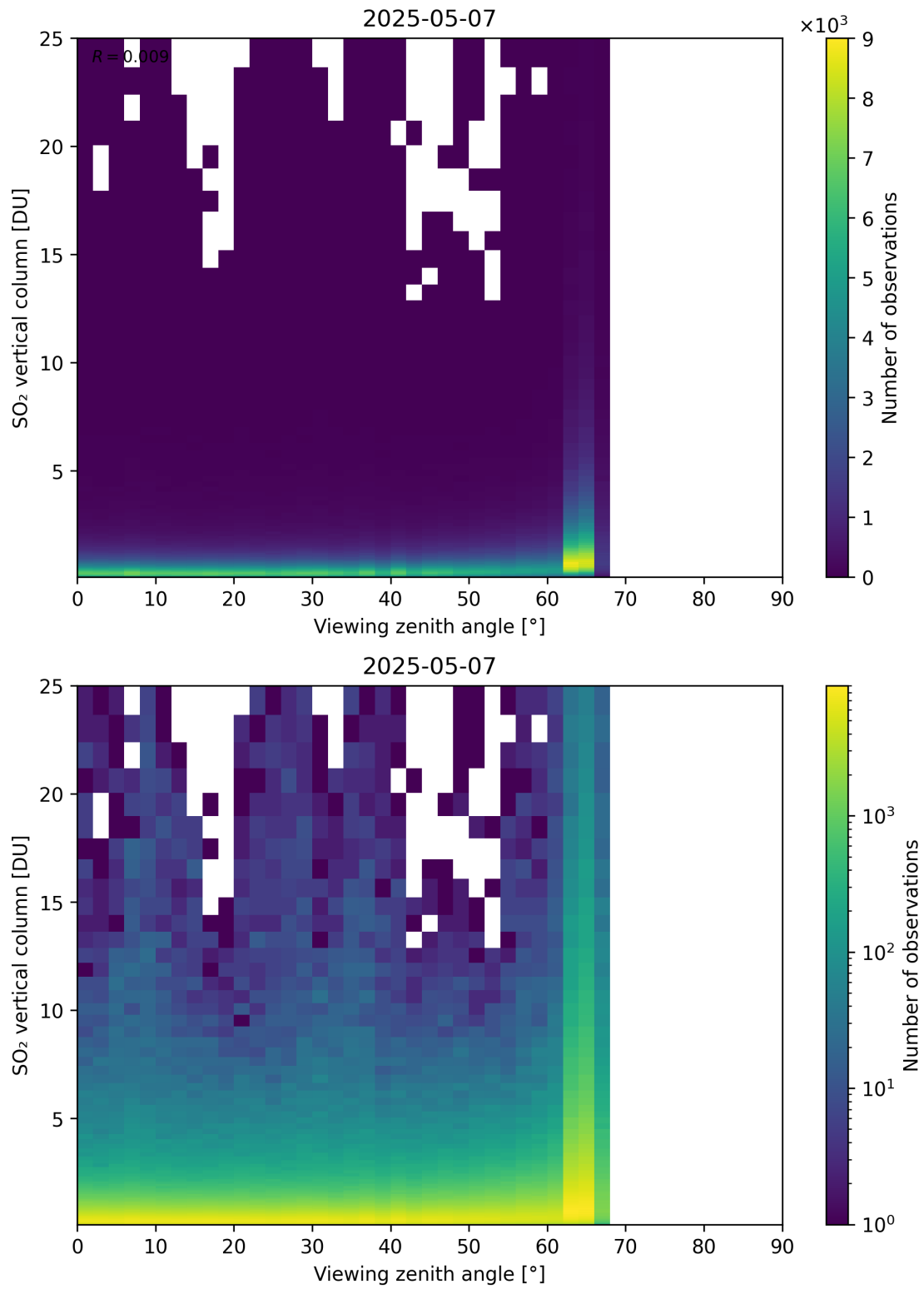
Figure 383: Scatter density plot of “Viewing zenith angle” against “SO 2 vertical column” for 2025-05-06 to 2025-05-08.
