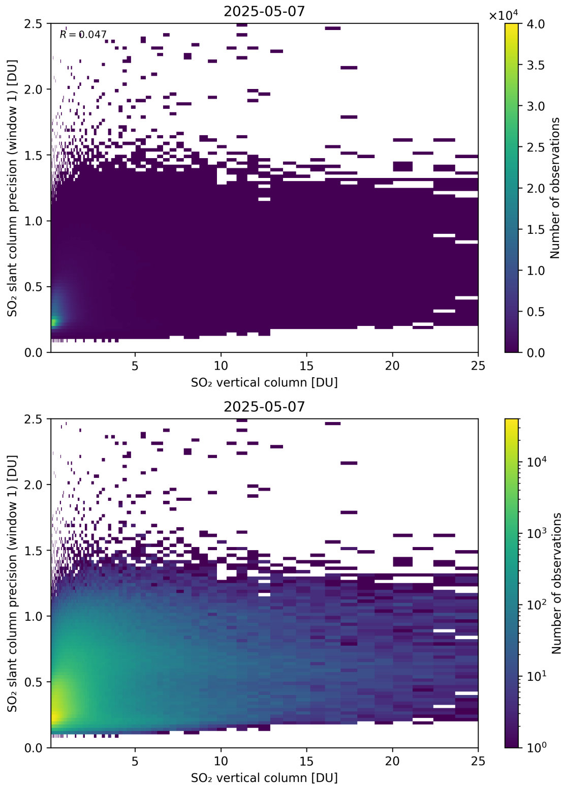
Figure 355: Scatter density plot of “SO 2 vertical column” against “SO 2 slant column precision (window 1)” for 2025-05-06 to 2025-05-08.
