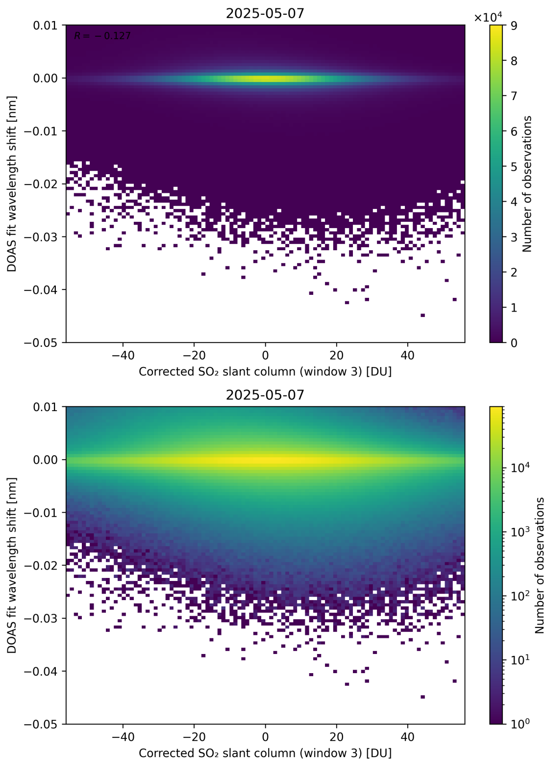
Figure 256: Scatter density plot of “Corrected SO 2 slant column (window 3)” against “DOAS fit wavelength shift” for 2025-05-06 to 2025-05-08.
