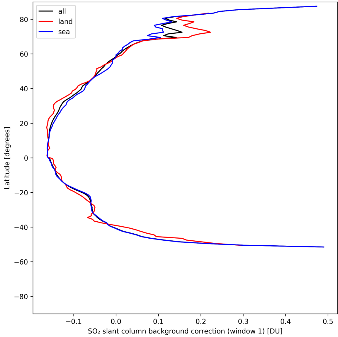
Figure 40: Zonal average of "SO 2 slant column background correction (window 1)" for 2025-05-06 to 2025-05-08.
