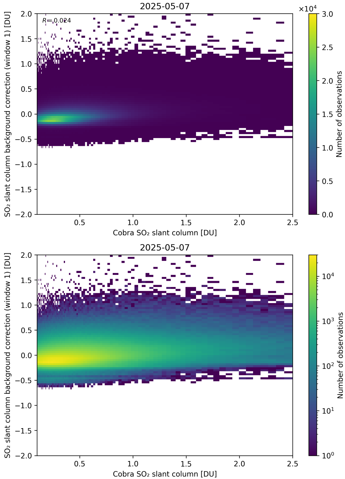
Figure 193: Scatter density plot of “Cobra SO 2 slant column” against “SO 2 slant column background correction (window 1)” for 2025-05-06 to 2025-05-08.
