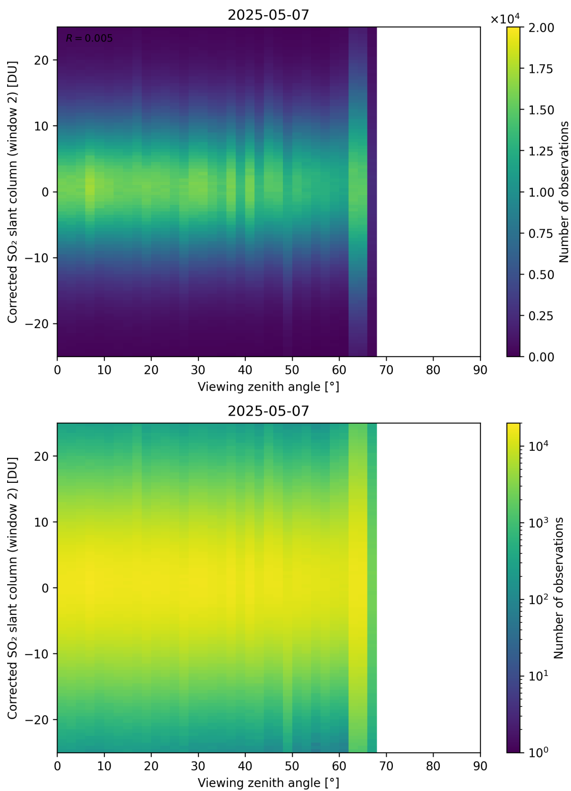
Figure 374: Scatter density plot of “Viewing zenith angle” against “Corrected SO 2 slant column (window 2)” for 2025-05-06 to 2025-05-08.
