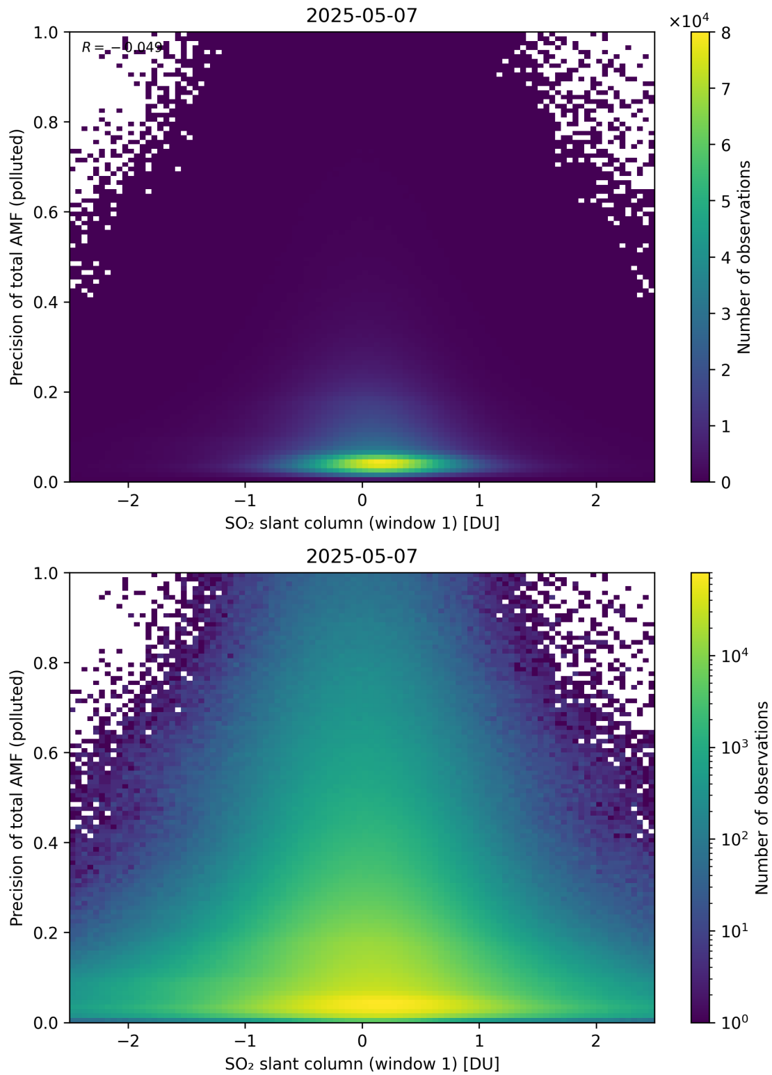
Figure 290: Scatter density plot of “SO 2 slant column (window 1)” against “Precision of total AMF (polluted)” for 2025-05-06 to 2025-05-08.
