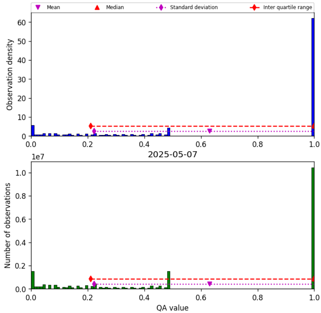
Figure 57: Histogram of “QA value” for 2025-05-06 to 2025-05-08
