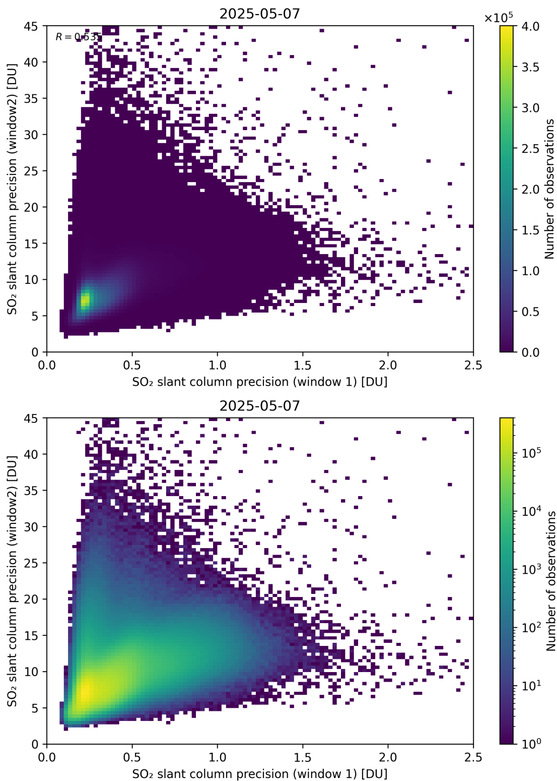
Figure 277: Scatter density plot of “SO 2 slant column precision (window 1)” against “SO 2 slant column precision (window2)” for 2025-05-06 to 2025-05-08.
