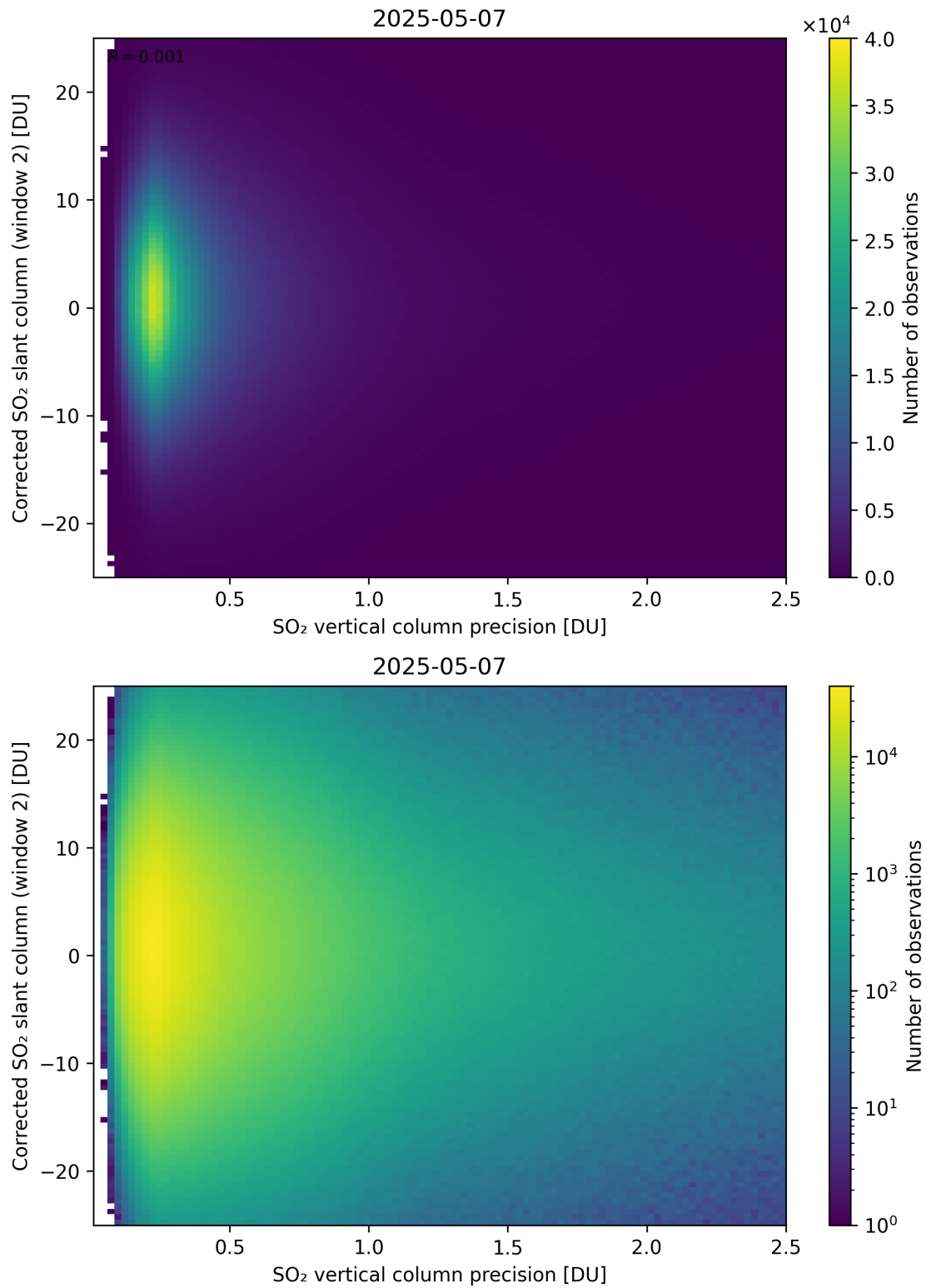
Figure 339: Scatter density plot of “SO 2 vertical column precision” against “Corrected SO 2 slant column (window 2)” for 2025-05-06 to 2025-05-08.
