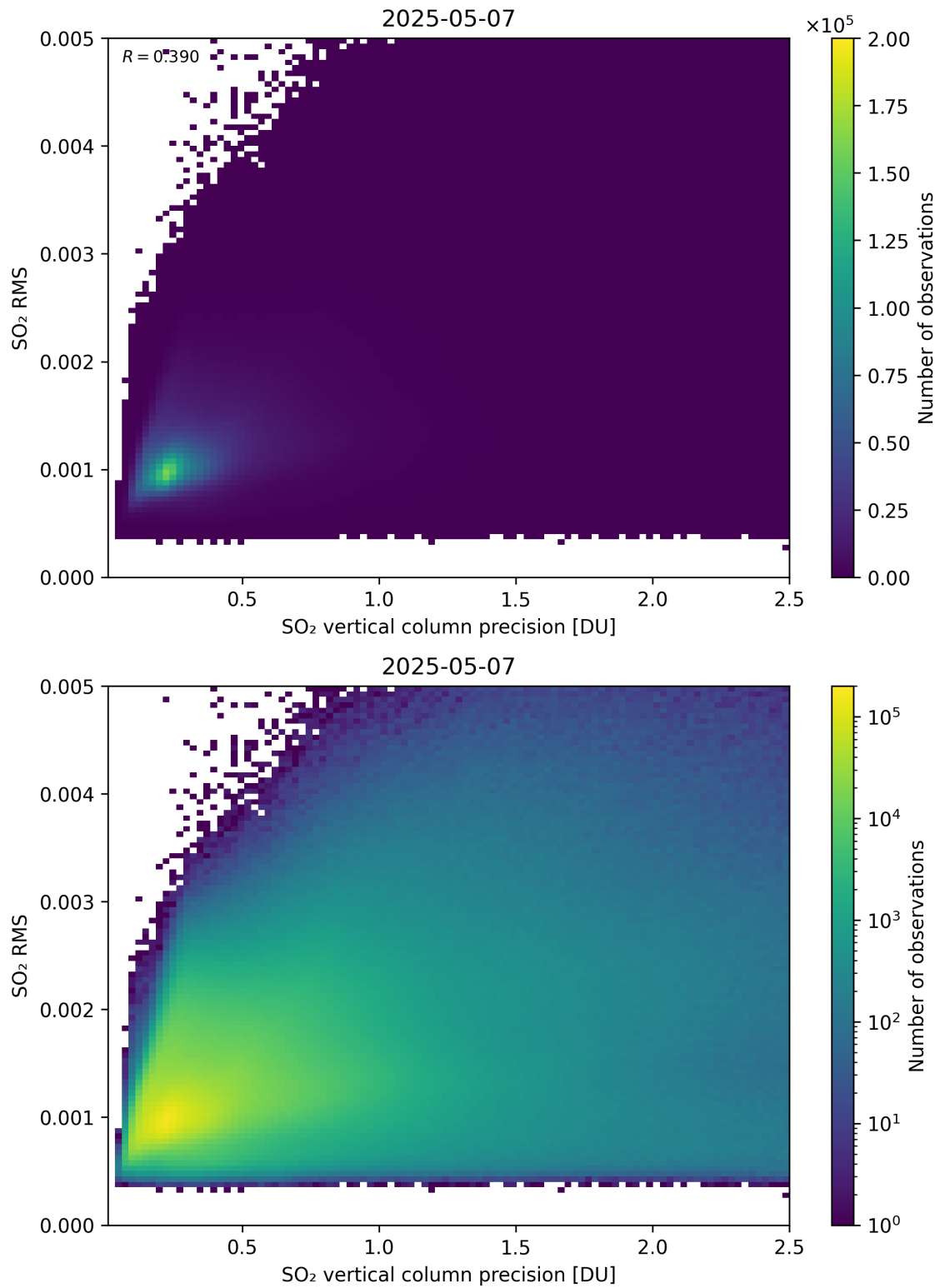
Figure 334: Scatter density plot of “SO 2 vertical column precision” against “SO 2 RMS” for 2025-05-06 to 2025-05-08.
