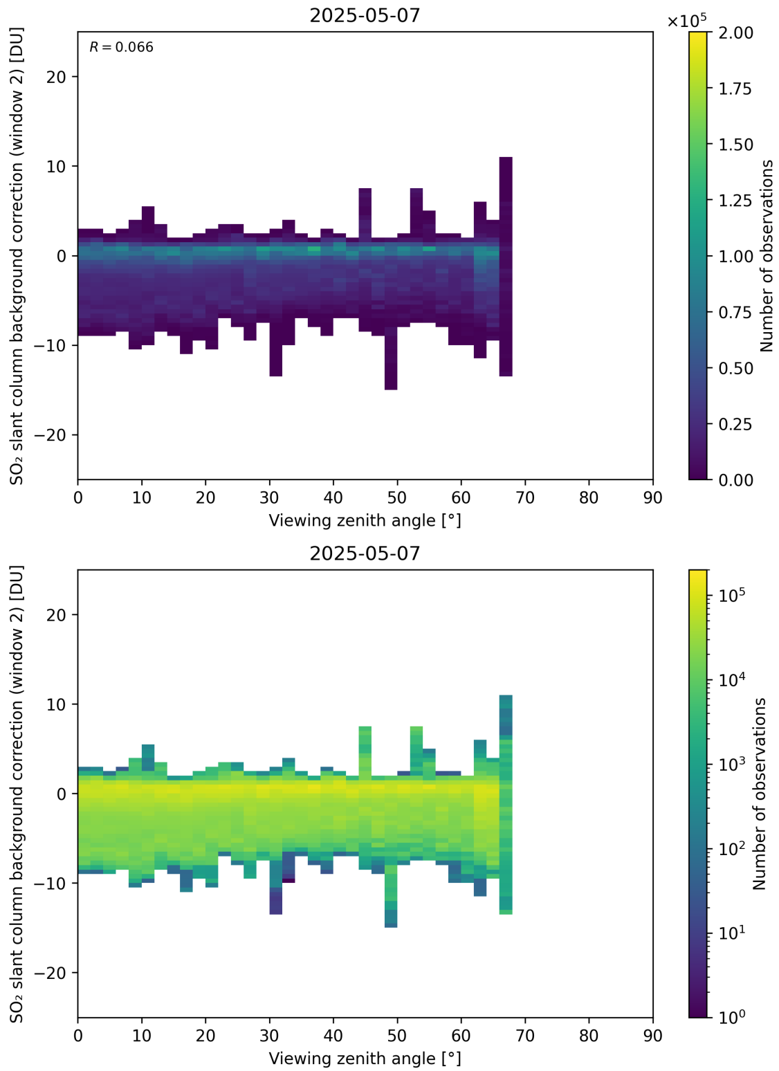
Figure 363: Scatter density plot of “Viewing zenith angle” against “SO 2 slant column background correction (window 2)” for 2025-05-06 to 2025-05-08.
