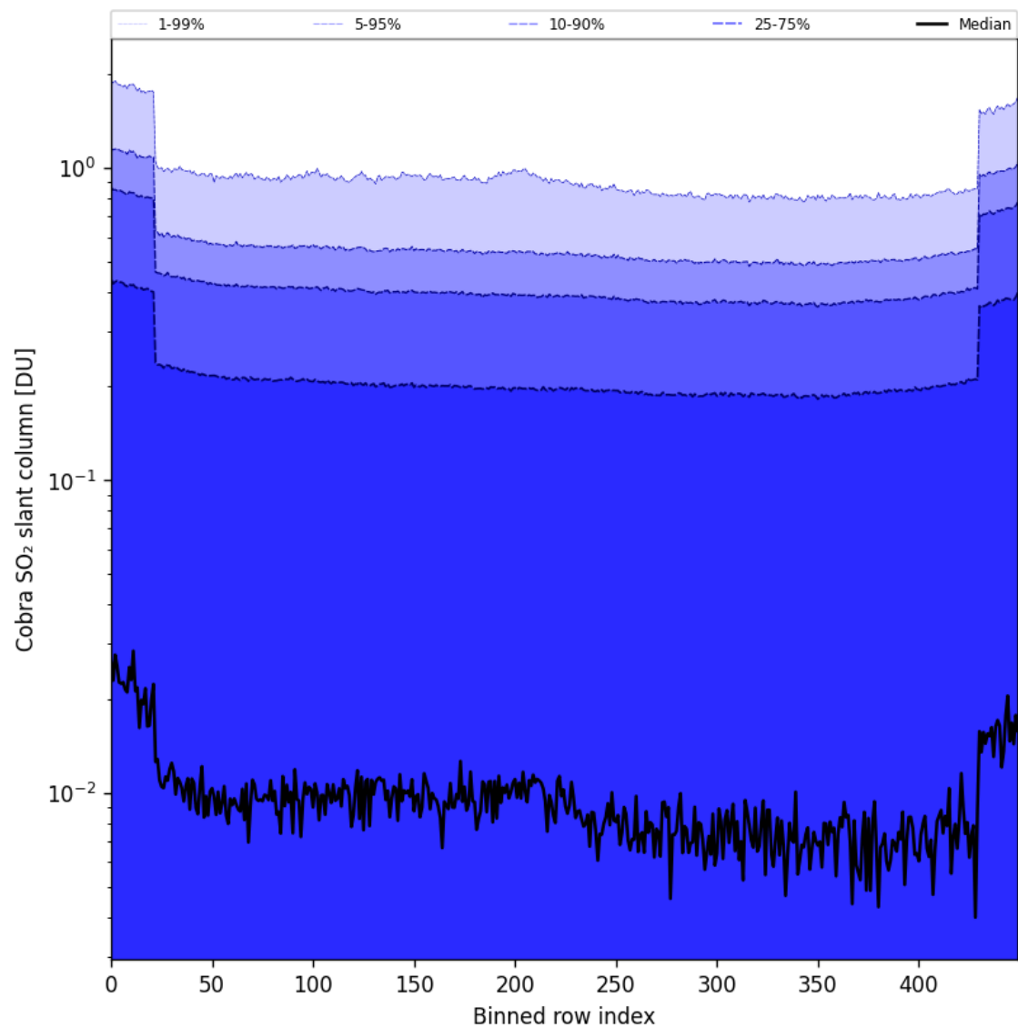
Figure 87: Along track statistics of "Cobra SO 2 slant column" for 2025-05-06 to 2025-05-08
