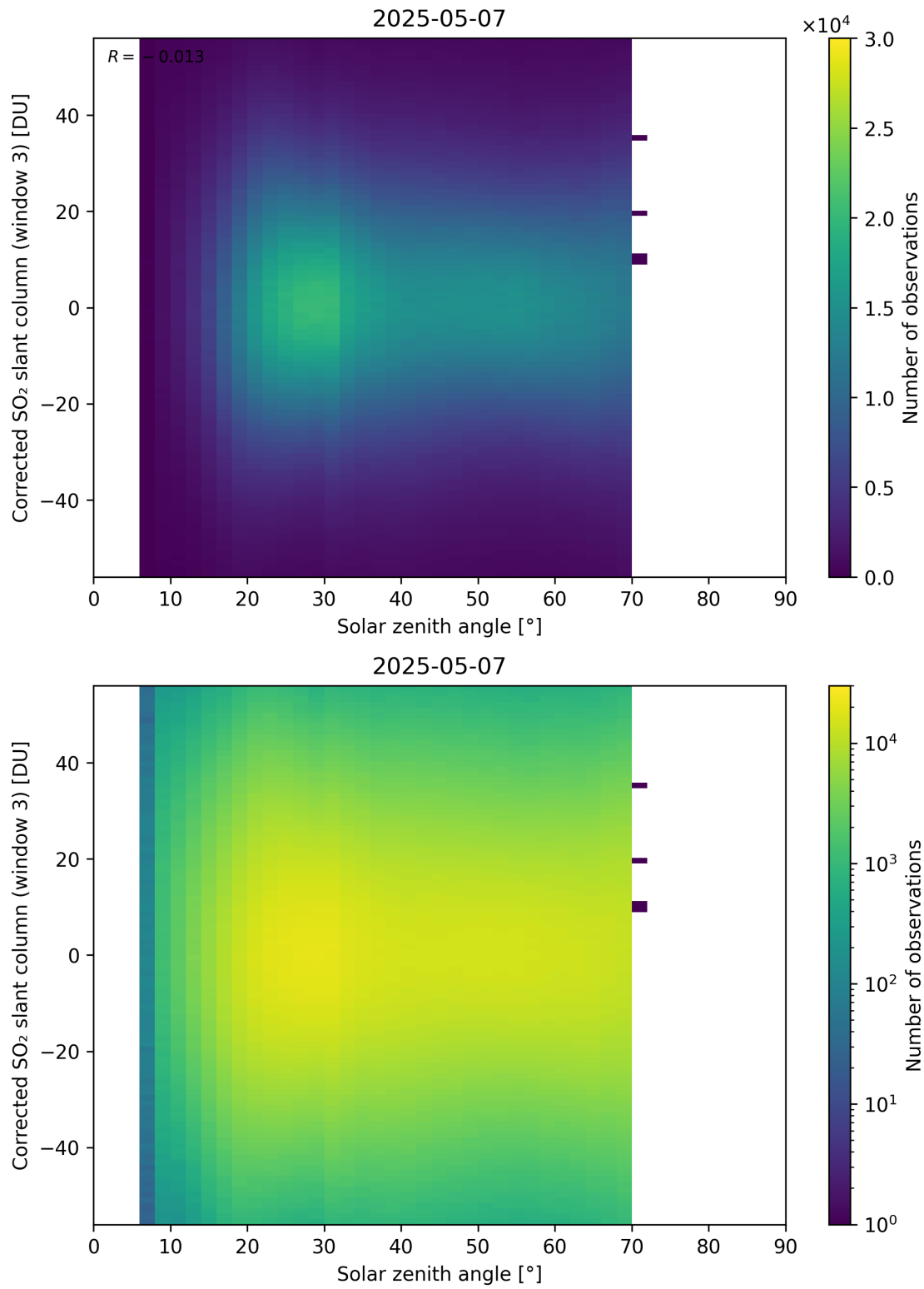
Figure 183: Scatter density plot of “Solar zenith angle” against “Corrected SO 2 slant column (window 3)” for 2025-05-06 to 2025-05-08.
