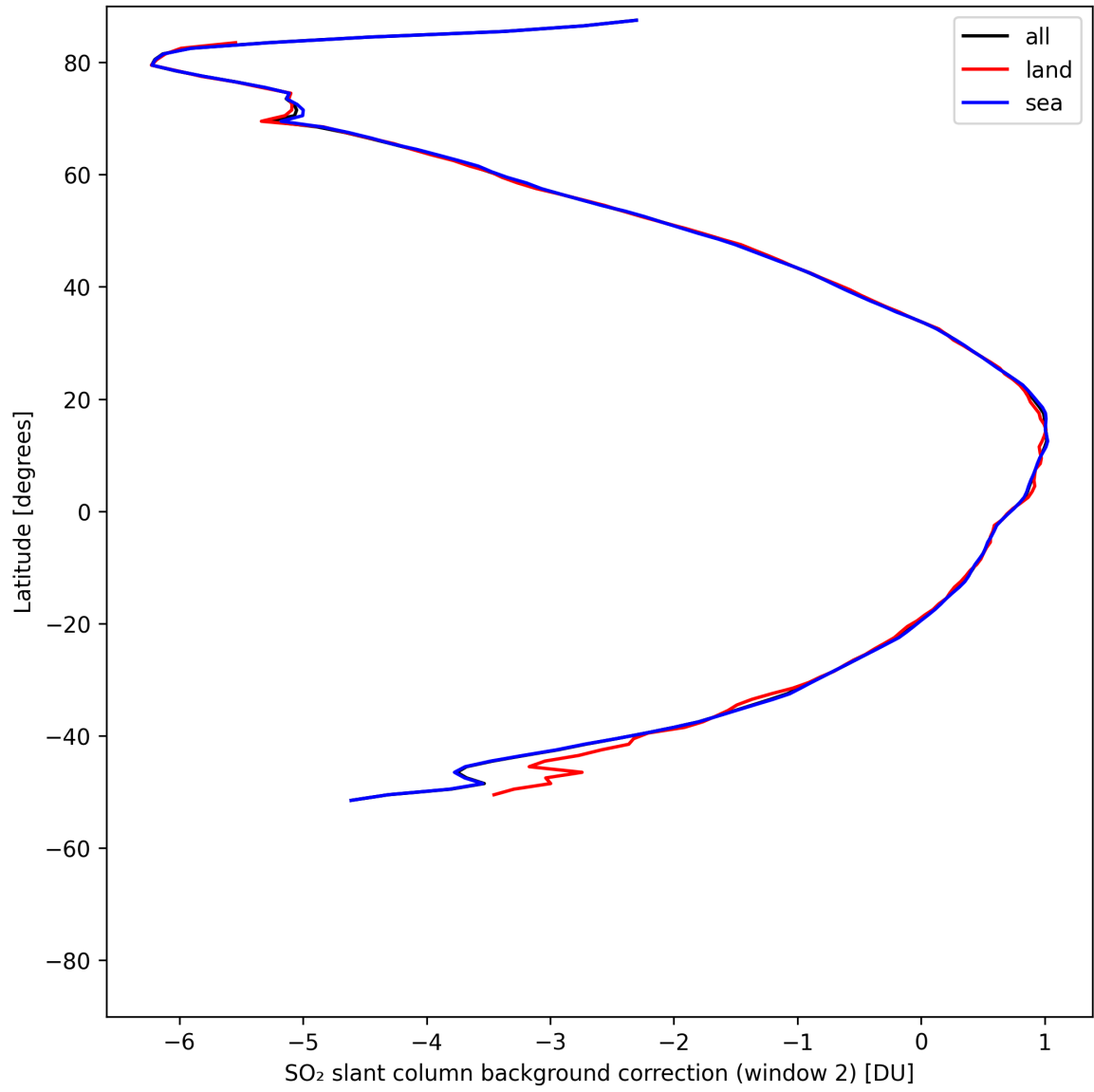
Figure 44: Zonal average of “SO 2 slant column background correction (window 2)” for 2025-05-06 to 2025-05-08.
