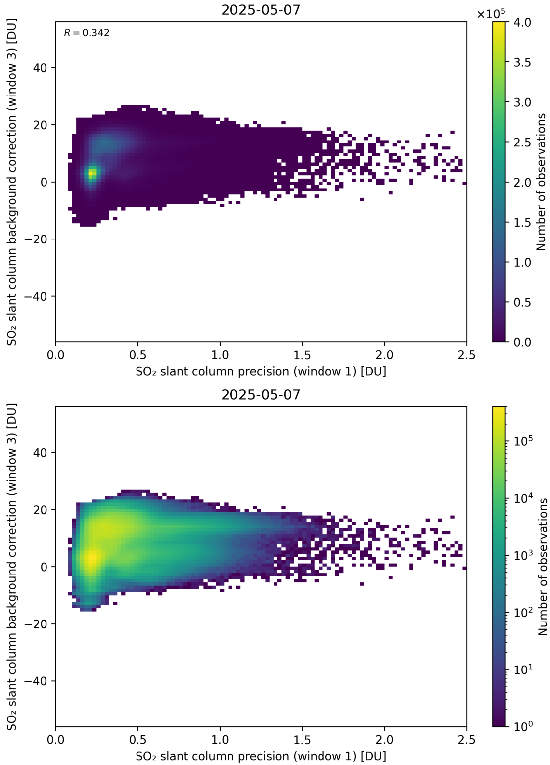
Figure 270: Scatter density plot of “SO 2 slant column precision (window 1)” against “SO 2 slant column background correction (window 3)” for 2025-05-06 to 2025-05-08.
