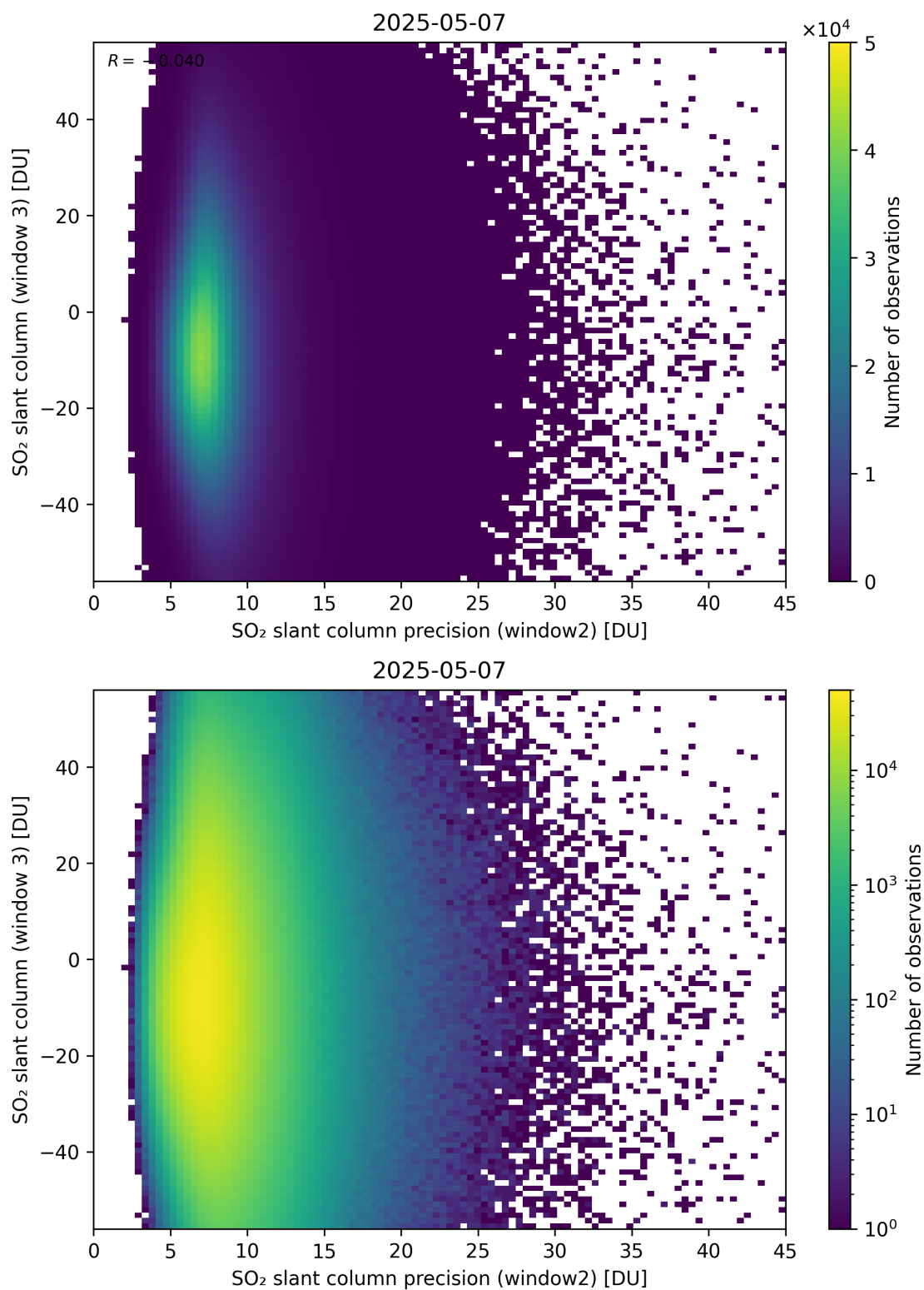
Figure 299: Scatter density plot of “SO 2 slant column precision (window2)” against “SO 2 slant column (window 3)” for 2025-05-06 to 2025-05-08.
