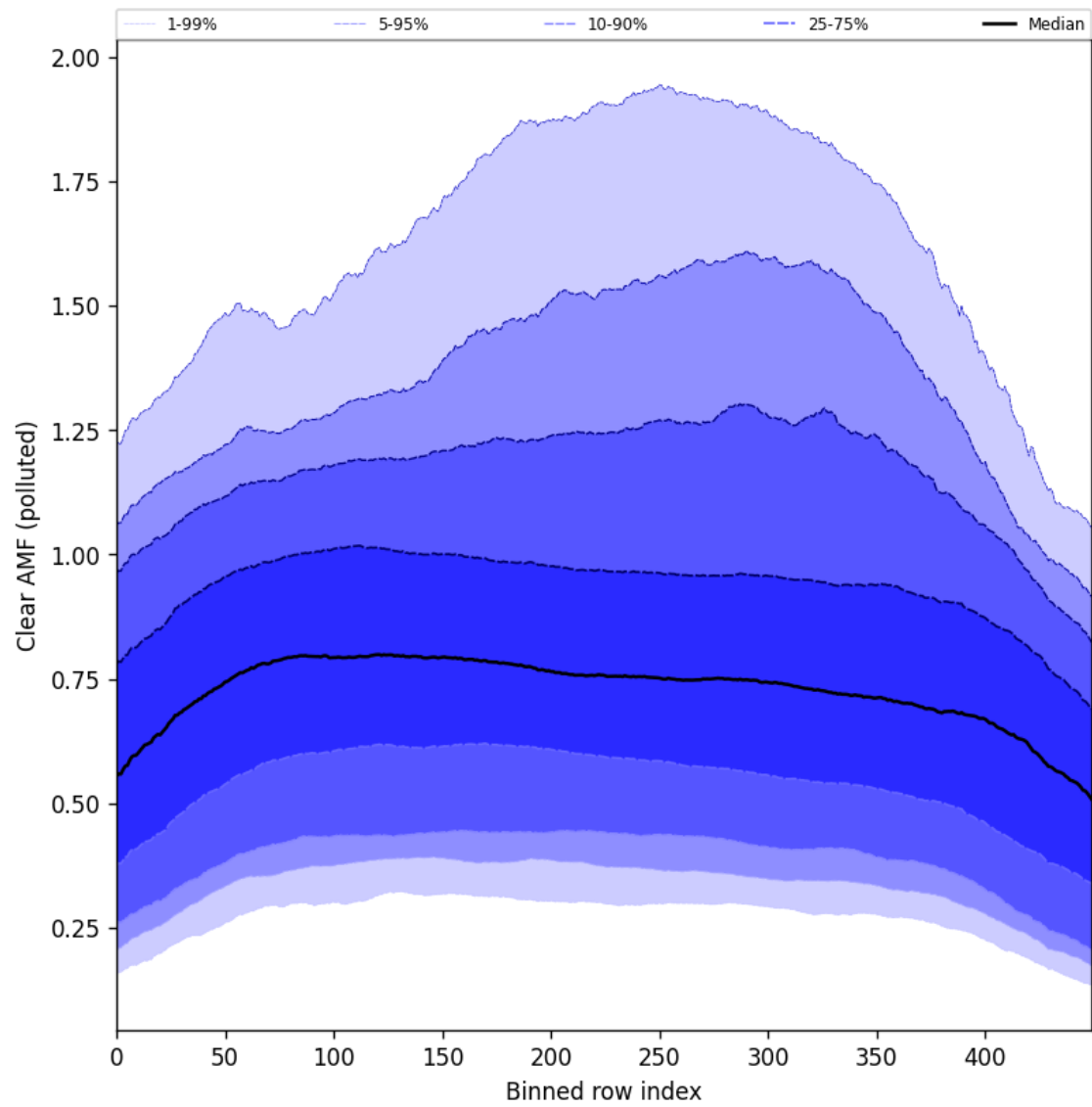
Figure 107: Along track statistics of “Clear AMF (polluted)” for 2025-05-06 to 2025-05-08
