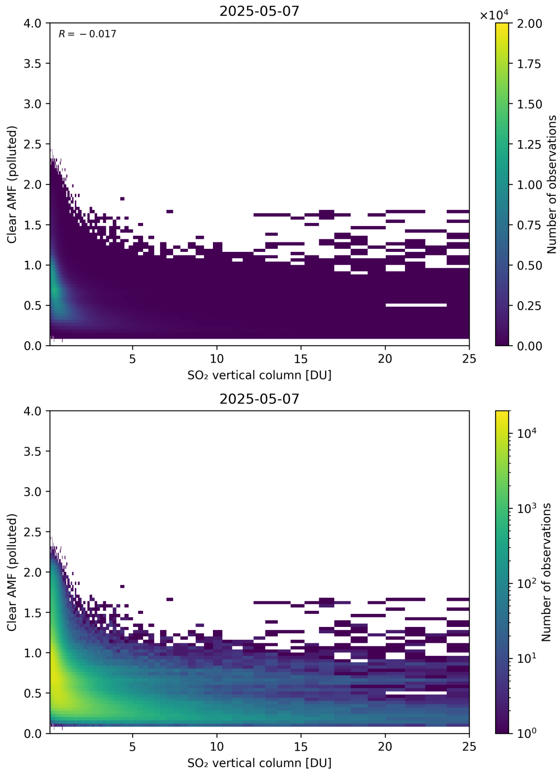
Figure 348: Scatter density plot of “SO 2 vertical column” against “Clear AMF (polluted)” for 2025-05-06 to 2025-05-08.
