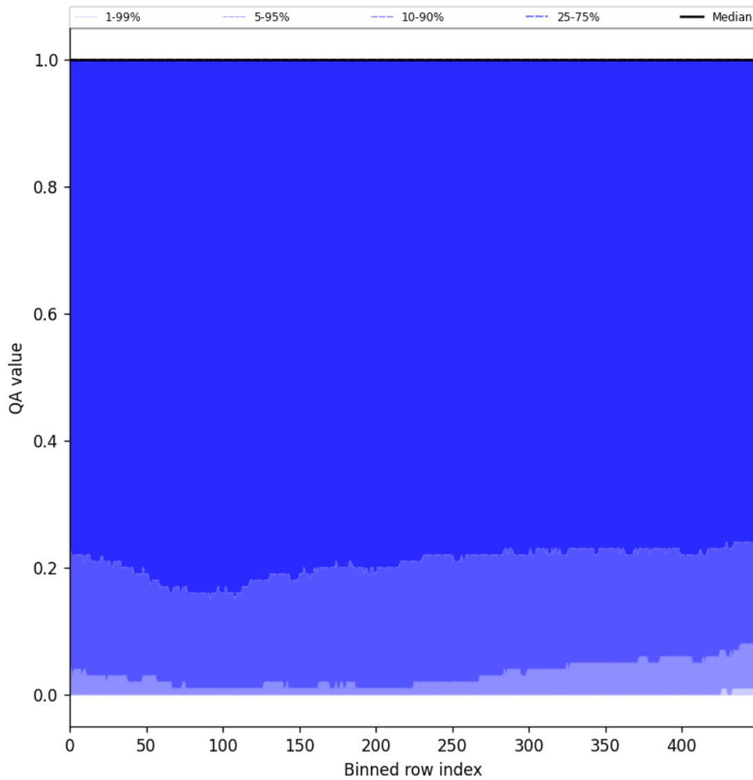
Figure 83: Along track statistics of “QA value” for 2025-05-06 to 2025-05-08
