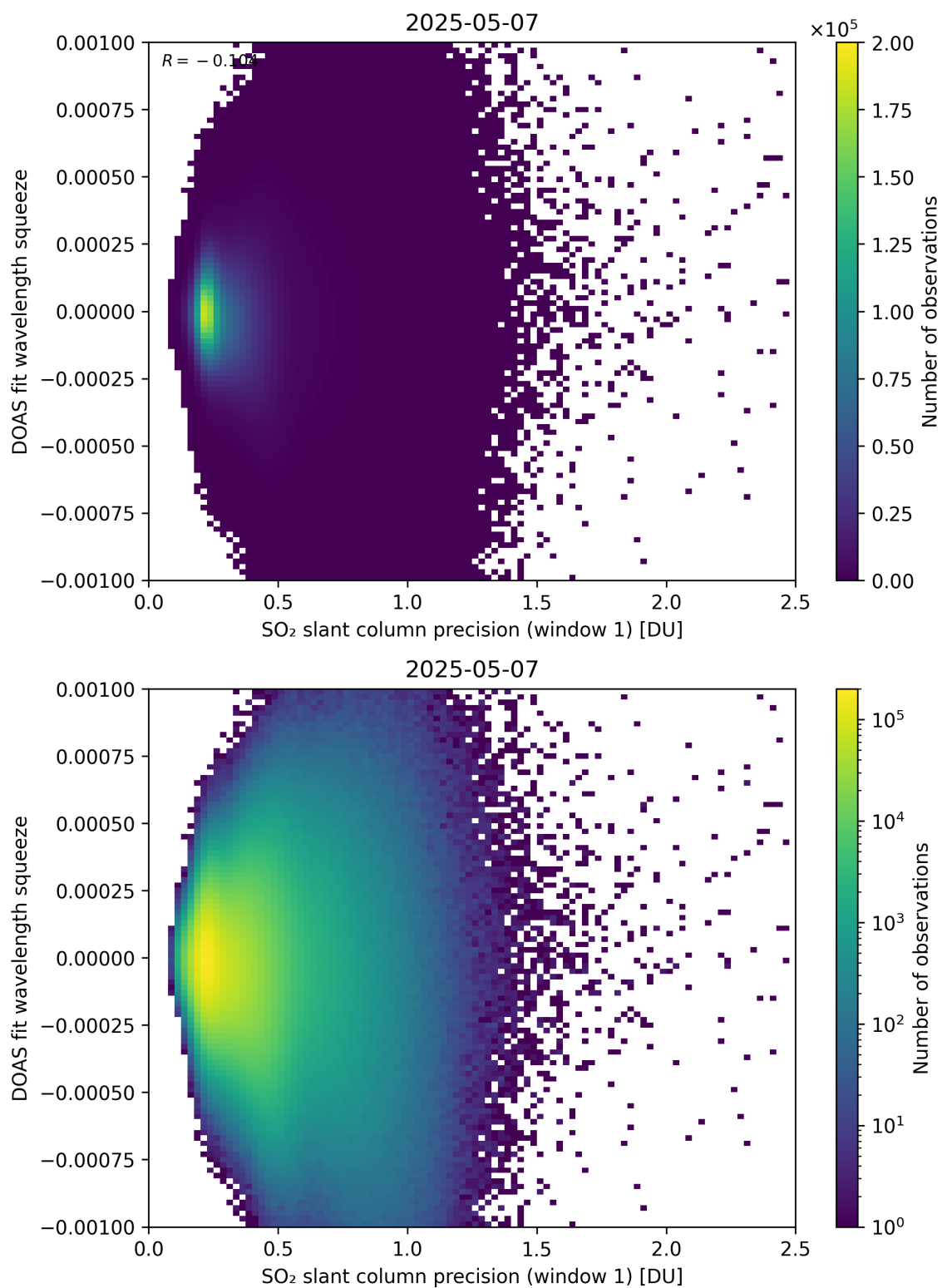
Figure 272: Scatter density plot of “SO 2 slant column precision (window 1)” against “DOAS fit wavelength squeeze” for 2025-05-06 to 2025-05-08.
