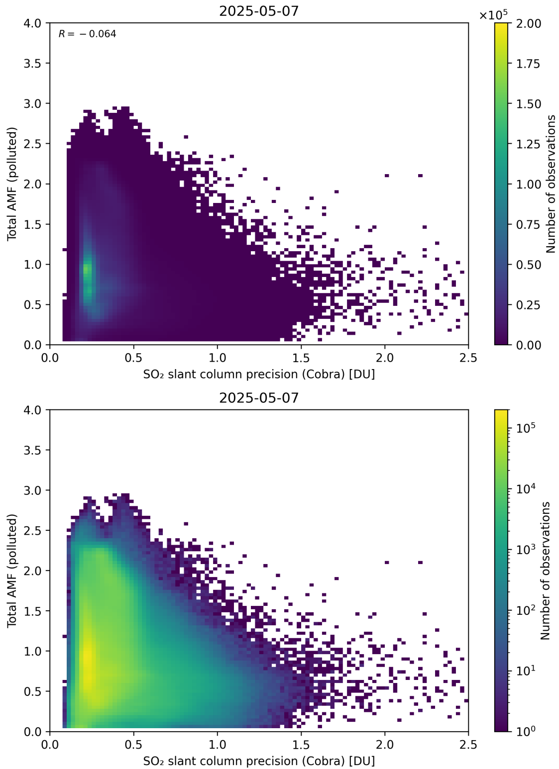
Figure 213: Scatter density plot of “SO 2 slant column precision (Cobra)” against “Total AMF (polluted)” for 2025-05-06 to 2025-05-08.
