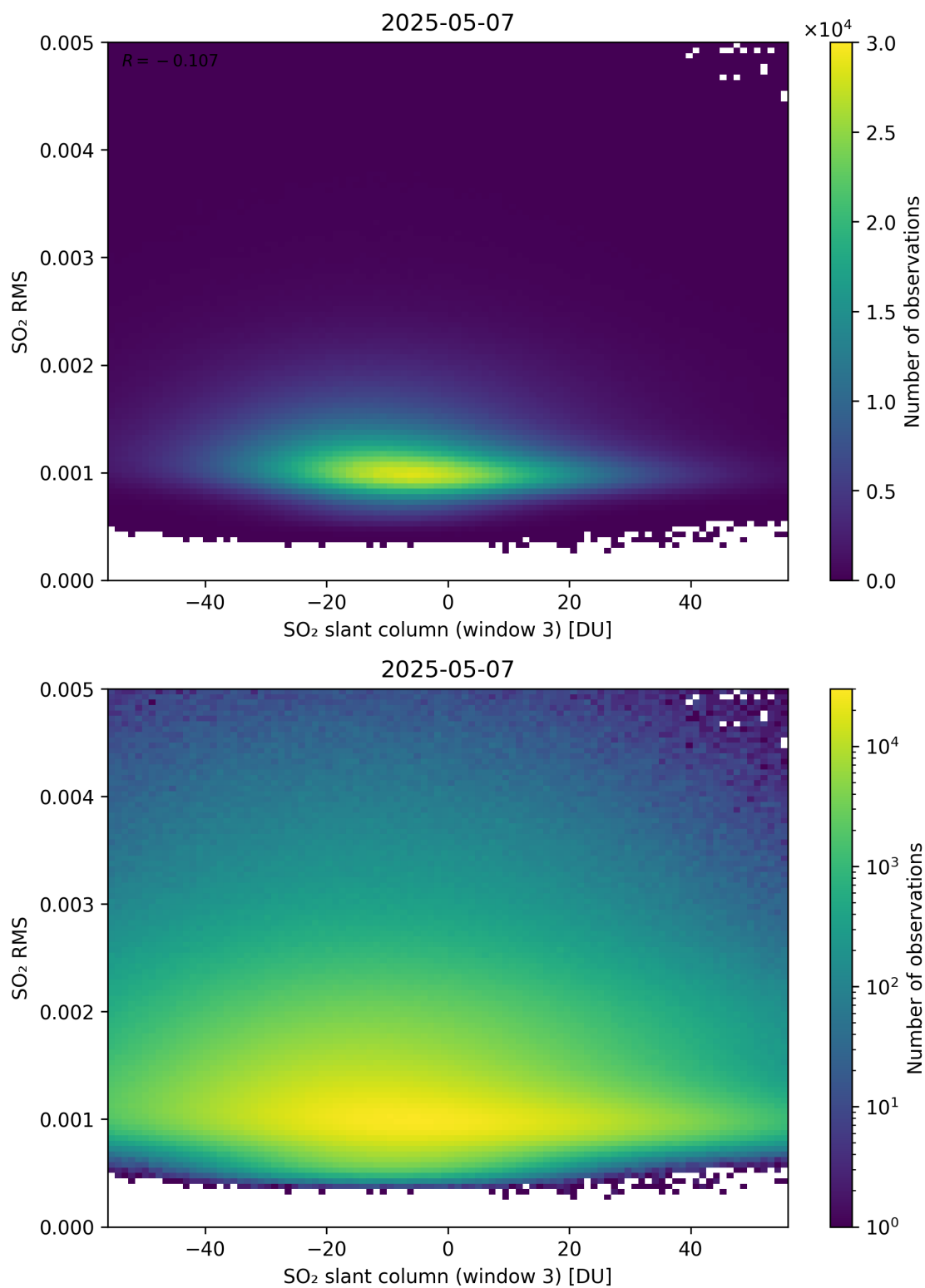
Figure 306: Scatter density plot of “SO 2 slant column (window 3)” against “SO 2 RMS” for 2025-05-06 to 2025-05-08.
