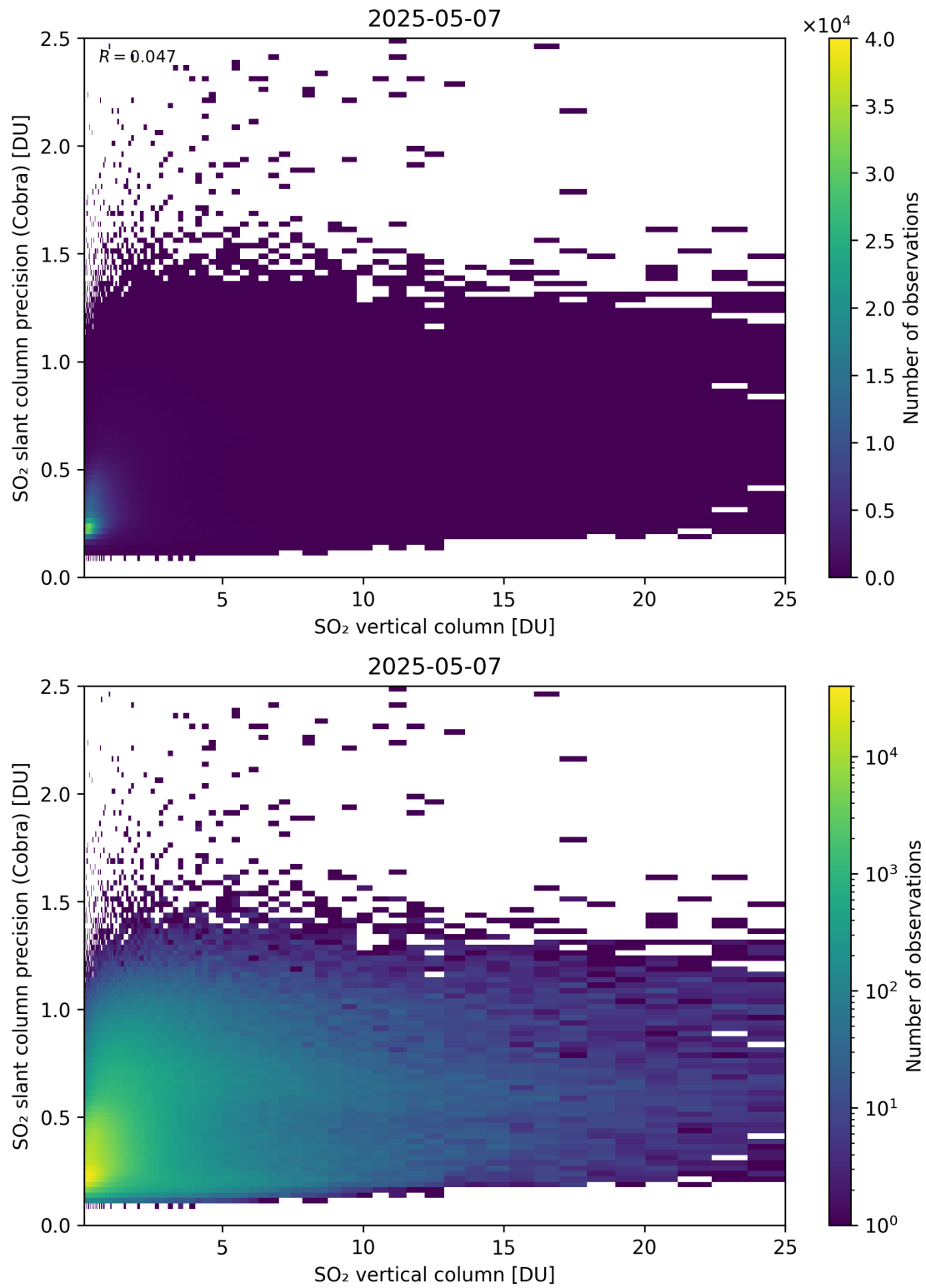
Figure 350: Scatter density plot of “SO 2 vertical column” against “SO 2 slant column precision (Cobra)” for 2025-05-06 to 2025-05-08.
