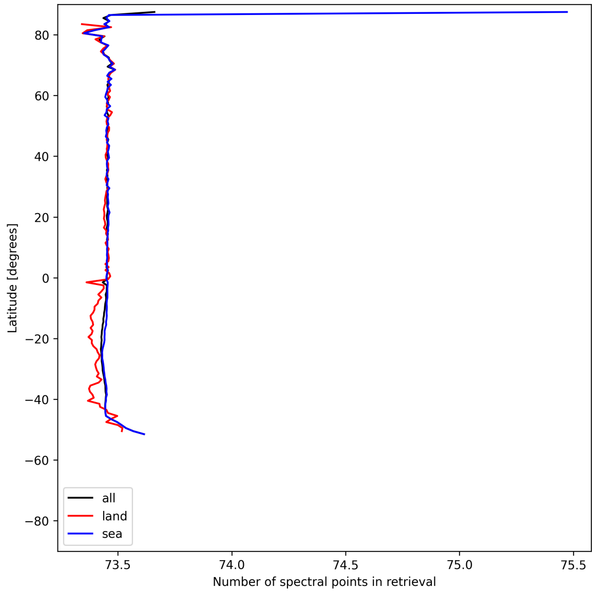
Figure 56: Zonal average of “Number of spectral points in retrieval” for 2025-05-06 to 2025-05-08.
