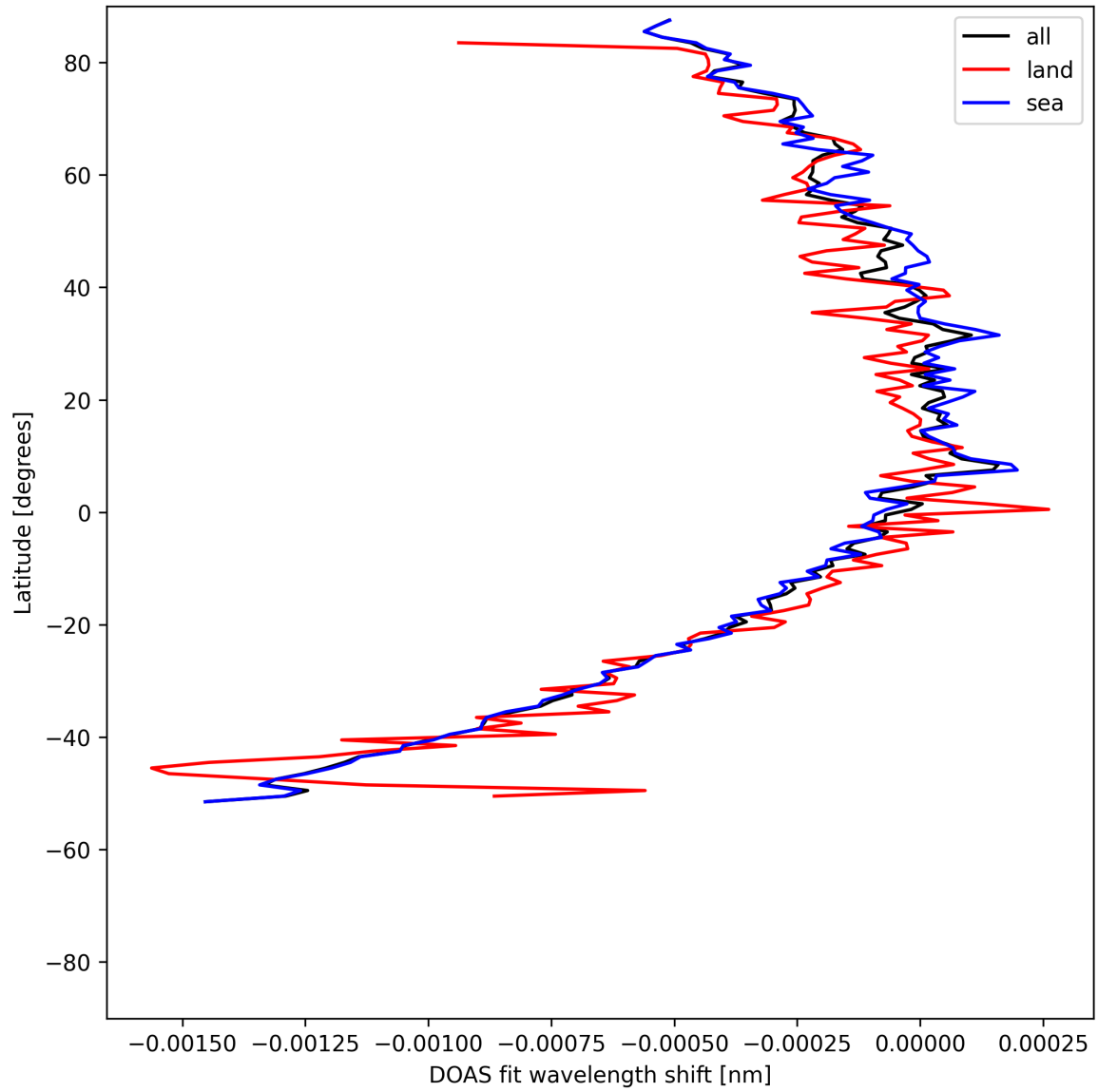
Figure 50: Zonal average of "DOAS fit wavelength shift" for 2025-05-06 to 2025-05-08.
