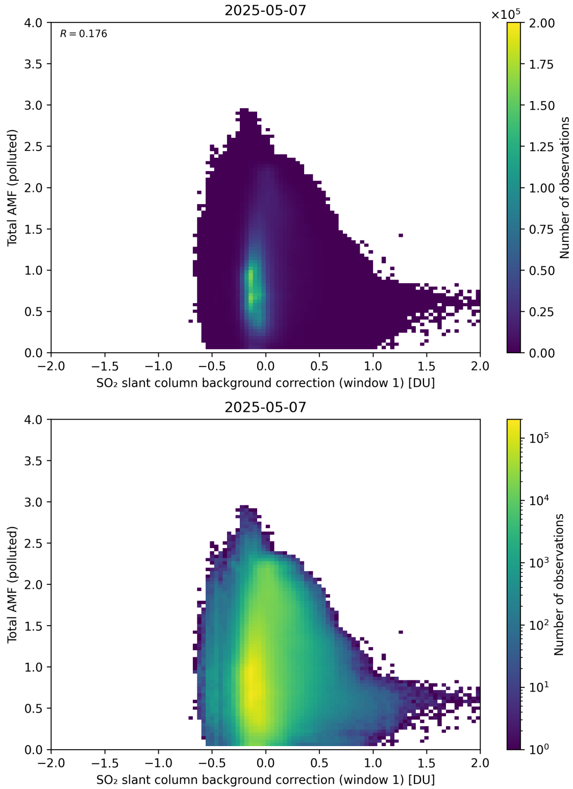
Figure 120: Scatter density plot of “SO 2 slant column background correction (window 1)” against “Total AMF (polluted)” for 2025-05-06 to 2025-05-08.
