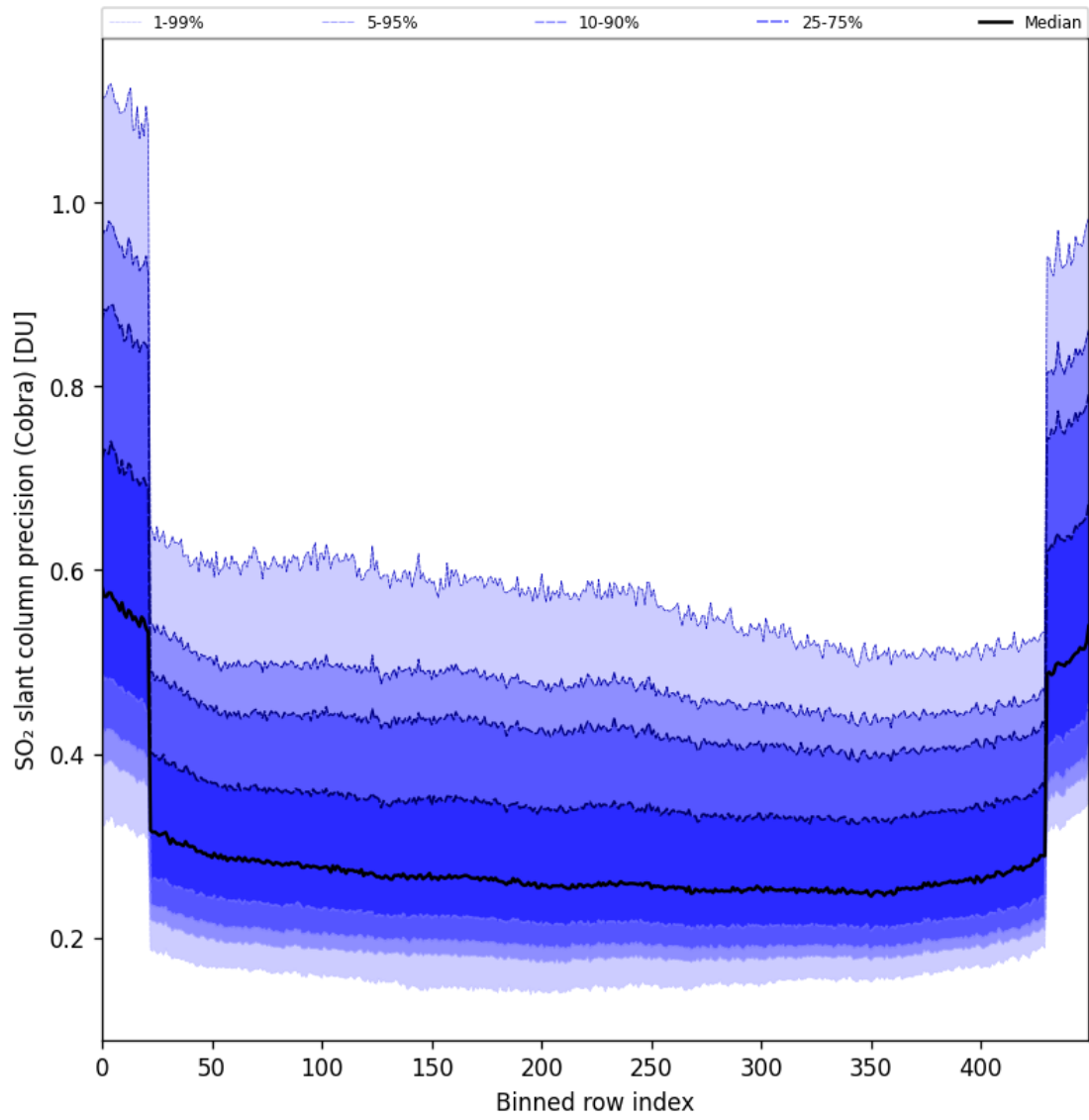
Figure 88: Along track statistics of “SO 2 slant column precision (Cobra)” for 2025-05-06 to 2025-05-08
