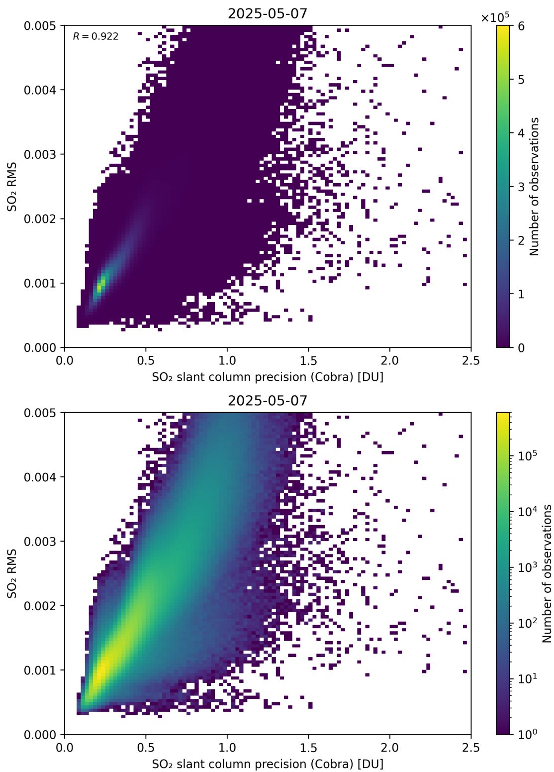
Figure 204: Scatter density plot of “SO 2 slant column precision (Cobra)” against “SO 2 RMS” for 2025-05-06 to 2025-05-08.
