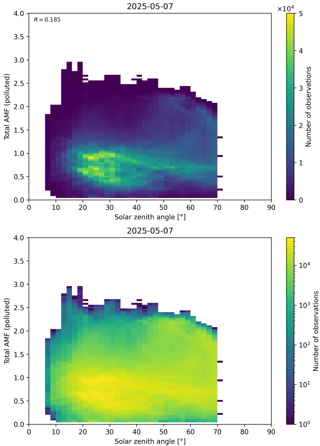
Figure 189: Scatter density plot of “Solar zenith angle” against “Total AMF (polluted)” for 2025-05-06 to 2025-05-08.
