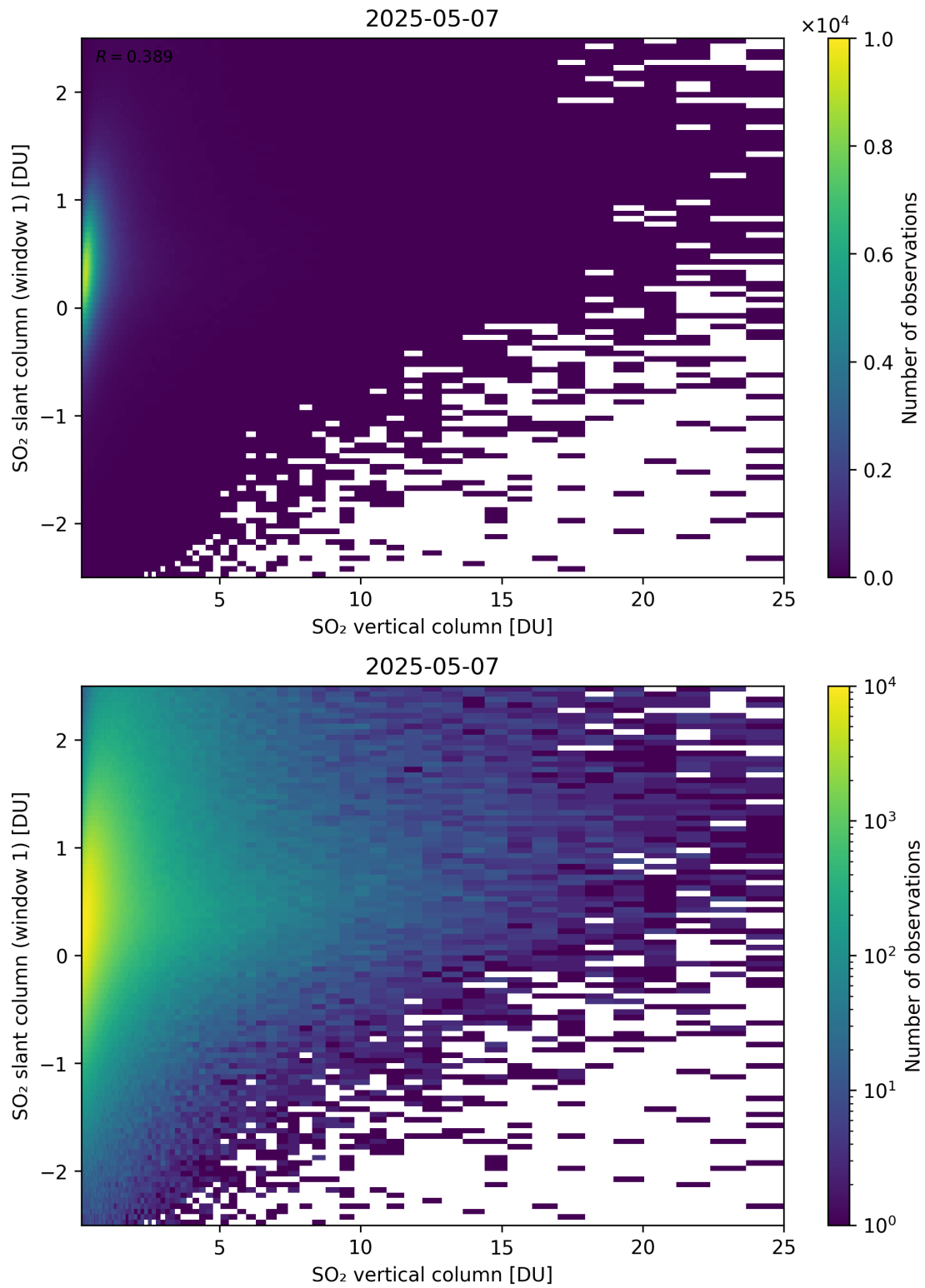
Figure 354: Scatter density plot of “SO 2 vertical column” against “SO 2 slant column (window 1)” for 2025-05-06 to 2025-05-08.
