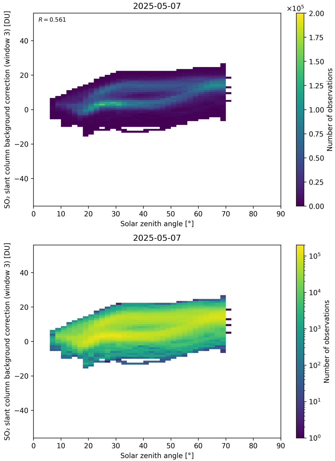
Figure 173: Scatter density plot of “Solar zenith angle” against “SO 2 slant column background correction (window 3)” for 2025-05-06 to 2025-05-08.
