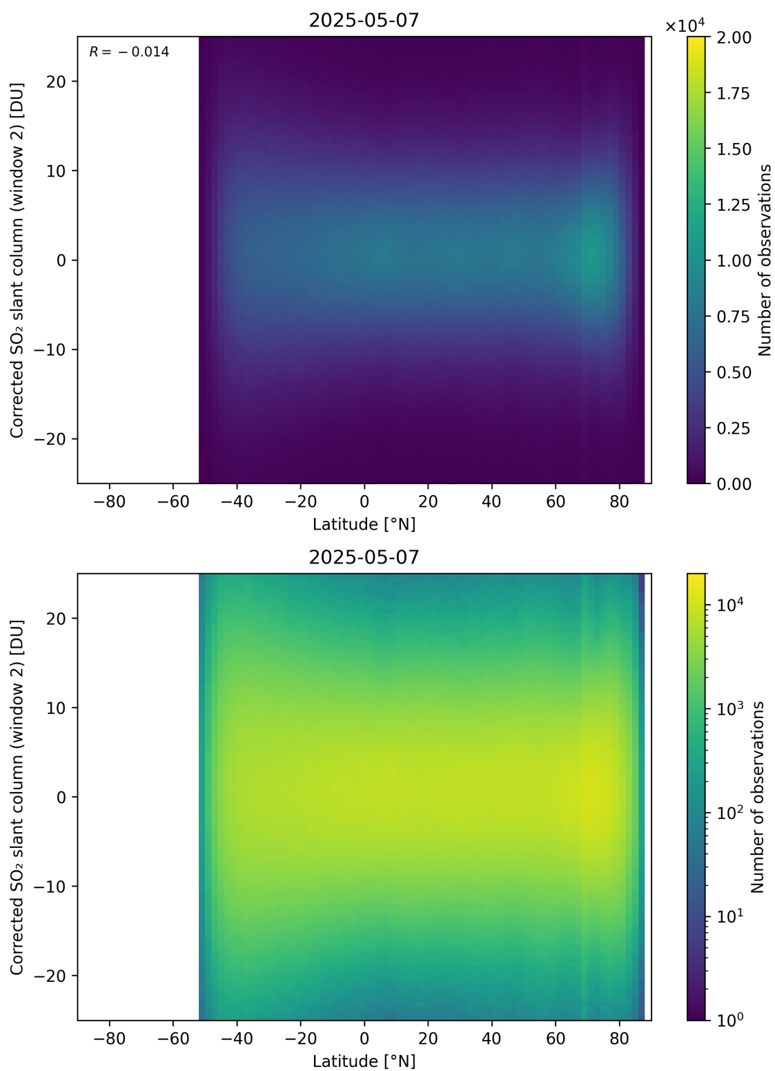
Figure 160: Scatter density plot of “Latitude” against “Corrected SO 2 slant column (window 2)” for 2025-05-06 to 2025-05-08.
