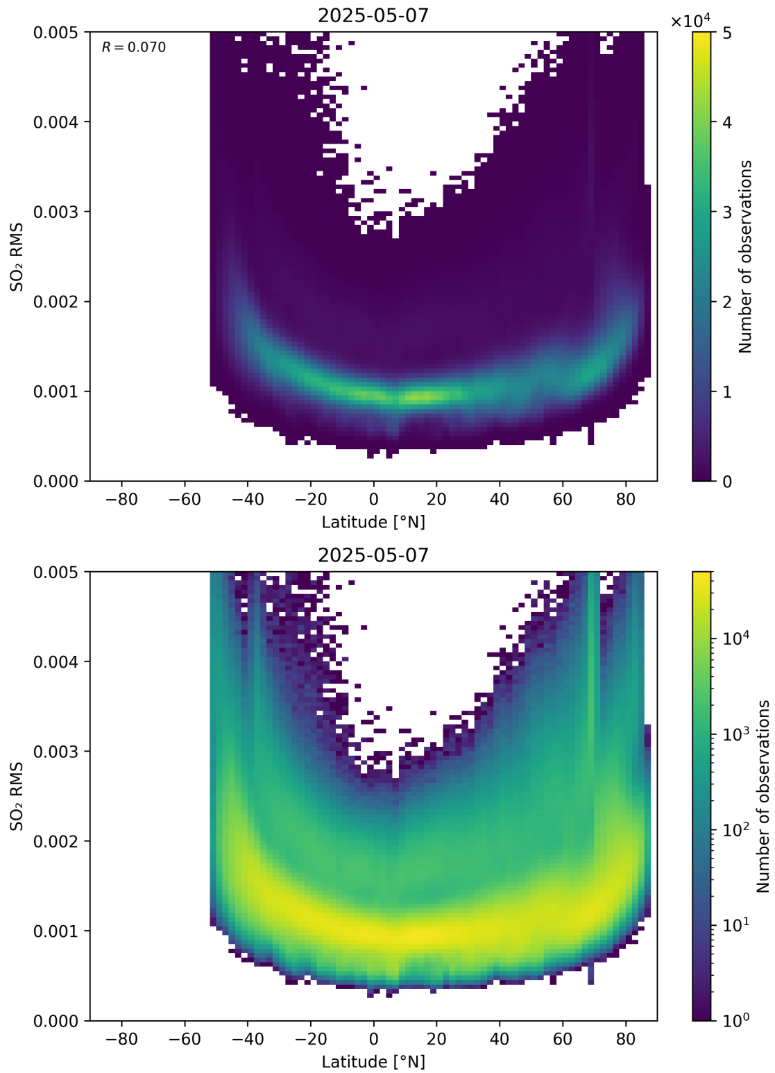
Figure 155: Scatter density plot of “Latitude” against “SO 2 RMS” for 2025-05-06 to 2025-05-08.
