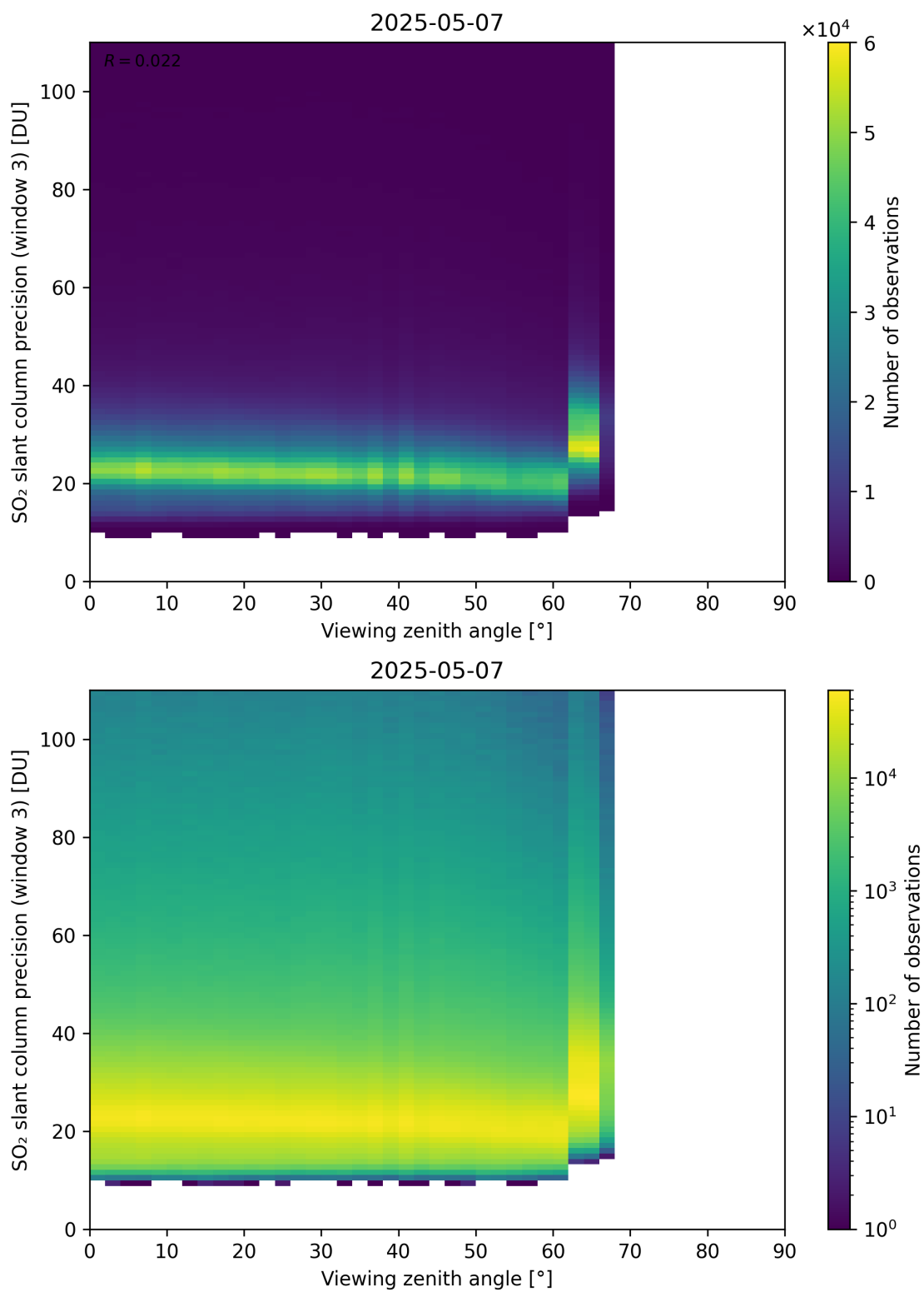
Figure 380: Scatter density plot of “Viewing zenith angle” against “SO 2 slant column precision (window 3)” for 2025-05-06 to 2025-05-08.
