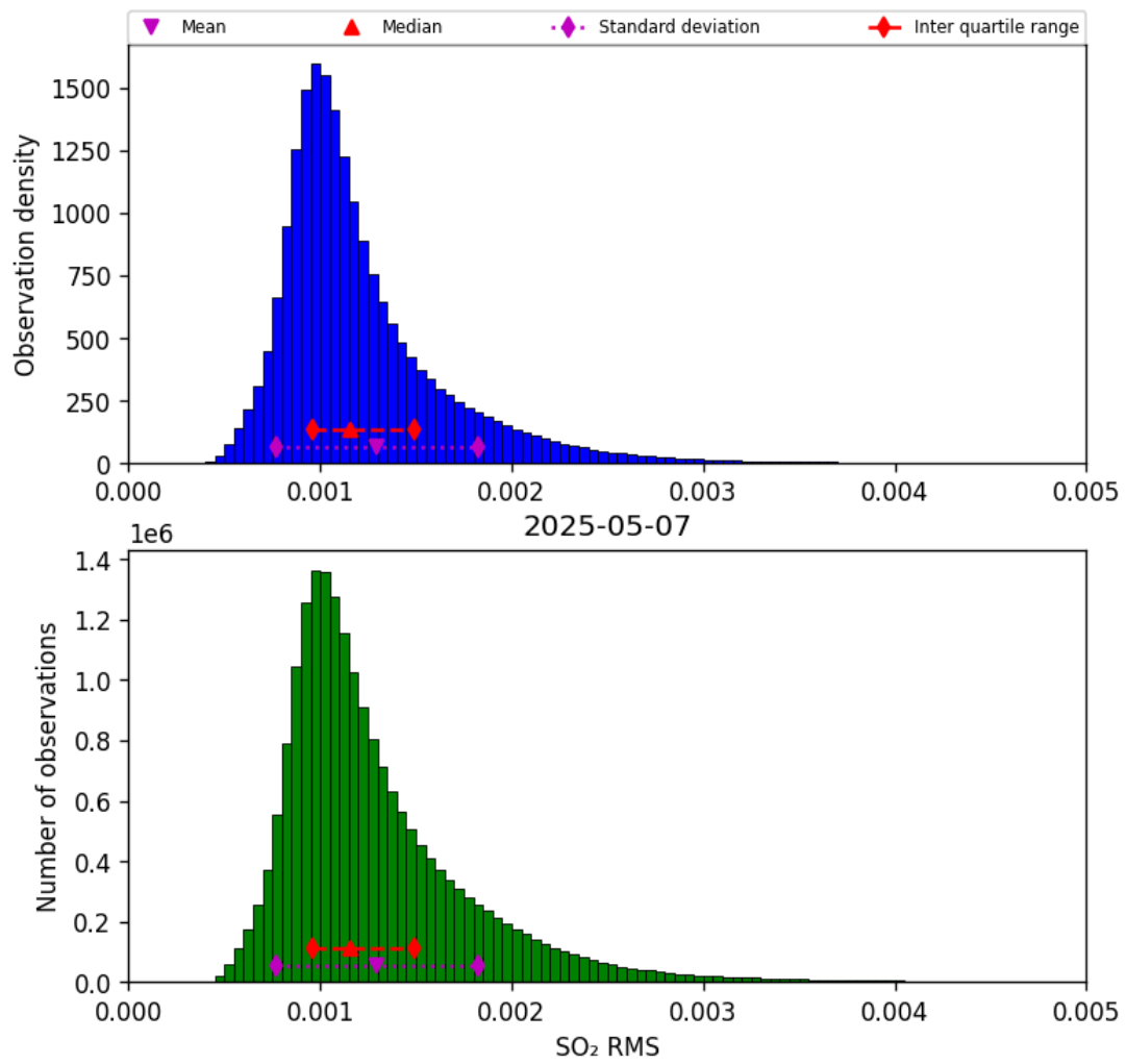
Figure 78: Histogram of “SO 2 RMS” for 2025-05-06 to 2025-05-08
