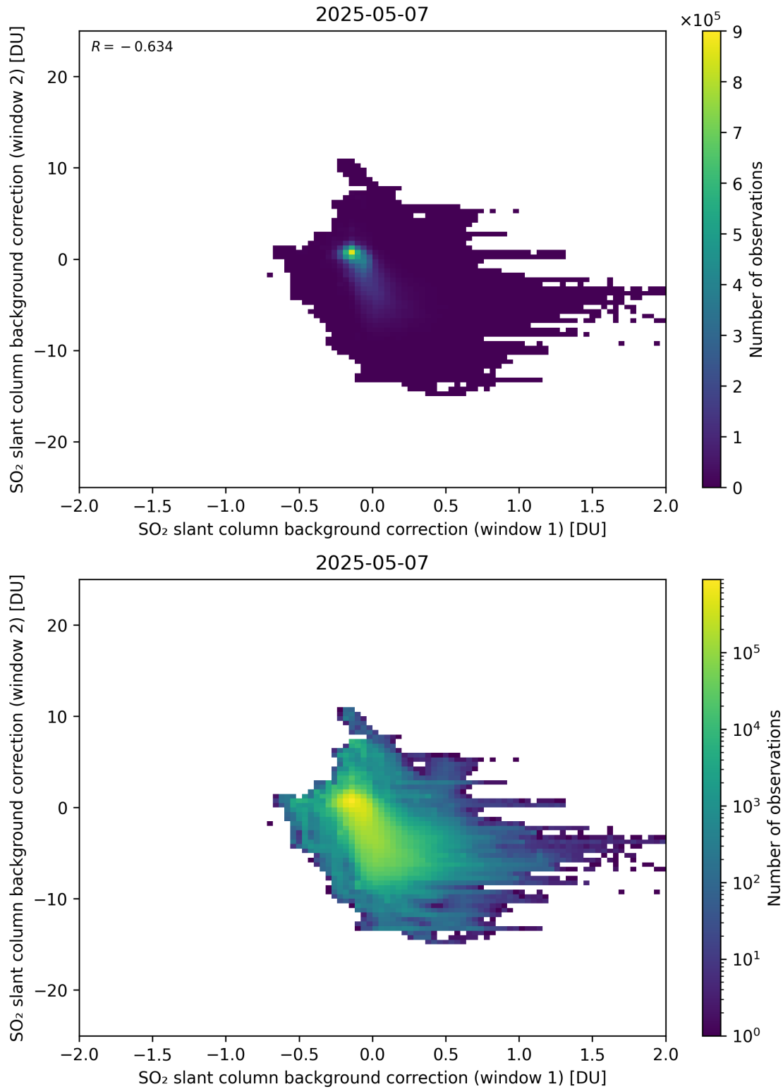
Figure 109: Scatter density plot of “SO 2 slant column background correction (window 1)” against “SO 2 slant column background correction (window 2)” for 2025-05-06 to 2025-05-08.
