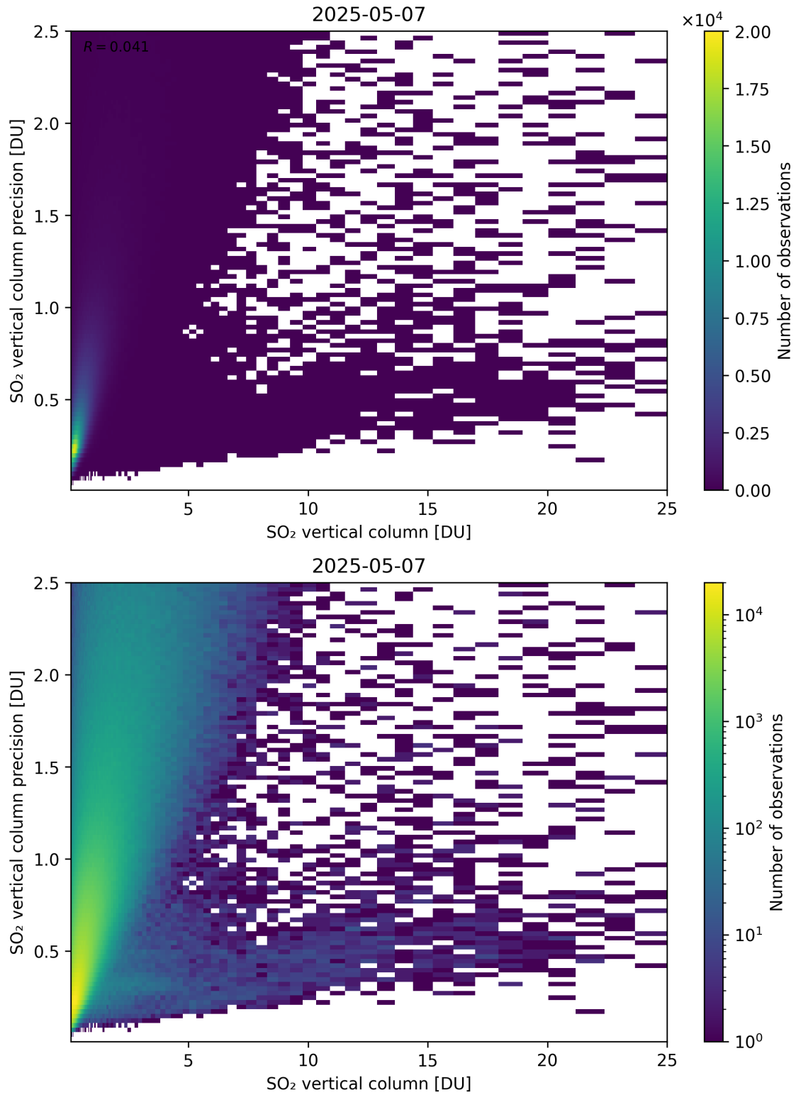
Figure 361: Scatter density plot of “SO 2 vertical column” against “SO 2 vertical column precision” for 2025-05-06 to 2025-05-08.
