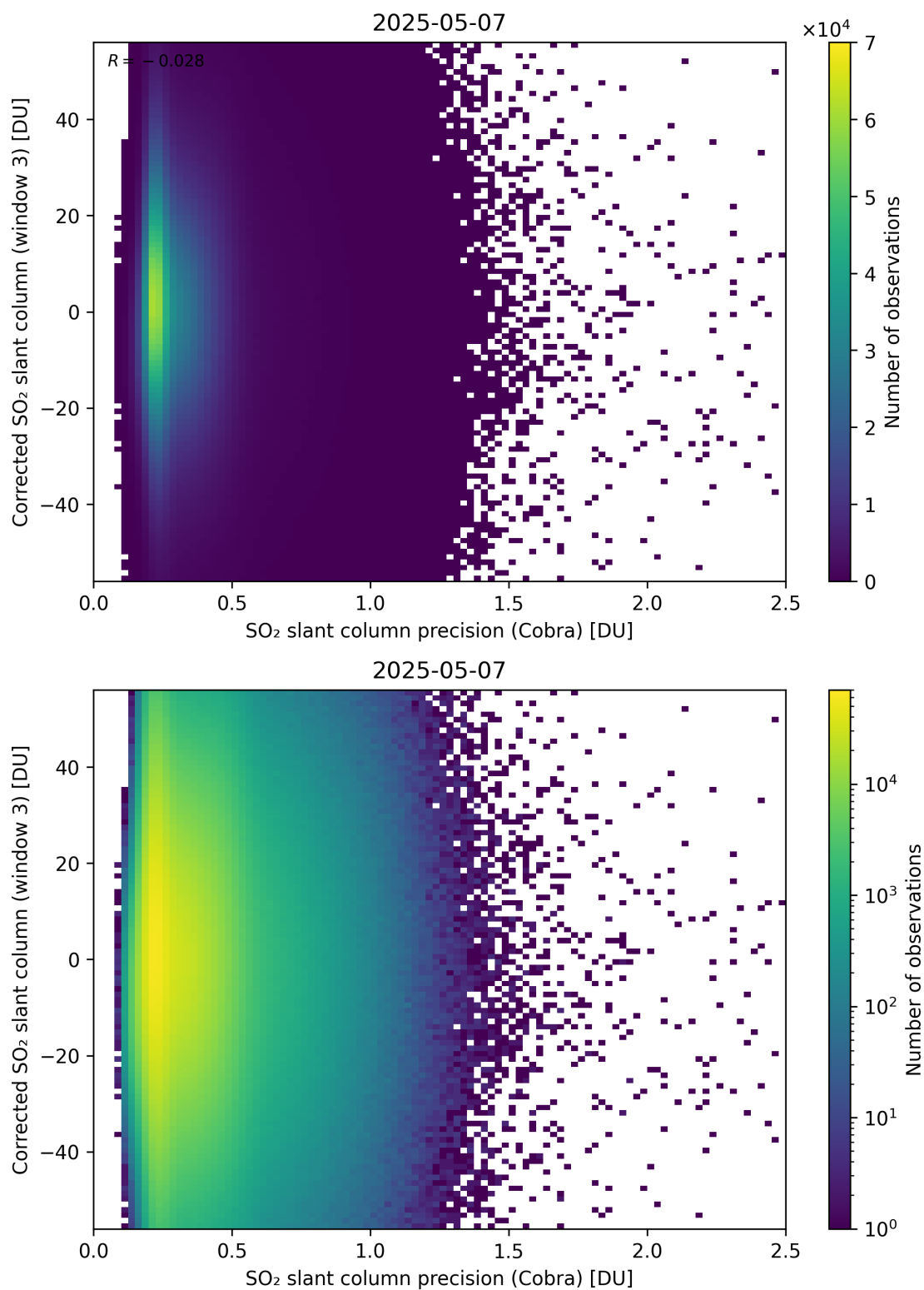
Figure 207: Scatter density plot of “SO 2 slant column precision (Cobra)” against “Corrected SO 2 slant column (window 3)” for 2025-05-06 to 2025-05-08.
