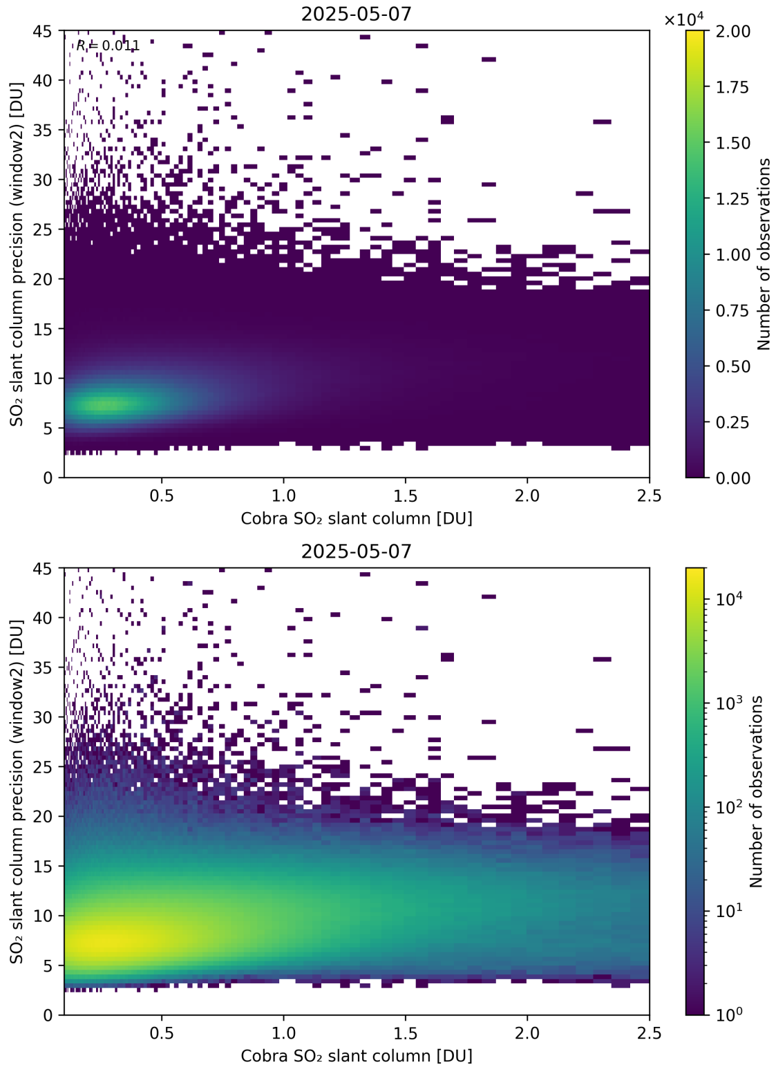
Figure 221: Scatter density plot of “Cobra SO 2 slant column” against “SO 2 slant column precision (window2)” for 2025-05-06 to 2025-05-08.
