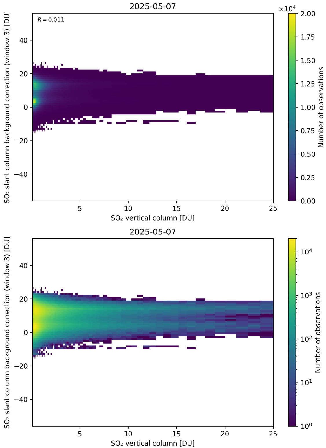
Figure 325: Scatter density plot of “SO 2 vertical column” against “SO 2 slant column background correction (window 3)” for 2025-05-06 to 2025-05-08.
