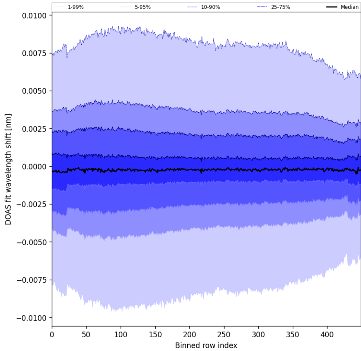
Figure 102: Along track statistics of “DOAS fit wavelength shift” for 2025-05-06 to 2025-05-08
