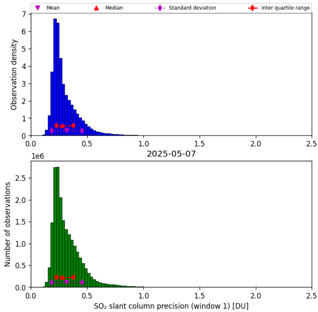
Figure 64: Histogram of “SO 2 slant column precision (window 1)” for 2025-05-06 to 2025-05-08
