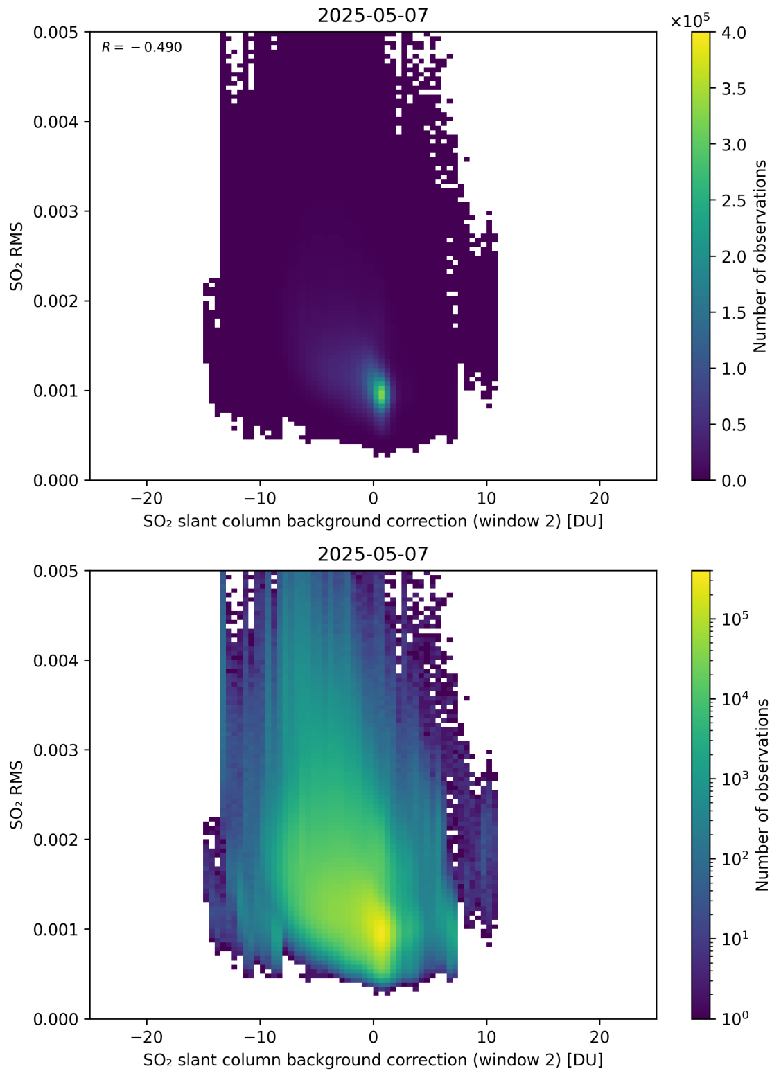
Figure 125: Scatter density plot of “SO 2 slant column background correction (window 2)” against “SO 2 RMS” for 2025-05-06 to 2025-05-08.
