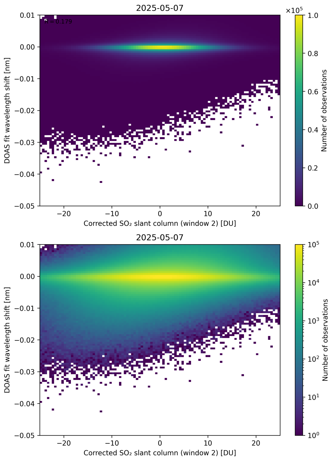
Figure 246: Scatter density plot of “Corrected SO 2 slant column (window 2)” against “DOAS fit wavelength shift” for 2025-05-06 to 2025-05-08.
