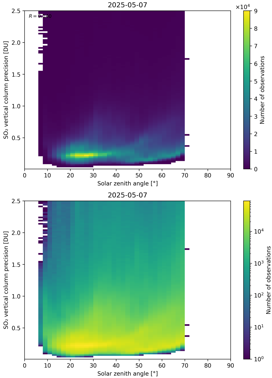
Figure 192: Scatter density plot of “Solar zenith angle” against “SO 2 vertical column precision” for 2025-05-06 to 2025-05-08.
