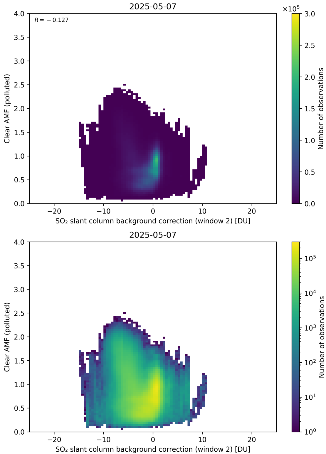
Figure 126: Scatter density plot of “SO 2 slant column background correction (window 2)” against “Clear AMF (polluted)” for 2025-05-06 to 2025-05-08.
