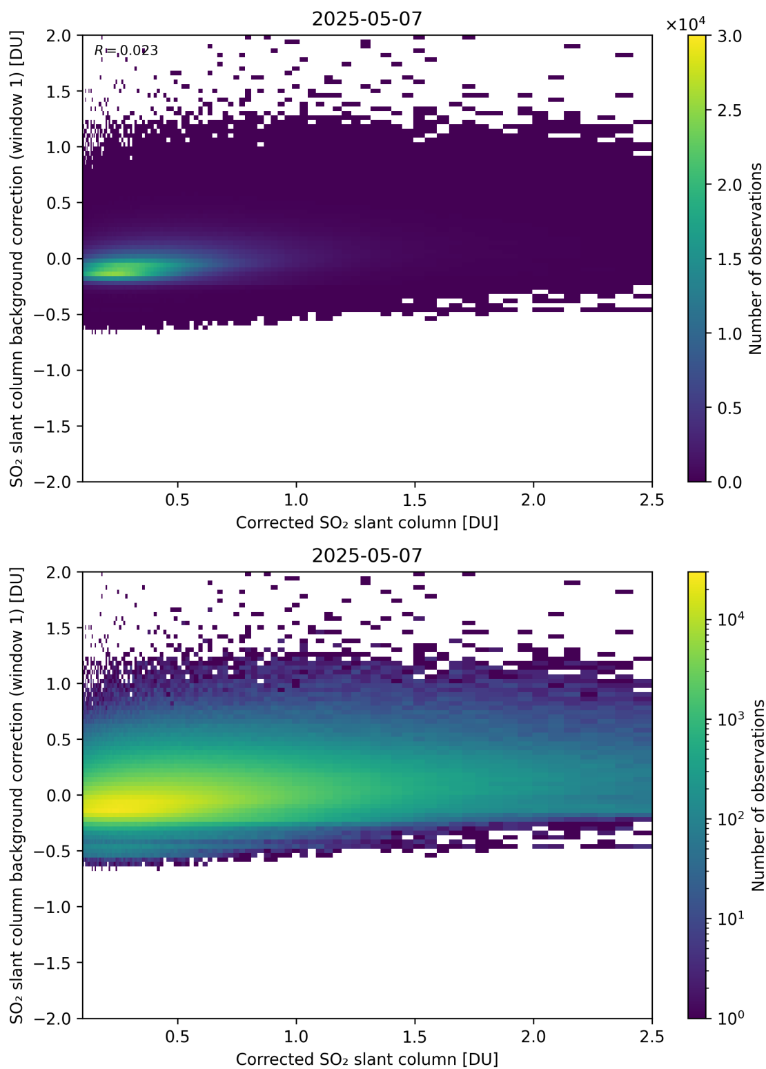
Figure 226: Scatter density plot of “Corrected SO 2 slant column” against “SO 2 slant column background correction (window 1)” for 2025-05-06 to 2025-05-08.
