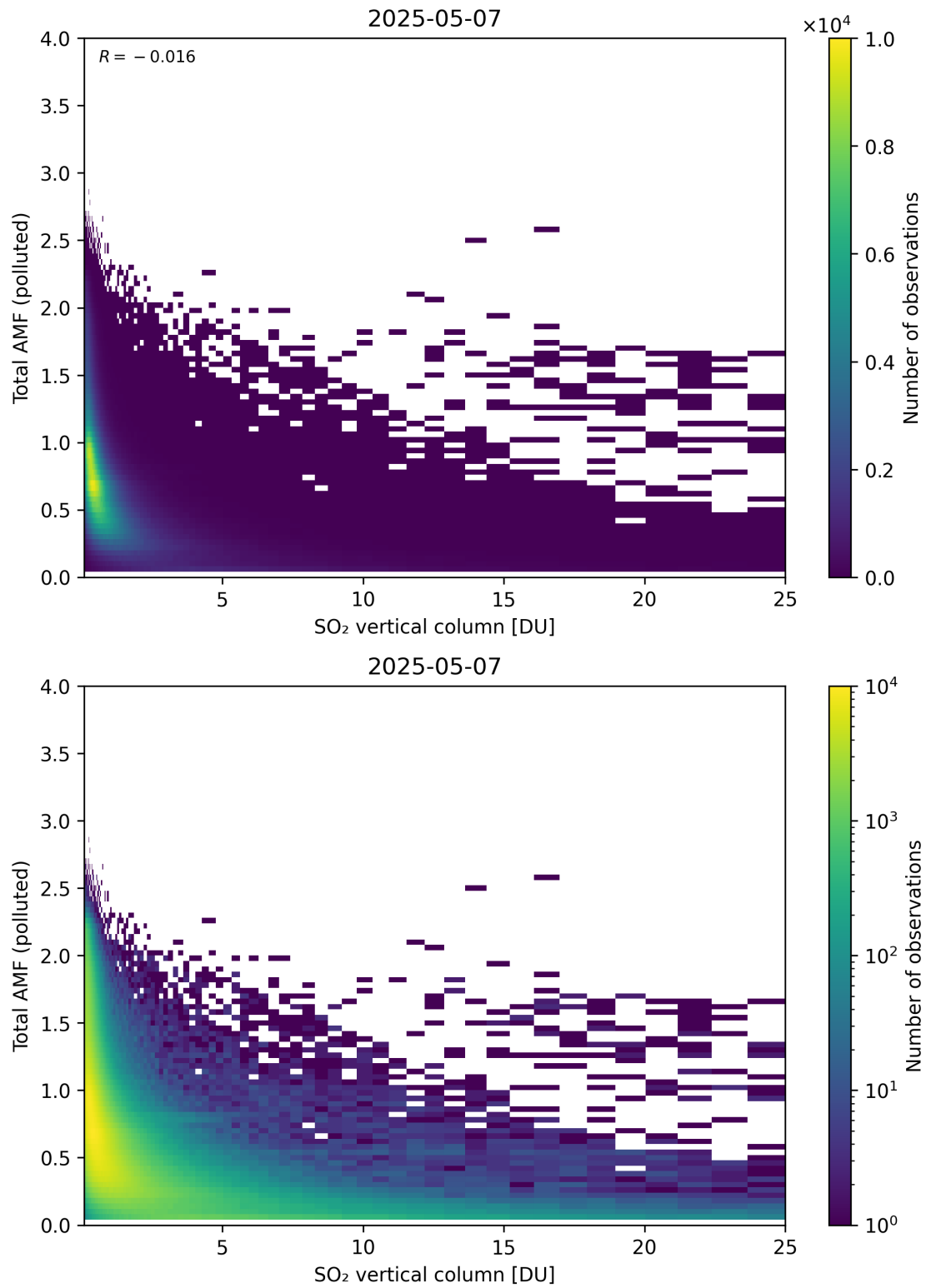
Figure 359: Scatter density plot of “SO 2 vertical column” against “Total AMF (polluted)” for 2025-05-06 to 2025-05-08.
