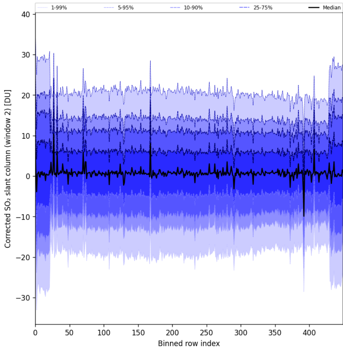
Figure 95: Along track statistics of “Corrected SO 2 slant column (window 2)” for 2025-05-06 to 2025-05-08
