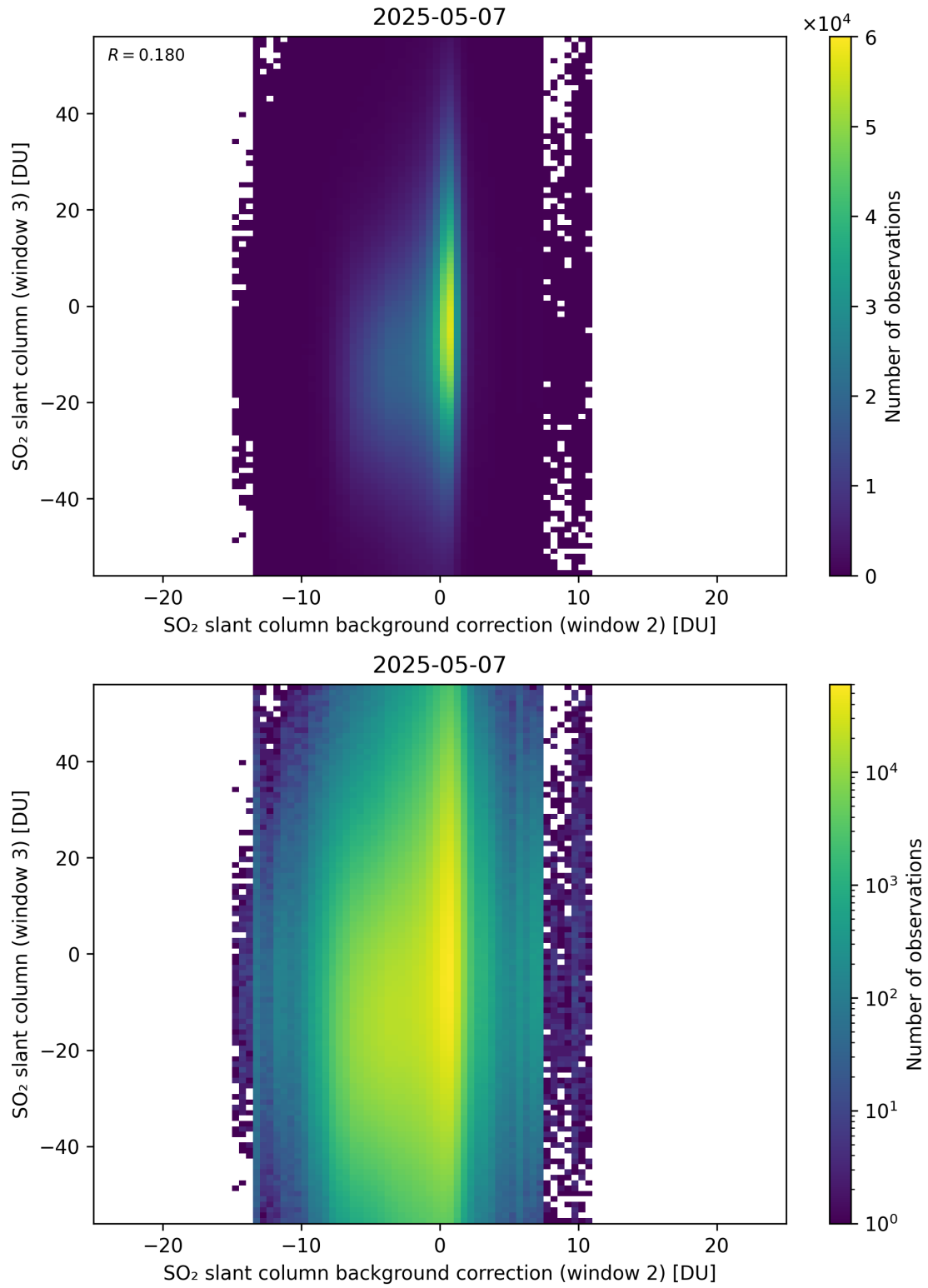
Figure 128: Scatter density plot of “SO 2 slant column background correction (window 2)” against “SO 2 slant column (window 3)” for 2025-05-06 to 2025-05-08.
