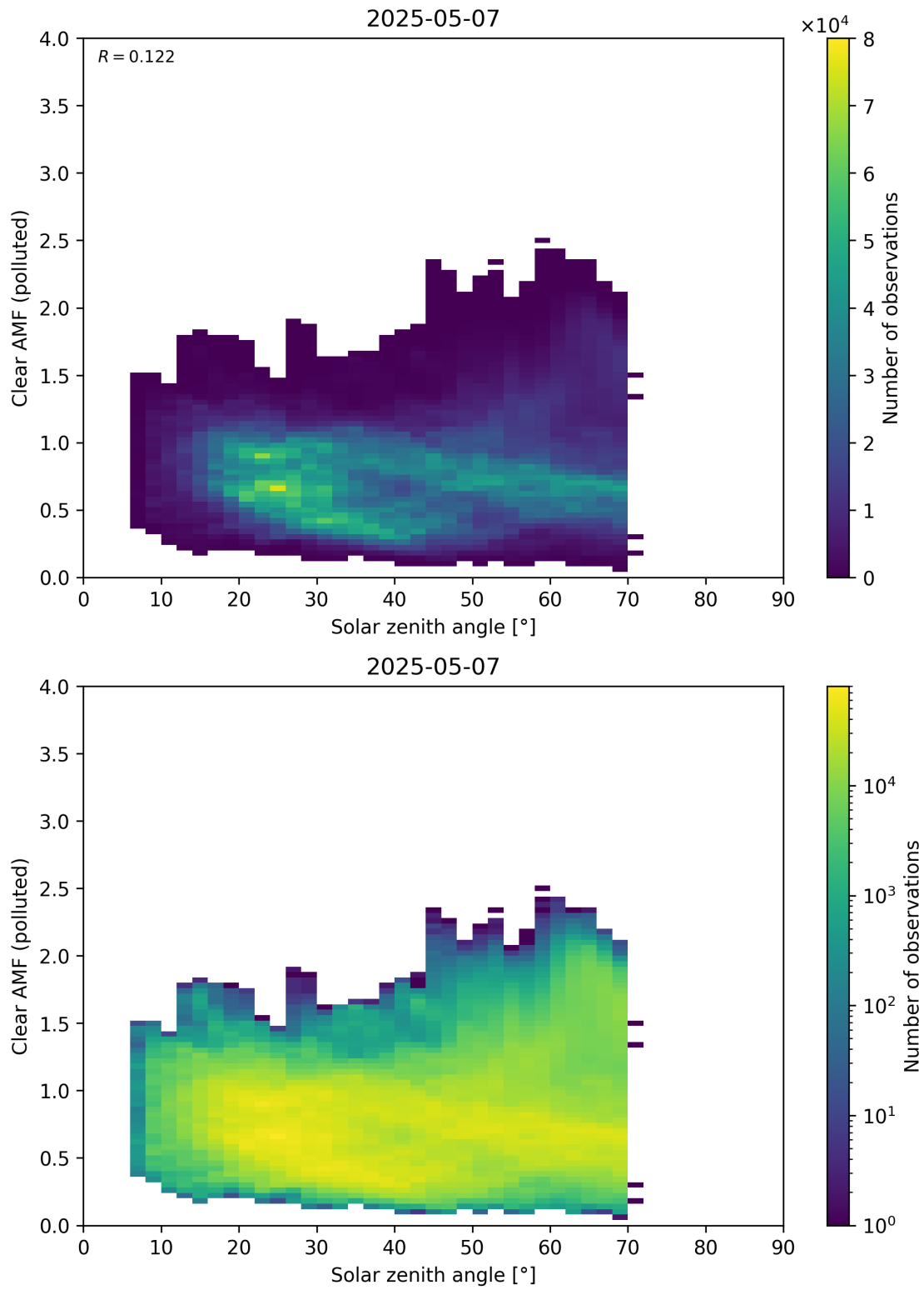
Figure 178: Scatter density plot of “Solar zenith angle” against “Clear AMF (polluted)” for 2025-05-06 to 2025-05-08.
