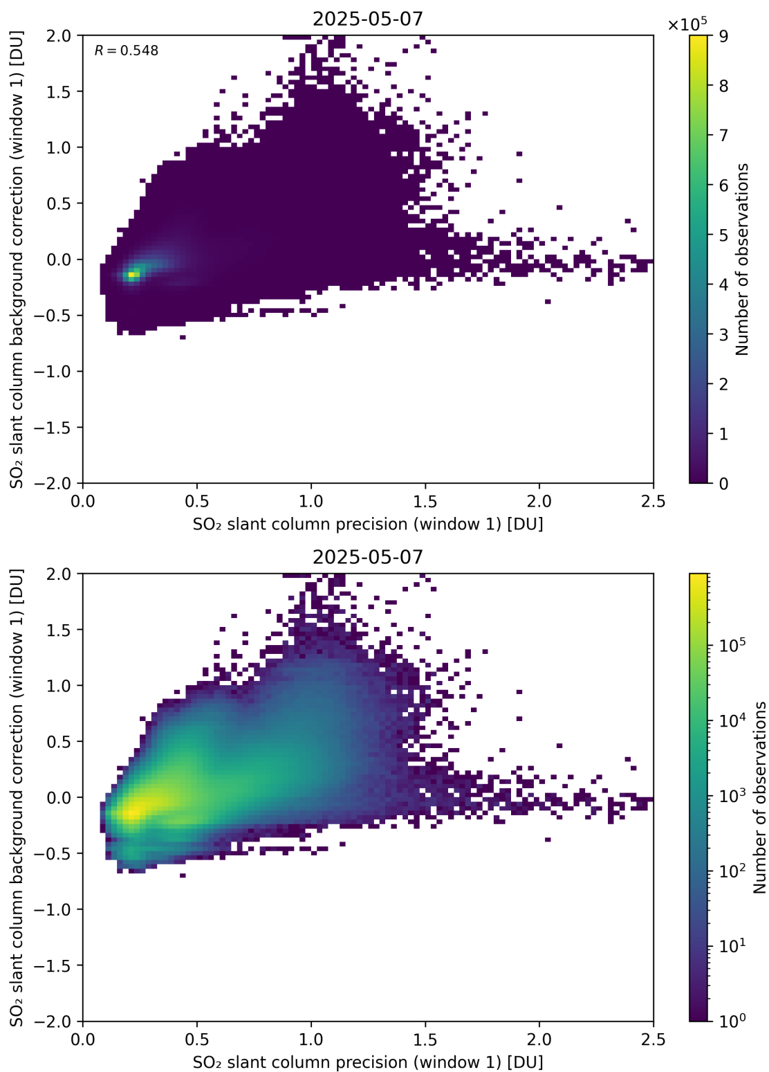
Figure 268: Scatter density plot of “SO 2 slant column precision (window 1)” against “SO 2 slant column background correction (window 1)” for 2025-05-06 to 2025-05-08.
