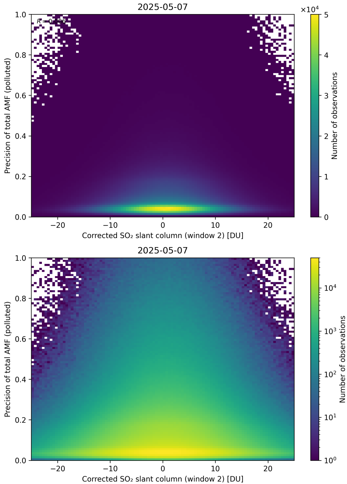
Figure 254: Scatter density plot of “Corrected SO 2 slant column (window 2)” against “Precision of total AMF (polluted)” for 2025-05-06 to 2025-05-08.
