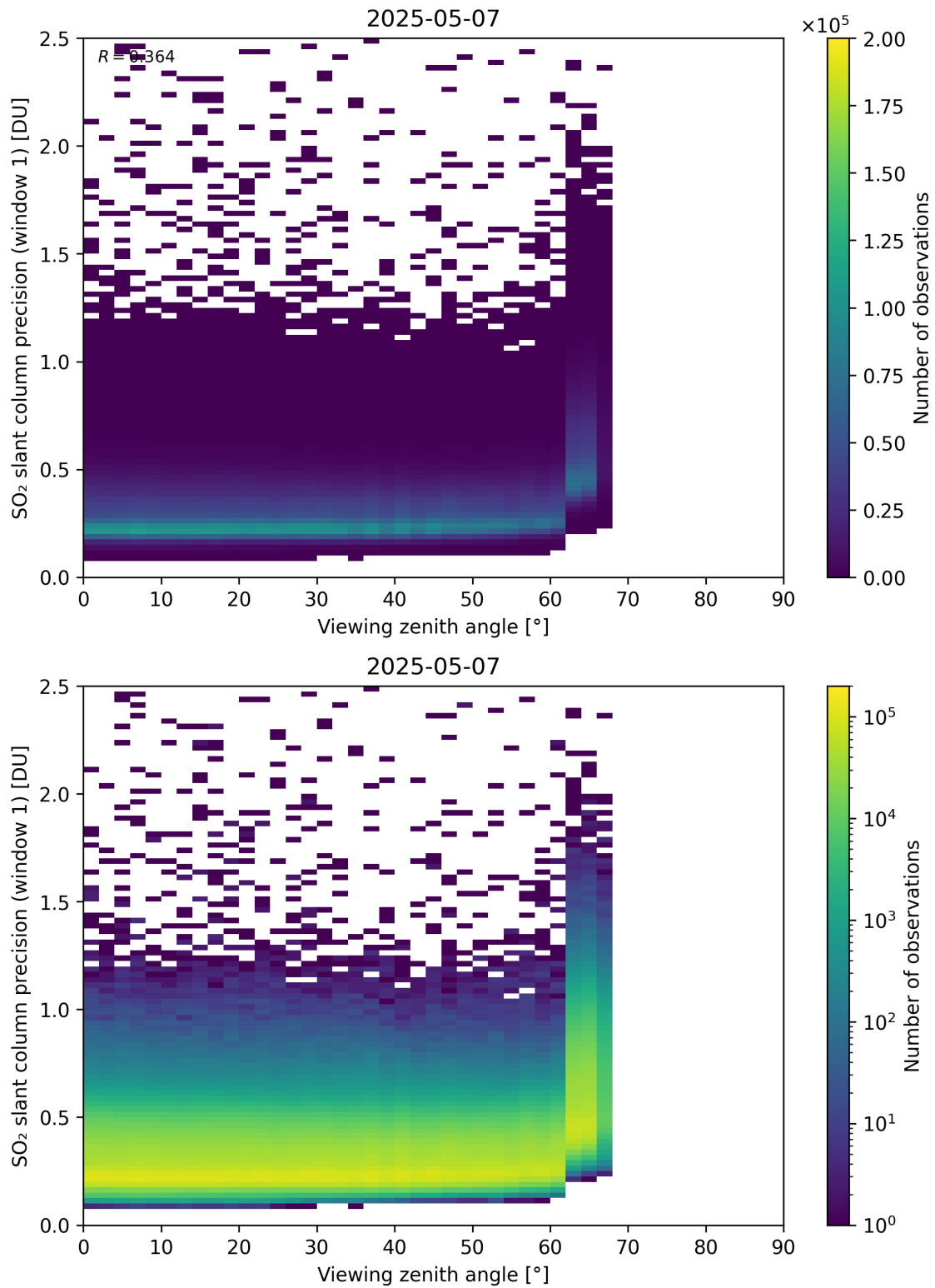
Figure 377: Scatter density plot of “Viewing zenith angle” against “SO 2 slant column precision (window 1)” for 2025-05-06 to 2025-05-08.
