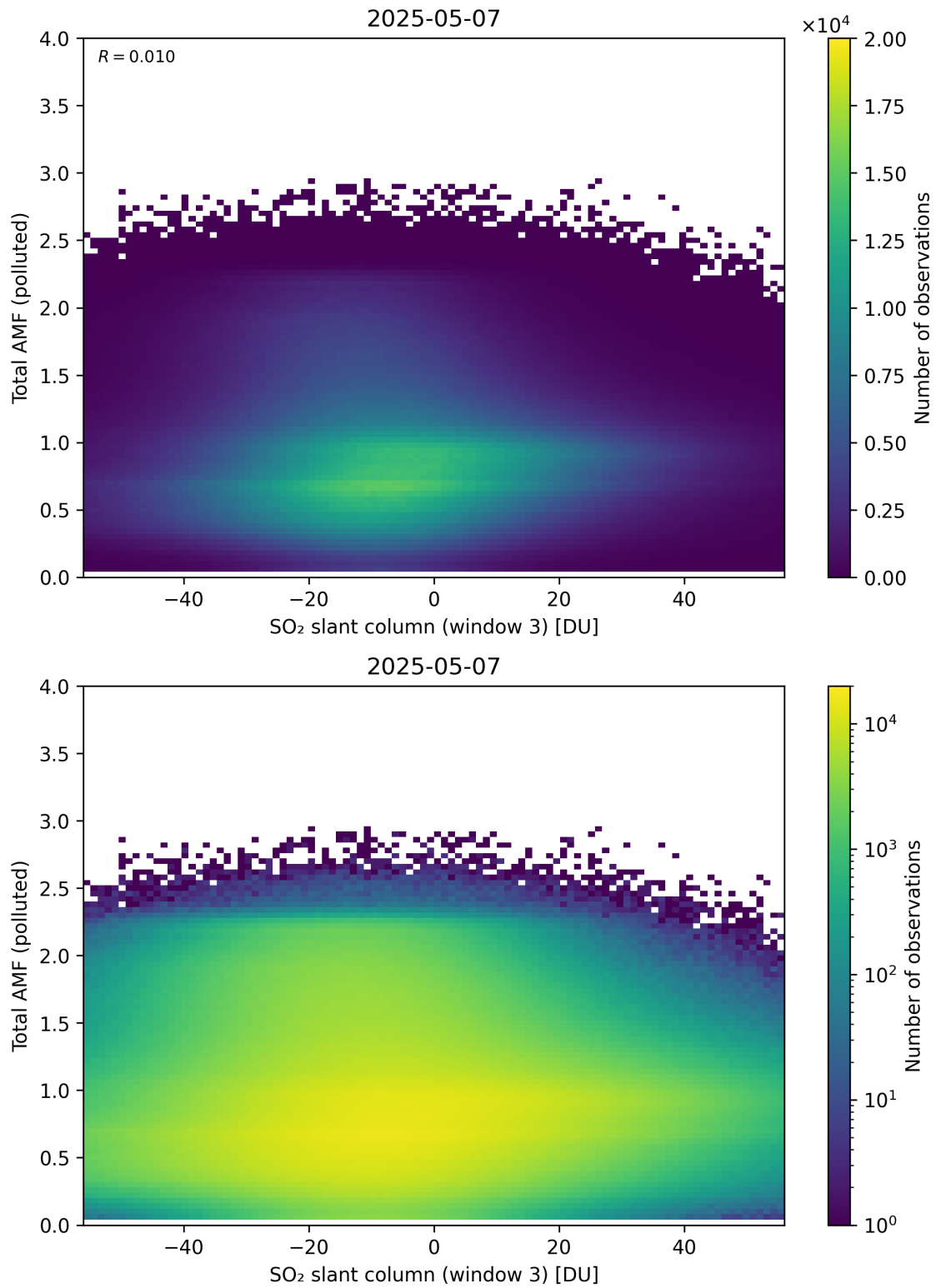
Figure 318: Scatter density plot of “SO 2 slant column (window 3)” against “Total AMF (polluted)” for 2025-05-06 to 2025-05-08.
