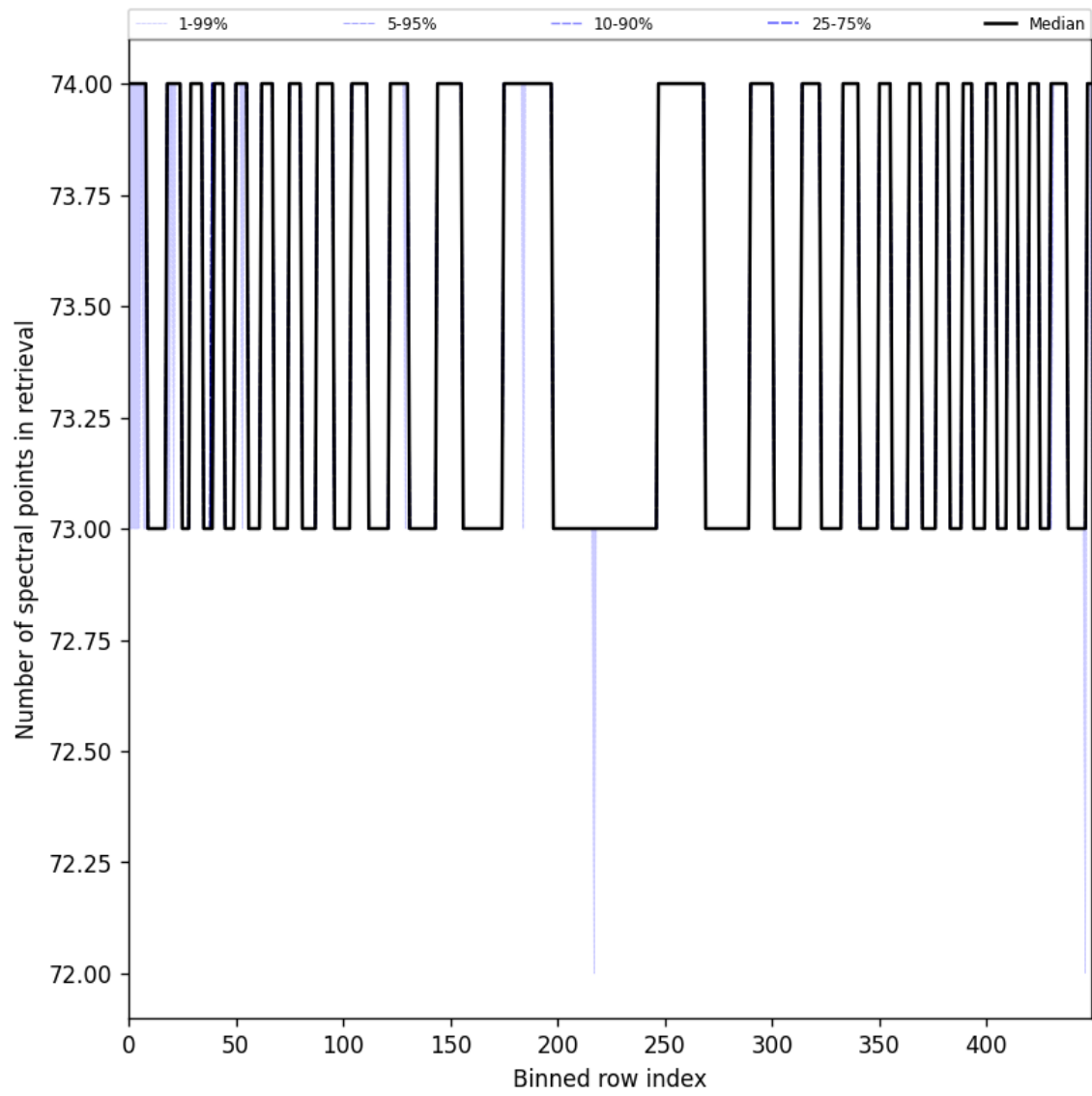
Figure 108: Along track statistics of “Number of spectral points in retrieval” for 2025-05-06 to 2025-05-08
