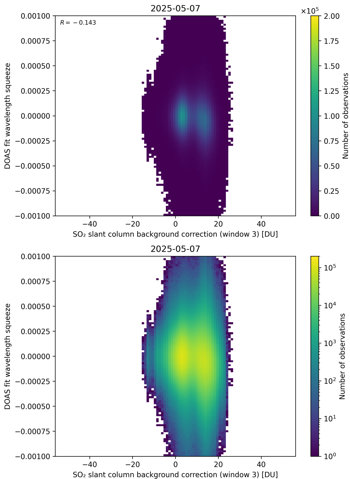
Figure 133: Scatter density plot of “SO 2 slant column background correction (window 3)” against “DOAS fit wavelength squeeze” for 2025-05-06 to 2025-05-08.
