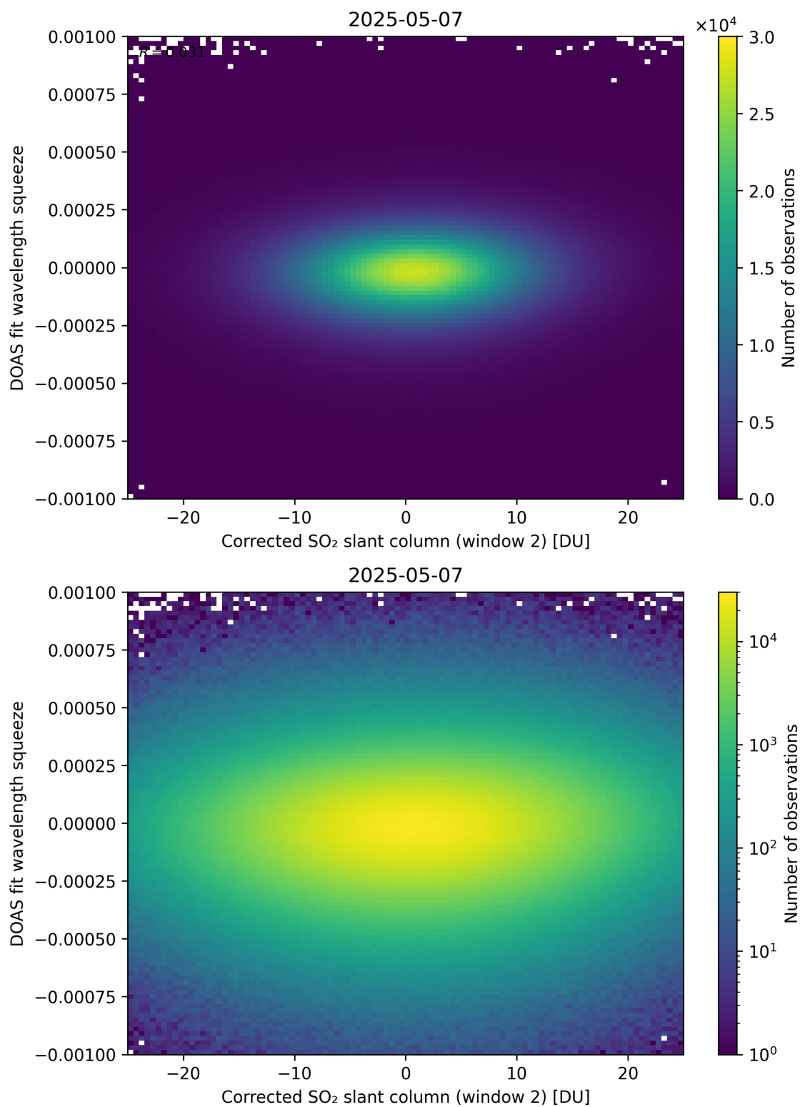
Figure 247: Scatter density plot of “Corrected SO 2 slant column (window 2)” against “DOAS fit wavelength squeeze” for 2025-05-06 to 2025-05-08.
