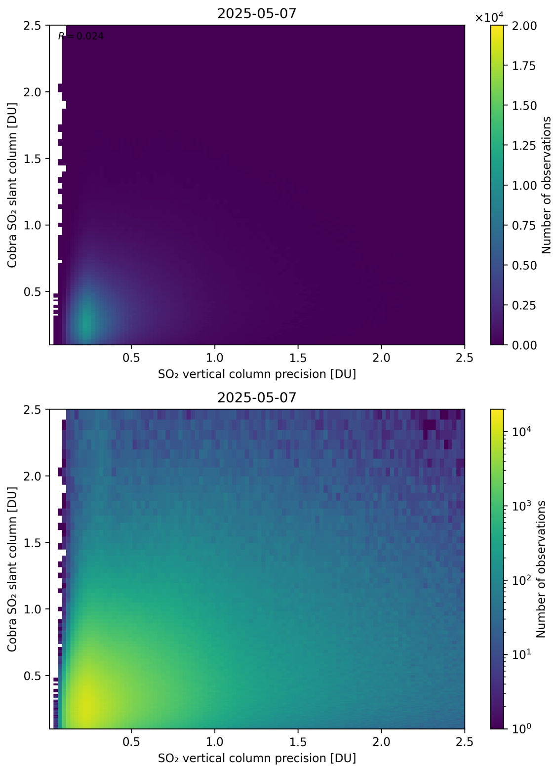
Figure 336: Scatter density plot of “SO 2 vertical column precision” against “Cobra SO 2 slant column” for 2025-05-06 to 2025-05-08.
