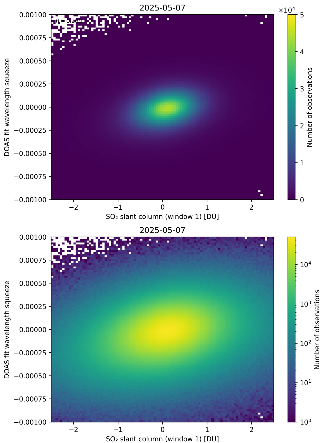
Figure 266: Scatter density plot of “SO 2 slant column (window 1)” against “DOAS fit wavelength squeeze” for 2025-05-06 to 2025-05-08.
