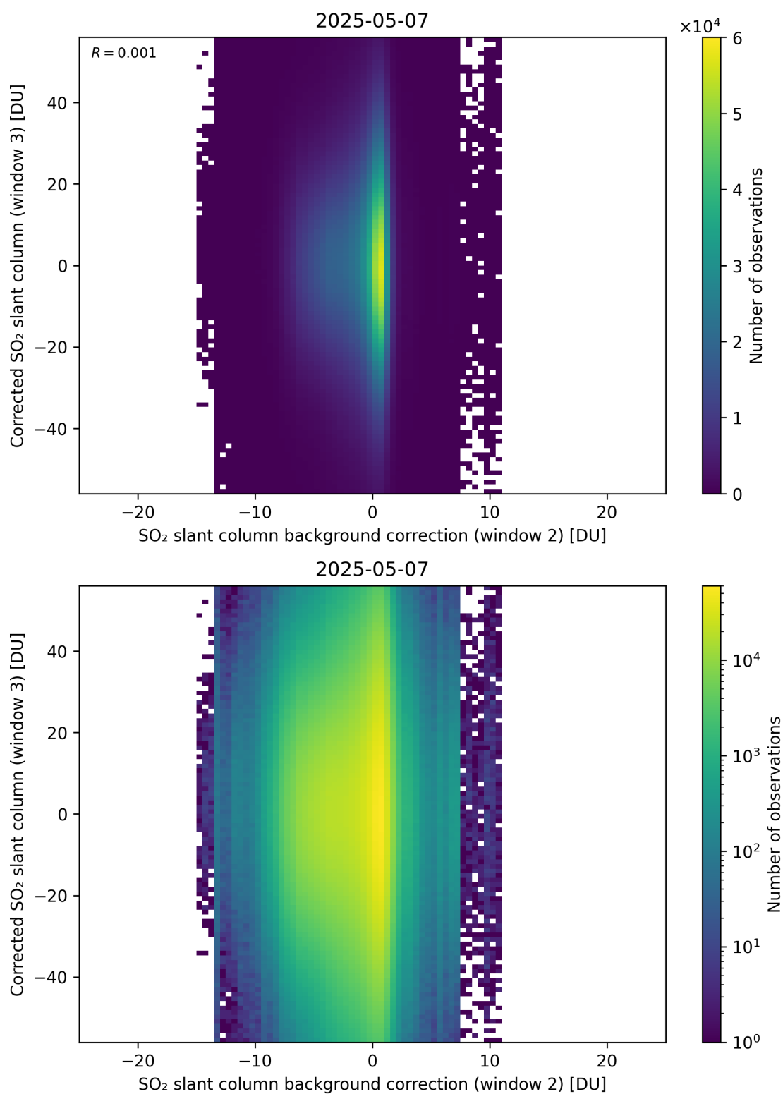
Figure 127: Scatter density plot of “SO 2 slant column background correction (window 2)” against “Corrected SO 2 slant column (window 3)” for 2025-05-06 to 2025-05-08.
