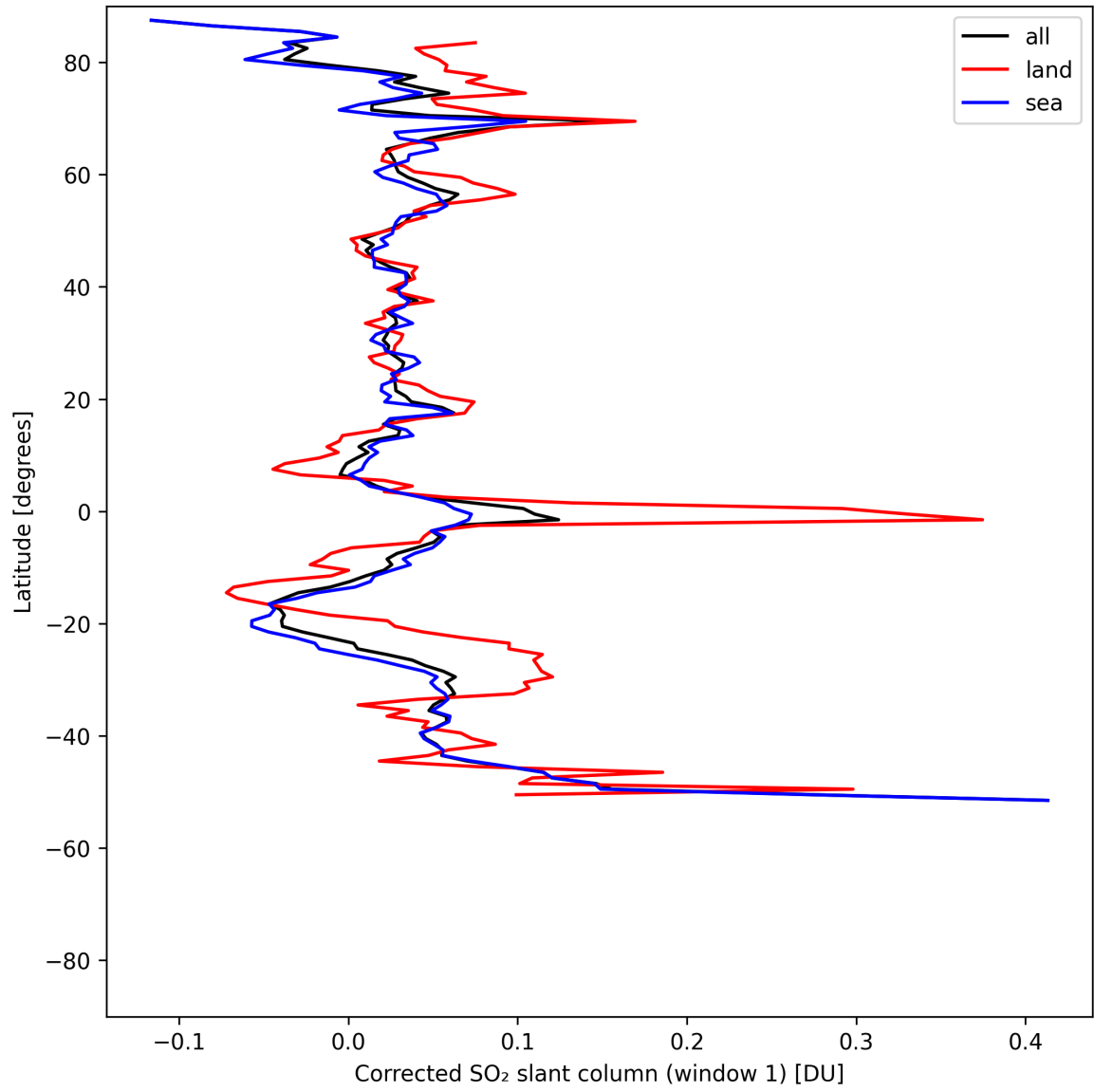
Figure 39: Zonal average of “Corrected SO 2 slant column (window 1)” for 2025-05-06 to 2025-05-08.
