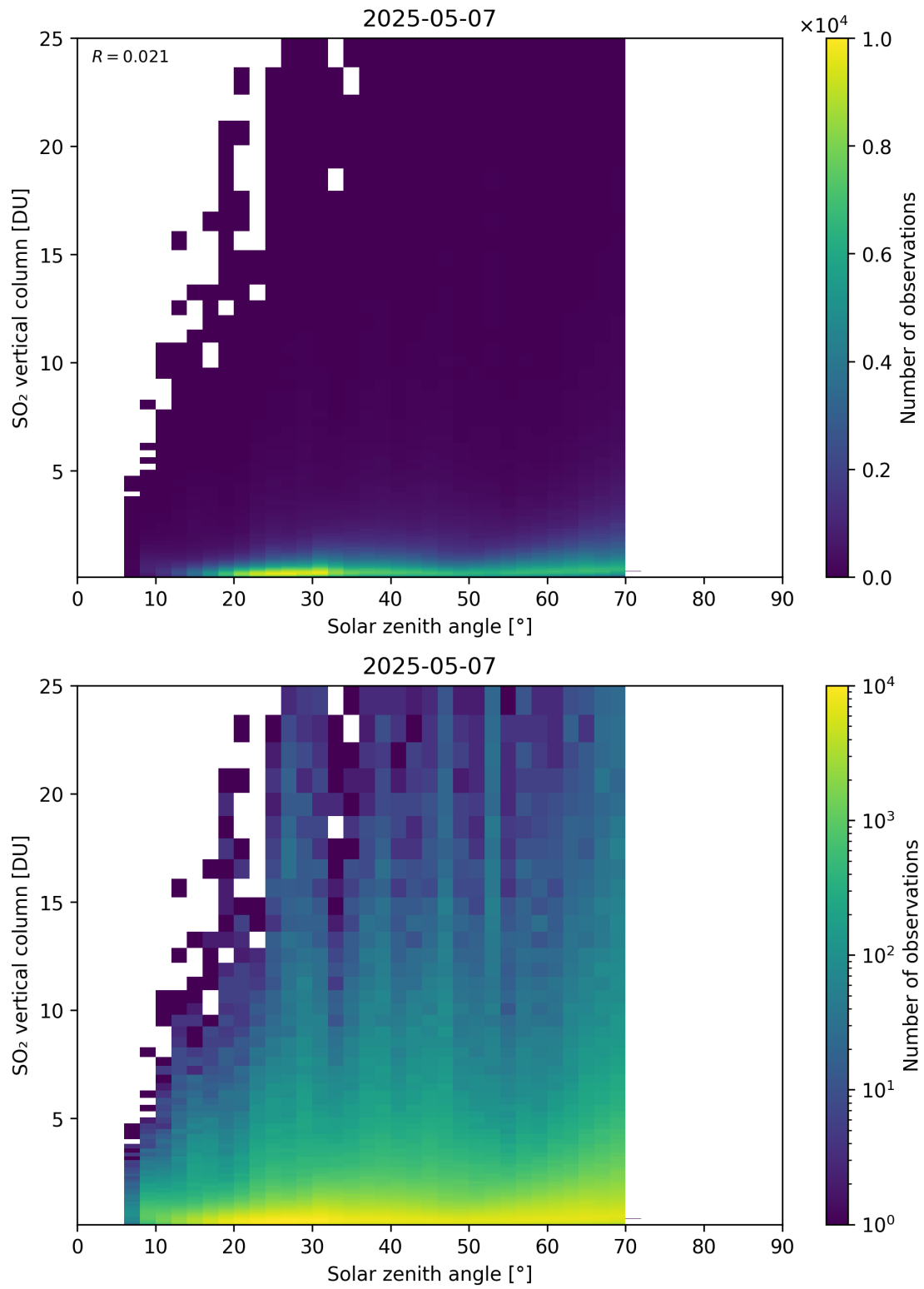
Figure 191: Scatter density plot of “Solar zenith angle” against “SO 2 vertical column” for 2025-05-06 to 2025-05-08.
