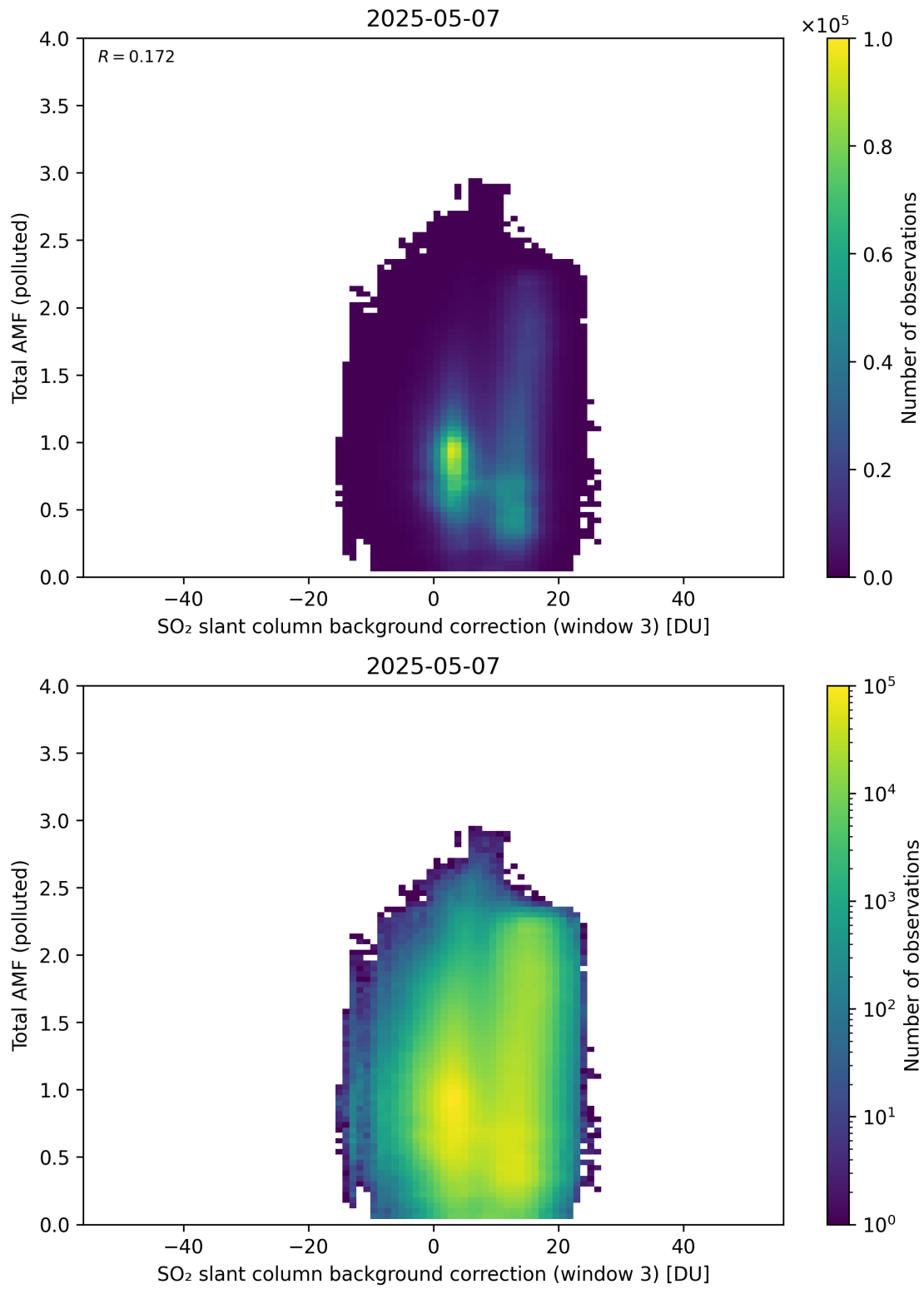
Figure 136: Scatter density plot of “SO 2 slant column background correction (window 3)” against “Total AMF (polluted)” for 2025-05-06 to 2025-05-08.
