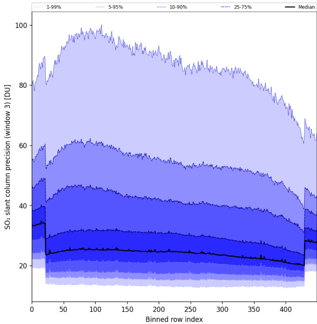
Figure 98: Along track statistics of “SO 2 slant column precision (window 3)” for 2025-05-06 to 2025-05-08
