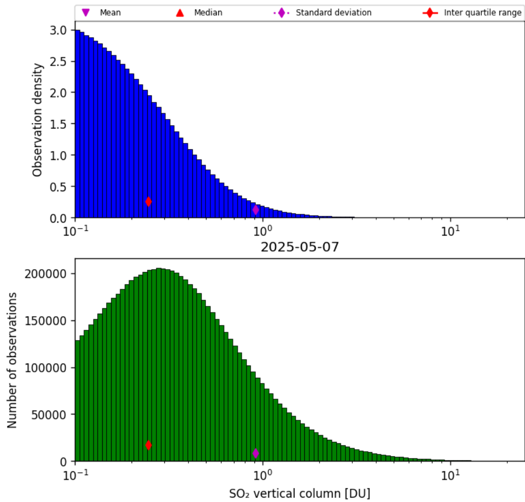
Figure 58: Histogram of “SO 2 vertical column” for 2025-05-06 to 2025-05-08
