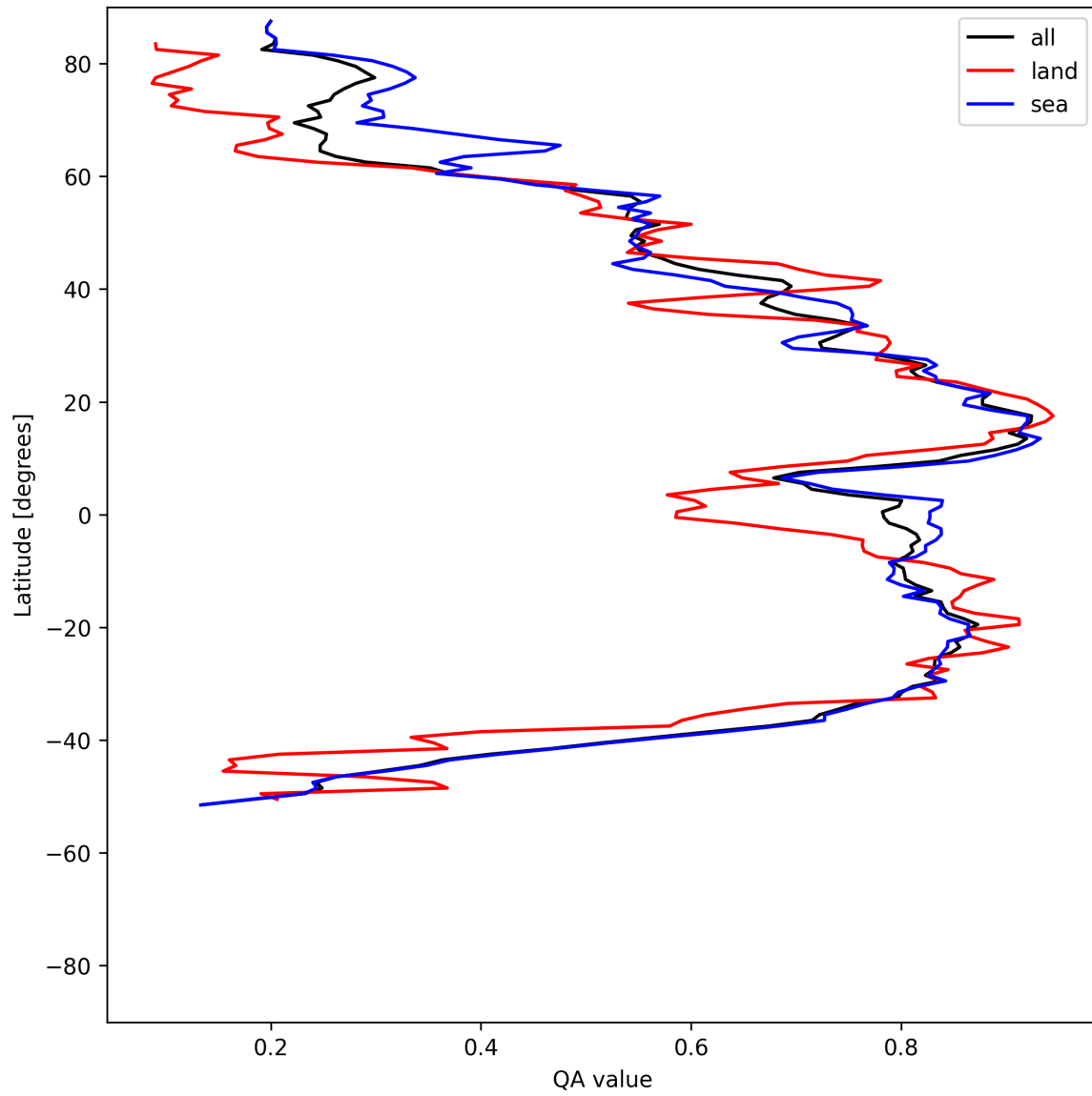
Figure 31: Zonal average of “QA value” for 2025-05-06 to 2025-05-08.
