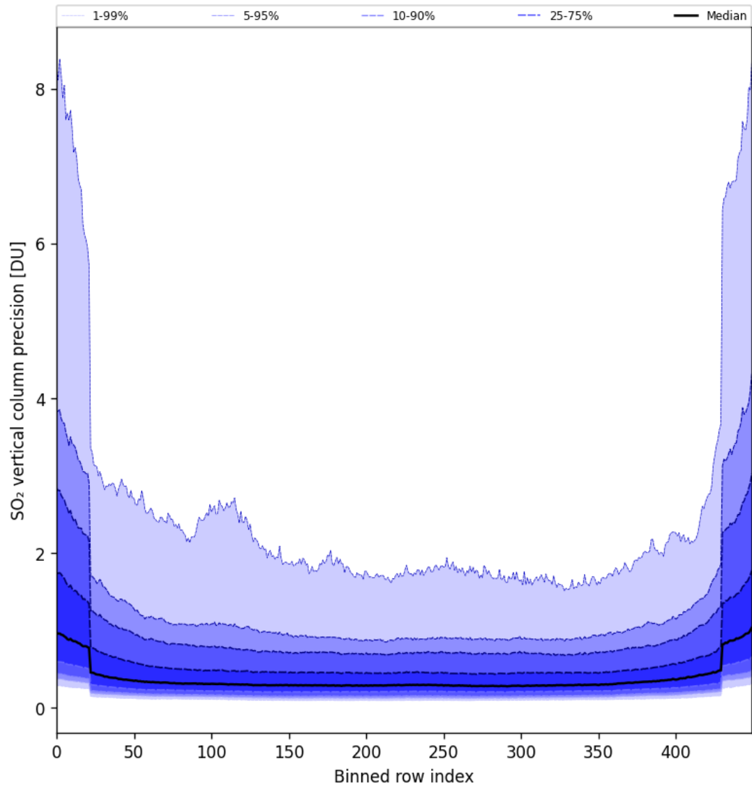
Figure 85: Along track statistics of “SO 2 vertical column precision” for 2025-05-06 to 2025-05-08
