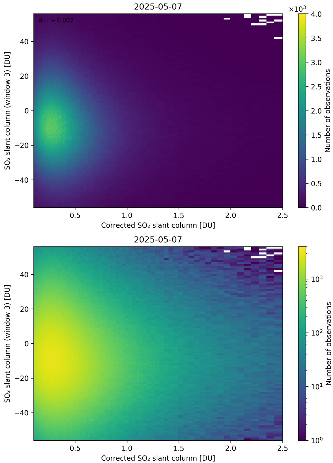
Figure 240: Scatter density plot of “Corrected SO 2 slant column” against “SO 2 slant column (window 3)” for 2025-05-06 to 2025-05-08.
