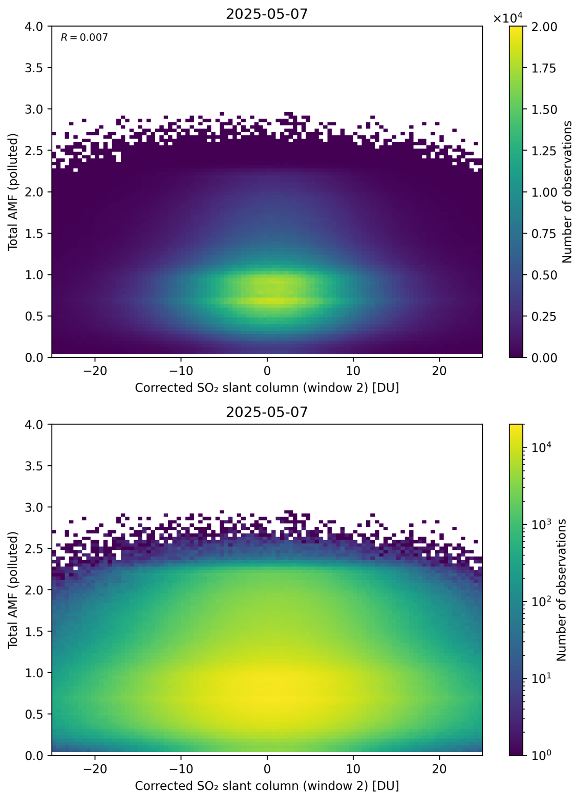
Figure 253: Scatter density plot of “Corrected SO 2 slant column (window 2)” against “Total AMF (polluted)” for 2025-05-06 to 2025-05-08.
