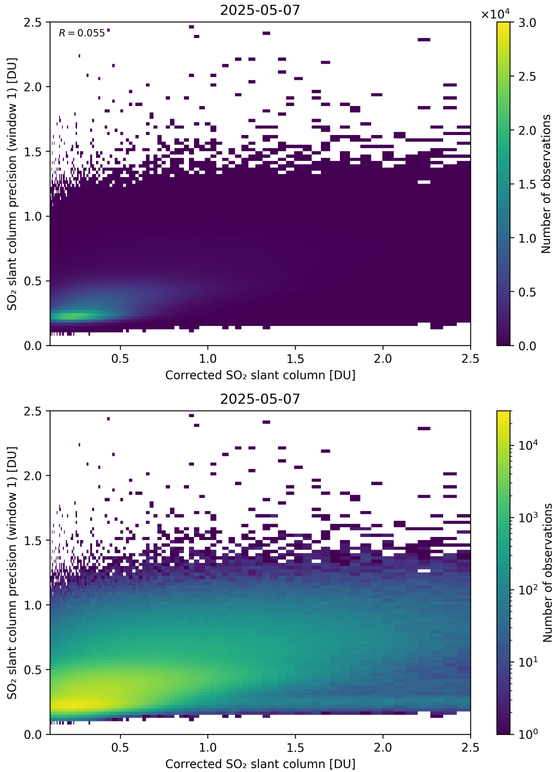
Figure 238: Scatter density plot of “Corrected SO 2 slant column” against “SO 2 slant column precision (window 1)” for 2025-05-06 to 2025-05-08.
