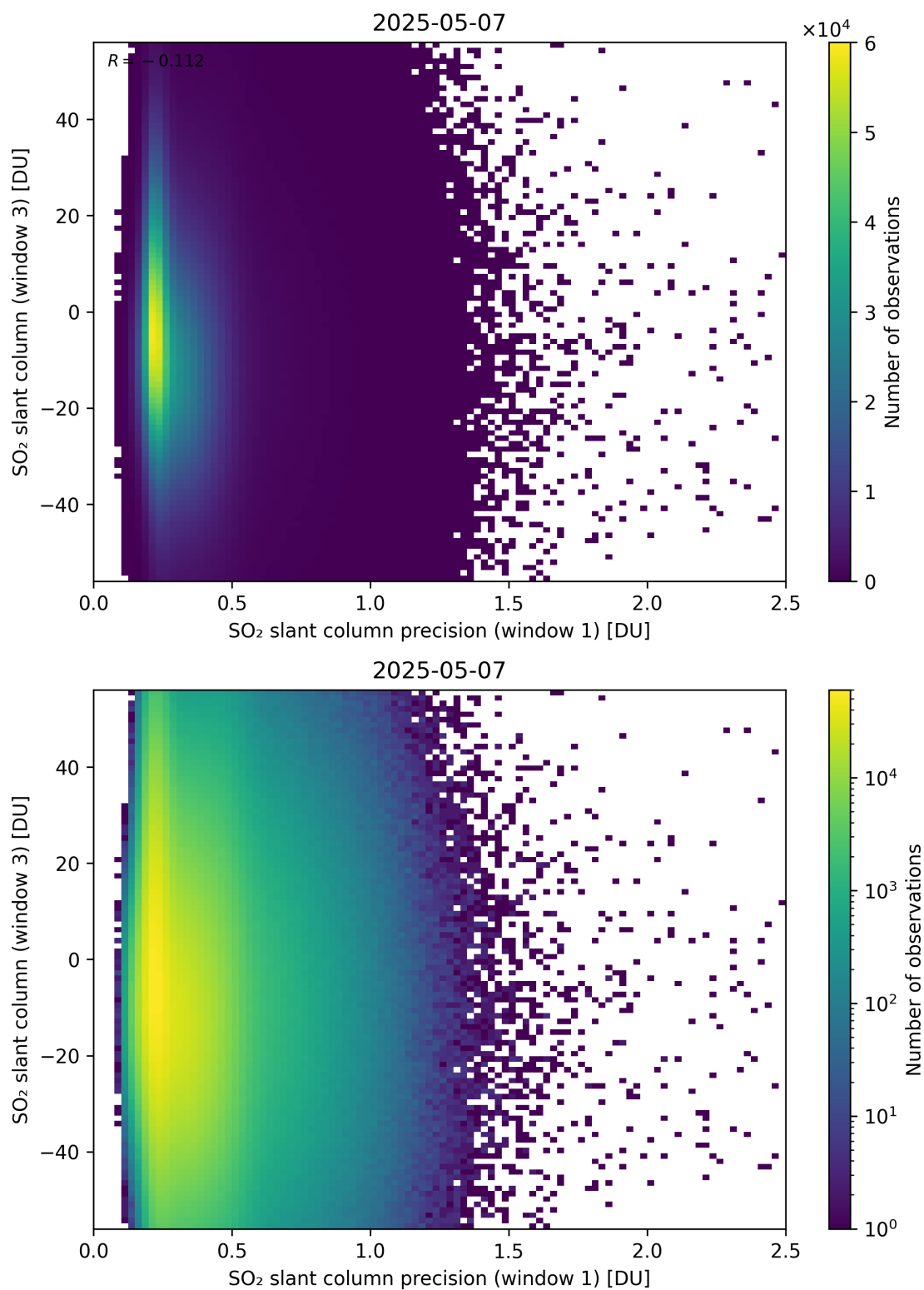
Figure 278: Scatter density plot of “SO 2 slant column precision (window 1)” against “SO 2 slant column (window 3)” for 2025-05-06 to 2025-05-08.
