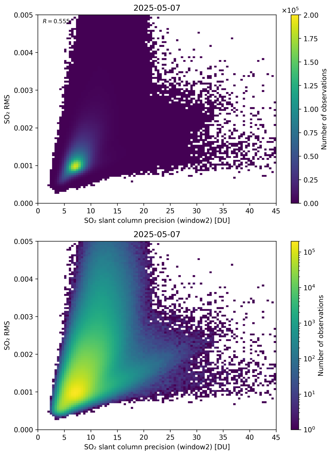
Figure 295: Scatter density plot of “SO 2 slant column precision (window2)” against “SO 2 RMS” for 2025-05-06 to 2025-05-08.
