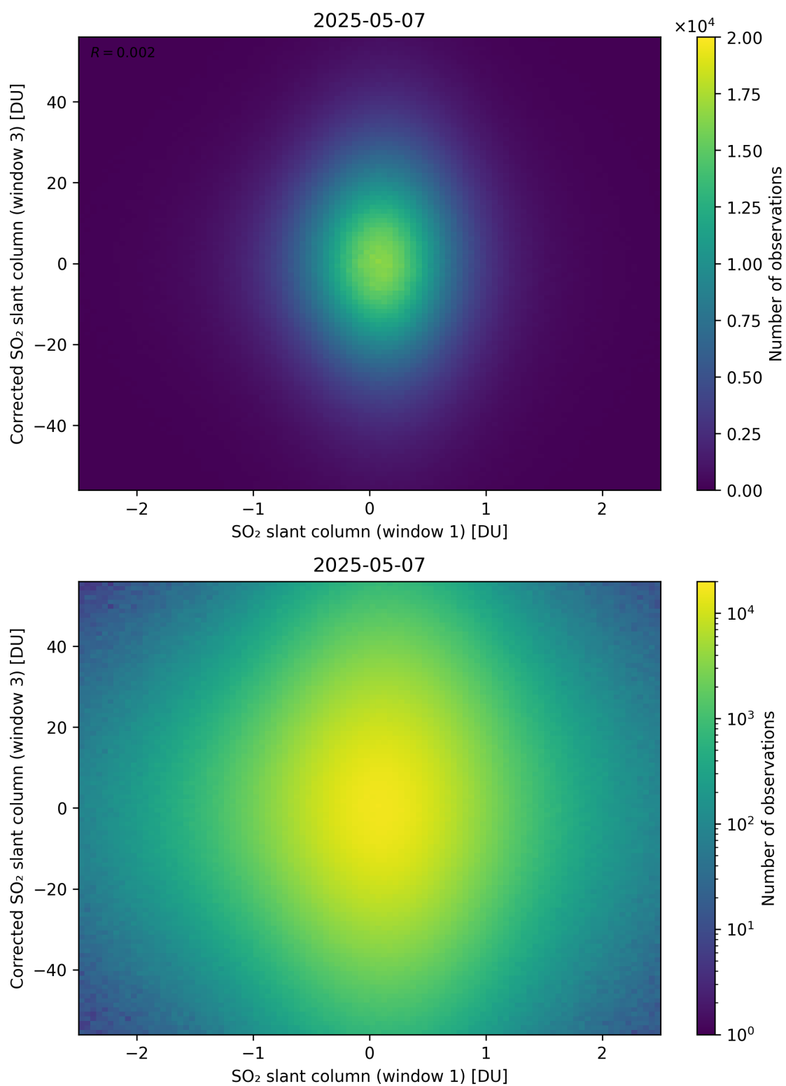
Figure 284: Scatter density plot of “SO 2 slant column (window 1)” against “Corrected SO 2 slant column (window 3)” for 2025-05-06 to 2025-05-08.
