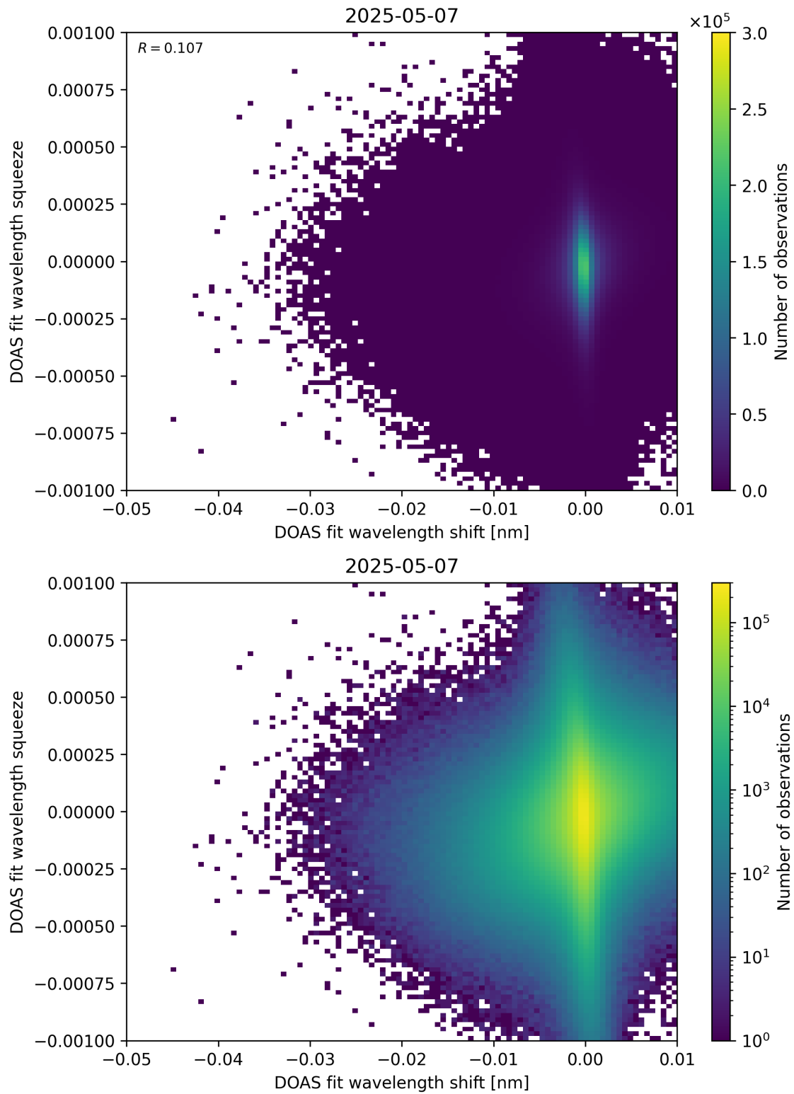
Figure 138: Scatter density plot of “DOAS fit wavelength shift” against “DOAS fit wavelength squeeze” for 2025-05-06 to 2025-05-08.
