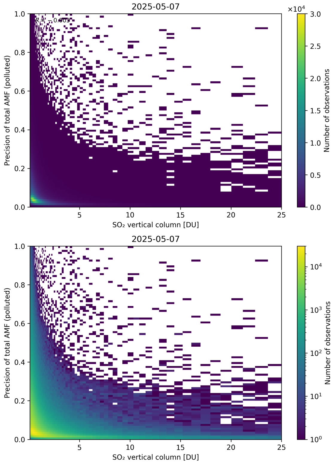
Figure 360: Scatter density plot of “SO 2 vertical column” against “Precision of total AMF (polluted)” for 2025-05-06 to 2025-05-08.
