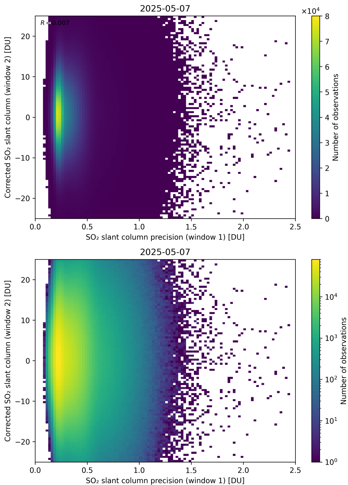
Figure 275: Scatter density plot of “SO 2 slant column precision (window 1)” against “Corrected SO 2 slant column (window 2)” for 2025-05-06 to 2025-05-08.
