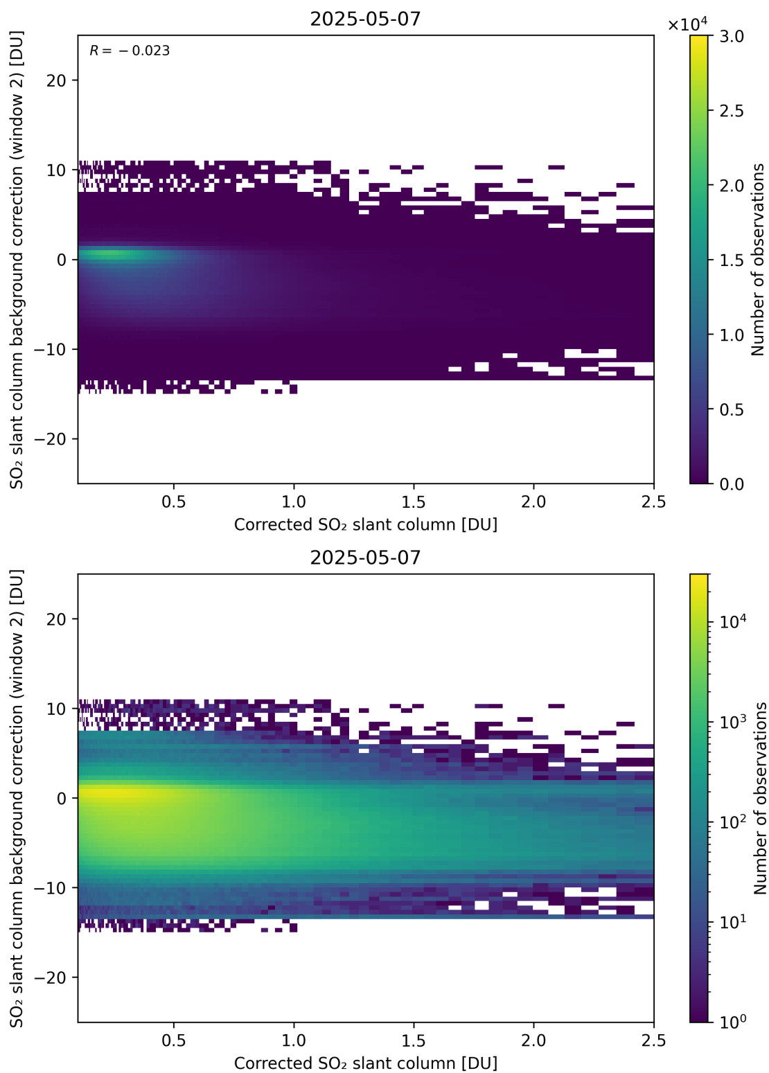
Figure 227: Scatter density plot of “Corrected SO 2 slant column” against “SO 2 slant column background correction (window 2)” for 2025-05-06 to 2025-05-08.
