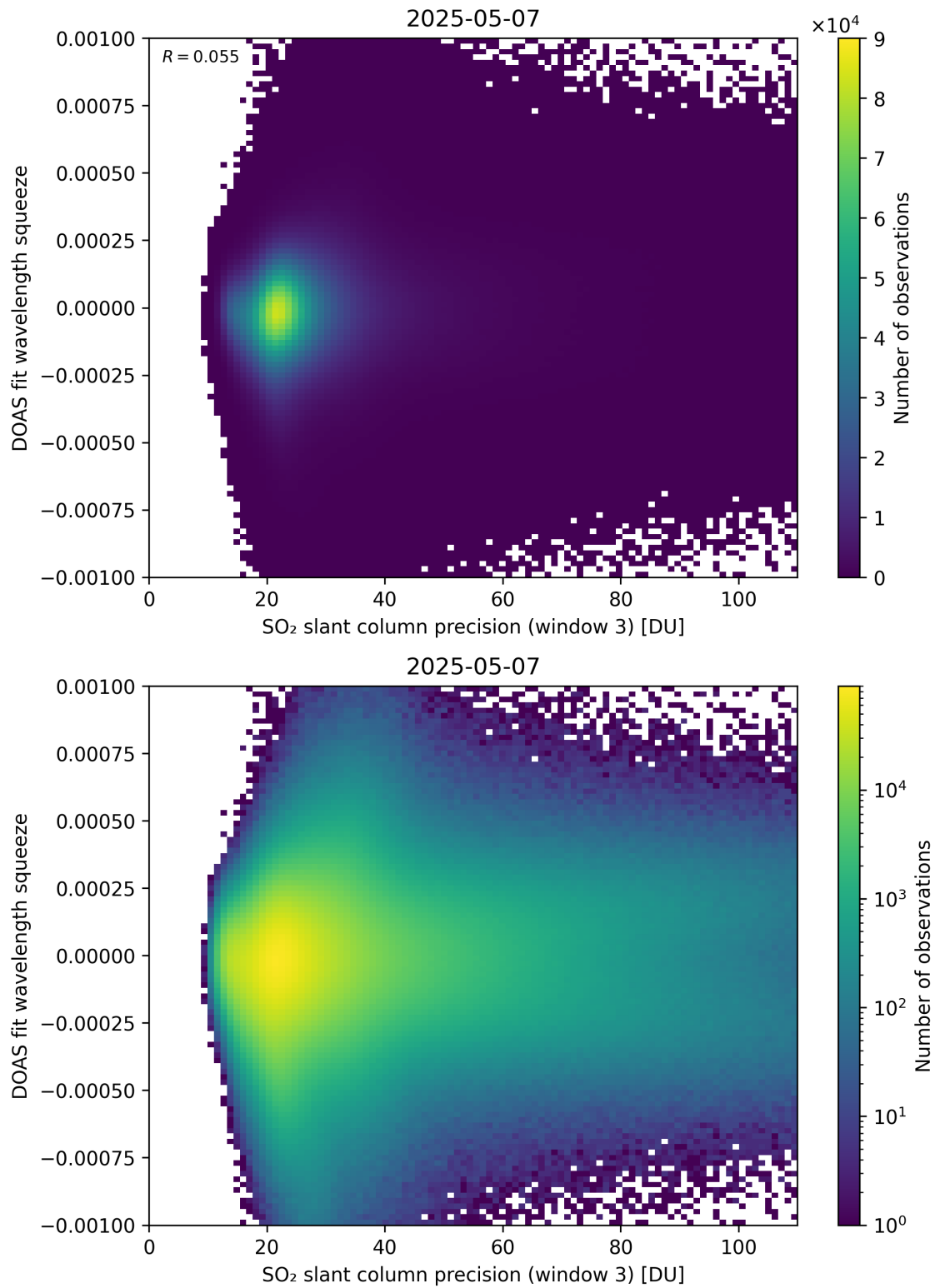
Figure 309: Scatter density plot of “SO 2 slant column precision (window 3)” against “DOAS fit wavelength squeeze” for 2025-05-06 to 2025-05-08.
