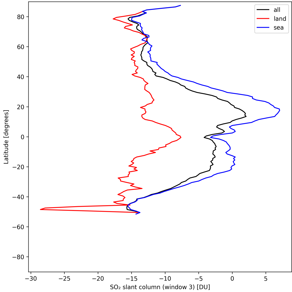
Figure 45: Zonal average of “SO 2 slant column (window 3)” for 2025-05-06 to 2025-05-08.
