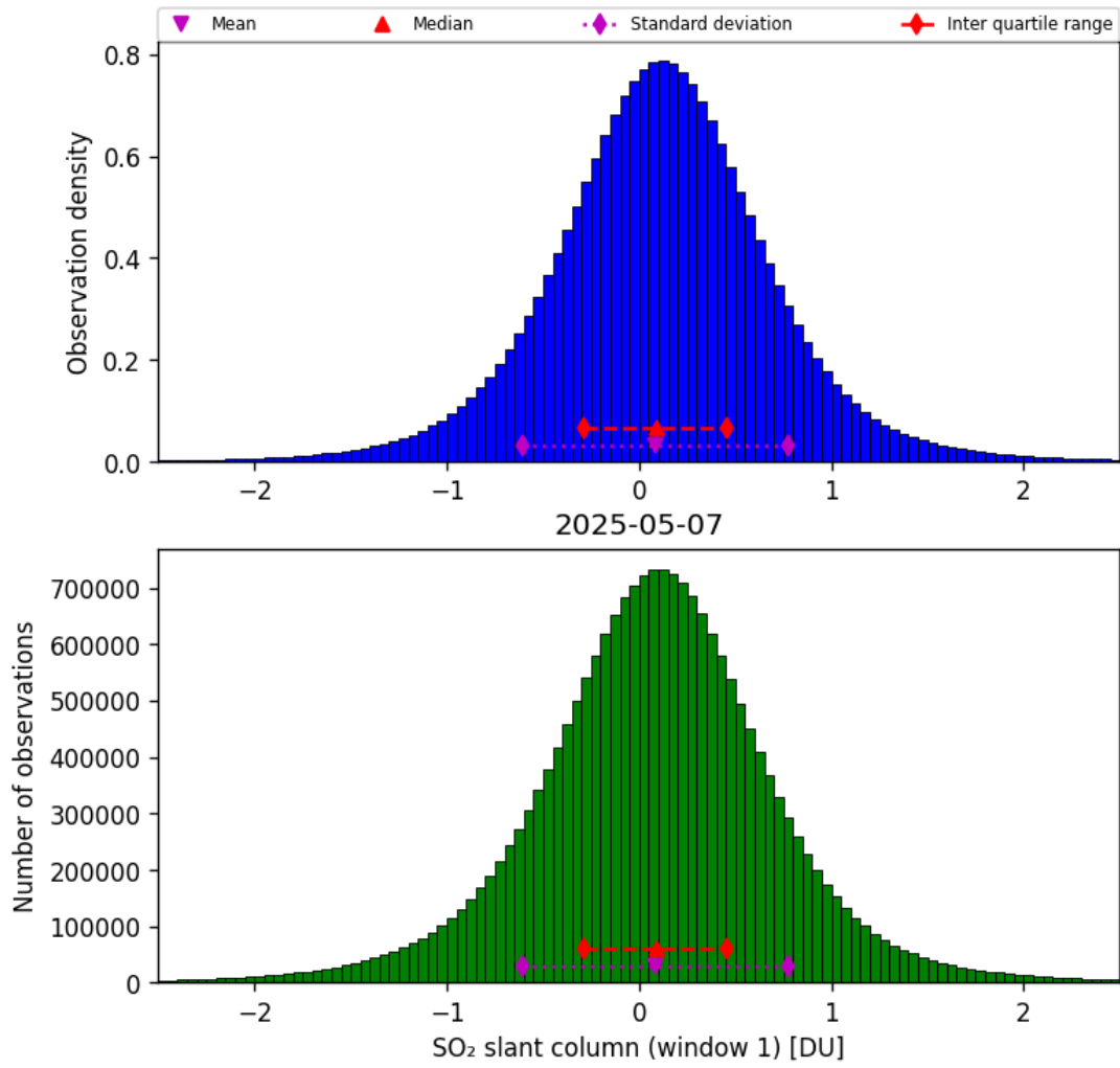
Figure 63: Histogram of “SO 2 slant column (window 1)” for 2025-05-06 to 2025-05-08
