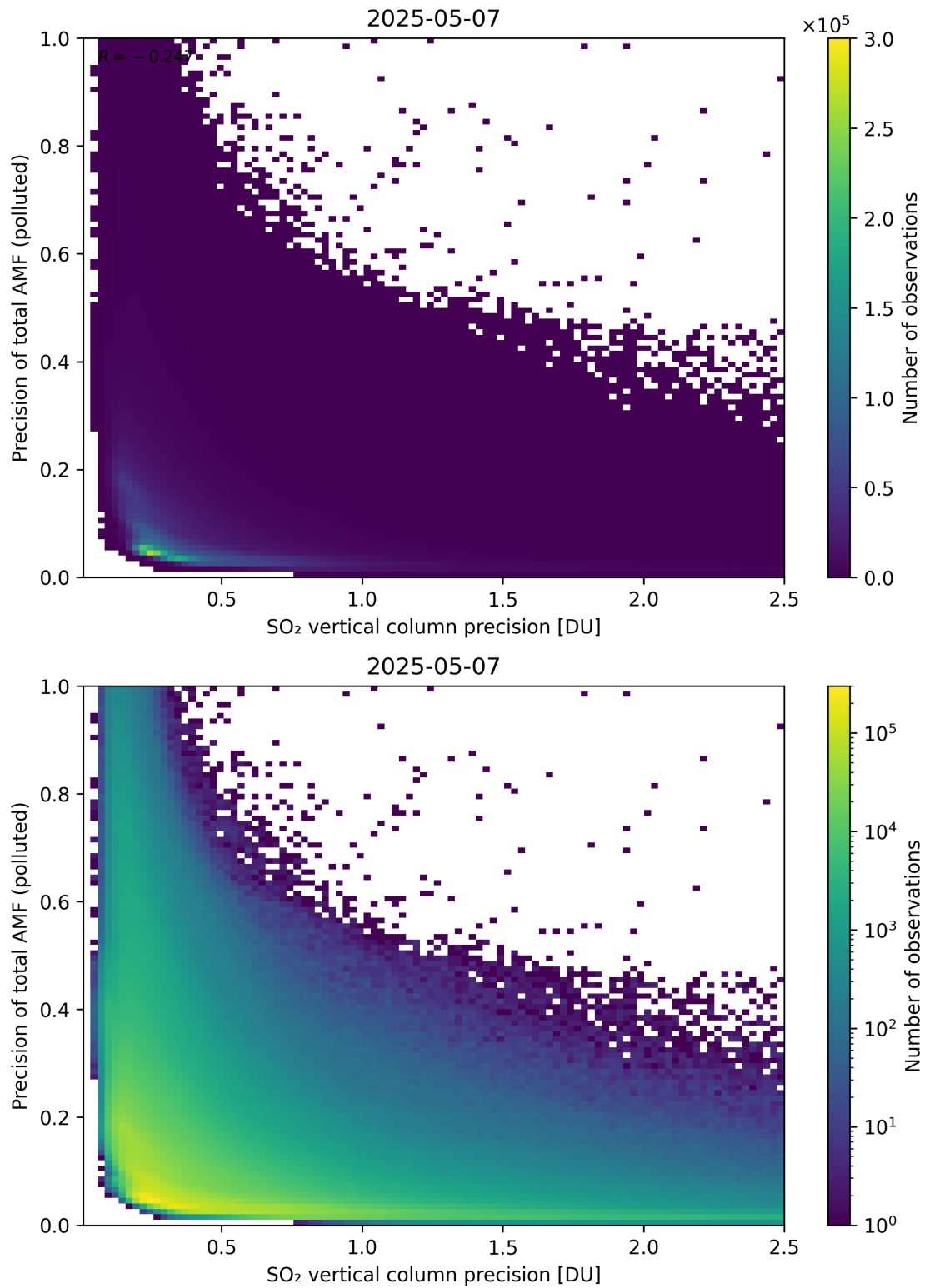
Figure 347: Scatter density plot of “SO 2 vertical column precision” against “Precision of total AMF (polluted)” for 2025-05-06 to 2025-05-08.
