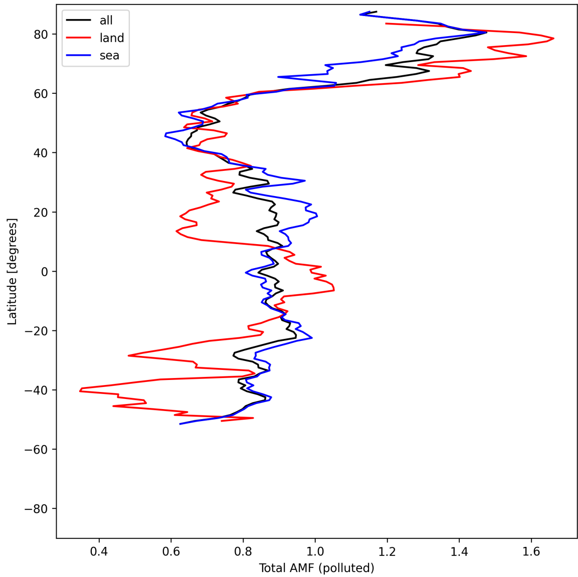
Figure 53: Zonal average of “Total AMF (polluted)” for 2025-05-06 to 2025-05-08.
