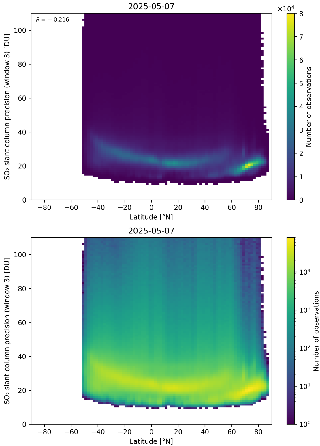
Figure 166: Scatter density plot of “Latitude” against “SO 2 slant column precision (window 3)” for 2025-05-06 to 2025-05-08.
