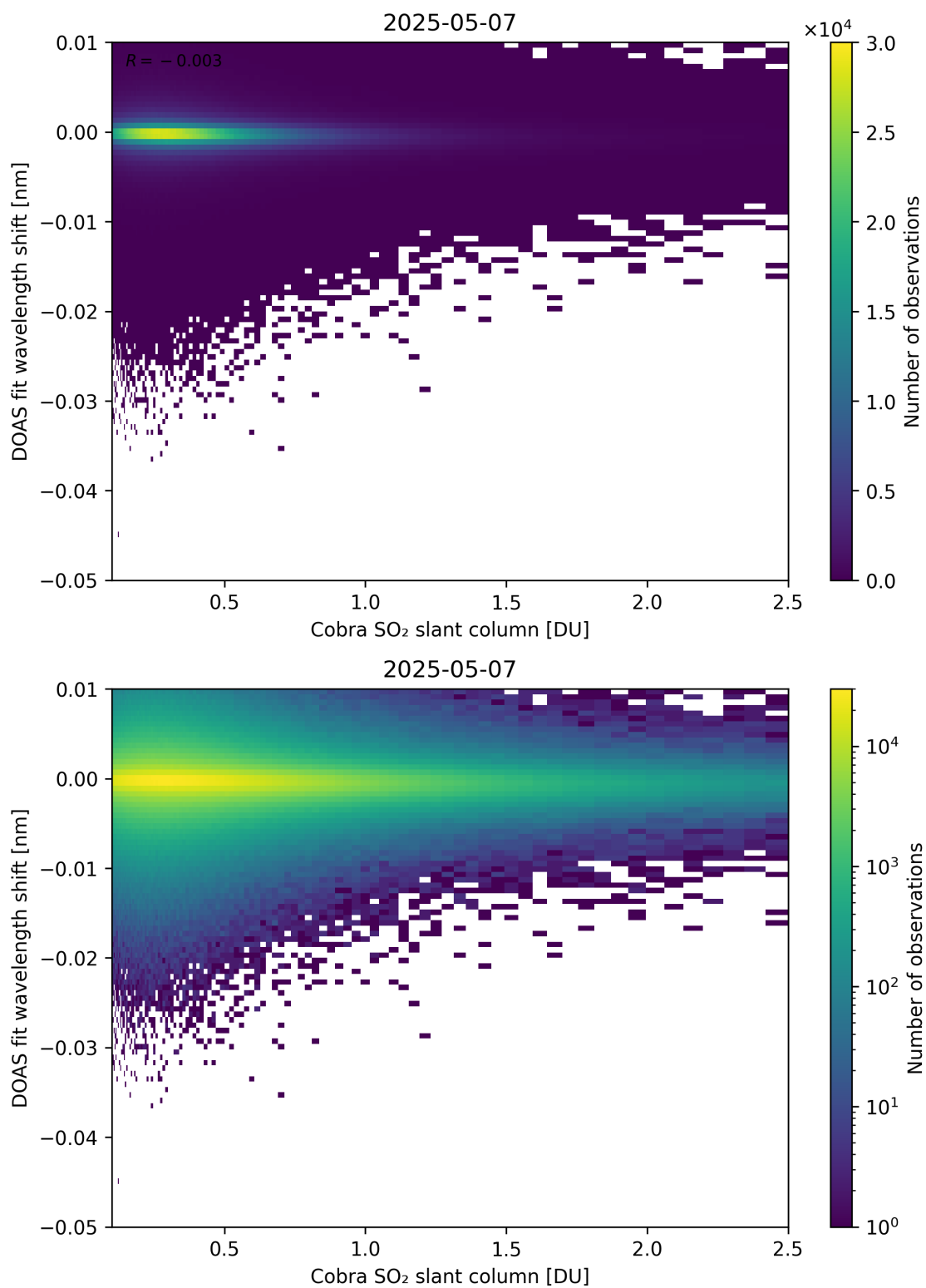
Figure 196: Scatter density plot of “Cobra SO 2 slant column” against “DOAS fit wavelength shift” for 2025-05-06 to 2025-05-08.
