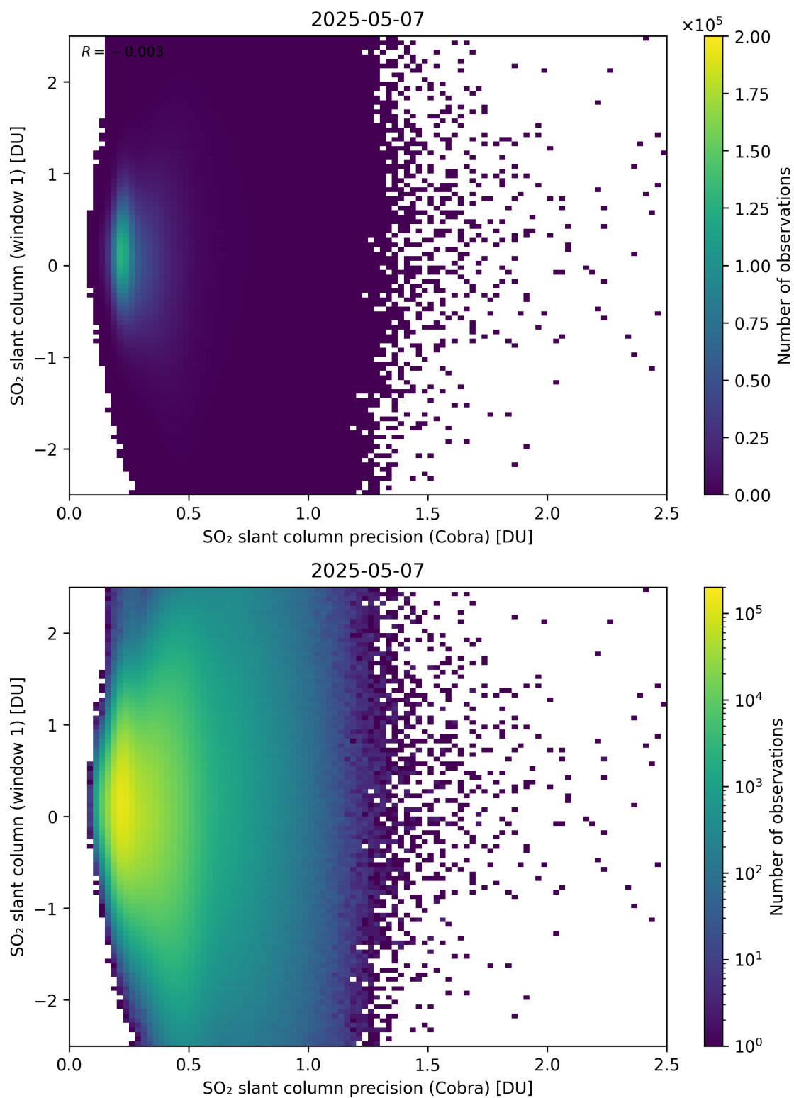
Figure 208: Scatter density plot of “SO 2 slant column precision (Cobra)” against “SO 2 slant column (window 1)” for 2025-05-06 to 2025-05-08.
