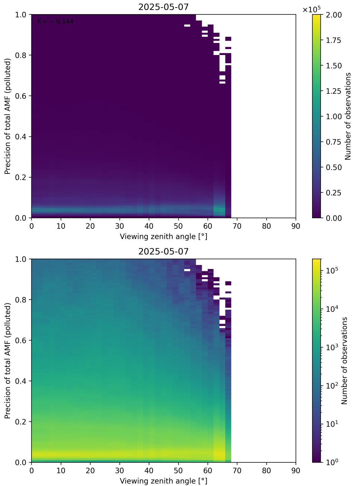
Figure 382: Scatter density plot of “Viewing zenith angle” against “Precision of total AMF (polluted)” for 2025-05-06 to 2025-05-08.
