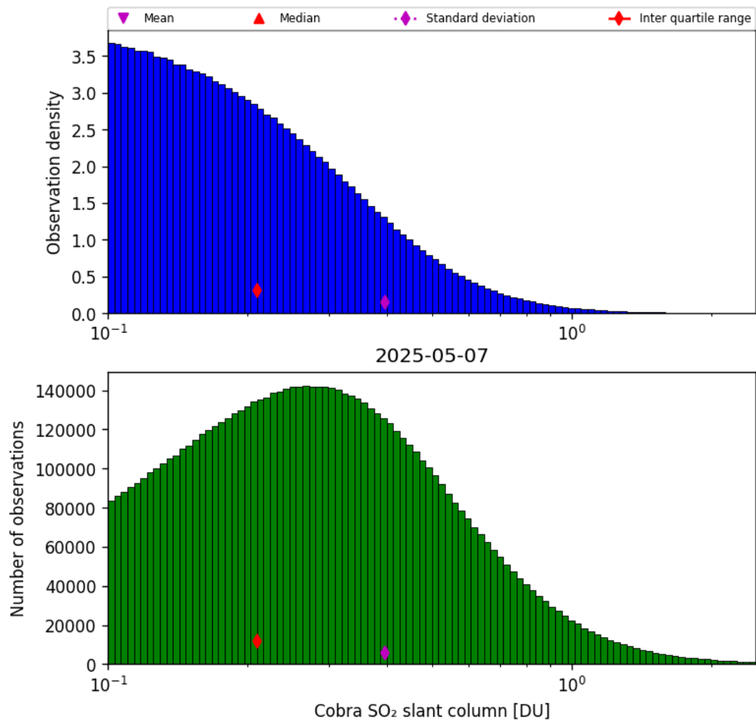
Figure 61: Histogram of “Cobra SO 2 slant column” for 2025-05-06 to 2025-05-08
