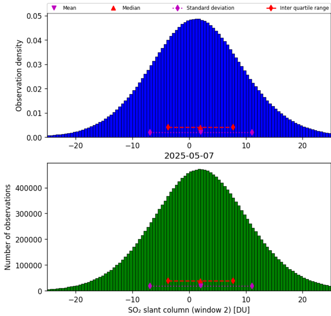
Figure 67: Histogram of “SO 2 slant column (window 2)” for 2025-05-06 to 2025-05-08
