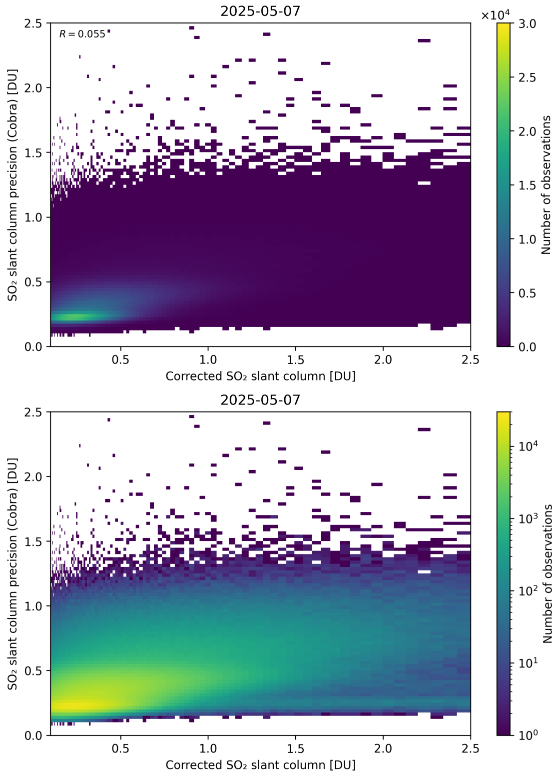
Figure 234: Scatter density plot of “Corrected SO 2 slant column” against “SO 2 slant column precision (Cobra)” for 2025-05-06 to 2025-05-08.
