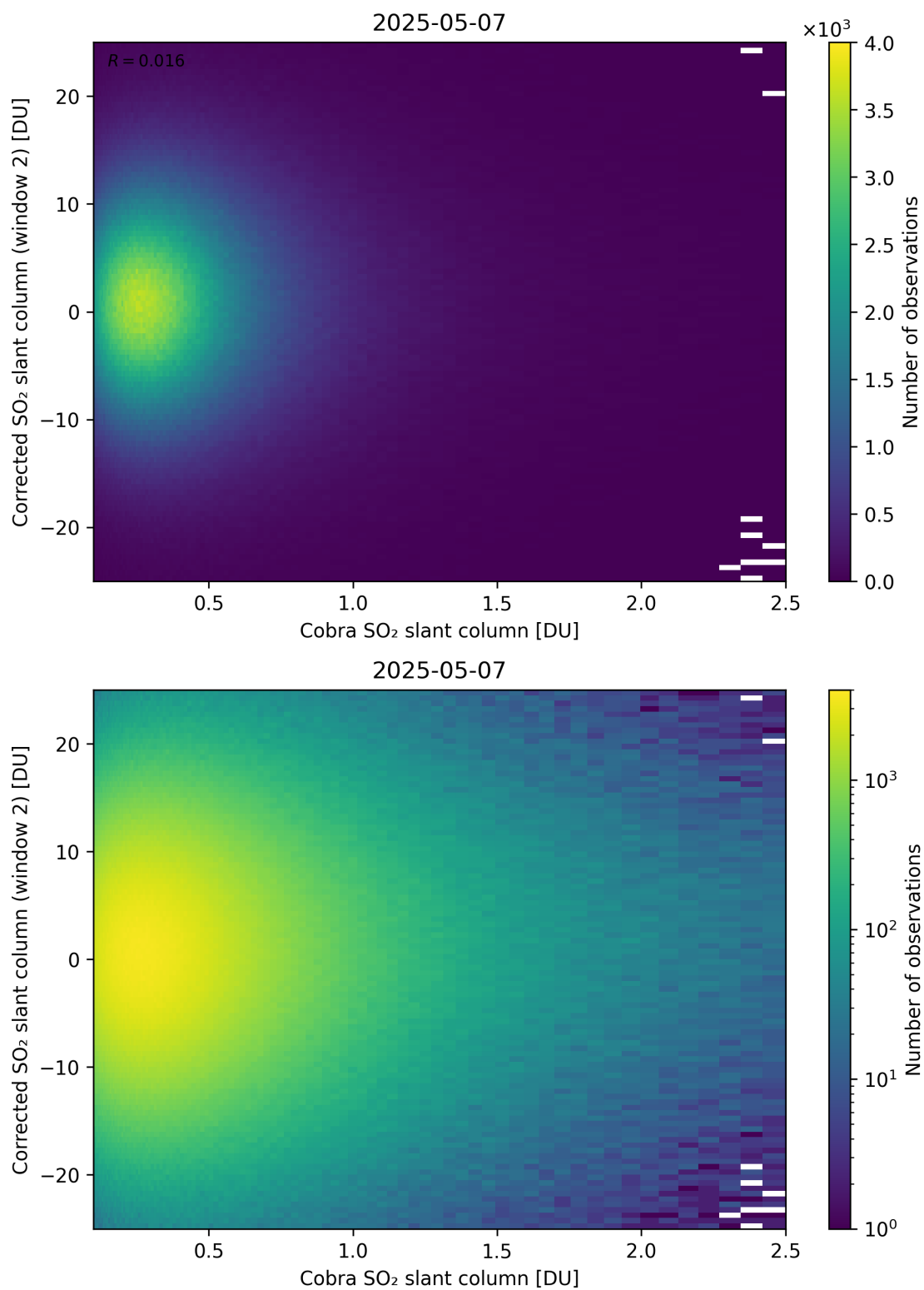
Figure 217: Scatter density plot of “Cobra SO 2 slant column” against “Corrected SO 2 slant column (window 2)” for 2025-05-06 to 2025-05-08.
