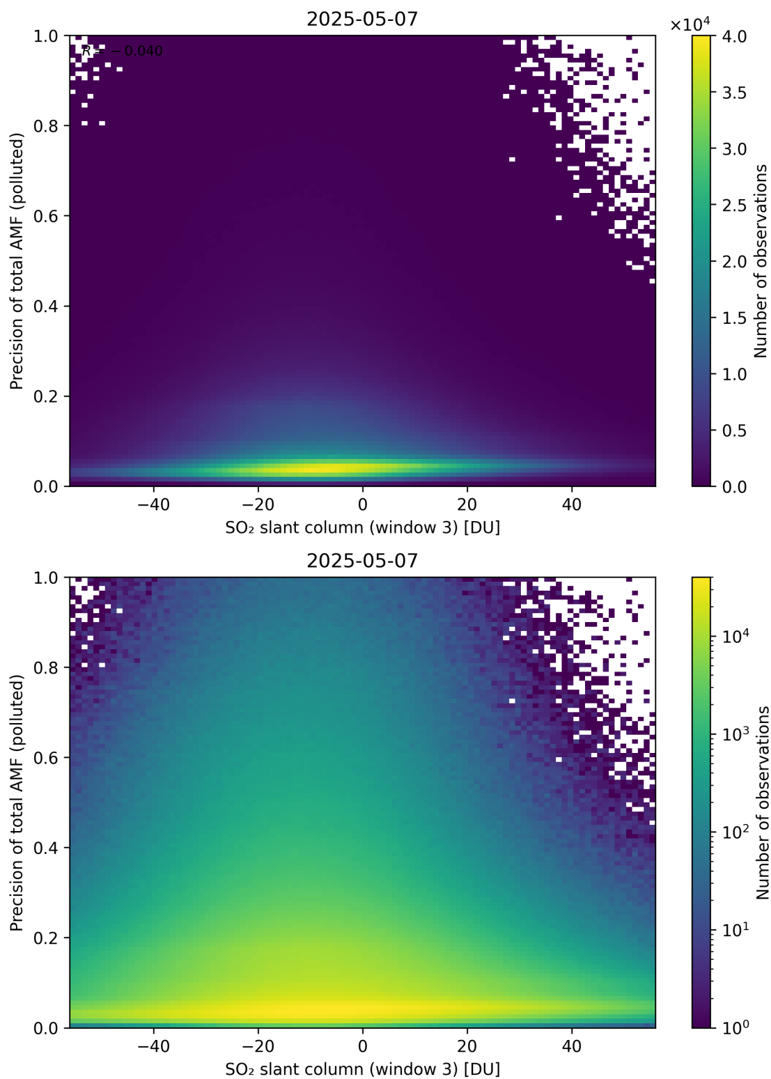
Figure 319: Scatter density plot of “SO 2 slant column (window 3)” against “Precision of total AMF (polluted)” for 2025-05-06 to 2025-05-08.
