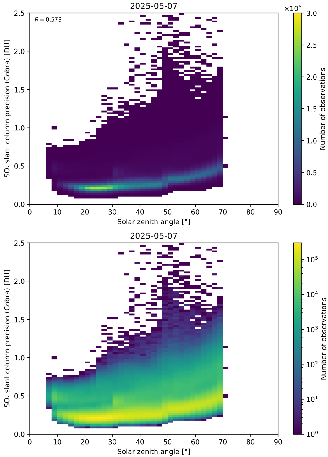
Figure 180: Scatter density plot of “Solar zenith angle” against “SO 2 slant column precision (Cobra)” for 2025-05-06 to 2025-05-08.
