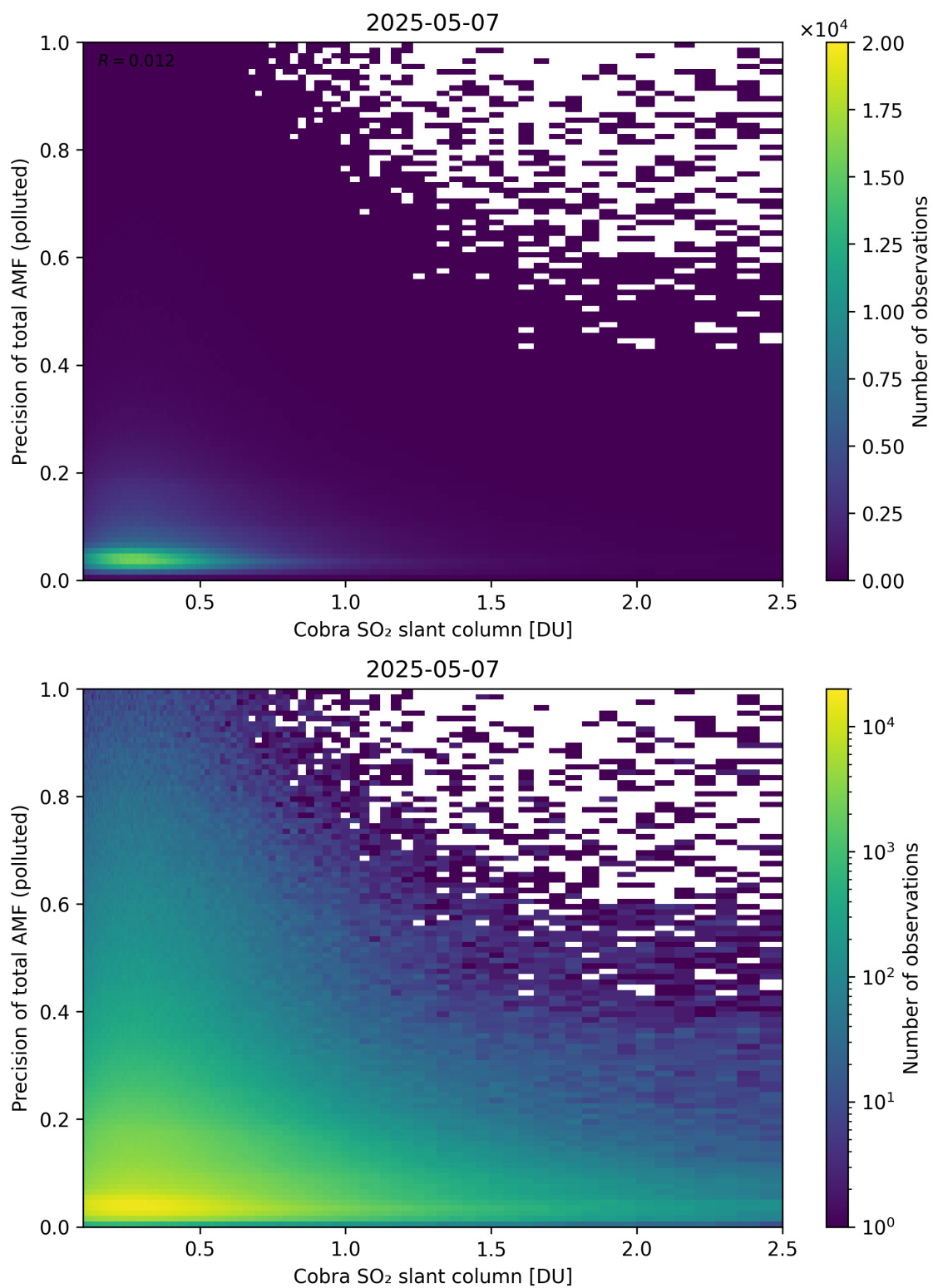
Figure 225: Scatter density plot of “Cobra SO 2 slant column” against “Precision of total AMF (polluted)” for 2025-05-06 to 2025-05-08.
