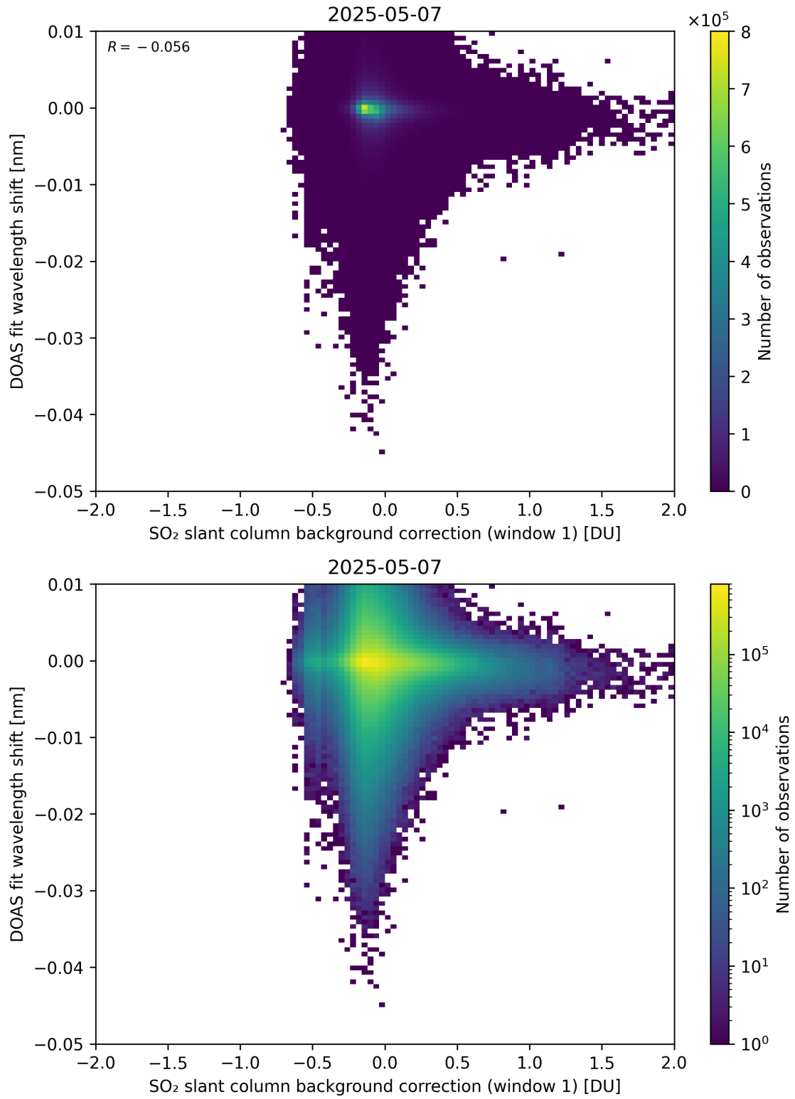
Figure 111: Scatter density plot of “SO 2 slant column background correction (window 1)” against “DOAS fit wavelength shift” for 2025-05-06 to 2025-05-08.
