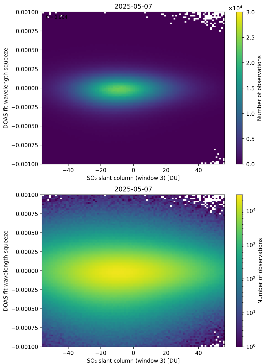
Figure 305: Scatter density plot of “SO 2 slant column (window 3)” against “DOAS fit wavelength squeeze” for 2025-05-06 to 2025-05-08.
