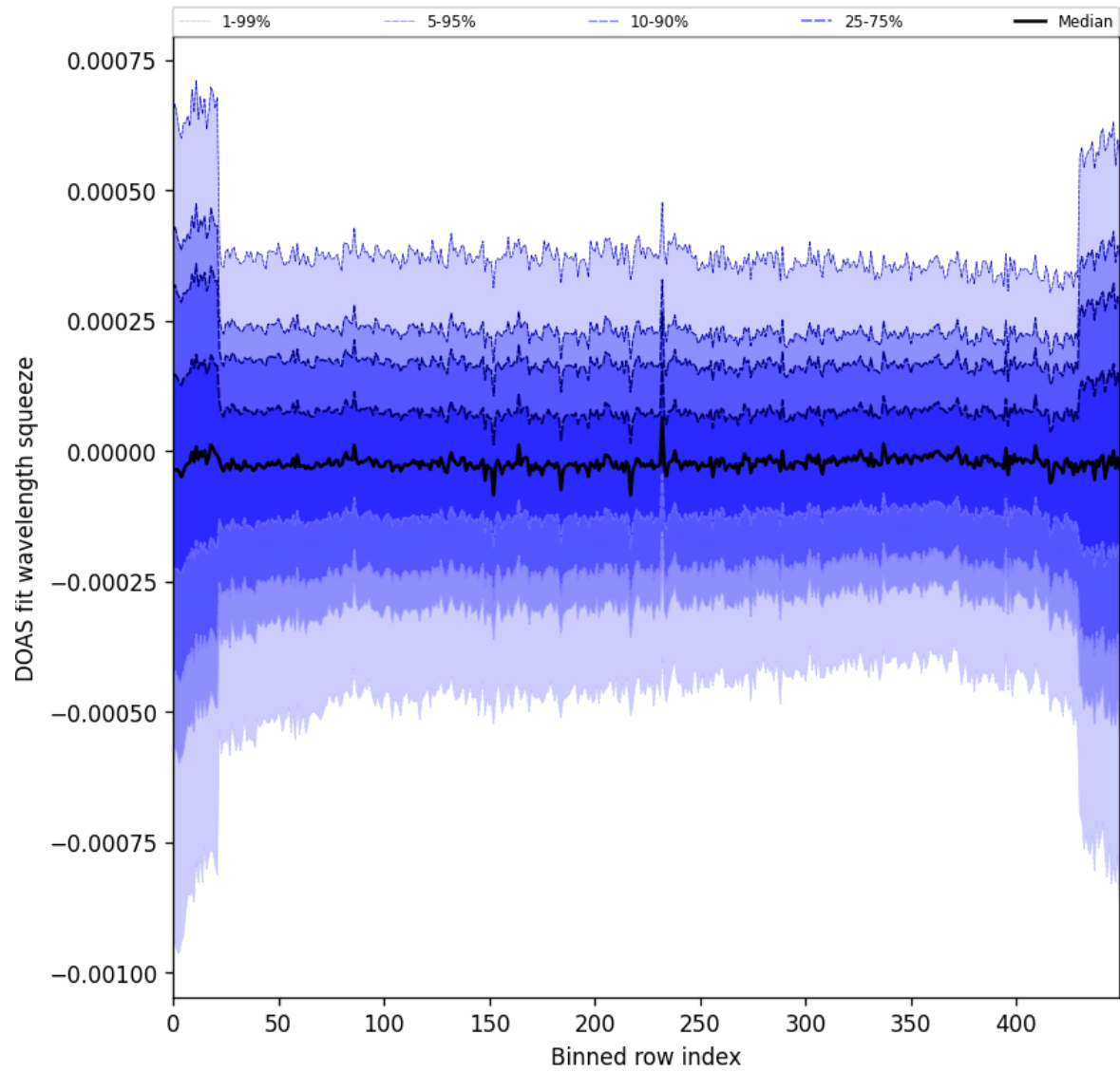
Figure 103: Along track statistics of “DOAS fit wavelength squeeze” for 2025-05-06 to 2025-05-08
