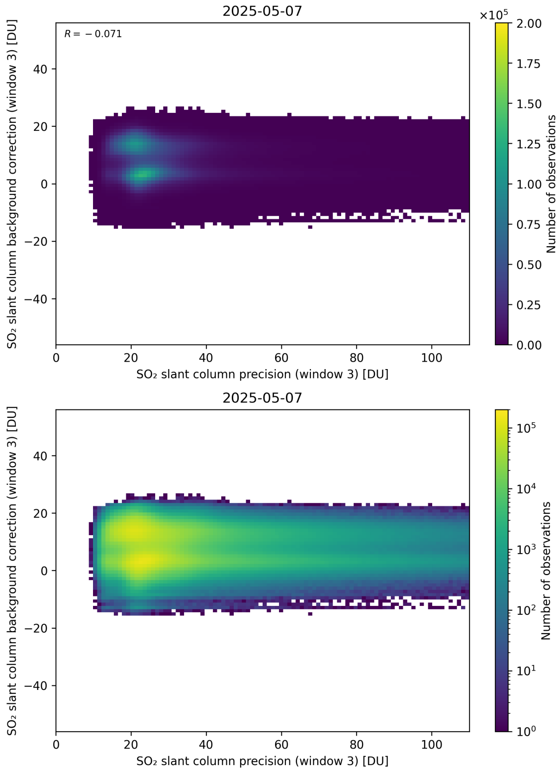
Figure 307: Scatter density plot of “SO 2 slant column precision (window 3)” against “SO 2 slant column background correction (window 3)” for 2025-05-06 to 2025-05-08.
