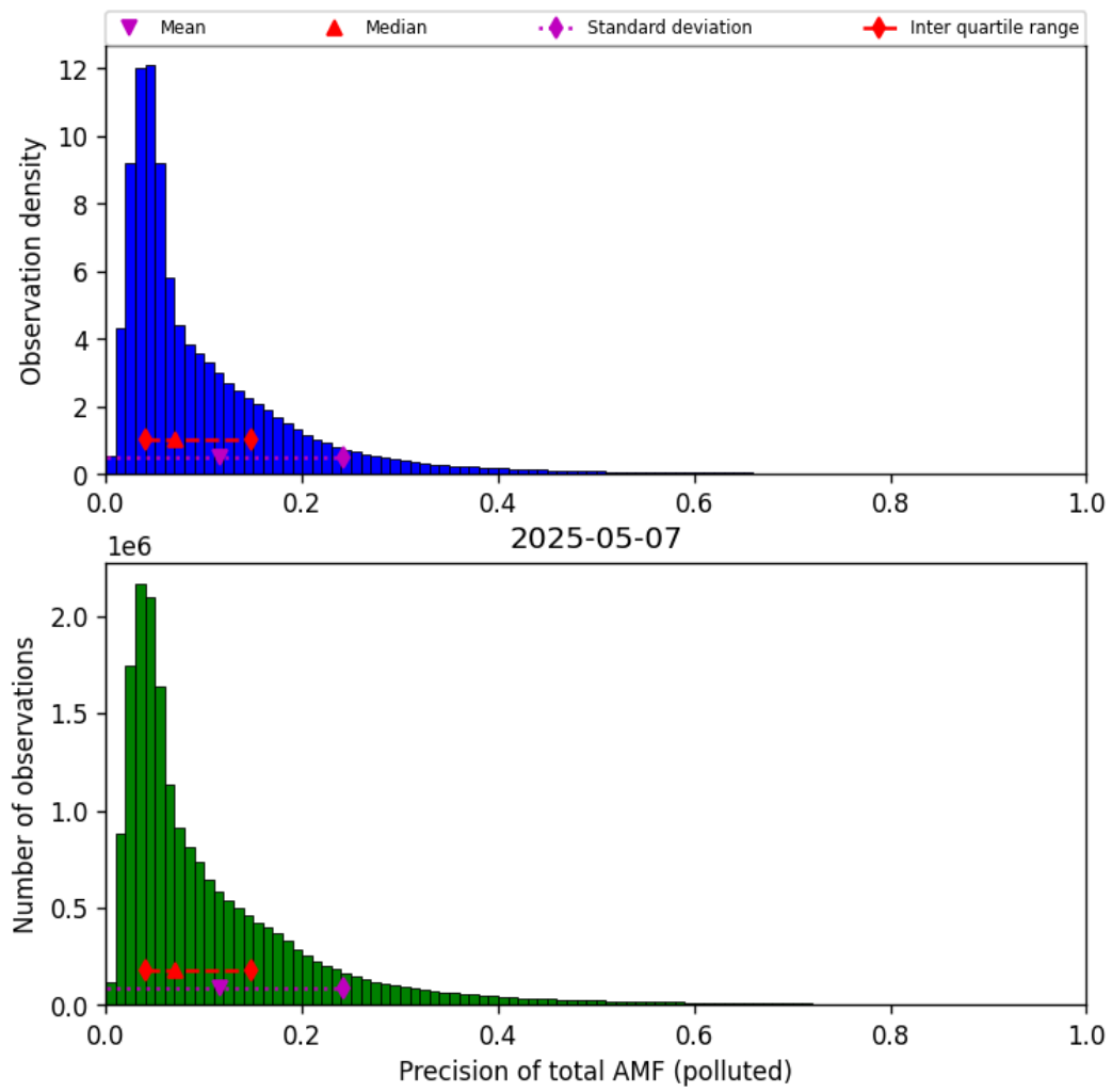
Figure 80: Histogram of “Precision of total AMF (polluted)” for 2025-05-06 to 2025-05-08
