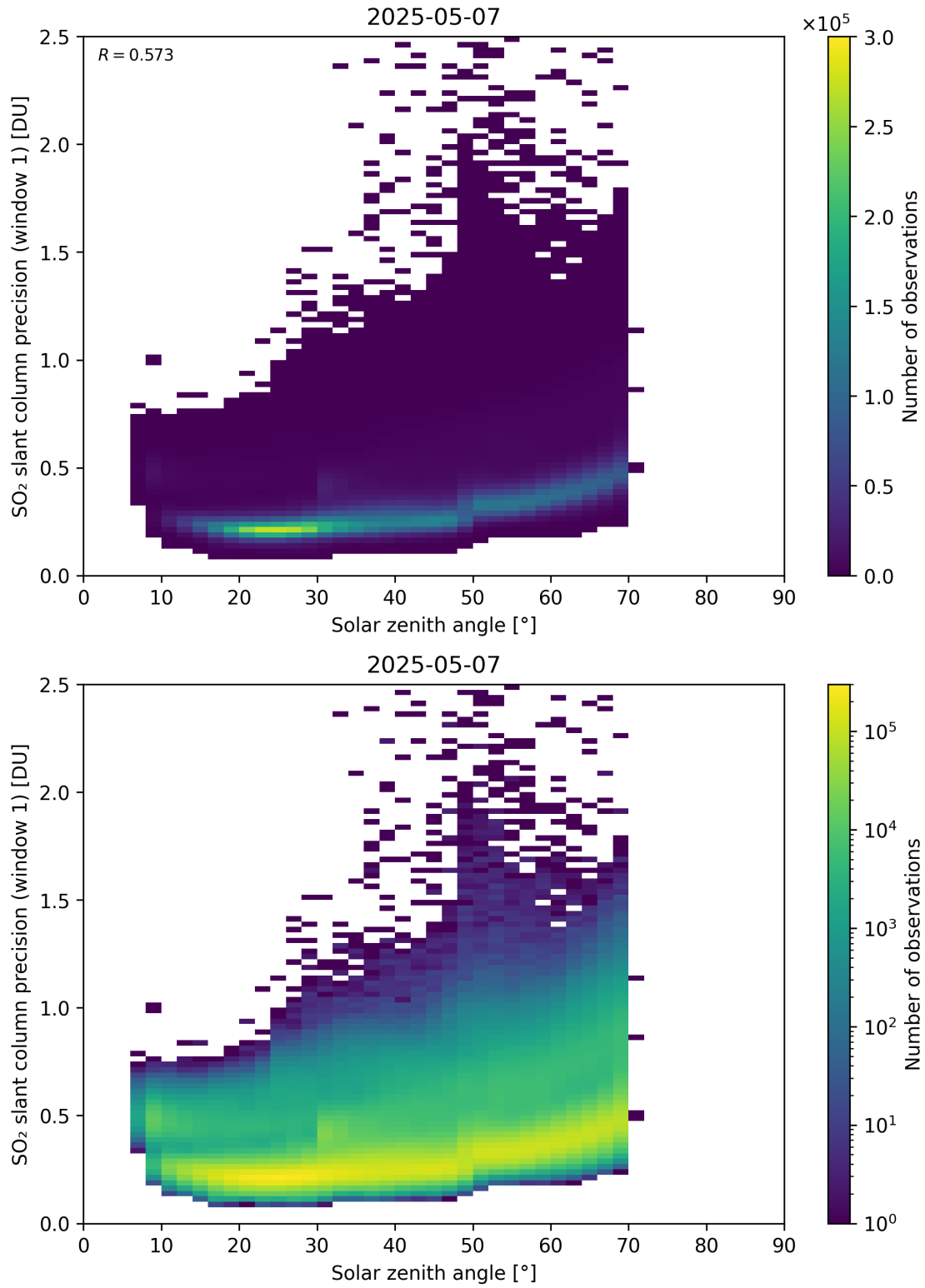
Figure 185: Scatter density plot of “Solar zenith angle” against “SO 2 slant column precision (window 1)” for 2025-05-06 to 2025-05-08.
