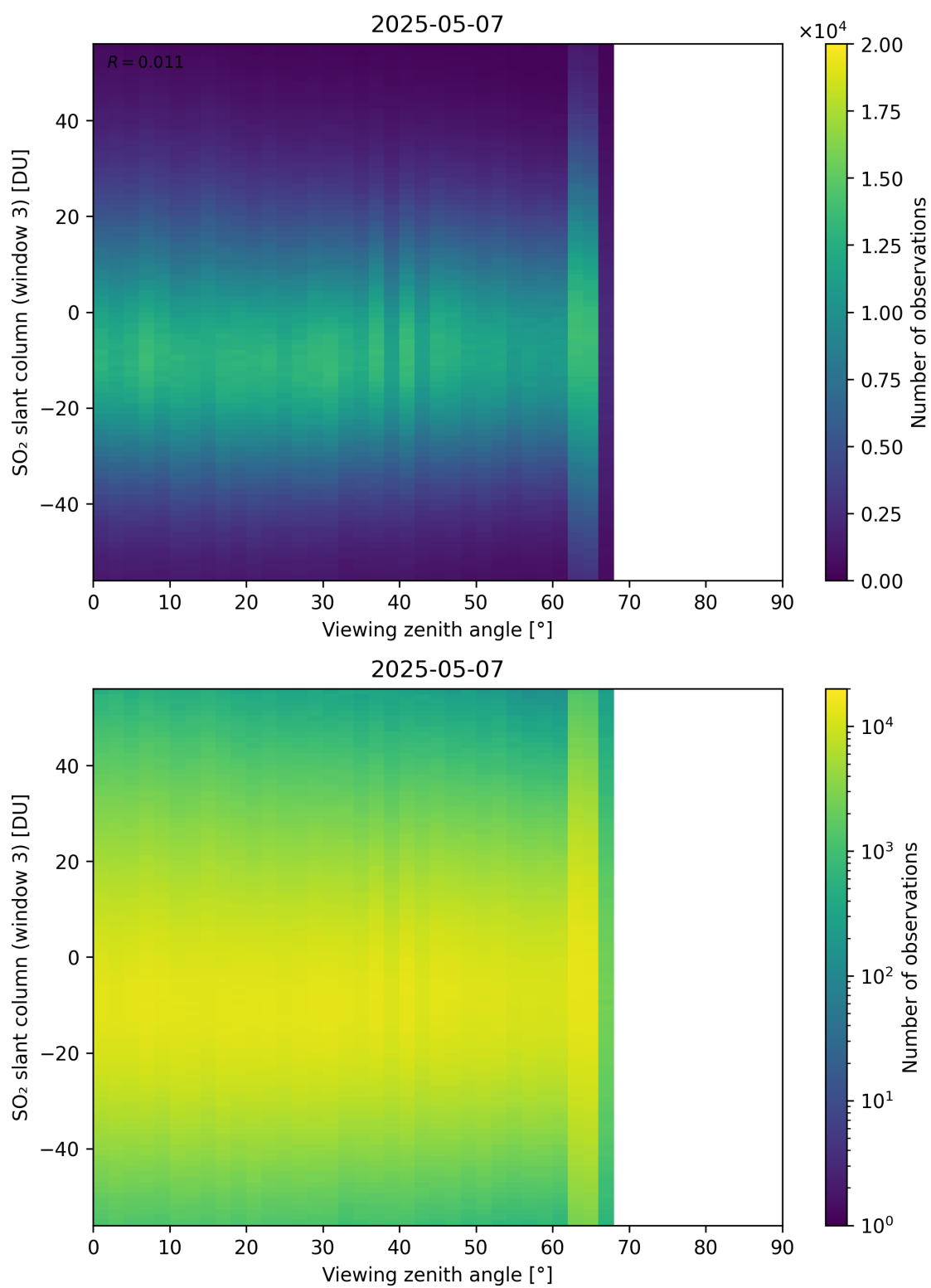
Figure 379: Scatter density plot of “Viewing zenith angle” against “SO 2 slant column (window 3)” for 2025-05-06 to 2025-05-08.
