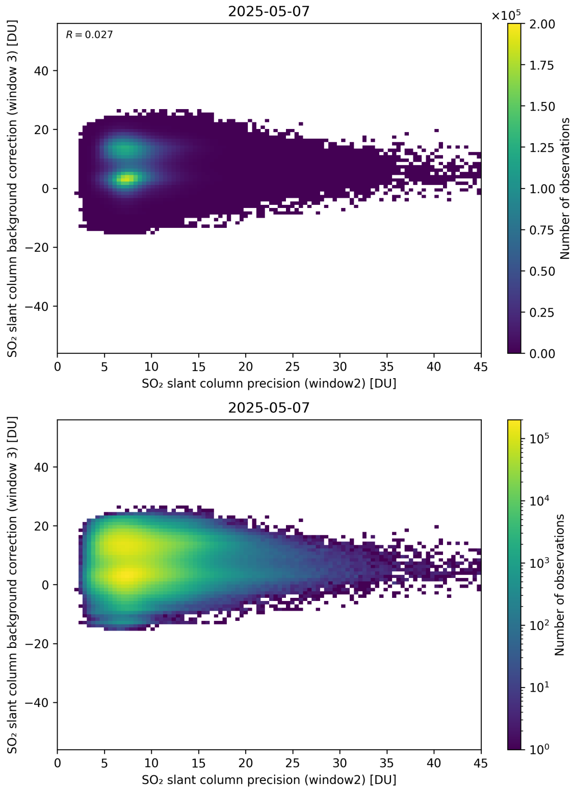
Figure 292: Scatter density plot of “SO 2 slant column precision (window2)” against “SO 2 slant column background correction (window 3)” for 2025-05-06 to 2025-05-08.
