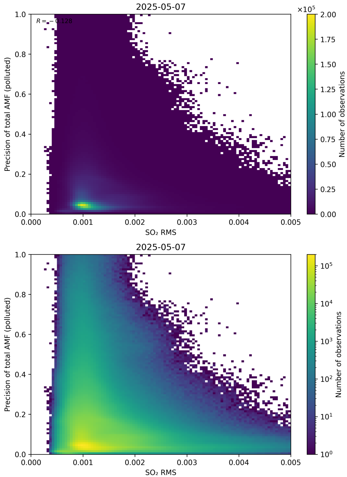
Figure 149: Scatter density plot of “SO 2 RMS” against “Precision of total AMF (polluted)” for 2025-05-06 to 2025-05-08.
