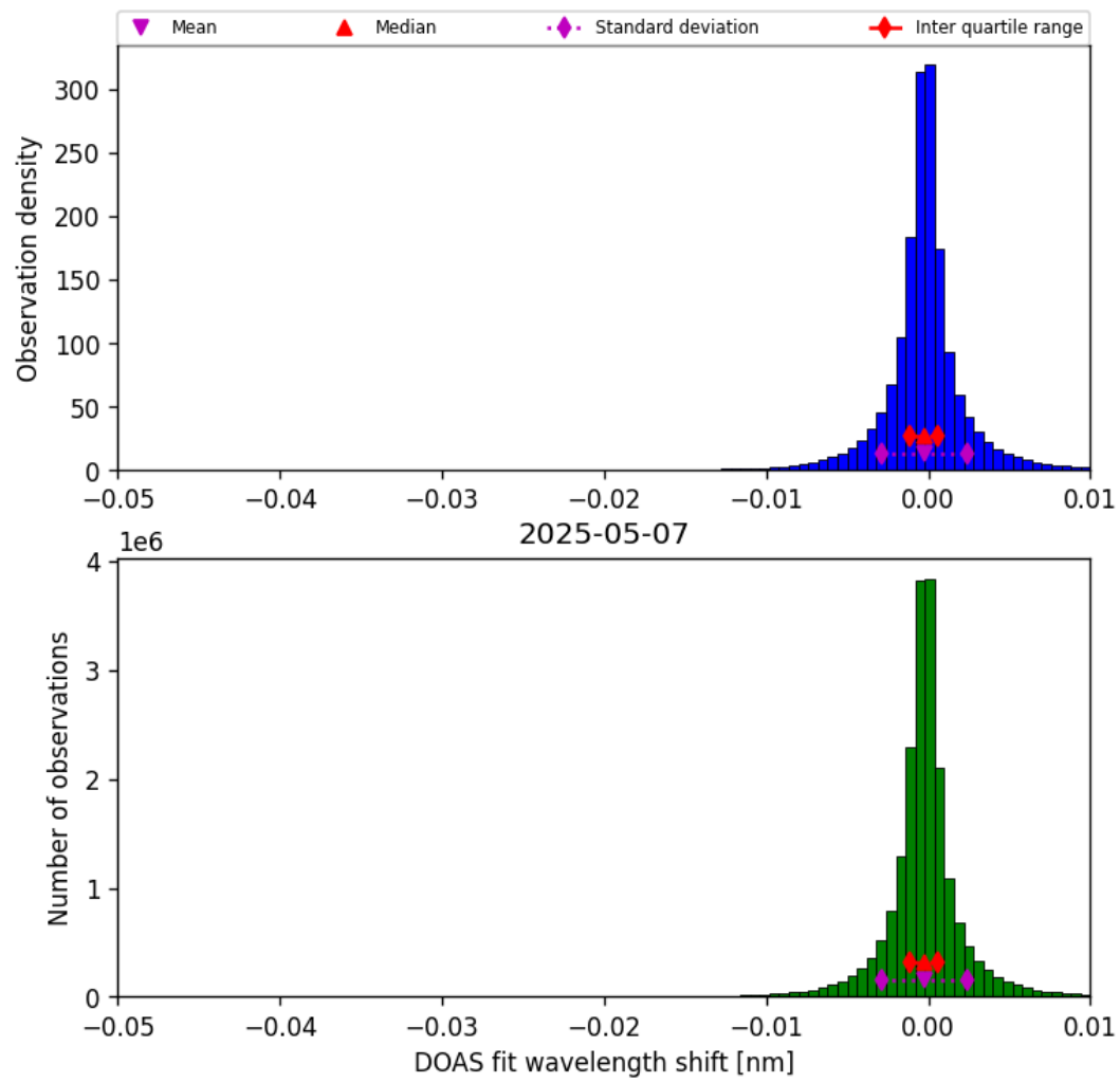
Figure 76: Histogram of “DOAS fit wavelength shift” for 2025-05-06 to 2025-05-08
