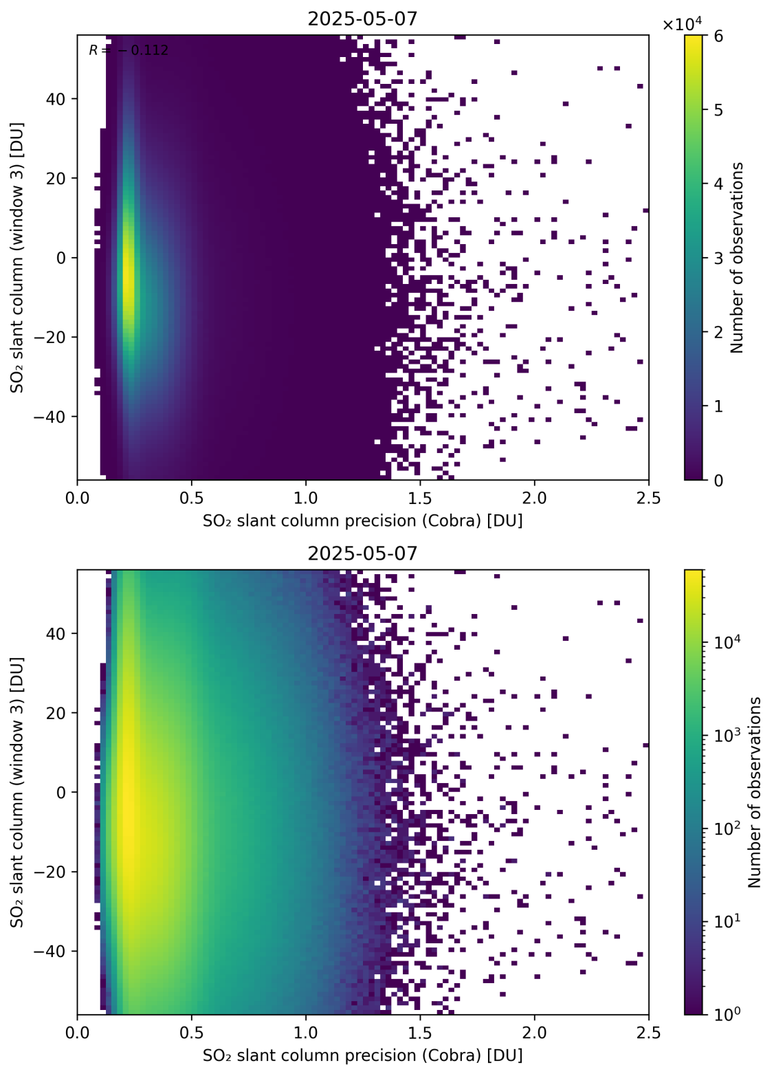
Figure 211: Scatter density plot of “SO 2 slant column precision (Cobra)” against “SO 2 slant column (window 3)” for 2025-05-06 to 2025-05-08.
