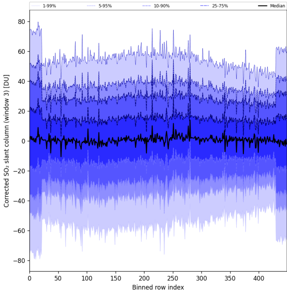
Figure 99: Along track statistics of “Corrected SO 2 slant column (window 3)” for 2025-05-06 to 2025-05-08
