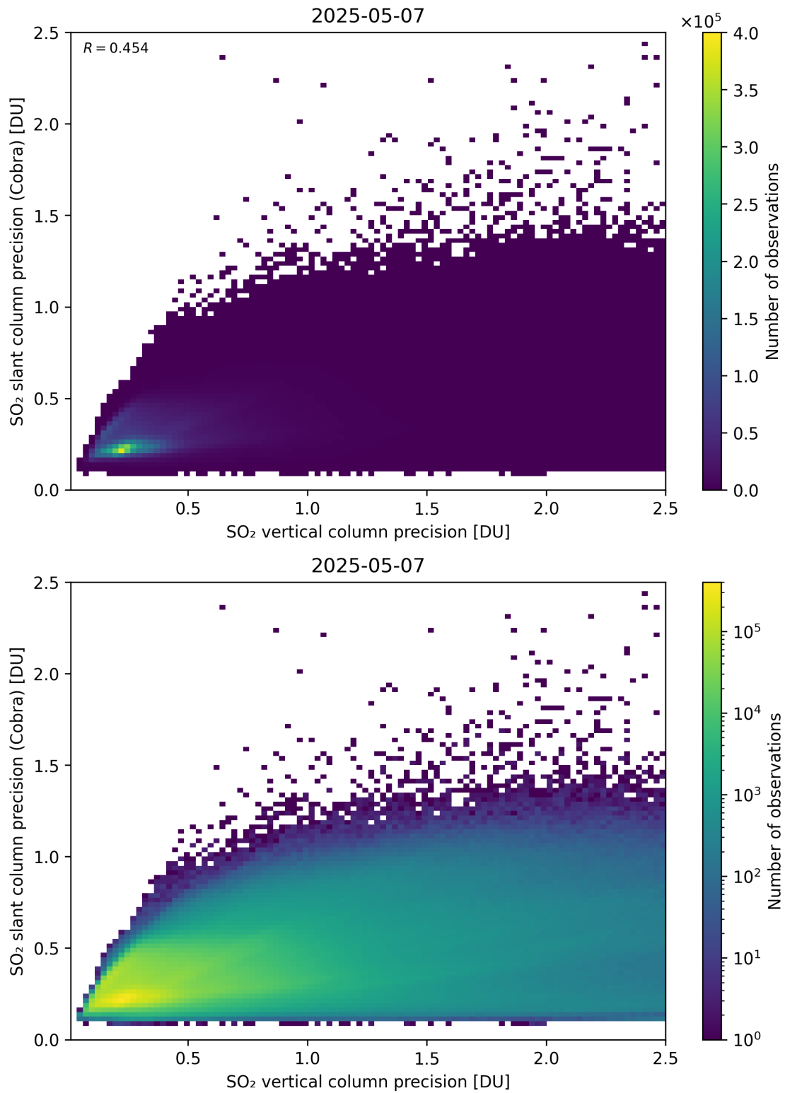
Figure 337: Scatter density plot of “SO 2 vertical column precision” against “SO 2 slant column precision (Cobra)” for 2025-05-06 to 2025-05-08.
