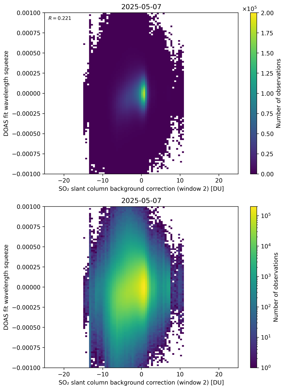
Figure 124: Scatter density plot of “SO 2 slant column background correction (window 2)” against “DOAS fit wavelength squeeze” for 2025-05-06 to 2025-05-08.
