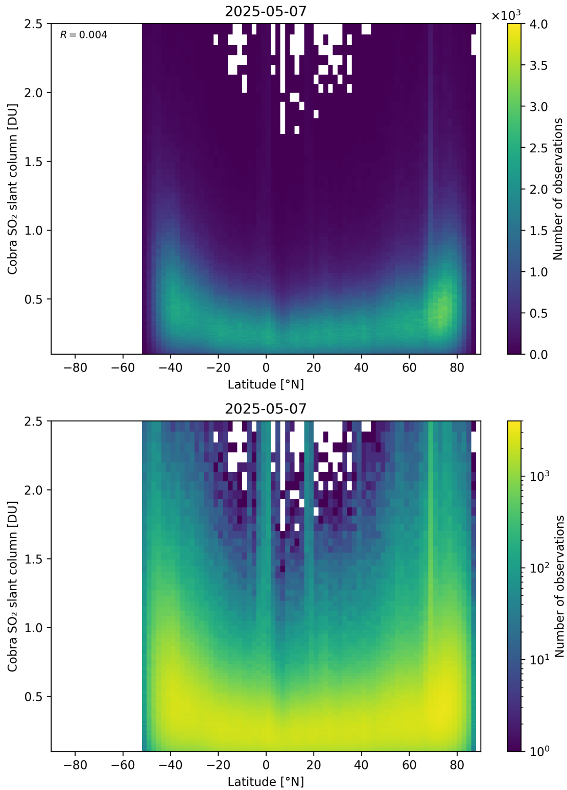
Figure 157: Scatter density plot of “Latitude” against “Cobra SO 2 slant column” for 2025-05-06 to 2025-05-08.
