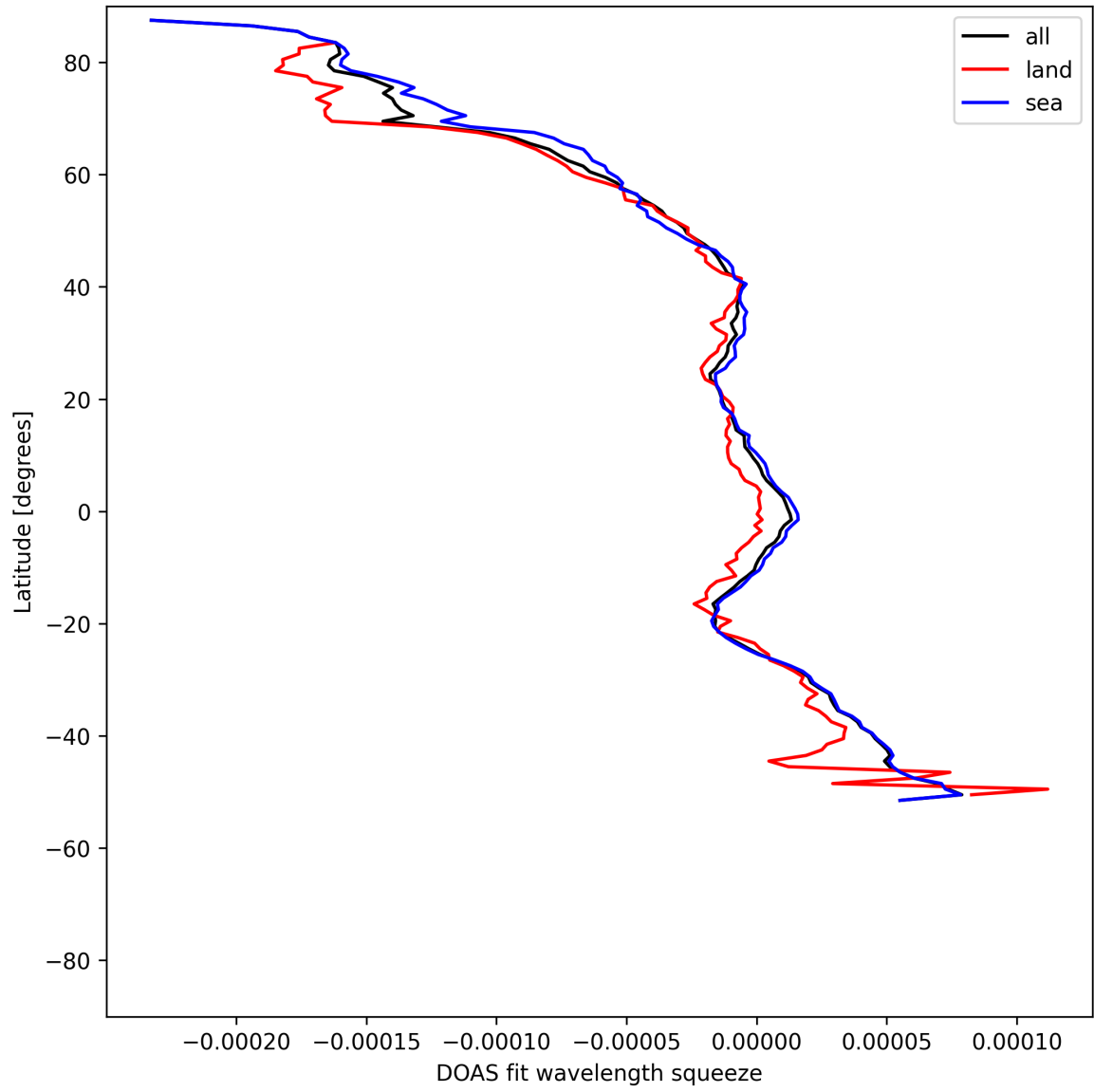
Figure 51: Zonal average of “DOAS fit wavelength squeeze” for 2025-05-06 to 2025-05-08.
