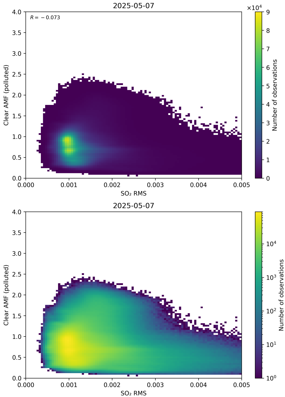
Figure 147: Scatter density plot of “SO 2 RMS” against “Clear AMF (polluted)” for 2025-05-06 to 2025-05-08.
