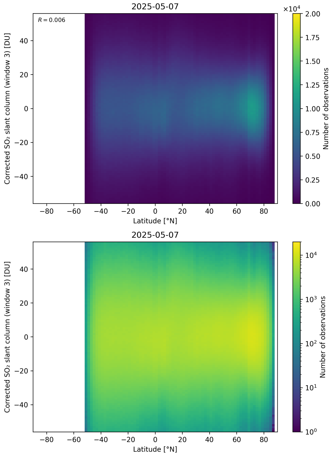
Figure 161: Scatter density plot of “Latitude” against “Corrected SO 2 slant column (window 3)” for 2025-05-06 to 2025-05-08.
