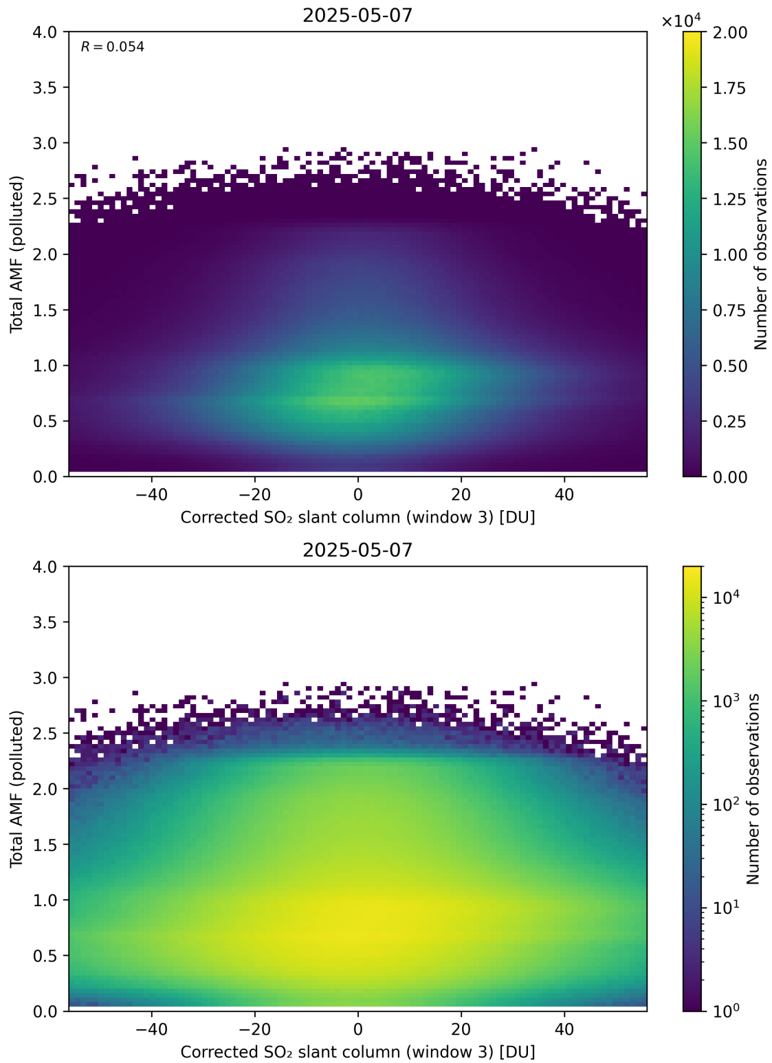
Figure 260: Scatter density plot of “Corrected SO 2 slant column (window 3)” against “Total AMF (polluted)” for 2025-05-06 to 2025-05-08.
