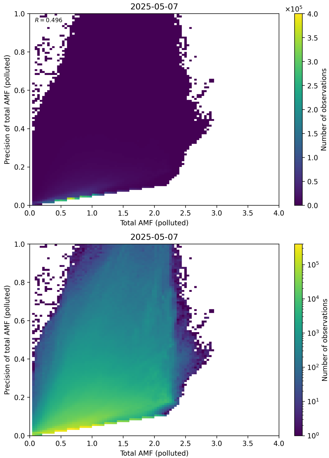
Figure 322: Scatter density plot of “Total AMF (polluted)” against “Precision of total AMF (polluted)” for 2025-05-06 to 2025-05-08.
