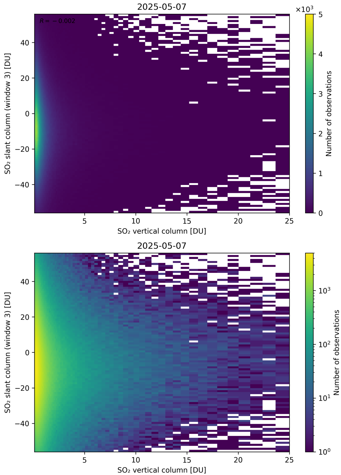
Figure 357: Scatter density plot of “SO 2 vertical column” against “SO 2 slant column (window 3)” for 2025-05-06 to 2025-05-08.
