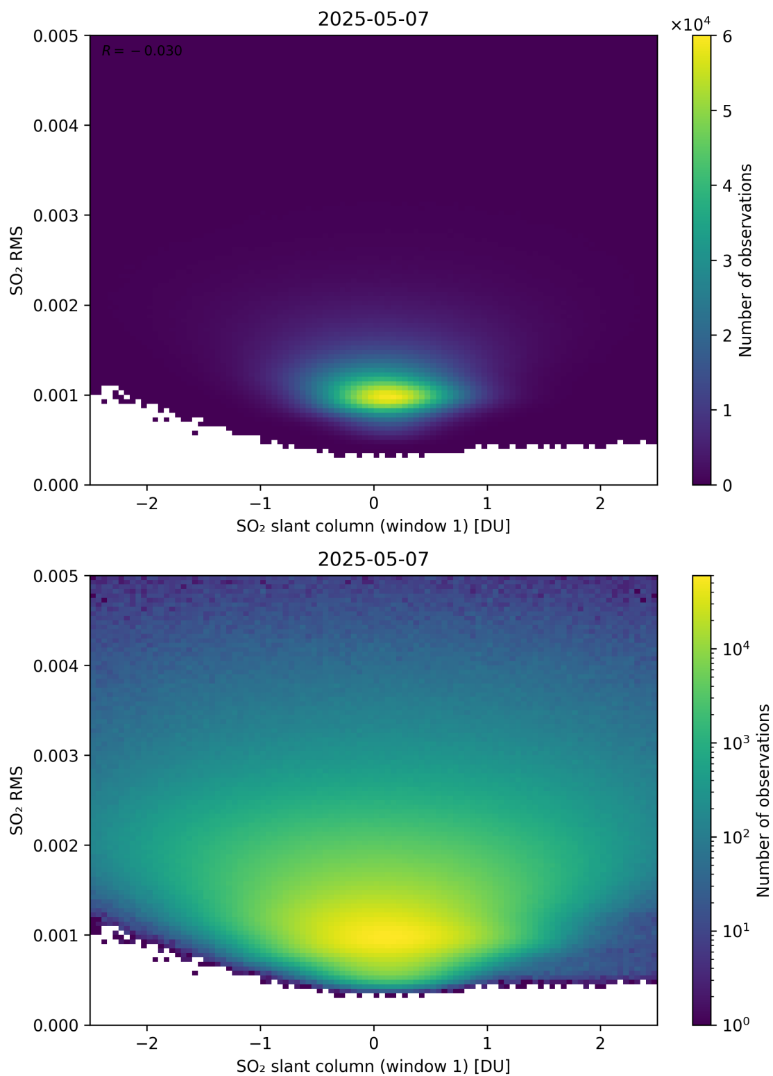
Figure 267: Scatter density plot of “SO 2 slant column (window 1)” against “SO 2 RMS” for 2025-05-06 to 2025-05-08.
