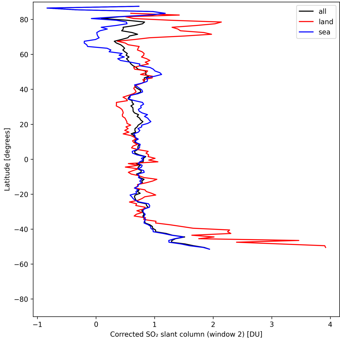
Figure 43: Zonal average of “Corrected SO 2 slant column (window 2)” for 2025-05-06 to 2025-05-08.
