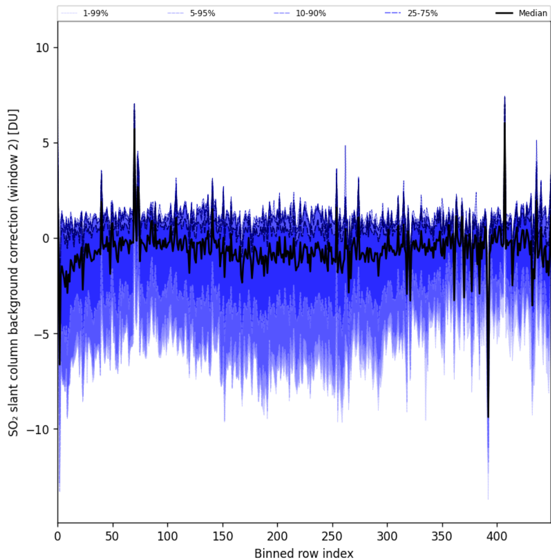
Figure 96: Along track statistics of “SO 2 slant column background correction (window 2)” for 2025-05-06 to 2025-05-08
