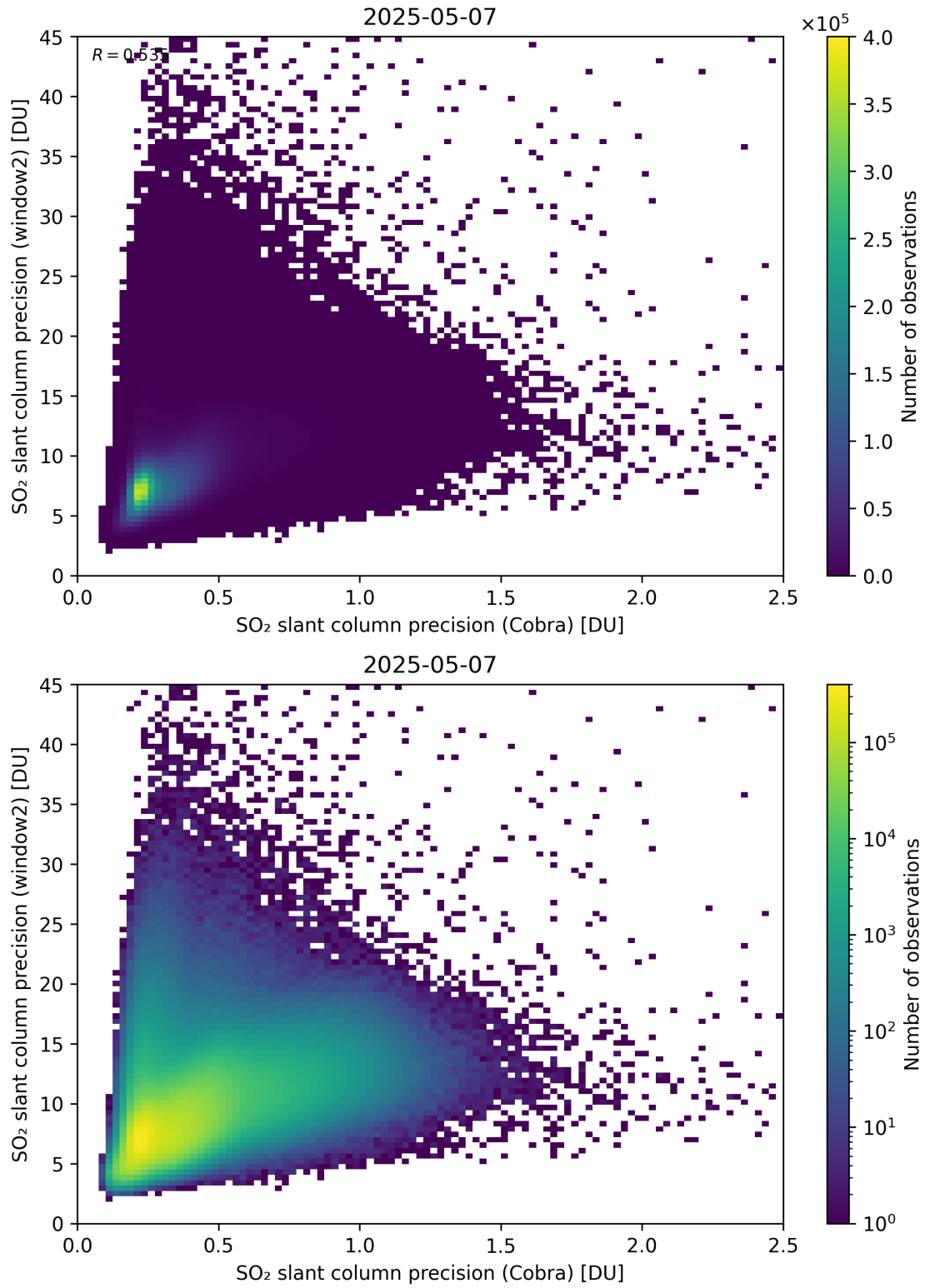
Figure 210: Scatter density plot of “SO 2 slant column precision (Cobra)” against “SO 2 slant column precision (window2)” for 2025-05-06 to 2025-05-08.
