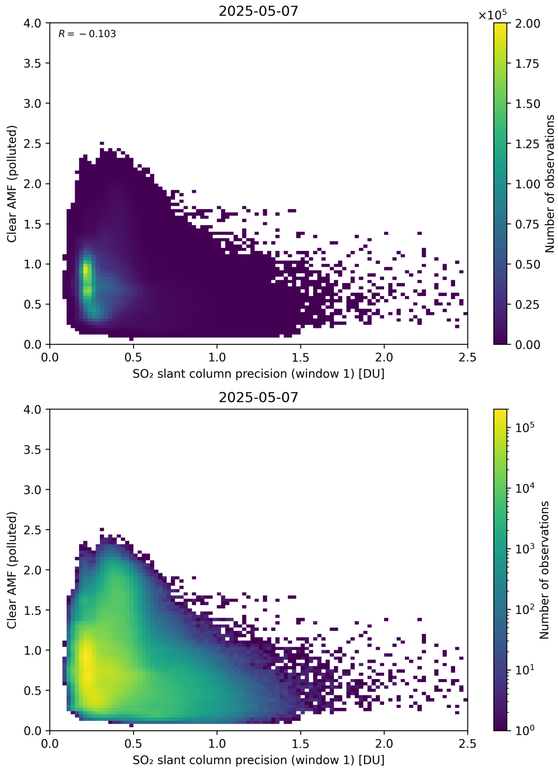
Figure 274: Scatter density plot of “SO 2 slant column precision (window 1)” against “Clear AMF (polluted)” for 2025-05-06 to 2025-05-08.
