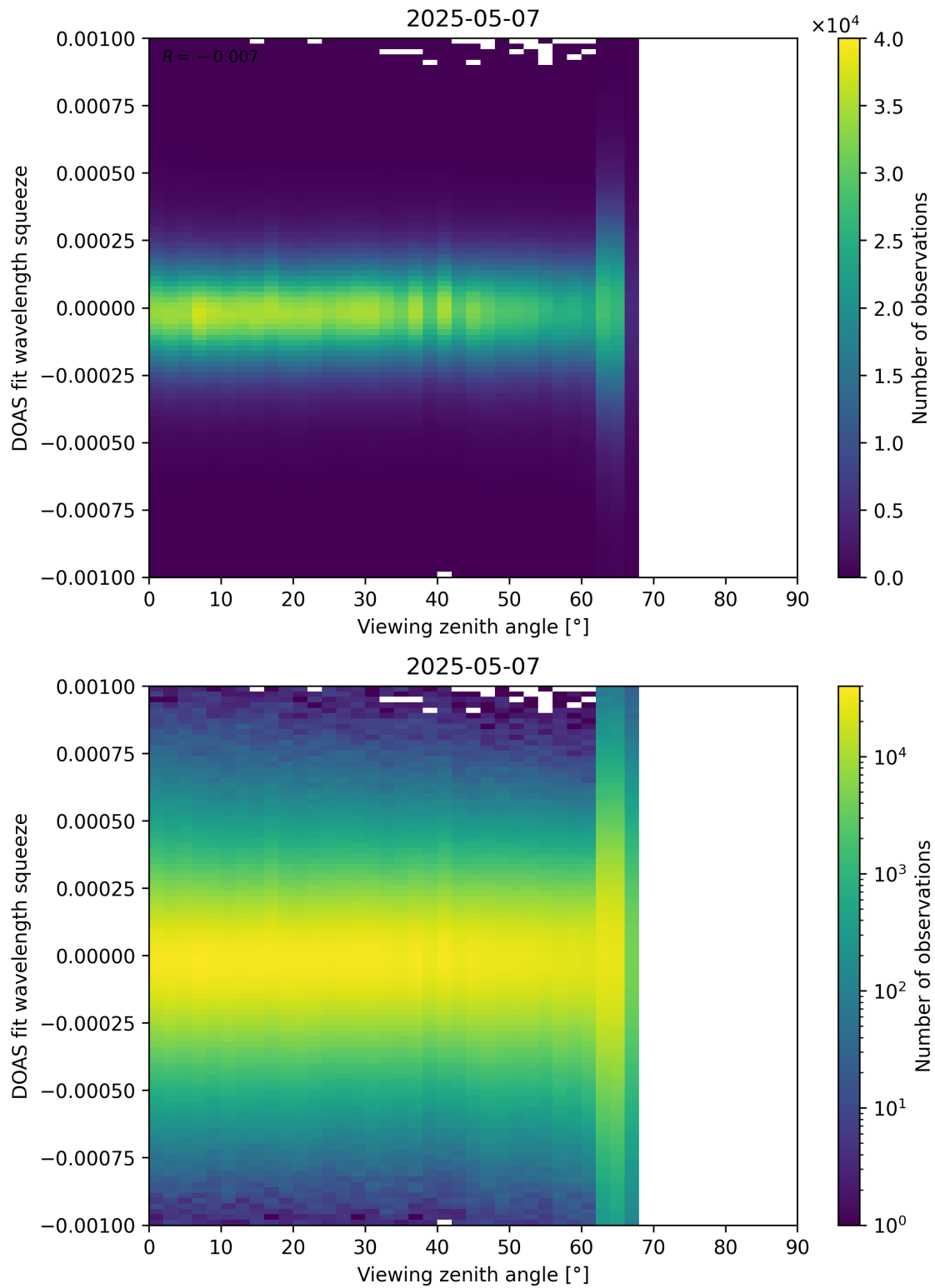
Figure 366: Scatter density plot of “Viewing zenith angle” against “DOAS fit wavelength squeeze” for 2025-05-06 to 2025-05-08.
