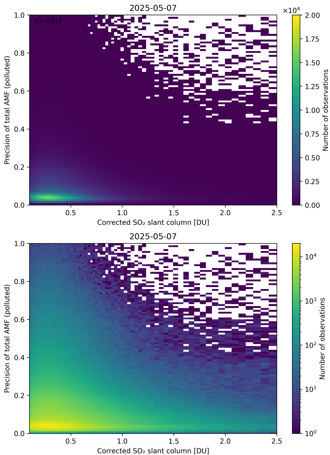
Figure 243: Scatter density plot of “Corrected SO 2 slant column” against “Precision of total AMF (polluted)” for 2025-05-06 to 2025-05-08.
