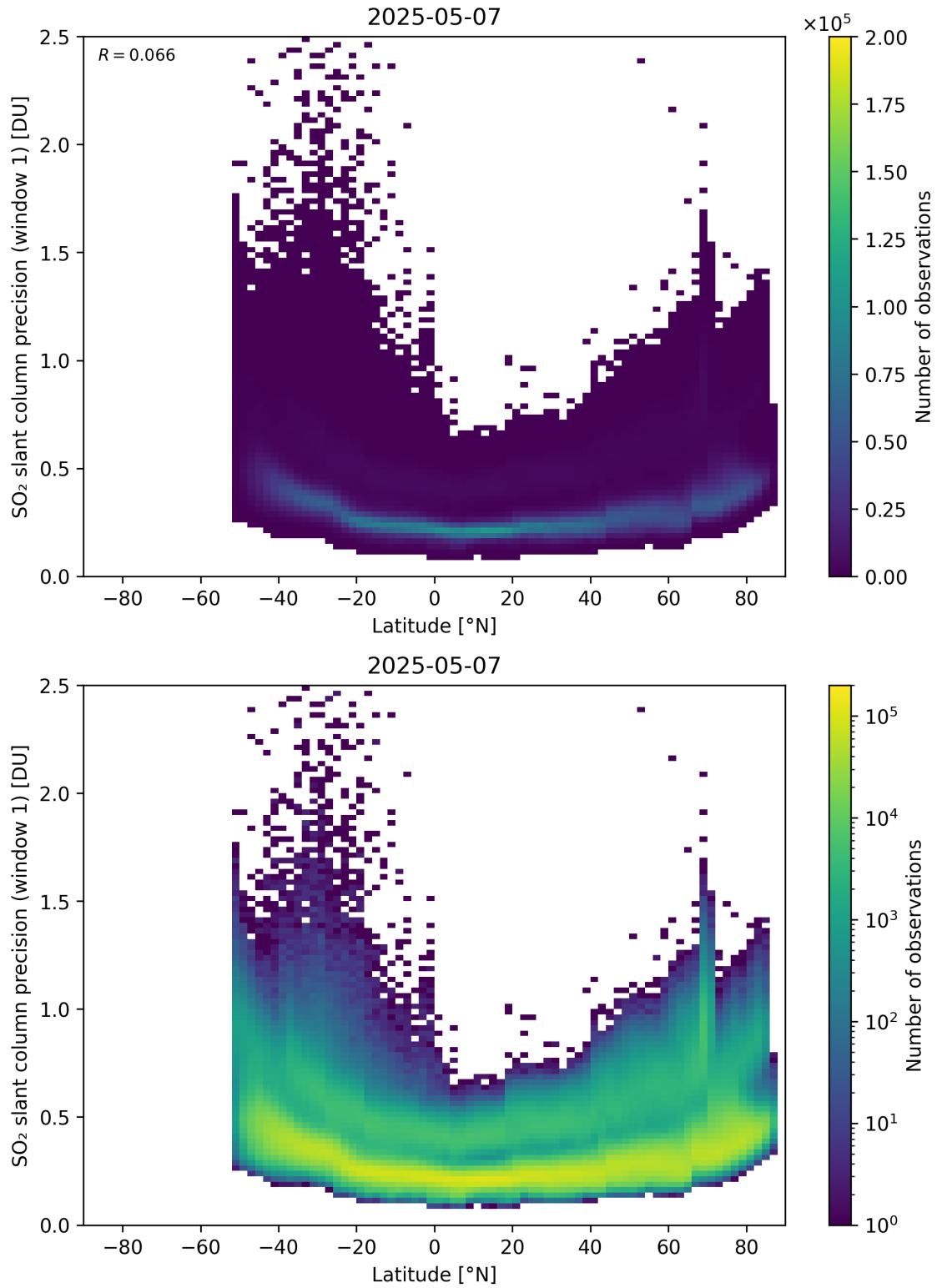
Figure 163: Scatter density plot of “Latitude” against “SO 2 slant column precision (window 1)” for 2025-05-06 to 2025-05-08.
