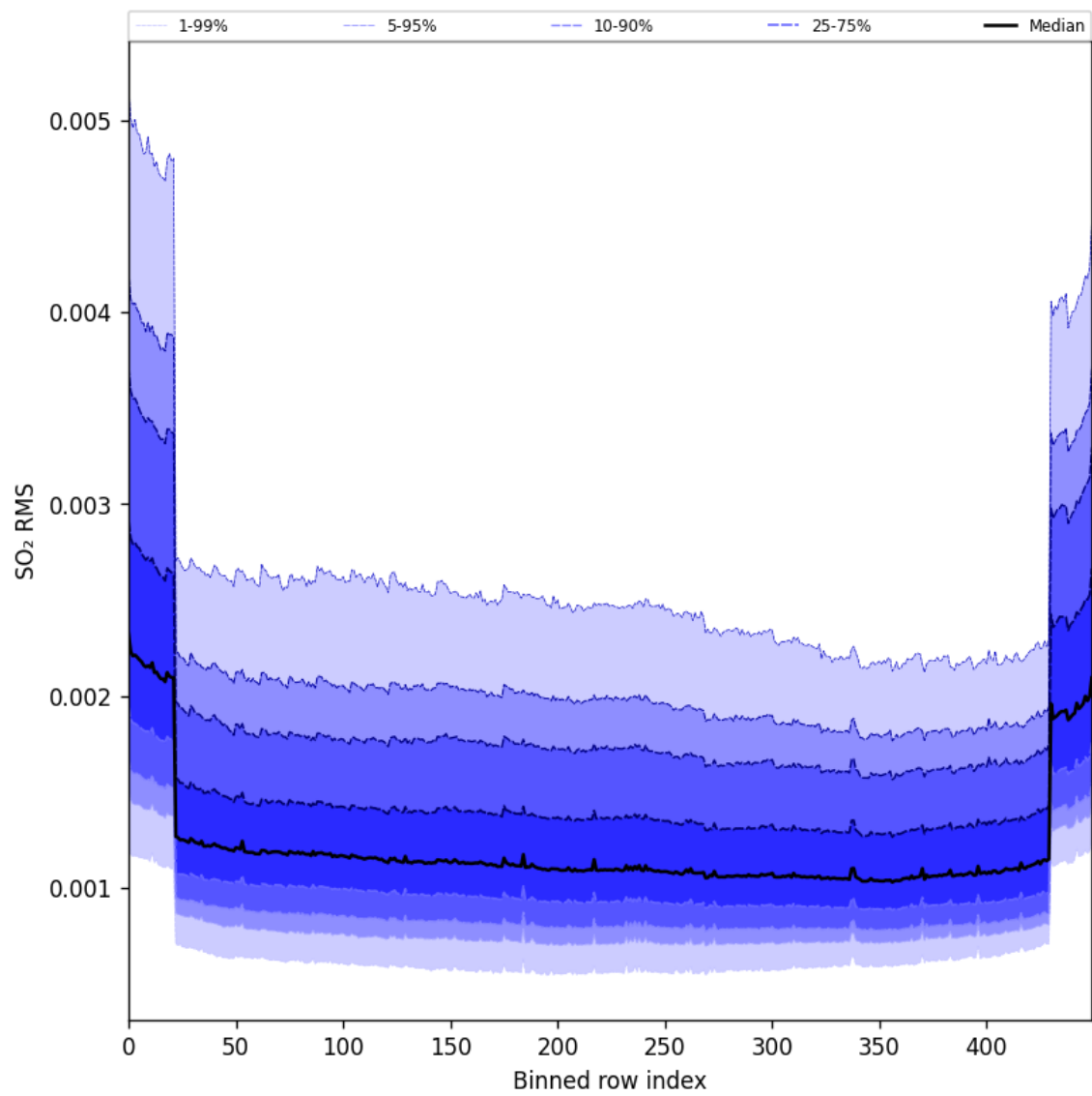
Figure 104: Along track statistics of “SO 2 RMS” for 2025-05-06 to 2025-05-08
