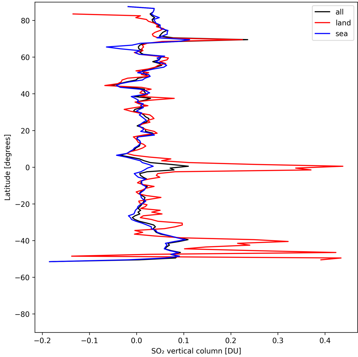
Figure 32: Zonal average of “SO 2 vertical column” for 2025-05-06 to 2025-05-08.
