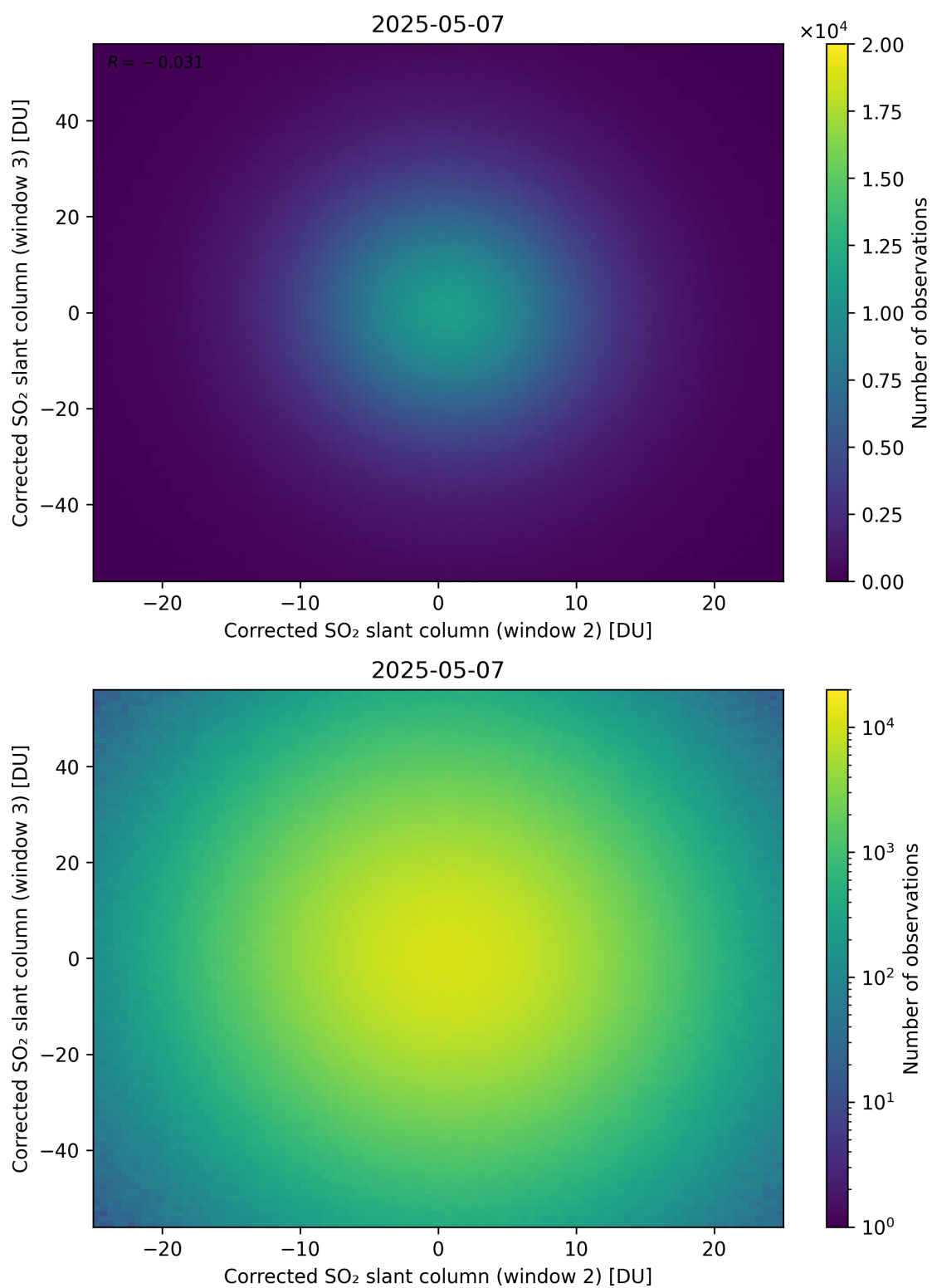
Figure 250: Scatter density plot of “Corrected SO 2 slant column (window 2)” against “Corrected SO 2 slant column (window 3)” for 2025-05-06 to 2025-05-08.
