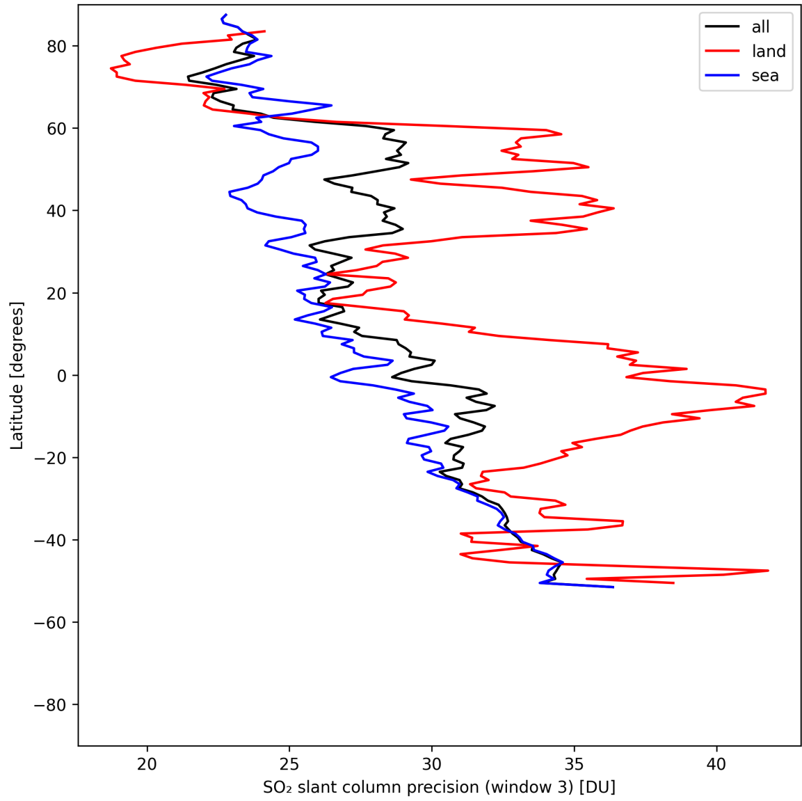
Figure 46: Zonal average of “SO 2 slant column precision (window 3)” for 2025-05-06 to 2025-05-08.
