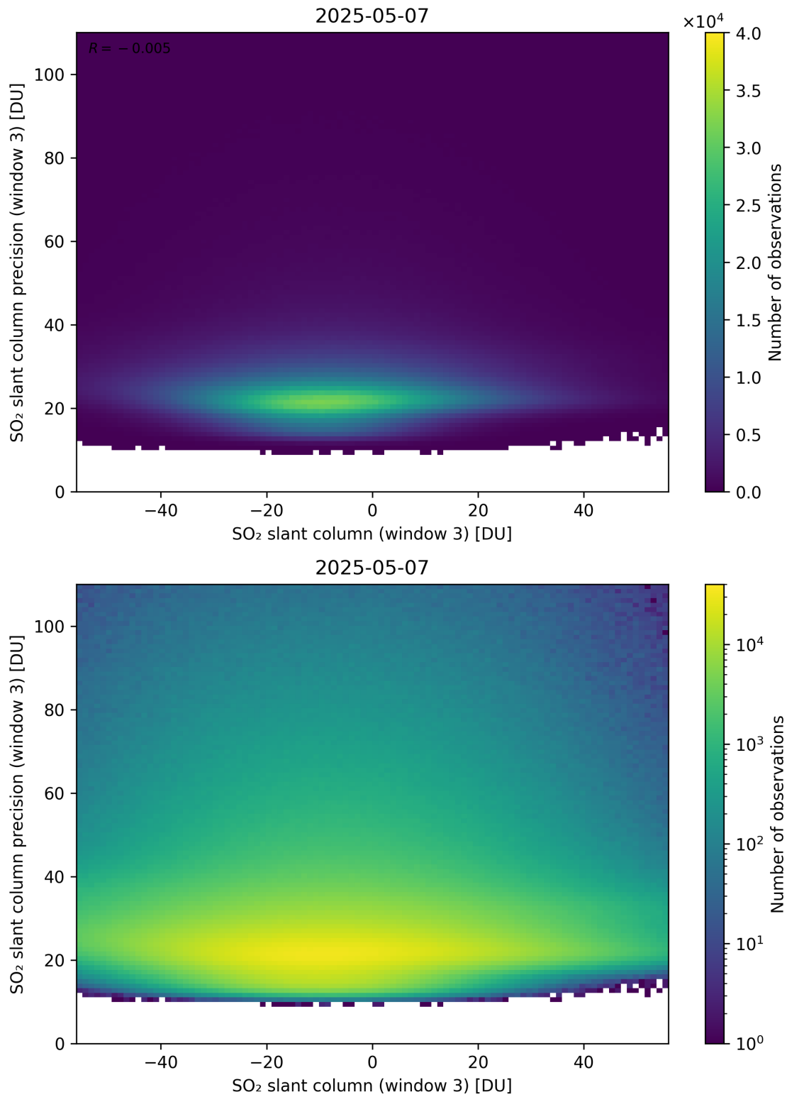
Figure 317: Scatter density plot of “SO 2 slant column (window 3)” against “SO 2 slant column precision (window 3)” for 2025-05-06 to 2025-05-08.
