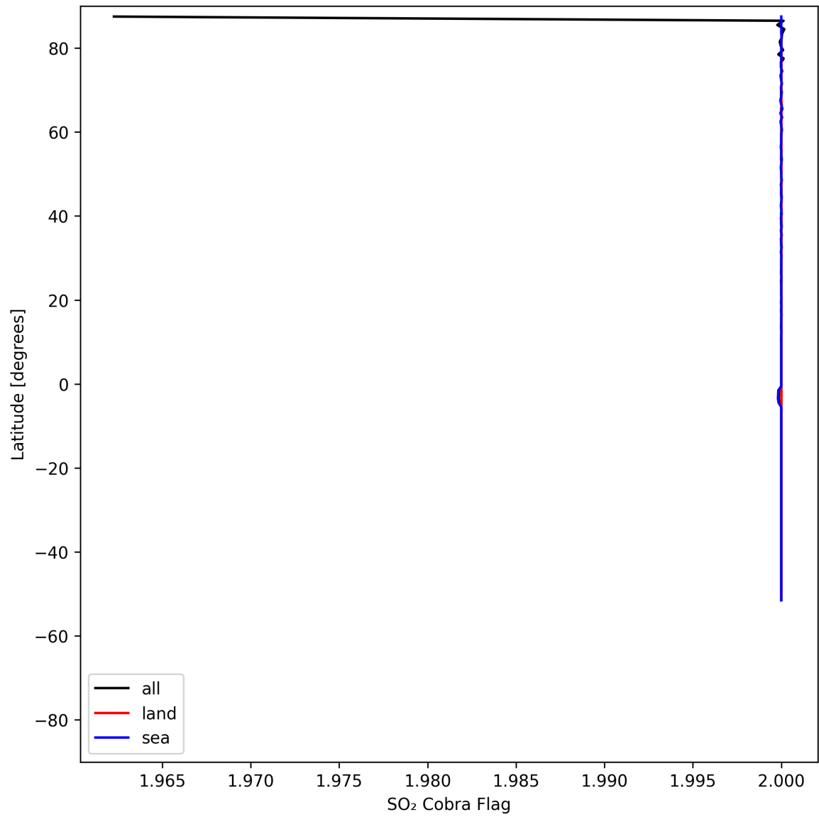
Figure 49: Zonal average of “SO 2 Cobra Flag” for 2025-05-06 to 2025-05-08.
