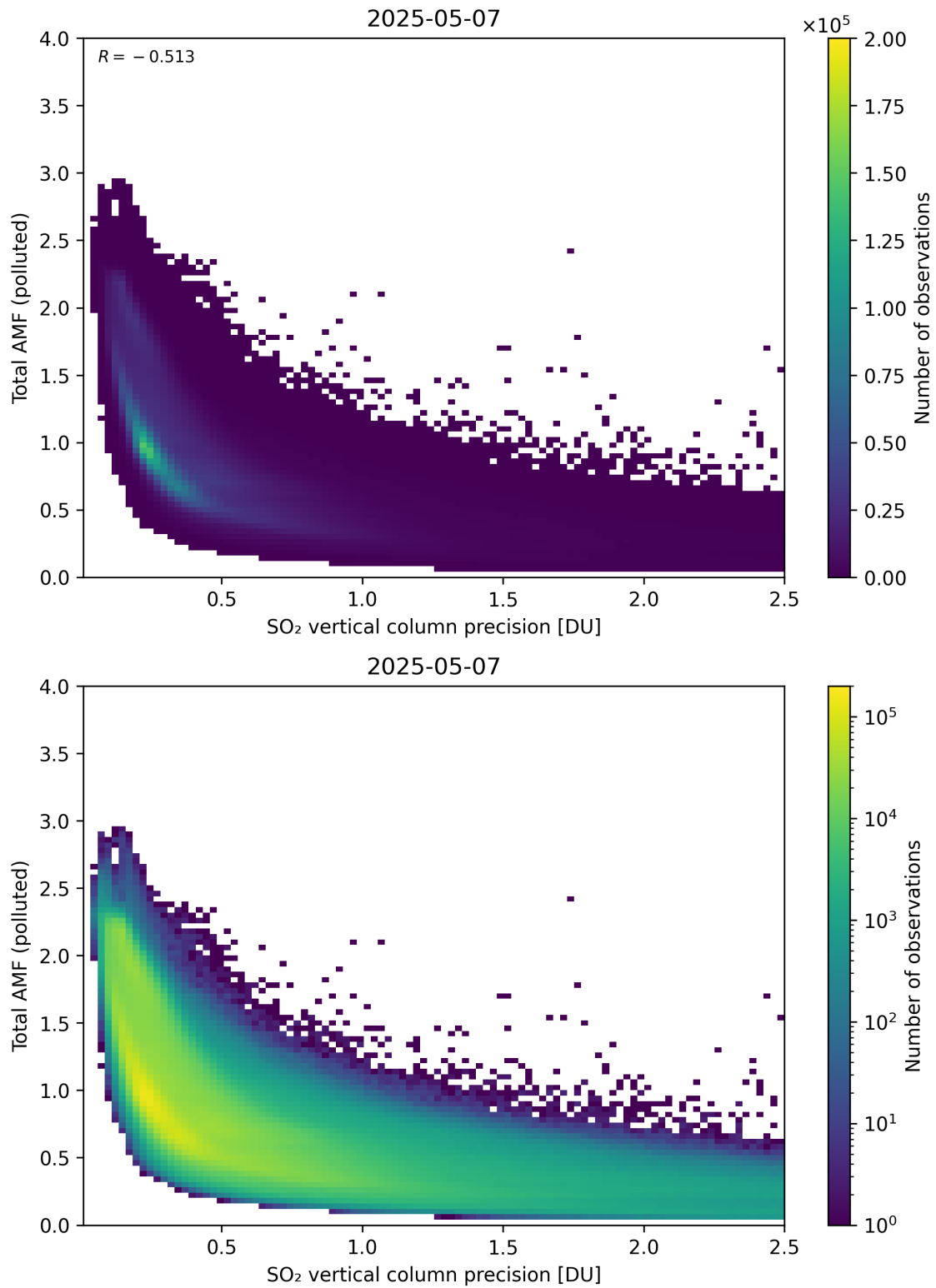
Figure 346: Scatter density plot of “SO 2 vertical column precision” against “Total AMF (polluted)” for 2025-05-06 to 2025-05-08.
