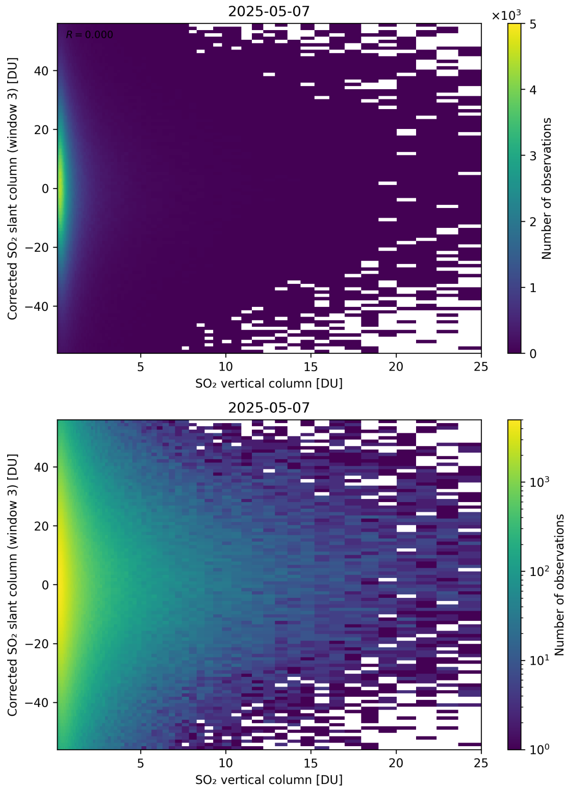
Figure 353: Scatter density plot of “SO 2 vertical column” against “Corrected SO 2 slant column (window 3)” for 2025-05-06 to 2025-05-08.
