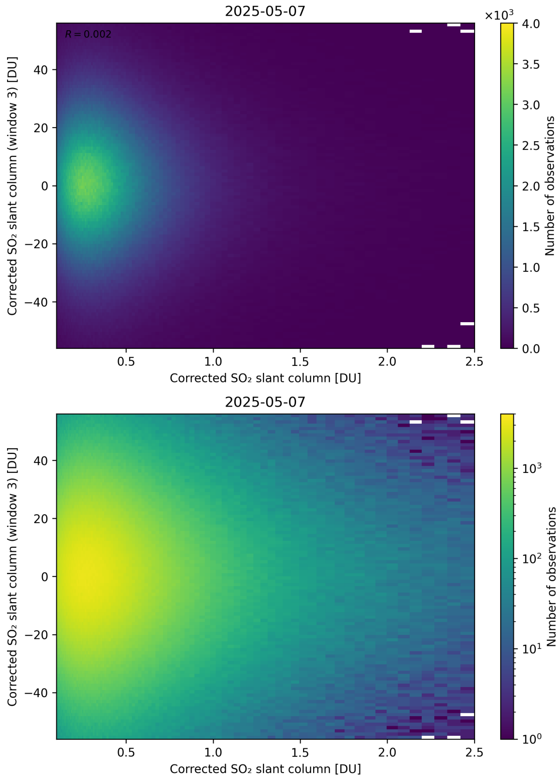
Figure 236: Scatter density plot of “Corrected SO 2 slant column” against “Corrected SO 2 slant column (window 3)” for 2025-05-06 to 2025-05-08.
