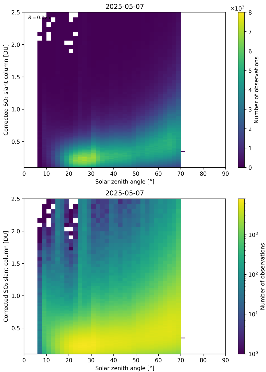
Figure 181: Scatter density plot of “Solar zenith angle” against “Corrected SO 2 slant column” for 2025-05-06 to 2025-05-08.
