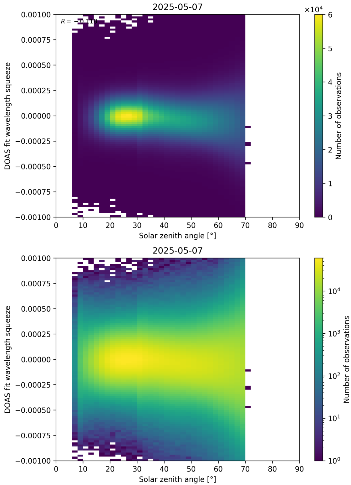
Figure 175: Scatter density plot of “Solar zenith angle” against “DOAS fit wavelength squeeze” for 2025-05-06 to 2025-05-08.
