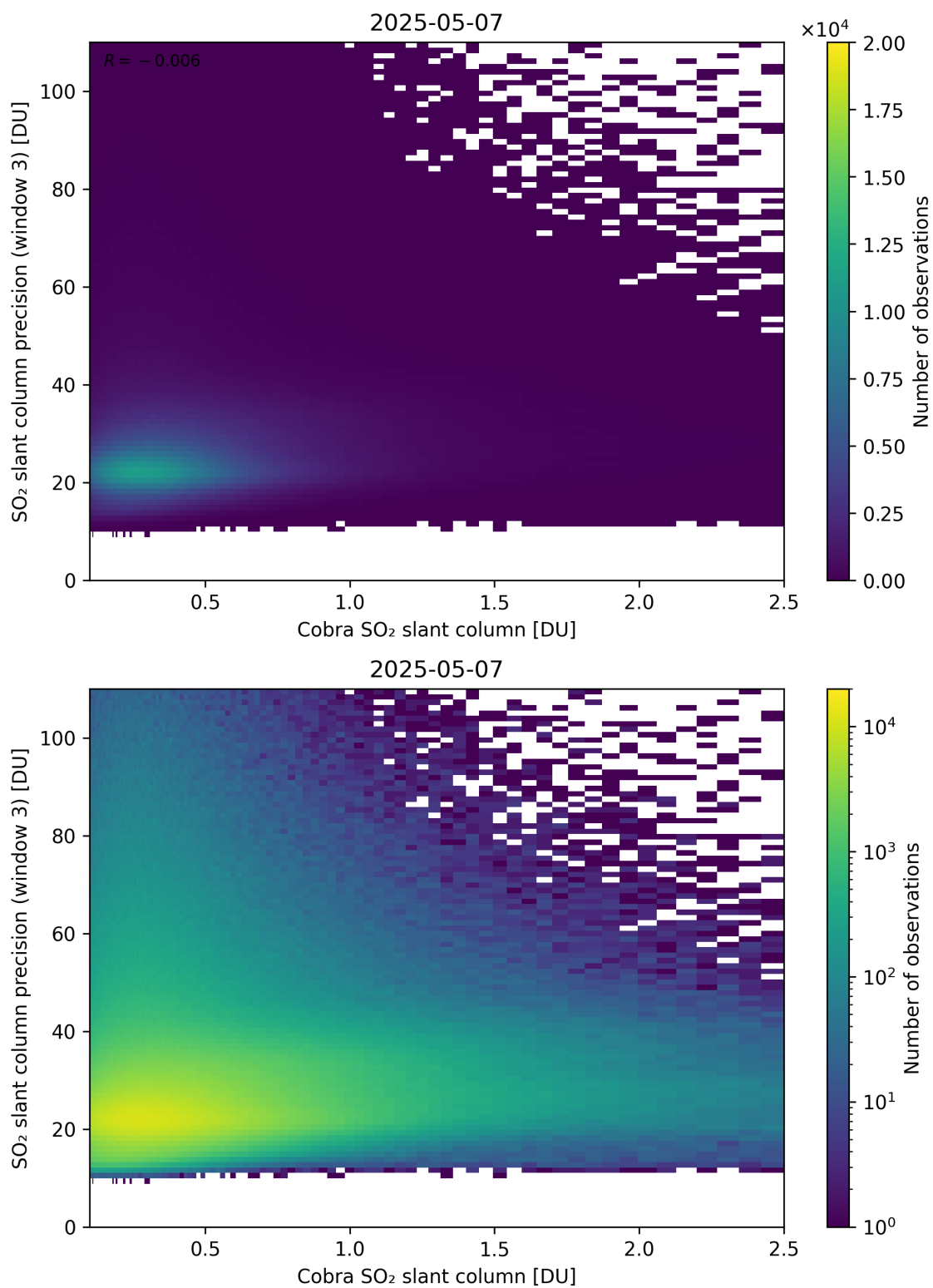
Figure 223: Scatter density plot of “Cobra SO 2 slant column” against “SO 2 slant column precision (window 3)” for 2025-05-06 to 2025-05-08.
