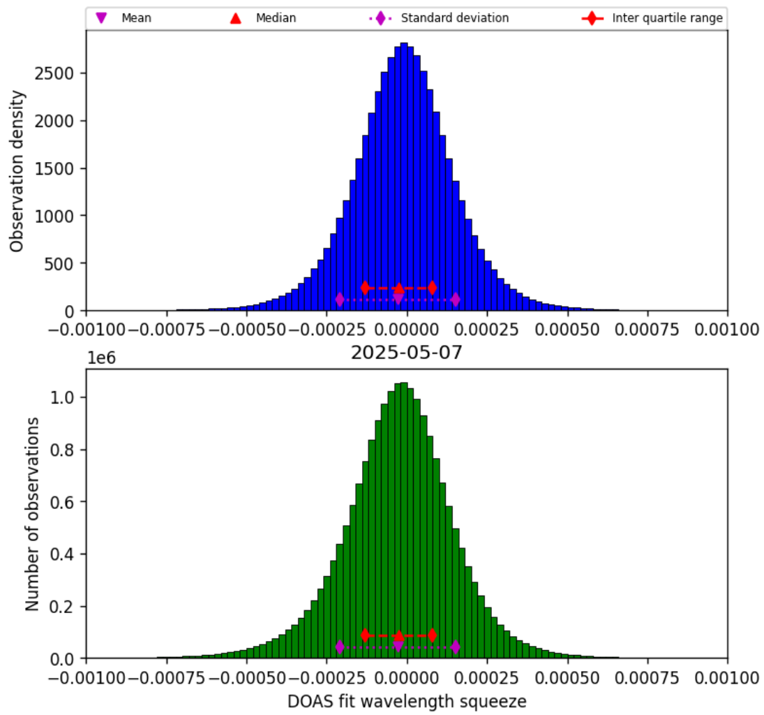
Figure 77: Histogram of “DOAS fit wavelength squeeze” for 2025-05-06 to 2025-05-08
