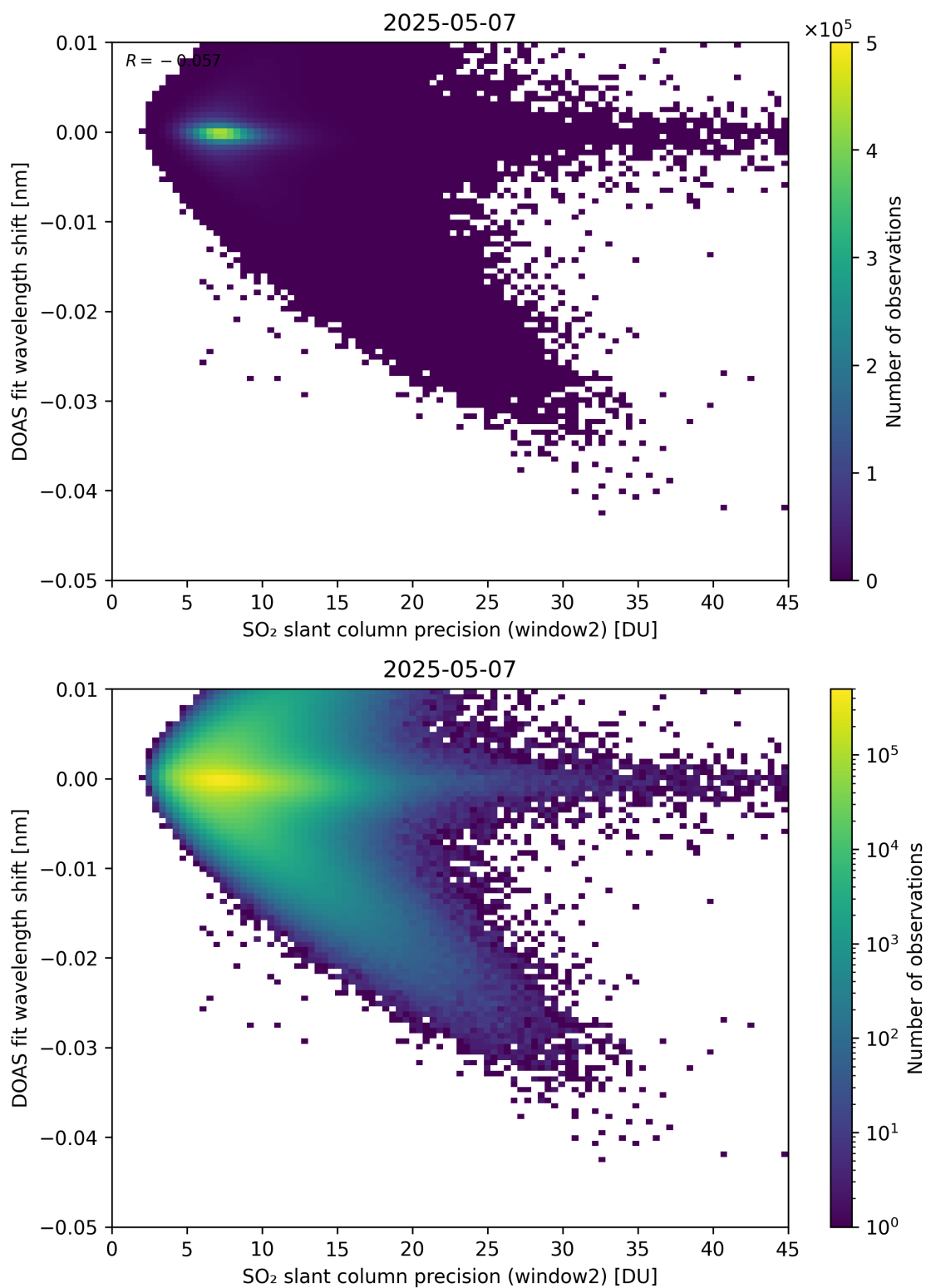
Figure 293: Scatter density plot of “SO 2 slant column precision (window2)” against “DOAS fit wavelength shift” for 2025-05-06 to 2025-05-08.
