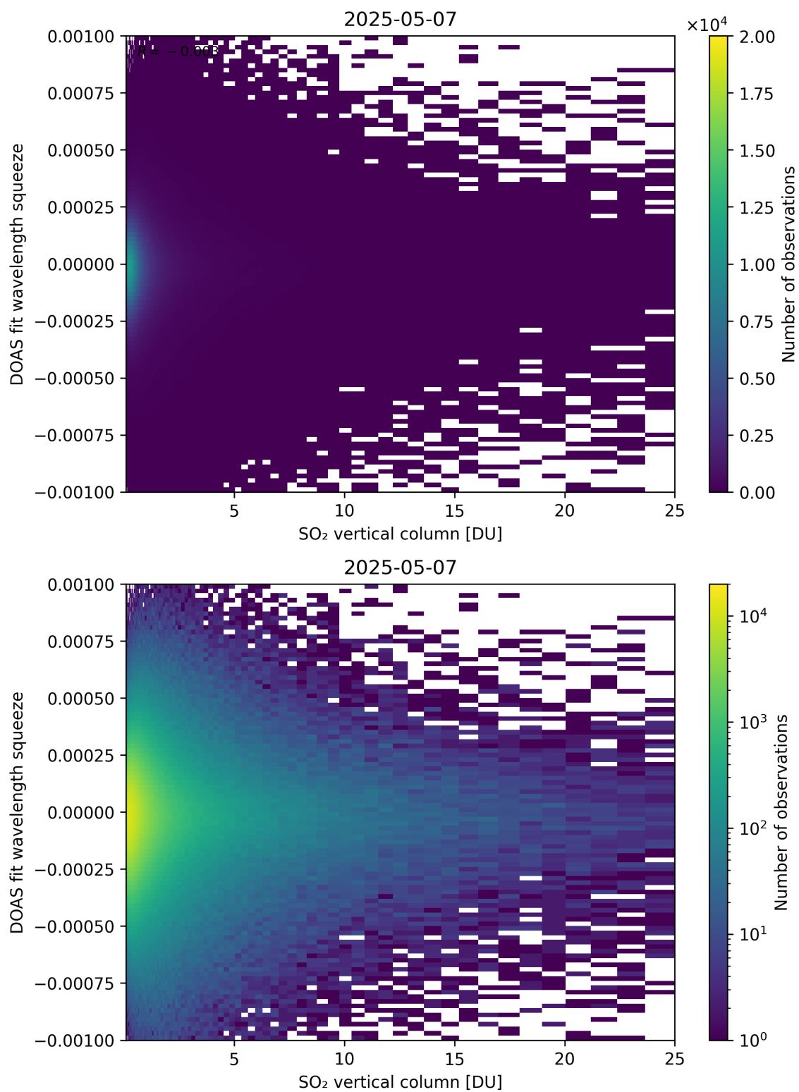
Figure 327: Scatter density plot of “SO 2 vertical column” against “DOAS fit wavelength squeeze” for 2025-05-06 to 2025-05-08.
