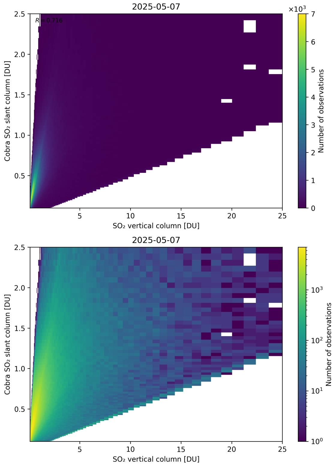
Figure 349: Scatter density plot of “SO 2 vertical column” against “Cobra SO 2 slant column” for 2025-05-06 to 2025-05-08.
