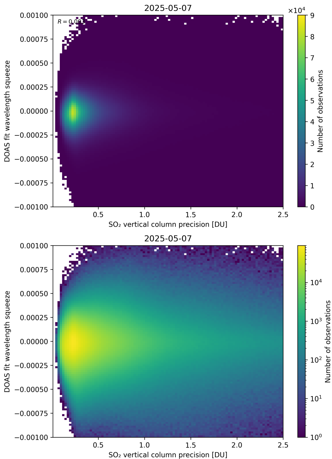
Figure 333: Scatter density plot of “SO 2 vertical column precision” against “DOAS fit wavelength squeeze” for 2025-05-06 to 2025-05-08.
