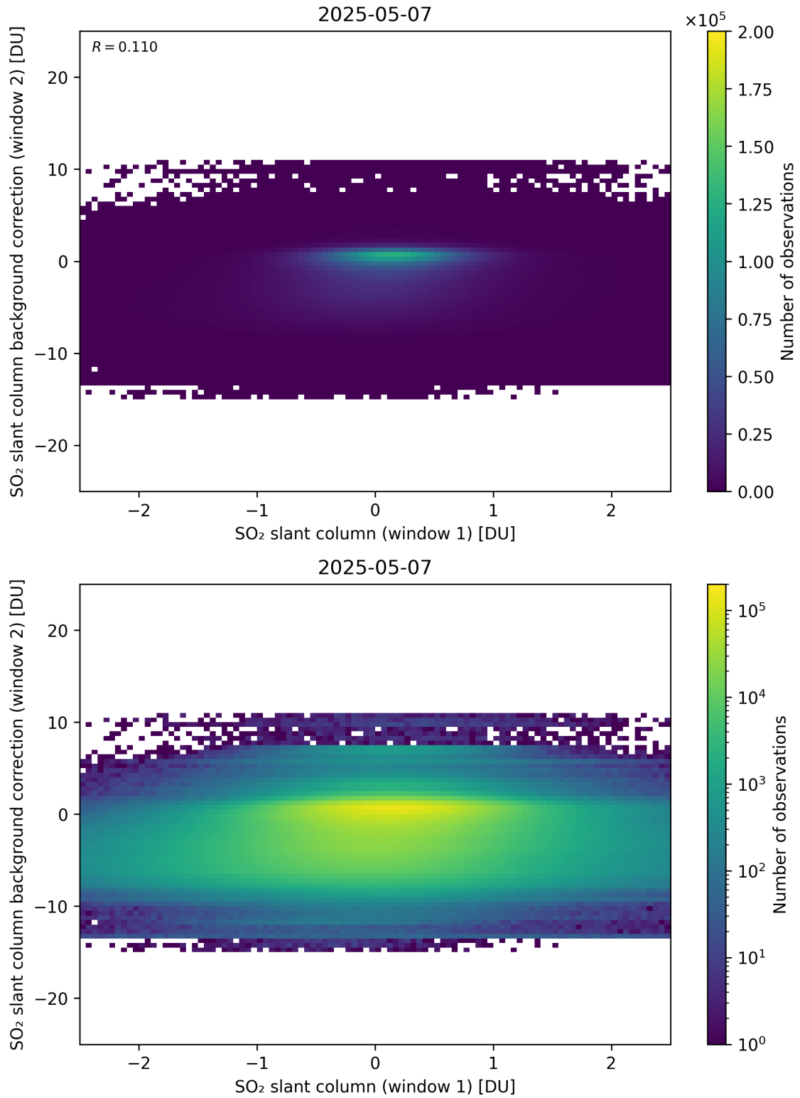
Figure 263: Scatter density plot of “SO 2 slant column (window 1)” against “SO 2 slant column background correction (window 2)” for 2025-05-06 to 2025-05-08.
