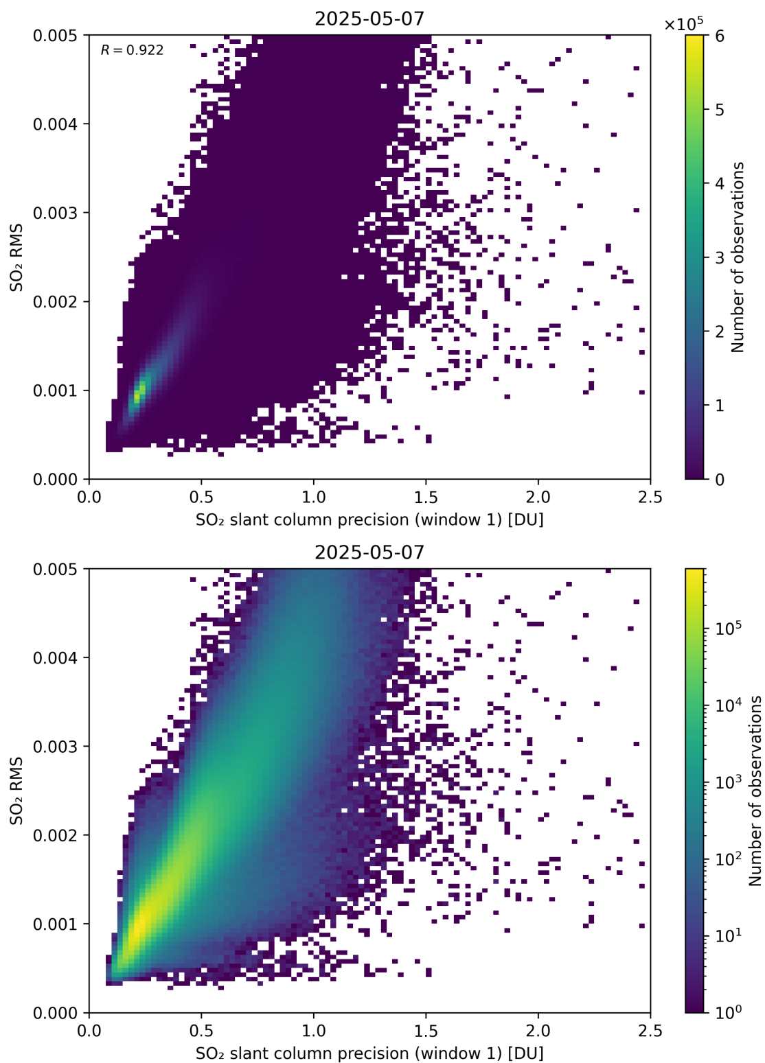
Figure 273: Scatter density plot of “SO 2 slant column precision (window 1)” against “SO 2 RMS” for 2025-05-06 to 2025-05-08.
