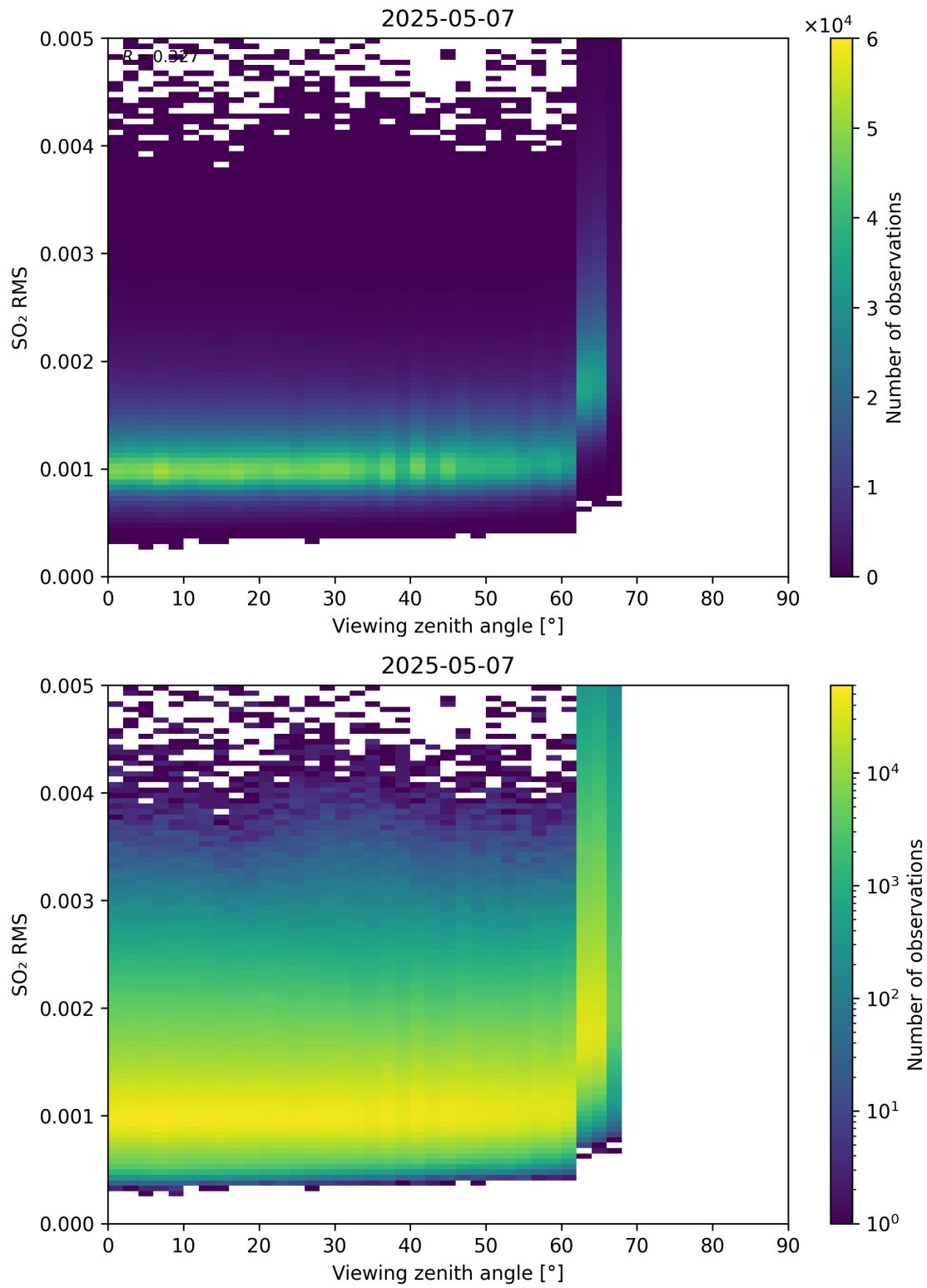
Figure 367: Scatter density plot of “Viewing zenith angle” against “SO 2 RMS” for 2025-05-06 to 2025-05-08.
