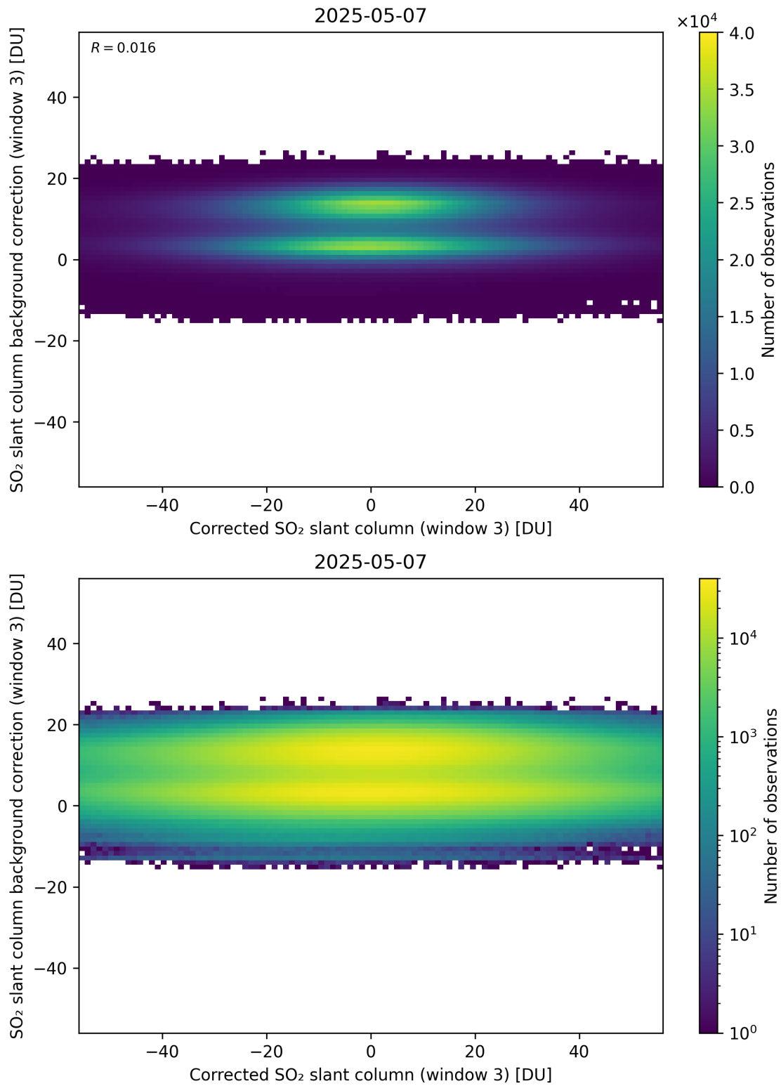
Figure 255: Scatter density plot of “Corrected SO 2 slant column (window 3)” against “SO 2 slant column background correction (window 3)” for 2025-05-06 to 2025-05-08.
