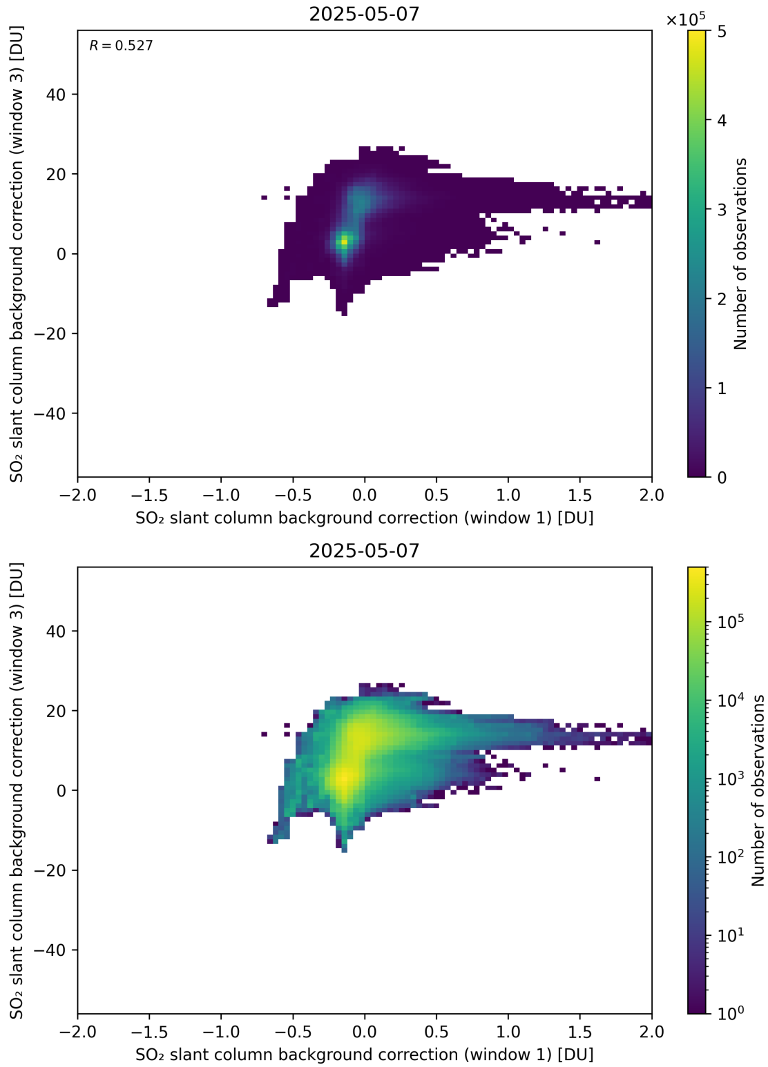
Figure 110: Scatter density plot of “SO 2 slant column background correction (window 1)” against “SO 2 slant column background correction (window 3)” for 2025-05-06 to 2025-05-08.
