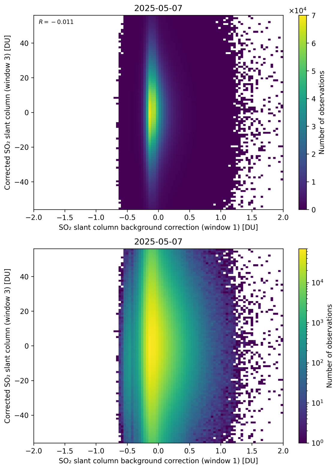
Figure 116: Scatter density plot of “SO 2 slant column background correction (window 1)” against “Corrected SO 2 slant column (window 3)” for 2025-05-06 to 2025-05-08.
