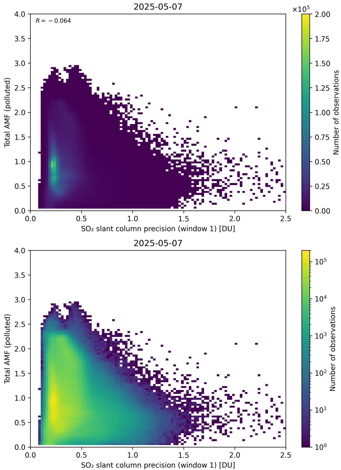
Figure 280: Scatter density plot of “SO 2 slant column precision (window 1)” against “Total AMF (polluted)” for 2025-05-06 to 2025-05-08.
