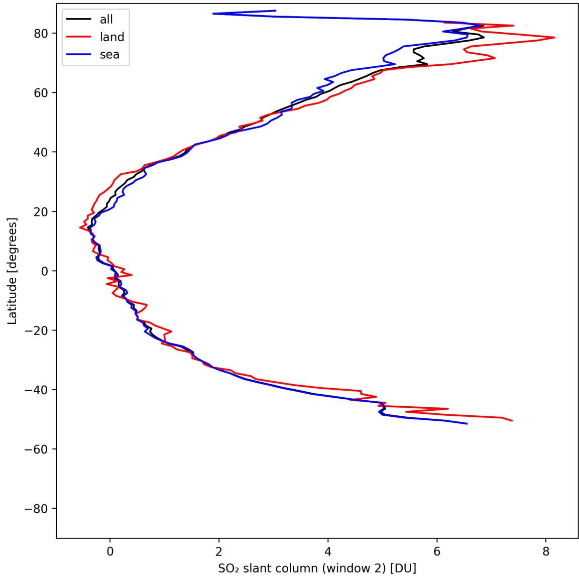
Figure 41: Zonal average of “SO 2 slant column (window 2)” for 2025-05-06 to 2025-05-08.
