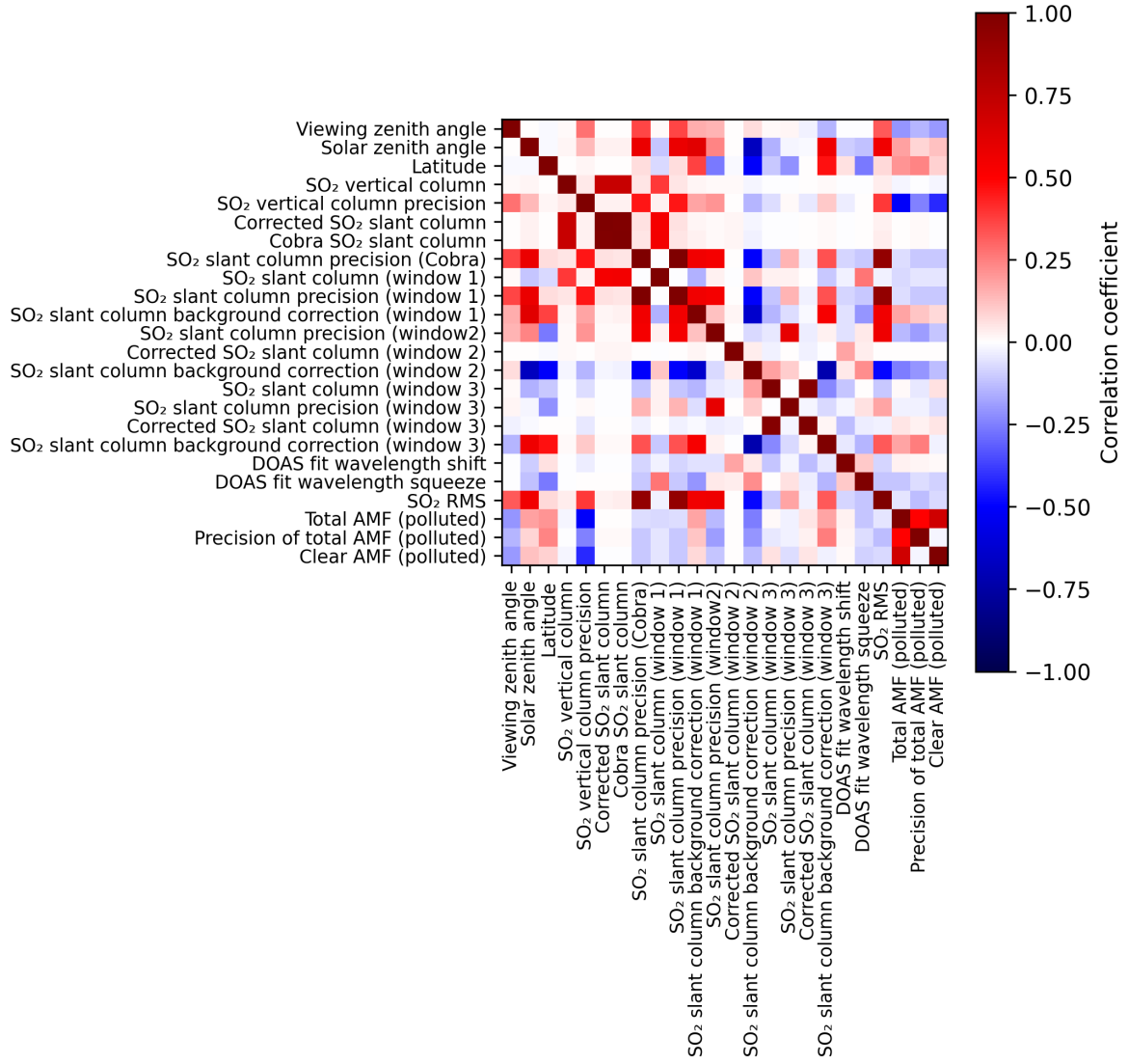
Figure 2: Map of correlation matrix for 2025-05-06 to 2025-05-08.
