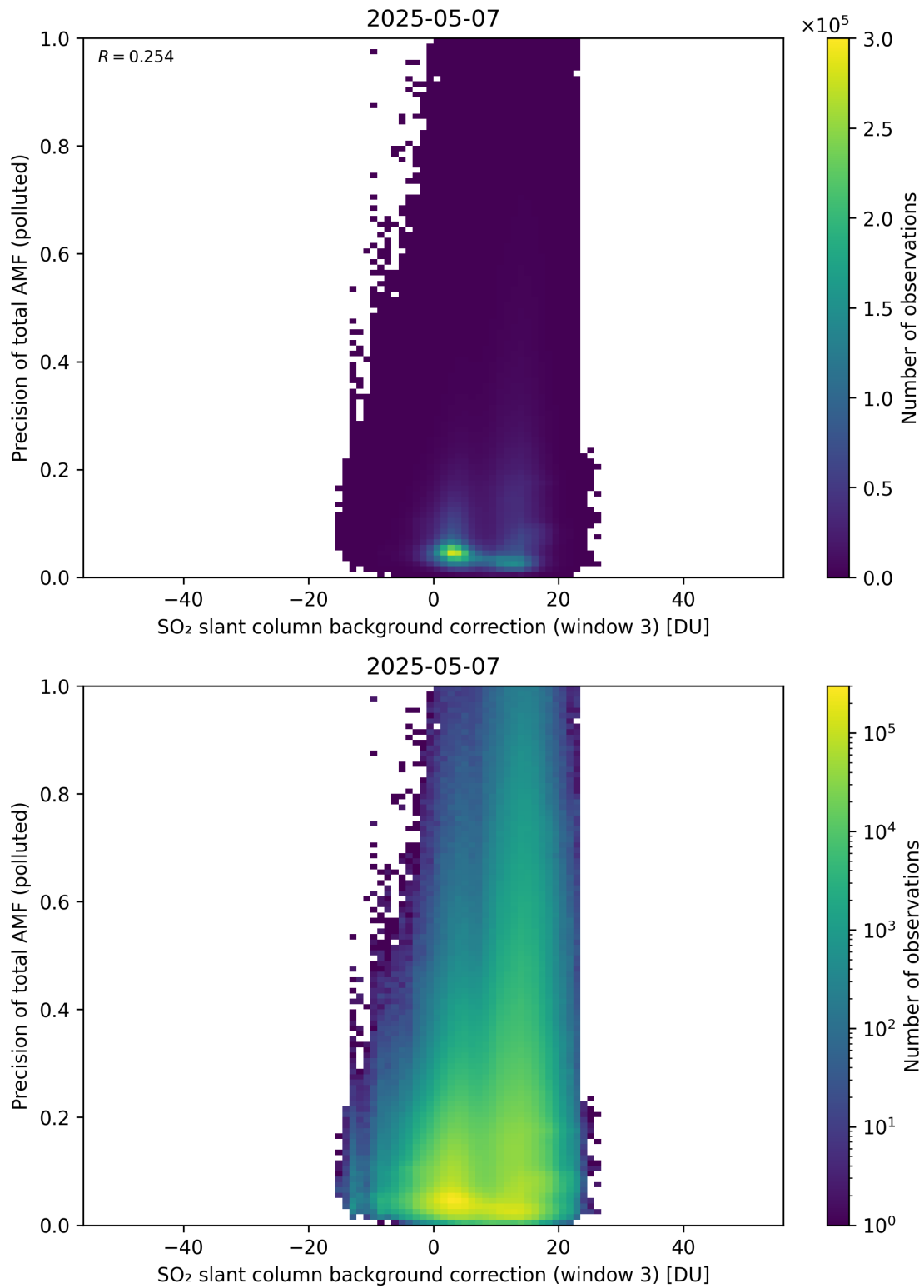
Figure 137: Scatter density plot of “SO 2 slant column background correction (window 3)” against “Precision of total AMF (polluted)” for 2025-05-06 to 2025-05-08.
