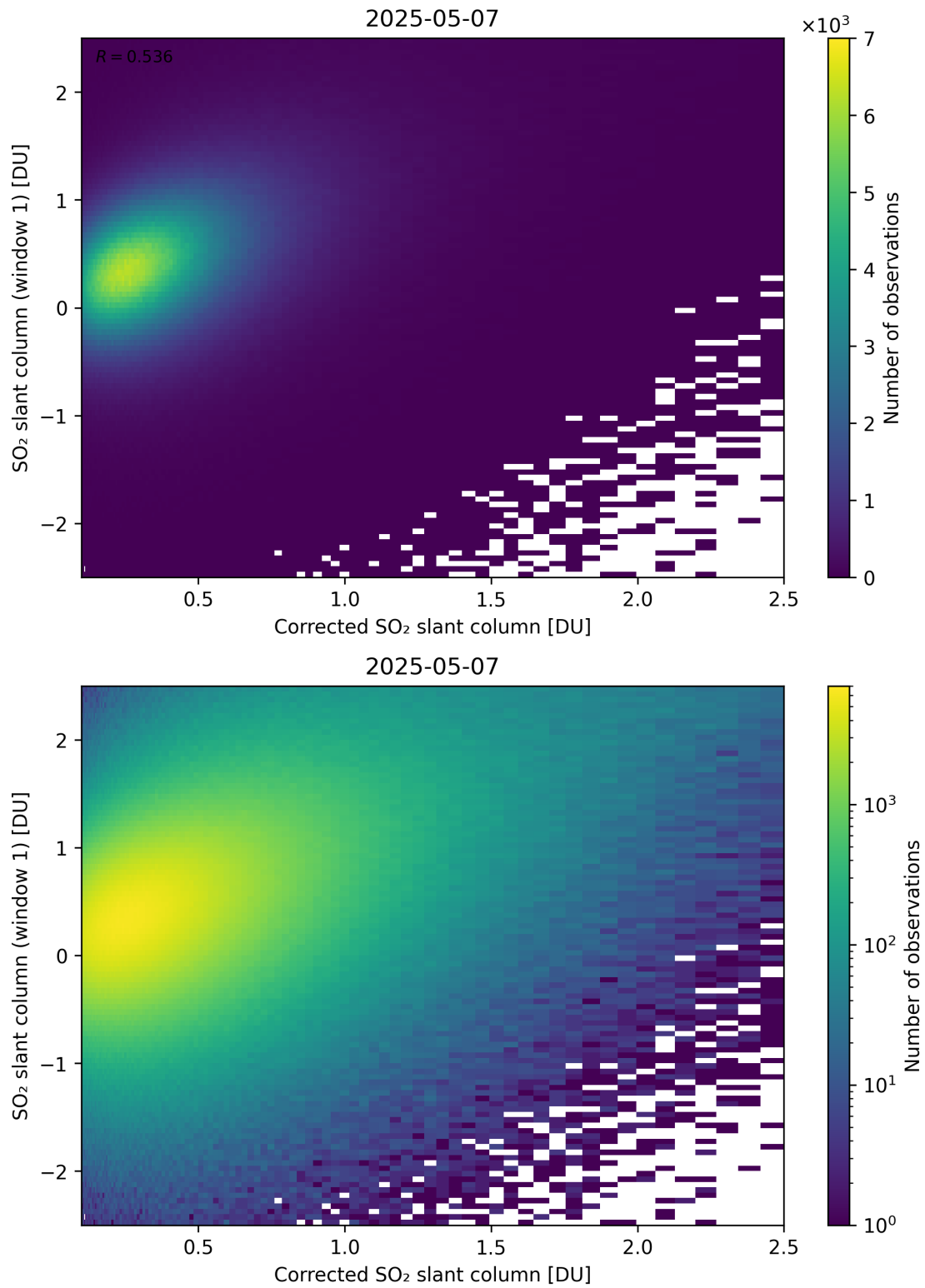
Figure 237: Scatter density plot of “Corrected SO 2 slant column” against “SO 2 slant column (window 1)” for 2025-05-06 to 2025-05-08.
