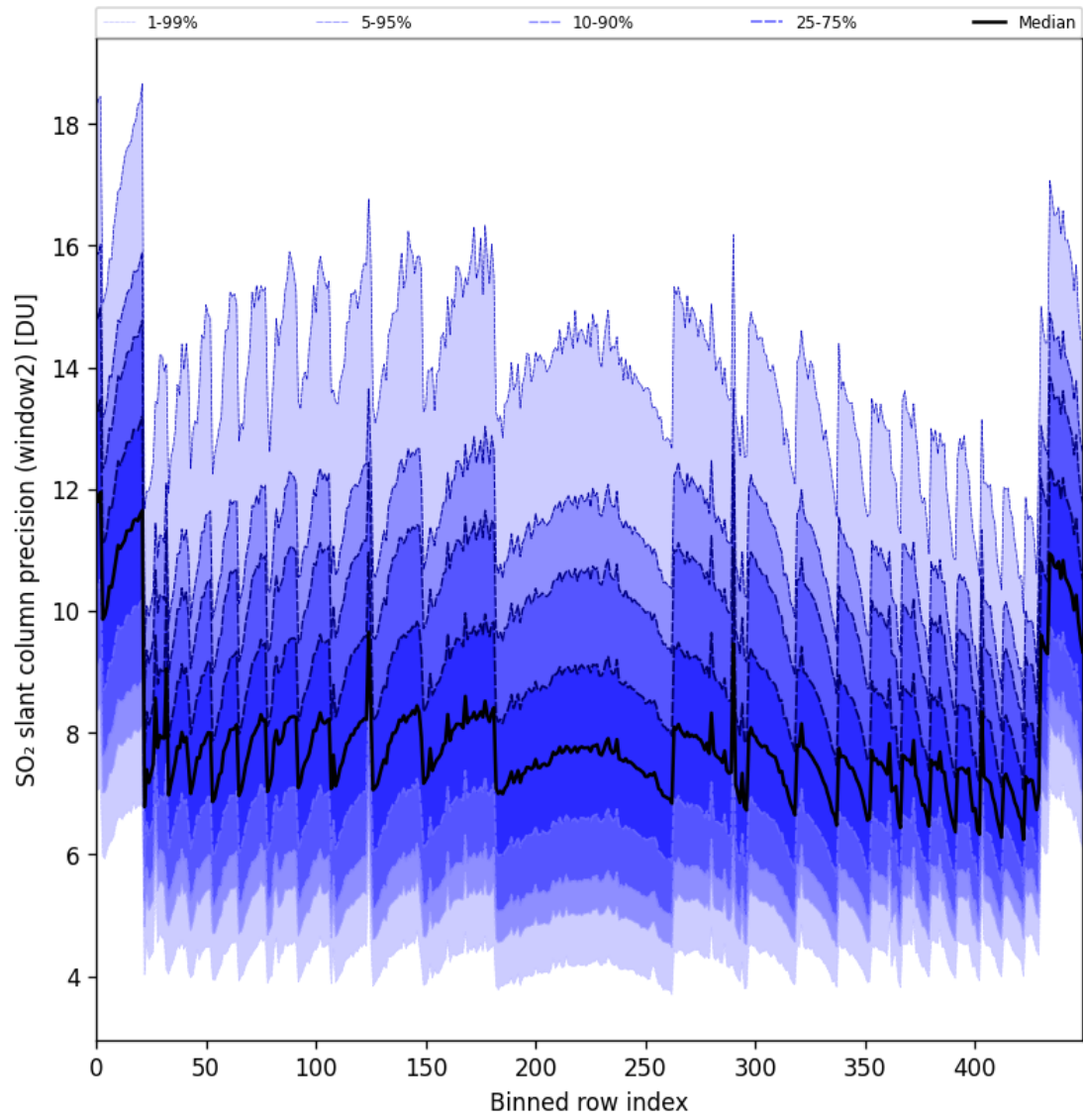
Figure 94: Along track statistics of “SO 2 slant column precision (window2)” for 2025-05-06 to 2025-05-08
