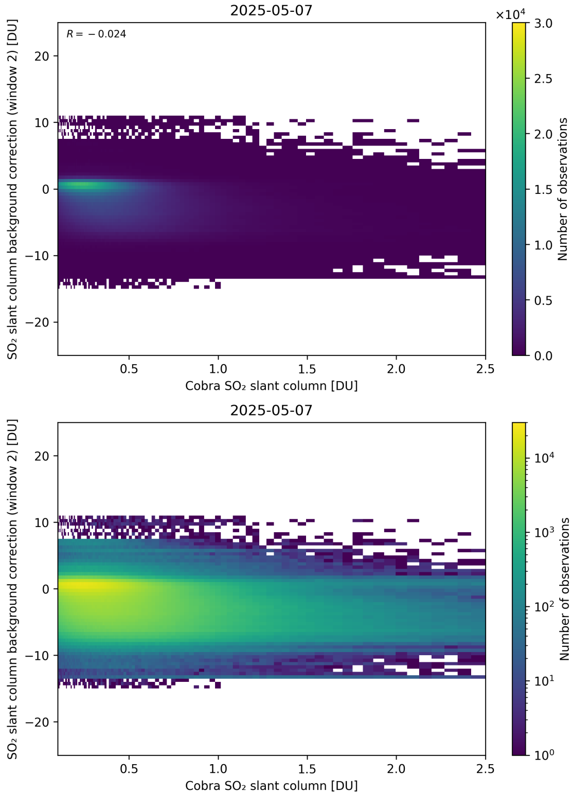
Figure 194: Scatter density plot of “Cobra SO 2 slant column” against “SO 2 slant column background correction (window 2)” for 2025-05-06 to 2025-05-08.
