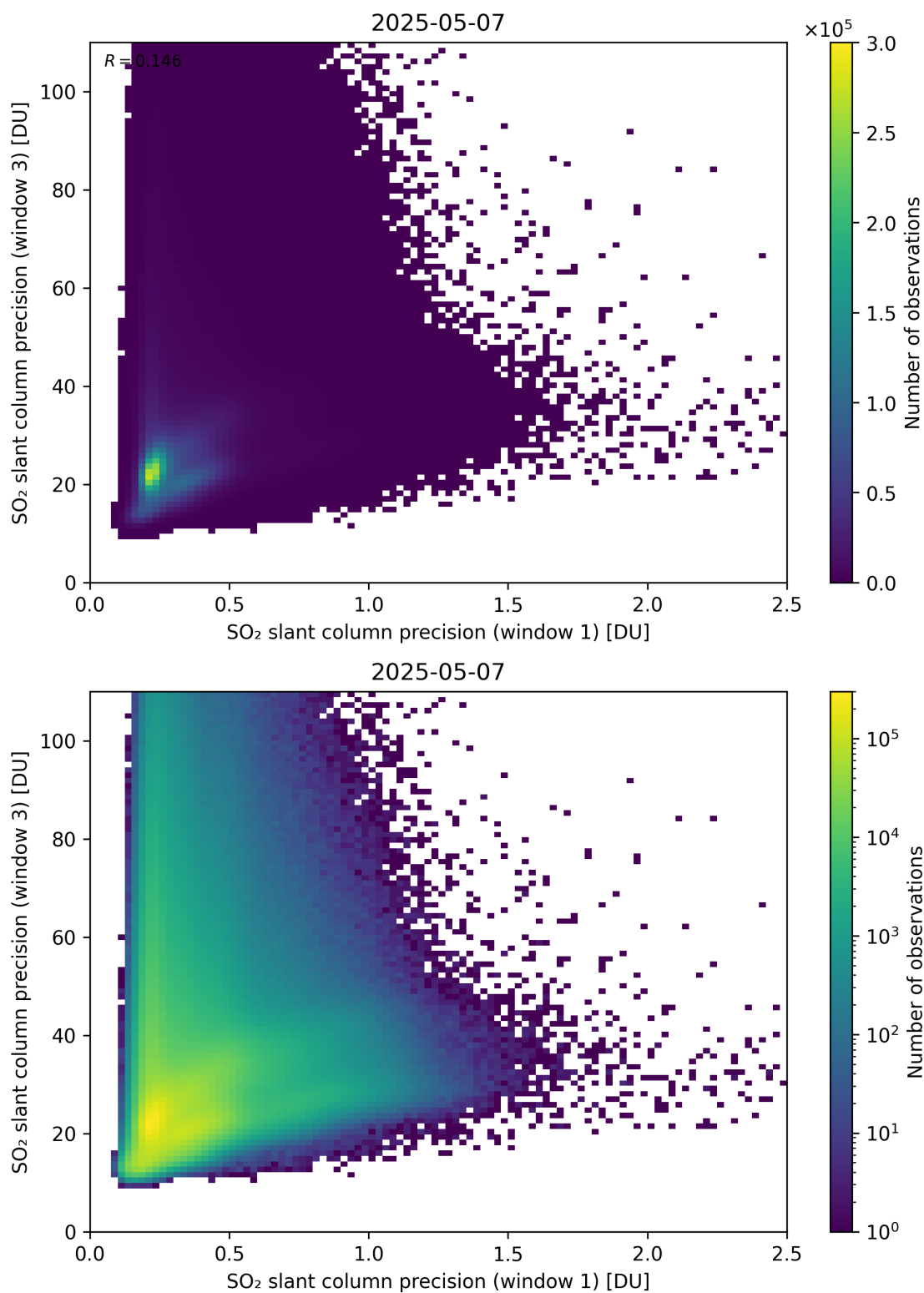
Figure 279: Scatter density plot of “SO 2 slant column precision (window 1)” against “SO 2 slant column precision (window 3)” for 2025-05-06 to 2025-05-08.
