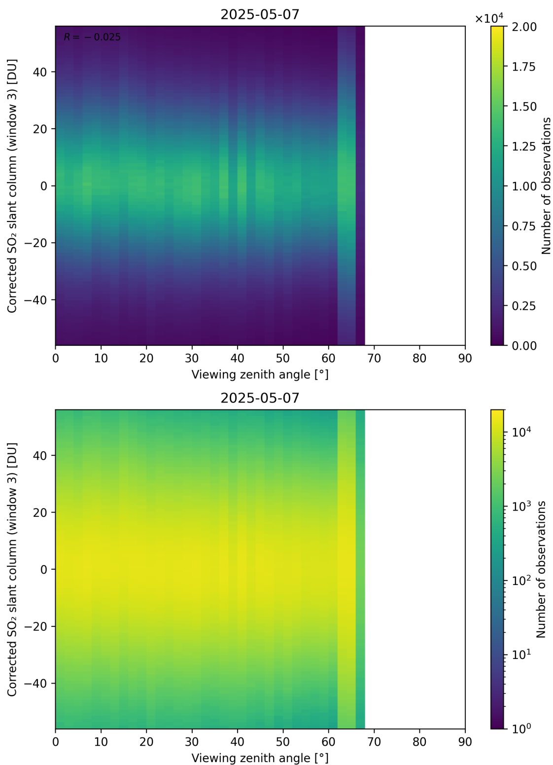
Figure 375: Scatter density plot of “Viewing zenith angle” against “Corrected SO 2 slant column (window 3)” for 2025-05-06 to 2025-05-08.
