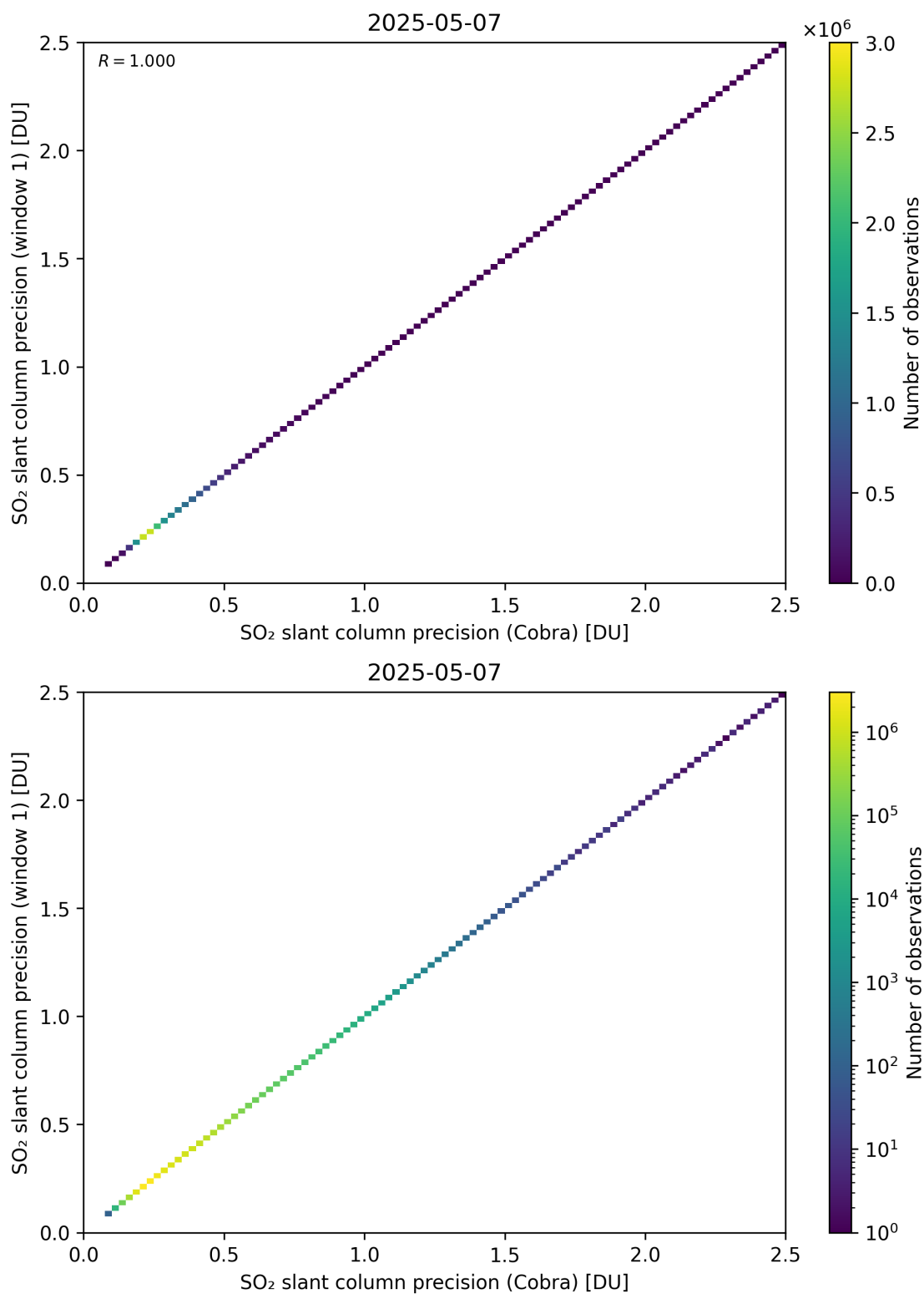
Figure 209: Scatter density plot of “SO 2 slant column precision (Cobra)” against “SO 2 slant column precision (window 1)” for 2025-05-06 to 2025-05-08.
