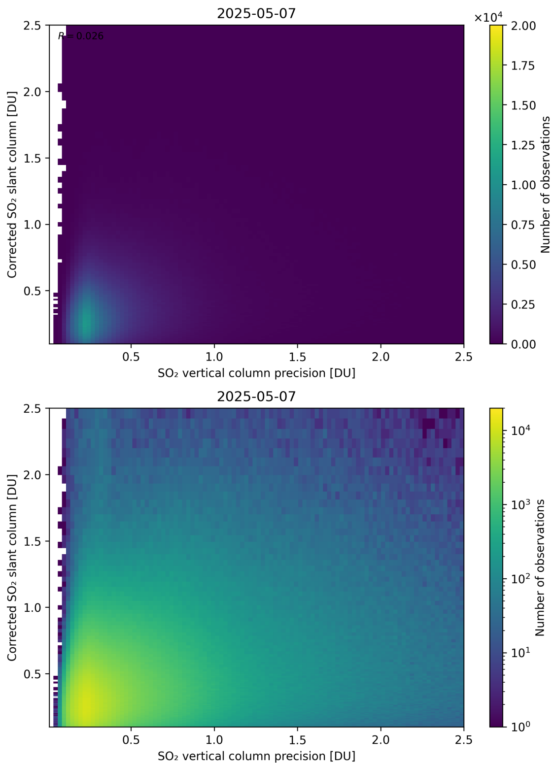
Figure 338: Scatter density plot of “SO 2 vertical column precision” against “Corrected SO 2 slant column” for 2025-05-06 to 2025-05-08.
