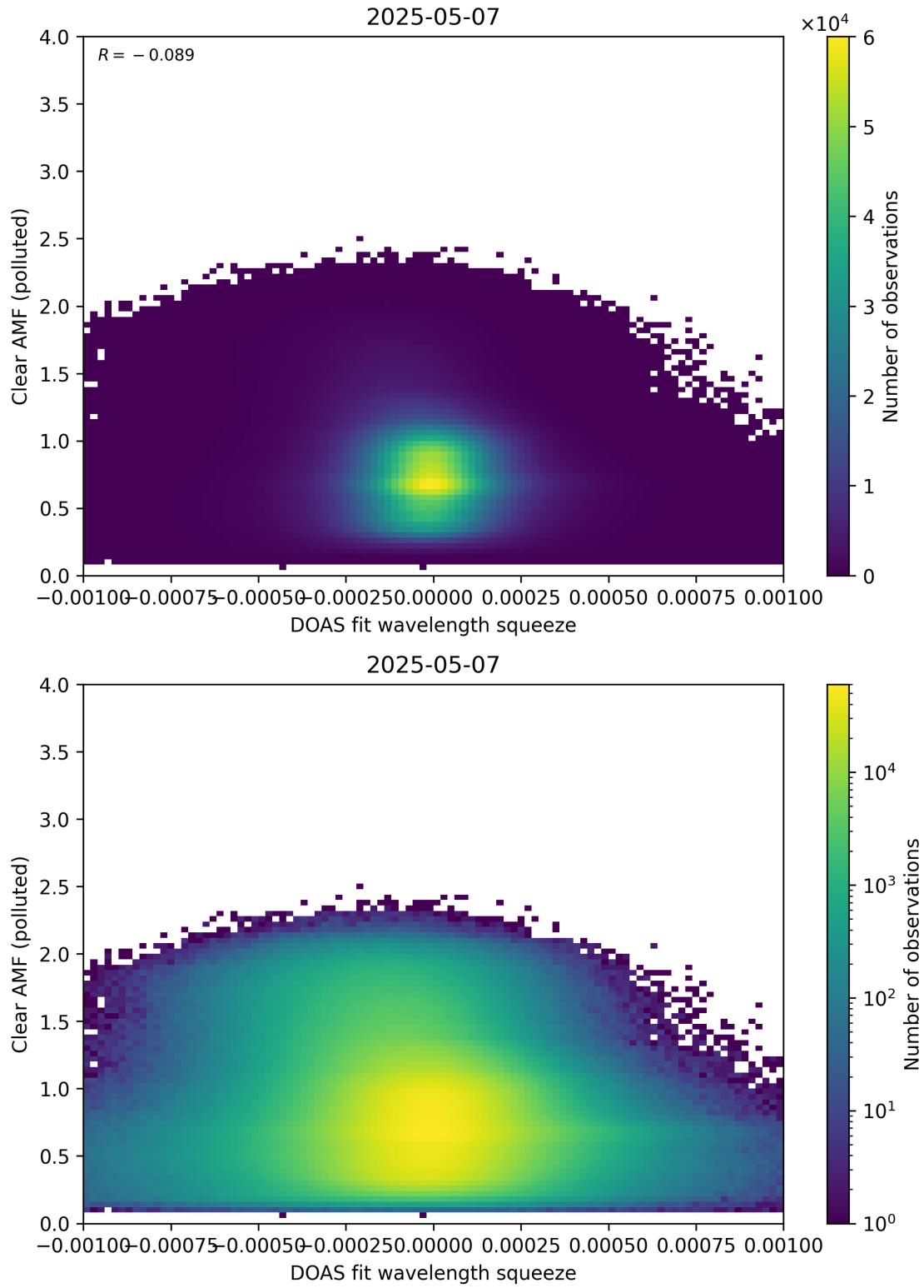
Figure 144: Scatter density plot of “DOAS fit wavelength squeeze” against “Clear AMF (polluted)” for 2025-05-06 to 2025-05-08.
