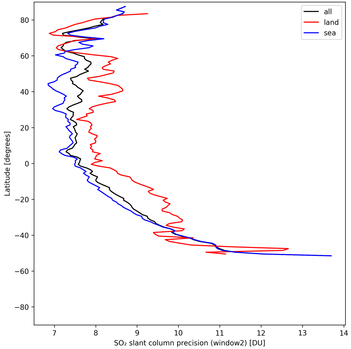
Figure 42: Zonal average of “SO 2 slant column precision (window2)” for 2025-05-06 to 2025-05-08.
