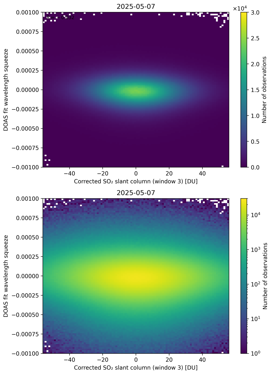
Figure 257: Scatter density plot of “Corrected SO 2 slant column (window 3)” against “DOAS fit wavelength squeeze” for 2025-05-06 to 2025-05-08.
