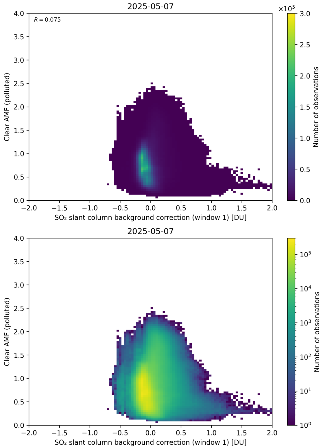
Figure 114: Scatter density plot of “SO 2 slant column background correction (window 1)” against “Clear AMF (polluted)” for 2025-05-06 to 2025-05-08.
