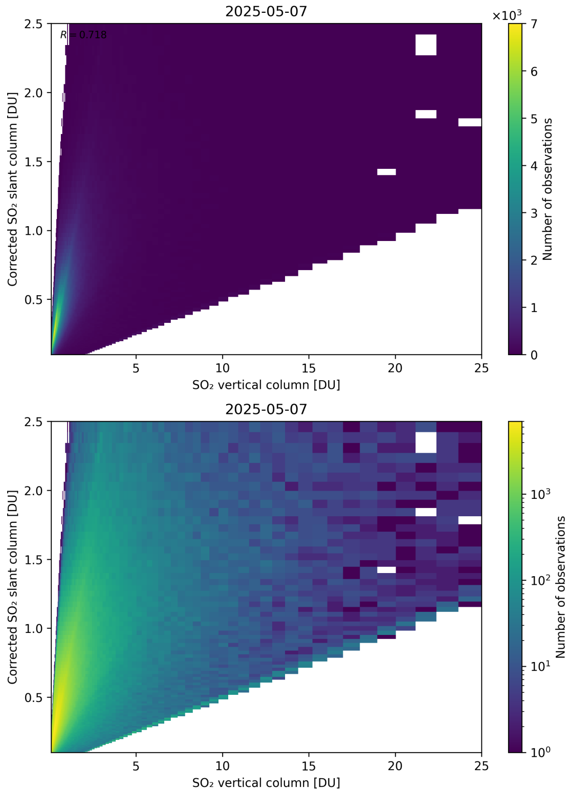
Figure 351: Scatter density plot of “SO 2 vertical column” against “Corrected SO 2 slant column” for 2025-05-06 to 2025-05-08.
