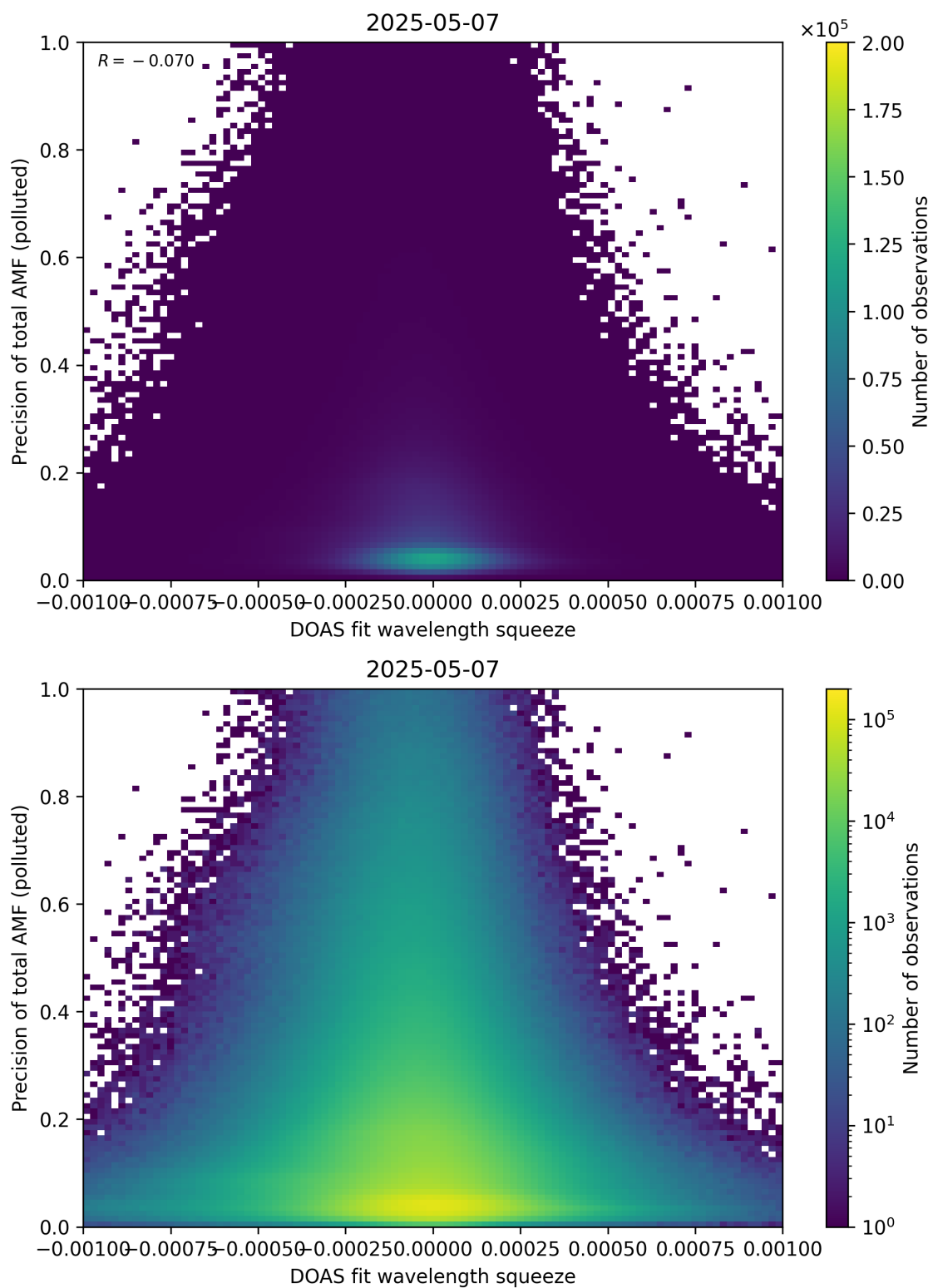
Figure 146: Scatter density plot of “DOAS fit wavelength squeeze” against “Precision of total AMF (polluted)” for 2025-05-06 to 2025-05-08.
