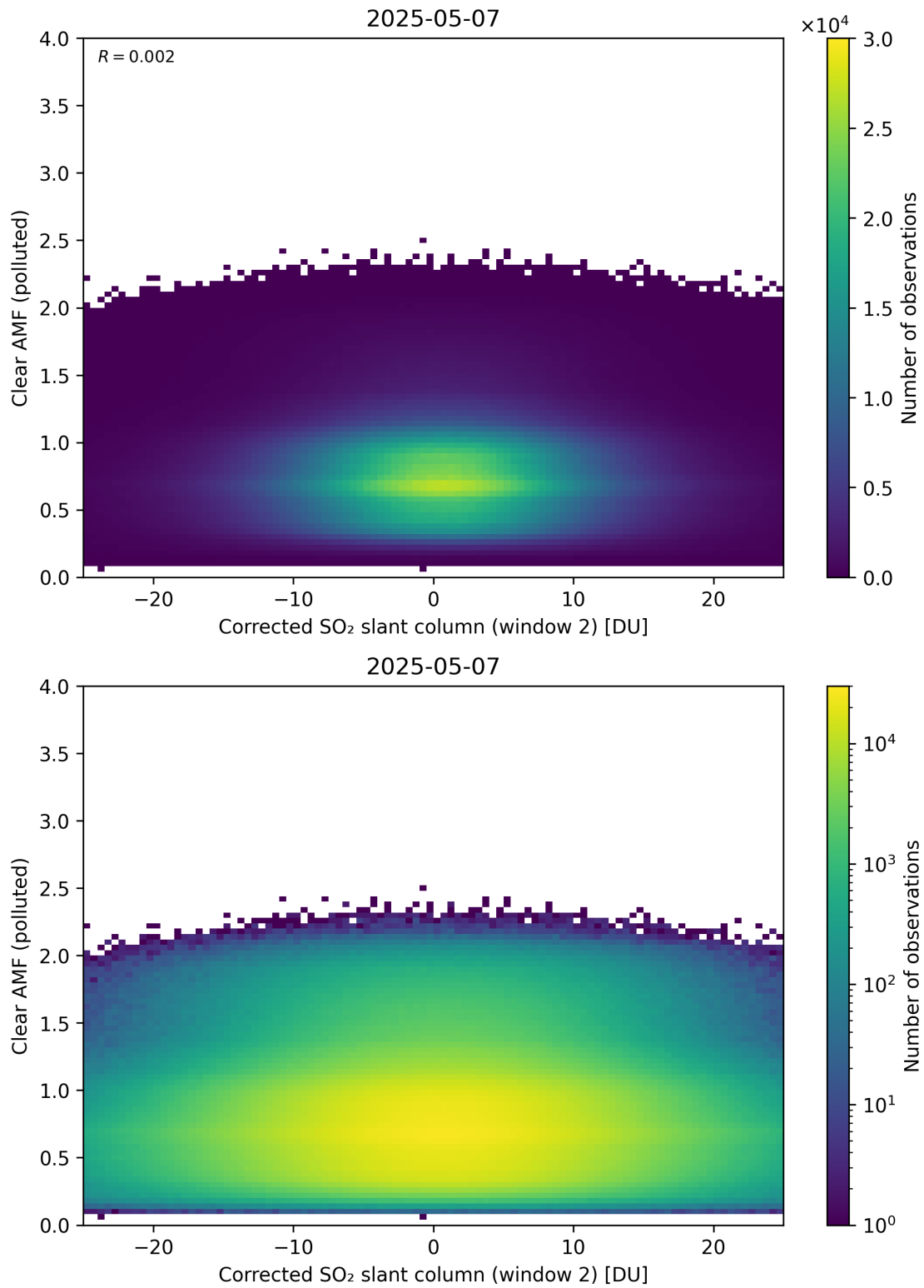
Figure 249: Scatter density plot of “Corrected SO 2 slant column (window 2)” against “Clear AMF (polluted)” for 2025-05-06 to 2025-05-08.
