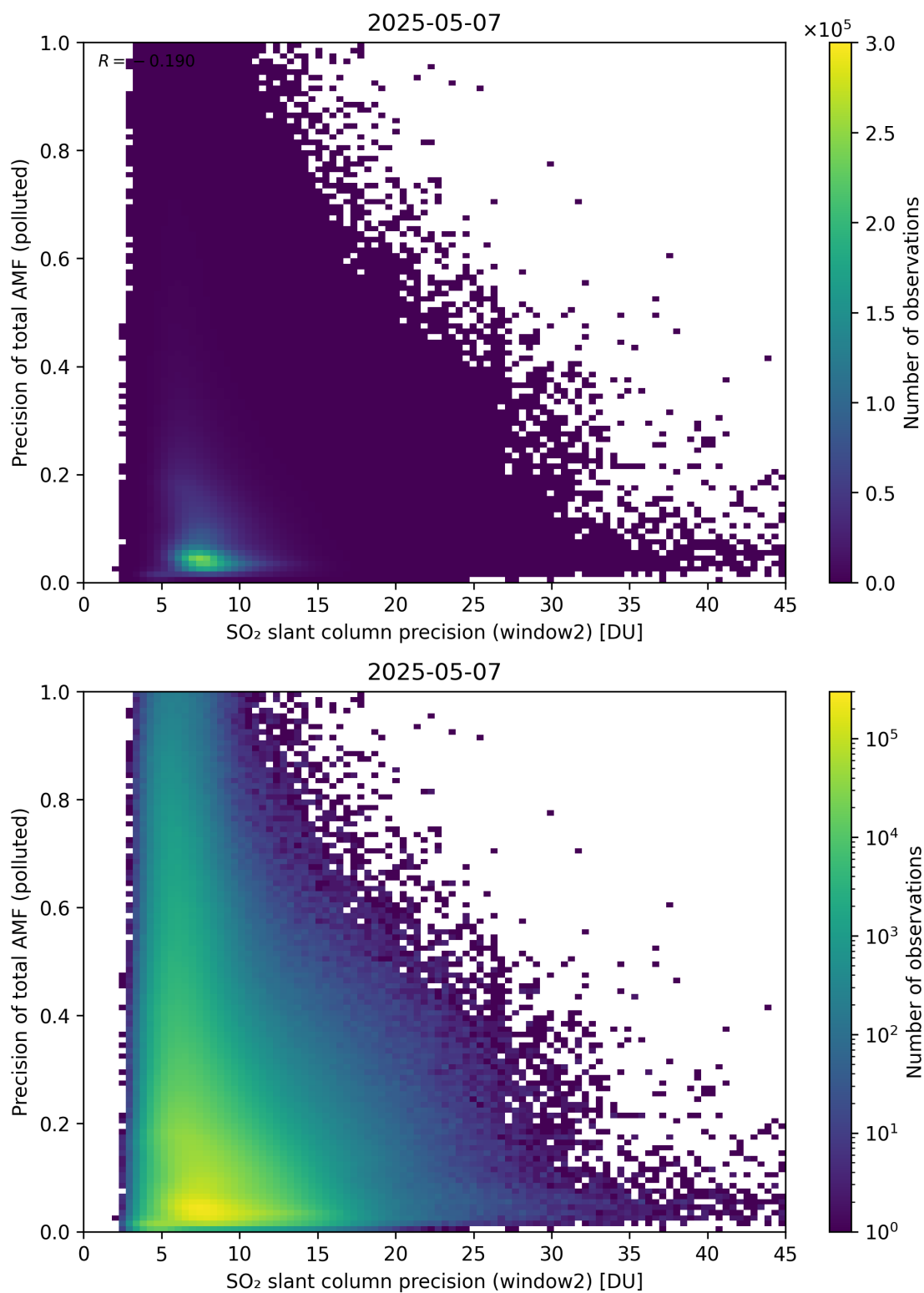
Figure 302: Scatter density plot of “SO 2 slant column precision (window2)” against “Precision of total AMF (polluted)” for 2025-05-06 to 2025-05-08.
