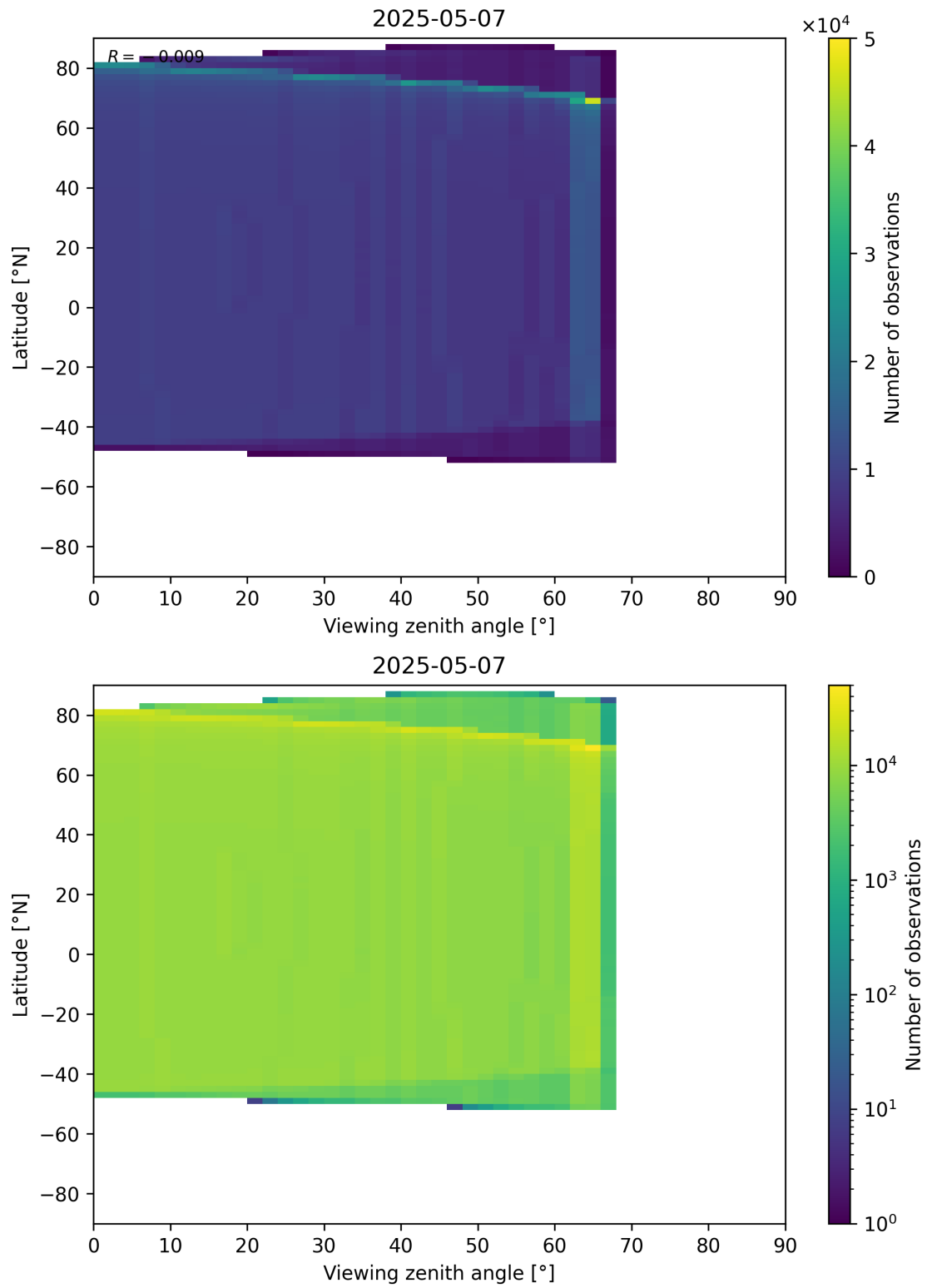
Figure 368: Scatter density plot of “Viewing zenith angle” against “Latitude” for 2025-05-06 to 2025-05-08.
