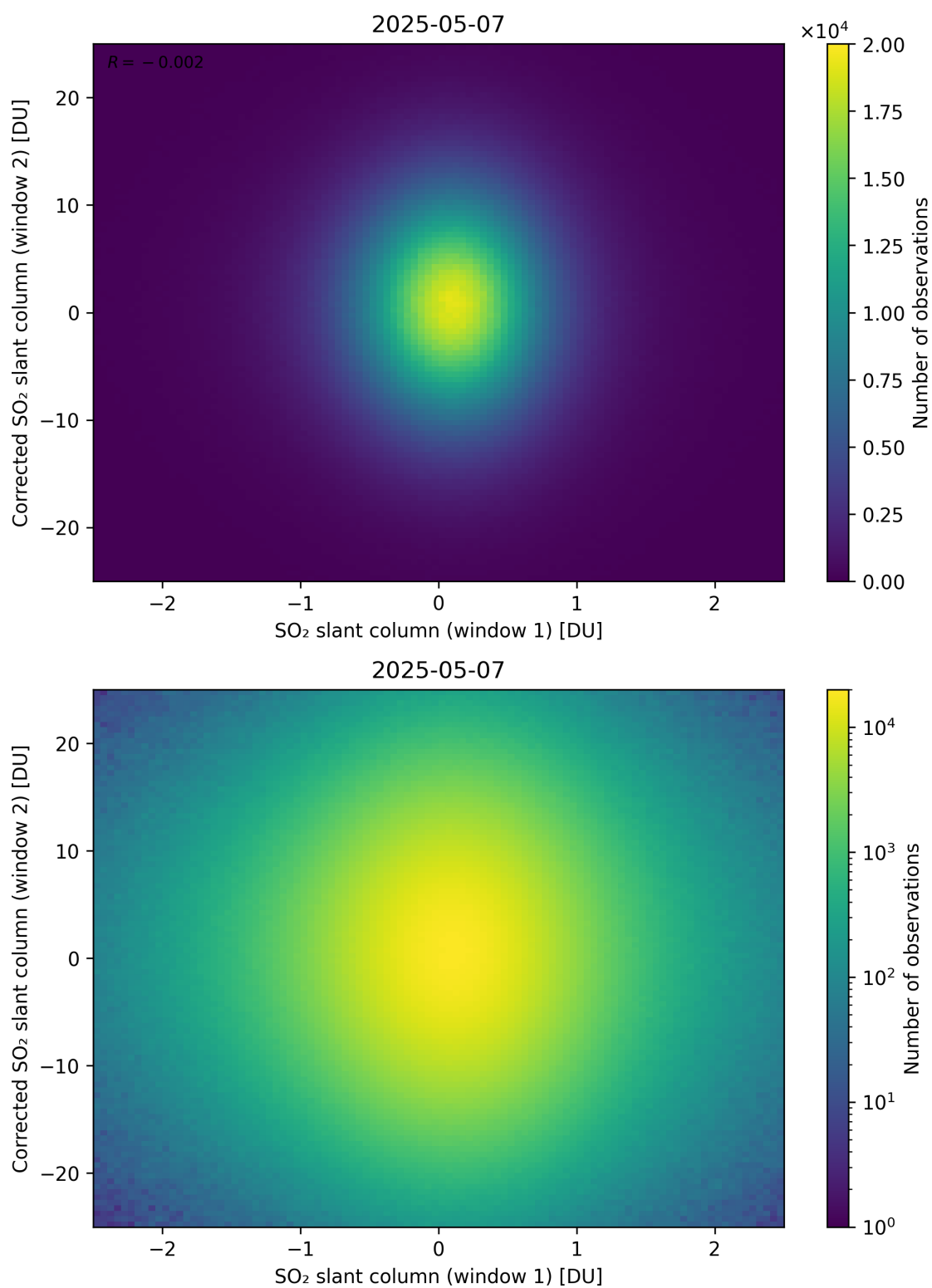
Figure 283: Scatter density plot of “SO 2 slant column (window 1)” against “Corrected SO 2 slant column (window 2)” for 2025-05-06 to 2025-05-08.
