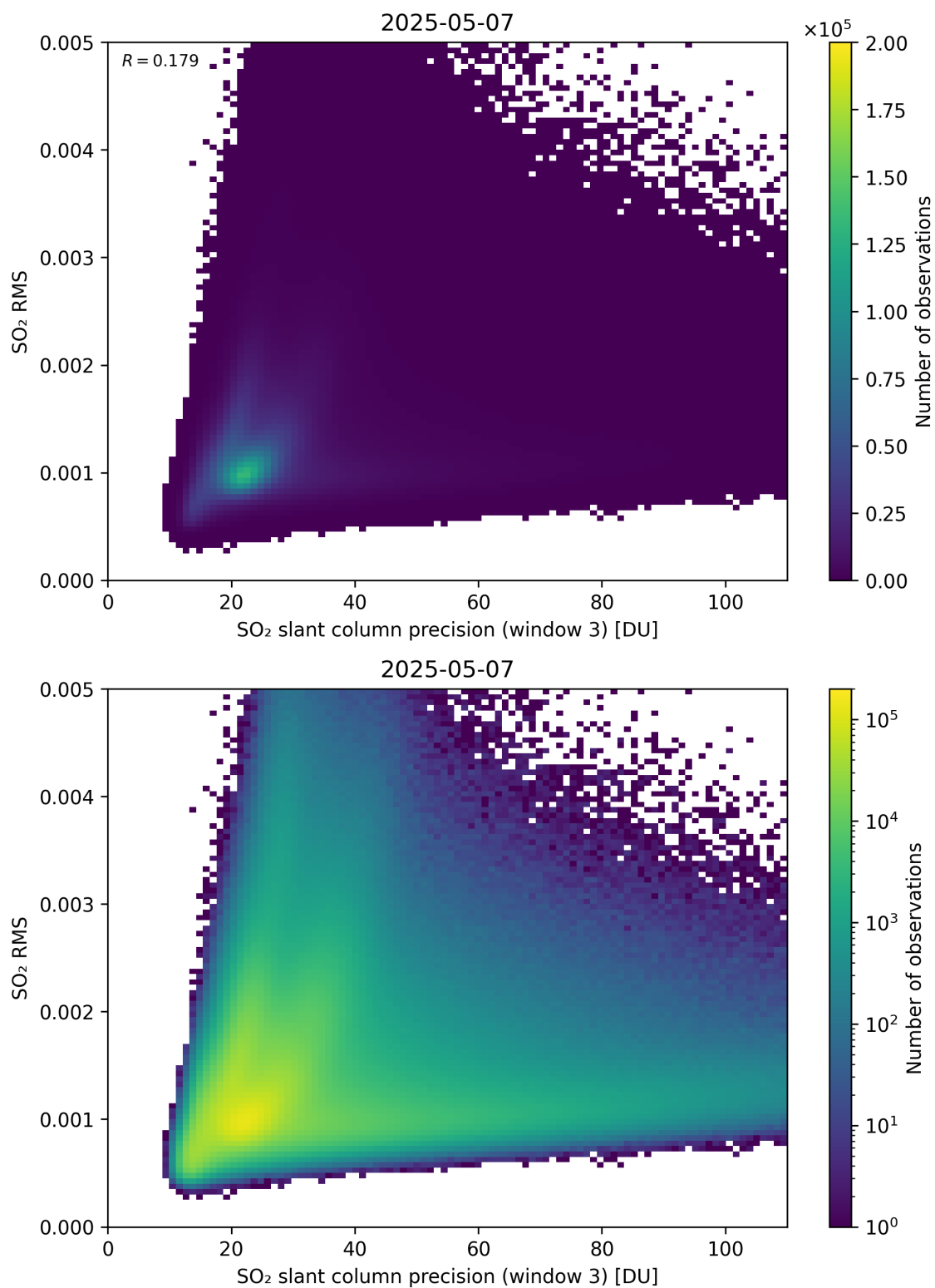
Figure 310: Scatter density plot of “SO 2 slant column precision (window 3)” against “SO 2 RMS” for 2025-05-06 to 2025-05-08.
