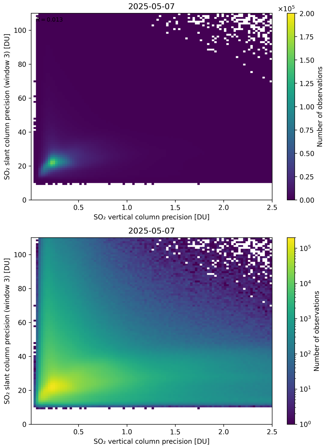
Figure 345: Scatter density plot of “SO 2 vertical column precision” against “SO 2 slant column precision (window 3)” for 2025-05-06 to 2025-05-08.
