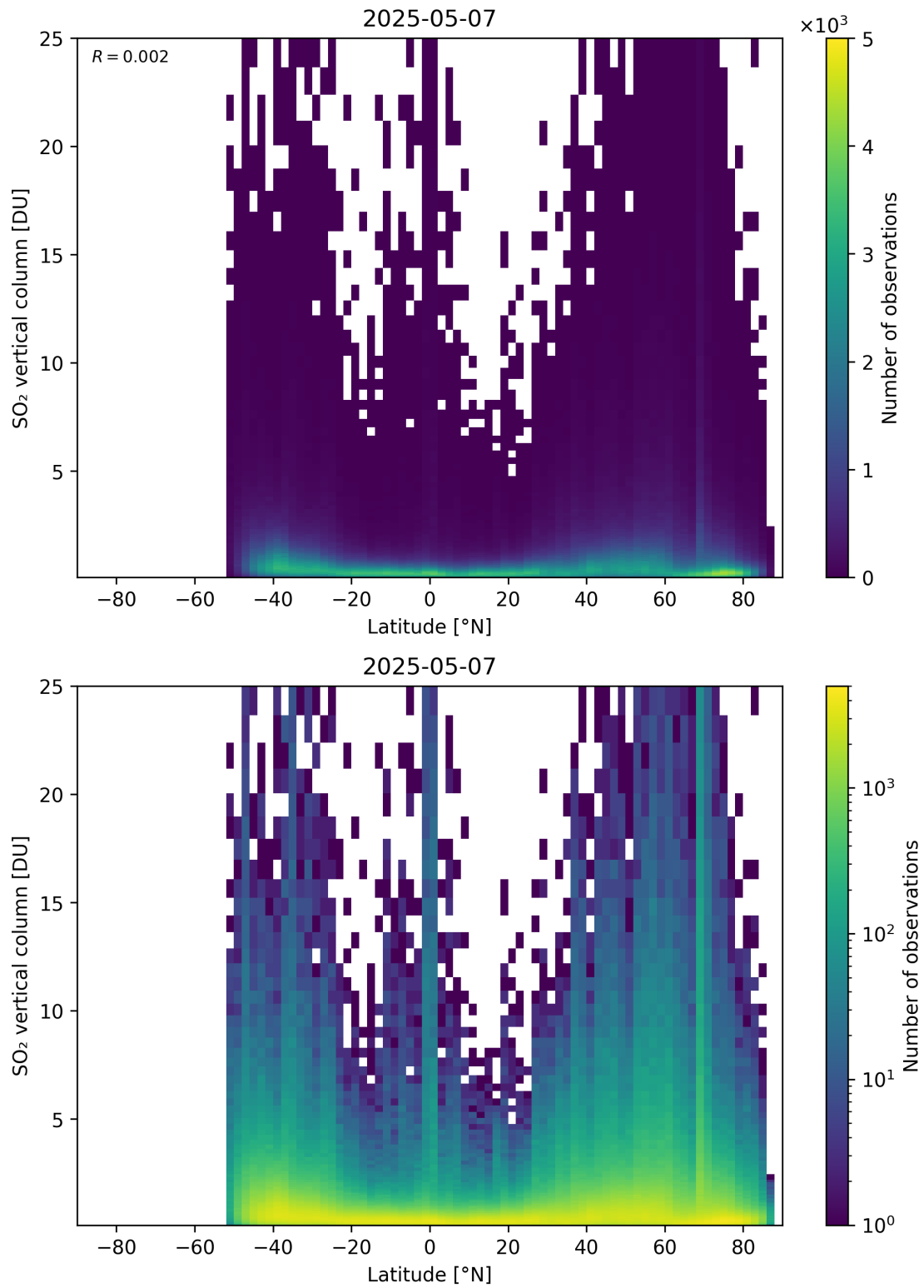
Figure 169: Scatter density plot of “Latitude” against “SO 2 vertical column” for 2025-05-06 to 2025-05-08.
