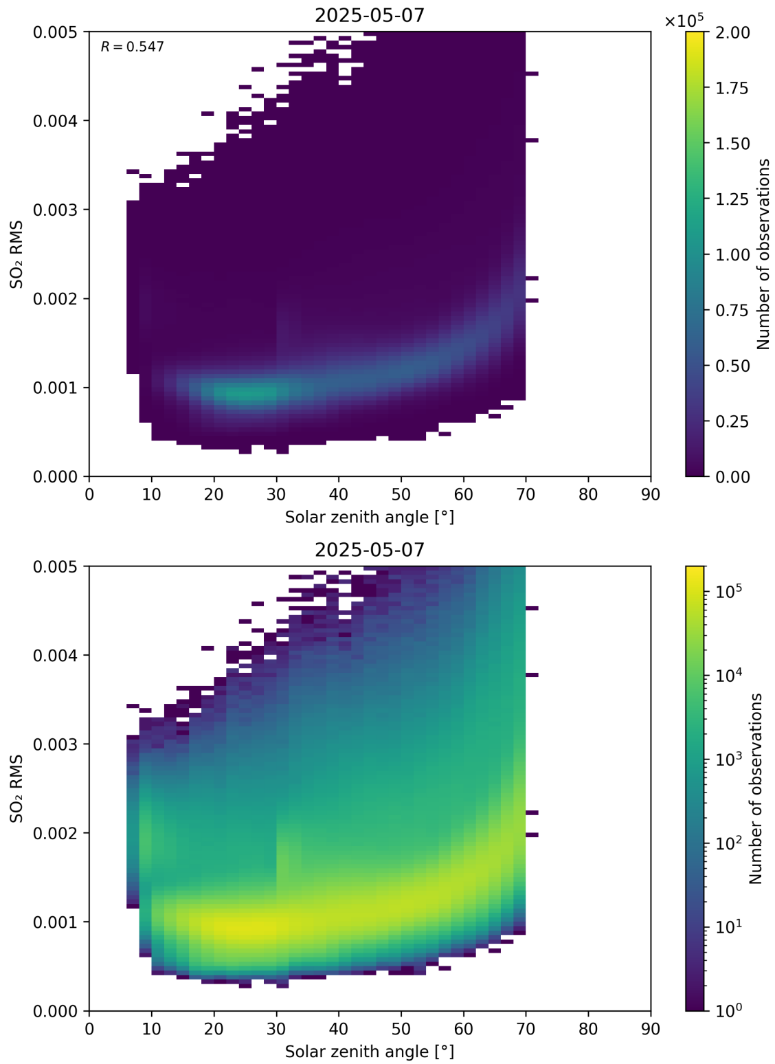
Figure 176: Scatter density plot of “Solar zenith angle” against “SO 2 RMS” for 2025-05-06 to 2025-05-08.
