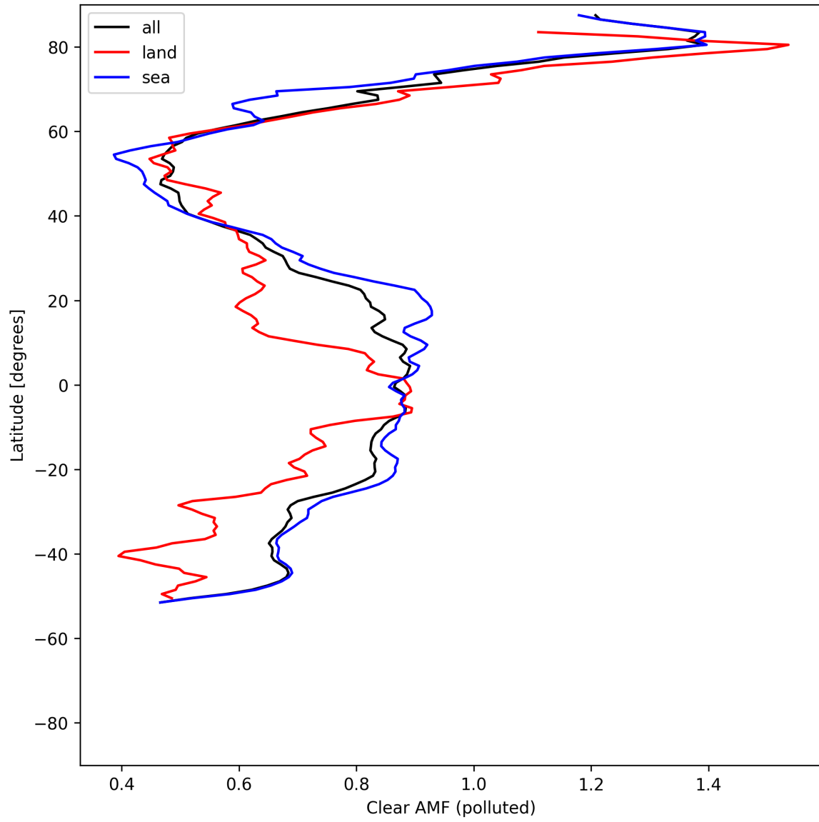
Figure 55: Zonal average of “Clear AMF (polluted)” for 2025-05-06 to 2025-05-08.
