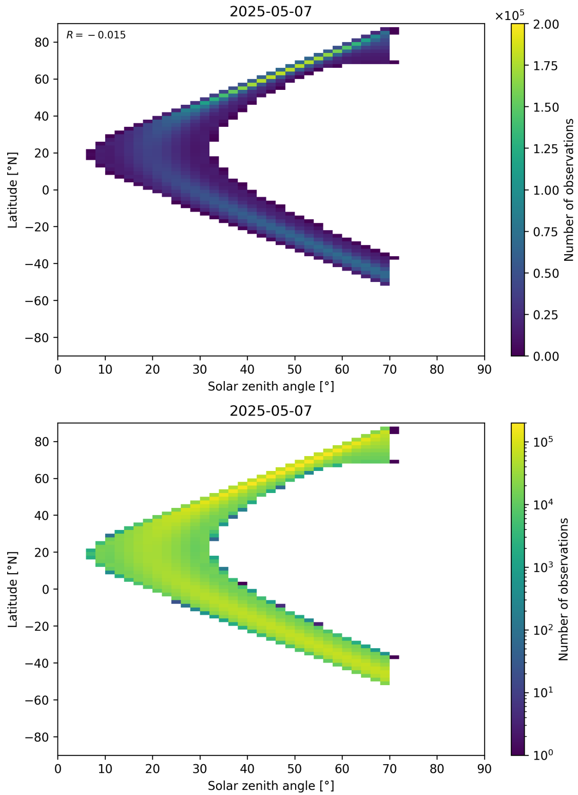
Figure 177: Scatter density plot of “Solar zenith angle” against “Latitude” for 2025-05-06 to 2025-05-08.
