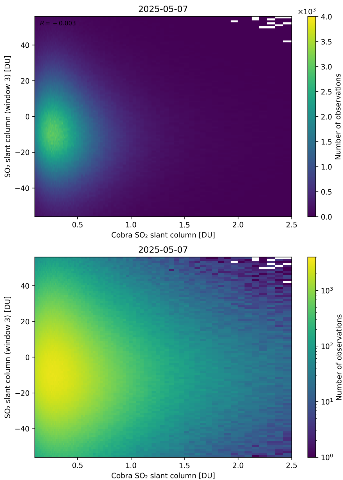
Figure 222: Scatter density plot of “Cobra SO 2 slant column” against “SO 2 slant column (window 3)” for 2025-05-06 to 2025-05-08.
