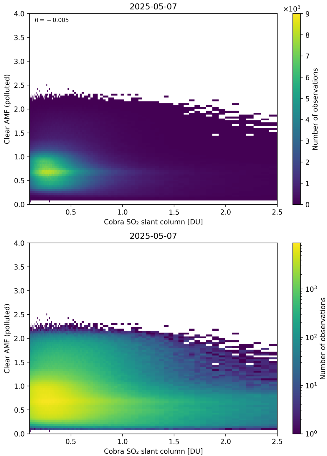
Figure 215: Scatter density plot of “Cobra SO 2 slant column” against “Clear AMF (polluted)” for 2025-05-06 to 2025-05-08.
