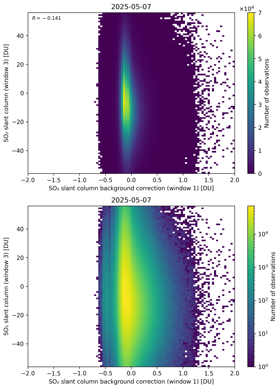
Figure 118: Scatter density plot of “SO 2 slant column background correction (window 1)” against “SO 2 slant column (window 3)” for 2025-05-06 to 2025-05-08.
