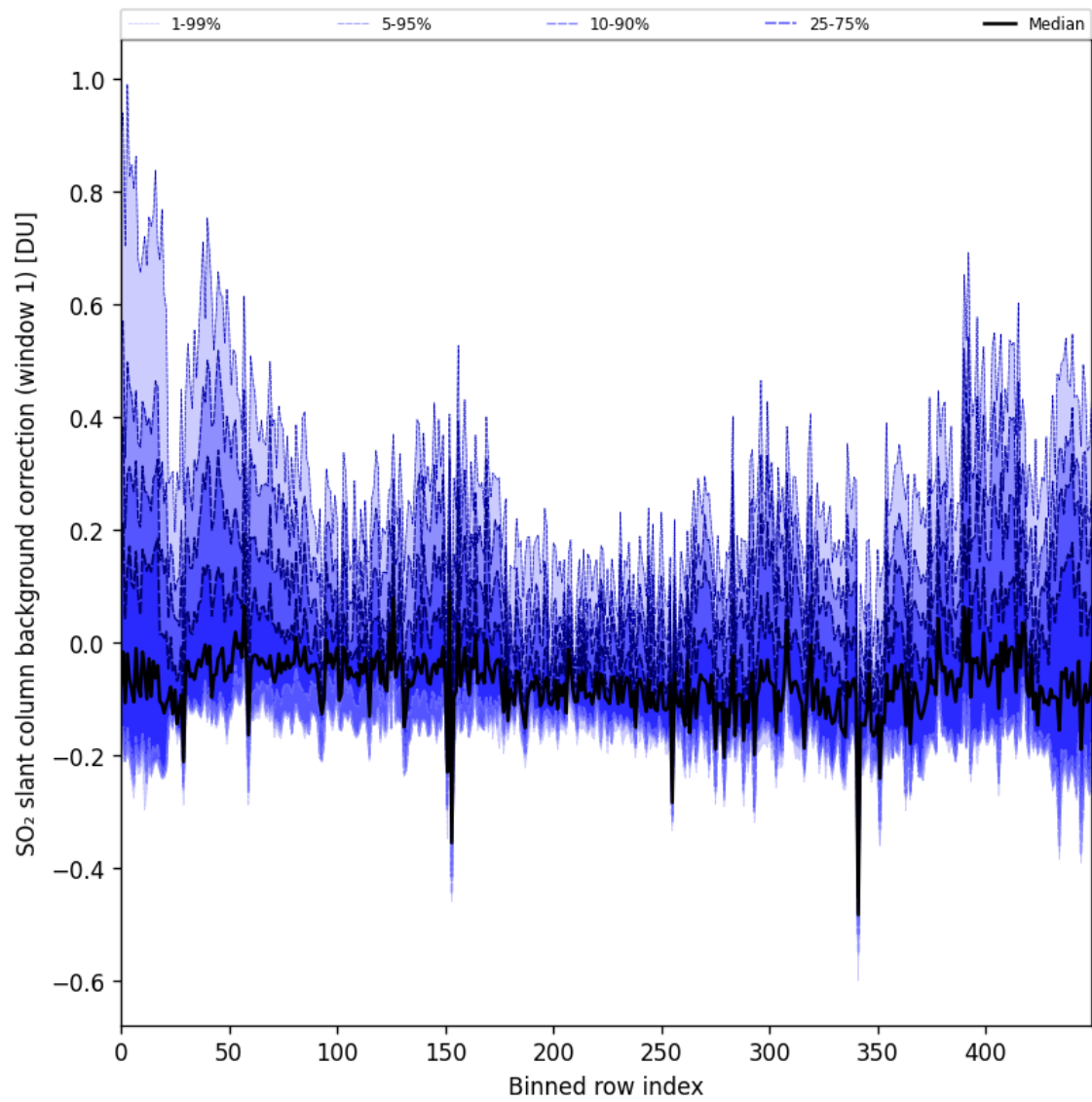
Figure 92: Along track statistics of “SO 2 slant column background correction (window 1)” for 2025-05-06 to 2025-05-08
