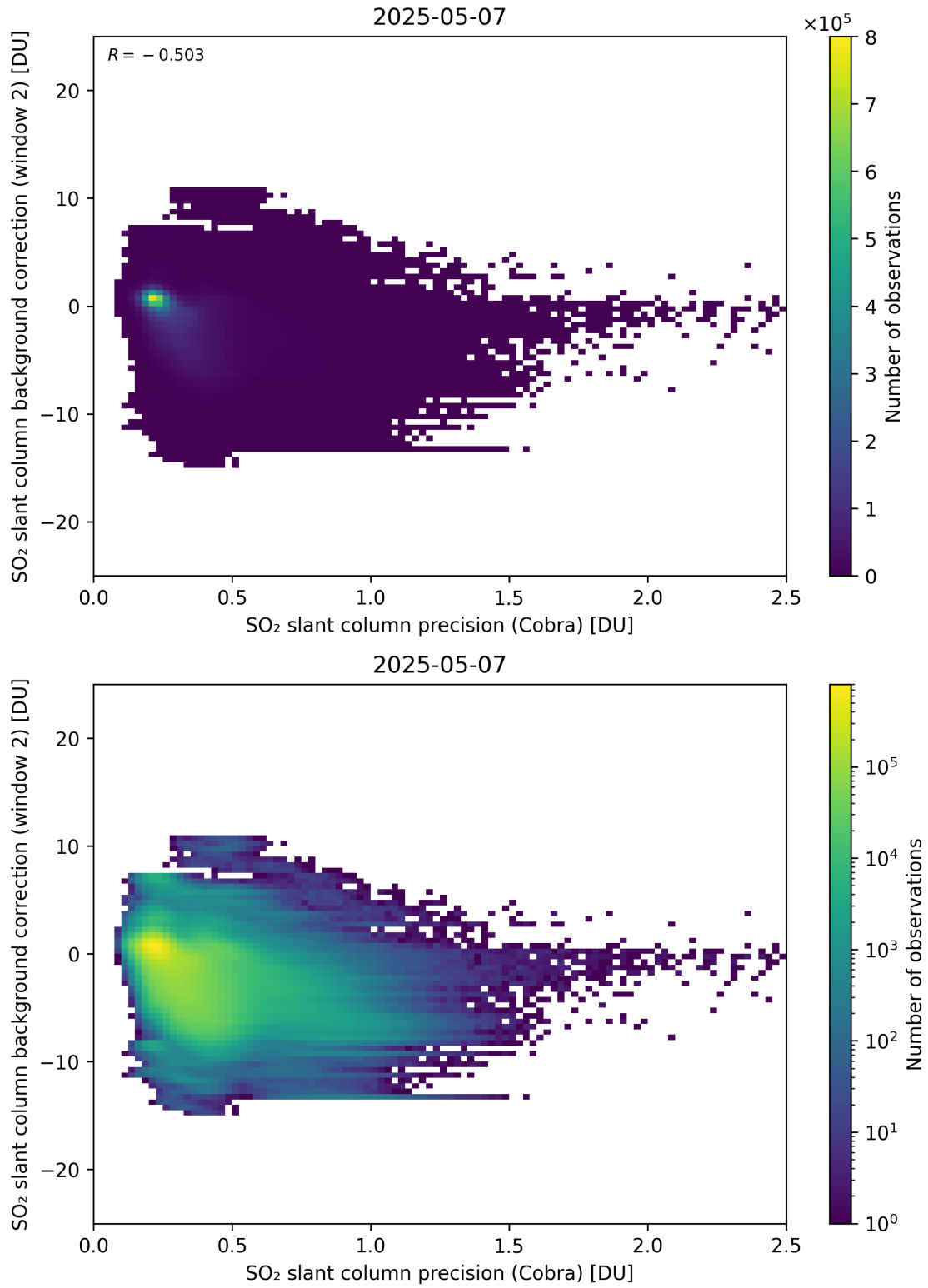
Figure 200: Scatter density plot of “SO 2 slant column precision (Cobra)” against “SO 2 slant column background correction (window 2)” for 2025-05-06 to 2025-05-08.
