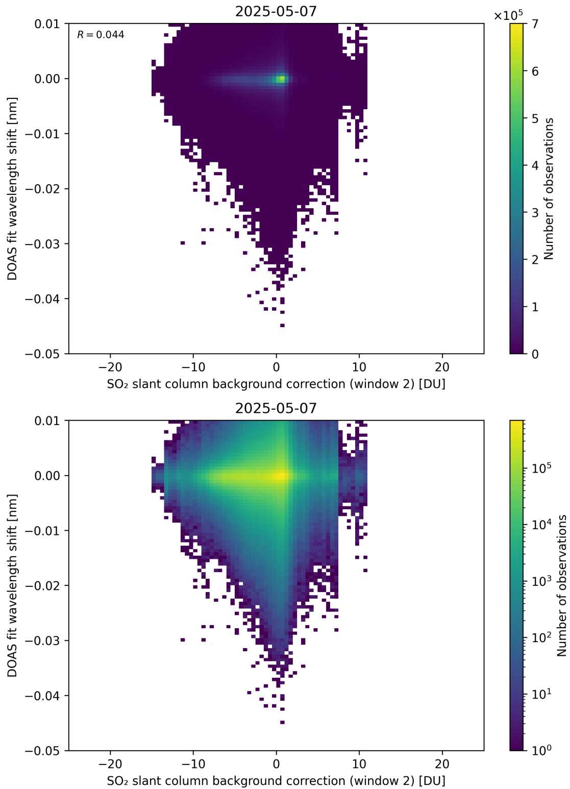
Figure 123: Scatter density plot of “SO 2 slant column background correction (window 2)” against “DOAS fit wavelength shift” for 2025-05-06 to 2025-05-08.
