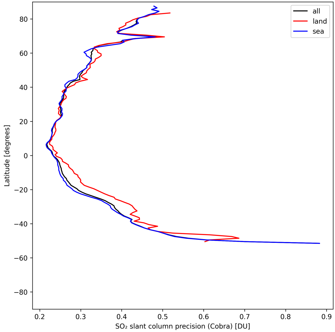
Figure 36: Zonal average of “SO 2 slant column precision (Cobra)” for 2025-05-06 to 2025-05-08.
