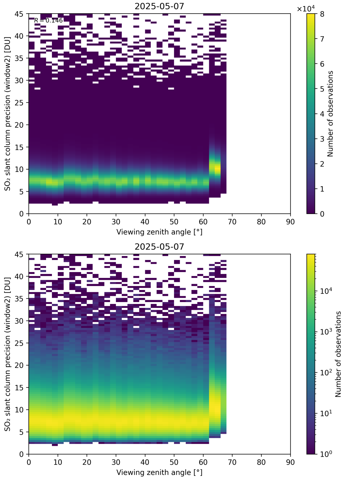
Figure 378: Scatter density plot of “Viewing zenith angle” against “SO 2 slant column precision (window2)” for 2025-05-06 to 2025-05-08.
