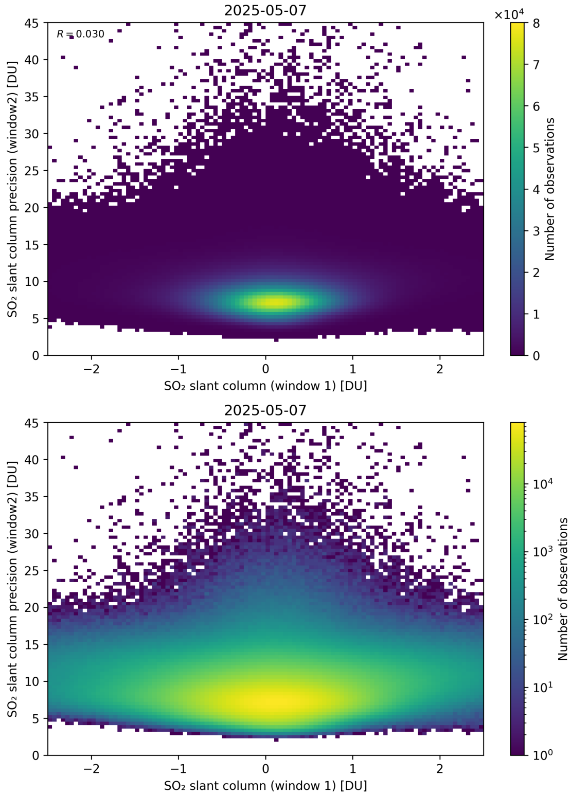
Figure 286: Scatter density plot of “SO 2 slant column (window 1)” against “SO 2 slant column precision (window2)” for 2025-05-06 to 2025-05-08.
