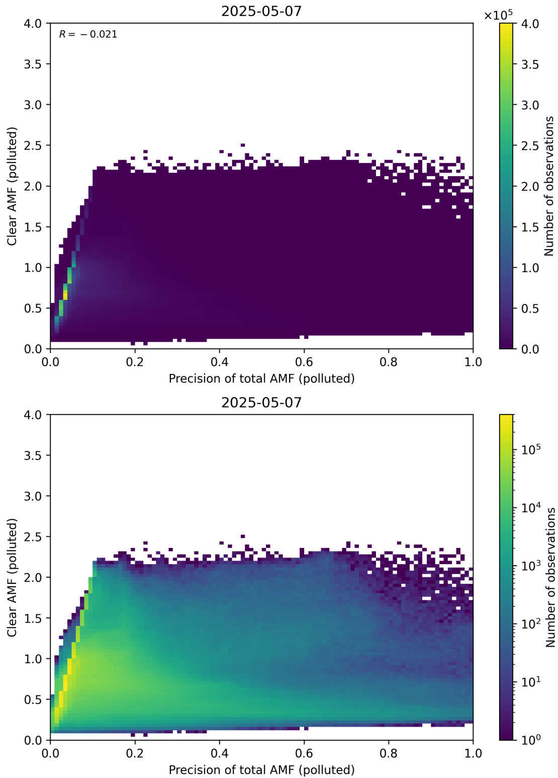
Figure 320: Scatter density plot of “Precision of total AMF (polluted)” against “Clear AMF (polluted)” for 2025-05-06 to 2025-05-08.
