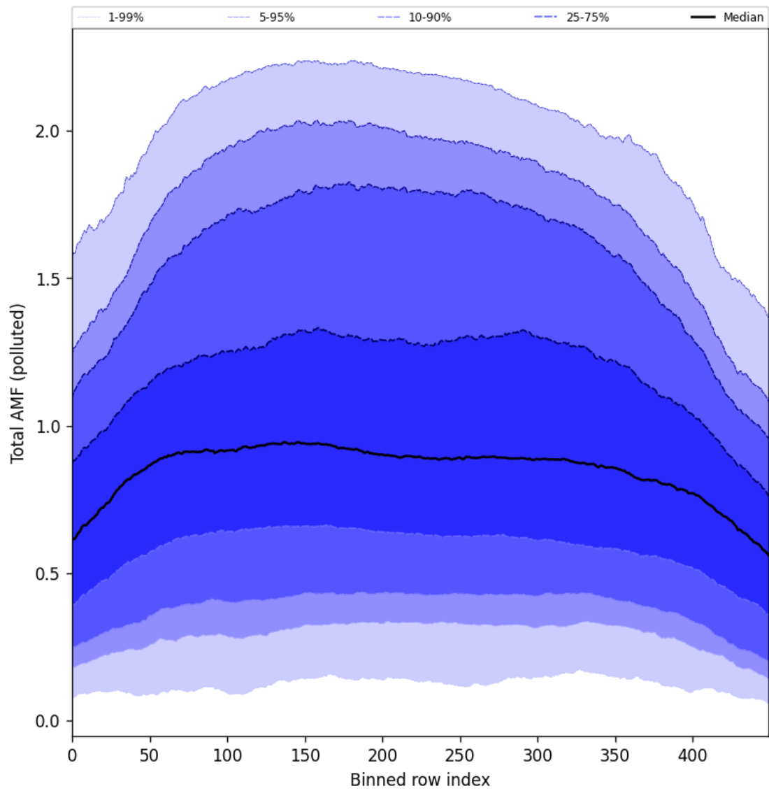
Figure 105: Along track statistics of “Total AMF (polluted)” for 2025-05-06 to 2025-05-08
