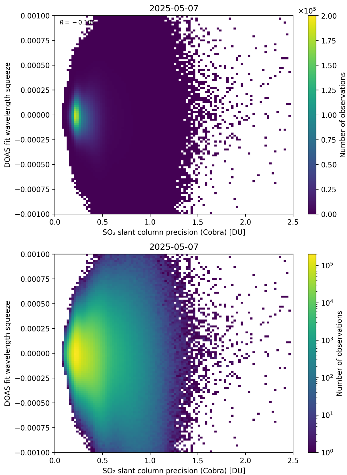
Figure 203: Scatter density plot of “SO 2 slant column precision (Cobra)” against “DOAS fit wavelength squeeze” for 2025-05-06 to 2025-05-08.
