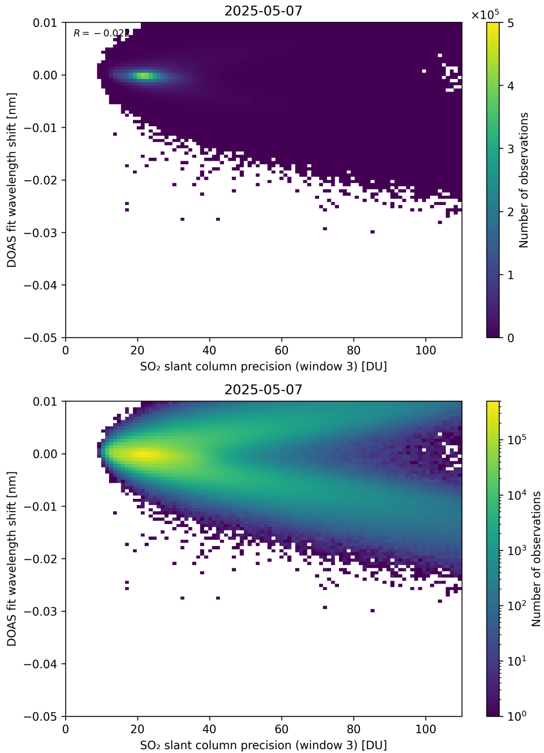
Figure 308: Scatter density plot of “SO 2 slant column precision (window 3)” against “DOAS fit wavelength shift” for 2025-05-06 to 2025-05-08.
