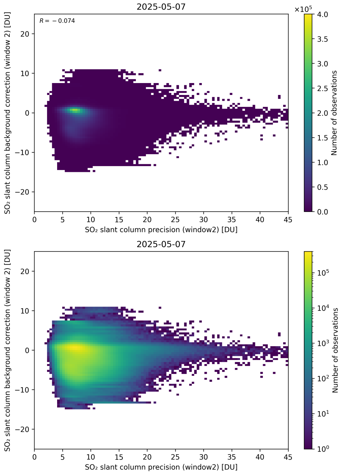
Figure 291: Scatter density plot of “SO 2 slant column precision (window2)” against “SO 2 slant column background correction (window 2)” for 2025-05-06 to 2025-05-08.
