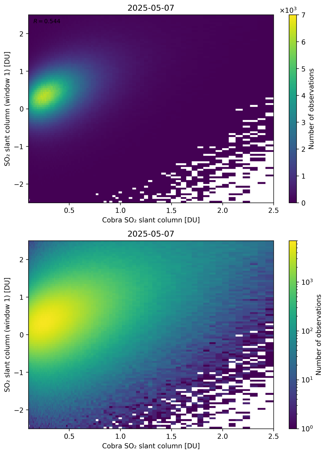
Figure 219: Scatter density plot of “Cobra SO 2 slant column” against “SO 2 slant column (window 1)” for 2025-05-06 to 2025-05-08.
