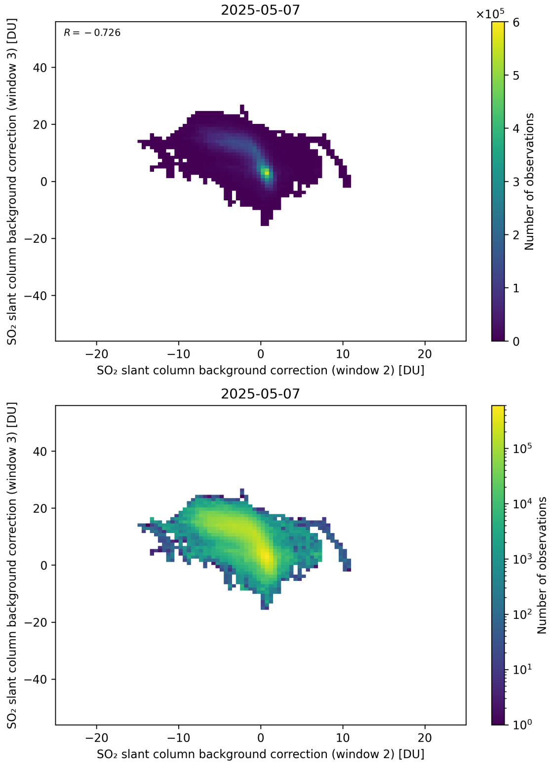
Figure 122: Scatter density plot of “SO 2 slant column background correction (window 2)” against “SO 2 slant column background correction (window 3)” for 2025-05-06 to 2025-05-08.
