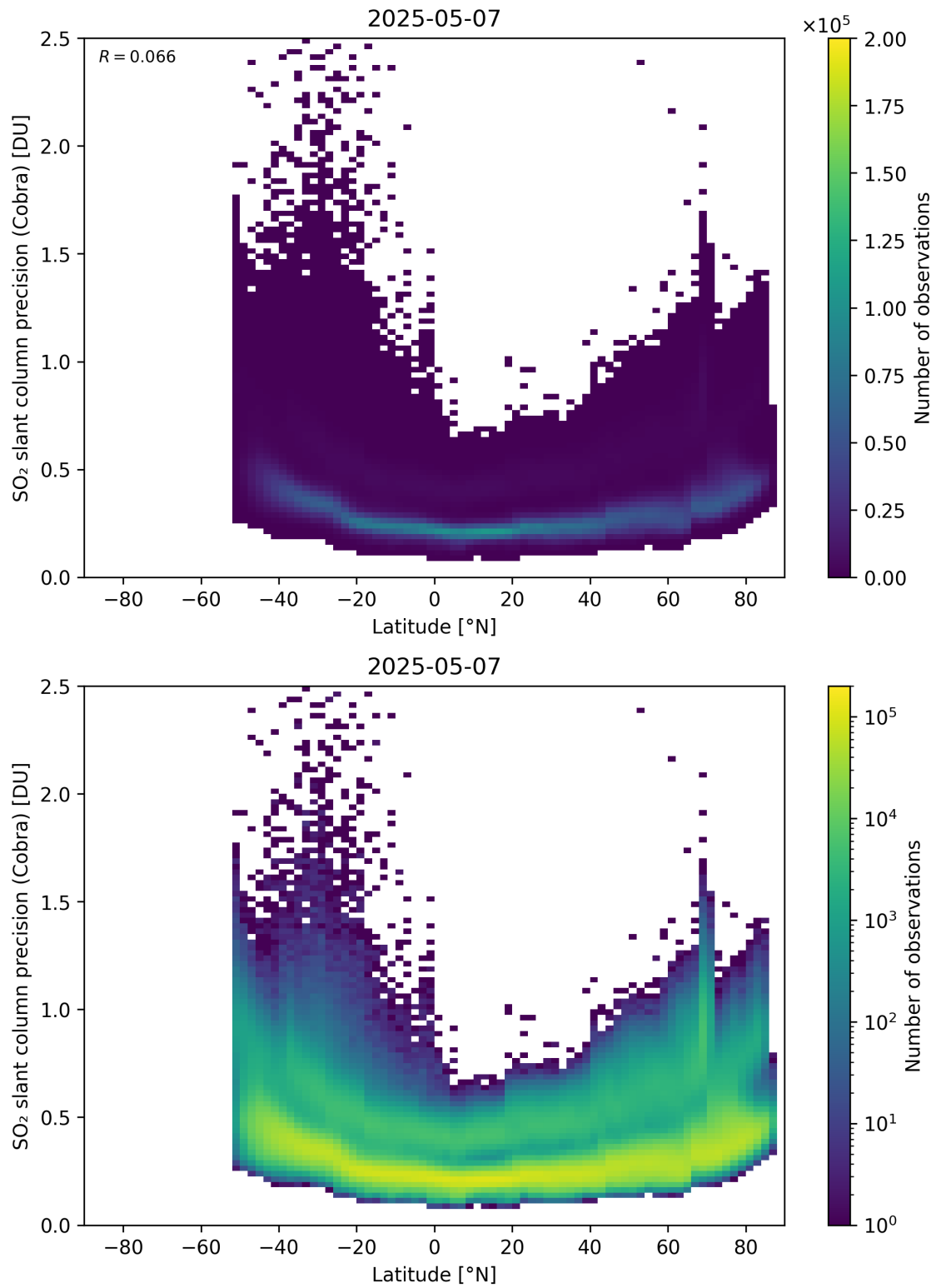
Figure 158: Scatter density plot of “Latitude” against “SO 2 slant column precision (Cobra)” for 2025-05-06 to 2025-05-08.
