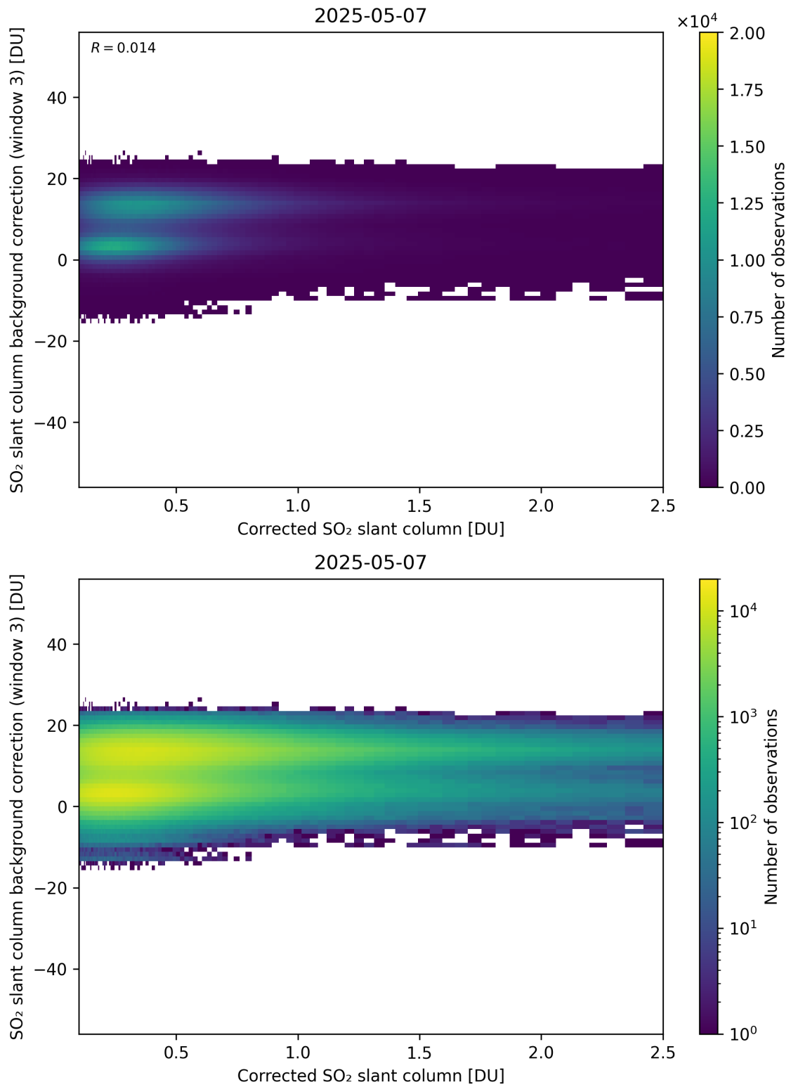
Figure 228: Scatter density plot of “Corrected SO 2 slant column” against “SO 2 slant column background correction (window 3)” for 2025-05-06 to 2025-05-08.
