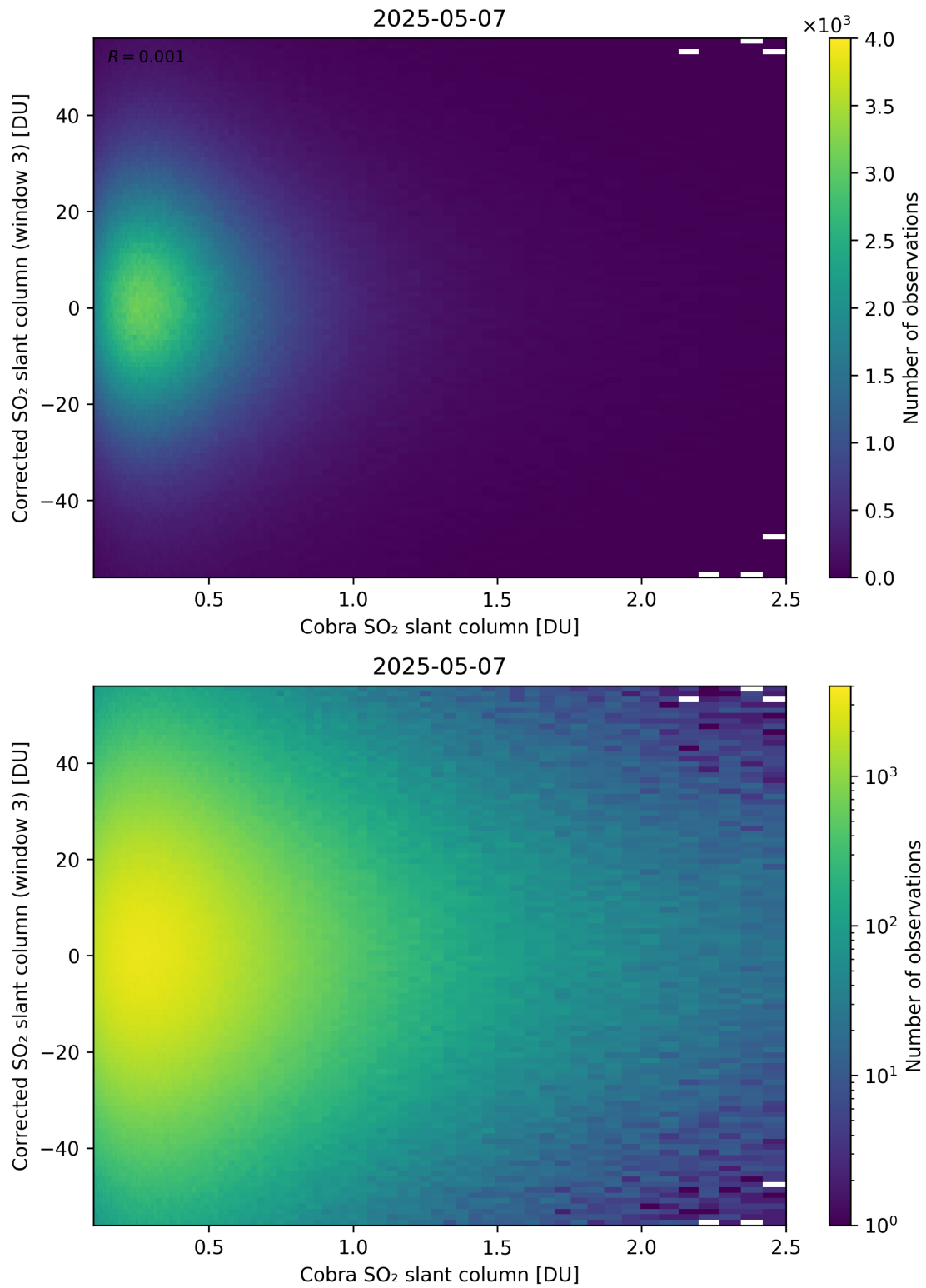
Figure 218: Scatter density plot of “Cobra SO 2 slant column” against “Corrected SO 2 slant column (window 3)” for 2025-05-06 to 2025-05-08.
