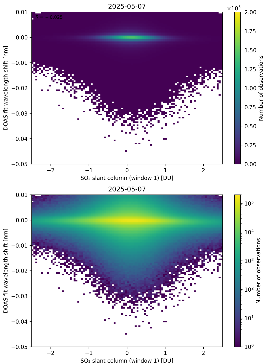
Figure 265: Scatter density plot of “SO 2 slant column (window 1)” against “DOAS fit wavelength shift” for 2025-05-06 to 2025-05-08.
