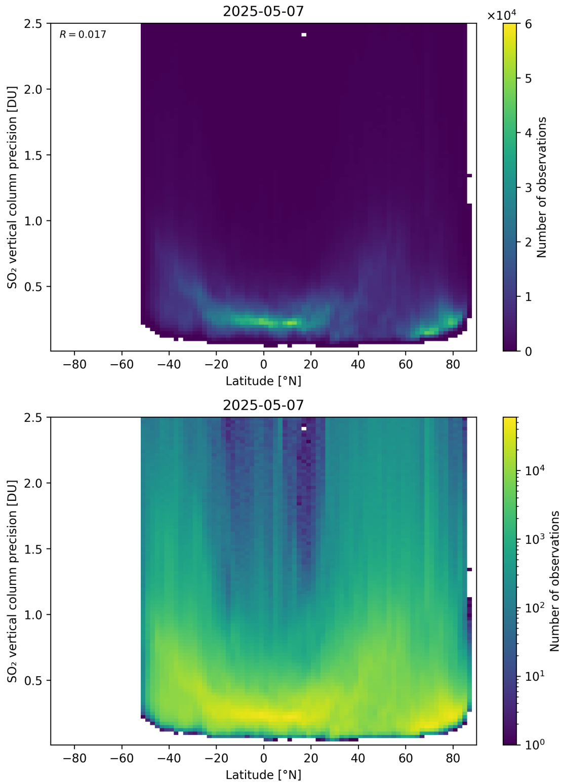
Figure 170: Scatter density plot of “Latitude” against “SO 2 vertical column precision” for 2025-05-06 to 2025-05-08.
