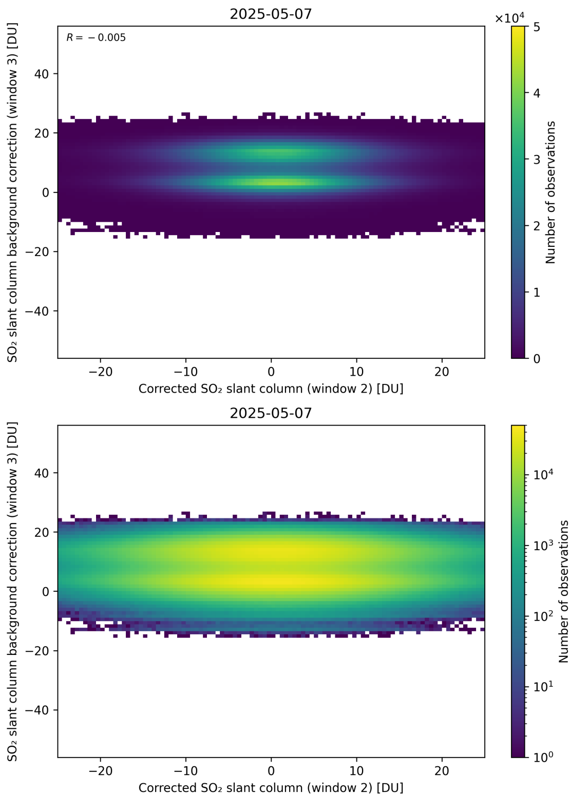
Figure 245: Scatter density plot of “Corrected SO 2 slant column (window 2)” against “SO 2 slant column background correction (window 3)” for 2025-05-06 to 2025-05-08.
