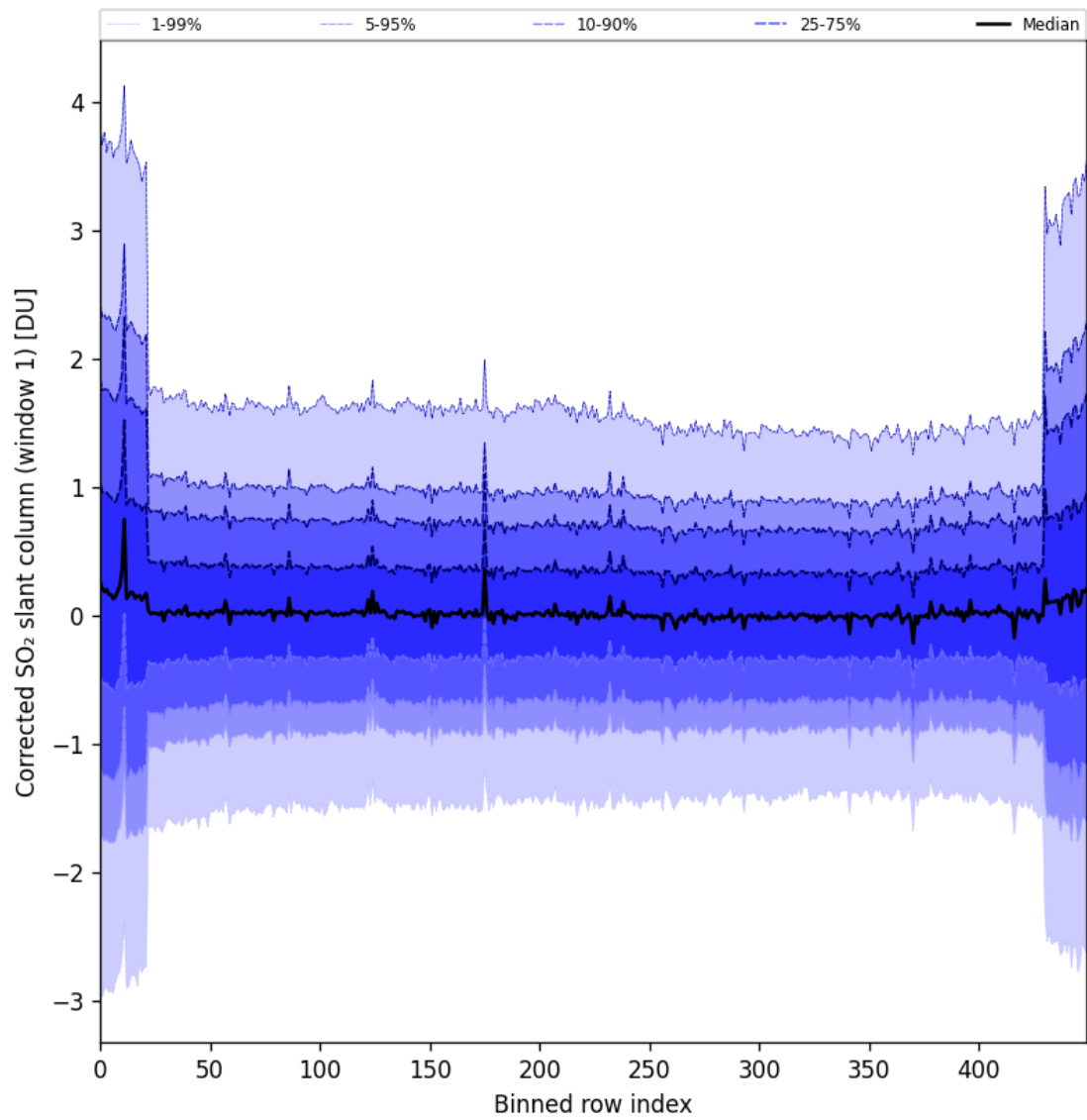
Figure 91: Along track statistics of “Corrected SO 2 slant column (window 1)” for 2025-05-06 to 2025-05-08
