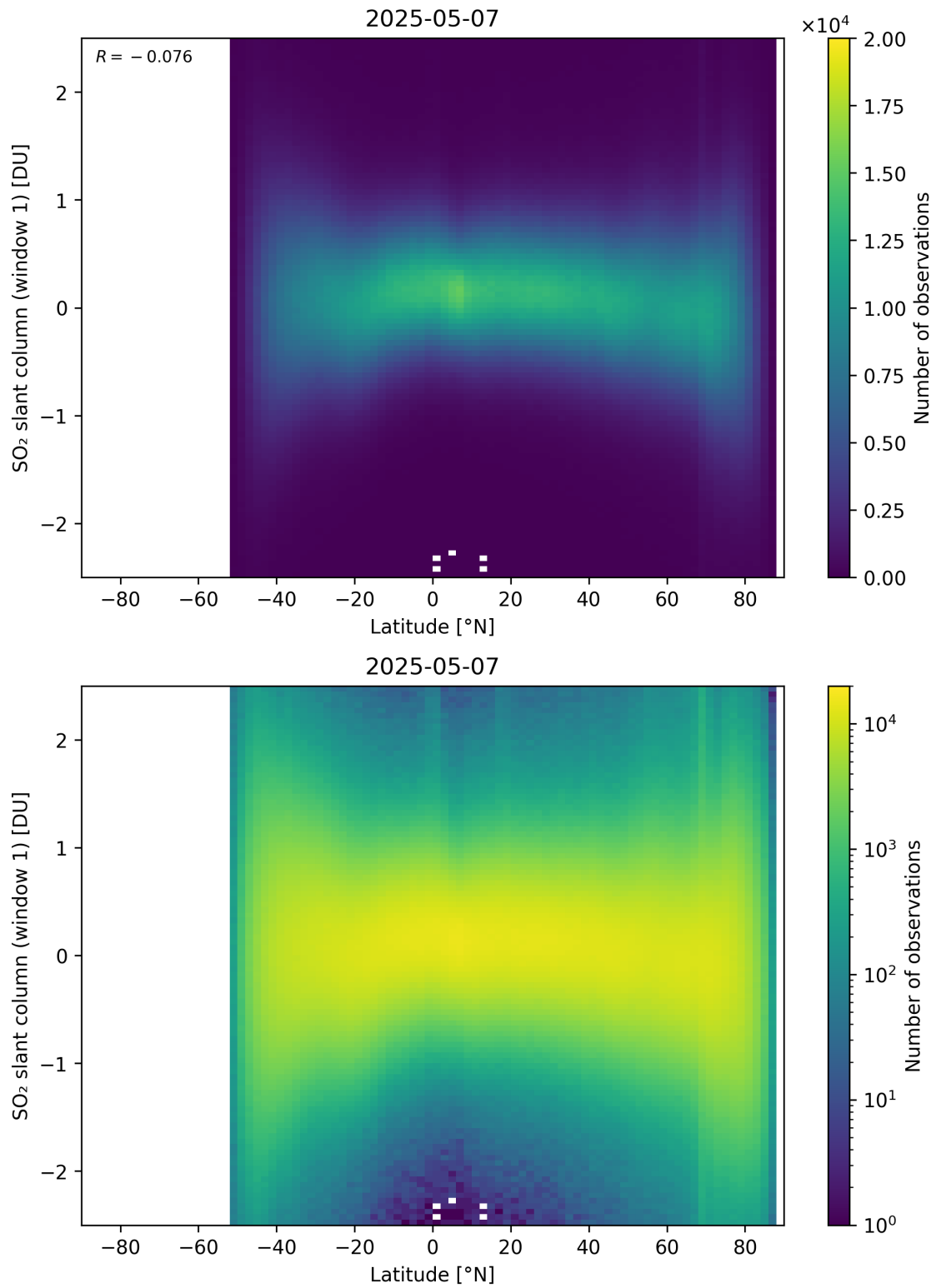
Figure 162: Scatter density plot of “Latitude” against “SO 2 slant column (window 1)” for 2025-05-06 to 2025-05-08.
