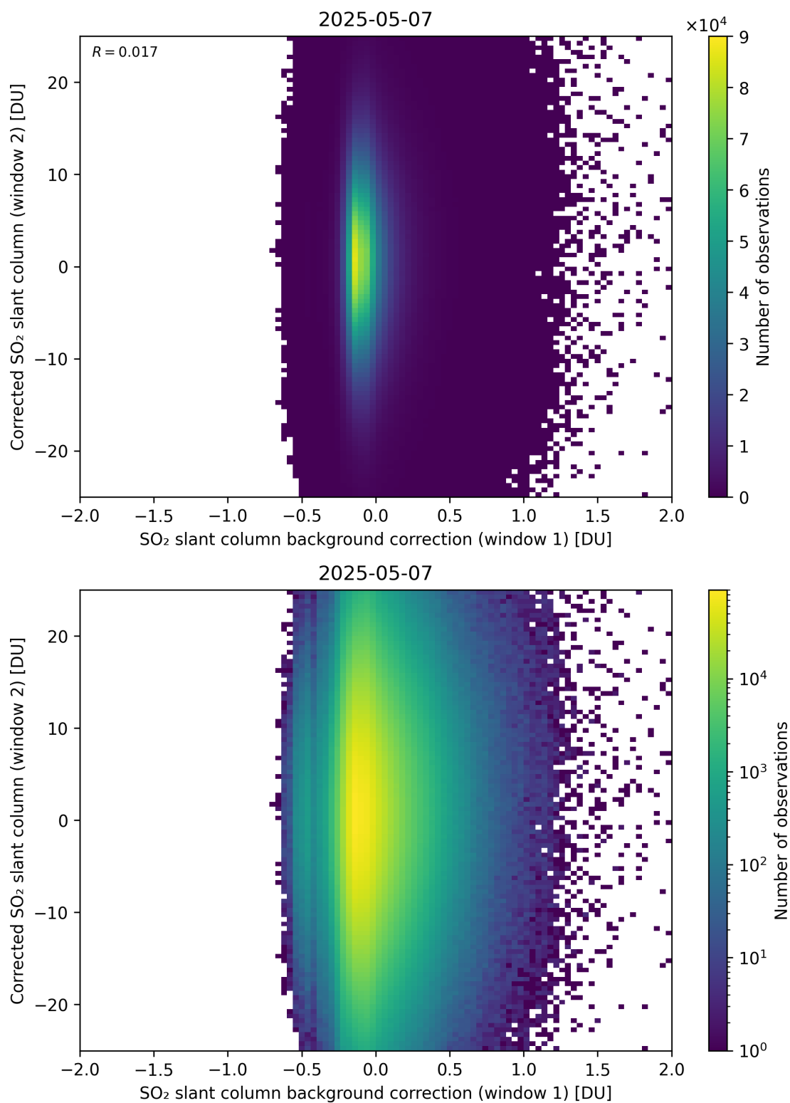
Figure 115: Scatter density plot of “SO 2 slant column background correction (window 1)” against “Corrected SO 2 slant column (window 2)” for 2025-05-06 to 2025-05-08.
