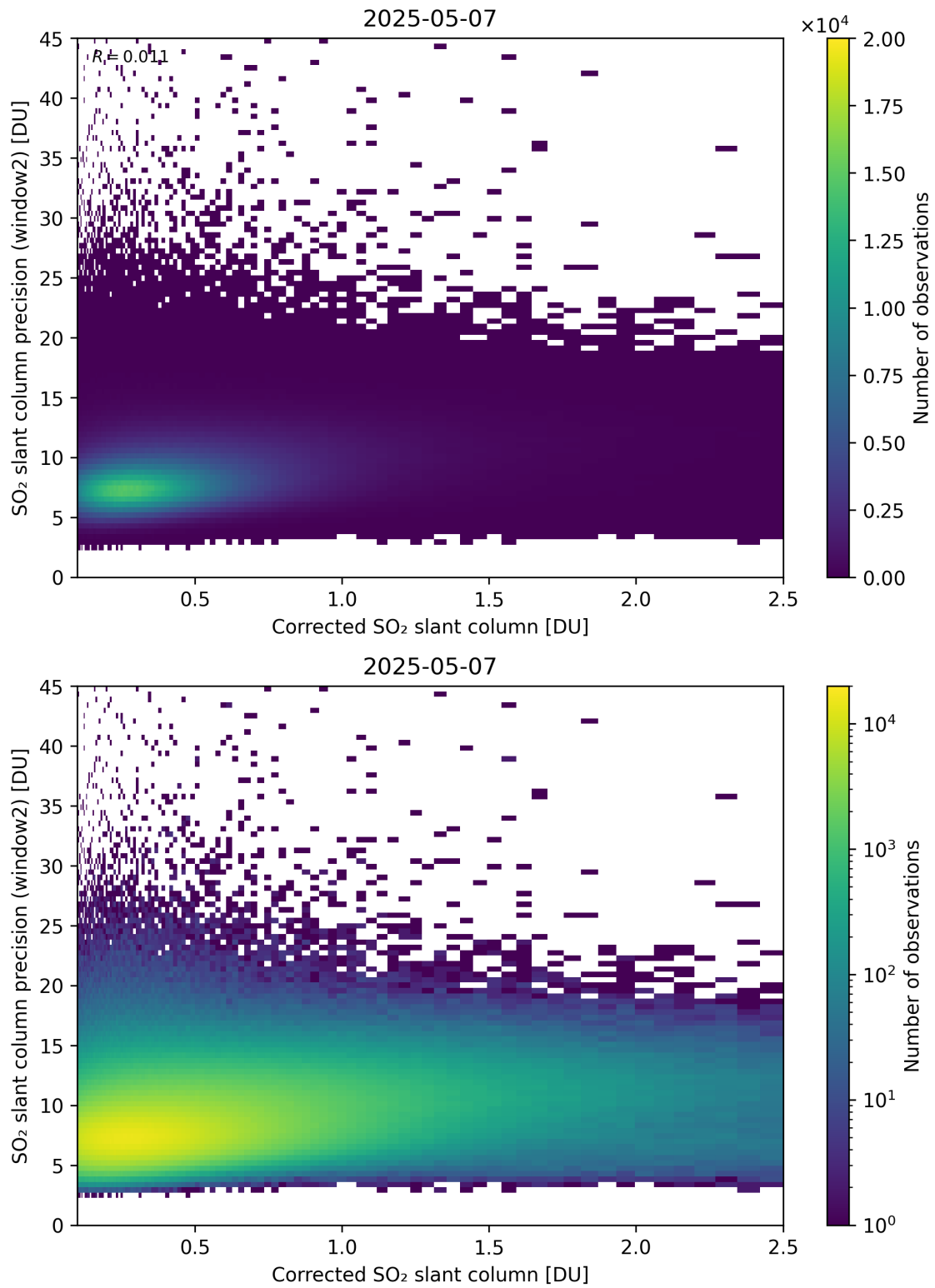
Figure 239: Scatter density plot of “Corrected SO 2 slant column” against “SO 2 slant column precision (window2)” for 2025-05-06 to 2025-05-08.
