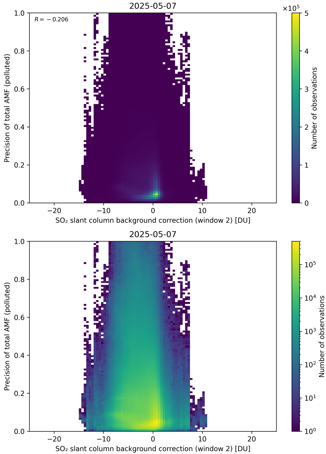
Figure 131: Scatter density plot of “SO 2 slant column background correction (window 2)” against “Precision of total AMF (polluted)” for 2025-05-06 to 2025-05-08.
