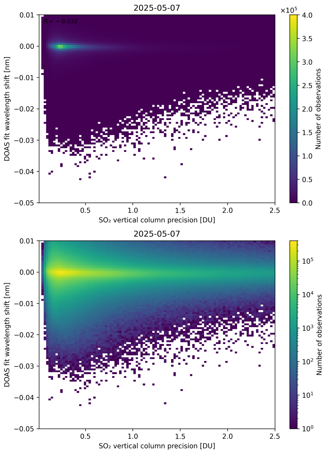
Figure 332: Scatter density plot of “SO 2 vertical column precision” against “DOAS fit wavelength shift” for 2025-05-06 to 2025-05-08.
