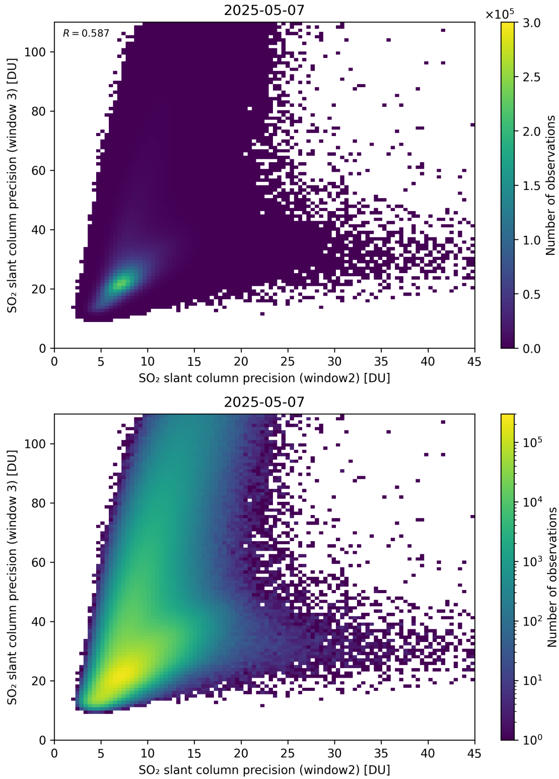
Figure 300: Scatter density plot of “SO 2 slant column precision (window2)” against “SO 2 slant column precision (window 3)” for 2025-05-06 to 2025-05-08.
