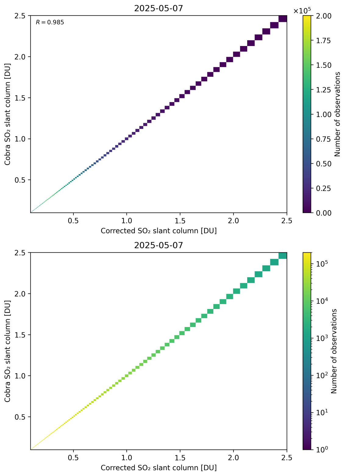
Figure 233: Scatter density plot of “Corrected SO 2 slant column” against “Cobra SO 2 slant column” for 2025-05-06 to 2025-05-08.
