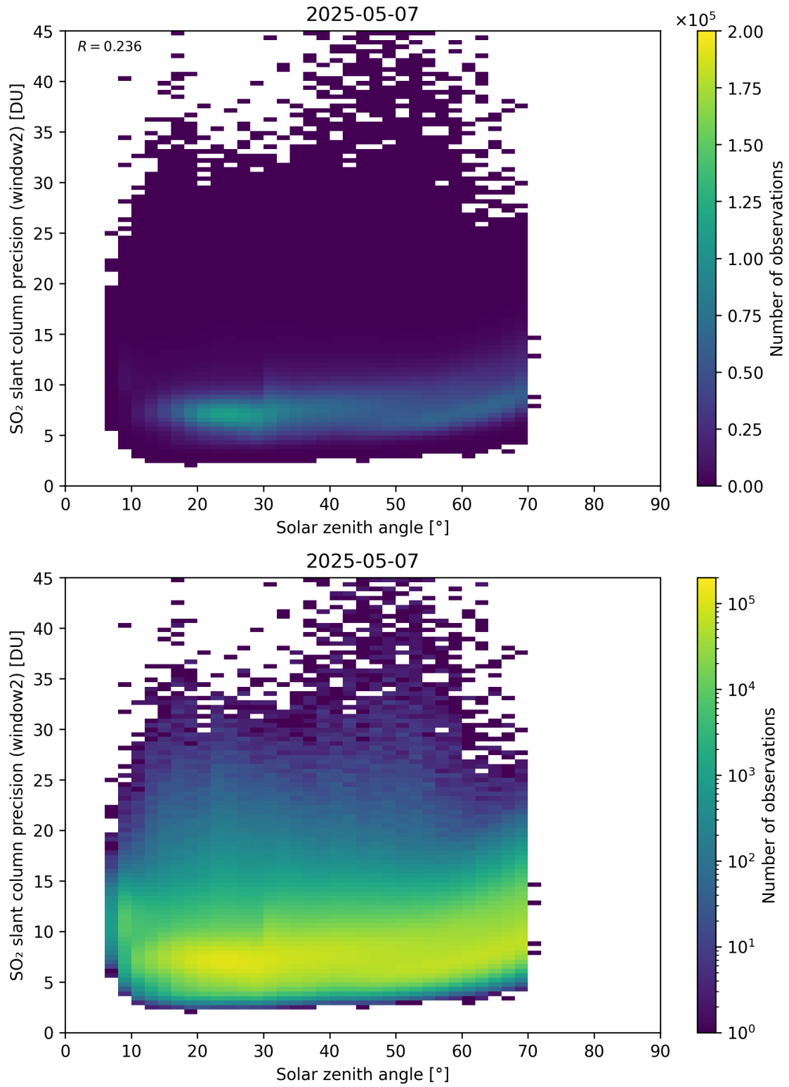
Figure 186: Scatter density plot of “Solar zenith angle” against “SO 2 slant column precision (window2)” for 2025-05-06 to 2025-05-08.
