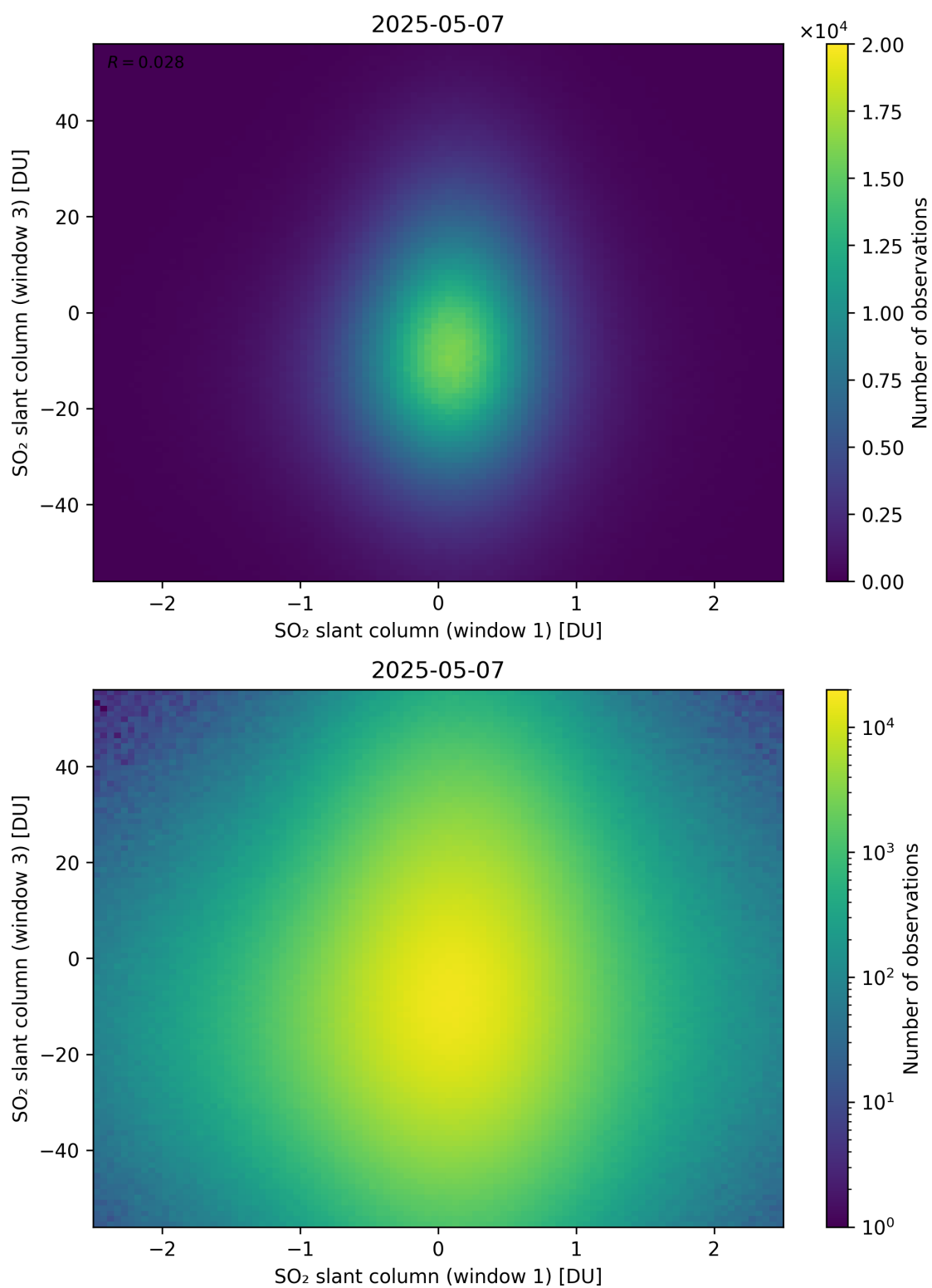
Figure 287: Scatter density plot of “SO 2 slant column (window 1)” against “SO 2 slant column (window 3)” for 2025-05-06 to 2025-05-08.
