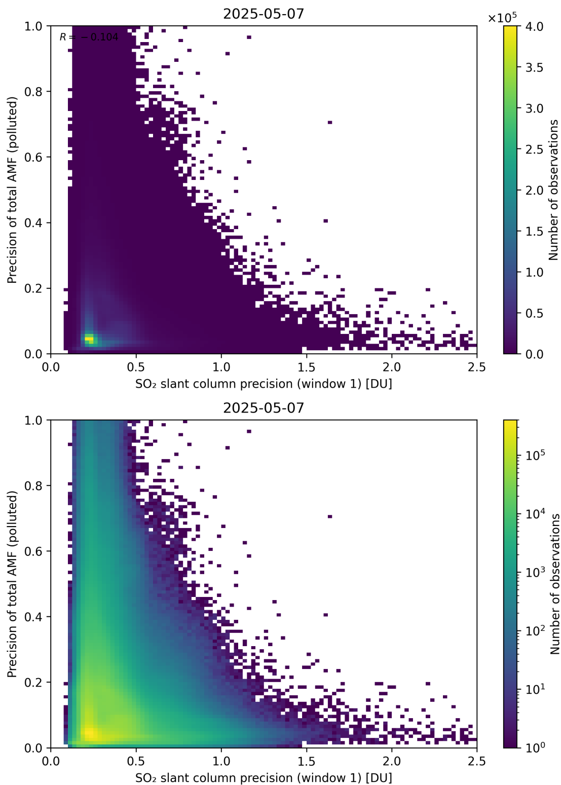
Figure 281: Scatter density plot of “SO 2 slant column precision (window 1)” against “Precision of total AMF (polluted)” for 2025-05-06 to 2025-05-08.
