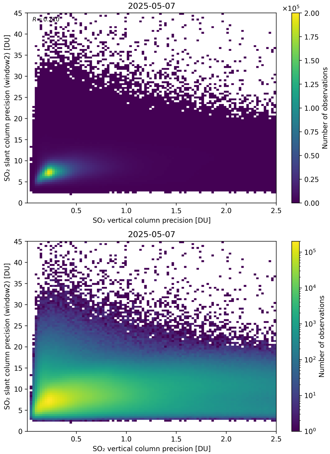
Figure 343: Scatter density plot of “SO 2 vertical column precision” against “SO 2 slant column precision (window2)” for 2025-05-06 to 2025-05-08.
