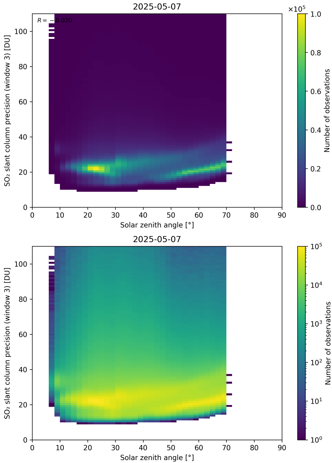
Figure 188: Scatter density plot of “Solar zenith angle” against “SO 2 slant column precision (window 3)” for 2025-05-06 to 2025-05-08.
