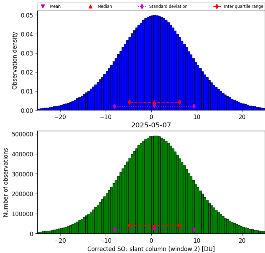
Figure 69: Histogram of “Corrected SO 2 slant column (window 2)” for 2025-05-06 to 2025-05-08
