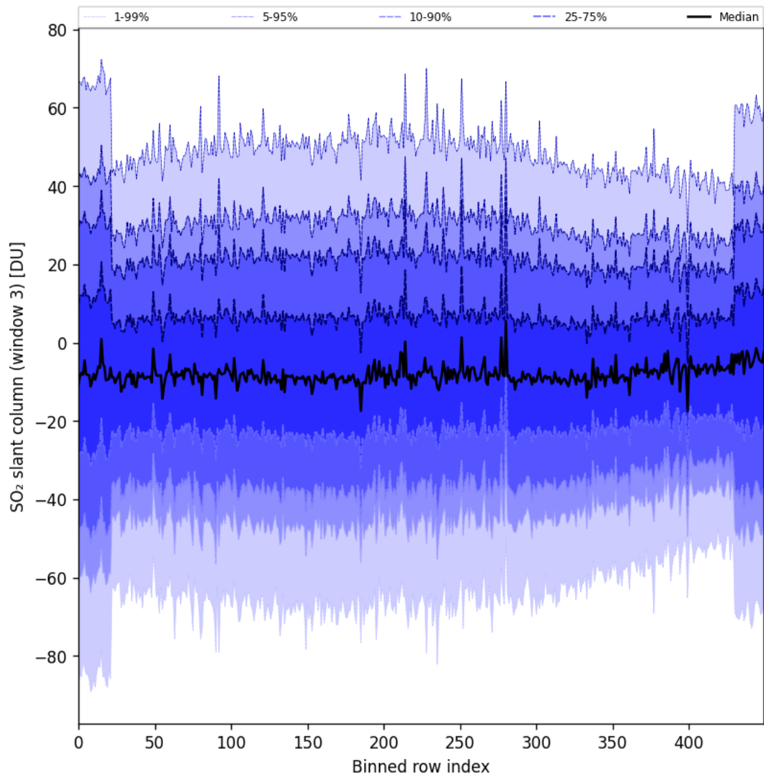
Figure 97: Along track statistics of “SO 2 slant column (window 3)” for 2025-05-06 to 2025-05-08
