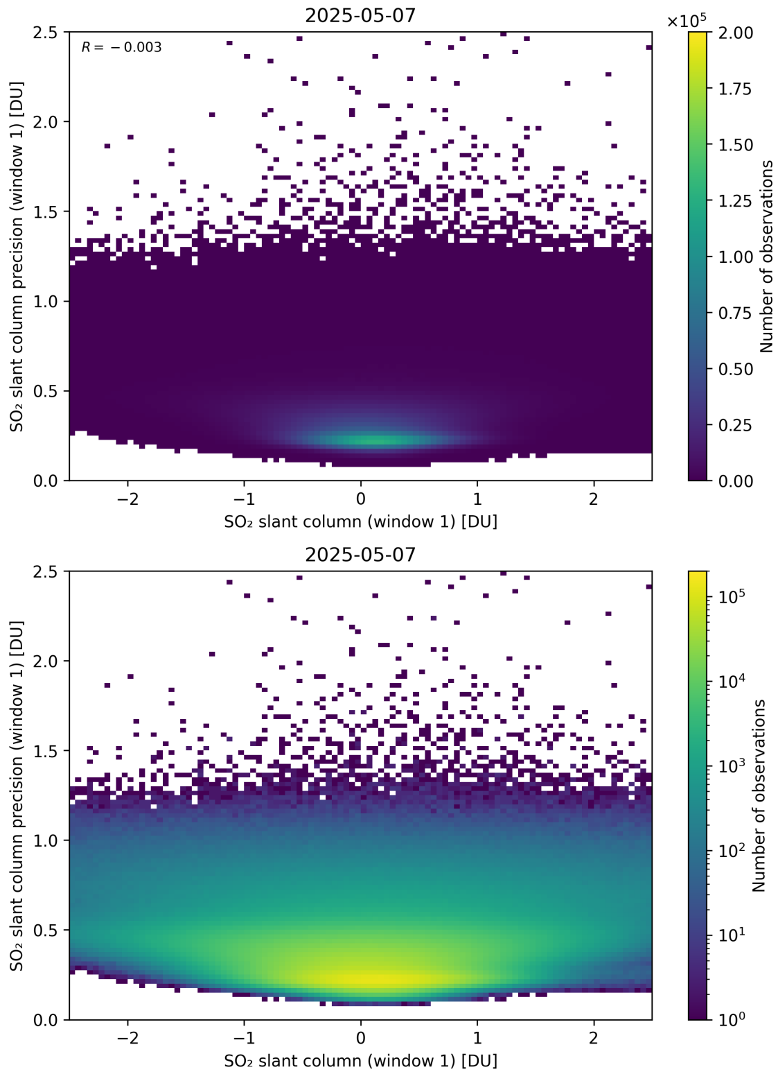
Figure 285: Scatter density plot of “SO 2 slant column (window 1)” against “SO 2 slant column precision (window 1)” for 2025-05-06 to 2025-05-08.
