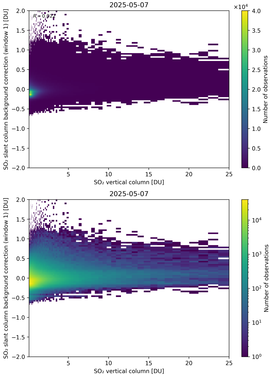
Figure 323: Scatter density plot of “SO 2 vertical column” against “SO 2 slant column background correction (window 1)” for 2025-05-06 to 2025-05-08.
