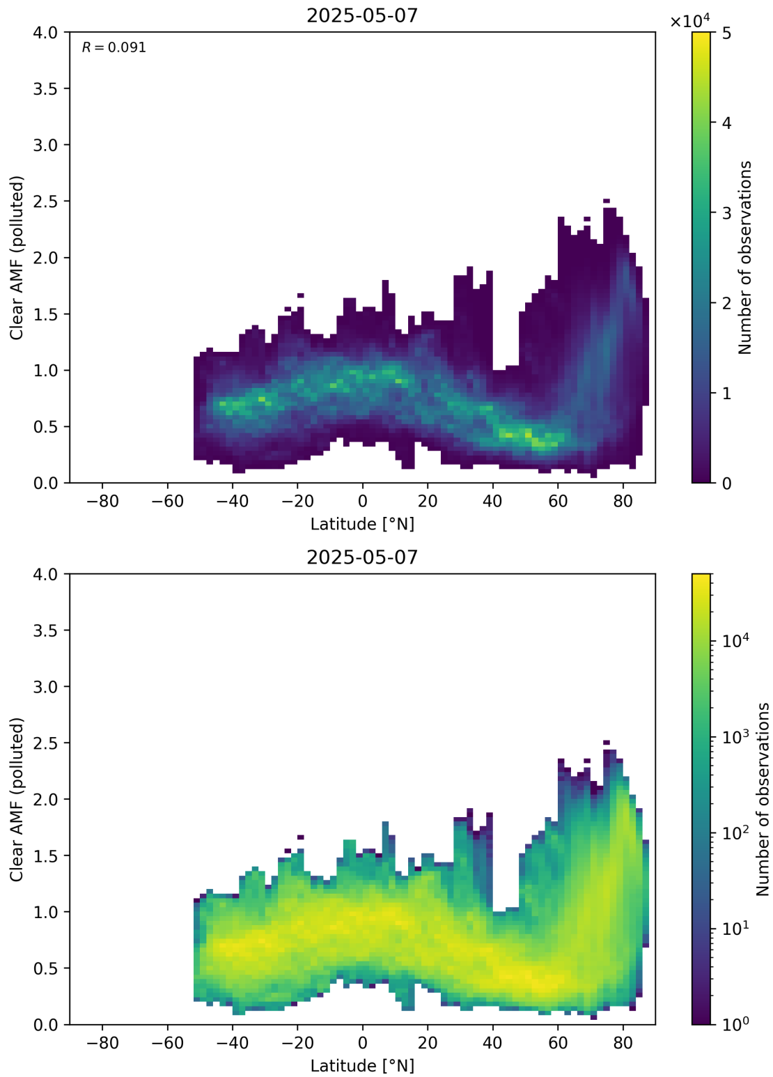
Figure 156: Scatter density plot of “Latitude” against “Clear AMF (polluted)” for 2025-05-06 to 2025-05-08.
