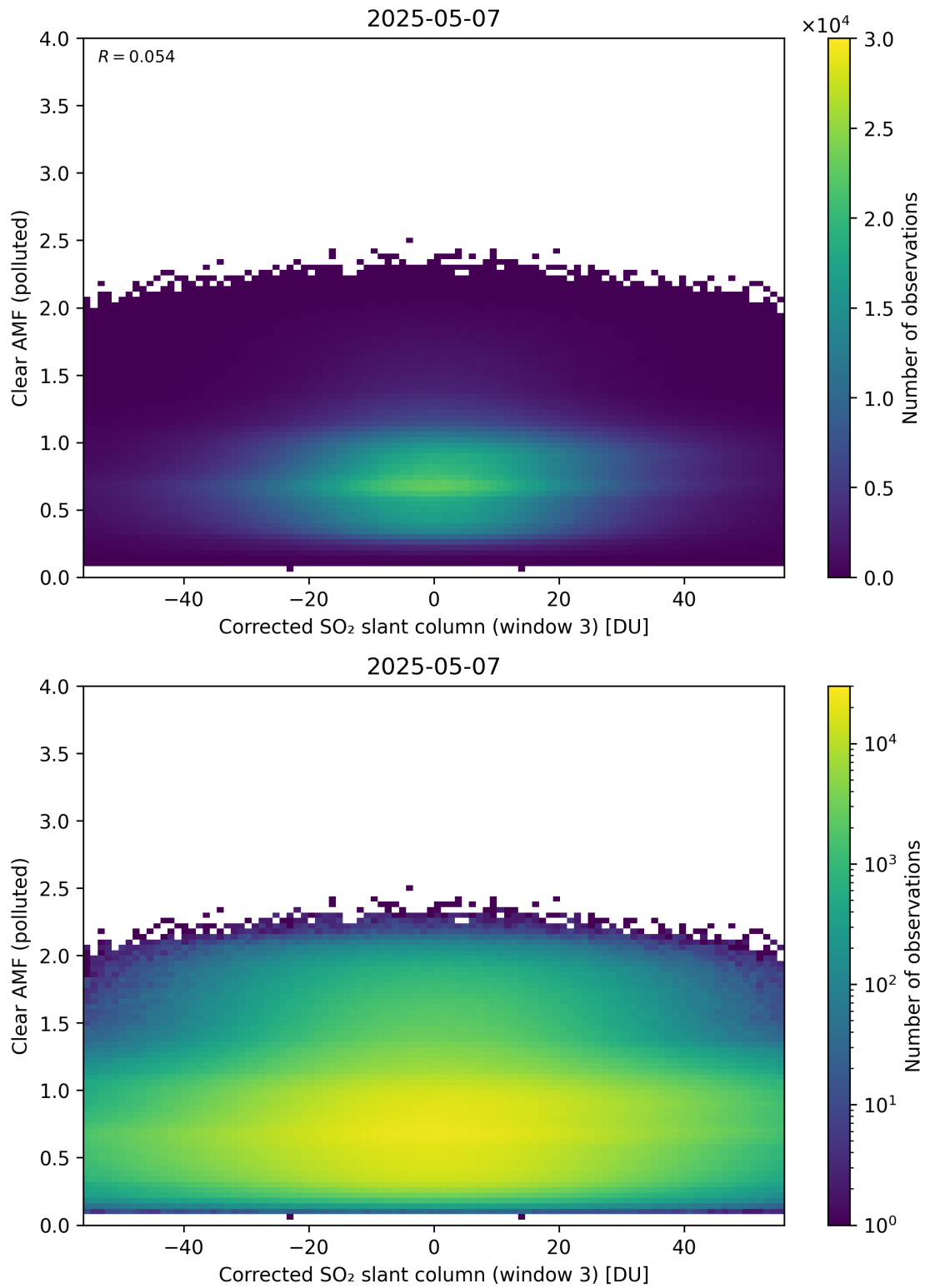
Figure 259: Scatter density plot of “Corrected SO 2 slant column (window 3)” against “Clear AMF (polluted)” for 2025-05-06 to 2025-05-08.
