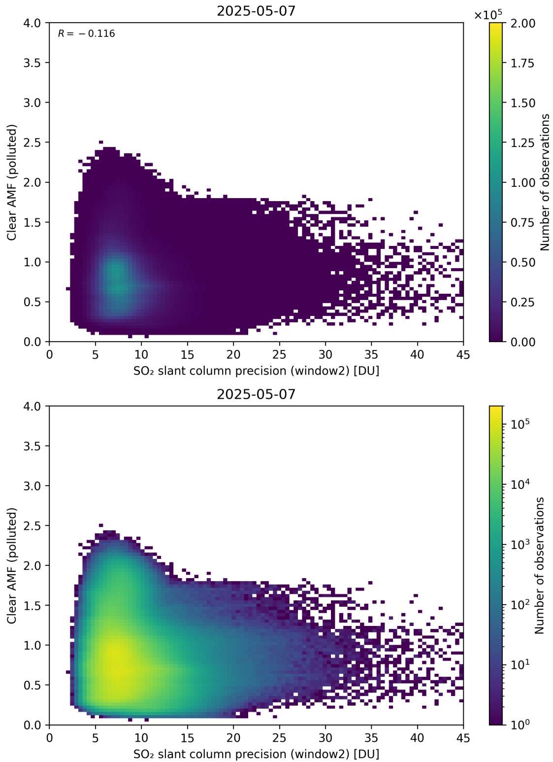
Figure 296: Scatter density plot of “SO 2 slant column precision (window2)” against “Clear AMF (polluted)” for 2025-05-06 to 2025-05-08.
