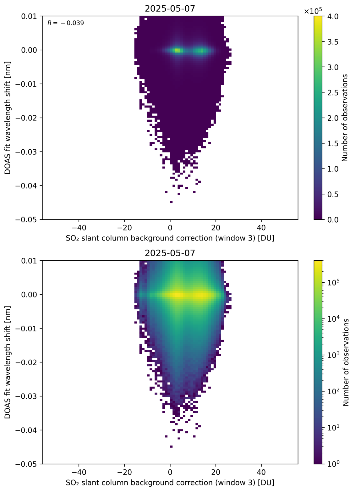
Figure 132: Scatter density plot of “SO 2 slant column background correction (window 3)” against “DOAS fit wavelength shift” for 2025-05-06 to 2025-05-08.
