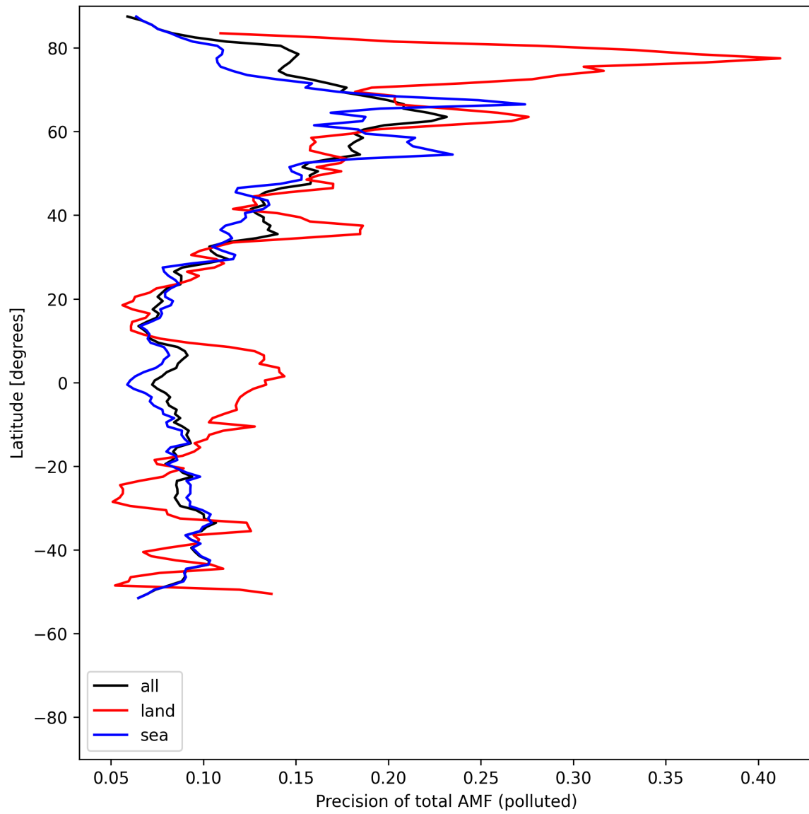
Figure 54: Zonal average of “Precision of total AMF (polluted)” for 2025-05-06 to 2025-05-08.
