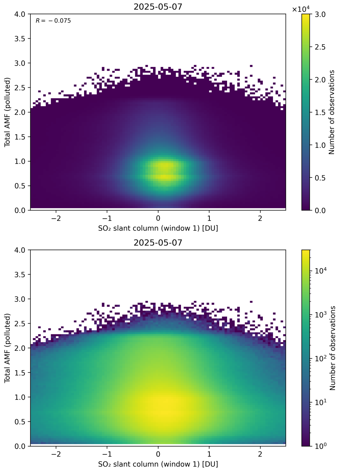
Figure 289: Scatter density plot of “SO 2 slant column (window 1)” against “Total AMF (polluted)” for 2025-05-06 to 2025-05-08.
