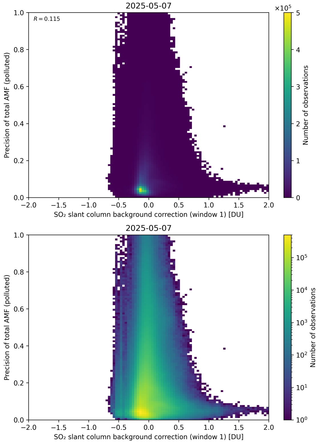
Figure 121: Scatter density plot of “SO 2 slant column background correction (window 1)” against “Precision of total AMF (polluted)” for 2025-05-06 to 2025-05-08.
