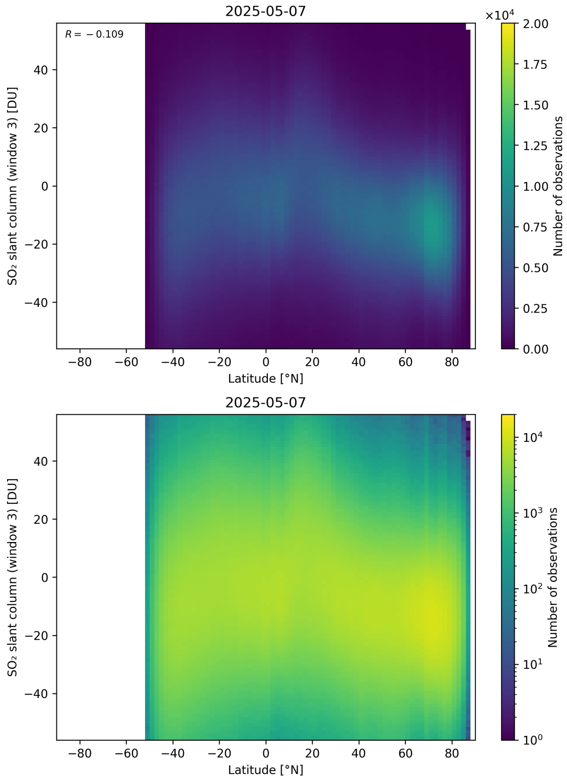
Figure 165: Scatter density plot of “Latitude” against “SO 2 slant column (window 3)” for 2025-05-06 to 2025-05-08.
