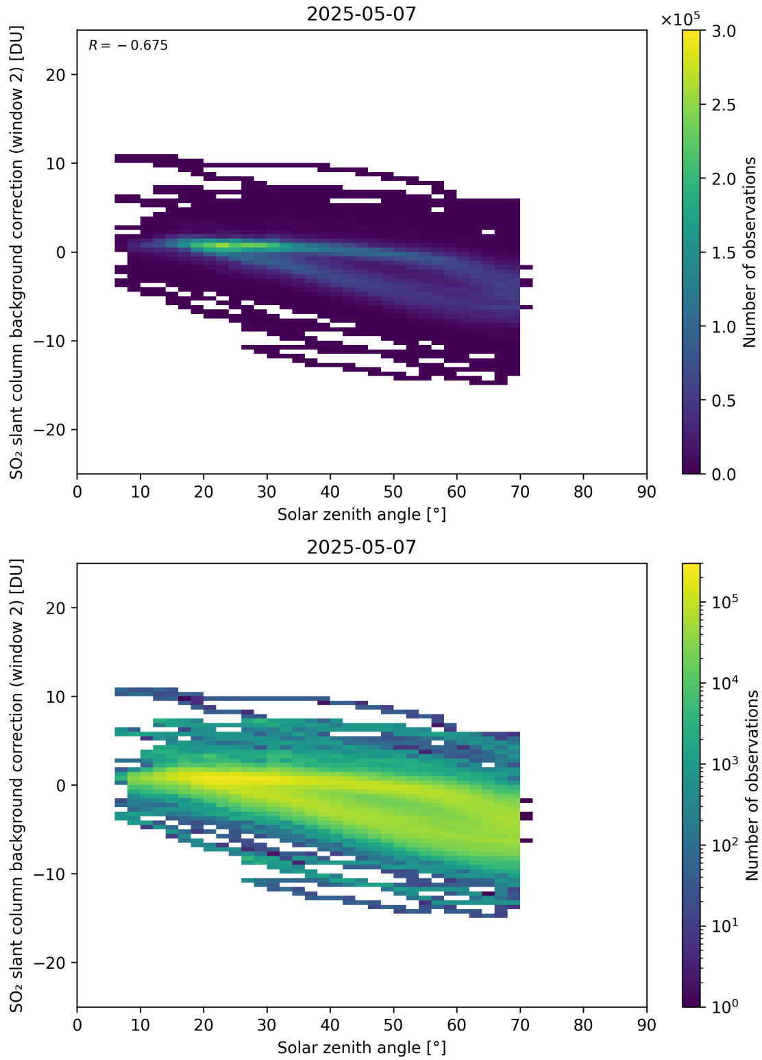
Figure 172: Scatter density plot of “Solar zenith angle” against “SO 2 slant column background correction (window 2)” for 2025-05-06 to 2025-05-08.
