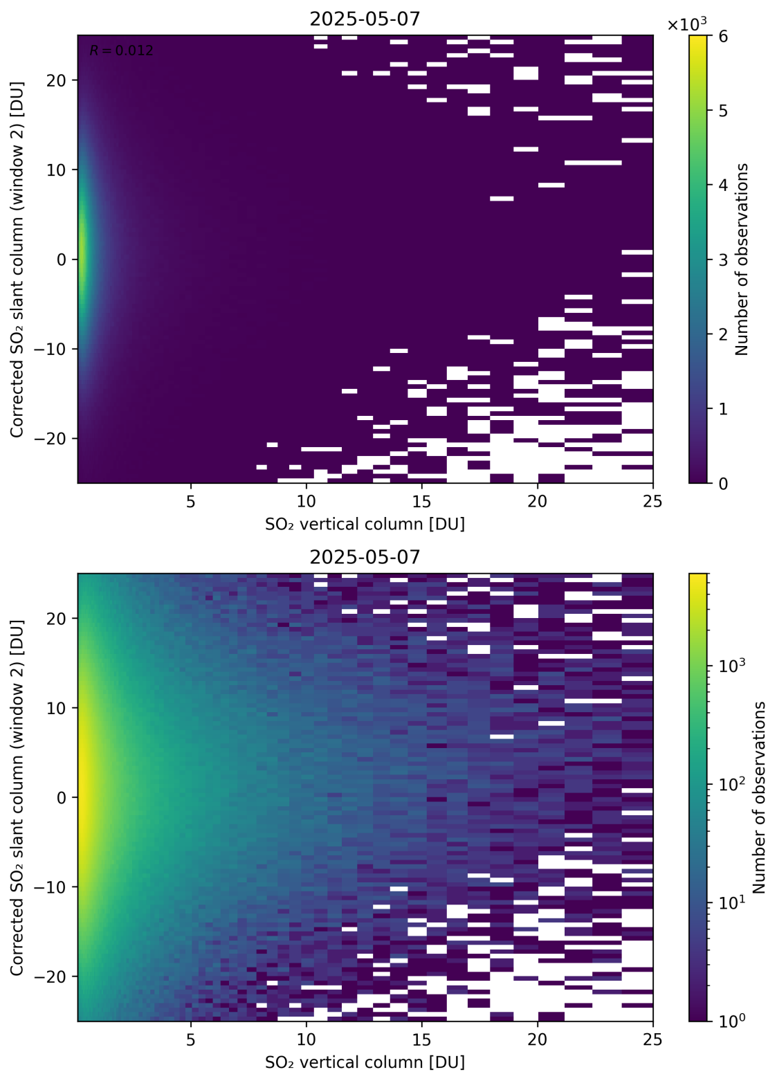
Figure 352: Scatter density plot of “SO 2 vertical column” against “Corrected SO 2 slant column (window 2)” for 2025-05-06 to 2025-05-08.
