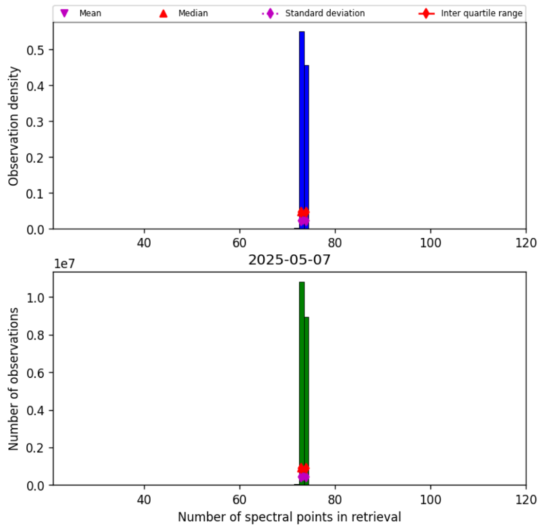
Figure 82: Histogram of “Number of spectral points in retrieval” for 2025-05-06 to 2025-05-08
