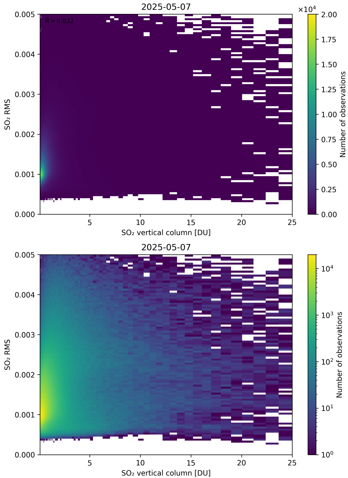
Figure 328: Scatter density plot of “SO 2 vertical column” against “SO 2 RMS” for 2025-05-06 to 2025-05-08.
