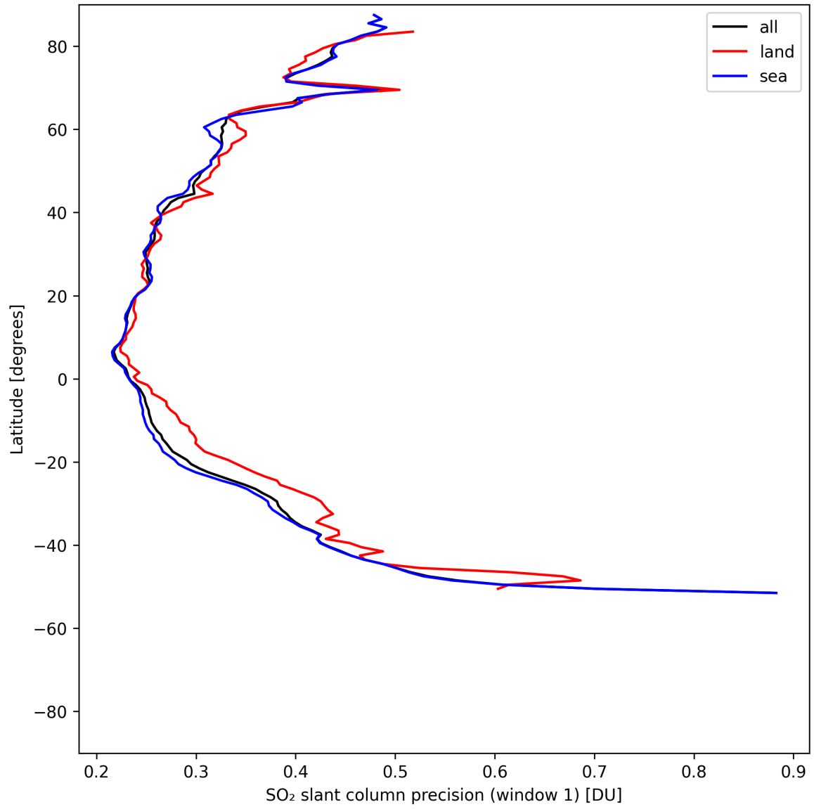
Figure 38: Zonal average of “SO 2 slant column precision (window 1)” for 2025-05-06 to 2025-05-08.
