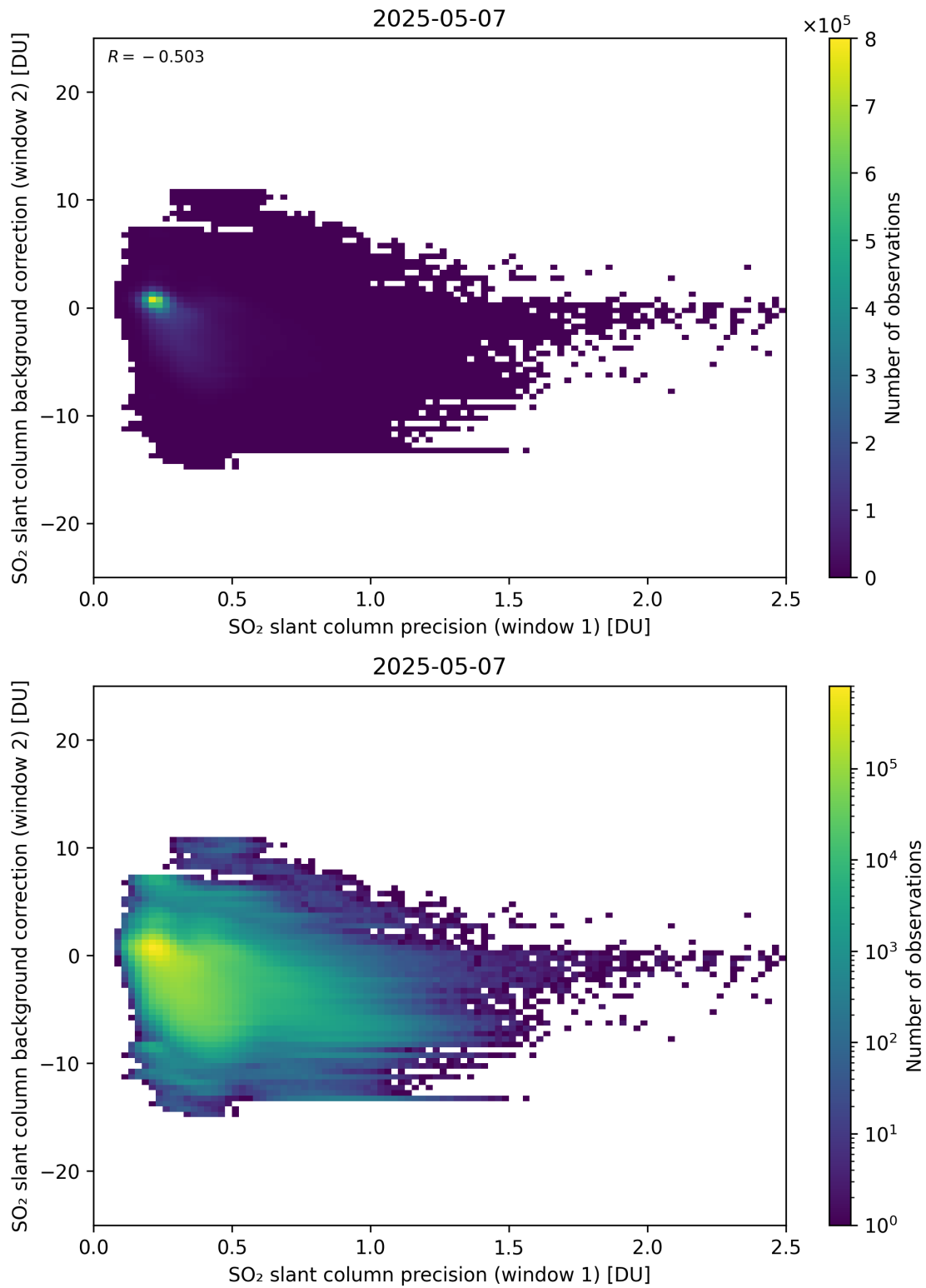
Figure 269: Scatter density plot of “SO 2 slant column precision (window 1)” against “SO 2 slant column background correction (window 2)” for 2025-05-06 to 2025-05-08.
