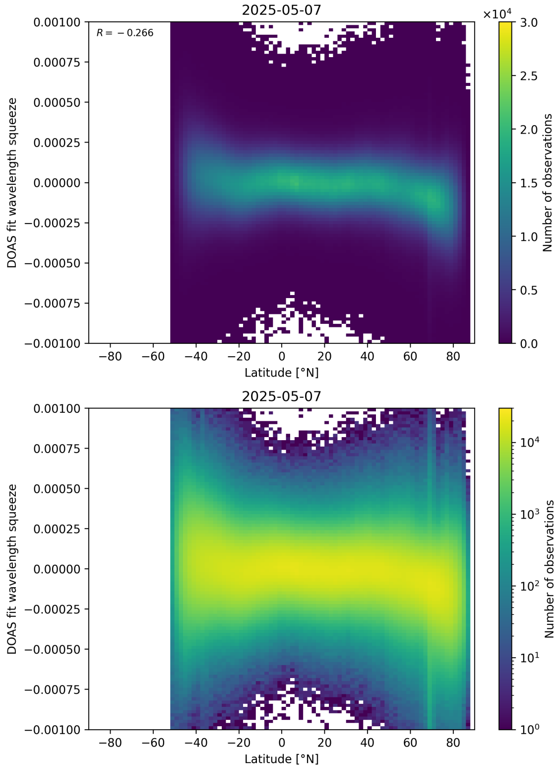
Figure 154: Scatter density plot of “Latitude” against “DOAS fit wavelength squeeze” for 2025-05-06 to 2025-05-08.
