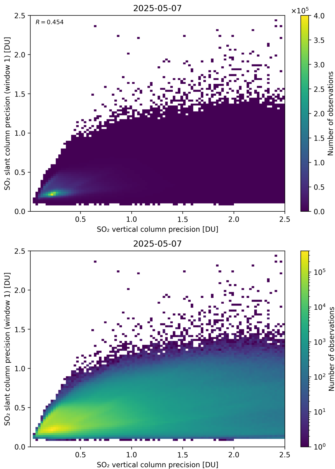
Figure 342: Scatter density plot of “SO 2 vertical column precision” against “SO 2 slant column precision (window 1)” for 2025-05-06 to 2025-05-08.
