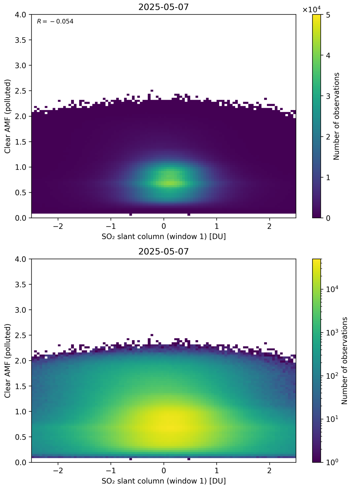
Figure 282: Scatter density plot of “SO 2 slant column (window 1)” against “Clear AMF (polluted)” for 2025-05-06 to 2025-05-08.
