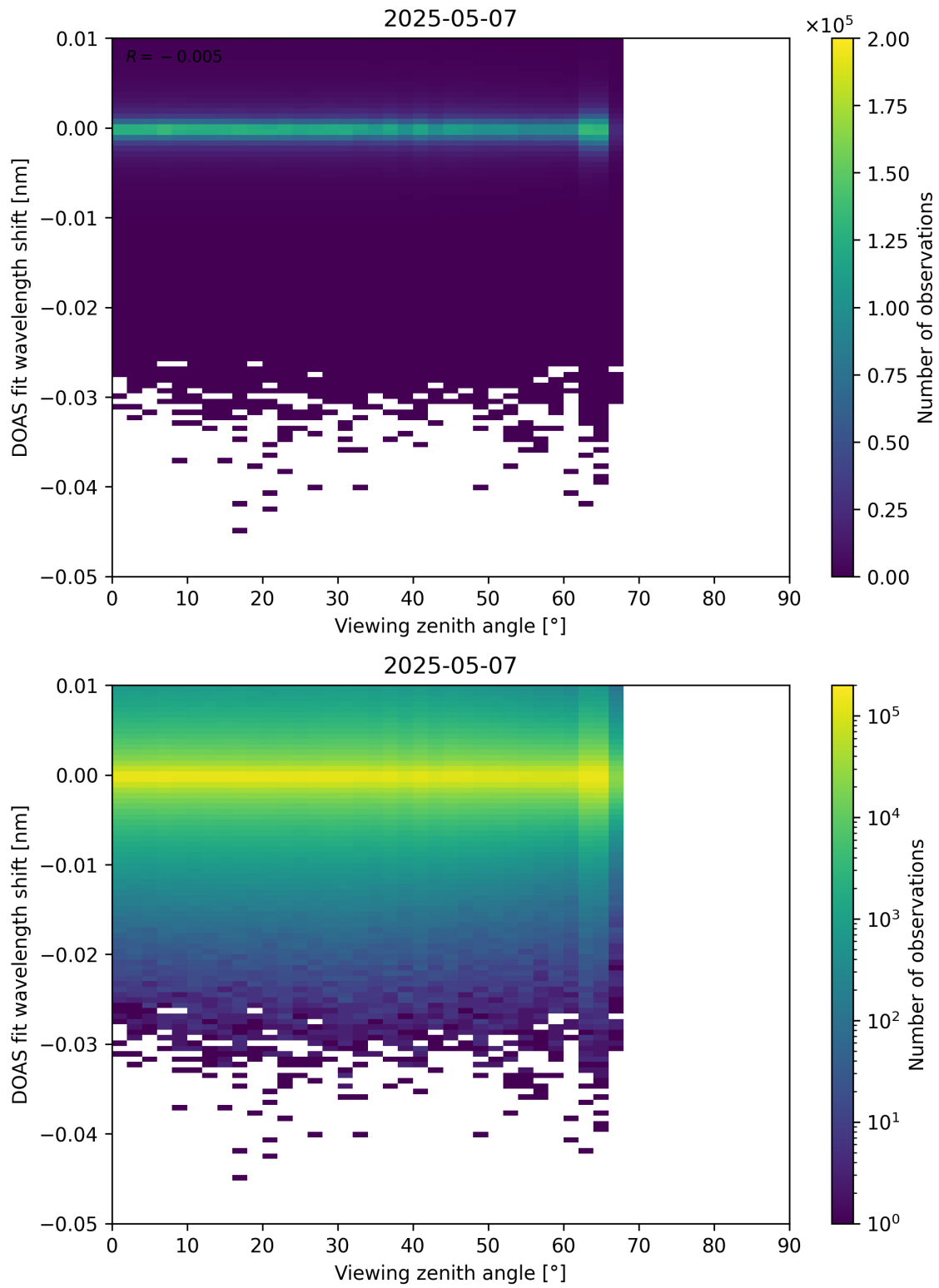
Figure 365: Scatter density plot of “Viewing zenith angle” against “DOAS fit wavelength shift” for 2025-05-06 to 2025-05-08.
