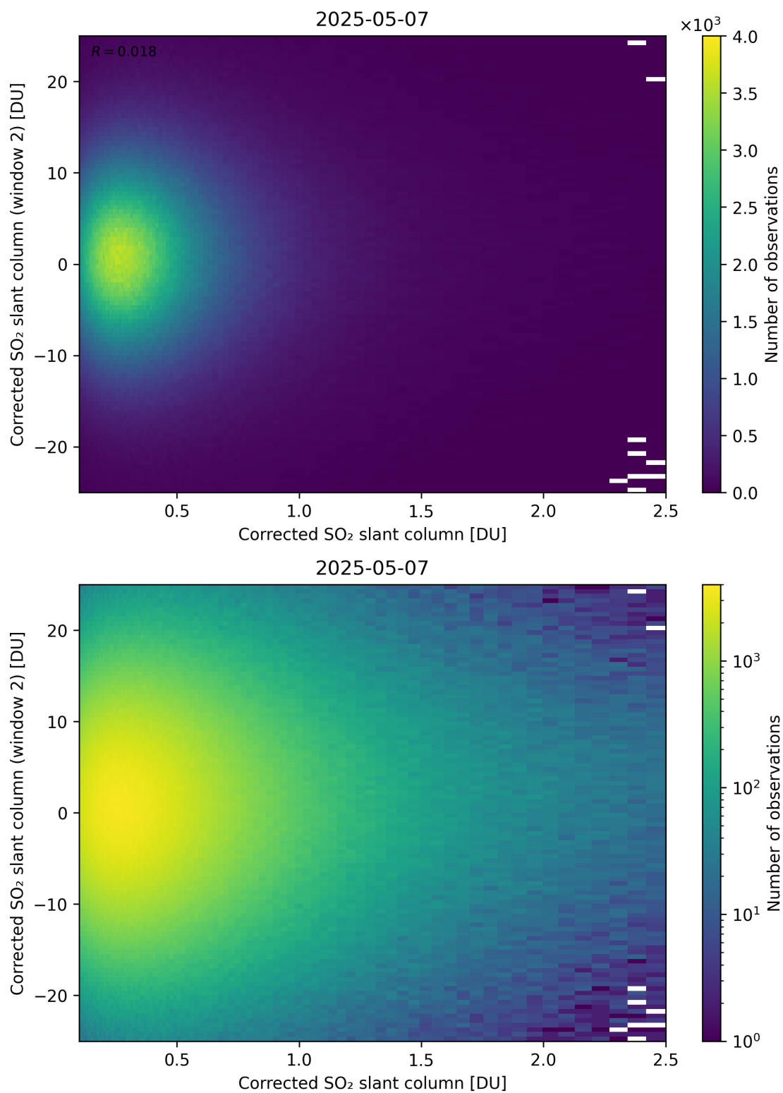
Figure 235: Scatter density plot of “Corrected SO 2 slant column” against “Corrected SO 2 slant column (window 2)” for 2025-05-06 to 2025-05-08.
