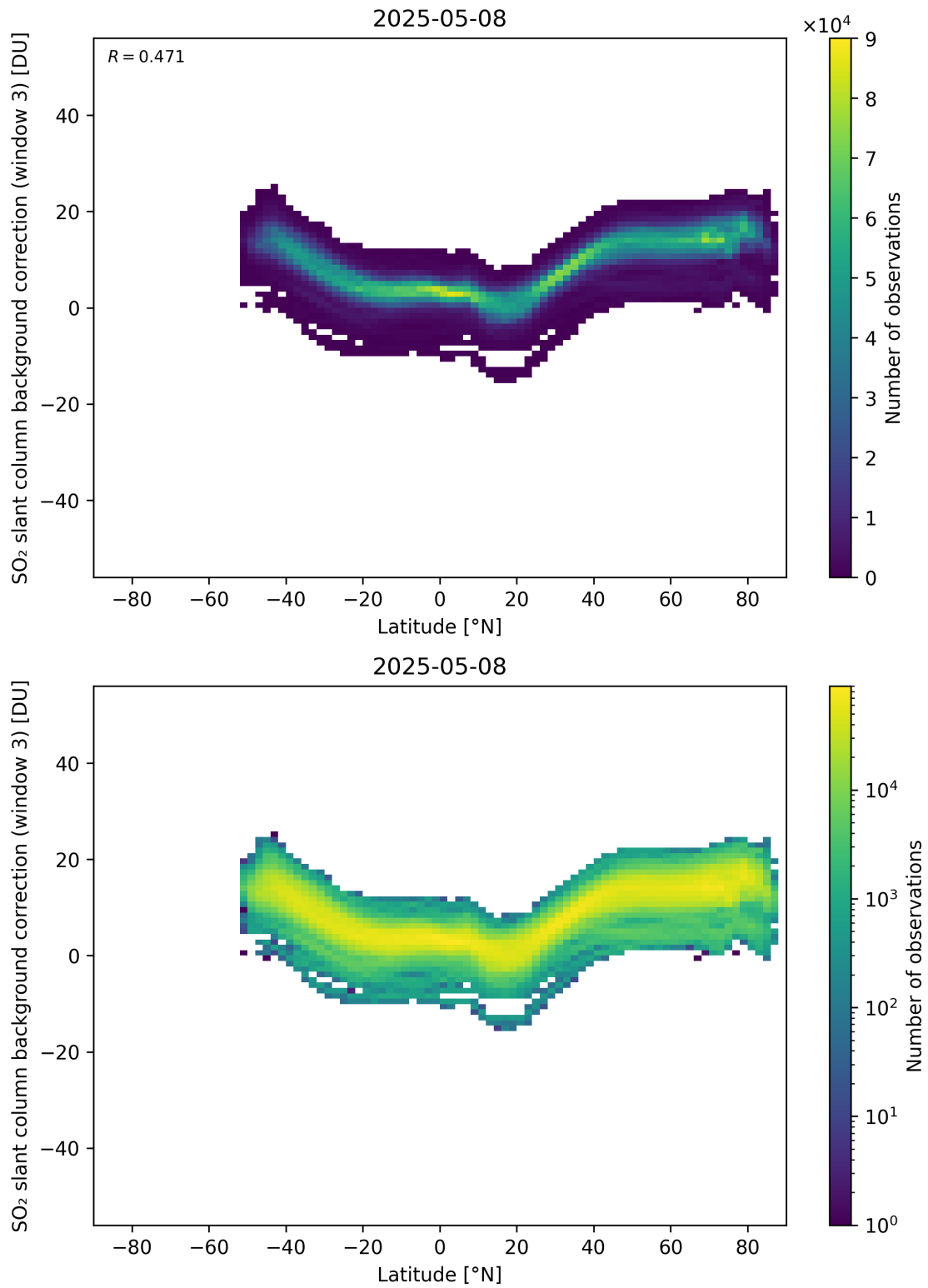
Figure 152: Scatter density plot of “Latitude” against “SO 2 slant column background correction (window 3)” for 2025-05-07 to 2025-05-09.
