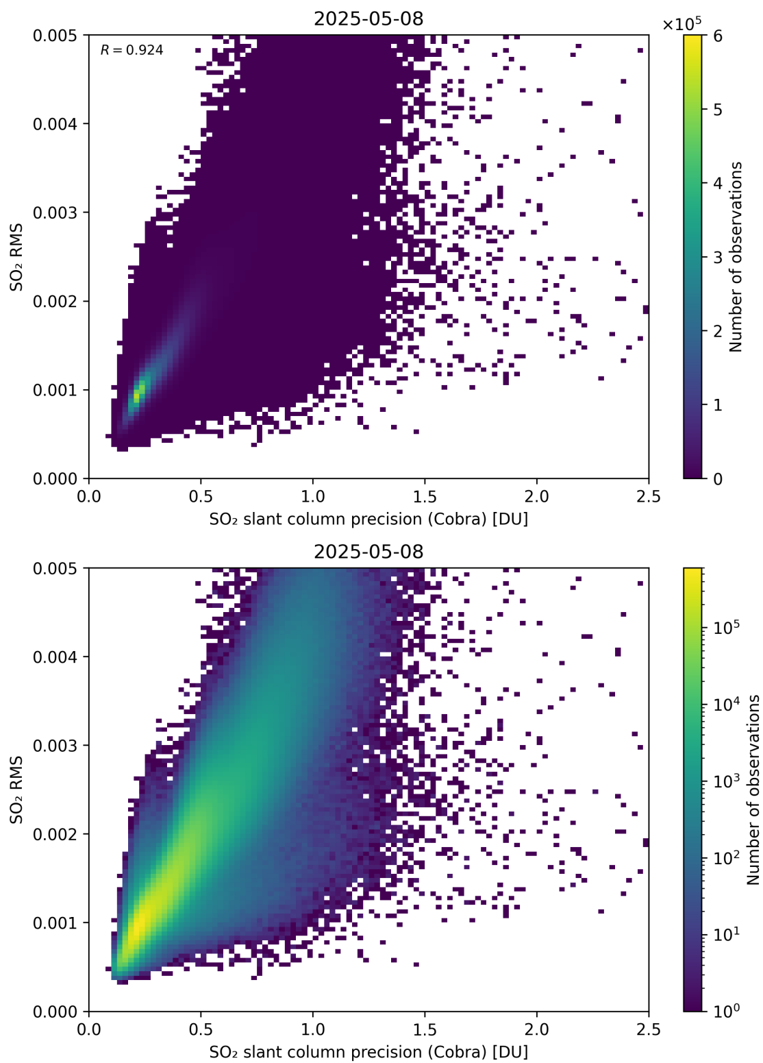
Figure 204: Scatter density plot of “SO 2 slant column precision (Cobra)” against “SO 2 RMS” for 2025-05-07 to 2025-05-09.
