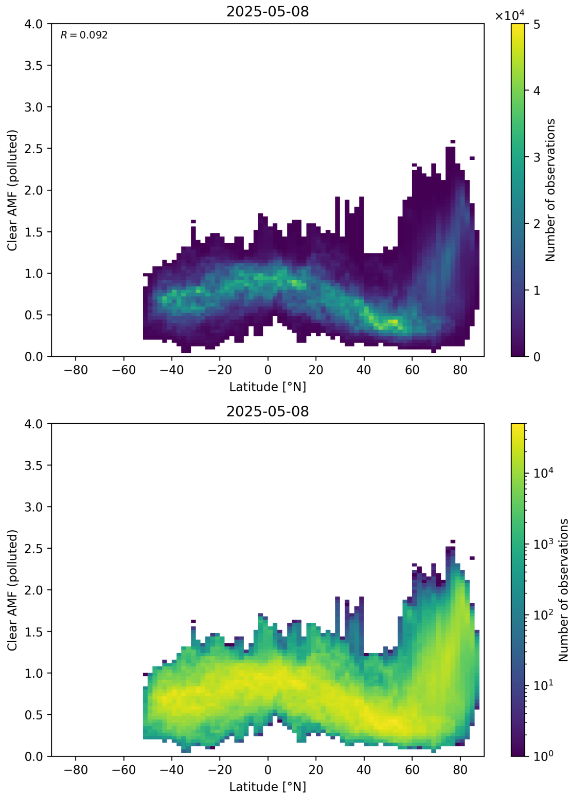
Figure 156: Scatter density plot of “Latitude” against “Clear AMF (polluted)” for 2025-05-07 to 2025-05-09.
