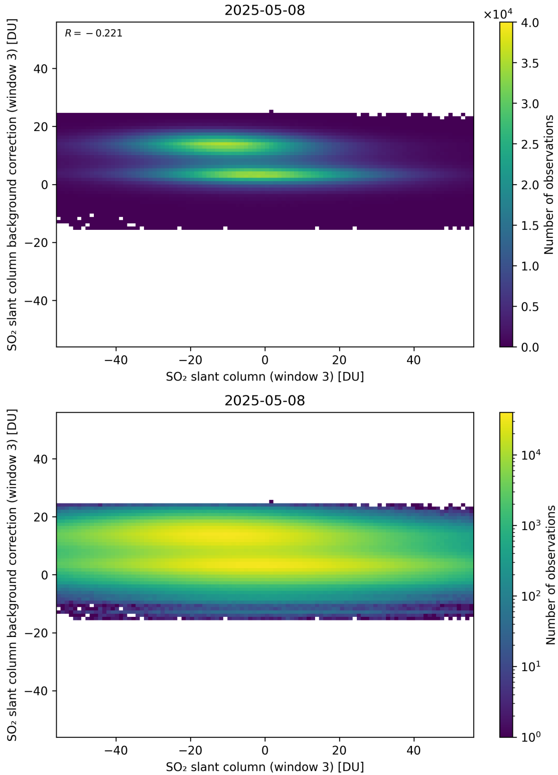
Figure 303: Scatter density plot of “SO 2 slant column (window 3)” against “SO 2 slant column background correction (window 3)” for 2025-05-07 to 2025-05-09.
