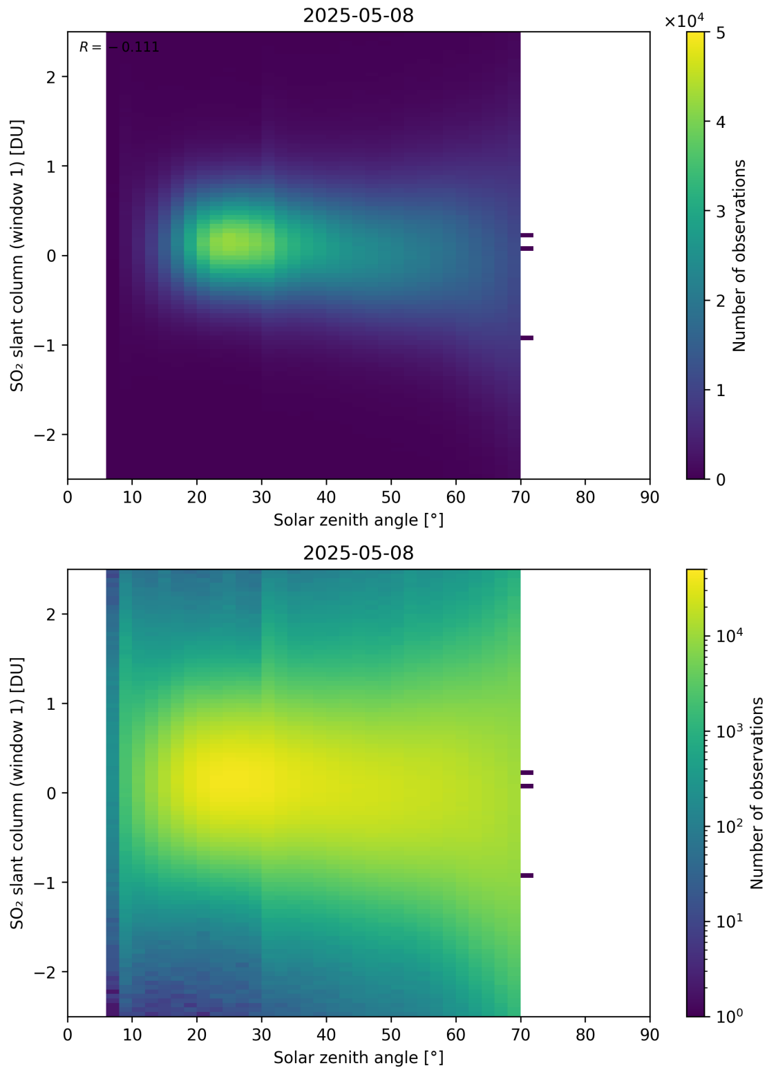
Figure 184: Scatter density plot of “Solar zenith angle” against “SO 2 slant column (window 1)” for 2025-05-07 to 2025-05-09.
