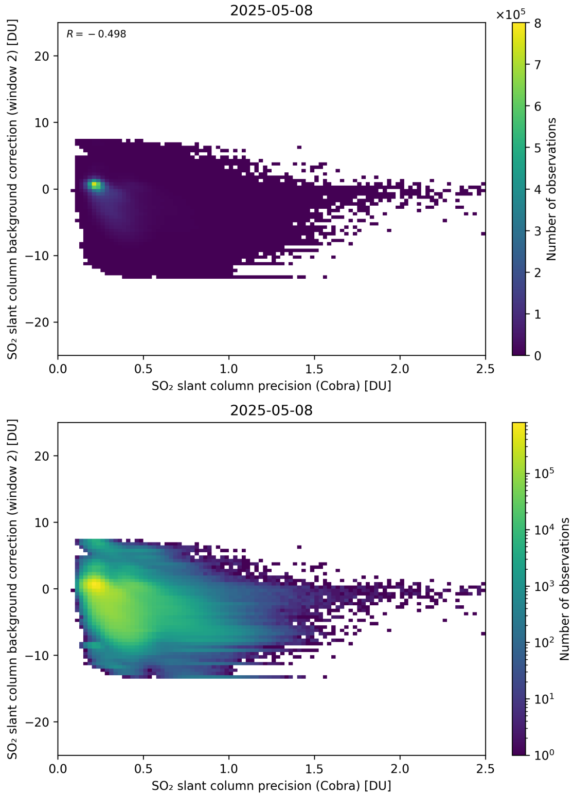
Figure 200: Scatter density plot of “SO 2 slant column precision (Cobra)” against “SO 2 slant column background correction (window 2)” for 2025-05-07 to 2025-05-09.
