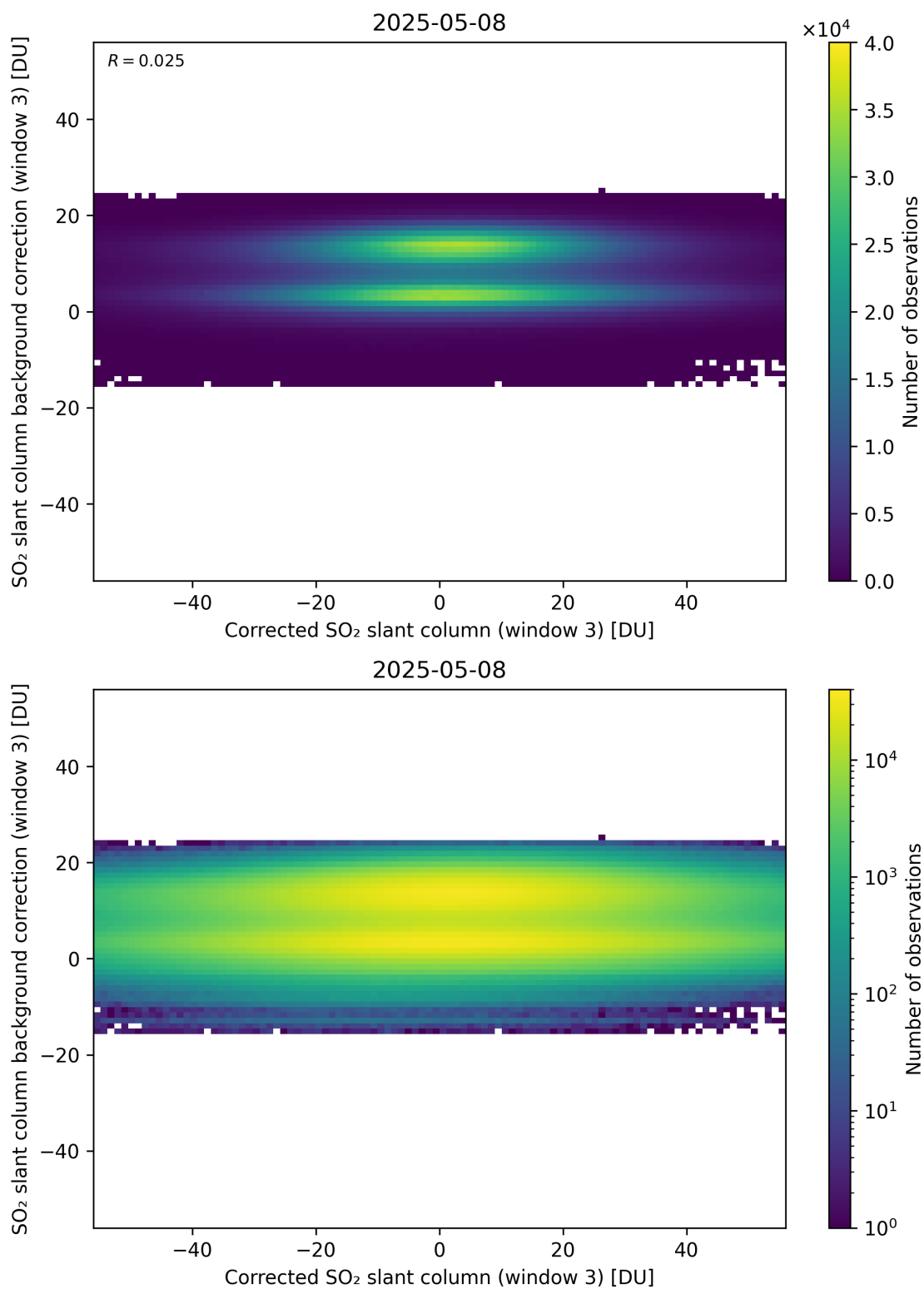
Figure 255: Scatter density plot of “Corrected SO 2 slant column (window 3)” against “SO 2 slant column background correction (window 3)” for 2025-05-07 to 2025-05-09.
