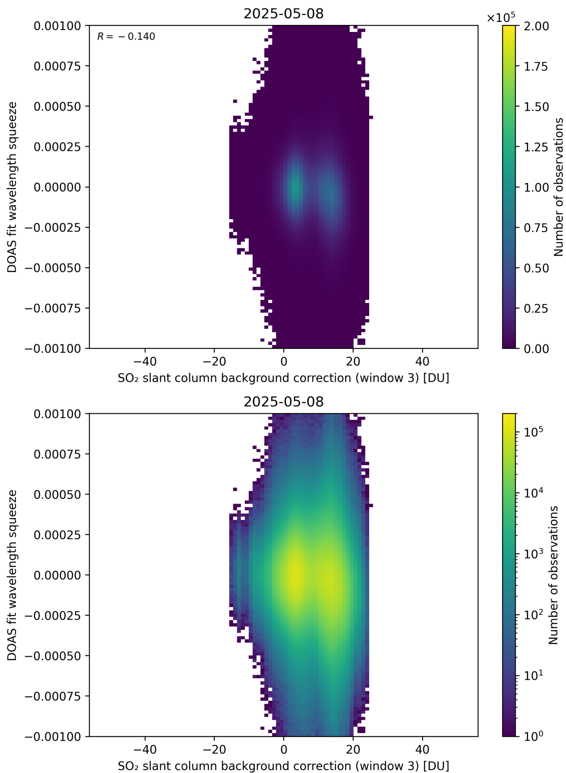
Figure 133: Scatter density plot of “SO 2 slant column background correction (window 3)” against “DOAS fit wavelength squeeze” for 2025-05-07 to 2025-05-09.
