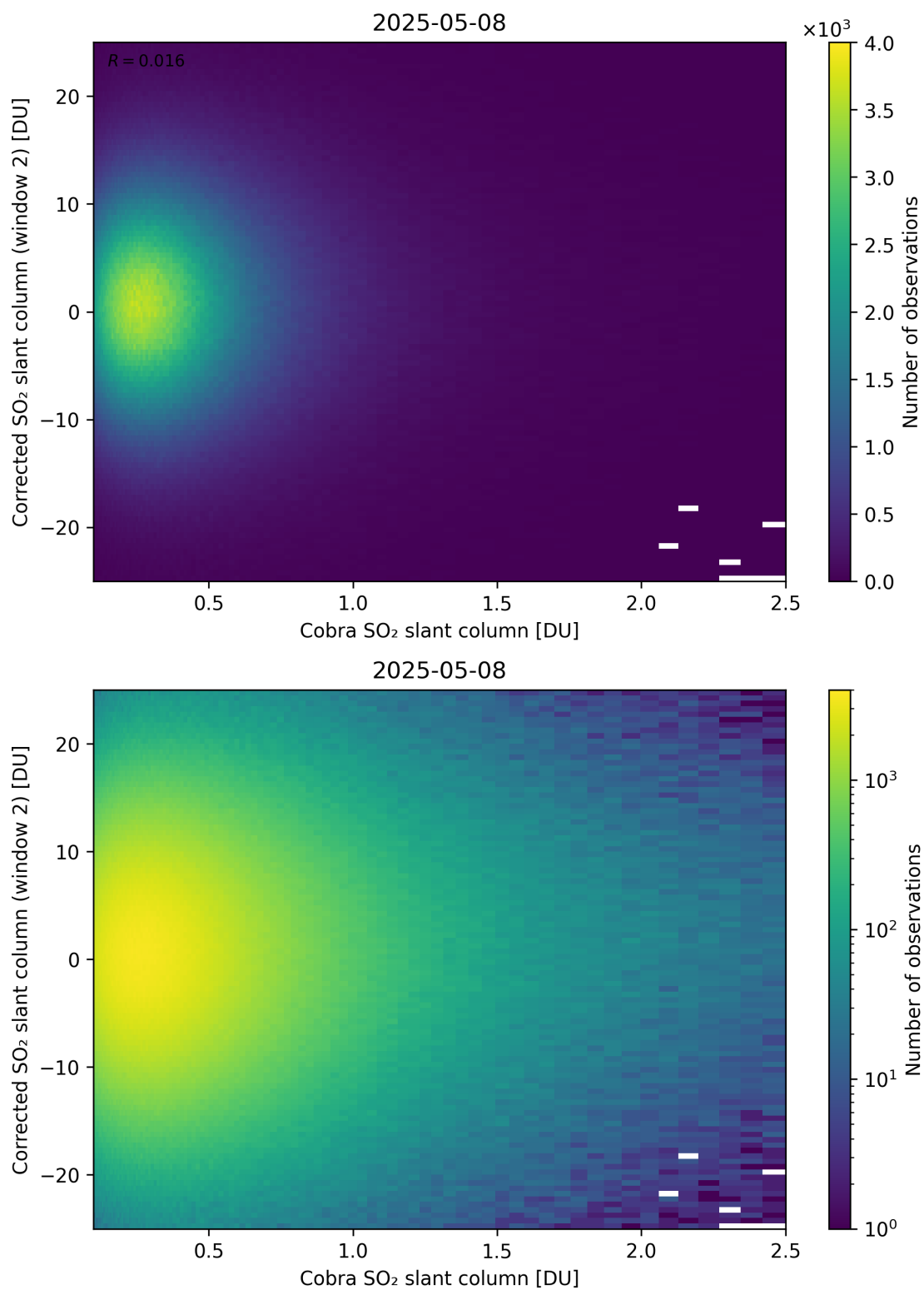
Figure 217: Scatter density plot of “Cobra SO 2 slant column” against “Corrected SO 2 slant column (window 2)” for 2025-05-07 to 2025-05-09.
