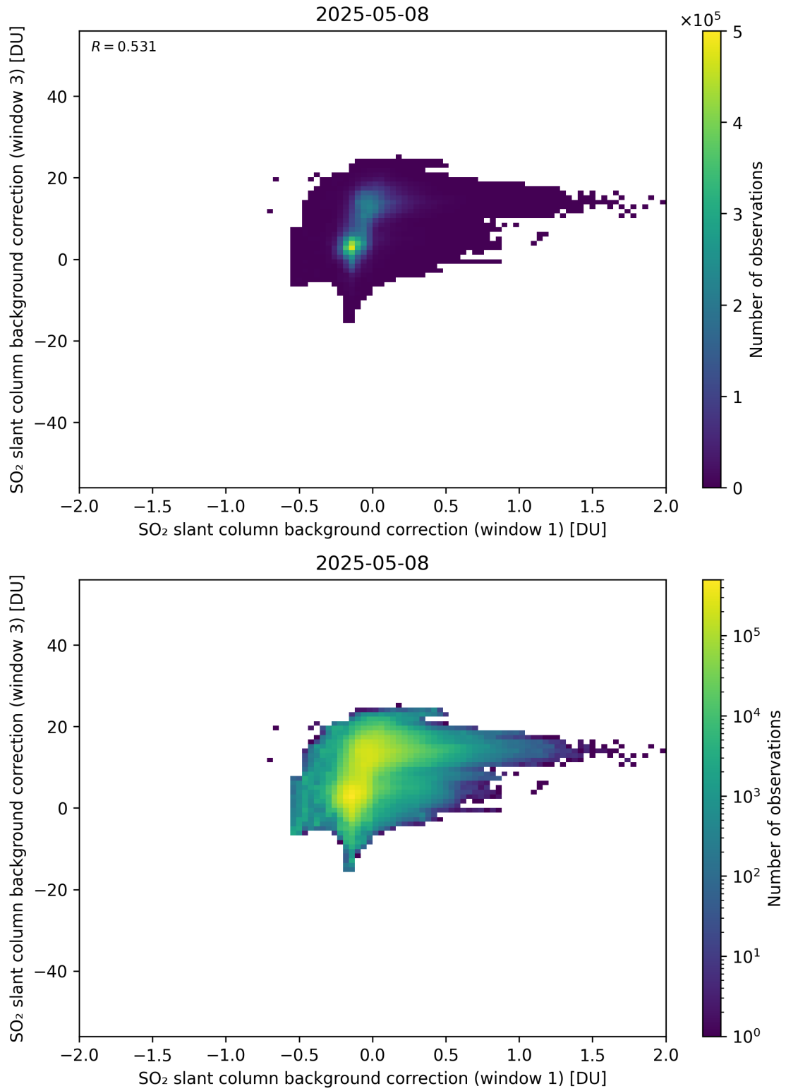
Figure 110: Scatter density plot of “SO 2 slant column background correction (window 1)” against “SO 2 slant column background correction (window 3)” for 2025-05-07 to 2025-05-09.
