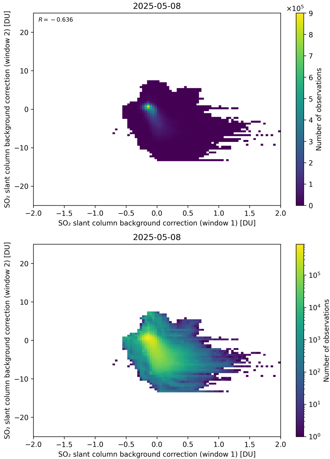
Figure 109: Scatter density plot of “SO 2 slant column background correction (window 1)” against “SO 2 slant column background correction (window 2)” for 2025-05-07 to 2025-05-09.
