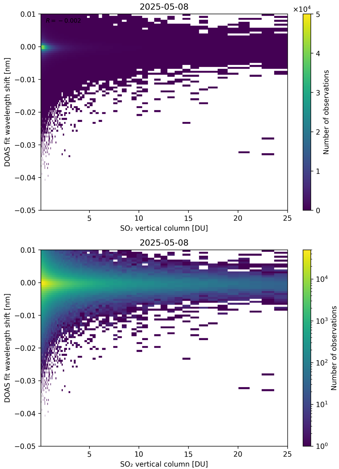
Figure 326: Scatter density plot of “SO 2 vertical column” against “DOAS fit wavelength shift” for 2025-05-07 to 2025-05-09.
