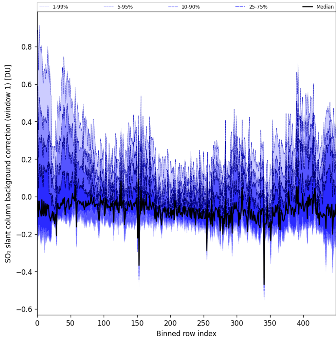
Figure 92: Along track statistics of “SO 2 slant column background correction (window 1)” for 2025-05-07 to 2025-05-09
