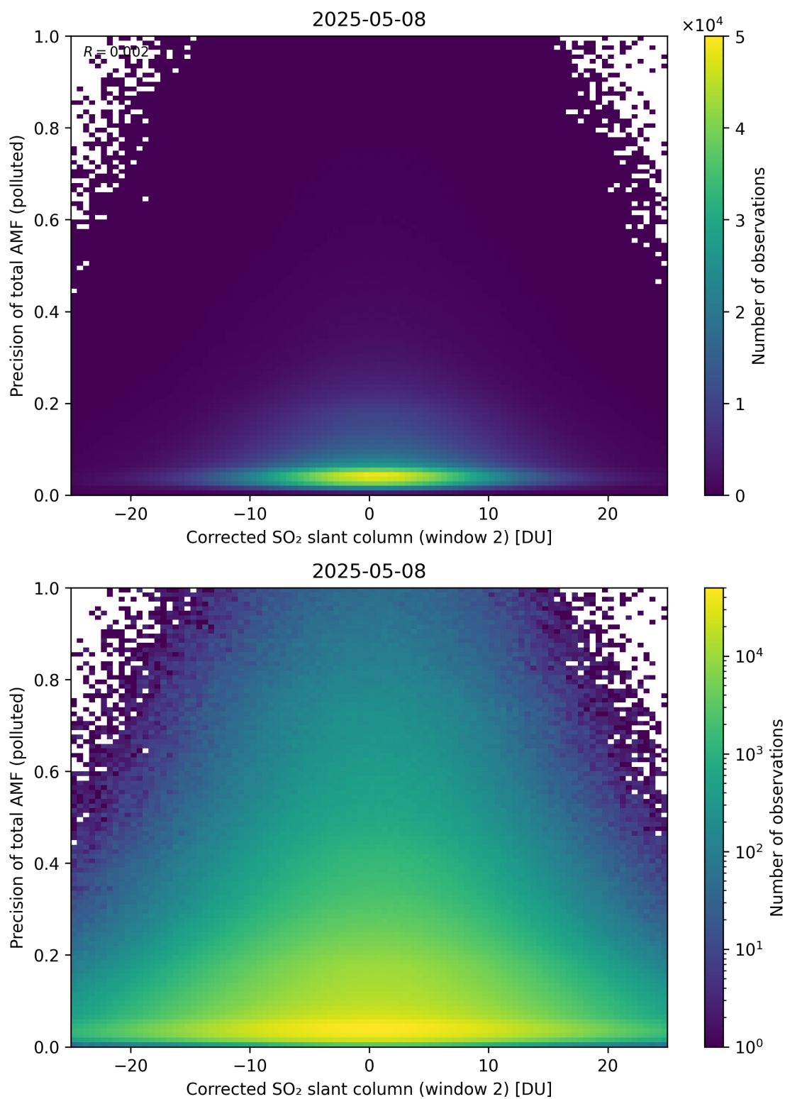
Figure 254: Scatter density plot of “Corrected SO 2 slant column (window 2)” against “Precision of total AMF (polluted)” for 2025-05-07 to 2025-05-09.
