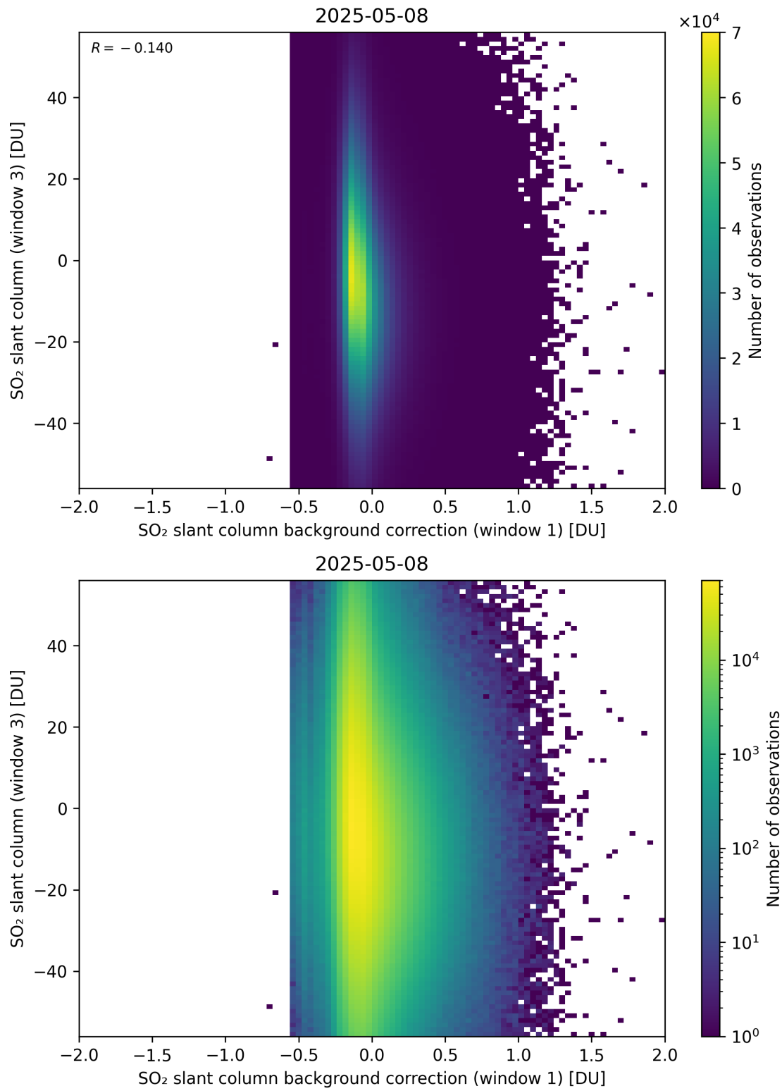
Figure 118: Scatter density plot of “SO 2 slant column background correction (window 1)” against “SO 2 slant column (window 3)” for 2025-05-07 to 2025-05-09.
