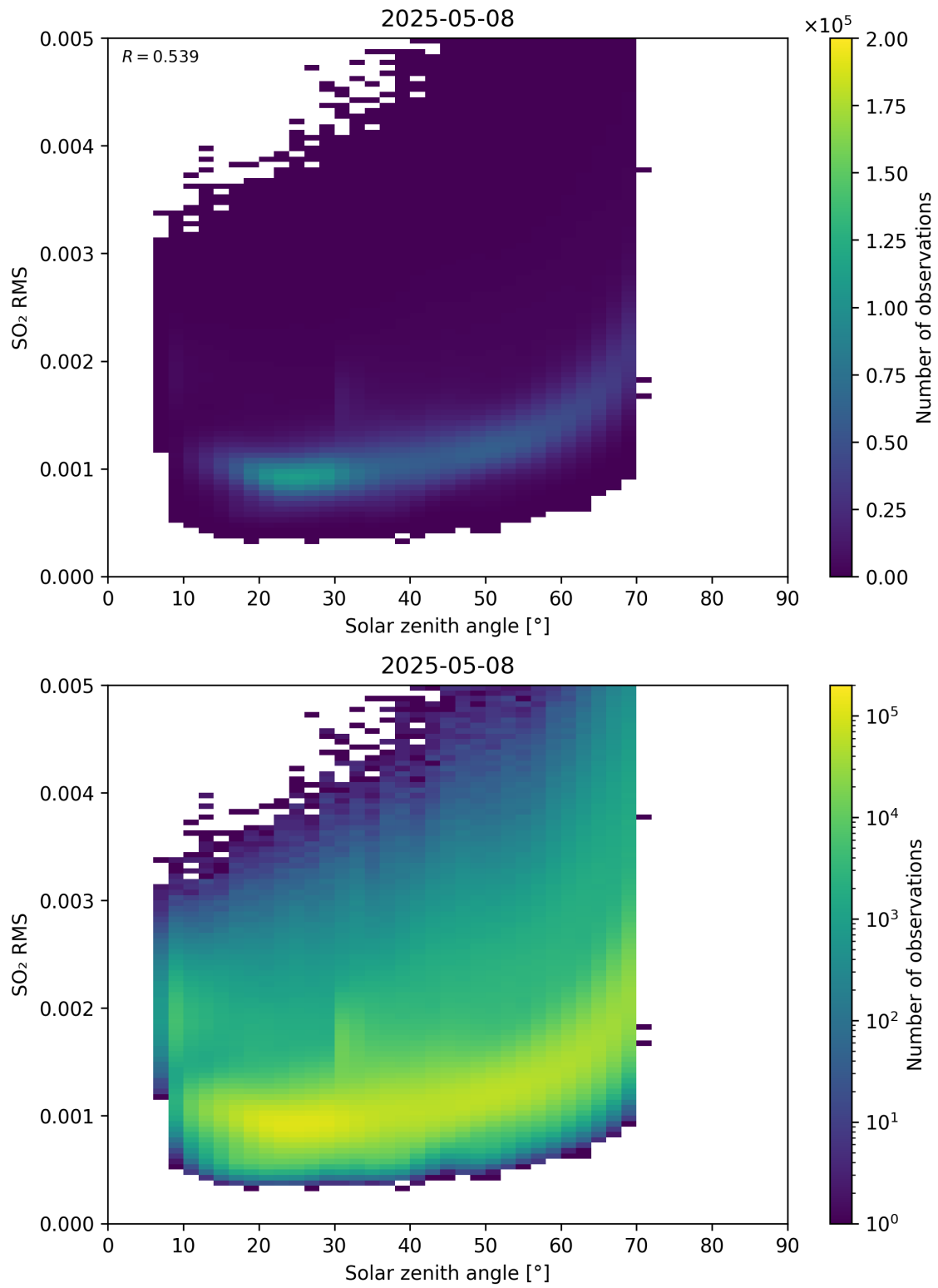
Figure 176: Scatter density plot of “Solar zenith angle” against “SO 2 RMS” for 2025-05-07 to 2025-05-09.
