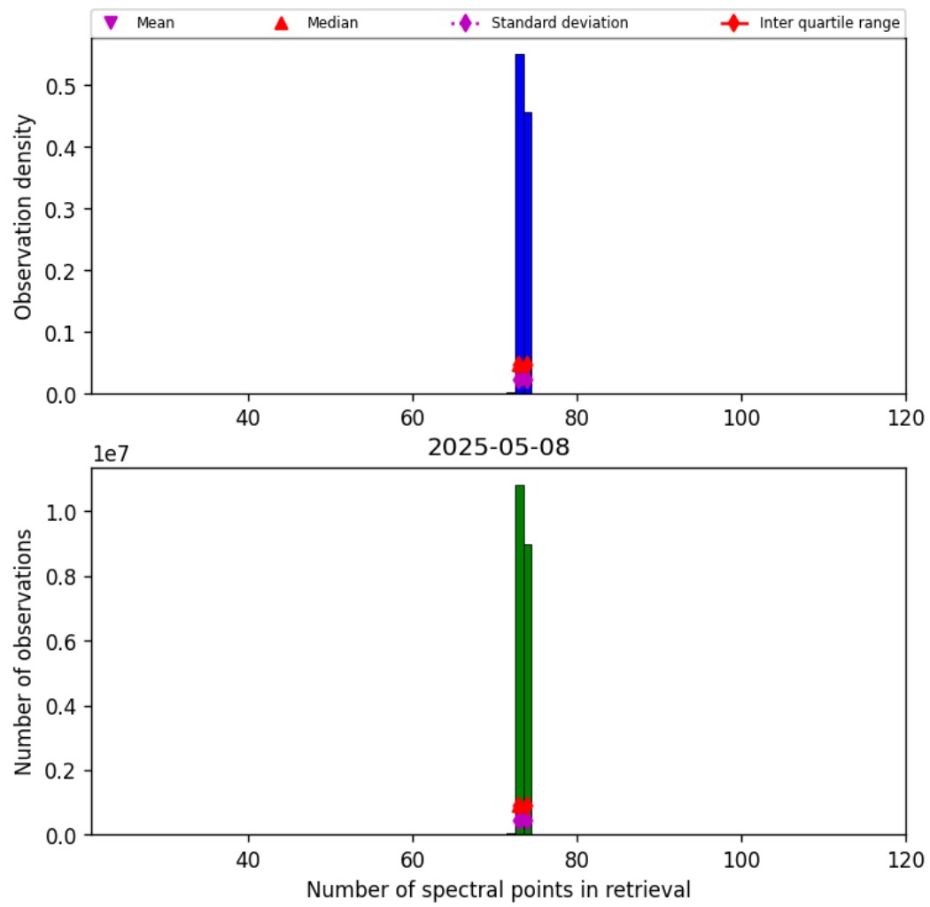
Figure 82: Histogram of “Number of spectral points in retrieval” for 2025-05-07 to 2025-05-09
