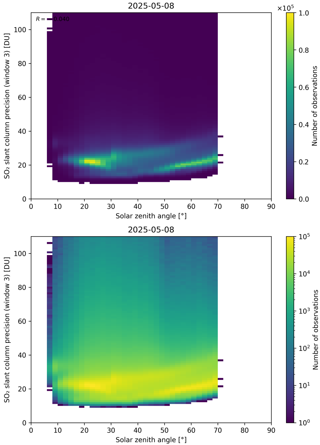
Figure 188: Scatter density plot of “Solar zenith angle” against “SO 2 slant column precision (window 3)” for 2025-05-07 to 2025-05-09.
