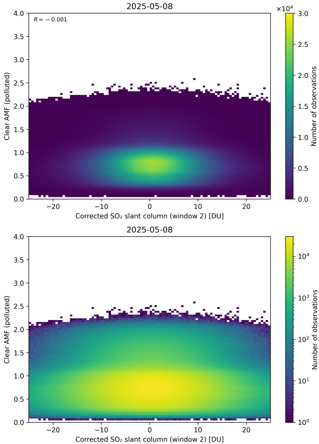
Figure 249: Scatter density plot of “Corrected SO 2 slant column (window 2)” against “Clear AMF (polluted)” for 2025-05-07 to 2025-05-09.
