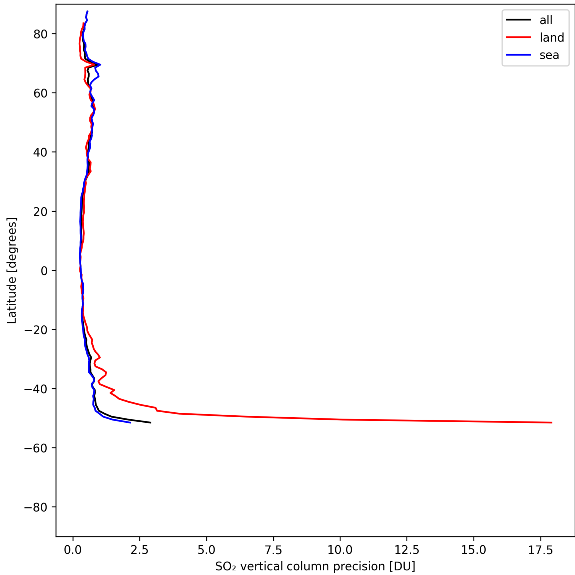
Figure 33: Zonal average of “SO 2 vertical column precision” for 2025-05-07 to 2025-05-09.
