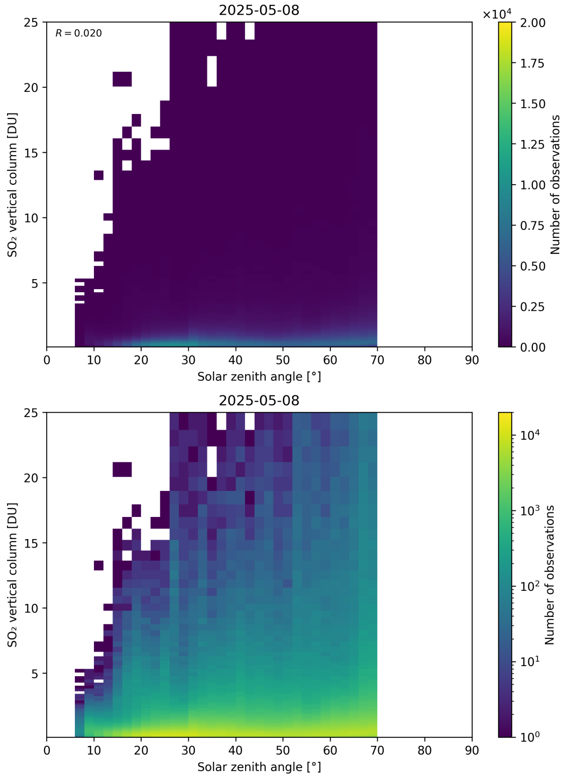
Figure 191: Scatter density plot of “Solar zenith angle” against “SO 2 vertical column” for 2025-05-07 to 2025-05-09.
