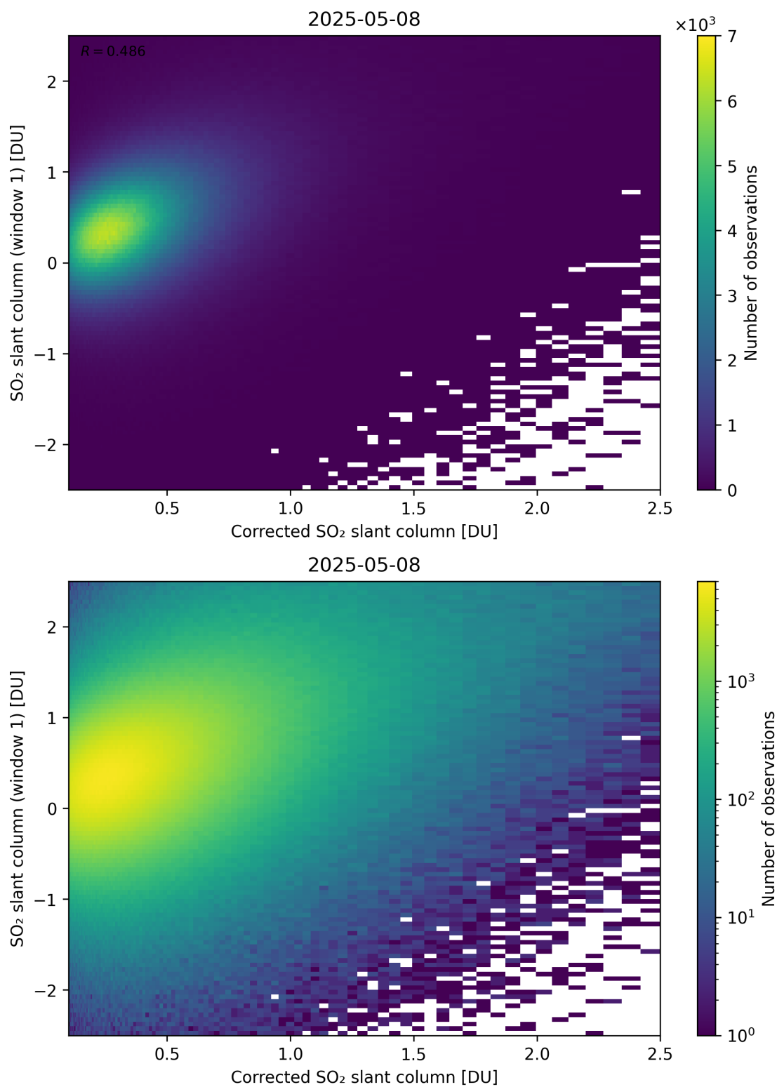
Figure 237: Scatter density plot of “Corrected SO 2 slant column” against “SO 2 slant column (window 1)” for 2025-05-07 to 2025-05-09.
