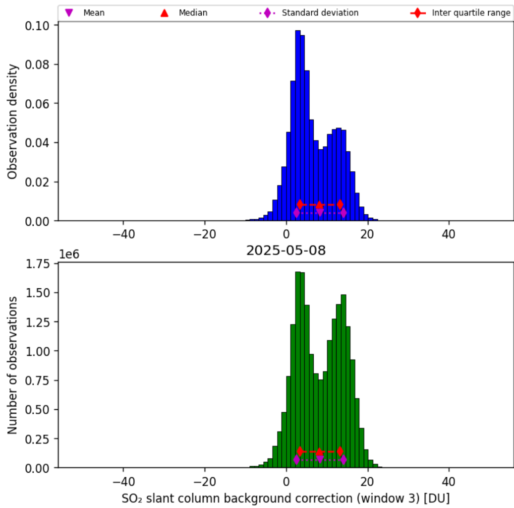
Figure 74: Histogram of “SO 2 slant column background correction (window 3)” for 2025-05-07 to 2025-05-09
