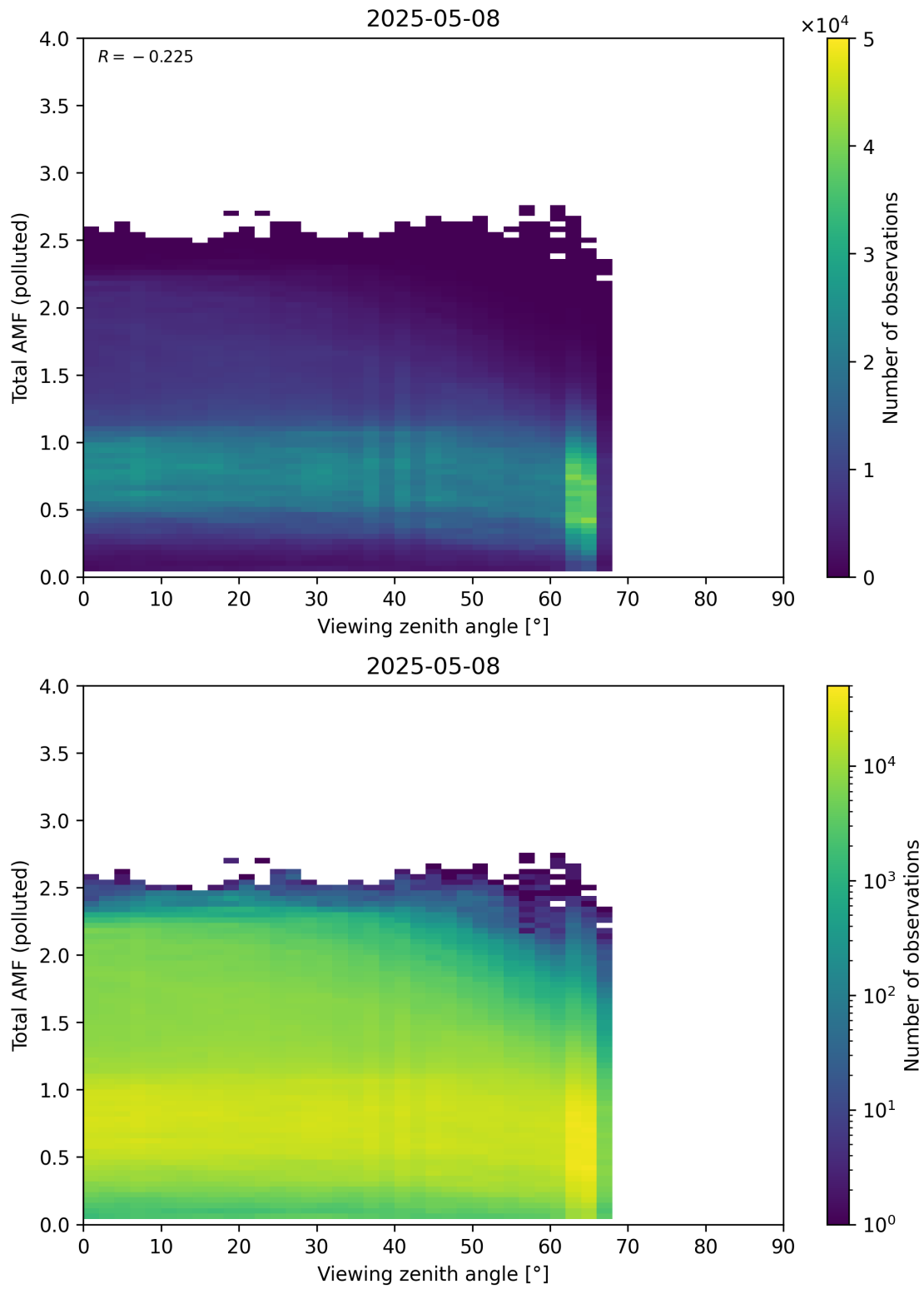
Figure 381: Scatter density plot of “Viewing zenith angle” against “Total AMF (polluted)” for 2025-05-07 to 2025-05-09.
