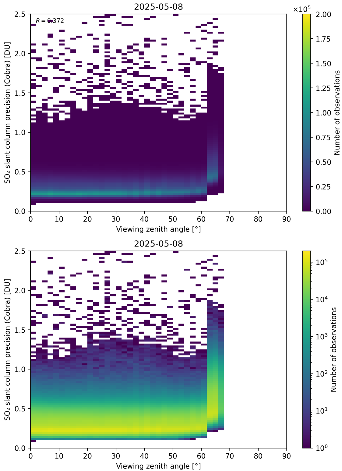
Figure 372: Scatter density plot of “Viewing zenith angle” against “SO 2 slant column precision (Cobra)” for 2025-05-07 to 2025-05-09.
