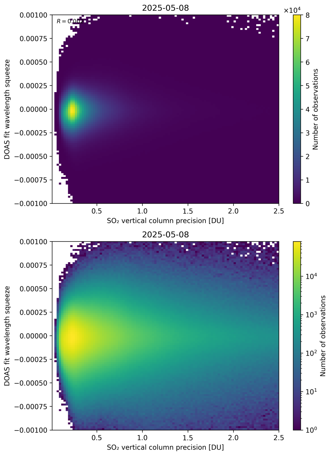
Figure 333: Scatter density plot of “SO 2 vertical column precision” against “DOAS fit wavelength squeeze” for 2025-05-07 to 2025-05-09.
