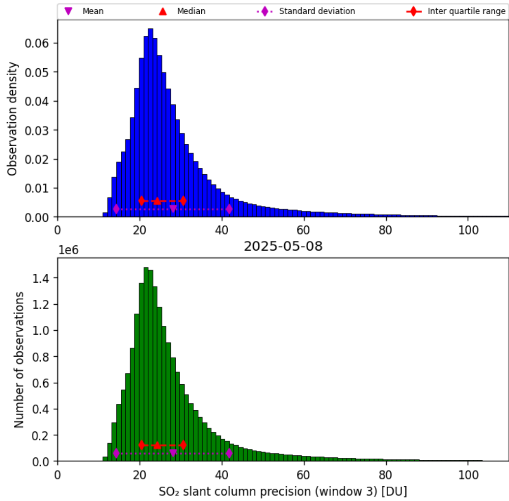
Figure 72: Histogram of “SO 2 slant column precision (window 3)” for 2025-05-07 to 2025-05-09
