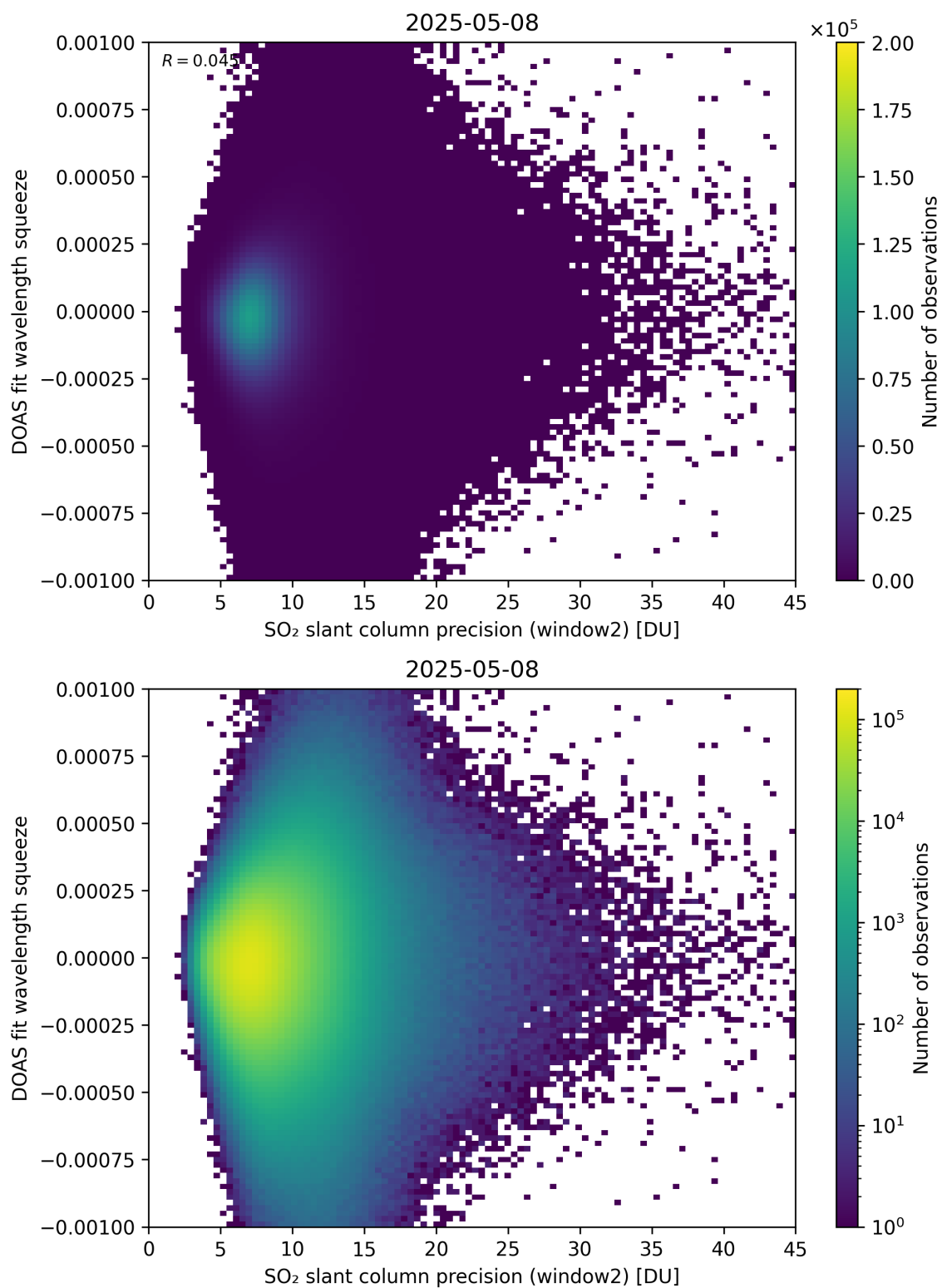
Figure 294: Scatter density plot of “SO 2 slant column precision (window2)” against “DOAS fit wavelength squeeze” for 2025-05-07 to 2025-05-09.
