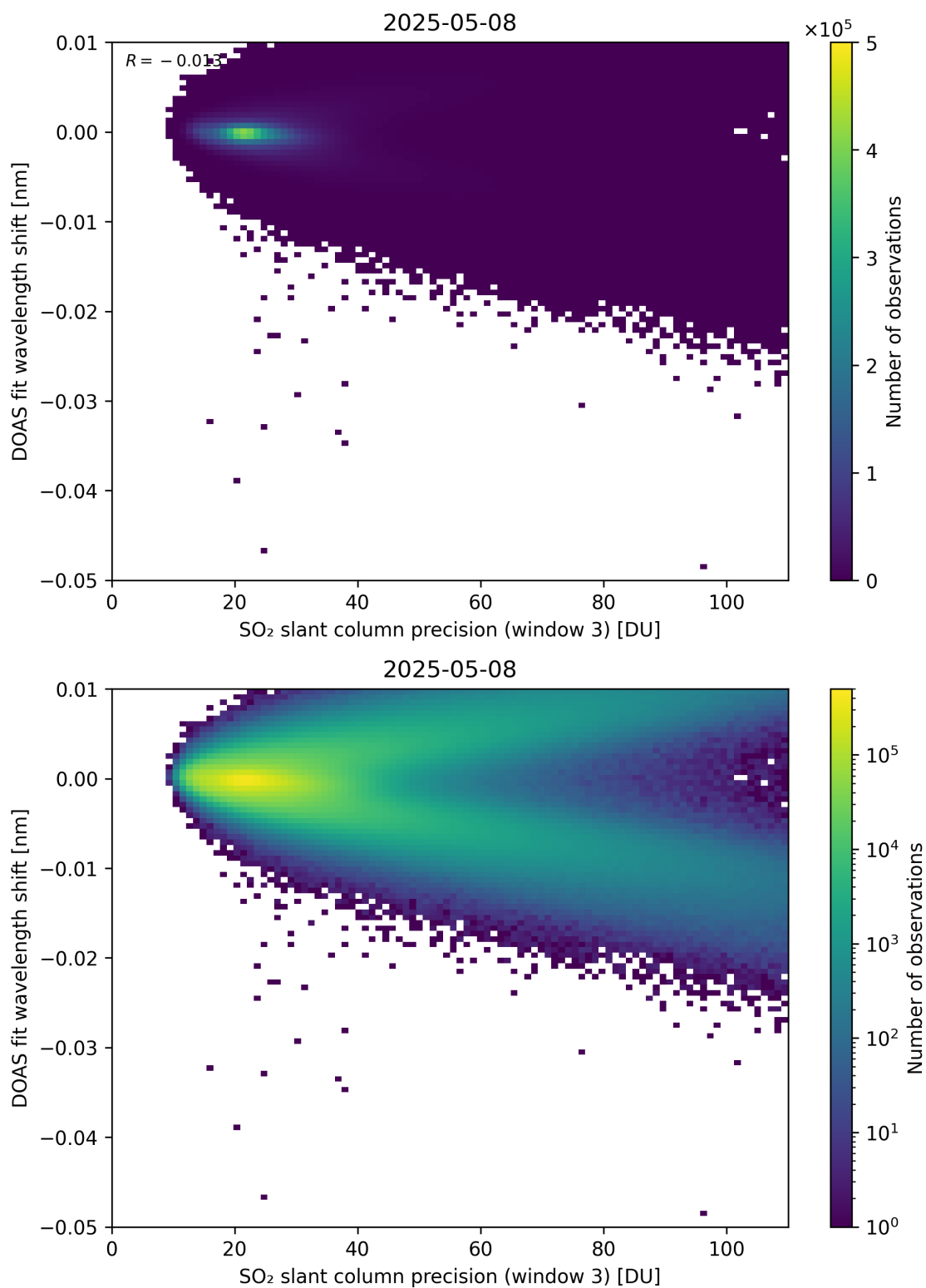
Figure 308: Scatter density plot of “SO 2 slant column precision (window 3)” against “DOAS fit wavelength shift” for 2025-05-07 to 2025-05-09.
