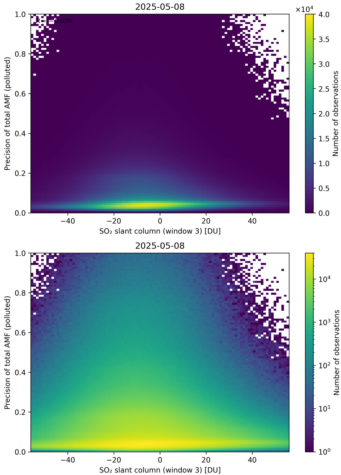
Figure 319: Scatter density plot of “SO 2 slant column (window 3)” against “Precision of total AMF (polluted)” for 2025-05-07 to 2025-05-09.
