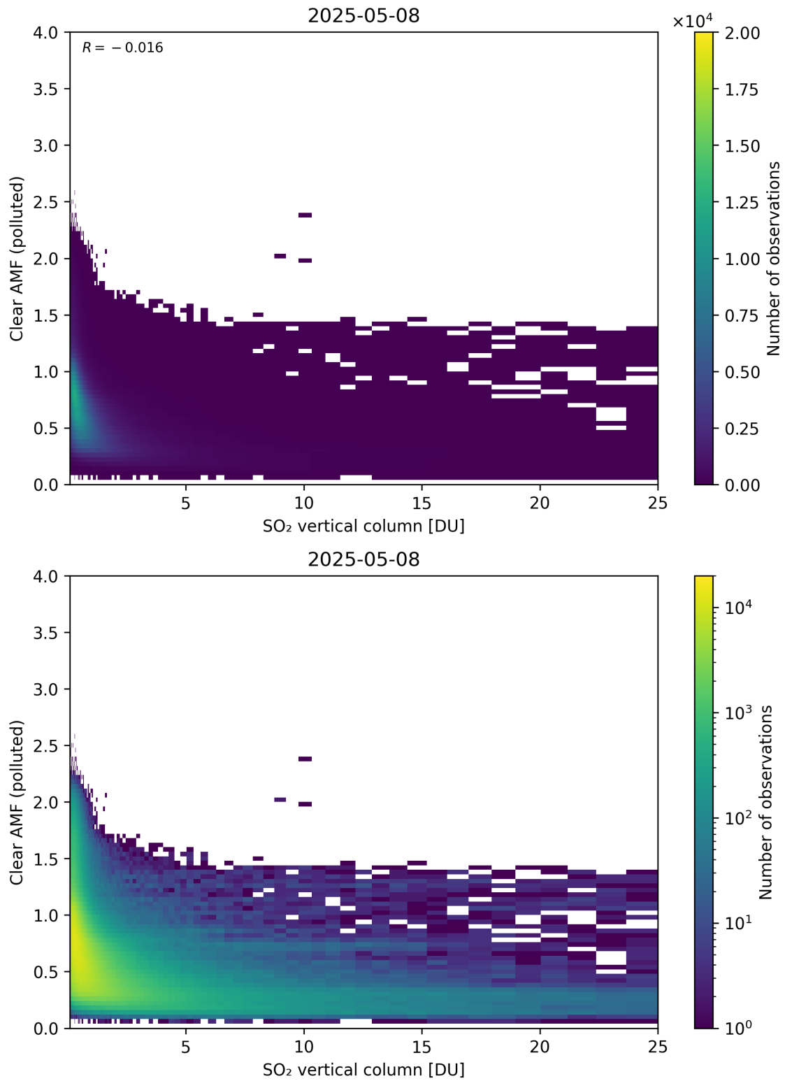
Figure 348: Scatter density plot of “SO 2 vertical column” against “Clear AMF (polluted)” for 2025-05-07 to 2025-05-09.
