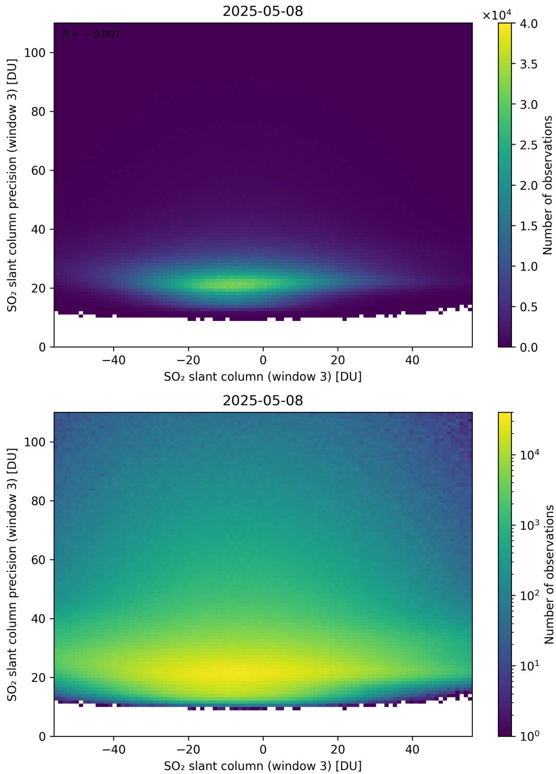
Figure 317: Scatter density plot of “SO 2 slant column (window 3)” against “SO 2 slant column precision (window 3)” for 2025-05-07 to 2025-05-09.
