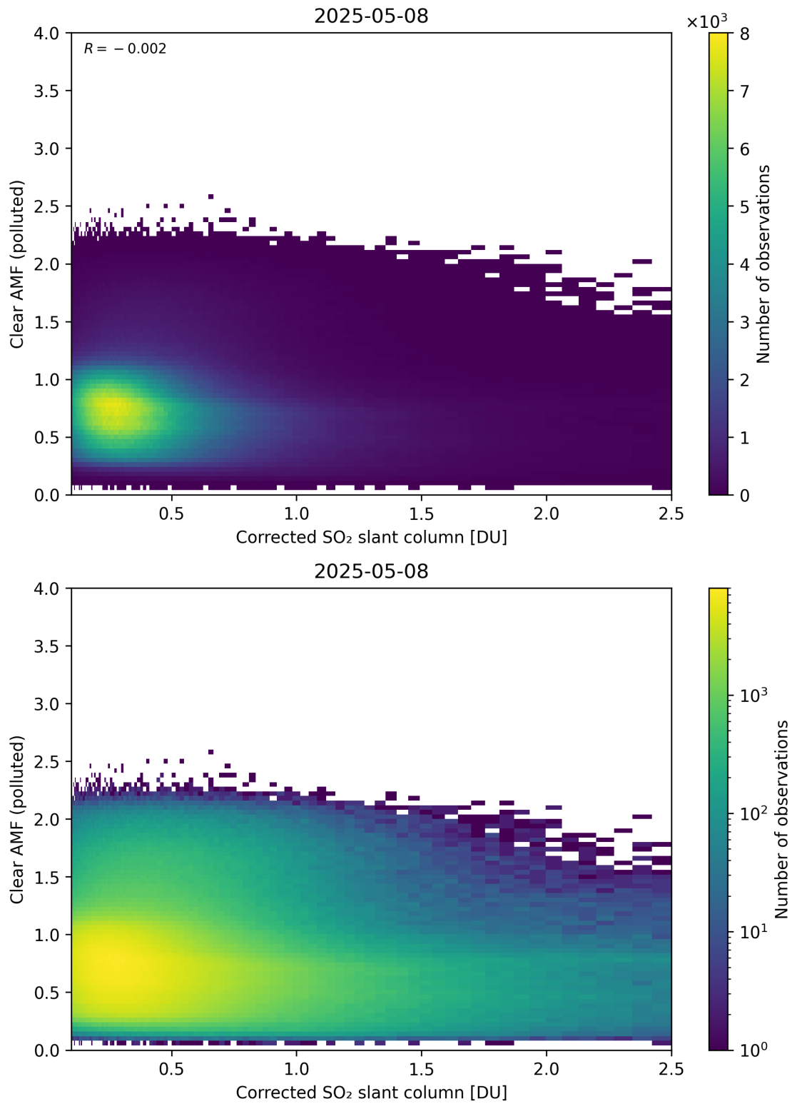
Figure 232: Scatter density plot of “Corrected SO 2 slant column” against “Clear AMF (polluted)” for 2025-05-07 to 2025-05-09.
