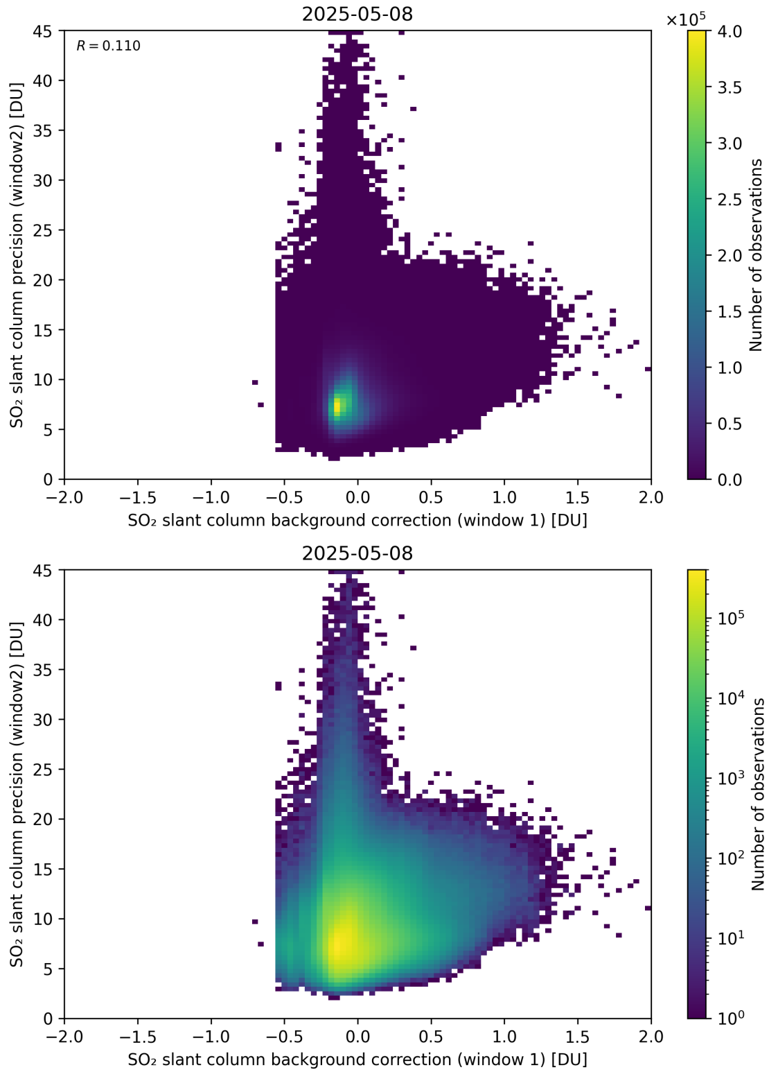
Figure 117: Scatter density plot of “SO 2 slant column background correction (window 1)” against “SO 2 slant column precision (window2)” for 2025-05-07 to 2025-05-09.
