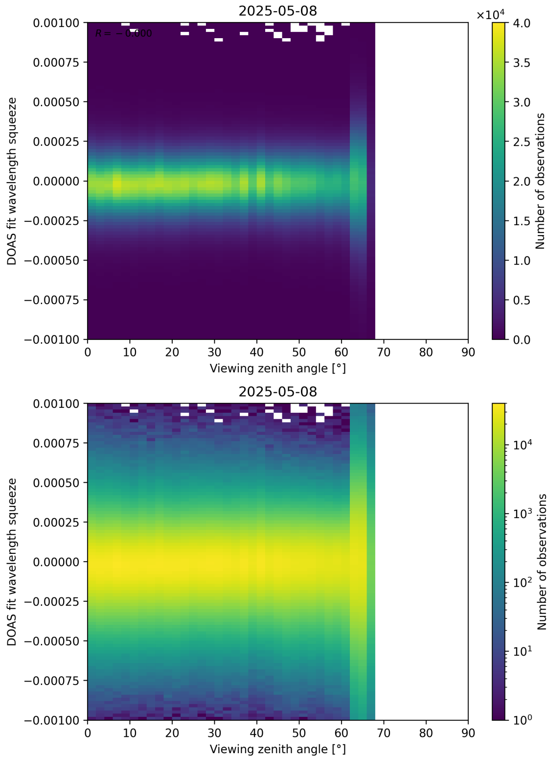
Figure 366: Scatter density plot of “Viewing zenith angle” against “DOAS fit wavelength squeeze” for 2025-05-07 to 2025-05-09.
