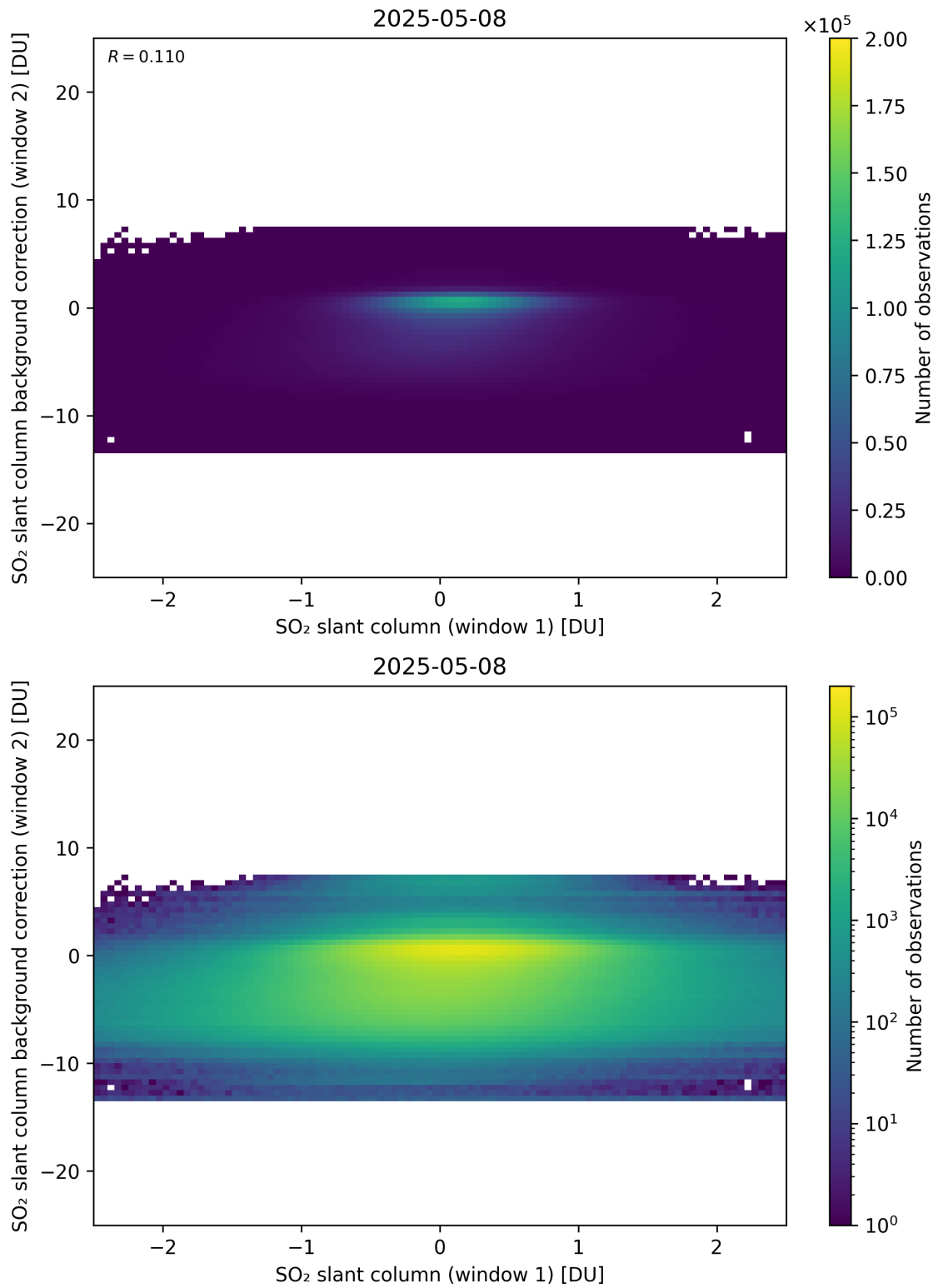
Figure 263: Scatter density plot of “SO 2 slant column (window 1)” against “SO 2 slant column background correction (window 2)” for 2025-05-07 to 2025-05-09.
