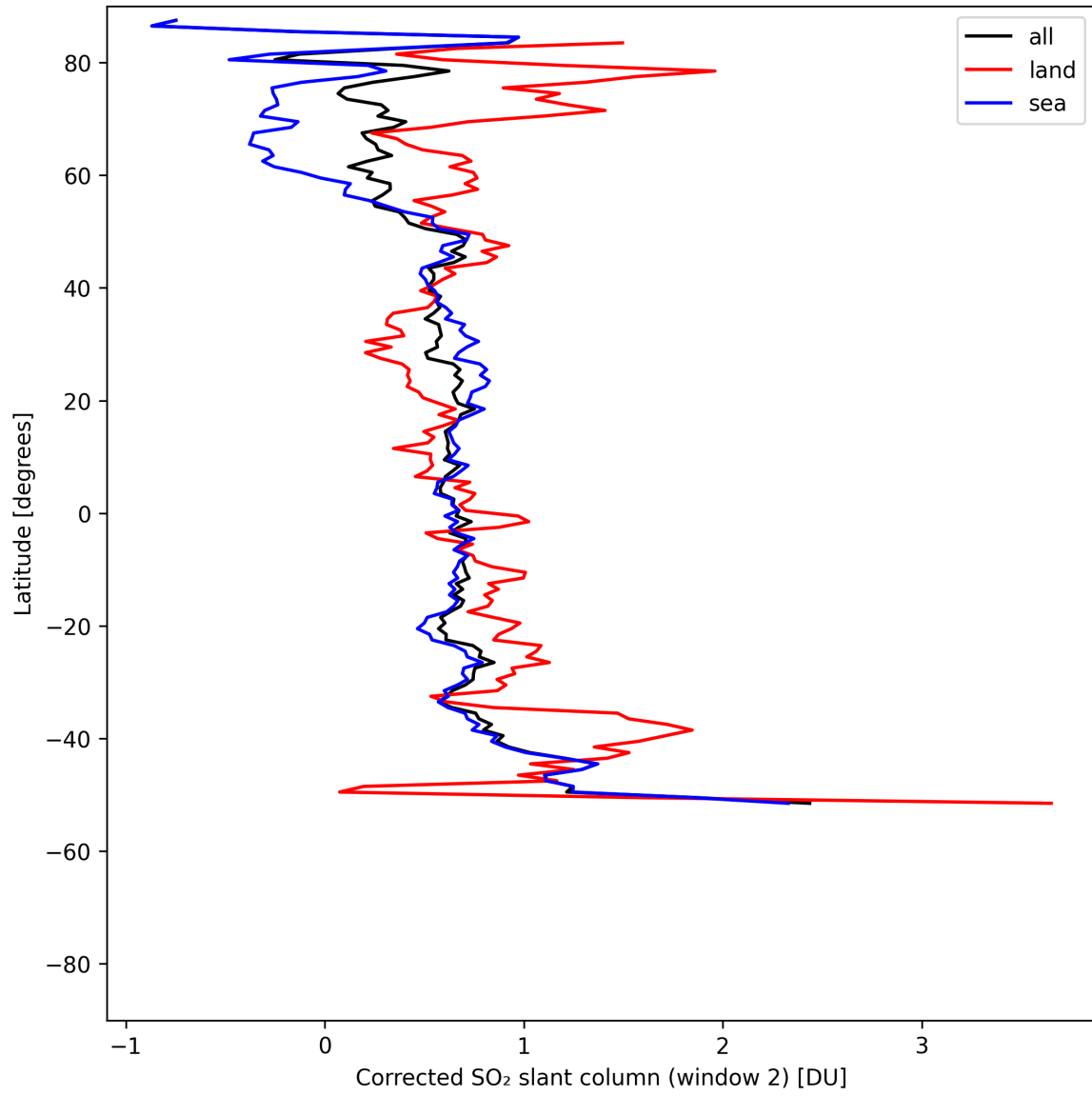
Figure 43: Zonal average of “Corrected SO 2 slant column (window 2)” for 2025-05-07 to 2025-05-09.
