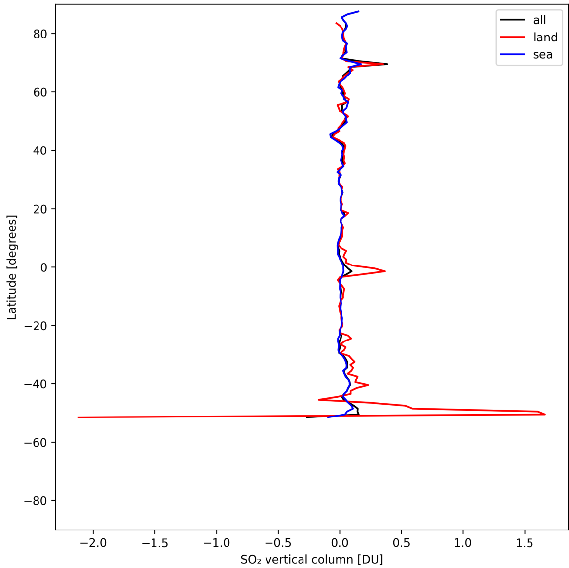
Figure 32: Zonal average of “SO 2 vertical column” for 2025-05-07 to 2025-05-09.
