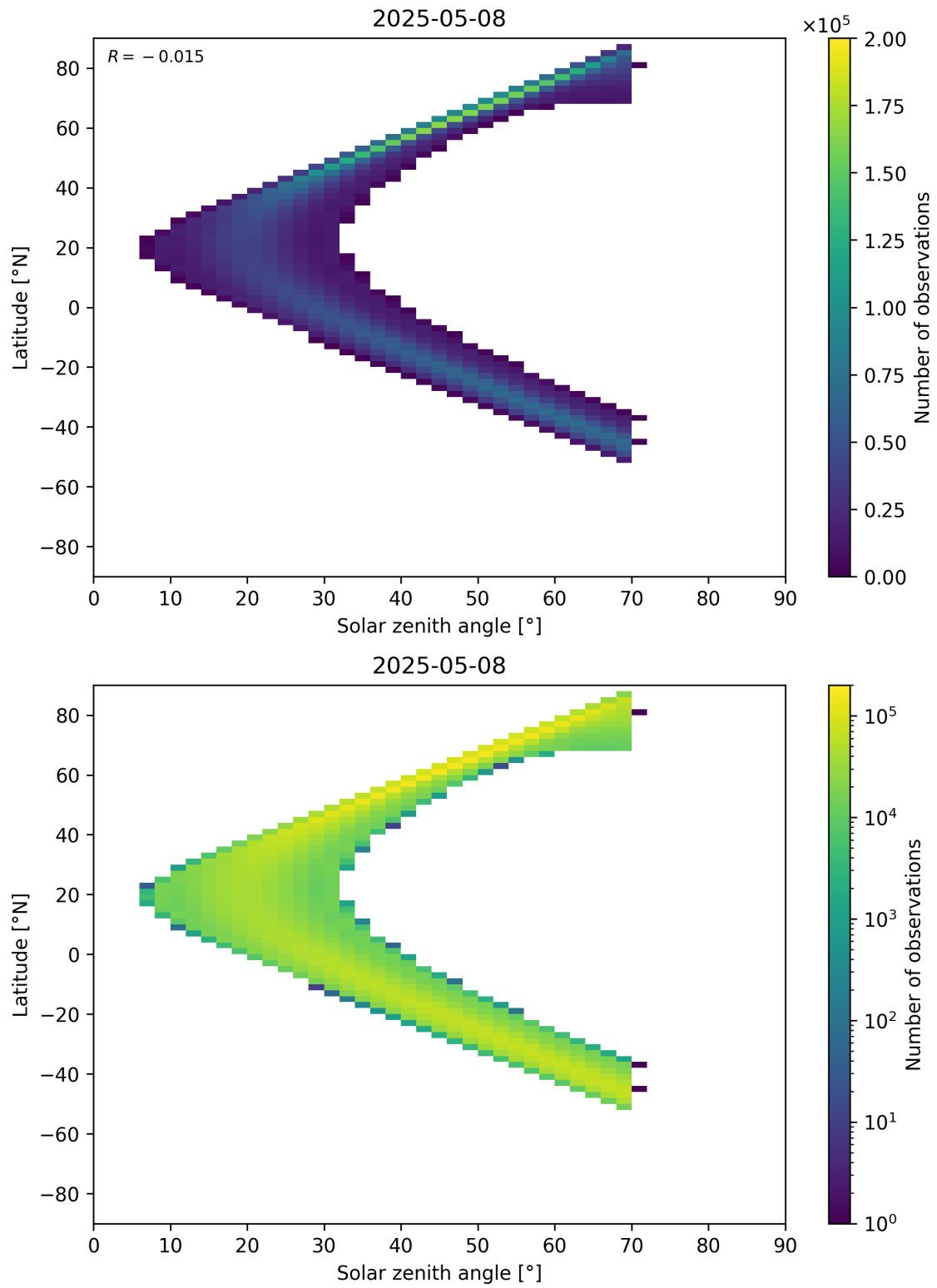
Figure 177: Scatter density plot of “Solar zenith angle” against “Latitude” for 2025-05-07 to 2025-05-09.
