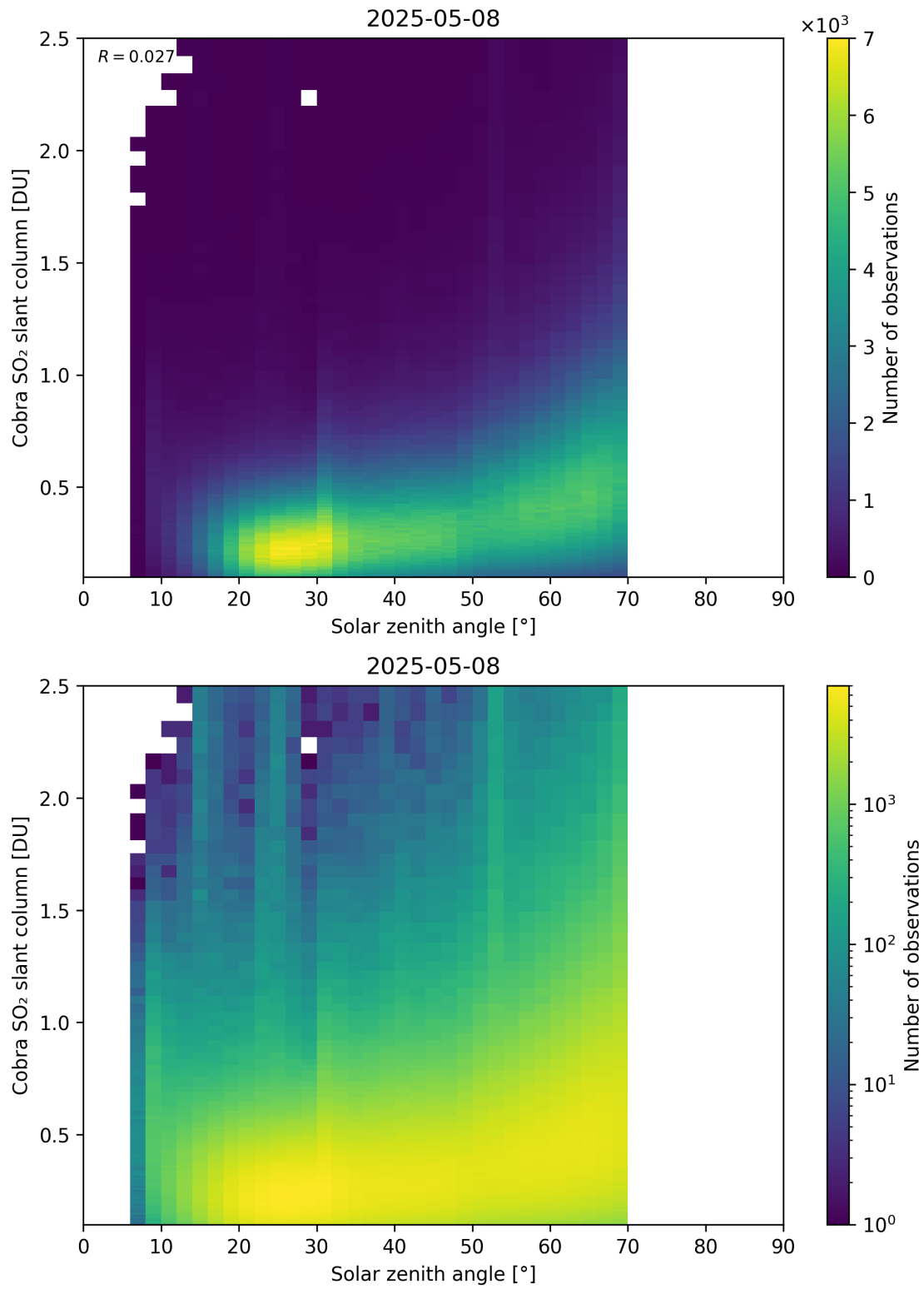
Figure 179: Scatter density plot of “Solar zenith angle” against “Cobra SO 2 slant column” for 2025-05-07 to 2025-05-09.
