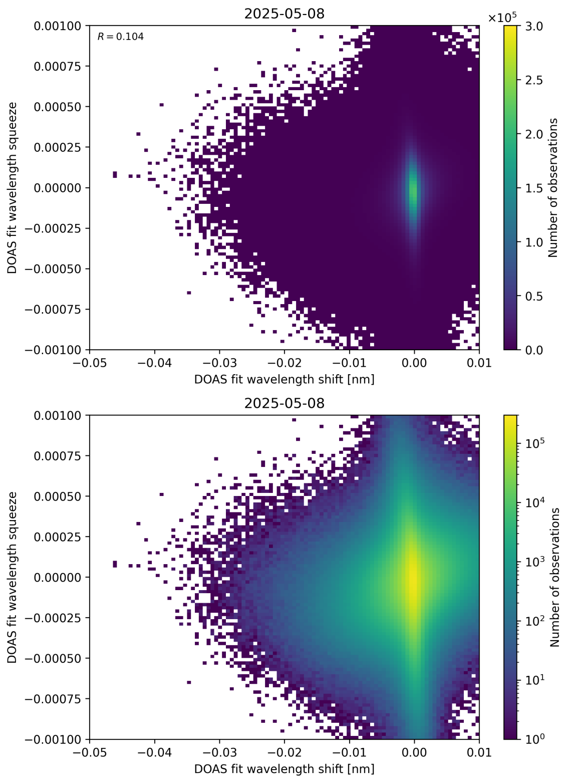
Figure 138: Scatter density plot of “DOAS fit wavelength shift” against “DOAS fit wavelength squeeze” for 2025-05-07 to 2025-05-09.
