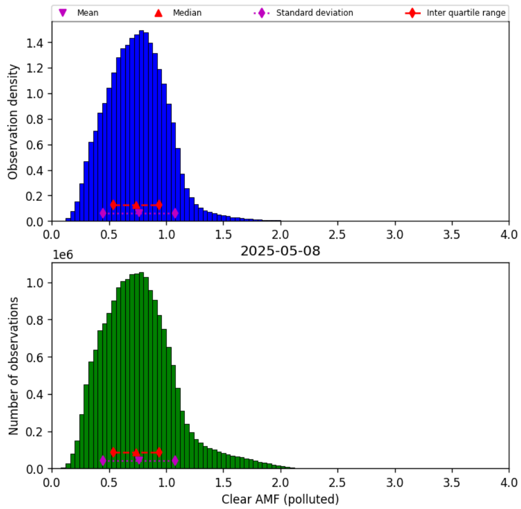
Figure 81: Histogram of “Clear AMF (polluted)” for 2025-05-07 to 2025-05-09
