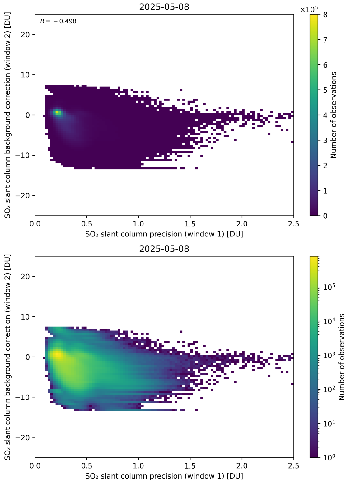
Figure 269: Scatter density plot of “SO 2 slant column precision (window 1)” against “SO 2 slant column background correction (window 2)” for 2025-05-07 to 2025-05-09.
