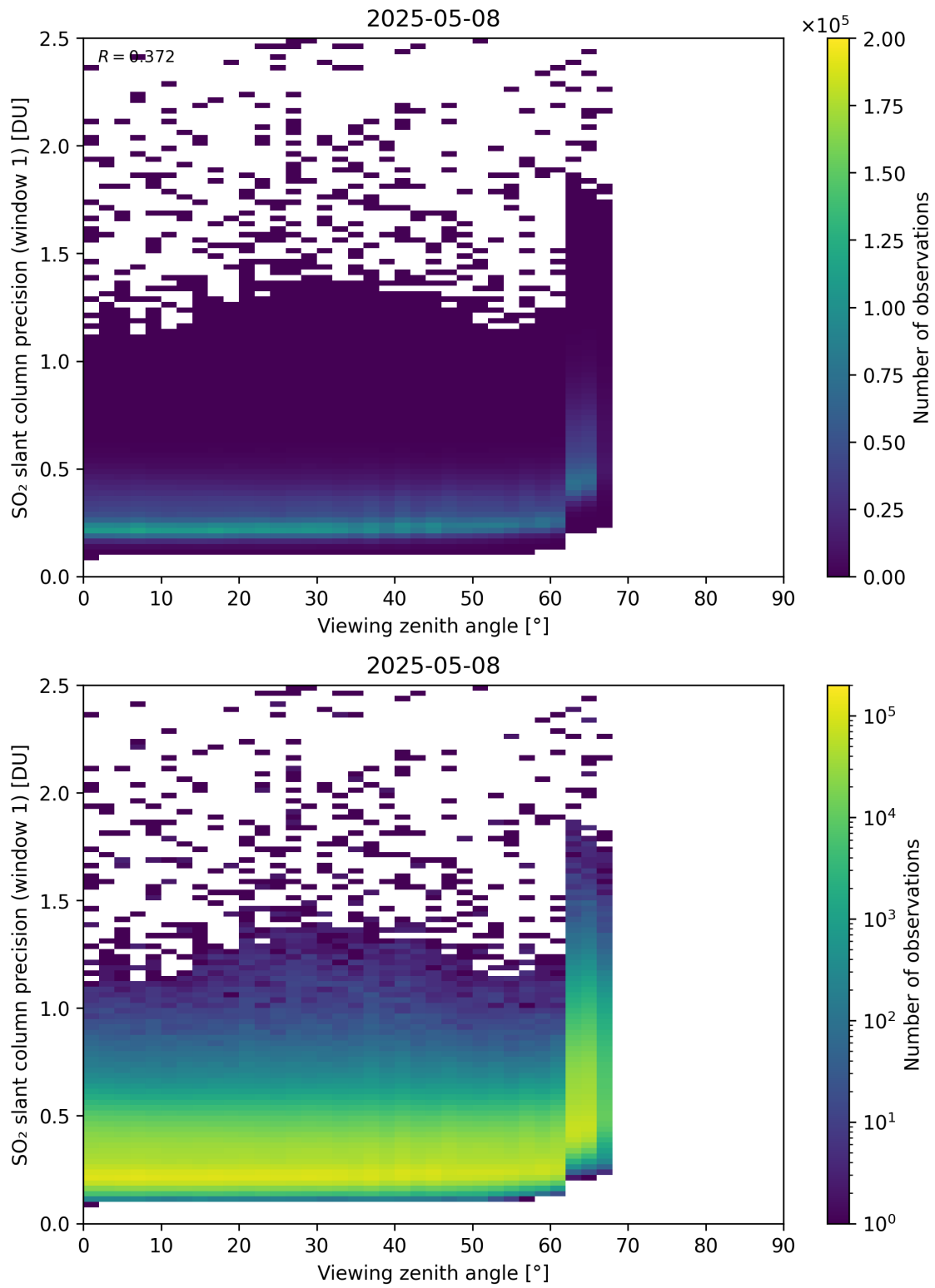
Figure 377: Scatter density plot of “Viewing zenith angle” against “SO 2 slant column precision (window 1)” for 2025-05-07 to 2025-05-09.
