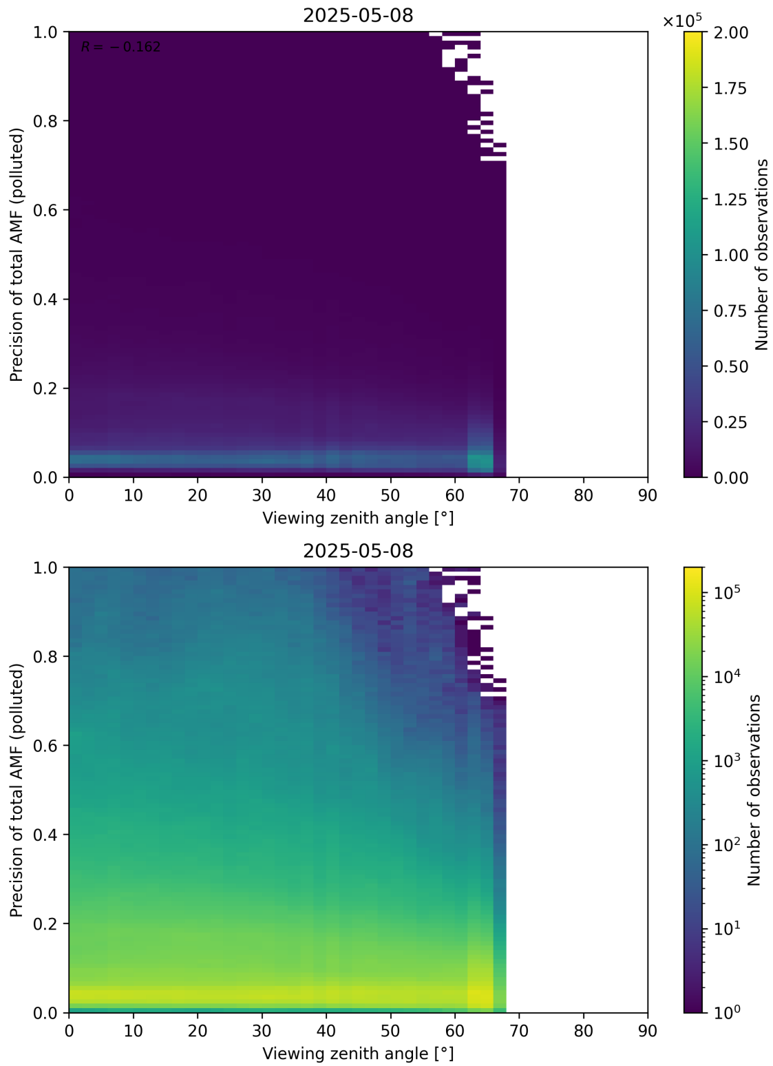
Figure 382: Scatter density plot of “Viewing zenith angle” against “Precision of total AMF (polluted)” for 2025-05-07 to 2025-05-09.
