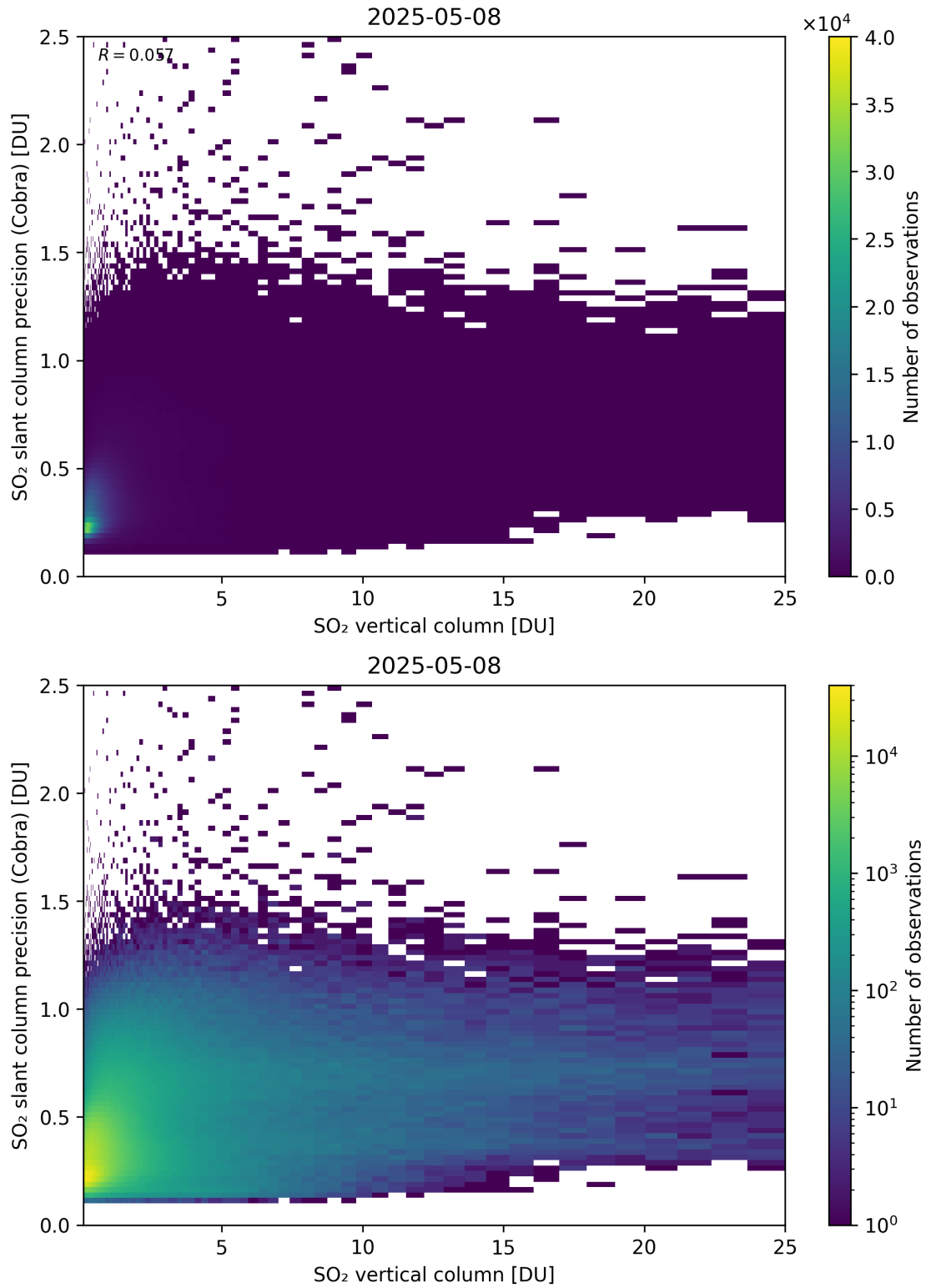
Figure 350: Scatter density plot of “SO 2 vertical column” against “SO 2 slant column precision (Cobra)” for 2025-05-07 to 2025-05-09.
