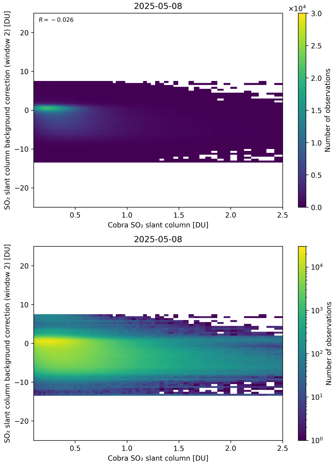
Figure 194: Scatter density plot of “Cobra SO 2 slant column” against “SO 2 slant column background correction (window 2)” for 2025-05-07 to 2025-05-09.
