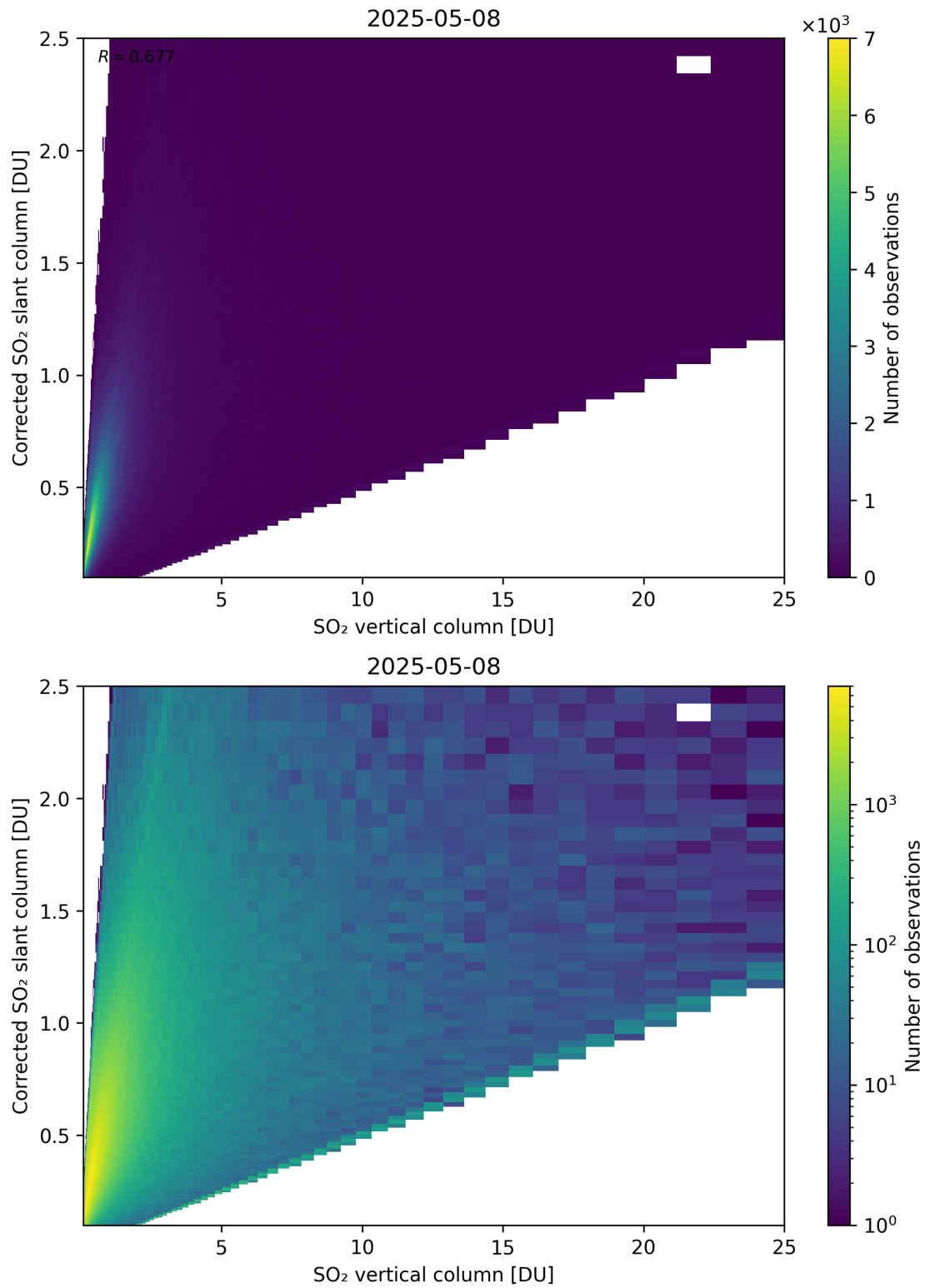
Figure 351: Scatter density plot of “SO 2 vertical column” against “Corrected SO 2 slant column” for 2025-05-07 to 2025-05-09.
