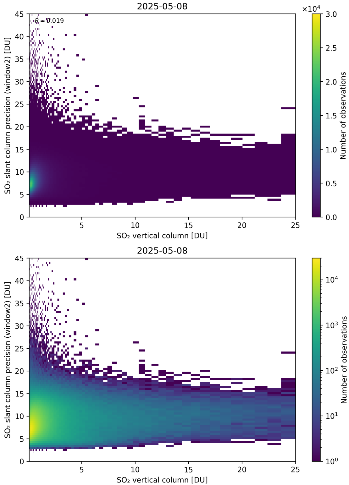
Figure 356: Scatter density plot of “SO 2 vertical column” against “SO 2 slant column precision (window2)” for 2025-05-07 to 2025-05-09.
