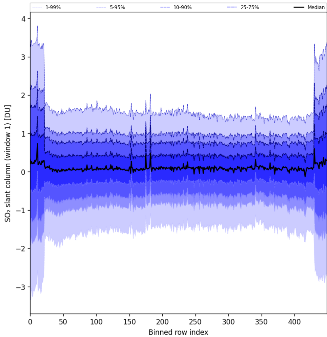
Figure 89: Along track statistics of “SO 2 slant column (window 1)” for 2025-05-07 to 2025-05-09
