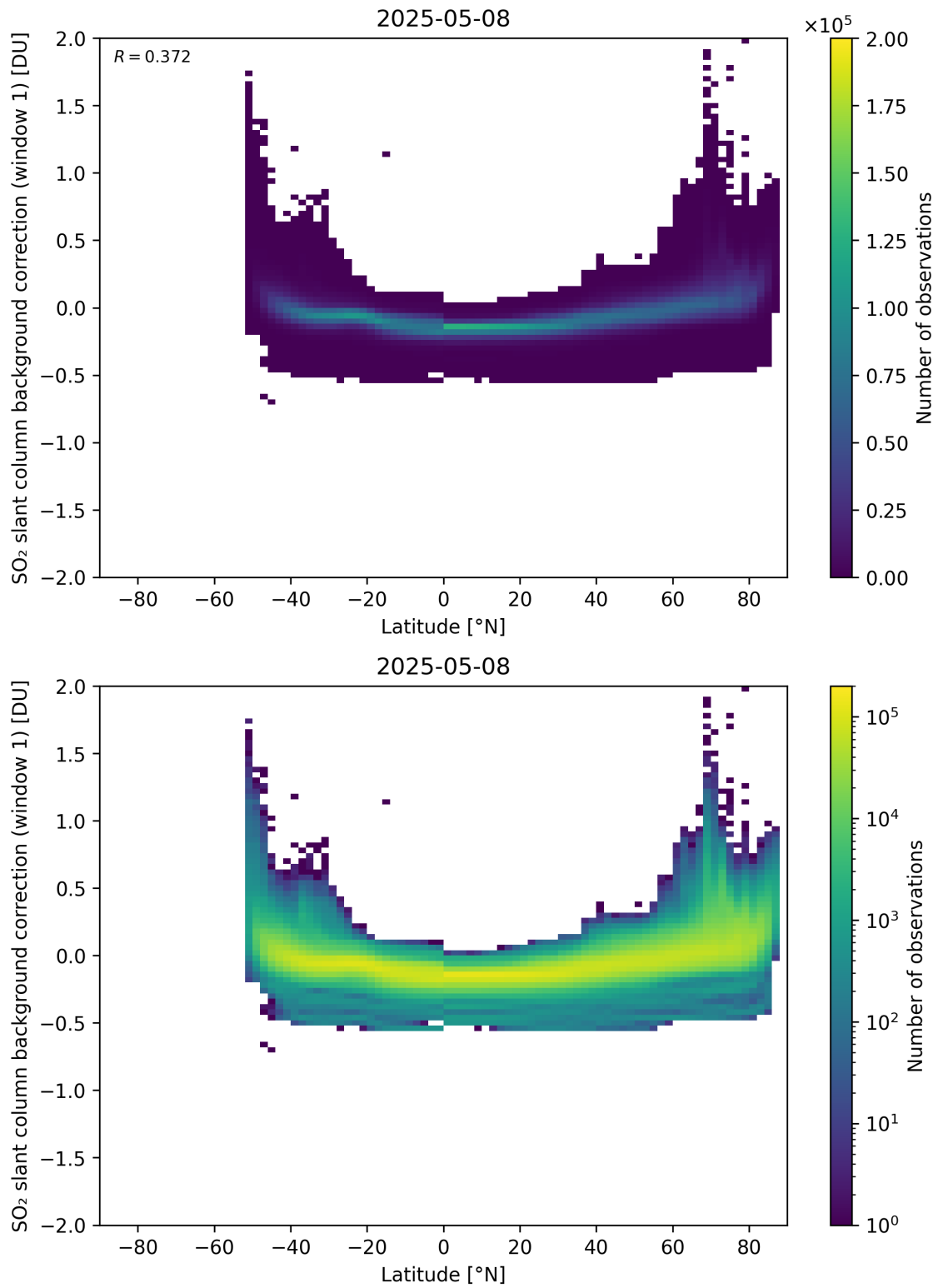
Figure 150: Scatter density plot of “Latitude” against “SO 2 slant column background correction (window 1)” for 2025-05-07 to 2025-05-09.
