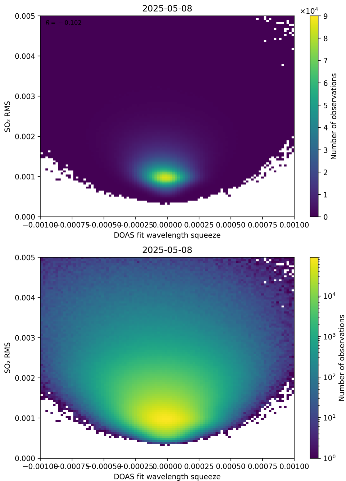
Figure 143: Scatter density plot of “DOAS fit wavelength squeeze” against “SO 2 RMS” for 2025-05-07 to 2025-05-09.
