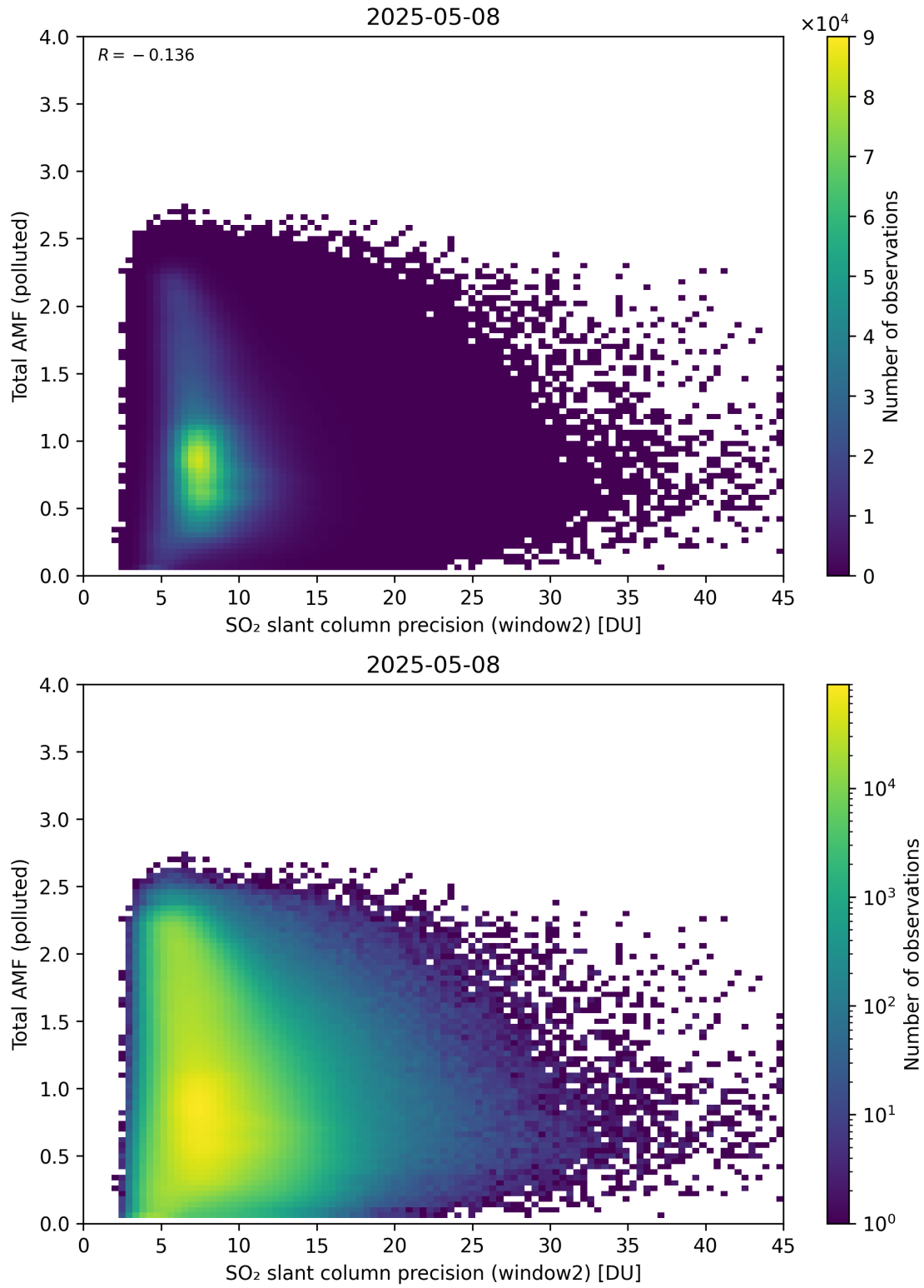
Figure 301: Scatter density plot of “SO 2 slant column precision (window2)” against “Total AMF (polluted)” for 2025-05-07 to 2025-05-09.
