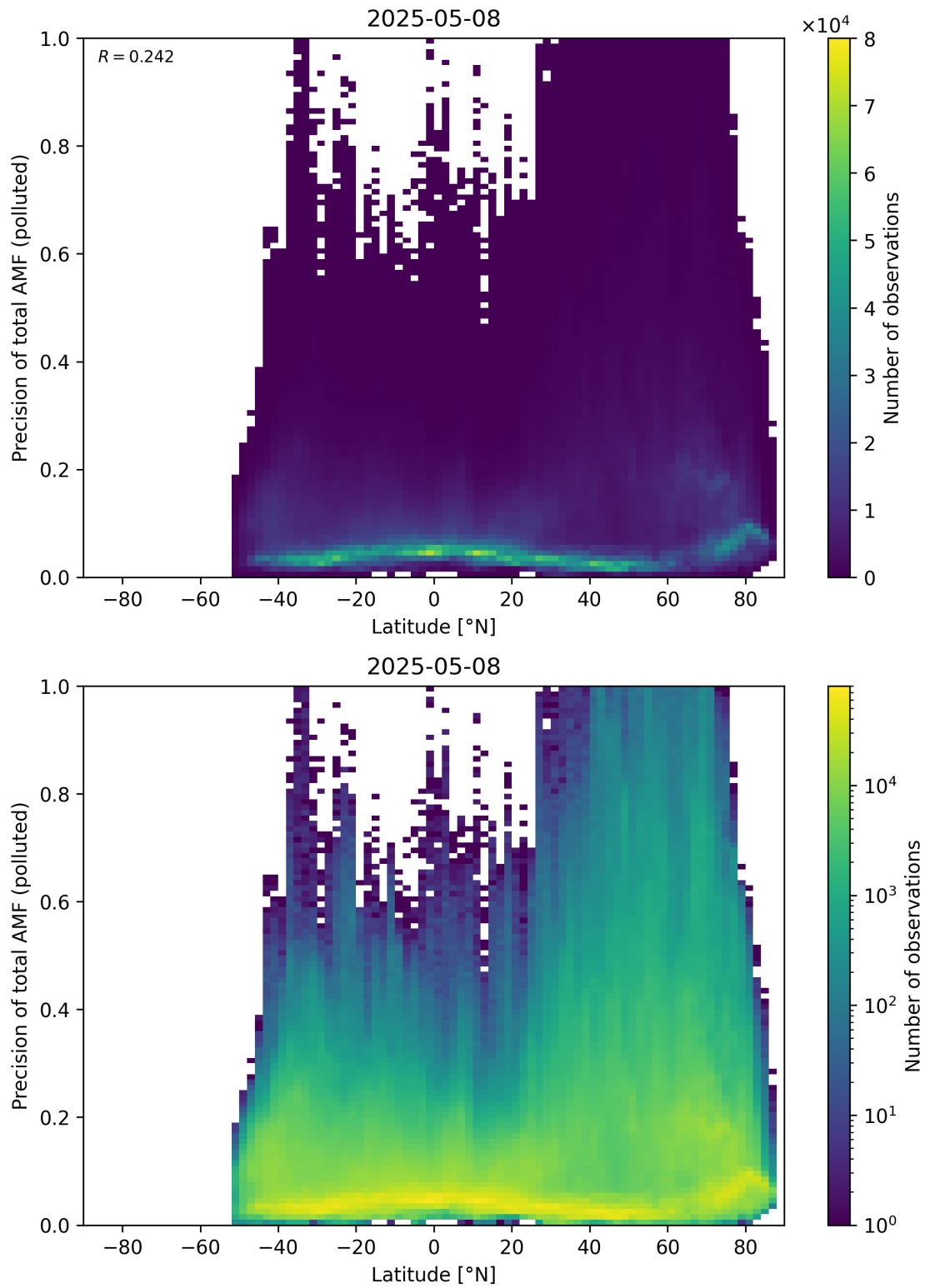
Figure 168: Scatter density plot of “Latitude” against “Precision of total AMF (polluted)” for 2025-05-07 to 2025-05-09.
