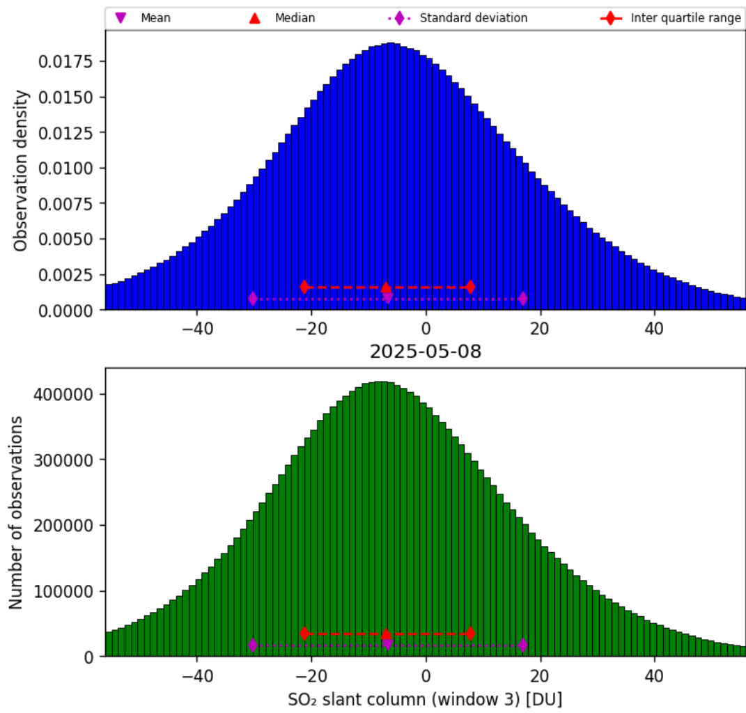
Figure 71: Histogram of “SO 2 slant column (window 3)” for 2025-05-07 to 2025-05-09
