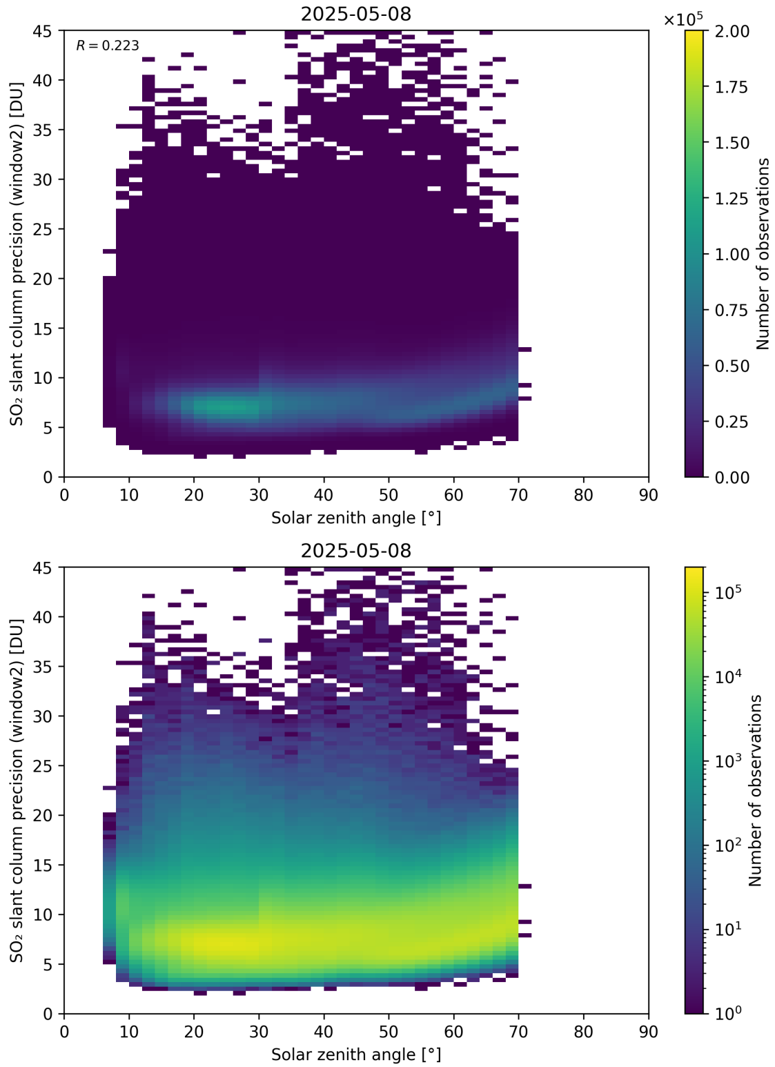
Figure 186: Scatter density plot of “Solar zenith angle” against “SO 2 slant column precision (window2)” for 2025-05-07 to 2025-05-09.
