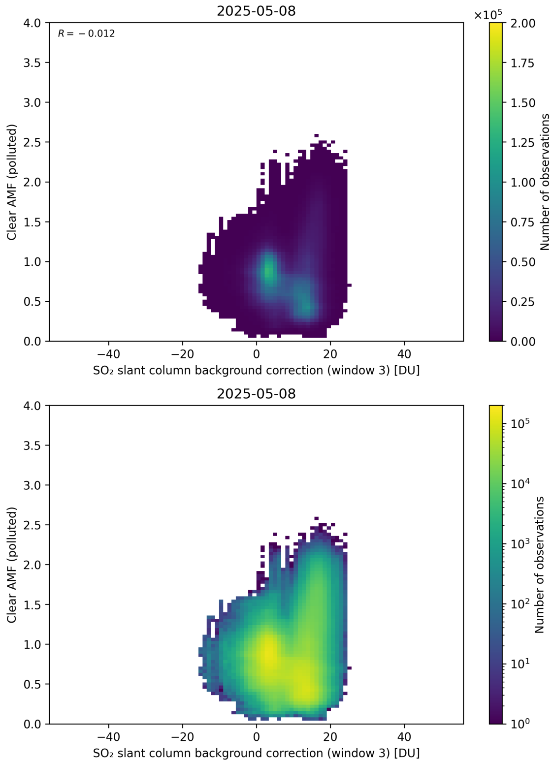
Figure 135: Scatter density plot of “SO 2 slant column background correction (window 3)” against “Clear AMF (polluted)” for 2025-05-07 to 2025-05-09.
