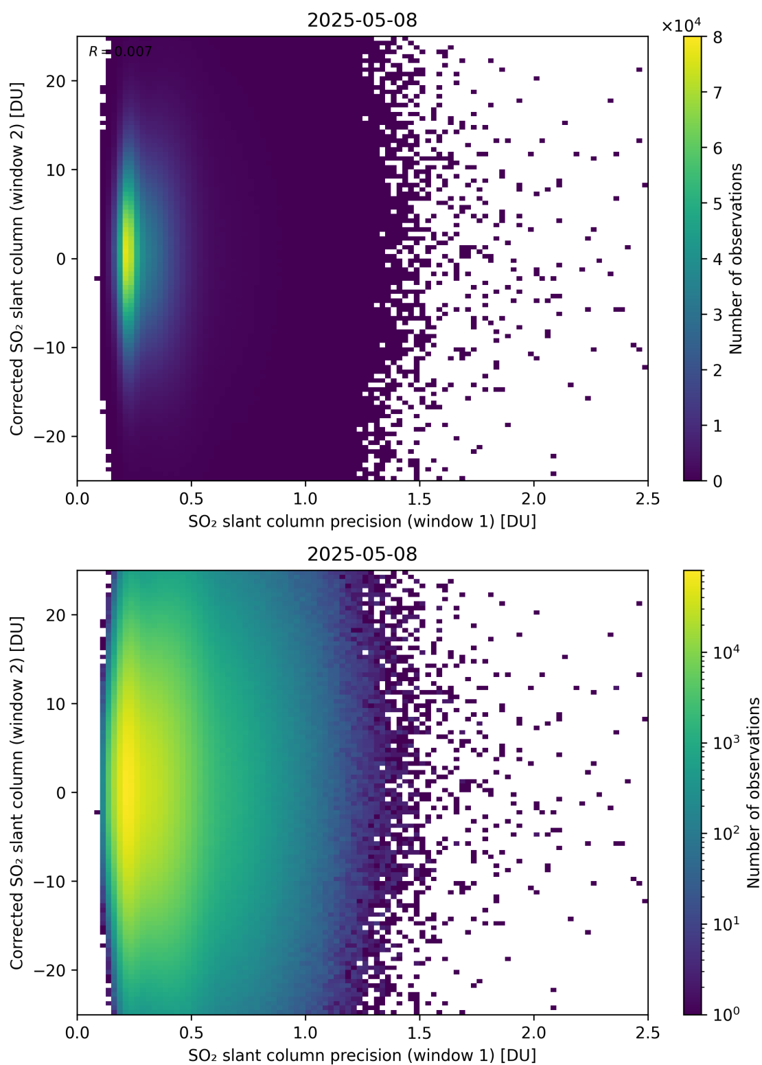
Figure 275: Scatter density plot of “SO 2 slant column precision (window 1)” against “Corrected SO 2 slant column (window 2)” for 2025-05-07 to 2025-05-09.
