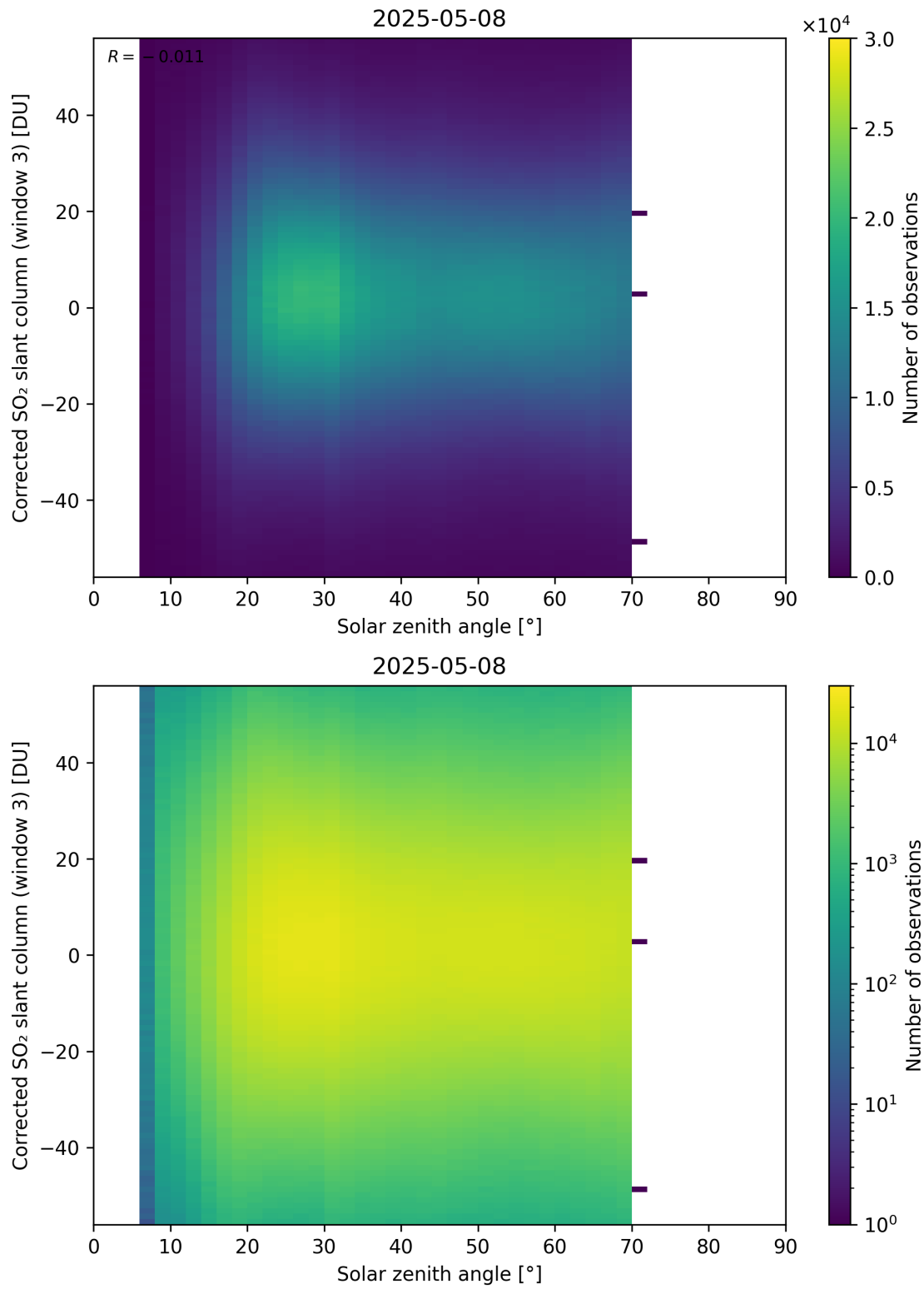
Figure 183: Scatter density plot of “Solar zenith angle” against “Corrected SO 2 slant column (window 3)” for 2025-05-07 to 2025-05-09.
