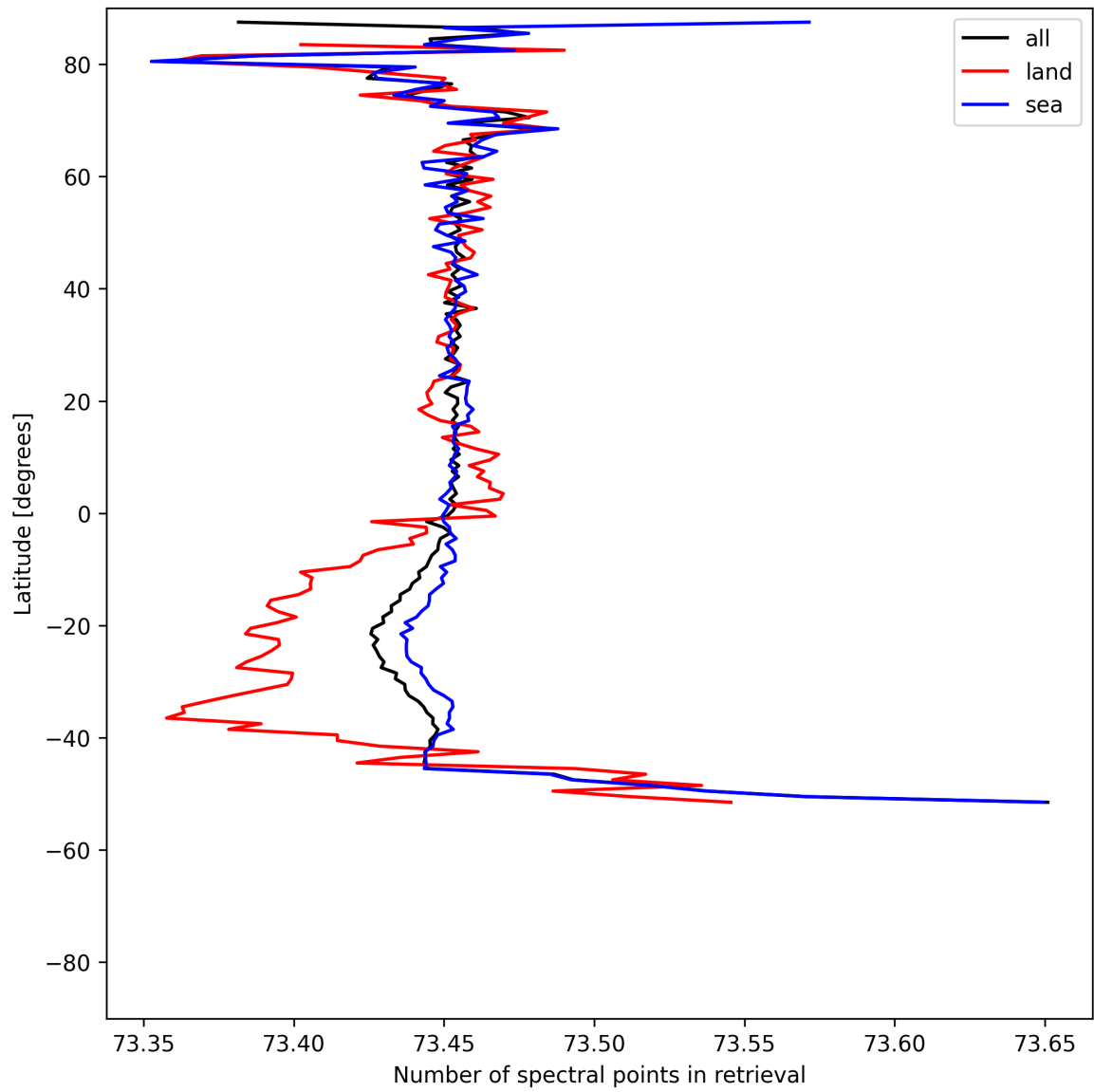
Figure 56: Zonal average of “Number of spectral points in retrieval” for 2025-05-07 to 2025-05-09.
