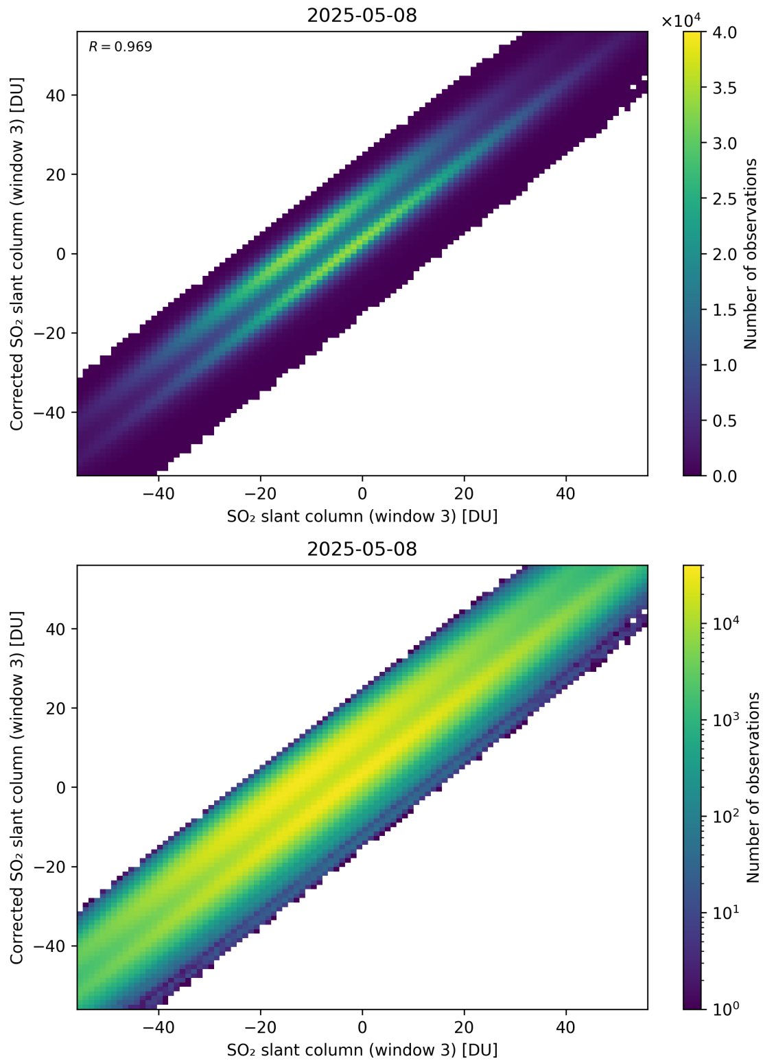
Figure 316: Scatter density plot of “SO 2 slant column (window 3)” against “Corrected SO 2 slant column (window 3)” for 2025-05-07 to 2025-05-09.
