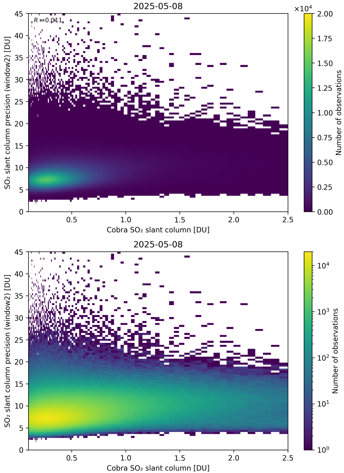
Figure 221: Scatter density plot of “Cobra SO 2 slant column” against “SO 2 slant column precision (window2)” for 2025-05-07 to 2025-05-09.
