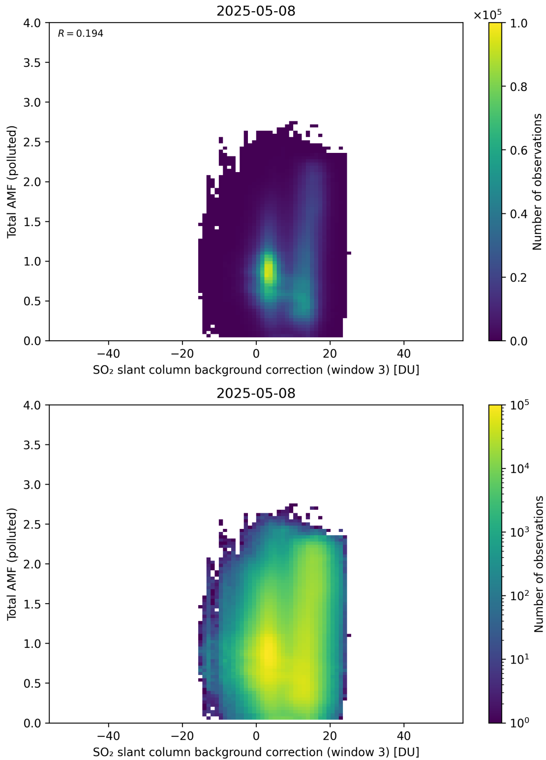
Figure 136: Scatter density plot of “SO 2 slant column background correction (window 3)” against “Total AMF (polluted)” for 2025-05-07 to 2025-05-09.
