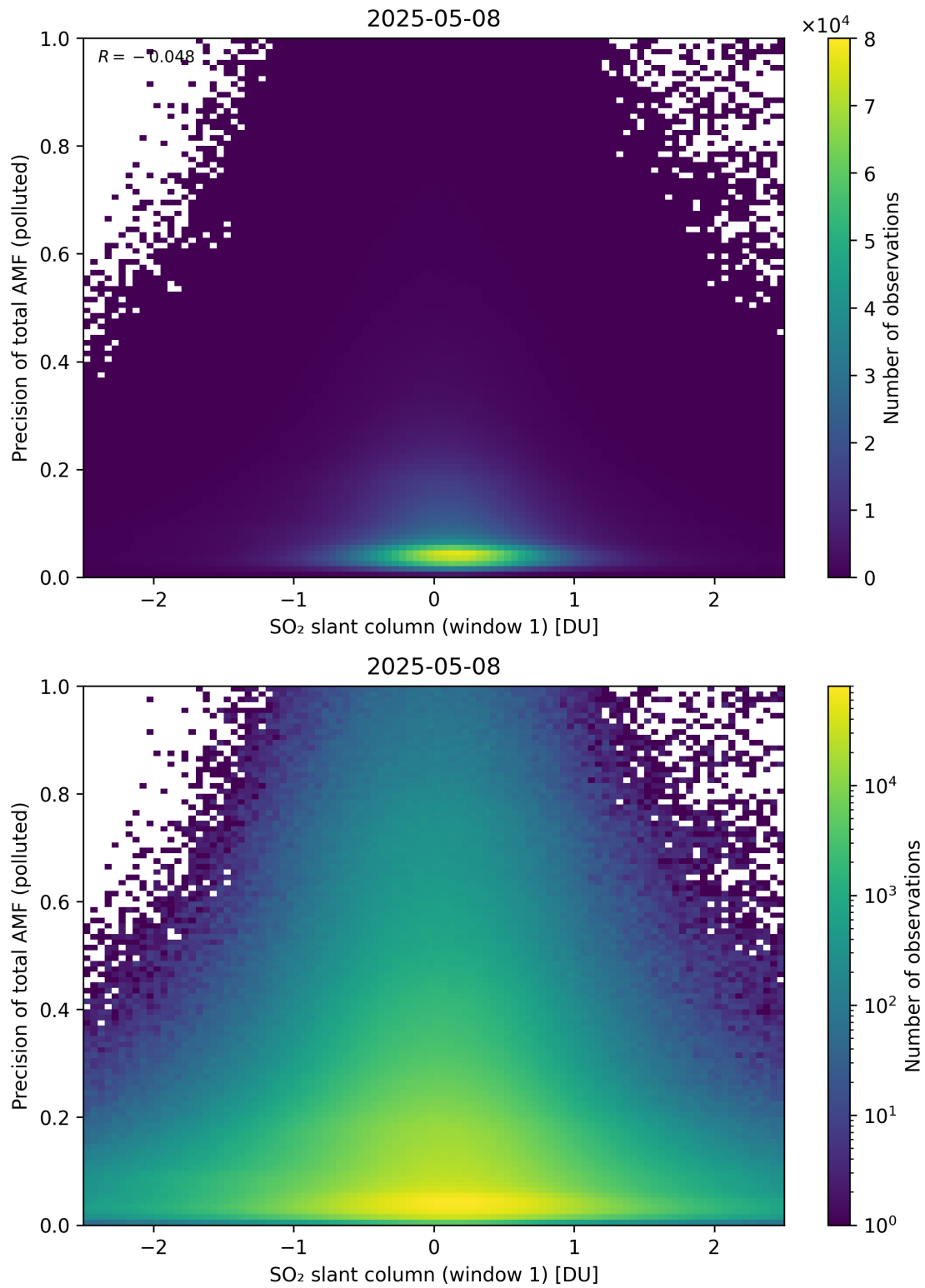
Figure 290: Scatter density plot of “SO 2 slant column (window 1)” against “Precision of total AMF (polluted)” for 2025-05-07 to 2025-05-09.
