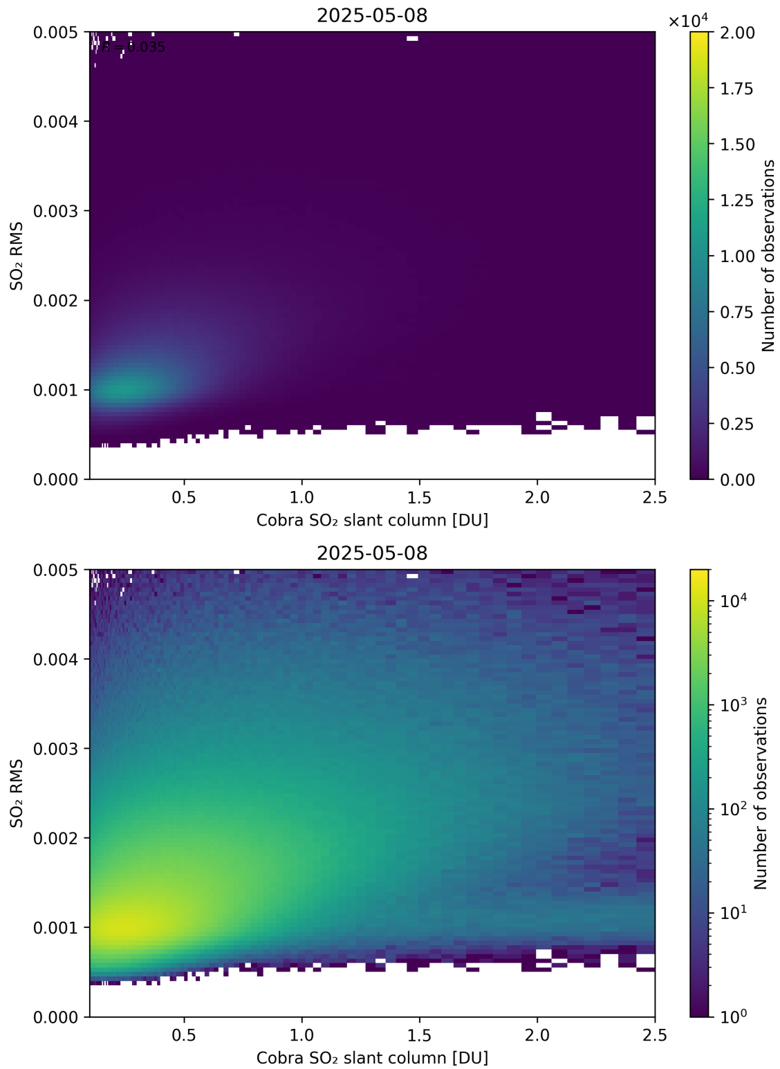
Figure 198: Scatter density plot of “Cobra SO 2 slant column” against “SO 2 RMS” for 2025-05-07 to 2025-05-09.
