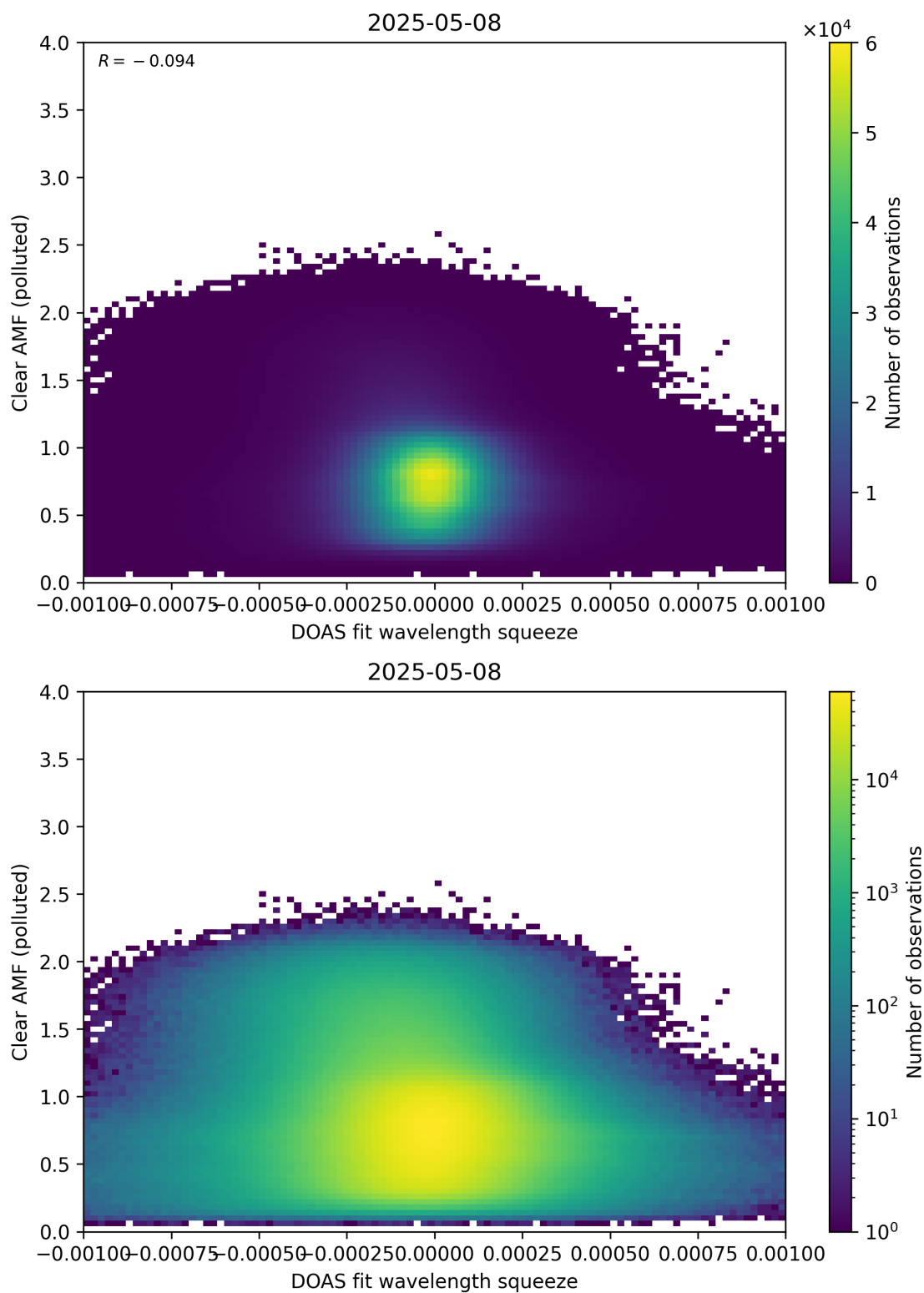
Figure 144: Scatter density plot of “DOAS fit wavelength squeeze” against “Clear AMF (polluted)” for 2025-05-07 to 2025-05-09.
