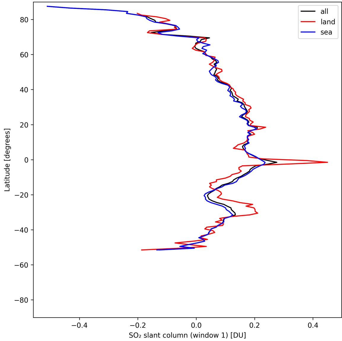
Figure 37: Zonal average of “SO 2 slant column (window 1)” for 2025-05-07 to 2025-05-09.
