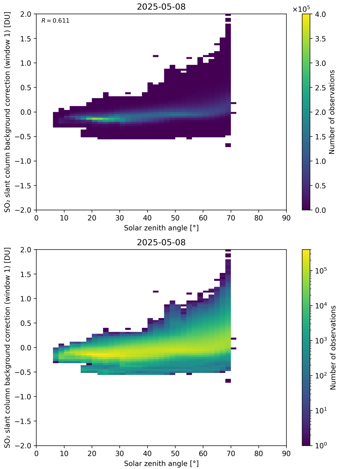
Figure 171: Scatter density plot of “Solar zenith angle” against “SO 2 slant column background correction (window 1)” for 2025-05-07 to 2025-05-09.
