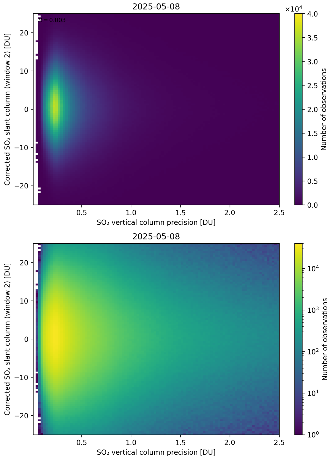
Figure 339: Scatter density plot of “SO 2 vertical column precision” against “Corrected SO 2 slant column (window 2)” for 2025-05-07 to 2025-05-09.
