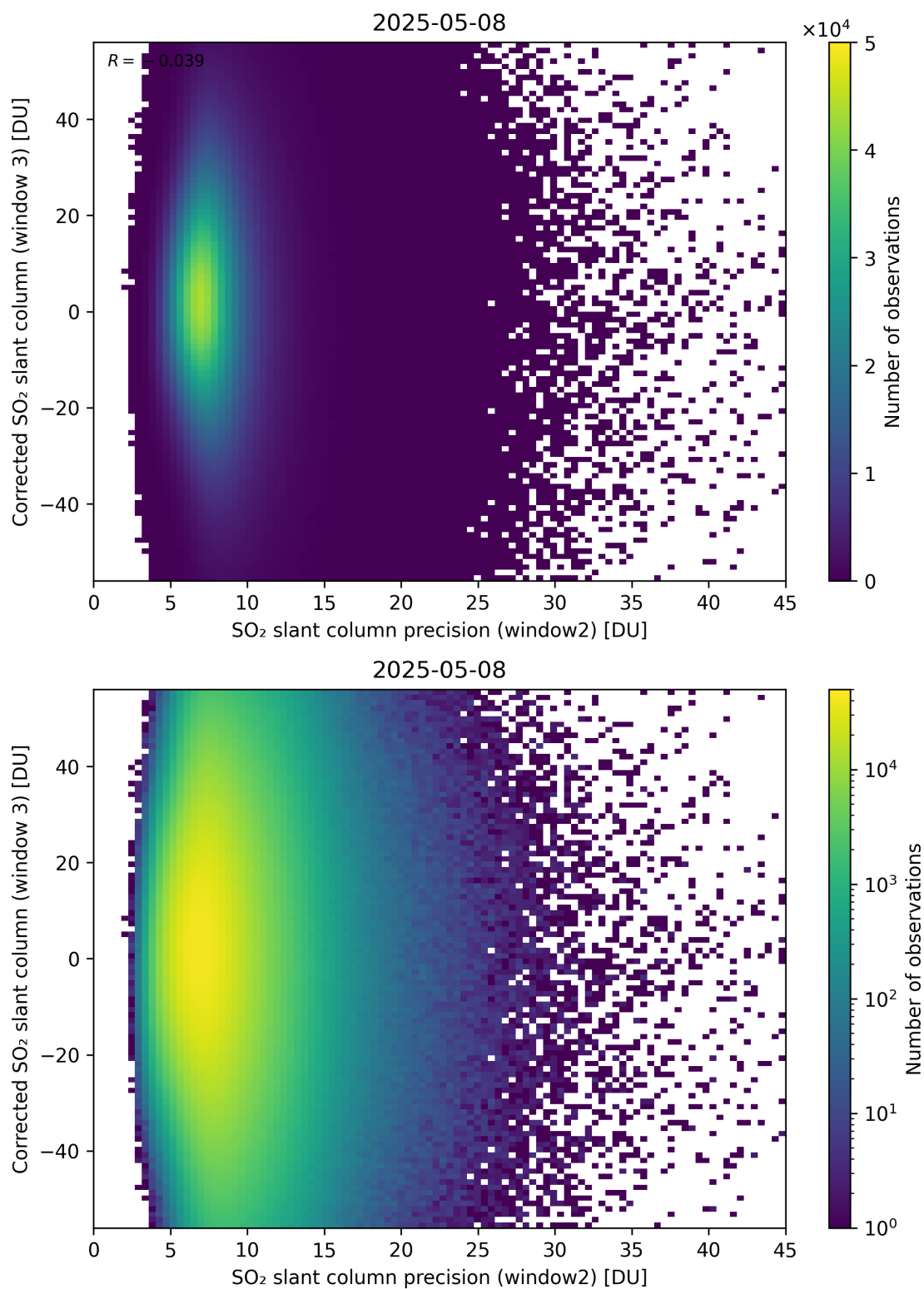
Figure 298: Scatter density plot of “SO 2 slant column precision (window2)” against “Corrected SO 2 slant column (window 3)” for 2025-05-07 to 2025-05-09.
