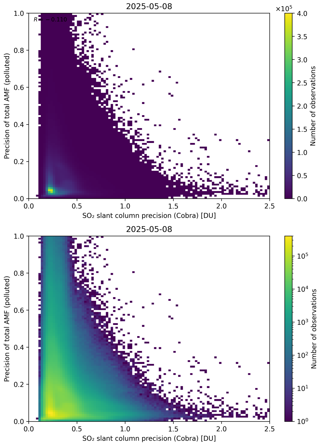
Figure 214: Scatter density plot of “SO 2 slant column precision (Cobra)” against “Precision of total AMF (polluted)” for 2025-05-07 to 2025-05-09.
