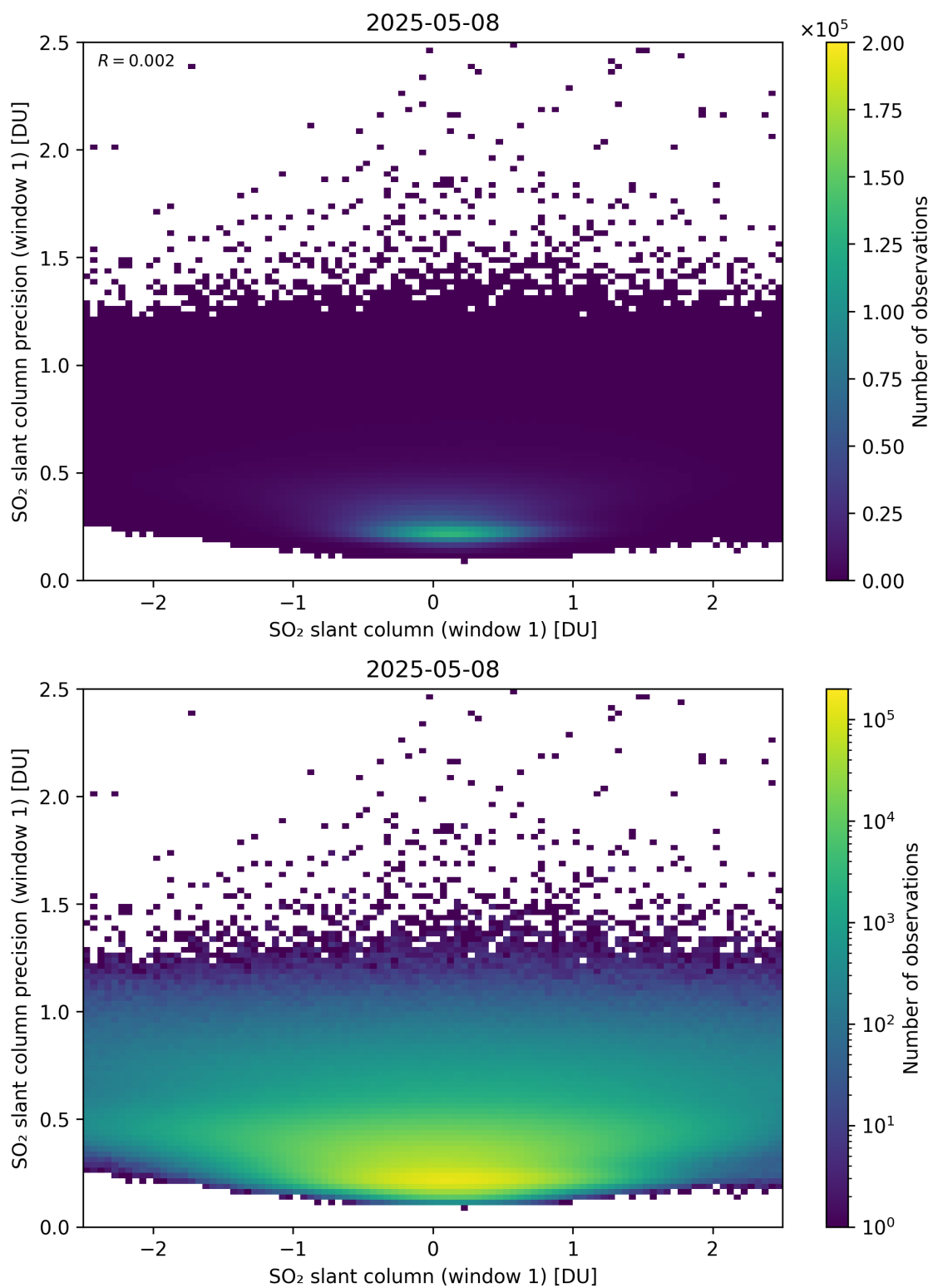
Figure 285: Scatter density plot of “SO 2 slant column (window 1)” against “SO 2 slant column precision (window 1)” for 2025-05-07 to 2025-05-09.
