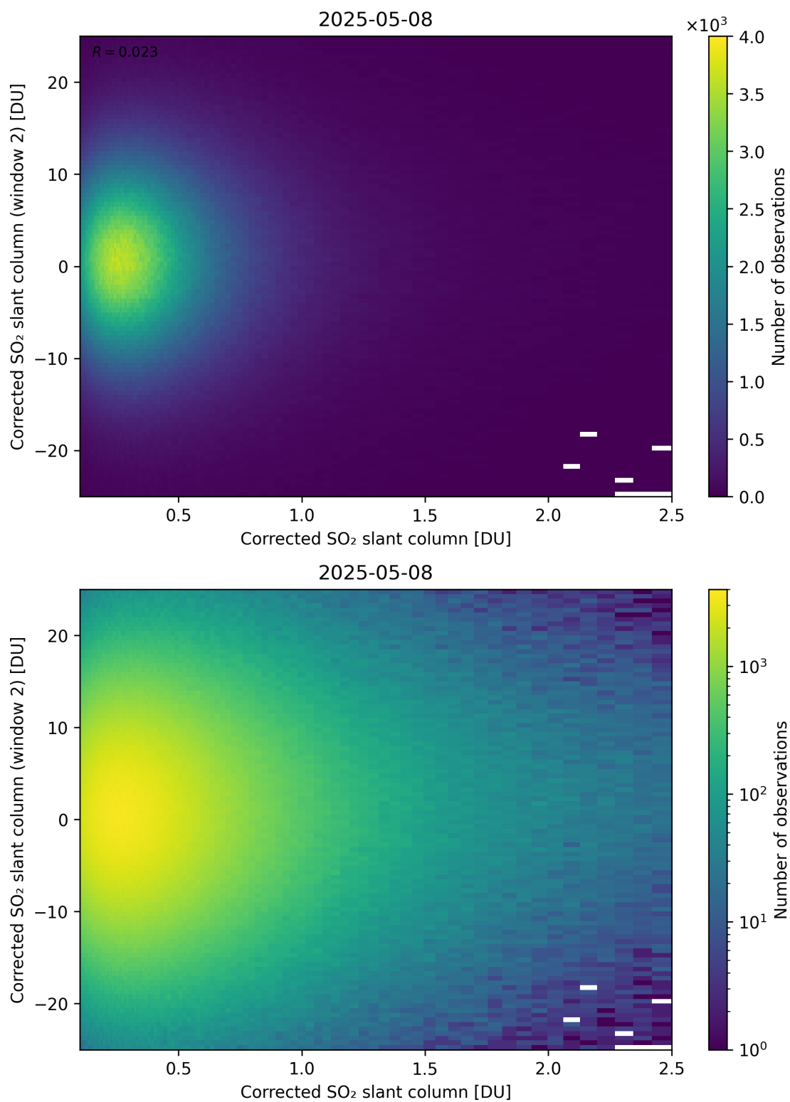
Figure 235: Scatter density plot of “Corrected SO 2 slant column” against “Corrected SO 2 slant column (window 2)” for 2025-05-07 to 2025-05-09.
