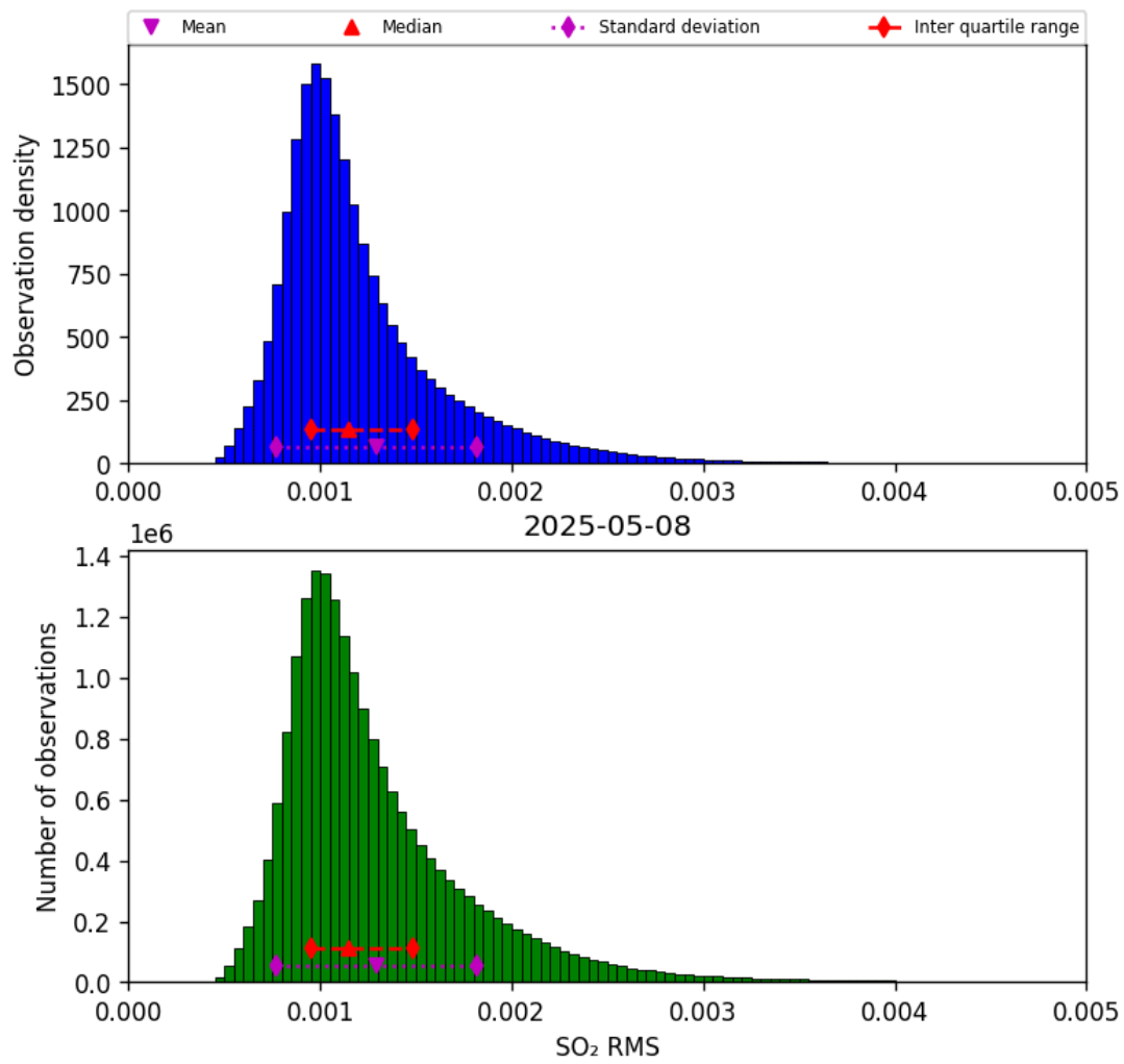
Figure 78: Histogram of “SO 2 RMS” for 2025-05-07 to 2025-05-09
