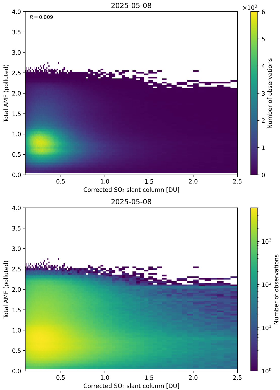
Figure 242: Scatter density plot of “Corrected SO 2 slant column” against “Total AMF (polluted)” for 2025-05-07 to 2025-05-09.
