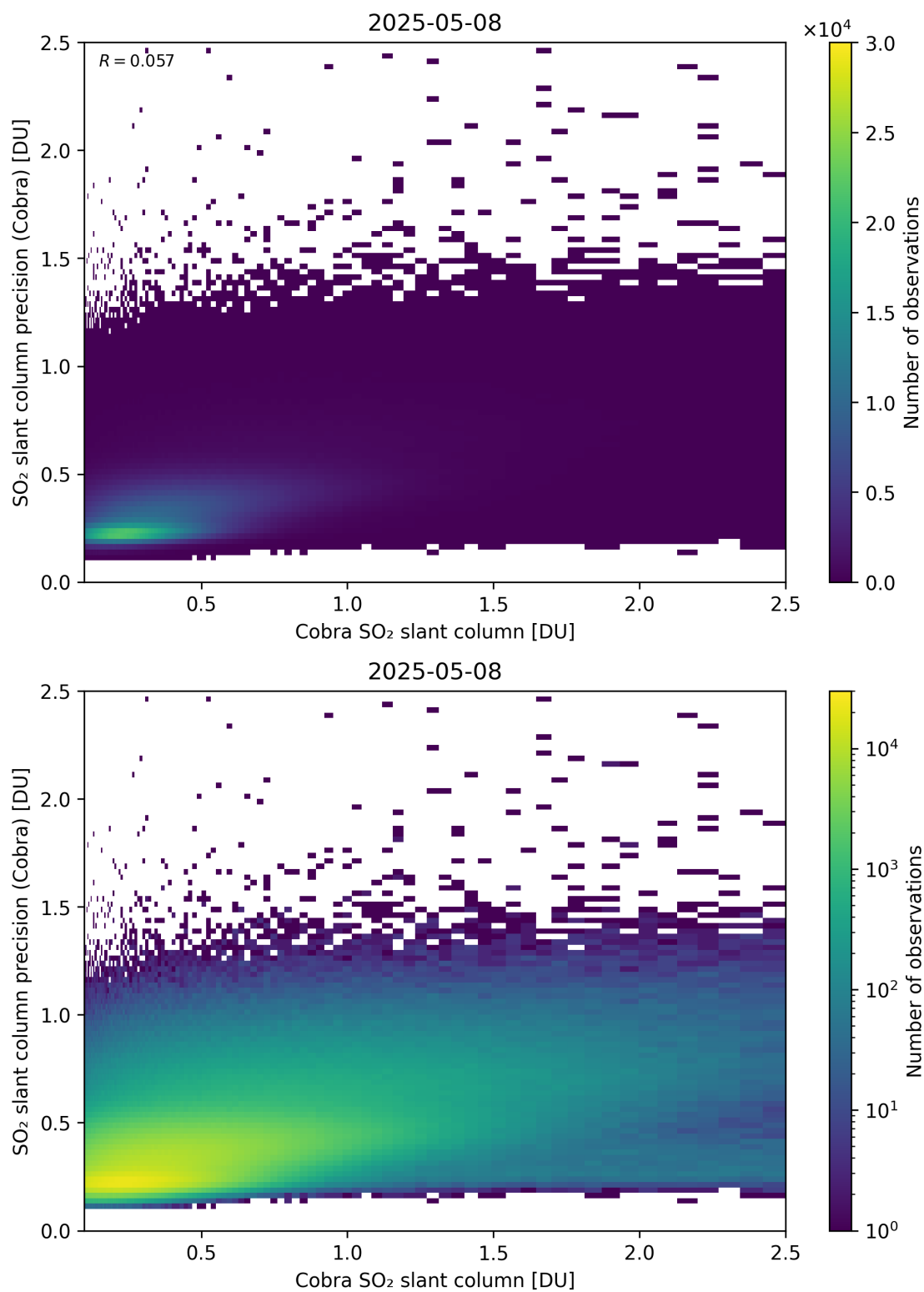
Figure 216: Scatter density plot of “Cobra SO 2 slant column” against “SO 2 slant column precision (Cobra)” for 2025-05-07 to 2025-05-09.
