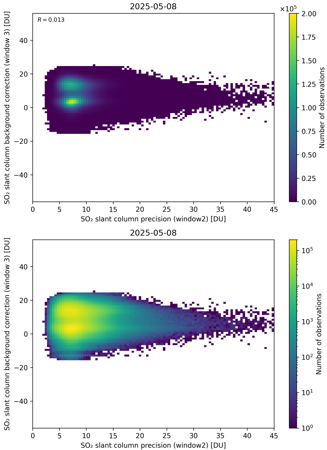
Figure 292: Scatter density plot of “SO 2 slant column precision (window2)” against “SO 2 slant column background correction (window 3)” for 2025-05-07 to 2025-05-09.
