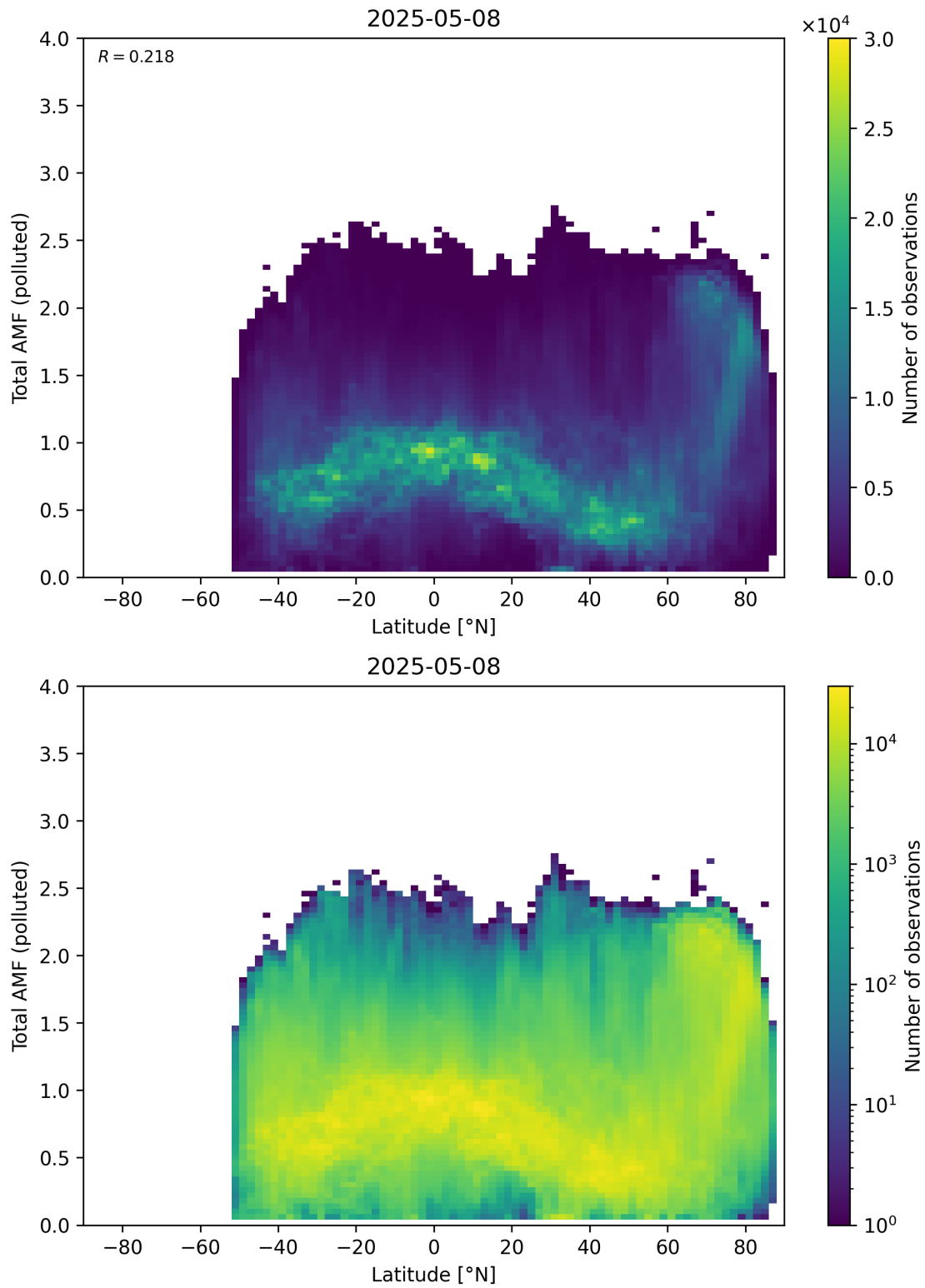
Figure 167: Scatter density plot of “Latitude” against “Total AMF (polluted)” for 2025-05-07 to 2025-05-09.
