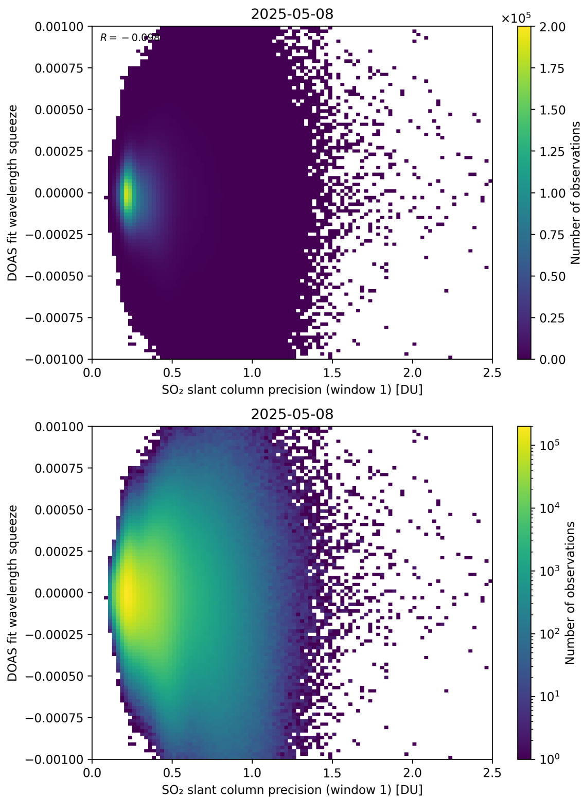
Figure 272: Scatter density plot of “SO 2 slant column precision (window 1)” against “DOAS fit wavelength squeeze” for 2025-05-07 to 2025-05-09.
