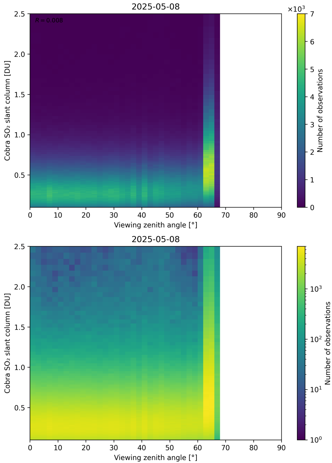
Figure 371: Scatter density plot of “Viewing zenith angle” against “Cobra SO 2 slant column” for 2025-05-07 to 2025-05-09.
