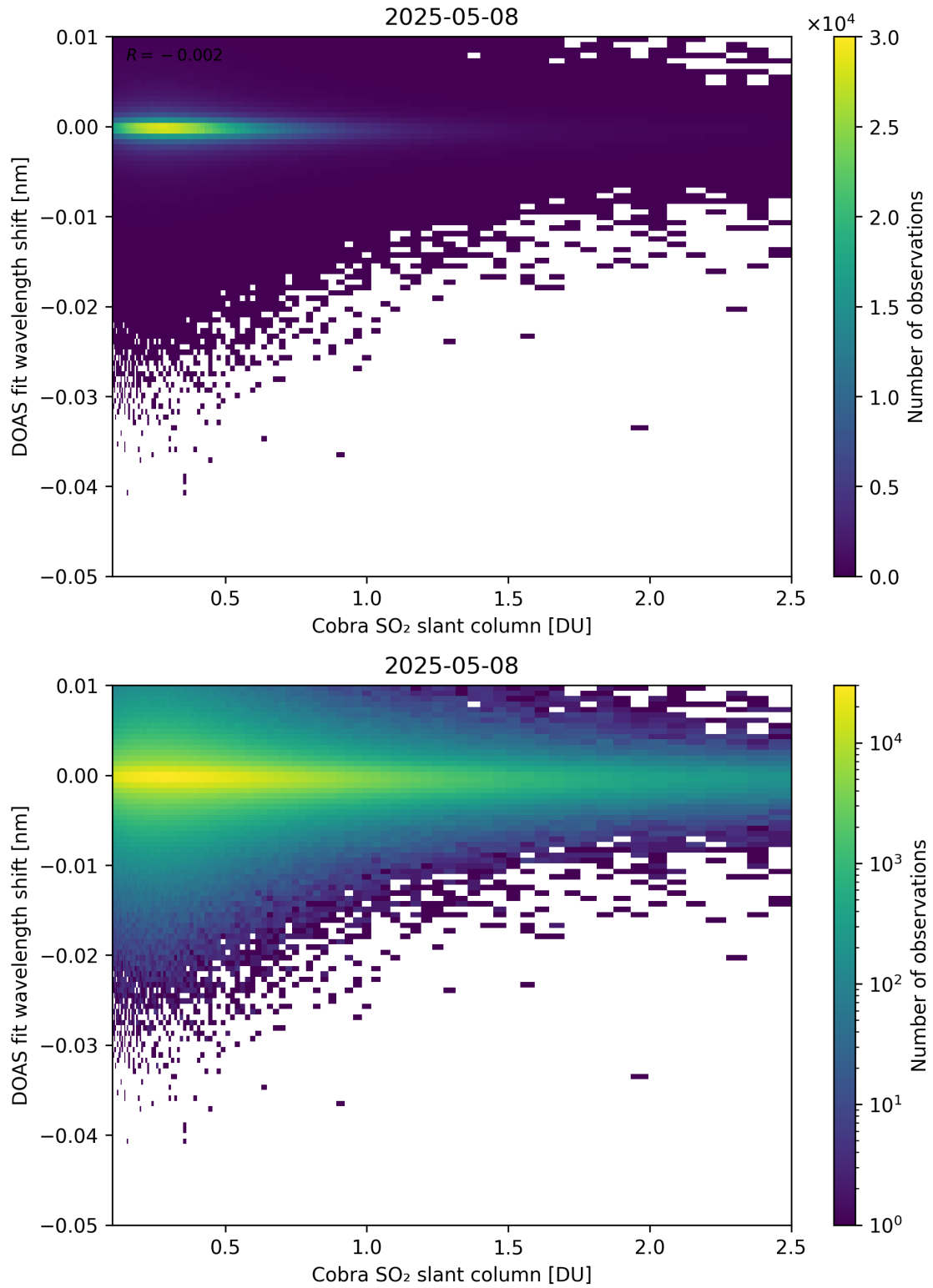
Figure 196: Scatter density plot of “Cobra SO 2 slant column” against “DOAS fit wavelength shift” for 2025-05-07 to 2025-05-09.
