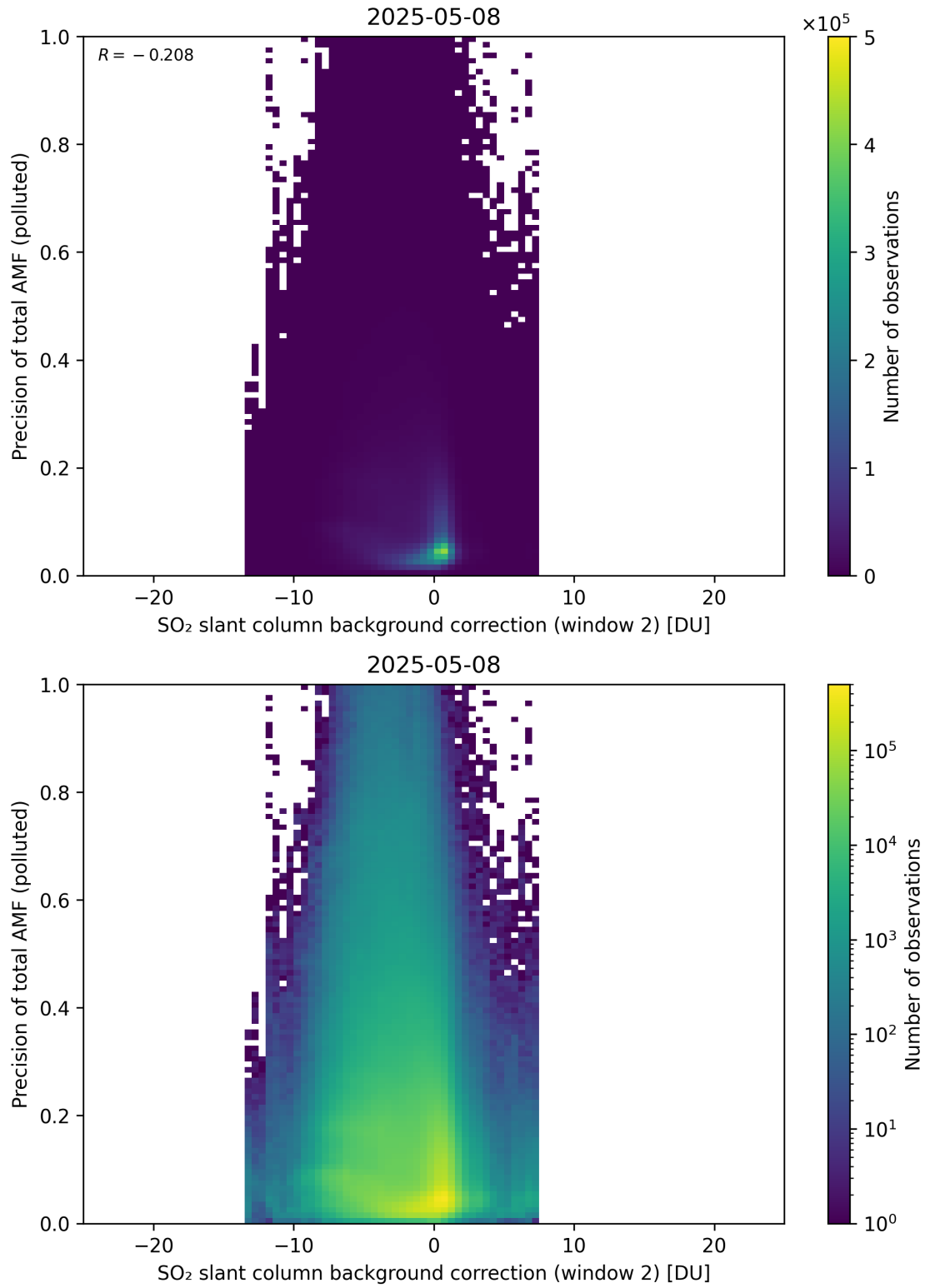
Figure 131: Scatter density plot of “SO 2 slant column background correction (window 2)” against “Precision of total AMF (polluted)” for 2025-05-07 to 2025-05-09.
