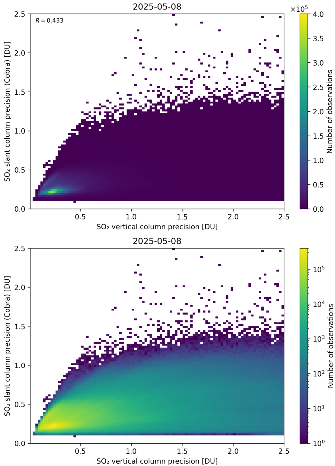
Figure 337: Scatter density plot of “SO 2 vertical column precision” against “SO 2 slant column precision (Cobra)” for 2025-05-07 to 2025-05-09.
