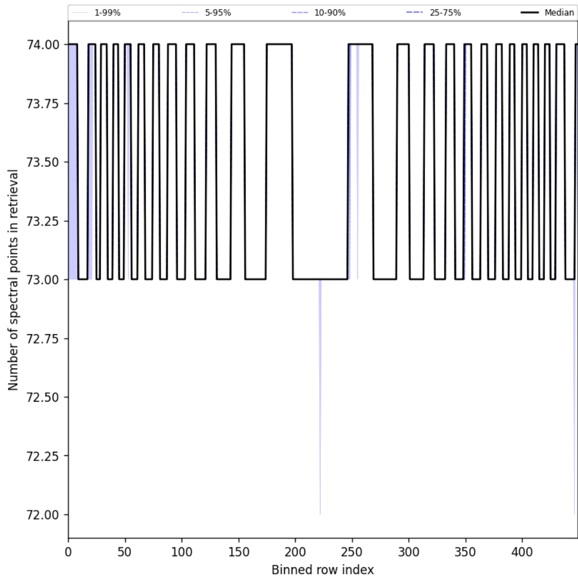
Figure 108: Along track statistics of “Number of spectral points in retrieval” for 2025-05-07 to 2025-05-09
