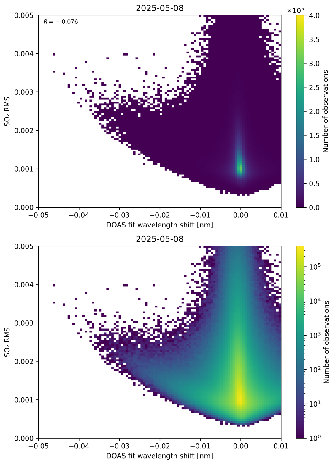
Figure 139: Scatter density plot of “DOAS fit wavelength shift” against “SO 2 RMS” for 2025-05-07 to 2025-05-09.
