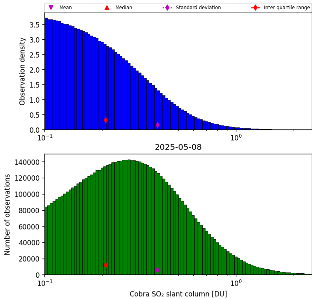
Figure 61: Histogram of “Cobra SO 2 slant column” for 2025-05-07 to 2025-05-09
