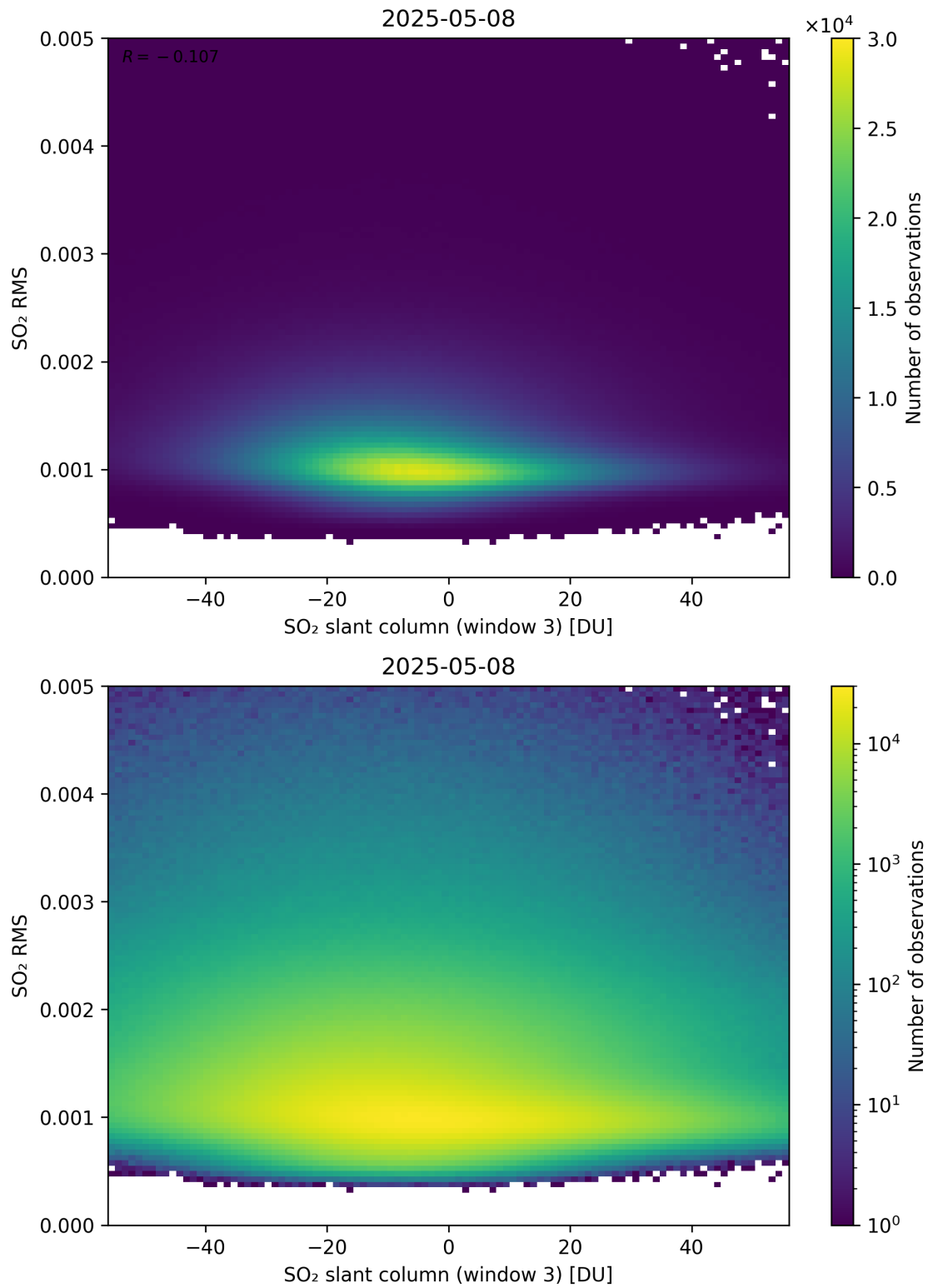
Figure 306: Scatter density plot of “SO 2 slant column (window 3)” against “SO 2 RMS” for 2025-05-07 to 2025-05-09.
