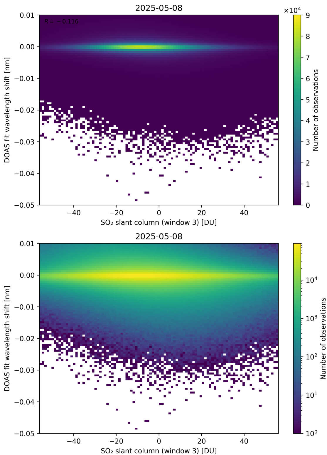
Figure 304: Scatter density plot of “SO 2 slant column (window 3)” against “DOAS fit wavelength shift” for 2025-05-07 to 2025-05-09.
