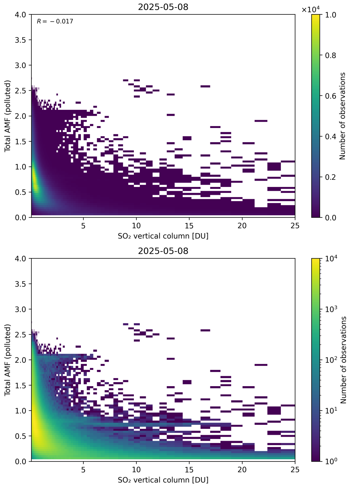
Figure 359: Scatter density plot of “SO 2 vertical column” against “Total AMF (polluted)” for 2025-05-07 to 2025-05-09.
