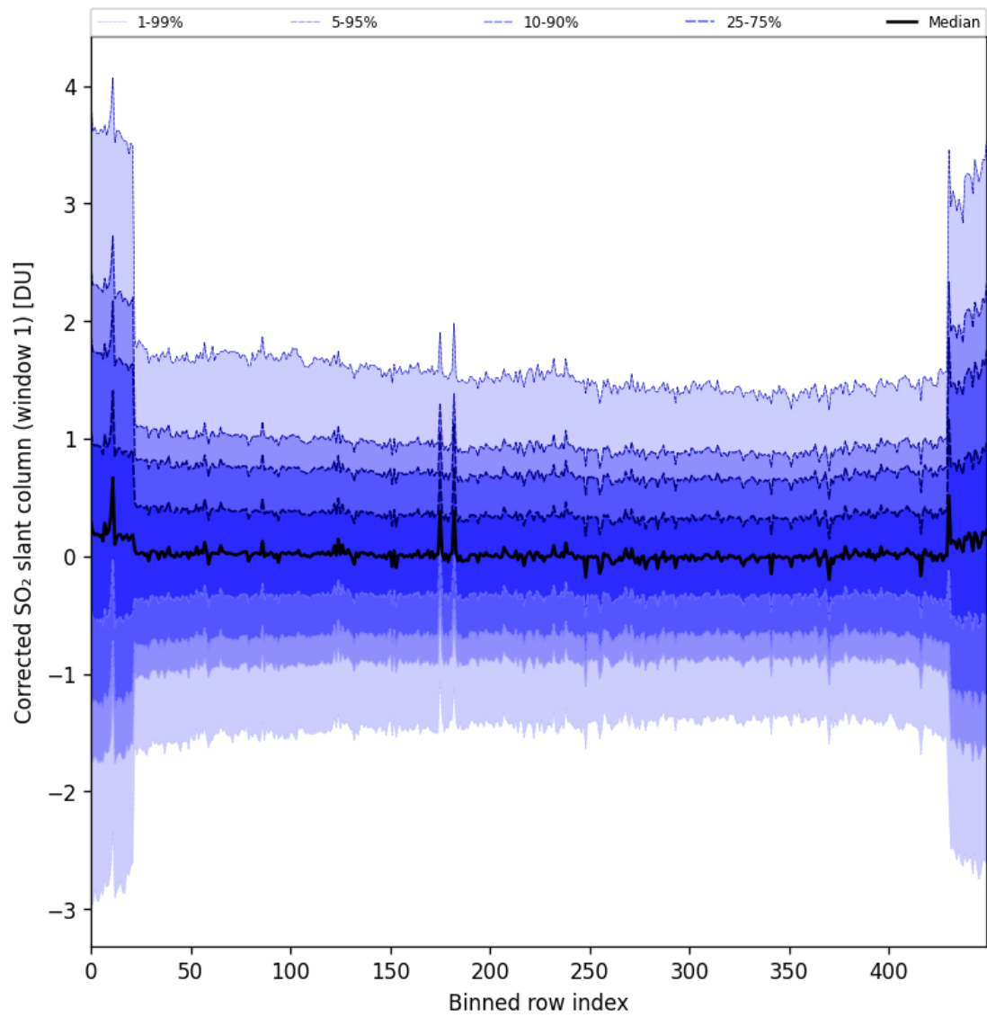
Figure 91: Along track statistics of “Corrected SO 2 slant column (window 1)” for 2025-05-07 to 2025-05-09
