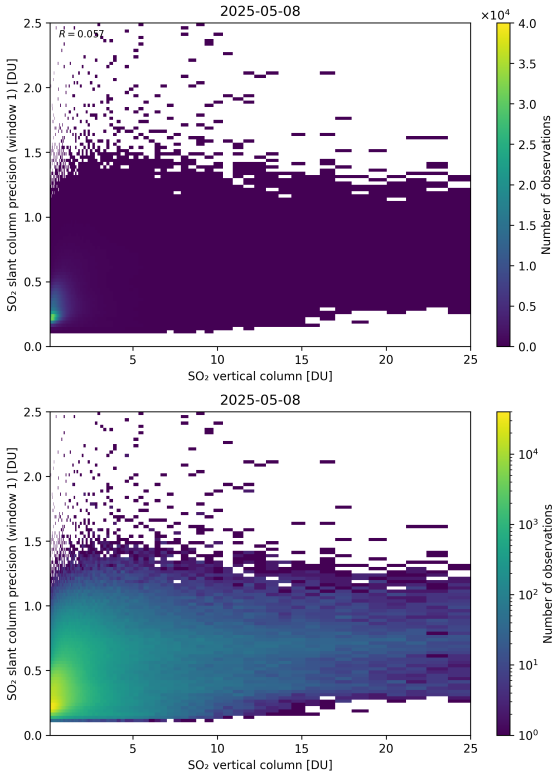
Figure 355: Scatter density plot of “SO 2 vertical column” against “SO 2 slant column precision (window 1)” for 2025-05-07 to 2025-05-09.
