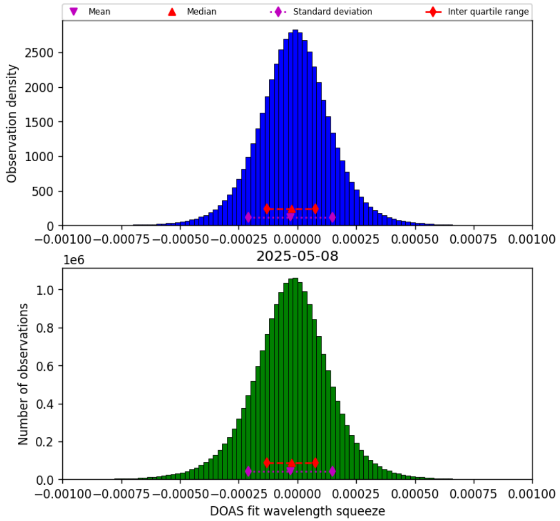
Figure 77: Histogram of “DOAS fit wavelength squeeze” for 2025-05-07 to 2025-05-09
