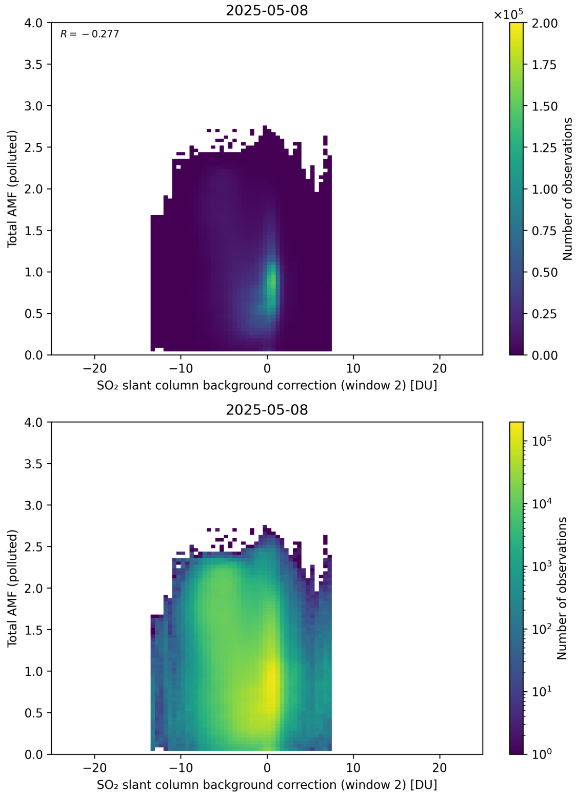
Figure 130: Scatter density plot of “SO 2 slant column background correction (window 2)” against “Total AMF (polluted)” for 2025-05-07 to 2025-05-09.
