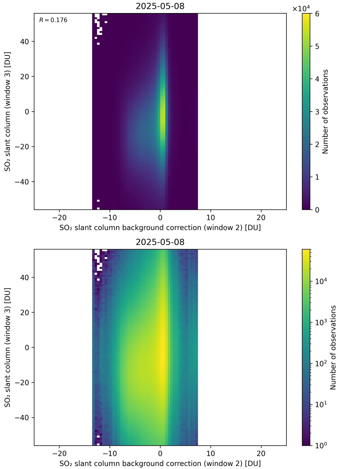
Figure 128: Scatter density plot of “SO 2 slant column background correction (window 2)” against “SO 2 slant column (window 3)” for 2025-05-07 to 2025-05-09.
