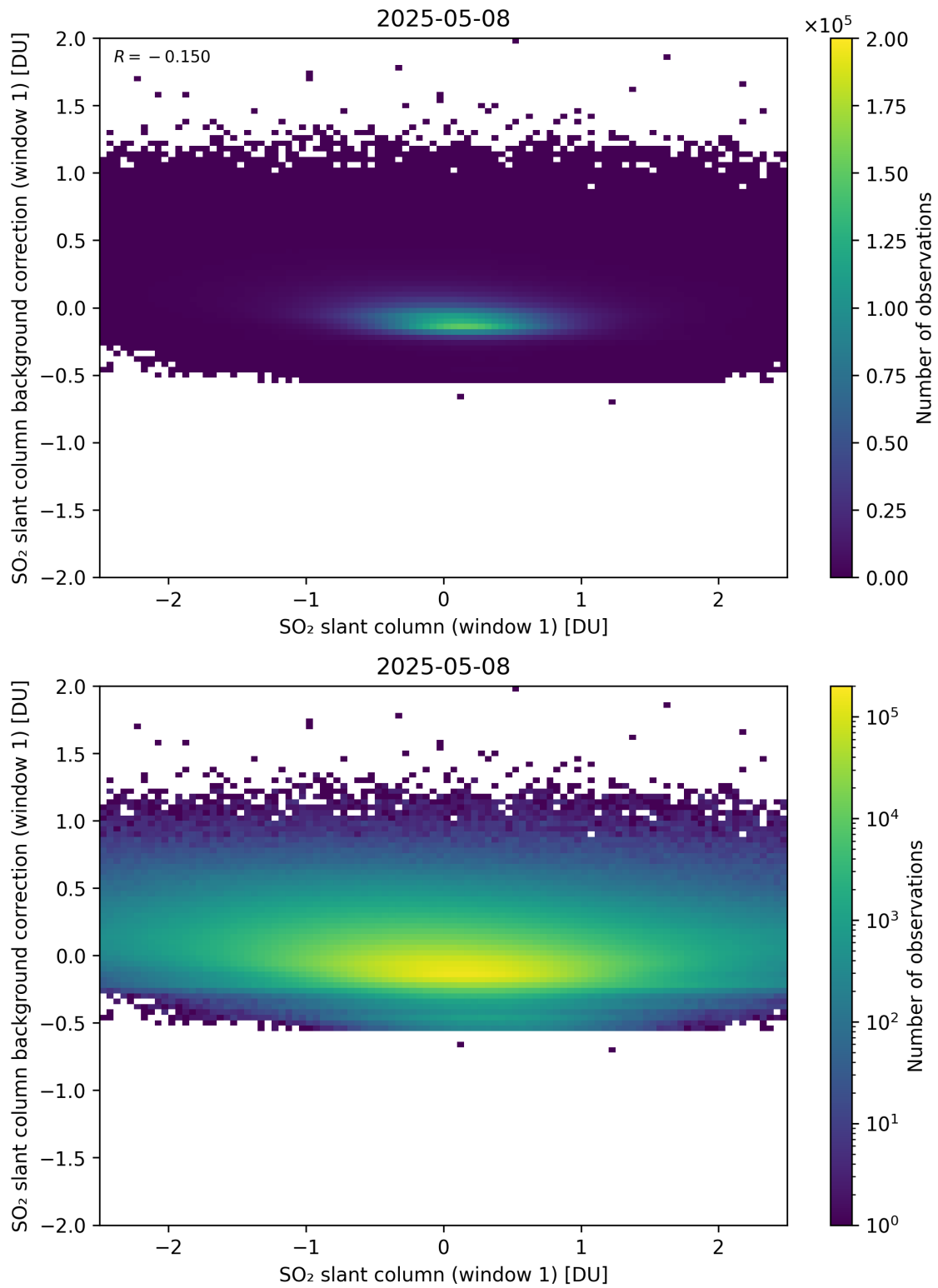
Figure 262: Scatter density plot of “SO 2 slant column (window 1)” against “SO 2 slant column background correction (window 1)” for 2025-05-07 to 2025-05-09.
