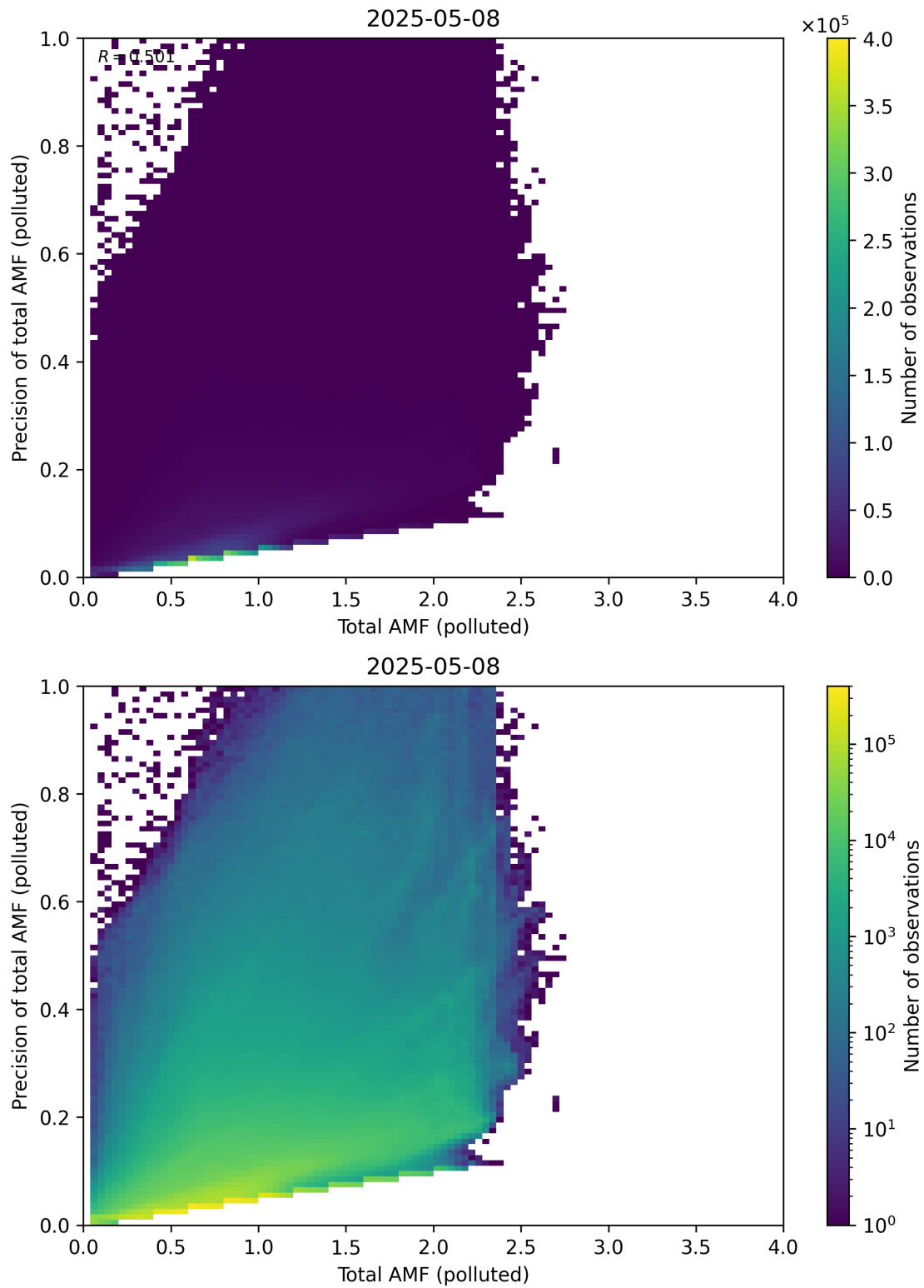
Figure 322: Scatter density plot of “Total AMF (polluted)” against “Precision of total AMF (polluted)” for 2025-05-07 to 2025-05-09.
