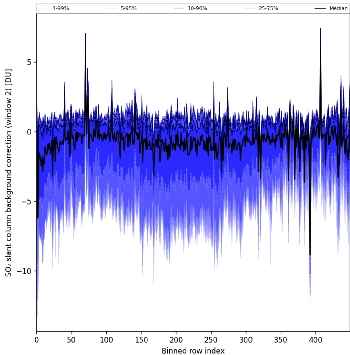
Figure 96: Along track statistics of “SO 2 slant column background correction (window 2)” for 2025-05-07 to 2025-05-09
