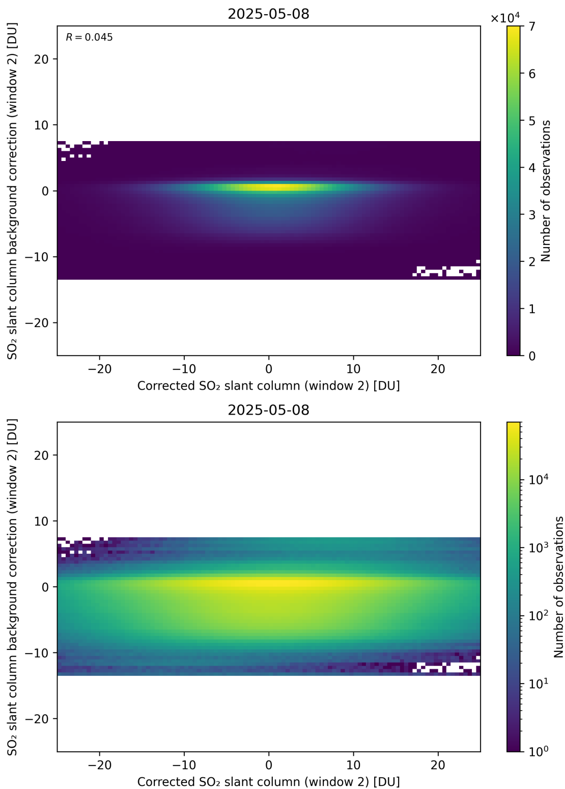
Figure 244: Scatter density plot of “Corrected SO 2 slant column (window 2)” against “SO 2 slant column background correction (window 2)” for 2025-05-07 to 2025-05-09.
