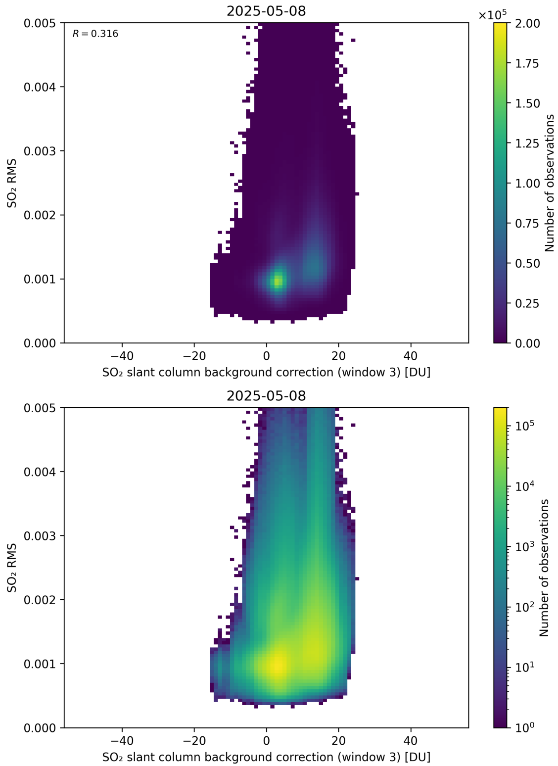
Figure 134: Scatter density plot of “SO 2 slant column background correction (window 3)” against “SO 2 RMS” for 2025-05-07 to 2025-05-09.
