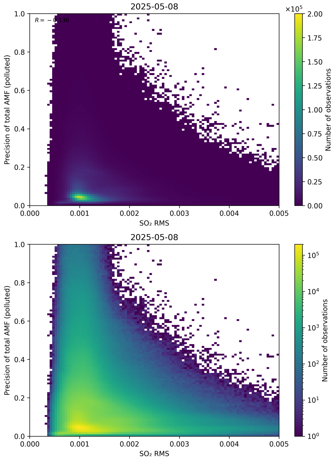
Figure 149: Scatter density plot of “SO 2 RMS” against “Precision of total AMF (polluted)” for 2025-05-07 to 2025-05-09.
