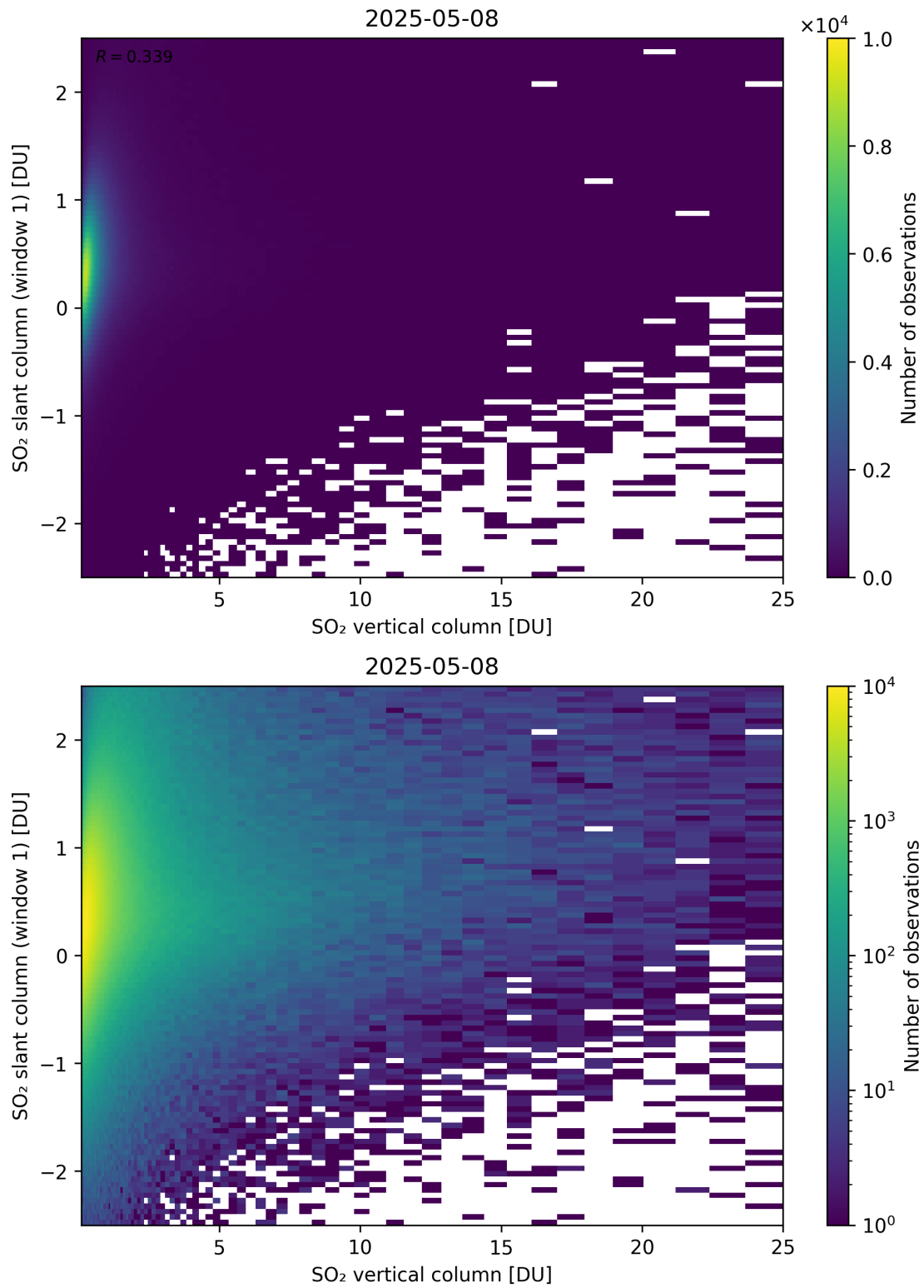
Figure 354: Scatter density plot of “SO 2 vertical column” against “SO 2 slant column (window 1)” for 2025-05-07 to 2025-05-09.
