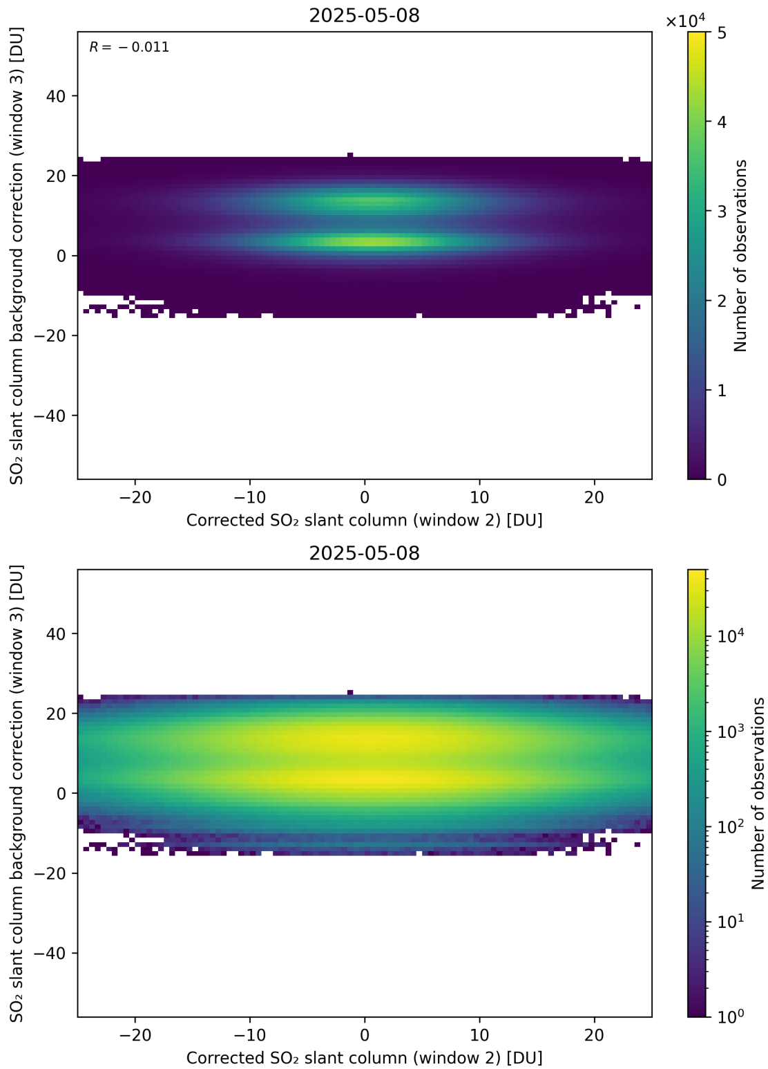
Figure 245: Scatter density plot of “Corrected SO 2 slant column (window 2)” against “SO 2 slant column background correction (window 3)” for 2025-05-07 to 2025-05-09.
