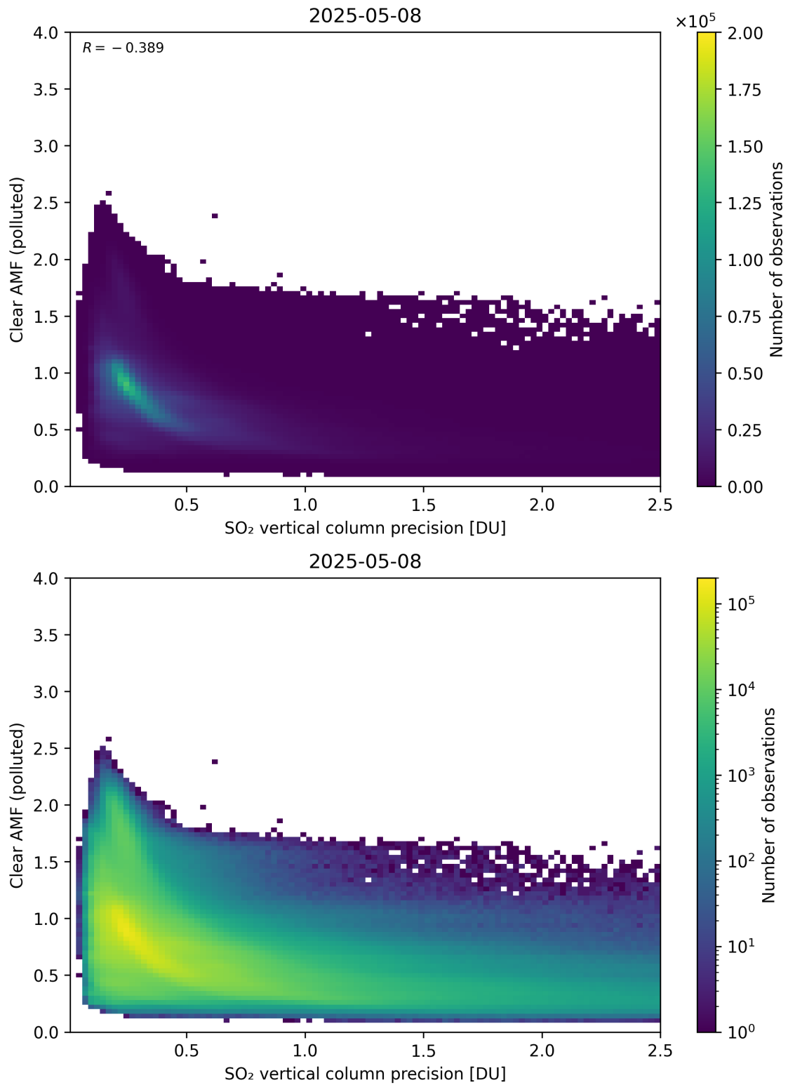
Figure 335: Scatter density plot of “SO 2 vertical column precision” against “Clear AMF (polluted)” for 2025-05-07 to 2025-05-09.
