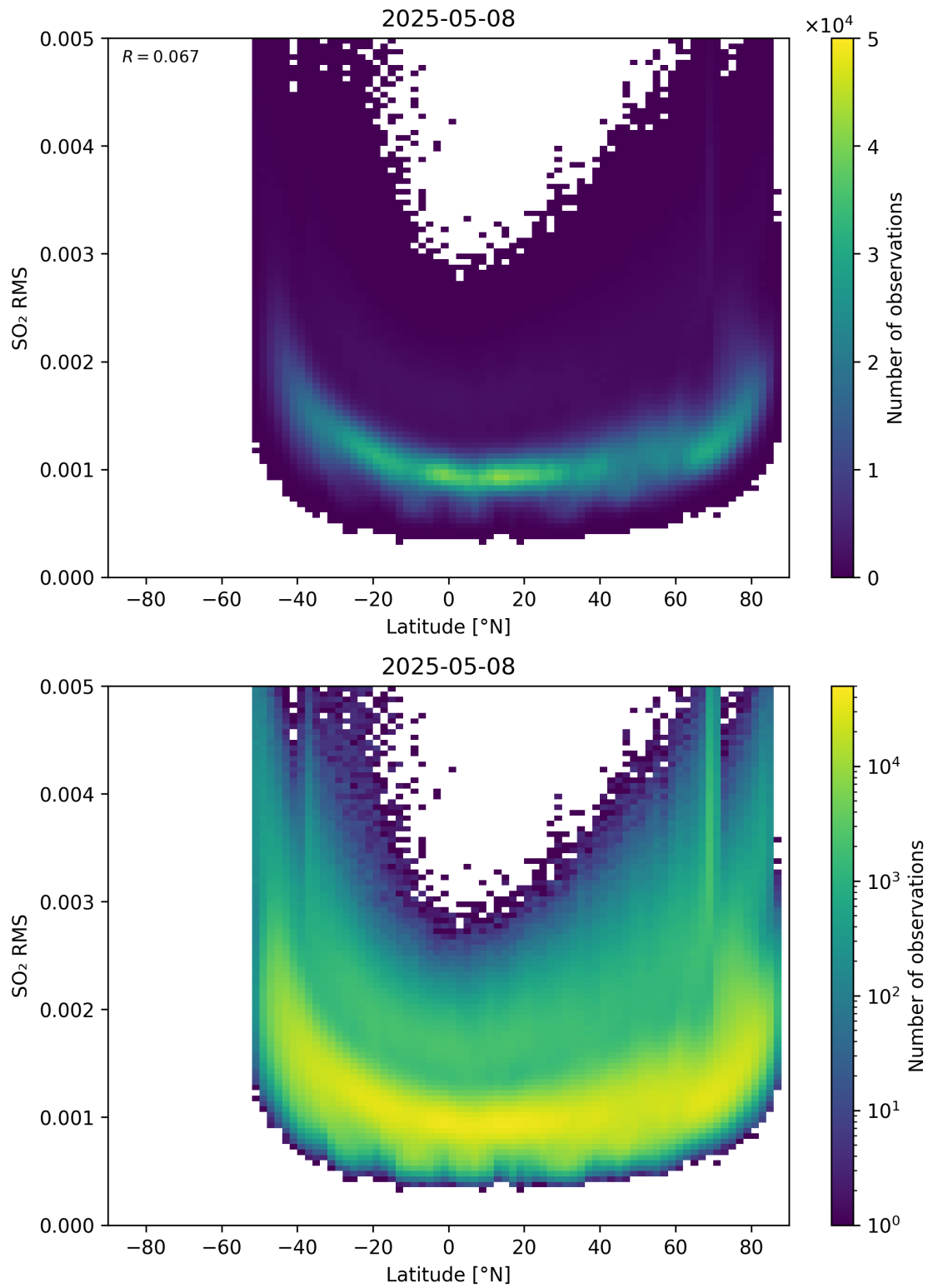
Figure 155: Scatter density plot of “Latitude” against “SO 2 RMS” for 2025-05-07 to 2025-05-09.
