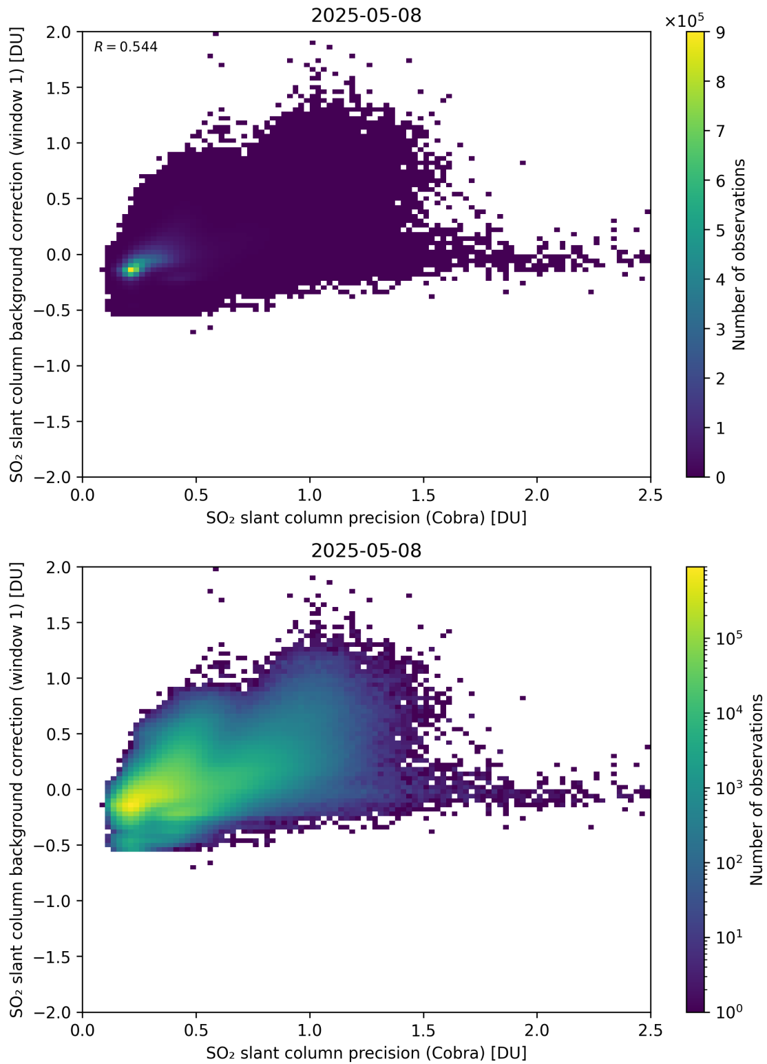
Figure 199: Scatter density plot of “SO 2 slant column precision (Cobra)” against “SO 2 slant column background correction (window 1)” for 2025-05-07 to 2025-05-09.
