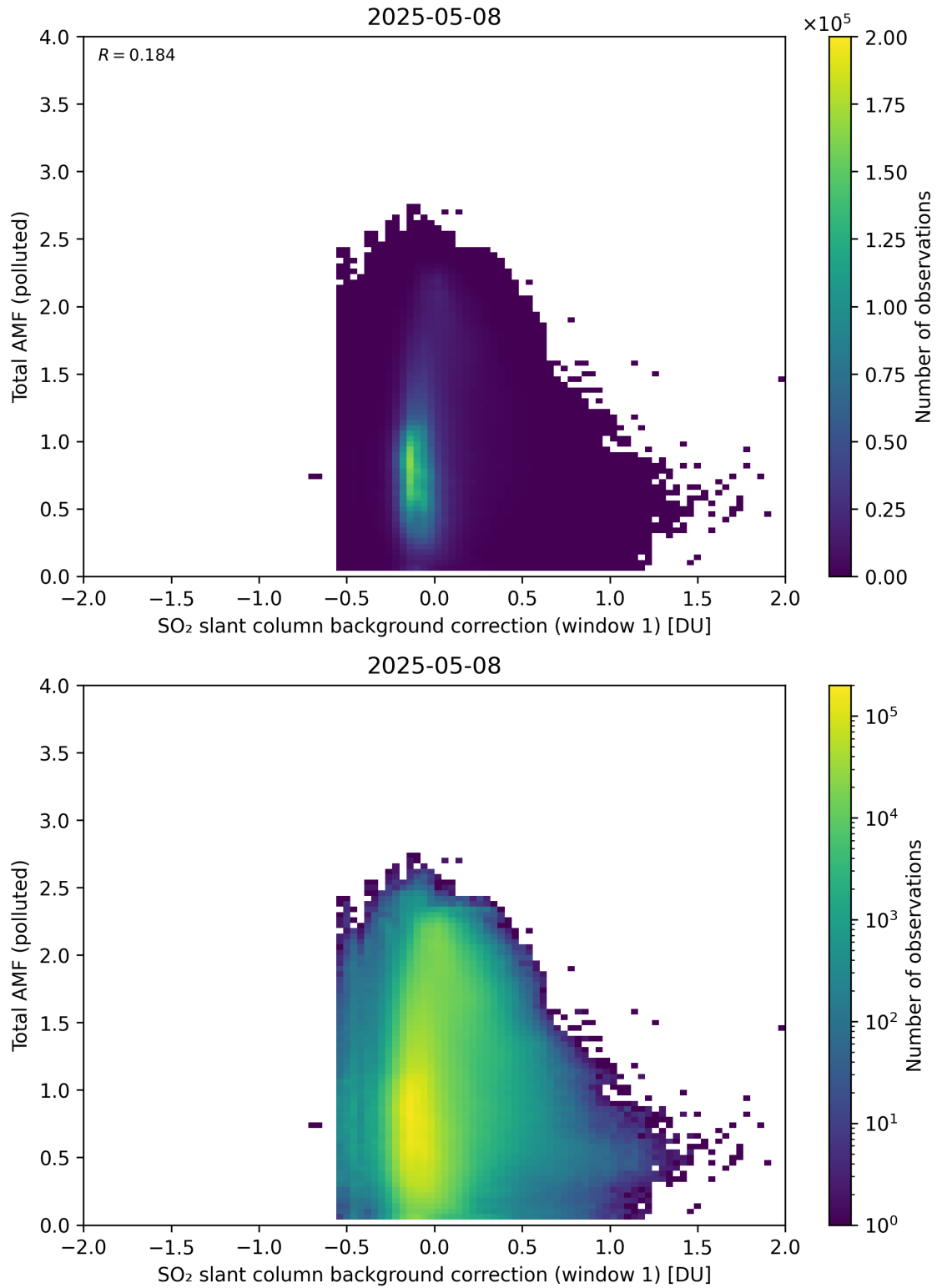
Figure 120: Scatter density plot of “SO 2 slant column background correction (window 1)” against “Total AMF (polluted)” for 2025-05-07 to 2025-05-09.
