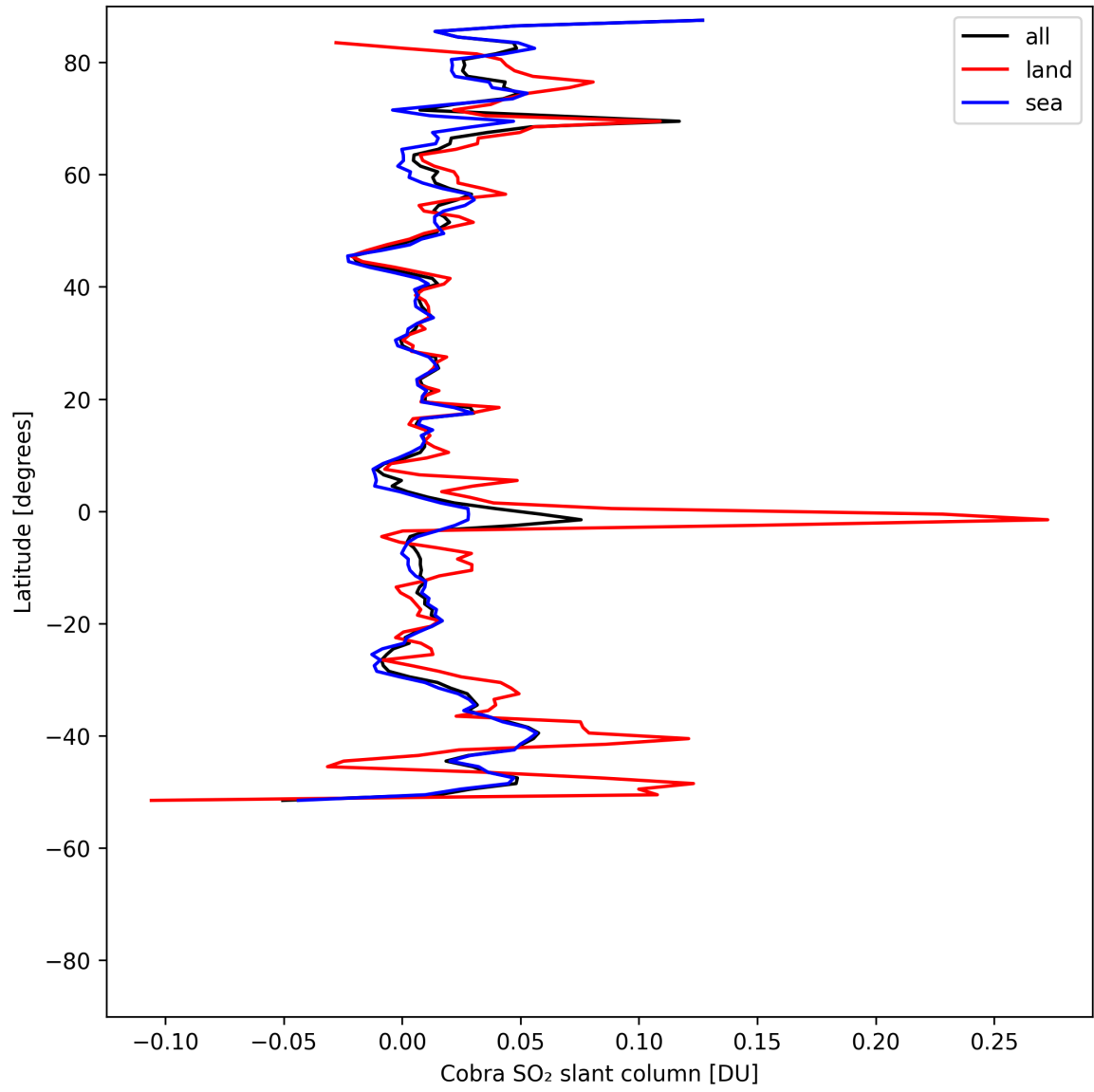
Figure 35: Zonal average of “Cobra SO 2 slant column” for 2025-05-07 to 2025-05-09.
