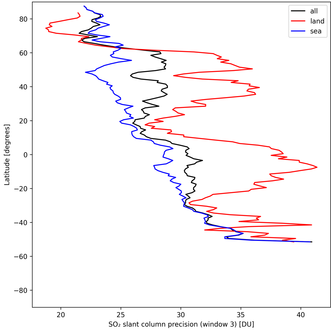
Figure 46: Zonal average of “SO 2 slant column precision (window 3)” for 2025-05-07 to 2025-05-09.
