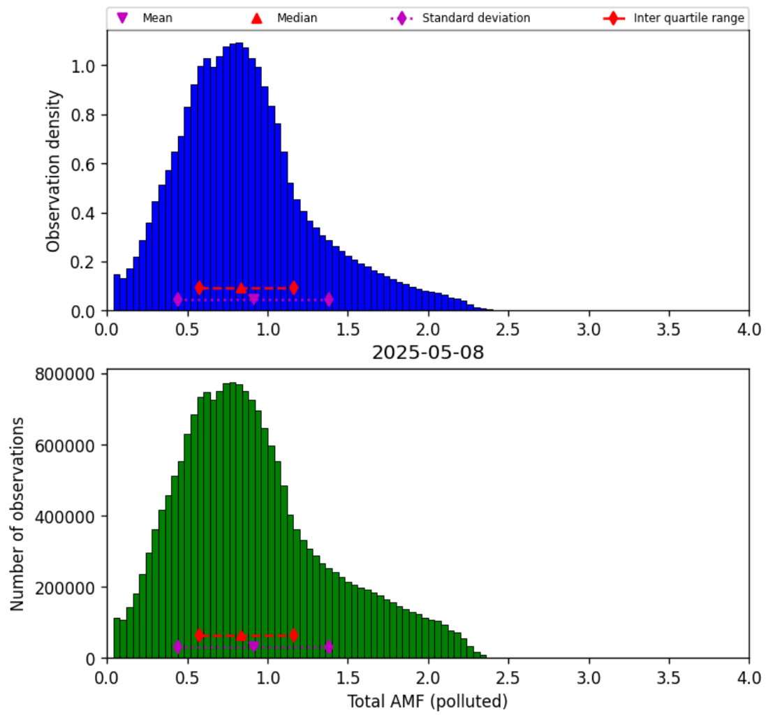
Figure 79: Histogram of “Total AMF (polluted)” for 2025-05-07 to 2025-05-09
