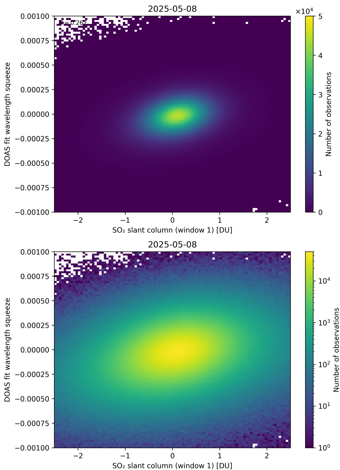
Figure 266: Scatter density plot of “SO 2 slant column (window 1)” against “DOAS fit wavelength squeeze” for 2025-05-07 to 2025-05-09.
