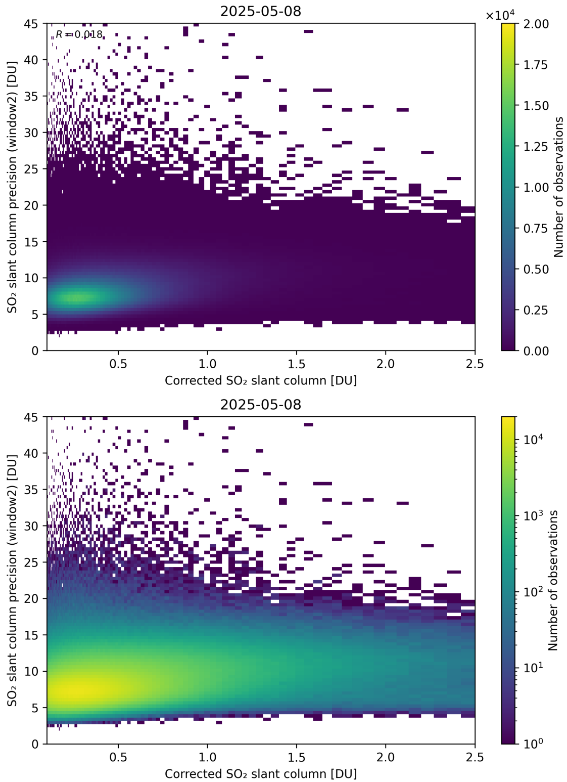
Figure 239: Scatter density plot of “Corrected SO 2 slant column” against “SO 2 slant column precision (window2)” for 2025-05-07 to 2025-05-09.
