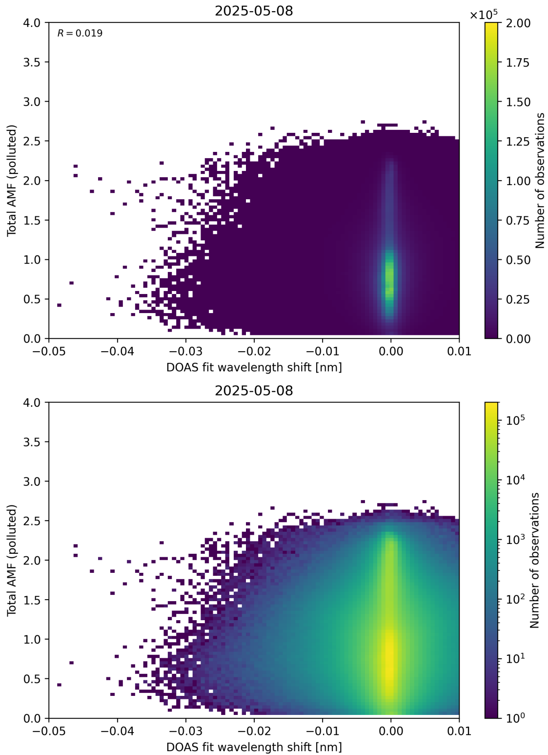
Figure 141: Scatter density plot of “DOAS fit wavelength shift” against “Total AMF (polluted)” for 2025-05-07 to 2025-05-09.
