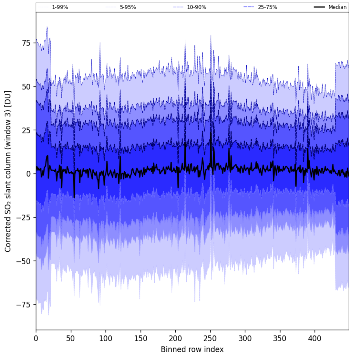
Figure 99: Along track statistics of “Corrected SO 2 slant column (window 3)” for 2025-05-07 to 2025-05-09
