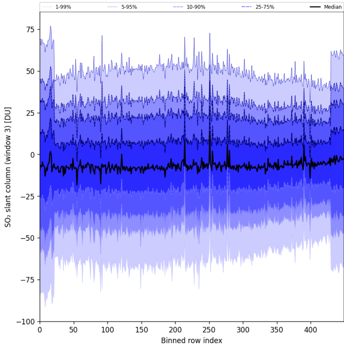
Figure 97: Along track statistics of “SO 2 slant column (window 3)” for 2025-05-07 to 2025-05-09
