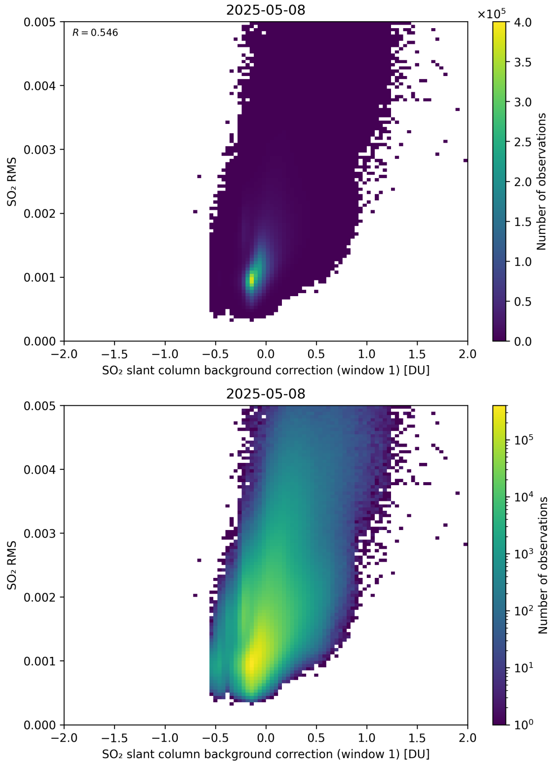
Figure 113: Scatter density plot of “SO 2 slant column background correction (window 1)” against “SO 2 RMS” for 2025-05-07 to 2025-05-09.
