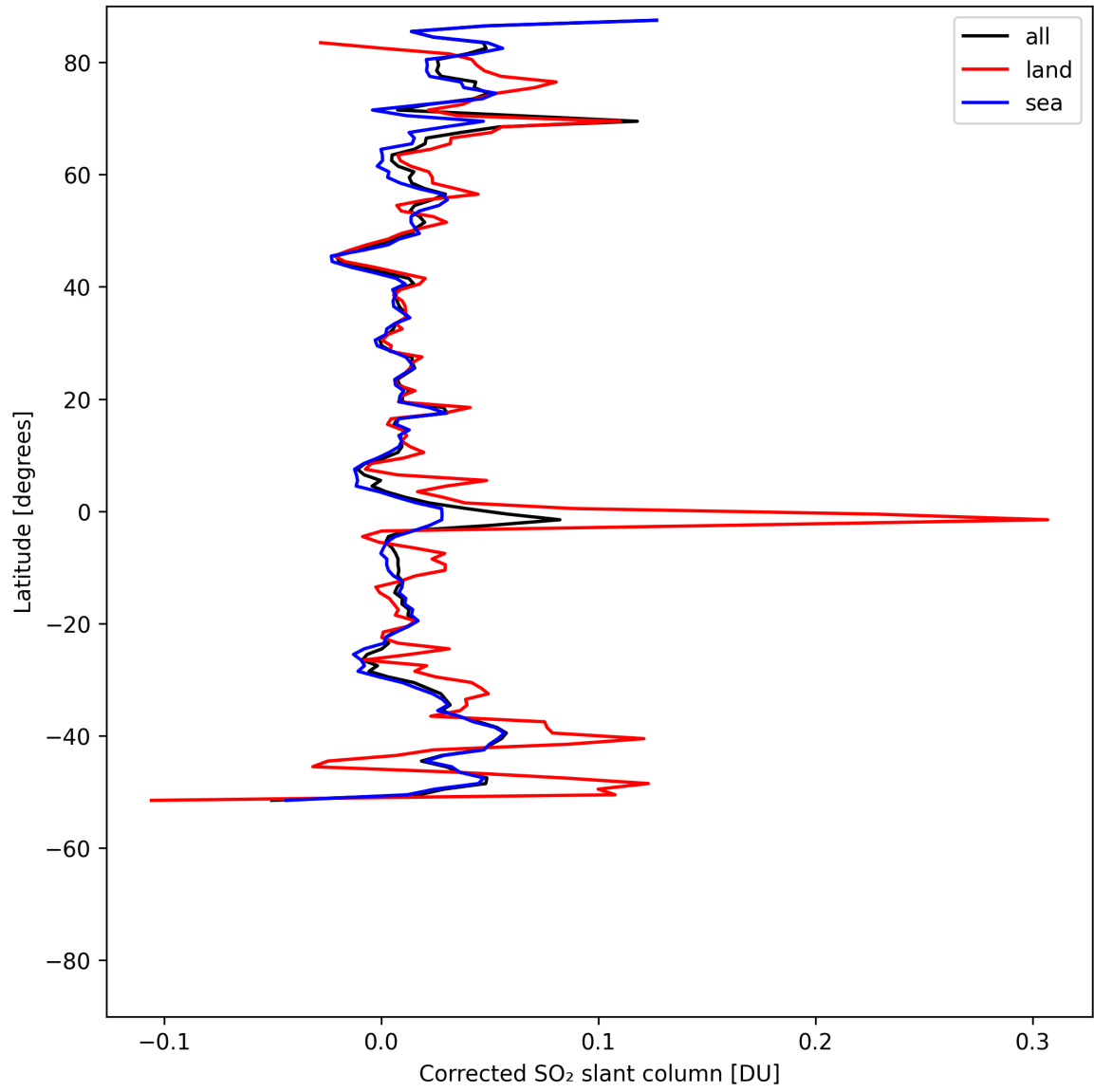
Figure 34: Zonal average of “Corrected SO 2 slant column” for 2025-05-07 to 2025-05-09.
