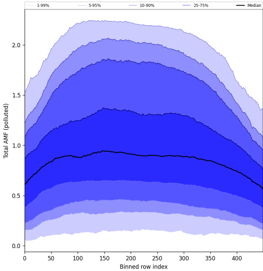
Figure 105: Along track statistics of “Total AMF (polluted)” for 2025-05-07 to 2025-05-09
