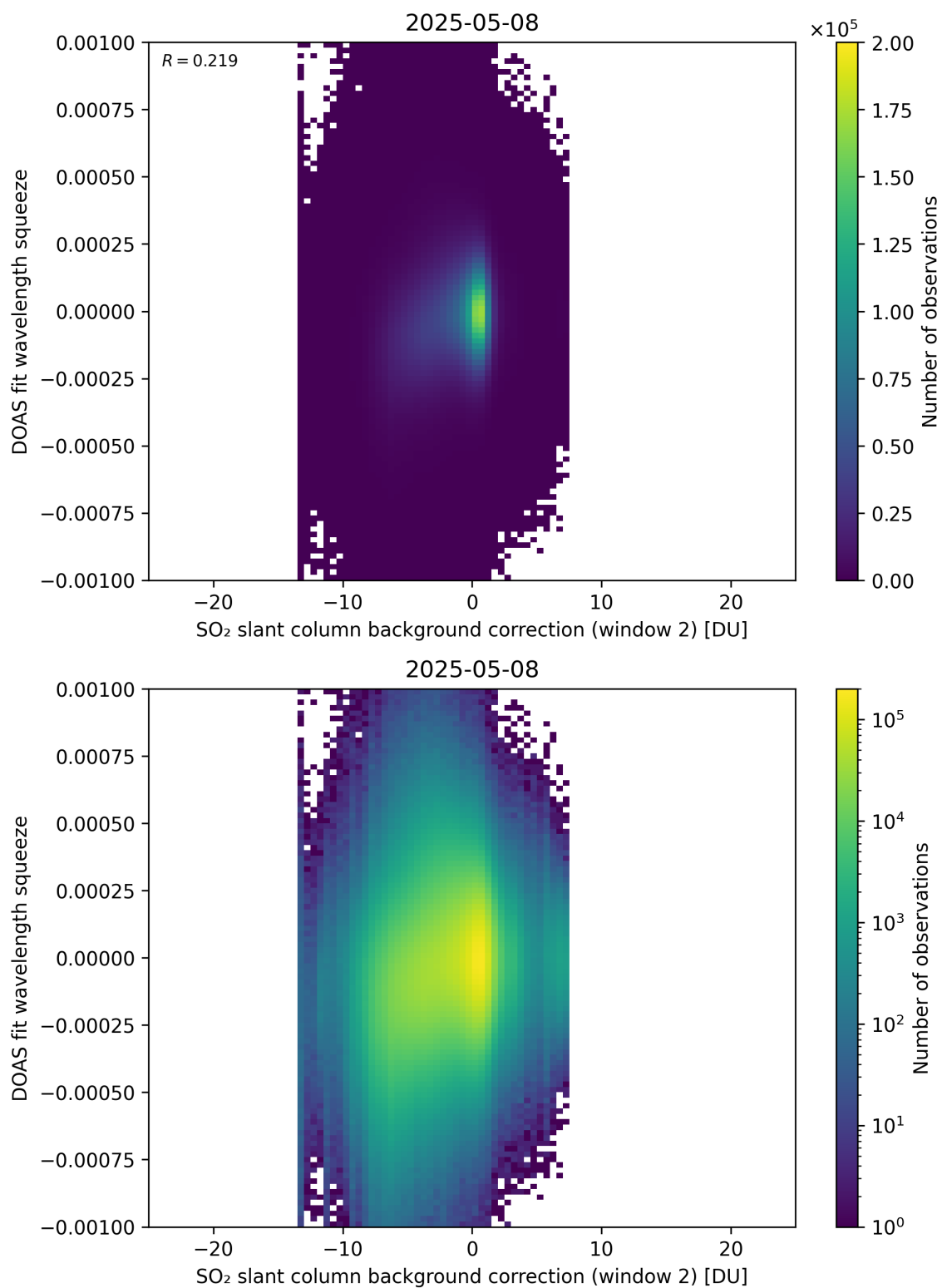
Figure 124: Scatter density plot of “SO 2 slant column background correction (window 2)” against “DOAS fit wavelength squeeze” for 2025-05-07 to 2025-05-09.
