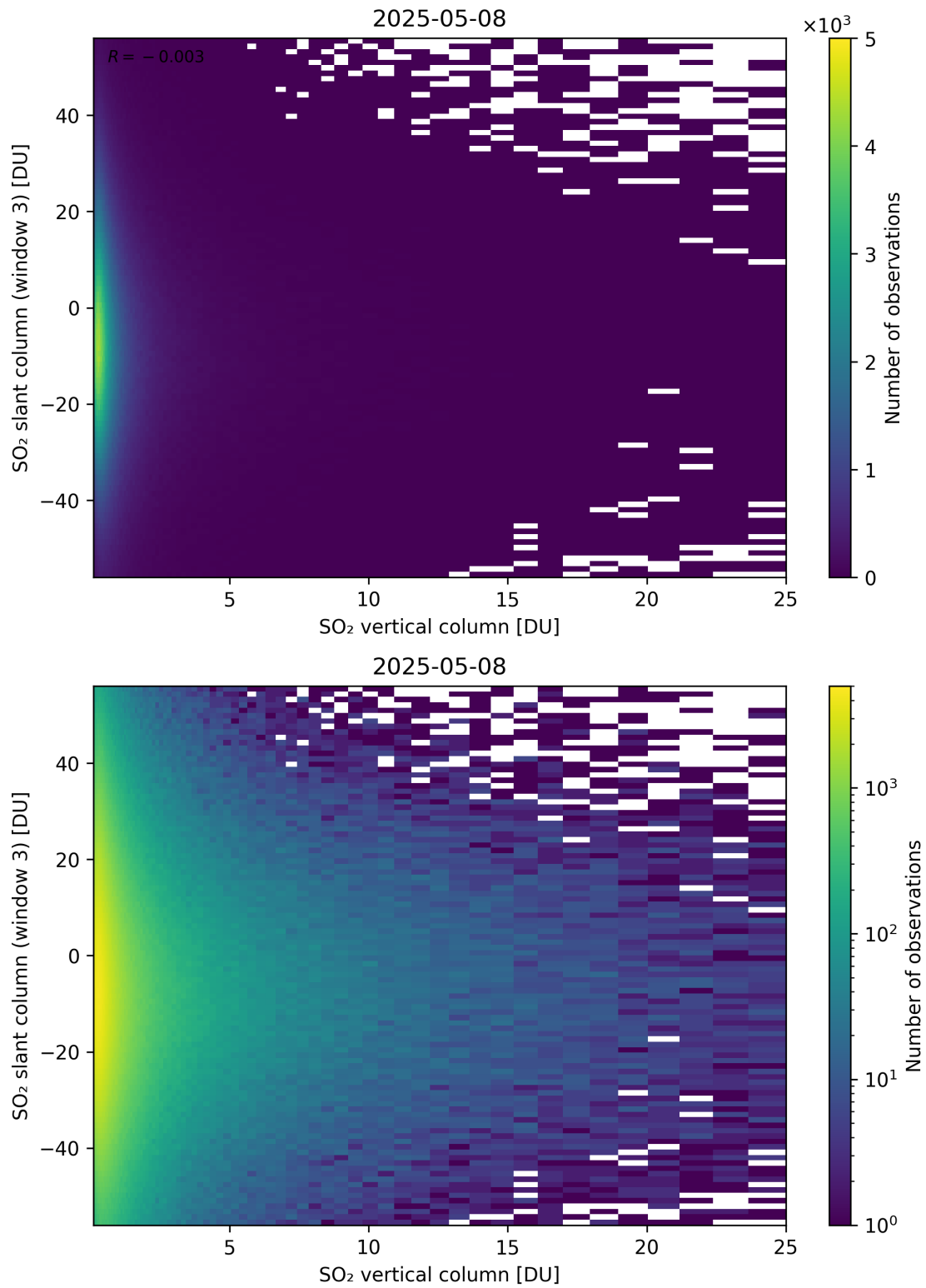
Figure 357: Scatter density plot of “SO 2 vertical column” against “SO 2 slant column (window 3)” for 2025-05-07 to 2025-05-09.
