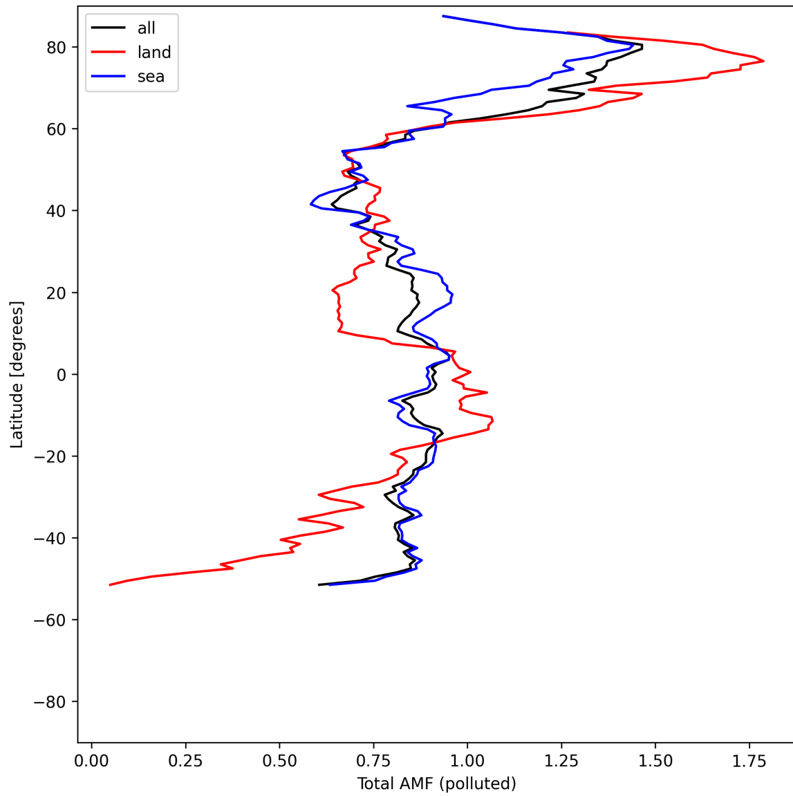
Figure 53: Zonal average of “Total AMF (polluted)” for 2025-05-07 to 2025-05-09.
