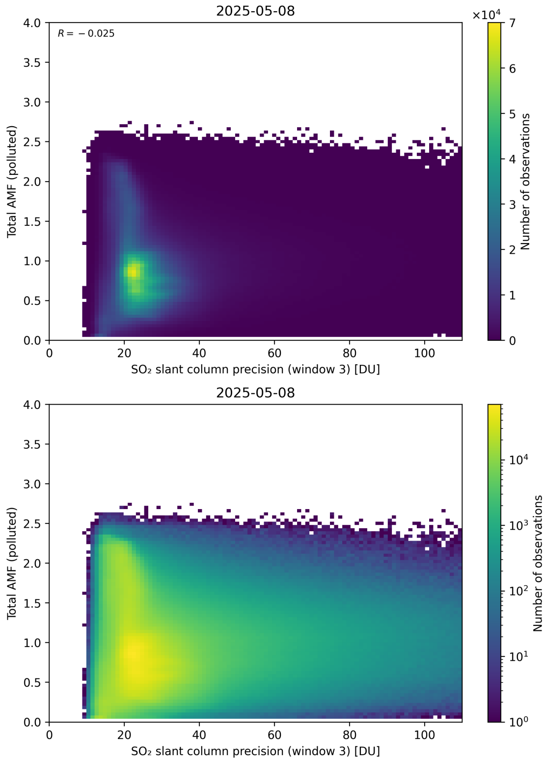
Figure 313: Scatter density plot of “SO 2 slant column precision (window 3)” against “Total AMF (polluted)” for 2025-05-07 to 2025-05-09.
