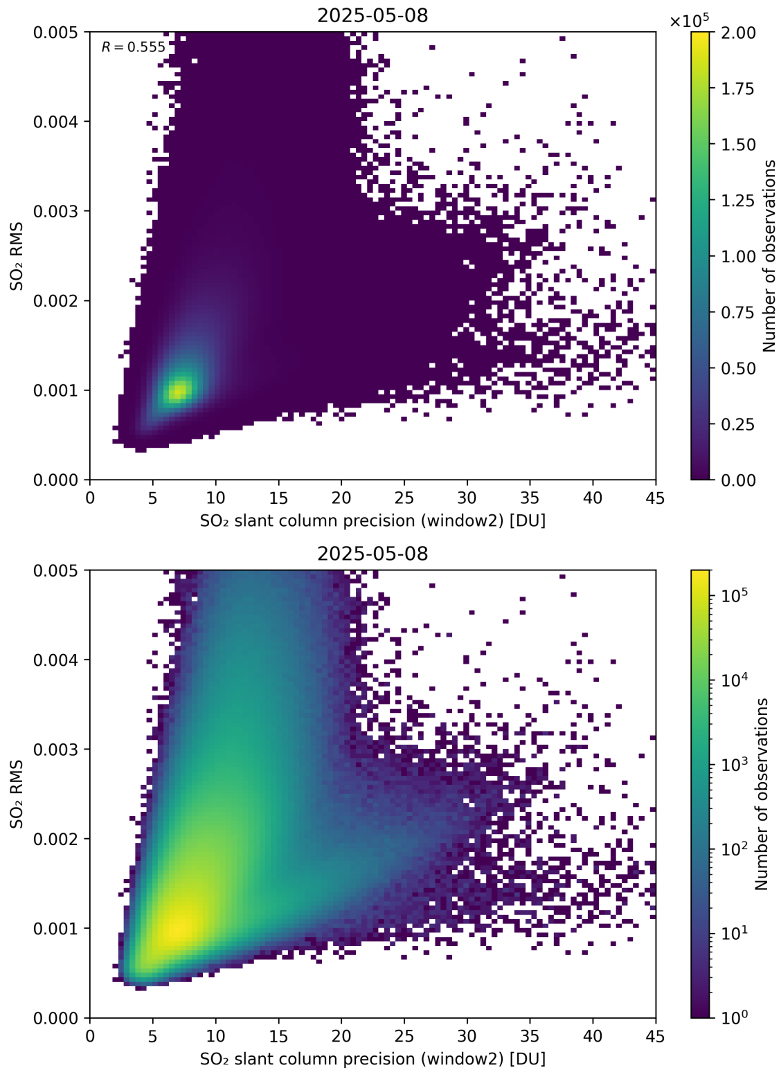
Figure 295: Scatter density plot of “SO 2 slant column precision (window2)” against “SO 2 RMS” for 2025-05-07 to 2025-05-09.
