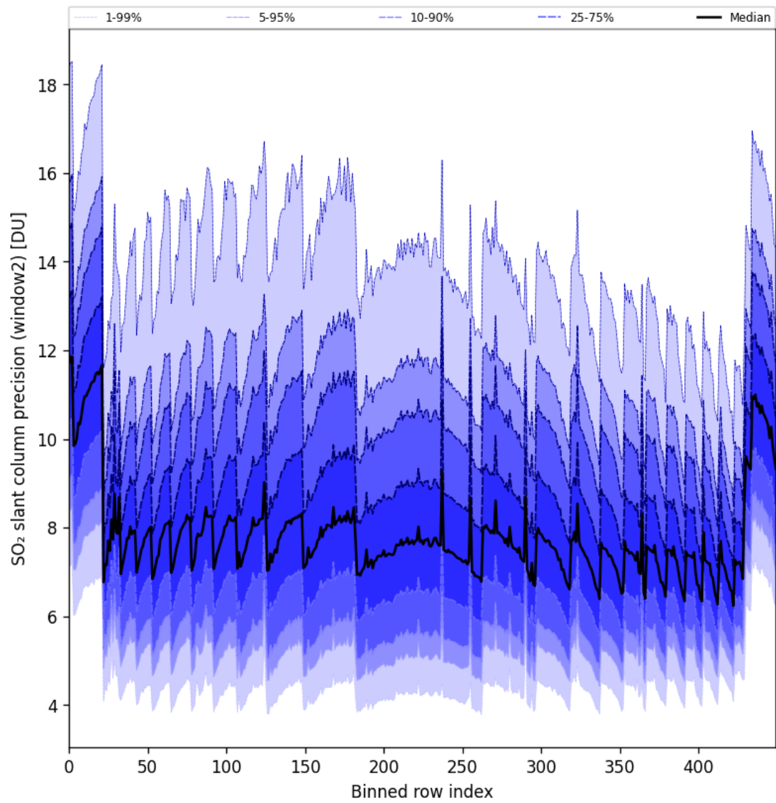
Figure 94: Along track statistics of “SO 2 slant column precision (window2)” for 2025-05-07 to 2025-05-09
