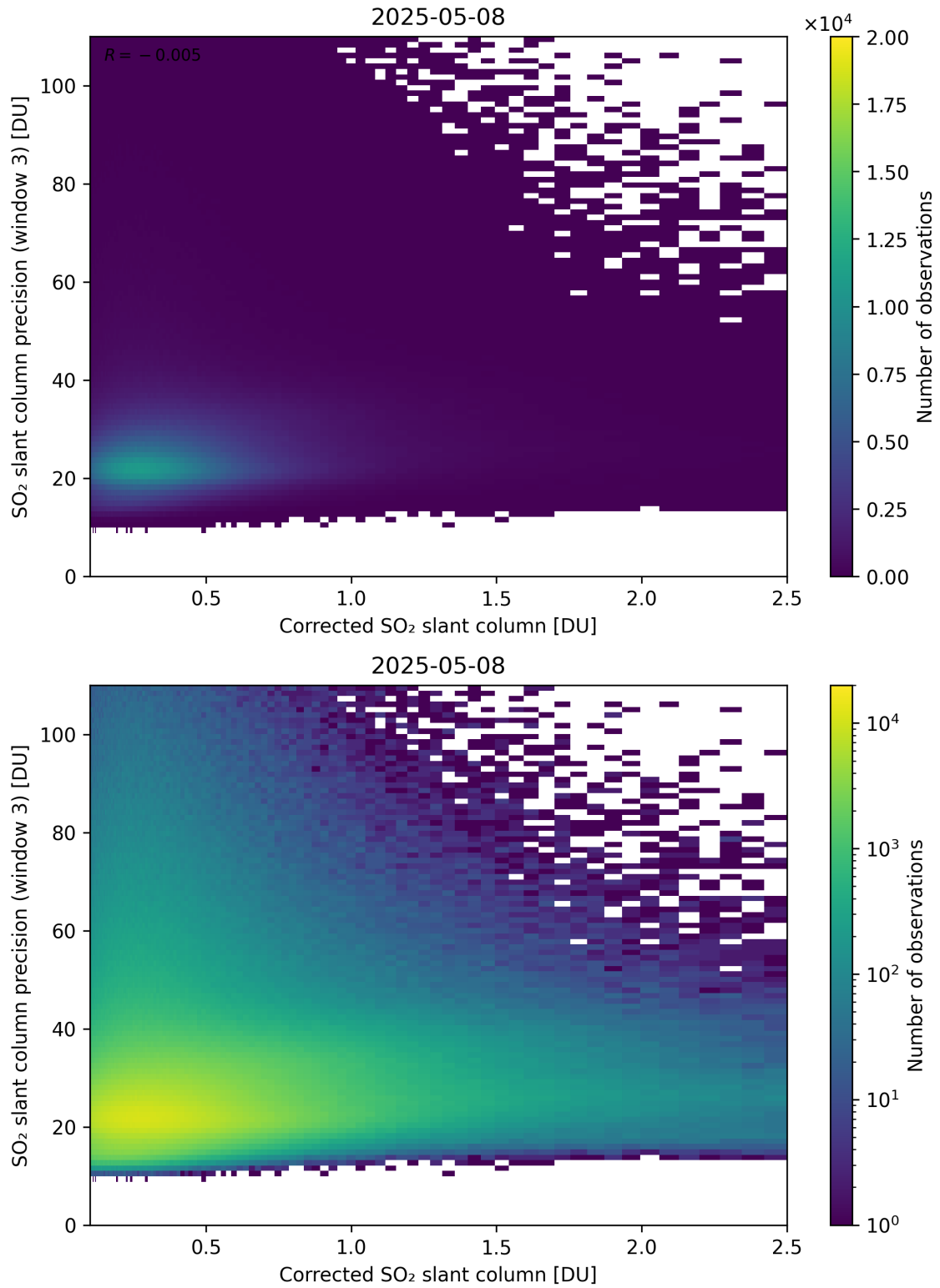
Figure 241: Scatter density plot of “Corrected SO 2 slant column” against “SO 2 slant column precision (window 3)” for 2025-05-07 to 2025-05-09.
