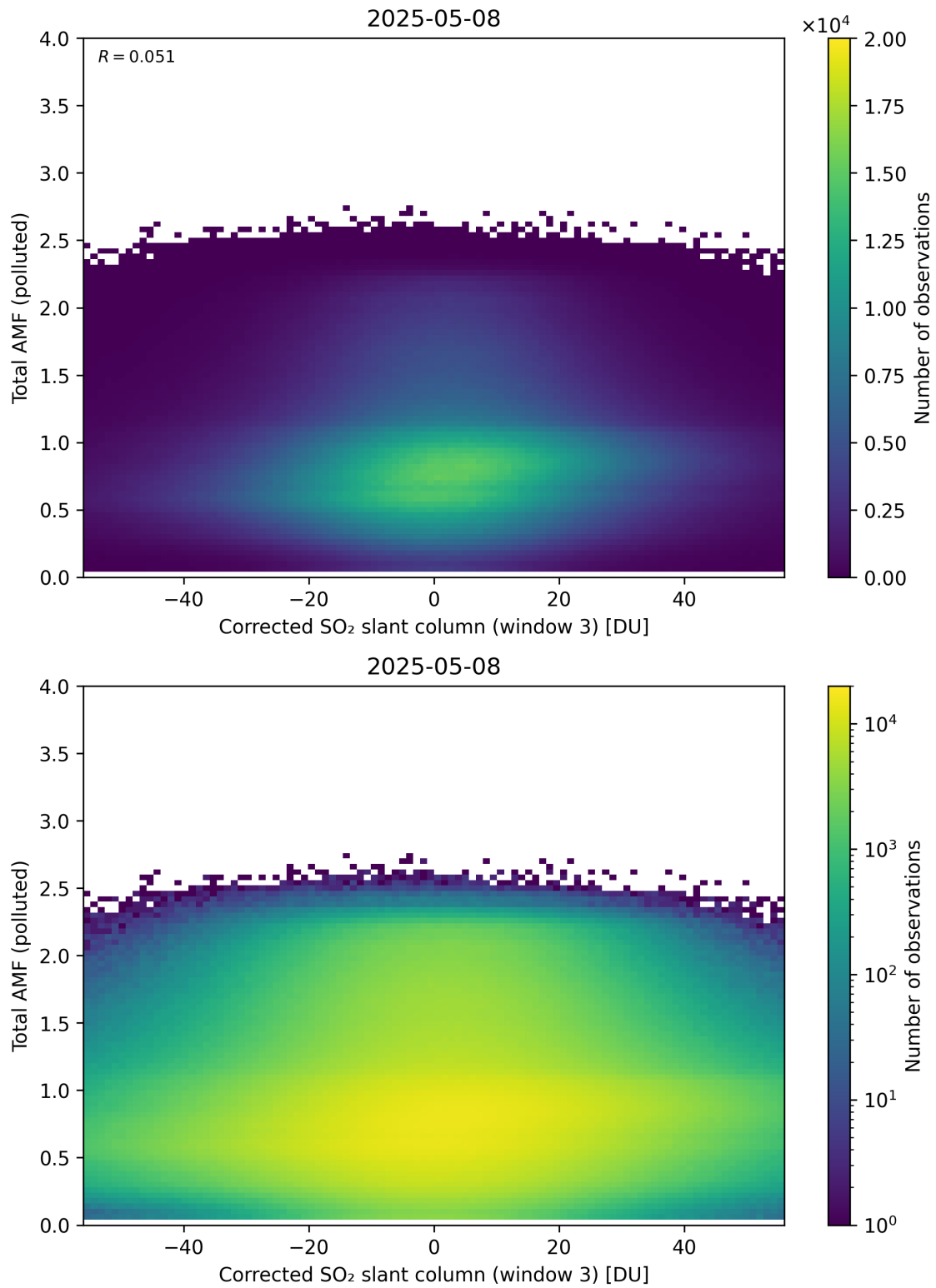
Figure 260: Scatter density plot of “Corrected SO 2 slant column (window 3)” against “Total AMF (polluted)” for 2025-05-07 to 2025-05-09.
