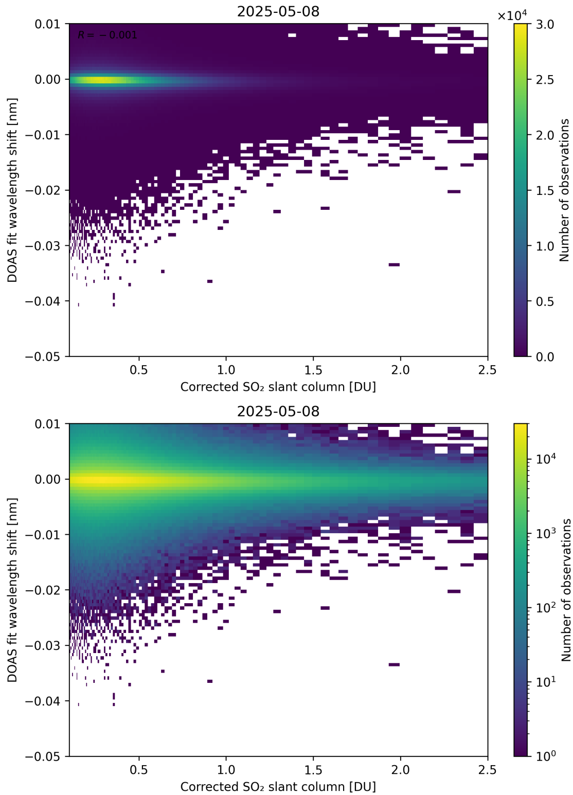
Figure 229: Scatter density plot of “Corrected SO 2 slant column” against “DOAS fit wavelength shift” for 2025-05-07 to 2025-05-09.
