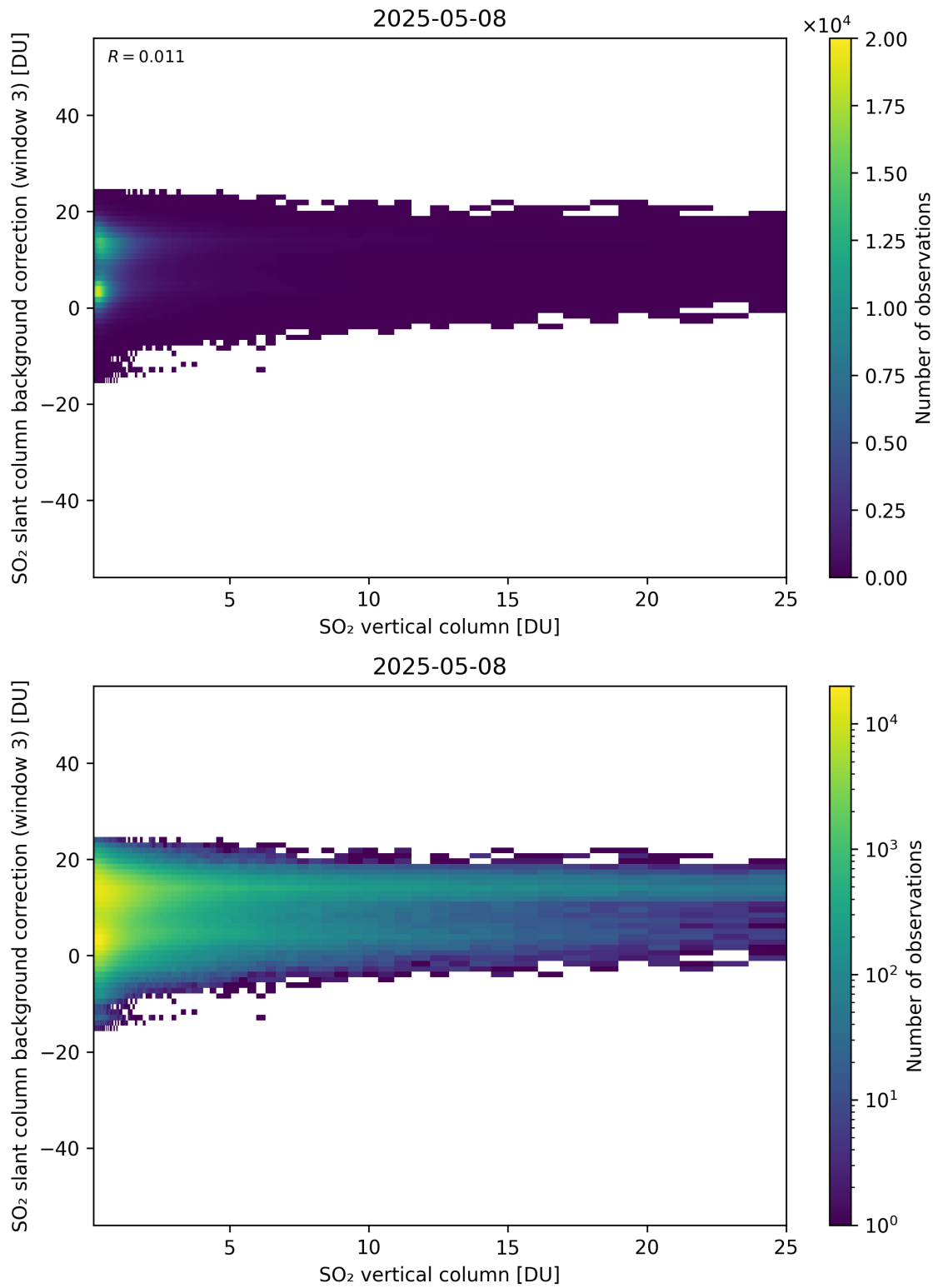
Figure 325: Scatter density plot of “SO 2 vertical column” against “SO 2 slant column background correction (window 3)” for 2025-05-07 to 2025-05-09.
