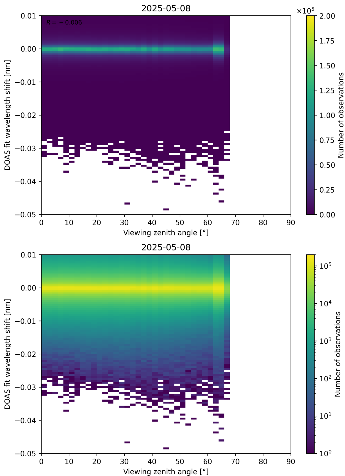
Figure 365: Scatter density plot of “Viewing zenith angle” against “DOAS fit wavelength shift” for 2025-05-07 to 2025-05-09.
