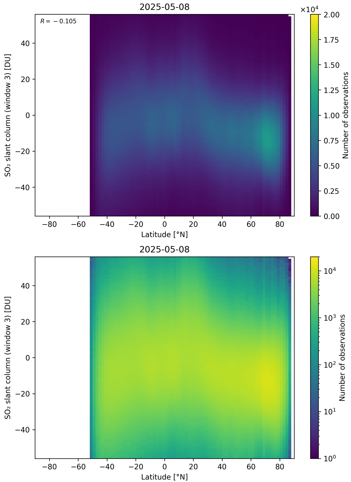
Figure 165: Scatter density plot of “Latitude” against “SO 2 slant column (window 3)” for 2025-05-07 to 2025-05-09.
