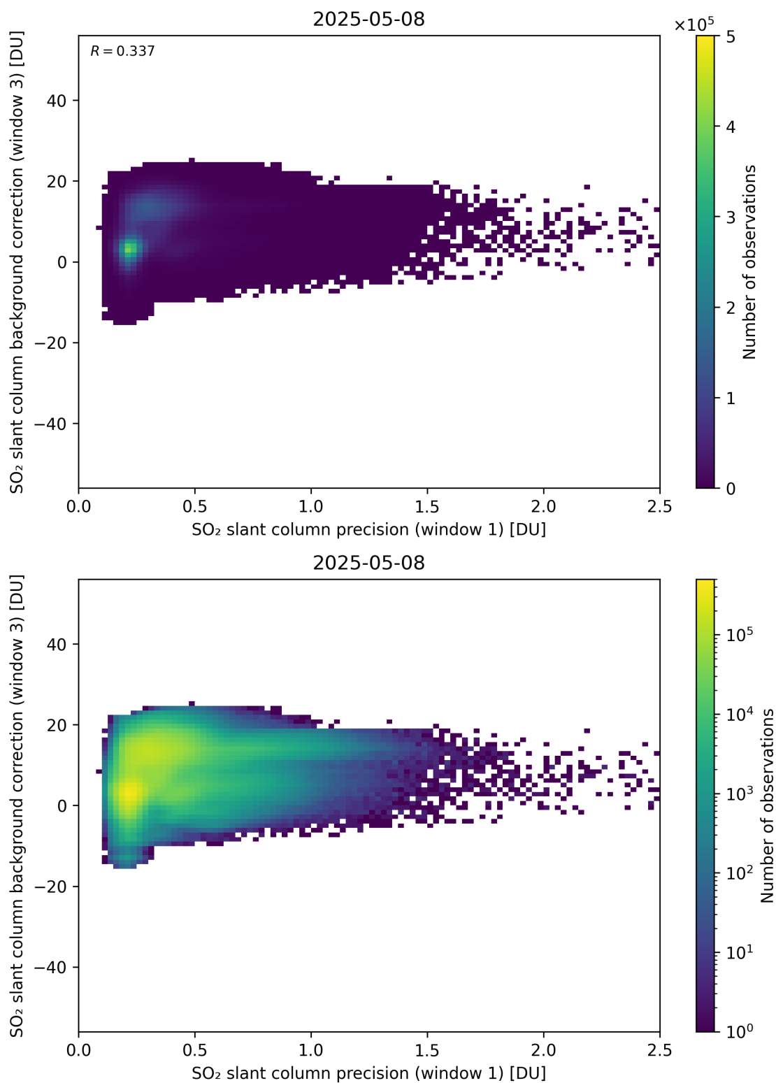
Figure 270: Scatter density plot of “SO 2 slant column precision (window 1)” against “SO 2 slant column background correction (window 3)” for 2025-05-07 to 2025-05-09.
