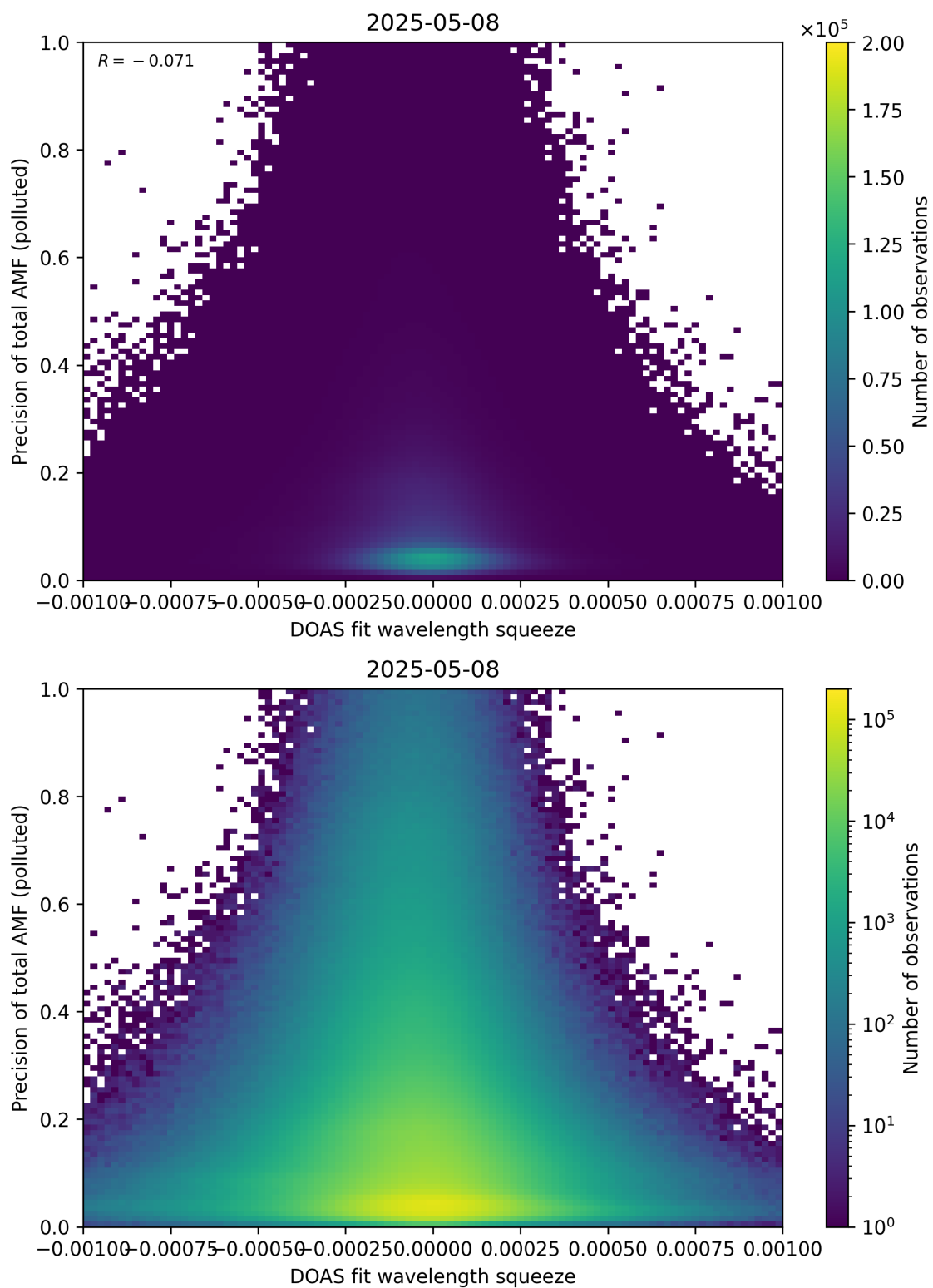
Figure 146: Scatter density plot of “DOAS fit wavelength squeeze” against “Precision of total AMF (polluted)” for 2025-05-07 to 2025-05-09.
