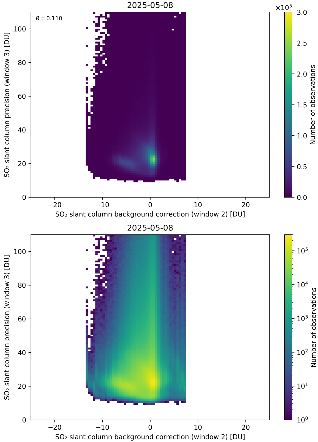
Figure 129: Scatter density plot of “SO 2 slant column background correction (window 2)” against “SO 2 slant column precision (window 3)” for 2025-05-07 to 2025-05-09.
