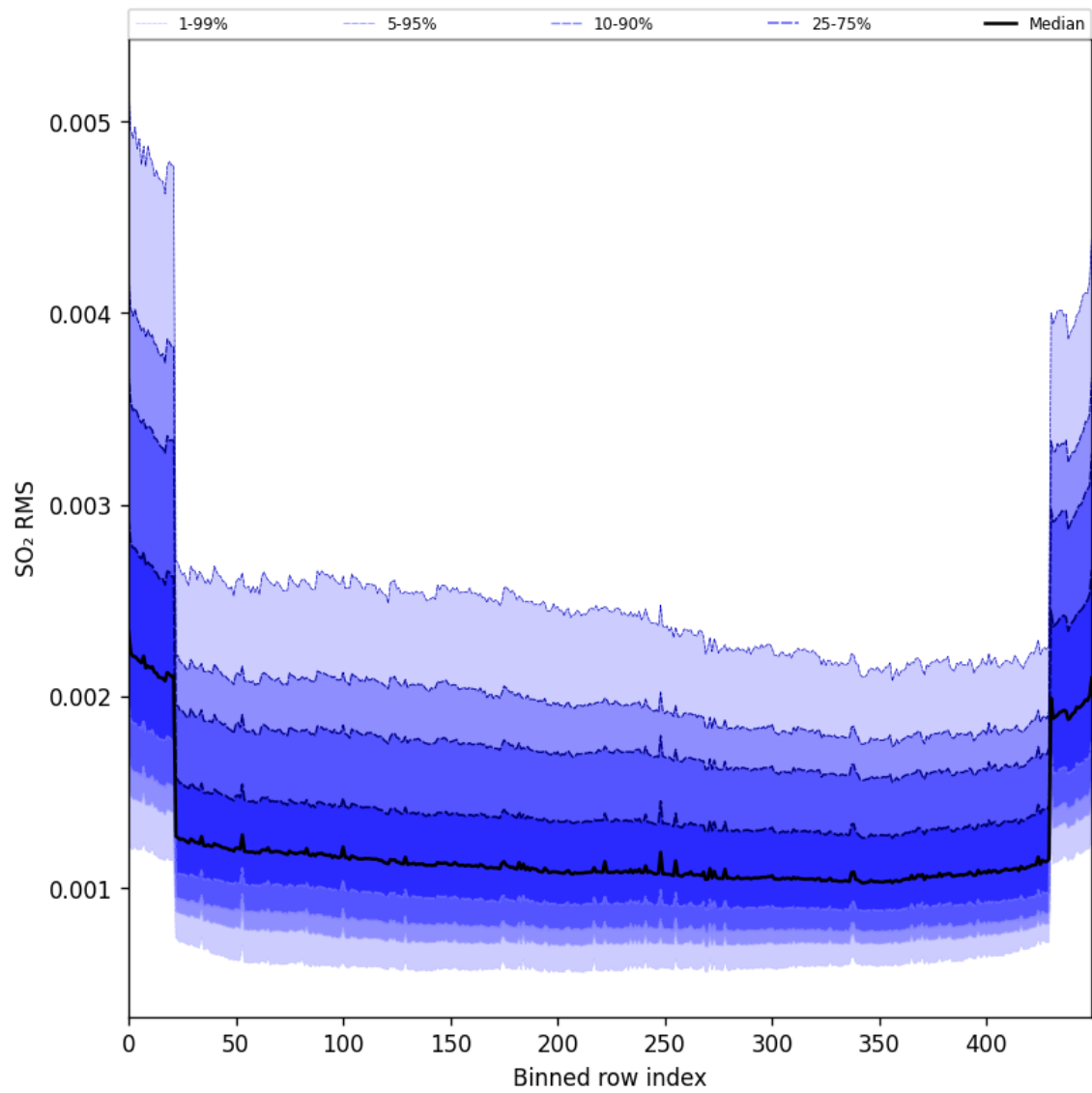
Figure 104: Along track statistics of “SO 2 RMS” for 2025-05-07 to 2025-05-09
