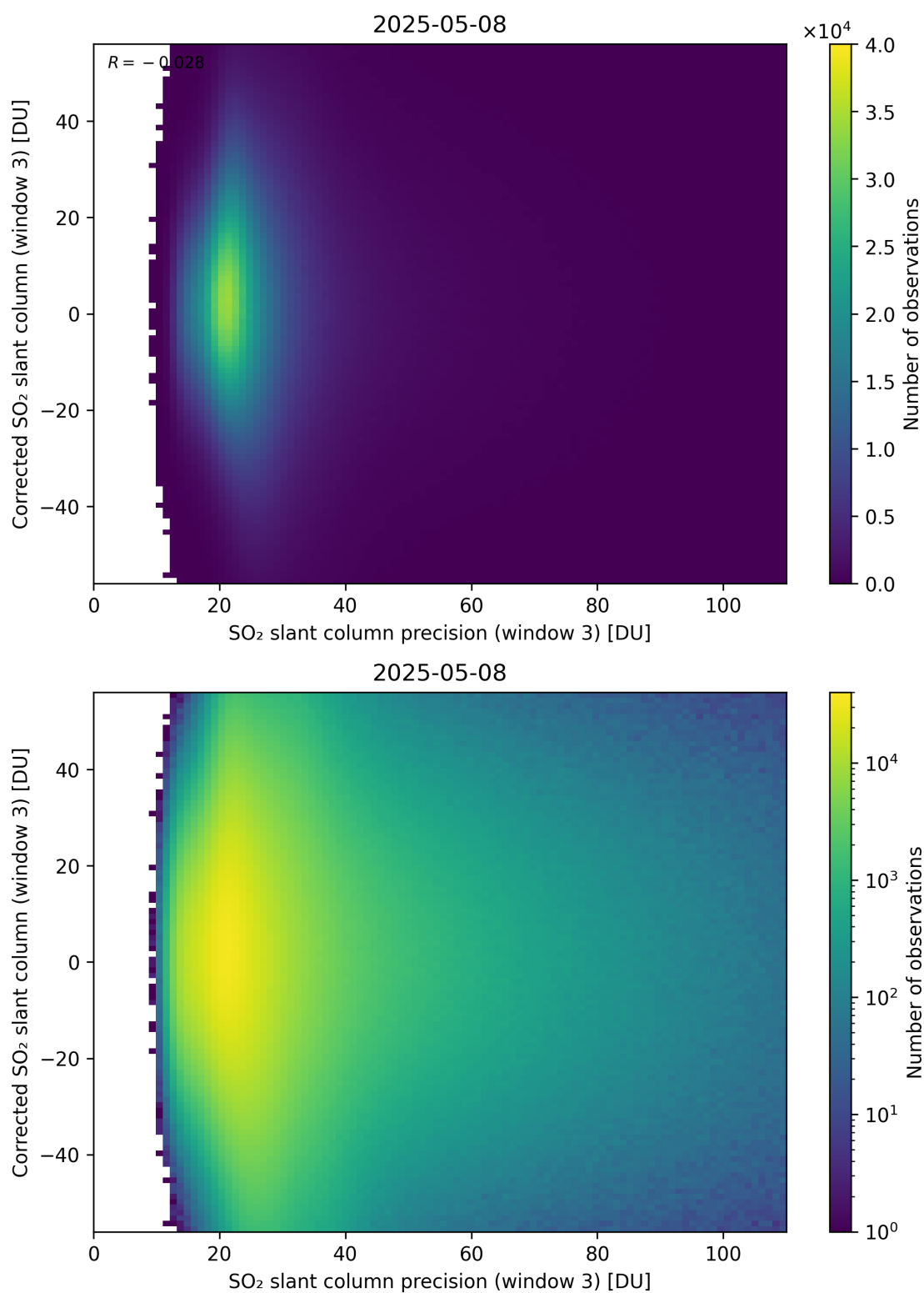
Figure 312: Scatter density plot of “SO 2 slant column precision (window 3)” against “Corrected SO 2 slant column (window 3)” for 2025-05-07 to 2025-05-09.
