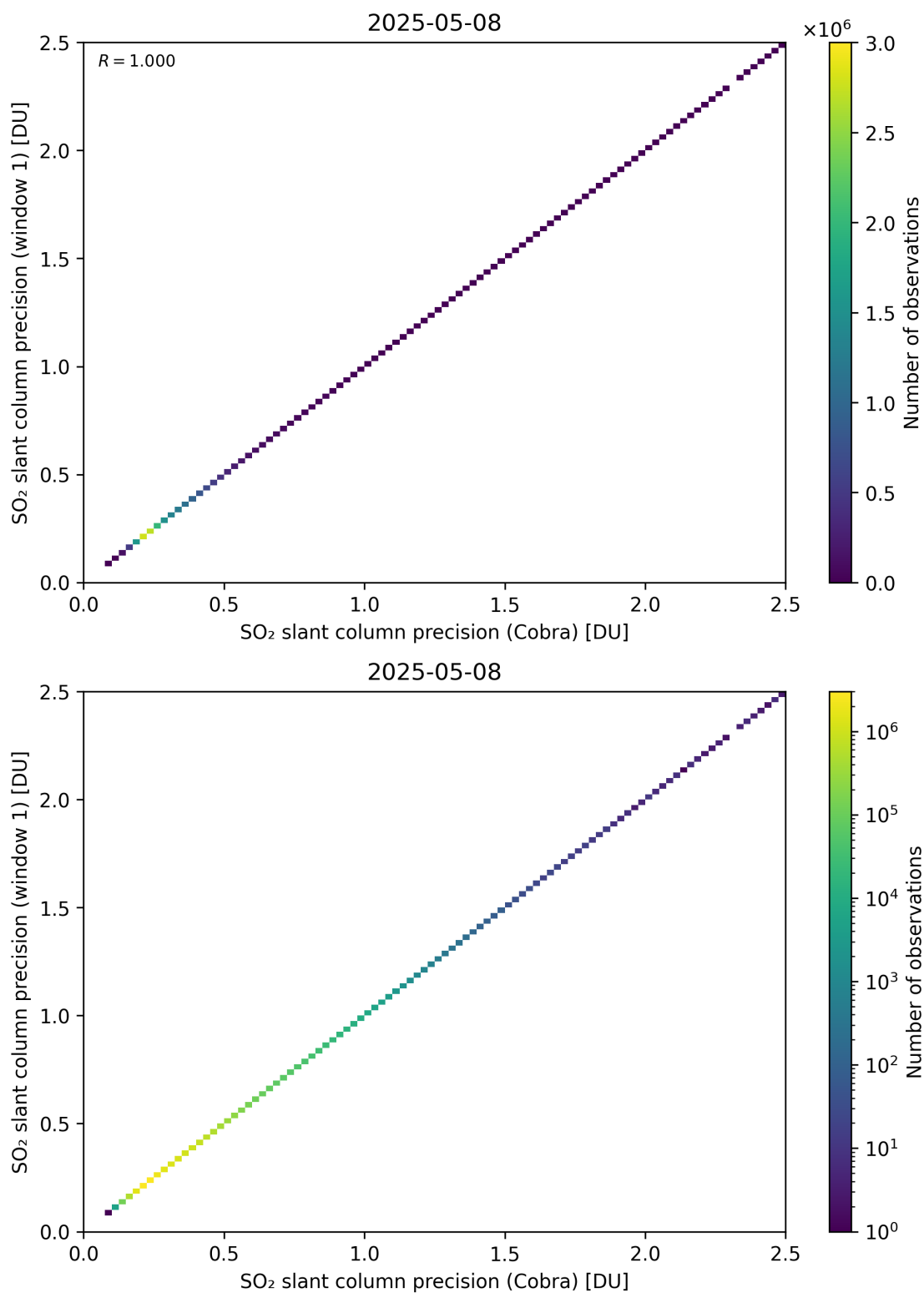
Figure 209: Scatter density plot of “SO 2 slant column precision (Cobra)” against “SO 2 slant column precision (window 1)” for 2025-05-07 to 2025-05-09.
