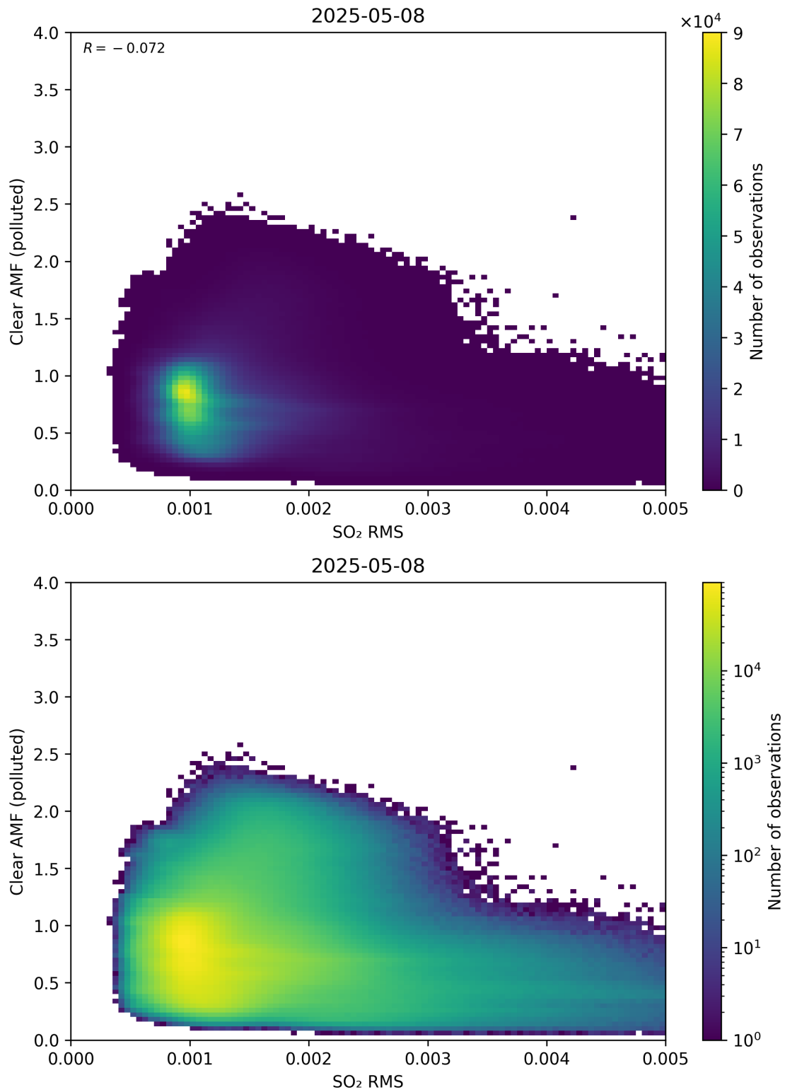
Figure 147: Scatter density plot of “SO 2 RMS” against “Clear AMF (polluted)” for 2025-05-07 to 2025-05-09.
