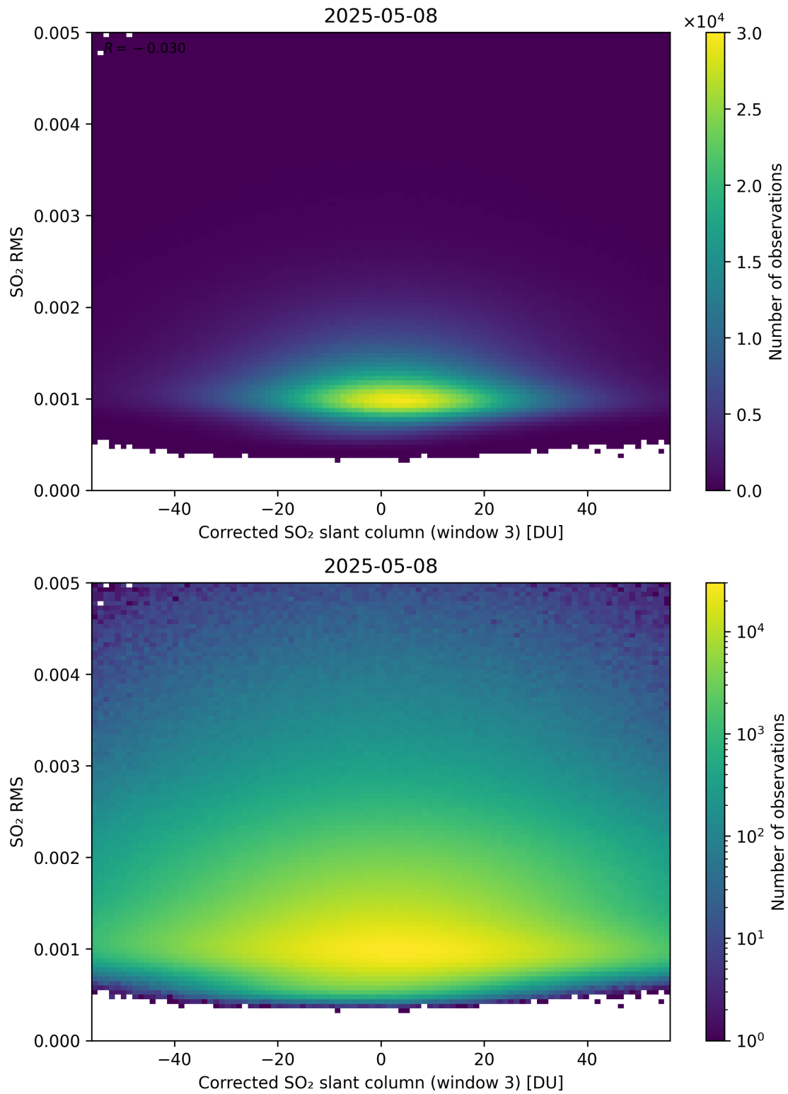
Figure 258: Scatter density plot of “Corrected SO 2 slant column (window 3)” against “SO 2 RMS” for 2025-05-07 to 2025-05-09.
