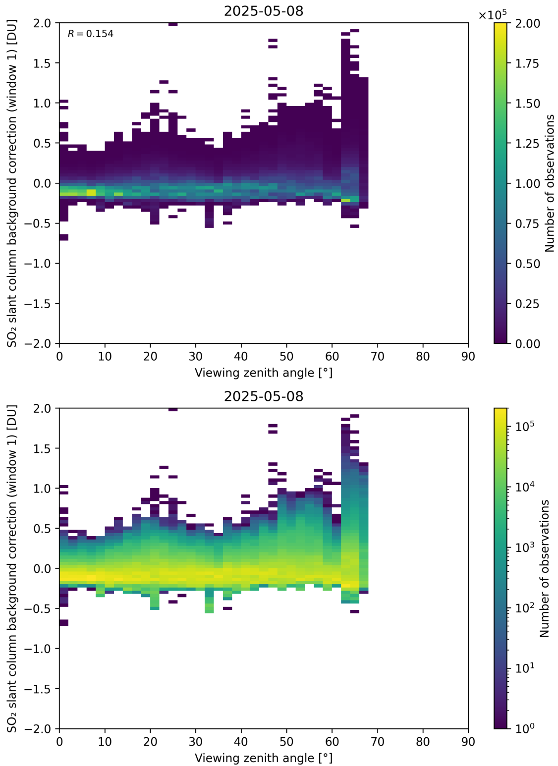
Figure 362: Scatter density plot of “Viewing zenith angle” against “SO 2 slant column background correction (window 1)” for 2025-05-07 to 2025-05-09.
