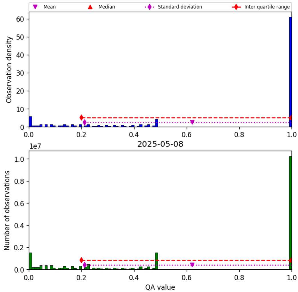
Figure 57: Histogram of “QA value” for 2025-05-07 to 2025-05-09
