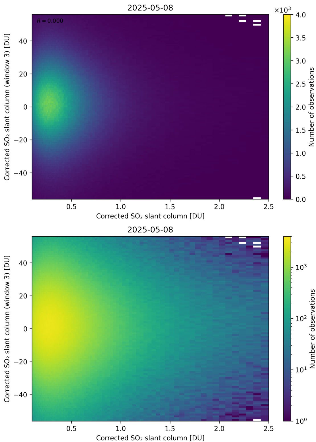
Figure 236: Scatter density plot of “Corrected SO 2 slant column” against “Corrected SO 2 slant column (window 3)” for 2025-05-07 to 2025-05-09.
