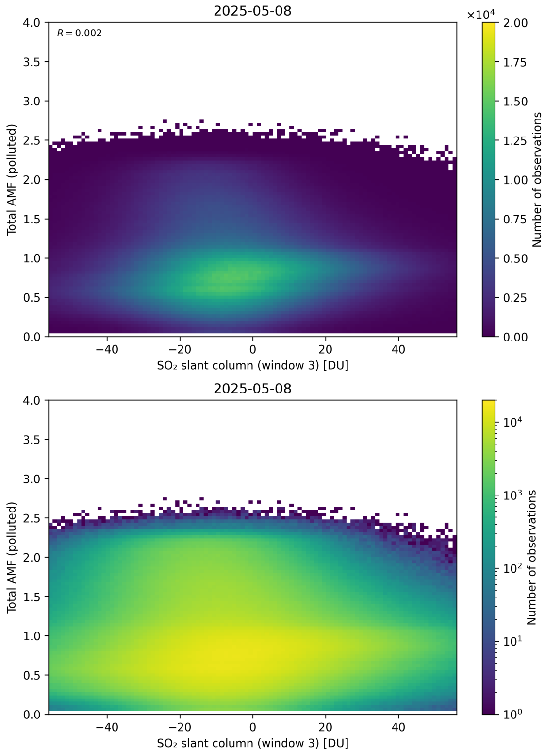
Figure 318: Scatter density plot of “SO 2 slant column (window 3)” against “Total AMF (polluted)” for 2025-05-07 to 2025-05-09.
