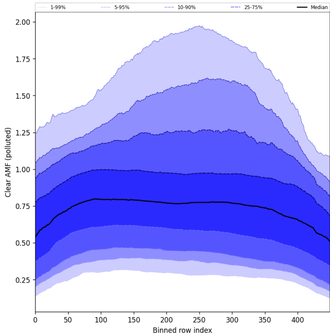
Figure 107: Along track statistics of “Clear AMF (polluted)” for 2025-05-07 to 2025-05-09
