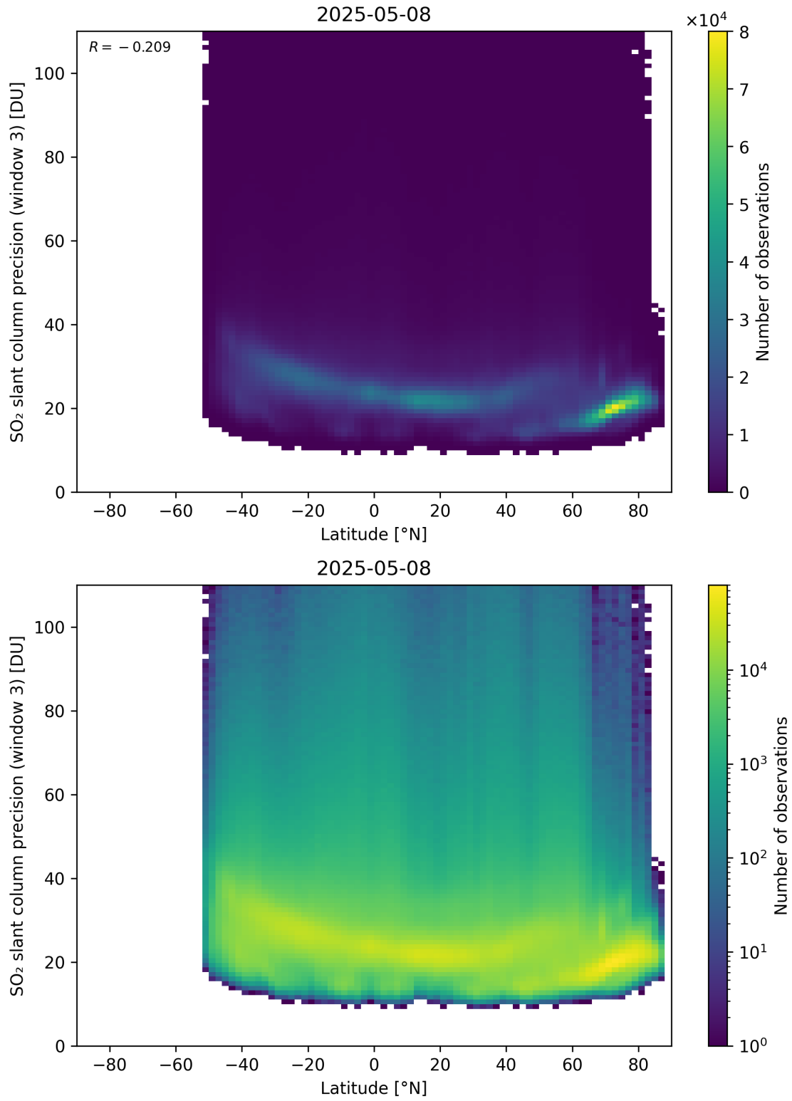
Figure 166: Scatter density plot of “Latitude” against “SO 2 slant column precision (window 3)” for 2025-05-07 to 2025-05-09.
