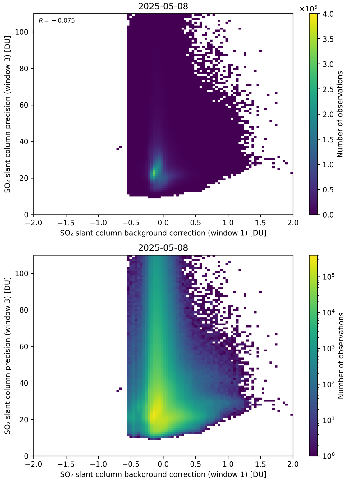
Figure 119: Scatter density plot of “SO 2 slant column background correction (window 1)” against “SO 2 slant column precision (window 3)” for 2025-05-07 to 2025-05-09.
