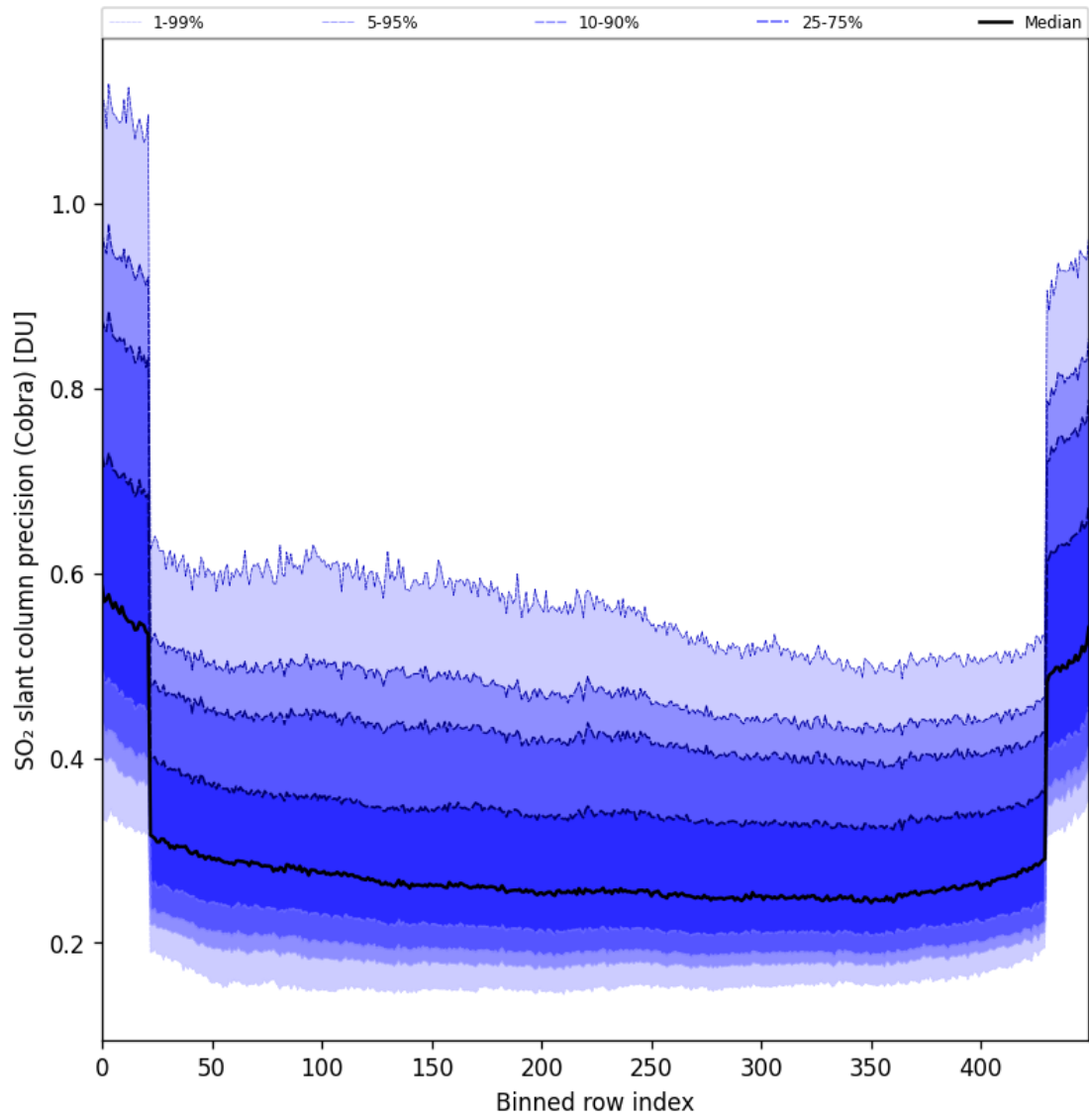
Figure 88: Along track statistics of “SO 2 slant column precision (Cobra)” for 2025-05-07 to 2025-05-09
