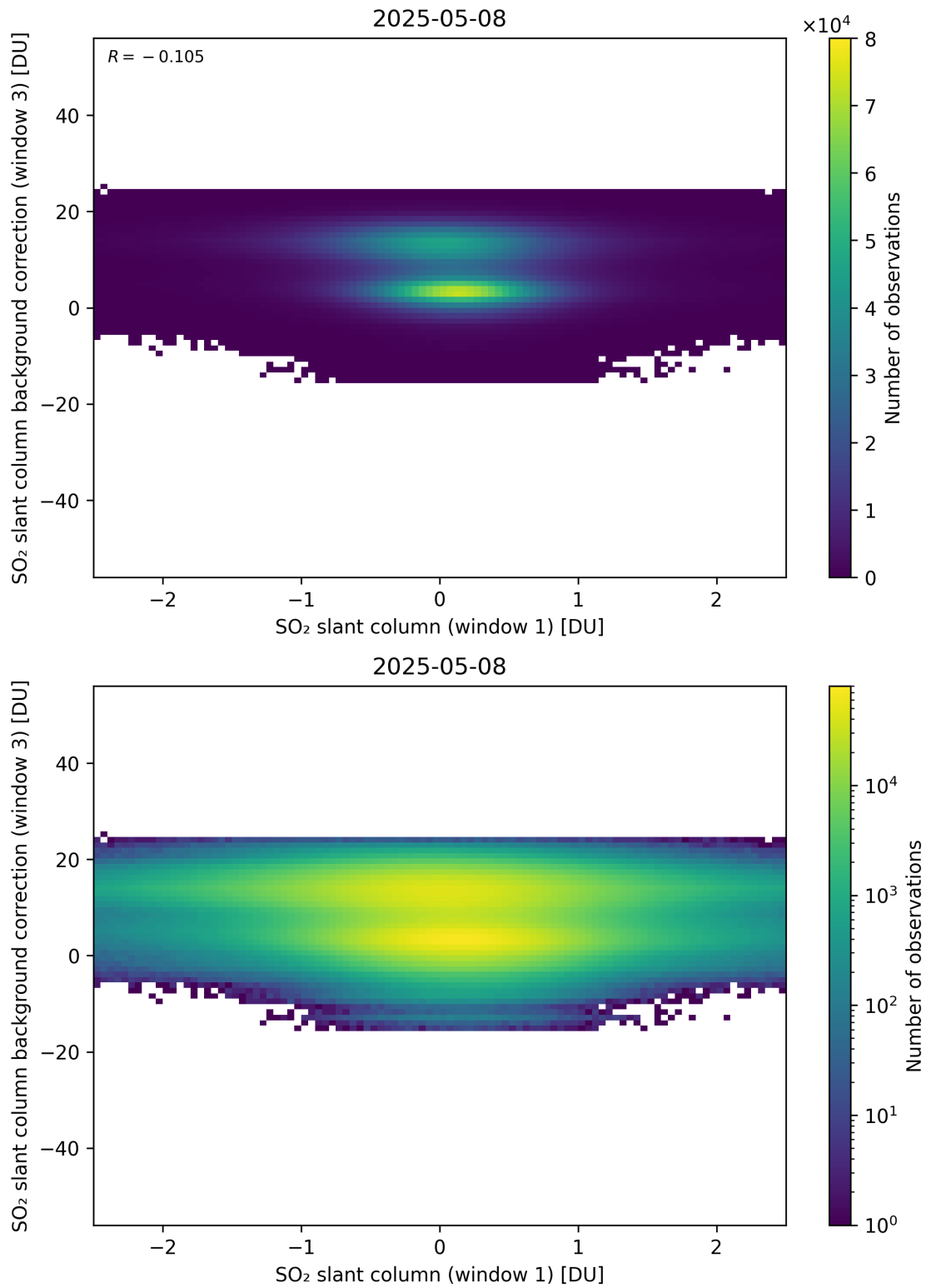
Figure 264: Scatter density plot of “SO 2 slant column (window 1)” against “SO 2 slant column background correction (window 3)” for 2025-05-07 to 2025-05-09.
