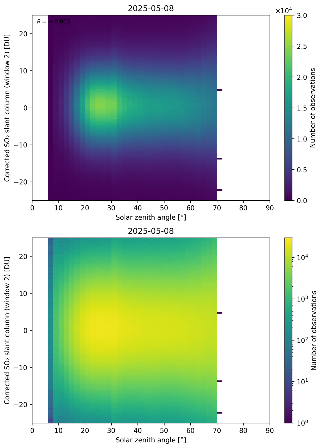
Figure 182: Scatter density plot of “Solar zenith angle” against “Corrected SO 2 slant column (window 2)” for 2025-05-07 to 2025-05-09.
