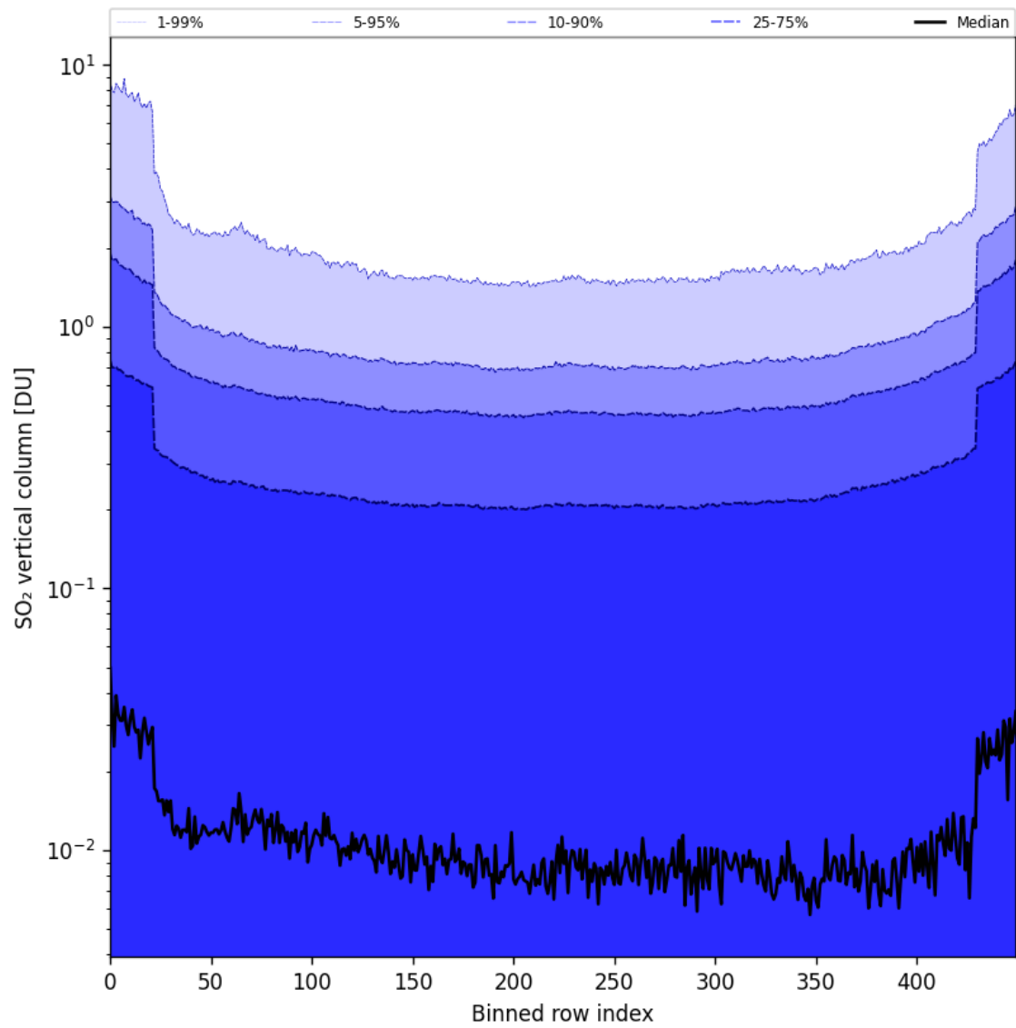
Figure 84: Along track statistics of “SO 2 vertical column” for 2025-05-07 to 2025-05-09
