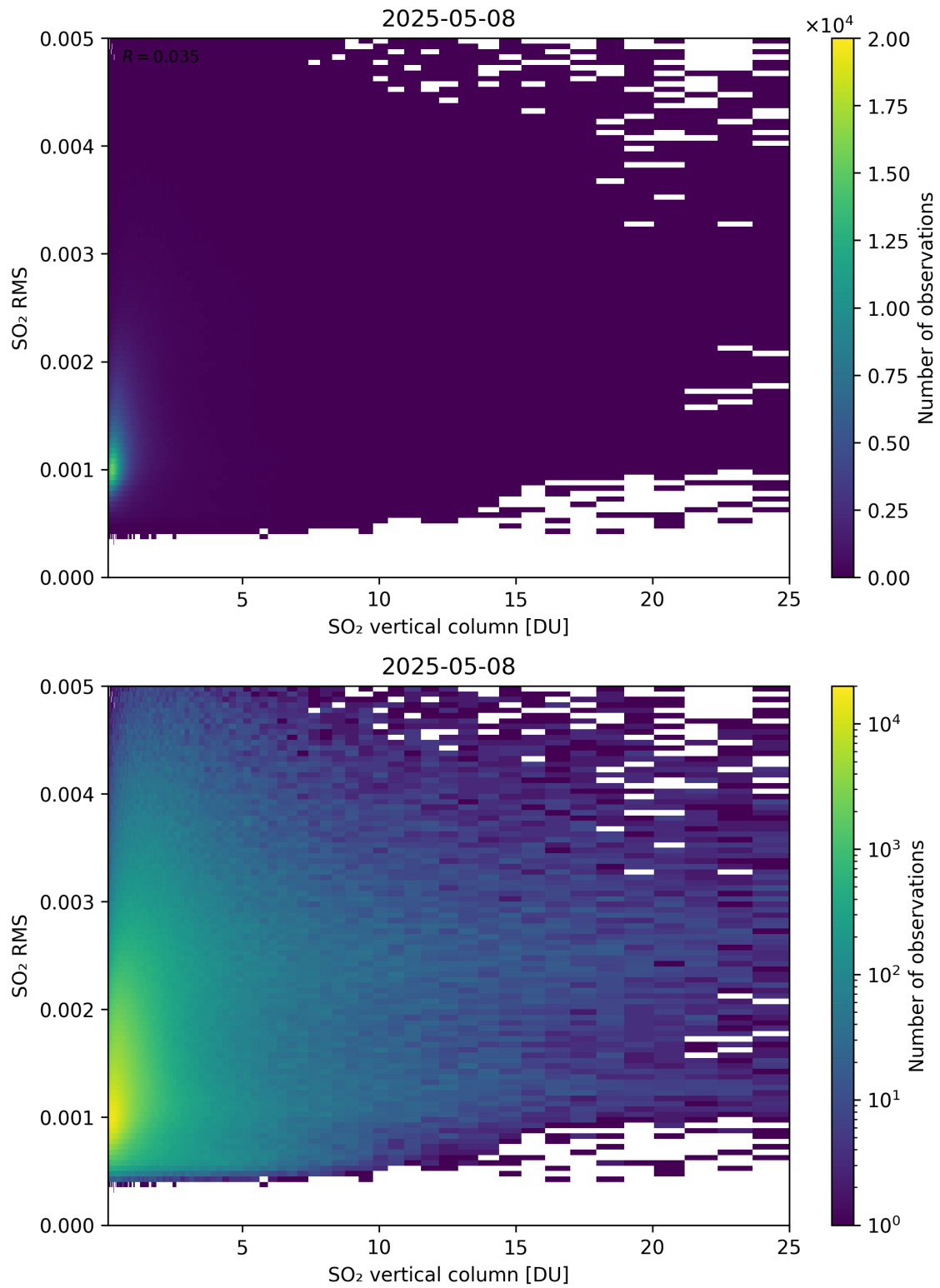
Figure 328: Scatter density plot of “SO 2 vertical column” against “SO 2 RMS” for 2025-05-07 to 2025-05-09.
