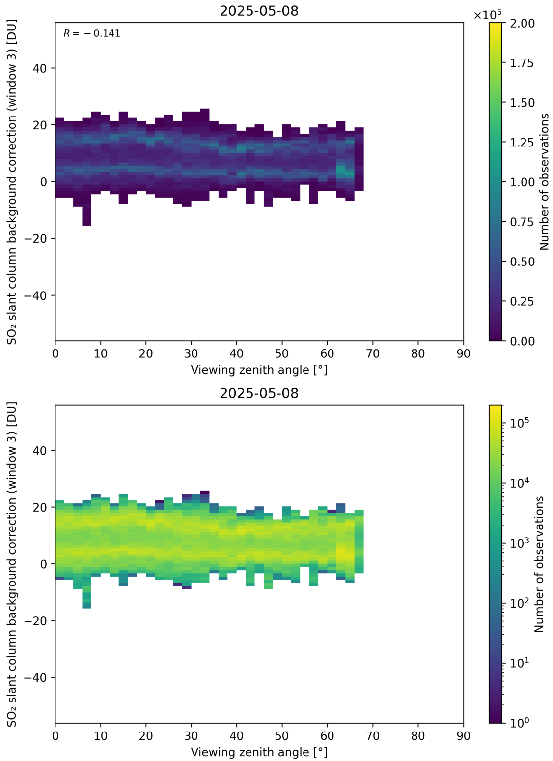
Figure 364: Scatter density plot of “Viewing zenith angle” against “SO 2 slant column background correction (window 3)” for 2025-05-07 to 2025-05-09.
