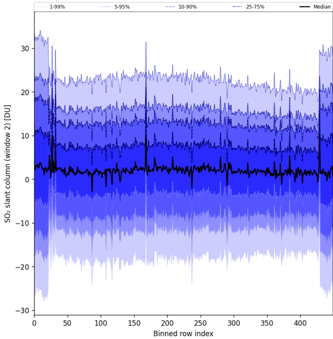
Figure 93: Along track statistics of “SO 2 slant column (window 2)” for 2025-05-07 to 2025-05-09
