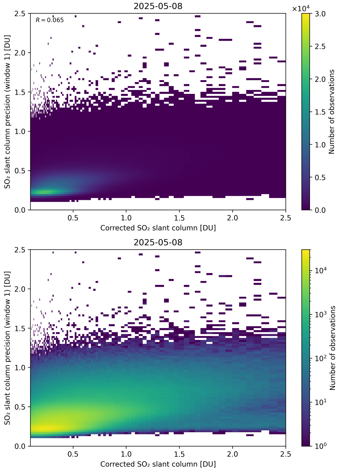
Figure 238: Scatter density plot of “Corrected SO 2 slant column” against “SO 2 slant column precision (window 1)” for 2025-05-07 to 2025-05-09.
