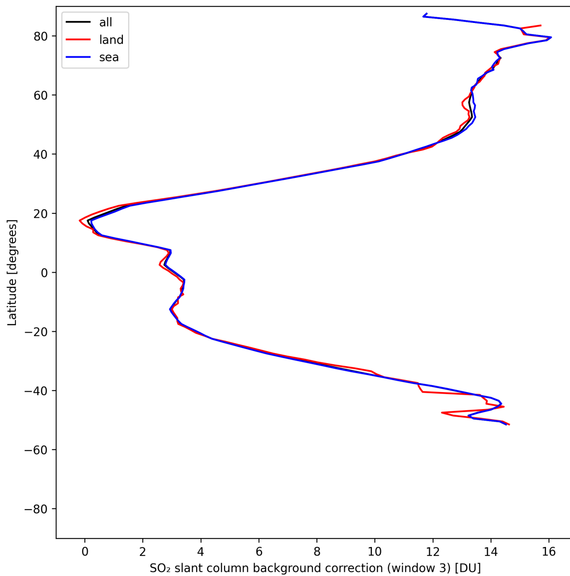
Figure 48: Zonal average of “SO 2 slant column background correction (window 3)” for 2025-05-07 to 2025-05-09.
