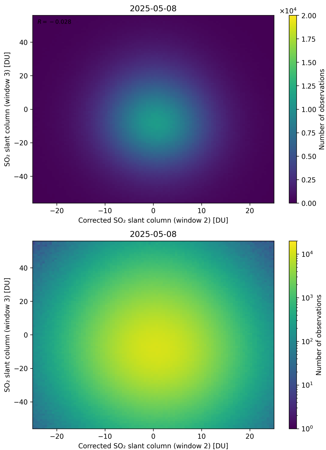
Figure 251: Scatter density plot of “Corrected SO 2 slant column (window 2)” against “SO 2 slant column (window 3)” for 2025-05-07 to 2025-05-09.
