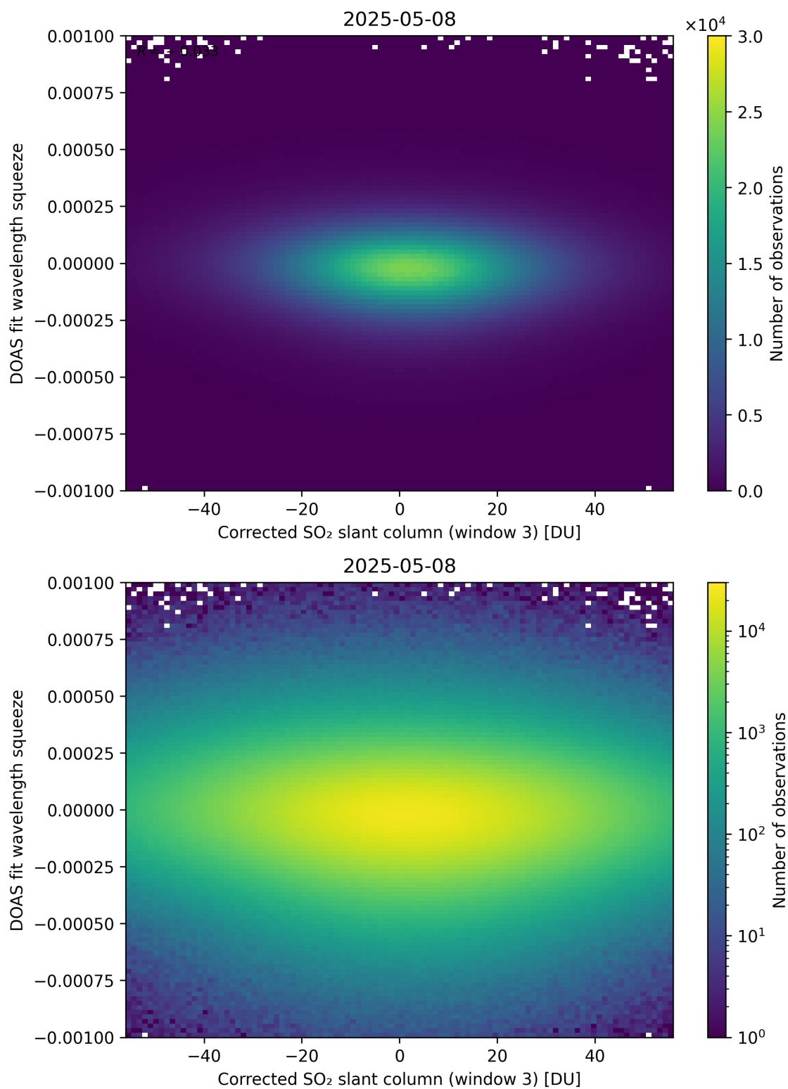
Figure 257: Scatter density plot of “Corrected SO 2 slant column (window 3)” against “DOAS fit wavelength squeeze” for 2025-05-07 to 2025-05-09.
