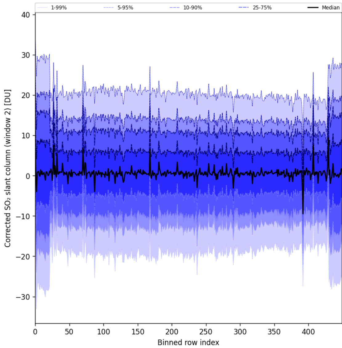
Figure 95: Along track statistics of “Corrected SO 2 slant column (window 2)” for 2025-05-07 to 2025-05-09
