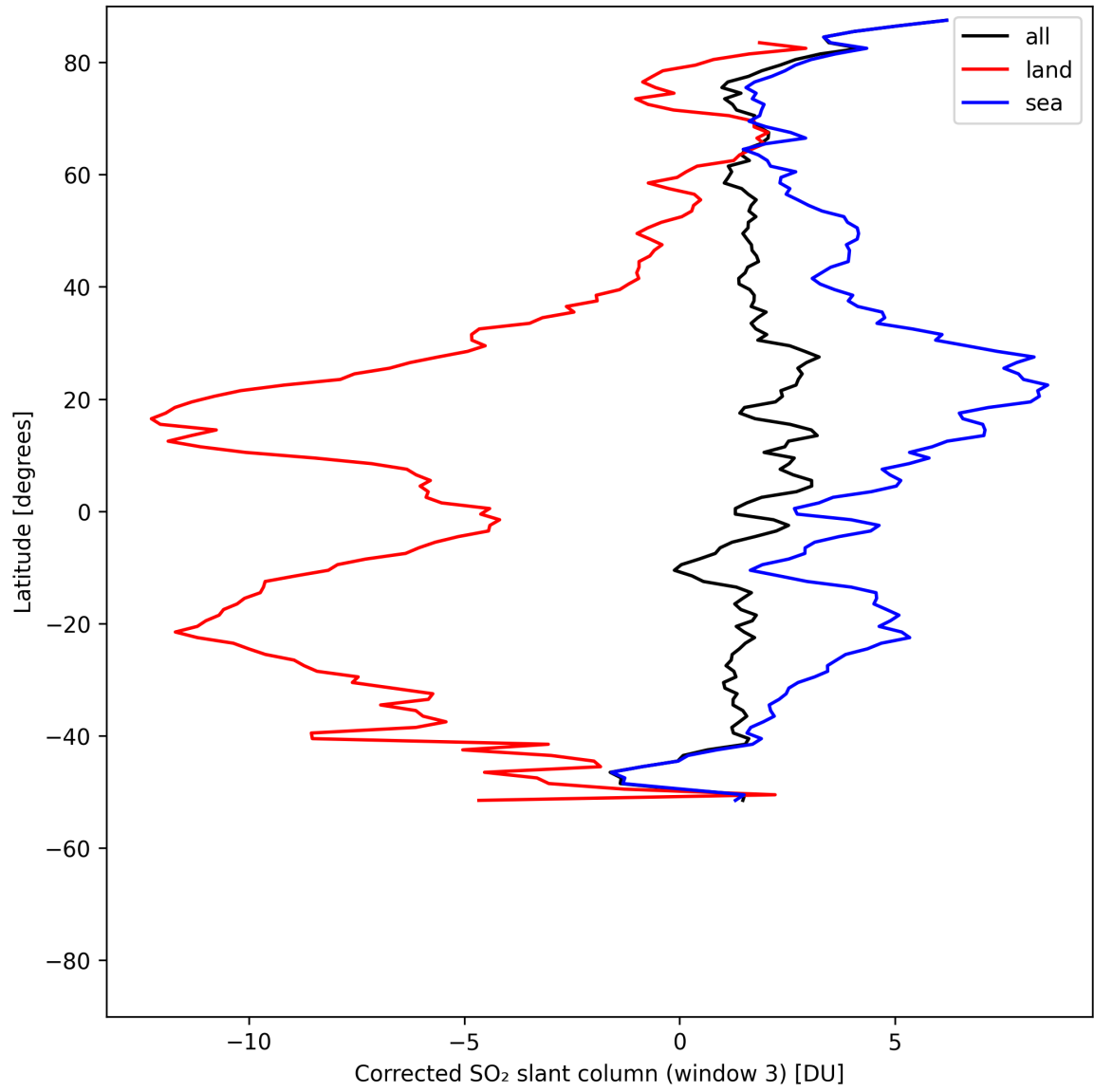
Figure 47: Zonal average of “Corrected SO 2 slant column (window 3)” for 2025-05-07 to 2025-05-09.
