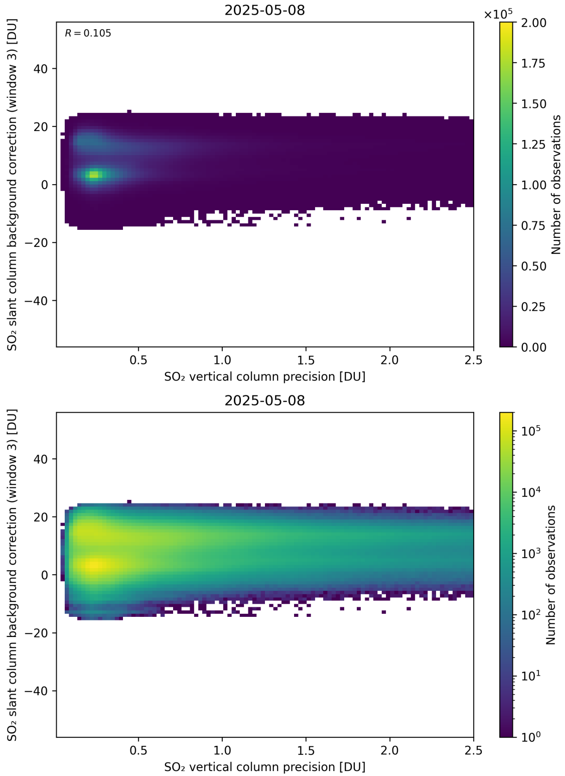
Figure 331: Scatter density plot of “SO 2 vertical column precision” against “SO 2 slant column background correction (window 3)” for 2025-05-07 to 2025-05-09.
