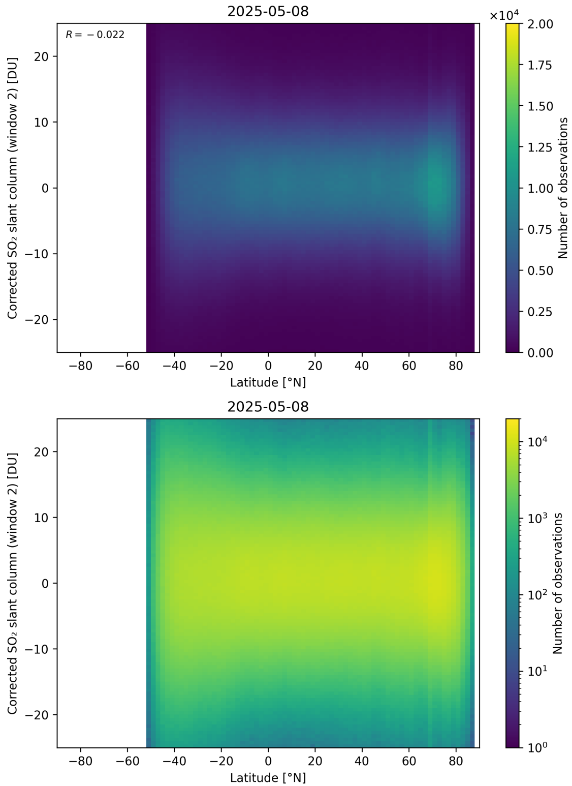
Figure 160: Scatter density plot of “Latitude” against “Corrected SO 2 slant column (window 2)” for 2025-05-07 to 2025-05-09.
