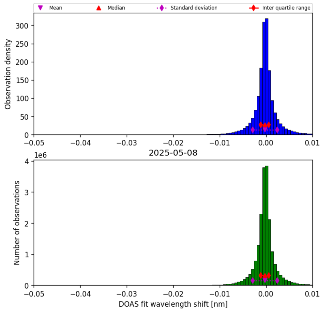
Figure 76: Histogram of “DOAS fit wavelength shift” for 2025-05-07 to 2025-05-09
