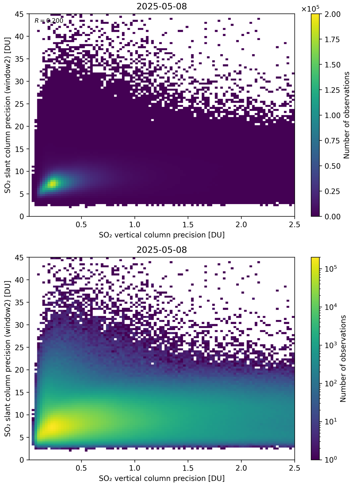
Figure 343: Scatter density plot of “SO 2 vertical column precision” against “SO 2 slant column precision (window2)” for 2025-05-07 to 2025-05-09.
