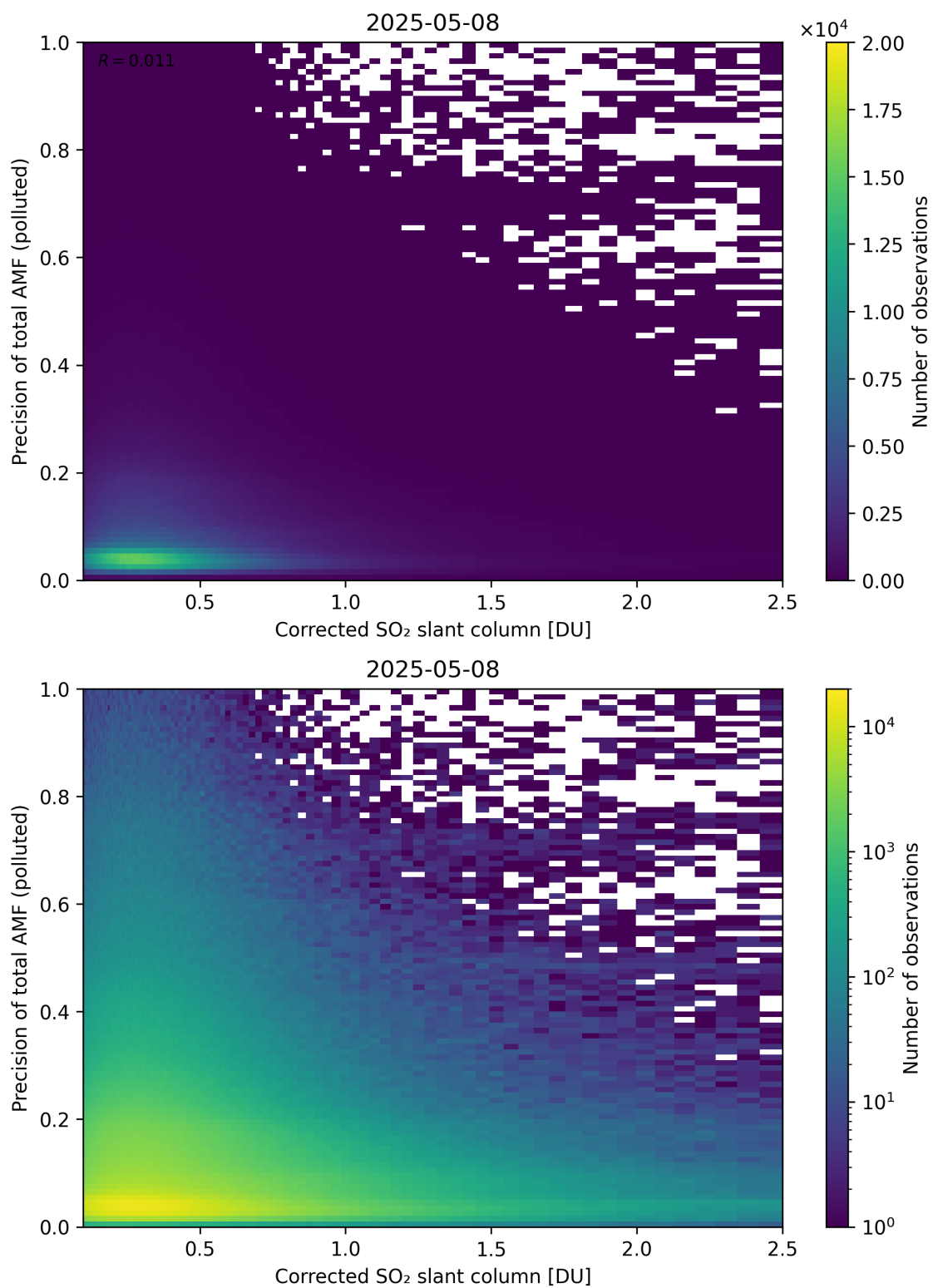
Figure 243: Scatter density plot of “Corrected SO 2 slant column” against “Precision of total AMF (polluted)” for 2025-05-07 to 2025-05-09.
