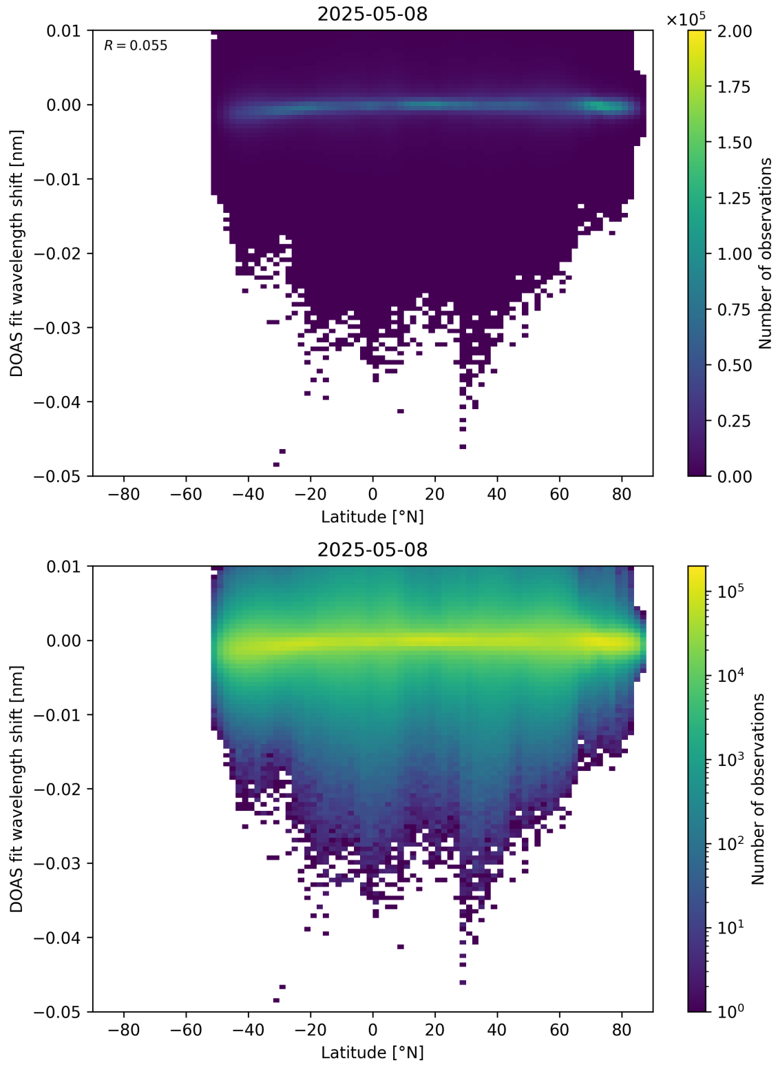
Figure 153: Scatter density plot of “Latitude” against “DOAS fit wavelength shift” for 2025-05-07 to 2025-05-09.
