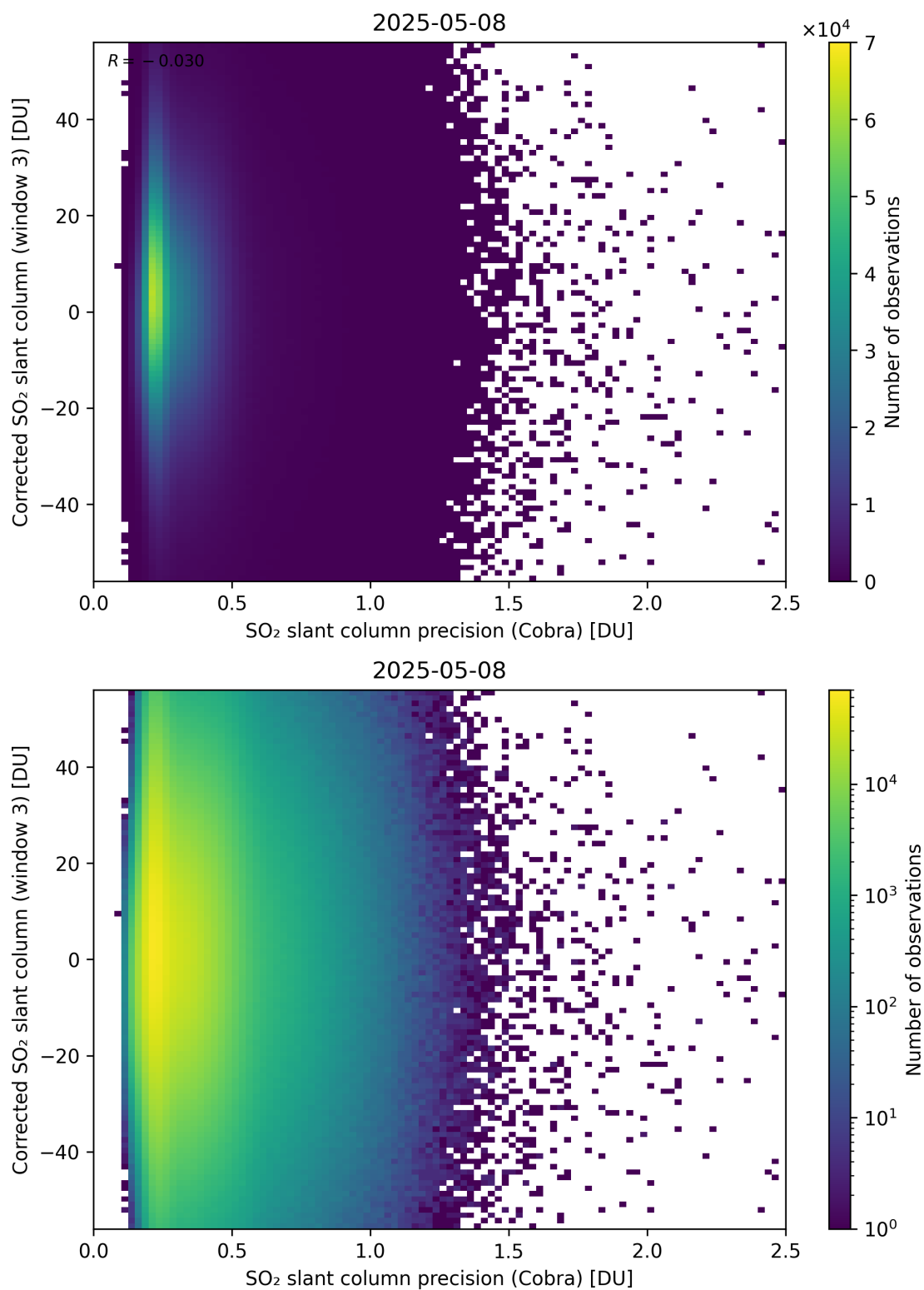
Figure 207: Scatter density plot of “SO 2 slant column precision (Cobra)” against “Corrected SO 2 slant column (window 3)” for 2025-05-07 to 2025-05-09.
