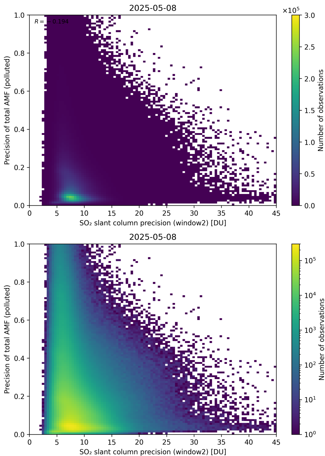
Figure 302: Scatter density plot of “SO 2 slant column precision (window2)” against “Precision of total AMF (polluted)” for 2025-05-07 to 2025-05-09.
