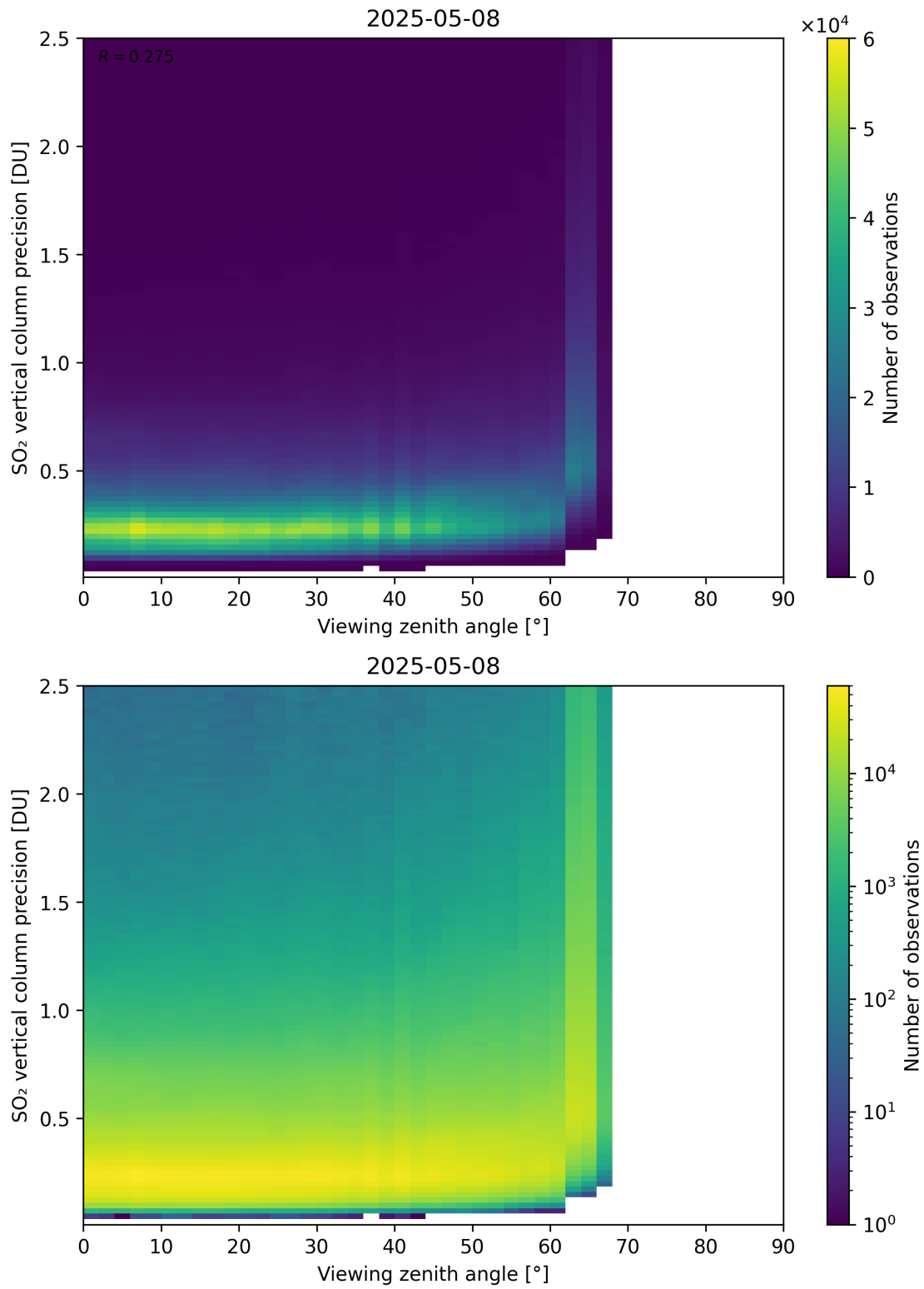
Figure 384: Scatter density plot of “Viewing zenith angle” against “SO 2 vertical column precision” for 2025-05-07 to 2025-05-09.
