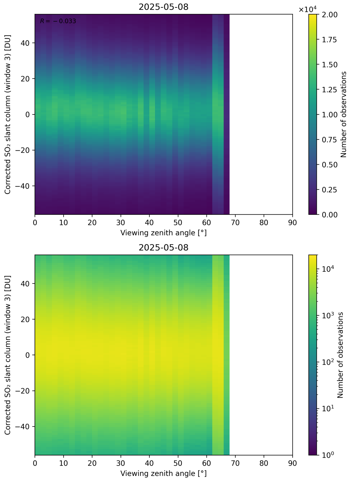
Figure 375: Scatter density plot of “Viewing zenith angle” against “Corrected SO 2 slant column (window 3)” for 2025-05-07 to 2025-05-09.
