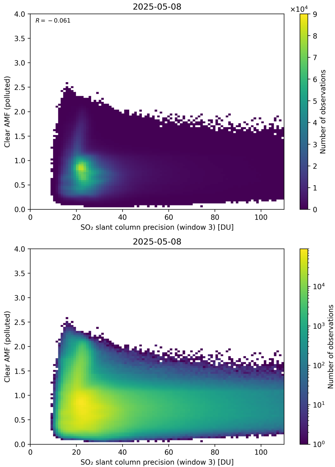
Figure 311: Scatter density plot of “SO 2 slant column precision (window 3)” against “Clear AMF (polluted)” for 2025-05-07 to 2025-05-09.
