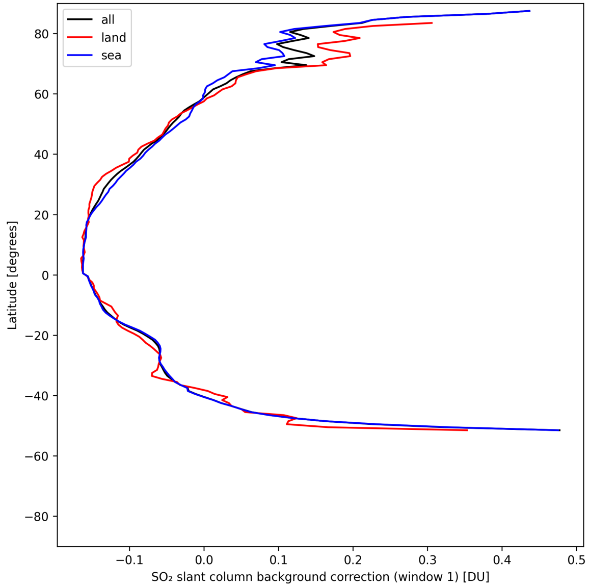
Figure 40: Zonal average of “SO 2 slant column background correction (window 1)” for 2025-05-07 to 2025-05-09.
