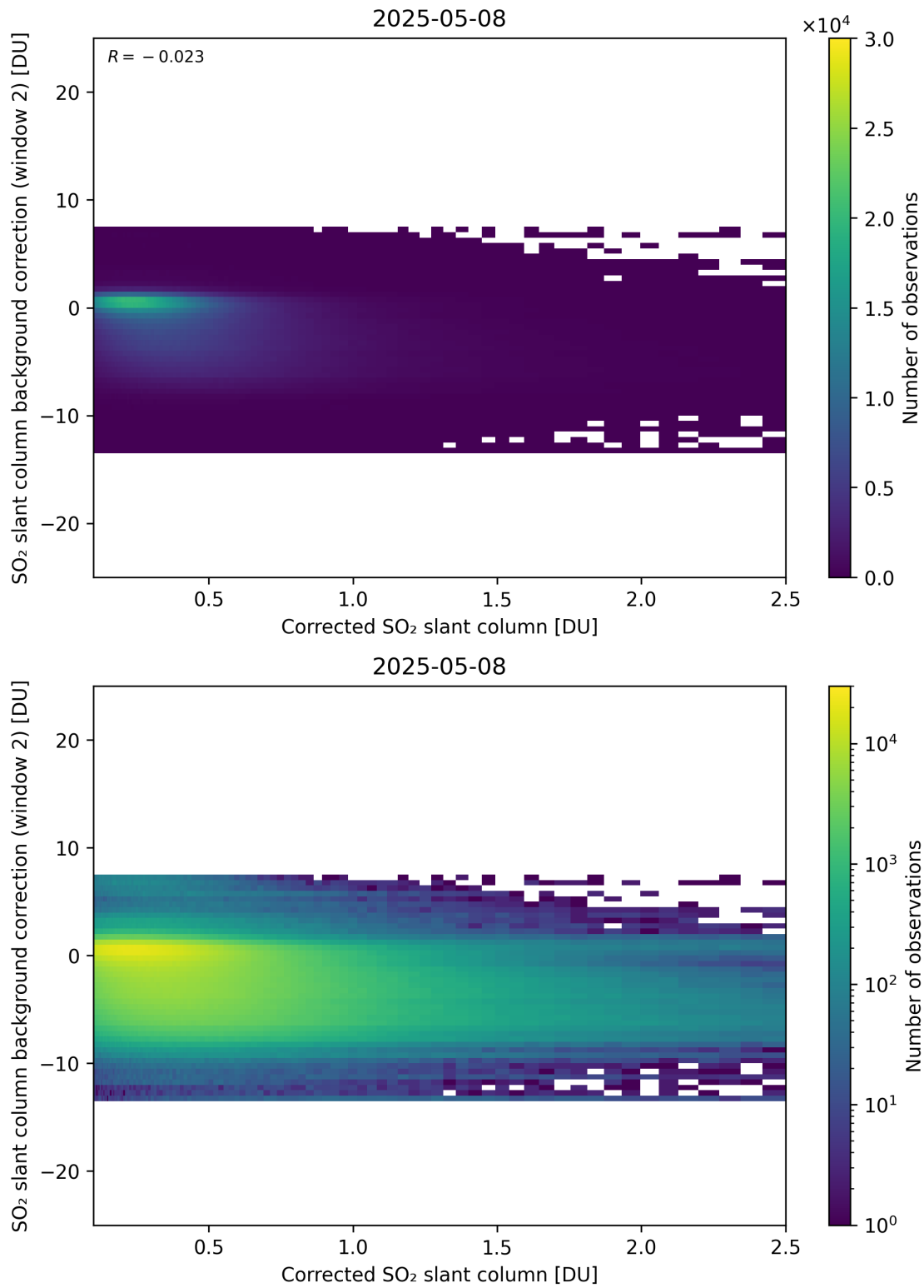
Figure 227: Scatter density plot of “Corrected SO 2 slant column” against “SO 2 slant column background correction (window 2)” for 2025-05-07 to 2025-05-09.
