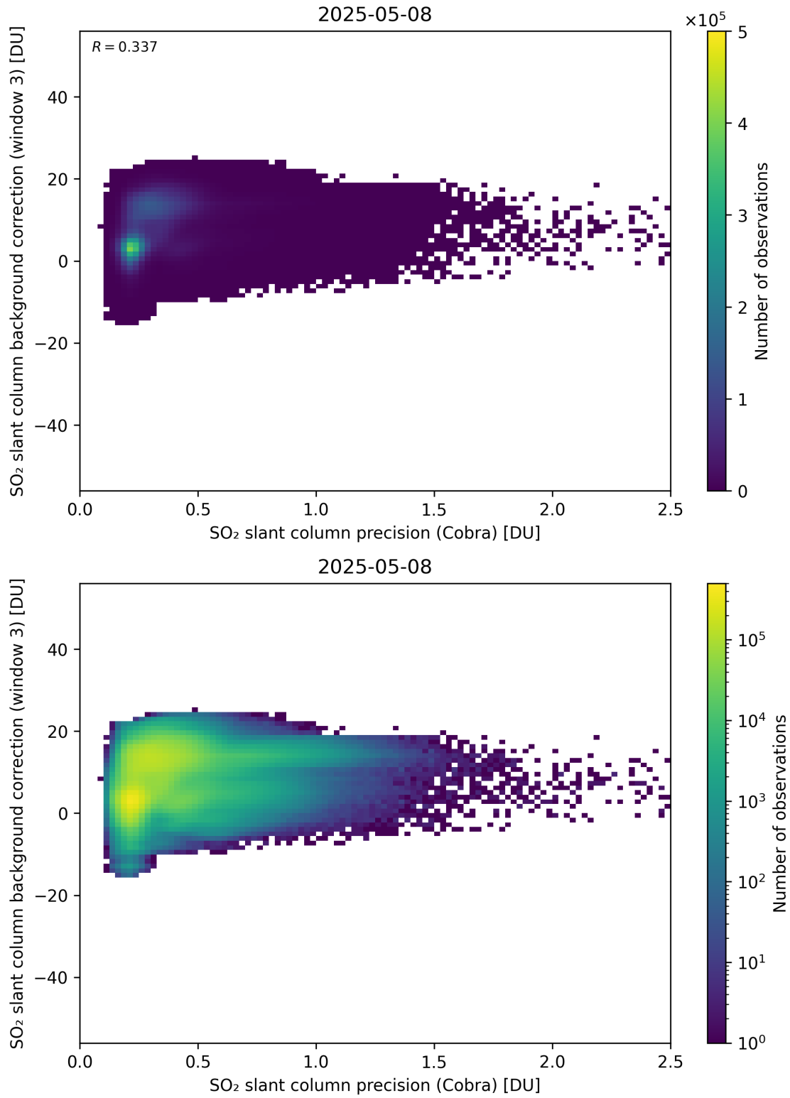
Figure 201: Scatter density plot of “SO 2 slant column precision (Cobra)” against “SO 2 slant column background correction (window 3)” for 2025-05-07 to 2025-05-09.
