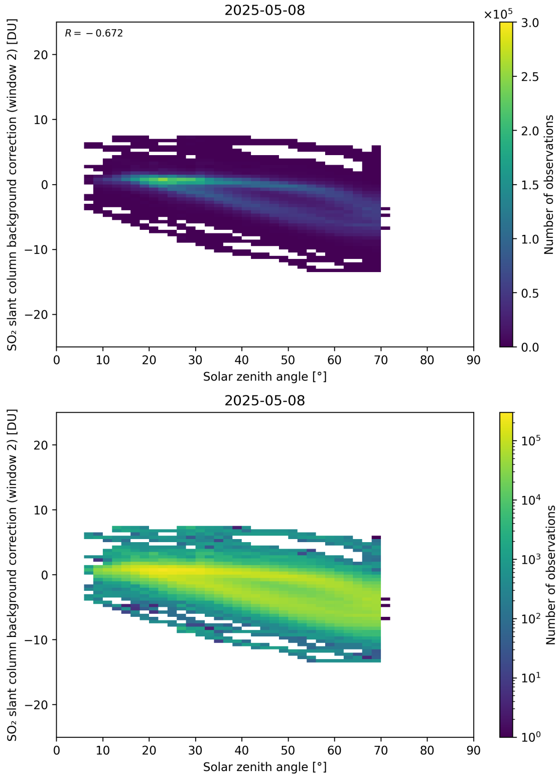
Figure 172: Scatter density plot of “Solar zenith angle” against “SO 2 slant column background correction (window 2)” for 2025-05-07 to 2025-05-09.
