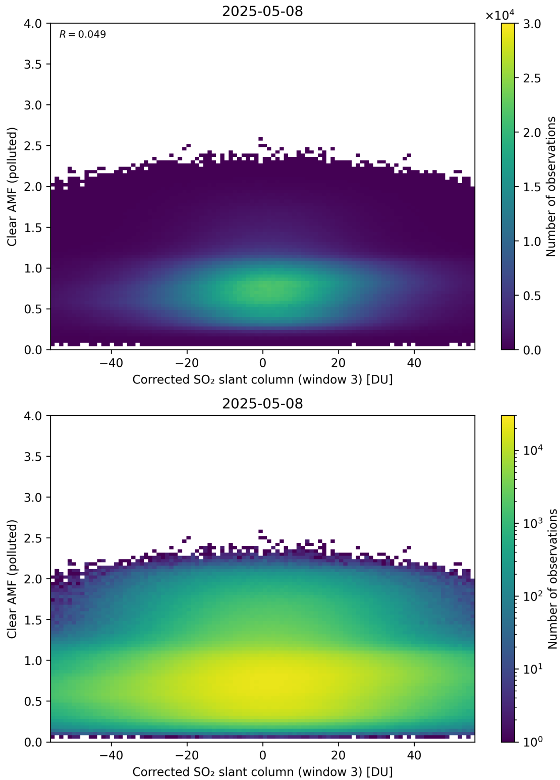
Figure 259: Scatter density plot of “Corrected SO 2 slant column (window 3)” against “Clear AMF (polluted)” for 2025-05-07 to 2025-05-09.
