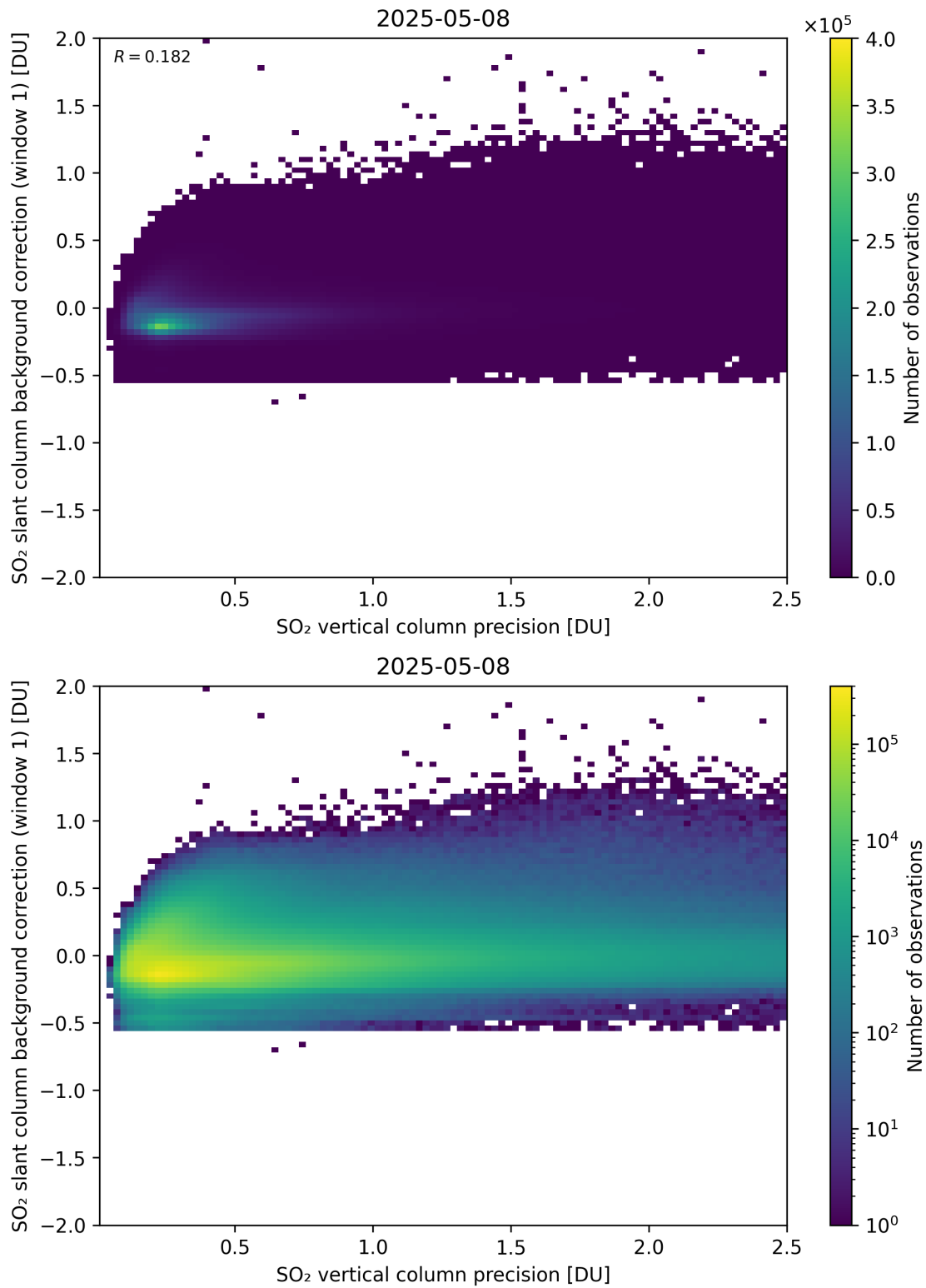
Figure 329: Scatter density plot of “SO 2 vertical column precision” against “SO 2 slant column background correction (window 1)” for 2025-05-07 to 2025-05-09.
