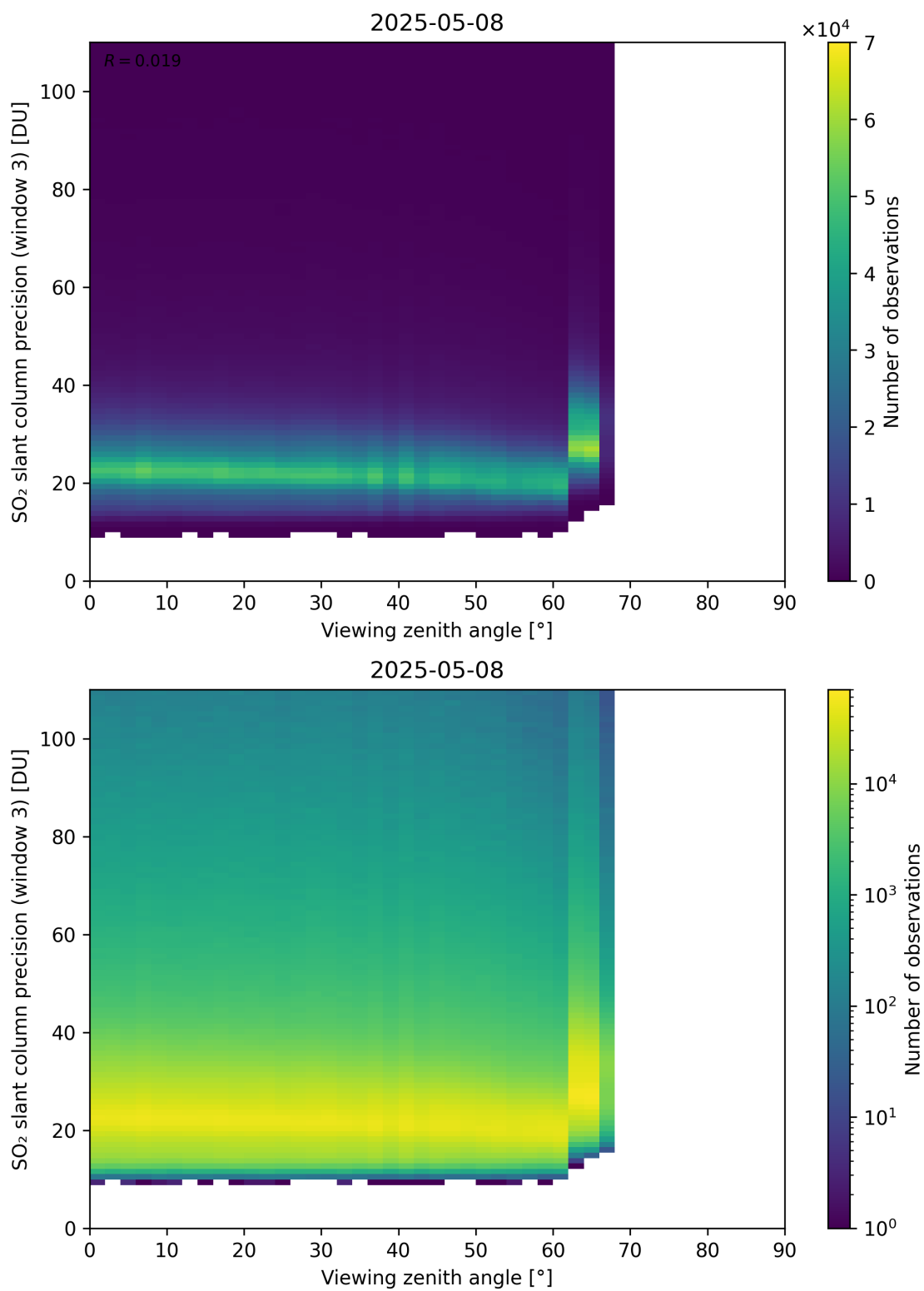
Figure 380: Scatter density plot of “Viewing zenith angle” against “SO 2 slant column precision (window 3)” for 2025-05-07 to 2025-05-09.
