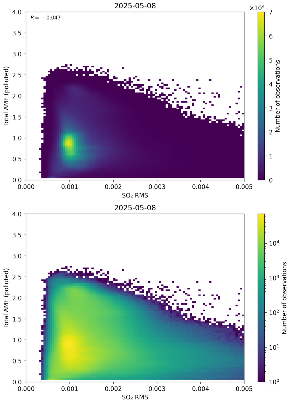
Figure 148: Scatter density plot of “SO 2 RMS” against “Total AMF (polluted)” for 2025-05-07 to 2025-05-09.
