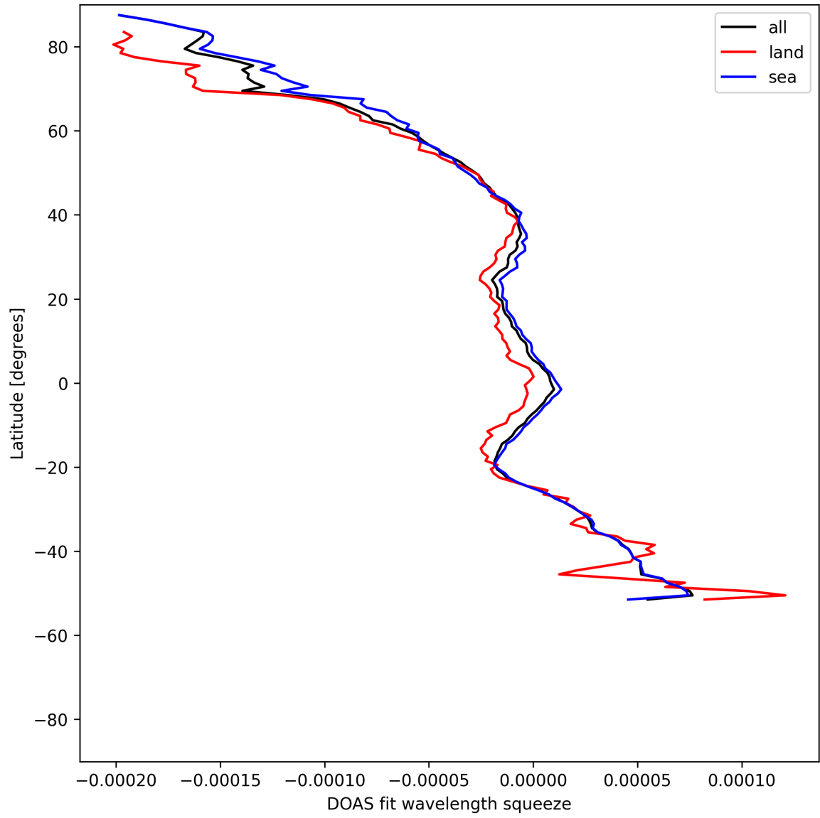
Figure 51: Zonal average of “DOAS fit wavelength squeeze” for 2025-05-07 to 2025-05-09.
