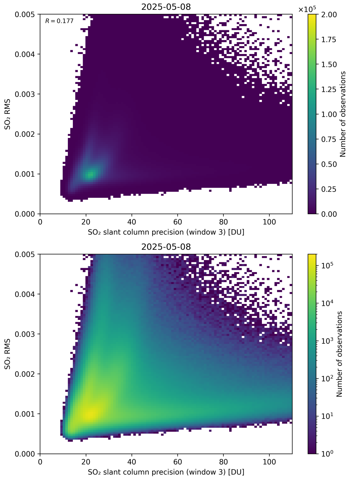
Figure 310: Scatter density plot of “SO 2 slant column precision (window 3)” against “SO 2 RMS” for 2025-05-07 to 2025-05-09.
