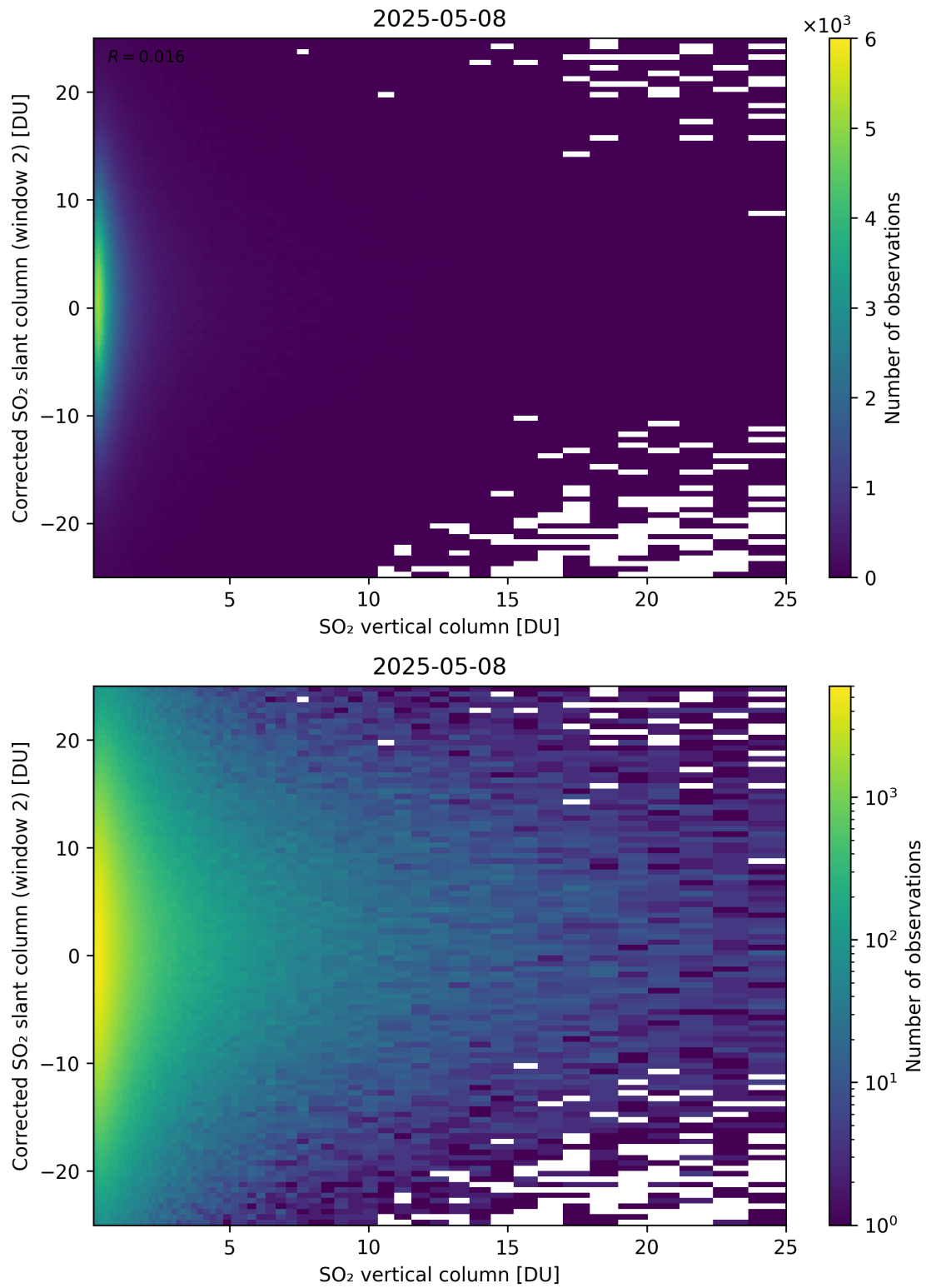
Figure 352: Scatter density plot of “SO 2 vertical column” against “Corrected SO 2 slant column (window 2)” for 2025-05-07 to 2025-05-09.
