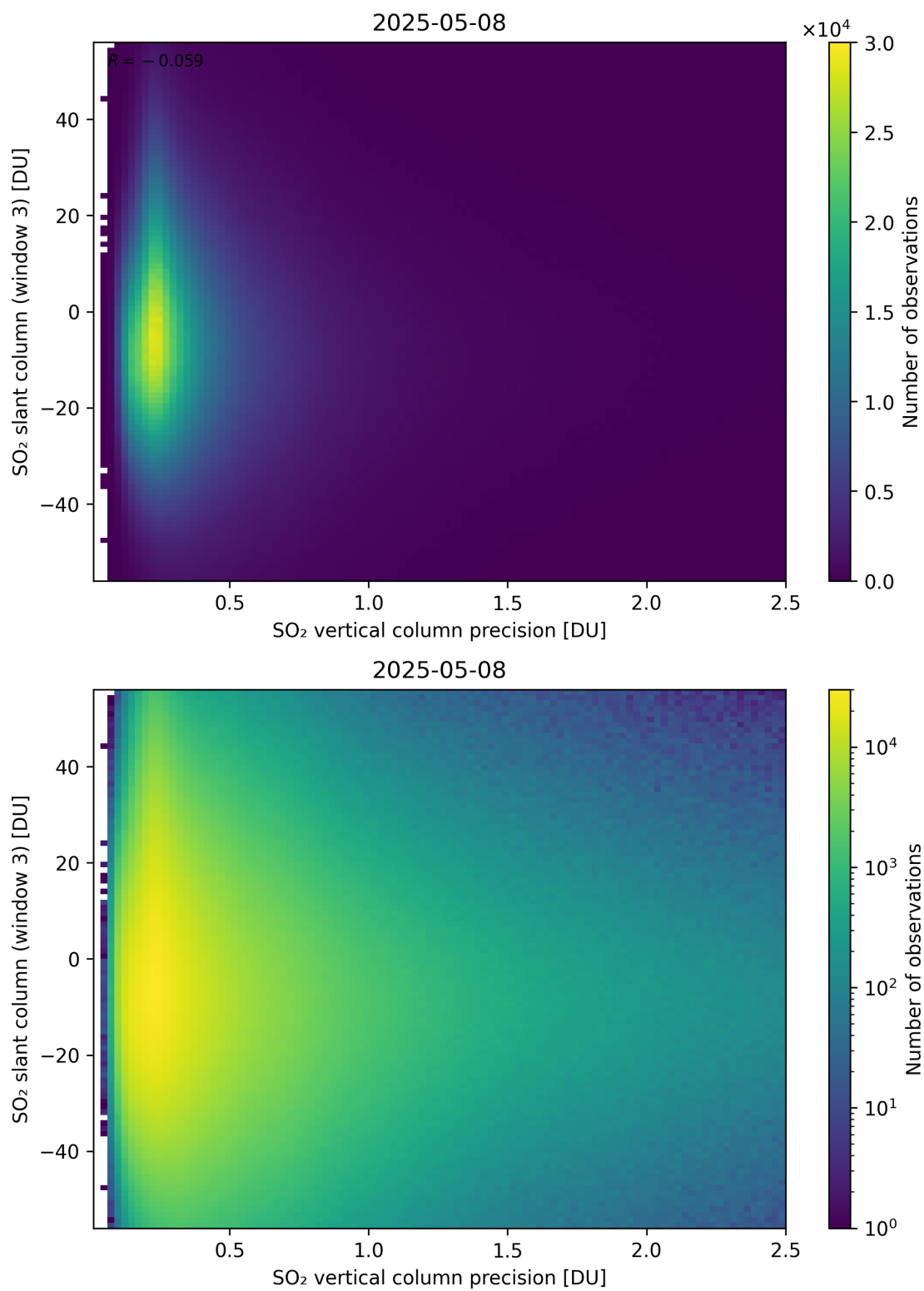
Figure 344: Scatter density plot of “SO 2 vertical column precision” against “SO 2 slant column (window 3)” for 2025-05-07 to 2025-05-09.
