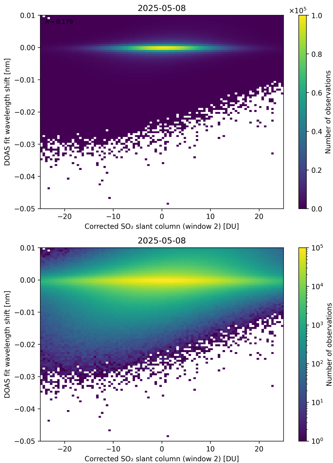
Figure 246: Scatter density plot of “Corrected SO 2 slant column (window 2)” against “DOAS fit wavelength shift” for 2025-05-07 to 2025-05-09.
