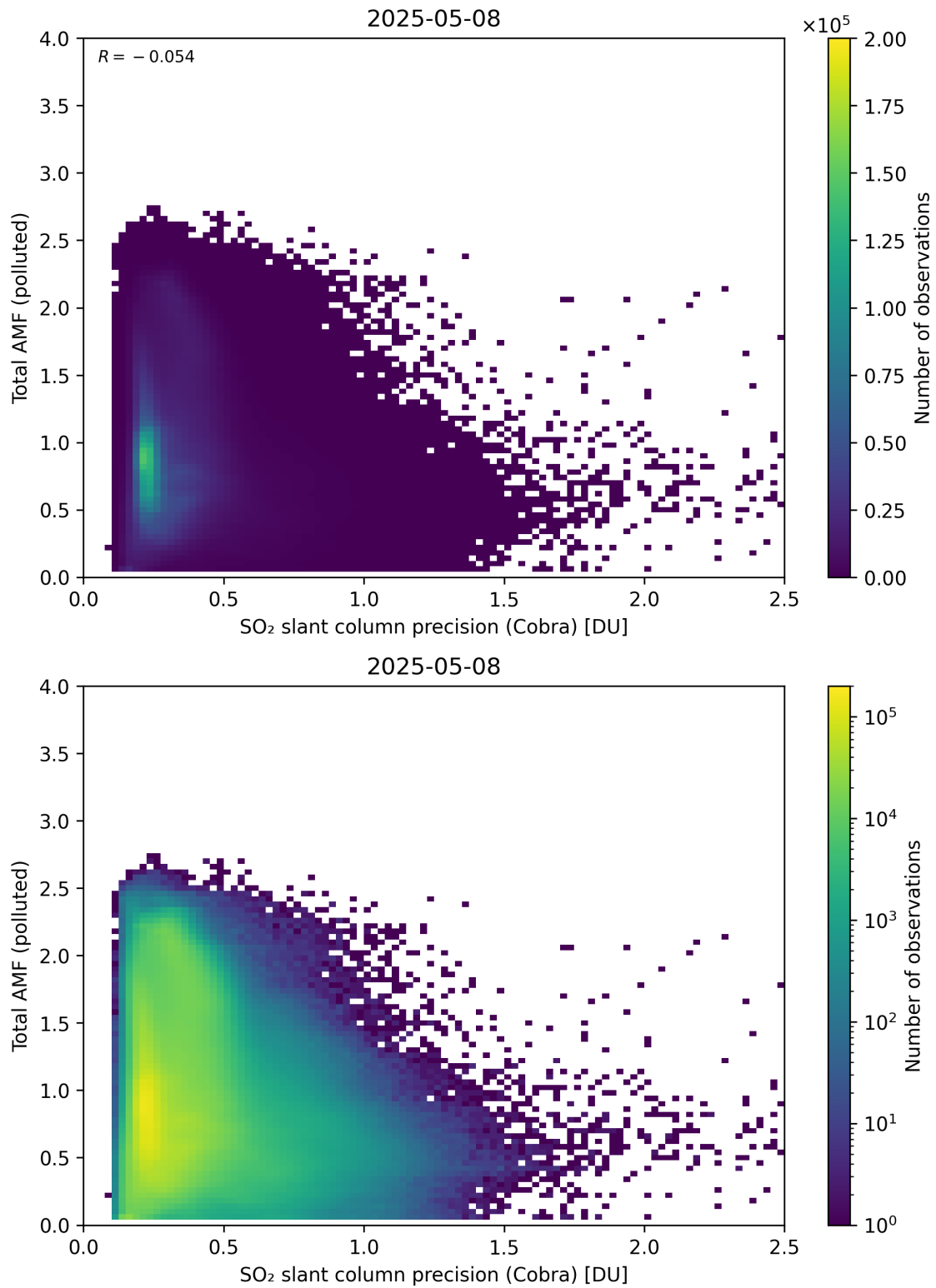
Figure 213: Scatter density plot of “SO 2 slant column precision (Cobra)” against “Total AMF (polluted)” for 2025-05-07 to 2025-05-09.
