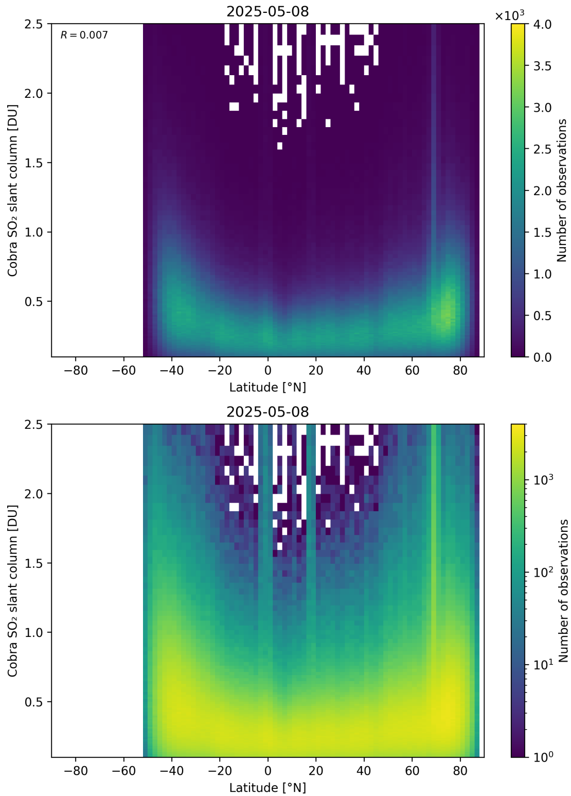
Figure 157: Scatter density plot of “Latitude” against “Cobra SO 2 slant column” for 2025-05-07 to 2025-05-09.
