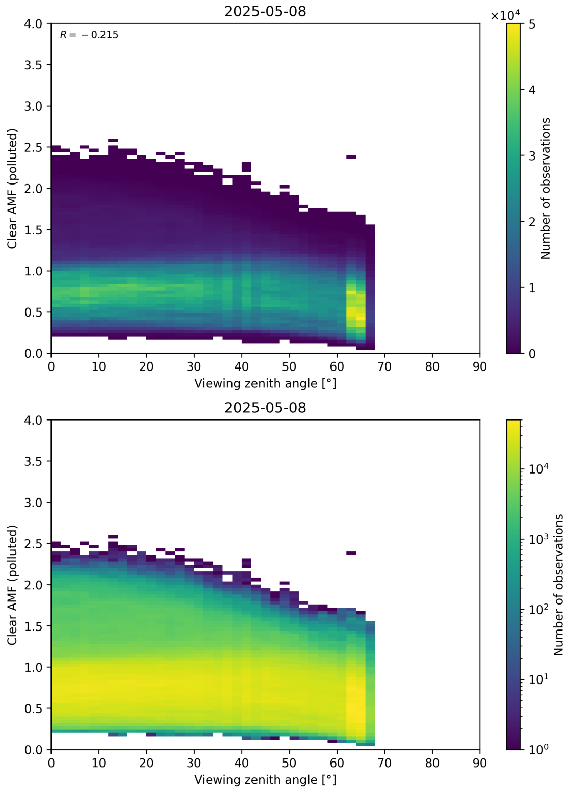
Figure 370: Scatter density plot of “Viewing zenith angle” against “Clear AMF (polluted)” for 2025-05-07 to 2025-05-09.
