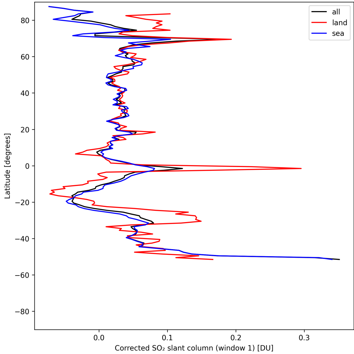
Figure 39: Zonal average of “Corrected SO 2 slant column (window 1)” for 2025-05-07 to 2025-05-09.
