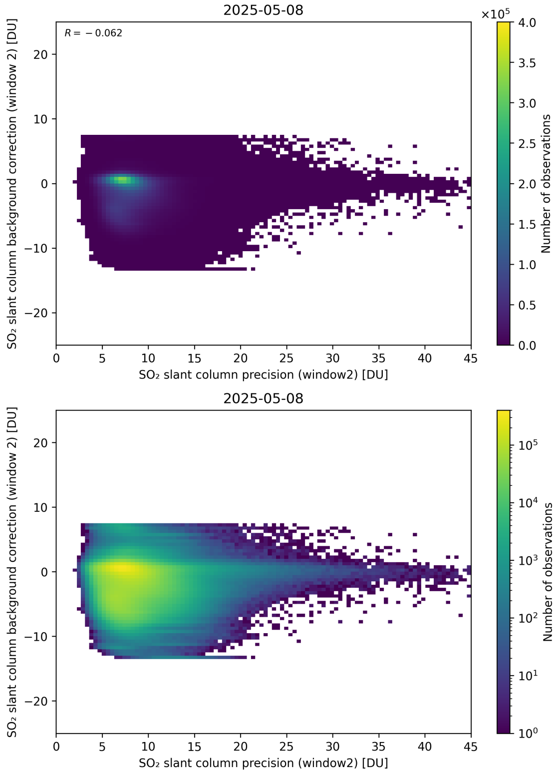
Figure 291: Scatter density plot of “SO 2 slant column precision (window2)” against “SO 2 slant column background correction (window 2)” for 2025-05-07 to 2025-05-09.
