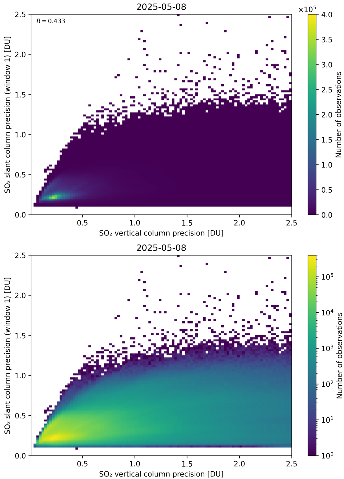
Figure 342: Scatter density plot of “SO 2 vertical column precision” against “SO 2 slant column precision (window 1)” for 2025-05-07 to 2025-05-09.
