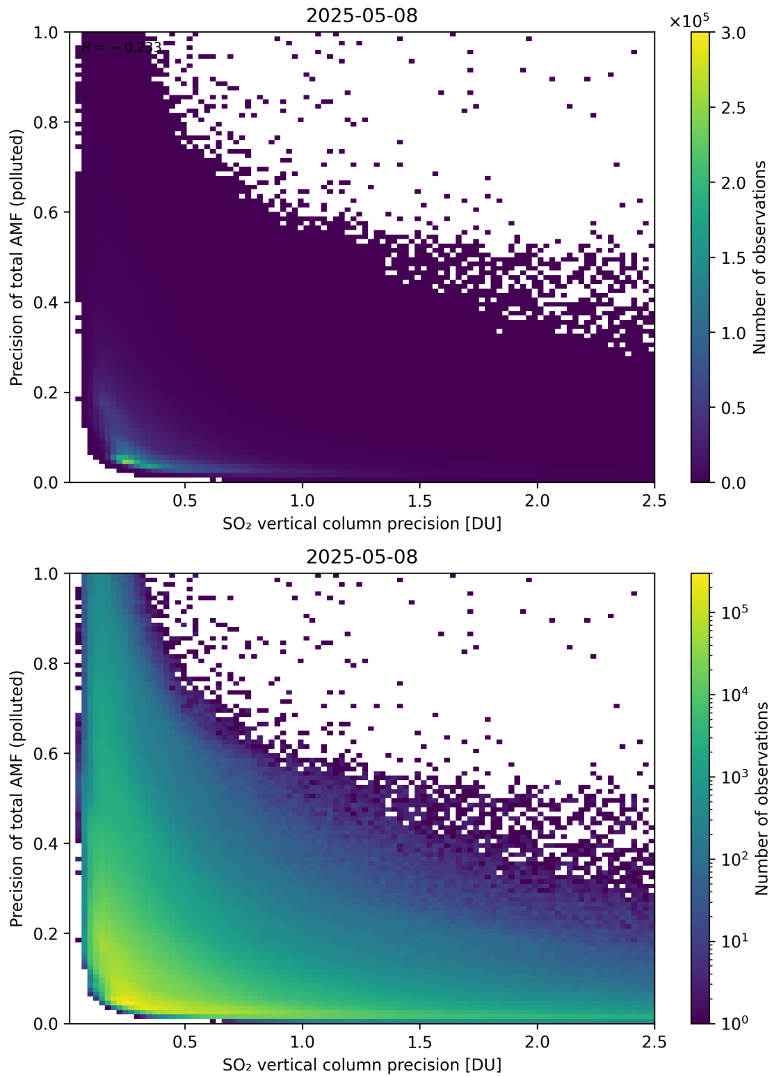
Figure 347: Scatter density plot of “SO 2 vertical column precision” against “Precision of total AMF (polluted)” for 2025-05-07 to 2025-05-09.
