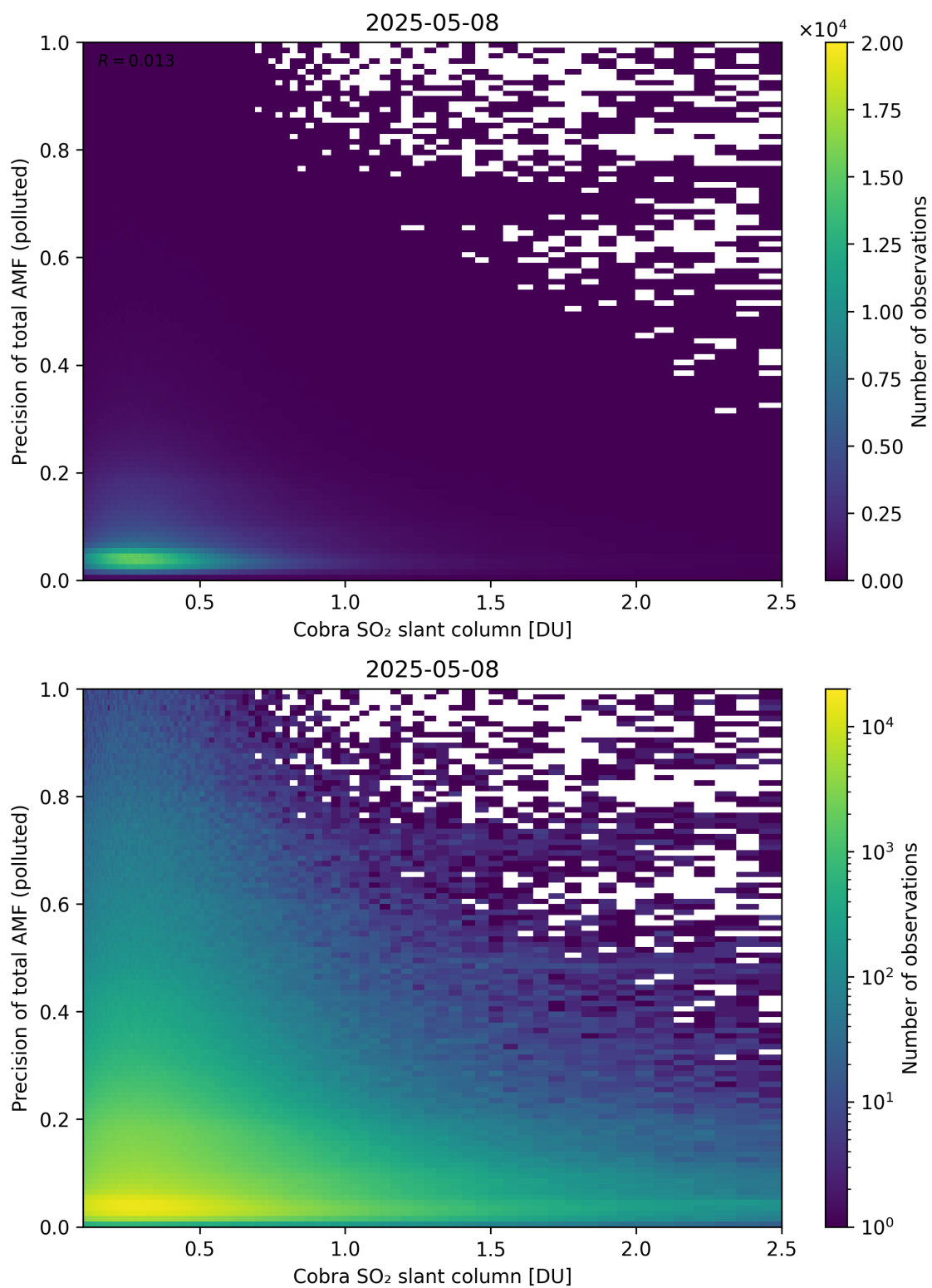
Figure 225: Scatter density plot of “Cobra SO 2 slant column” against “Precision of total AMF (polluted)” for 2025-05-07 to 2025-05-09.
