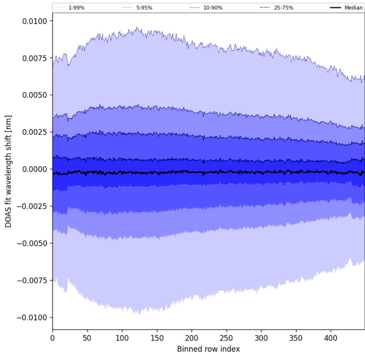
Figure 102: Along track statistics of “DOAS fit wavelength shift” for 2025-05-07 to 2025-05-09
