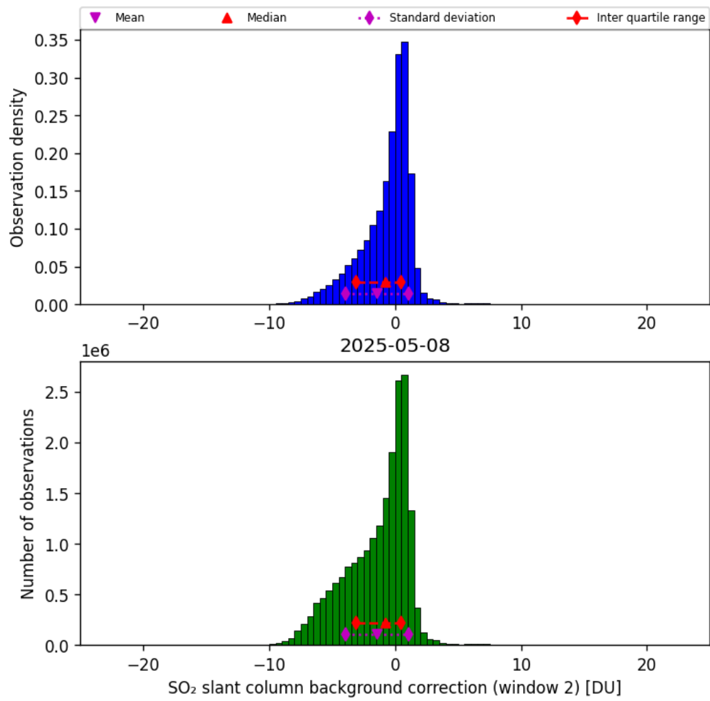
Figure 70: Histogram of “SO 2 slant column background correction (window 2)” for 2025-05-07 to 2025-05-09
