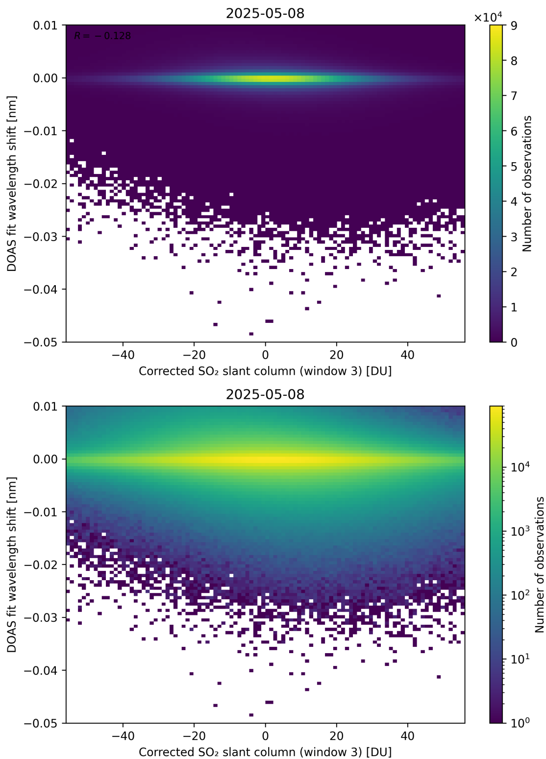
Figure 256: Scatter density plot of “Corrected SO 2 slant column (window 3)” against “DOAS fit wavelength shift” for 2025-05-07 to 2025-05-09.
