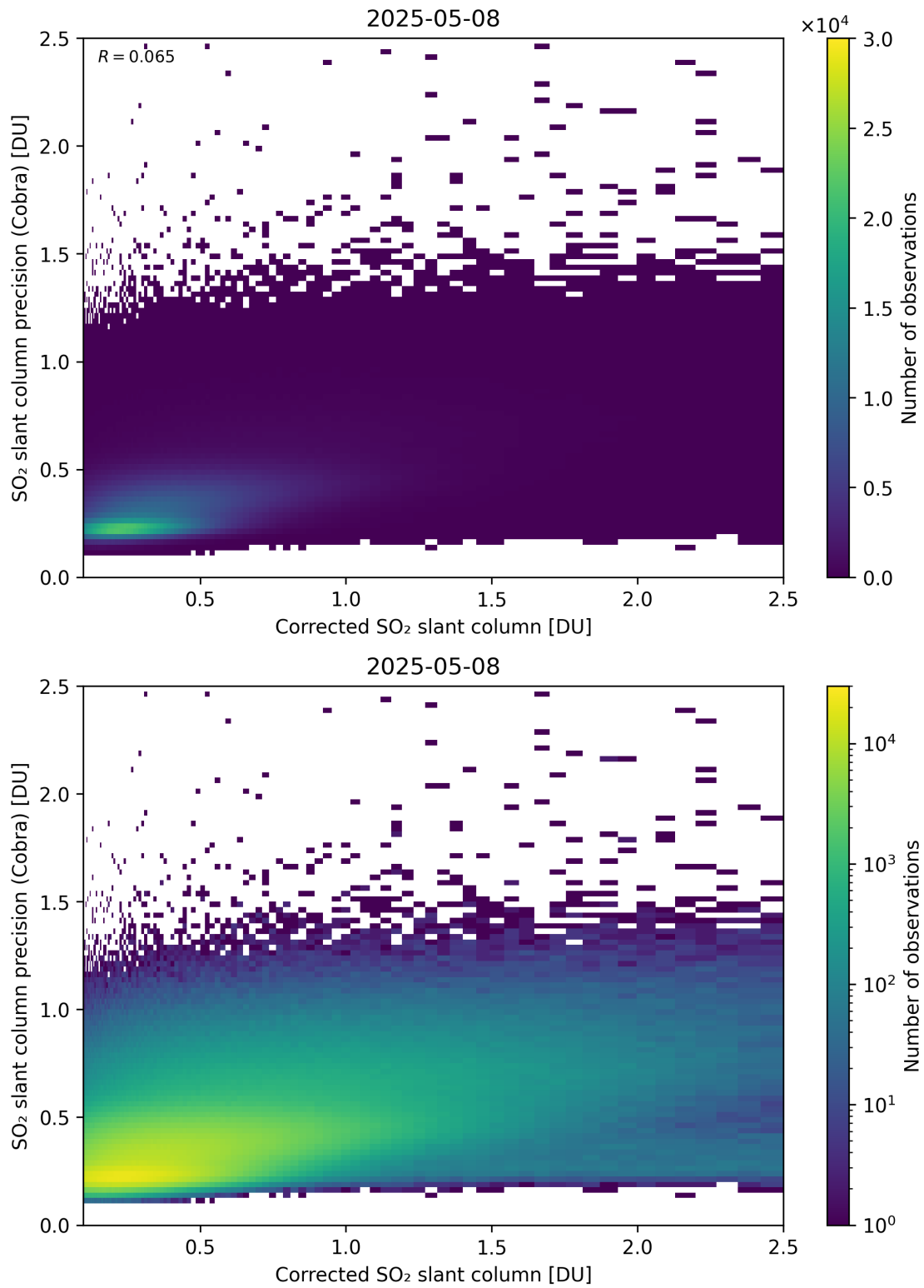
Figure 234: Scatter density plot of “Corrected SO 2 slant column” against “SO 2 slant column precision (Cobra)” for 2025-05-07 to 2025-05-09.
