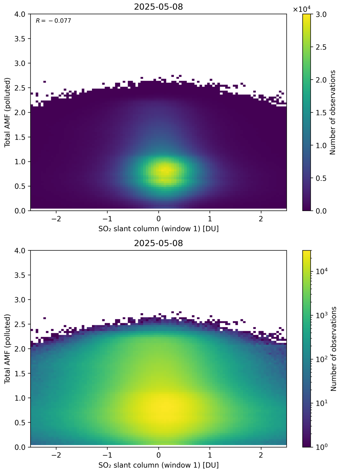
Figure 289: Scatter density plot of “SO 2 slant column (window 1)” against “Total AMF (polluted)” for 2025-05-07 to 2025-05-09.
