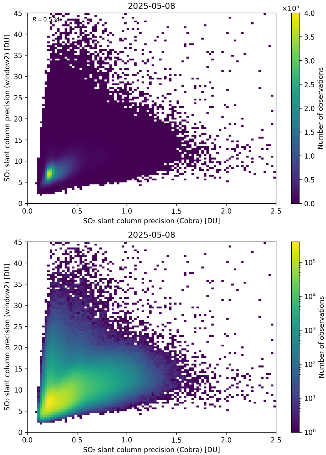
Figure 210: Scatter density plot of “SO 2 slant column precision (Cobra)” against “SO 2 slant column precision (window2)” for 2025-05-07 to 2025-05-09.
