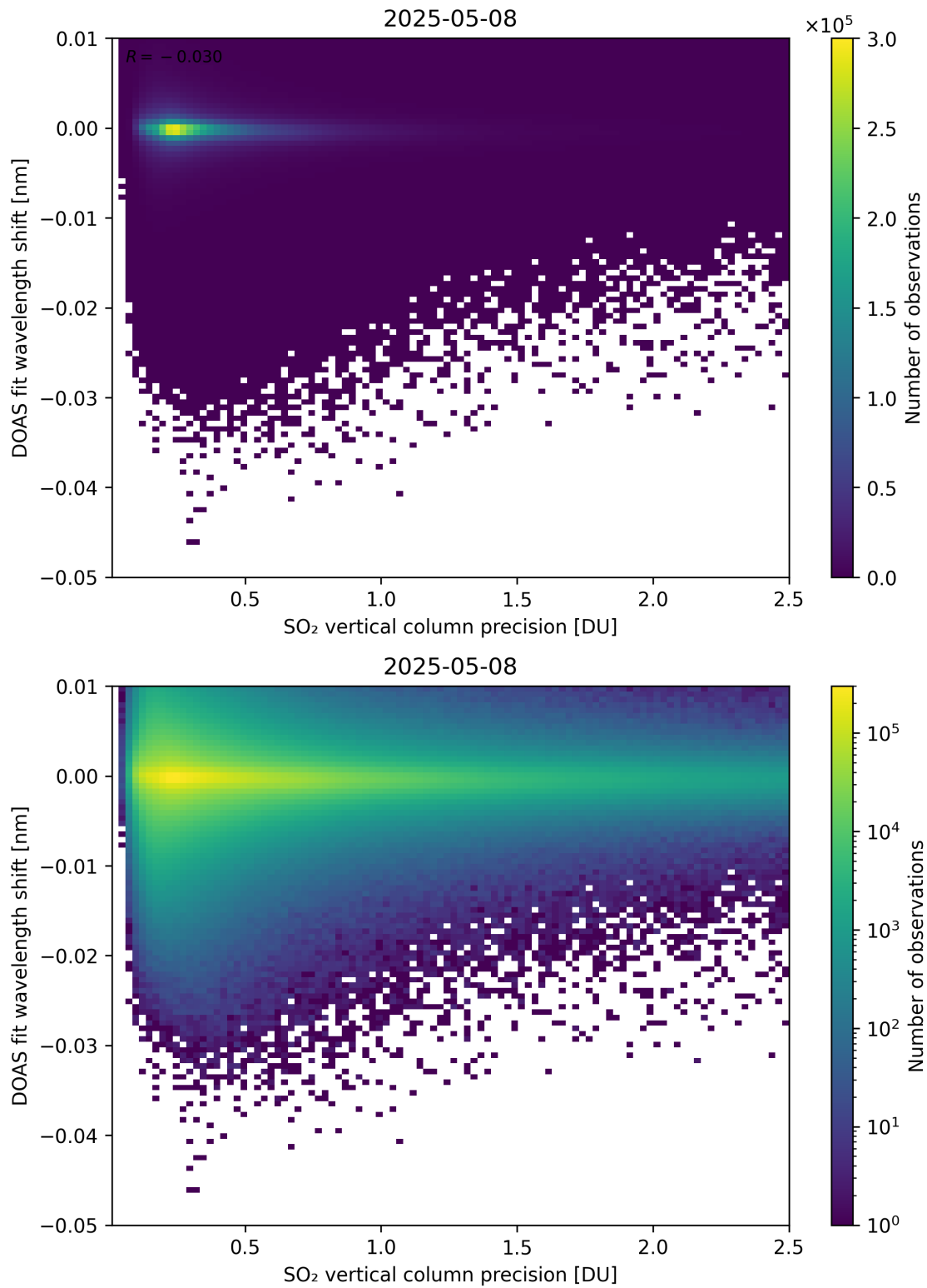
Figure 332: Scatter density plot of “SO 2 vertical column precision” against “DOAS fit wavelength shift” for 2025-05-07 to 2025-05-09.
