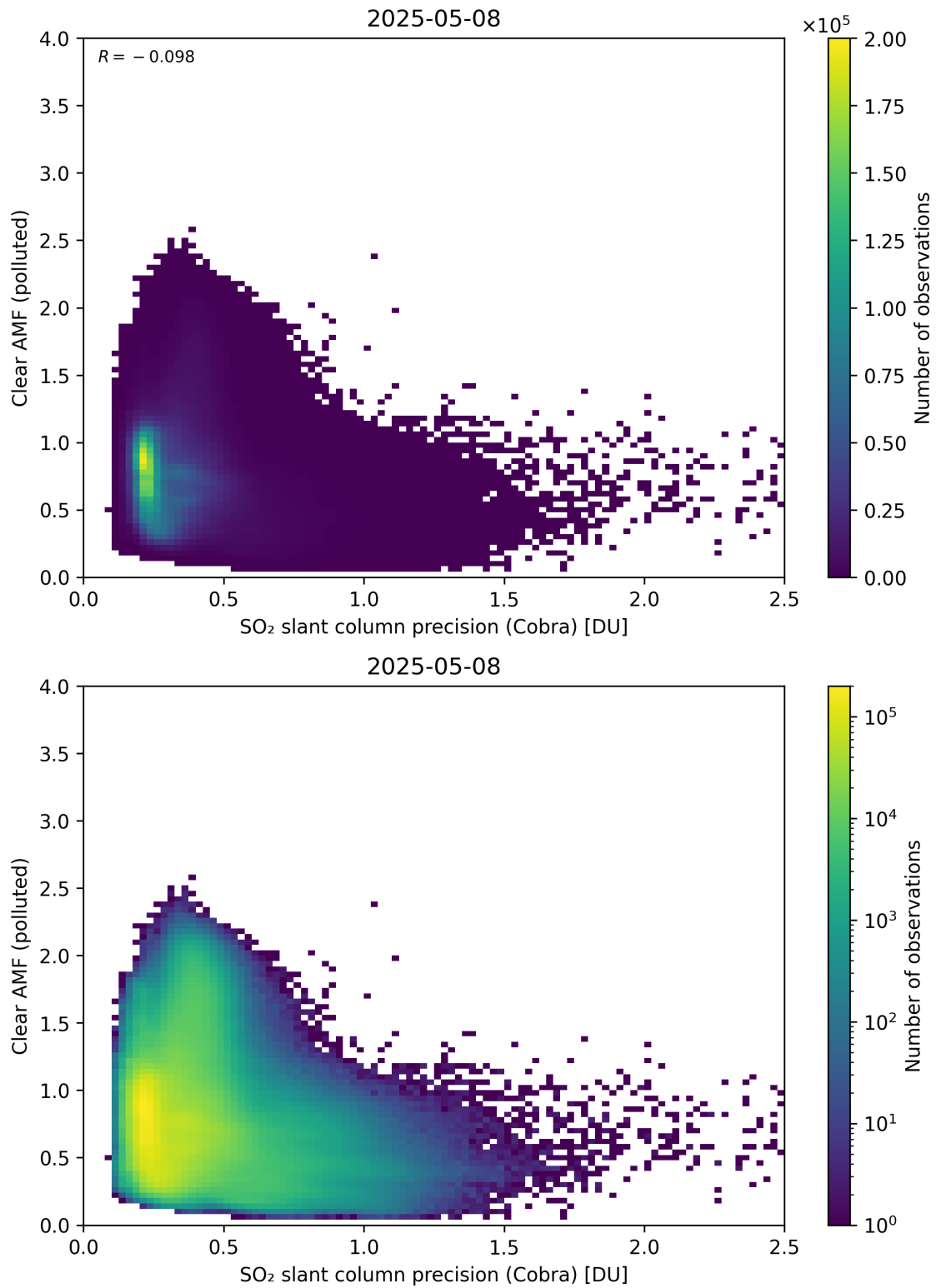
Figure 205: Scatter density plot of “SO 2 slant column precision (Cobra)” against “Clear AMF (polluted)” for 2025-05-07 to 2025-05-09.
