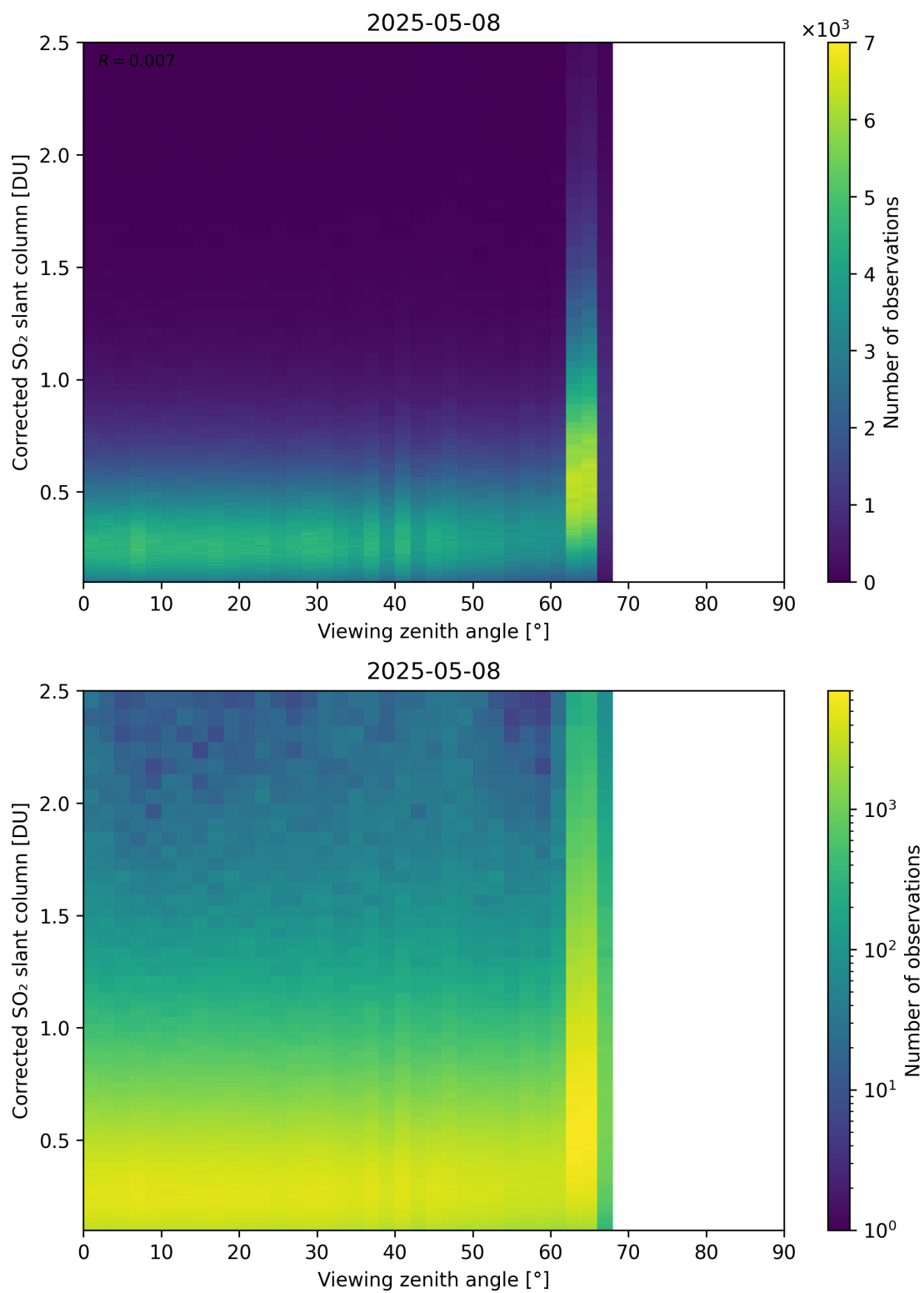
Figure 373: Scatter density plot of “Viewing zenith angle” against “Corrected SO 2 slant column” for 2025-05-07 to 2025-05-09.
