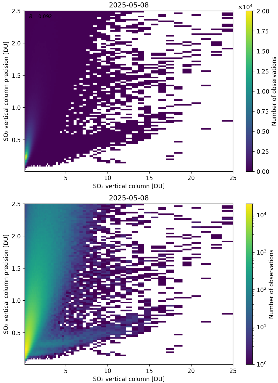
Figure 361: Scatter density plot of “SO 2 vertical column” against “SO 2 vertical column precision” for 2025-05-07 to 2025-05-09.
