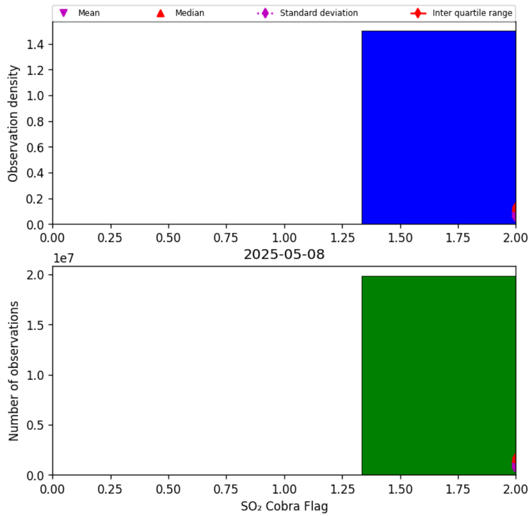
Figure 75: Histogram of “SO 2 Cobra Flag” for 2025-05-07 to 2025-05-09
