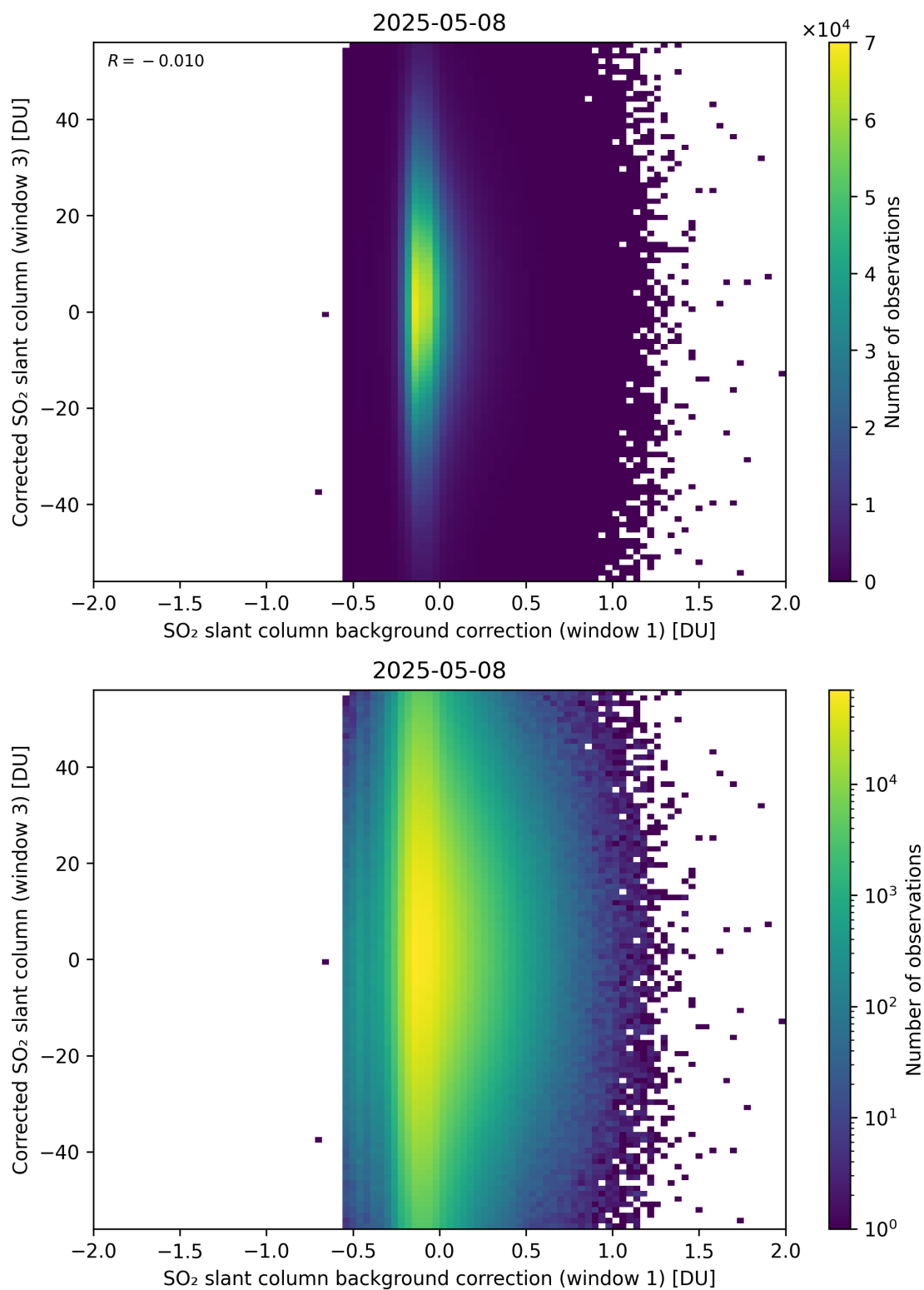
Figure 116: Scatter density plot of “SO 2 slant column background correction (window 1)” against “Corrected SO 2 slant column (window 3)” for 2025-05-07 to 2025-05-09.
