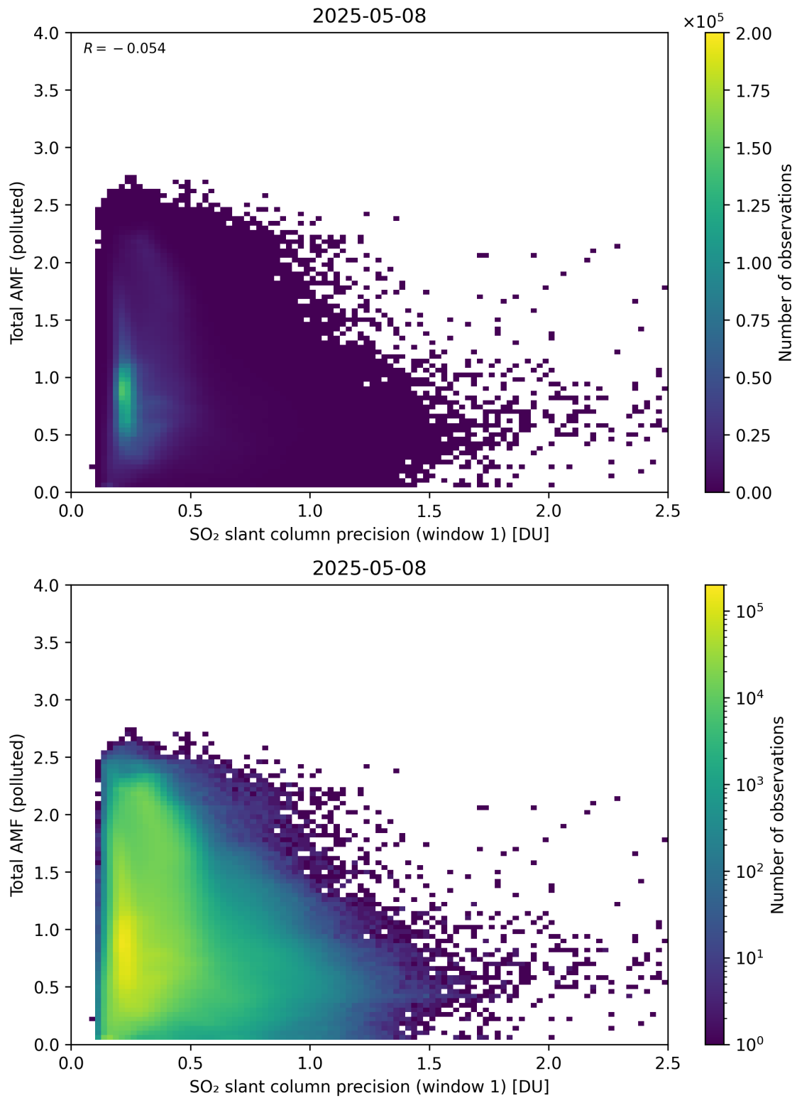
Figure 280: Scatter density plot of “SO 2 slant column precision (window 1)” against “Total AMF (polluted)” for 2025-05-07 to 2025-05-09.
