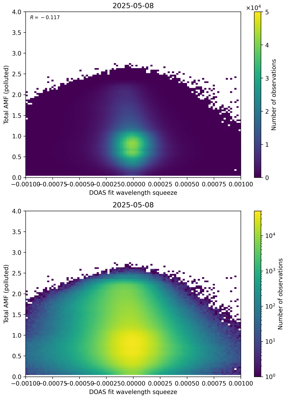
Figure 145: Scatter density plot of “DOAS fit wavelength squeeze” against “Total AMF (polluted)” for 2025-05-07 to 2025-05-09.
