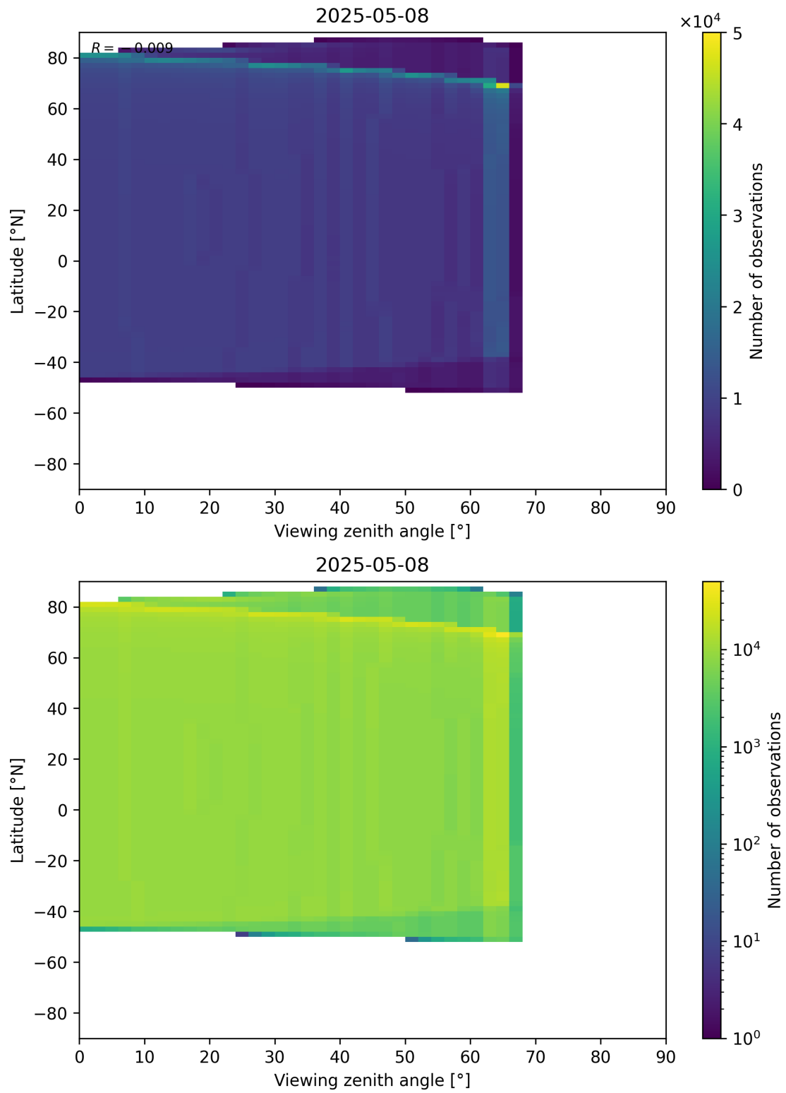
Figure 368: Scatter density plot of “Viewing zenith angle” against “Latitude” for 2025-05-07 to 2025-05-09.
