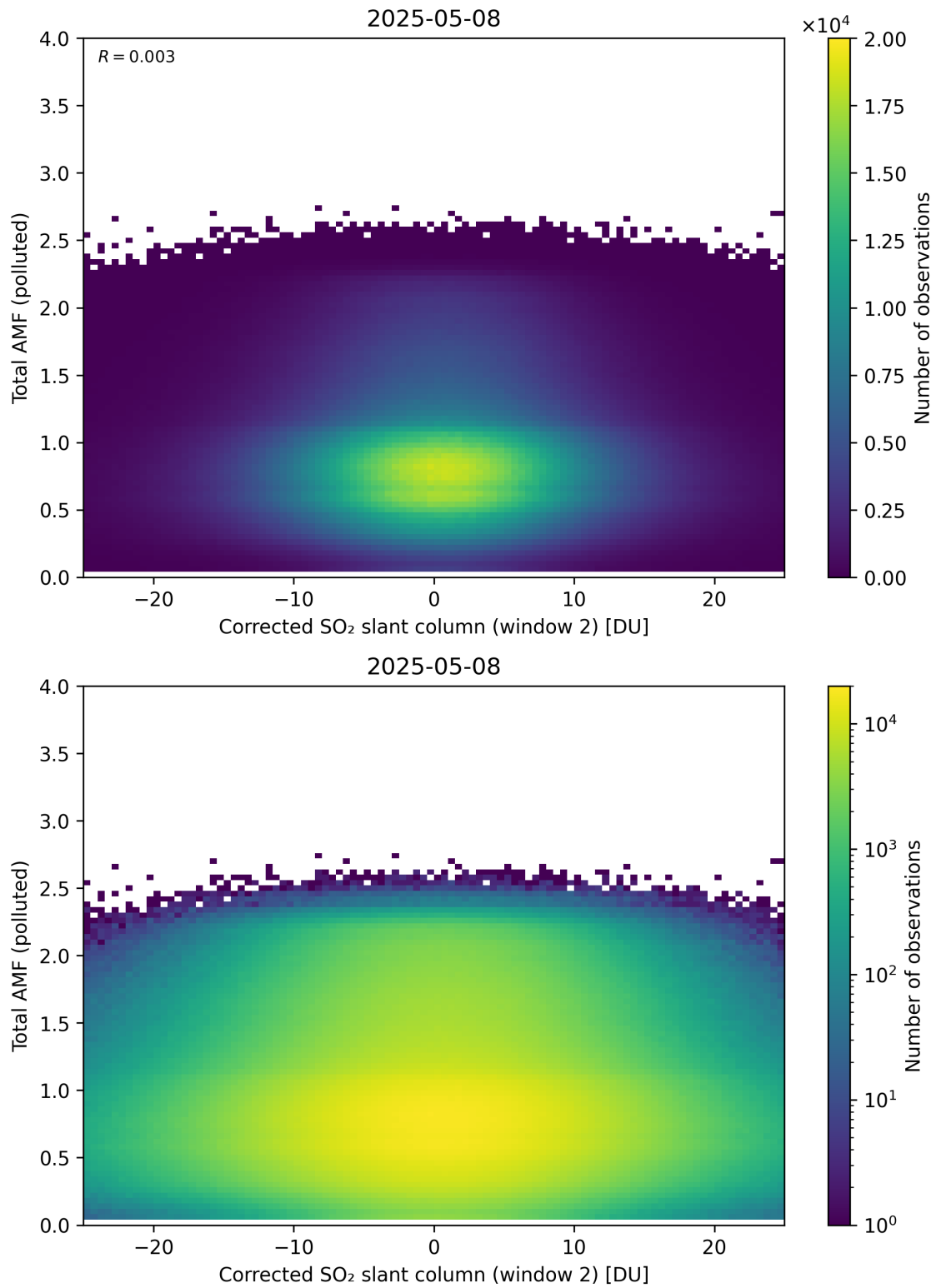
Figure 253: Scatter density plot of “Corrected SO 2 slant column (window 2)” against “Total AMF (polluted)” for 2025-05-07 to 2025-05-09.
