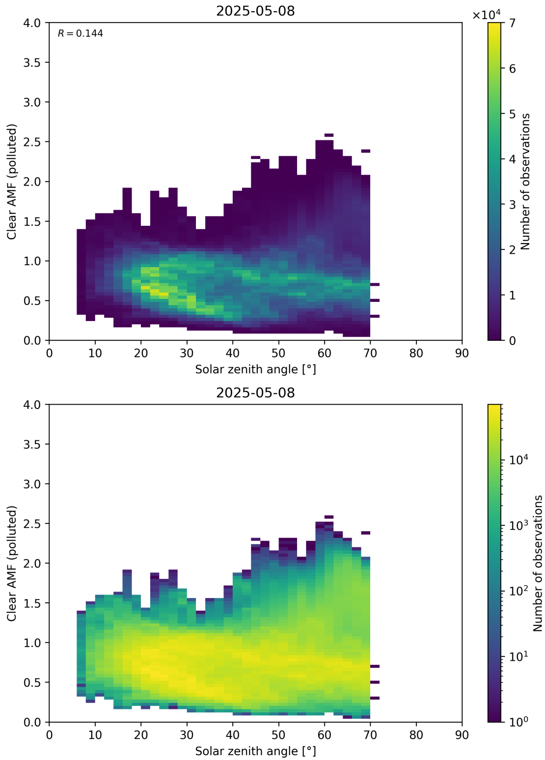
Figure 178: Scatter density plot of “Solar zenith angle” against “Clear AMF (polluted)” for 2025-05-07 to 2025-05-09.
