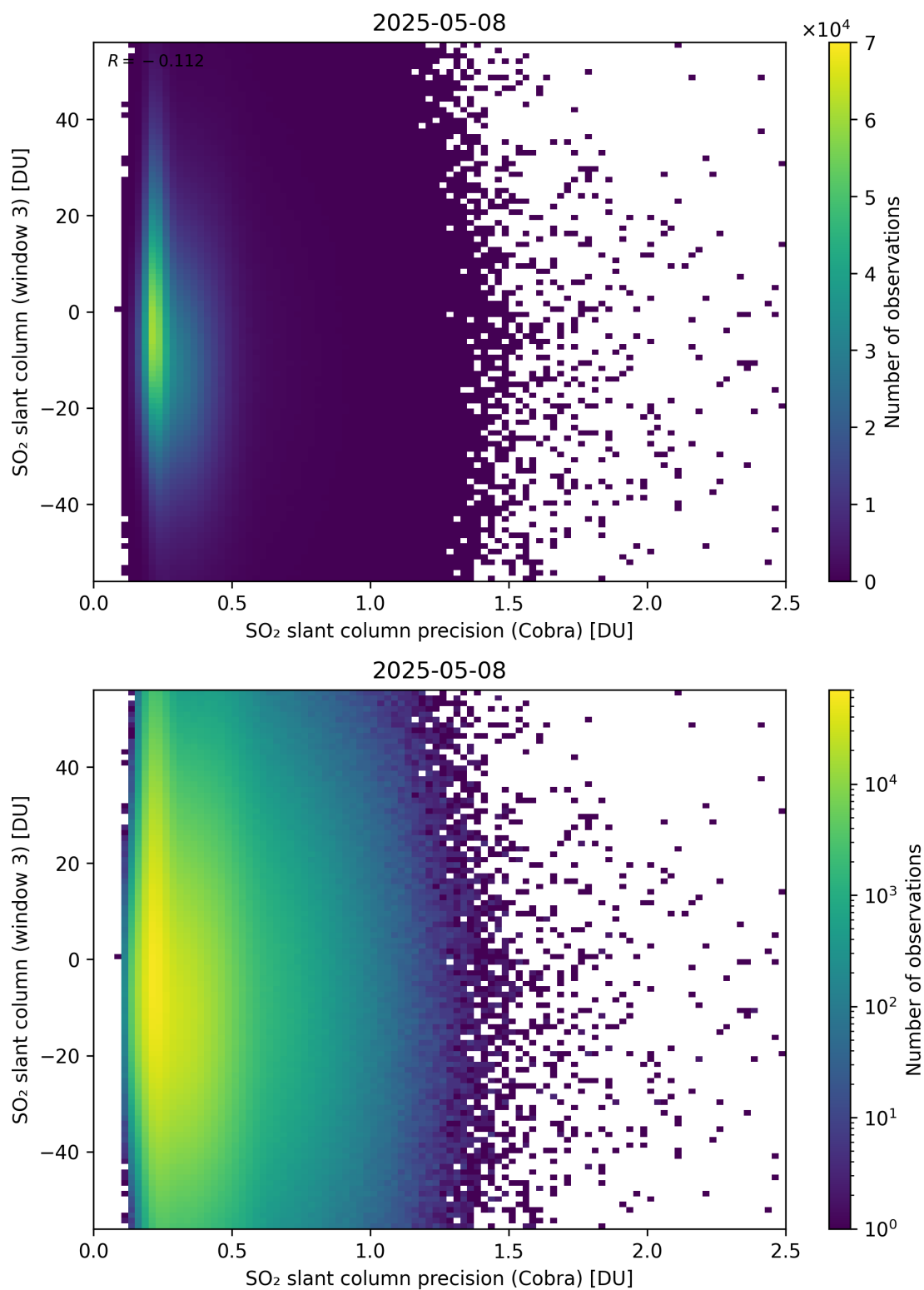
Figure 211: Scatter density plot of “SO 2 slant column precision (Cobra)” against “SO 2 slant column (window 3)” for 2025-05-07 to 2025-05-09.
