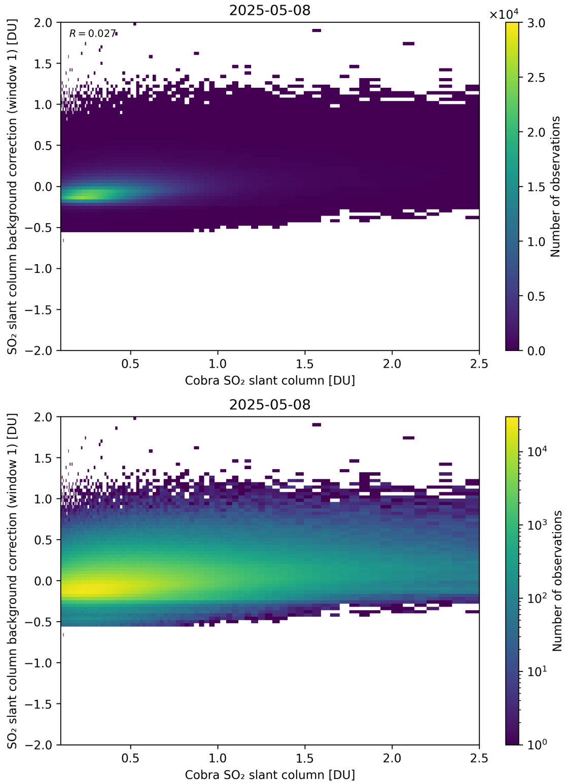
Figure 193: Scatter density plot of “Cobra SO 2 slant column” against “SO 2 slant column background correction (window 1)” for 2025-05-07 to 2025-05-09.
