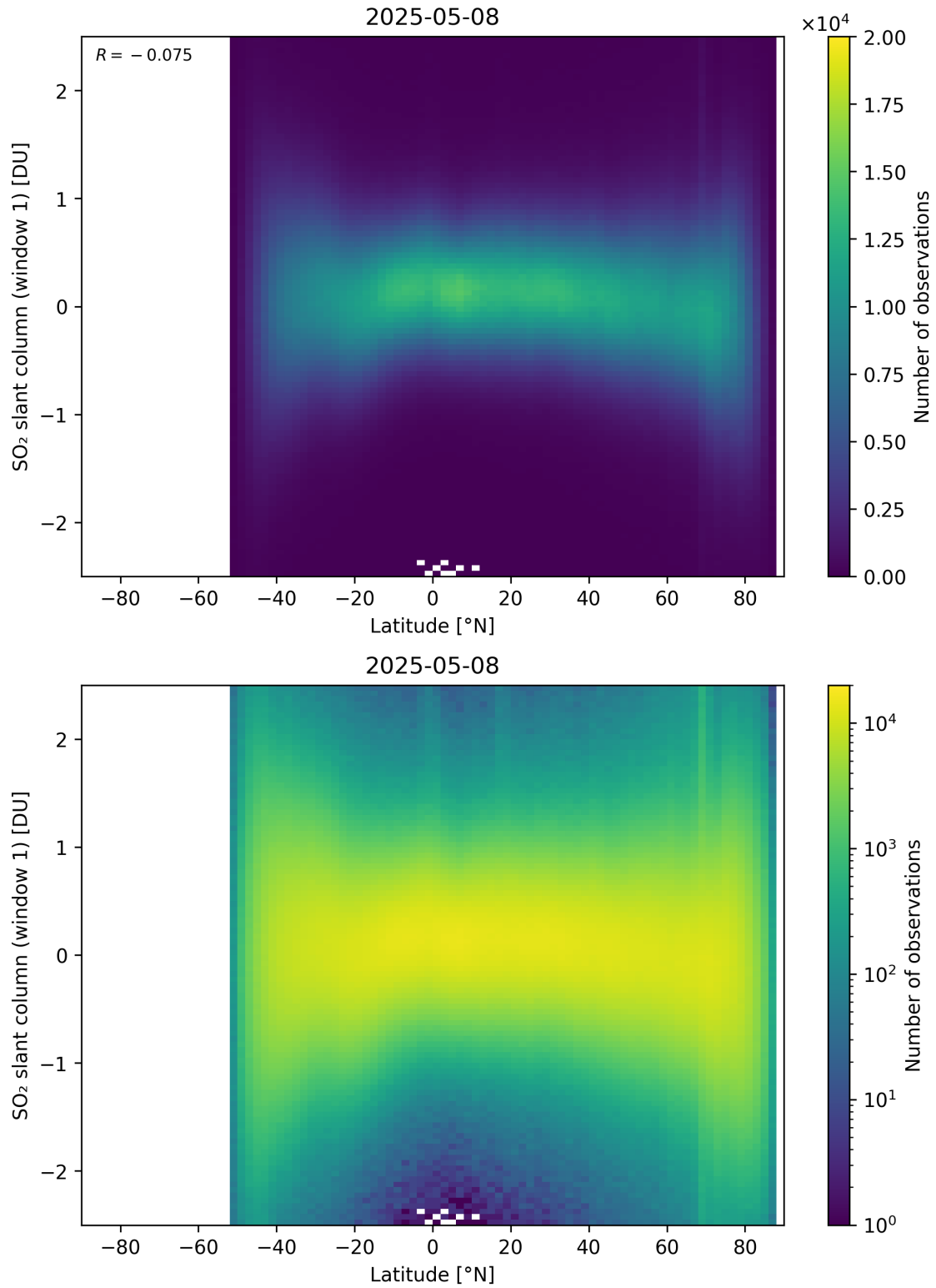
Figure 162: Scatter density plot of “Latitude” against “SO 2 slant column (window 1)” for 2025-05-07 to 2025-05-09.
