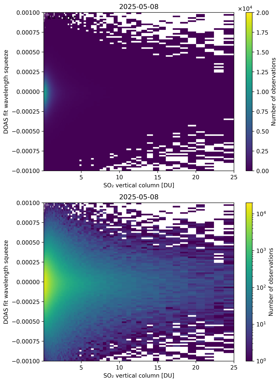
Figure 327: Scatter density plot of “SO 2 vertical column” against “DOAS fit wavelength squeeze” for 2025-05-07 to 2025-05-09.
