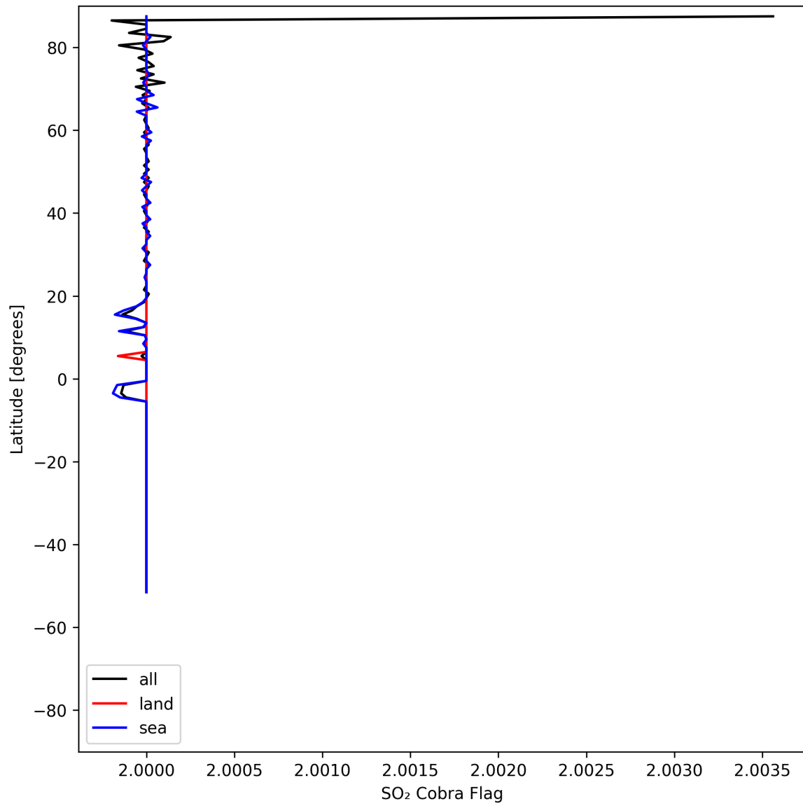
Figure 49: Zonal average of “SO 2 Cobra Flag” for 2025-05-07 to 2025-05-09.
