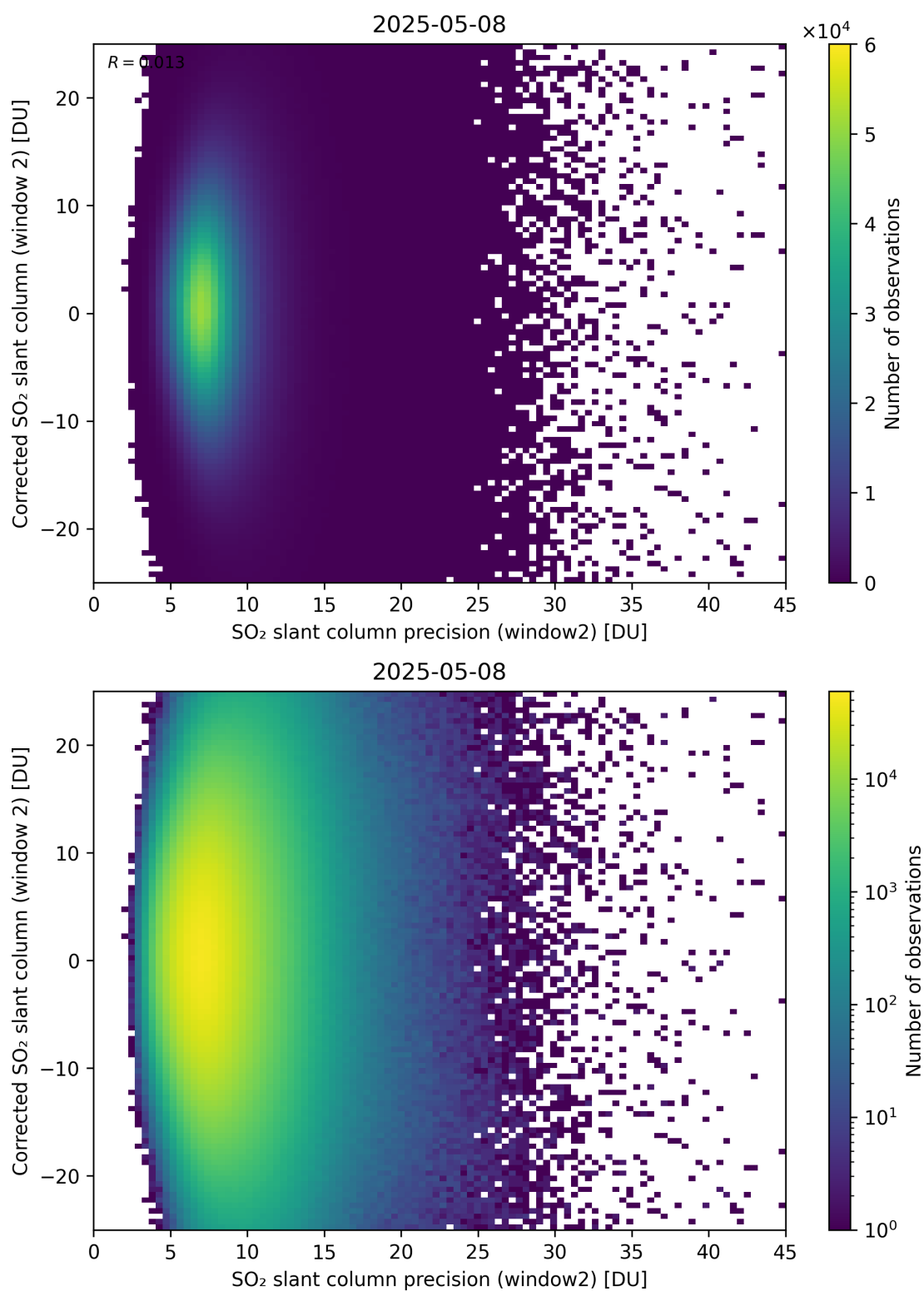
Figure 297: Scatter density plot of “SO 2 slant column precision (window2)” against “Corrected SO 2 slant column (window 2)” for 2025-05-07 to 2025-05-09.
