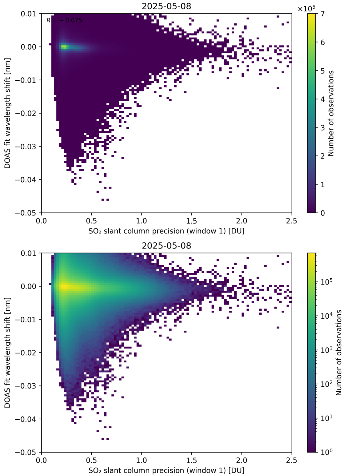
Figure 271: Scatter density plot of “SO 2 slant column precision (window 1)” against “DOAS fit wavelength shift” for 2025-05-07 to 2025-05-09.
