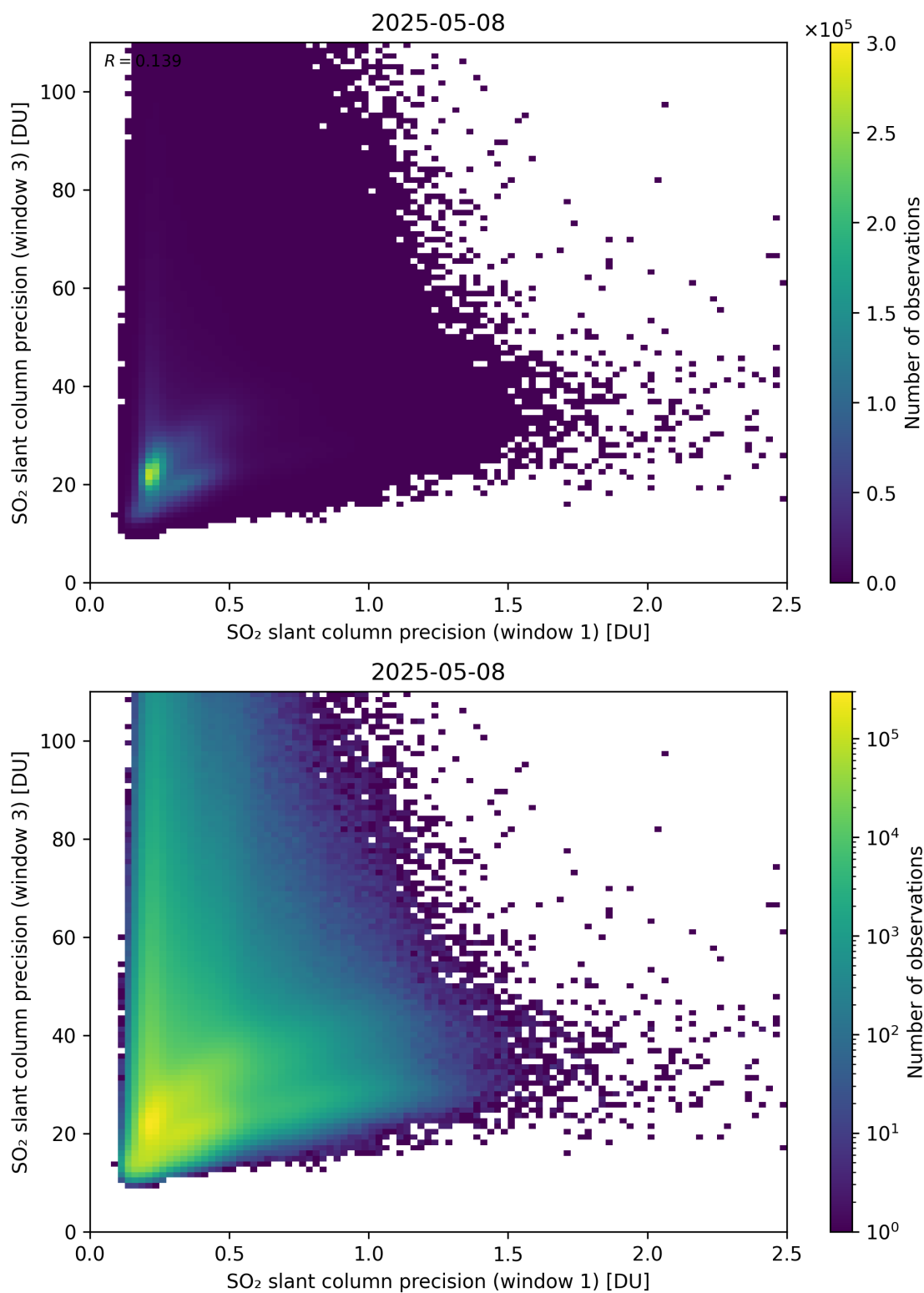
Figure 279: Scatter density plot of “SO 2 slant column precision (window 1)” against “SO 2 slant column precision (window 3)” for 2025-05-07 to 2025-05-09.
