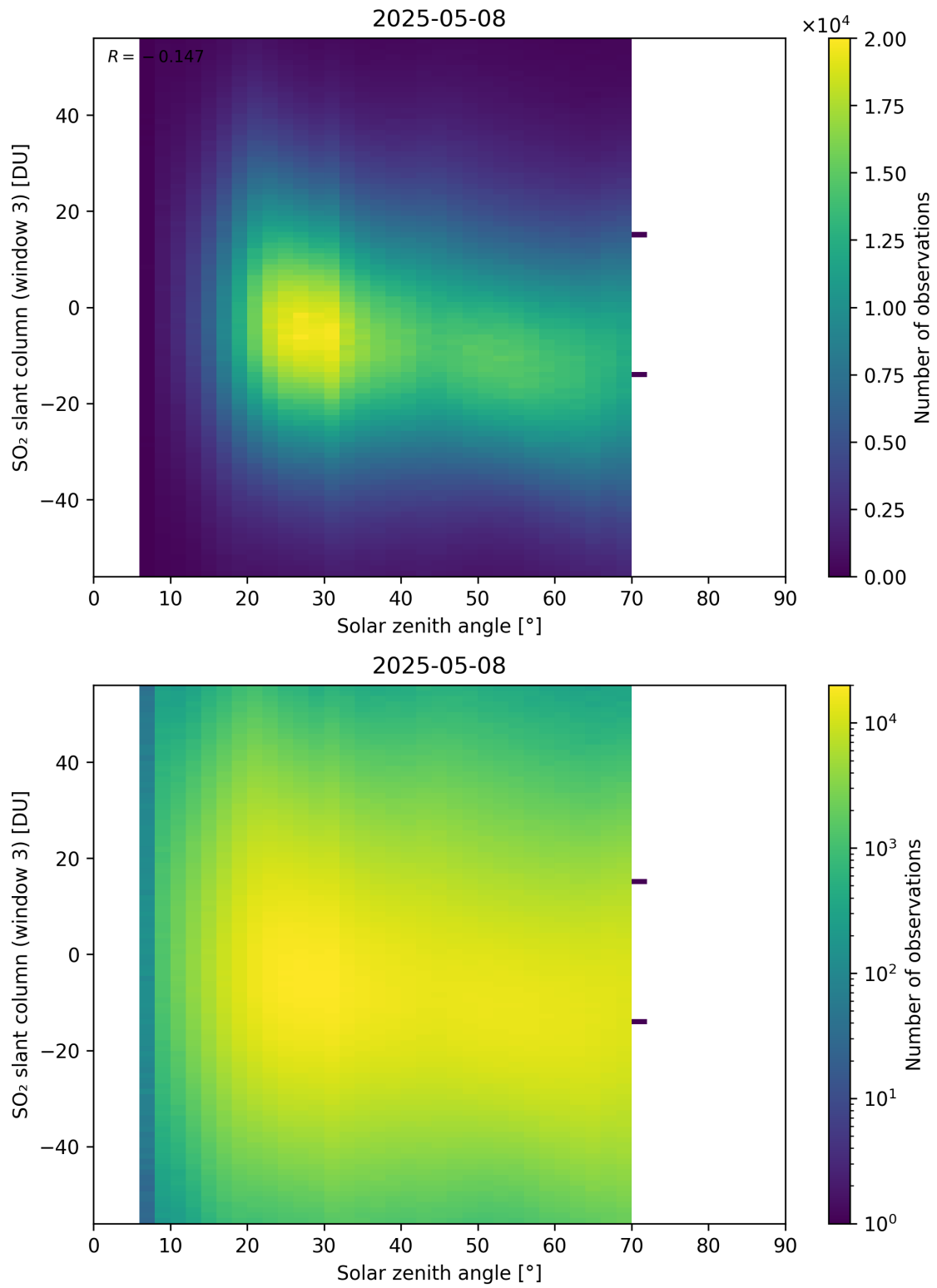
Figure 187: Scatter density plot of “Solar zenith angle” against “SO 2 slant column (window 3)” for 2025-05-07 to 2025-05-09.
