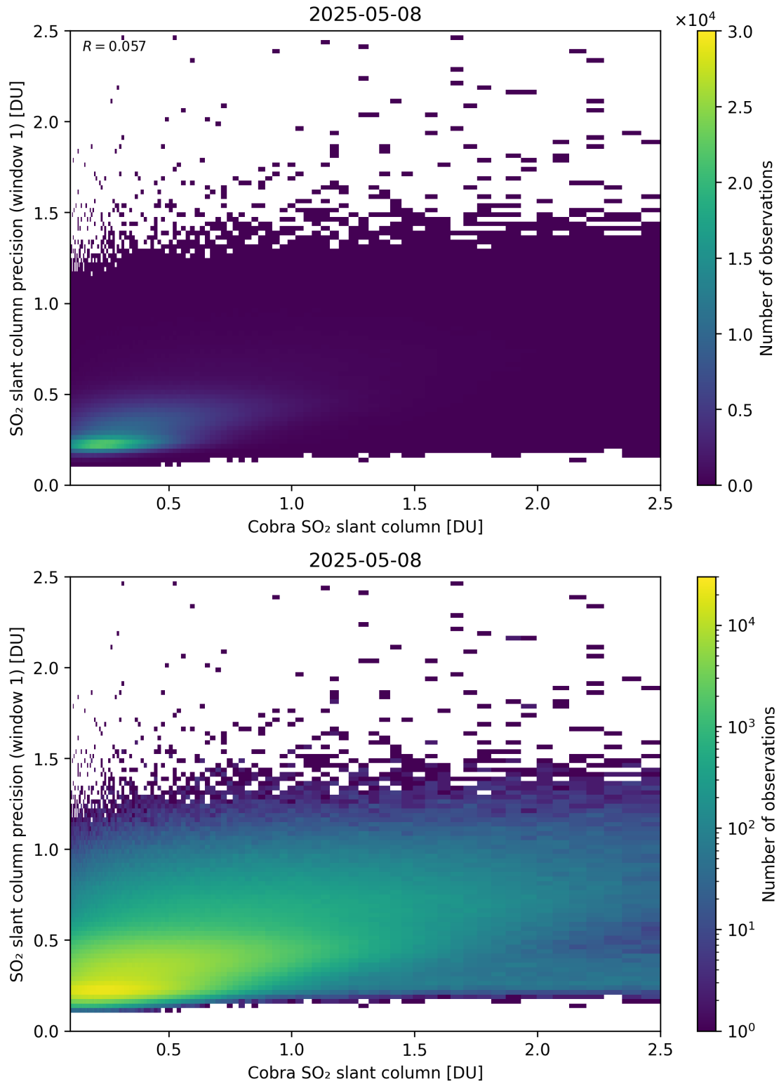
Figure 220: Scatter density plot of “Cobra SO 2 slant column” against “SO 2 slant column precision (window 1)” for 2025-05-07 to 2025-05-09.
