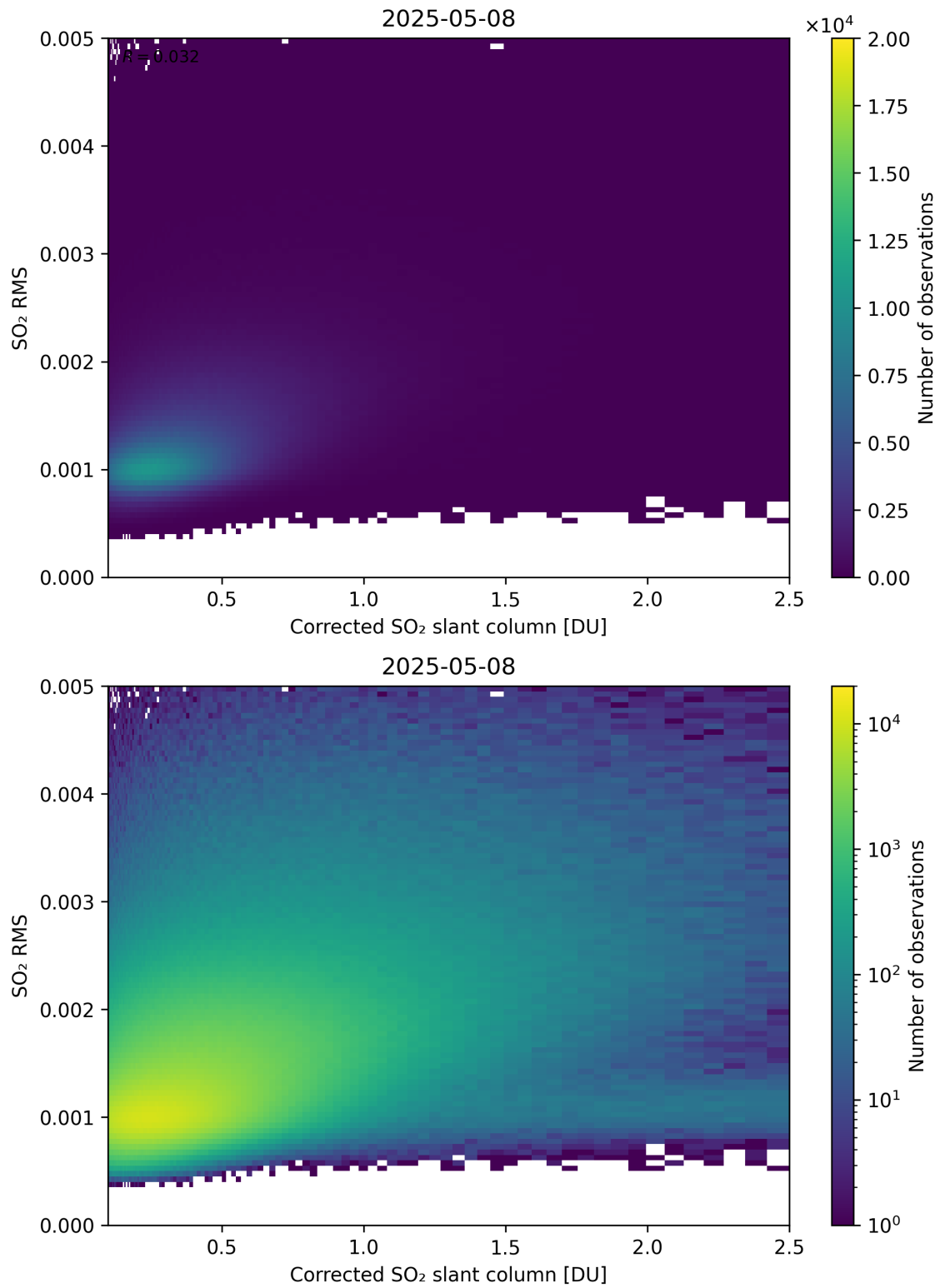
Figure 231: Scatter density plot of “Corrected SO 2 slant column” against “SO 2 RMS” for 2025-05-07 to 2025-05-09.
