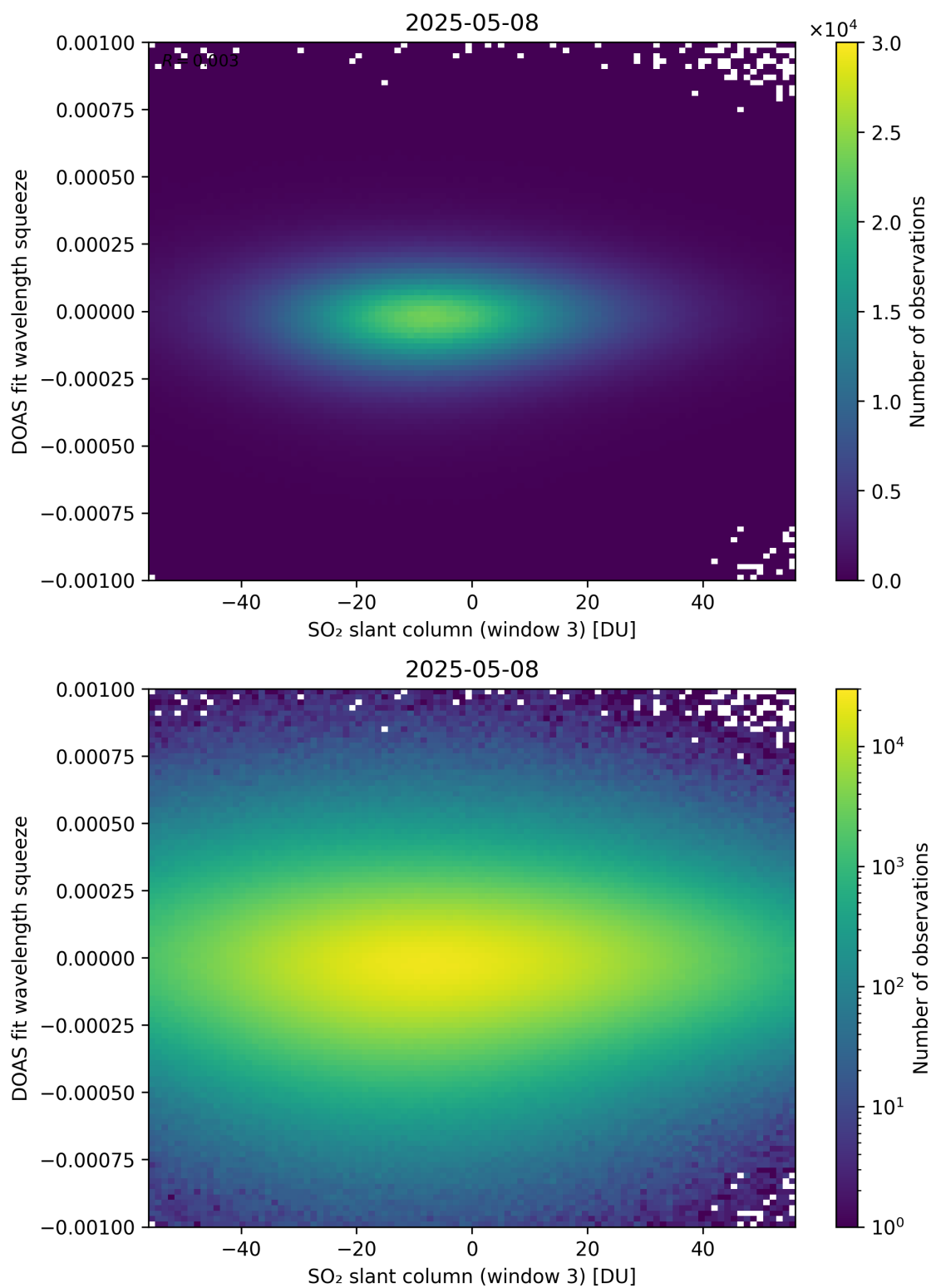
Figure 305: Scatter density plot of “SO 2 slant column (window 3)” against “DOAS fit wavelength squeeze” for 2025-05-07 to 2025-05-09.
