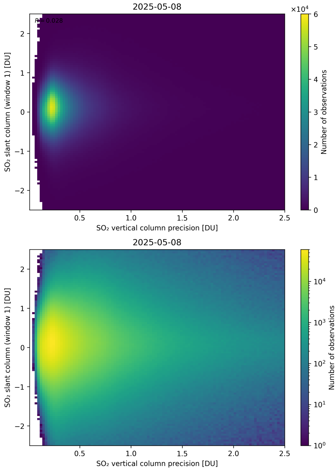
Figure 341: Scatter density plot of “SO 2 vertical column precision” against “SO 2 slant column (window 1)” for 2025-05-07 to 2025-05-09.
