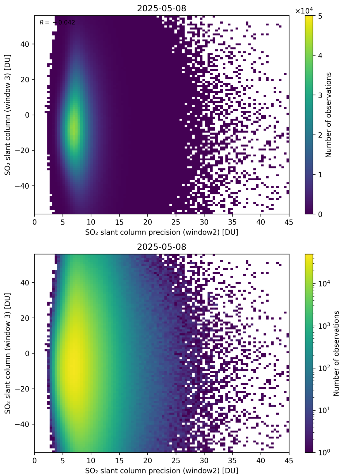
Figure 299: Scatter density plot of “SO 2 slant column precision (window2)” against “SO 2 slant column (window 3)” for 2025-05-07 to 2025-05-09.
