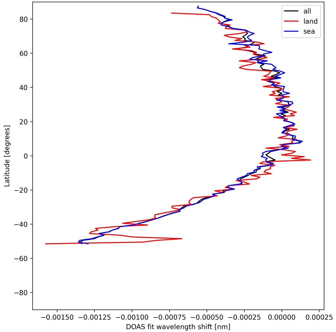
Figure 50: Zonal average of “DOAS fit wavelength shift” for 2025-05-07 to 2025-05-09.
