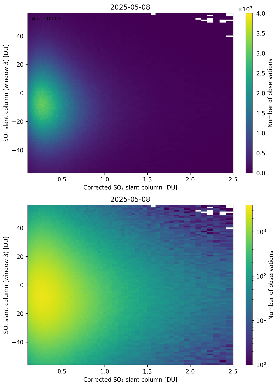
Figure 240: Scatter density plot of “Corrected SO 2 slant column” against “SO 2 slant column (window 3)” for 2025-05-07 to 2025-05-09.
