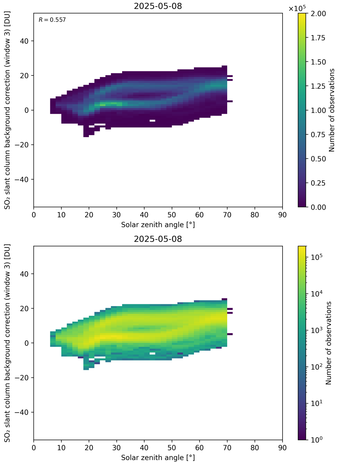
Figure 173: Scatter density plot of “Solar zenith angle” against “SO 2 slant column background correction (window 3)” for 2025-05-07 to 2025-05-09.
