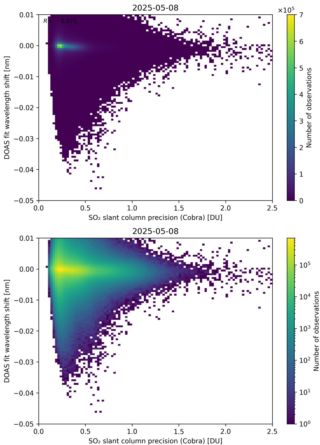
Figure 202: Scatter density plot of “SO 2 slant column precision (Cobra)” against “DOAS fit wavelength shift” for 2025-05-07 to 2025-05-09.
