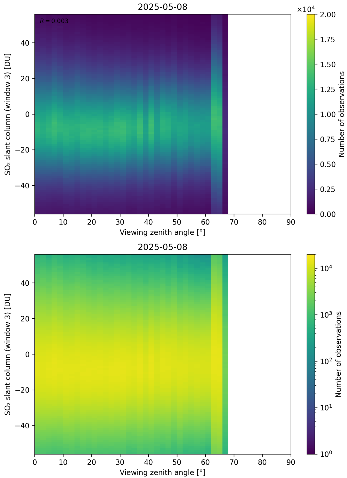
Figure 379: Scatter density plot of “Viewing zenith angle” against “SO 2 slant column (window 3)” for 2025-05-07 to 2025-05-09.
