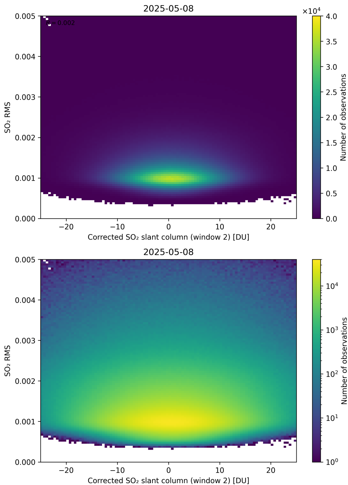
Figure 248: Scatter density plot of “Corrected SO 2 slant column (window 2)” against “SO 2 RMS” for 2025-05-07 to 2025-05-09.
