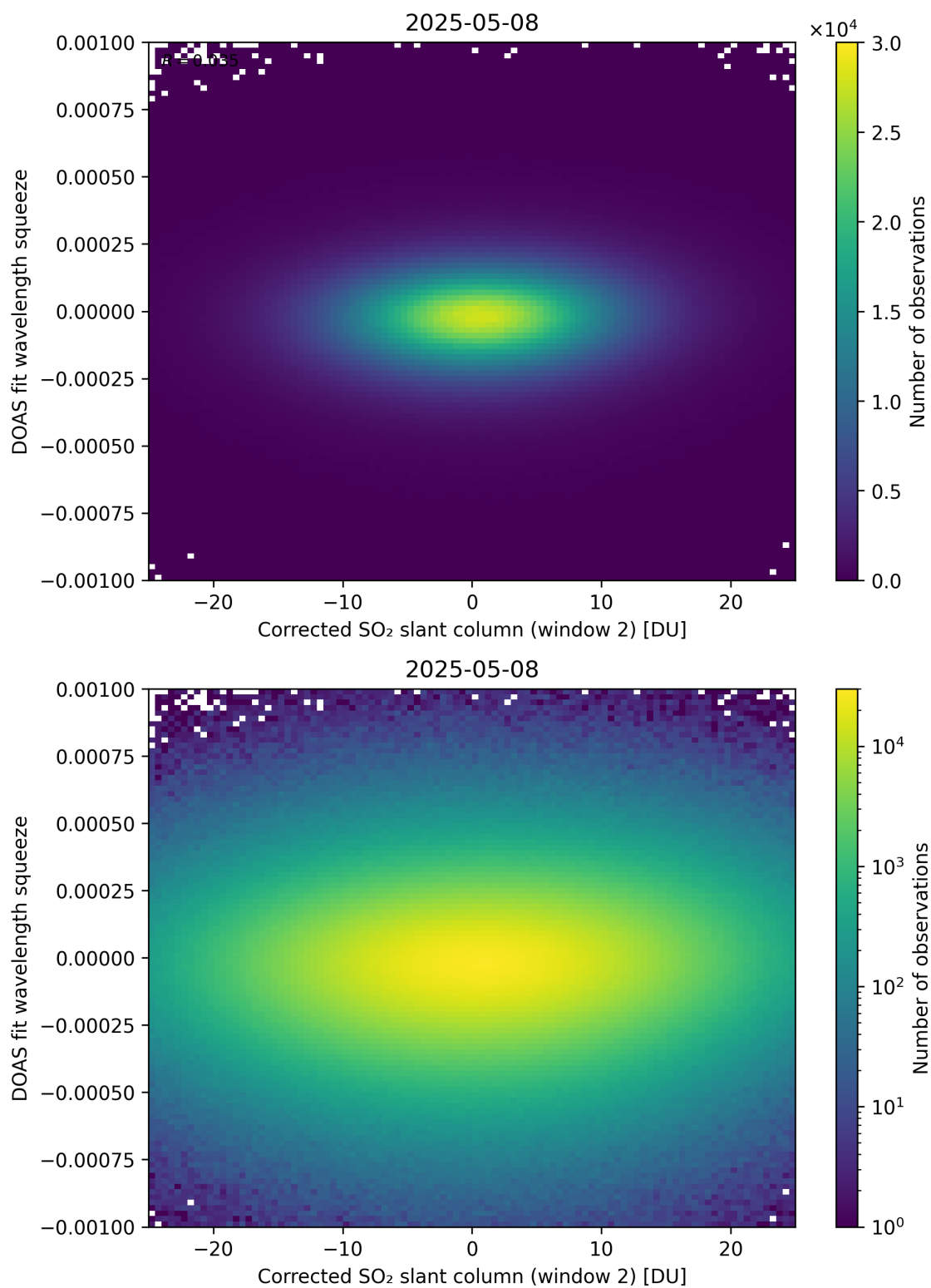
Figure 247: Scatter density plot of “Corrected SO 2 slant column (window 2)” against “DOAS fit wavelength squeeze” for 2025-05-07 to 2025-05-09.
