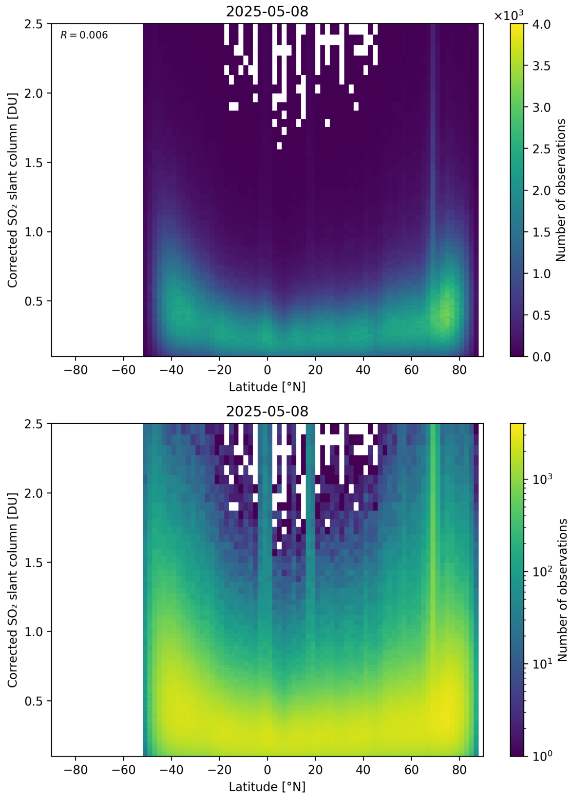
Figure 159: Scatter density plot of “Latitude” against “Corrected SO 2 slant column” for 2025-05-07 to 2025-05-09.
