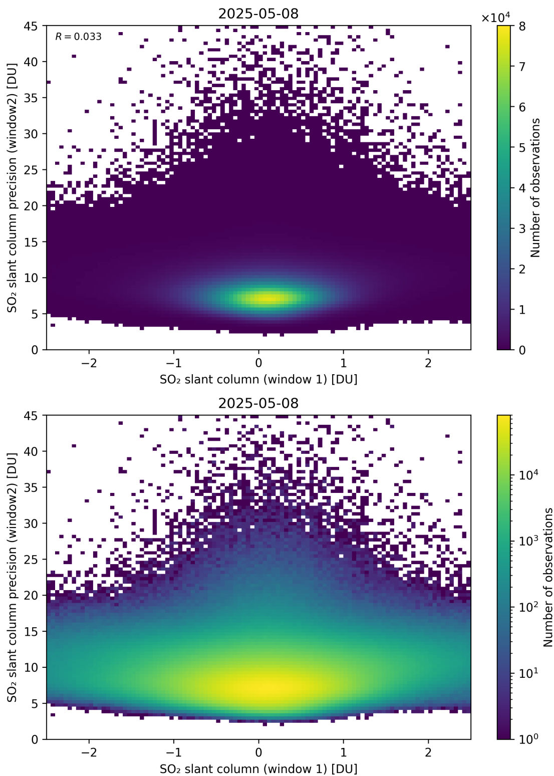
Figure 286: Scatter density plot of “SO 2 slant column (window 1)” against “SO 2 slant column precision (window2)” for 2025-05-07 to 2025-05-09.
