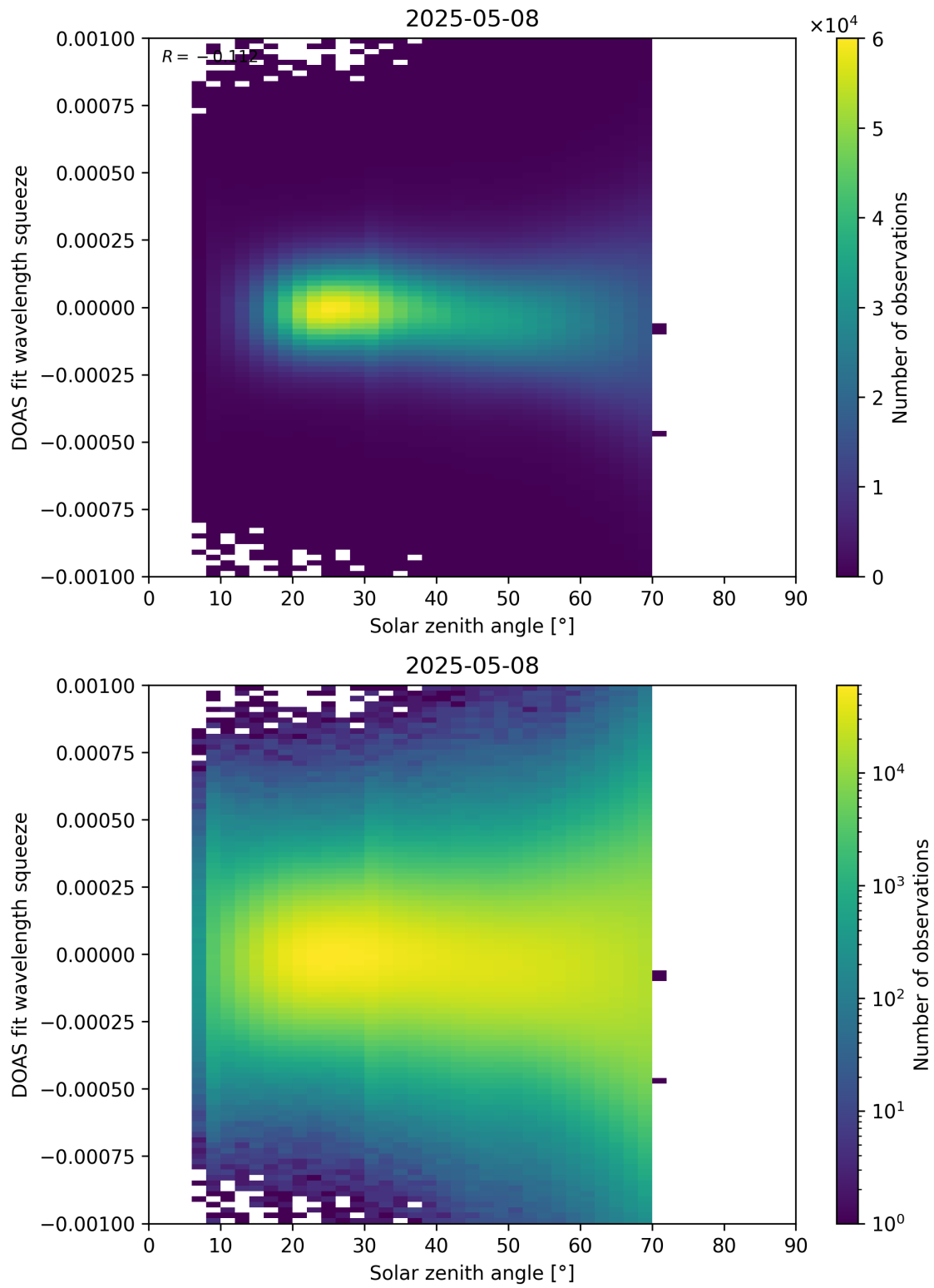
Figure 175: Scatter density plot of “Solar zenith angle” against “DOAS fit wavelength squeeze” for 2025-05-07 to 2025-05-09.
