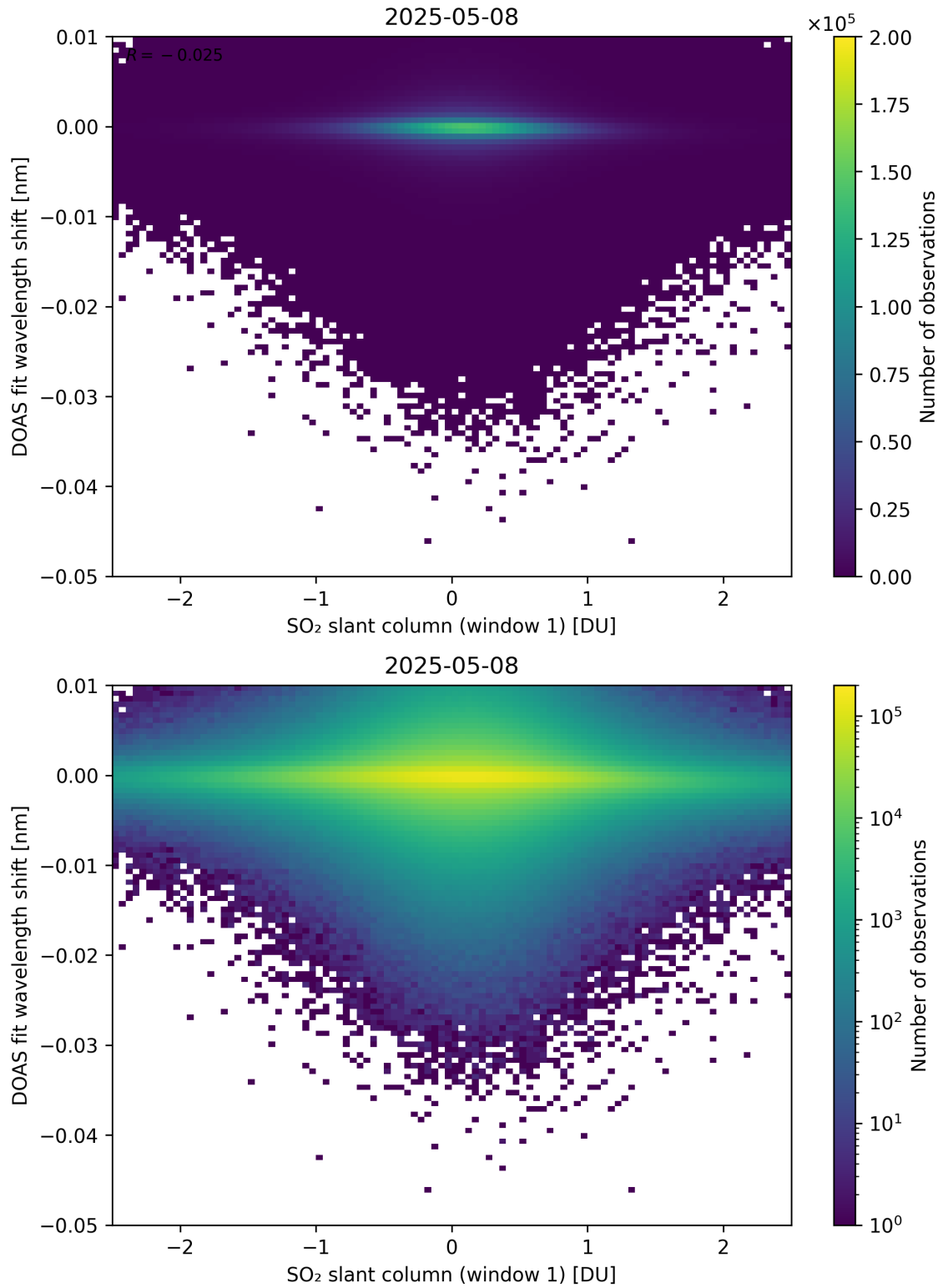
Figure 265: Scatter density plot of “SO 2 slant column (window 1)” against “DOAS fit wavelength shift” for 2025-05-07 to 2025-05-09.
