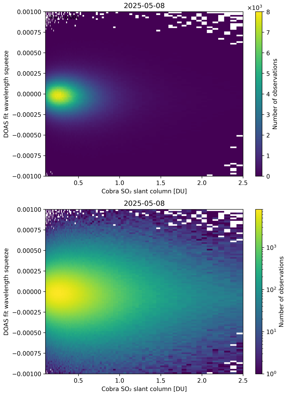
Figure 197: Scatter density plot of “Cobra SO 2 slant column” against “DOAS fit wavelength squeeze” for 2025-05-07 to 2025-05-09.
