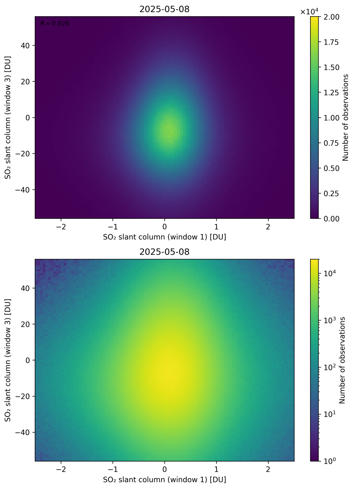
Figure 287: Scatter density plot of “SO 2 slant column (window 1)” against “SO 2 slant column (window 3)” for 2025-05-07 to 2025-05-09.
