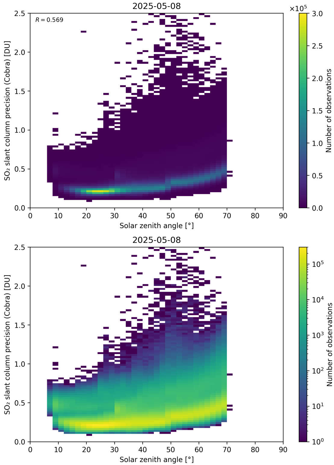
Figure 180: Scatter density plot of “Solar zenith angle” against “SO 2 slant column precision (Cobra)” for 2025-05-07 to 2025-05-09.
