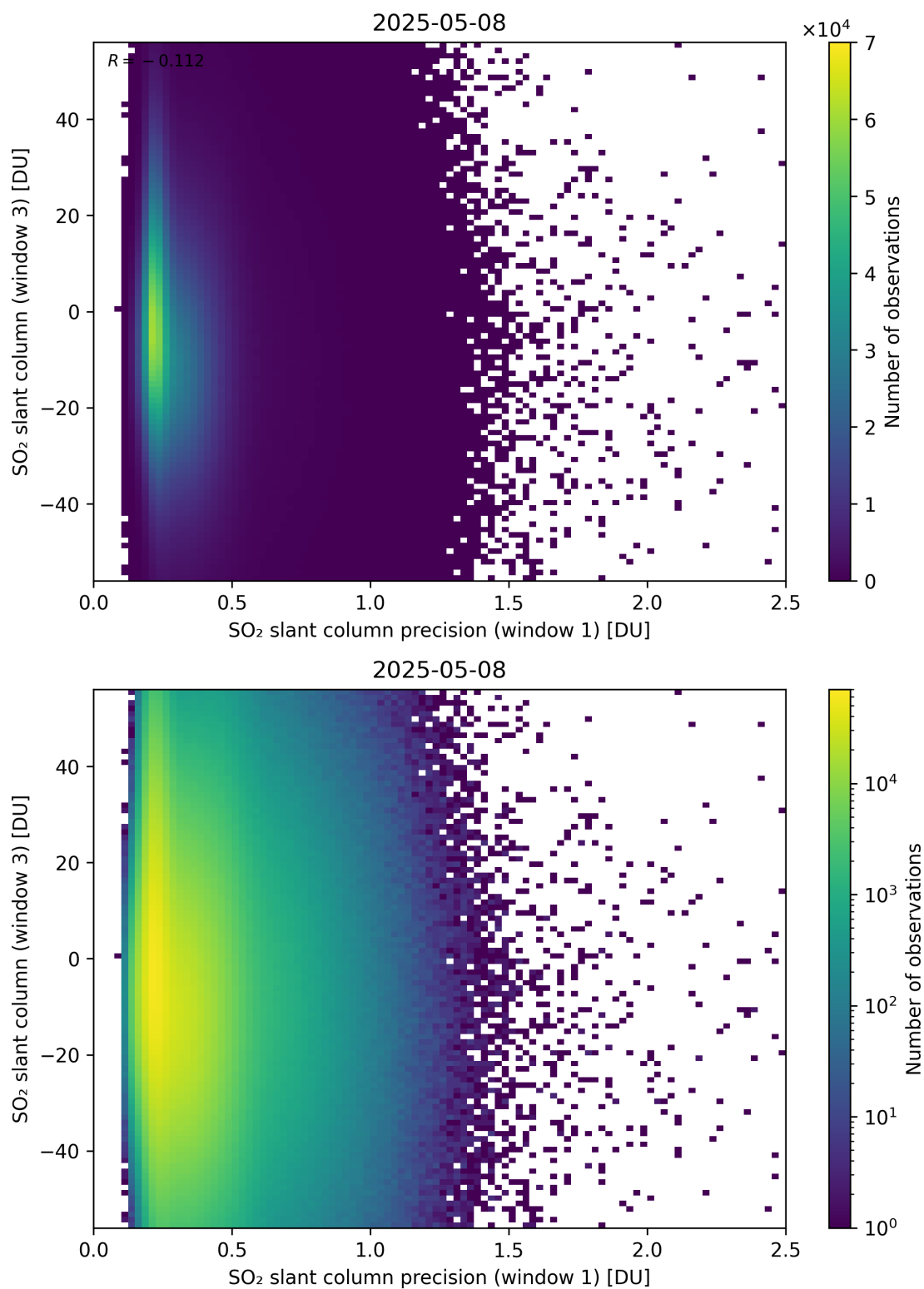
Figure 278: Scatter density plot of “SO 2 slant column precision (window 1)” against “SO 2 slant column (window 3)” for 2025-05-07 to 2025-05-09.
