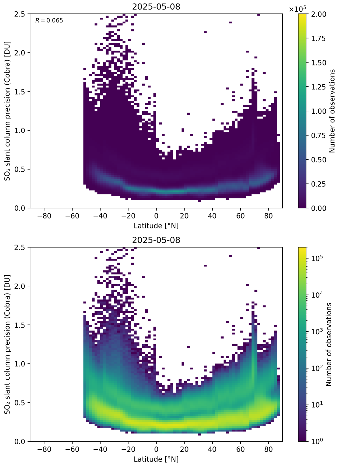
Figure 158: Scatter density plot of “Latitude” against “SO 2 slant column precision (Cobra)” for 2025-05-07 to 2025-05-09.
