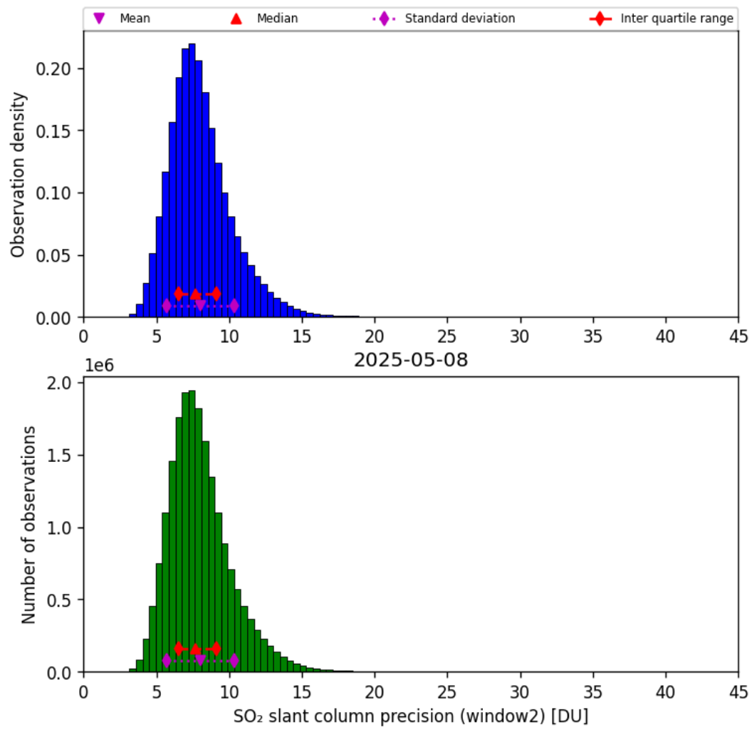
Figure 68: Histogram of “SO 2 slant column precision (window2)” for 2025-05-07 to 2025-05-09
