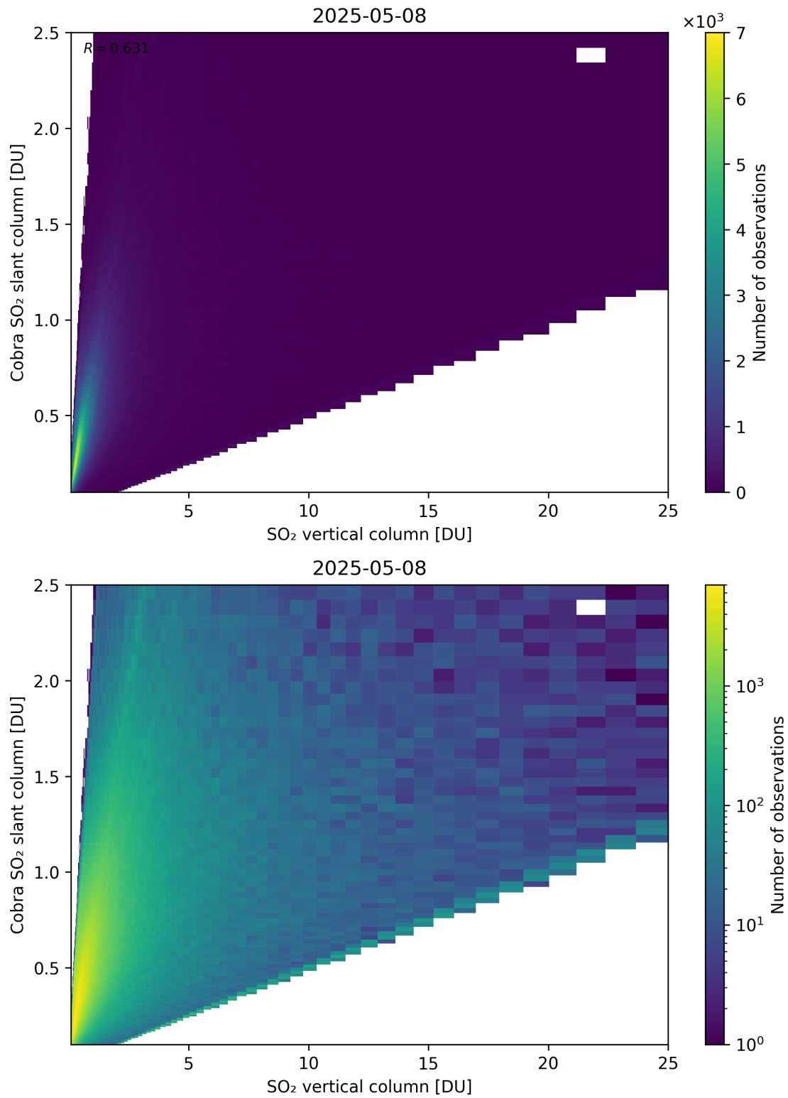
Figure 349: Scatter density plot of “SO 2 vertical column” against “Cobra SO 2 slant column” for 2025-05-07 to 2025-05-09.
