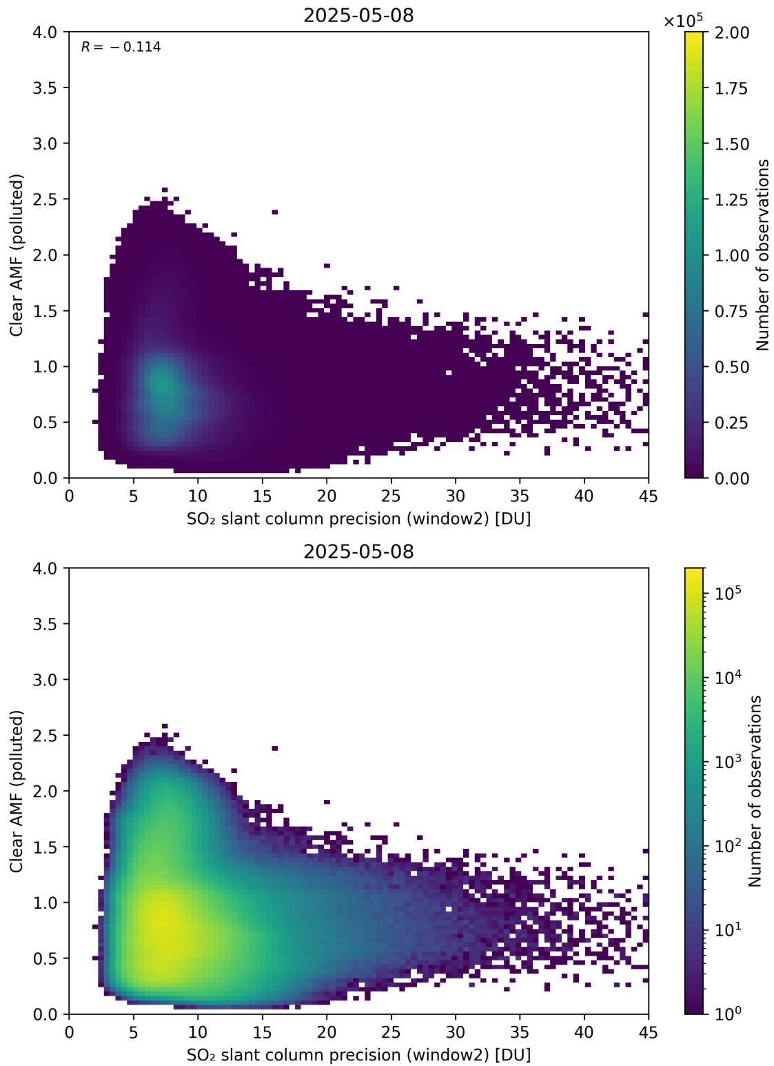
Figure 296: Scatter density plot of “SO 2 slant column precision (window2)” against “Clear AMF (polluted)” for 2025-05-07 to 2025-05-09.
