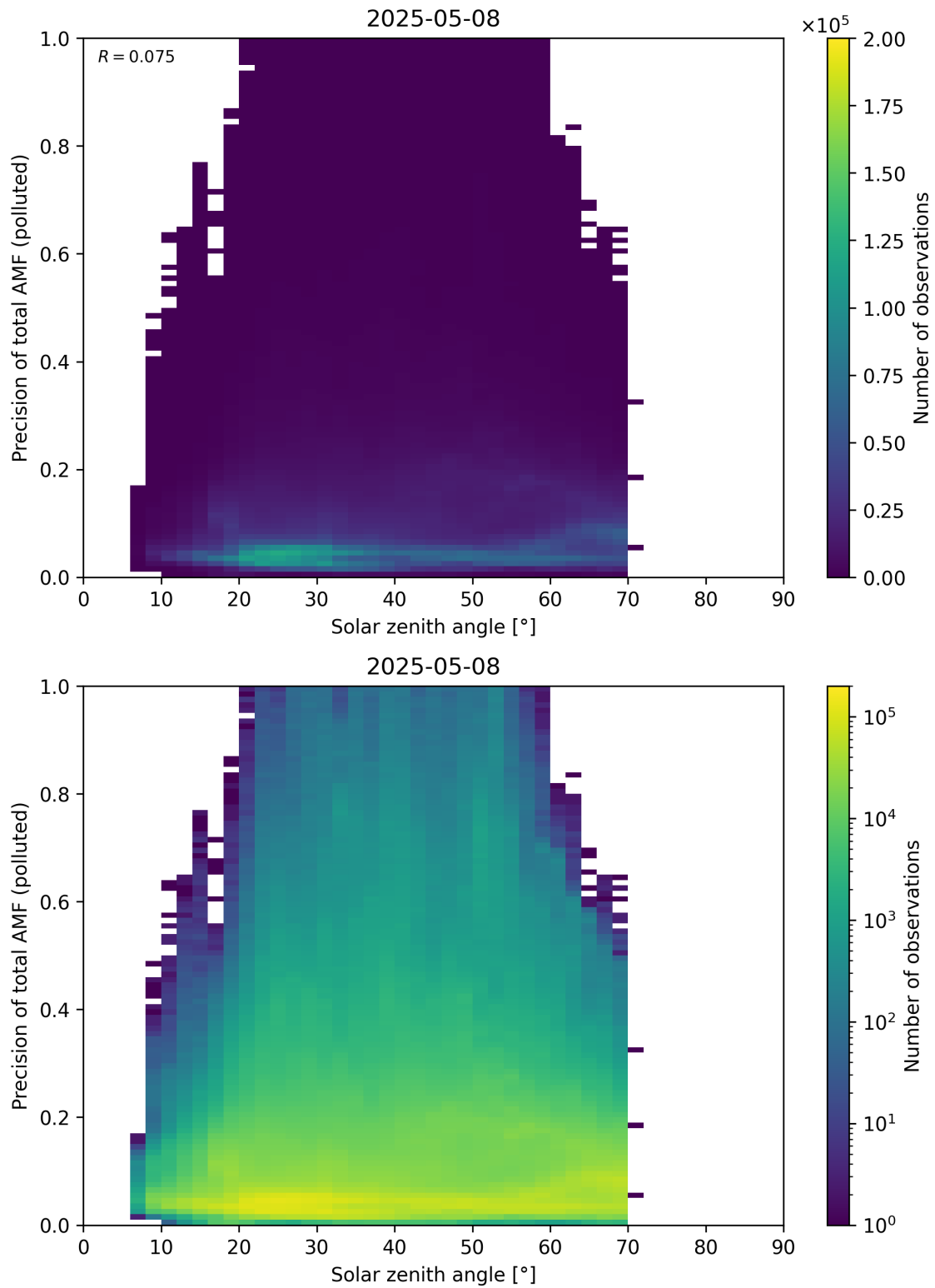
Figure 190: Scatter density plot of “Solar zenith angle” against “Precision of total AMF (polluted)” for 2025-05-07 to 2025-05-09.
