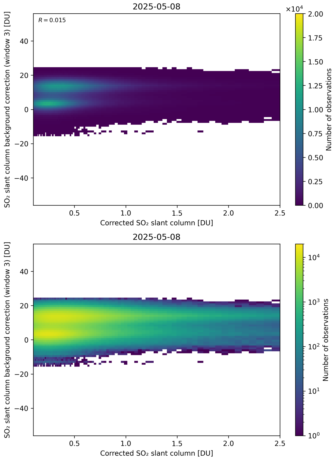
Figure 228: Scatter density plot of “Corrected SO 2 slant column” against “SO 2 slant column background correction (window 3)” for 2025-05-07 to 2025-05-09.
