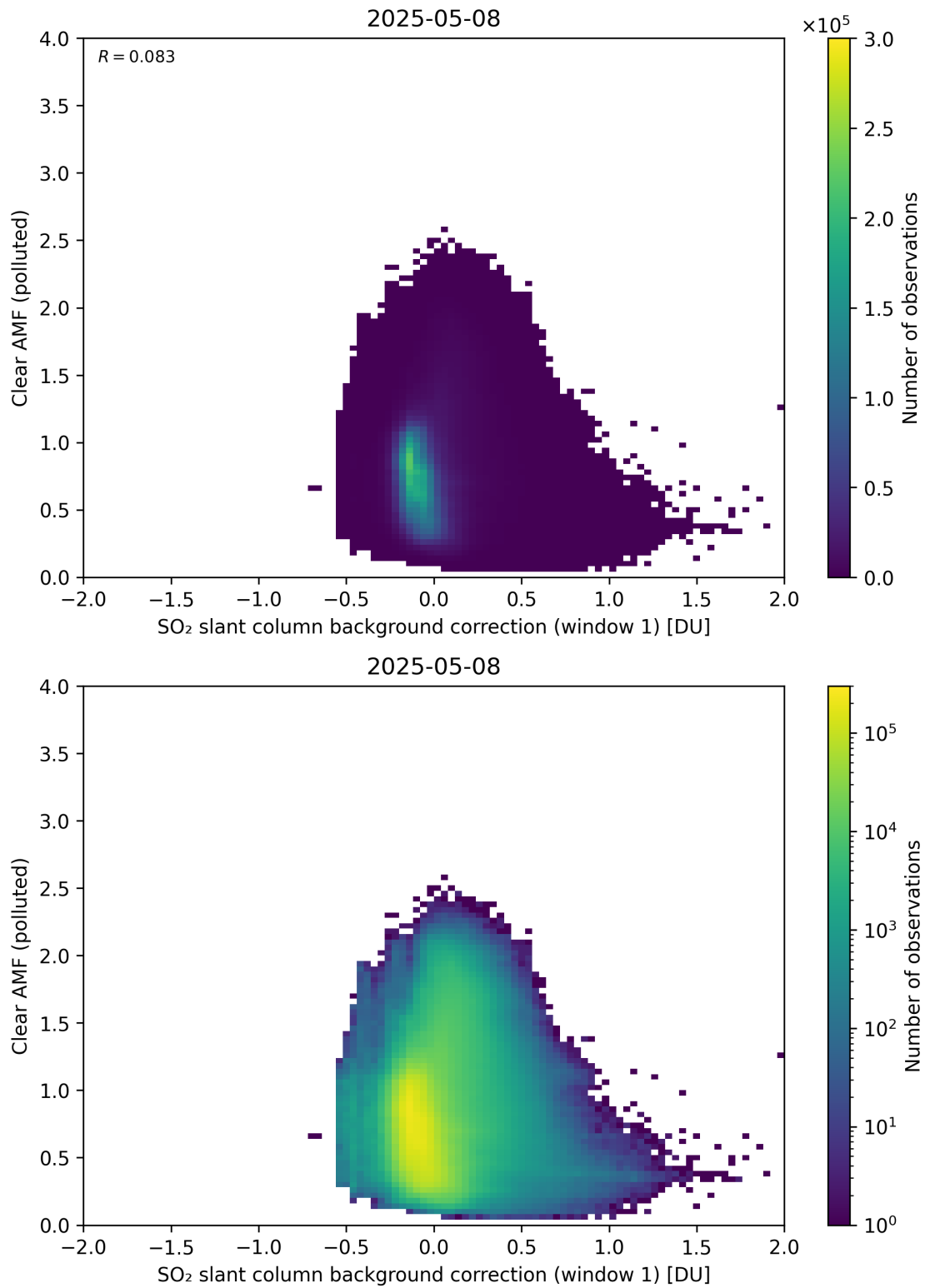
Figure 114: Scatter density plot of “SO 2 slant column background correction (window 1)” against “Clear AMF (polluted)” for 2025-05-07 to 2025-05-09.
