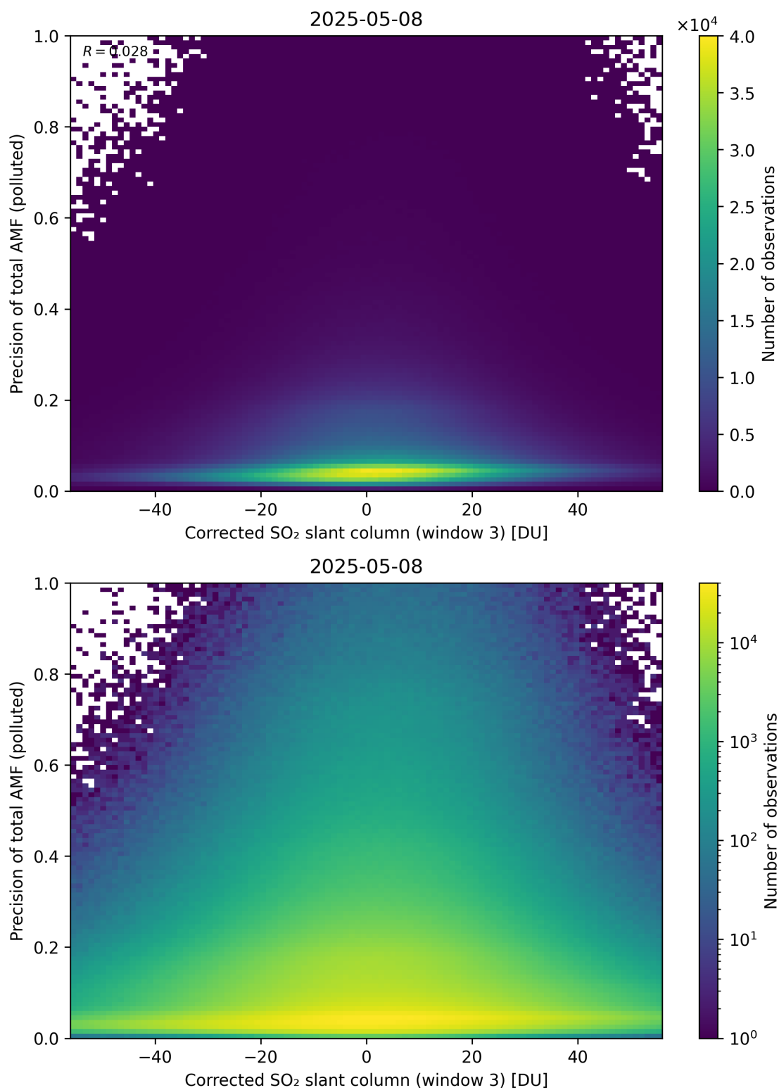
Figure 261: Scatter density plot of “Corrected SO 2 slant column (window 3)” against “Precision of total AMF (polluted)” for 2025-05-07 to 2025-05-09.
