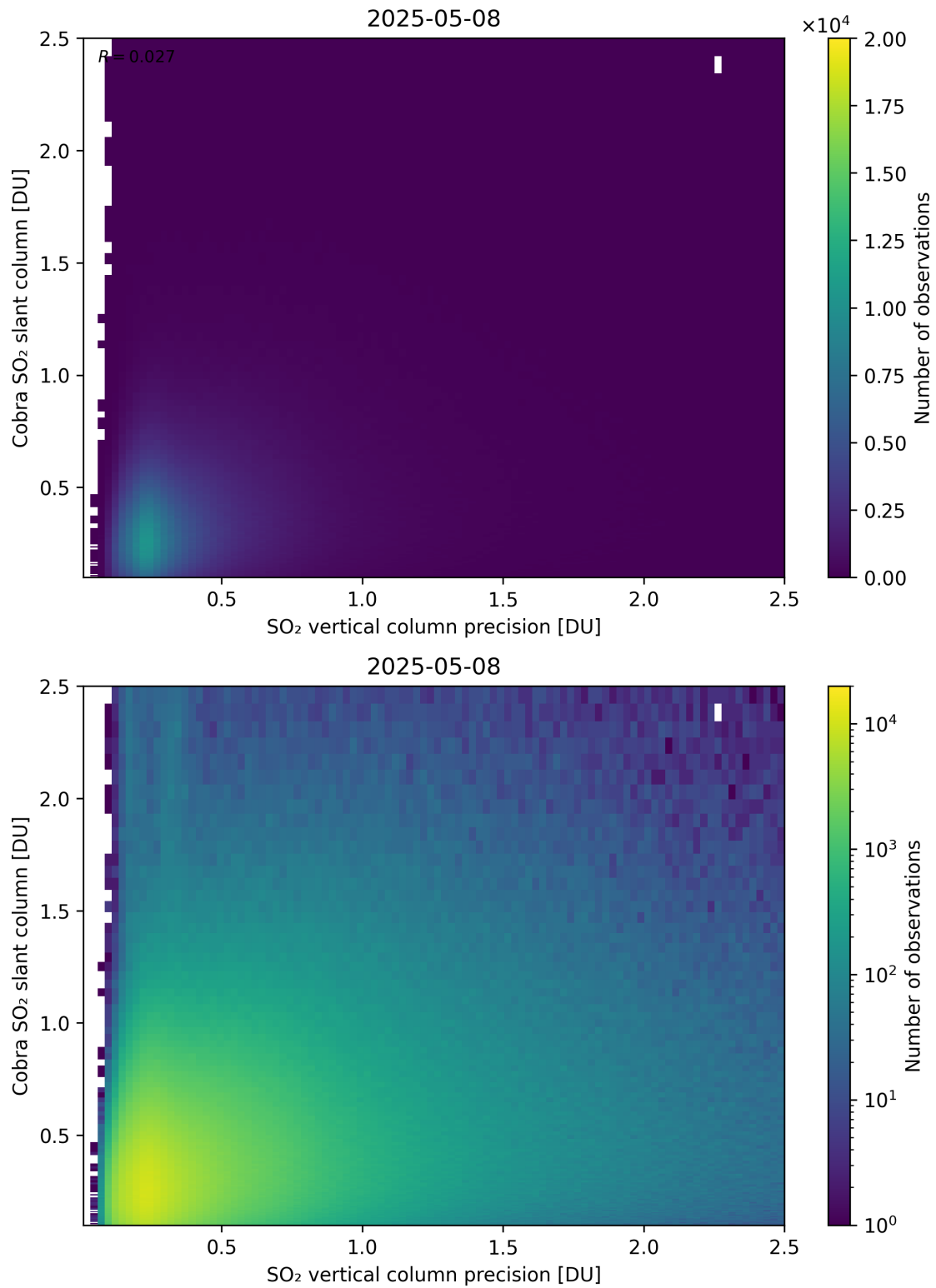
Figure 336: Scatter density plot of “SO 2 vertical column precision” against “Cobra SO 2 slant column” for 2025-05-07 to 2025-05-09.
