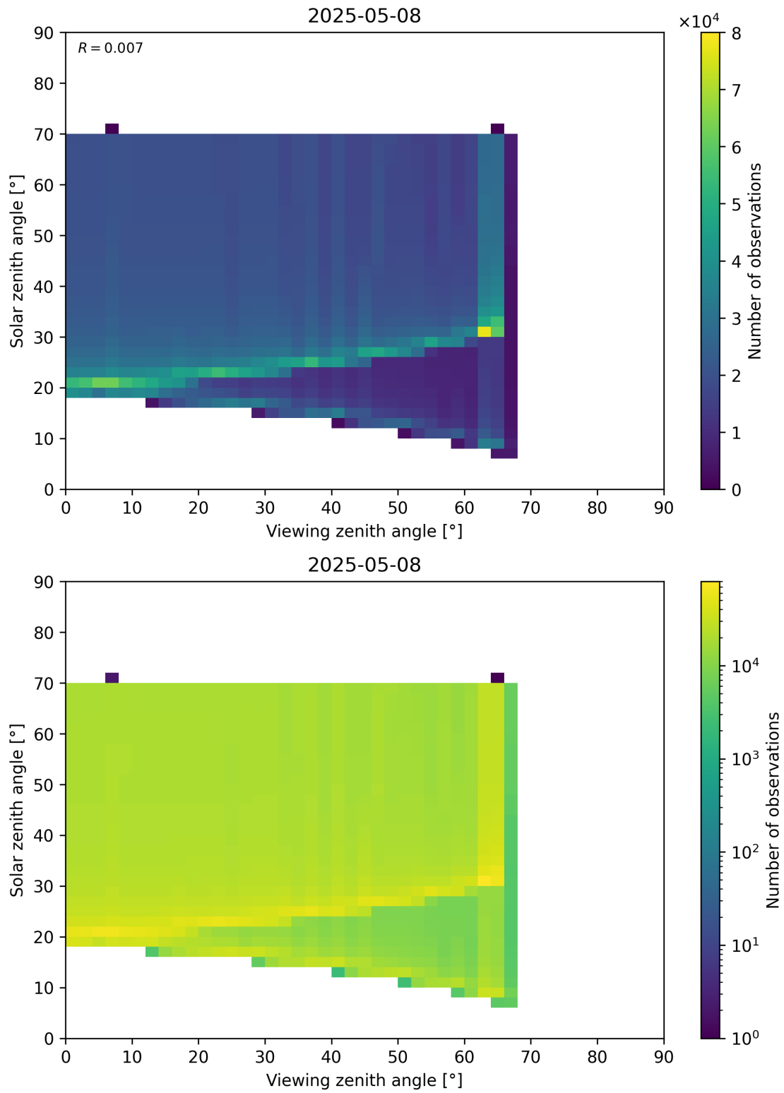
Figure 369: Scatter density plot of “Viewing zenith angle” against “Solar zenith angle” for 2025-05-07 to 2025-05-09.
