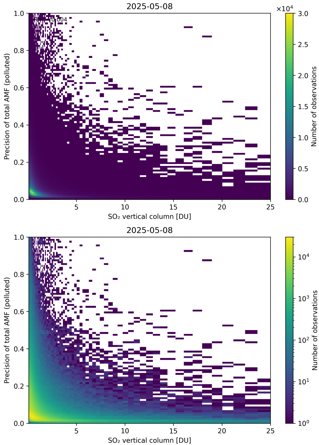
Figure 360: Scatter density plot of “SO 2 vertical column” against “Precision of total AMF (polluted)” for 2025-05-07 to 2025-05-09.
