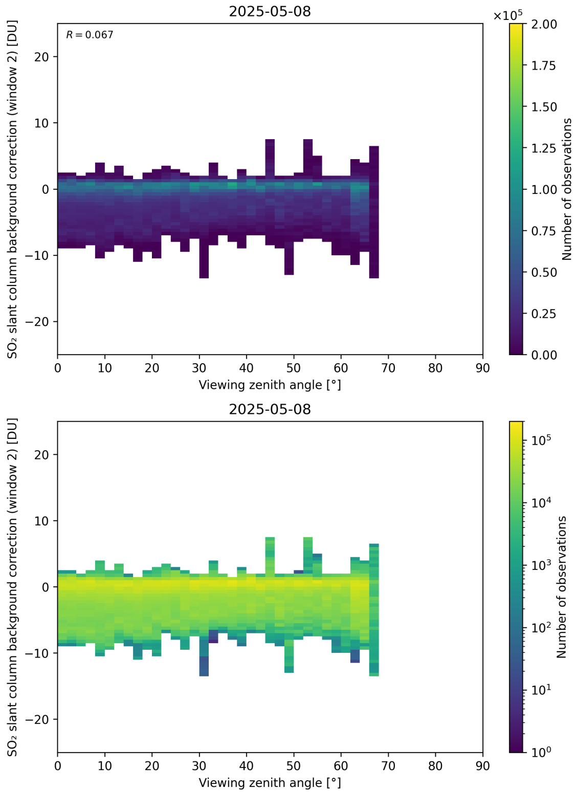
Figure 363: Scatter density plot of “Viewing zenith angle” against “SO 2 slant column background correction (window 2)” for 2025-05-07 to 2025-05-09.
