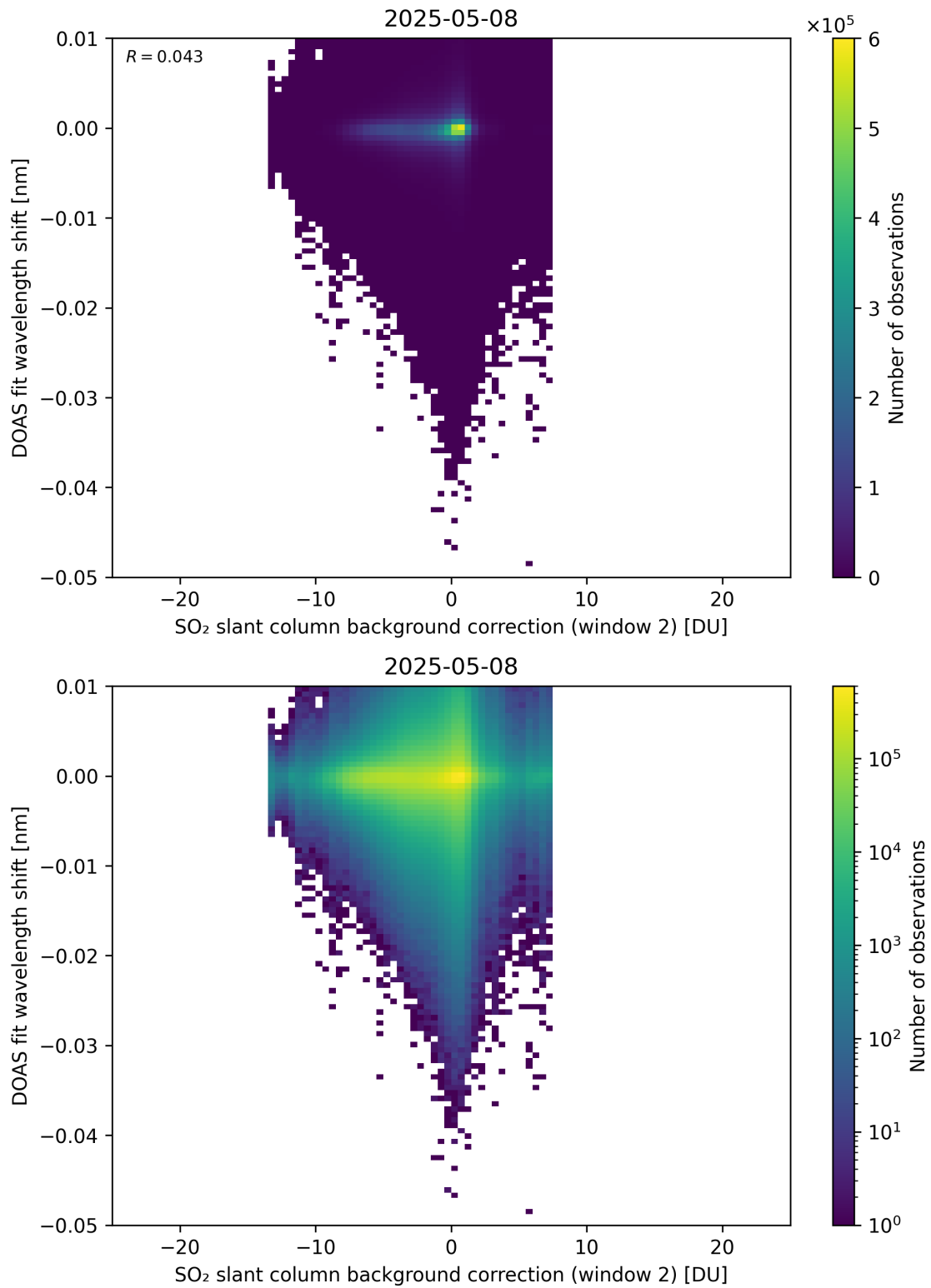
Figure 123: Scatter density plot of “SO 2 slant column background correction (window 2)” against “DOAS fit wavelength shift” for 2025-05-07 to 2025-05-09.
