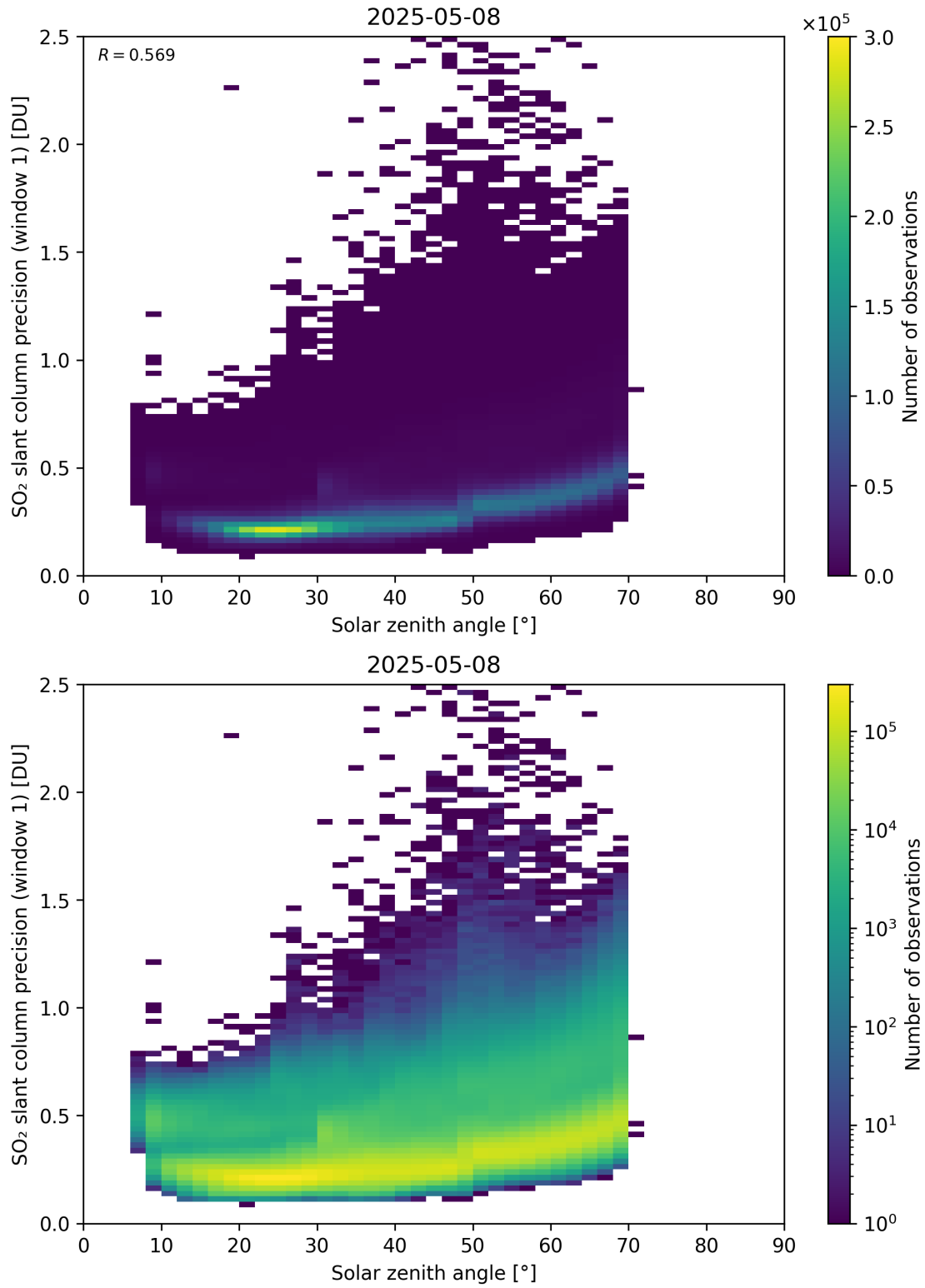
Figure 185: Scatter density plot of “Solar zenith angle” against “SO 2 slant column precision (window 1)” for 2025-05-07 to 2025-05-09.
