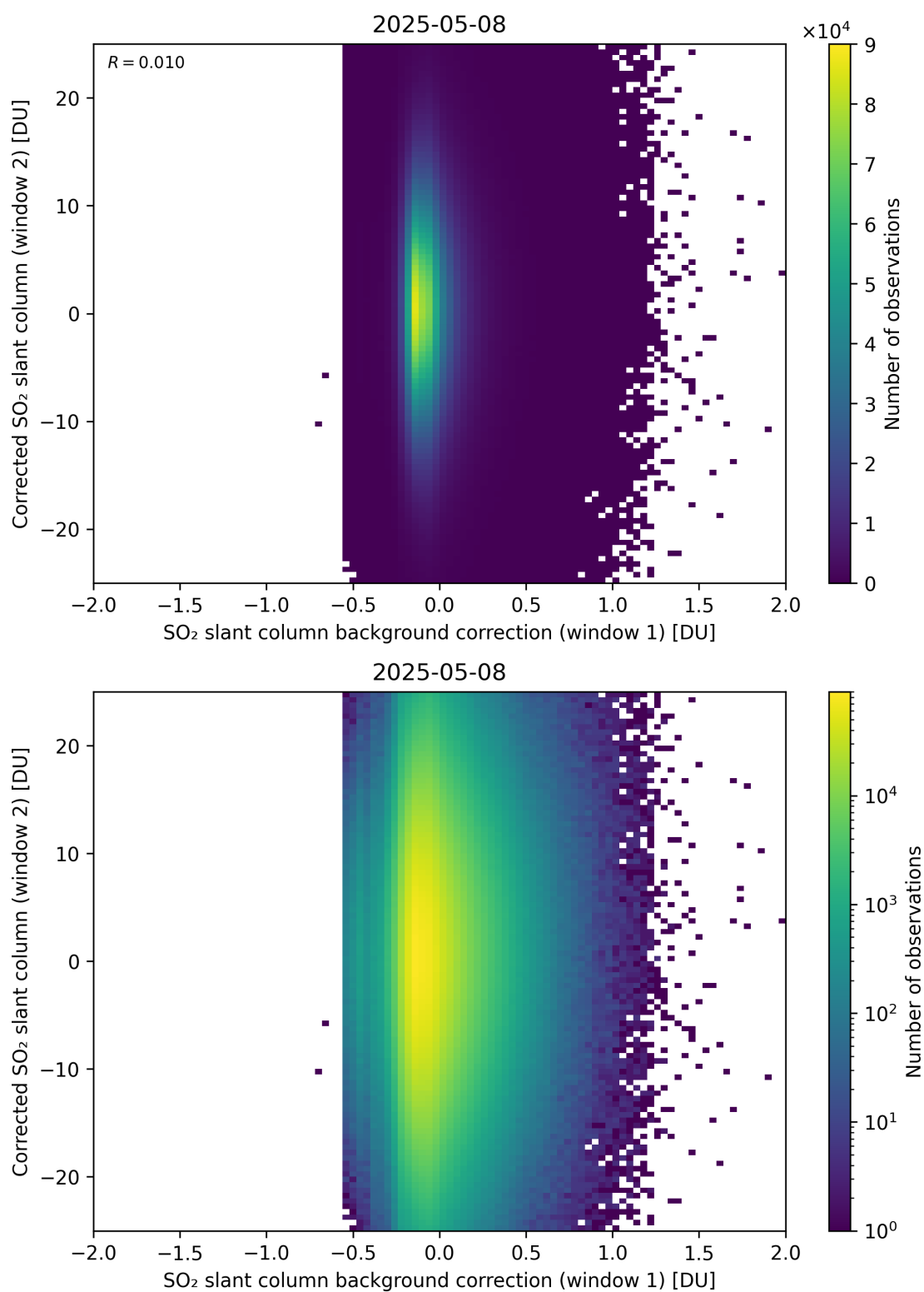
Figure 115: Scatter density plot of “SO 2 slant column background correction (window 1)” against “Corrected SO 2 slant column (window 2)” for 2025-05-07 to 2025-05-09.
