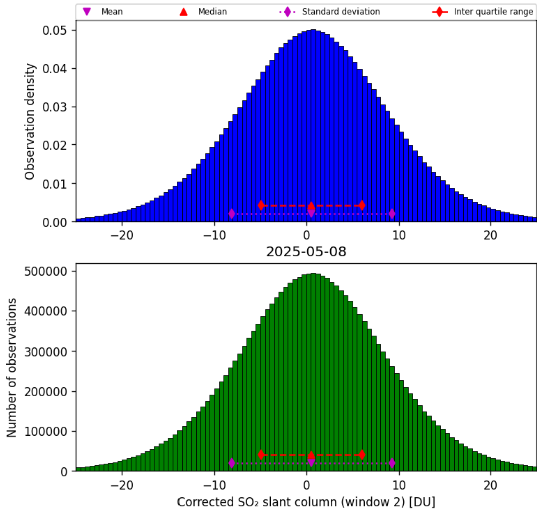
Figure 69: Histogram of “Corrected SO 2 slant column (window 2)” for 2025-05-07 to 2025-05-09
