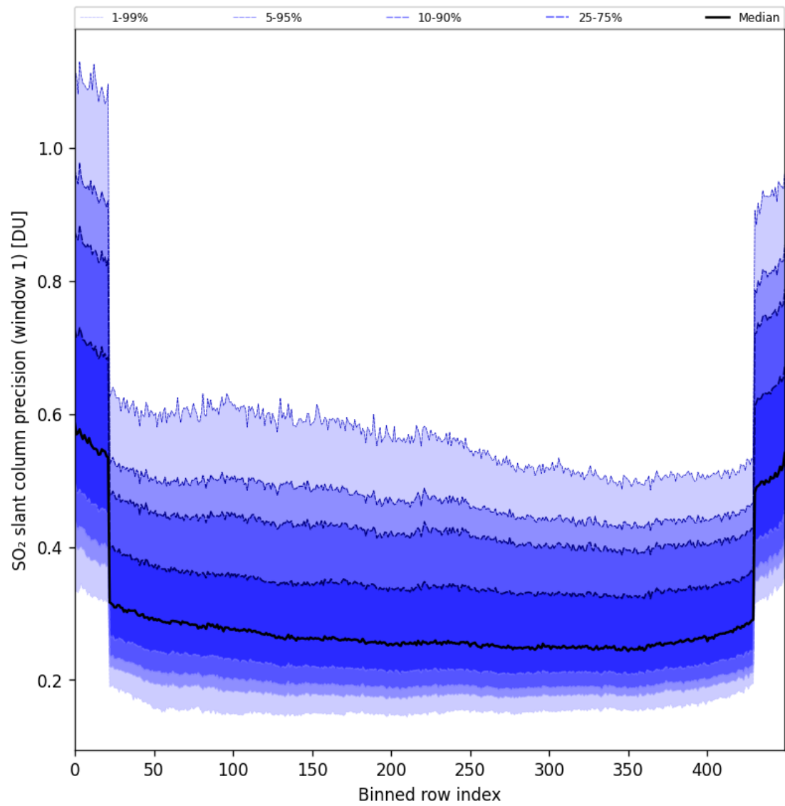
Figure 90: Along track statistics of “SO 2 slant column precision (window 1)” for 2025-05-07 to 2025-05-09
