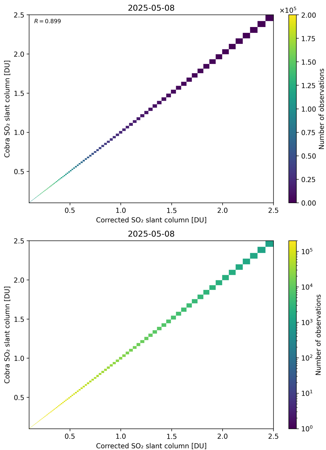
Figure 233: Scatter density plot of “Corrected SO 2 slant column” against “Cobra SO 2 slant column” for 2025-05-07 to 2025-05-09.
