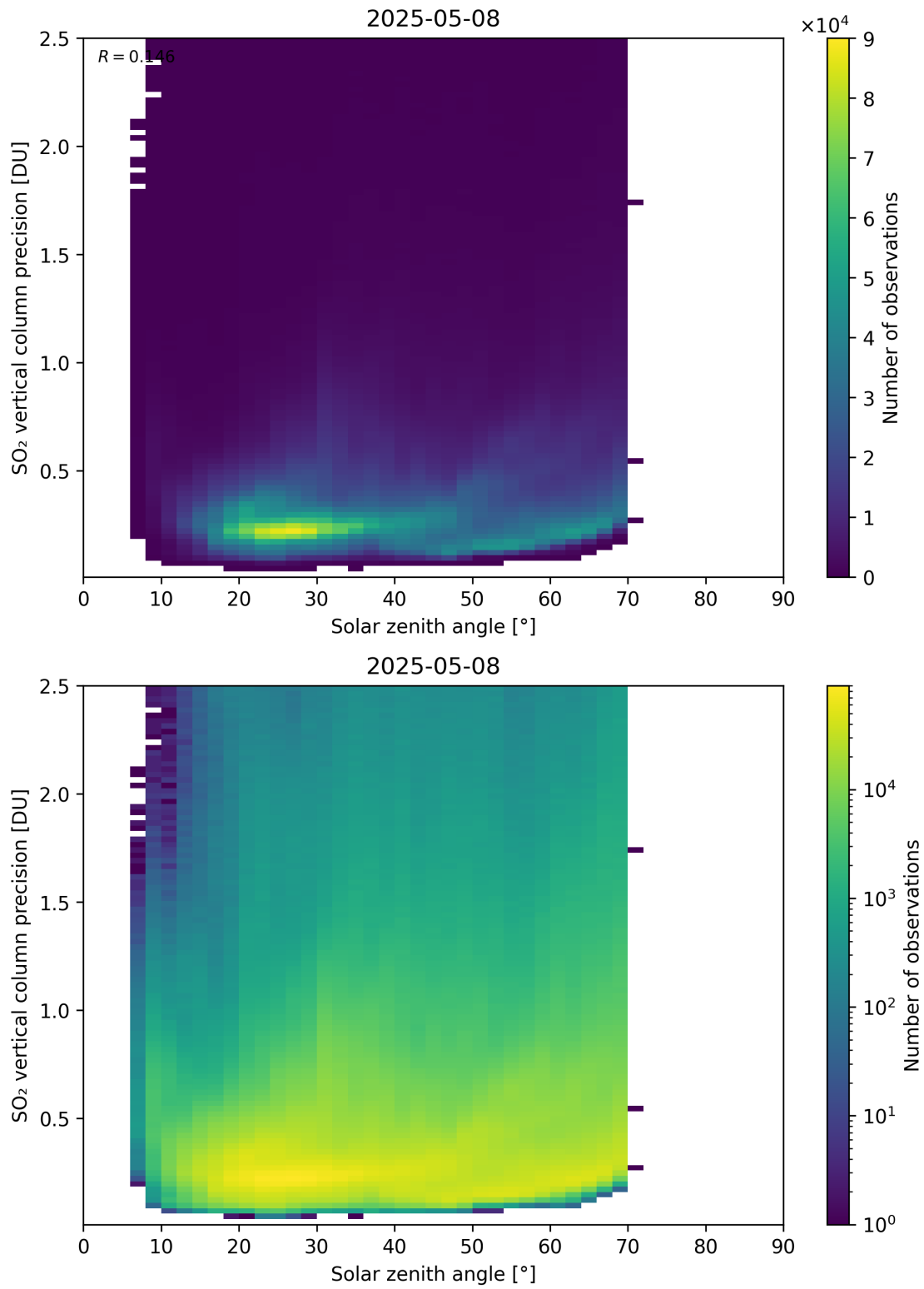
Figure 192: Scatter density plot of “Solar zenith angle” against “SO 2 vertical column precision” for 2025-05-07 to 2025-05-09.
