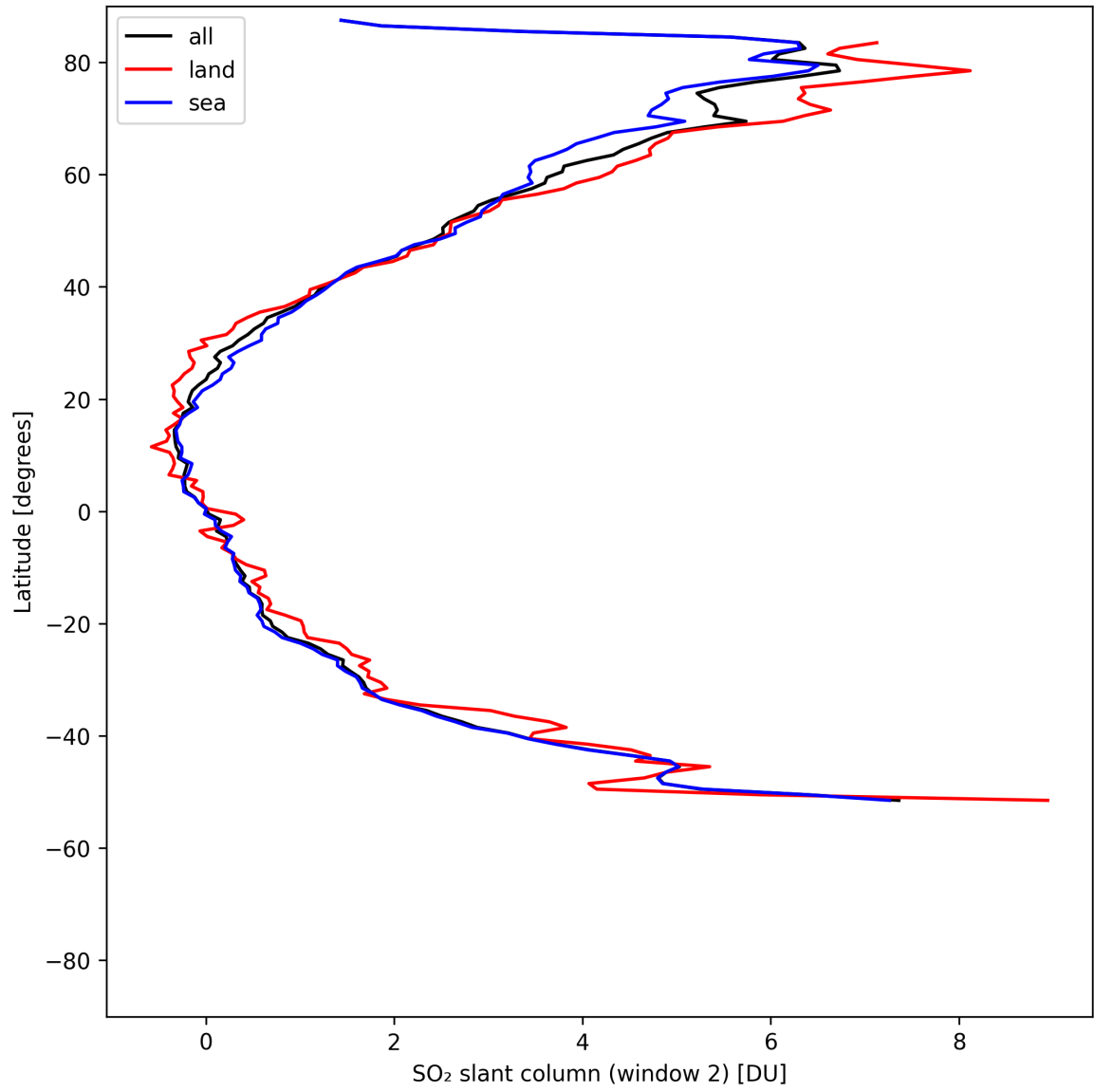
Figure 41: Zonal average of “SO 2 slant column (window 2)” for 2025-05-07 to 2025-05-09.
