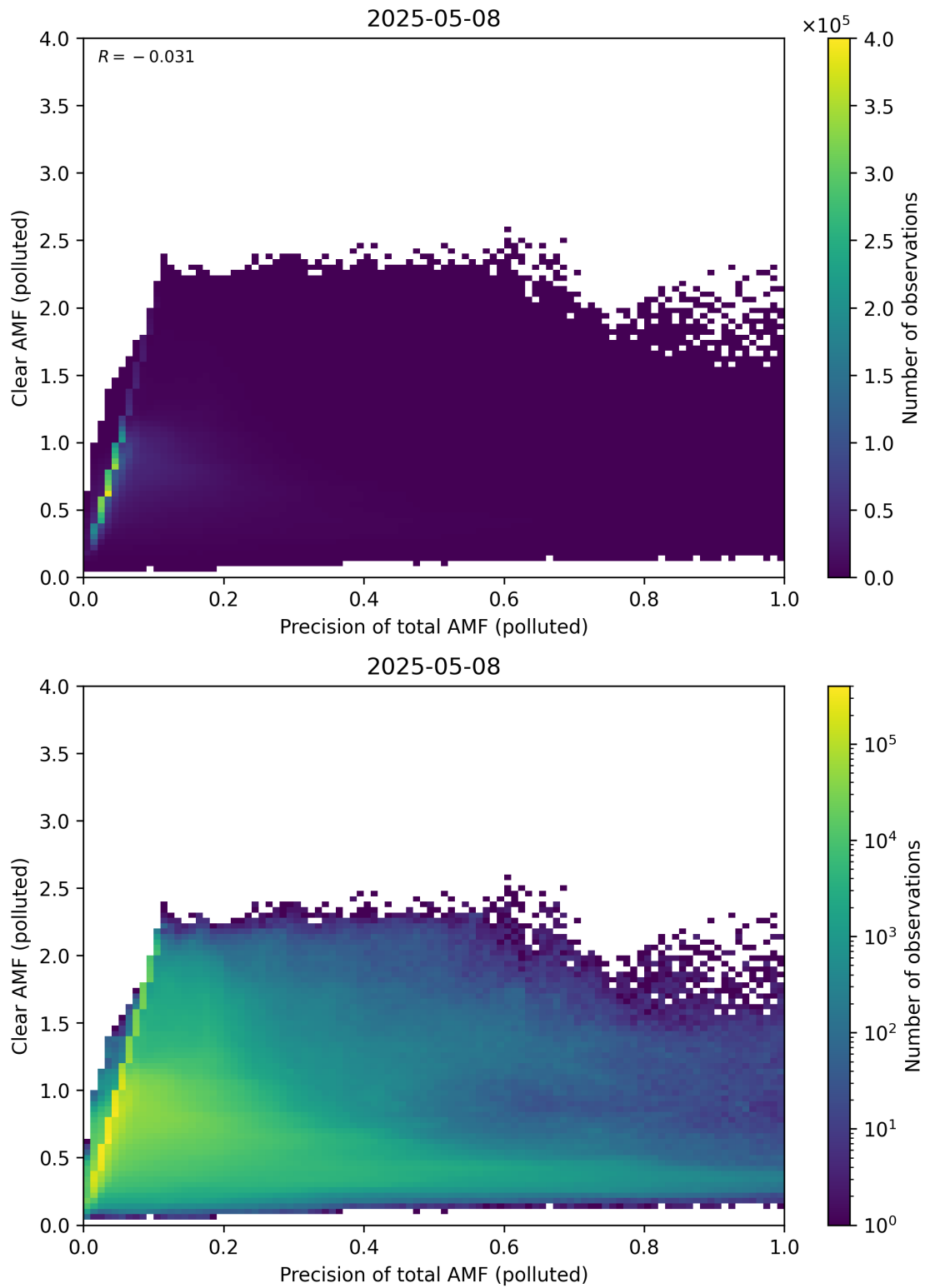
Figure 320: Scatter density plot of “Precision of total AMF (polluted)” against “Clear AMF (polluted)” for 2025-05-07 to 2025-05-09.
