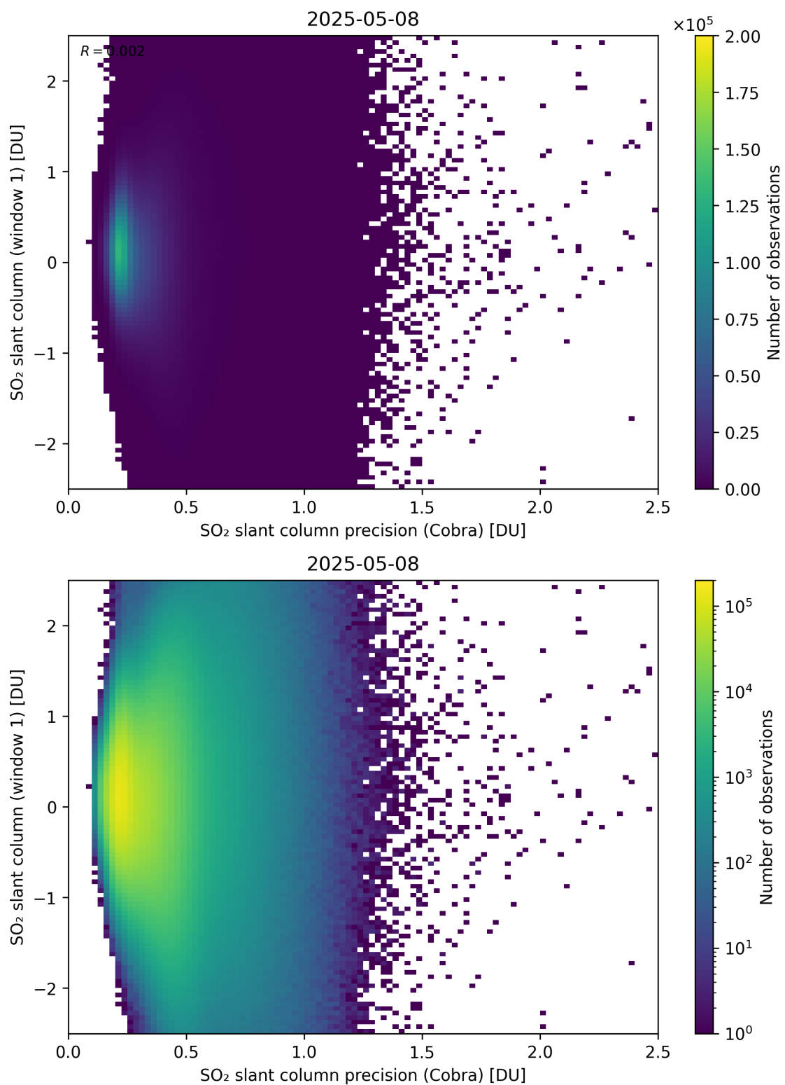
Figure 208: Scatter density plot of “SO 2 slant column precision (Cobra)” against “SO 2 slant column (window 1)” for 2025-05-07 to 2025-05-09.
