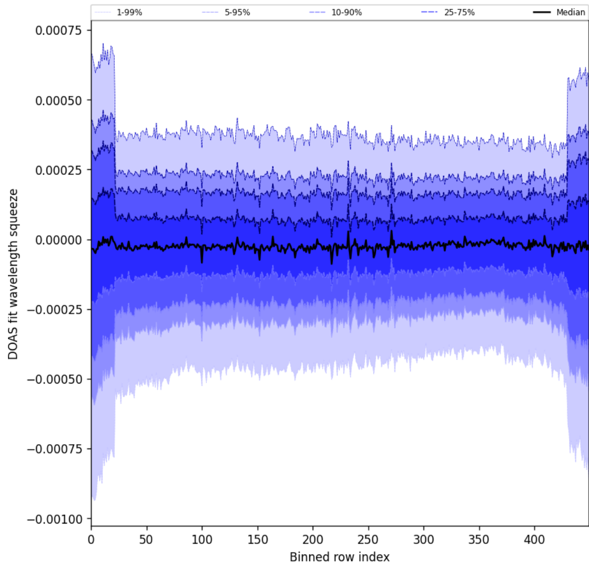
Figure 103: Along track statistics of “DOAS fit wavelength squeeze” for 2025-05-07 to 2025-05-09
