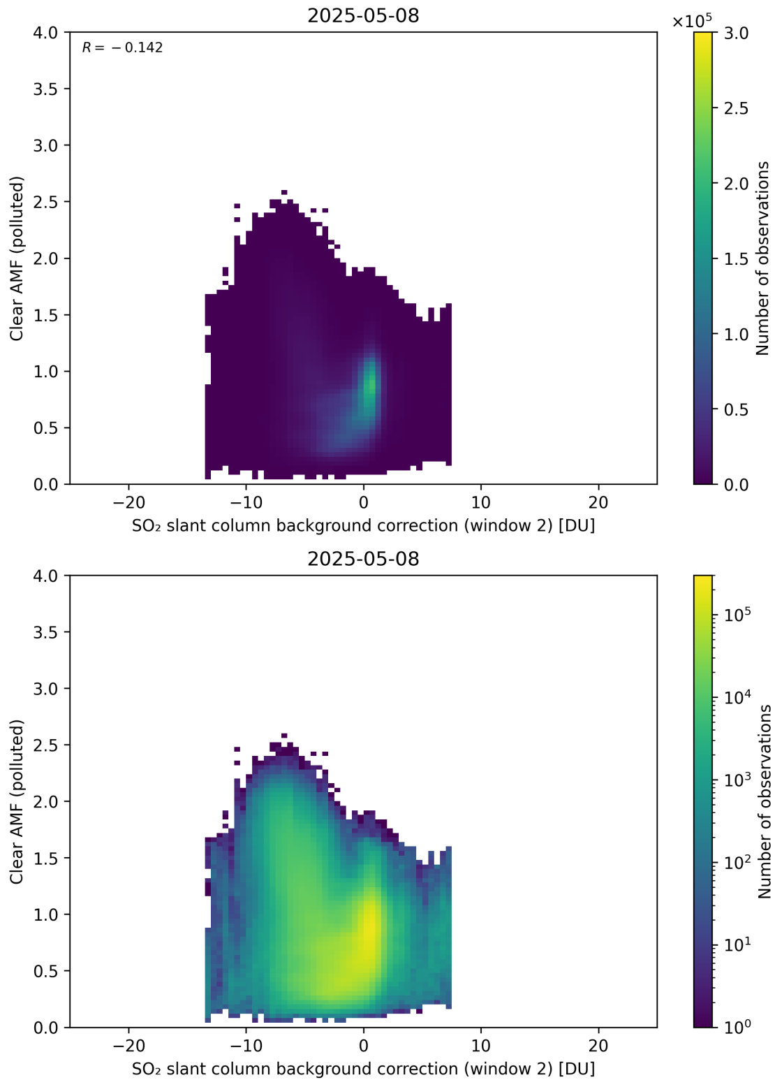
Figure 126: Scatter density plot of “SO 2 slant column background correction (window 2)” against “Clear AMF (polluted)” for 2025-05-07 to 2025-05-09.
