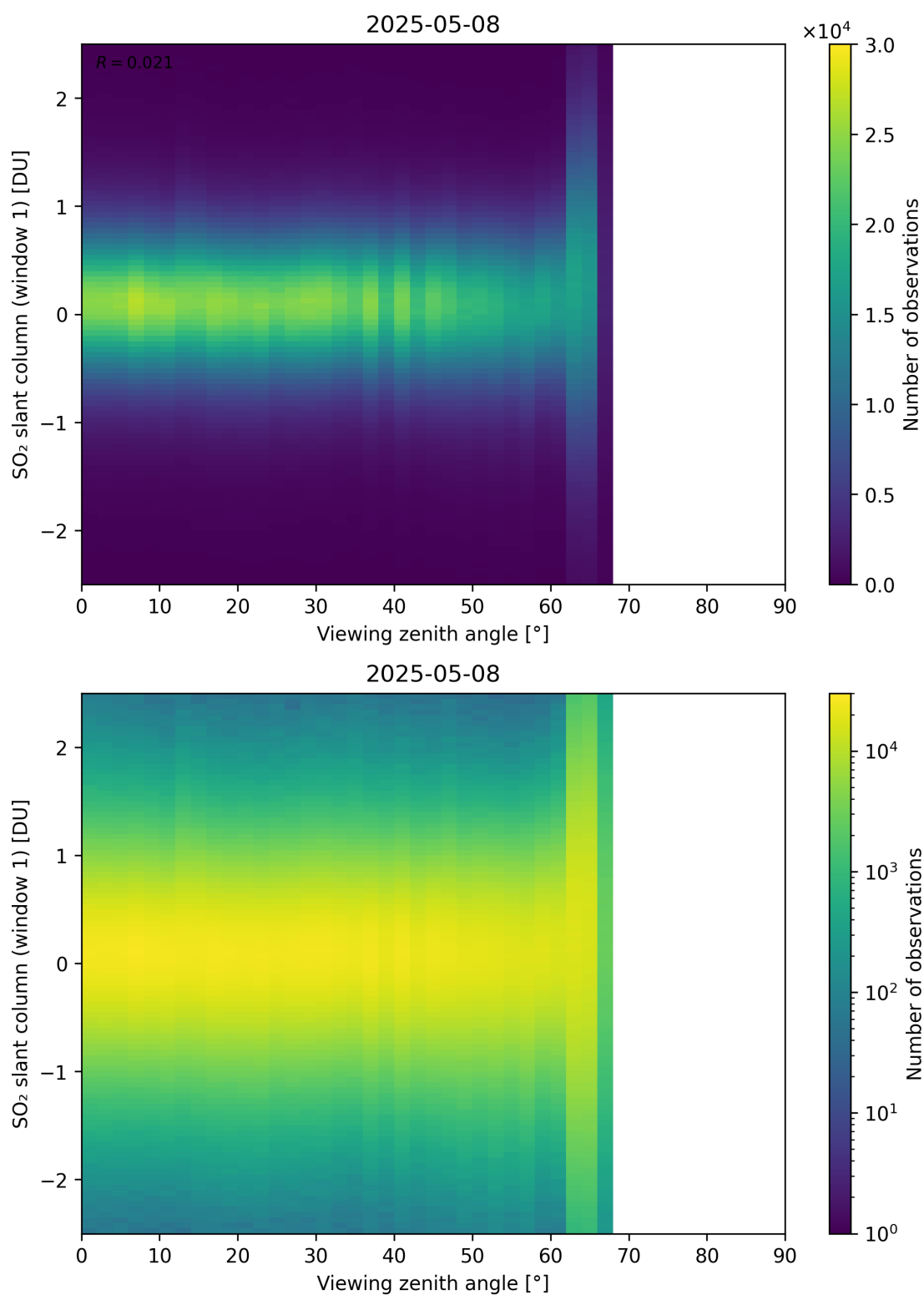
Figure 376: Scatter density plot of “Viewing zenith angle” against “SO 2 slant column (window 1)” for 2025-05-07 to 2025-05-09.
