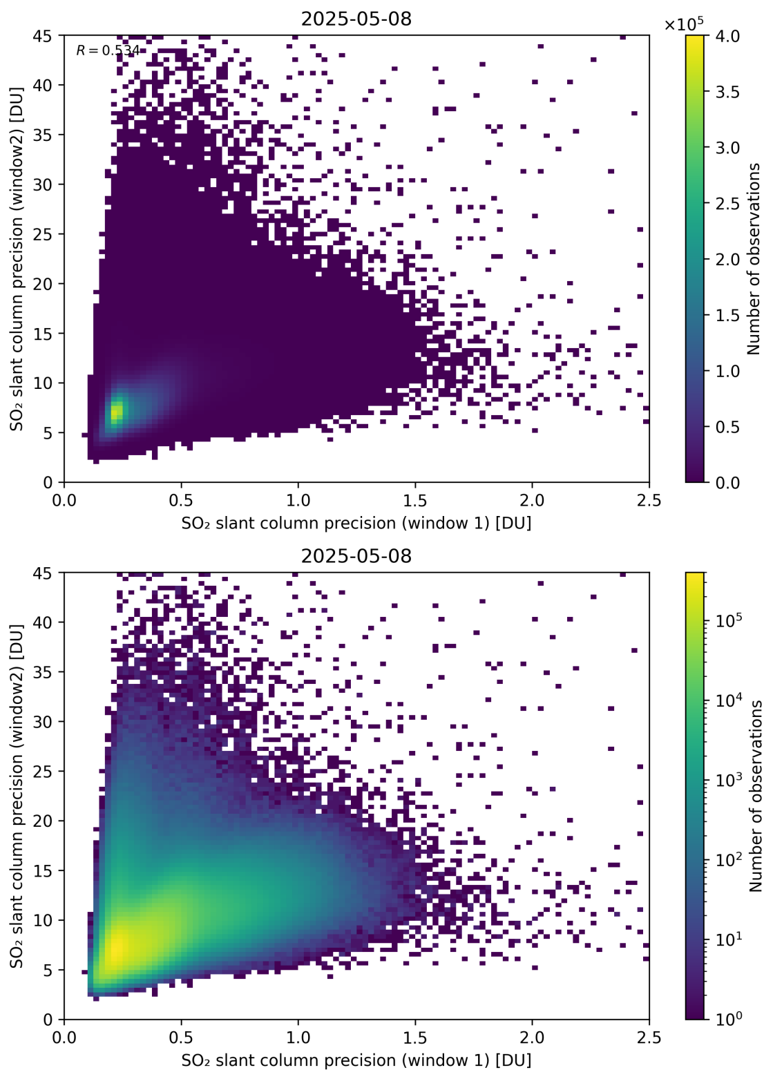
Figure 277: Scatter density plot of “SO 2 slant column precision (window 1)” against “SO 2 slant column precision (window2)” for 2025-05-07 to 2025-05-09.
