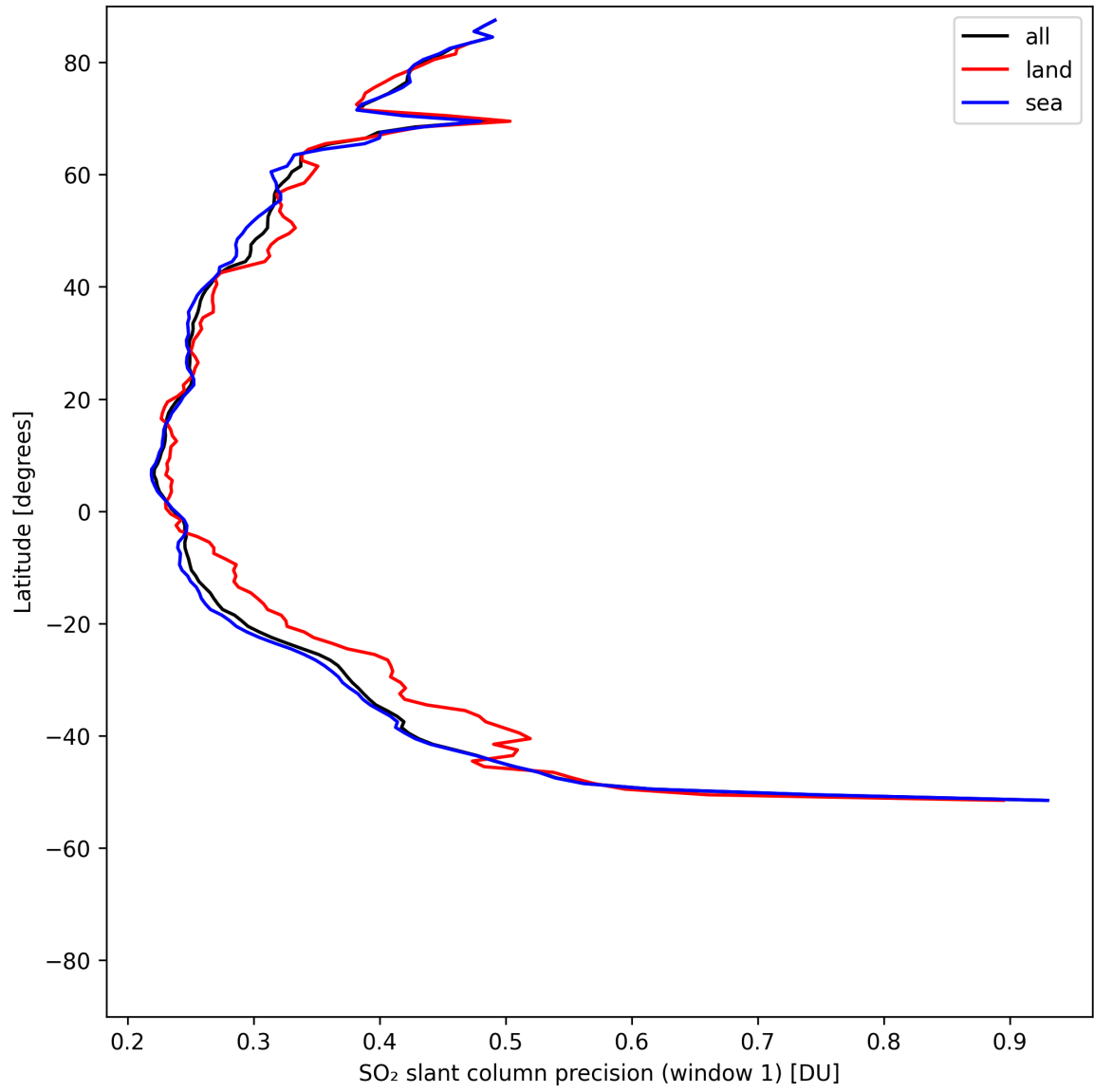
Figure 38: Zonal average of “SO 2 slant column precision (window 1)” for 2025-05-07 to 2025-05-09.
