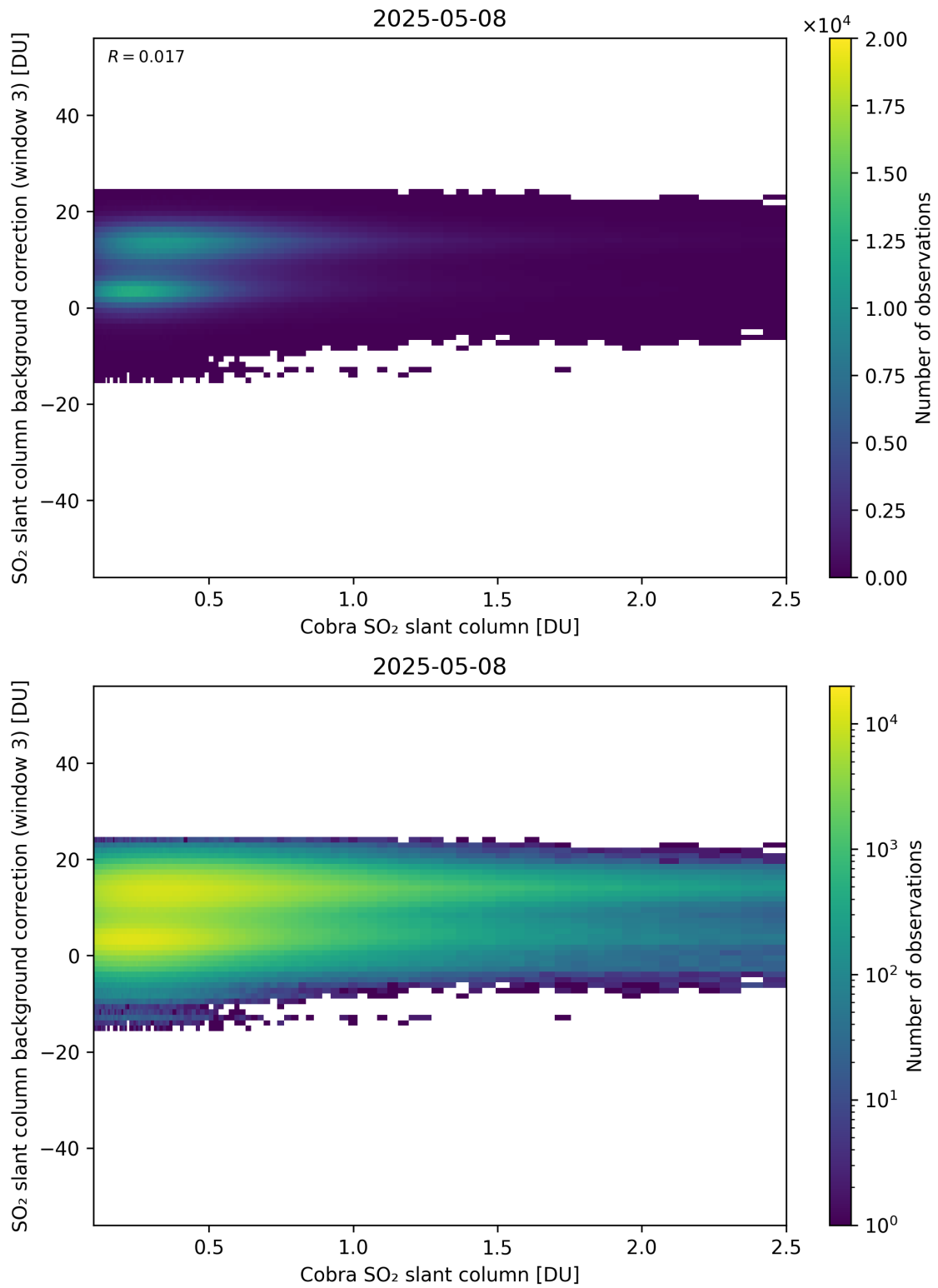
Figure 195: Scatter density plot of “Cobra SO 2 slant column” against “SO 2 slant column background correction (window 3)” for 2025-05-07 to 2025-05-09.
