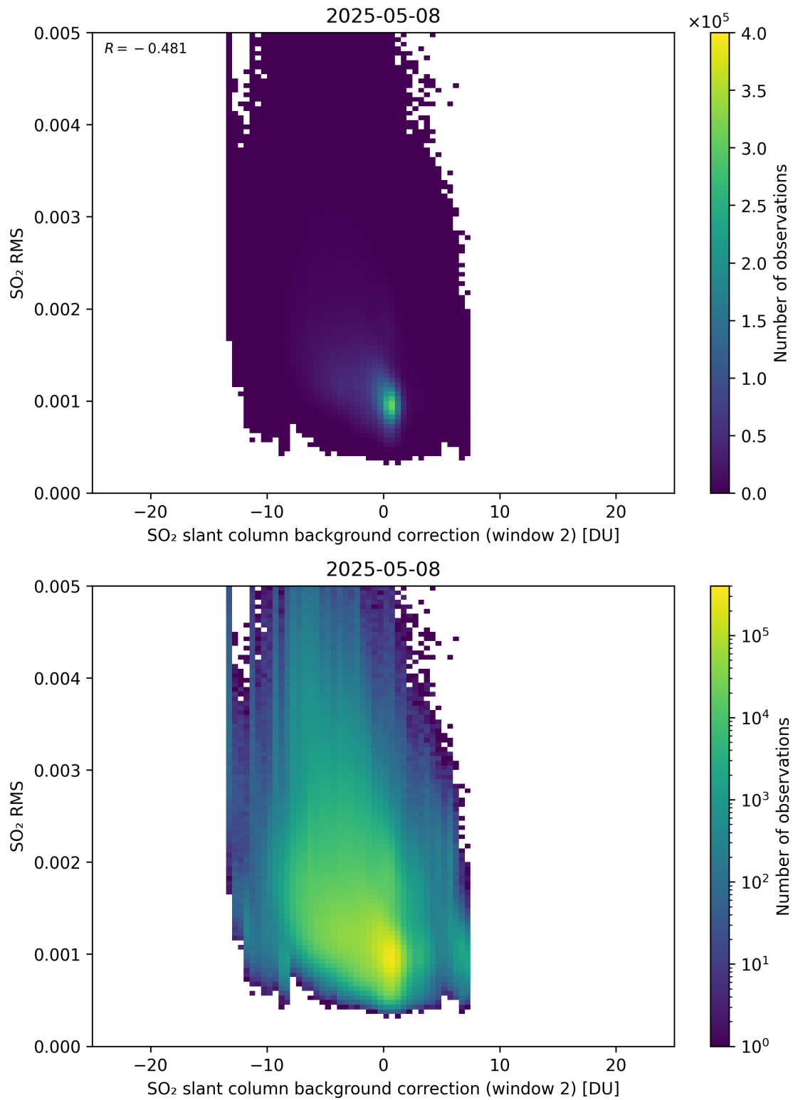
Figure 125: Scatter density plot of “SO 2 slant column background correction (window 2)” against “SO 2 RMS” for 2025-05-07 to 2025-05-09.
