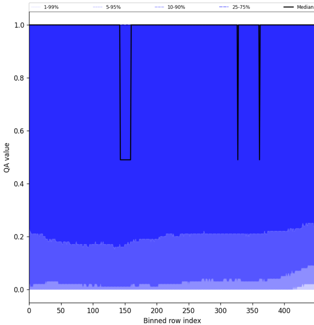
Figure 83: Along track statistics of “QA value” for 2025-05-07 to 2025-05-09
