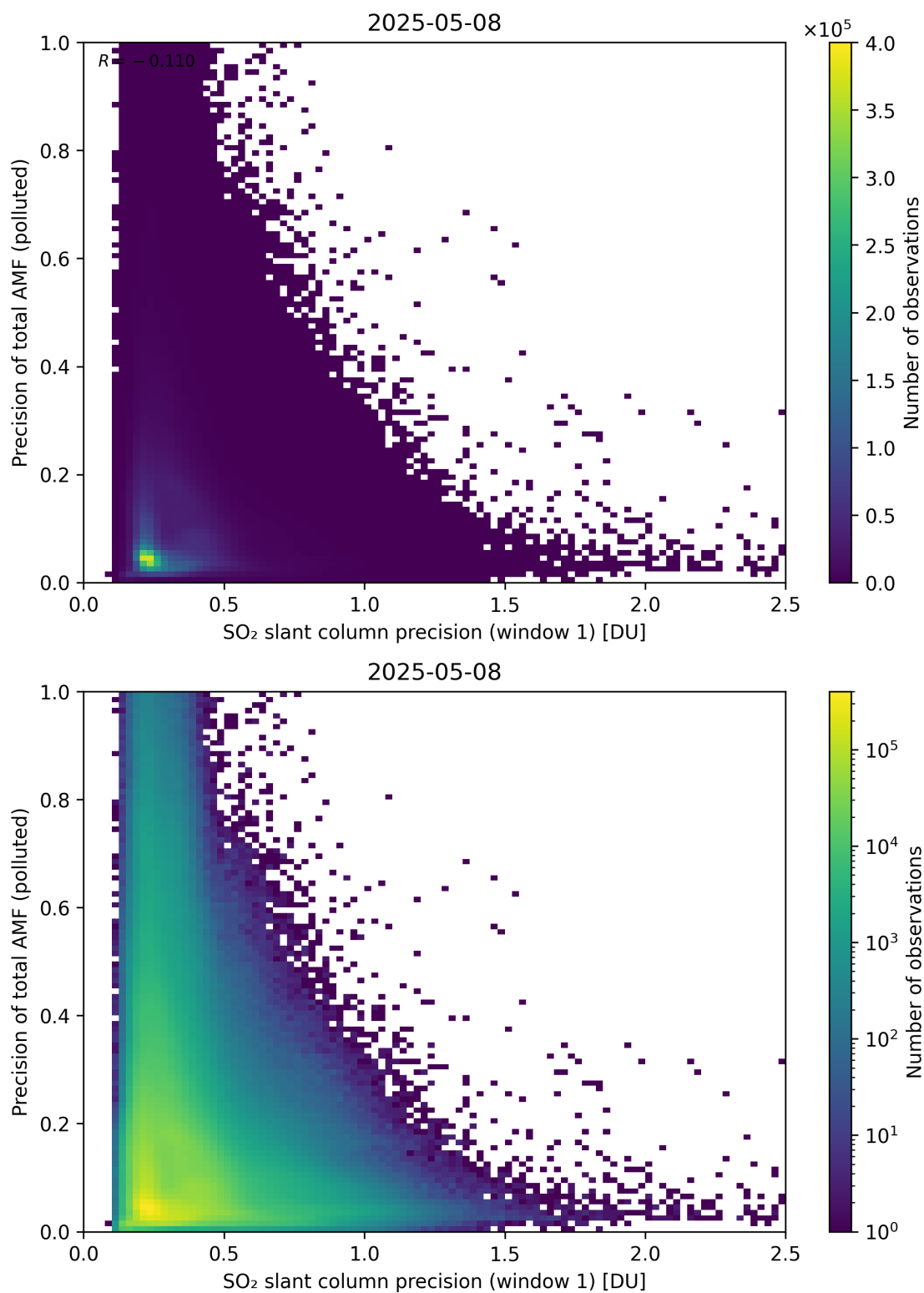
Figure 281: Scatter density plot of “SO 2 slant column precision (window 1)” against “Precision of total AMF (polluted)” for 2025-05-07 to 2025-05-09.
