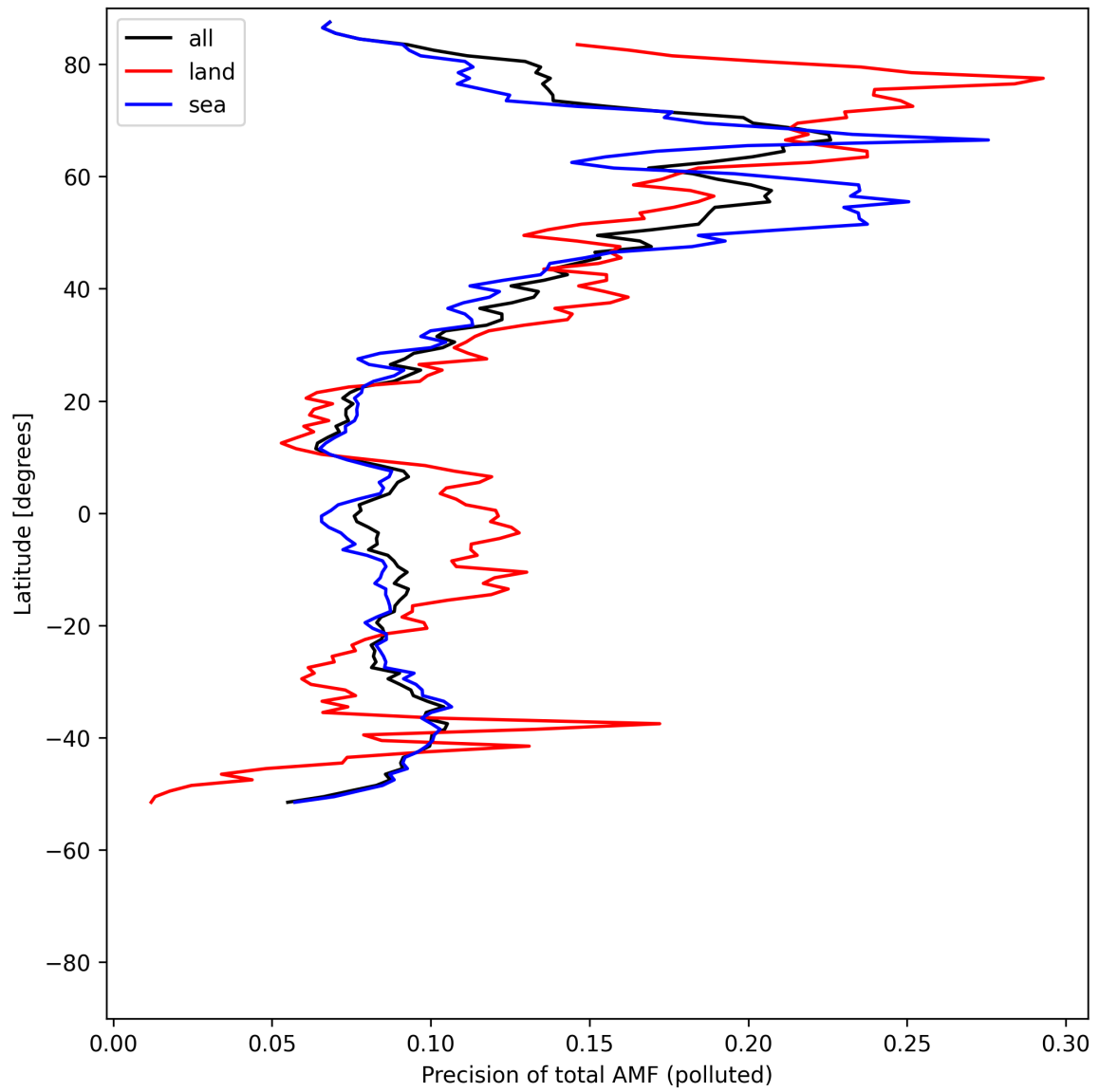
Figure 54: Zonal average of “Precision of total AMF (polluted)” for 2025-05-07 to 2025-05-09.
