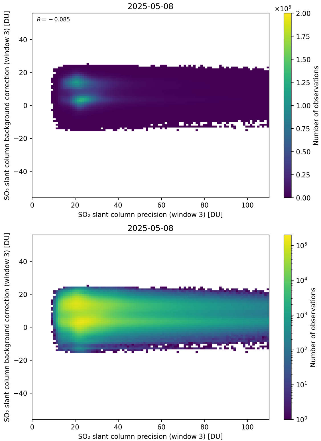
Figure 307: Scatter density plot of “SO 2 slant column precision (window 3)” against “SO 2 slant column background correction (window 3)” for 2025-05-07 to 2025-05-09.
