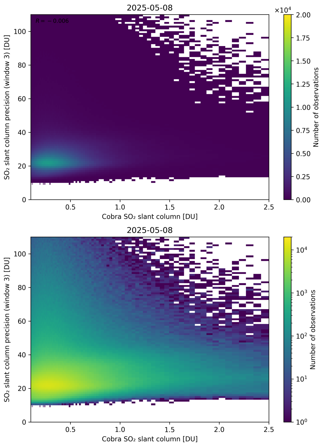
Figure 223: Scatter density plot of “Cobra SO 2 slant column” against “SO 2 slant column precision (window 3)” for 2025-05-07 to 2025-05-09.
