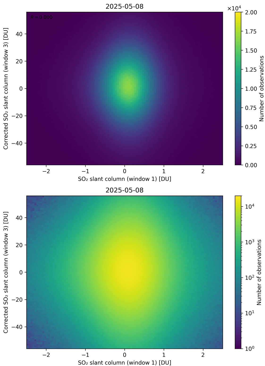
Figure 284: Scatter density plot of “SO 2 slant column (window 1)” against “Corrected SO 2 slant column (window 3)” for 2025-05-07 to 2025-05-09.
