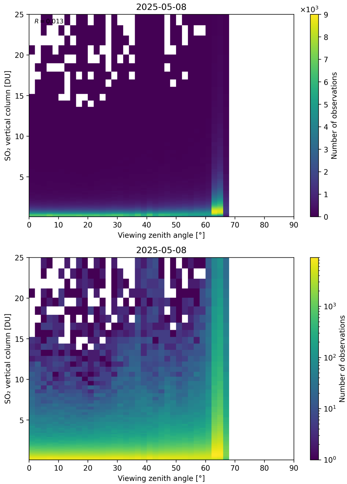
Figure 383: Scatter density plot of “Viewing zenith angle” against “SO 2 vertical column” for 2025-05-07 to 2025-05-09.
