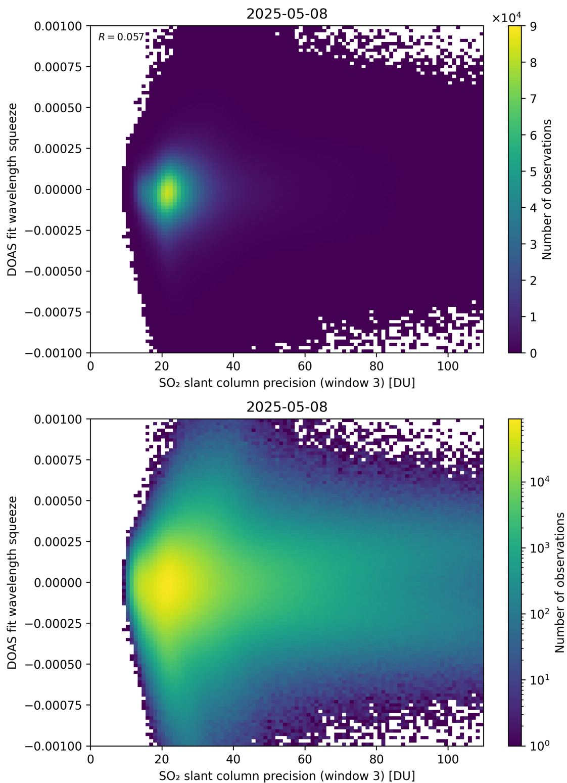
Figure 309: Scatter density plot of “SO 2 slant column precision (window 3)” against “DOAS fit wavelength squeeze” for 2025-05-07 to 2025-05-09.
