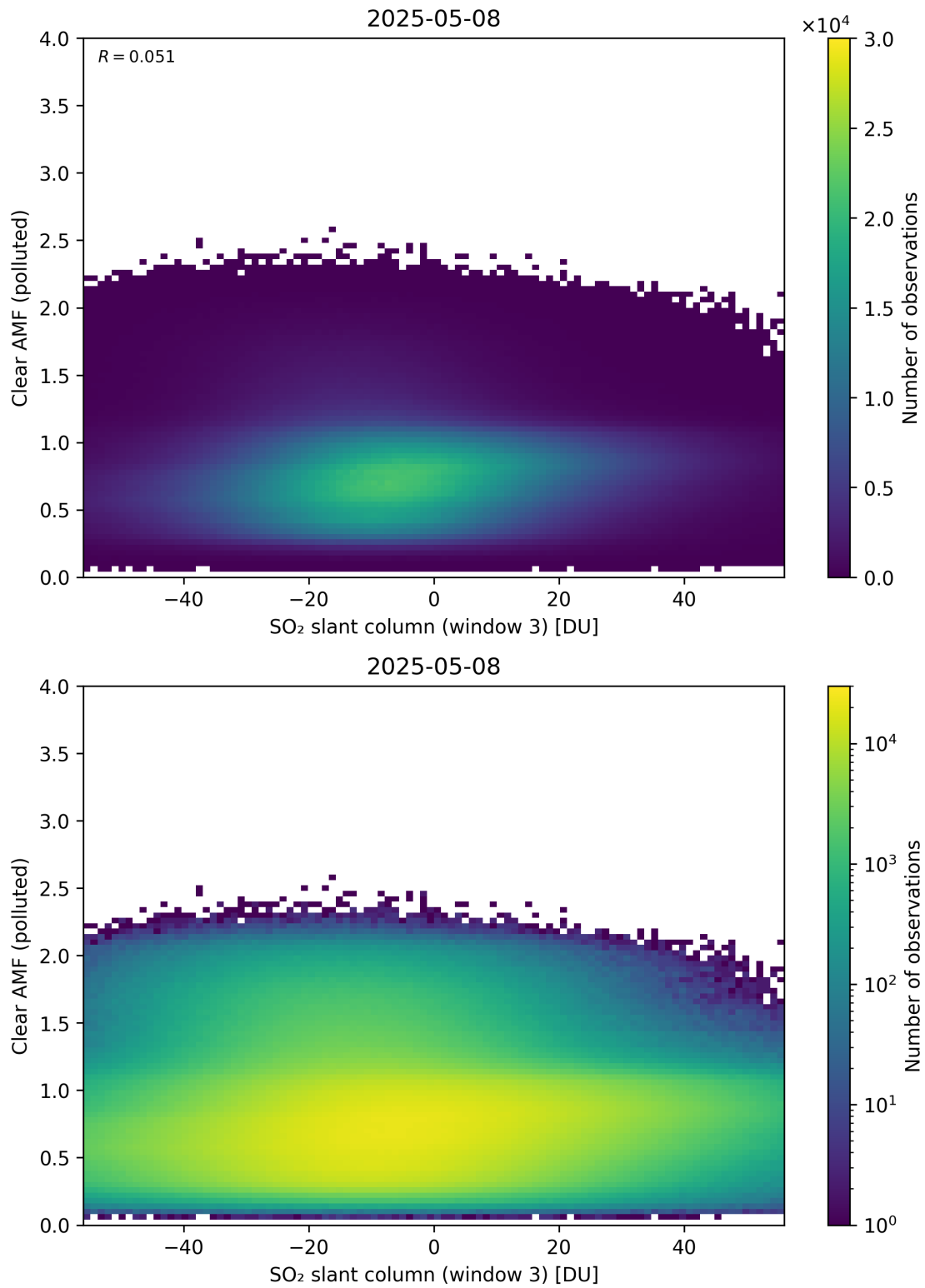
Figure 315: Scatter density plot of “SO 2 slant column (window 3)” against “Clear AMF (polluted)” for 2025-05-07 to 2025-05-09.
