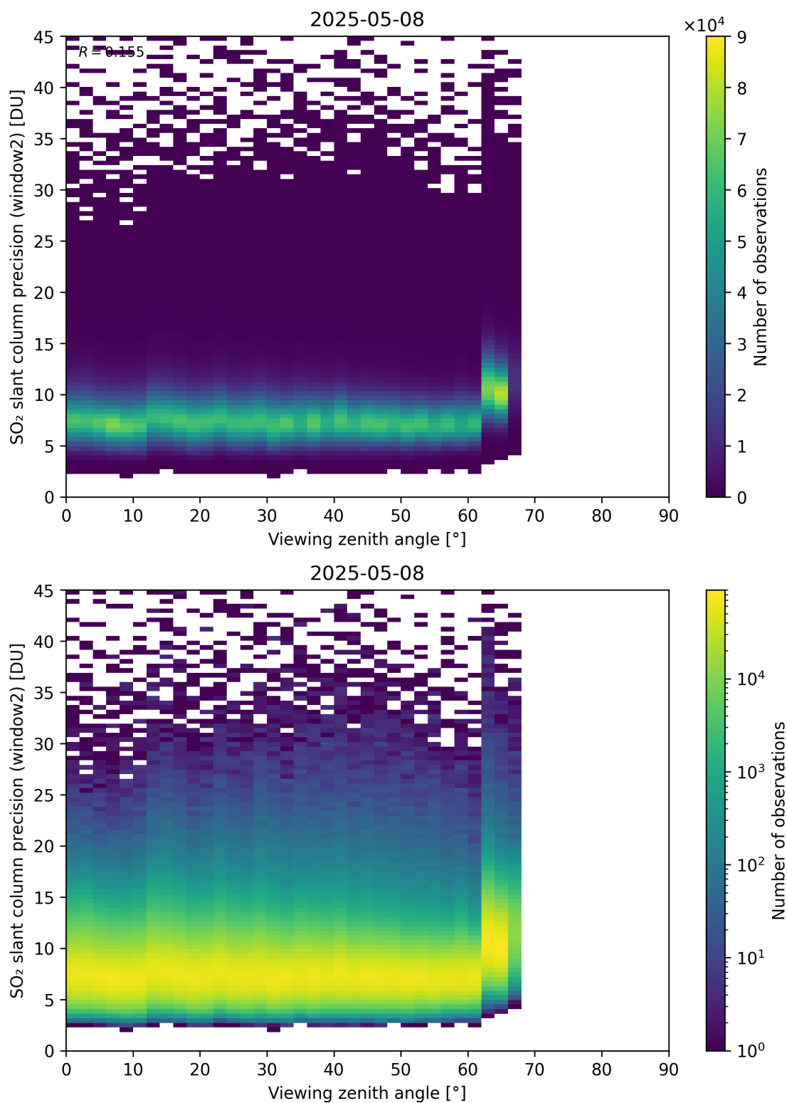
Figure 378: Scatter density plot of “Viewing zenith angle” against “SO 2 slant column precision (window2)” for 2025-05-07 to 2025-05-09.
