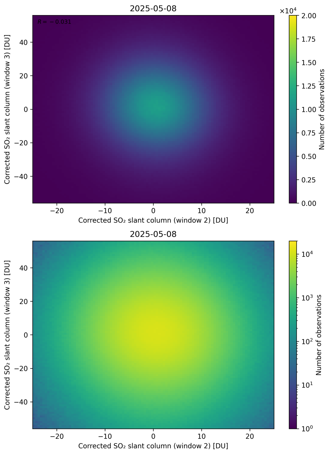
Figure 250: Scatter density plot of “Corrected SO 2 slant column (window 2)” against “Corrected SO 2 slant column (window 3)” for 2025-05-07 to 2025-05-09.
