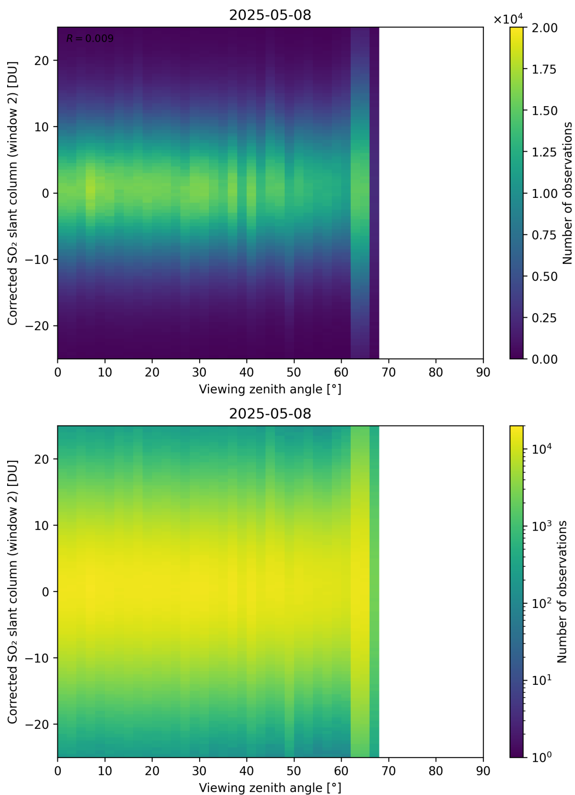
Figure 374: Scatter density plot of “Viewing zenith angle” against “Corrected SO 2 slant column (window 2)” for 2025-05-07 to 2025-05-09.
