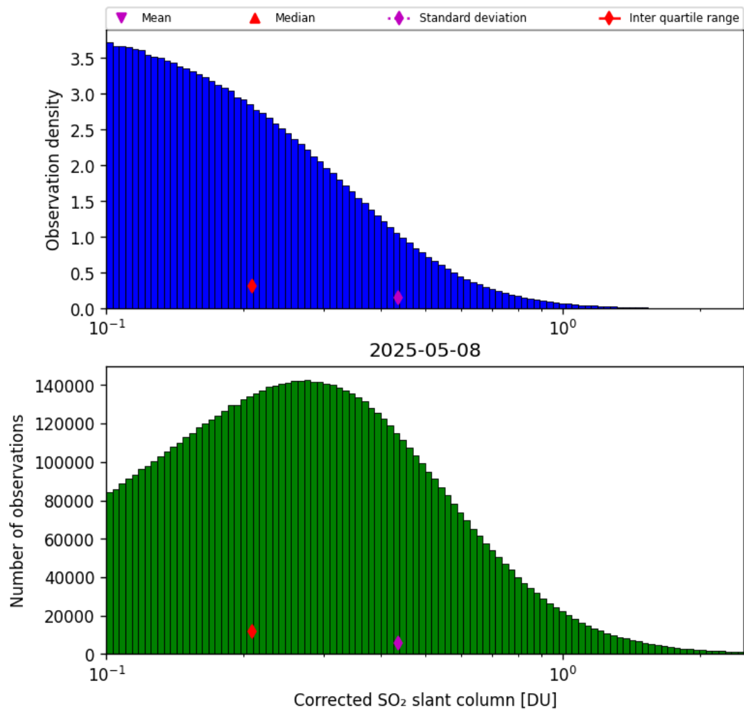
Figure 60: Histogram of “Corrected SO 2 slant column” for 2025-05-07 to 2025-05-09
