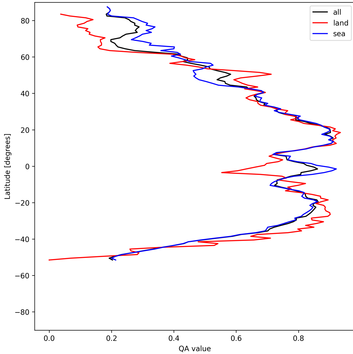
Figure 31: Zonal average of “QA value” for 2025-05-07 to 2025-05-09.
