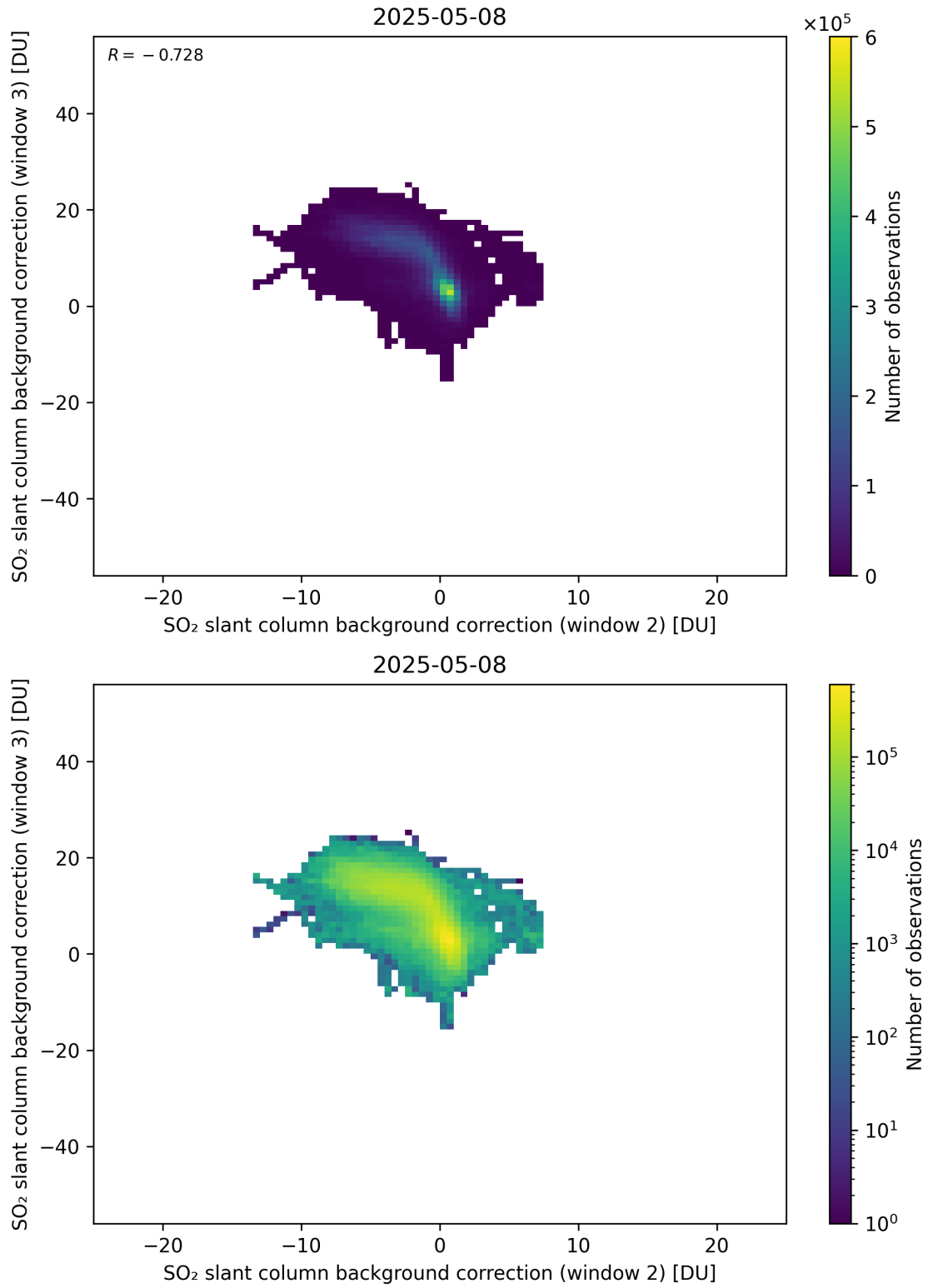
Figure 122: Scatter density plot of “SO 2 slant column background correction (window 2)” against “SO 2 slant column background correction (window 3)” for 2025-05-07 to 2025-05-09.
