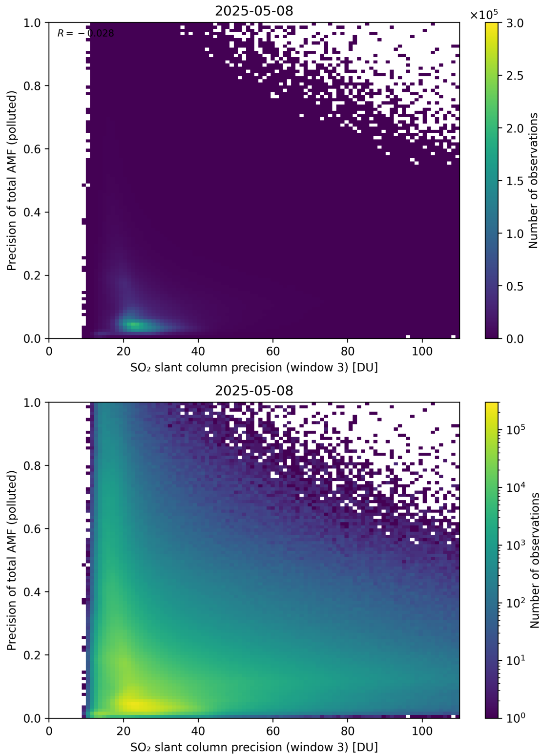
Figure 314: Scatter density plot of “SO 2 slant column precision (window 3)” against “Precision of total AMF (polluted)” for 2025-05-07 to 2025-05-09.
