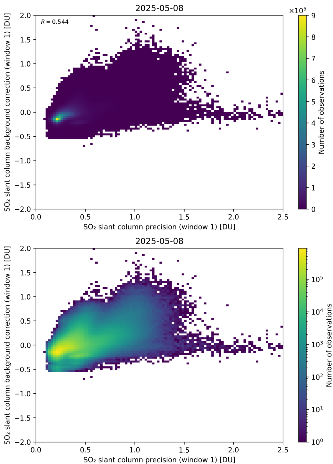
Figure 268: Scatter density plot of “SO 2 slant column precision (window 1)” against “SO 2 slant column background correction (window 1)” for 2025-05-07 to 2025-05-09.
