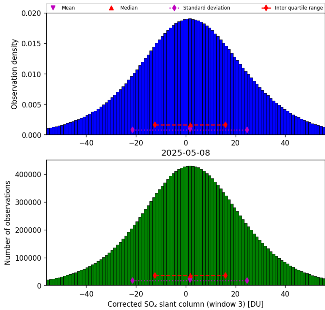
Figure 73: Histogram of “Corrected SO 2 slant column (window 3)” for 2025-05-07 to 2025-05-09
