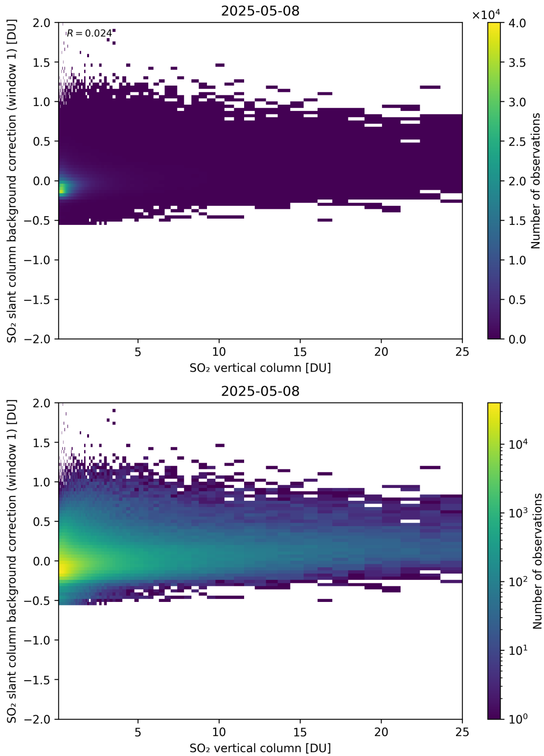
Figure 323: Scatter density plot of “SO 2 vertical column” against “SO 2 slant column background correction (window 1)” for 2025-05-07 to 2025-05-09.
