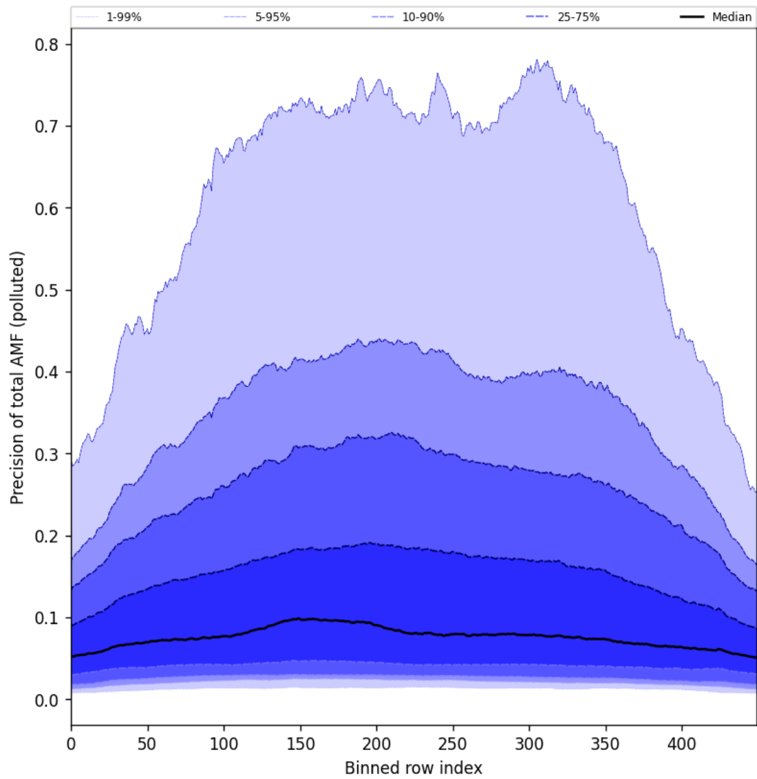
Figure 106: Along track statistics of “Precision of total AMF (polluted)” for 2025-05-07 to 2025-05-09
