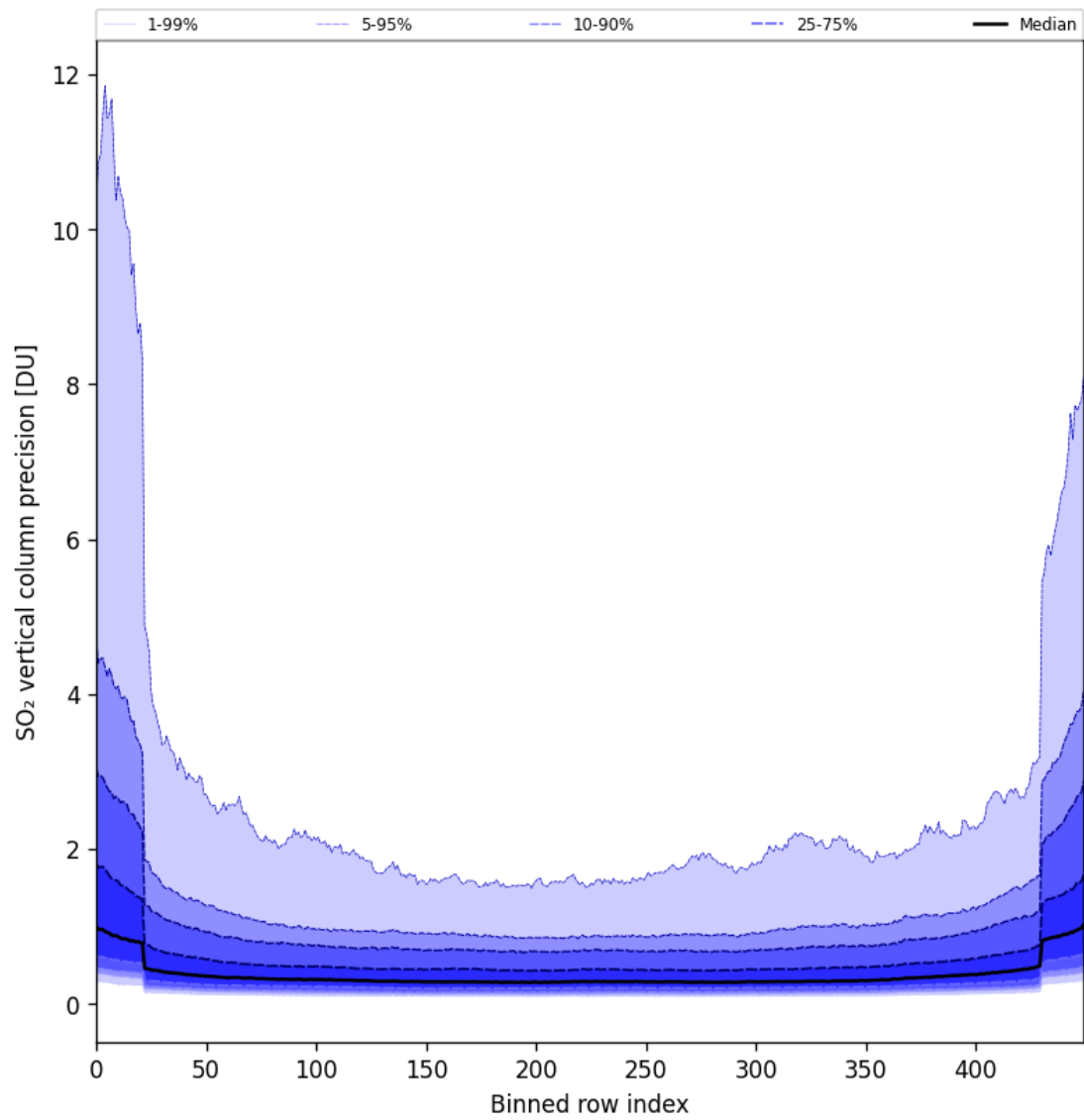
Figure 85: Along track statistics of “SO 2 vertical column precision” for 2025-05-07 to 2025-05-09
