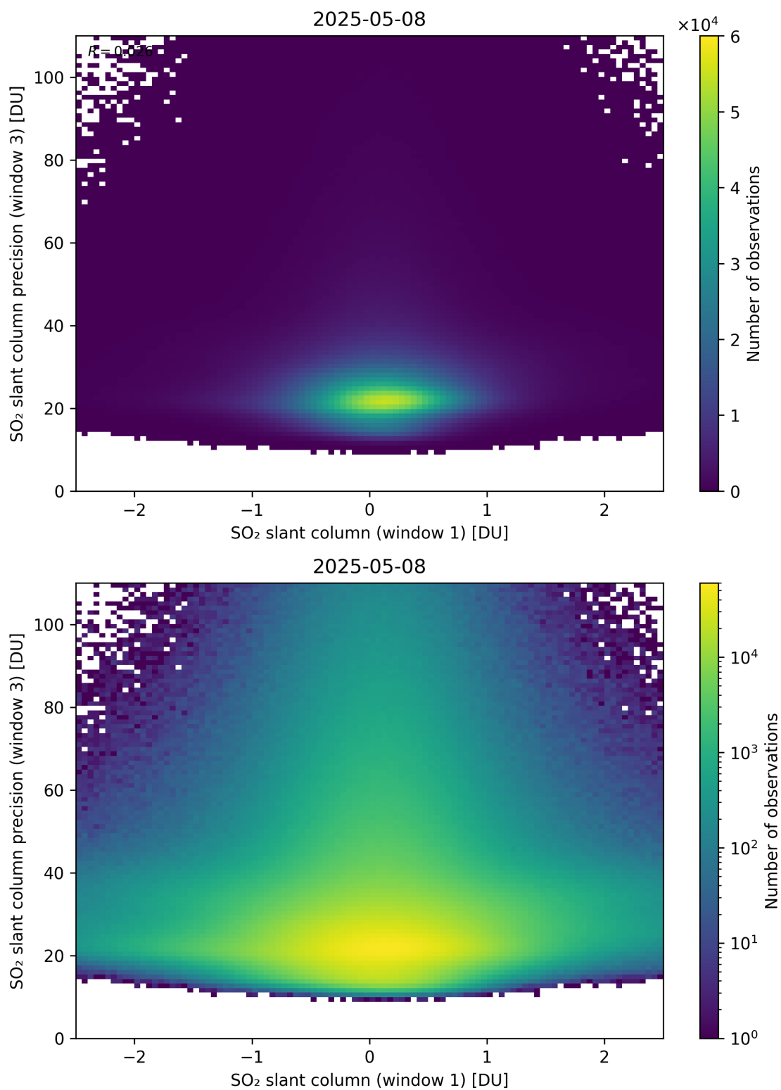
Figure 288: Scatter density plot of “SO 2 slant column (window 1)” against “SO 2 slant column precision (window 3)” for 2025-05-07 to 2025-05-09.
