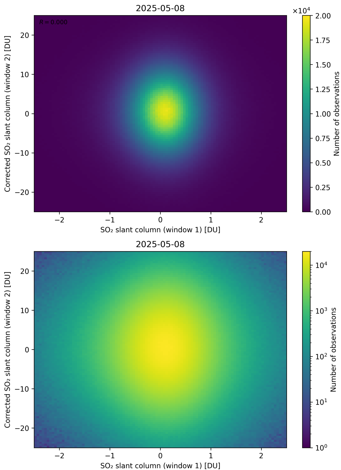
Figure 283: Scatter density plot of “SO 2 slant column (window 1)” against “Corrected SO 2 slant column (window 2)” for 2025-05-07 to 2025-05-09.
