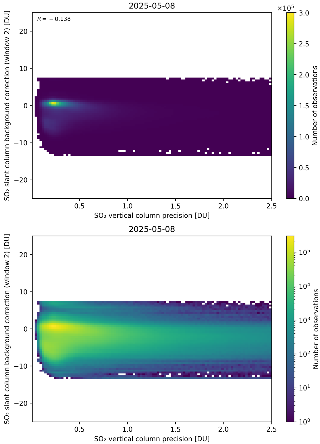
Figure 330: Scatter density plot of “SO 2 vertical column precision” against “SO 2 slant column background correction (window 2)” for 2025-05-07 to 2025-05-09.
