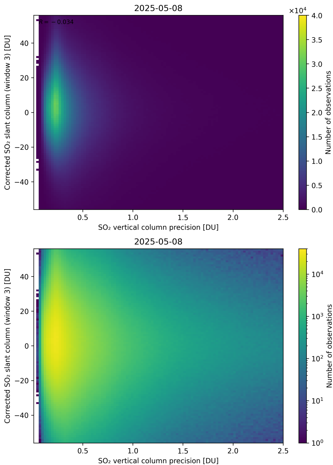
Figure 340: Scatter density plot of “SO 2 vertical column precision” against “Corrected SO 2 slant column (window 3)” for 2025-05-07 to 2025-05-09.
