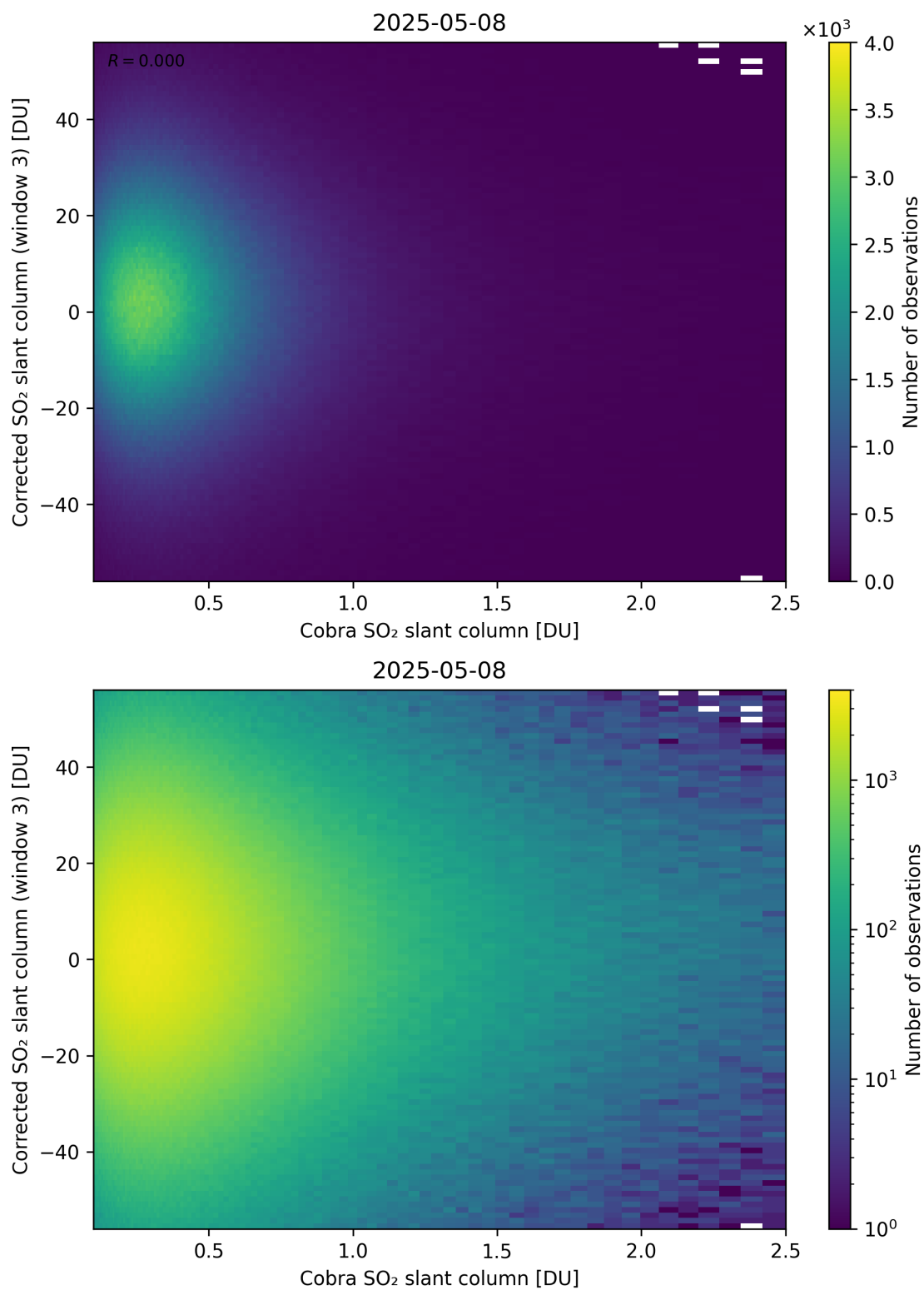
Figure 218: Scatter density plot of “Cobra SO 2 slant column” against “Corrected SO 2 slant column (window 3)” for 2025-05-07 to 2025-05-09.
