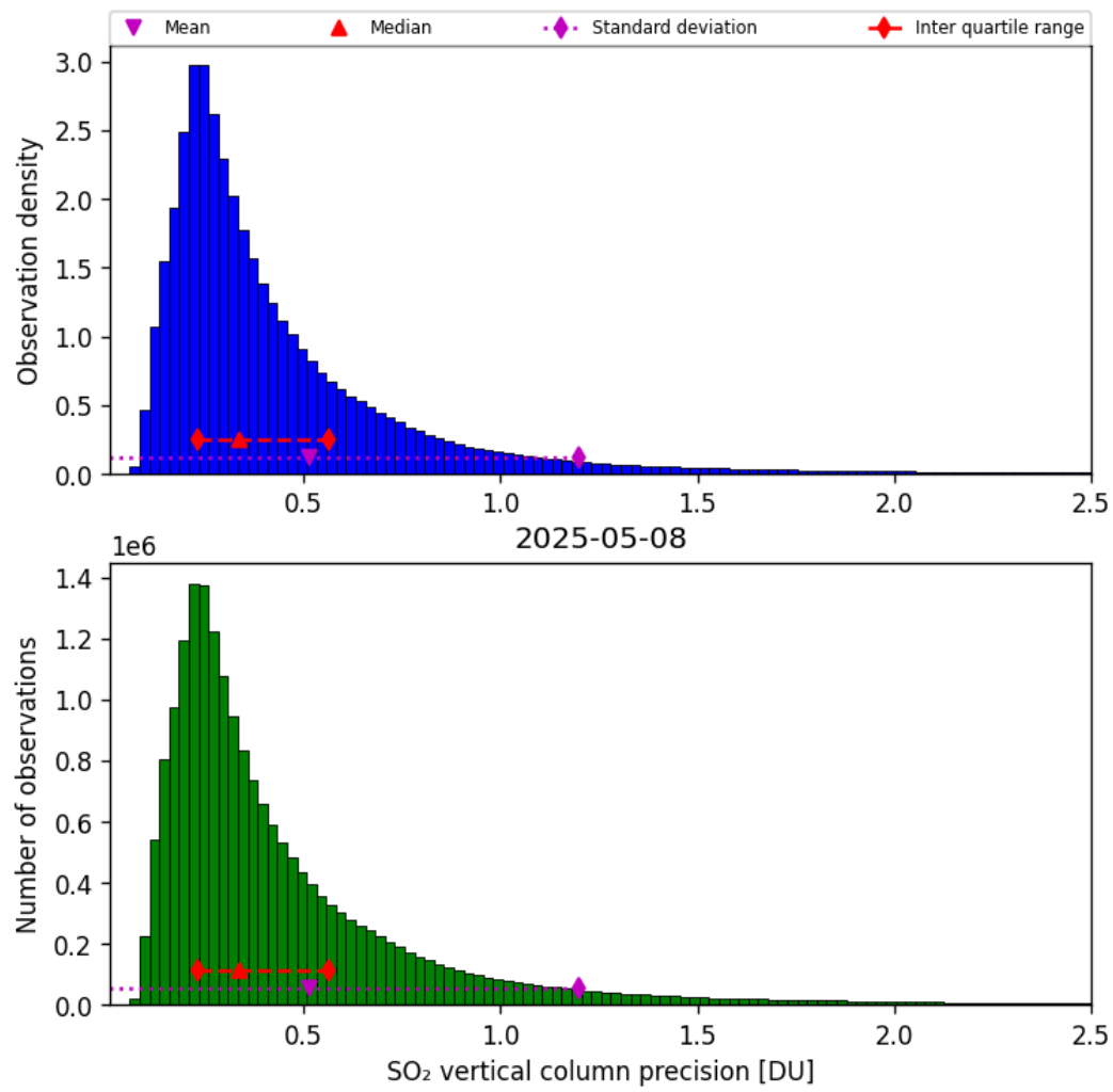
Figure 59: Histogram of “SO 2 vertical column precision” for 2025-05-07 to 2025-05-09
