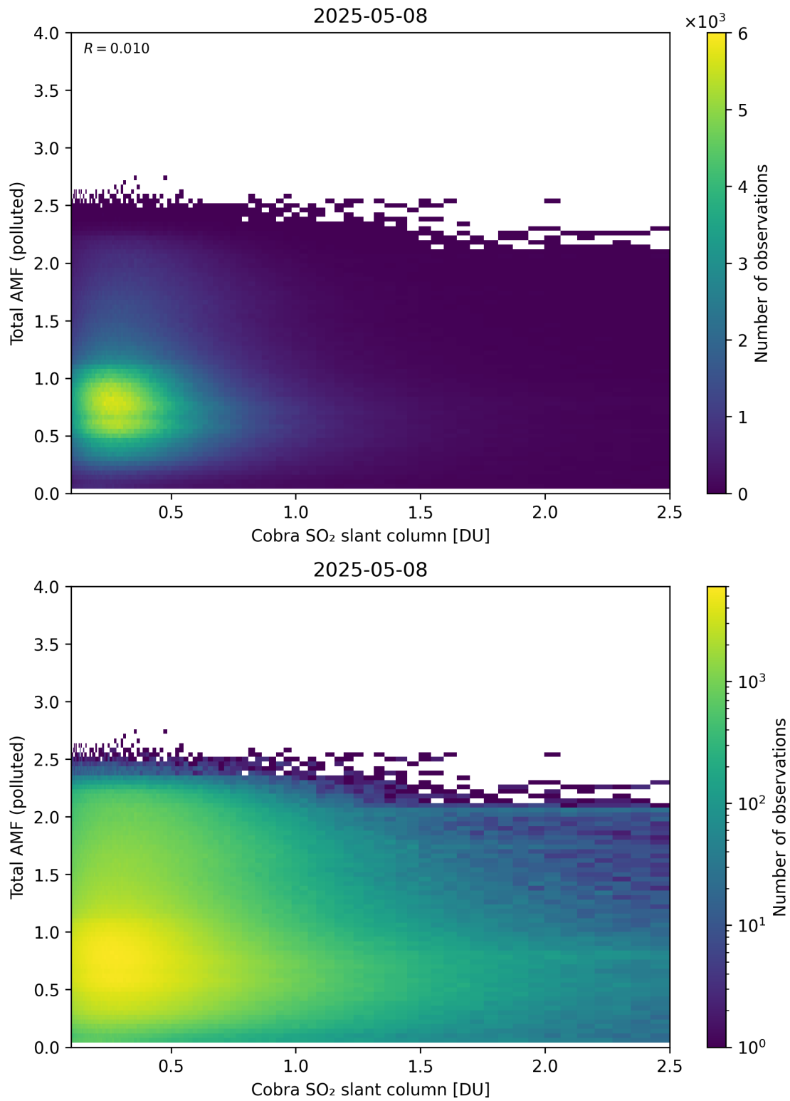
Figure 224: Scatter density plot of “Cobra SO 2 slant column” against “Total AMF (polluted)” for 2025-05-07 to 2025-05-09.
