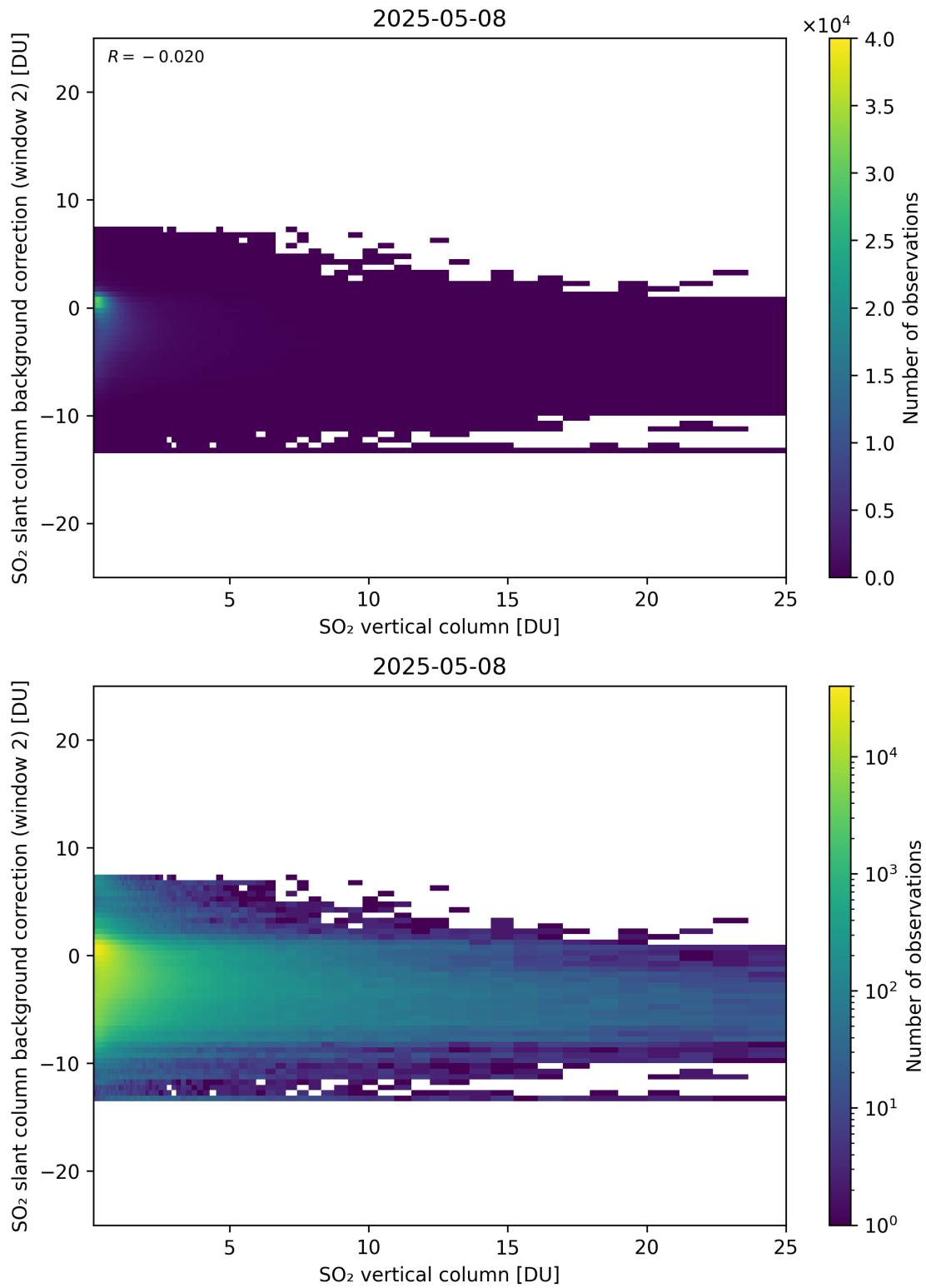
Figure 324: Scatter density plot of “SO 2 vertical column” against “SO 2 slant column background correction (window 2)” for 2025-05-07 to 2025-05-09.
