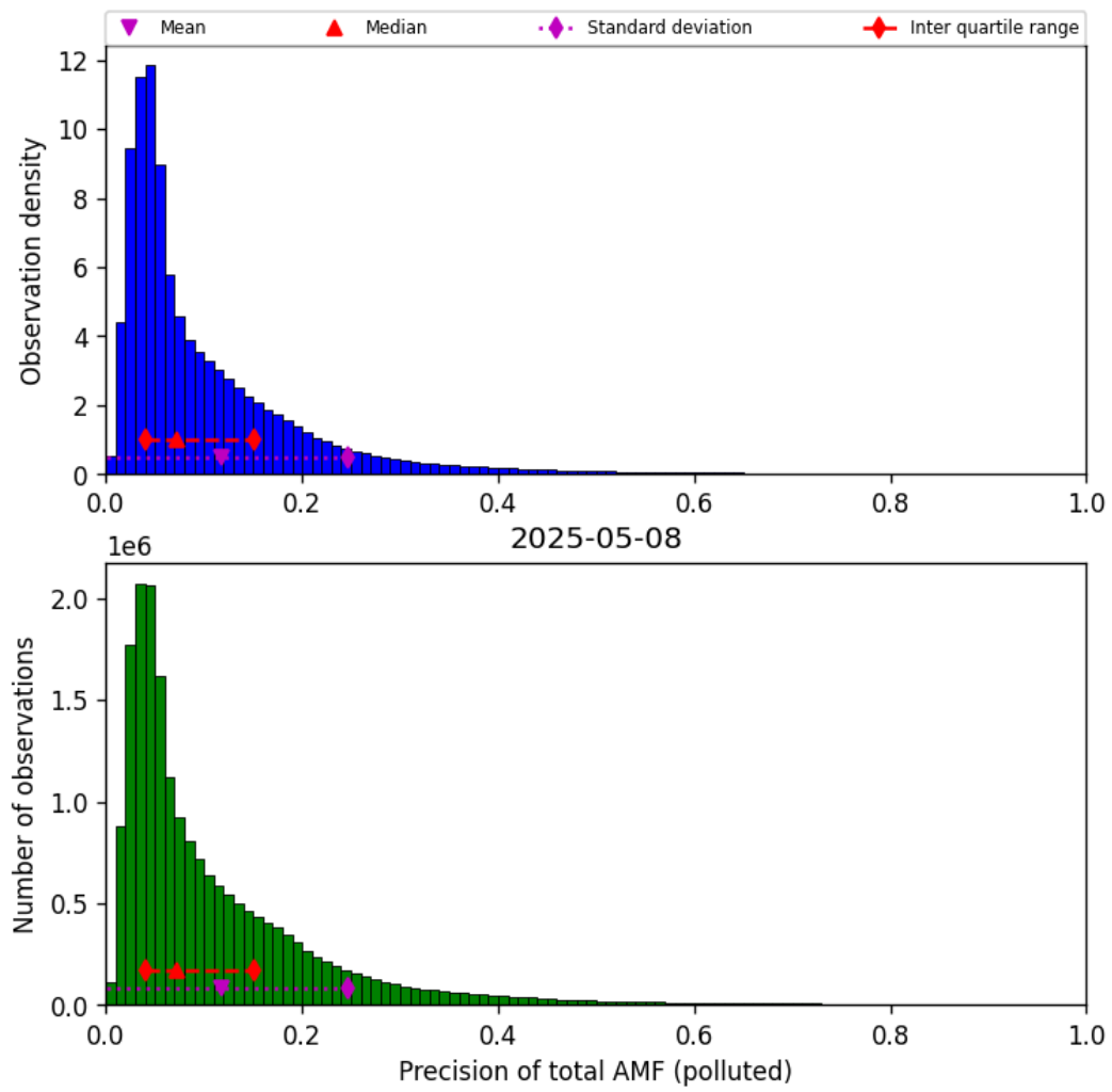
Figure 80: Histogram of “Precision of total AMF (polluted)” for 2025-05-07 to 2025-05-09
