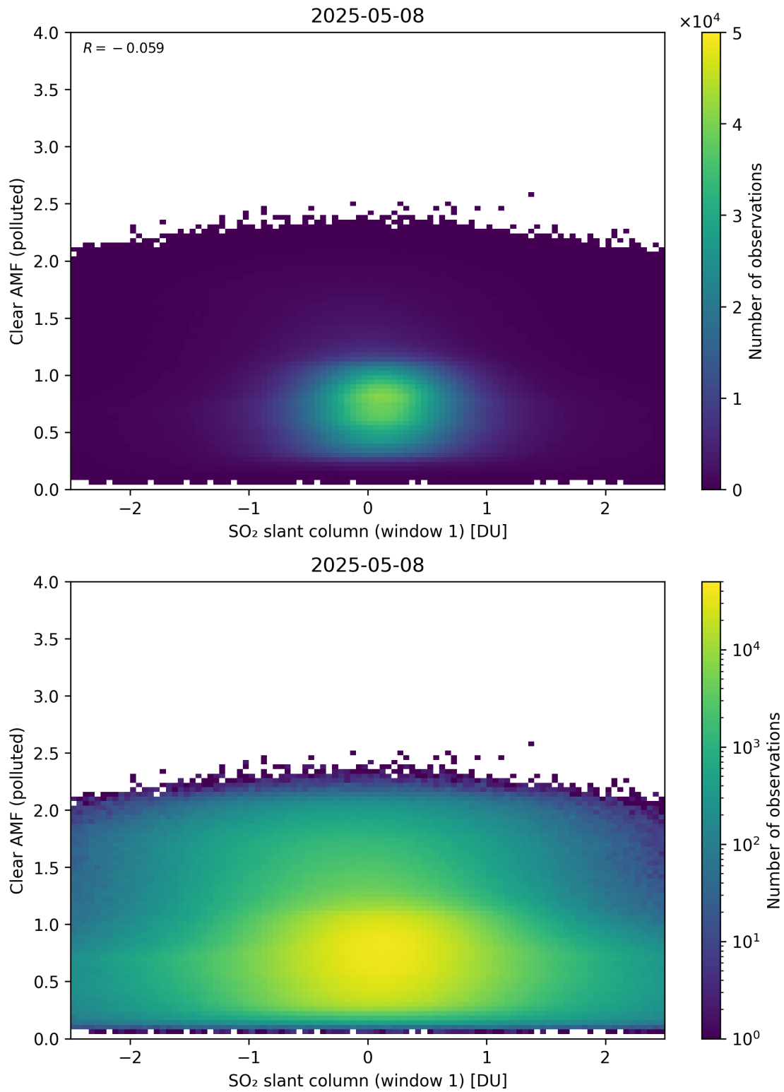
Figure 282: Scatter density plot of “SO 2 slant column (window 1)” against “Clear AMF (polluted)” for 2025-05-07 to 2025-05-09.
