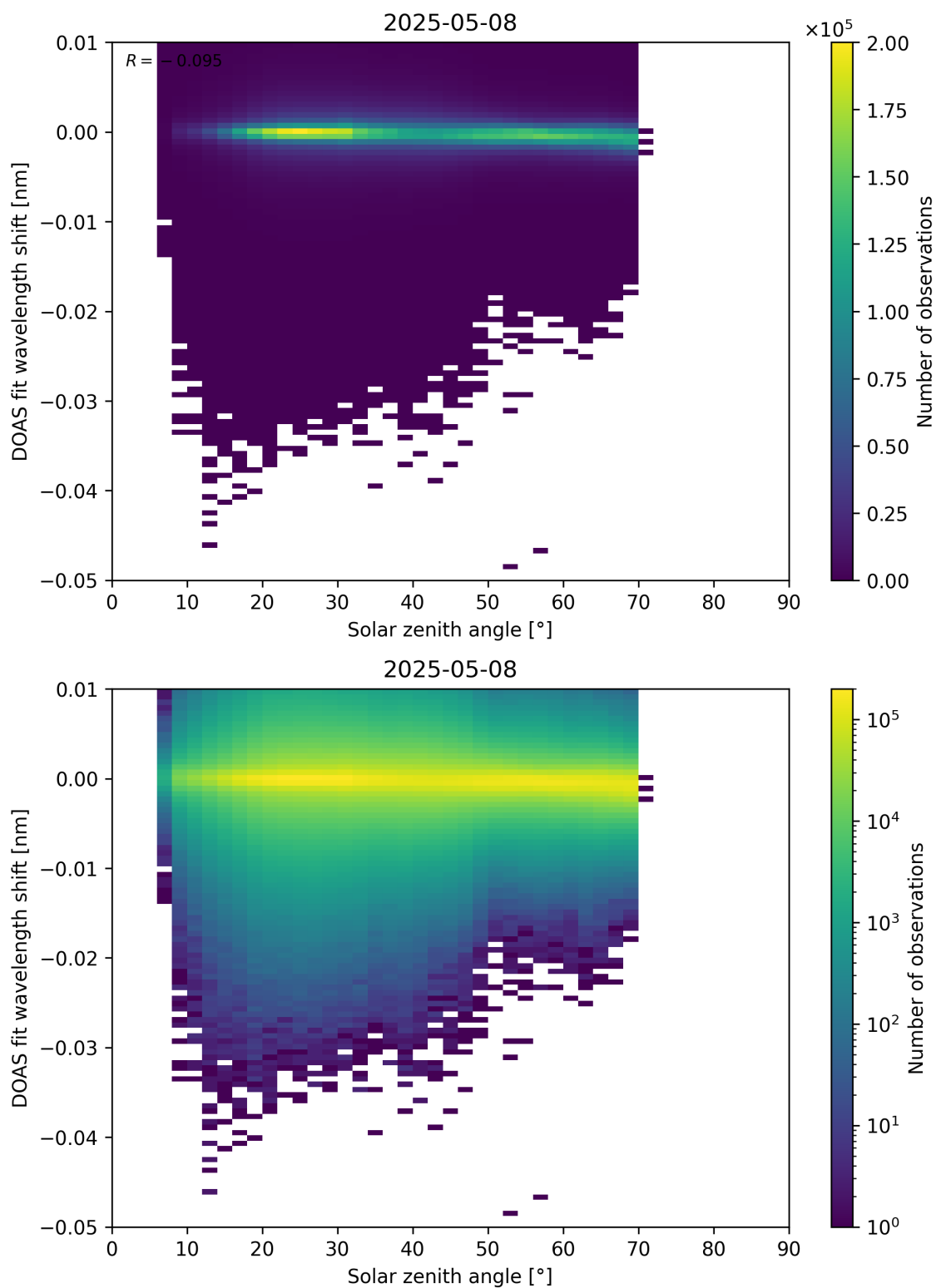
Figure 174: Scatter density plot of “Solar zenith angle” against “DOAS fit wavelength shift” for 2025-05-07 to 2025-05-09.
