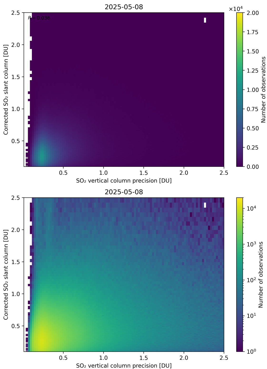
Figure 338: Scatter density plot of “SO 2 vertical column precision” against “Corrected SO 2 slant column” for 2025-05-07 to 2025-05-09.
