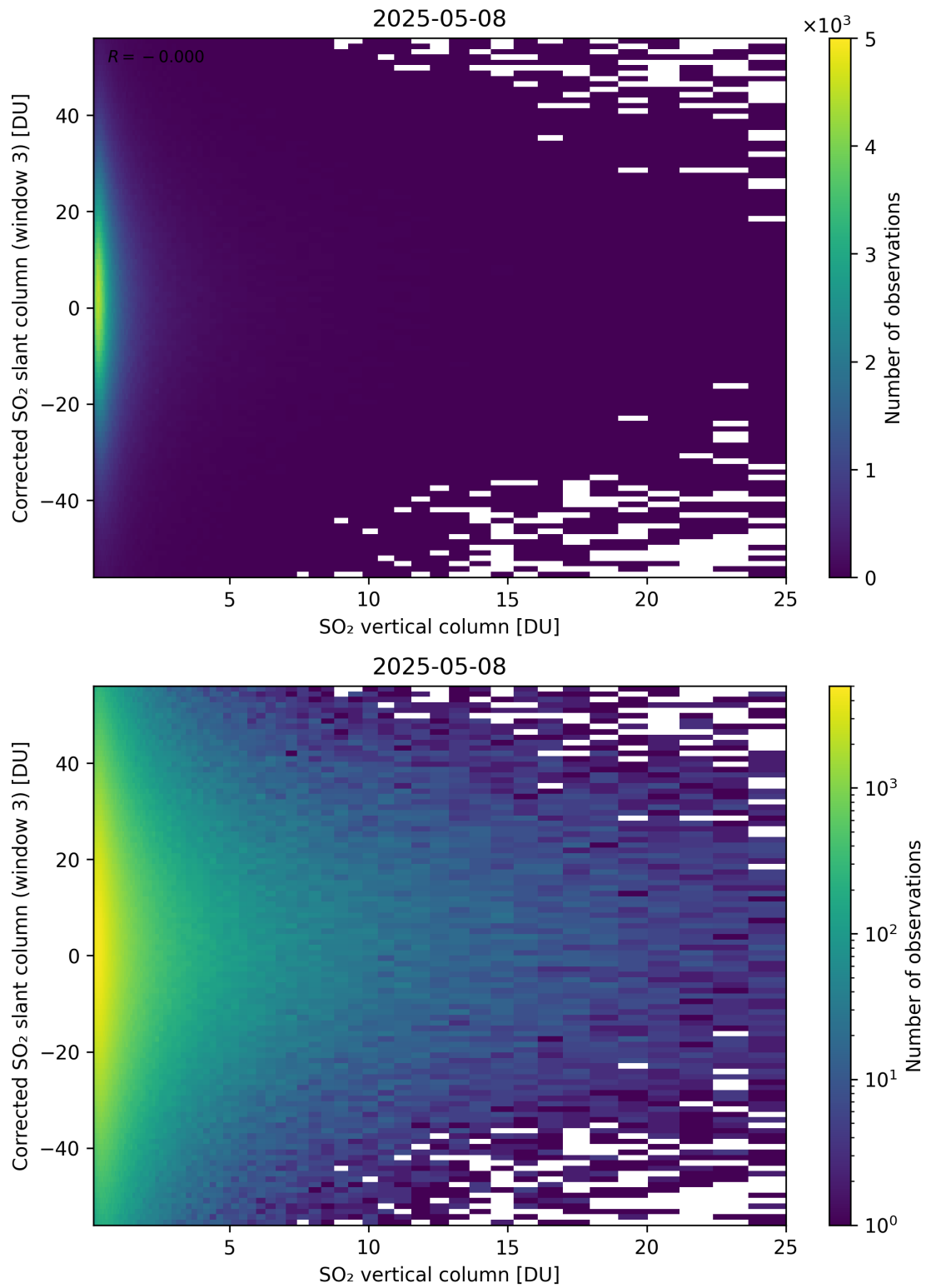
Figure 353: Scatter density plot of “SO 2 vertical column” against “Corrected SO 2 slant column (window 3)” for 2025-05-07 to 2025-05-09.
