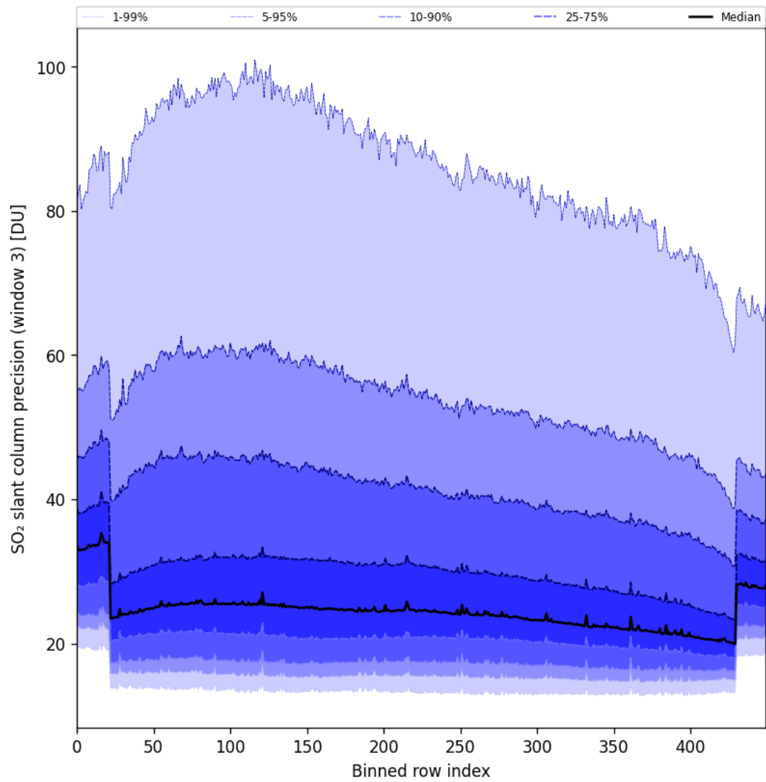
Figure 98: Along track statistics of “SO 2 slant column precision (window 3)” for 2025-05-07 to 2025-05-09
