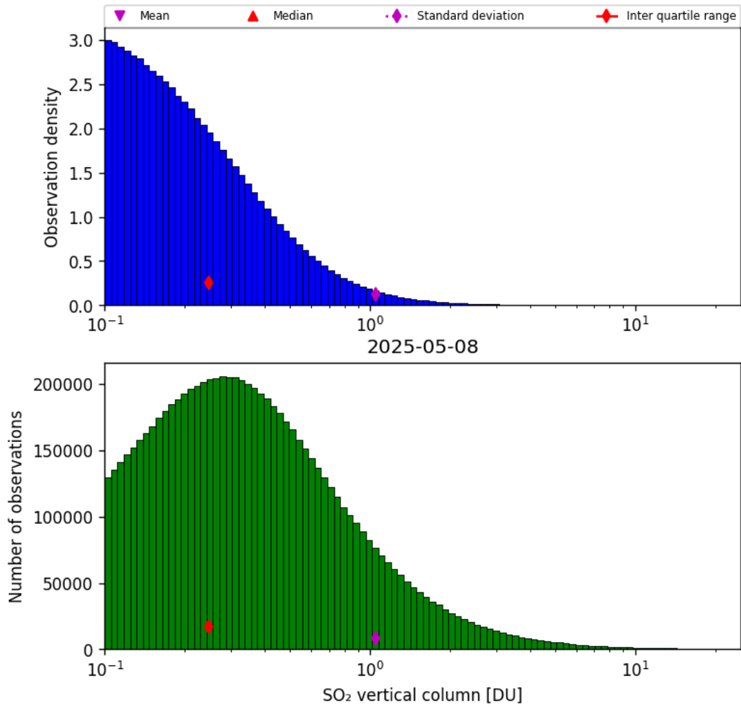
Figure 58: Histogram of “SO 2 vertical column” for 2025-05-07 to 2025-05-09
