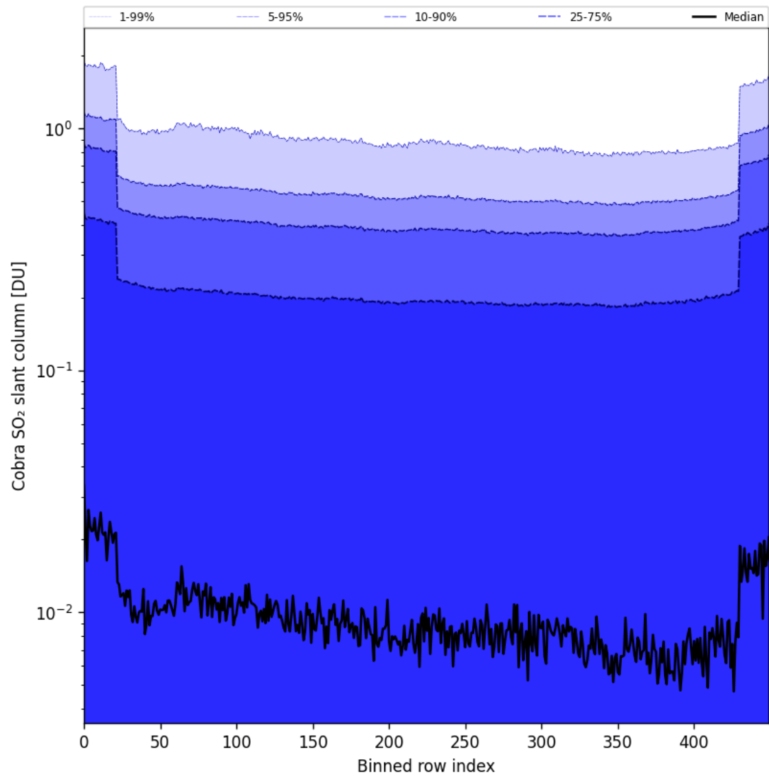
Figure 87: Along track statistics of "Cobra SO 2 slant column" for 2025-05-07 to 2025-05-09
