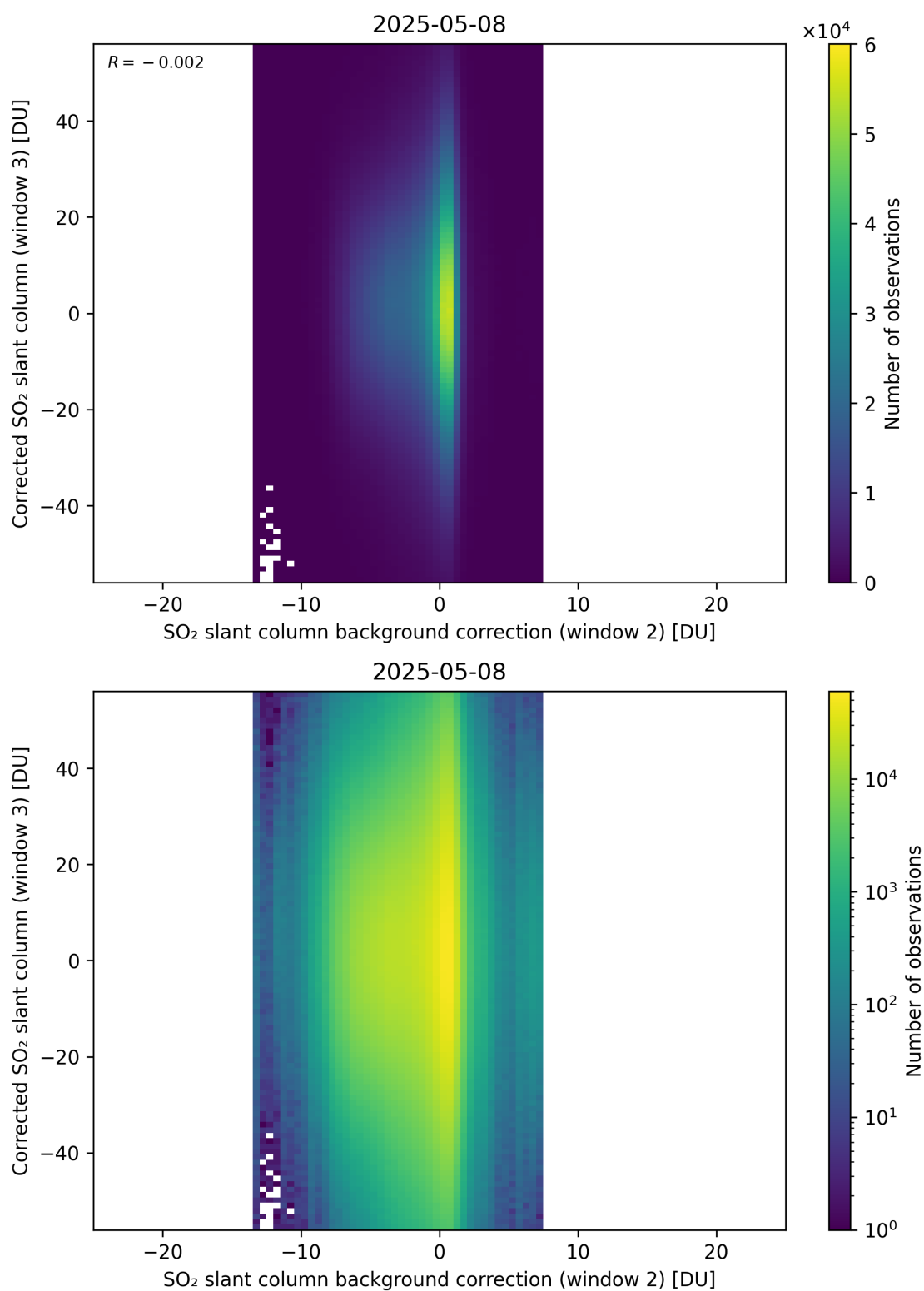
Figure 127: Scatter density plot of “SO 2 slant column background correction (window 2)” against “Corrected SO 2 slant column (window 3)” for 2025-05-07 to 2025-05-09.
