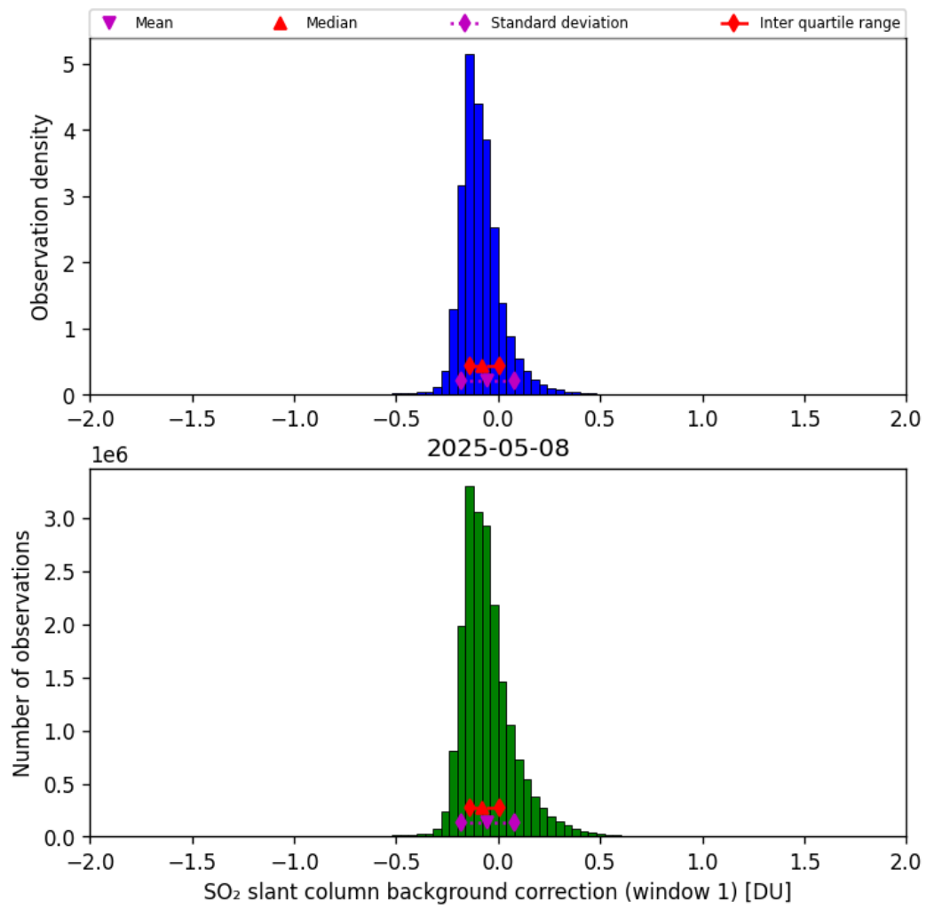
Figure 66: Histogram of “SO 2 slant column background correction (window 1)” for 2025-05-07 to 2025-05-09
