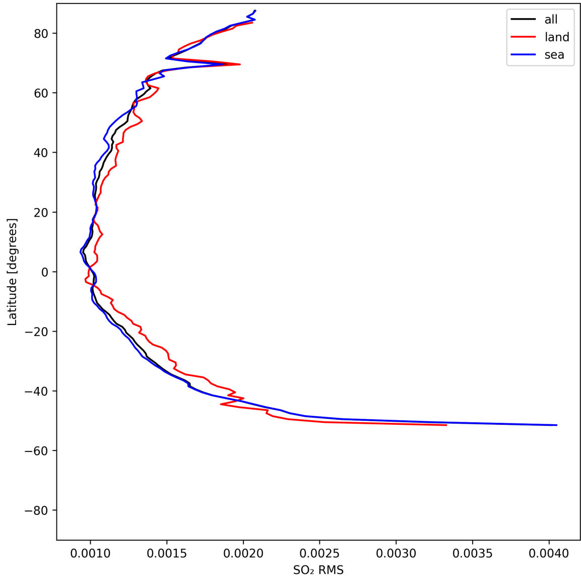
Figure 52: Zonal average of “SO 2 RMS” for 2025-05-07 to 2025-05-09.
