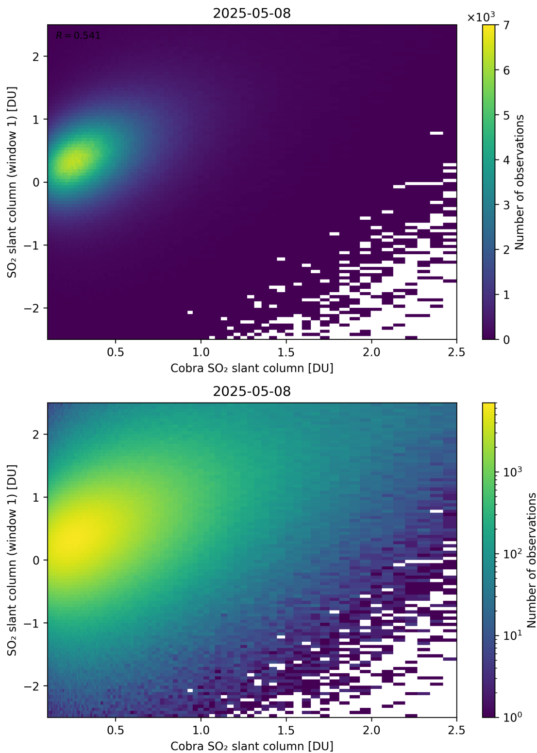
Figure 219: Scatter density plot of “Cobra SO 2 slant column” against “SO 2 slant column (window 1)” for 2025-05-07 to 2025-05-09.
