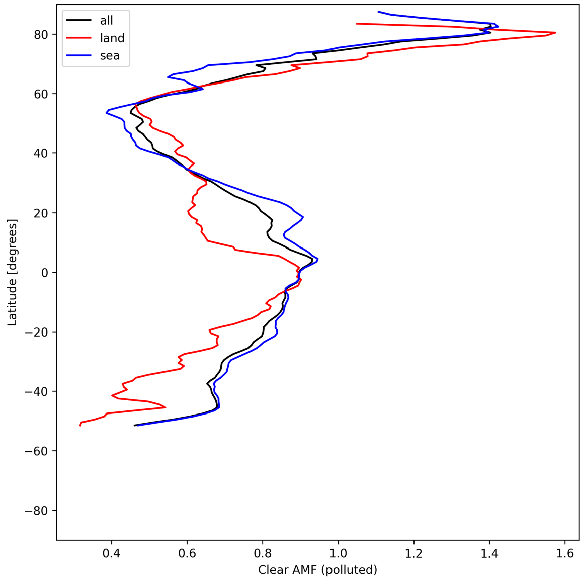
Figure 55: Zonal average of “Clear AMF (polluted)” for 2025-05-07 to 2025-05-09.
