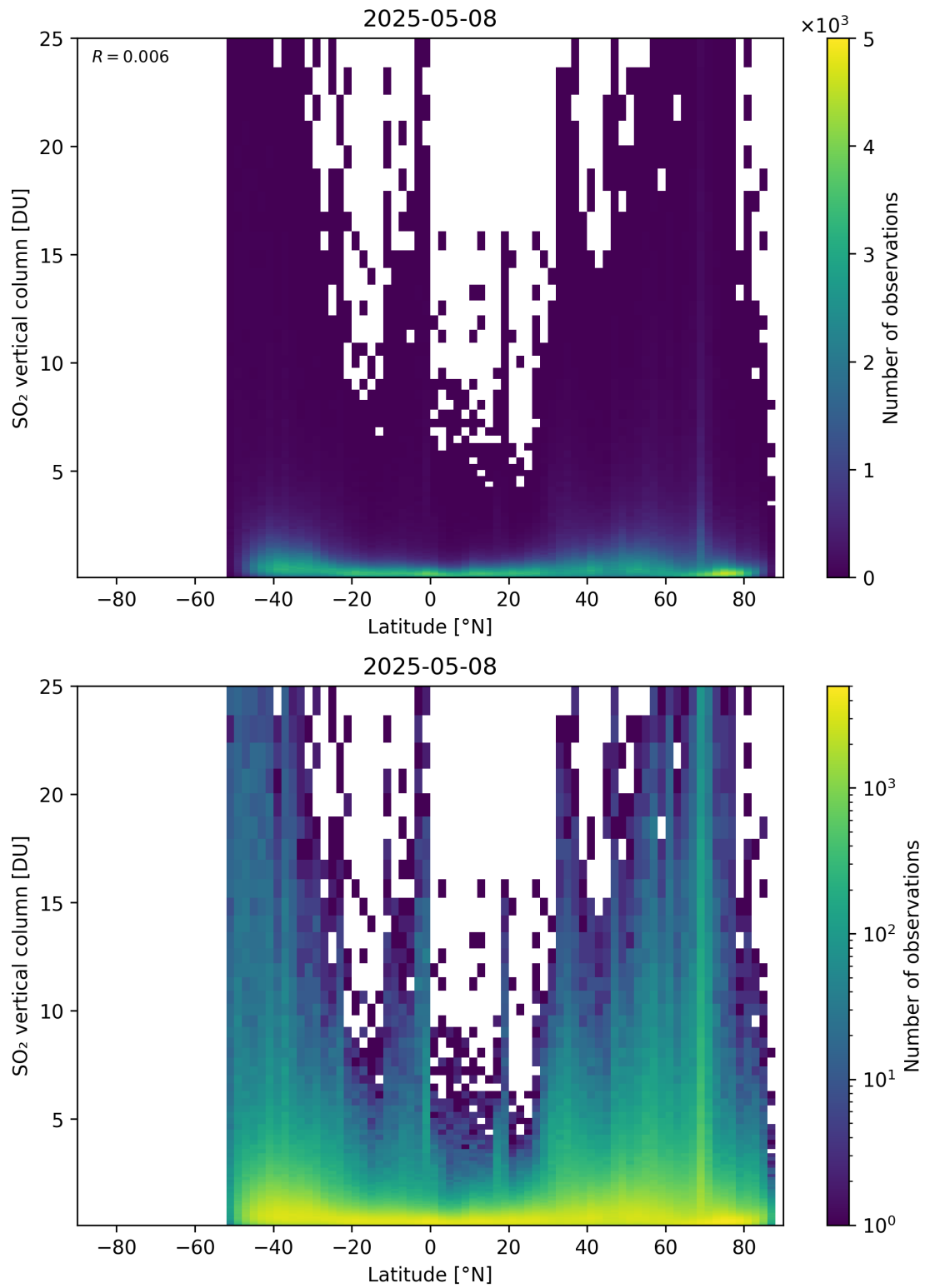
Figure 169: Scatter density plot of “Latitude” against “SO 2 vertical column” for 2025-05-07 to 2025-05-09.
