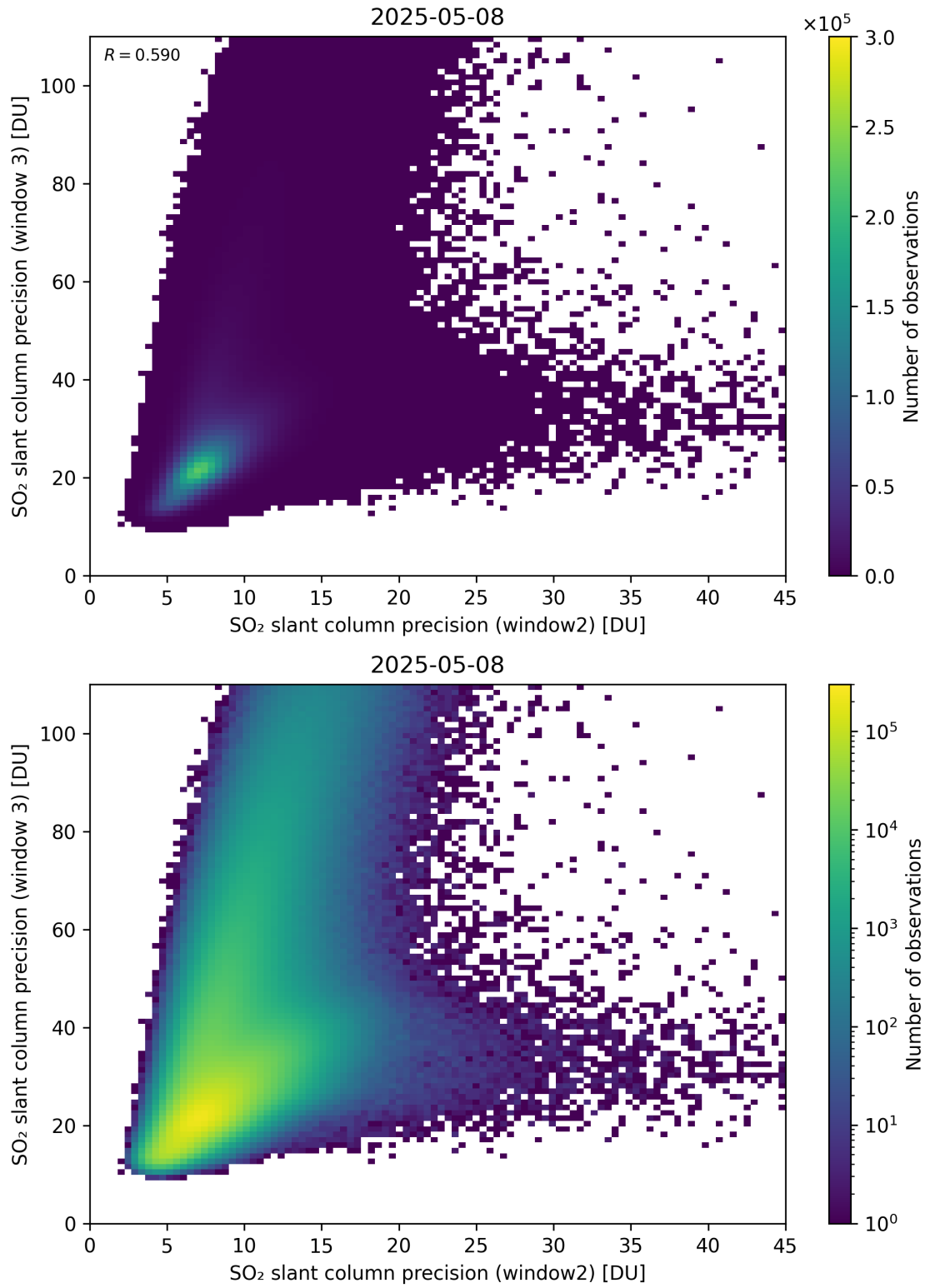
Figure 300: Scatter density plot of “SO 2 slant column precision (window2)” against “SO 2 slant column precision (window 3)” for 2025-05-07 to 2025-05-09.
