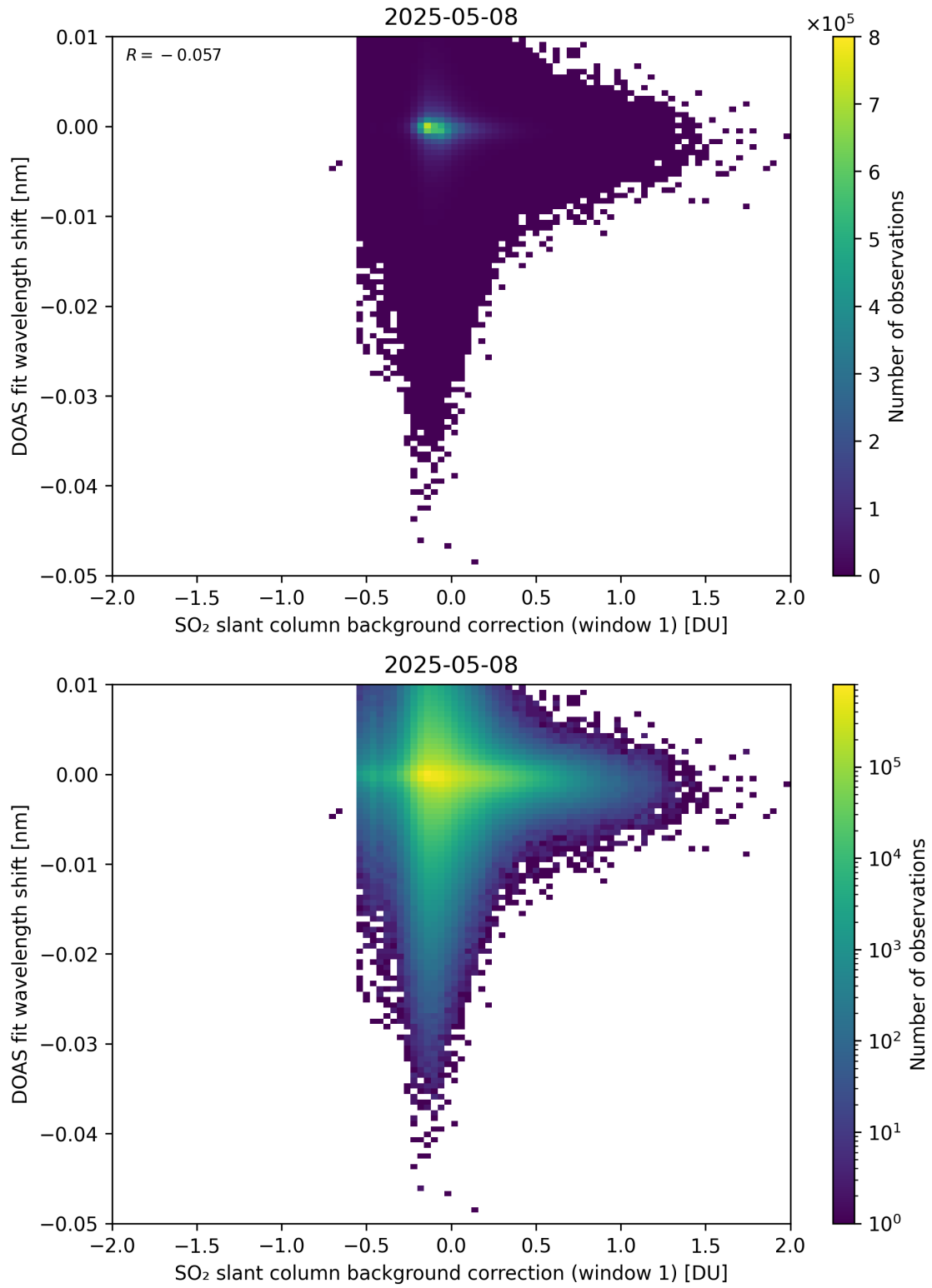
Figure 111: Scatter density plot of “SO 2 slant column background correction (window 1)” against “DOAS fit wavelength shift” for 2025-05-07 to 2025-05-09.
