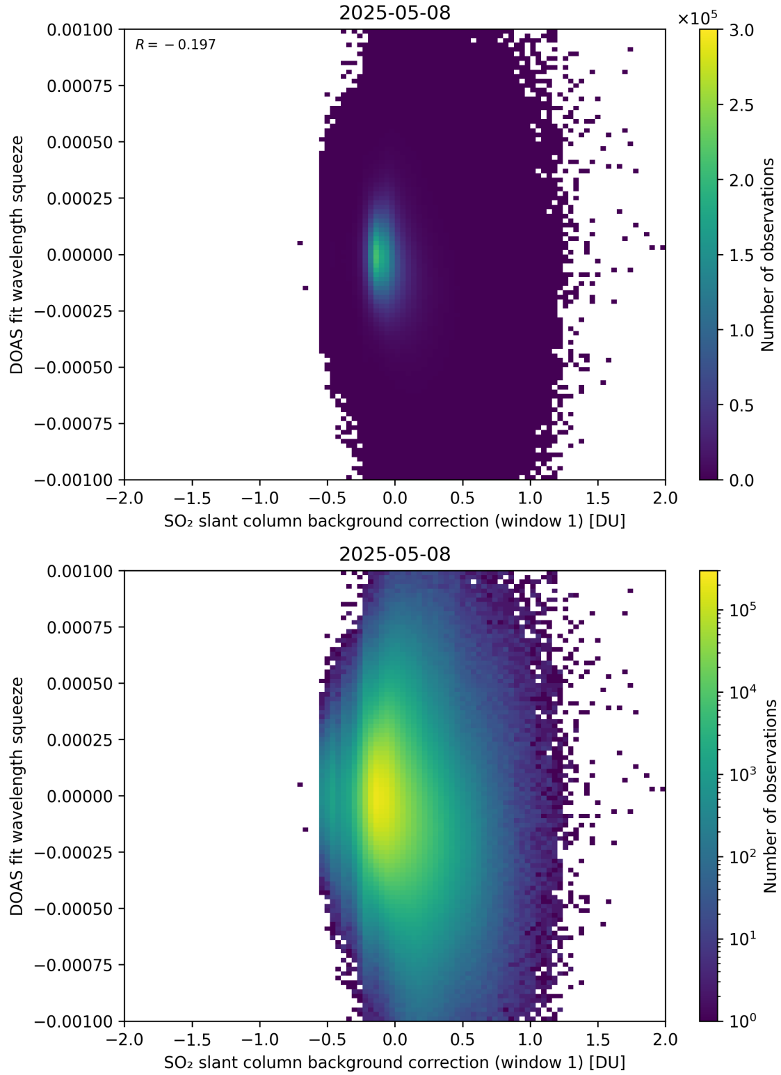
Figure 112: Scatter density plot of “SO 2 slant column background correction (window 1)” against “DOAS fit wavelength squeeze” for 2025-05-07 to 2025-05-09.
