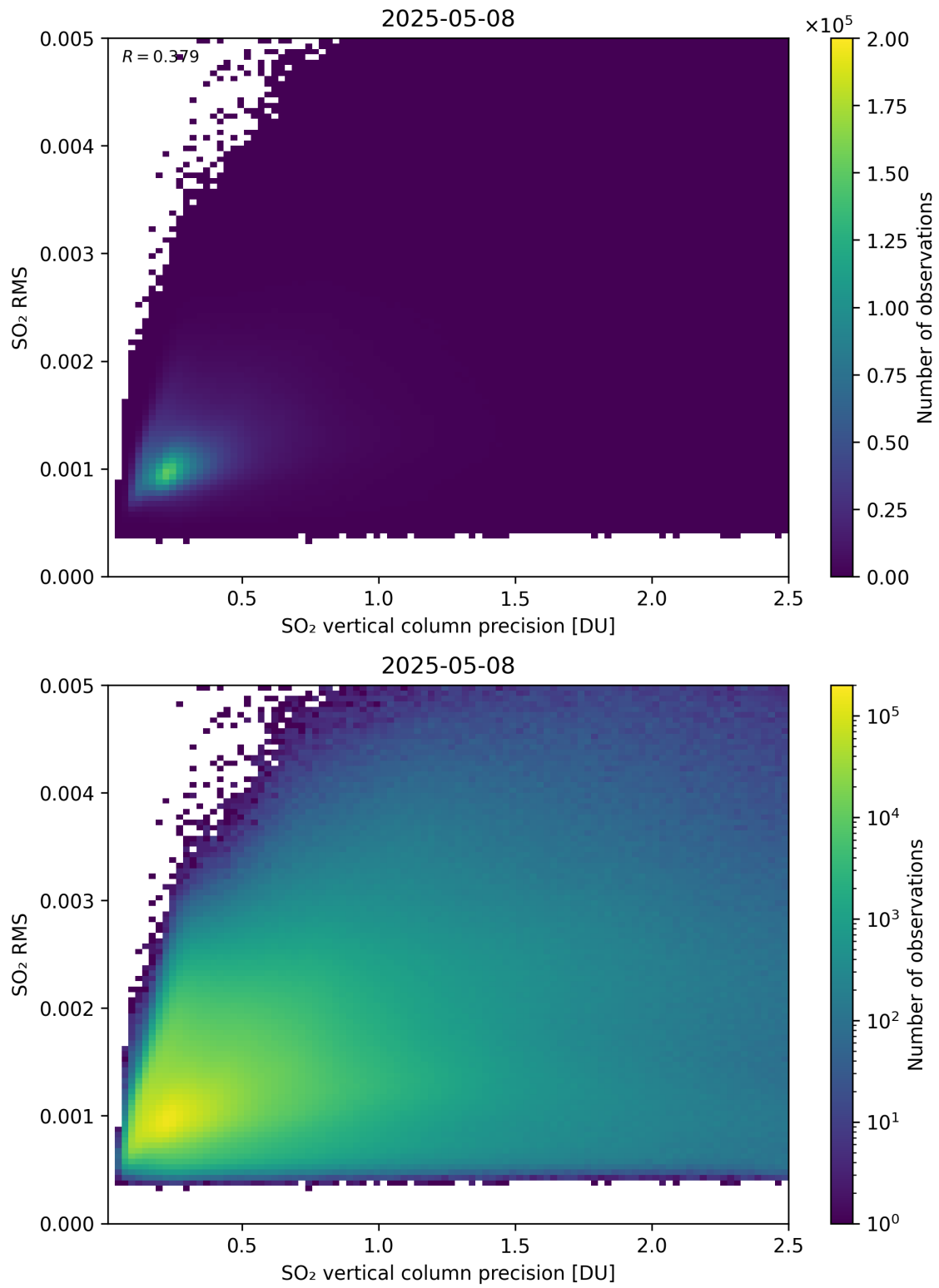
Figure 334: Scatter density plot of “SO 2 vertical column precision” against “SO 2 RMS” for 2025-05-07 to 2025-05-09.
