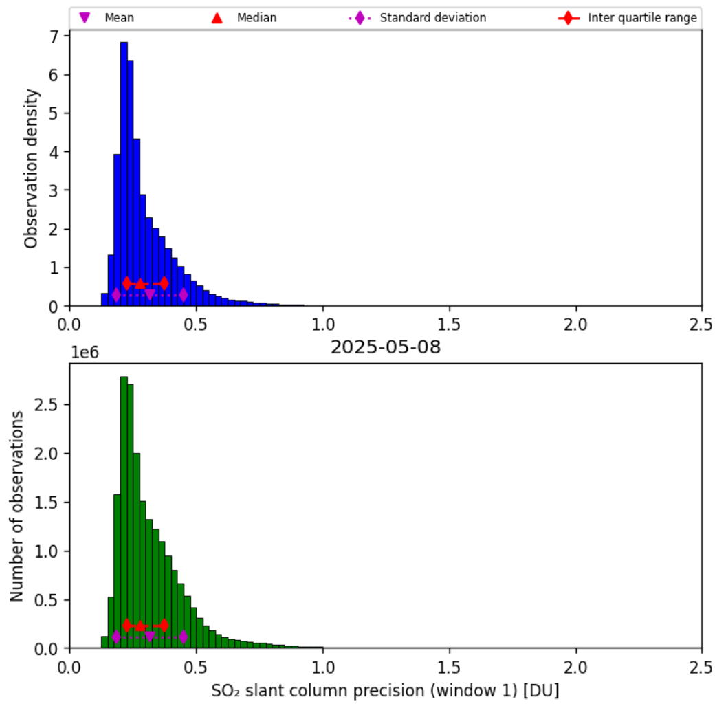
Figure 64: Histogram of “SO 2 slant column precision (window 1)” for 2025-05-07 to 2025-05-09
