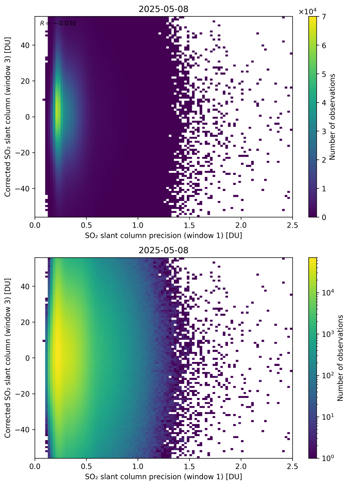
Figure 276: Scatter density plot of “SO 2 slant column precision (window 1)” against “Corrected SO 2 slant column (window 3)” for 2025-05-07 to 2025-05-09.
