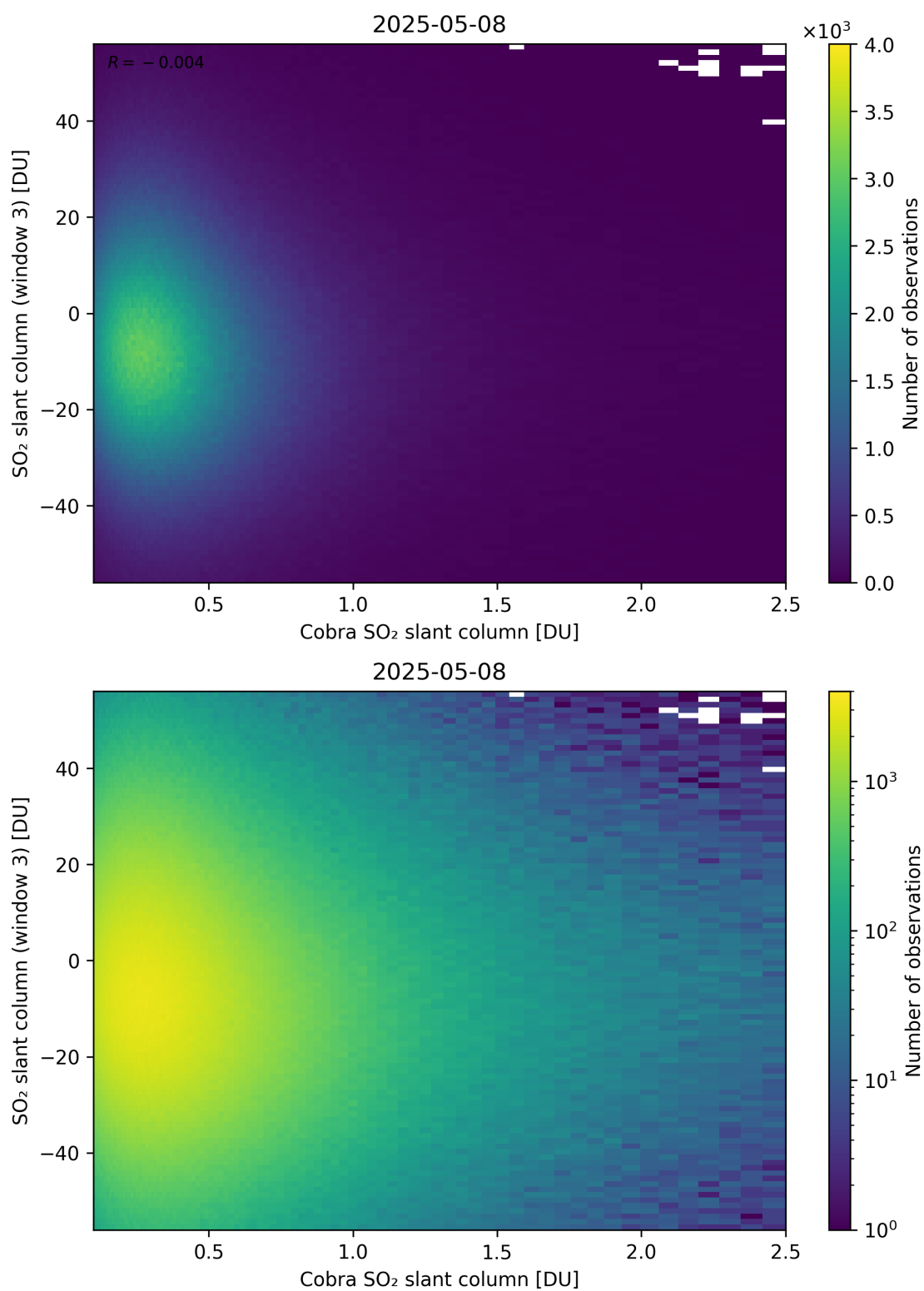
Figure 222: Scatter density plot of “Cobra SO 2 slant column” against “SO 2 slant column (window 3)” for 2025-05-07 to 2025-05-09.
