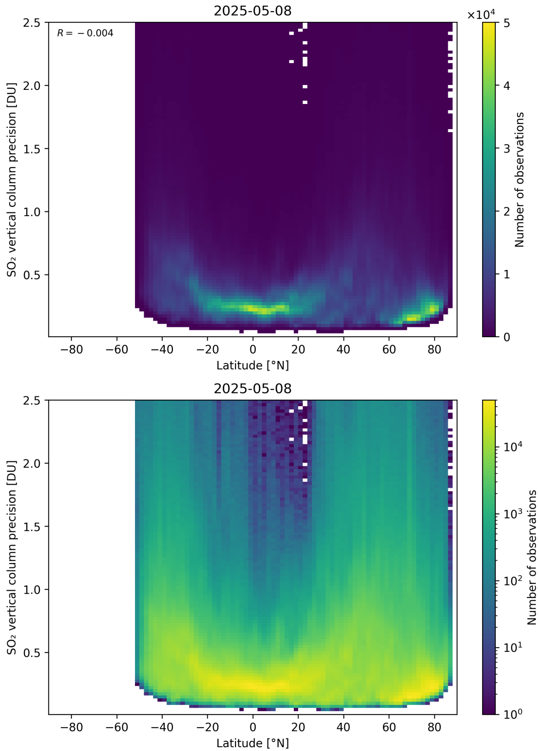
Figure 170: Scatter density plot of “Latitude” against “SO 2 vertical column precision” for 2025-05-07 to 2025-05-09.
