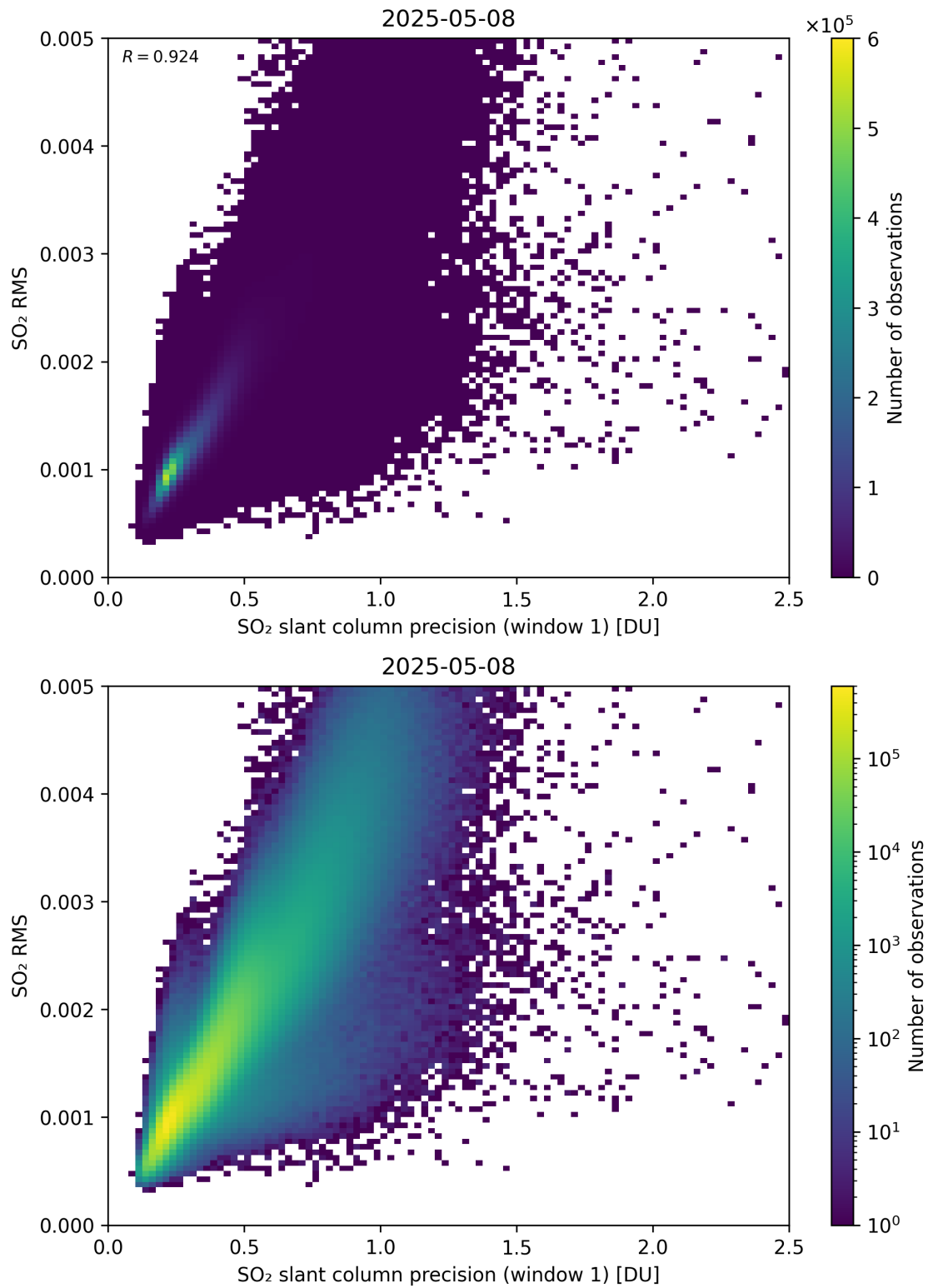
Figure 273: Scatter density plot of “SO 2 slant column precision (window 1)” against “SO 2 RMS” for 2025-05-07 to 2025-05-09.
