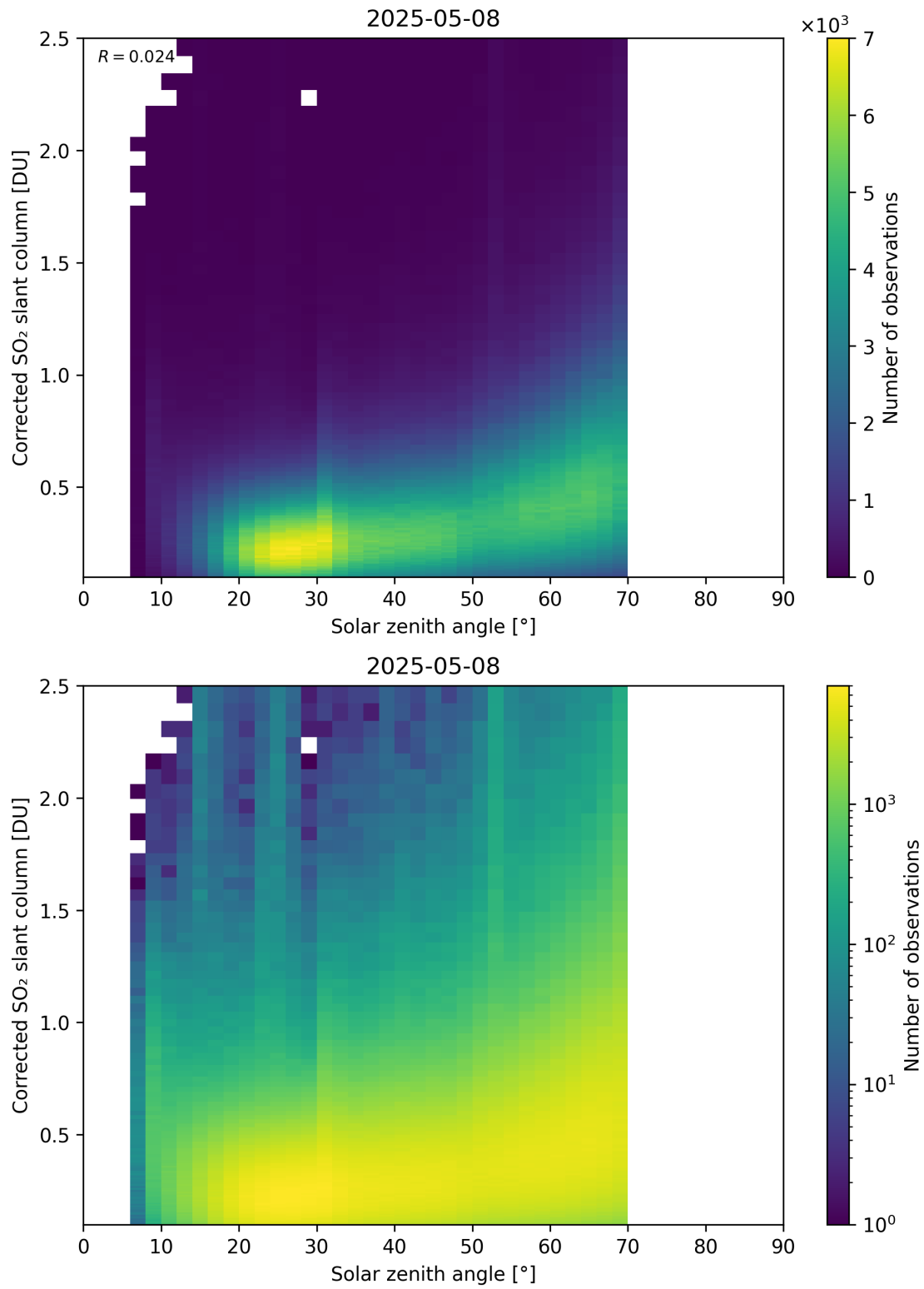
Figure 181: Scatter density plot of “Solar zenith angle” against “Corrected SO 2 slant column” for 2025-05-07 to 2025-05-09.
