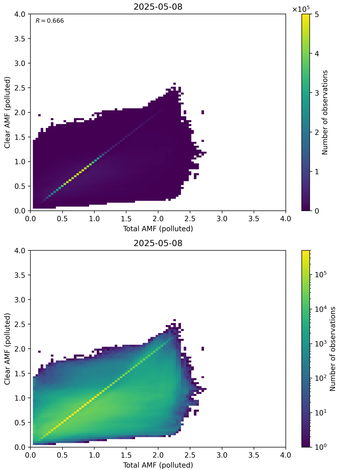
Figure 321: Scatter density plot of “Total AMF (polluted)” against “Clear AMF (polluted)” for 2025-05-07 to 2025-05-09.
