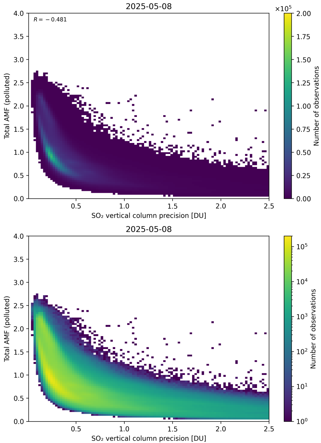
Figure 346: Scatter density plot of “SO 2 vertical column precision” against “Total AMF (polluted)” for 2025-05-07 to 2025-05-09.
