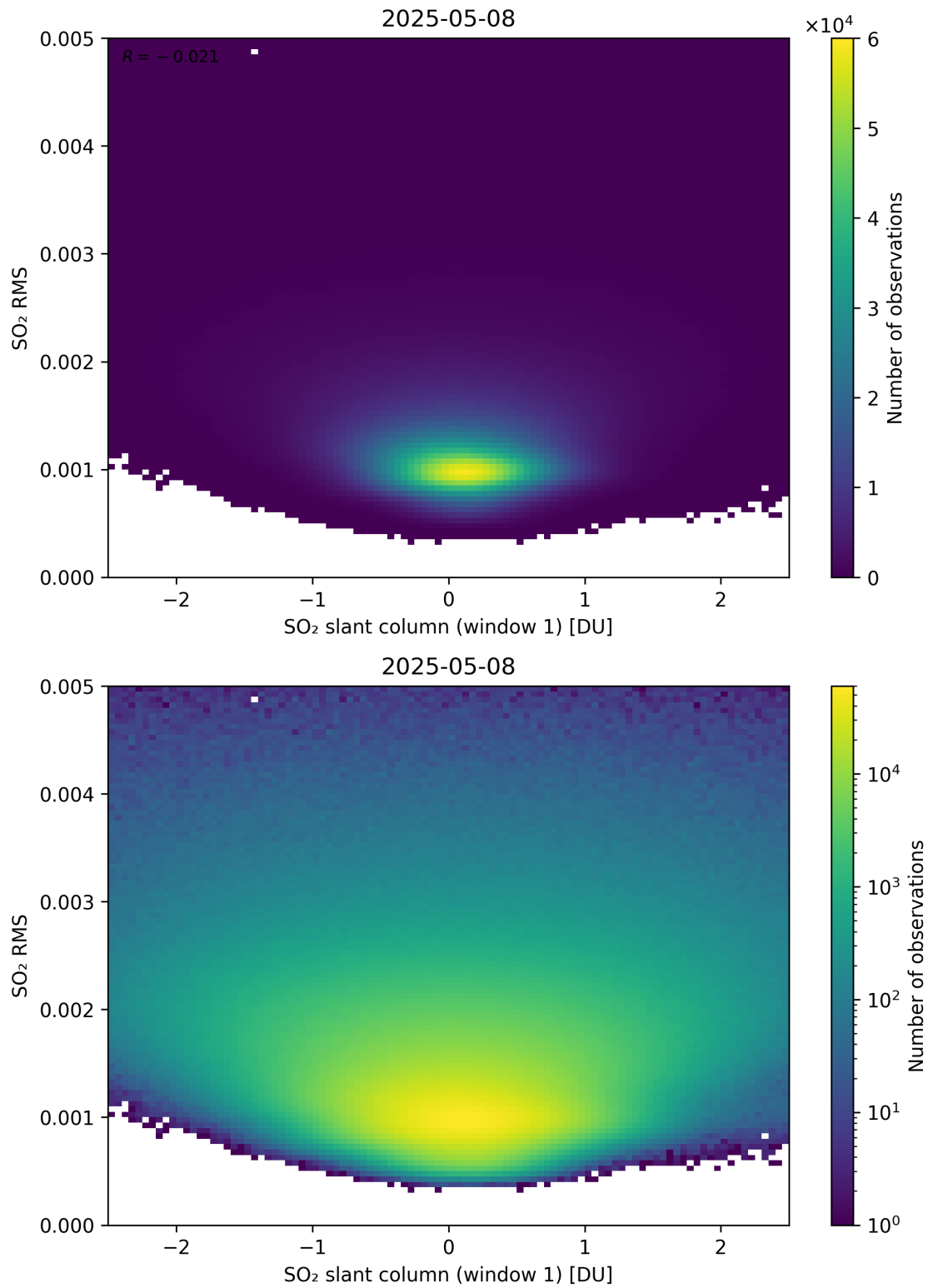
Figure 267: Scatter density plot of “SO 2 slant column (window 1)” against “SO 2 RMS” for 2025-05-07 to 2025-05-09.
