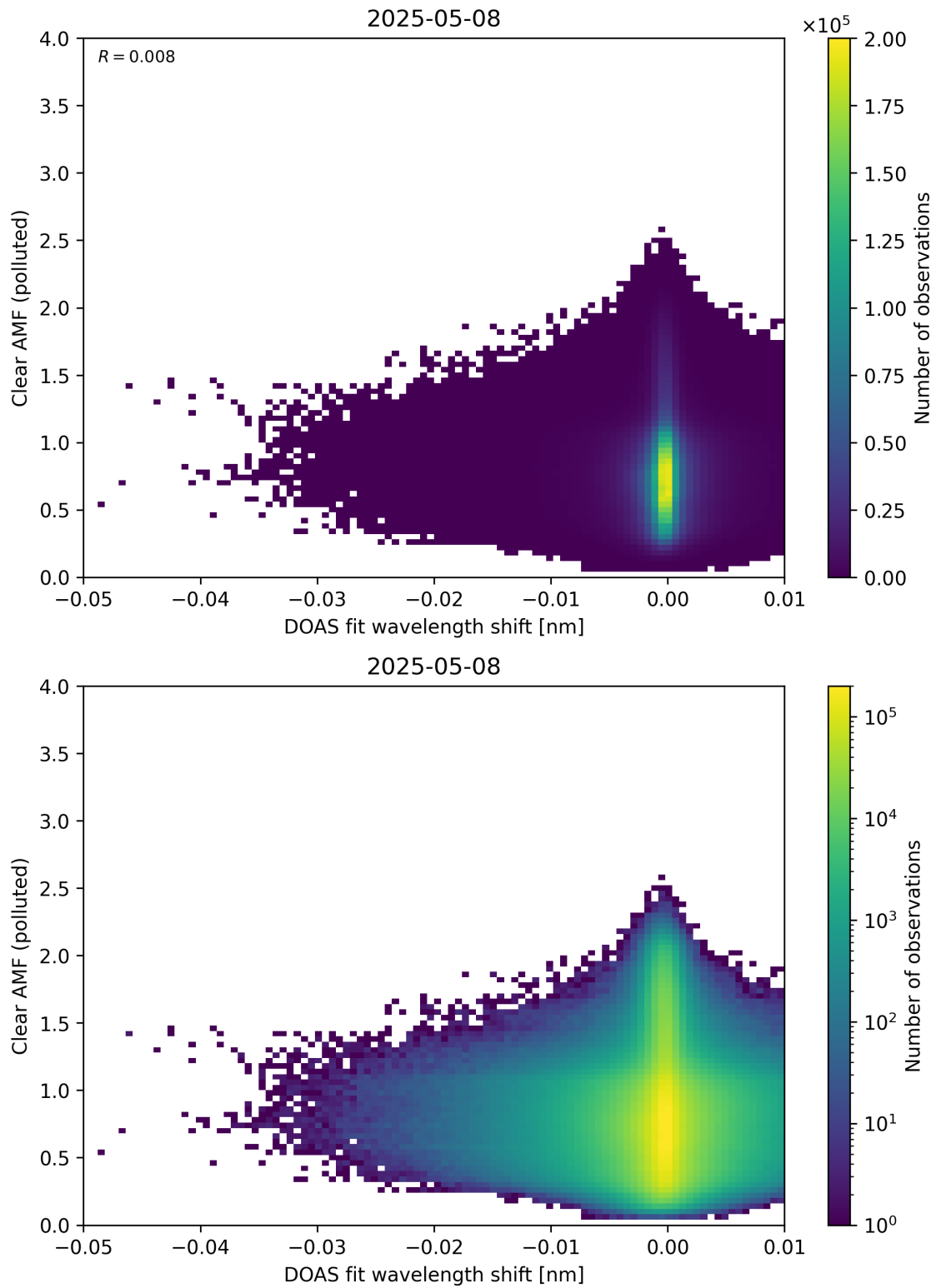
Figure 140: Scatter density plot of “DOAS fit wavelength shift” against “Clear AMF (polluted)” for 2025-05-07 to 2025-05-09.
