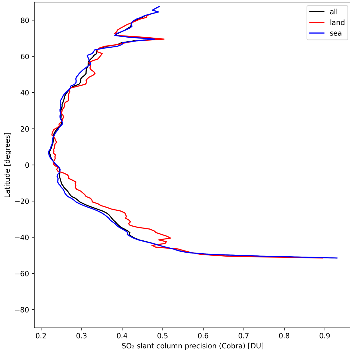
Figure 36: Zonal average of “SO 2 slant column precision (Cobra)” for 2025-05-07 to 2025-05-09.
