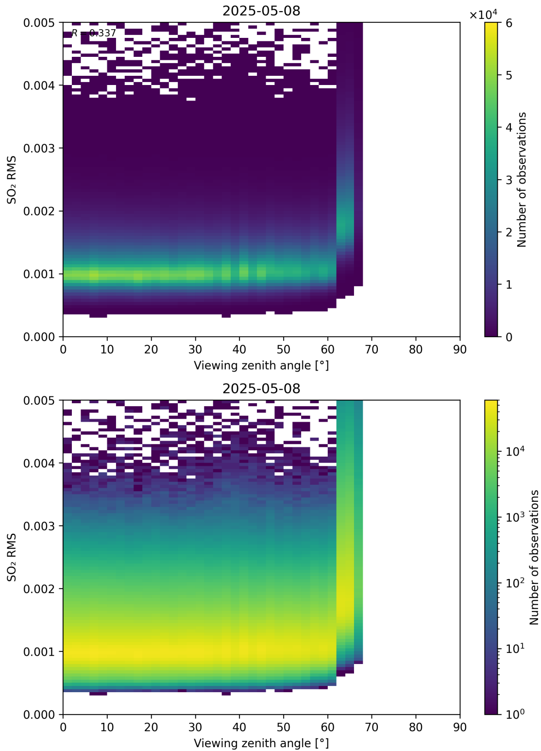
Figure 367: Scatter density plot of “Viewing zenith angle” against “SO 2 RMS” for 2025-05-07 to 2025-05-09.
