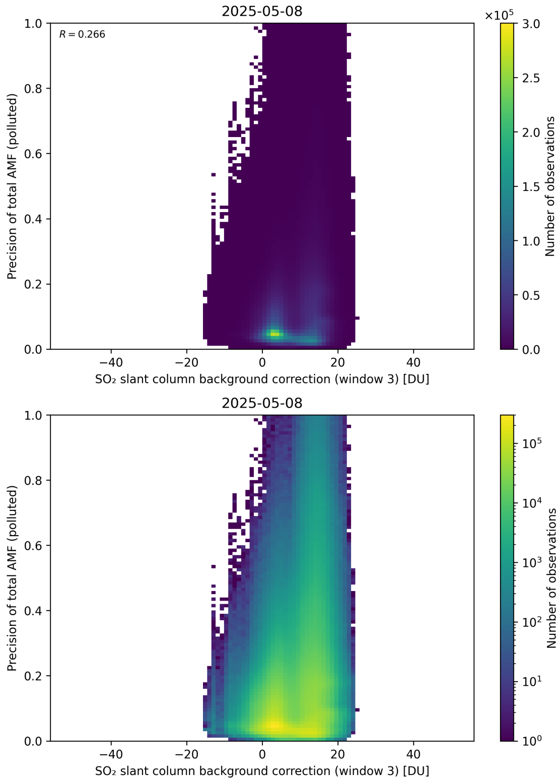
Figure 137: Scatter density plot of “SO 2 slant column background correction (window 3)” against “Precision of total AMF (polluted)” for 2025-05-07 to 2025-05-09.
