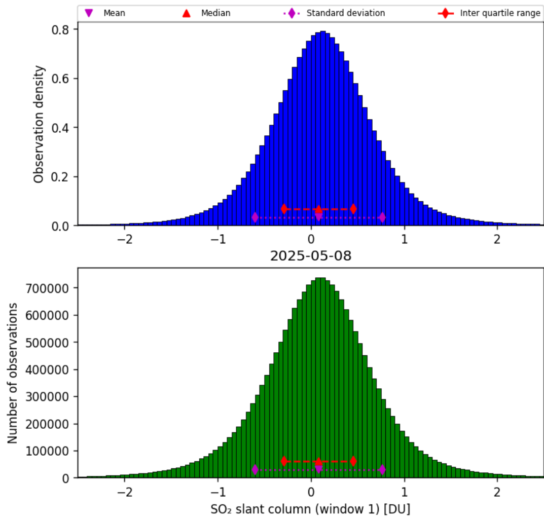
Figure 63: Histogram of “SO 2 slant column (window 1)” for 2025-05-07 to 2025-05-09
