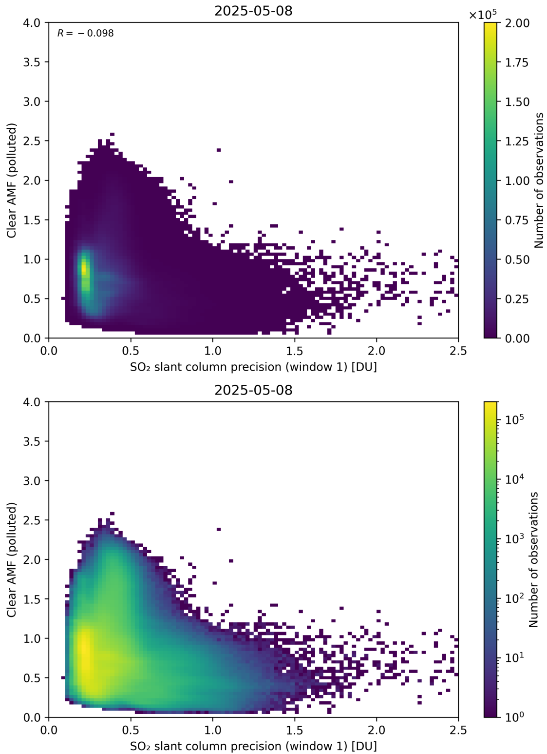
Figure 274: Scatter density plot of “SO 2 slant column precision (window 1)” against “Clear AMF (polluted)” for 2025-05-07 to 2025-05-09.
