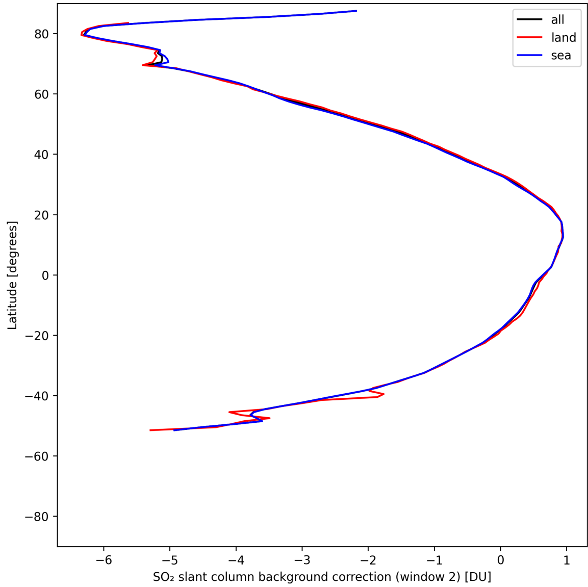
Figure 44: Zonal average of “SO 2 slant column background correction (window 2)” for 2025-05-07 to 2025-05-09.
