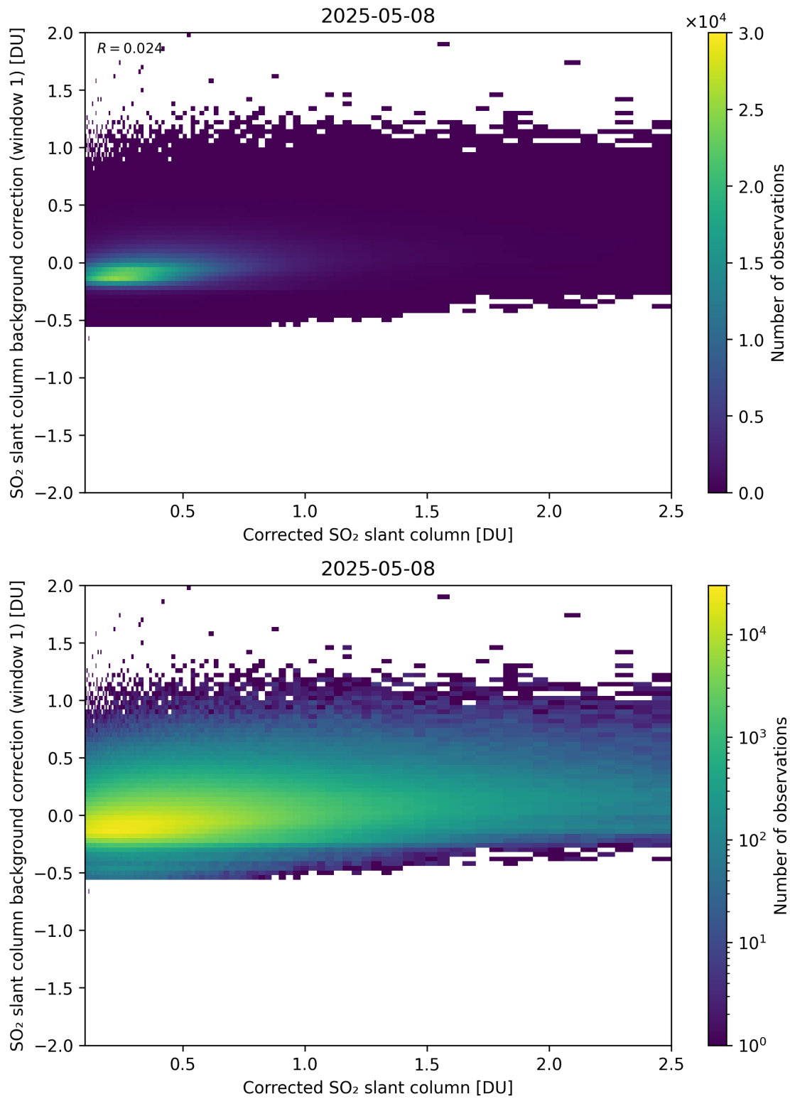
Figure 226: Scatter density plot of “Corrected SO 2 slant column” against “SO 2 slant column background correction (window 1)” for 2025-05-07 to 2025-05-09.
