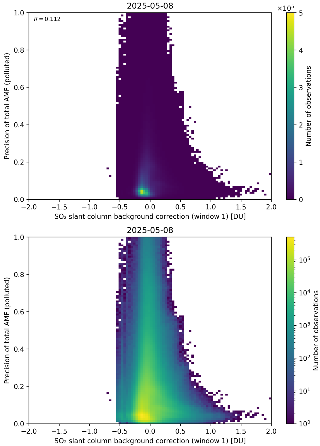
Figure 121: Scatter density plot of “SO 2 slant column background correction (window 1)” against “Precision of total AMF (polluted)” for 2025-05-07 to 2025-05-09.
