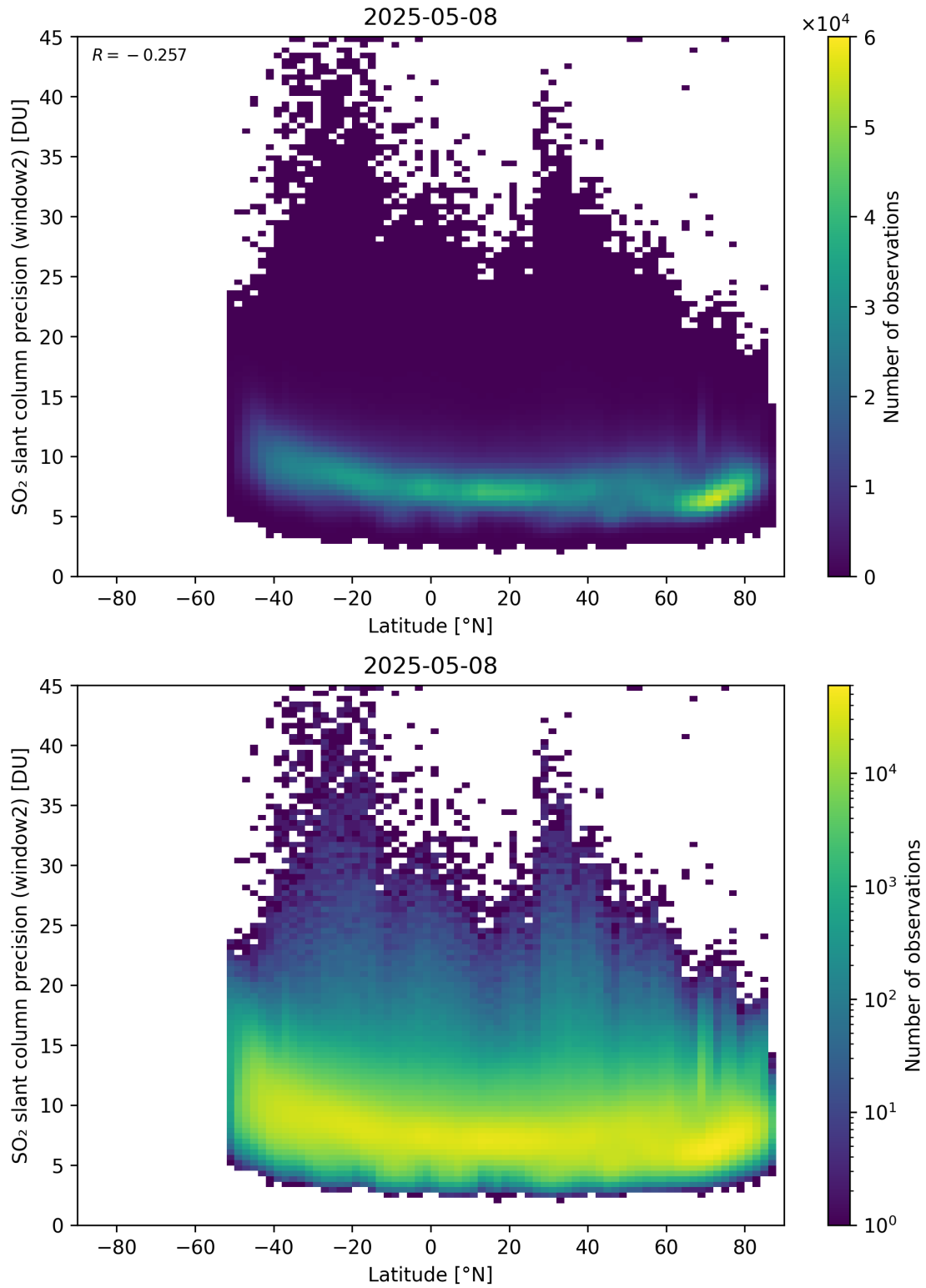
Figure 164: Scatter density plot of “Latitude” against “SO 2 slant column precision (window2)” for 2025-05-07 to 2025-05-09.
