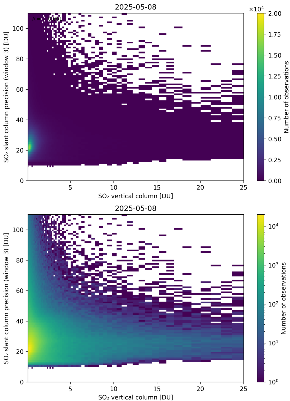
Figure 358: Scatter density plot of “SO 2 vertical column” against “SO 2 slant column precision (window 3)” for 2025-05-07 to 2025-05-09.
