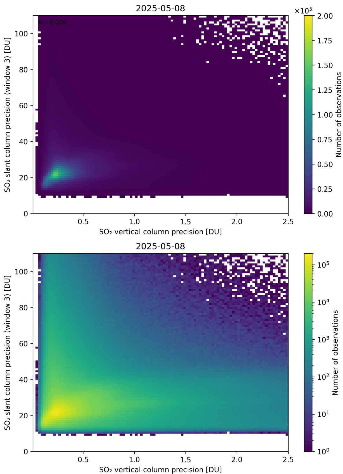
Figure 345: Scatter density plot of “SO 2 vertical column precision” against “SO 2 slant column precision (window 3)” for 2025-05-07 to 2025-05-09.
