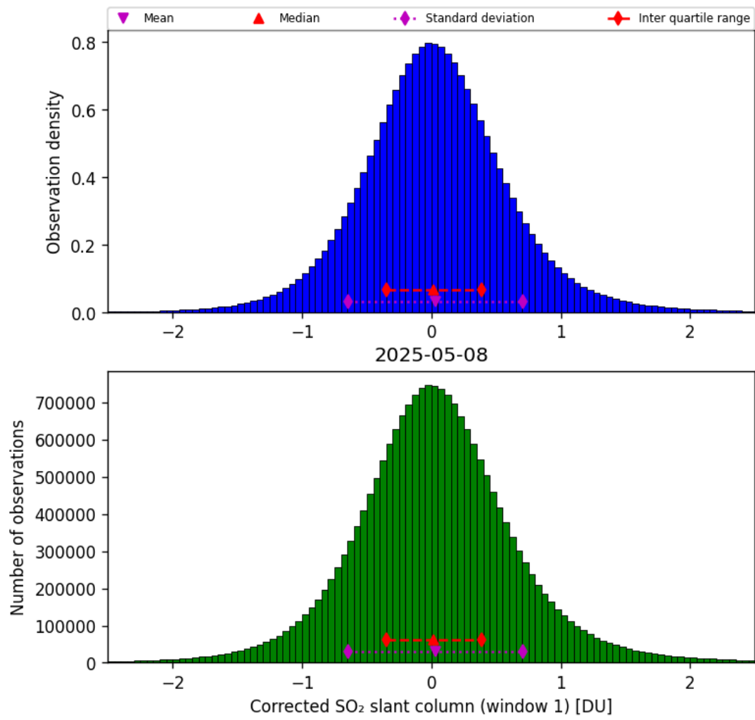
Figure 65: Histogram of “Corrected SO 2 slant column (window 1)” for 2025-05-07 to 2025-05-09
