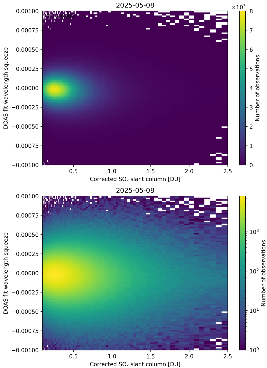
Figure 230: Scatter density plot of “Corrected SO 2 slant column” against “DOAS fit wavelength squeeze” for 2025-05-07 to 2025-05-09.
