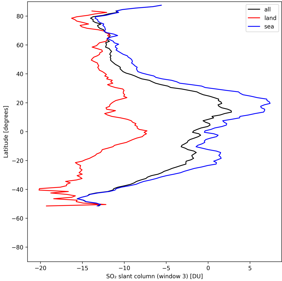
Figure 45: Zonal average of “SO 2 slant column (window 3)” for 2025-05-07 to 2025-05-09.
