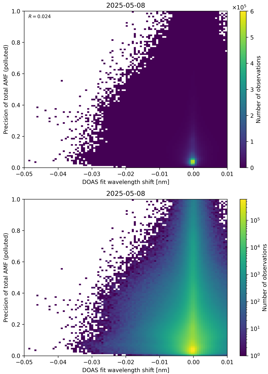
Figure 142: Scatter density plot of “DOAS fit wavelength shift” against “Precision of total AMF (polluted)” for 2025-05-07 to 2025-05-09.
