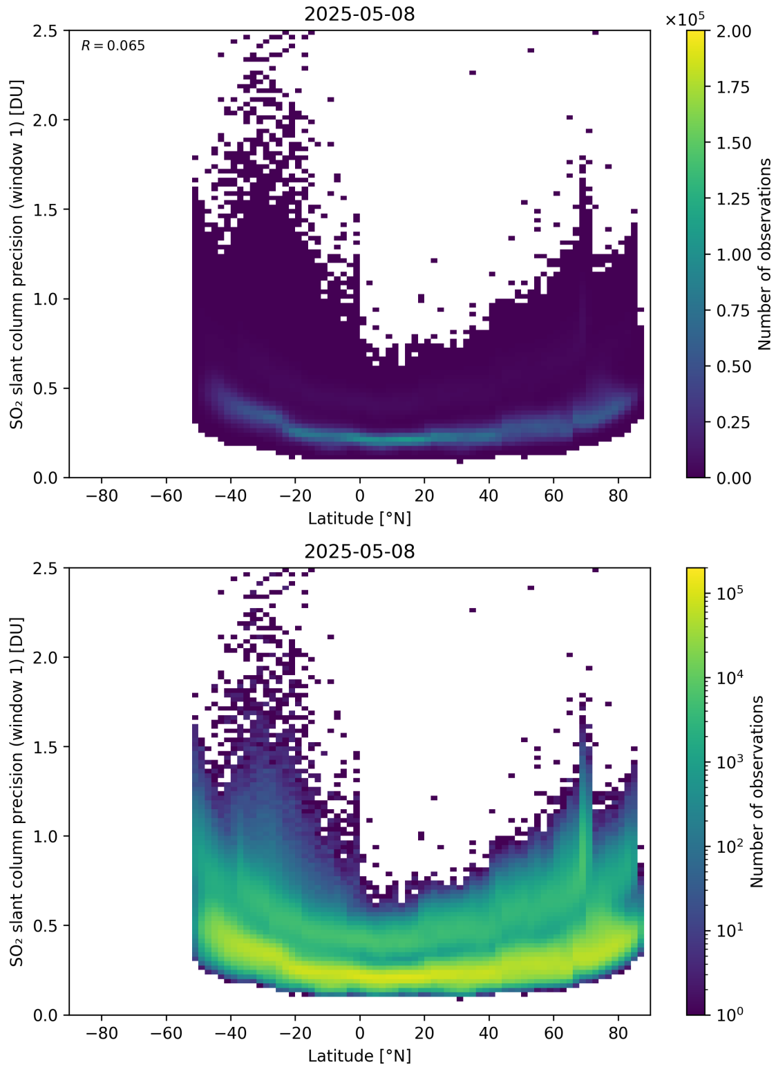
Figure 163: Scatter density plot of “Latitude” against “SO 2 slant column precision (window 1)” for 2025-05-07 to 2025-05-09.
