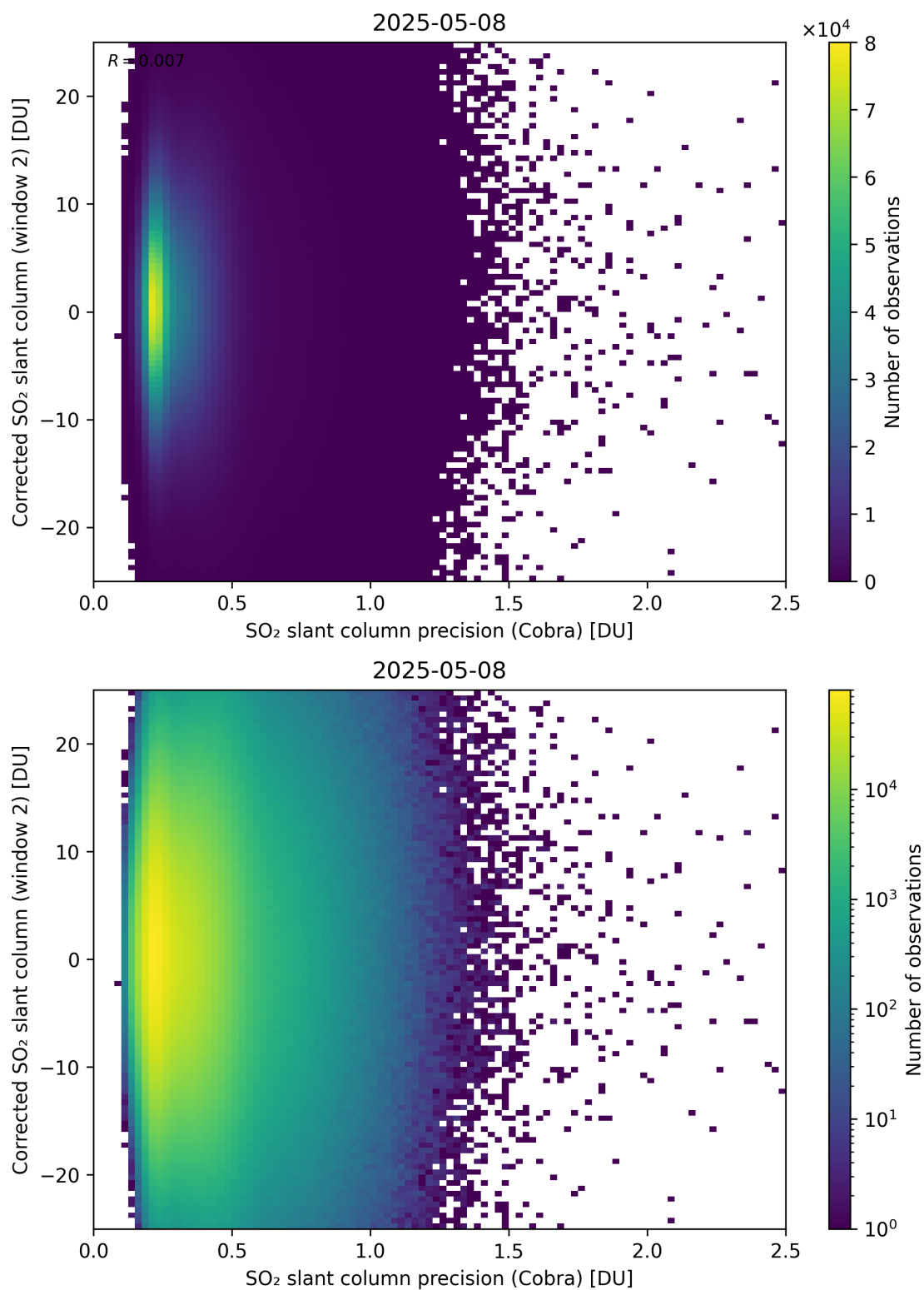
Figure 206: Scatter density plot of “SO 2 slant column precision (Cobra)” against “Corrected SO 2 slant column (window 2)” for 2025-05-07 to 2025-05-09.
