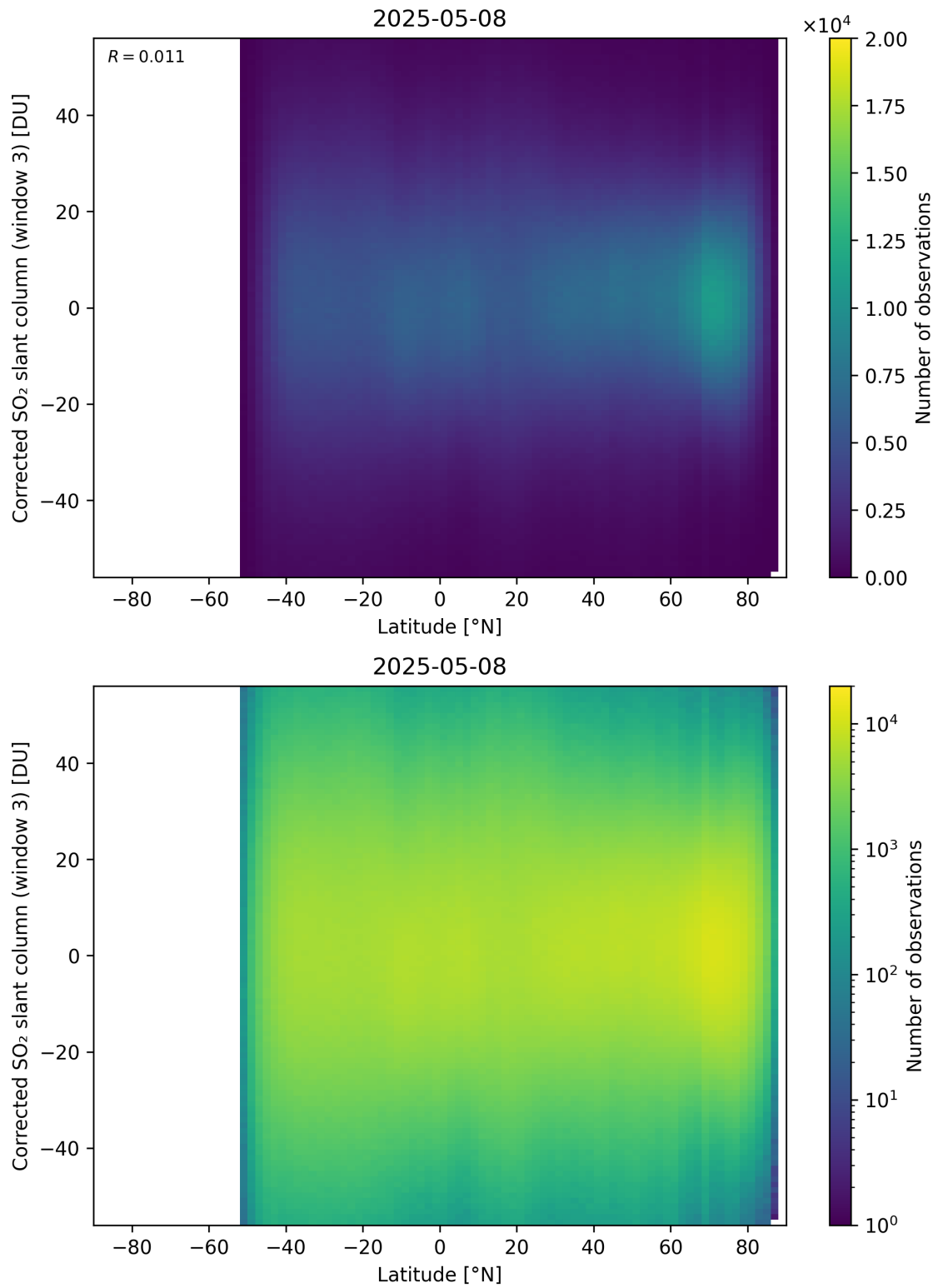
Figure 161: Scatter density plot of “Latitude” against “Corrected SO 2 slant column (window 3)” for 2025-05-07 to 2025-05-09.
