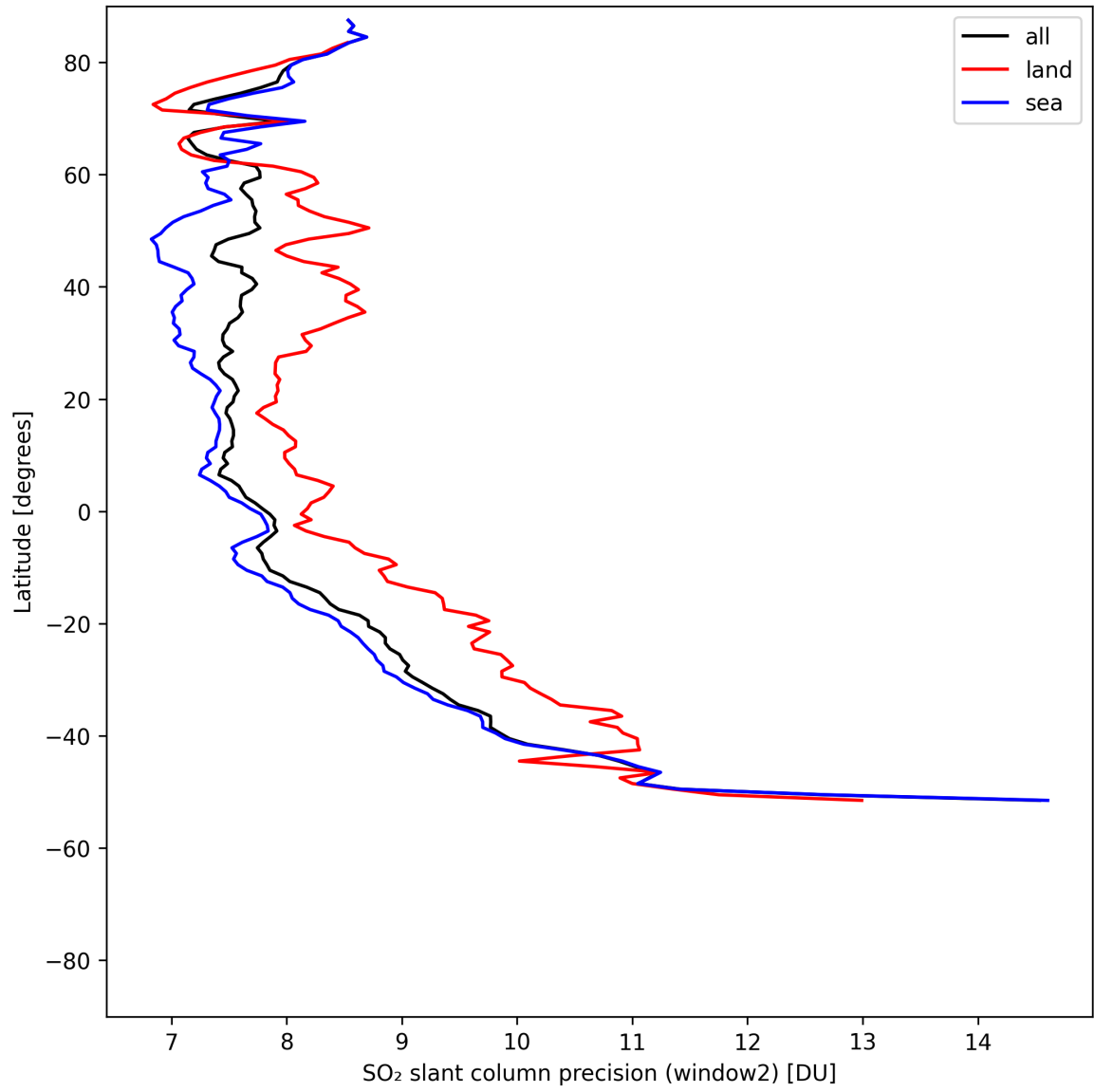
Figure 42: Zonal average of “SO 2 slant column precision (window2)” for 2025-05-07 to 2025-05-09.
