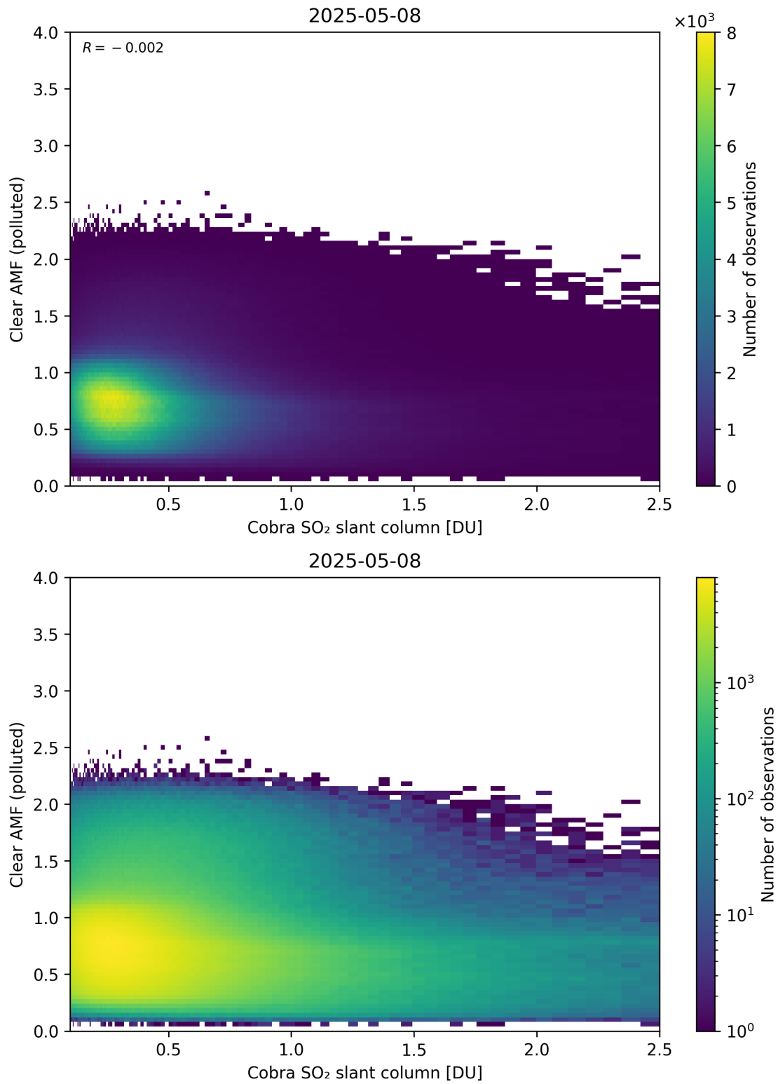
Figure 215: Scatter density plot of “Cobra SO 2 slant column” against “Clear AMF (polluted)” for 2025-05-07 to 2025-05-09.
