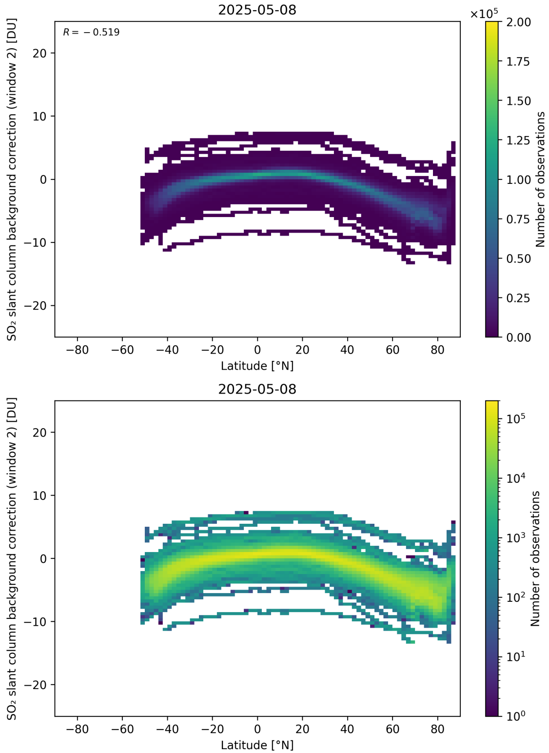
Figure 151: Scatter density plot of “Latitude” against “SO 2 slant column background correction (window 2)” for 2025-05-07 to 2025-05-09.
