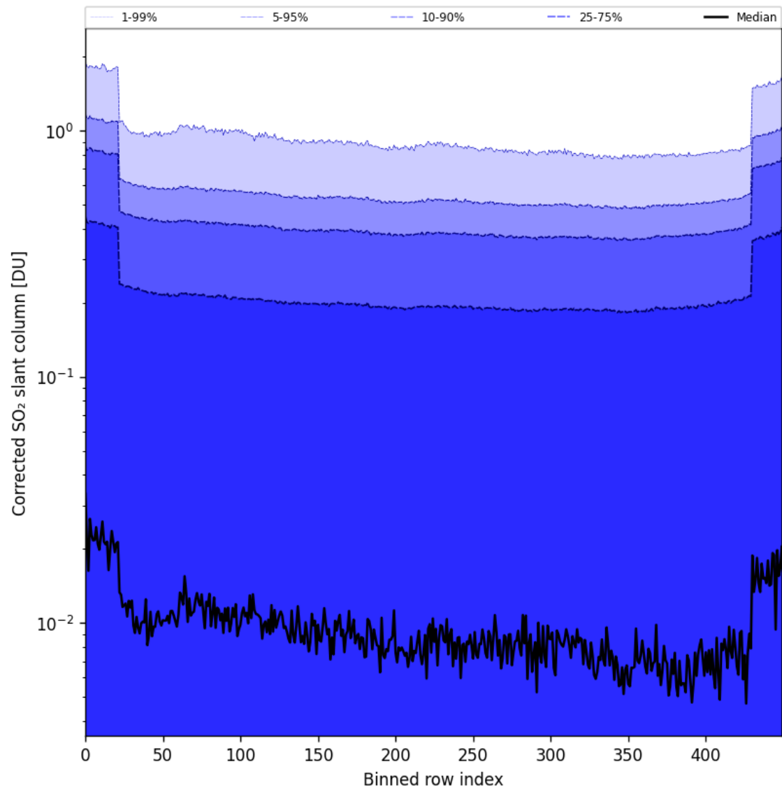
Figure 86: Along track statistics of “Corrected SO 2 slant column” for 2025-05-07 to 2025-05-09
