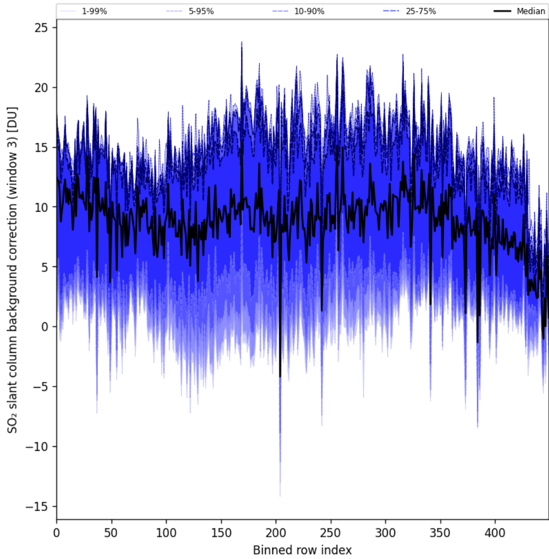
Figure 100: Along track statistics of “SO 2 slant column background correction (window 3)” for 2025-05-07 to 2025-05-09
