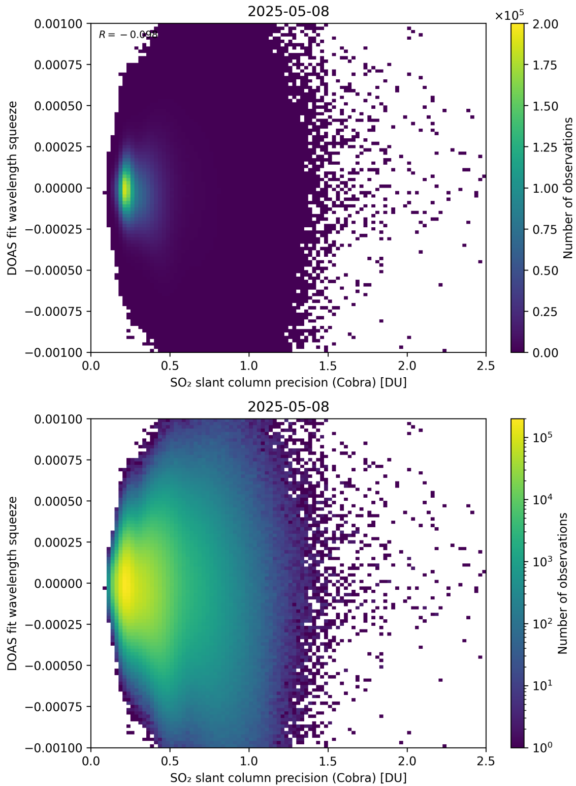
Figure 203: Scatter density plot of “SO 2 slant column precision (Cobra)” against “DOAS fit wavelength squeeze” for 2025-05-07 to 2025-05-09.
