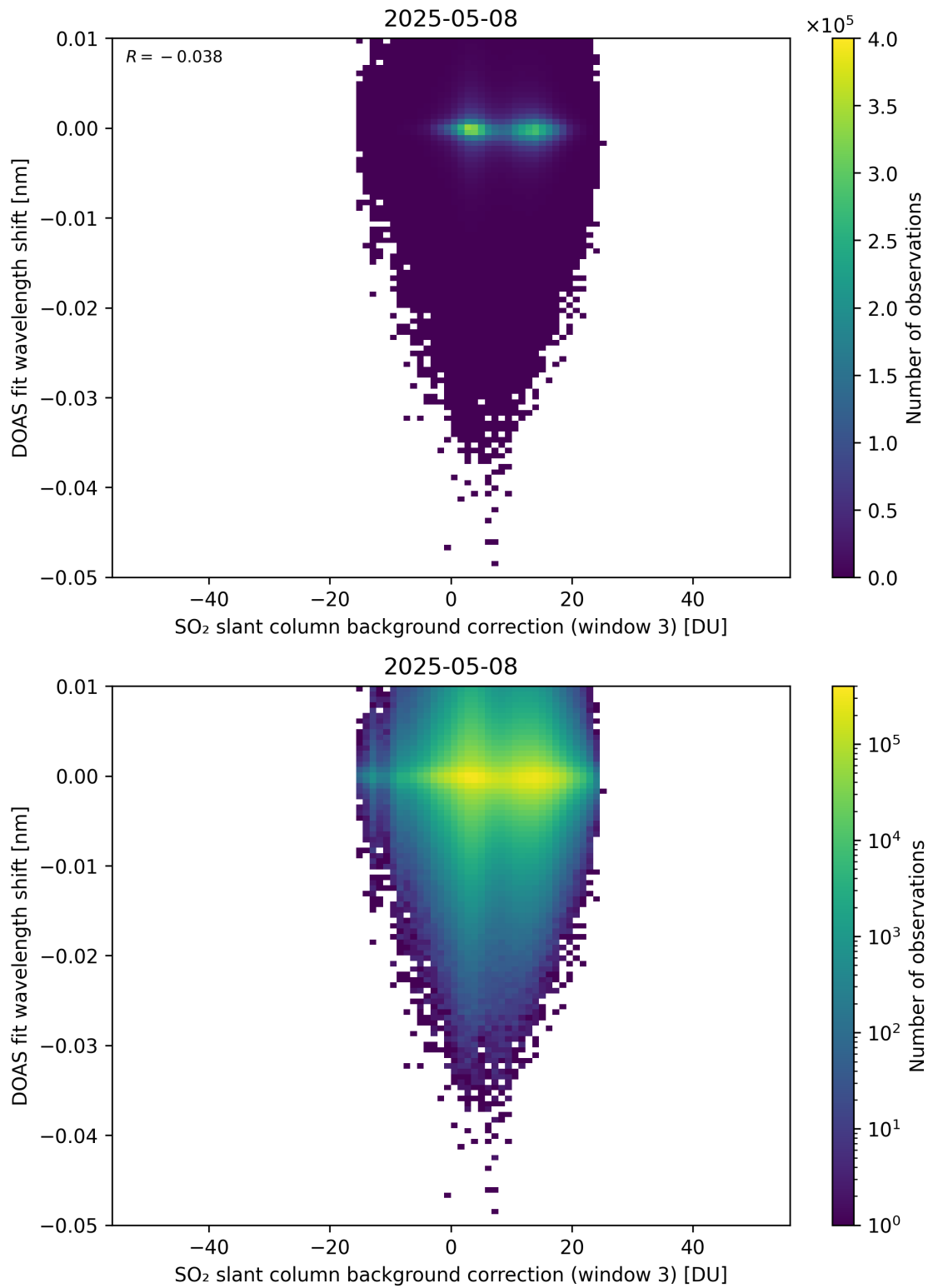
Figure 132: Scatter density plot of “SO 2 slant column background correction (window 3)” against “DOAS fit wavelength shift” for 2025-05-07 to 2025-05-09.
