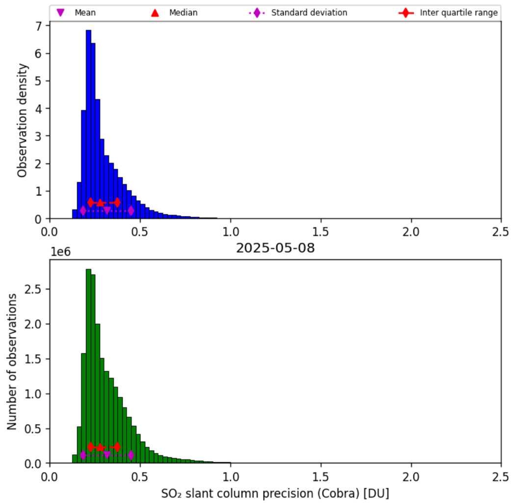
Figure 62: Histogram of “SO 2 slant column precision (Cobra)” for 2025-05-07 to 2025-05-09
