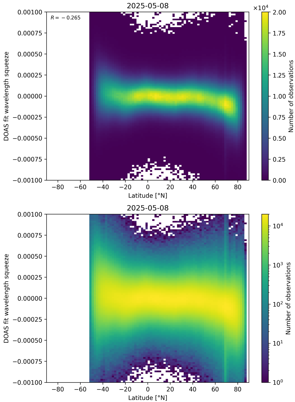
Figure 154: Scatter density plot of “Latitude” against “DOAS fit wavelength squeeze” for 2025-05-07 to 2025-05-09.
