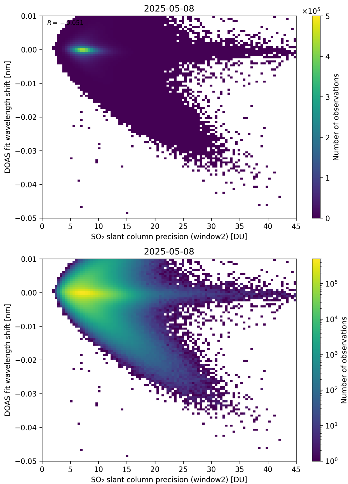
Figure 293: Scatter density plot of “SO 2 slant column precision (window2)” against “DOAS fit wavelength shift” for 2025-05-07 to 2025-05-09.
