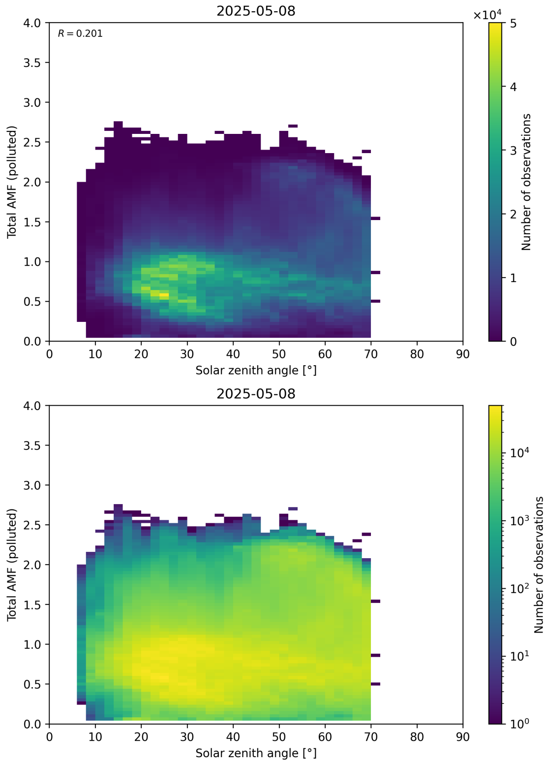
Figure 189: Scatter density plot of “Solar zenith angle” against “Total AMF (polluted)” for 2025-05-07 to 2025-05-09.
