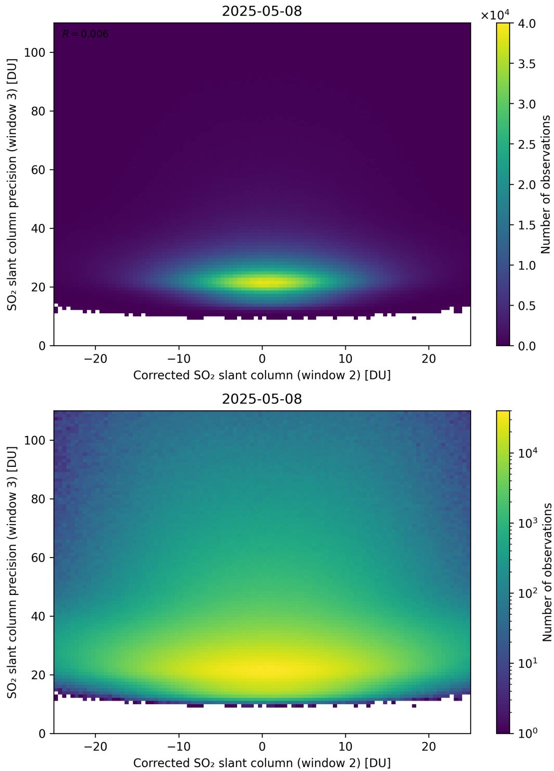
Figure 252: Scatter density plot of “Corrected SO 2 slant column (window 2)” against “SO 2 slant column precision (window 3)” for 2025-05-07 to 2025-05-09.
