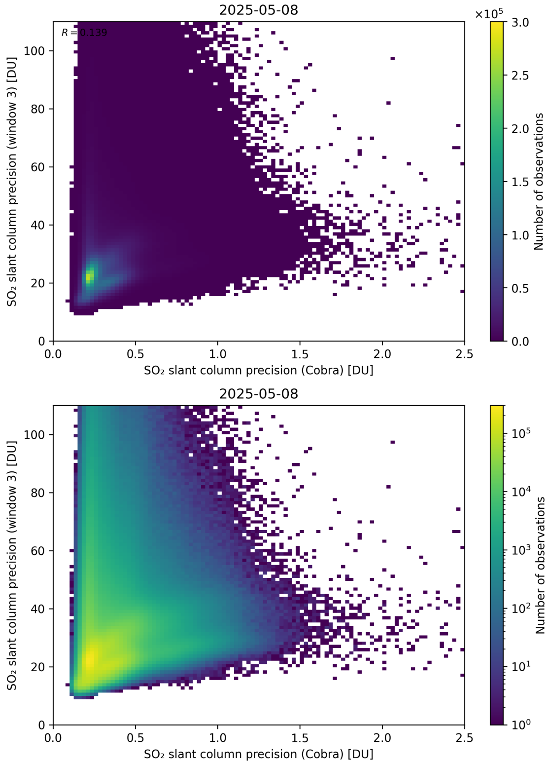
Figure 212: Scatter density plot of “SO 2 slant column precision (Cobra)” against “SO 2 slant column precision (window 3)” for 2025-05-07 to 2025-05-09.
