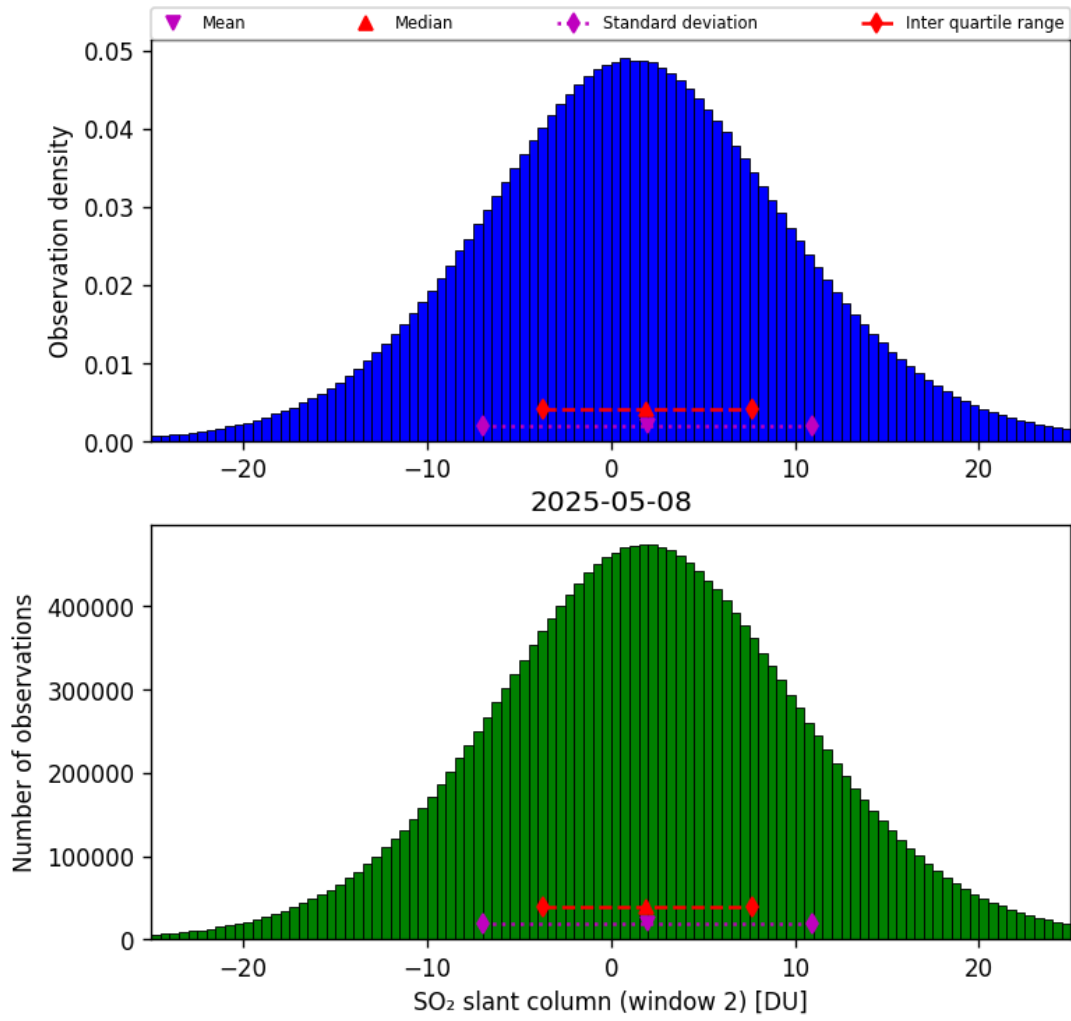
Figure 67: Histogram of “SO 2 slant column (window 2)” for 2025-05-07 to 2025-05-09
