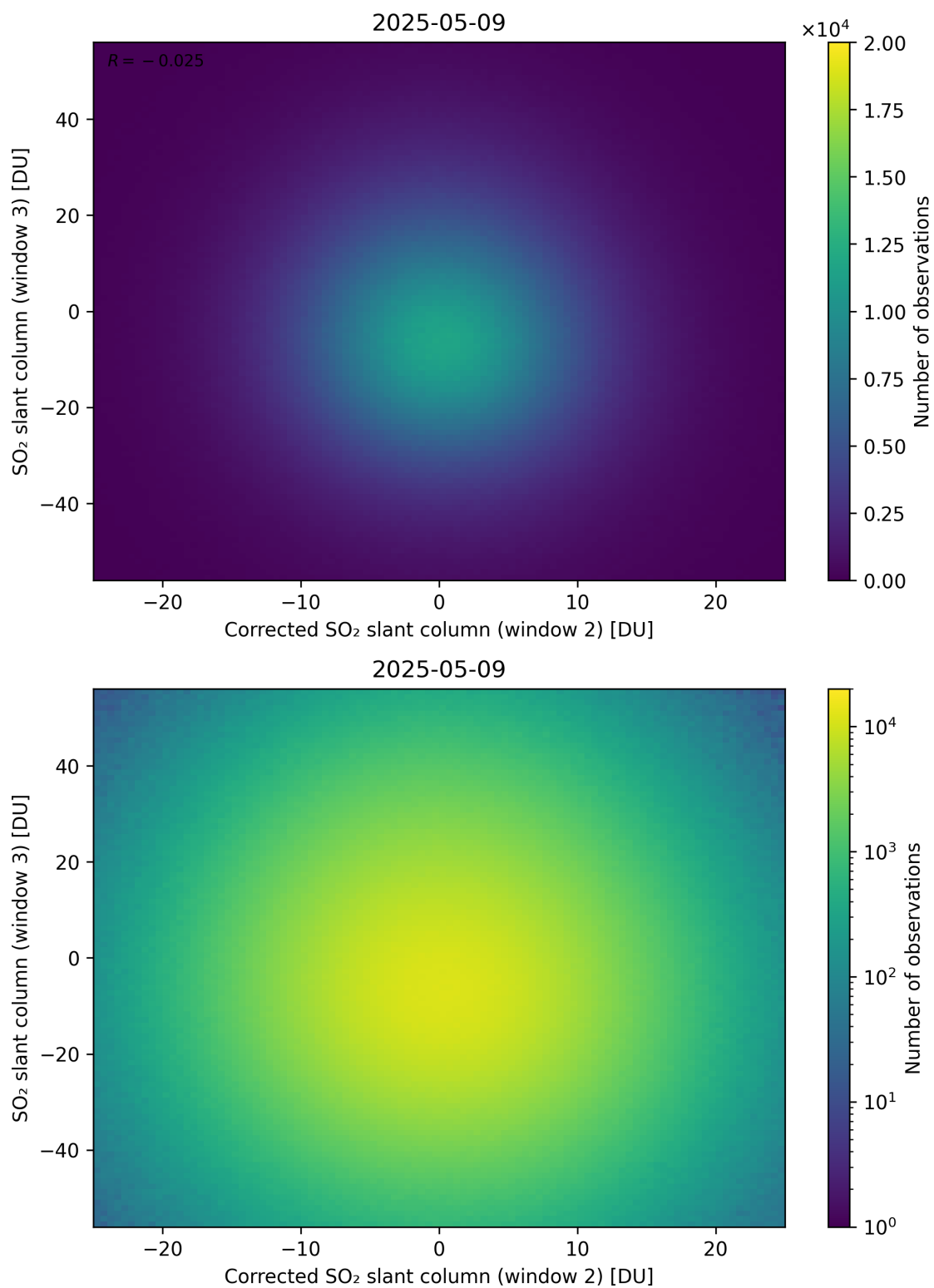
Figure 251: Scatter density plot of “Corrected SO 2 slant column (window 2)” against “SO 2 slant column (window 3)” for 2025-05-08 to 2025-05-10.
