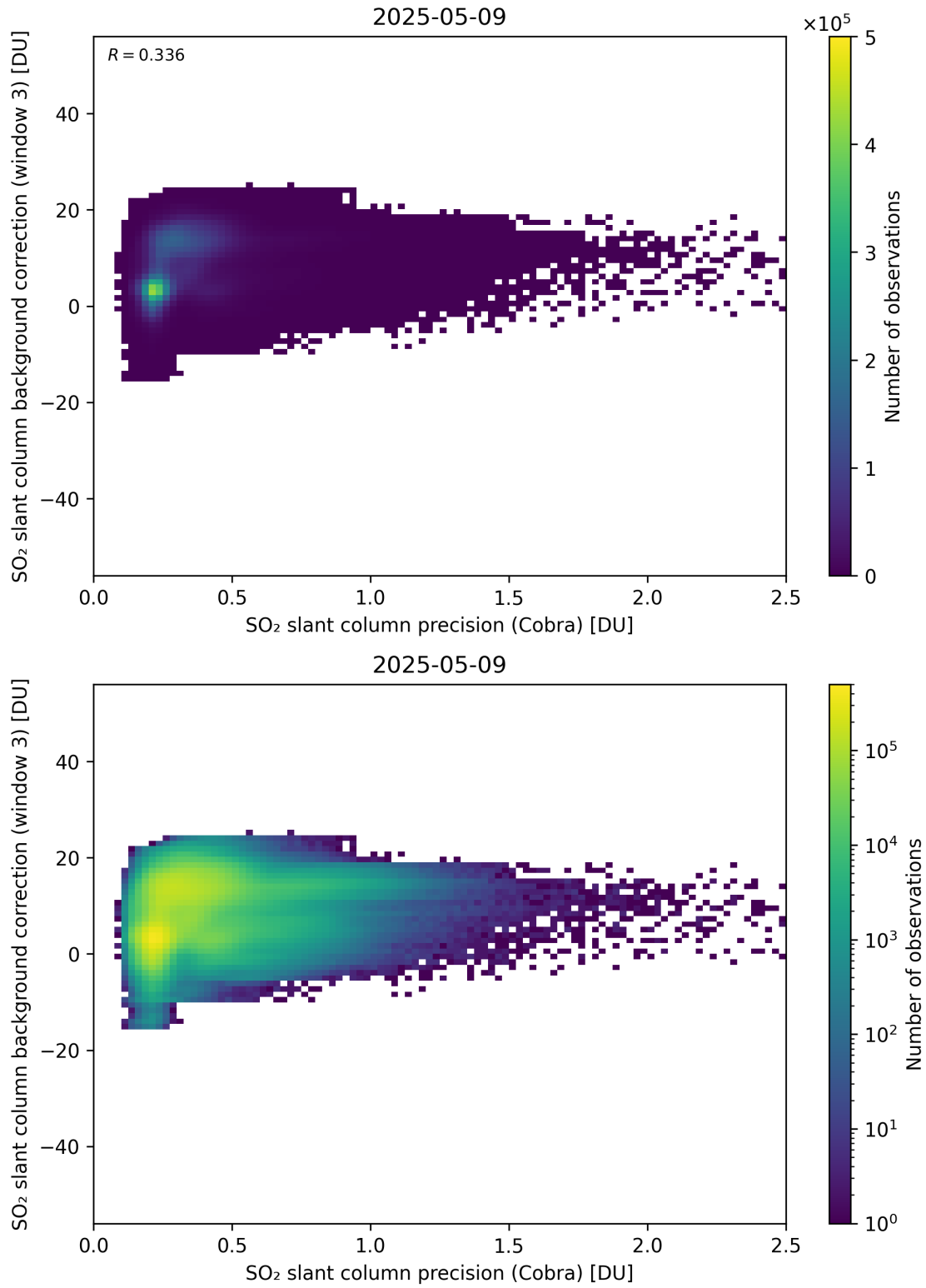
Figure 201: Scatter density plot of “SO 2 slant column precision (Cobra)” against “SO 2 slant column background correction (window 3)” for 2025-05-08 to 2025-05-10.
