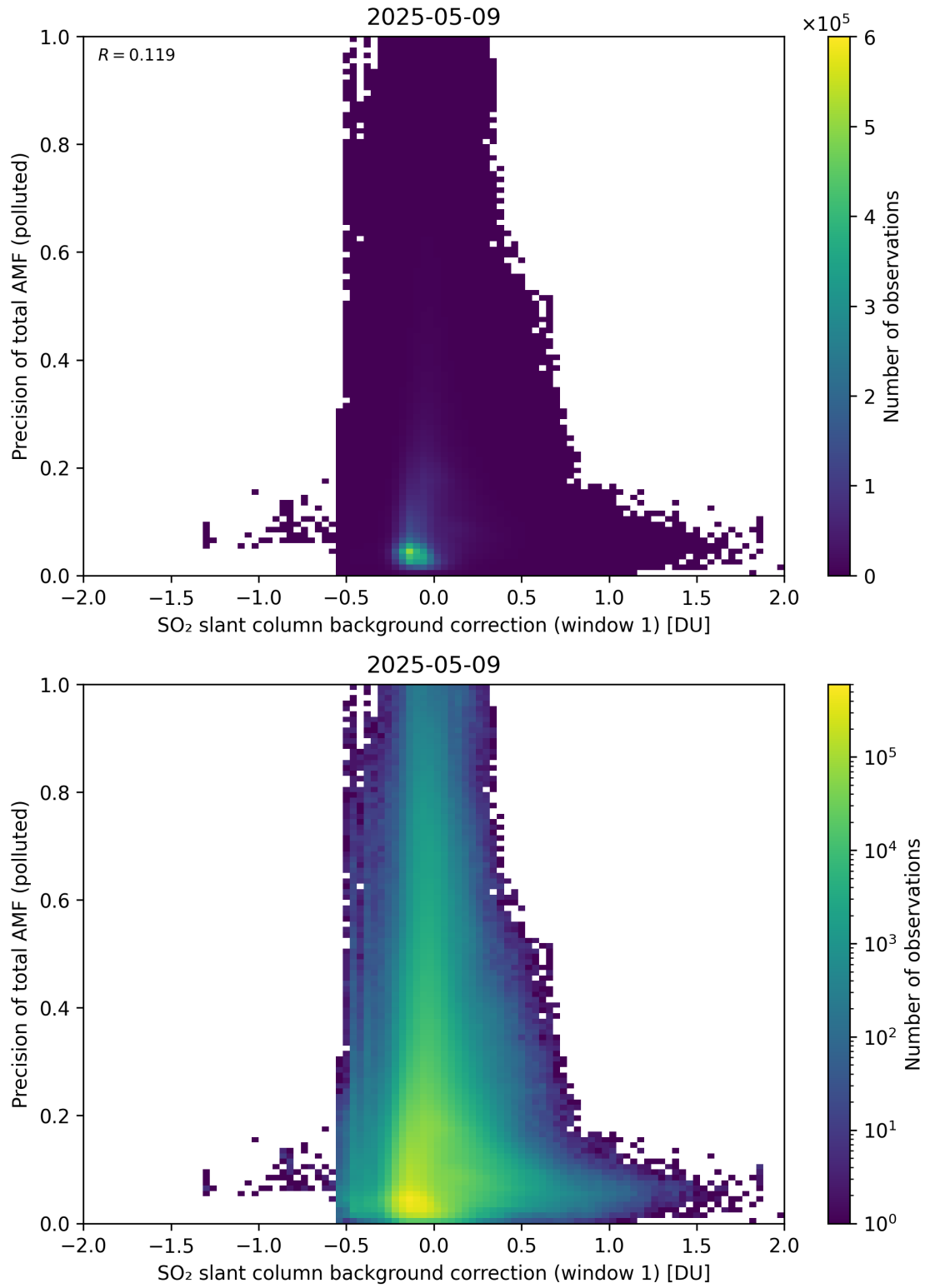
Figure 121: Scatter density plot of “SO 2 slant column background correction (window 1)” against “Precision of total AMF (polluted)” for 2025-05-08 to 2025-05-10.
