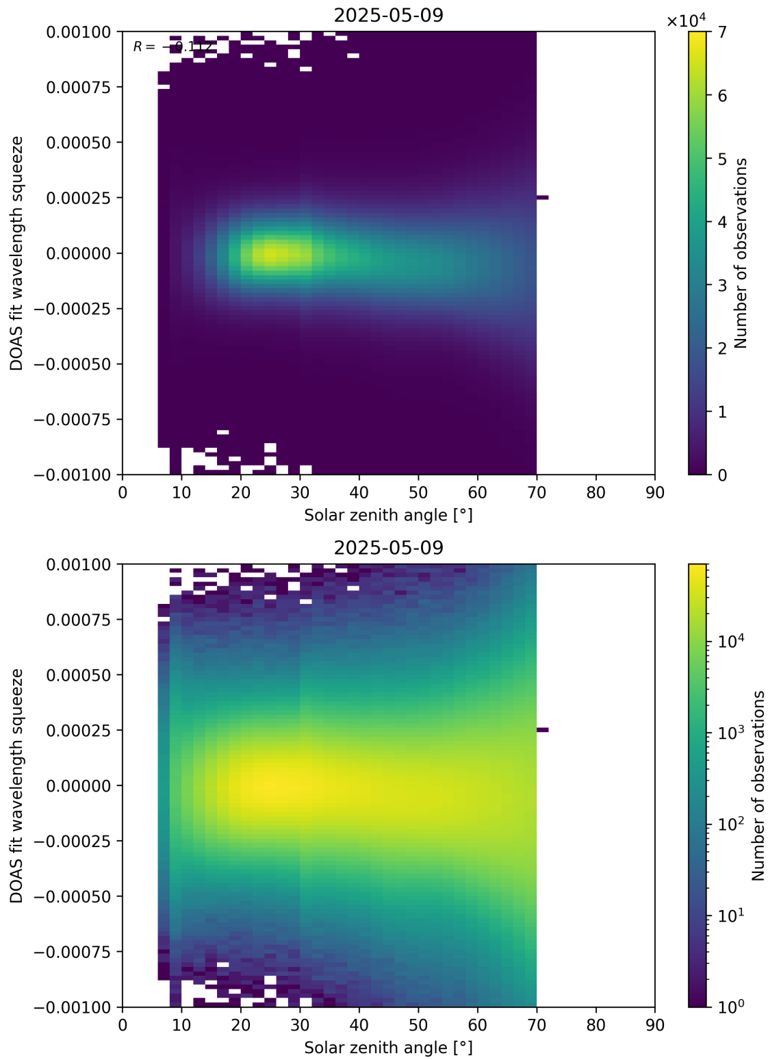
Figure 175: Scatter density plot of “Solar zenith angle” against “DOAS fit wavelength squeeze” for 2025-05-08 to 2025-05-10.
