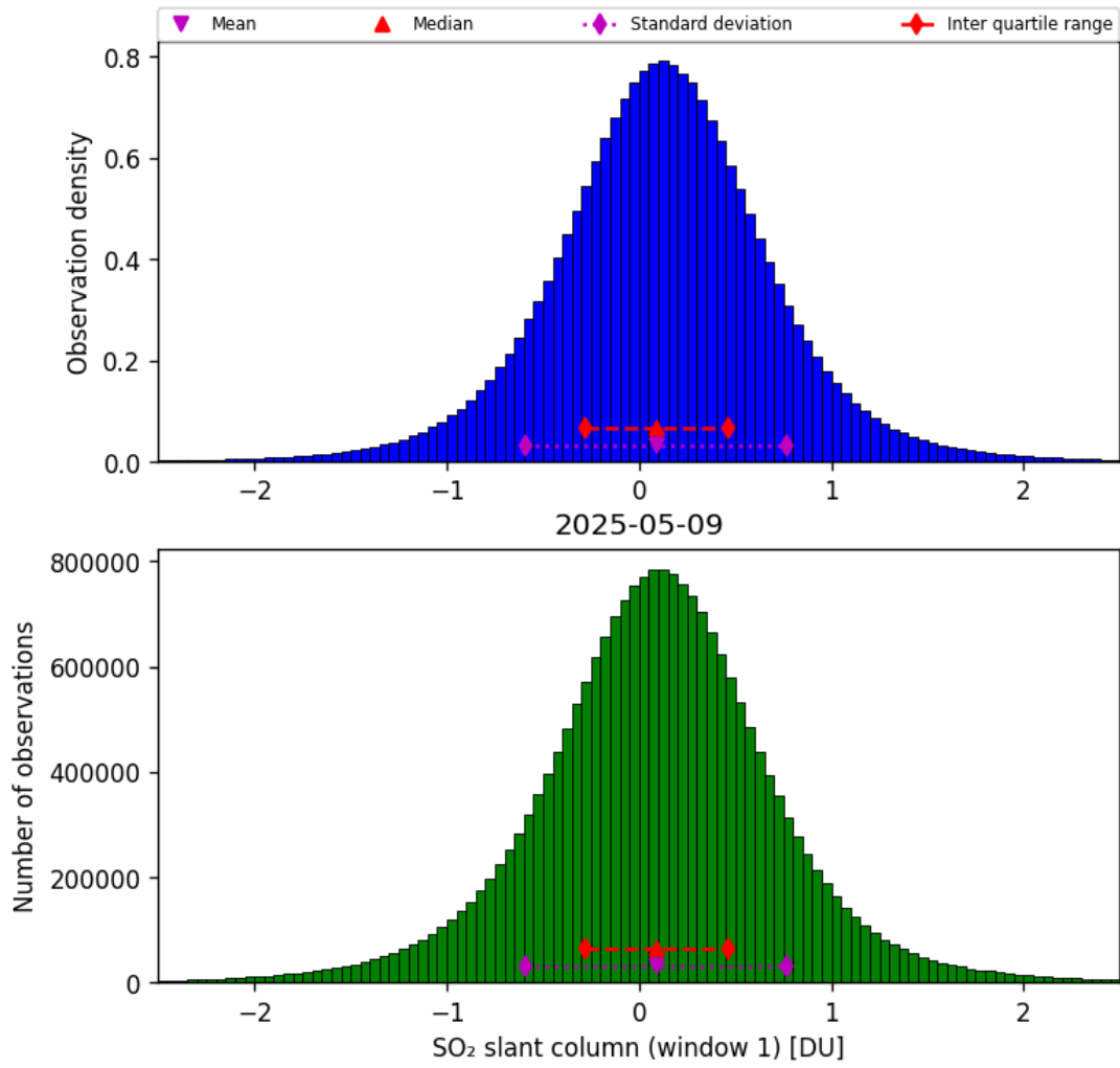
Figure 63: Histogram of “SO 2 slant column (window 1)” for 2025-05-08 to 2025-05-10
