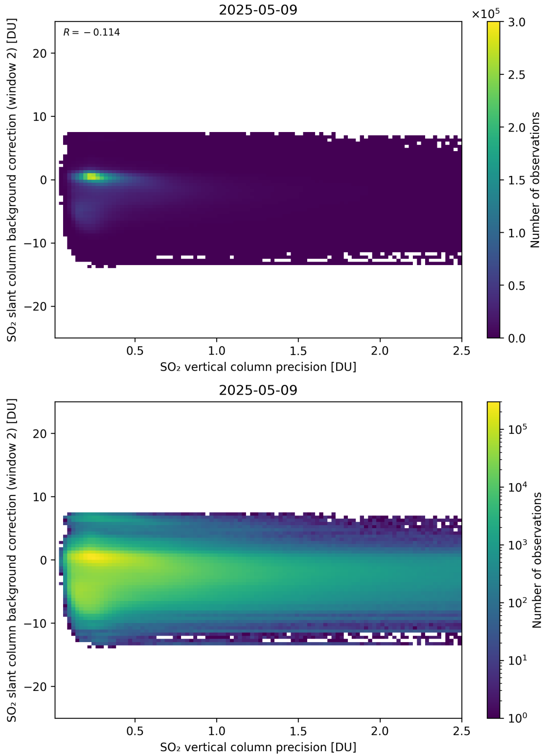
Figure 330: Scatter density plot of “SO 2 vertical column precision” against “SO 2 slant column background correction (window 2)” for 2025-05-08 to 2025-05-10.
