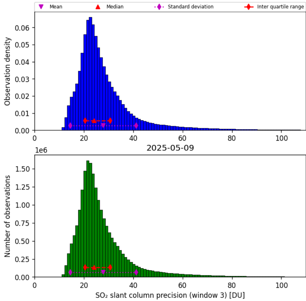
Figure 72: Histogram of “SO 2 slant column precision (window 3)” for 2025-05-08 to 2025-05-10
