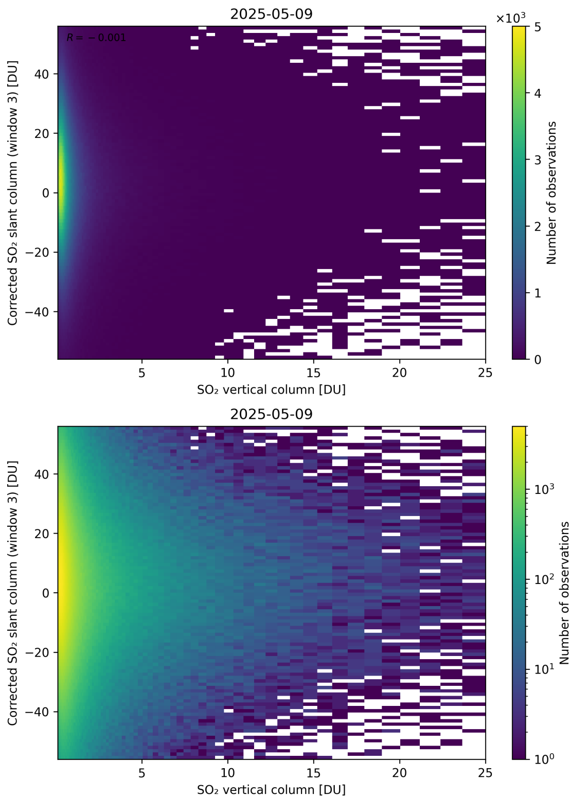
Figure 353: Scatter density plot of “SO 2 vertical column” against “Corrected SO 2 slant column (window 3)” for 2025-05-08 to 2025-05-10.
