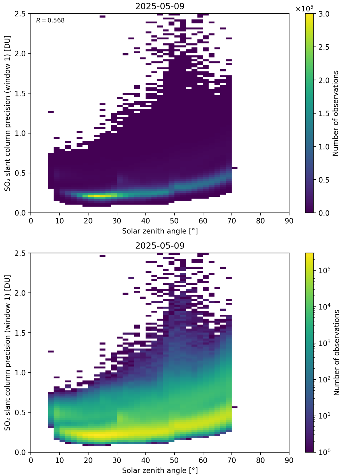
Figure 185: Scatter density plot of “Solar zenith angle” against “SO 2 slant column precision (window 1)” for 2025-05-08 to 2025-05-10.
