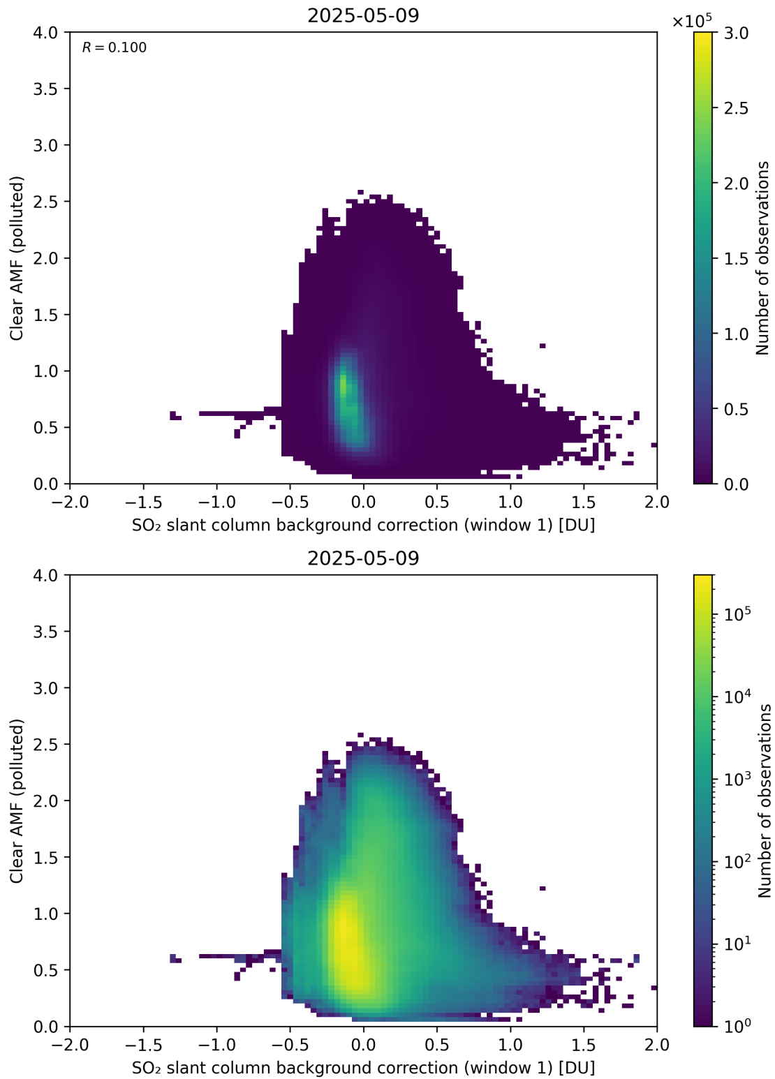
Figure 114: Scatter density plot of “SO 2 slant column background correction (window 1)” against “Clear AMF (polluted)” for 2025-05-08 to 2025-05-10.
