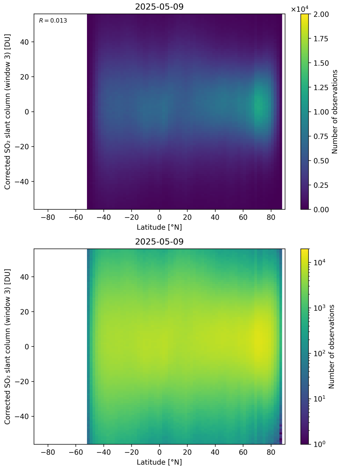
Figure 161: Scatter density plot of “Latitude” against “Corrected SO 2 slant column (window 3)” for 2025-05-08 to 2025-05-10.
