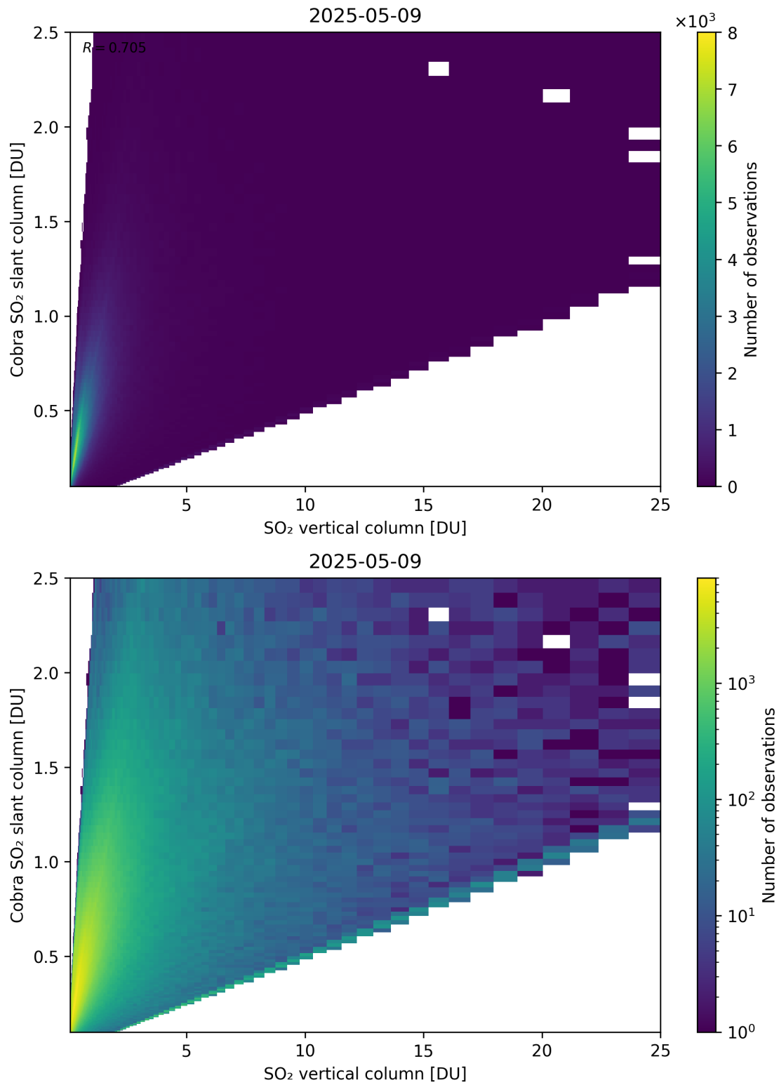
Figure 349: Scatter density plot of “SO 2 vertical column” against “Cobra SO 2 slant column” for 2025-05-08 to 2025-05-10.
