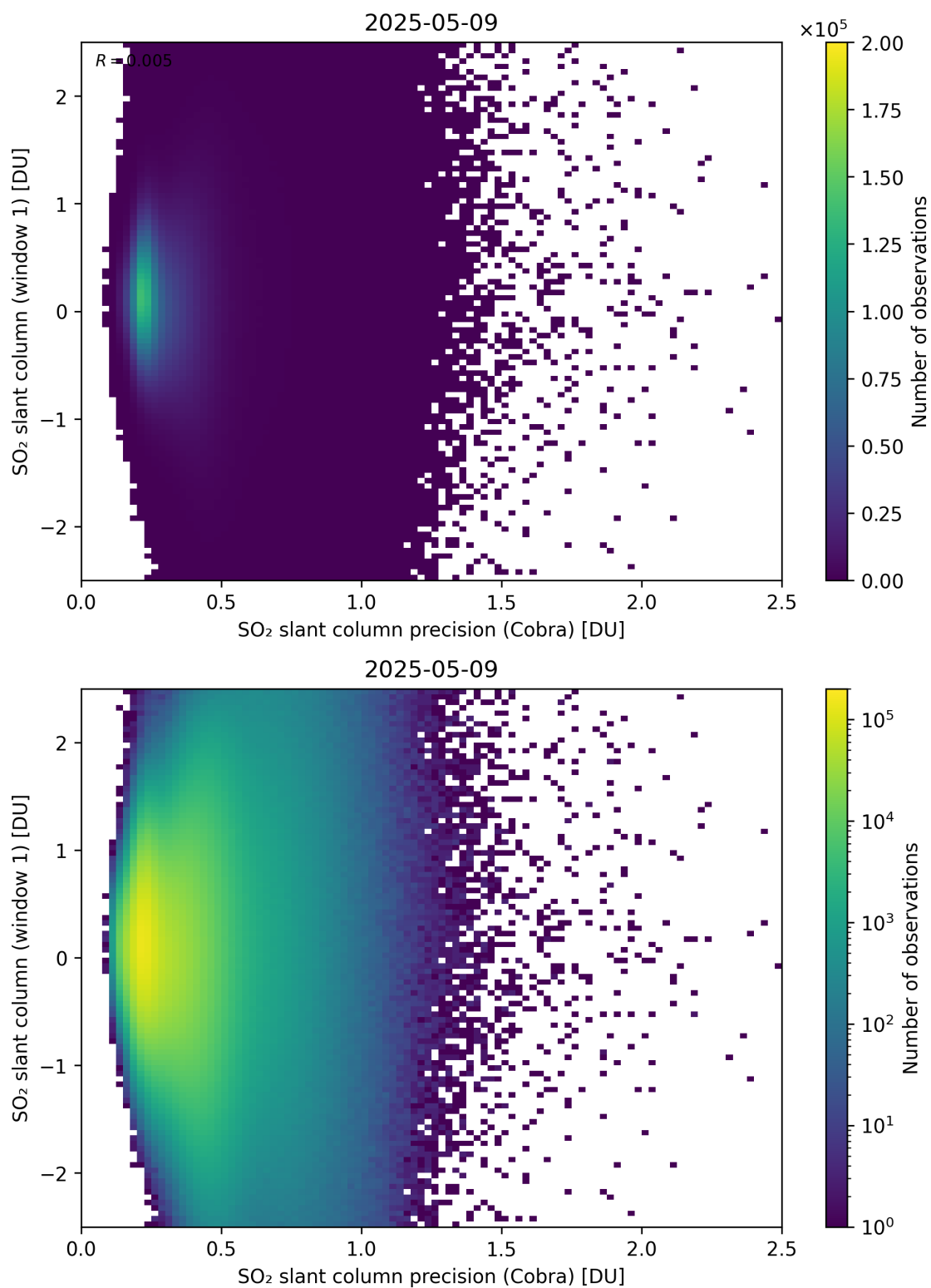
Figure 208: Scatter density plot of “SO 2 slant column precision (Cobra)” against “SO 2 slant column (window 1)” for 2025-05-08 to 2025-05-10.
