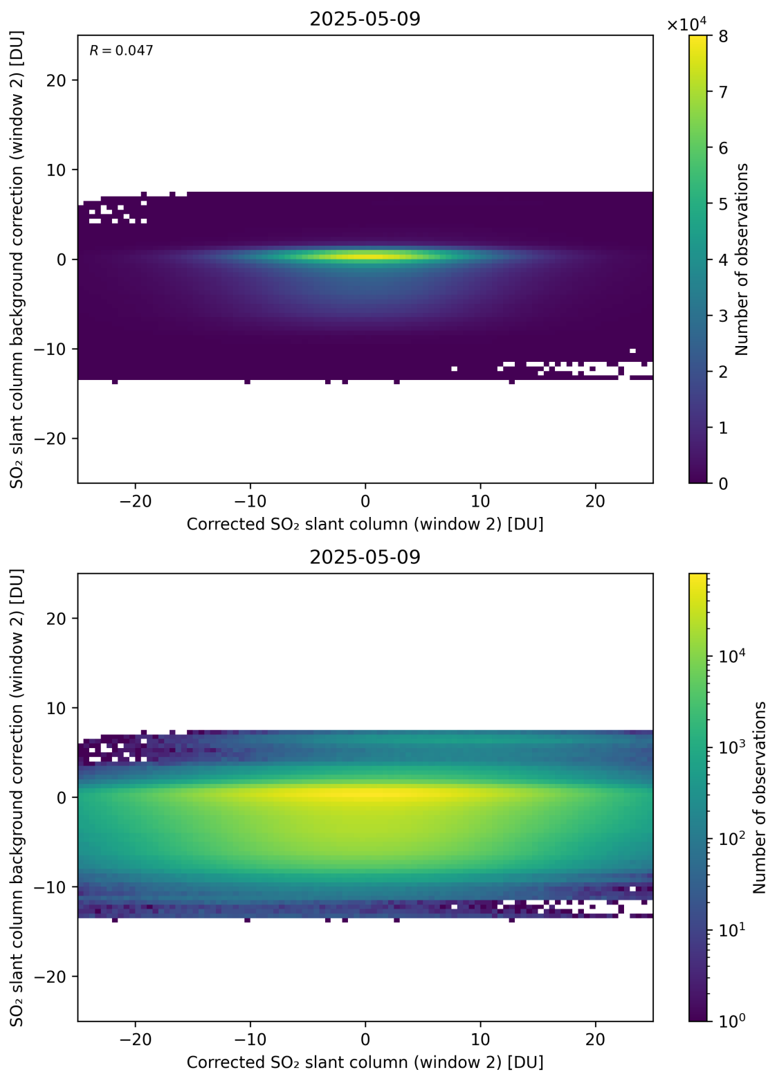
Figure 244: Scatter density plot of “Corrected SO 2 slant column (window 2)” against “SO 2 slant column background correction (window 2)” for 2025-05-08 to 2025-05-10.
