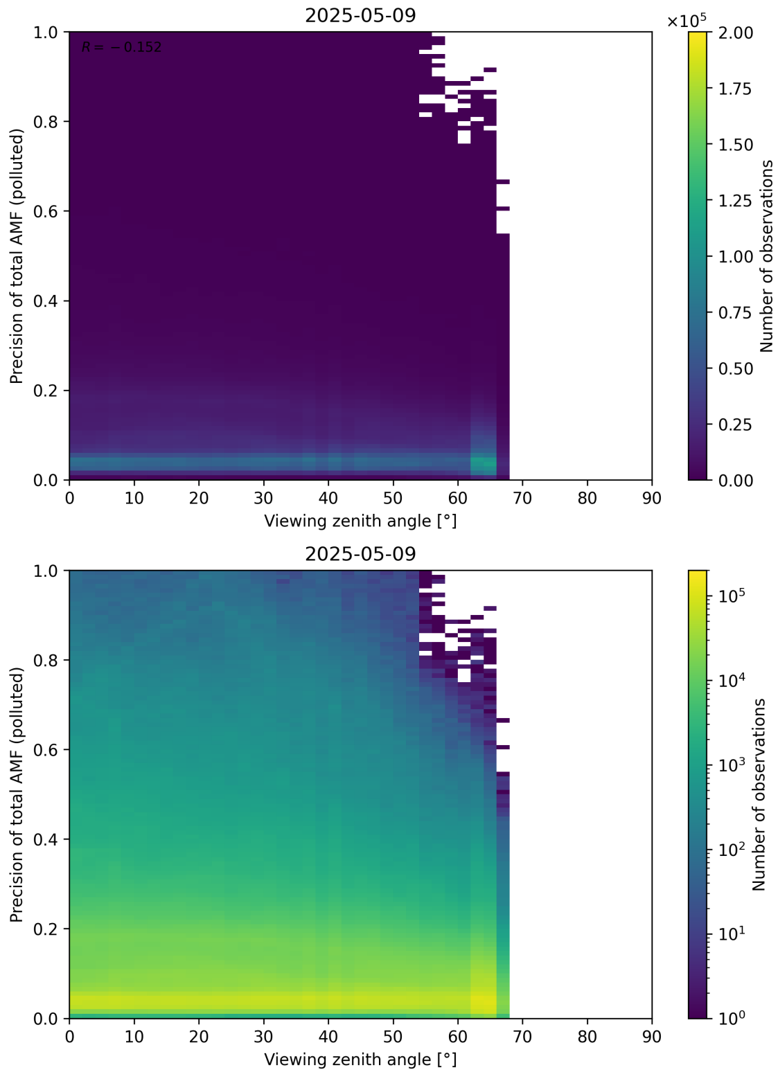
Figure 382: Scatter density plot of “Viewing zenith angle” against “Precision of total AMF (polluted)” for 2025-05-08 to 2025-05-10.
