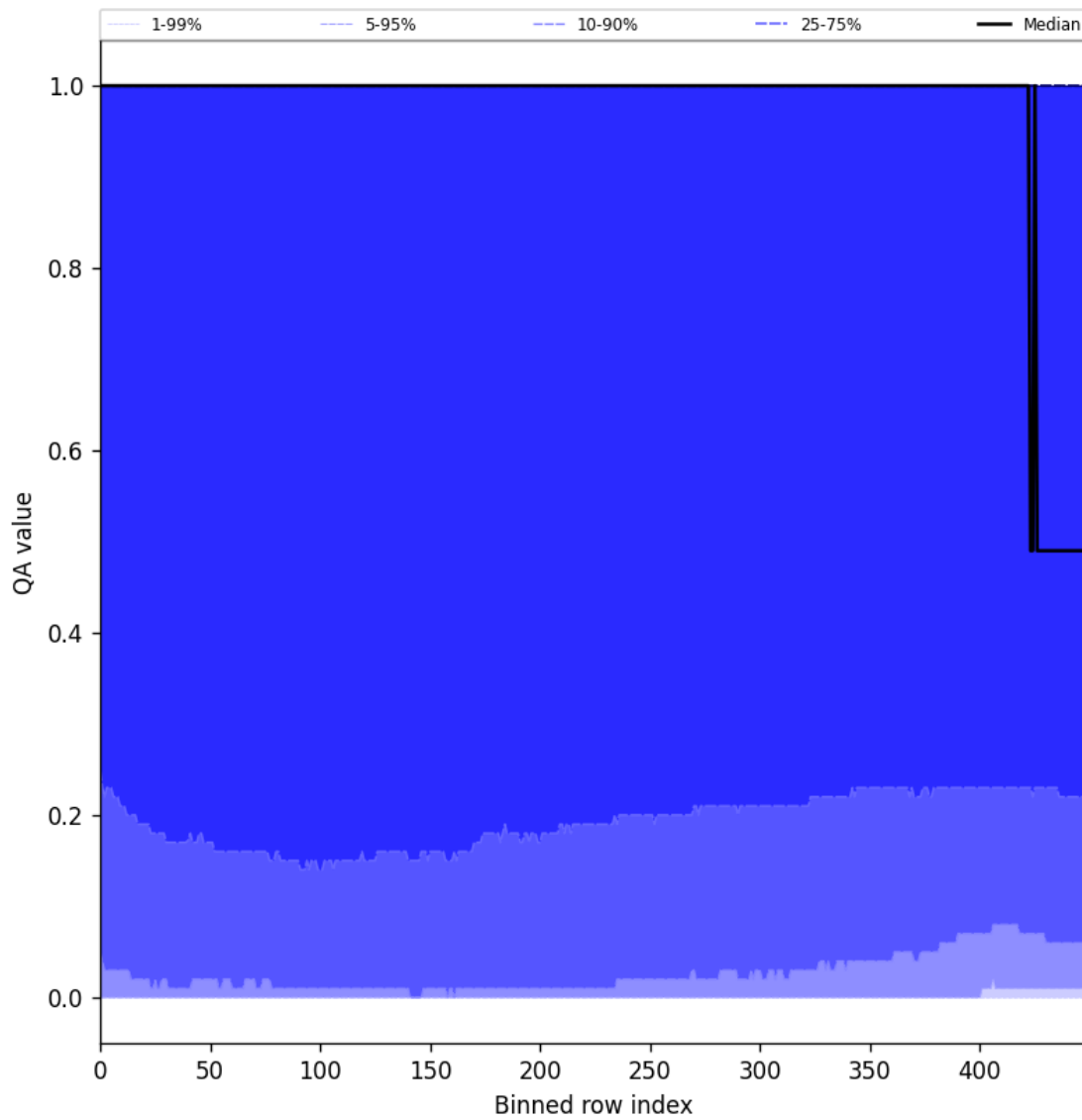
Figure 83: Along track statistics of “QA value” for 2025-05-08 to 2025-05-10
