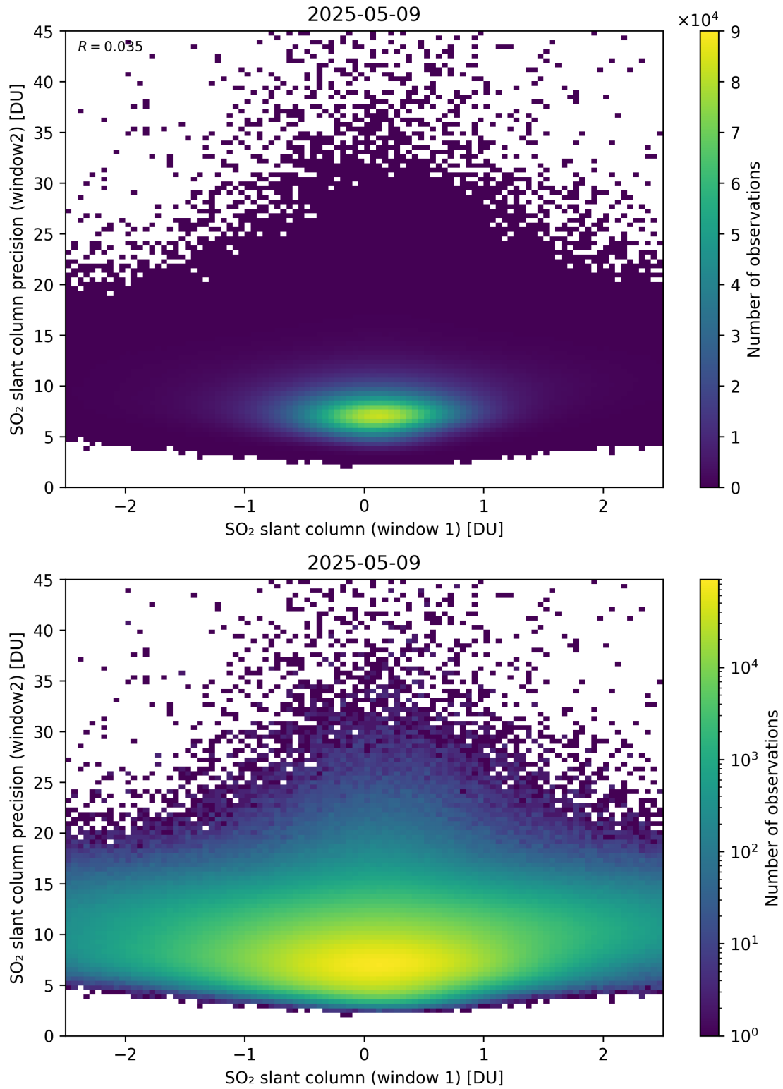
Figure 286: Scatter density plot of “SO 2 slant column (window 1)” against “SO 2 slant column precision (window2)” for 2025-05-08 to 2025-05-10.
