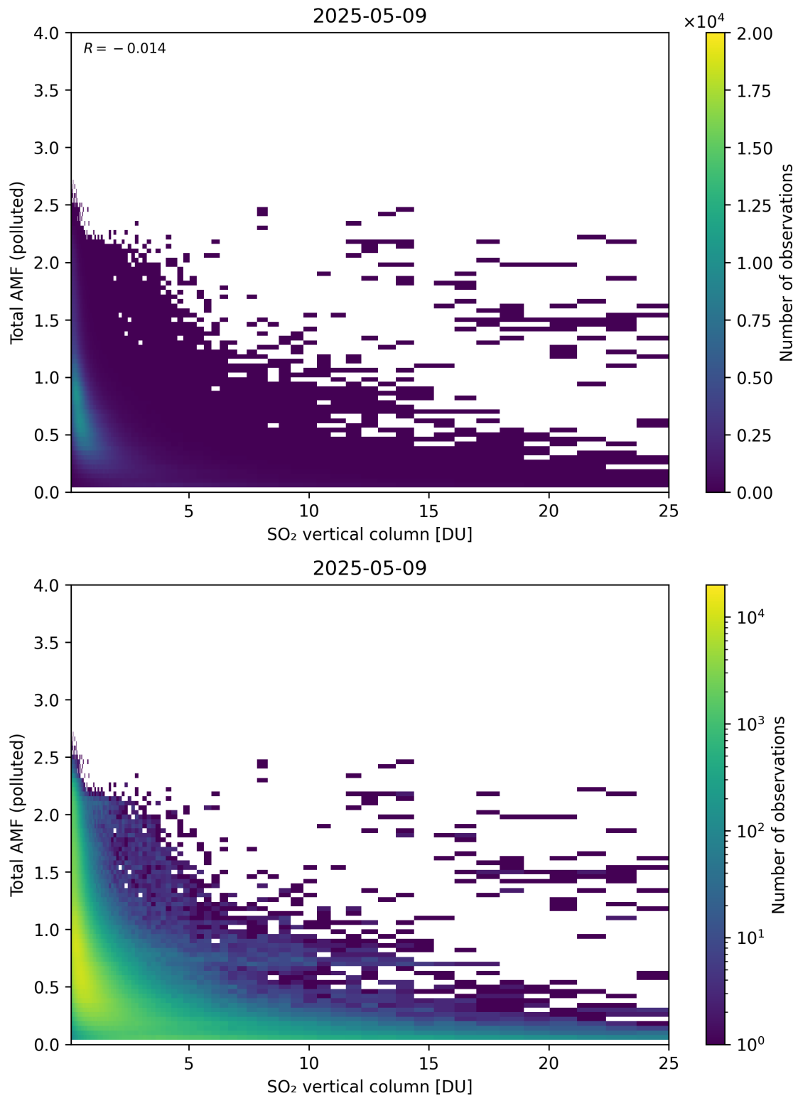
Figure 359: Scatter density plot of “SO 2 vertical column” against “Total AMF (polluted)” for 2025-05-08 to 2025-05-10.
