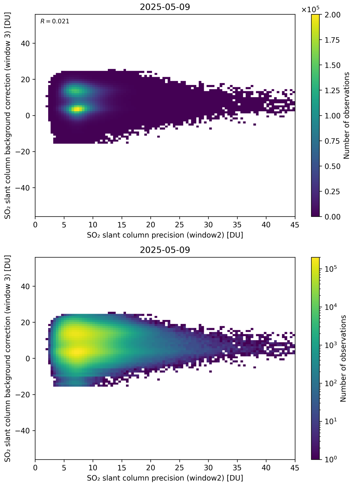
Figure 292: Scatter density plot of “SO 2 slant column precision (window2)” against “SO 2 slant column background correction (window 3)” for 2025-05-08 to 2025-05-10.
