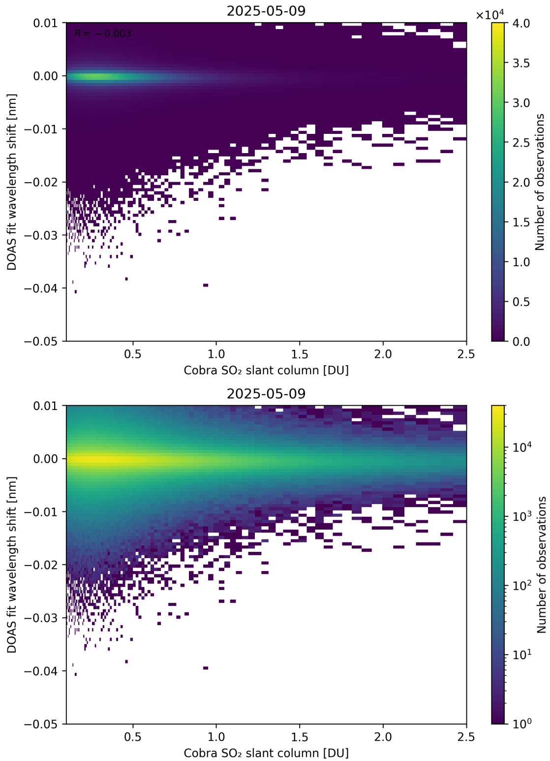
Figure 196: Scatter density plot of “Cobra SO 2 slant column” against “DOAS fit wavelength shift” for 2025-05-08 to 2025-05-10.
