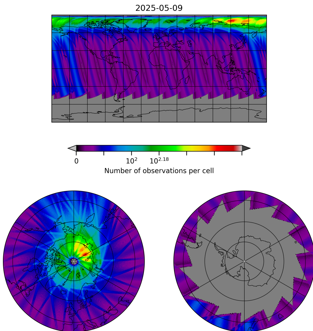
Figure 30: Map of the number of observations for 2025-05-08 to 2025-05-10
