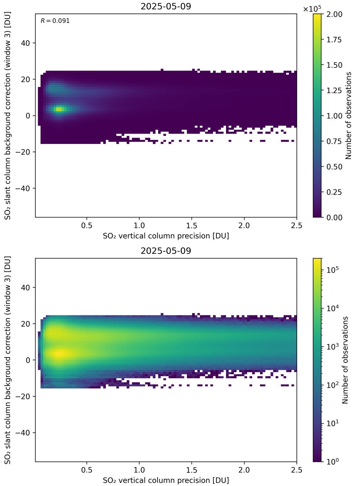
Figure 331: Scatter density plot of “SO 2 vertical column precision” against “SO 2 slant column background correction (window 3)” for 2025-05-08 to 2025-05-10.
