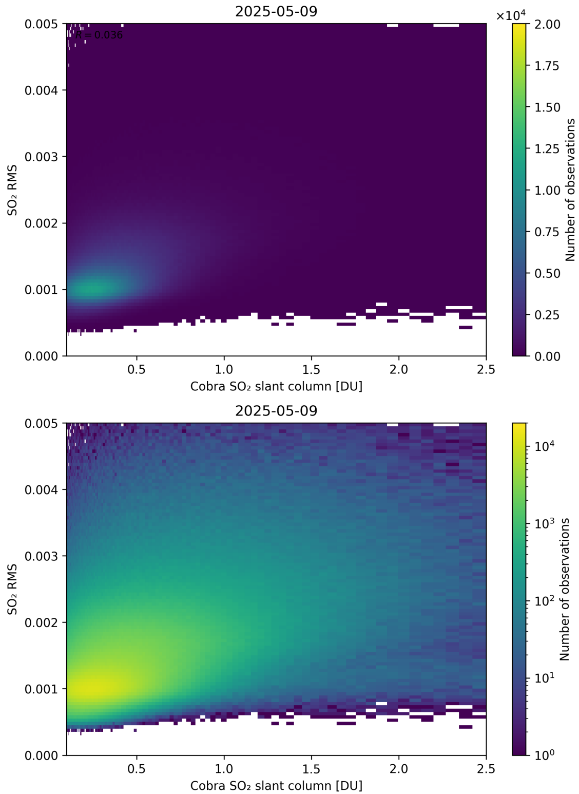
Figure 198: Scatter density plot of “Cobra SO 2 slant column” against “SO 2 RMS” for 2025-05-08 to 2025-05-10.
