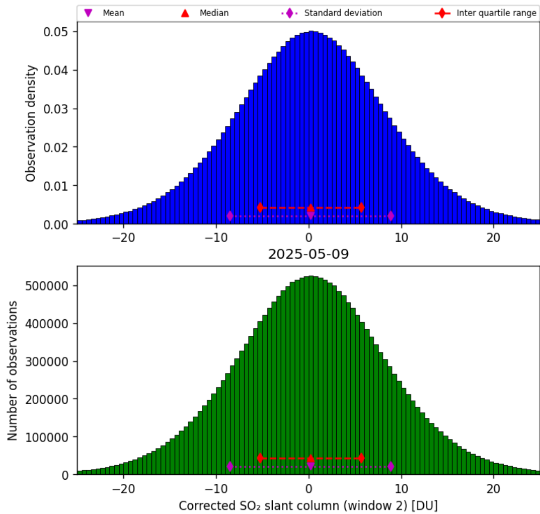
Figure 69: Histogram of “Corrected SO 2 slant column (window 2)” for 2025-05-08 to 2025-05-10
