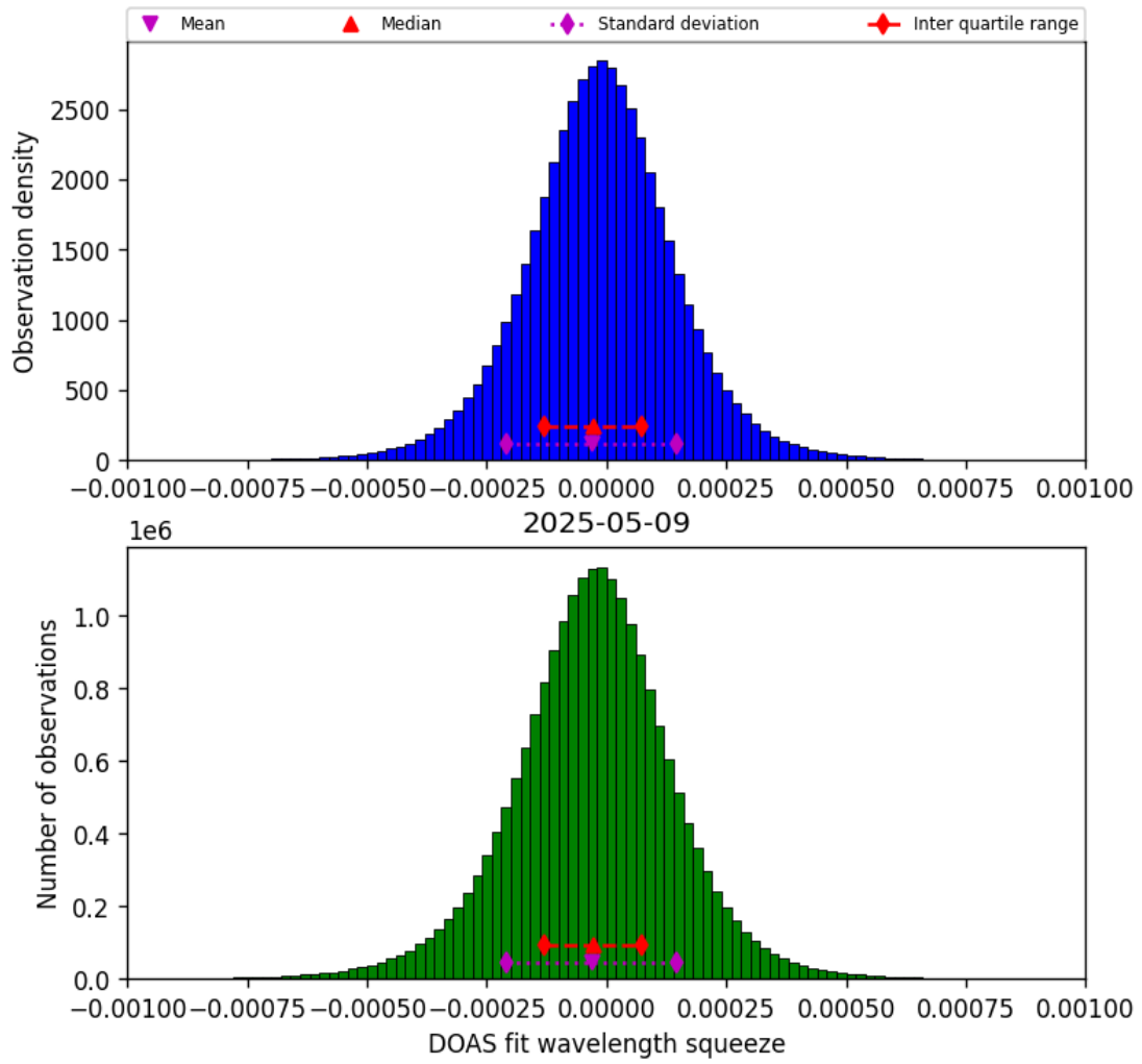
Figure 77: Histogram of “DOAS fit wavelength squeeze” for 2025-05-08 to 2025-05-10
