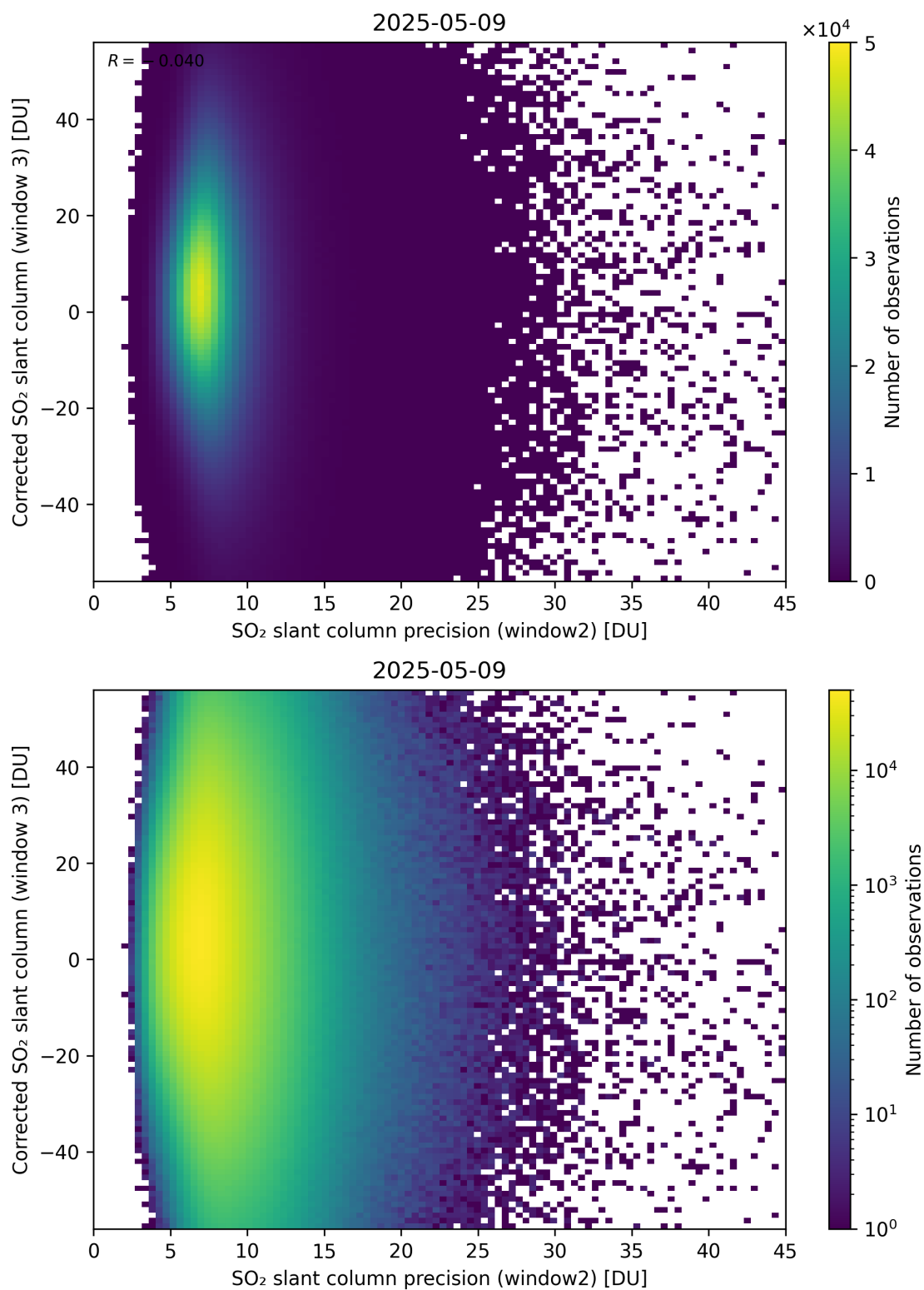
Figure 298: Scatter density plot of “SO 2 slant column precision (window2)” against “Corrected SO 2 slant column (window 3)” for 2025-05-08 to 2025-05-10.
