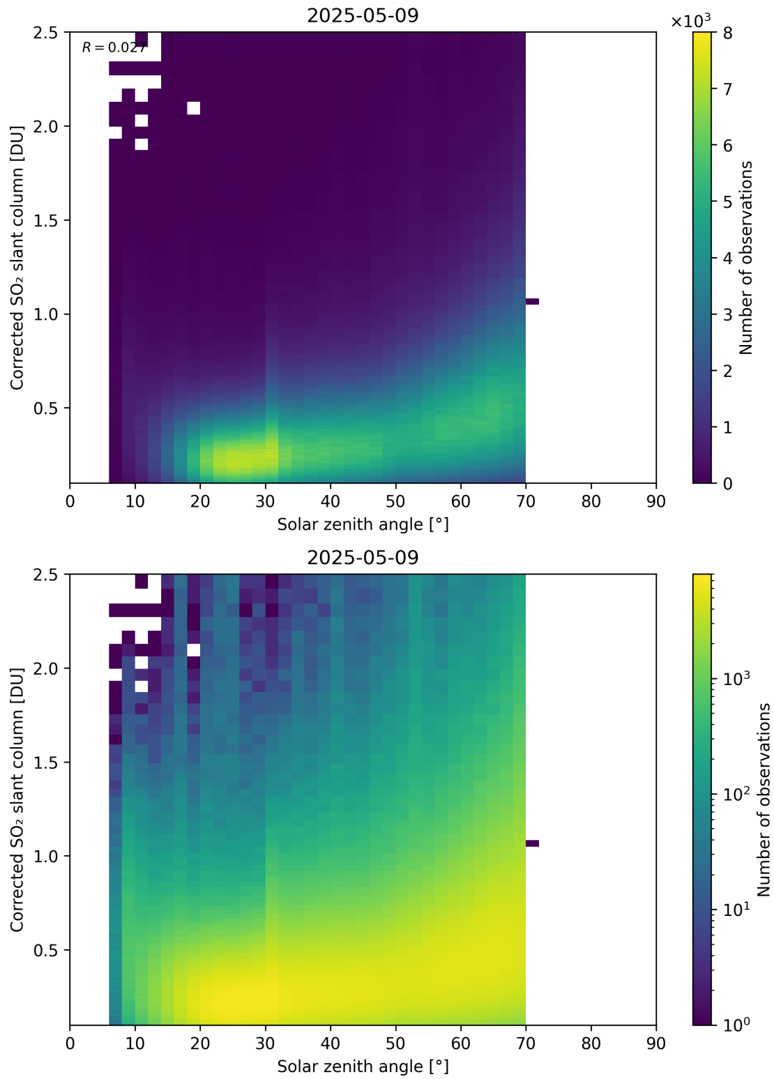
Figure 181: Scatter density plot of “Solar zenith angle” against “Corrected SO 2 slant column” for 2025-05-08 to 2025-05-10.
