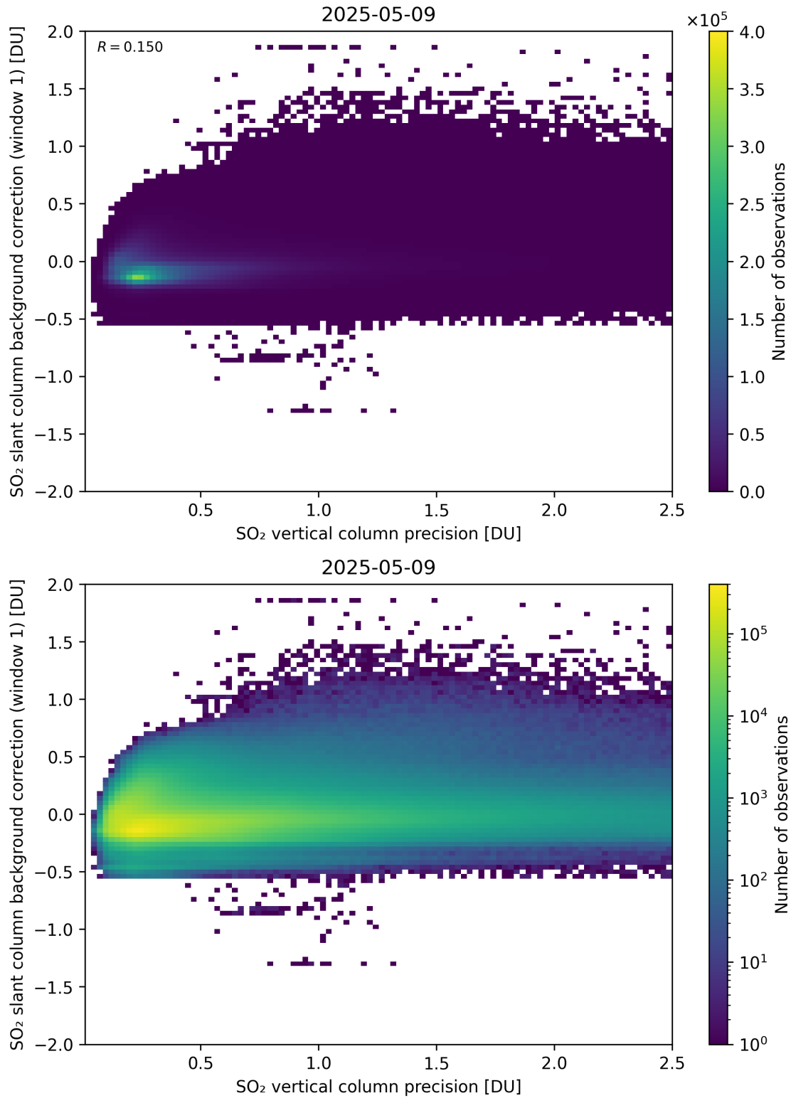
Figure 329: Scatter density plot of “SO 2 vertical column precision” against “SO 2 slant column background correction (window 1)” for 2025-05-08 to 2025-05-10.
