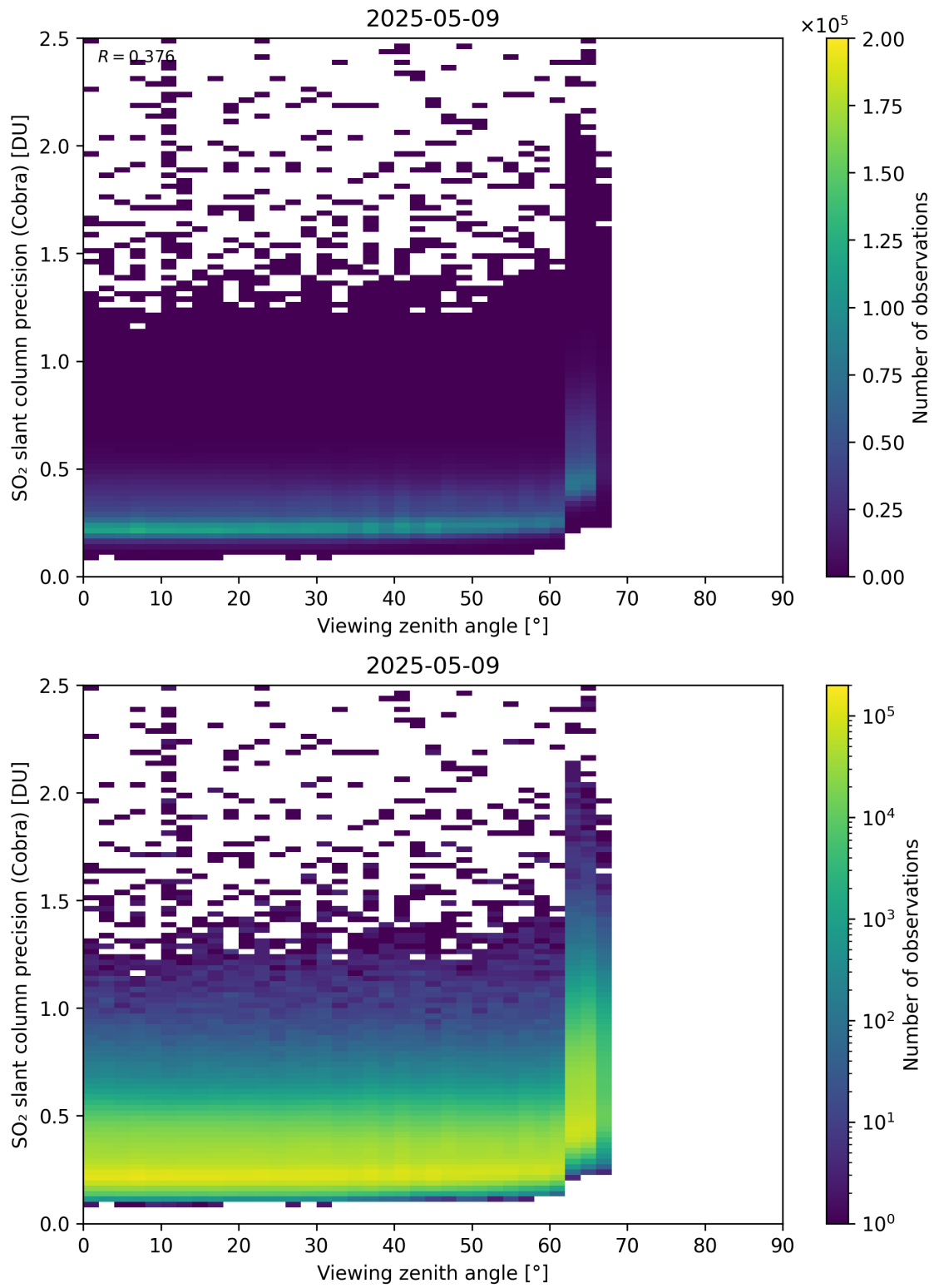
Figure 372: Scatter density plot of “Viewing zenith angle” against “SO 2 slant column precision (Cobra)” for 2025-05-08 to 2025-05-10.
