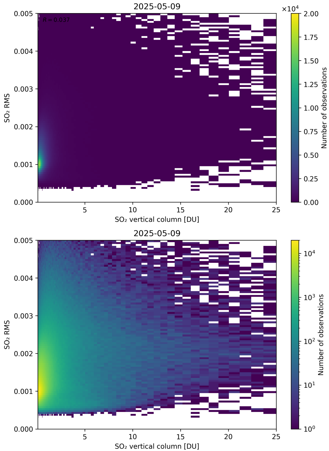
Figure 328: Scatter density plot of “SO 2 vertical column” against “SO 2 RMS” for 2025-05-08 to 2025-05-10.
