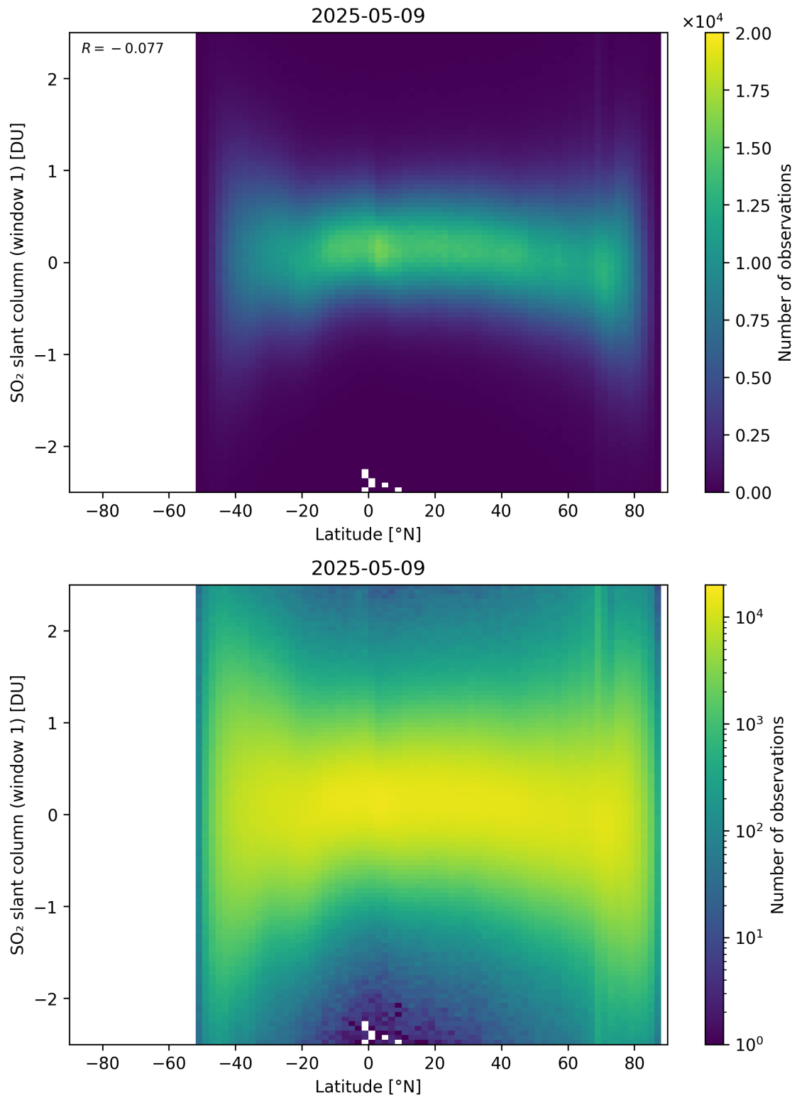
Figure 162: Scatter density plot of “Latitude” against “SO 2 slant column (window 1)” for 2025-05-08 to 2025-05-10.
