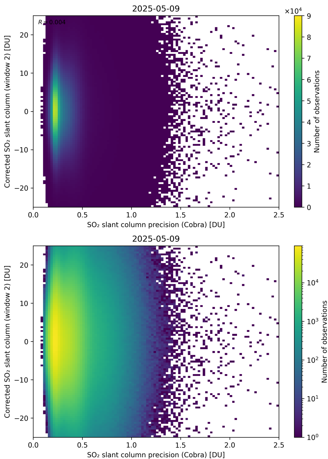
Figure 206: Scatter density plot of “SO 2 slant column precision (Cobra)” against “Corrected SO 2 slant column (window 2)” for 2025-05-08 to 2025-05-10.
