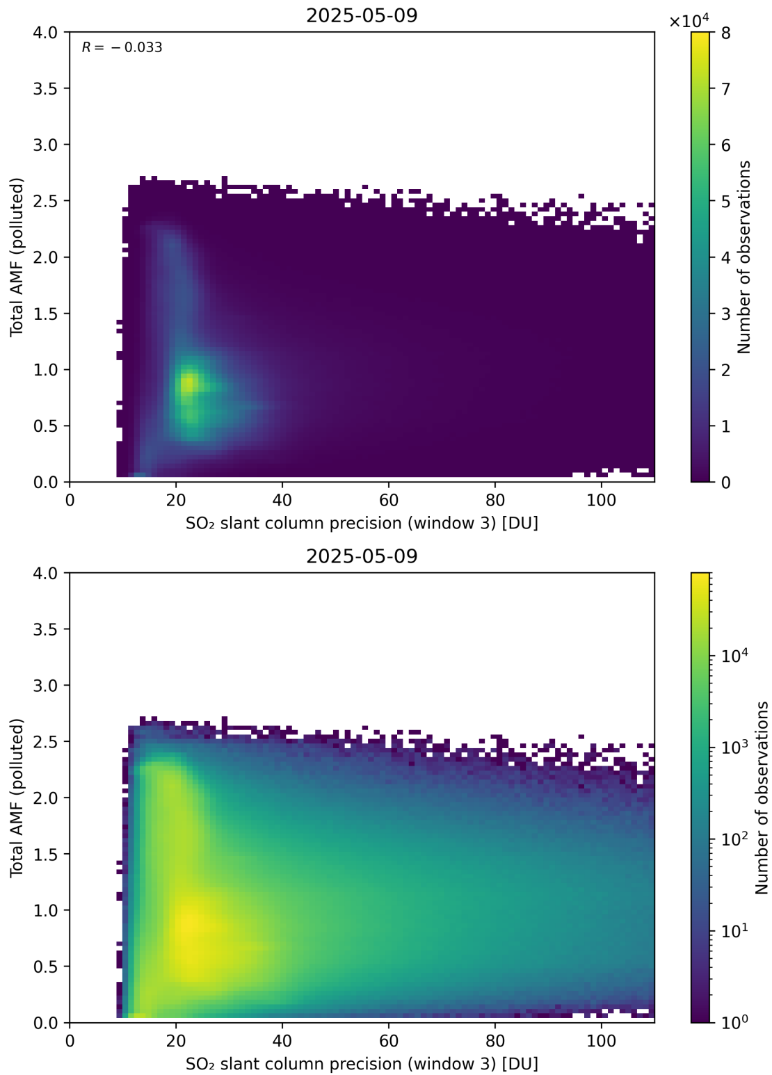
Figure 313: Scatter density plot of “SO 2 slant column precision (window 3)” against “Total AMF (polluted)” for 2025-05-08 to 2025-05-10.
