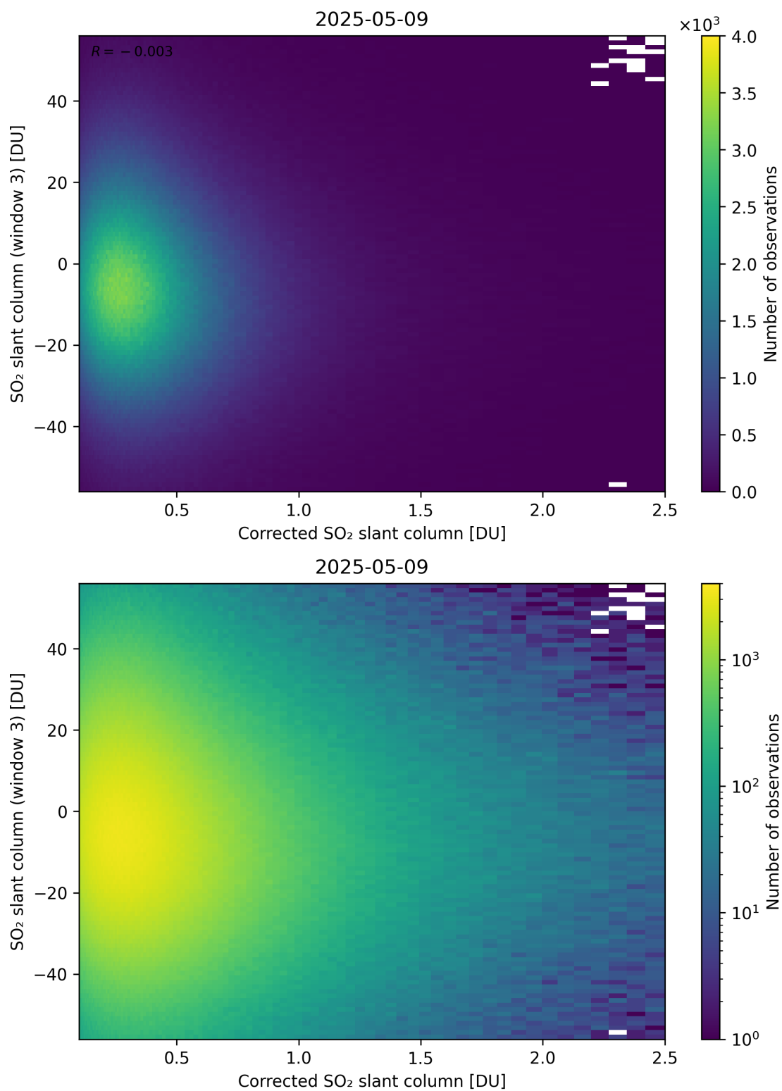
Figure 240: Scatter density plot of “Corrected SO 2 slant column” against “SO 2 slant column (window 3)” for 2025-05-08 to 2025-05-10.
