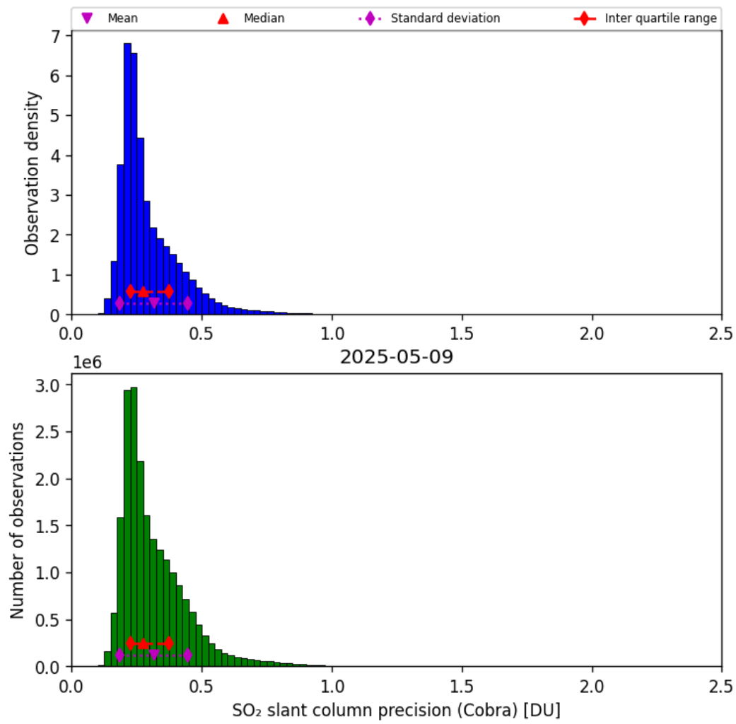
Figure 62: Histogram of “SO 2 slant column precision (Cobra)” for 2025-05-08 to 2025-05-10
