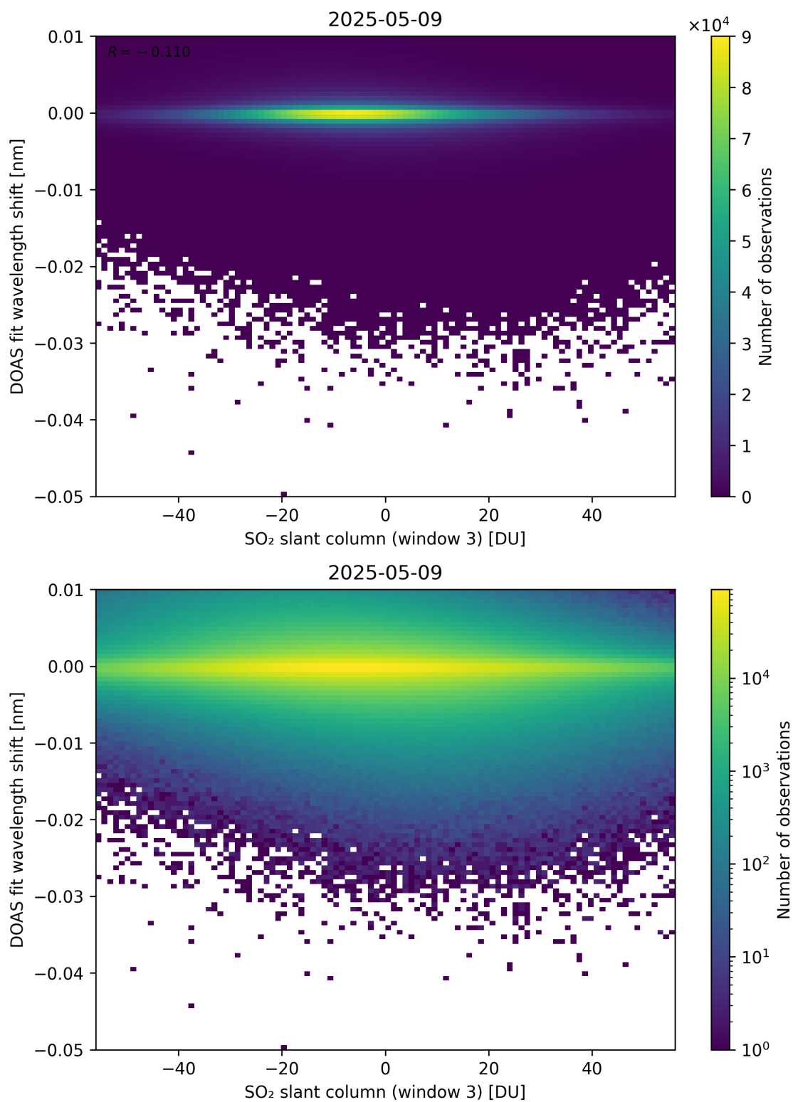
Figure 304: Scatter density plot of “SO 2 slant column (window 3)” against “DOAS fit wavelength shift” for 2025-05-08 to 2025-05-10.
