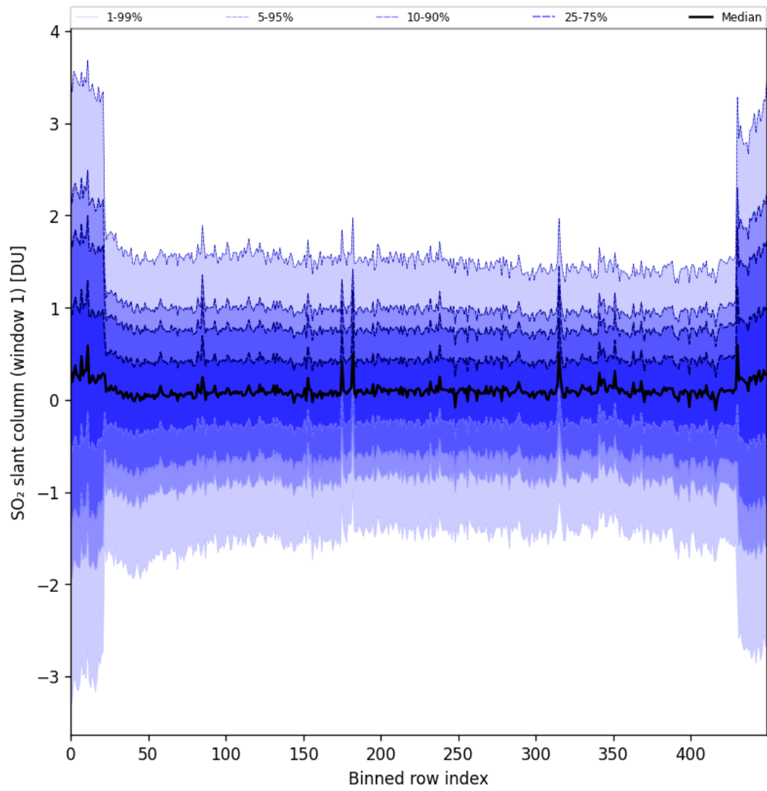
Figure 89: Along track statistics of “SO 2 slant column (window 1)” for 2025-05-08 to 2025-05-10
