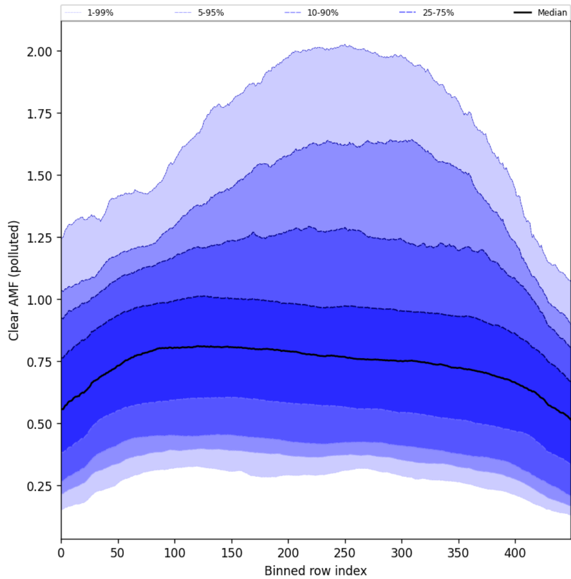
Figure 107: Along track statistics of “Clear AMF (polluted)” for 2025-05-08 to 2025-05-10
