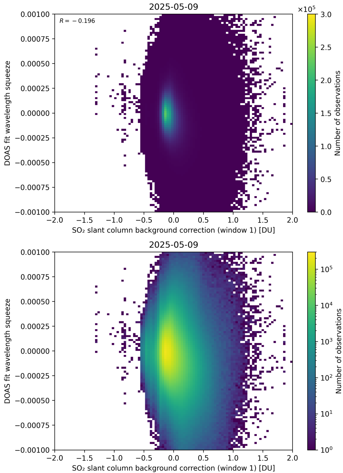
Figure 112: Scatter density plot of “SO 2 slant column background correction (window 1)” against “DOAS fit wavelength squeeze” for 2025-05-08 to 2025-05-10.
