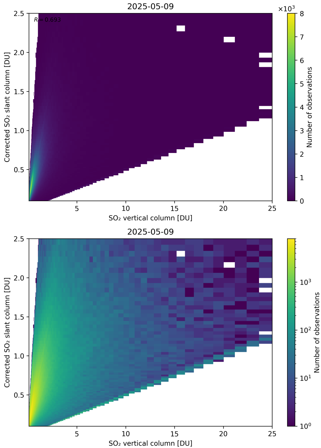
Figure 351: Scatter density plot of “SO 2 vertical column” against “Corrected SO 2 slant column” for 2025-05-08 to 2025-05-10.
