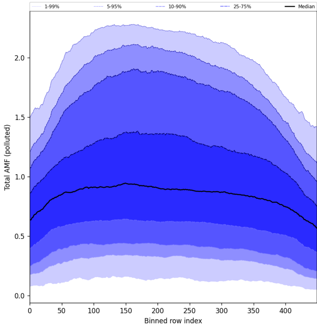
Figure 105: Along track statistics of “Total AMF (polluted)” for 2025-05-08 to 2025-05-10
