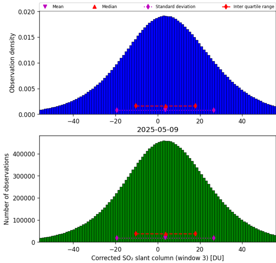
Figure 73: Histogram of “Corrected SO 2 slant column (window 3)” for 2025-05-08 to 2025-05-10
