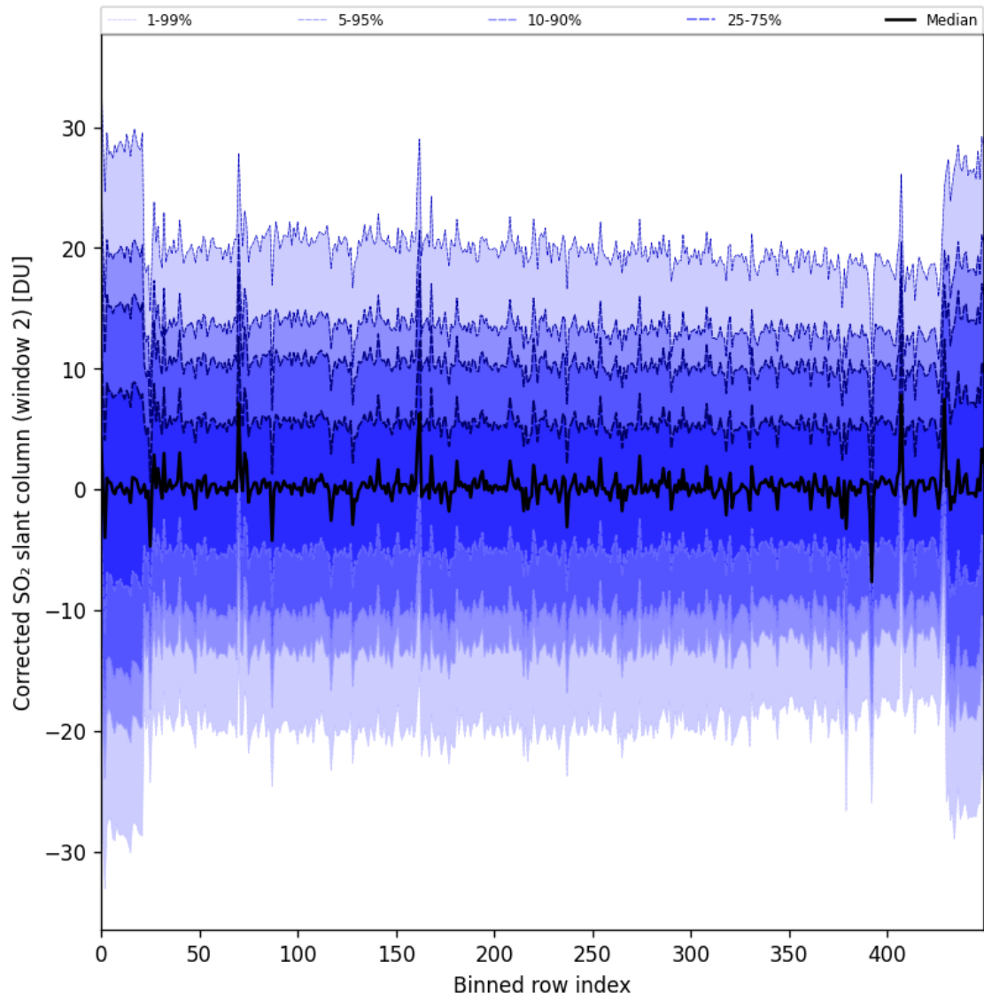
Figure 95: Along track statistics of "Corrected SO 2 slant column (window 2)" for 2025-05-08 to 2025-05-10
