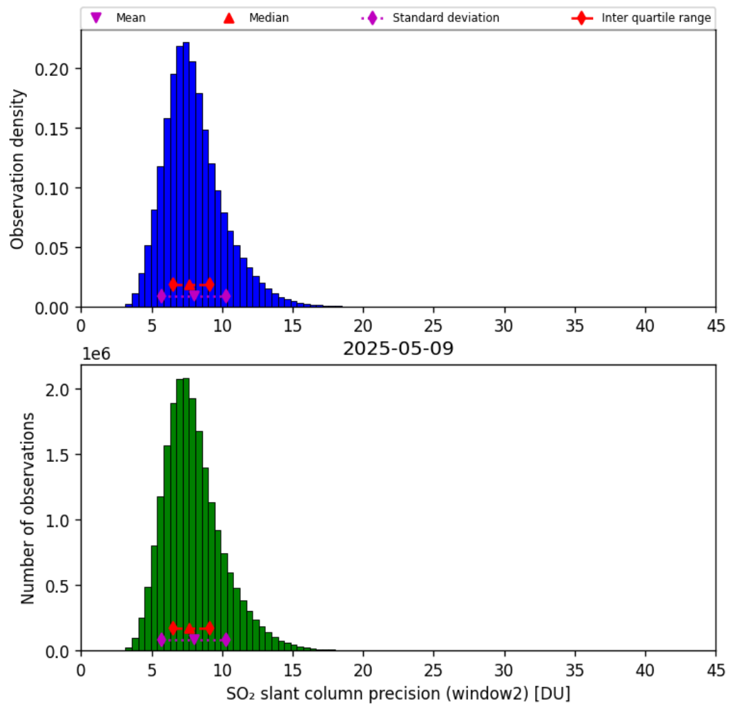
Figure 68: Histogram of “SO 2 slant column precision (window2)” for 2025-05-08 to 2025-05-10
