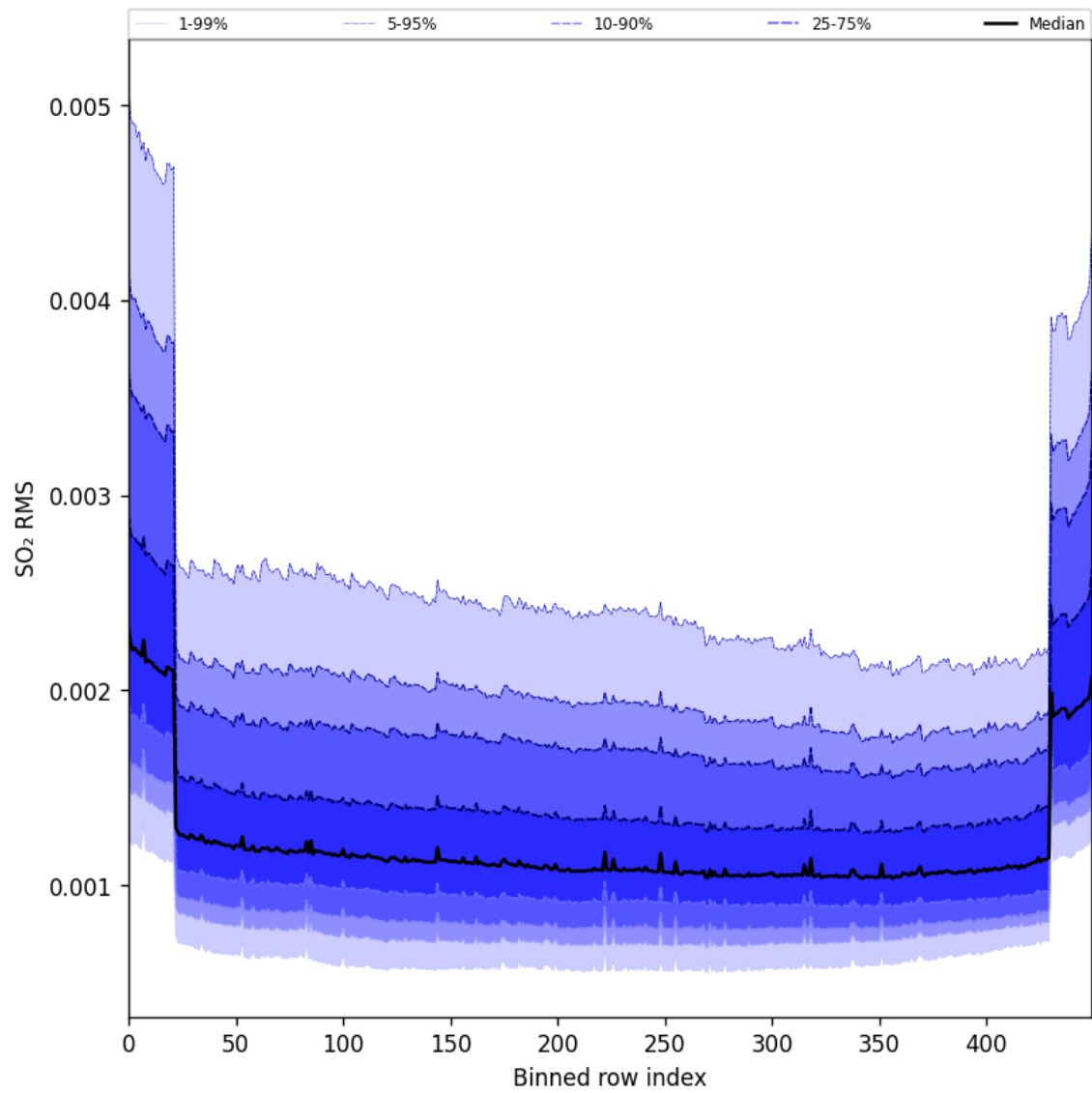
Figure 104: Along track statistics of “SO 2 RMS” for 2025-05-08 to 2025-05-10
