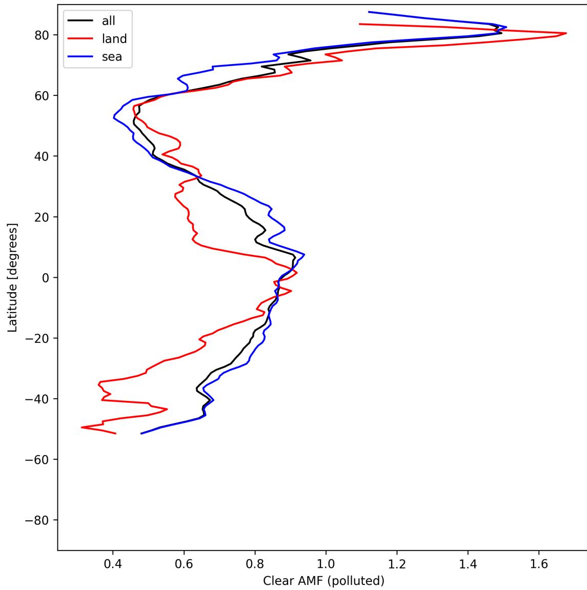
Figure 55: Zonal average of “Clear AMF (polluted)” for 2025-05-08 to 2025-05-10.
