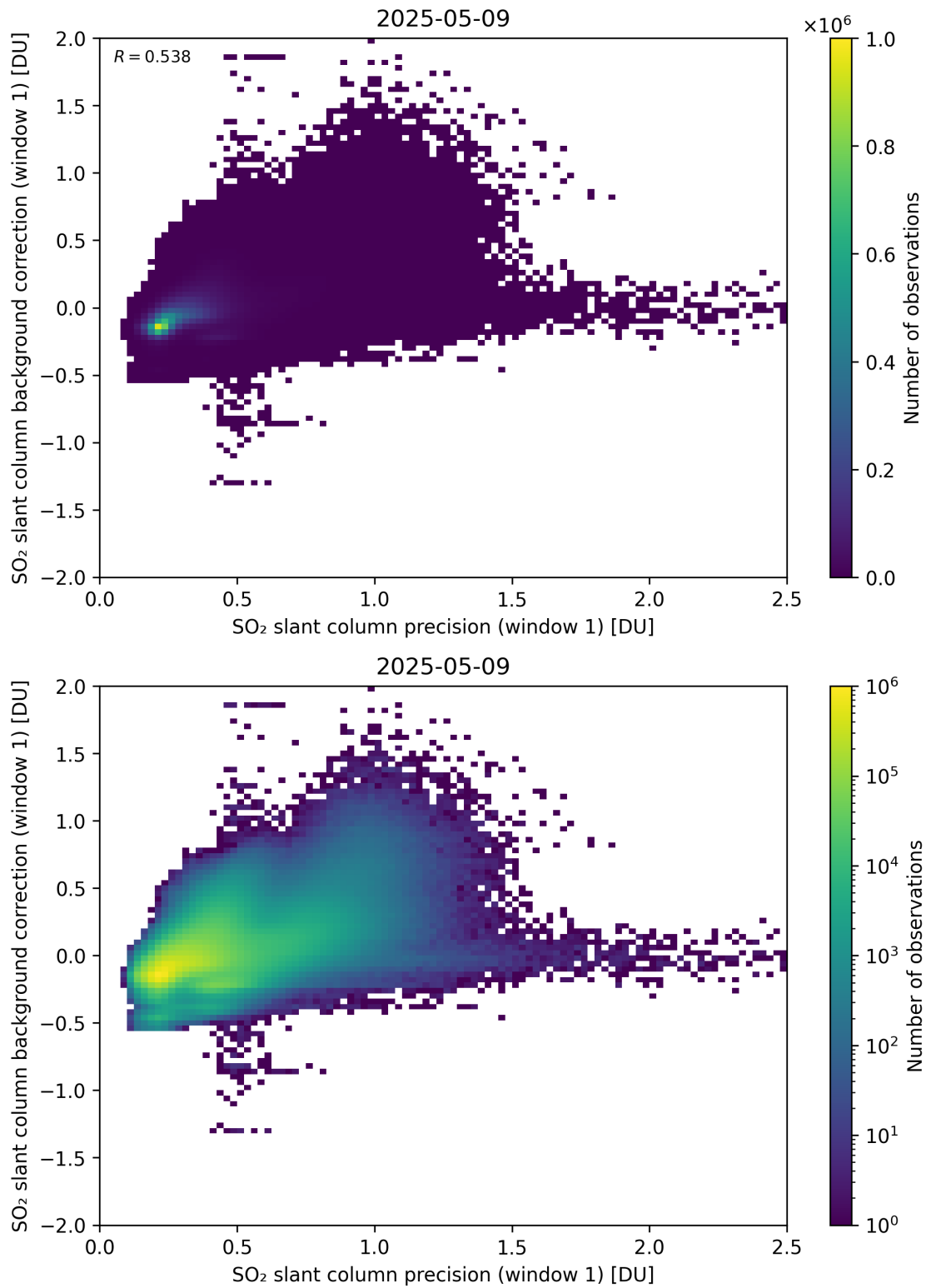
Figure 268: Scatter density plot of “SO 2 slant column precision (window 1)” against “SO 2 slant column background correction (window 1)” for 2025-05-08 to 2025-05-10.
