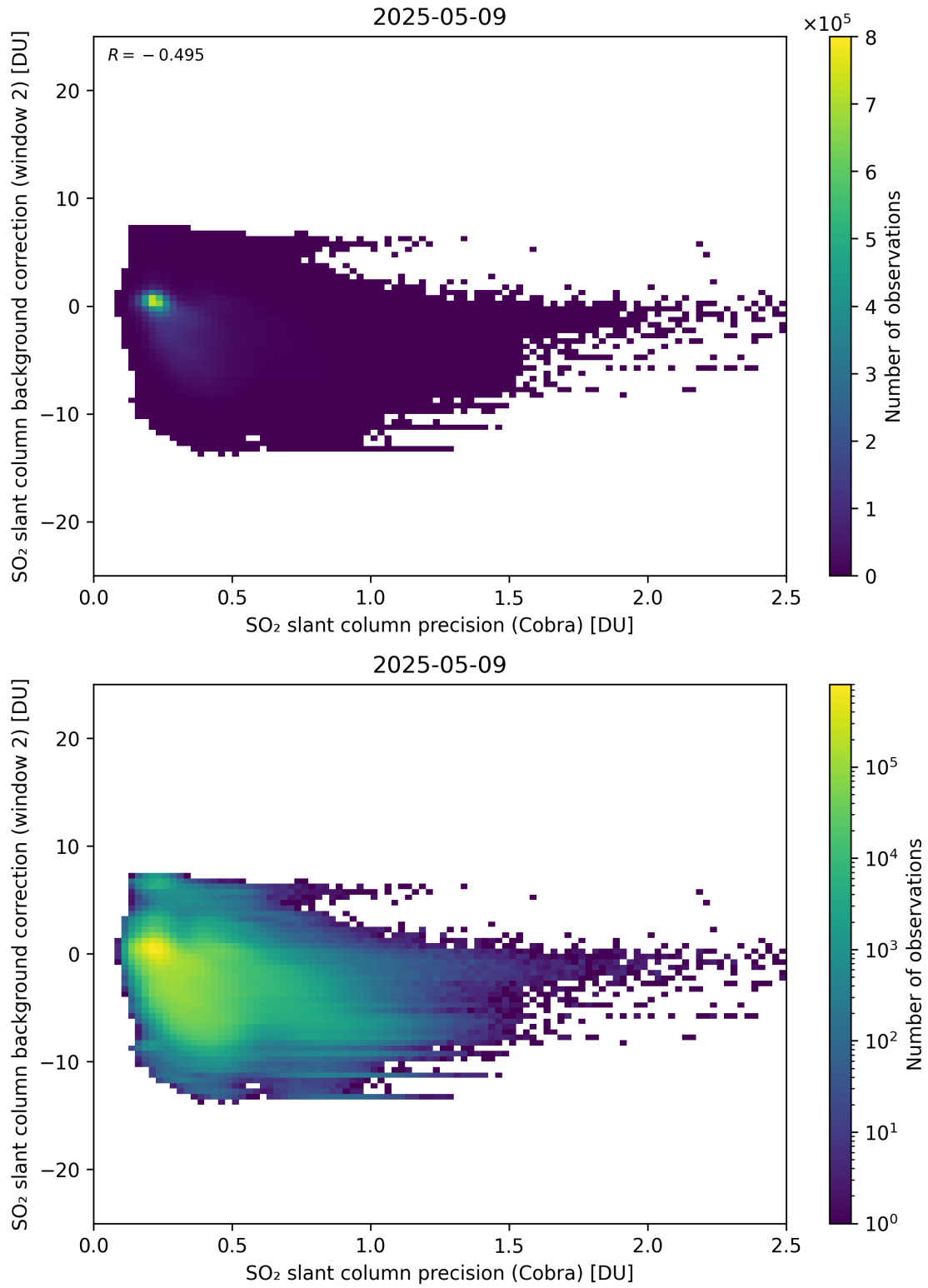
Figure 200: Scatter density plot of “SO 2 slant column precision (Cobra)” against “SO 2 slant column background correction (window 2)” for 2025-05-08 to 2025-05-10.
