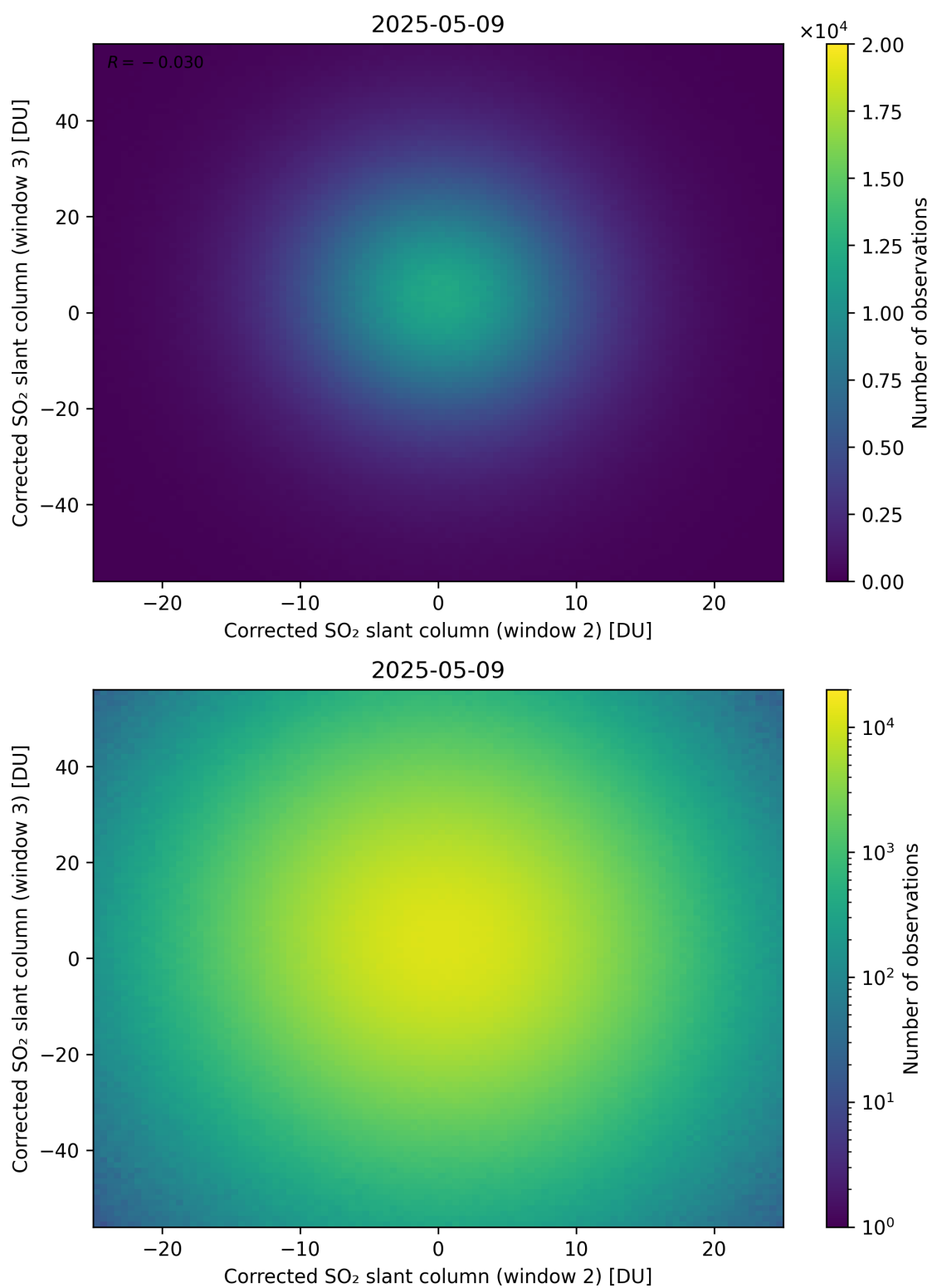
Figure 250: Scatter density plot of “Corrected SO 2 slant column (window 2)” against “Corrected SO 2 slant column (window 3)” for 2025-05-08 to 2025-05-10.
