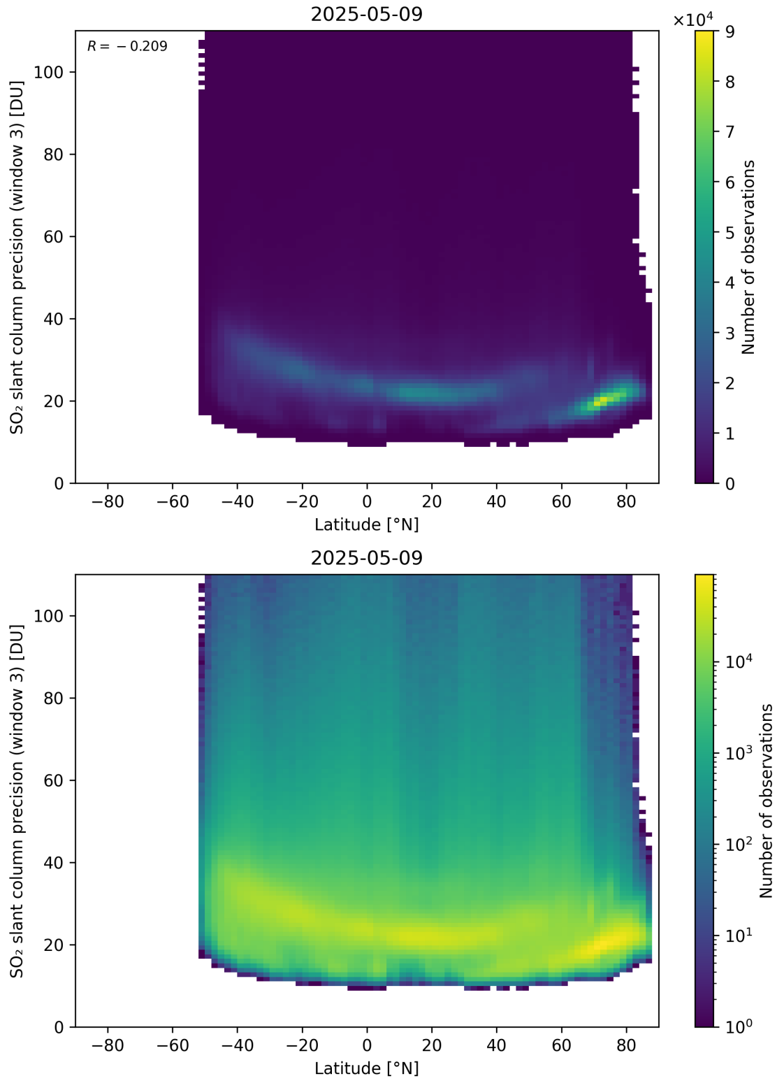
Figure 166: Scatter density plot of “Latitude” against “SO 2 slant column precision (window 3)” for 2025-05-08 to 2025-05-10.
