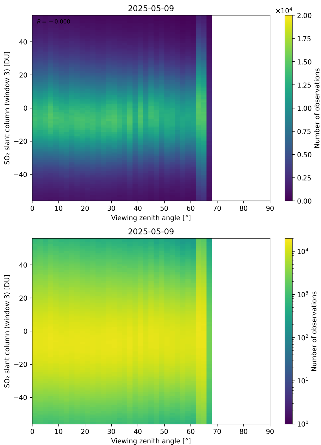
Figure 379: Scatter density plot of “Viewing zenith angle” against “SO 2 slant column (window 3)” for 2025-05-08 to 2025-05-10.
