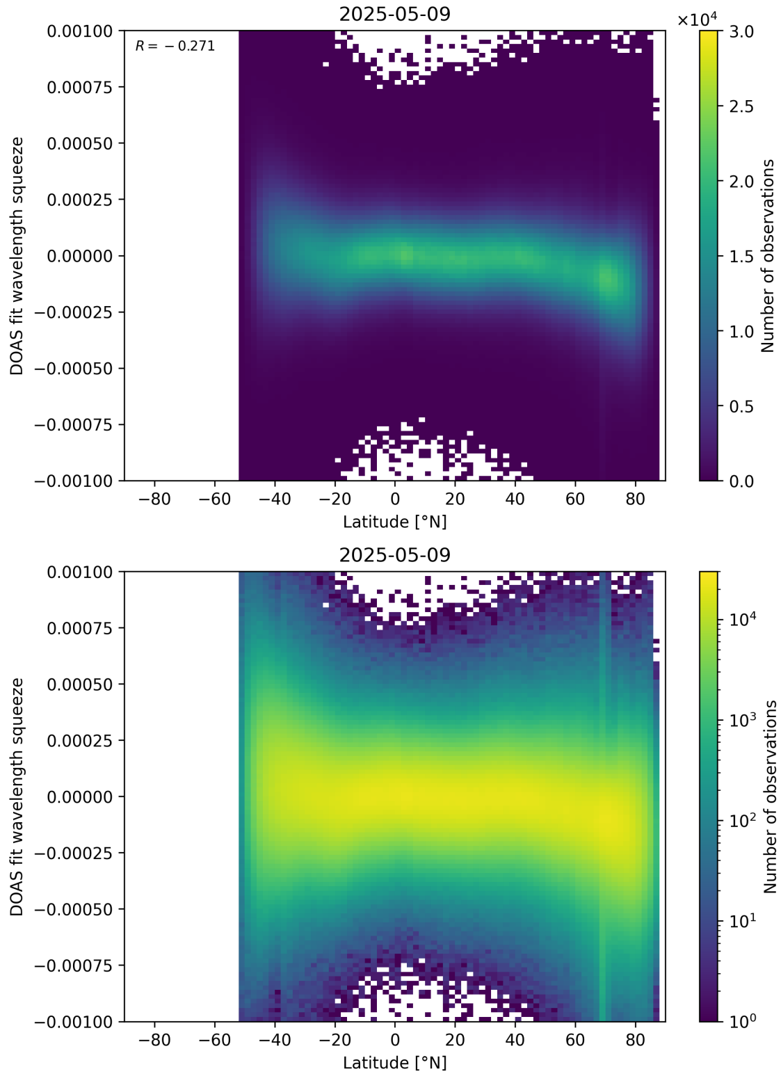
Figure 154: Scatter density plot of “Latitude” against “DOAS fit wavelength squeeze” for 2025-05-08 to 2025-05-10.
