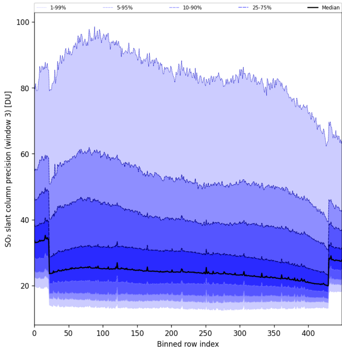
Figure 98: Along track statistics of “SO 2 slant column precision (window 3)” for 2025-05-08 to 2025-05-10
