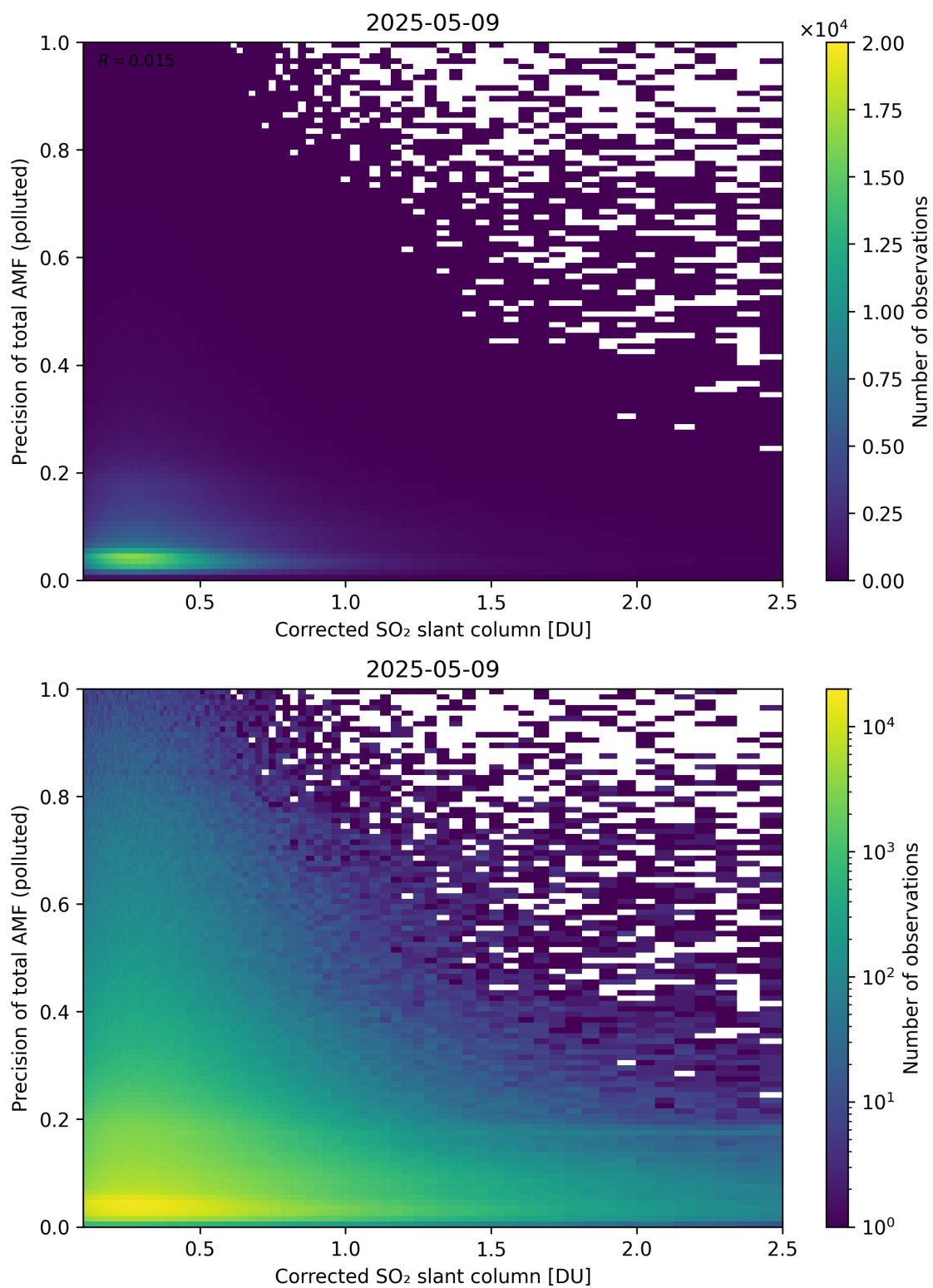
Figure 243: Scatter density plot of “Corrected SO 2 slant column” against “Precision of total AMF (polluted)” for 2025-05-08 to 2025-05-10.
