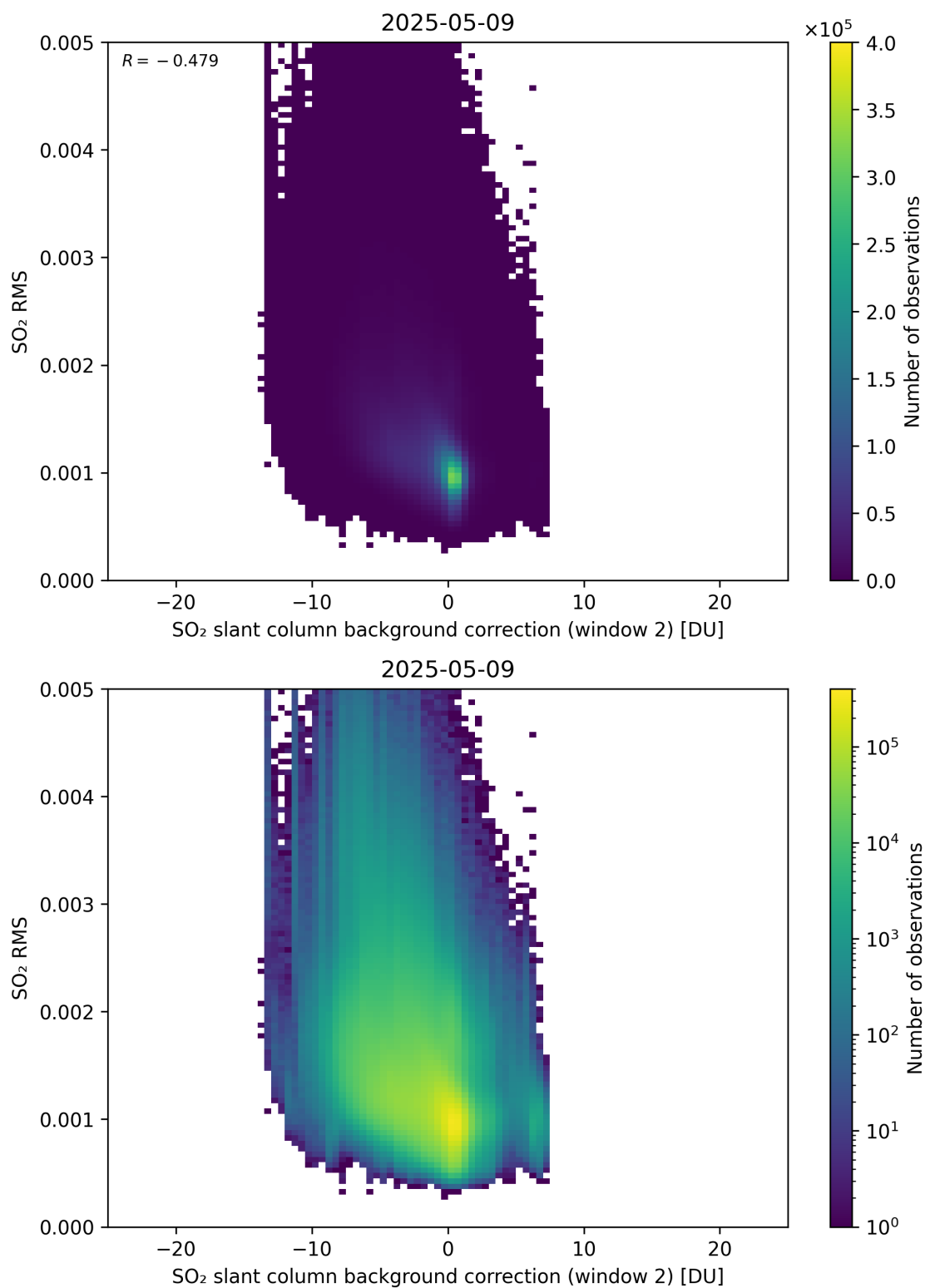
Figure 125: Scatter density plot of “SO 2 slant column background correction (window 2)” against “SO 2 RMS” for 2025-05-08 to 2025-05-10.
