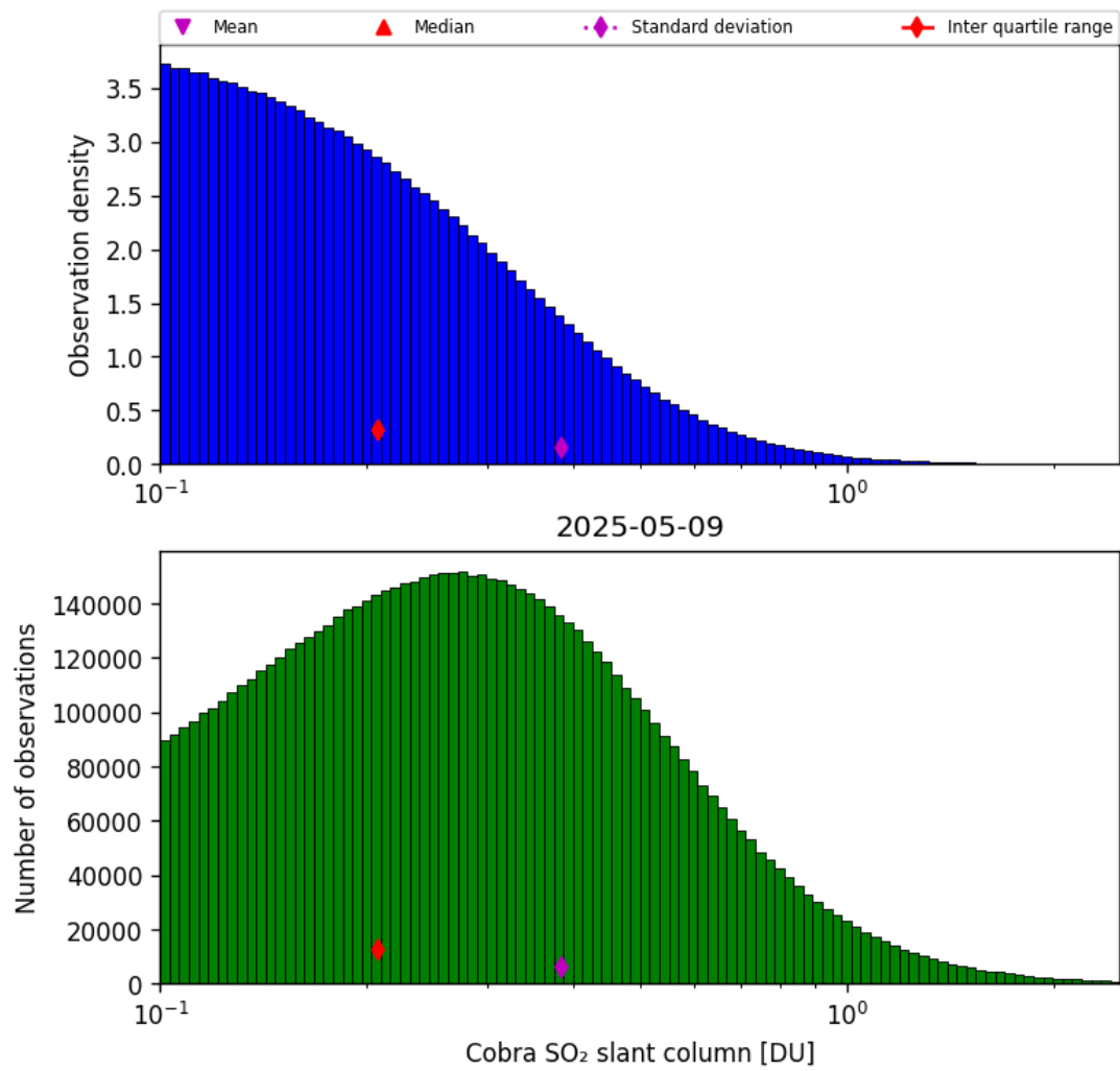
Figure 61: Histogram of “Cobra SO 2 slant column” for 2025-05-08 to 2025-05-10
