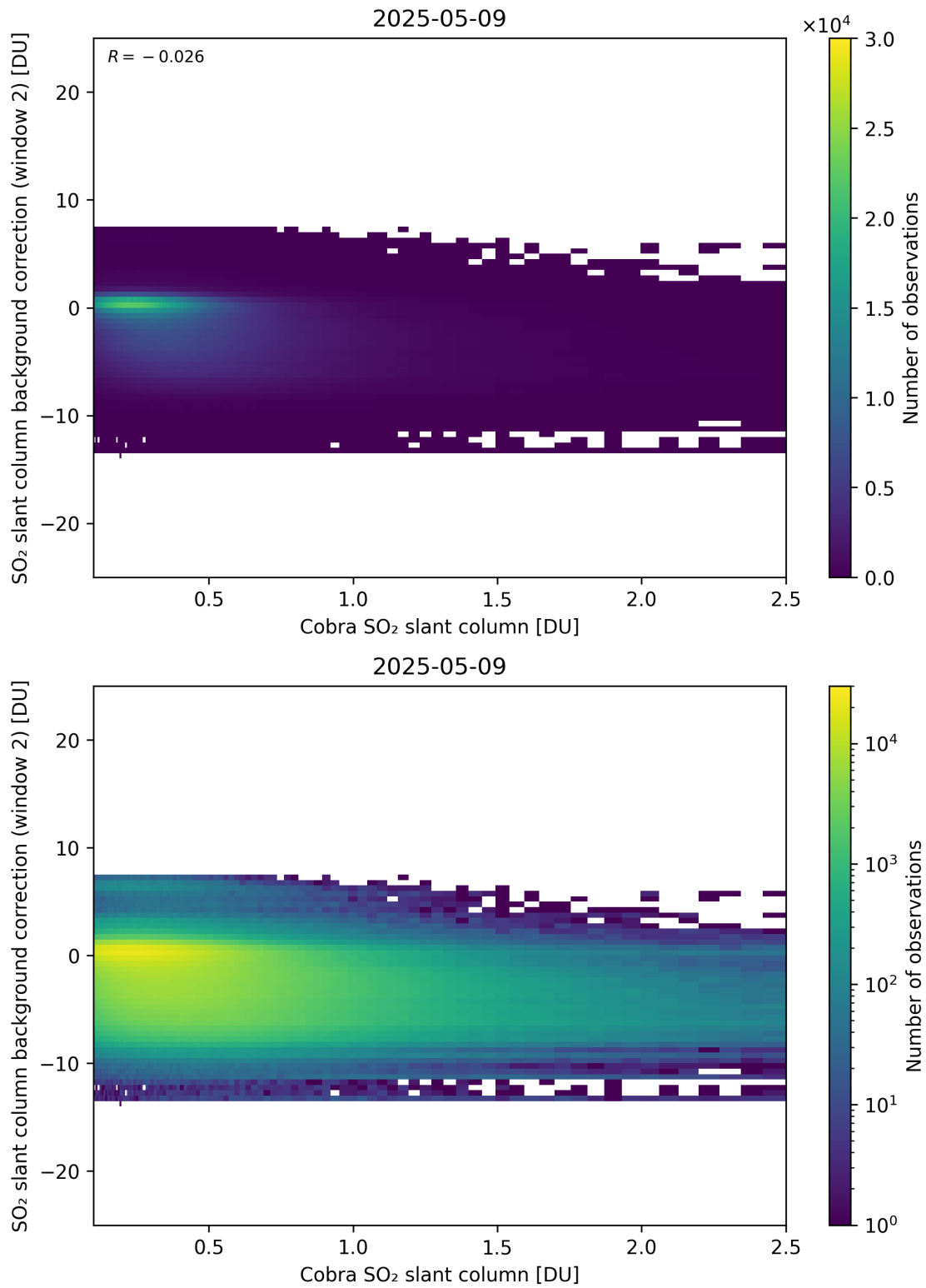
Figure 194: Scatter density plot of “Cobra SO 2 slant column” against “SO 2 slant column background correction (window 2)” for 2025-05-08 to 2025-05-10.
