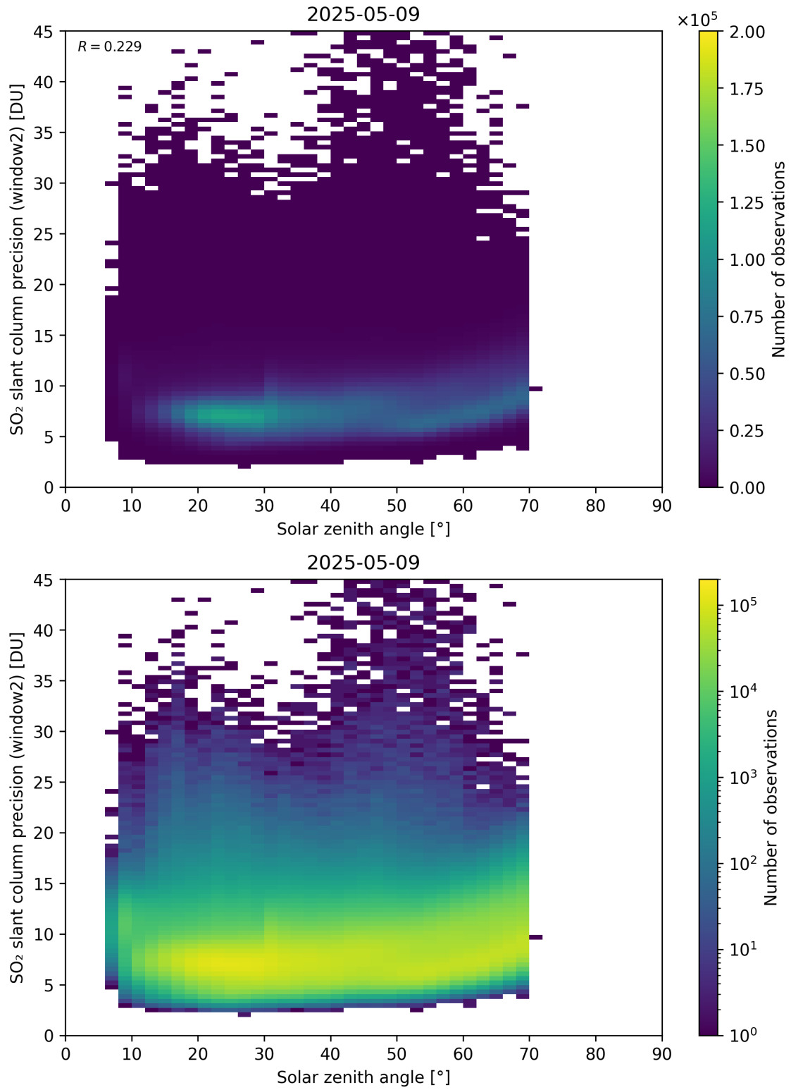
Figure 186: Scatter density plot of “Solar zenith angle” against “SO 2 slant column precision (window2)” for 2025-05-08 to 2025-05-10.
