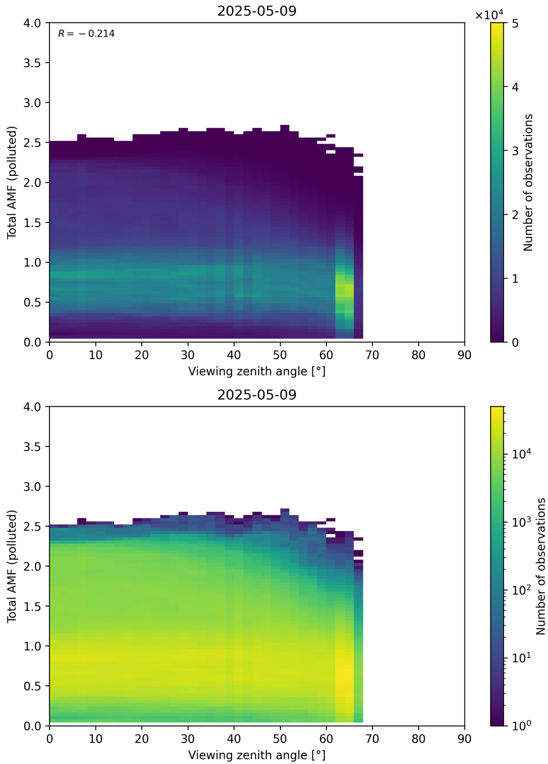
Figure 381: Scatter density plot of “Viewing zenith angle” against “Total AMF (polluted)” for 2025-05-08 to 2025-05-10.
