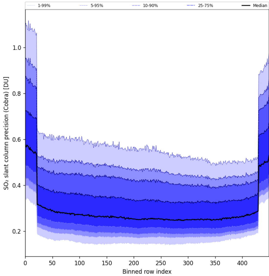
Figure 88: Along track statistics of “SO 2 slant column precision (Cobra)” for 2025-05-08 to 2025-05-10
