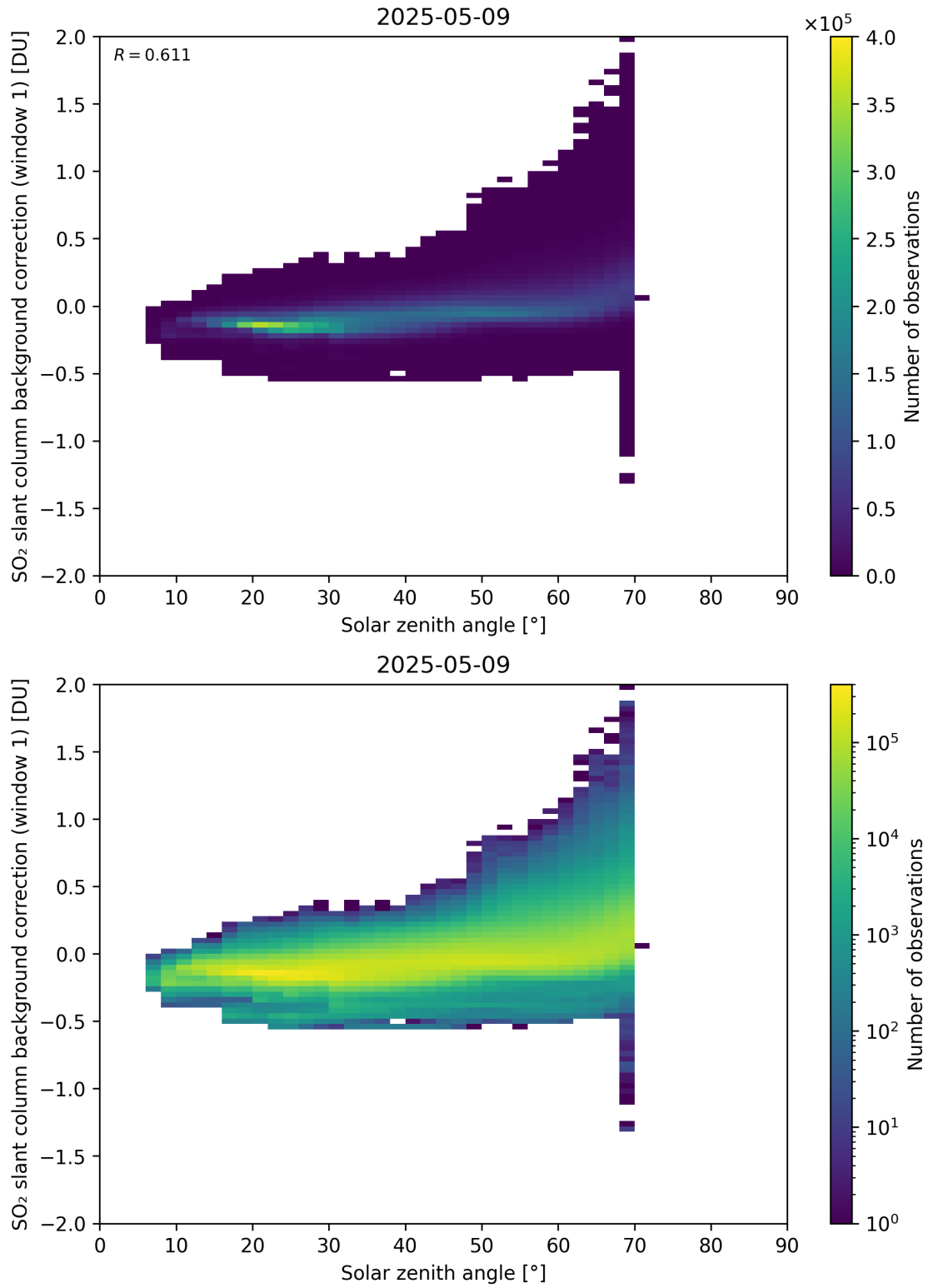
Figure 171: Scatter density plot of “Solar zenith angle” against “SO 2 slant column background correction (window 1)” for 2025-05-08 to 2025-05-10.
