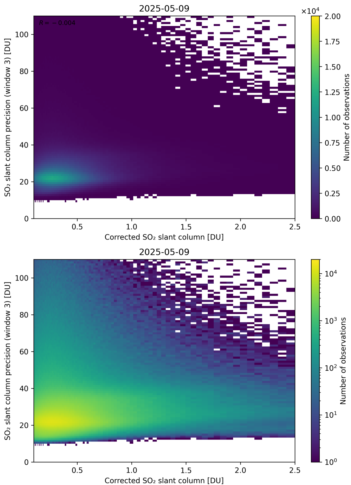
Figure 241: Scatter density plot of “Corrected SO 2 slant column” against “SO 2 slant column precision (window 3)” for 2025-05-08 to 2025-05-10.
