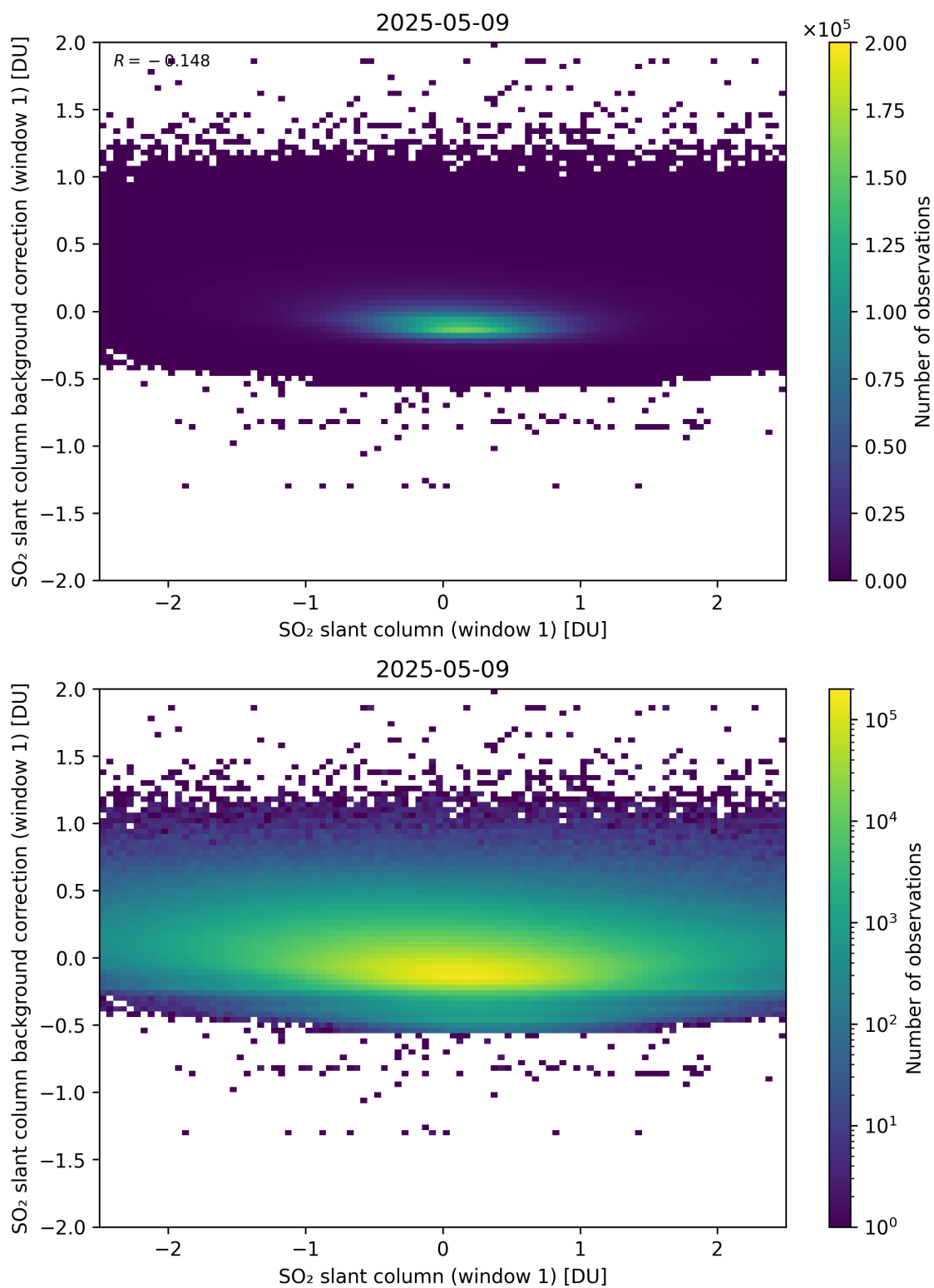
Figure 262: Scatter density plot of “SO 2 slant column (window 1)” against “SO 2 slant column background correction (window 1)” for 2025-05-08 to 2025-05-10.
