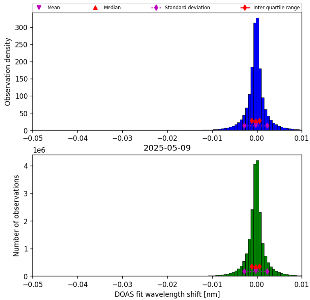
Figure 76: Histogram of “DOAS fit wavelength shift” for 2025-05-08 to 2025-05-10
