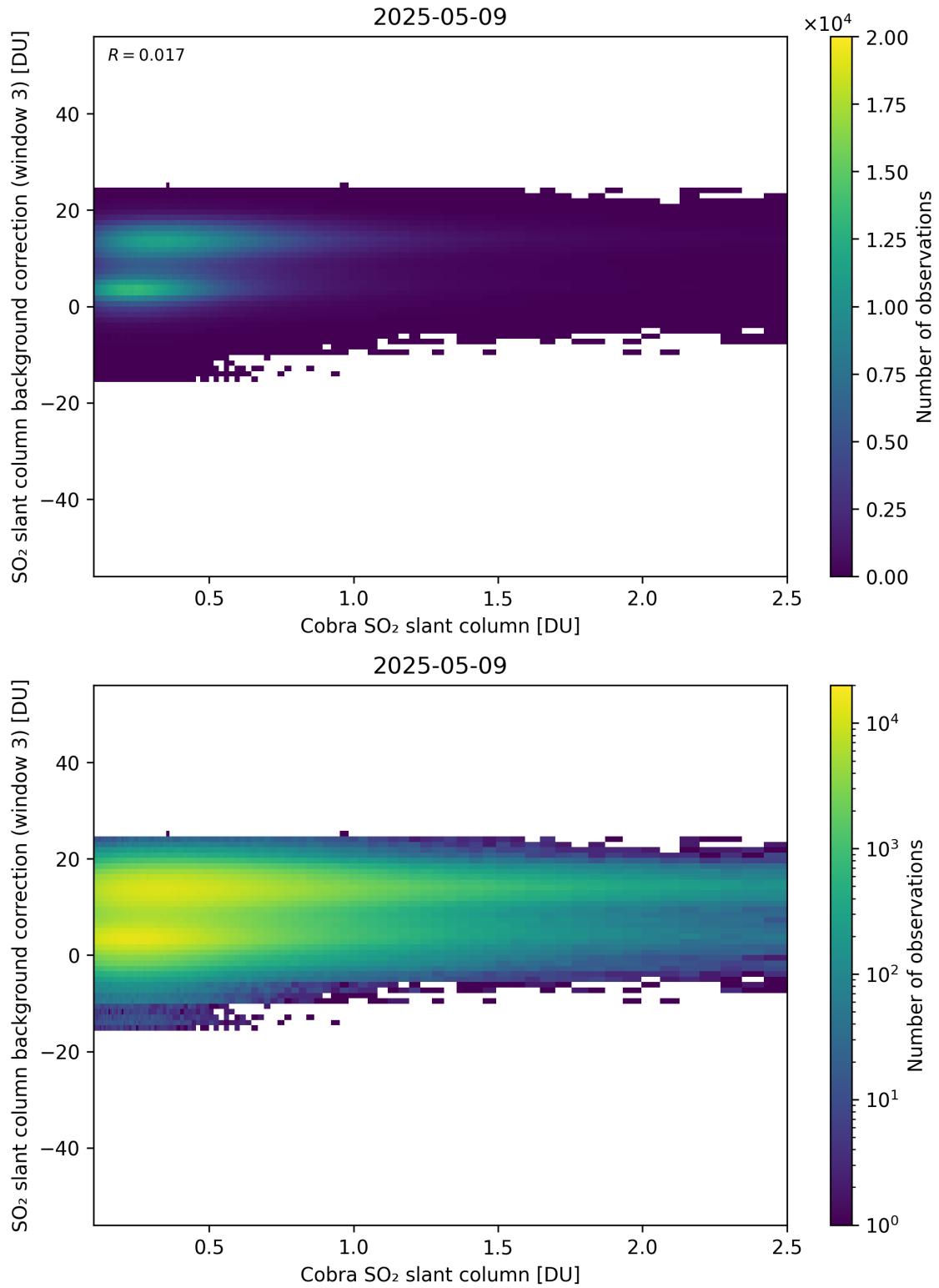
Figure 195: Scatter density plot of “Cobra SO 2 slant column” against “SO 2 slant column background correction (window 3)” for 2025-05-08 to 2025-05-10.
