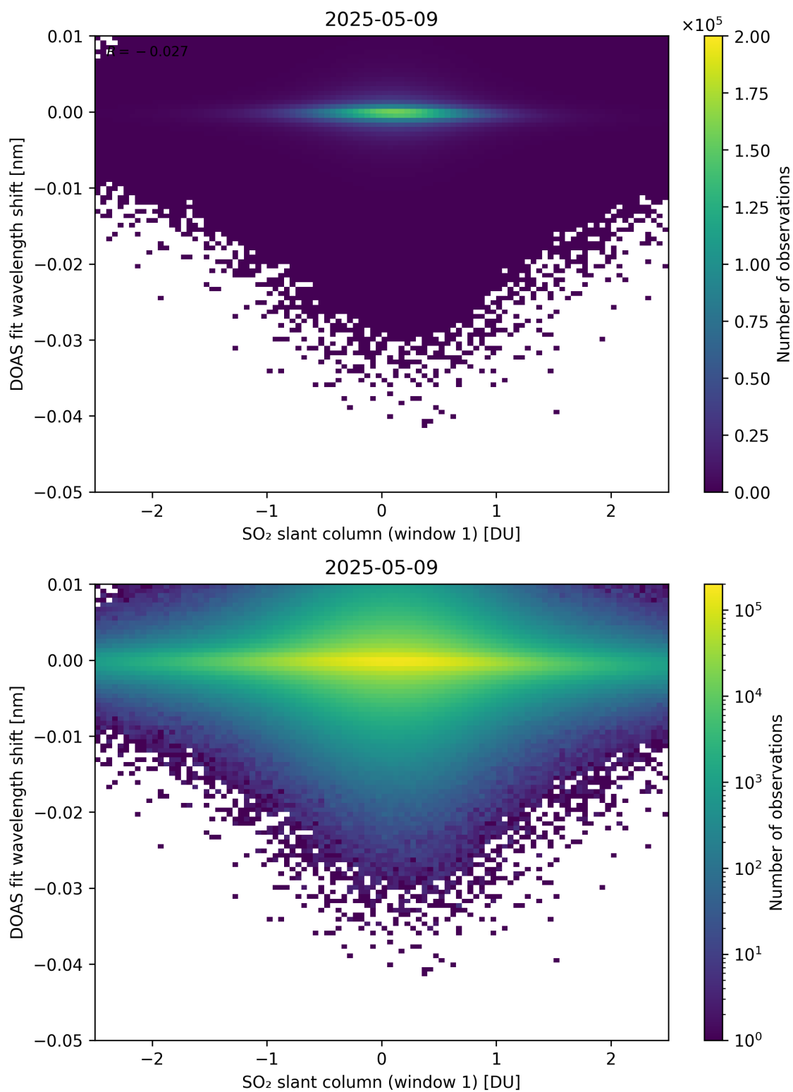
Figure 265: Scatter density plot of “SO 2 slant column (window 1)” against “DOAS fit wavelength shift” for 2025-05-08 to 2025-05-10.
