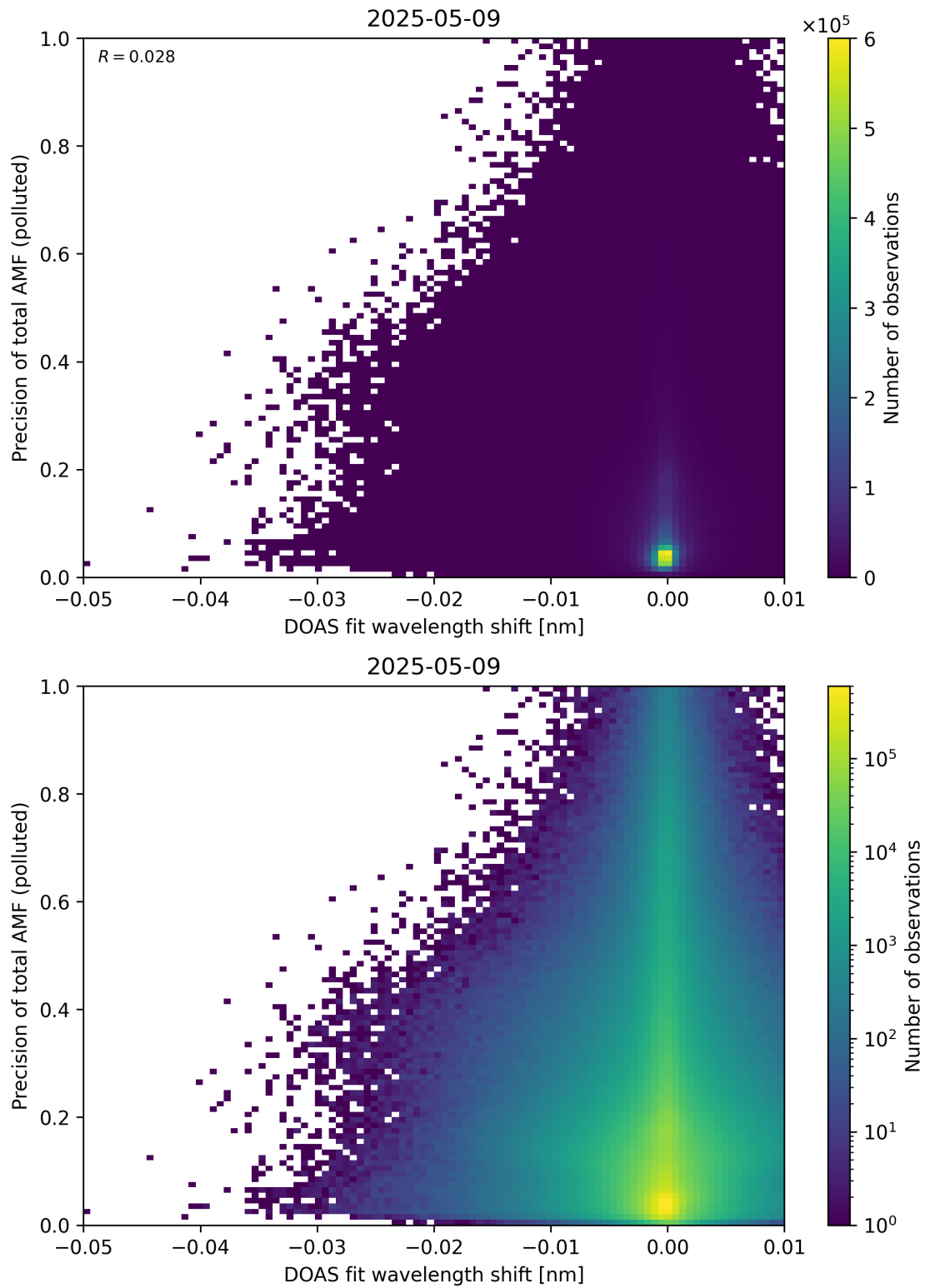
Figure 142: Scatter density plot of “DOAS fit wavelength shift” against “Precision of total AMF (polluted)” for 2025-05-08 to 2025-05-10.
