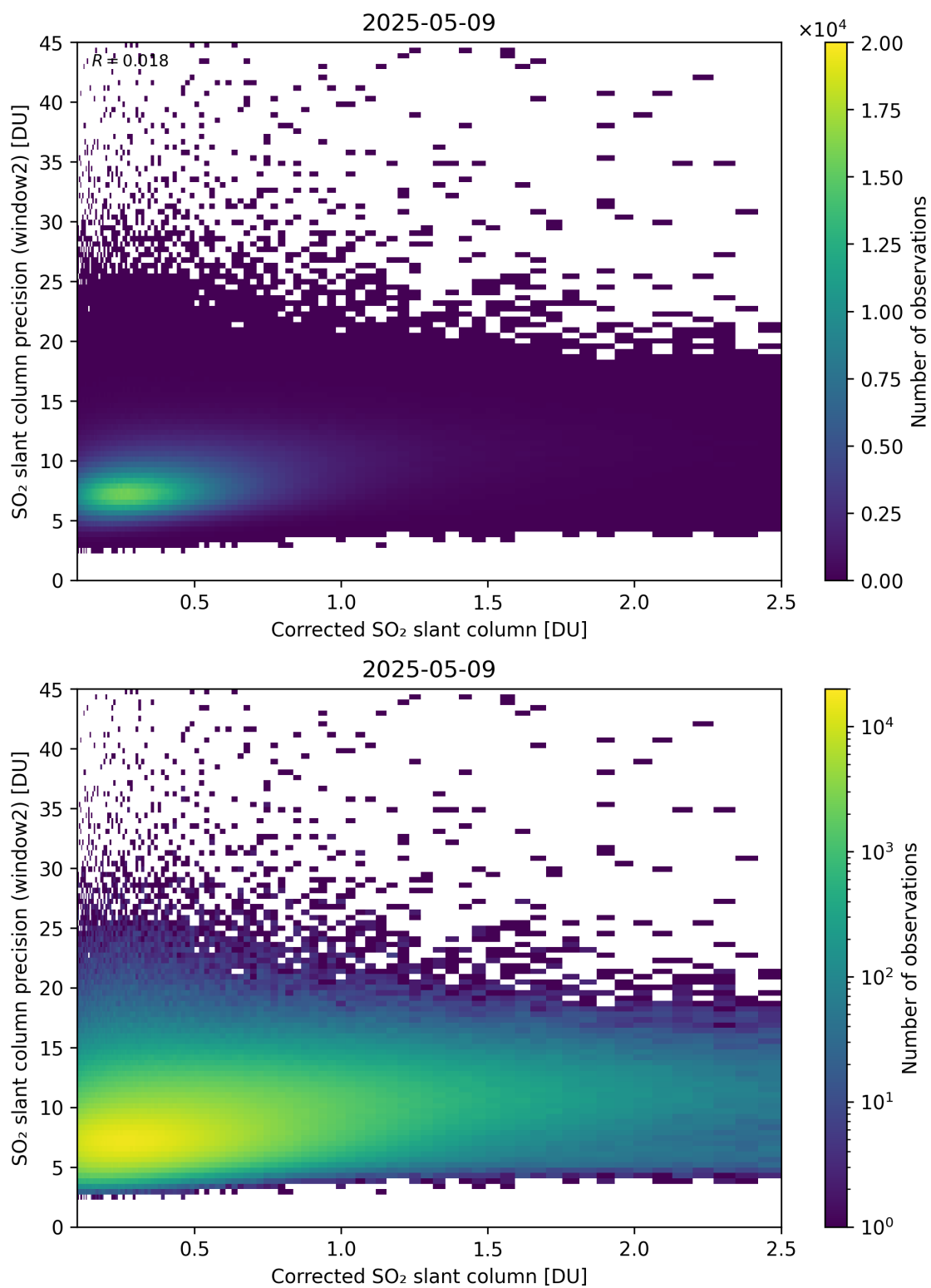
Figure 239: Scatter density plot of “Corrected SO 2 slant column” against “SO 2 slant column precision (window2)” for 2025-05-08 to 2025-05-10.
