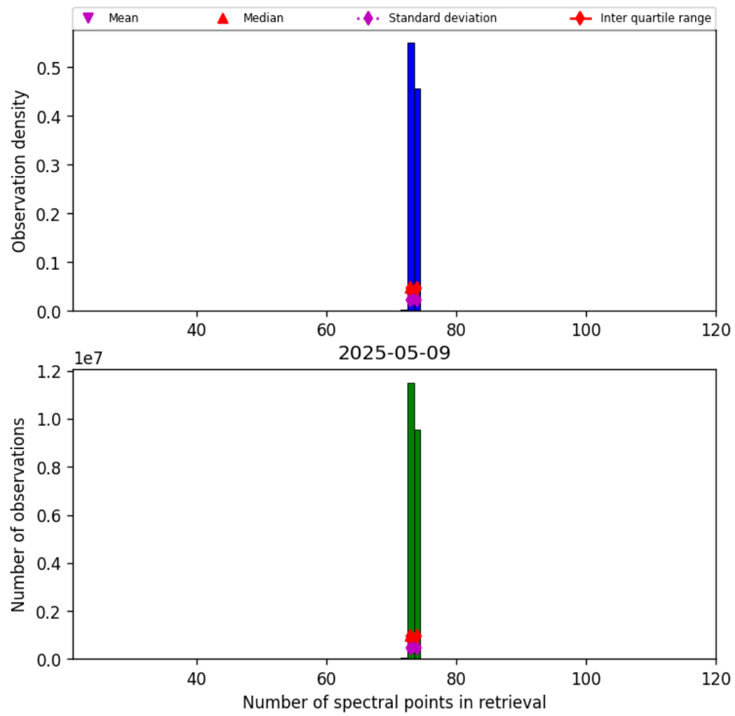
Figure 82: Histogram of “Number of spectral points in retrieval” for 2025-05-08 to 2025-05-10
