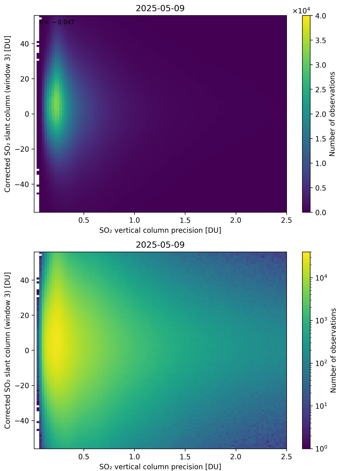
Figure 340: Scatter density plot of “SO 2 vertical column precision” against “Corrected SO 2 slant column (window 3)” for 2025-05-08 to 2025-05-10.
