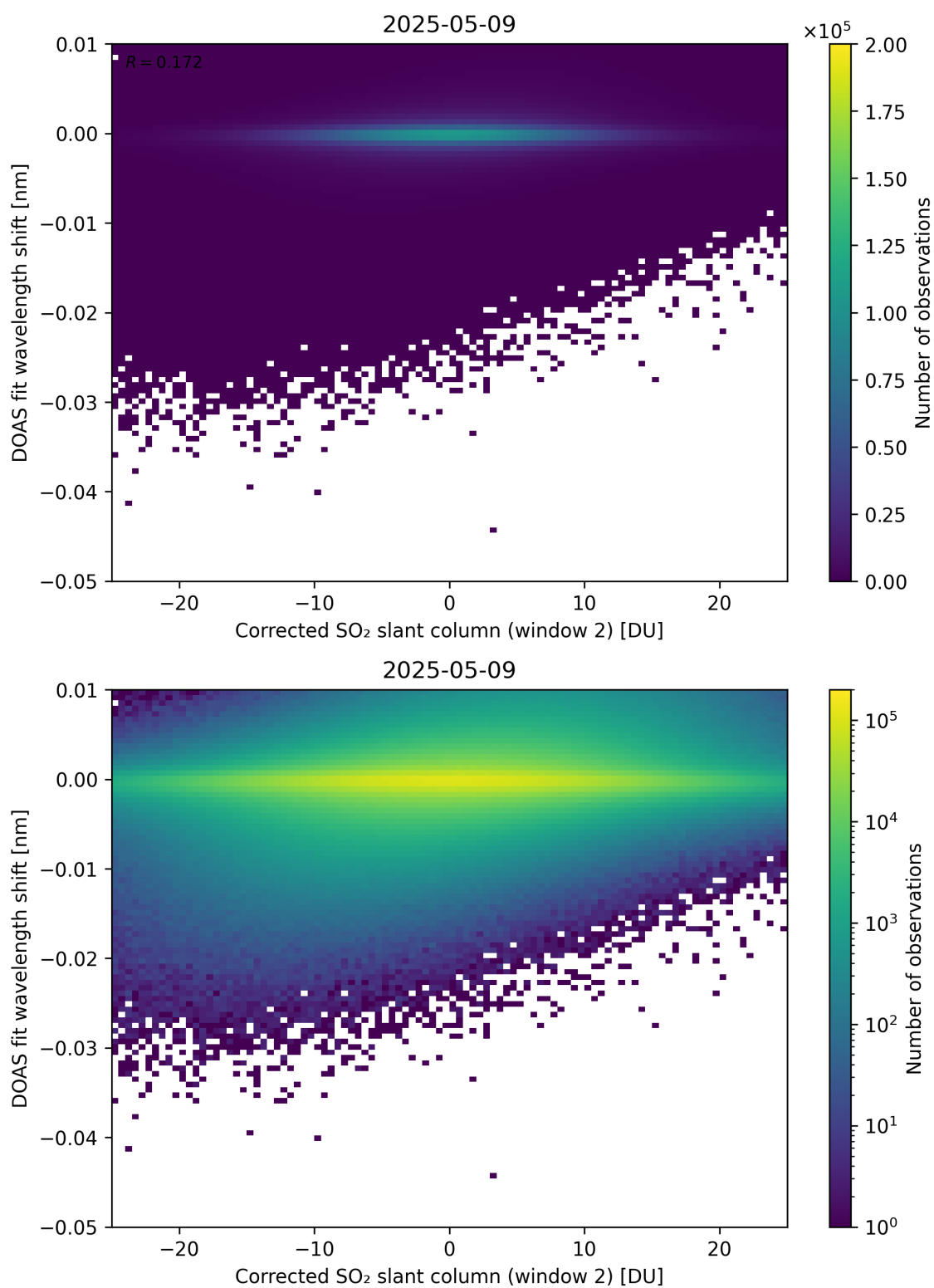
Figure 246: Scatter density plot of “Corrected SO 2 slant column (window 2)” against “DOAS fit wavelength shift” for 2025-05-08 to 2025-05-10.
