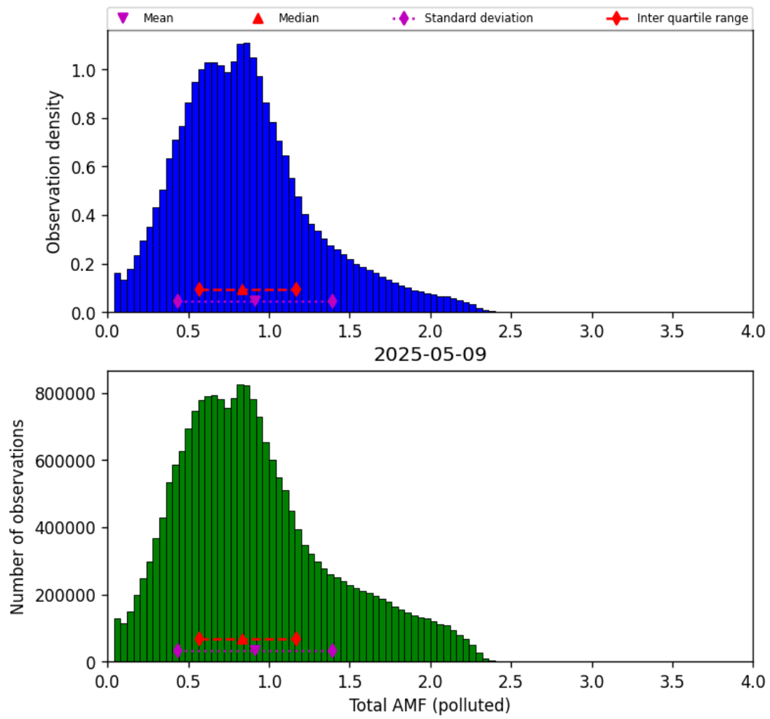
Figure 79: Histogram of “Total AMF (polluted)” for 2025-05-08 to 2025-05-10
