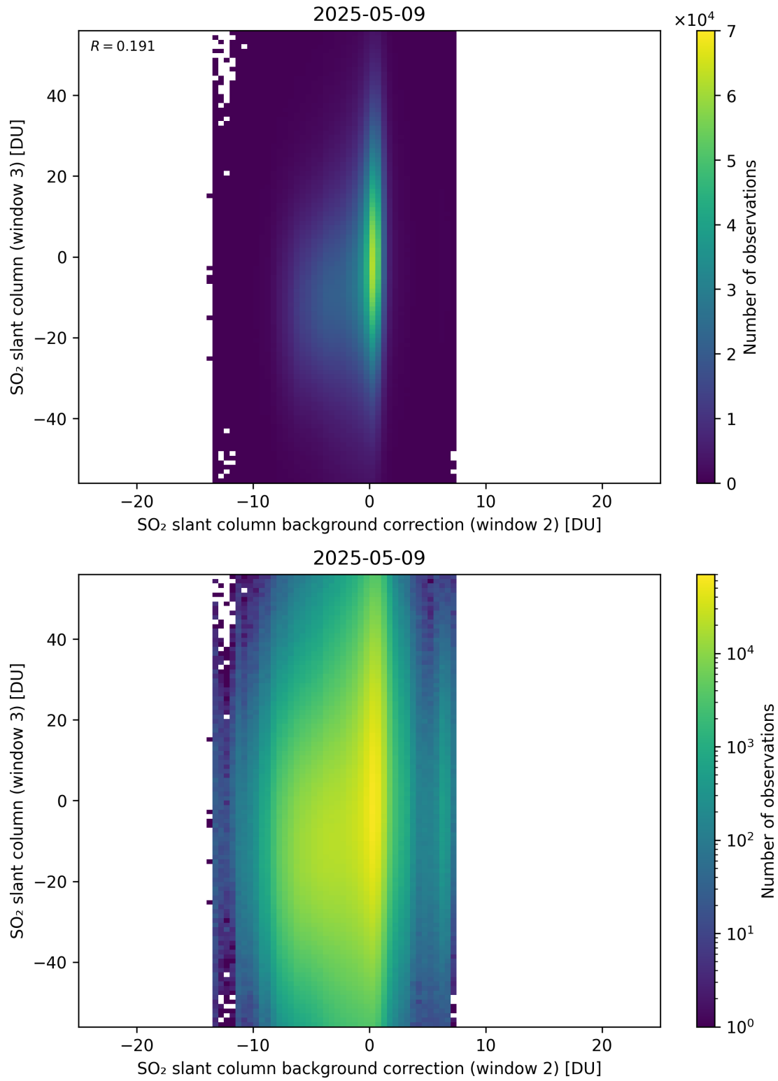
Figure 128: Scatter density plot of “SO 2 slant column background correction (window 2)” against “SO 2 slant column (window 3)” for 2025-05-08 to 2025-05-10.
