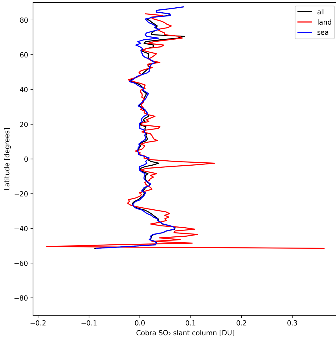
Figure 35: Zonal average of “Cobra SO 2 slant column” for 2025-05-08 to 2025-05-10.
