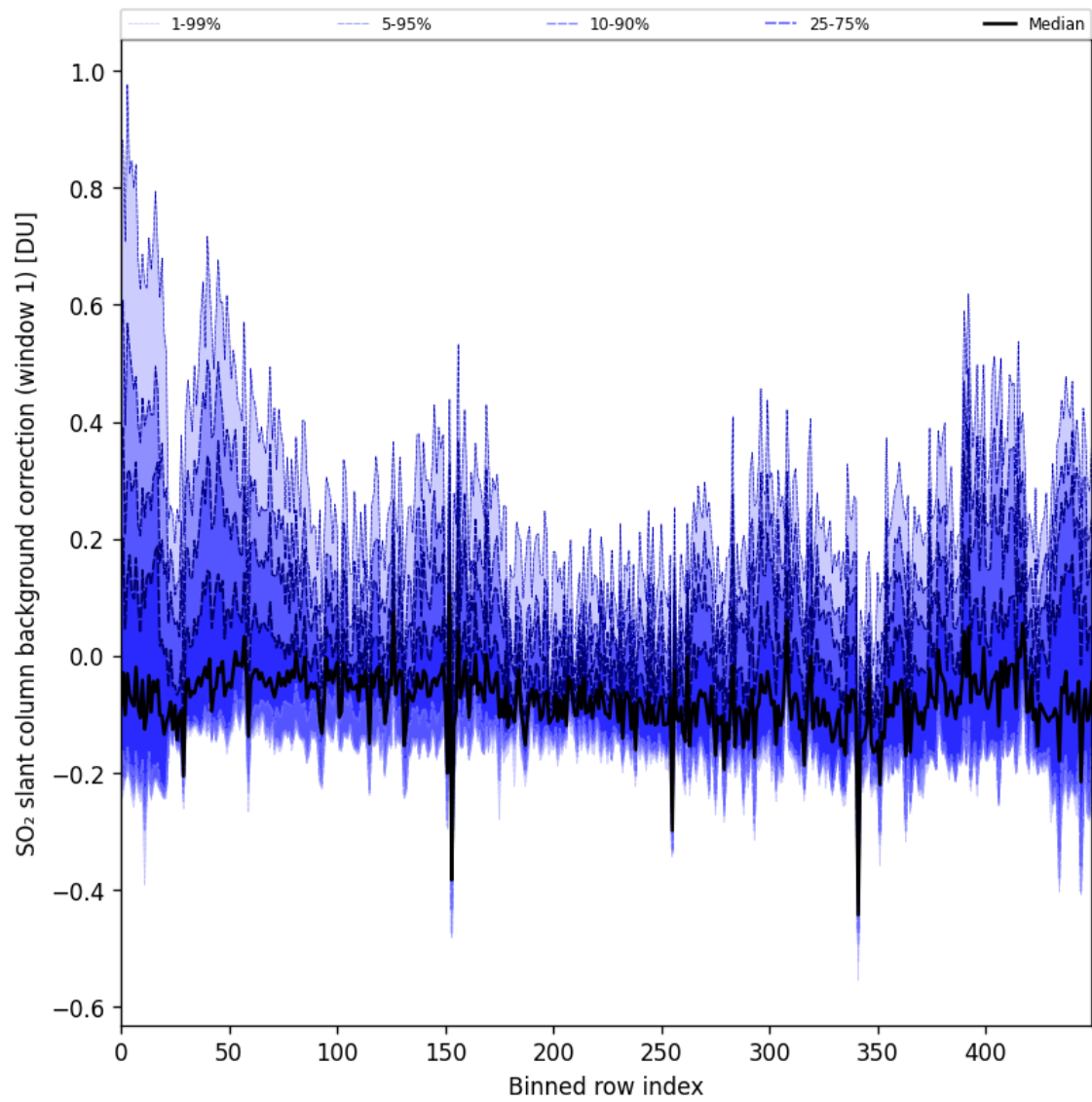
Figure 92: Along track statistics of “SO 2 slant column background correction (window 1)” for 2025-05-08 to 2025-05-10
