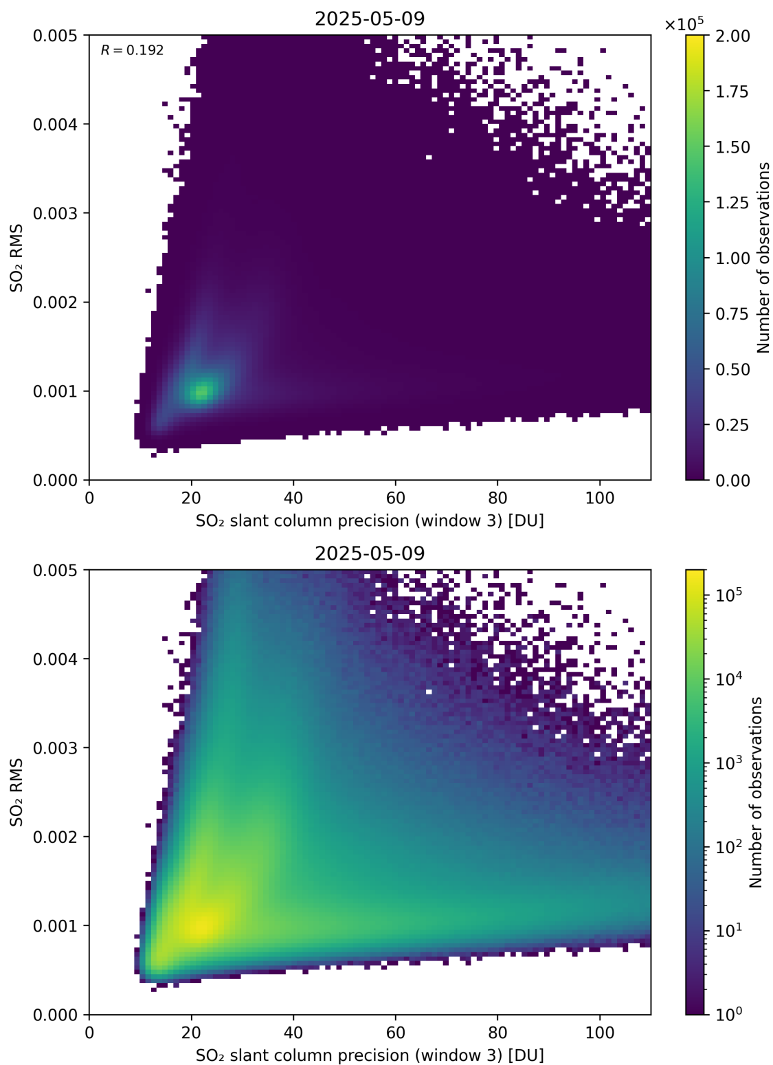
Figure 310: Scatter density plot of “SO 2 slant column precision (window 3)” against “SO 2 RMS” for 2025-05-08 to 2025-05-10.
