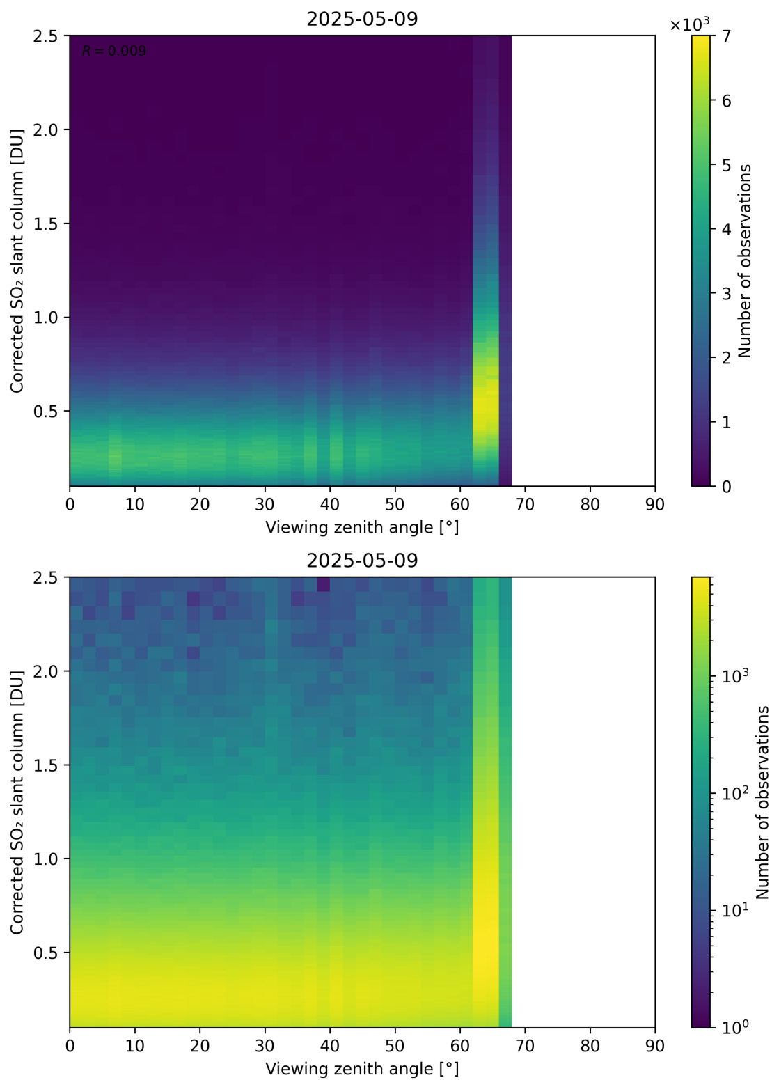
Figure 373: Scatter density plot of “Viewing zenith angle” against “Corrected SO 2 slant column” for 2025-05-08 to 2025-05-10.
