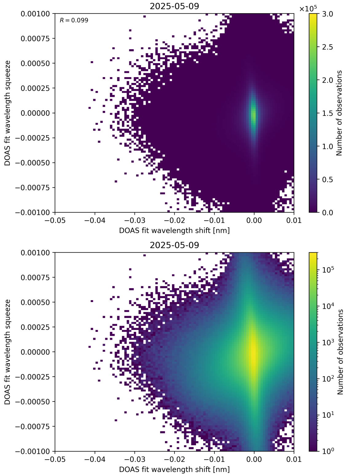
Figure 138: Scatter density plot of “DOAS fit wavelength shift” against “DOAS fit wavelength squeeze” for 2025-05-08 to 2025-05-10.
