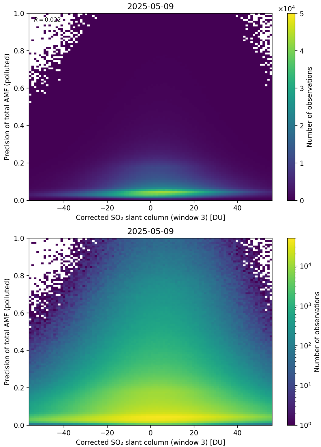
Figure 261: Scatter density plot of “Corrected SO 2 slant column (window 3)” against “Precision of total AMF (polluted)” for 2025-05-08 to 2025-05-10.
