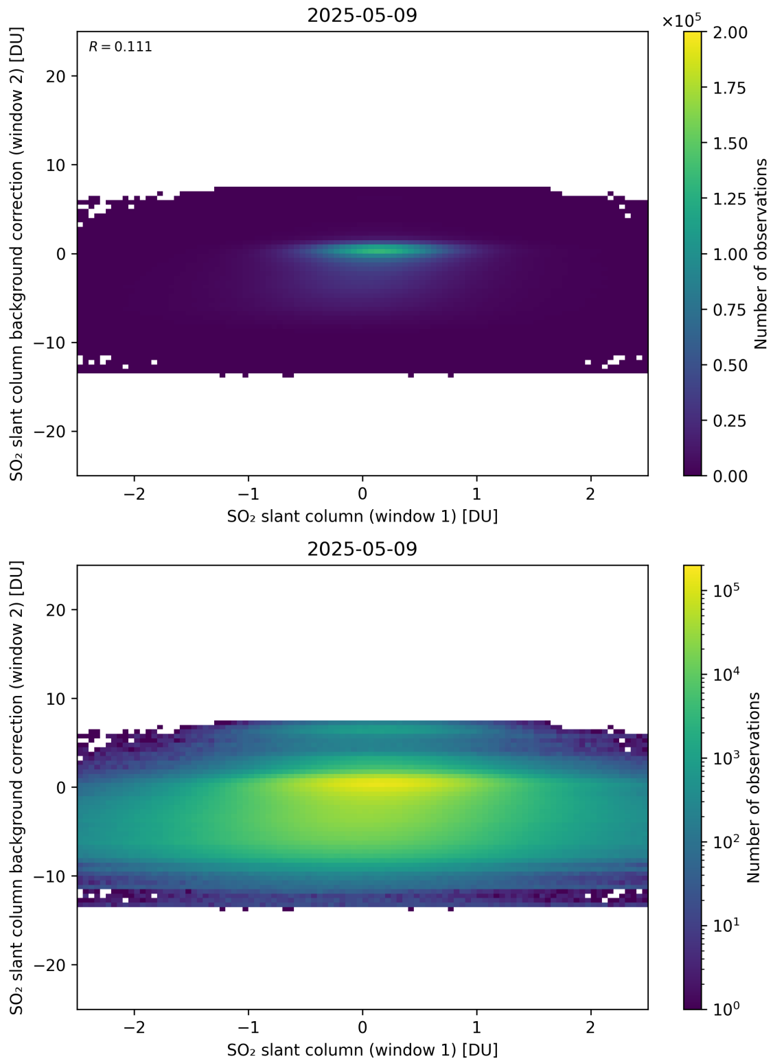
Figure 263: Scatter density plot of “SO 2 slant column (window 1)” against “SO 2 slant column background correction (window 2)” for 2025-05-08 to 2025-05-10.
