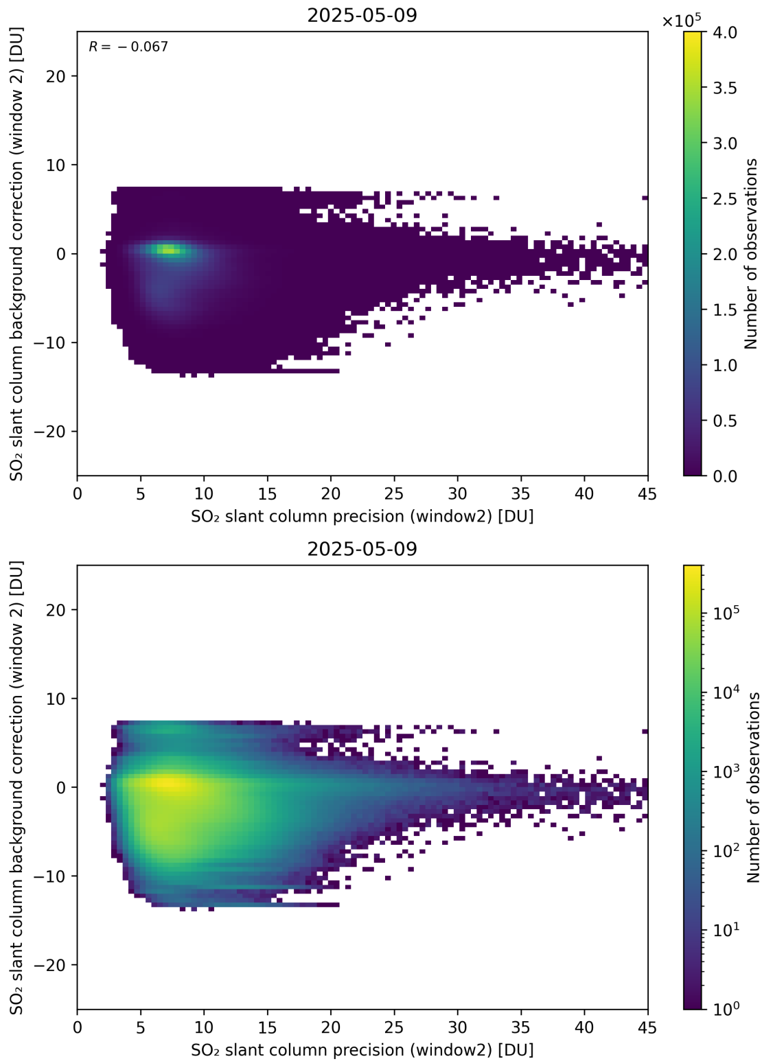
Figure 291: Scatter density plot of “SO 2 slant column precision (window2)” against “SO 2 slant column background correction (window 2)” for 2025-05-08 to 2025-05-10.
