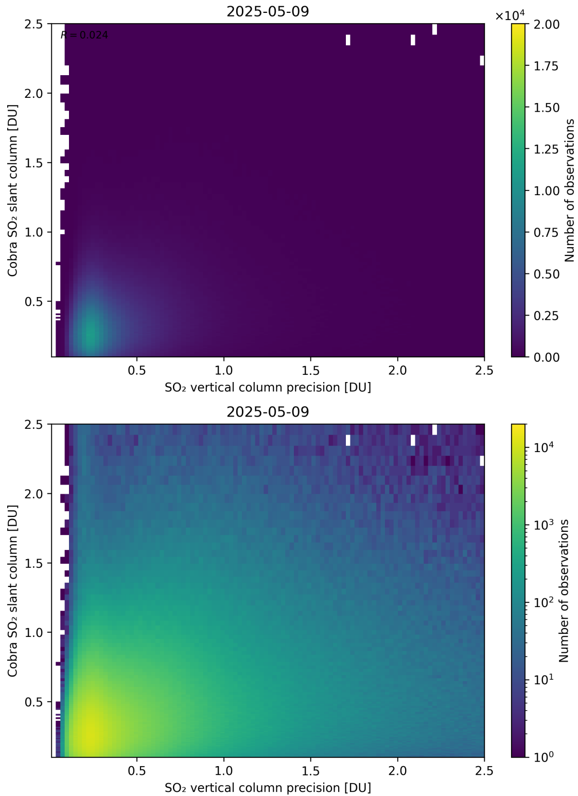
Figure 336: Scatter density plot of “SO 2 vertical column precision” against “Cobra SO 2 slant column” for 2025-05-08 to 2025-05-10.
