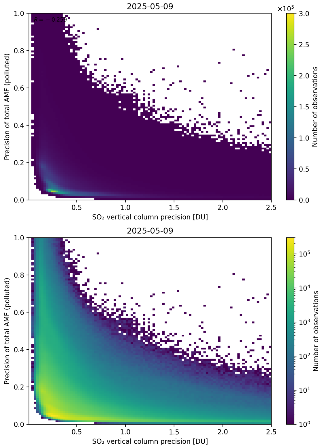
Figure 347: Scatter density plot of “SO 2 vertical column precision” against “Precision of total AMF (polluted)” for 2025-05-08 to 2025-05-10.
