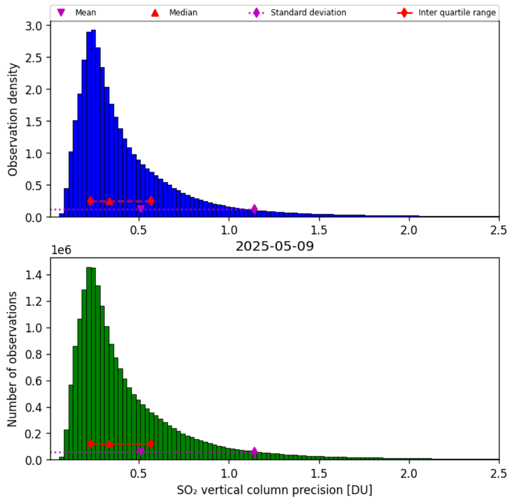
Figure 59: Histogram of “SO 2 vertical column precision” for 2025-05-08 to 2025-05-10
