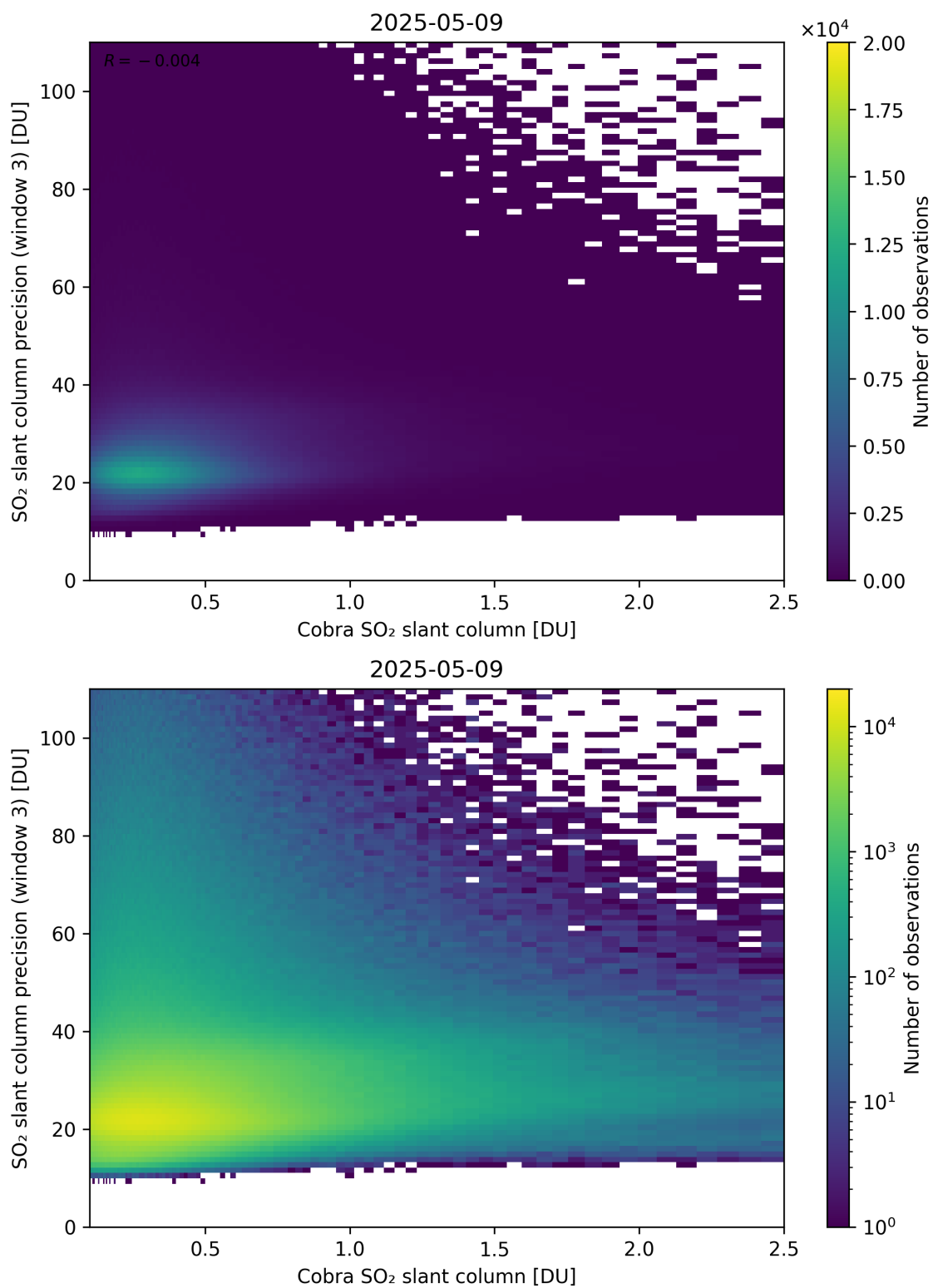
Figure 223: Scatter density plot of “Cobra SO 2 slant column” against “SO 2 slant column precision (window 3)” for 2025-05-08 to 2025-05-10.
