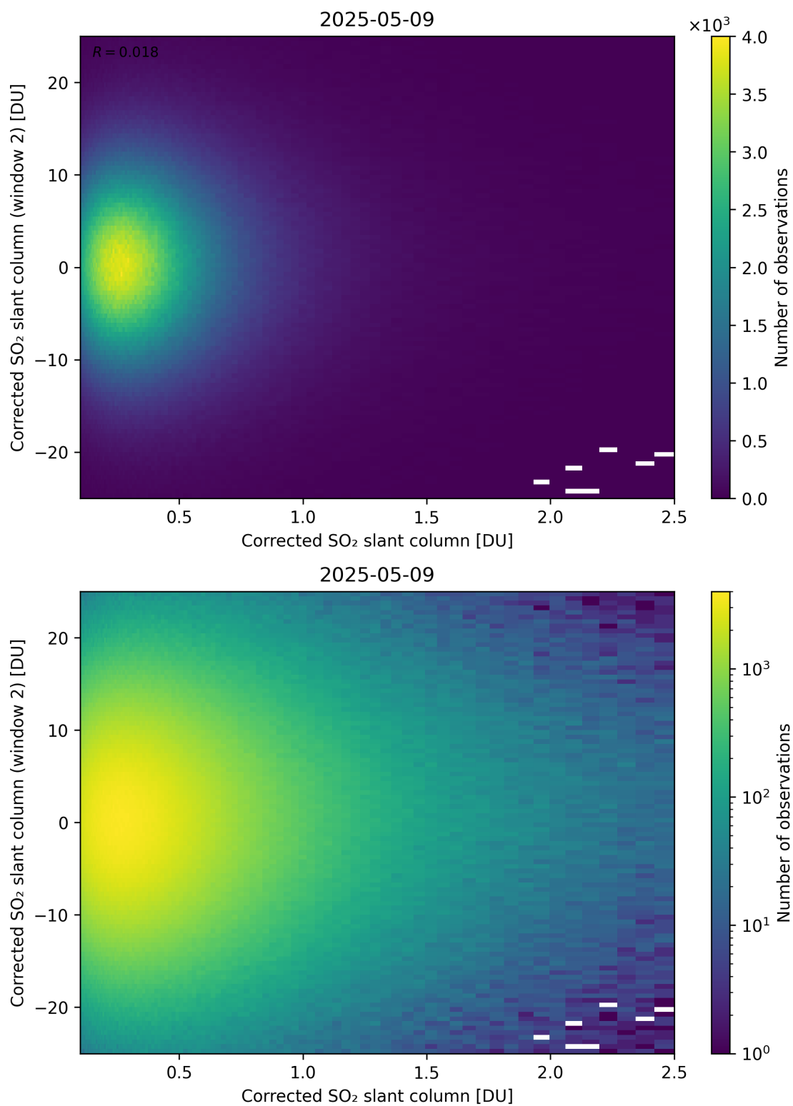
Figure 235: Scatter density plot of “Corrected SO 2 slant column” against “Corrected SO 2 slant column (window 2)” for 2025-05-08 to 2025-05-10.
