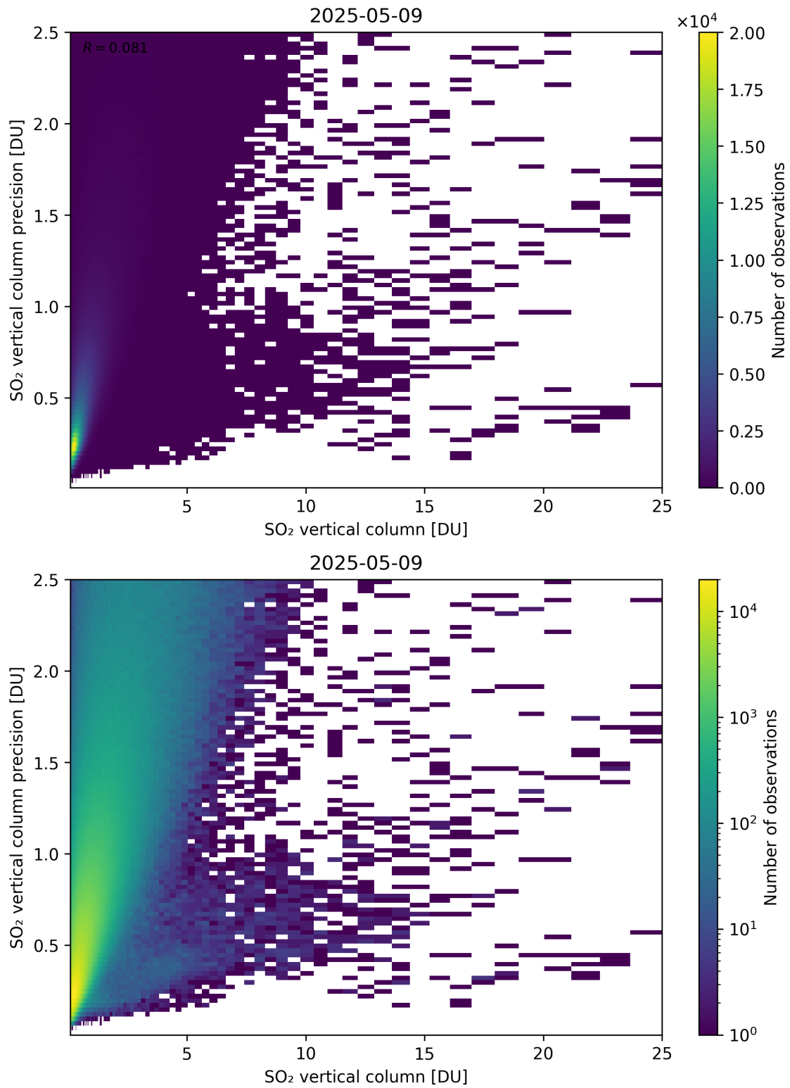
Figure 361: Scatter density plot of “SO 2 vertical column” against “SO 2 vertical column precision” for 2025-05-08 to 2025-05-10.
