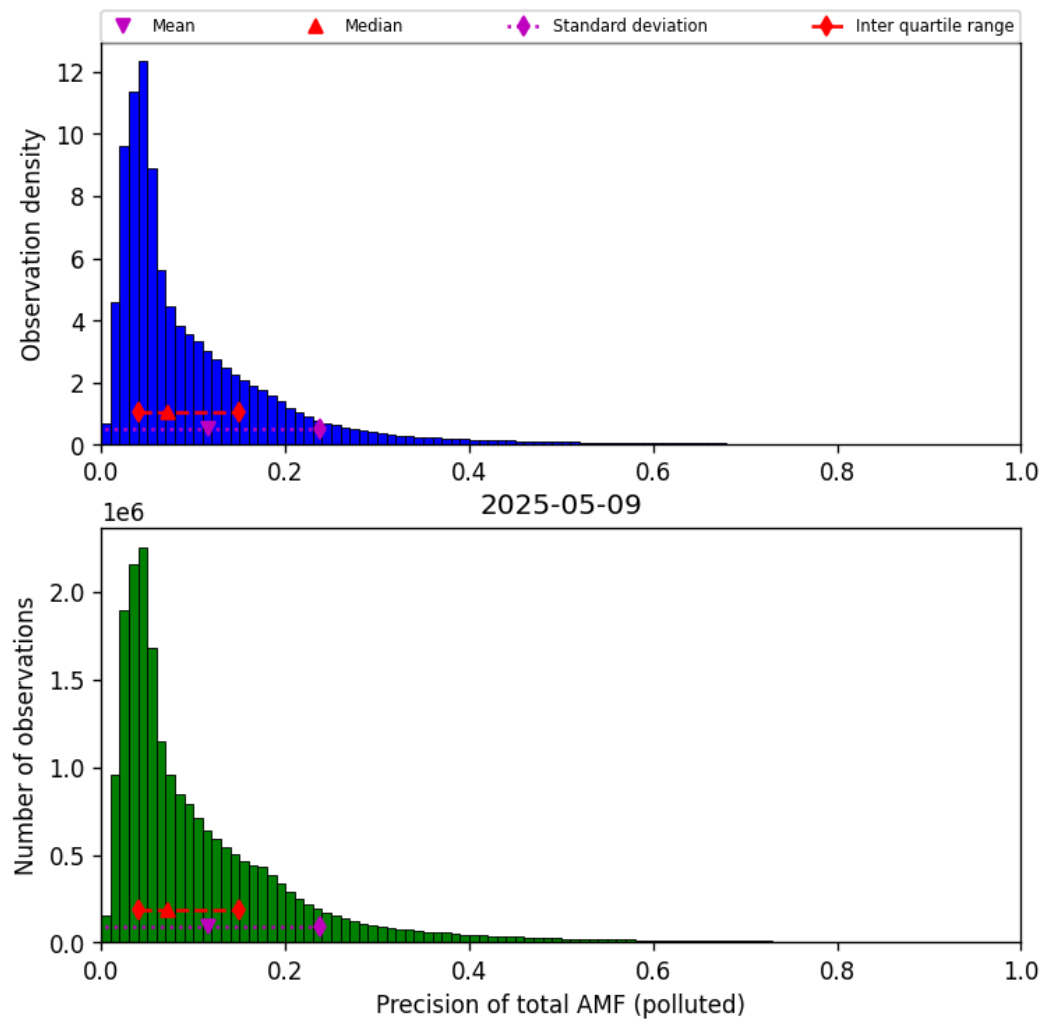
Figure 80: Histogram of “Precision of total AMF (polluted)” for 2025-05-08 to 2025-05-10
