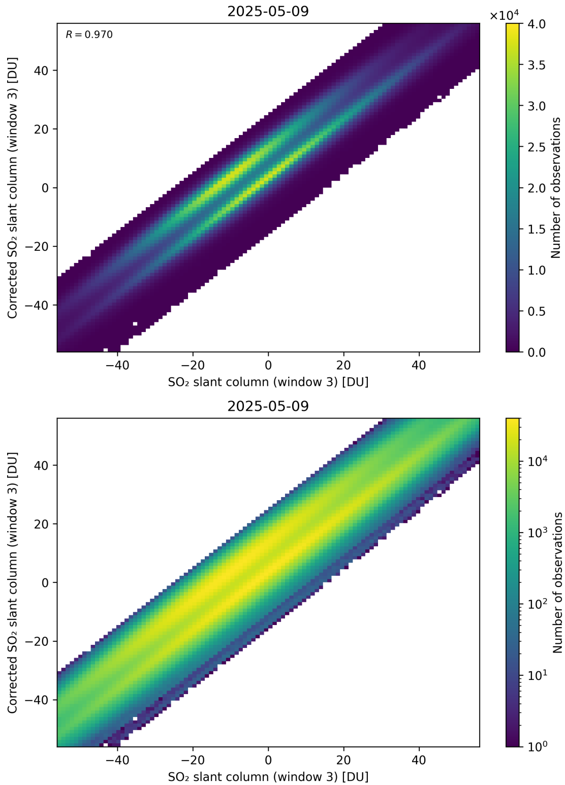
Figure 316: Scatter density plot of “SO 2 slant column (window 3)” against “Corrected SO 2 slant column (window 3)” for 2025-05-08 to 2025-05-10.
