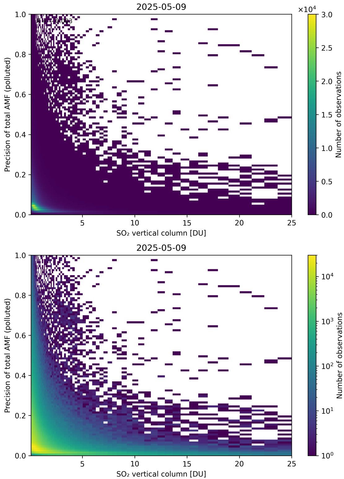
Figure 360: Scatter density plot of “SO 2 vertical column” against “Precision of total AMF (polluted)” for 2025-05-08 to 2025-05-10.
