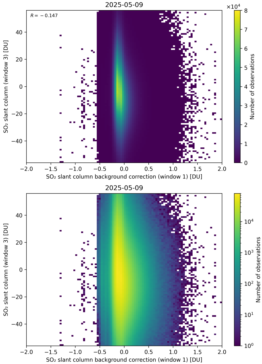
Figure 118: Scatter density plot of “SO 2 slant column background correction (window 1)” against “SO 2 slant column (window 3)” for 2025-05-08 to 2025-05-10.
