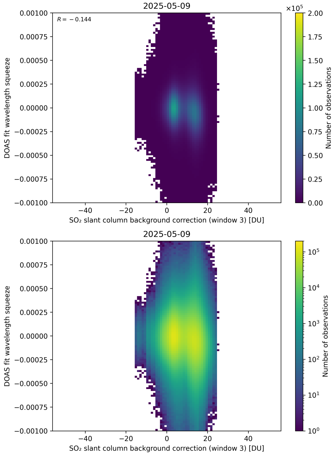
Figure 133: Scatter density plot of “SO 2 slant column background correction (window 3)” against “DOAS fit wavelength squeeze” for 2025-05-08 to 2025-05-10.
