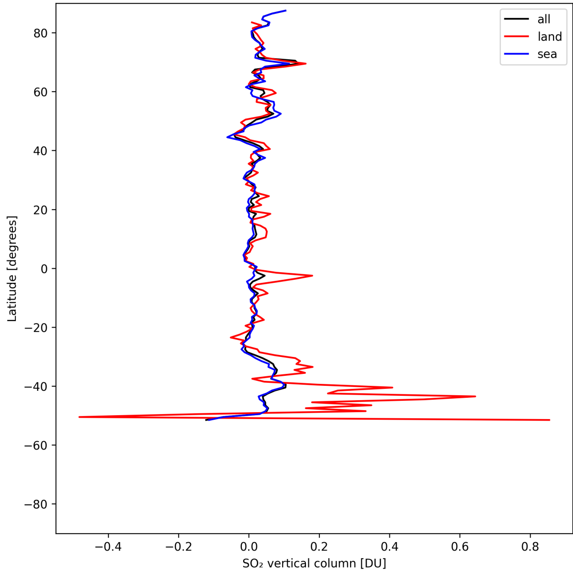
Figure 32: Zonal average of “SO 2 vertical column” for 2025-05-08 to 2025-05-10.
