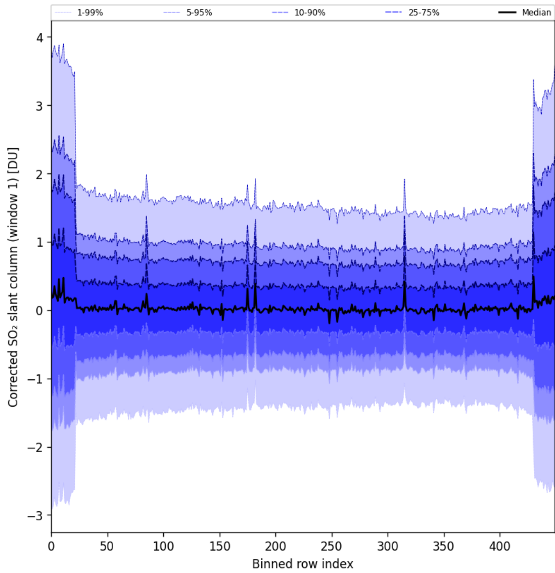
Figure 91: Along track statistics of "Corrected SO 2 slant column (window 1)" for 2025-05-08 to 2025-05-10
