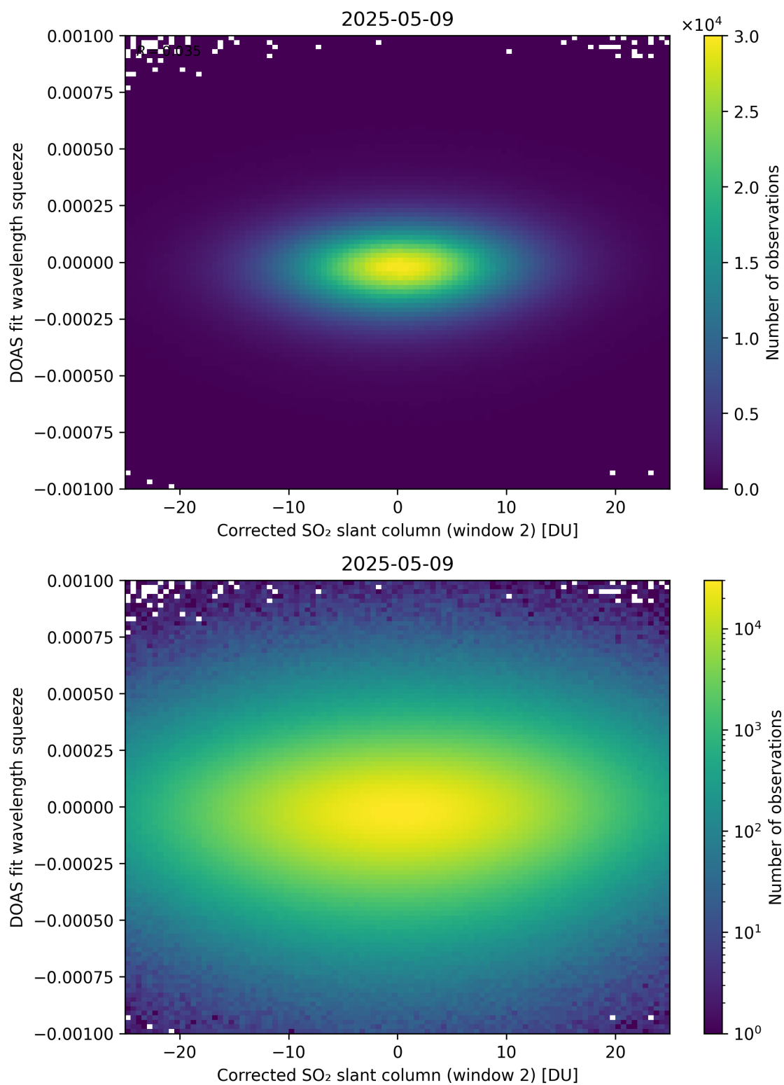
Figure 247: Scatter density plot of “Corrected SO 2 slant column (window 2)” against “DOAS fit wavelength squeeze” for 2025-05-08 to 2025-05-10.
