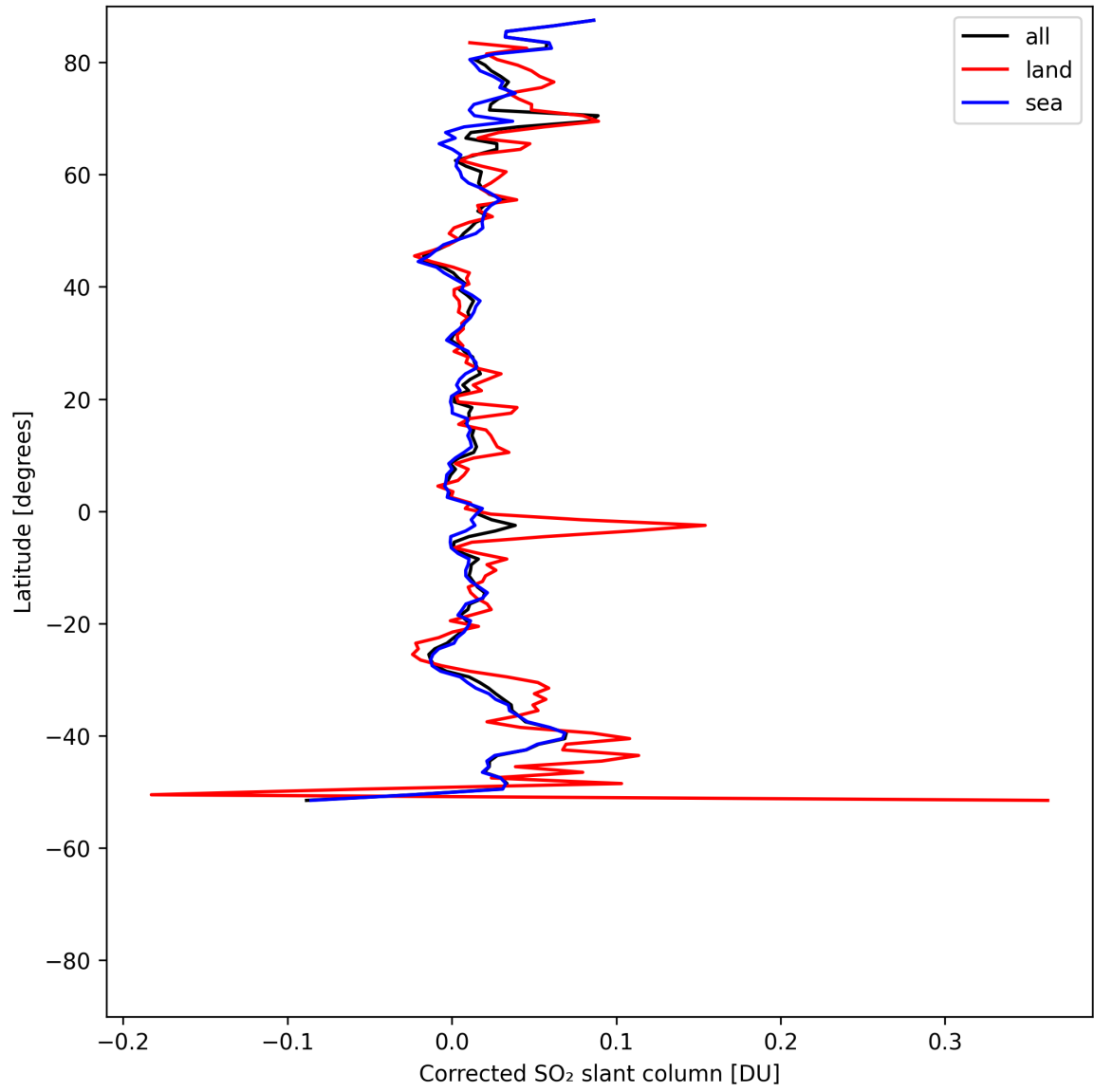
Figure 34: Zonal average of “Corrected SO 2 slant column” for 2025-05-08 to 2025-05-10.
