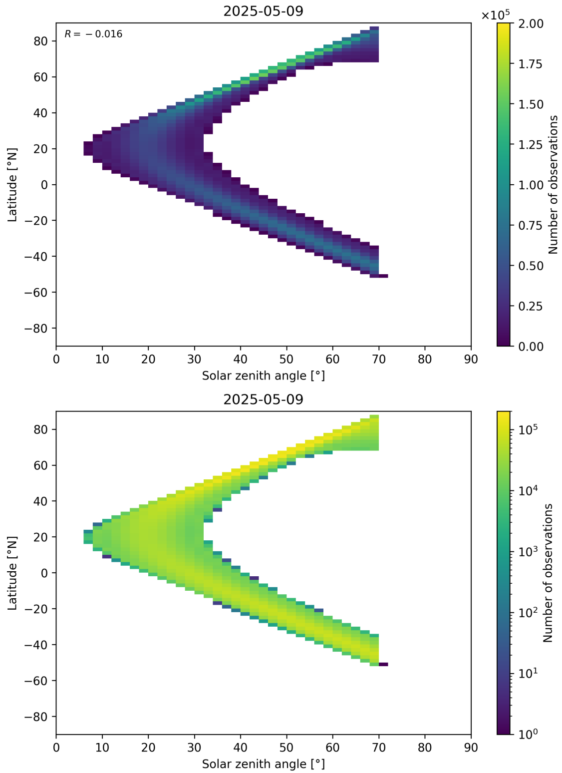
Figure 177: Scatter density plot of “Solar zenith angle” against “Latitude” for 2025-05-08 to 2025-05-10.
