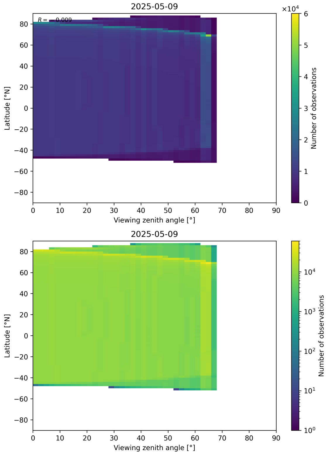
Figure 368: Scatter density plot of “Viewing zenith angle” against “Latitude” for 2025-05-08 to 2025-05-10.
