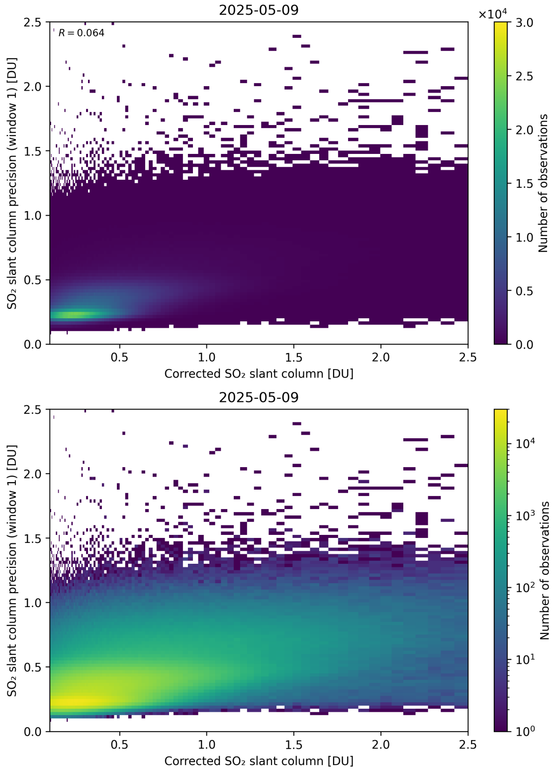
Figure 238: Scatter density plot of “Corrected SO 2 slant column” against “SO 2 slant column precision (window 1)” for 2025-05-08 to 2025-05-10.
