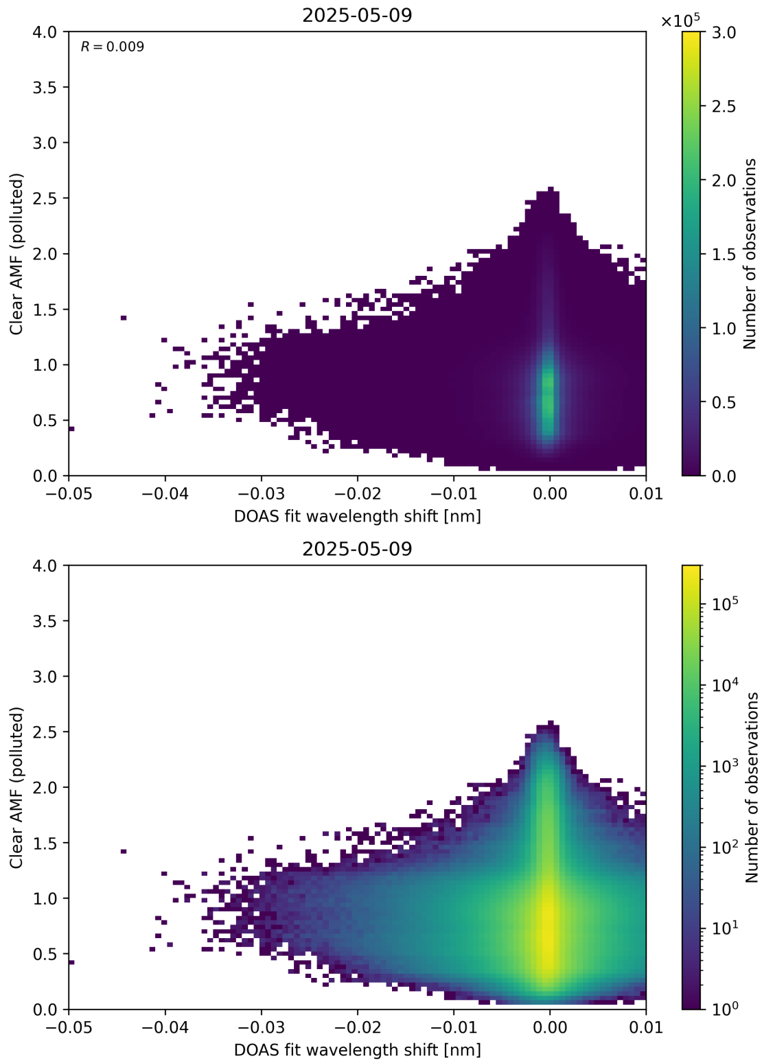
Figure 140: Scatter density plot of “DOAS fit wavelength shift” against “Clear AMF (polluted)” for 2025-05-08 to 2025-05-10.
