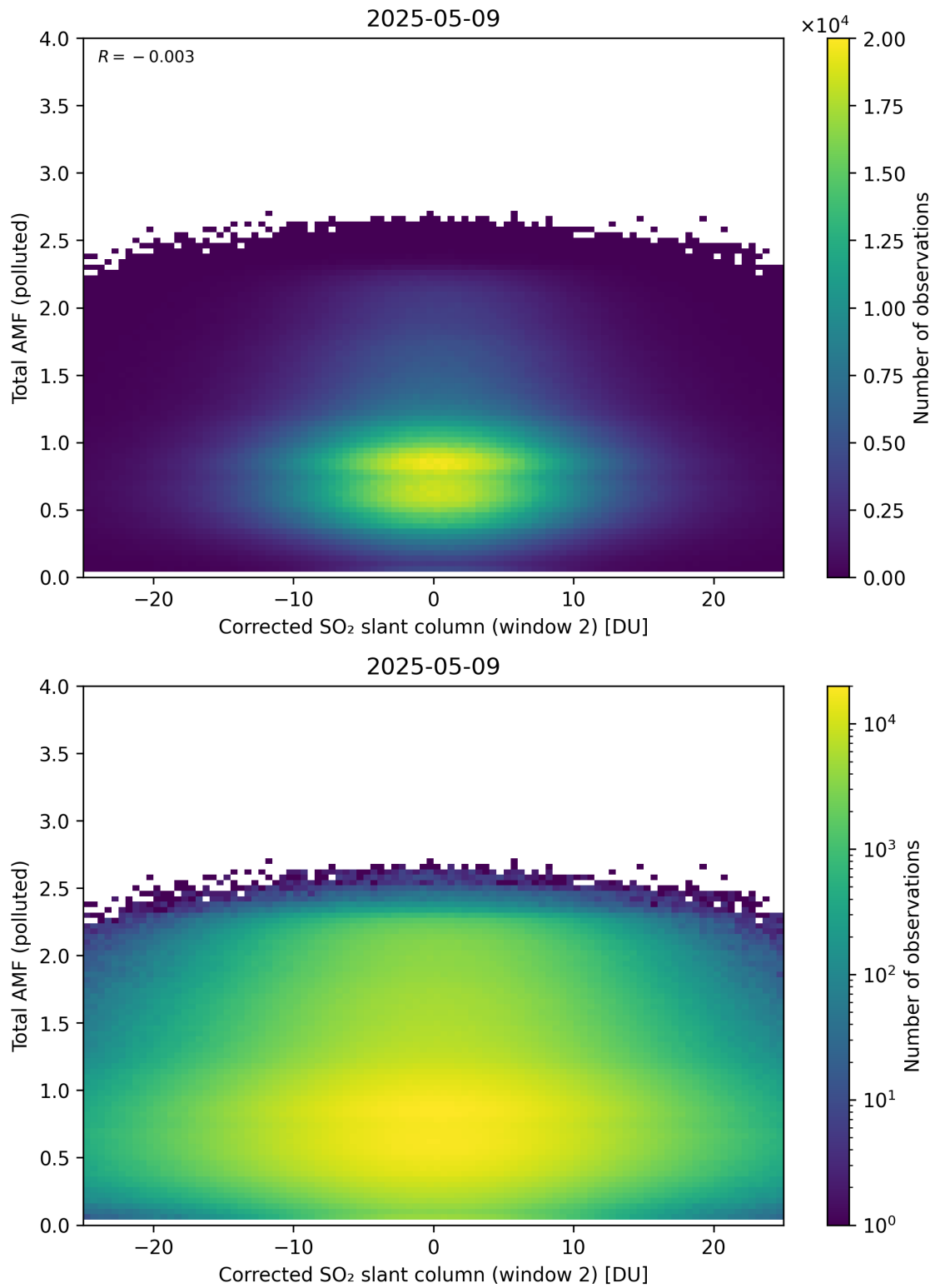
Figure 253: Scatter density plot of “Corrected SO 2 slant column (window 2)” against “Total AMF (polluted)” for 2025-05-08 to 2025-05-10.
