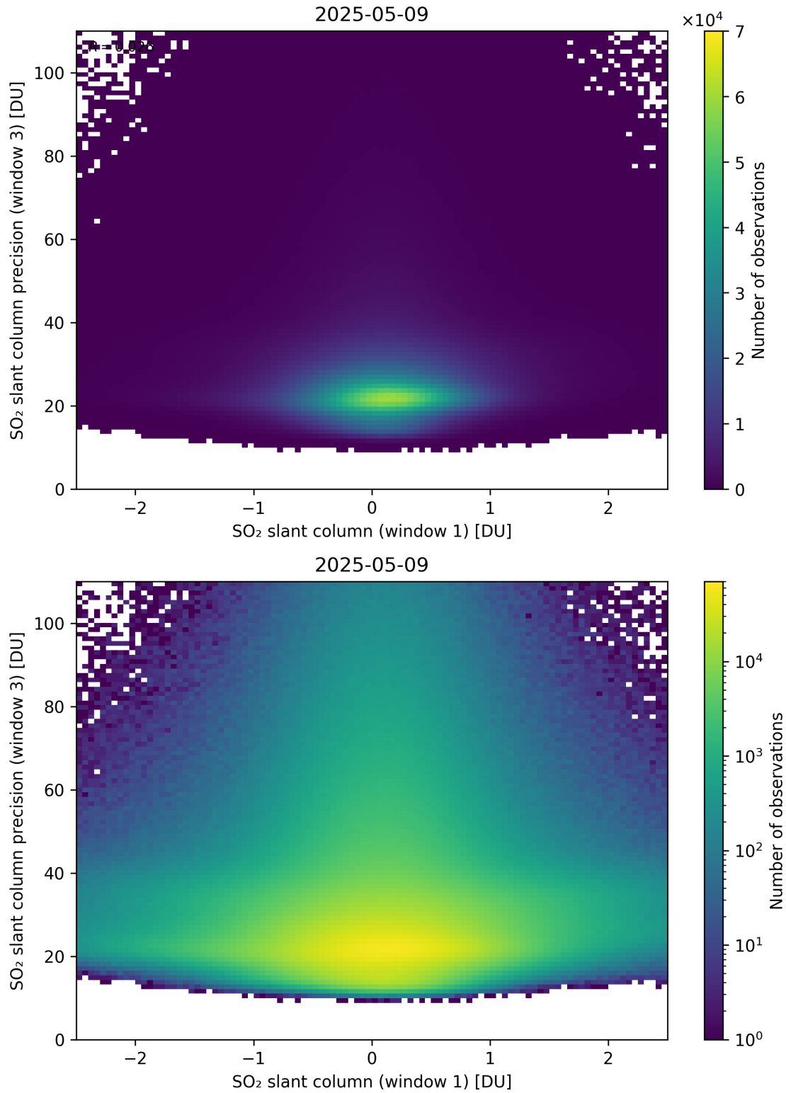
Figure 288: Scatter density plot of “SO 2 slant column (window 1)” against “SO 2 slant column precision (window 3)” for 2025-05-08 to 2025-05-10.
