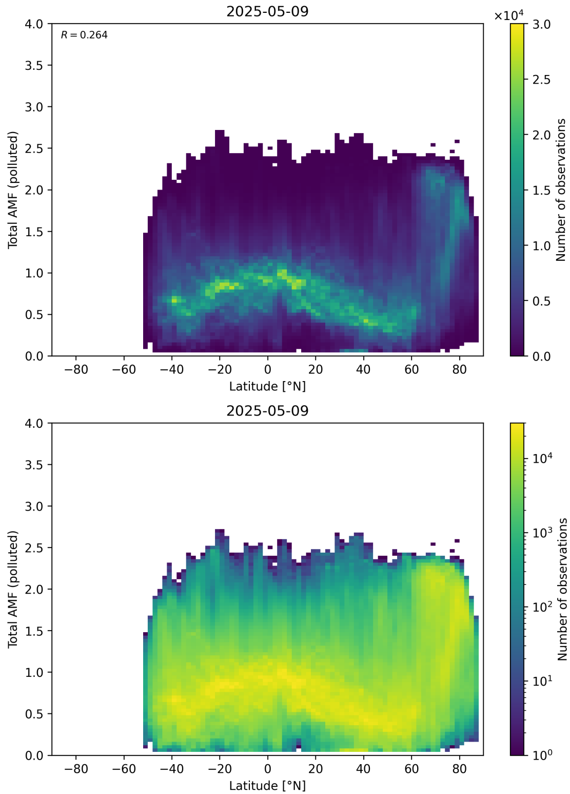
Figure 167: Scatter density plot of “Latitude” against “Total AMF (polluted)” for 2025-05-08 to 2025-05-10.
