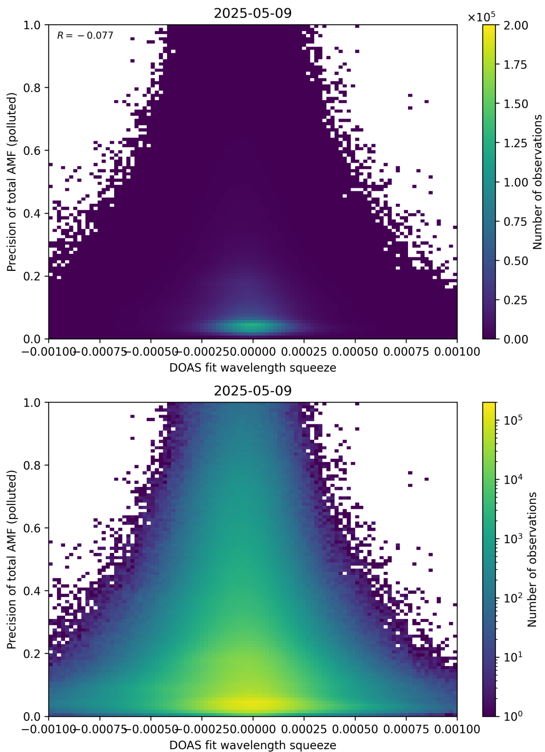
Figure 146: Scatter density plot of “DOAS fit wavelength squeeze” against “Precision of total AMF (polluted)” for 2025-05-08 to 2025-05-10.
