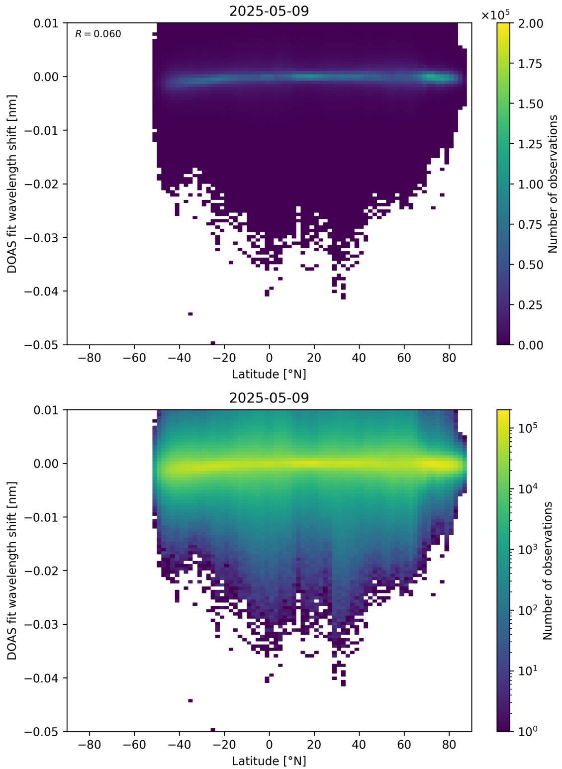
Figure 153: Scatter density plot of “Latitude” against “DOAS fit wavelength shift” for 2025-05-08 to 2025-05-10.
