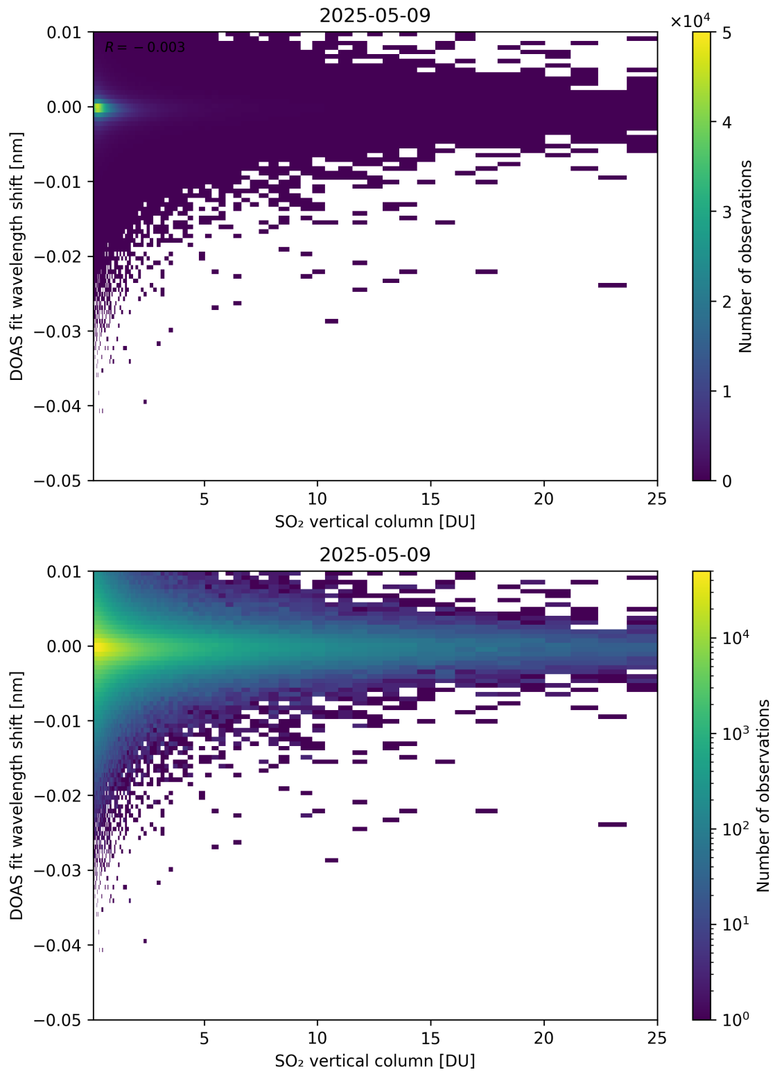
Figure 326: Scatter density plot of “SO 2 vertical column” against “DOAS fit wavelength shift” for 2025-05-08 to 2025-05-10.
