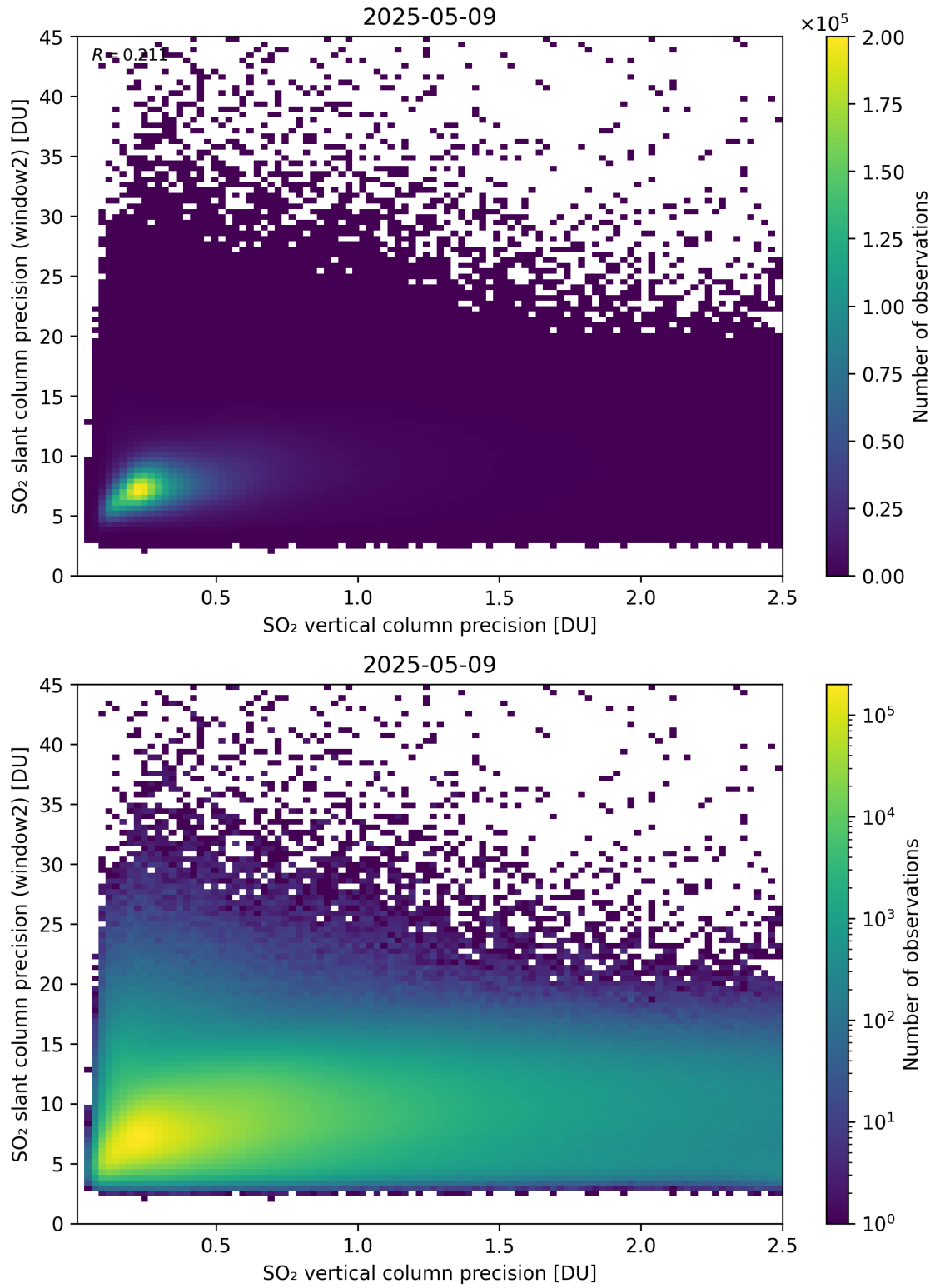
Figure 343: Scatter density plot of “SO 2 vertical column precision” against “SO 2 slant column precision (window2)” for 2025-05-08 to 2025-05-10.
