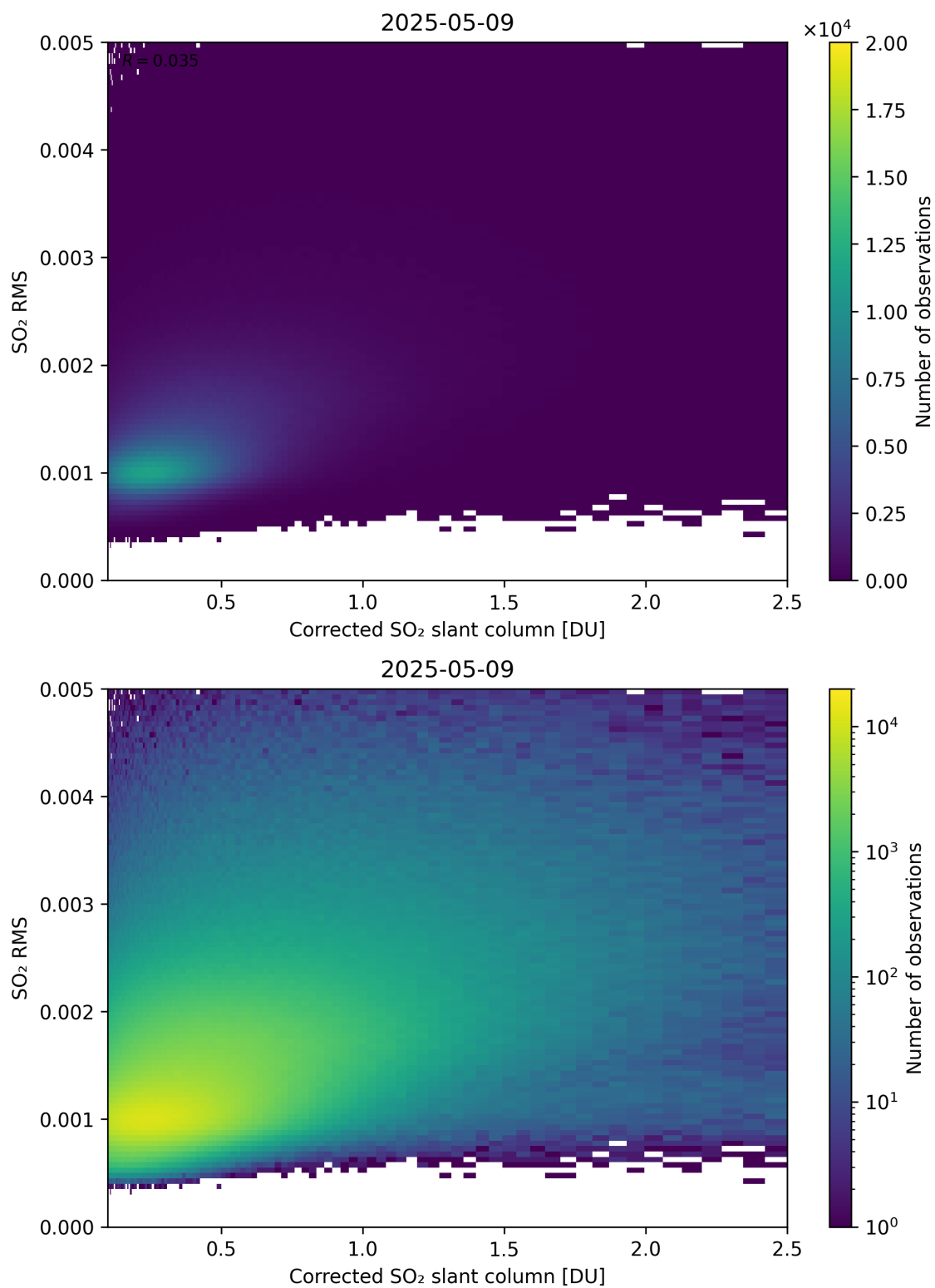
Figure 231: Scatter density plot of “Corrected SO 2 slant column” against “SO 2 RMS” for 2025-05-08 to 2025-05-10.
