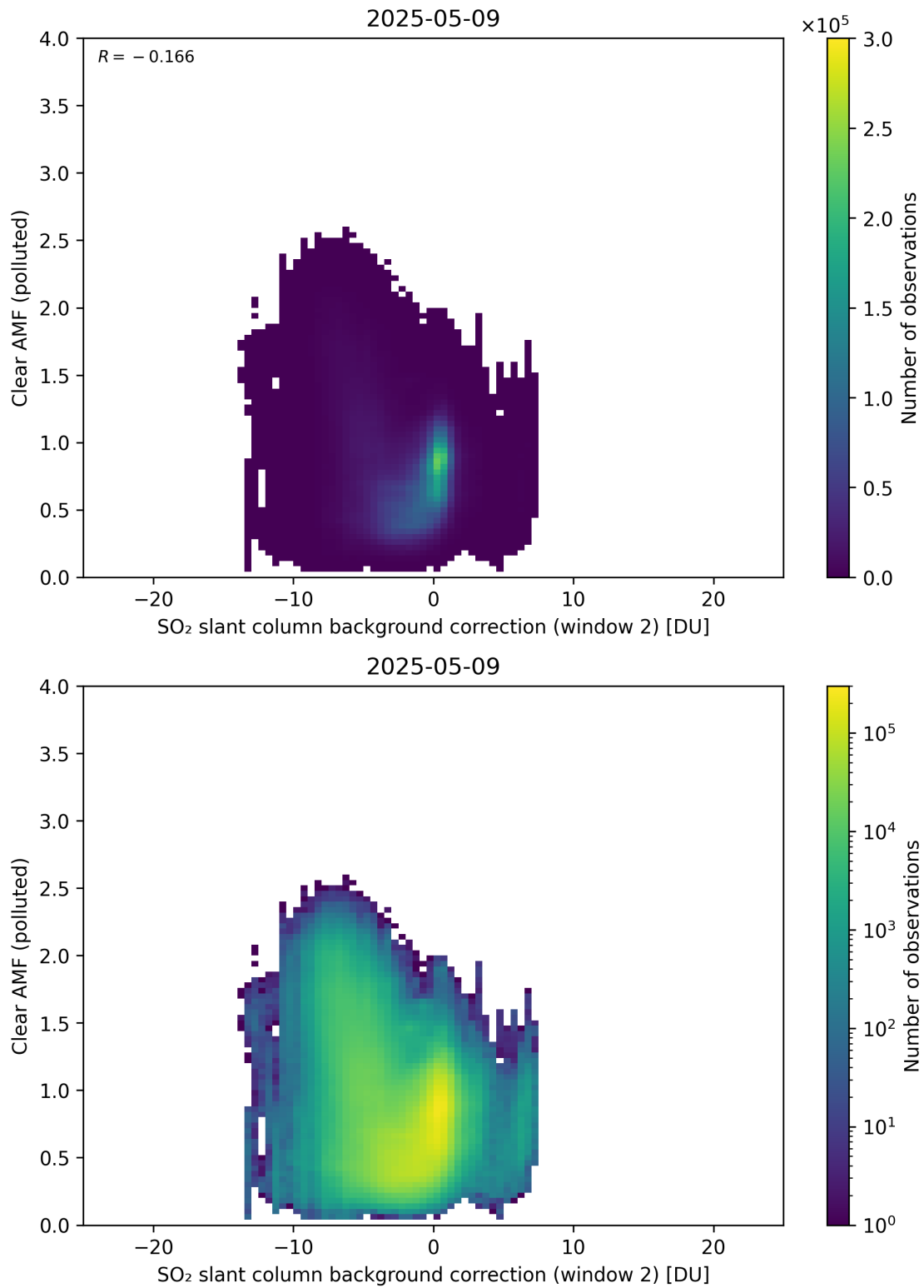
Figure 126: Scatter density plot of “SO 2 slant column background correction (window 2)” against “Clear AMF (polluted)” for 2025-05-08 to 2025-05-10.
