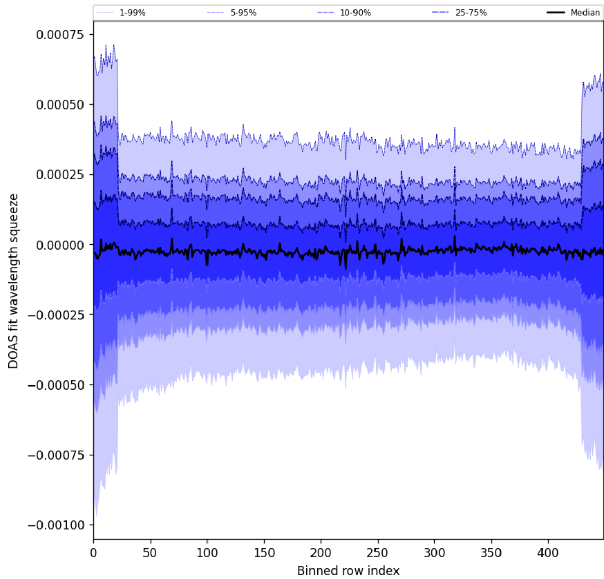
Figure 103: Along track statistics of “DOAS fit wavelength squeeze” for 2025-05-08 to 2025-05-10
