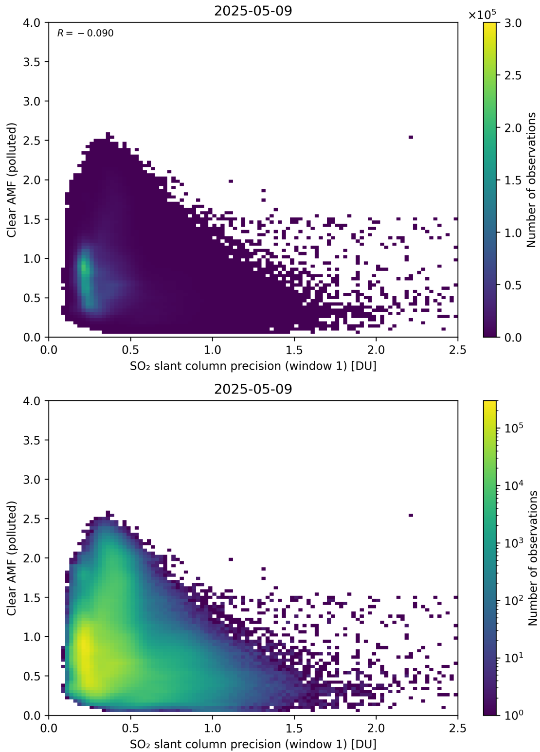
Figure 274: Scatter density plot of “SO 2 slant column precision (window 1)” against “Clear AMF (polluted)” for 2025-05-08 to 2025-05-10.
