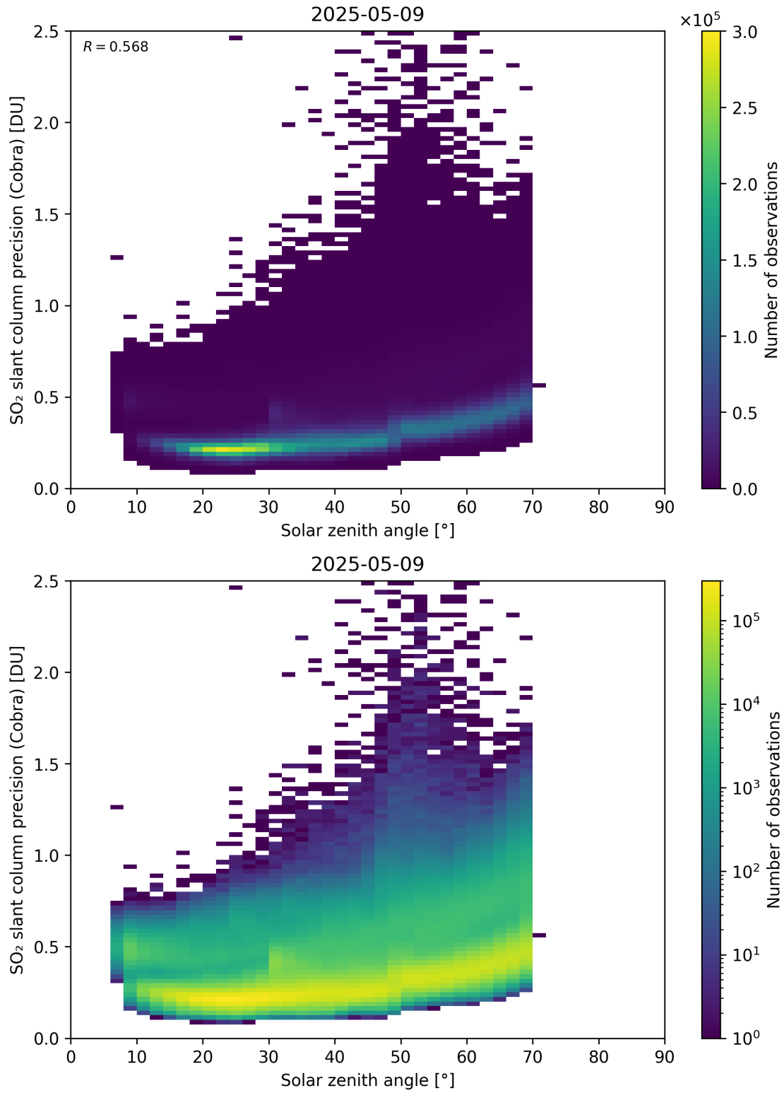
Figure 180: Scatter density plot of “Solar zenith angle” against “SO 2 slant column precision (Cobra)” for 2025-05-08 to 2025-05-10.
