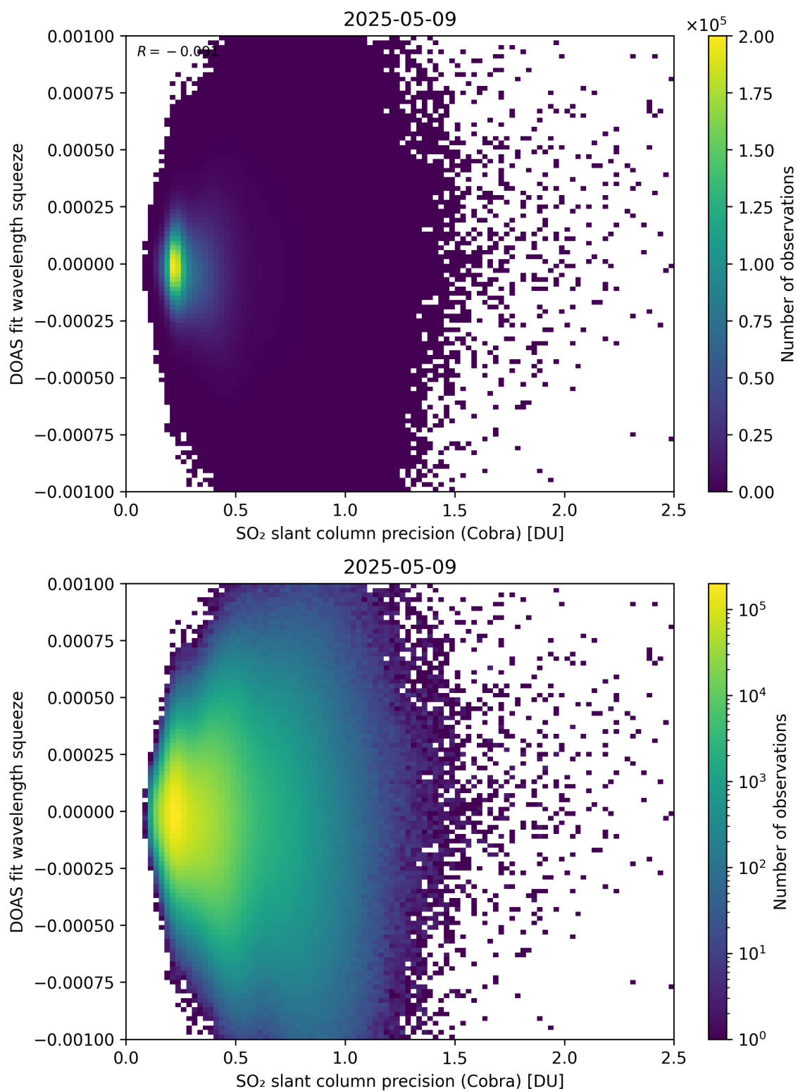
Figure 203: Scatter density plot of “SO 2 slant column precision (Cobra)” against “DOAS fit wavelength squeeze” for 2025-05-08 to 2025-05-10.
