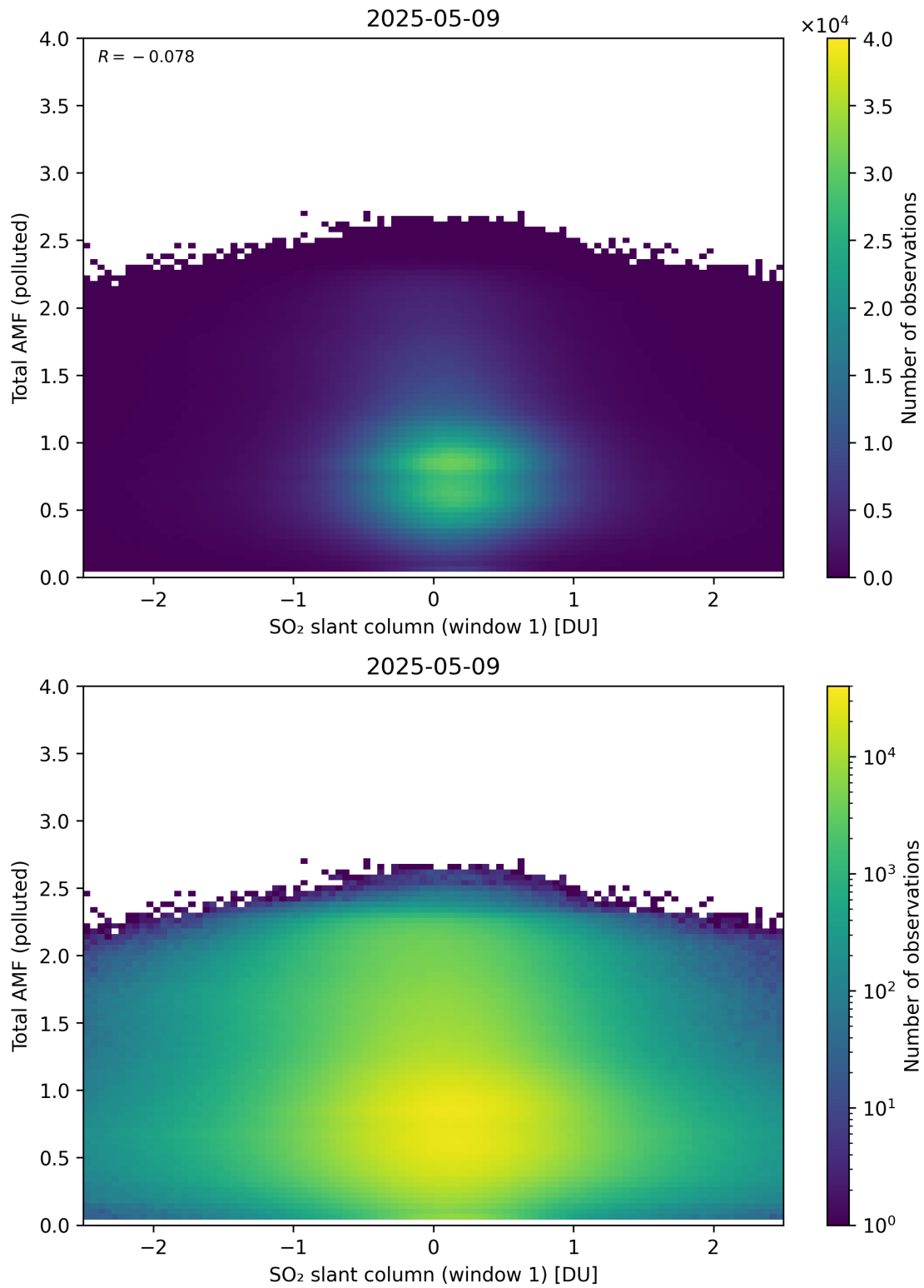
Figure 289: Scatter density plot of “SO 2 slant column (window 1)” against “Total AMF (polluted)” for 2025-05-08 to 2025-05-10.
