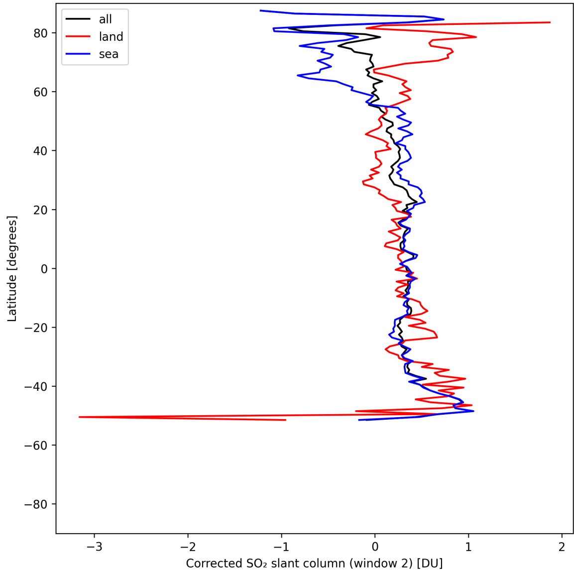
Figure 43: Zonal average of “Corrected SO 2 slant column (window 2)” for 2025-05-08 to 2025-05-10.
