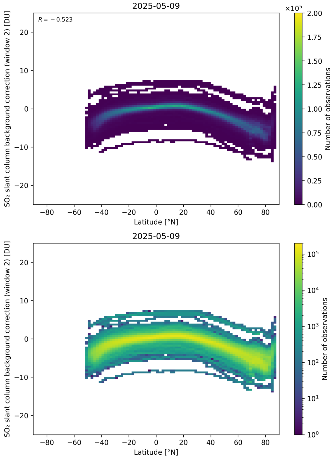
Figure 151: Scatter density plot of “Latitude” against “SO 2 slant column background correction (window 2)” for 2025-05-08 to 2025-05-10.
