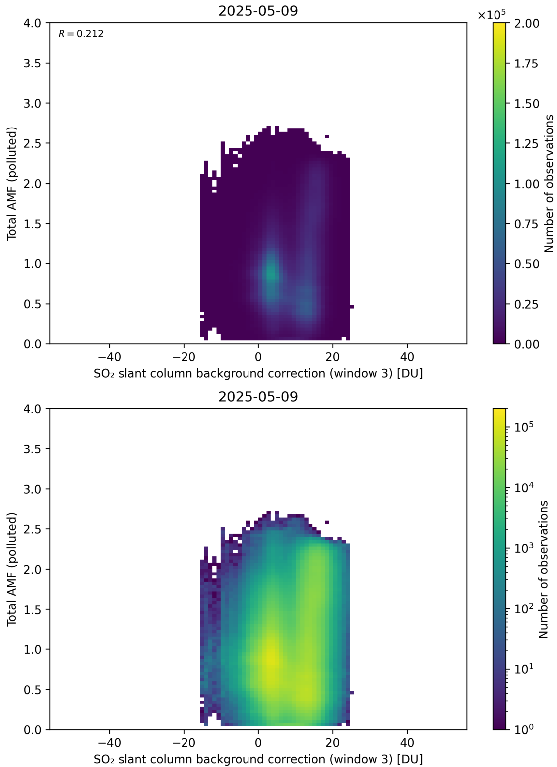
Figure 136: Scatter density plot of “SO 2 slant column background correction (window 3)” against “Total AMF (polluted)” for 2025-05-08 to 2025-05-10.
