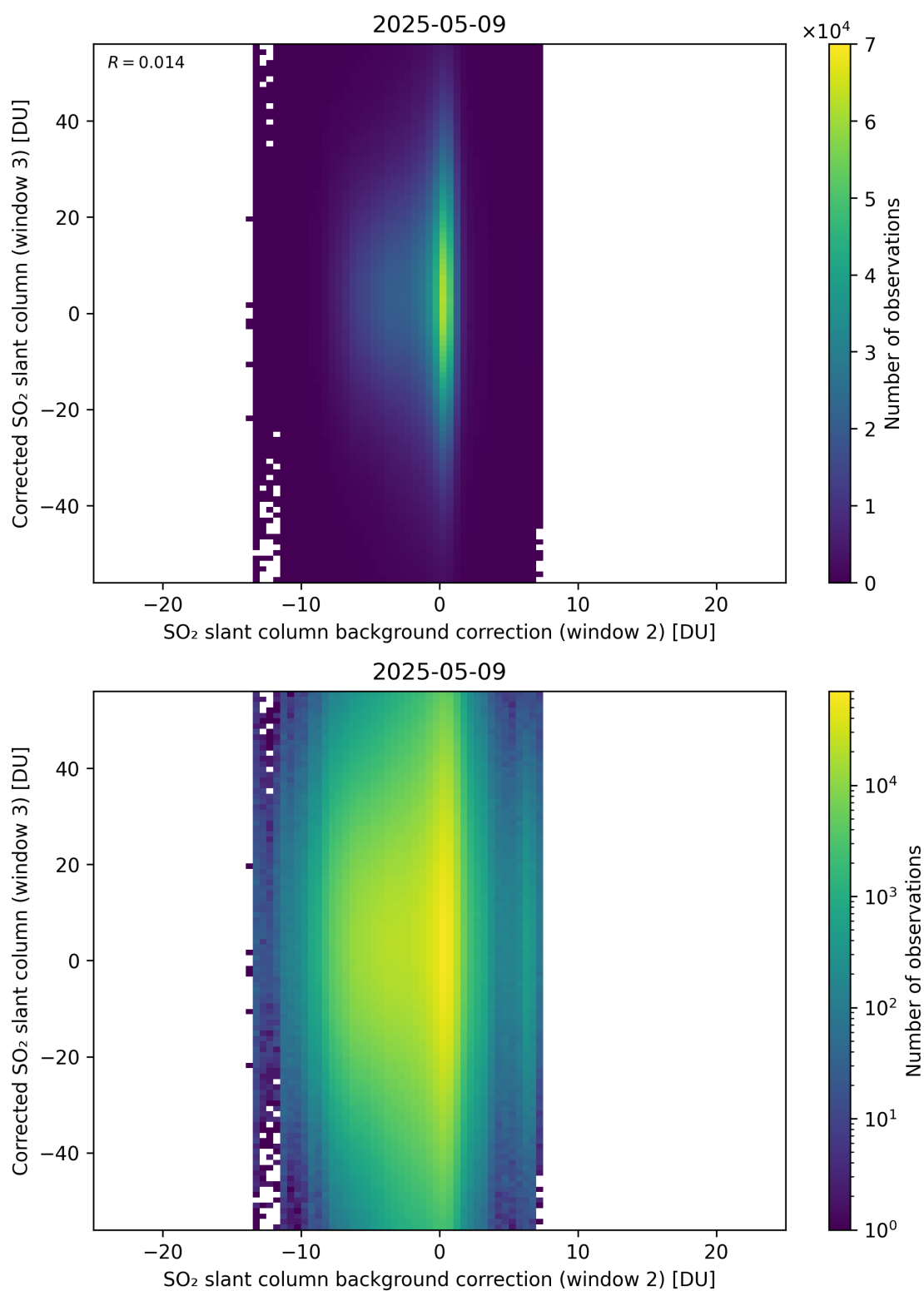
Figure 127: Scatter density plot of “SO 2 slant column background correction (window 2)” against “Corrected SO 2 slant column (window 3)” for 2025-05-08 to 2025-05-10.
