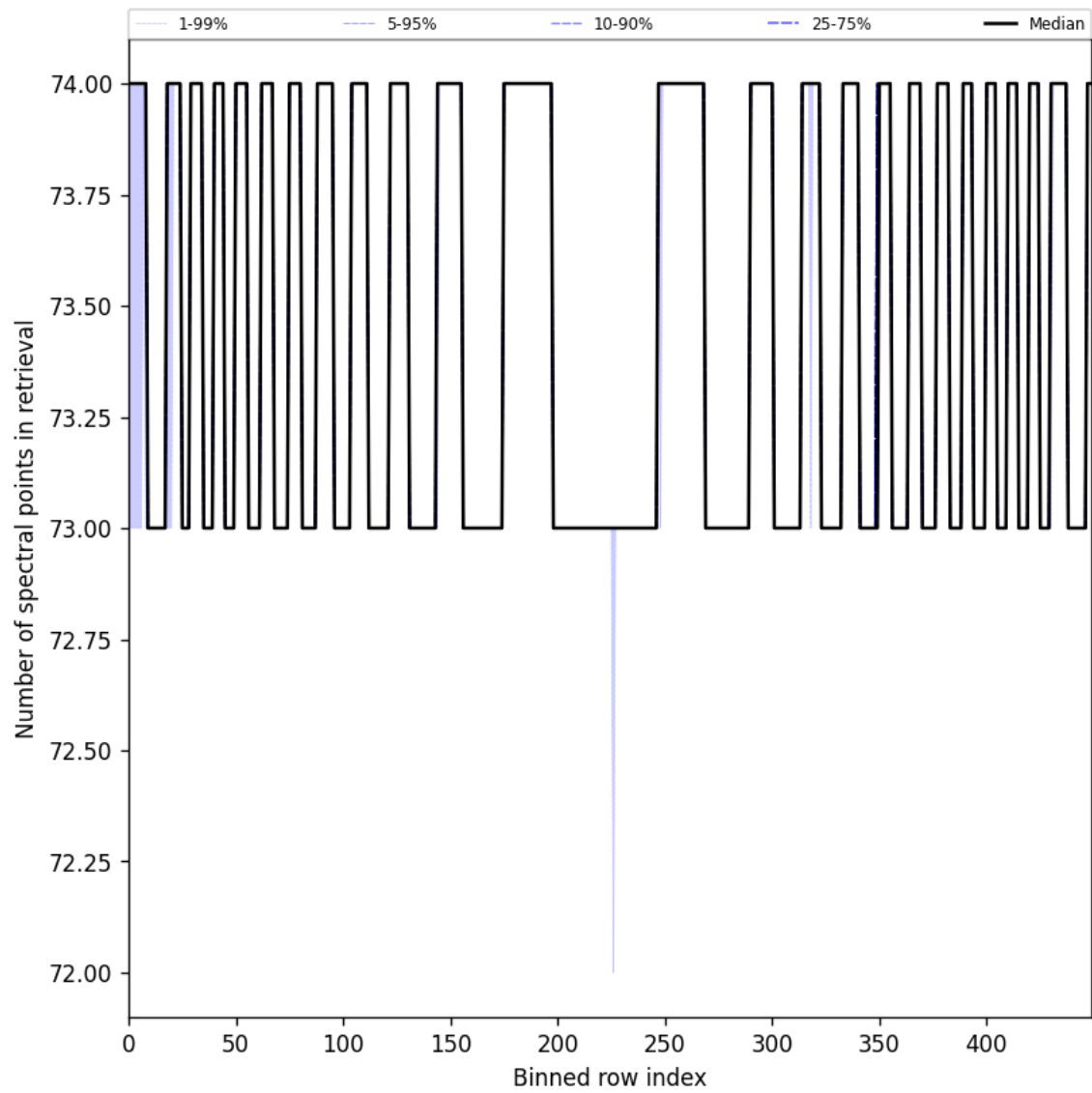
Figure 108: Along track statistics of “Number of spectral points in retrieval” for 2025-05-08 to 2025-05-10
