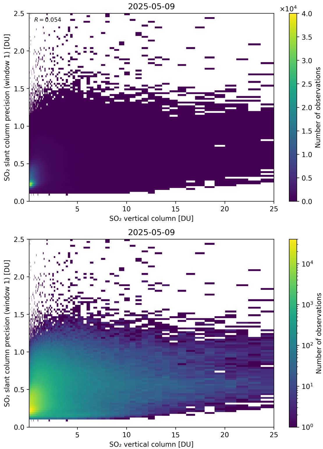
Figure 355: Scatter density plot of “SO 2 vertical column” against “SO 2 slant column precision (window 1)” for 2025-05-08 to 2025-05-10.
