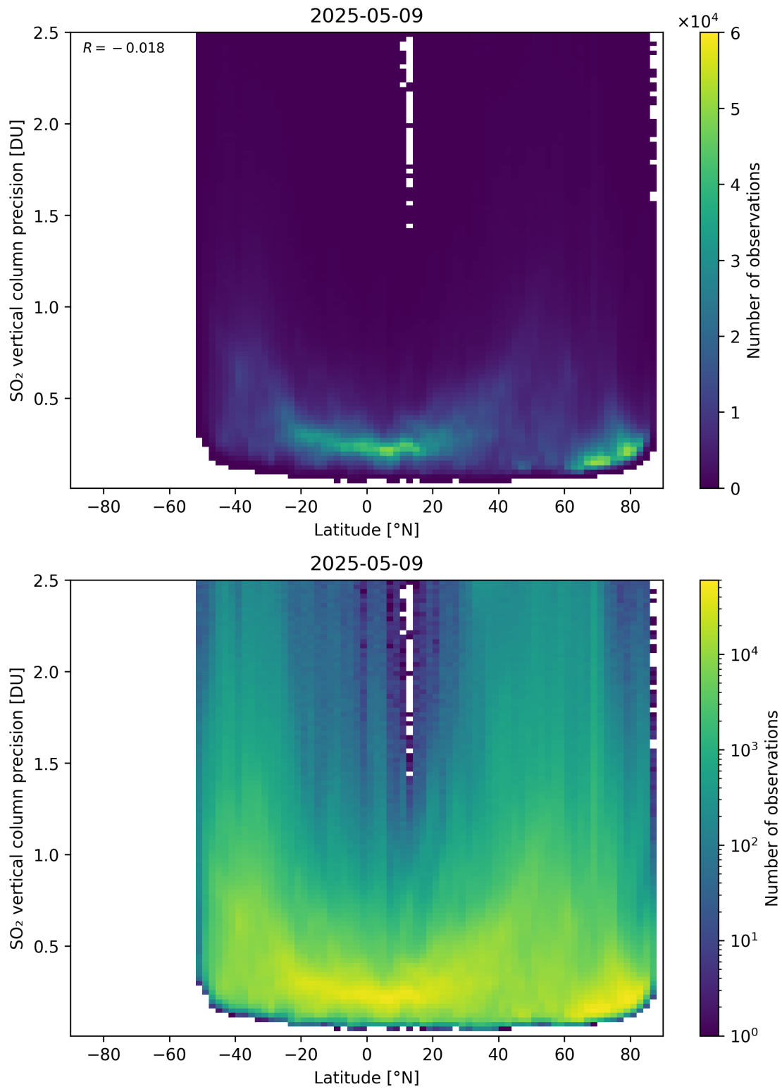
Figure 170: Scatter density plot of “Latitude” against “SO 2 vertical column precision” for 2025-05-08 to 2025-05-10.
