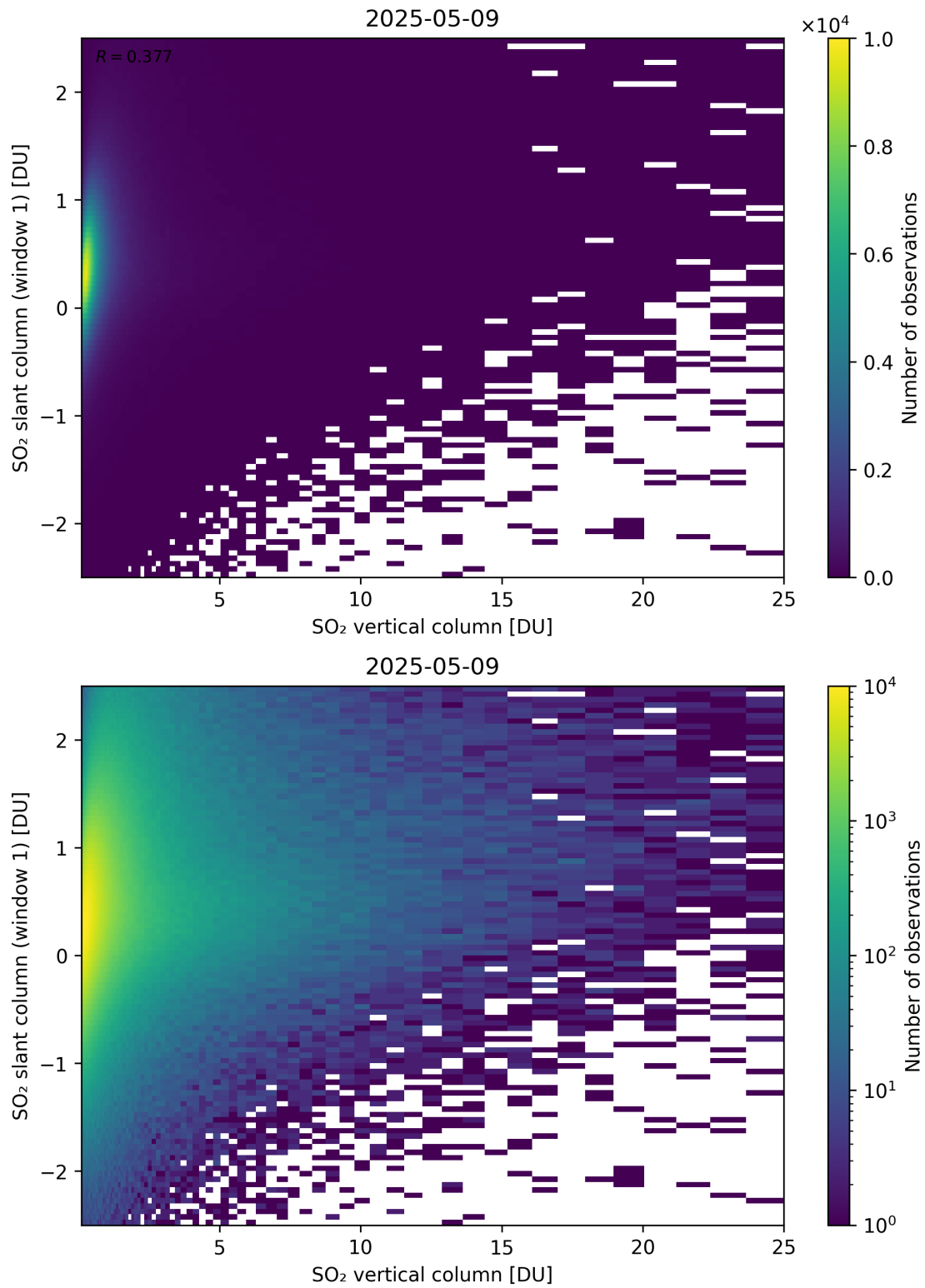
Figure 354: Scatter density plot of “SO 2 vertical column” against “SO 2 slant column (window 1)” for 2025-05-08 to 2025-05-10.
