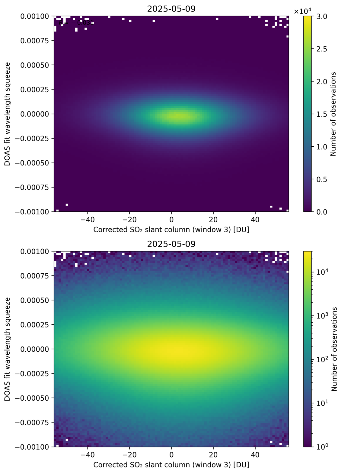
Figure 257: Scatter density plot of “Corrected SO 2 slant column (window 3)” against “DOAS fit wavelength squeeze” for 2025-05-08 to 2025-05-10.
