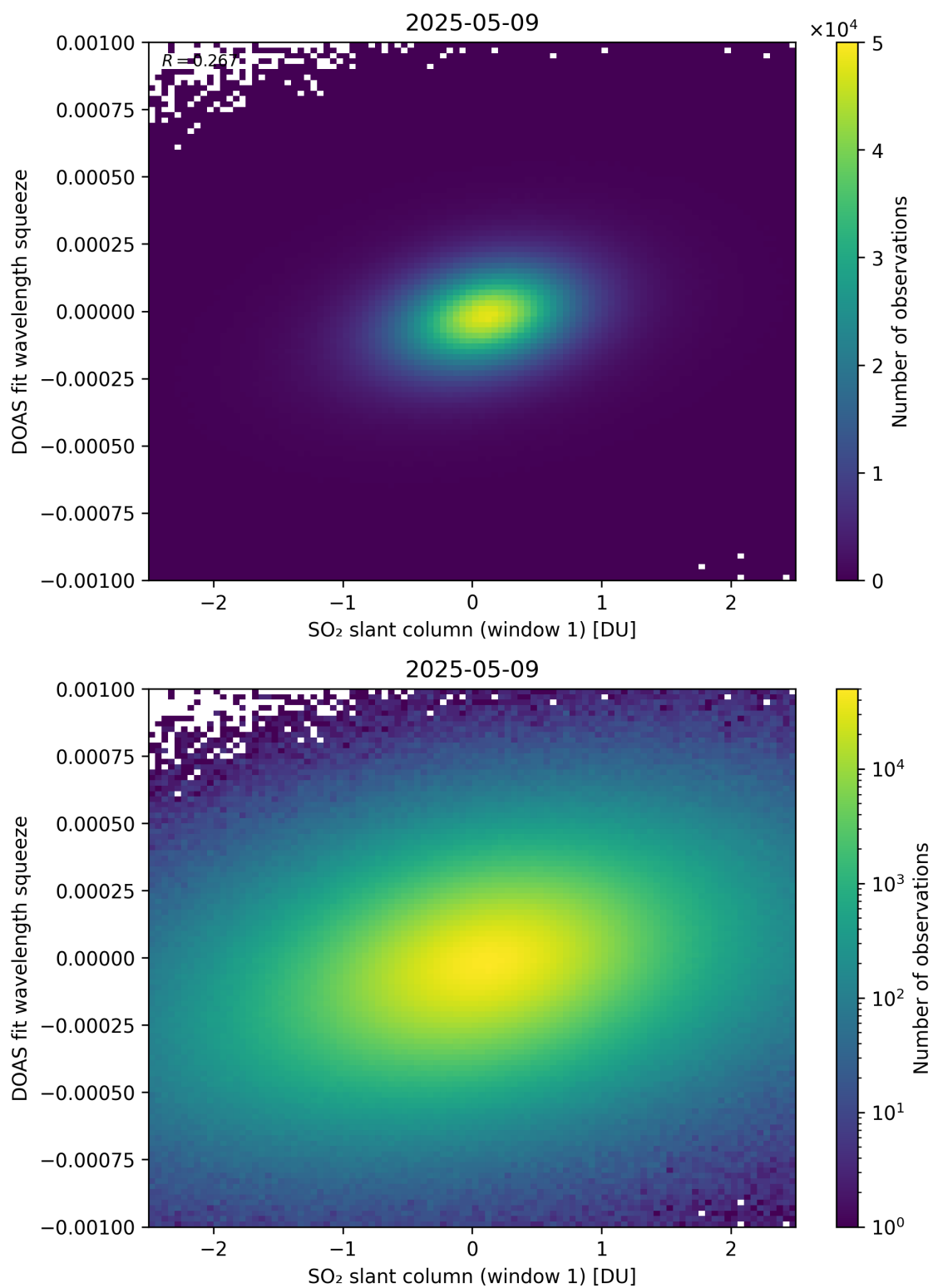
Figure 266: Scatter density plot of “SO 2 slant column (window 1)” against “DOAS fit wavelength squeeze” for 2025-05-08 to 2025-05-10.
