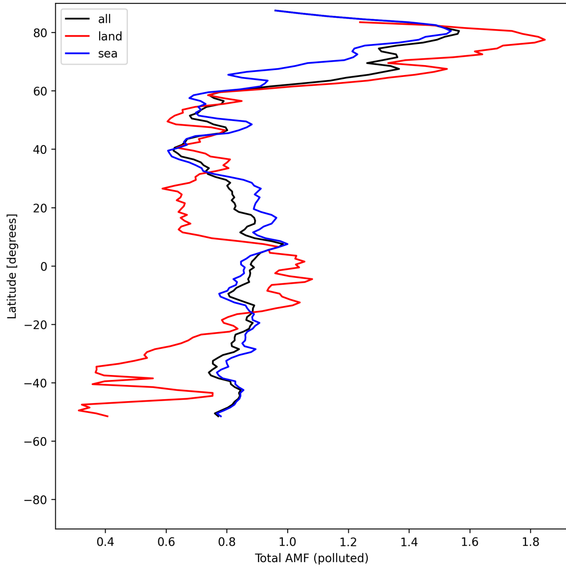
Figure 53: Zonal average of “Total AMF (polluted)” for 2025-05-08 to 2025-05-10.
