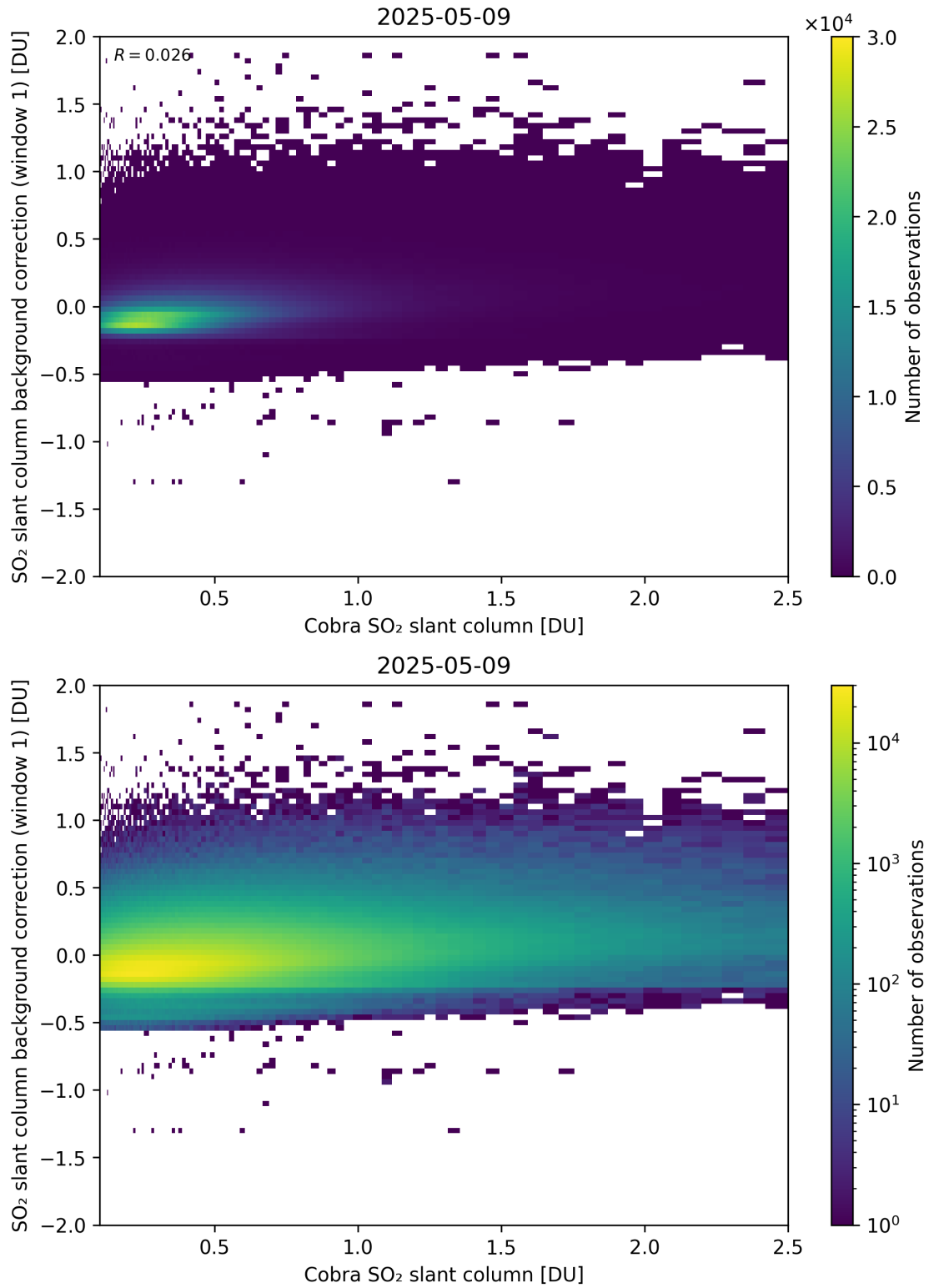
Figure 193: Scatter density plot of “Cobra SO 2 slant column” against “SO 2 slant column background correction (window 1)” for 2025-05-08 to 2025-05-10.
