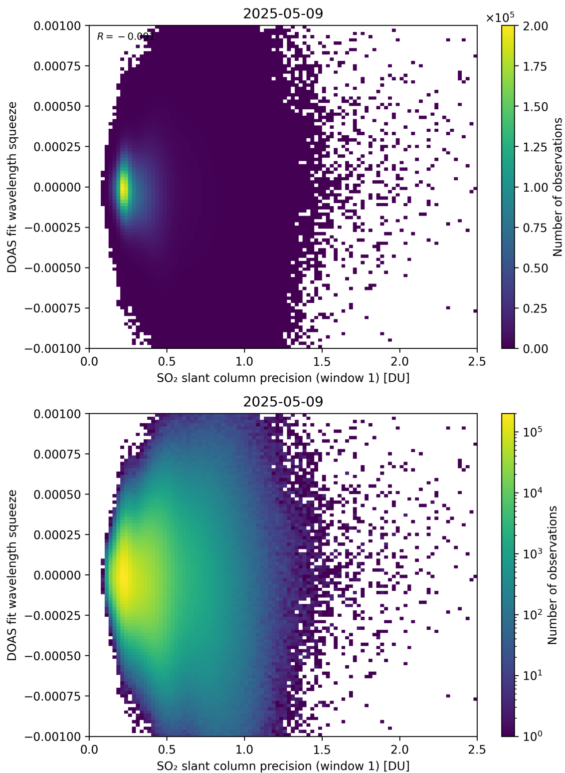
Figure 272: Scatter density plot of “SO 2 slant column precision (window 1)” against “DOAS fit wavelength squeeze” for 2025-05-08 to 2025-05-10.
