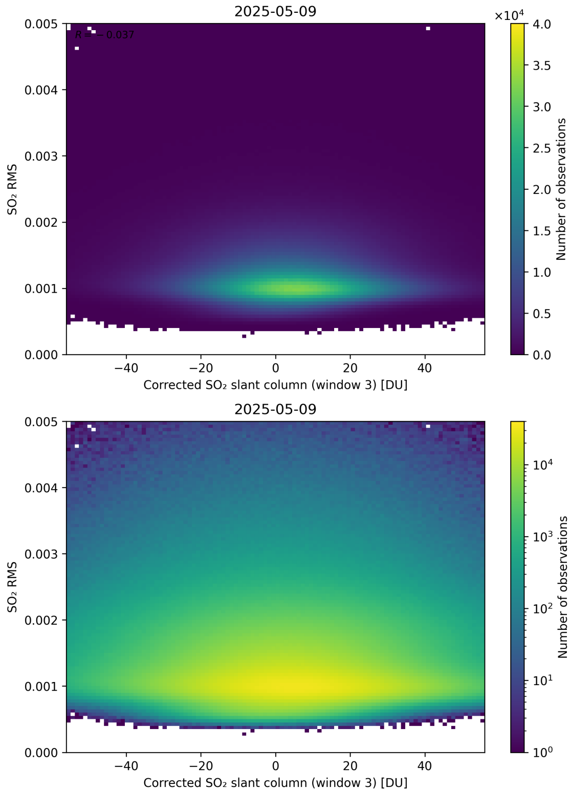
Figure 258: Scatter density plot of “Corrected SO 2 slant column (window 3)” against “SO 2 RMS” for 2025-05-08 to 2025-05-10.
