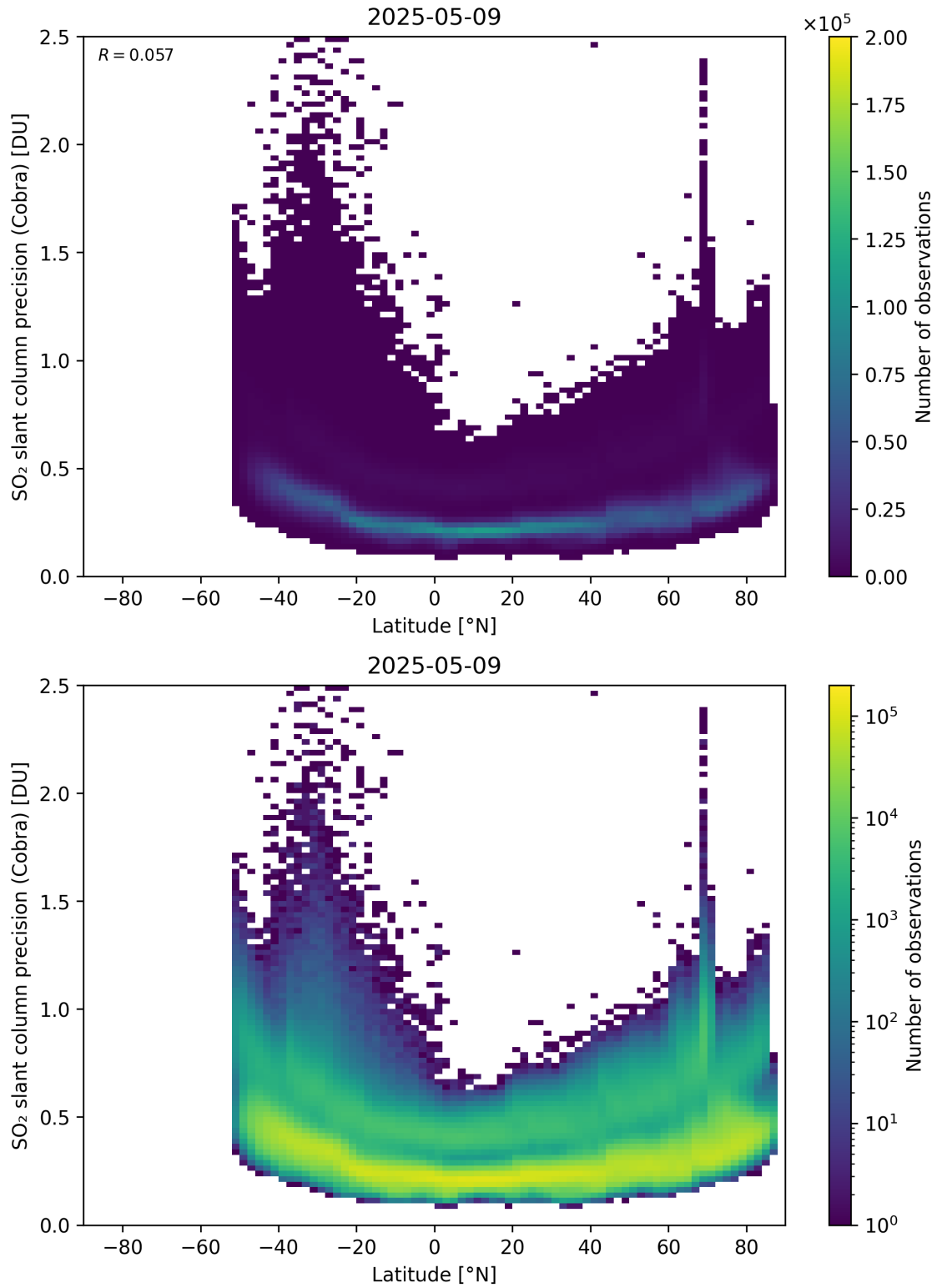
Figure 158: Scatter density plot of “Latitude” against “SO 2 slant column precision (Cobra)” for 2025-05-08 to 2025-05-10.
