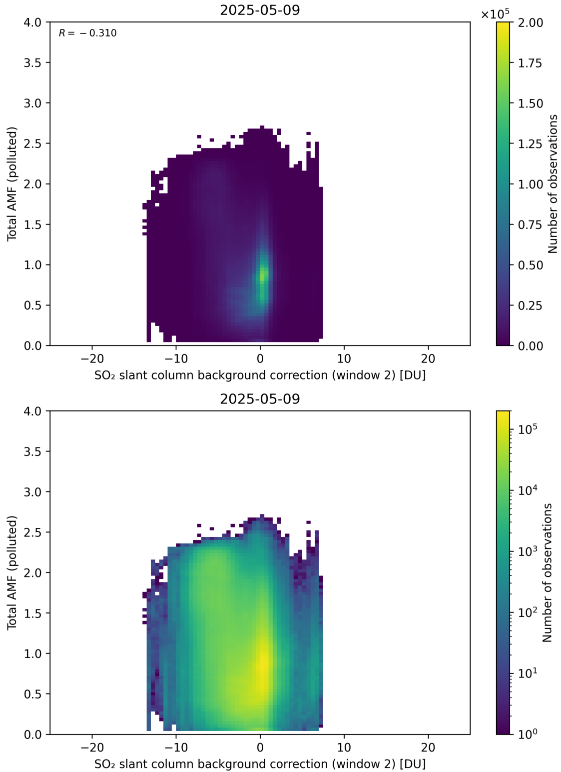
Figure 130: Scatter density plot of “SO 2 slant column background correction (window 2)” against “Total AMF (polluted)” for 2025-05-08 to 2025-05-10.
