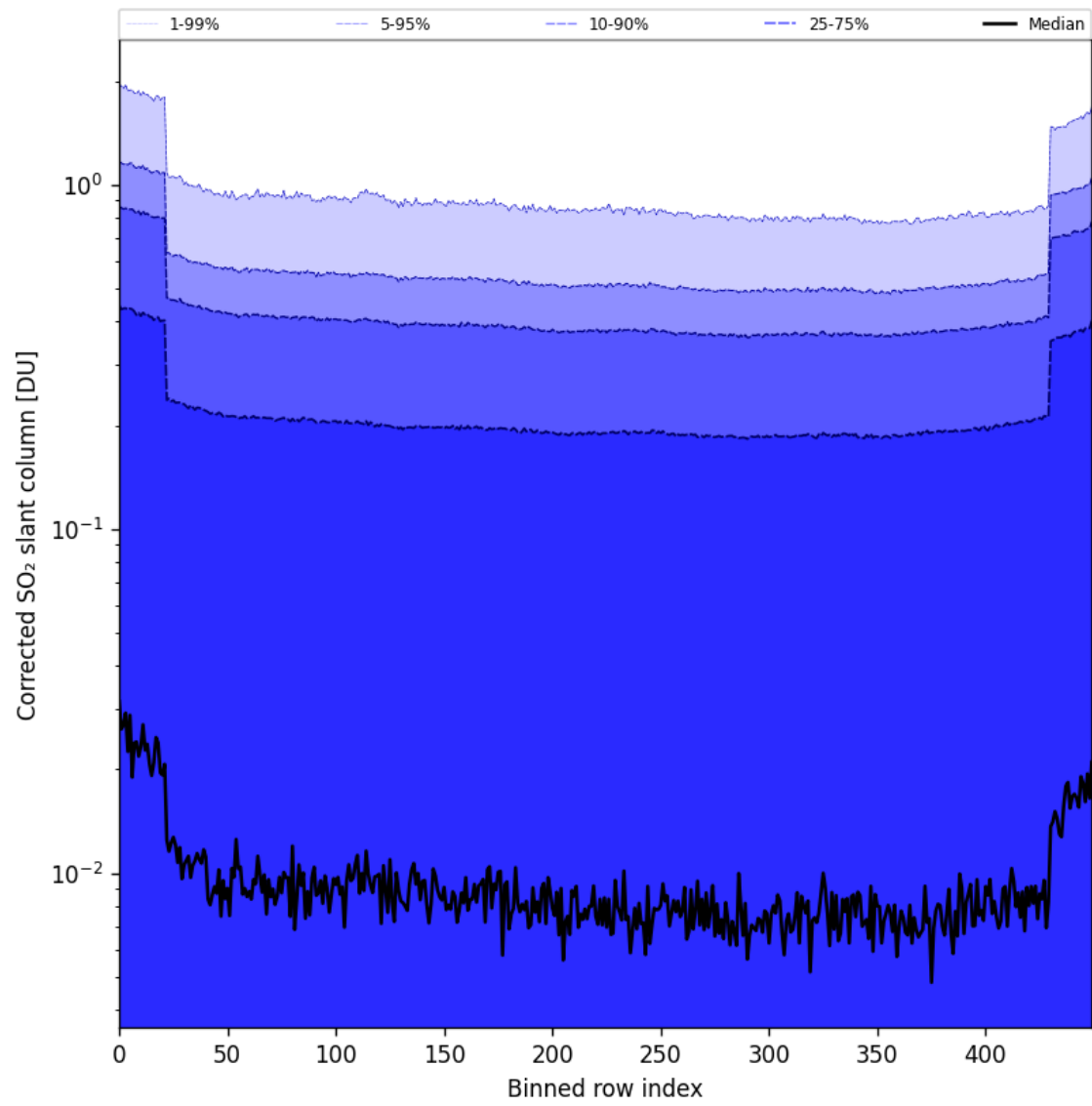
Figure 86: Along track statistics of “Corrected SO 2 slant column” for 2025-05-08 to 2025-05-10
