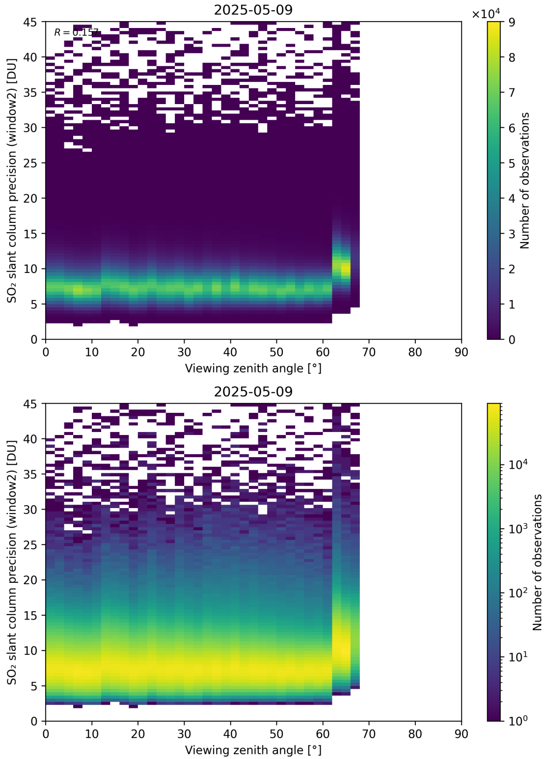
Figure 378: Scatter density plot of “Viewing zenith angle” against “SO 2 slant column precision (window2)” for 2025-05-08 to 2025-05-10.
