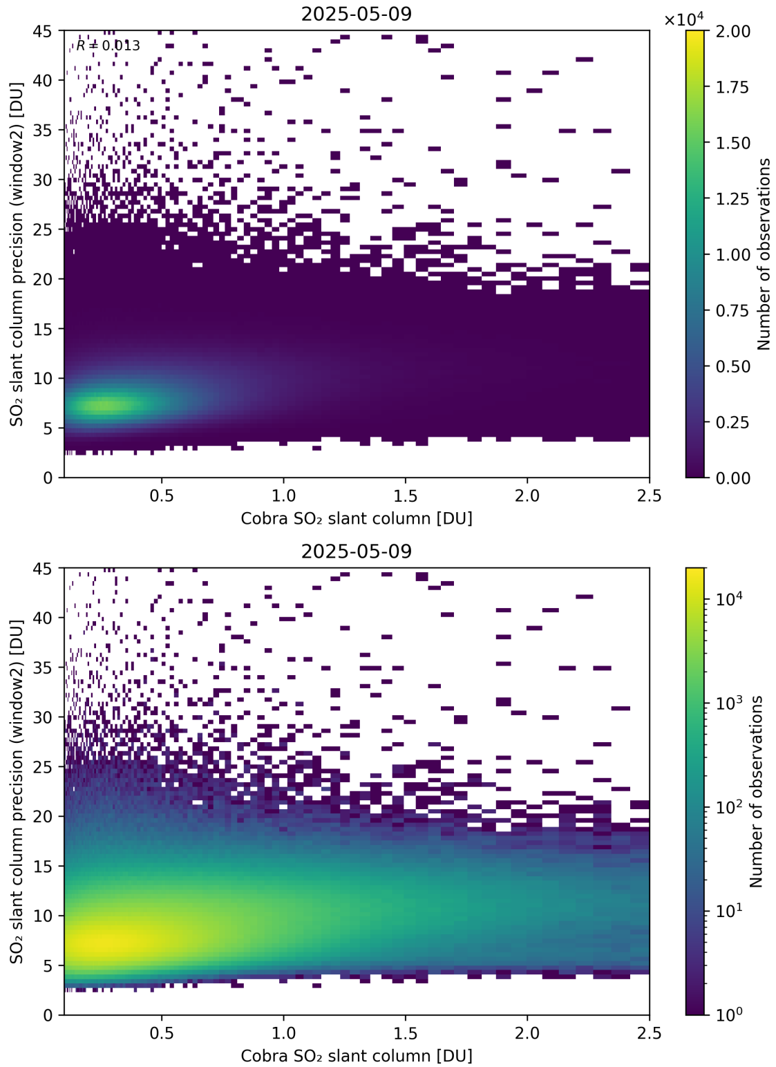
Figure 221: Scatter density plot of “Cobra SO 2 slant column” against “SO 2 slant column precision (window2)” for 2025-05-08 to 2025-05-10.
