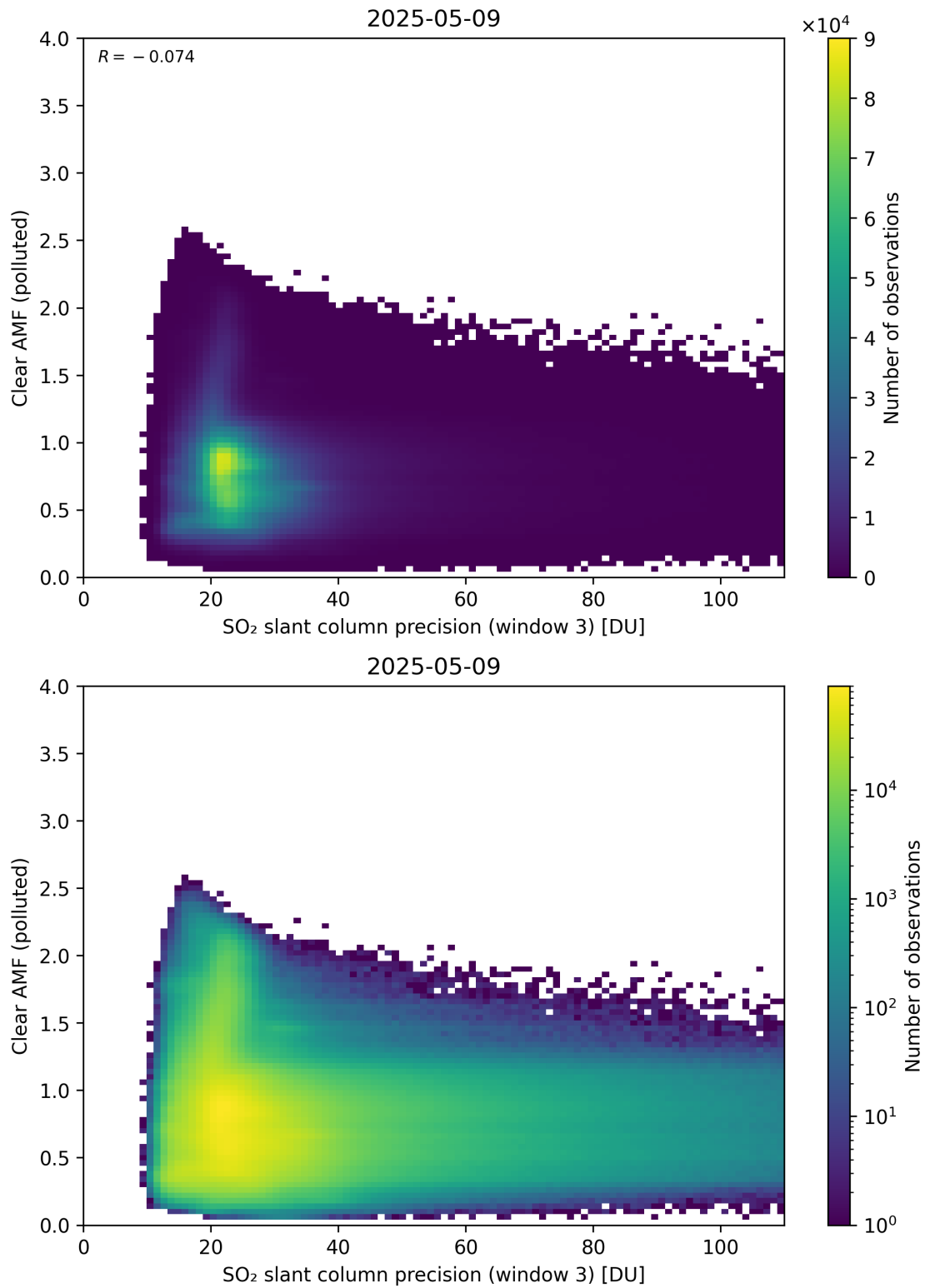
Figure 311: Scatter density plot of “SO 2 slant column precision (window 3)” against “Clear AMF (polluted)” for 2025-05-08 to 2025-05-10.
