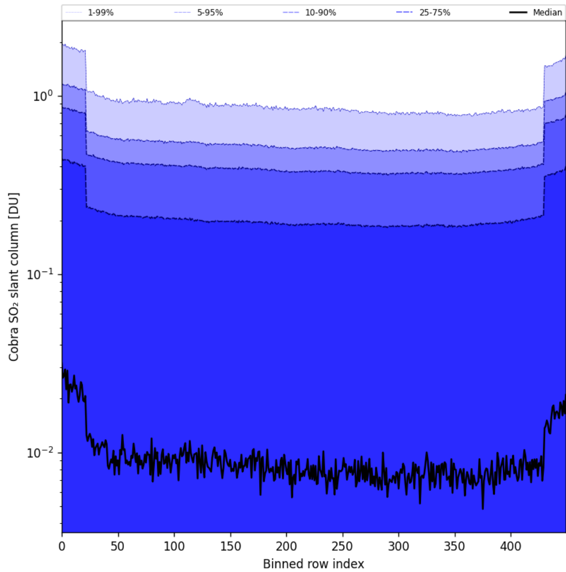
Figure 87: Along track statistics of "Cobra SO 2 slant column" for 2025-05-08 to 2025-05-10
