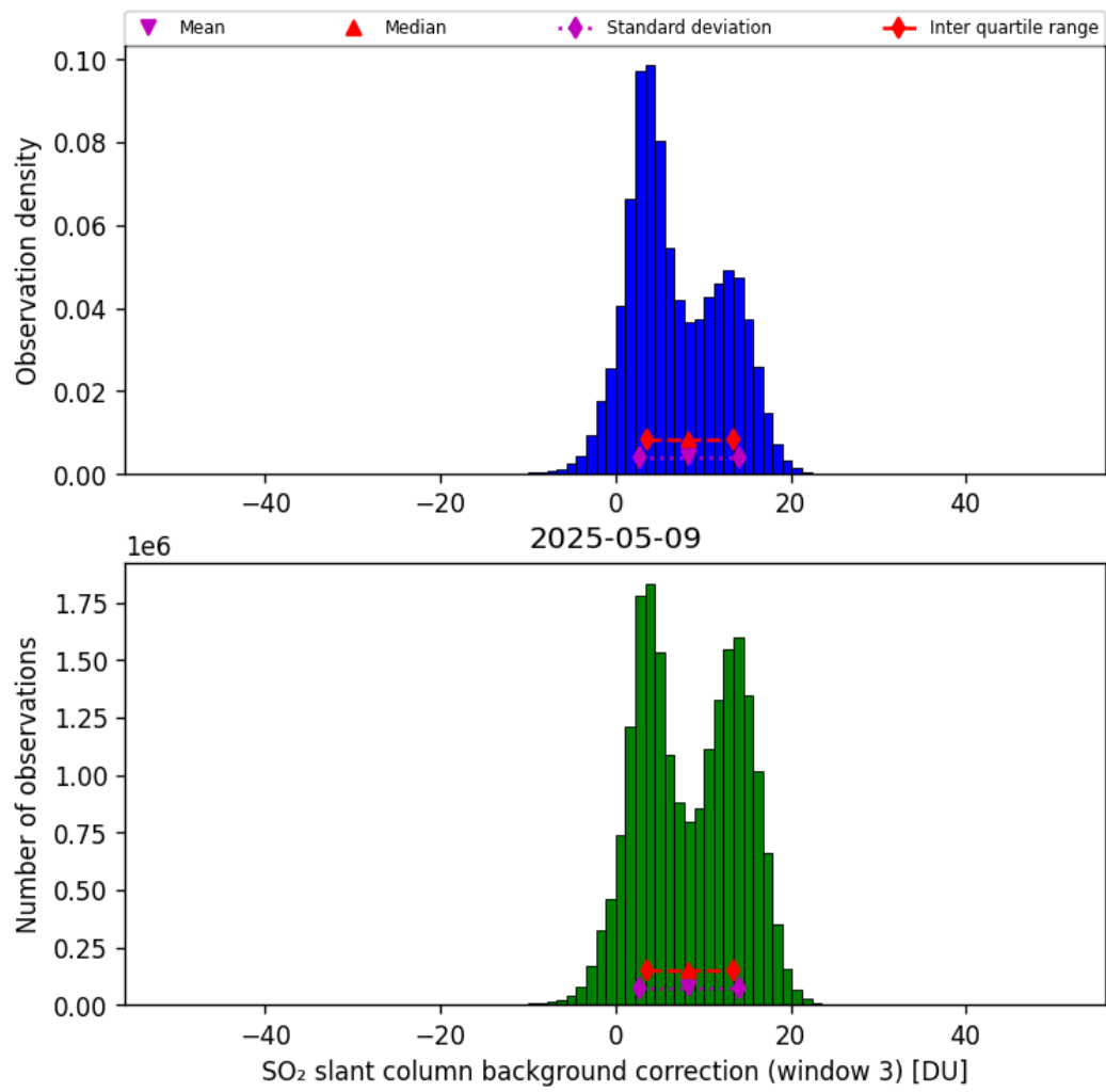
Figure 74: Histogram of “SO 2 slant column background correction (window 3)” for 2025-05-08 to 2025-05-10
