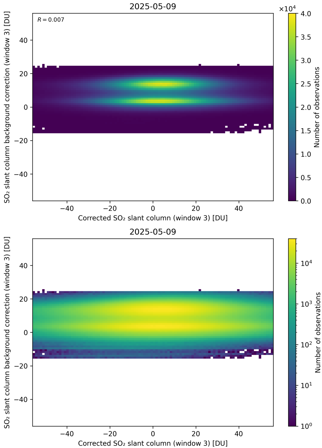
Figure 255: Scatter density plot of “Corrected SO 2 slant column (window 3)” against “SO 2 slant column background correction (window 3)” for 2025-05-08 to 2025-05-10.
