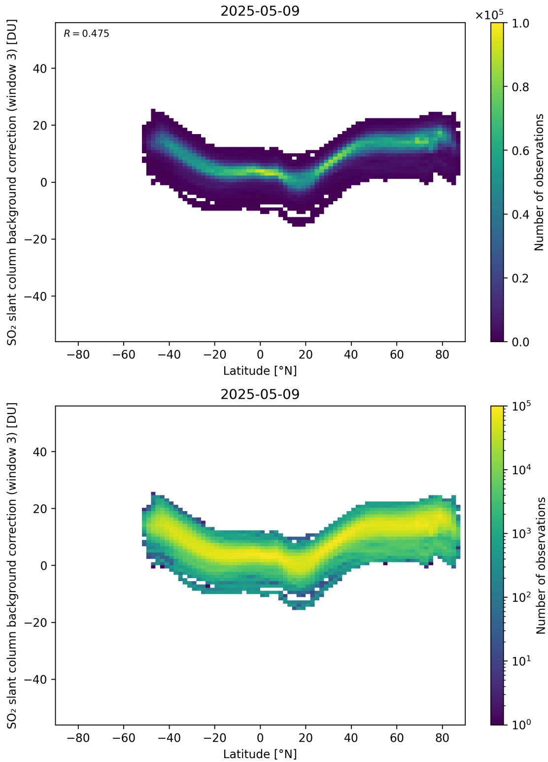
Figure 152: Scatter density plot of “Latitude” against “SO 2 slant column background correction (window 3)” for 2025-05-08 to 2025-05-10.
