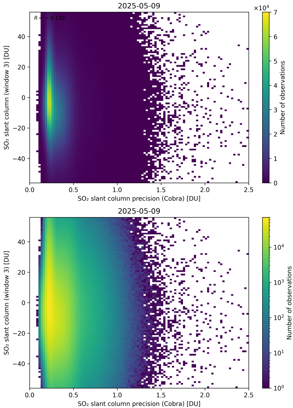
Figure 211: Scatter density plot of “SO 2 slant column precision (Cobra)” against “SO 2 slant column (window 3)” for 2025-05-08 to 2025-05-10.
