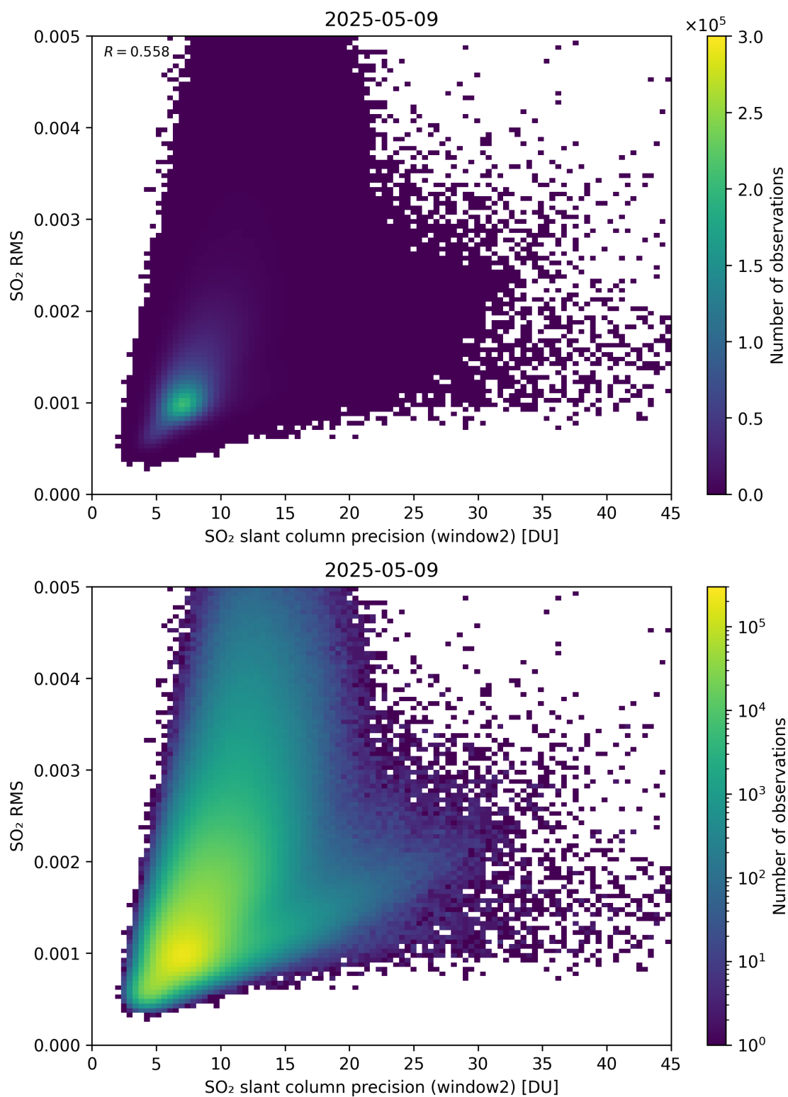
Figure 295: Scatter density plot of “SO 2 slant column precision (window2)” against “SO 2 RMS” for 2025-05-08 to 2025-05-10.
