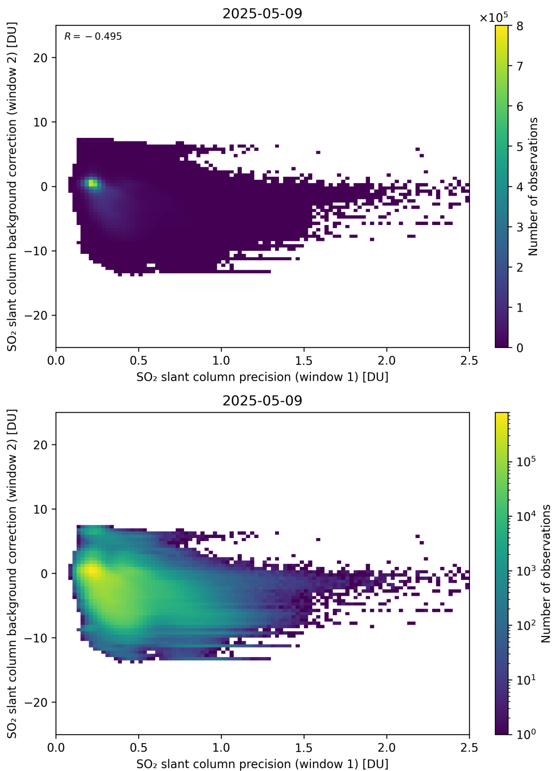
Figure 269: Scatter density plot of “SO 2 slant column precision (window 1)” against “SO 2 slant column background correction (window 2)” for 2025-05-08 to 2025-05-10.
