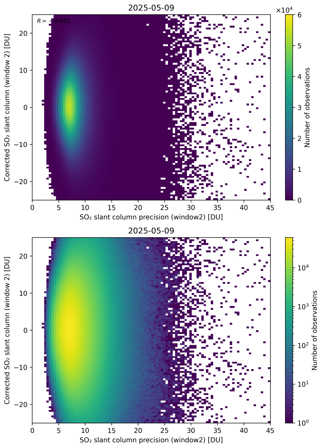
Figure 297: Scatter density plot of “SO 2 slant column precision (window2)” against “Corrected SO 2 slant column (window 2)” for 2025-05-08 to 2025-05-10.
