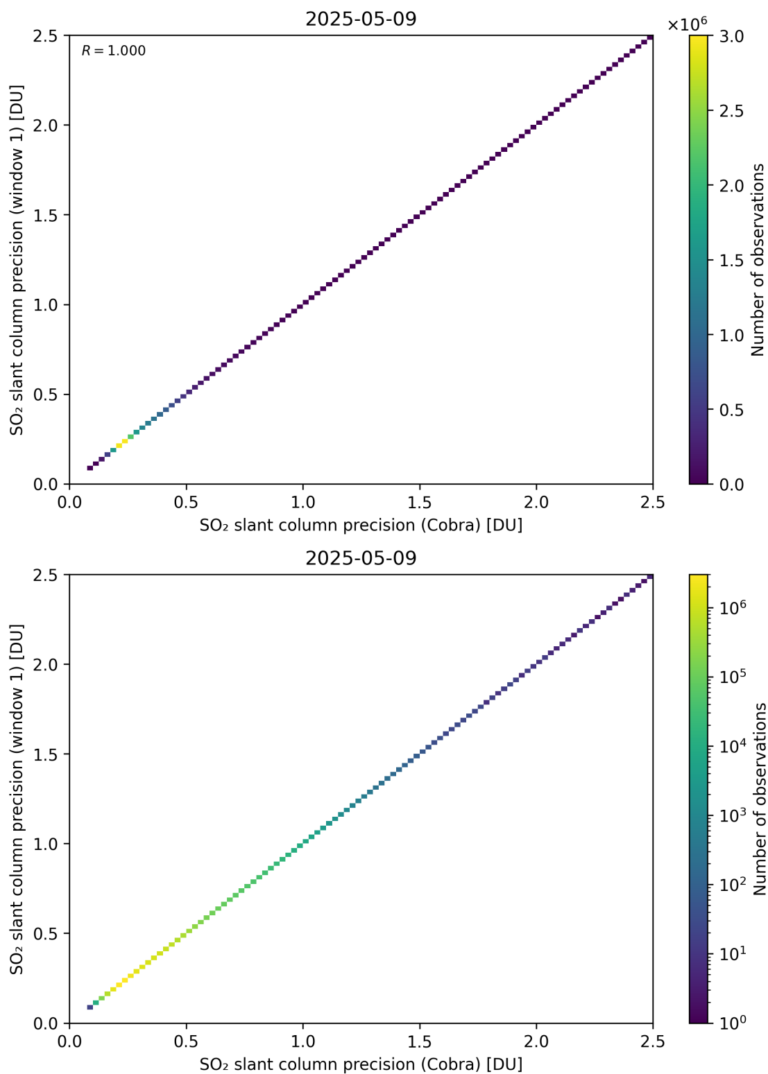
Figure 209: Scatter density plot of “SO 2 slant column precision (Cobra)” against “SO 2 slant column precision (window 1)” for 2025-05-08 to 2025-05-10.
