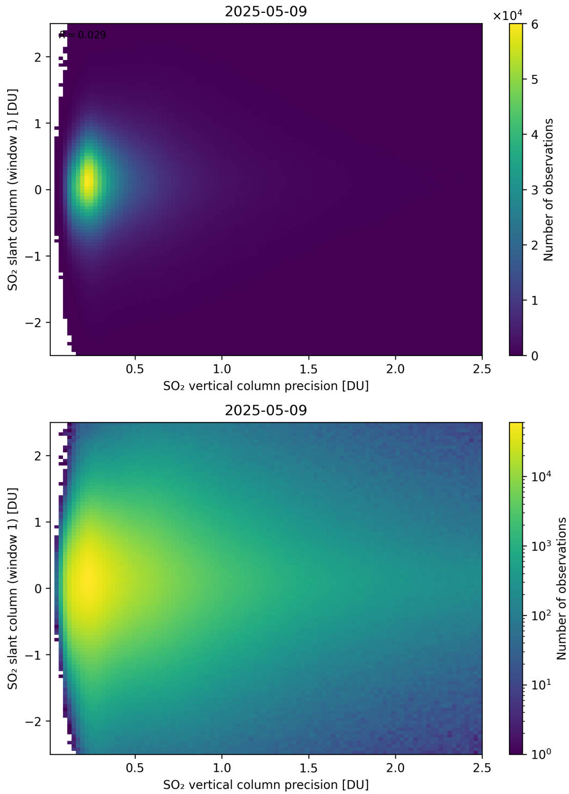
Figure 341: Scatter density plot of “SO 2 vertical column precision” against “SO 2 slant column (window 1)” for 2025-05-08 to 2025-05-10.
