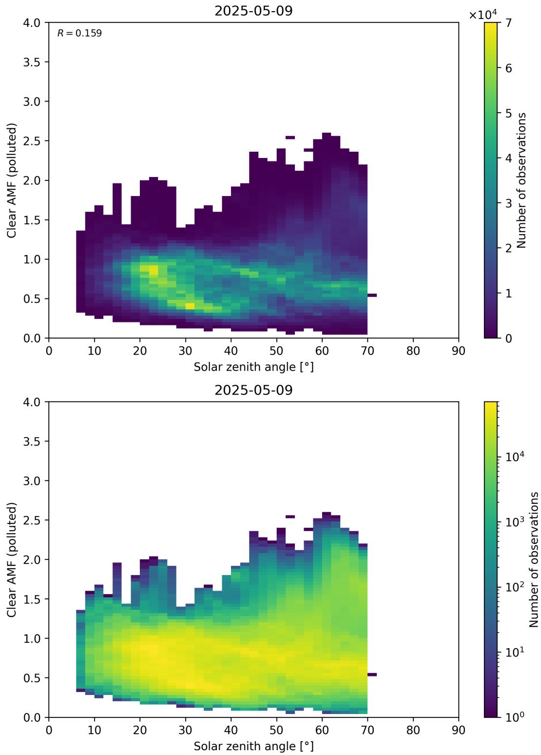
Figure 178: Scatter density plot of “Solar zenith angle” against “Clear AMF (polluted)” for 2025-05-08 to 2025-05-10.
