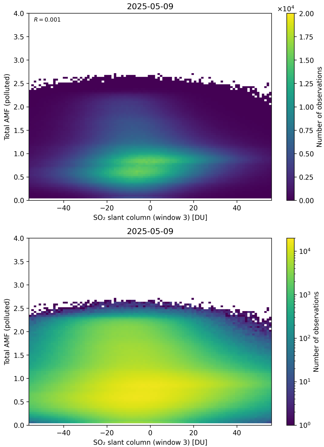
Figure 318: Scatter density plot of “SO 2 slant column (window 3)” against “Total AMF (polluted)” for 2025-05-08 to 2025-05-10.
