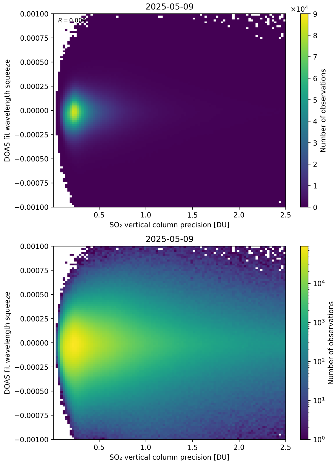
Figure 333: Scatter density plot of “SO 2 vertical column precision” against “DOAS fit wavelength squeeze” for 2025-05-08 to 2025-05-10.
