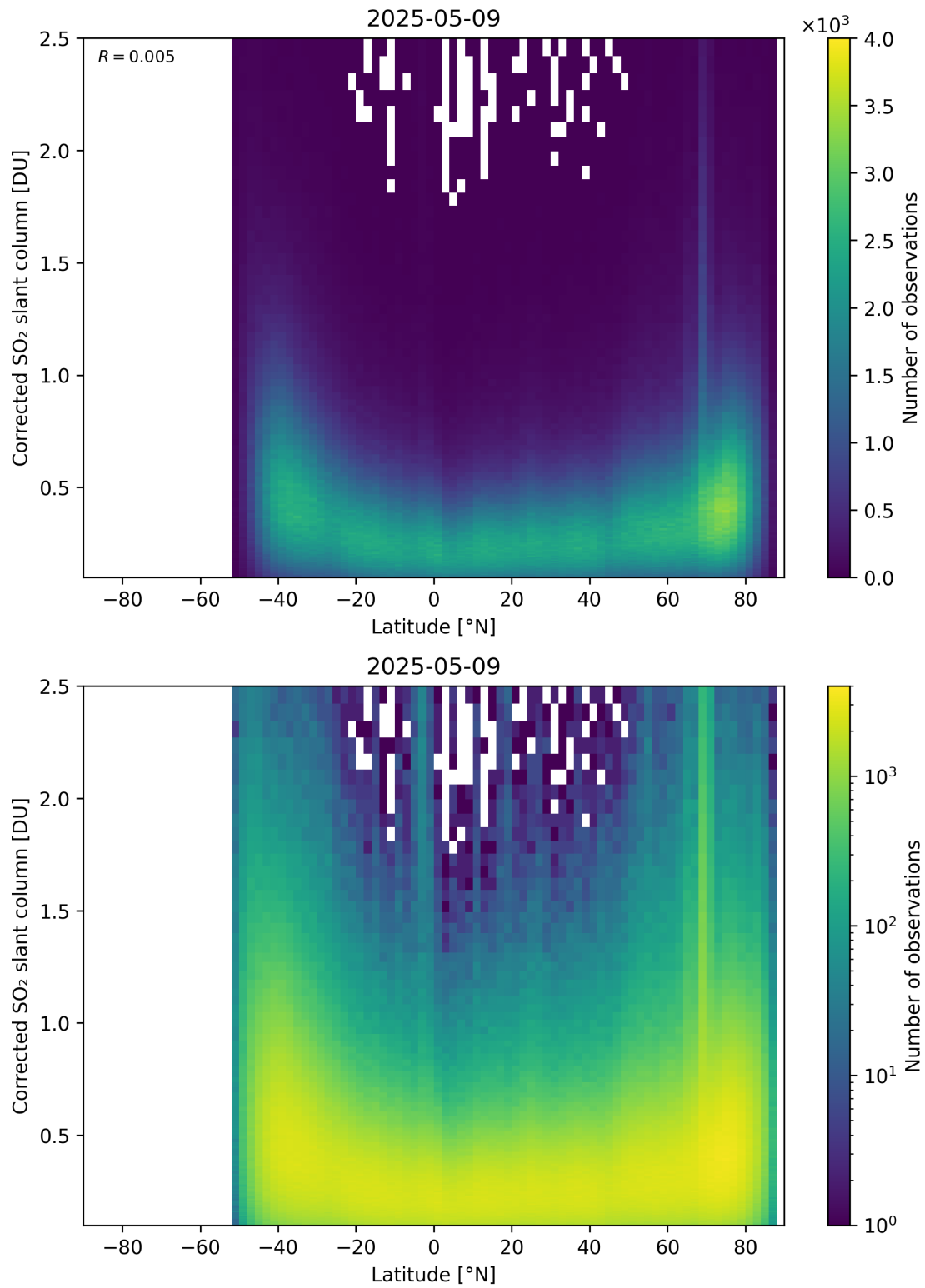
Figure 159: Scatter density plot of “Latitude” against “Corrected SO 2 slant column” for 2025-05-08 to 2025-05-10.
