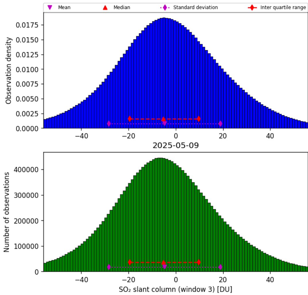
Figure 71: Histogram of “SO 2 slant column (window 3)” for 2025-05-08 to 2025-05-10
