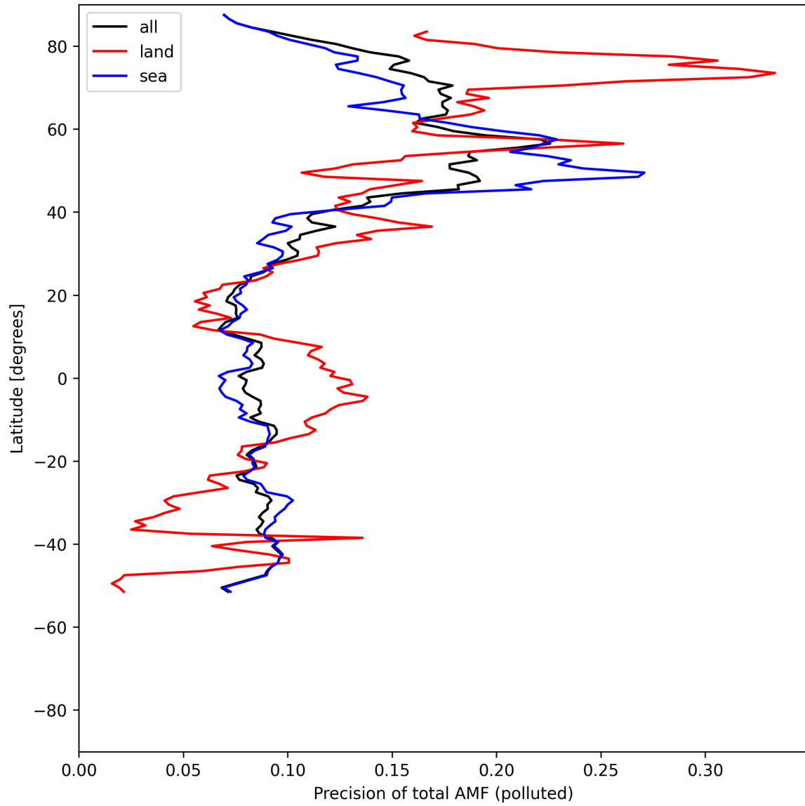
Figure 54: Zonal average of “Precision of total AMF (polluted)” for 2025-05-08 to 2025-05-10.
