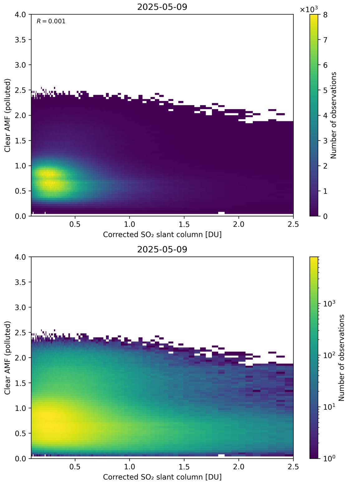
Figure 232: Scatter density plot of “Corrected SO 2 slant column” against “Clear AMF (polluted)” for 2025-05-08 to 2025-05-10.
