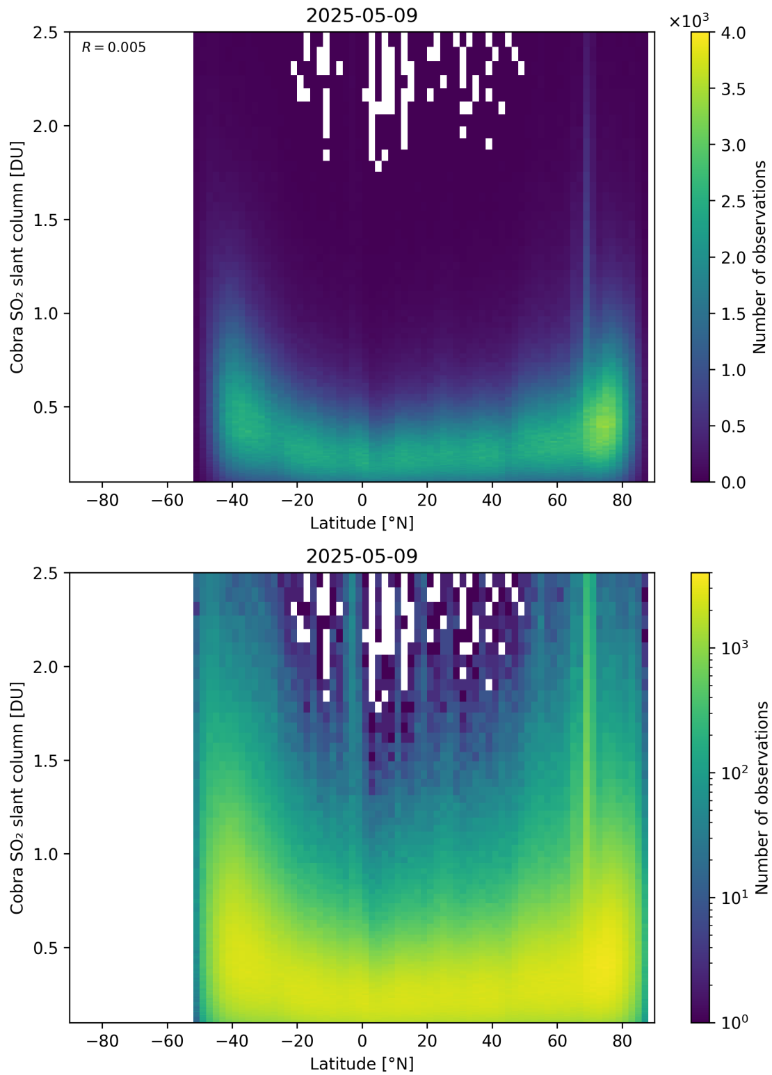
Figure 157: Scatter density plot of “Latitude” against “Cobra SO 2 slant column” for 2025-05-08 to 2025-05-10.
