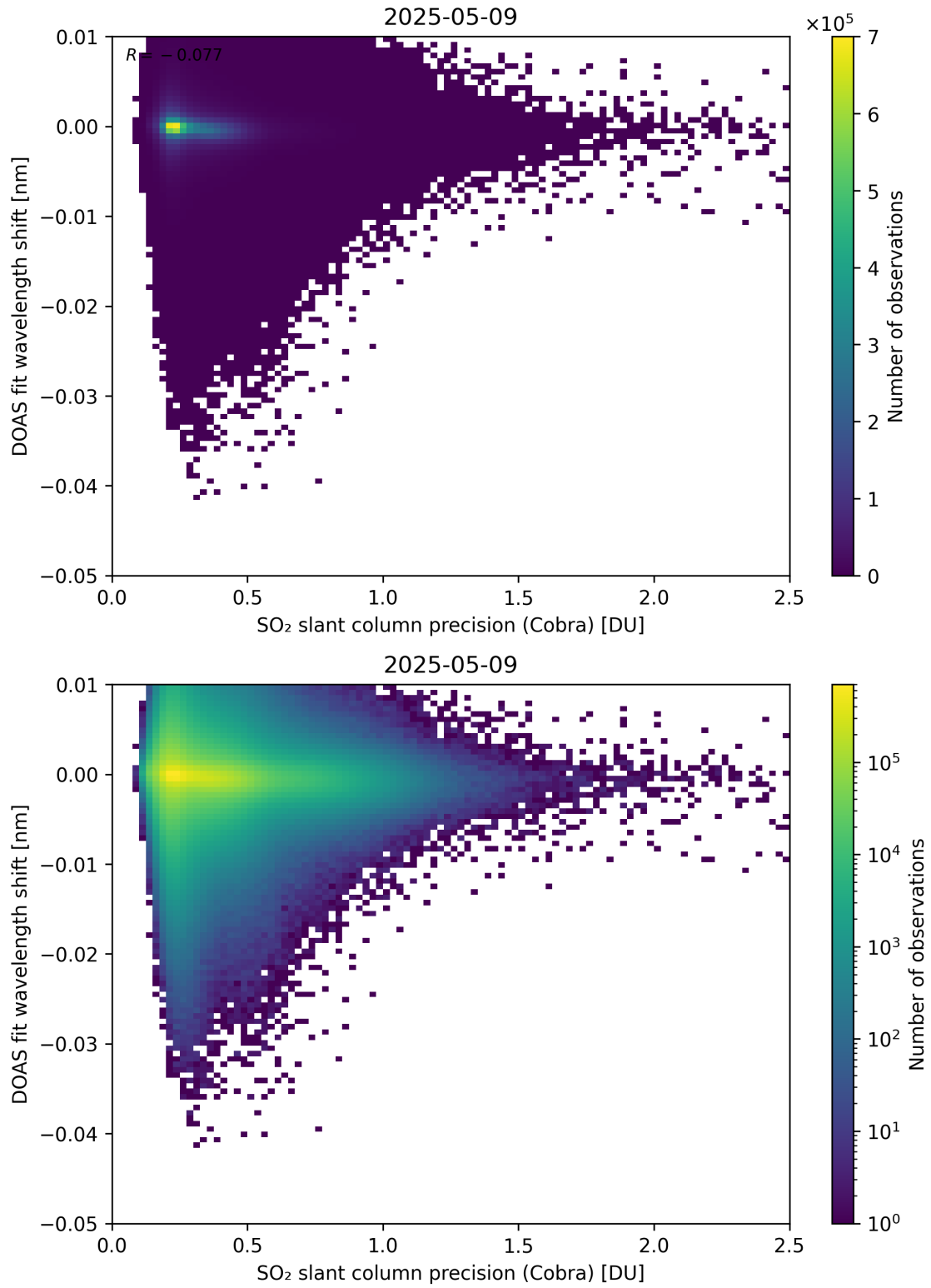
Figure 202: Scatter density plot of “SO 2 slant column precision (Cobra)” against “DOAS fit wavelength shift” for 2025-05-08 to 2025-05-10.
