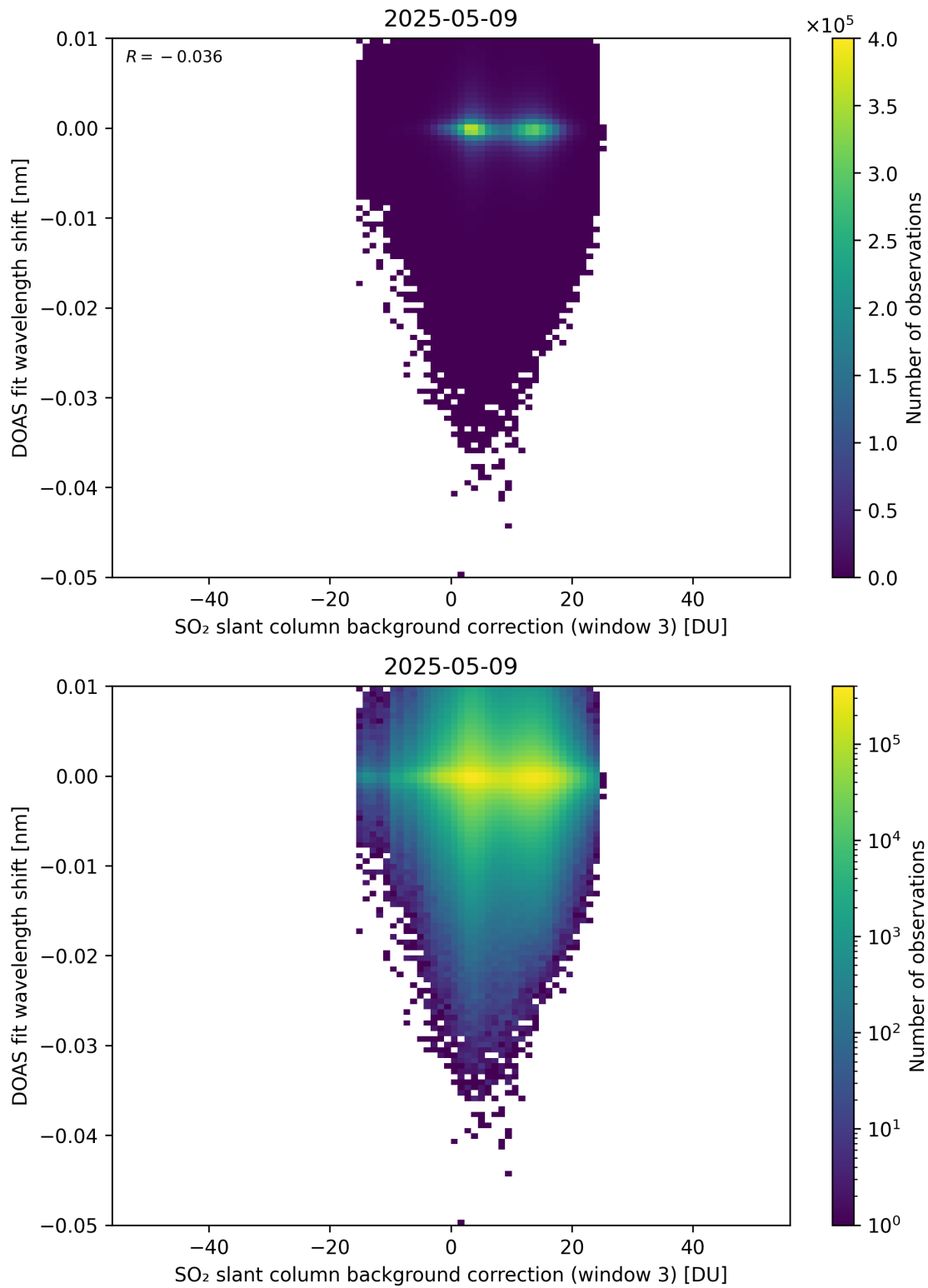
Figure 132: Scatter density plot of “SO 2 slant column background correction (window 3)” against “DOAS fit wavelength shift” for 2025-05-08 to 2025-05-10.
