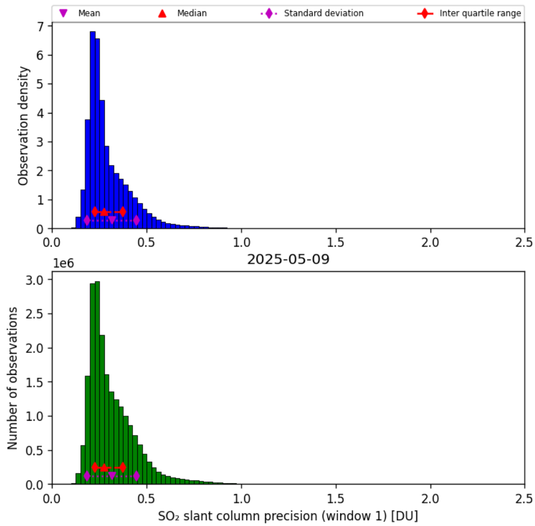
Figure 64: Histogram of “SO 2 slant column precision (window 1)” for 2025-05-08 to 2025-05-10
