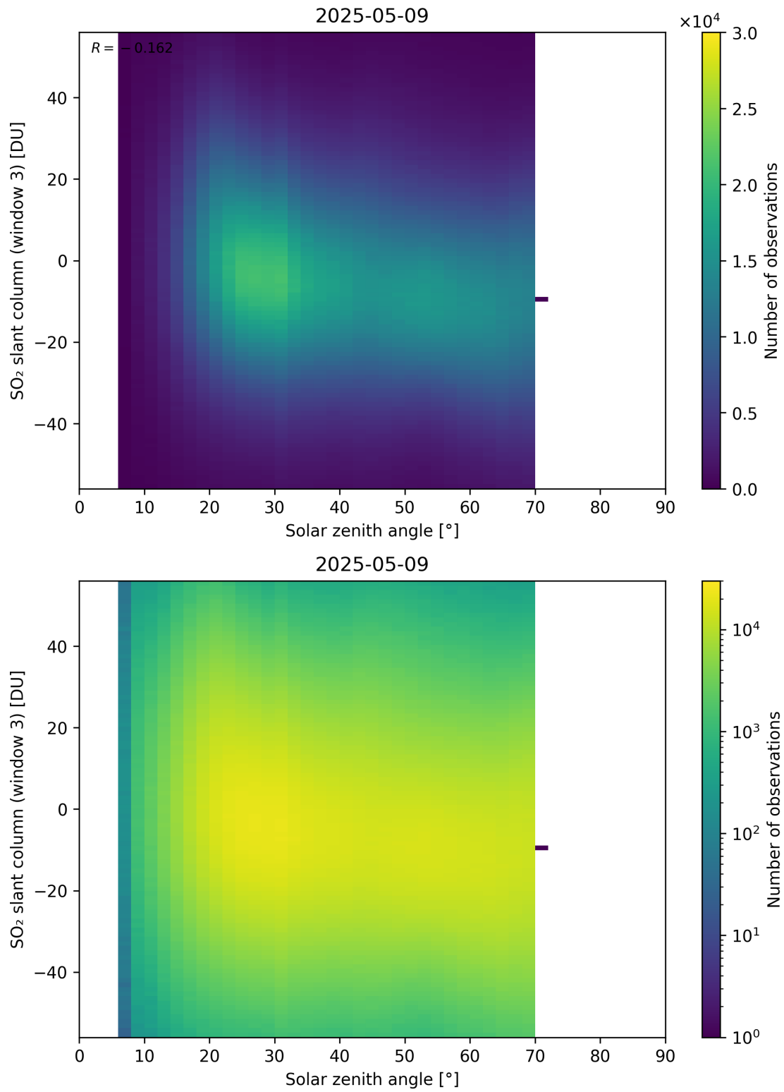
Figure 187: Scatter density plot of “Solar zenith angle” against “SO 2 slant column (window 3)” for 2025-05-08 to 2025-05-10.
