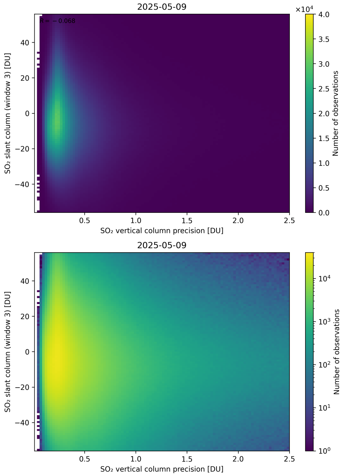
Figure 344: Scatter density plot of “SO 2 vertical column precision” against “SO 2 slant column (window 3)” for 2025-05-08 to 2025-05-10.
