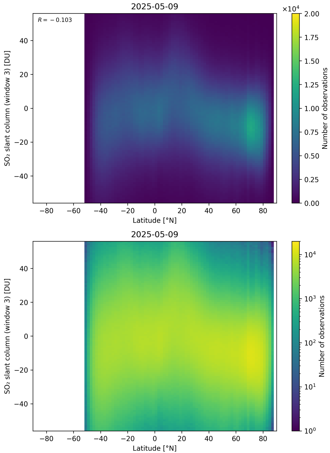
Figure 165: Scatter density plot of “Latitude” against “SO 2 slant column (window 3)” for 2025-05-08 to 2025-05-10.
