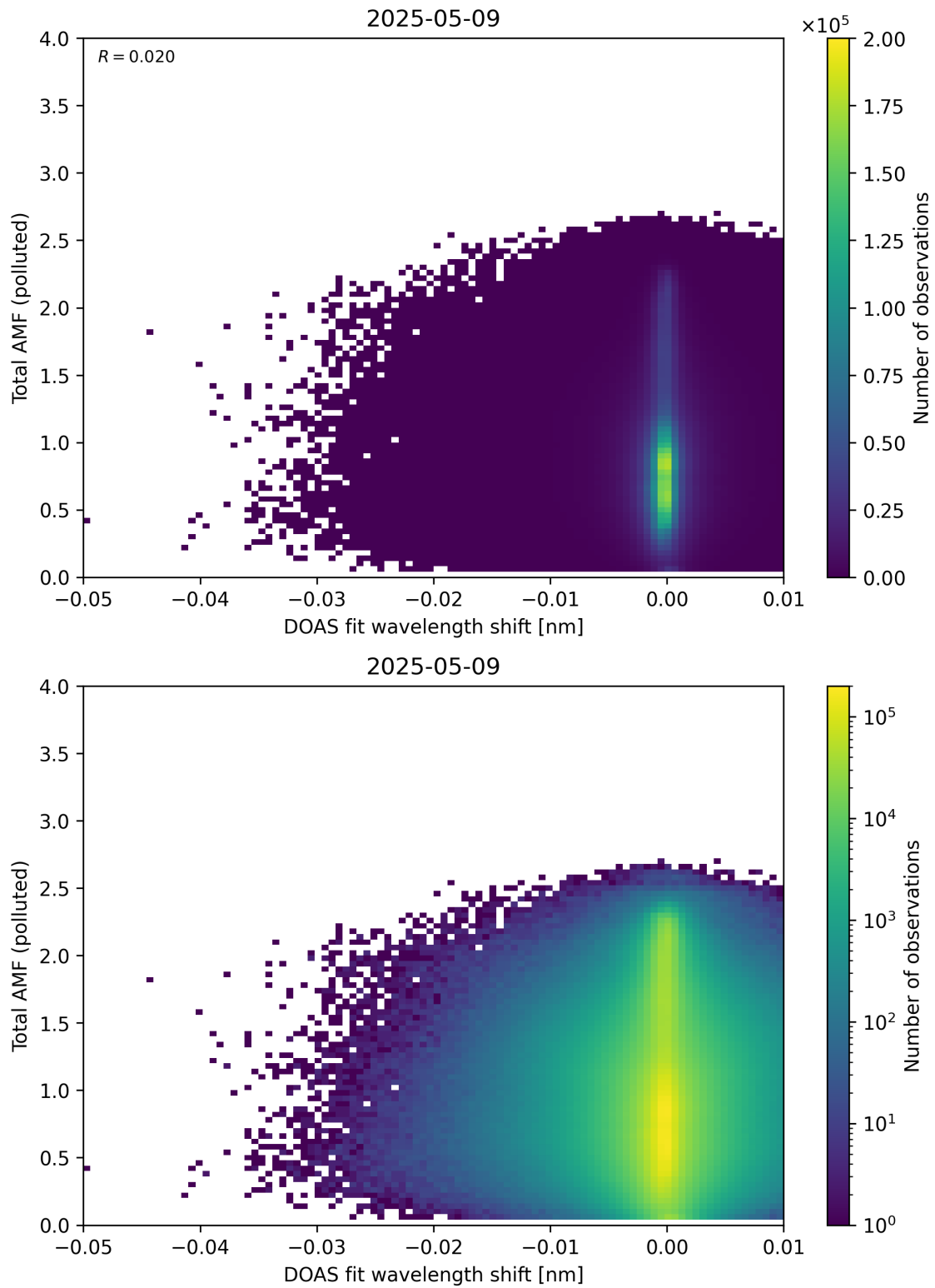
Figure 141: Scatter density plot of “DOAS fit wavelength shift” against “Total AMF (polluted)” for 2025-05-08 to 2025-05-10.
