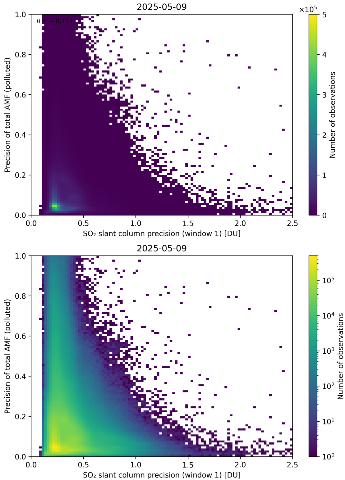
Figure 281: Scatter density plot of “SO 2 slant column precision (window 1)” against “Precision of total AMF (polluted)” for 2025-05-08 to 2025-05-10.
