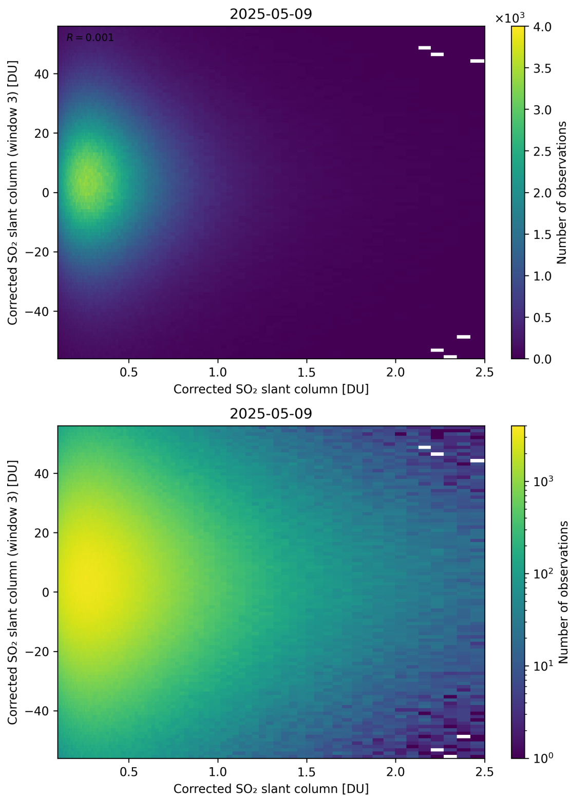
Figure 236: Scatter density plot of “Corrected SO 2 slant column” against “Corrected SO 2 slant column (window 3)” for 2025-05-08 to 2025-05-10.
