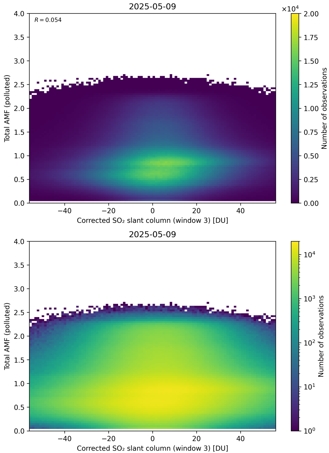
Figure 260: Scatter density plot of “Corrected SO 2 slant column (window 3)” against “Total AMF (polluted)” for 2025-05-08 to 2025-05-10.
