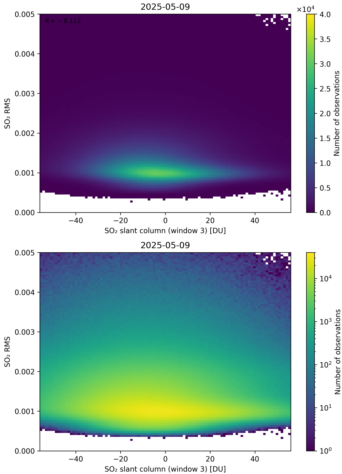
Figure 306: Scatter density plot of “SO 2 slant column (window 3)” against “SO 2 RMS” for 2025-05-08 to 2025-05-10.
