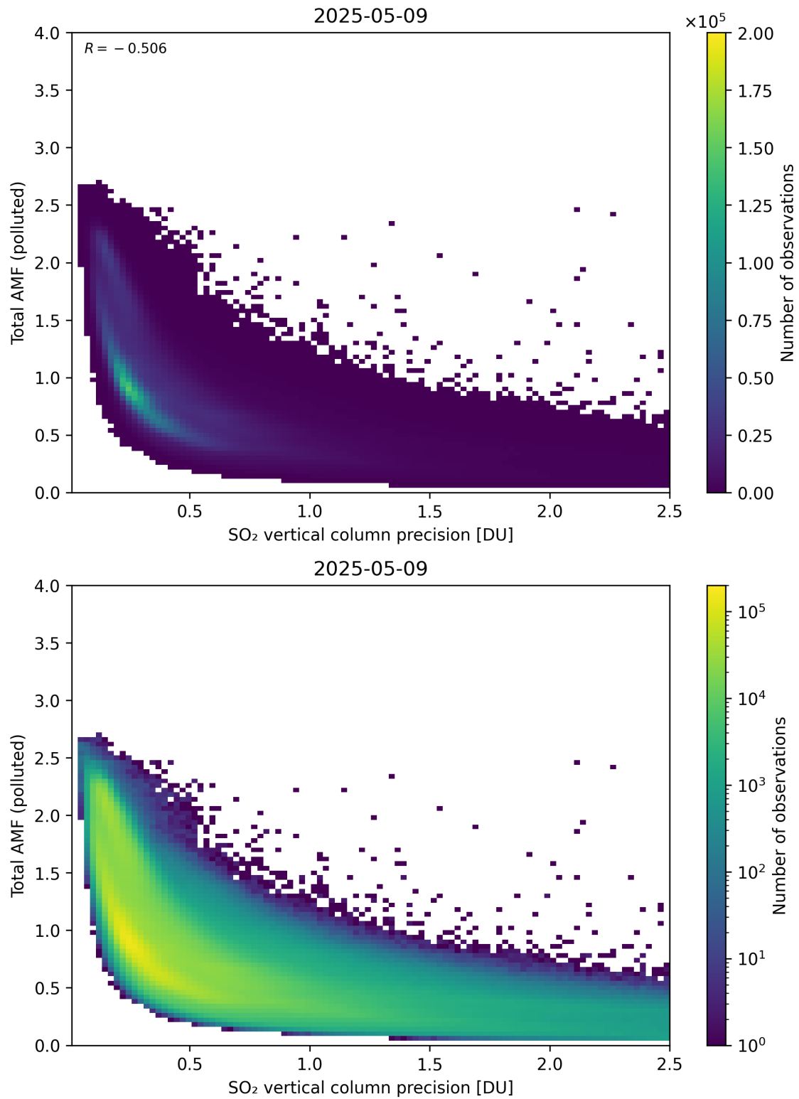
Figure 346: Scatter density plot of “SO 2 vertical column precision” against “Total AMF (polluted)” for 2025-05-08 to 2025-05-10.
