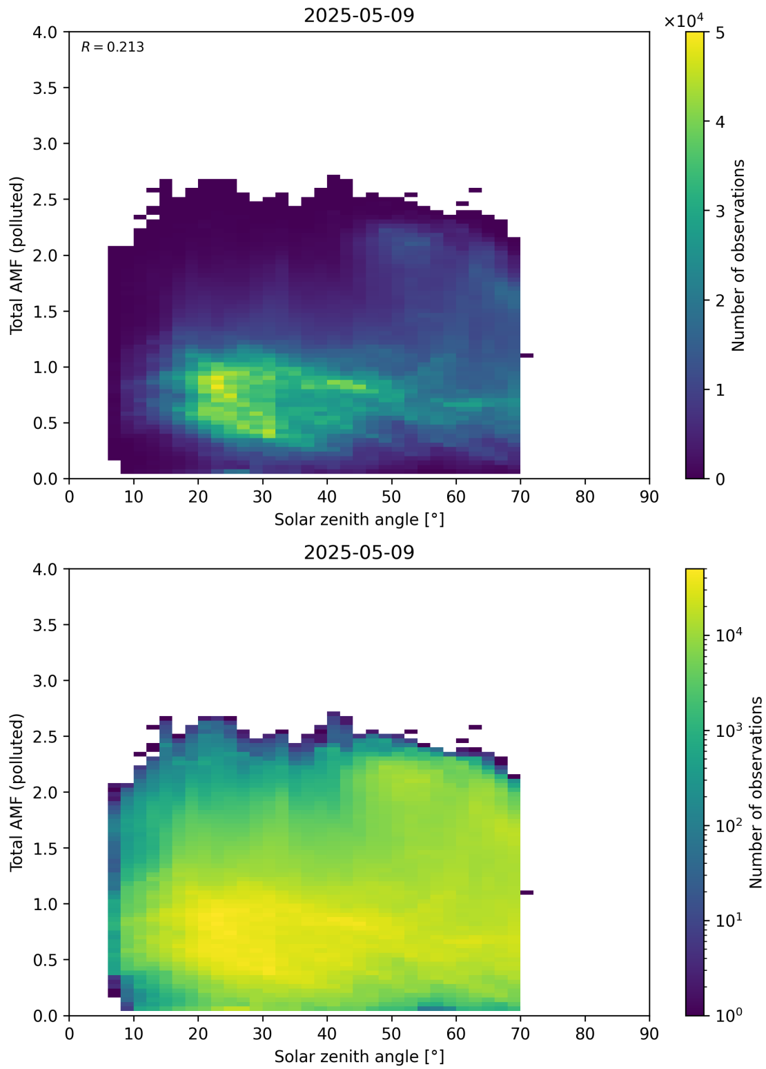
Figure 189: Scatter density plot of “Solar zenith angle” against “Total AMF (polluted)” for 2025-05-08 to 2025-05-10.
