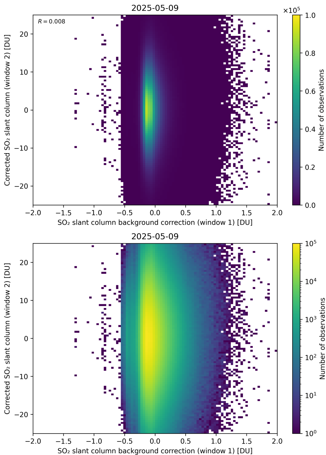
Figure 115: Scatter density plot of “SO 2 slant column background correction (window 1)” against “Corrected SO 2 slant column (window 2)” for 2025-05-08 to 2025-05-10.
