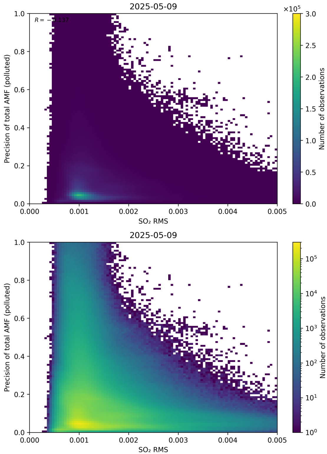
Figure 149: Scatter density plot of “SO 2 RMS” against “Precision of total AMF (polluted)” for 2025-05-08 to 2025-05-10.
