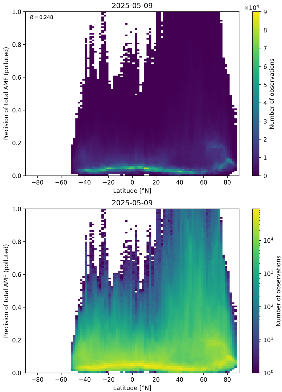
Figure 168: Scatter density plot of “Latitude” against “Precision of total AMF (polluted)” for 2025-05-08 to 2025-05-10.
