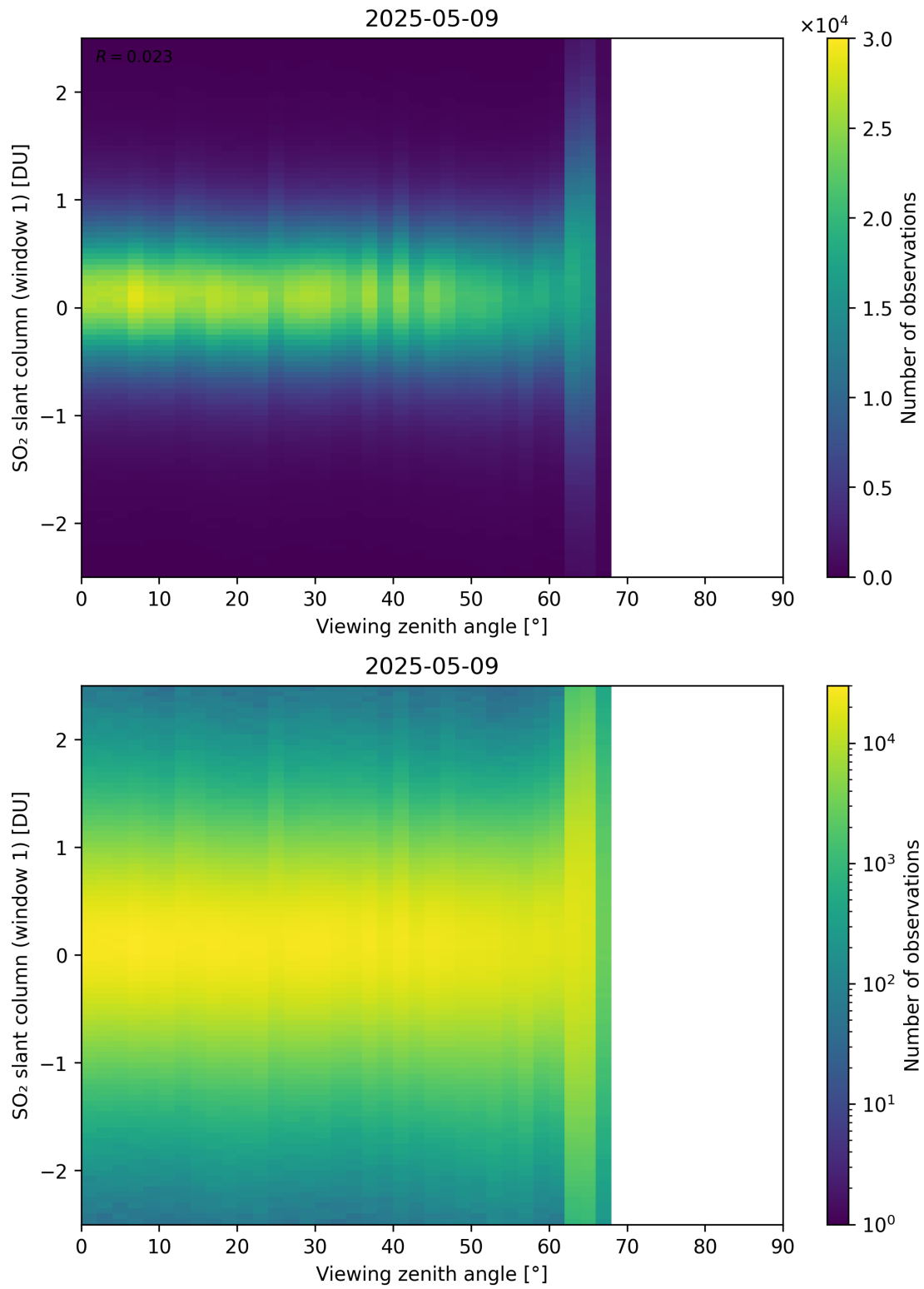
Figure 376: Scatter density plot of “Viewing zenith angle” against “SO 2 slant column (window 1)” for 2025-05-08 to 2025-05-10.
