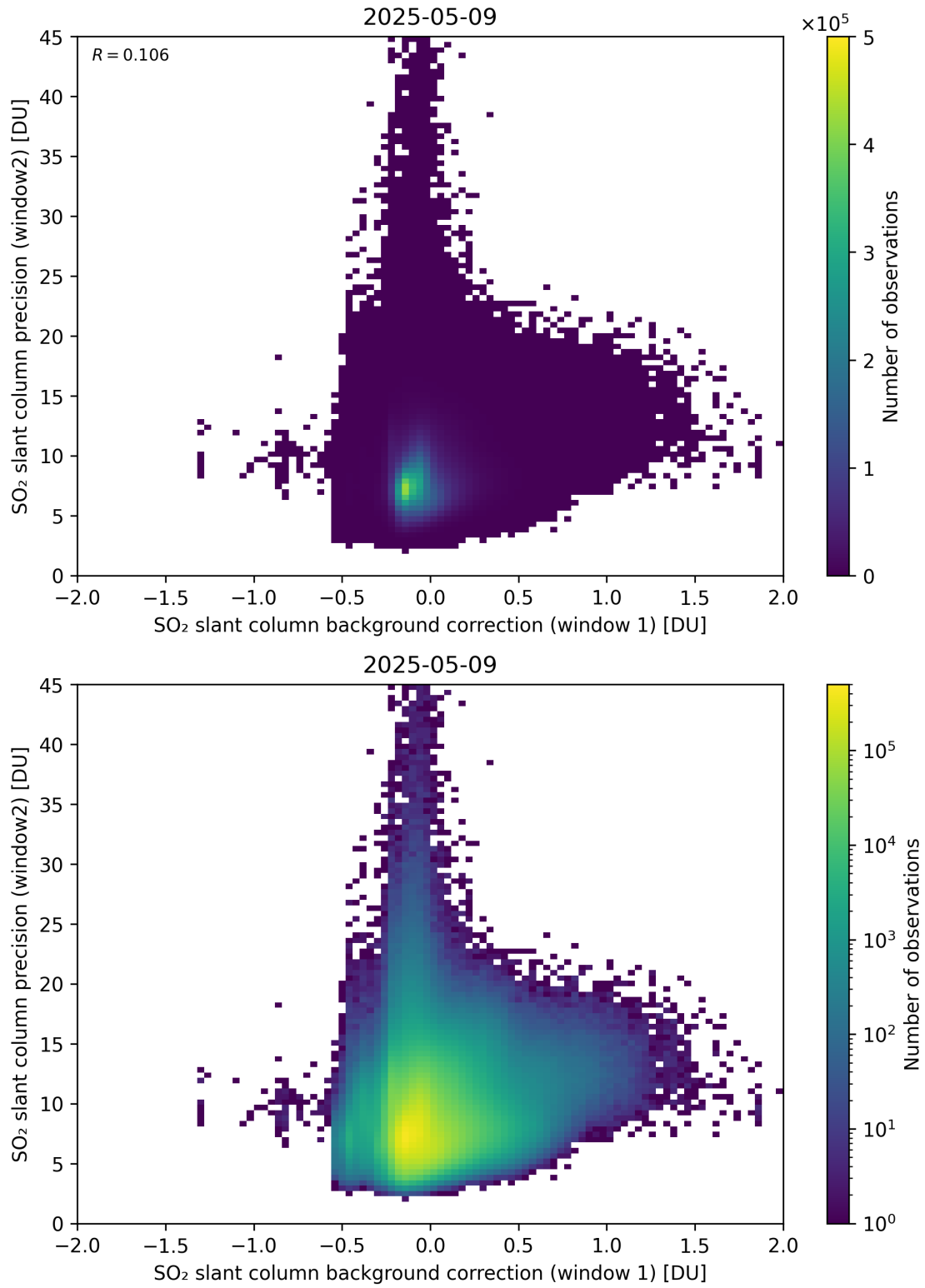
Figure 117: Scatter density plot of “SO 2 slant column background correction (window 1)” against “SO 2 slant column precision (window2)” for 2025-05-08 to 2025-05-10.
