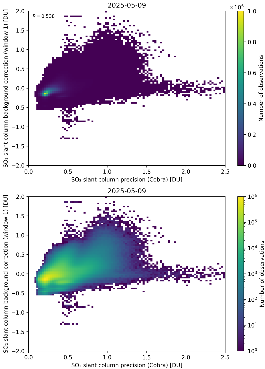
Figure 199: Scatter density plot of “SO 2 slant column precision (Cobra)” against “SO 2 slant column background correction (window 1)” for 2025-05-08 to 2025-05-10.
