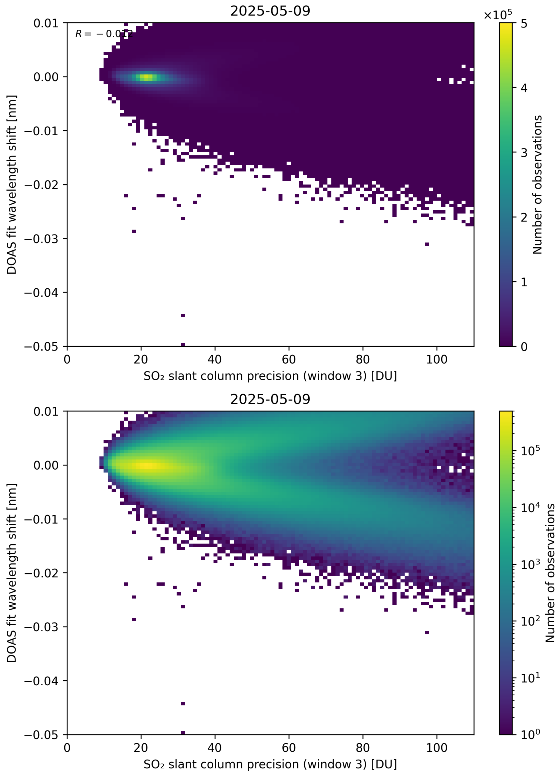
Figure 308: Scatter density plot of “SO 2 slant column precision (window 3)” against “DOAS fit wavelength shift” for 2025-05-08 to 2025-05-10.
