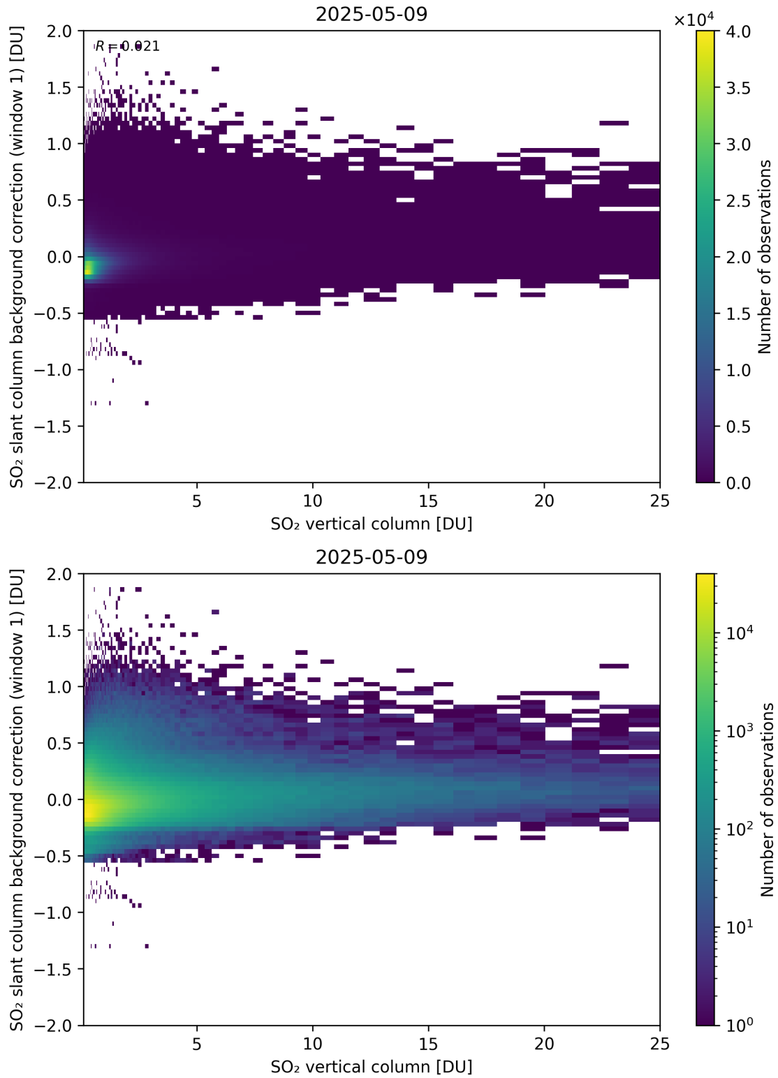
Figure 323: Scatter density plot of “SO 2 vertical column” against “SO 2 slant column background correction (window 1)” for 2025-05-08 to 2025-05-10.
