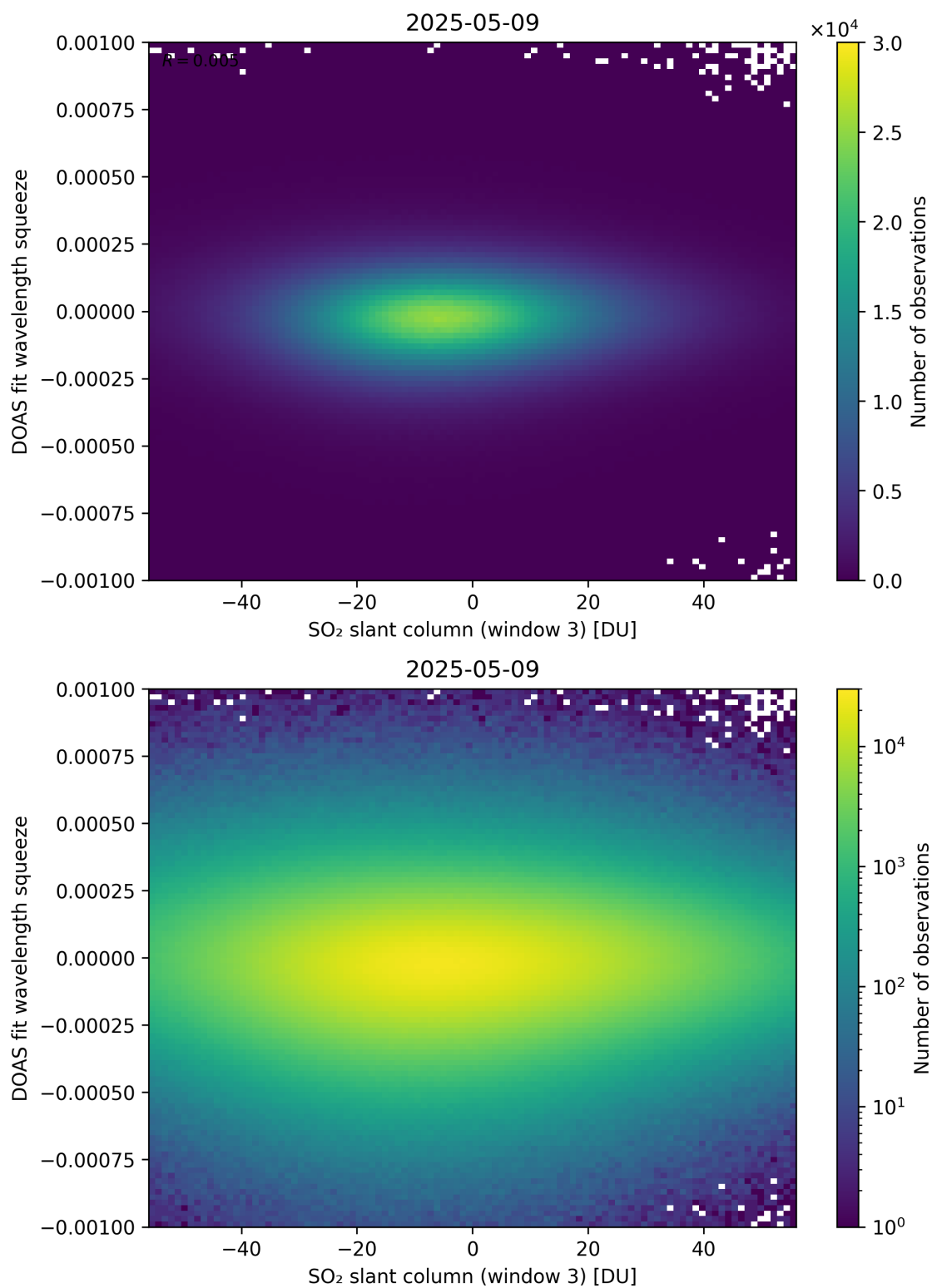
Figure 305: Scatter density plot of “SO 2 slant column (window 3)” against “DOAS fit wavelength squeeze” for 2025-05-08 to 2025-05-10.
