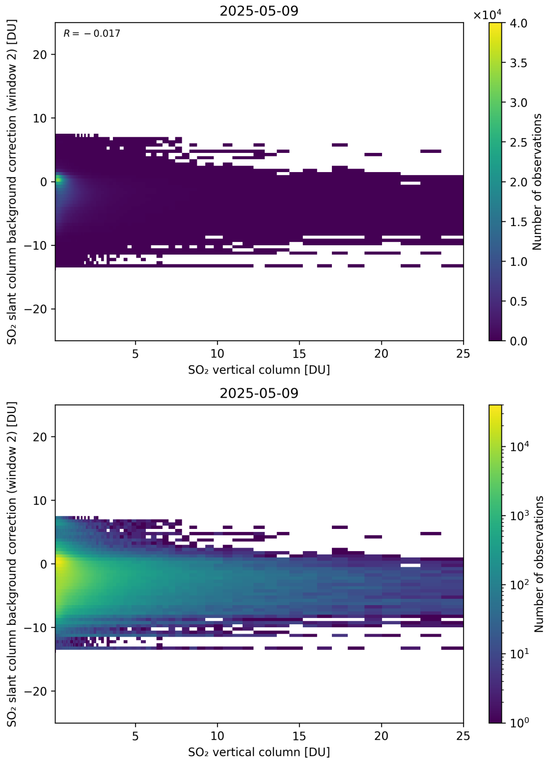
Figure 324: Scatter density plot of “SO 2 vertical column” against “SO 2 slant column background correction (window 2)” for 2025-05-08 to 2025-05-10.
