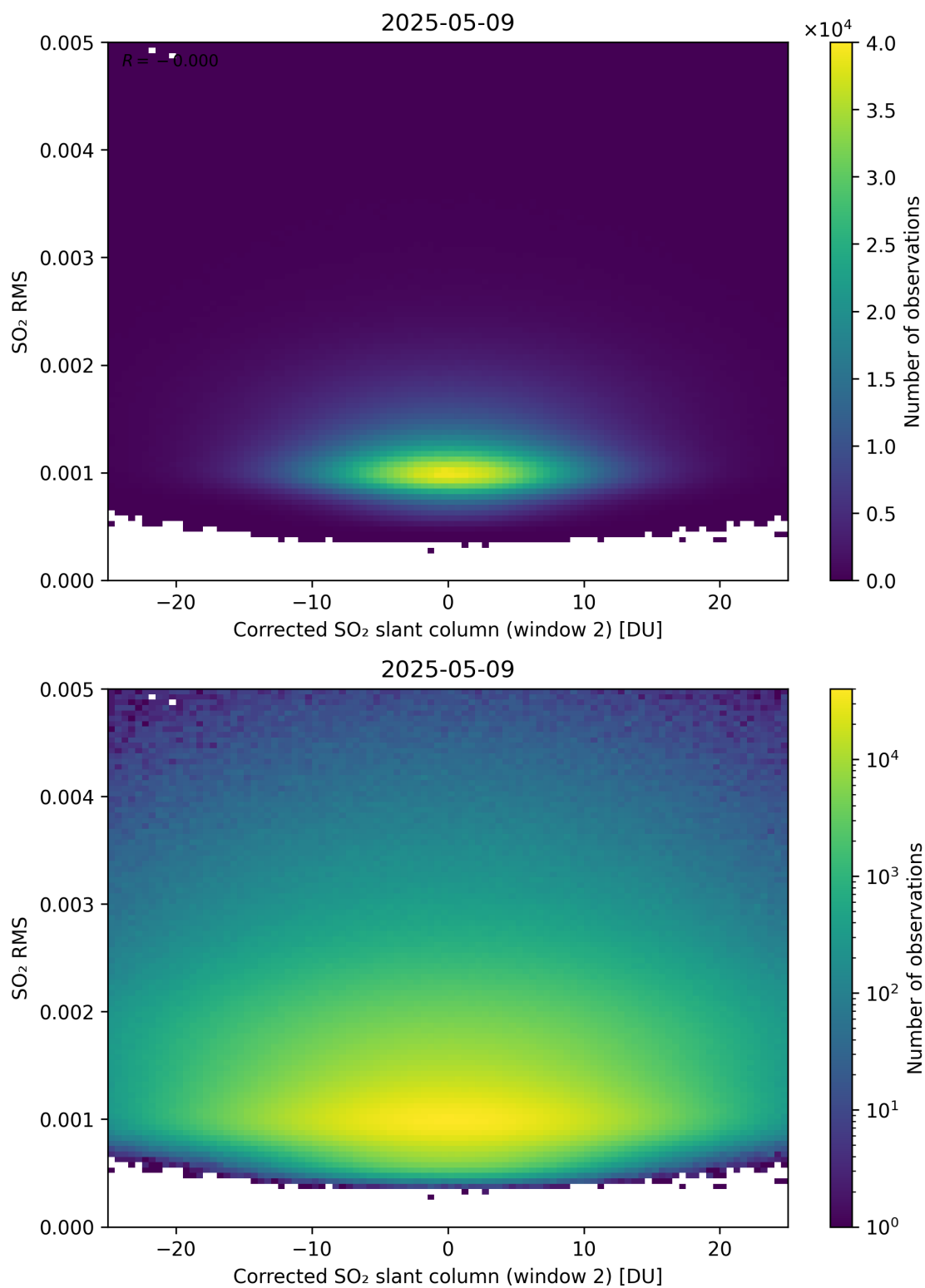
Figure 248: Scatter density plot of “Corrected SO 2 slant column (window 2)” against “SO 2 RMS” for 2025-05-08 to 2025-05-10.
