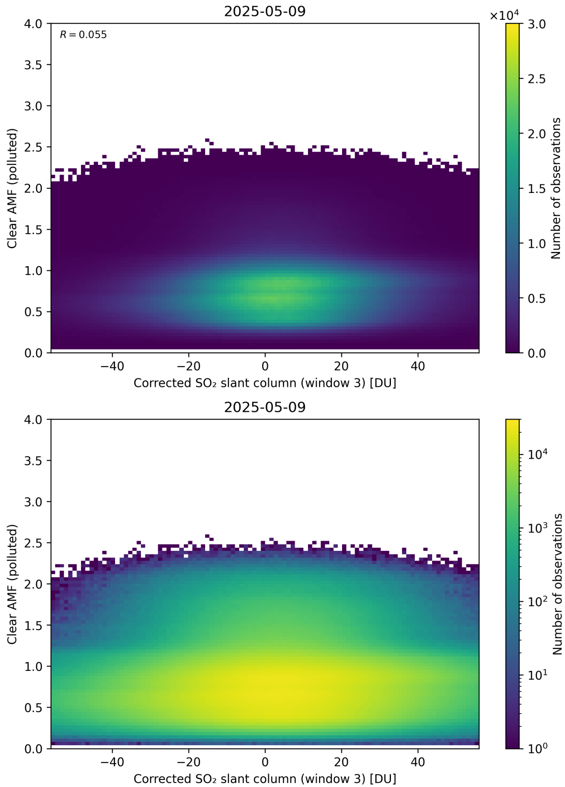
Figure 259: Scatter density plot of “Corrected SO 2 slant column (window 3)” against “Clear AMF (polluted)” for 2025-05-08 to 2025-05-10.
