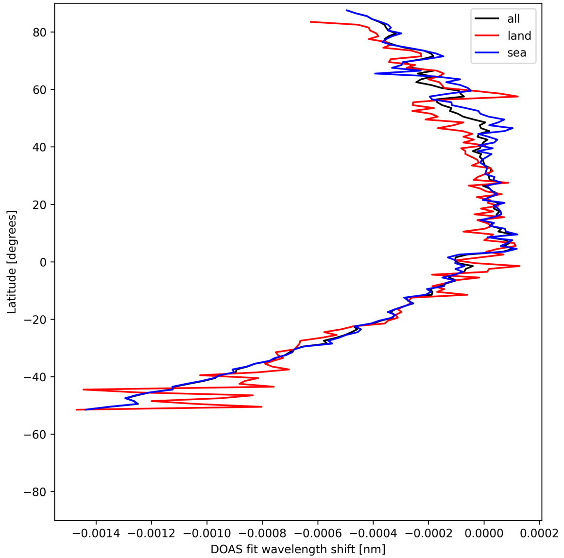
Figure 50: Zonal average of “DOAS fit wavelength shift” for 2025-05-08 to 2025-05-10.
