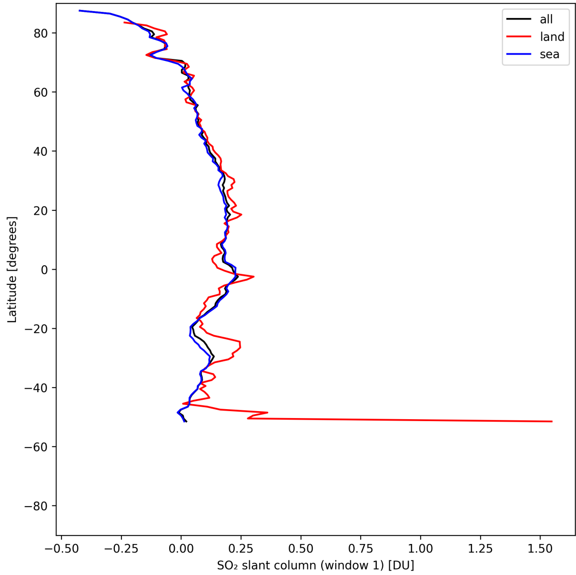
Figure 37: Zonal average of “SO 2 slant column (window 1)” for 2025-05-08 to 2025-05-10.
