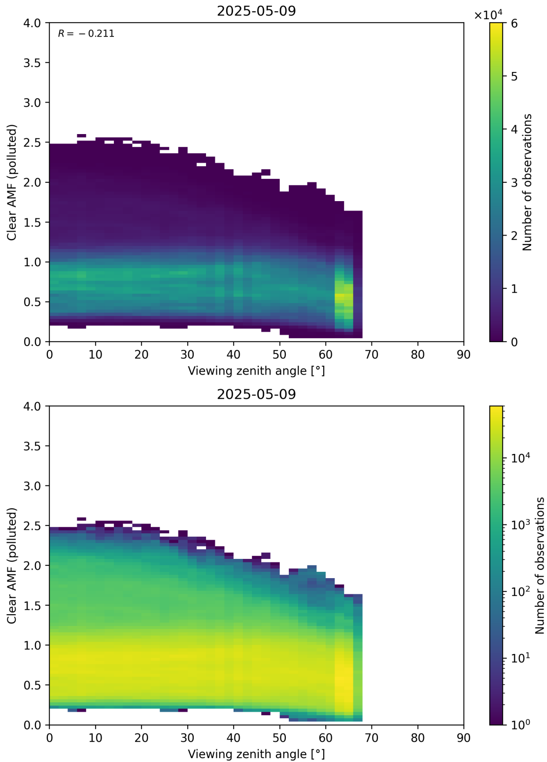
Figure 370: Scatter density plot of “Viewing zenith angle” against “Clear AMF (polluted)” for 2025-05-08 to 2025-05-10.
