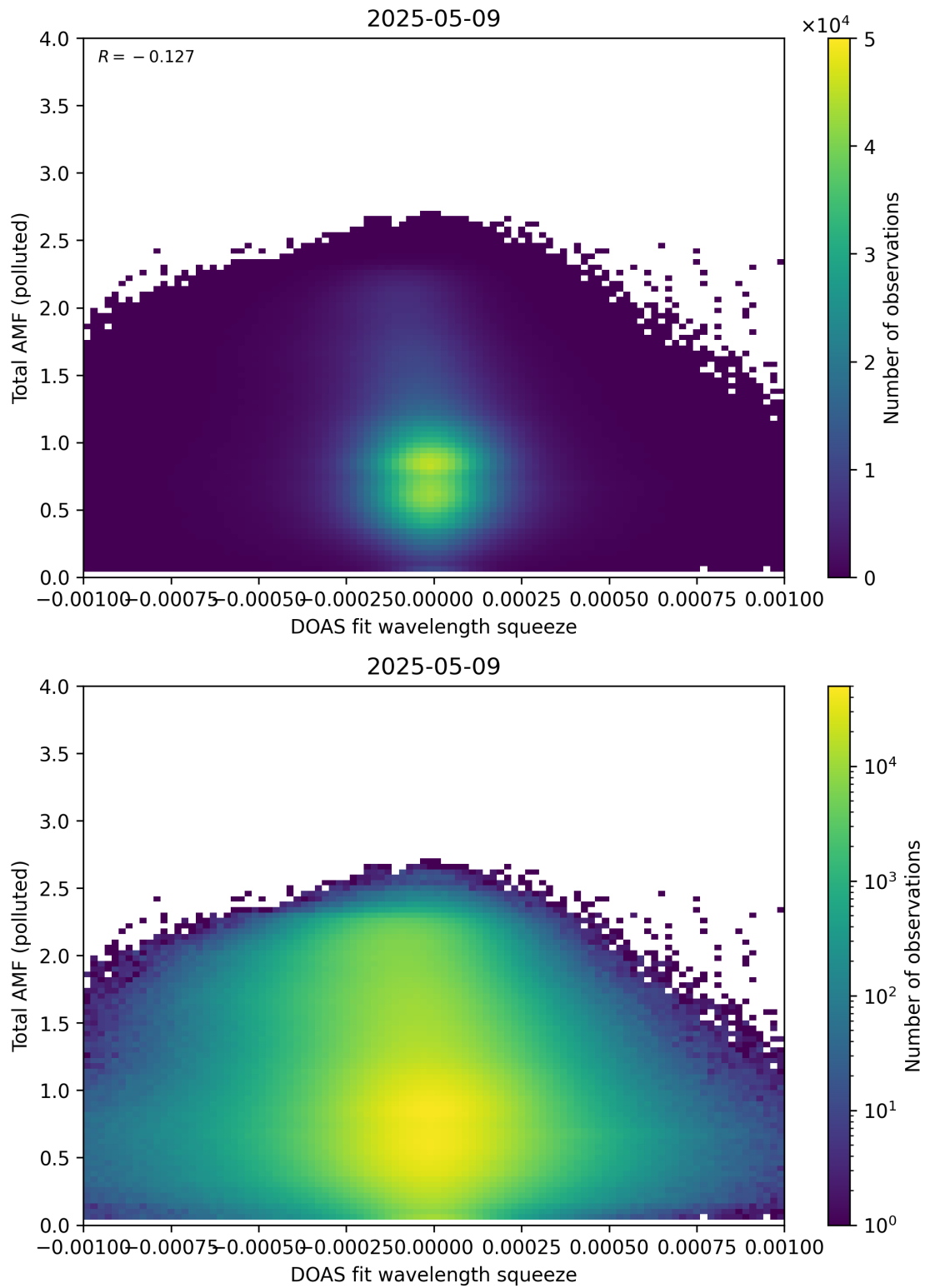
Figure 145: Scatter density plot of “DOAS fit wavelength squeeze” against “Total AMF (polluted)” for 2025-05-08 to 2025-05-10.
