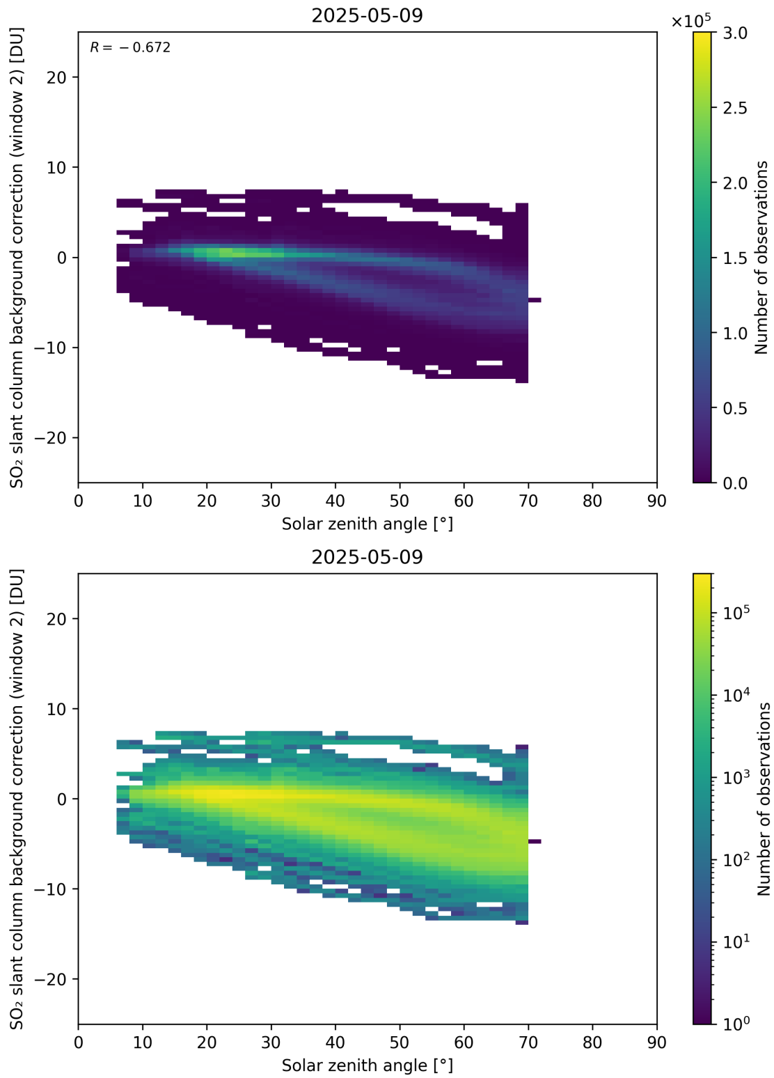
Figure 172: Scatter density plot of “Solar zenith angle” against “SO 2 slant column background correction (window 2)” for 2025-05-08 to 2025-05-10.
