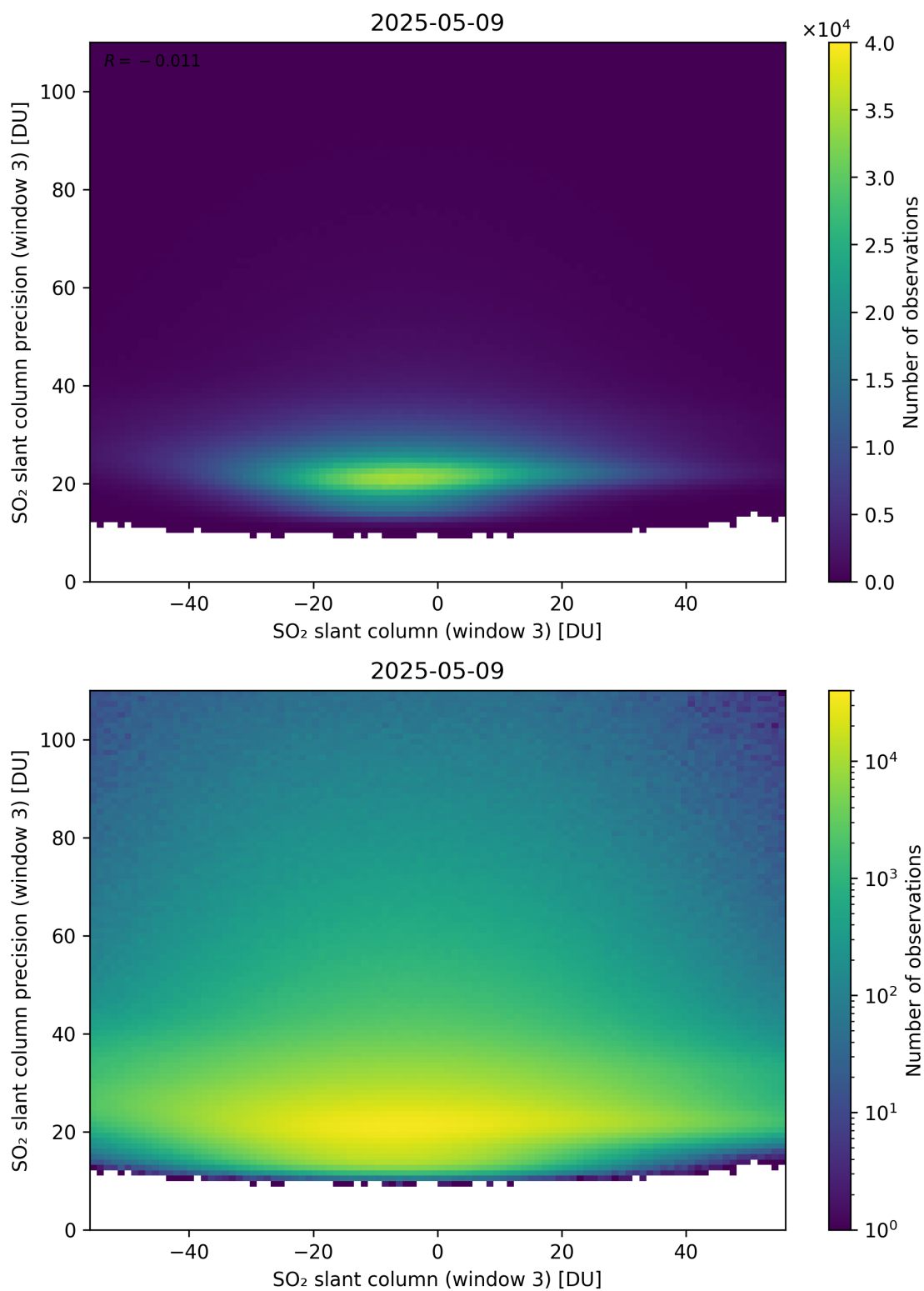
Figure 317: Scatter density plot of “SO 2 slant column (window 3)” against “SO 2 slant column precision (window 3)” for 2025-05-08 to 2025-05-10.
