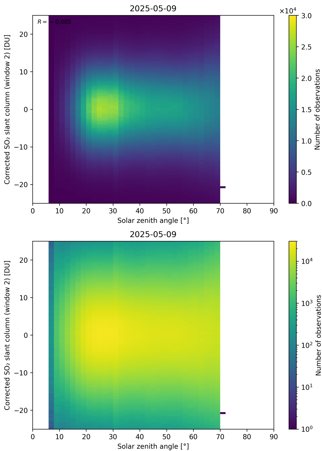
Figure 182: Scatter density plot of “Solar zenith angle” against “Corrected SO 2 slant column (window 2)” for 2025-05-08 to 2025-05-10.
