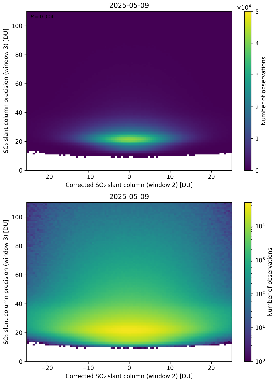
Figure 252: Scatter density plot of “Corrected SO 2 slant column (window 2)” against “SO 2 slant column precision (window 3)” for 2025-05-08 to 2025-05-10.
