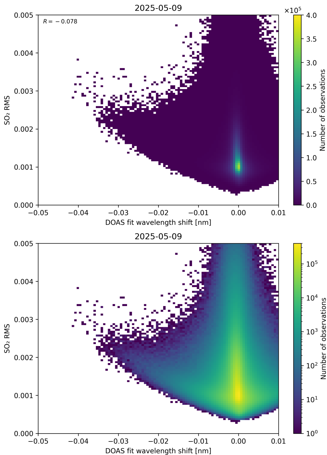
Figure 139: Scatter density plot of “DOAS fit wavelength shift” against “SO 2 RMS” for 2025-05-08 to 2025-05-10.
