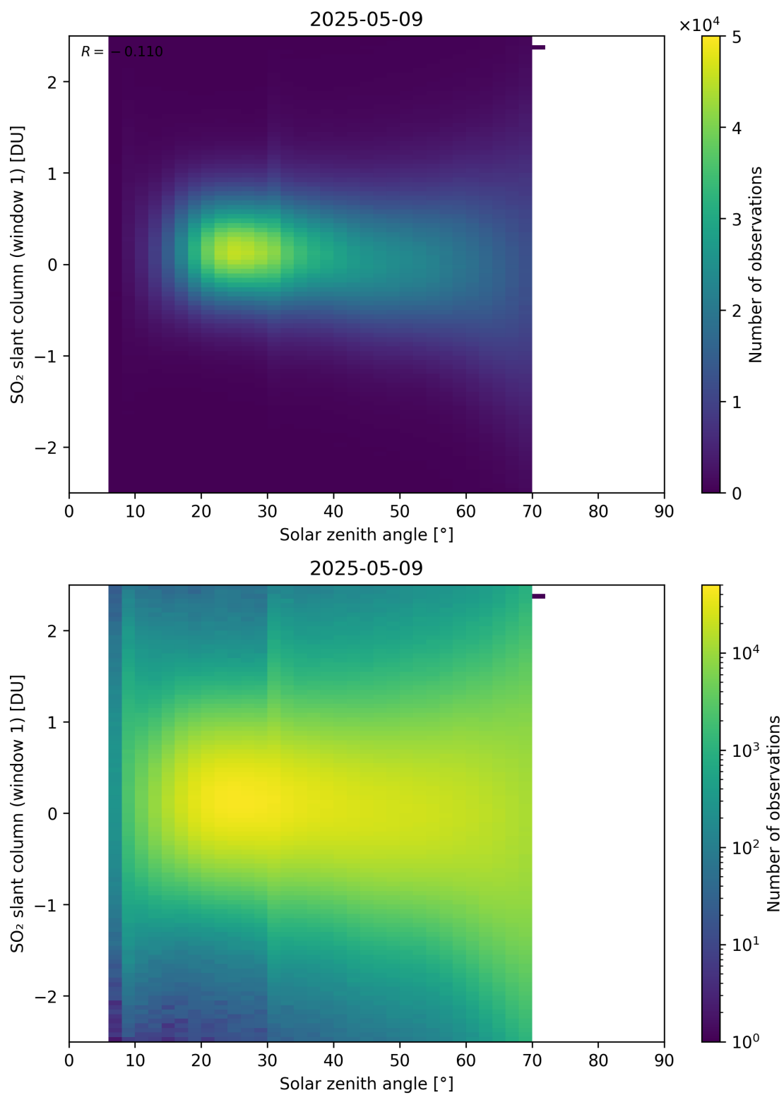
Figure 184: Scatter density plot of “Solar zenith angle” against “SO 2 slant column (window 1)” for 2025-05-08 to 2025-05-10.
