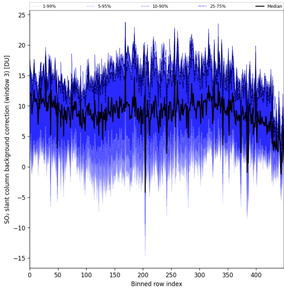
Figure 100: Along track statistics of “SO 2 slant column background correction (window 3)” for 2025-05-08 to 2025-05-10
