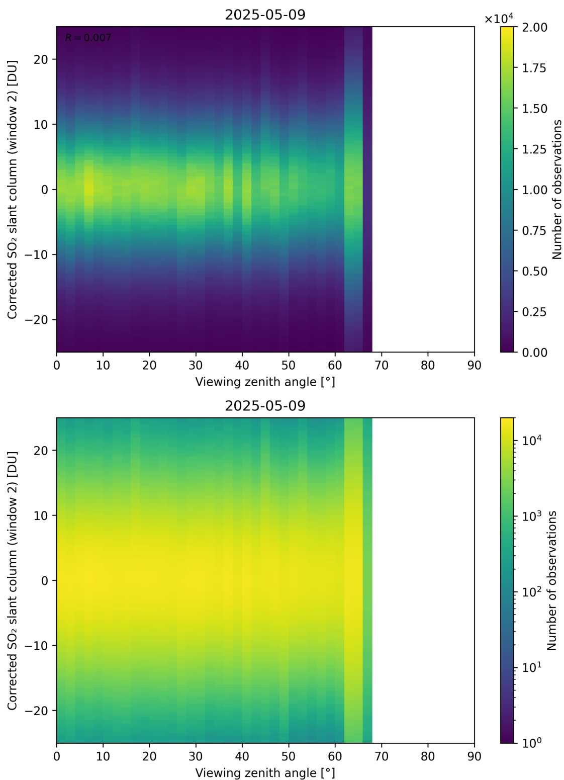
Figure 374: Scatter density plot of “Viewing zenith angle” against “Corrected SO 2 slant column (window 2)” for 2025-05-08 to 2025-05-10.
