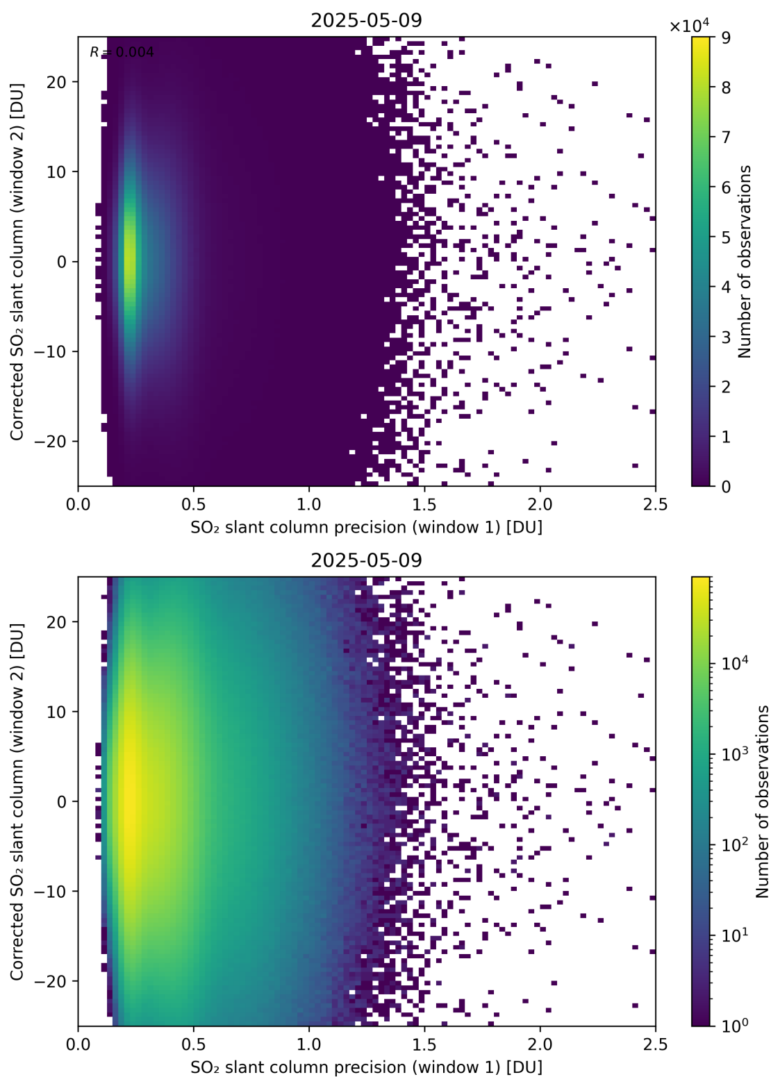
Figure 275: Scatter density plot of “SO 2 slant column precision (window 1)” against “Corrected SO 2 slant column (window 2)” for 2025-05-08 to 2025-05-10.
