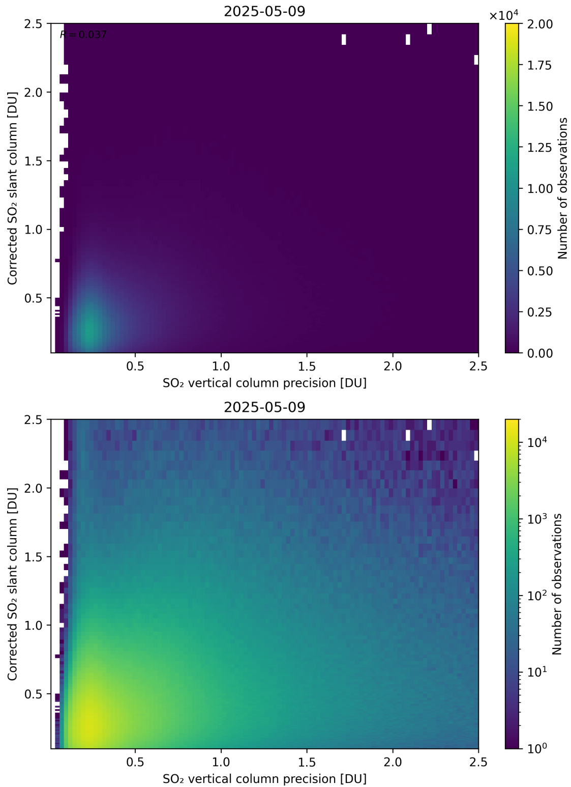
Figure 338: Scatter density plot of “SO 2 vertical column precision” against “Corrected SO 2 slant column” for 2025-05-08 to 2025-05-10.
