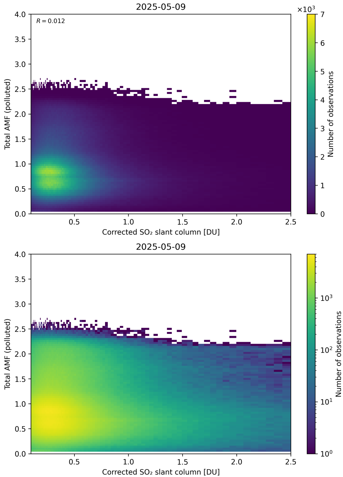
Figure 242: Scatter density plot of “Corrected SO 2 slant column” against “Total AMF (polluted)” for 2025-05-08 to 2025-05-10.
