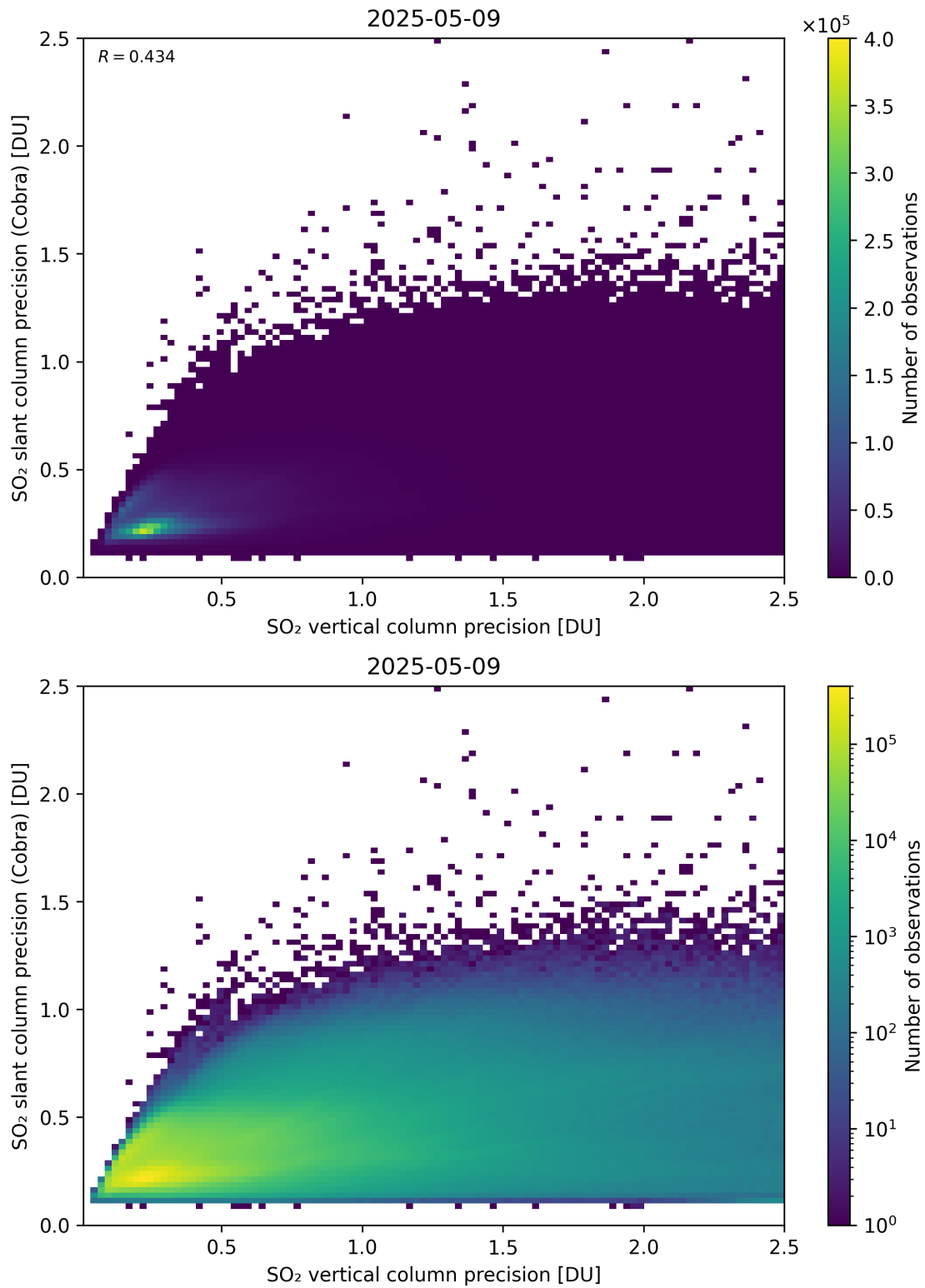
Figure 337: Scatter density plot of “SO 2 vertical column precision” against “SO 2 slant column precision (Cobra)” for 2025-05-08 to 2025-05-10.
