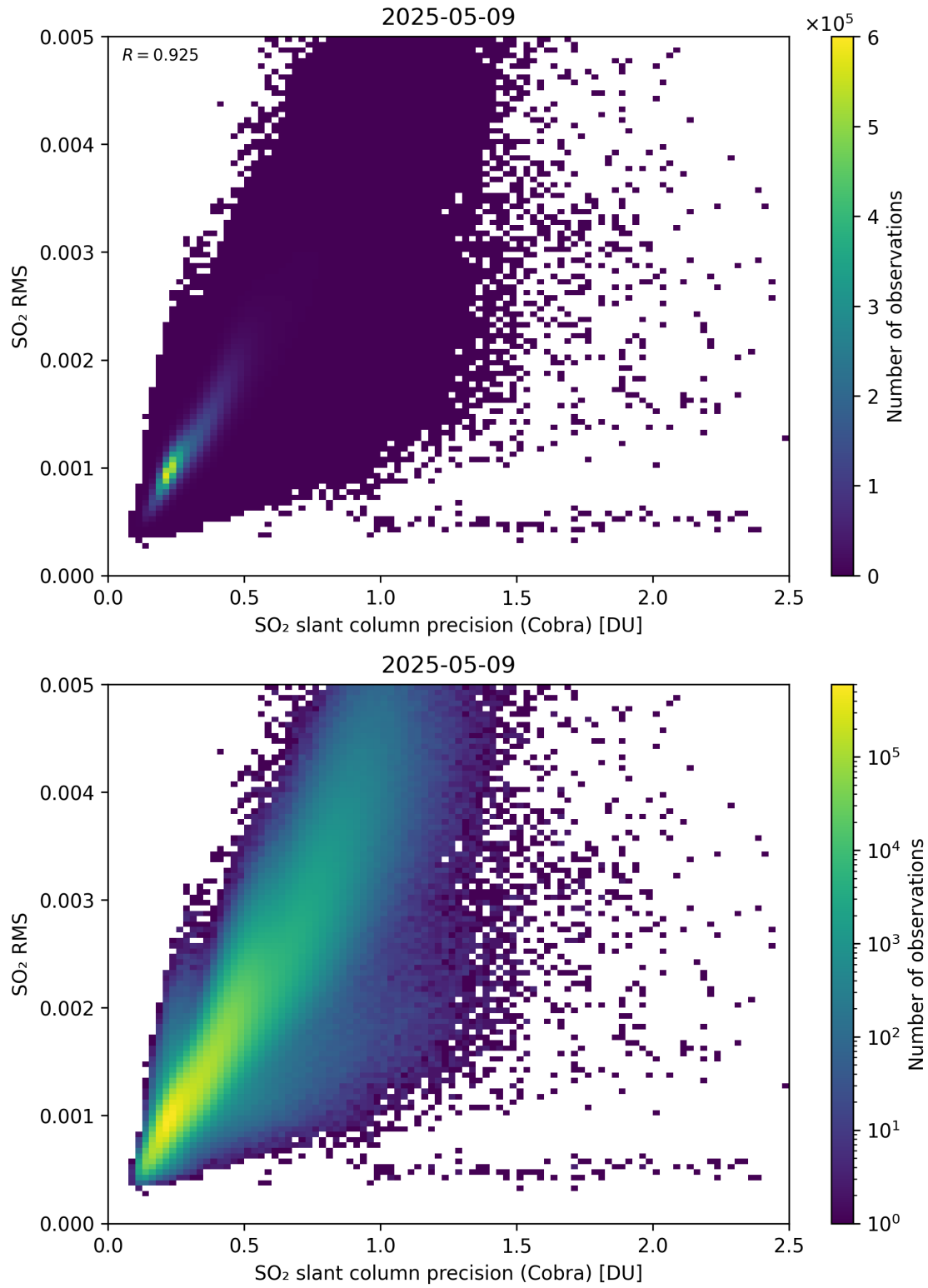
Figure 204: Scatter density plot of “SO 2 slant column precision (Cobra)” against “SO 2 RMS” for 2025-05-08 to 2025-05-10.
