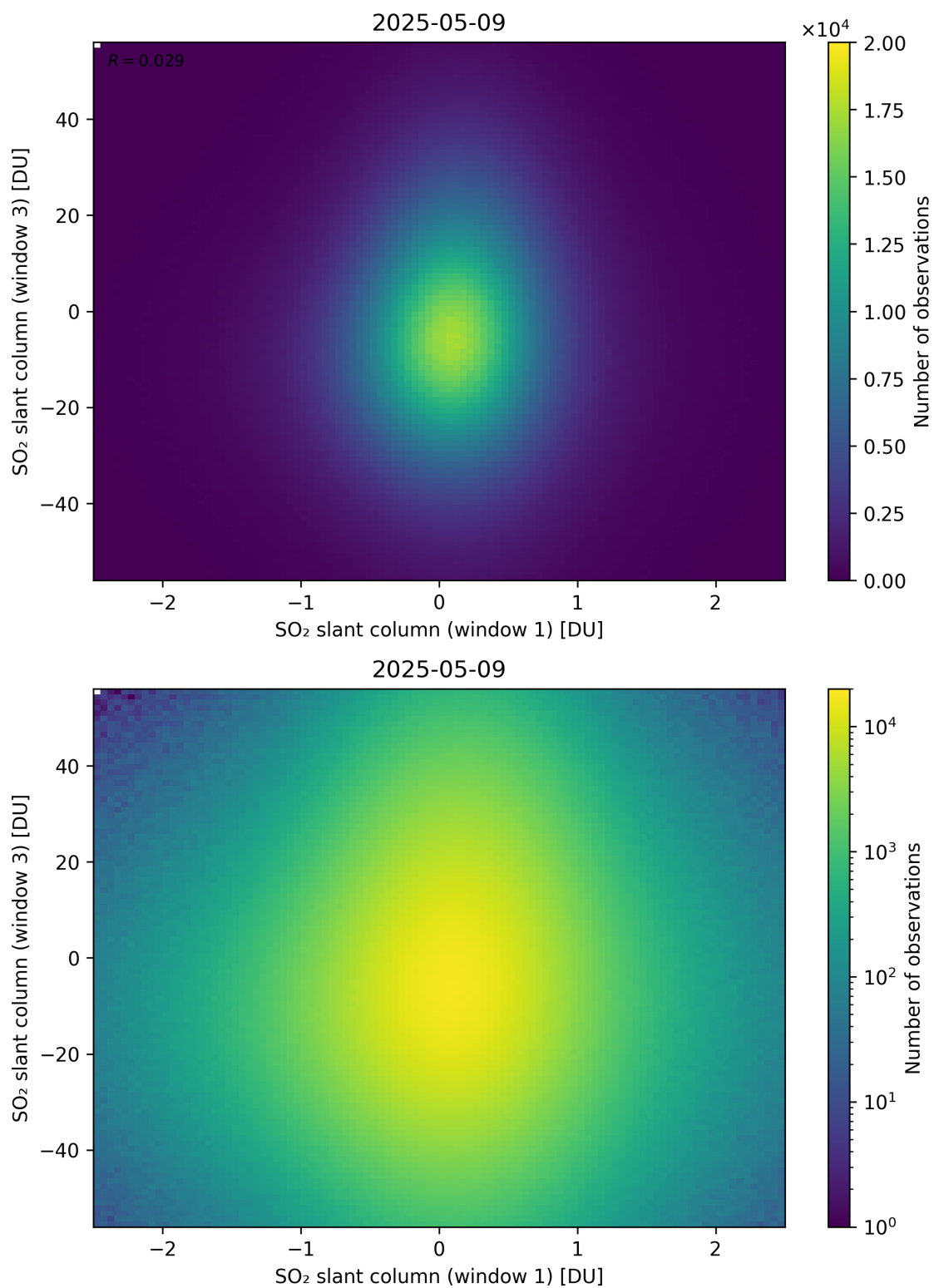
Figure 287: Scatter density plot of “SO 2 slant column (window 1)” against “SO 2 slant column (window 3)” for 2025-05-08 to 2025-05-10.
