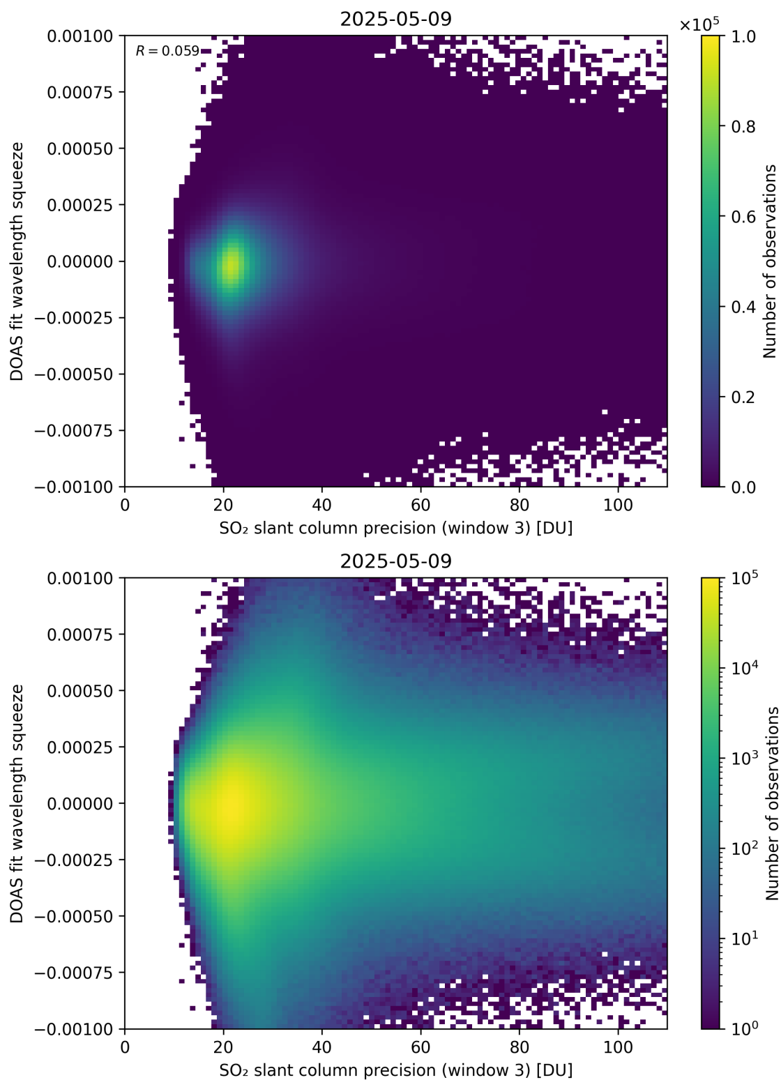
Figure 309: Scatter density plot of “SO 2 slant column precision (window 3)” against “DOAS fit wavelength squeeze” for 2025-05-08 to 2025-05-10.
