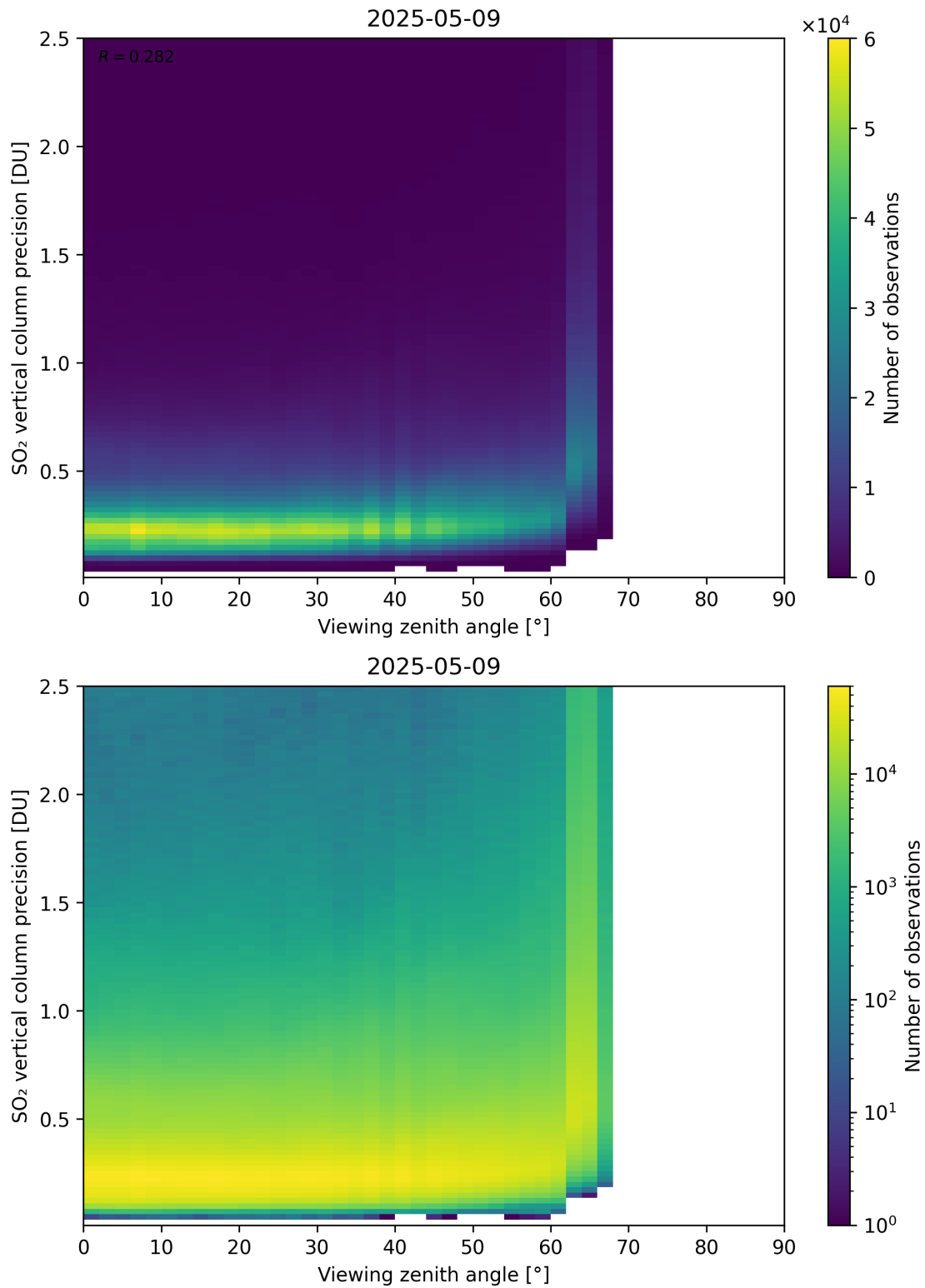
Figure 384: Scatter density plot of “Viewing zenith angle” against “SO 2 vertical column precision” for 2025-05-08 to 2025-05-10.
