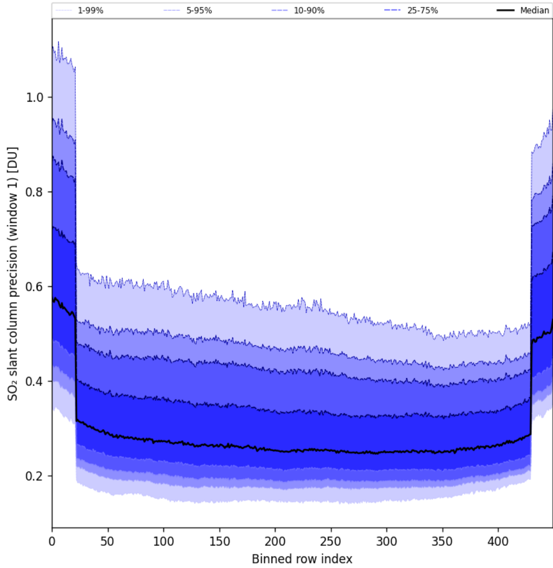
Figure 90: Along track statistics of “SO 2 slant column precision (window 1)” for 2025-05-08 to 2025-05-10
