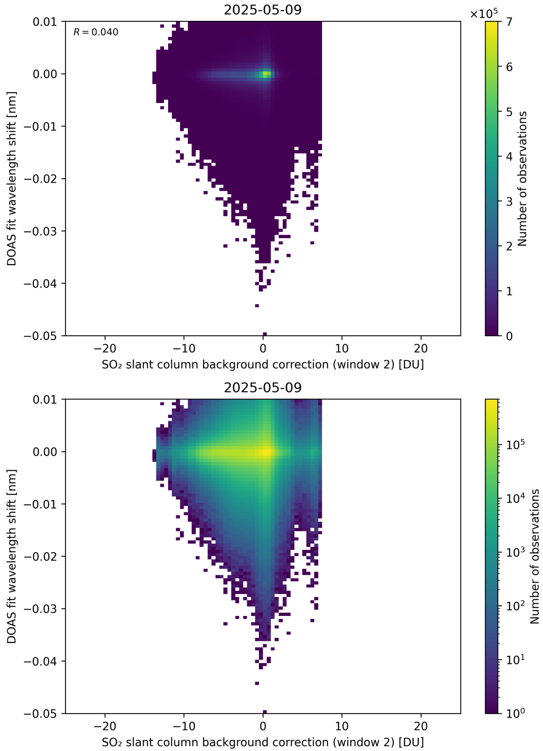
Figure 123: Scatter density plot of “SO 2 slant column background correction (window 2)” against “DOAS fit wavelength shift” for 2025-05-08 to 2025-05-10.
