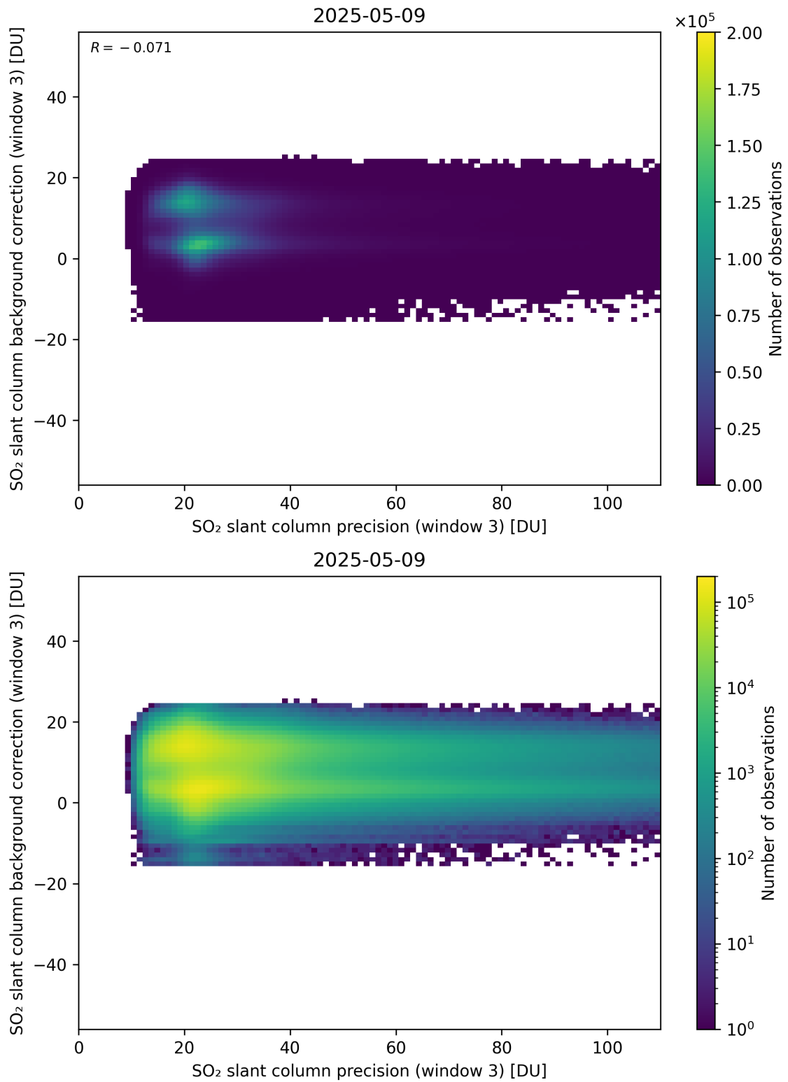
Figure 307: Scatter density plot of “SO 2 slant column precision (window 3)” against “SO 2 slant column background correction (window 3)” for 2025-05-08 to 2025-05-10.
