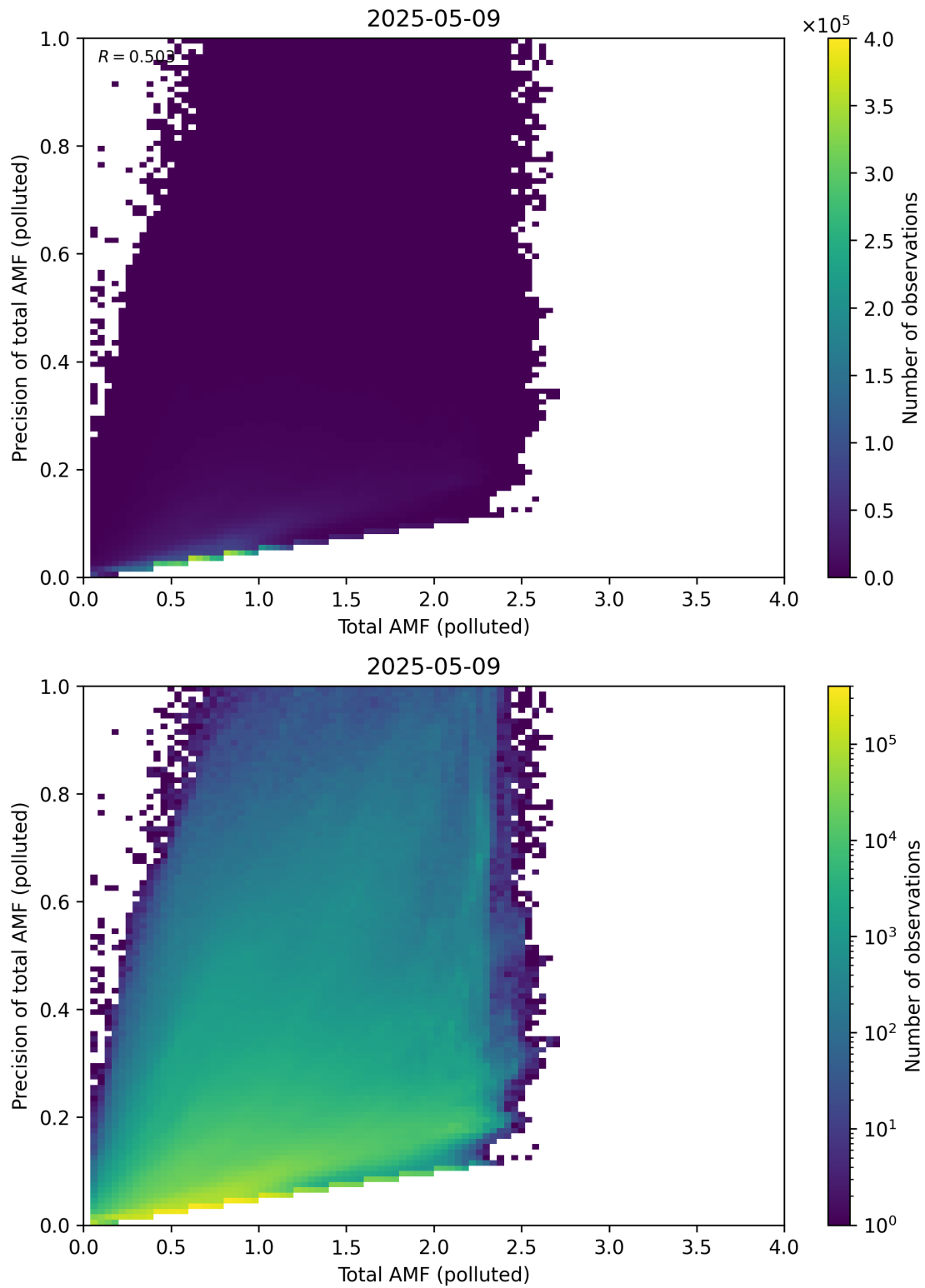
Figure 322: Scatter density plot of “Total AMF (polluted)” against “Precision of total AMF (polluted)” for 2025-05-08 to 2025-05-10.
