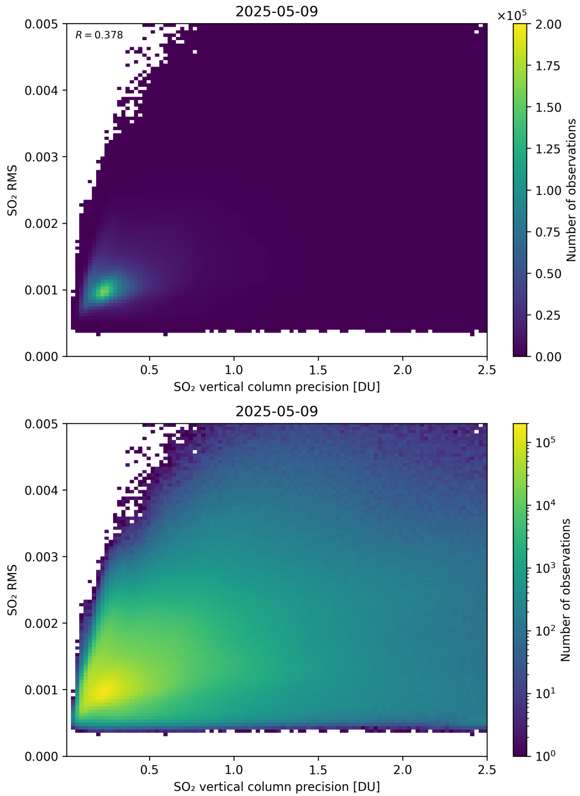
Figure 334: Scatter density plot of “SO 2 vertical column precision” against “SO 2 RMS” for 2025-05-08 to 2025-05-10.
