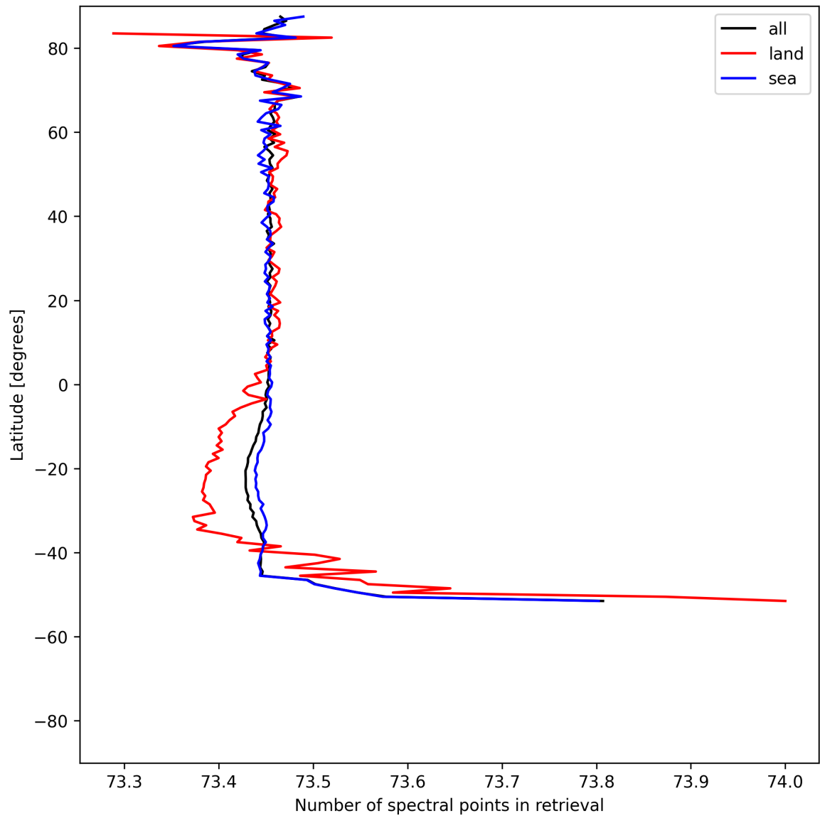
Figure 56: Zonal average of “Number of spectral points in retrieval” for 2025-05-08 to 2025-05-10.
