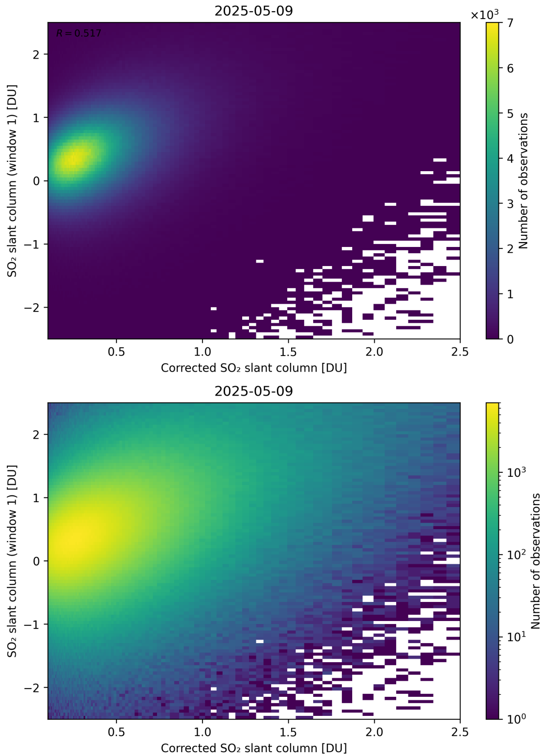
Figure 237: Scatter density plot of “Corrected SO 2 slant column” against “SO 2 slant column (window 1)” for 2025-05-08 to 2025-05-10.
