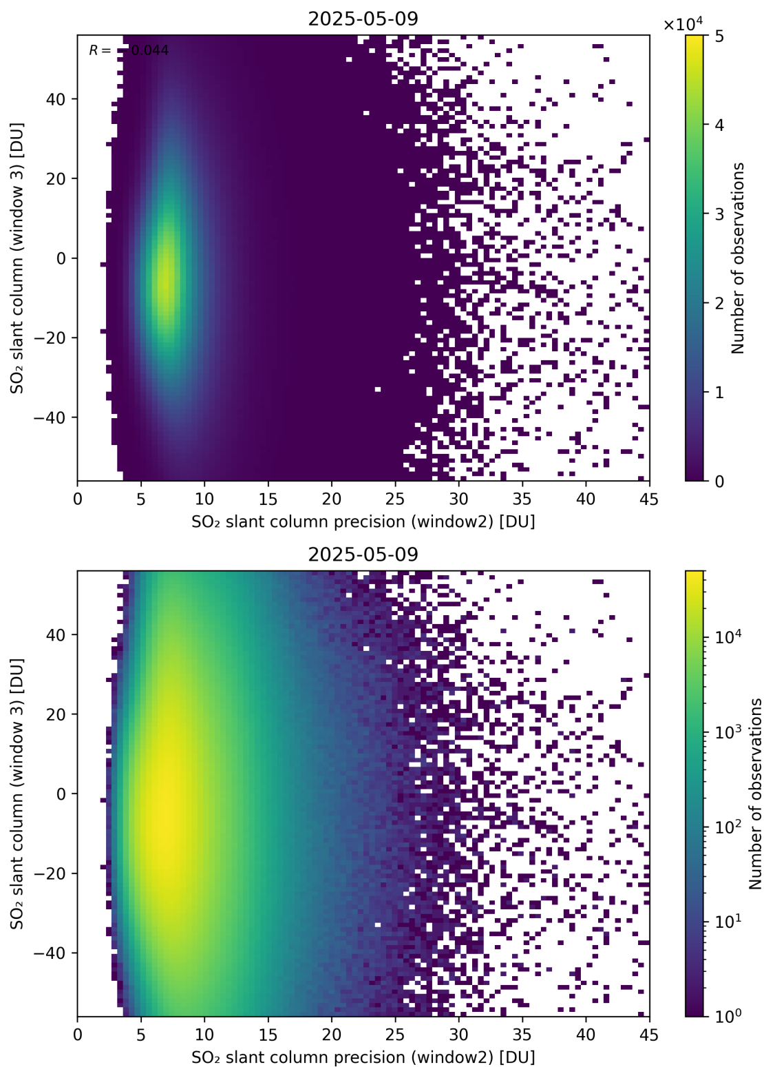
Figure 299: Scatter density plot of “SO 2 slant column precision (window2)” against “SO 2 slant column (window 3)” for 2025-05-08 to 2025-05-10.
