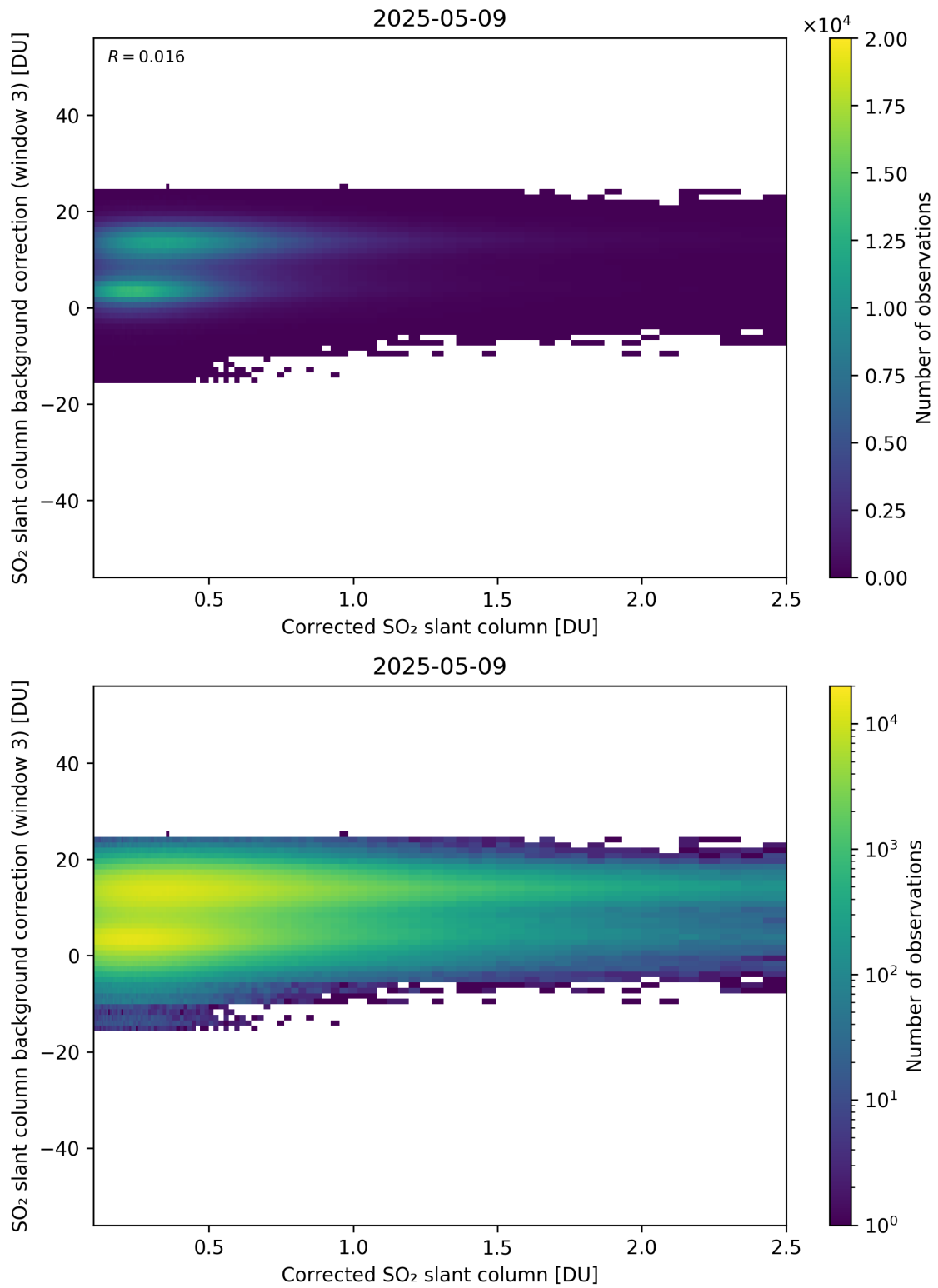
Figure 228: Scatter density plot of “Corrected SO 2 slant column” against “SO 2 slant column background correction (window 3)” for 2025-05-08 to 2025-05-10.
