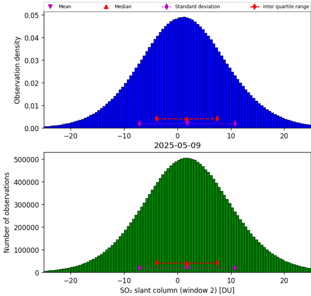
Figure 67: Histogram of “SO 2 slant column (window 2)” for 2025-05-08 to 2025-05-10
