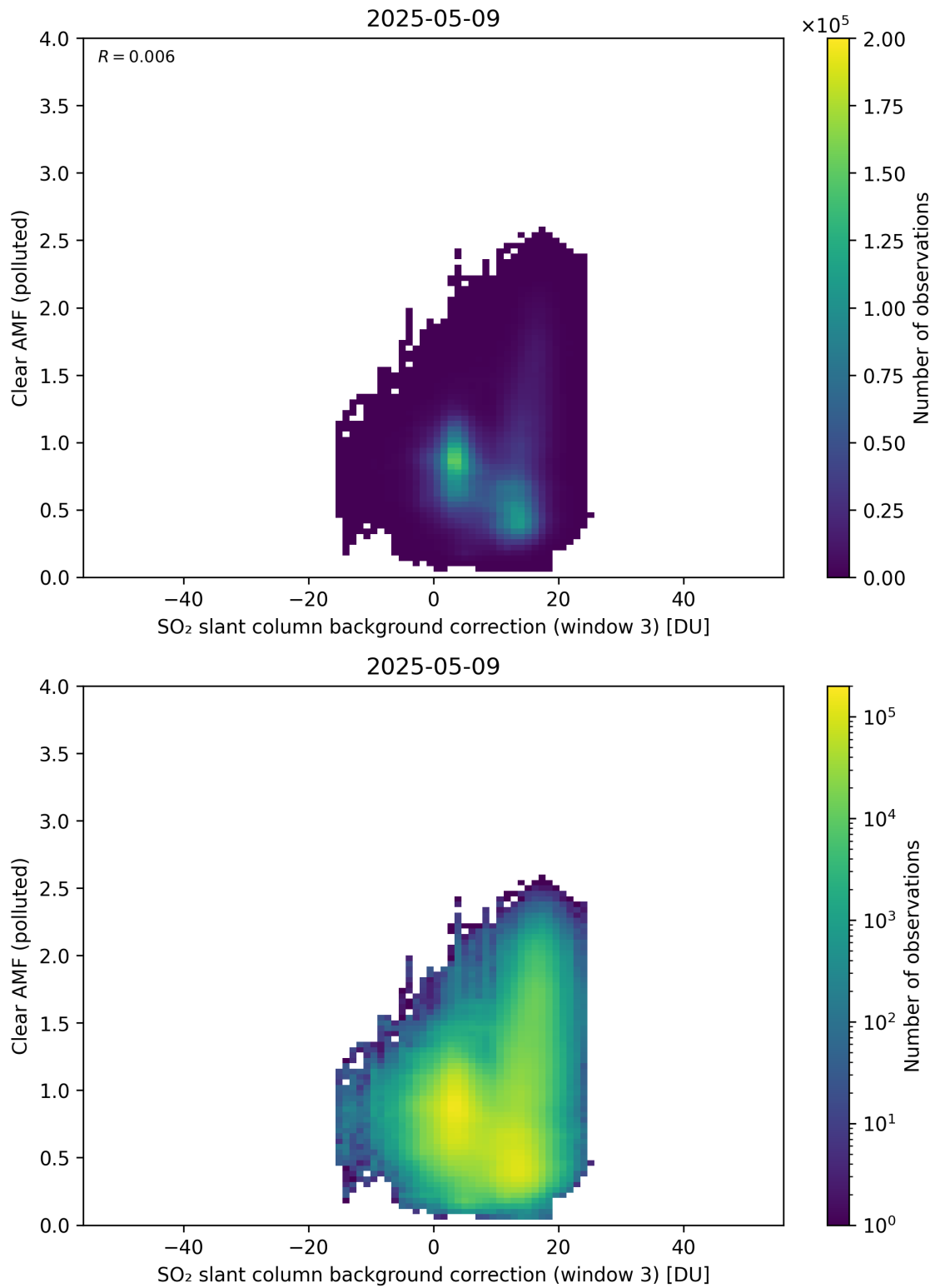
Figure 135: Scatter density plot of “SO 2 slant column background correction (window 3)” against “Clear AMF (polluted)” for 2025-05-08 to 2025-05-10.
