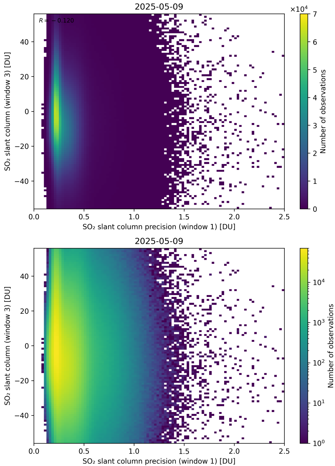
Figure 278: Scatter density plot of “SO 2 slant column precision (window 1)” against “SO 2 slant column (window 3)” for 2025-05-08 to 2025-05-10.
