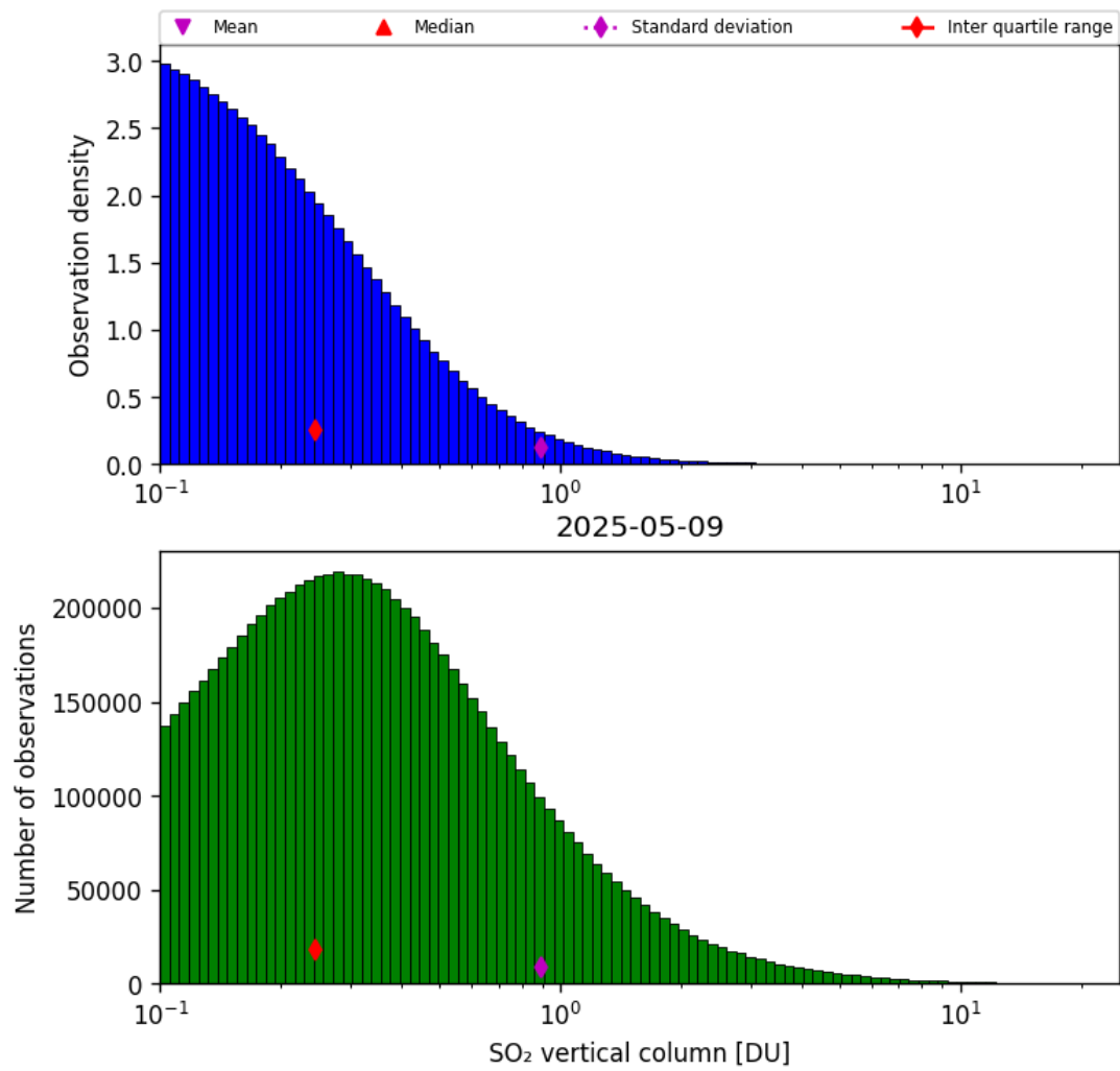
Figure 58: Histogram of “SO 2 vertical column” for 2025-05-08 to 2025-05-10
