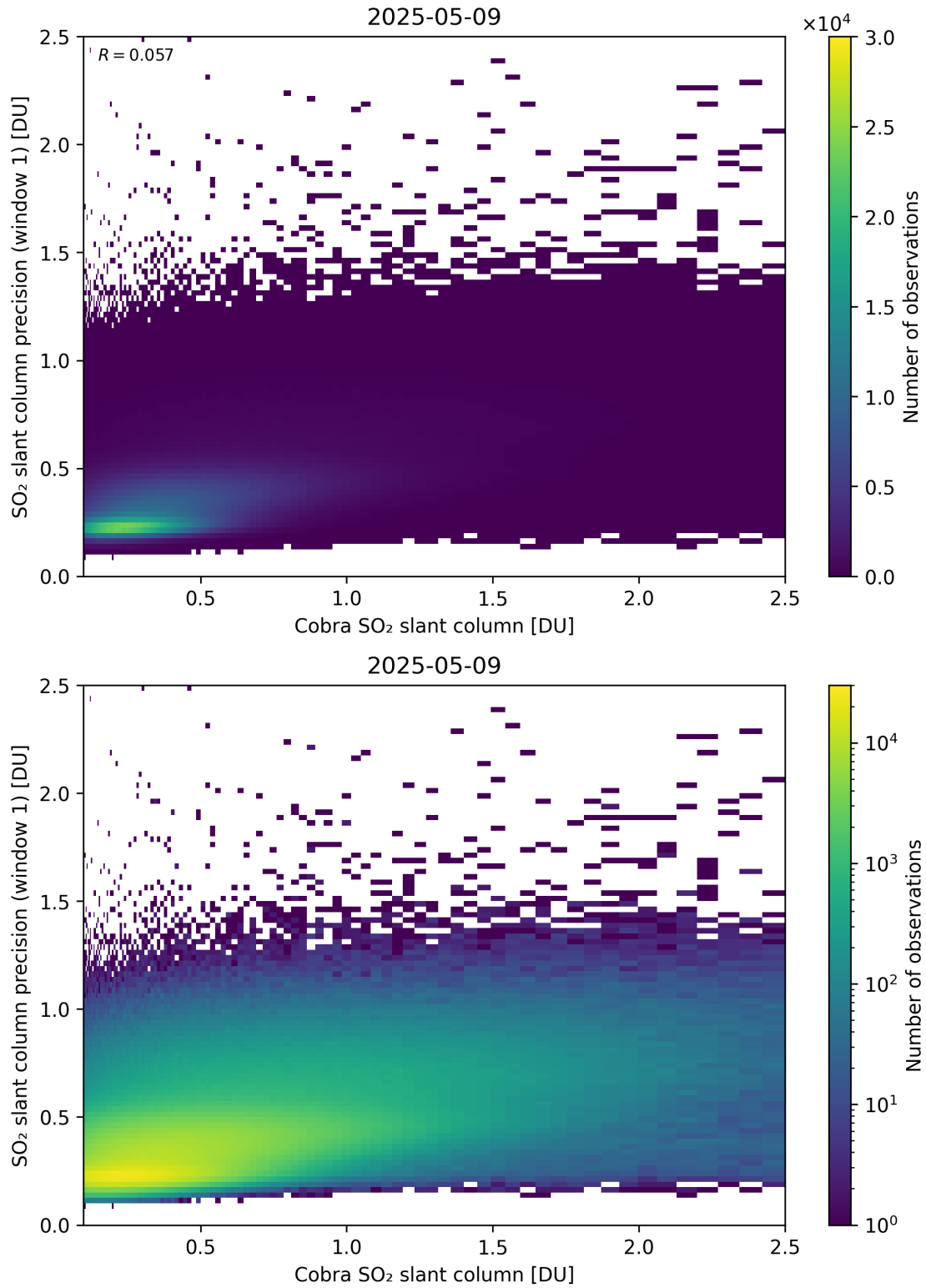
Figure 220: Scatter density plot of “Cobra SO 2 slant column” against “SO 2 slant column precision (window 1)” for 2025-05-08 to 2025-05-10.
