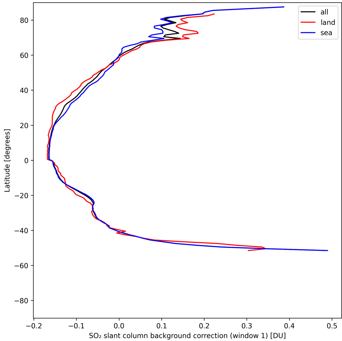
Figure 40: Zonal average of “SO 2 slant column background correction (window 1)” for 2025-05-08 to 2025-05-10.
