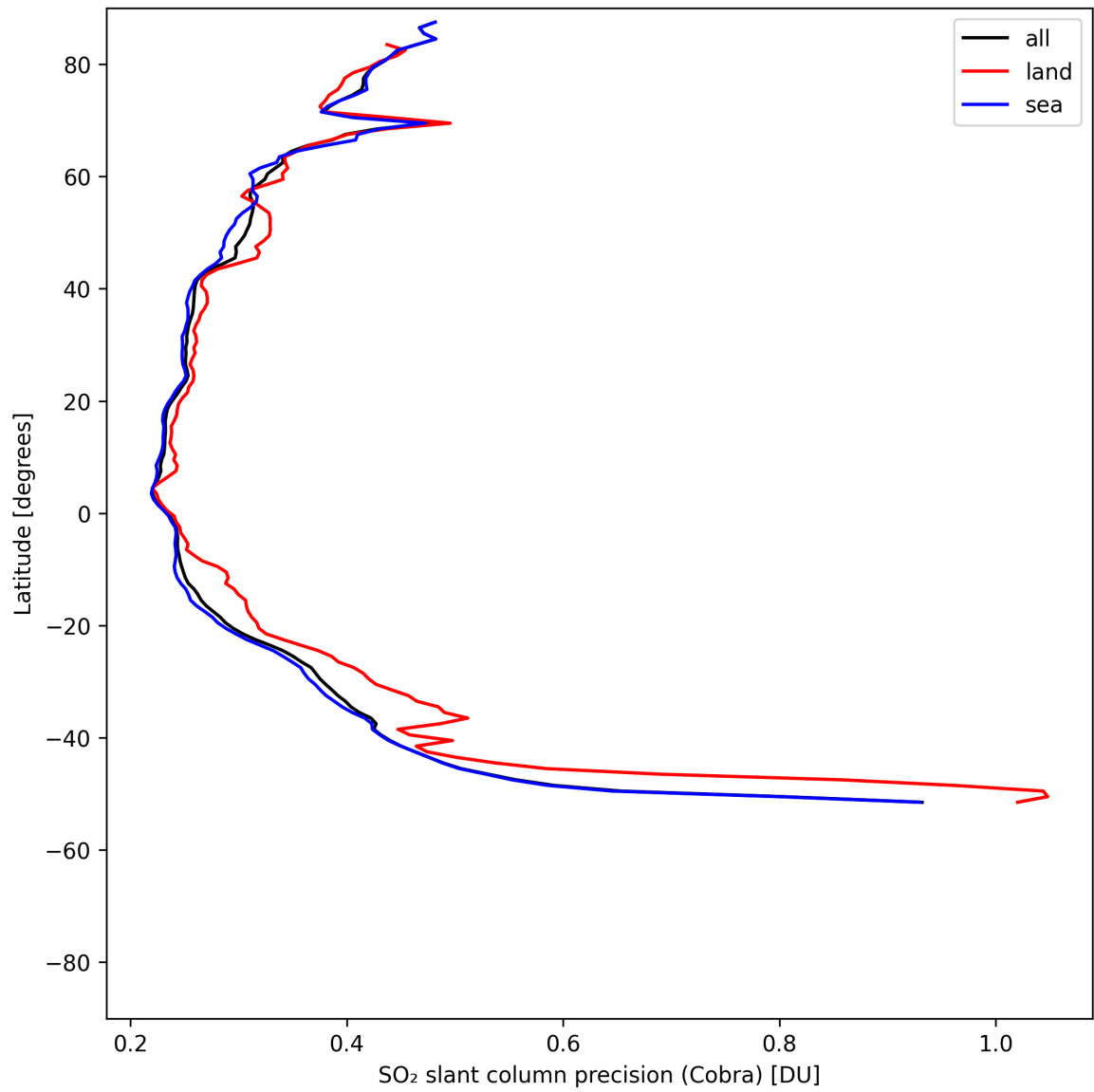
Figure 36: Zonal average of “SO 2 slant column precision (Cobra)” for 2025-05-08 to 2025-05-10.
