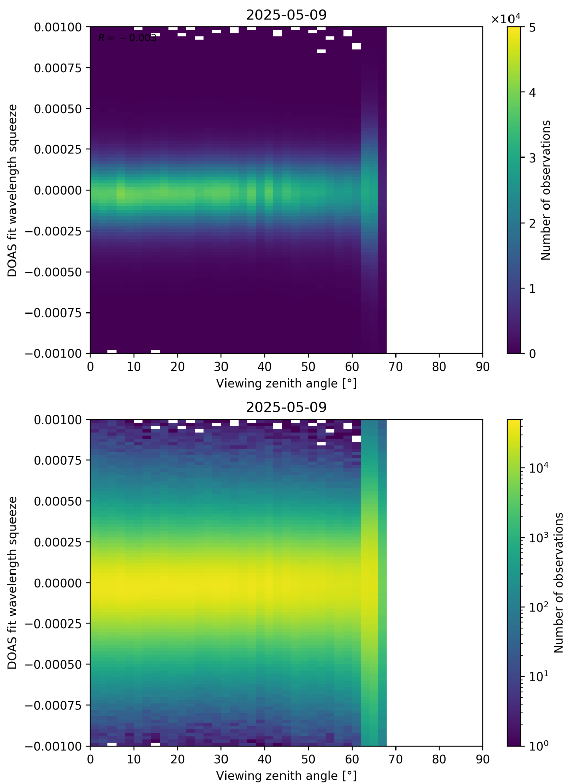
Figure 366: Scatter density plot of “Viewing zenith angle” against “DOAS fit wavelength squeeze” for 2025-05-08 to 2025-05-10.
