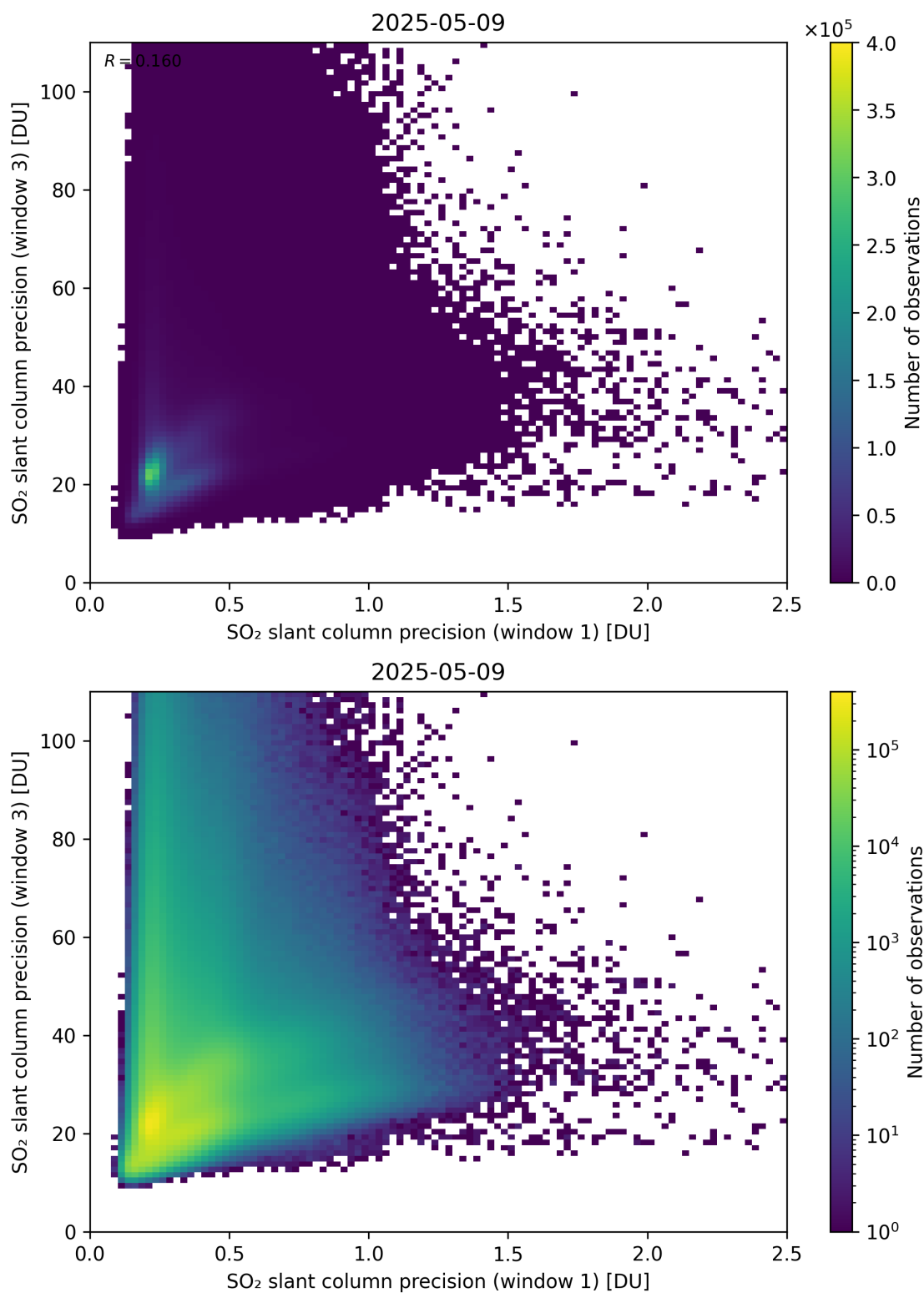
Figure 279: Scatter density plot of “SO 2 slant column precision (window 1)” against “SO 2 slant column precision (window 3)” for 2025-05-08 to 2025-05-10.
