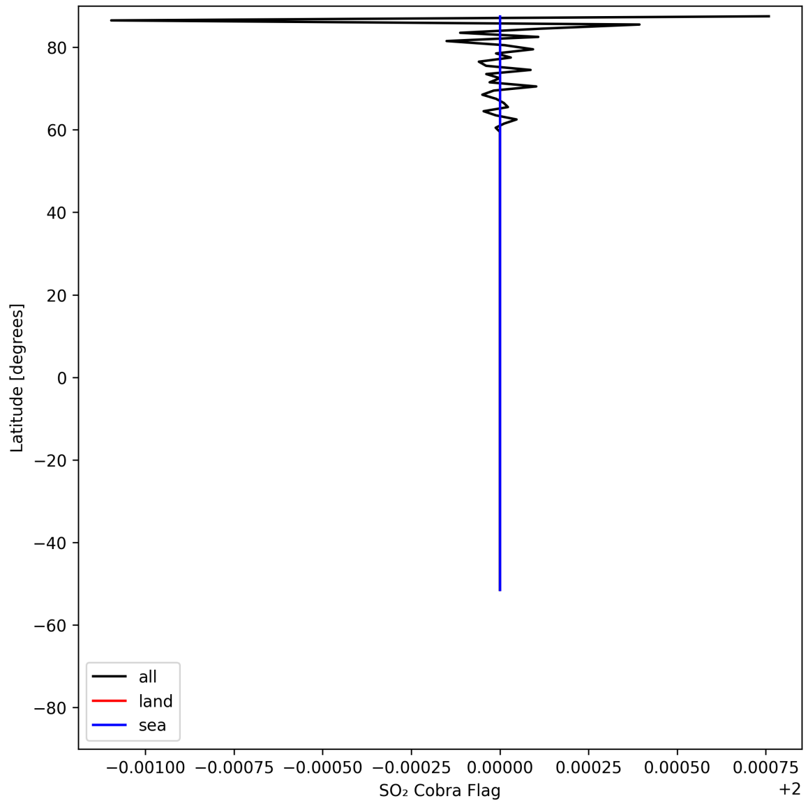
Figure 49: Zonal average of "SO 2 Cobra Flag" for 2025-05-08 to 2025-05-10.
