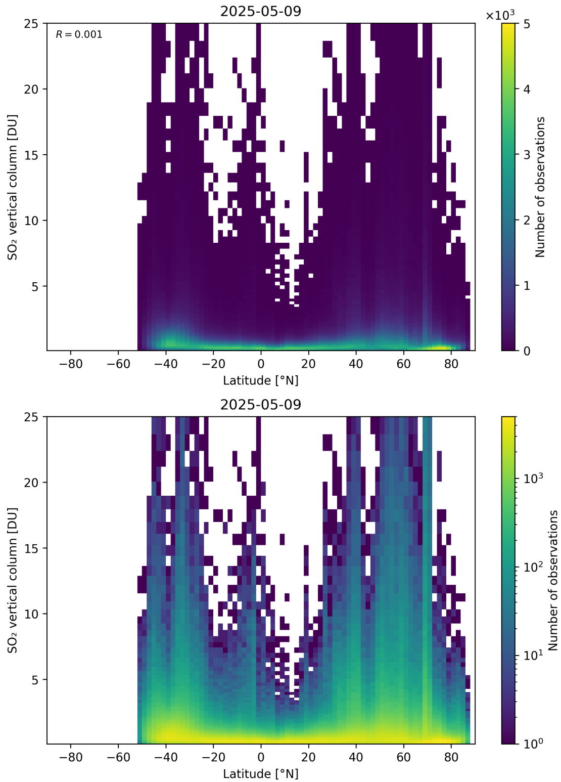
Figure 169: Scatter density plot of “Latitude” against “SO 2 vertical column” for 2025-05-08 to 2025-05-10.
