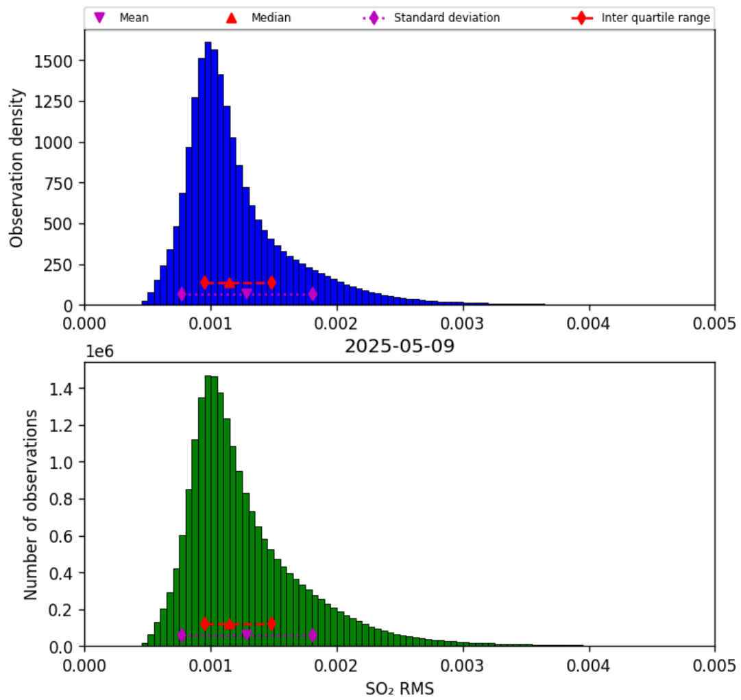
Figure 78: Histogram of “SO 2 RMS” for 2025-05-08 to 2025-05-10
