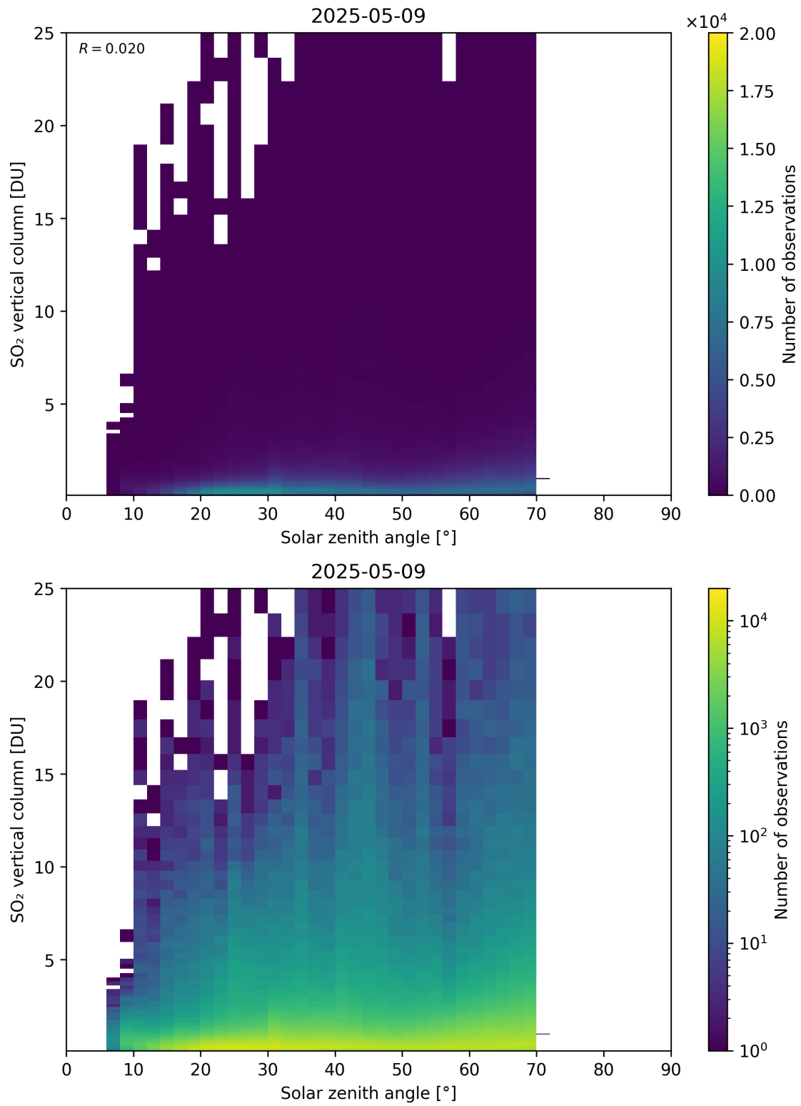
Figure 191: Scatter density plot of “Solar zenith angle” against “SO 2 vertical column” for 2025-05-08 to 2025-05-10.
