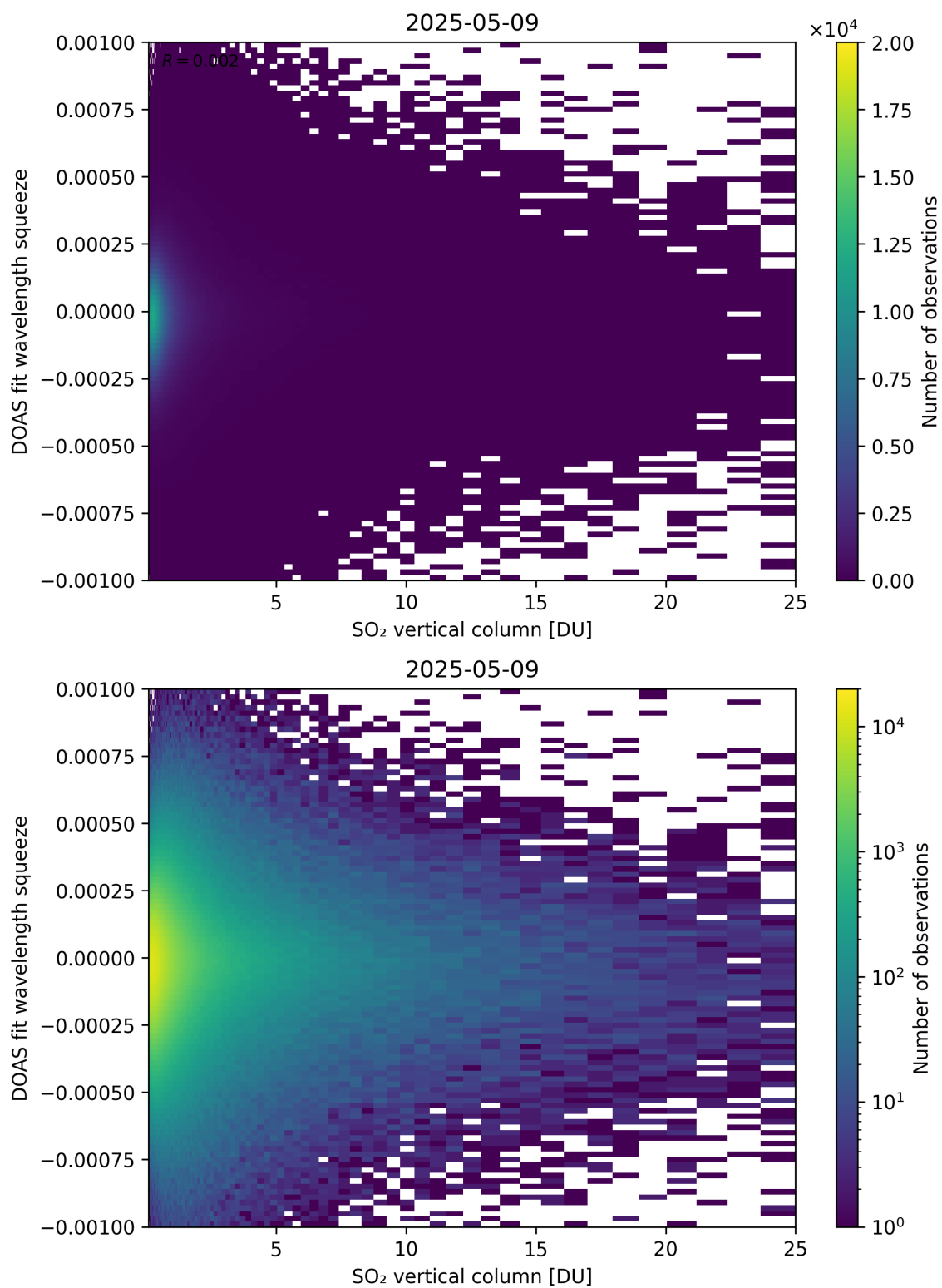
Figure 327: Scatter density plot of “SO 2 vertical column” against “DOAS fit wavelength squeeze” for 2025-05-08 to 2025-05-10.
