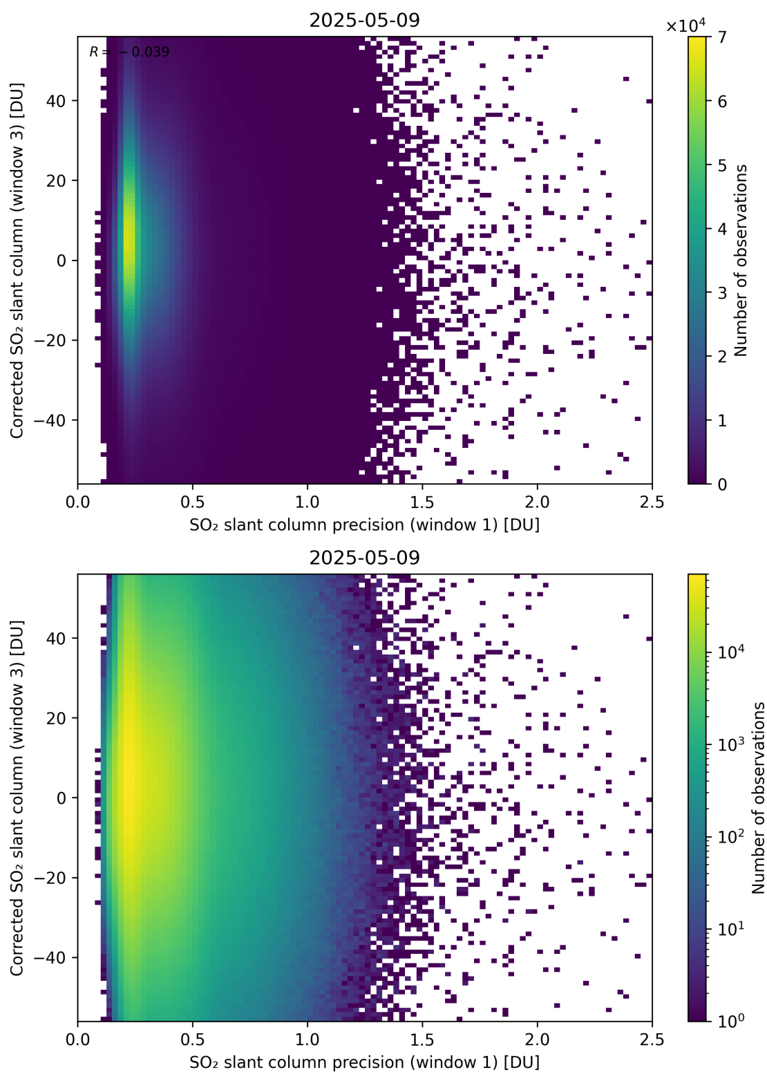
Figure 276: Scatter density plot of “SO 2 slant column precision (window 1)” against “Corrected SO 2 slant column (window 3)” for 2025-05-08 to 2025-05-10.
