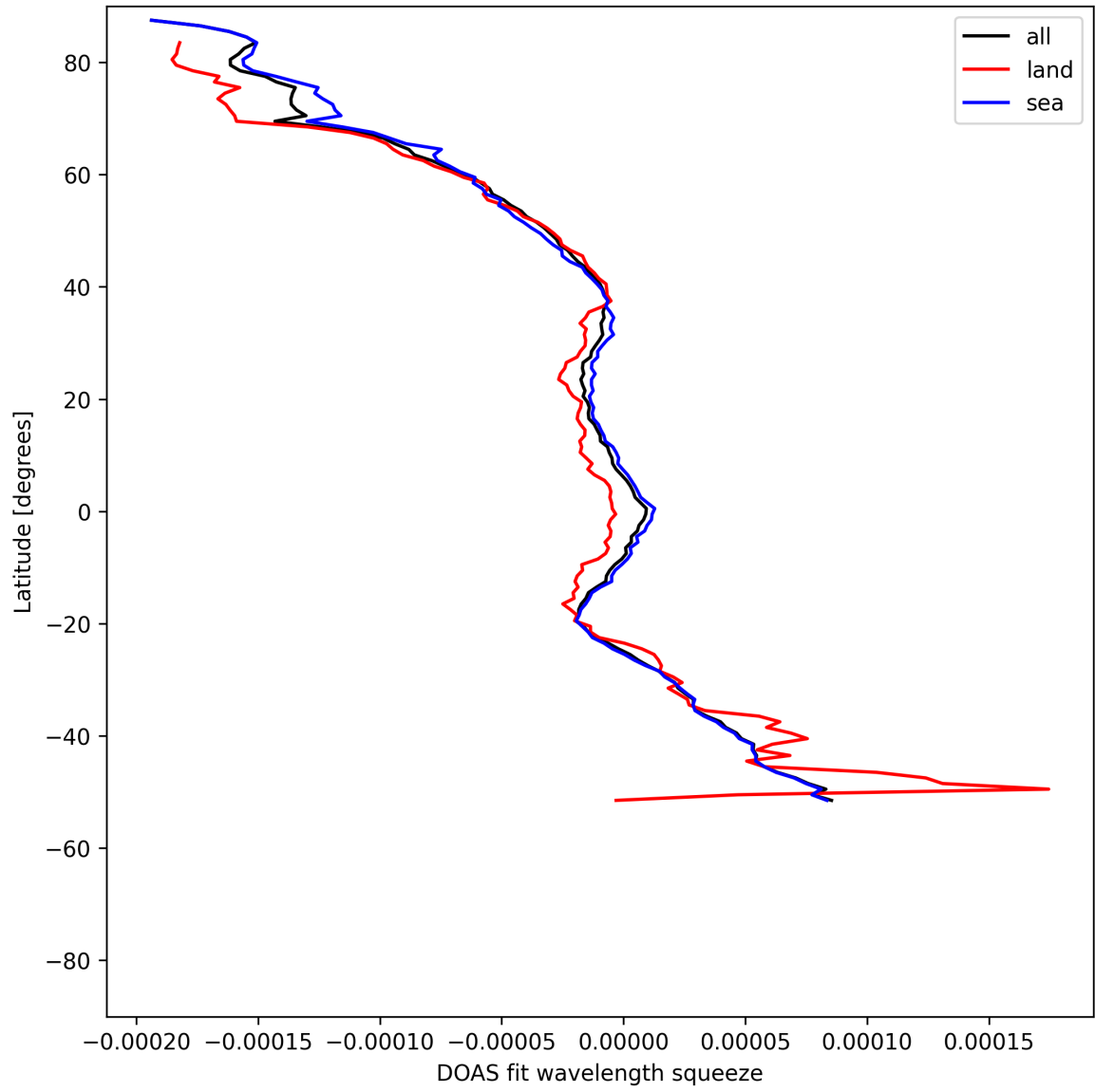
Figure 51: Zonal average of “DOAS fit wavelength squeeze” for 2025-05-08 to 2025-05-10.
