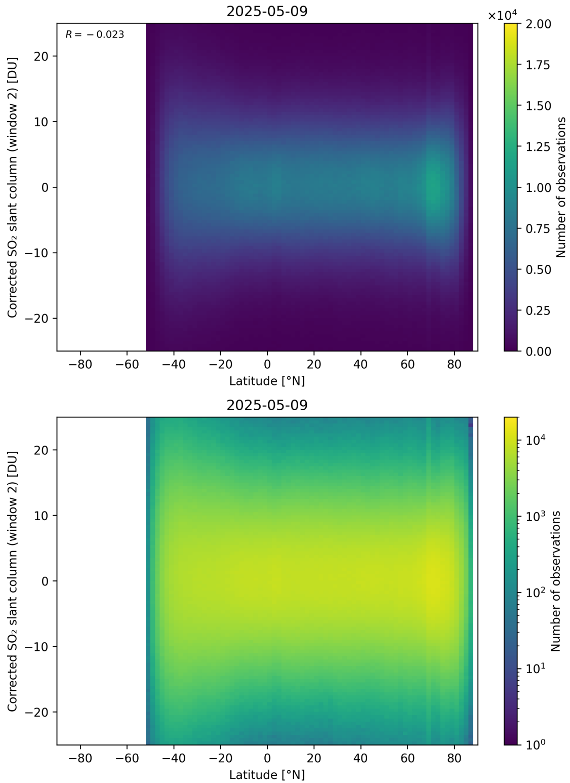
Figure 160: Scatter density plot of “Latitude” against “Corrected SO 2 slant column (window 2)” for 2025-05-08 to 2025-05-10.
