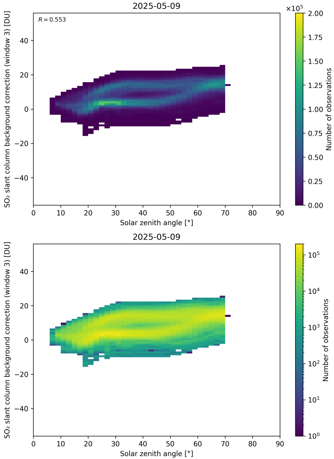
Figure 173: Scatter density plot of “Solar zenith angle” against “SO 2 slant column background correction (window 3)” for 2025-05-08 to 2025-05-10.
