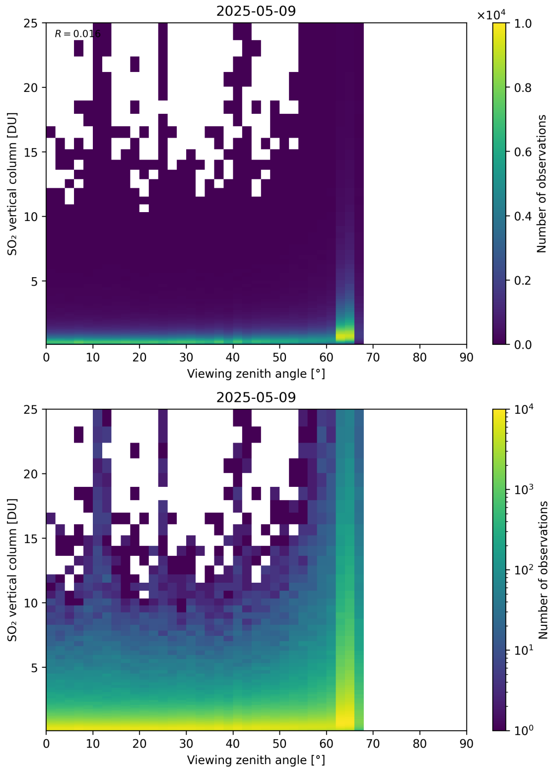
Figure 383: Scatter density plot of “Viewing zenith angle” against “SO 2 vertical column” for 2025-05-08 to 2025-05-10.
