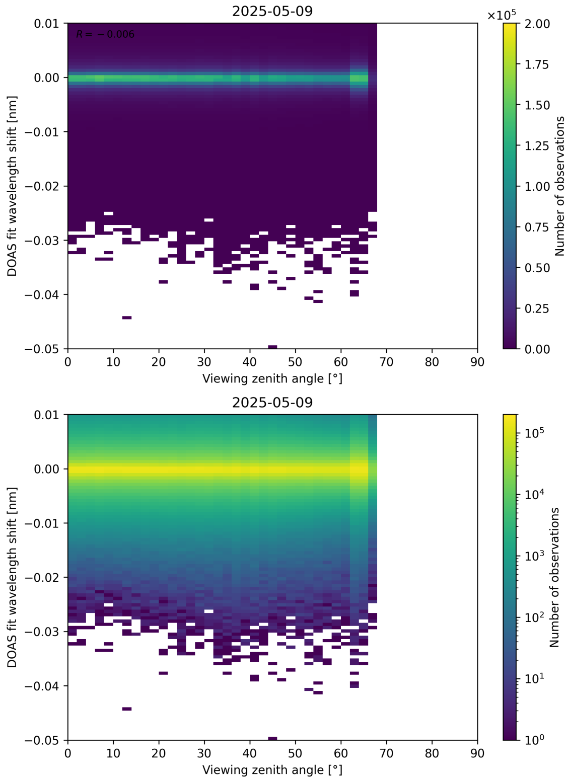
Figure 365: Scatter density plot of “Viewing zenith angle” against “DOAS fit wavelength shift” for 2025-05-08 to 2025-05-10.
