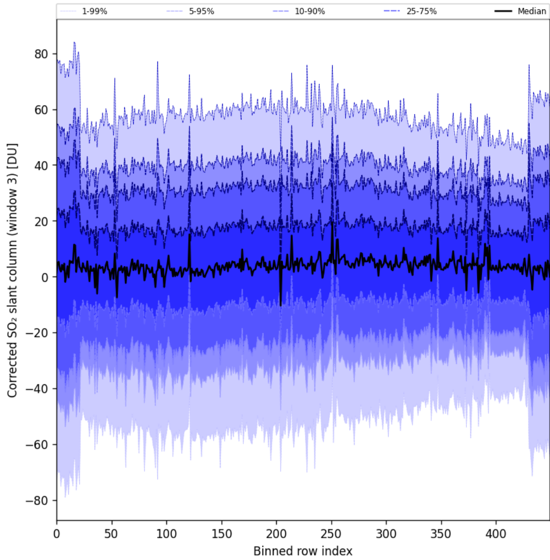
Figure 99: Along track statistics of “Corrected SO 2 slant column (window 3)” for 2025-05-08 to 2025-05-10
