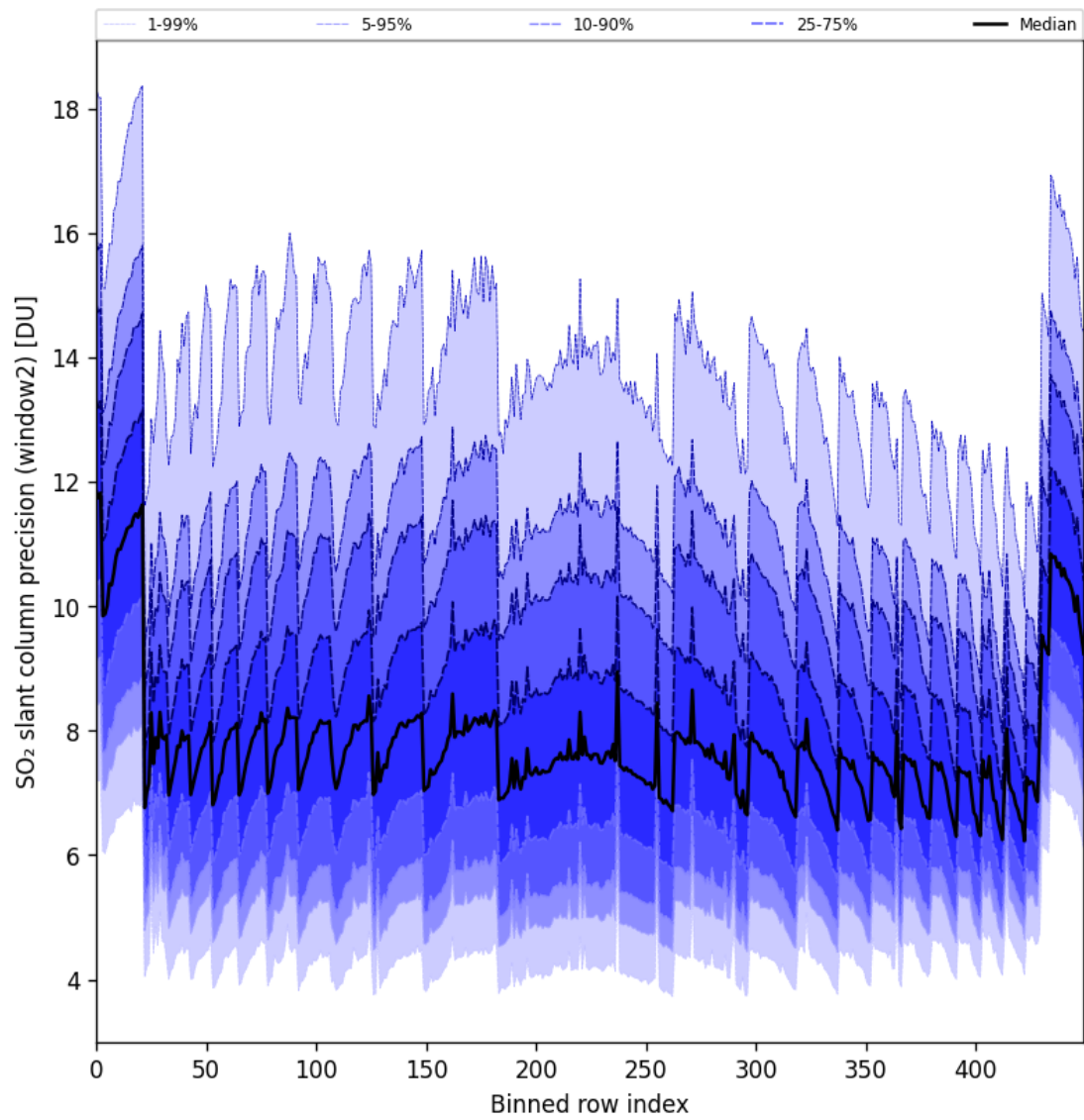
Figure 94: Along track statistics of “SO 2 slant column precision (window2)” for 2025-05-08 to 2025-05-10
