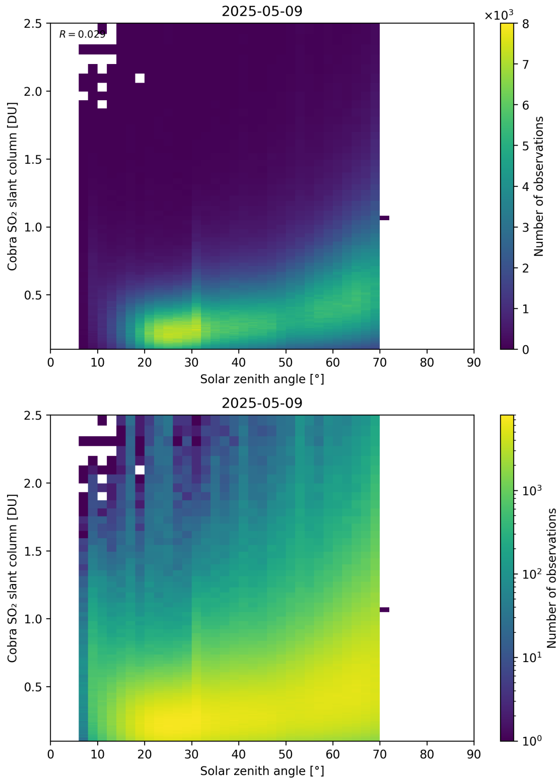
Figure 179: Scatter density plot of “Solar zenith angle” against “Cobra SO 2 slant column” for 2025-05-08 to 2025-05-10.
