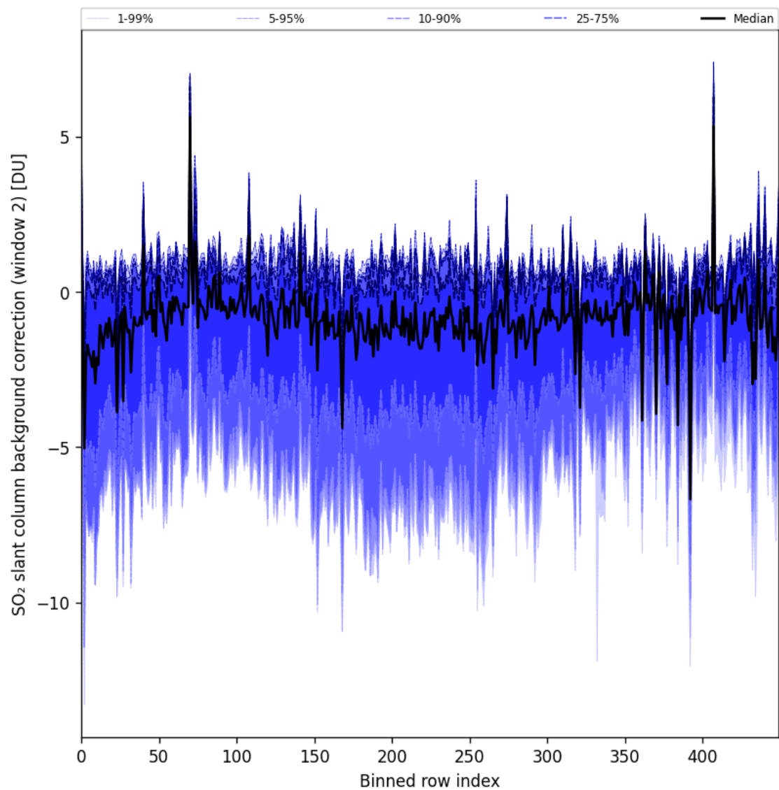
Figure 96: Along track statistics of “SO 2 slant column background correction (window 2)” for 2025-05-08 to 2025-05-10
