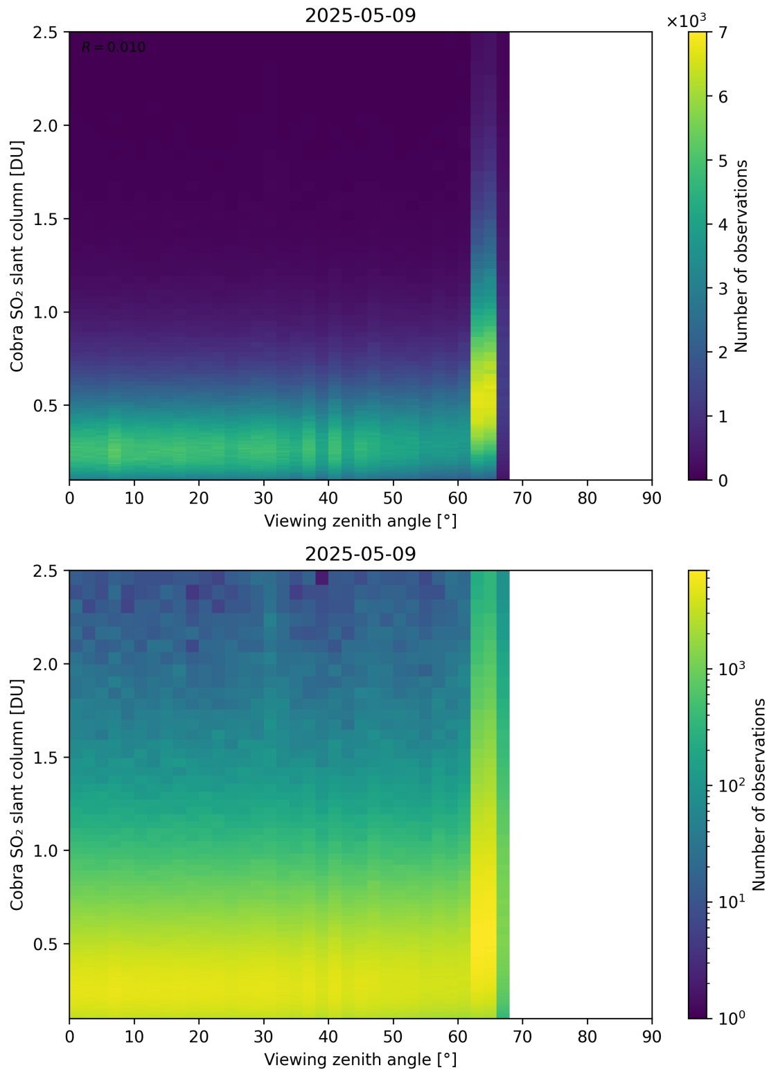
Figure 371: Scatter density plot of “Viewing zenith angle” against “Cobra SO 2 slant column” for 2025-05-08 to 2025-05-10.
