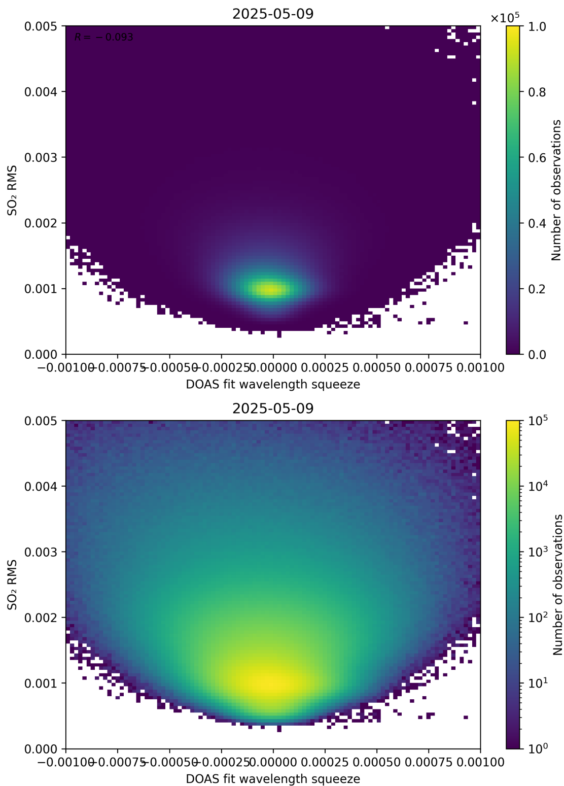
Figure 143: Scatter density plot of “DOAS fit wavelength squeeze” against “SO 2 RMS” for 2025-05-08 to 2025-05-10.
