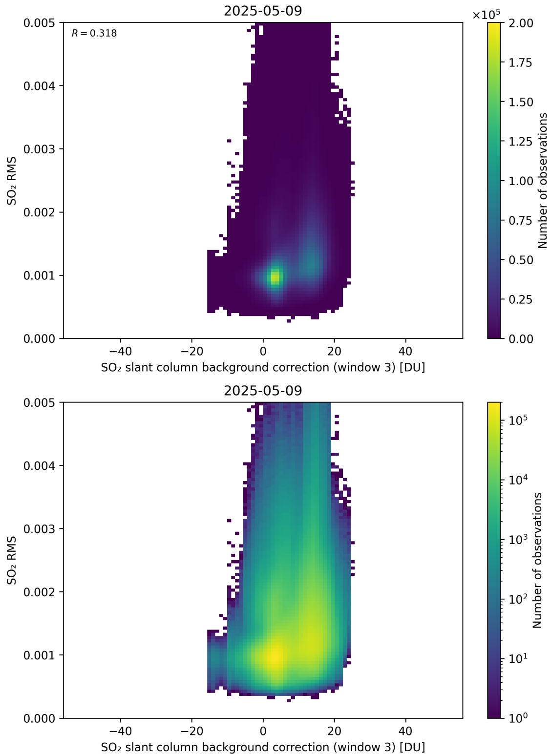
Figure 134: Scatter density plot of “SO 2 slant column background correction (window 3)” against “SO 2 RMS” for 2025-05-08 to 2025-05-10.
