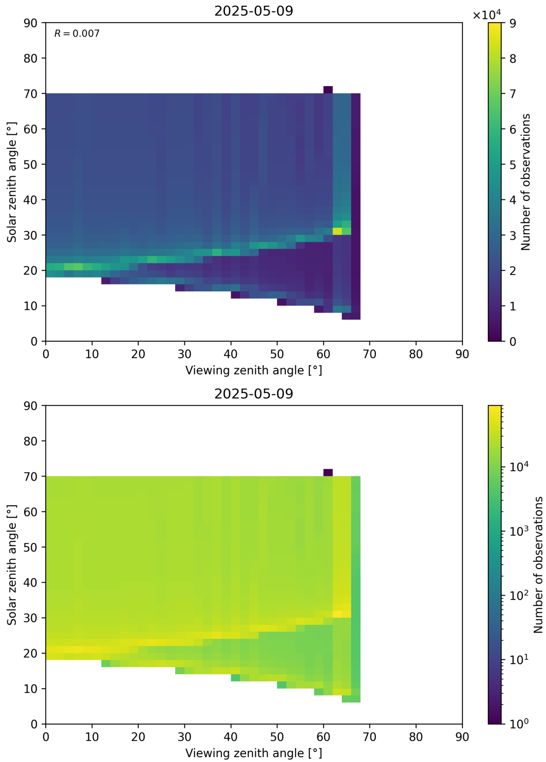
Figure 369: Scatter density plot of “Viewing zenith angle” against “Solar zenith angle” for 2025-05-08 to 2025-05-10.
