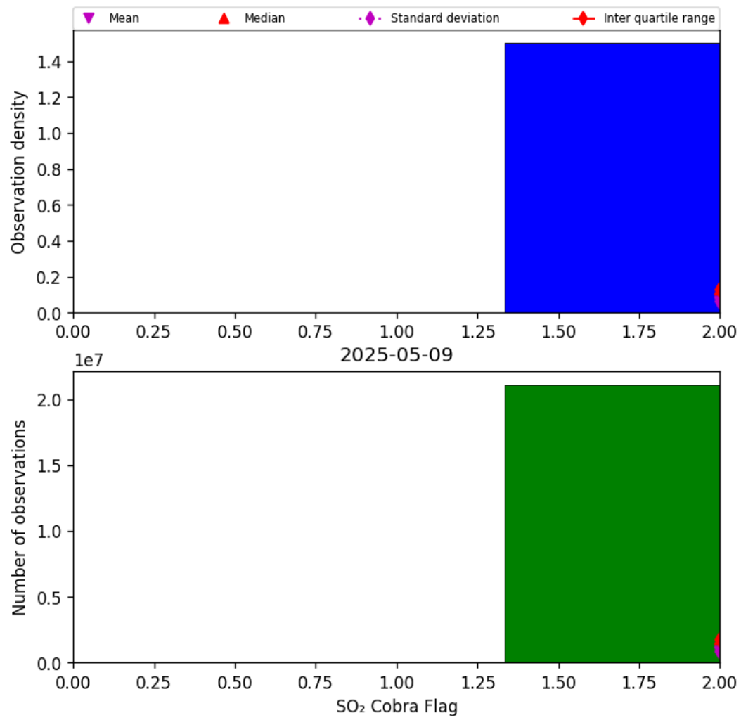
Figure 75: Histogram of “SO 2 Cobra Flag” for 2025-05-08 to 2025-05-10
