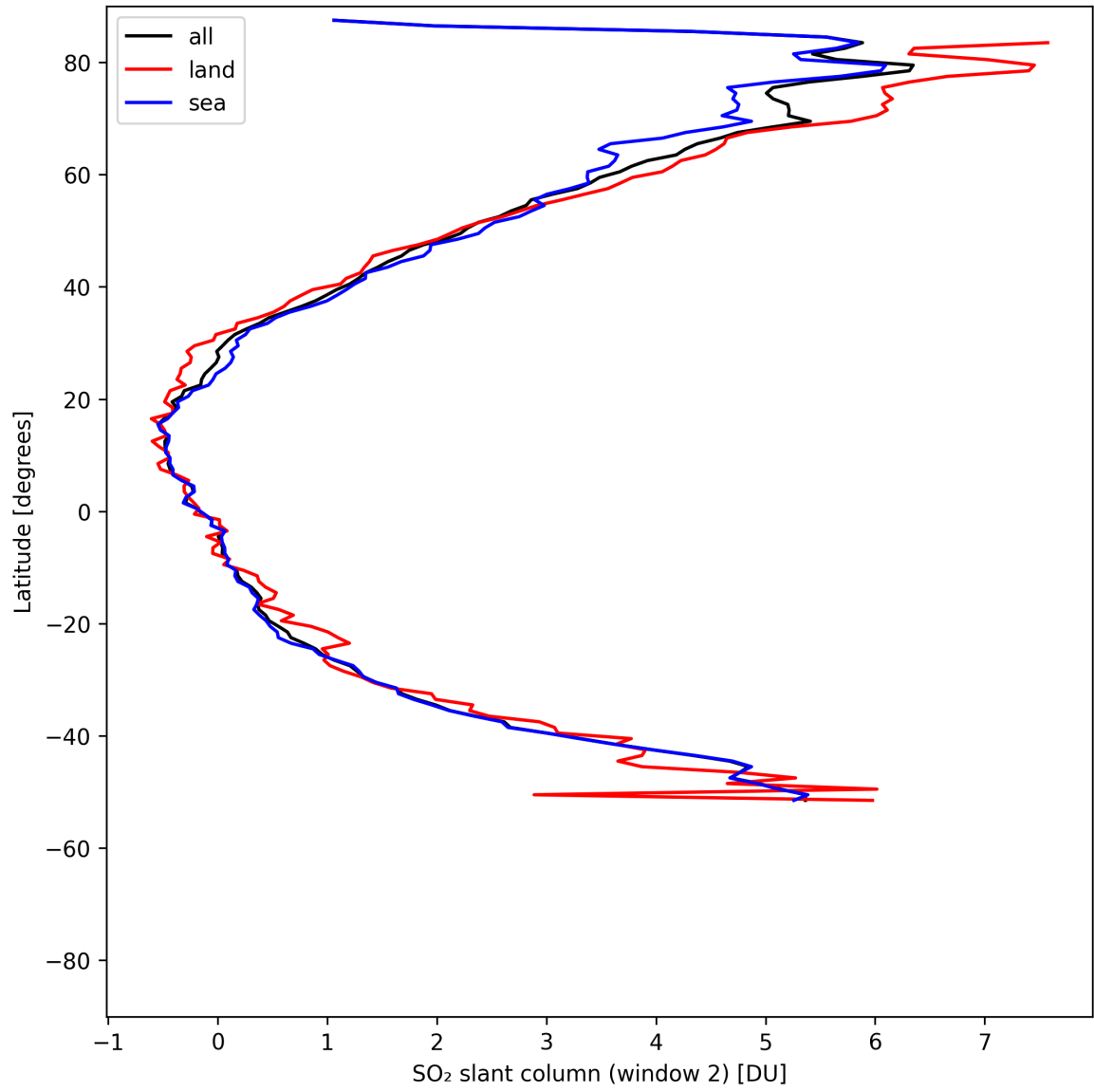
Figure 41: Zonal average of “SO 2 slant column (window 2)” for 2025-05-08 to 2025-05-10.
