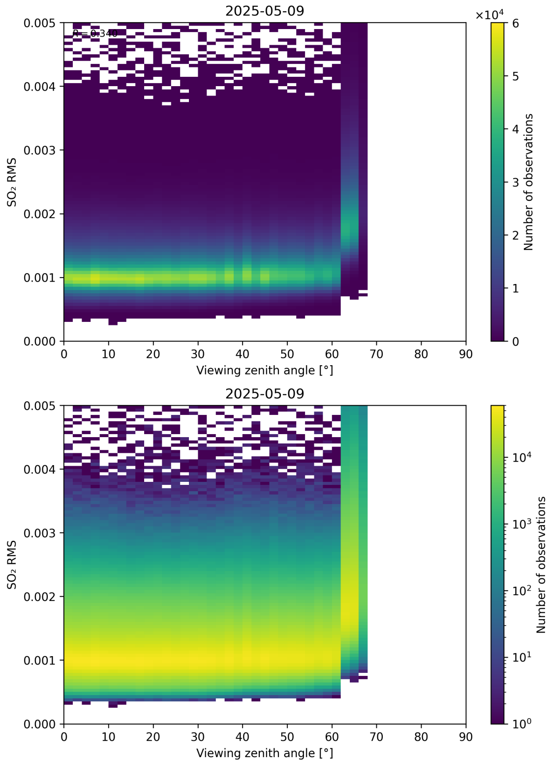
Figure 367: Scatter density plot of “Viewing zenith angle” against “SO 2 RMS” for 2025-05-08 to 2025-05-10.
