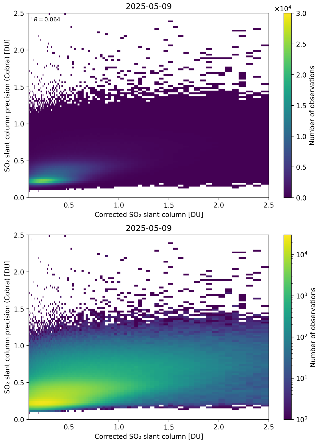
Figure 234: Scatter density plot of “Corrected SO 2 slant column” against “SO 2 slant column precision (Cobra)” for 2025-05-08 to 2025-05-10.
