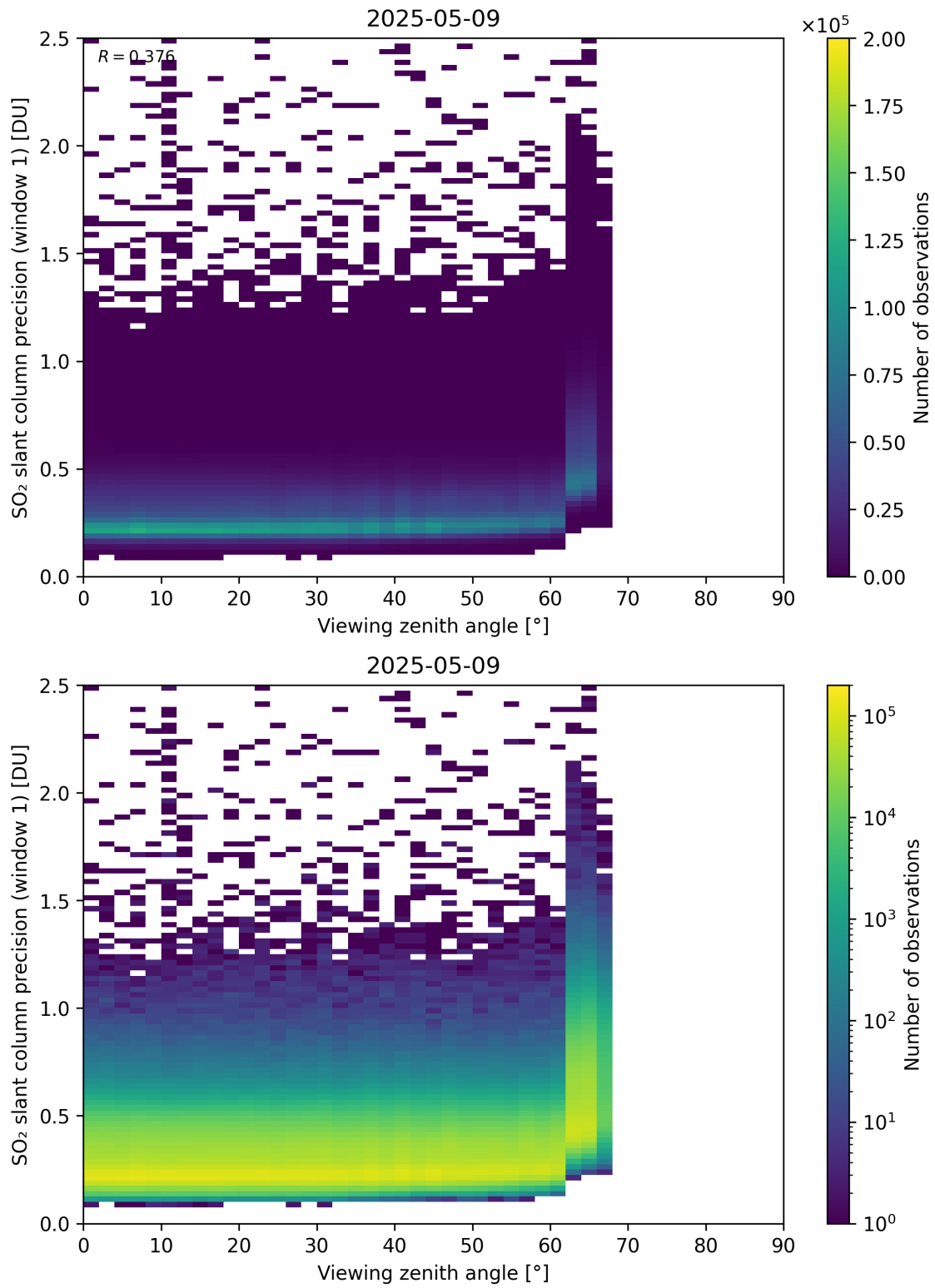
Figure 377: Scatter density plot of “Viewing zenith angle” against “SO 2 slant column precision (window 1)” for 2025-05-08 to 2025-05-10.
