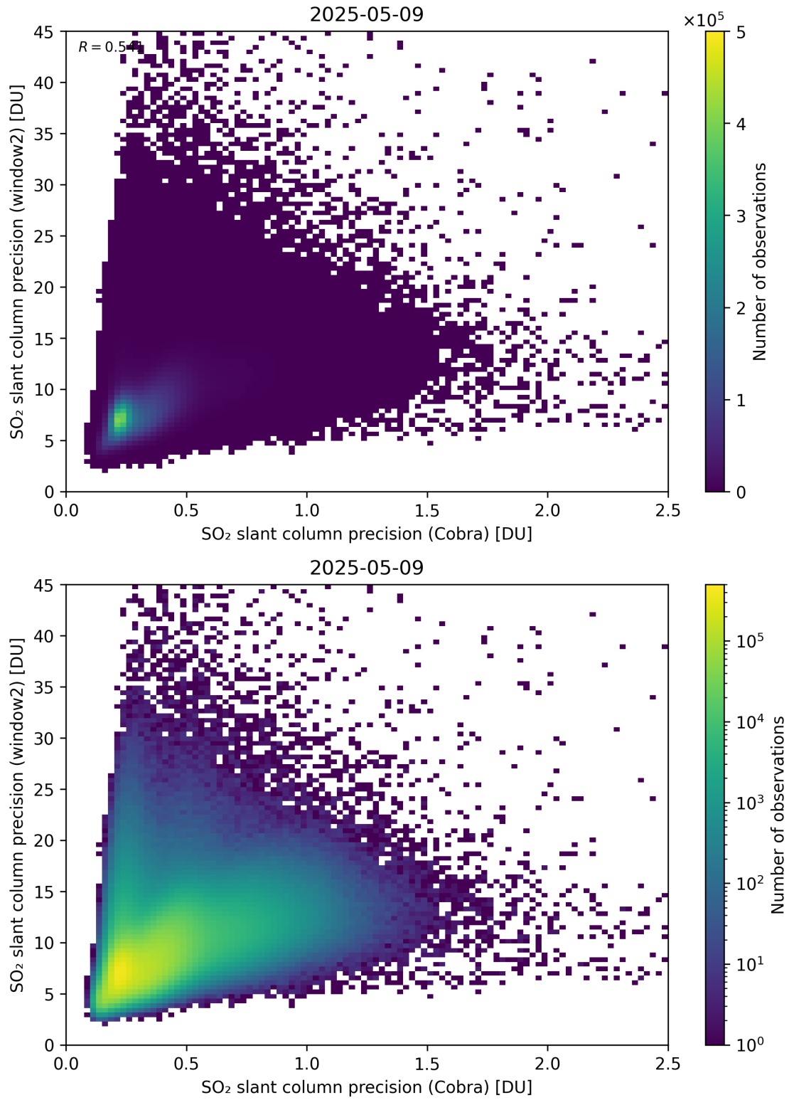
Figure 210: Scatter density plot of “SO 2 slant column precision (Cobra)” against “SO 2 slant column precision (window2)” for 2025-05-08 to 2025-05-10.
