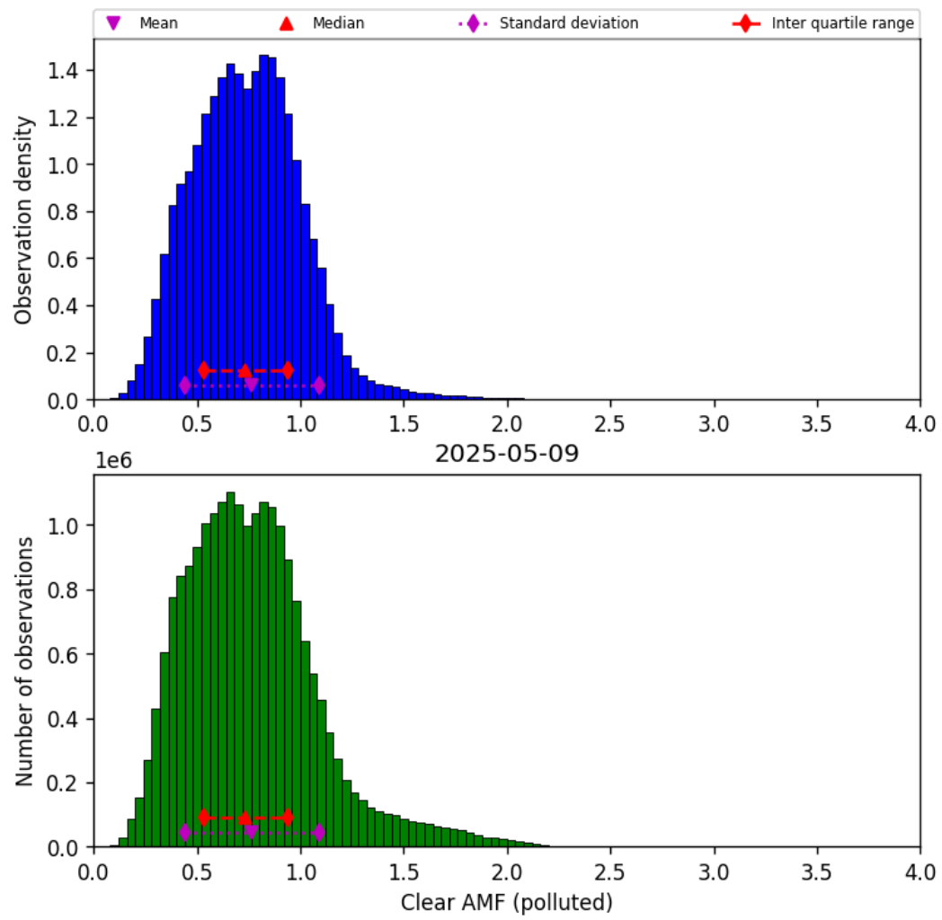
Figure 81: Histogram of “Clear AMF (polluted)” for 2025-05-08 to 2025-05-10
