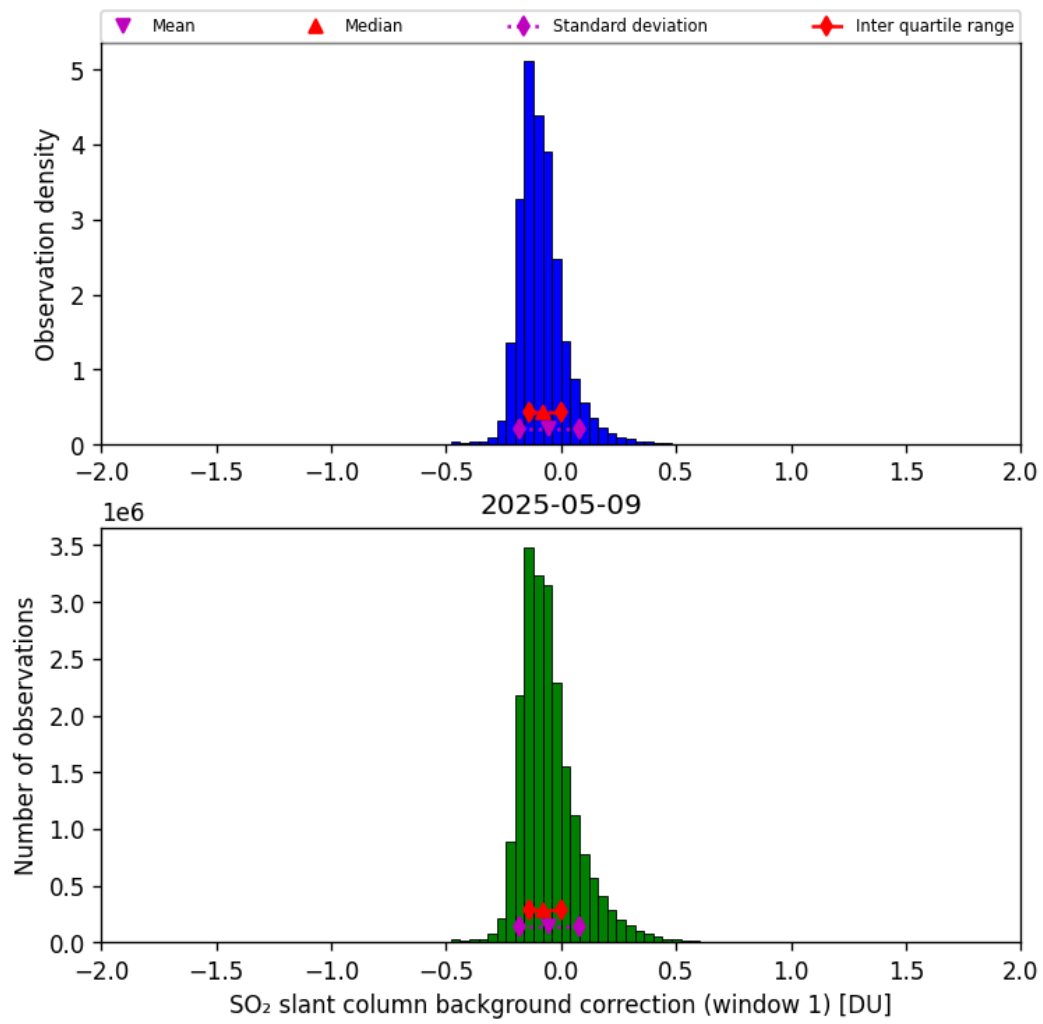
Figure 66: Histogram of “SO 2 slant column background correction (window 1)” for 2025-05-08 to 2025-05-10
