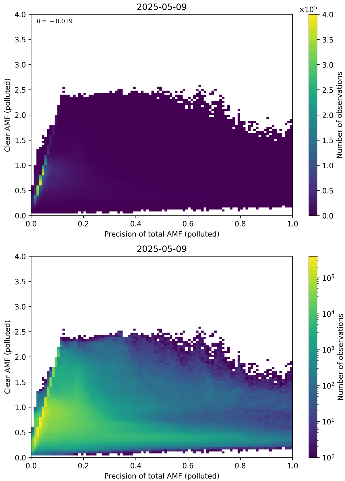
Figure 320: Scatter density plot of “Precision of total AMF (polluted)” against “Clear AMF (polluted)” for 2025-05-08 to 2025-05-10.
