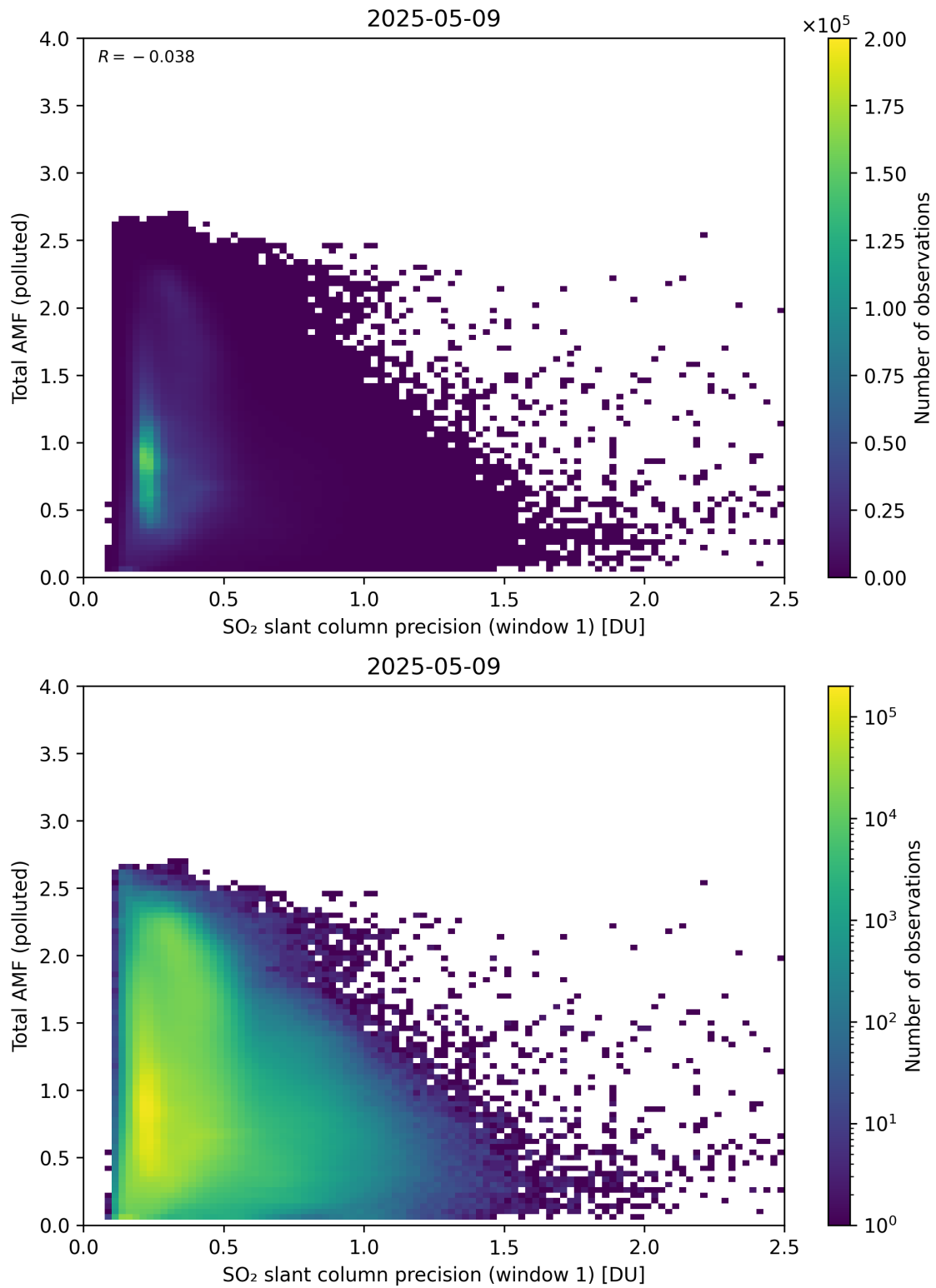
Figure 280: Scatter density plot of “SO 2 slant column precision (window 1)” against “Total AMF (polluted)” for 2025-05-08 to 2025-05-10.
