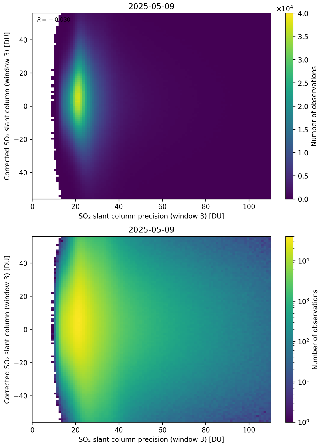
Figure 312: Scatter density plot of “SO 2 slant column precision (window 3)” against “Corrected SO 2 slant column (window 3)” for 2025-05-08 to 2025-05-10.
