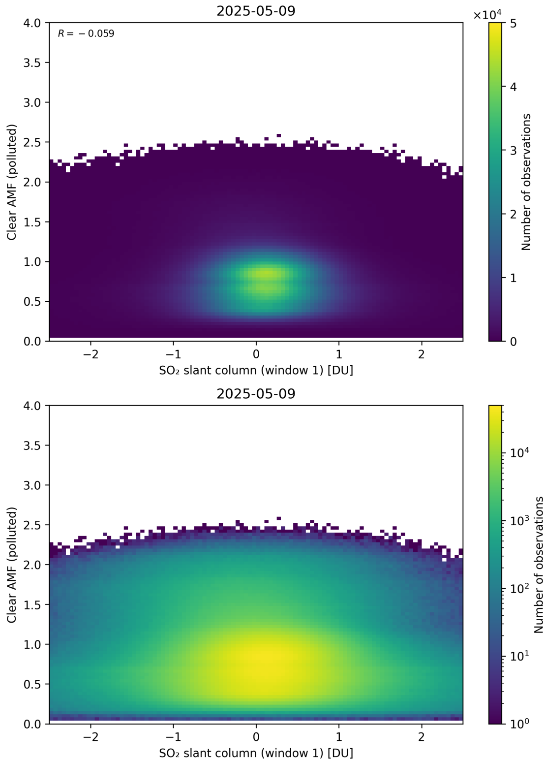
Figure 282: Scatter density plot of “SO 2 slant column (window 1)” against “Clear AMF (polluted)” for 2025-05-08 to 2025-05-10.
