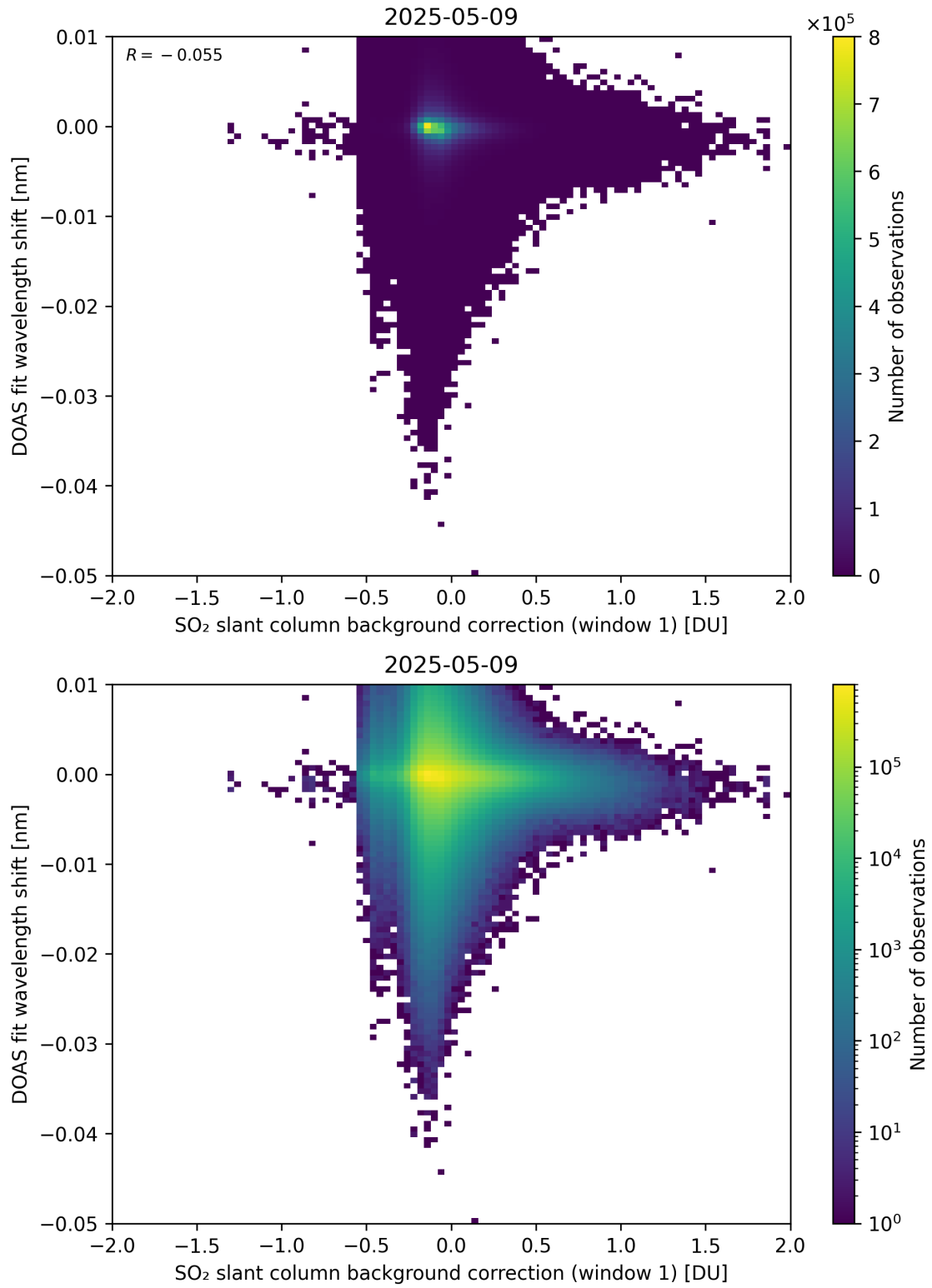
Figure 111: Scatter density plot of “SO 2 slant column background correction (window 1)” against “DOAS fit wavelength shift” for 2025-05-08 to 2025-05-10.
