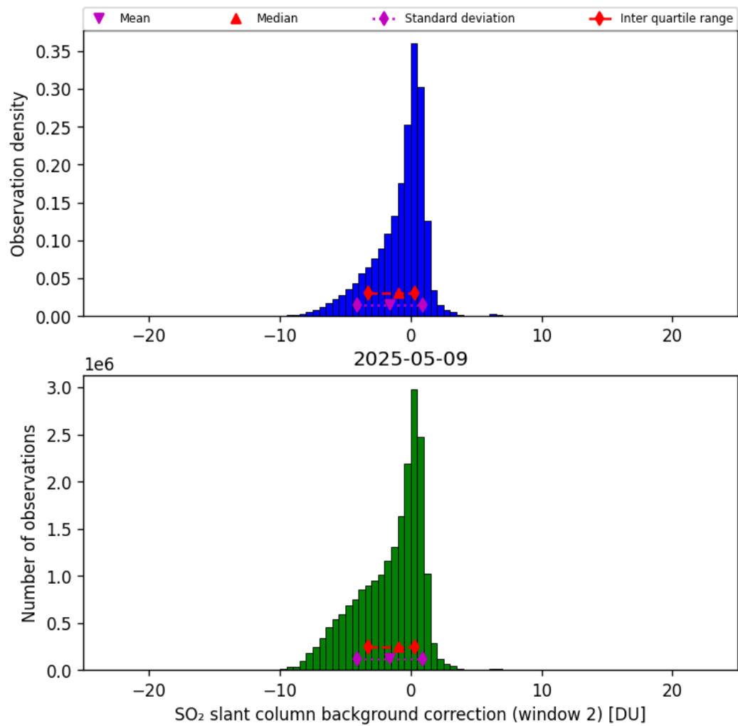
Figure 70: Histogram of “SO 2 slant column background correction (window 2)” for 2025-05-08 to 2025-05-10
