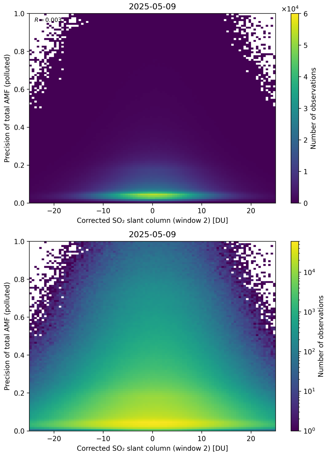
Figure 254: Scatter density plot of “Corrected SO 2 slant column (window 2)” against “Precision of total AMF (polluted)” for 2025-05-08 to 2025-05-10.
