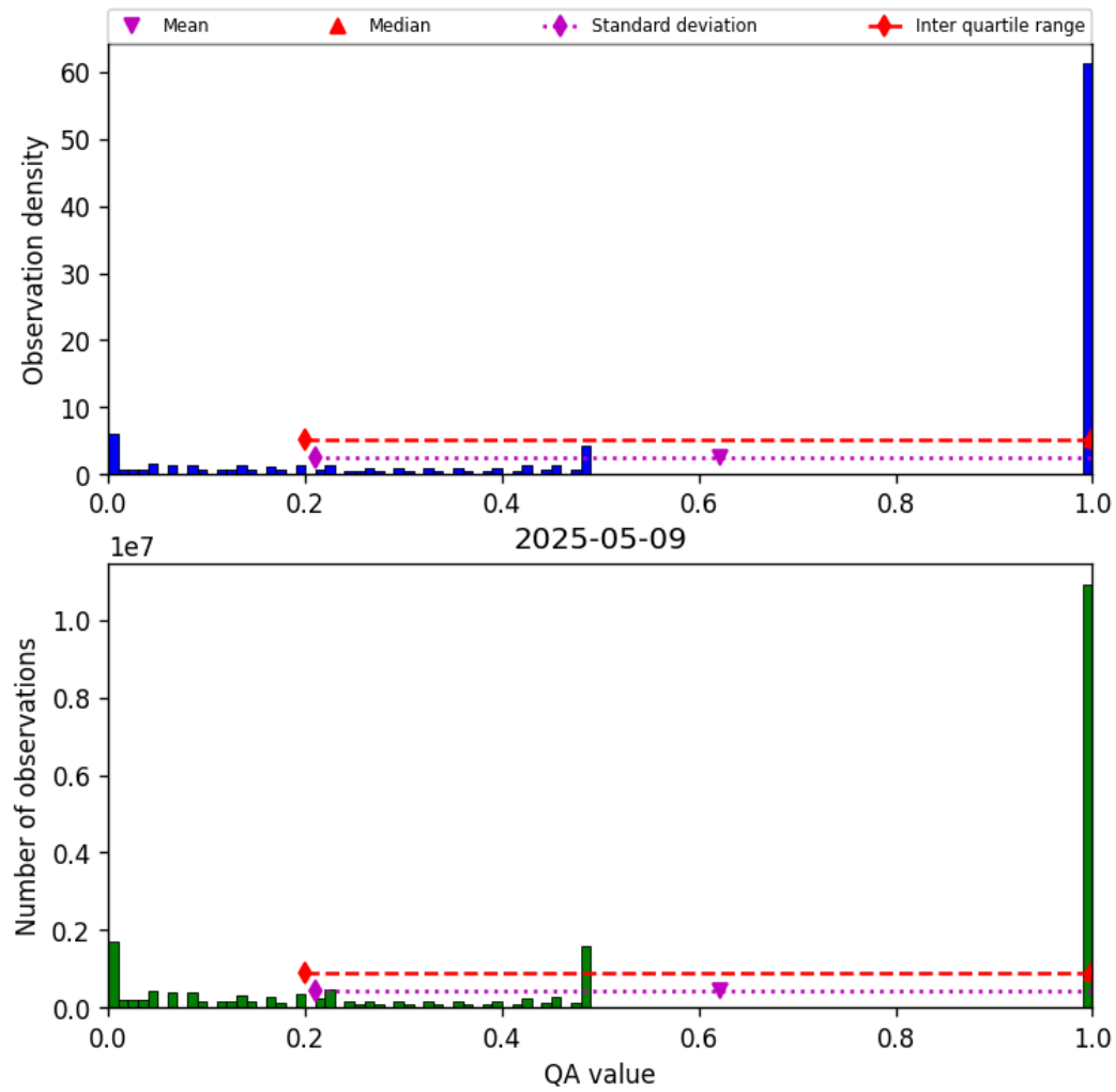
Figure 57: Histogram of “QA value” for 2025-05-08 to 2025-05-10
