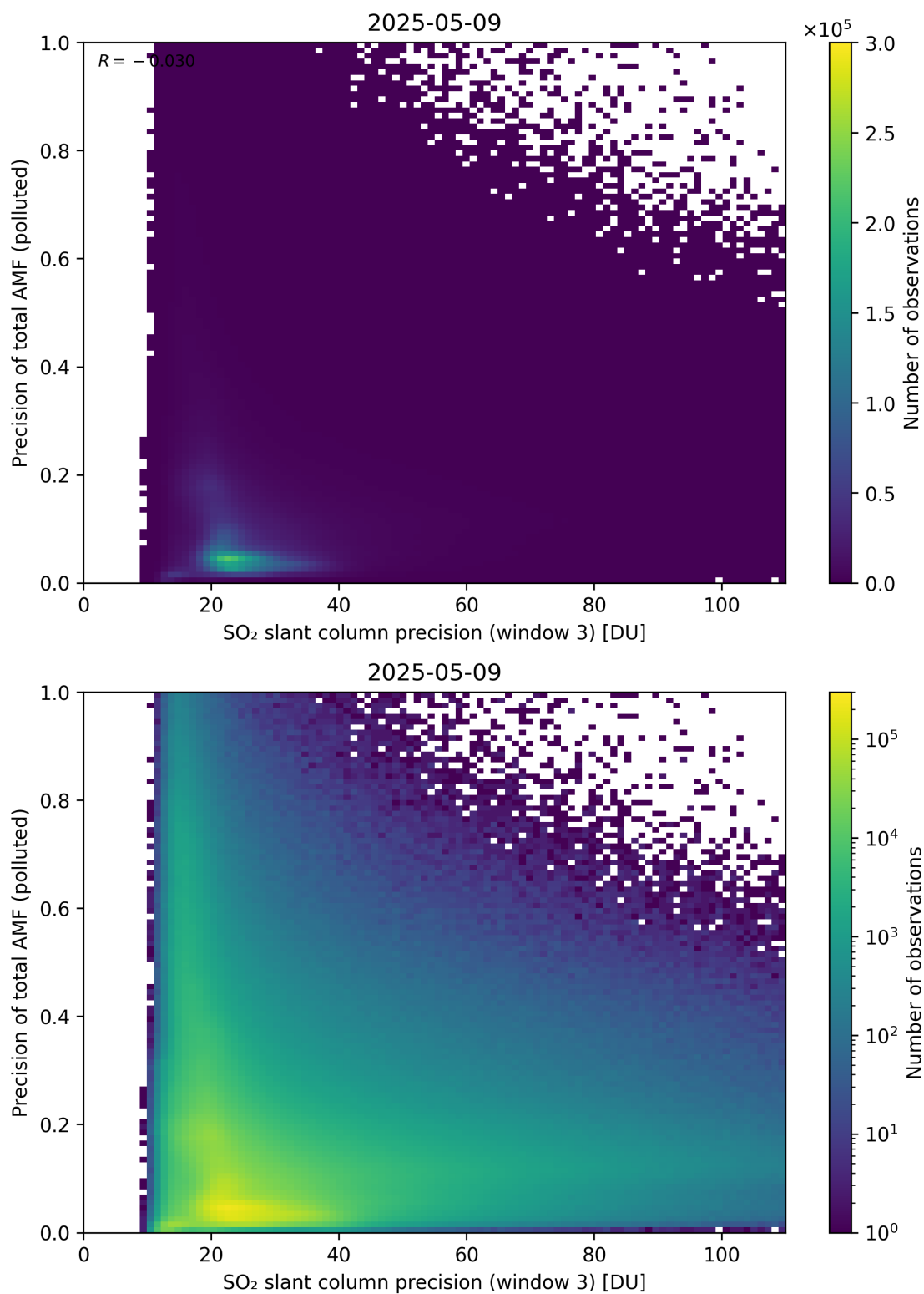
Figure 314: Scatter density plot of “SO 2 slant column precision (window 3)” against “Precision of total AMF (polluted)” for 2025-05-08 to 2025-05-10.
