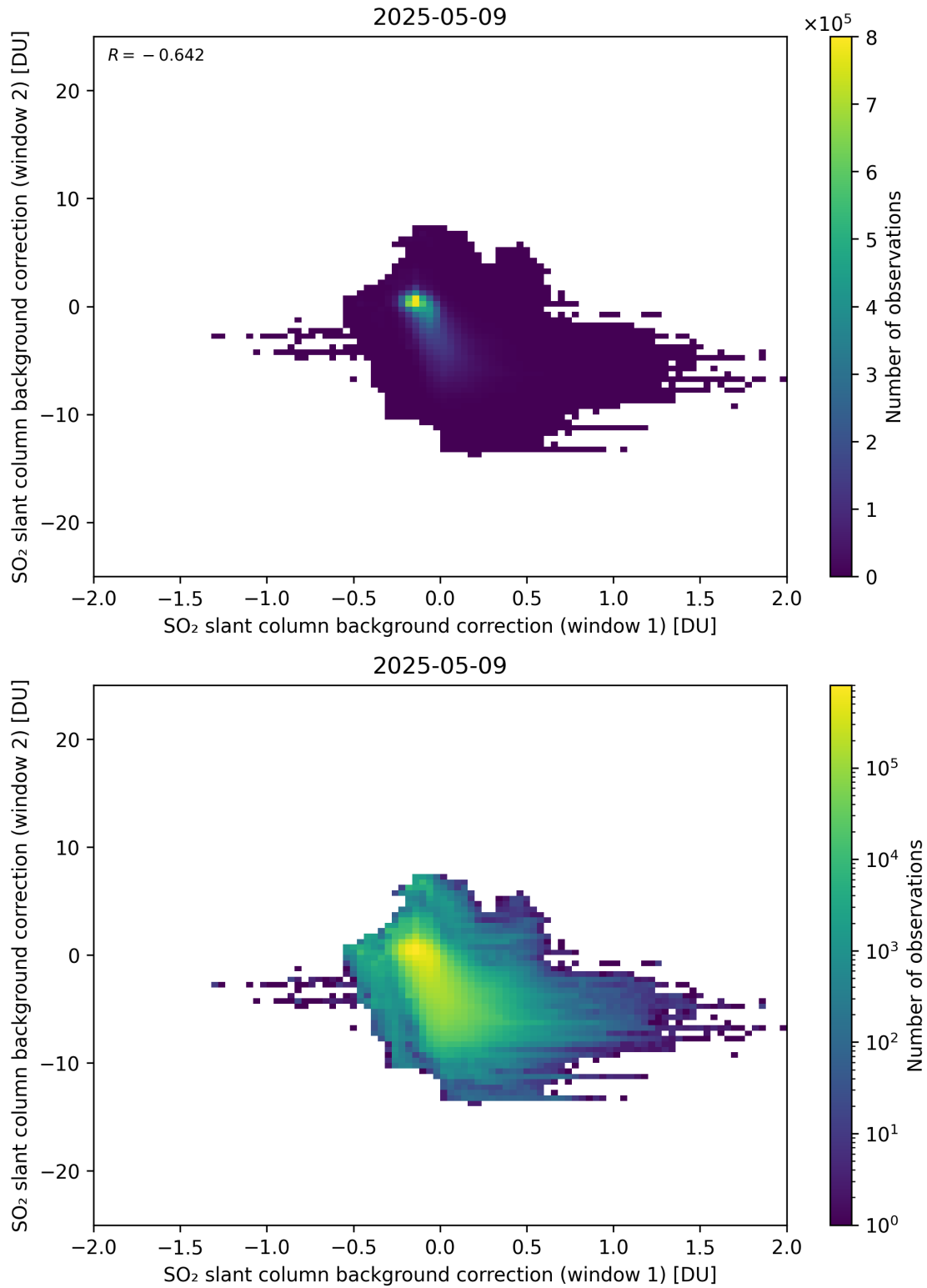
Figure 109: Scatter density plot of “SO 2 slant column background correction (window 1)” against “SO 2 slant column background correction (window 2)” for 2025-05-08 to 2025-05-10.
