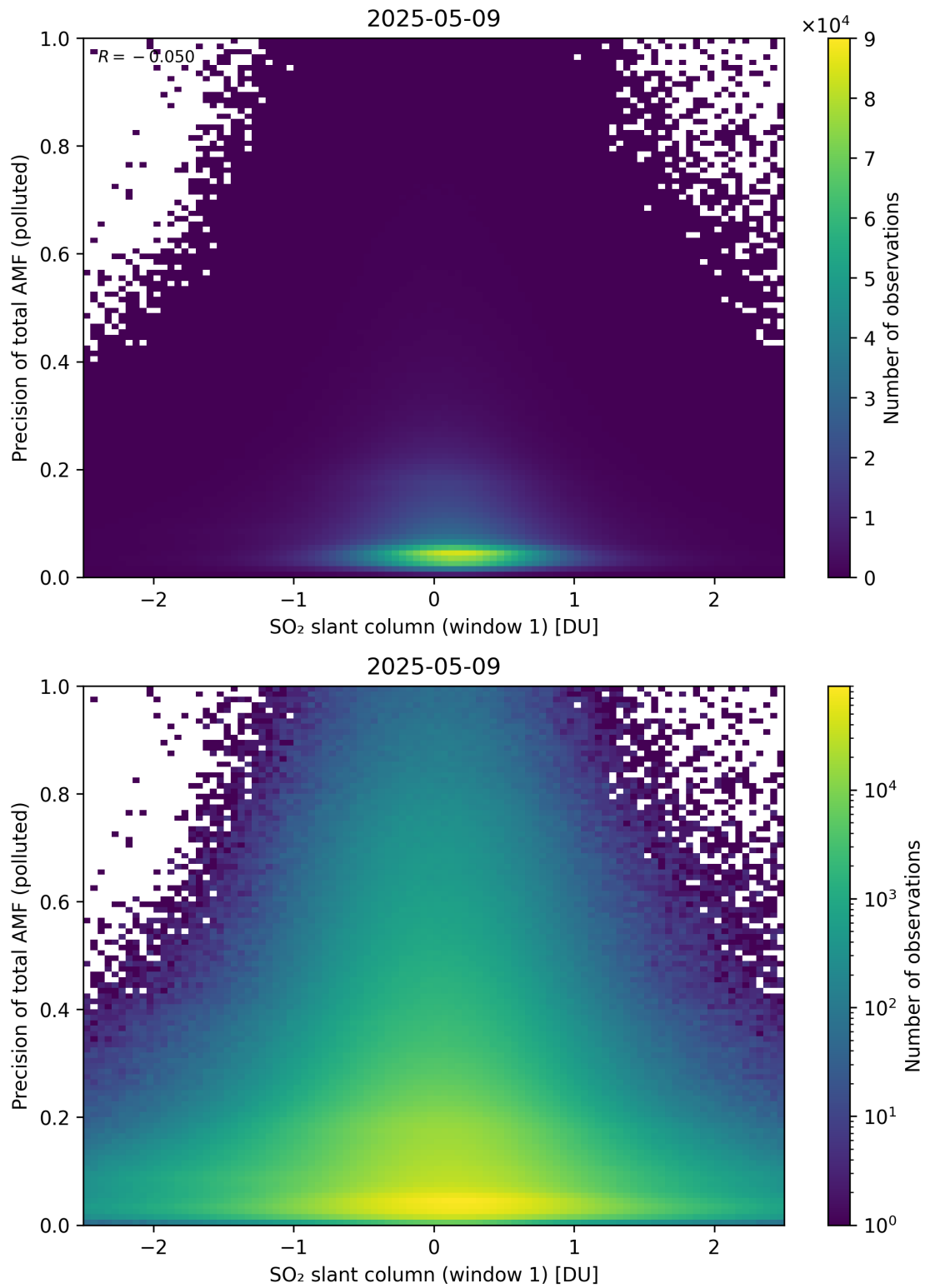
Figure 290: Scatter density plot of “SO 2 slant column (window 1)” against “Precision of total AMF (polluted)” for 2025-05-08 to 2025-05-10.
