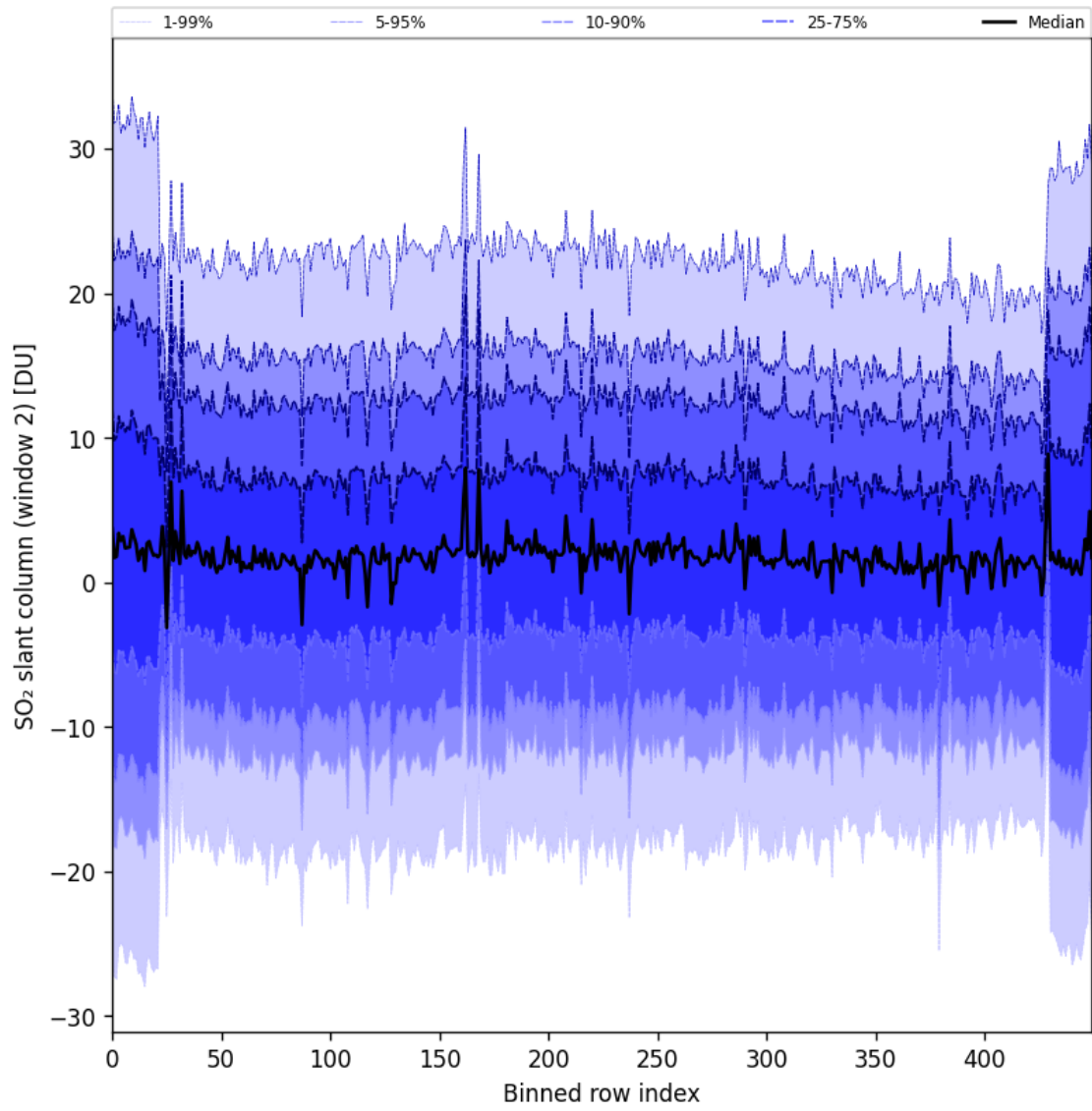
Figure 93: Along track statistics of “SO 2 slant column (window 2)” for 2025-05-08 to 2025-05-10
