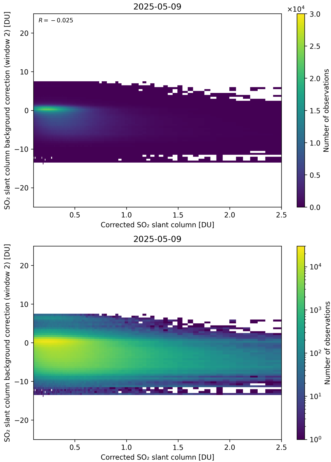
Figure 227: Scatter density plot of “Corrected SO 2 slant column” against “SO 2 slant column background correction (window 2)” for 2025-05-08 to 2025-05-10.
