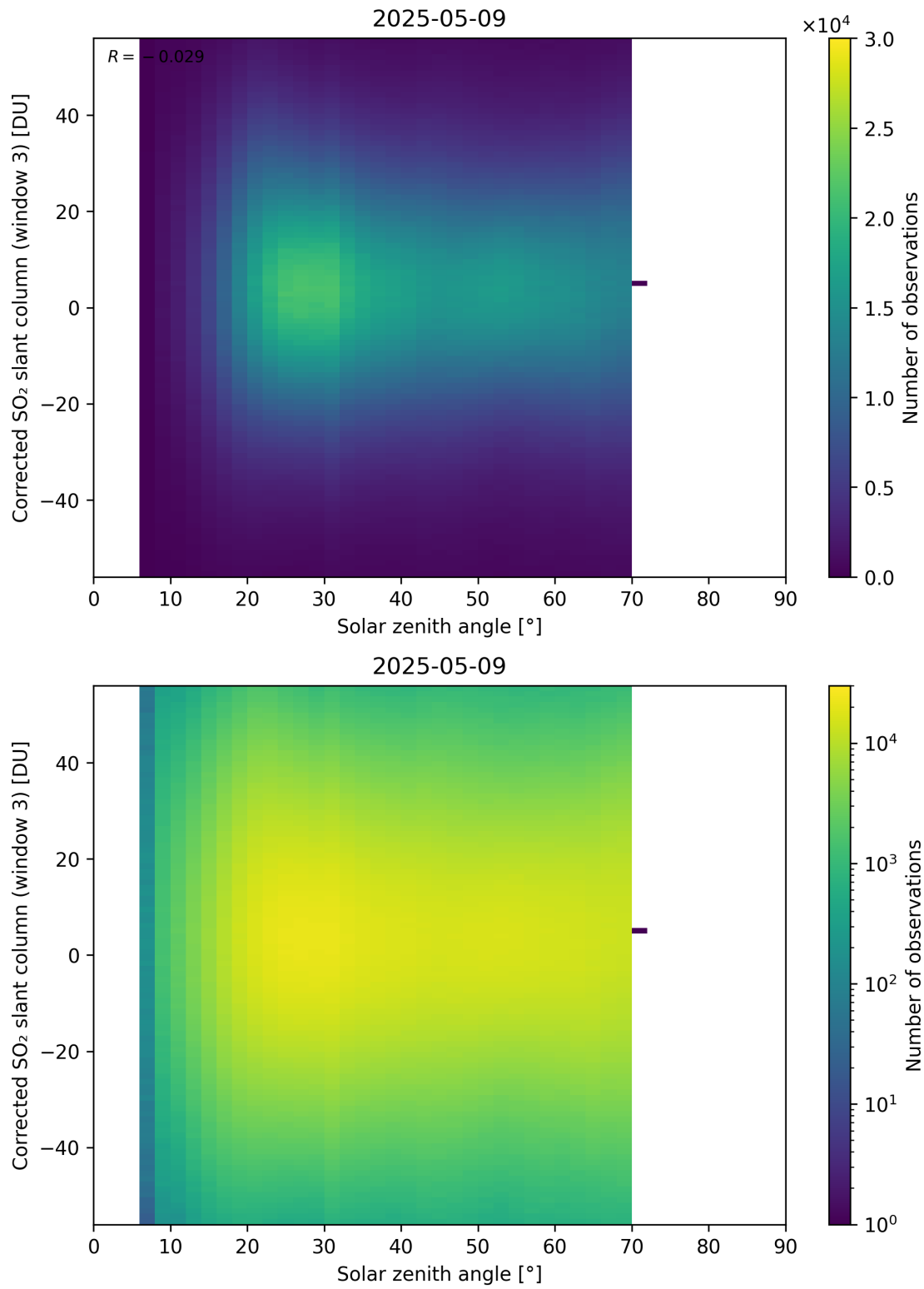
Figure 183: Scatter density plot of “Solar zenith angle” against “Corrected SO 2 slant column (window 3)” for 2025-05-08 to 2025-05-10.
