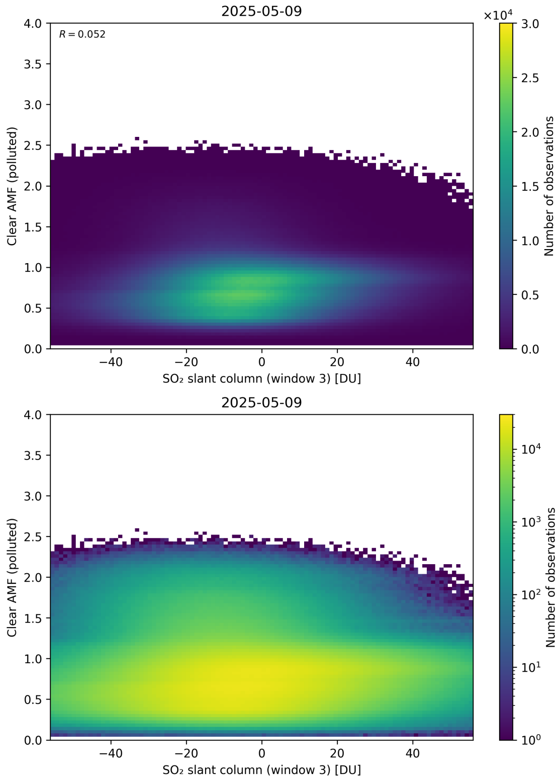
Figure 315: Scatter density plot of “SO 2 slant column (window 3)” against “Clear AMF (polluted)” for 2025-05-08 to 2025-05-10.
