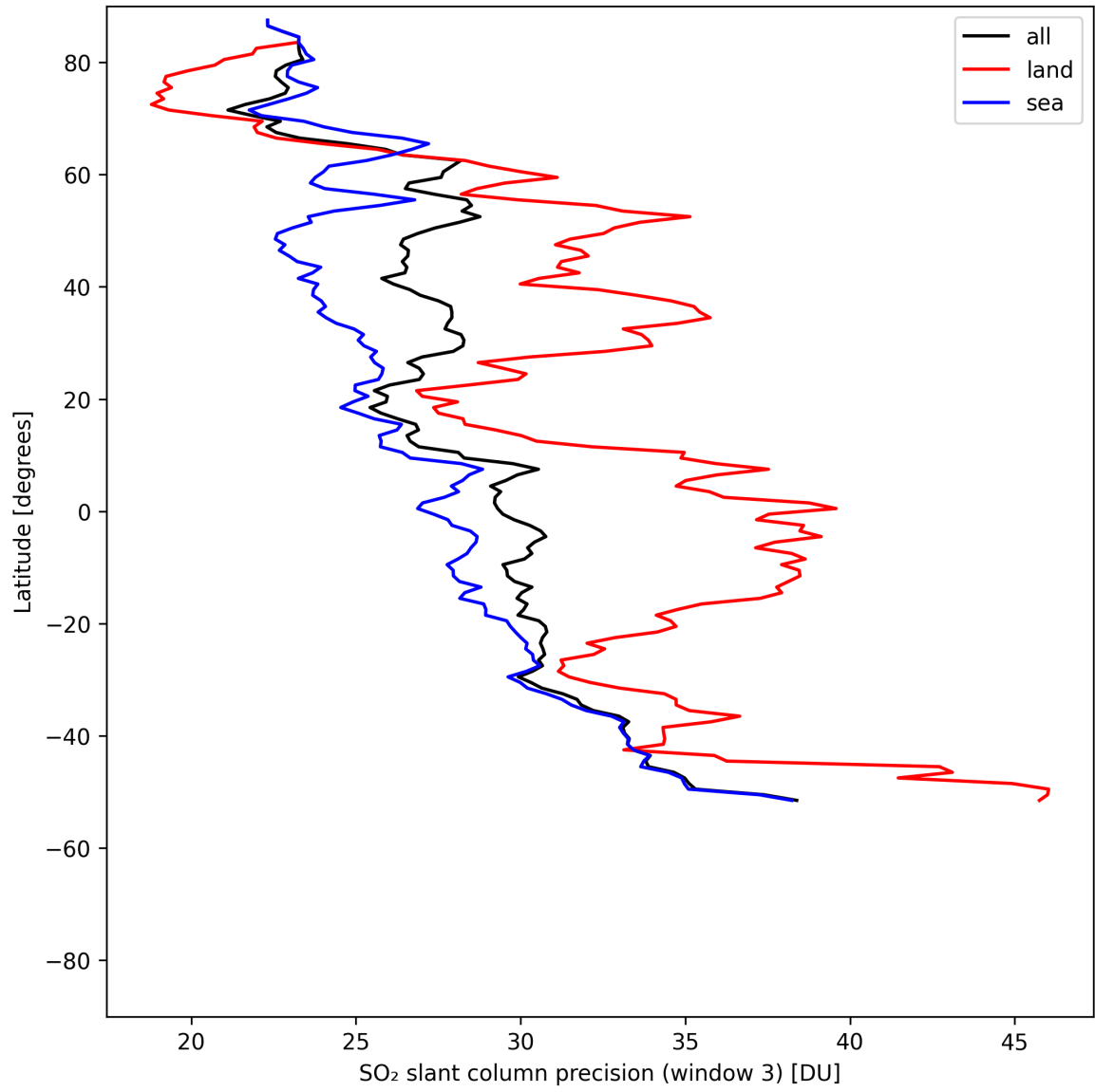
Figure 46: Zonal average of “SO 2 slant column precision (window 3)” for 2025-05-08 to 2025-05-10.
