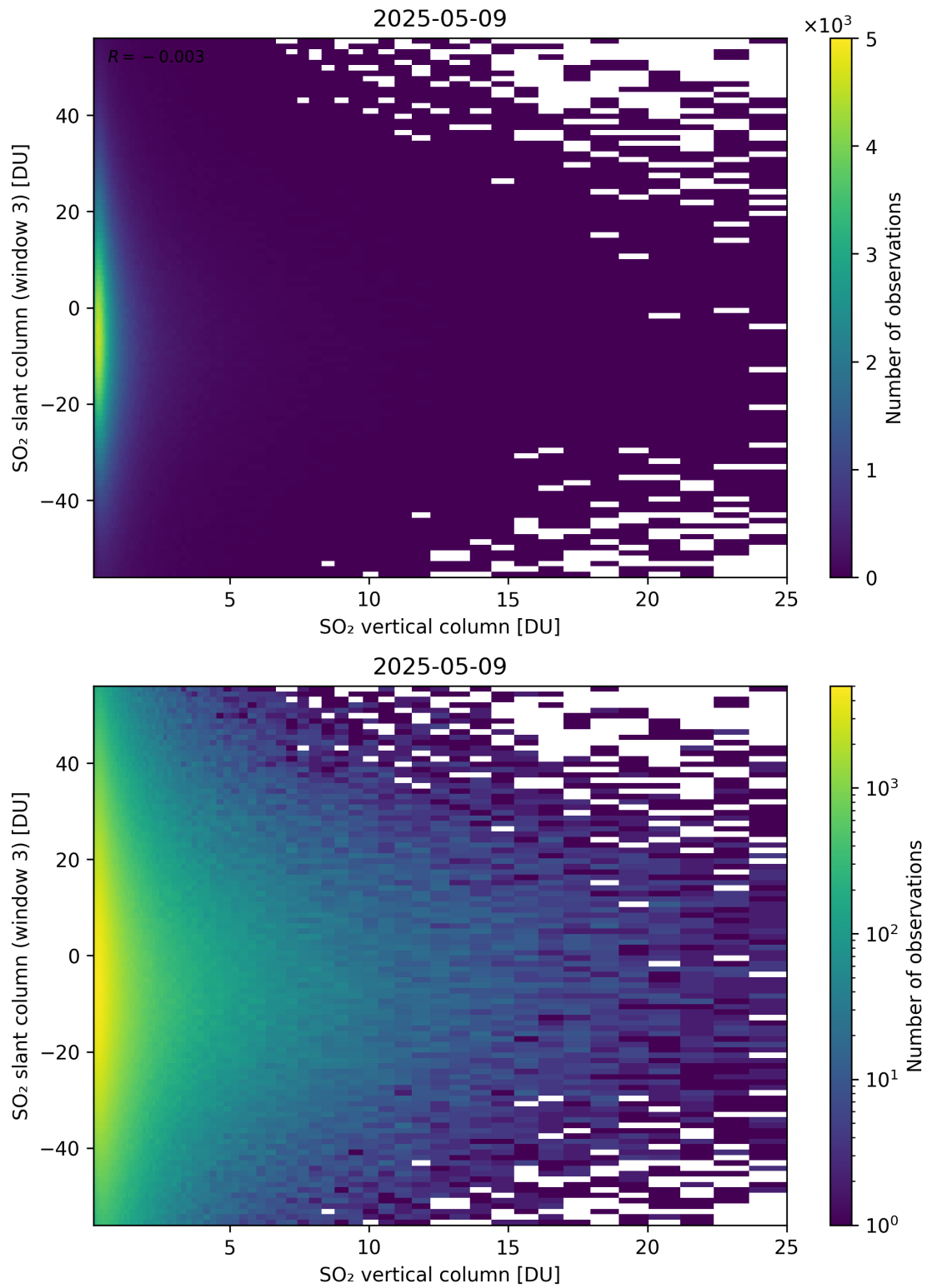
Figure 357: Scatter density plot of “SO 2 vertical column” against “SO 2 slant column (window 3)” for 2025-05-08 to 2025-05-10.
