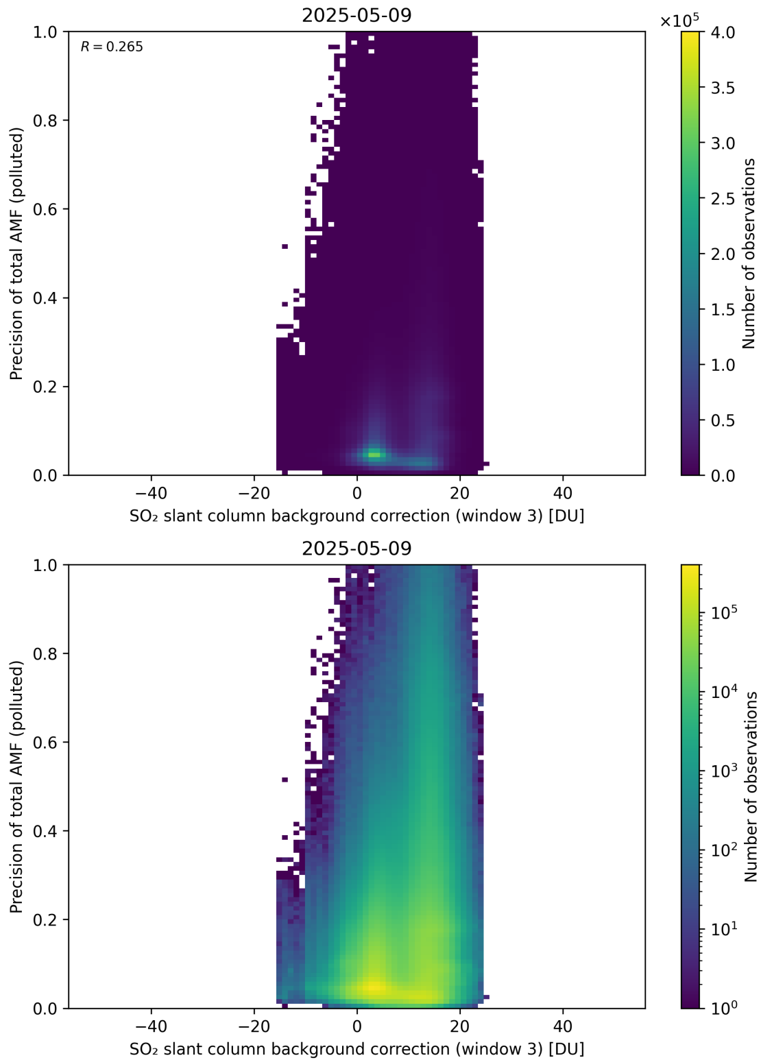
Figure 137: Scatter density plot of “SO 2 slant column background correction (window 3)” against “Precision of total AMF (polluted)” for 2025-05-08 to 2025-05-10.
