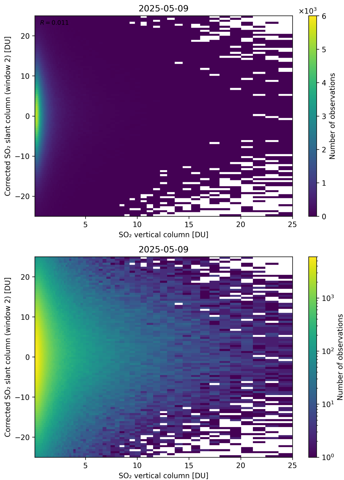
Figure 352: Scatter density plot of “SO 2 vertical column” against “Corrected SO 2 slant column (window 2)” for 2025-05-08 to 2025-05-10.
