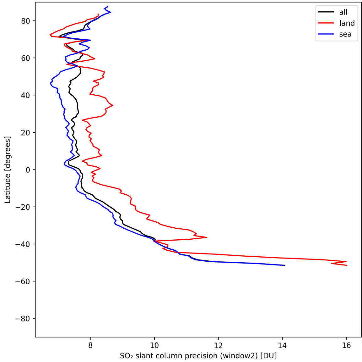
Figure 42: Zonal average of “SO 2 slant column precision (window2)” for 2025-05-08 to 2025-05-10.
