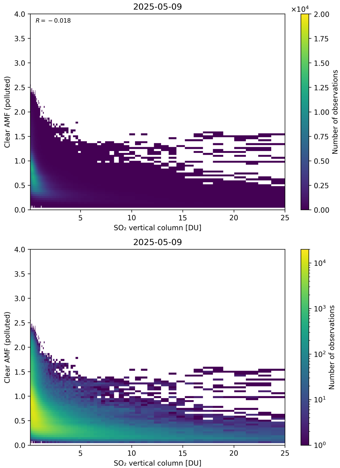
Figure 348: Scatter density plot of “SO 2 vertical column” against “Clear AMF (polluted)” for 2025-05-08 to 2025-05-10.
