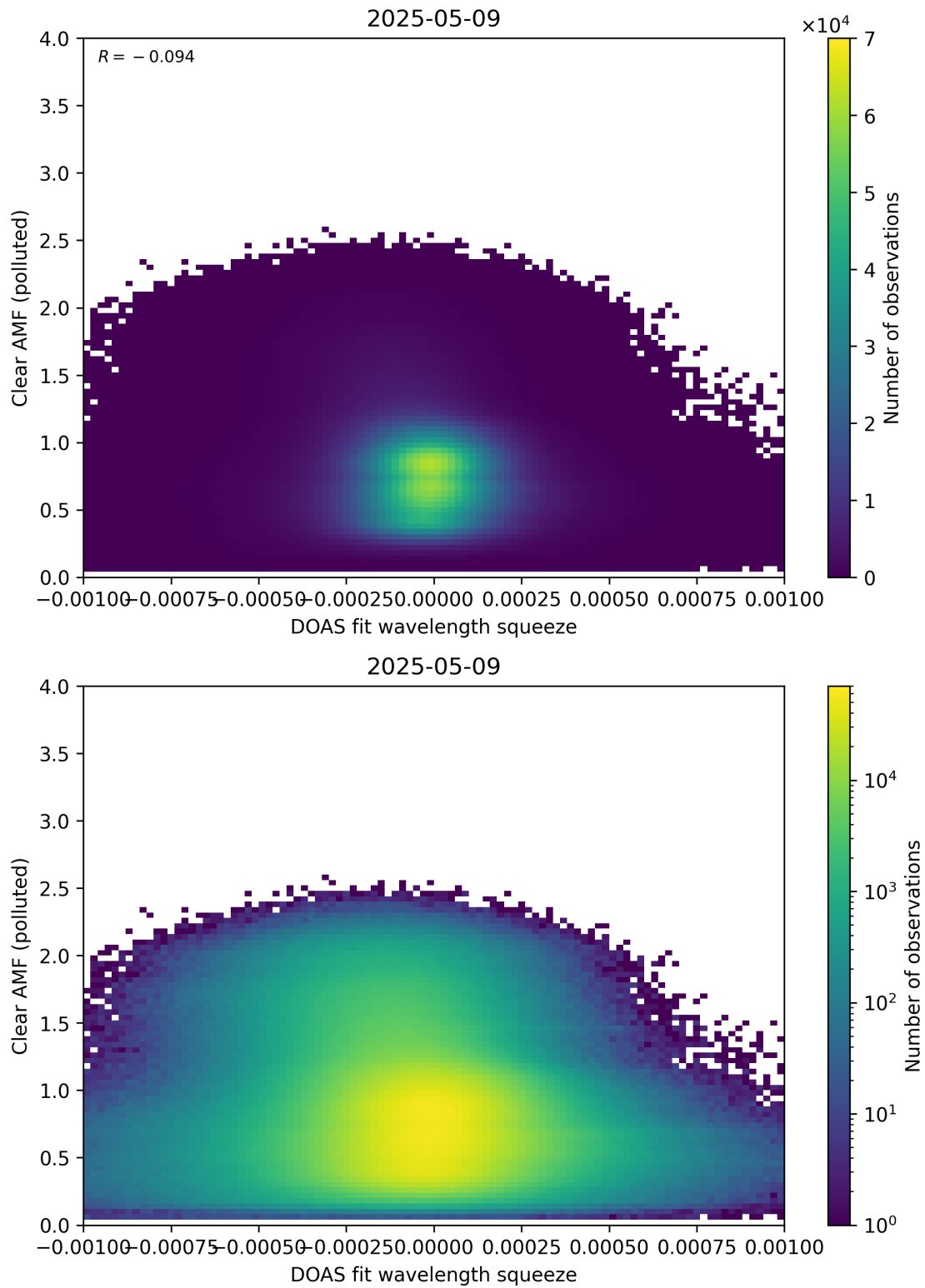
Figure 144: Scatter density plot of “DOAS fit wavelength squeeze” against “Clear AMF (polluted)” for 2025-05-08 to 2025-05-10.
