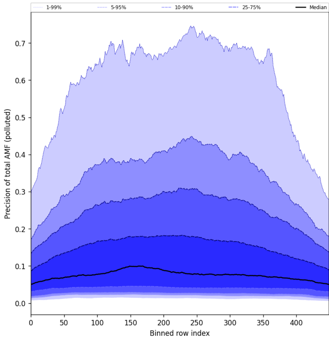
Figure 106: Along track statistics of “Precision of total AMF (polluted)” for 2025-05-08 to 2025-05-10
