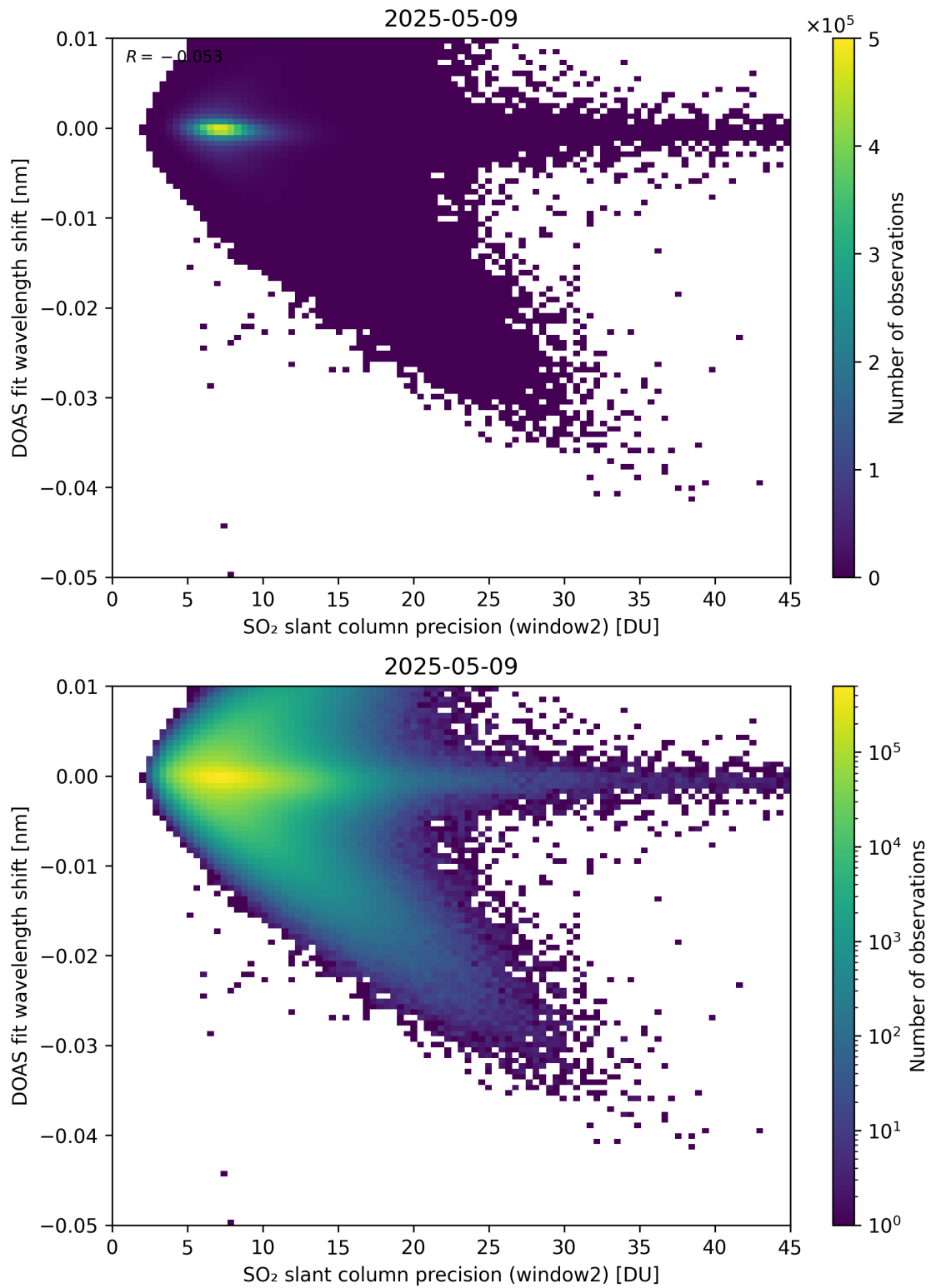
Figure 293: Scatter density plot of “SO 2 slant column precision (window2)” against “DOAS fit wavelength shift” for 2025-05-08 to 2025-05-10.
