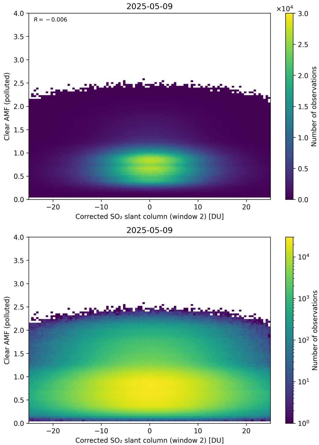
Figure 249: Scatter density plot of “Corrected SO 2 slant column (window 2)” against “Clear AMF (polluted)” for 2025-05-08 to 2025-05-10.
