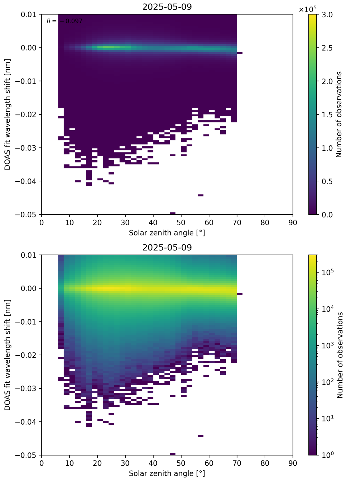
Figure 174: Scatter density plot of “Solar zenith angle” against “DOAS fit wavelength shift” for 2025-05-08 to 2025-05-10.
