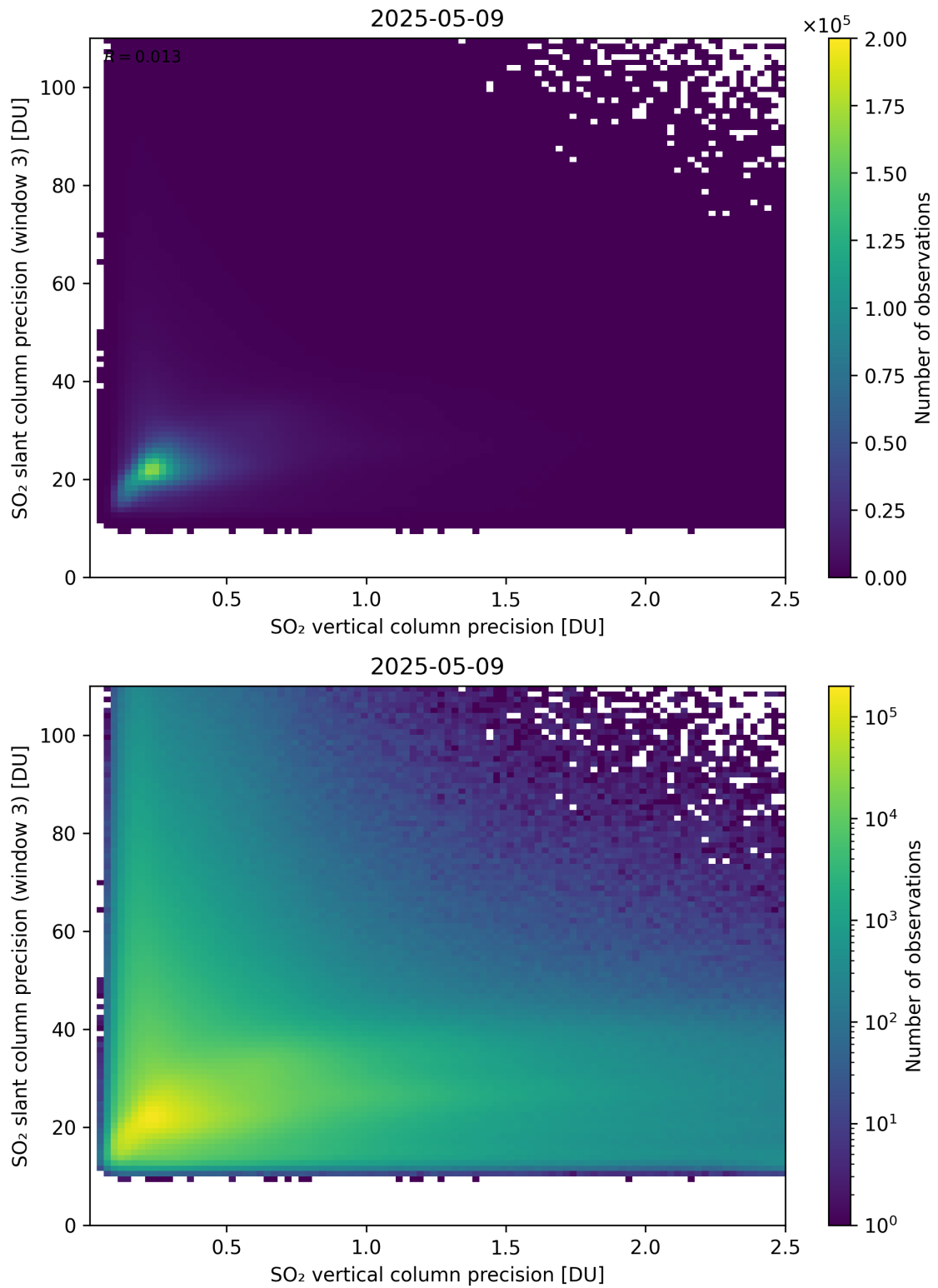
Figure 345: Scatter density plot of “SO 2 vertical column precision” against “SO 2 slant column precision (window 3)” for 2025-05-08 to 2025-05-10.
