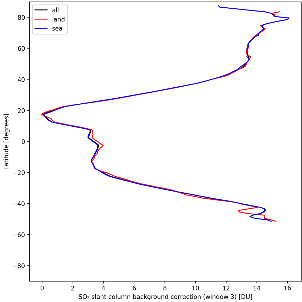
Figure 48: Zonal average of “SO 2 slant column background correction (window 3)” for 2025-05-08 to 2025-05-10.
