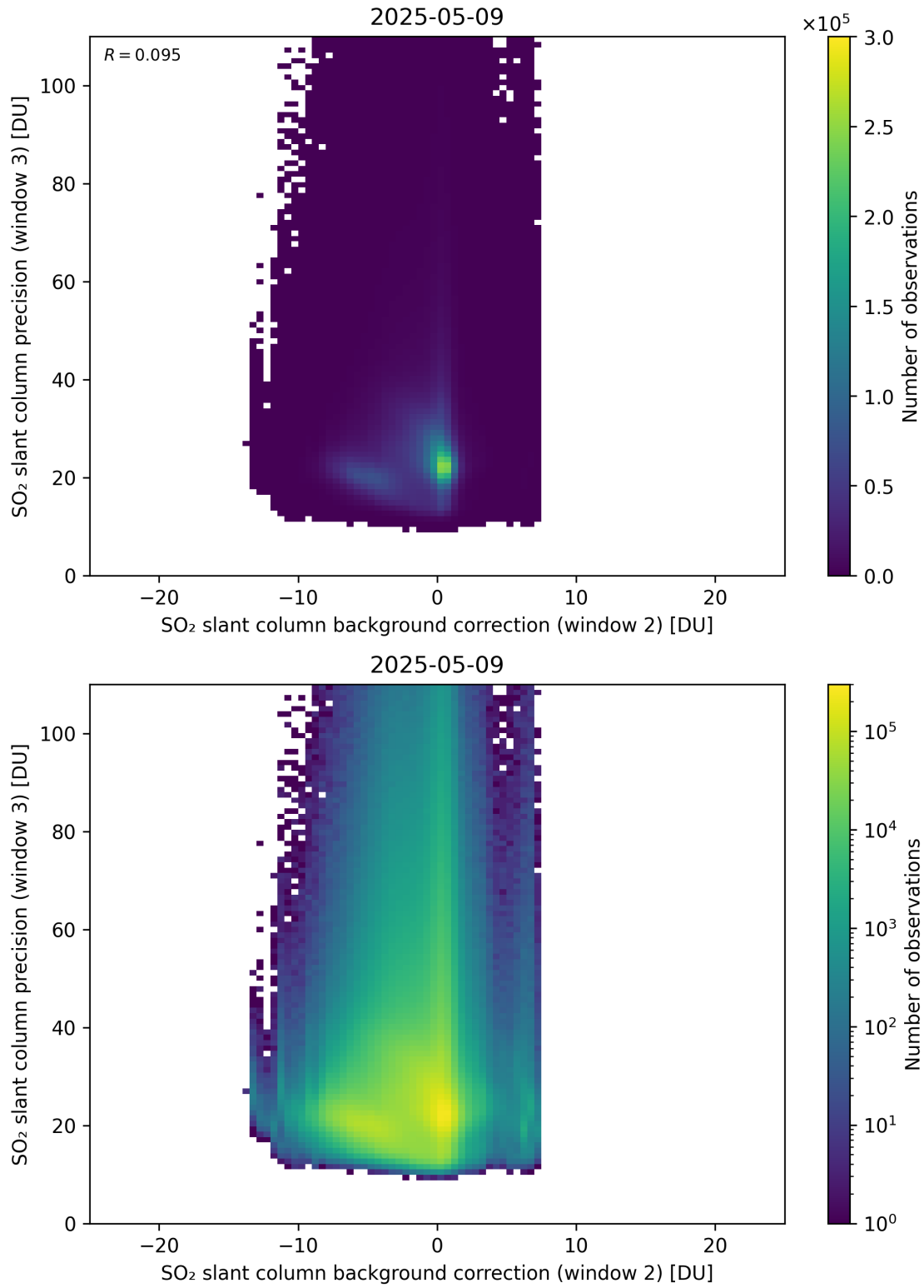
Figure 129: Scatter density plot of “SO 2 slant column background correction (window 2)” against “SO 2 slant column precision (window 3)” for 2025-05-08 to 2025-05-10.
