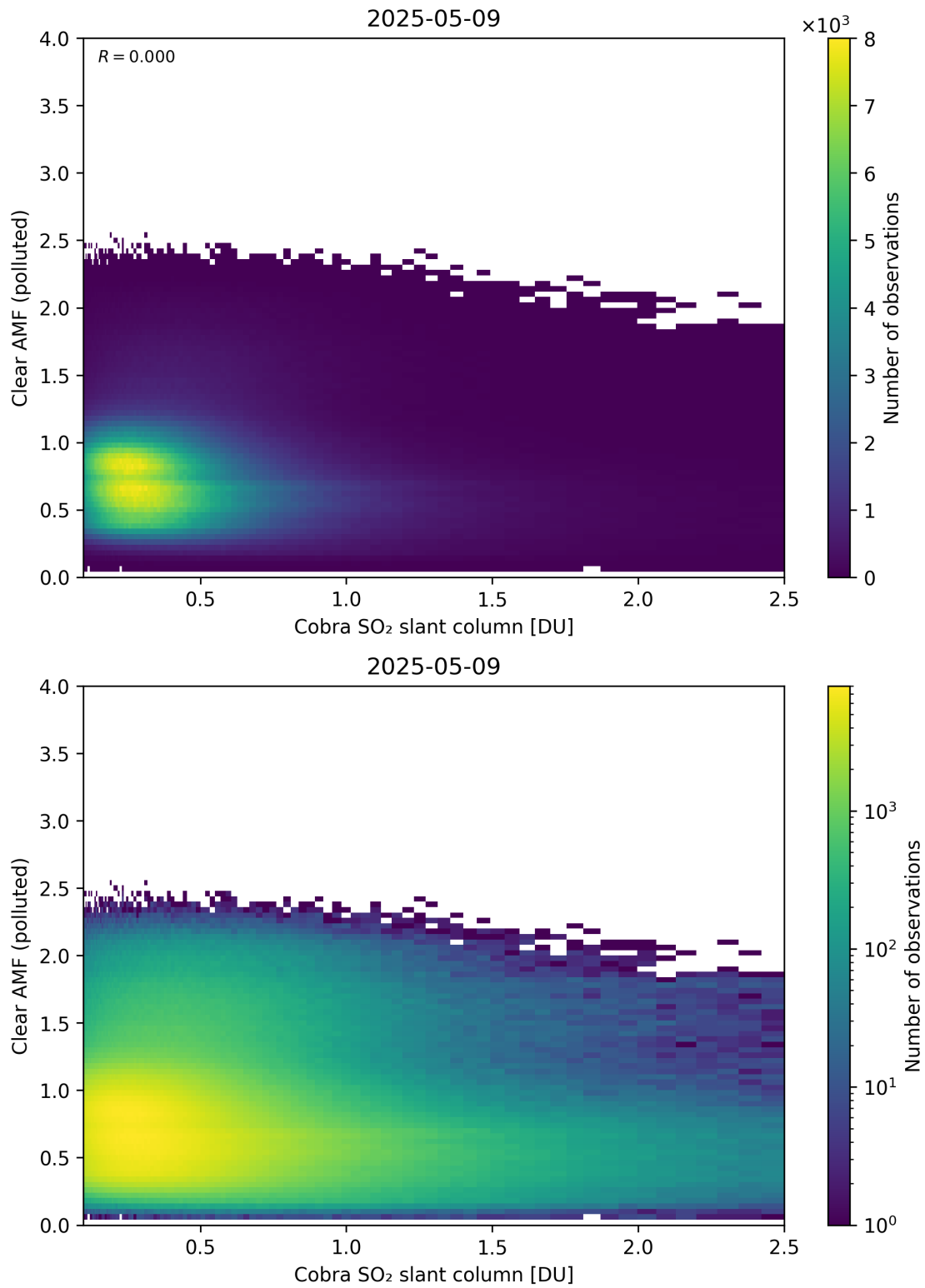
Figure 215: Scatter density plot of “Cobra SO 2 slant column” against “Clear AMF (polluted)” for 2025-05-08 to 2025-05-10.
