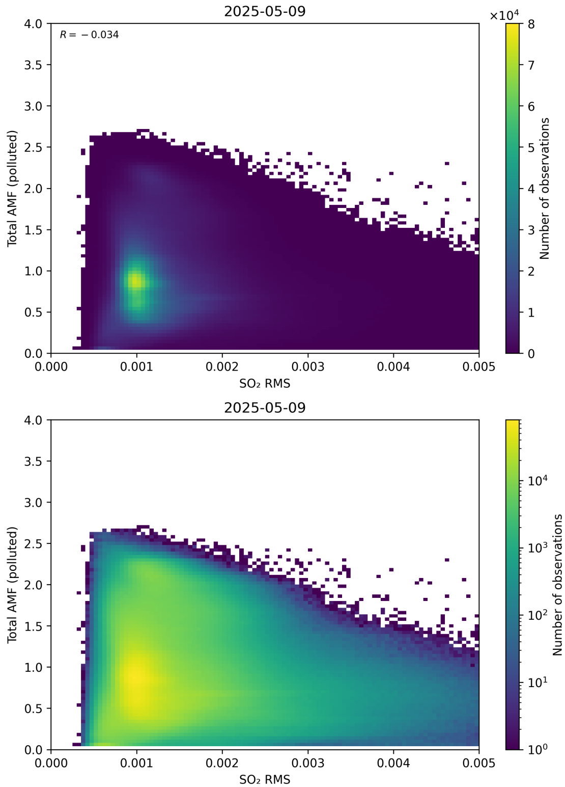
Figure 148: Scatter density plot of “SO 2 RMS” against “Total AMF (polluted)” for 2025-05-08 to 2025-05-10.
