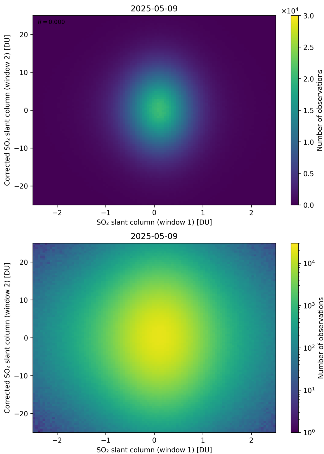
Figure 283: Scatter density plot of “SO 2 slant column (window 1)” against “Corrected SO 2 slant column (window 2)” for 2025-05-08 to 2025-05-10.
