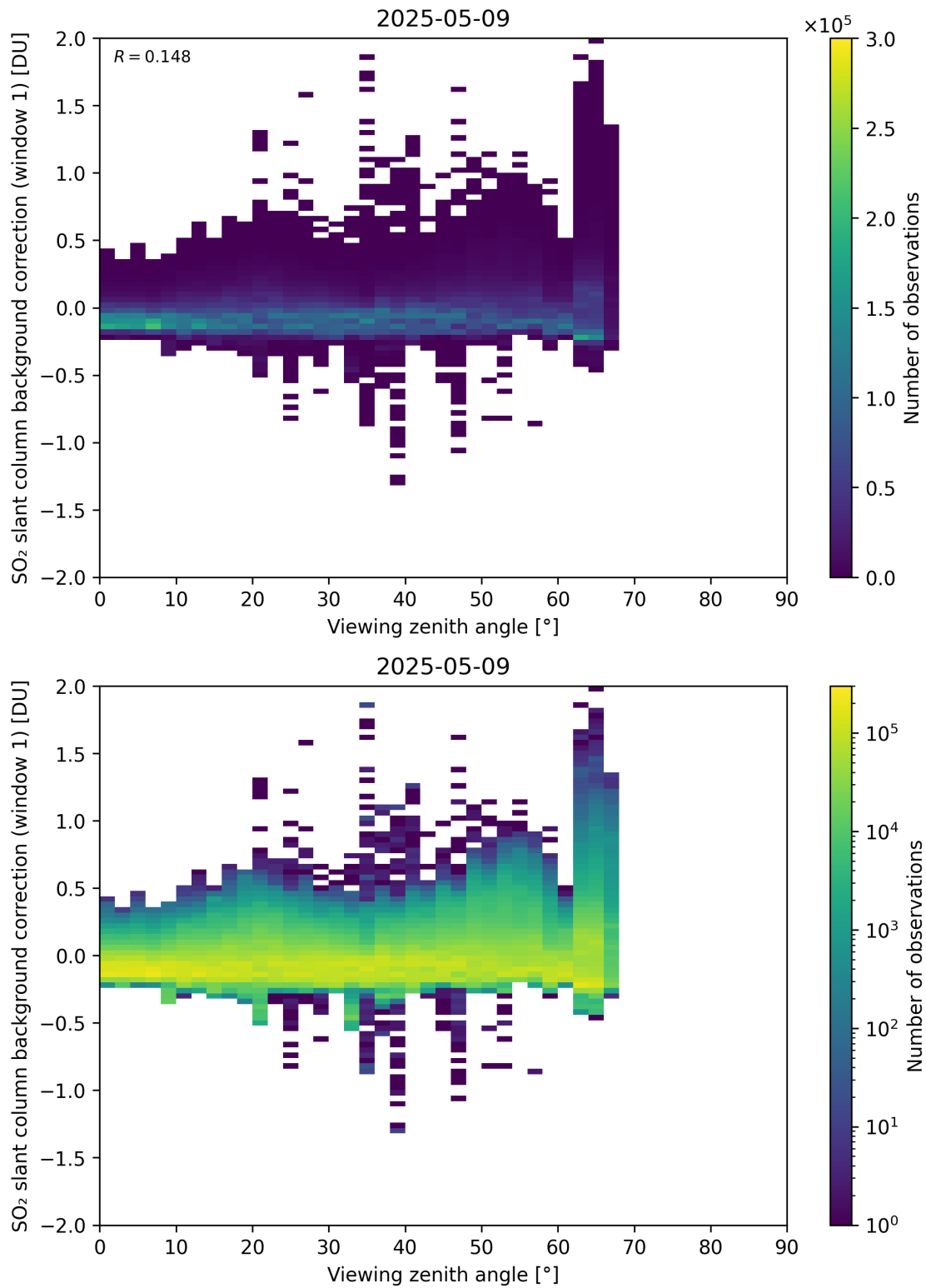
Figure 362: Scatter density plot of “Viewing zenith angle” against “SO 2 slant column background correction (window 1)” for 2025-05-08 to 2025-05-10.
