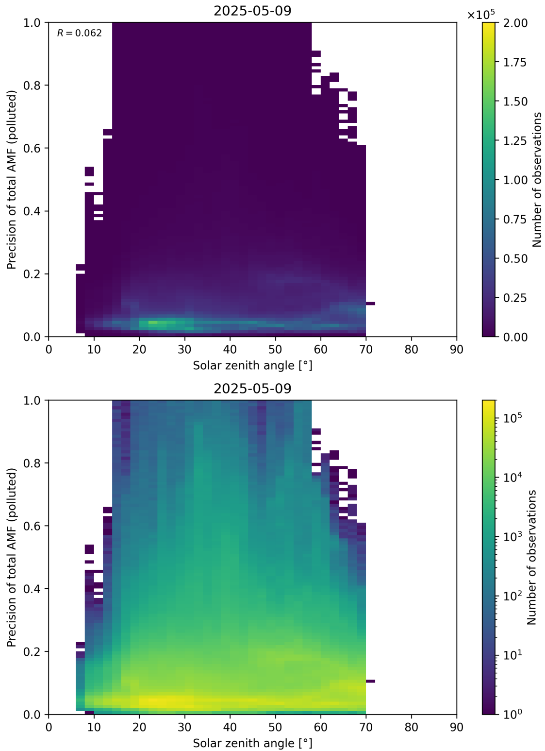
Figure 190: Scatter density plot of “Solar zenith angle” against “Precision of total AMF (polluted)” for 2025-05-08 to 2025-05-10.
