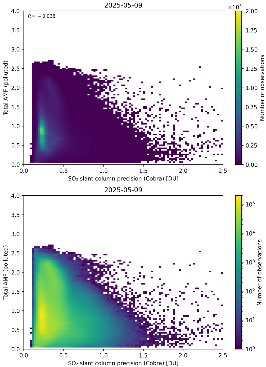
Figure 213: Scatter density plot of “SO 2 slant column precision (Cobra)” against “Total AMF (polluted)” for 2025-05-08 to 2025-05-10.
