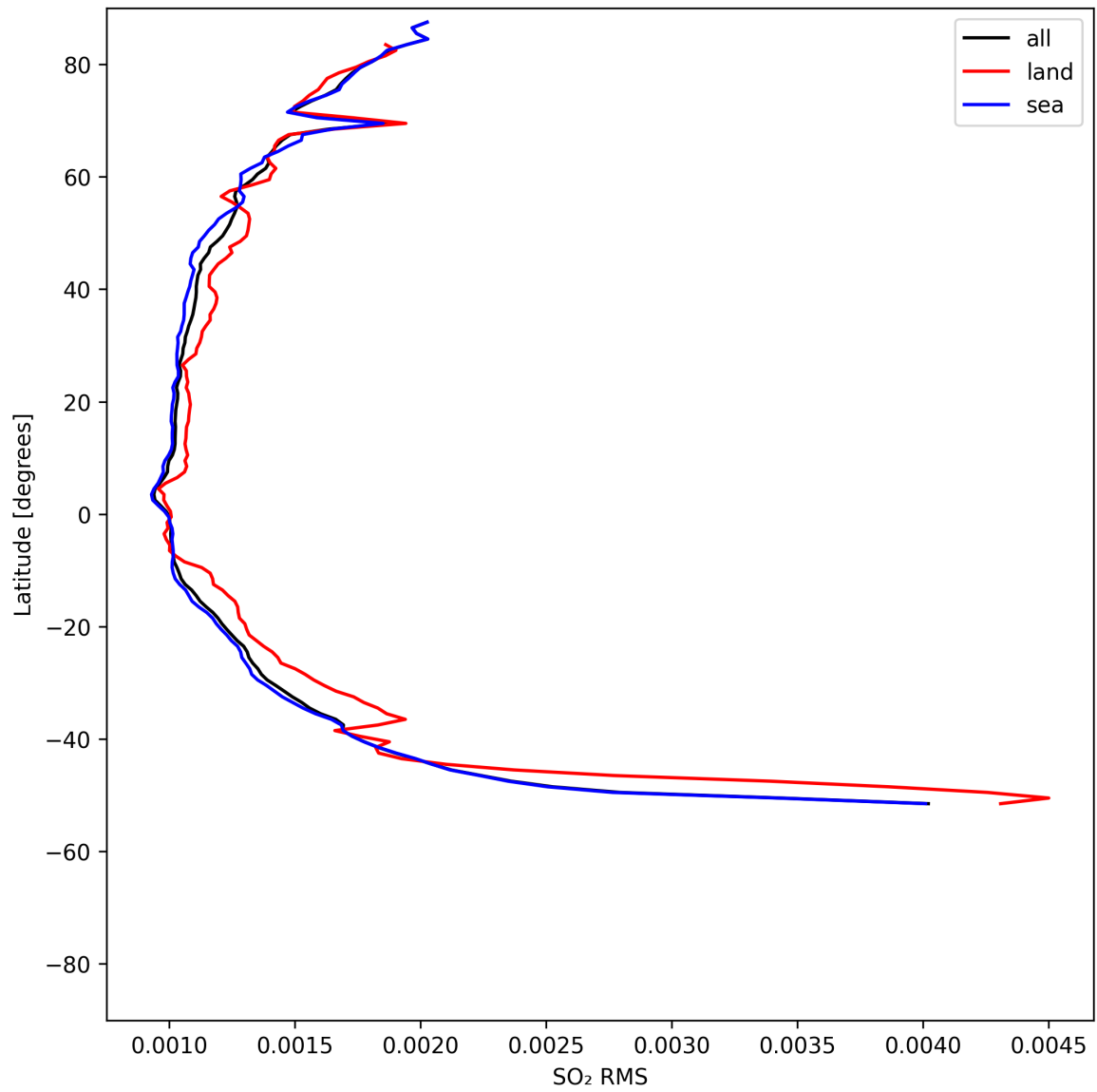
Figure 52: Zonal average of “SO 2 RMS” for 2025-05-08 to 2025-05-10.
