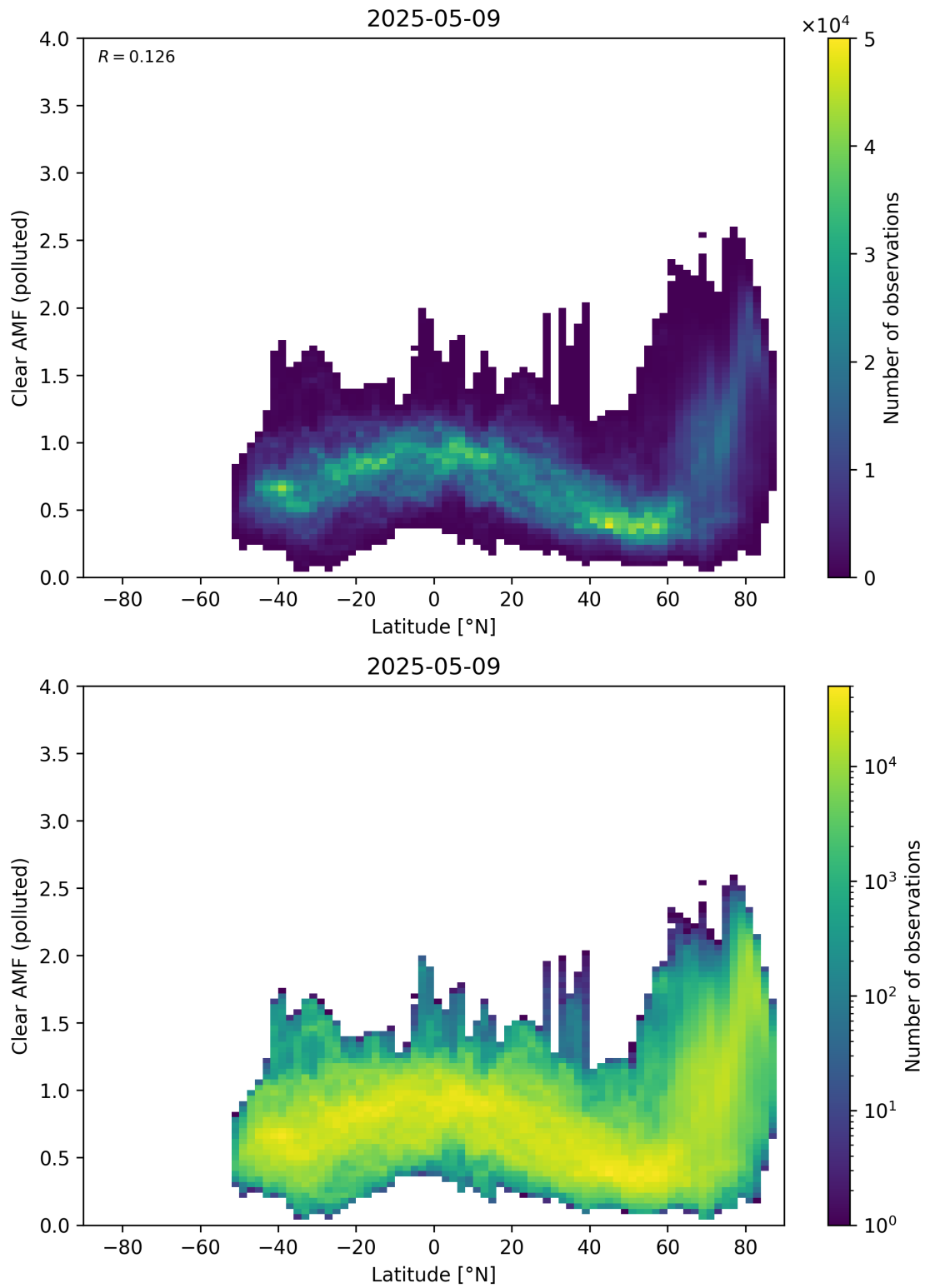
Figure 156: Scatter density plot of “Latitude” against “Clear AMF (polluted)” for 2025-05-08 to 2025-05-10.
