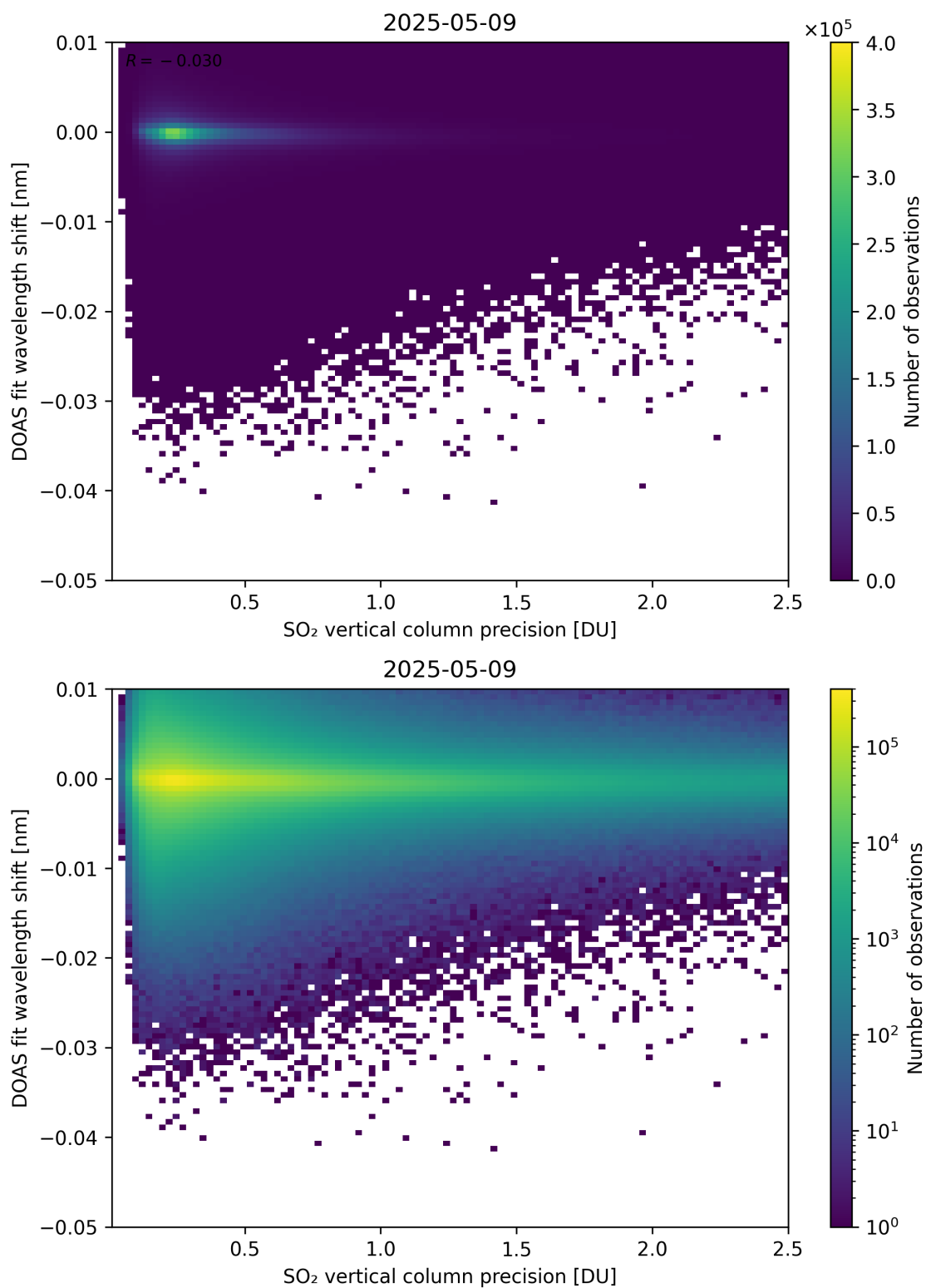
Figure 332: Scatter density plot of “SO 2 vertical column precision” against “DOAS fit wavelength shift” for 2025-05-08 to 2025-05-10.
