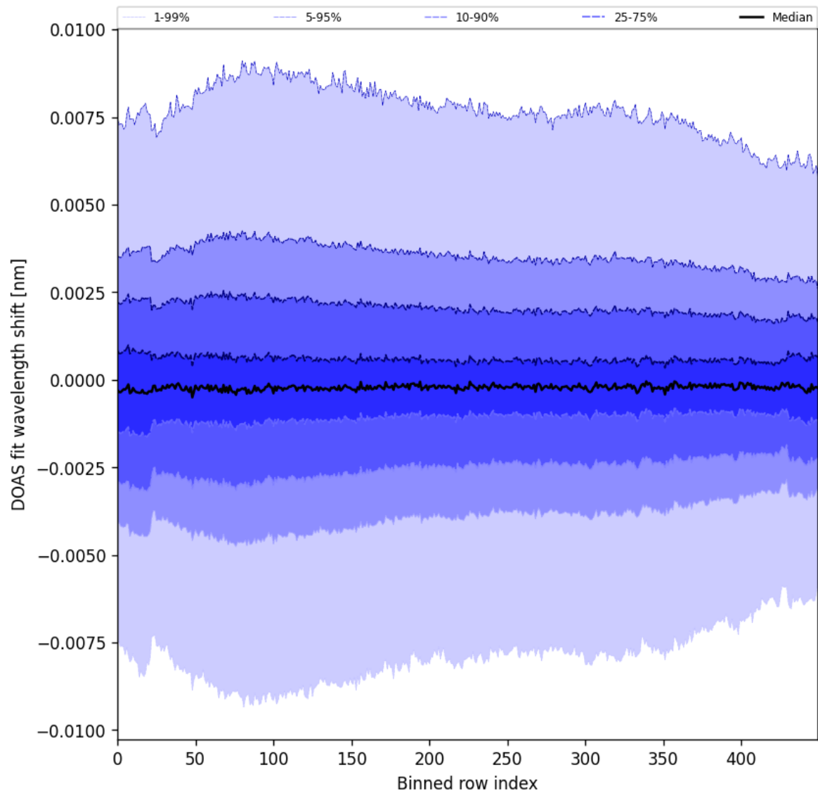
Figure 102: Along track statistics of “DOAS fit wavelength shift” for 2025-05-08 to 2025-05-10
