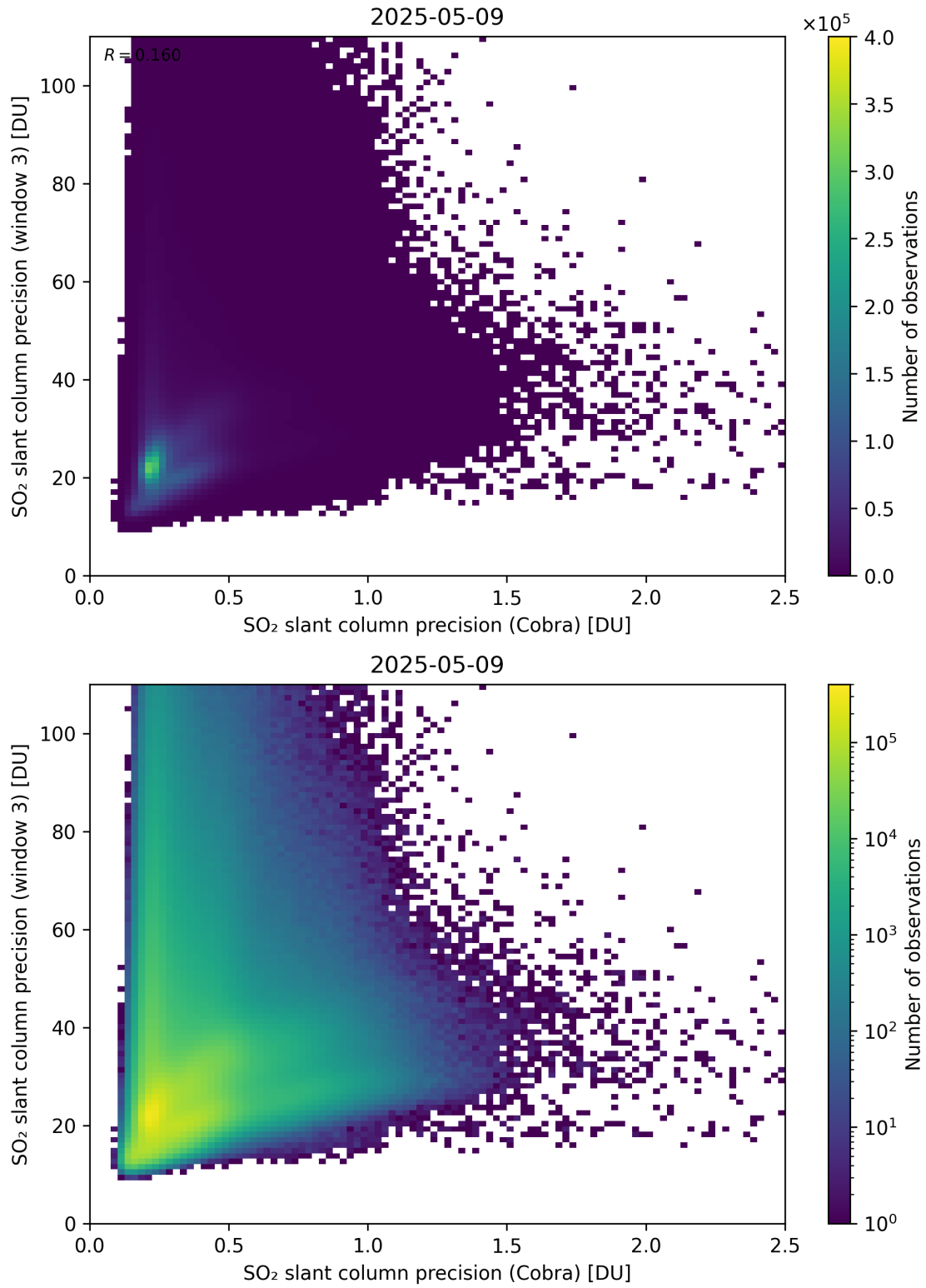
Figure 212: Scatter density plot of “SO 2 slant column precision (Cobra)” against “SO 2 slant column precision (window 3)” for 2025-05-08 to 2025-05-10.
