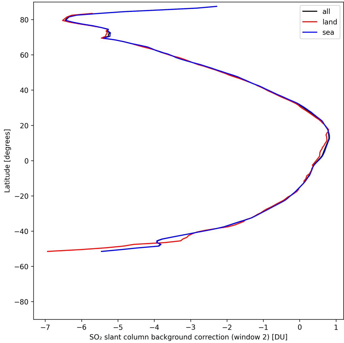
Figure 44: Zonal average of “SO 2 slant column background correction (window 2)” for 2025-05-08 to 2025-05-10.
