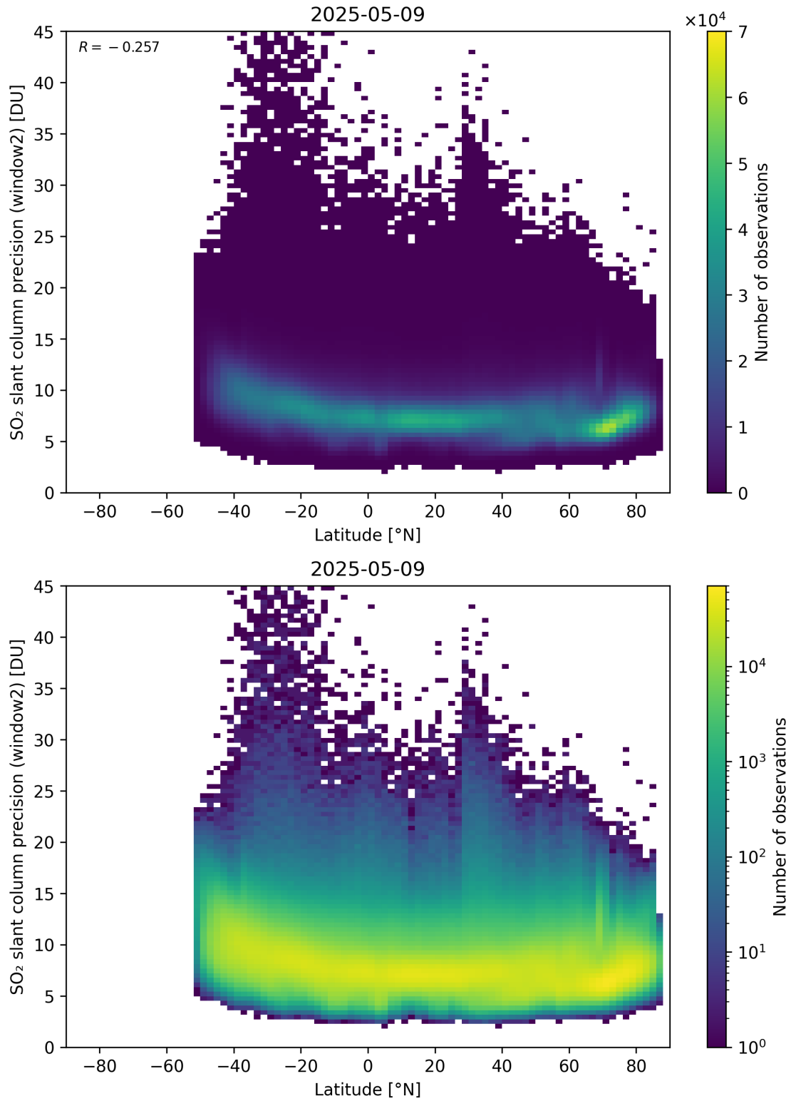
Figure 164: Scatter density plot of “Latitude” against “SO 2 slant column precision (window2)” for 2025-05-08 to 2025-05-10.
