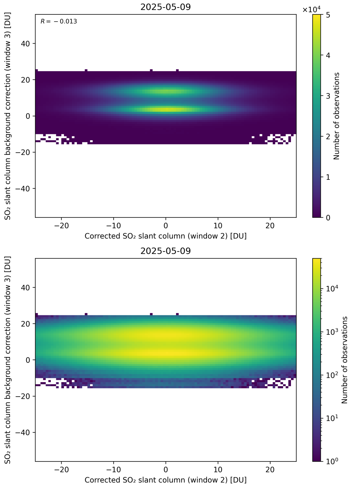
Figure 245: Scatter density plot of “Corrected SO 2 slant column (window 2)” against “SO 2 slant column background correction (window 3)” for 2025-05-08 to 2025-05-10.
