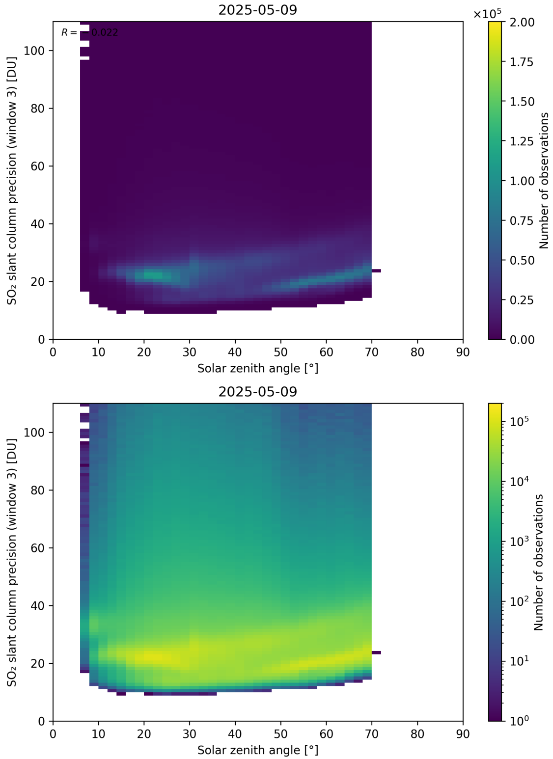
Figure 188: Scatter density plot of “Solar zenith angle” against “SO 2 slant column precision (window 3)” for 2025-05-08 to 2025-05-10.
