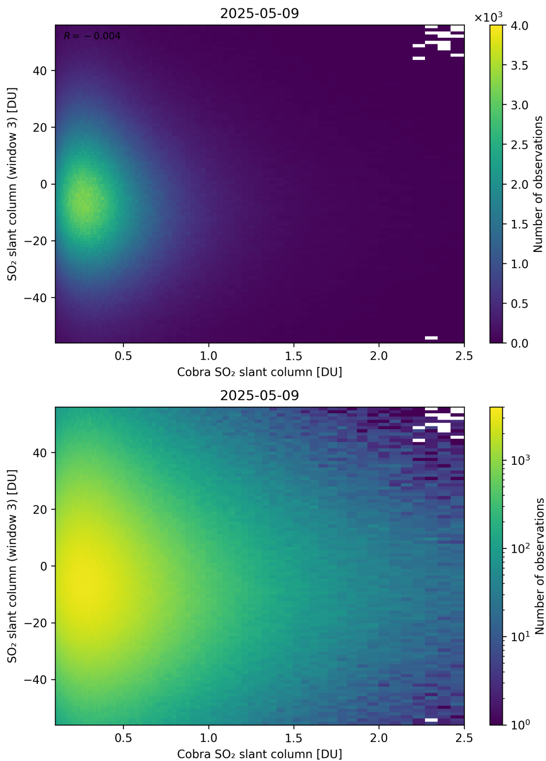
Figure 222: Scatter density plot of “Cobra SO 2 slant column” against “SO 2 slant column (window 3)” for 2025-05-08 to 2025-05-10.
