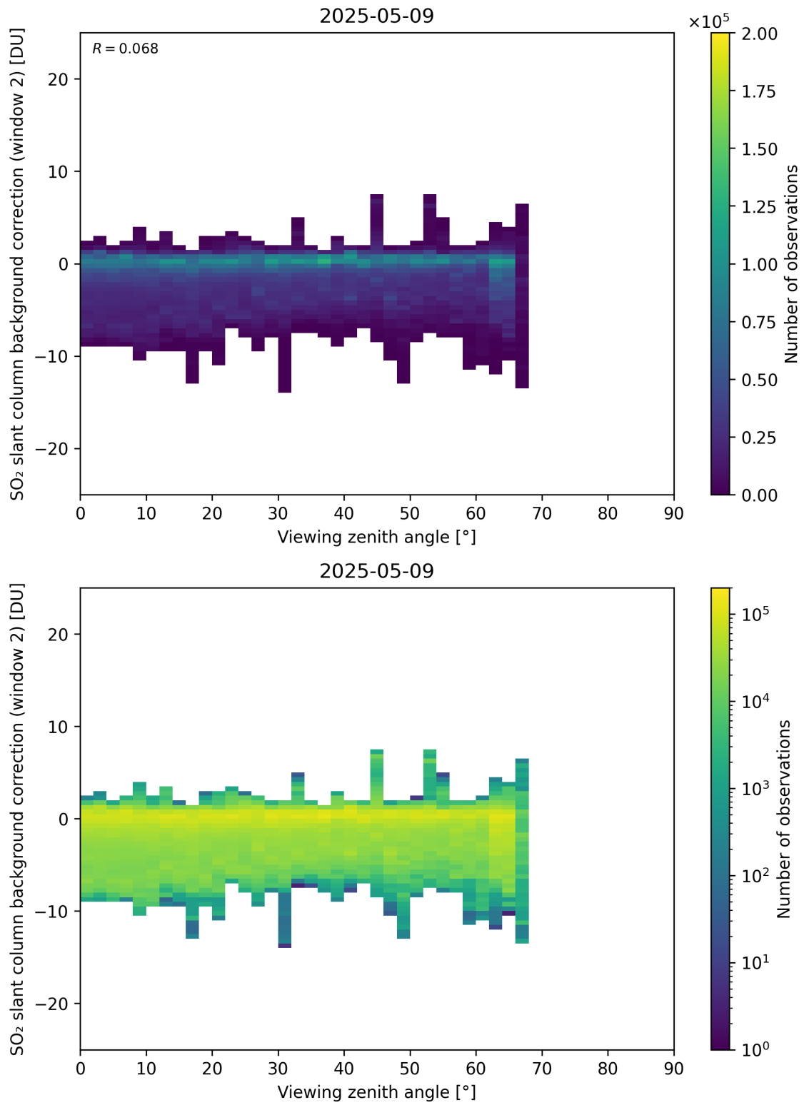
Figure 363: Scatter density plot of “Viewing zenith angle” against “SO 2 slant column background correction (window 2)” for 2025-05-08 to 2025-05-10.
