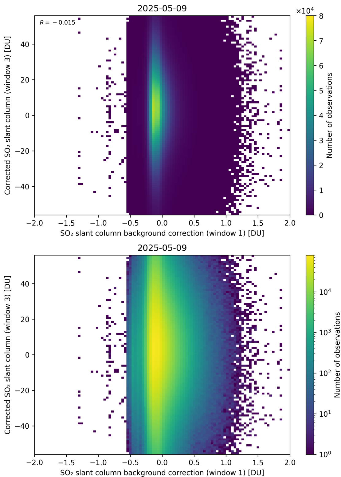
Figure 116: Scatter density plot of “SO 2 slant column background correction (window 1)” against “Corrected SO 2 slant column (window 3)” for 2025-05-08 to 2025-05-10.
