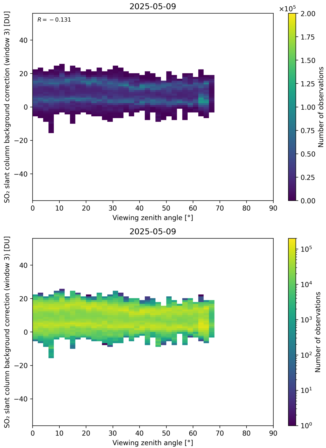
Figure 364: Scatter density plot of “Viewing zenith angle” against “SO 2 slant column background correction (window 3)” for 2025-05-08 to 2025-05-10.
