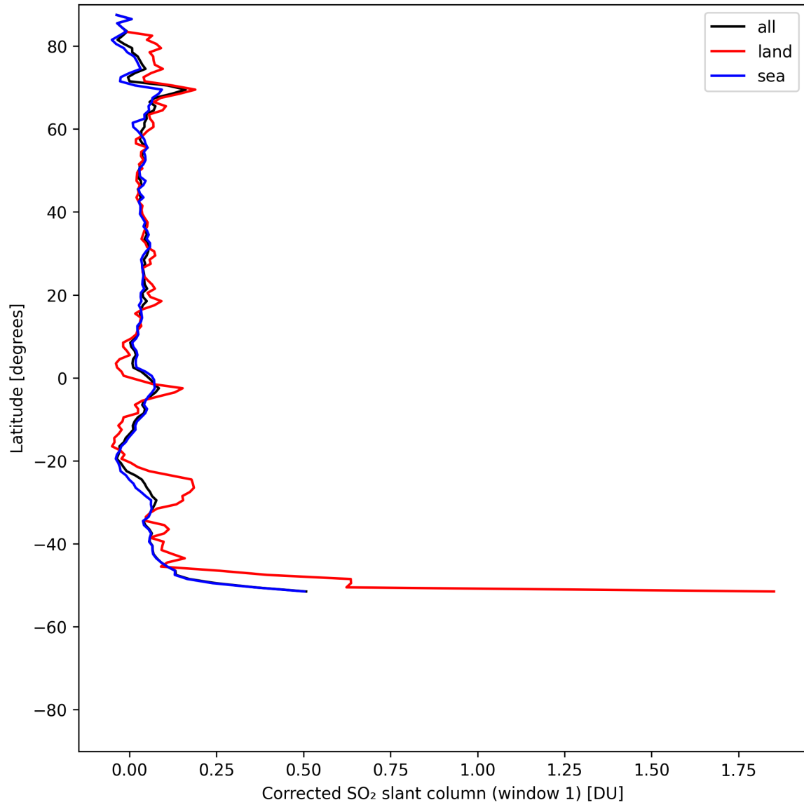
Figure 39: Zonal average of “Corrected SO 2 slant column (window 1)” for 2025-05-08 to 2025-05-10.
