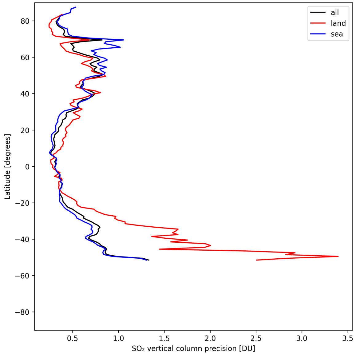
Figure 33: Zonal average of “SO 2 vertical column precision” for 2025-05-08 to 2025-05-10.
