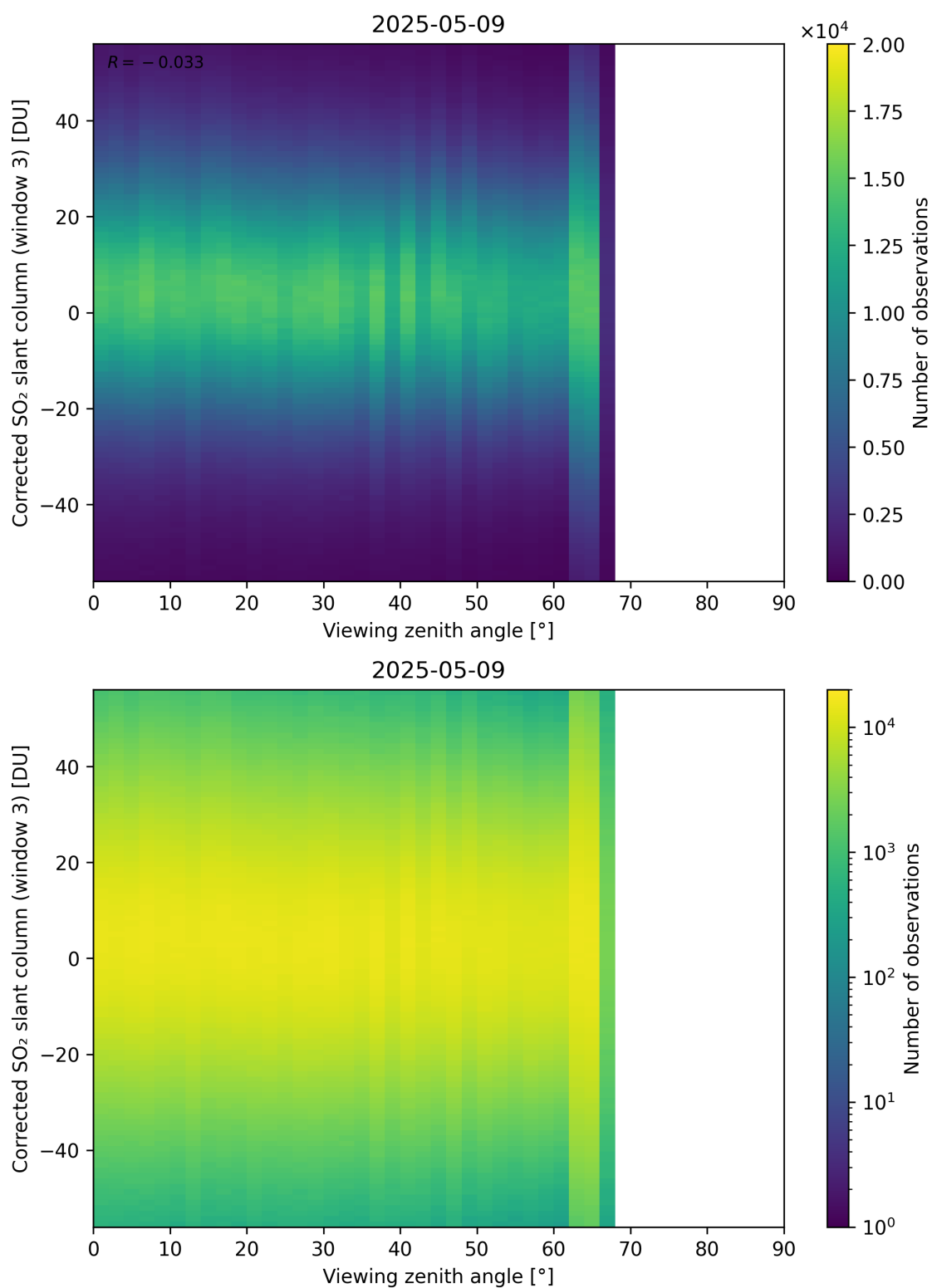
Figure 375: Scatter density plot of “Viewing zenith angle” against “Corrected SO 2 slant column (window 3)” for 2025-05-08 to 2025-05-10.
