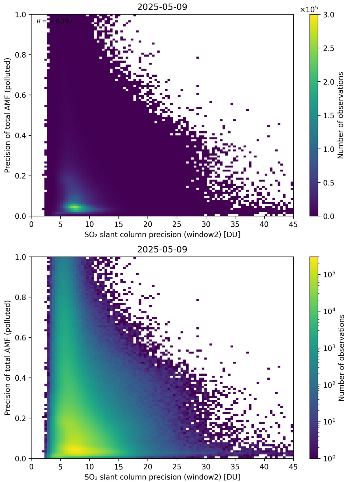
Figure 302: Scatter density plot of “SO 2 slant column precision (window2)” against “Precision of total AMF (polluted)” for 2025-05-08 to 2025-05-10.
