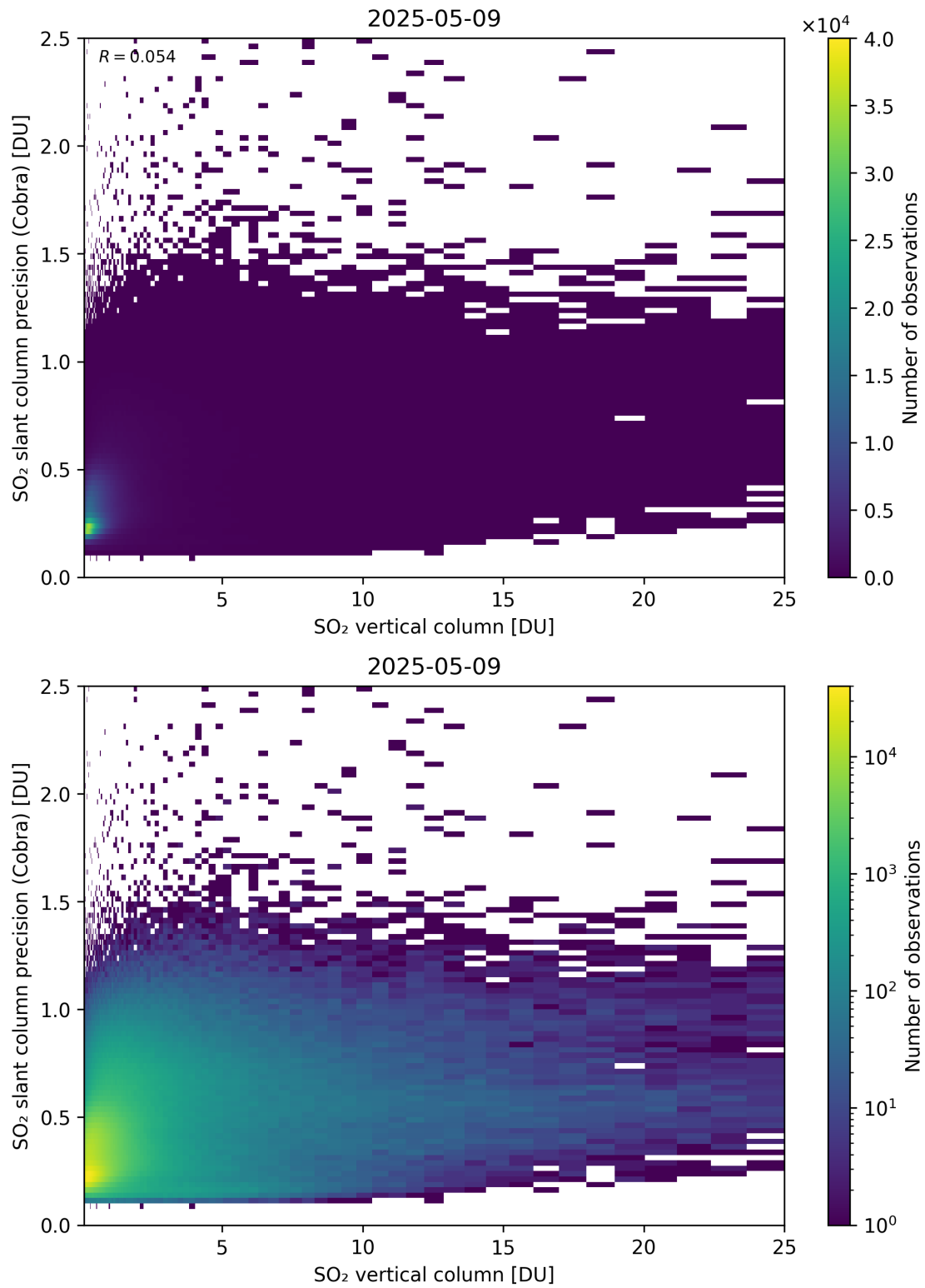
Figure 350: Scatter density plot of “SO 2 vertical column” against “SO 2 slant column precision (Cobra)” for 2025-05-08 to 2025-05-10.
