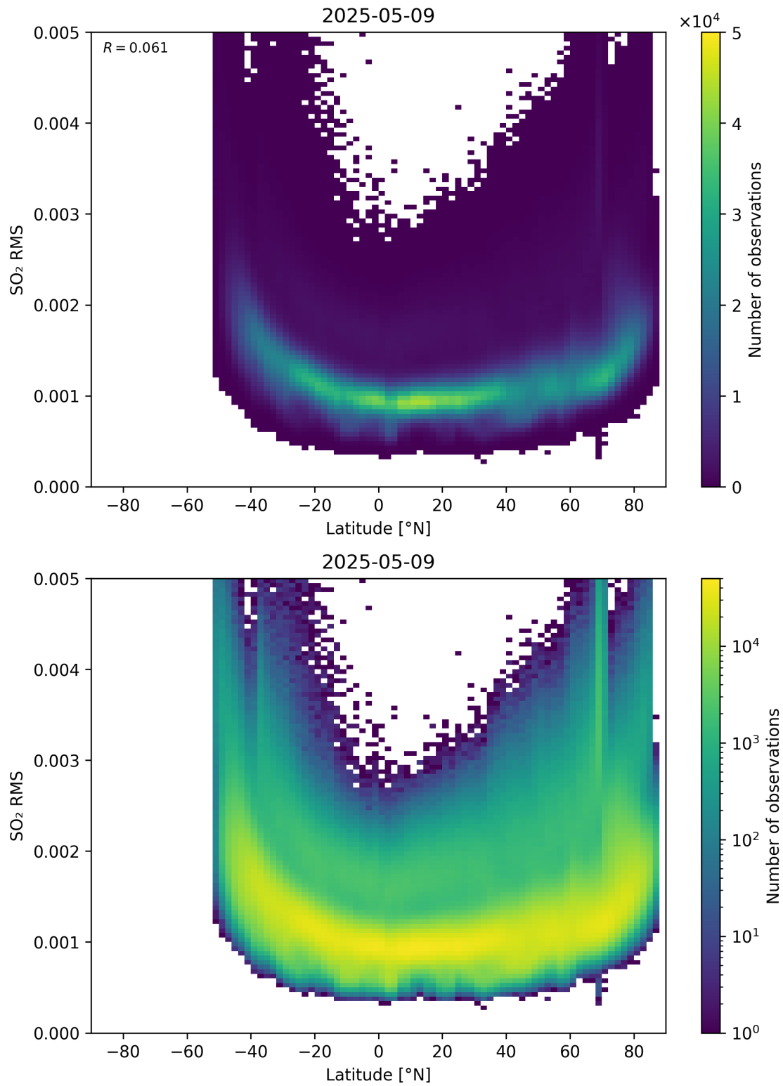
Figure 155: Scatter density plot of “Latitude” against “SO 2 RMS” for 2025-05-08 to 2025-05-10.
