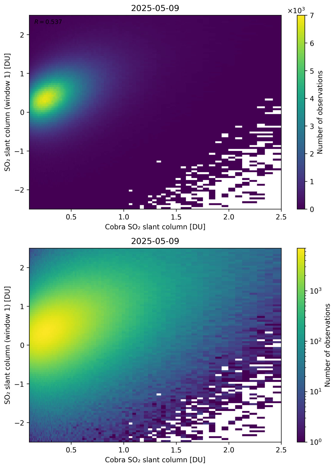
Figure 219: Scatter density plot of “Cobra SO 2 slant column” against “SO 2 slant column (window 1)” for 2025-05-08 to 2025-05-10.
