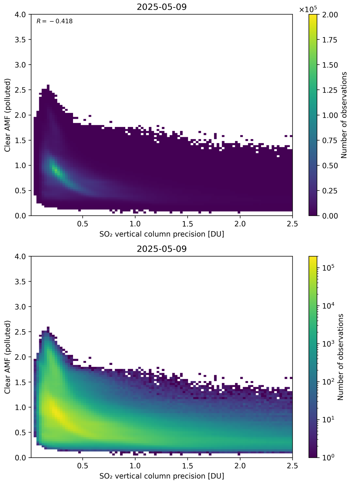
Figure 335: Scatter density plot of “SO 2 vertical column precision” against “Clear AMF (polluted)” for 2025-05-08 to 2025-05-10.
