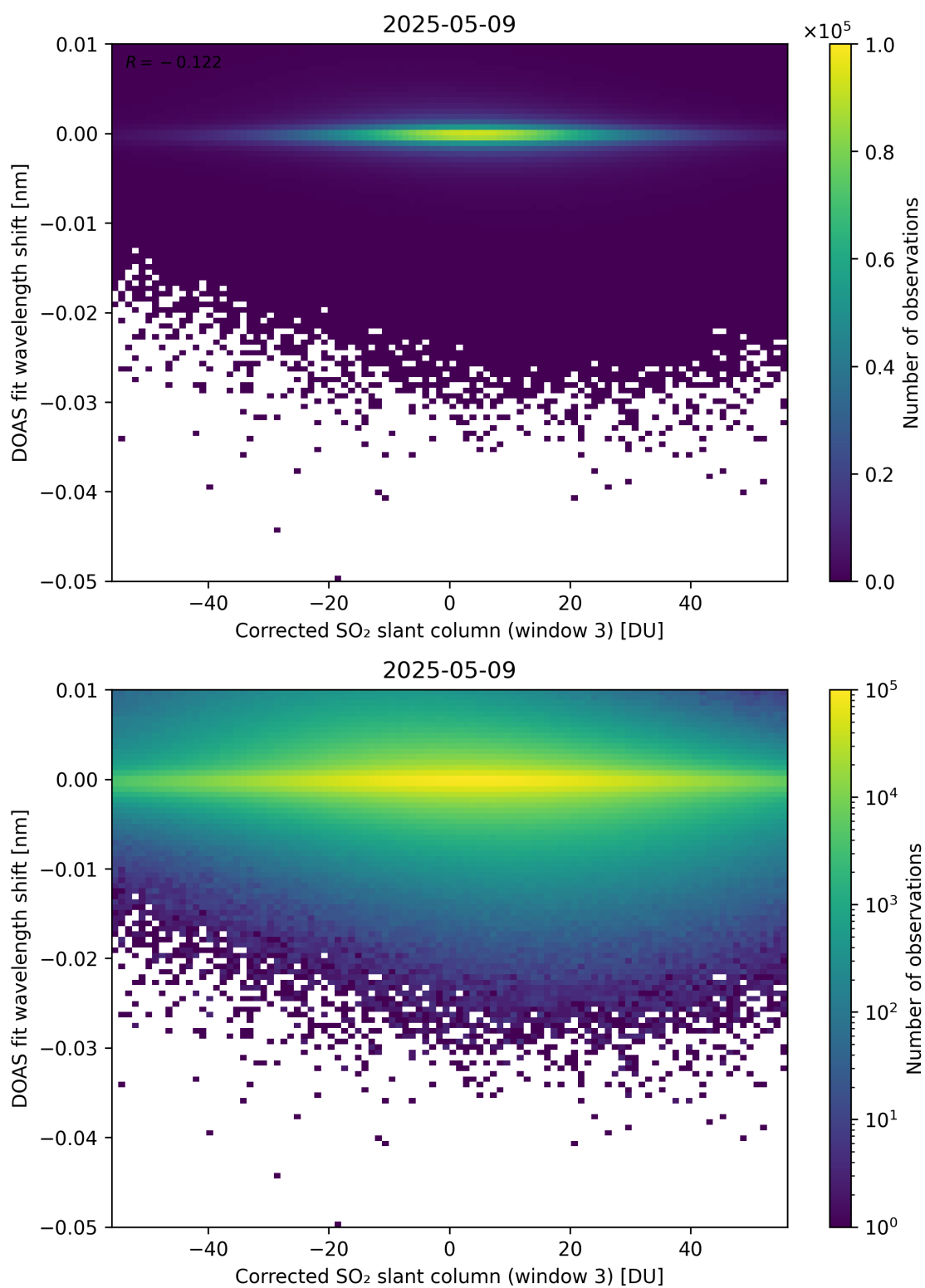
Figure 256: Scatter density plot of “Corrected SO 2 slant column (window 3)” against “DOAS fit wavelength shift” for 2025-05-08 to 2025-05-10.
