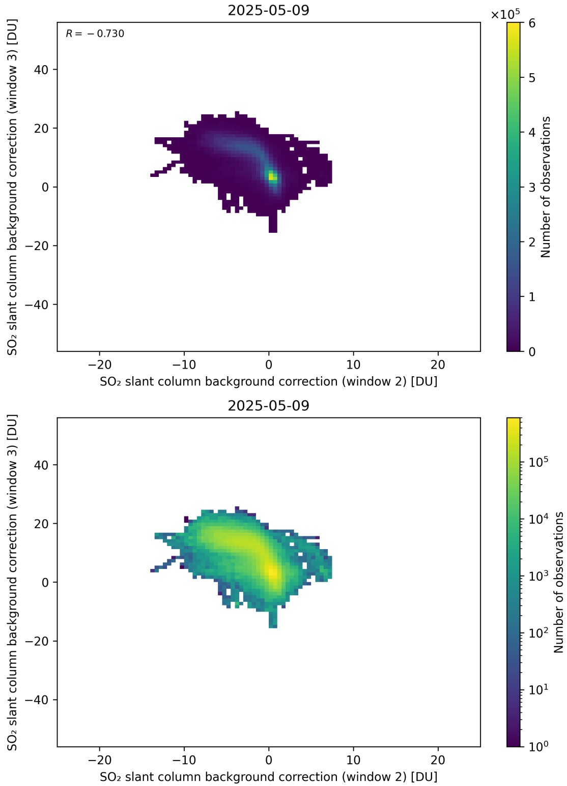
Figure 122: Scatter density plot of “SO 2 slant column background correction (window 2)” against “SO 2 slant column background correction (window 3)” for 2025-05-08 to 2025-05-10.
