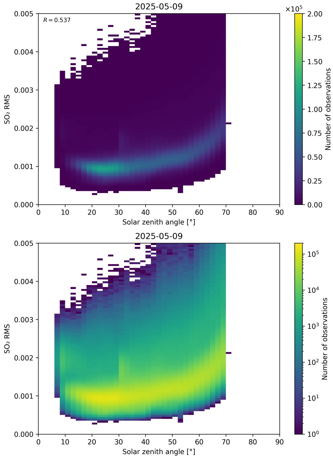
Figure 176: Scatter density plot of “Solar zenith angle” against “SO 2 RMS” for 2025-05-08 to 2025-05-10.
