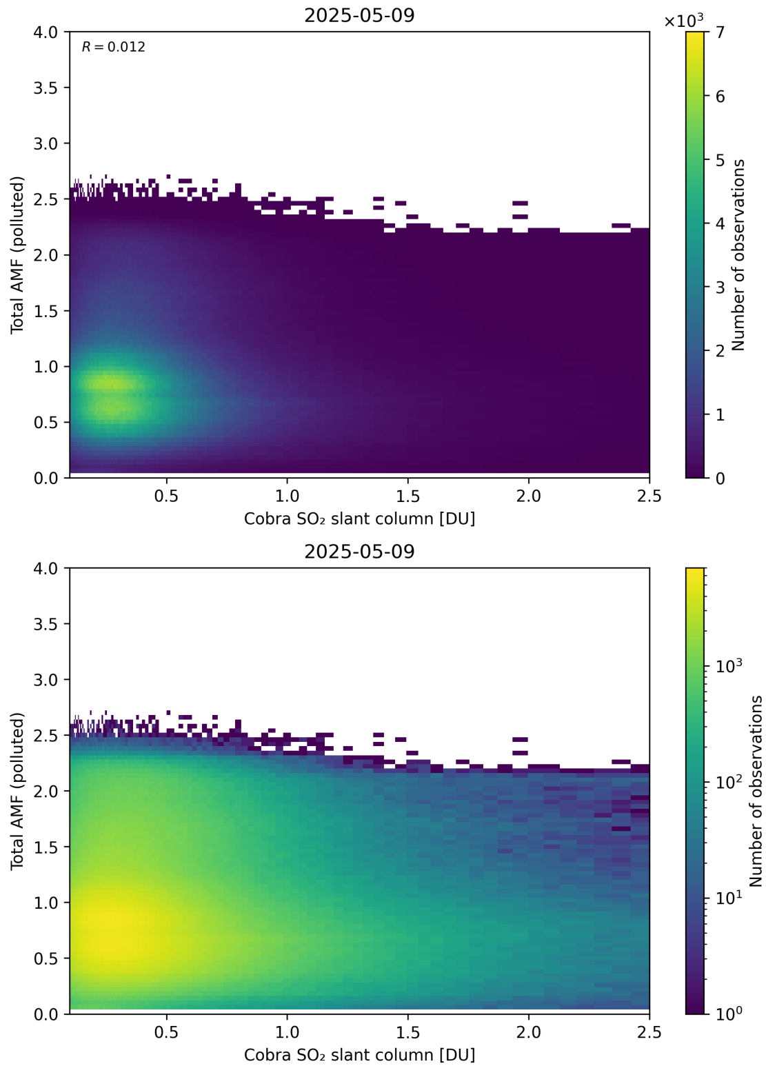
Figure 224: Scatter density plot of “Cobra SO 2 slant column” against “Total AMF (polluted)” for 2025-05-08 to 2025-05-10.
