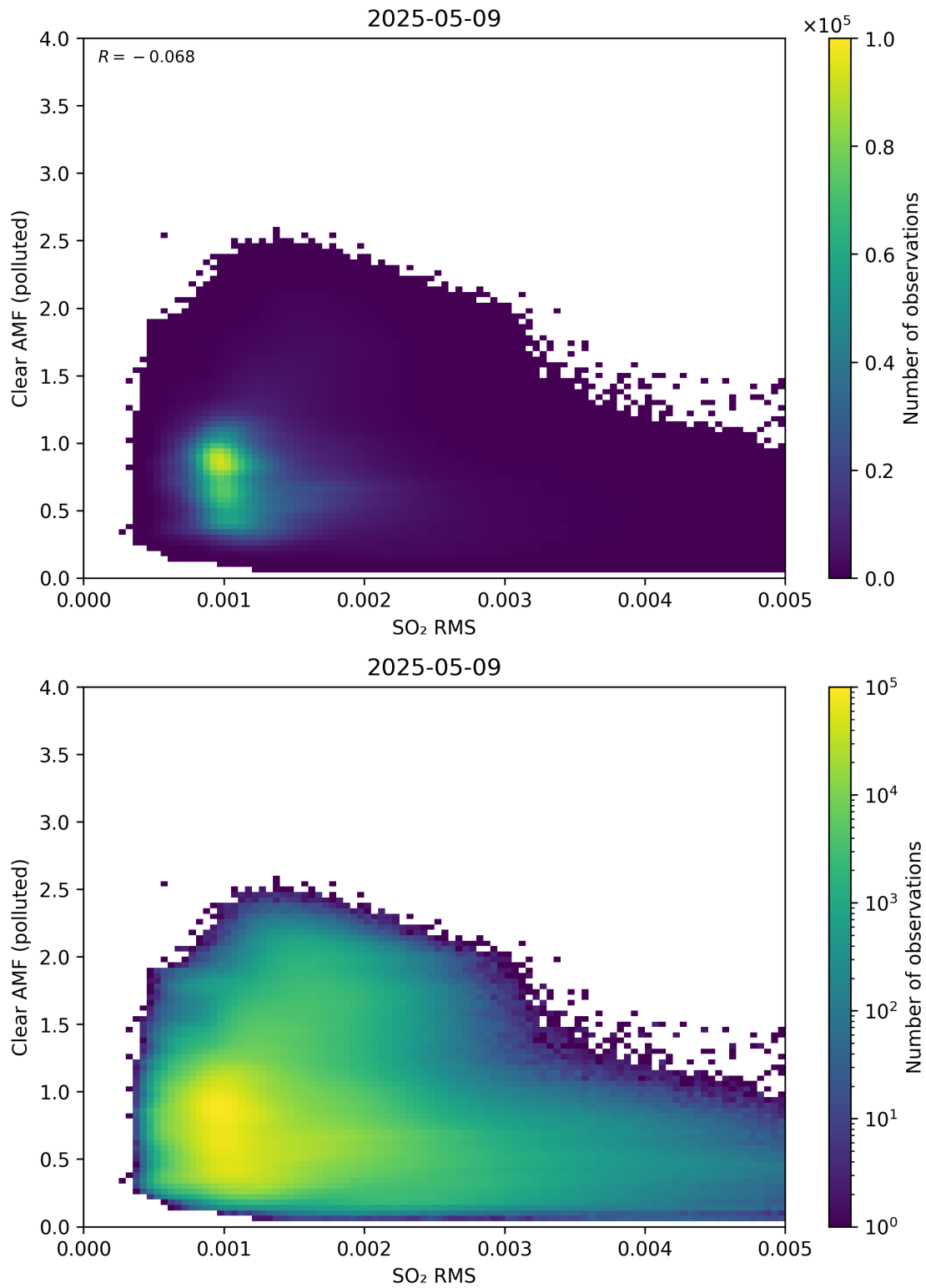
Figure 147: Scatter density plot of “SO 2 RMS” against “Clear AMF (polluted)” for 2025-05-08 to 2025-05-10.
