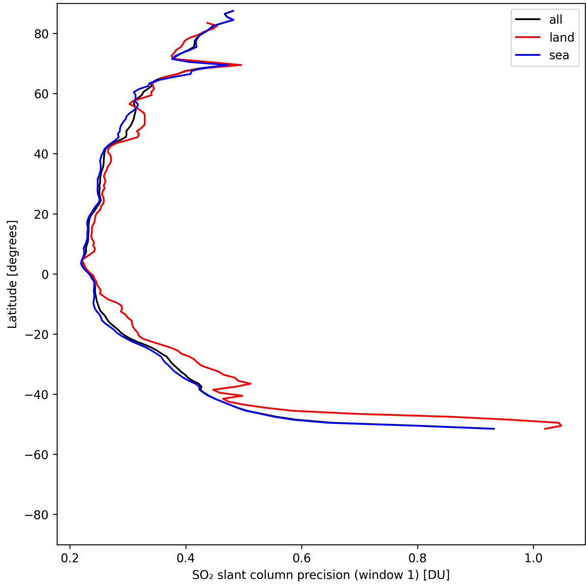
Figure 38: Zonal average of “SO 2 slant column precision (window 1)” for 2025-05-08 to 2025-05-10.
