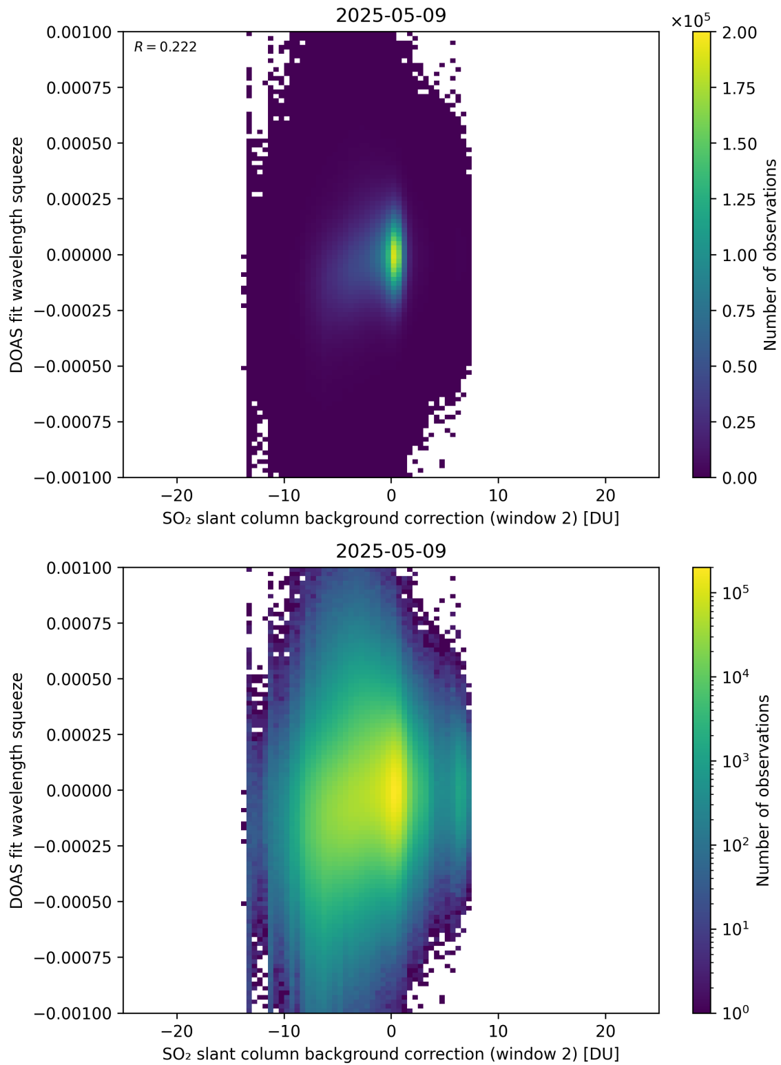
Figure 124: Scatter density plot of “SO 2 slant column background correction (window 2)” against “DOAS fit wavelength squeeze” for 2025-05-08 to 2025-05-10.
