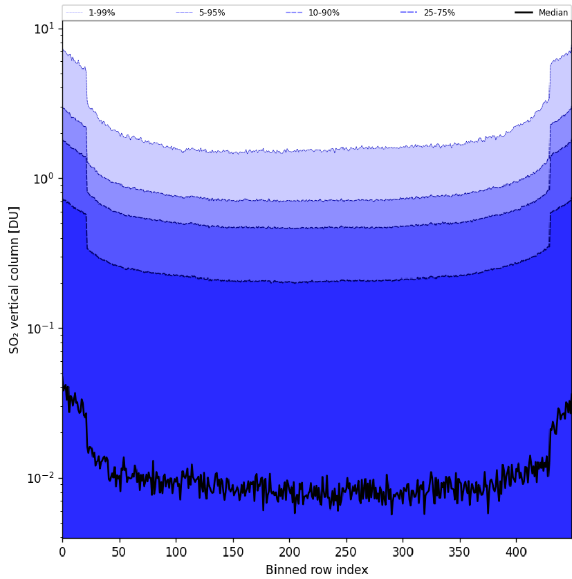
Figure 84: Along track statistics of “SO 2 vertical column” for 2025-05-08 to 2025-05-10
