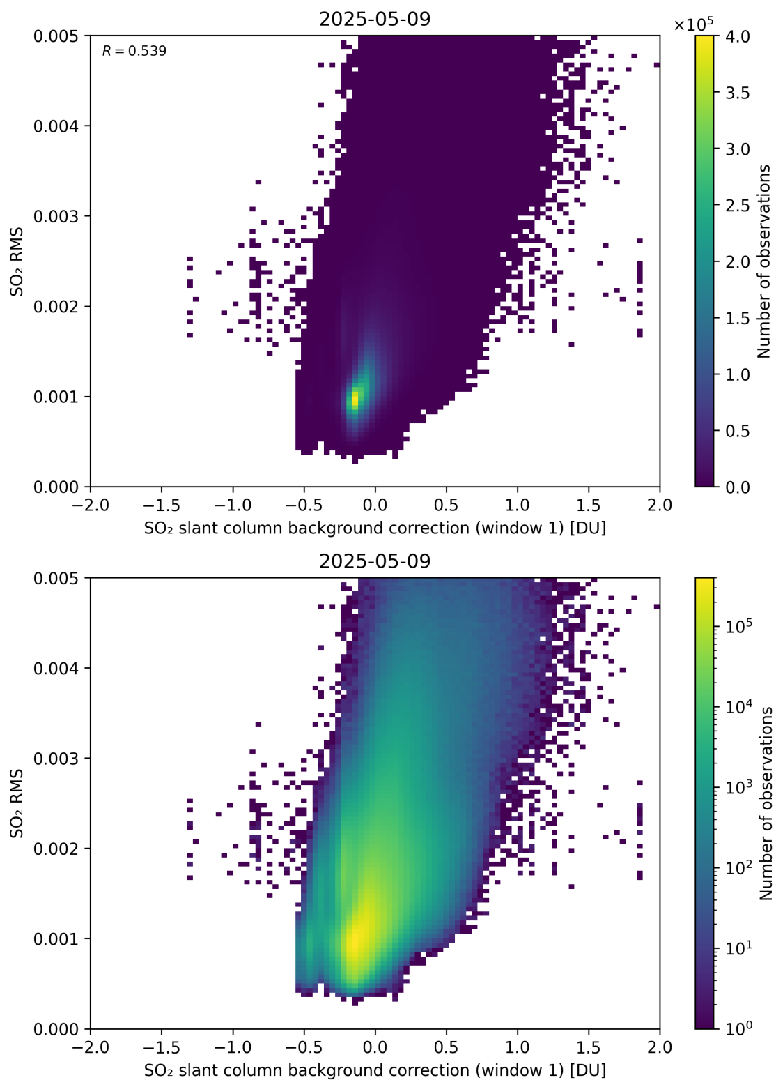
Figure 113: Scatter density plot of “SO 2 slant column background correction (window 1)” against “SO 2 RMS” for 2025-05-08 to 2025-05-10.
