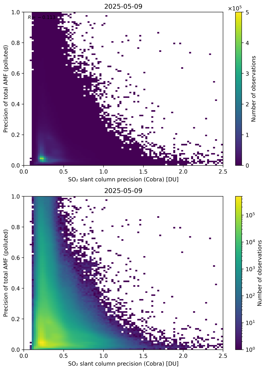
Figure 214: Scatter density plot of “SO 2 slant column precision (Cobra)” against “Precision of total AMF (polluted)” for 2025-05-08 to 2025-05-10.
