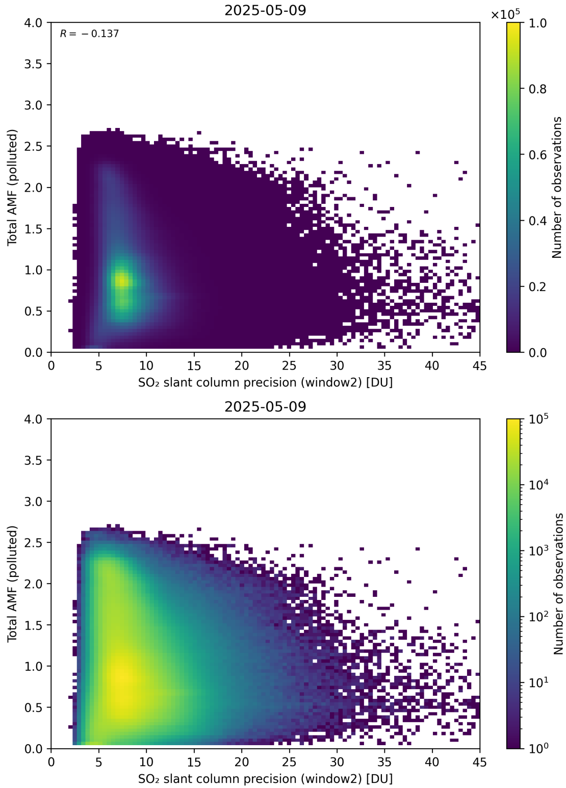
Figure 301: Scatter density plot of “SO 2 slant column precision (window2)” against “Total AMF (polluted)” for 2025-05-08 to 2025-05-10.
