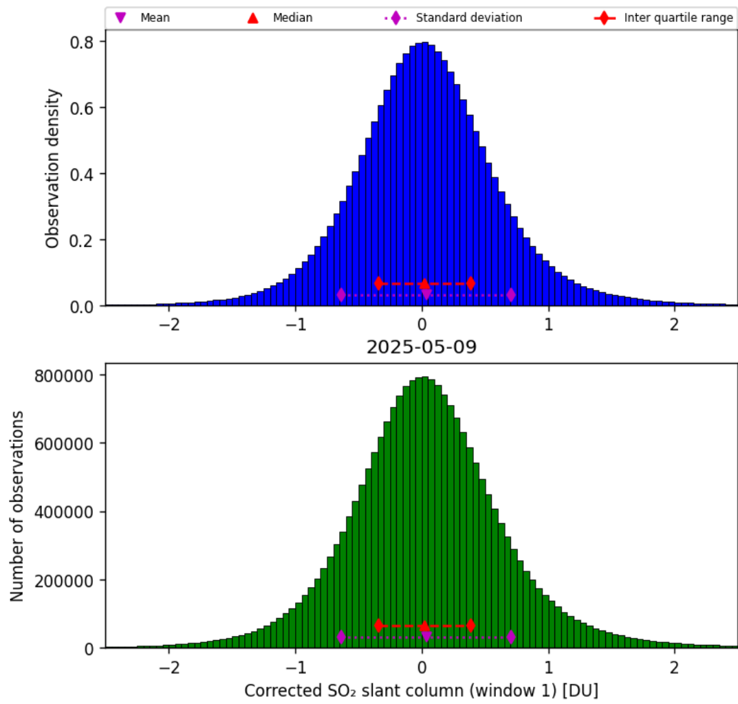
Figure 65: Histogram of “Corrected SO 2 slant column (window 1)” for 2025-05-08 to 2025-05-10
