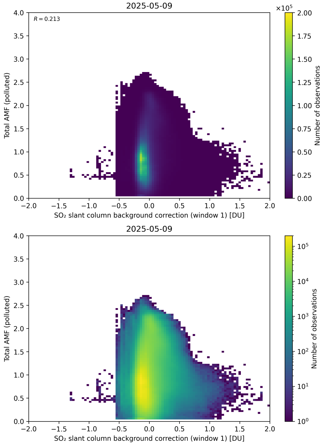
Figure 120: Scatter density plot of “SO 2 slant column background correction (window 1)” against “Total AMF (polluted)” for 2025-05-08 to 2025-05-10.
