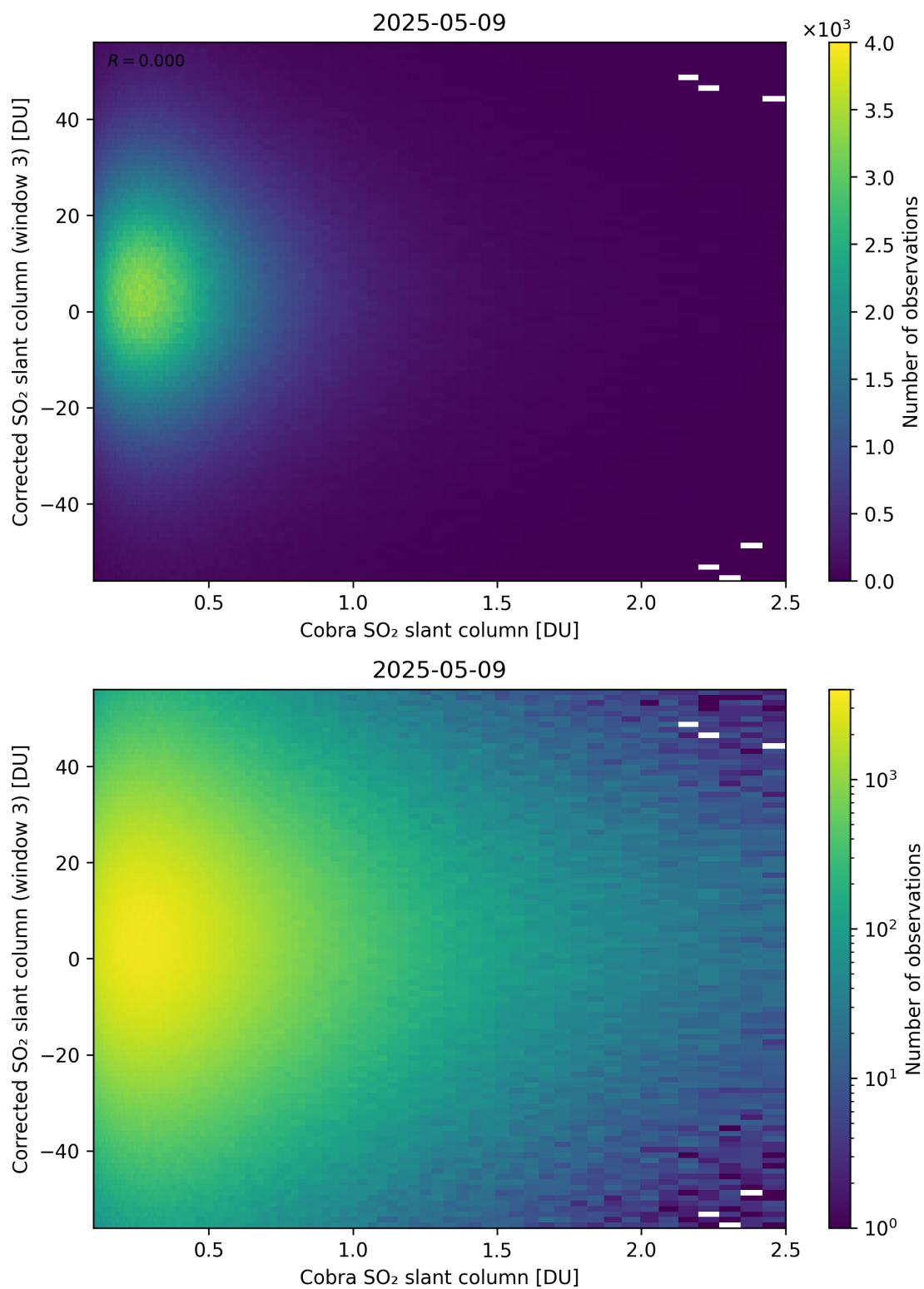
Figure 218: Scatter density plot of “Cobra SO 2 slant column” against “Corrected SO 2 slant column (window 3)” for 2025-05-08 to 2025-05-10.
