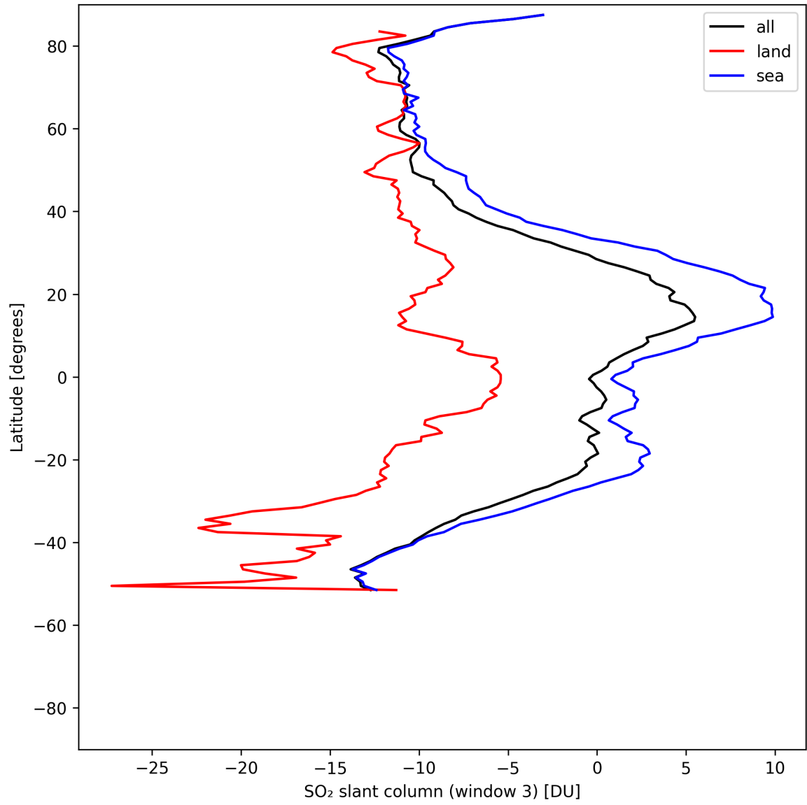
Figure 45: Zonal average of “SO 2 slant column (window 3)” for 2025-05-08 to 2025-05-10.
