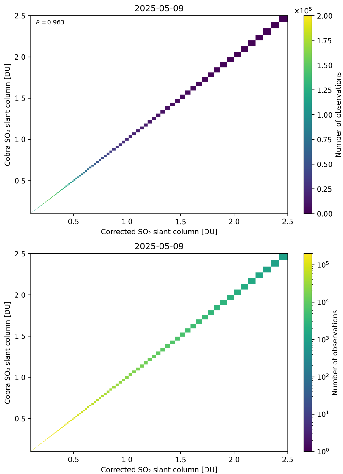
Figure 233: Scatter density plot of “Corrected SO 2 slant column” against “Cobra SO 2 slant column” for 2025-05-08 to 2025-05-10.
