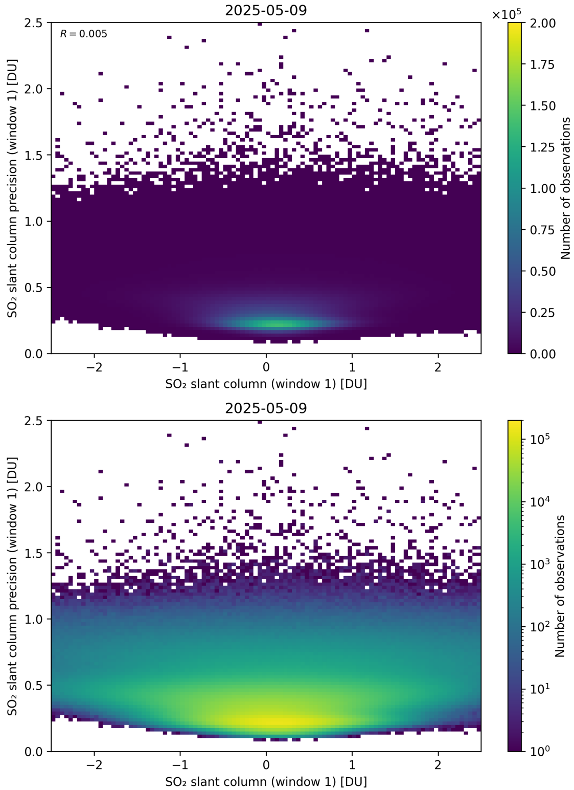
Figure 285: Scatter density plot of “SO 2 slant column (window 1)” against “SO 2 slant column precision (window 1)” for 2025-05-08 to 2025-05-10.
