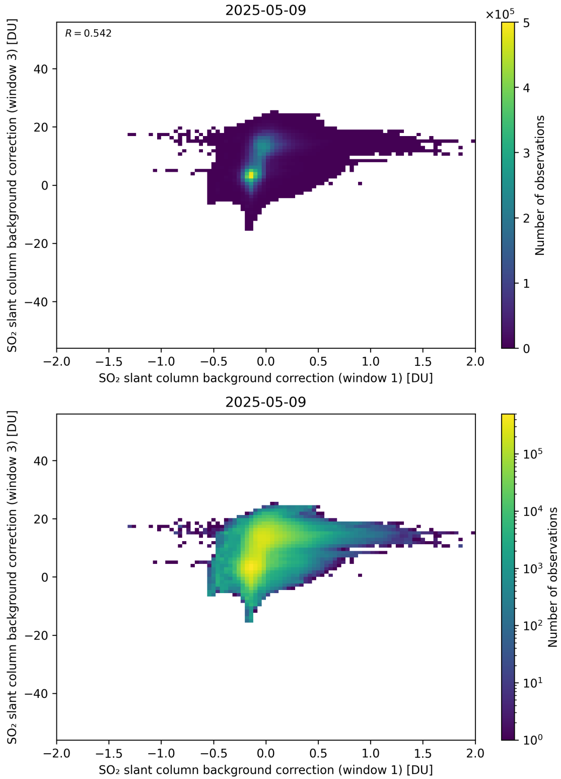
Figure 110: Scatter density plot of “SO 2 slant column background correction (window 1)” against “SO 2 slant column background correction (window 3)” for 2025-05-08 to 2025-05-10.
