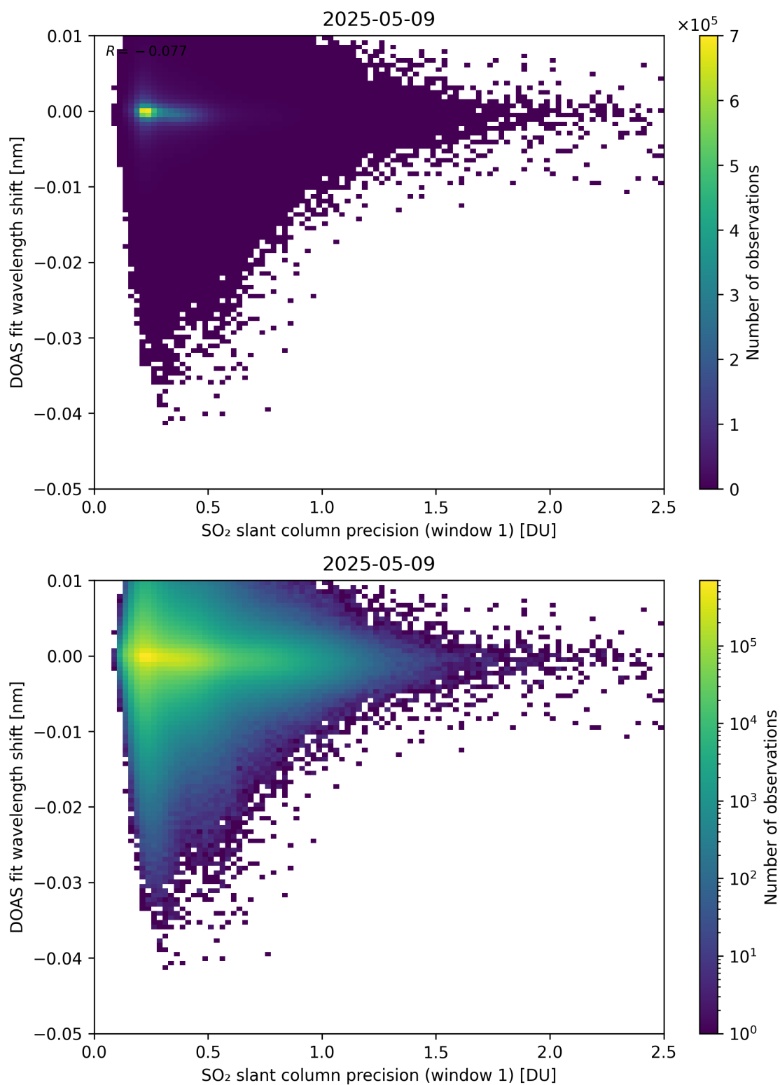
Figure 271: Scatter density plot of “SO 2 slant column precision (window 1)” against “DOAS fit wavelength shift” for 2025-05-08 to 2025-05-10.
