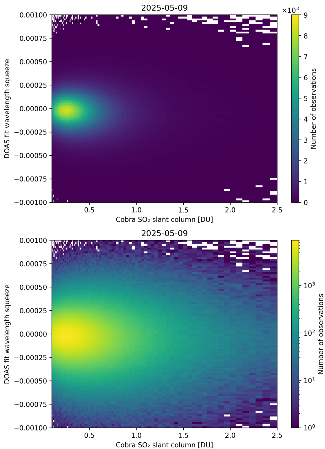
Figure 197: Scatter density plot of “Cobra SO 2 slant column” against “DOAS fit wavelength squeeze” for 2025-05-08 to 2025-05-10.
