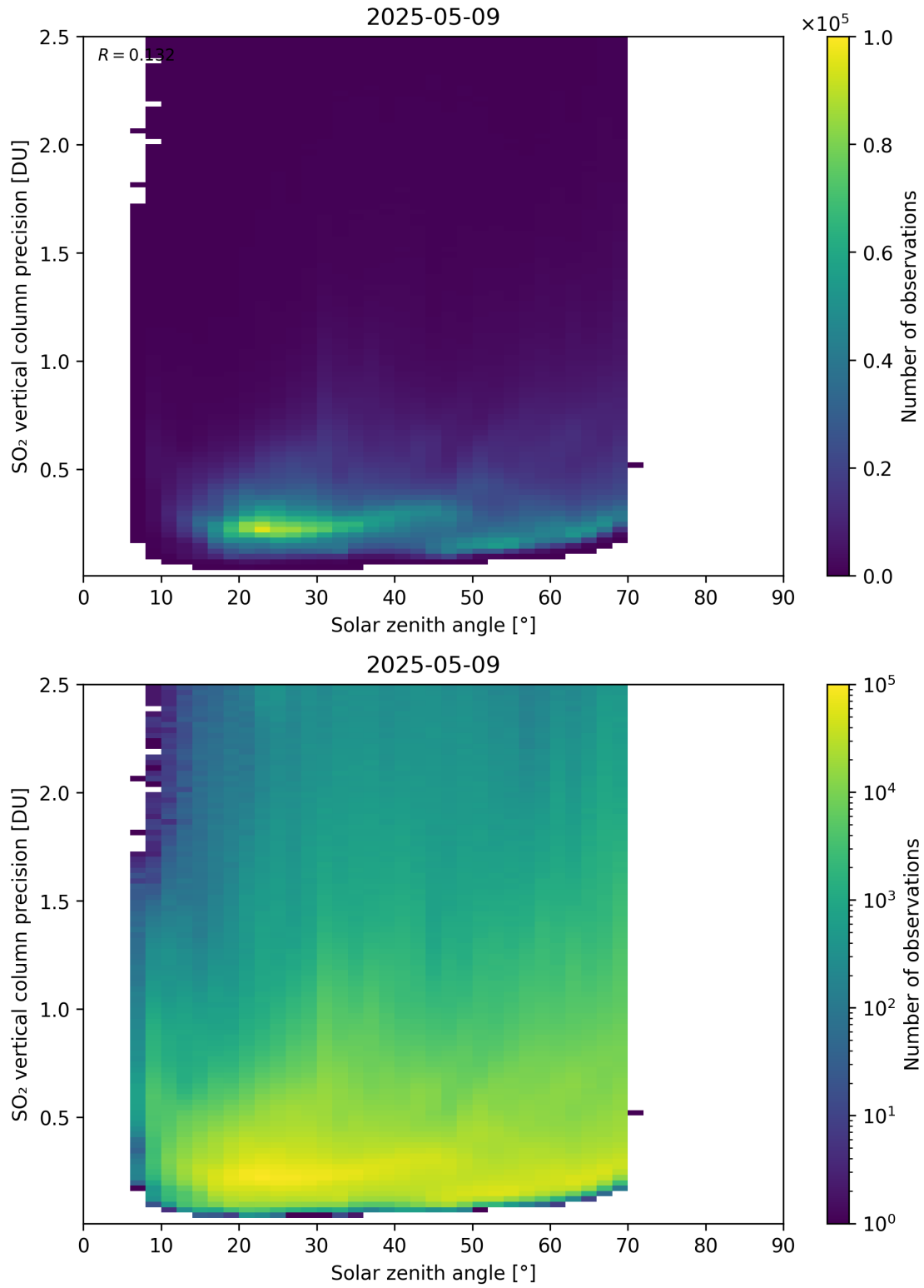
Figure 192: Scatter density plot of “Solar zenith angle” against “SO 2 vertical column precision” for 2025-05-08 to 2025-05-10.
