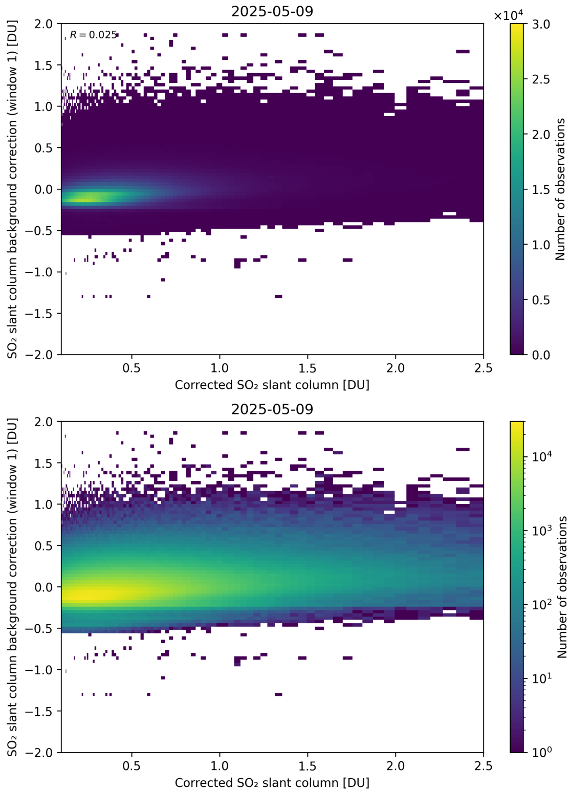
Figure 226: Scatter density plot of “Corrected SO 2 slant column” against “SO 2 slant column background correction (window 1)” for 2025-05-08 to 2025-05-10.
