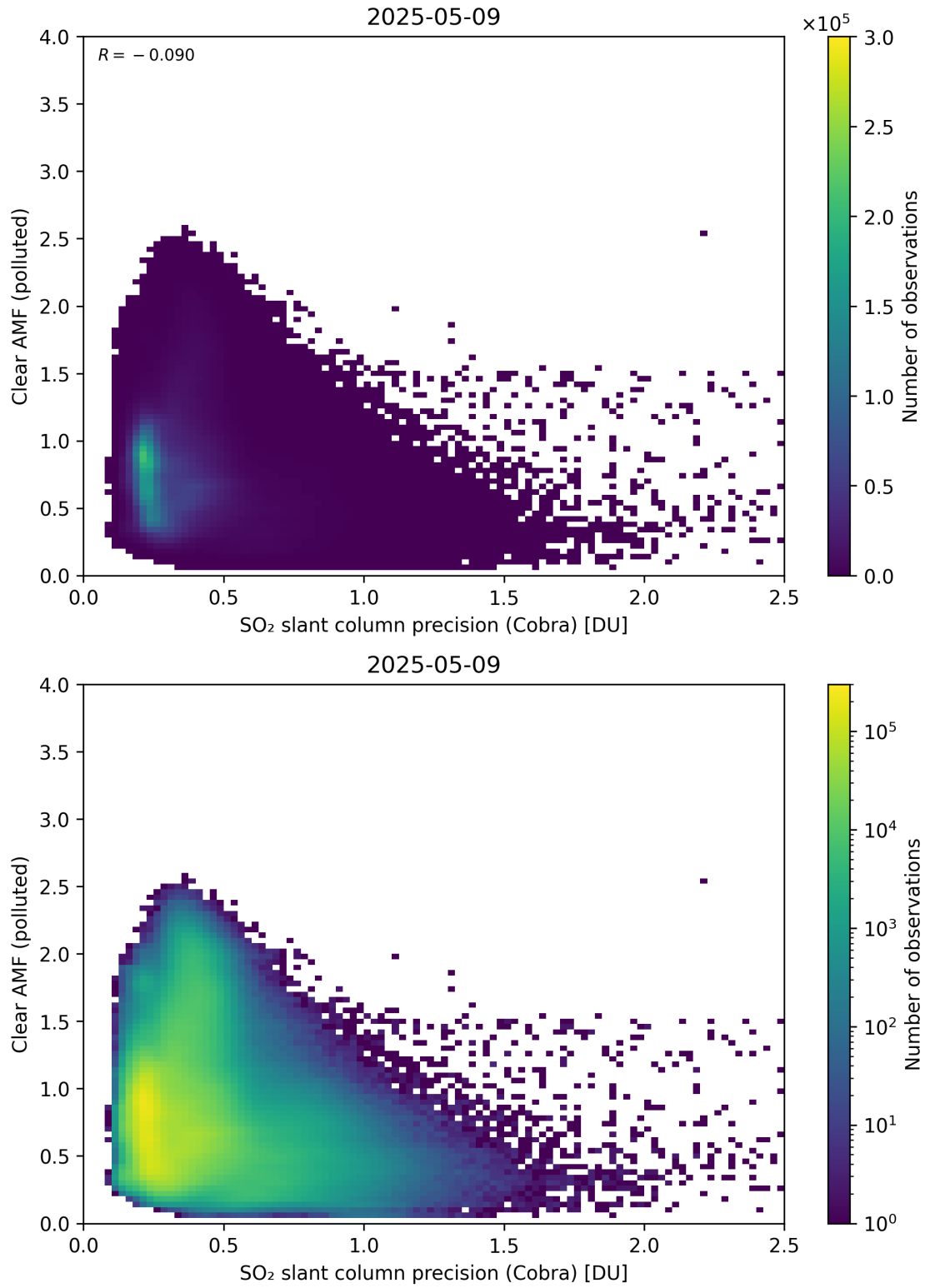
Figure 205: Scatter density plot of “SO 2 slant column precision (Cobra)” against “Clear AMF (polluted)” for 2025-05-08 to 2025-05-10.
