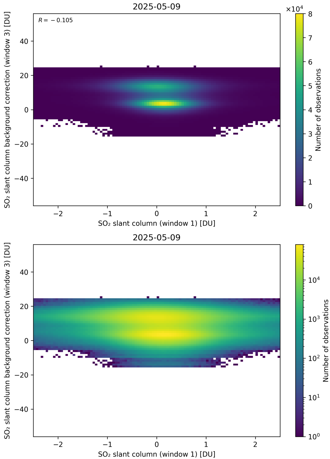
Figure 264: Scatter density plot of “SO 2 slant column (window 1)” against “SO 2 slant column background correction (window 3)” for 2025-05-08 to 2025-05-10.
