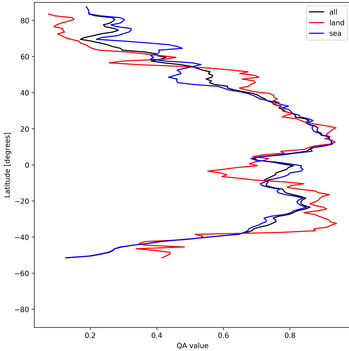
Figure 31: Zonal average of “QA value” for 2025-05-08 to 2025-05-10.
