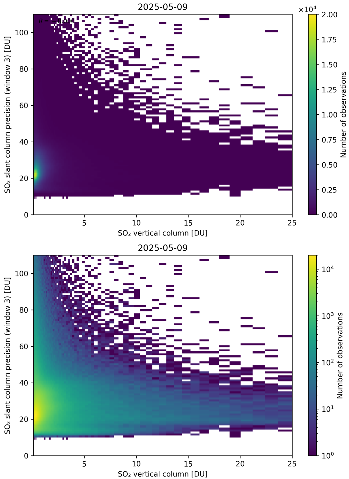
Figure 358: Scatter density plot of “SO 2 vertical column” against “SO 2 slant column precision (window 3)” for 2025-05-08 to 2025-05-10.
