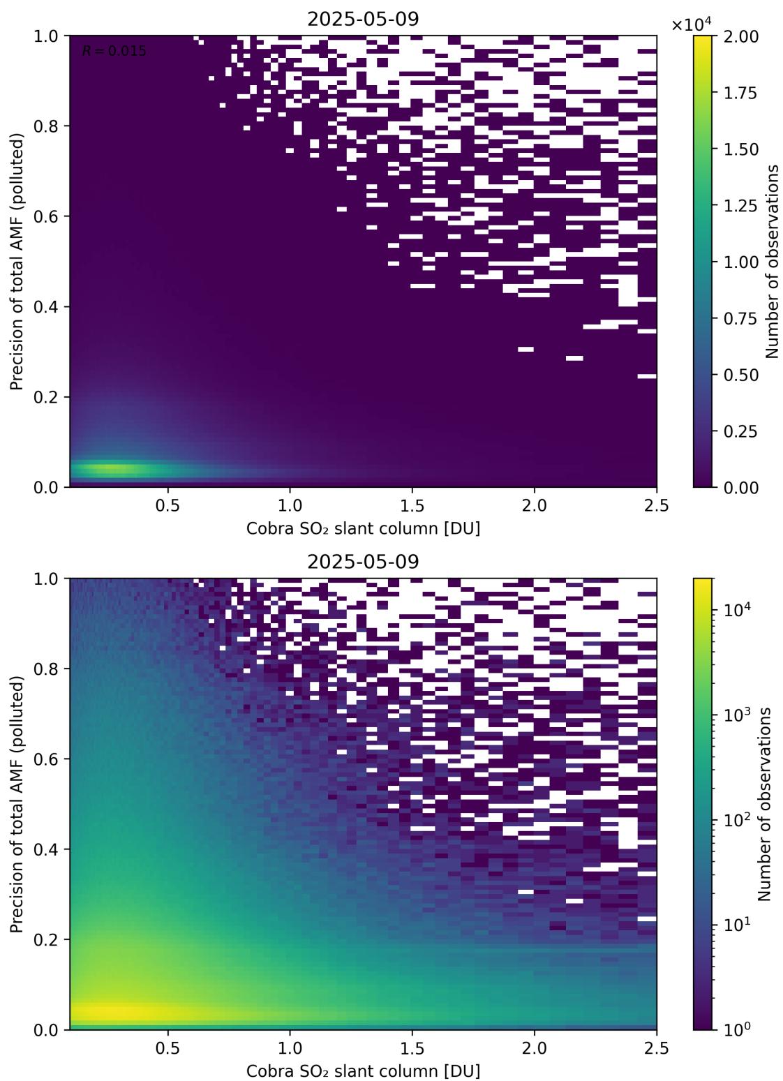
Figure 225: Scatter density plot of “Cobra SO 2 slant column” against “Precision of total AMF (polluted)” for 2025-05-08 to 2025-05-10.
