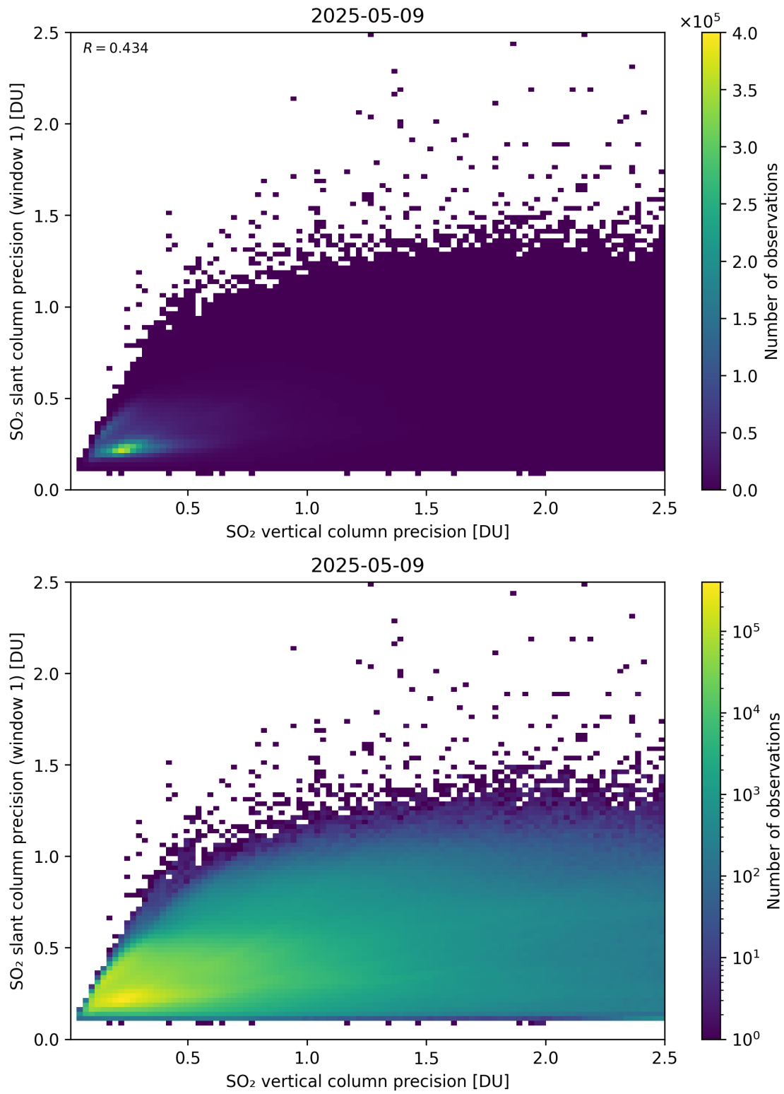
Figure 342: Scatter density plot of “SO 2 vertical column precision” against “SO 2 slant column precision (window 1)” for 2025-05-08 to 2025-05-10.
