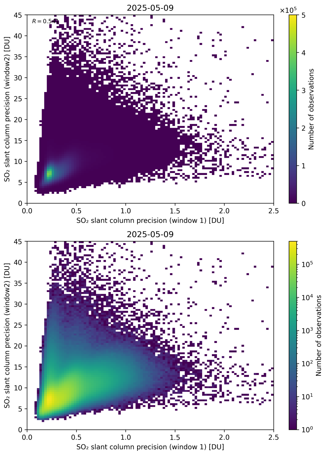
Figure 277: Scatter density plot of “SO 2 slant column precision (window 1)” against “SO 2 slant column precision (window2)” for 2025-05-08 to 2025-05-10.
