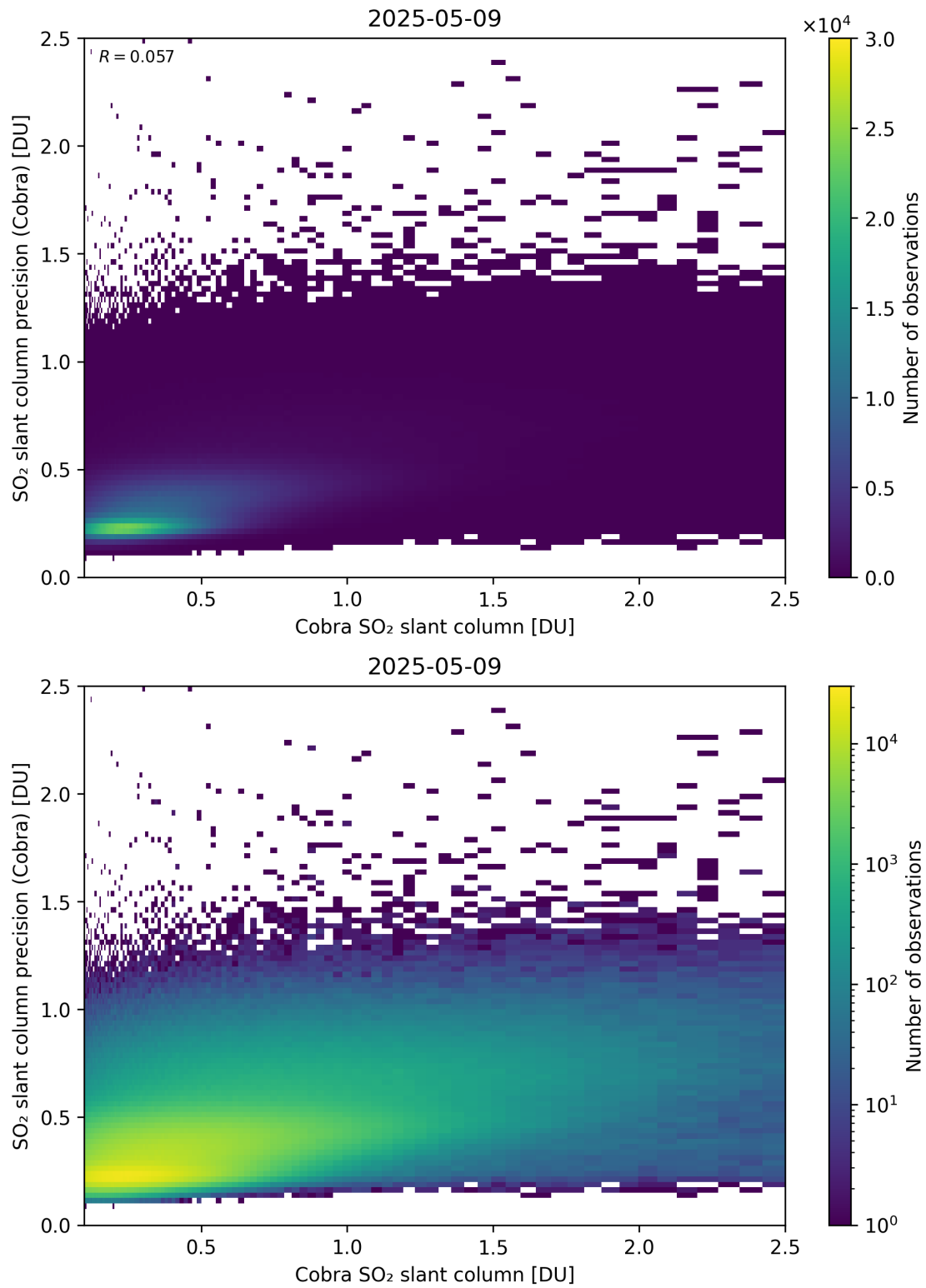
Figure 216: Scatter density plot of “Cobra SO 2 slant column” against “SO 2 slant column precision (Cobra)” for 2025-05-08 to 2025-05-10.
