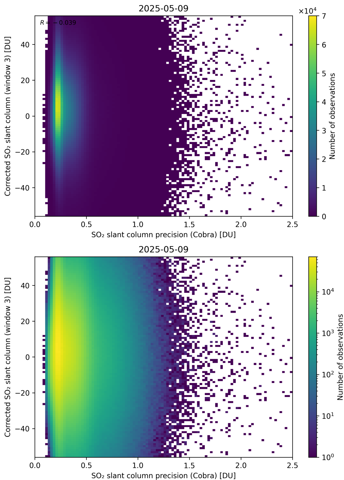
Figure 207: Scatter density plot of “SO 2 slant column precision (Cobra)” against “Corrected SO 2 slant column (window 3)” for 2025-05-08 to 2025-05-10.
