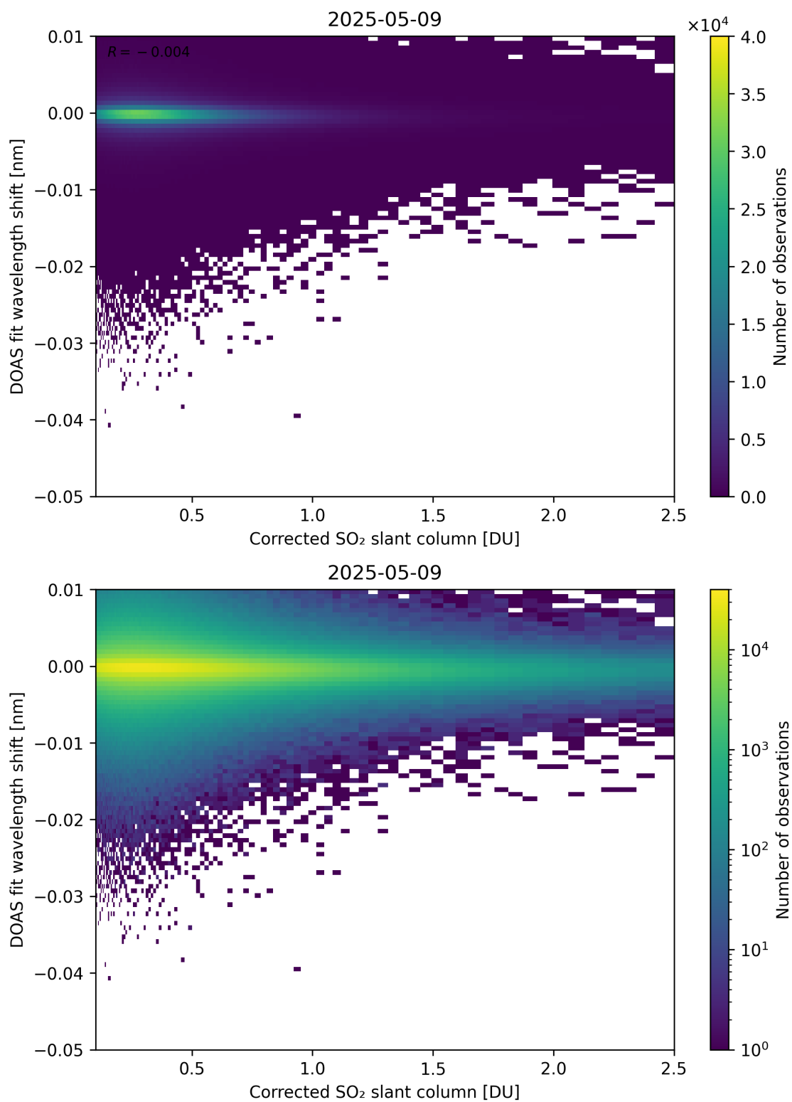
Figure 229: Scatter density plot of “Corrected SO 2 slant column” against “DOAS fit wavelength shift” for 2025-05-08 to 2025-05-10.
