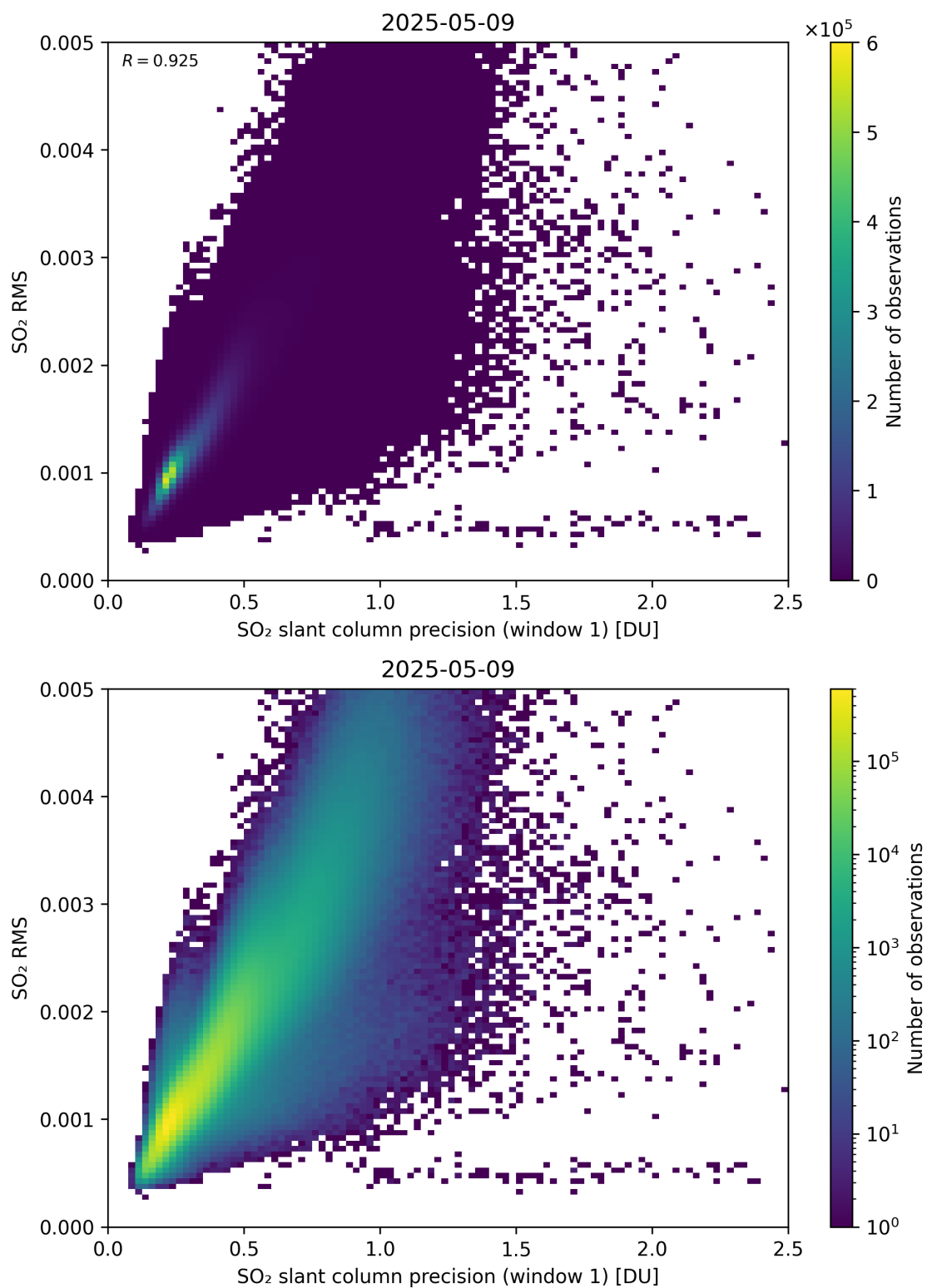
Figure 273: Scatter density plot of “SO 2 slant column precision (window 1)” against “SO 2 RMS” for 2025-05-08 to 2025-05-10.
