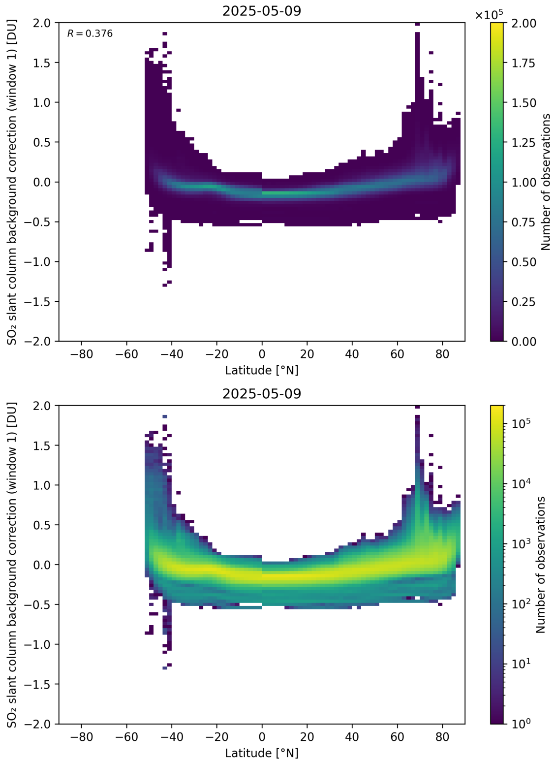
Figure 150: Scatter density plot of “Latitude” against “SO 2 slant column background correction (window 1)” for 2025-05-08 to 2025-05-10.
