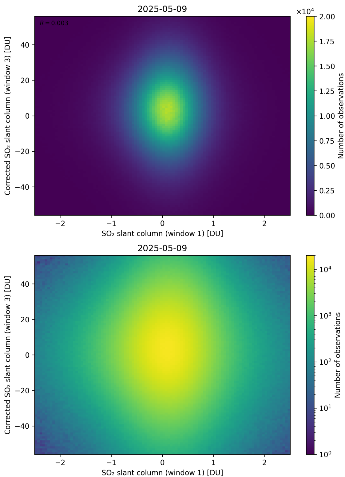
Figure 284: Scatter density plot of “SO 2 slant column (window 1)” against “Corrected SO 2 slant column (window 3)” for 2025-05-08 to 2025-05-10.
