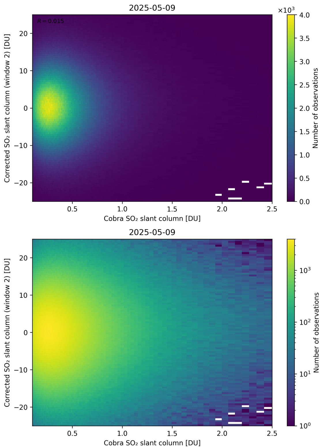
Figure 217: Scatter density plot of “Cobra SO 2 slant column” against “Corrected SO 2 slant column (window 2)” for 2025-05-08 to 2025-05-10.
