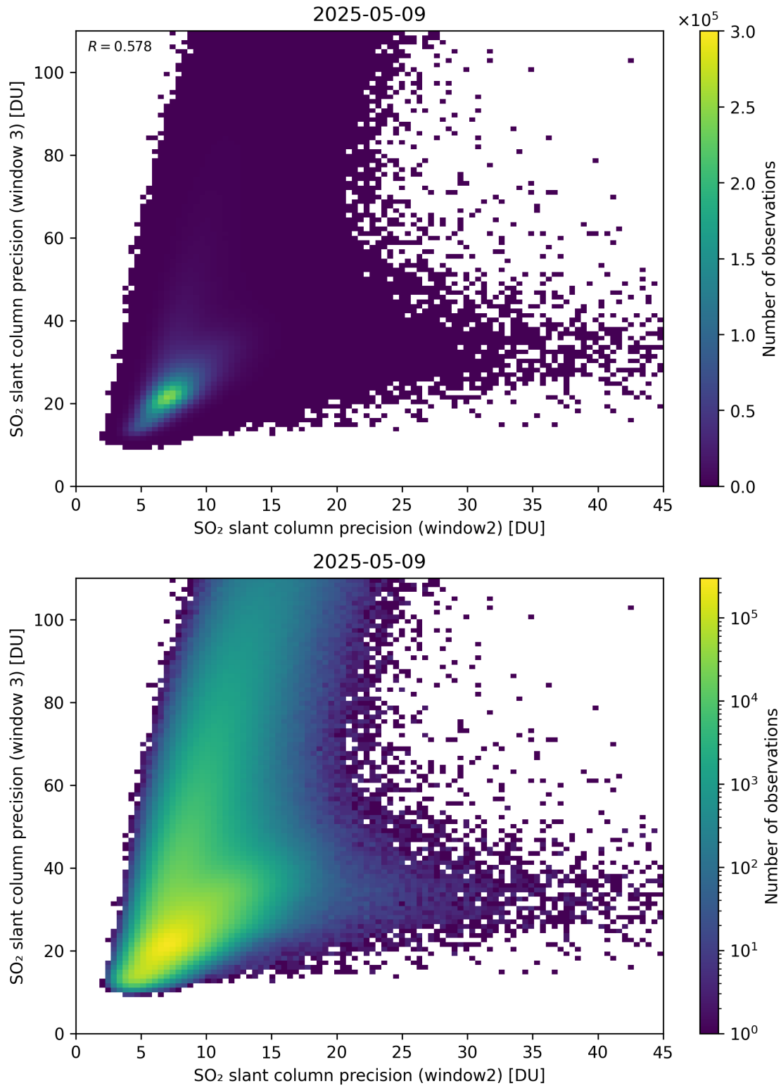
Figure 300: Scatter density plot of “SO 2 slant column precision (window2)” against “SO 2 slant column precision (window 3)” for 2025-05-08 to 2025-05-10.
