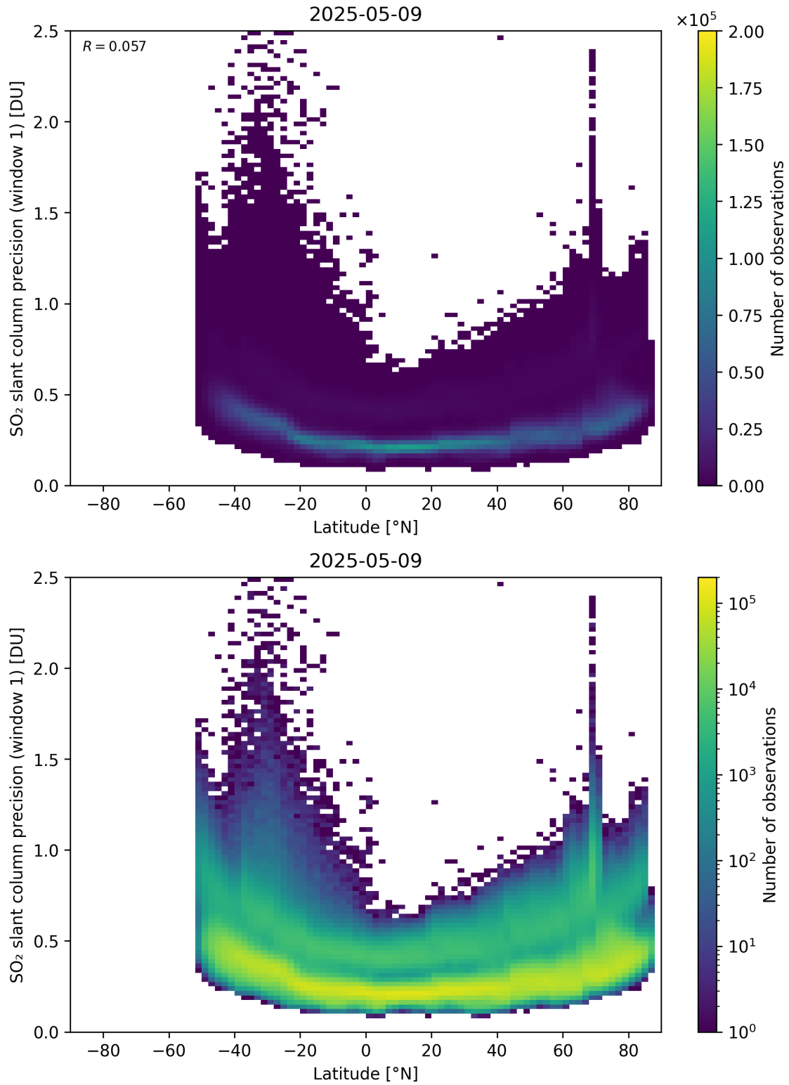
Figure 163: Scatter density plot of “Latitude” against “SO 2 slant column precision (window 1)” for 2025-05-08 to 2025-05-10.
