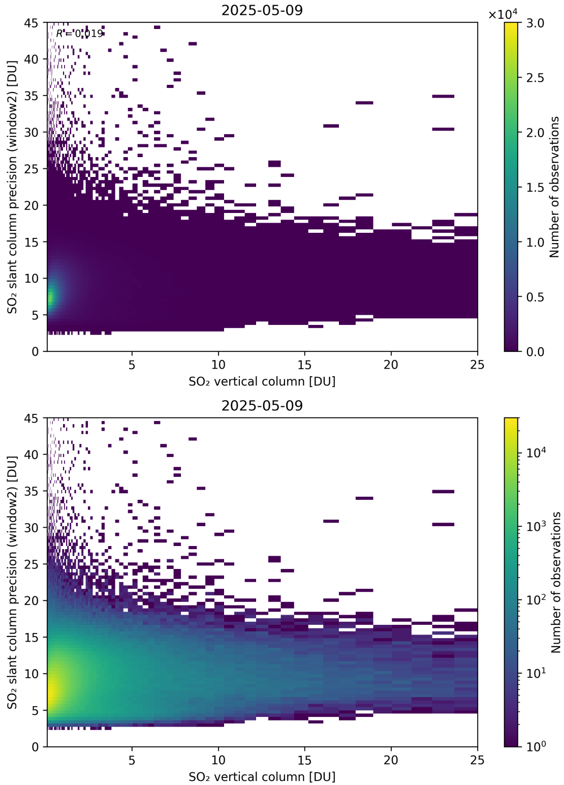
Figure 356: Scatter density plot of “SO 2 vertical column” against “SO 2 slant column precision (window2)” for 2025-05-08 to 2025-05-10.
