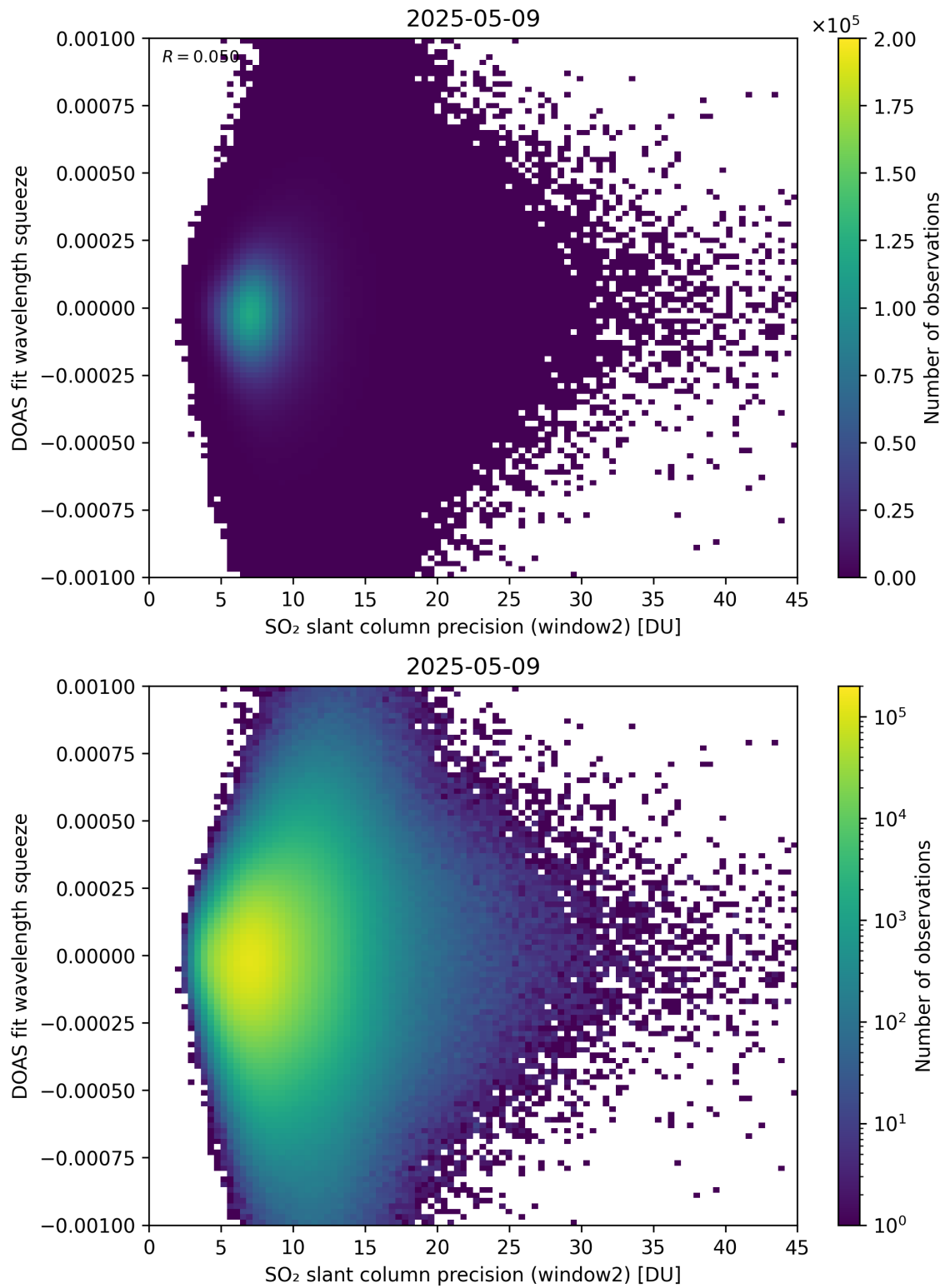
Figure 294: Scatter density plot of “SO 2 slant column precision (window2)” against “DOAS fit wavelength squeeze” for 2025-05-08 to 2025-05-10.
