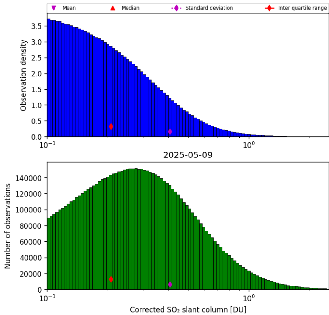
Figure 60: Histogram of "Corrected SO 2 slant column" for 2025-05-08 to 2025-05-10
