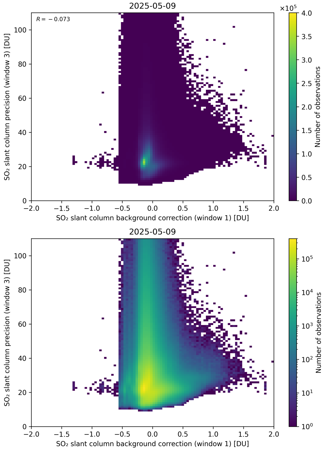
Figure 119: Scatter density plot of “SO 2 slant column background correction (window 1)” against “SO 2 slant column precision (window 3)” for 2025-05-08 to 2025-05-10.
