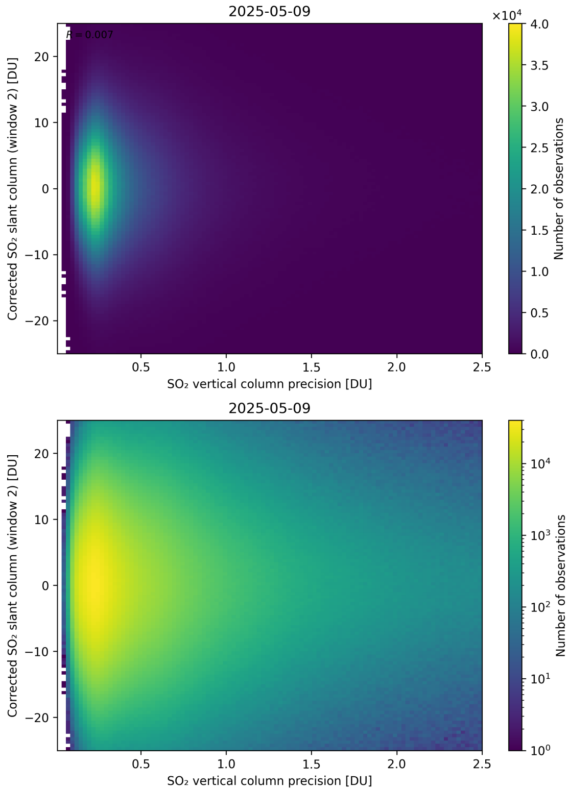
Figure 339: Scatter density plot of “SO 2 vertical column precision” against “Corrected SO 2 slant column (window 2)” for 2025-05-08 to 2025-05-10.
