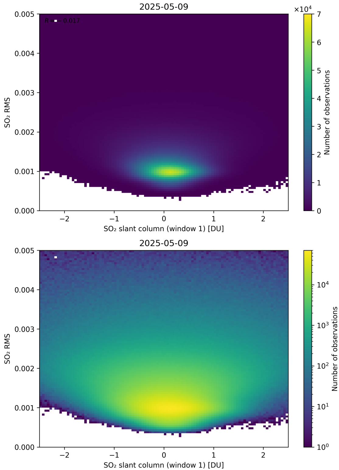
Figure 267: Scatter density plot of “SO 2 slant column (window 1)” against “SO 2 RMS” for 2025-05-08 to 2025-05-10.
