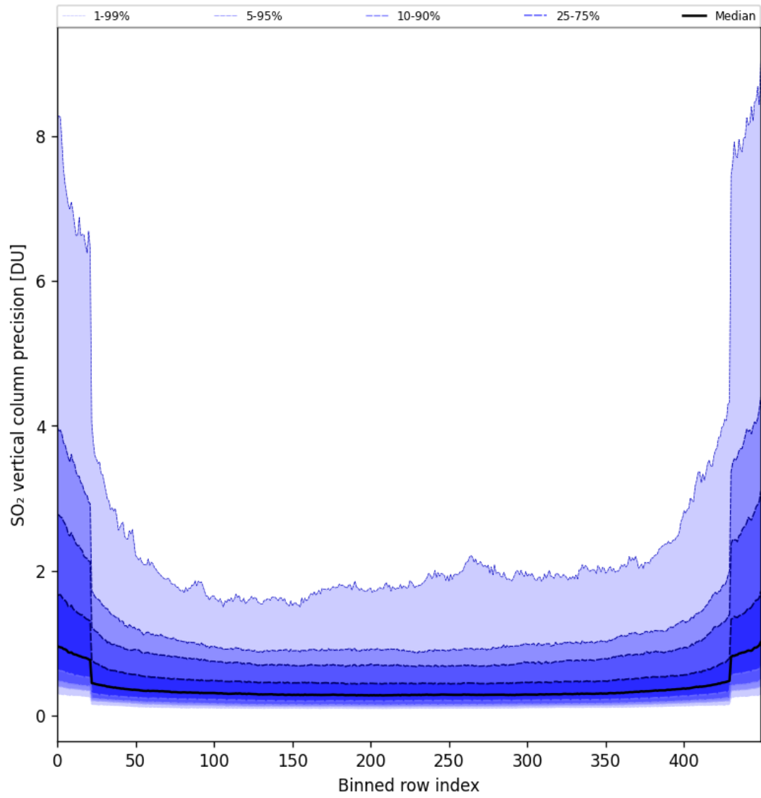
Figure 85: Along track statistics of “SO 2 vertical column precision” for 2025-05-08 to 2025-05-10
