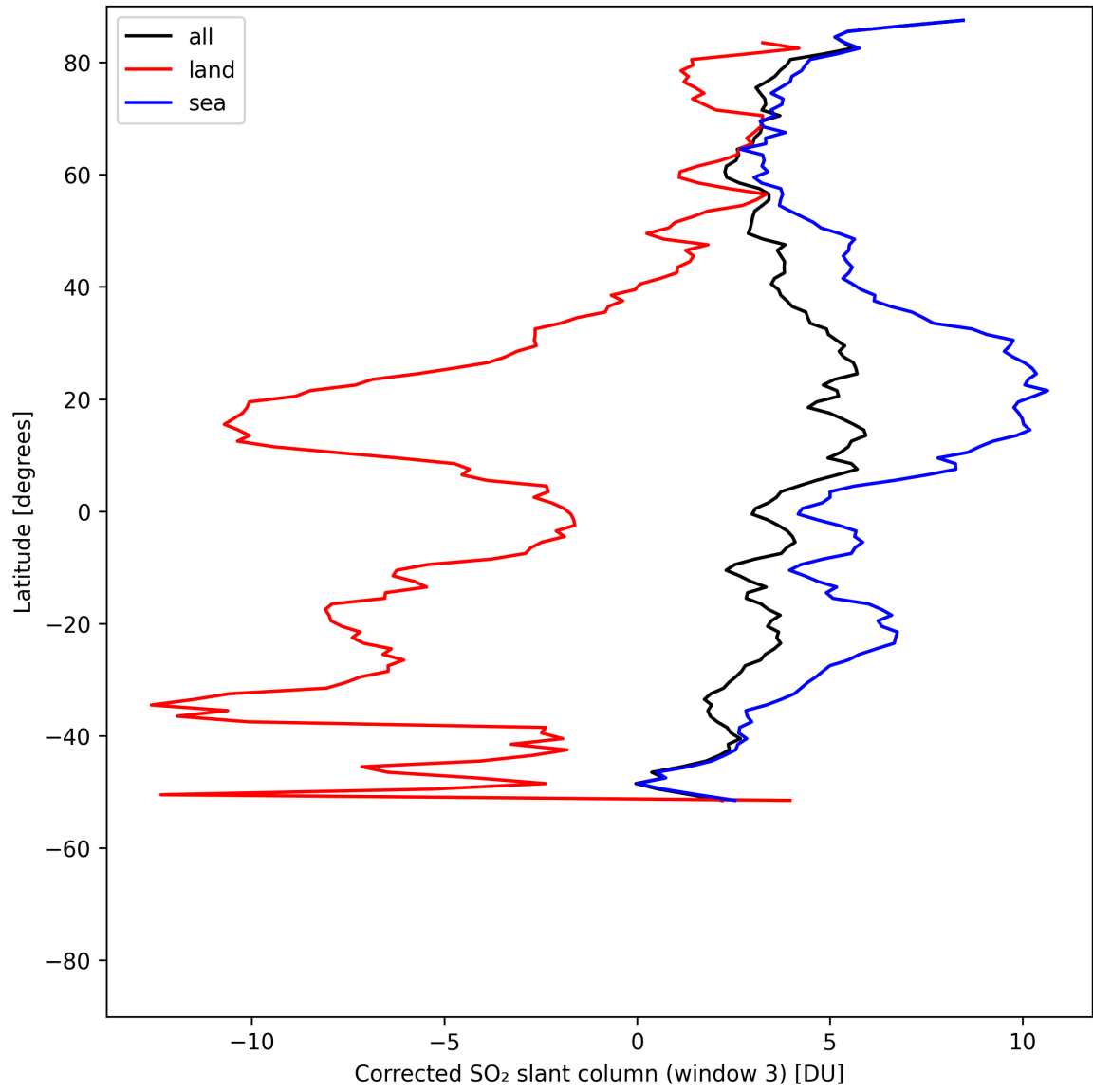
Figure 47: Zonal average of “Corrected SO 2 slant column (window 3)” for 2025-05-08 to 2025-05-10.
