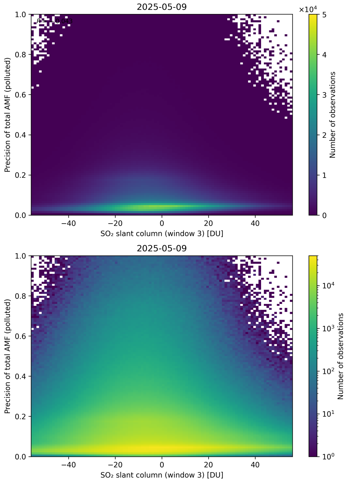
Figure 319: Scatter density plot of “SO 2 slant column (window 3)” against “Precision of total AMF (polluted)” for 2025-05-08 to 2025-05-10.
