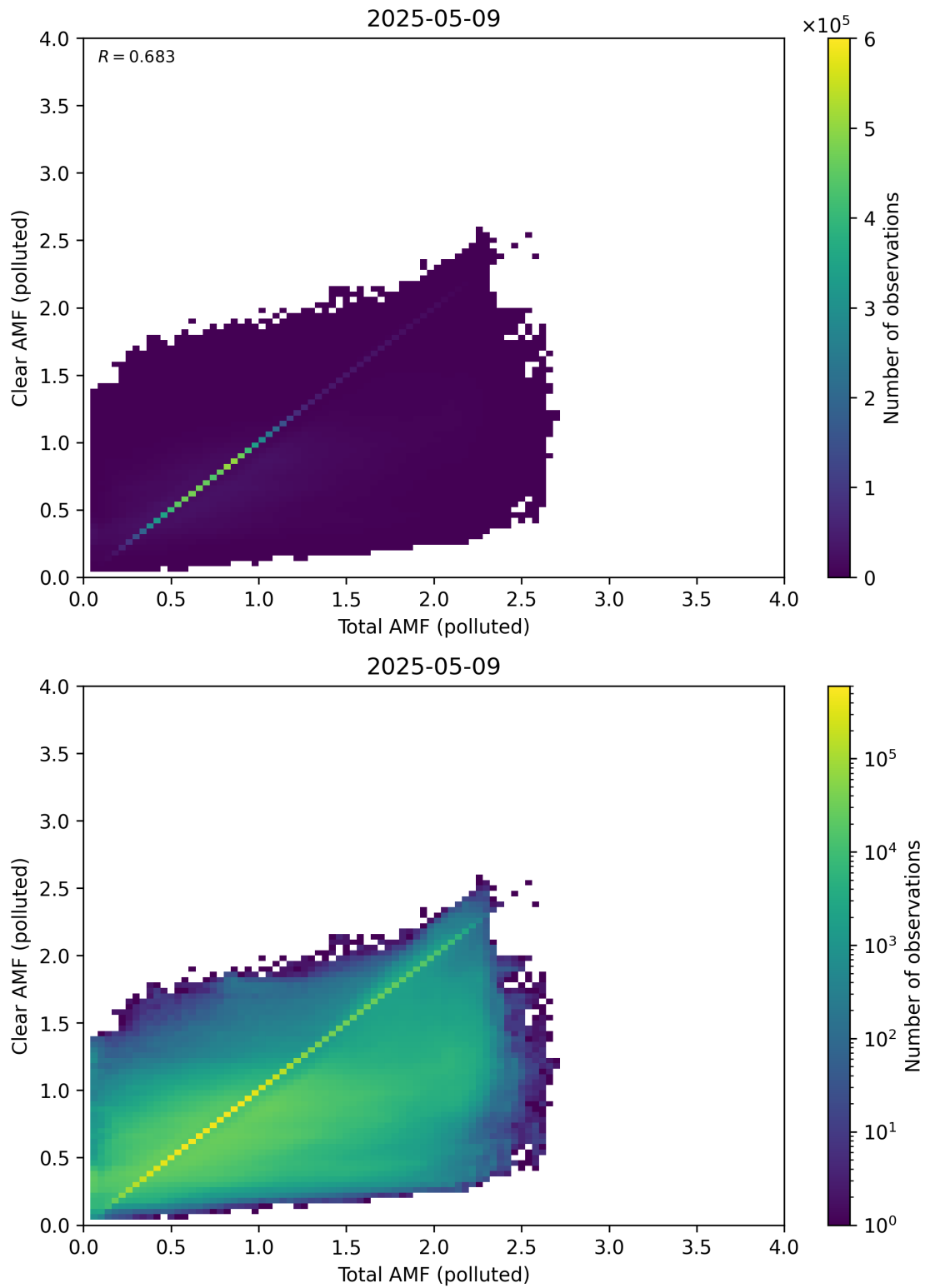
Figure 321: Scatter density plot of “Total AMF (polluted)” against “Clear AMF (polluted)” for 2025-05-08 to 2025-05-10.
