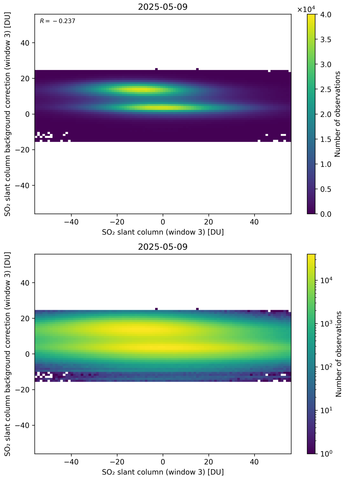
Figure 303: Scatter density plot of “SO 2 slant column (window 3)” against “SO 2 slant column background correction (window 3)” for 2025-05-08 to 2025-05-10.
