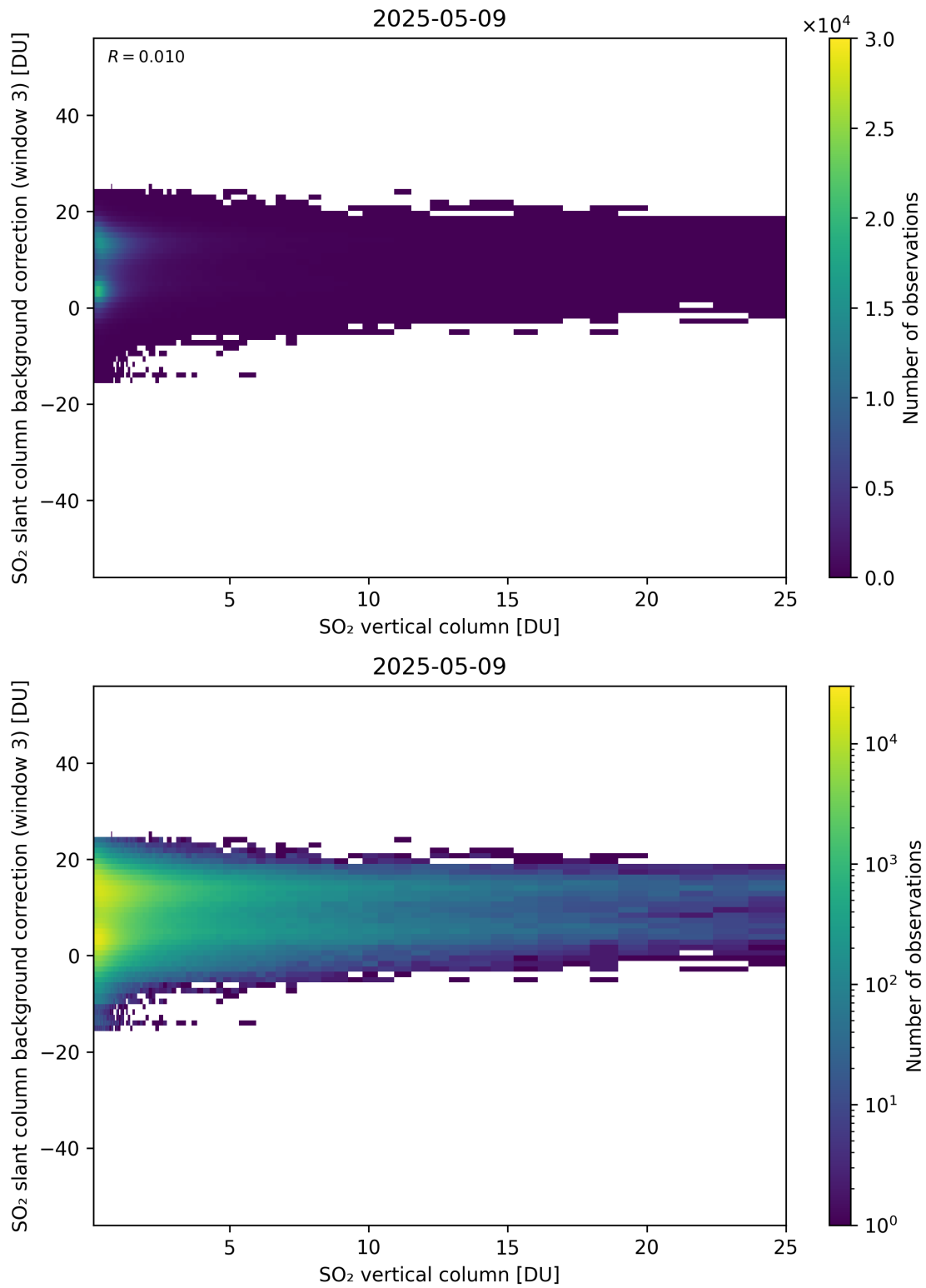
Figure 325: Scatter density plot of “SO 2 vertical column” against “SO 2 slant column background correction (window 3)” for 2025-05-08 to 2025-05-10.
