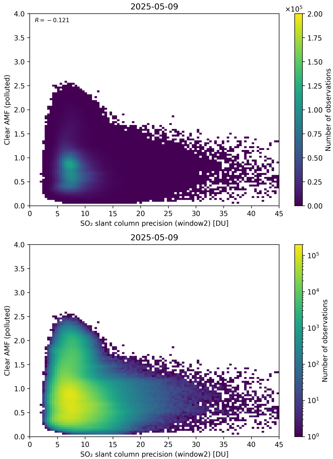
Figure 296: Scatter density plot of “SO 2 slant column precision (window2)” against “Clear AMF (polluted)” for 2025-05-08 to 2025-05-10.
