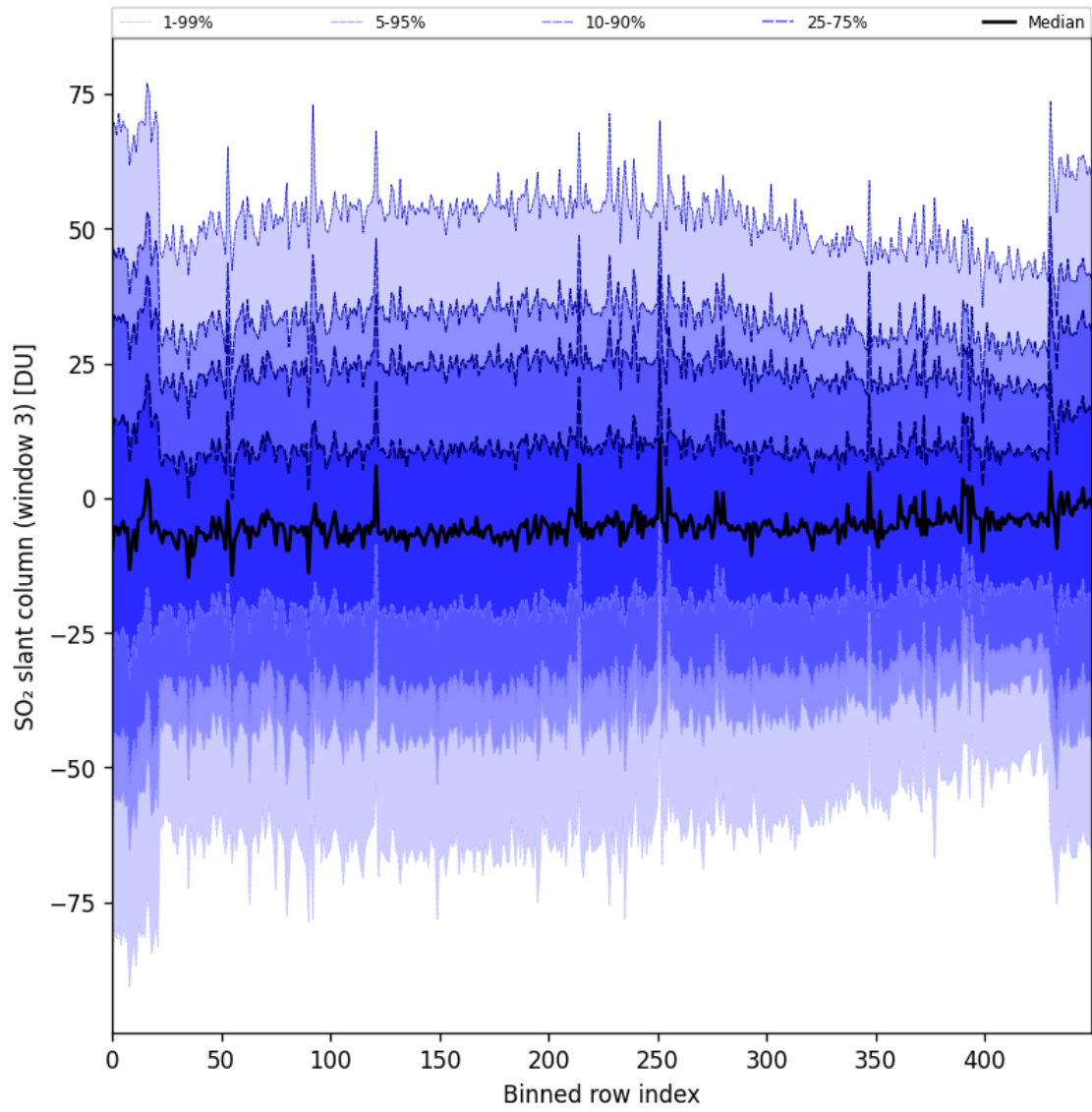
Figure 97: Along track statistics of “SO 2 slant column (window 3)” for 2025-05-08 to 2025-05-10
