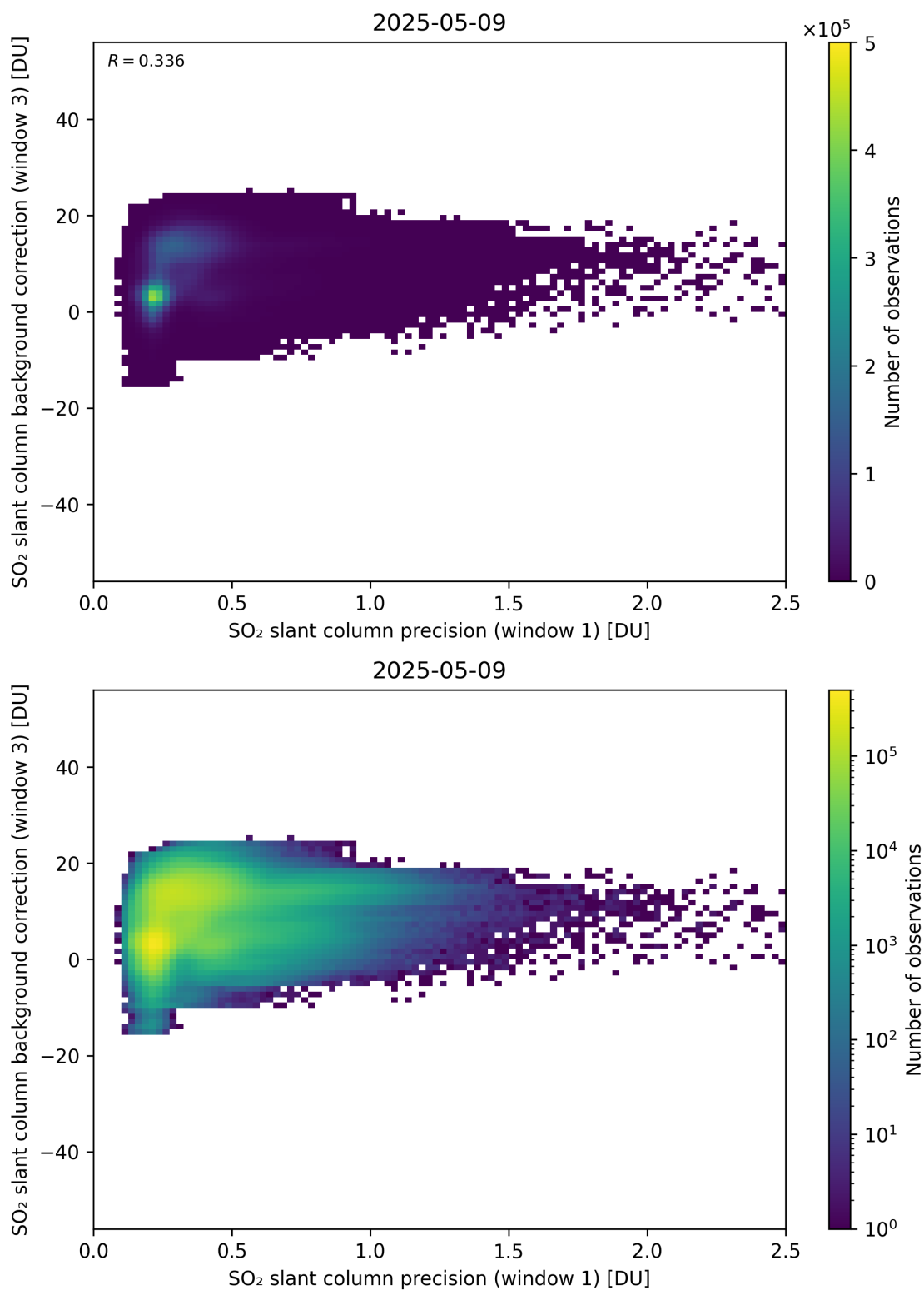
Figure 270: Scatter density plot of “SO 2 slant column precision (window 1)” against “SO 2 slant column background correction (window 3)” for 2025-05-08 to 2025-05-10.
