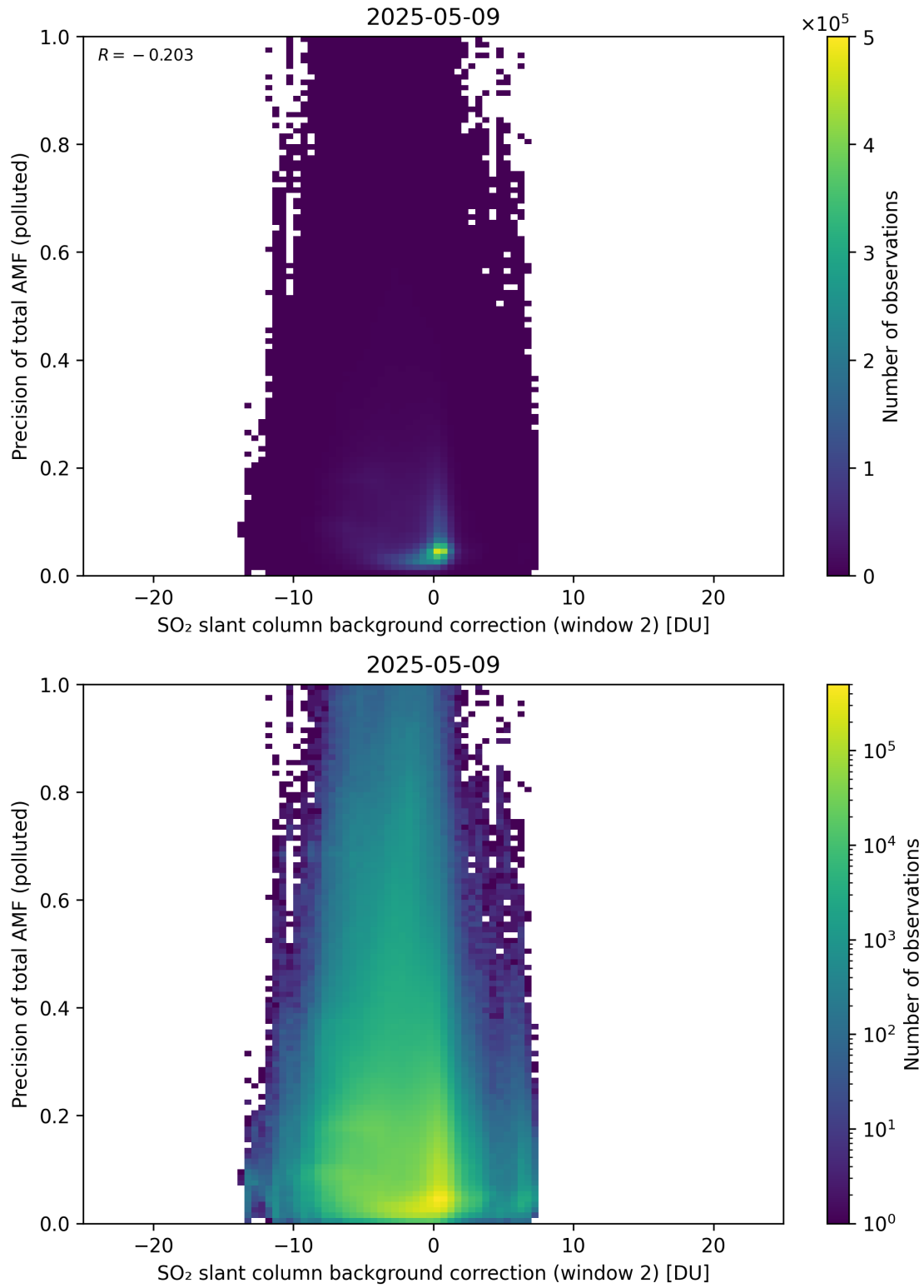
Figure 131: Scatter density plot of “SO 2 slant column background correction (window 2)” against “Precision of total AMF (polluted)” for 2025-05-08 to 2025-05-10.
