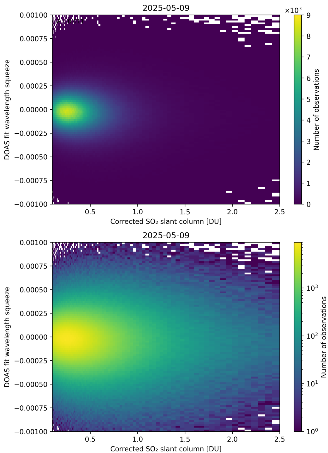
Figure 230: Scatter density plot of “Corrected SO 2 slant column” against “DOAS fit wavelength squeeze” for 2025-05-08 to 2025-05-10.
