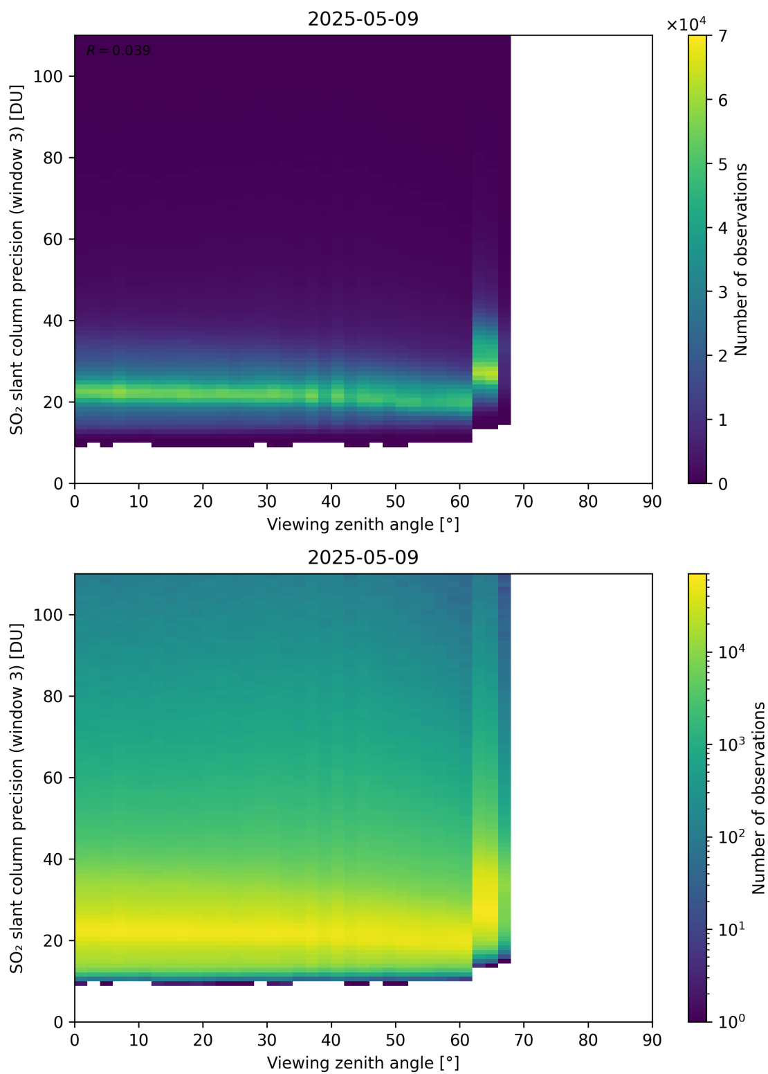
Figure 380: Scatter density plot of “Viewing zenith angle” against “SO 2 slant column precision (window 3)” for 2025-05-08 to 2025-05-10.
