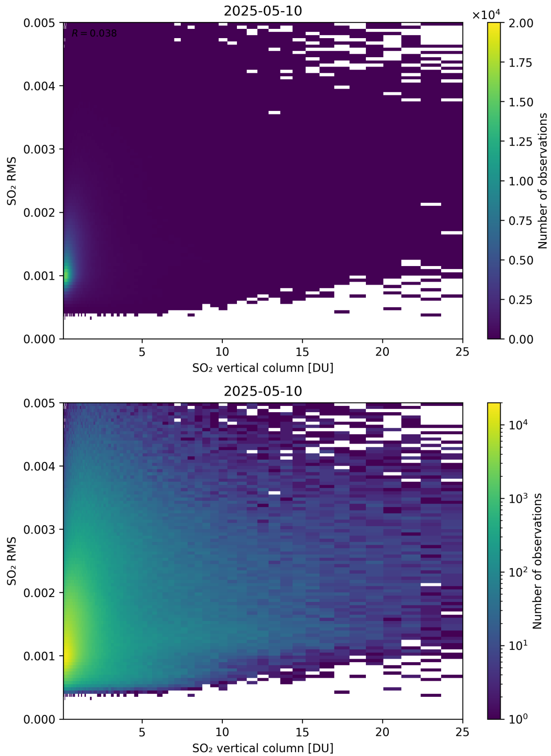
Figure 328: Scatter density plot of “SO 2 vertical column” against “SO 2 RMS” for 2025-05-10 to 2025-05-11.
