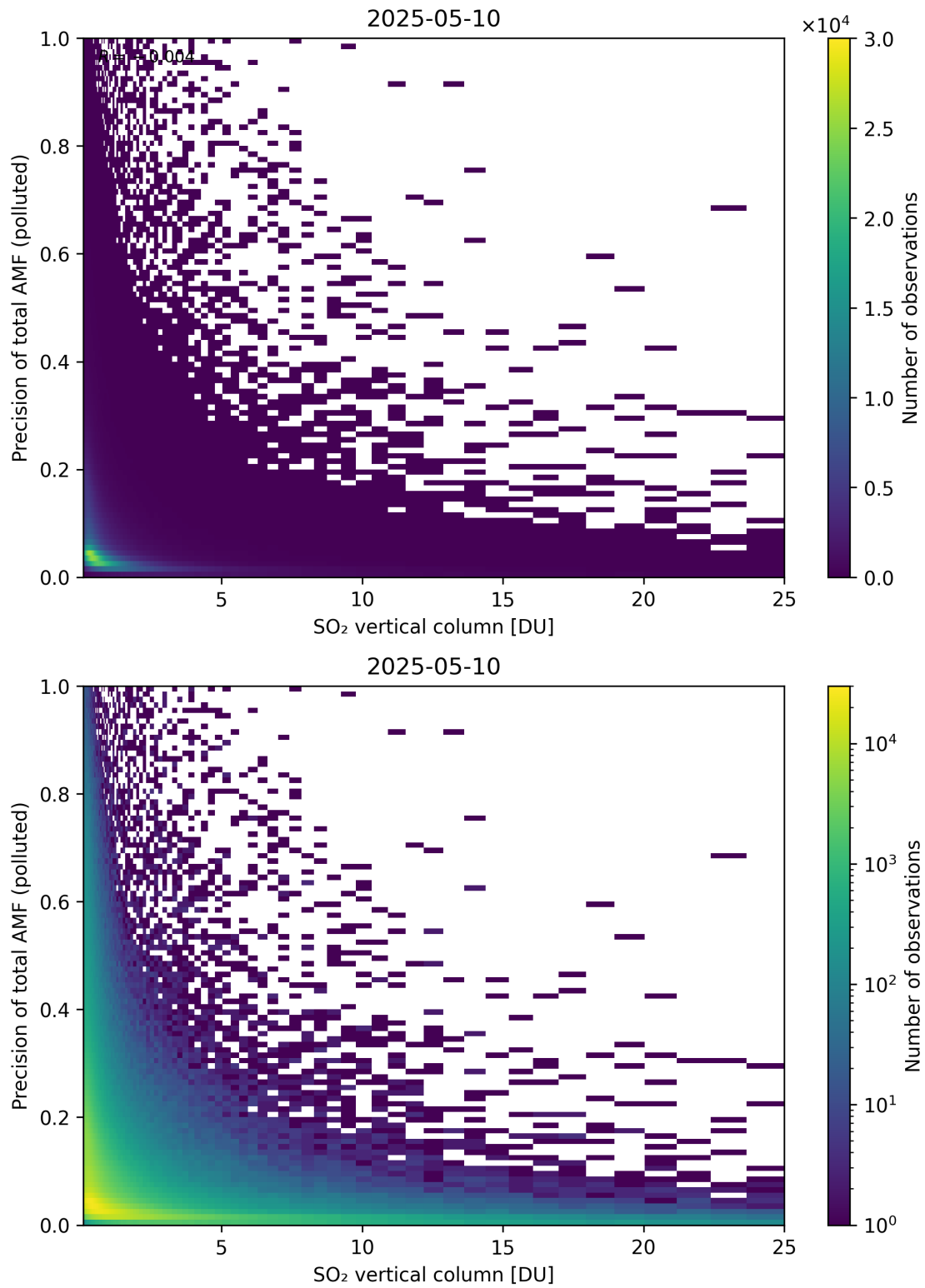
Figure 360: Scatter density plot of “SO 2 vertical column” against “Precision of total AMF (polluted)” for 2025-05-10 to 2025-05-11.
