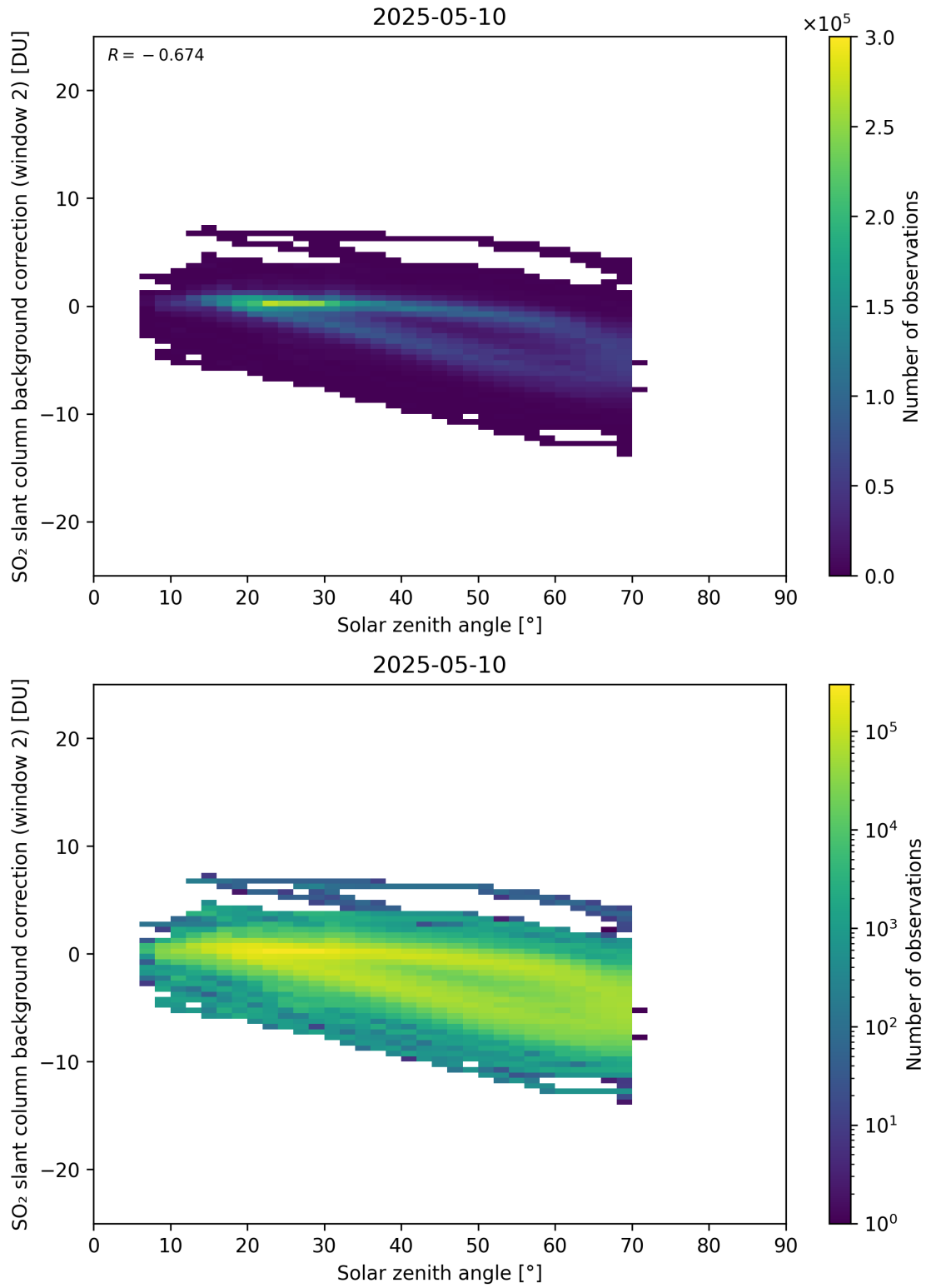
Figure 172: Scatter density plot of “Solar zenith angle” against “SO 2 slant column background correction (window 2)” for 2025-05-10 to 2025-05-11.
