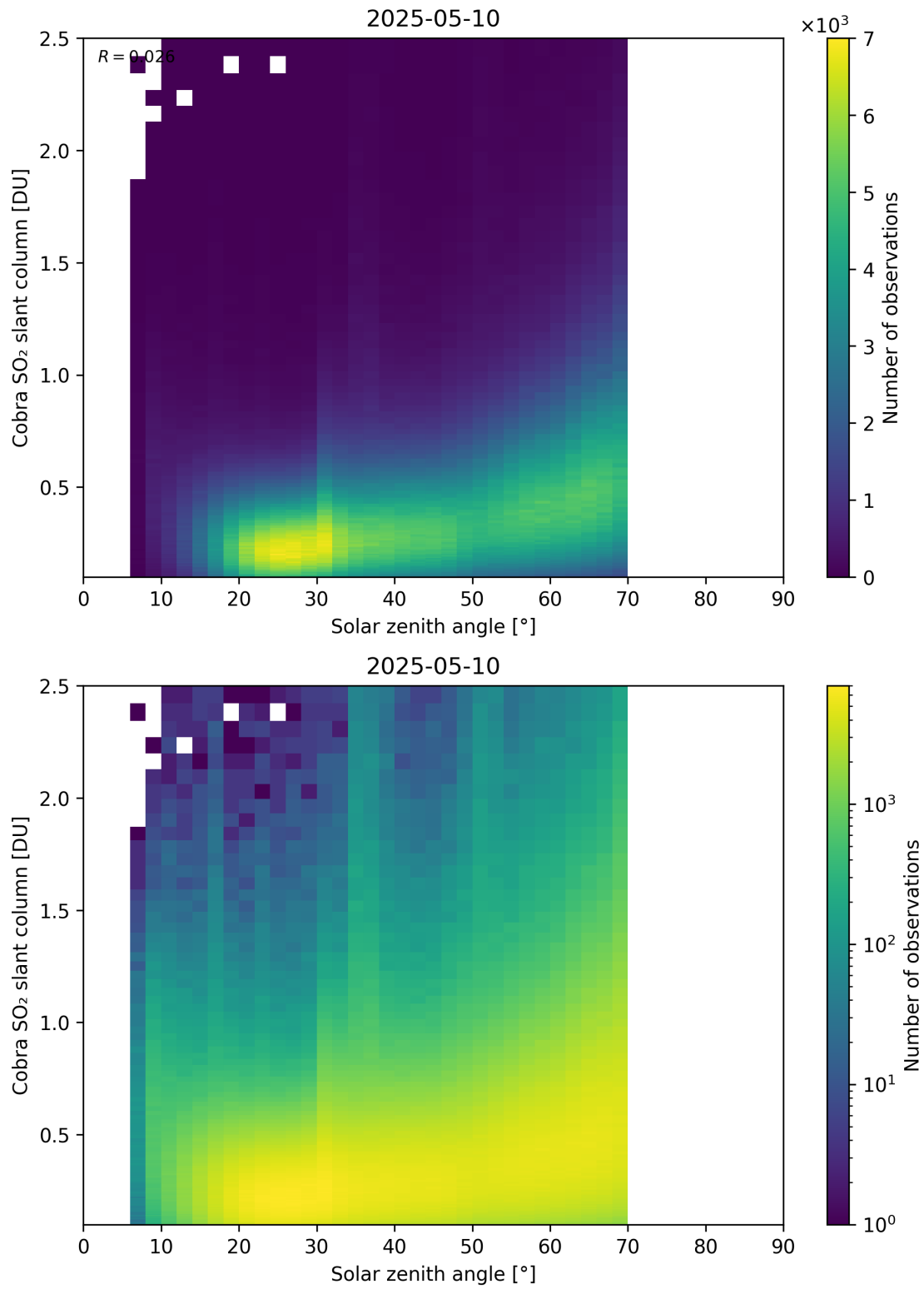
Figure 179: Scatter density plot of “Solar zenith angle” against “Cobra SO 2 slant column” for 2025-05-10 to 2025-05-11.
