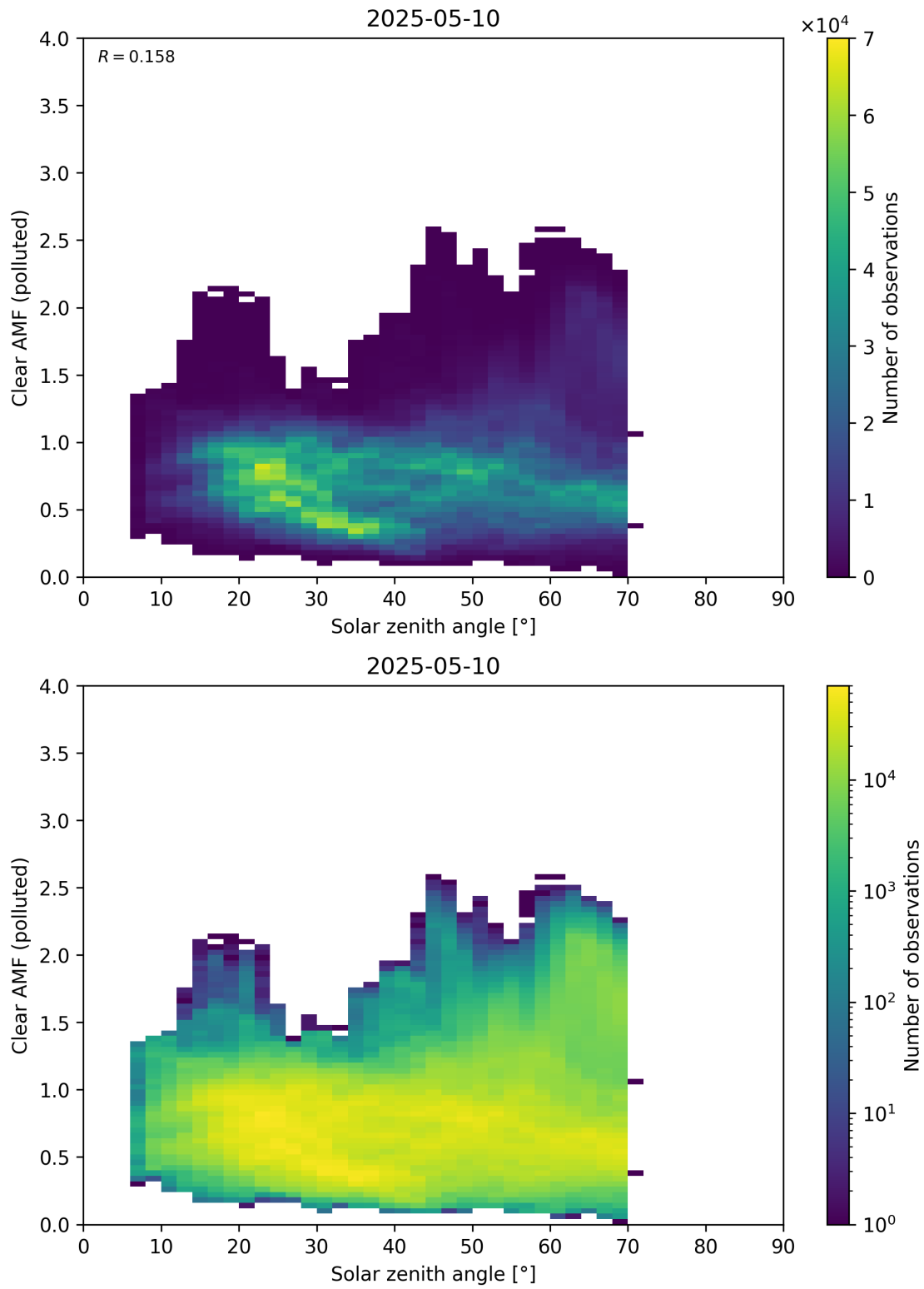
Figure 178: Scatter density plot of “Solar zenith angle” against “Clear AMF (polluted)” for 2025-05-10 to 2025-05-11.
