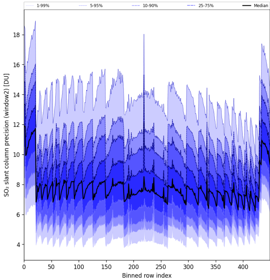
Figure 94: Along track statistics of “SO 2 slant column precision (window2)” for 2025-05-10 to 2025-05-11
