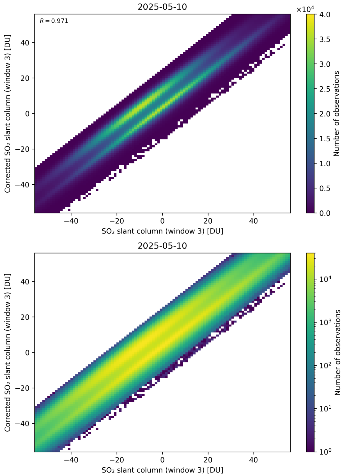
Figure 316: Scatter density plot of “SO 2 slant column (window 3)” against “Corrected SO 2 slant column (window 3)” for 2025-05-10 to 2025-05-11.
