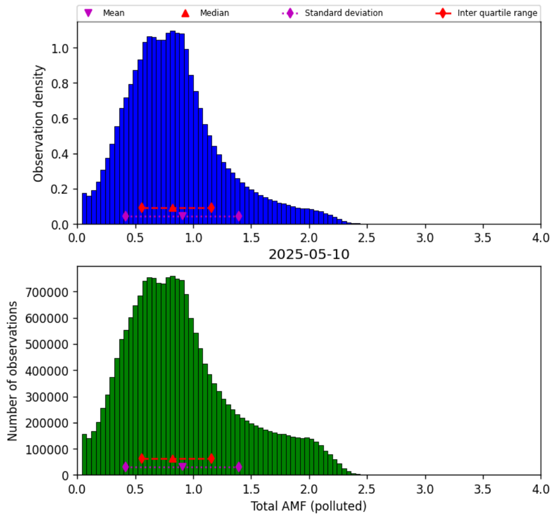
Figure 79: Histogram of “Total AMF (polluted)” for 2025-05-10 to 2025-05-11
