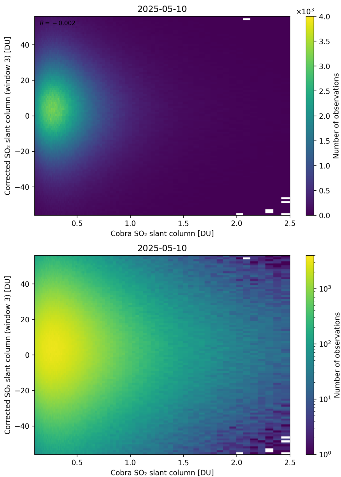
Figure 218: Scatter density plot of “Cobra SO 2 slant column” against “Corrected SO 2 slant column (window 3)” for 2025-05-10 to 2025-05-11.
