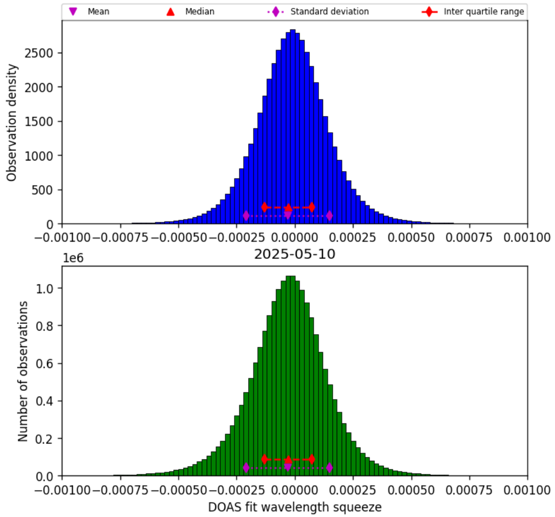
Figure 77: Histogram of “DOAS fit wavelength squeeze” for 2025-05-10 to 2025-05-11
