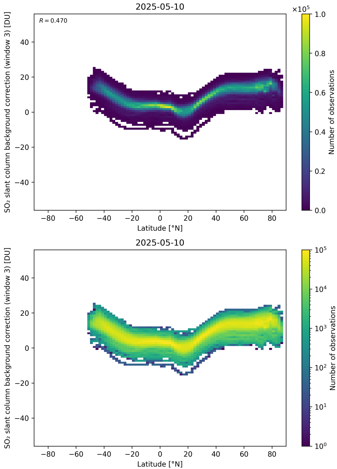
Figure 152: Scatter density plot of “Latitude” against “SO 2 slant column background correction (window 3)” for 2025-05-10 to 2025-05-11.
