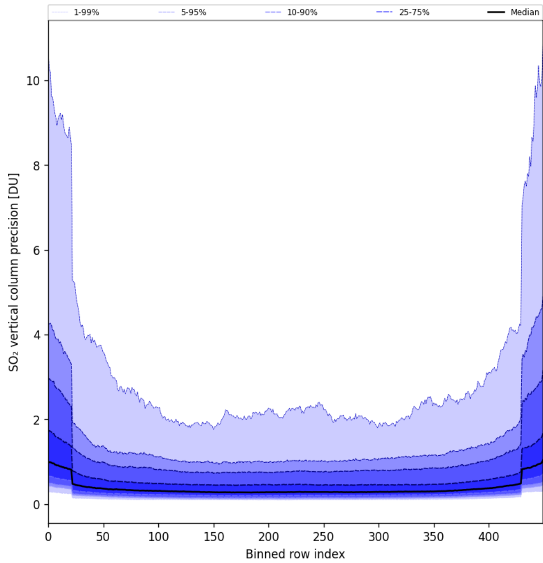
Figure 85: Along track statistics of “SO 2 vertical column precision” for 2025-05-10 to 2025-05-11
