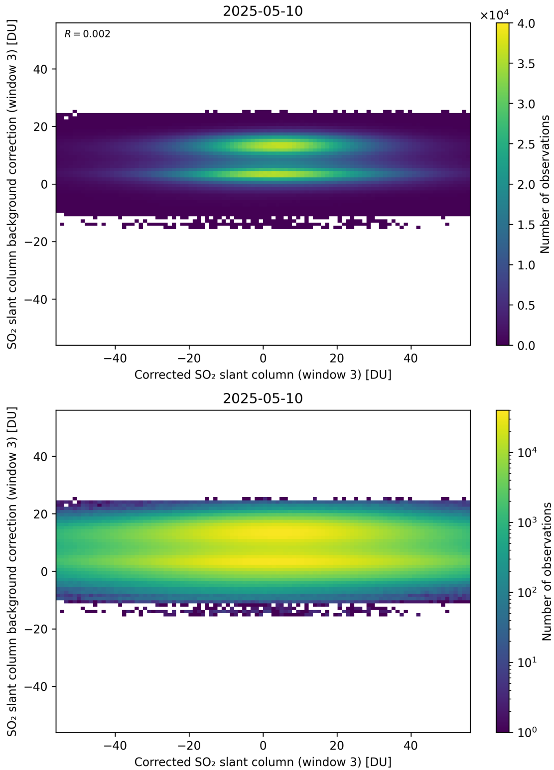
Figure 255: Scatter density plot of “Corrected SO 2 slant column (window 3)” against “SO 2 slant column background correction (window 3)” for 2025-05-10 to 2025-05-11.
