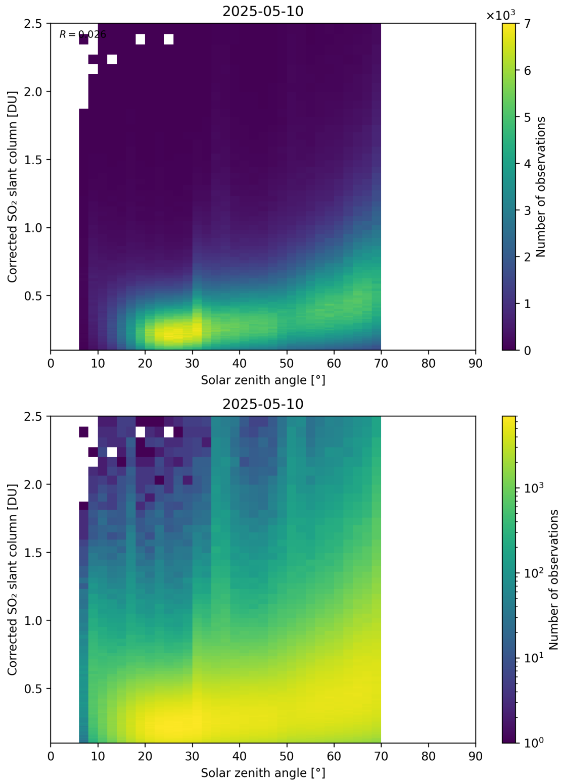
Figure 181: Scatter density plot of “Solar zenith angle” against “Corrected SO 2 slant column” for 2025-05-10 to 2025-05-11.
