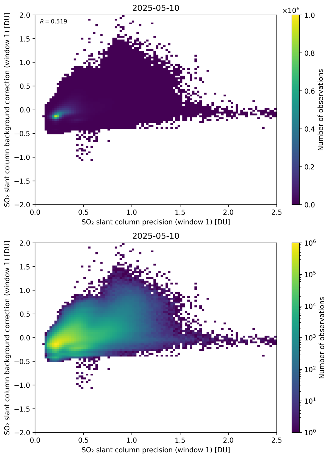
Figure 268: Scatter density plot of “SO 2 slant column precision (window 1)” against “SO 2 slant column background correction (window 1)” for 2025-05-10 to 2025-05-11.
