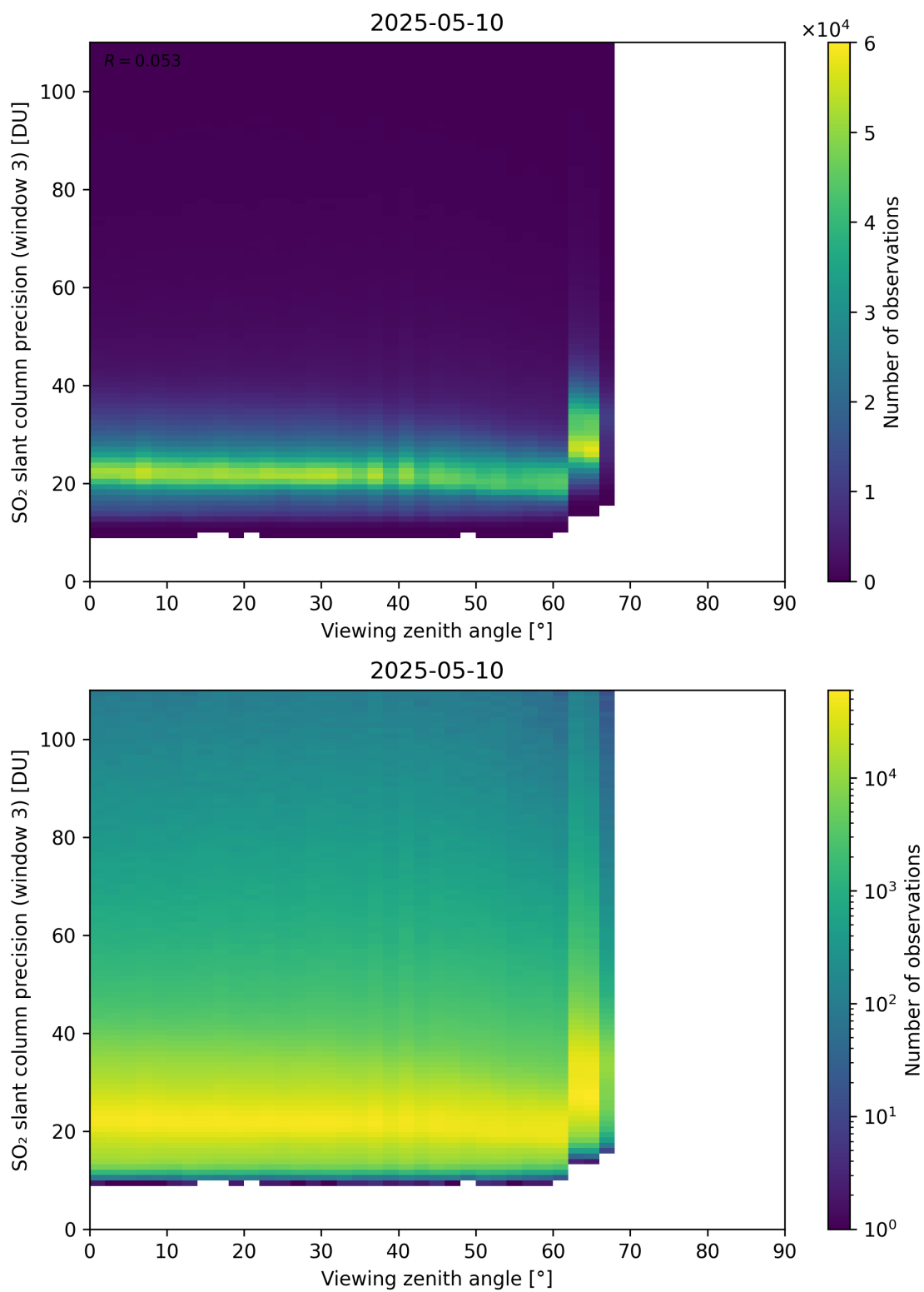
Figure 380: Scatter density plot of “Viewing zenith angle” against “SO 2 slant column precision (window 3)” for 2025-05-10 to 2025-05-11.
