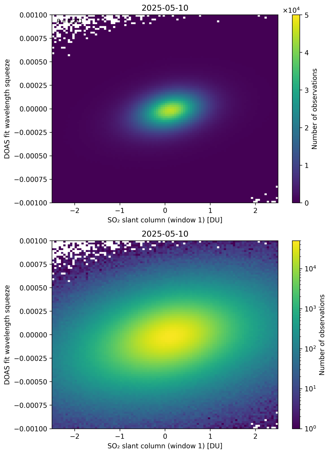
Figure 266: Scatter density plot of “SO 2 slant column (window 1)” against “DOAS fit wavelength squeeze” for 2025-05-10 to 2025-05-11.
