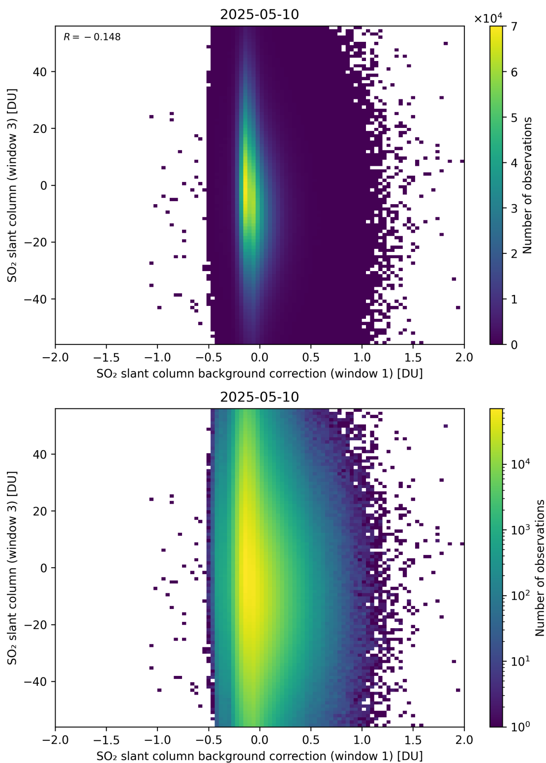
Figure 118: Scatter density plot of “SO 2 slant column background correction (window 1)” against “SO 2 slant column (window 3)” for 2025-05-10 to 2025-05-11.
