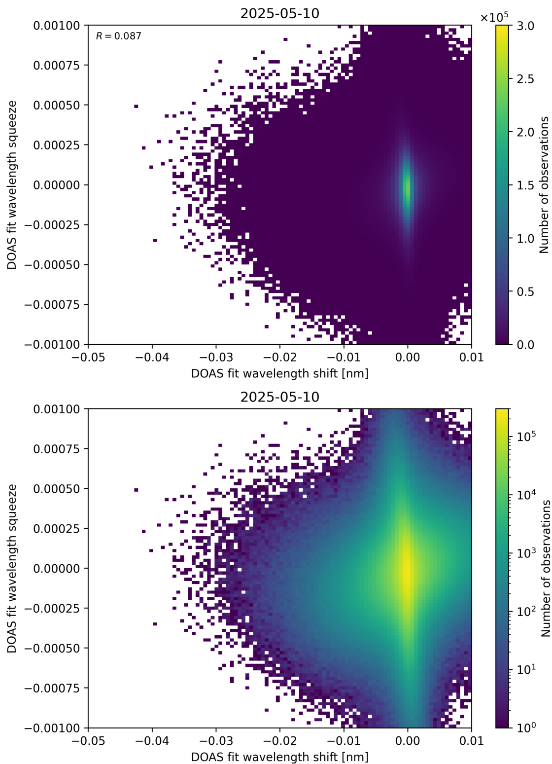
Figure 138: Scatter density plot of “DOAS fit wavelength shift” against “DOAS fit wavelength squeeze” for 2025-05-10 to 2025-05-11.
