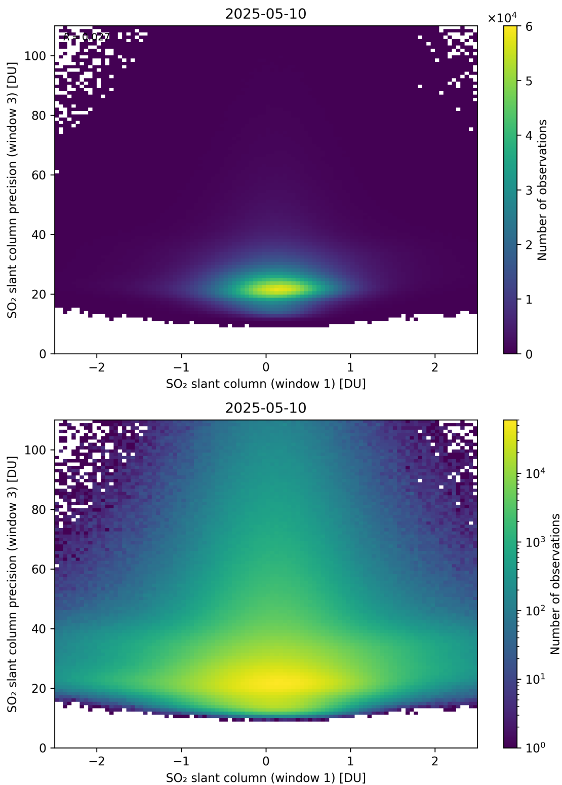
Figure 288: Scatter density plot of “SO 2 slant column (window 1)” against “SO 2 slant column precision (window 3)” for 2025-05-10 to 2025-05-11.
