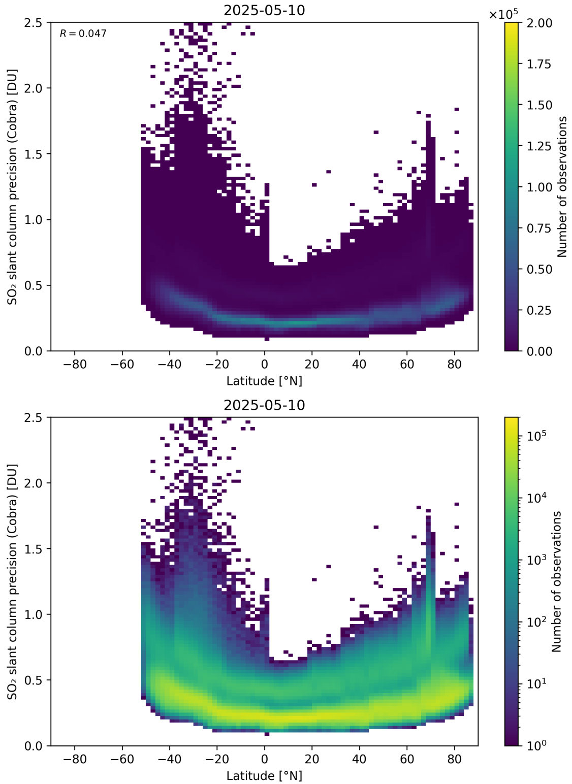
Figure 158: Scatter density plot of “Latitude” against “SO 2 slant column precision (Cobra)” for 2025-05-10 to 2025-05-11.
