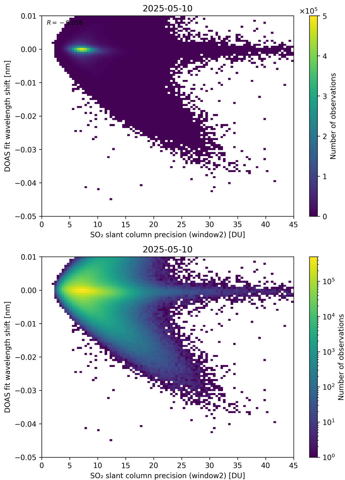
Figure 293: Scatter density plot of “SO 2 slant column precision (window2)” against “DOAS fit wavelength shift” for 2025-05-10 to 2025-05-11.
