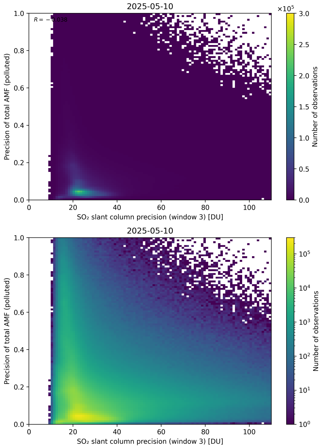
Figure 314: Scatter density plot of “SO 2 slant column precision (window 3)” against “Precision of total AMF (polluted)” for 2025-05-10 to 2025-05-11.
