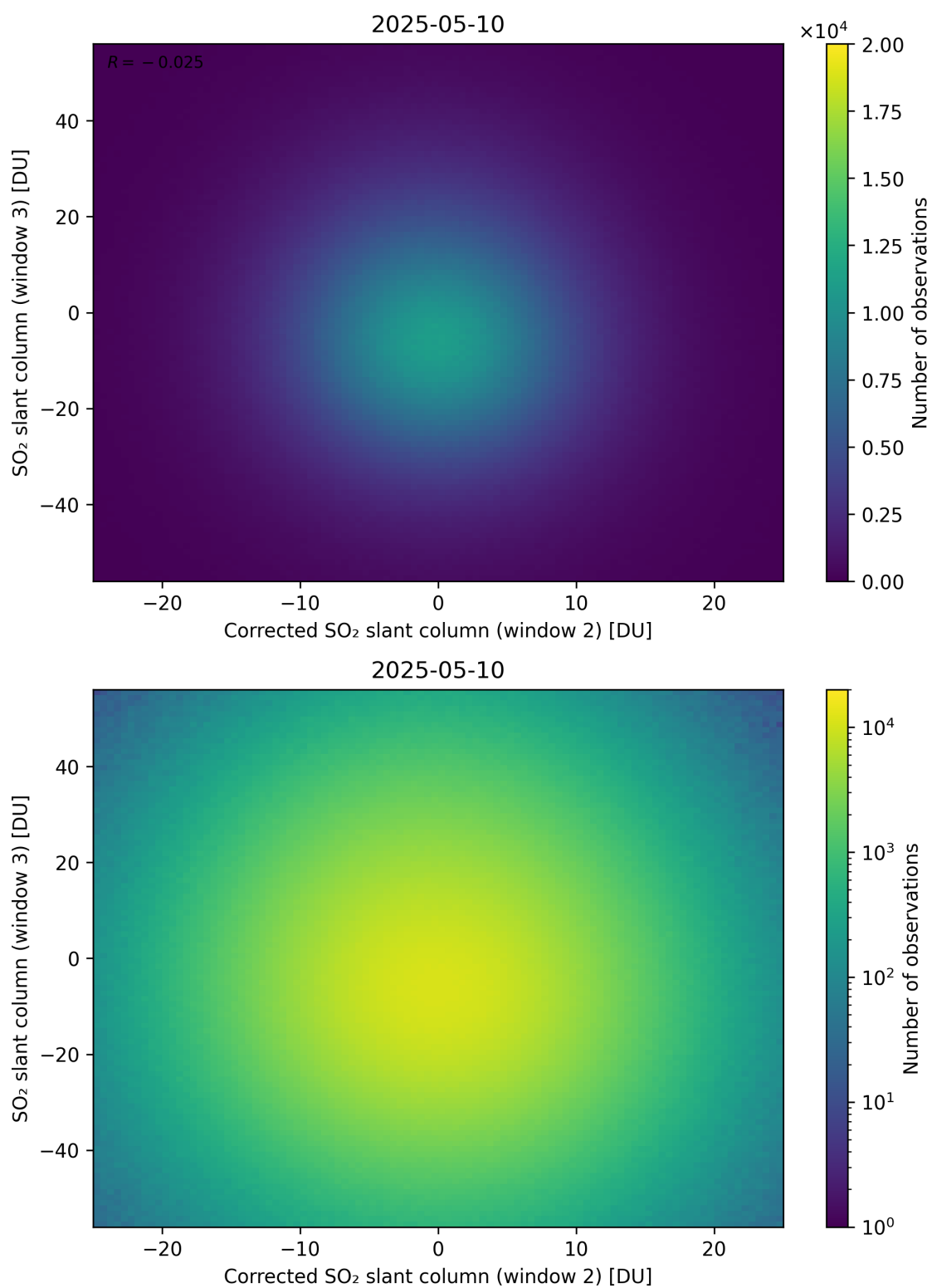
Figure 251: Scatter density plot of “Corrected SO 2 slant column (window 2)” against “SO 2 slant column (window 3)” for 2025-05-10 to 2025-05-11.
