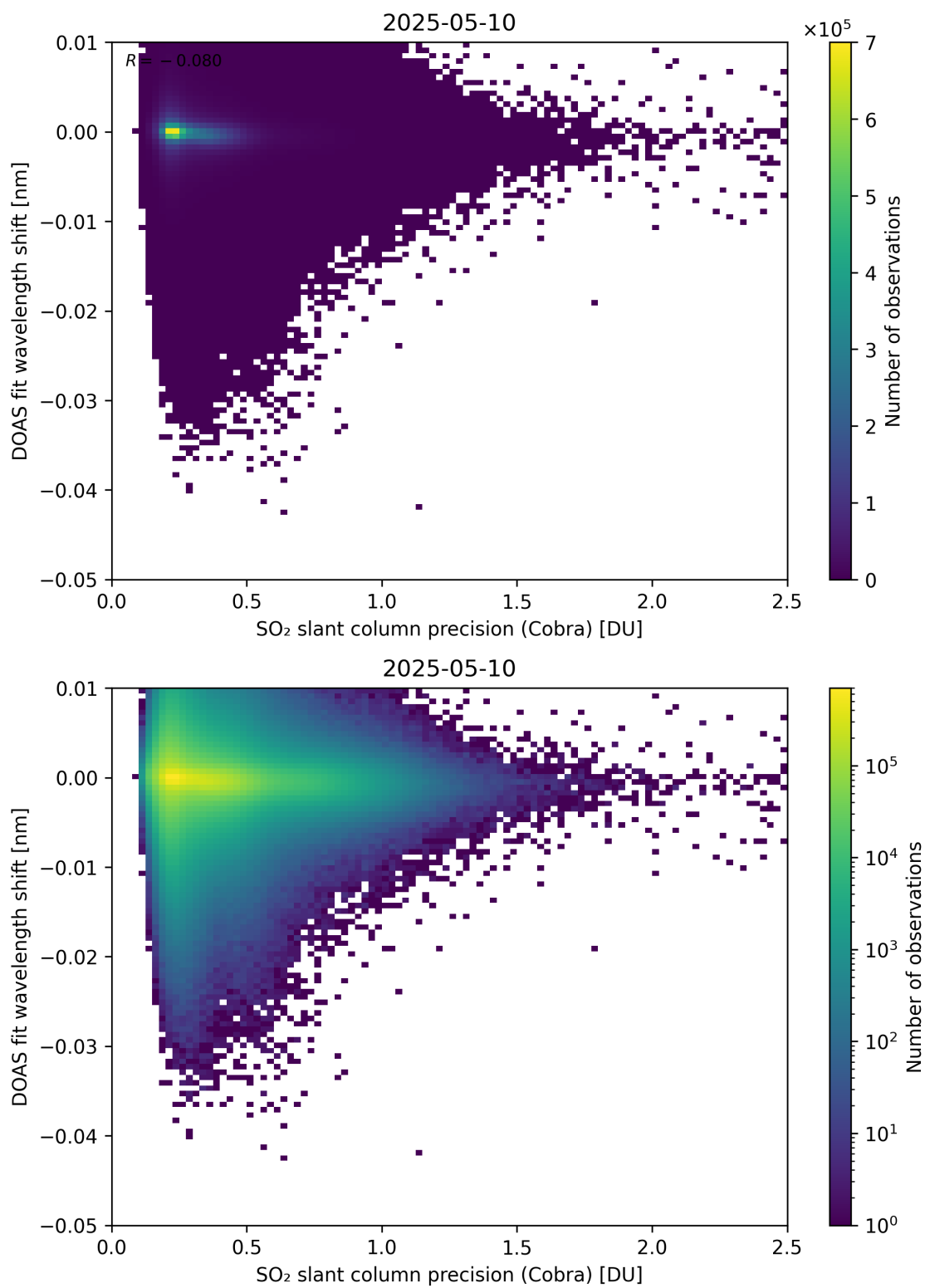
Figure 202: Scatter density plot of “SO 2 slant column precision (Cobra)” against “DOAS fit wavelength shift” for 2025-05-10 to 2025-05-11.
