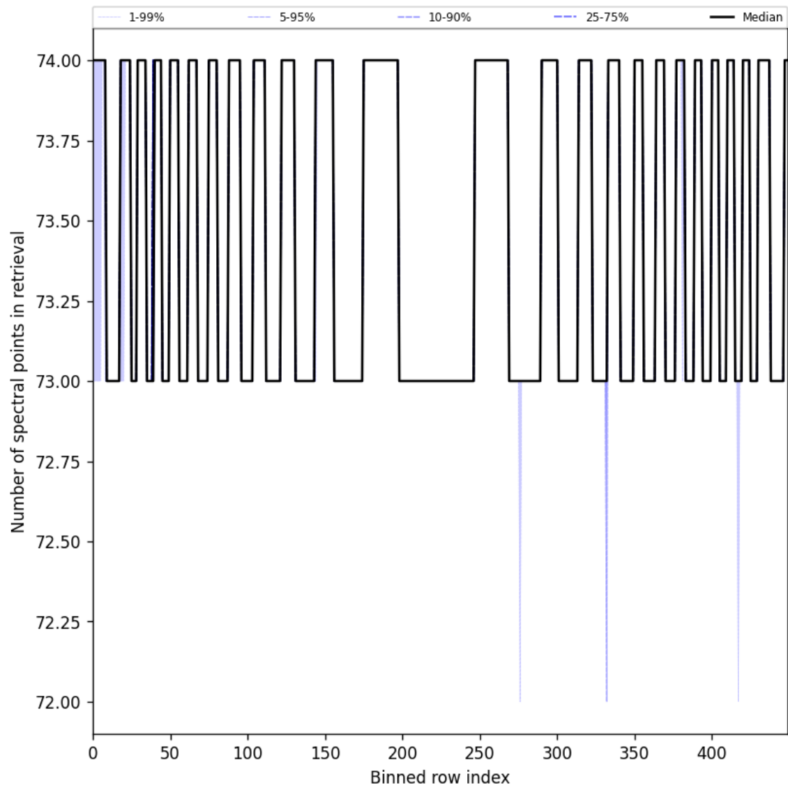
Figure 108: Along track statistics of “Number of spectral points in retrieval” for 2025-05-10 to 2025-05-11
