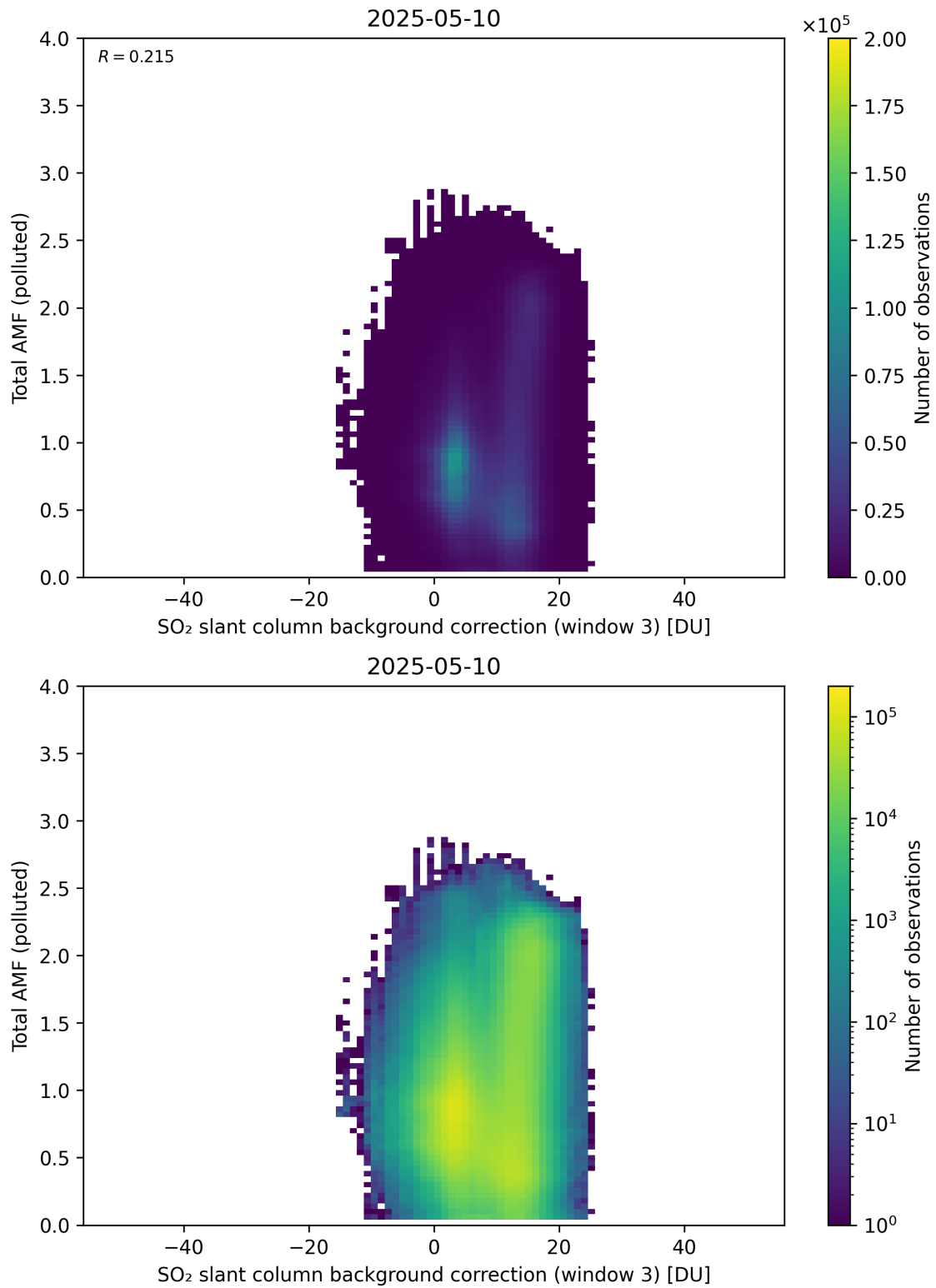
Figure 136: Scatter density plot of “SO 2 slant column background correction (window 3)” against “Total AMF (polluted)” for 2025-05-10 to 2025-05-11.
