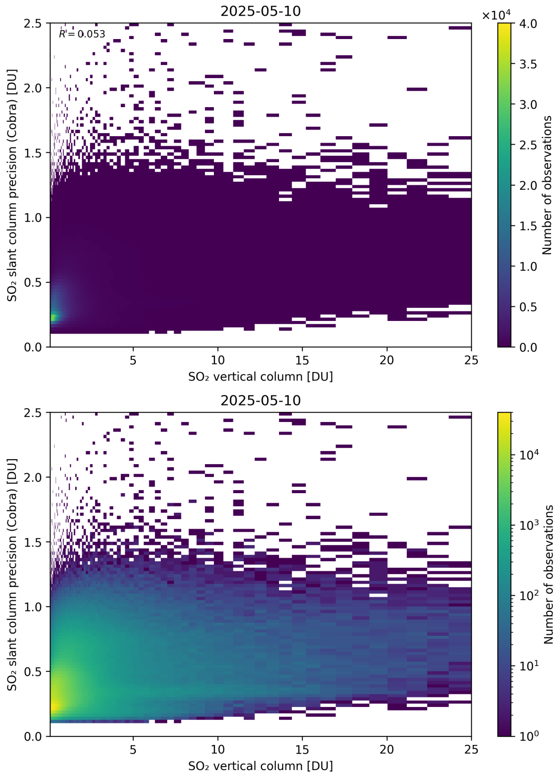
Figure 350: Scatter density plot of “SO 2 vertical column” against “SO 2 slant column precision (Cobra)” for 2025-05-10 to 2025-05-11.
