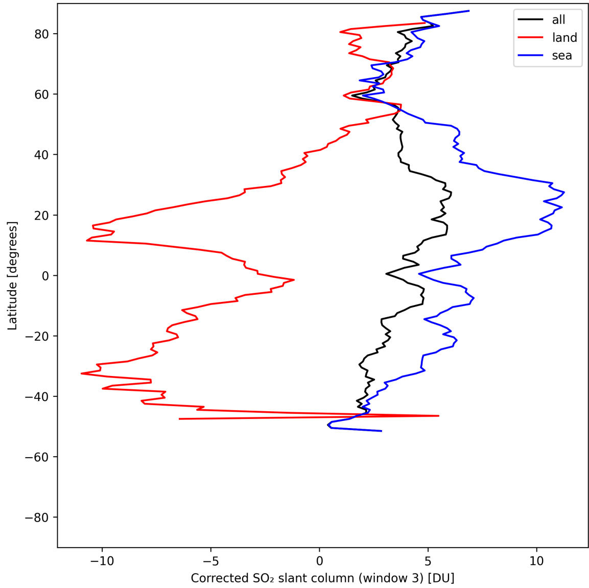
Figure 47: Zonal average of “Corrected SO 2 slant column (window 3)” for 2025-05-10 to 2025-05-11.
