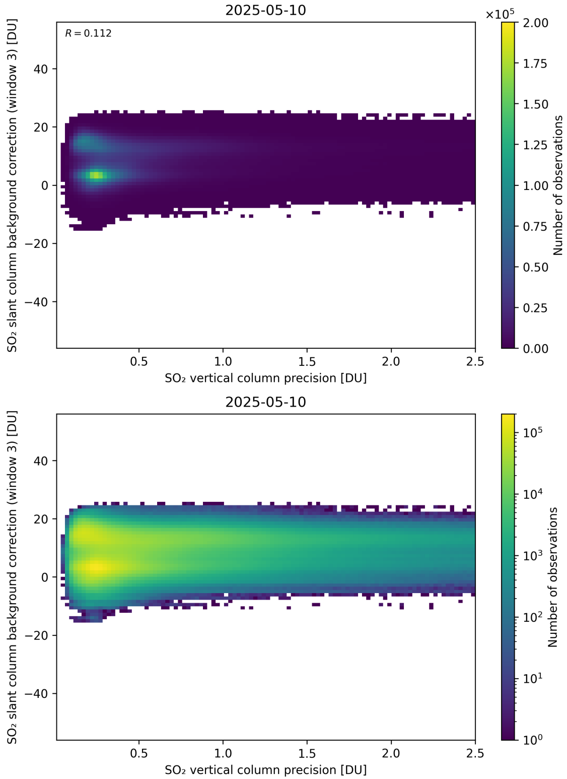
Figure 331: Scatter density plot of “SO 2 vertical column precision” against “SO 2 slant column background correction (window 3)” for 2025-05-10 to 2025-05-11.
