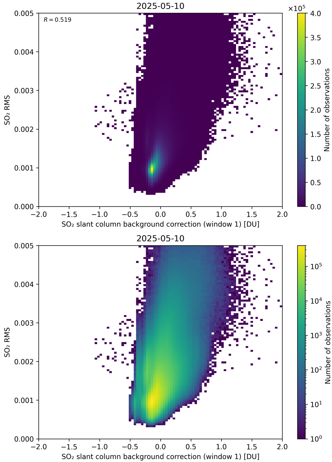
Figure 113: Scatter density plot of “SO 2 slant column background correction (window 1)” against “SO 2 RMS” for 2025-05-10 to 2025-05-11.
