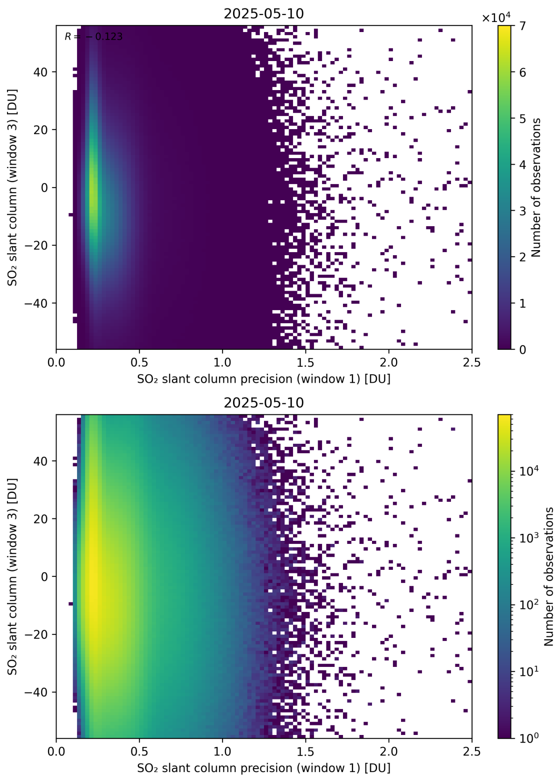
Figure 278: Scatter density plot of “SO 2 slant column precision (window 1)” against “SO 2 slant column (window 3)” for 2025-05-10 to 2025-05-11.
