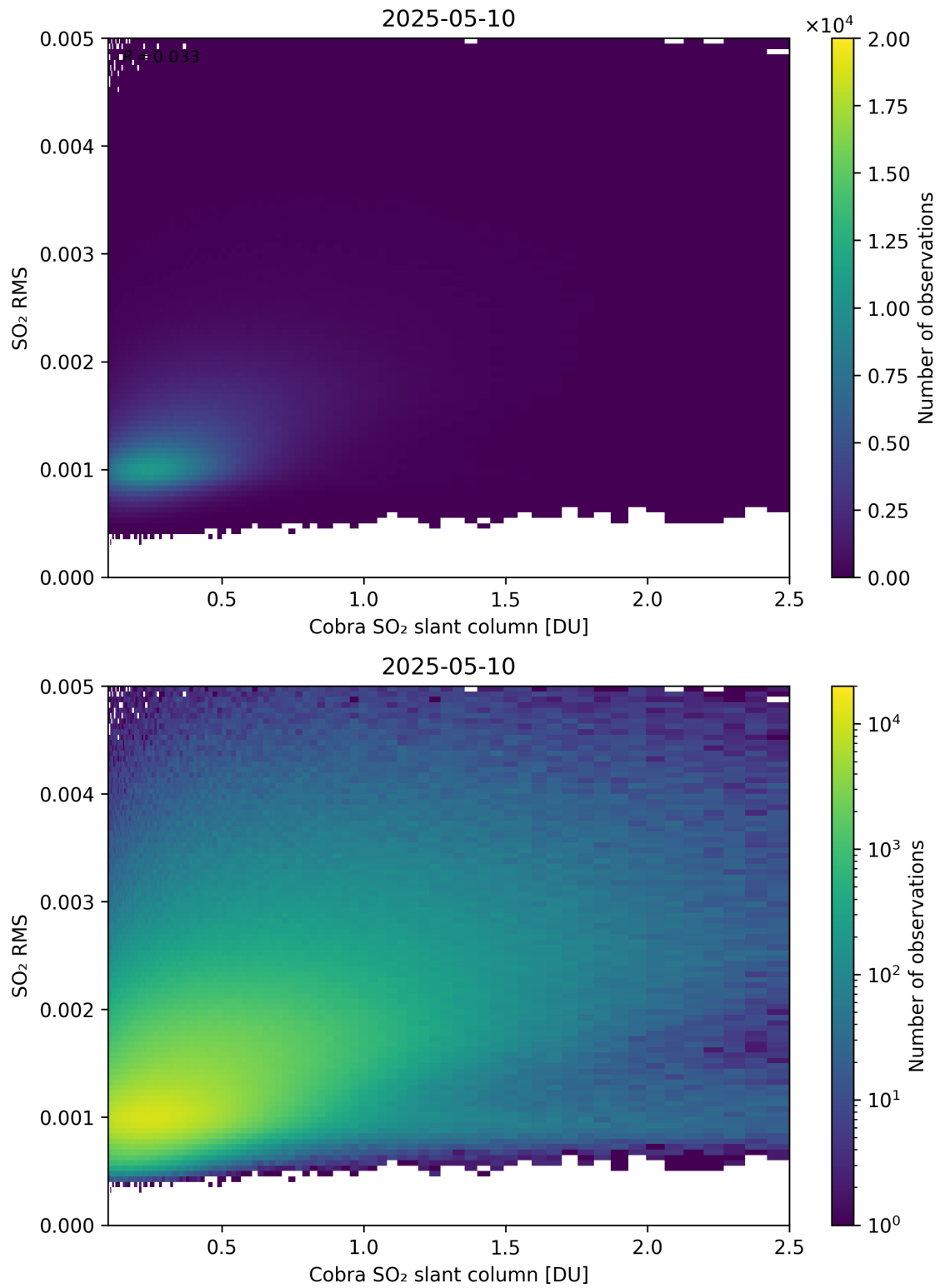
Figure 198: Scatter density plot of “Cobra SO 2 slant column” against “SO 2 RMS” for 2025-05-10 to 2025-05-11.
