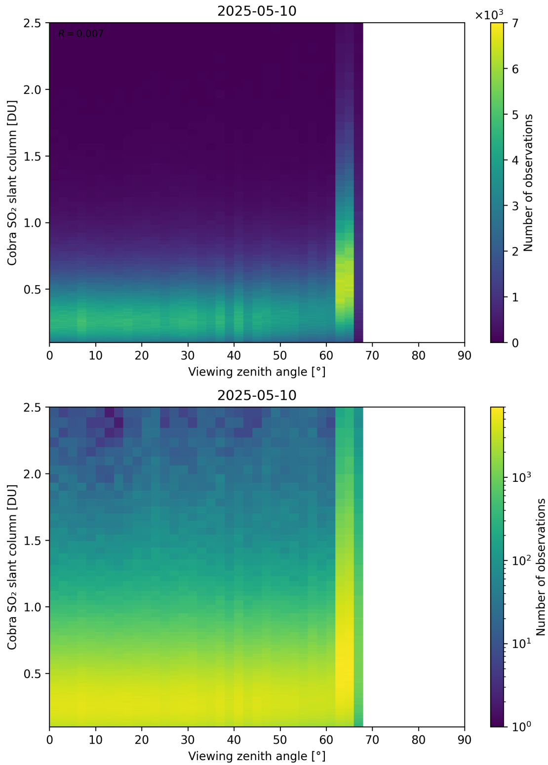
Figure 371: Scatter density plot of “Viewing zenith angle” against “Cobra SO 2 slant column” for 2025-05-10 to 2025-05-11.
