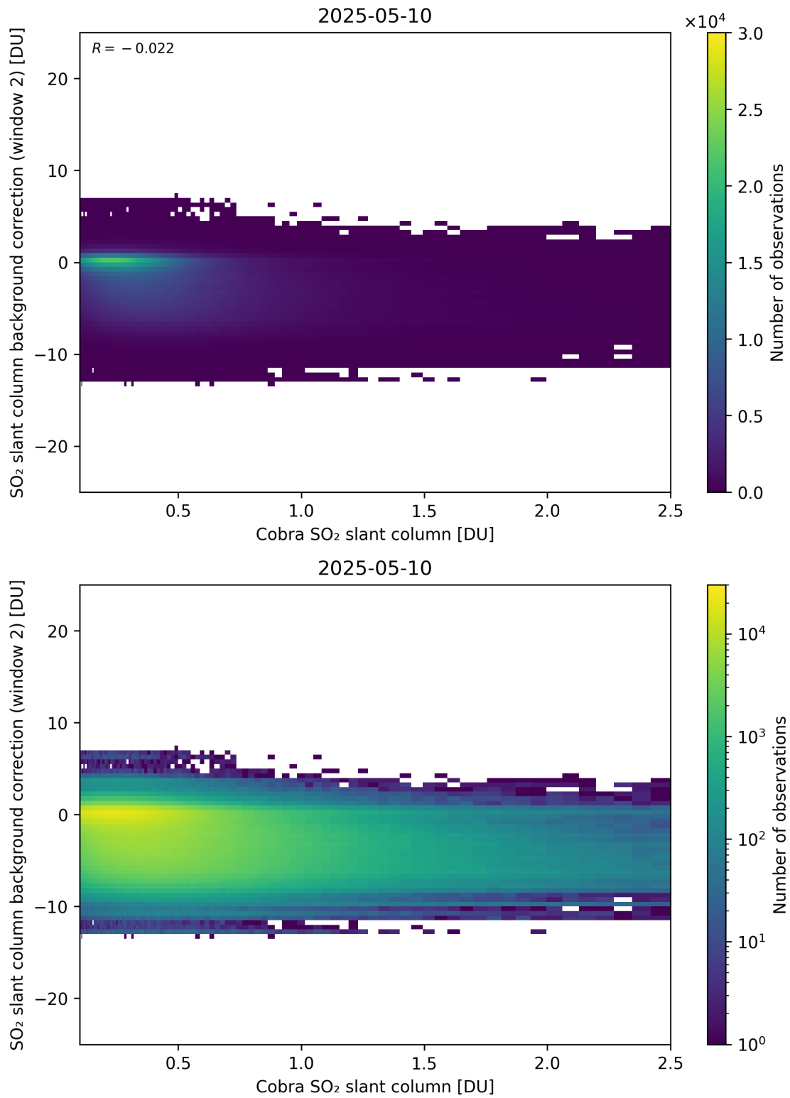
Figure 194: Scatter density plot of “Cobra SO 2 slant column” against “SO 2 slant column background correction (window 2)” for 2025-05-10 to 2025-05-11.
