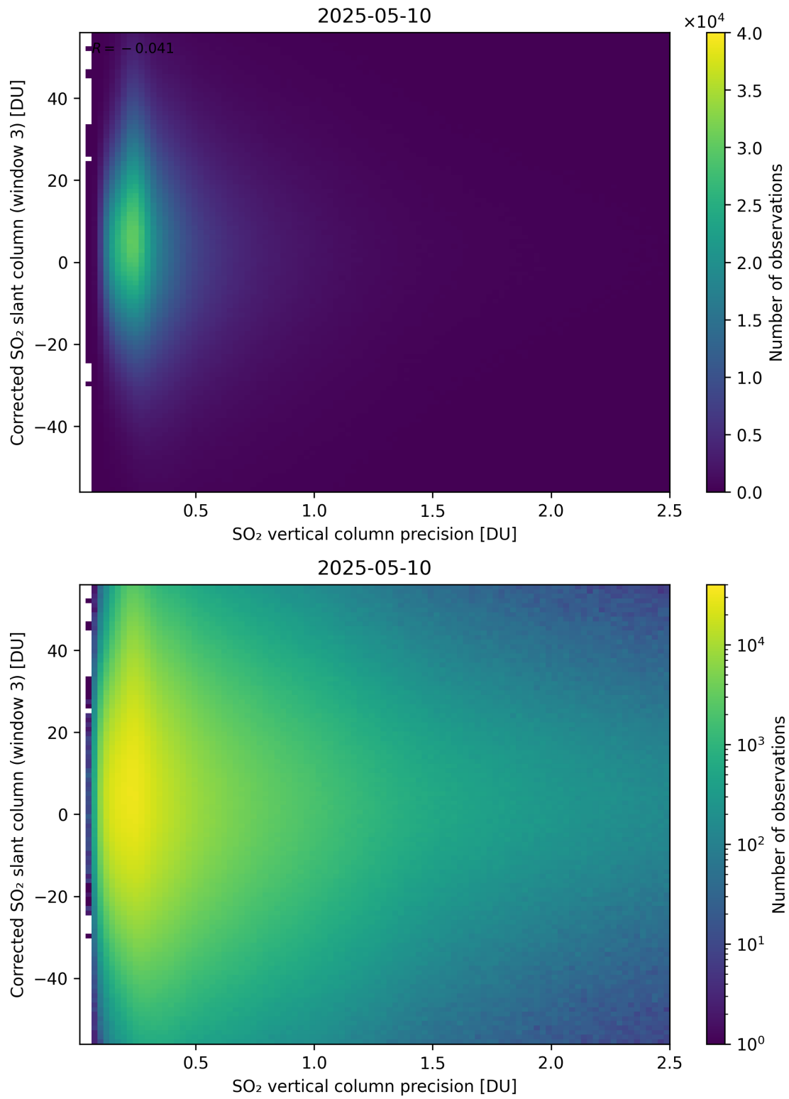
Figure 340: Scatter density plot of “SO 2 vertical column precision” against “Corrected SO 2 slant column (window 3)” for 2025-05-10 to 2025-05-11.
