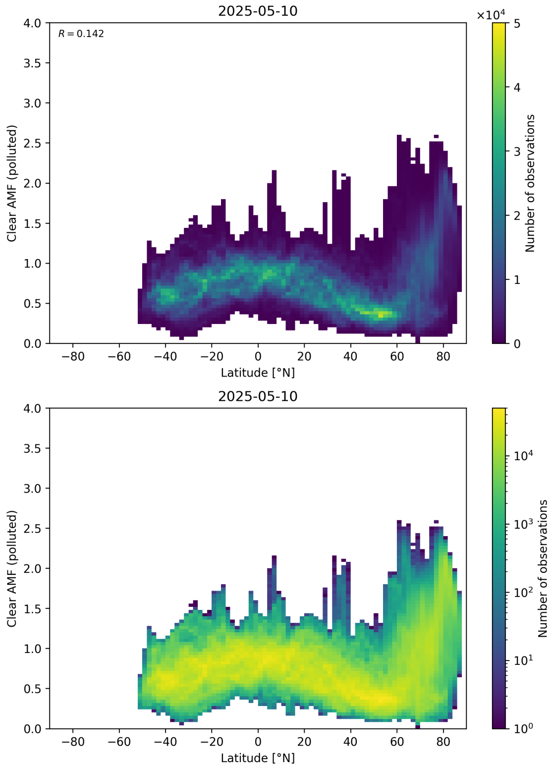
Figure 156: Scatter density plot of “Latitude” against “Clear AMF (polluted)” for 2025-05-10 to 2025-05-11.
