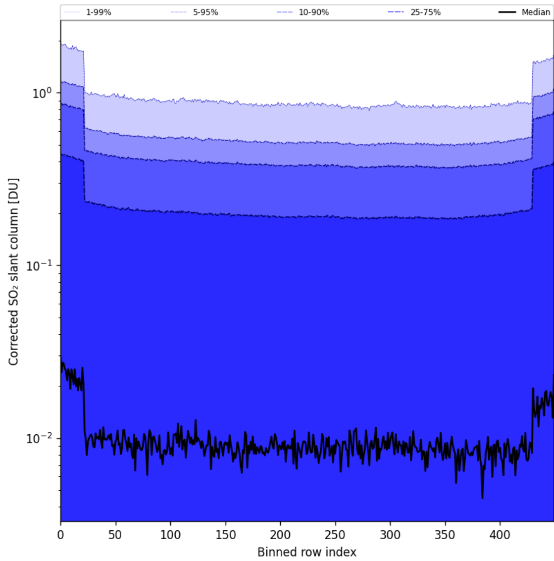
Figure 86: Along track statistics of “Corrected SO 2 slant column” for 2025-05-10 to 2025-05-11
