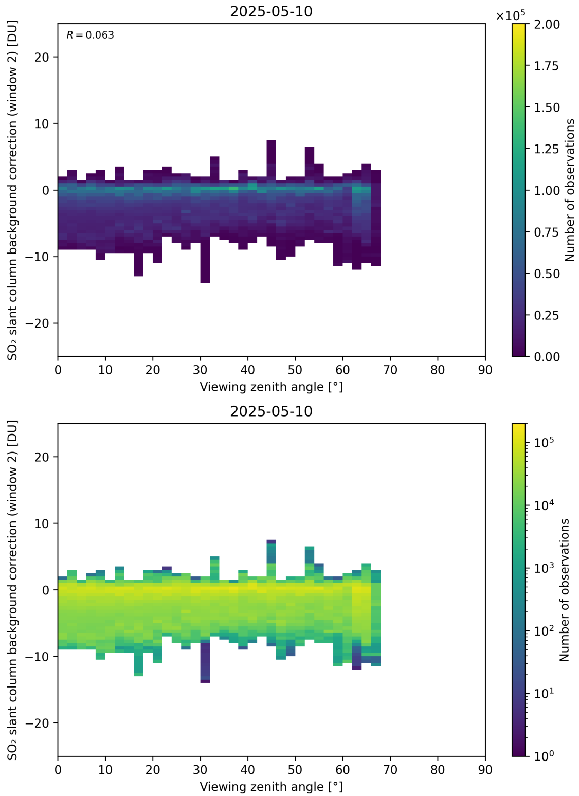
Figure 363: Scatter density plot of “Viewing zenith angle” against “SO 2 slant column background correction (window 2)” for 2025-05-10 to 2025-05-11.
