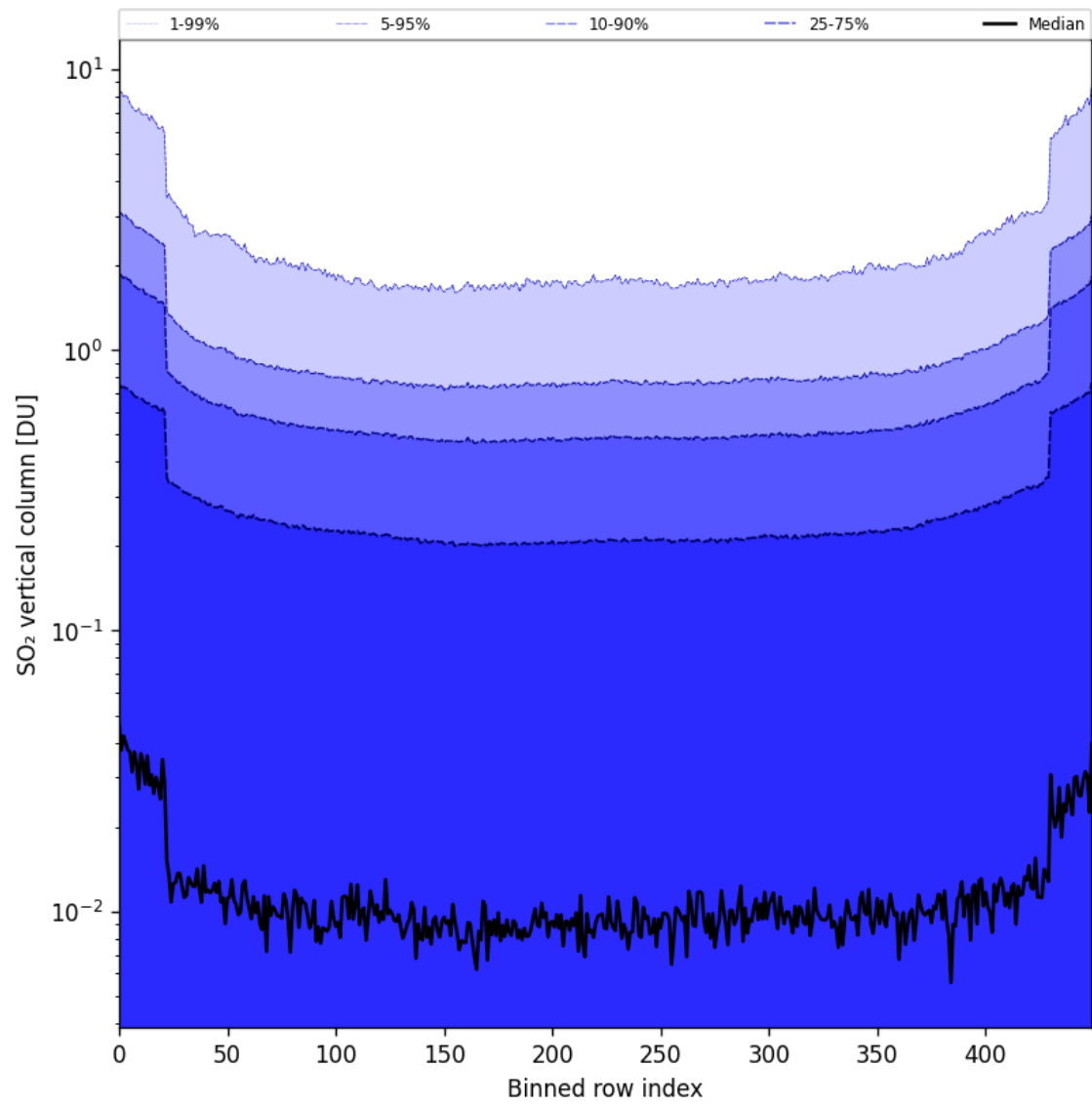
Figure 84: Along track statistics of “SO 2 vertical column” for 2025-05-10 to 2025-05-11
