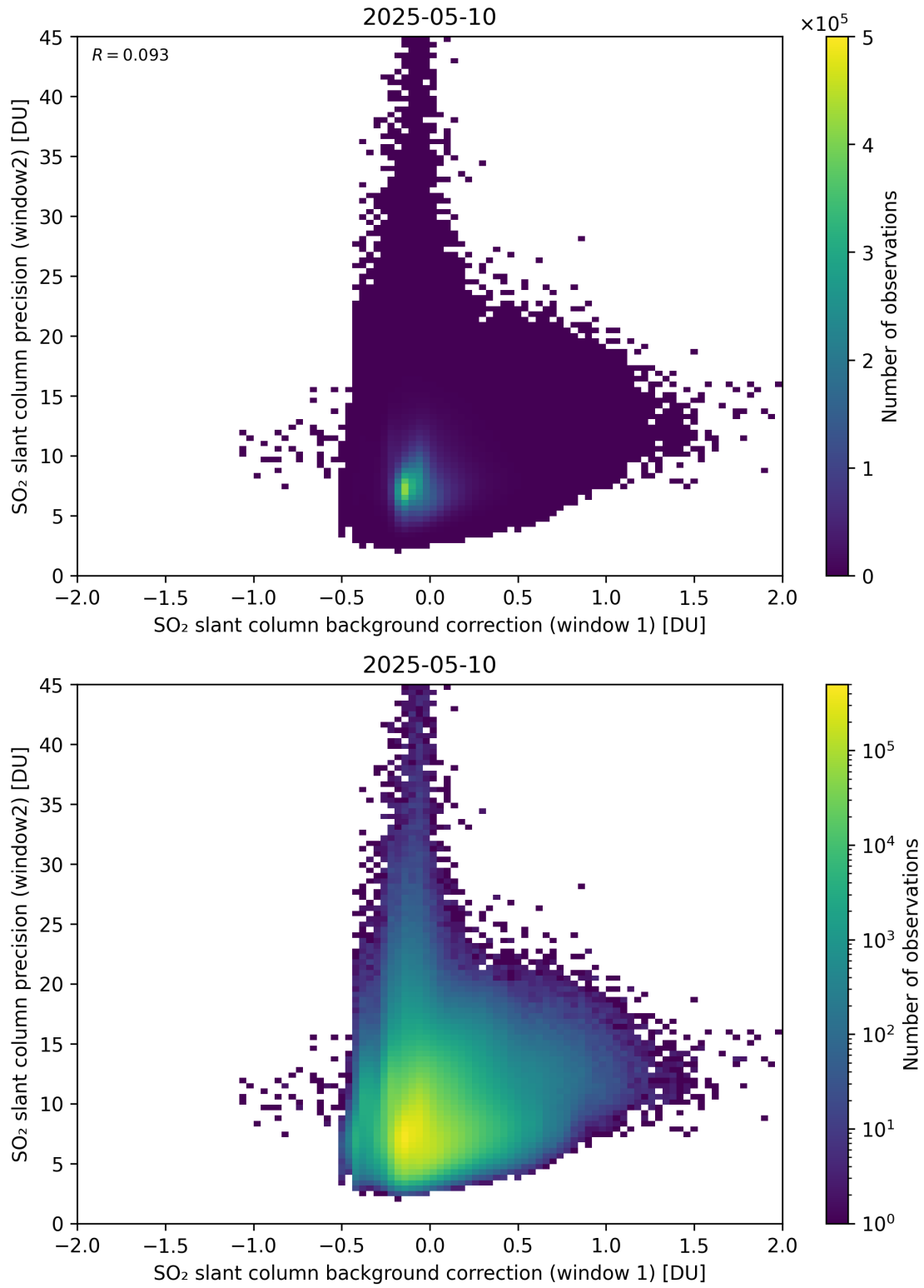
Figure 117: Scatter density plot of “SO 2 slant column background correction (window 1)” against “SO 2 slant column precision (window2)” for 2025-05-10 to 2025-05-11.
