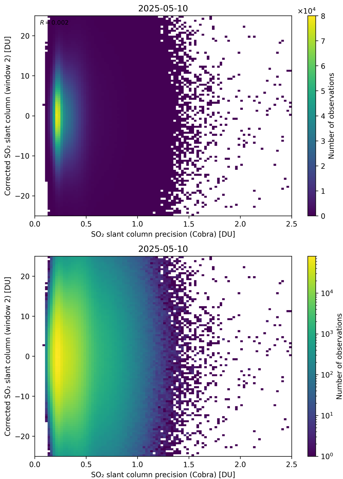
Figure 206: Scatter density plot of “SO 2 slant column precision (Cobra)” against “Corrected SO 2 slant column (window 2)” for 2025-05-10 to 2025-05-11.
