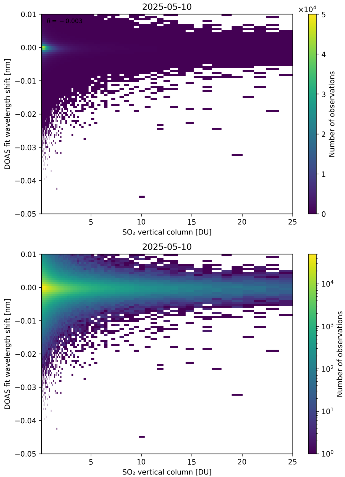
Figure 326: Scatter density plot of “SO 2 vertical column” against “DOAS fit wavelength shift” for 2025-05-10 to 2025-05-11.
