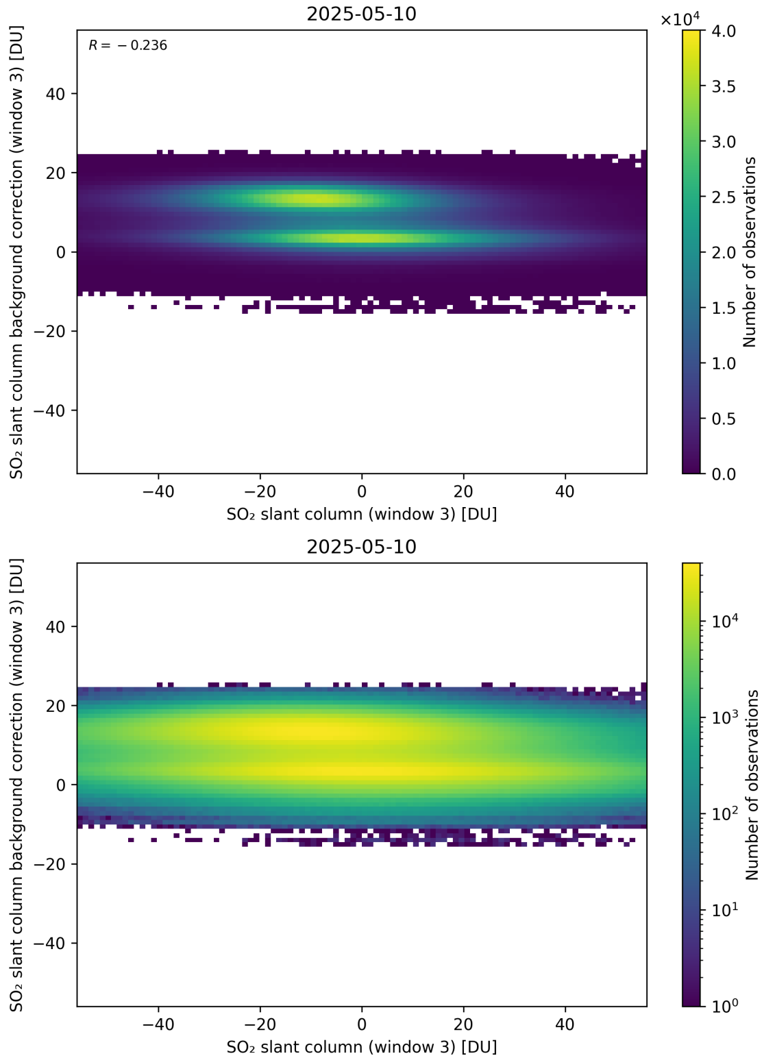
Figure 303: Scatter density plot of “SO 2 slant column (window 3)” against “SO 2 slant column background correction (window 3)” for 2025-05-10 to 2025-05-11.
