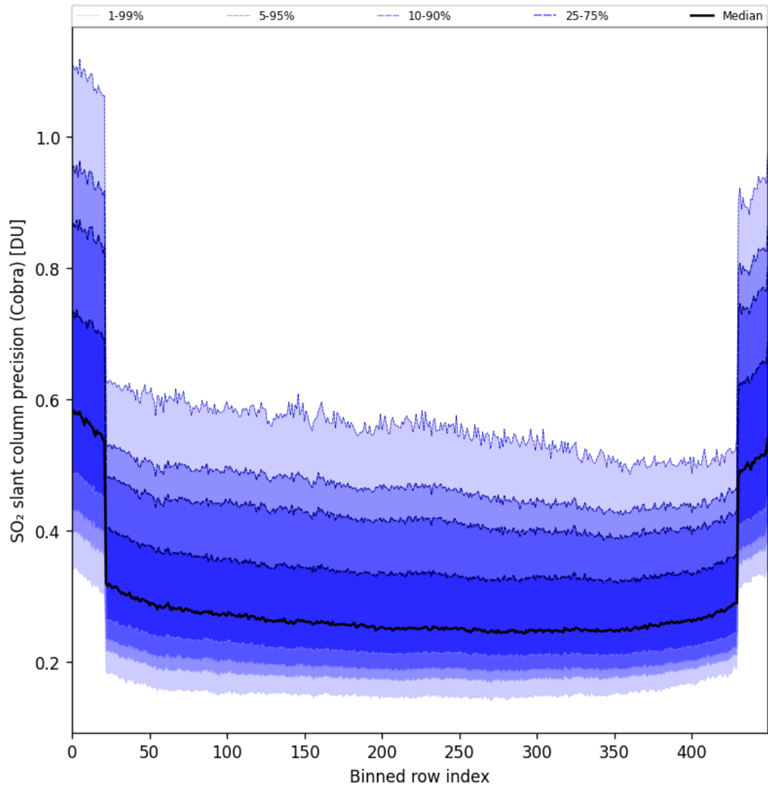
Figure 88: Along track statistics of “SO 2 slant column precision (Cobra)” for 2025-05-10 to 2025-05-11
