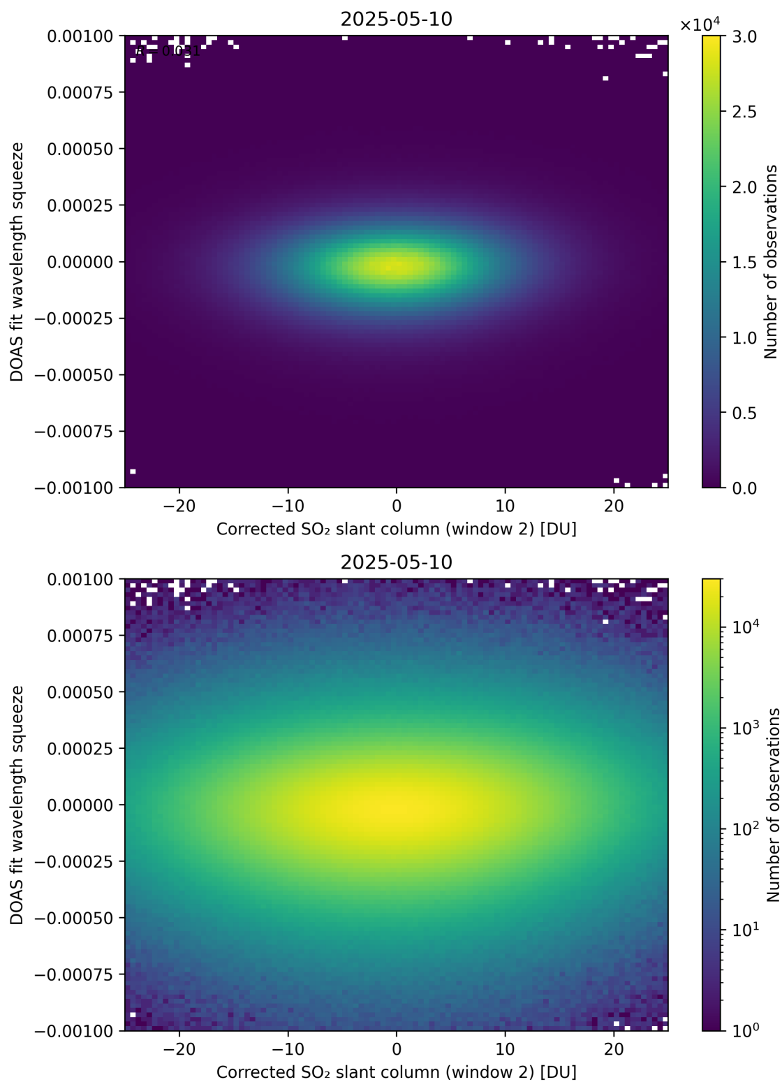
Figure 247: Scatter density plot of “Corrected SO 2 slant column (window 2)” against “DOAS fit wavelength squeeze” for 2025-05-10 to 2025-05-11.
