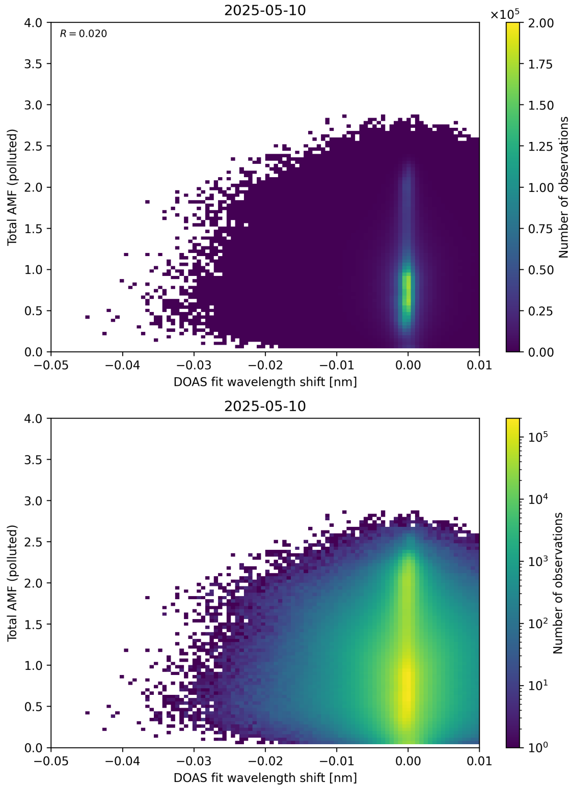
Figure 141: Scatter density plot of “DOAS fit wavelength shift” against “Total AMF (polluted)” for 2025-05-10 to 2025-05-11.
