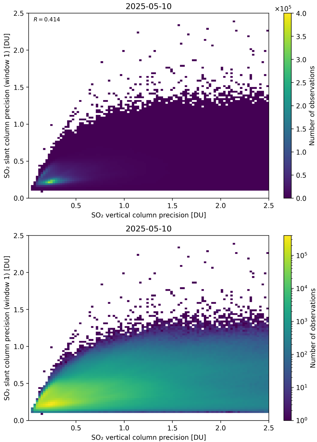
Figure 342: Scatter density plot of “SO 2 vertical column precision” against “SO 2 slant column precision (window 1)” for 2025-05-10 to 2025-05-11.
