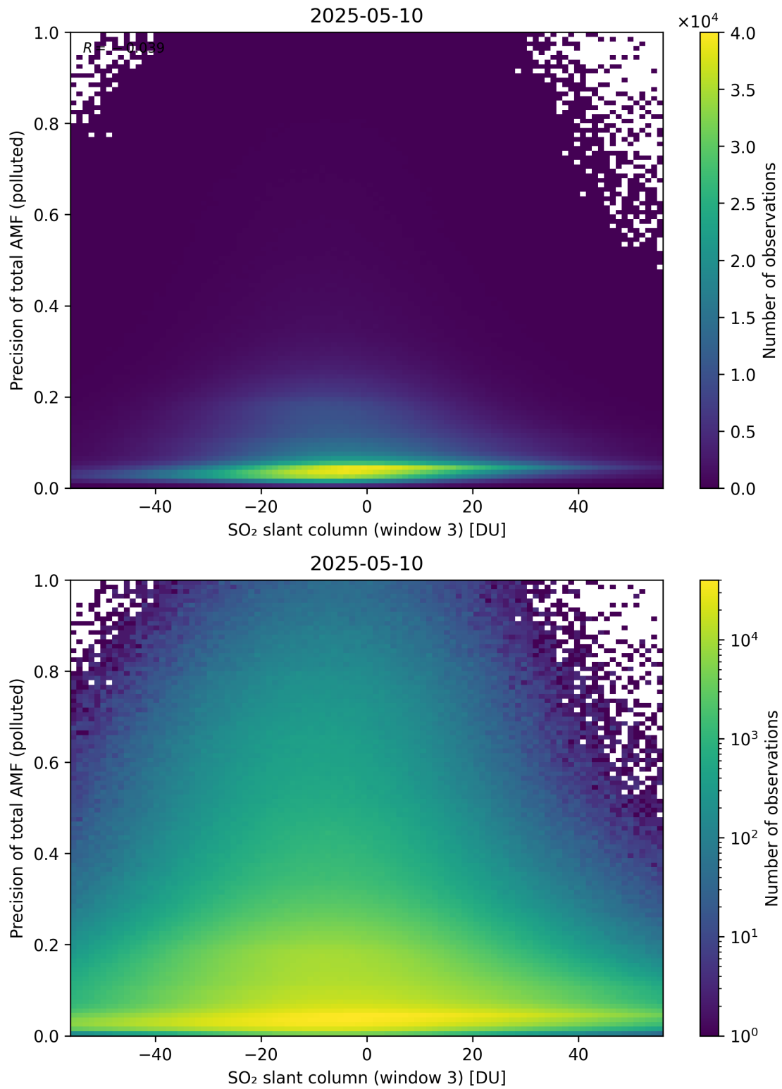
Figure 319: Scatter density plot of “SO 2 slant column (window 3)” against “Precision of total AMF (polluted)” for 2025-05-10 to 2025-05-11.
