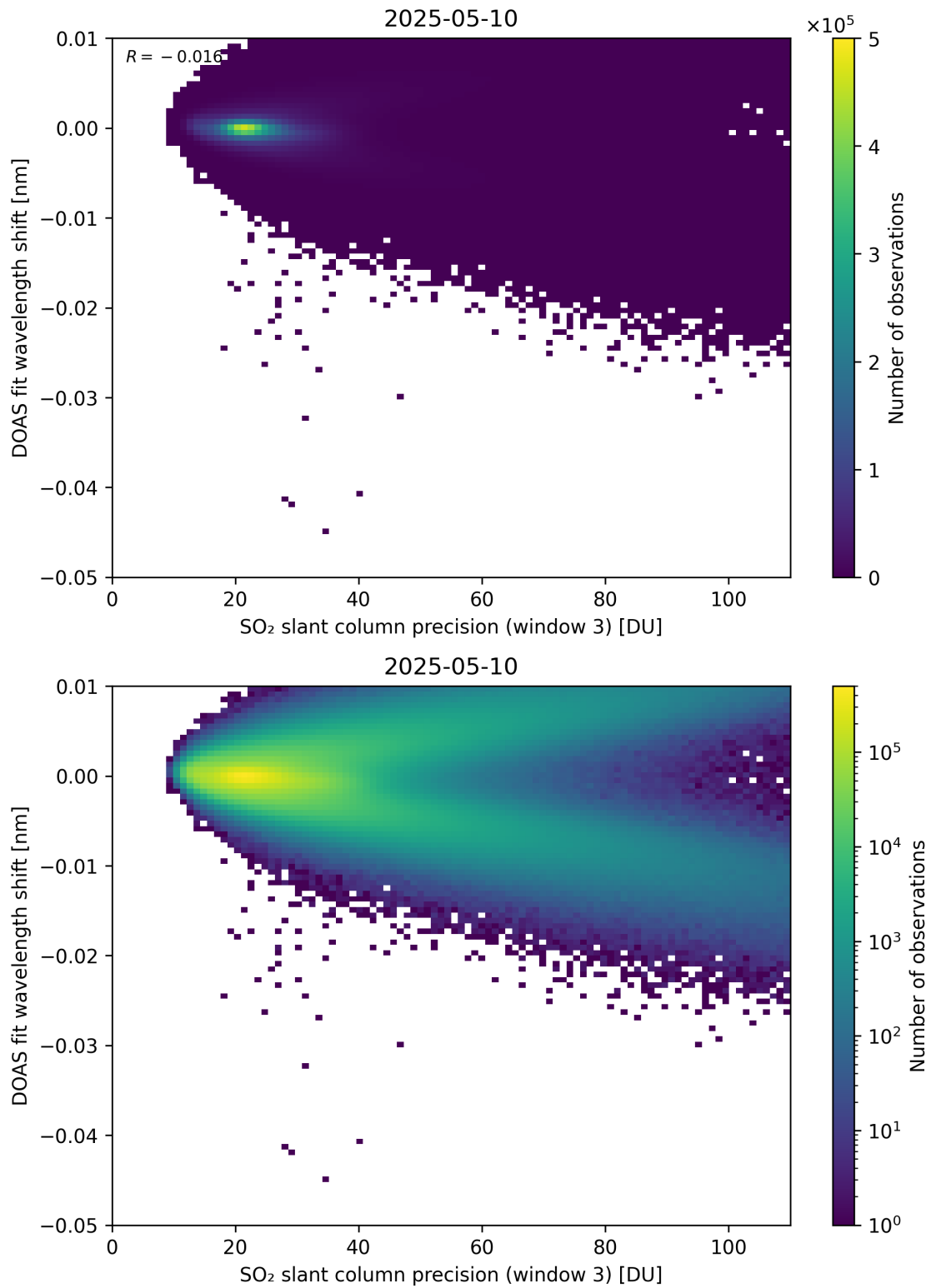
Figure 308: Scatter density plot of “SO 2 slant column precision (window 3)” against “DOAS fit wavelength shift” for 2025-05-10 to 2025-05-11.
