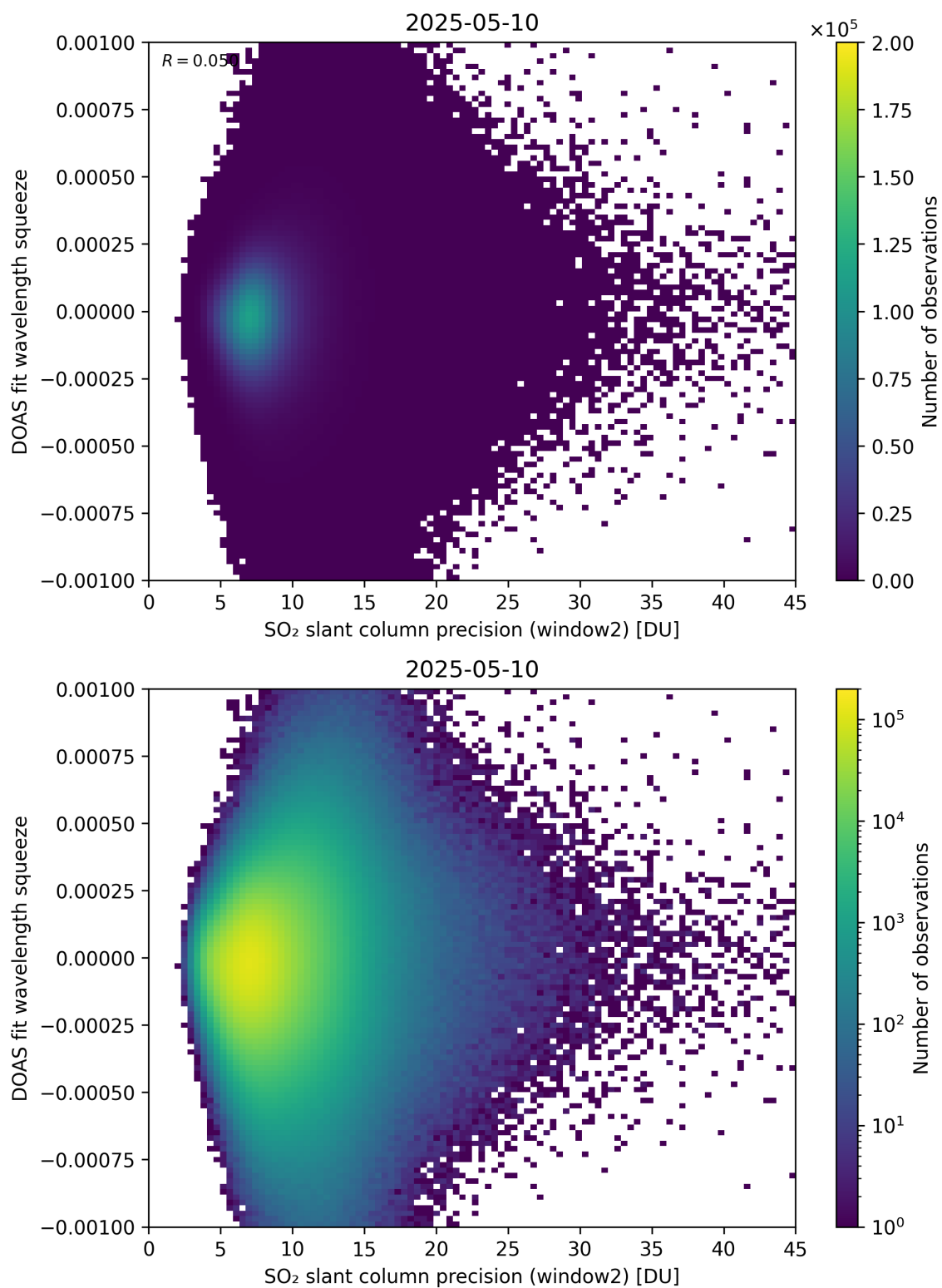
Figure 294: Scatter density plot of “SO 2 slant column precision (window2)” against “DOAS fit wavelength squeeze” for 2025-05-10 to 2025-05-11.
