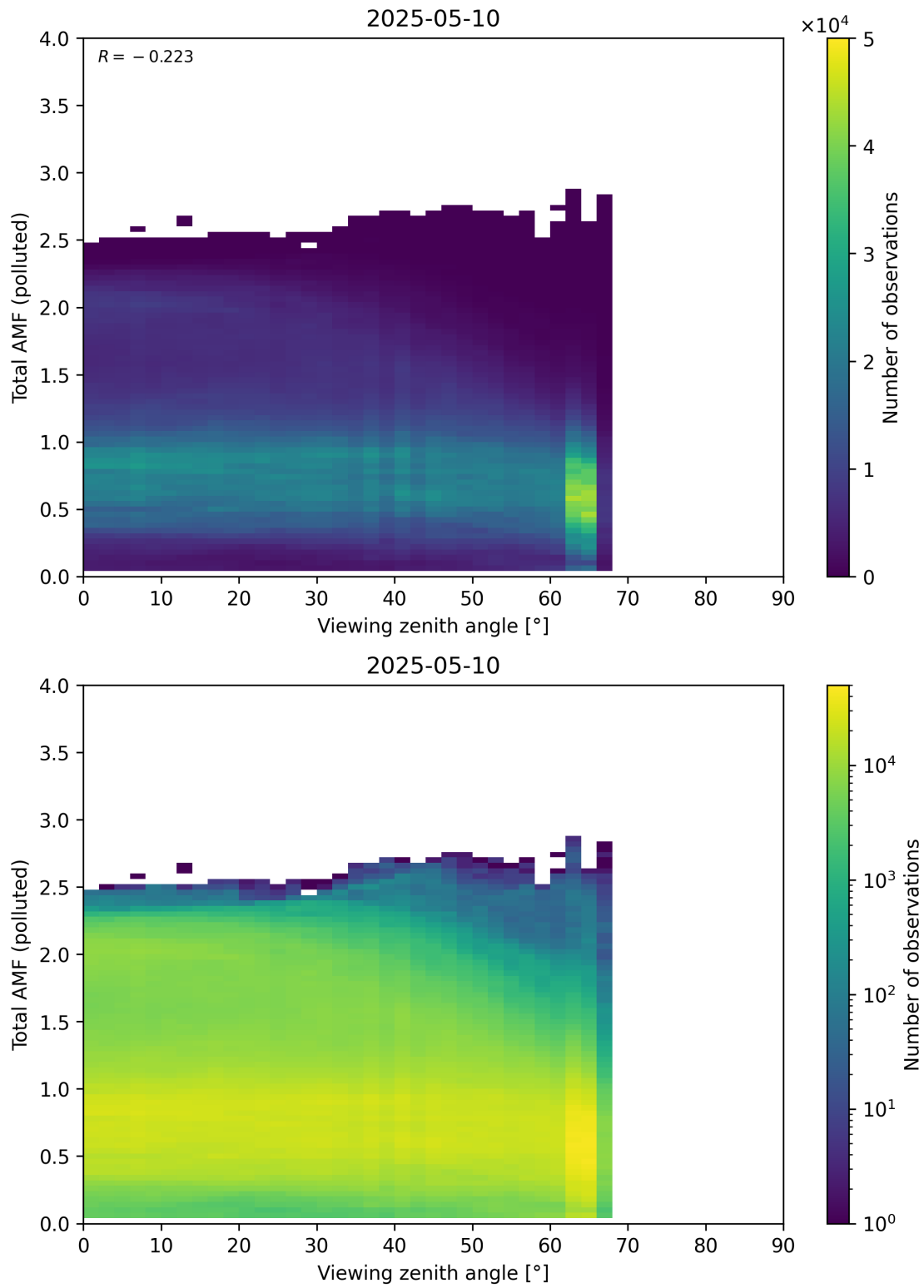
Figure 381: Scatter density plot of “Viewing zenith angle” against “Total AMF (polluted)” for 2025-05-10 to 2025-05-11.
