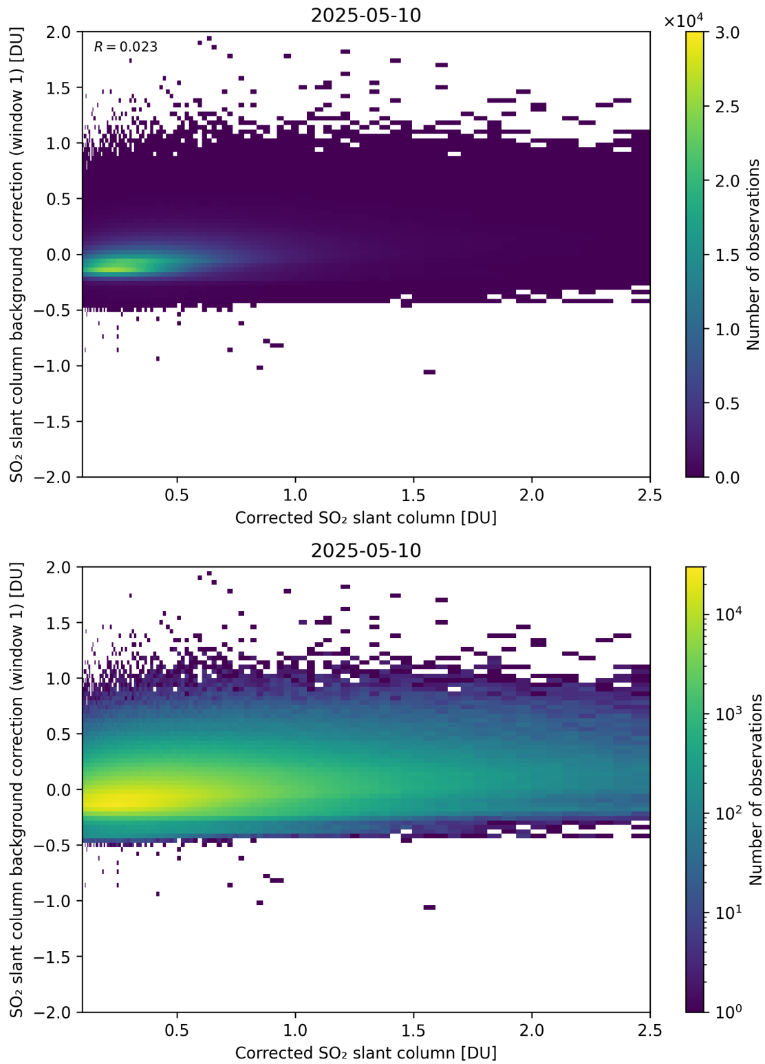
Figure 226: Scatter density plot of “Corrected SO 2 slant column” against “SO 2 slant column background correction (window 1)” for 2025-05-10 to 2025-05-11.
