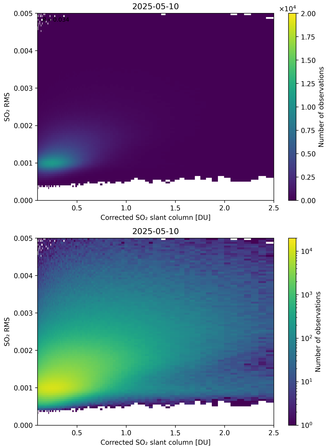
Figure 231: Scatter density plot of “Corrected SO 2 slant column” against “SO 2 RMS” for 2025-05-10 to 2025-05-11.
