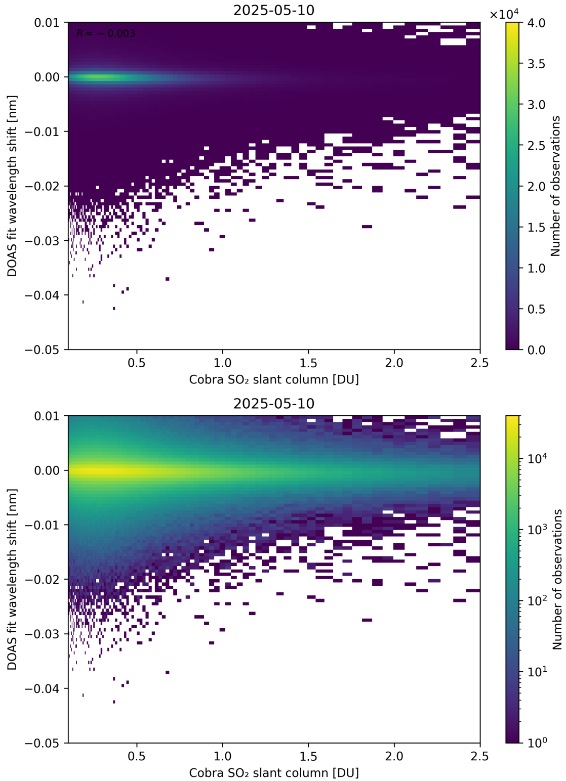
Figure 196: Scatter density plot of “Cobra SO 2 slant column” against “DOAS fit wavelength shift” for 2025-05-10 to 2025-05-11.
