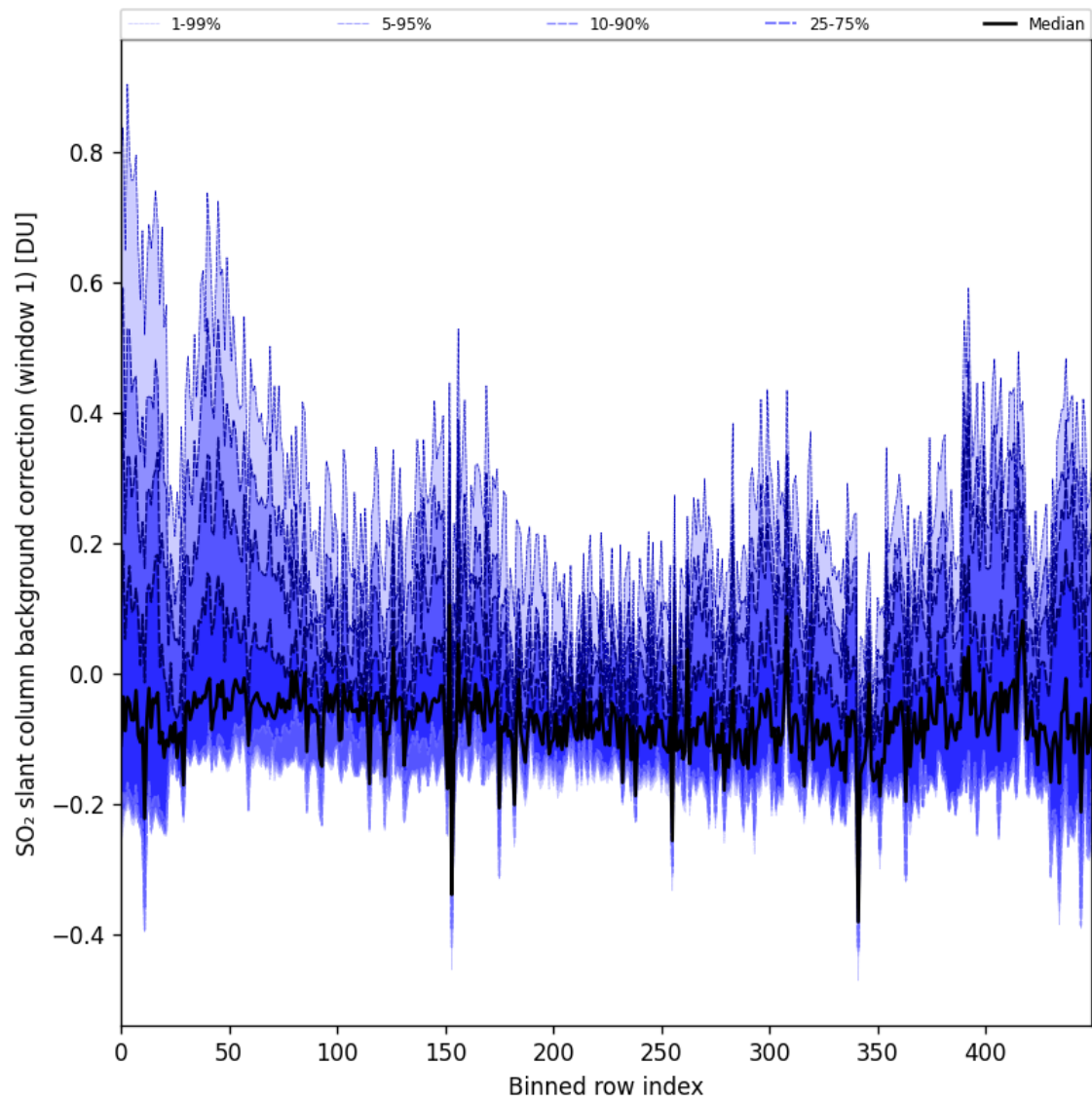
Figure 92: Along track statistics of “SO 2 slant column background correction (window 1)” for 2025-05-10 to 2025-05-11
