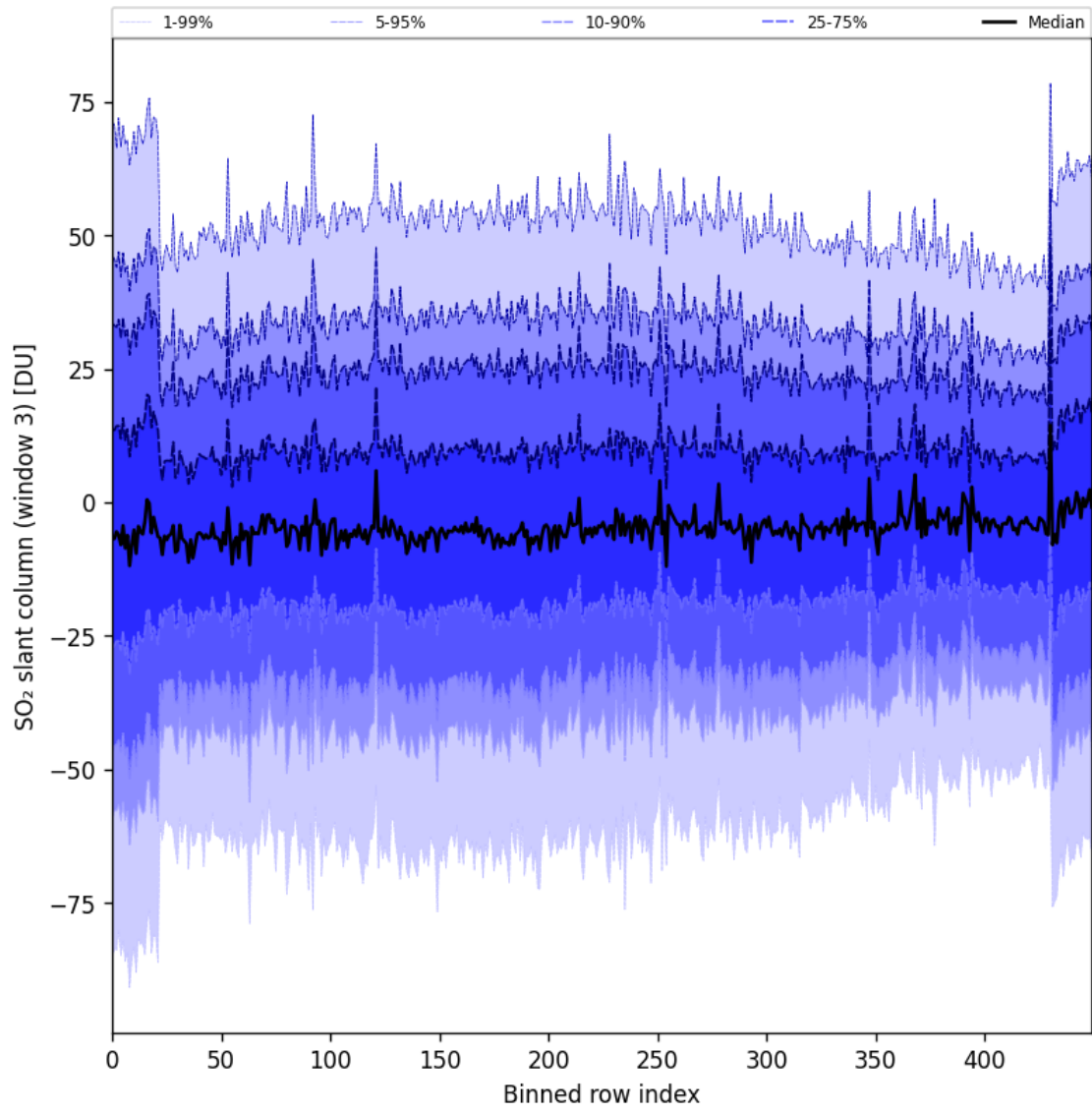
Figure 97: Along track statistics of “SO 2 slant column (window 3)” for 2025-05-10 to 2025-05-11
