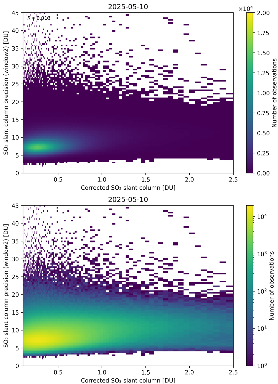
Figure 239: Scatter density plot of “Corrected SO 2 slant column” against “SO 2 slant column precision (window2)” for 2025-05-10 to 2025-05-11.
