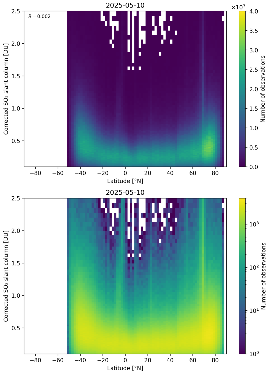
Figure 159: Scatter density plot of “Latitude” against “Corrected SO 2 slant column” for 2025-05-10 to 2025-05-11.
