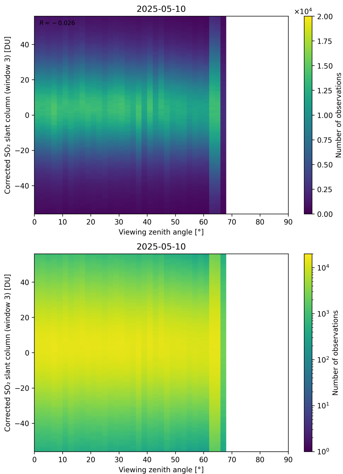
Figure 375: Scatter density plot of “Viewing zenith angle” against “Corrected SO 2 slant column (window 3)” for 2025-05-10 to 2025-05-11.
