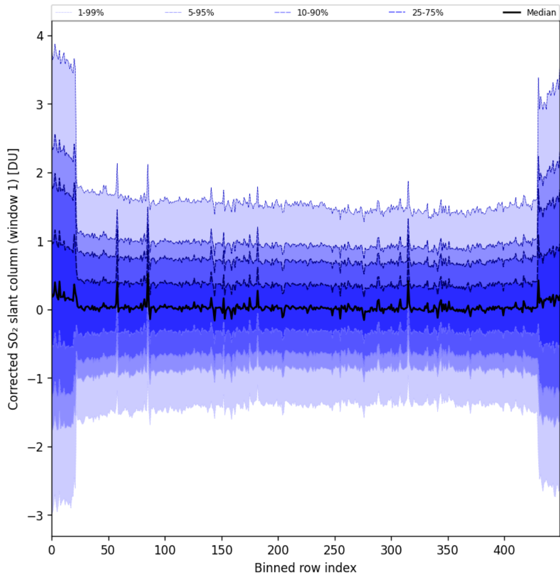
Figure 91: Along track statistics of “Corrected SO 2 slant column (window 1)” for 2025-05-10 to 2025-05-11
