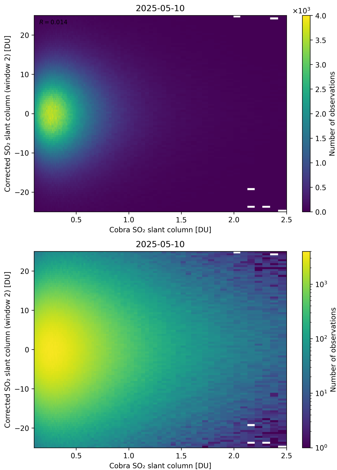
Figure 217: Scatter density plot of “Cobra SO 2 slant column” against “Corrected SO 2 slant column (window 2)” for 2025-05-10 to 2025-05-11.
