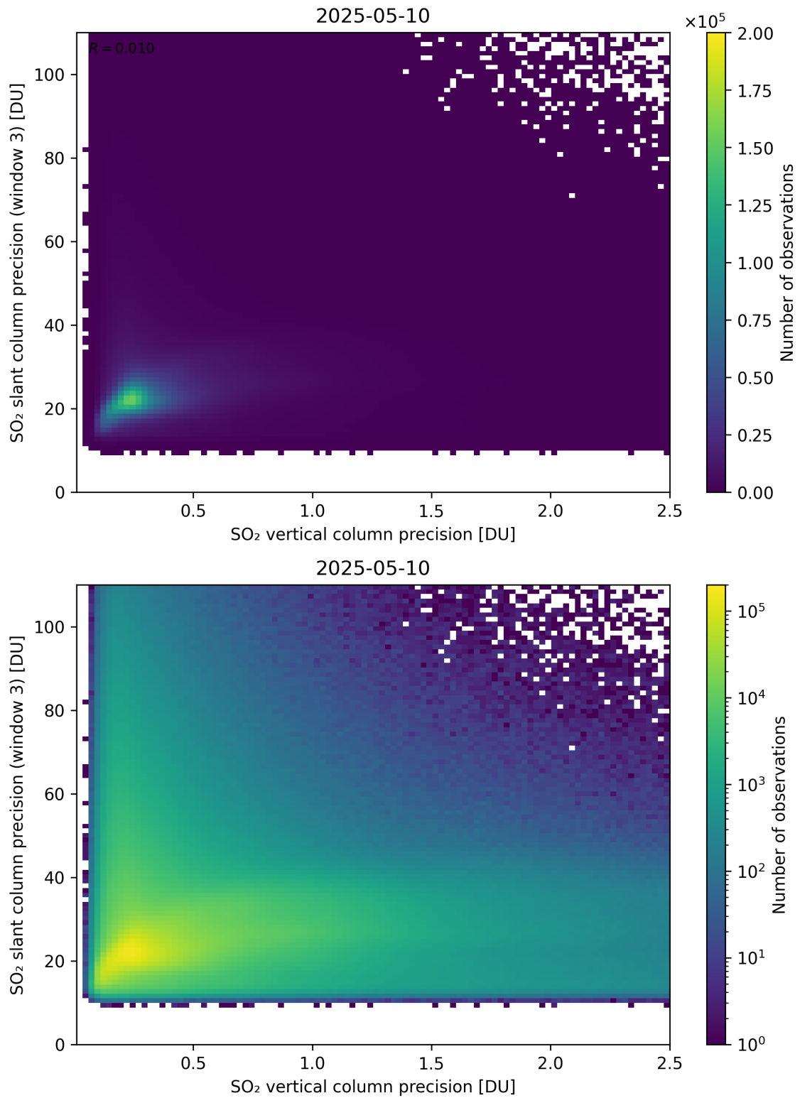
Figure 345: Scatter density plot of “SO 2 vertical column precision” against “SO 2 slant column precision (window 3)” for 2025-05-10 to 2025-05-11.
