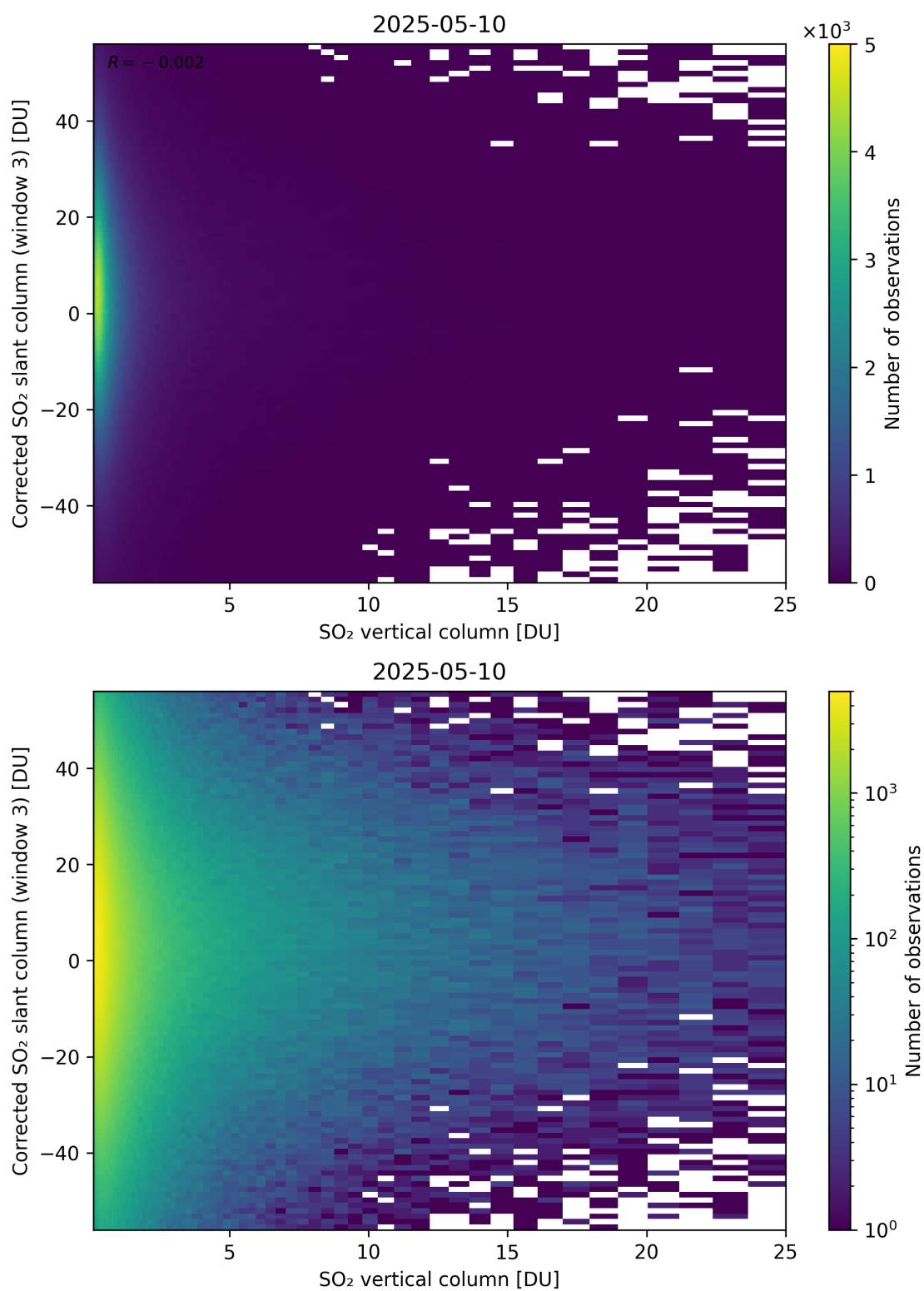
Figure 353: Scatter density plot of “SO 2 vertical column” against “Corrected SO 2 slant column (window 3)” for 2025-05-10 to 2025-05-11.
