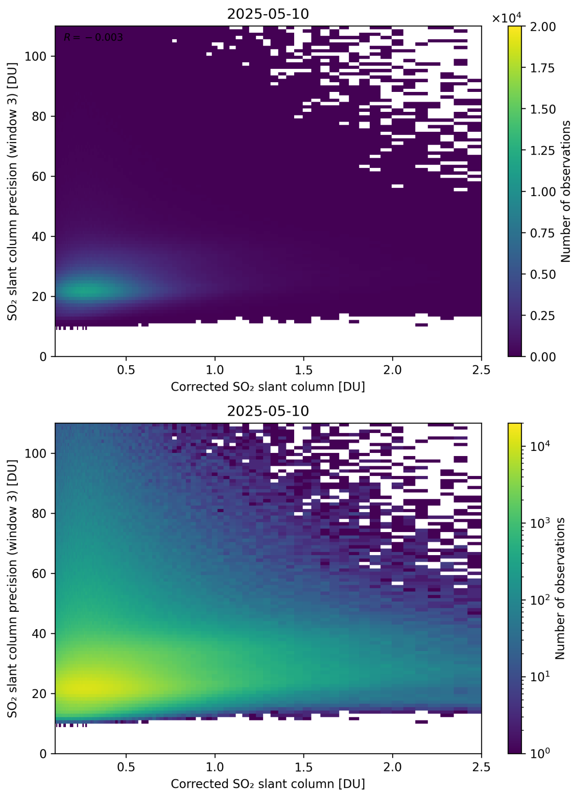
Figure 241: Scatter density plot of “Corrected SO 2 slant column” against “SO 2 slant column precision (window 3)” for 2025-05-10 to 2025-05-11.
