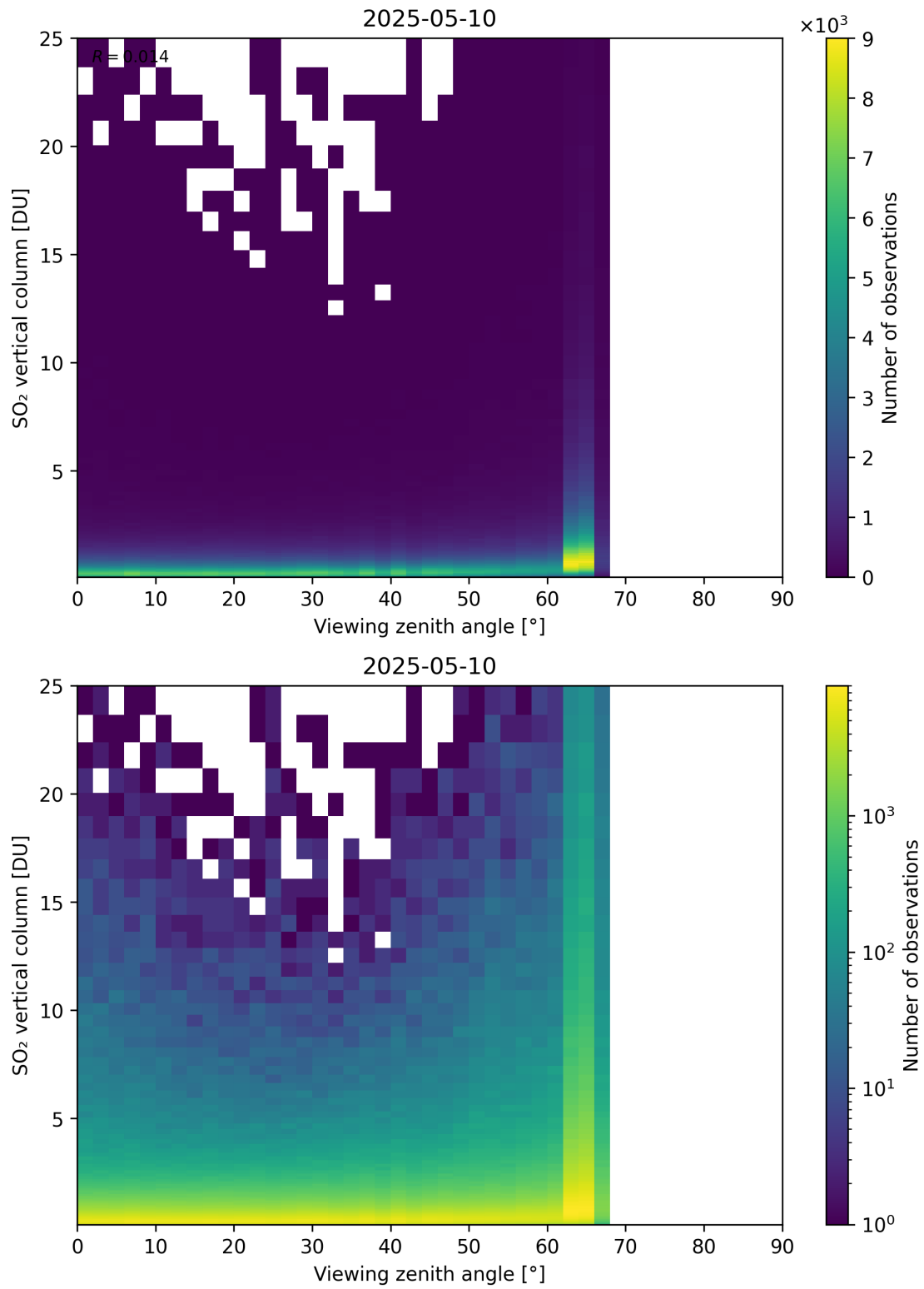
Figure 383: Scatter density plot of “Viewing zenith angle” against “SO 2 vertical column” for 2025-05-10 to 2025-05-11.
