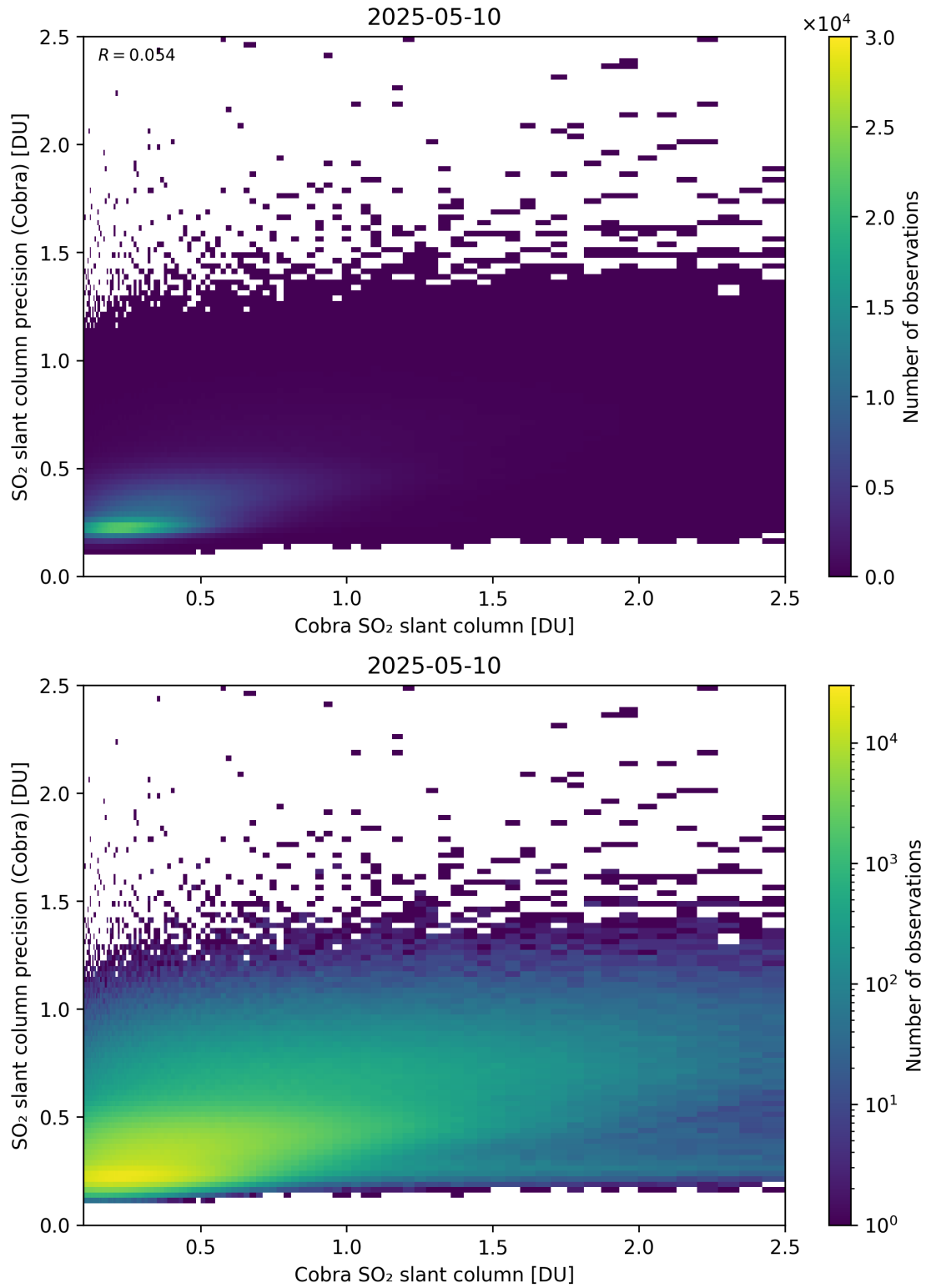
Figure 216: Scatter density plot of “Cobra SO 2 slant column” against “SO 2 slant column precision (Cobra)” for 2025-05-10 to 2025-05-11.
