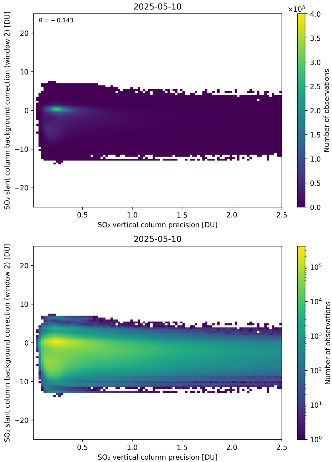
Figure 330: Scatter density plot of “SO 2 vertical column precision” against “SO 2 slant column background correction (window 2)” for 2025-05-10 to 2025-05-11.
