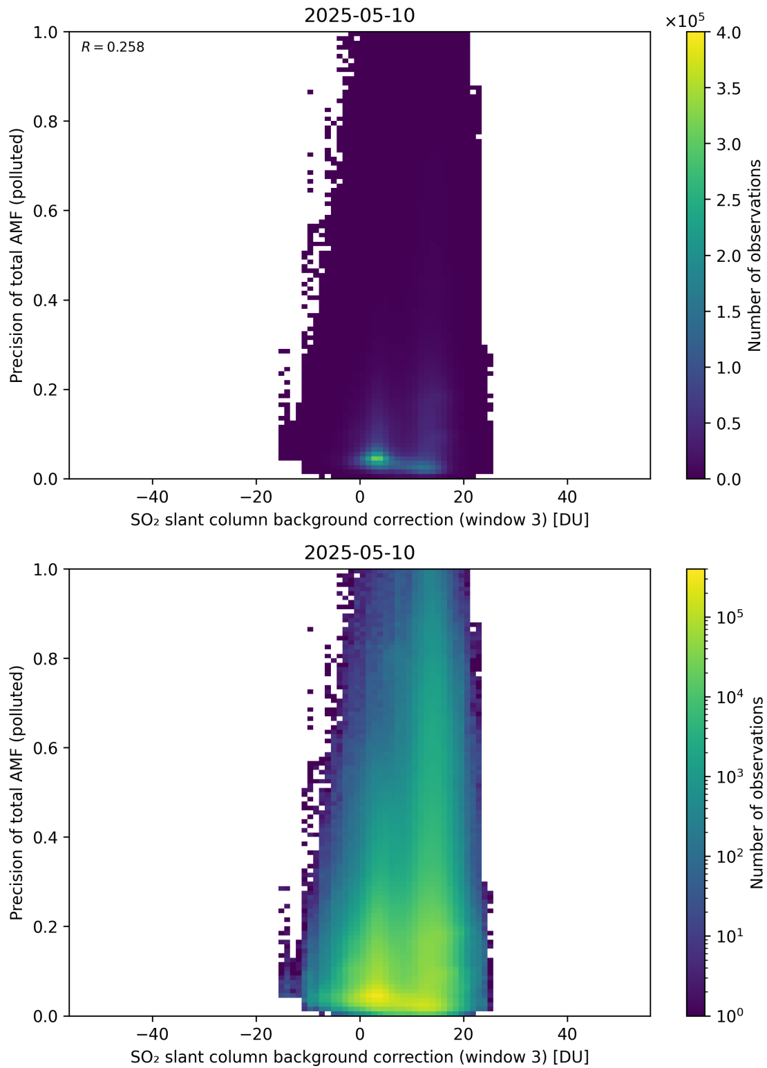
Figure 137: Scatter density plot of “SO 2 slant column background correction (window 3)” against “Precision of total AMF (polluted)” for 2025-05-10 to 2025-05-11.
