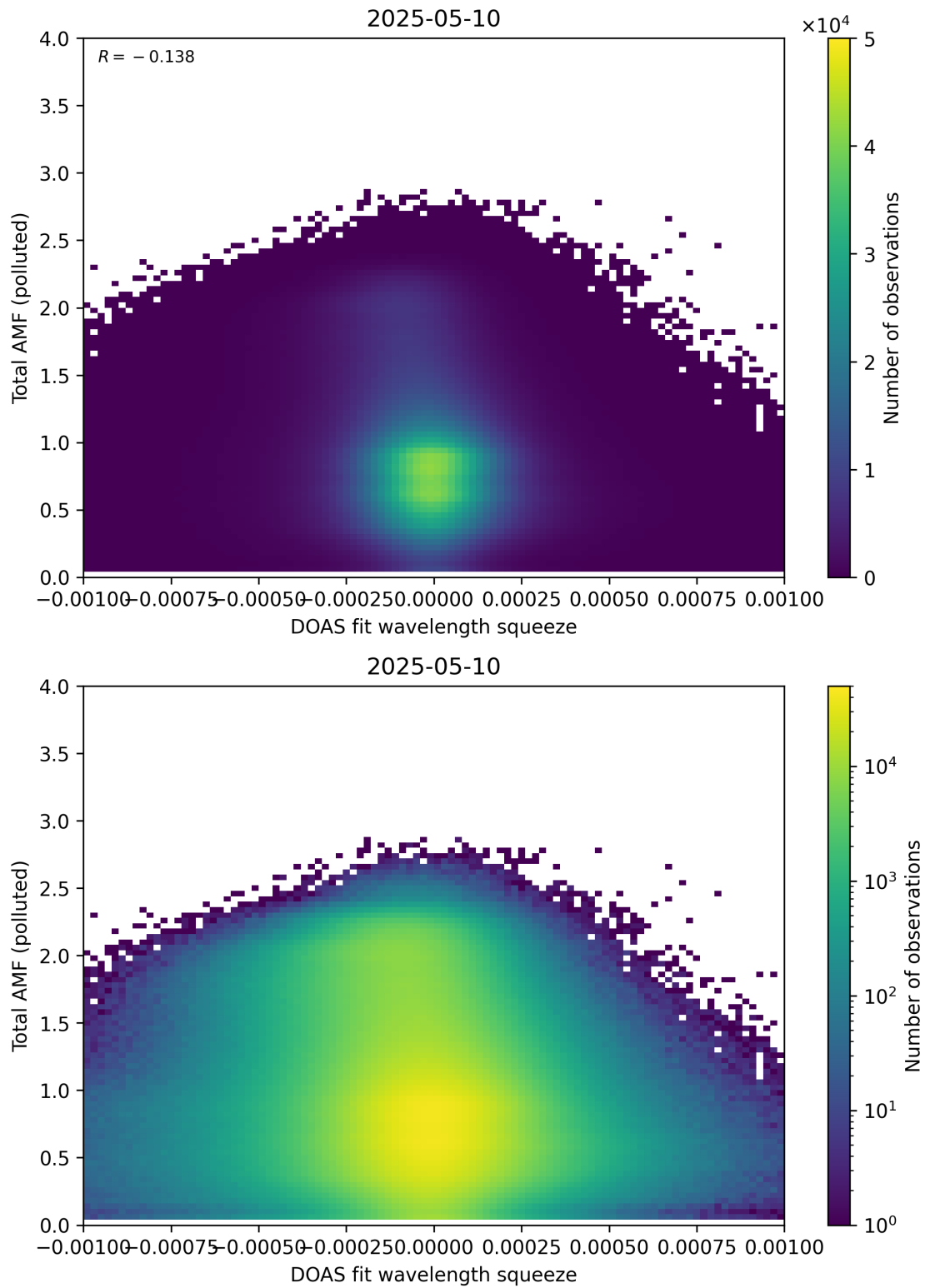
Figure 145: Scatter density plot of “DOAS fit wavelength squeeze” against “Total AMF (polluted)” for 2025-05-10 to 2025-05-11.
