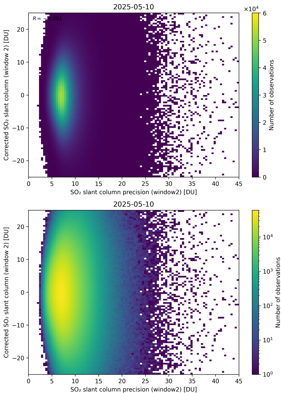
Figure 297: Scatter density plot of “SO 2 slant column precision (window2)” against “Corrected SO 2 slant column (window 2)” for 2025-05-10 to 2025-05-11.
