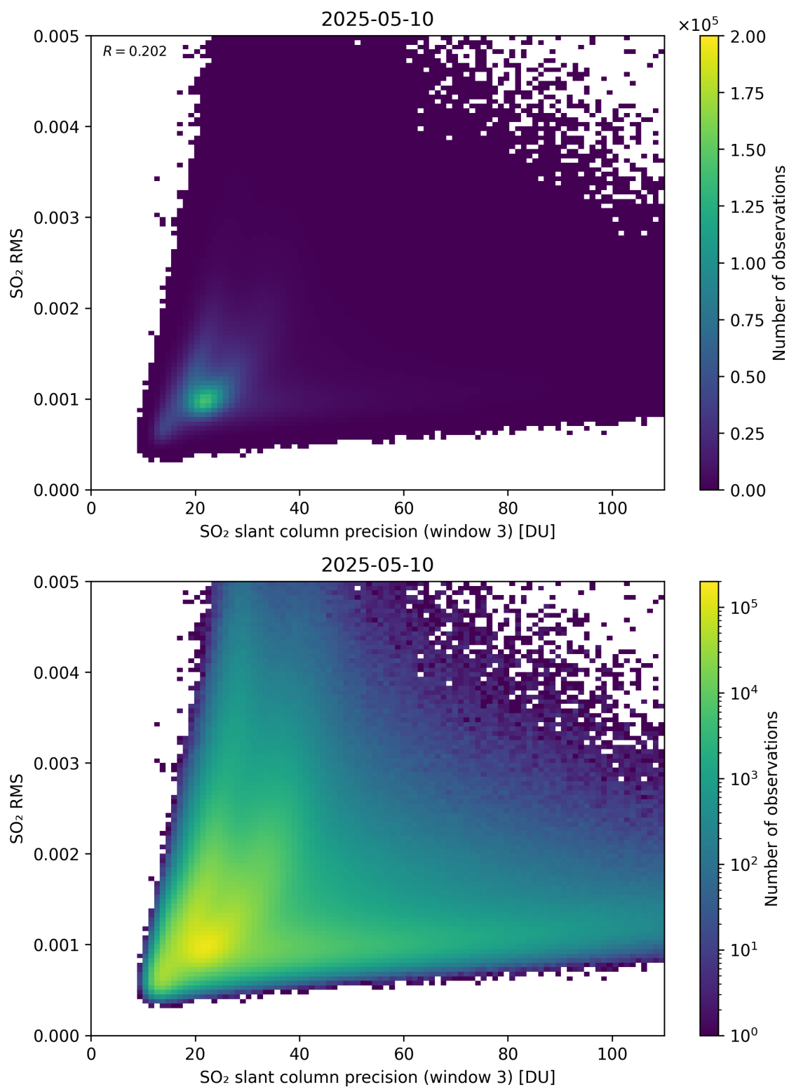
Figure 310: Scatter density plot of “SO 2 slant column precision (window 3)” against “SO 2 RMS” for 2025-05-10 to 2025-05-11.
