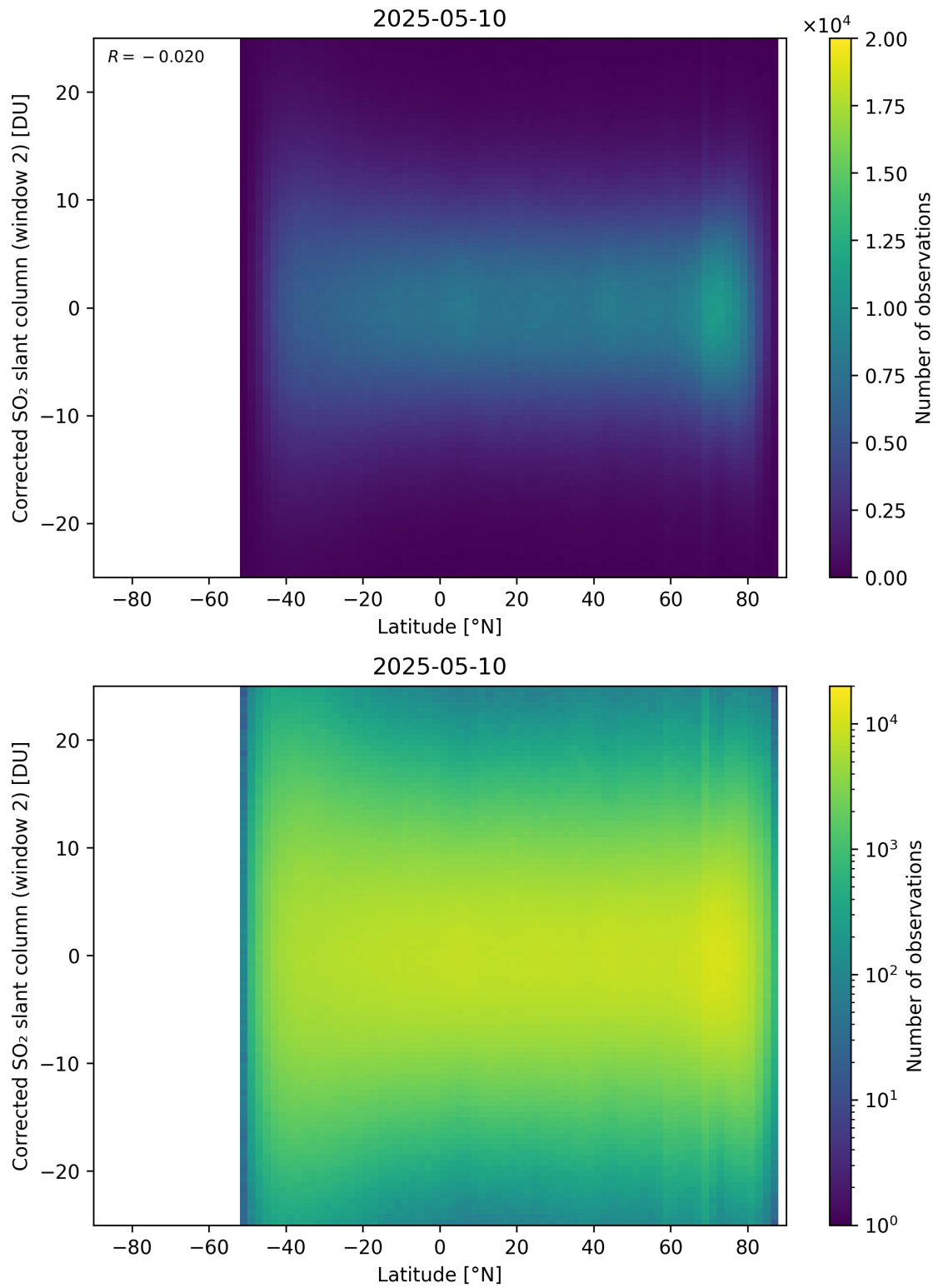
Figure 160: Scatter density plot of “Latitude” against “Corrected SO 2 slant column (window 2)” for 2025-05-10 to 2025-05-11.
