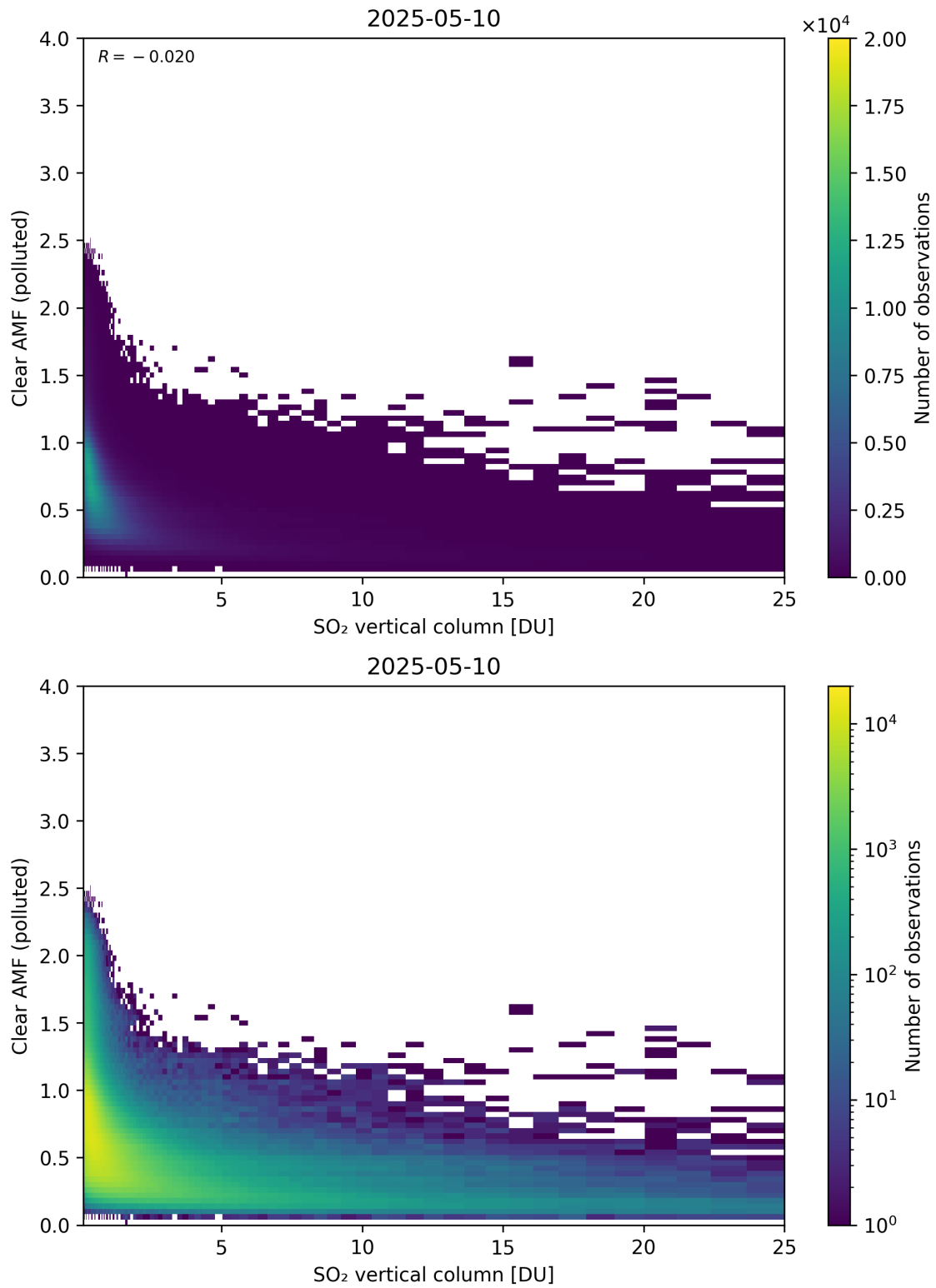
Figure 348: Scatter density plot of “SO 2 vertical column” against “Clear AMF (polluted)” for 2025-05-10 to 2025-05-11.
