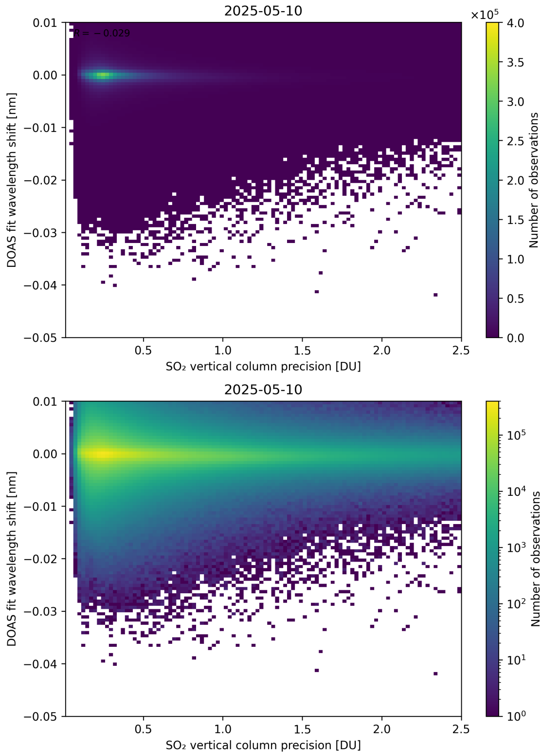
Figure 332: Scatter density plot of “SO 2 vertical column precision” against “DOAS fit wavelength shift” for 2025-05-10 to 2025-05-11.
