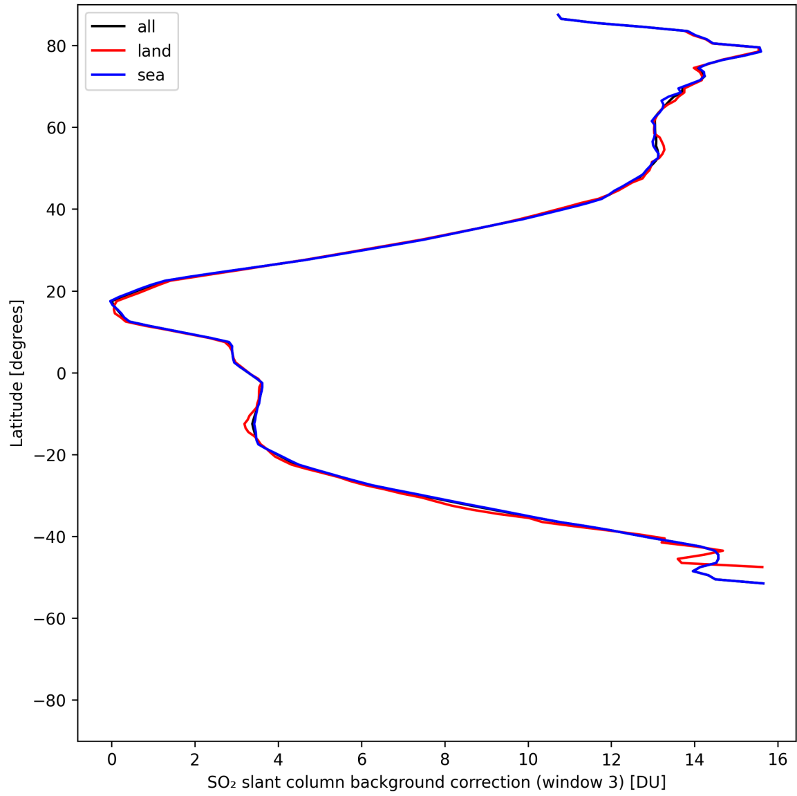
Figure 48: Zonal average of “SO 2 slant column background correction (window 3)” for 2025-05-10 to 2025-05-11.
