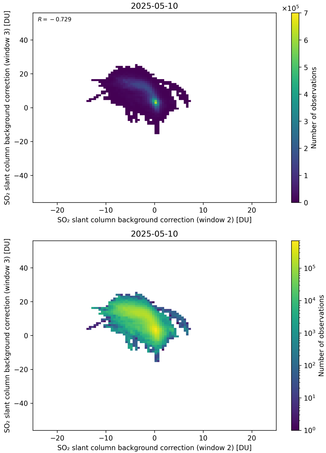
Figure 122: Scatter density plot of “SO 2 slant column background correction (window 2)” against “SO 2 slant column background correction (window 3)” for 2025-05-10 to 2025-05-11.
