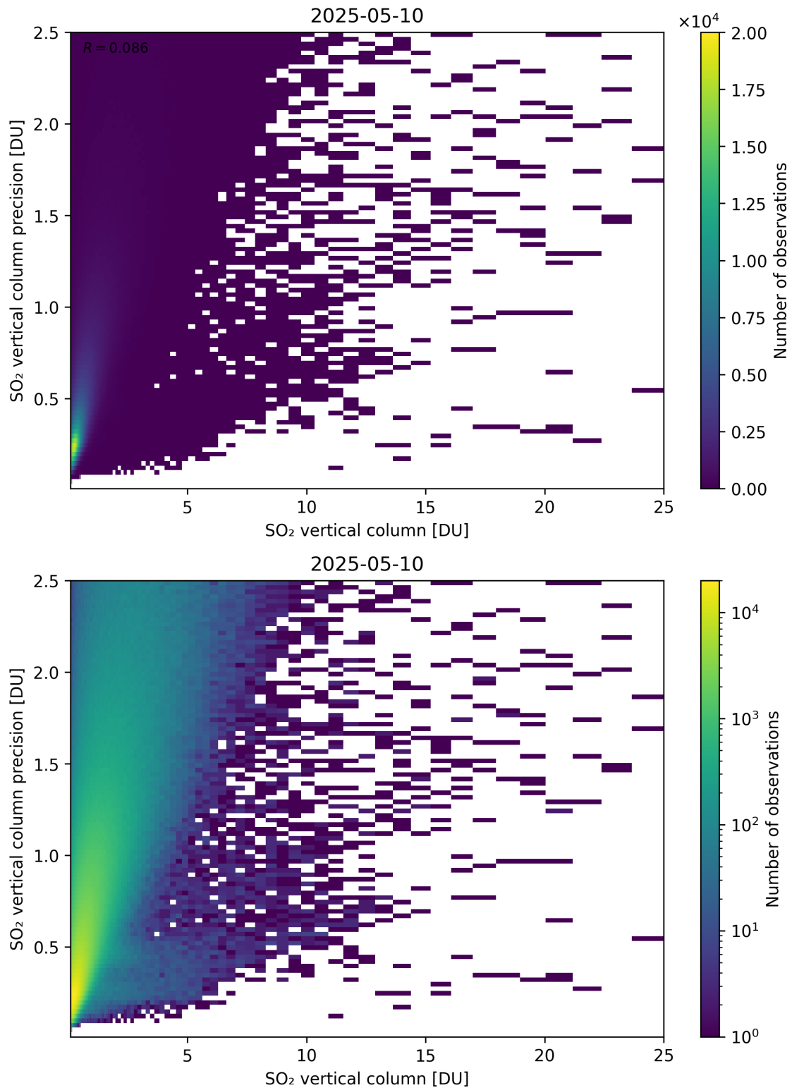
Figure 361: Scatter density plot of “SO 2 vertical column” against “SO 2 vertical column precision” for 2025-05-10 to 2025-05-11.
