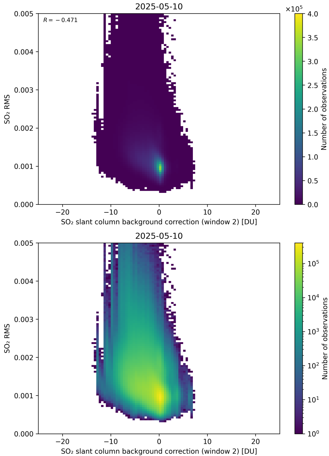
Figure 125: Scatter density plot of “SO 2 slant column background correction (window 2)” against “SO 2 RMS” for 2025-05-10 to 2025-05-11.
