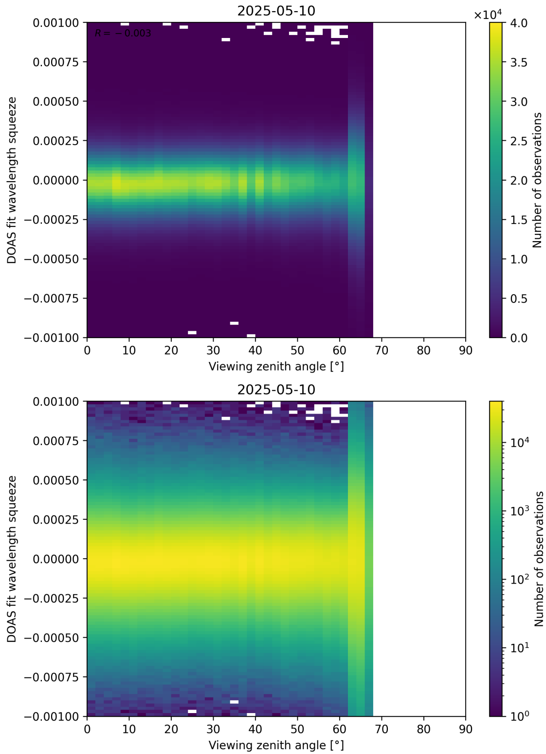
Figure 366: Scatter density plot of “Viewing zenith angle” against “DOAS fit wavelength squeeze” for 2025-05-10 to 2025-05-11.
