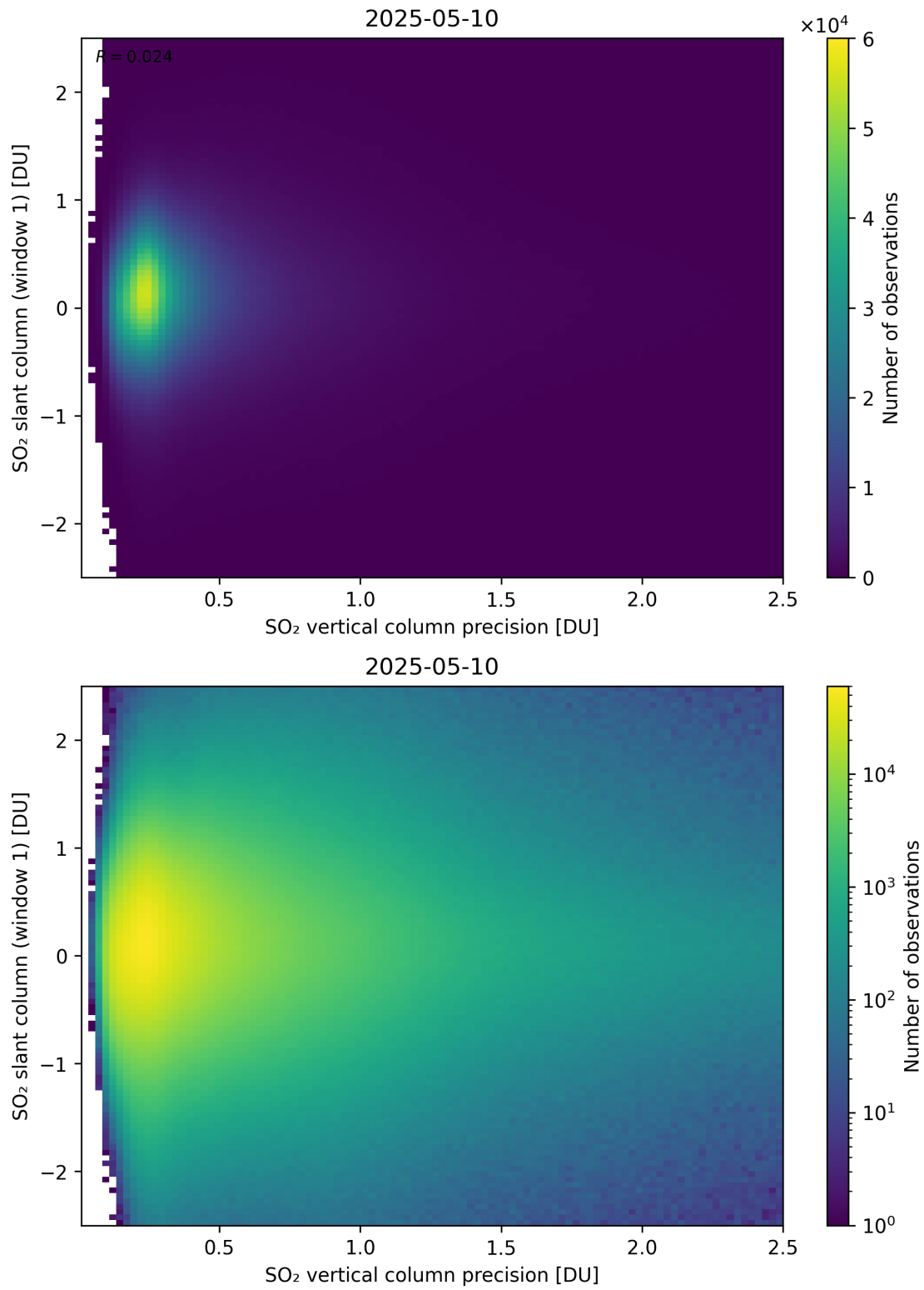
Figure 341: Scatter density plot of “SO 2 vertical column precision” against “SO 2 slant column (window 1)” for 2025-05-10 to 2025-05-11.
