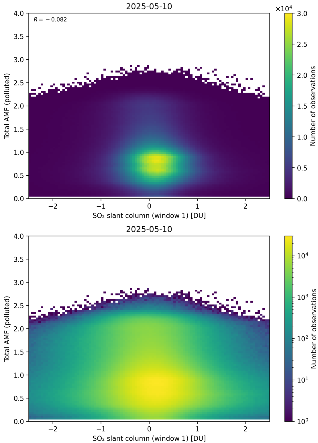
Figure 289: Scatter density plot of “SO 2 slant column (window 1)” against “Total AMF (polluted)” for 2025-05-10 to 2025-05-11.
