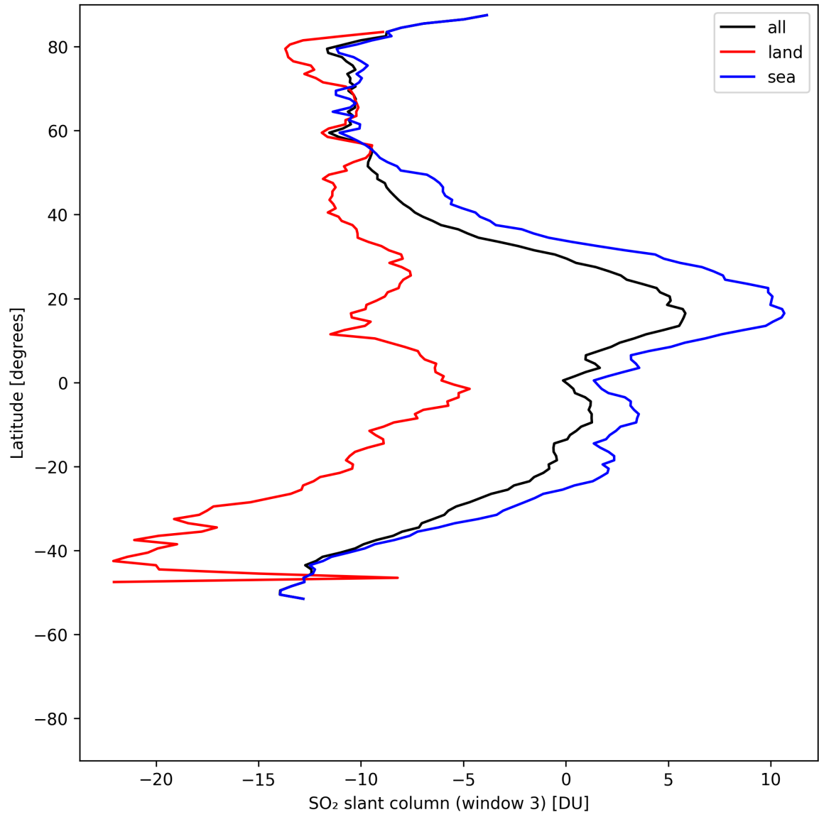
Figure 45: Zonal average of “SO 2 slant column (window 3)” for 2025-05-10 to 2025-05-11.
