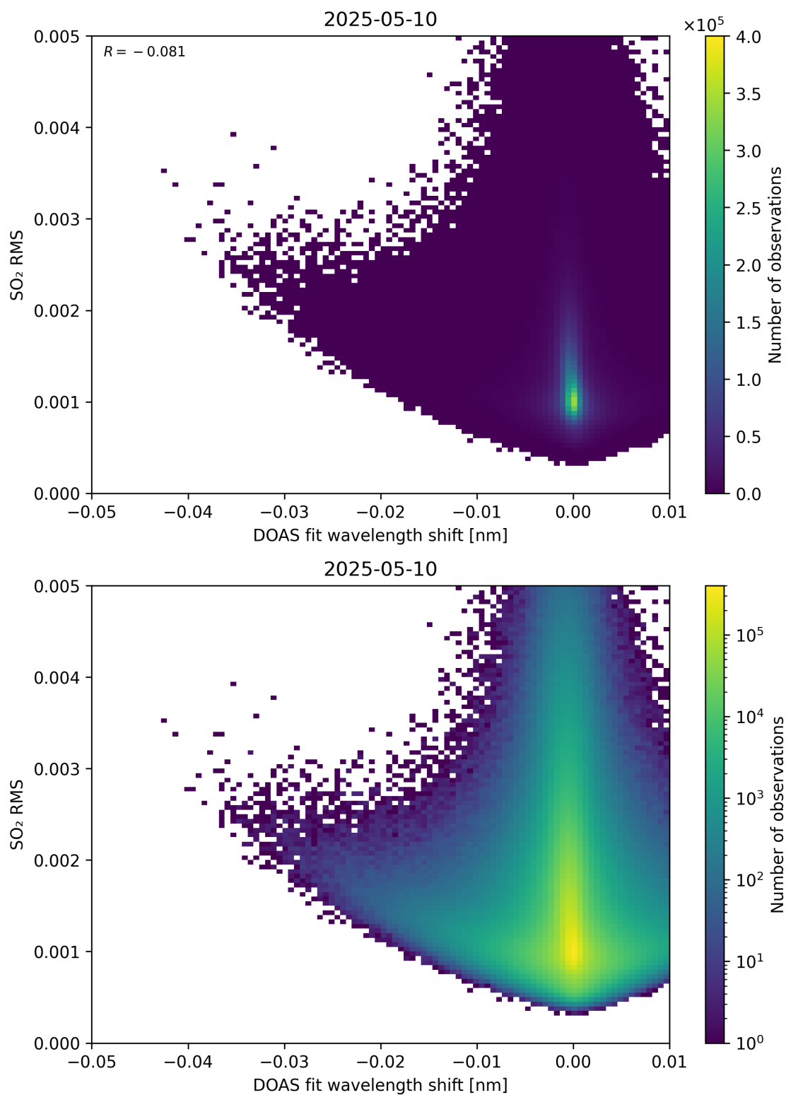
Figure 139: Scatter density plot of “DOAS fit wavelength shift” against “SO 2 RMS” for 2025-05-10 to 2025-05-11.
