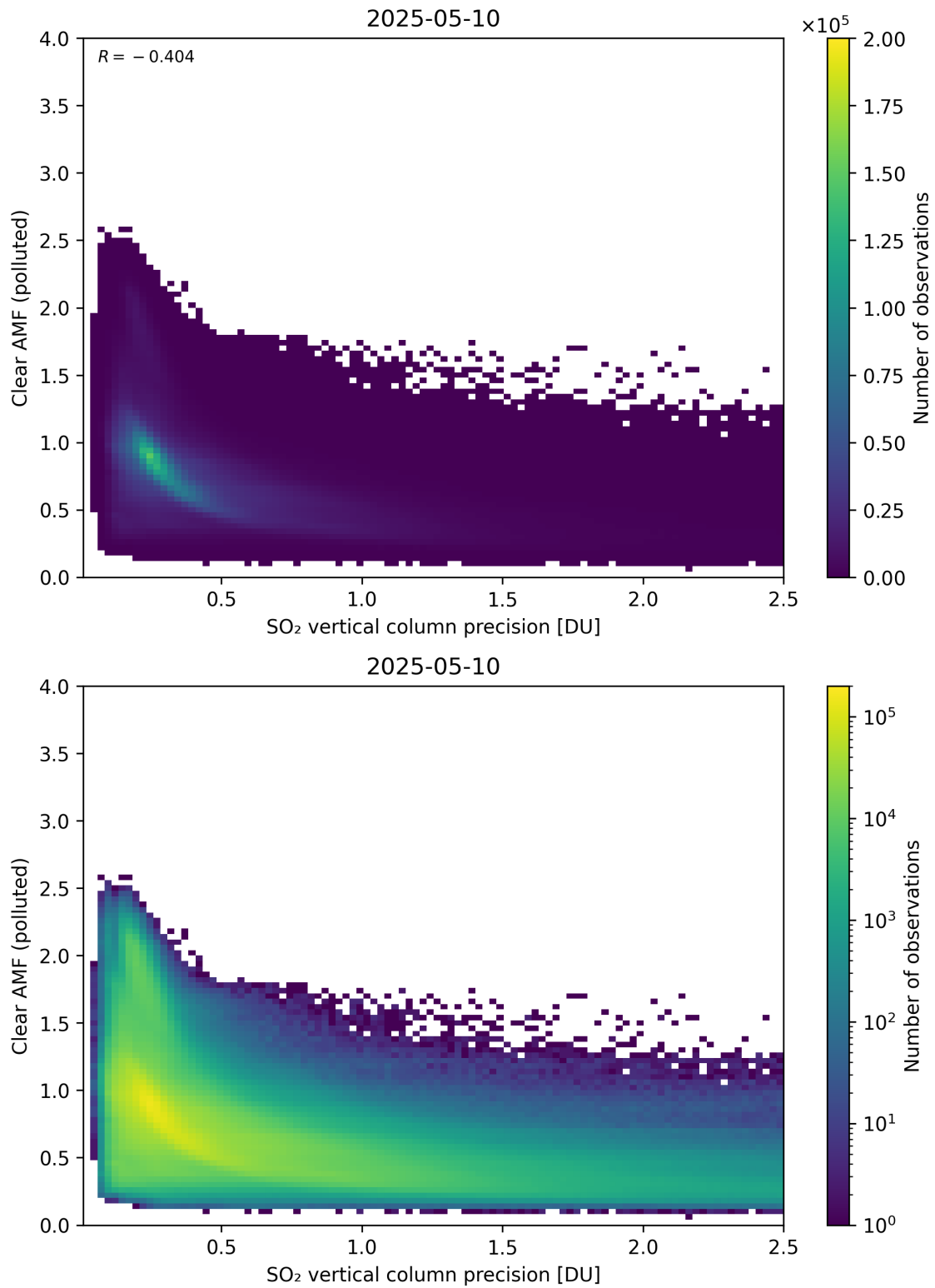
Figure 335: Scatter density plot of “SO 2 vertical column precision” against “Clear AMF (polluted)” for 2025-05-10 to 2025-05-11.
