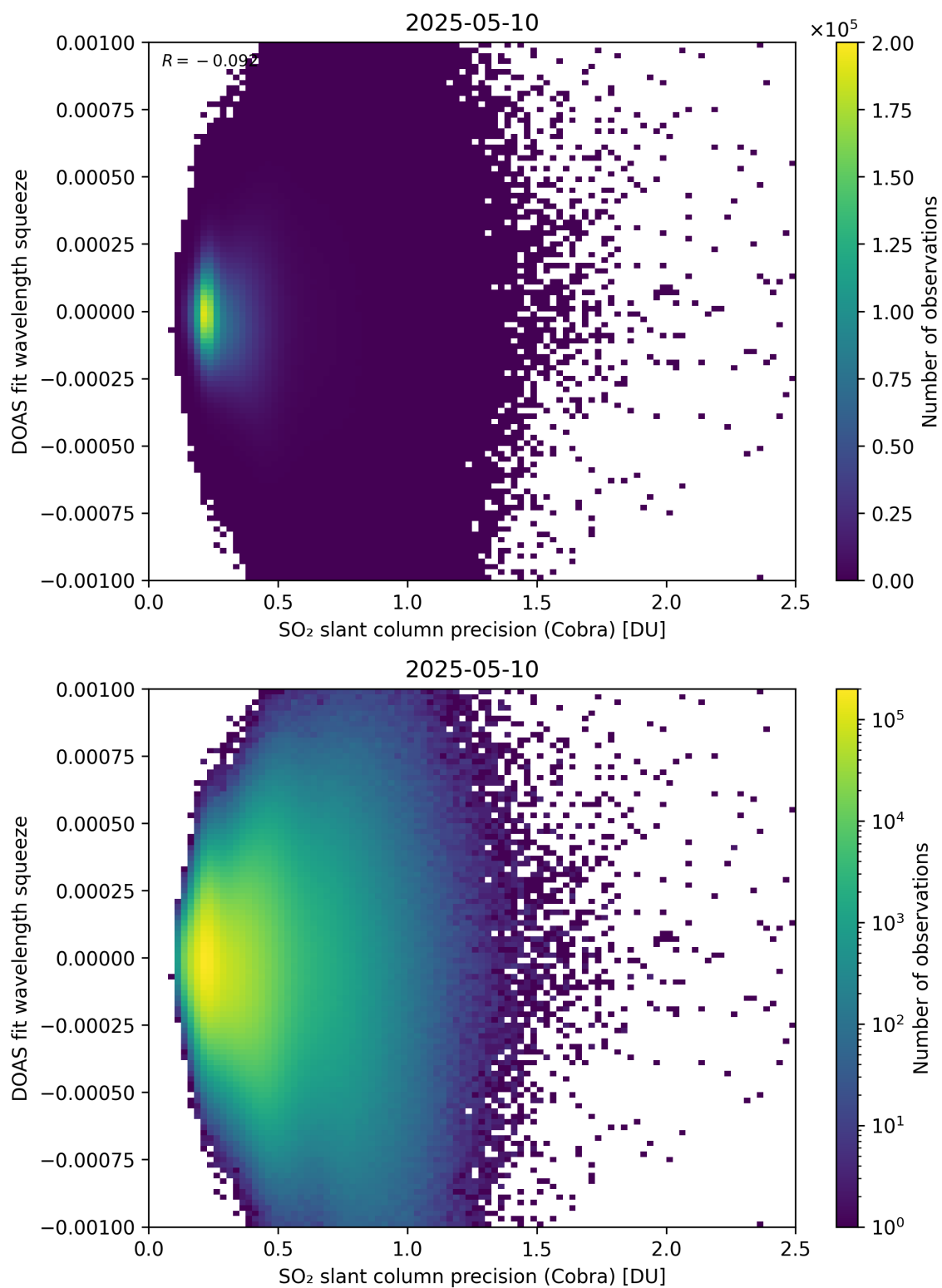
Figure 203: Scatter density plot of “SO 2 slant column precision (Cobra)” against “DOAS fit wavelength squeeze” for 2025-05-10 to 2025-05-11.
