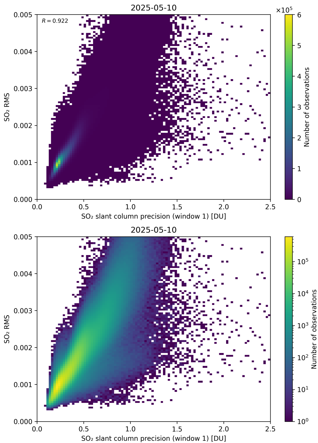
Figure 273: Scatter density plot of “SO 2 slant column precision (window 1)” against “SO 2 RMS” for 2025-05-10 to 2025-05-11.
