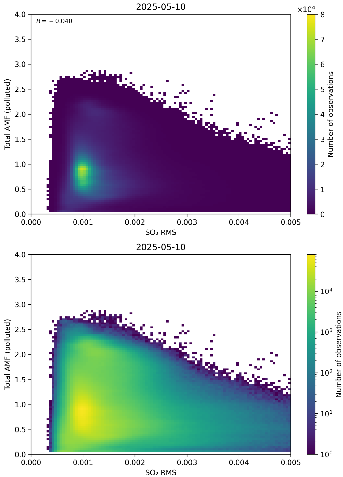
Figure 148: Scatter density plot of “SO 2 RMS” against “Total AMF (polluted)” for 2025-05-10 to 2025-05-11.
