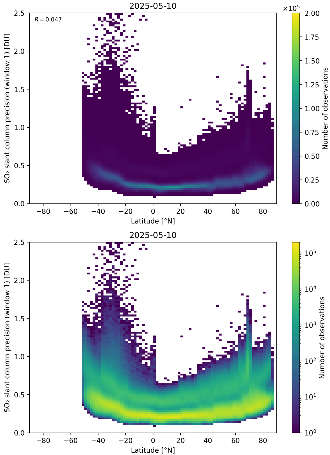
Figure 163: Scatter density plot of “Latitude” against “SO 2 slant column precision (window 1)” for 2025-05-10 to 2025-05-11.
