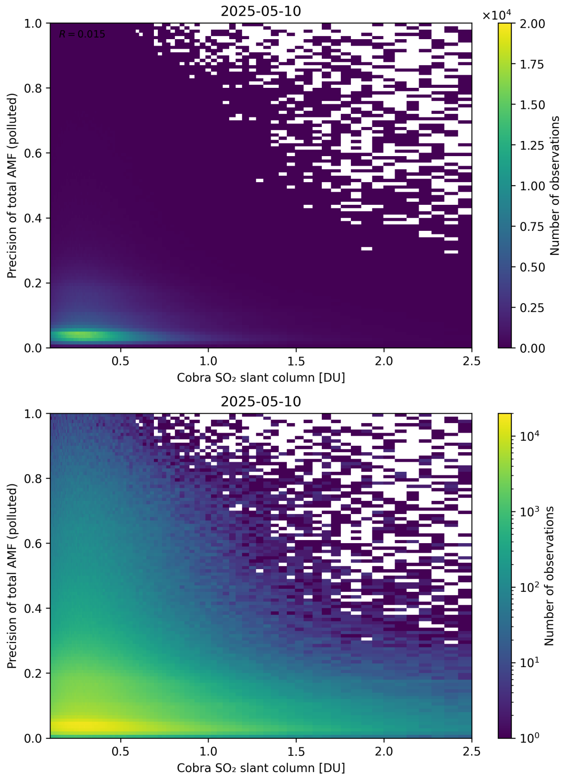
Figure 225: Scatter density plot of “Cobra SO 2 slant column” against “Precision of total AMF (polluted)” for 2025-05-10 to 2025-05-11.
