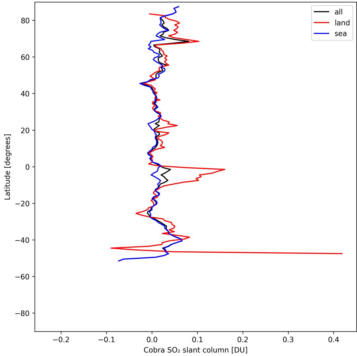
Figure 35: Zonal average of “Cobra SO 2 slant column” for 2025-05-10 to 2025-05-11.
