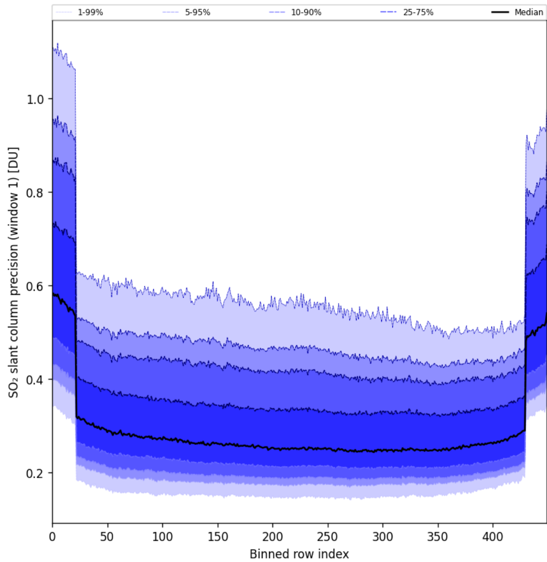
Figure 90: Along track statistics of “SO 2 slant column precision (window 1)” for 2025-05-10 to 2025-05-11
