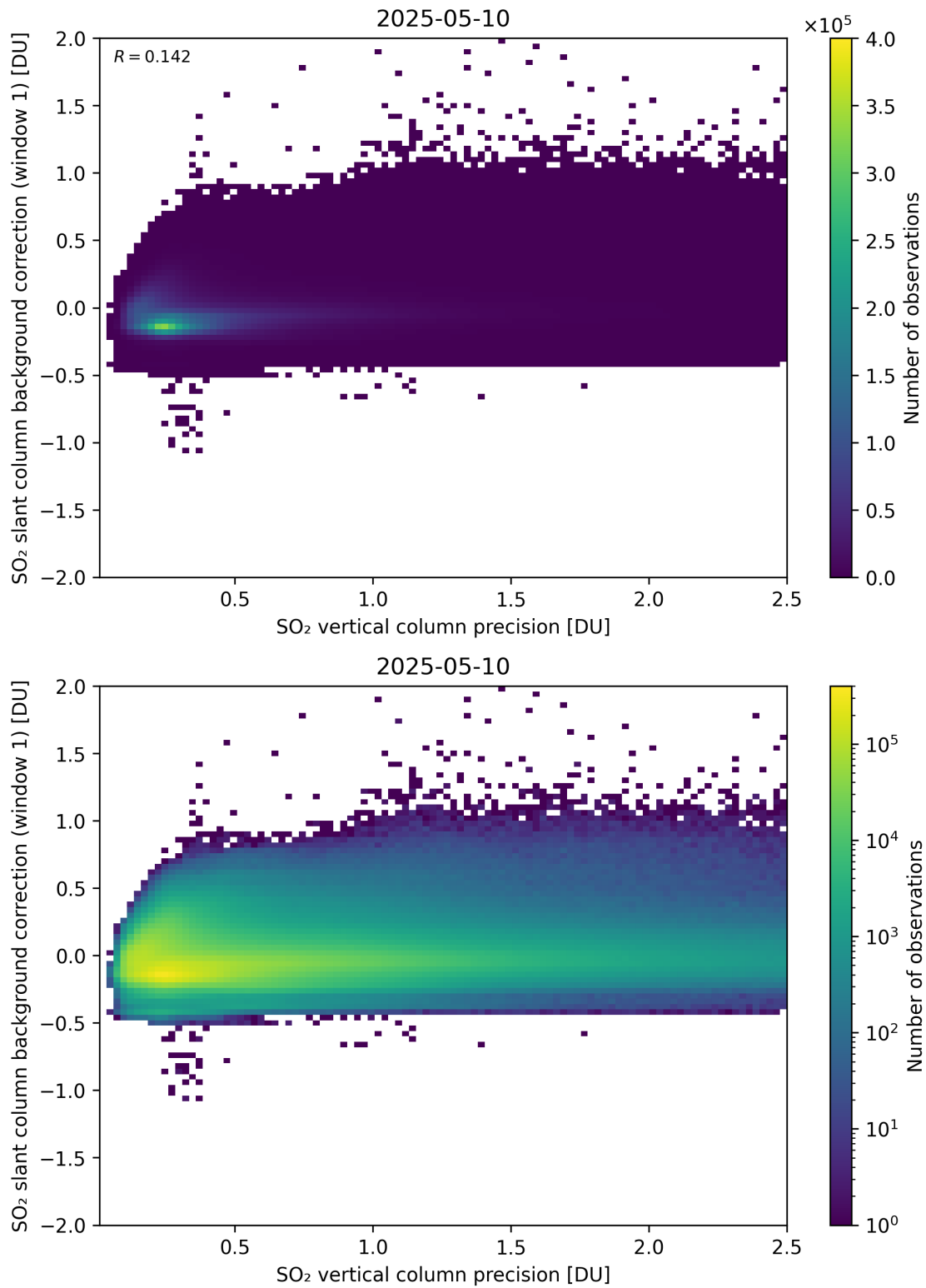
Figure 329: Scatter density plot of “SO 2 vertical column precision” against “SO 2 slant column background correction (window 1)” for 2025-05-10 to 2025-05-11.
