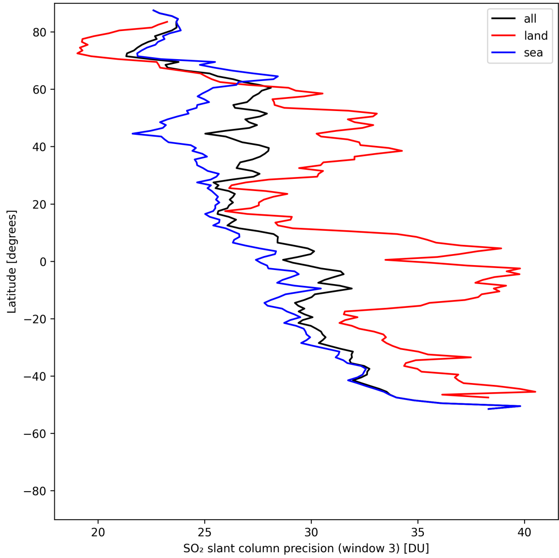
Figure 46: Zonal average of “SO 2 slant column precision (window 3)” for 2025-05-10 to 2025-05-11.
