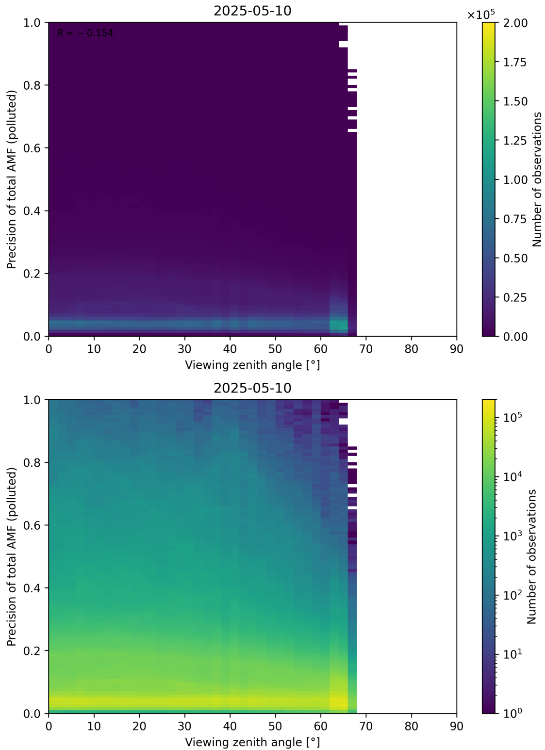
Figure 382: Scatter density plot of “Viewing zenith angle” against “Precision of total AMF (polluted)” for 2025-05-10 to 2025-05-11.
