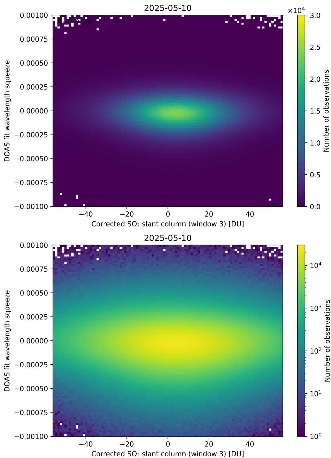
Figure 257: Scatter density plot of “Corrected SO 2 slant column (window 3)” against “DOAS fit wavelength squeeze” for 2025-05-10 to 2025-05-11.
