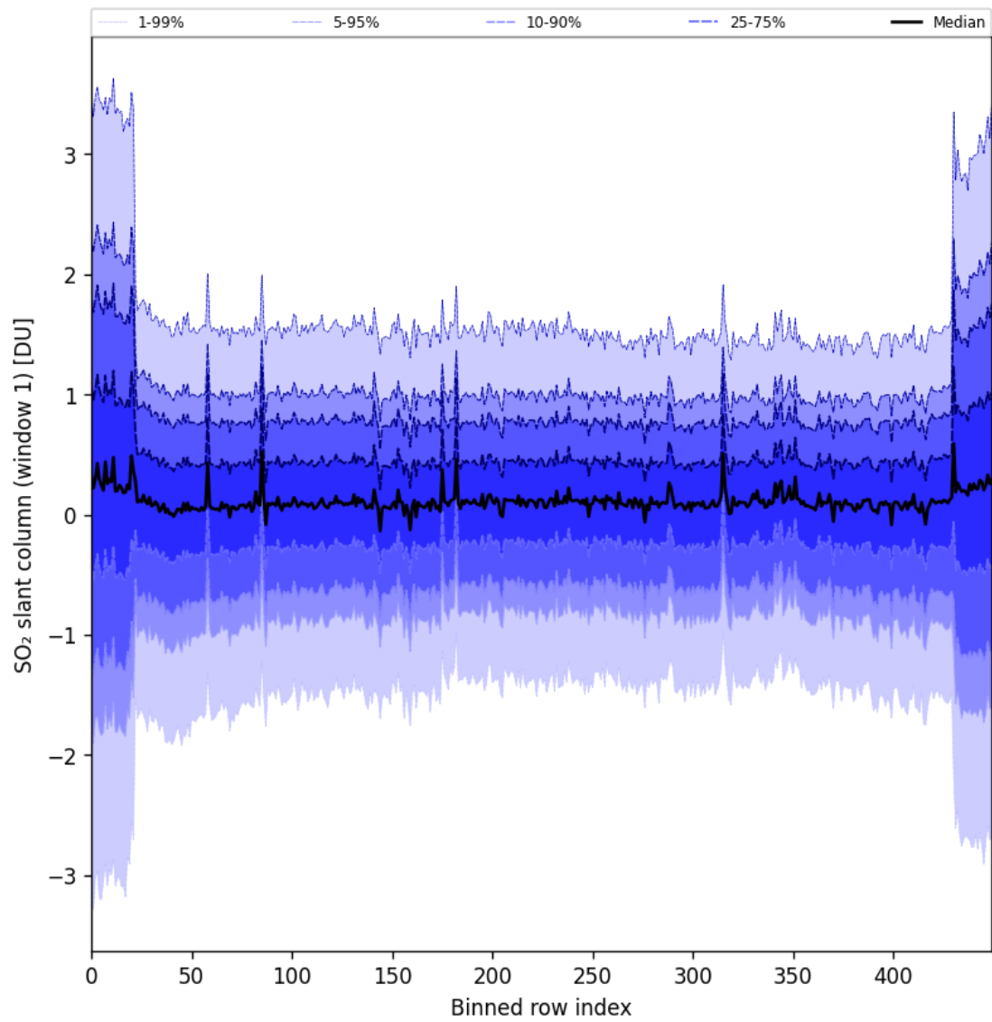
Figure 89: Along track statistics of “SO 2 slant column (window 1)” for 2025-05-10 to 2025-05-11
