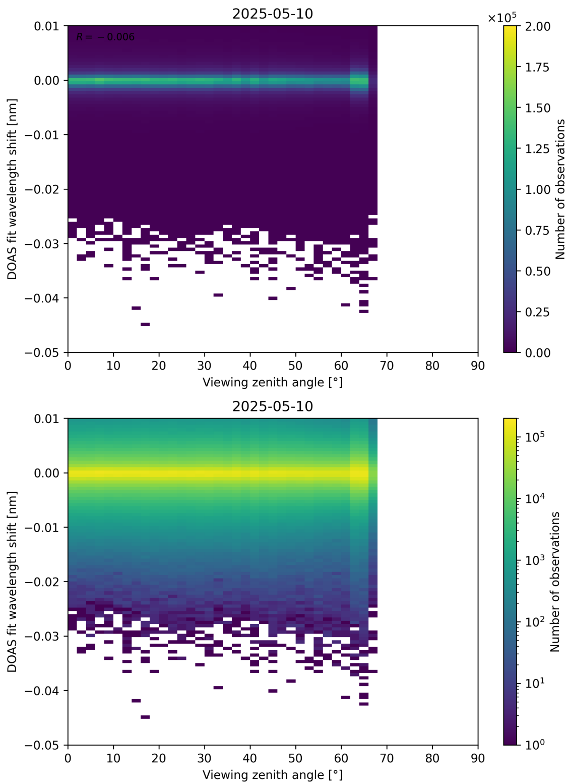
Figure 365: Scatter density plot of “Viewing zenith angle” against “DOAS fit wavelength shift” for 2025-05-10 to 2025-05-11.
