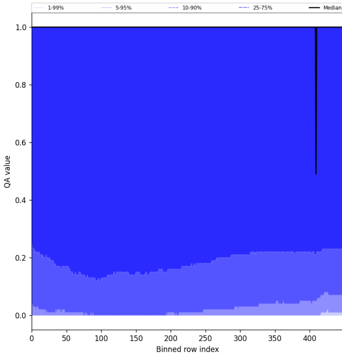
Figure 83: Along track statistics of “QA value” for 2025-05-10 to 2025-05-11
