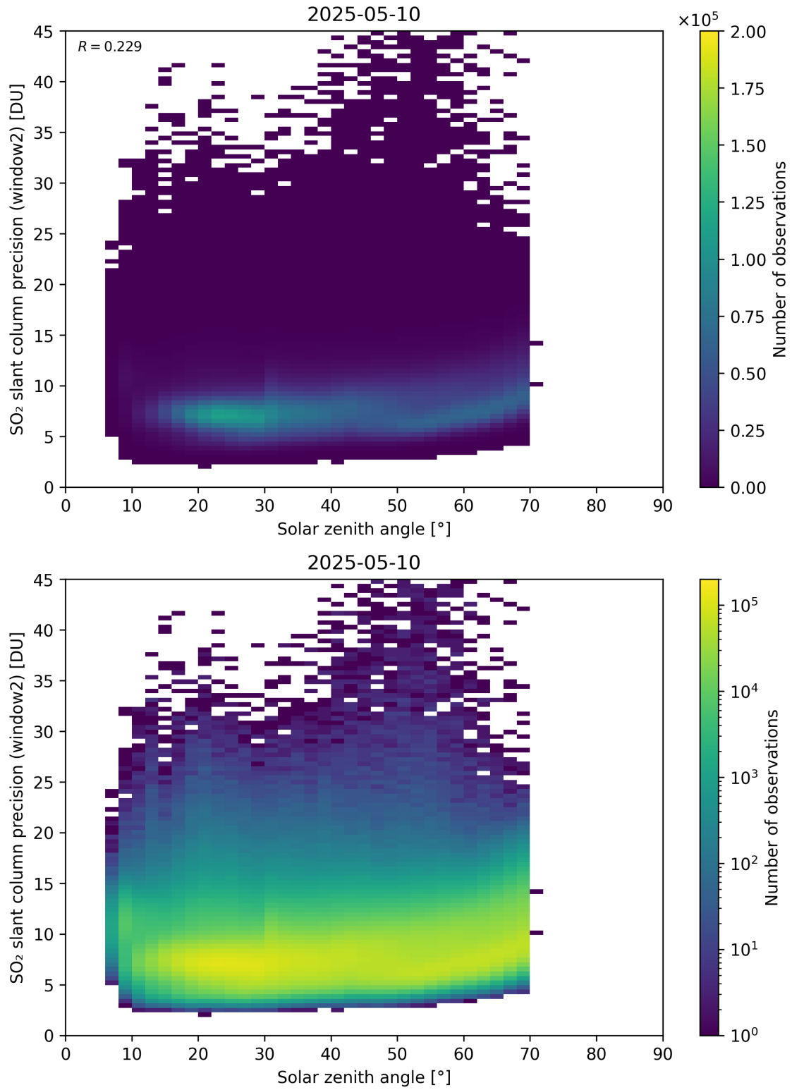
Figure 186: Scatter density plot of “Solar zenith angle” against “SO 2 slant column precision (window2)” for 2025-05-10 to 2025-05-11.
