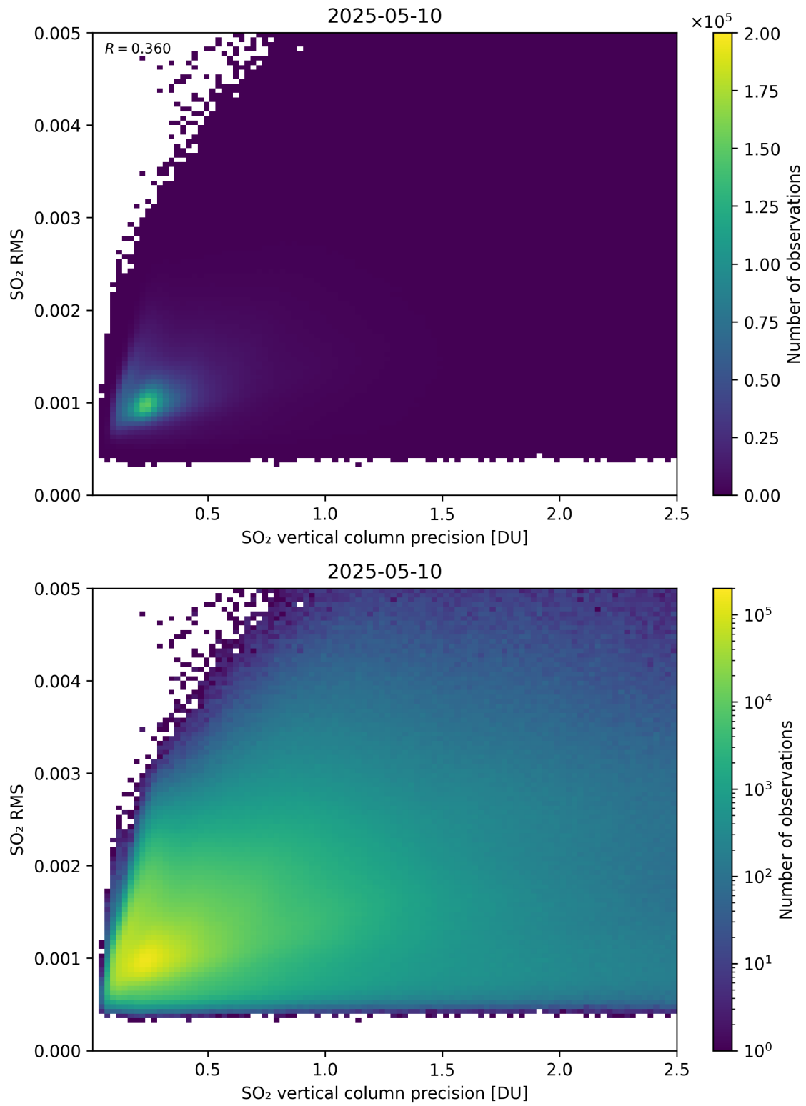
Figure 334: Scatter density plot of “SO 2 vertical column precision” against “SO 2 RMS” for 2025-05-10 to 2025-05-11.
