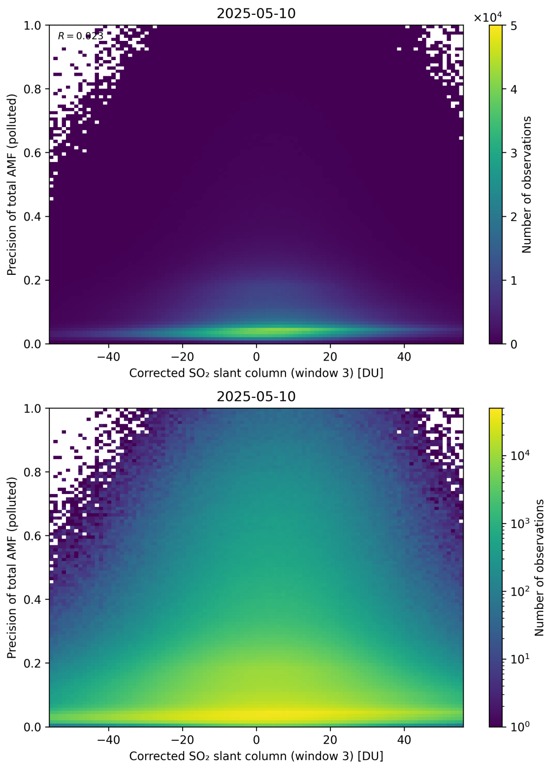
Figure 261: Scatter density plot of “Corrected SO 2 slant column (window 3)” against “Precision of total AMF (polluted)” for 2025-05-10 to 2025-05-11.
