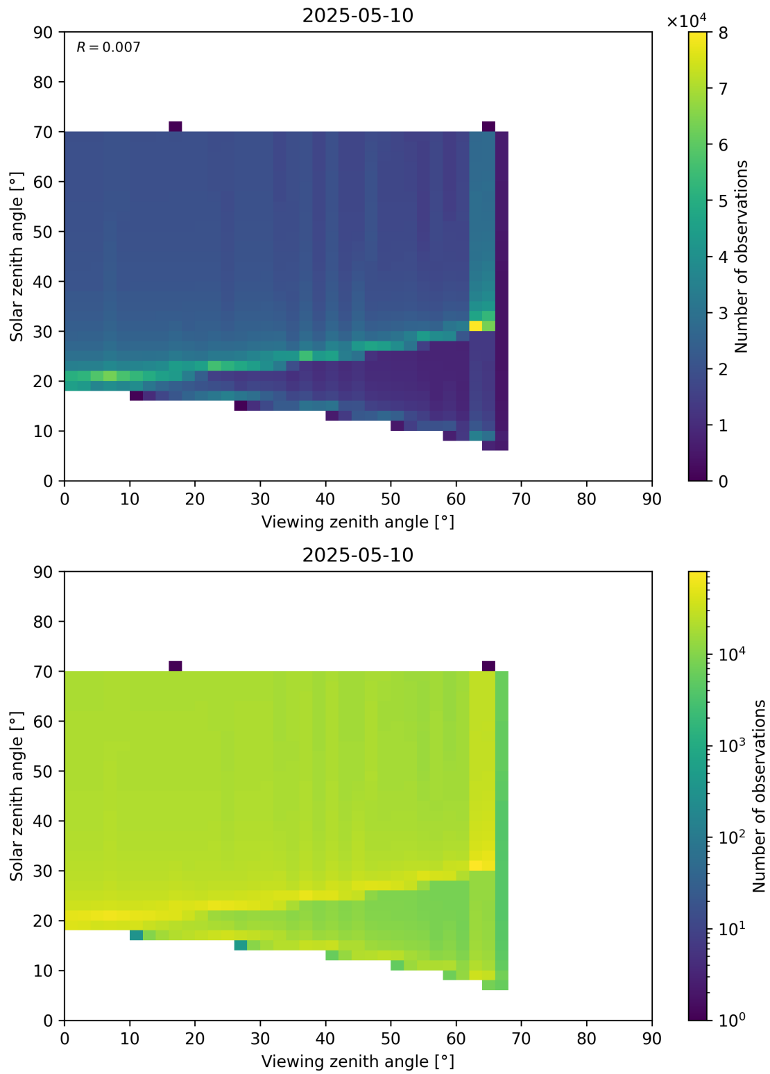
Figure 369: Scatter density plot of “Viewing zenith angle” against “Solar zenith angle” for 2025-05-10 to 2025-05-11.
