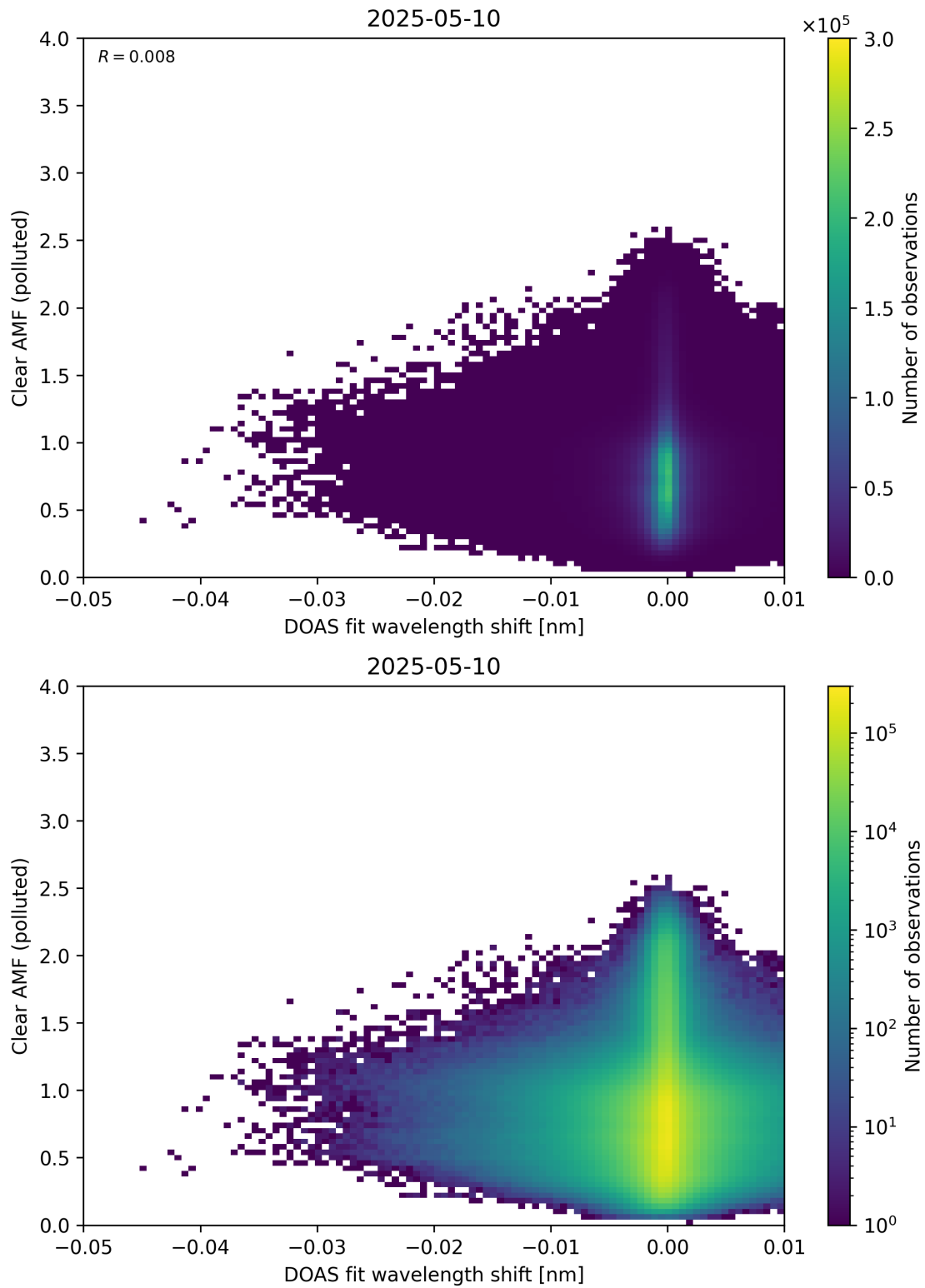
Figure 140: Scatter density plot of “DOAS fit wavelength shift” against “Clear AMF (polluted)” for 2025-05-10 to 2025-05-11.
