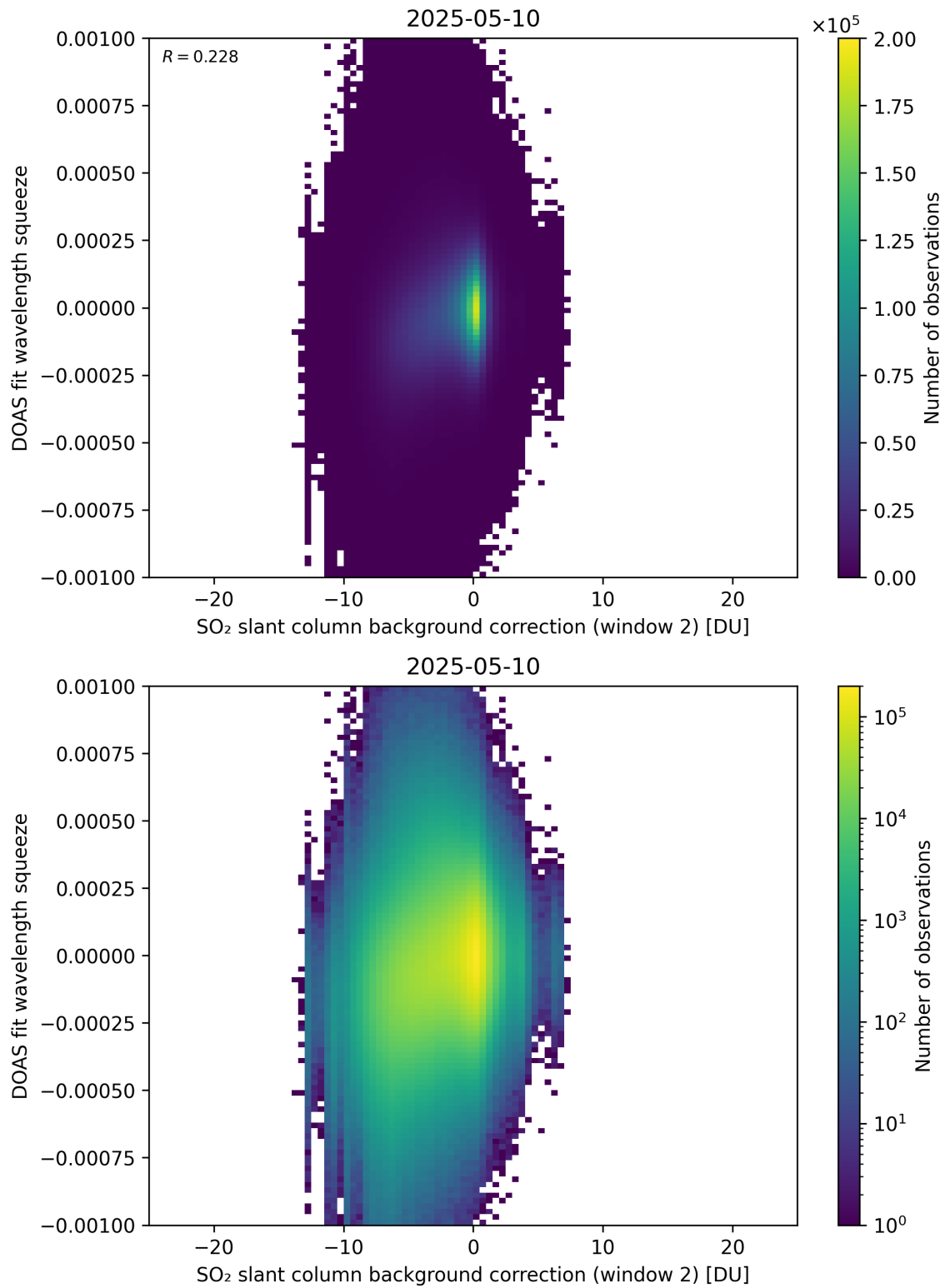
Figure 124: Scatter density plot of “SO 2 slant column background correction (window 2)” against “DOAS fit wavelength squeeze” for 2025-05-10 to 2025-05-11.
