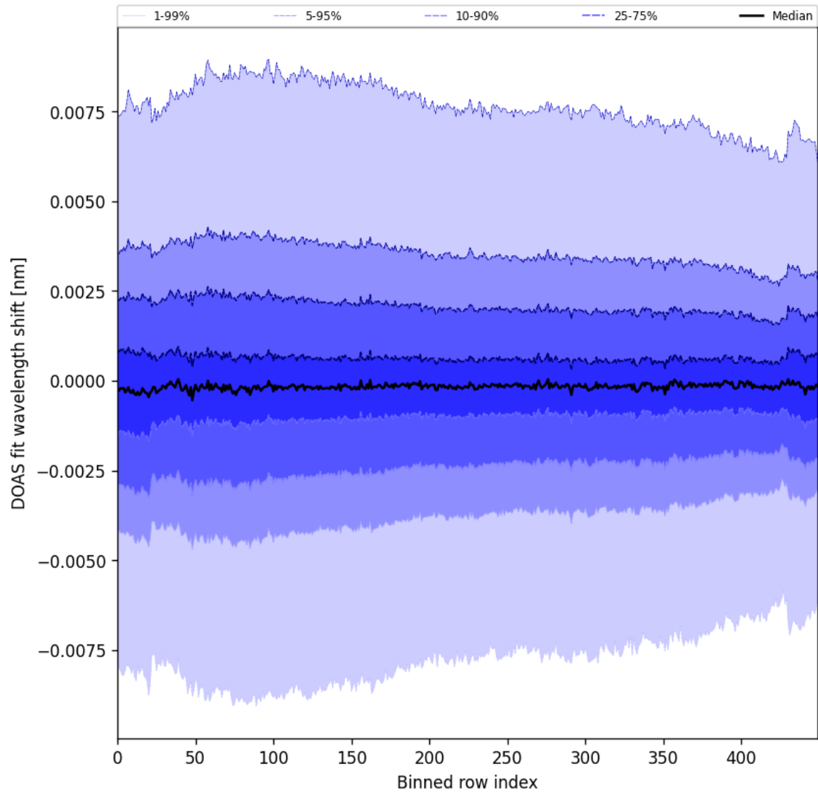
Figure 102: Along track statistics of “DOAS fit wavelength shift” for 2025-05-10 to 2025-05-11
