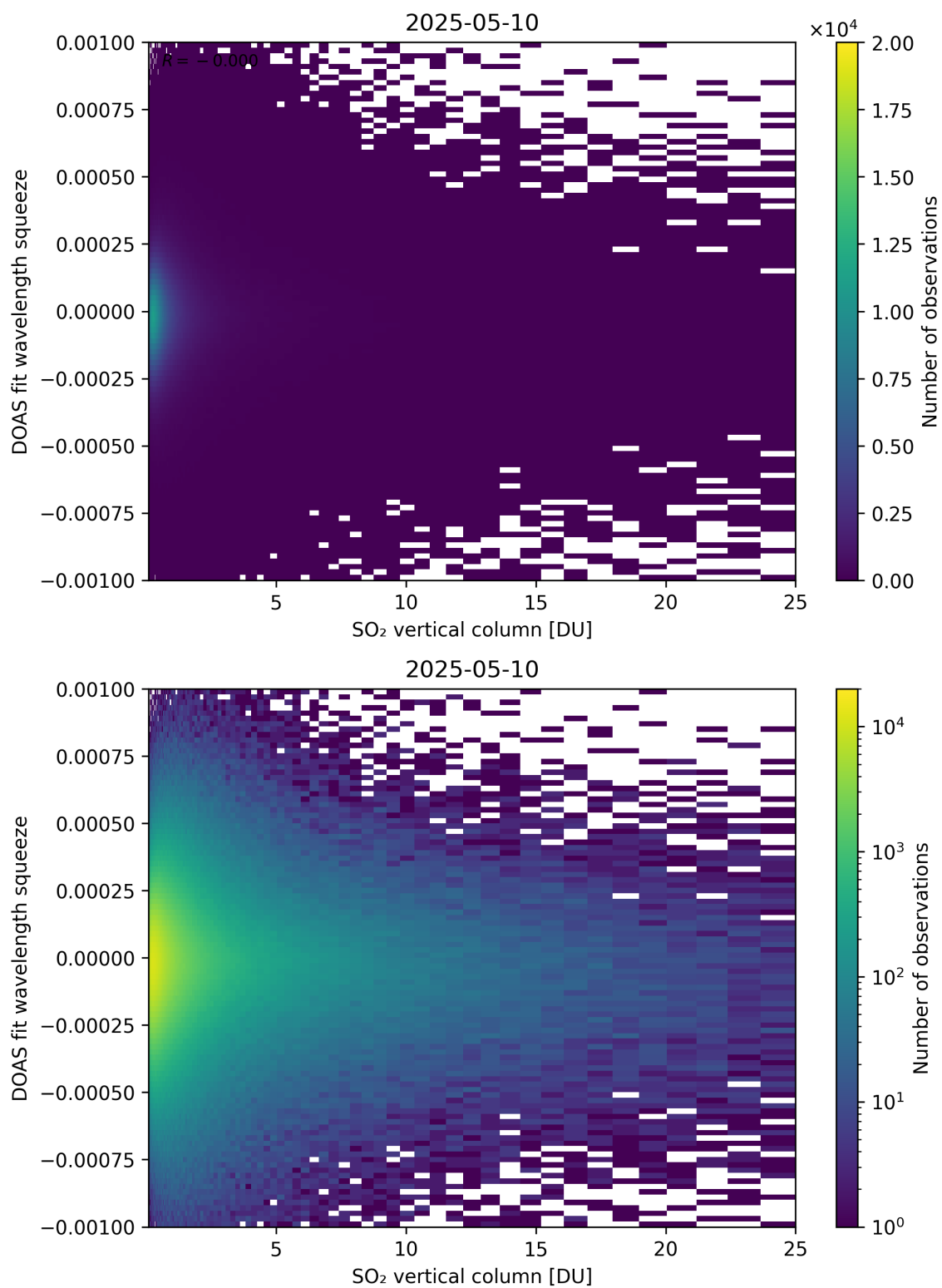
Figure 327: Scatter density plot of “SO 2 vertical column” against “DOAS fit wavelength squeeze” for 2025-05-10 to 2025-05-11.
