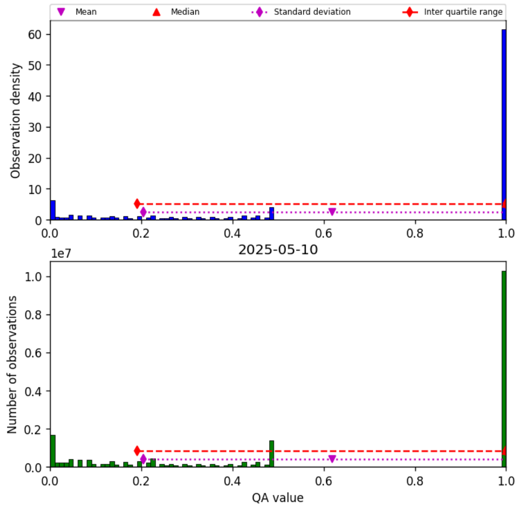
Figure 57: Histogram of “QA value” for 2025-05-10 to 2025-05-11
