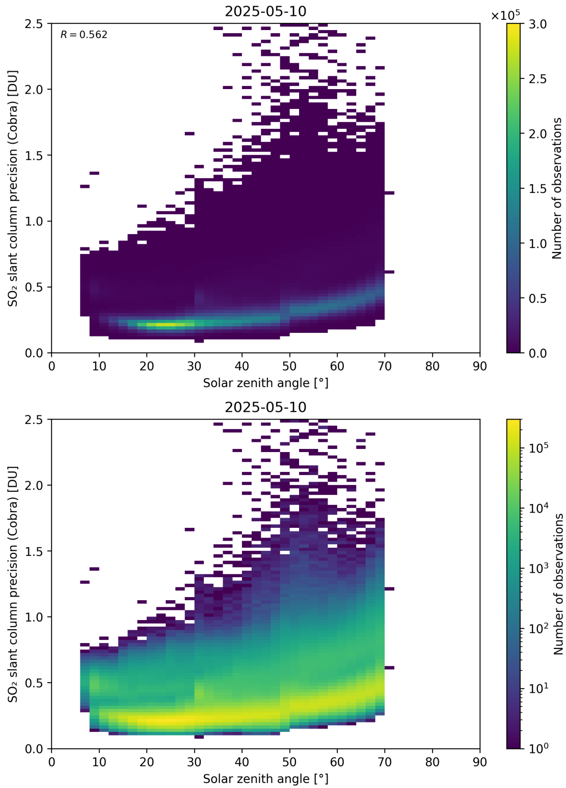
Figure 180: Scatter density plot of “Solar zenith angle” against “SO 2 slant column precision (Cobra)” for 2025-05-10 to 2025-05-11.
