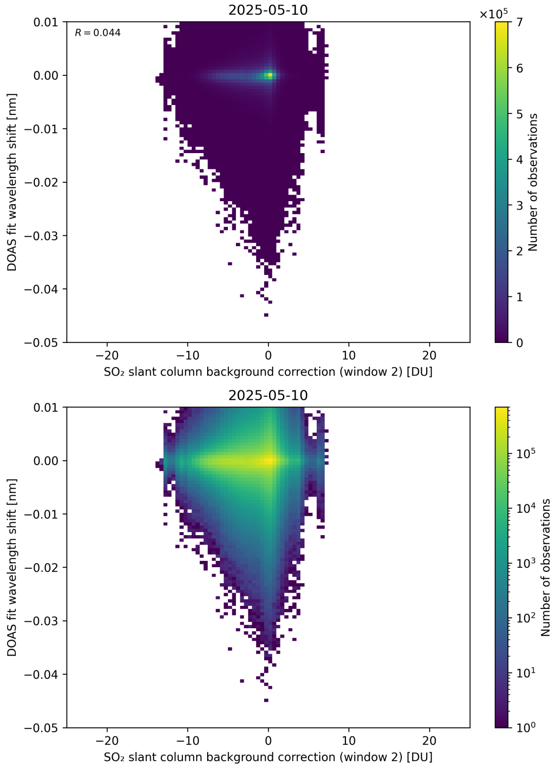
Figure 123: Scatter density plot of “SO 2 slant column background correction (window 2)” against “DOAS fit wavelength shift” for 2025-05-10 to 2025-05-11.
