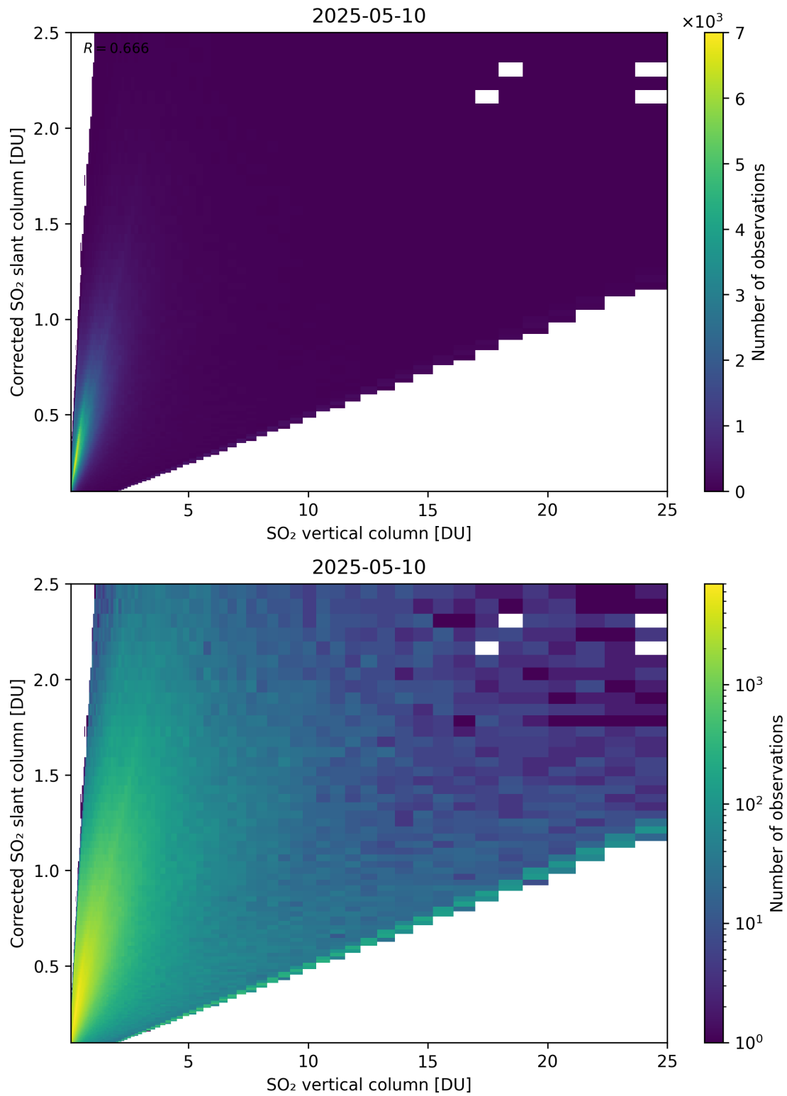
Figure 351: Scatter density plot of “SO 2 vertical column” against “Corrected SO 2 slant column” for 2025-05-10 to 2025-05-11.
