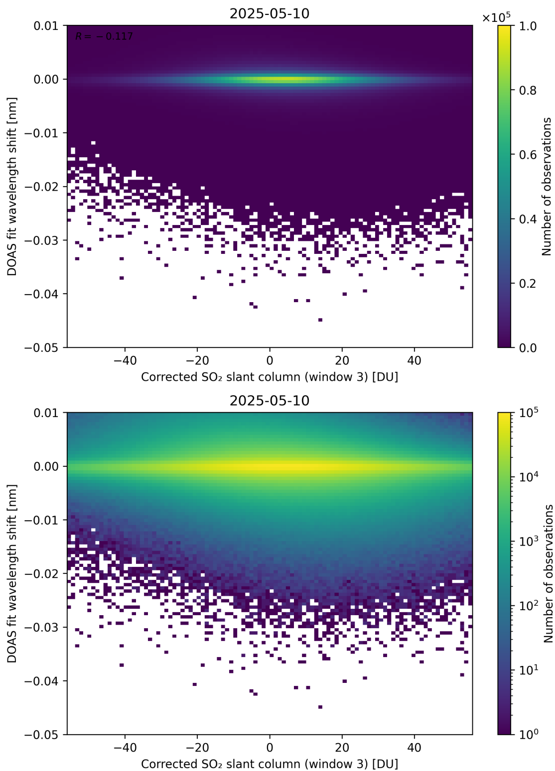
Figure 256: Scatter density plot of “Corrected SO 2 slant column (window 3)” against “DOAS fit wavelength shift” for 2025-05-10 to 2025-05-11.
