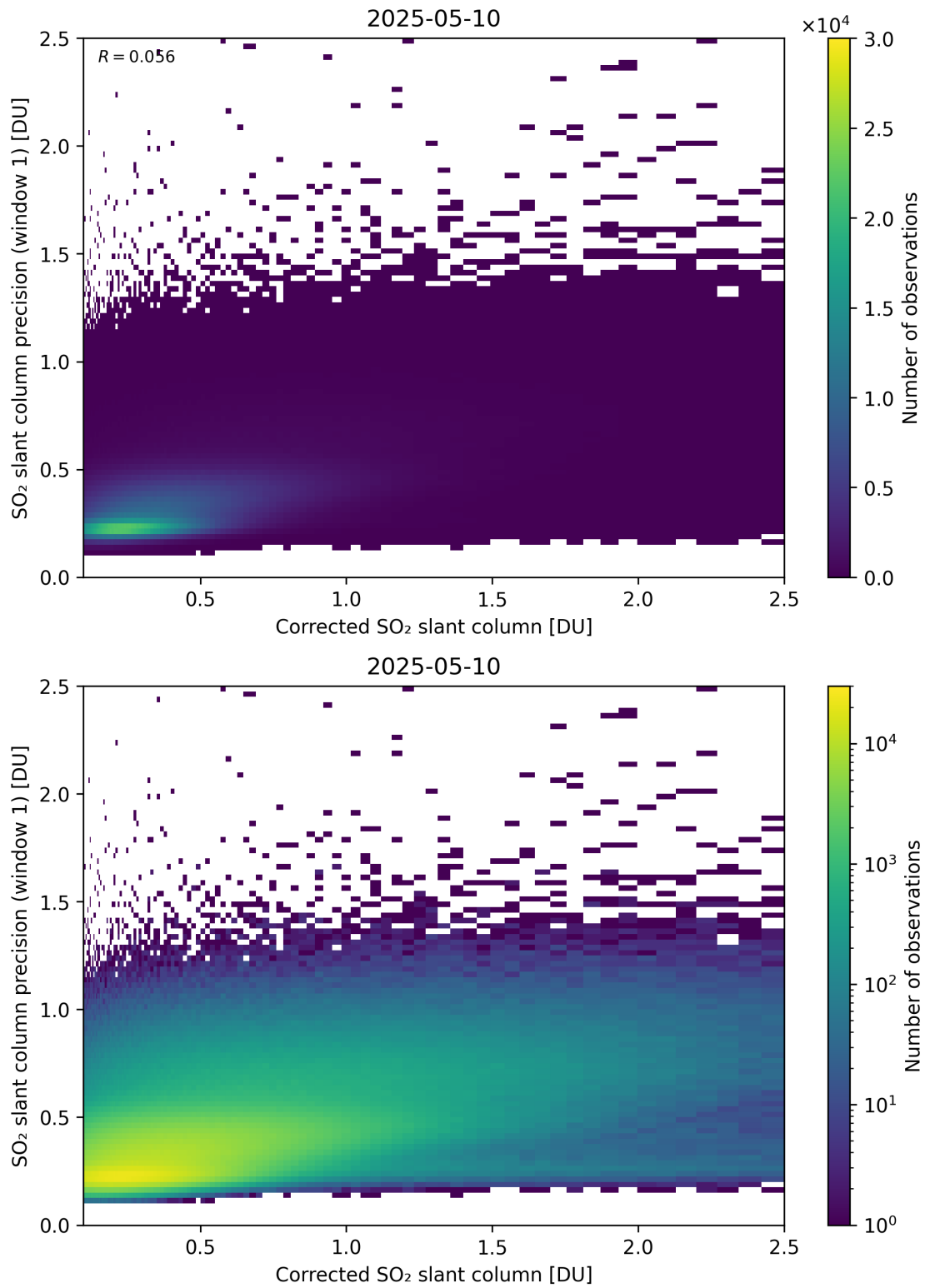
Figure 238: Scatter density plot of “Corrected SO 2 slant column” against “SO 2 slant column precision (window 1)” for 2025-05-10 to 2025-05-11.
