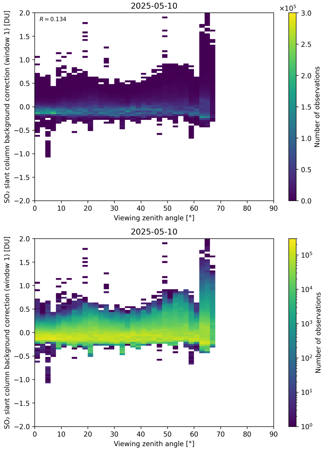
Figure 362: Scatter density plot of “Viewing zenith angle” against “SO 2 slant column background correction (window 1)” for 2025-05-10 to 2025-05-11.
