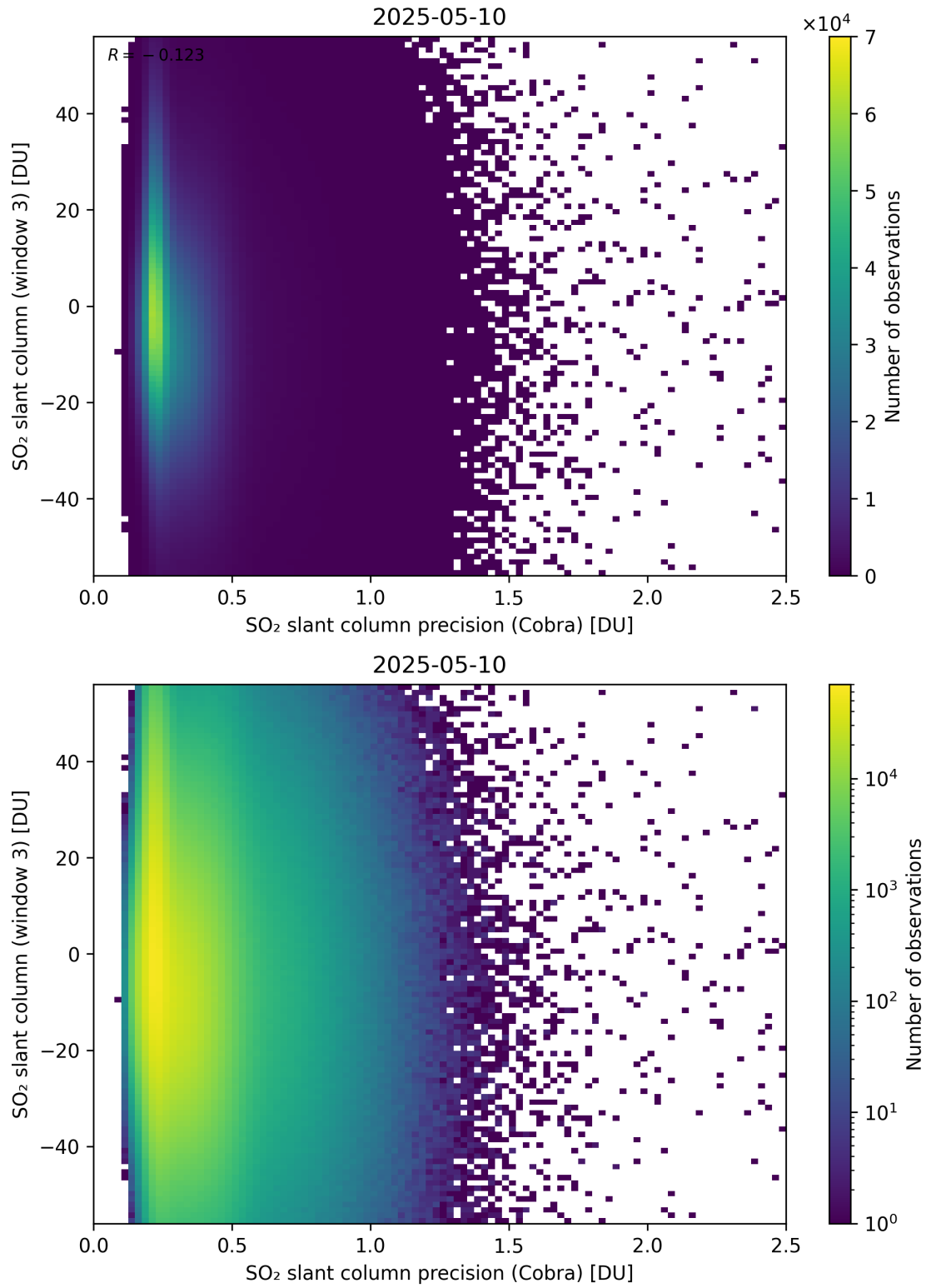
Figure 211: Scatter density plot of “SO 2 slant column precision (Cobra)” against “SO 2 slant column (window 3)” for 2025-05-10 to 2025-05-11.
