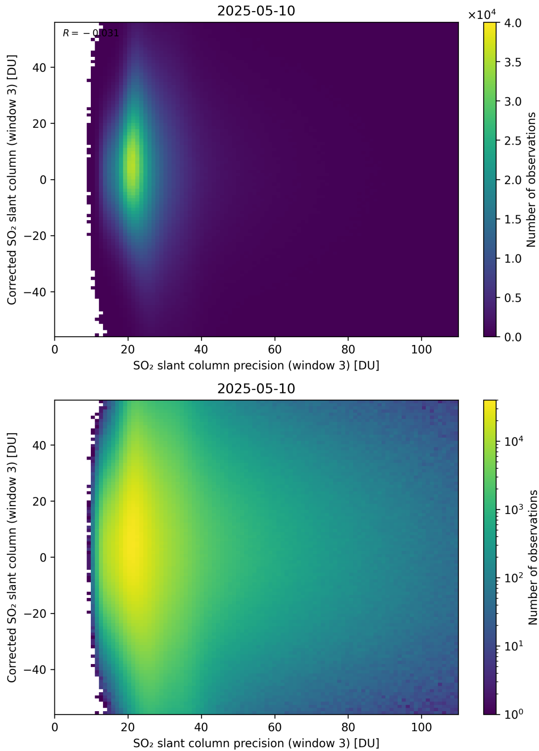
Figure 312: Scatter density plot of “SO 2 slant column precision (window 3)” against “Corrected SO 2 slant column (window 3)” for 2025-05-10 to 2025-05-11.
