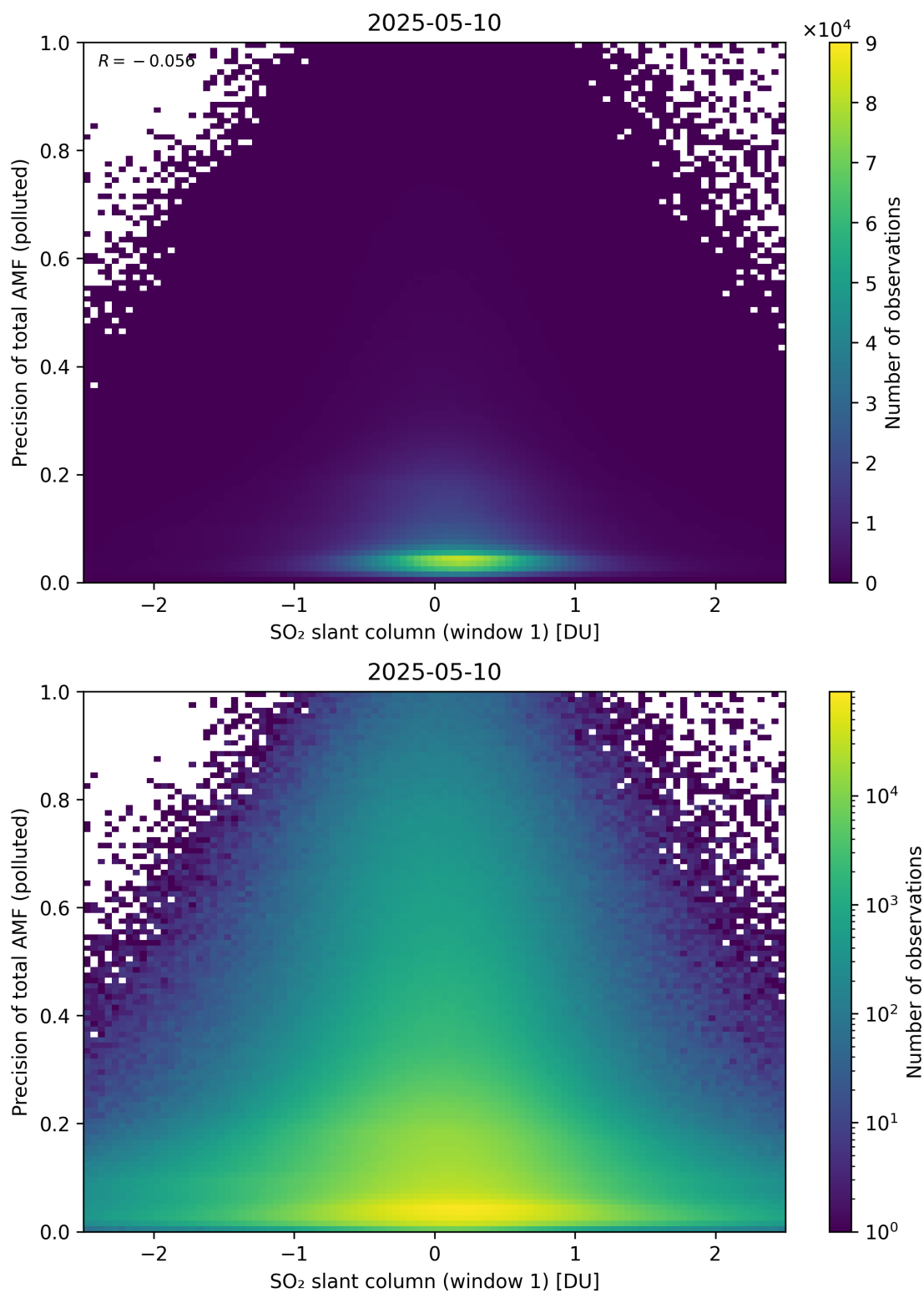
Figure 290: Scatter density plot of “SO 2 slant column (window 1)” against “Precision of total AMF (polluted)” for 2025-05-10 to 2025-05-11.
