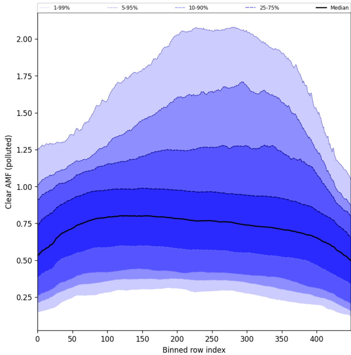
Figure 107: Along track statistics of “Clear AMF (polluted)” for 2025-05-10 to 2025-05-11
