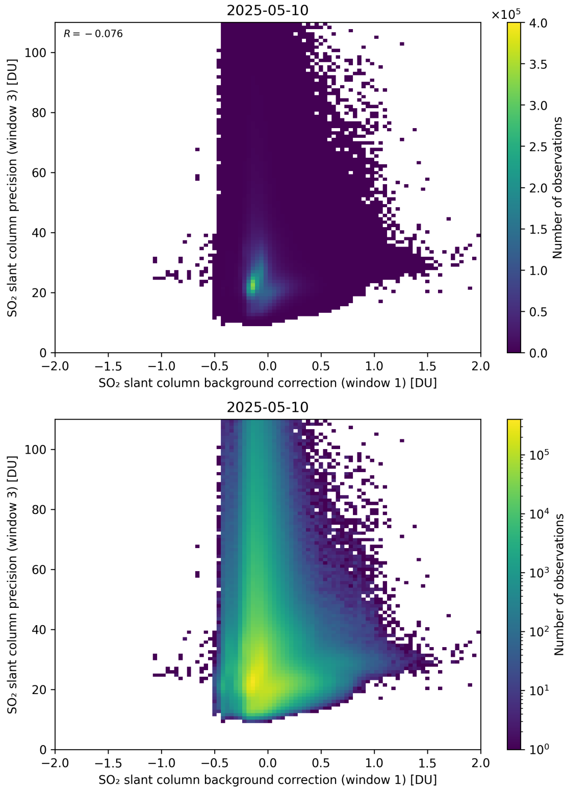
Figure 119: Scatter density plot of “SO 2 slant column background correction (window 1)” against “SO 2 slant column precision (window 3)” for 2025-05-10 to 2025-05-11.
