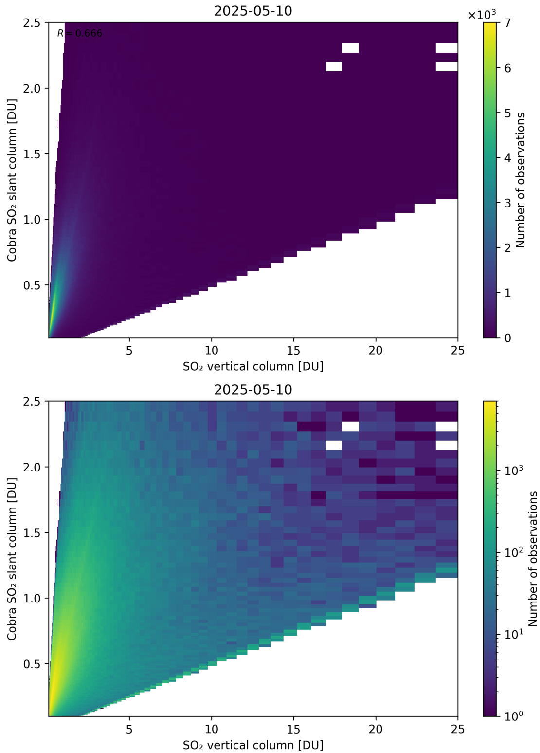
Figure 349: Scatter density plot of “SO 2 vertical column” against “Cobra SO 2 slant column” for 2025-05-10 to 2025-05-11.
