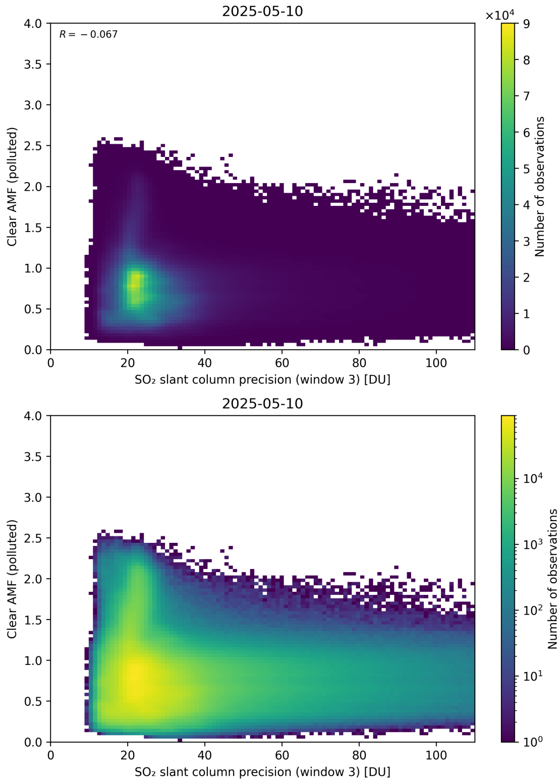
Figure 311: Scatter density plot of “SO 2 slant column precision (window 3)” against “Clear AMF (polluted)” for 2025-05-10 to 2025-05-11.
