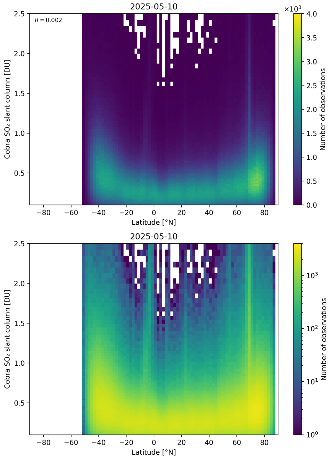
Figure 157: Scatter density plot of “Latitude” against “Cobra SO 2 slant column” for 2025-05-10 to 2025-05-11.
