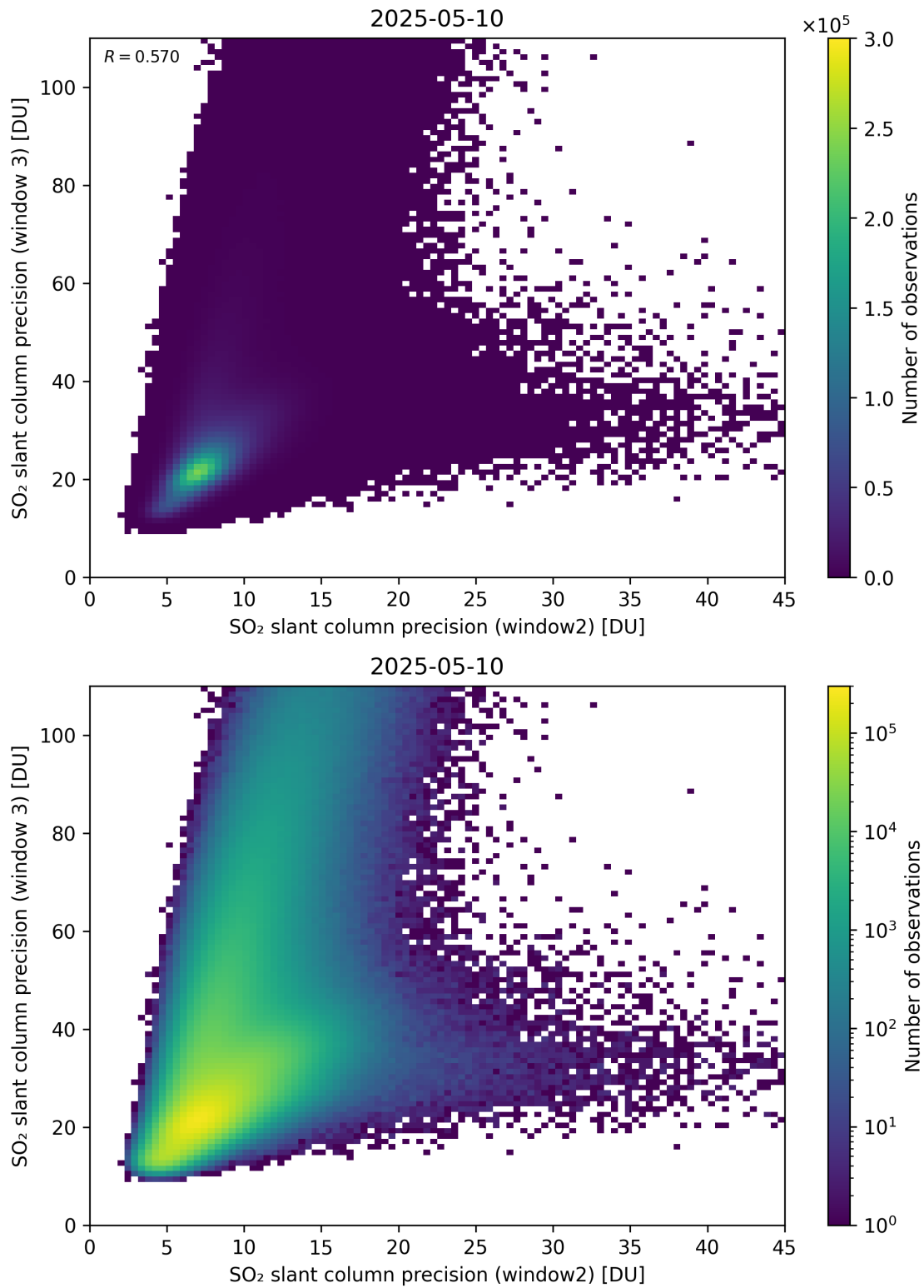
Figure 300: Scatter density plot of “SO 2 slant column precision (window2)” against “SO 2 slant column precision (window 3)” for 2025-05-10 to 2025-05-11.
