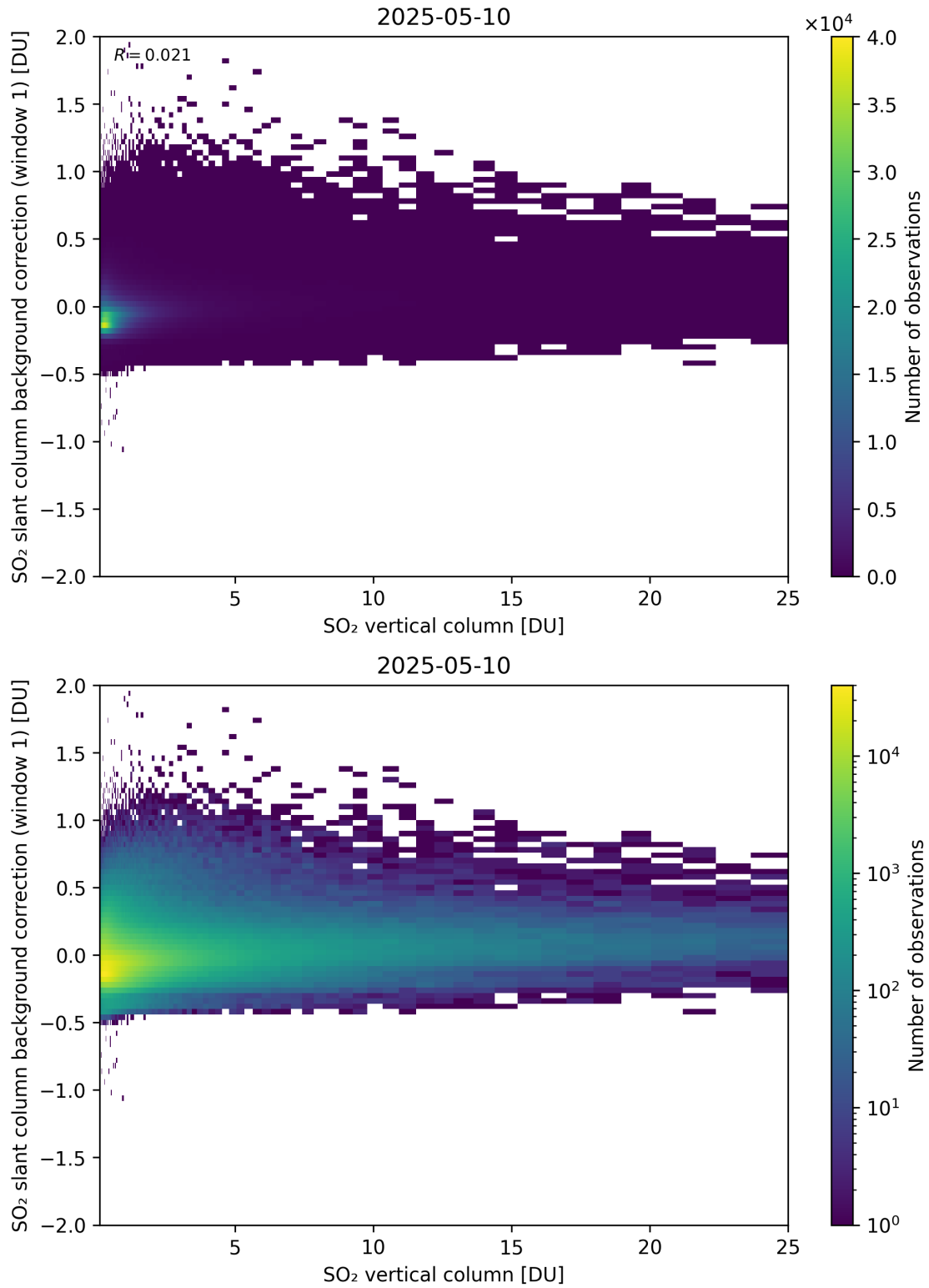
Figure 323: Scatter density plot of “SO 2 vertical column” against “SO 2 slant column background correction (window 1)” for 2025-05-10 to 2025-05-11.
