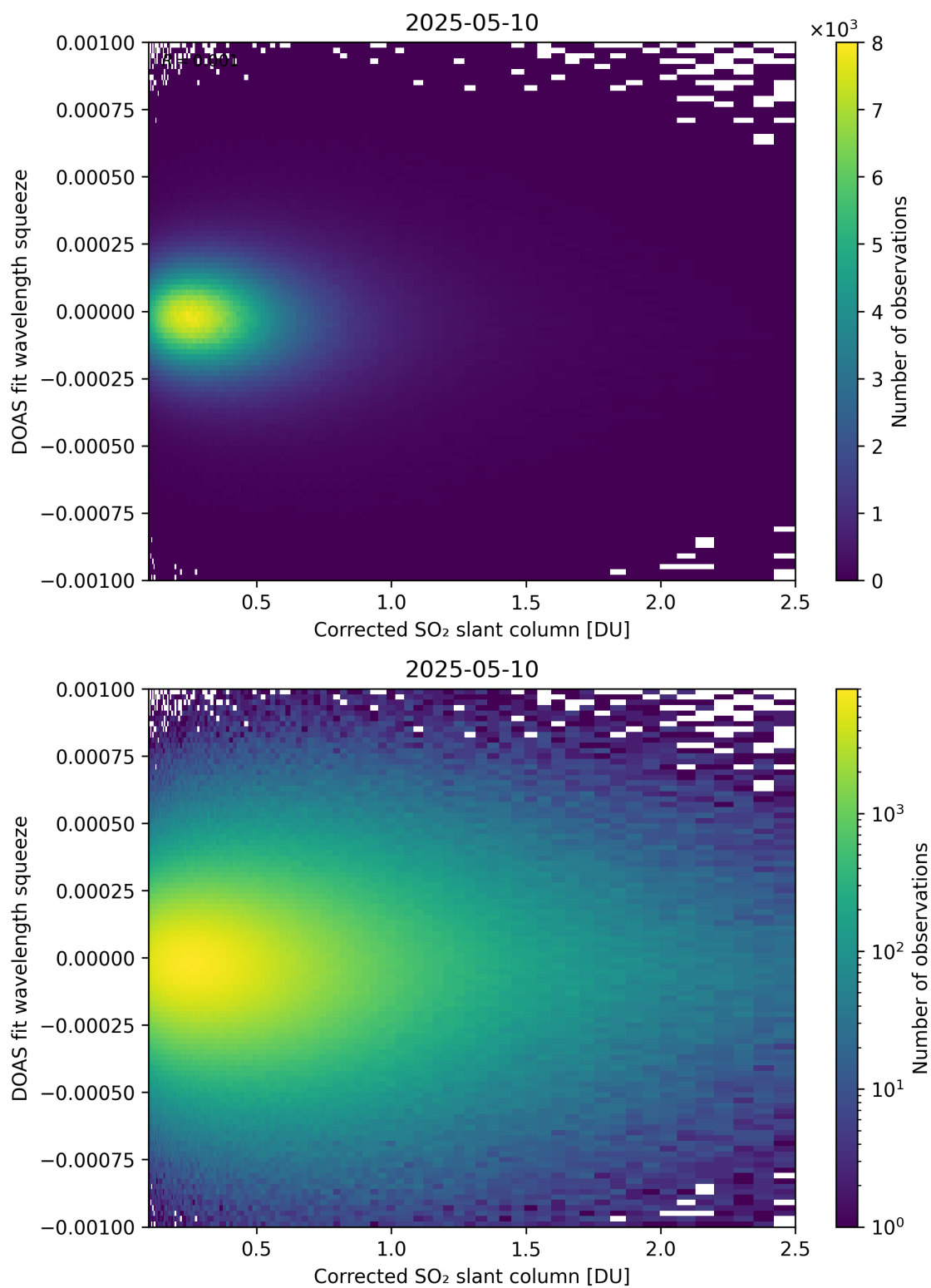
Figure 230: Scatter density plot of “Corrected SO 2 slant column” against “DOAS fit wavelength squeeze” for 2025-05-10 to 2025-05-11.
