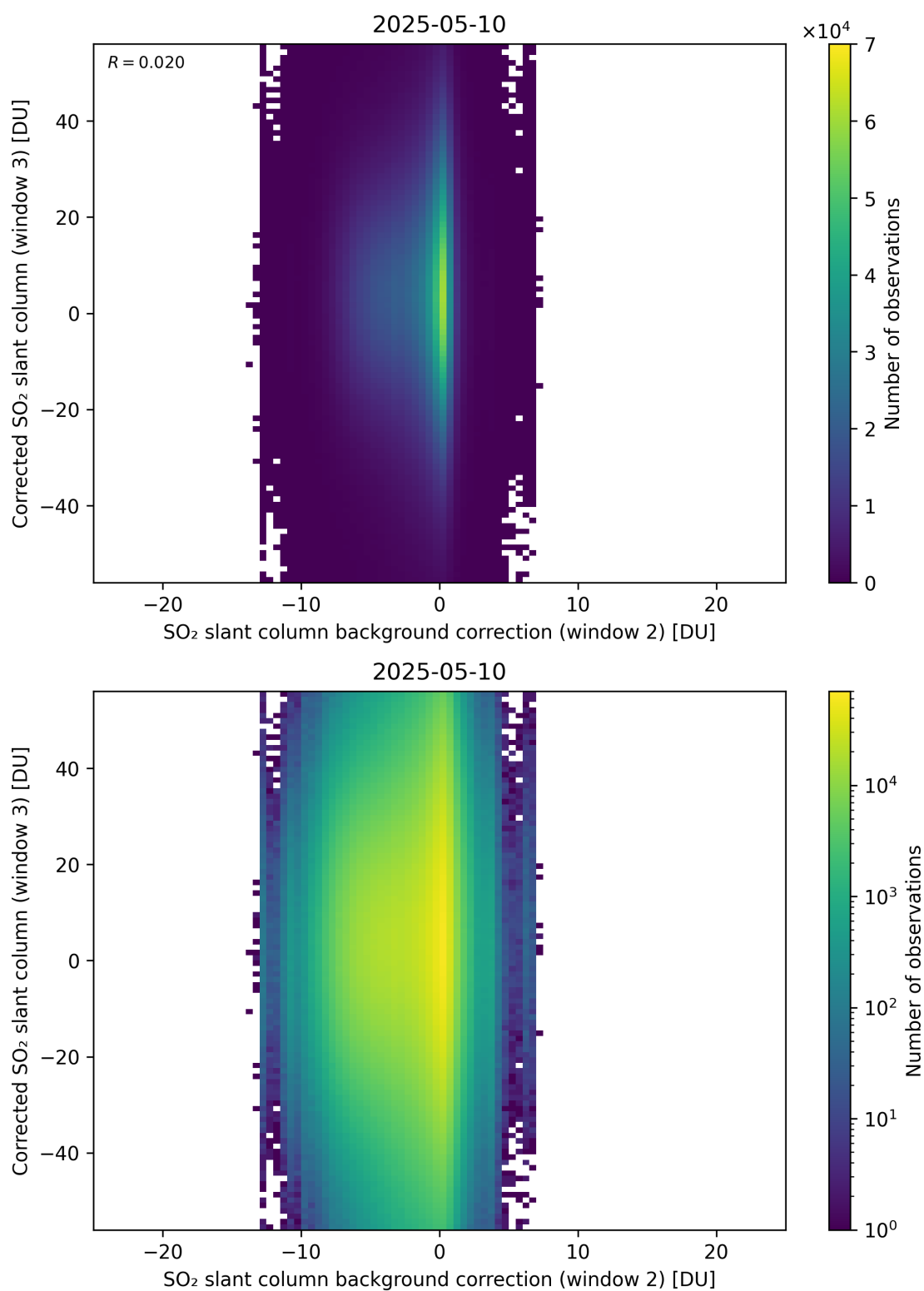
Figure 127: Scatter density plot of “SO 2 slant column background correction (window 2)” against “Corrected SO 2 slant column (window 3)” for 2025-05-10 to 2025-05-11.
