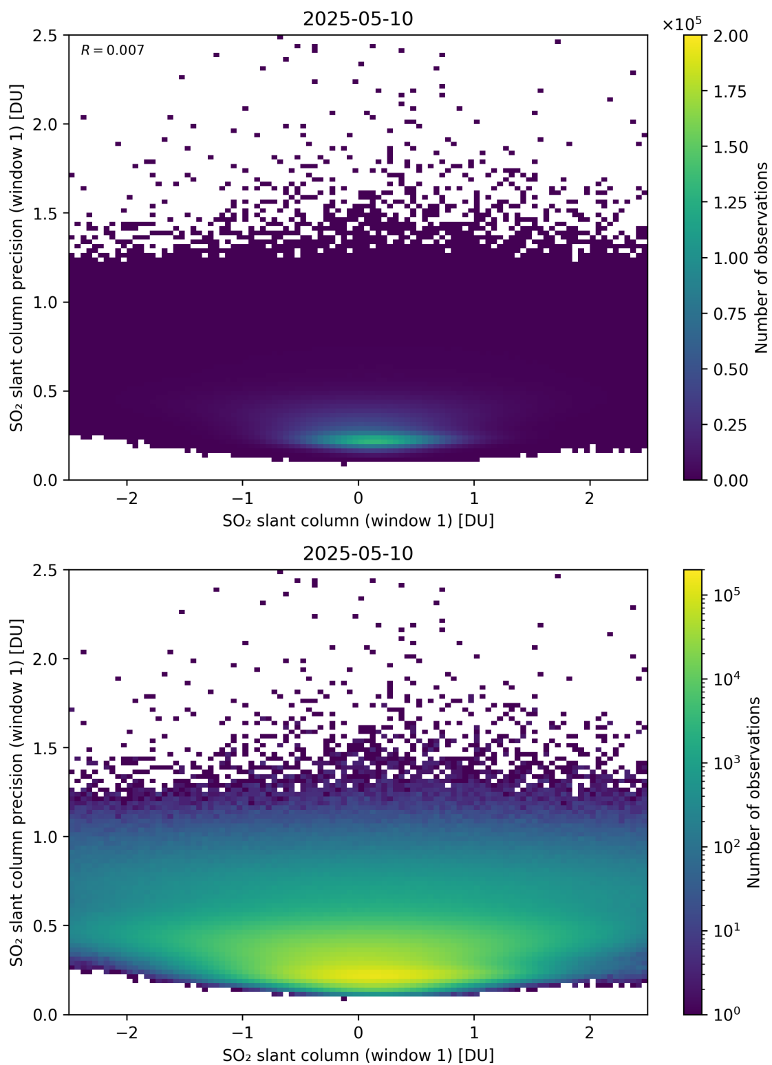
Figure 285: Scatter density plot of “SO 2 slant column (window 1)” against “SO 2 slant column precision (window 1)” for 2025-05-10 to 2025-05-11.
