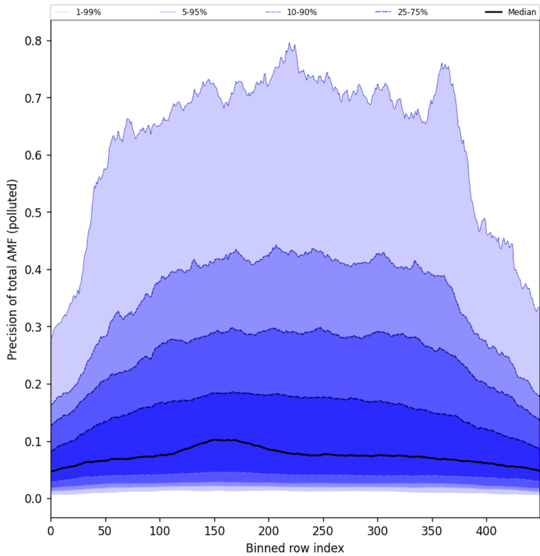
Figure 106: Along track statistics of “Precision of total AMF (polluted)” for 2025-05-10 to 2025-05-11
