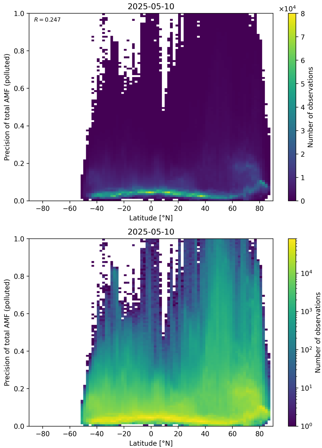
Figure 168: Scatter density plot of “Latitude” against “Precision of total AMF (polluted)” for 2025-05-10 to 2025-05-11.
