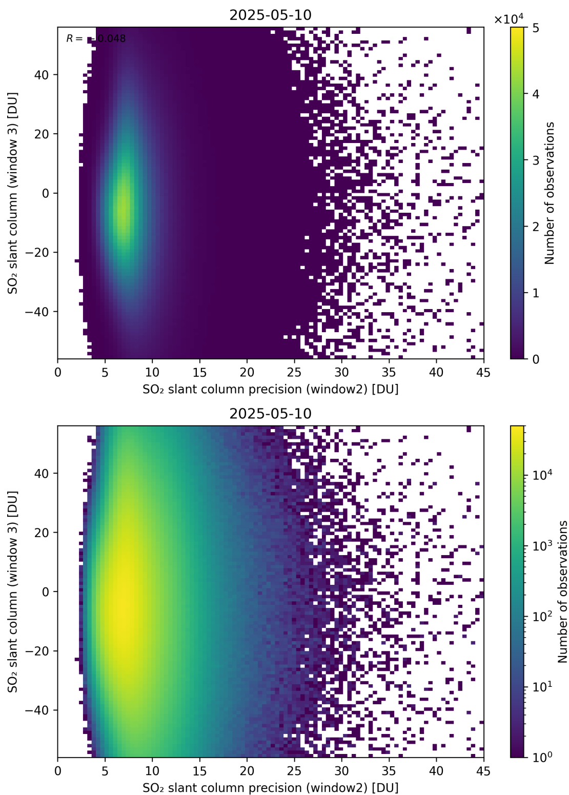
Figure 299: Scatter density plot of “SO 2 slant column precision (window2)” against “SO 2 slant column (window 3)” for 2025-05-10 to 2025-05-11.
