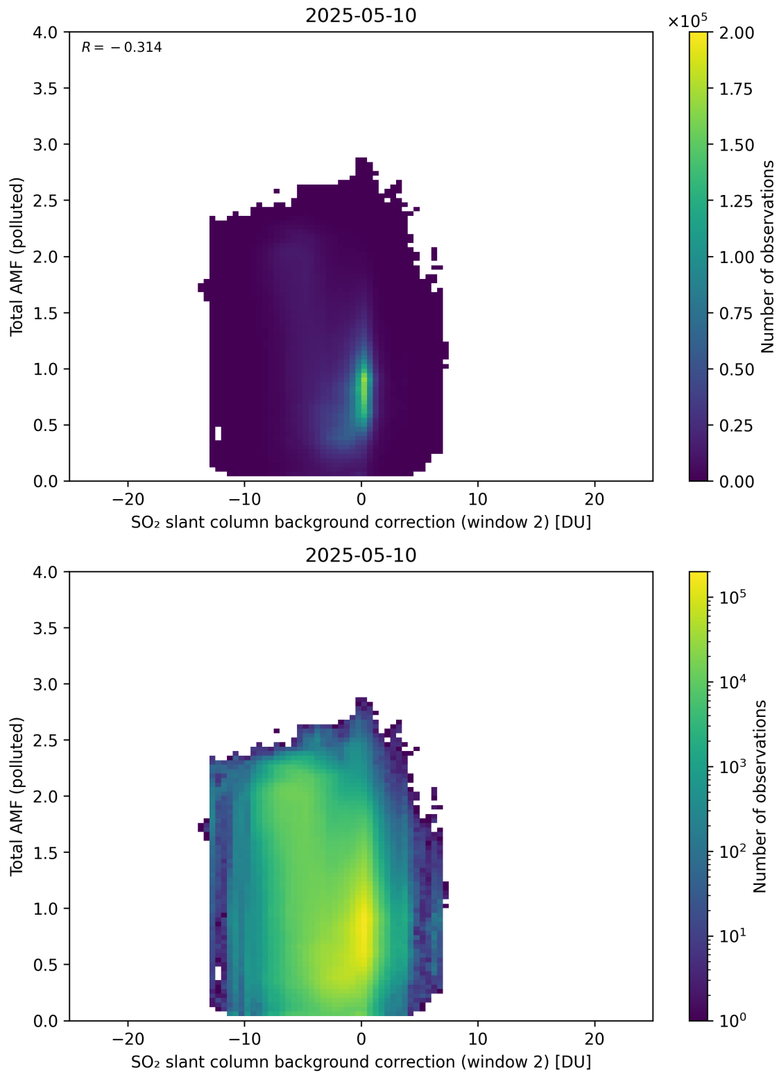
Figure 130: Scatter density plot of “SO 2 slant column background correction (window 2)” against “Total AMF (polluted)” for 2025-05-10 to 2025-05-11.
