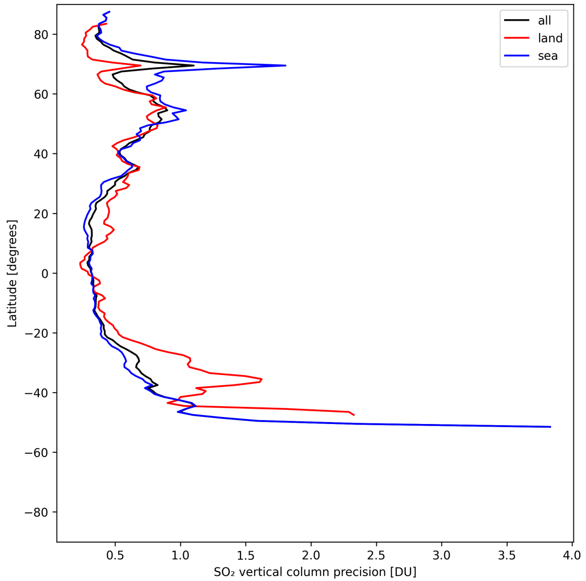
Figure 33: Zonal average of “SO 2 vertical column precision” for 2025-05-10 to 2025-05-11.
