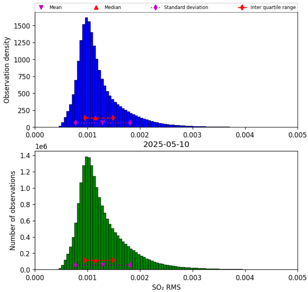
Figure 78: Histogram of "SO 2 RMS" for 2025-05-10 to 2025-05-11
