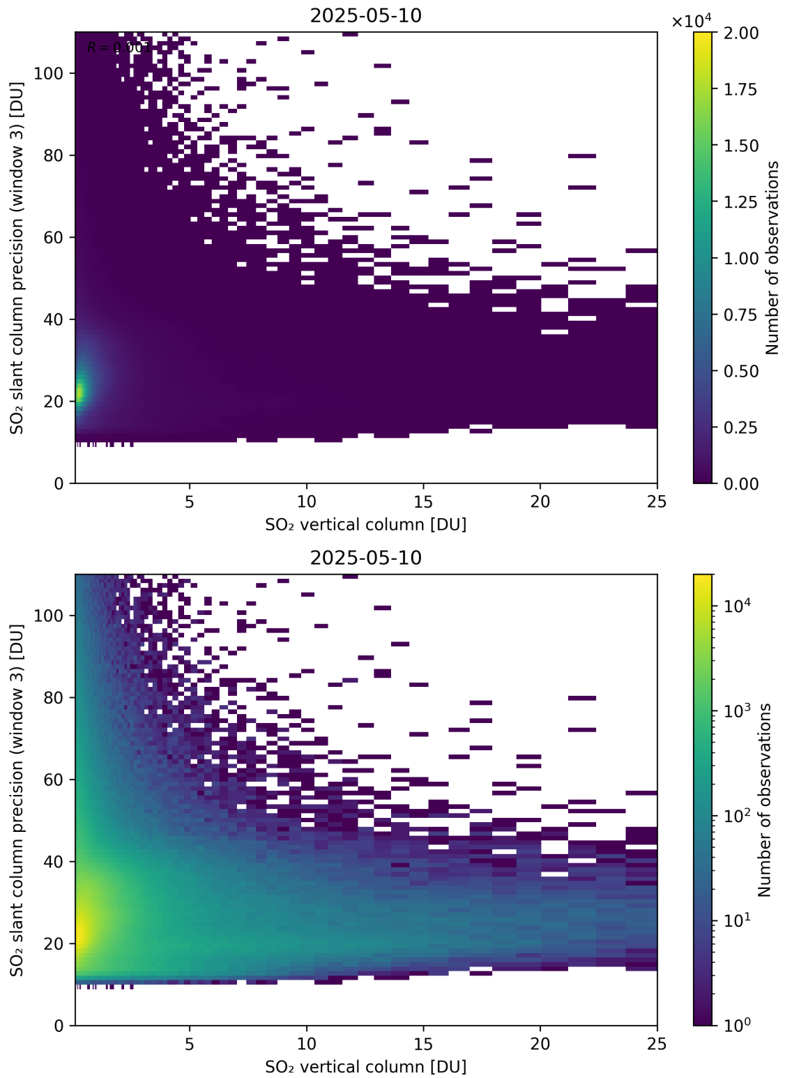
Figure 358: Scatter density plot of “SO 2 vertical column” against “SO 2 slant column precision (window 3)” for 2025-05-10 to 2025-05-11.
