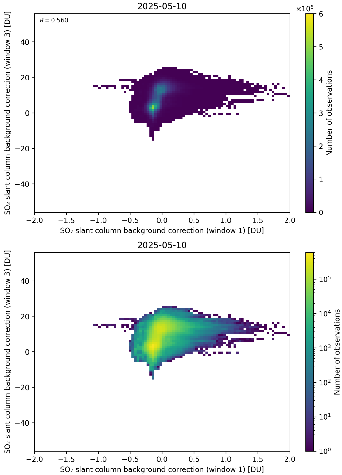
Figure 110: Scatter density plot of “SO 2 slant column background correction (window 1)” against “SO 2 slant column background correction (window 3)” for 2025-05-10 to 2025-05-11.
