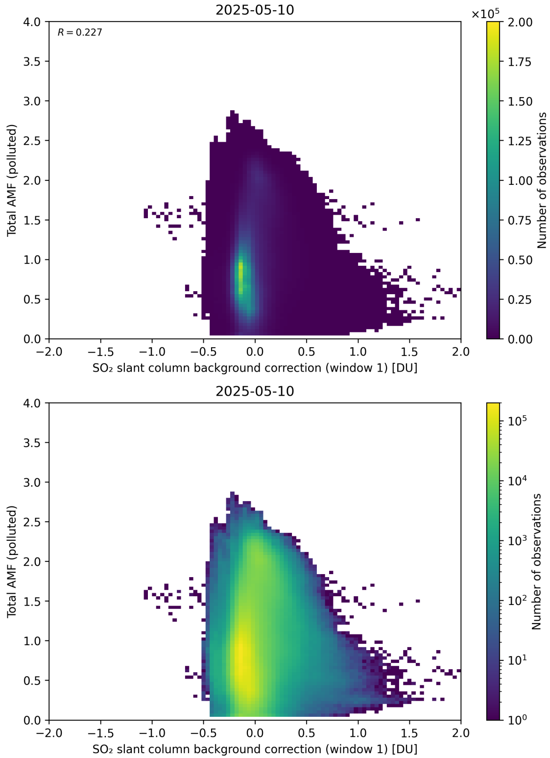
Figure 120: Scatter density plot of “SO 2 slant column background correction (window 1)” against “Total AMF (polluted)” for 2025-05-10 to 2025-05-11.
