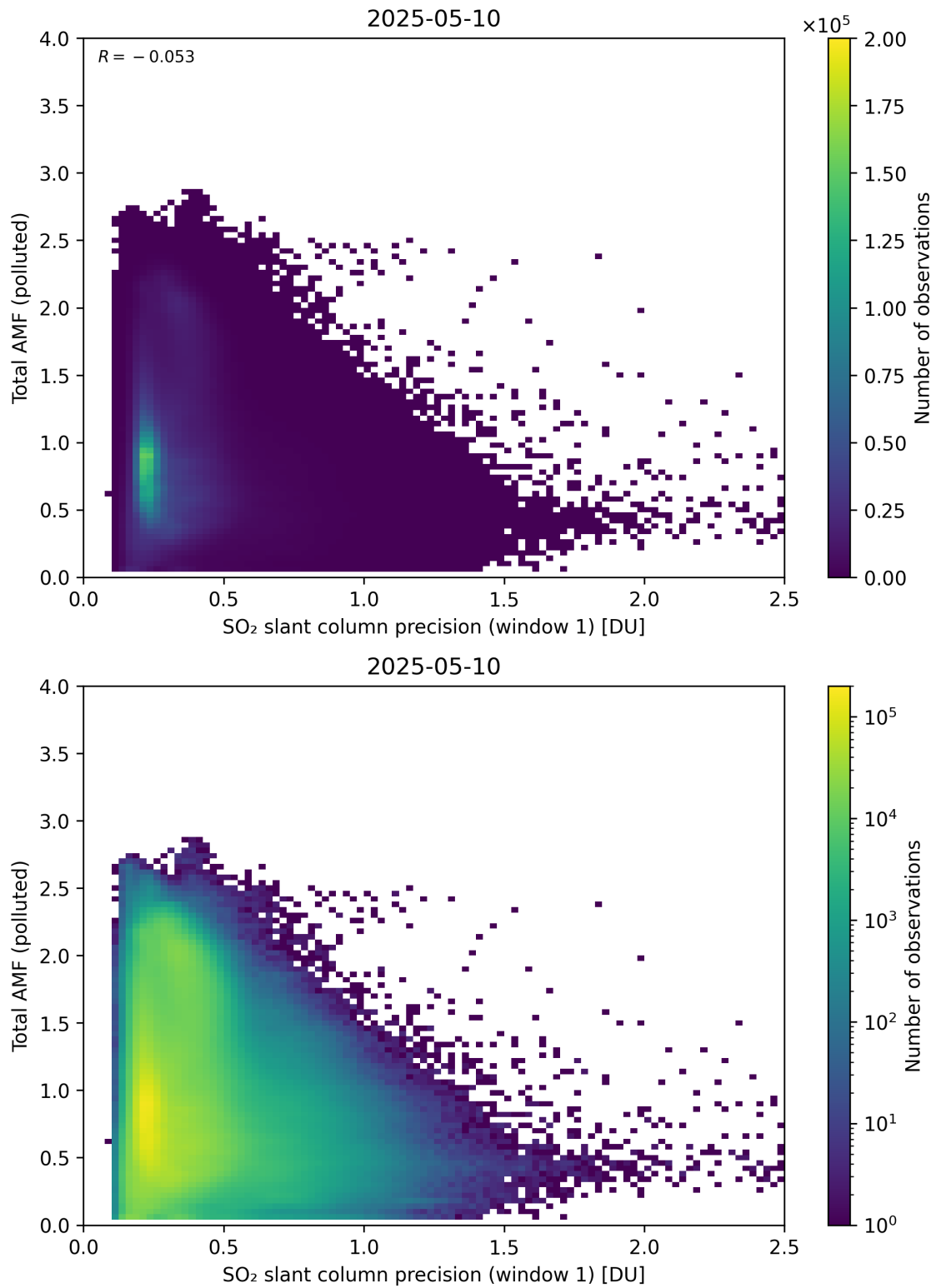
Figure 280: Scatter density plot of “SO 2 slant column precision (window 1)” against “Total AMF (polluted)” for 2025-05-10 to 2025-05-11.
