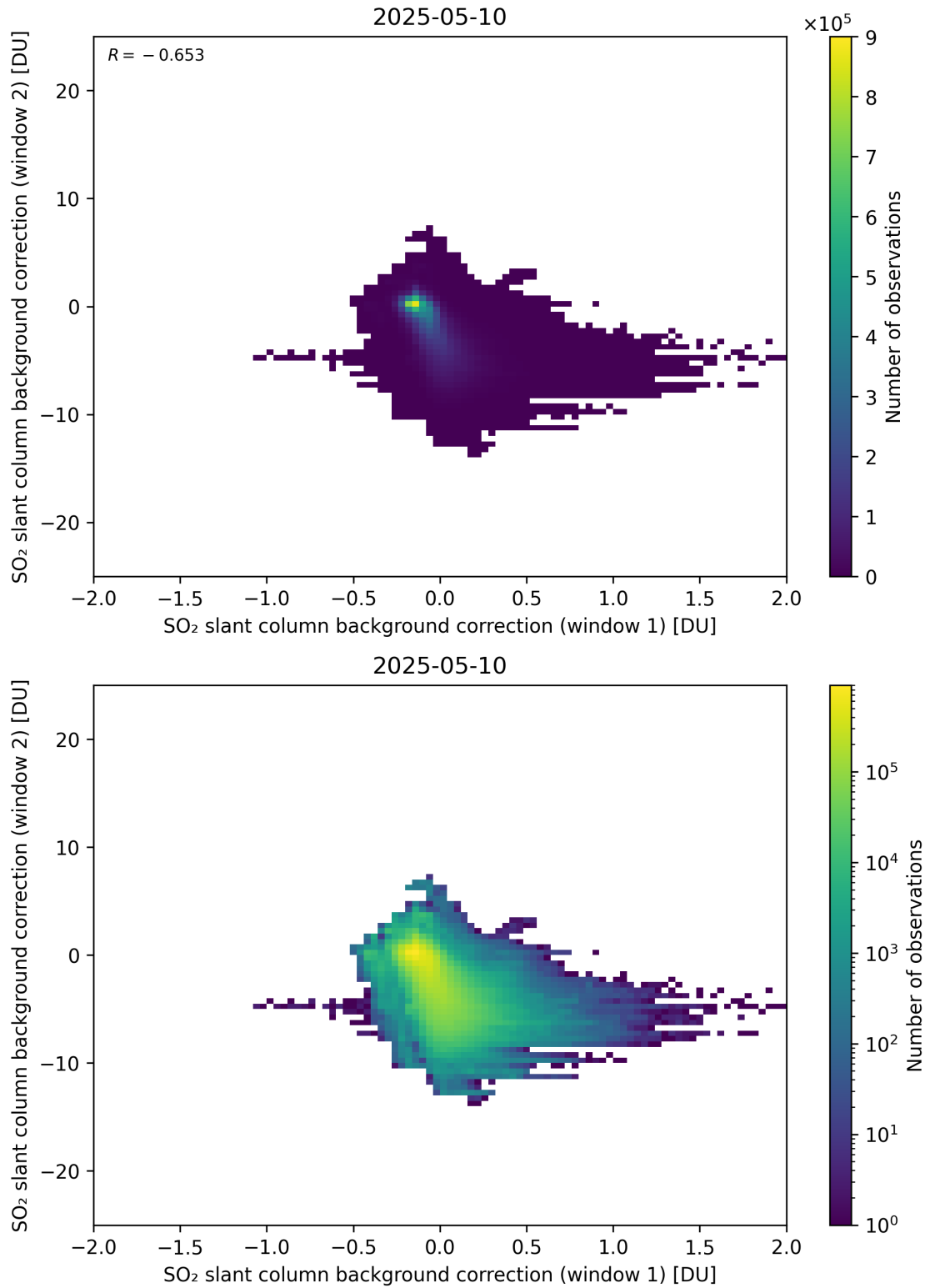
Figure 109: Scatter density plot of “SO 2 slant column background correction (window 1)” against “SO 2 slant column background correction (window 2)” for 2025-05-10 to 2025-05-11.
