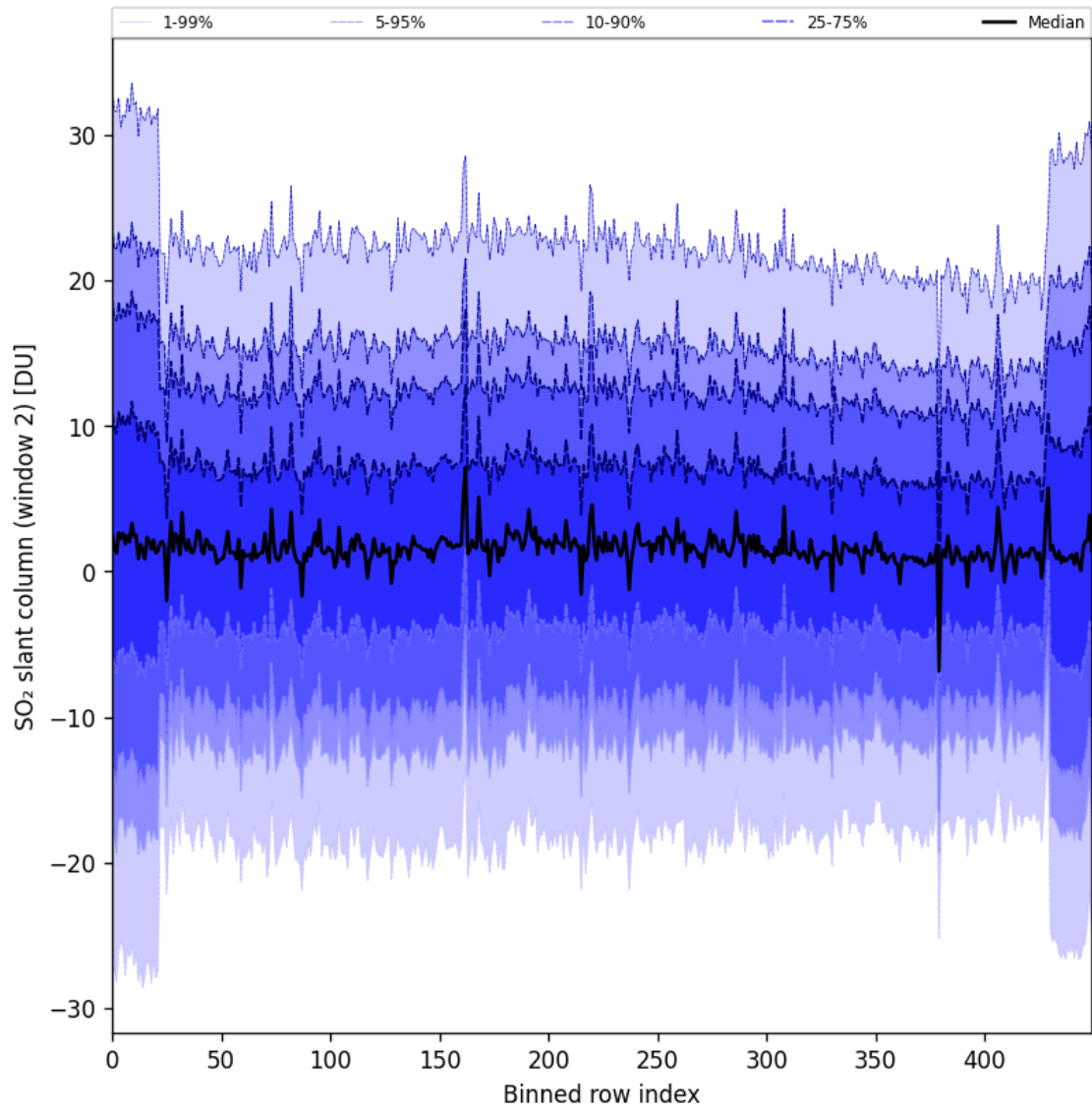
Figure 93: Along track statistics of “SO 2 slant column (window 2)” for 2025-05-10 to 2025-05-11
