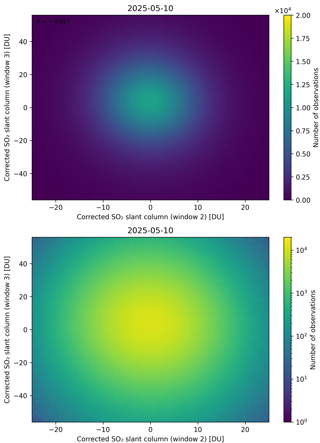
Figure 250: Scatter density plot of “Corrected SO 2 slant column (window 2)” against “Corrected SO 2 slant column (window 3)” for 2025-05-10 to 2025-05-11.
