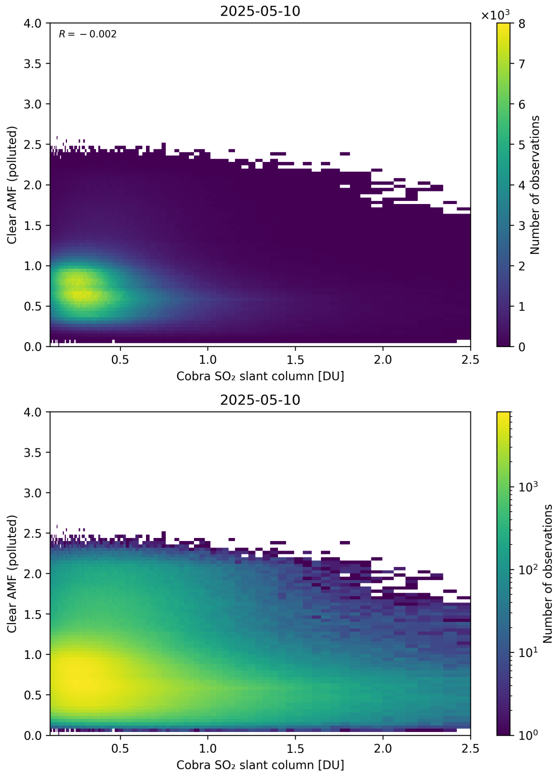
Figure 215: Scatter density plot of “Cobra SO 2 slant column” against “Clear AMF (polluted)” for 2025-05-10 to 2025-05-11.
