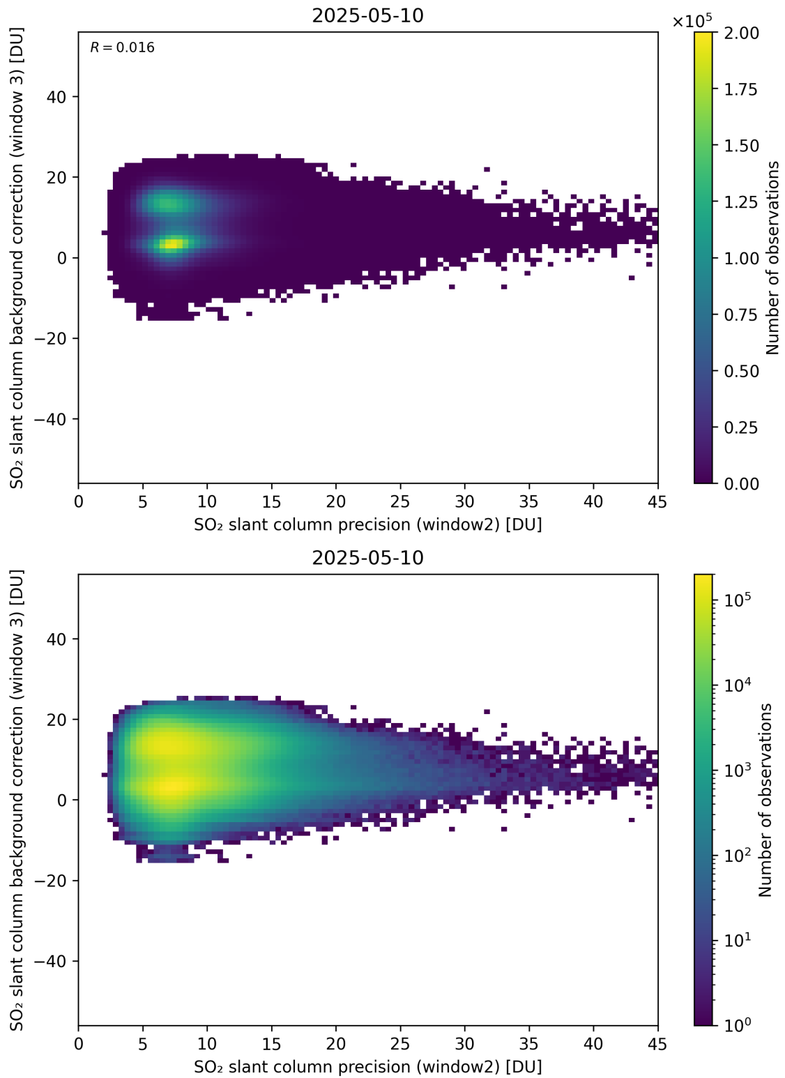
Figure 292: Scatter density plot of “SO 2 slant column precision (window2)” against “SO 2 slant column background correction (window 3)” for 2025-05-10 to 2025-05-11.
