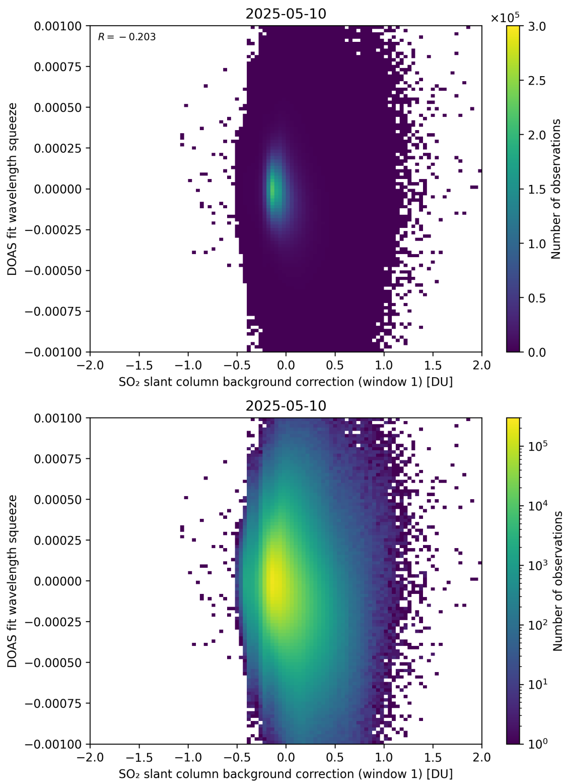
Figure 112: Scatter density plot of “SO 2 slant column background correction (window 1)” against “DOAS fit wavelength squeeze” for 2025-05-10 to 2025-05-11.
