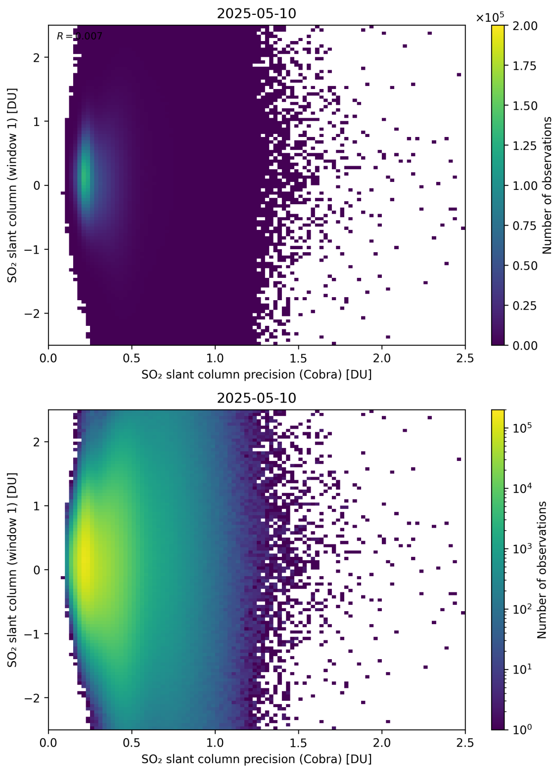
Figure 208: Scatter density plot of “SO 2 slant column precision (Cobra)” against “SO 2 slant column (window 1)” for 2025-05-10 to 2025-05-11.
