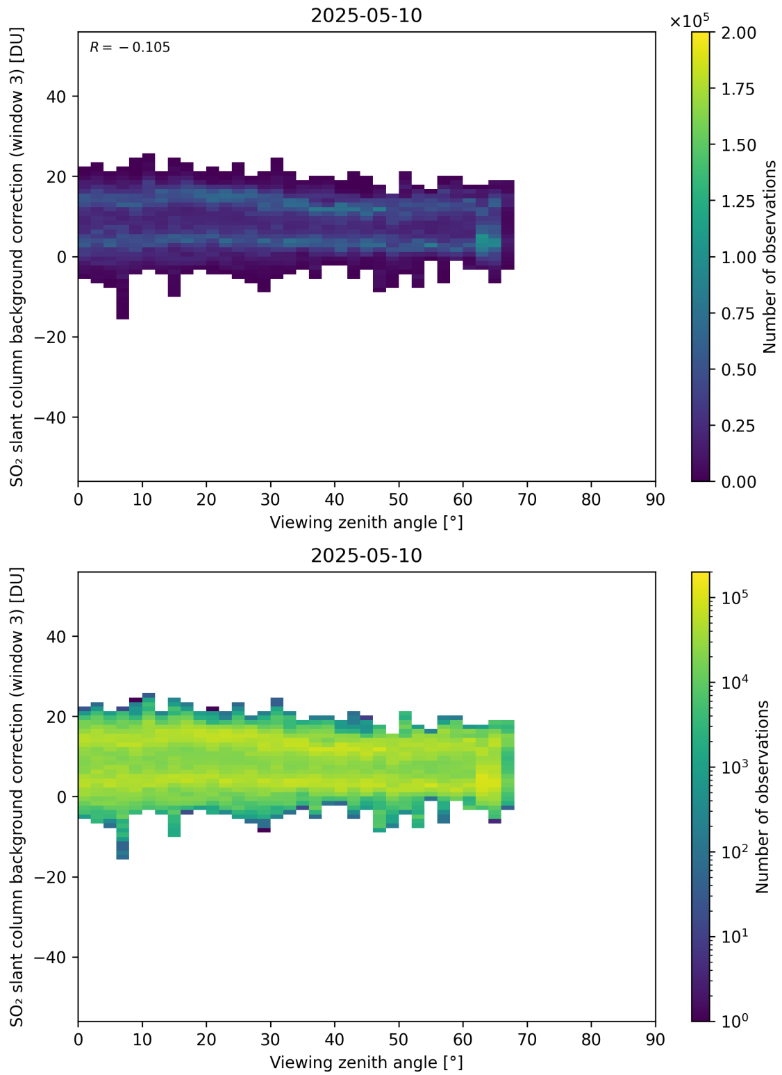
Figure 364: Scatter density plot of “Viewing zenith angle” against “SO 2 slant column background correction (window 3)” for 2025-05-10 to 2025-05-11.
