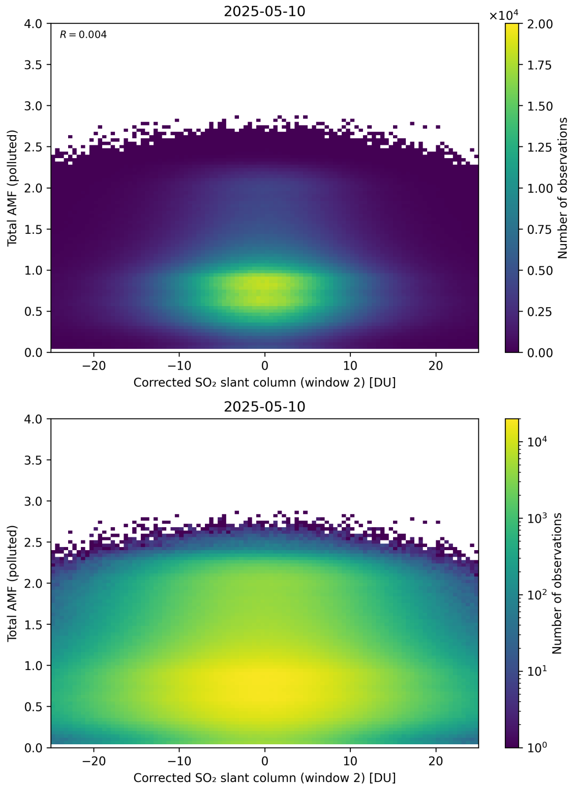
Figure 253: Scatter density plot of “Corrected SO 2 slant column (window 2)” against “Total AMF (polluted)” for 2025-05-10 to 2025-05-11.
