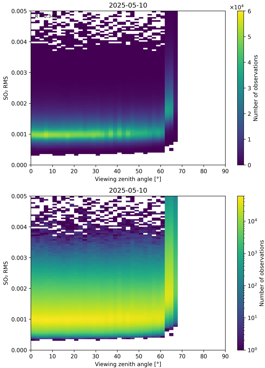
Figure 367: Scatter density plot of “Viewing zenith angle” against “SO 2 RMS” for 2025-05-10 to 2025-05-11.
