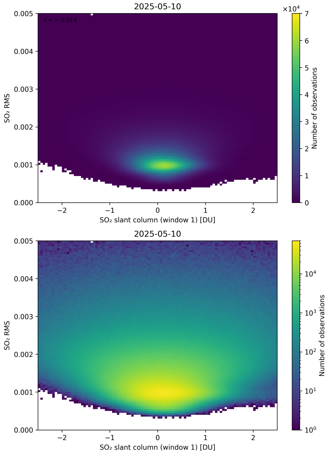
Figure 267: Scatter density plot of “SO 2 slant column (window 1)” against “SO 2 RMS” for 2025-05-10 to 2025-05-11.
