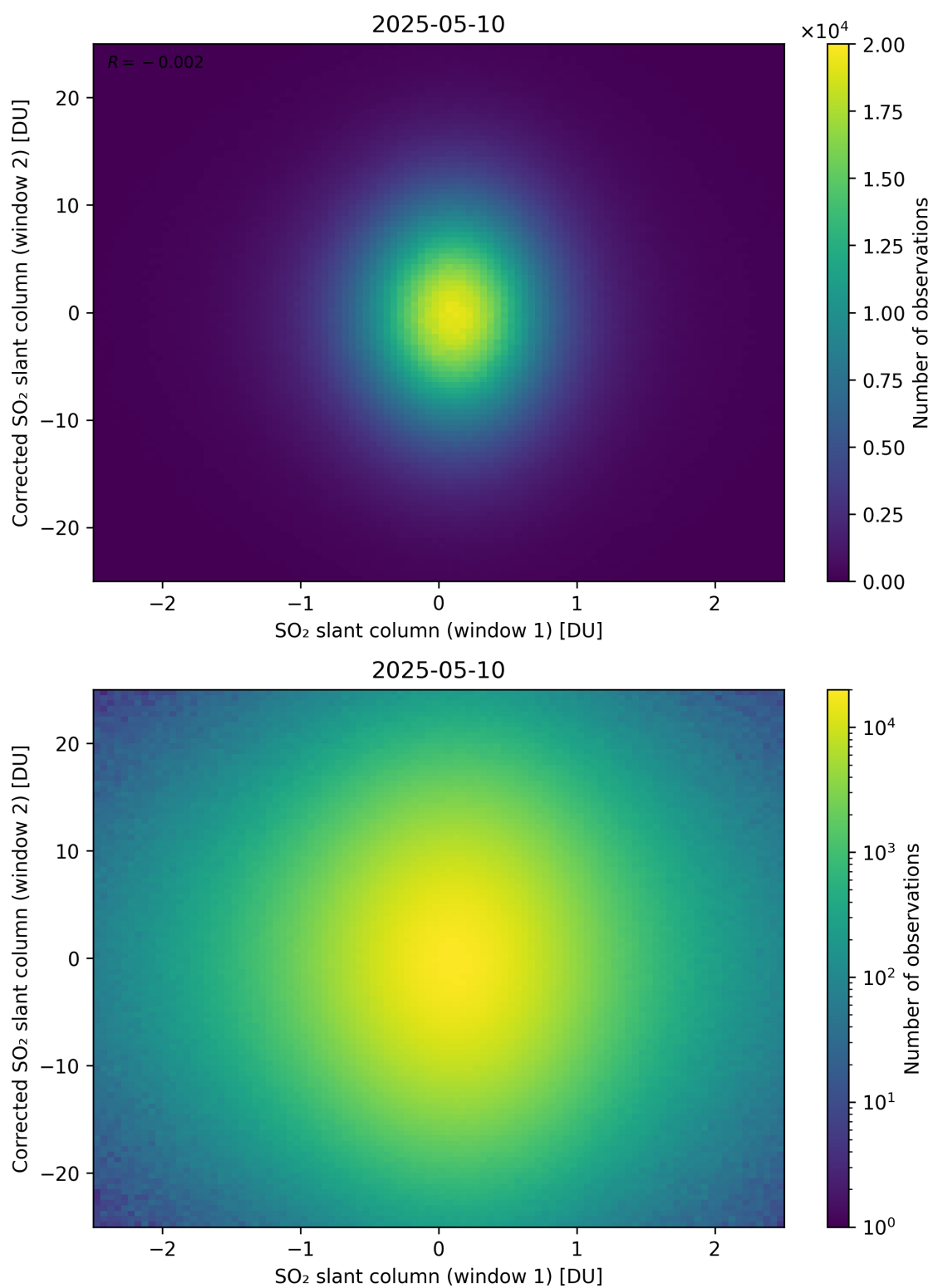
Figure 283: Scatter density plot of “SO 2 slant column (window 1)” against “Corrected SO 2 slant column (window 2)” for 2025-05-10 to 2025-05-11.
