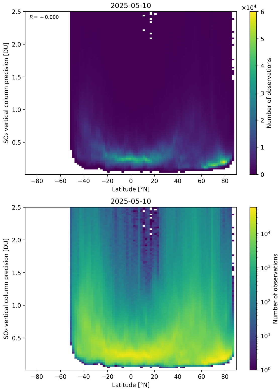
Figure 170: Scatter density plot of “Latitude” against “SO 2 vertical column precision” for 2025-05-10 to 2025-05-11.
