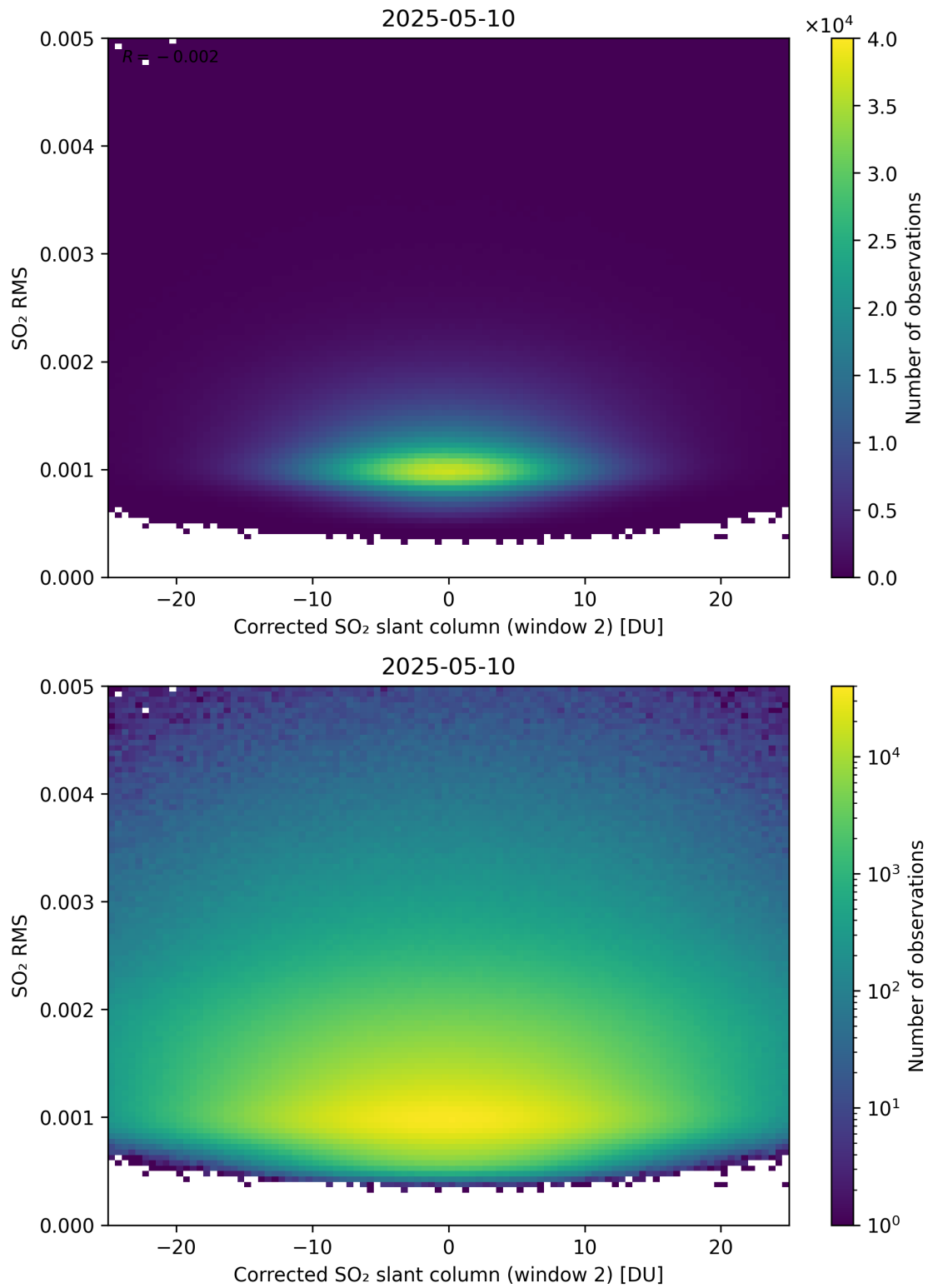
Figure 248: Scatter density plot of “Corrected SO 2 slant column (window 2)” against “SO 2 RMS” for 2025-05-10 to 2025-05-11.
