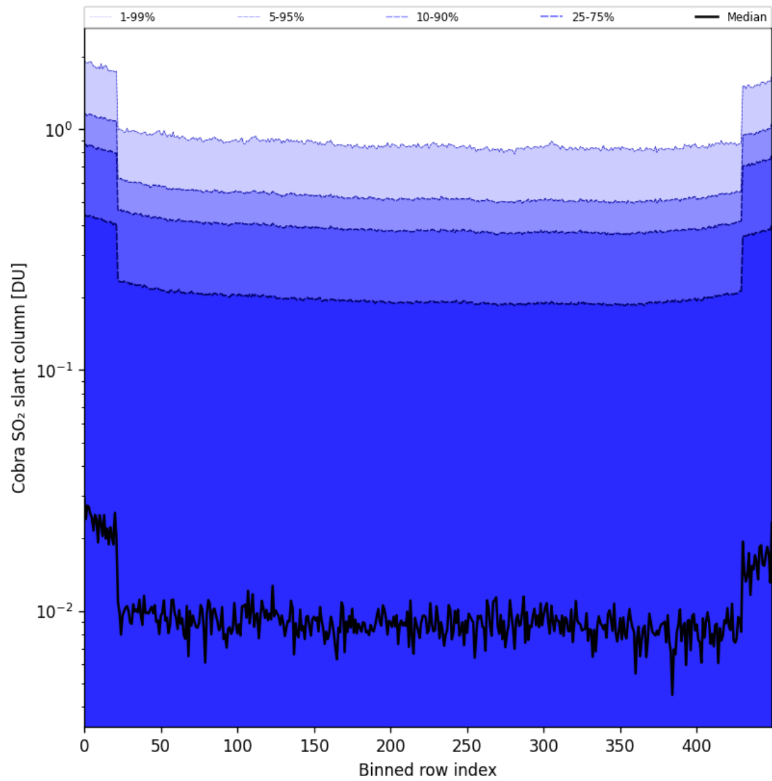
Figure 87: Along track statistics of “Cobra SO 2 slant column” for 2025-05-10 to 2025-05-11
