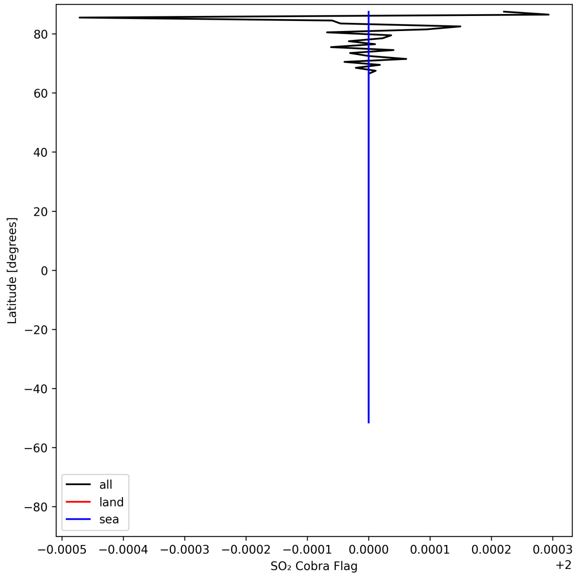
Figure 49: Zonal average of "SO 2 Cobra Flag" for 2025-05-10 to 2025-05-11.
