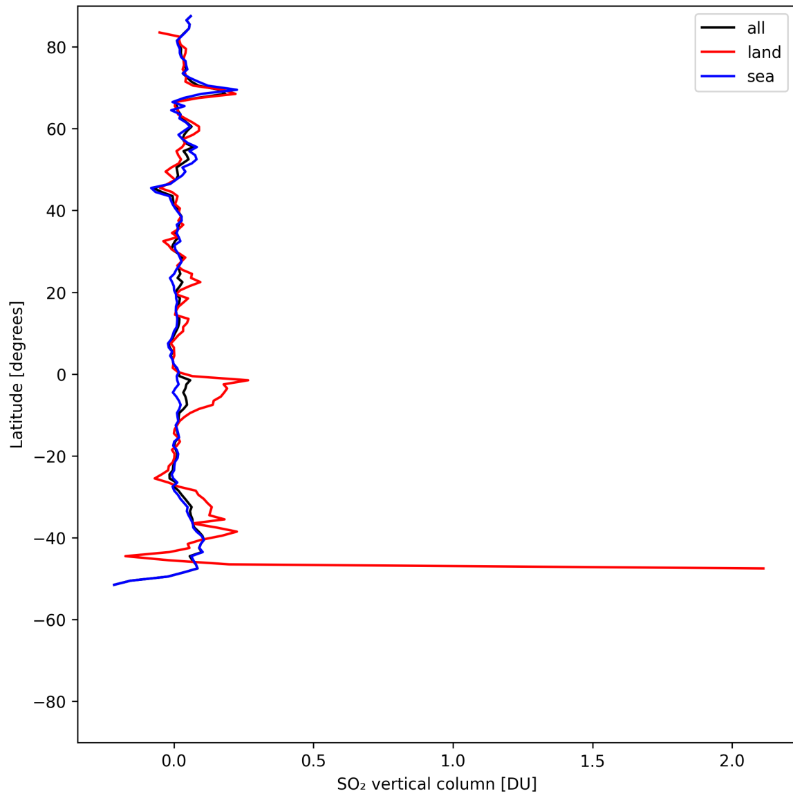
Figure 32: Zonal average of “SO 2 vertical column” for 2025-05-10 to 2025-05-11.
