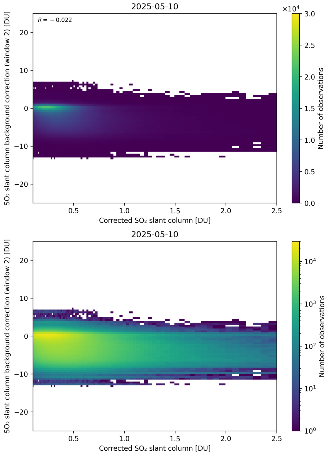
Figure 227: Scatter density plot of “Corrected SO 2 slant column” against “SO 2 slant column background correction (window 2)” for 2025-05-10 to 2025-05-11.
