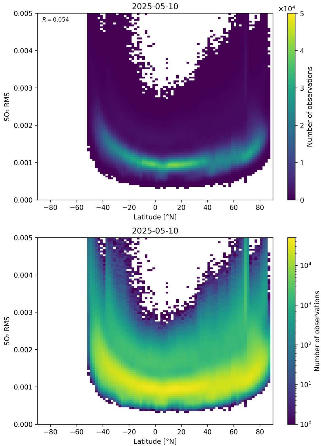
Figure 155: Scatter density plot of “Latitude” against “SO 2 RMS” for 2025-05-10 to 2025-05-11.
