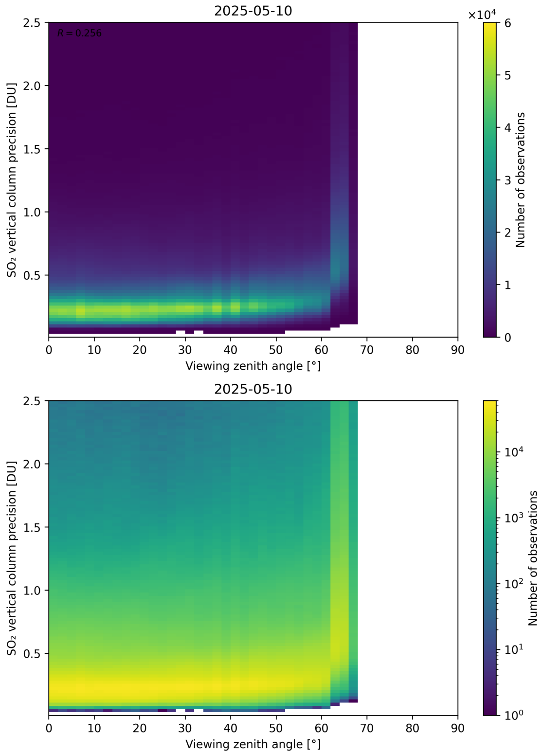
Figure 384: Scatter density plot of “Viewing zenith angle” against “SO 2 vertical column precision” for 2025-05-10 to 2025-05-11.
