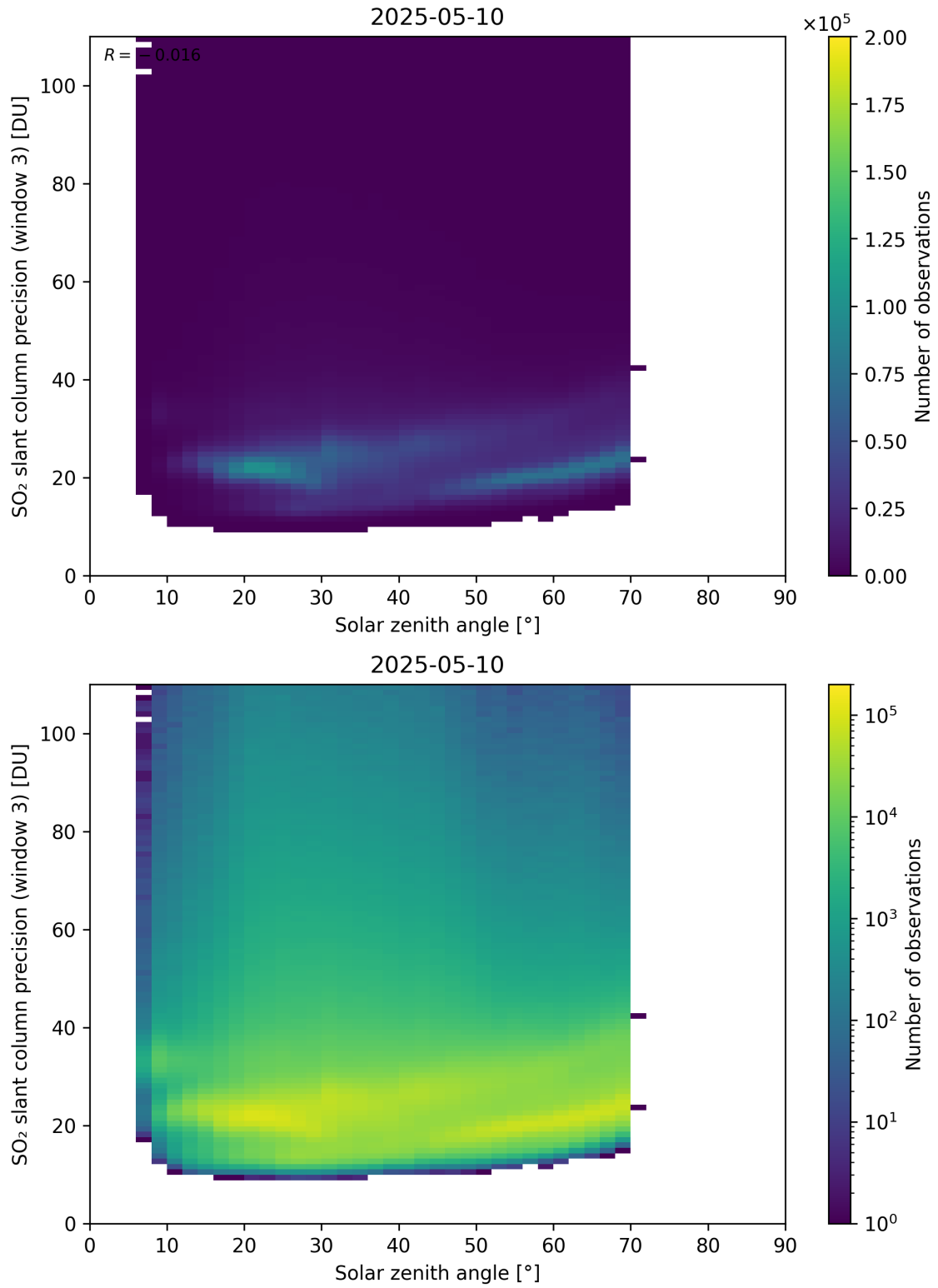
Figure 188: Scatter density plot of “Solar zenith angle” against “SO 2 slant column precision (window 3)” for 2025-05-10 to 2025-05-11.
