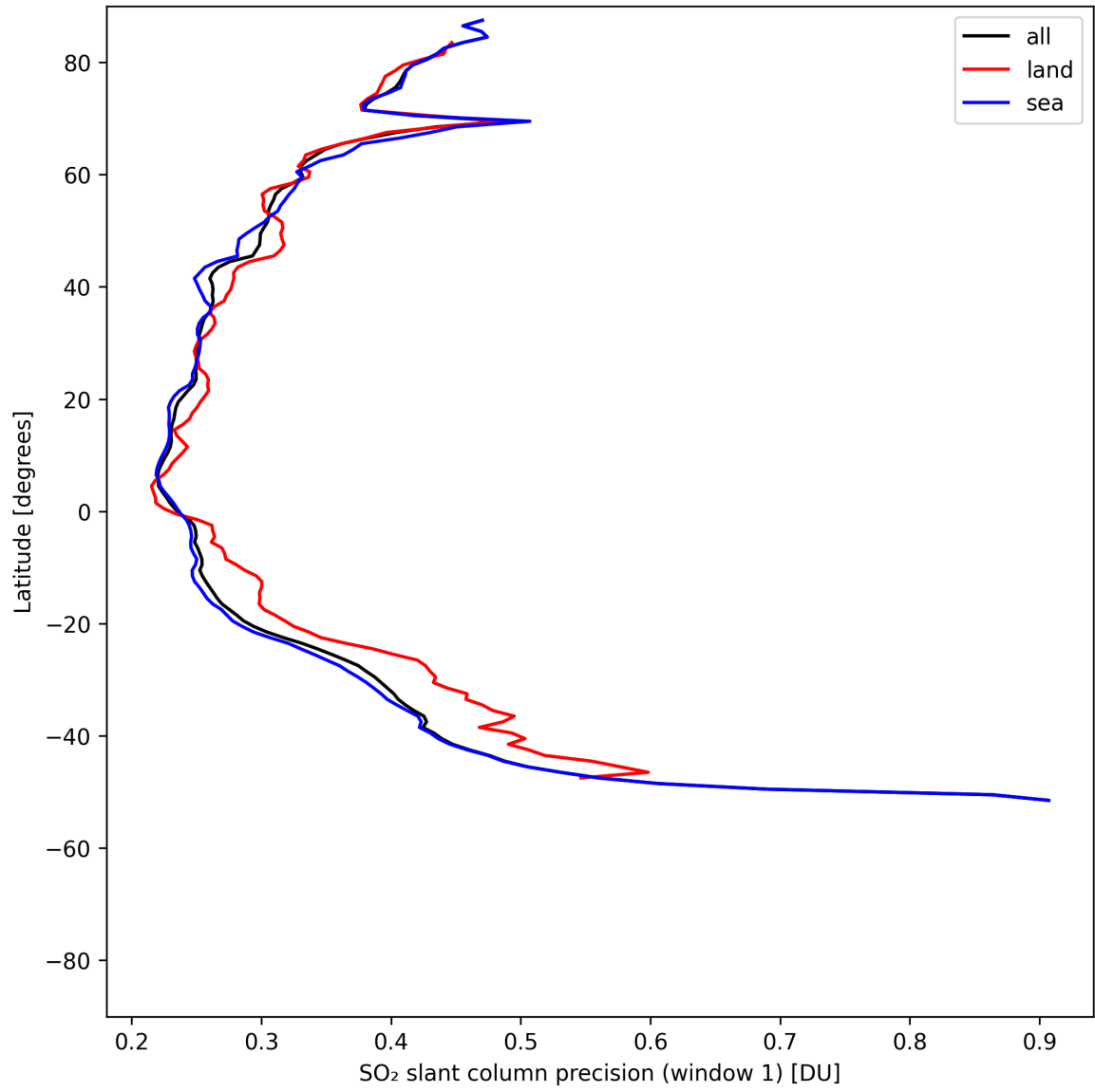
Figure 38: Zonal average of “SO 2 slant column precision (window 1)” for 2025-05-10 to 2025-05-11.
