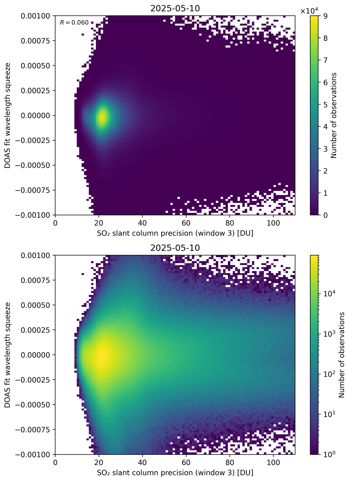
Figure 309: Scatter density plot of “SO 2 slant column precision (window 3)” against “DOAS fit wavelength squeeze” for 2025-05-10 to 2025-05-11.
