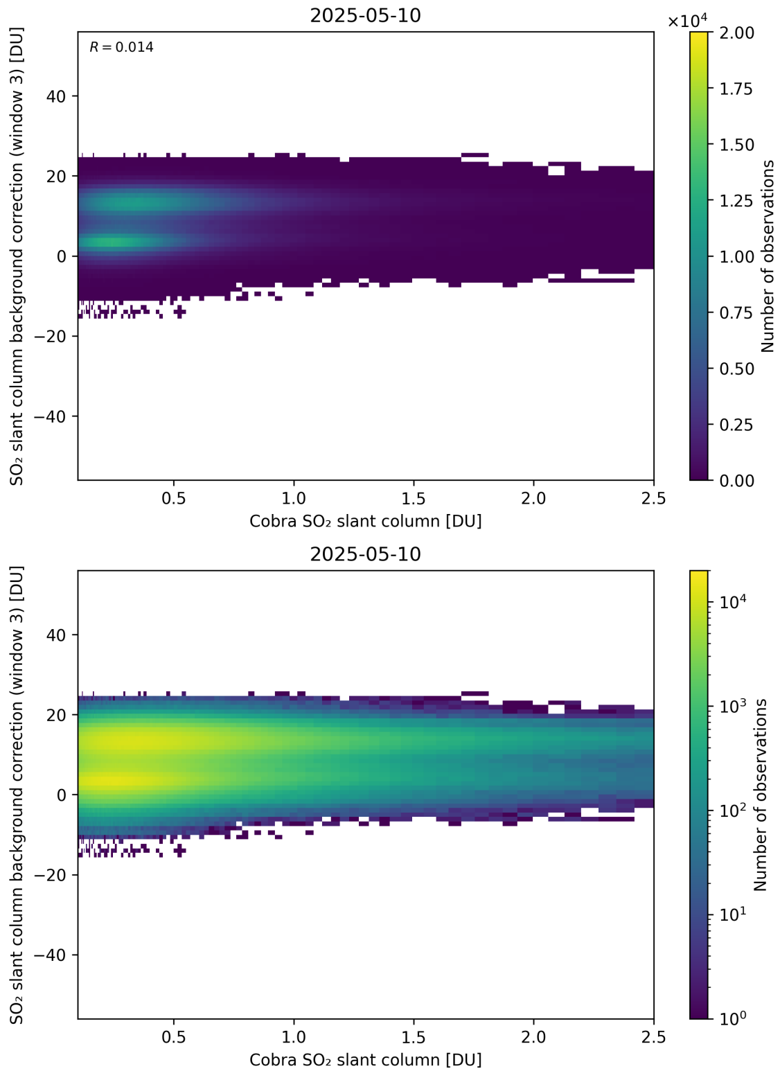
Figure 195: Scatter density plot of “Cobra SO 2 slant column” against “SO 2 slant column background correction (window 3)” for 2025-05-10 to 2025-05-11.
