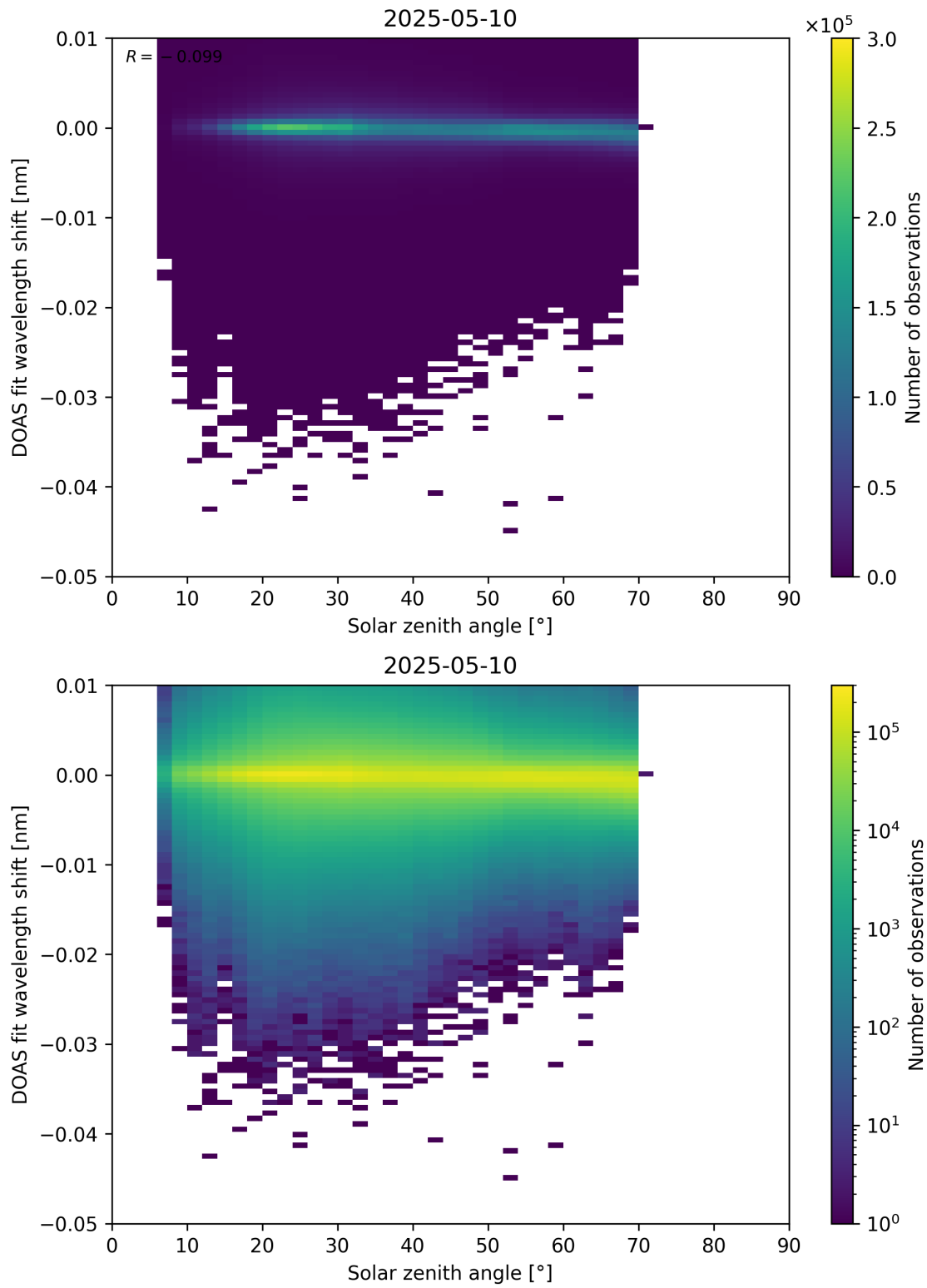
Figure 174: Scatter density plot of “Solar zenith angle” against “DOAS fit wavelength shift” for 2025-05-10 to 2025-05-11.
