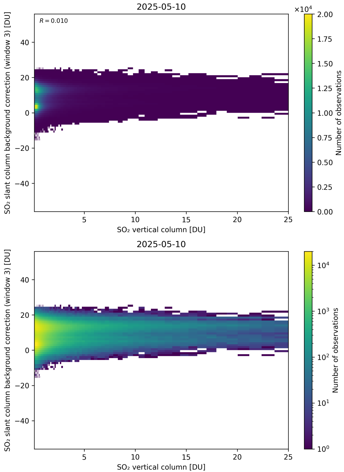
Figure 325: Scatter density plot of “SO 2 vertical column” against “SO 2 slant column background correction (window 3)” for 2025-05-10 to 2025-05-11.
