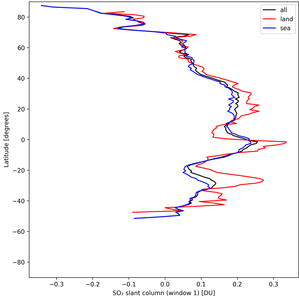
Figure 37: Zonal average of “SO 2 slant column (window 1)” for 2025-05-10 to 2025-05-11.
