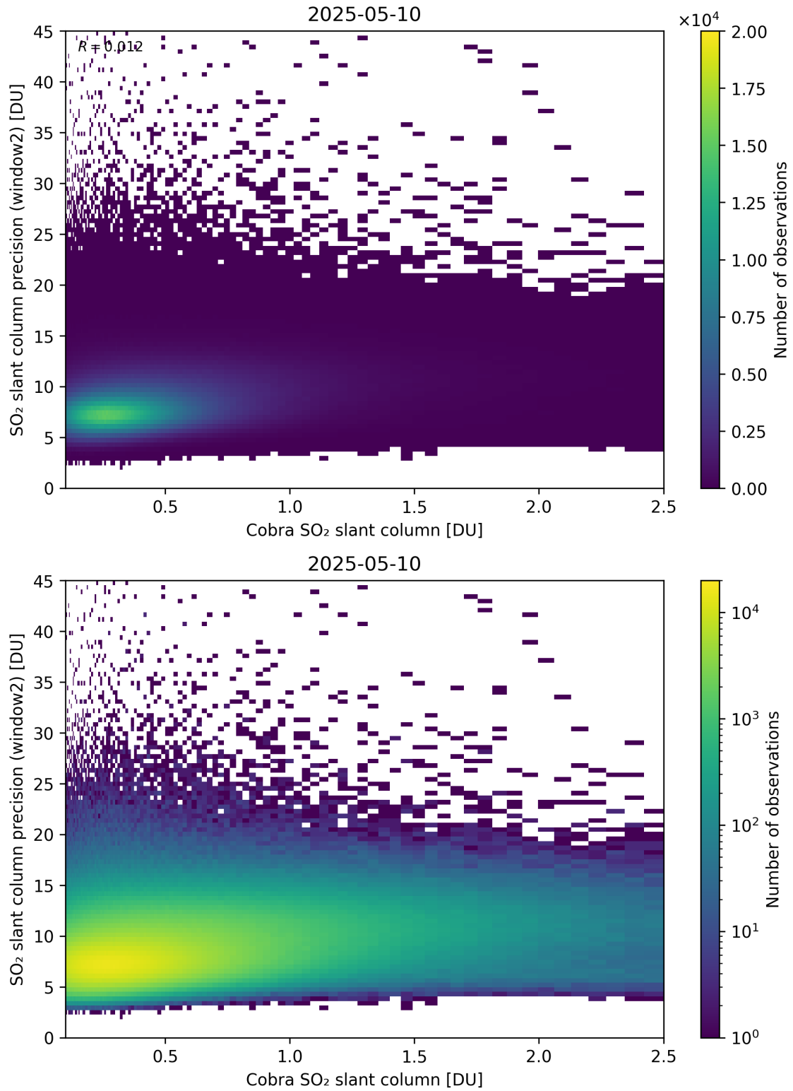
Figure 221: Scatter density plot of “Cobra SO 2 slant column” against “SO 2 slant column precision (window2)” for 2025-05-10 to 2025-05-11.
