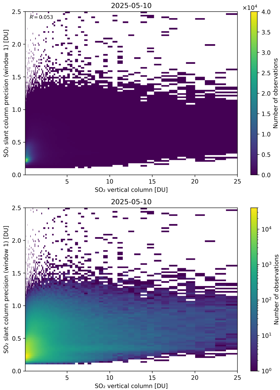
Figure 355: Scatter density plot of “SO 2 vertical column” against “SO 2 slant column precision (window 1)” for 2025-05-10 to 2025-05-11.
