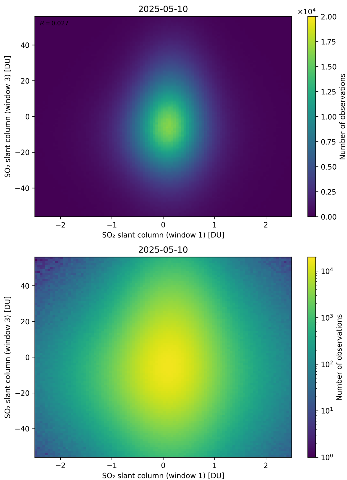
Figure 287: Scatter density plot of “SO 2 slant column (window 1)” against “SO 2 slant column (window 3)” for 2025-05-10 to 2025-05-11.
