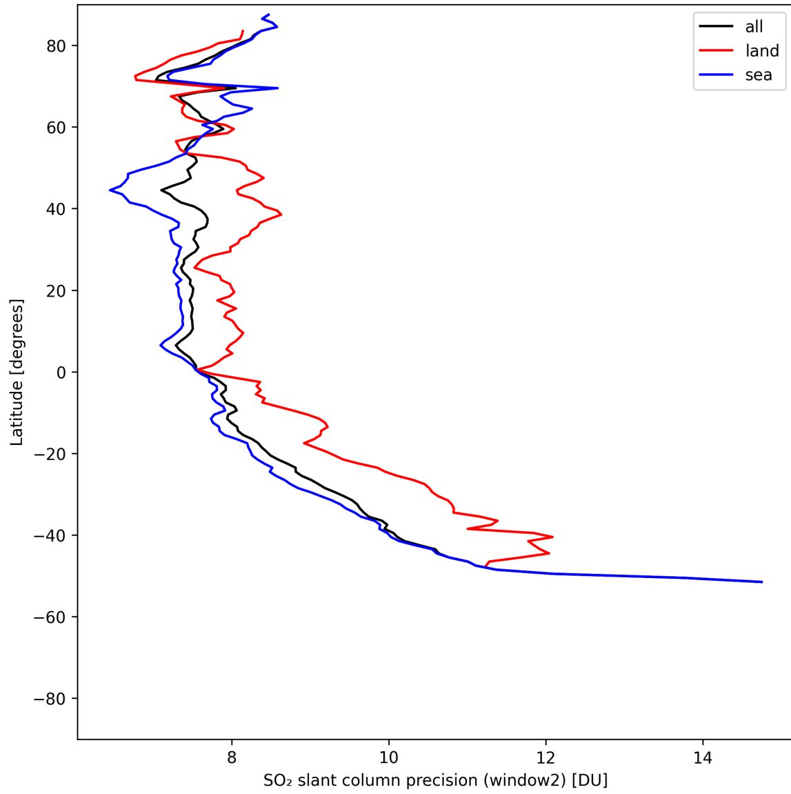
Figure 42: Zonal average of “SO 2 slant column precision (window2)” for 2025-05-10 to 2025-05-11.
