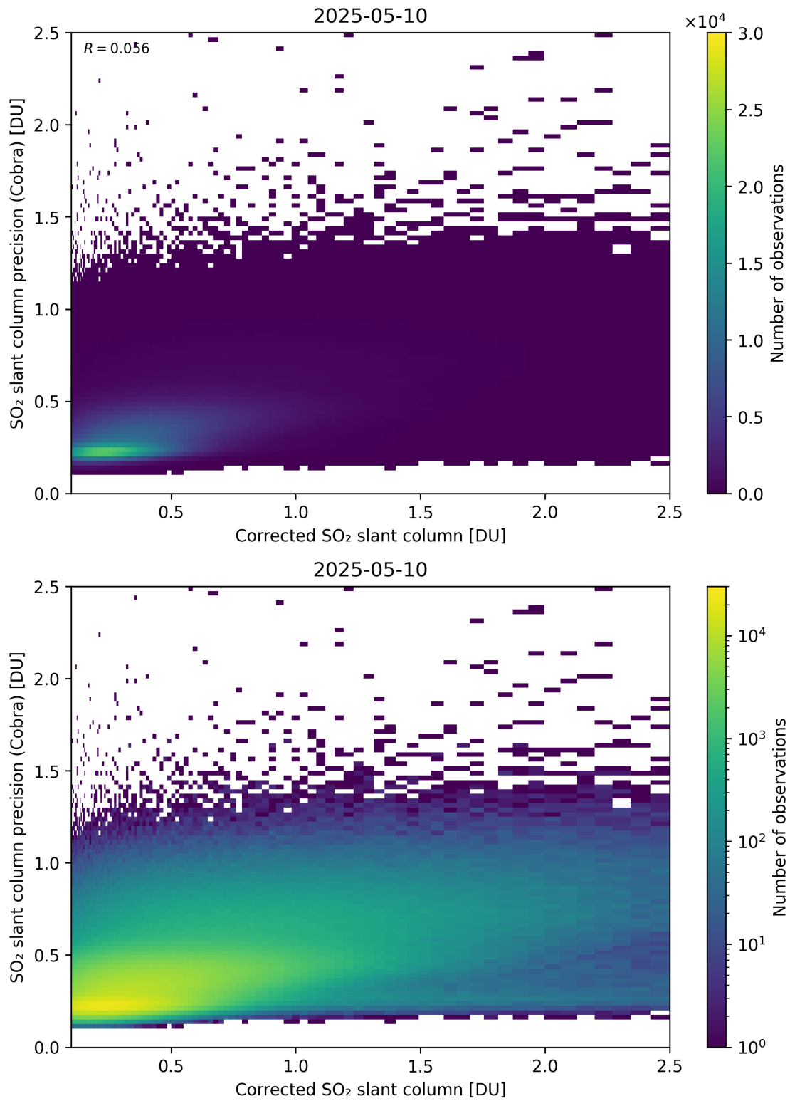
Figure 234: Scatter density plot of “Corrected SO 2 slant column” against “SO 2 slant column precision (Cobra)” for 2025-05-10 to 2025-05-11.
