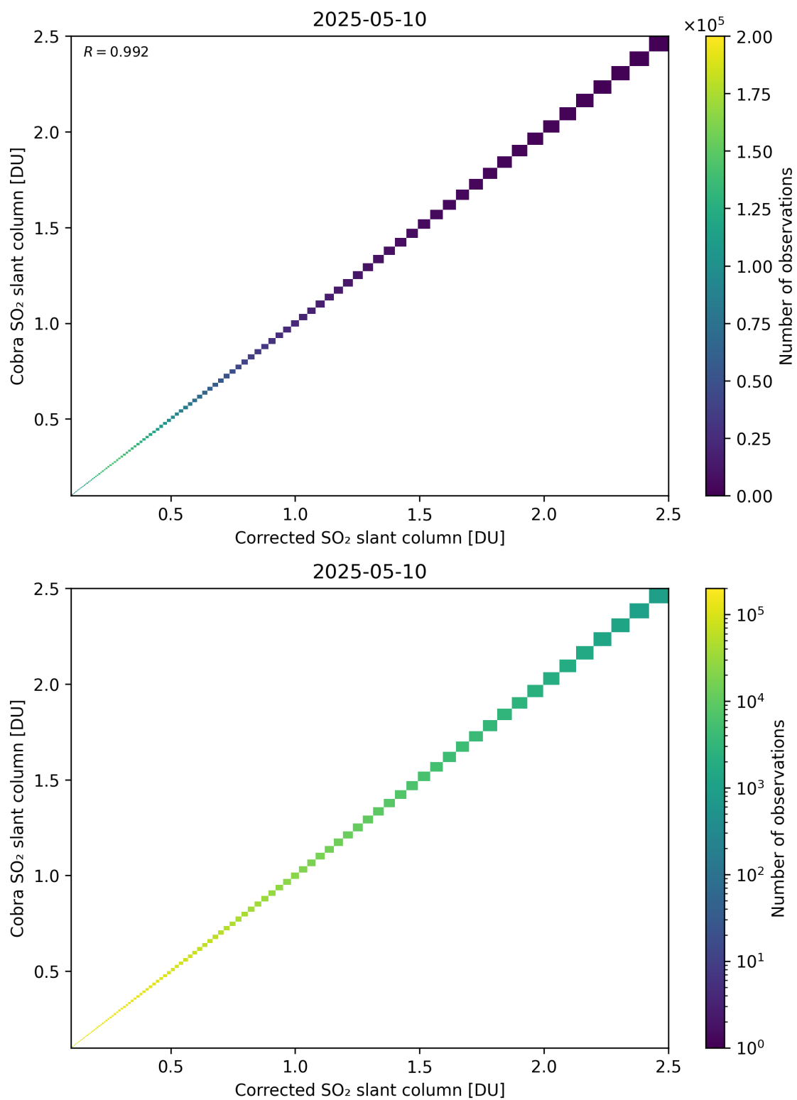
Figure 233: Scatter density plot of “Corrected SO 2 slant column” against “Cobra SO 2 slant column” for 2025-05-10 to 2025-05-11.
