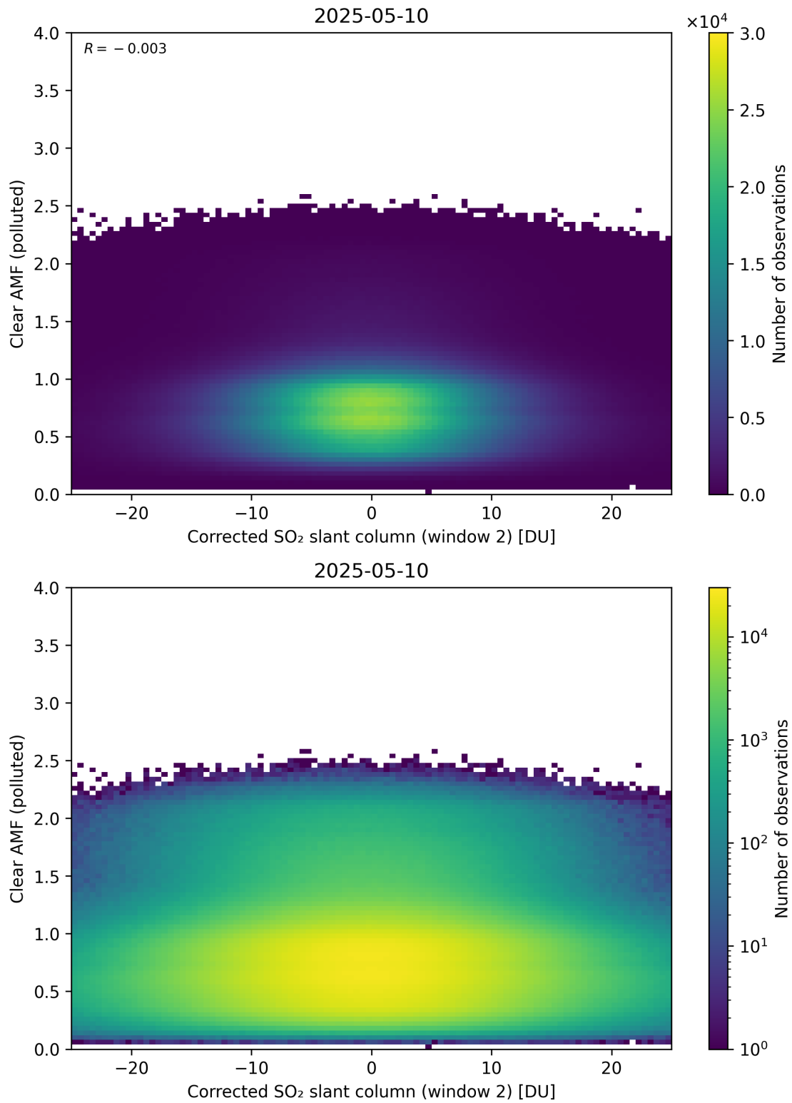
Figure 249: Scatter density plot of “Corrected SO 2 slant column (window 2)” against “Clear AMF (polluted)” for 2025-05-10 to 2025-05-11.
