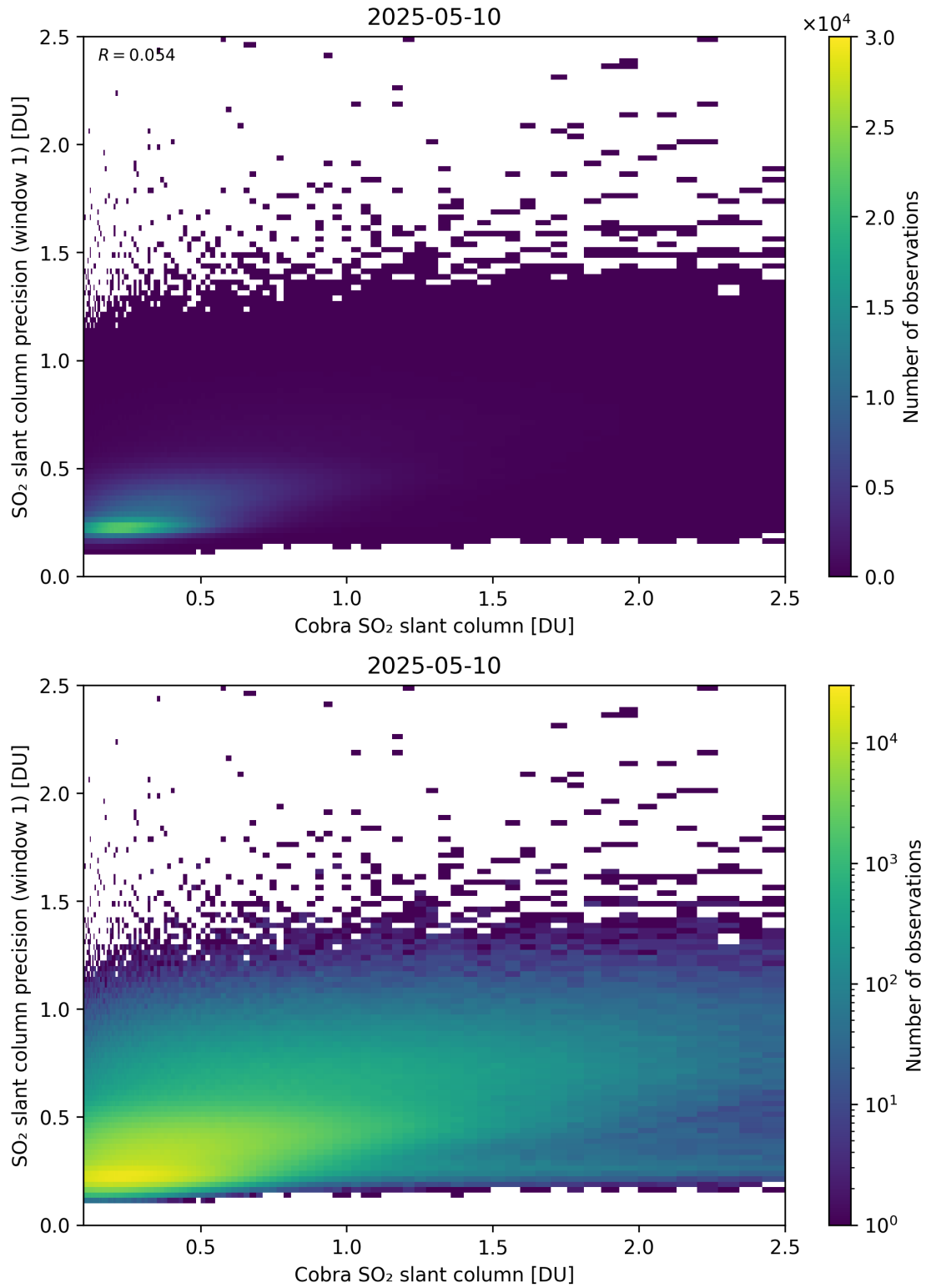
Figure 220: Scatter density plot of “Cobra SO 2 slant column” against “SO 2 slant column precision (window 1)” for 2025-05-10 to 2025-05-11.
