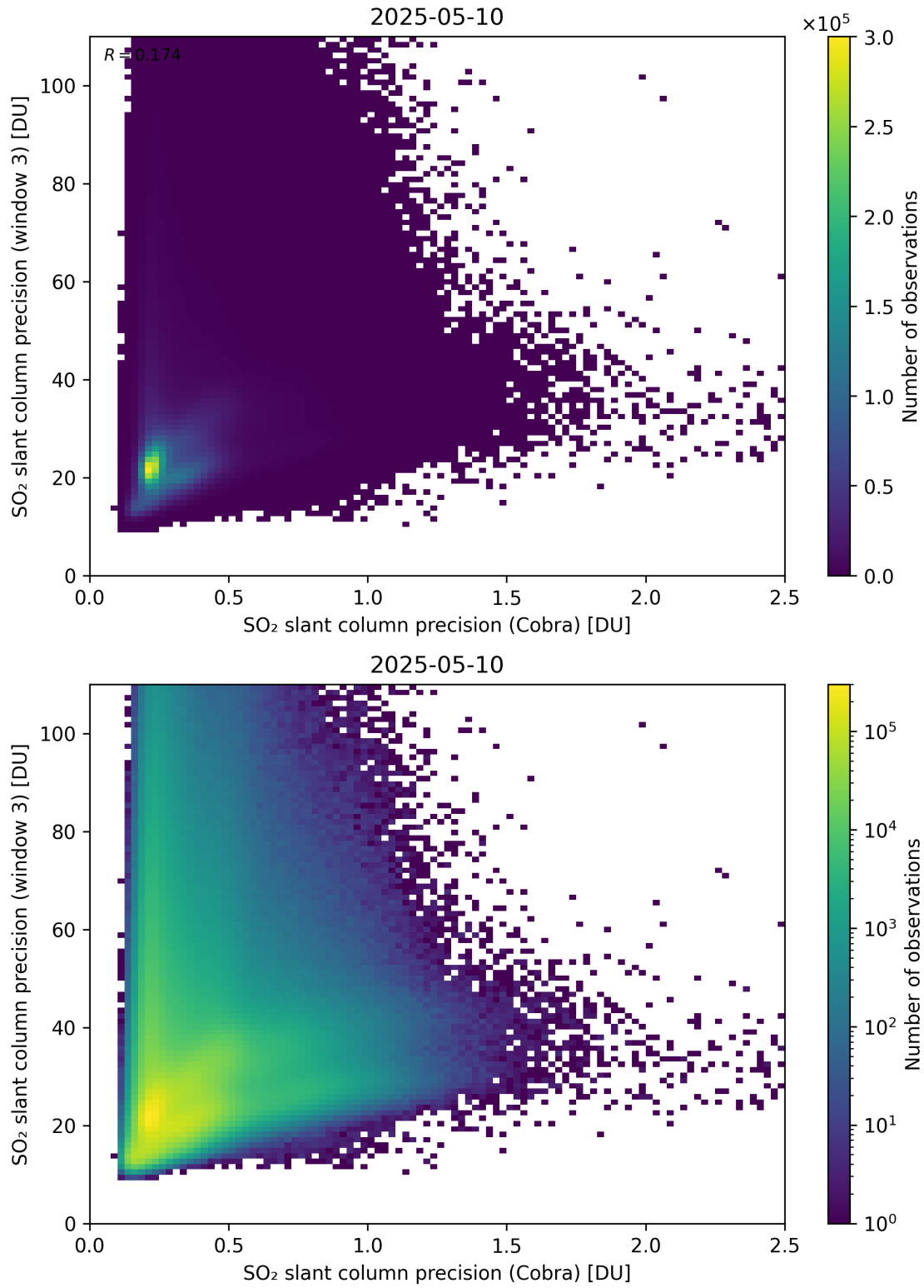
Figure 212: Scatter density plot of “SO 2 slant column precision (Cobra)” against “SO 2 slant column precision (window 3)” for 2025-05-10 to 2025-05-11.
