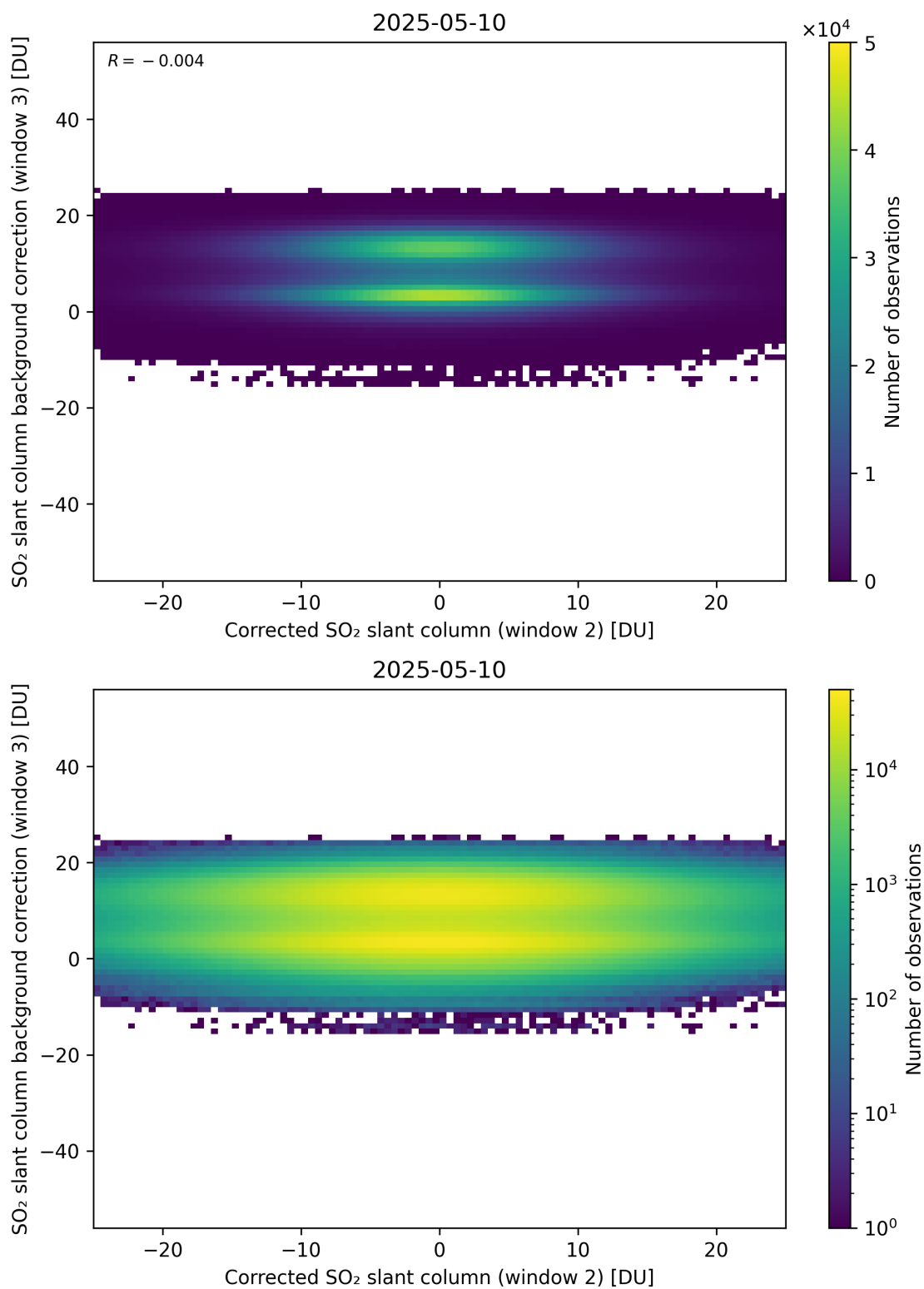
Figure 245: Scatter density plot of “Corrected SO 2 slant column (window 2)” against “SO 2 slant column background correction (window 3)” for 2025-05-10 to 2025-05-11.
