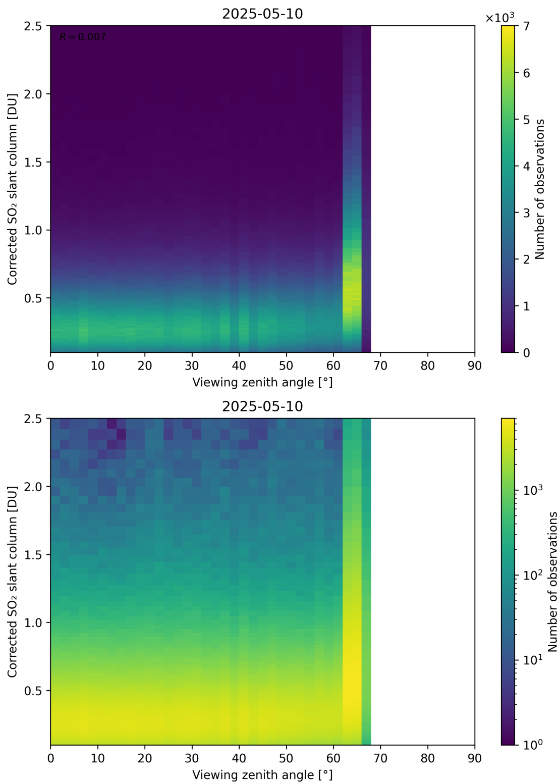
Figure 373: Scatter density plot of “Viewing zenith angle” against “Corrected SO 2 slant column” for 2025-05-10 to 2025-05-11.
