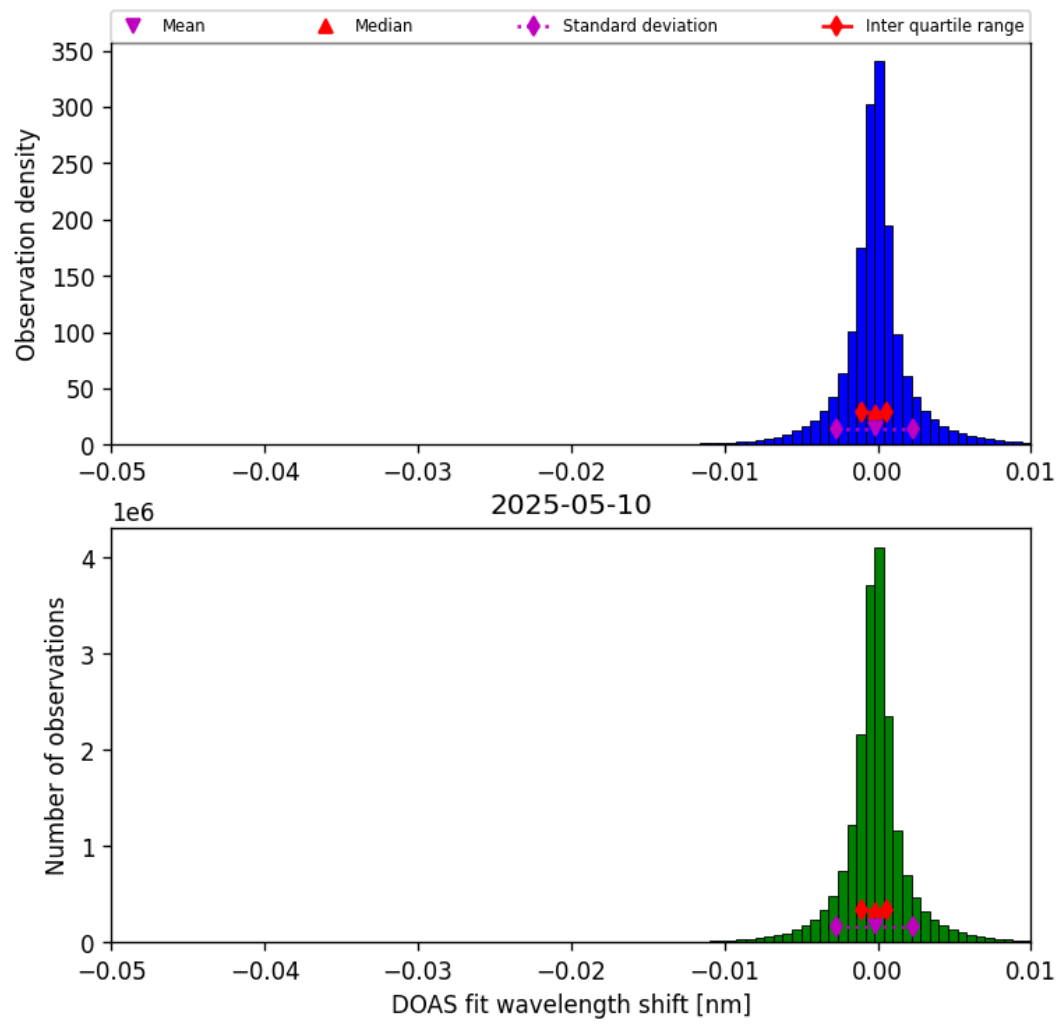
Figure 76: Histogram of “DOAS fit wavelength shift” for 2025-05-10 to 2025-05-11
