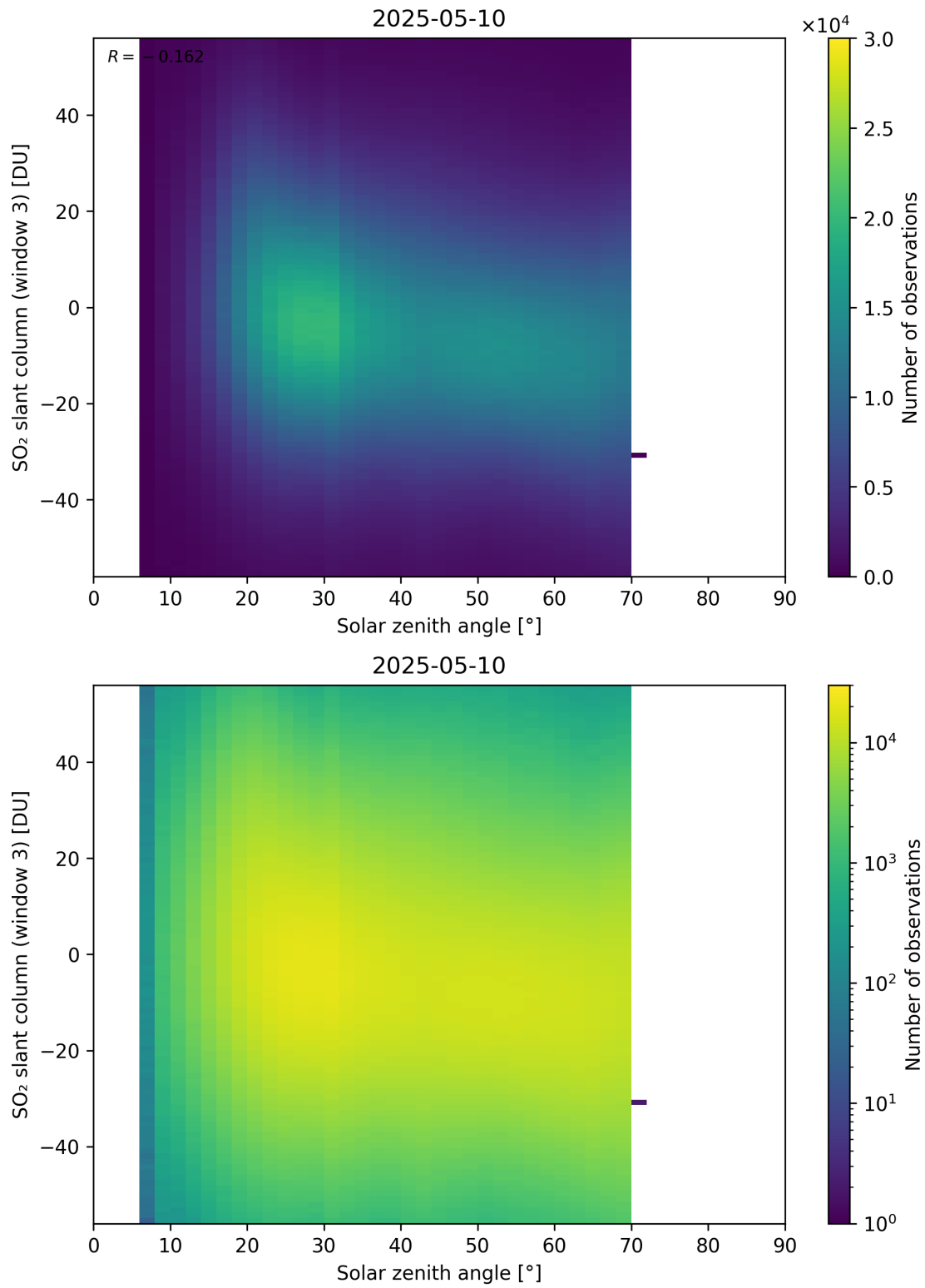
Figure 187: Scatter density plot of “Solar zenith angle” against “SO 2 slant column (window 3)” for 2025-05-10 to 2025-05-11.
