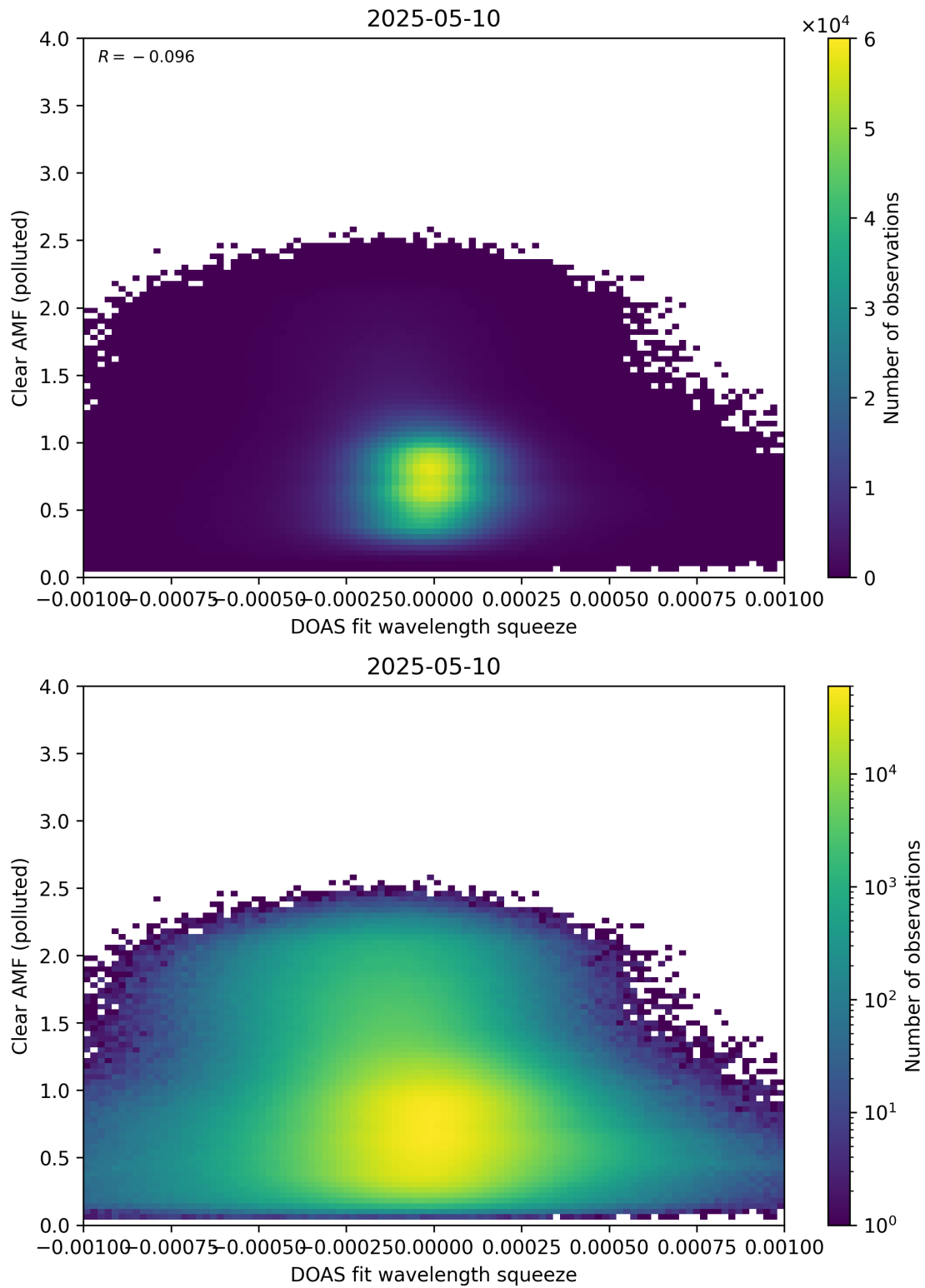
Figure 144: Scatter density plot of “DOAS fit wavelength squeeze” against “Clear AMF (polluted)” for 2025-05-10 to 2025-05-11.
