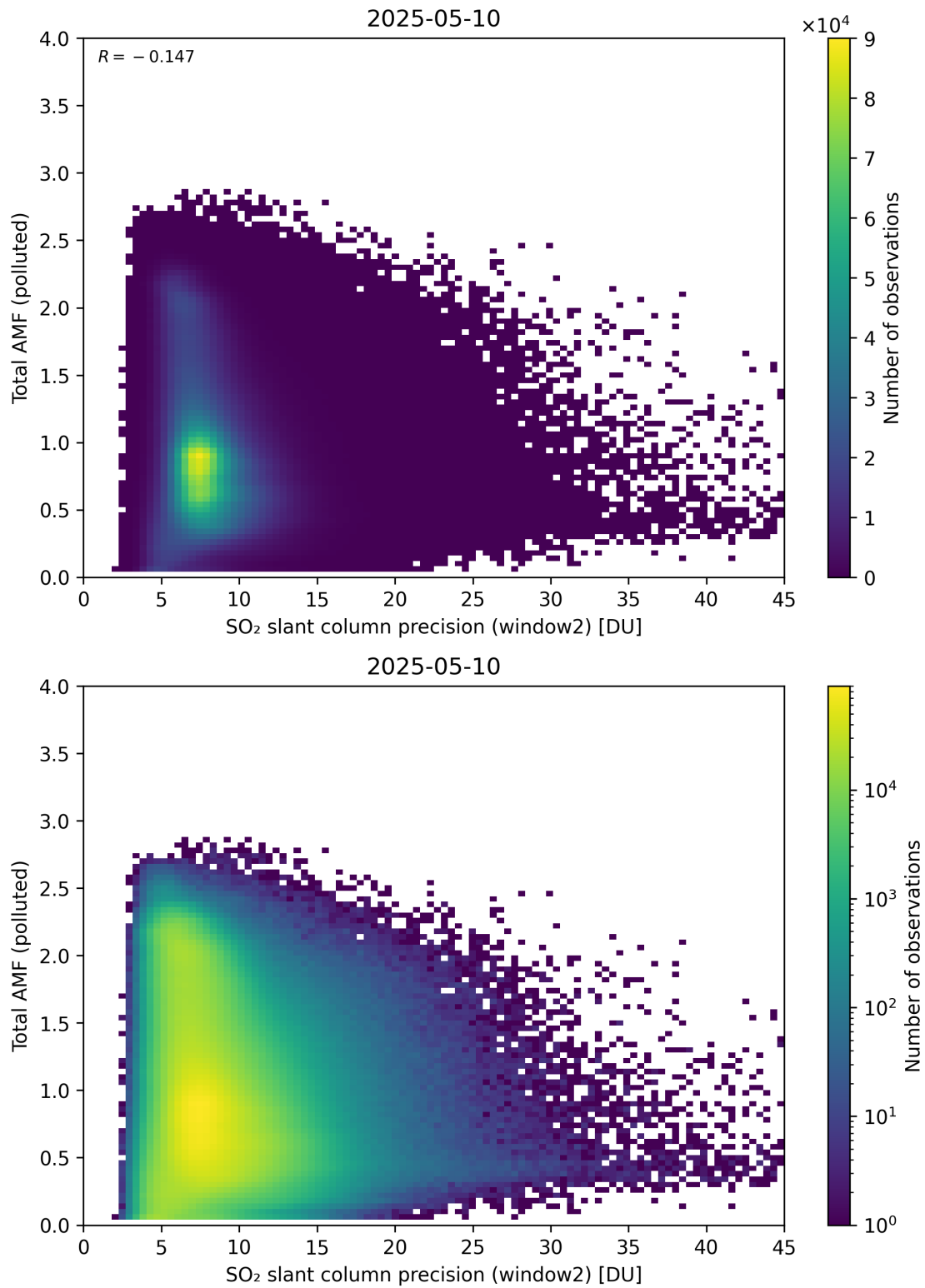
Figure 301: Scatter density plot of “SO 2 slant column precision (window2)” against “Total AMF (polluted)” for 2025-05-10 to 2025-05-11.
