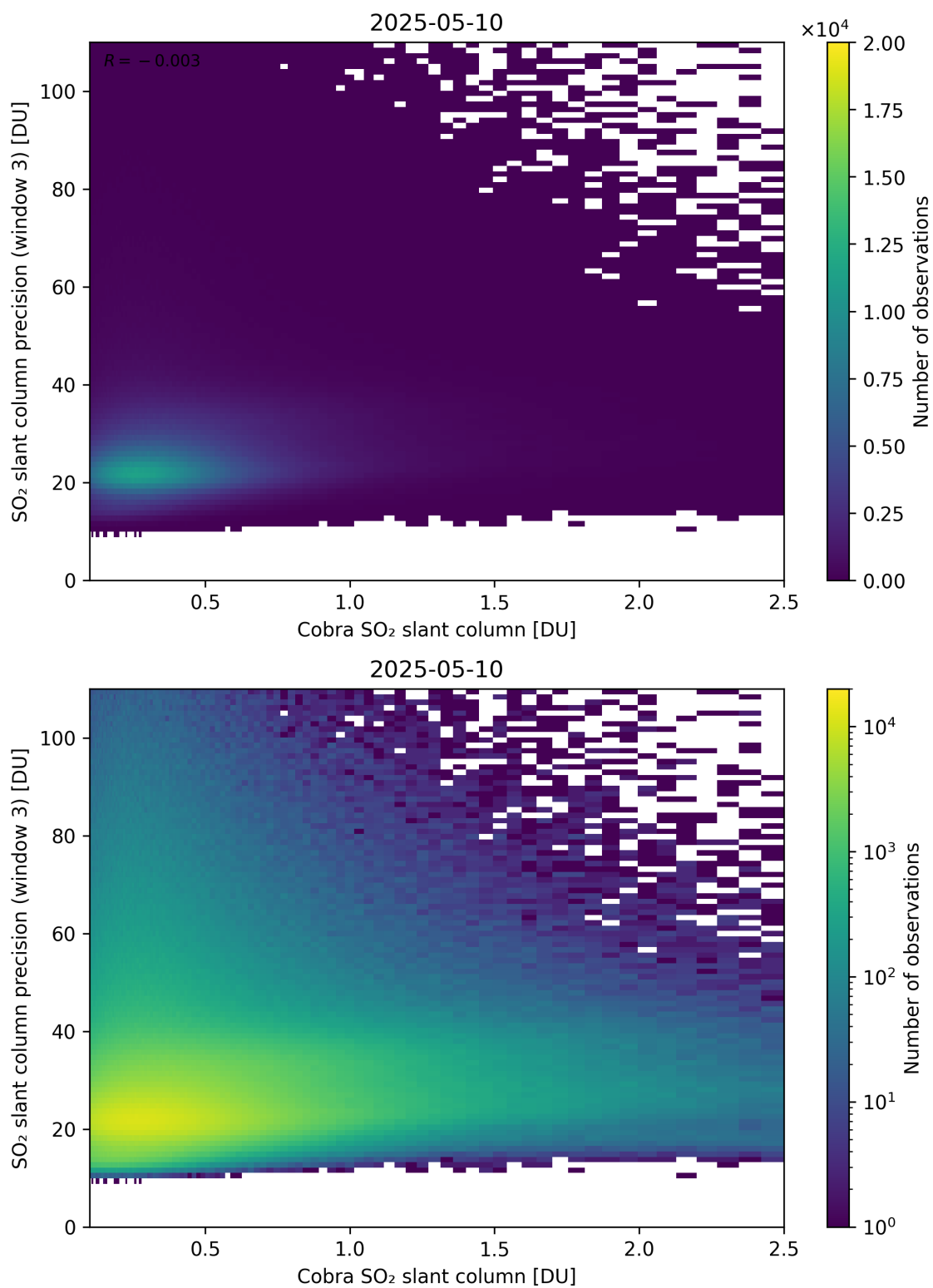
Figure 223: Scatter density plot of “Cobra SO 2 slant column” against “SO 2 slant column precision (window 3)” for 2025-05-10 to 2025-05-11.
