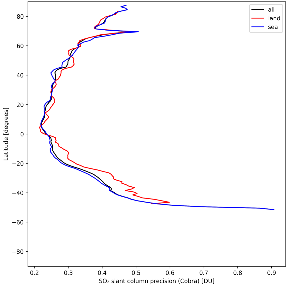
Figure 36: Zonal average of “SO 2 slant column precision (Cobra)” for 2025-05-10 to 2025-05-11.
