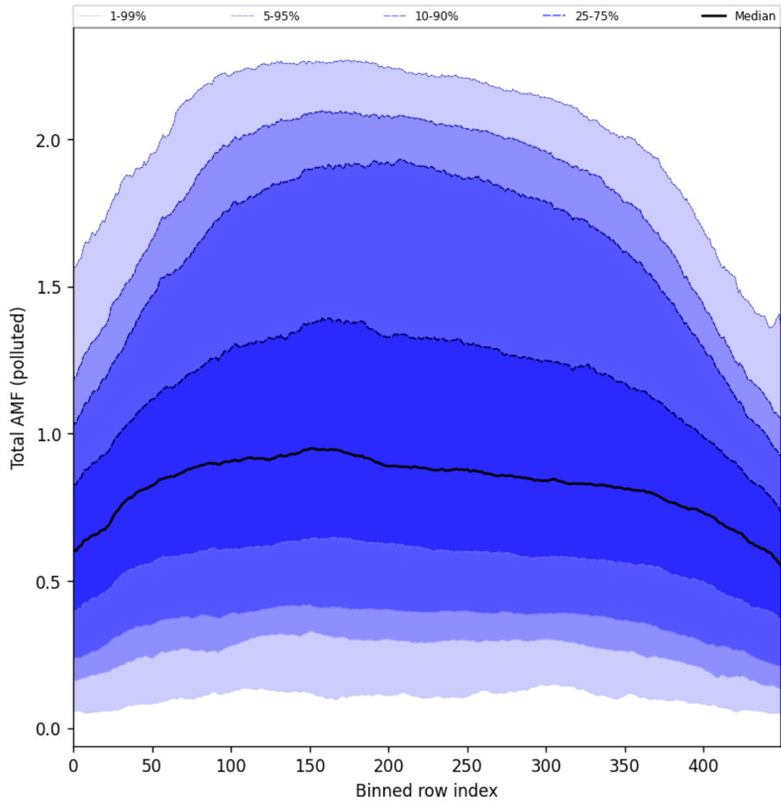
Figure 105: Along track statistics of “Total AMF (polluted)” for 2025-05-10 to 2025-05-11
