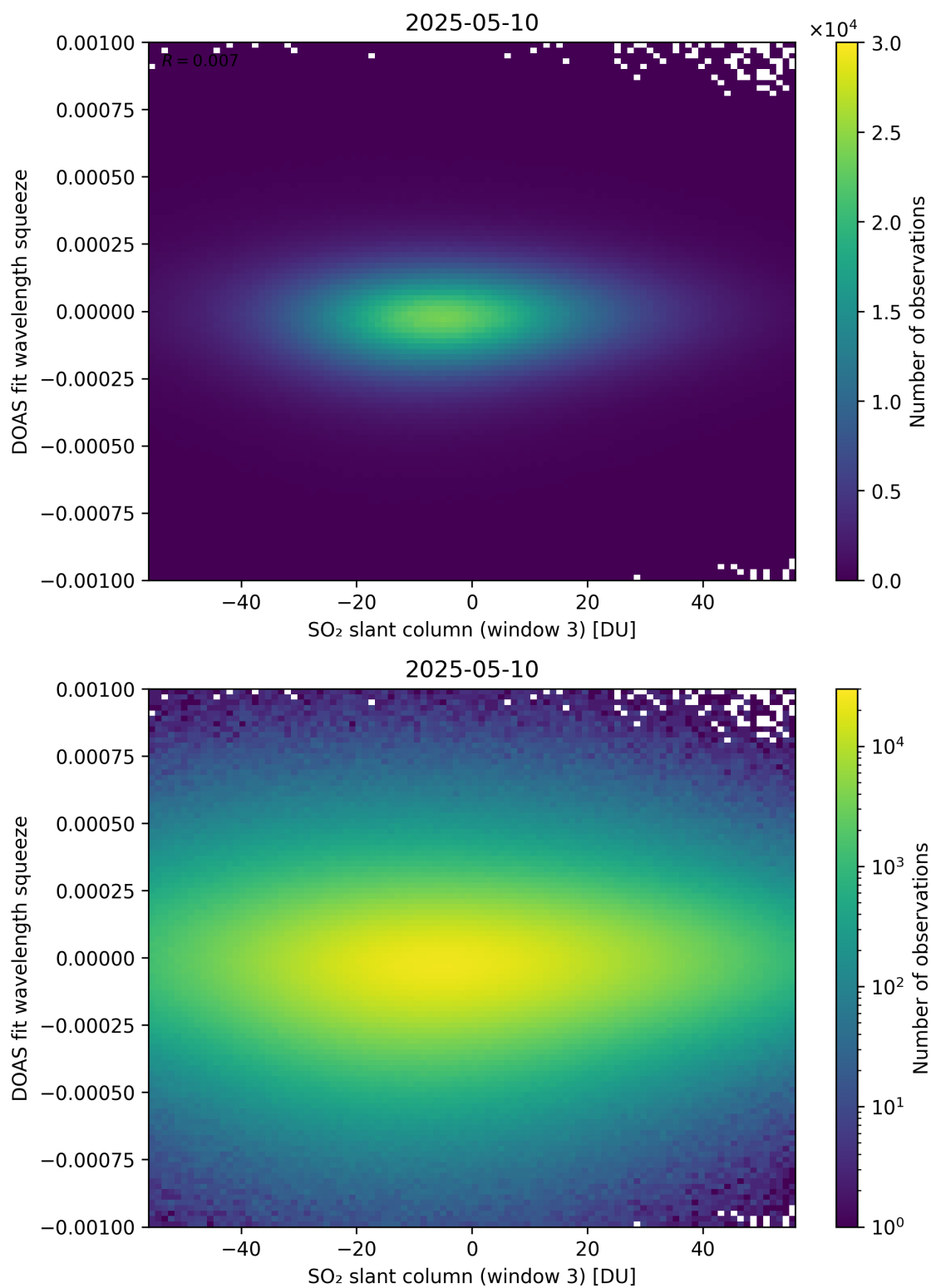
Figure 305: Scatter density plot of “SO 2 slant column (window 3)” against “DOAS fit wavelength squeeze” for 2025-05-10 to 2025-05-11.
