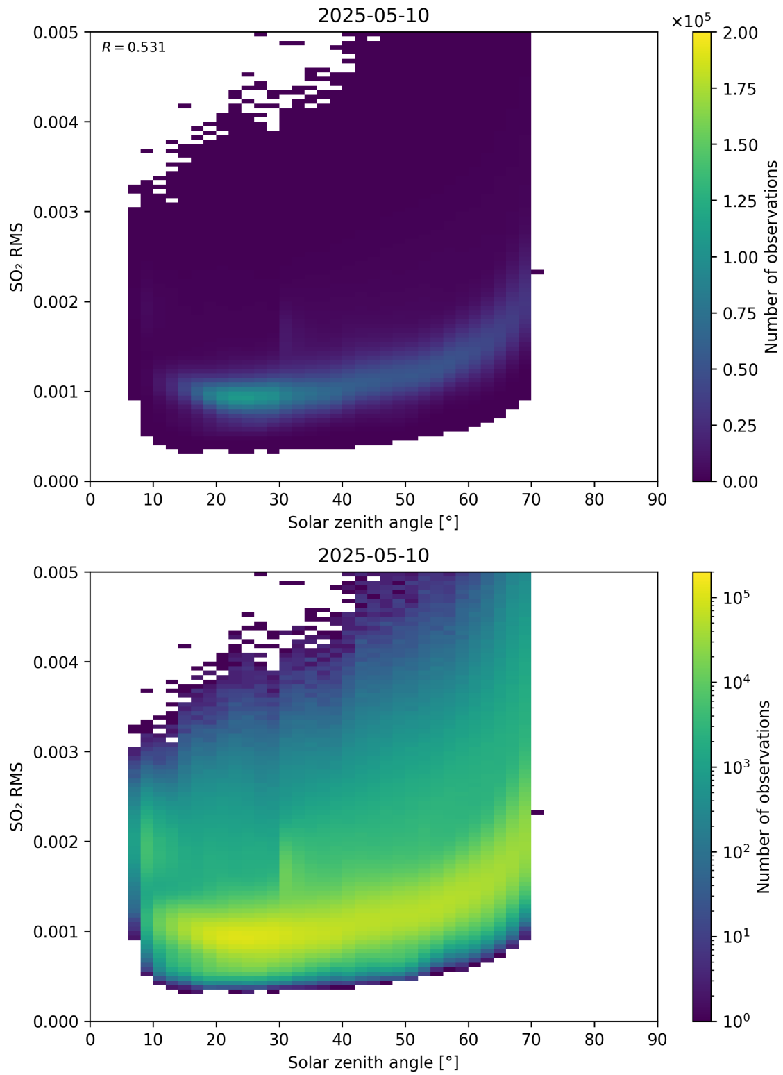
Figure 176: Scatter density plot of “Solar zenith angle” against “SO 2 RMS” for 2025-05-10 to 2025-05-11.
