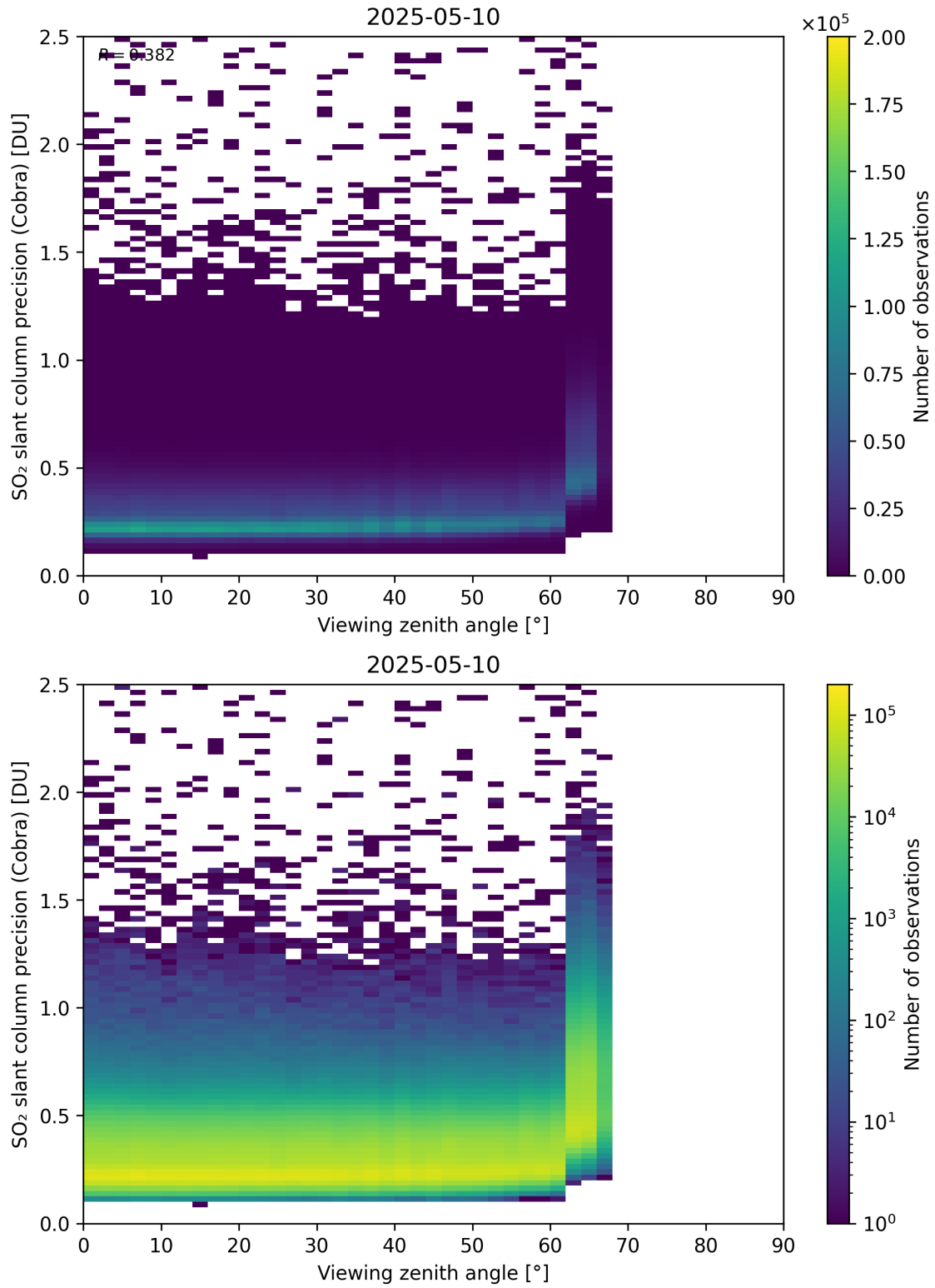
Figure 372: Scatter density plot of “Viewing zenith angle” against “SO 2 slant column precision (Cobra)” for 2025-05-10 to 2025-05-11.
