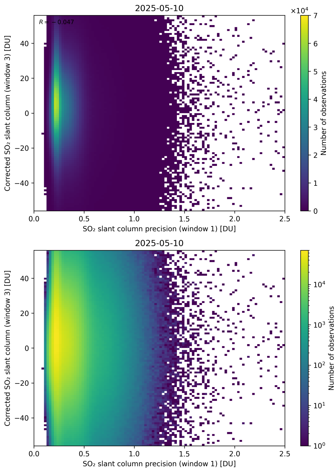
Figure 276: Scatter density plot of “SO 2 slant column precision (window 1)” against “Corrected SO 2 slant column (window 3)” for 2025-05-10 to 2025-05-11.
