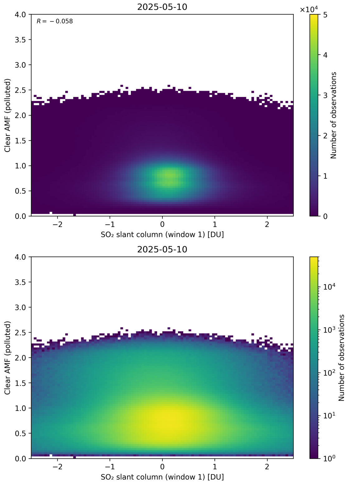
Figure 282: Scatter density plot of “SO 2 slant column (window 1)” against “Clear AMF (polluted)” for 2025-05-10 to 2025-05-11.
