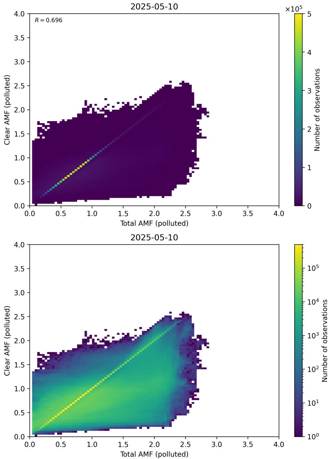
Figure 321: Scatter density plot of “Total AMF (polluted)” against “Clear AMF (polluted)” for 2025-05-10 to 2025-05-11.
