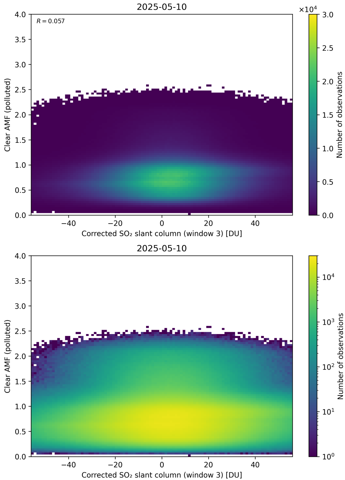
Figure 259: Scatter density plot of “Corrected SO 2 slant column (window 3)” against “Clear AMF (polluted)” for 2025-05-10 to 2025-05-11.
