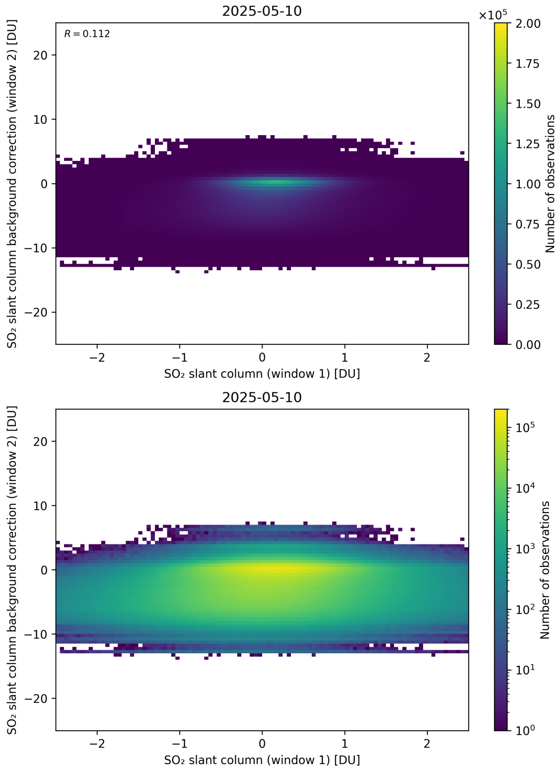
Figure 263: Scatter density plot of “SO 2 slant column (window 1)” against “SO 2 slant column background correction (window 2)” for 2025-05-10 to 2025-05-11.
