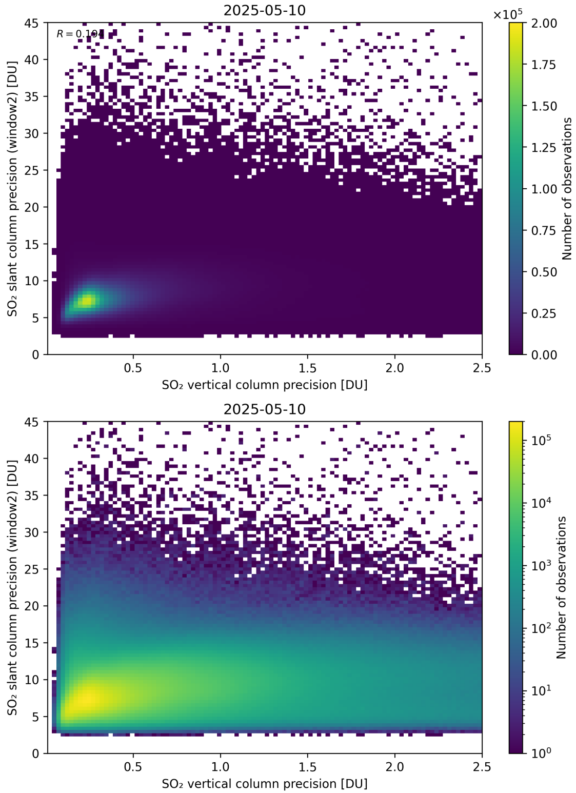
Figure 343: Scatter density plot of “SO 2 vertical column precision” against “SO 2 slant column precision (window2)” for 2025-05-10 to 2025-05-11.
