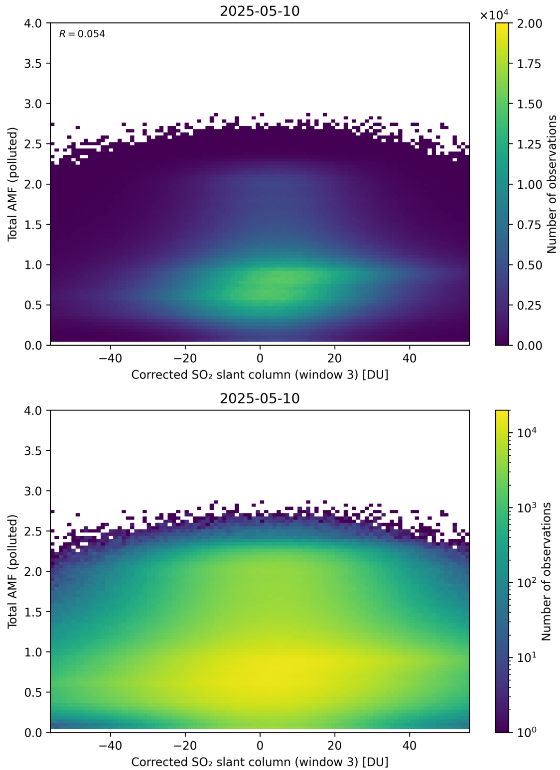
Figure 260: Scatter density plot of “Corrected SO 2 slant column (window 3)” against “Total AMF (polluted)” for 2025-05-10 to 2025-05-11.
