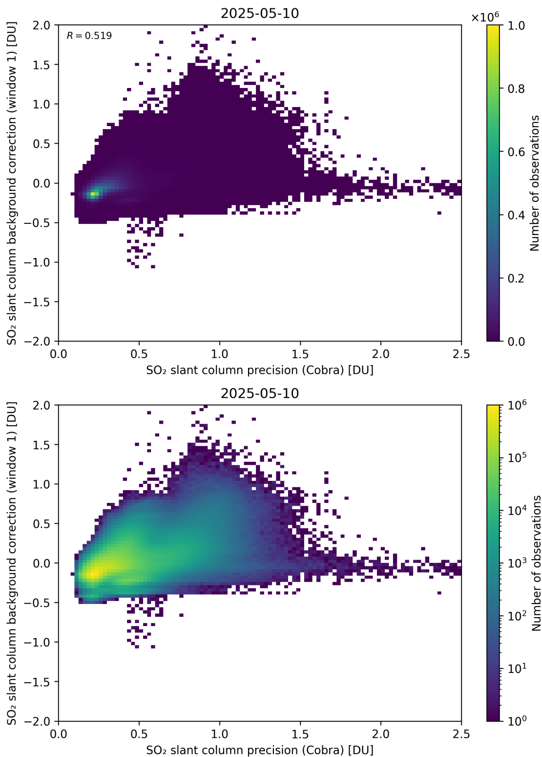
Figure 199: Scatter density plot of “SO 2 slant column precision (Cobra)” against “SO 2 slant column background correction (window 1)” for 2025-05-10 to 2025-05-11.
