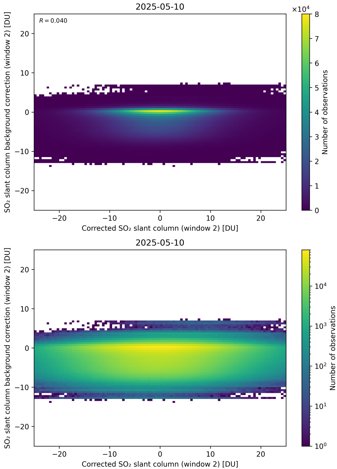
Figure 244: Scatter density plot of “Corrected SO 2 slant column (window 2)” against “SO 2 slant column background correction (window 2)” for 2025-05-10 to 2025-05-11.
