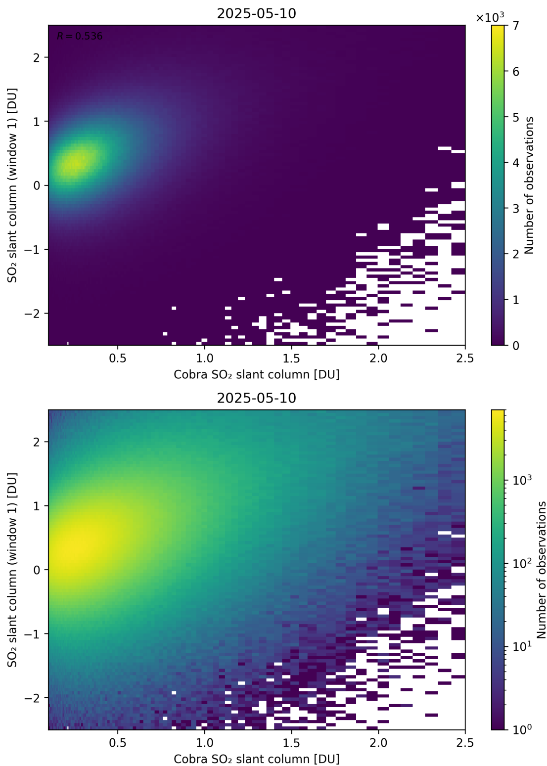
Figure 219: Scatter density plot of “Cobra SO 2 slant column” against “SO 2 slant column (window 1)” for 2025-05-10 to 2025-05-11.
