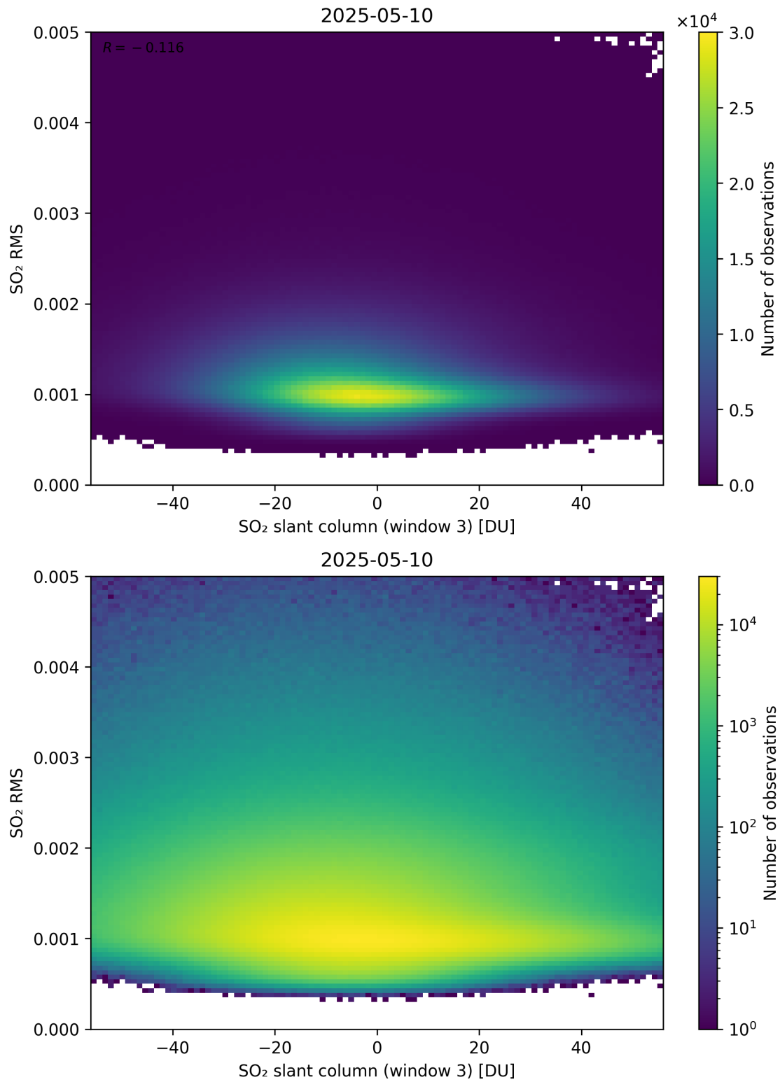
Figure 306: Scatter density plot of “SO 2 slant column (window 3)” against “SO 2 RMS” for 2025-05-10 to 2025-05-11.
