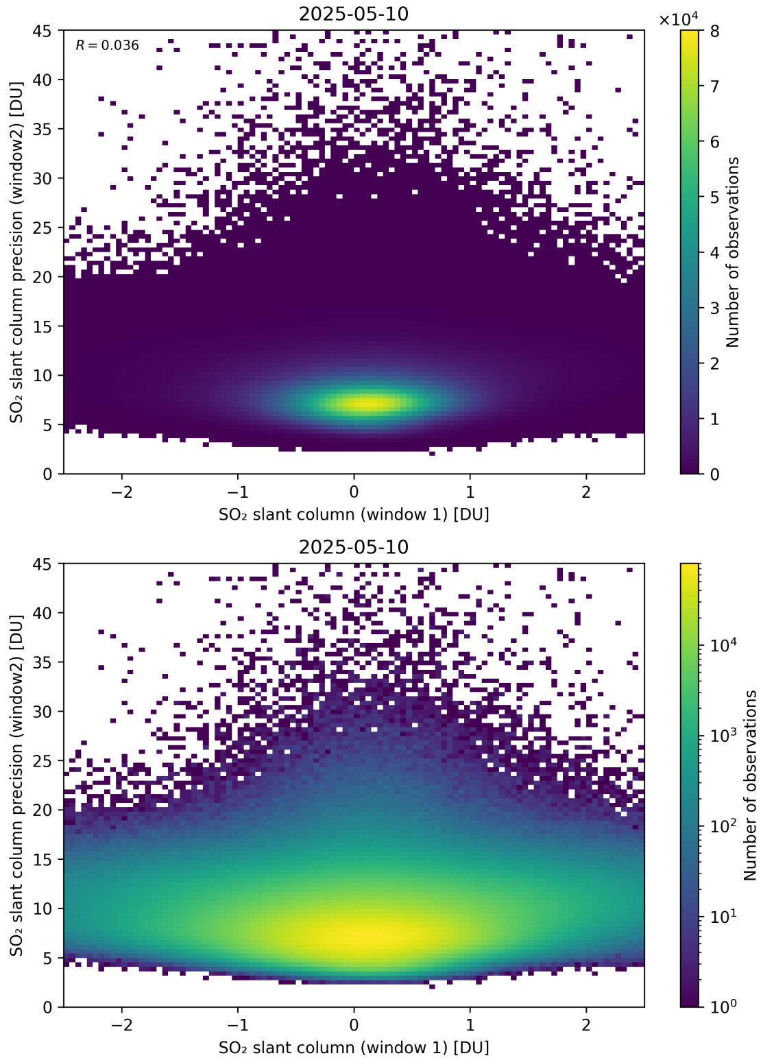
Figure 286: Scatter density plot of “SO 2 slant column (window 1)” against “SO 2 slant column precision (window2)” for 2025-05-10 to 2025-05-11.
