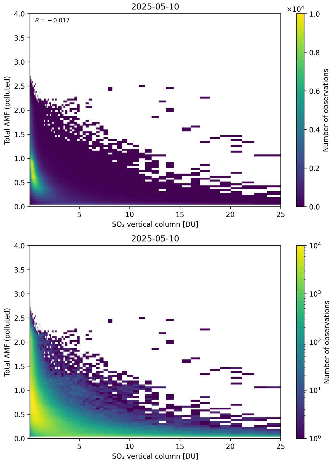
Figure 359: Scatter density plot of “SO 2 vertical column” against “Total AMF (polluted)” for 2025-05-10 to 2025-05-11.
