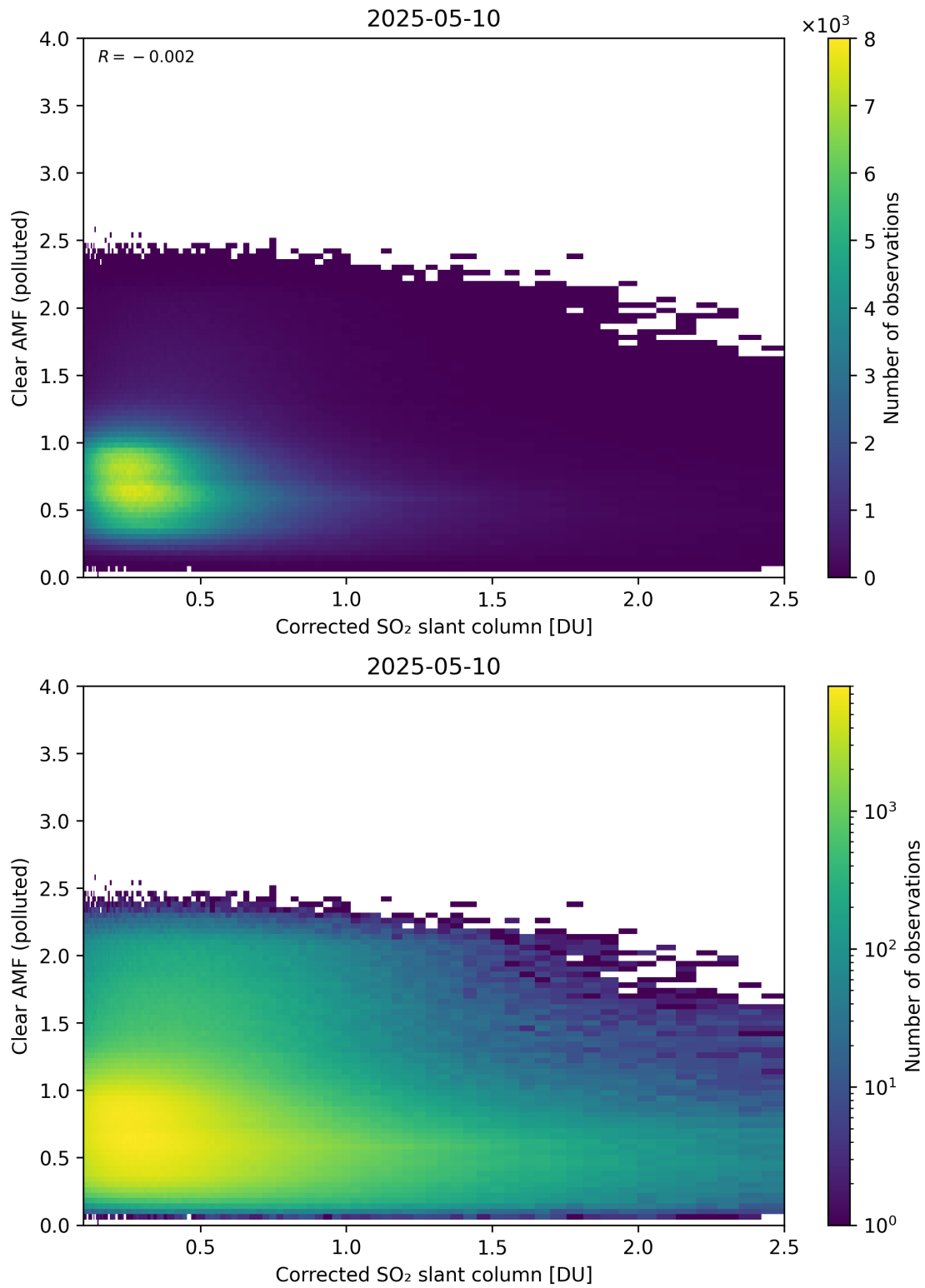
Figure 232: Scatter density plot of “Corrected SO 2 slant column” against “Clear AMF (polluted)” for 2025-05-10 to 2025-05-11.
