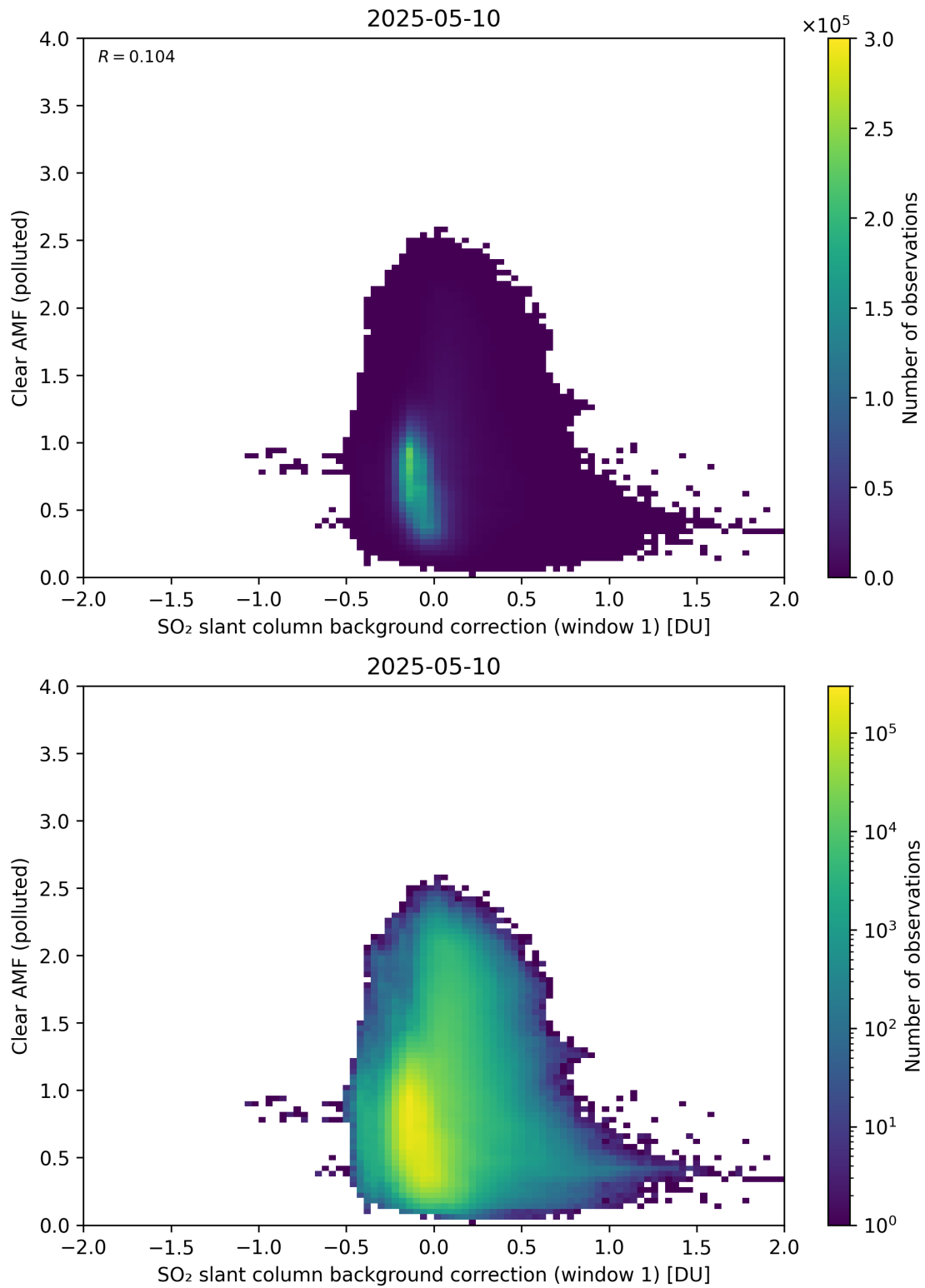
Figure 114: Scatter density plot of “SO 2 slant column background correction (window 1)” against “Clear AMF (polluted)” for 2025-05-10 to 2025-05-11.
