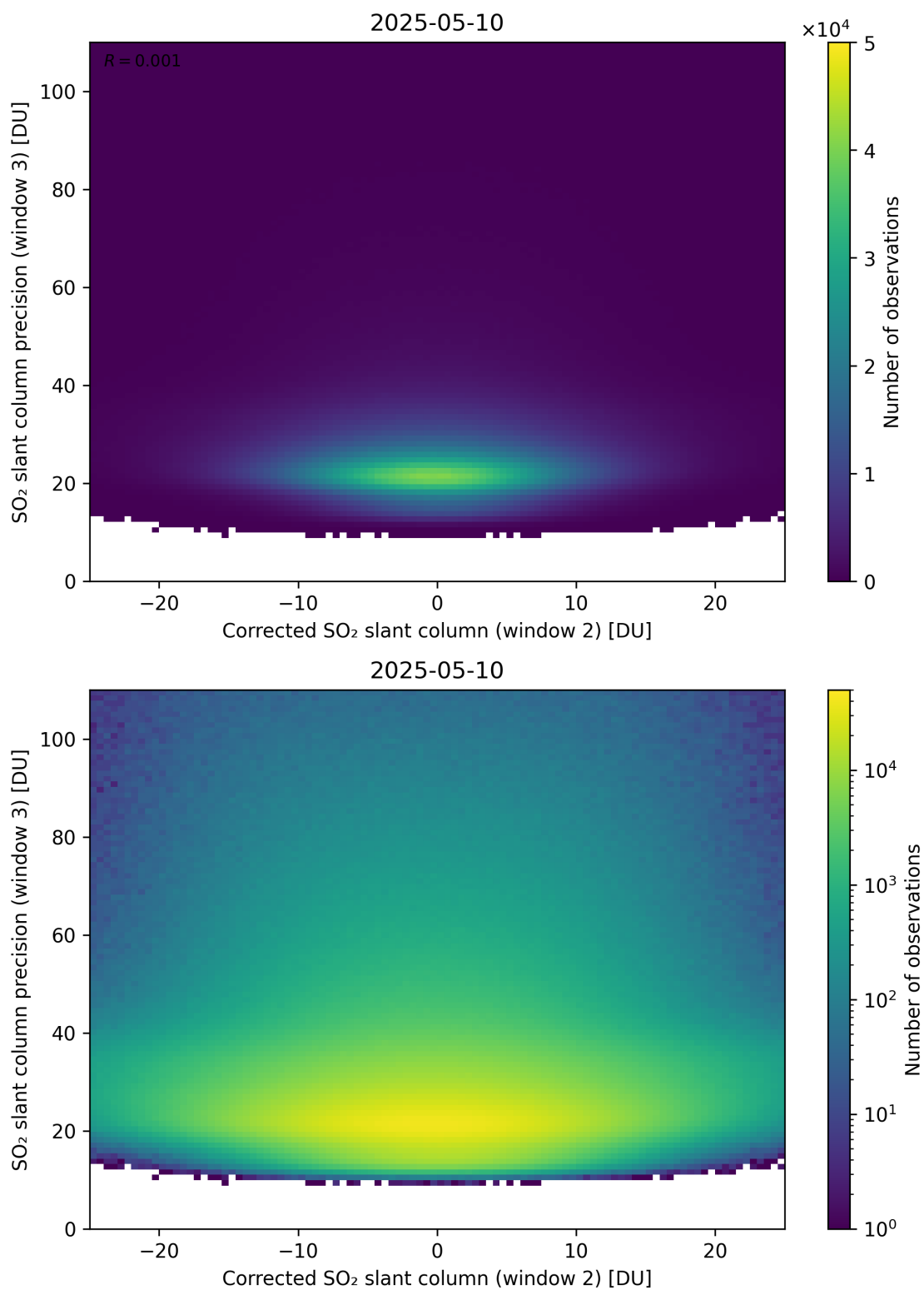
Figure 252: Scatter density plot of “Corrected SO 2 slant column (window 2)” against “SO 2 slant column precision (window 3)” for 2025-05-10 to 2025-05-11.
