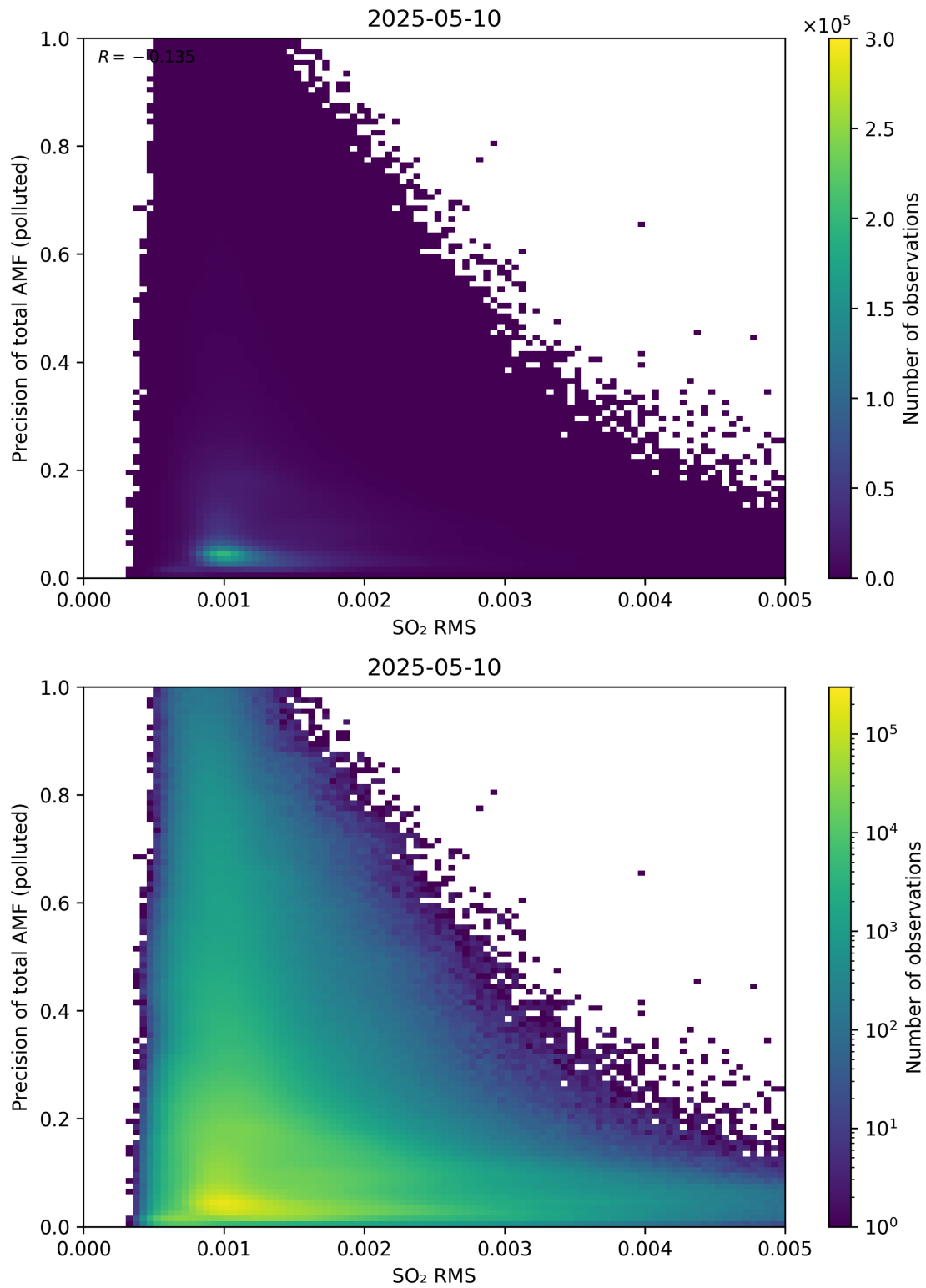
Figure 149: Scatter density plot of “SO 2 RMS” against “Precision of total AMF (polluted)” for 2025-05-10 to 2025-05-11.
