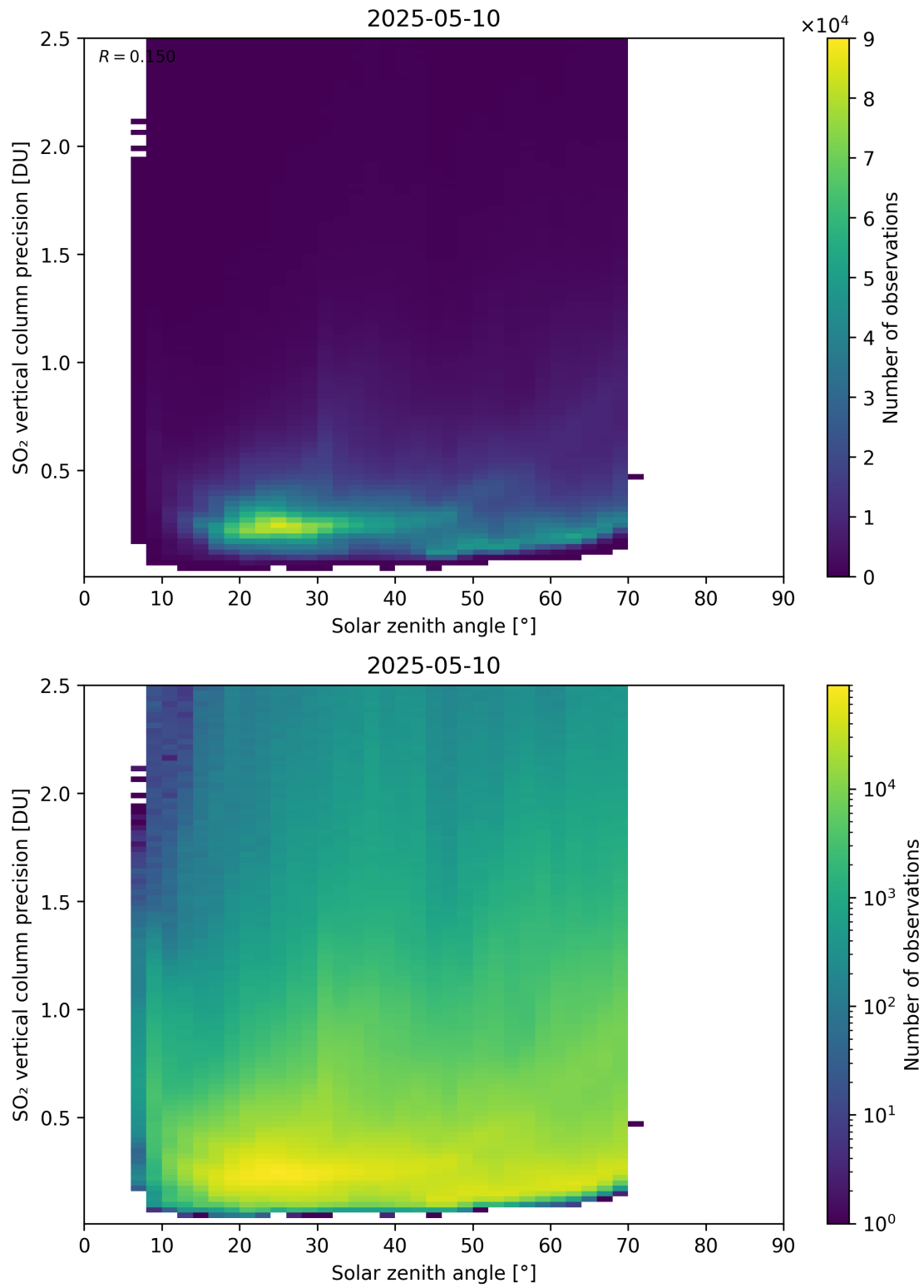
Figure 192: Scatter density plot of “Solar zenith angle” against “SO 2 vertical column precision” for 2025-05-10 to 2025-05-11.
