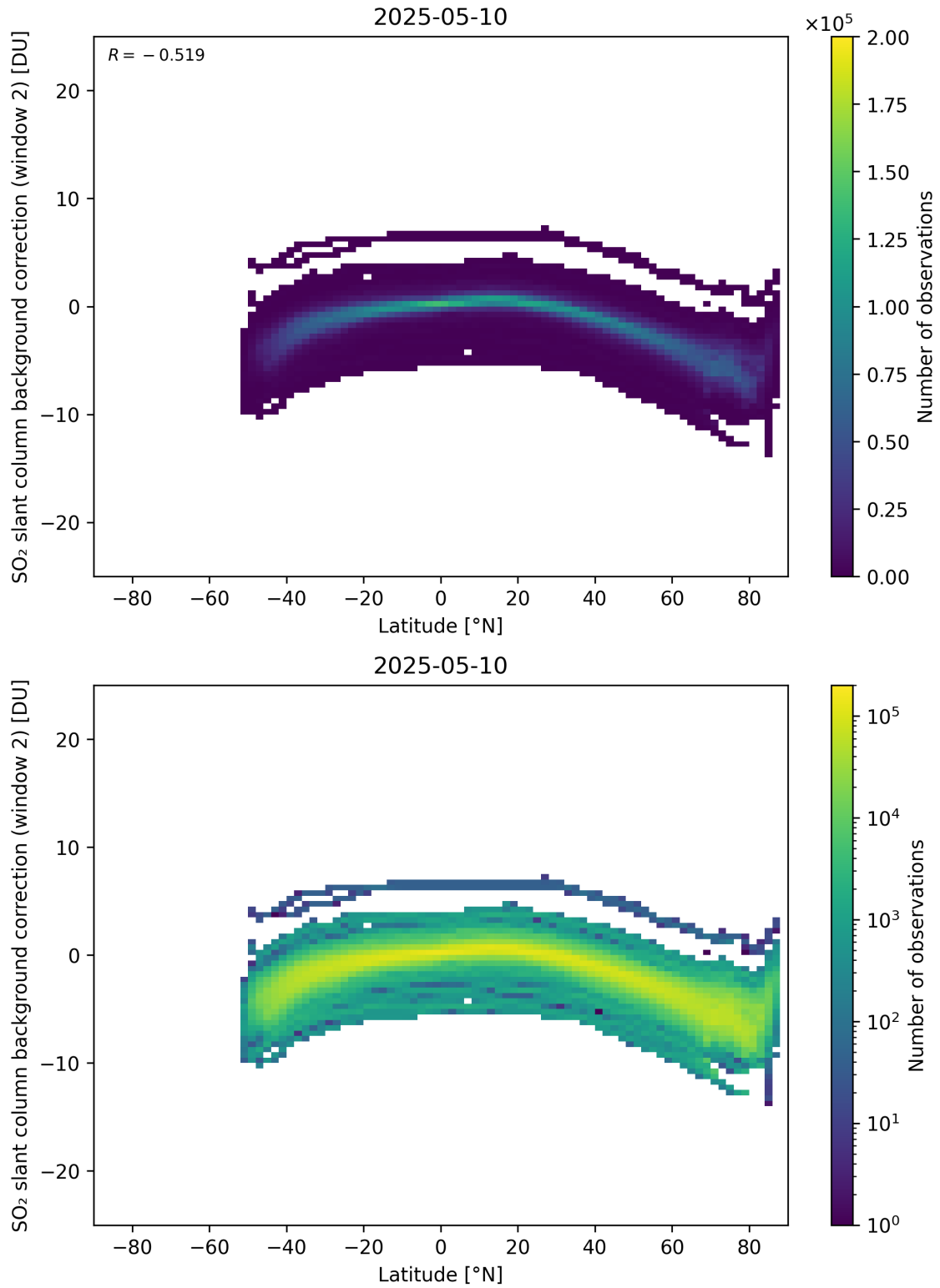
Figure 151: Scatter density plot of “Latitude” against “SO 2 slant column background correction (window 2)” for 2025-05-10 to 2025-05-11.
