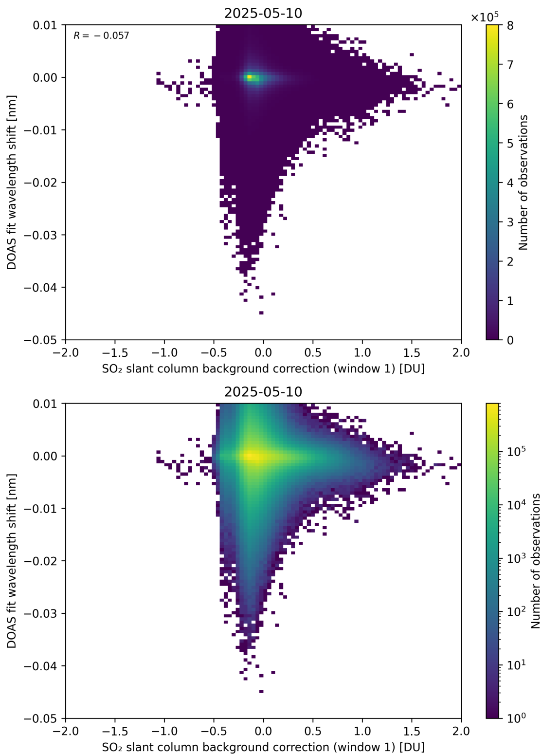
Figure 111: Scatter density plot of “SO 2 slant column background correction (window 1)” against “DOAS fit wavelength shift” for 2025-05-10 to 2025-05-11.
