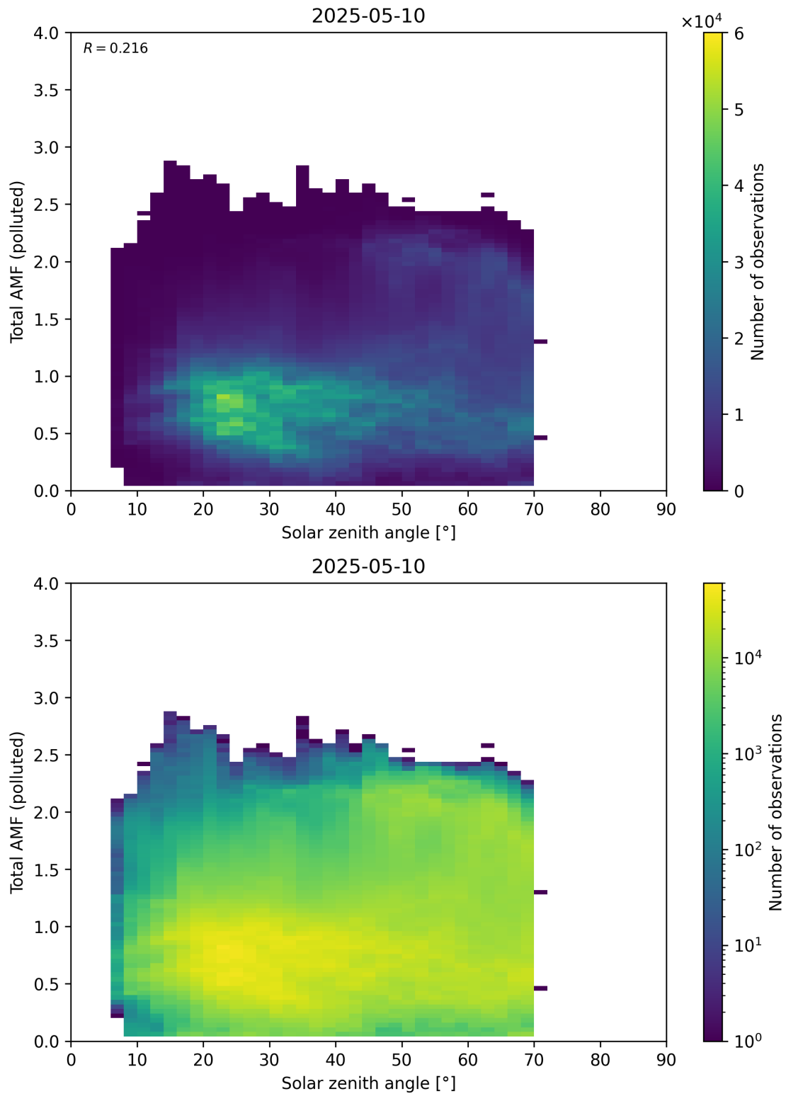
Figure 189: Scatter density plot of “Solar zenith angle” against “Total AMF (polluted)” for 2025-05-10 to 2025-05-11.
