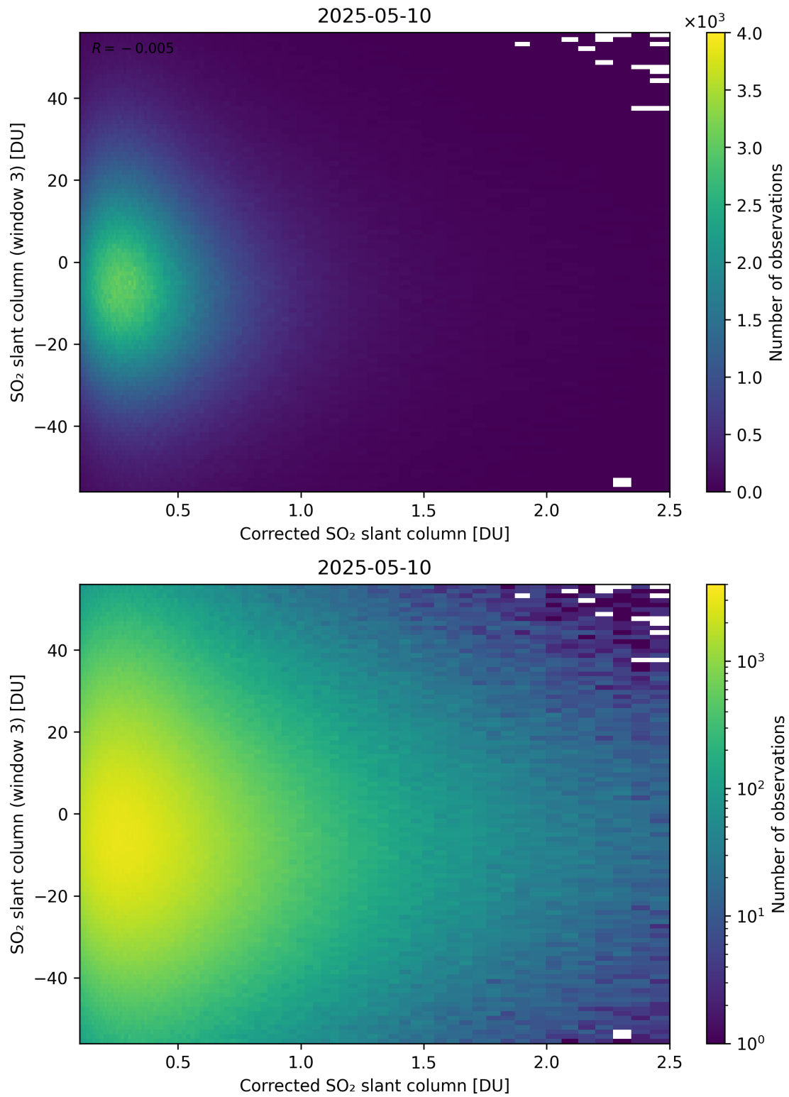
Figure 240: Scatter density plot of “Corrected SO 2 slant column” against “SO 2 slant column (window 3)” for 2025-05-10 to 2025-05-11.
