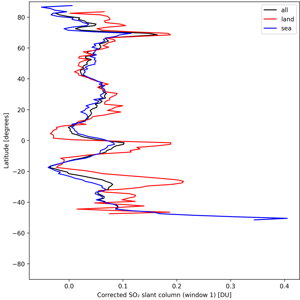
Figure 39: Zonal average of “Corrected SO 2 slant column (window 1)” for 2025-05-10 to 2025-05-11.
