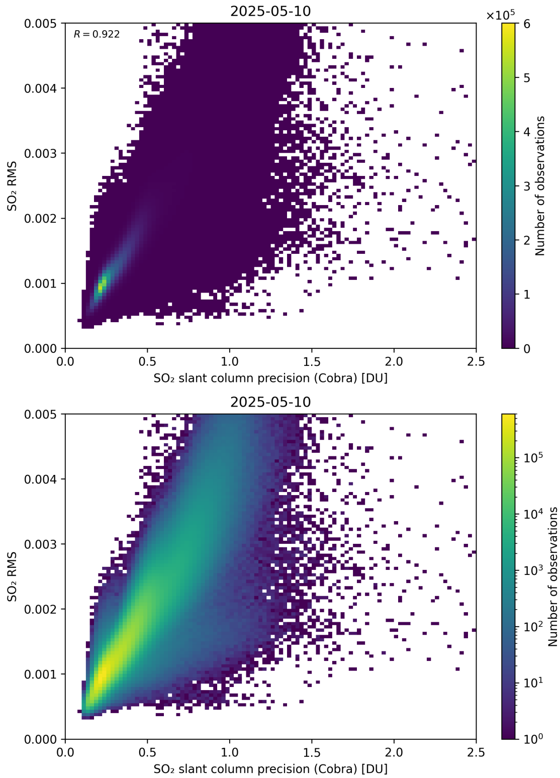
Figure 204: Scatter density plot of “SO 2 slant column precision (Cobra)” against “SO 2 RMS” for 2025-05-10 to 2025-05-11.
