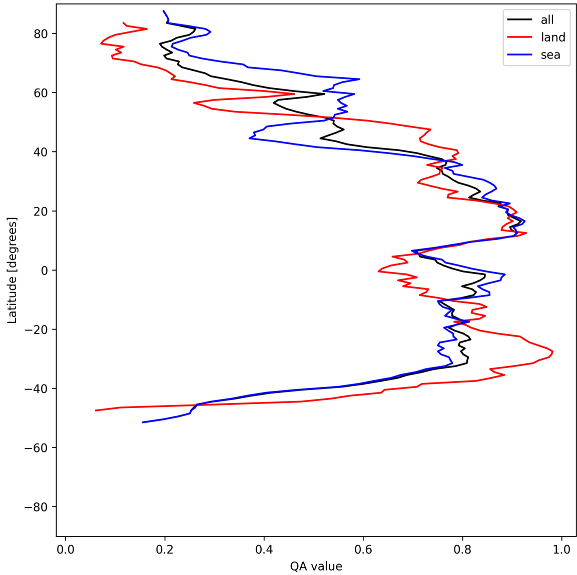
Figure 31: Zonal average of “QA value” for 2025-05-10 to 2025-05-11.
