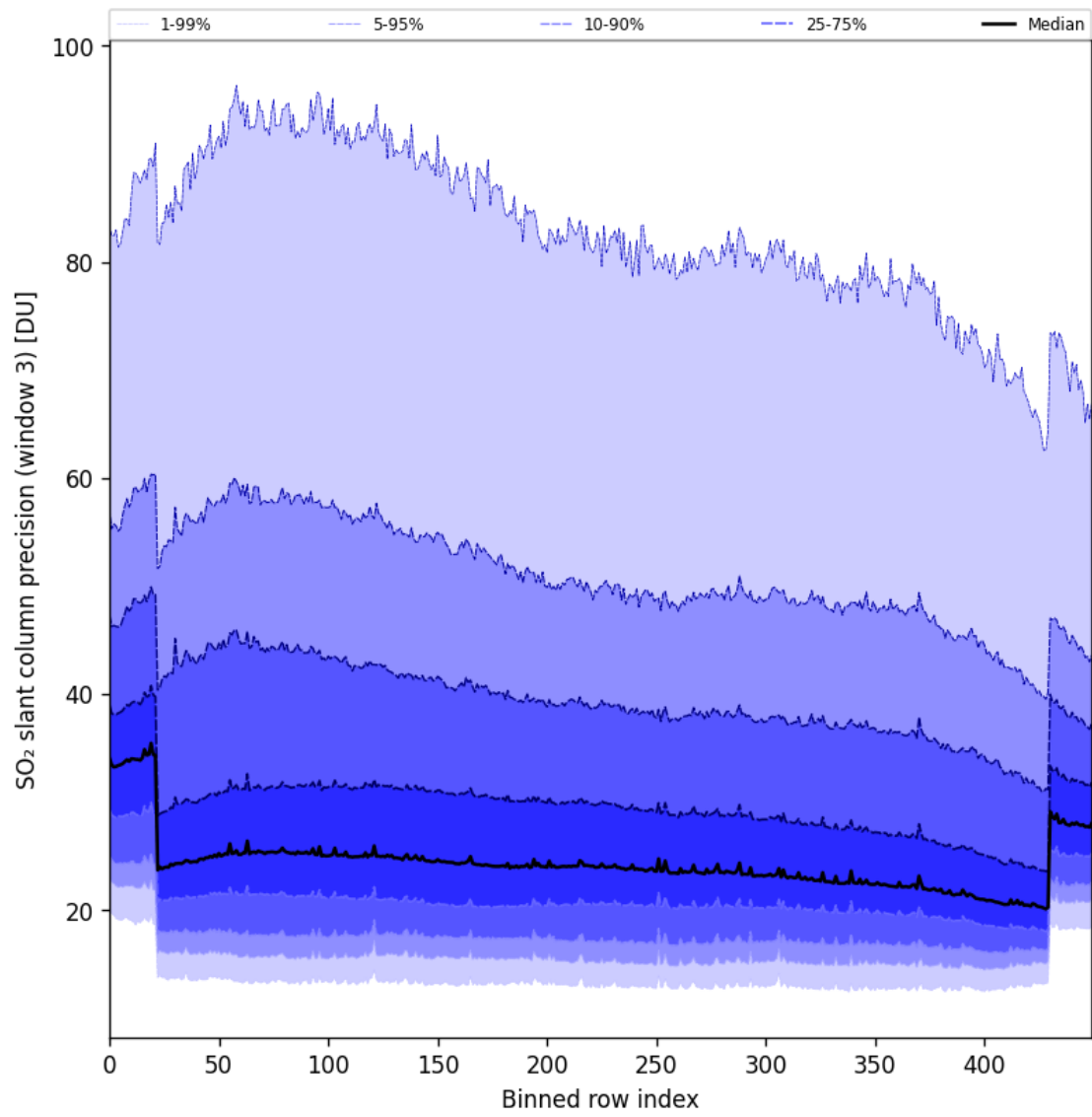
Figure 98: Along track statistics of “SO 2 slant column precision (window 3)” for 2025-05-10 to 2025-05-11
