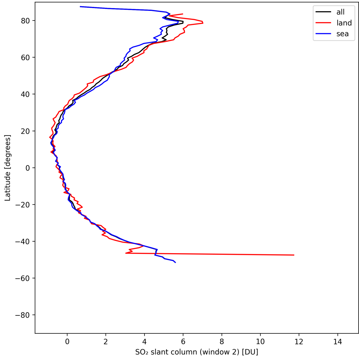
Figure 41: Zonal average of “SO 2 slant column (window 2)” for 2025-05-10 to 2025-05-11.
