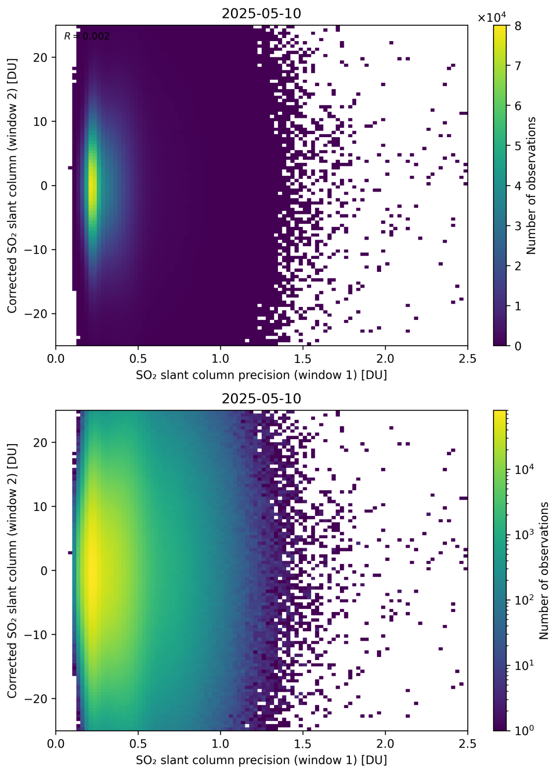
Figure 275: Scatter density plot of “SO 2 slant column precision (window 1)” against “Corrected SO 2 slant column (window 2)” for 2025-05-10 to 2025-05-11.
