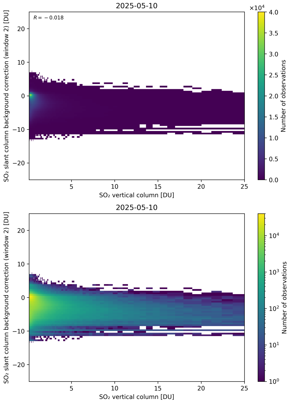
Figure 324: Scatter density plot of “SO 2 vertical column” against “SO 2 slant column background correction (window 2)” for 2025-05-10 to 2025-05-11.
