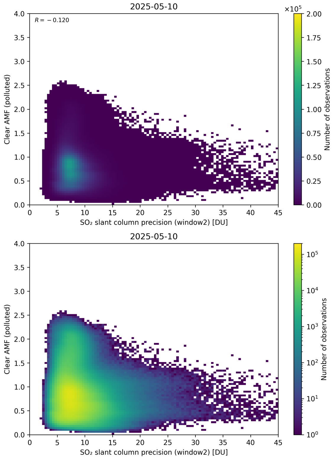
Figure 296: Scatter density plot of “SO 2 slant column precision (window2)” against “Clear AMF (polluted)” for 2025-05-10 to 2025-05-11.
