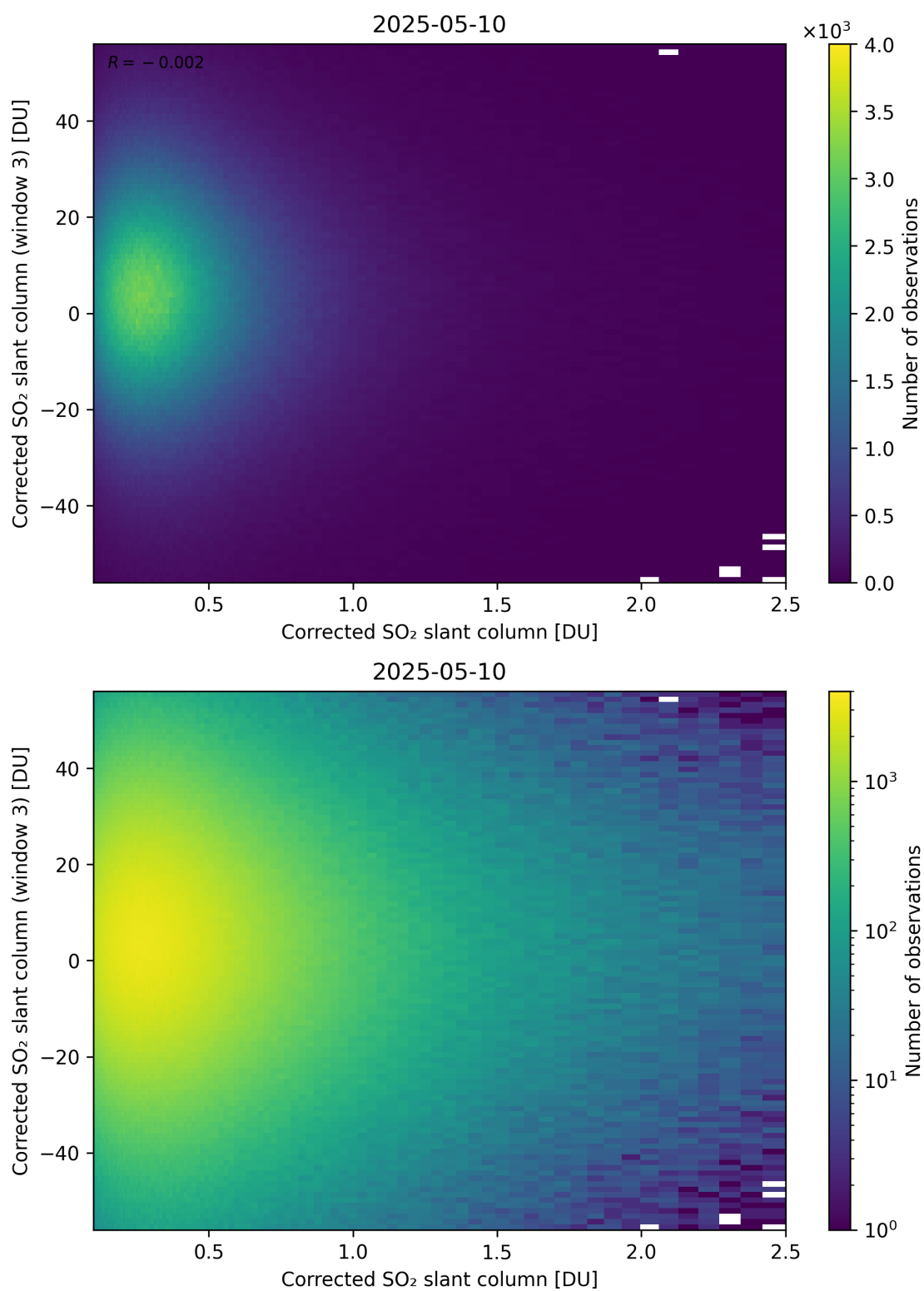
Figure 236: Scatter density plot of “Corrected SO 2 slant column” against “Corrected SO 2 slant column (window 3)” for 2025-05-10 to 2025-05-11.
