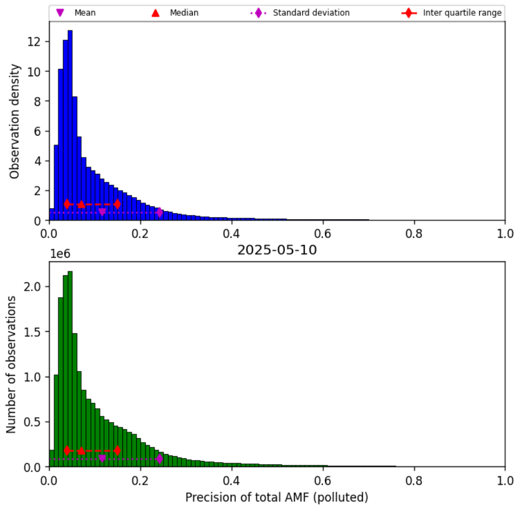
Figure 80: Histogram of “Precision of total AMF (polluted)” for 2025-05-10 to 2025-05-11
