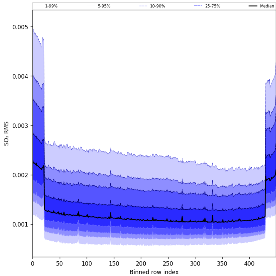
Figure 104: Along track statistics of “SO 2 RMS” for 2025-05-10 to 2025-05-11
