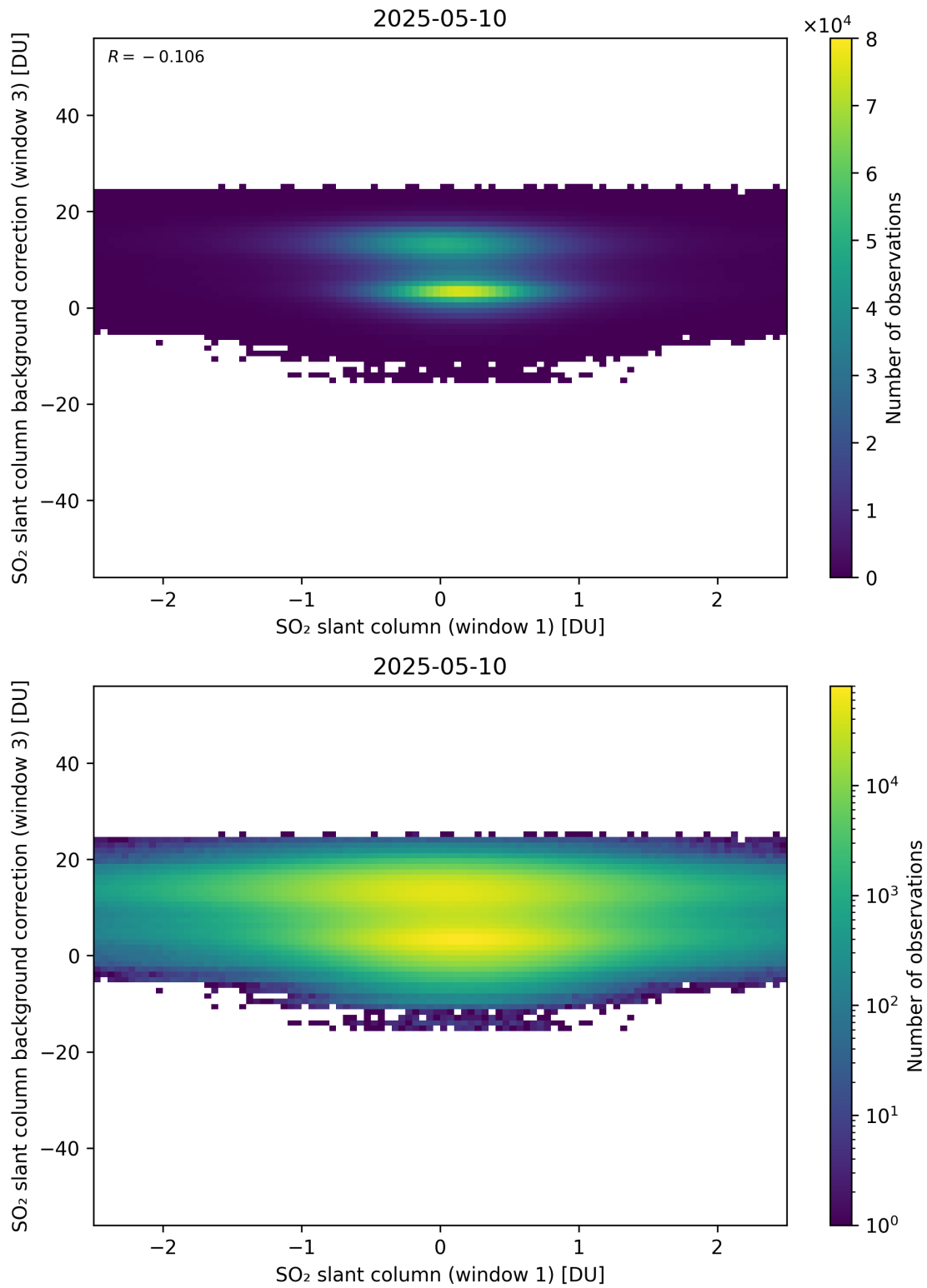
Figure 264: Scatter density plot of “SO 2 slant column (window 1)” against “SO 2 slant column background correction (window 3)” for 2025-05-10 to 2025-05-11.
