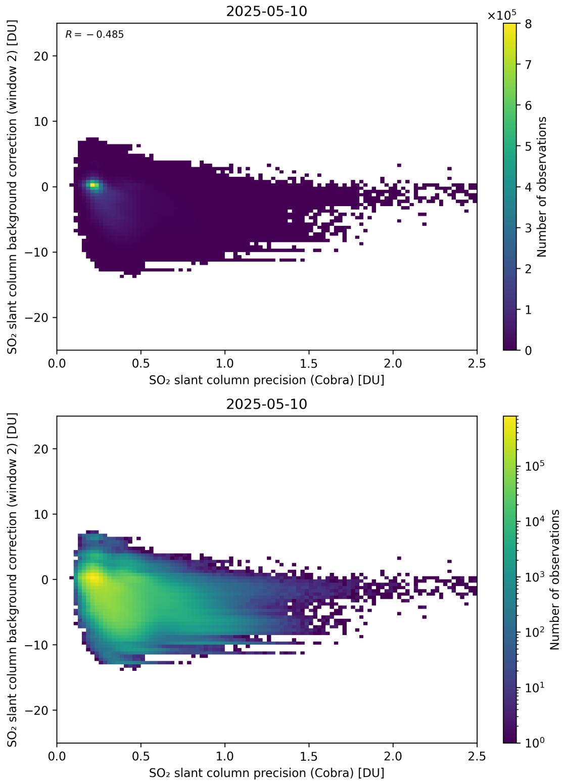
Figure 200: Scatter density plot of “SO 2 slant column precision (Cobra)” against “SO 2 slant column background correction (window 2)” for 2025-05-10 to 2025-05-11.
