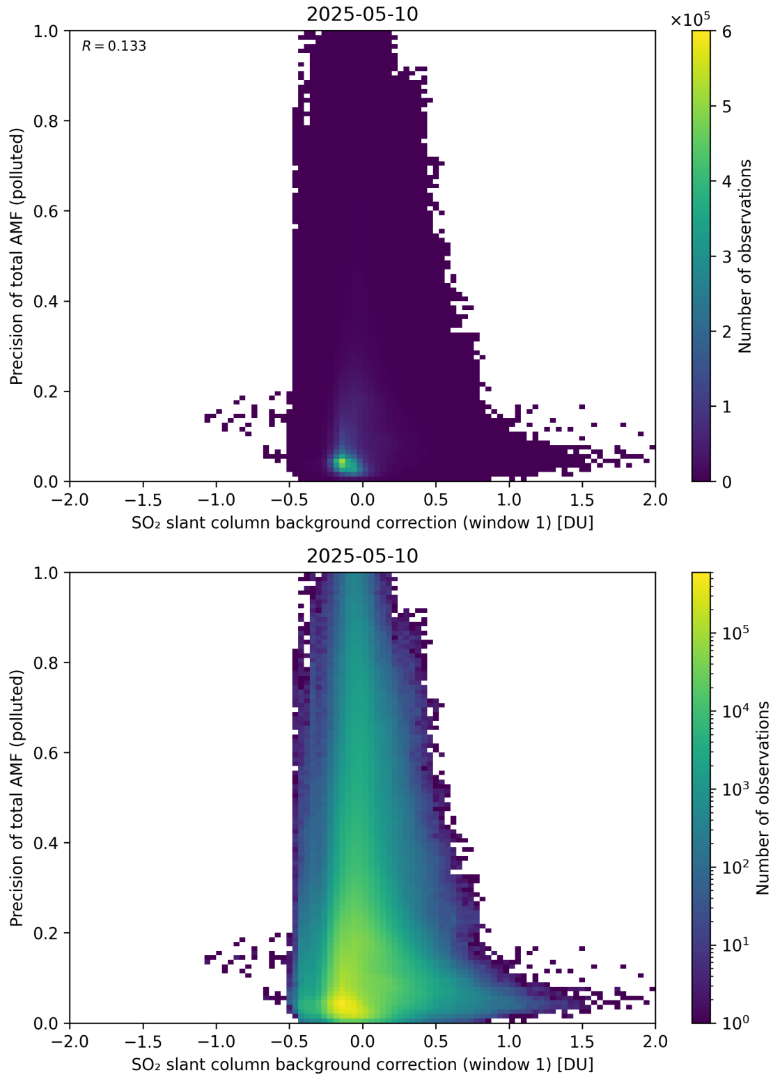
Figure 121: Scatter density plot of “SO 2 slant column background correction (window 1)” against “Precision of total AMF (polluted)” for 2025-05-10 to 2025-05-11.
