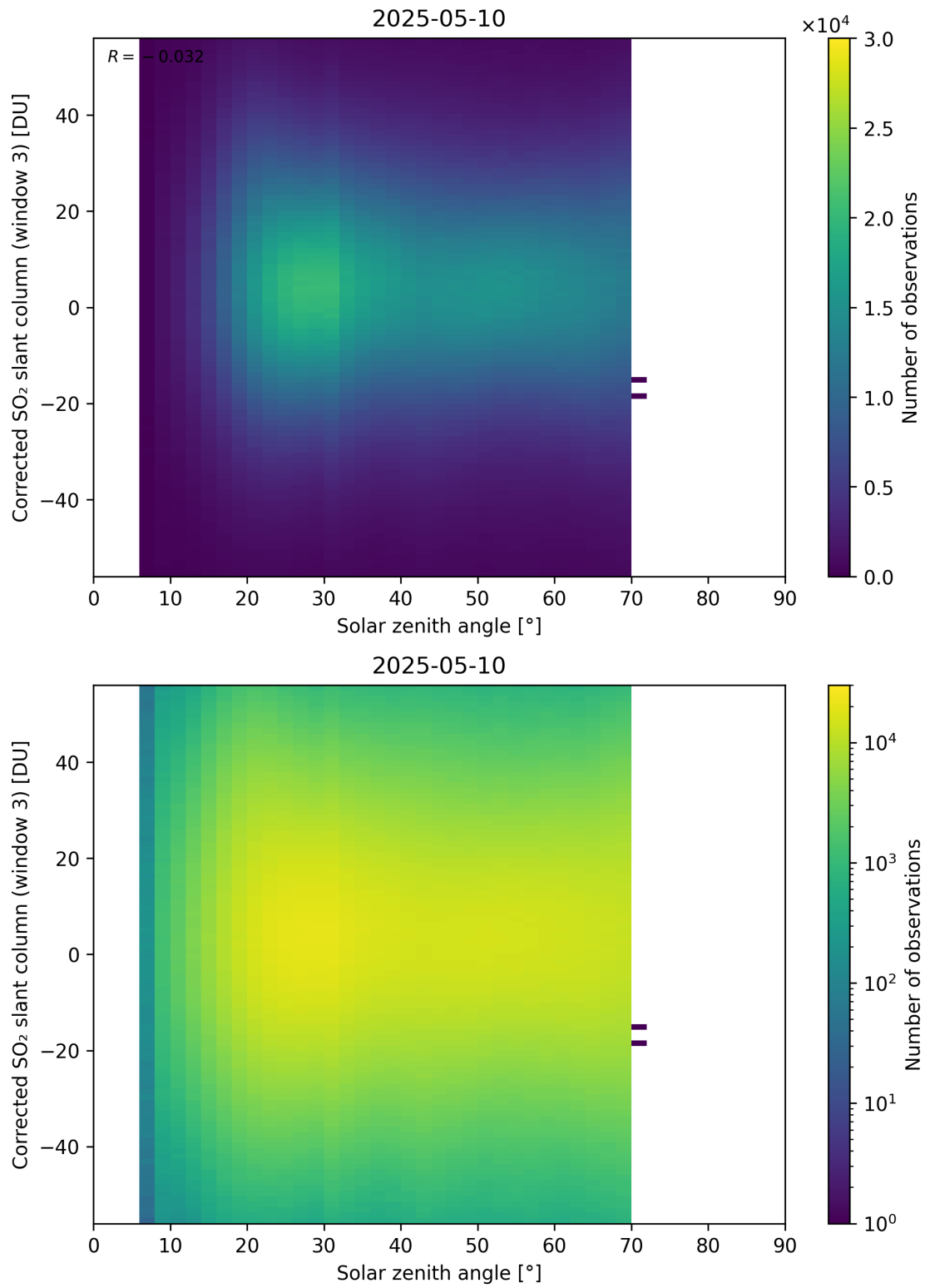
Figure 183: Scatter density plot of “Solar zenith angle” against “Corrected SO 2 slant column (window 3)” for 2025-05-10 to 2025-05-11.
