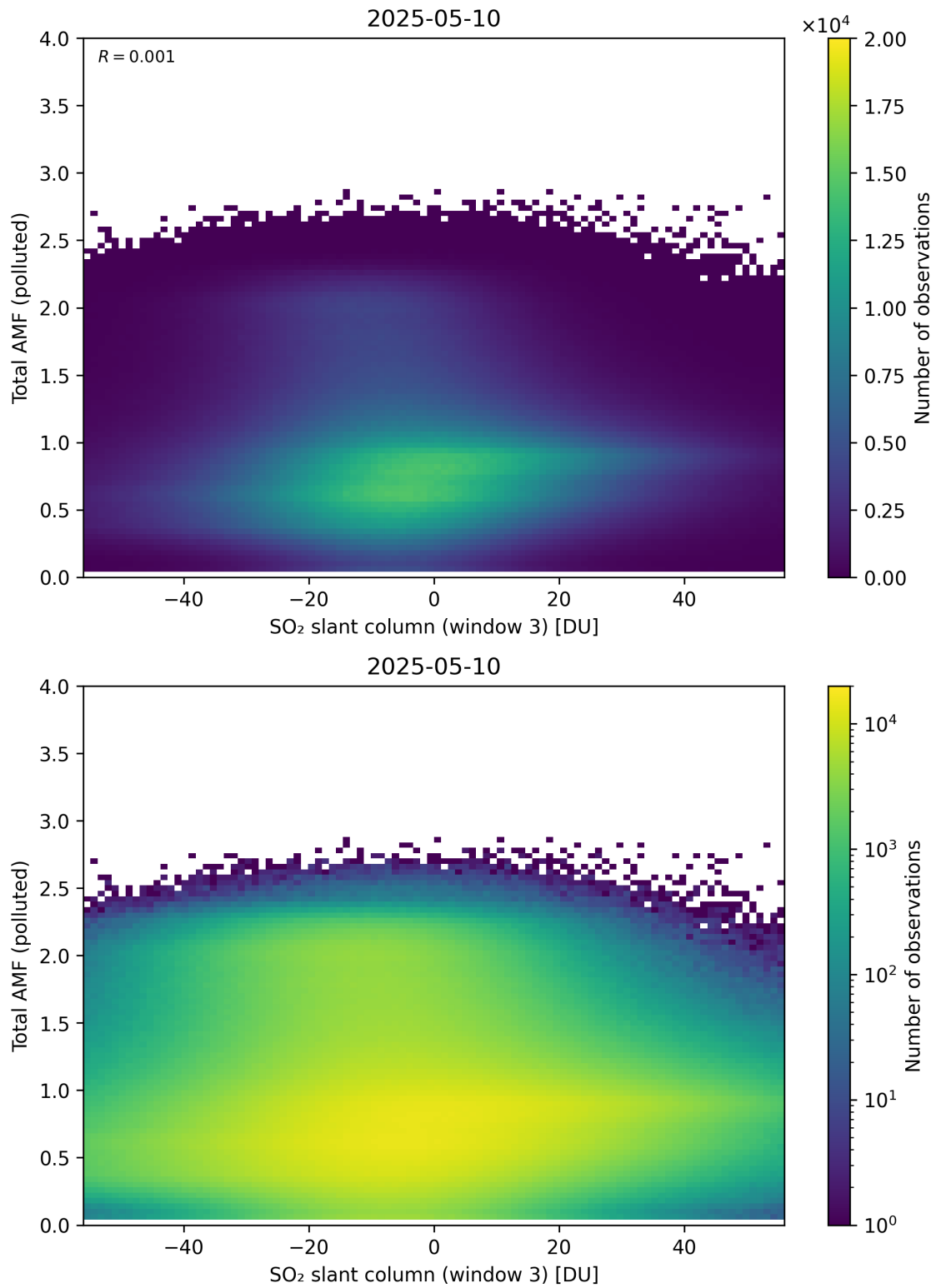
Figure 318: Scatter density plot of “SO 2 slant column (window 3)” against “Total AMF (polluted)” for 2025-05-10 to 2025-05-11.
