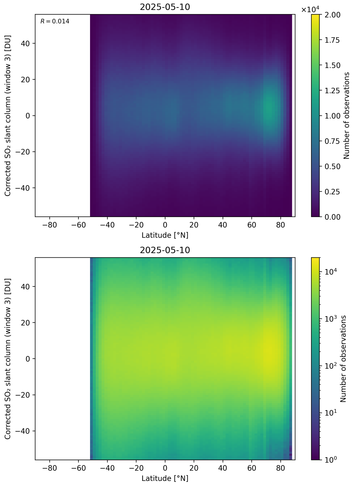
Figure 161: Scatter density plot of “Latitude” against “Corrected SO 2 slant column (window 3)” for 2025-05-10 to 2025-05-11.
