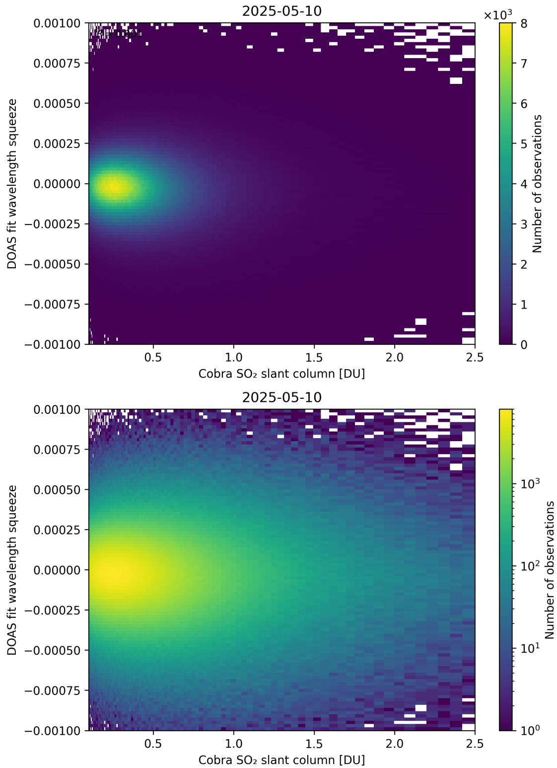
Figure 197: Scatter density plot of “Cobra SO 2 slant column” against “DOAS fit wavelength squeeze” for 2025-05-10 to 2025-05-11.
