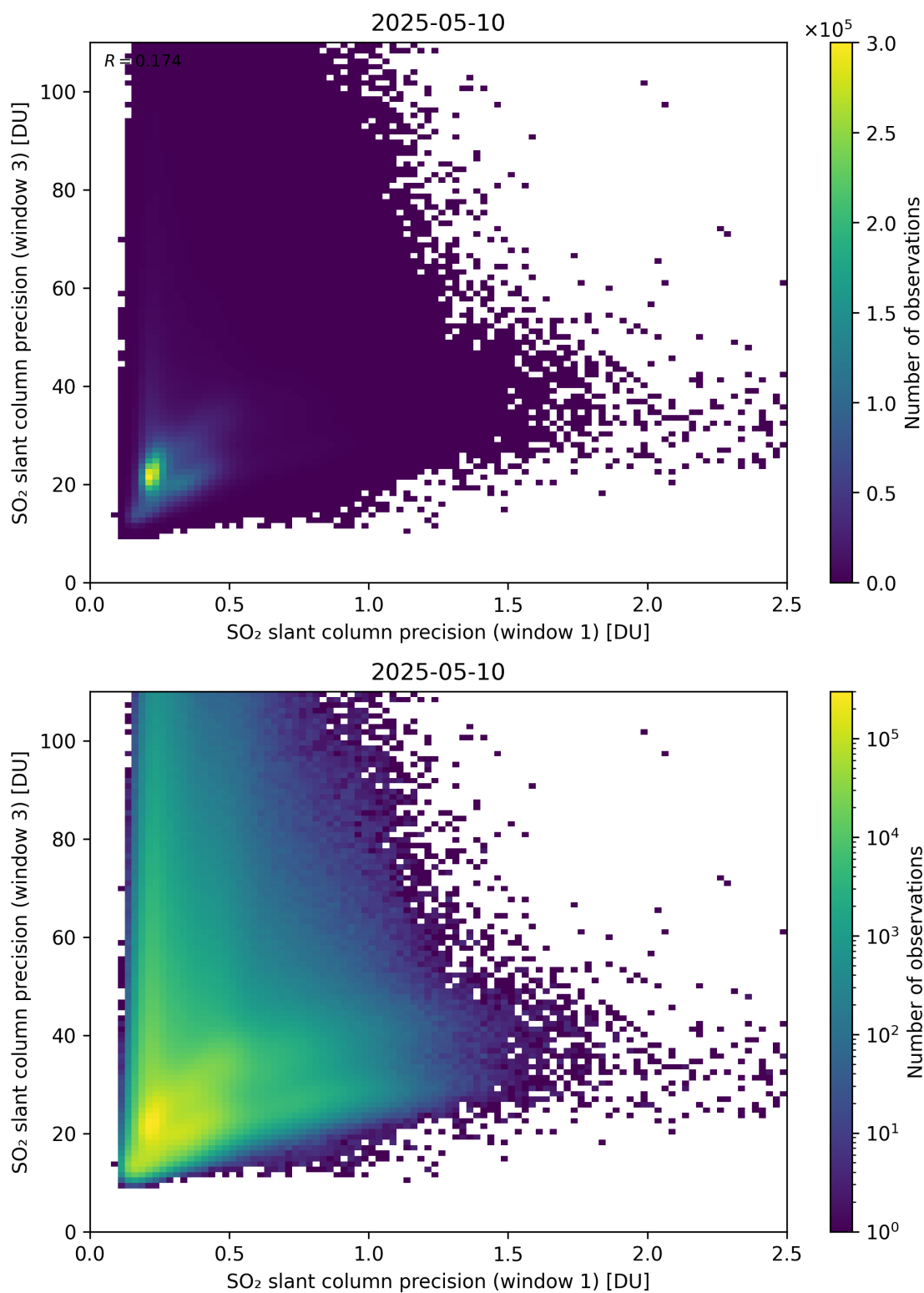
Figure 279: Scatter density plot of “SO 2 slant column precision (window 1)” against “SO 2 slant column precision (window 3)” for 2025-05-10 to 2025-05-11.
