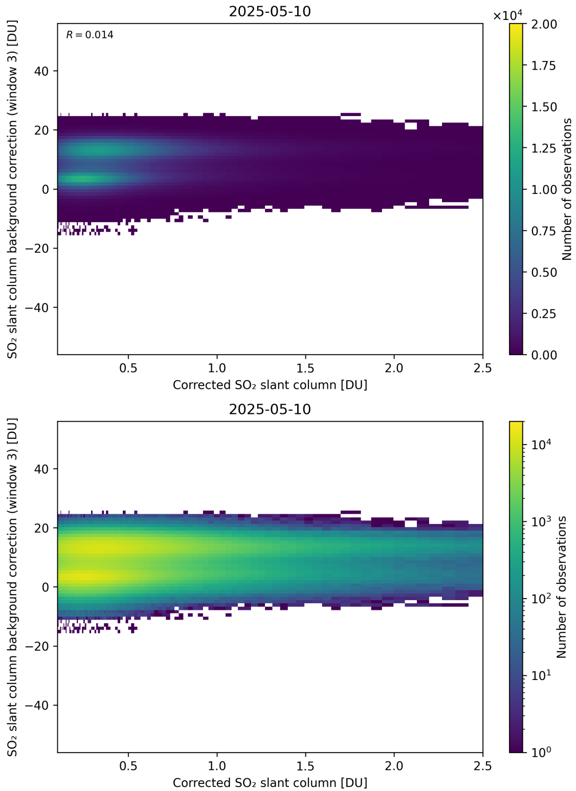
Figure 228: Scatter density plot of “Corrected SO 2 slant column” against “SO 2 slant column background correction (window 3)” for 2025-05-10 to 2025-05-11.
