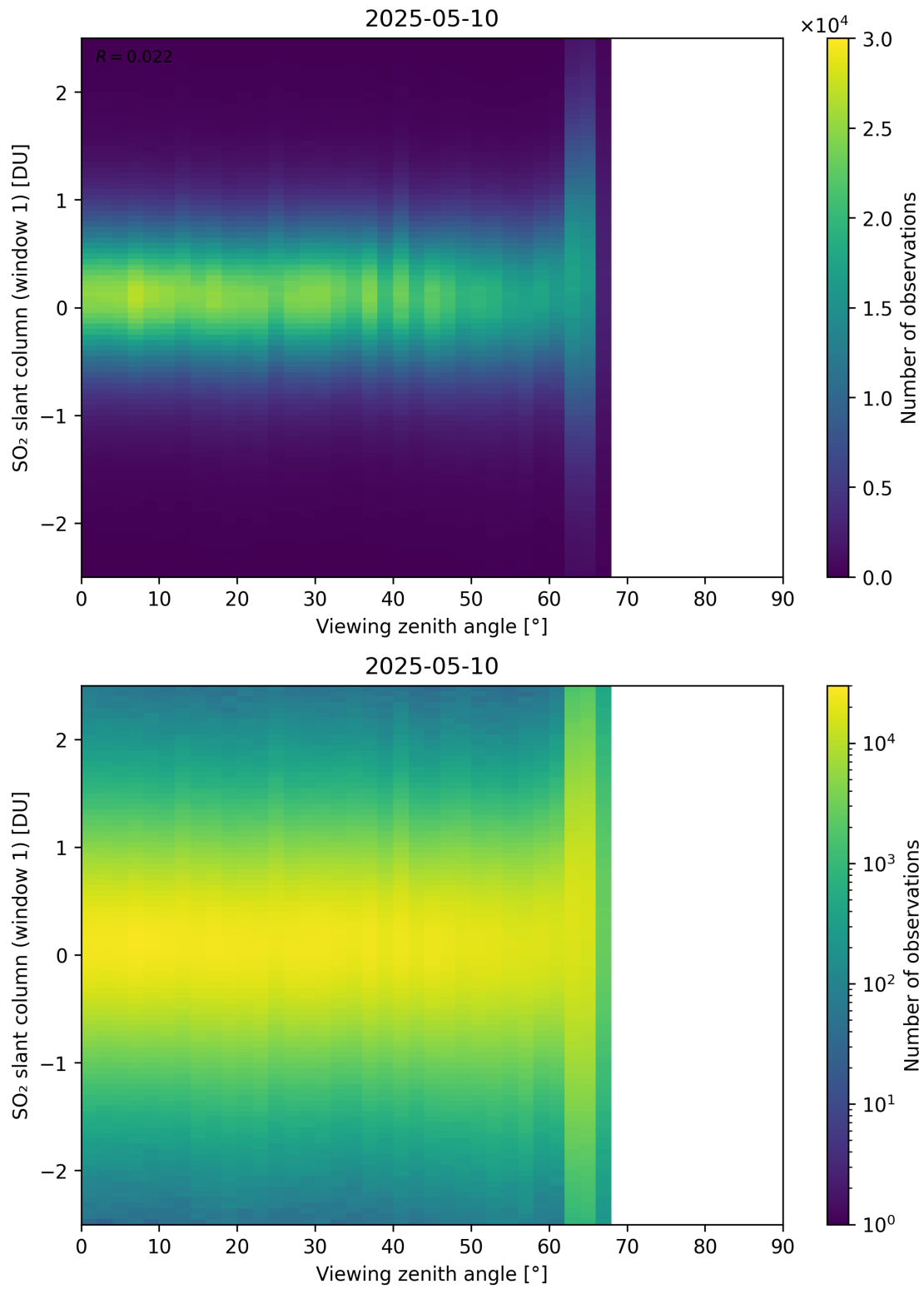
Figure 376: Scatter density plot of “Viewing zenith angle” against “SO 2 slant column (window 1)” for 2025-05-10 to 2025-05-11.
