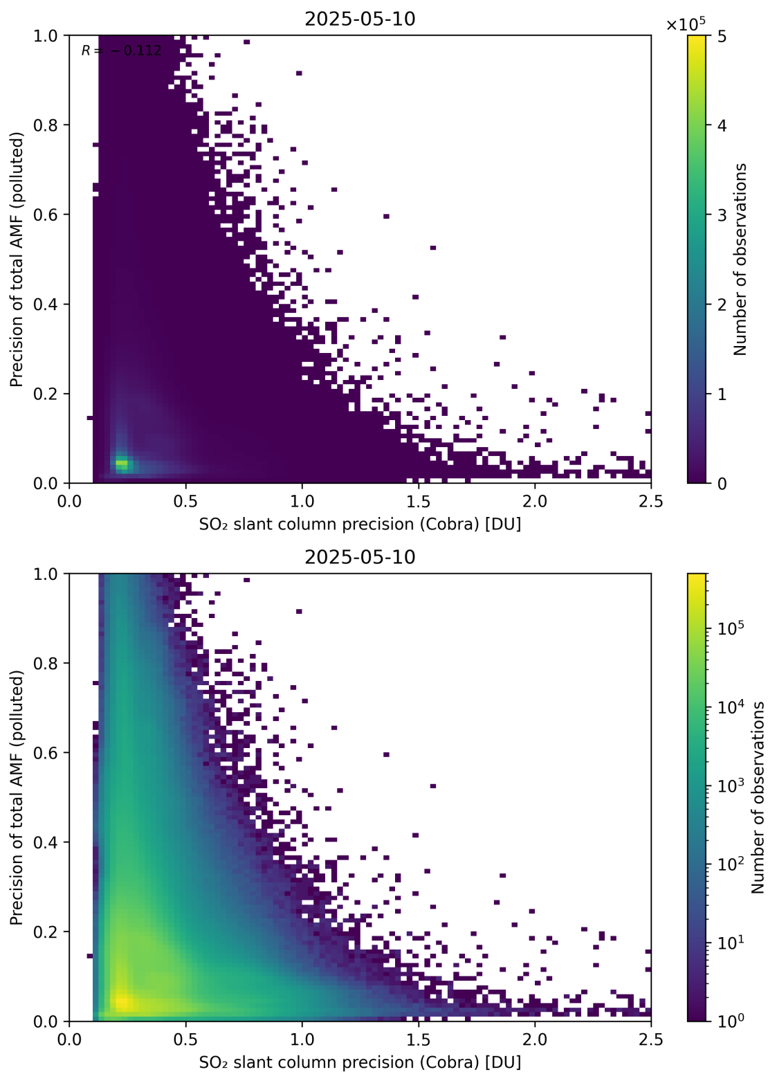
Figure 214: Scatter density plot of “SO 2 slant column precision (Cobra)” against “Precision of total AMF (polluted)” for 2025-05-10 to 2025-05-11.
