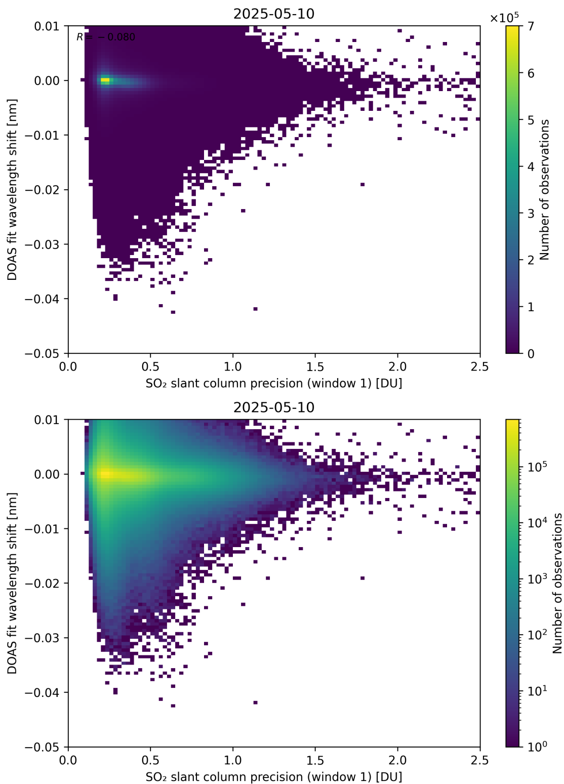
Figure 271: Scatter density plot of “SO 2 slant column precision (window 1)” against “DOAS fit wavelength shift” for 2025-05-10 to 2025-05-11.
