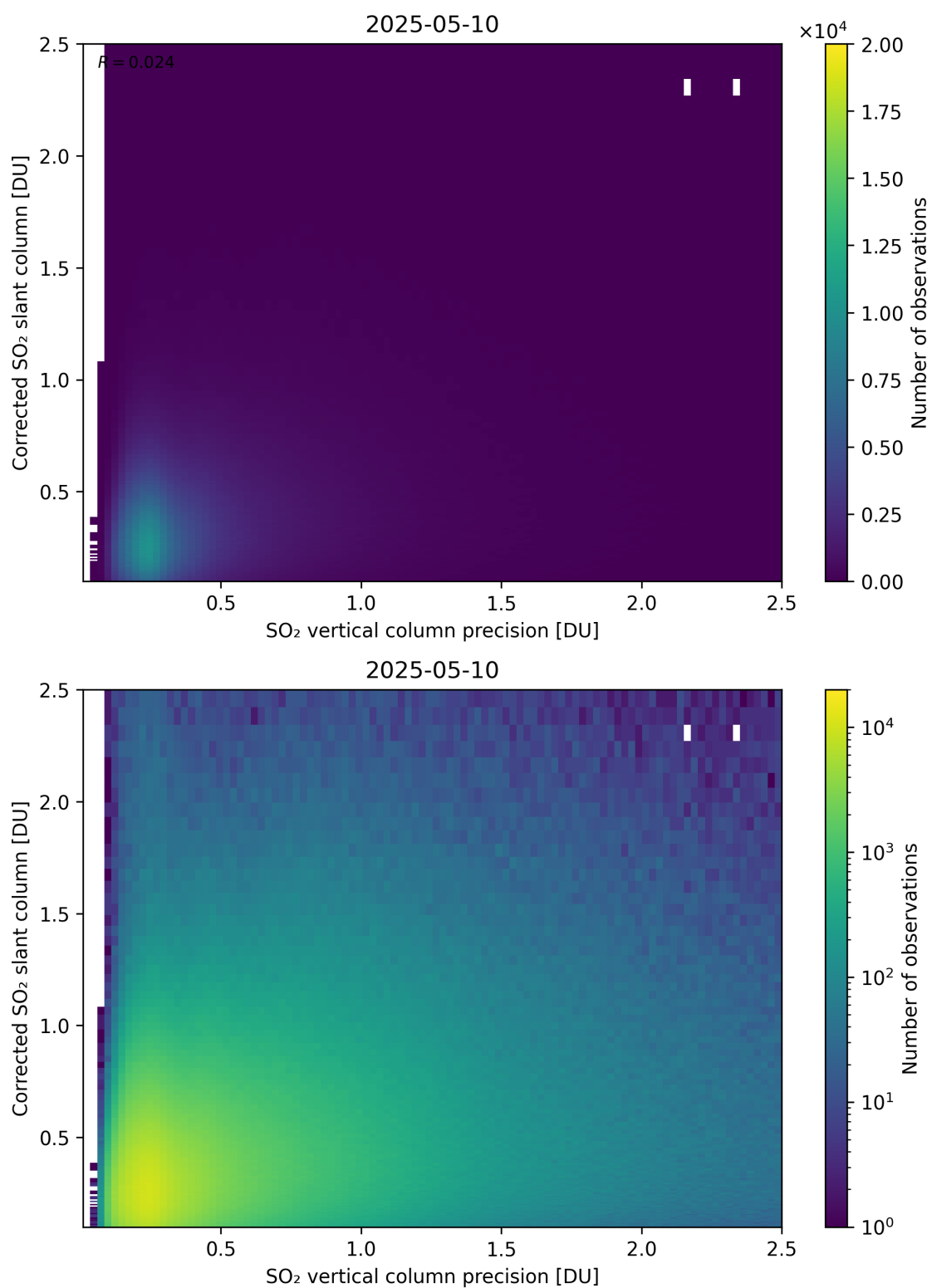
Figure 338: Scatter density plot of “SO 2 vertical column precision” against “Corrected SO 2 slant column” for 2025-05-10 to 2025-05-11.
