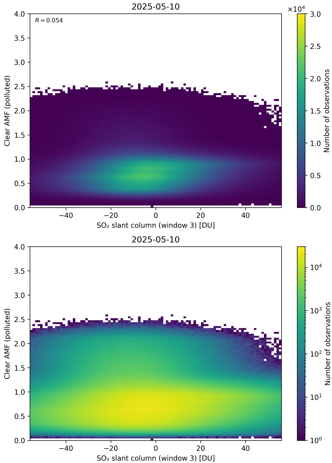
Figure 315: Scatter density plot of “SO 2 slant column (window 3)” against “Clear AMF (polluted)” for 2025-05-10 to 2025-05-11.
