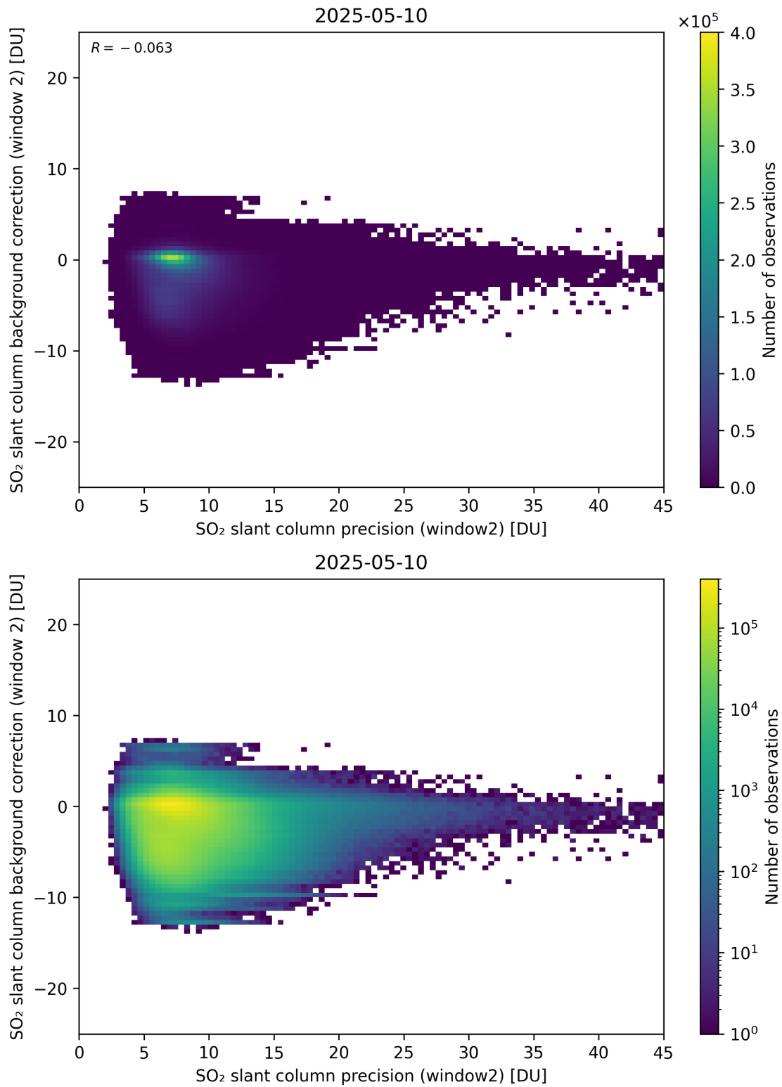
Figure 291: Scatter density plot of “SO 2 slant column precision (window2)” against “SO 2 slant column background correction (window 2)” for 2025-05-10 to 2025-05-11.
