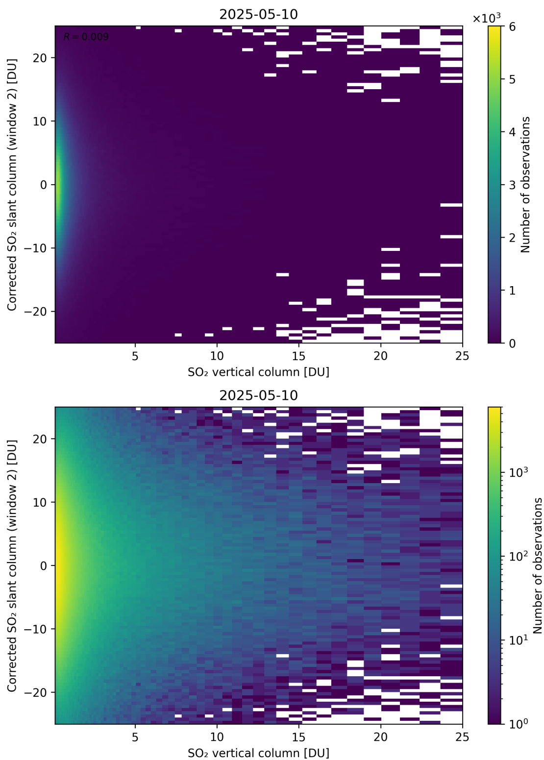
Figure 352: Scatter density plot of “SO 2 vertical column” against “Corrected SO 2 slant column (window 2)” for 2025-05-10 to 2025-05-11.
