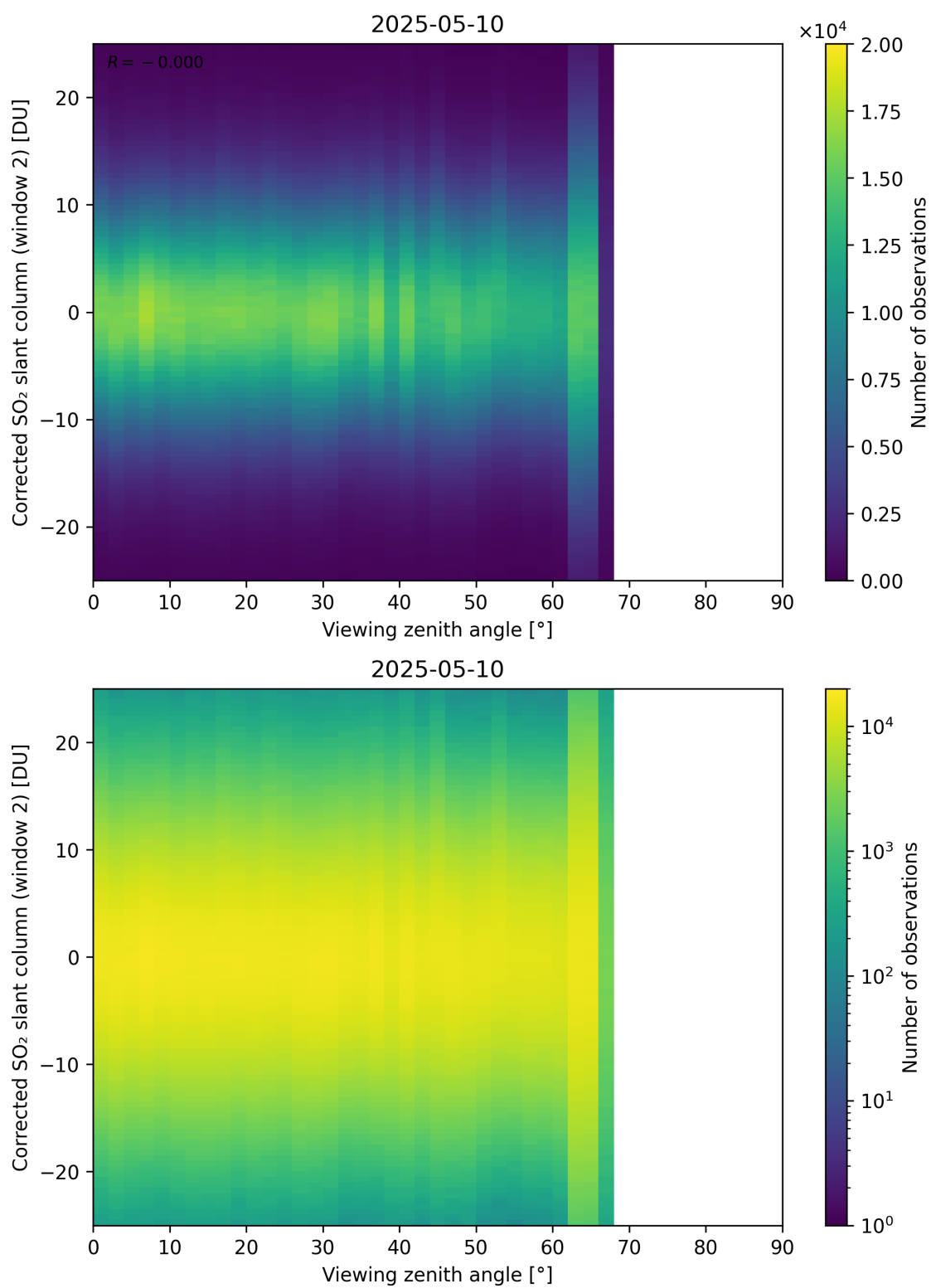
Figure 374: Scatter density plot of “Viewing zenith angle” against “Corrected SO 2 slant column (window 2)” for 2025-05-10 to 2025-05-11.
