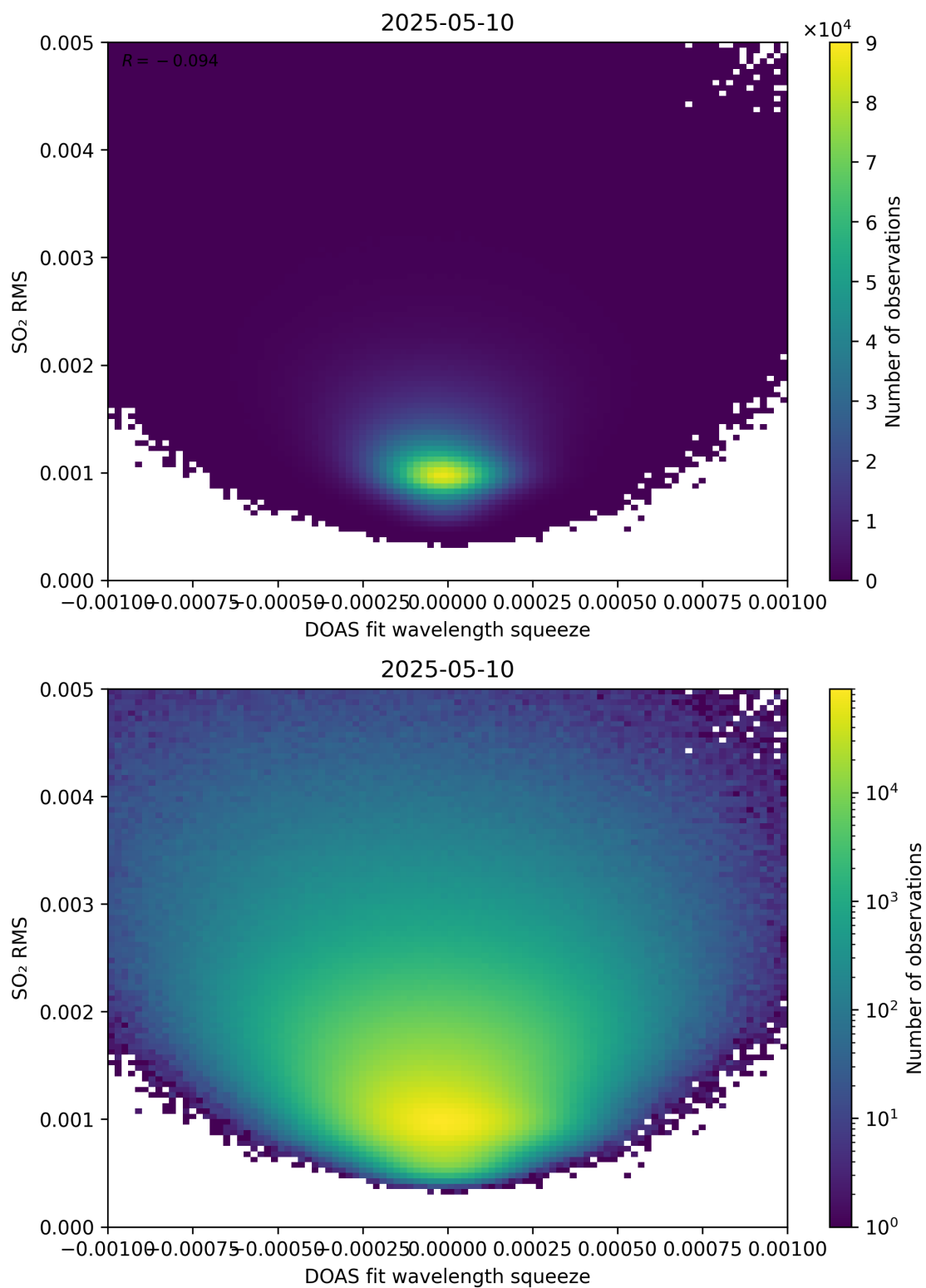
Figure 143: Scatter density plot of “DOAS fit wavelength squeeze” against “SO 2 RMS” for 2025-05-10 to 2025-05-11.
