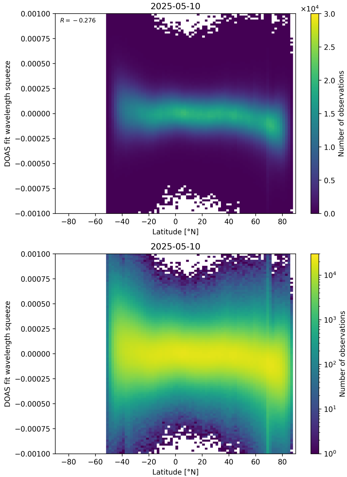
Figure 154: Scatter density plot of “Latitude” against “DOAS fit wavelength squeeze” for 2025-05-10 to 2025-05-11.
