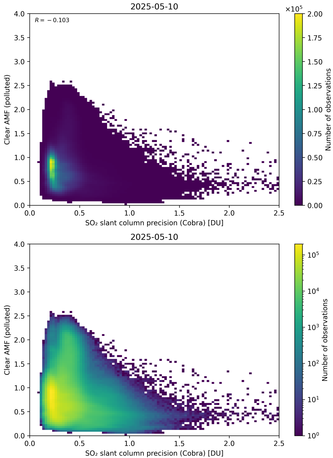
Figure 205: Scatter density plot of “SO 2 slant column precision (Cobra)” against “Clear AMF (polluted)” for 2025-05-10 to 2025-05-11.
