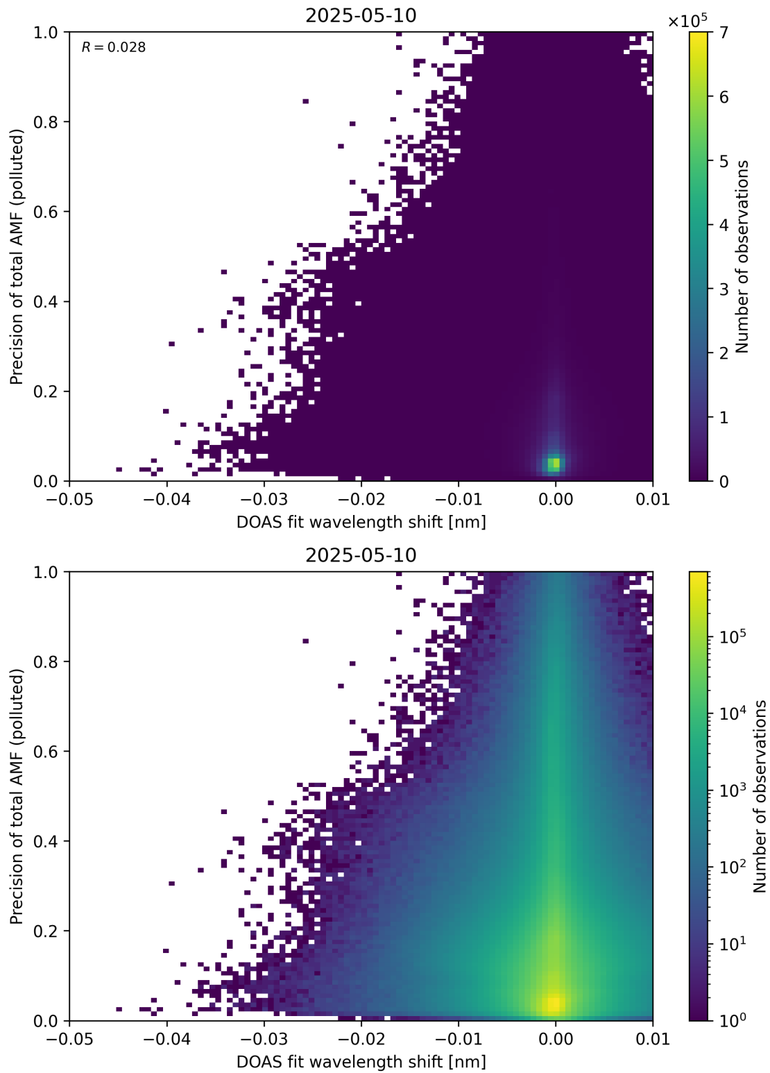
Figure 142: Scatter density plot of “DOAS fit wavelength shift” against “Precision of total AMF (polluted)” for 2025-05-10 to 2025-05-11.
