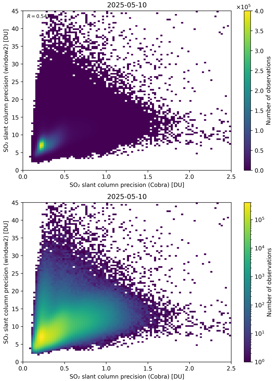
Figure 210: Scatter density plot of “SO 2 slant column precision (Cobra)” against “SO 2 slant column precision (window2)” for 2025-05-10 to 2025-05-11.
