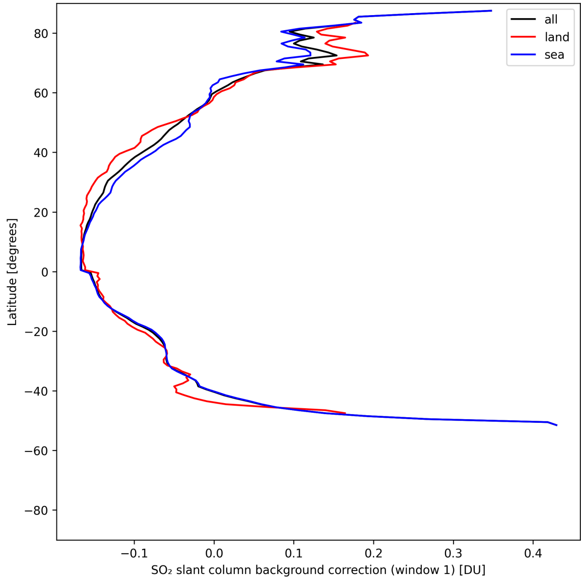
Figure 40: Zonal average of “SO 2 slant column background correction (window 1)” for 2025-05-10 to 2025-05-11.
