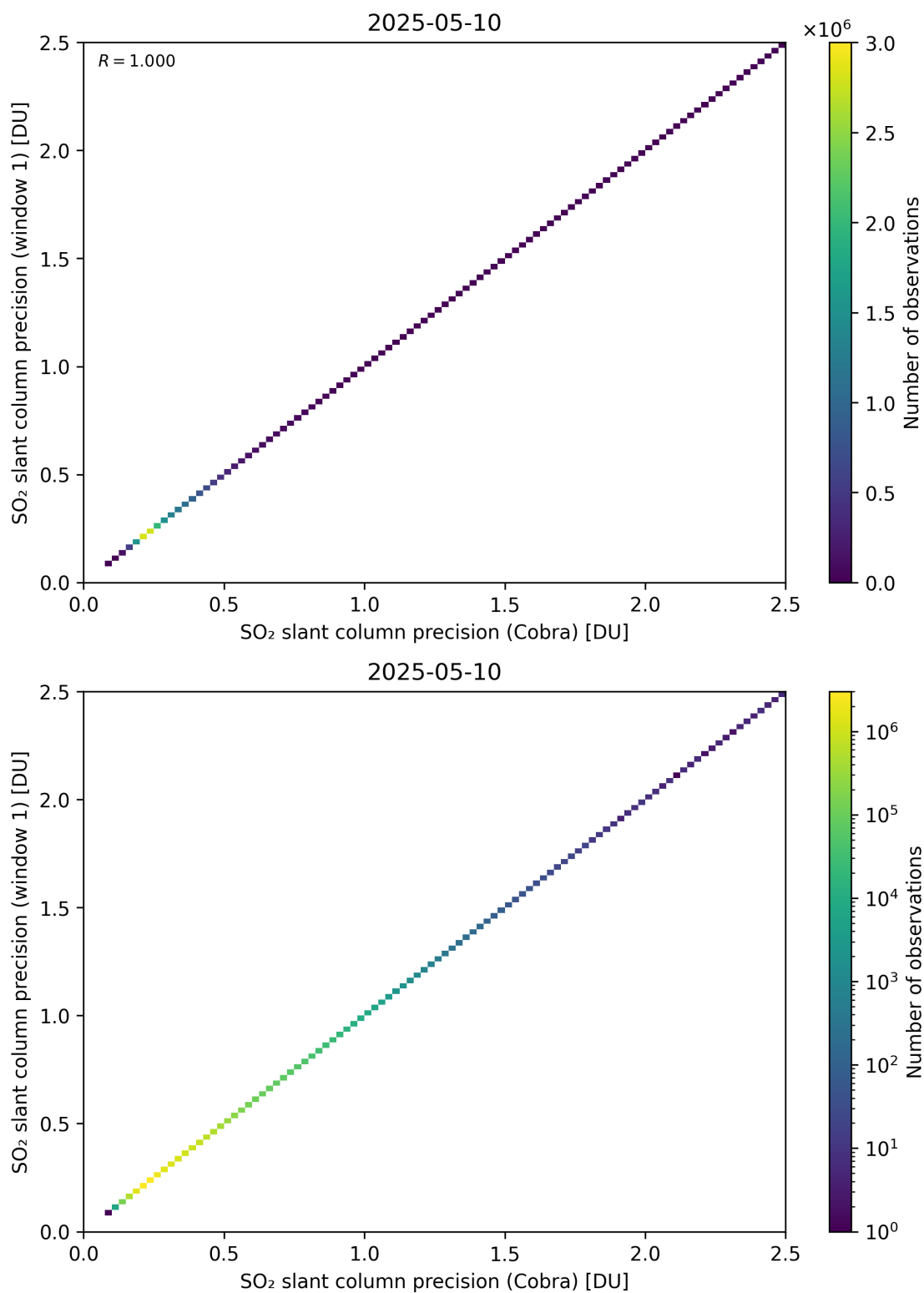
Figure 209: Scatter density plot of “SO 2 slant column precision (Cobra)” against “SO 2 slant column precision (window 1)” for 2025-05-10 to 2025-05-11.
