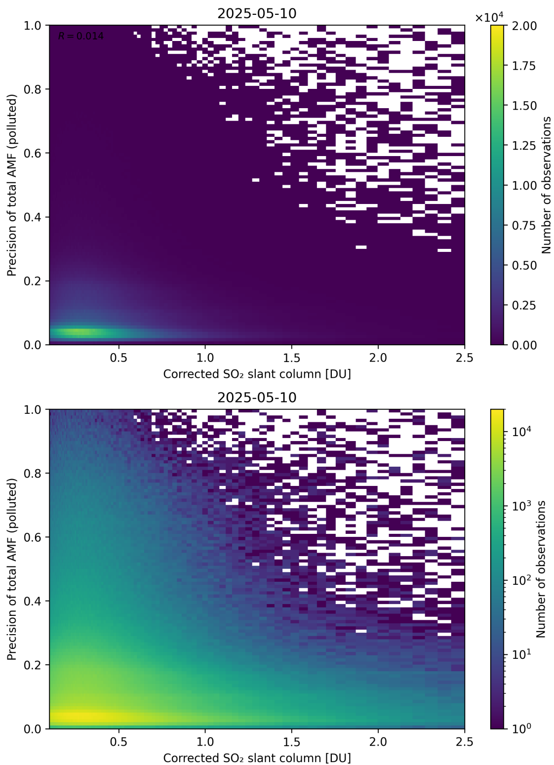
Figure 243: Scatter density plot of “Corrected SO 2 slant column” against “Precision of total AMF (polluted)” for 2025-05-10 to 2025-05-11.
