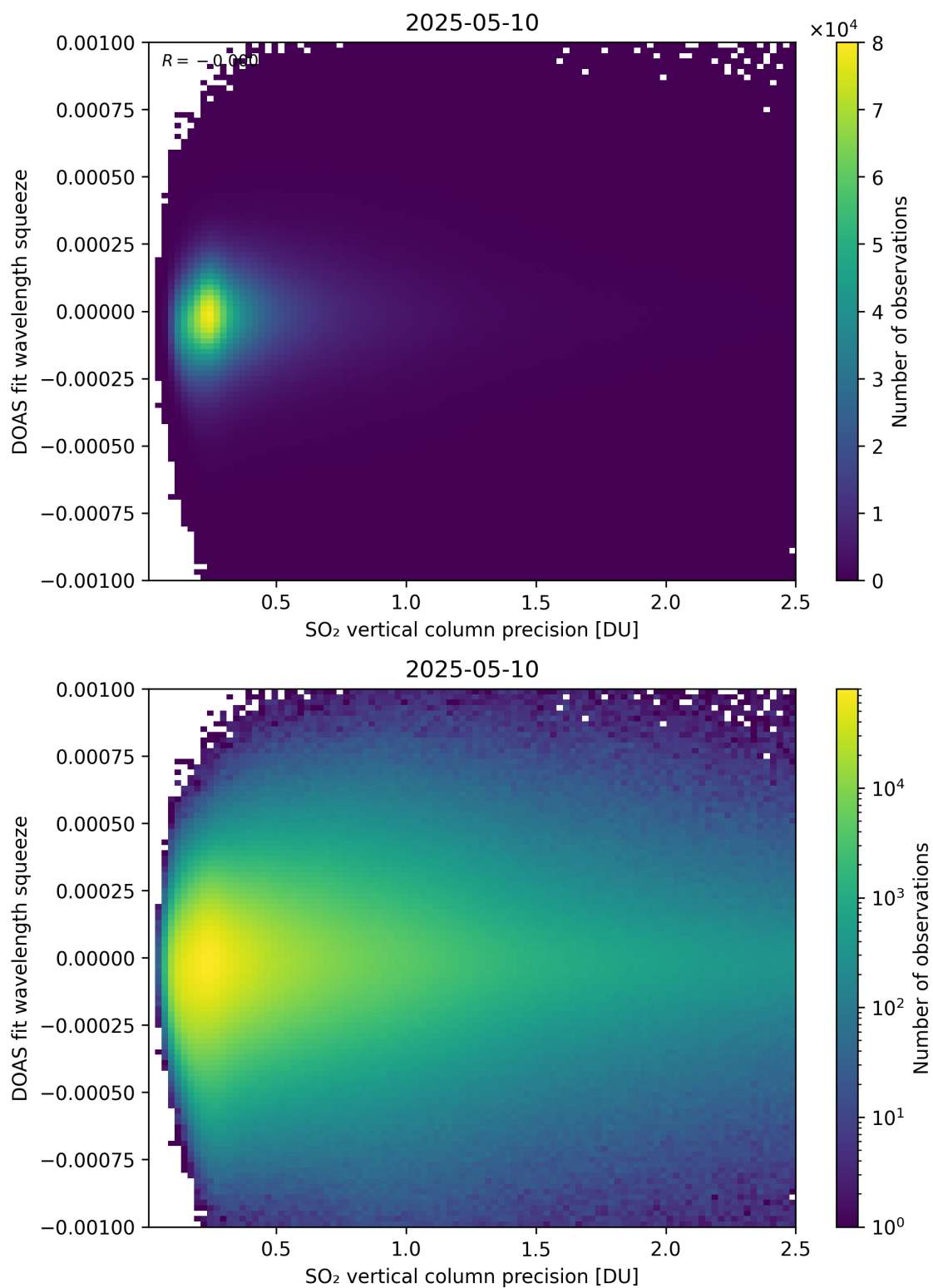
Figure 333: Scatter density plot of “SO 2 vertical column precision” against “DOAS fit wavelength squeeze” for 2025-05-10 to 2025-05-11.
