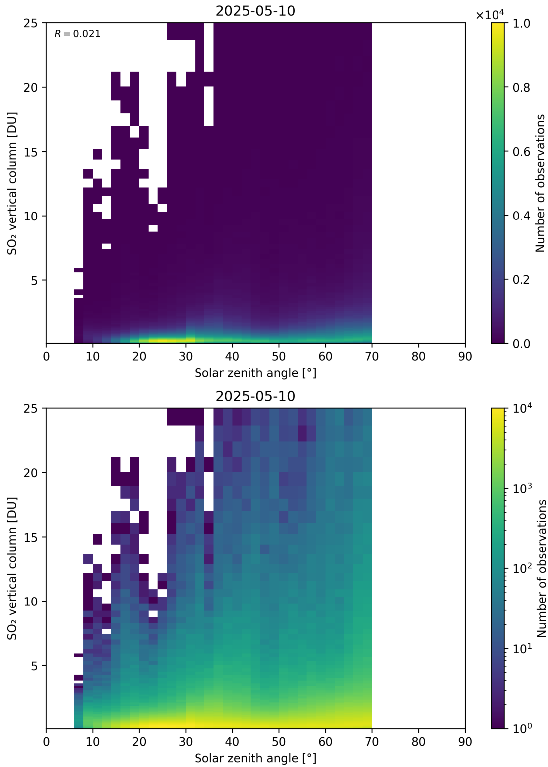
Figure 191: Scatter density plot of “Solar zenith angle” against “SO 2 vertical column” for 2025-05-10 to 2025-05-11.
