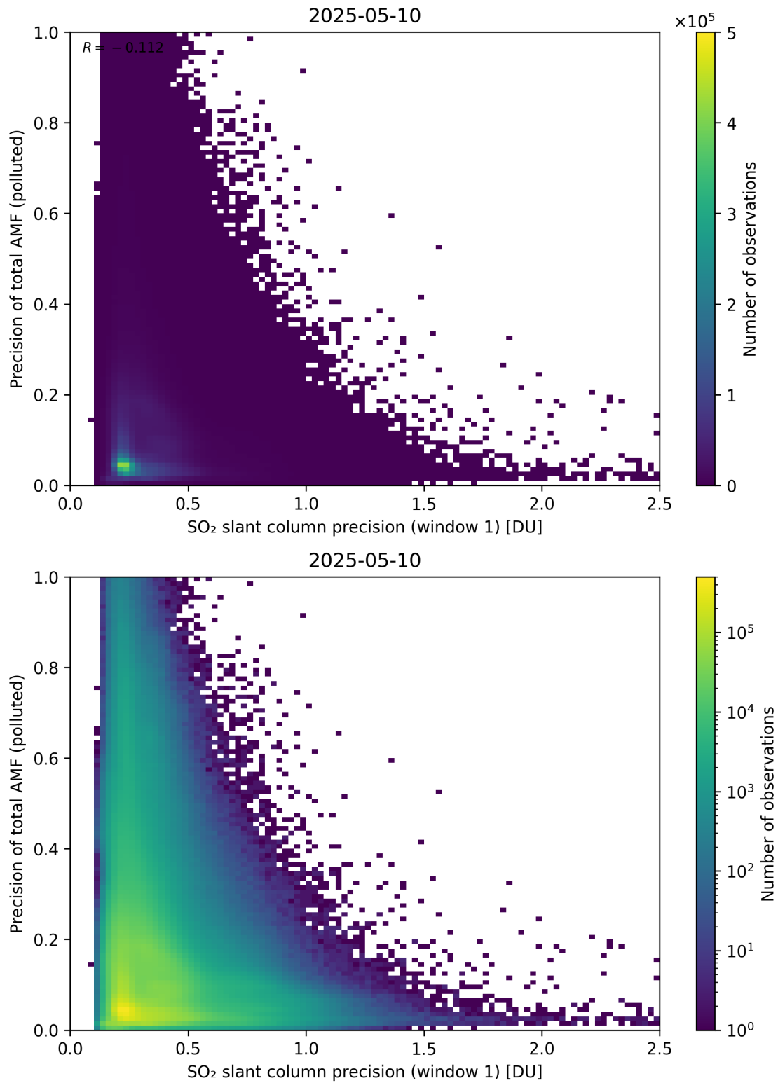
Figure 281: Scatter density plot of “SO 2 slant column precision (window 1)” against “Precision of total AMF (polluted)” for 2025-05-10 to 2025-05-11.
