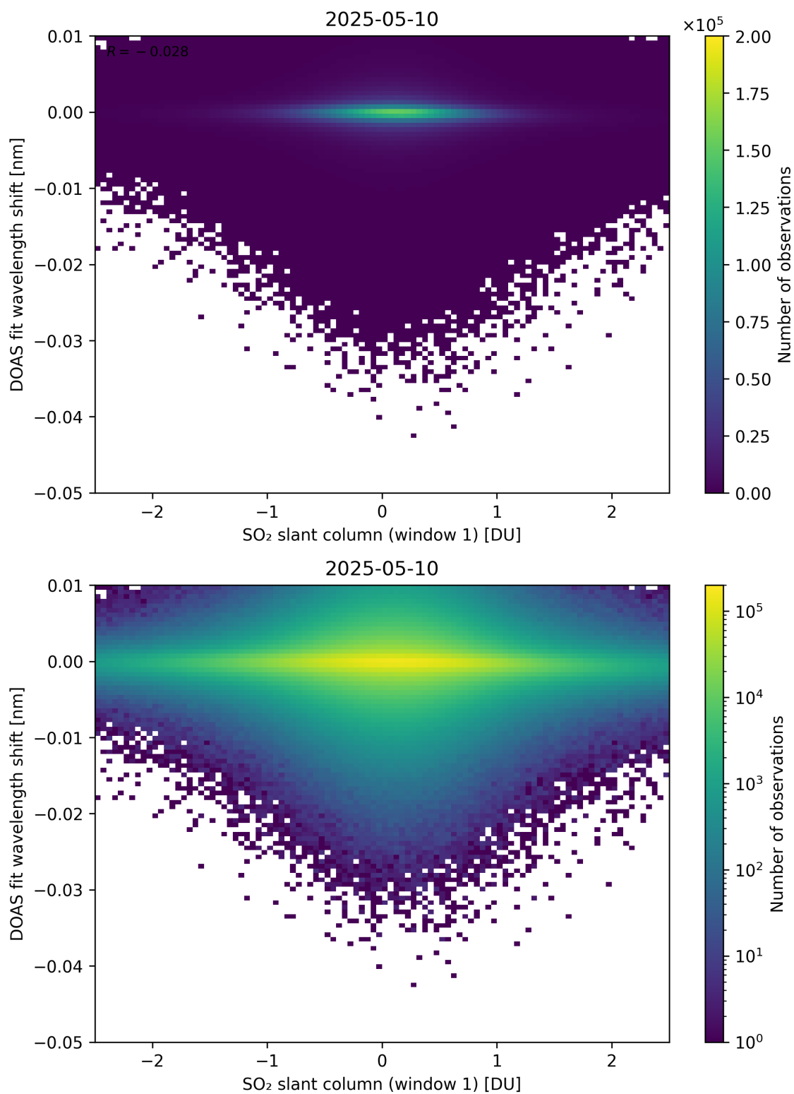
Figure 265: Scatter density plot of “SO 2 slant column (window 1)” against “DOAS fit wavelength shift” for 2025-05-10 to 2025-05-11.
