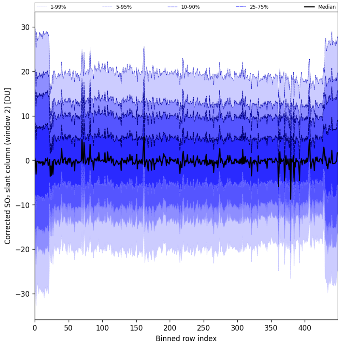
Figure 95: Along track statistics of “Corrected SO 2 slant column (window 2)” for 2025-05-10 to 2025-05-11
