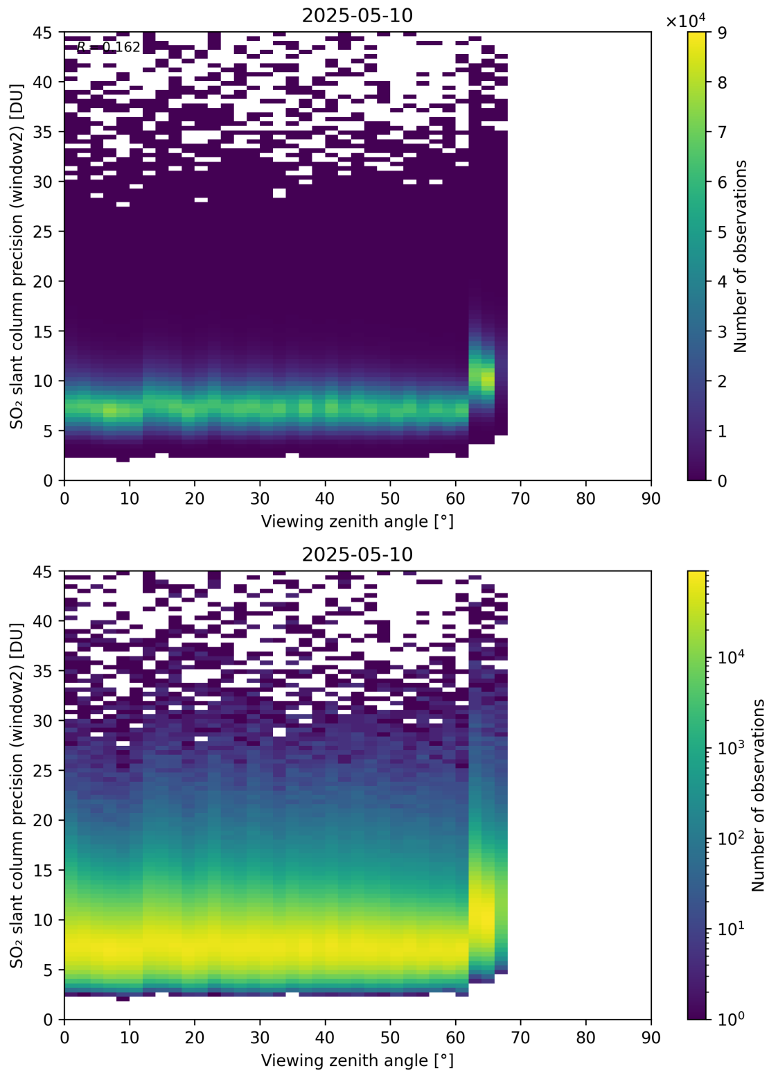
Figure 378: Scatter density plot of “Viewing zenith angle” against “SO 2 slant column precision (window2)” for 2025-05-10 to 2025-05-11.
