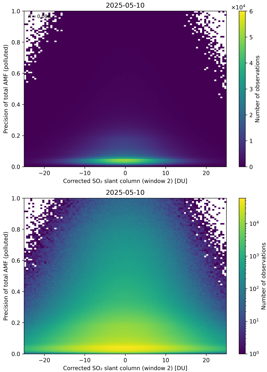
Figure 254: Scatter density plot of “Corrected SO 2 slant column (window 2)” against “Precision of total AMF (polluted)” for 2025-05-10 to 2025-05-11.
