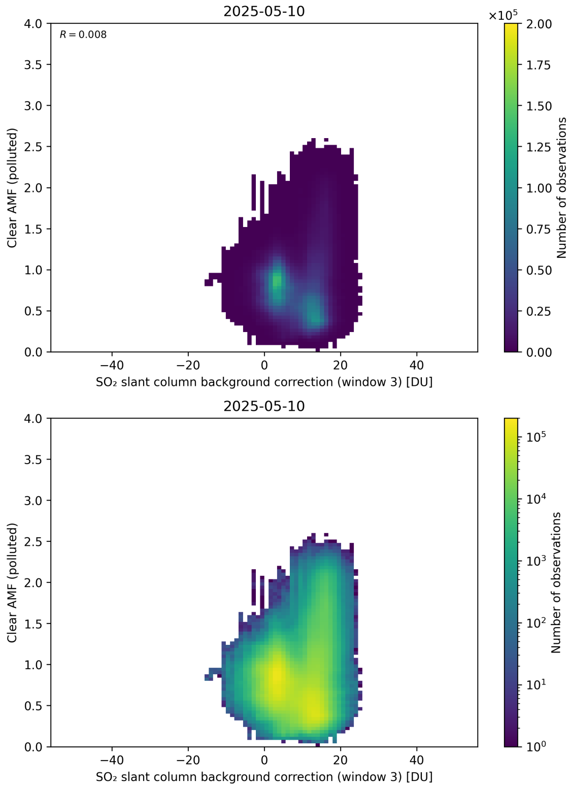
Figure 135: Scatter density plot of “SO 2 slant column background correction (window 3)” against “Clear AMF (polluted)” for 2025-05-10 to 2025-05-11.
