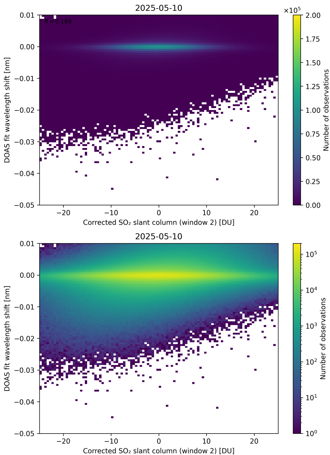
Figure 246: Scatter density plot of “Corrected SO 2 slant column (window 2)” against “DOAS fit wavelength shift” for 2025-05-10 to 2025-05-11.
