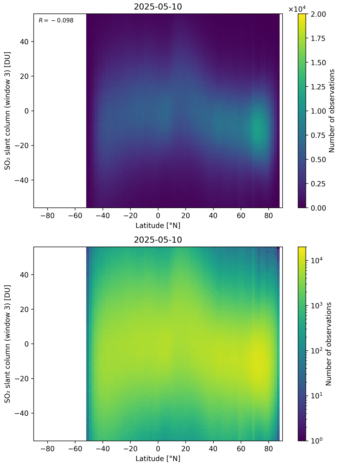
Figure 165: Scatter density plot of “Latitude” against “SO 2 slant column (window 3)” for 2025-05-10 to 2025-05-11.
