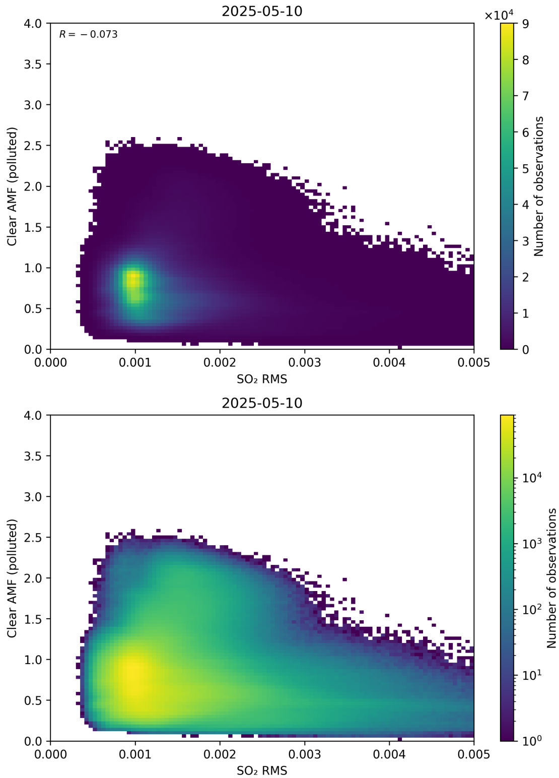
Figure 147: Scatter density plot of “SO 2 RMS” against “Clear AMF (polluted)” for 2025-05-10 to 2025-05-11.
