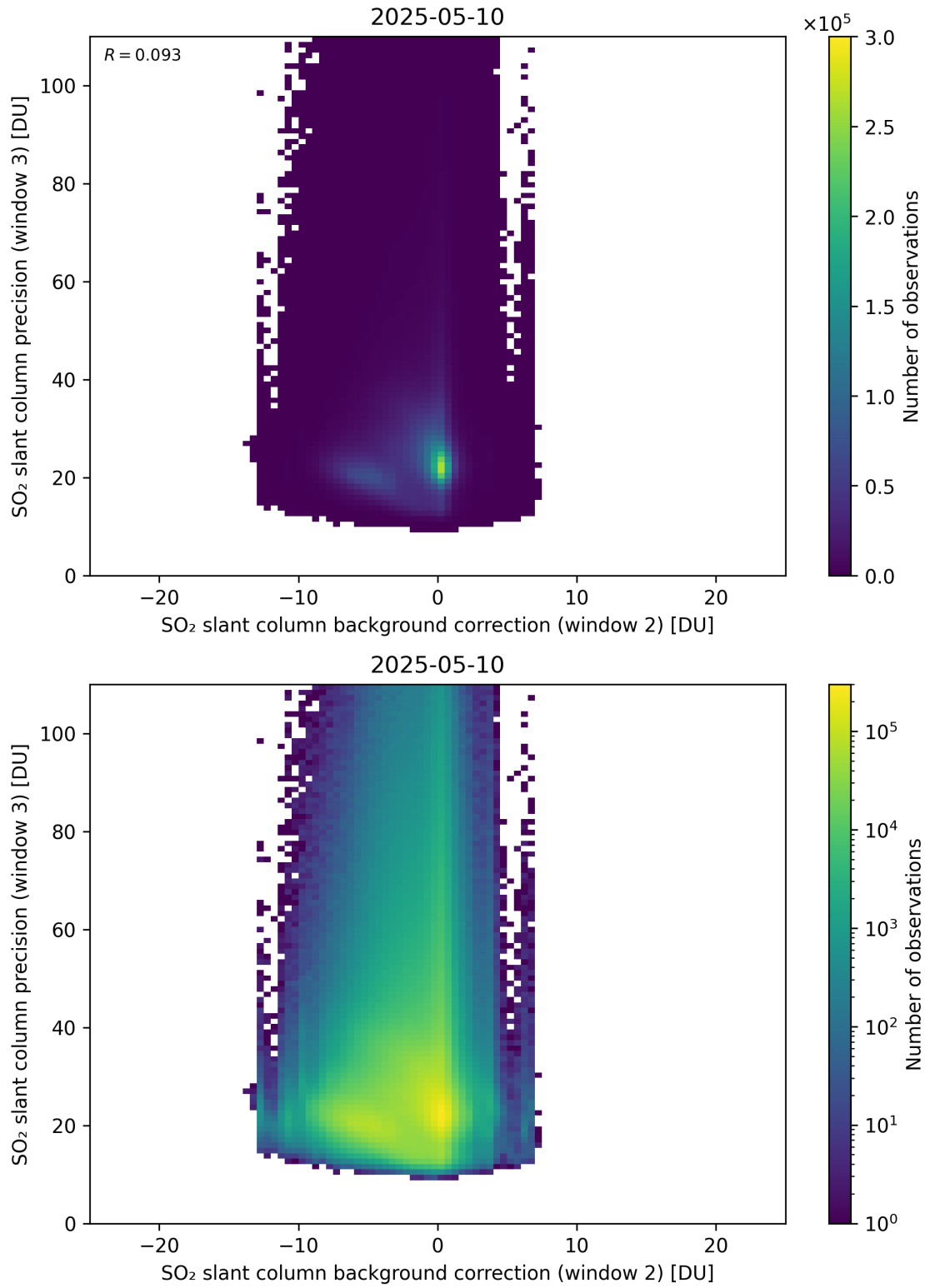
Figure 129: Scatter density plot of “SO 2 slant column background correction (window 2)” against “SO 2 slant column precision (window 3)” for 2025-05-10 to 2025-05-11.
