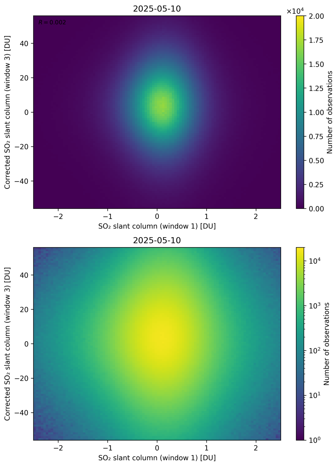
Figure 284: Scatter density plot of “SO 2 slant column (window 1)” against “Corrected SO 2 slant column (window 3)” for 2025-05-10 to 2025-05-11.
