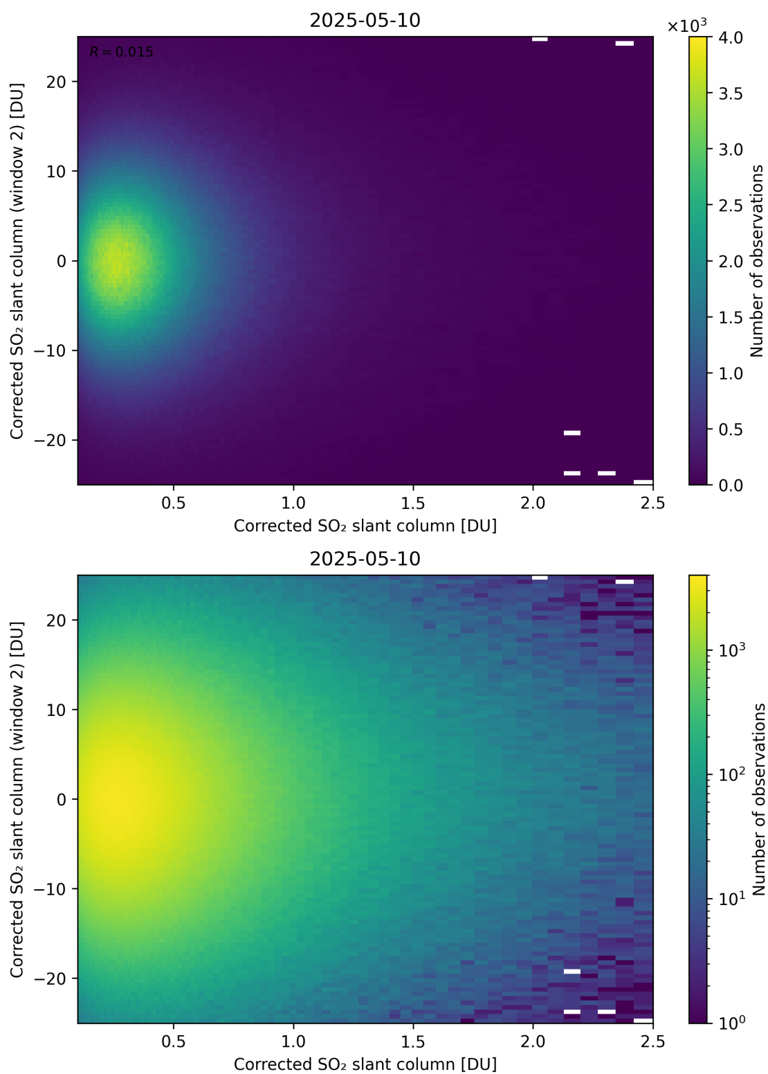
Figure 235: Scatter density plot of “Corrected SO 2 slant column” against “Corrected SO 2 slant column (window 2)” for 2025-05-10 to 2025-05-11.
