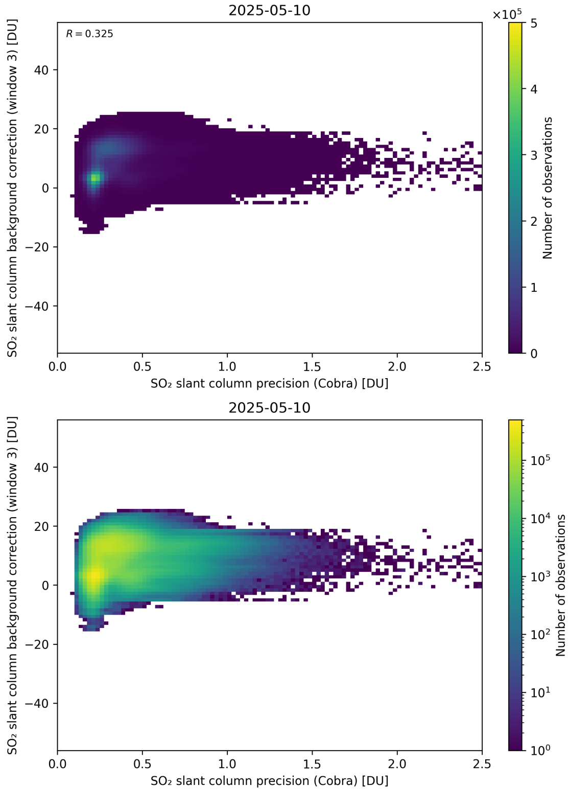
Figure 201: Scatter density plot of “SO 2 slant column precision (Cobra)” against “SO 2 slant column background correction (window 3)” for 2025-05-10 to 2025-05-11.
