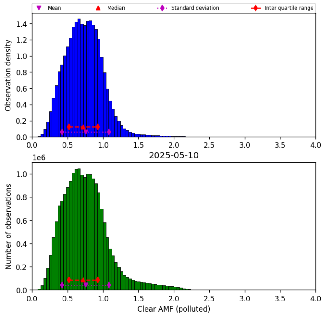
Figure 81: Histogram of “Clear AMF (polluted)” for 2025-05-10 to 2025-05-11
