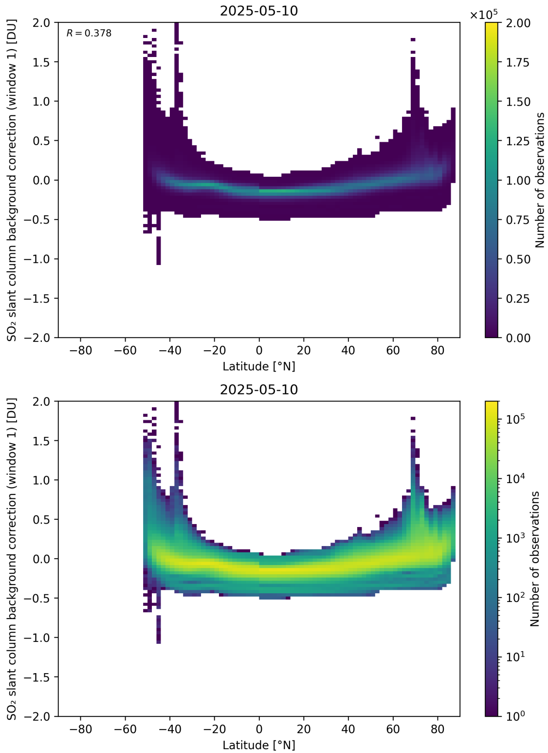
Figure 150: Scatter density plot of “Latitude” against “SO 2 slant column background correction (window 1)” for 2025-05-10 to 2025-05-11.
