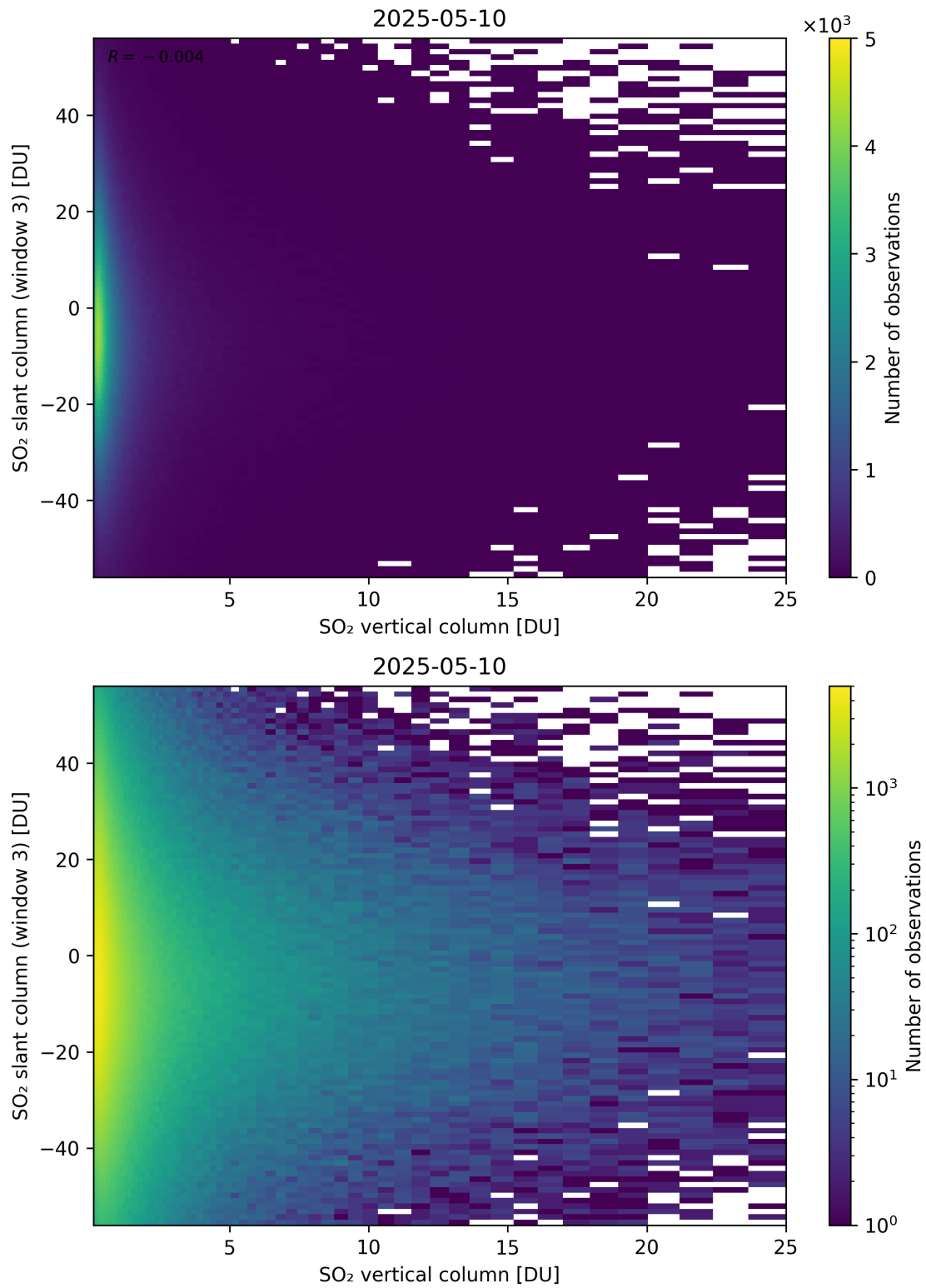
Figure 357: Scatter density plot of “SO 2 vertical column” against “SO 2 slant column (window 3)” for 2025-05-10 to 2025-05-11.
