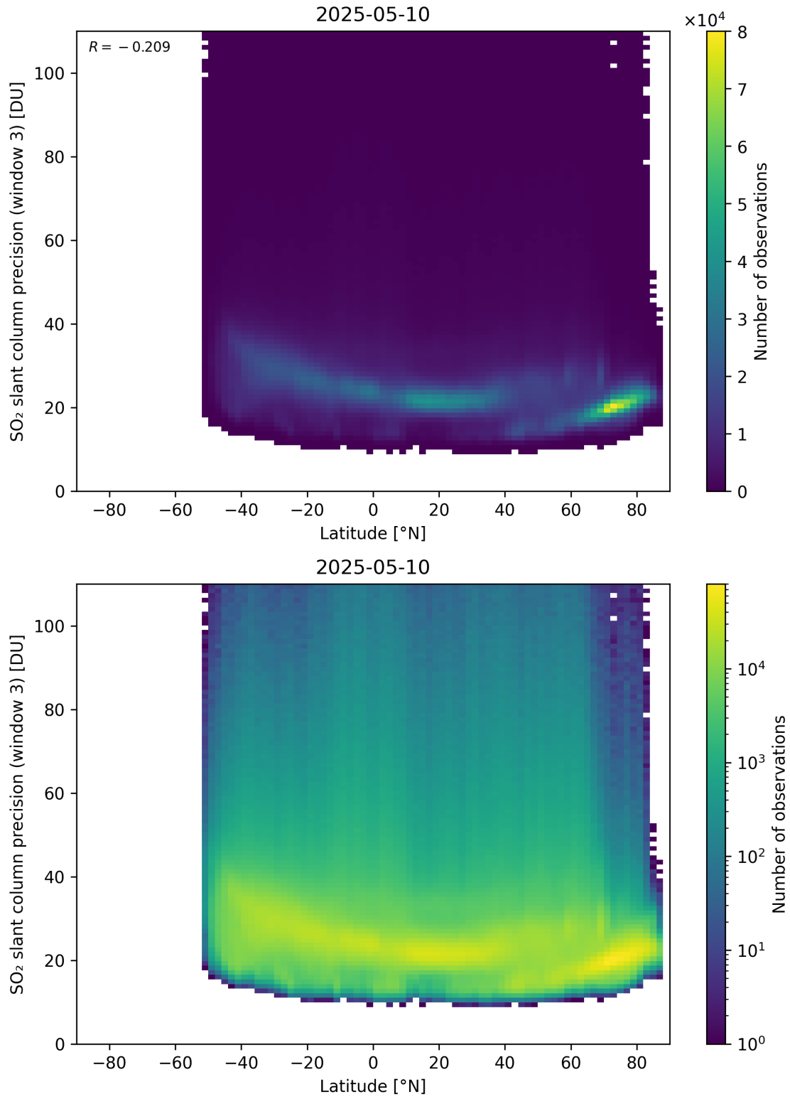
Figure 166: Scatter density plot of “Latitude” against “SO 2 slant column precision (window 3)” for 2025-05-10 to 2025-05-11.
