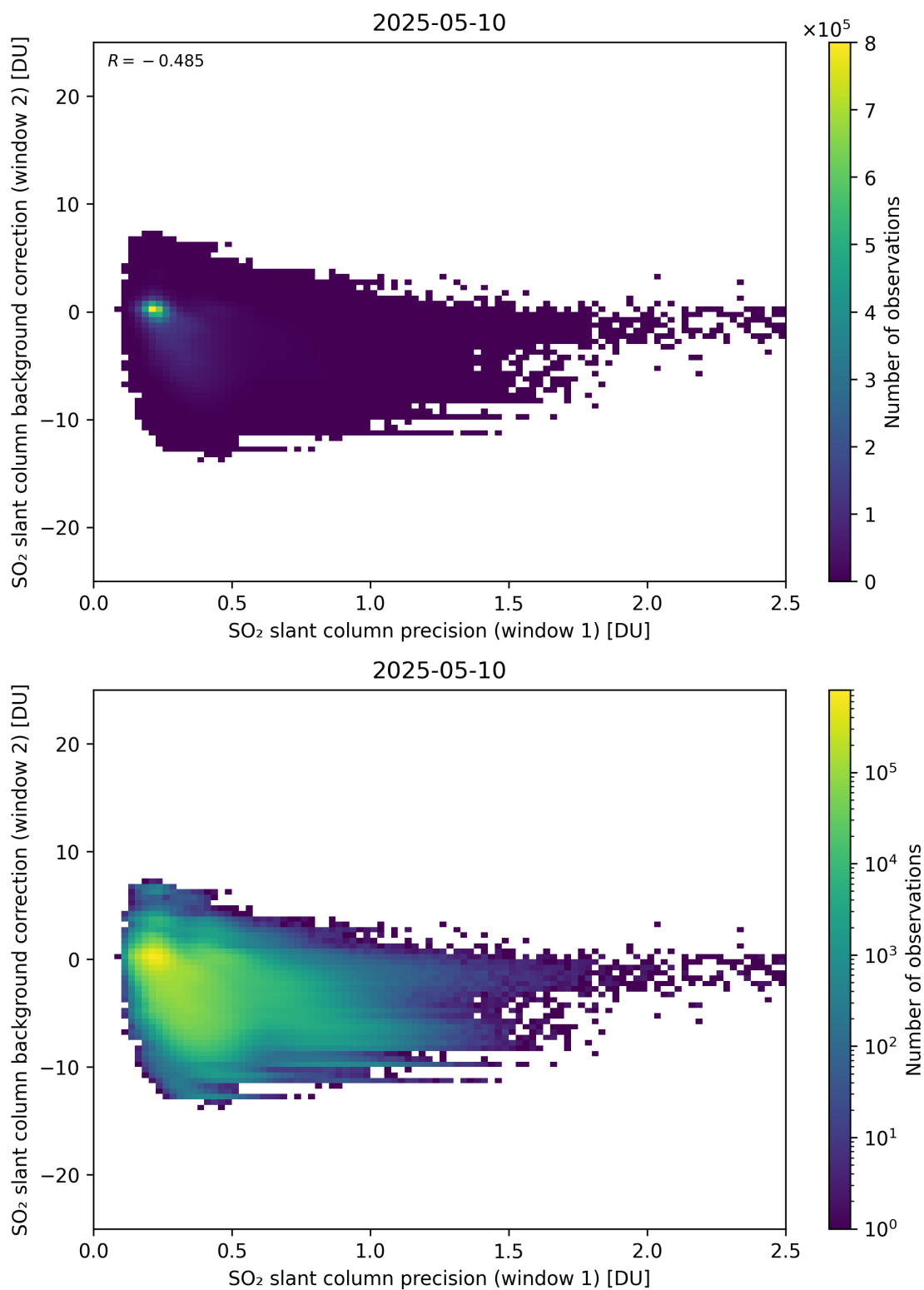
Figure 269: Scatter density plot of “SO 2 slant column precision (window 1)” against “SO 2 slant column background correction (window 2)” for 2025-05-10 to 2025-05-11.
