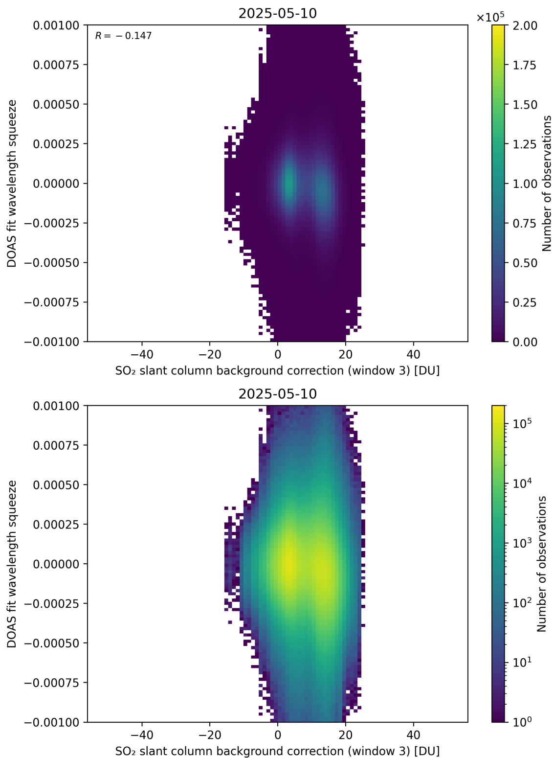
Figure 133: Scatter density plot of “SO 2 slant column background correction (window 3)” against “DOAS fit wavelength squeeze” for 2025-05-10 to 2025-05-11.
