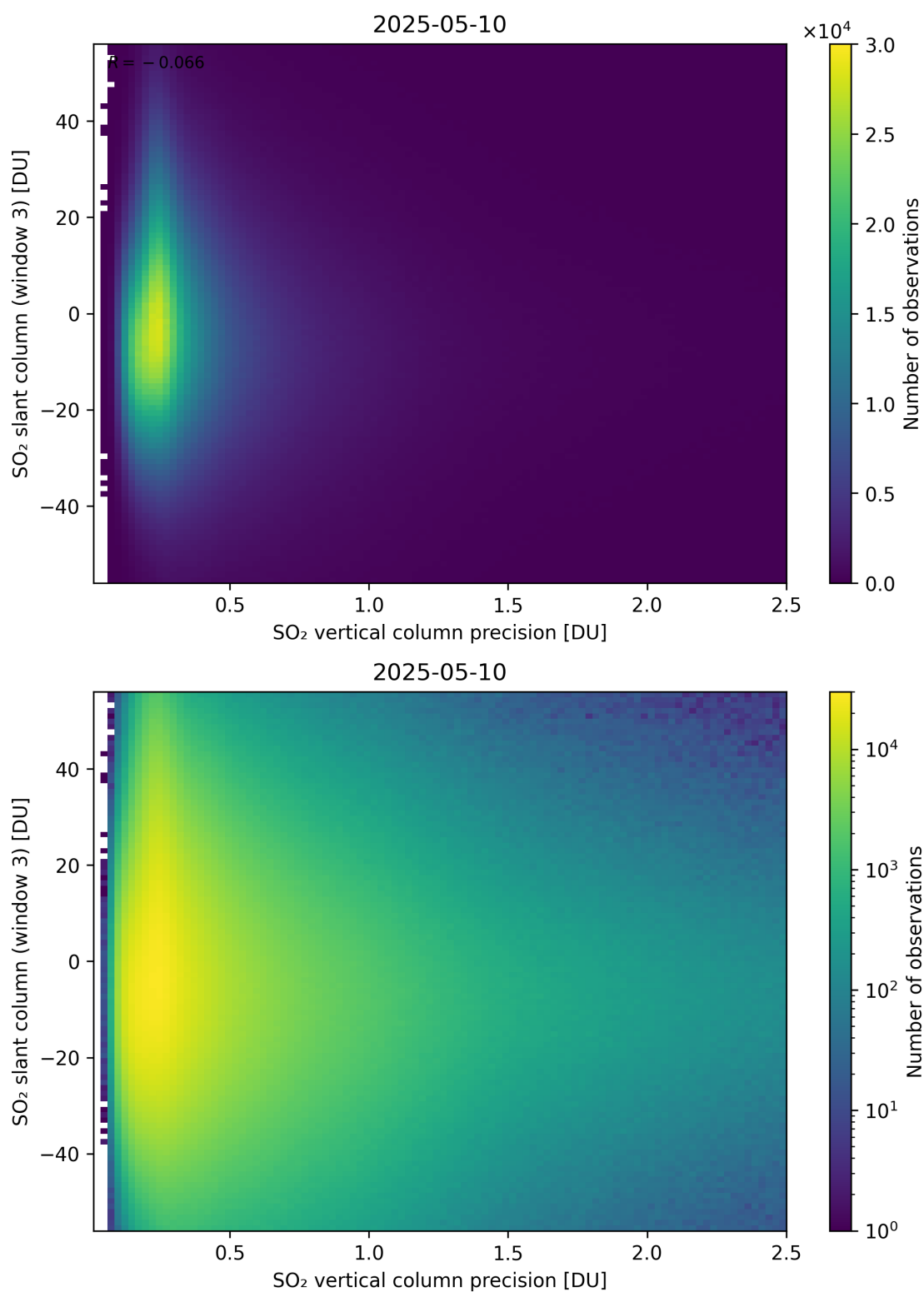
Figure 344: Scatter density plot of “SO 2 vertical column precision” against “SO 2 slant column (window 3)” for 2025-05-10 to 2025-05-11.
