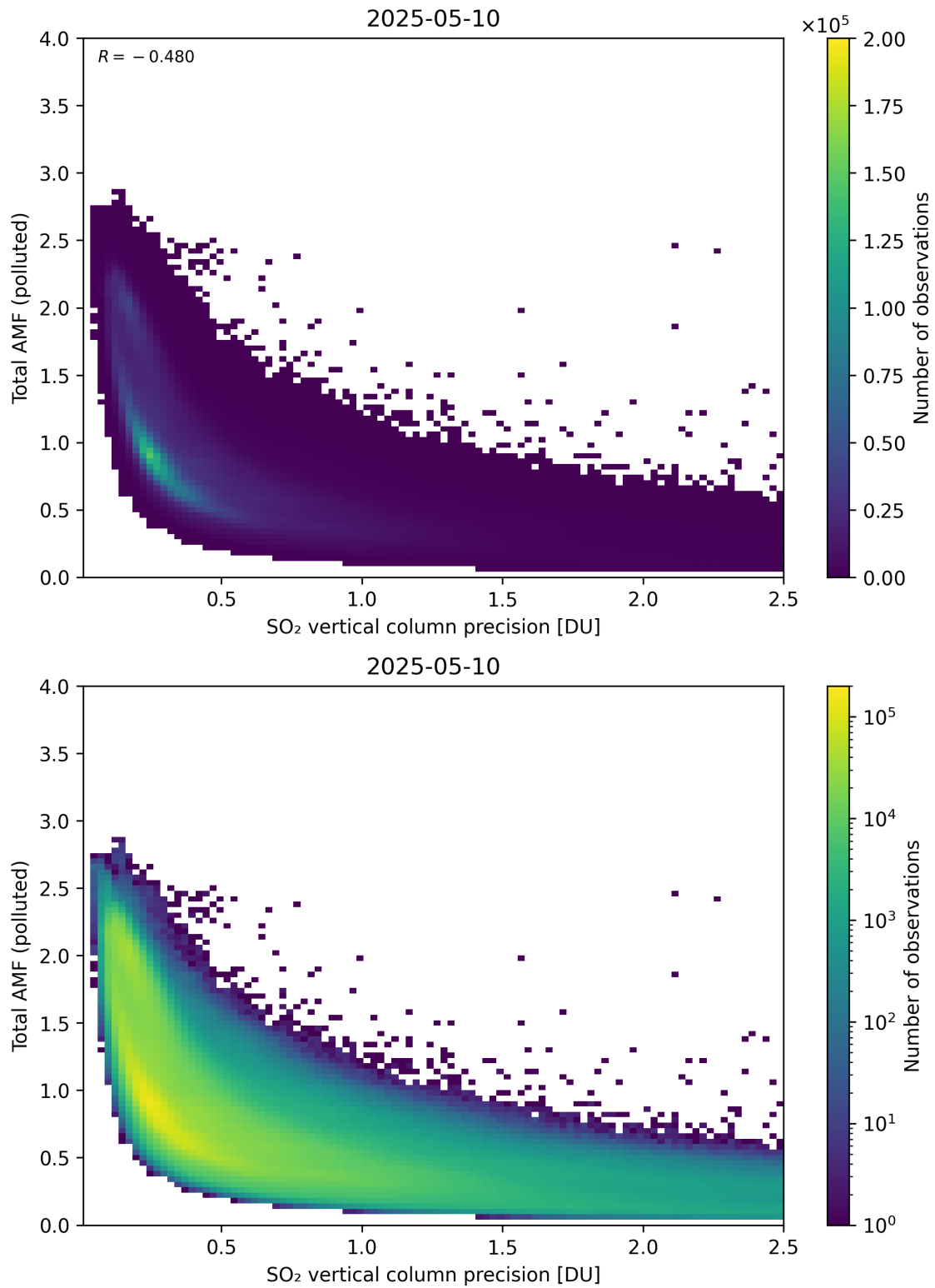
Figure 346: Scatter density plot of “SO 2 vertical column precision” against “Total AMF (polluted)” for 2025-05-10 to 2025-05-11.
