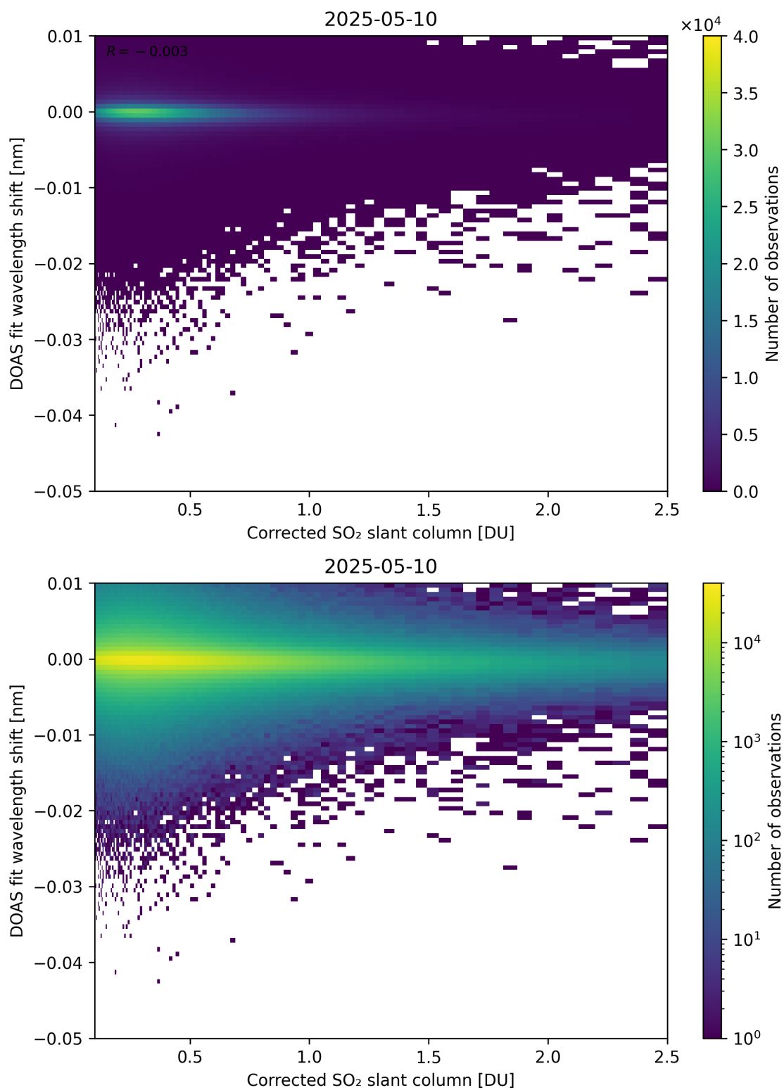
Figure 229: Scatter density plot of “Corrected SO 2 slant column” against “DOAS fit wavelength shift” for 2025-05-10 to 2025-05-11.
