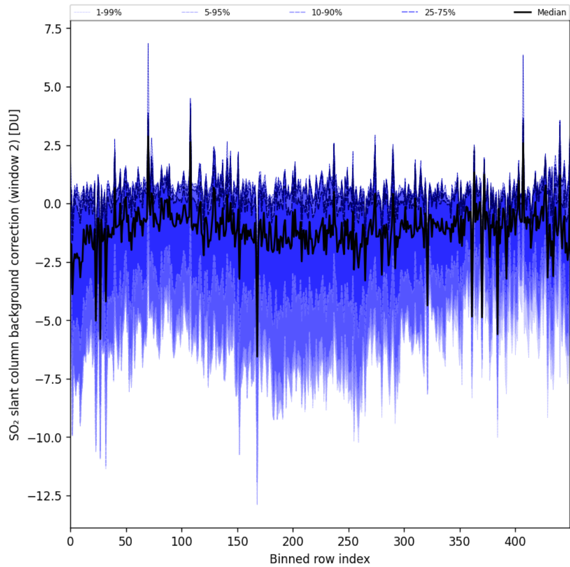
Figure 96: Along track statistics of “SO 2 slant column background correction (window 2)” for 2025-05-10 to 2025-05-11
