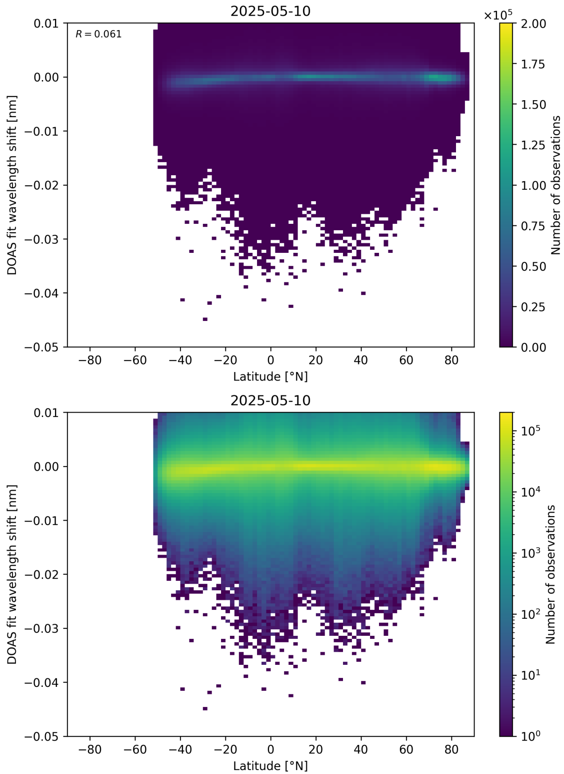
Figure 153: Scatter density plot of “Latitude” against “DOAS fit wavelength shift” for 2025-05-10 to 2025-05-11.
