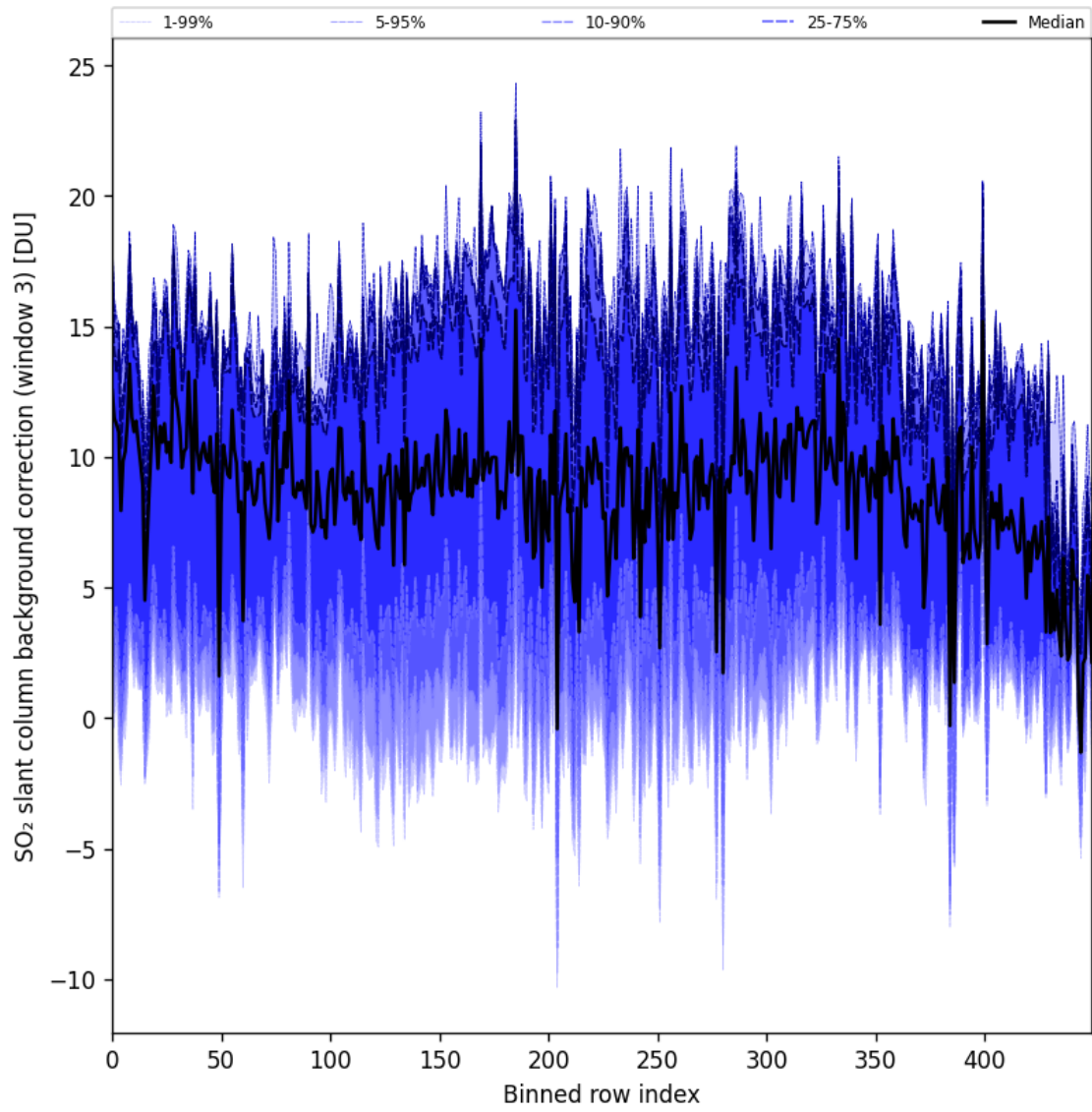
Figure 100: Along track statistics of “SO 2 slant column background correction (window 3)” for 2025-05-10 to 2025-05-11
