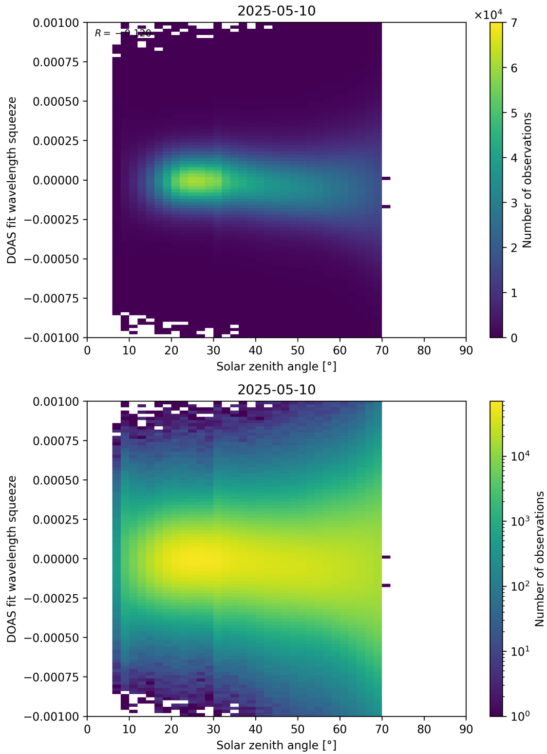
Figure 175: Scatter density plot of “Solar zenith angle” against “DOAS fit wavelength squeeze” for 2025-05-10 to 2025-05-11.
