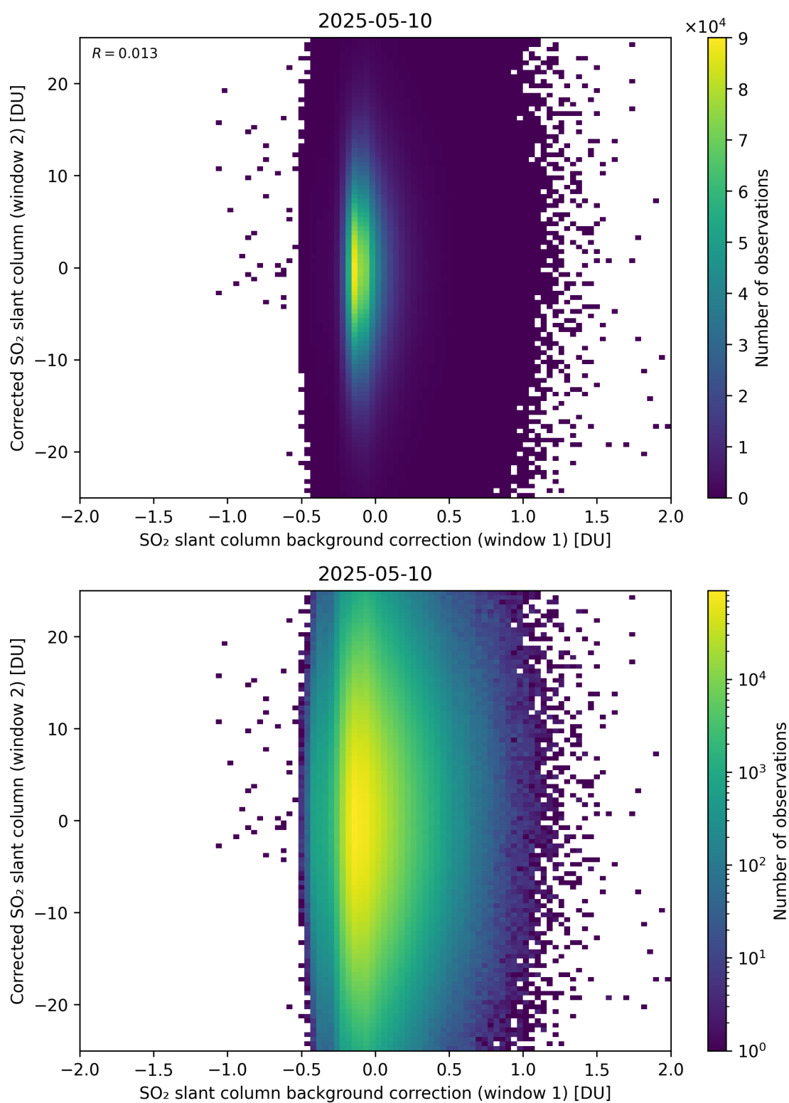
Figure 115: Scatter density plot of “SO 2 slant column background correction (window 1)” against “Corrected SO 2 slant column (window 2)” for 2025-05-10 to 2025-05-11.
