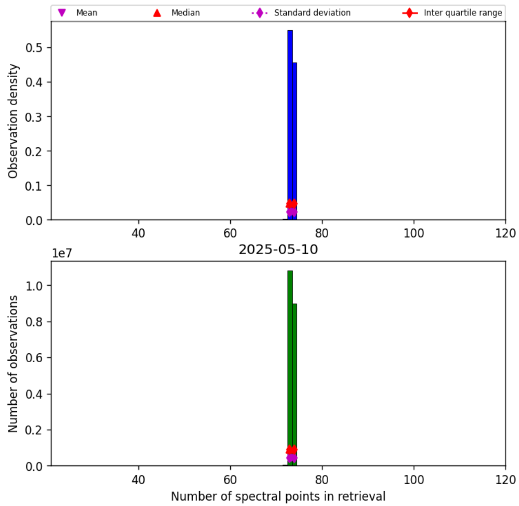
Figure 82: Histogram of “Number of spectral points in retrieval” for 2025-05-10 to 2025-05-11
