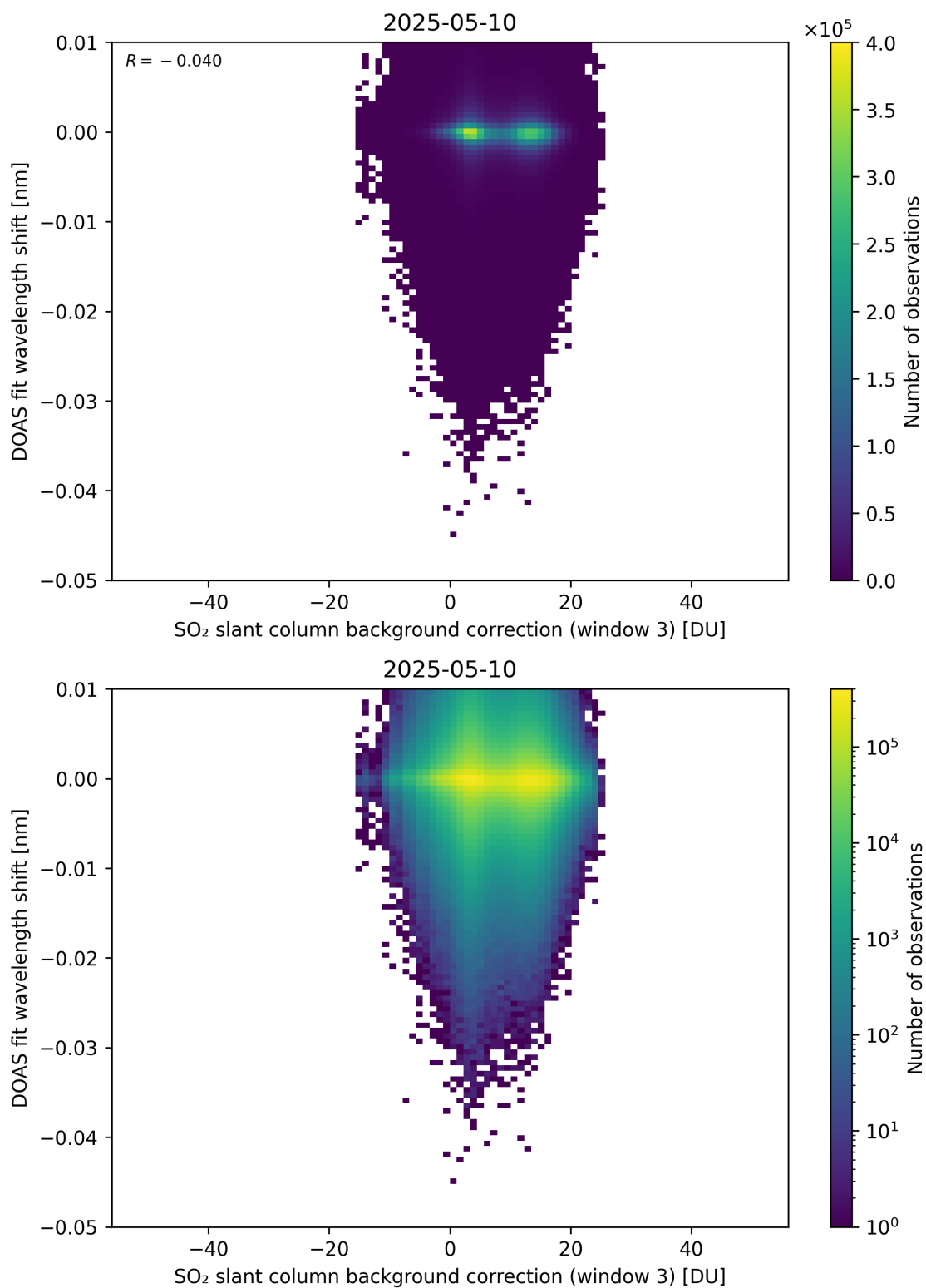
Figure 132: Scatter density plot of “SO 2 slant column background correction (window 3)” against “DOAS fit wavelength shift” for 2025-05-10 to 2025-05-11.
