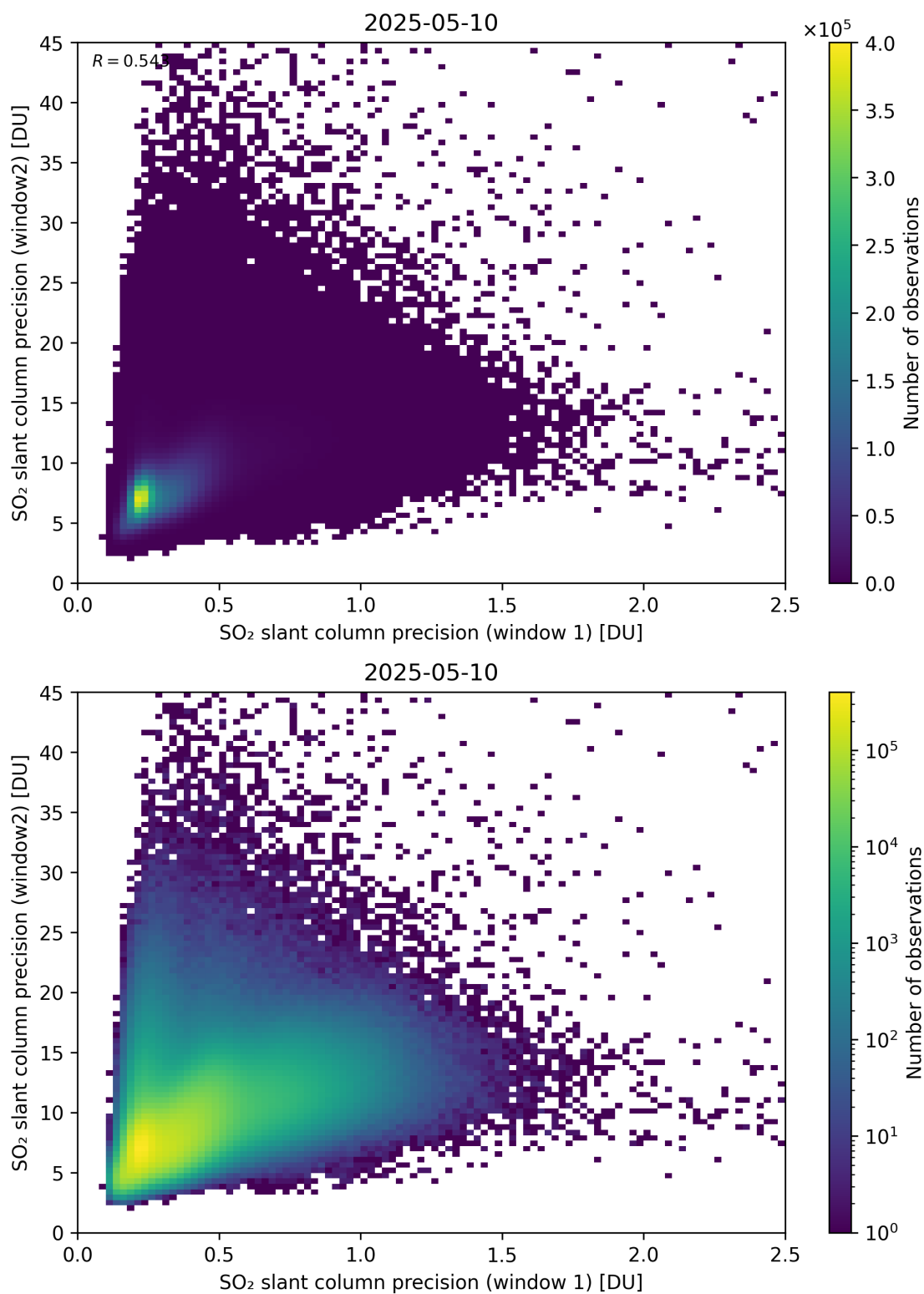
Figure 277: Scatter density plot of “SO 2 slant column precision (window 1)” against “SO 2 slant column precision (window2)” for 2025-05-10 to 2025-05-11.
