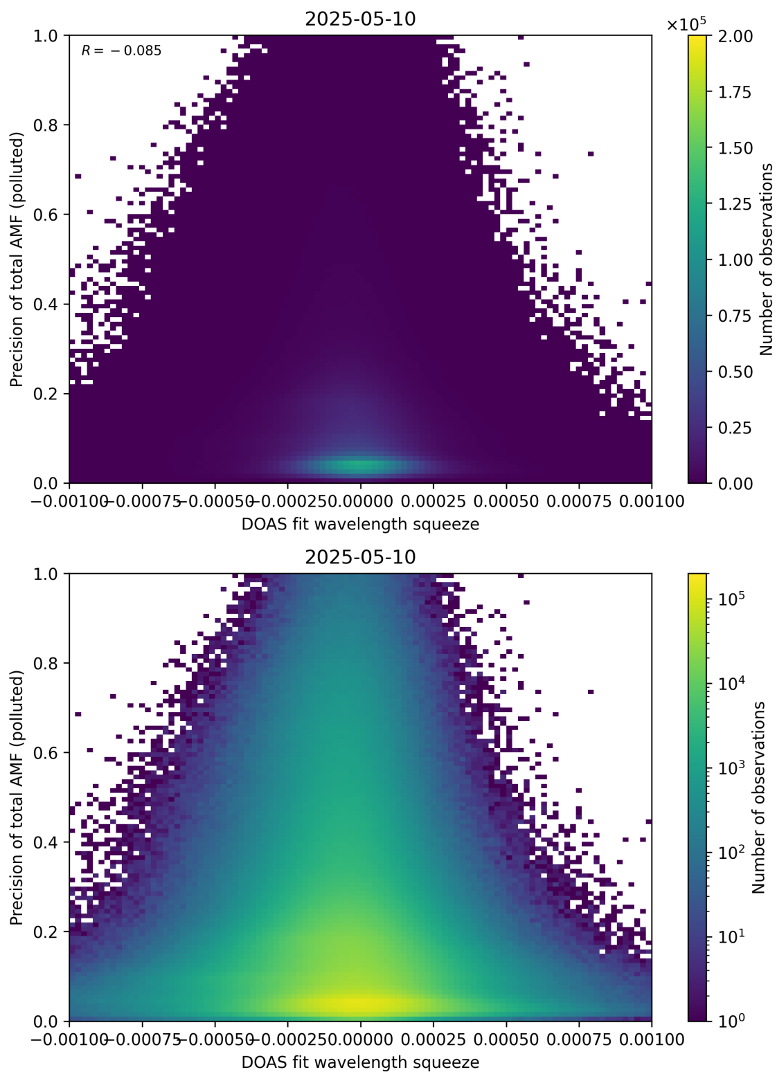
Figure 146: Scatter density plot of “DOAS fit wavelength squeeze” against “Precision of total AMF (polluted)” for 2025-05-10 to 2025-05-11.
