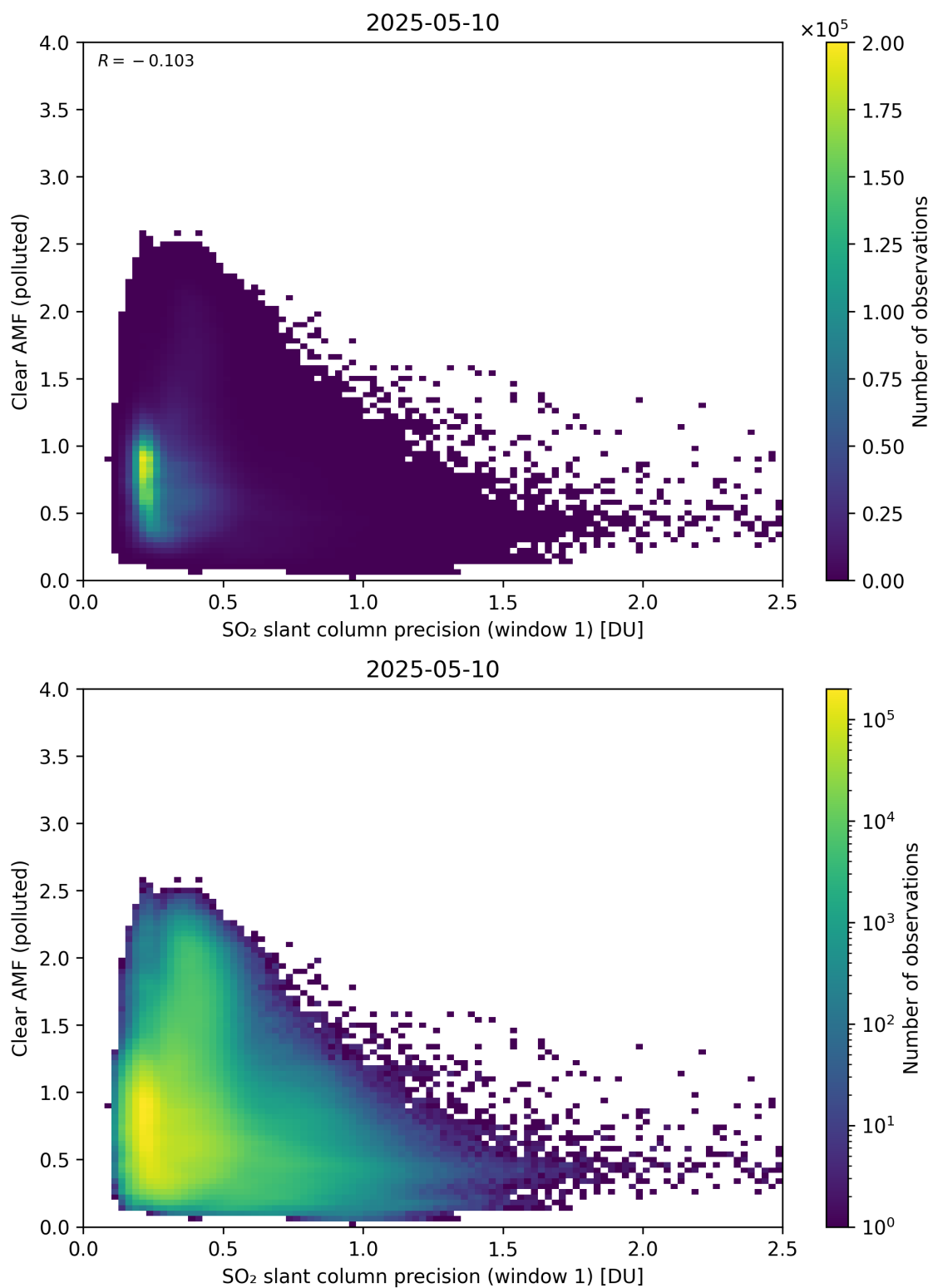
Figure 274: Scatter density plot of “SO 2 slant column precision (window 1)” against “Clear AMF (polluted)” for 2025-05-10 to 2025-05-11.
