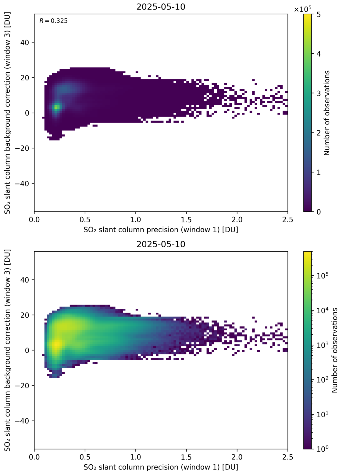
Figure 270: Scatter density plot of “SO 2 slant column precision (window 1)” against “SO 2 slant column background correction (window 3)” for 2025-05-10 to 2025-05-11.
