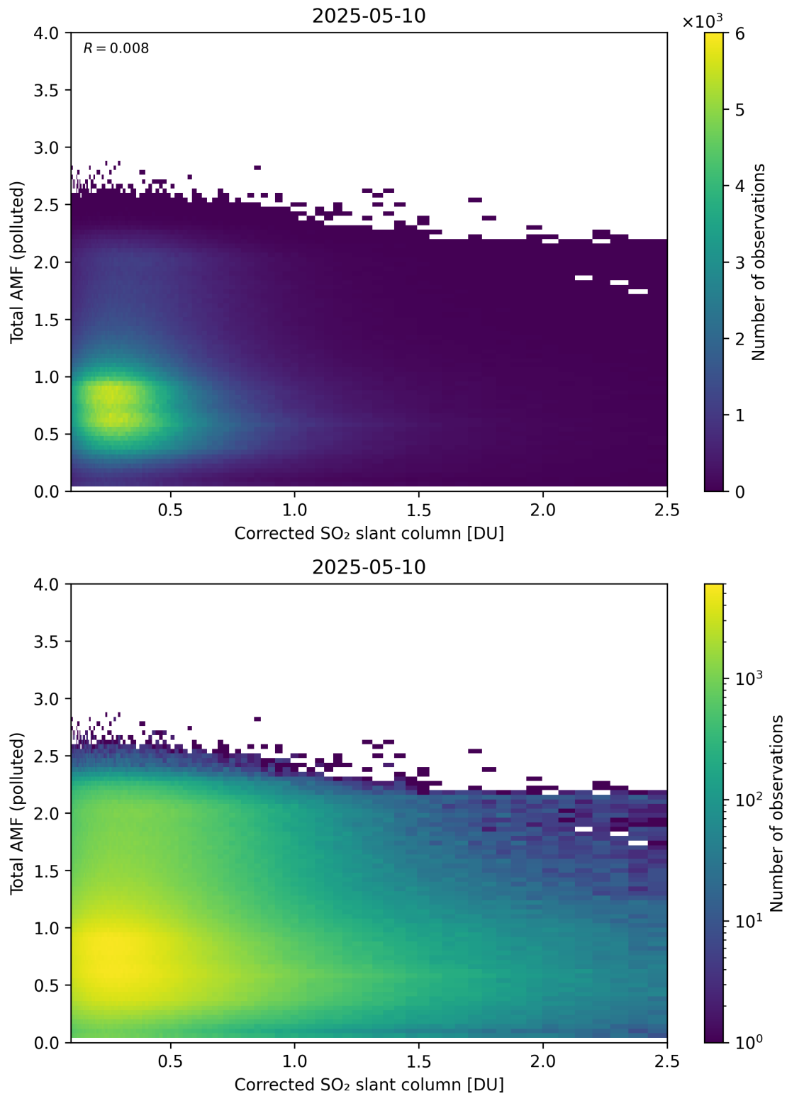
Figure 242: Scatter density plot of “Corrected SO 2 slant column” against “Total AMF (polluted)” for 2025-05-10 to 2025-05-11.
