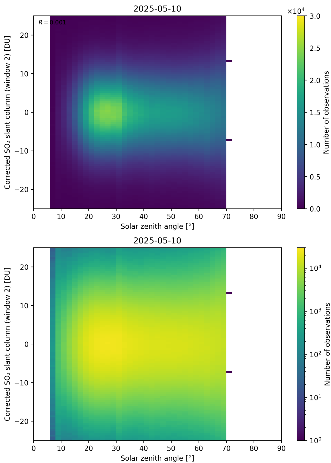
Figure 182: Scatter density plot of “Solar zenith angle” against “Corrected SO 2 slant column (window 2)” for 2025-05-10 to 2025-05-11.
