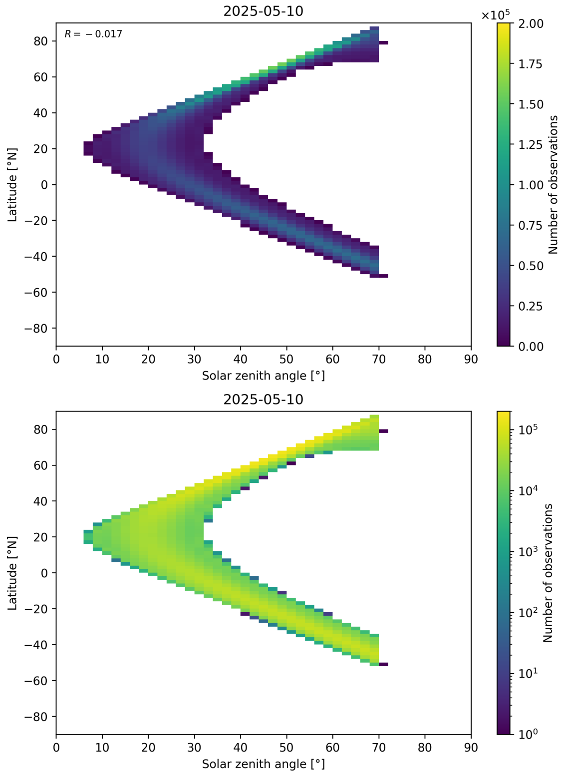
Figure 177: Scatter density plot of “Solar zenith angle” against “Latitude” for 2025-05-10 to 2025-05-11.
