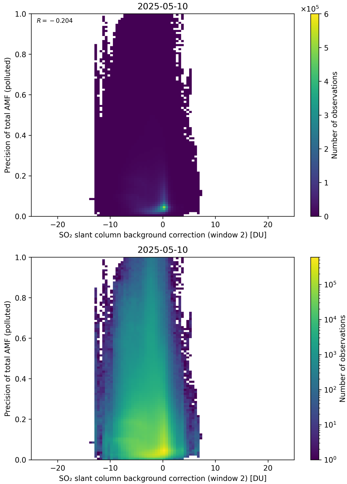
Figure 131: Scatter density plot of “SO 2 slant column background correction (window 2)” against “Precision of total AMF (polluted)” for 2025-05-10 to 2025-05-11.
