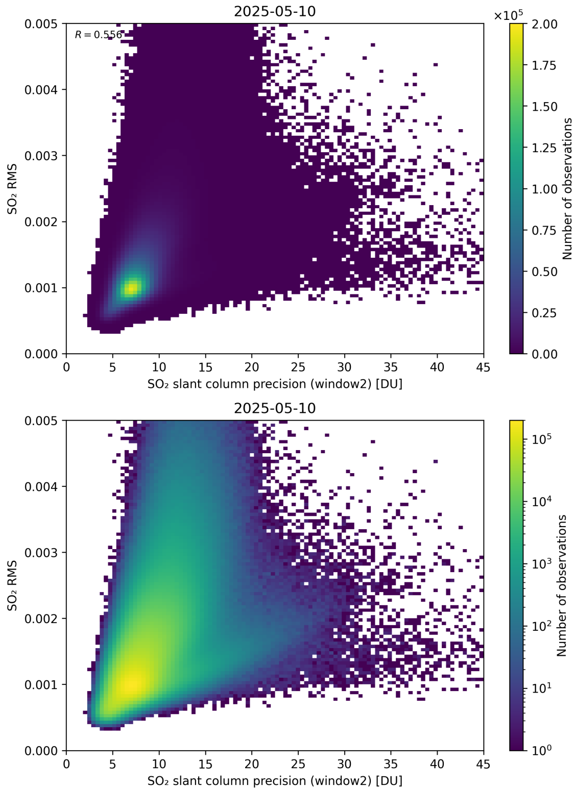
Figure 295: Scatter density plot of “SO 2 slant column precision (window2)” against “SO 2 RMS” for 2025-05-10 to 2025-05-11.
