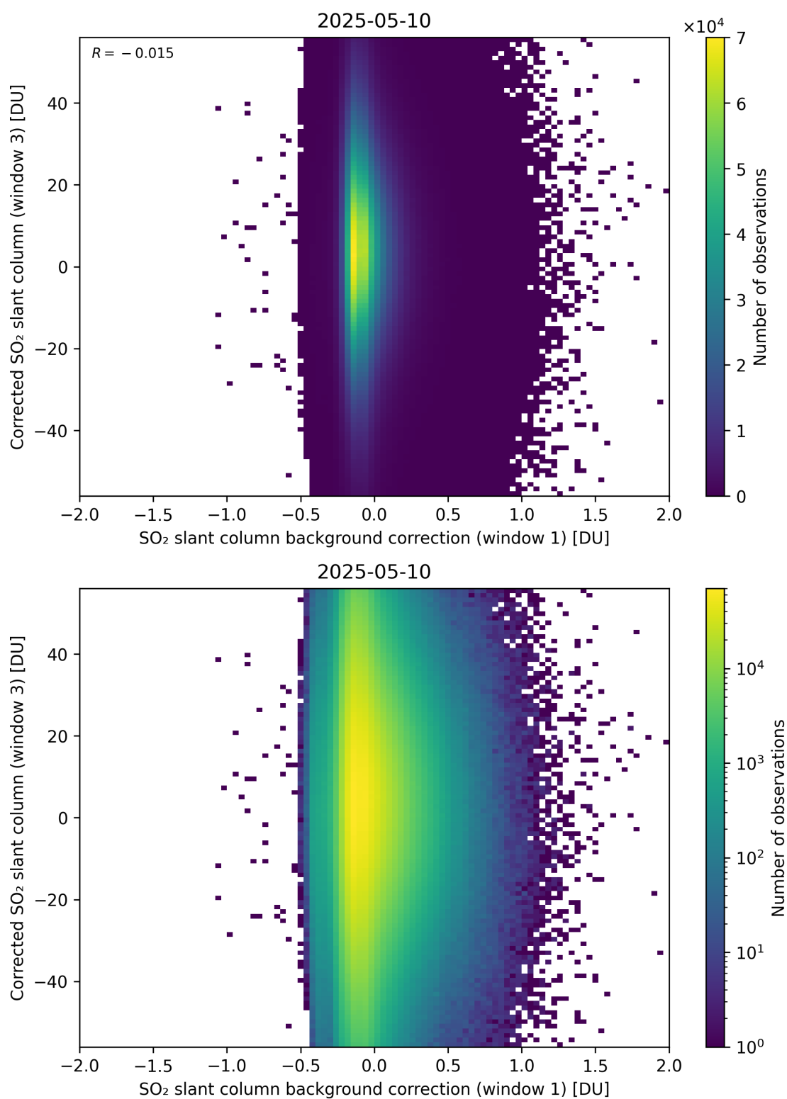
Figure 116: Scatter density plot of “SO 2 slant column background correction (window 1)” against “Corrected SO 2 slant column (window 3)” for 2025-05-10 to 2025-05-11.
