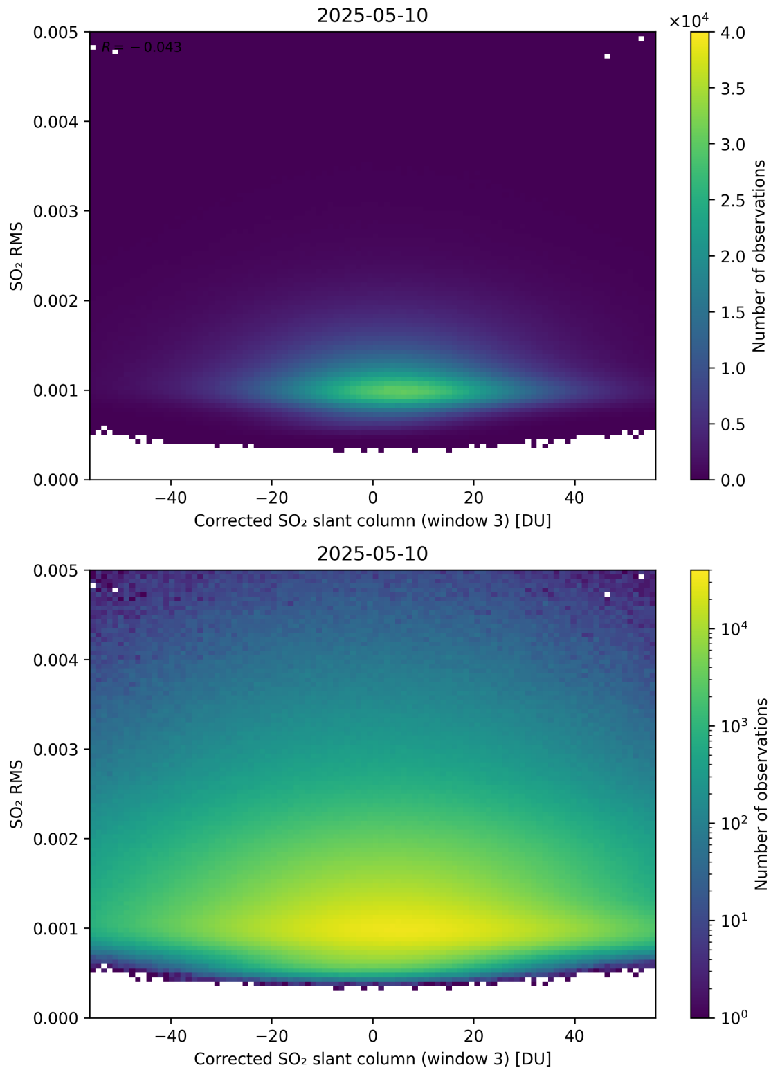
Figure 258: Scatter density plot of “Corrected SO 2 slant column (window 3)” against “SO 2 RMS” for 2025-05-10 to 2025-05-11.
