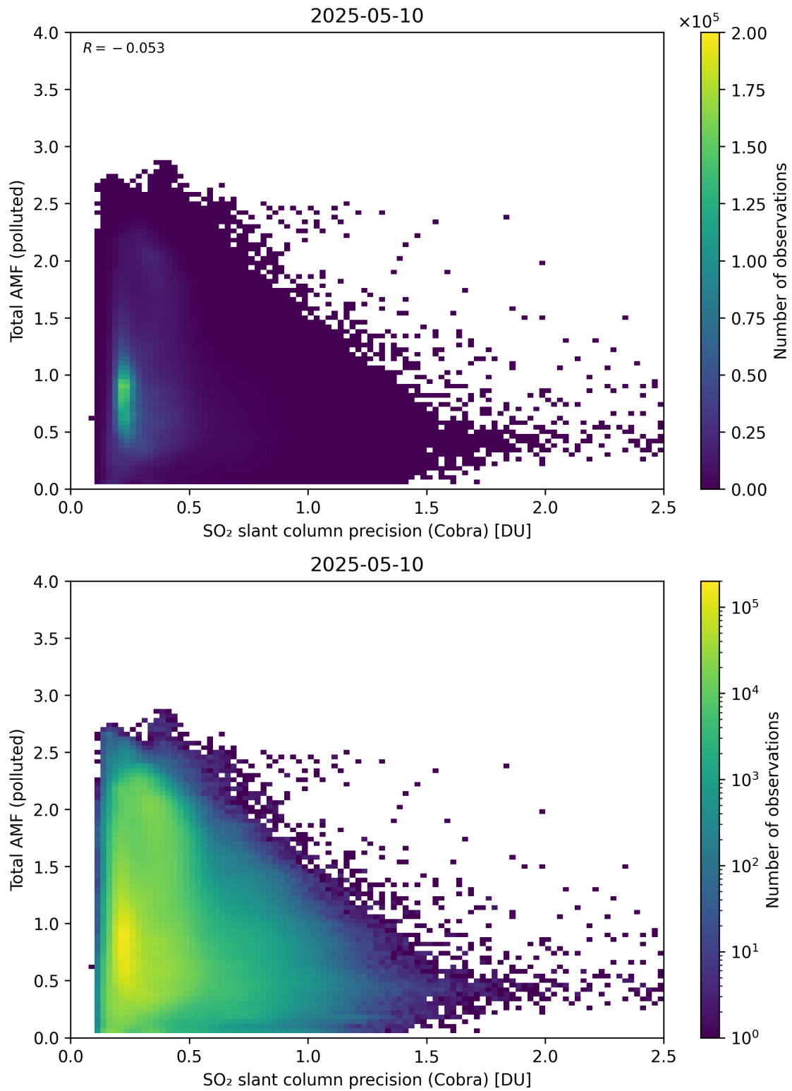
Figure 213: Scatter density plot of “SO 2 slant column precision (Cobra)” against “Total AMF (polluted)” for 2025-05-10 to 2025-05-11.
