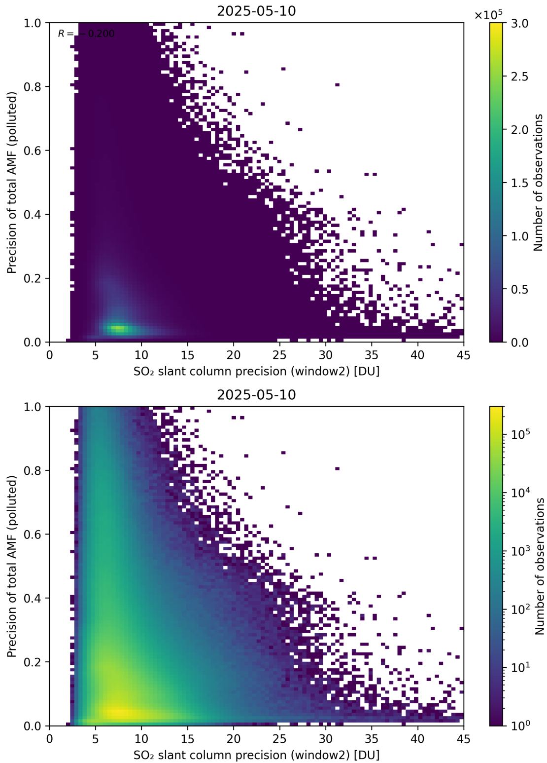
Figure 302: Scatter density plot of “SO 2 slant column precision (window2)” against “Precision of total AMF (polluted)” for 2025-05-10 to 2025-05-11.
