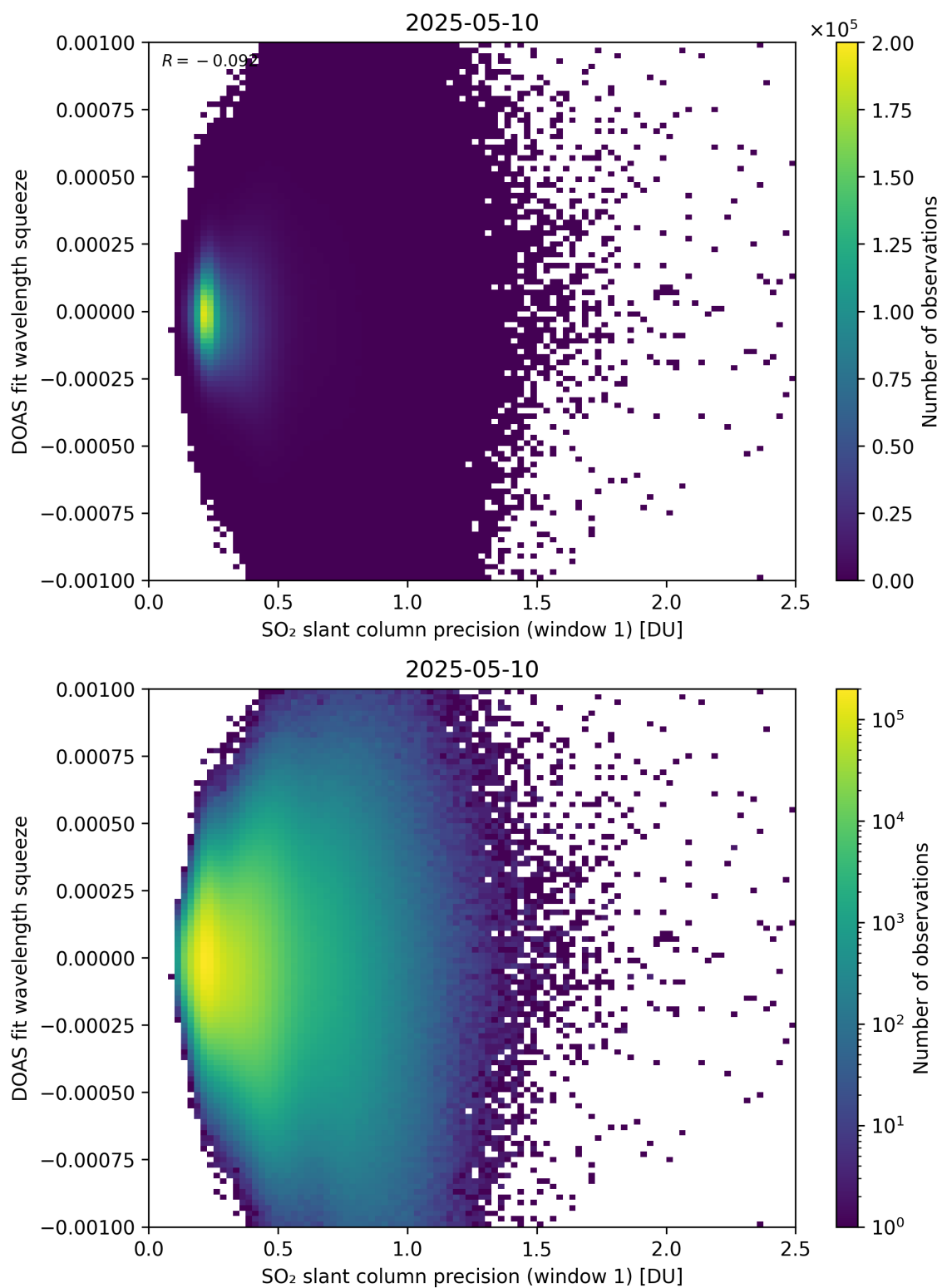
Figure 272: Scatter density plot of “SO 2 slant column precision (window 1)” against “DOAS fit wavelength squeeze” for 2025-05-10 to 2025-05-11.
