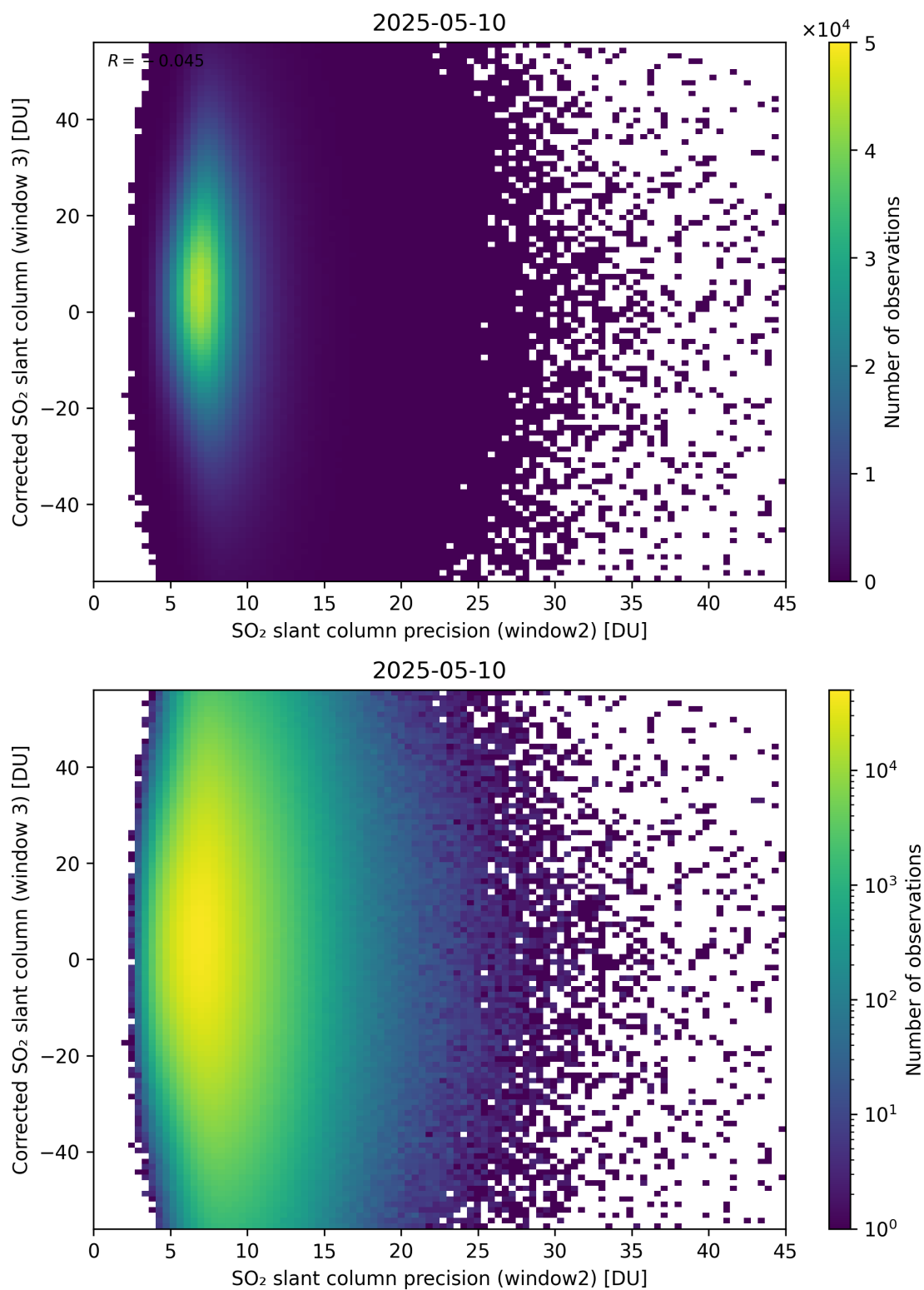
Figure 298: Scatter density plot of “SO 2 slant column precision (window2)” against “Corrected SO 2 slant column (window 3)” for 2025-05-10 to 2025-05-11.
