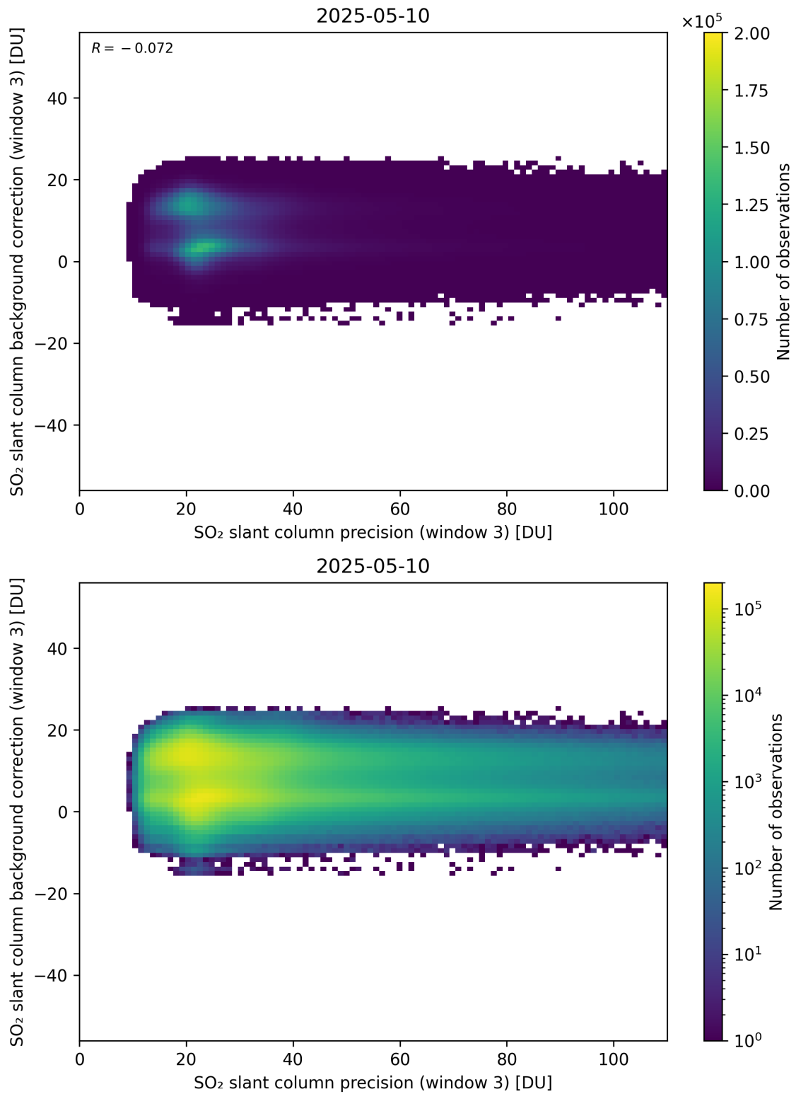
Figure 307: Scatter density plot of “SO 2 slant column precision (window 3)” against “SO 2 slant column background correction (window 3)” for 2025-05-10 to 2025-05-11.
