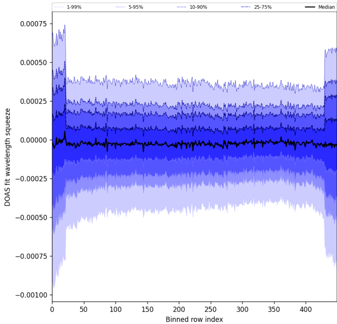
Figure 103: Along track statistics of “DOAS fit wavelength squeeze” for 2025-05-10 to 2025-05-11
