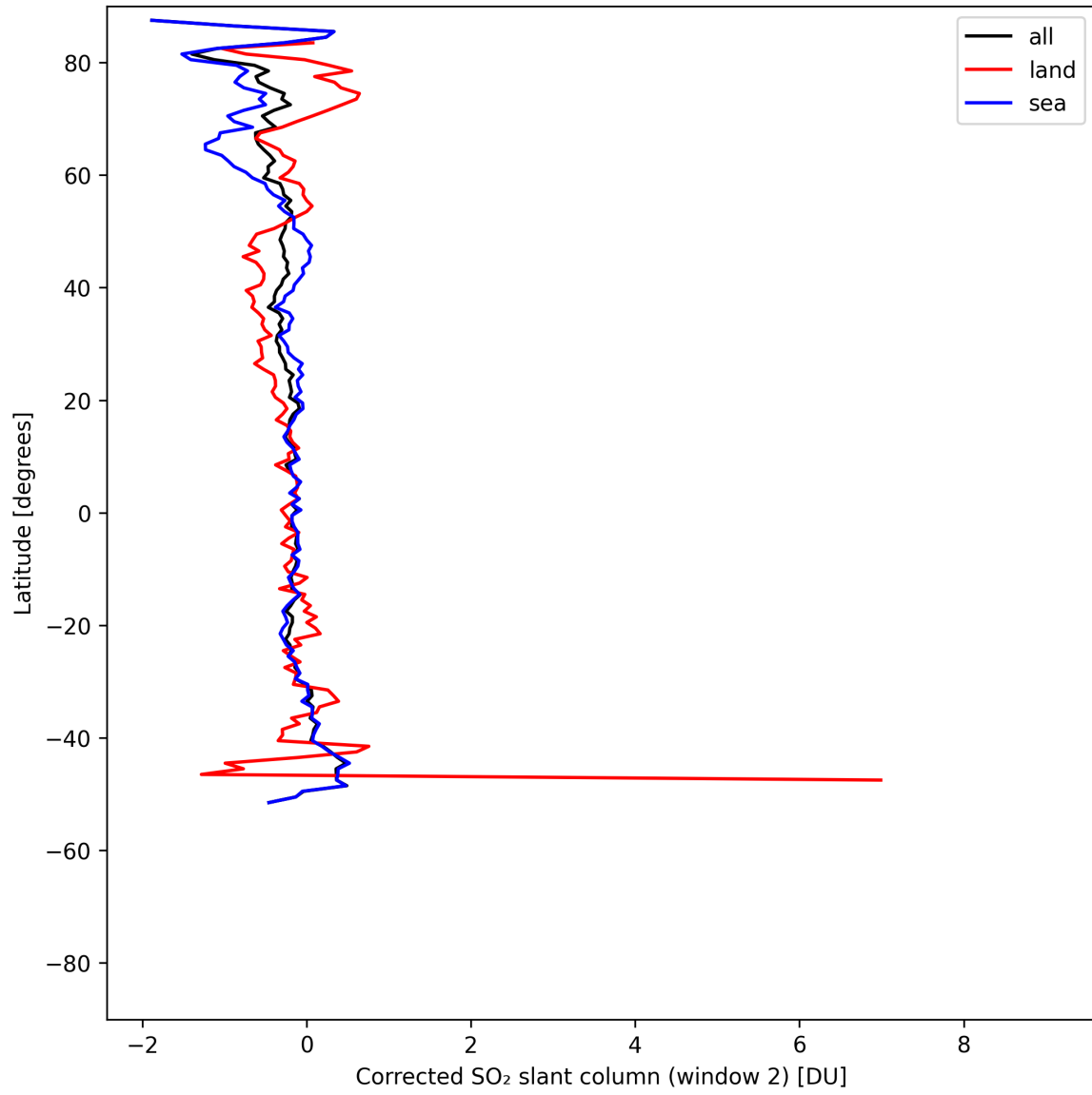
Figure 43: Zonal average of “Corrected SO 2 slant column (window 2)” for 2025-05-10 to 2025-05-11.
