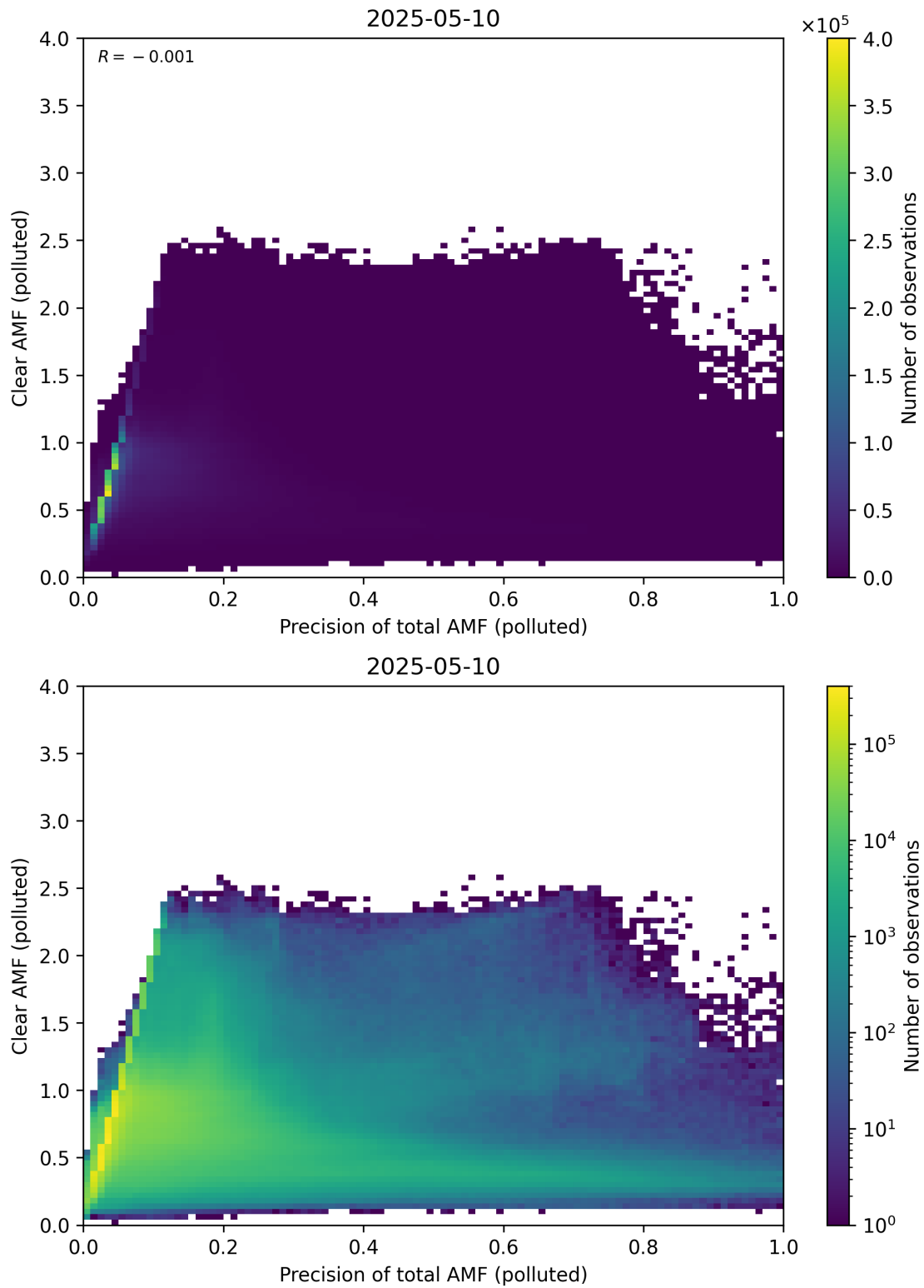
Figure 320: Scatter density plot of “Precision of total AMF (polluted)” against “Clear AMF (polluted)” for 2025-05-10 to 2025-05-11.
