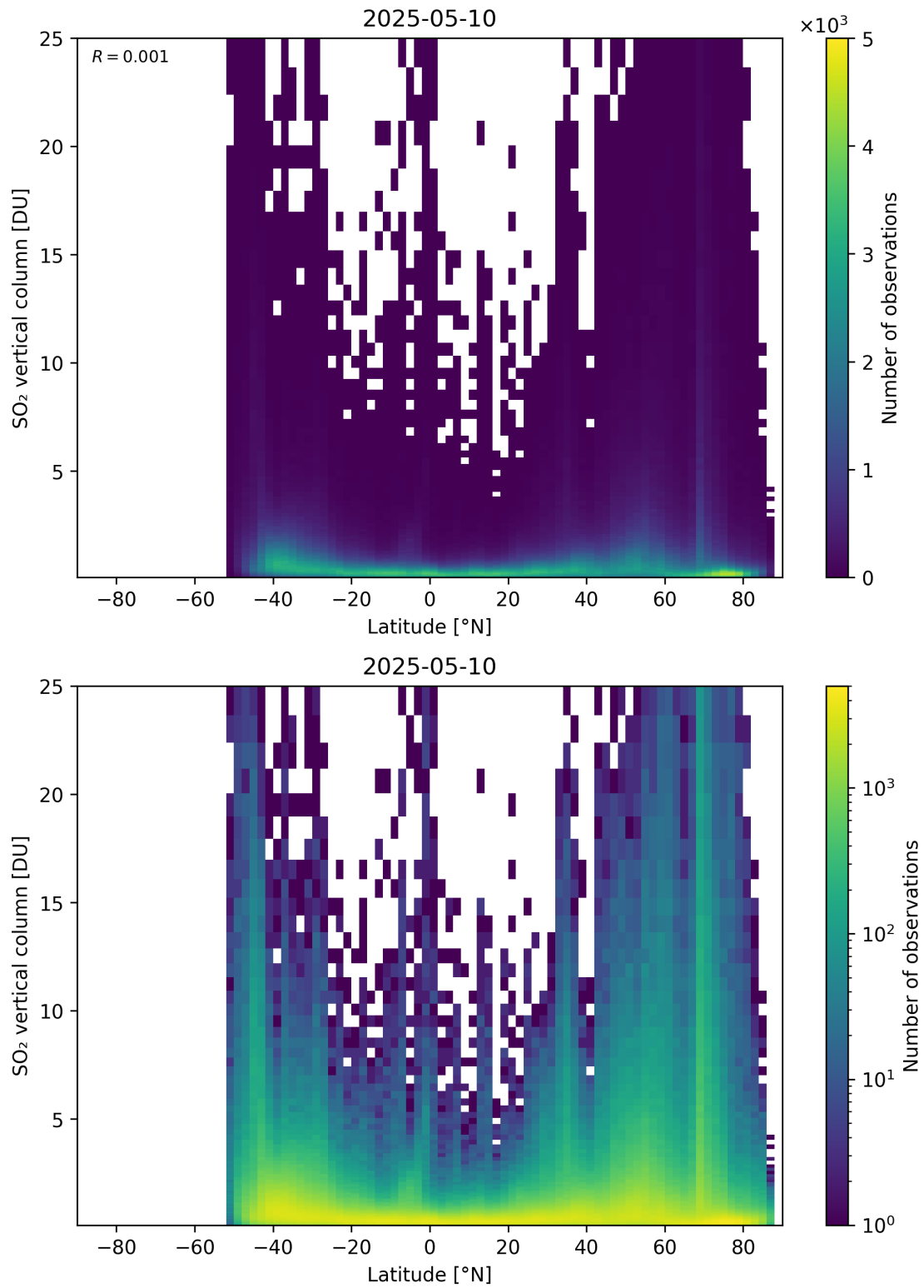
Figure 169: Scatter density plot of “Latitude” against “SO 2 vertical column” for 2025-05-10 to 2025-05-11.
