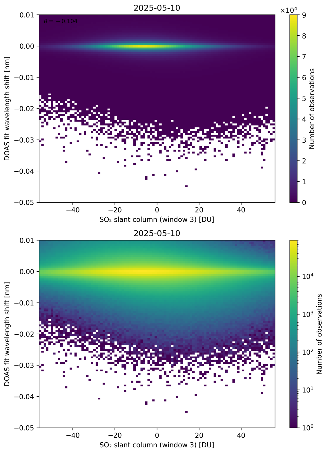
Figure 304: Scatter density plot of “SO 2 slant column (window 3)” against “DOAS fit wavelength shift” for 2025-05-10 to 2025-05-11.
