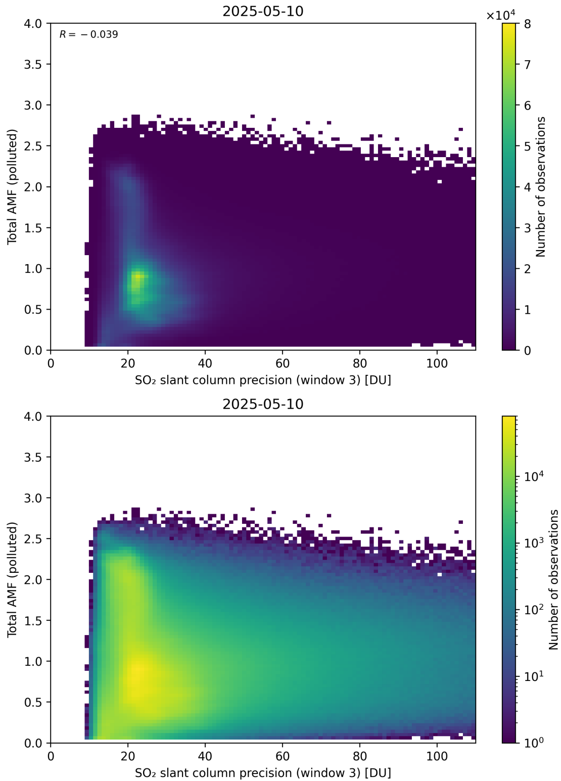
Figure 313: Scatter density plot of “SO 2 slant column precision (window 3)” against “Total AMF (polluted)” for 2025-05-10 to 2025-05-11.
