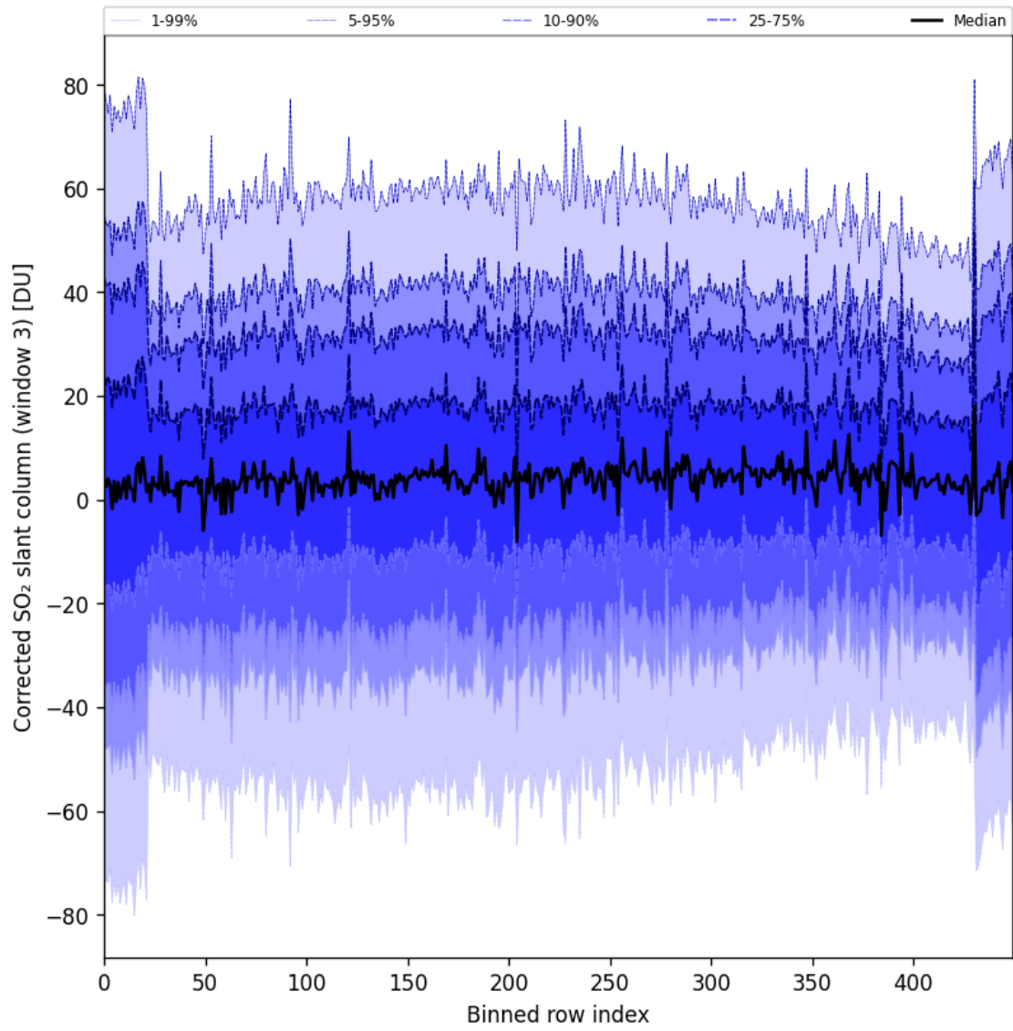
Figure 99: Along track statistics of “Corrected SO 2 slant column (window 3)” for 2025-05-10 to 2025-05-11
