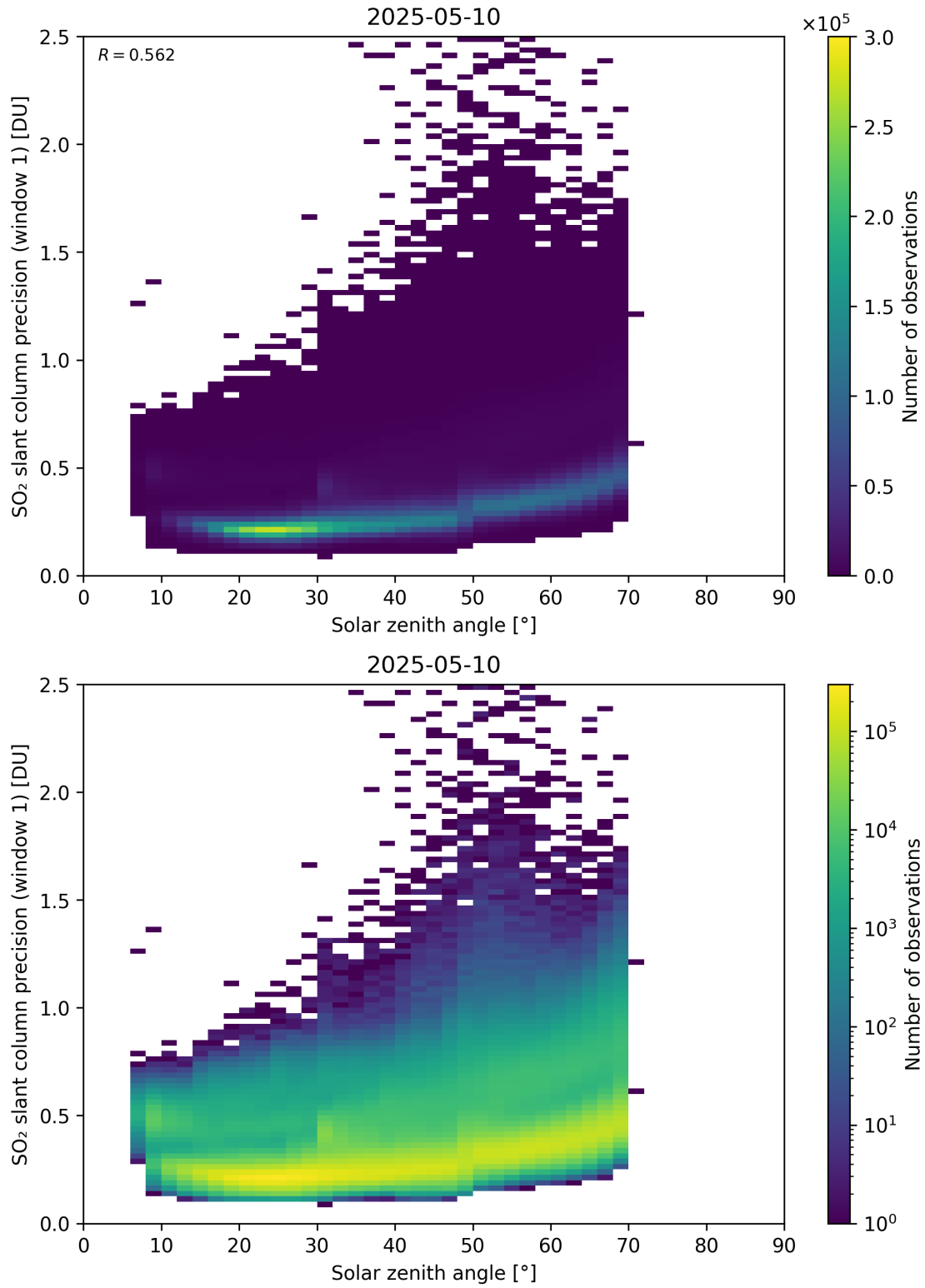
Figure 185: Scatter density plot of “Solar zenith angle” against “SO 2 slant column precision (window 1)” for 2025-05-10 to 2025-05-11.
