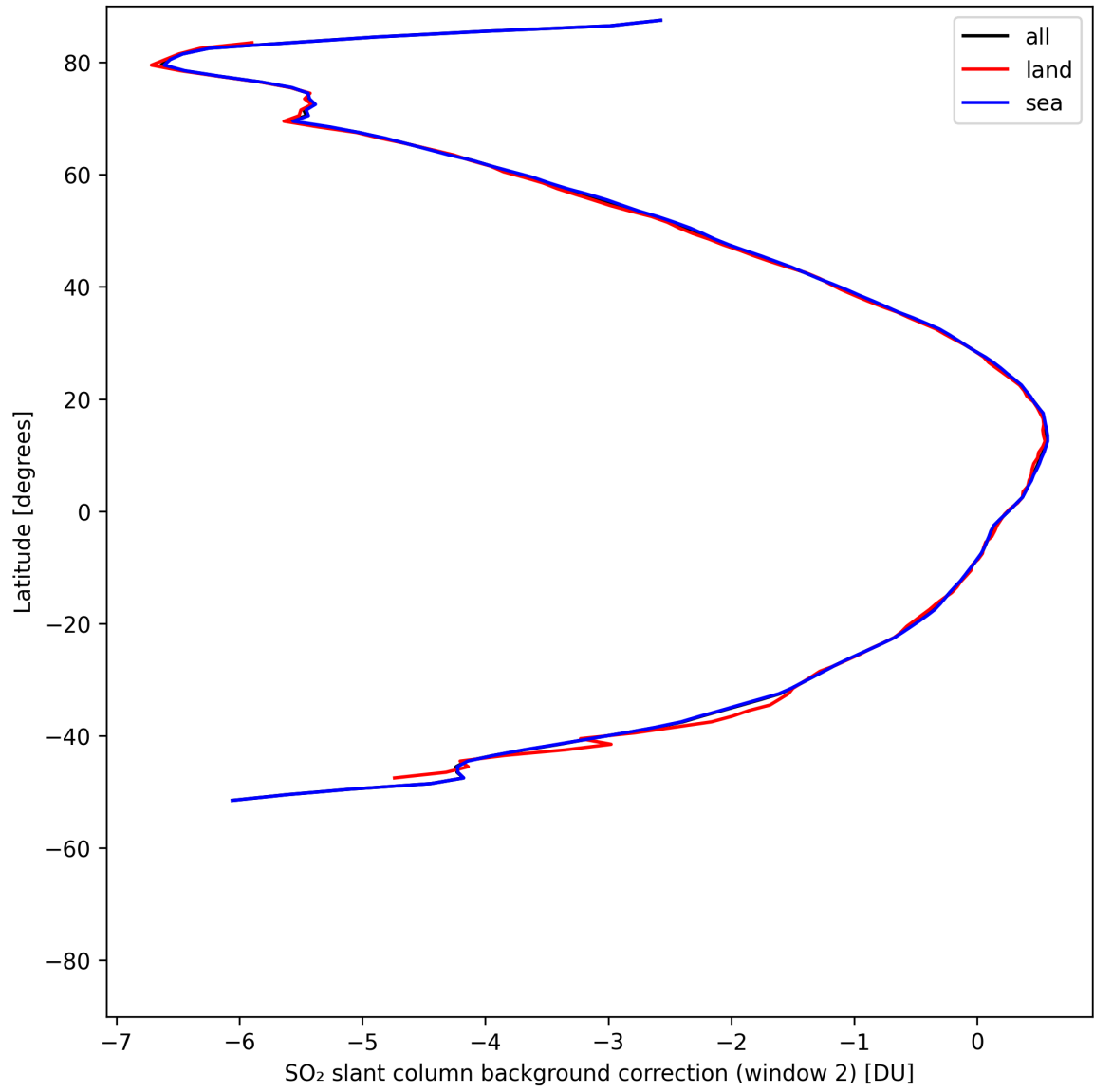
Figure 44: Zonal average of “SO 2 slant column background correction (window 2)” for 2025-05-10 to 2025-05-11.
