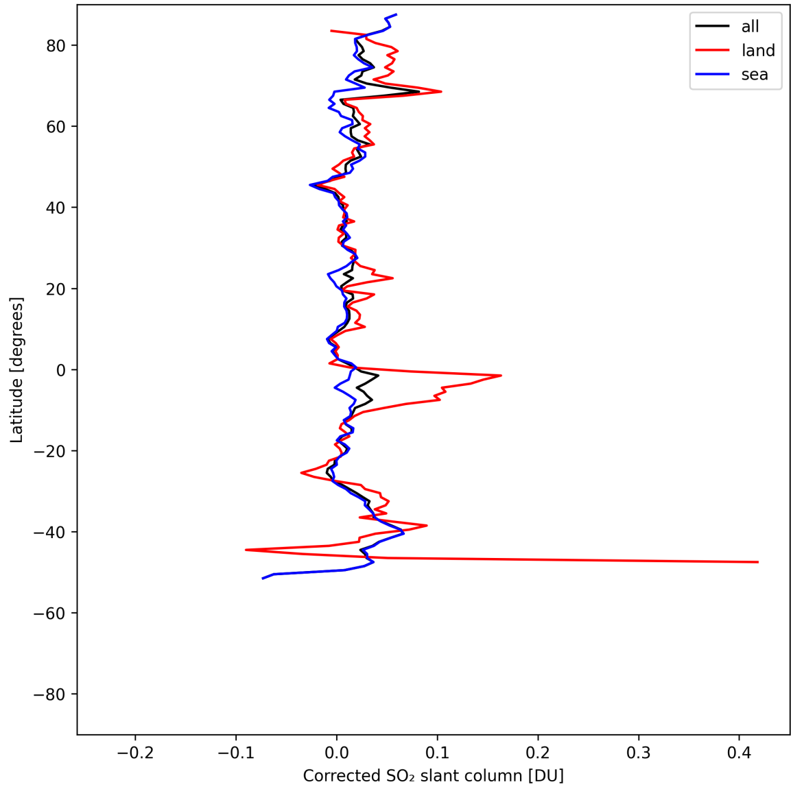
Figure 34: Zonal average of “Corrected SO 2 slant column” for 2025-05-10 to 2025-05-11.
