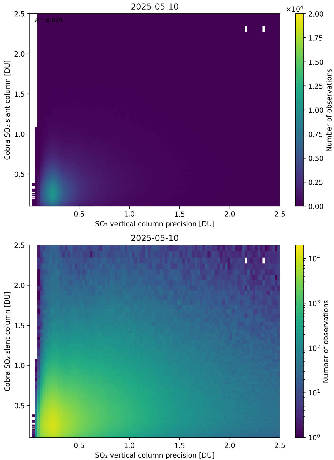
Figure 336: Scatter density plot of “SO 2 vertical column precision” against “Cobra SO 2 slant column” for 2025-05-10 to 2025-05-11.
