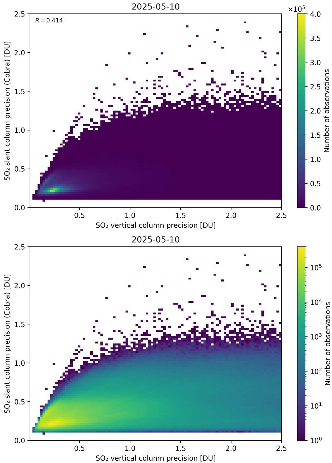
Figure 337: Scatter density plot of “SO 2 vertical column precision” against “SO 2 slant column precision (Cobra)” for 2025-05-10 to 2025-05-11.
