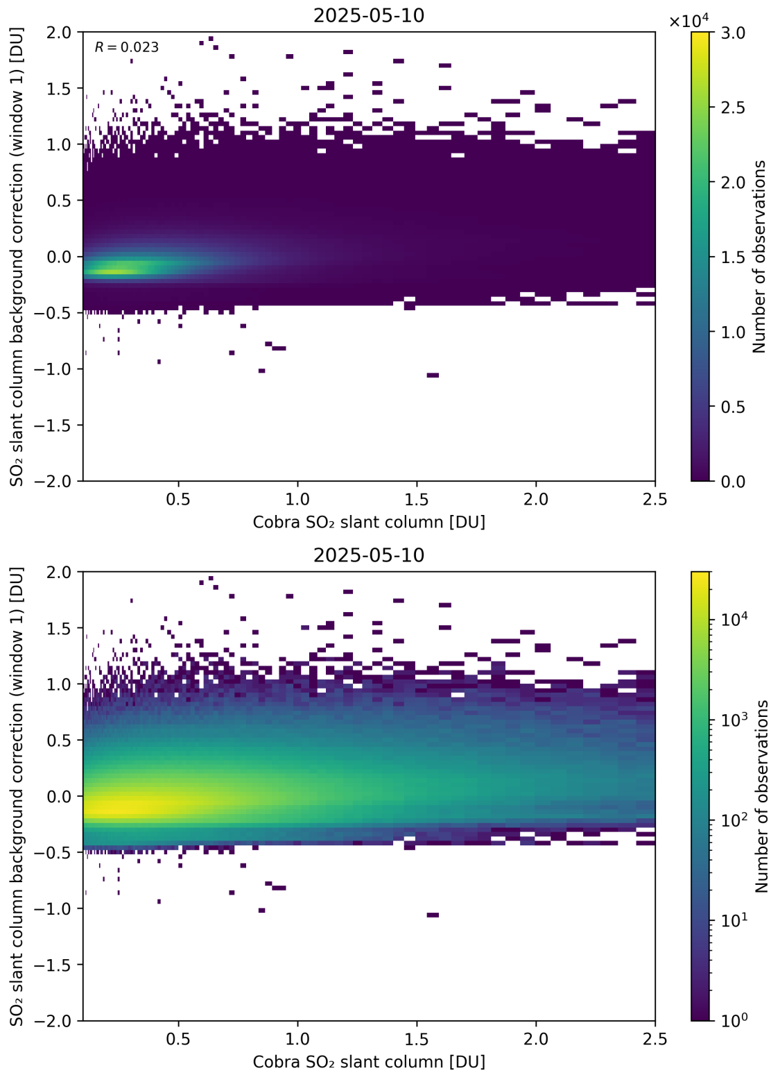
Figure 193: Scatter density plot of “Cobra SO 2 slant column” against “SO 2 slant column background correction (window 1)” for 2025-05-10 to 2025-05-11.
