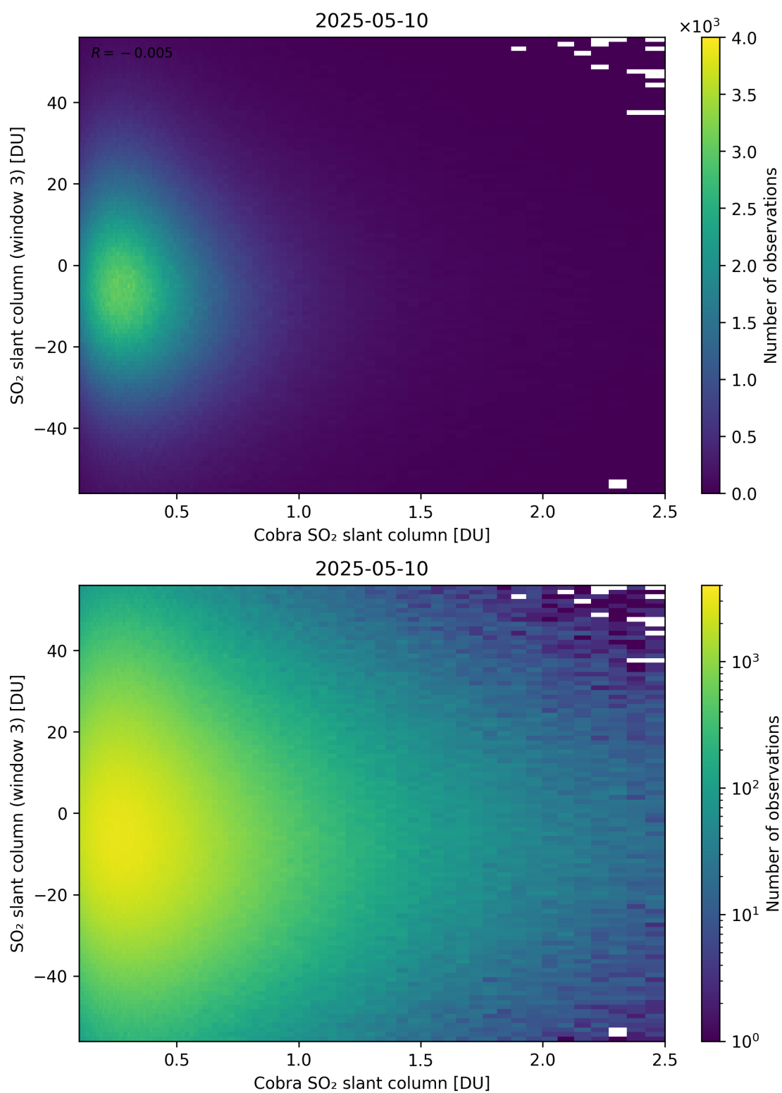
Figure 222: Scatter density plot of “Cobra SO 2 slant column” against “SO 2 slant column (window 3)” for 2025-05-10 to 2025-05-11.
