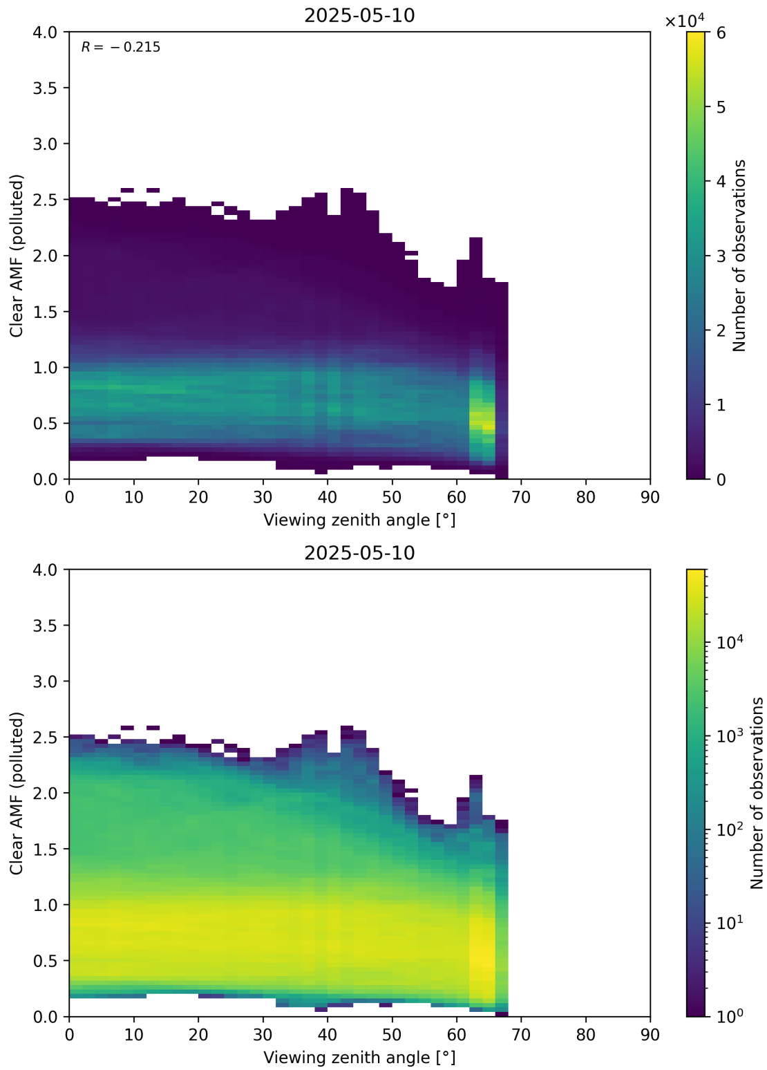
Figure 370: Scatter density plot of “Viewing zenith angle” against “Clear AMF (polluted)” for 2025-05-10 to 2025-05-11.
