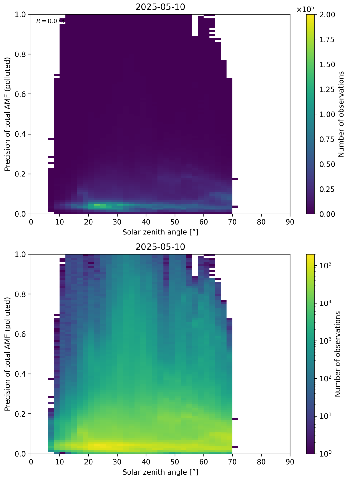
Figure 190: Scatter density plot of “Solar zenith angle” against “Precision of total AMF (polluted)” for 2025-05-10 to 2025-05-11.
