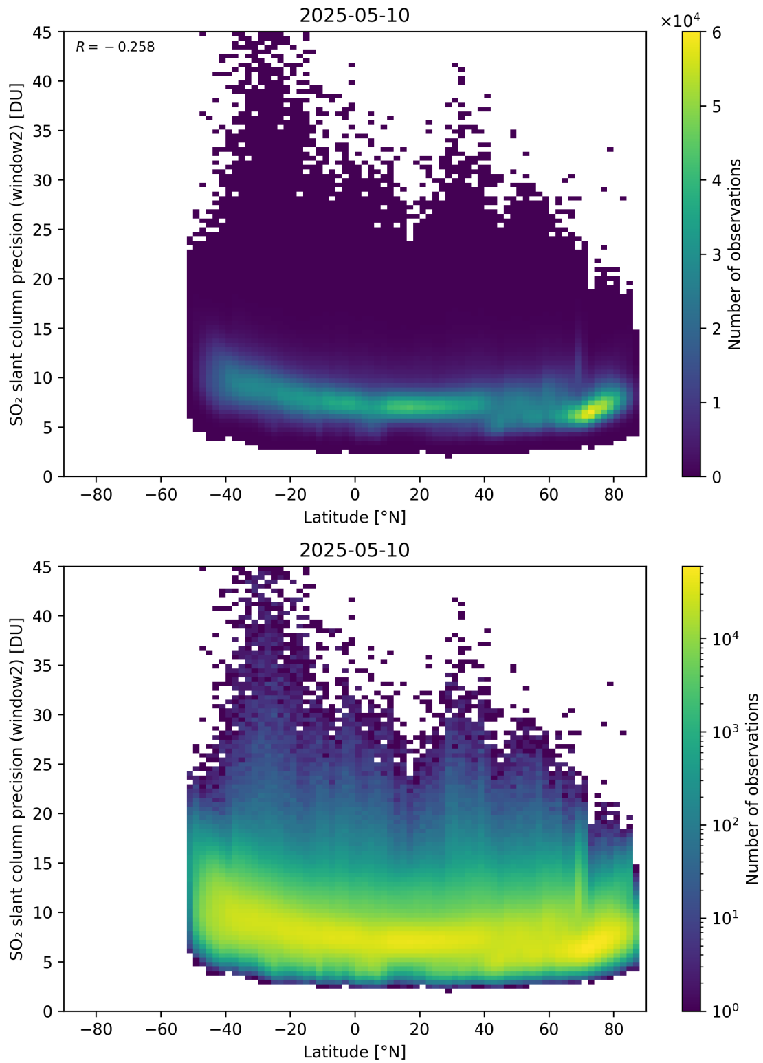
Figure 164: Scatter density plot of “Latitude” against “SO 2 slant column precision (window2)” for 2025-05-10 to 2025-05-11.
