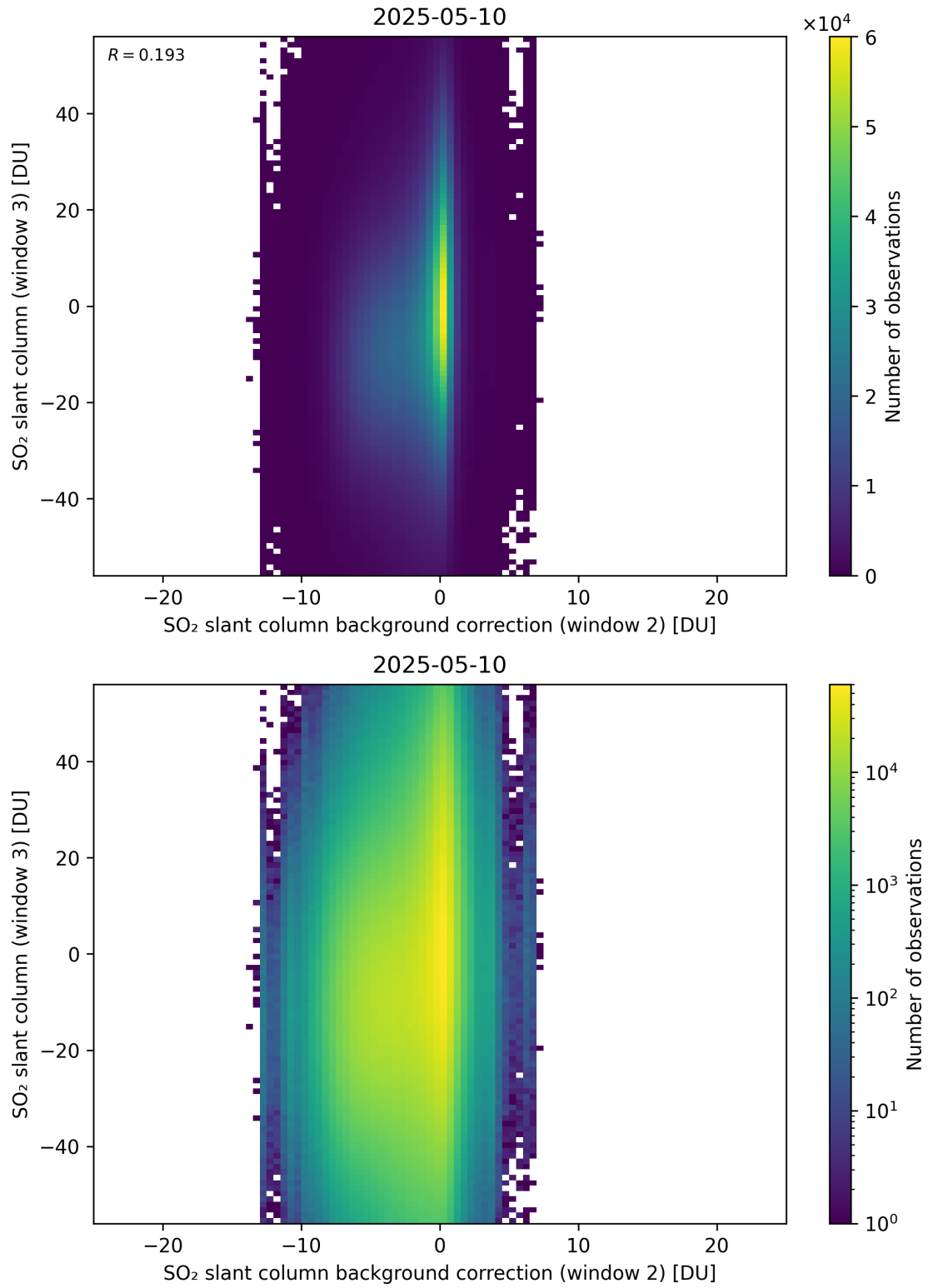
Figure 128: Scatter density plot of “SO 2 slant column background correction (window 2)” against “SO 2 slant column (window 3)” for 2025-05-10 to 2025-05-11.
