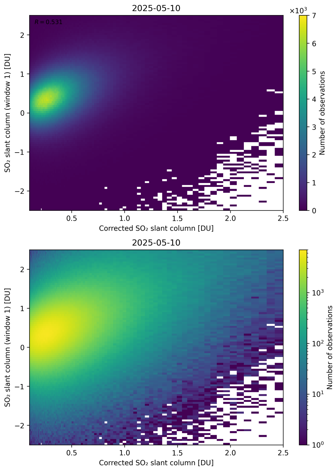
Figure 237: Scatter density plot of “Corrected SO 2 slant column” against “SO 2 slant column (window 1)” for 2025-05-10 to 2025-05-11.
