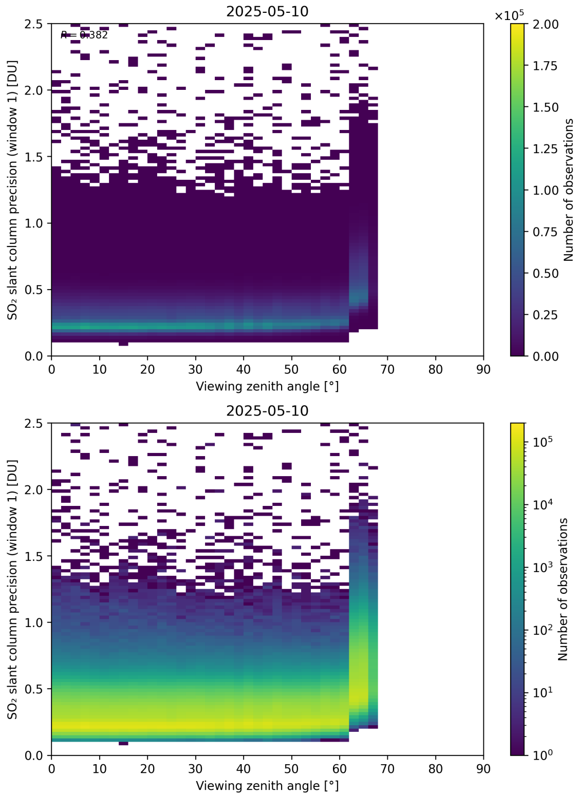
Figure 377: Scatter density plot of “Viewing zenith angle” against “SO 2 slant column precision (window 1)” for 2025-05-10 to 2025-05-11.
