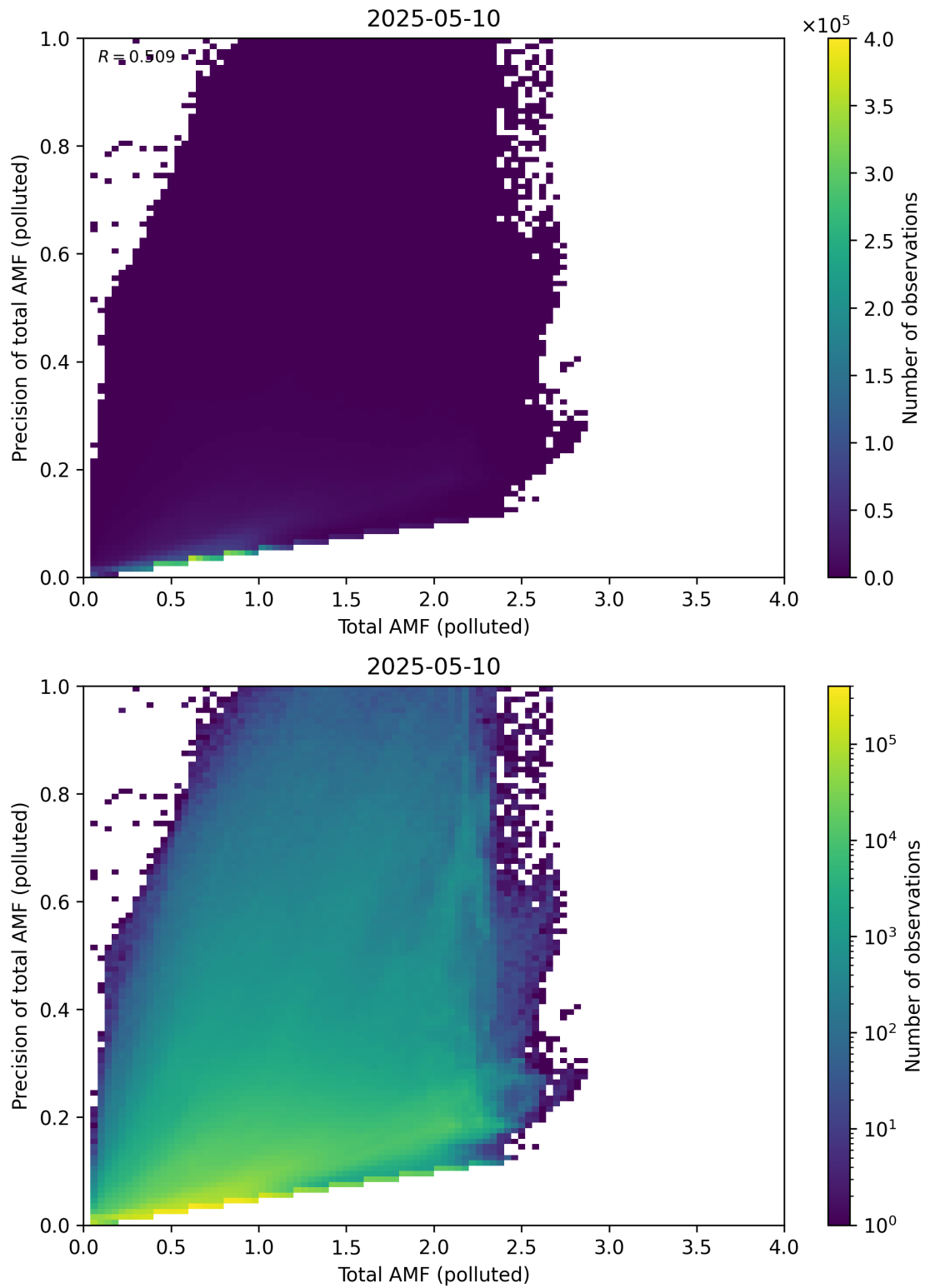
Figure 322: Scatter density plot of “Total AMF (polluted)” against “Precision of total AMF (polluted)” for 2025-05-10 to 2025-05-11.
