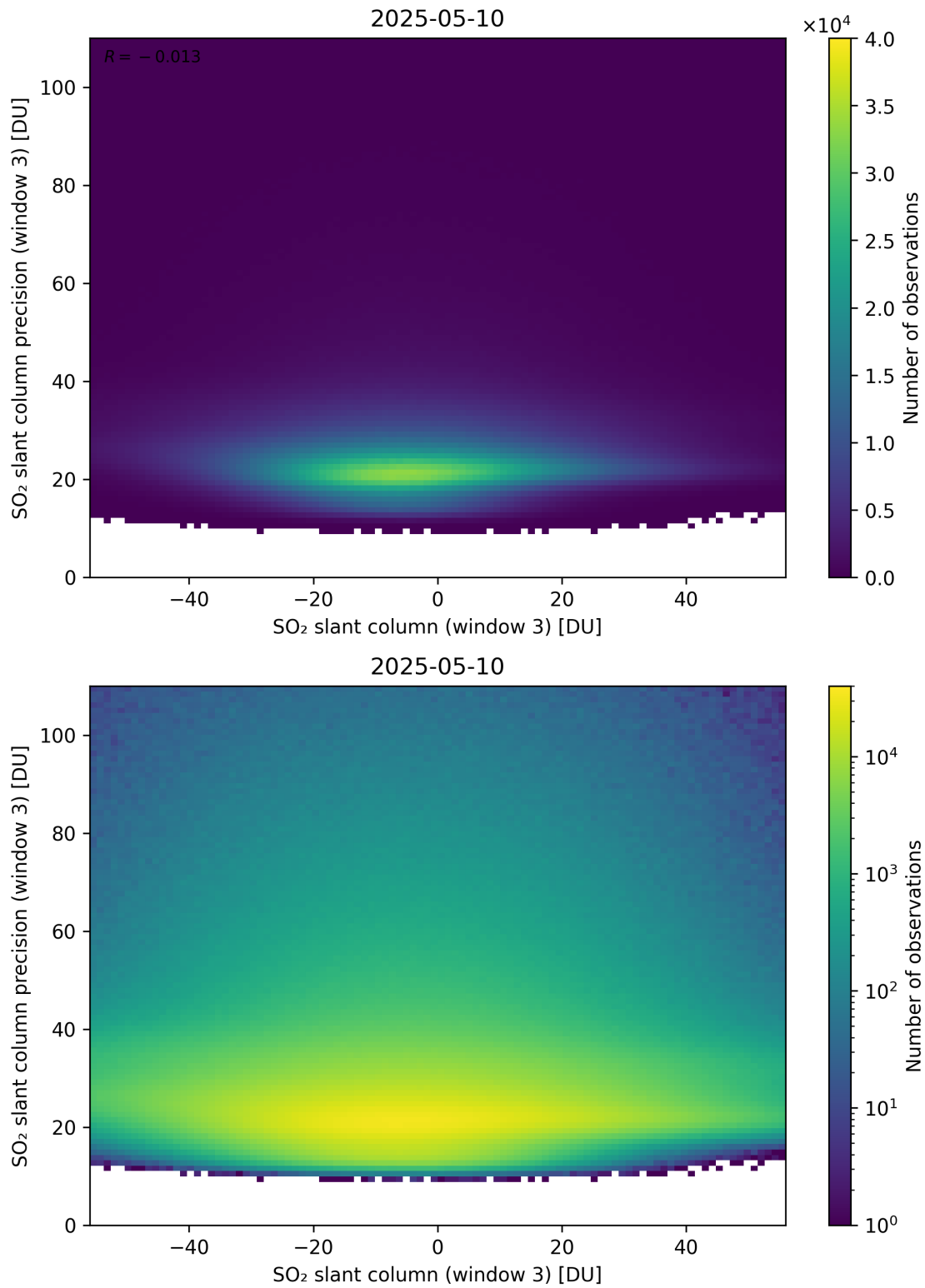
Figure 317: Scatter density plot of “SO 2 slant column (window 3)” against “SO 2 slant column precision (window 3)” for 2025-05-10 to 2025-05-11.
