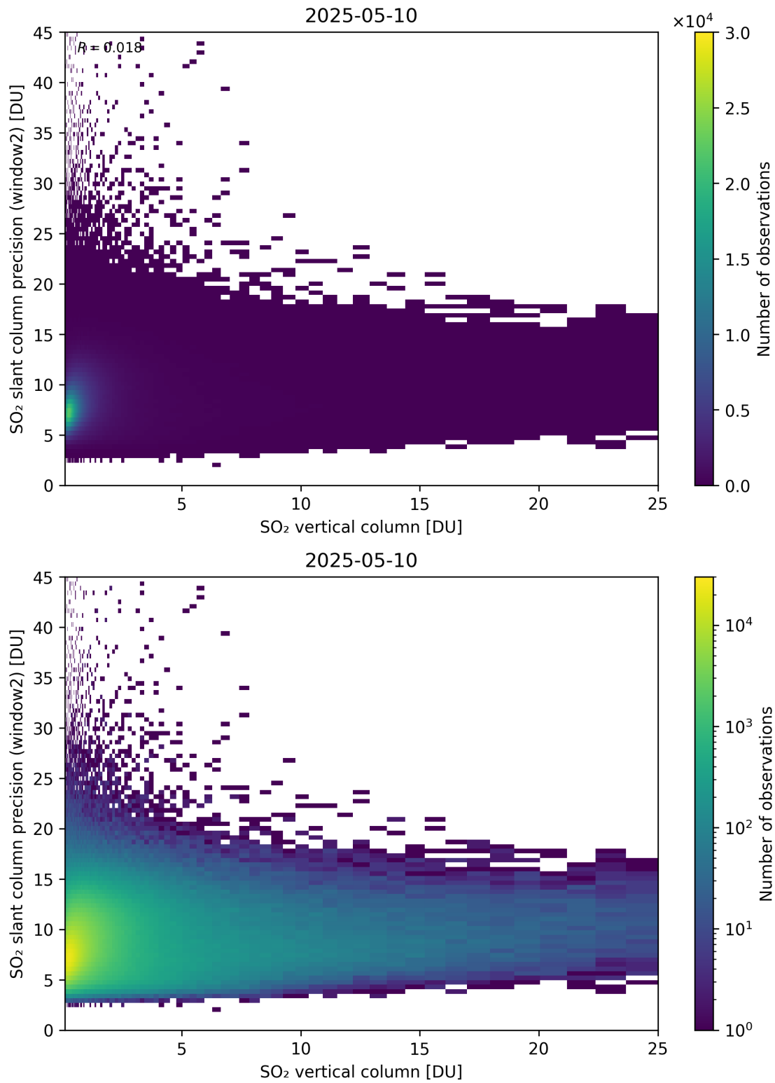
Figure 356: Scatter density plot of “SO 2 vertical column” against “SO 2 slant column precision (window2)” for 2025-05-10 to 2025-05-11.
