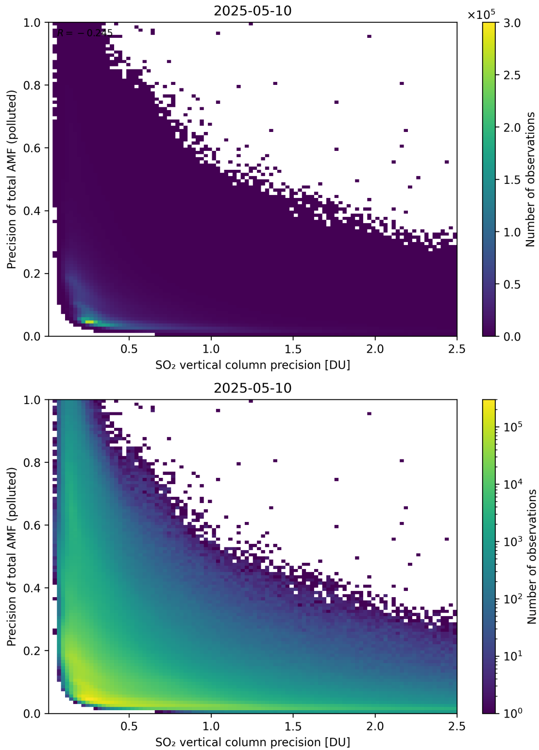
Figure 347: Scatter density plot of “SO 2 vertical column precision” against “Precision of total AMF (polluted)” for 2025-05-10 to 2025-05-11.
