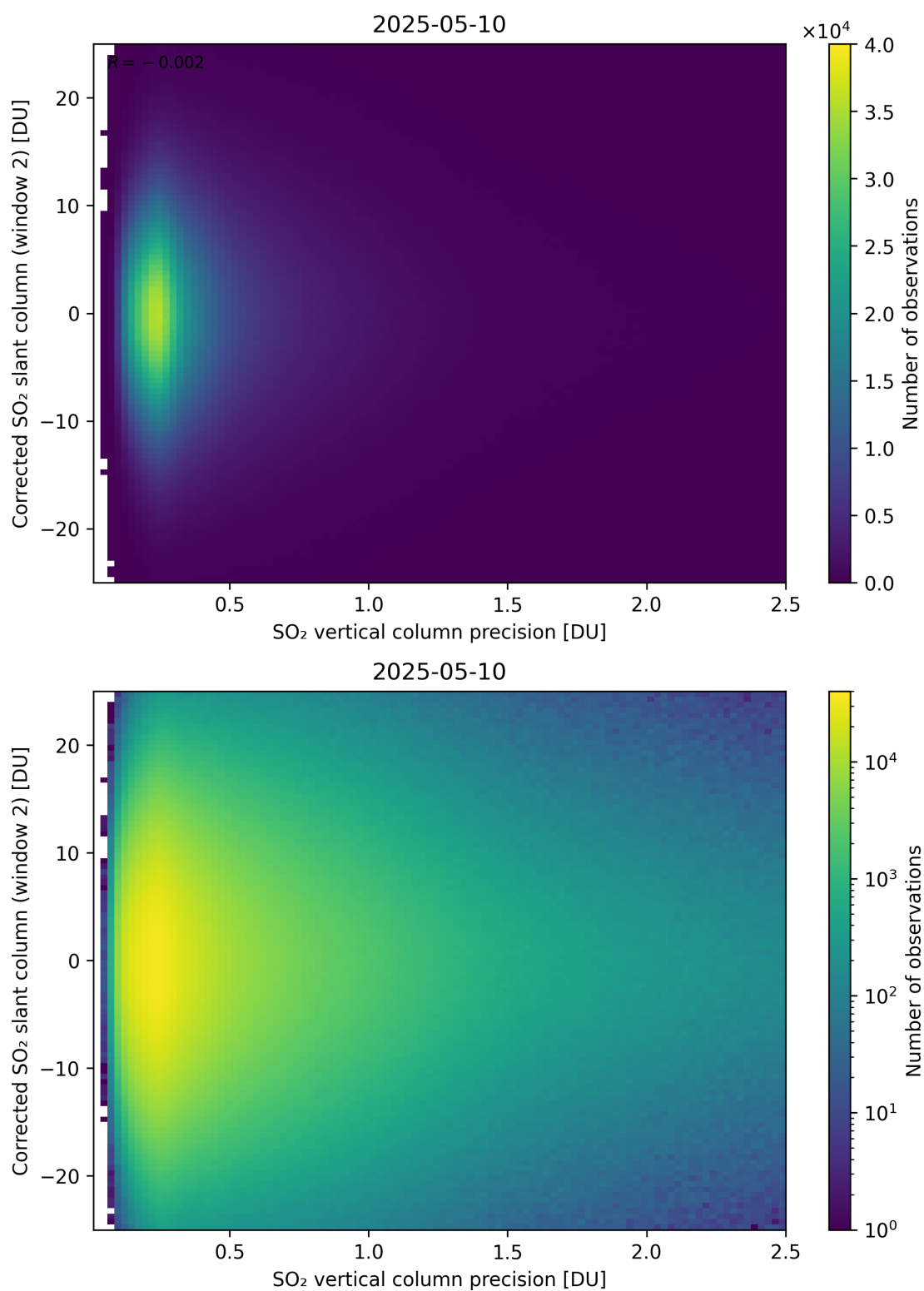
Figure 339: Scatter density plot of “SO 2 vertical column precision” against “Corrected SO 2 slant column (window 2)” for 2025-05-10 to 2025-05-11.
