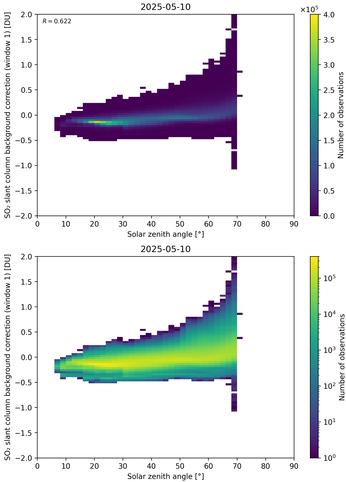
Figure 171: Scatter density plot of “Solar zenith angle” against “SO 2 slant column background correction (window 1)” for 2025-05-10 to 2025-05-11.
