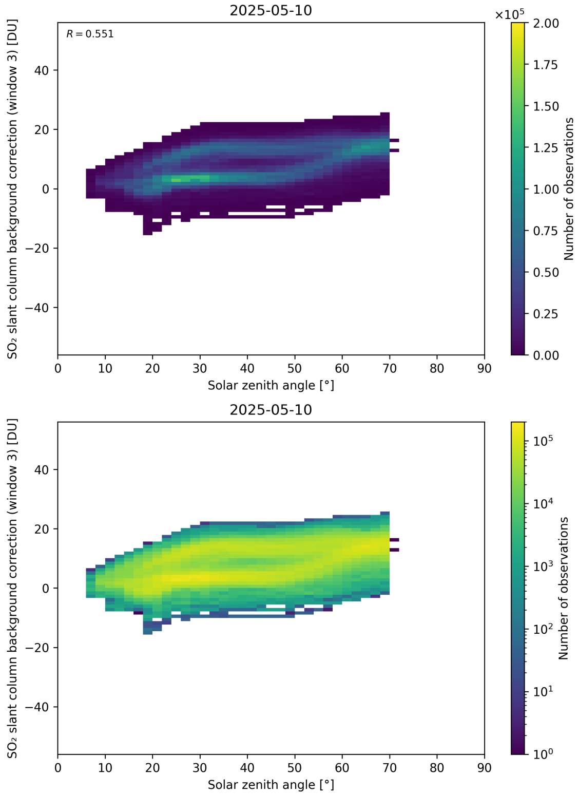
Figure 173: Scatter density plot of “Solar zenith angle” against “SO 2 slant column background correction (window 3)” for 2025-05-10 to 2025-05-11.
