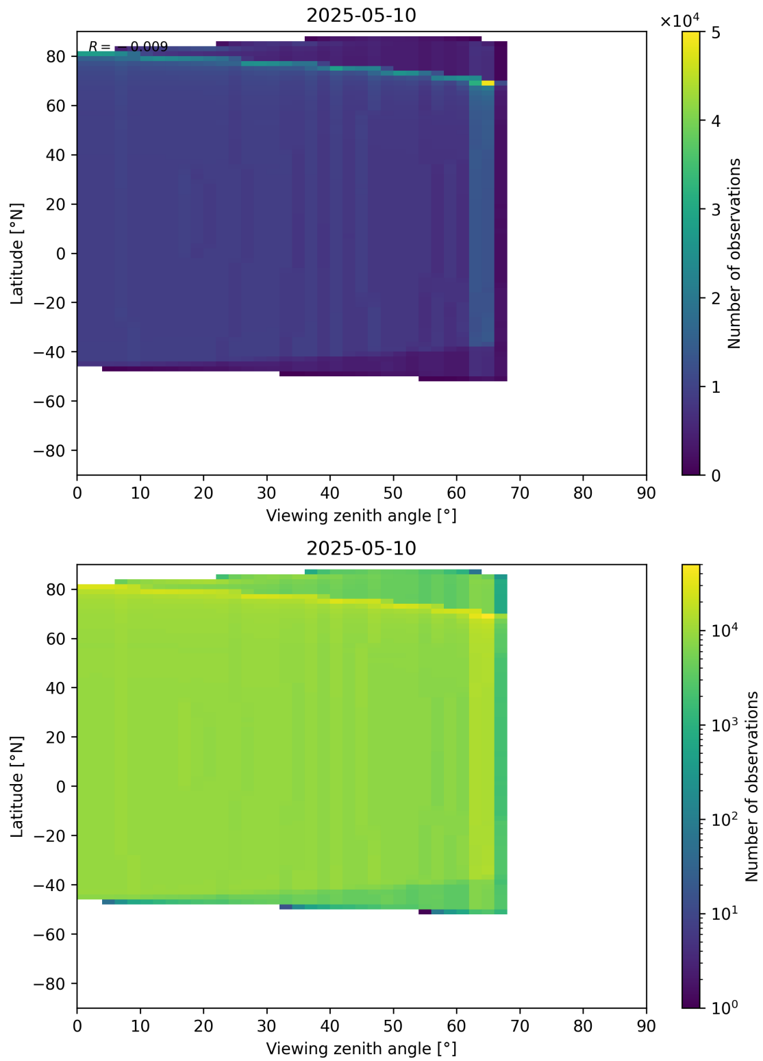
Figure 368: Scatter density plot of “Viewing zenith angle” against “Latitude” for 2025-05-10 to 2025-05-11.
