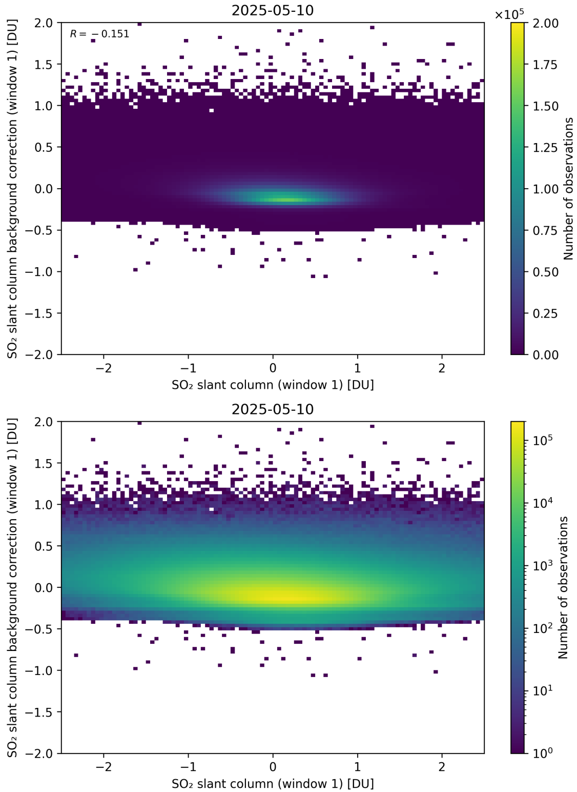
Figure 262: Scatter density plot of “SO 2 slant column (window 1)” against “SO 2 slant column background correction (window 1)” for 2025-05-10 to 2025-05-11.
