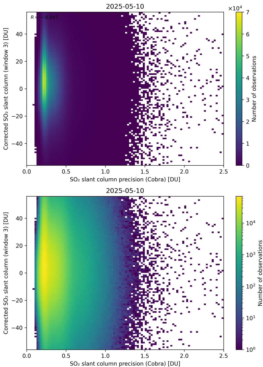
Figure 207: Scatter density plot of “SO 2 slant column precision (Cobra)” against “Corrected SO 2 slant column (window 3)” for 2025-05-10 to 2025-05-11.
