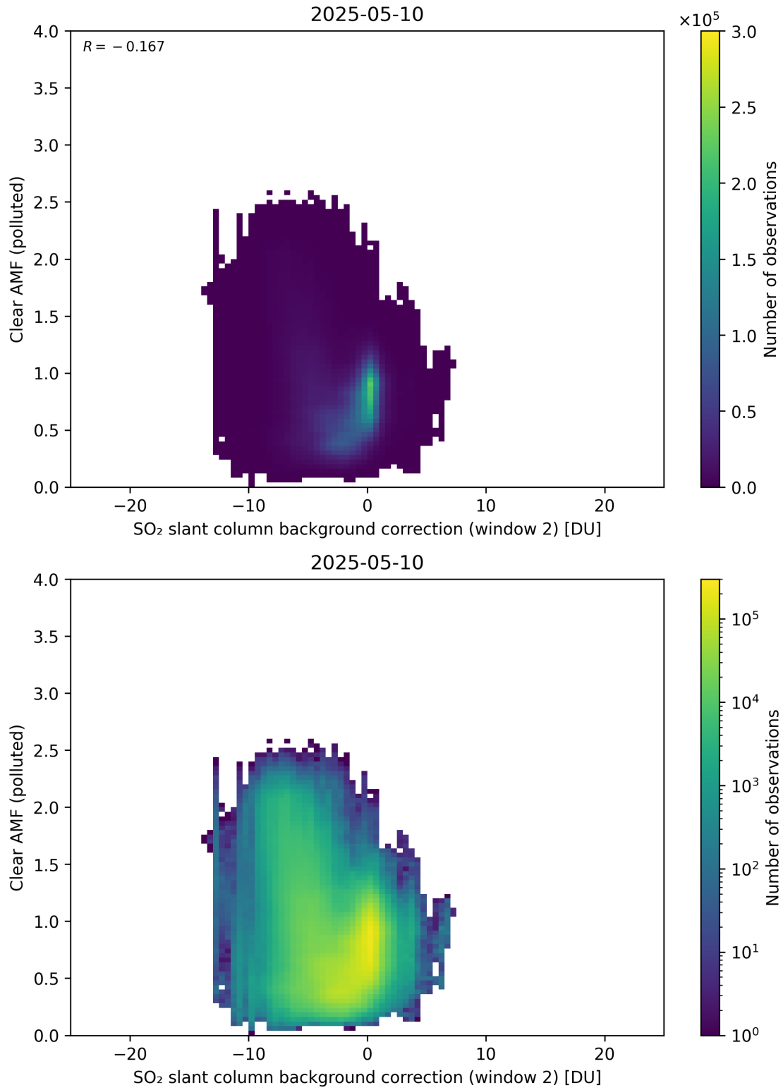
Figure 126: Scatter density plot of “SO 2 slant column background correction (window 2)” against “Clear AMF (polluted)” for 2025-05-10 to 2025-05-11.
