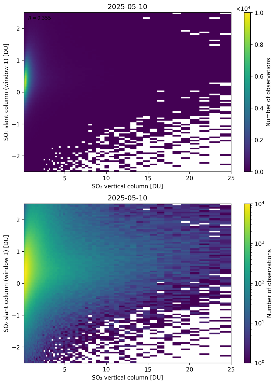
Figure 354: Scatter density plot of “SO 2 vertical column” against “SO 2 slant column (window 1)” for 2025-05-10 to 2025-05-11.
