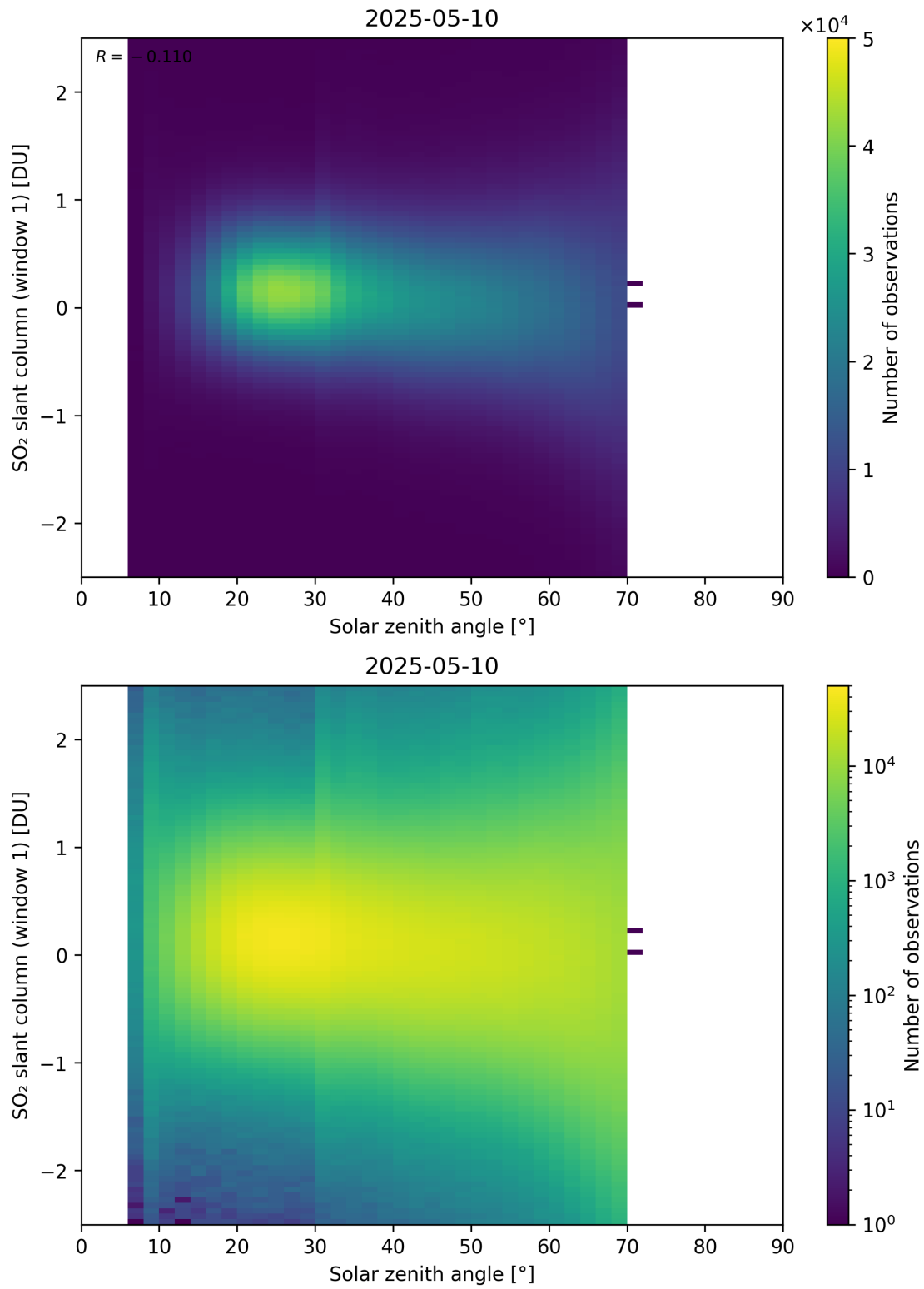
Figure 184: Scatter density plot of “Solar zenith angle” against “SO 2 slant column (window 1)” for 2025-05-10 to 2025-05-11.
