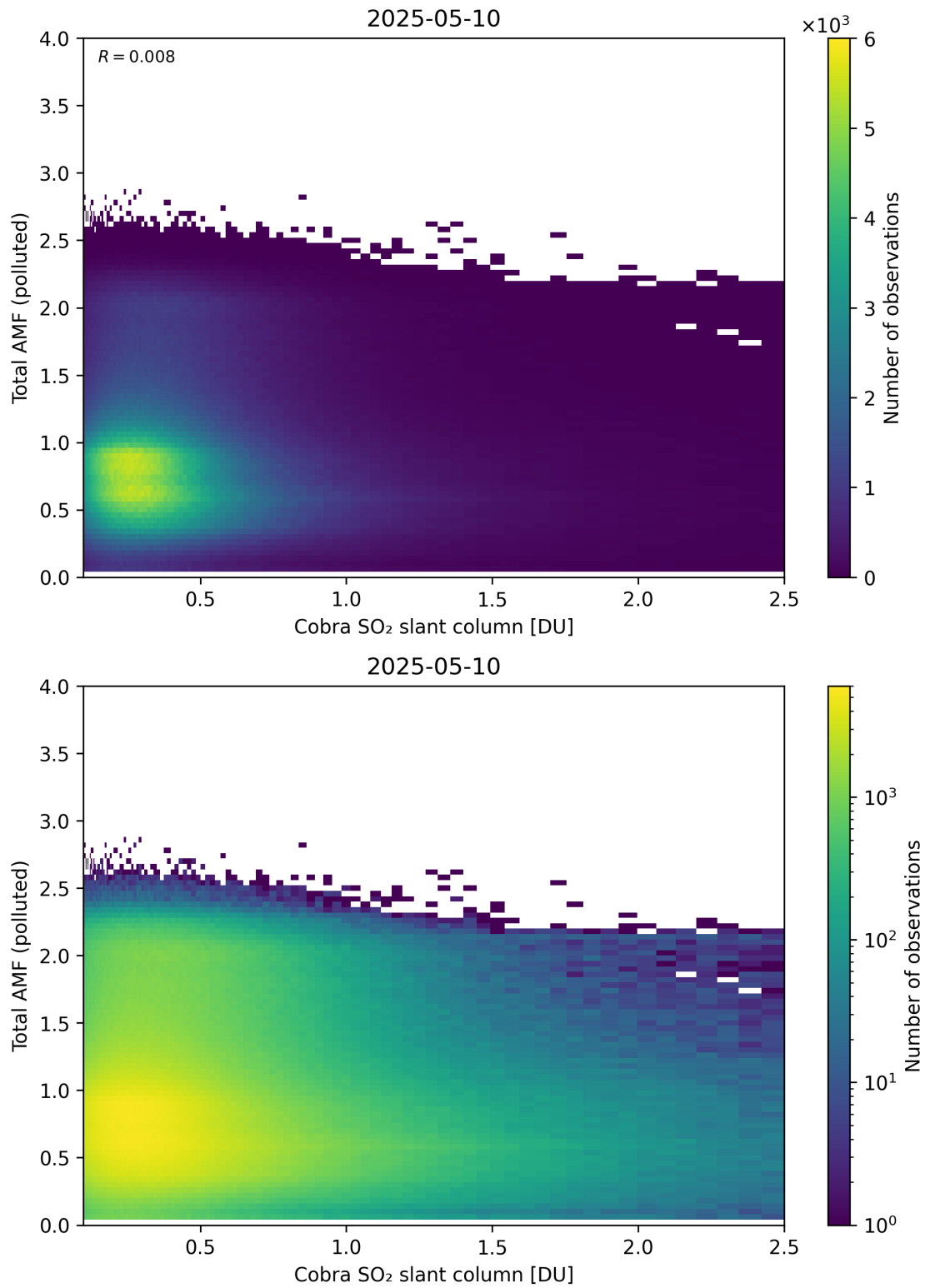
Figure 224: Scatter density plot of “Cobra SO 2 slant column” against “Total AMF (polluted)” for 2025-05-10 to 2025-05-11.
