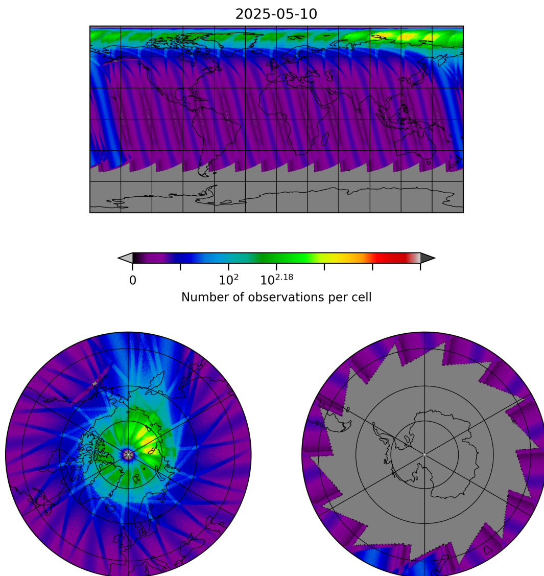
Figure 30: Map of the number of observations for 2025-05-10 to 2025-05-11
