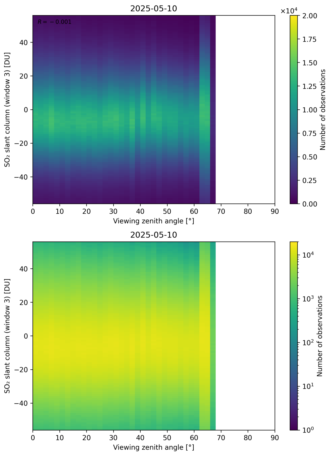
Figure 379: Scatter density plot of “Viewing zenith angle” against “SO 2 slant column (window 3)” for 2025-05-10 to 2025-05-11.
