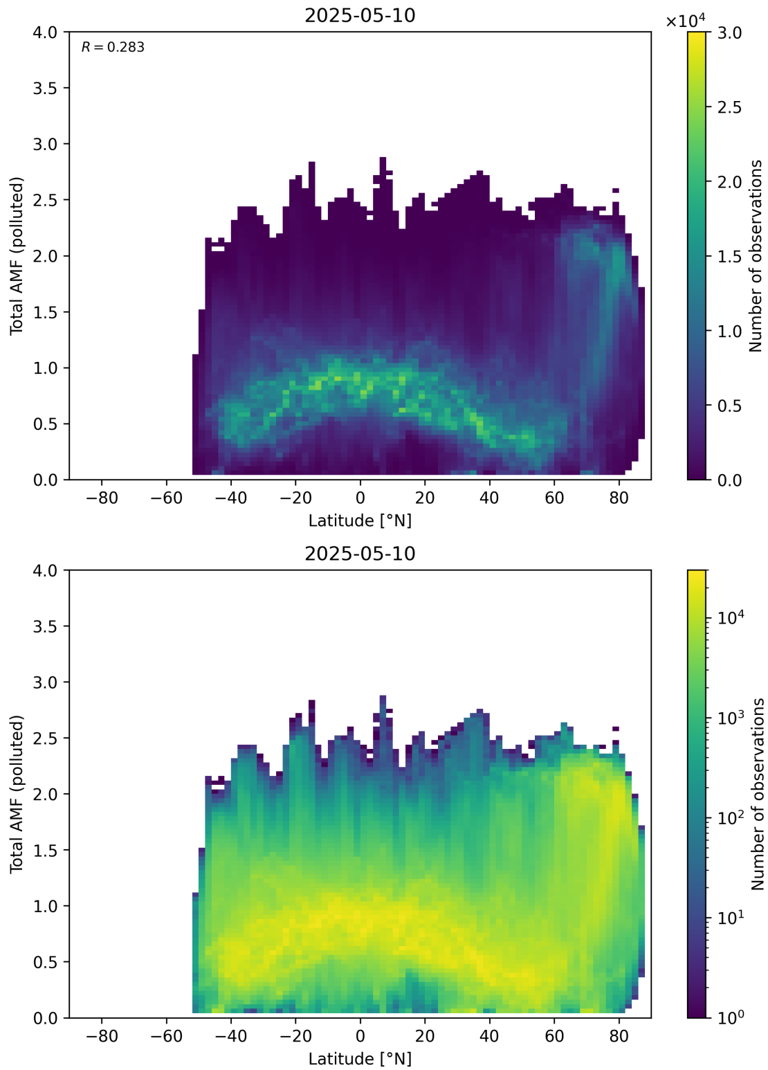
Figure 167: Scatter density plot of “Latitude” against “Total AMF (polluted)” for 2025-05-10 to 2025-05-11.
