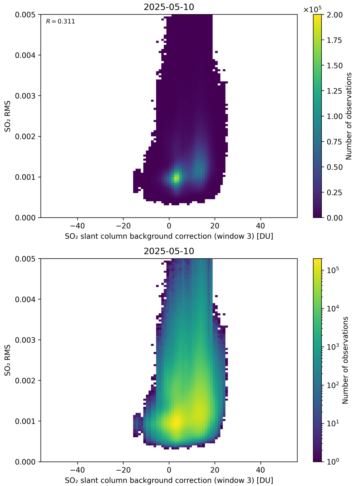
Figure 134: Scatter density plot of “SO 2 slant column background correction (window 3)” against “SO 2 RMS” for 2025-05-10 to 2025-05-11.
