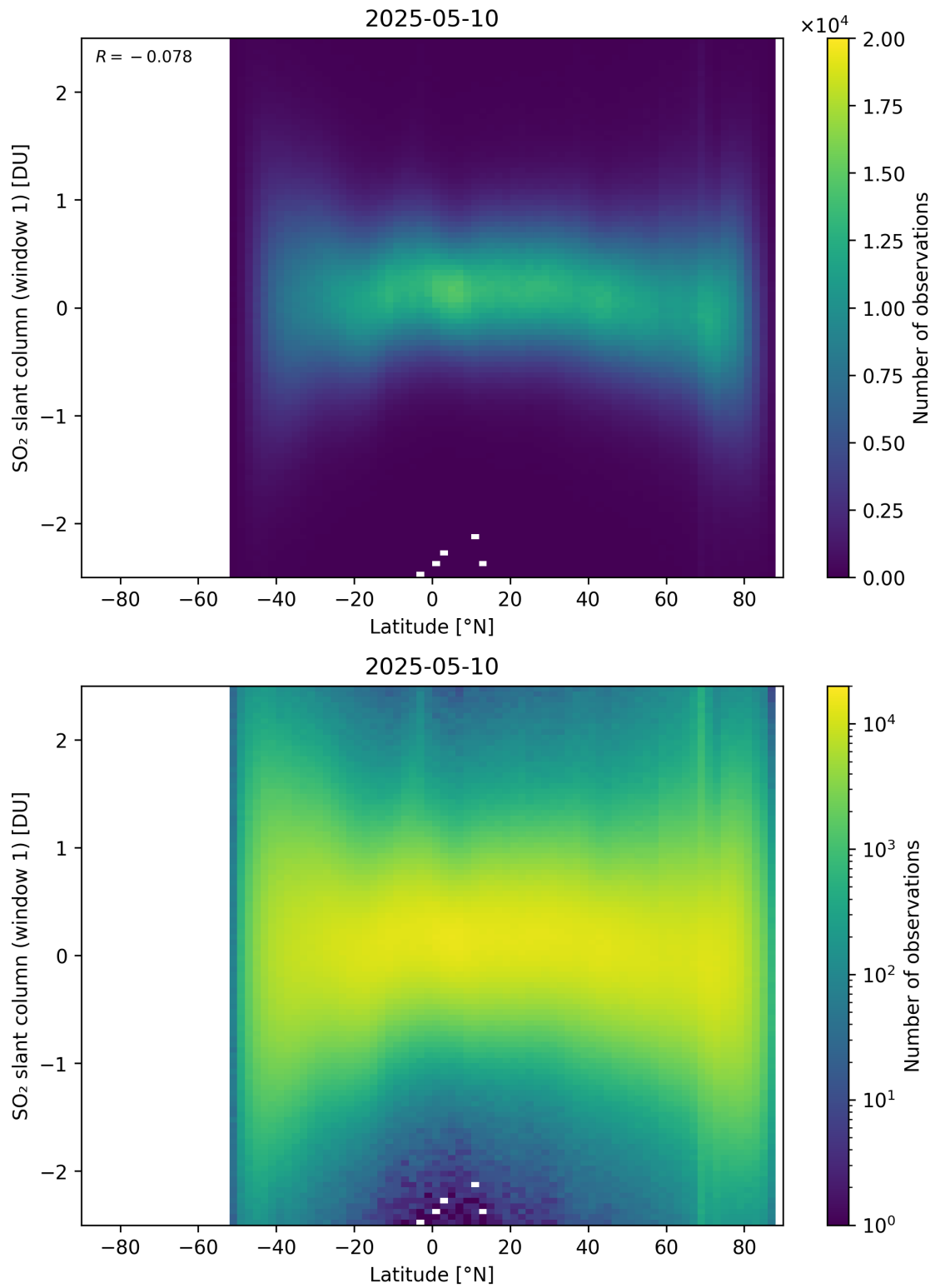
Figure 162: Scatter density plot of “Latitude” against “SO 2 slant column (window 1)” for 2025-05-10 to 2025-05-11.
