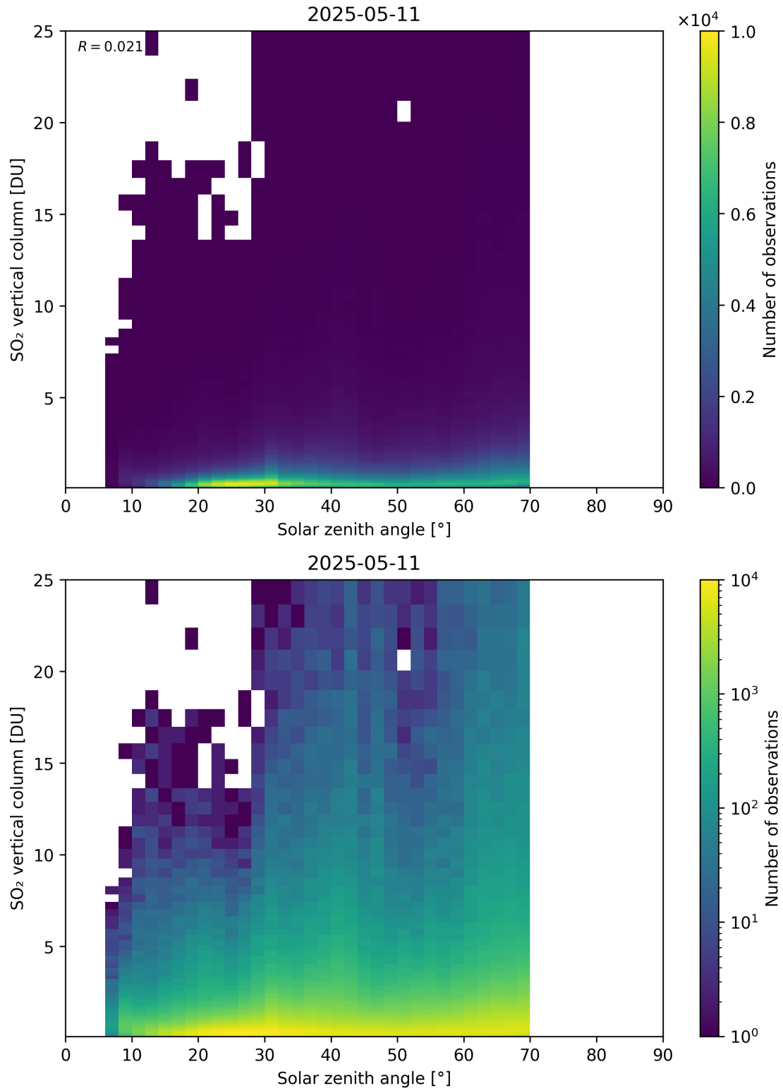
Figure 191: Scatter density plot of “Solar zenith angle” against “SO 2 vertical column” for 2025-05-10 to 2025-05-12.
