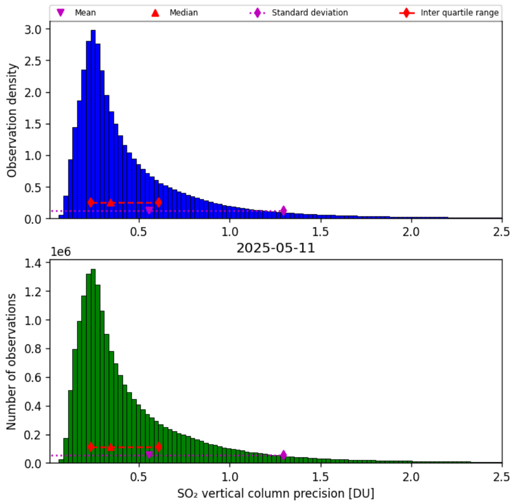
Figure 59: Histogram of “SO 2 vertical column precision” for 2025-05-10 to 2025-05-12
