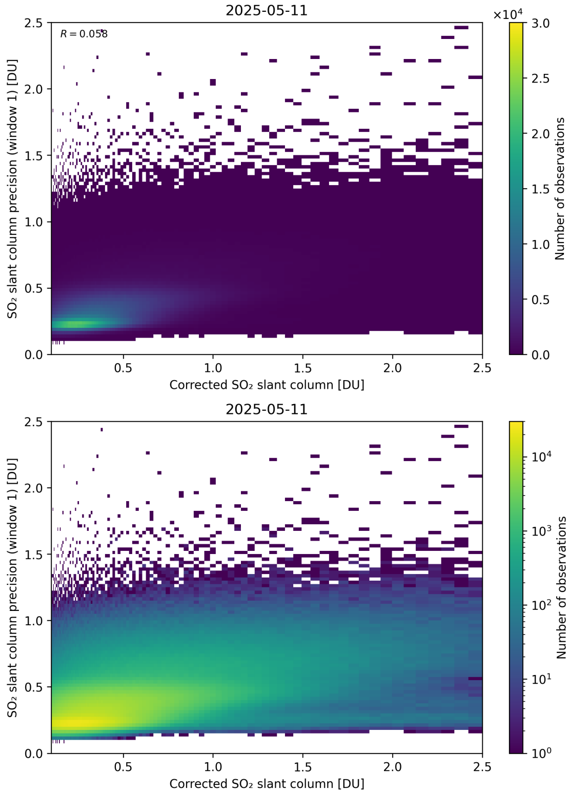
Figure 238: Scatter density plot of “Corrected SO 2 slant column” against “SO 2 slant column precision (window 1)” for 2025-05-10 to 2025-05-12.
