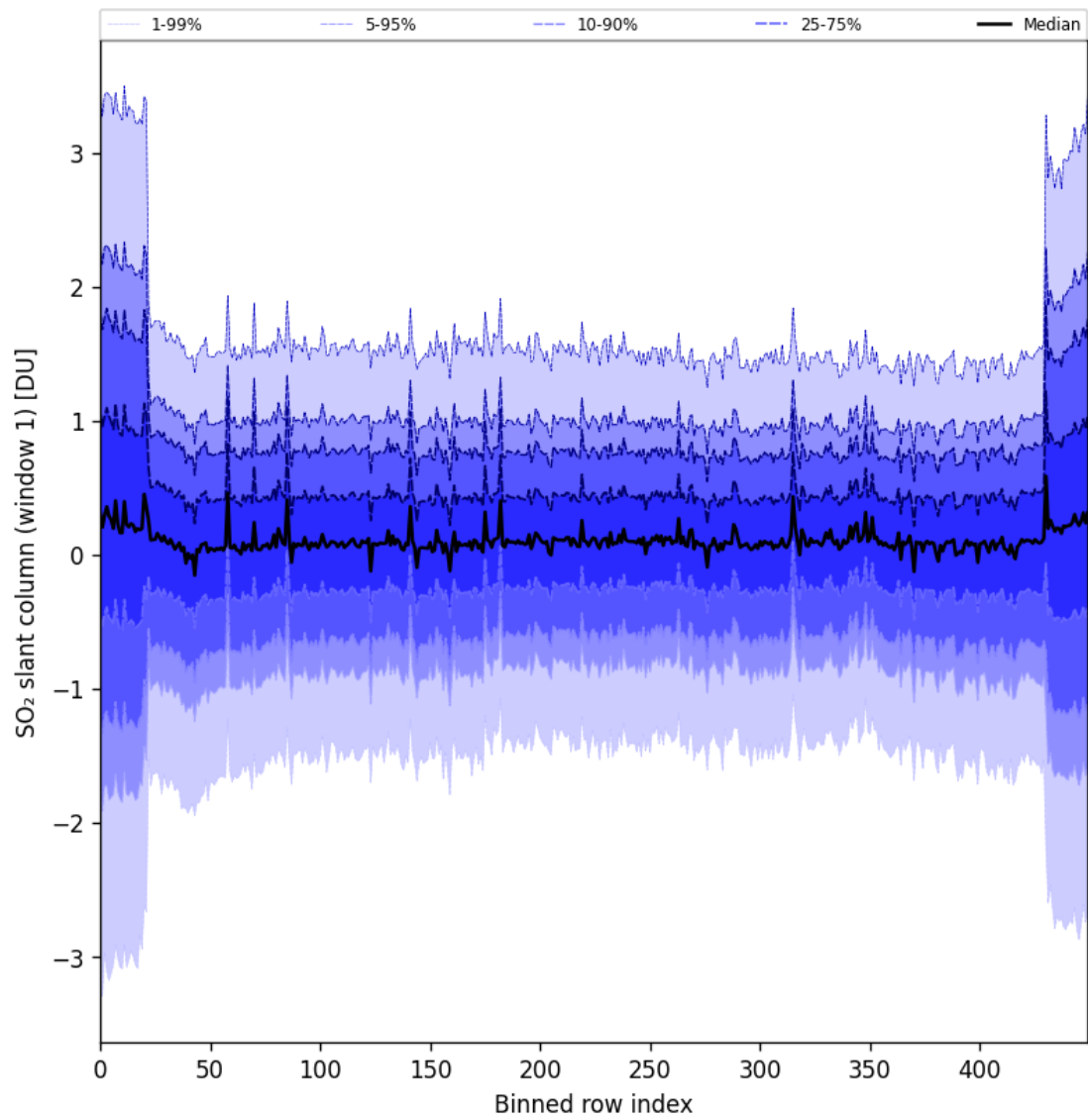
Figure 89: Along track statistics of “SO 2 slant column (window 1)” for 2025-05-10 to 2025-05-12
