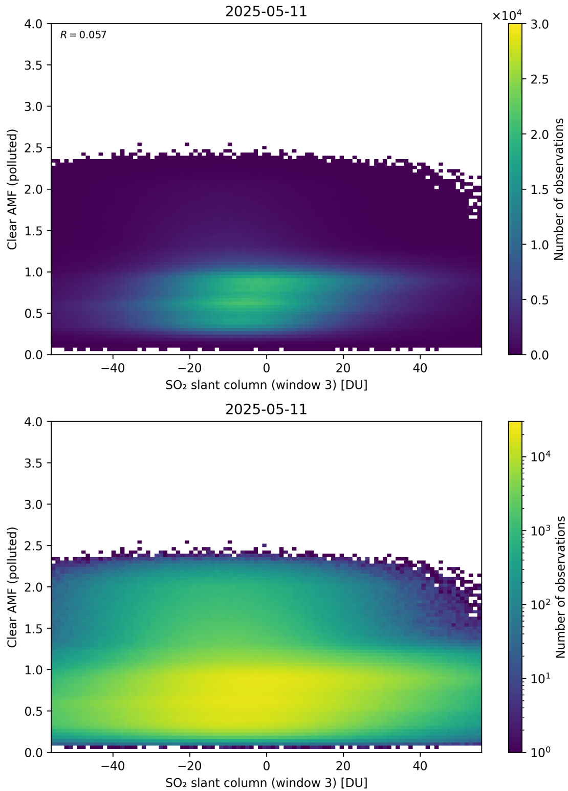
Figure 315: Scatter density plot of “SO 2 slant column (window 3)” against “Clear AMF (polluted)” for 2025-05-10 to 2025-05-12.
