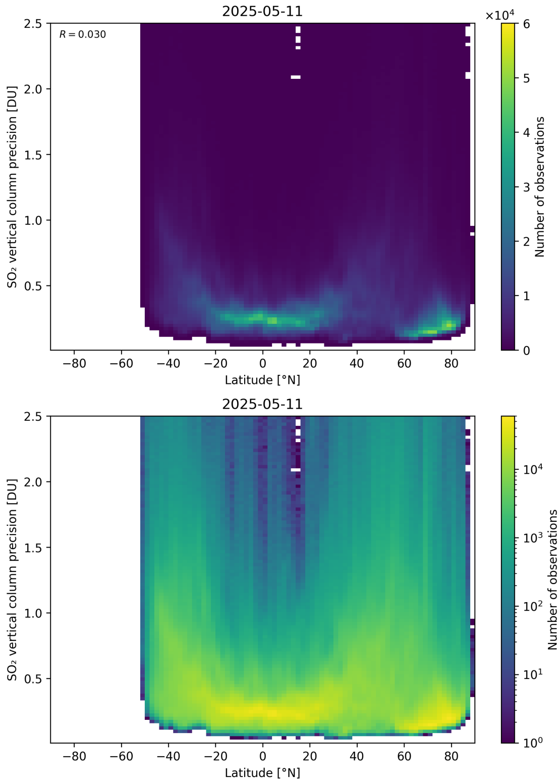
Figure 170: Scatter density plot of “Latitude” against “SO 2 vertical column precision” for 2025-05-10 to 2025-05-12.
