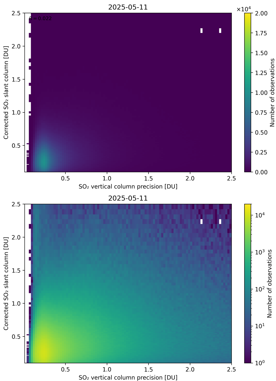
Figure 338: Scatter density plot of “SO 2 vertical column precision” against “Corrected SO 2 slant column” for 2025-05-10 to 2025-05-12.
