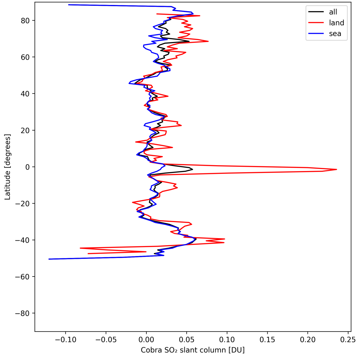
Figure 35: Zonal average of “Cobra SO 2 slant column” for 2025-05-10 to 2025-05-12.
