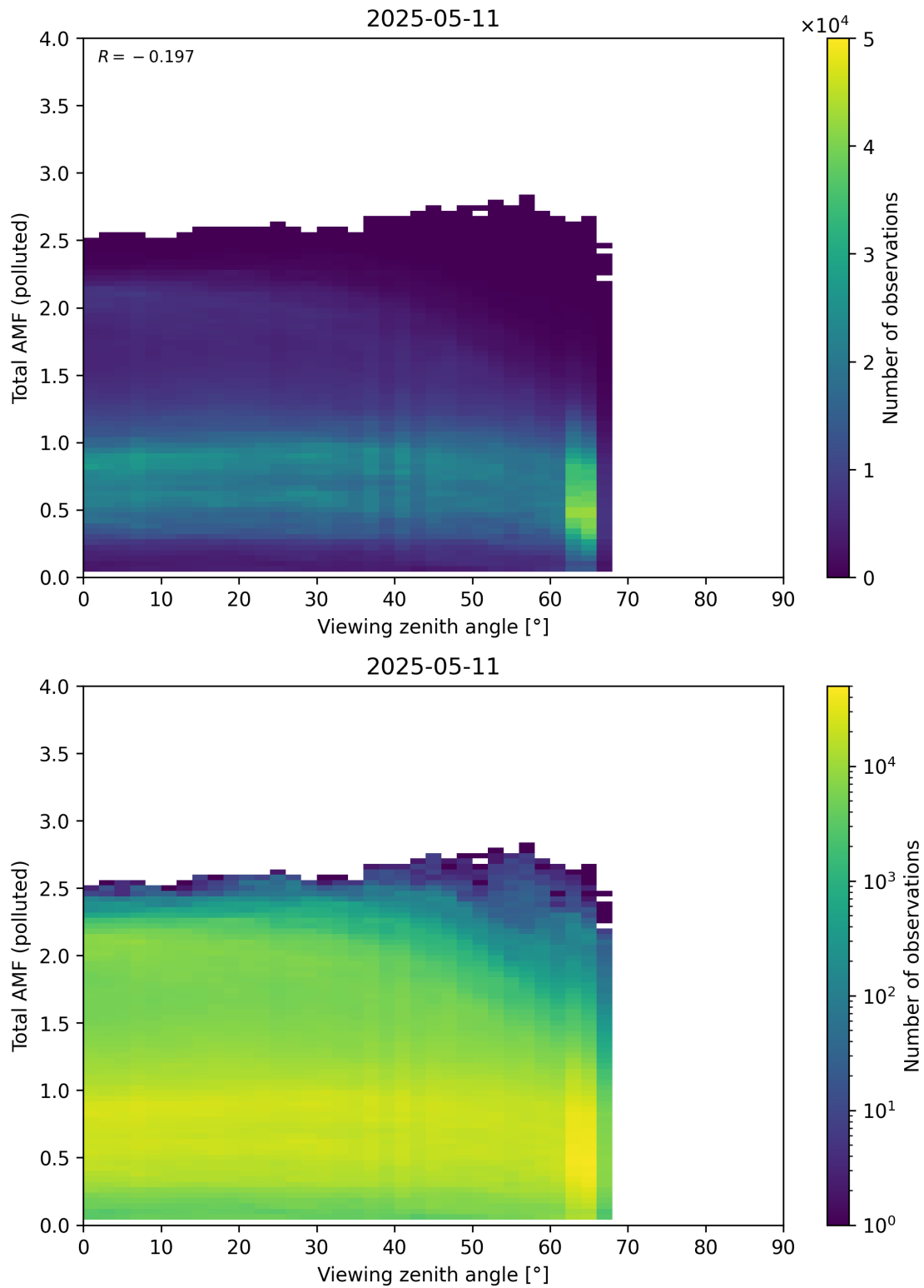
Figure 381: Scatter density plot of “Viewing zenith angle” against “Total AMF (polluted)” for 2025-05-10 to 2025-05-12.
