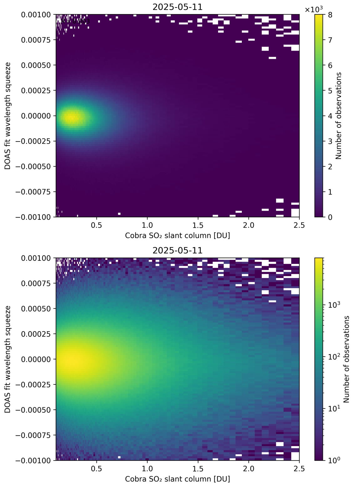
Figure 197: Scatter density plot of “Cobra SO 2 slant column” against “DOAS fit wavelength squeeze” for 2025-05-10 to 2025-05-12.
