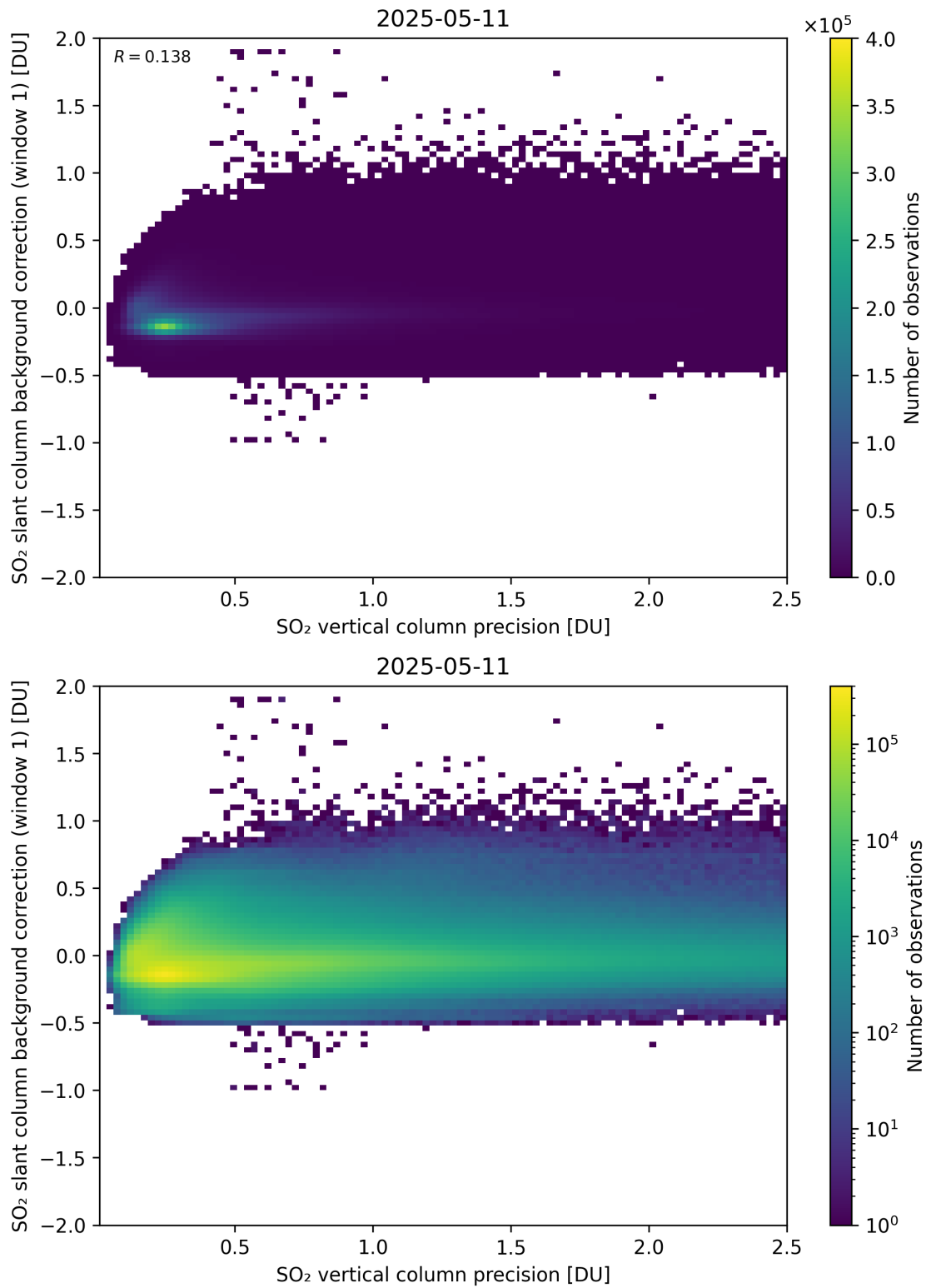
Figure 329: Scatter density plot of “SO 2 vertical column precision” against “SO 2 slant column background correction (window 1)” for 2025-05-10 to 2025-05-12.
