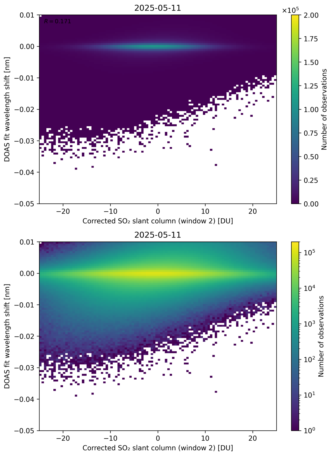
Figure 246: Scatter density plot of “Corrected SO 2 slant column (window 2)” against “DOAS fit wavelength shift” for 2025-05-10 to 2025-05-12.
