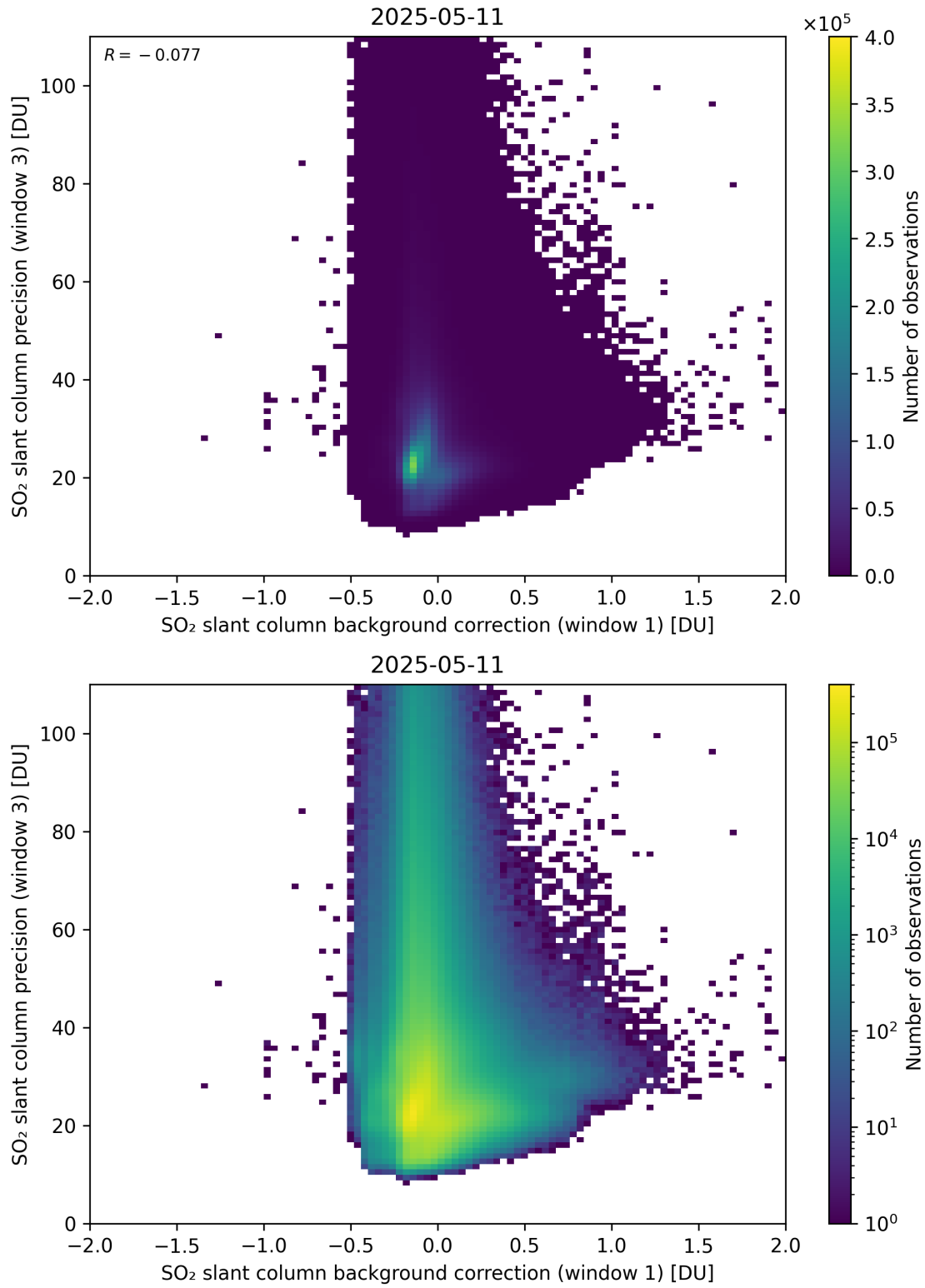
Figure 119: Scatter density plot of “SO 2 slant column background correction (window 1)” against “SO 2 slant column precision (window 3)” for 2025-05-10 to 2025-05-12.
