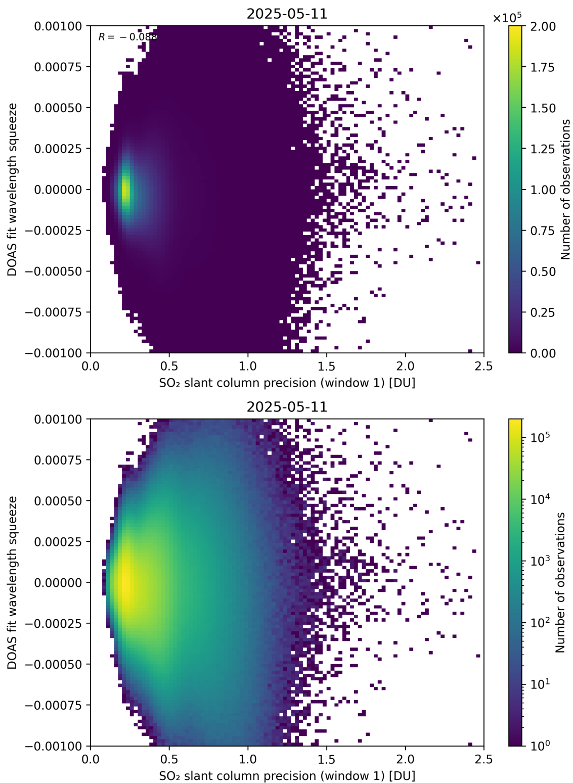
Figure 272: Scatter density plot of “SO 2 slant column precision (window 1)” against “DOAS fit wavelength squeeze” for 2025-05-10 to 2025-05-12.
