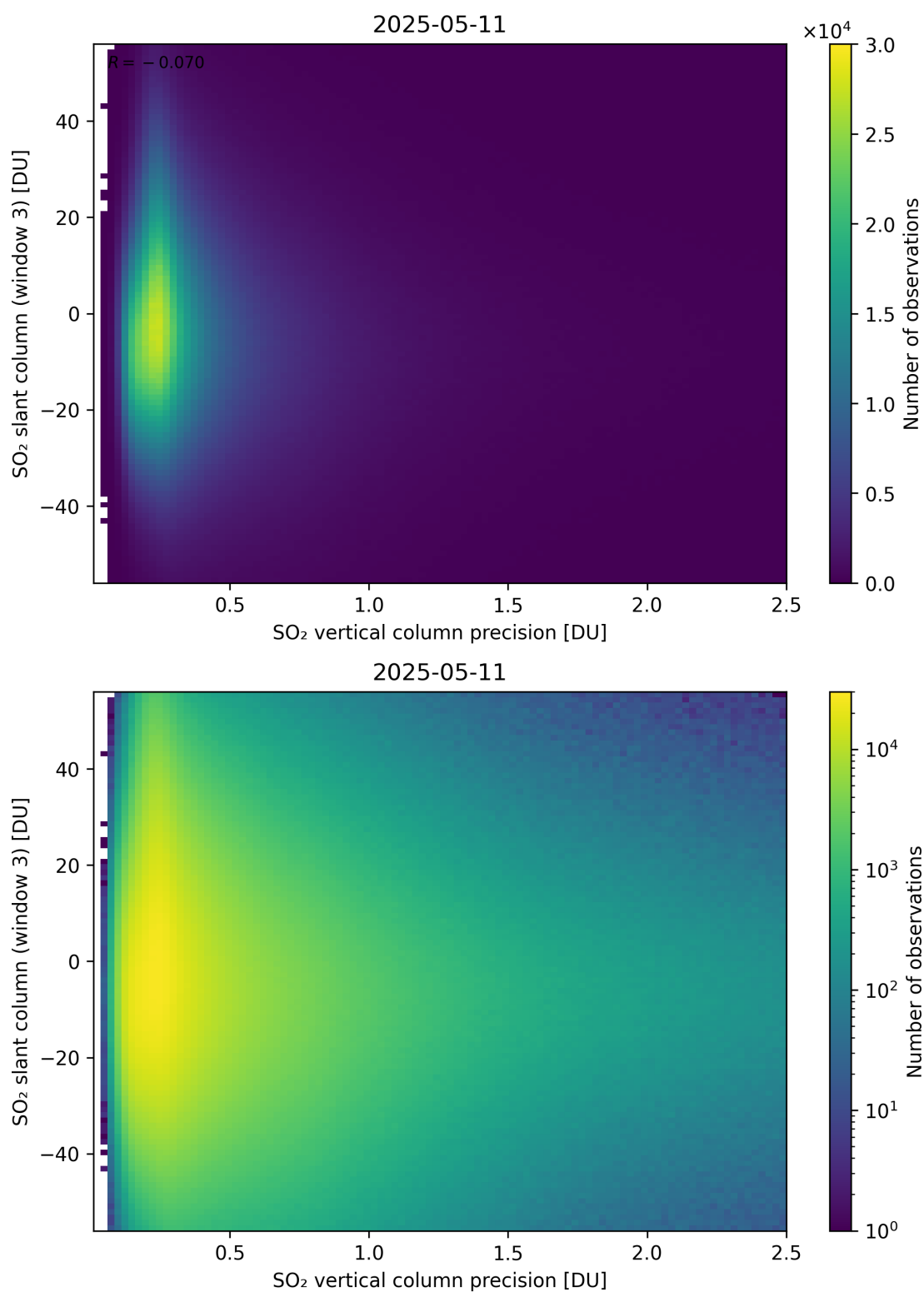
Figure 344: Scatter density plot of “SO 2 vertical column precision” against “SO 2 slant column (window 3)” for 2025-05-10 to 2025-05-12.
