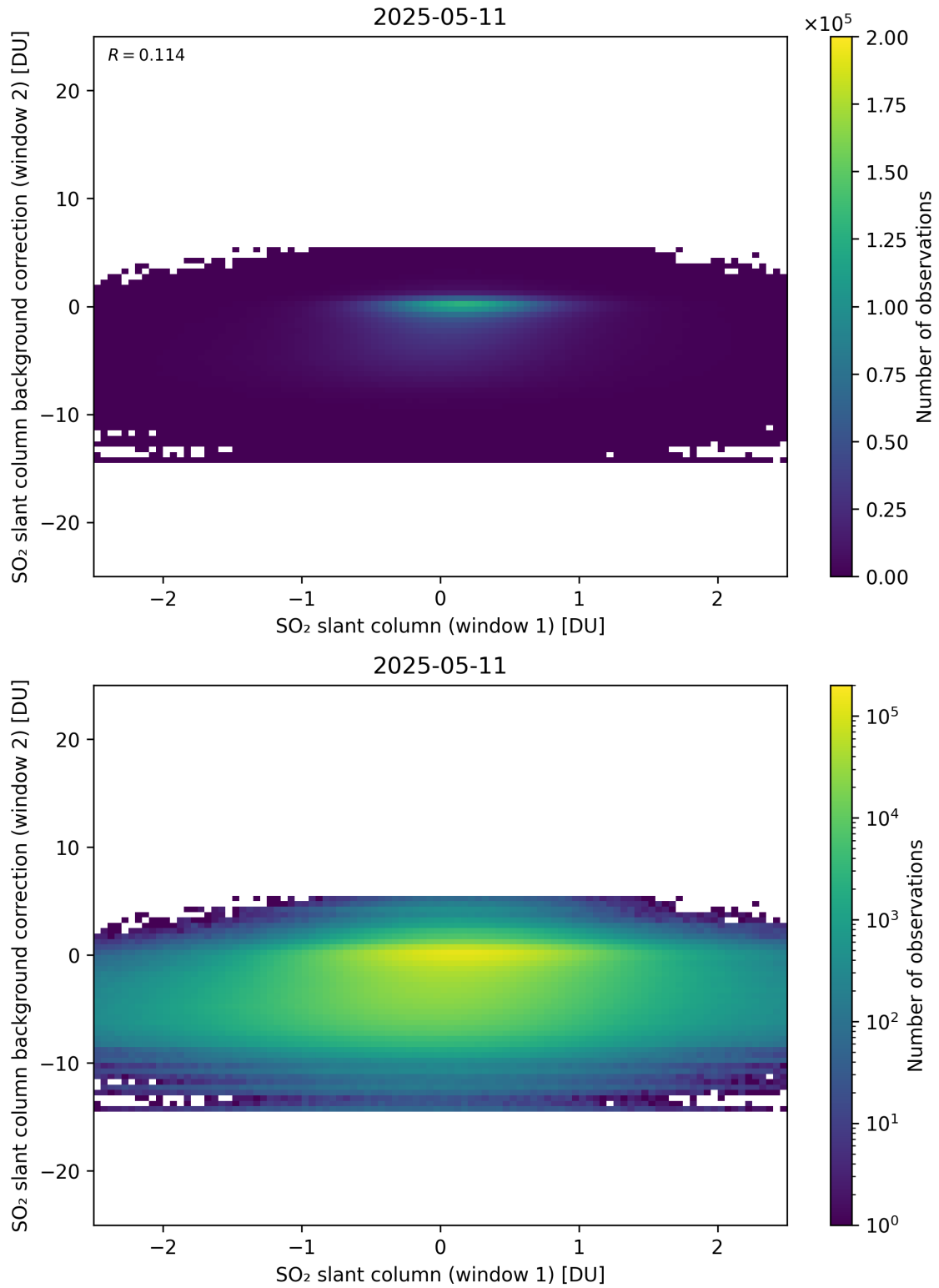
Figure 263: Scatter density plot of “SO 2 slant column (window 1)” against “SO 2 slant column background correction (window 2)” for 2025-05-10 to 2025-05-12.
