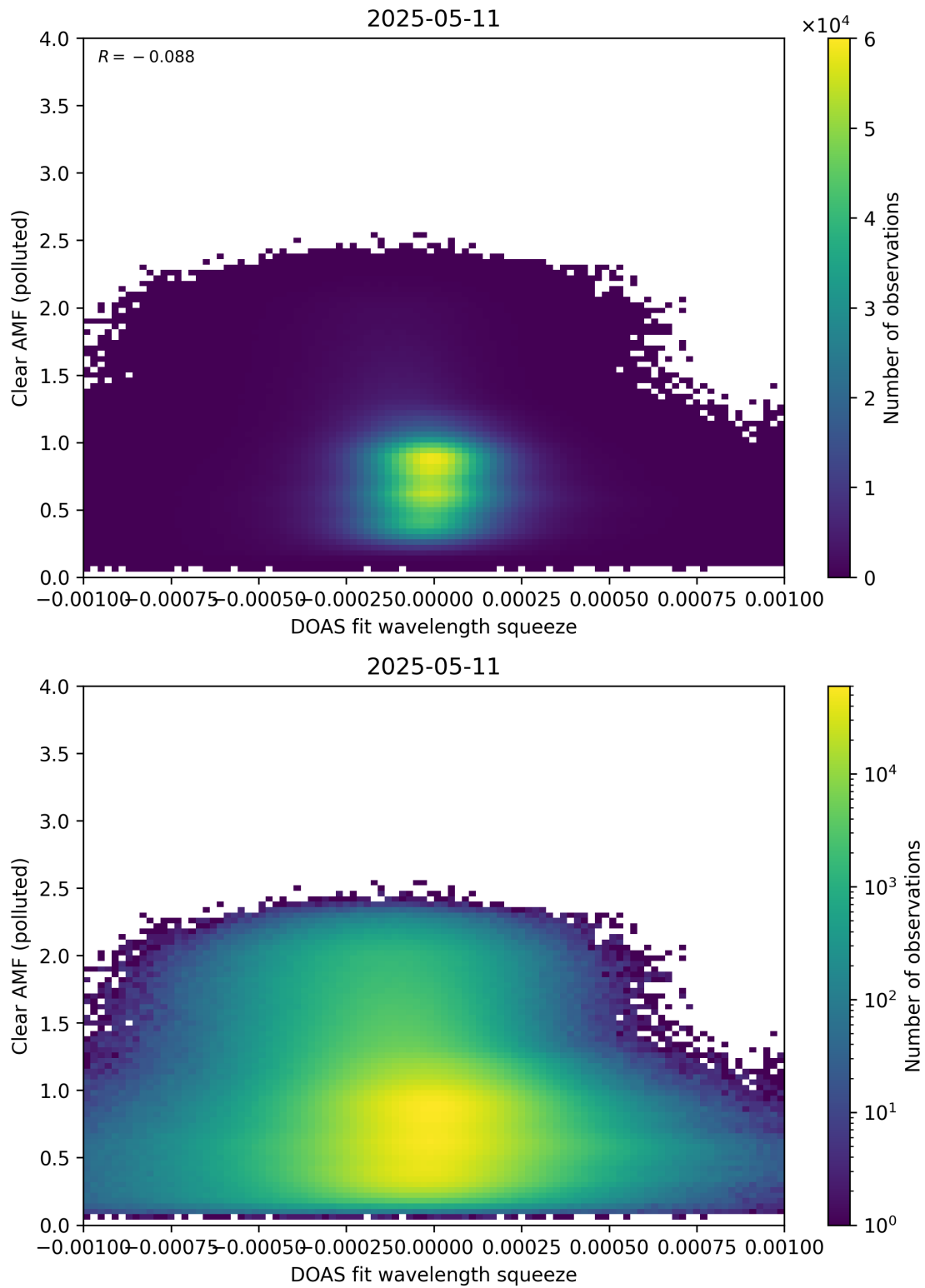
Figure 144: Scatter density plot of “DOAS fit wavelength squeeze” against “Clear AMF (polluted)” for 2025-05-10 to 2025-05-12.
