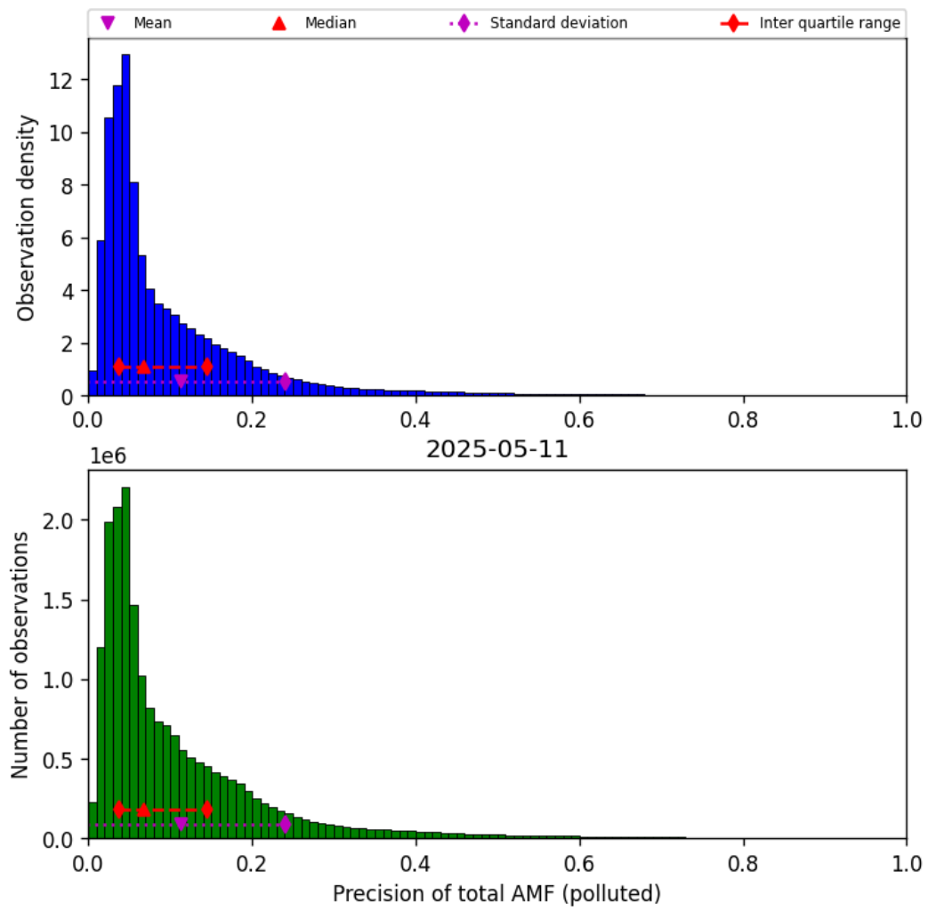
Figure 80: Histogram of “Precision of total AMF (polluted)” for 2025-05-10 to 2025-05-12
