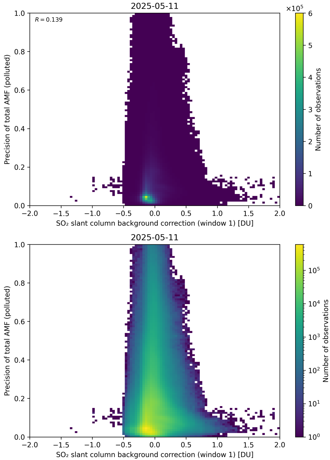
Figure 121: Scatter density plot of “SO 2 slant column background correction (window 1)” against “Precision of total AMF (polluted)” for 2025-05-10 to 2025-05-12.
