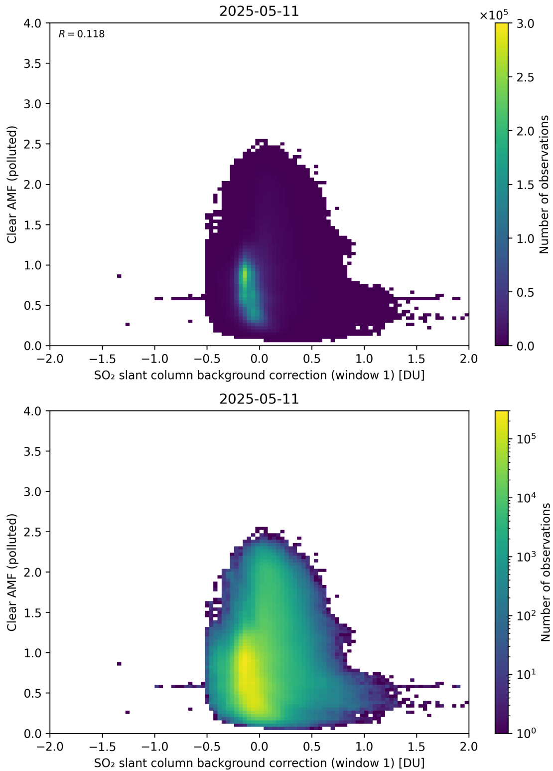
Figure 114: Scatter density plot of “SO 2 slant column background correction (window 1)” against “Clear AMF (polluted)” for 2025-05-10 to 2025-05-12.
