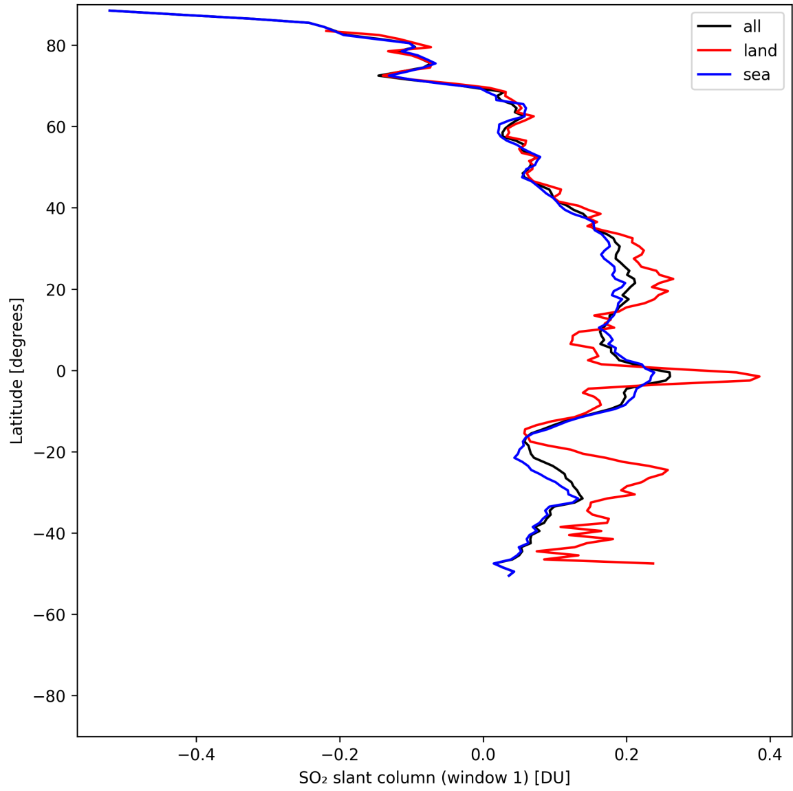
Figure 37: Zonal average of “SO 2 slant column (window 1)” for 2025-05-10 to 2025-05-12.
