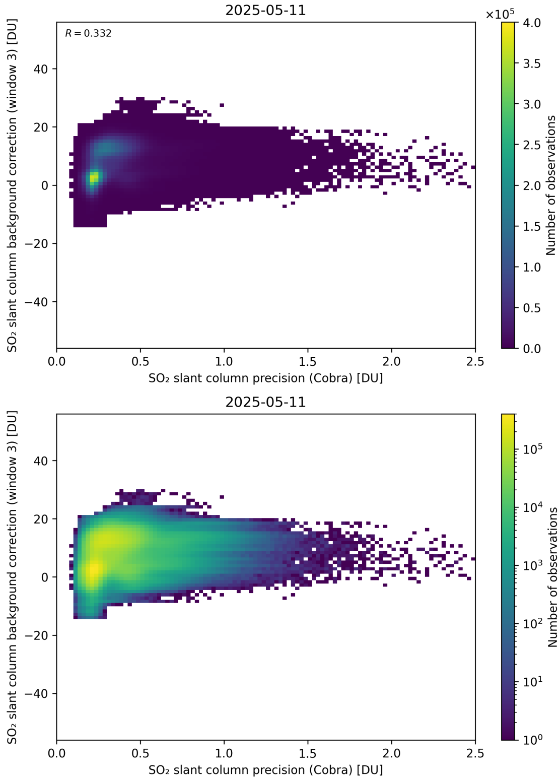
Figure 201: Scatter density plot of “SO 2 slant column precision (Cobra)” against “SO 2 slant column background correction (window 3)” for 2025-05-10 to 2025-05-12.
