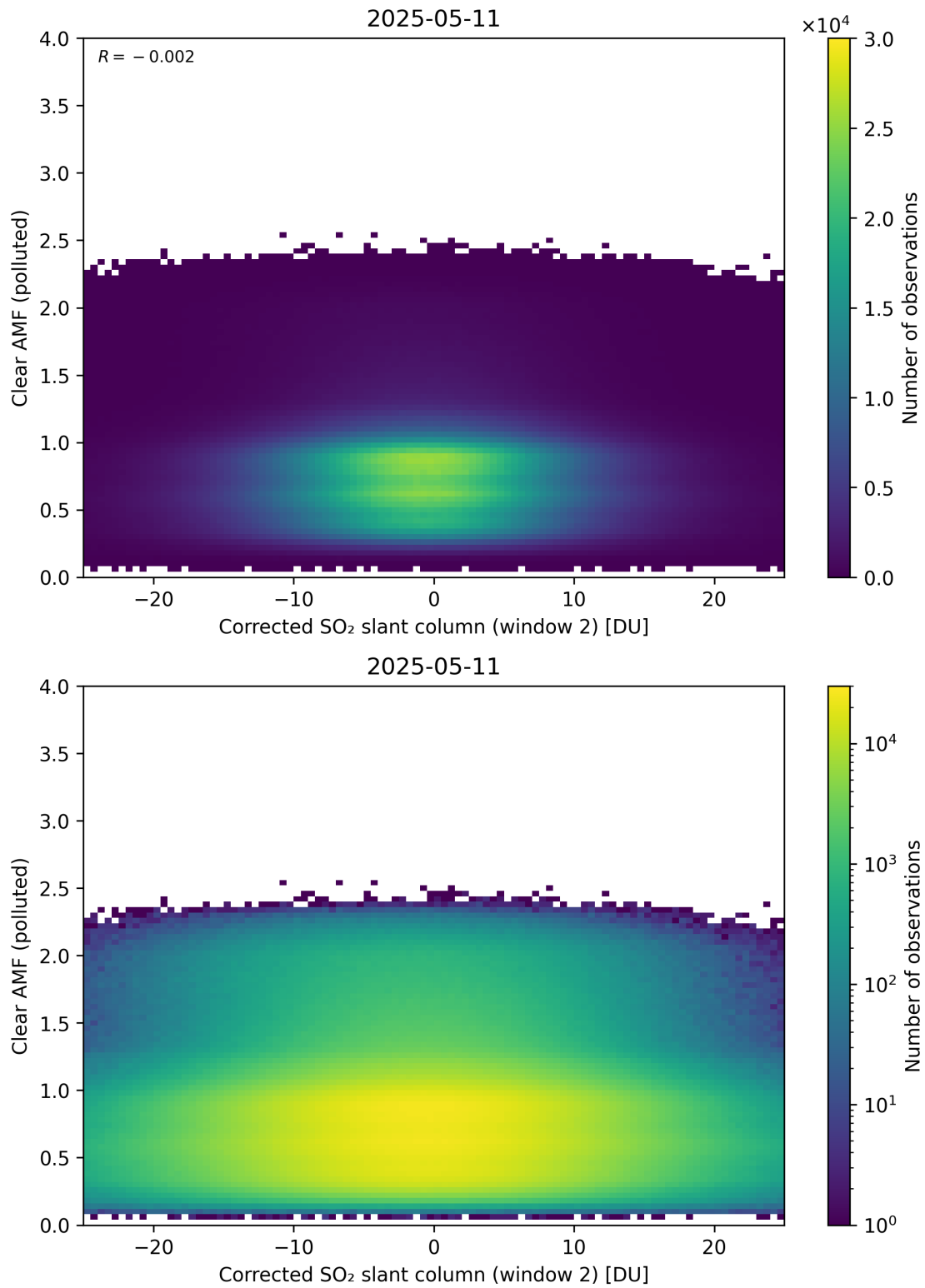
Figure 249: Scatter density plot of “Corrected SO 2 slant column (window 2)” against “Clear AMF (polluted)” for 2025-05-10 to 2025-05-12.
