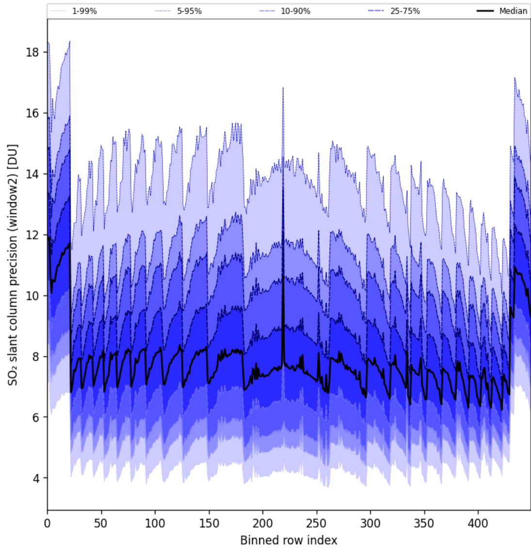
Figure 94: Along track statistics of “SO 2 slant column precision (window2)” for 2025-05-10 to 2025-05-12
