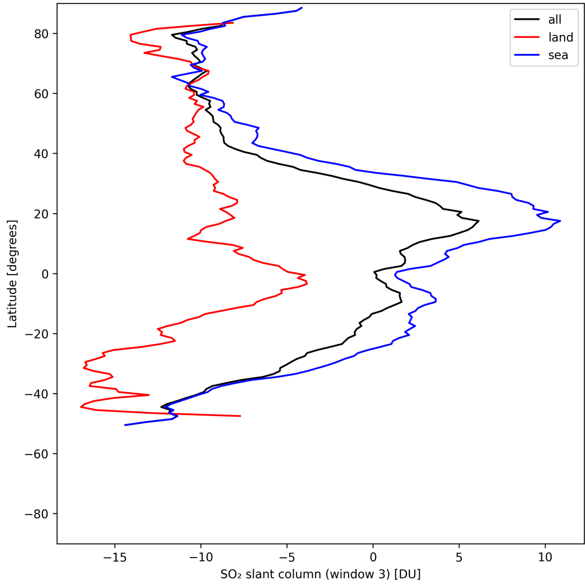
Figure 45: Zonal average of “SO 2 slant column (window 3)” for 2025-05-10 to 2025-05-12.
