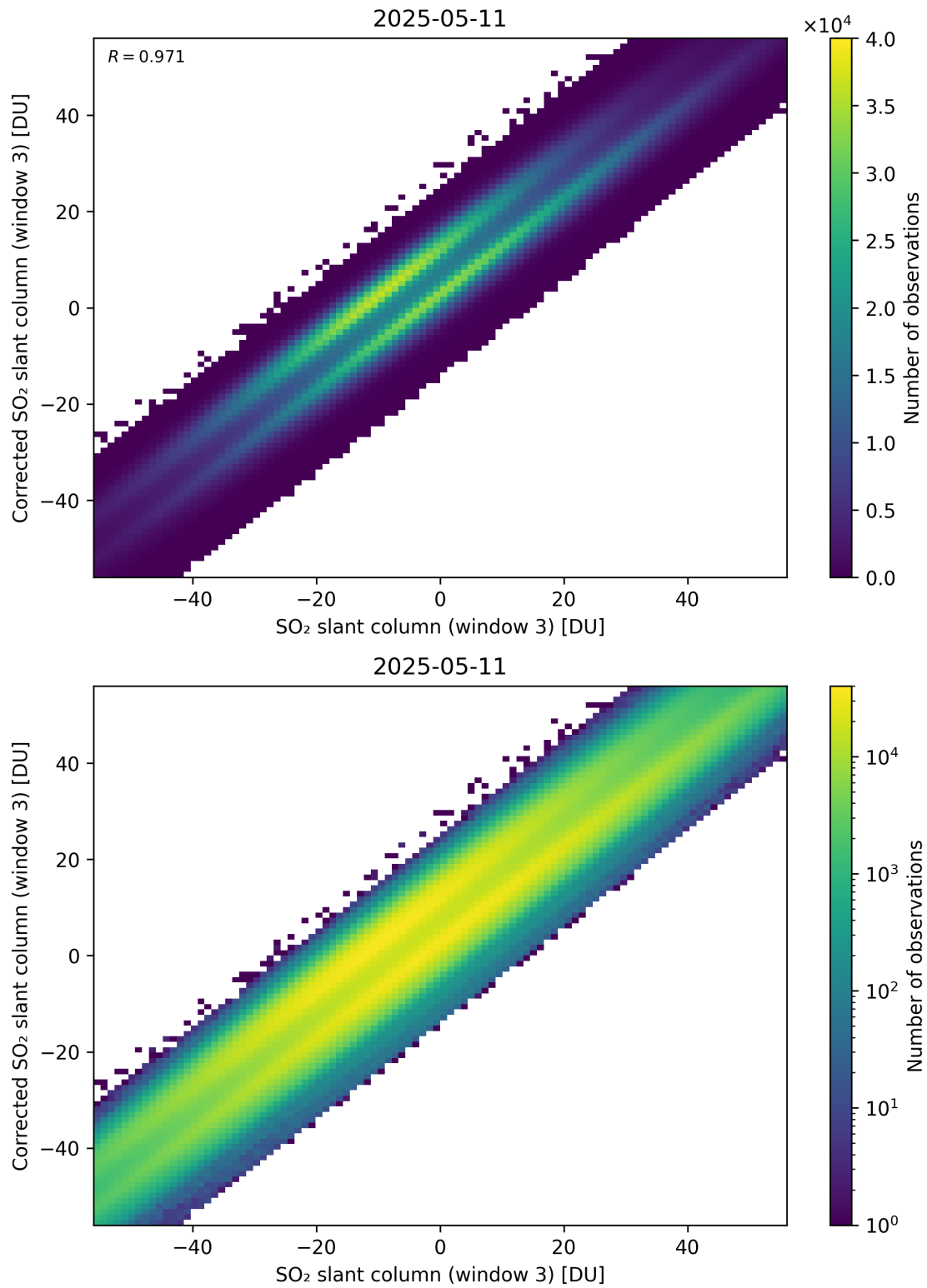
Figure 316: Scatter density plot of “SO 2 slant column (window 3)” against “Corrected SO 2 slant column (window 3)” for 2025-05-10 to 2025-05-12.
