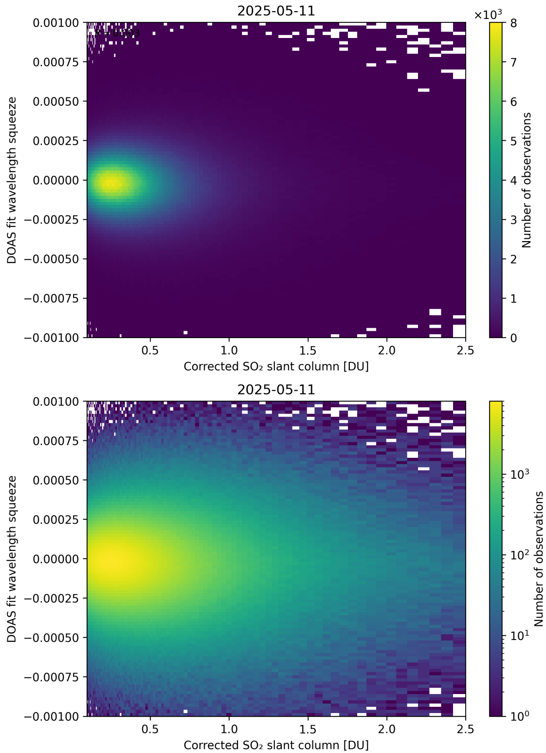
Figure 230: Scatter density plot of “Corrected SO 2 slant column” against “DOAS fit wavelength squeeze” for 2025-05-10 to 2025-05-12.
