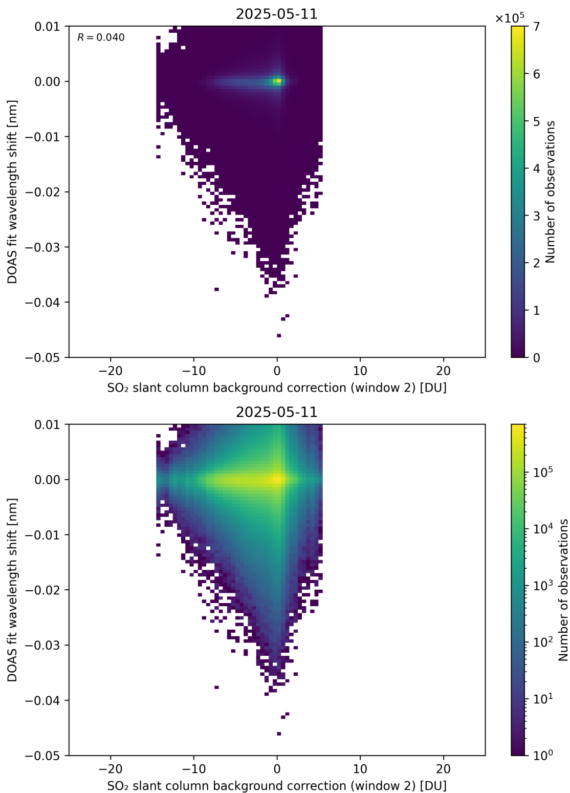
Figure 123: Scatter density plot of “SO 2 slant column background correction (window 2)” against “DOAS fit wavelength shift” for 2025-05-10 to 2025-05-12.
