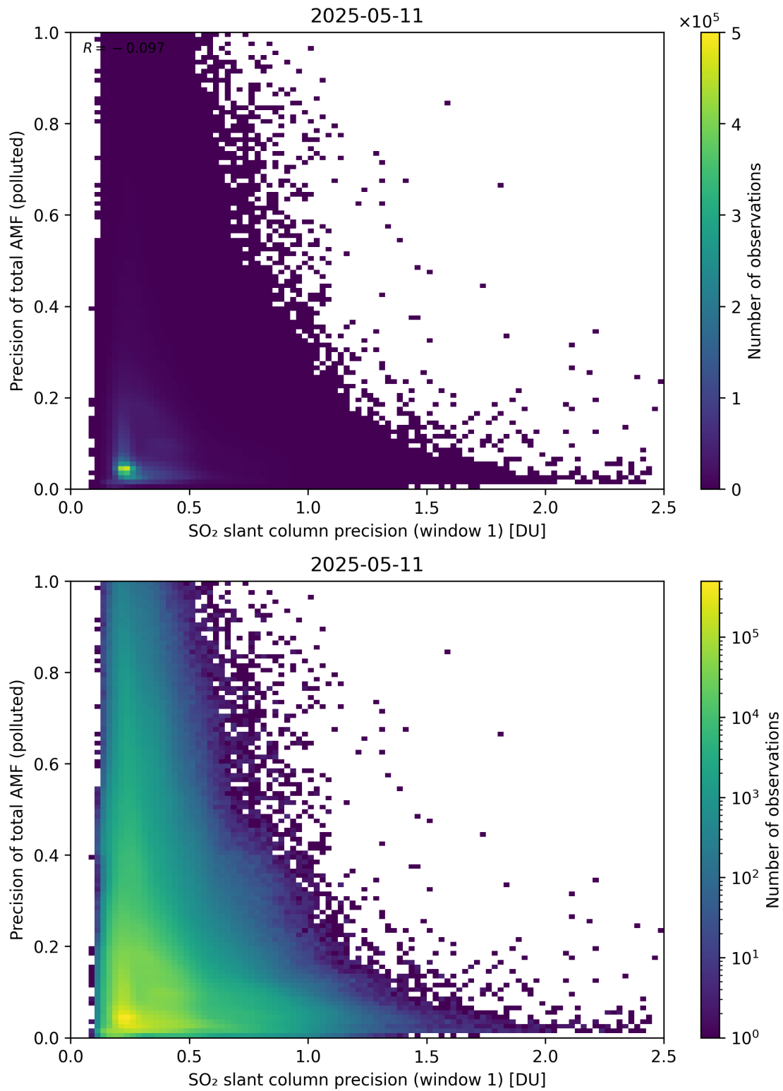
Figure 281: Scatter density plot of “SO 2 slant column precision (window 1)” against “Precision of total AMF (polluted)” for 2025-05-10 to 2025-05-12.
