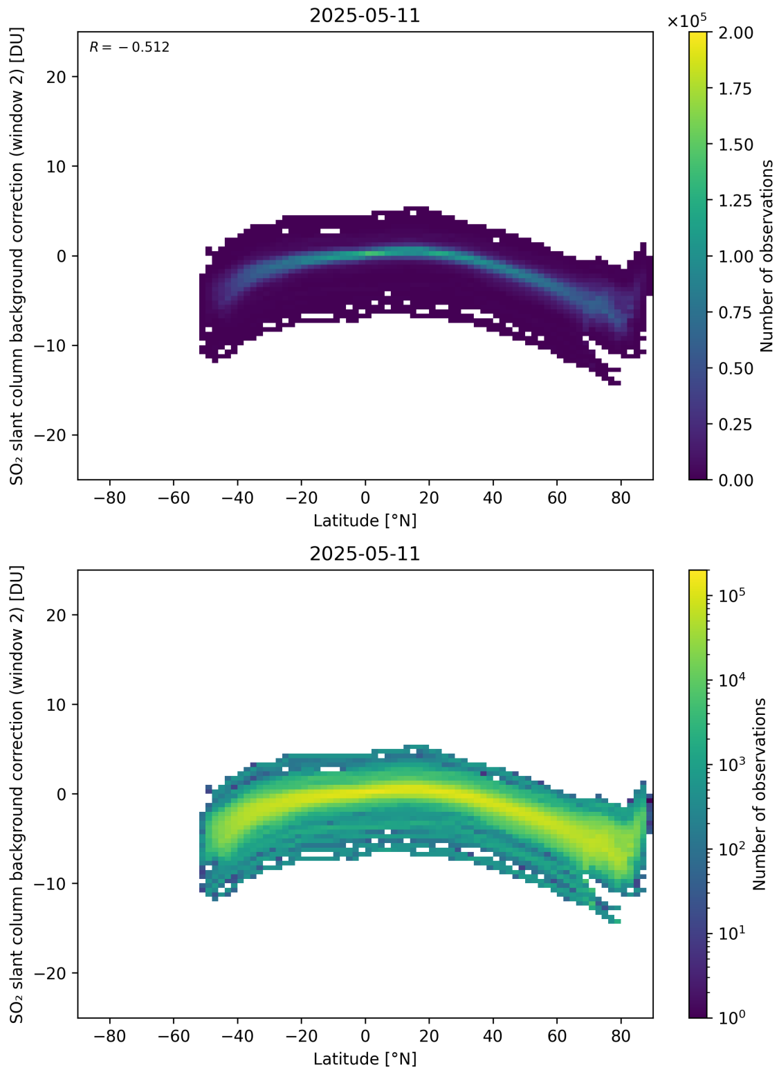
Figure 151: Scatter density plot of “Latitude” against “SO 2 slant column background correction (window 2)” for 2025-05-10 to 2025-05-12.
