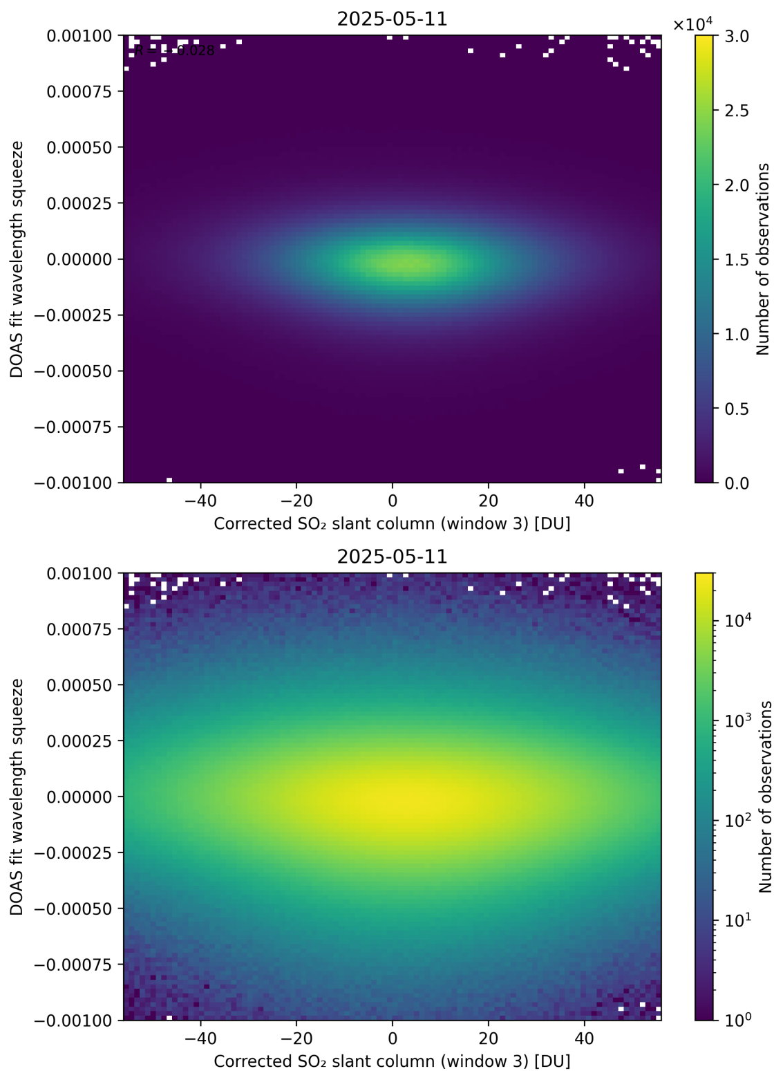
Figure 257: Scatter density plot of “Corrected SO 2 slant column (window 3)” against “DOAS fit wavelength squeeze” for 2025-05-10 to 2025-05-12.
