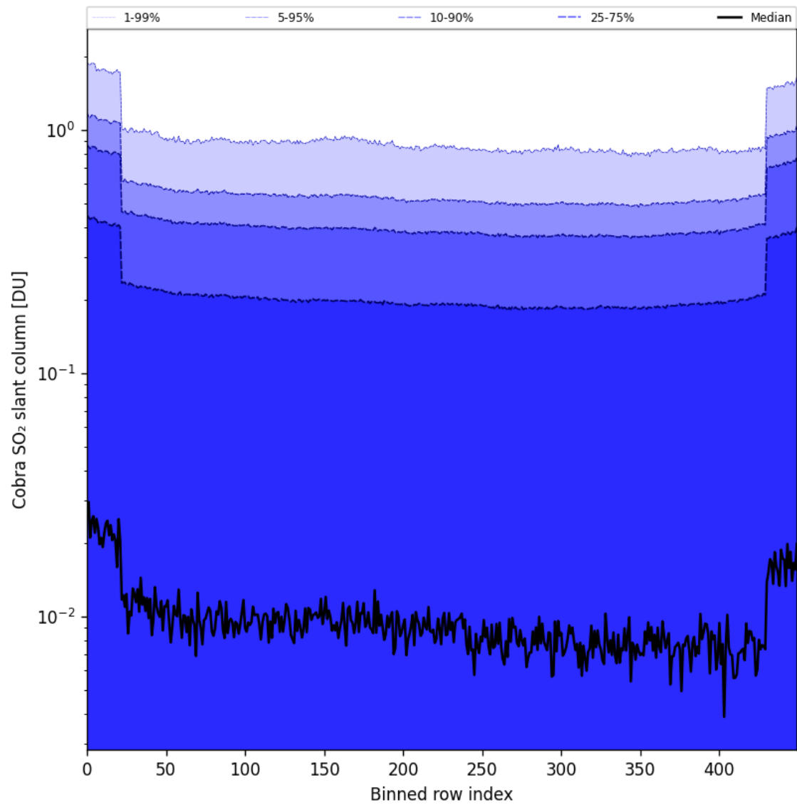
Figure 87: Along track statistics of “Cobra SO 2 slant column” for 2025-05-10 to 2025-05-12
