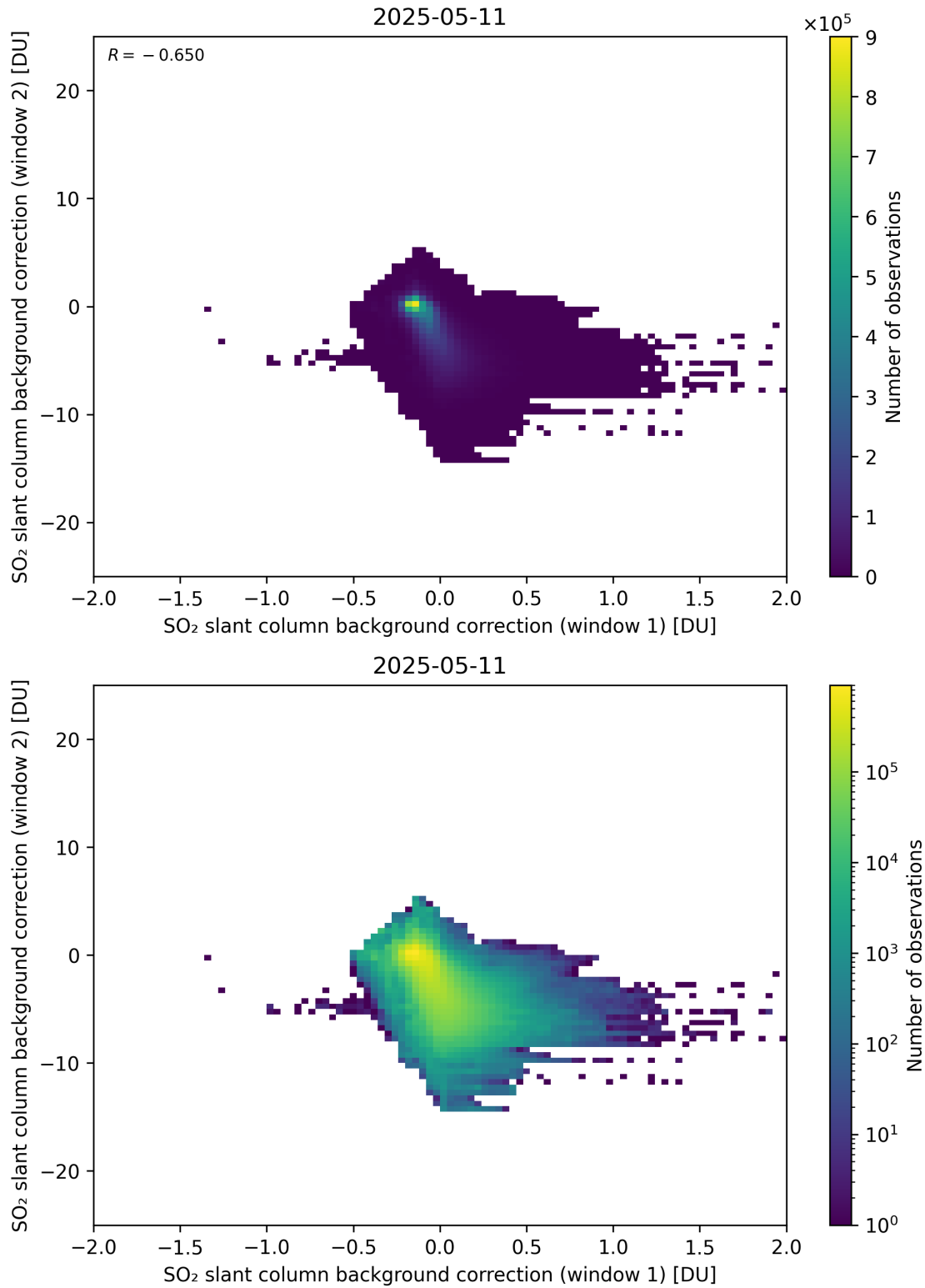
Figure 109: Scatter density plot of “SO 2 slant column background correction (window 1)” against “SO 2 slant column background correction (window 2)” for 2025-05-10 to 2025-05-12.
