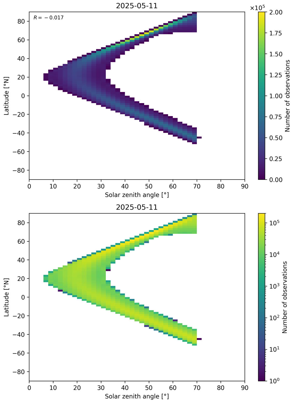
Figure 177: Scatter density plot of “Solar zenith angle” against “Latitude” for 2025-05-10 to 2025-05-12.
