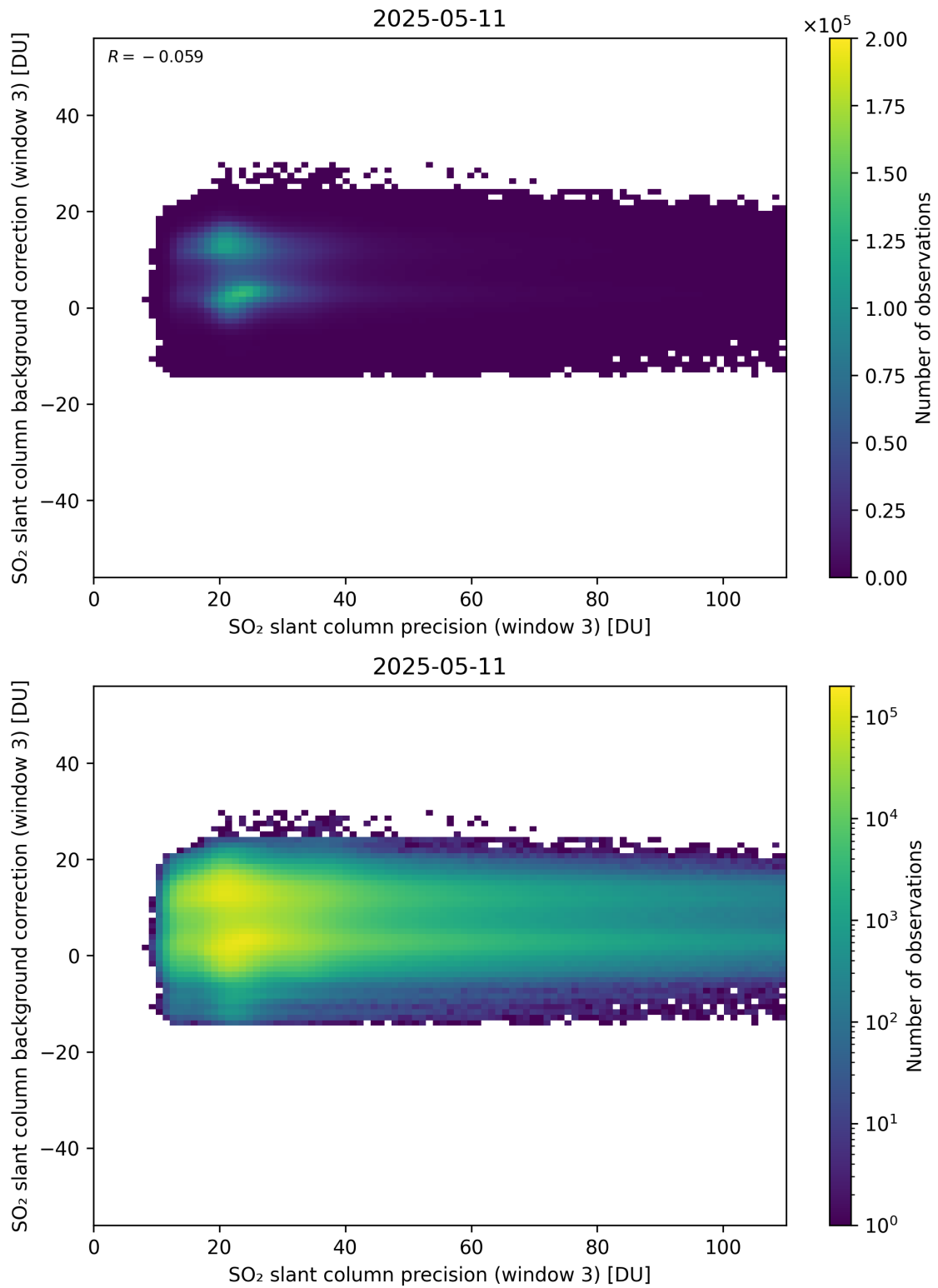
Figure 307: Scatter density plot of “SO 2 slant column precision (window 3)” against “SO 2 slant column background correction (window 3)” for 2025-05-10 to 2025-05-12.
