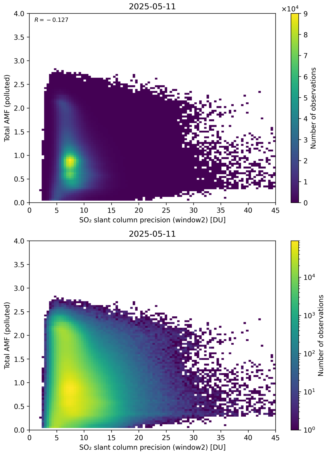
Figure 301: Scatter density plot of “SO 2 slant column precision (window2)” against “Total AMF (polluted)” for 2025-05-10 to 2025-05-12.
