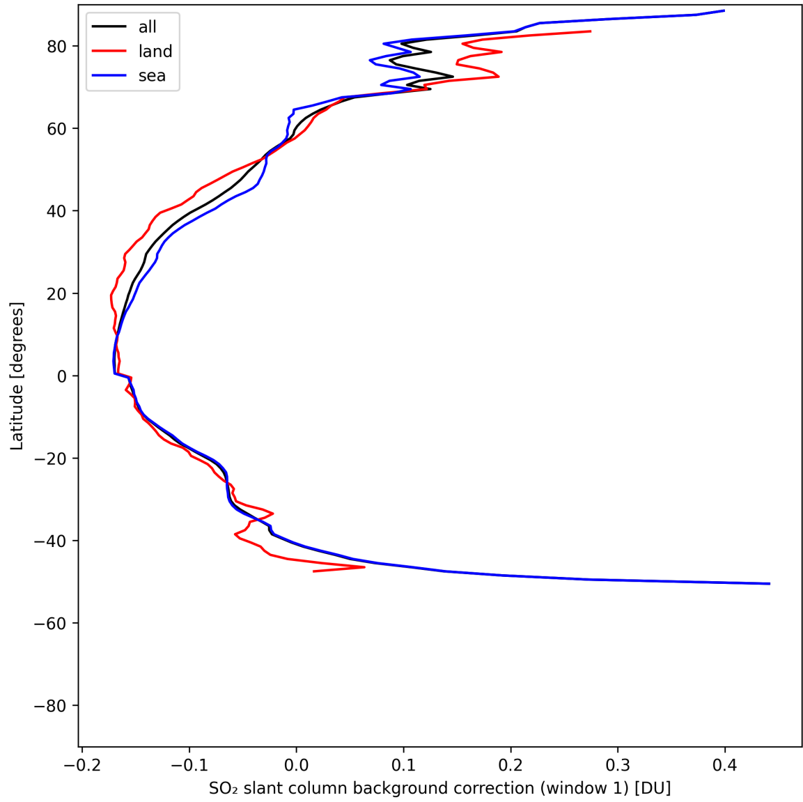
Figure 40: Zonal average of "SO 2 slant column background correction (window 1)" for 2025-05-10 to 2025-05-12.
