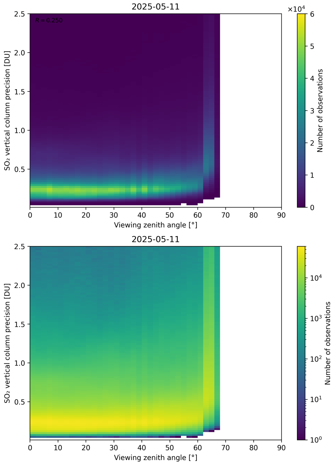
Figure 384: Scatter density plot of “Viewing zenith angle” against “SO 2 vertical column precision” for 2025-05-10 to 2025-05-12.
