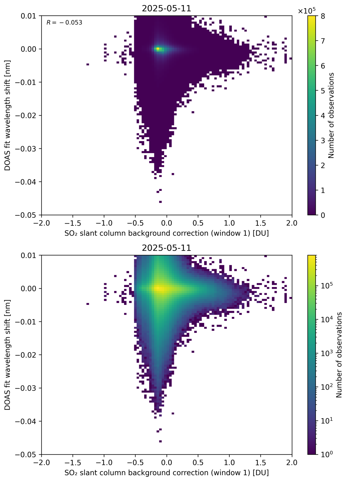
Figure 111: Scatter density plot of “SO 2 slant column background correction (window 1)” against “DOAS fit wavelength shift” for 2025-05-10 to 2025-05-12.
