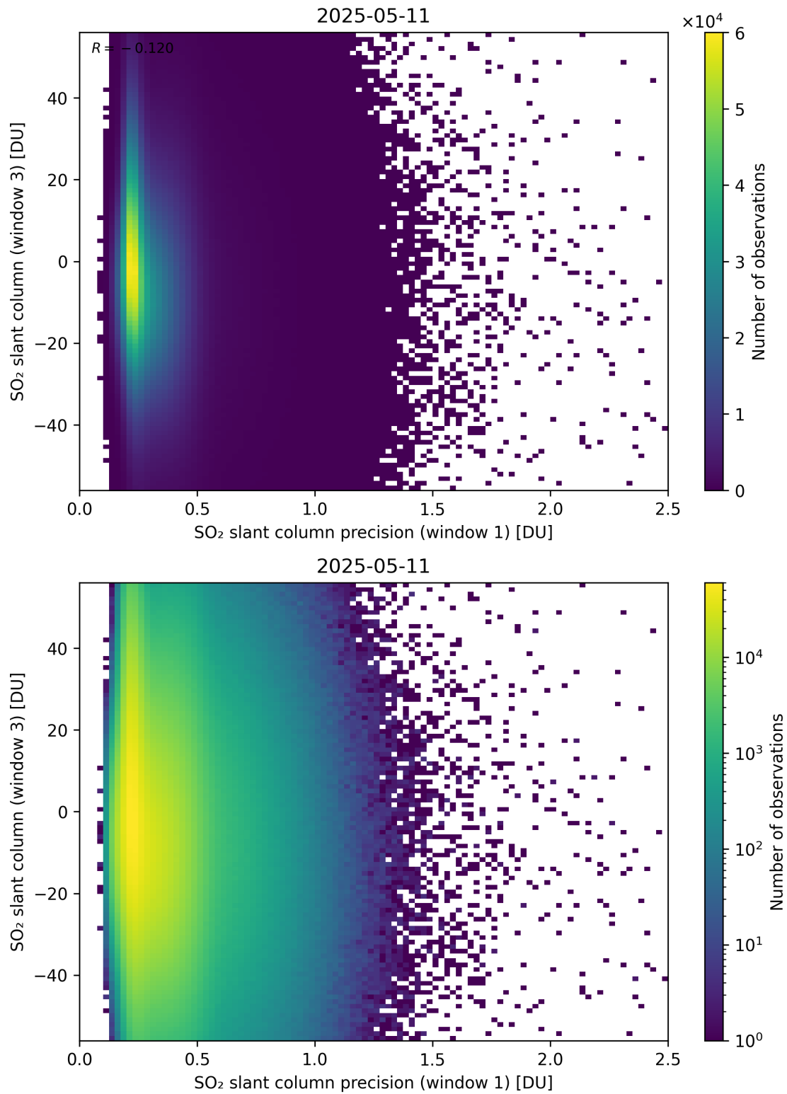
Figure 278: Scatter density plot of “SO 2 slant column precision (window 1)” against “SO 2 slant column (window 3)” for 2025-05-10 to 2025-05-12.
