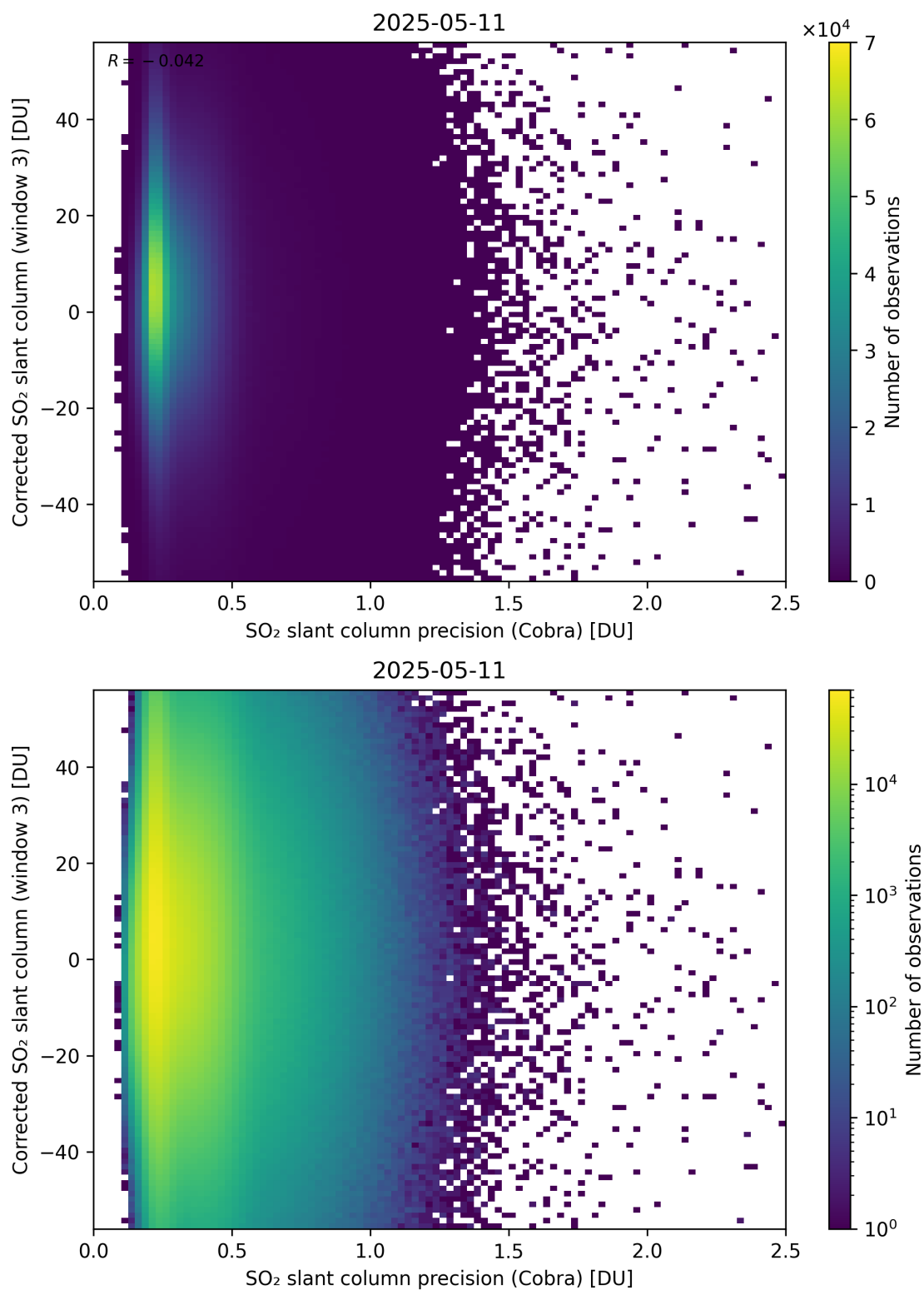
Figure 207: Scatter density plot of “SO 2 slant column precision (Cobra)” against “Corrected SO 2 slant column (window 3)” for 2025-05-10 to 2025-05-12.
