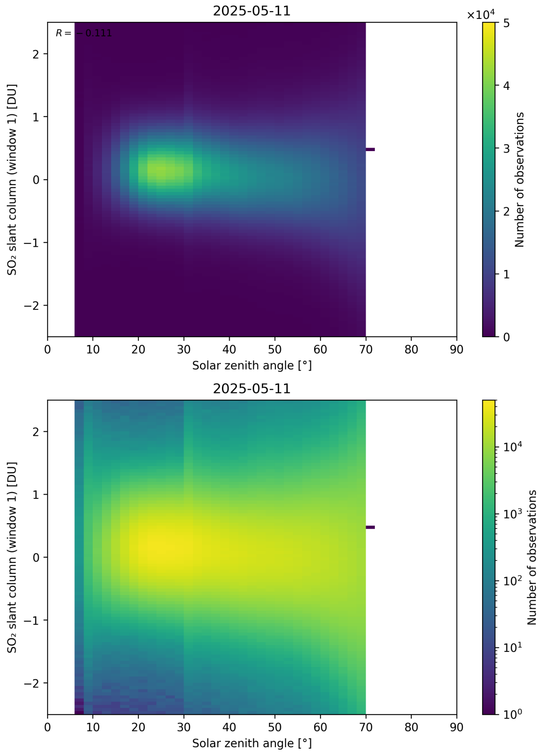
Figure 184: Scatter density plot of “Solar zenith angle” against “SO 2 slant column (window 1)” for 2025-05-10 to 2025-05-12.
