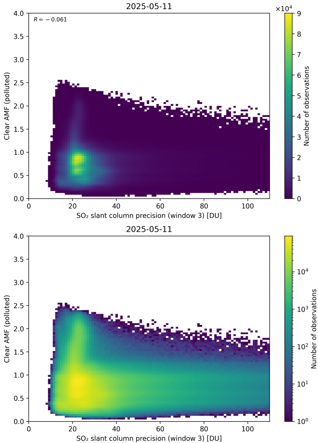
Figure 311: Scatter density plot of “SO 2 slant column precision (window 3)” against “Clear AMF (polluted)” for 2025-05-10 to 2025-05-12.
