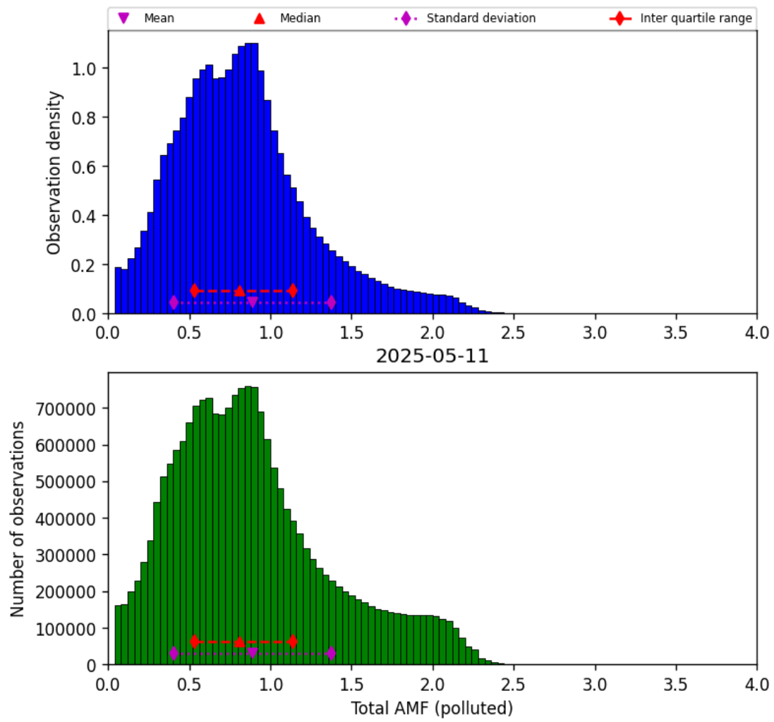
Figure 79: Histogram of “Total AMF (polluted)” for 2025-05-10 to 2025-05-12
