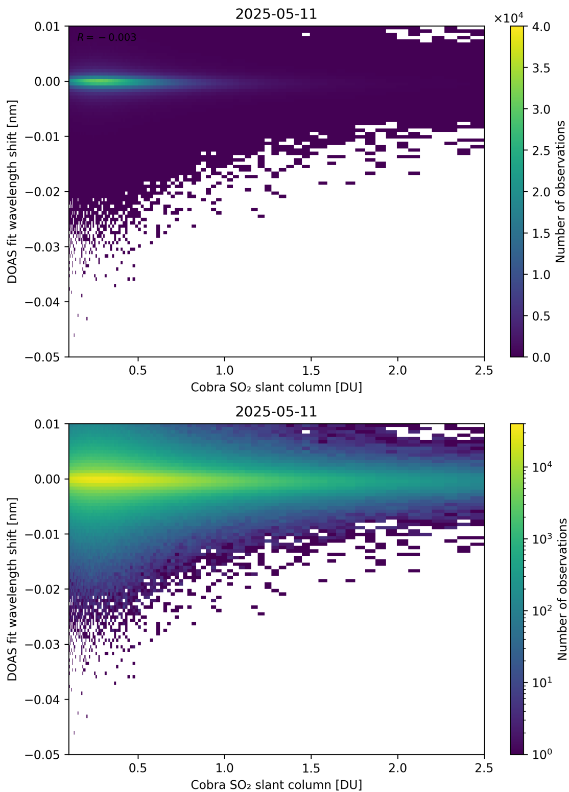
Figure 196: Scatter density plot of “Cobra SO 2 slant column” against “DOAS fit wavelength shift” for 2025-05-10 to 2025-05-12.
