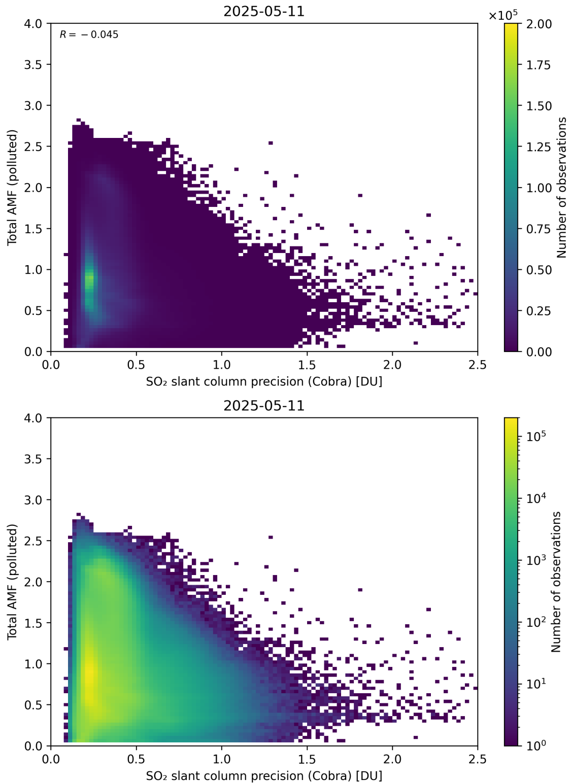
Figure 213: Scatter density plot of “SO 2 slant column precision (Cobra)” against “Total AMF (polluted)” for 2025-05-10 to 2025-05-12.
