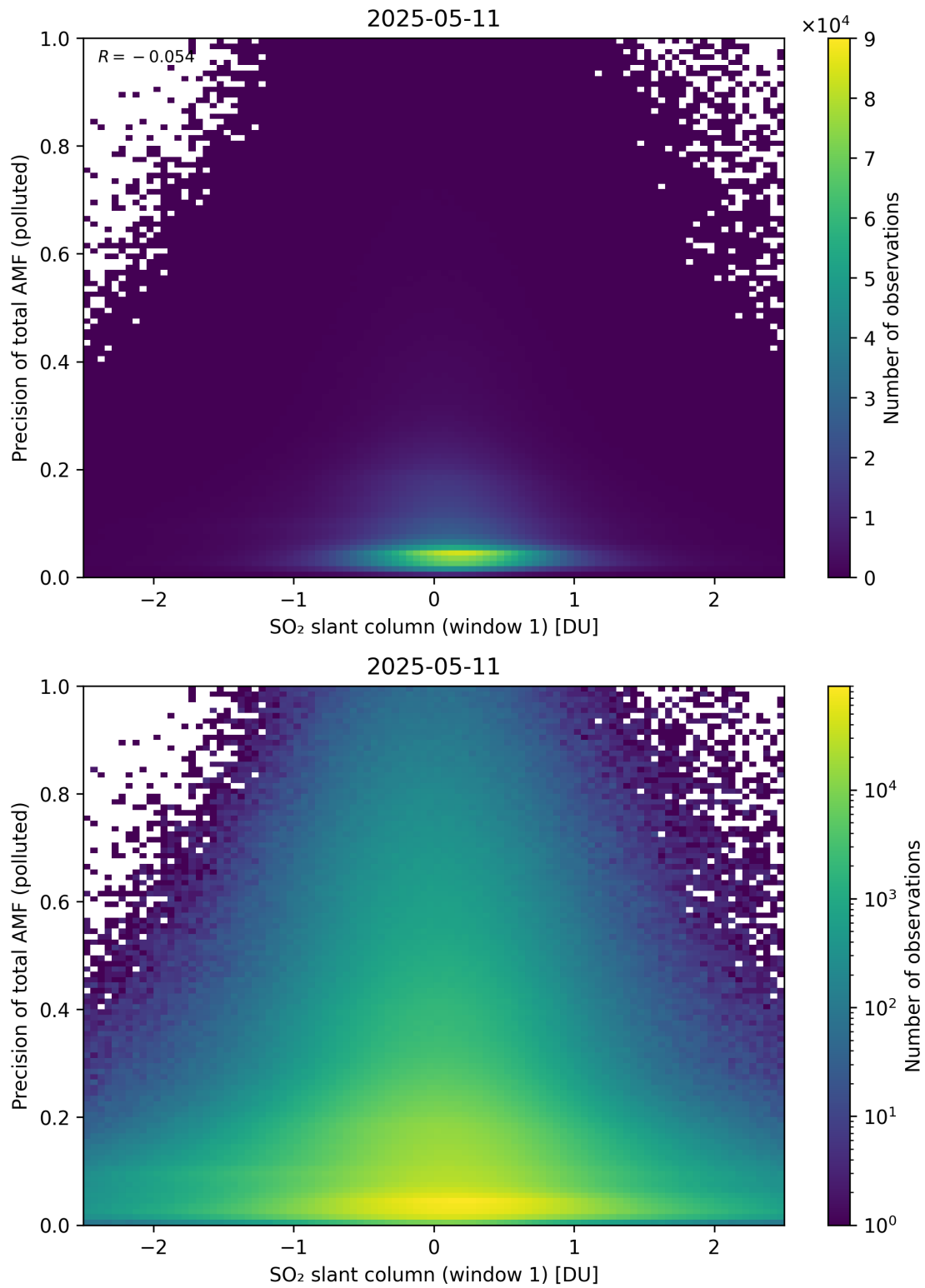
Figure 290: Scatter density plot of “SO 2 slant column (window 1)” against “Precision of total AMF (polluted)” for 2025-05-10 to 2025-05-12.
