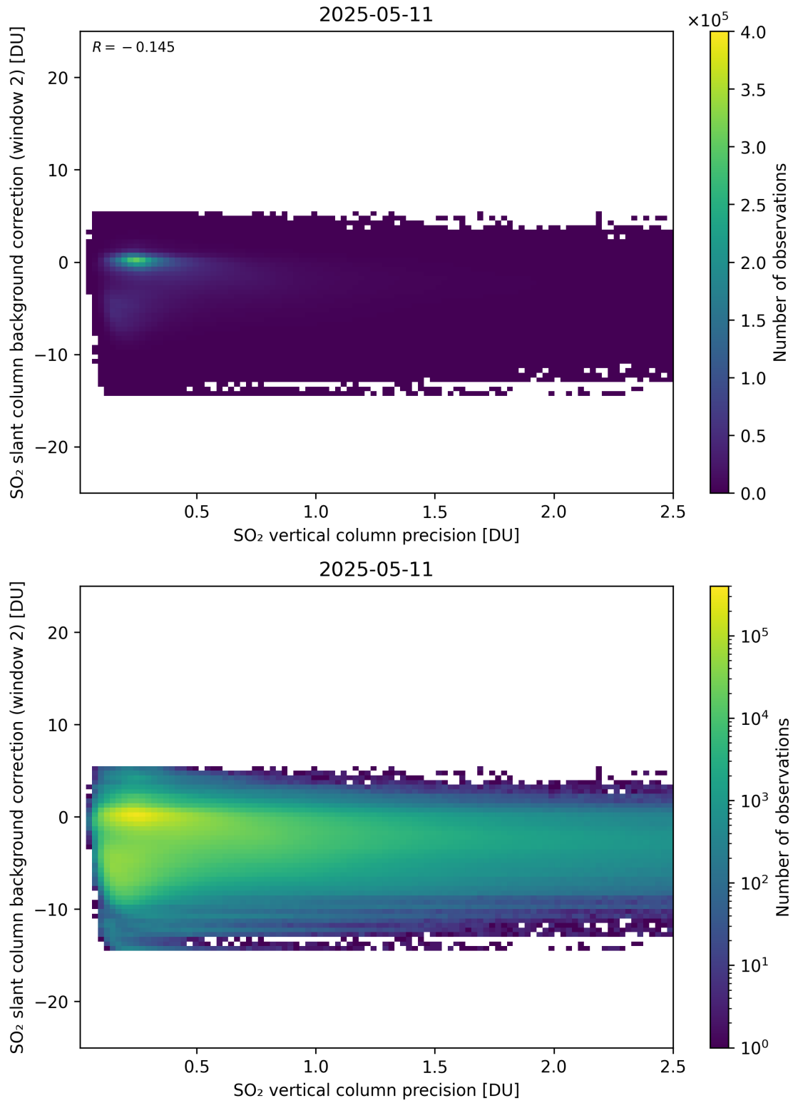
Figure 330: Scatter density plot of “SO 2 vertical column precision” against “SO 2 slant column background correction (window 2)” for 2025-05-10 to 2025-05-12.
