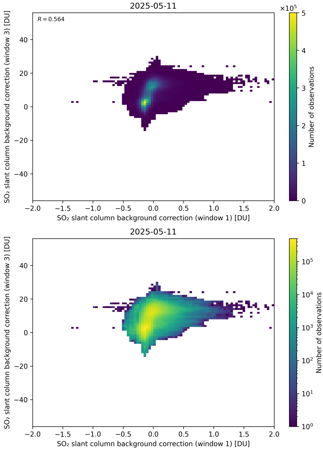
Figure 110: Scatter density plot of “SO 2 slant column background correction (window 1)” against “SO 2 slant column background correction (window 3)” for 2025-05-10 to 2025-05-12.
