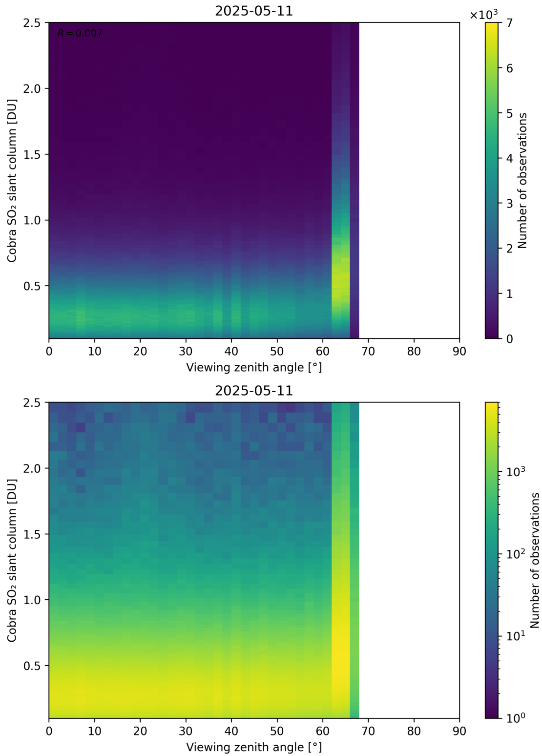
Figure 371: Scatter density plot of “Viewing zenith angle” against “Cobra SO 2 slant column” for 2025-05-10 to 2025-05-12.
