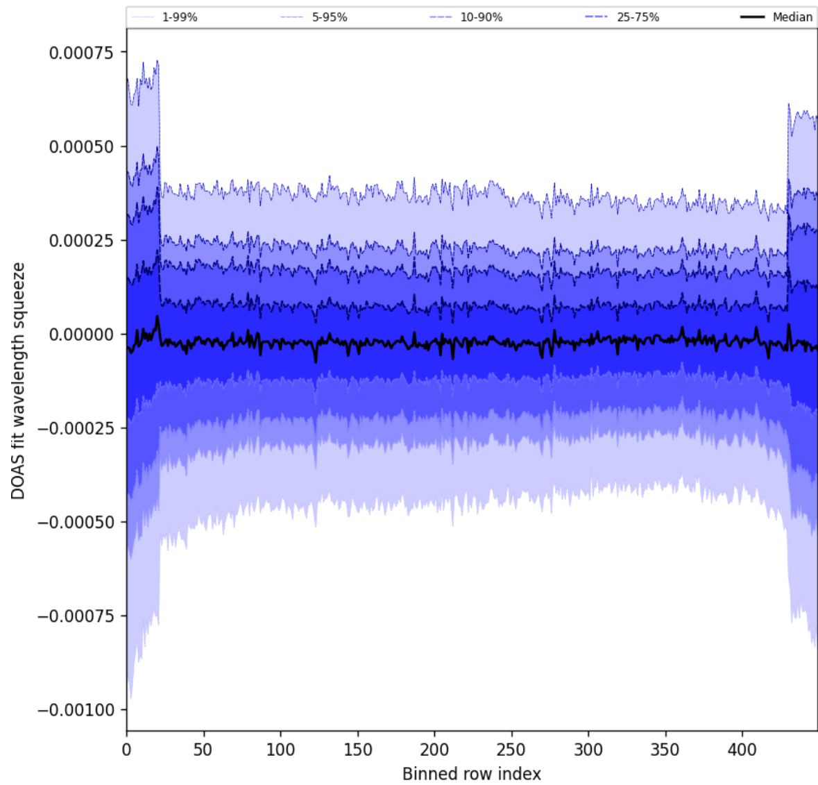
Figure 103: Along track statistics of “DOAS fit wavelength squeeze” for 2025-05-10 to 2025-05-12
