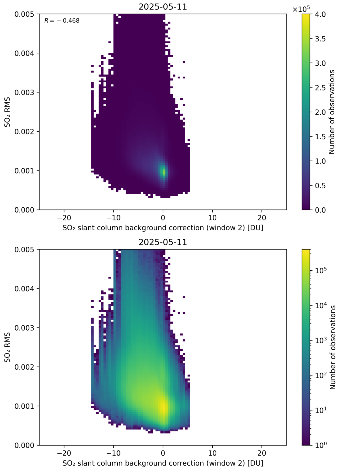
Figure 125: Scatter density plot of “SO 2 slant column background correction (window 2)” against “SO 2 RMS” for 2025-05-10 to 2025-05-12.
