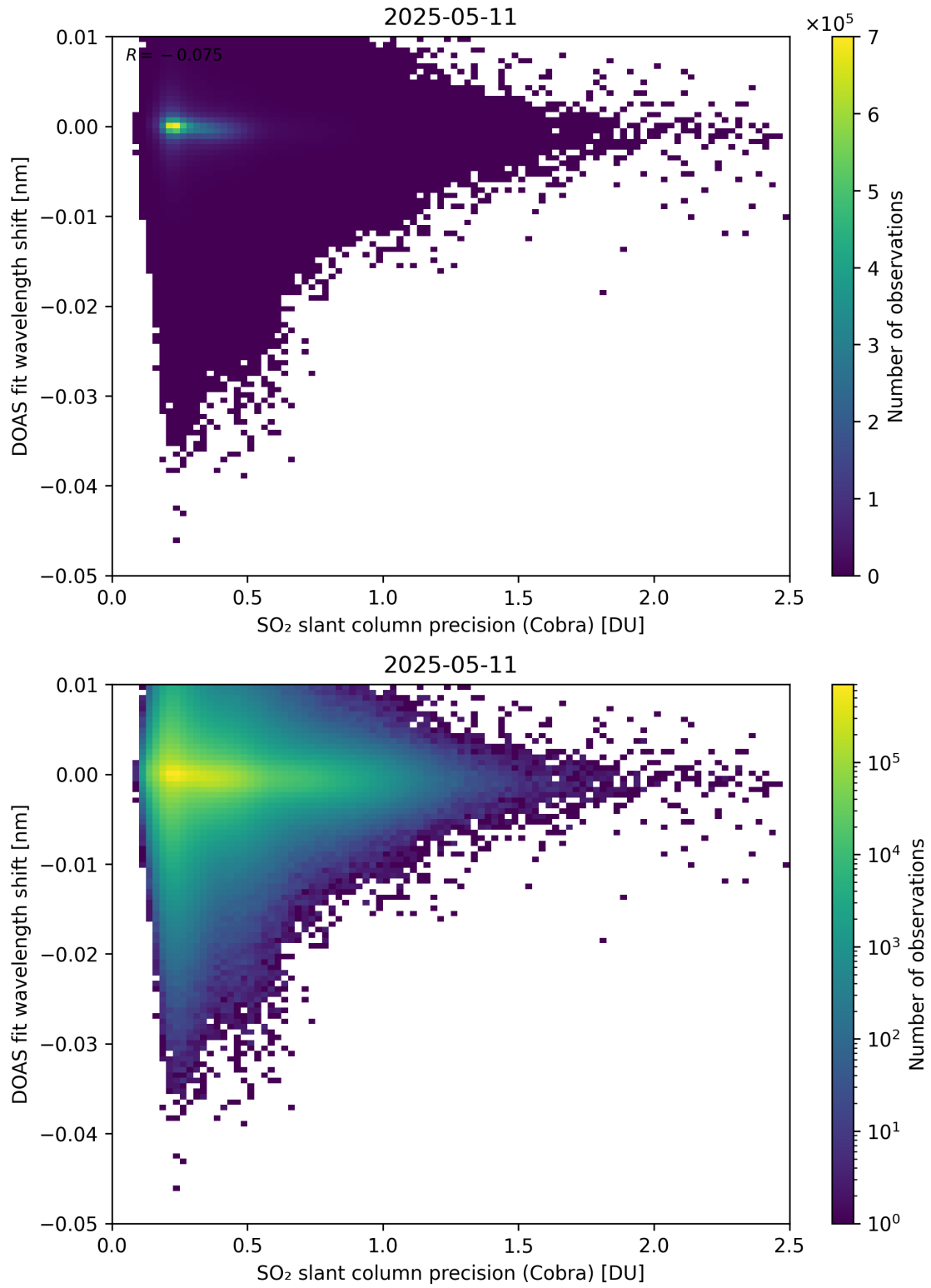
Figure 202: Scatter density plot of “SO 2 slant column precision (Cobra)” against “DOAS fit wavelength shift” for 2025-05-10 to 2025-05-12.
