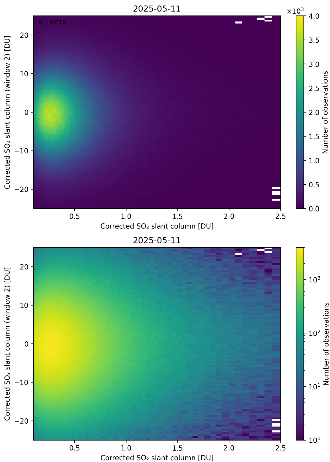
Figure 235: Scatter density plot of “Corrected SO 2 slant column” against “Corrected SO 2 slant column (window 2)” for 2025-05-10 to 2025-05-12.
