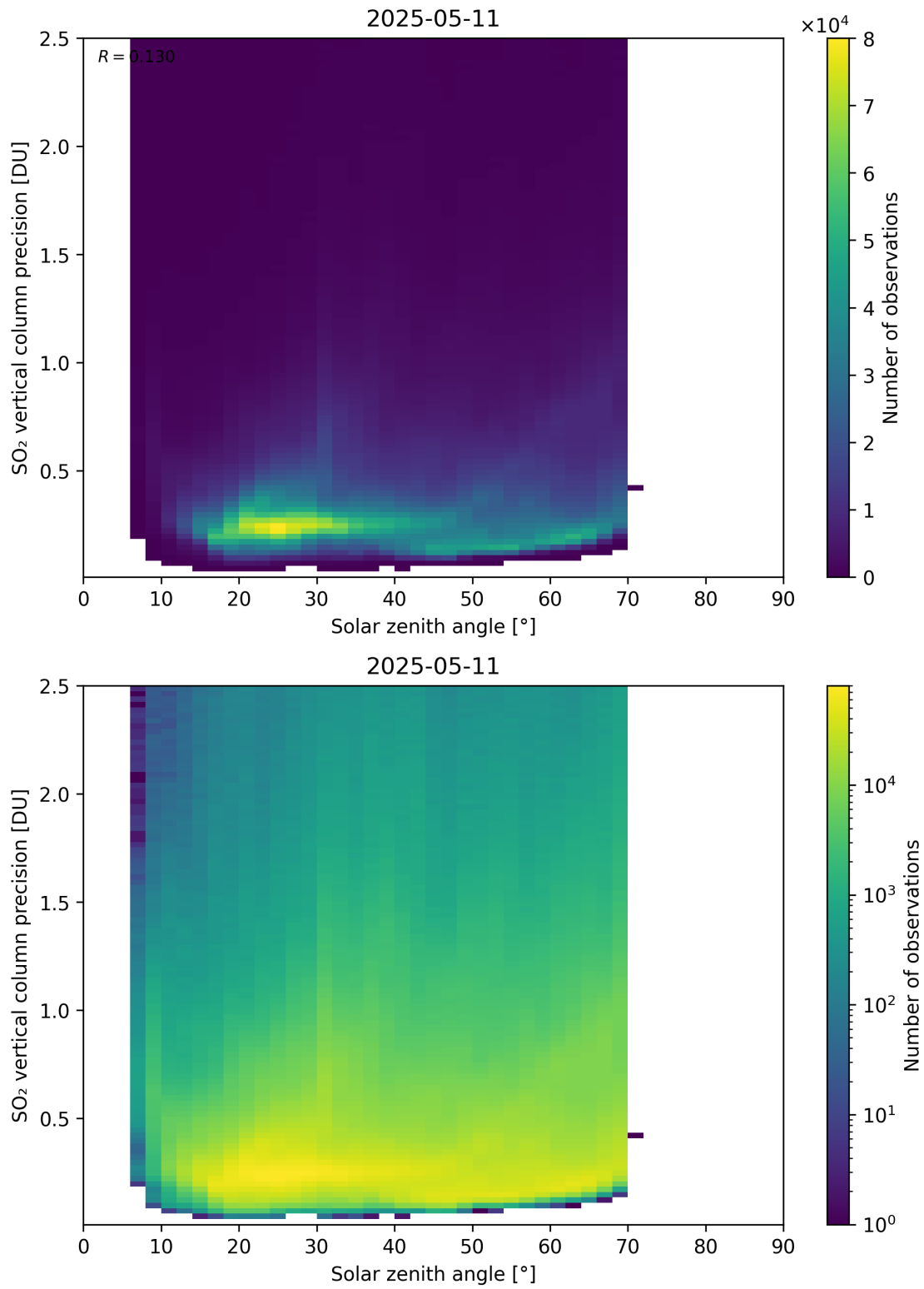
Figure 192: Scatter density plot of “Solar zenith angle” against “SO 2 vertical column precision” for 2025-05-10 to 2025-05-12.
