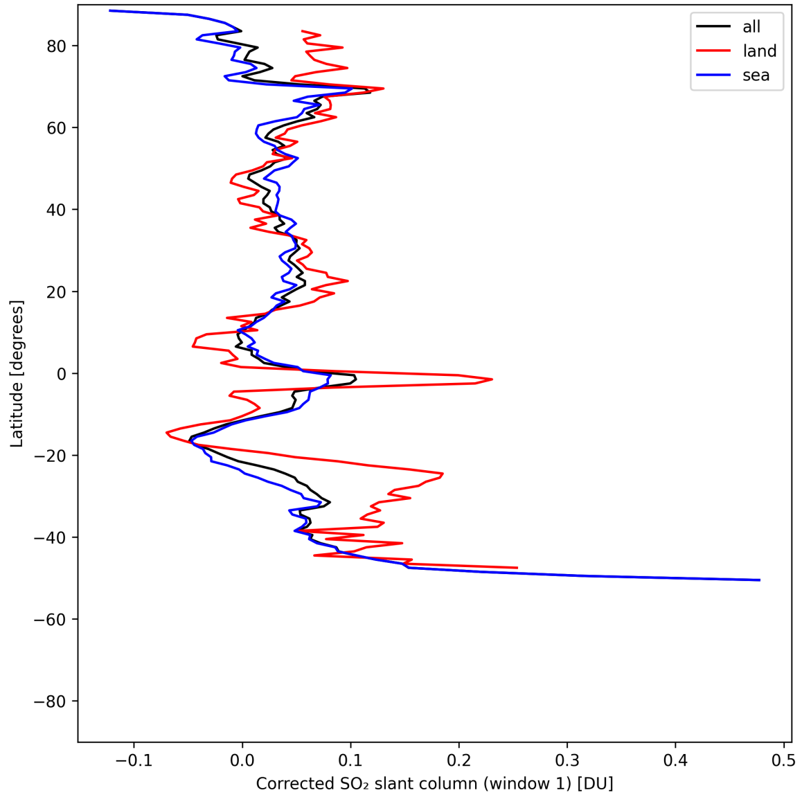
Figure 39: Zonal average of “Corrected SO 2 slant column (window 1)” for 2025-05-10 to 2025-05-12.
