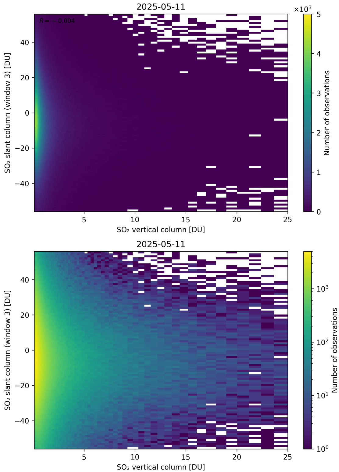
Figure 357: Scatter density plot of “SO 2 vertical column” against “SO 2 slant column (window 3)” for 2025-05-10 to 2025-05-12.
