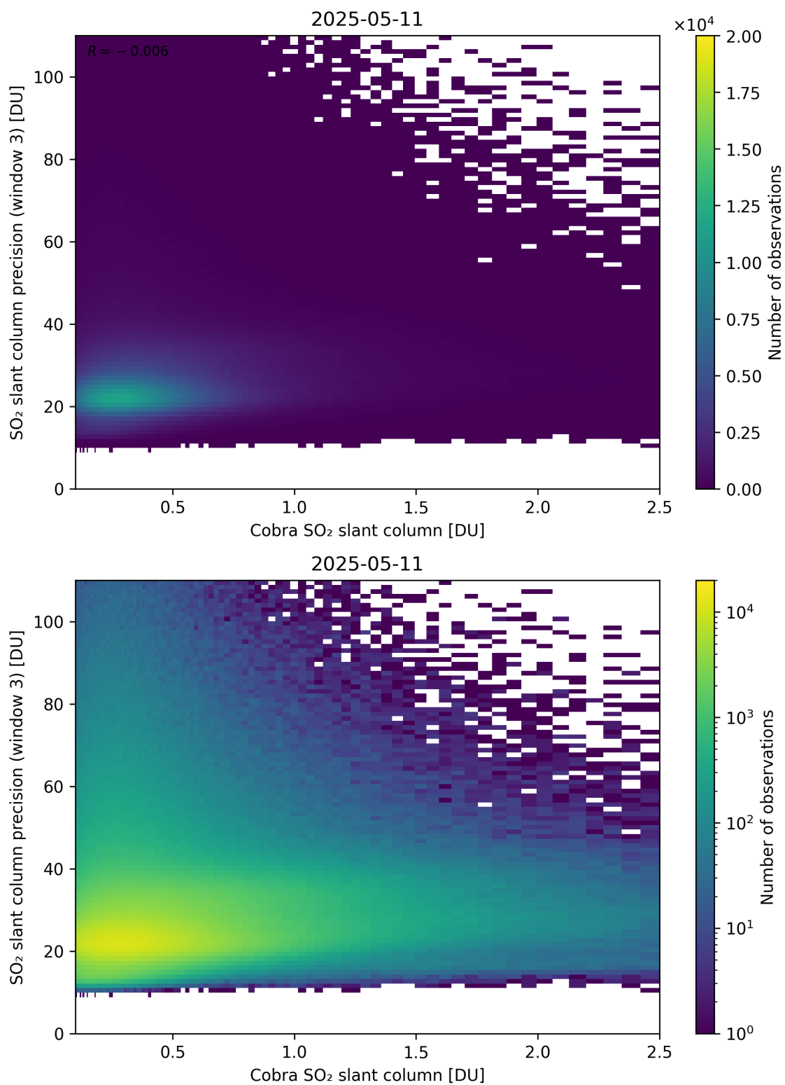
Figure 223: Scatter density plot of “Cobra SO 2 slant column” against “SO 2 slant column precision (window 3)” for 2025-05-10 to 2025-05-12.
