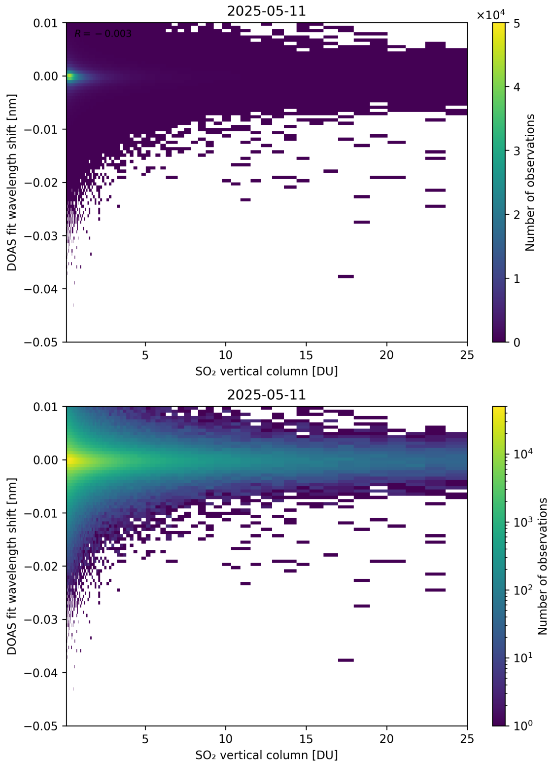
Figure 326: Scatter density plot of “SO 2 vertical column” against “DOAS fit wavelength shift” for 2025-05-10 to 2025-05-12.
