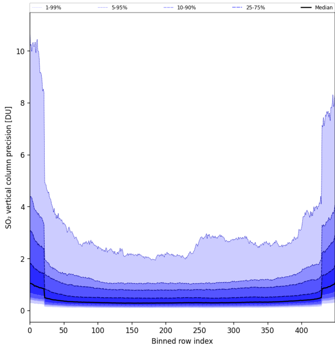
Figure 85: Along track statistics of “SO 2 vertical column precision” for 2025-05-10 to 2025-05-12
