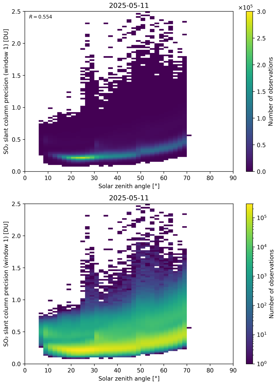
Figure 185: Scatter density plot of “Solar zenith angle” against “SO 2 slant column precision (window 1)” for 2025-05-10 to 2025-05-12.
