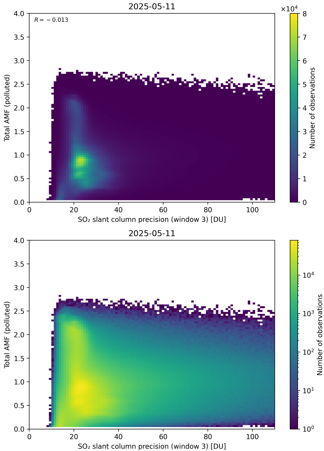
Figure 313: Scatter density plot of “SO 2 slant column precision (window 3)” against “Total AMF (polluted)” for 2025-05-10 to 2025-05-12.
