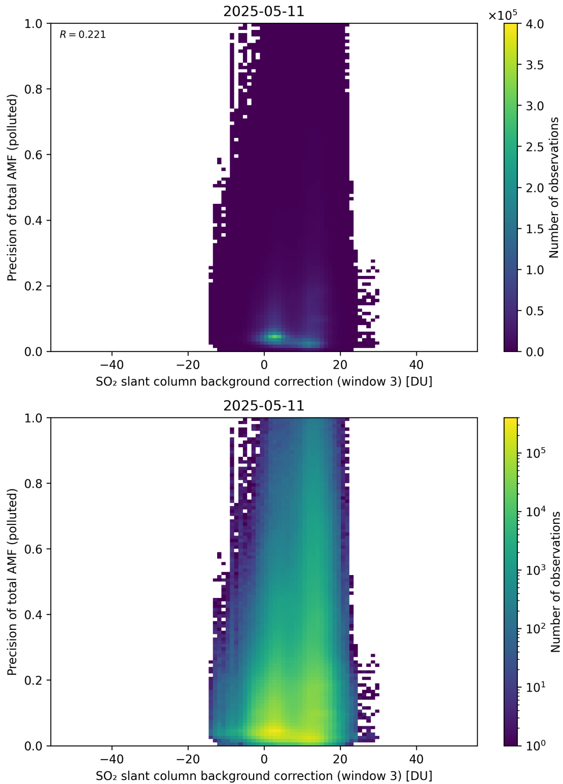
Figure 137: Scatter density plot of “SO 2 slant column background correction (window 3)” against “Precision of total AMF (polluted)” for 2025-05-10 to 2025-05-12.
