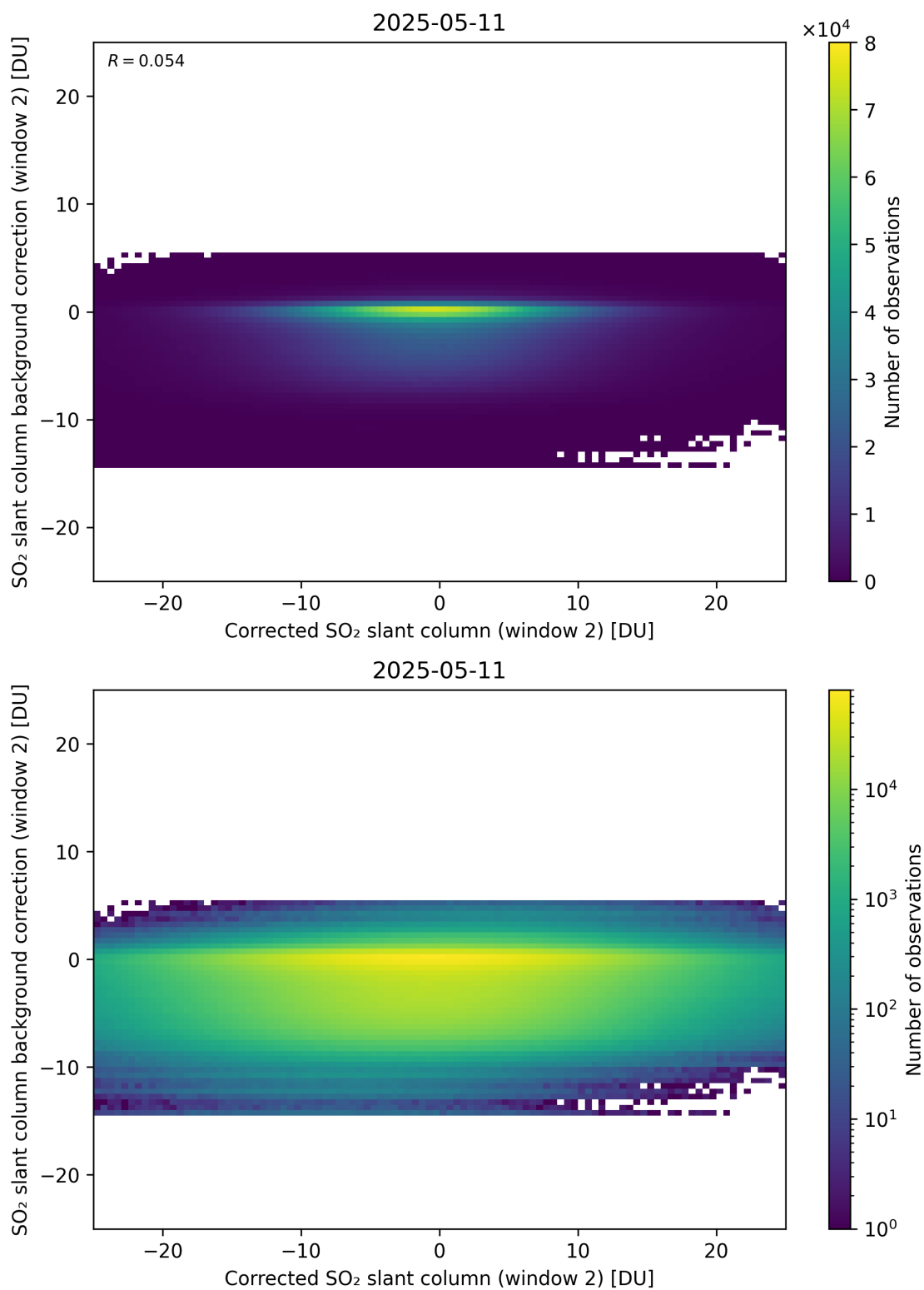
Figure 244: Scatter density plot of “Corrected SO 2 slant column (window 2)” against “SO 2 slant column background correction (window 2)” for 2025-05-10 to 2025-05-12.
