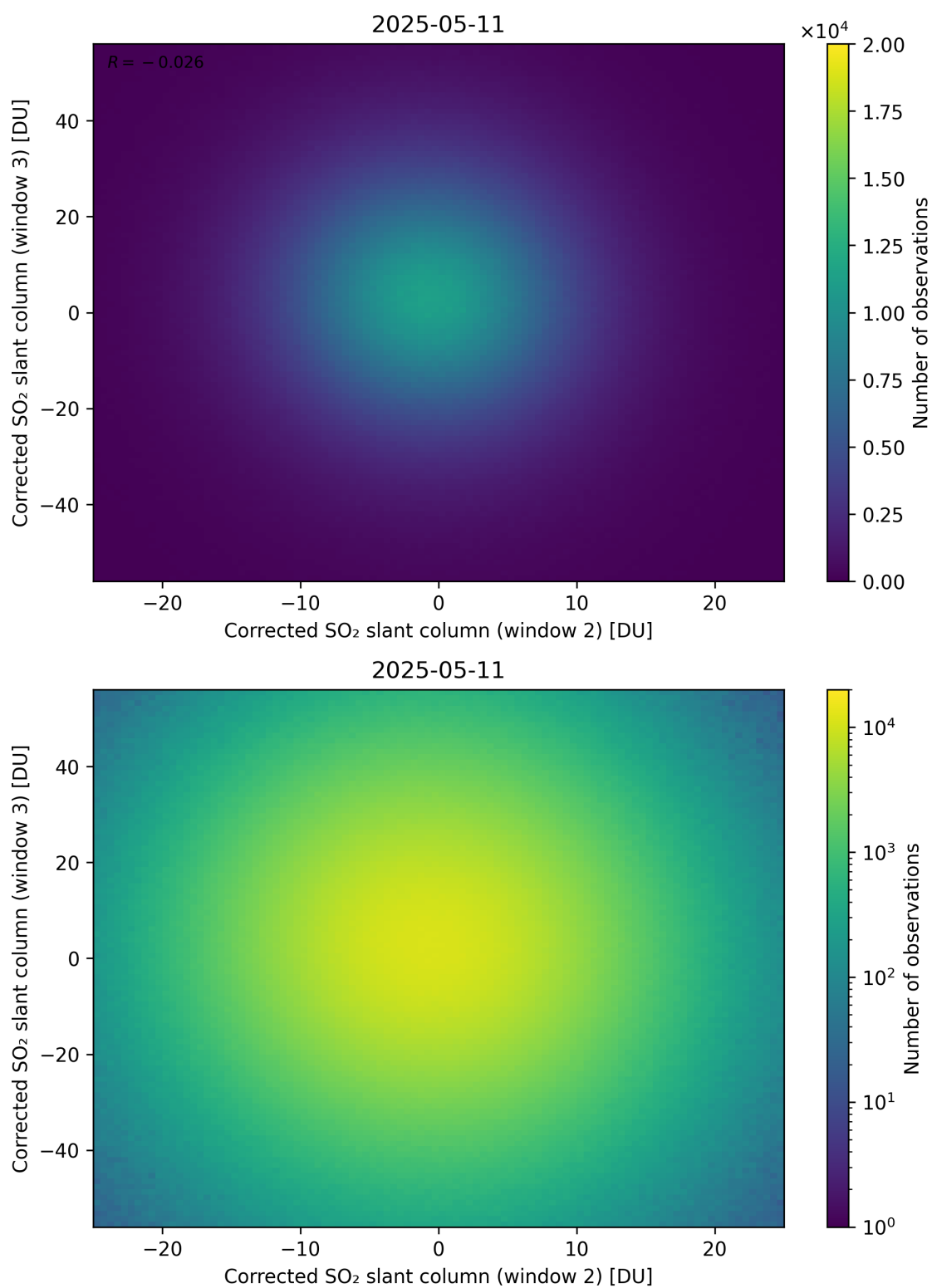
Figure 250: Scatter density plot of “Corrected SO 2 slant column (window 2)” against “Corrected SO 2 slant column (window 3)” for 2025-05-10 to 2025-05-12.
