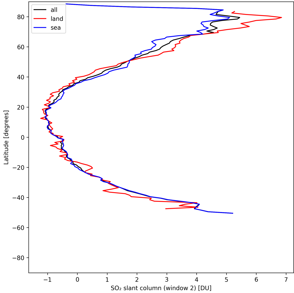
Figure 41: Zonal average of “SO 2 slant column (window 2)” for 2025-05-10 to 2025-05-12.
