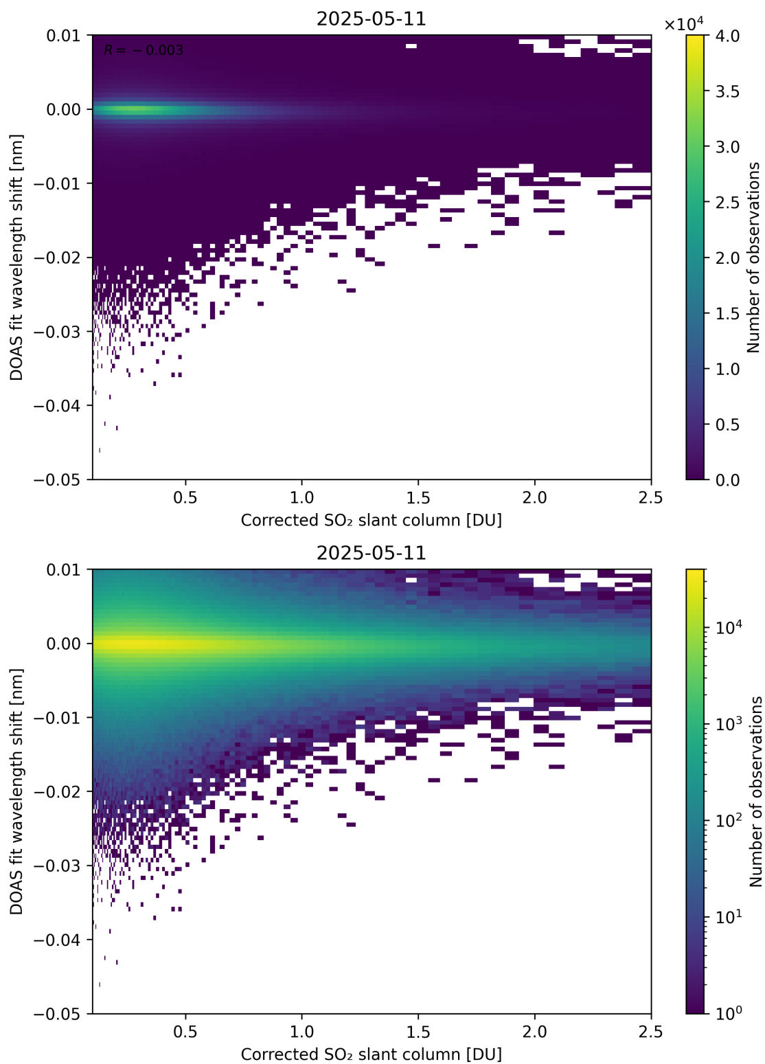
Figure 229: Scatter density plot of “Corrected SO 2 slant column” against “DOAS fit wavelength shift” for 2025-05-10 to 2025-05-12.
