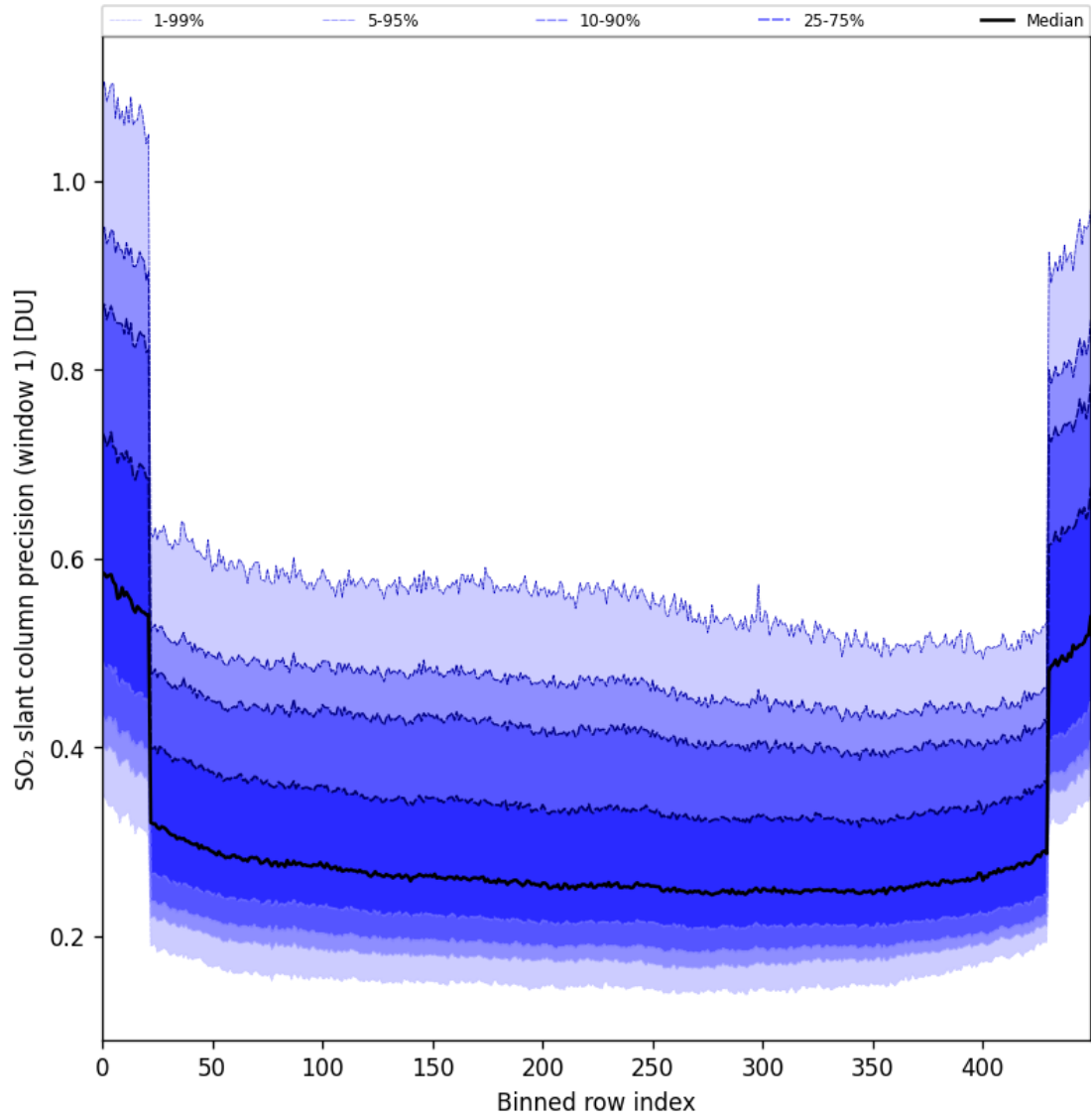
Figure 90: Along track statistics of “SO 2 slant column precision (window 1)” for 2025-05-10 to 2025-05-12
