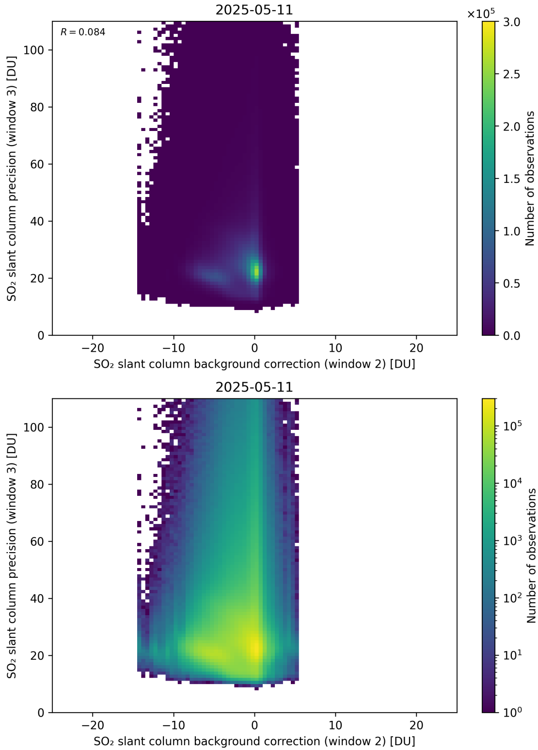
Figure 129: Scatter density plot of “SO 2 slant column background correction (window 2)” against “SO 2 slant column precision (window 3)” for 2025-05-10 to 2025-05-12.
