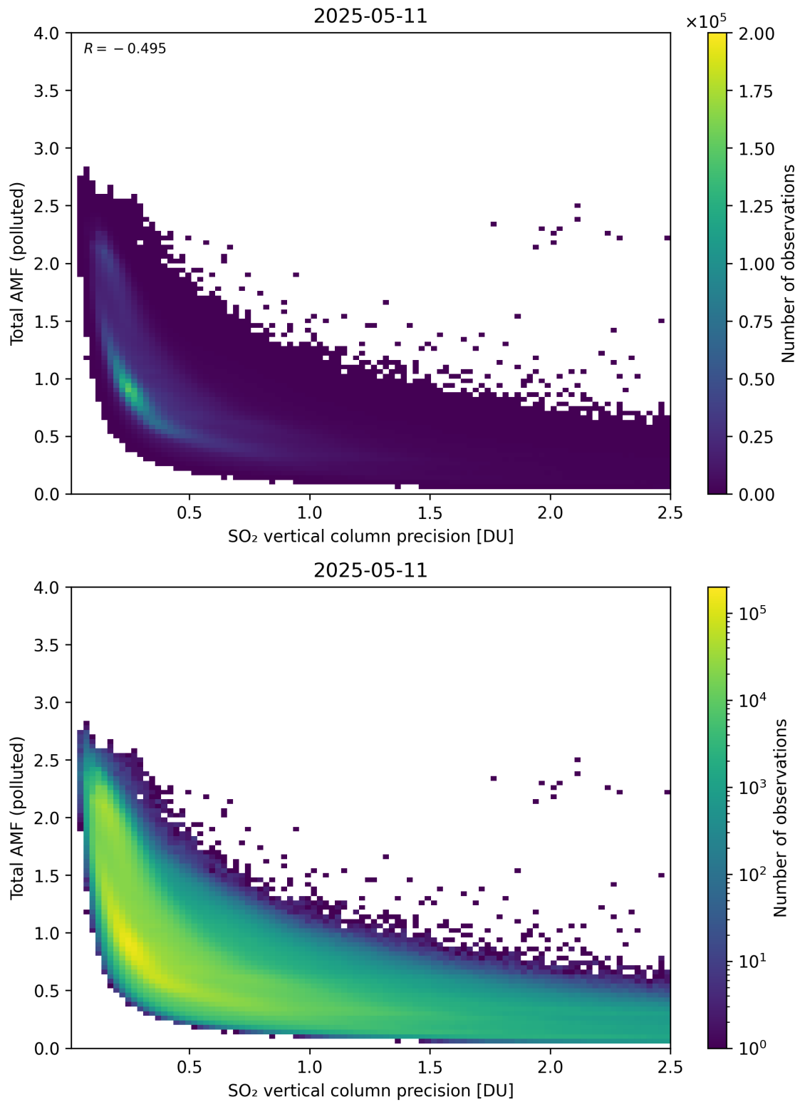
Figure 346: Scatter density plot of “SO 2 vertical column precision” against “Total AMF (polluted)” for 2025-05-10 to 2025-05-12.
