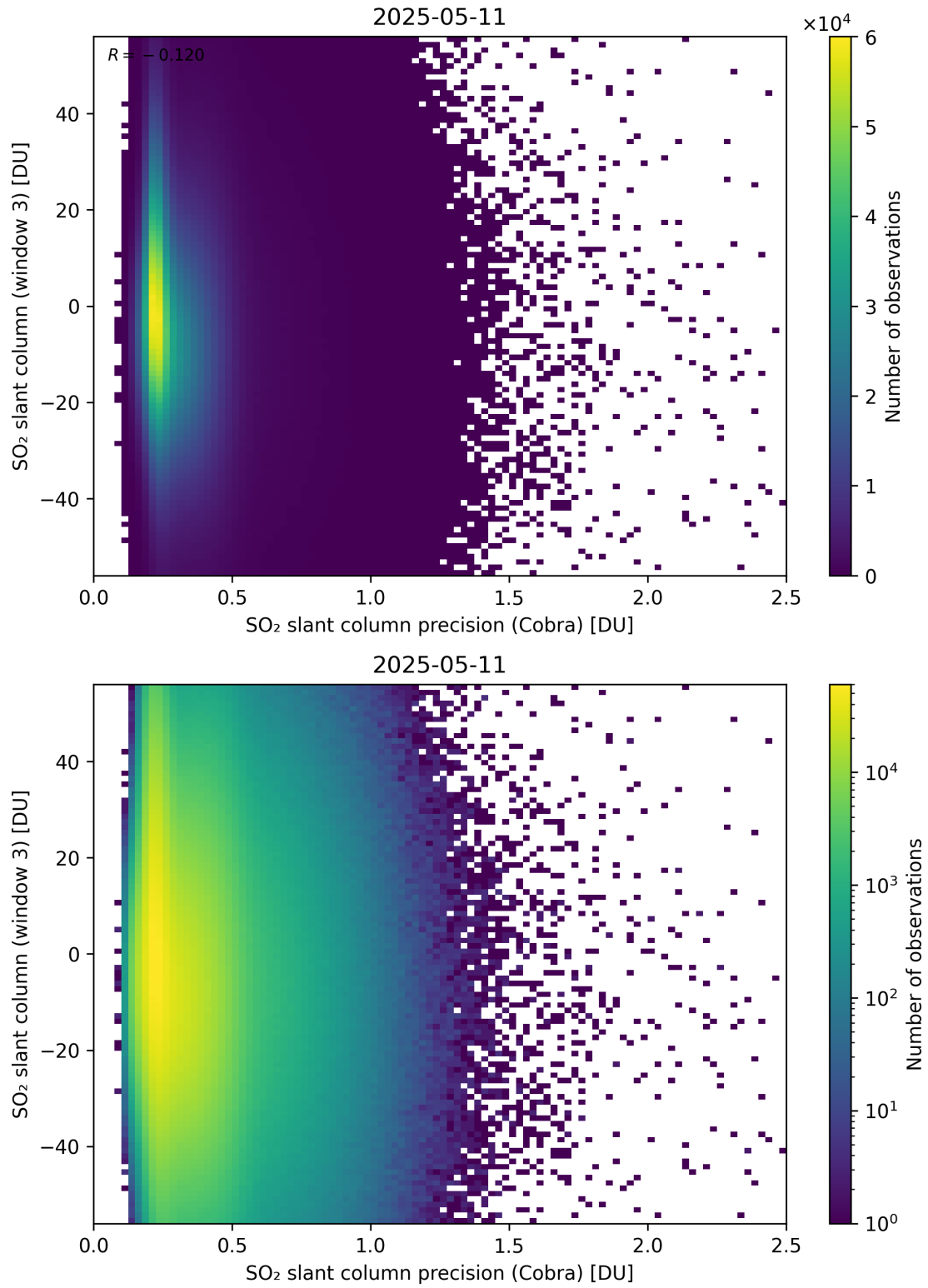
Figure 211: Scatter density plot of “SO 2 slant column precision (Cobra)” against “SO 2 slant column (window 3)” for 2025-05-10 to 2025-05-12.
