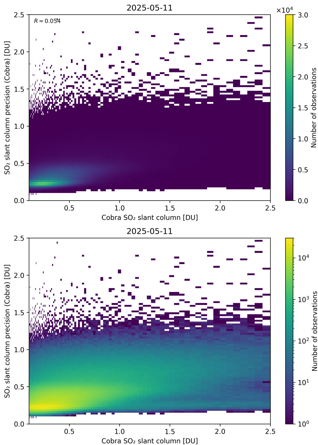
Figure 216: Scatter density plot of “Cobra SO 2 slant column” against “SO 2 slant column precision (Cobra)” for 2025-05-10 to 2025-05-12.
