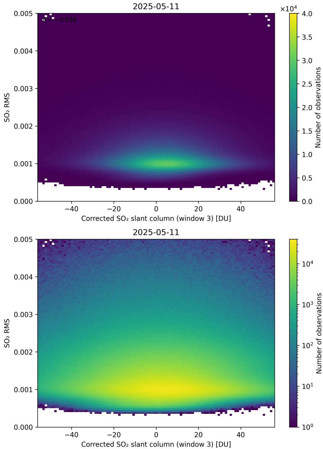
Figure 258: Scatter density plot of “Corrected SO 2 slant column (window 3)” against “SO 2 RMS” for 2025-05-10 to 2025-05-12.
