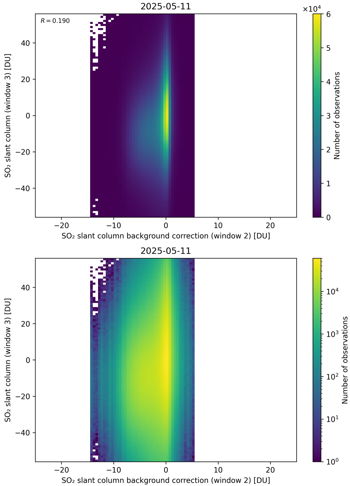
Figure 128: Scatter density plot of “SO 2 slant column background correction (window 2)” against “SO 2 slant column (window 3)” for 2025-05-10 to 2025-05-12.
