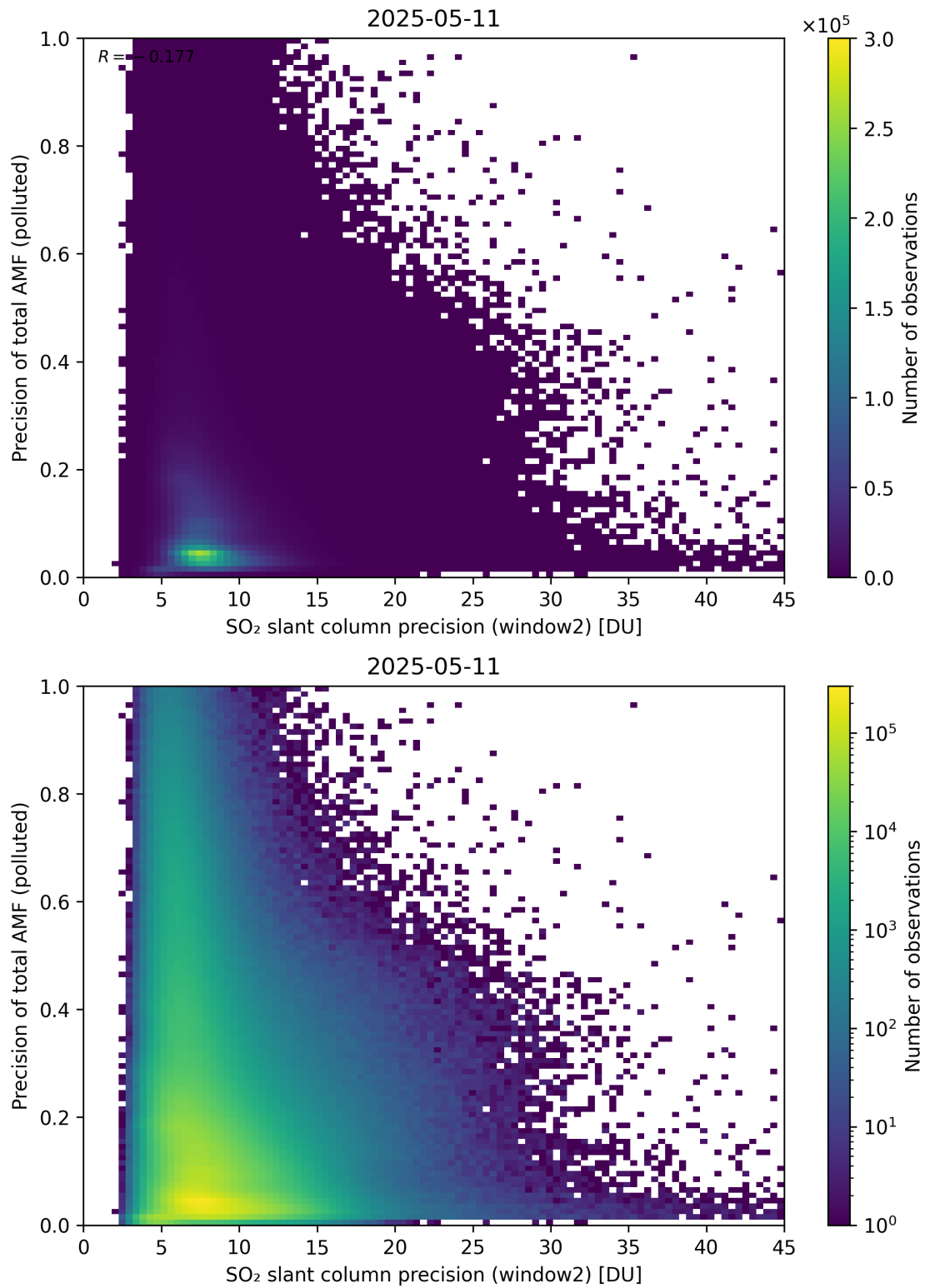
Figure 302: Scatter density plot of “SO 2 slant column precision (window2)” against “Precision of total AMF (polluted)” for 2025-05-10 to 2025-05-12.
