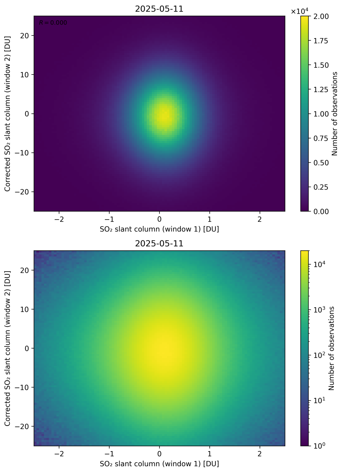
Figure 283: Scatter density plot of “SO 2 slant column (window 1)” against “Corrected SO 2 slant column (window 2)” for 2025-05-10 to 2025-05-12.
