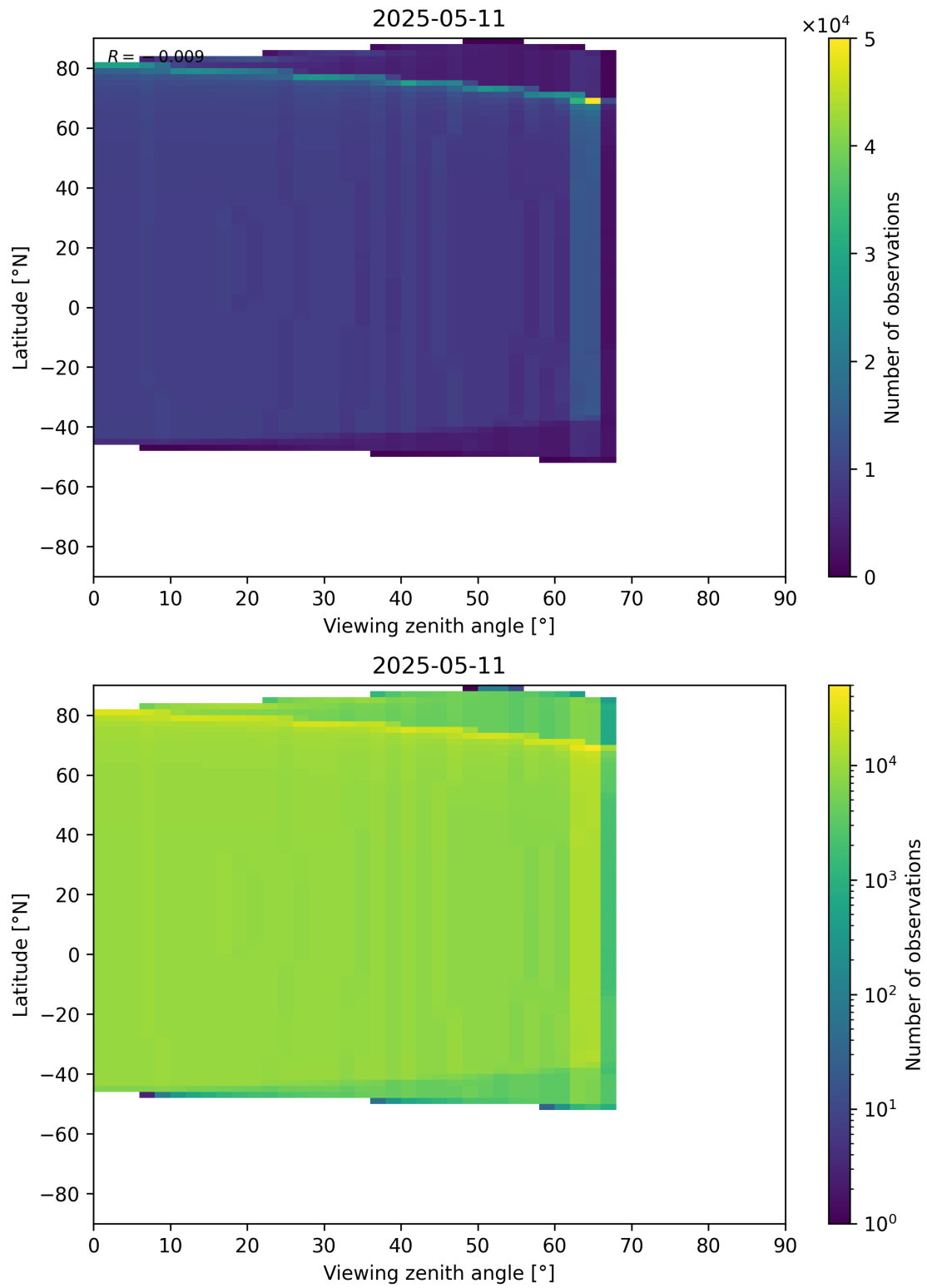
Figure 368: Scatter density plot of “Viewing zenith angle” against “Latitude” for 2025-05-10 to 2025-05-12.
