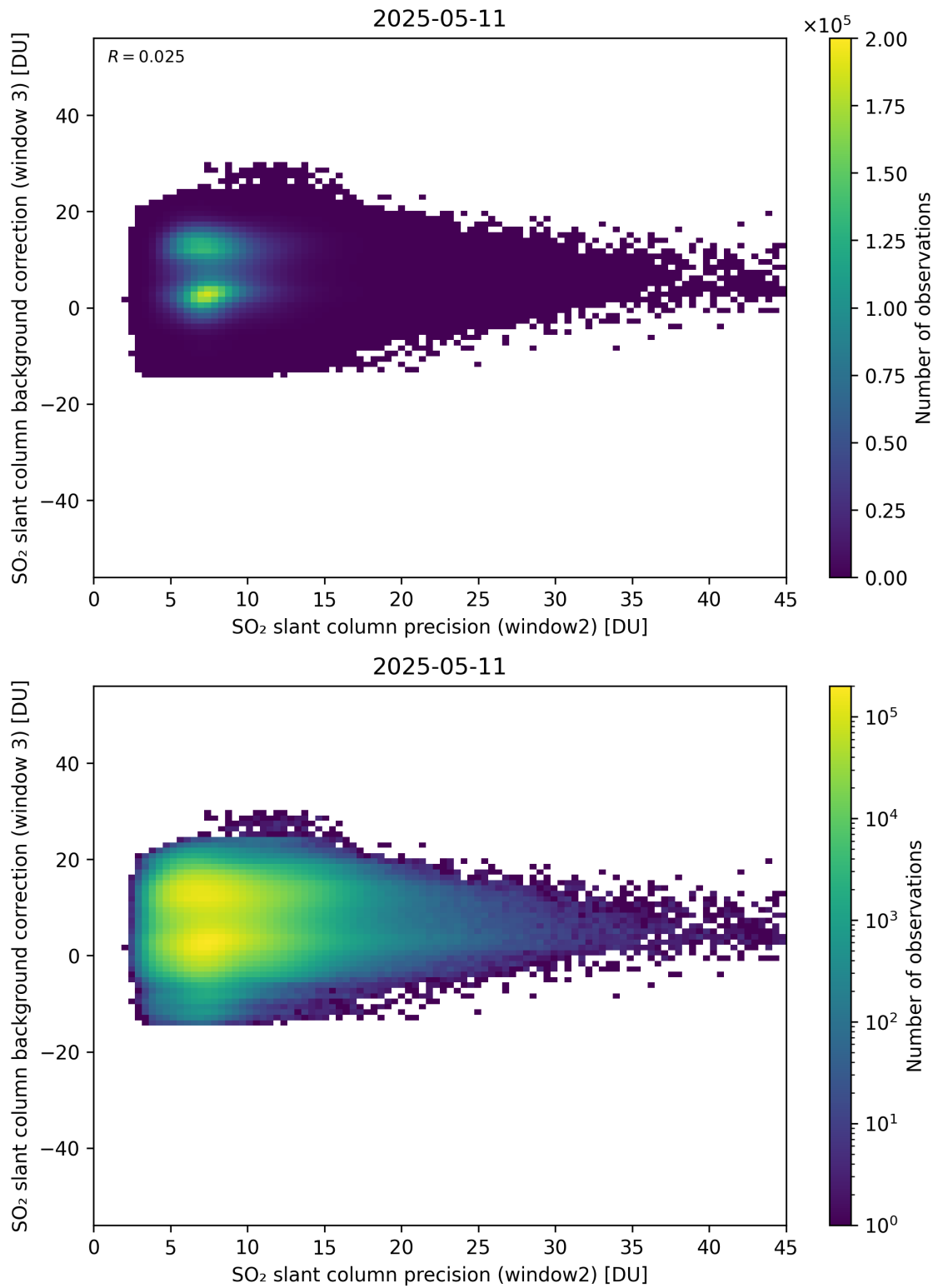
Figure 292: Scatter density plot of “SO 2 slant column precision (window2)” against “SO 2 slant column background correction (window 3)” for 2025-05-10 to 2025-05-12.
