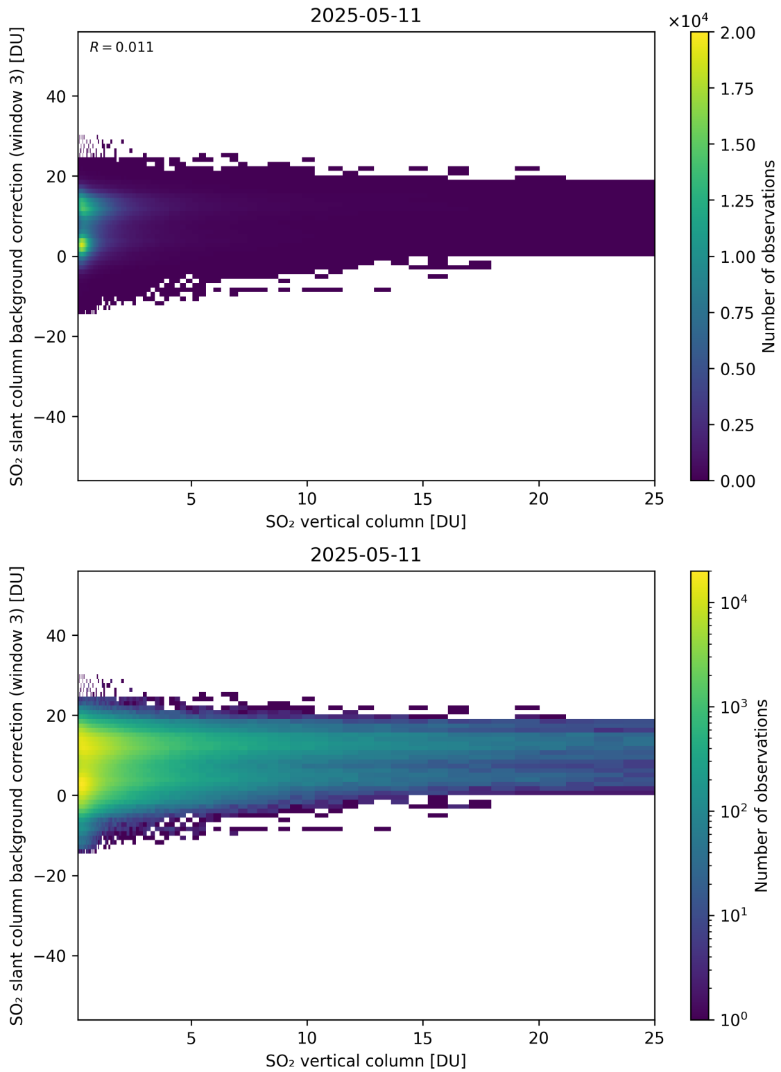
Figure 325: Scatter density plot of “SO 2 vertical column” against “SO 2 slant column background correction (window 3)” for 2025-05-10 to 2025-05-12.
