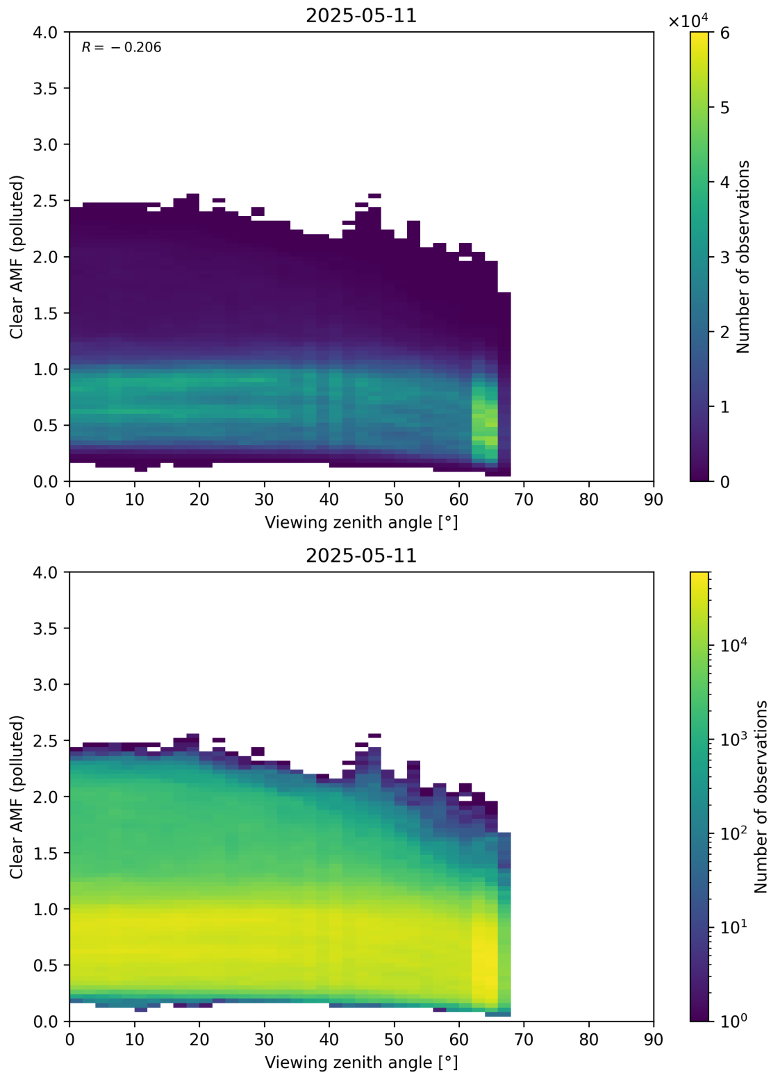
Figure 370: Scatter density plot of “Viewing zenith angle” against “Clear AMF (polluted)” for 2025-05-10 to 2025-05-12.
