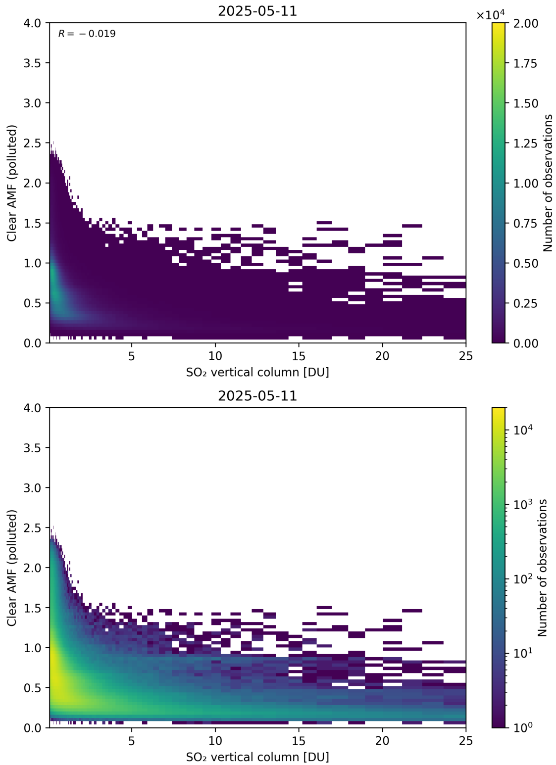
Figure 348: Scatter density plot of “SO 2 vertical column” against “Clear AMF (polluted)” for 2025-05-10 to 2025-05-12.
