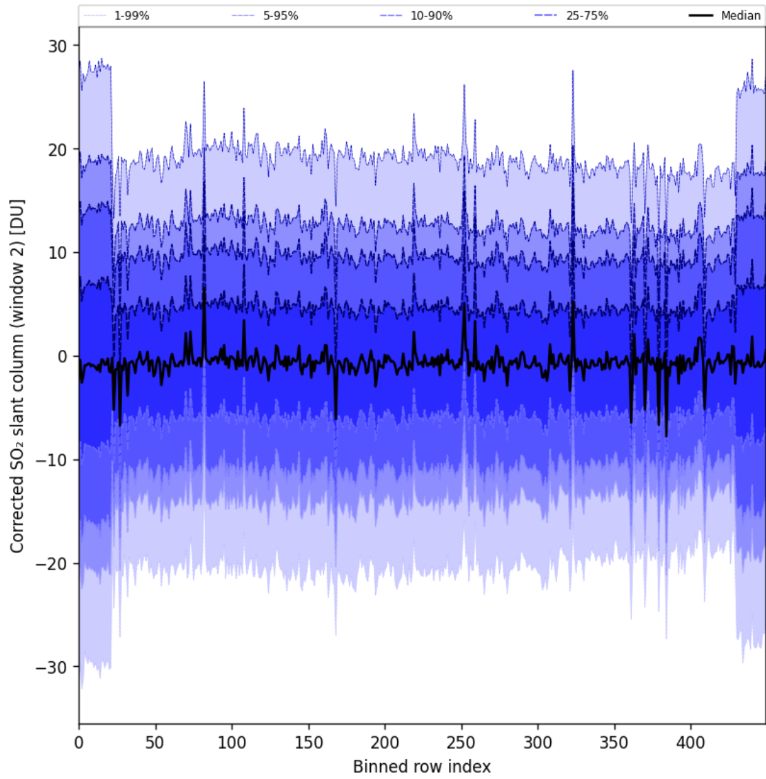
Figure 95: Along track statistics of “Corrected SO 2 slant column (window 2)” for 2025-05-10 to 2025-05-12
