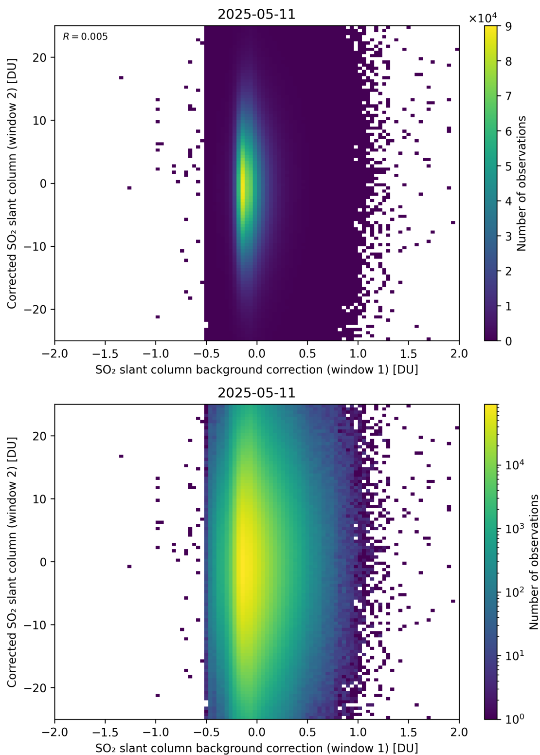
Figure 115: Scatter density plot of “SO 2 slant column background correction (window 1)” against “Corrected SO 2 slant column (window 2)” for 2025-05-10 to 2025-05-12.
