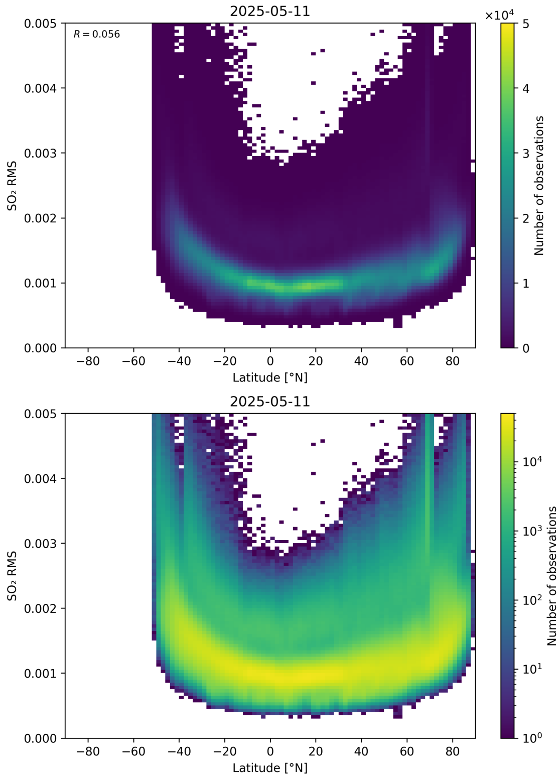
Figure 155: Scatter density plot of “Latitude” against “SO 2 RMS” for 2025-05-10 to 2025-05-12.
