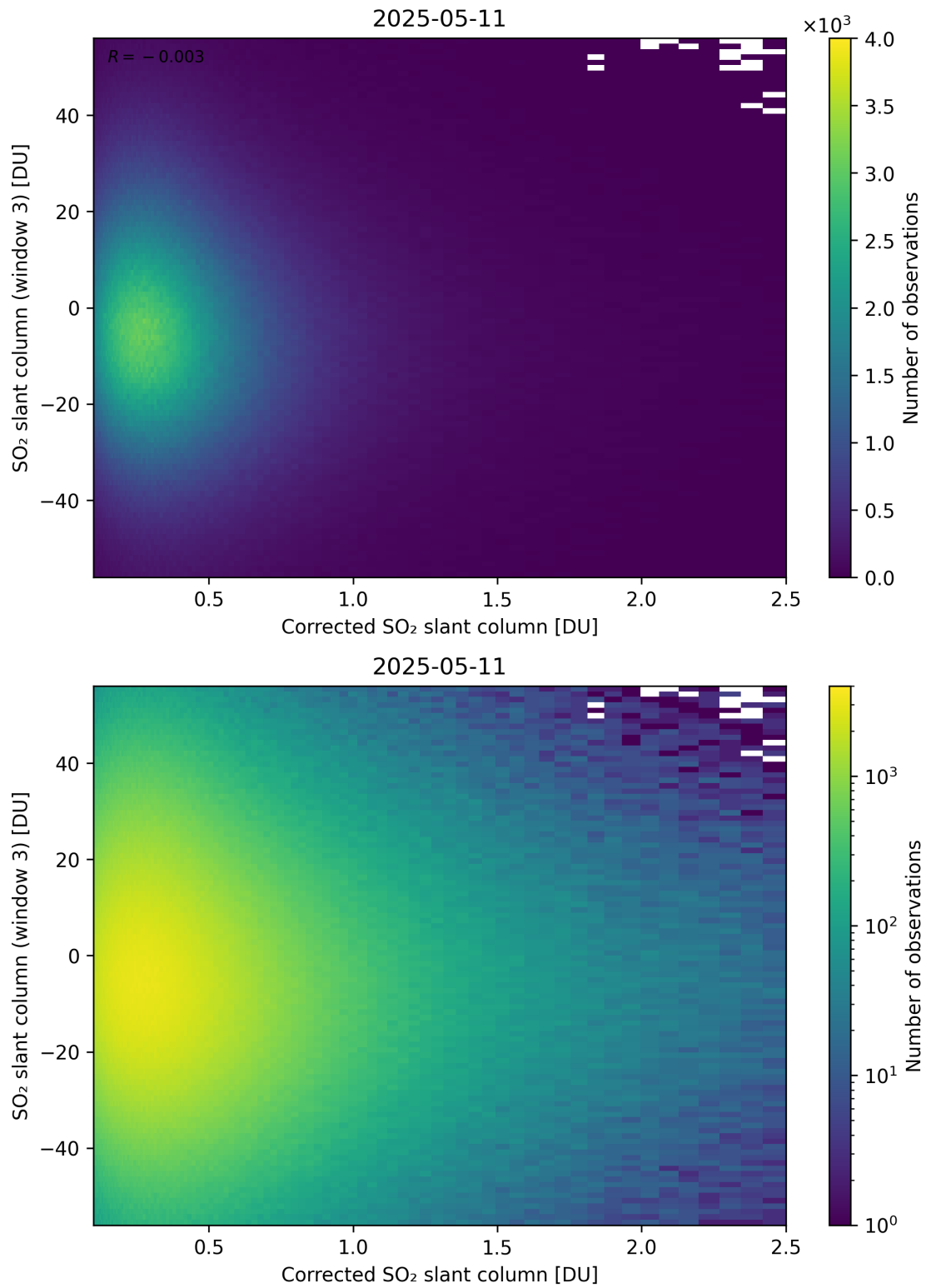
Figure 240: Scatter density plot of “Corrected SO 2 slant column” against “SO 2 slant column (window 3)” for 2025-05-10 to 2025-05-12.
