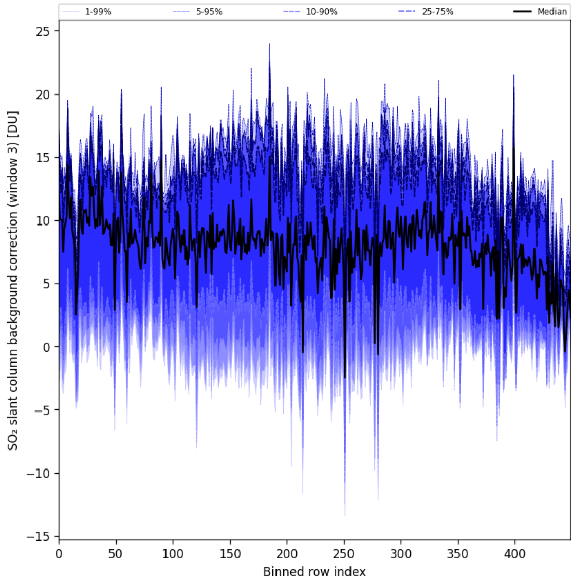
Figure 100: Along track statistics of “SO 2 slant column background correction (window 3)” for 2025-05-10 to 2025-05-12
