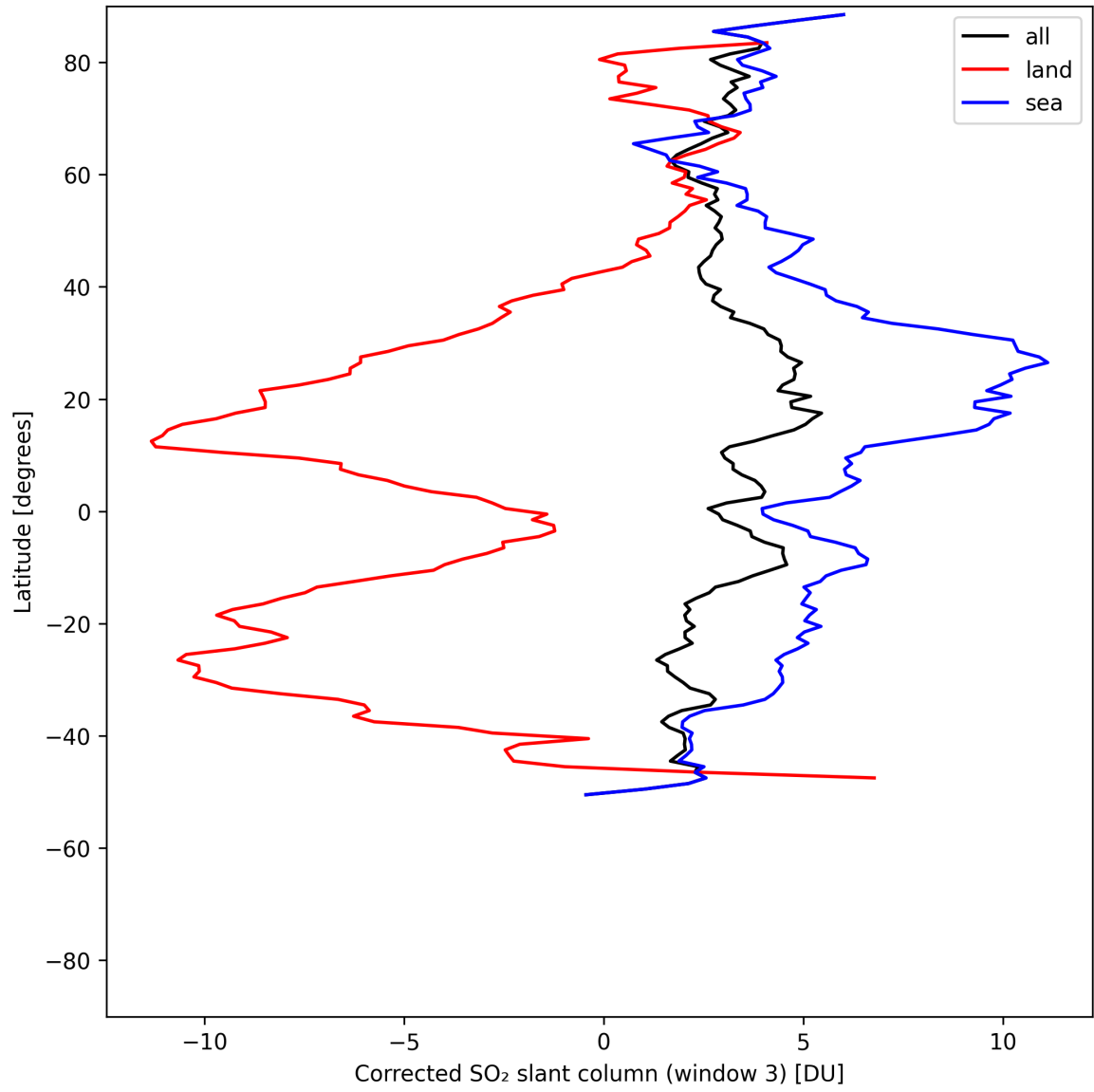
Figure 47: Zonal average of “Corrected SO 2 slant column (window 3)” for 2025-05-10 to 2025-05-12.
