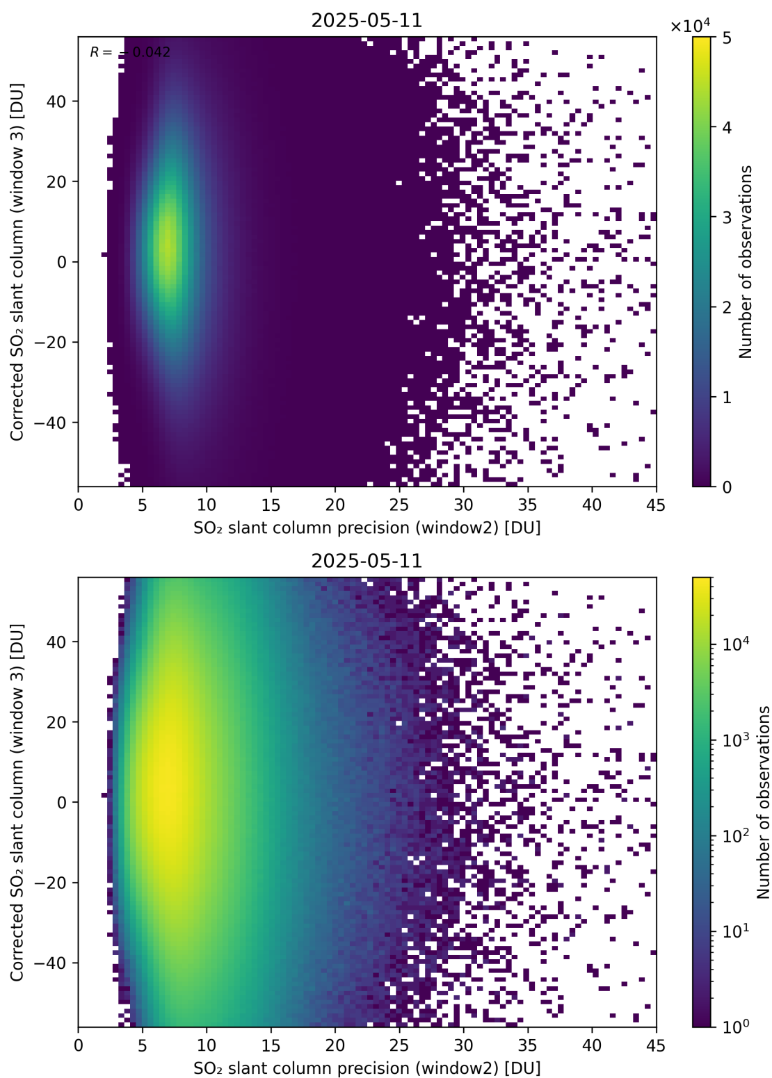
Figure 298: Scatter density plot of “SO 2 slant column precision (window2)” against “Corrected SO 2 slant column (window 3)” for 2025-05-10 to 2025-05-12.
