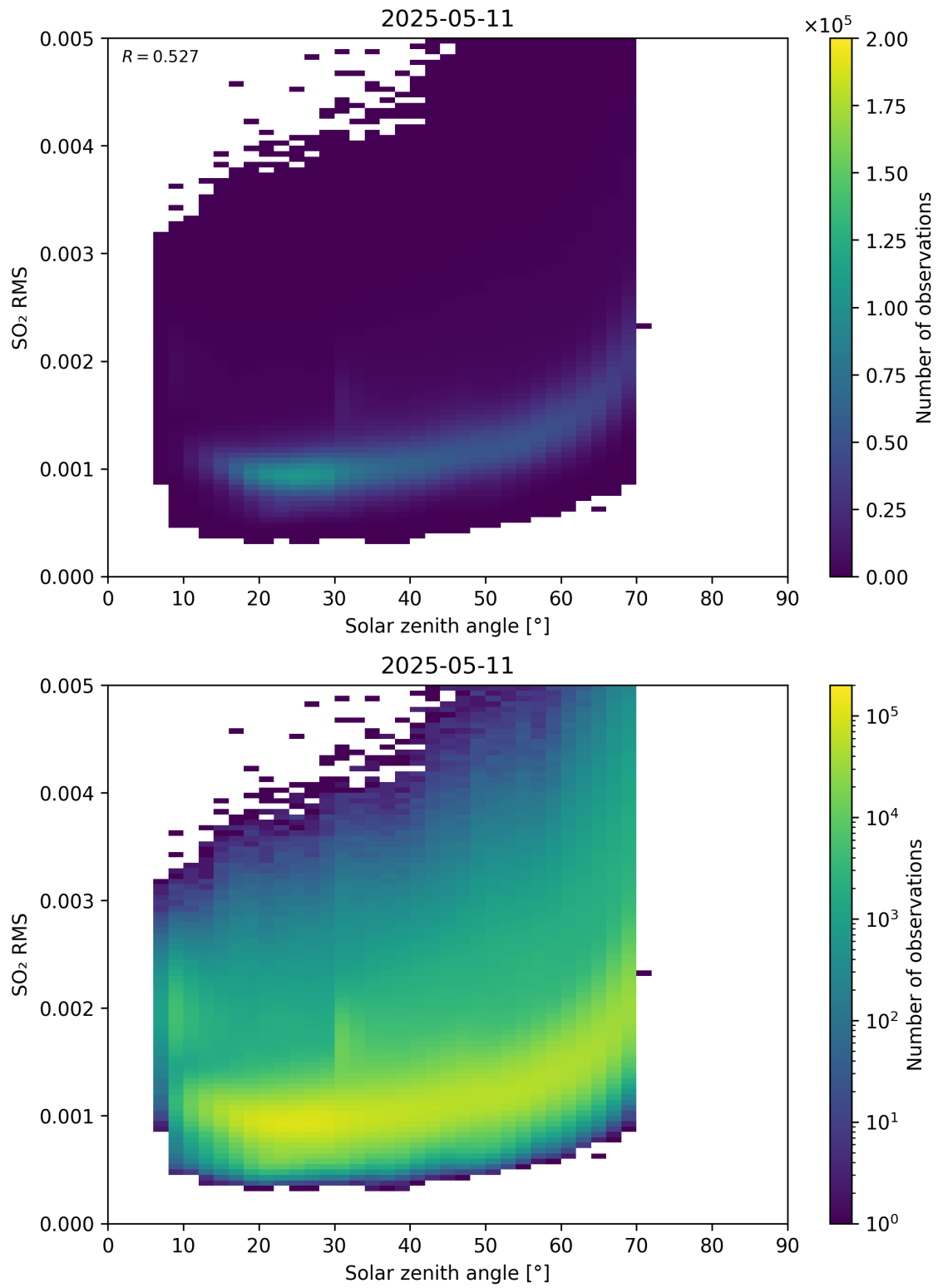
Figure 176: Scatter density plot of “Solar zenith angle” against “SO 2 RMS” for 2025-05-10 to 2025-05-12.
