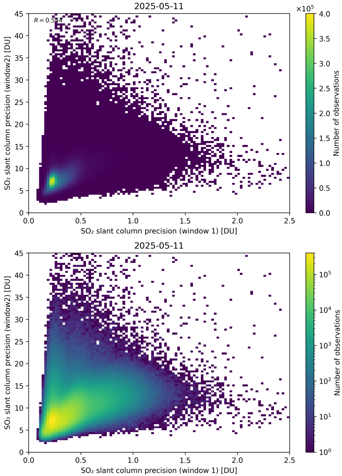
Figure 277: Scatter density plot of “SO 2 slant column precision (window 1)” against “SO 2 slant column precision (window2)” for 2025-05-10 to 2025-05-12.
