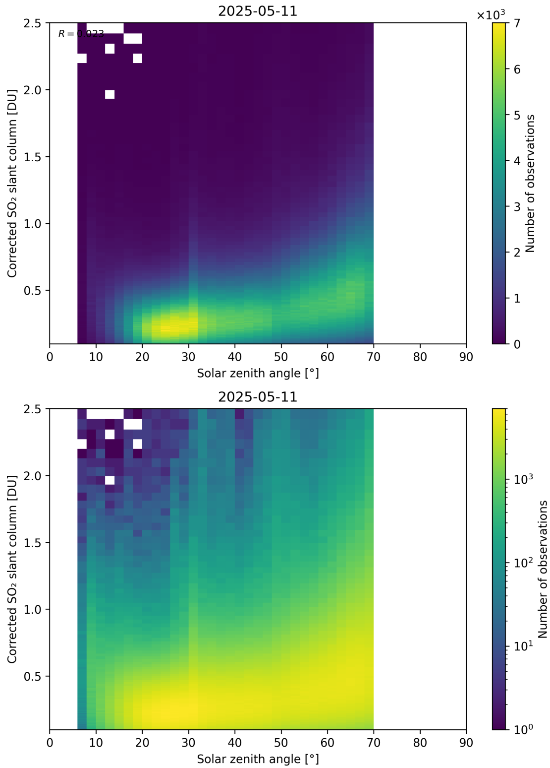
Figure 181: Scatter density plot of “Solar zenith angle” against “Corrected SO 2 slant column” for 2025-05-10 to 2025-05-12.
