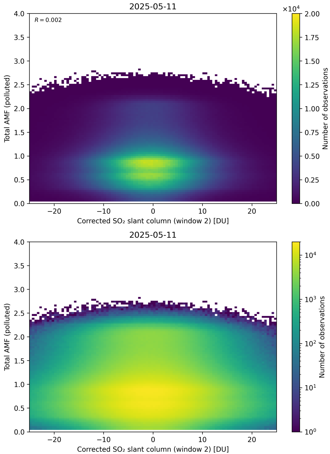
Figure 253: Scatter density plot of “Corrected SO 2 slant column (window 2)” against “Total AMF (polluted)” for 2025-05-10 to 2025-05-12.
