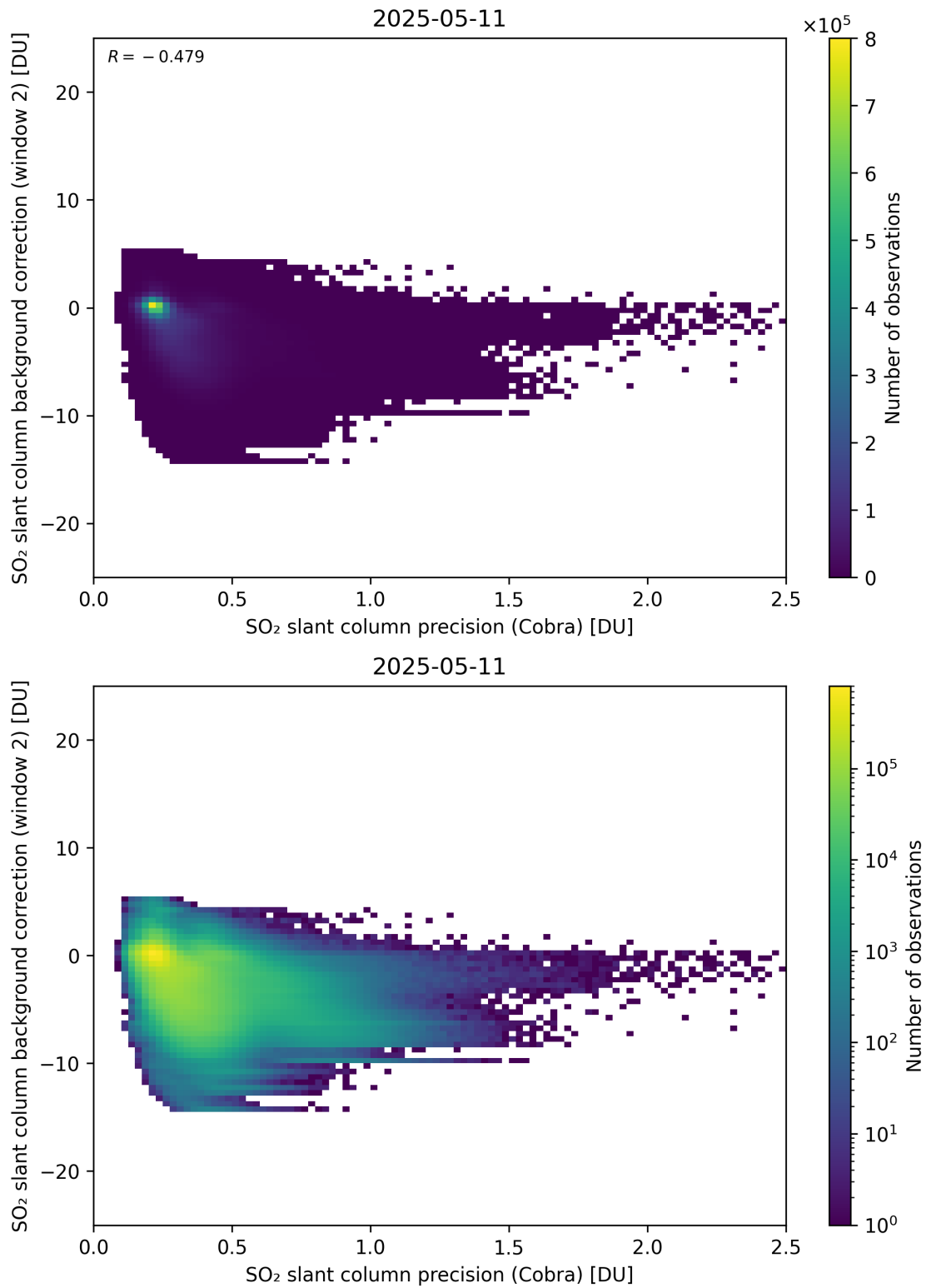
Figure 200: Scatter density plot of “SO 2 slant column precision (Cobra)” against “SO 2 slant column background correction (window 2)” for 2025-05-10 to 2025-05-12.
