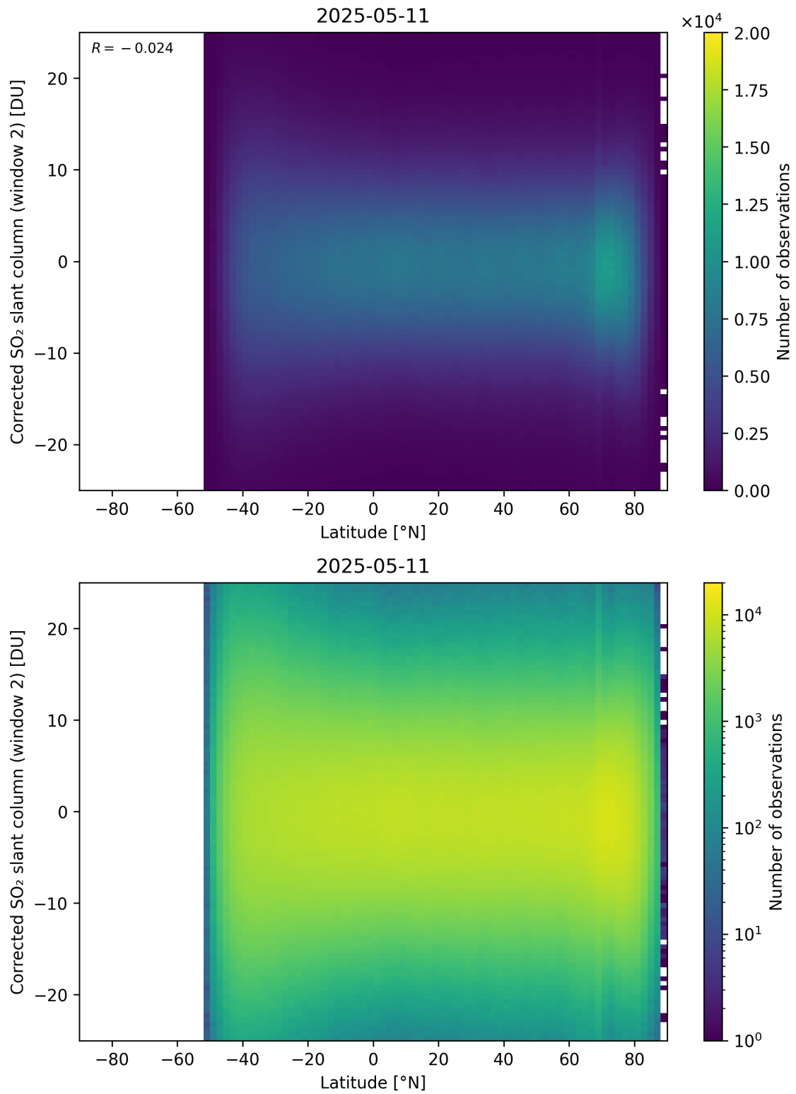
Figure 160: Scatter density plot of “Latitude” against “Corrected SO 2 slant column (window 2)” for 2025-05-10 to 2025-05-12.
