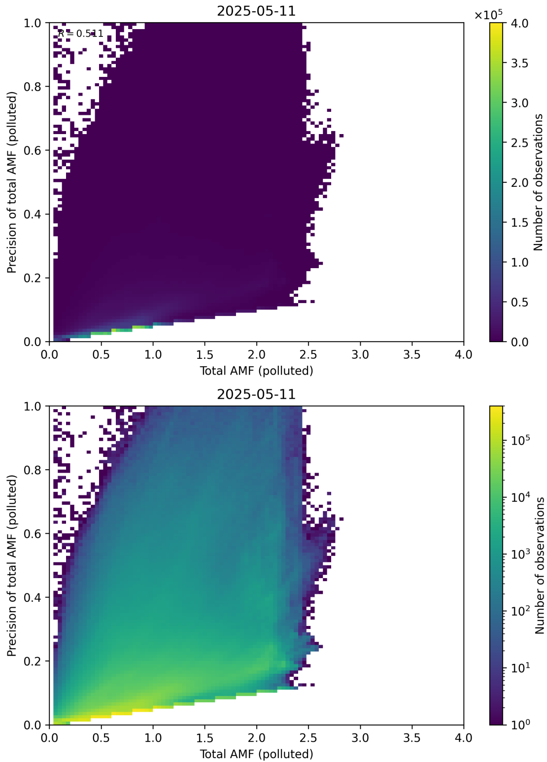
Figure 322: Scatter density plot of “Total AMF (polluted)” against “Precision of total AMF (polluted)” for 2025-05-10 to 2025-05-12.
