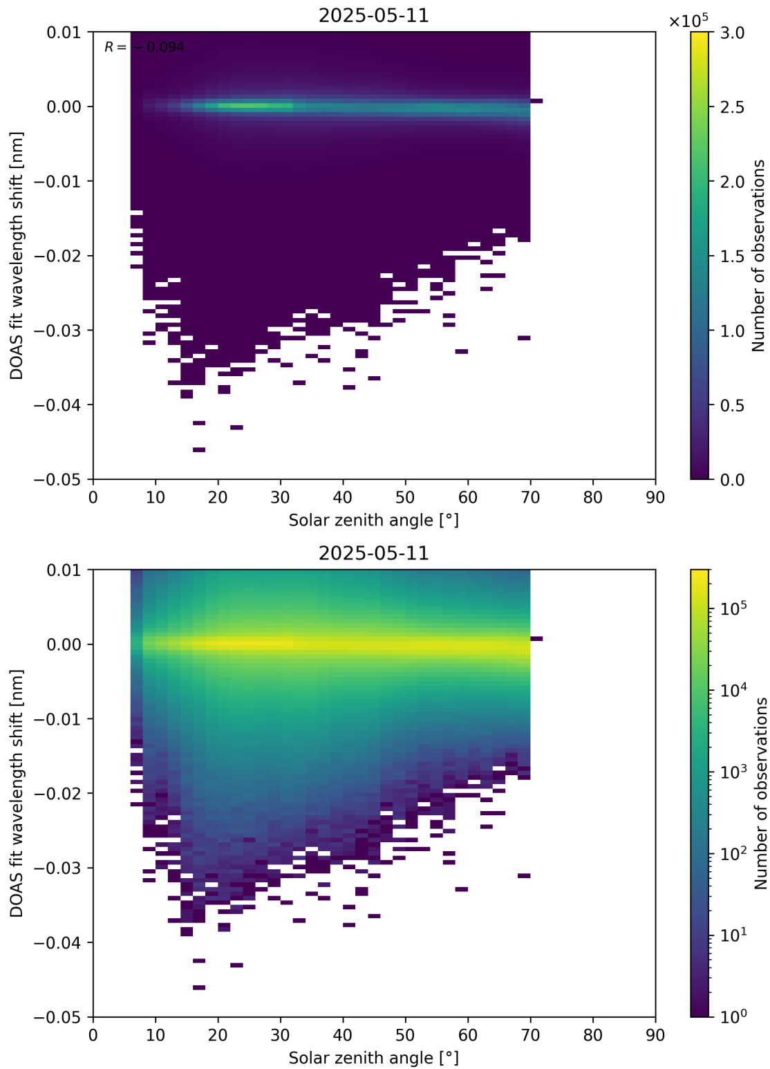
Figure 174: Scatter density plot of “Solar zenith angle” against “DOAS fit wavelength shift” for 2025-05-10 to 2025-05-12.
