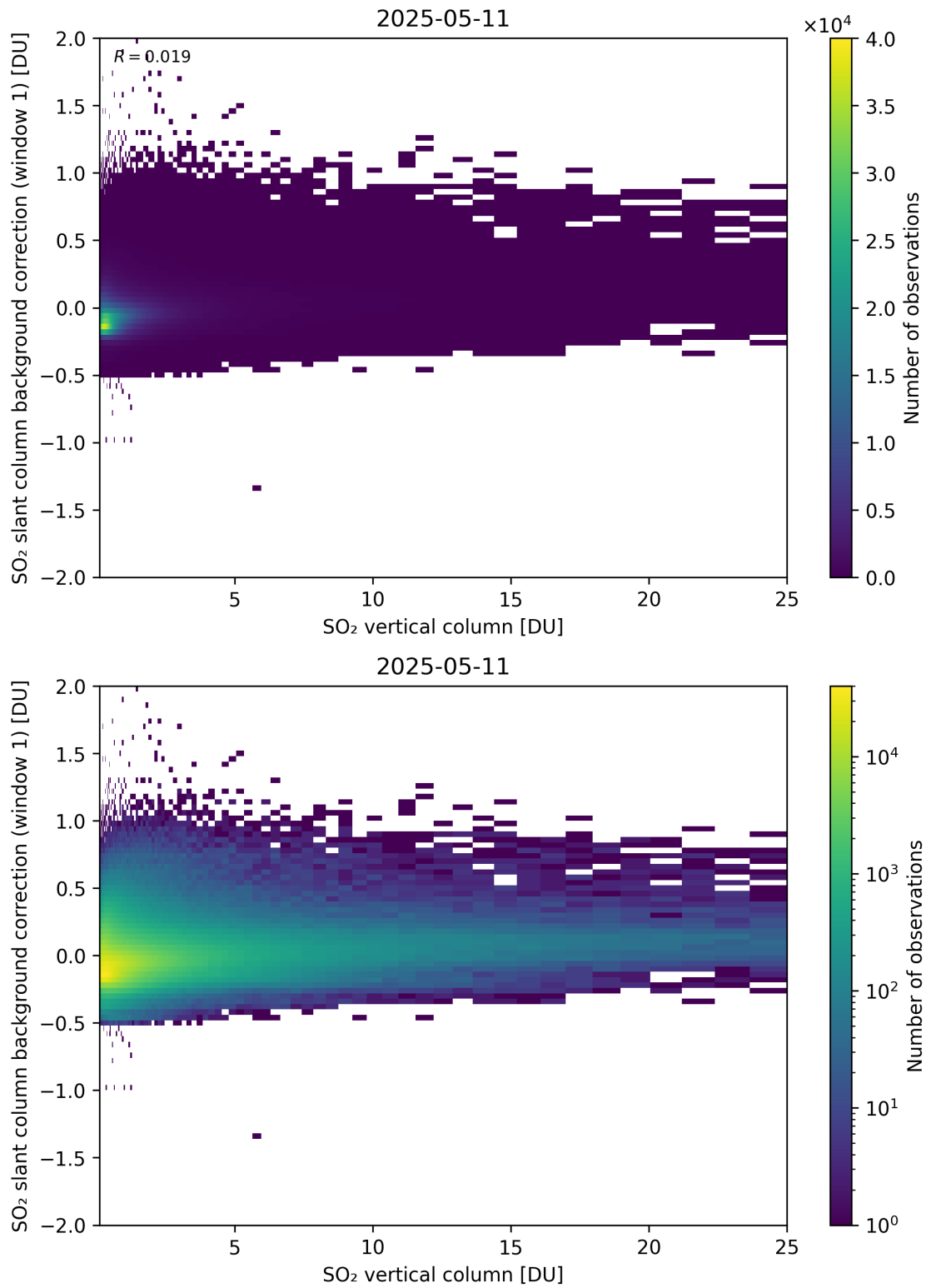
Figure 323: Scatter density plot of “SO 2 vertical column” against “SO 2 slant column background correction (window 1)” for 2025-05-10 to 2025-05-12.
