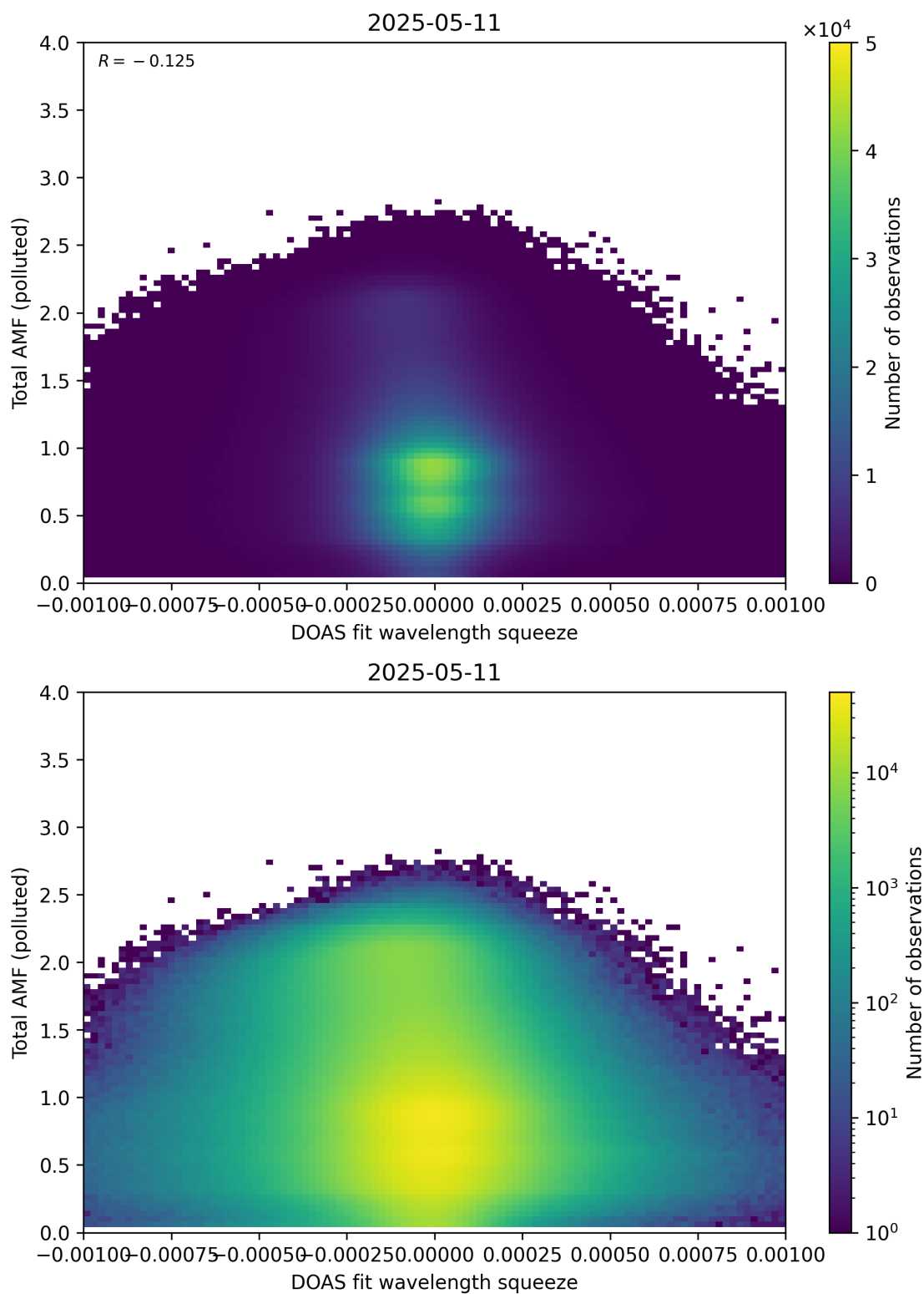
Figure 145: Scatter density plot of “DOAS fit wavelength squeeze” against “Total AMF (polluted)” for 2025-05-10 to 2025-05-12.
