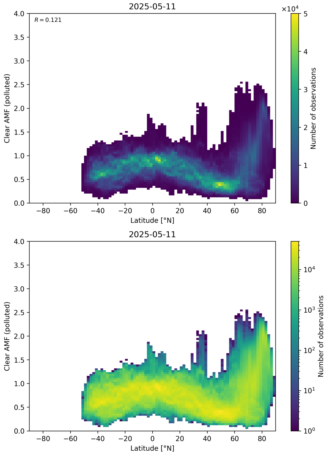
Figure 156: Scatter density plot of “Latitude” against “Clear AMF (polluted)” for 2025-05-10 to 2025-05-12.
