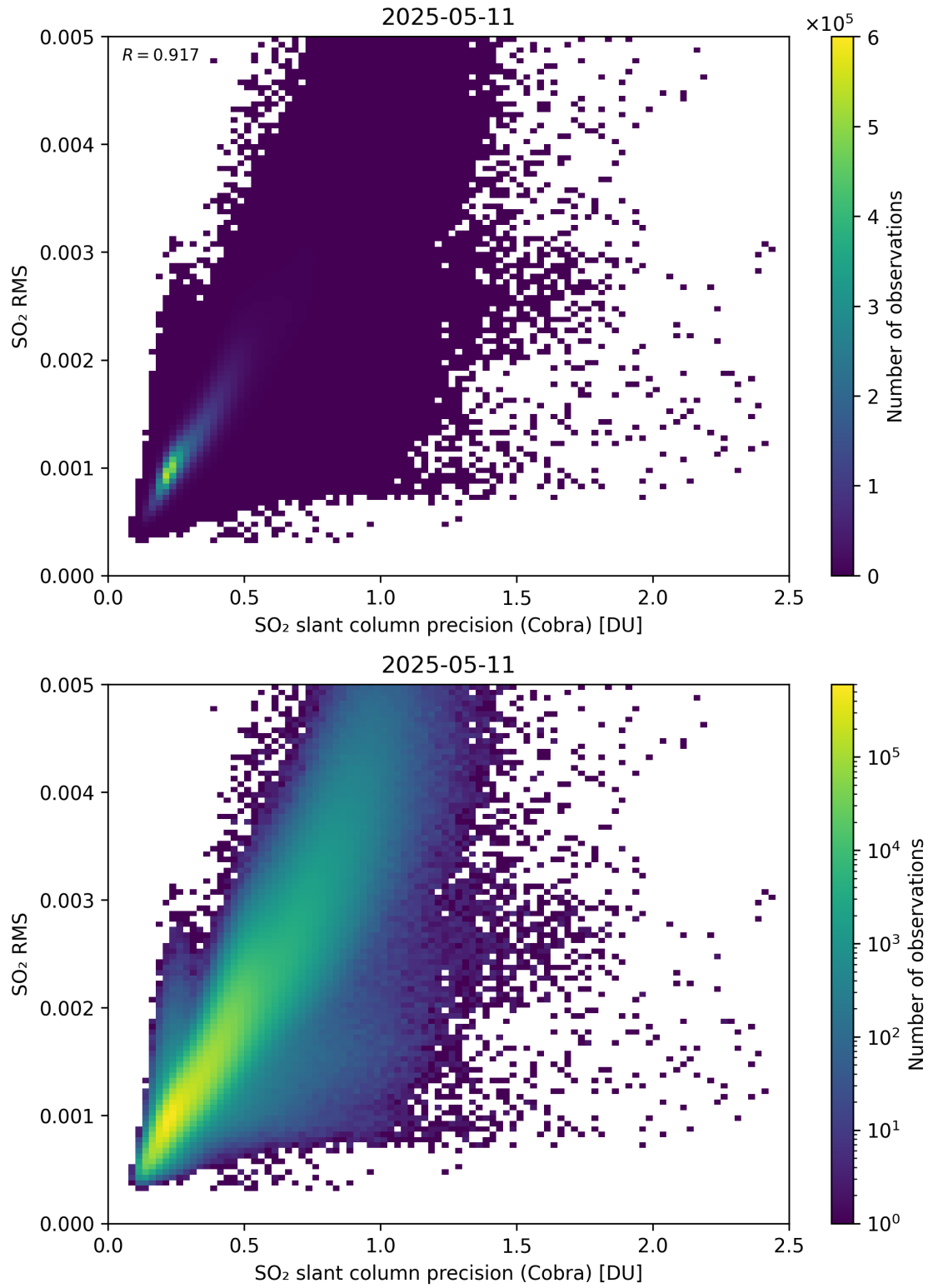
Figure 204: Scatter density plot of “SO 2 slant column precision (Cobra)” against “SO 2 RMS” for 2025-05-10 to 2025-05-12.
