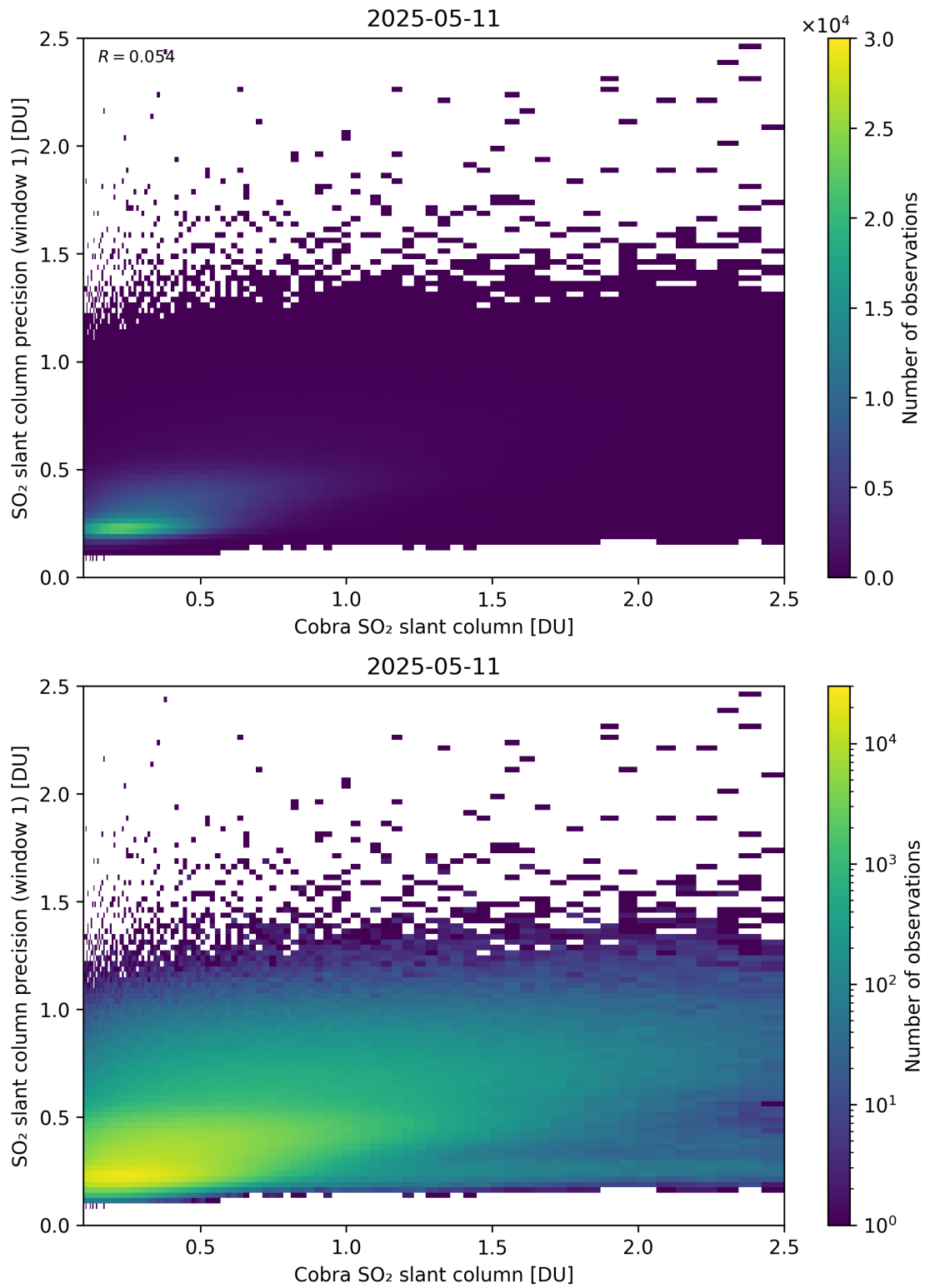
Figure 220: Scatter density plot of “Cobra SO 2 slant column” against “SO 2 slant column precision (window 1)” for 2025-05-10 to 2025-05-12.
