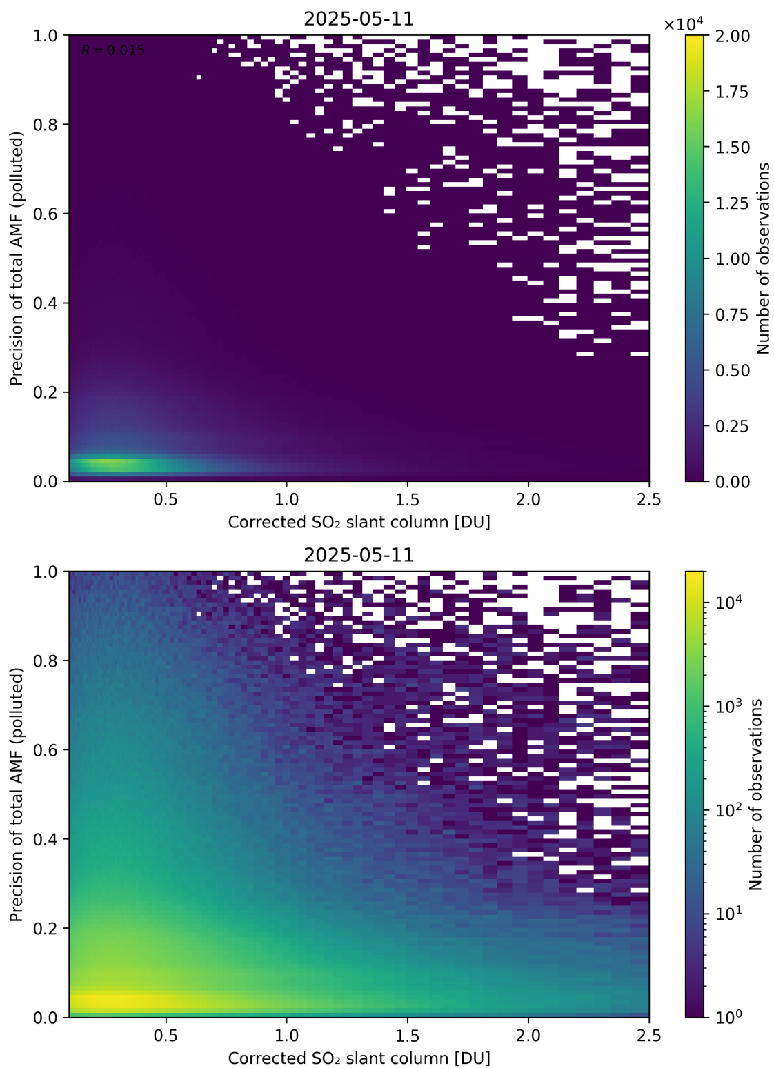
Figure 243: Scatter density plot of “Corrected SO 2 slant column” against “Precision of total AMF (polluted)” for 2025-05-10 to 2025-05-12.
