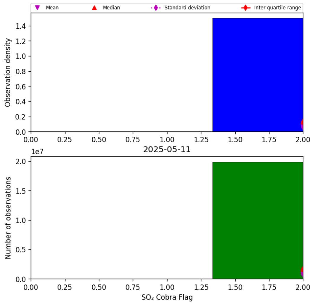
Figure 75: Histogram of "SO 2 Cobra Flag" for 2025-05-10 to 2025-05-12
