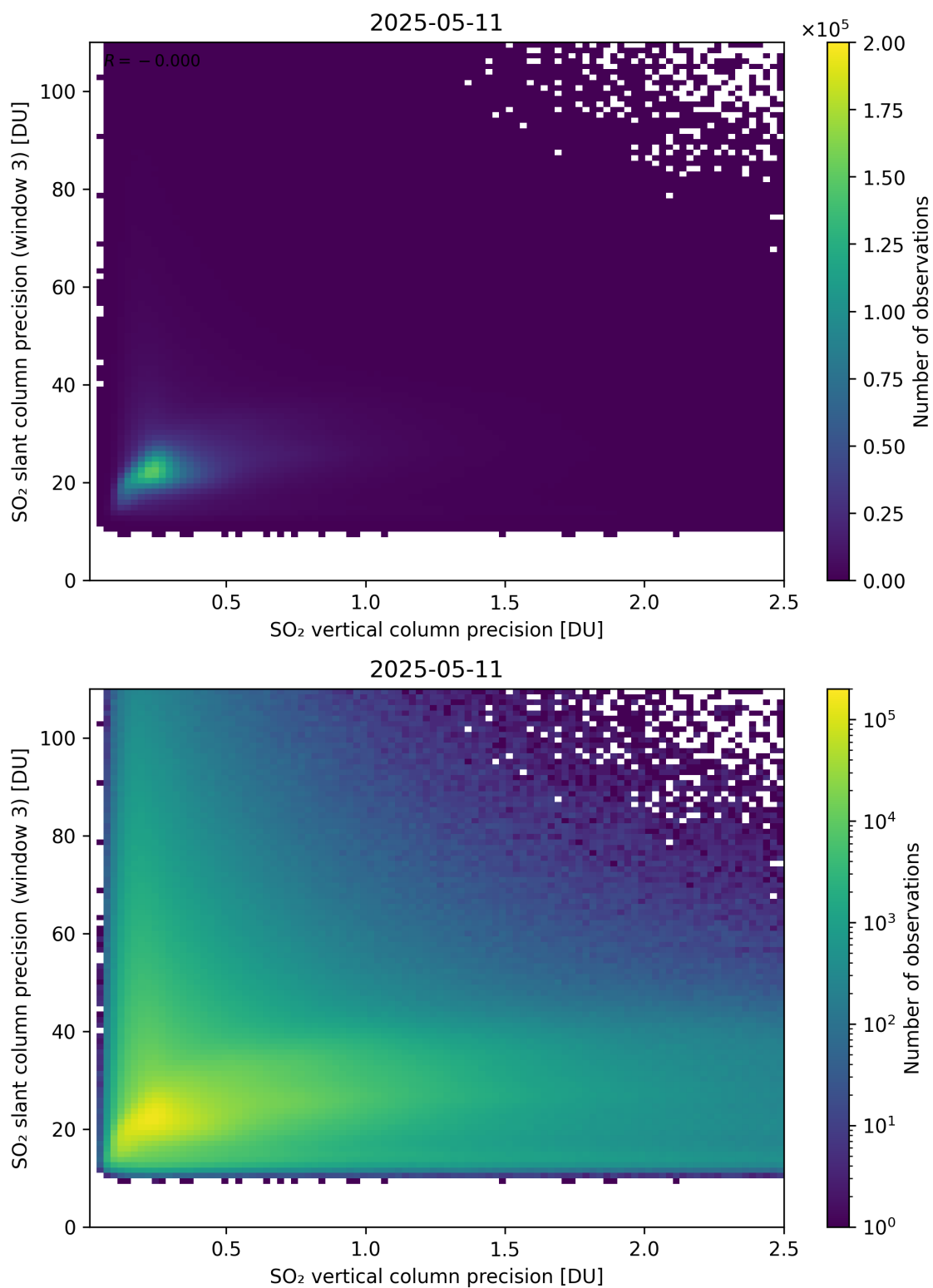
Figure 345: Scatter density plot of “SO 2 vertical column precision” against “SO 2 slant column precision (window 3)” for 2025-05-10 to 2025-05-12.
