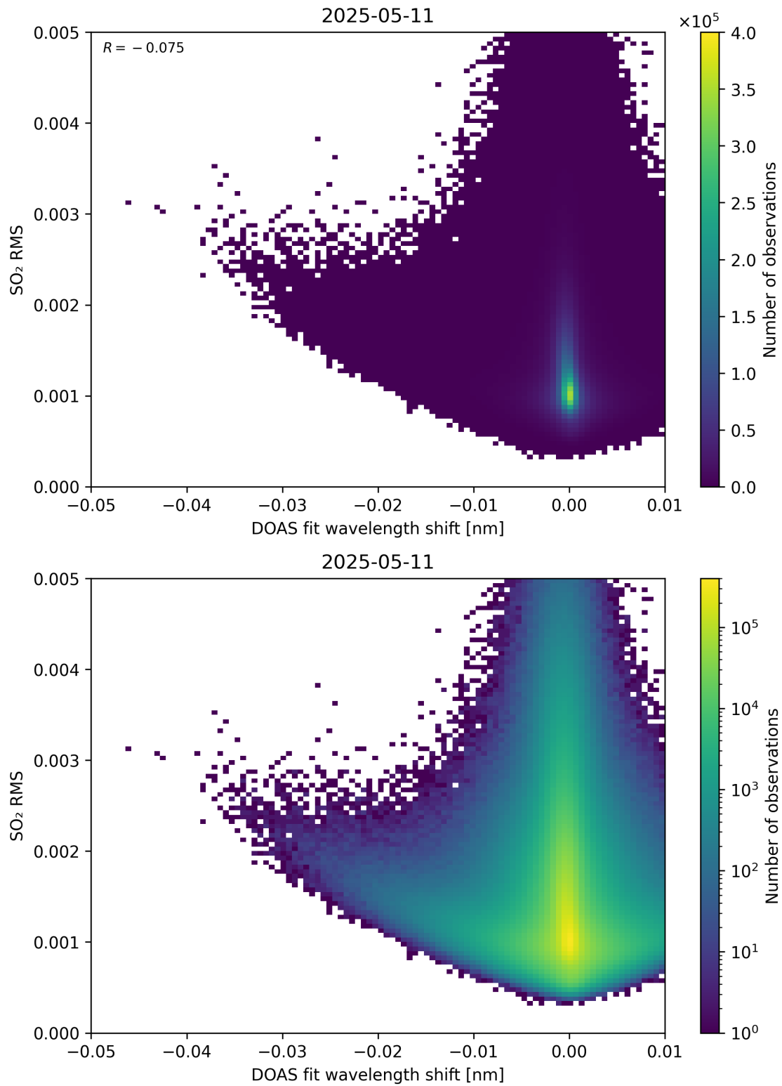
Figure 139: Scatter density plot of “DOAS fit wavelength shift” against “SO 2 RMS” for 2025-05-10 to 2025-05-12.
