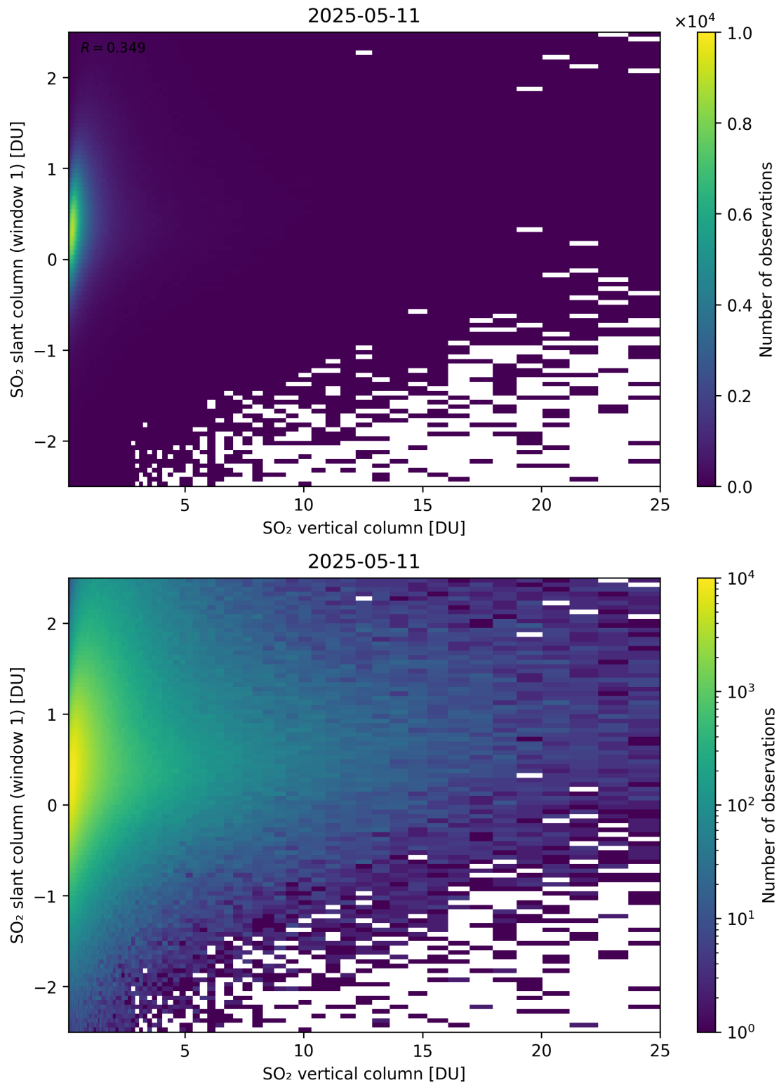
Figure 354: Scatter density plot of “SO 2 vertical column” against “SO 2 slant column (window 1)” for 2025-05-10 to 2025-05-12.
