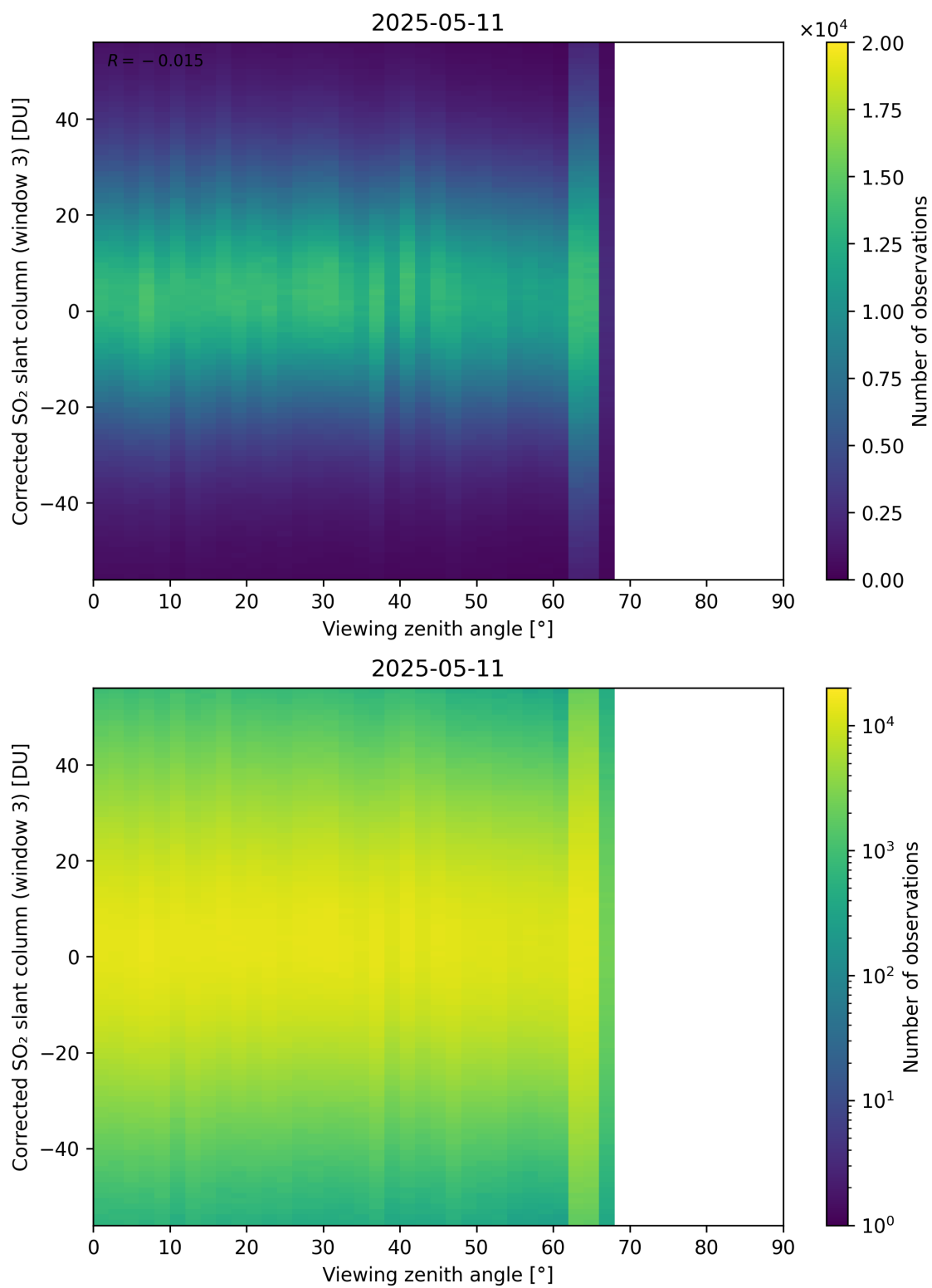
Figure 375: Scatter density plot of “Viewing zenith angle” against “Corrected SO 2 slant column (window 3)” for 2025-05-10 to 2025-05-12.
