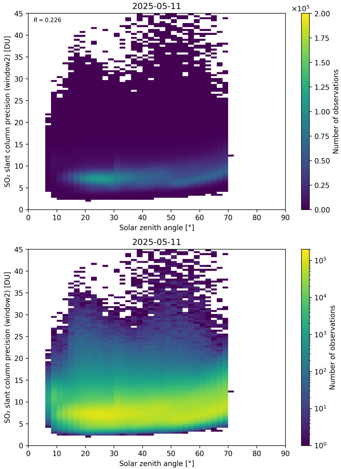
Figure 186: Scatter density plot of “Solar zenith angle” against “SO 2 slant column precision (window2)” for 2025-05-10 to 2025-05-12.
