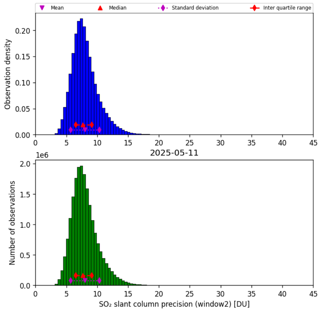
Figure 68: Histogram of “SO 2 slant column precision (window2)” for 2025-05-10 to 2025-05-12
