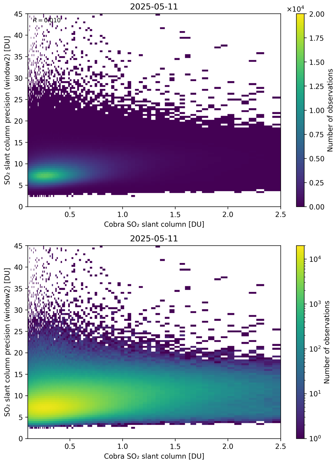
Figure 221: Scatter density plot of “Cobra SO 2 slant column” against “SO 2 slant column precision (window2)” for 2025-05-10 to 2025-05-12.
