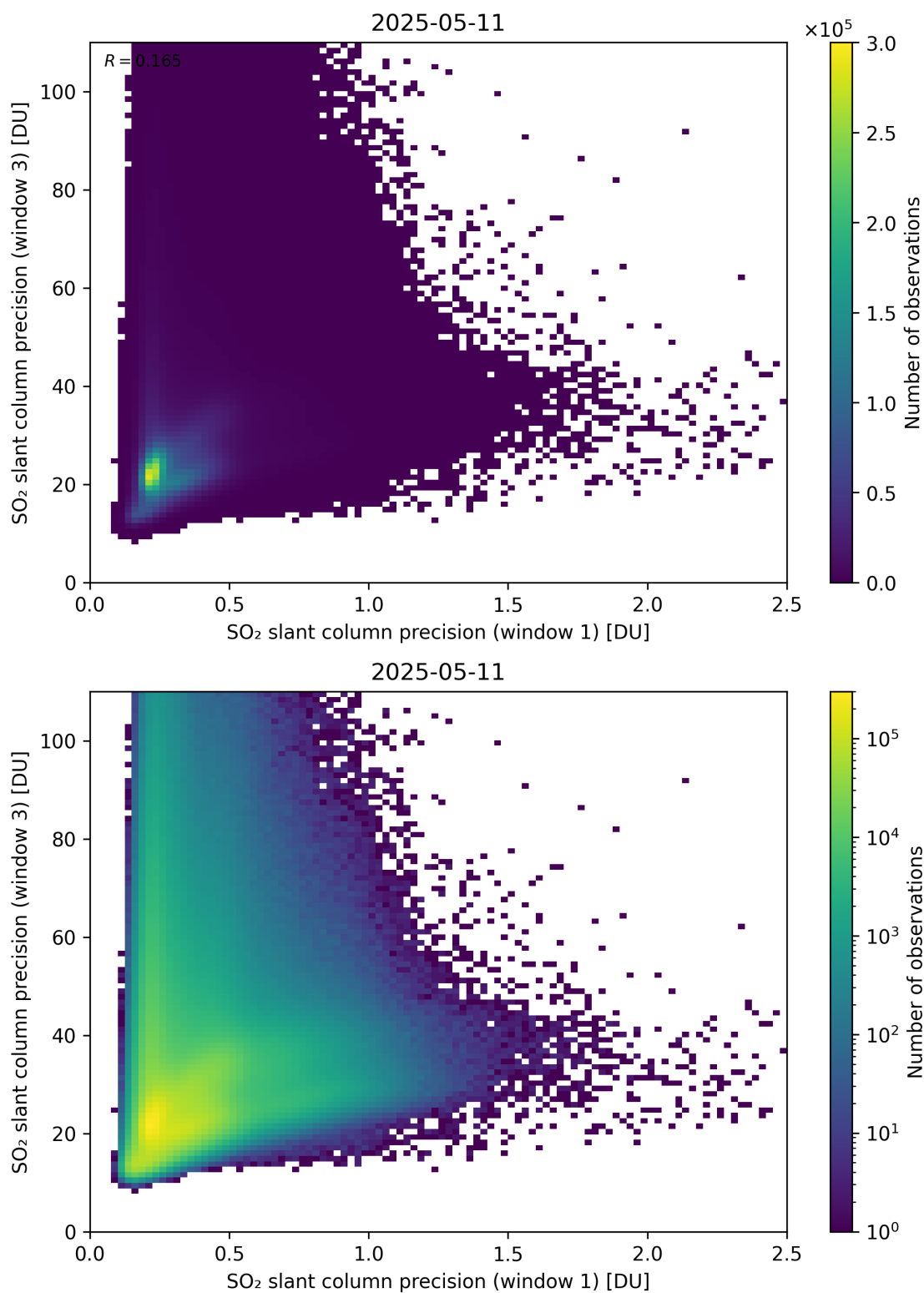
Figure 279: Scatter density plot of “SO 2 slant column precision (window 1)” against “SO 2 slant column precision (window 3)” for 2025-05-10 to 2025-05-12.
