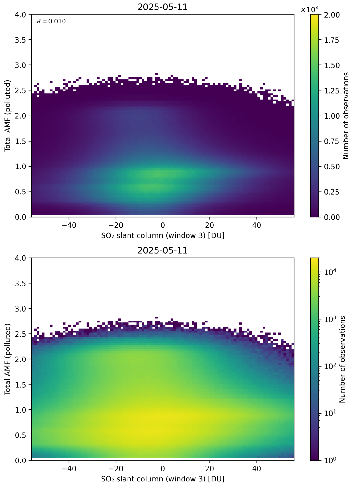
Figure 318: Scatter density plot of “SO 2 slant column (window 3)” against “Total AMF (polluted)” for 2025-05-10 to 2025-05-12.
