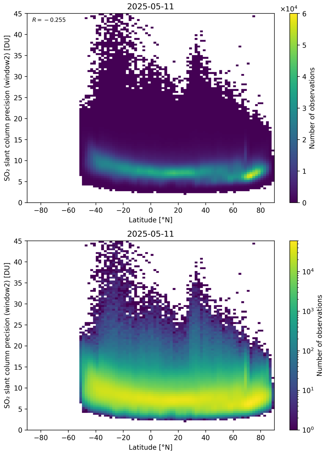
Figure 164: Scatter density plot of “Latitude” against “SO 2 slant column precision (window2)” for 2025-05-10 to 2025-05-12.
