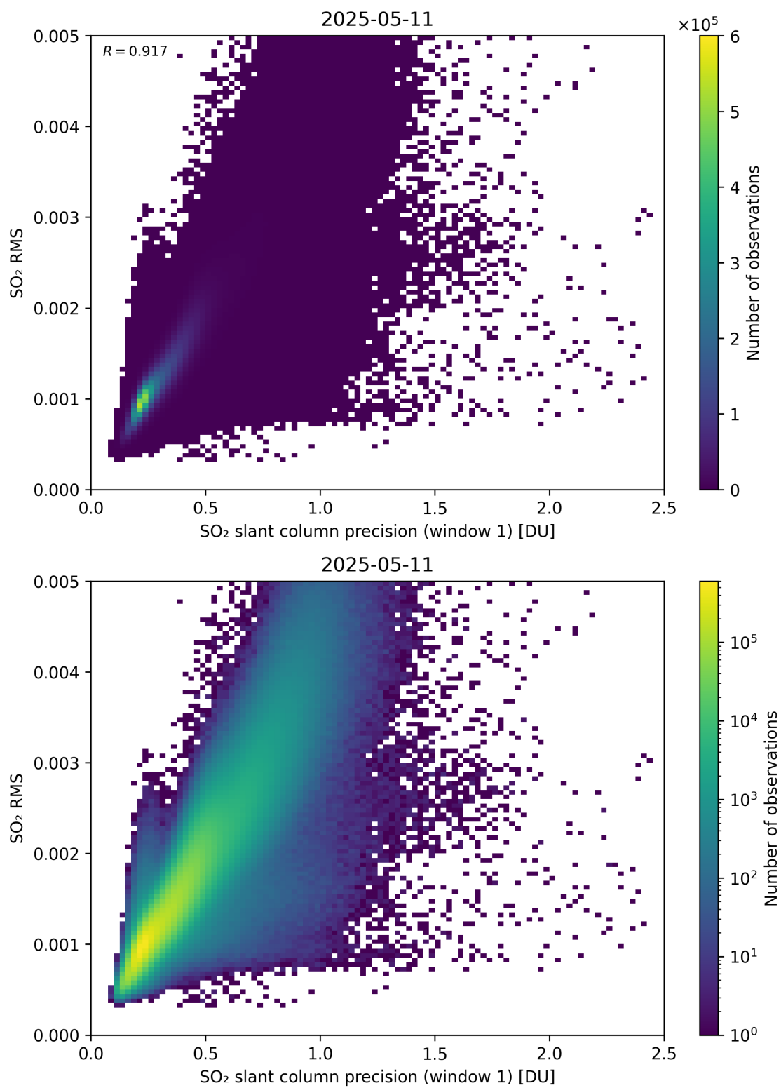
Figure 273: Scatter density plot of “SO 2 slant column precision (window 1)” against “SO 2 RMS” for 2025-05-10 to 2025-05-12.
