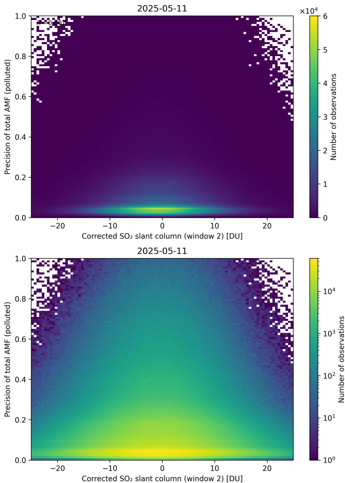
Figure 254: Scatter density plot of “Corrected SO 2 slant column (window 2)” against “Precision of total AMF (polluted)” for 2025-05-10 to 2025-05-12.
