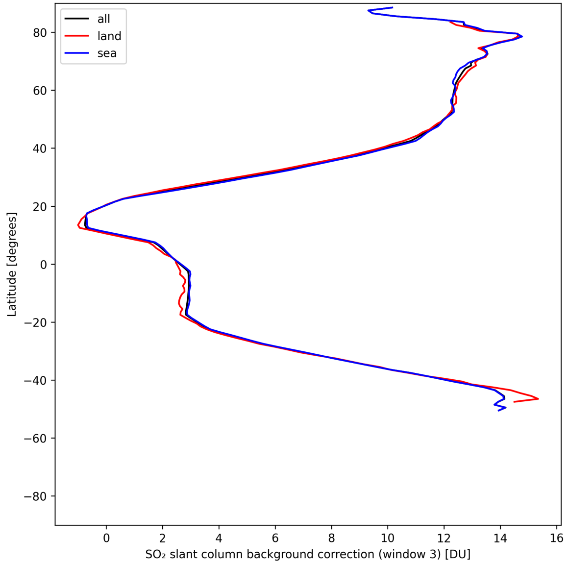
Figure 48: Zonal average of “SO 2 slant column background correction (window 3)” for 2025-05-10 to 2025-05-12.
