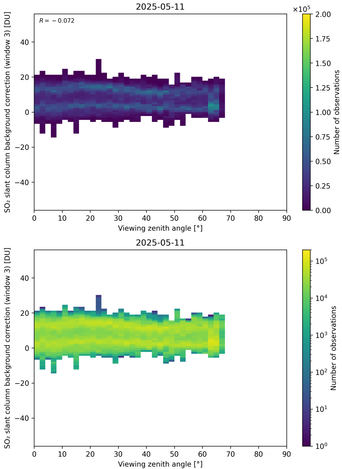
Figure 364: Scatter density plot of “Viewing zenith angle” against “SO 2 slant column background correction (window 3)” for 2025-05-10 to 2025-05-12.
