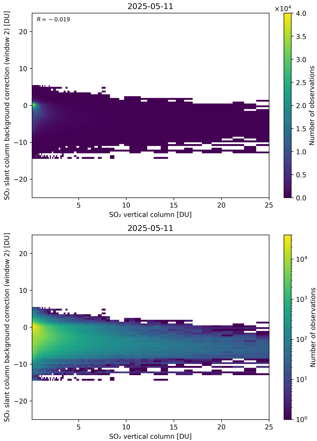
Figure 324: Scatter density plot of “SO 2 vertical column” against “SO 2 slant column background correction (window 2)” for 2025-05-10 to 2025-05-12.
