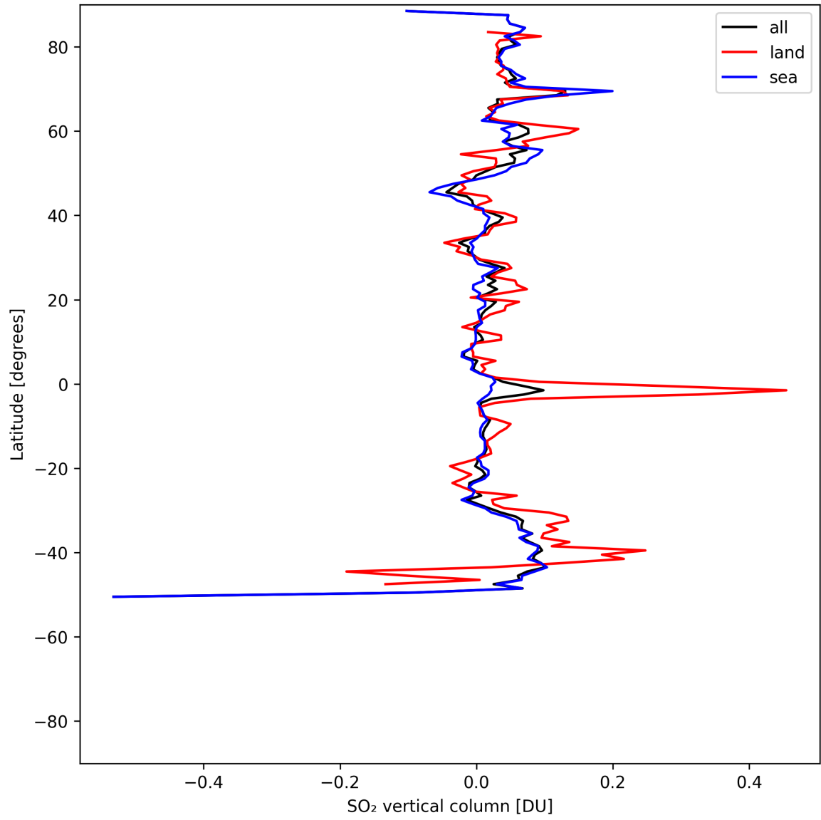
Figure 32: Zonal average of “SO 2 vertical column” for 2025-05-10 to 2025-05-12.
