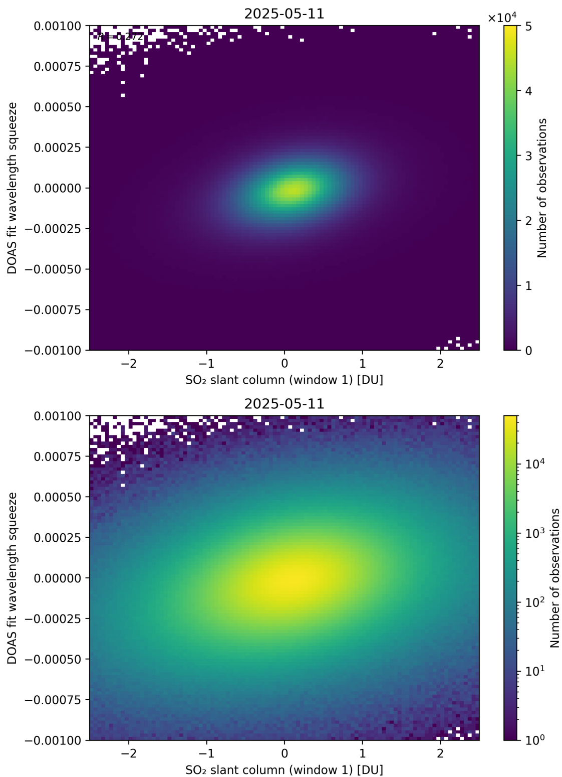
Figure 266: Scatter density plot of “SO 2 slant column (window 1)” against “DOAS fit wavelength squeeze” for 2025-05-10 to 2025-05-12.
