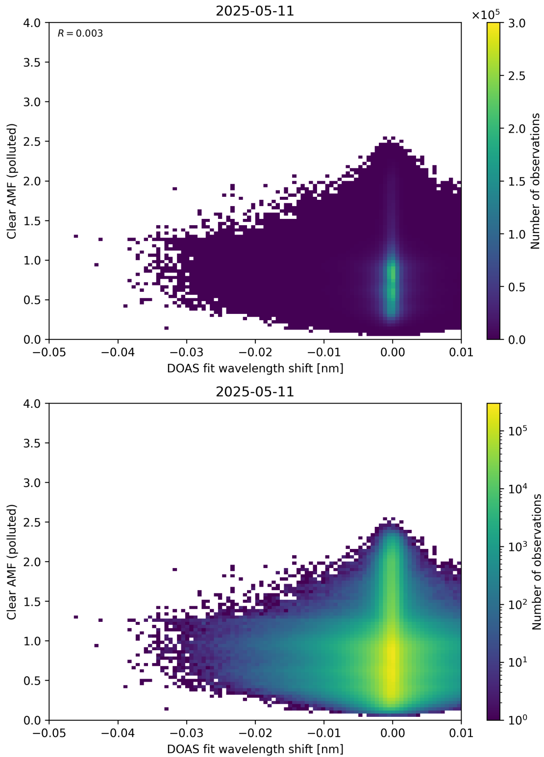
Figure 140: Scatter density plot of “DOAS fit wavelength shift” against “Clear AMF (polluted)” for 2025-05-10 to 2025-05-12.
