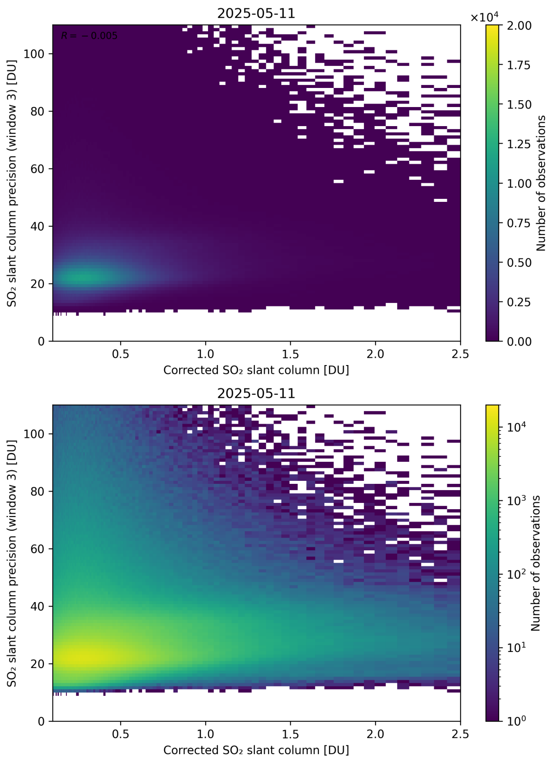
Figure 241: Scatter density plot of “Corrected SO 2 slant column” against “SO 2 slant column precision (window 3)” for 2025-05-10 to 2025-05-12.
