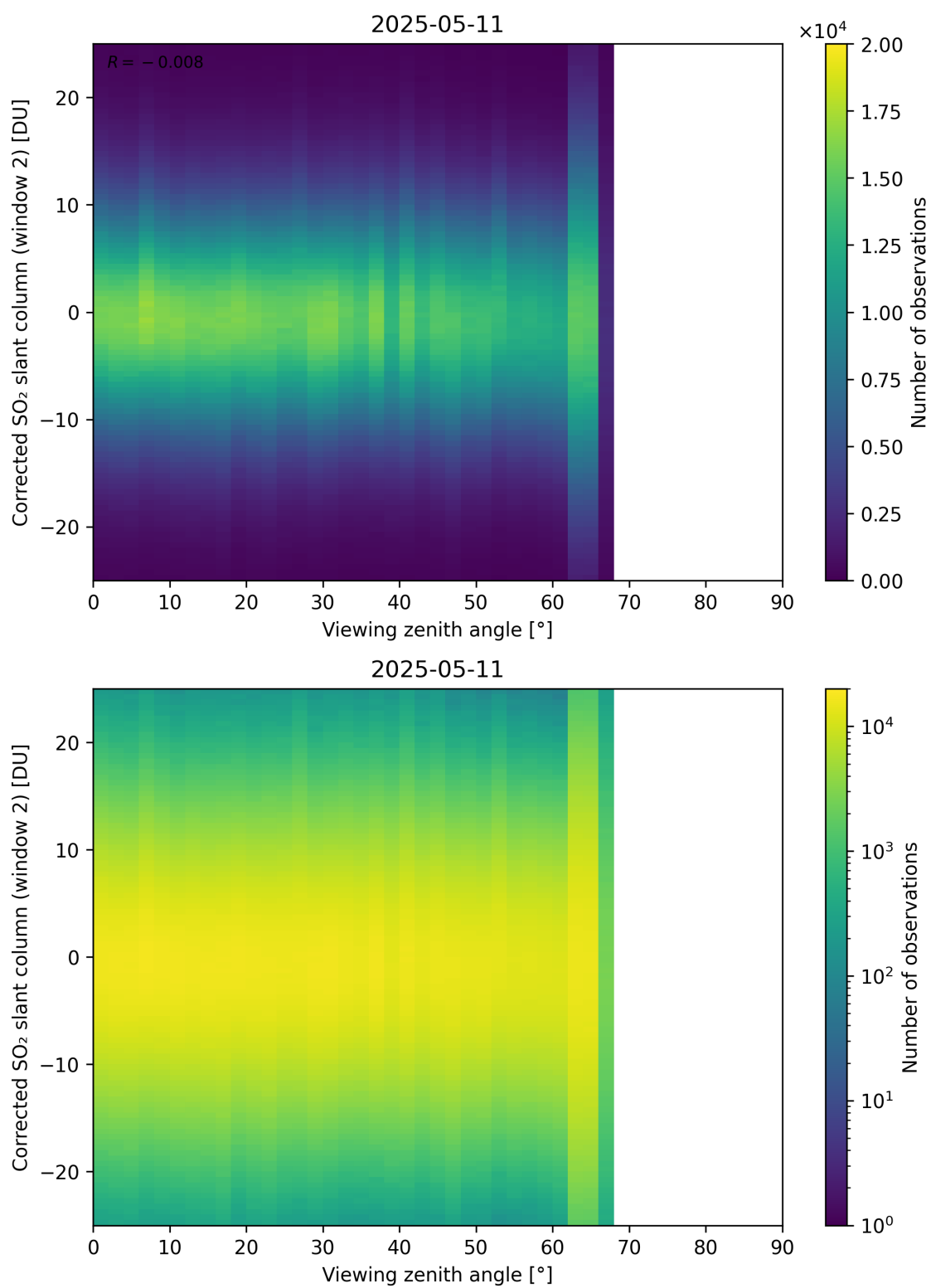
Figure 374: Scatter density plot of “Viewing zenith angle” against “Corrected SO 2 slant column (window 2)” for 2025-05-10 to 2025-05-12.
