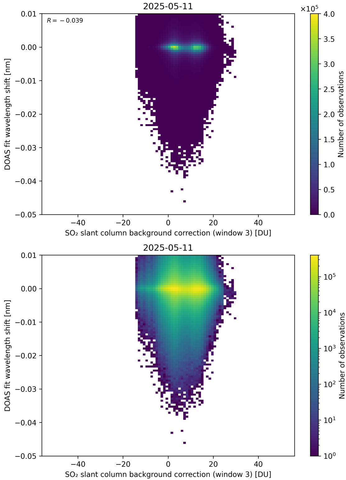
Figure 132: Scatter density plot of “SO 2 slant column background correction (window 3)” against “DOAS fit wavelength shift” for 2025-05-10 to 2025-05-12.
