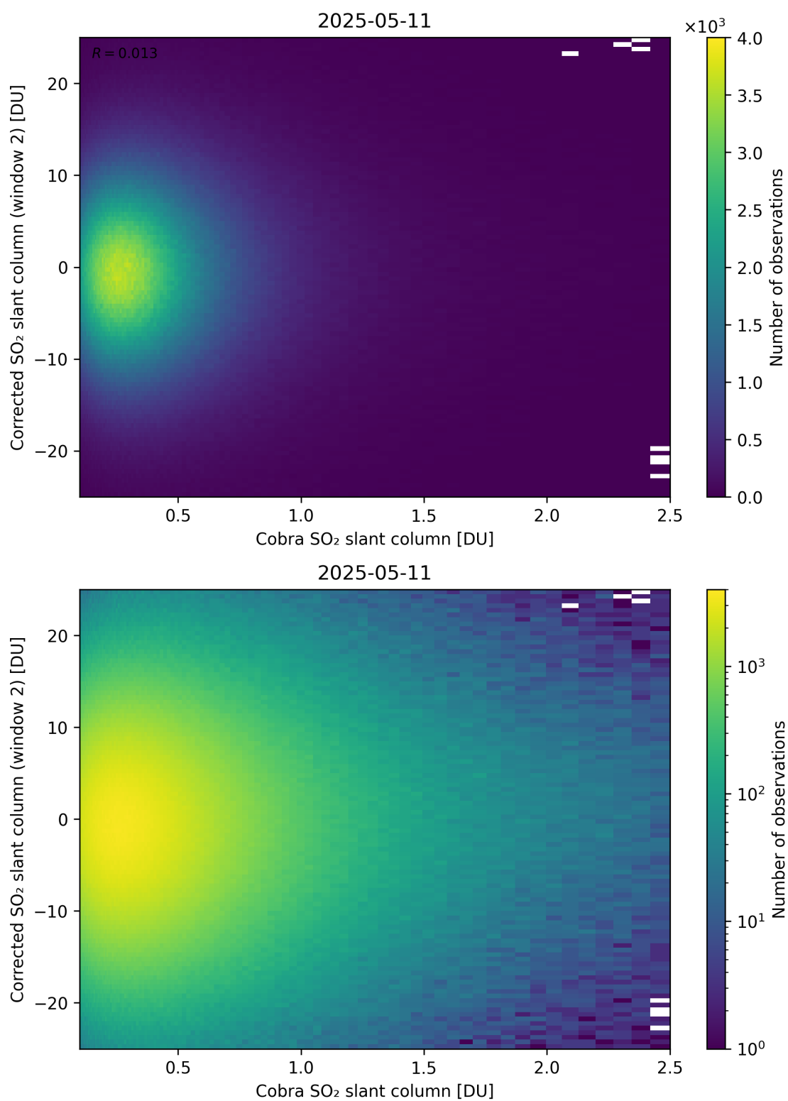
Figure 217: Scatter density plot of “Cobra SO 2 slant column” against “Corrected SO 2 slant column (window 2)” for 2025-05-10 to 2025-05-12.
