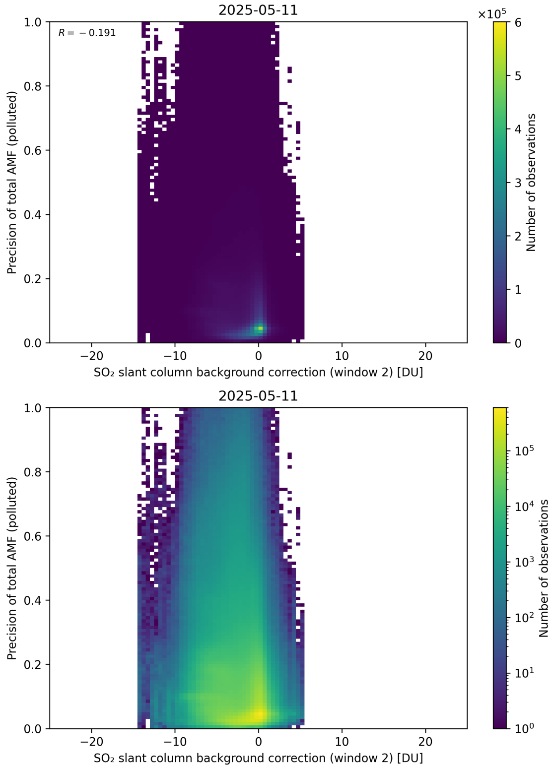
Figure 131: Scatter density plot of “SO 2 slant column background correction (window 2)” against “Precision of total AMF (polluted)” for 2025-05-10 to 2025-05-12.
