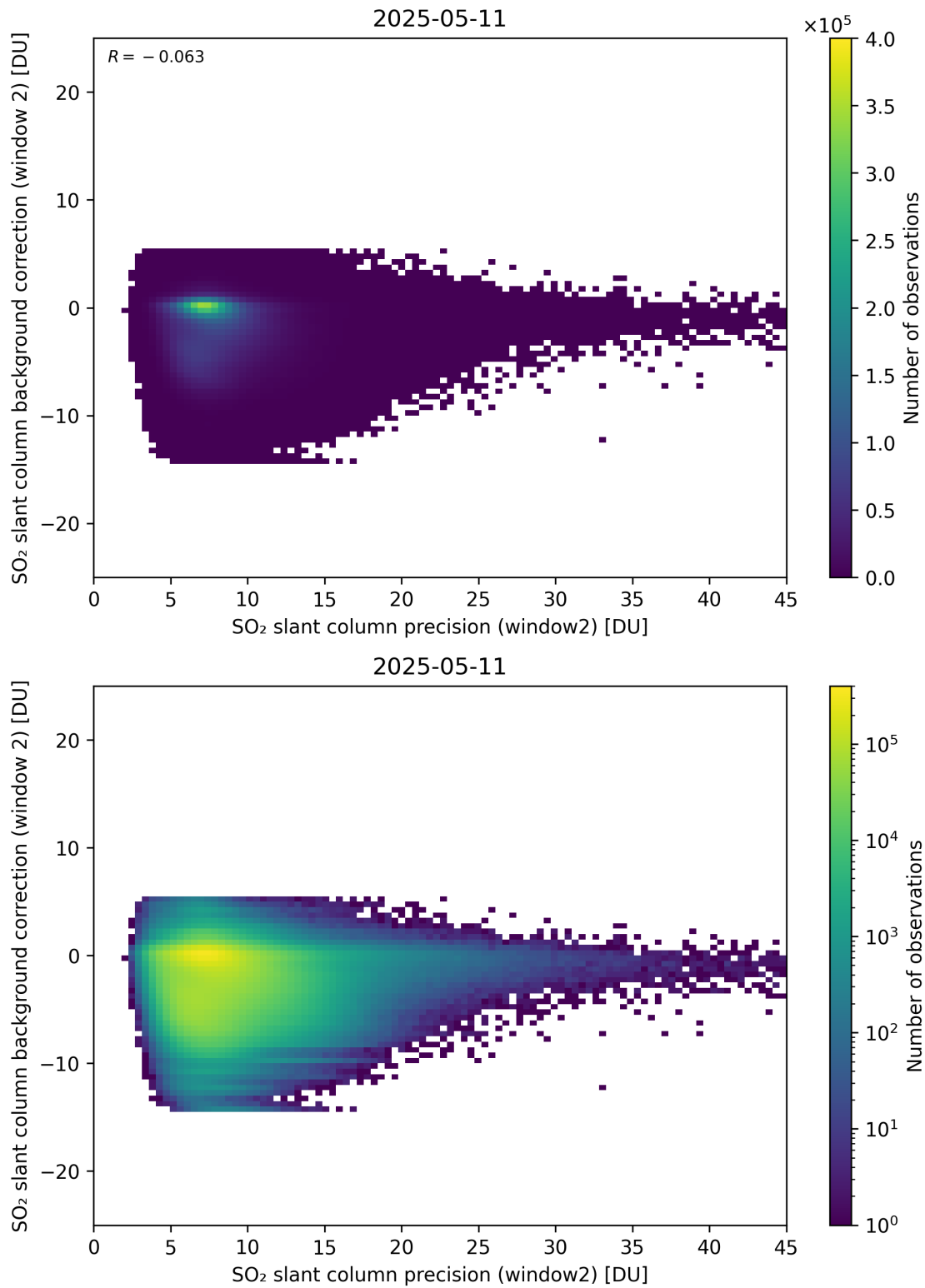
Figure 291: Scatter density plot of “SO 2 slant column precision (window2)” against “SO 2 slant column background correction (window 2)” for 2025-05-10 to 2025-05-12.
