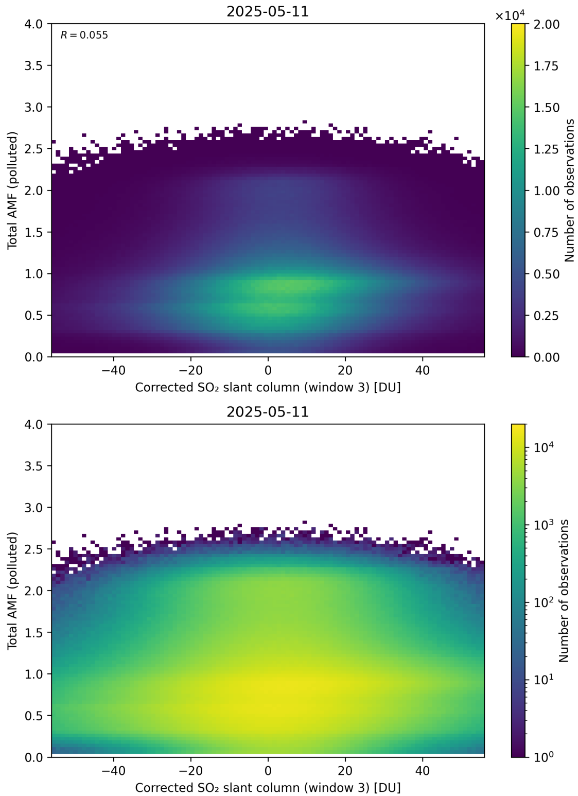
Figure 260: Scatter density plot of “Corrected SO 2 slant column (window 3)” against “Total AMF (polluted)” for 2025-05-10 to 2025-05-12.
