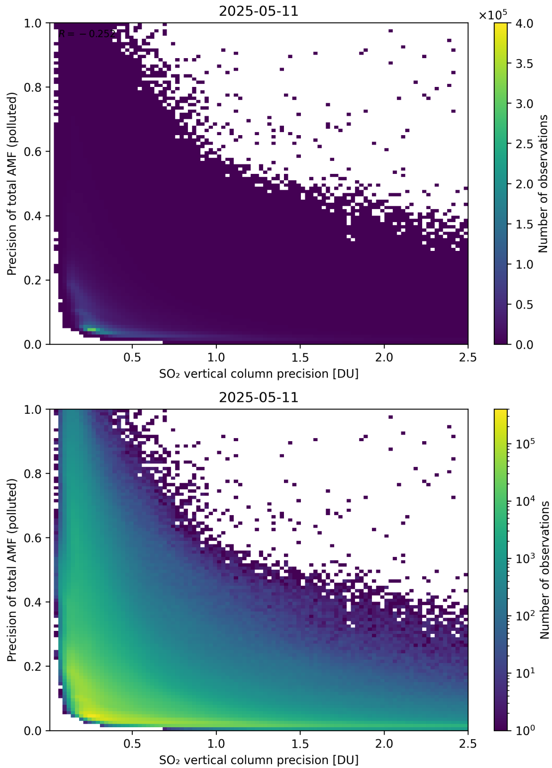
Figure 347: Scatter density plot of “SO 2 vertical column precision” against “Precision of total AMF (polluted)” for 2025-05-10 to 2025-05-12.
