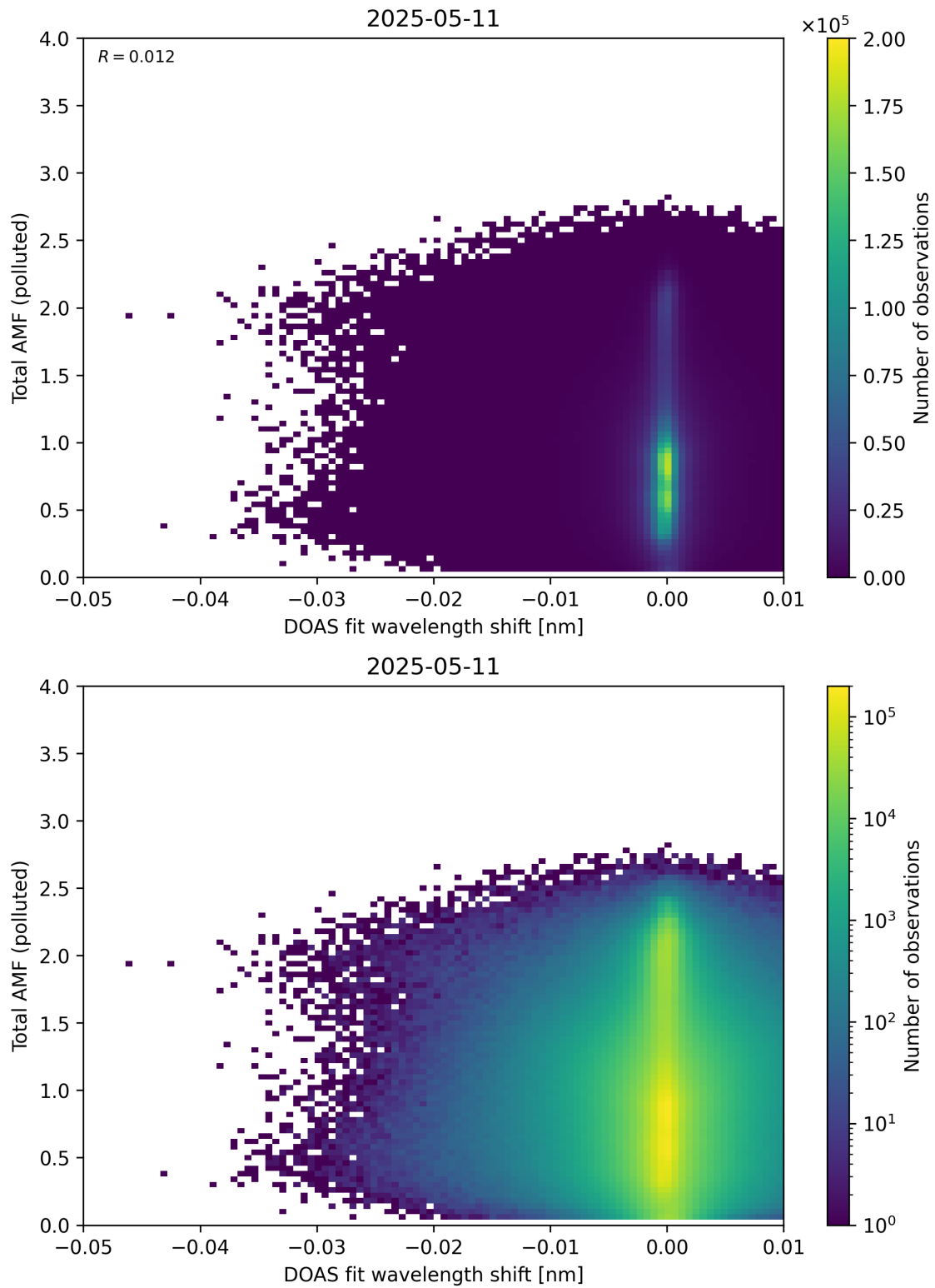
Figure 141: Scatter density plot of “DOAS fit wavelength shift” against “Total AMF (polluted)” for 2025-05-10 to 2025-05-12.
