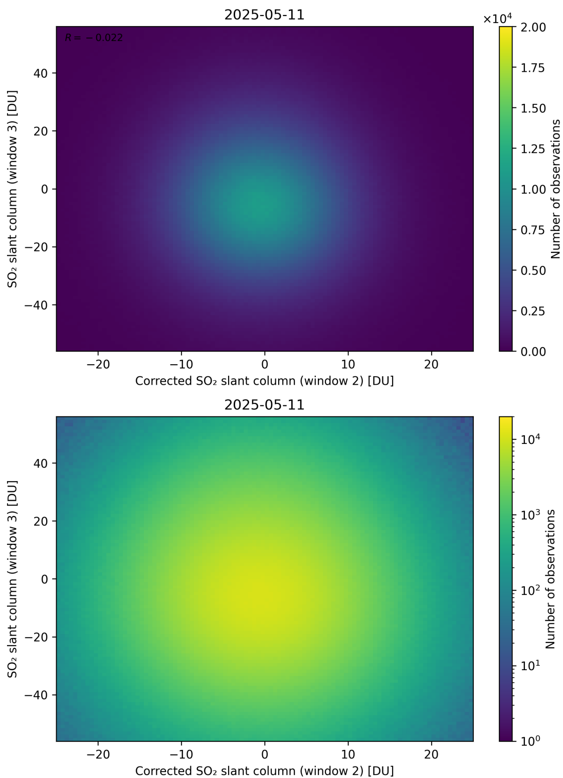
Figure 251: Scatter density plot of “Corrected SO 2 slant column (window 2)” against “SO 2 slant column (window 3)” for 2025-05-10 to 2025-05-12.
