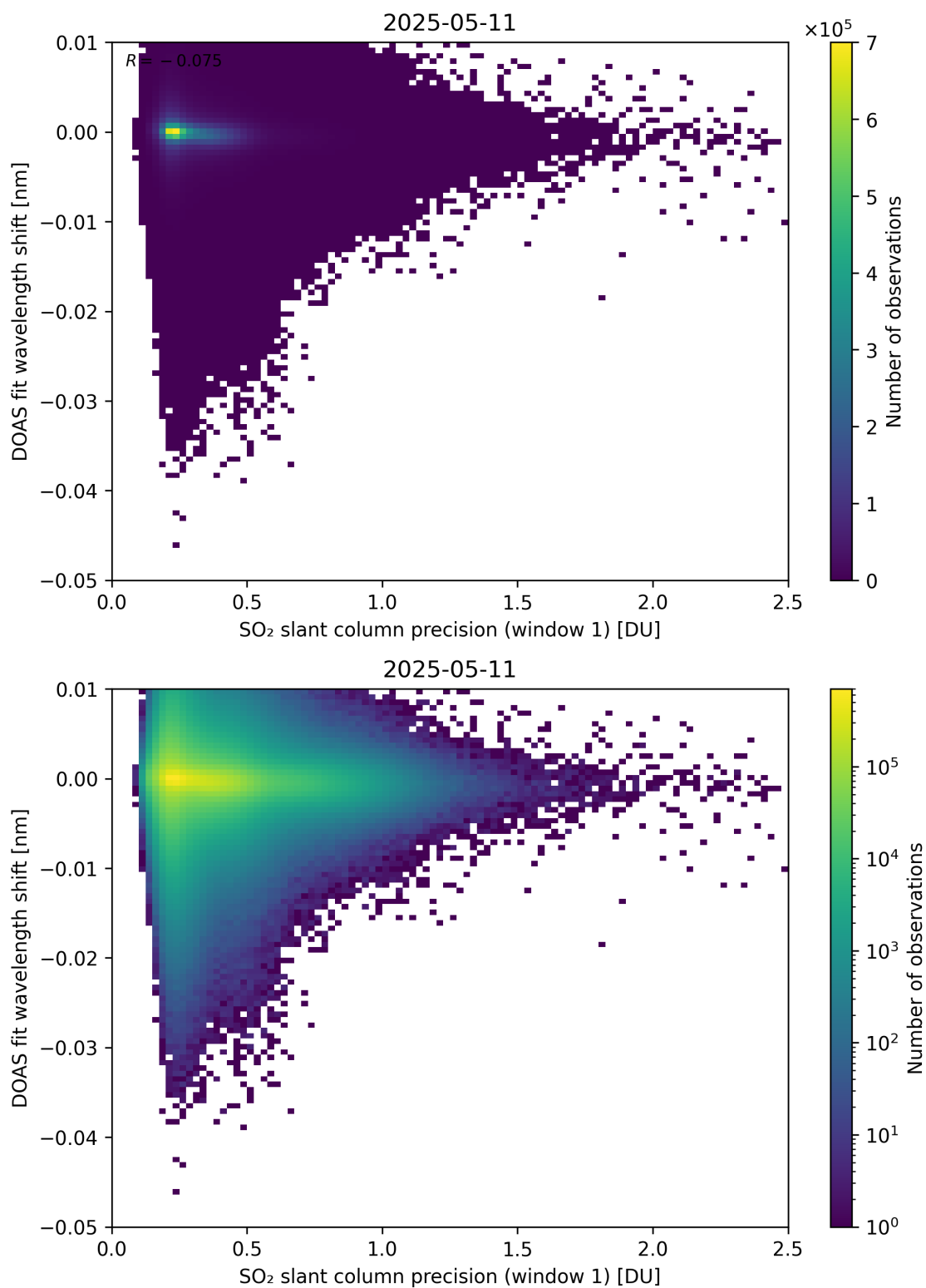
Figure 271: Scatter density plot of “SO 2 slant column precision (window 1)” against “DOAS fit wavelength shift” for 2025-05-10 to 2025-05-12.
