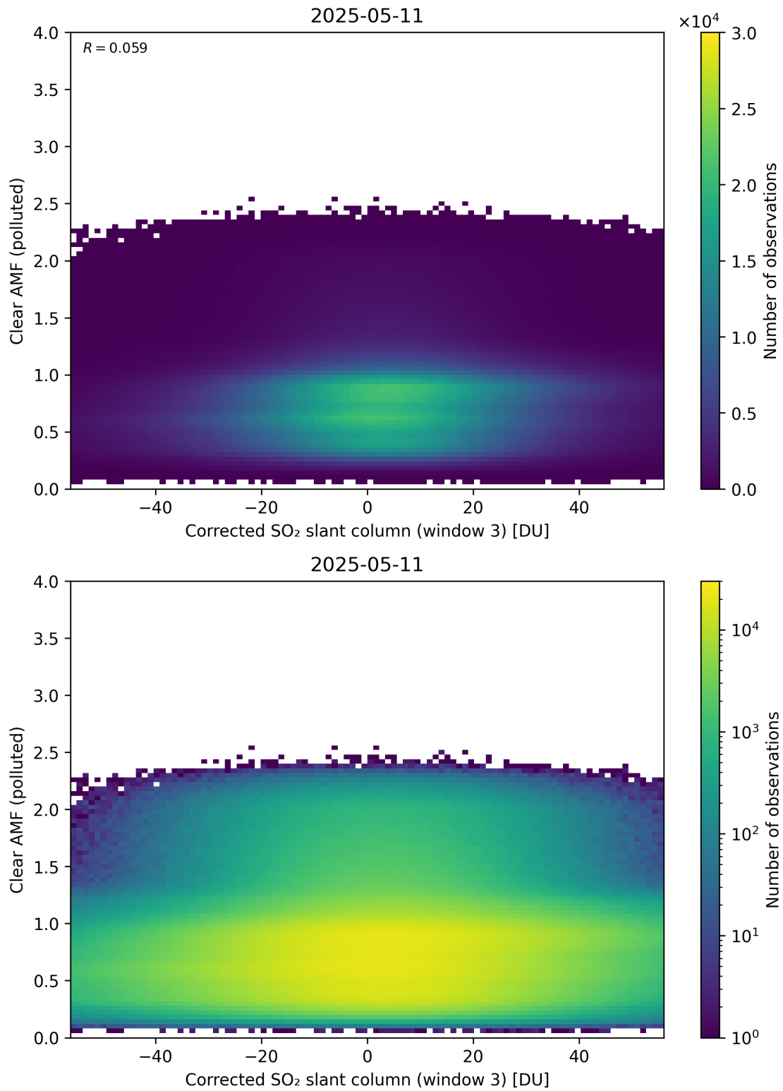
Figure 259: Scatter density plot of “Corrected SO 2 slant column (window 3)” against “Clear AMF (polluted)” for 2025-05-10 to 2025-05-12.
