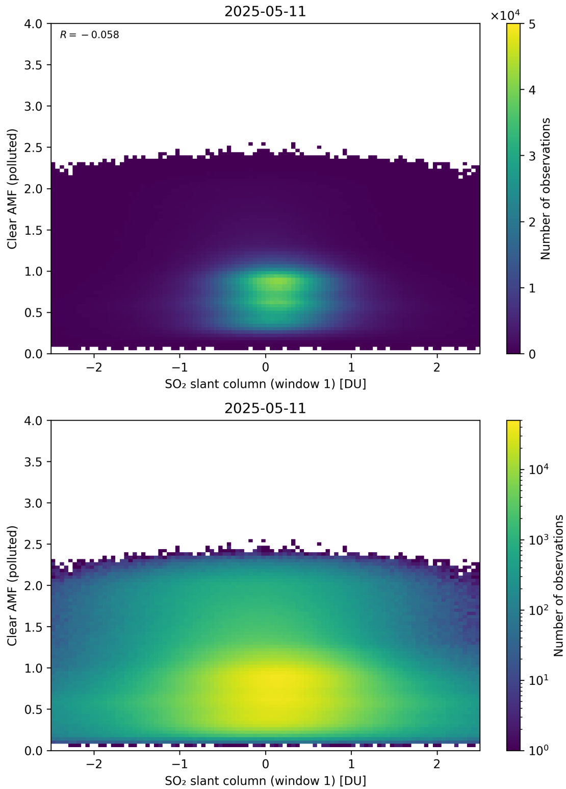
Figure 282: Scatter density plot of “SO 2 slant column (window 1)” against “Clear AMF (polluted)” for 2025-05-10 to 2025-05-12.
