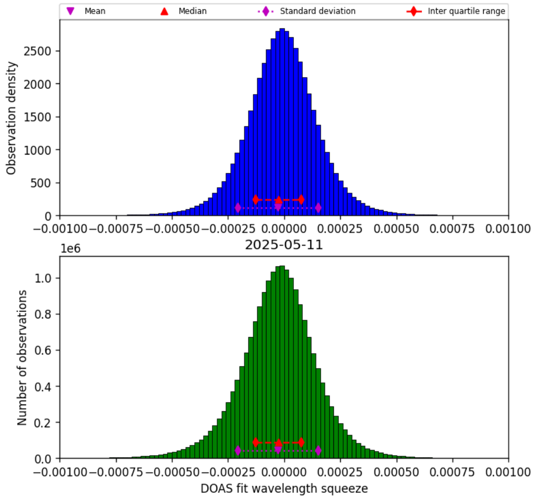
Figure 77: Histogram of “DOAS fit wavelength squeeze” for 2025-05-10 to 2025-05-12
