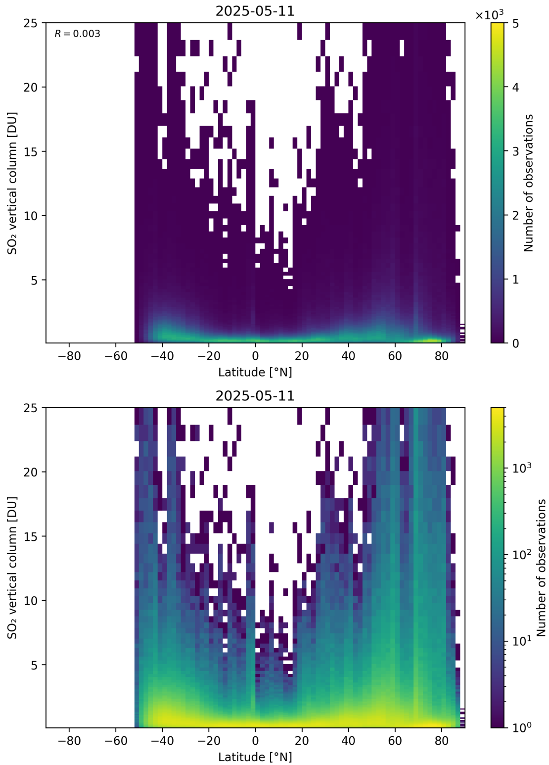
Figure 169: Scatter density plot of “Latitude” against “SO 2 vertical column” for 2025-05-10 to 2025-05-12.
