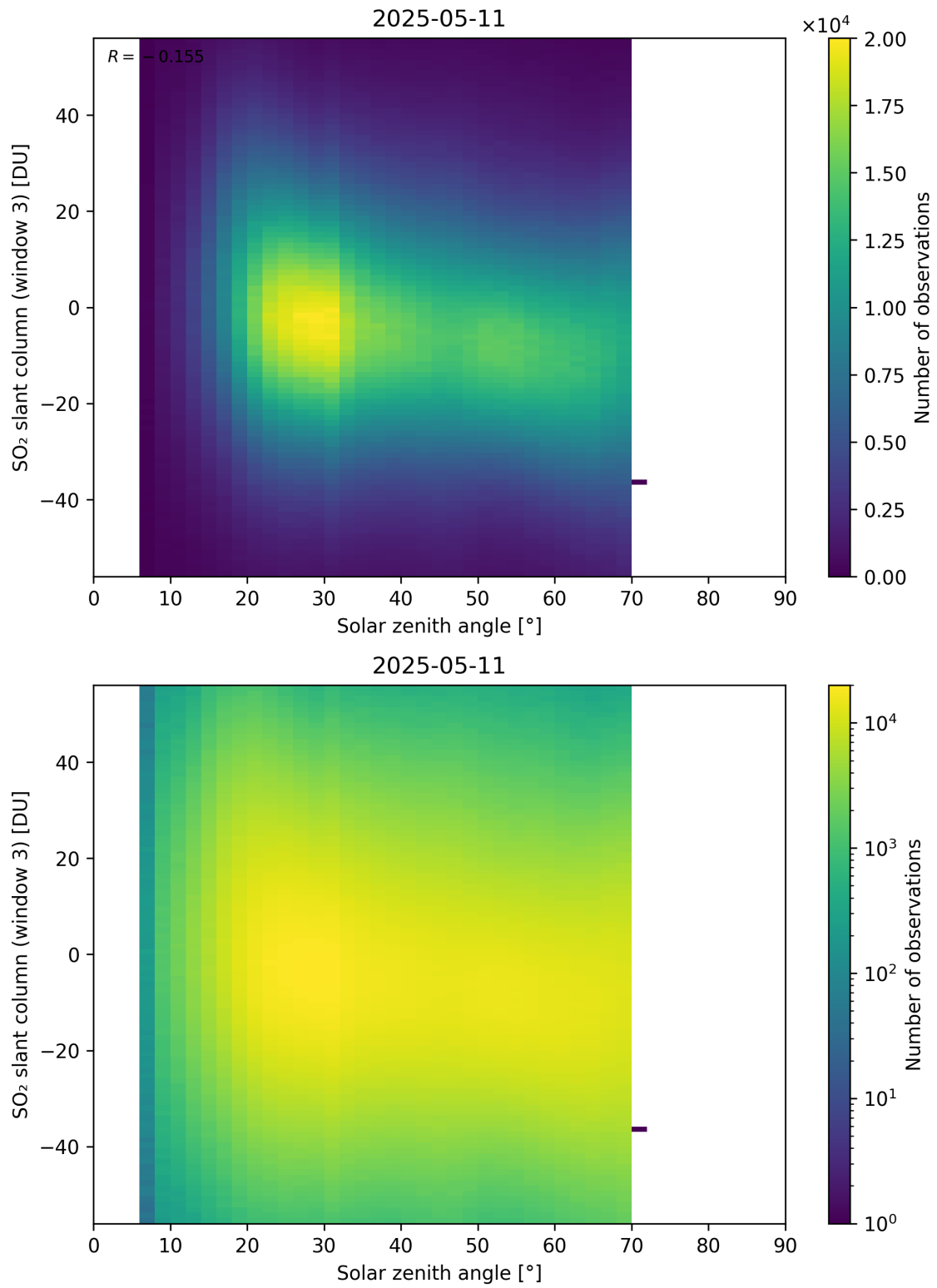
Figure 187: Scatter density plot of “Solar zenith angle” against “SO 2 slant column (window 3)” for 2025-05-10 to 2025-05-12.
