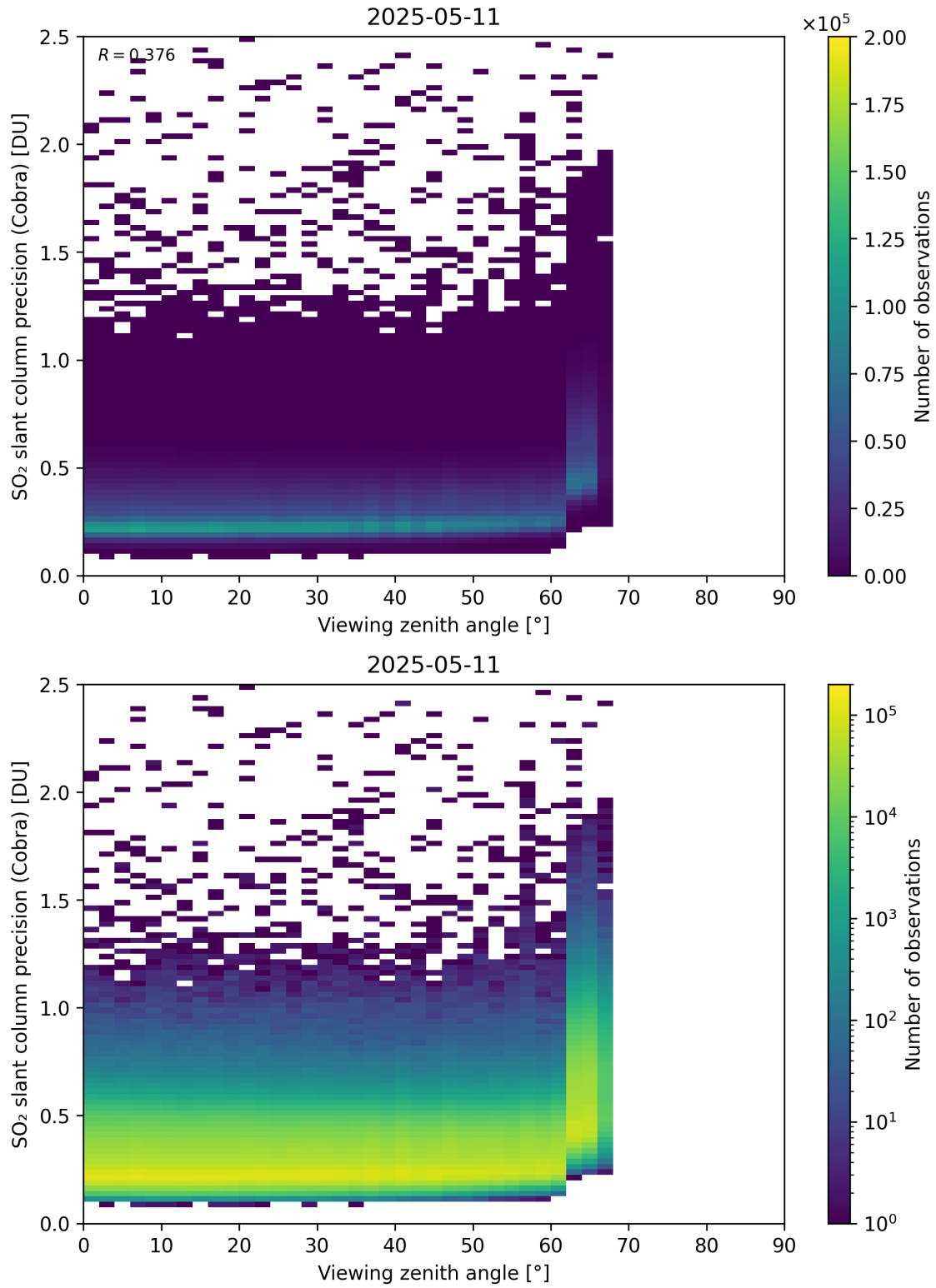
Figure 372: Scatter density plot of “Viewing zenith angle” against “SO 2 slant column precision (Cobra)” for 2025-05-10 to 2025-05-12.
