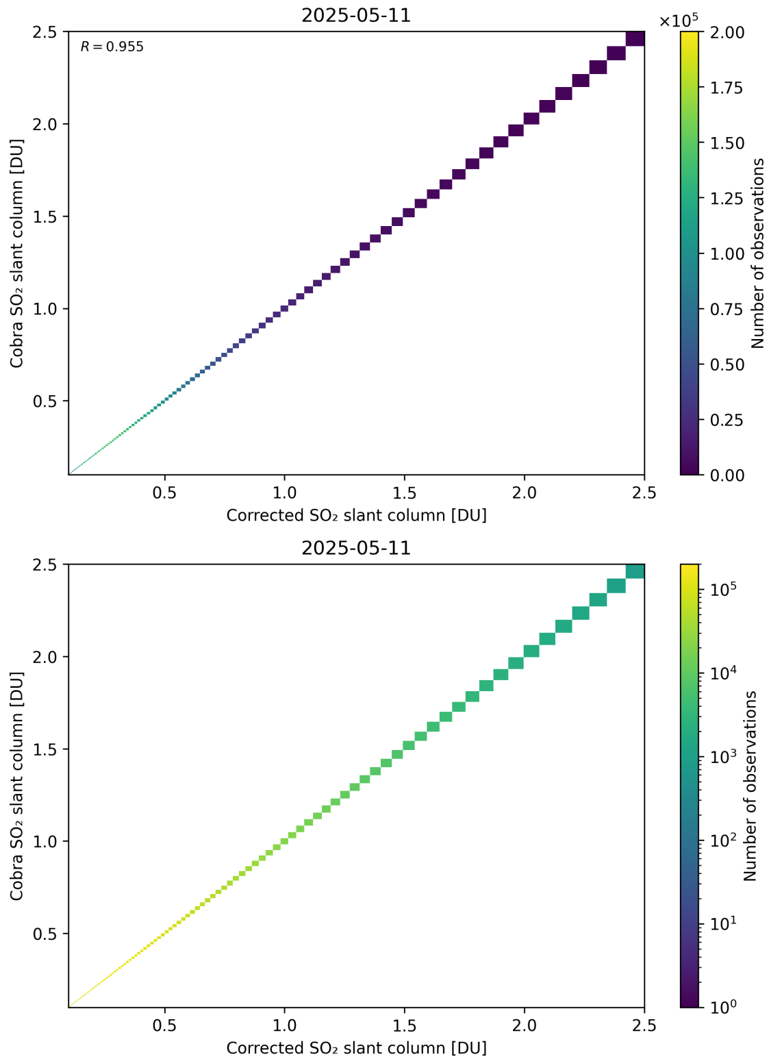
Figure 233: Scatter density plot of “Corrected SO 2 slant column” against “Cobra SO 2 slant column” for 2025-05-10 to 2025-05-12.
