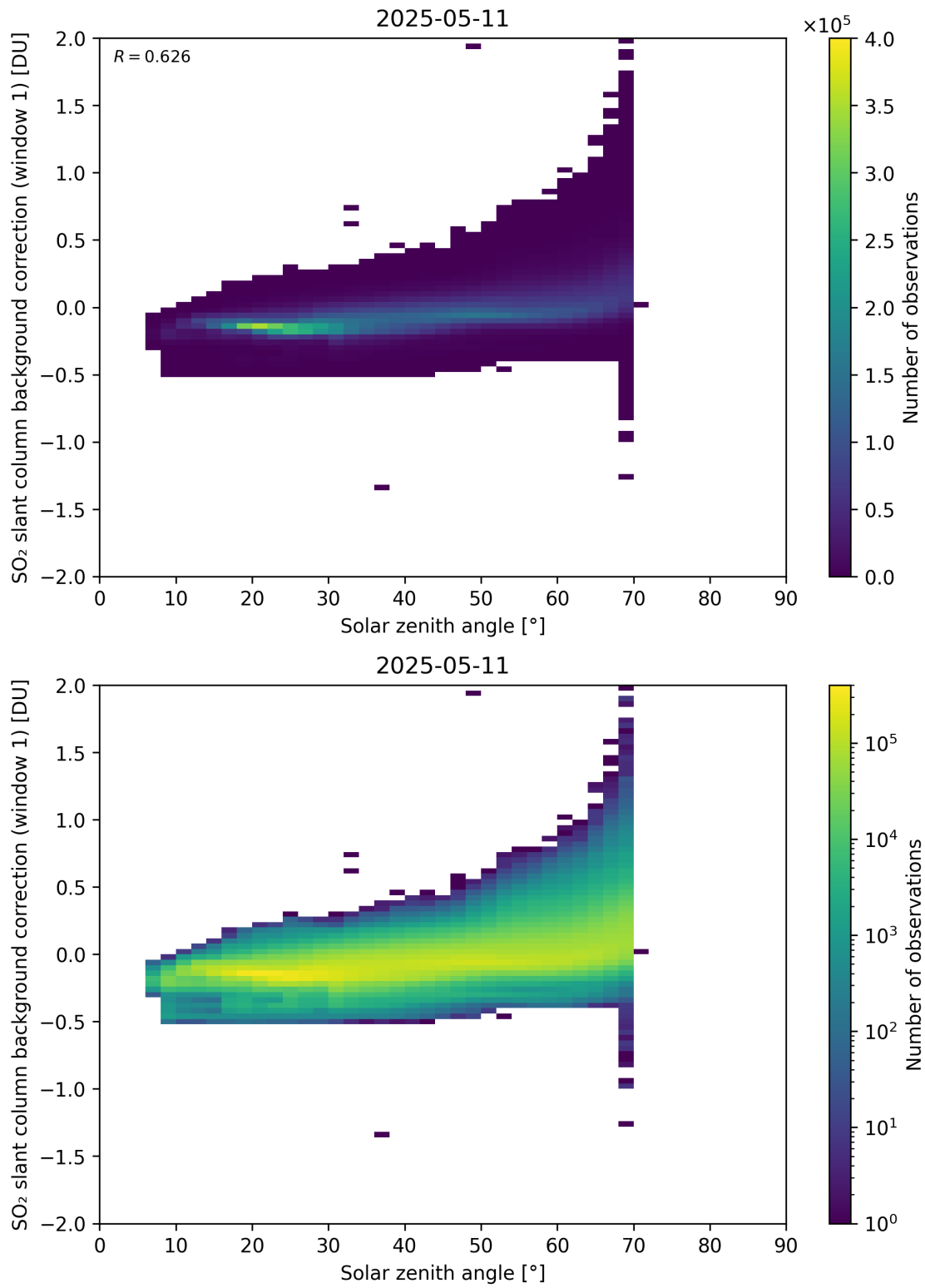
Figure 171: Scatter density plot of “Solar zenith angle” against “SO 2 slant column background correction (window 1)” for 2025-05-10 to 2025-05-12.
