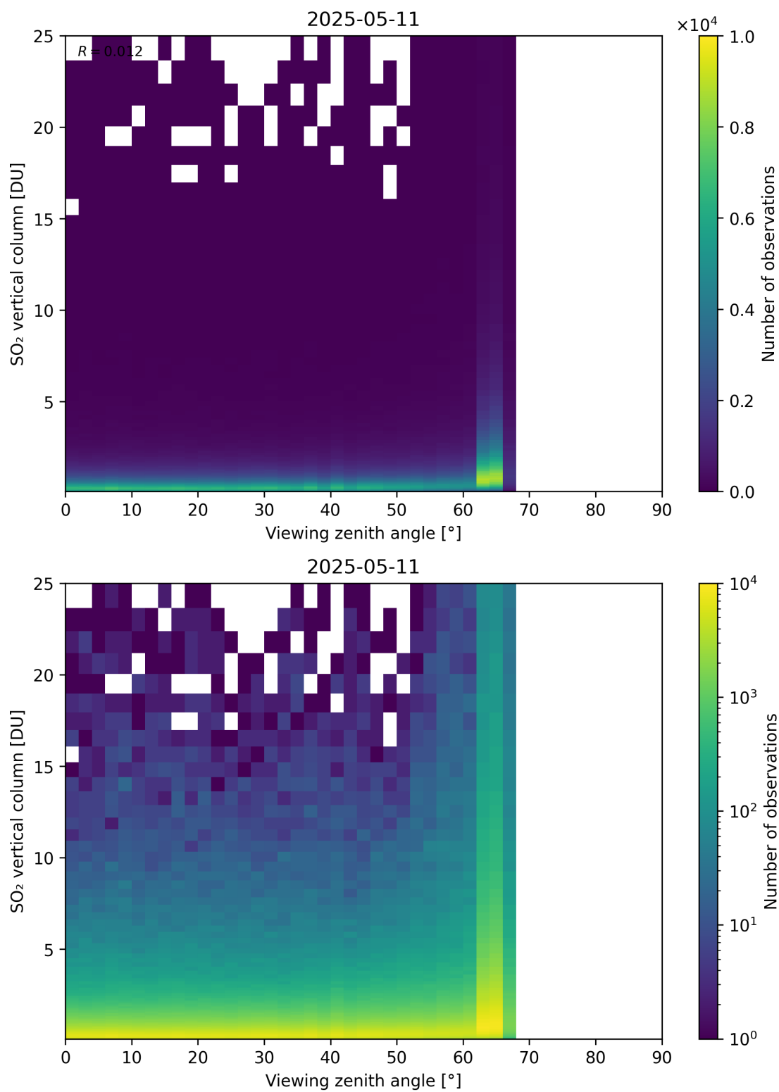
Figure 383: Scatter density plot of “Viewing zenith angle” against “SO 2 vertical column” for 2025-05-10 to 2025-05-12.
