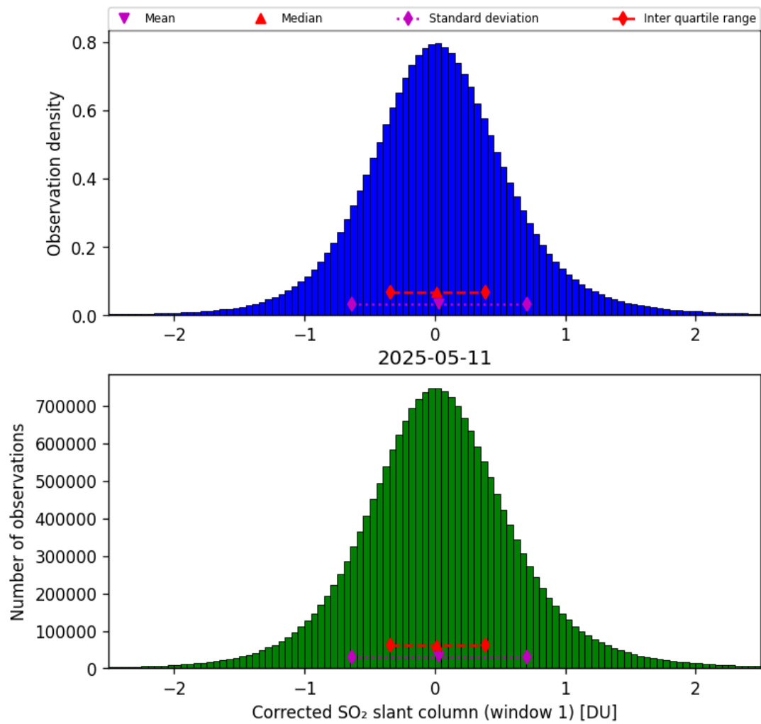
Figure 65: Histogram of “Corrected SO 2 slant column (window 1)” for 2025-05-10 to 2025-05-12
