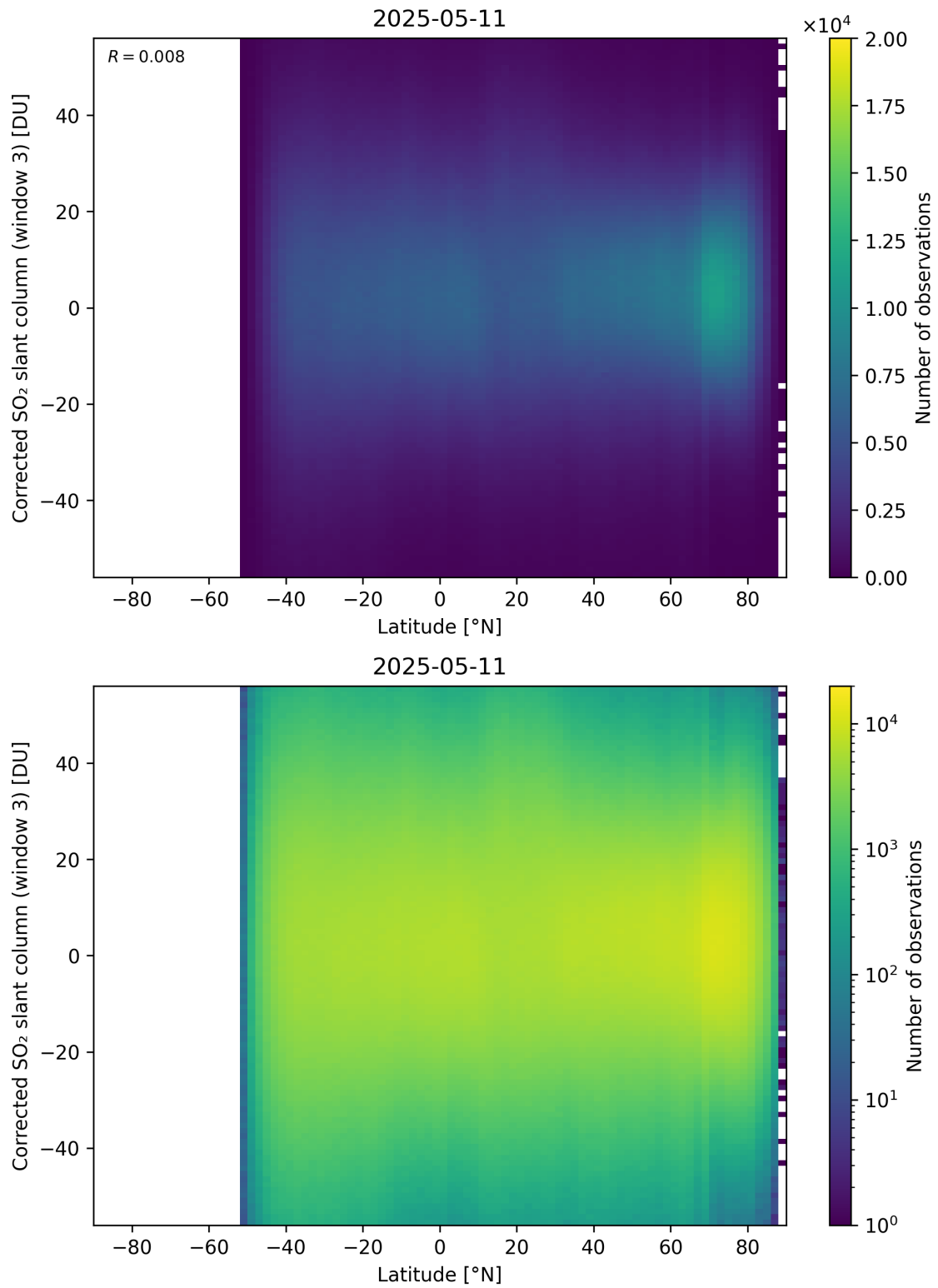
Figure 161: Scatter density plot of “Latitude” against “Corrected SO 2 slant column (window 3)” for 2025-05-10 to 2025-05-12.
