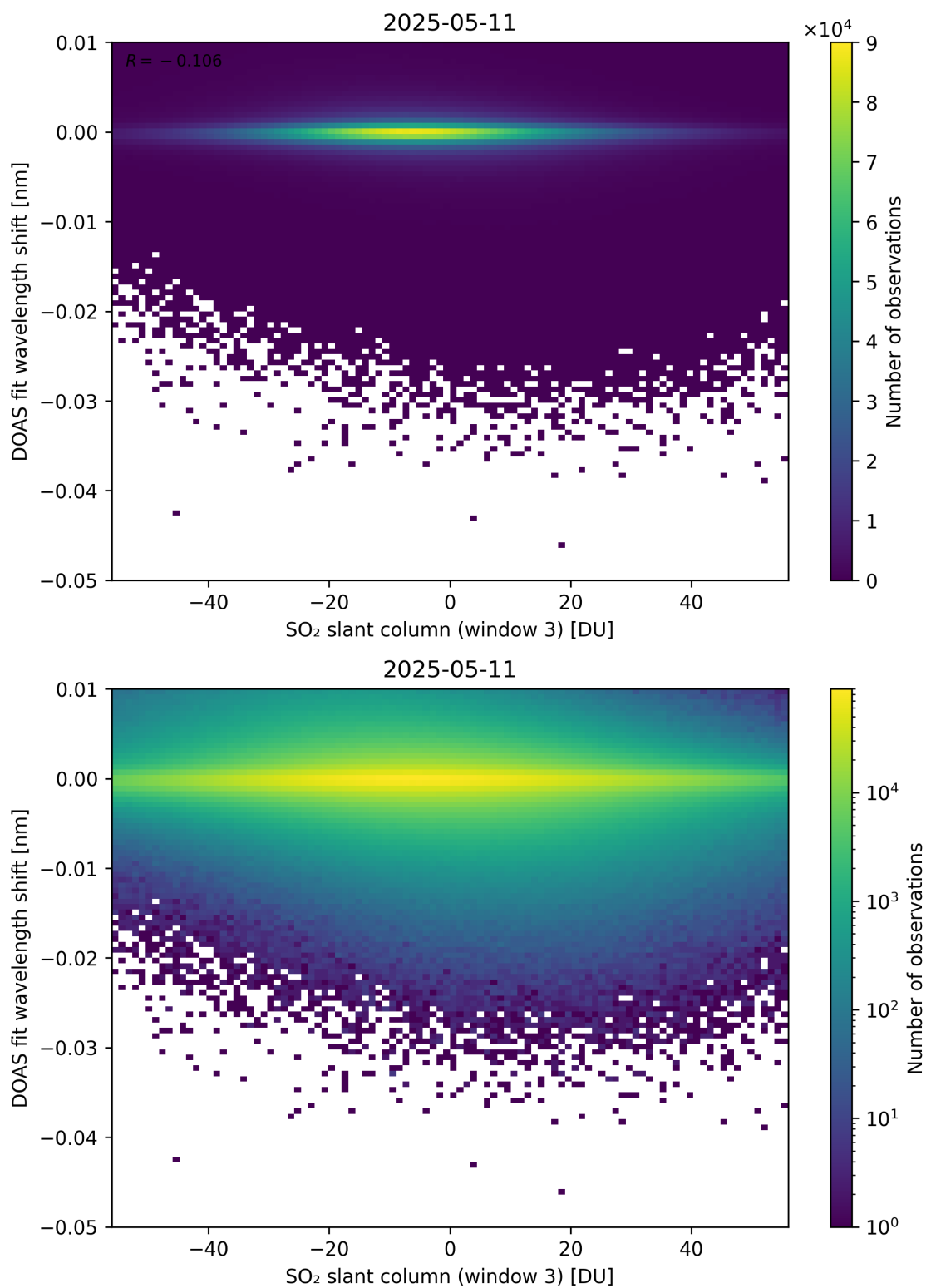
Figure 304: Scatter density plot of “SO 2 slant column (window 3)” against “DOAS fit wavelength shift” for 2025-05-10 to 2025-05-12.
