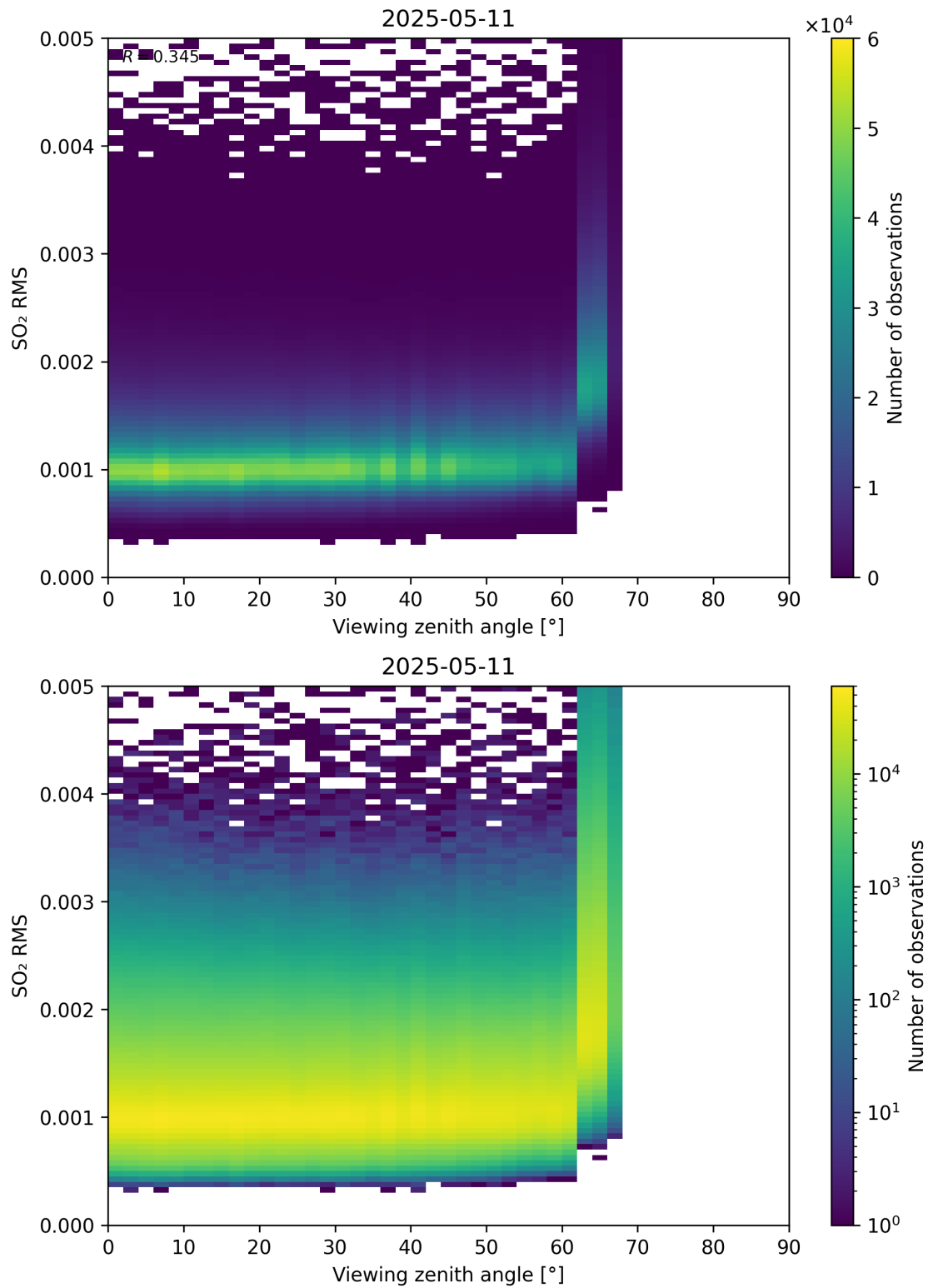
Figure 367: Scatter density plot of “Viewing zenith angle” against “SO 2 RMS” for 2025-05-10 to 2025-05-12.
