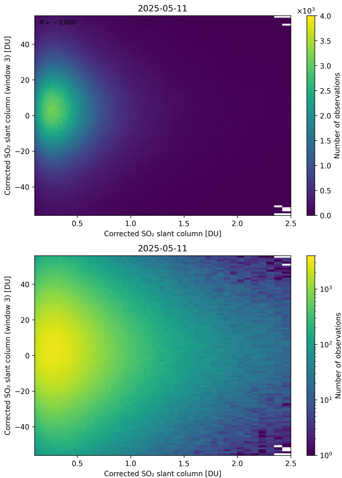
Figure 236: Scatter density plot of “Corrected SO 2 slant column” against “Corrected SO 2 slant column (window 3)” for 2025-05-10 to 2025-05-12.
