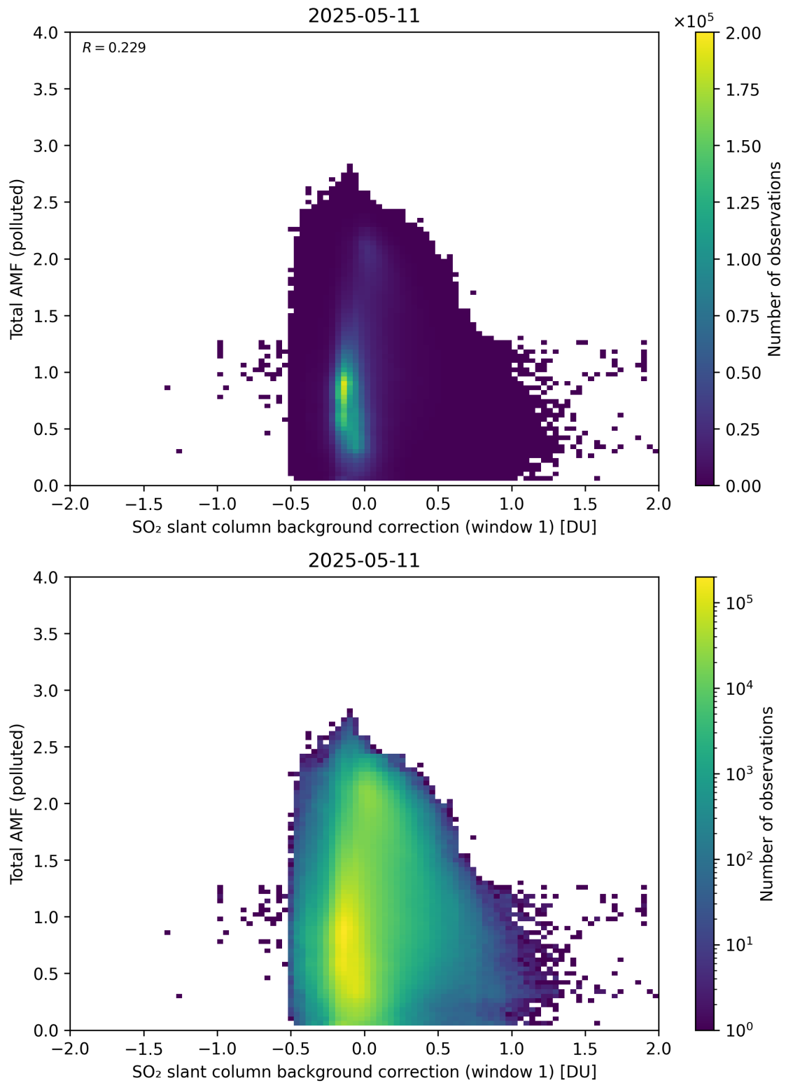
Figure 120: Scatter density plot of “SO 2 slant column background correction (window 1)” against “Total AMF (polluted)” for 2025-05-10 to 2025-05-12.
