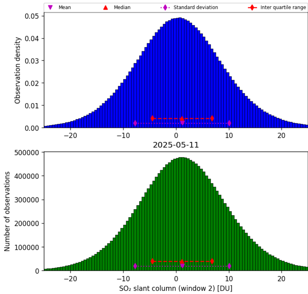
Figure 67: Histogram of “SO 2 slant column (window 2)” for 2025-05-10 to 2025-05-12
