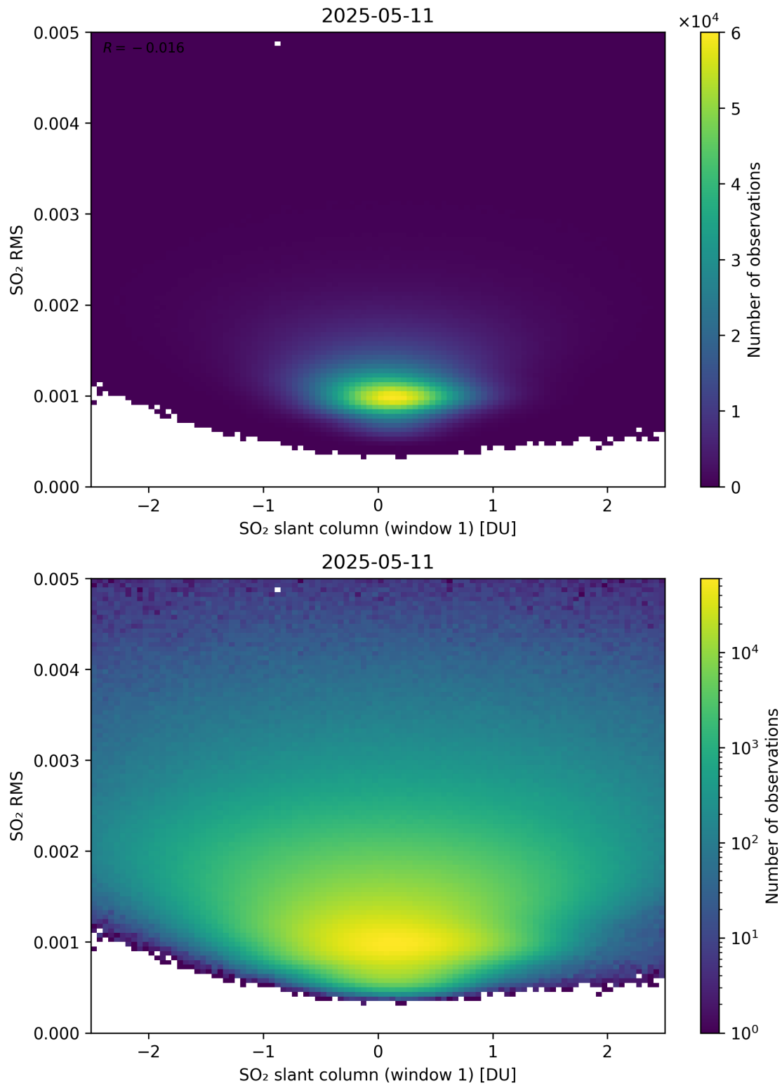
Figure 267: Scatter density plot of “SO 2 slant column (window 1)” against “SO 2 RMS” for 2025-05-10 to 2025-05-12.
