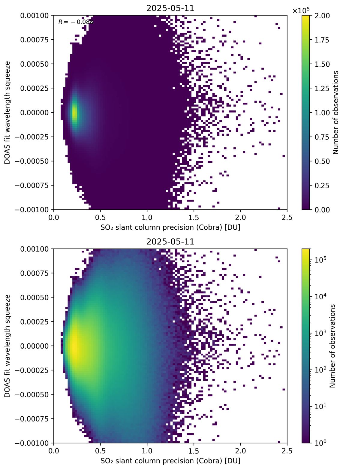
Figure 203: Scatter density plot of “SO 2 slant column precision (Cobra)” against “DOAS fit wavelength squeeze” for 2025-05-10 to 2025-05-12.
