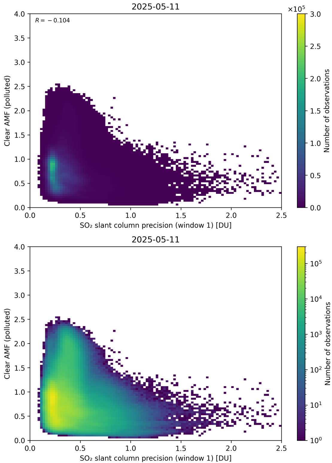
Figure 274: Scatter density plot of “SO 2 slant column precision (window 1)” against “Clear AMF (polluted)” for 2025-05-10 to 2025-05-12.
