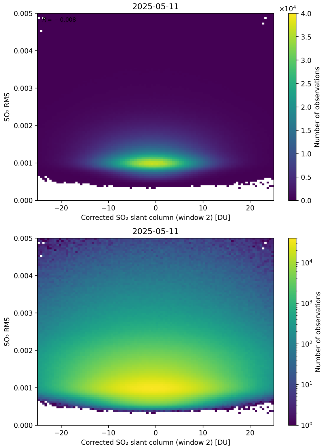
Figure 248: Scatter density plot of “Corrected SO 2 slant column (window 2)” against “SO 2 RMS” for 2025-05-10 to 2025-05-12.
