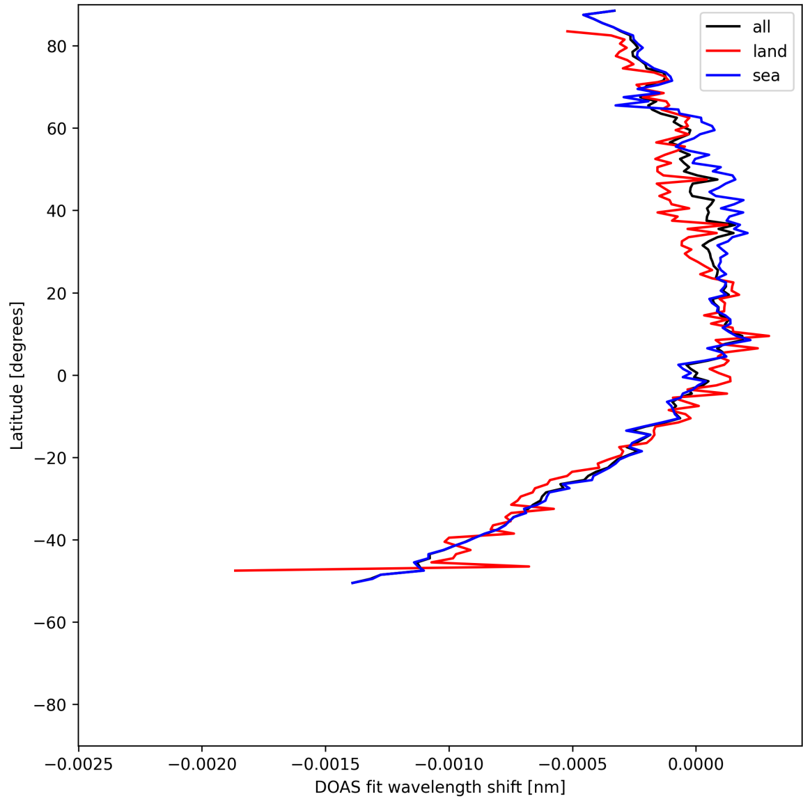
Figure 50: Zonal average of “DOAS fit wavelength shift” for 2025-05-10 to 2025-05-12.
