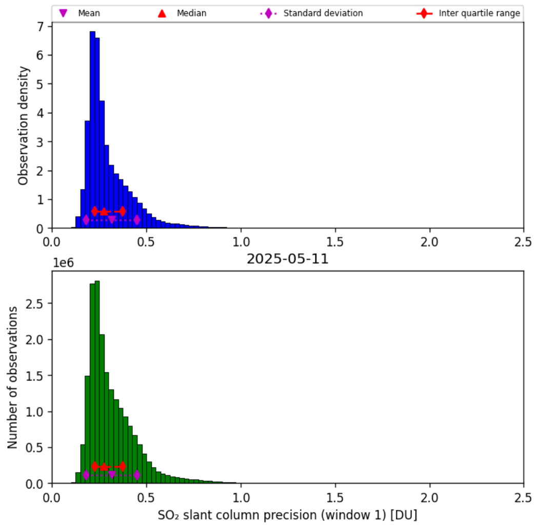
Figure 64: Histogram of “SO 2 slant column precision (window 1)” for 2025-05-10 to 2025-05-12
