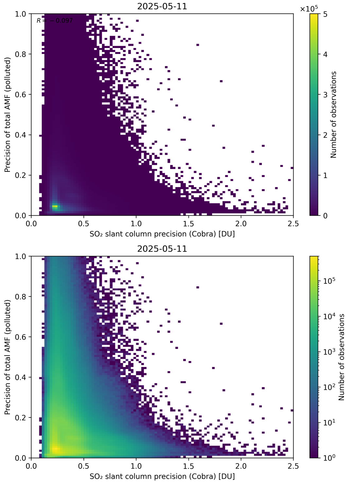
Figure 214: Scatter density plot of “SO 2 slant column precision (Cobra)” against “Precision of total AMF (polluted)” for 2025-05-10 to 2025-05-12.
