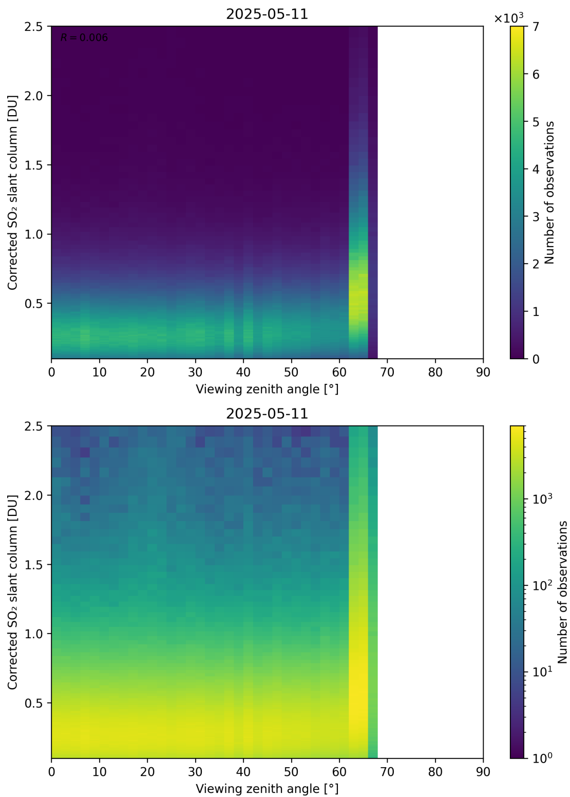
Figure 373: Scatter density plot of “Viewing zenith angle” against “Corrected SO 2 slant column” for 2025-05-10 to 2025-05-12.
