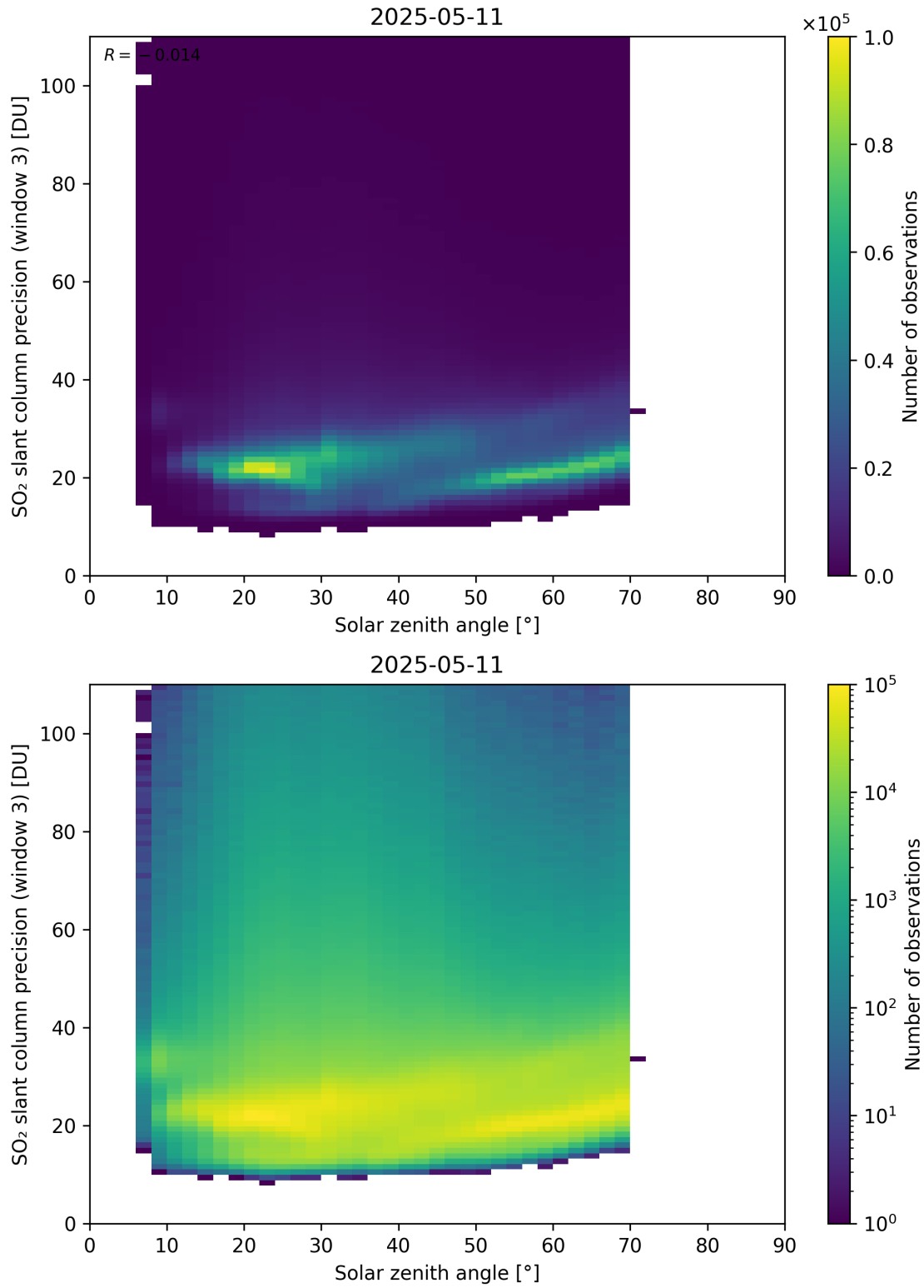
Figure 188: Scatter density plot of “Solar zenith angle” against “SO 2 slant column precision (window 3)” for 2025-05-10 to 2025-05-12.
