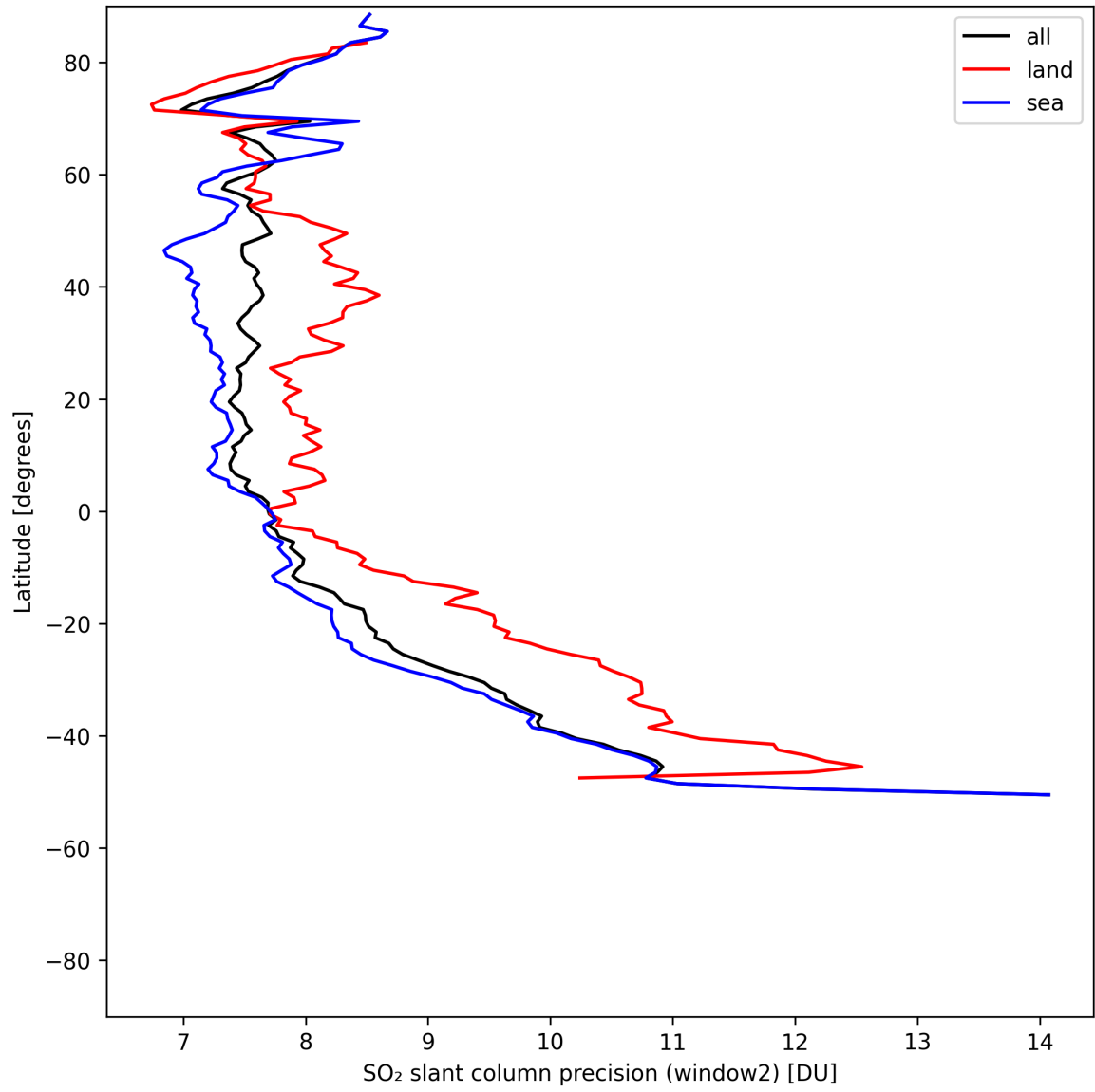
Figure 42: Zonal average of “SO 2 slant column precision (window2)” for 2025-05-10 to 2025-05-12.
