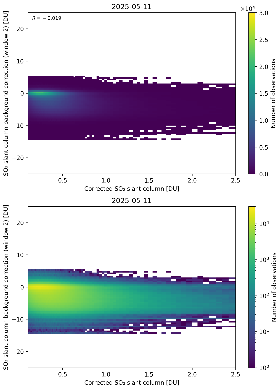
Figure 227: Scatter density plot of “Corrected SO 2 slant column” against “SO 2 slant column background correction (window 2)” for 2025-05-10 to 2025-05-12.
