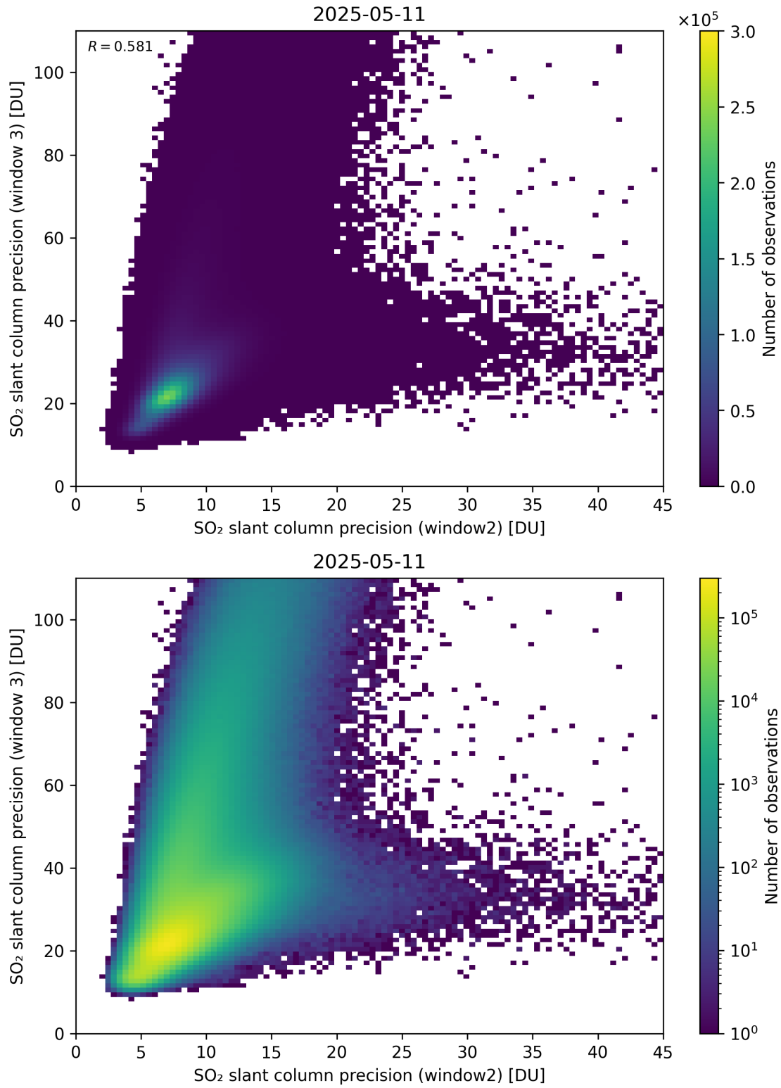
Figure 300: Scatter density plot of “SO 2 slant column precision (window2)” against “SO 2 slant column precision (window 3)” for 2025-05-10 to 2025-05-12.
