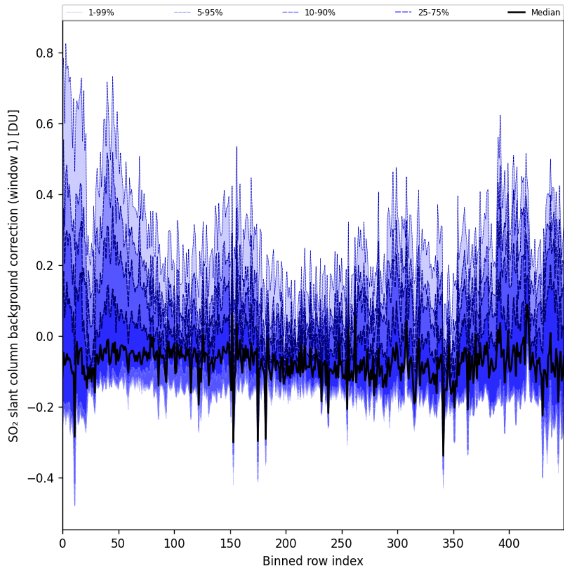
Figure 92: Along track statistics of “SO 2 slant column background correction (window 1)” for 2025-05-10 to 2025-05-12
