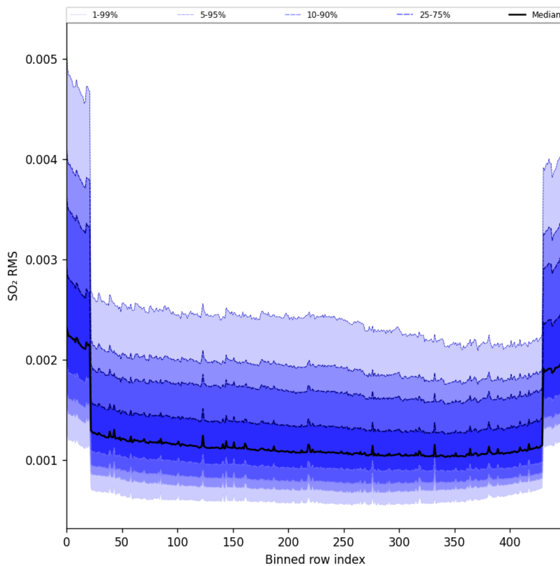
Figure 104: Along track statistics of “SO 2 RMS” for 2025-05-10 to 2025-05-12
