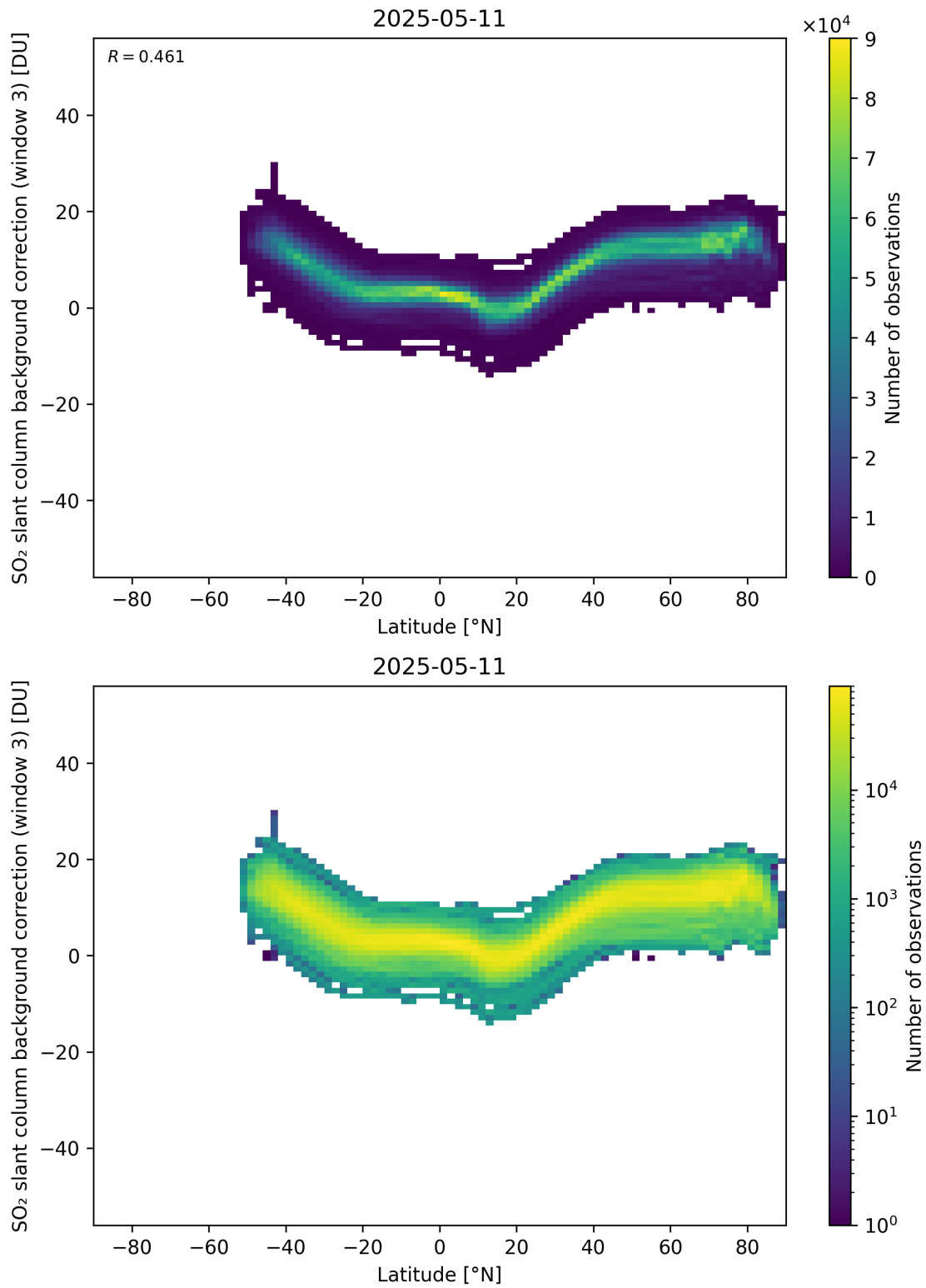
Figure 152: Scatter density plot of “Latitude” against “SO 2 slant column background correction (window 3)” for 2025-05-10 to 2025-05-12.
