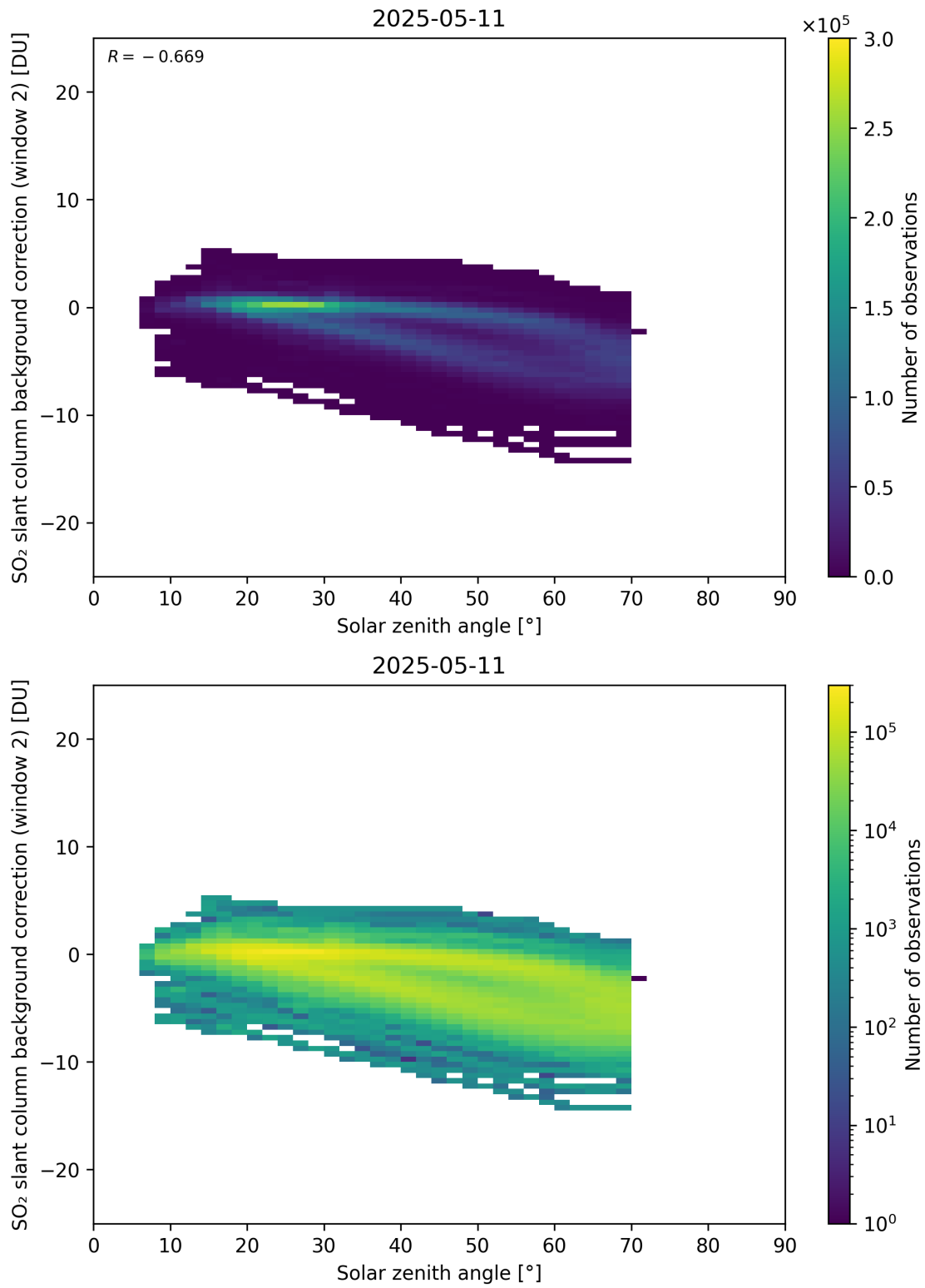
Figure 172: Scatter density plot of “Solar zenith angle” against “SO 2 slant column background correction (window 2)” for 2025-05-10 to 2025-05-12.
