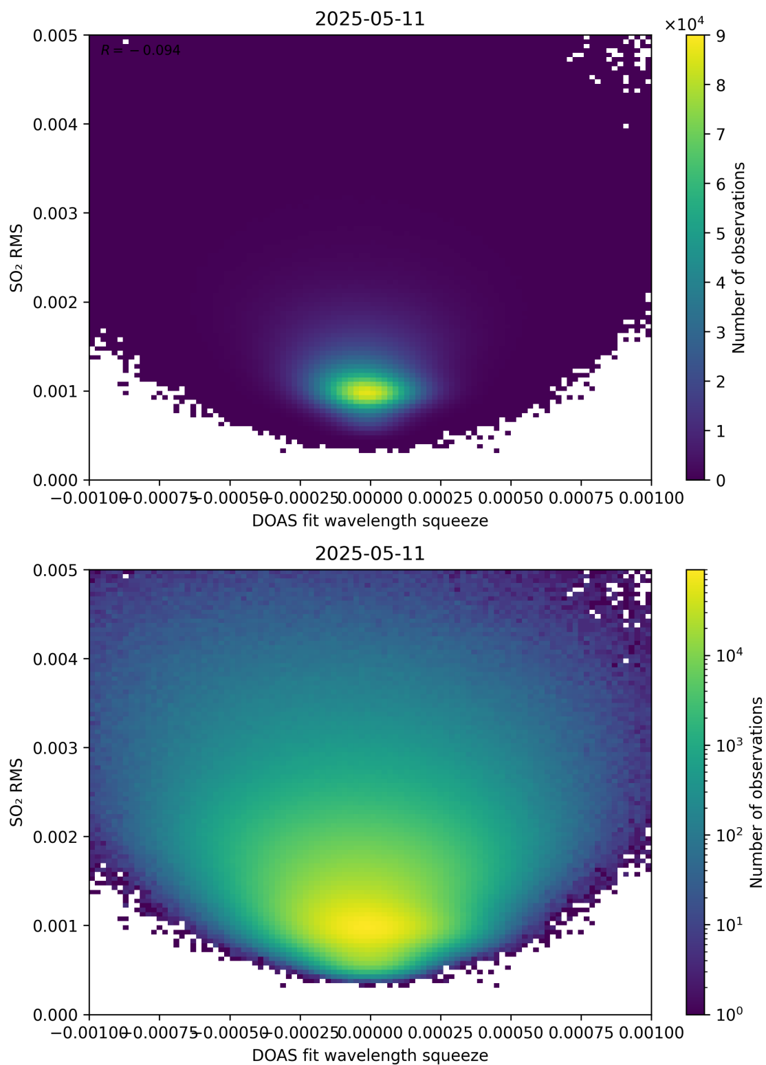
Figure 143: Scatter density plot of “DOAS fit wavelength squeeze” against “SO 2 RMS” for 2025-05-10 to 2025-05-12.
