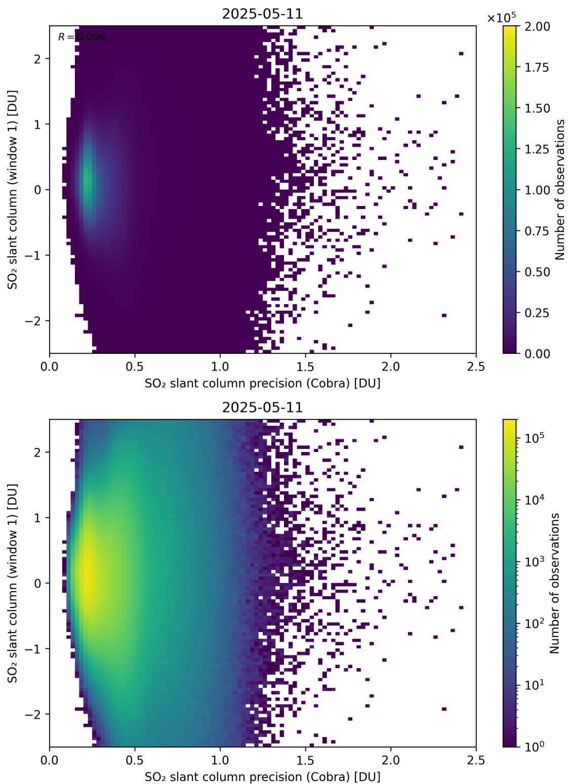
Figure 208: Scatter density plot of “SO 2 slant column precision (Cobra)” against “SO 2 slant column (window 1)” for 2025-05-10 to 2025-05-12.
