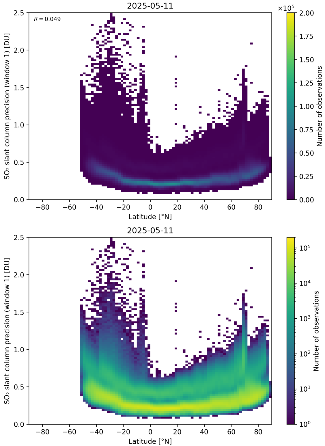
Figure 163: Scatter density plot of “Latitude” against “SO 2 slant column precision (window 1)” for 2025-05-10 to 2025-05-12.
