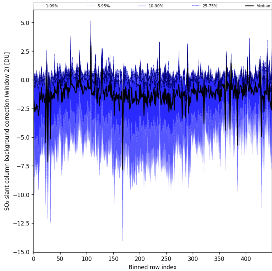
Figure 96: Along track statistics of “SO 2 slant column background correction (window 2)” for 2025-05-10 to 2025-05-12
