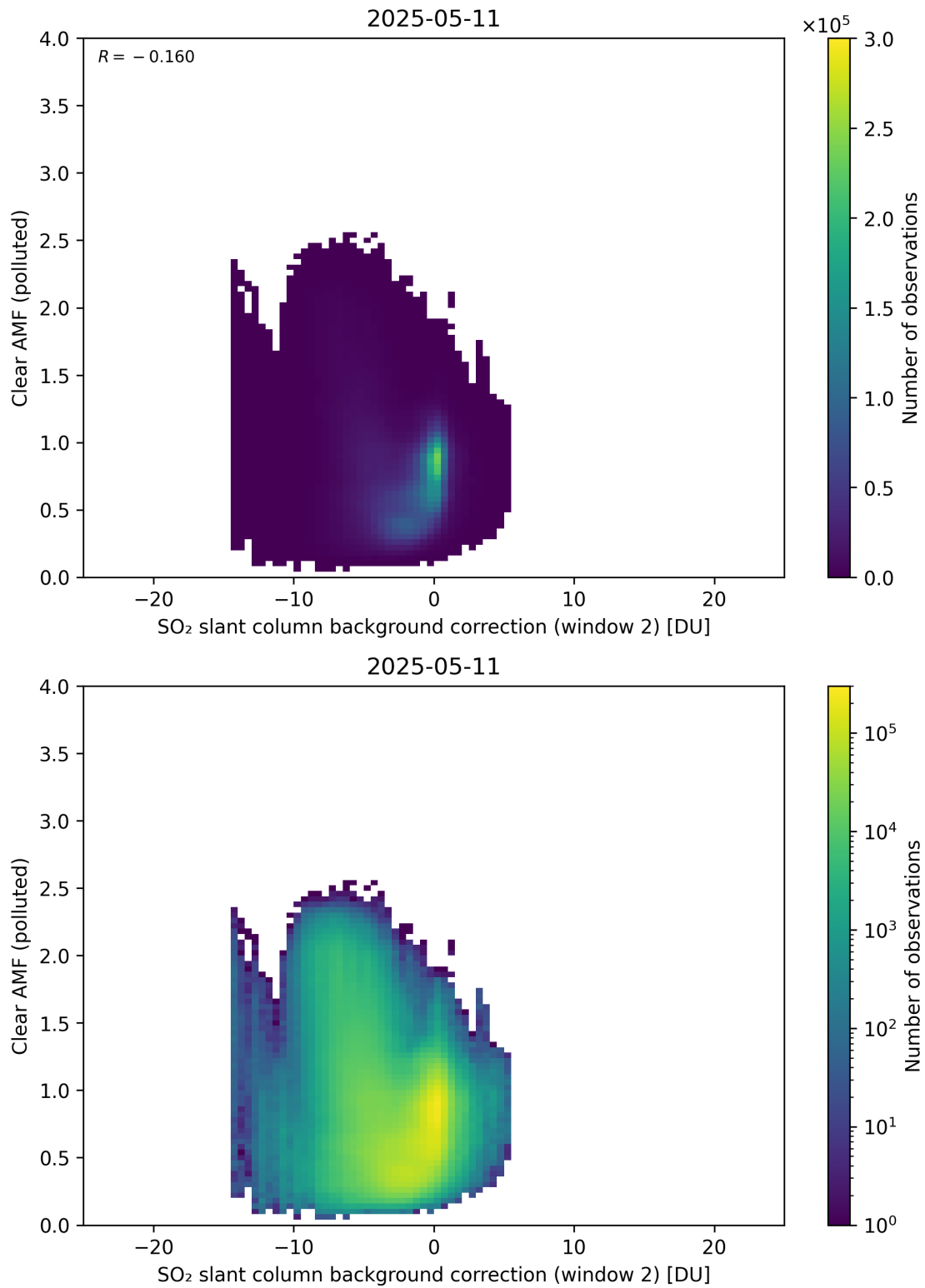
Figure 126: Scatter density plot of “SO 2 slant column background correction (window 2)” against “Clear AMF (polluted)” for 2025-05-10 to 2025-05-12.
