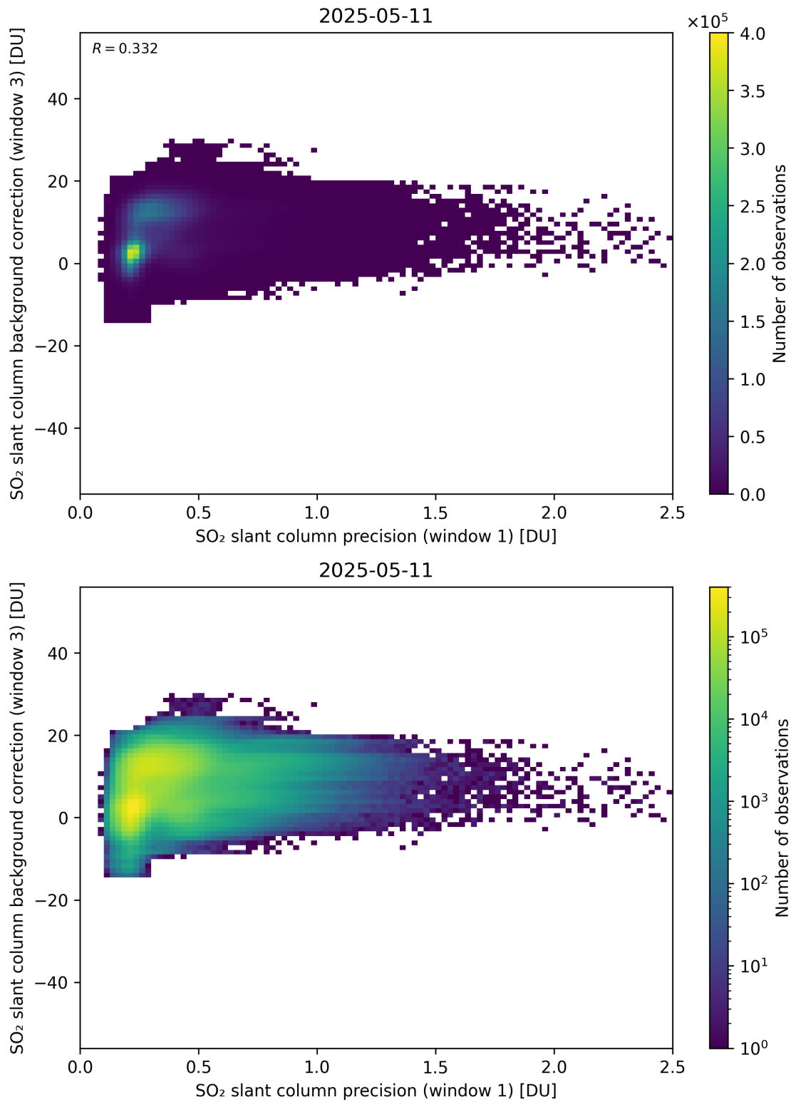
Figure 270: Scatter density plot of “SO 2 slant column precision (window 1)” against “SO 2 slant column background correction (window 3)” for 2025-05-10 to 2025-05-12.
