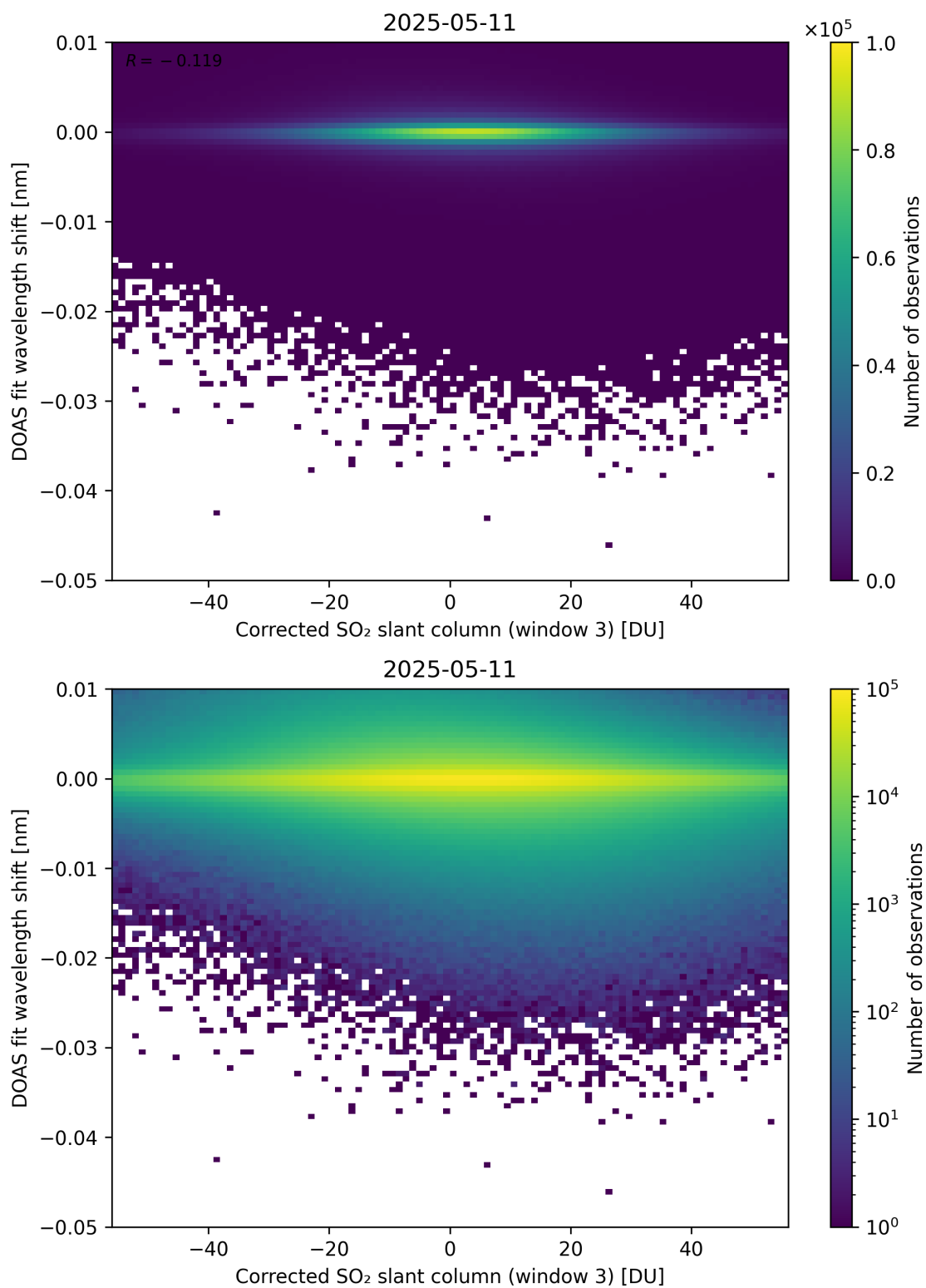
Figure 256: Scatter density plot of “Corrected SO 2 slant column (window 3)” against “DOAS fit wavelength shift” for 2025-05-10 to 2025-05-12.
