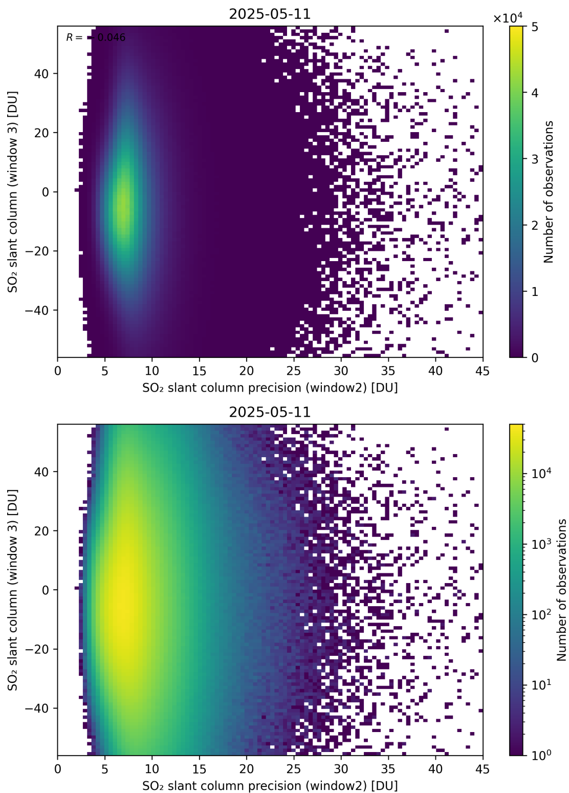
Figure 299: Scatter density plot of “SO 2 slant column precision (window2)” against “SO 2 slant column (window 3)” for 2025-05-10 to 2025-05-12.
