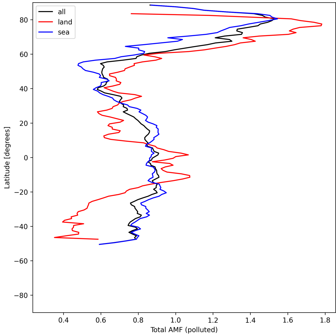
Figure 53: Zonal average of “Total AMF (polluted)” for 2025-05-10 to 2025-05-12.
