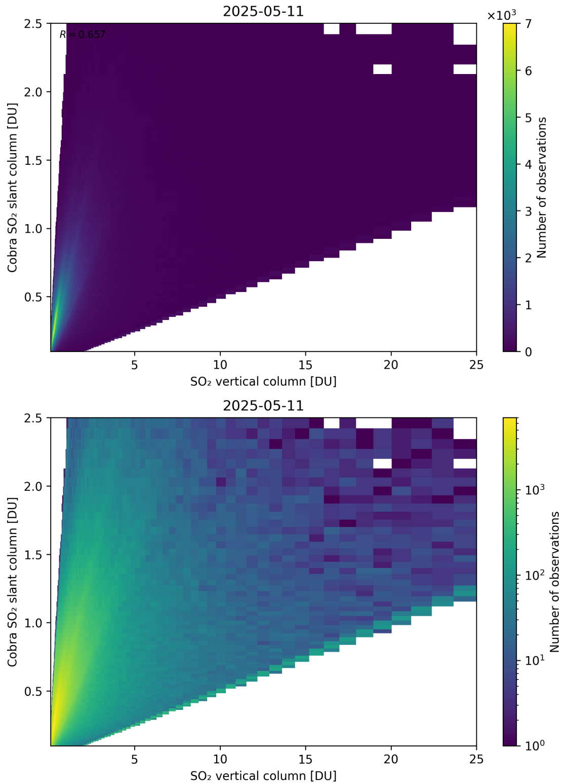
Figure 349: Scatter density plot of “SO 2 vertical column” against “Cobra SO 2 slant column” for 2025-05-10 to 2025-05-12.
