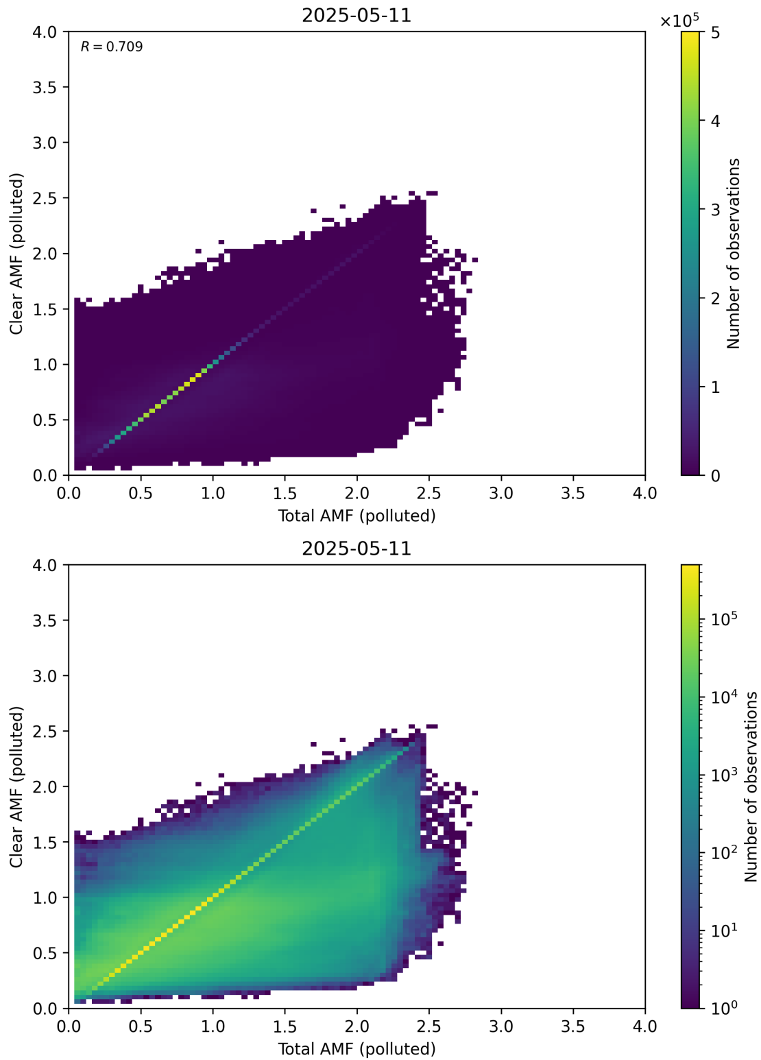
Figure 321: Scatter density plot of “Total AMF (polluted)” against “Clear AMF (polluted)” for 2025-05-10 to 2025-05-12.
