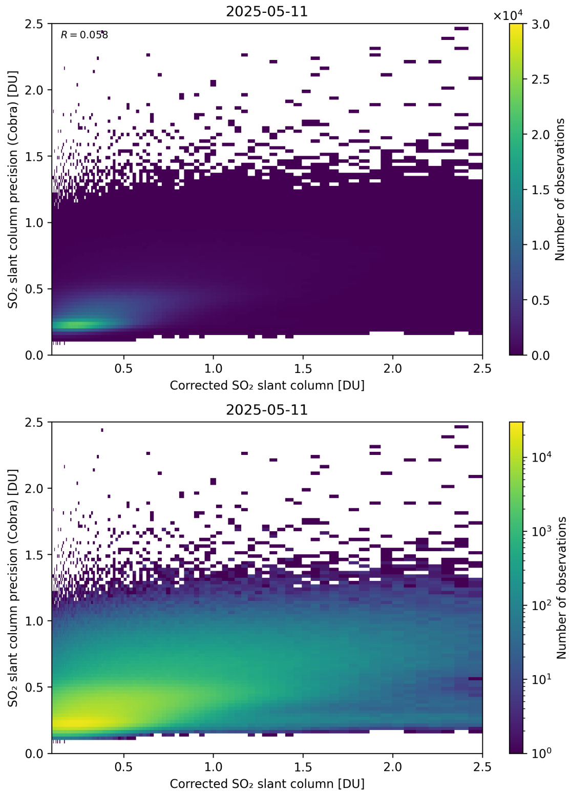
Figure 234: Scatter density plot of “Corrected SO 2 slant column” against “SO 2 slant column precision (Cobra)” for 2025-05-10 to 2025-05-12.
