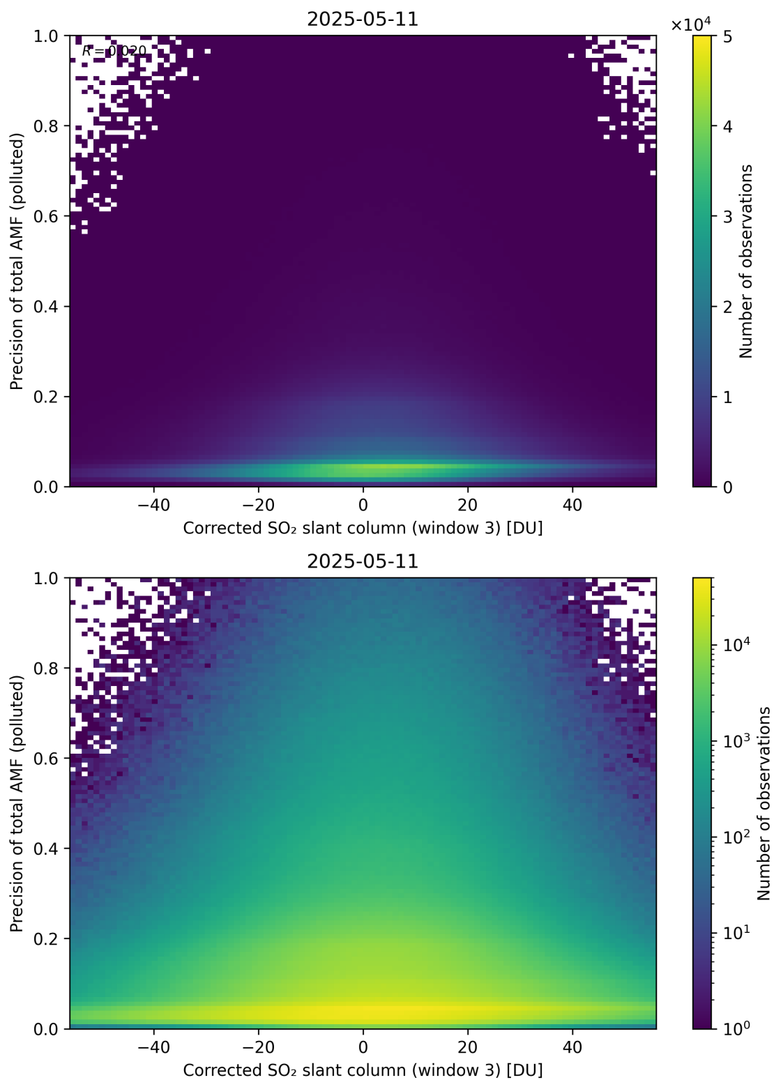
Figure 261: Scatter density plot of “Corrected SO 2 slant column (window 3)” against “Precision of total AMF (polluted)” for 2025-05-10 to 2025-05-12.
