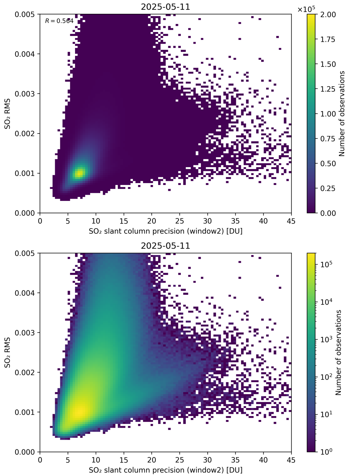
Figure 295: Scatter density plot of “SO 2 slant column precision (window2)” against “SO 2 RMS” for 2025-05-10 to 2025-05-12.
