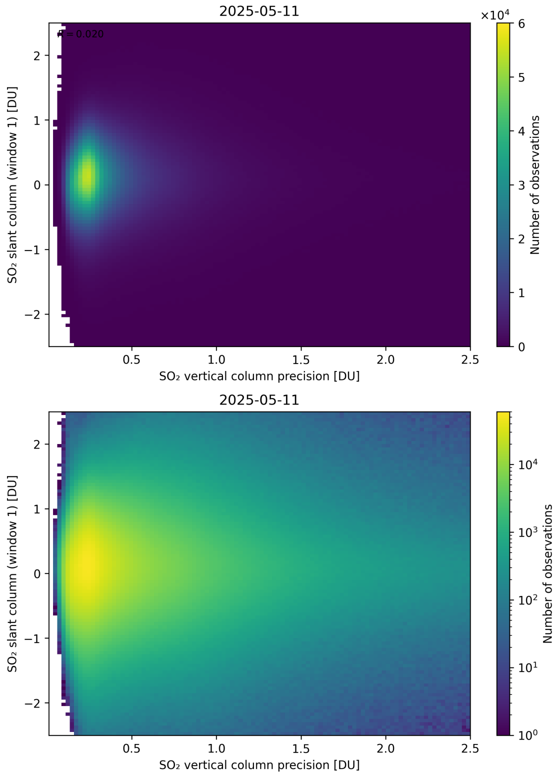
Figure 341: Scatter density plot of “SO 2 vertical column precision” against “SO 2 slant column (window 1)” for 2025-05-10 to 2025-05-12.
