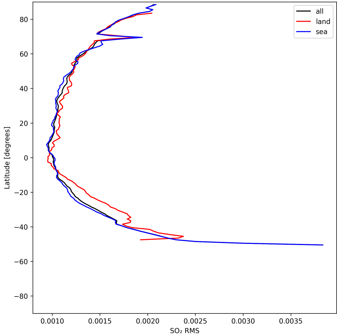
Figure 52: Zonal average of “SO 2 RMS” for 2025-05-10 to 2025-05-12.
