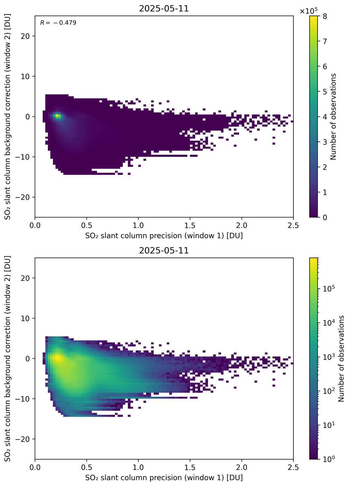
Figure 269: Scatter density plot of “SO 2 slant column precision (window 1)” against “SO 2 slant column background correction (window 2)” for 2025-05-10 to 2025-05-12.
