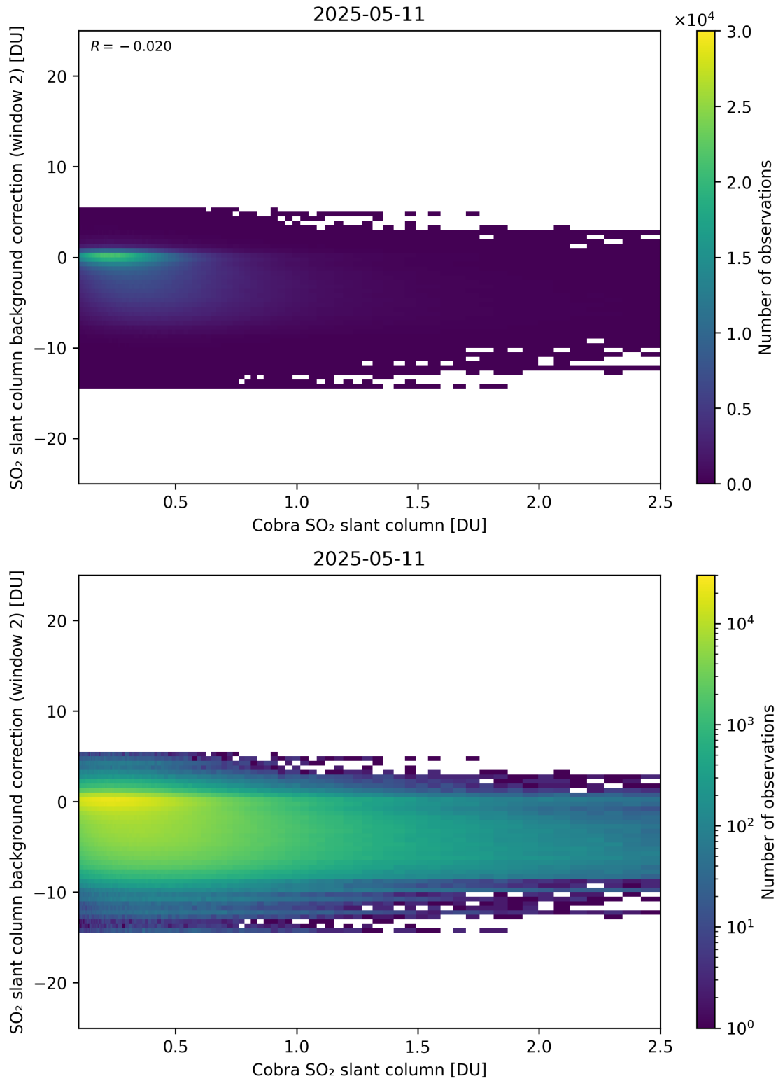
Figure 194: Scatter density plot of “Cobra SO 2 slant column” against “SO 2 slant column background correction (window 2)” for 2025-05-10 to 2025-05-12.
