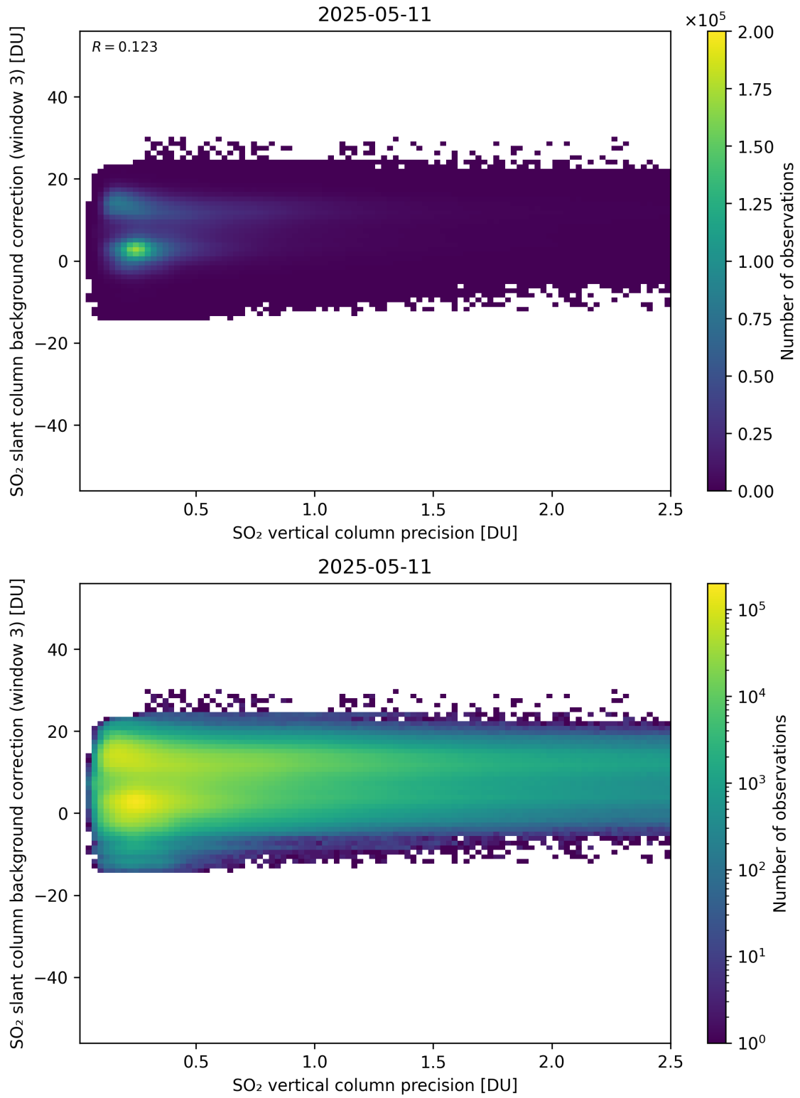
Figure 331: Scatter density plot of “SO 2 vertical column precision” against “SO 2 slant column background correction (window 3)” for 2025-05-10 to 2025-05-12.
