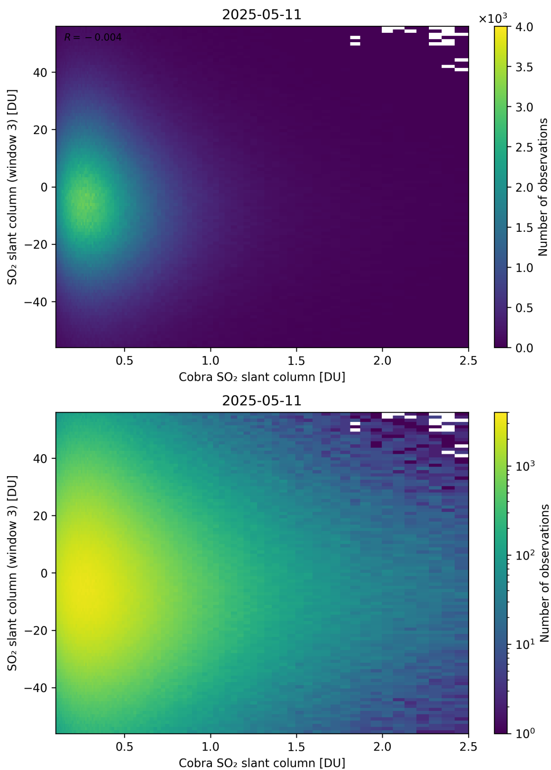
Figure 222: Scatter density plot of “Cobra SO 2 slant column” against “SO 2 slant column (window 3)” for 2025-05-10 to 2025-05-12.
