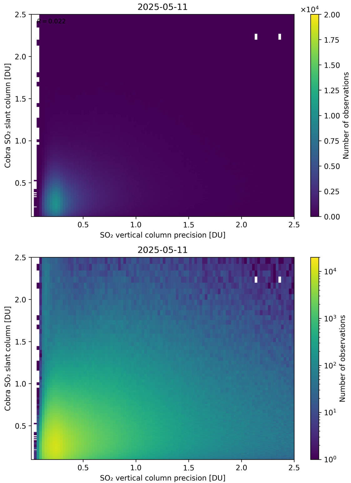
Figure 336: Scatter density plot of “SO 2 vertical column precision” against “Cobra SO 2 slant column” for 2025-05-10 to 2025-05-12.
