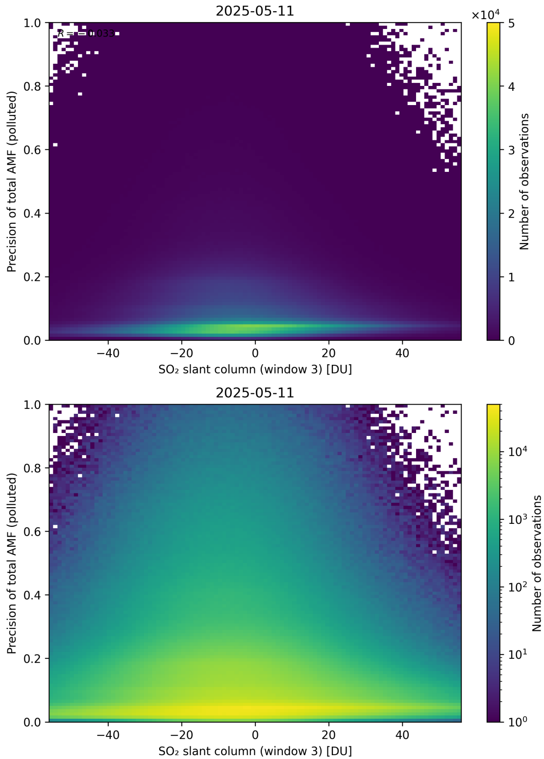
Figure 319: Scatter density plot of “SO 2 slant column (window 3)” against “Precision of total AMF (polluted)” for 2025-05-10 to 2025-05-12.
