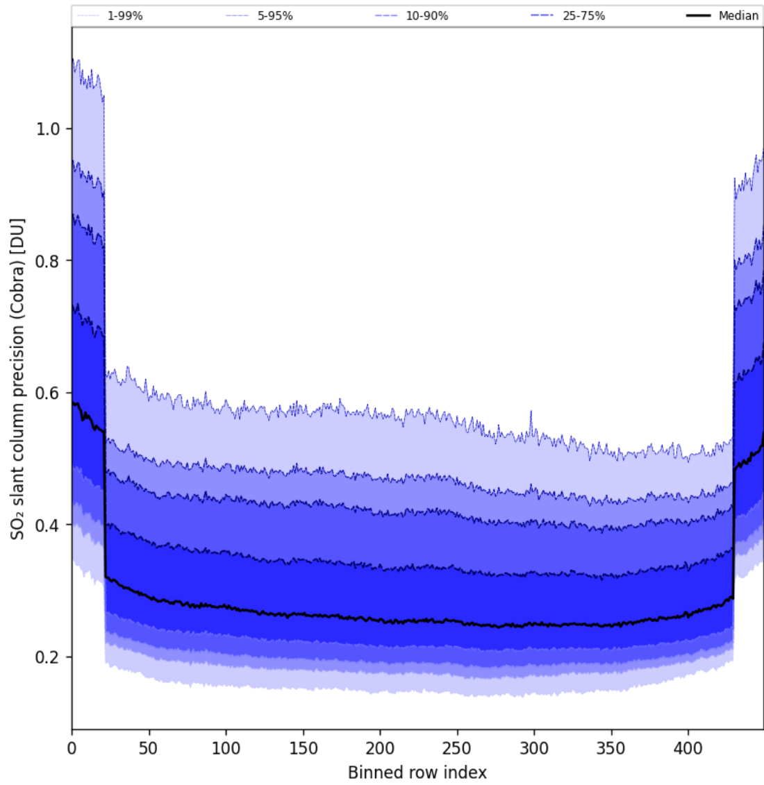
Figure 88: Along track statistics of “SO 2 slant column precision (Cobra)” for 2025-05-10 to 2025-05-12
