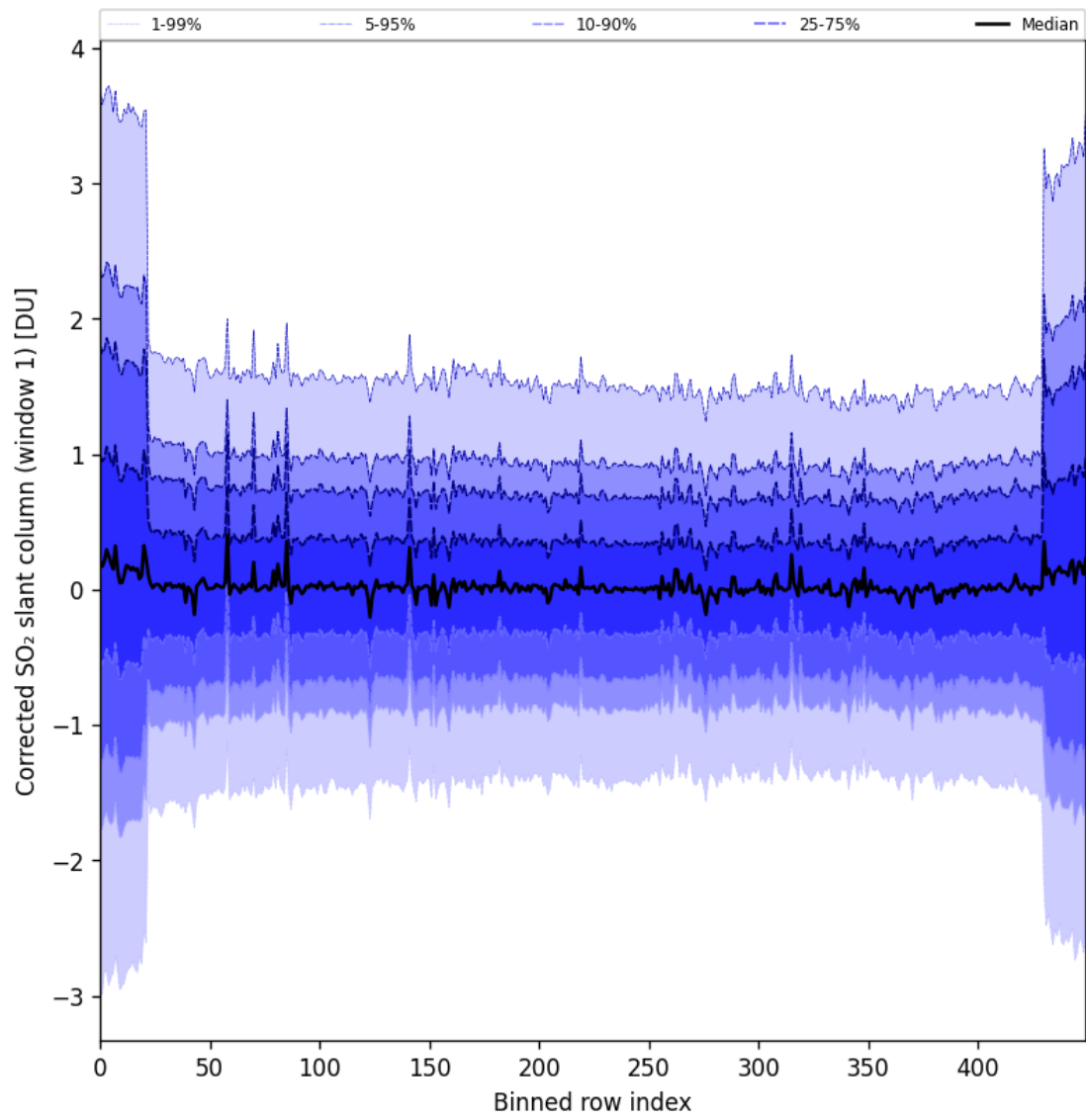
Figure 91: Along track statistics of “Corrected SO 2 slant column (window 1)” for 2025-05-10 to 2025-05-12
