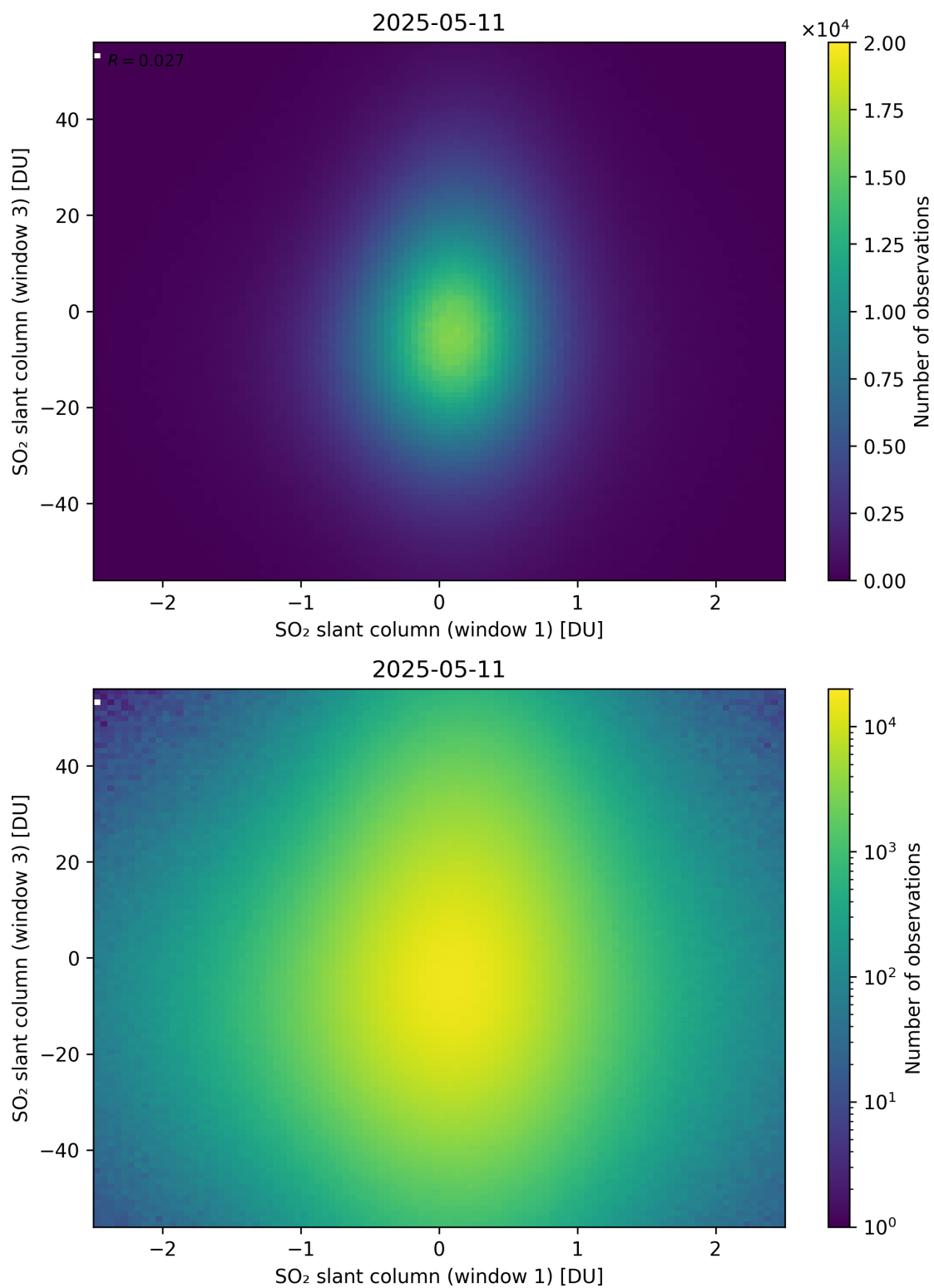
Figure 287: Scatter density plot of “SO 2 slant column (window 1)” against “SO 2 slant column (window 3)” for 2025-05-10 to 2025-05-12.
