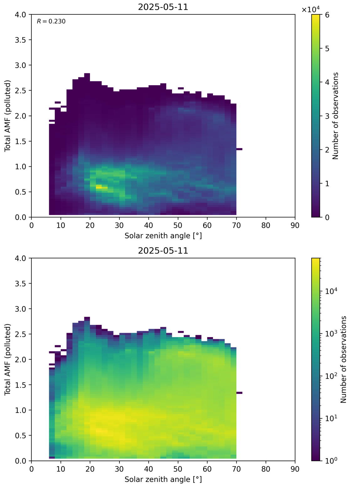
Figure 189: Scatter density plot of “Solar zenith angle” against “Total AMF (polluted)” for 2025-05-10 to 2025-05-12.
