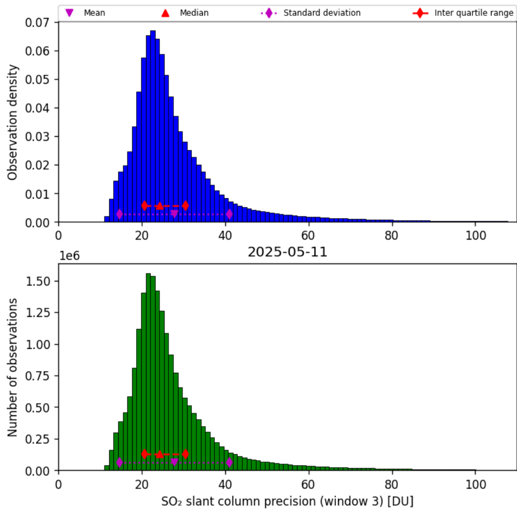
Figure 72: Histogram of “SO 2 slant column precision (window 3)” for 2025-05-10 to 2025-05-12
