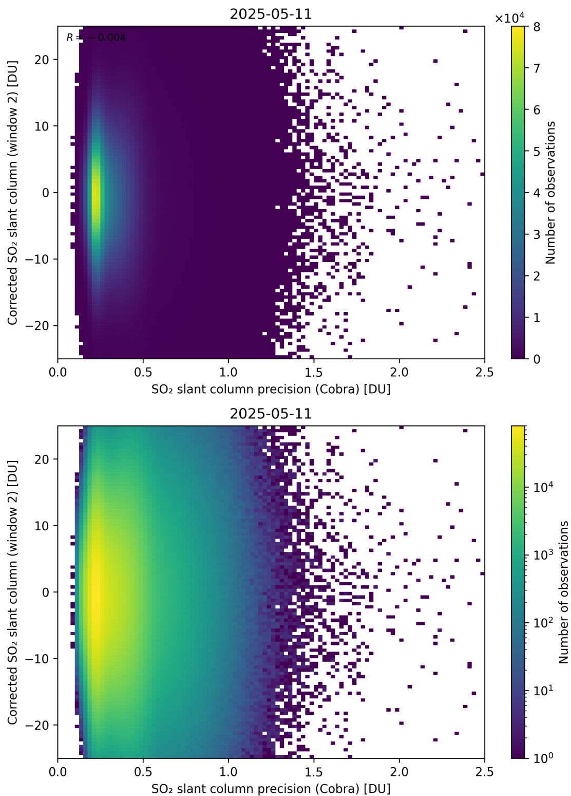
Figure 206: Scatter density plot of “SO 2 slant column precision (Cobra)” against “Corrected SO 2 slant column (window 2)” for 2025-05-10 to 2025-05-12.
