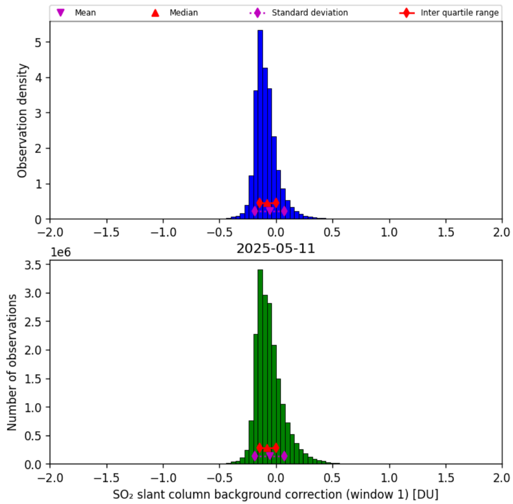
Figure 66: Histogram of “SO 2 slant column background correction (window 1)” for 2025-05-10 to 2025-05-12
