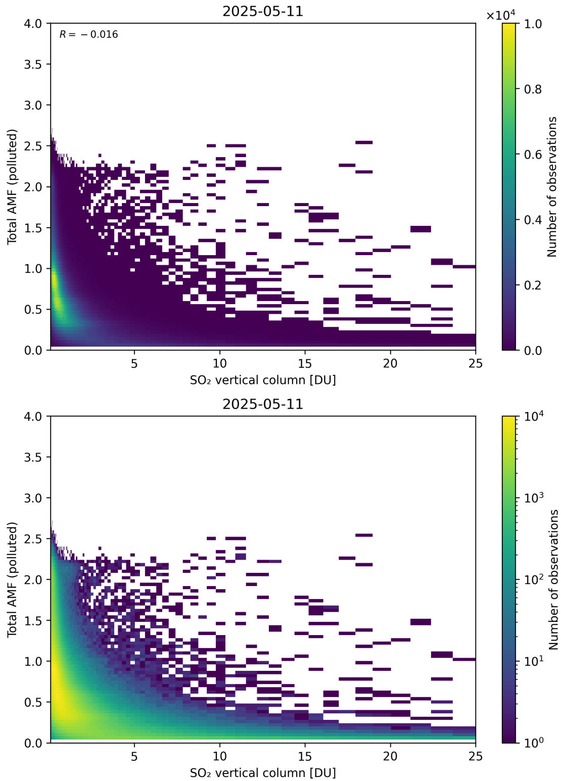
Figure 359: Scatter density plot of “SO 2 vertical column” against “Total AMF (polluted)” for 2025-05-10 to 2025-05-12.
