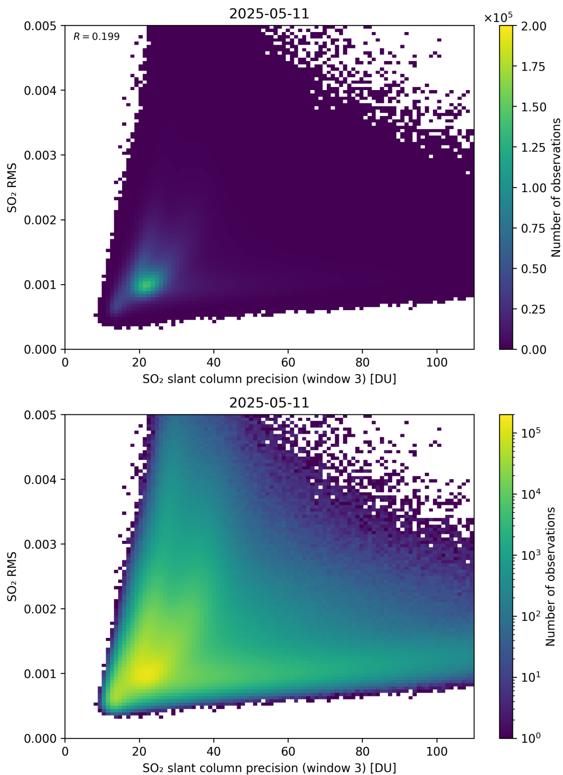
Figure 310: Scatter density plot of “SO 2 slant column precision (window 3)” against “SO 2 RMS” for 2025-05-10 to 2025-05-12.
