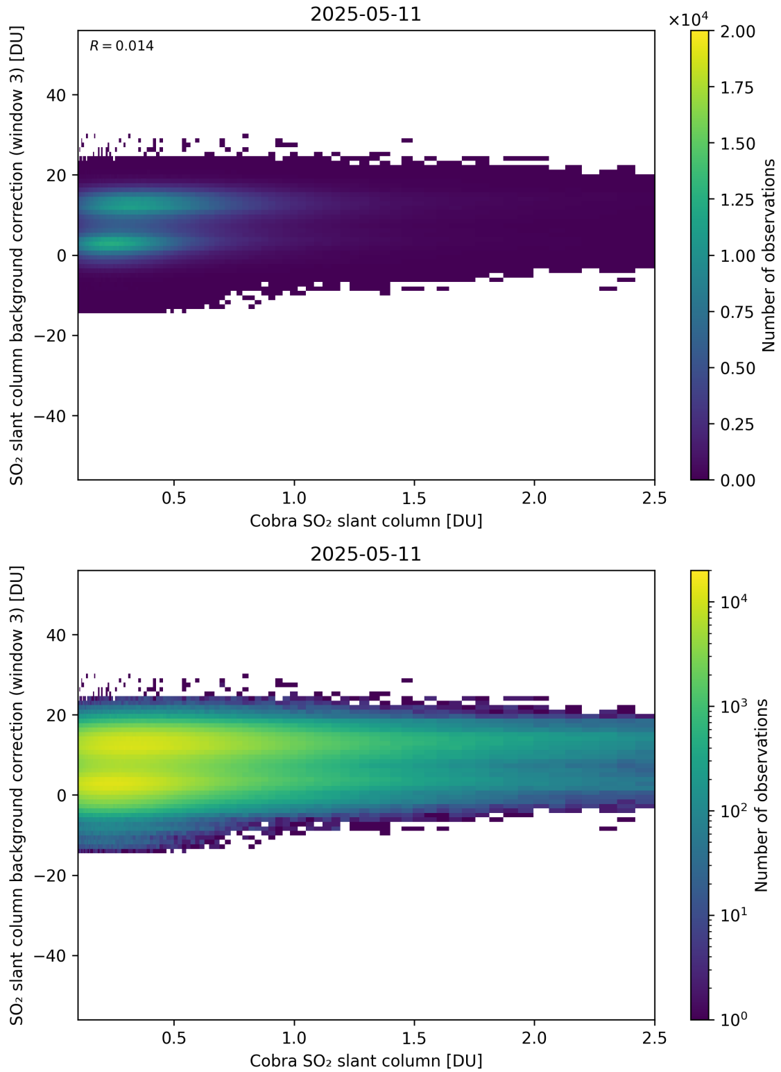
Figure 195: Scatter density plot of “Cobra SO 2 slant column” against “SO 2 slant column background correction (window 3)” for 2025-05-10 to 2025-05-12.
