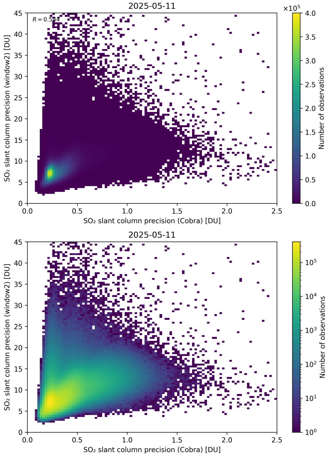
Figure 210: Scatter density plot of “SO 2 slant column precision (Cobra)” against “SO 2 slant column precision (window2)” for 2025-05-10 to 2025-05-12.
