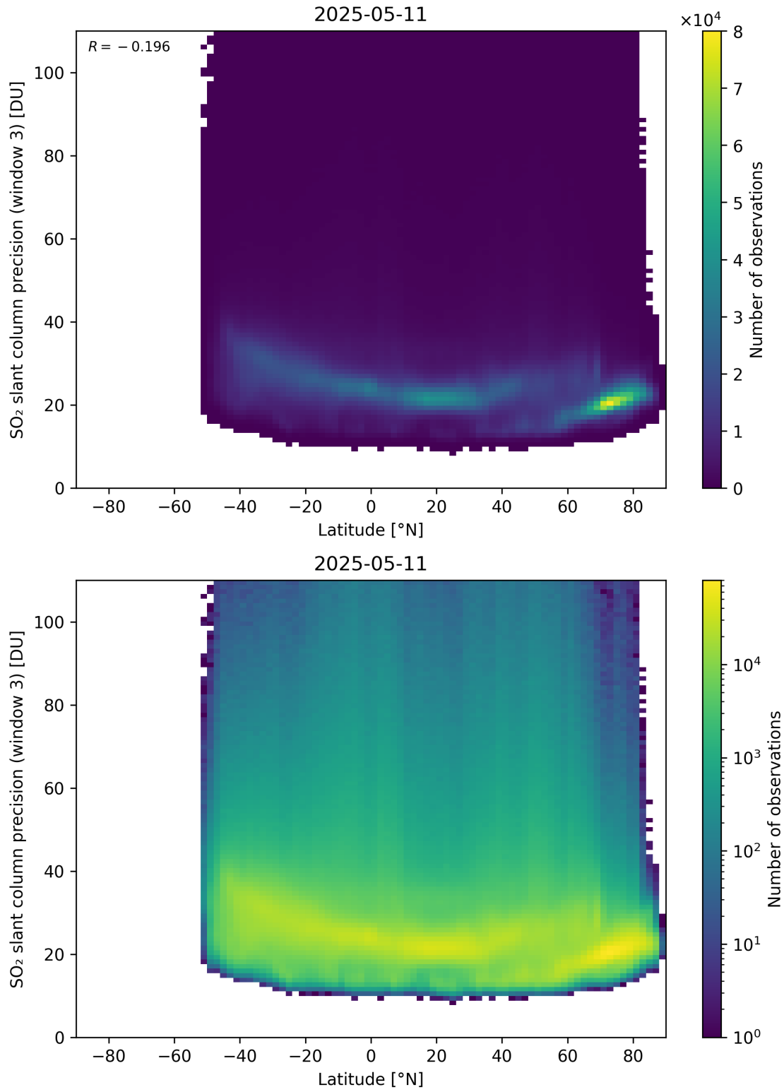
Figure 166: Scatter density plot of “Latitude” against “SO 2 slant column precision (window 3)” for 2025-05-10 to 2025-05-12.
