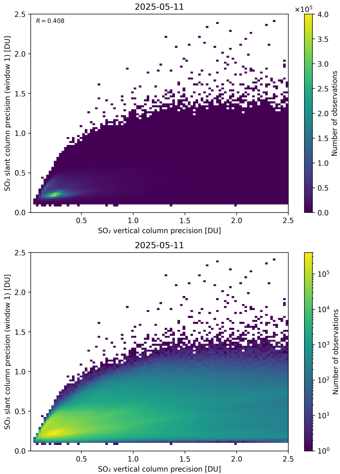
Figure 342: Scatter density plot of “SO 2 vertical column precision” against “SO 2 slant column precision (window 1)” for 2025-05-10 to 2025-05-12.
