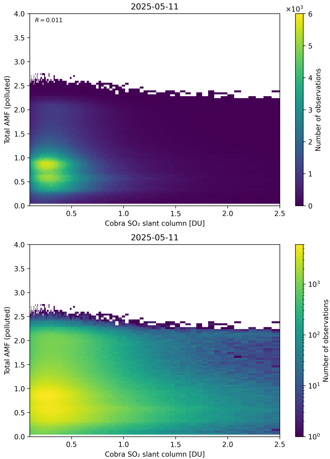
Figure 224: Scatter density plot of “Cobra SO 2 slant column” against “Total AMF (polluted)” for 2025-05-10 to 2025-05-12.
