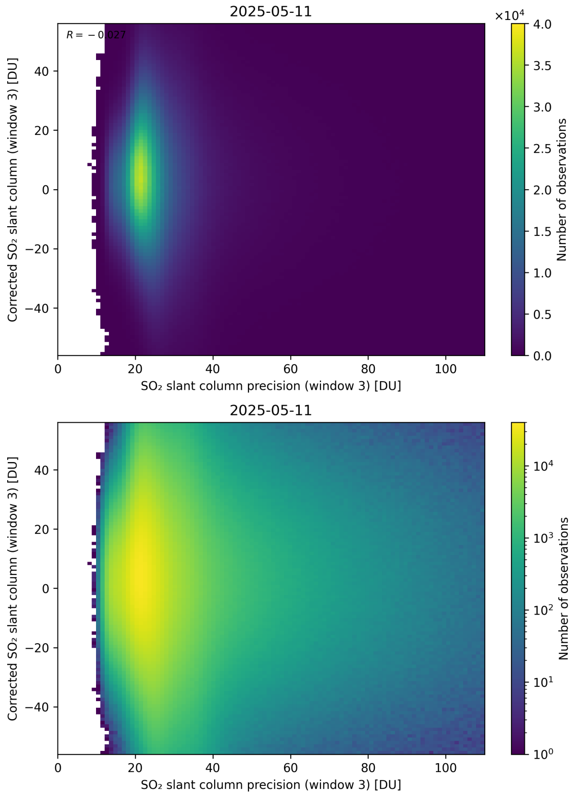
Figure 312: Scatter density plot of “SO 2 slant column precision (window 3)” against “Corrected SO 2 slant column (window 3)” for 2025-05-10 to 2025-05-12.
