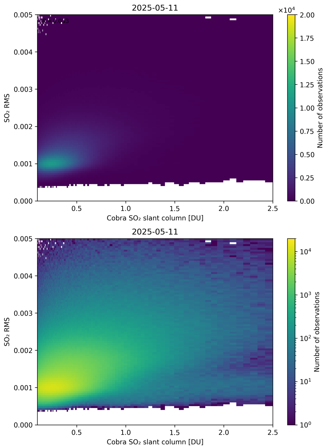
Figure 198: Scatter density plot of “Cobra SO 2 slant column” against “SO 2 RMS” for 2025-05-10 to 2025-05-12.
