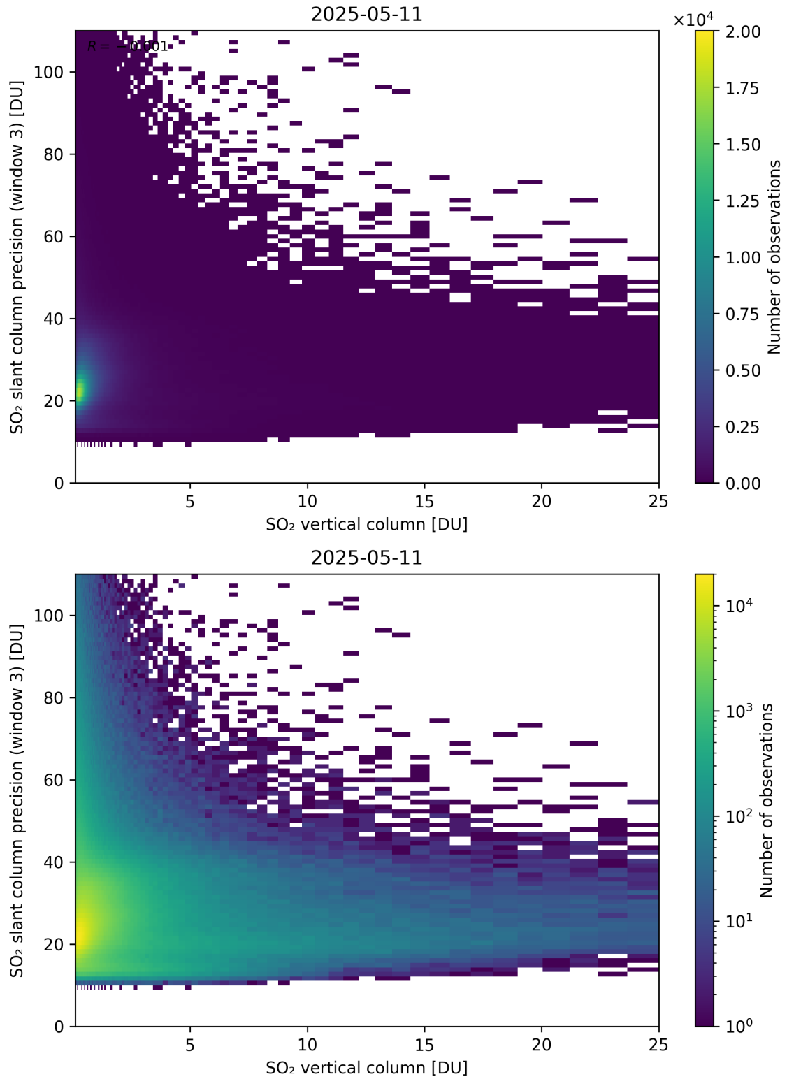
Figure 358: Scatter density plot of “SO 2 vertical column” against “SO 2 slant column precision (window 3)” for 2025-05-10 to 2025-05-12.
