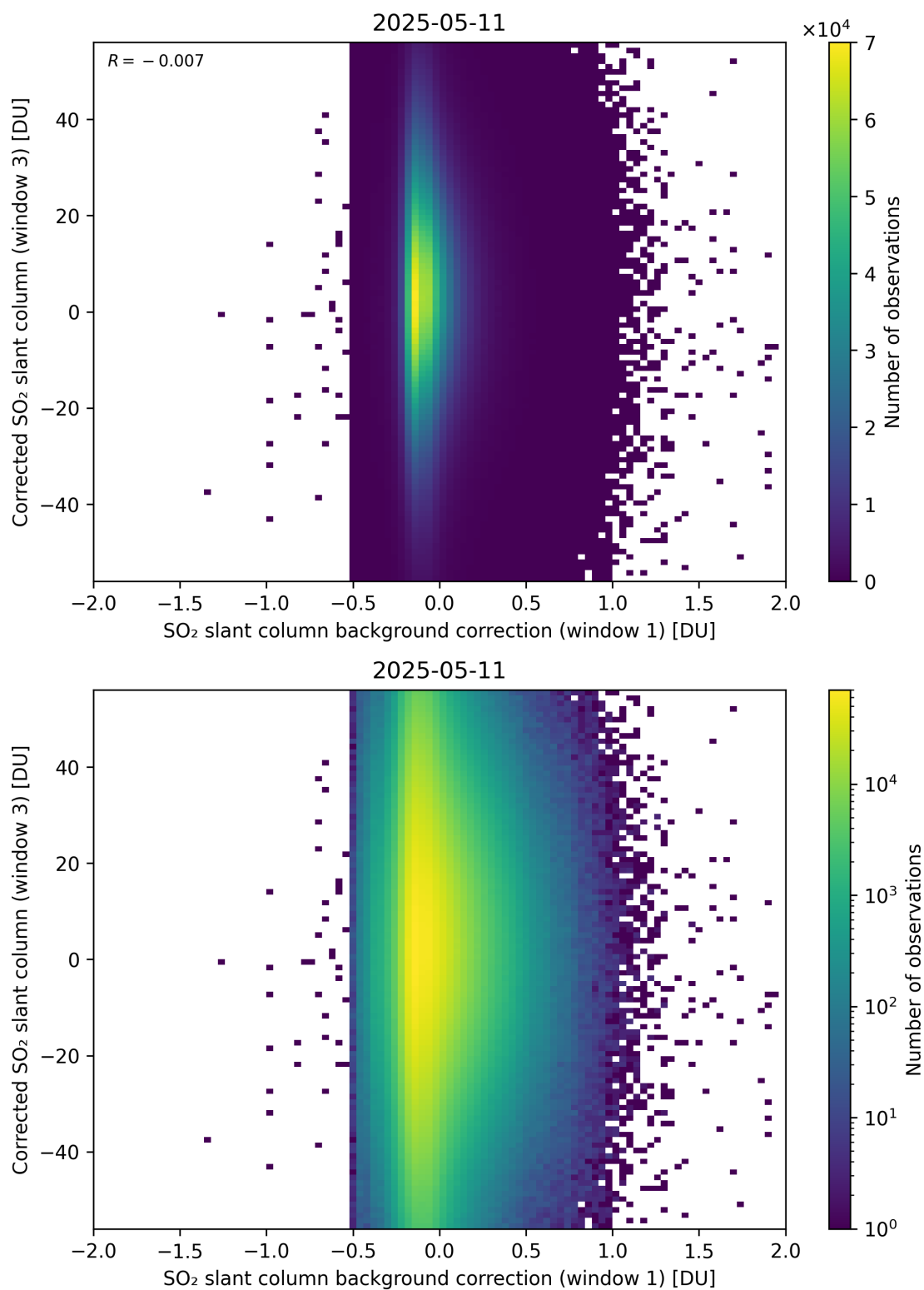
Figure 116: Scatter density plot of “SO 2 slant column background correction (window 1)” against “Corrected SO 2 slant column (window 3)” for 2025-05-10 to 2025-05-12.
