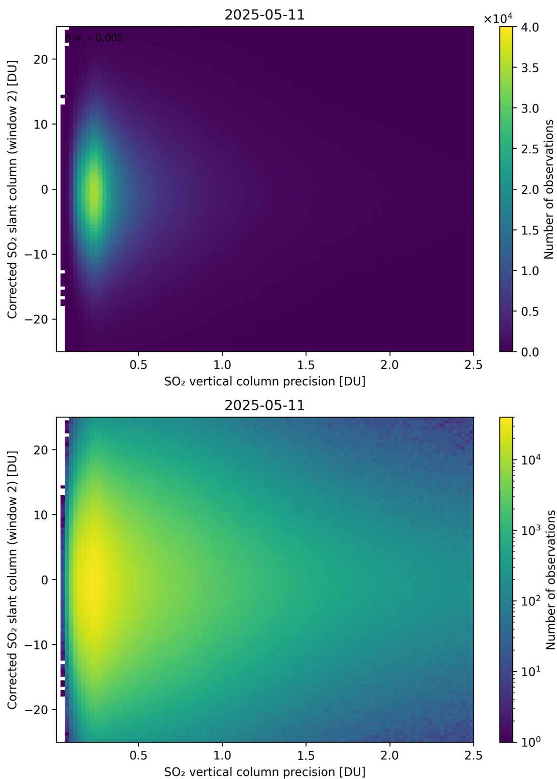
Figure 339: Scatter density plot of “SO 2 vertical column precision” against “Corrected SO 2 slant column (window 2)” for 2025-05-10 to 2025-05-12.
