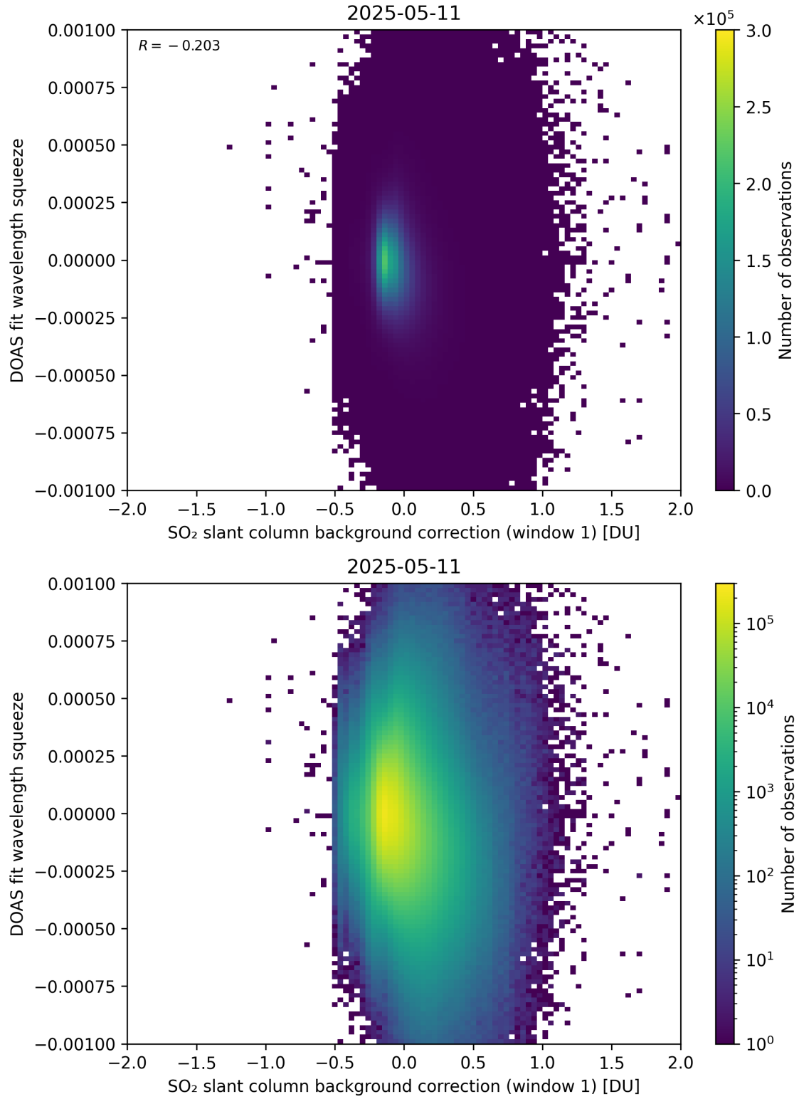
Figure 112: Scatter density plot of “SO 2 slant column background correction (window 1)” against “DOAS fit wavelength squeeze” for 2025-05-10 to 2025-05-12.
