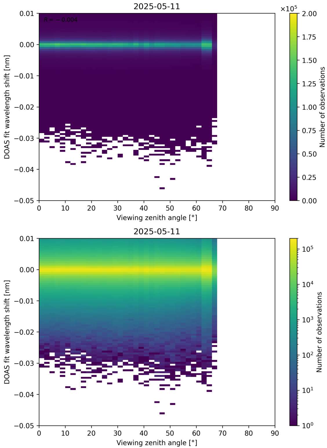
Figure 365: Scatter density plot of “Viewing zenith angle” against “DOAS fit wavelength shift” for 2025-05-10 to 2025-05-12.
