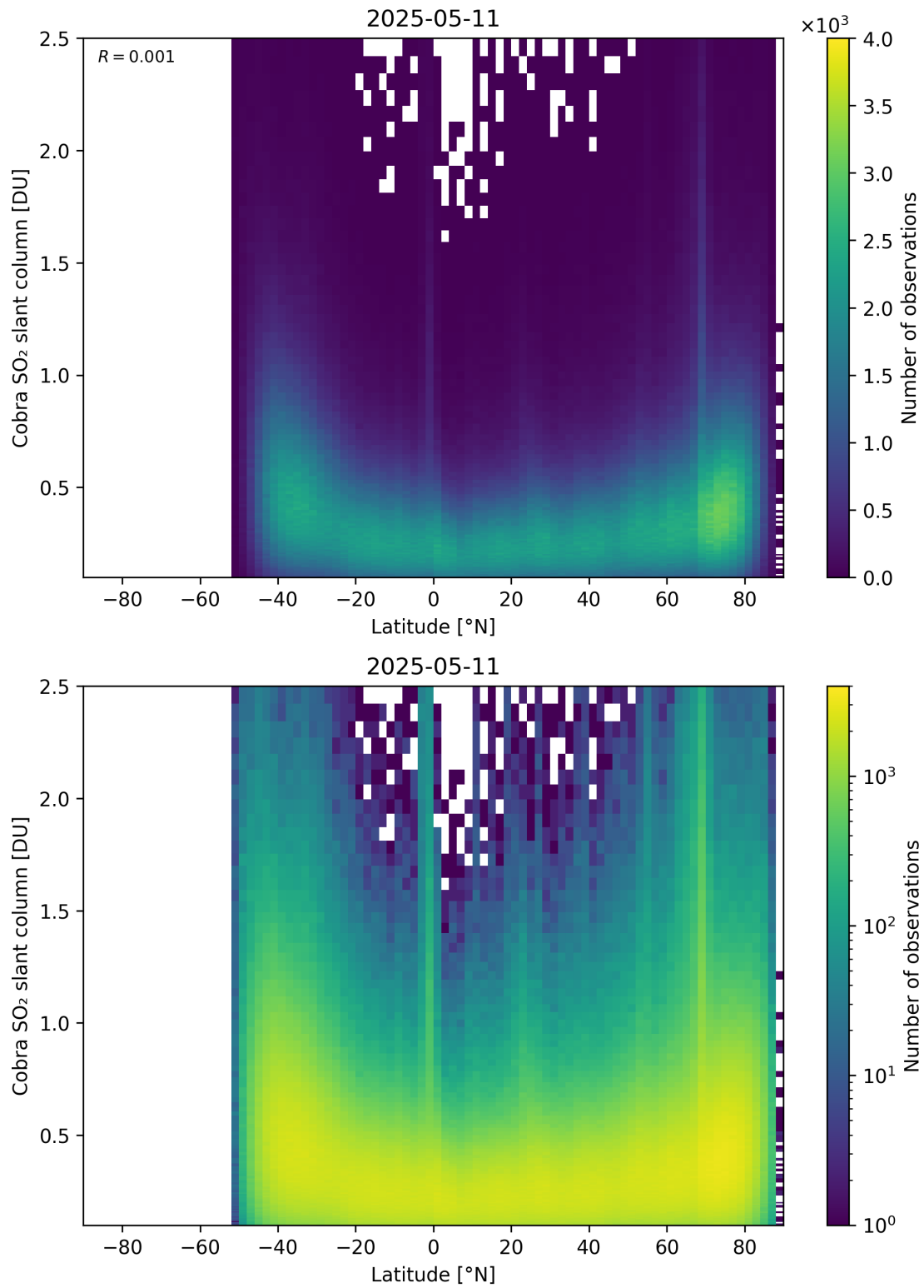
Figure 157: Scatter density plot of “Latitude” against “Cobra SO 2 slant column” for 2025-05-10 to 2025-05-12.
