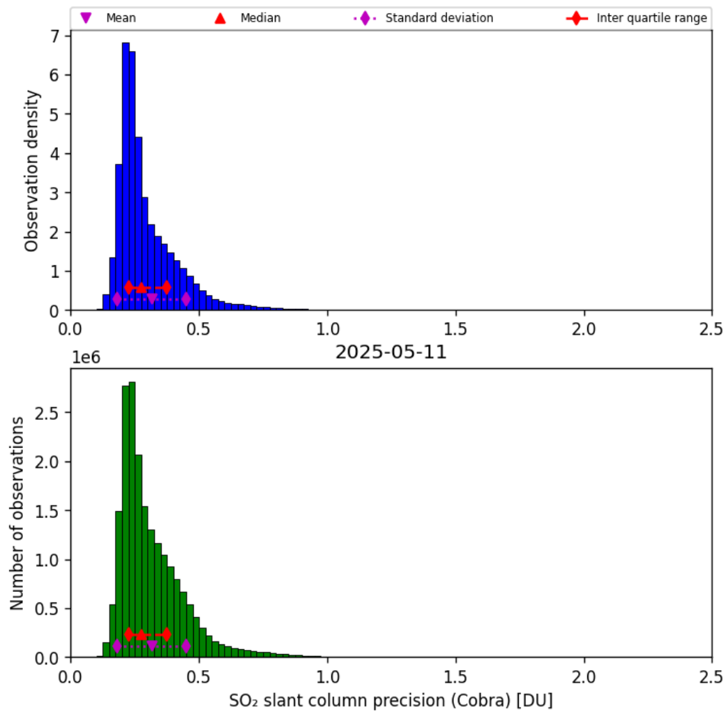
Figure 62: Histogram of “SO 2 slant column precision (Cobra)” for 2025-05-10 to 2025-05-12
