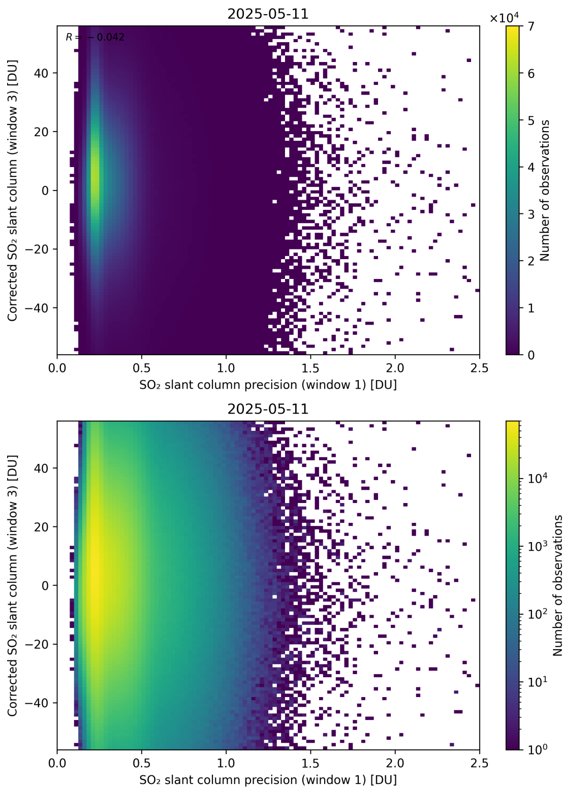
Figure 276: Scatter density plot of “SO 2 slant column precision (window 1)” against “Corrected SO 2 slant column (window 3)” for 2025-05-10 to 2025-05-12.
