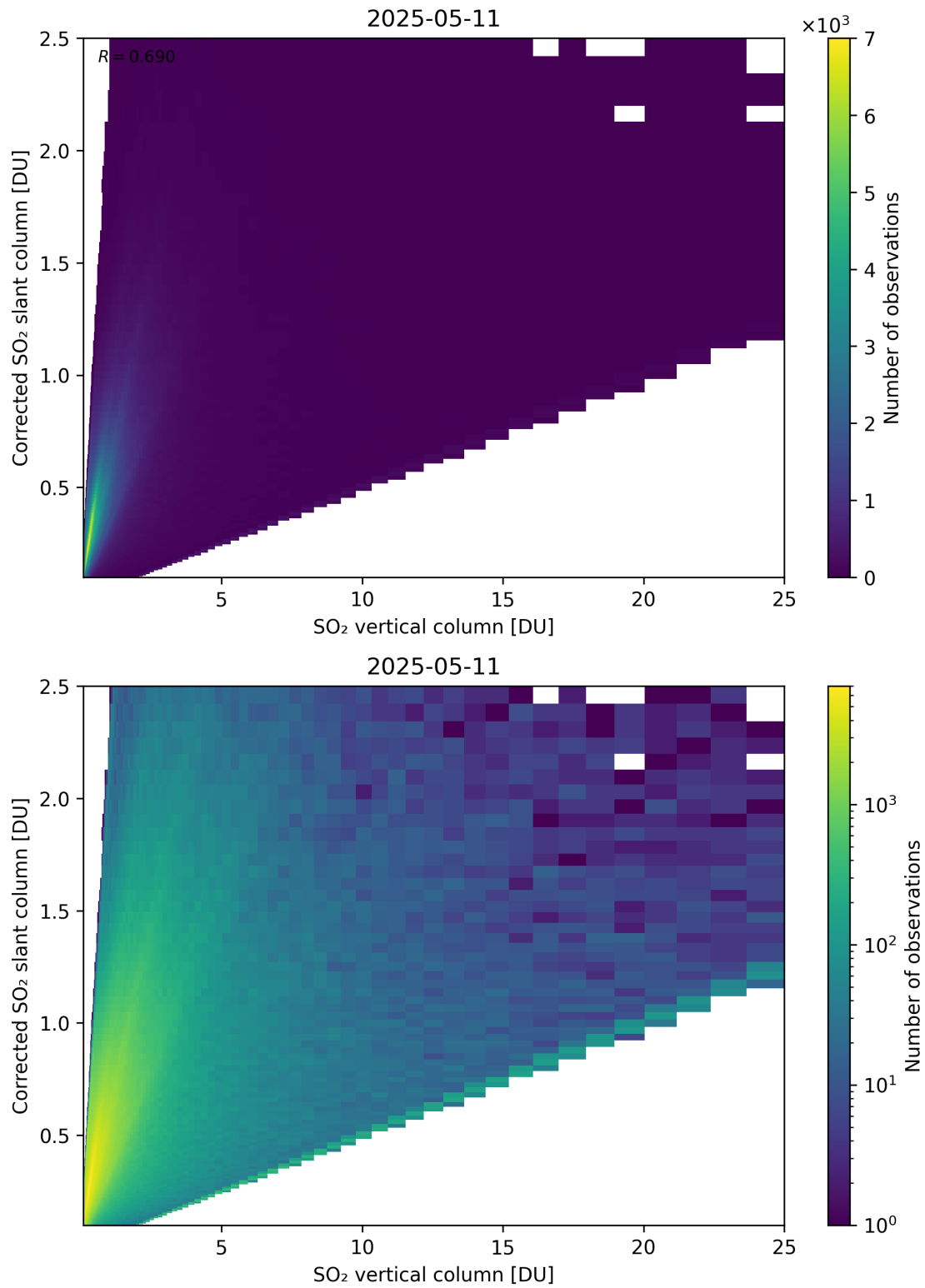
Figure 351: Scatter density plot of “SO 2 vertical column” against “Corrected SO 2 slant column” for 2025-05-10 to 2025-05-12.
