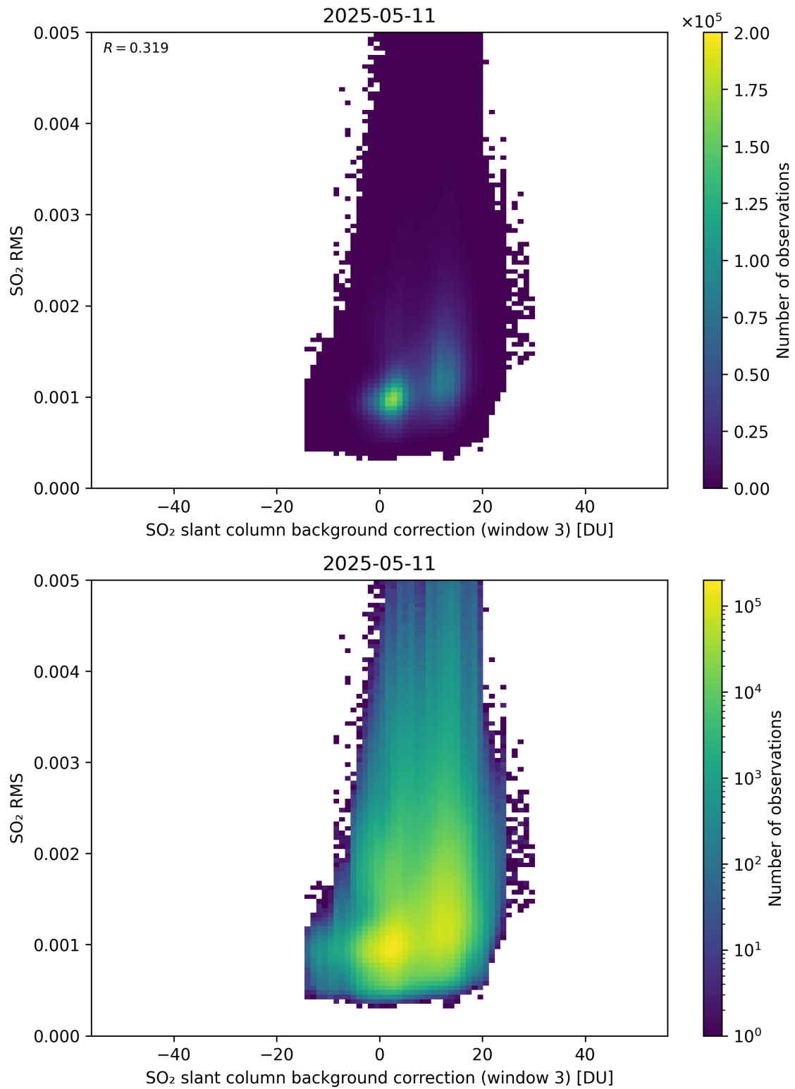
Figure 134: Scatter density plot of “SO 2 slant column background correction (window 3)” against “SO 2 RMS” for 2025-05-10 to 2025-05-12.
