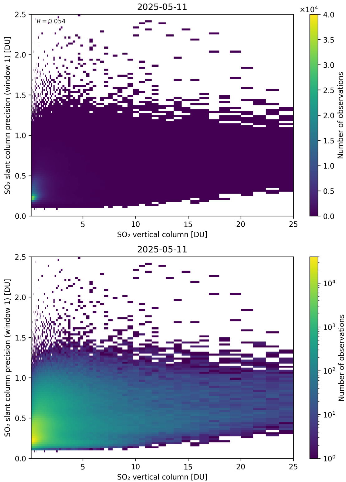
Figure 355: Scatter density plot of “SO 2 vertical column” against “SO 2 slant column precision (window 1)” for 2025-05-10 to 2025-05-12.
