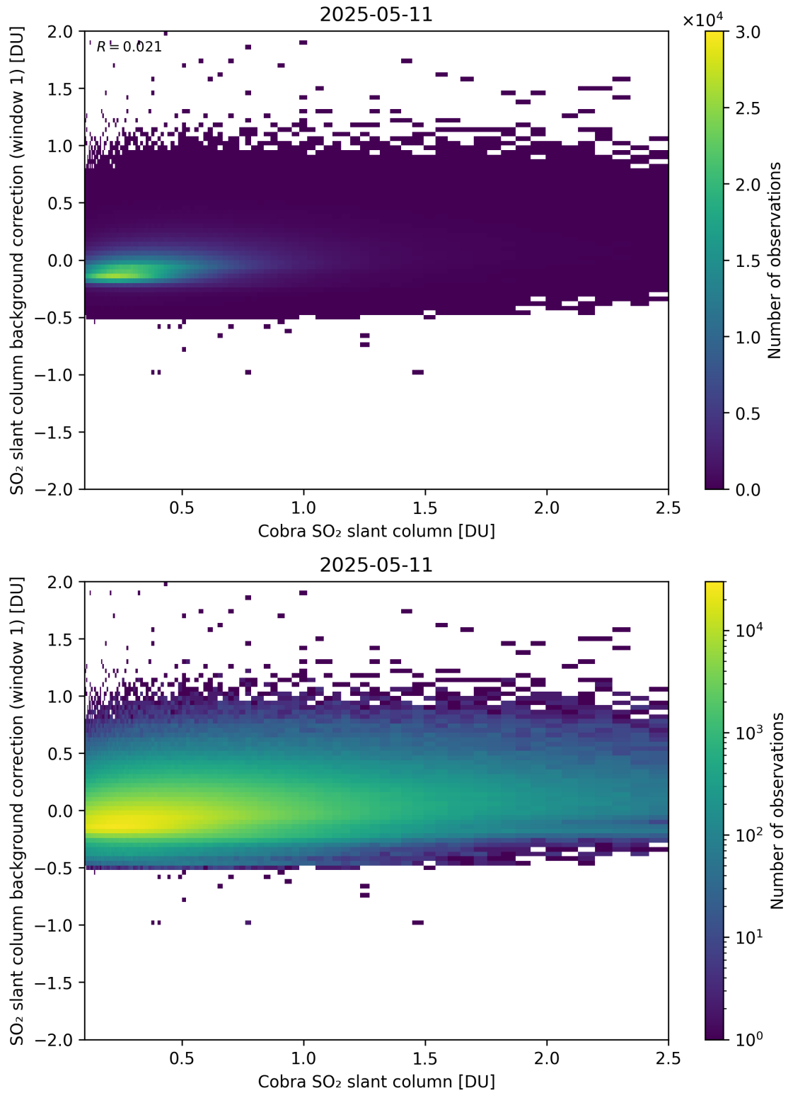
Figure 193: Scatter density plot of “Cobra SO 2 slant column” against “SO 2 slant column background correction (window 1)” for 2025-05-10 to 2025-05-12.
