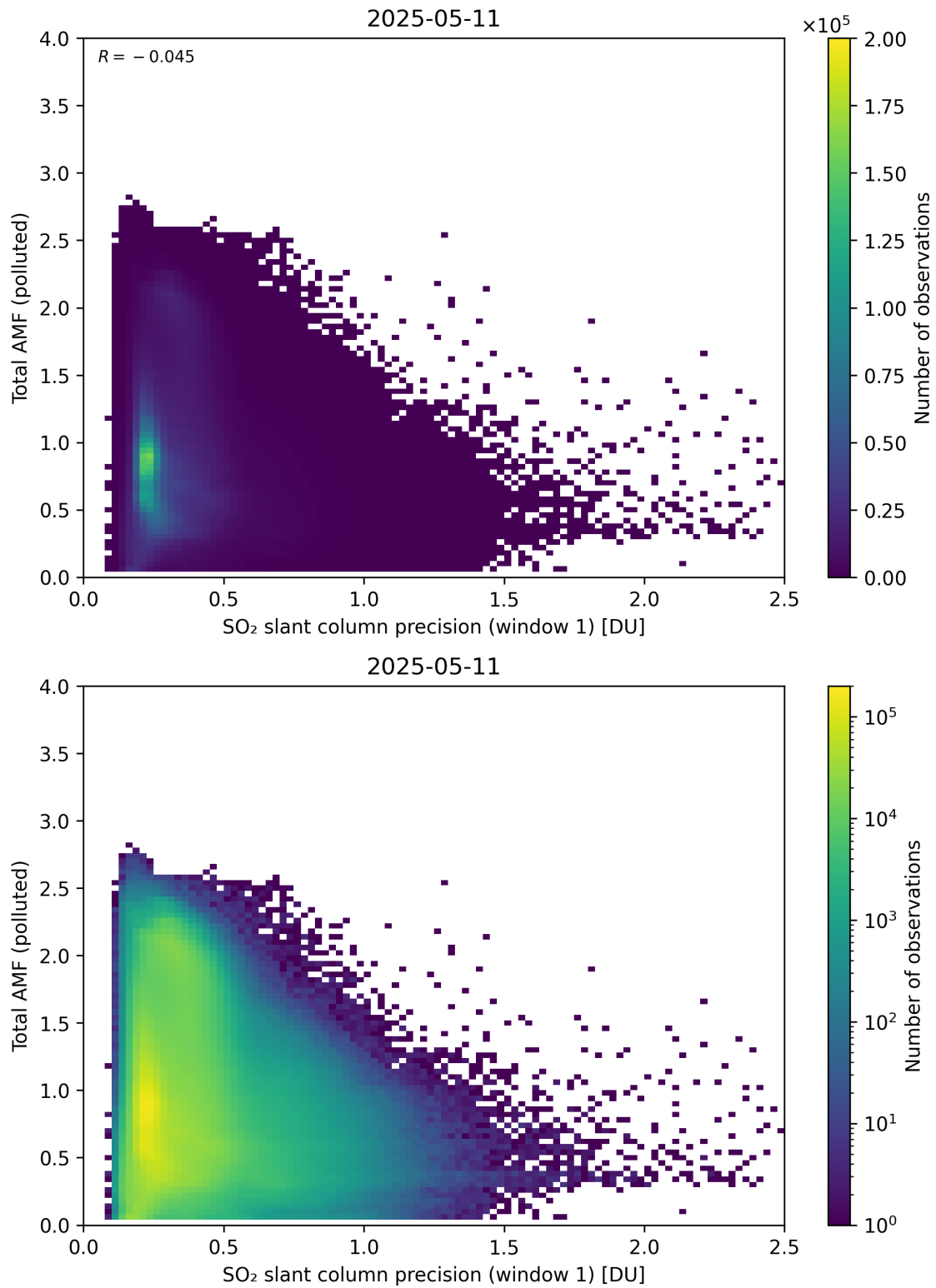
Figure 280: Scatter density plot of “SO 2 slant column precision (window 1)” against “Total AMF (polluted)” for 2025-05-10 to 2025-05-12.
