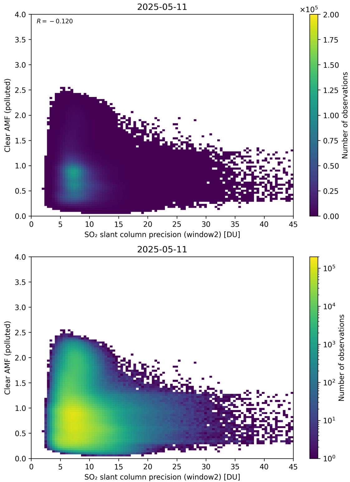
Figure 296: Scatter density plot of “SO 2 slant column precision (window2)” against “Clear AMF (polluted)” for 2025-05-10 to 2025-05-12.
