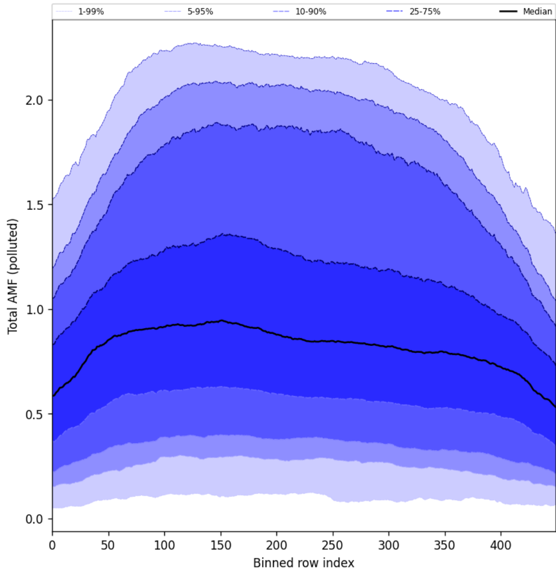
Figure 105: Along track statistics of “Total AMF (polluted)” for 2025-05-10 to 2025-05-12
