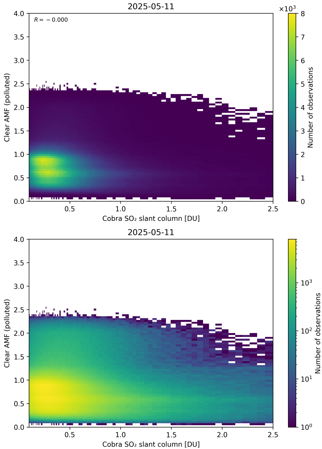
Figure 215: Scatter density plot of “Cobra SO 2 slant column” against “Clear AMF (polluted)” for 2025-05-10 to 2025-05-12.
