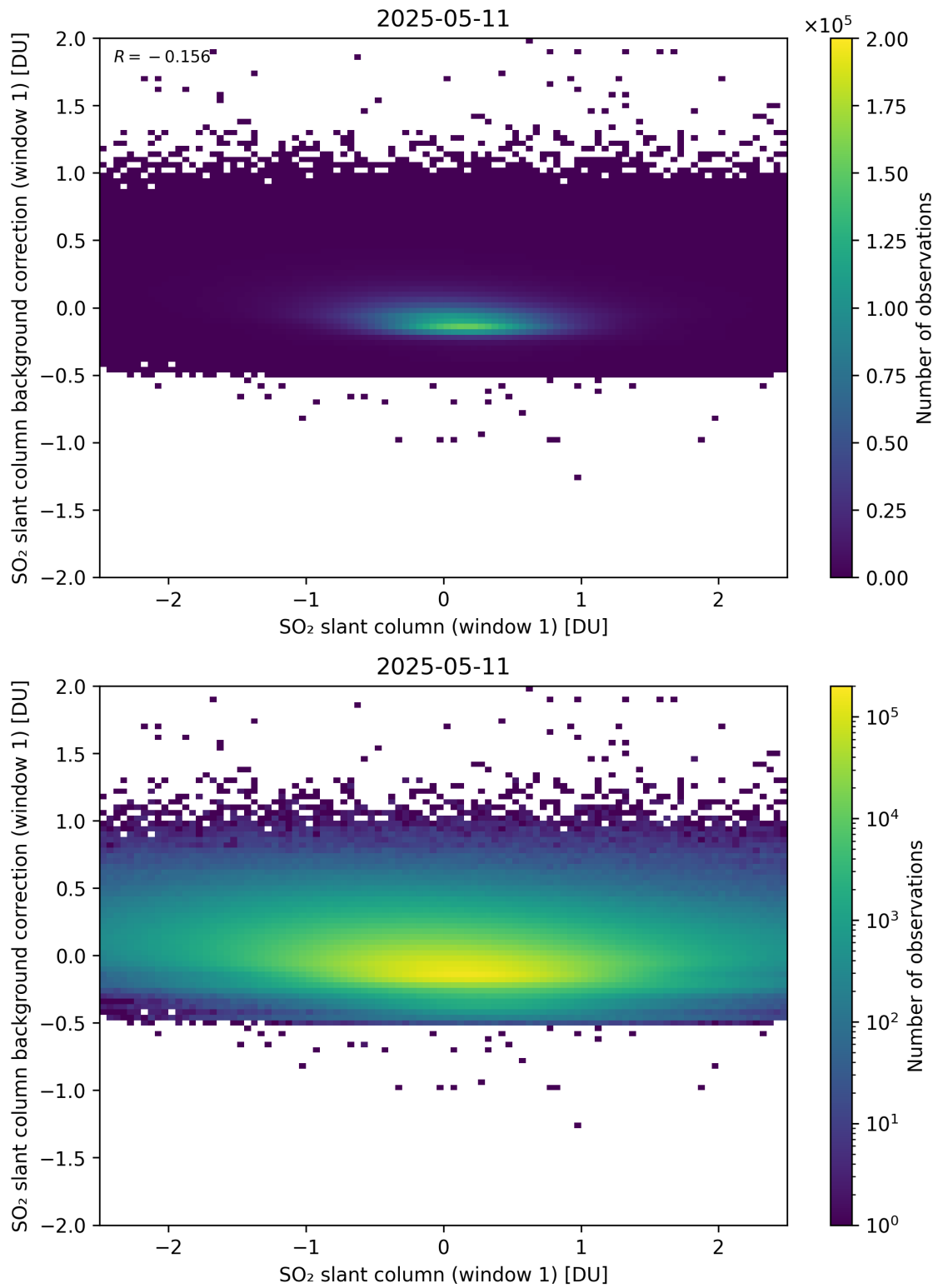
Figure 262: Scatter density plot of “SO 2 slant column (window 1)” against “SO 2 slant column background correction (window 1)” for 2025-05-10 to 2025-05-12.
