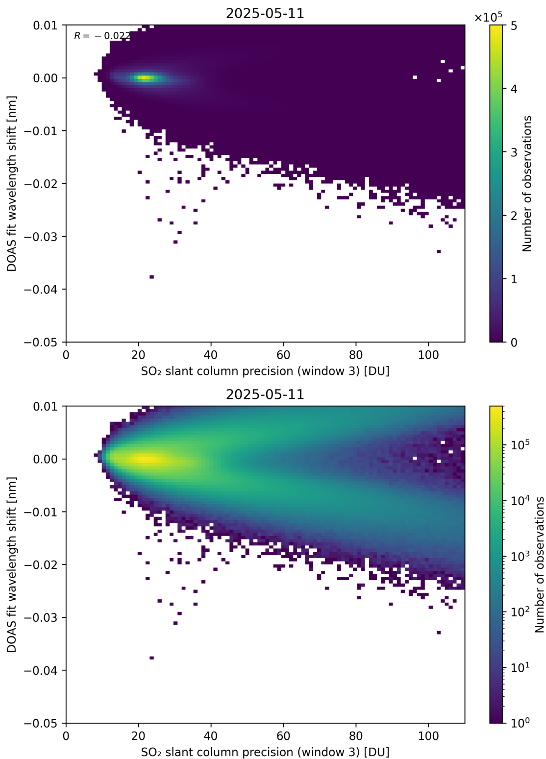
Figure 308: Scatter density plot of “SO 2 slant column precision (window 3)” against “DOAS fit wavelength shift” for 2025-05-10 to 2025-05-12.
