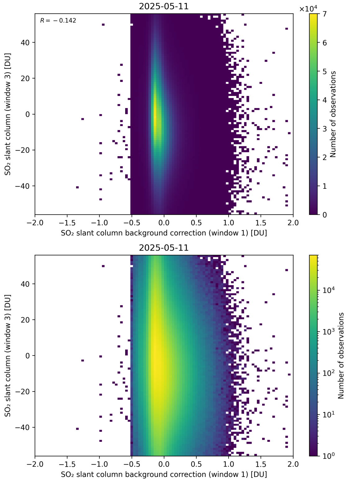
Figure 118: Scatter density plot of “SO 2 slant column background correction (window 1)” against “SO 2 slant column (window 3)” for 2025-05-10 to 2025-05-12.
