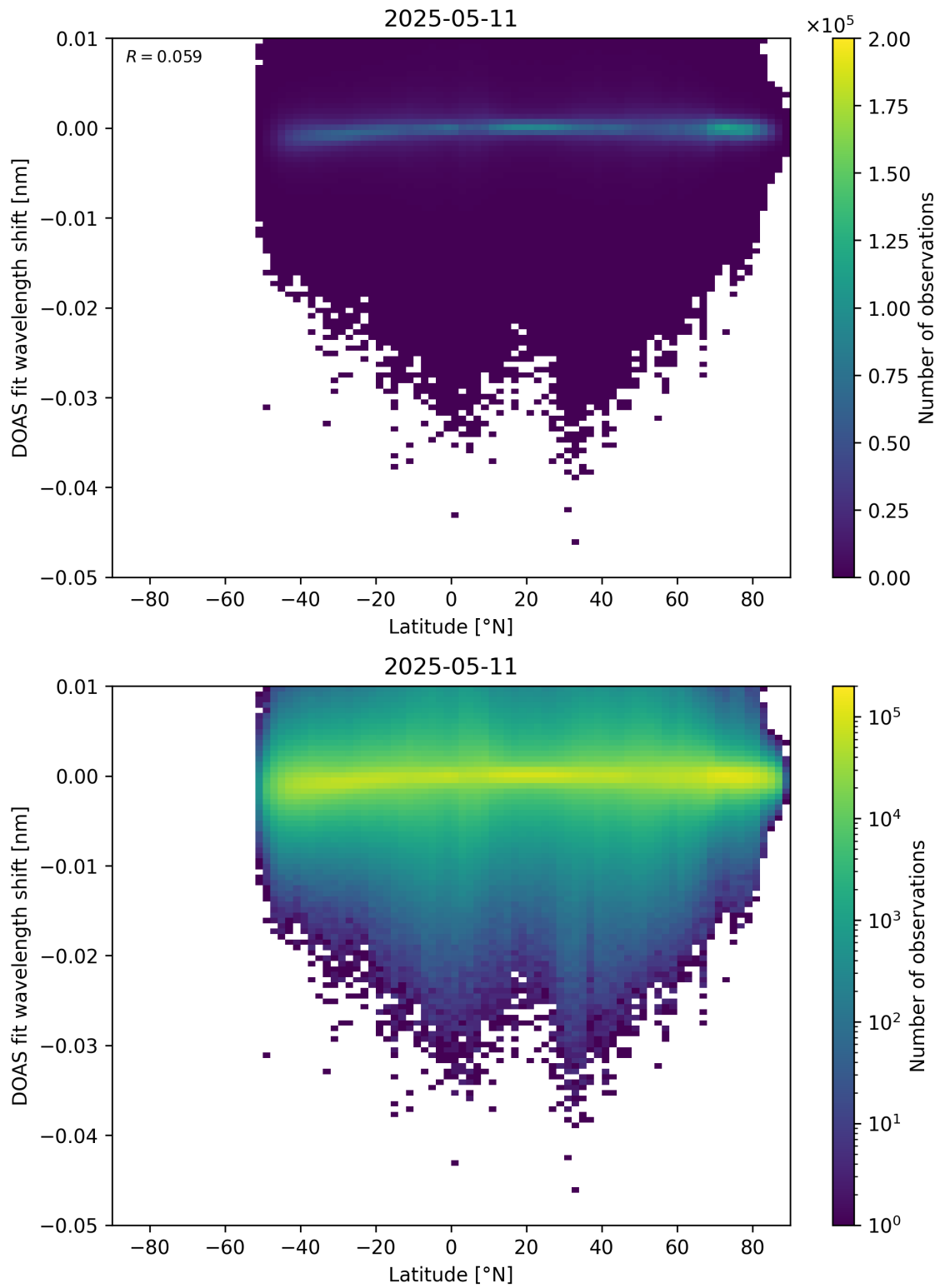
Figure 153: Scatter density plot of “Latitude” against “DOAS fit wavelength shift” for 2025-05-10 to 2025-05-12.
