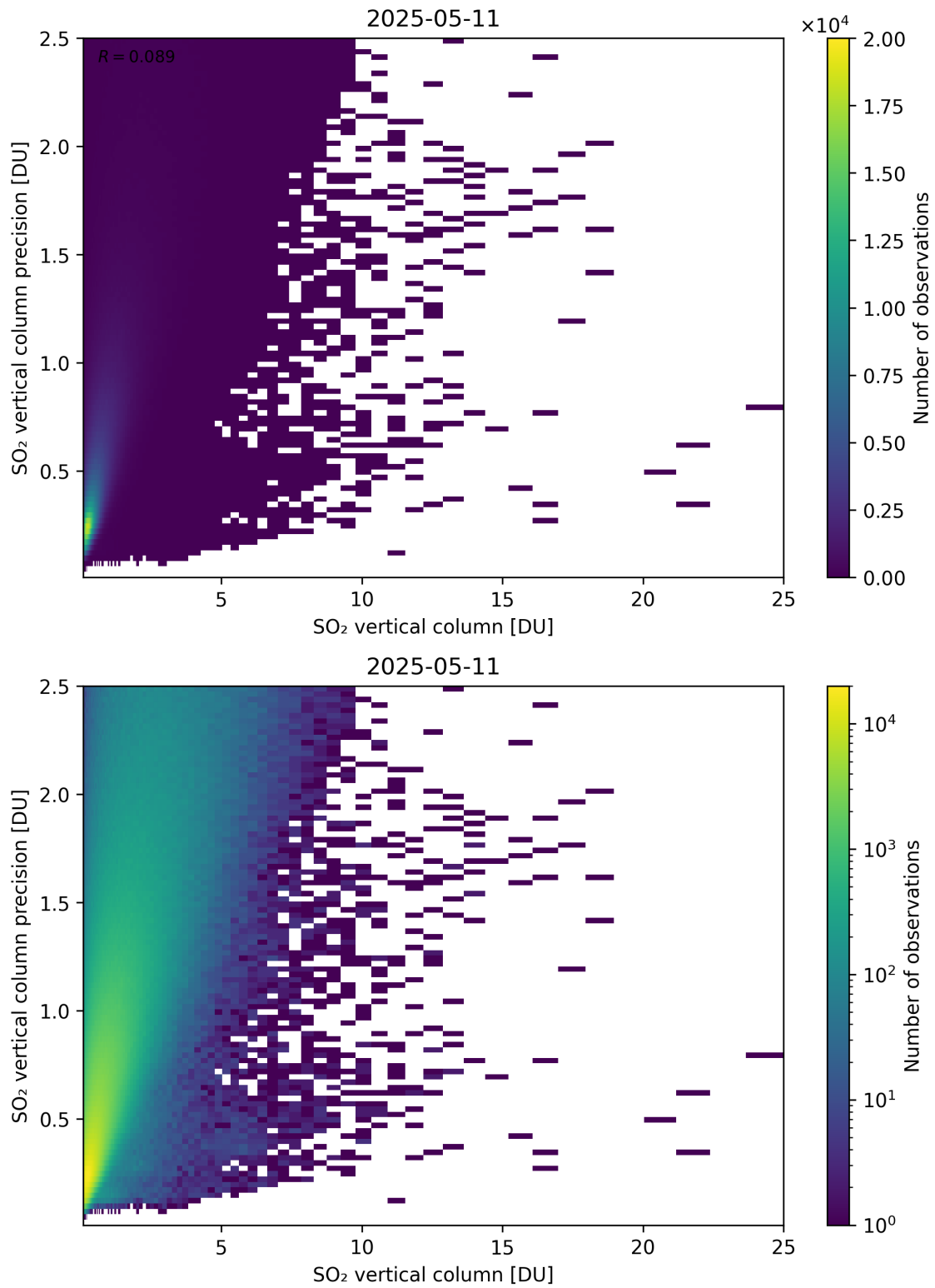
Figure 361: Scatter density plot of “SO 2 vertical column” against “SO 2 vertical column precision” for 2025-05-10 to 2025-05-12.
