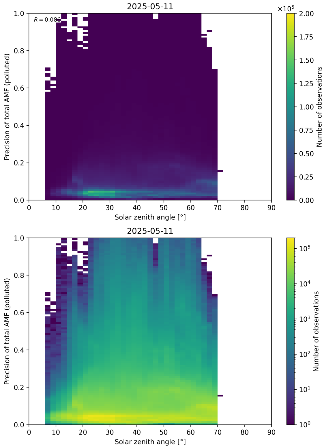
Figure 190: Scatter density plot of “Solar zenith angle” against “Precision of total AMF (polluted)” for 2025-05-10 to 2025-05-12.
