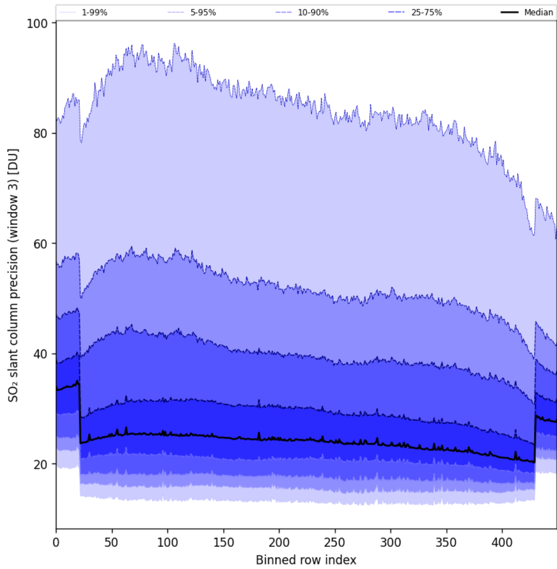
Figure 98: Along track statistics of “SO 2 slant column precision (window 3)” for 2025-05-10 to 2025-05-12
