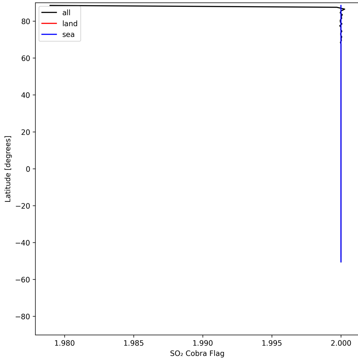
Figure 49: Zonal average of “SO 2 Cobra Flag” for 2025-05-10 to 2025-05-12.
