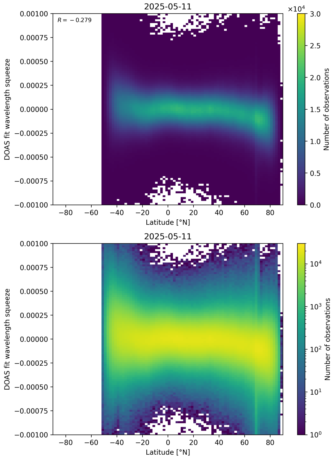
Figure 154: Scatter density plot of “Latitude” against “DOAS fit wavelength squeeze” for 2025-05-10 to 2025-05-12.
