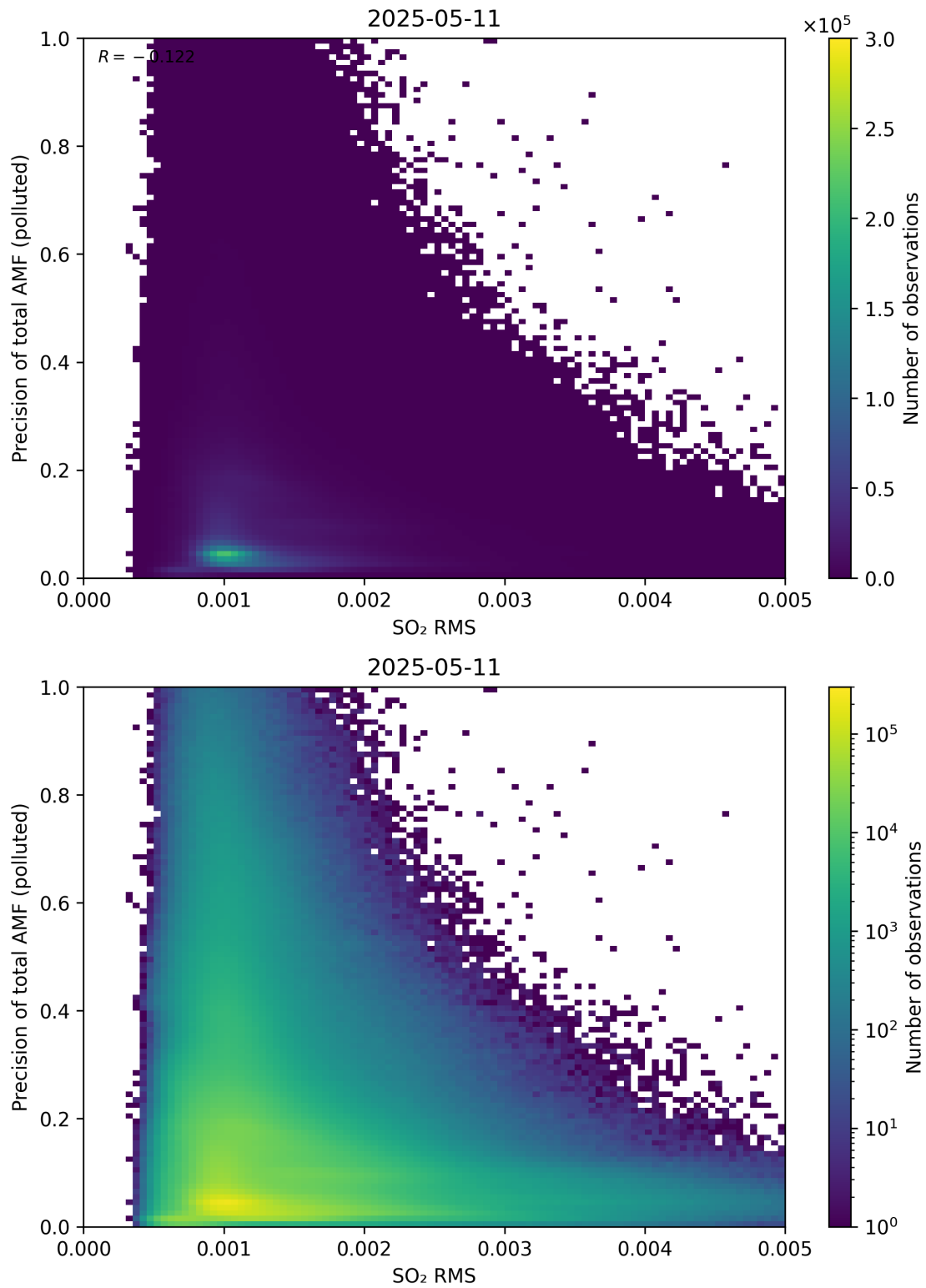
Figure 149: Scatter density plot of “SO 2 RMS” against “Precision of total AMF (polluted)” for 2025-05-10 to 2025-05-12.
