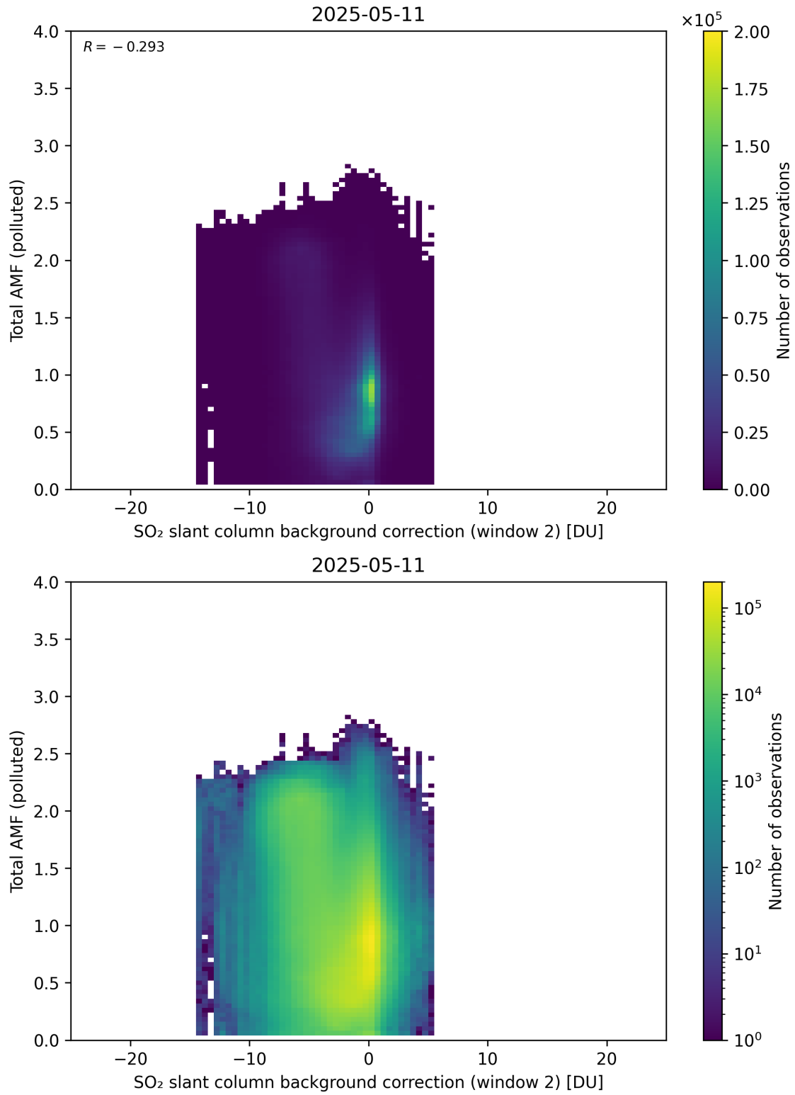
Figure 130: Scatter density plot of “SO 2 slant column background correction (window 2)” against “Total AMF (polluted)” for 2025-05-10 to 2025-05-12.
