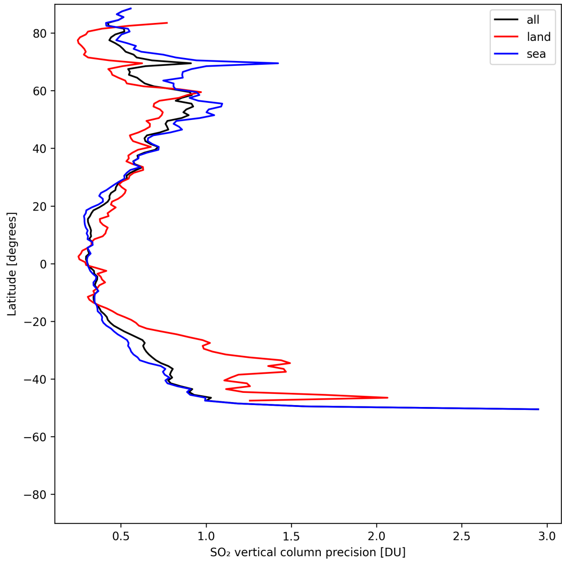
Figure 33: Zonal average of “SO 2 vertical column precision” for 2025-05-10 to 2025-05-12.
