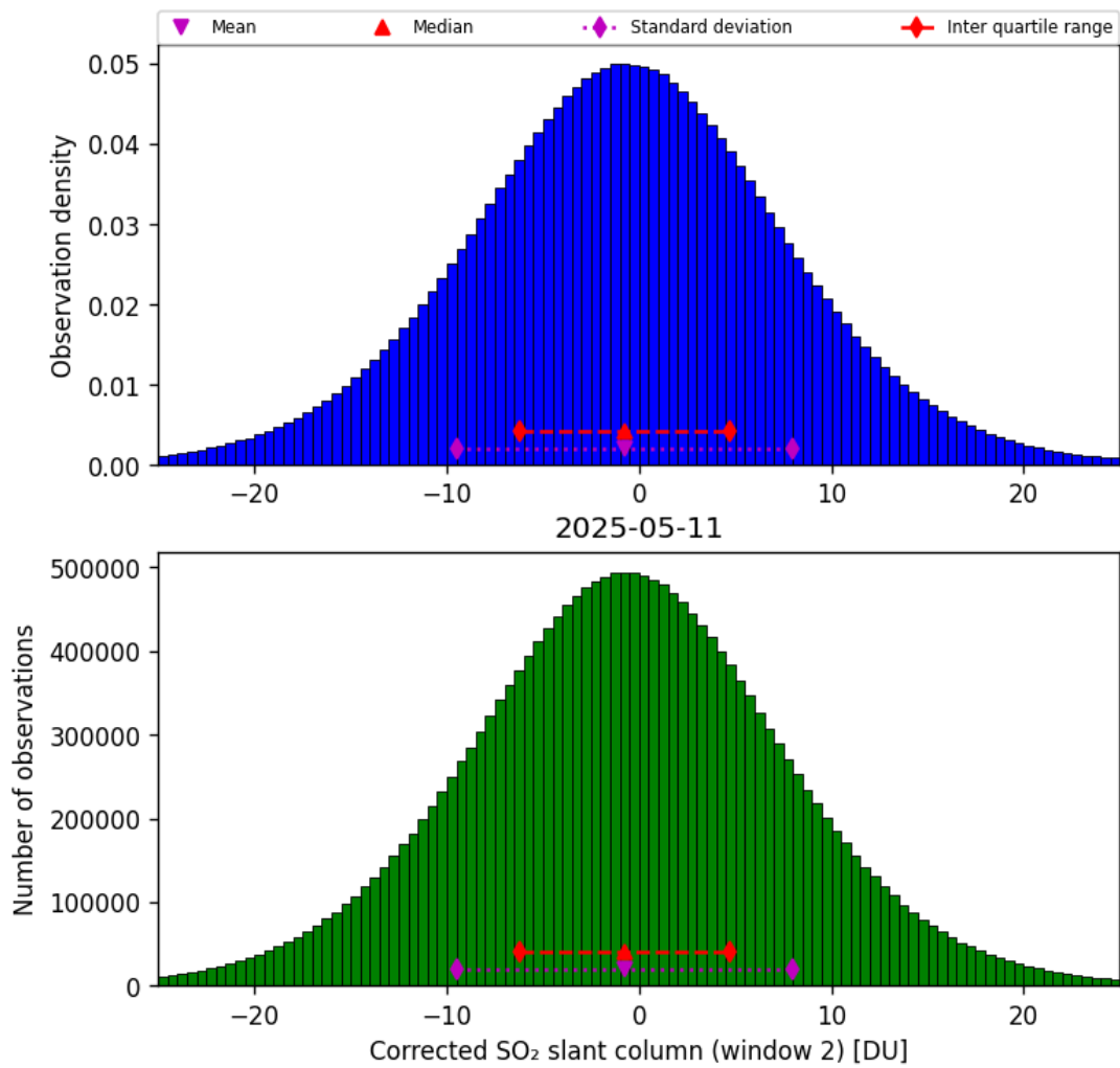
Figure 69: Histogram of “Corrected SO 2 slant column (window 2)” for 2025-05-10 to 2025-05-12
