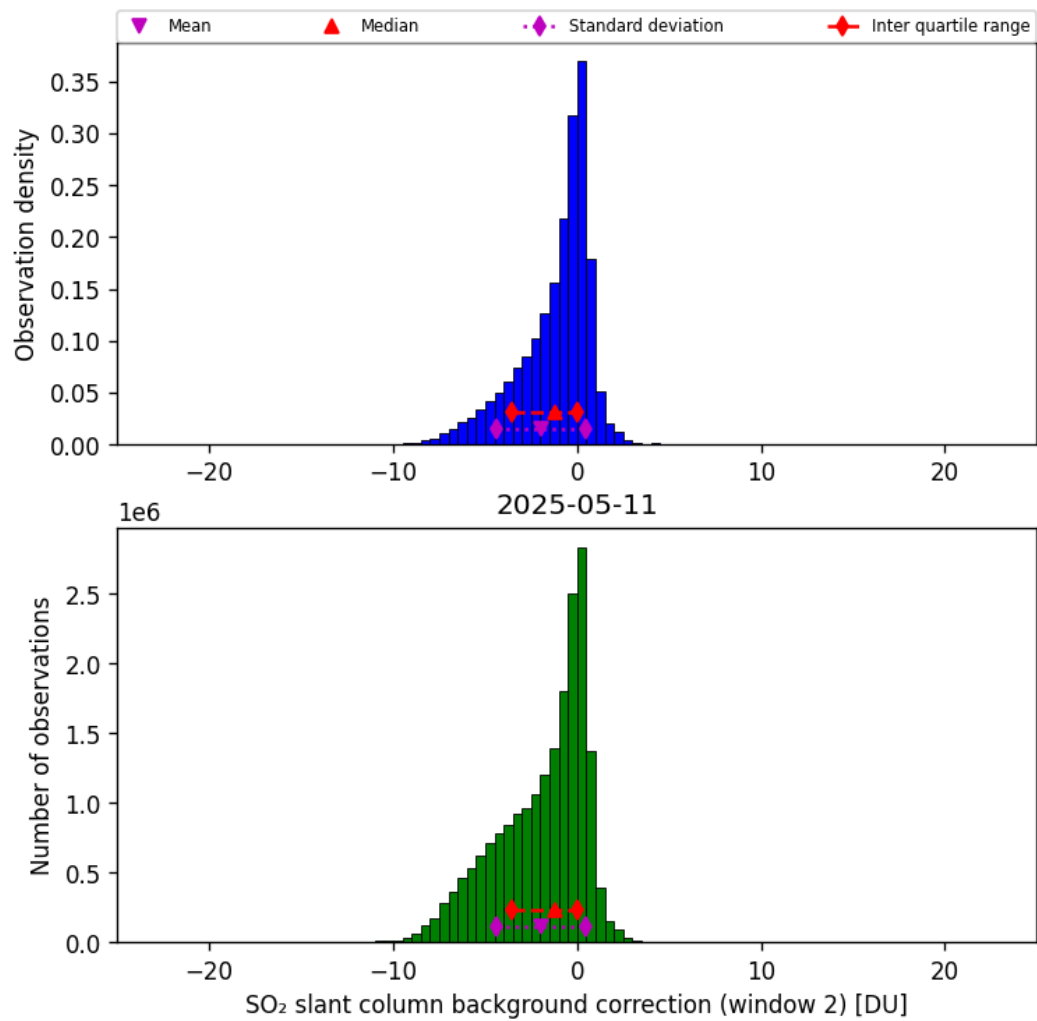
Figure 70: Histogram of “SO 2 slant column background correction (window 2)” for 2025-05-10 to 2025-05-12
