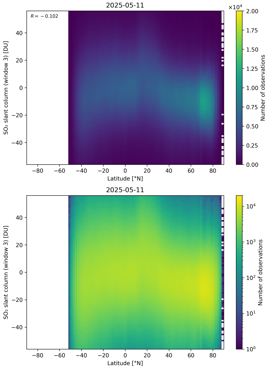
Figure 165: Scatter density plot of “Latitude” against “SO 2 slant column (window 3)” for 2025-05-10 to 2025-05-12.
