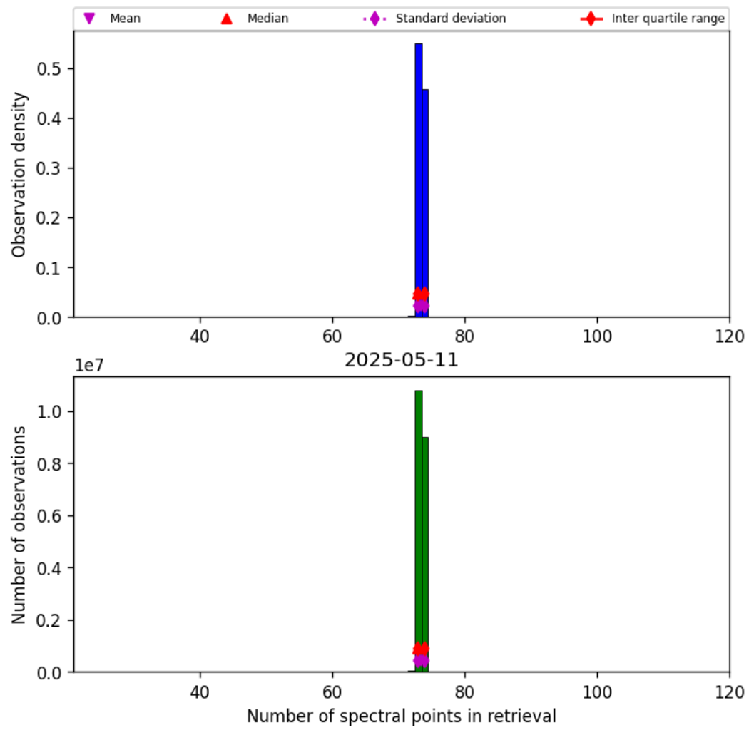
Figure 82: Histogram of “Number of spectral points in retrieval” for 2025-05-10 to 2025-05-12
