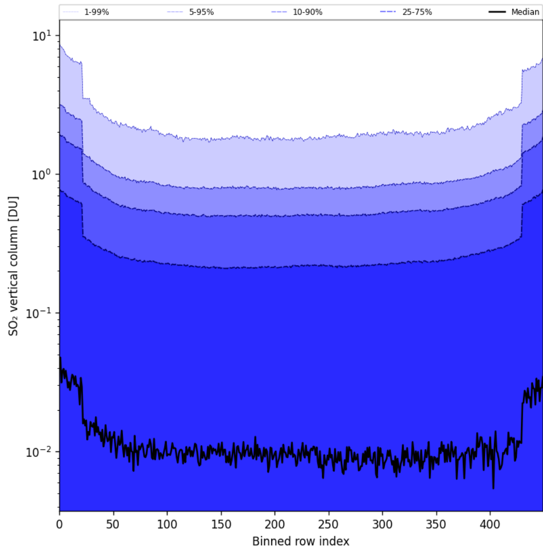
Figure 84: Along track statistics of “SO 2 vertical column” for 2025-05-10 to 2025-05-12
