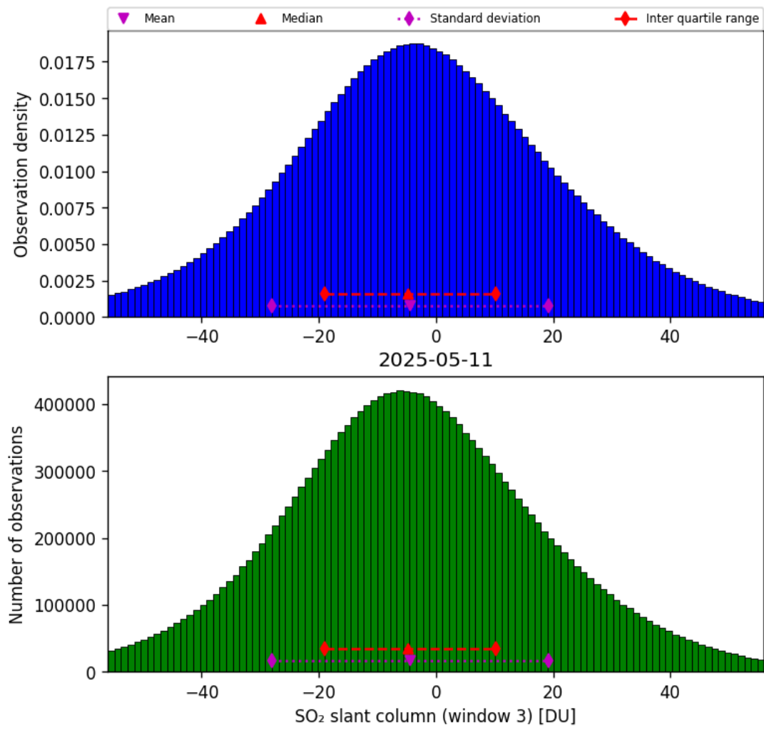
Figure 71: Histogram of “SO 2 slant column (window 3)” for 2025-05-10 to 2025-05-12
