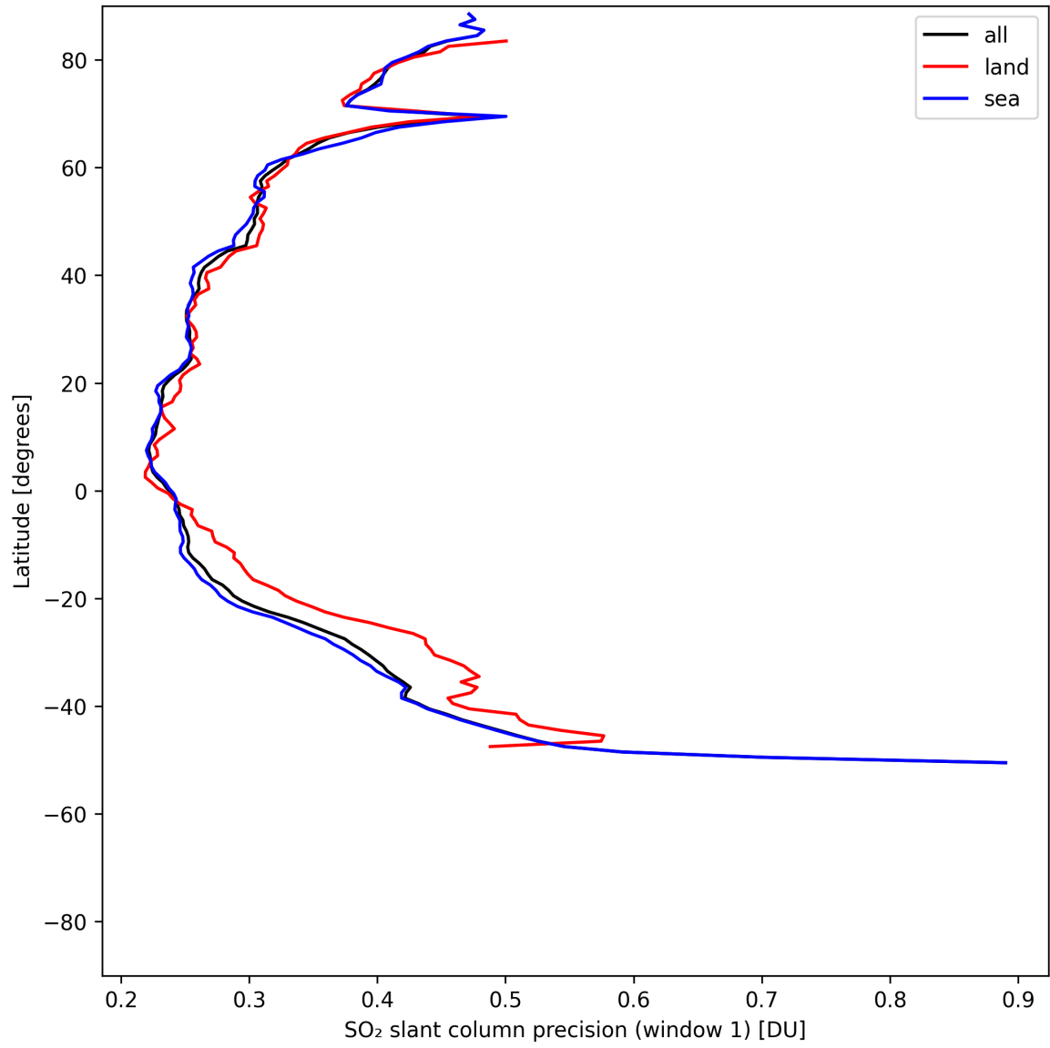
Figure 38: Zonal average of “SO 2 slant column precision (window 1)” for 2025-05-10 to 2025-05-12.
