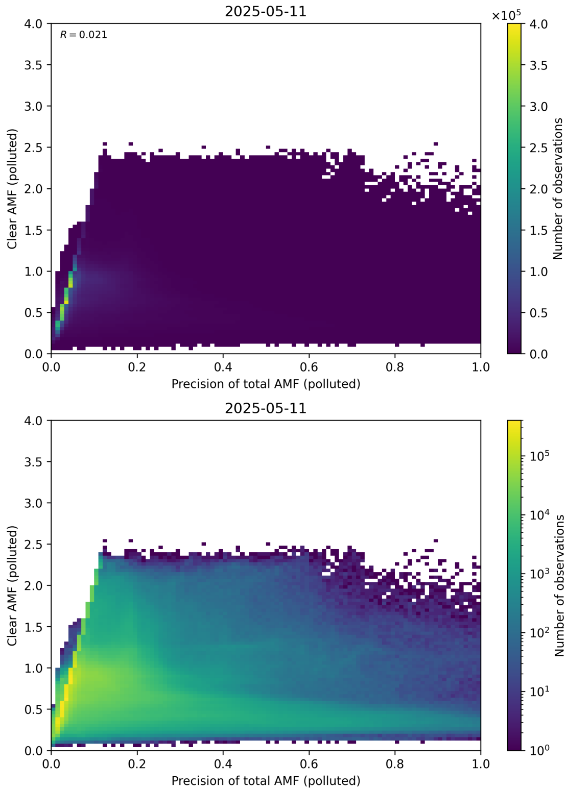
Figure 320: Scatter density plot of “Precision of total AMF (polluted)” against “Clear AMF (polluted)” for 2025-05-10 to 2025-05-12.
