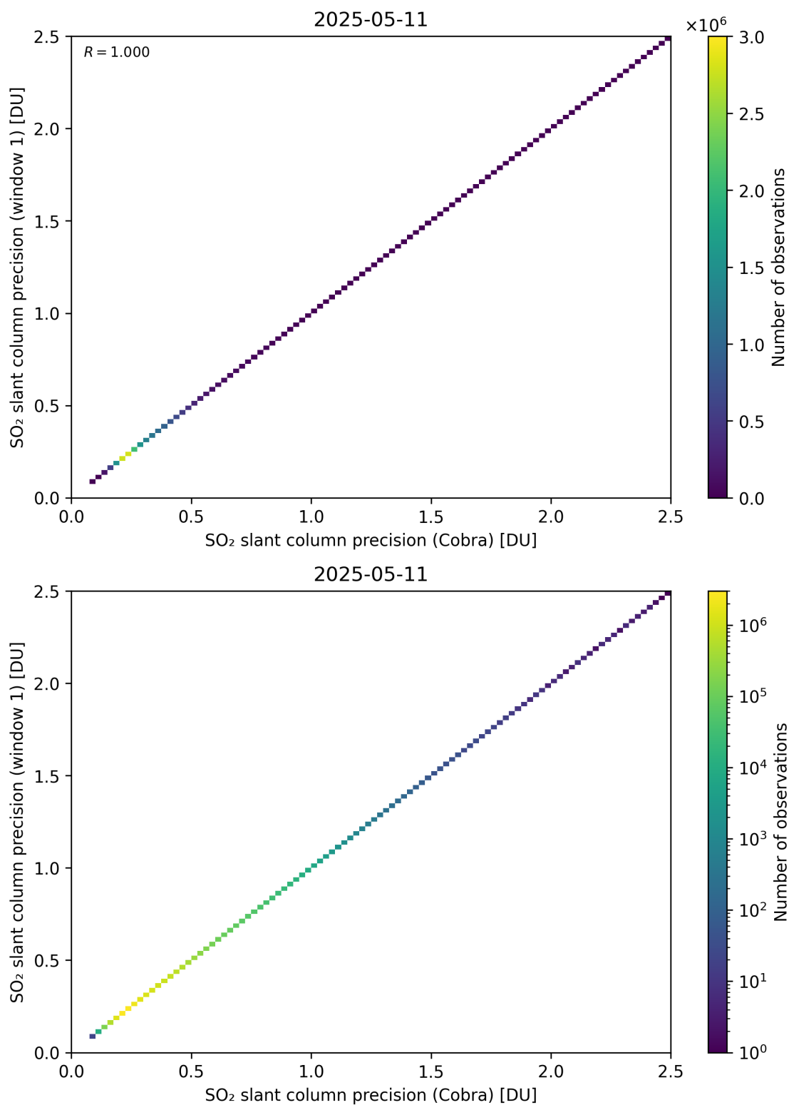
Figure 209: Scatter density plot of “SO 2 slant column precision (Cobra)” against “SO 2 slant column precision (window 1)” for 2025-05-10 to 2025-05-12.
