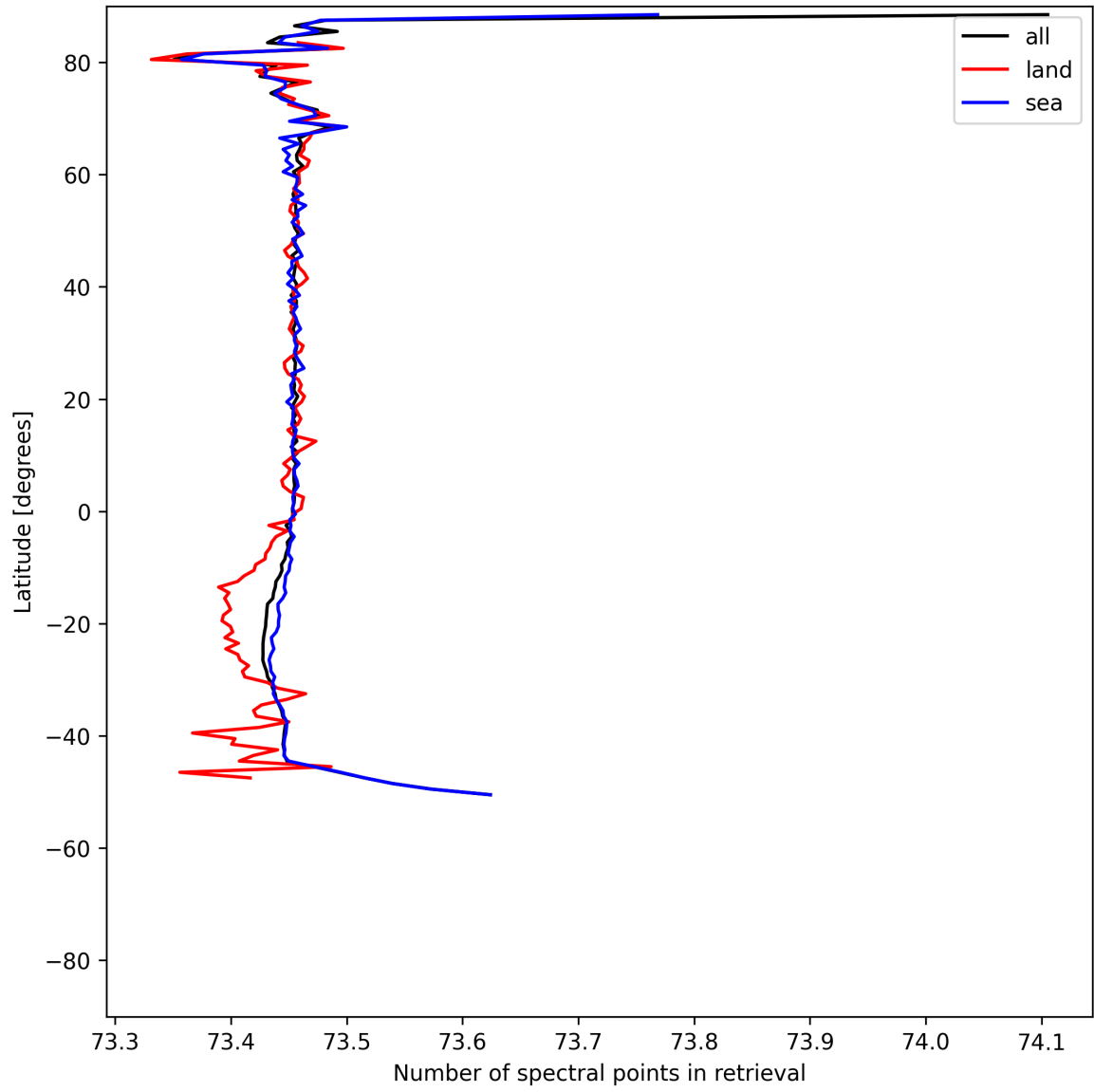
Figure 56: Zonal average of “Number of spectral points in retrieval” for 2025-05-10 to 2025-05-12.
