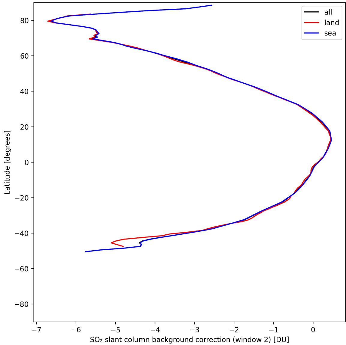
Figure 44: Zonal average of “SO 2 slant column background correction (window 2)” for 2025-05-10 to 2025-05-12.
