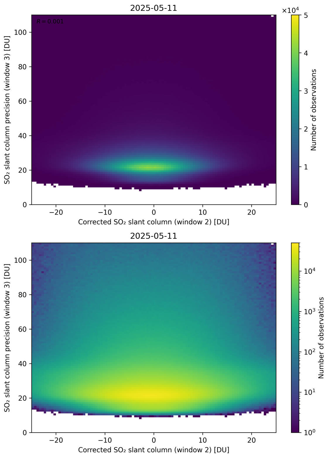
Figure 252: Scatter density plot of “Corrected SO 2 slant column (window 2)” against “SO 2 slant column precision (window 3)” for 2025-05-10 to 2025-05-12.
