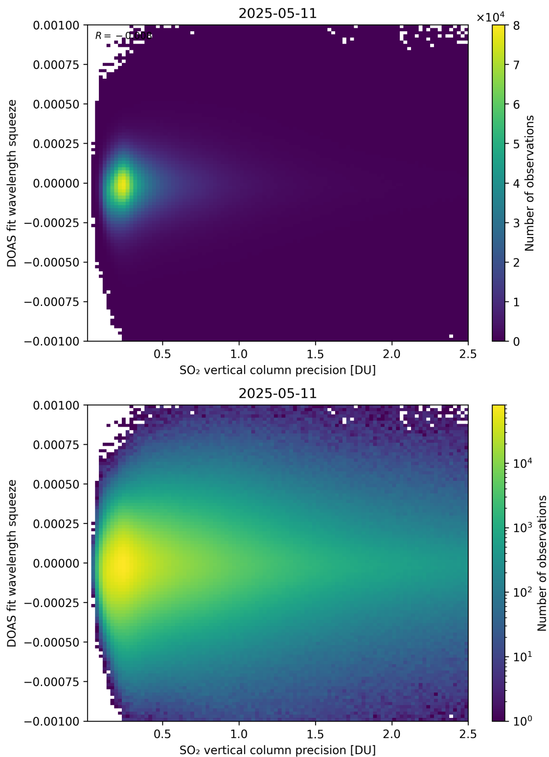
Figure 333: Scatter density plot of “SO 2 vertical column precision” against “DOAS fit wavelength squeeze” for 2025-05-10 to 2025-05-12.
