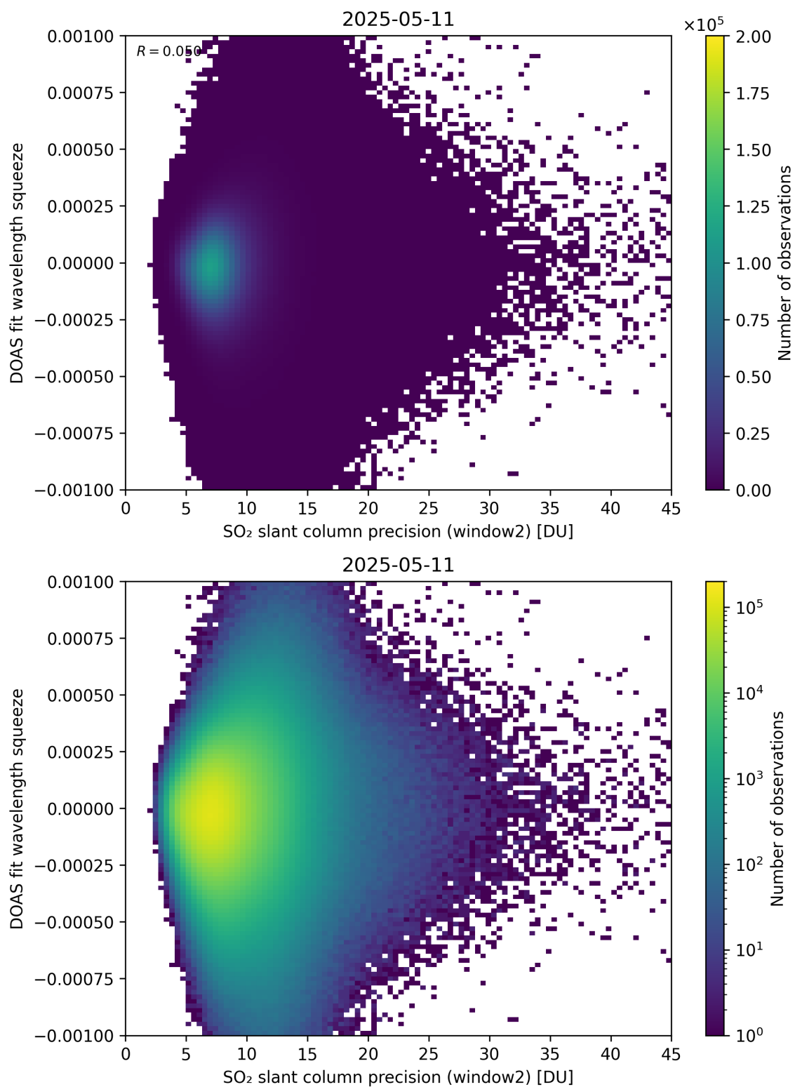
Figure 294: Scatter density plot of “SO 2 slant column precision (window2)” against “DOAS fit wavelength squeeze” for 2025-05-10 to 2025-05-12.
