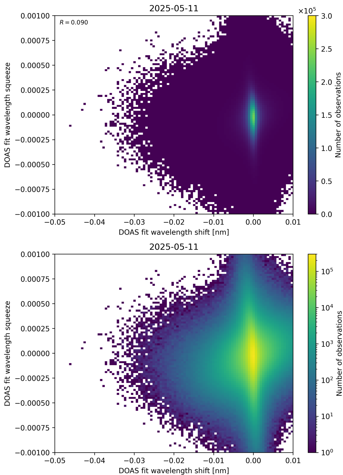
Figure 138: Scatter density plot of “DOAS fit wavelength shift” against “DOAS fit wavelength squeeze” for 2025-05-10 to 2025-05-12.
