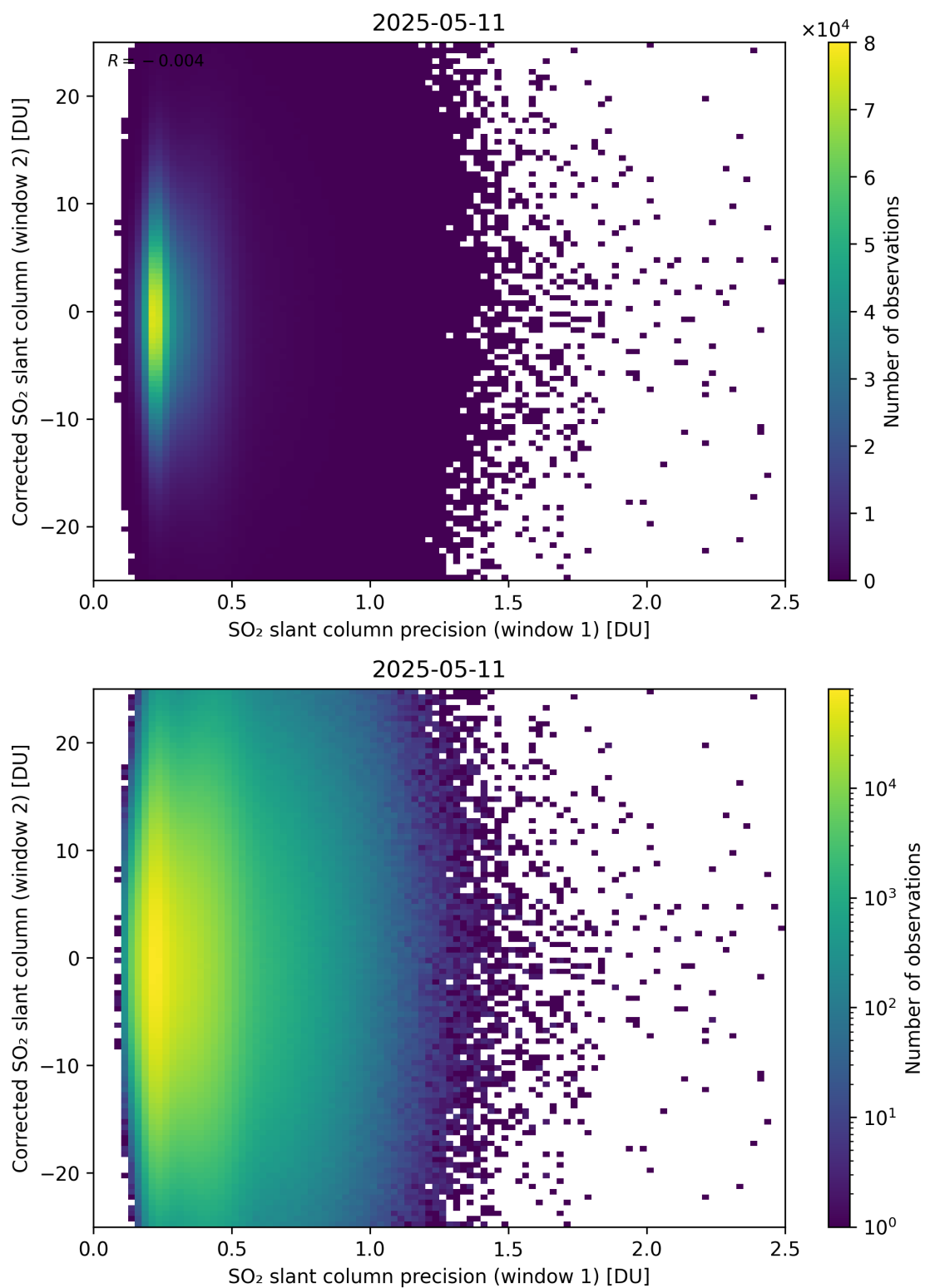
Figure 275: Scatter density plot of “SO 2 slant column precision (window 1)” against “Corrected SO 2 slant column (window 2)” for 2025-05-10 to 2025-05-12.
