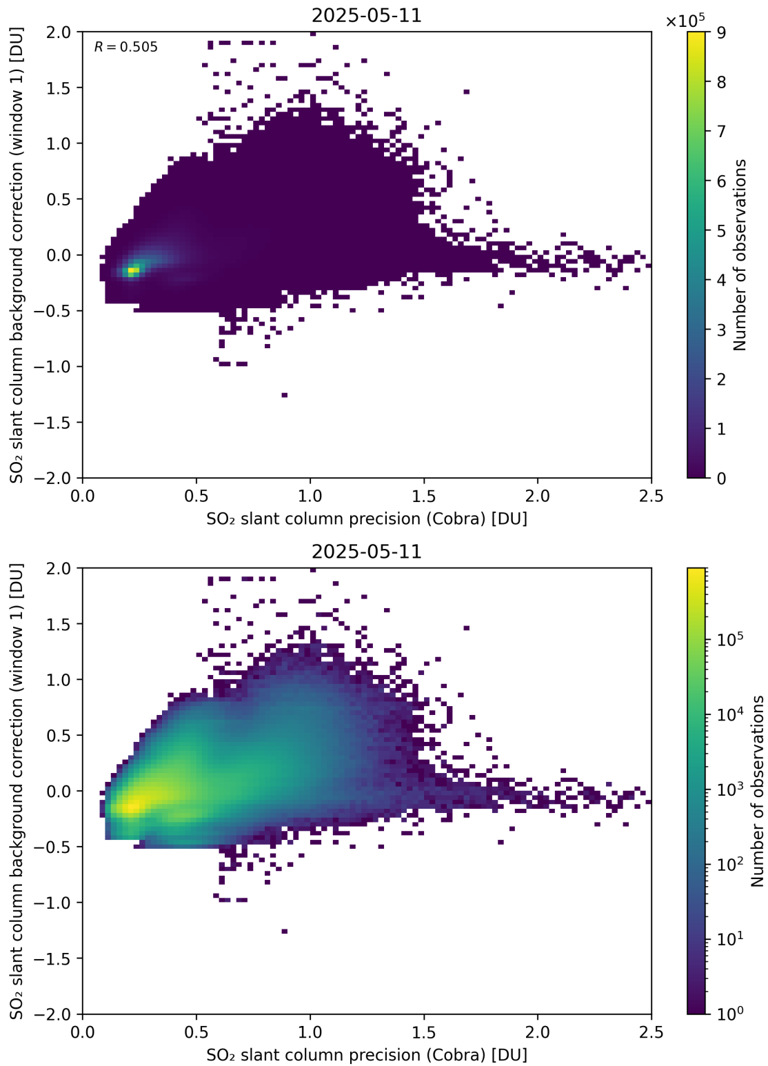
Figure 199: Scatter density plot of “SO 2 slant column precision (Cobra)” against “SO 2 slant column background correction (window 1)” for 2025-05-10 to 2025-05-12.
