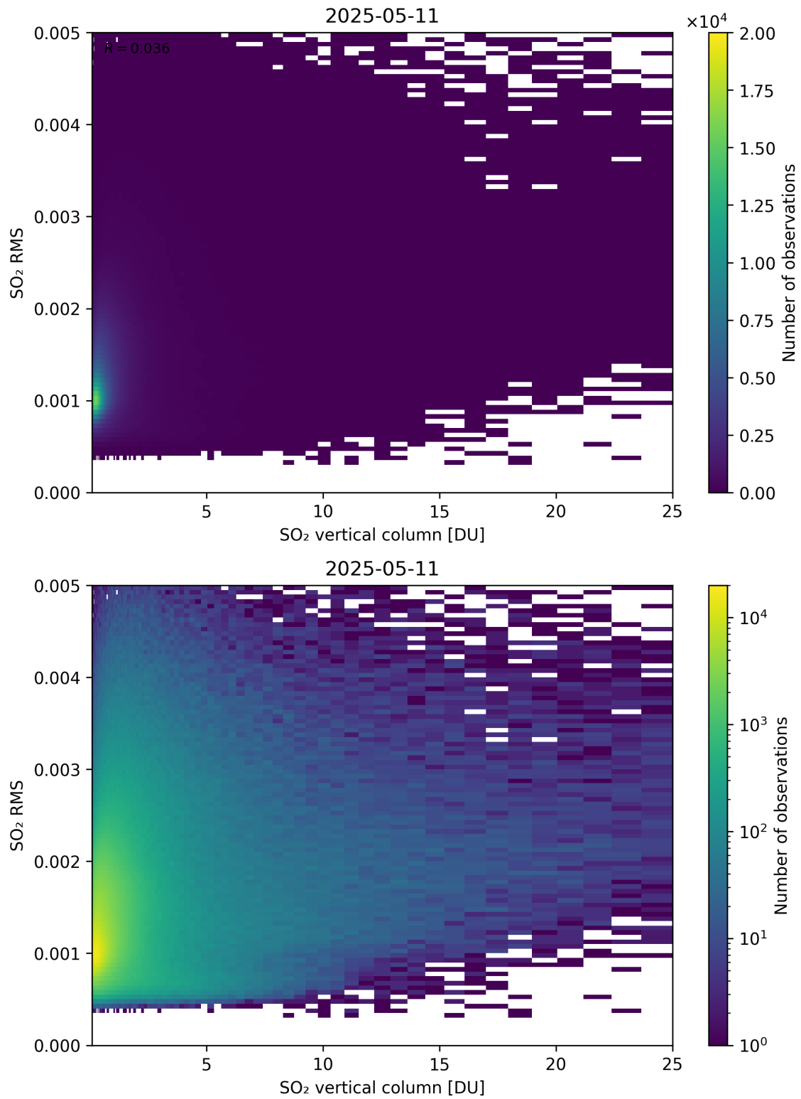
Figure 328: Scatter density plot of “SO 2 vertical column” against “SO 2 RMS” for 2025-05-10 to 2025-05-12.
