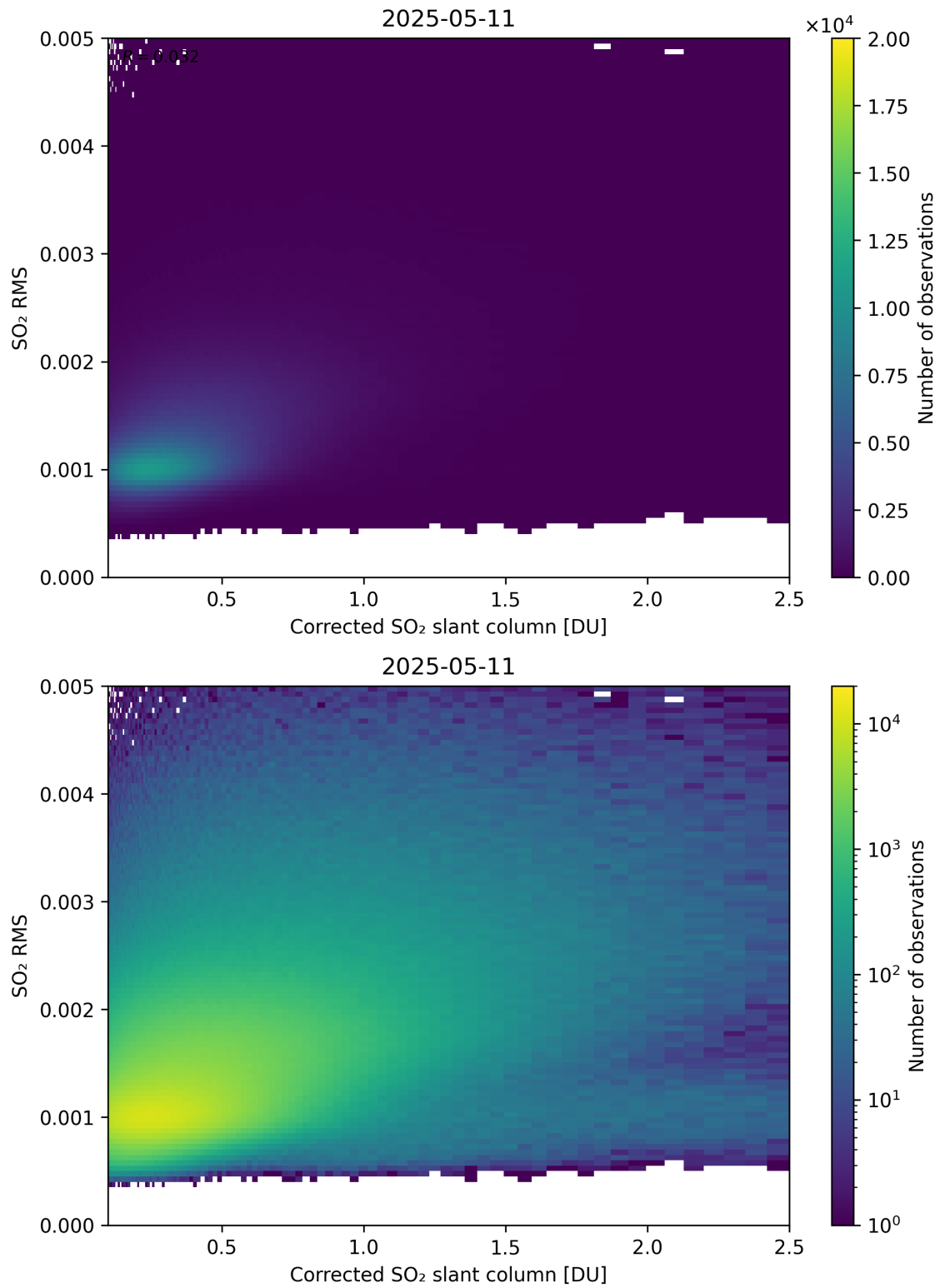
Figure 231: Scatter density plot of “Corrected SO 2 slant column” against “SO 2 RMS” for 2025-05-10 to 2025-05-12.
