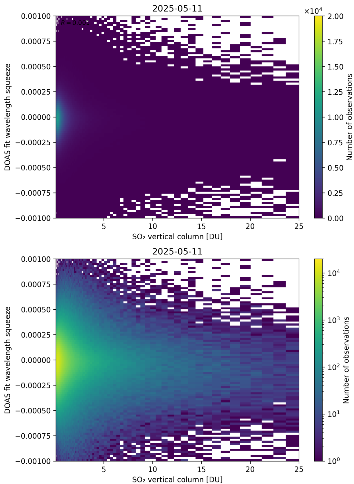
Figure 327: Scatter density plot of “SO 2 vertical column” against “DOAS fit wavelength squeeze” for 2025-05-10 to 2025-05-12.
