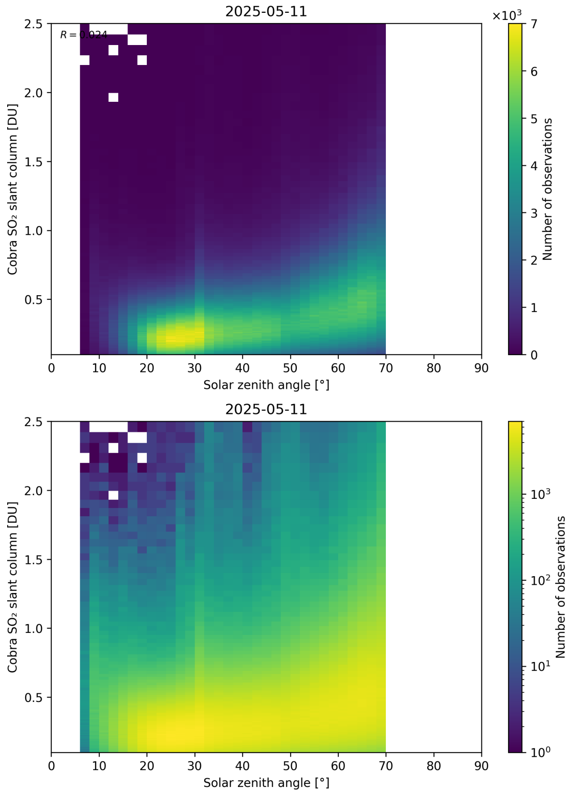
Figure 179: Scatter density plot of “Solar zenith angle” against “Cobra SO 2 slant column” for 2025-05-10 to 2025-05-12.
