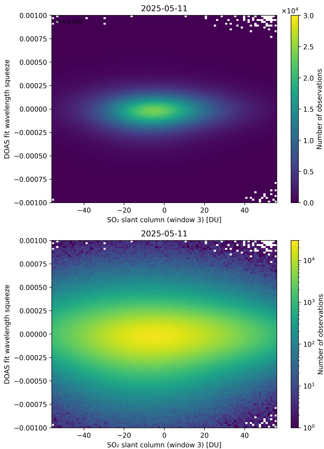
Figure 305: Scatter density plot of “SO 2 slant column (window 3)” against “DOAS fit wavelength squeeze” for 2025-05-10 to 2025-05-12.
