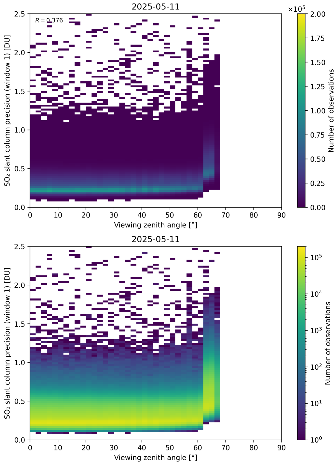
Figure 377: Scatter density plot of “Viewing zenith angle” against “SO 2 slant column precision (window 1)” for 2025-05-10 to 2025-05-12.
