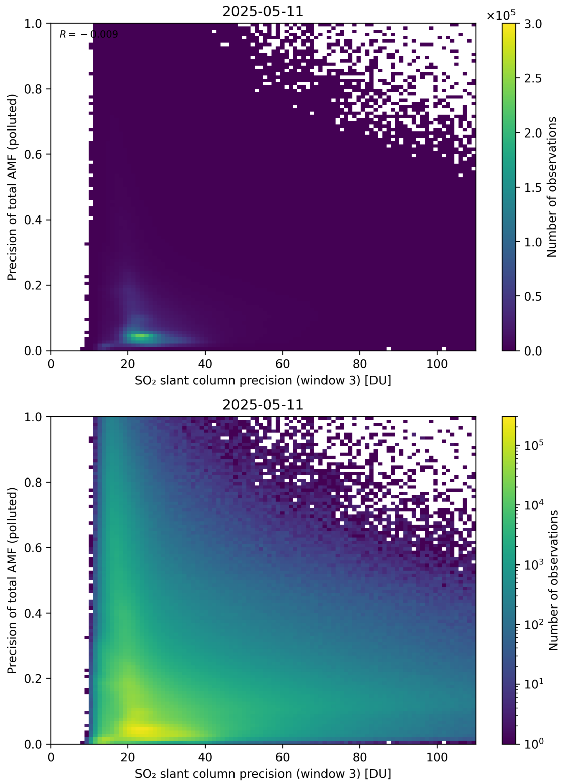
Figure 314: Scatter density plot of “SO 2 slant column precision (window 3)” against “Precision of total AMF (polluted)” for 2025-05-10 to 2025-05-12.
