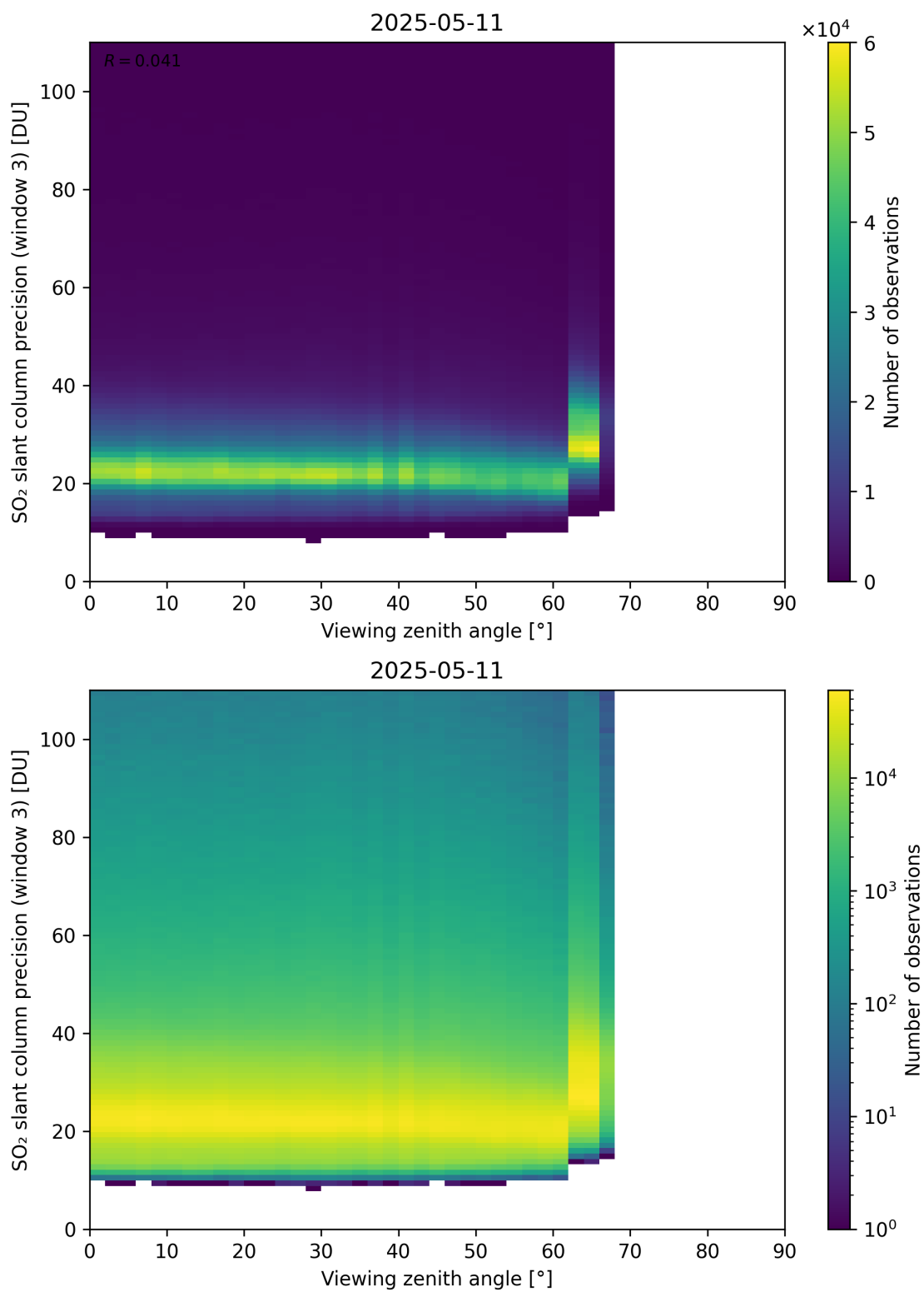
Figure 380: Scatter density plot of “Viewing zenith angle” against “SO 2 slant column precision (window 3)” for 2025-05-10 to 2025-05-12.
