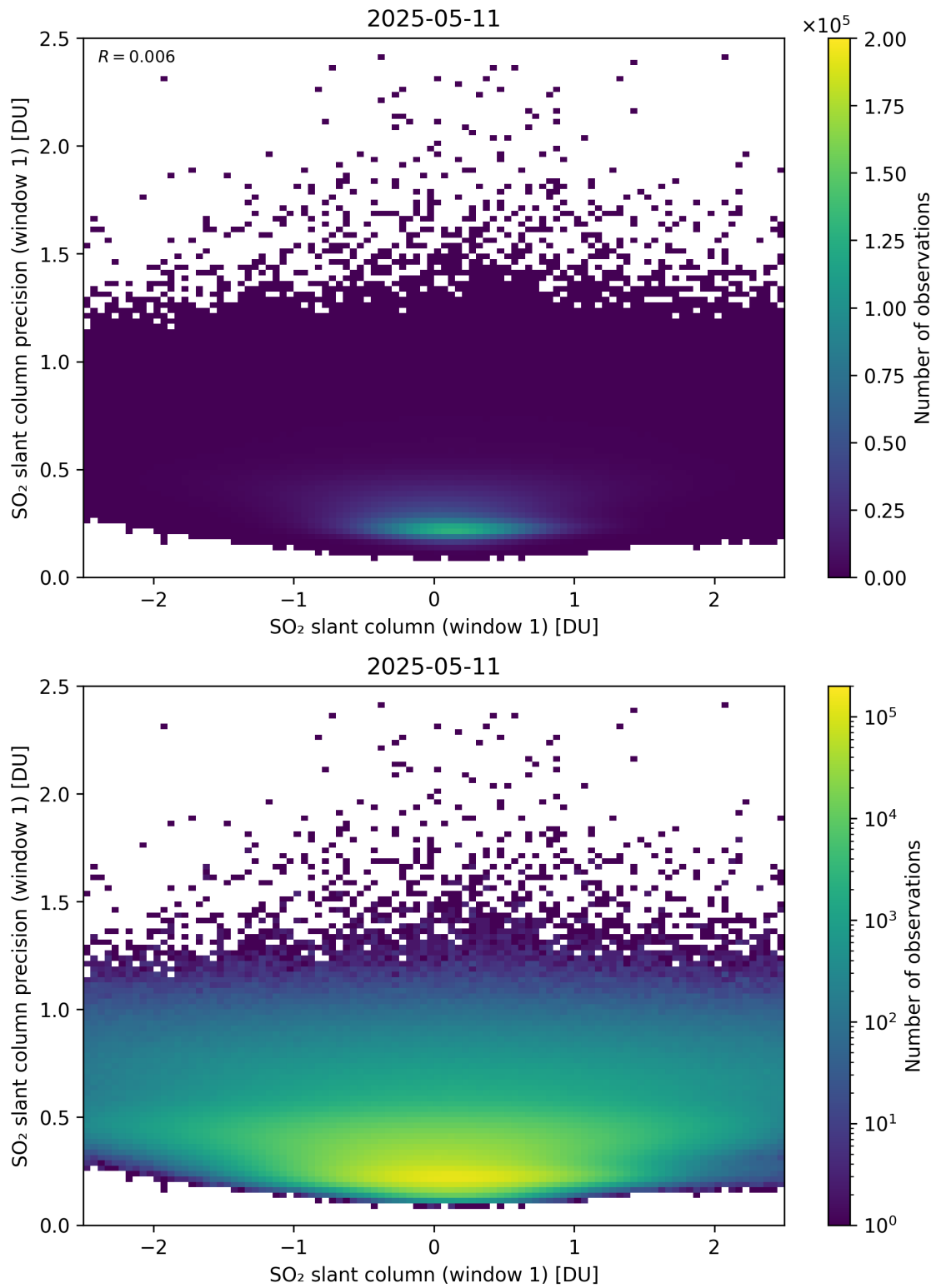
Figure 285: Scatter density plot of “SO 2 slant column (window 1)” against “SO 2 slant column precision (window 1)” for 2025-05-10 to 2025-05-12.
