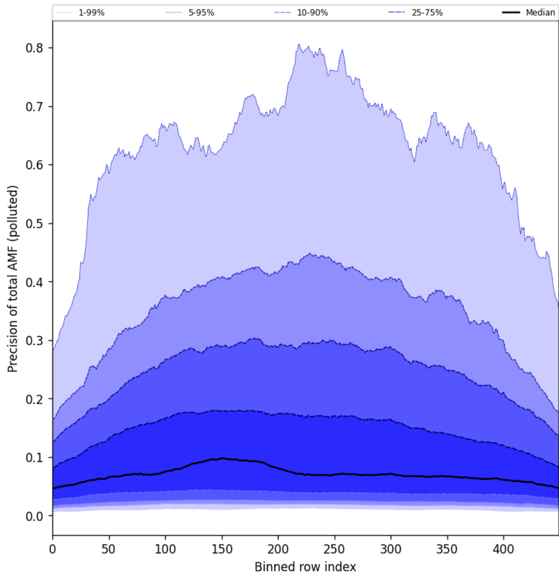
Figure 106: Along track statistics of “Precision of total AMF (polluted)” for 2025-05-10 to 2025-05-12
