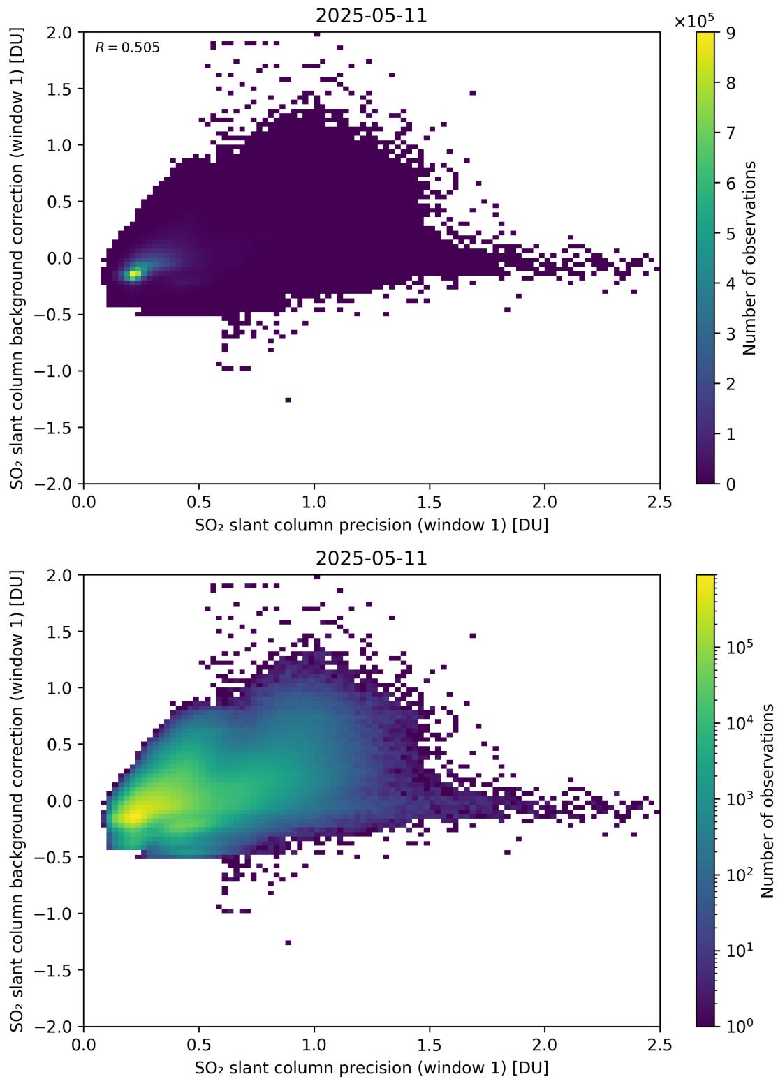
Figure 268: Scatter density plot of “SO 2 slant column precision (window 1)” against “SO 2 slant column background correction (window 1)” for 2025-05-10 to 2025-05-12.
