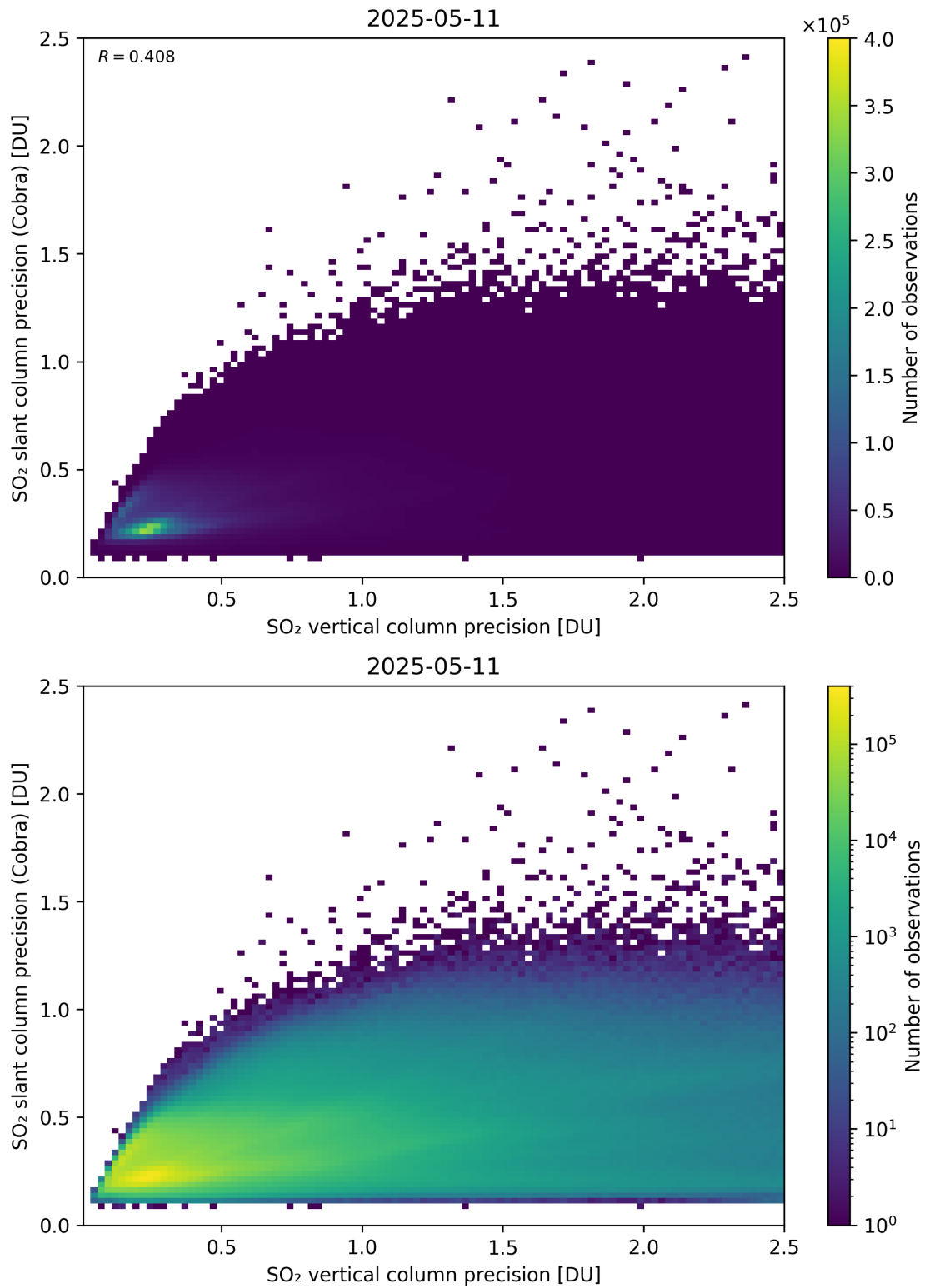
Figure 337: Scatter density plot of “SO 2 vertical column precision” against “SO 2 slant column precision (Cobra)” for 2025-05-10 to 2025-05-12.
