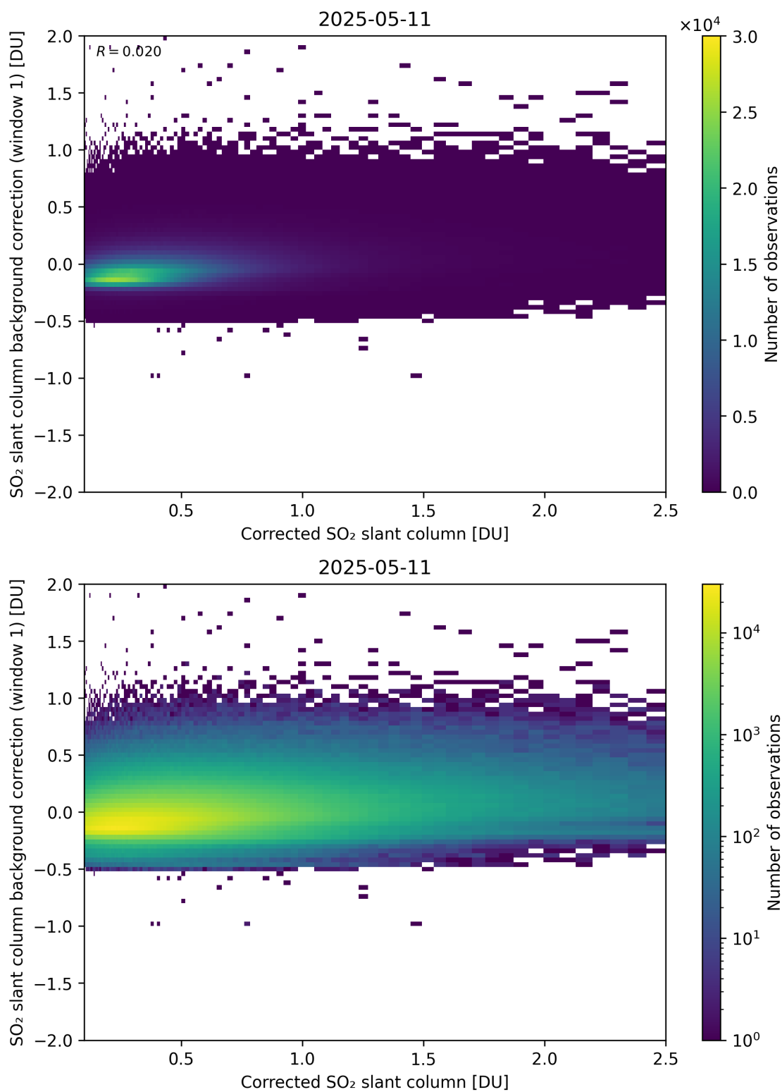
Figure 226: Scatter density plot of “Corrected SO 2 slant column” against “SO 2 slant column background correction (window 1)” for 2025-05-10 to 2025-05-12.
