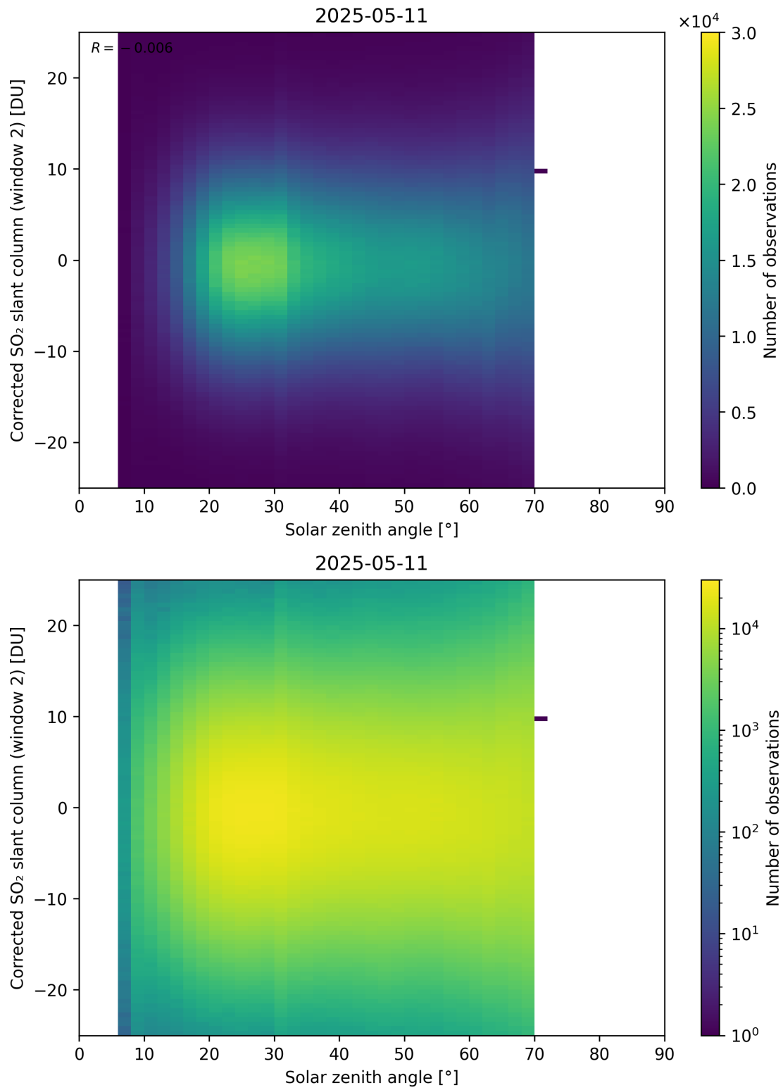
Figure 182: Scatter density plot of “Solar zenith angle” against “Corrected SO 2 slant column (window 2)” for 2025-05-10 to 2025-05-12.
