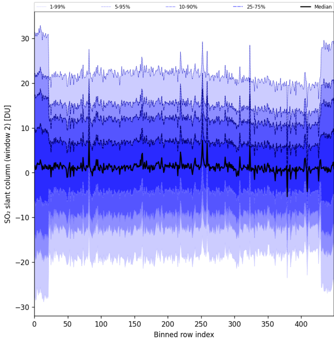
Figure 93: Along track statistics of “SO 2 slant column (window 2)” for 2025-05-10 to 2025-05-12
