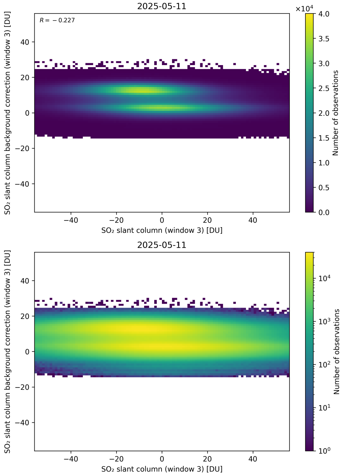
Figure 303: Scatter density plot of “SO 2 slant column (window 3)” against “SO 2 slant column background correction (window 3)” for 2025-05-10 to 2025-05-12.
