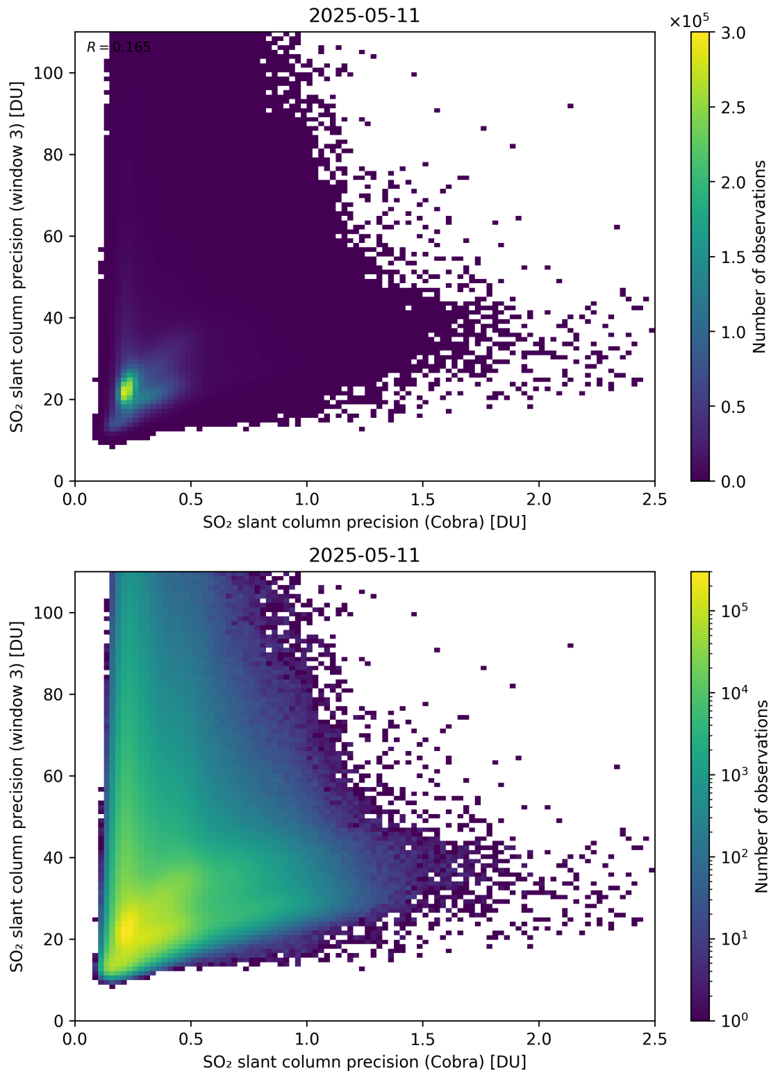
Figure 212: Scatter density plot of “SO 2 slant column precision (Cobra)” against “SO 2 slant column precision (window 3)” for 2025-05-10 to 2025-05-12.
