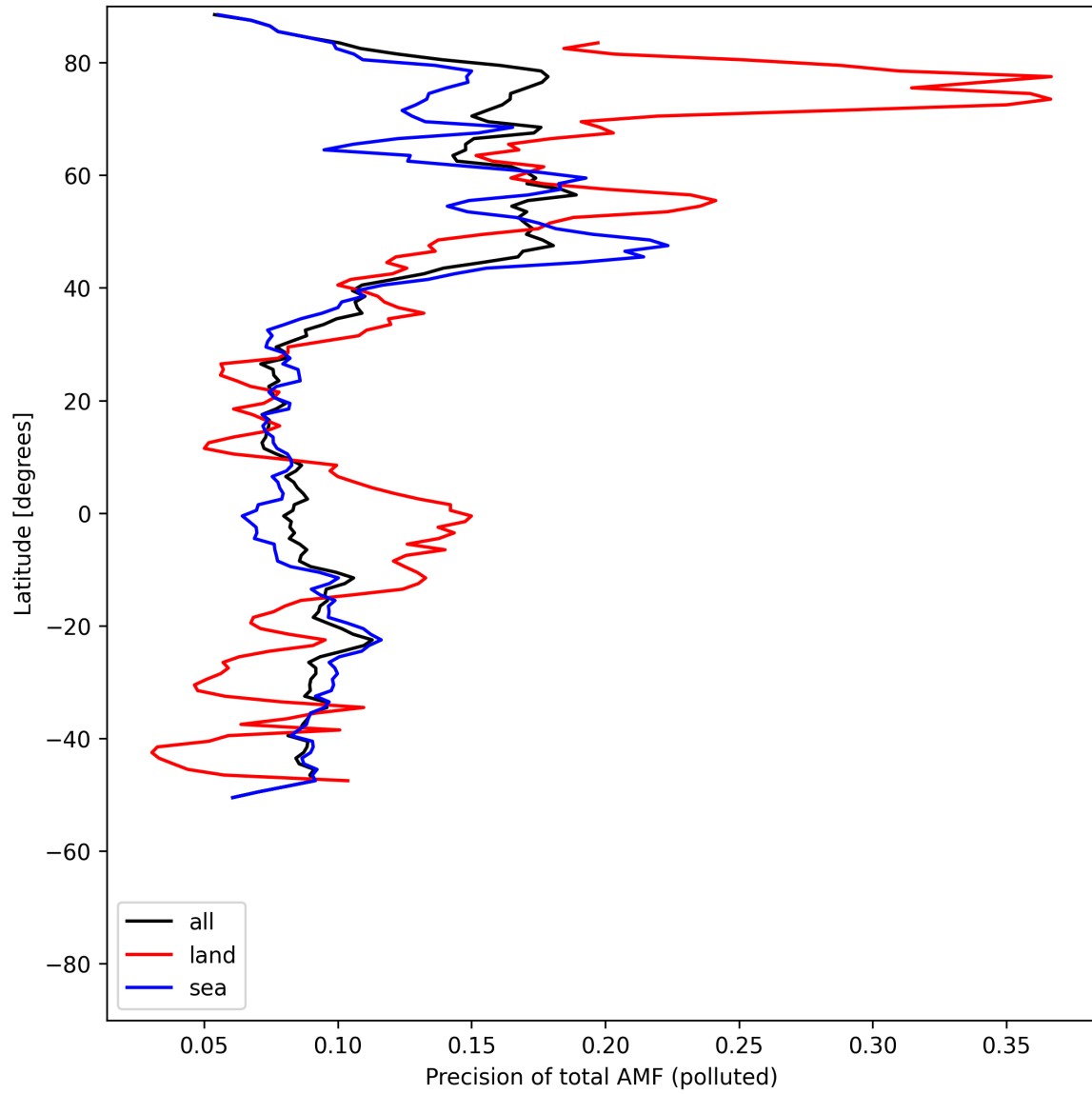
Figure 54: Zonal average of “Precision of total AMF (polluted)” for 2025-05-10 to 2025-05-12.
