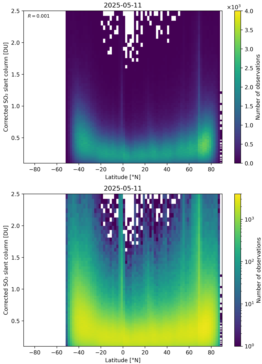
Figure 159: Scatter density plot of “Latitude” against “Corrected SO 2 slant column” for 2025-05-10 to 2025-05-12.
