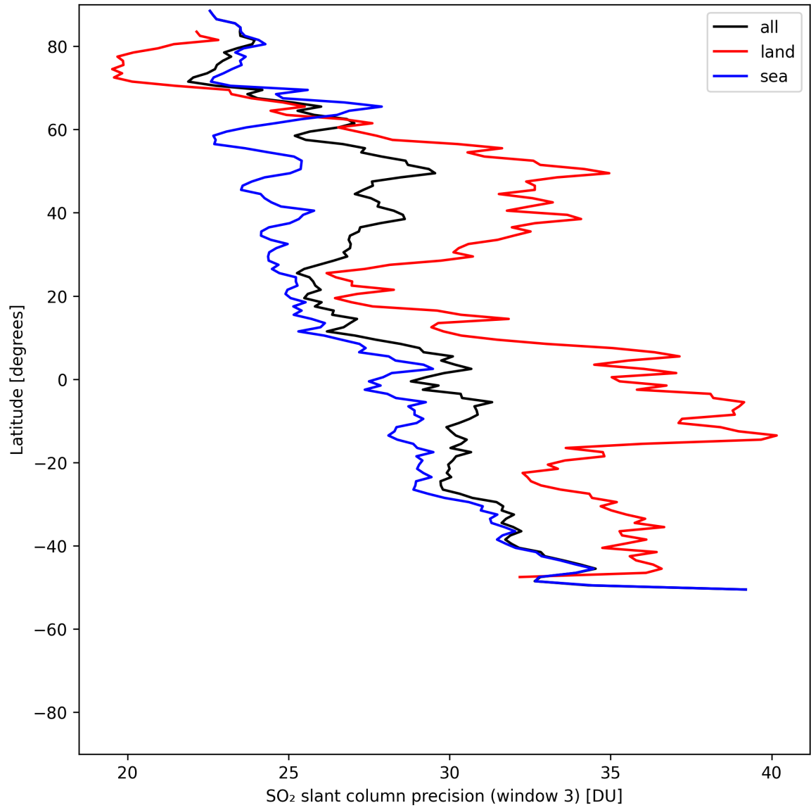
Figure 46: Zonal average of “SO 2 slant column precision (window 3)” for 2025-05-10 to 2025-05-12.
