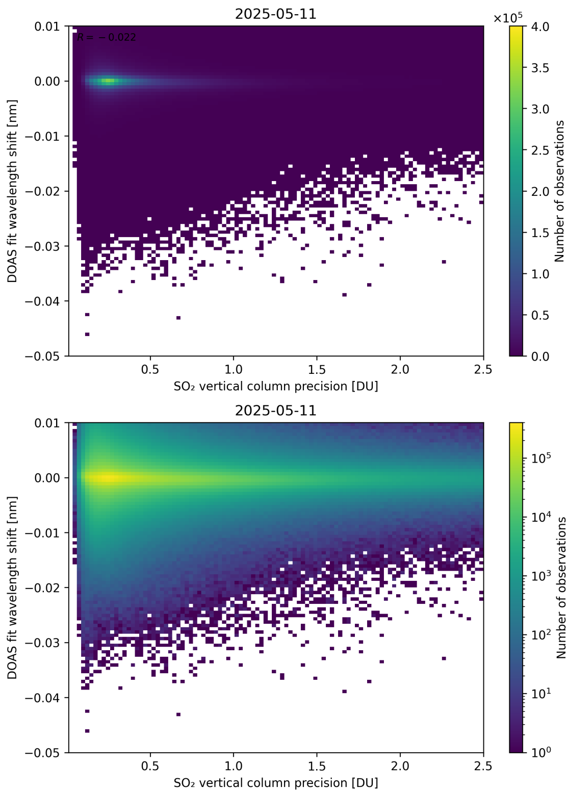
Figure 332: Scatter density plot of “SO 2 vertical column precision” against “DOAS fit wavelength shift” for 2025-05-10 to 2025-05-12.
