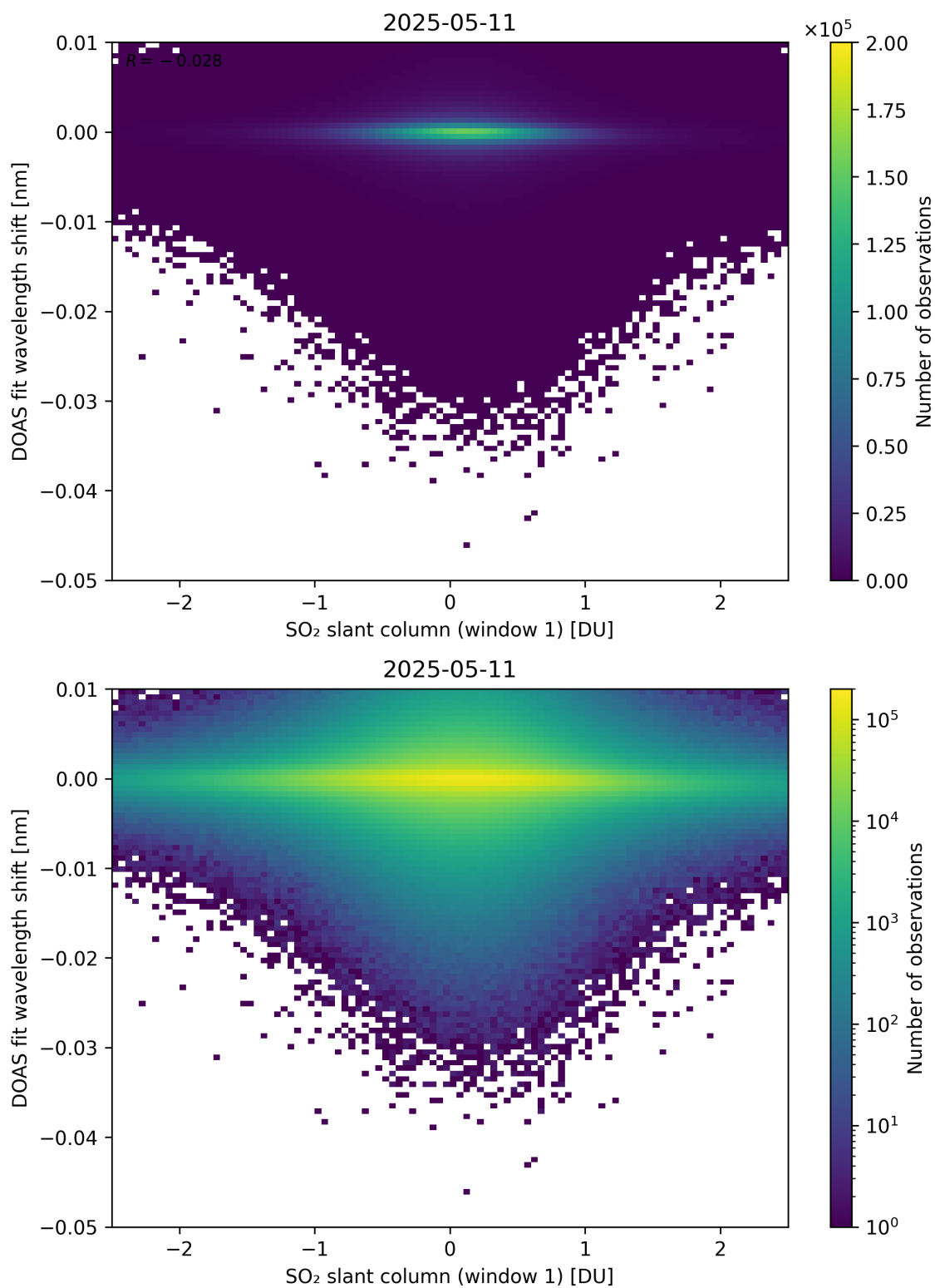
Figure 265: Scatter density plot of “SO 2 slant column (window 1)” against “DOAS fit wavelength shift” for 2025-05-10 to 2025-05-12.
