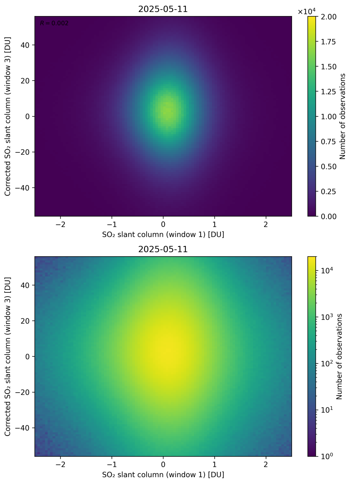
Figure 284: Scatter density plot of “SO 2 slant column (window 1)” against “Corrected SO 2 slant column (window 3)” for 2025-05-10 to 2025-05-12.
