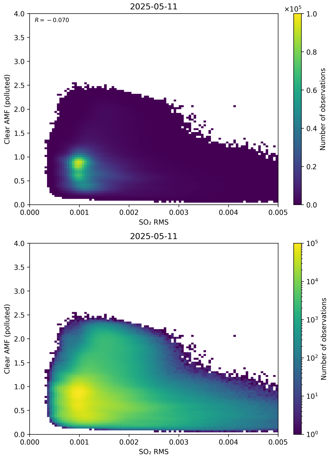
Figure 147: Scatter density plot of “SO 2 RMS” against “Clear AMF (polluted)” for 2025-05-10 to 2025-05-12.
