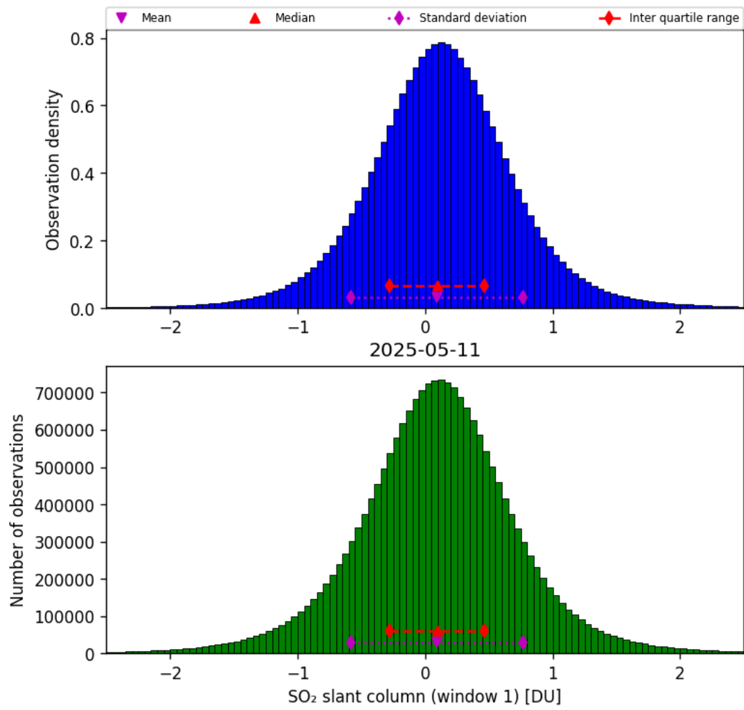
Figure 63: Histogram of “SO 2 slant column (window 1)” for 2025-05-10 to 2025-05-12
