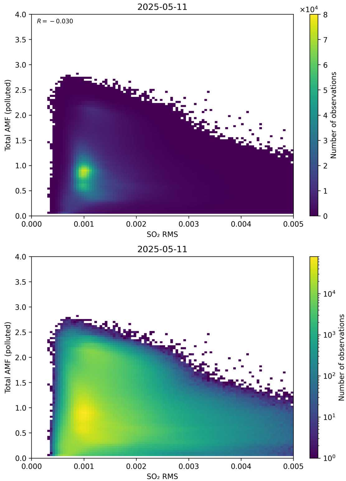
Figure 148: Scatter density plot of “SO 2 RMS” against “Total AMF (polluted)” for 2025-05-10 to 2025-05-12.
