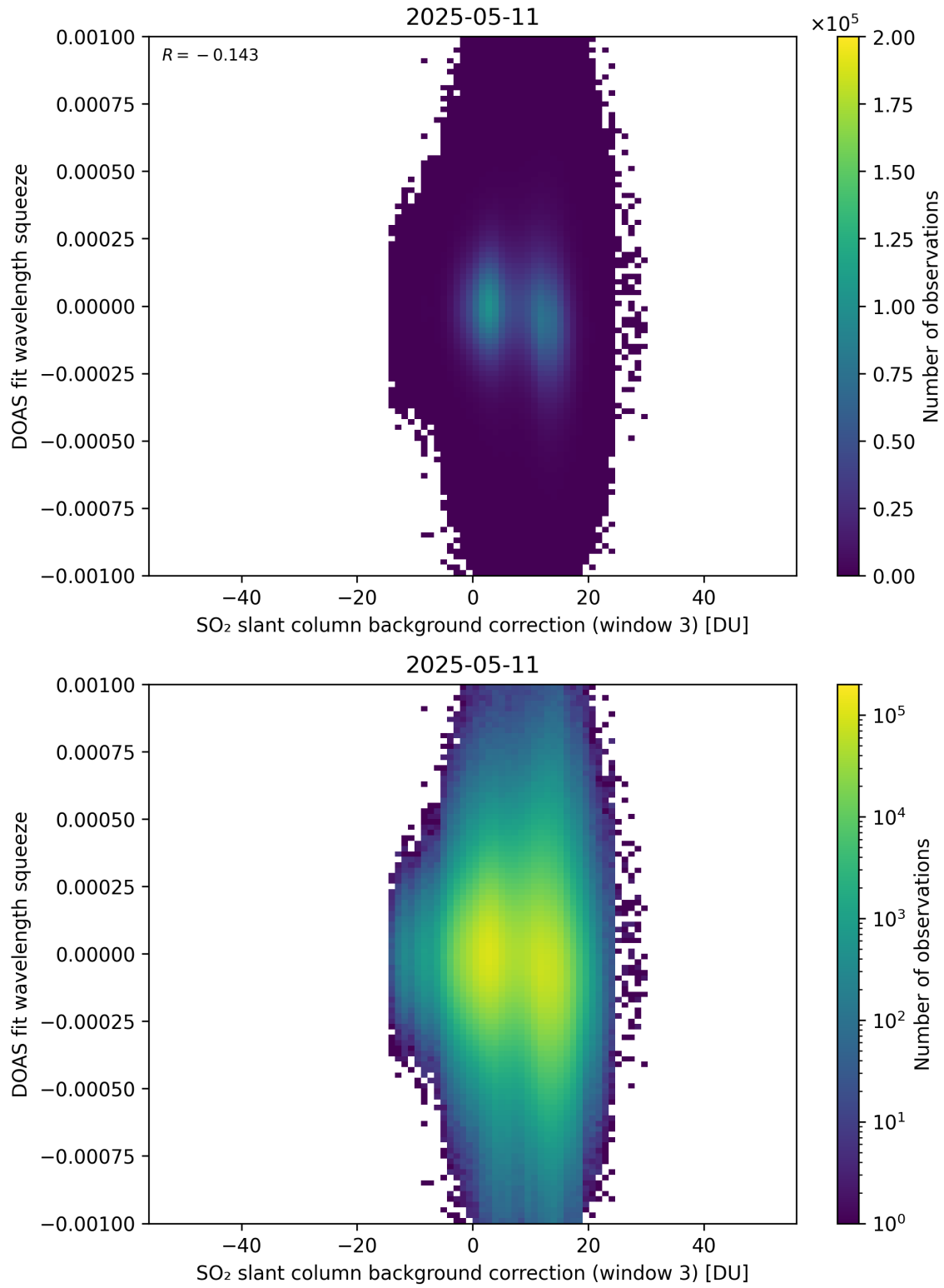
Figure 133: Scatter density plot of “SO 2 slant column background correction (window 3)” against “DOAS fit wavelength squeeze” for 2025-05-10 to 2025-05-12.
