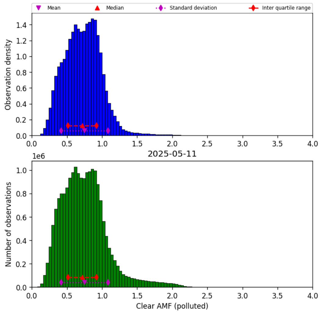
Figure 81: Histogram of “Clear AMF (polluted)” for 2025-05-10 to 2025-05-12
