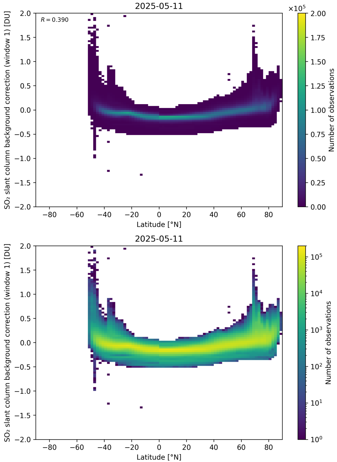
Figure 150: Scatter density plot of “Latitude” against “SO 2 slant column background correction (window 1)” for 2025-05-10 to 2025-05-12.
