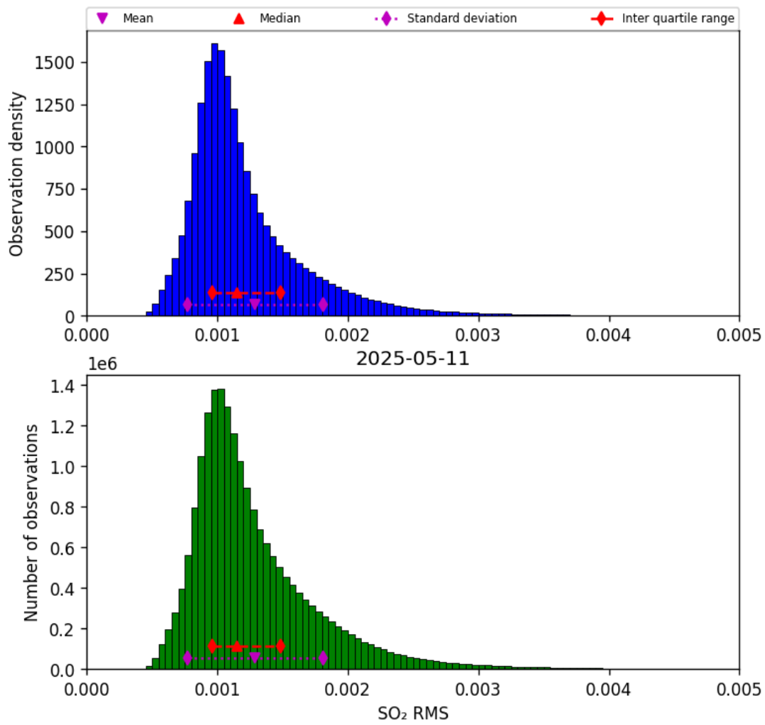
Figure 78: Histogram of “SO 2 RMS” for 2025-05-10 to 2025-05-12
