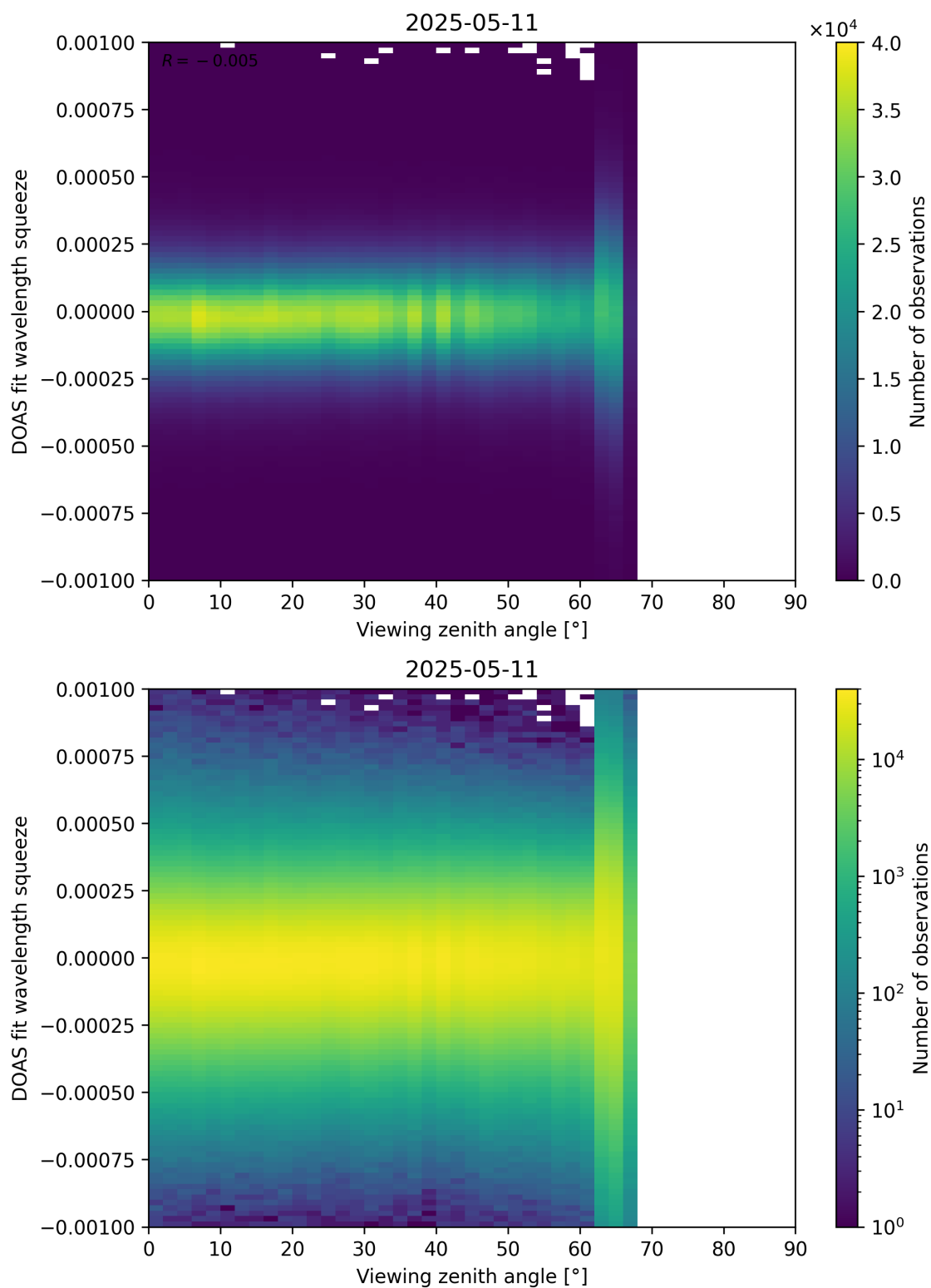
Figure 366: Scatter density plot of “Viewing zenith angle” against “DOAS fit wavelength squeeze” for 2025-05-10 to 2025-05-12.
