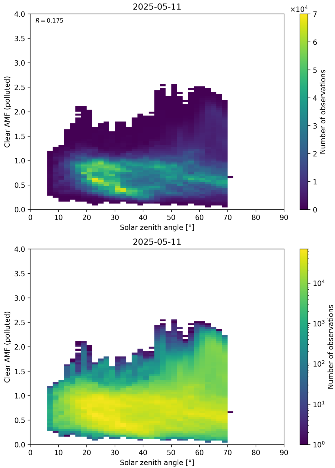
Figure 178: Scatter density plot of “Solar zenith angle” against “Clear AMF (polluted)” for 2025-05-10 to 2025-05-12.
