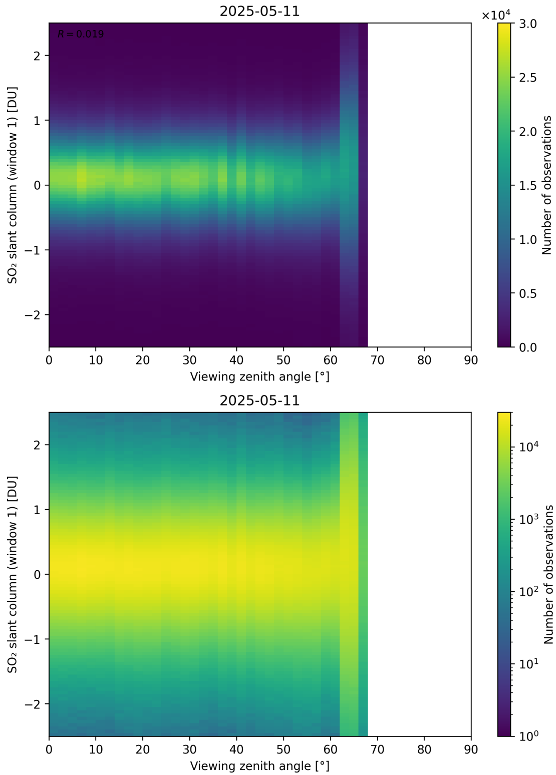
Figure 376: Scatter density plot of “Viewing zenith angle” against “SO 2 slant column (window 1)” for 2025-05-10 to 2025-05-12.
