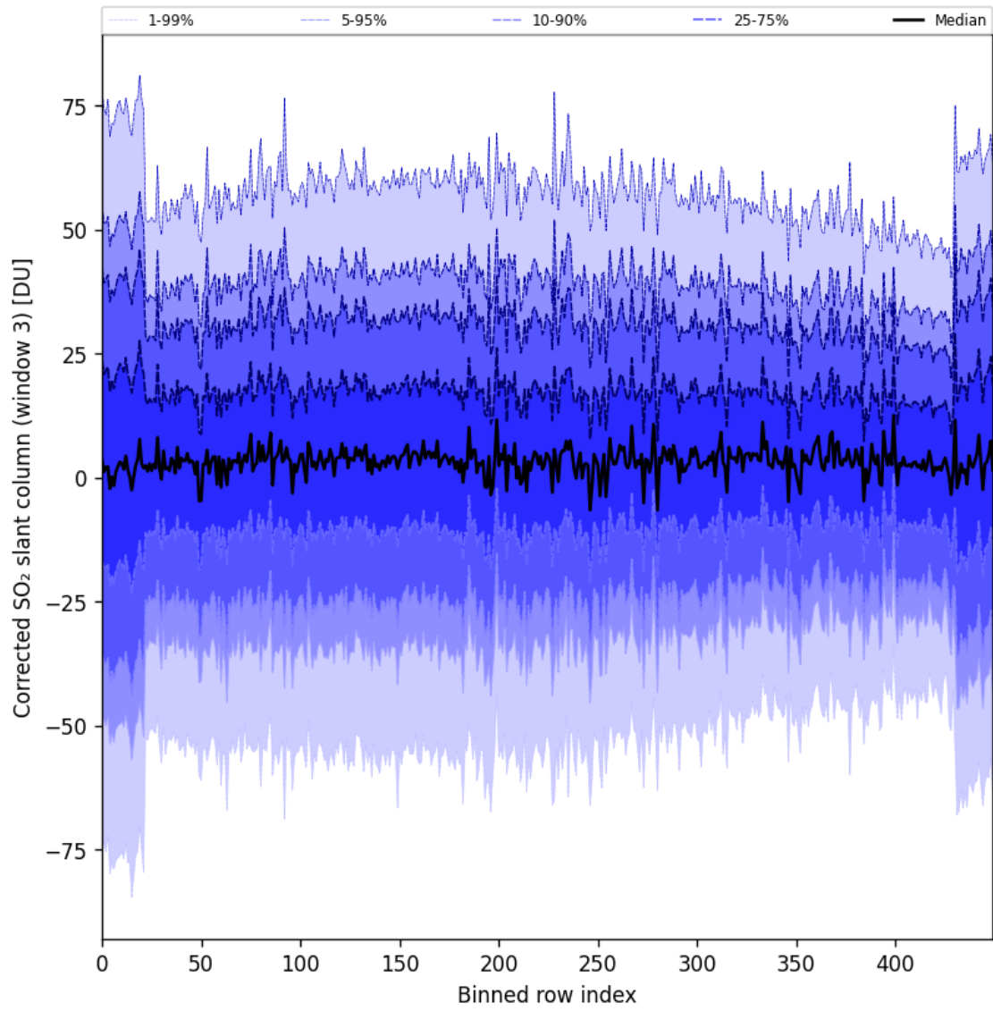
Figure 99: Along track statistics of “Corrected SO 2 slant column (window 3)” for 2025-05-10 to 2025-05-12
