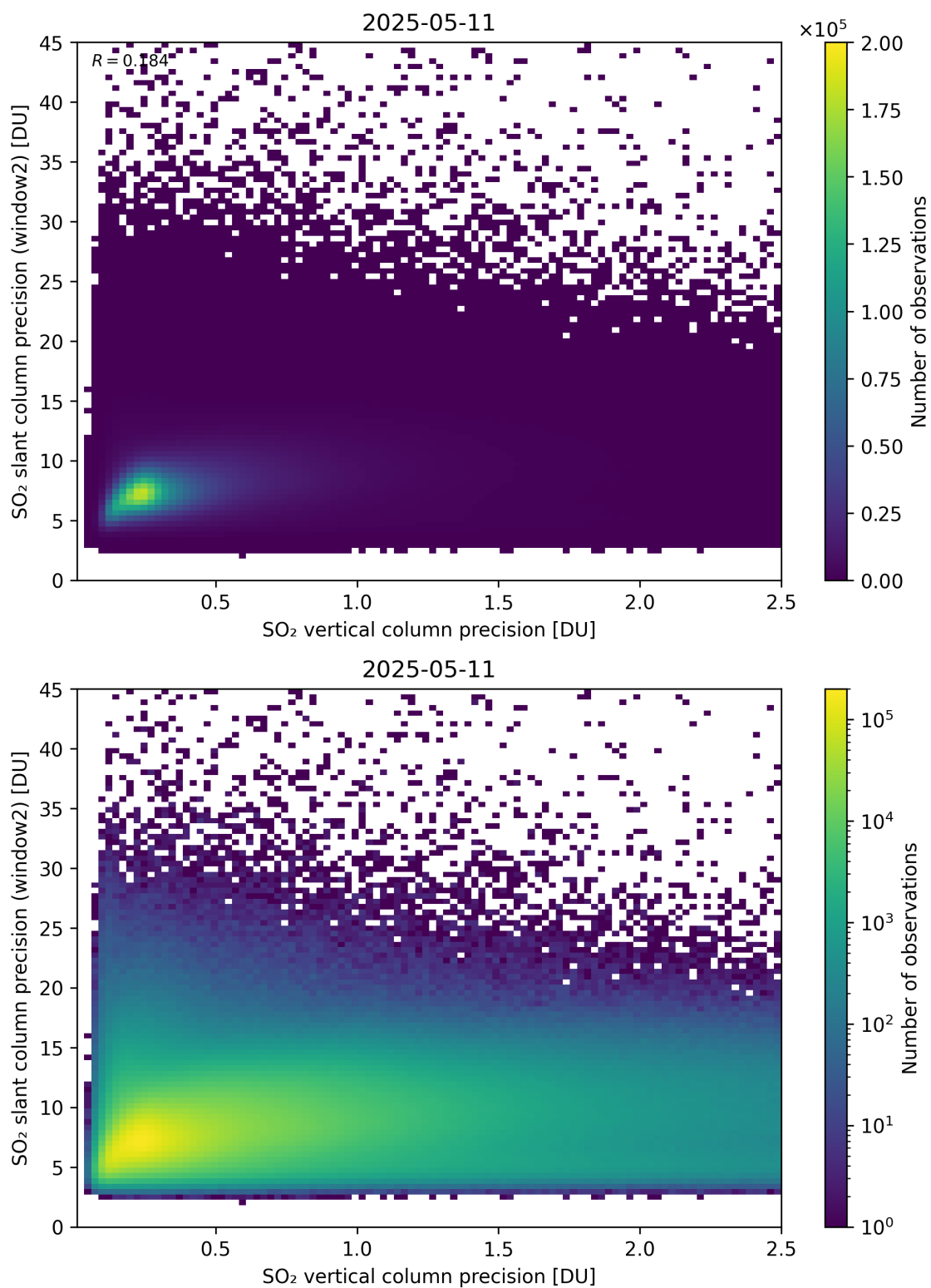
Figure 343: Scatter density plot of “SO 2 vertical column precision” against “SO 2 slant column precision (window2)” for 2025-05-10 to 2025-05-12.
