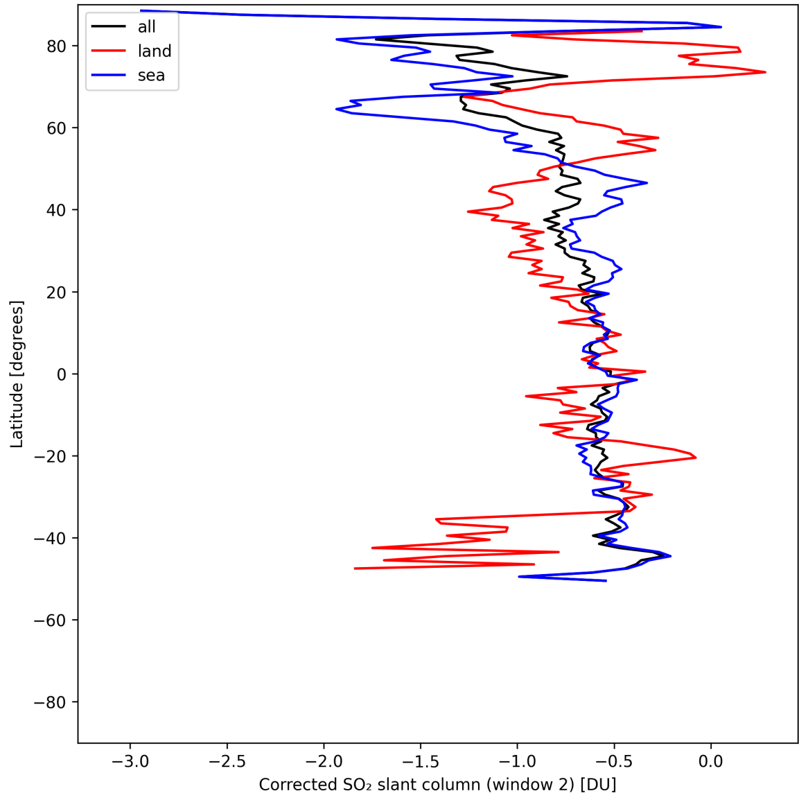
Figure 43: Zonal average of “Corrected SO 2 slant column (window 2)” for 2025-05-10 to 2025-05-12.
