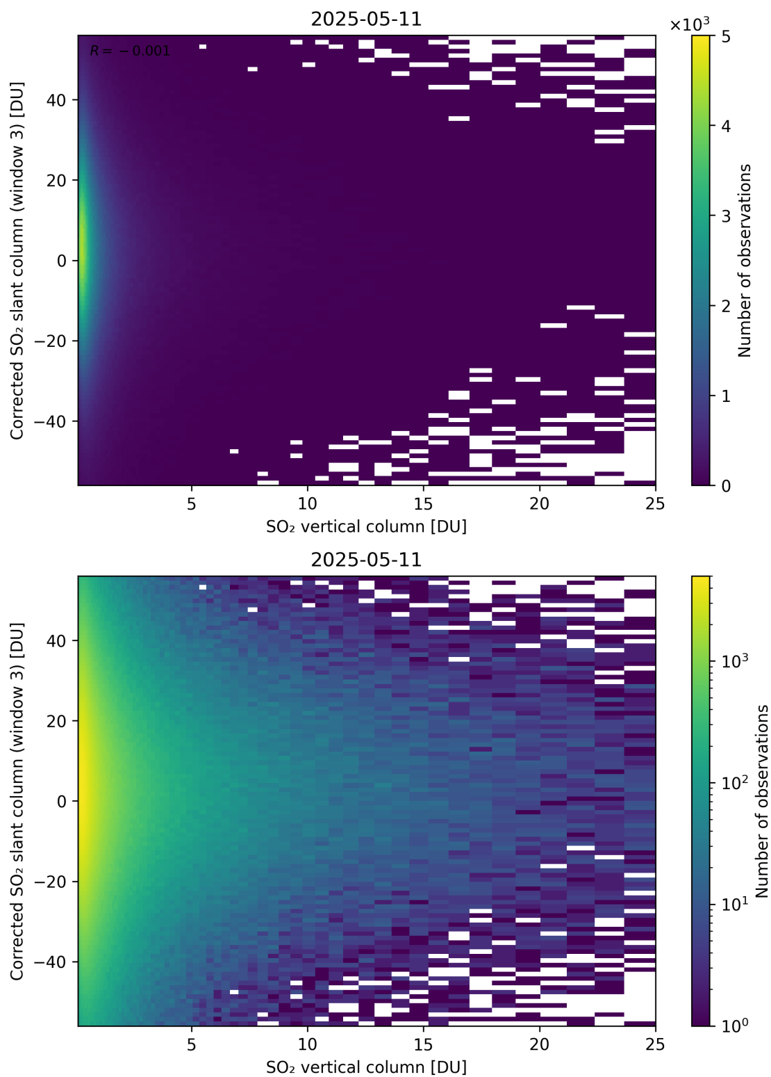
Figure 353: Scatter density plot of “SO 2 vertical column” against “Corrected SO 2 slant column (window 3)” for 2025-05-10 to 2025-05-12.
