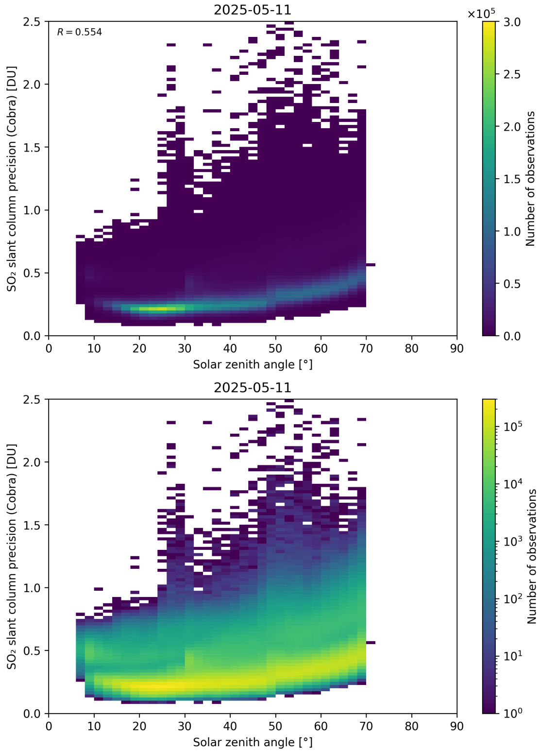
Figure 180: Scatter density plot of “Solar zenith angle” against “SO 2 slant column precision (Cobra)” for 2025-05-10 to 2025-05-12.
