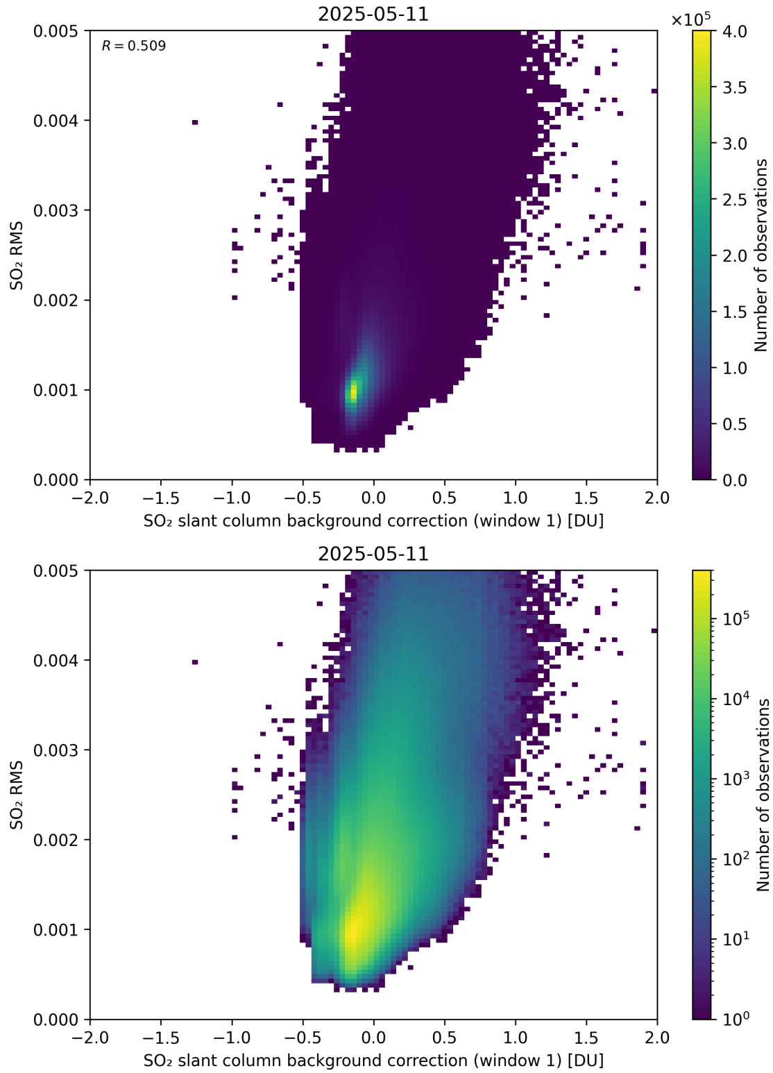
Figure 113: Scatter density plot of “SO 2 slant column background correction (window 1)” against “SO 2 RMS” for 2025-05-10 to 2025-05-12.
