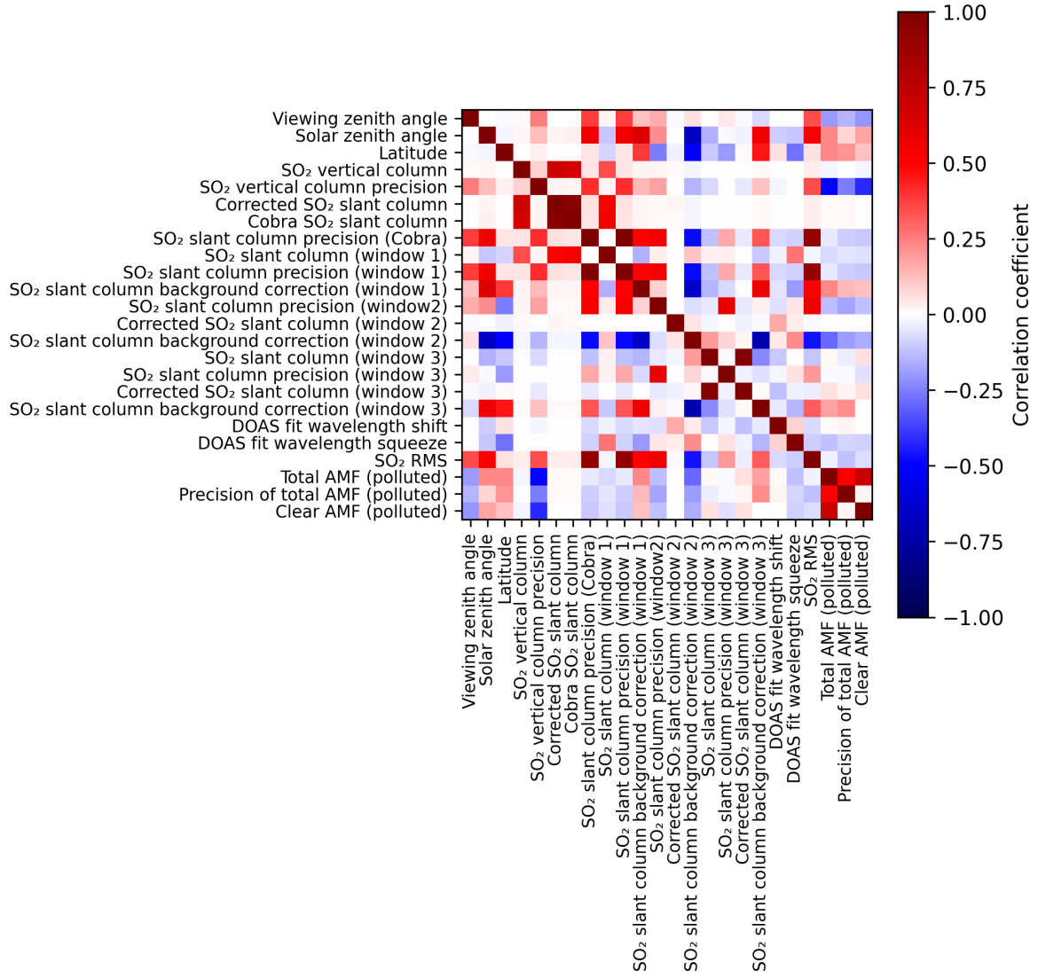
Figure 2: Map of correlation matrix for 2025-05-10 to 2025-05-12.
