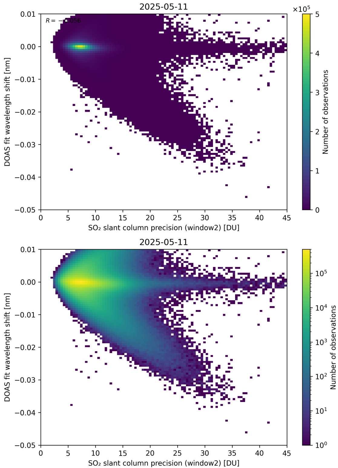
Figure 293: Scatter density plot of “SO 2 slant column precision (window2)” against “DOAS fit wavelength shift” for 2025-05-10 to 2025-05-12.
