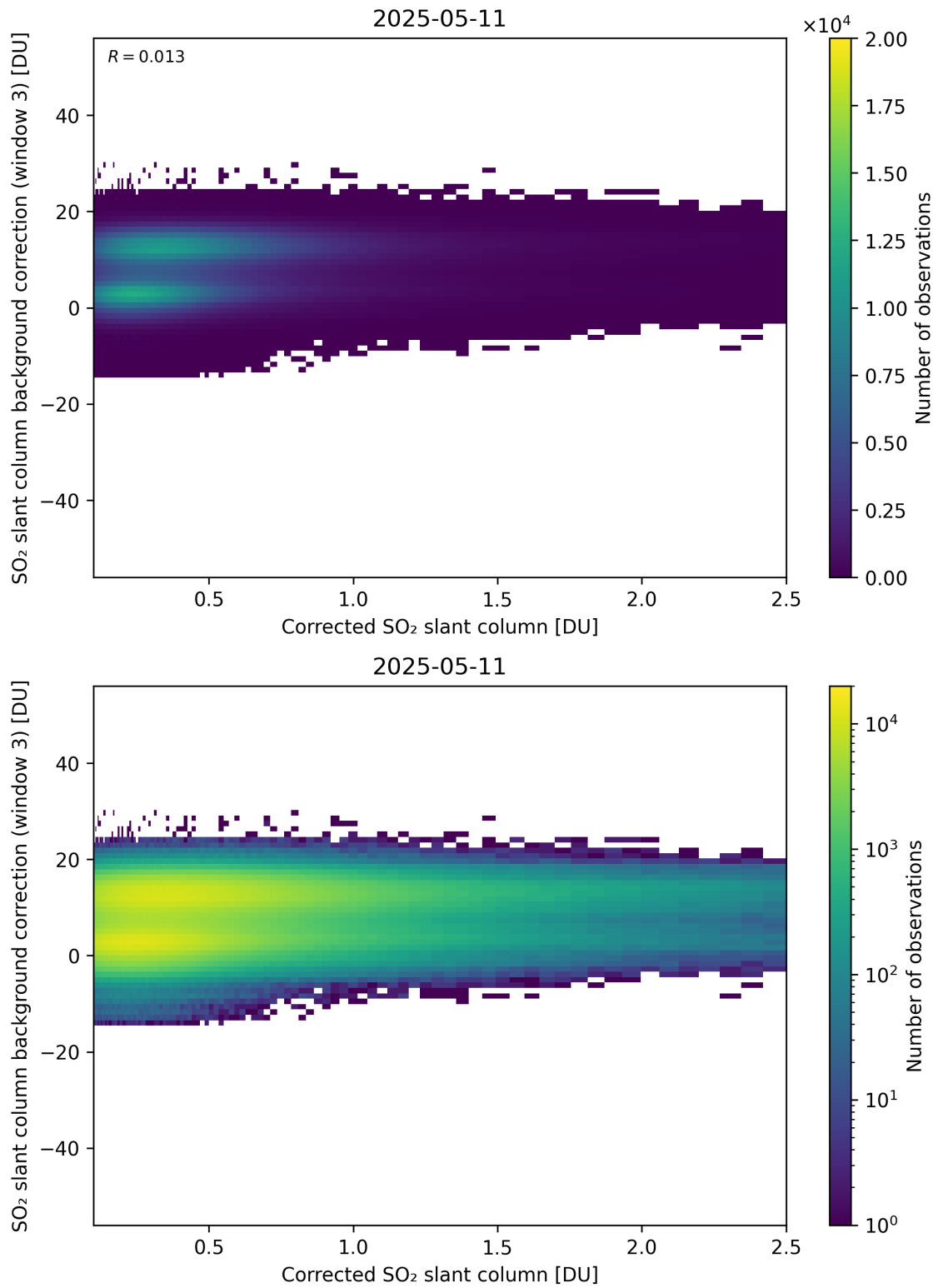
Figure 228: Scatter density plot of “Corrected SO 2 slant column” against “SO 2 slant column background correction (window 3)” for 2025-05-10 to 2025-05-12.
