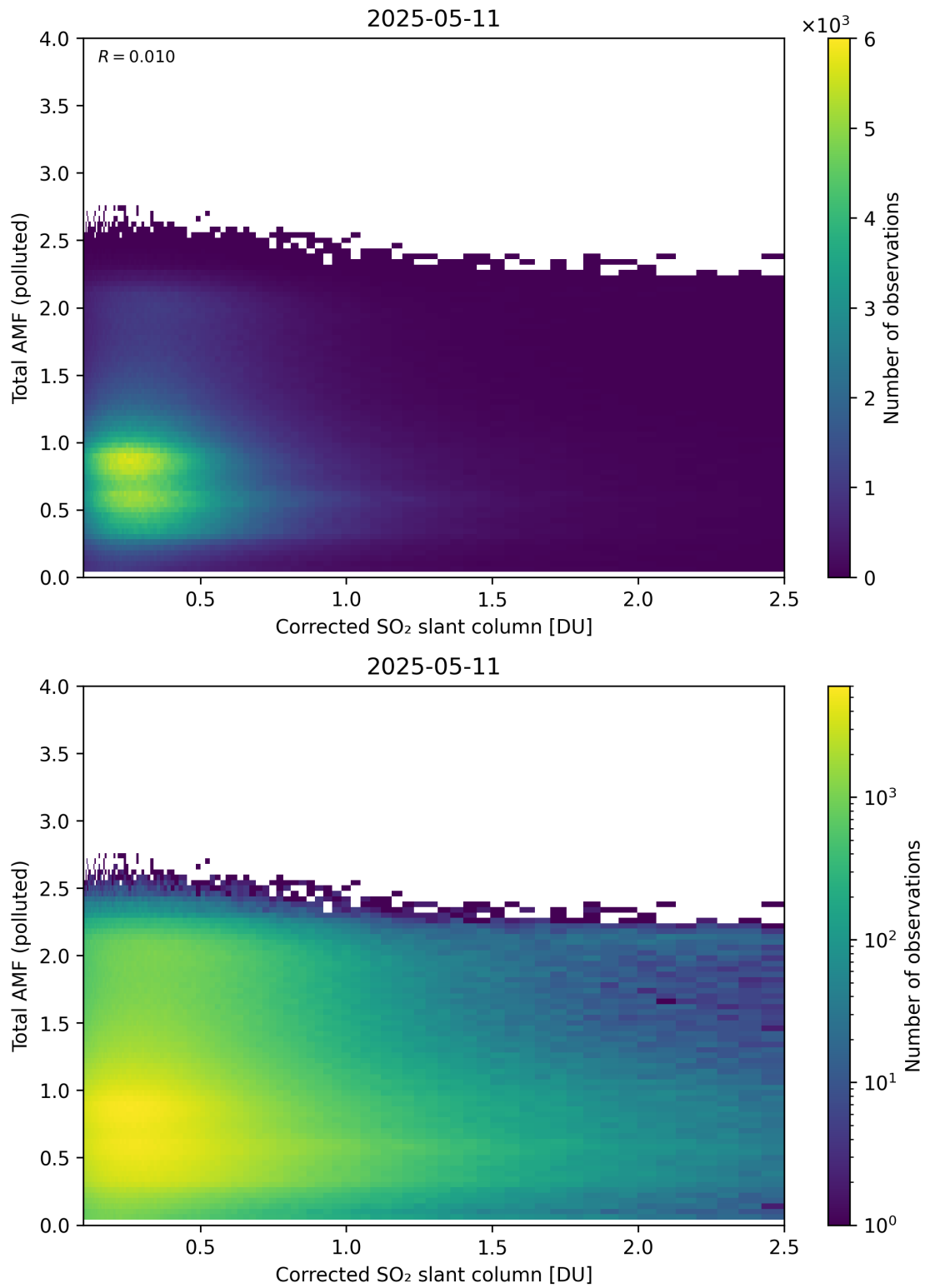
Figure 242: Scatter density plot of “Corrected SO 2 slant column” against “Total AMF (polluted)” for 2025-05-10 to 2025-05-12.
