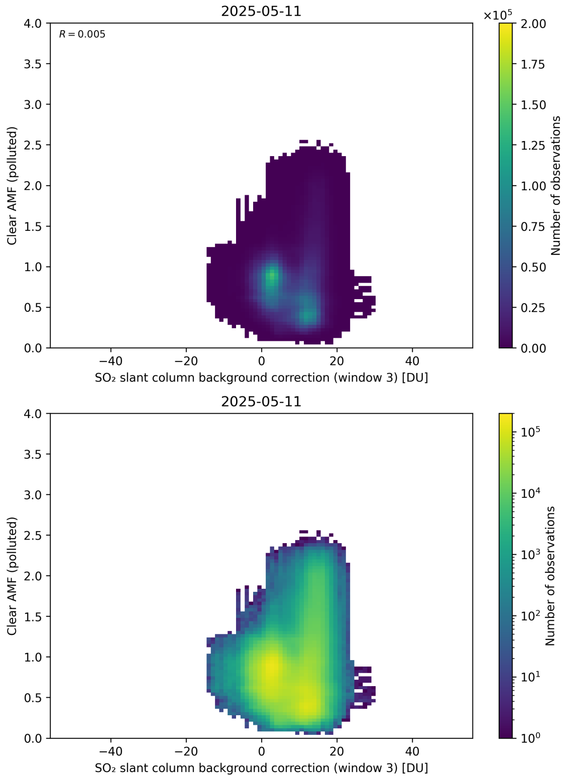
Figure 135: Scatter density plot of “SO 2 slant column background correction (window 3)” against “Clear AMF (polluted)” for 2025-05-10 to 2025-05-12.
