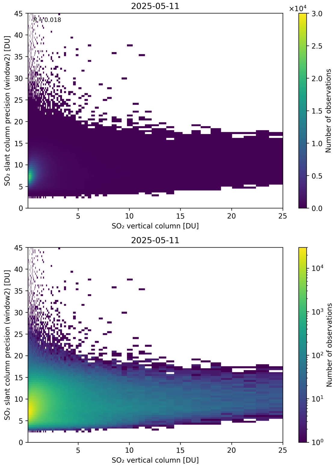
Figure 356: Scatter density plot of “SO 2 vertical column” against “SO 2 slant column precision (window2)” for 2025-05-10 to 2025-05-12.
