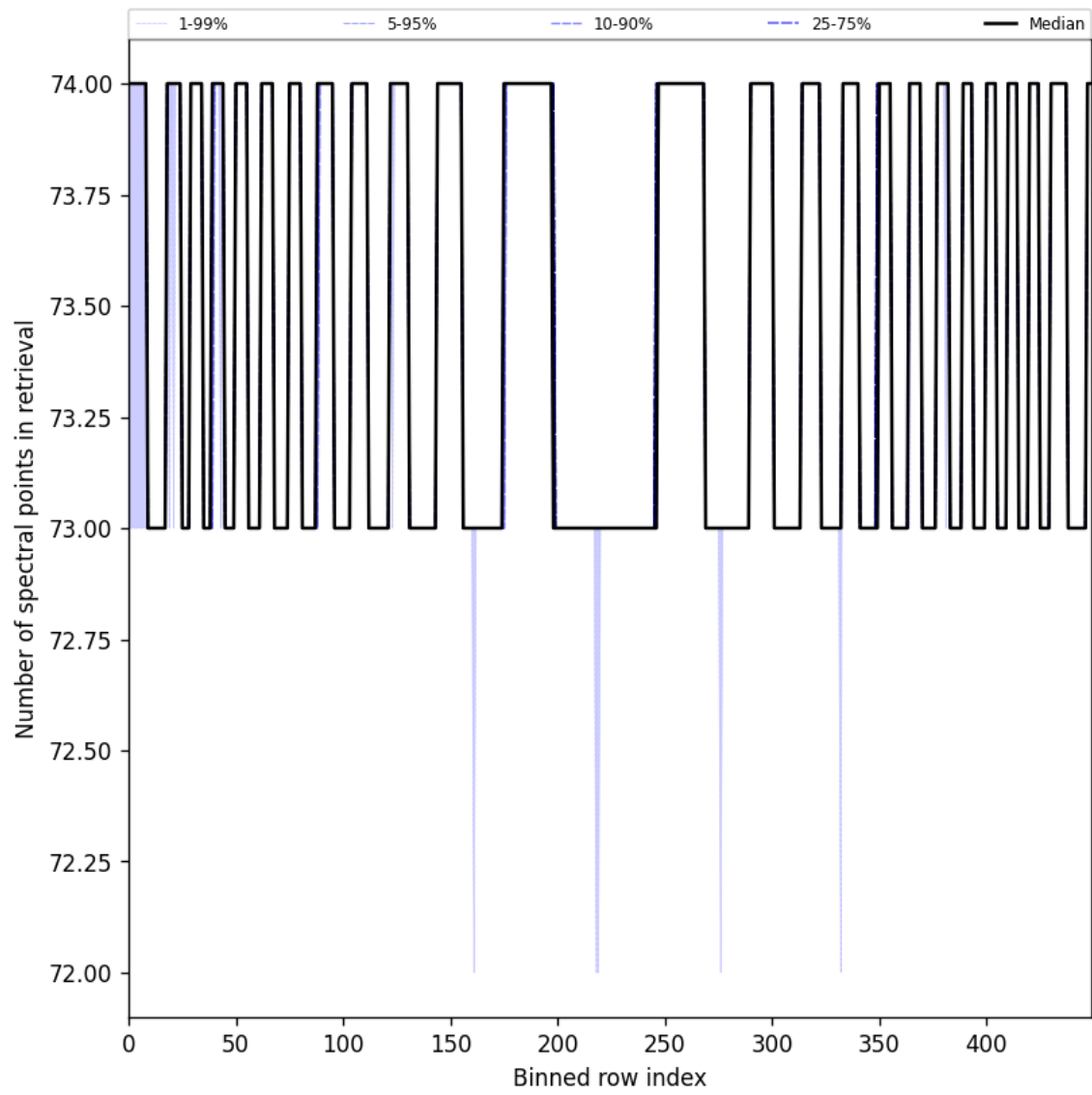
Figure 108: Along track statistics of “Number of spectral points in retrieval” for 2025-05-10 to 2025-05-12
