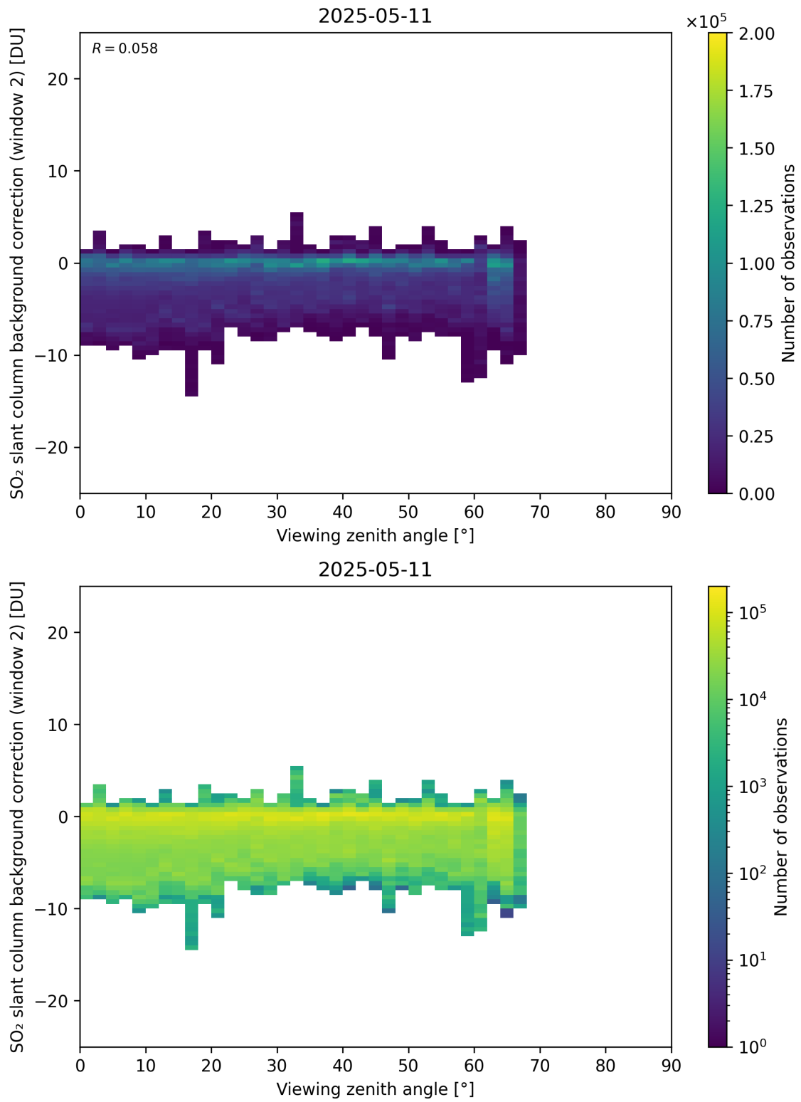
Figure 363: Scatter density plot of “Viewing zenith angle” against “SO 2 slant column background correction (window 2)” for 2025-05-10 to 2025-05-12.
