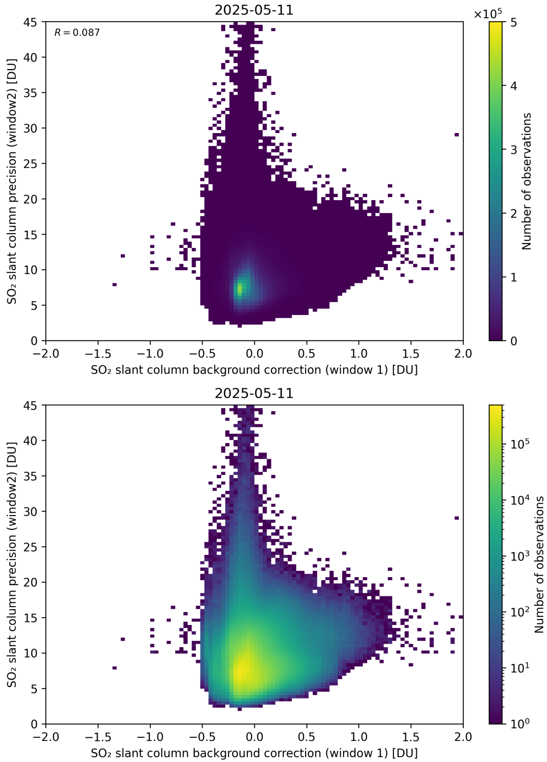
Figure 117: Scatter density plot of “SO 2 slant column background correction (window 1)” against “SO 2 slant column precision (window2)” for 2025-05-10 to 2025-05-12.
