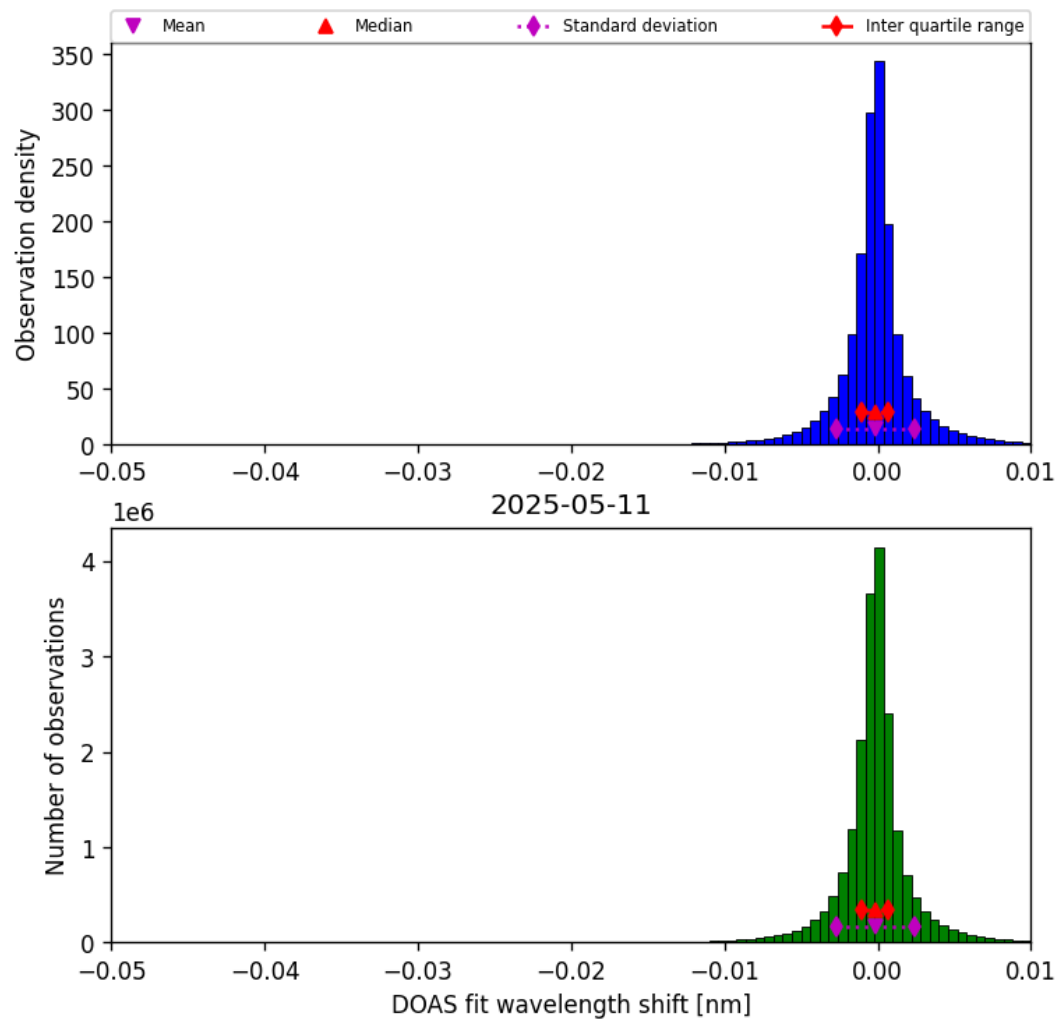
Figure 76: Histogram of “DOAS fit wavelength shift” for 2025-05-10 to 2025-05-12
