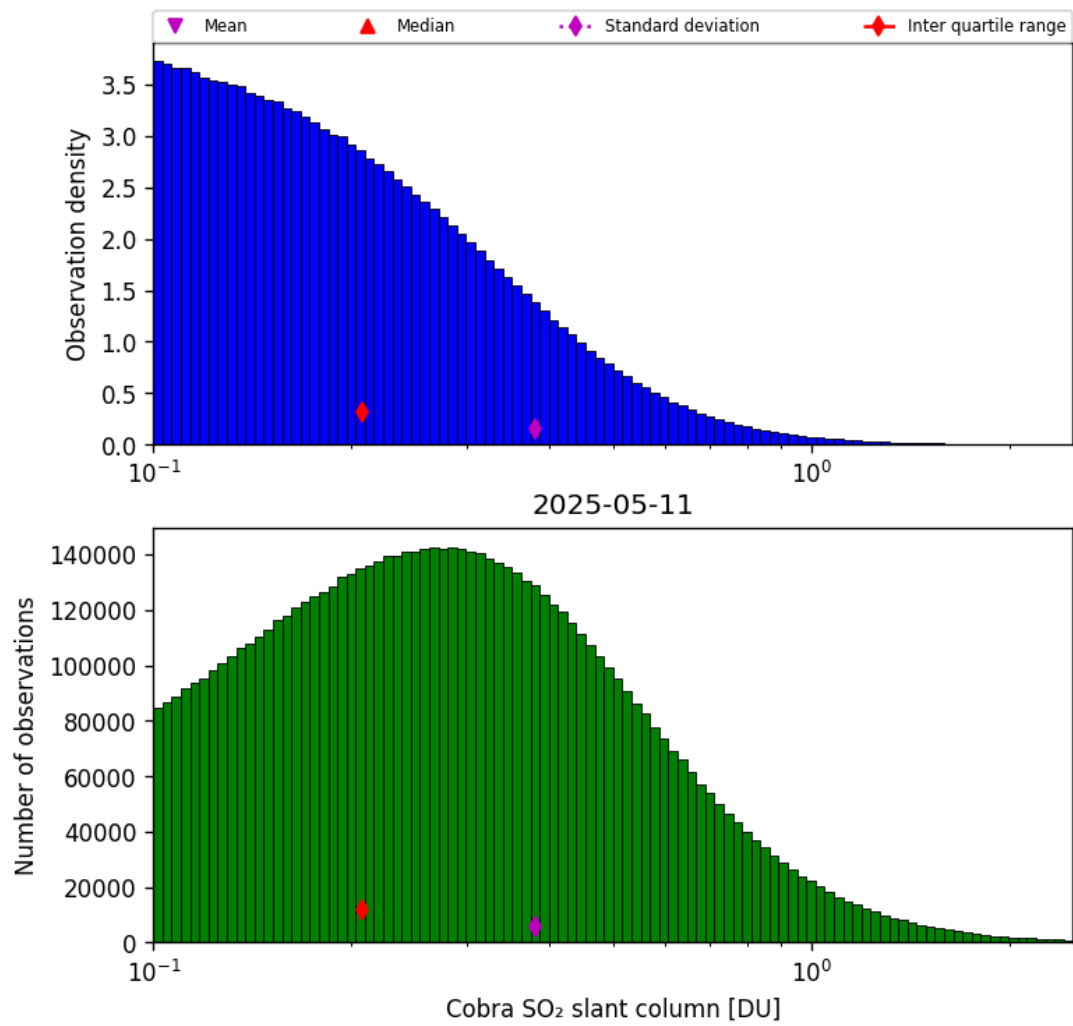
Figure 61: Histogram of “Cobra SO 2 slant column” for 2025-05-10 to 2025-05-12
