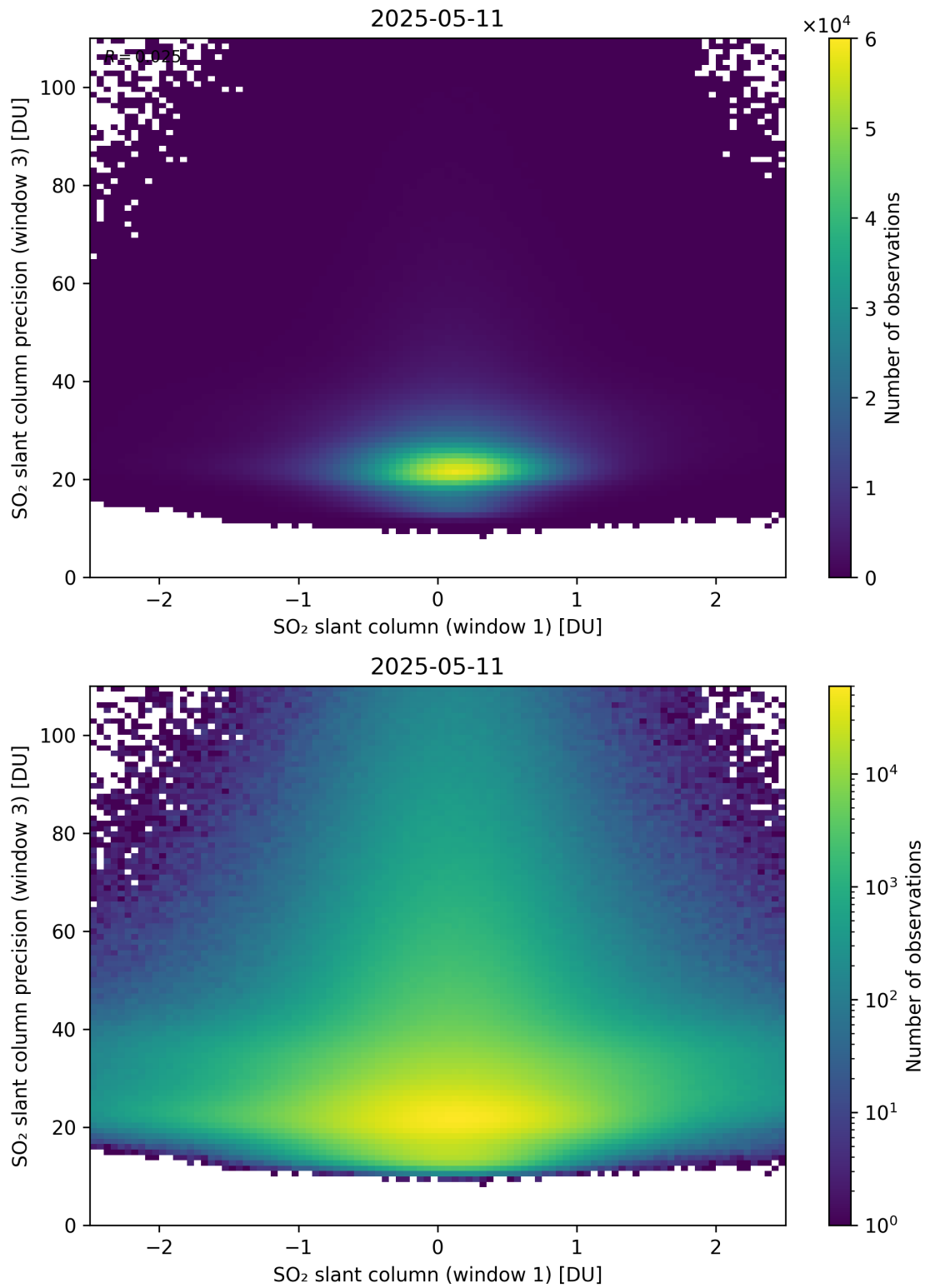
Figure 288: Scatter density plot of “SO 2 slant column (window 1)” against “SO 2 slant column precision (window 3)” for 2025-05-10 to 2025-05-12.
