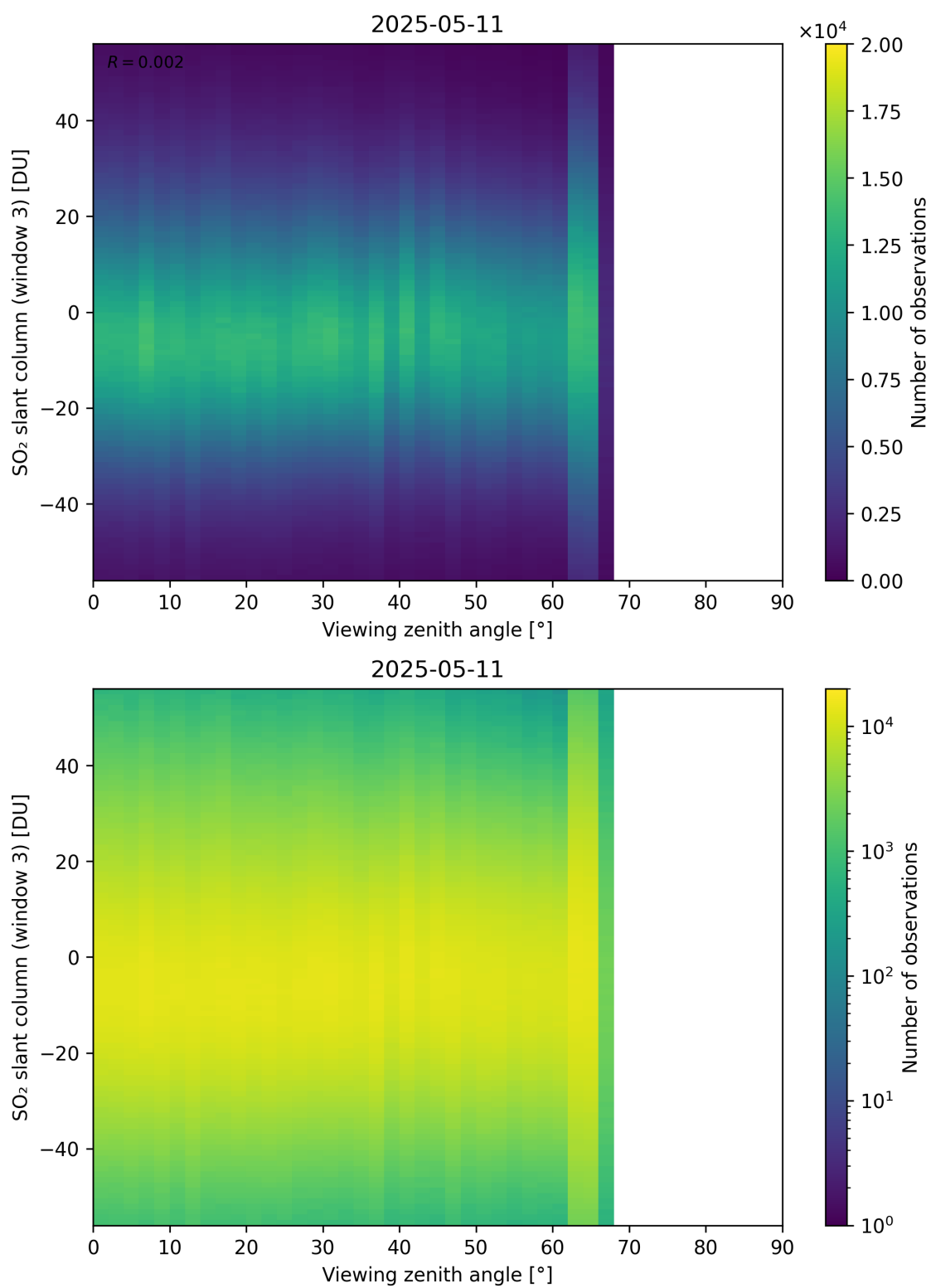
Figure 379: Scatter density plot of “Viewing zenith angle” against “SO 2 slant column (window 3)” for 2025-05-10 to 2025-05-12.
