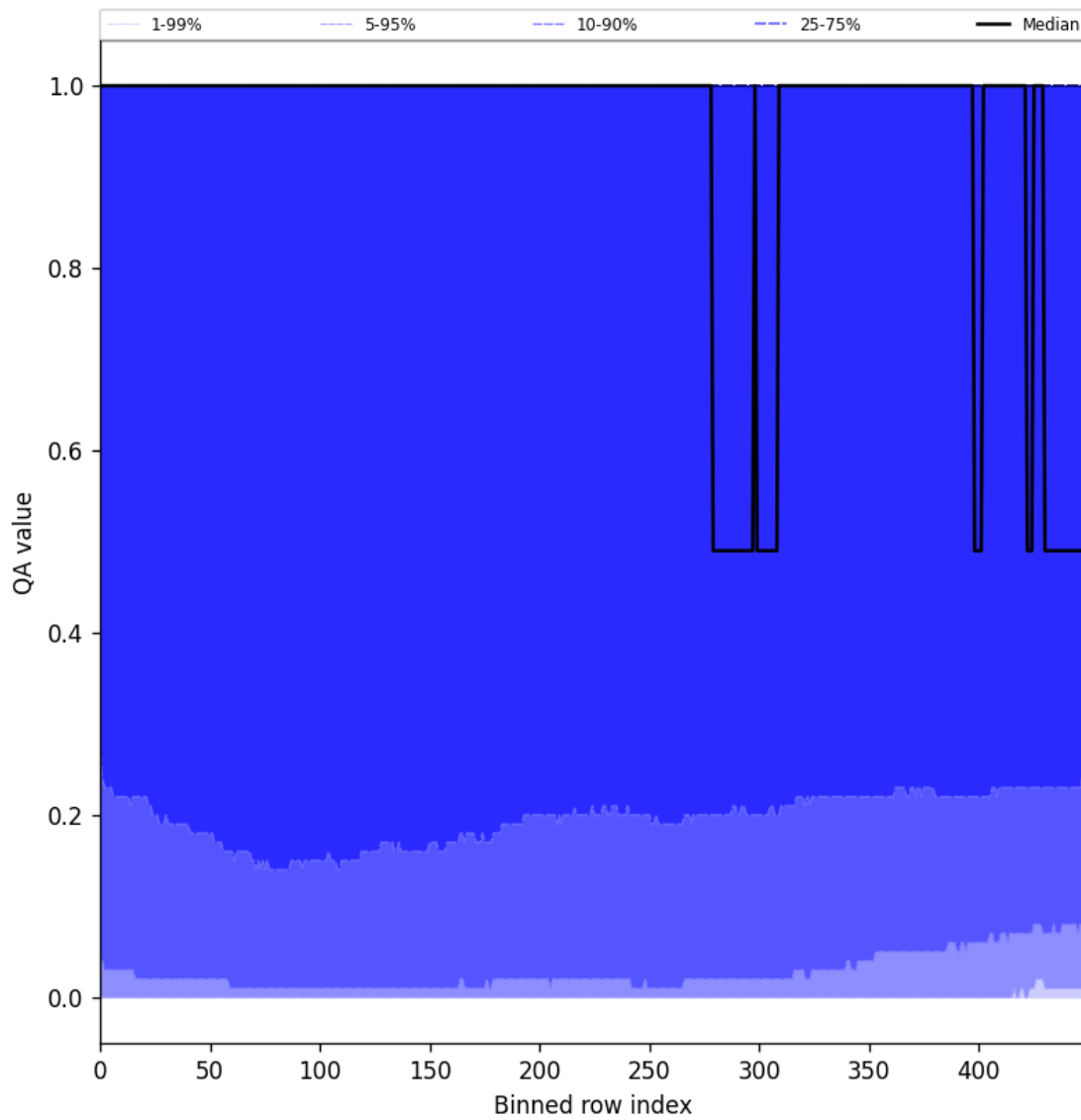
Figure 83: Along track statistics of “QA value” for 2025-05-10 to 2025-05-12
