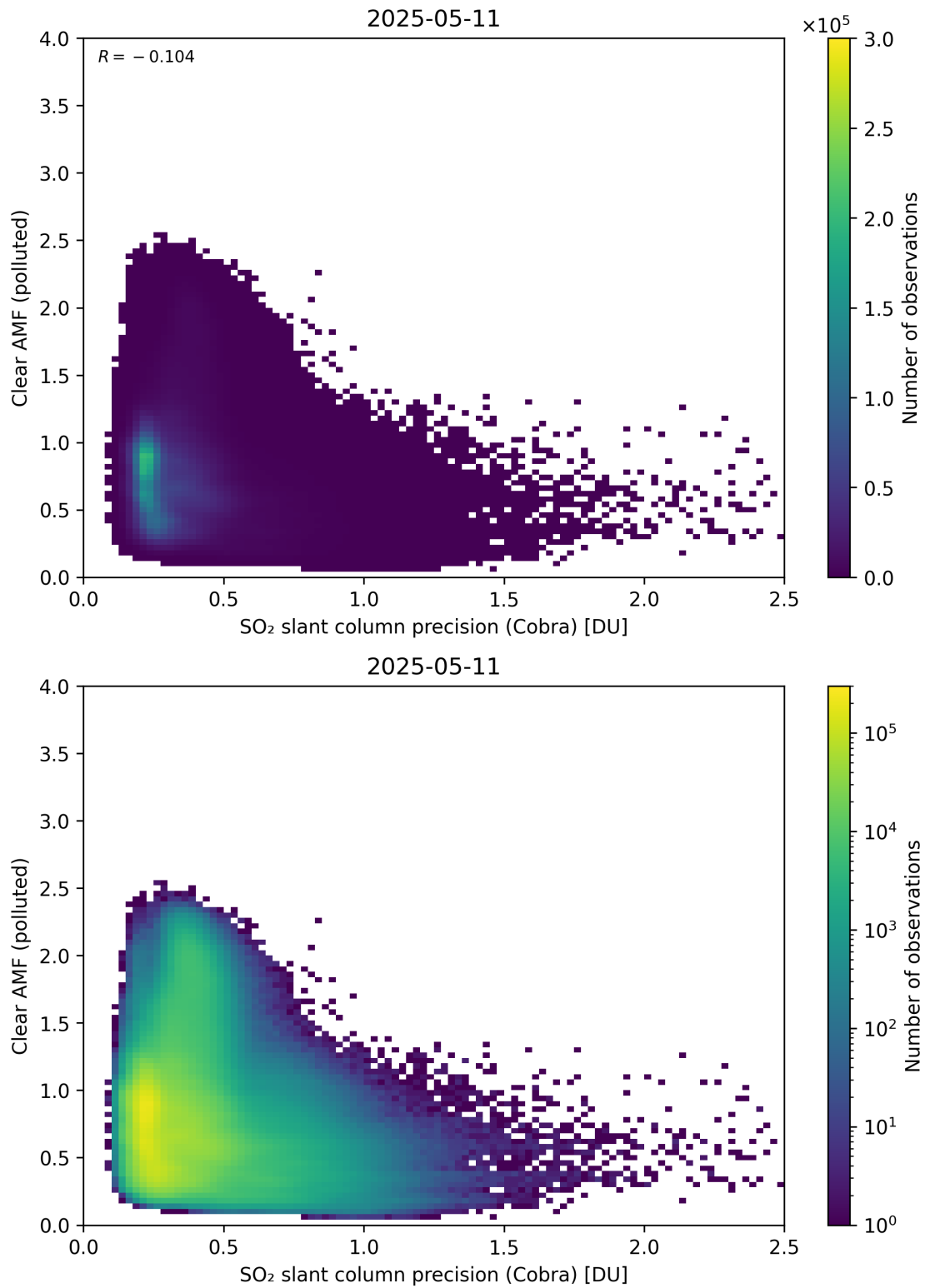
Figure 205: Scatter density plot of “SO 2 slant column precision (Cobra)” against “Clear AMF (polluted)” for 2025-05-10 to 2025-05-12.
