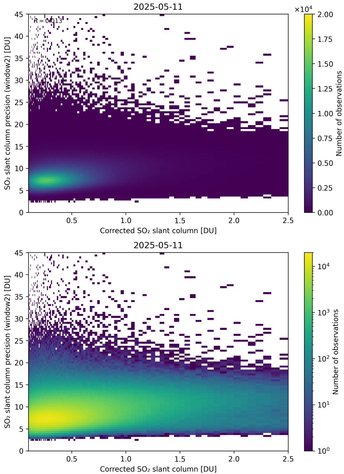
Figure 239: Scatter density plot of “Corrected SO 2 slant column” against “SO 2 slant column precision (window2)” for 2025-05-10 to 2025-05-12.
