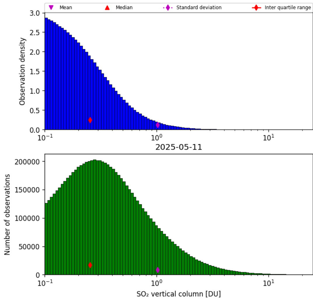
Figure 58: Histogram of “SO 2 vertical column” for 2025-05-10 to 2025-05-12
