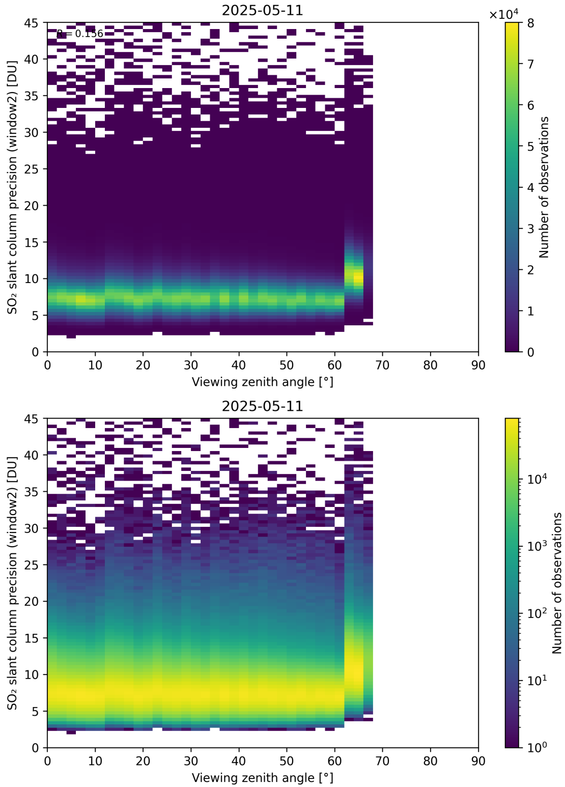
Figure 378: Scatter density plot of “Viewing zenith angle” against “SO 2 slant column precision (window2)” for 2025-05-10 to 2025-05-12.
