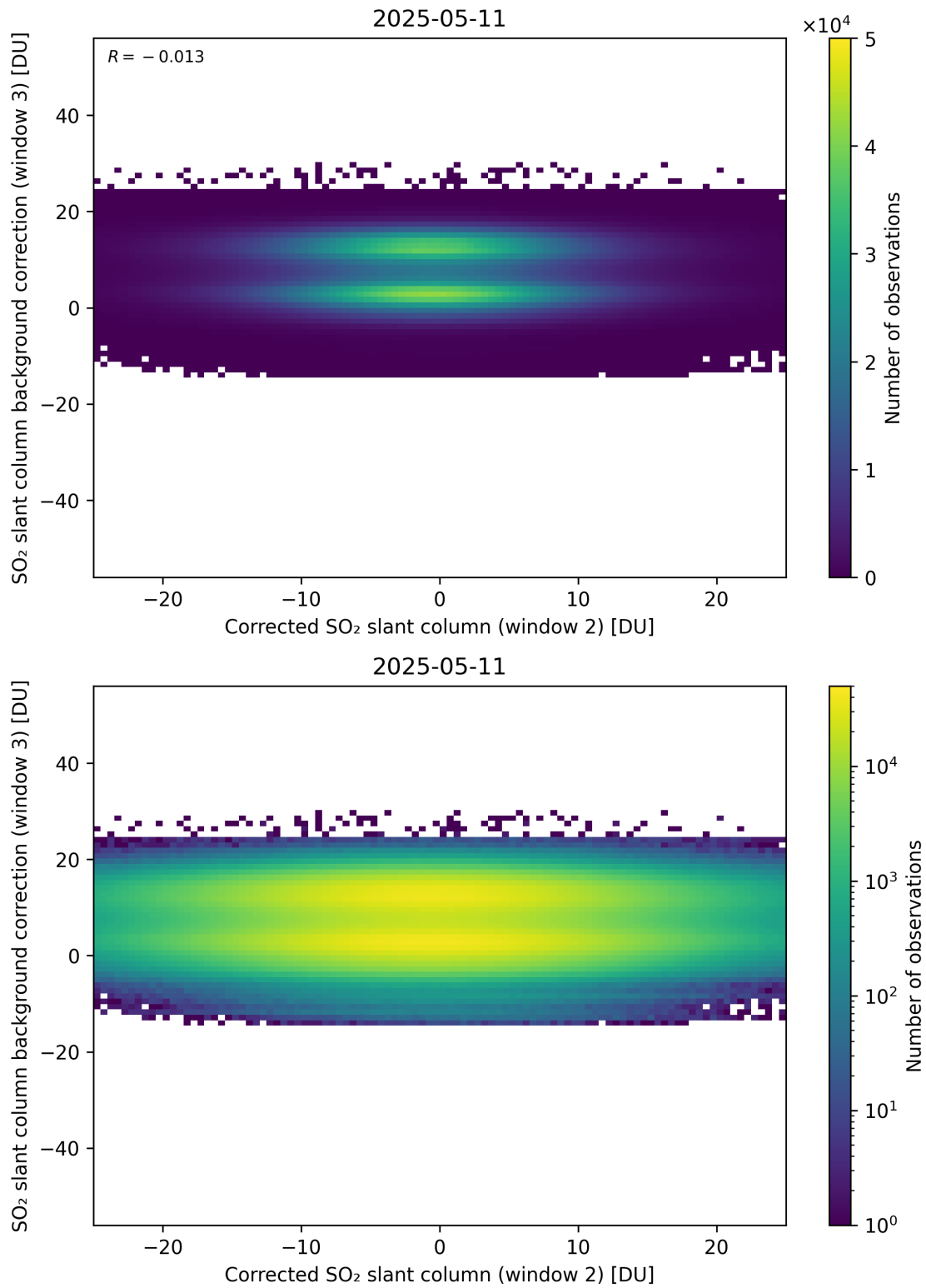
Figure 245: Scatter density plot of “Corrected SO 2 slant column (window 2)” against “SO 2 slant column background correction (window 3)” for 2025-05-10 to 2025-05-12.
