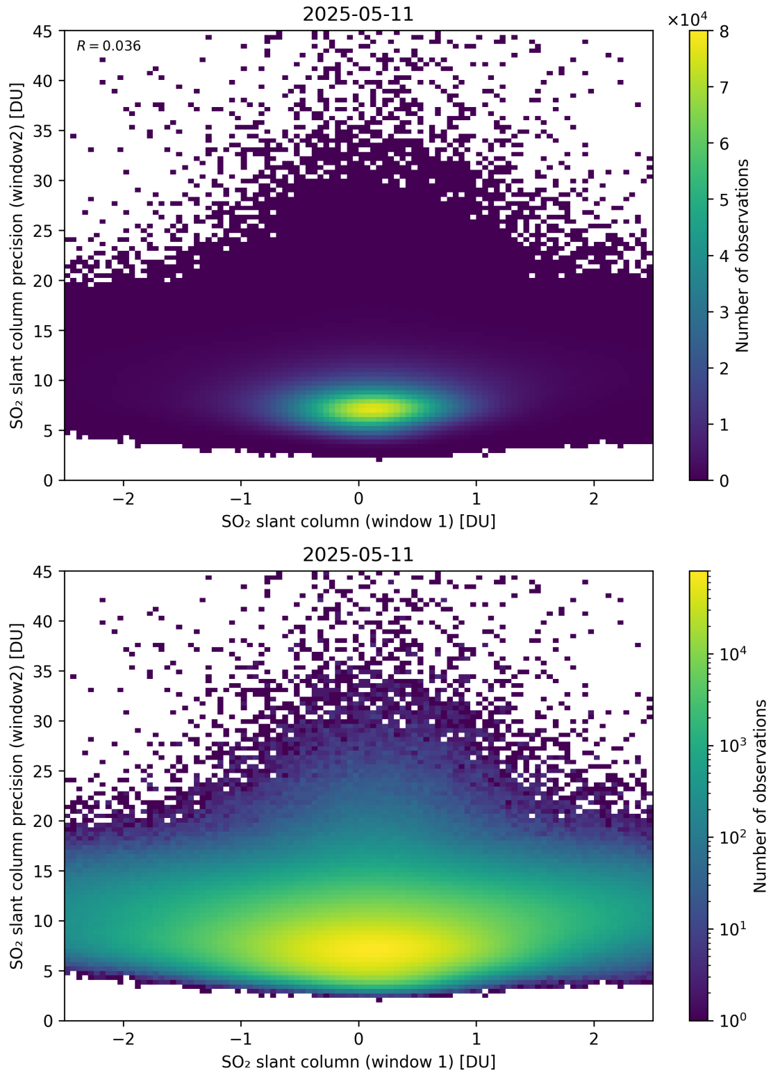
Figure 286: Scatter density plot of “SO 2 slant column (window 1)” against “SO 2 slant column precision (window2)” for 2025-05-10 to 2025-05-12.
