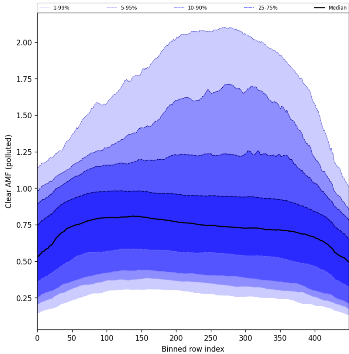
Figure 107: Along track statistics of “Clear AMF (polluted)” for 2025-05-10 to 2025-05-12
