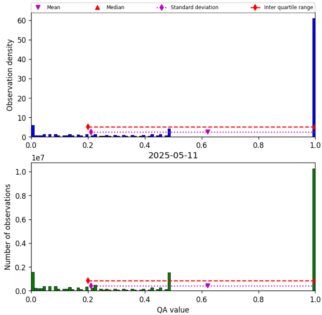
Figure 57: Histogram of “QA value” for 2025-05-10 to 2025-05-12
