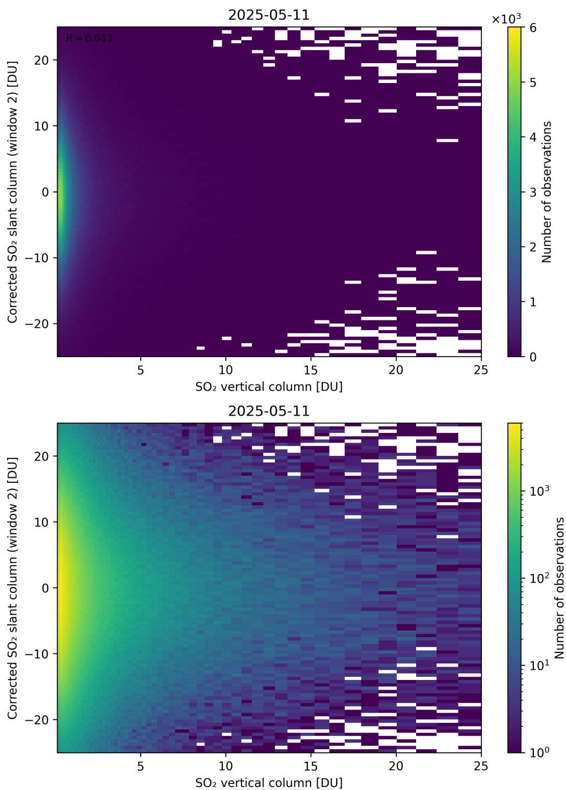
Figure 352: Scatter density plot of “SO 2 vertical column” against “Corrected SO 2 slant column (window 2)” for 2025-05-10 to 2025-05-12.
