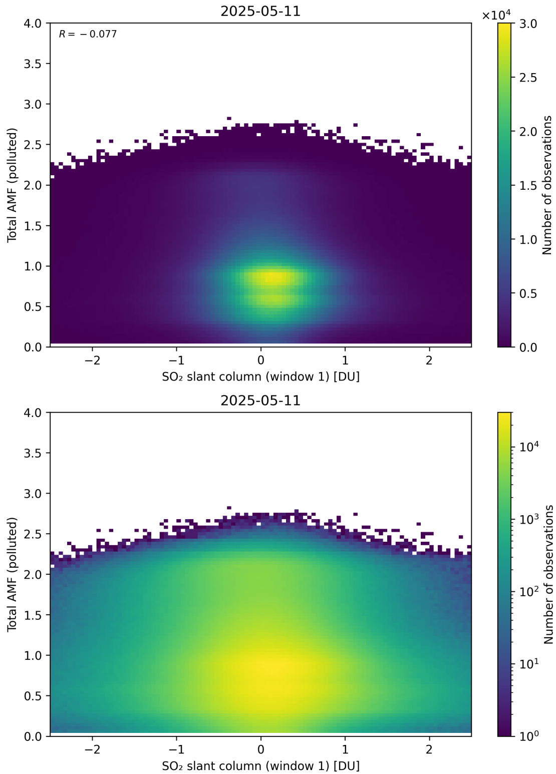
Figure 289: Scatter density plot of “SO 2 slant column (window 1)” against “Total AMF (polluted)” for 2025-05-10 to 2025-05-12.
