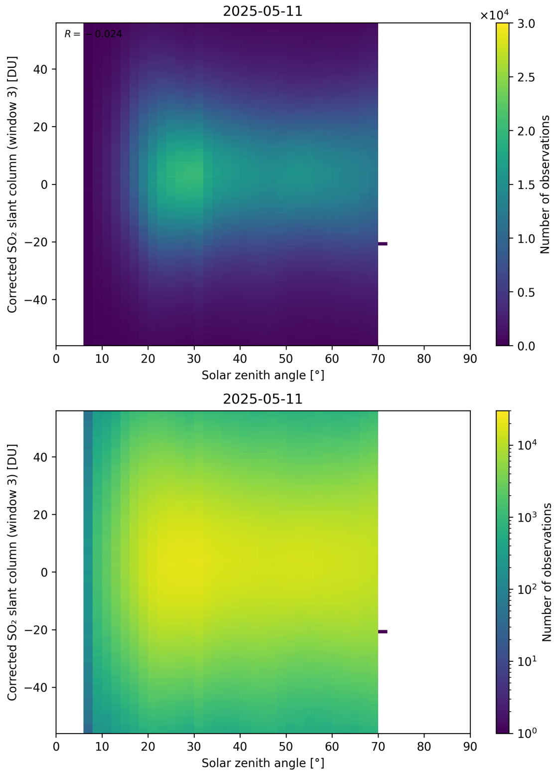
Figure 183: Scatter density plot of “Solar zenith angle” against “Corrected SO 2 slant column (window 3)” for 2025-05-10 to 2025-05-12.
