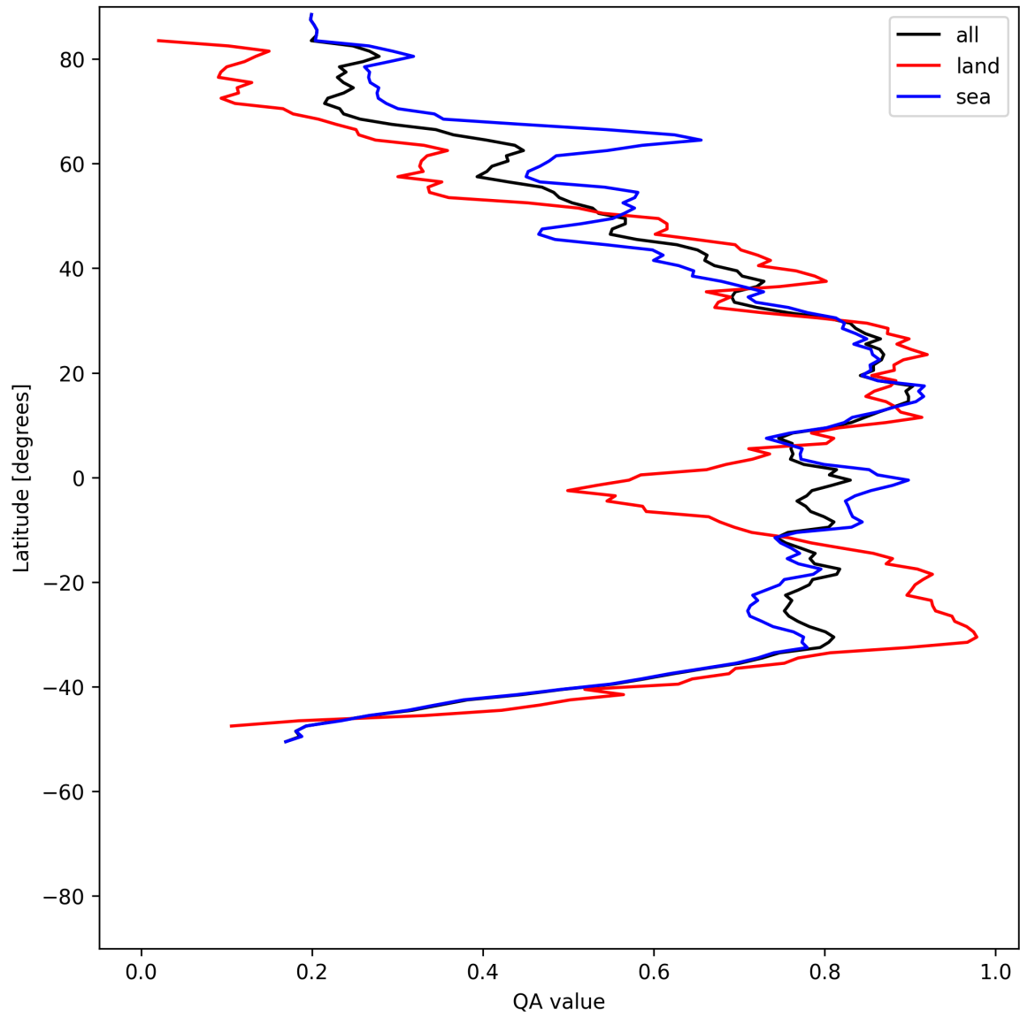
Figure 31: Zonal average of “QA value” for 2025-05-10 to 2025-05-12.
