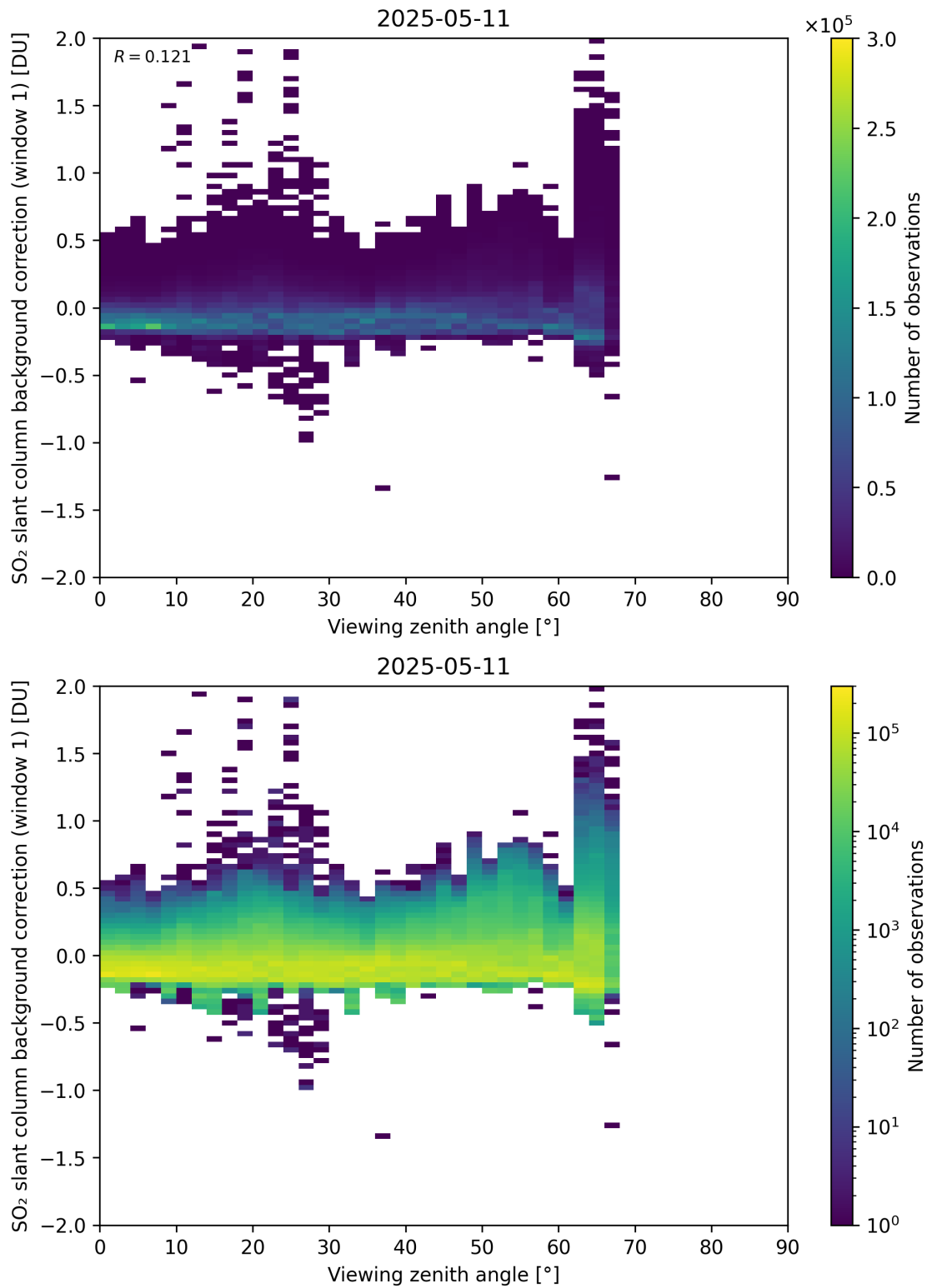
Figure 362: Scatter density plot of “Viewing zenith angle” against “SO 2 slant column background correction (window 1)” for 2025-05-10 to 2025-05-12.
