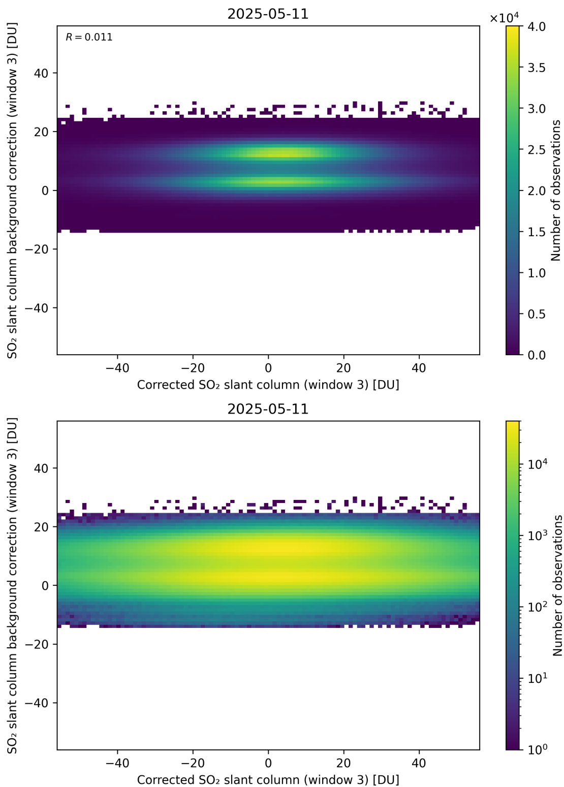
Figure 255: Scatter density plot of “Corrected SO 2 slant column (window 3)” against “SO 2 slant column background correction (window 3)” for 2025-05-10 to 2025-05-12.
