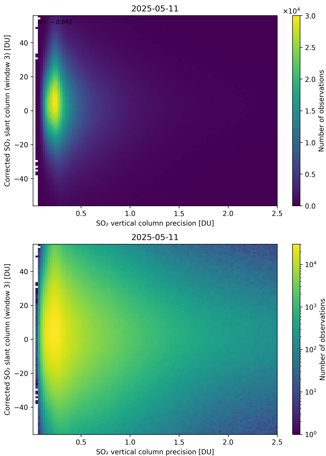
Figure 340: Scatter density plot of “SO 2 vertical column precision” against “Corrected SO 2 slant column (window 3)” for 2025-05-10 to 2025-05-12.
