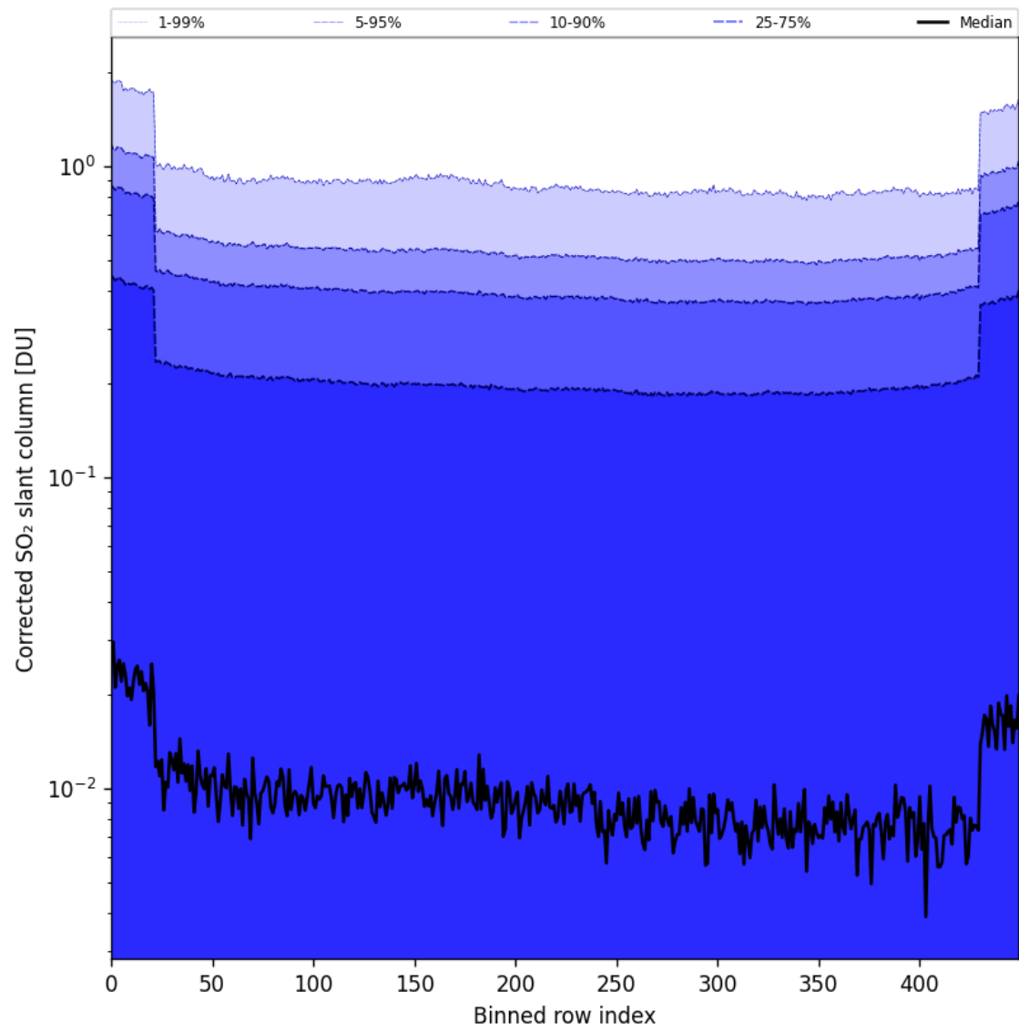
Figure 86: Along track statistics of “Corrected SO 2 slant column” for 2025-05-10 to 2025-05-12
