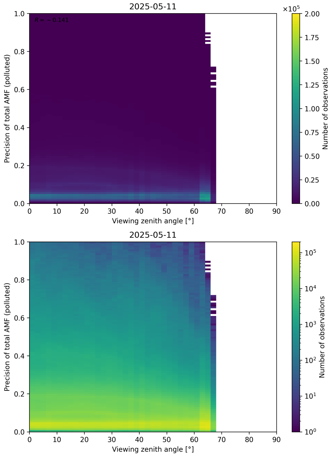
Figure 382: Scatter density plot of “Viewing zenith angle” against “Precision of total AMF (polluted)” for 2025-05-10 to 2025-05-12.
