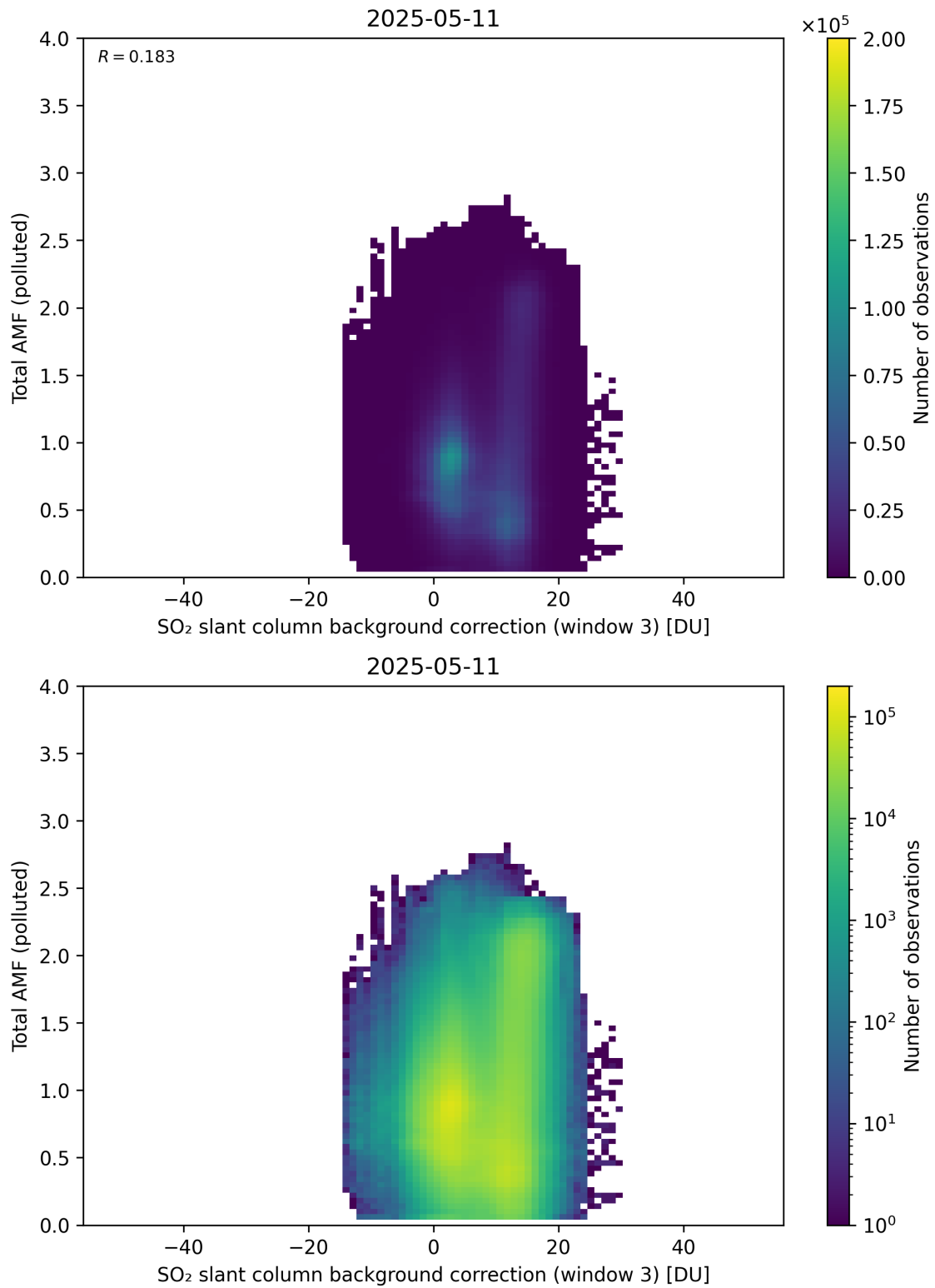
Figure 136: Scatter density plot of “SO 2 slant column background correction (window 3)” against “Total AMF (polluted)” for 2025-05-10 to 2025-05-12.
