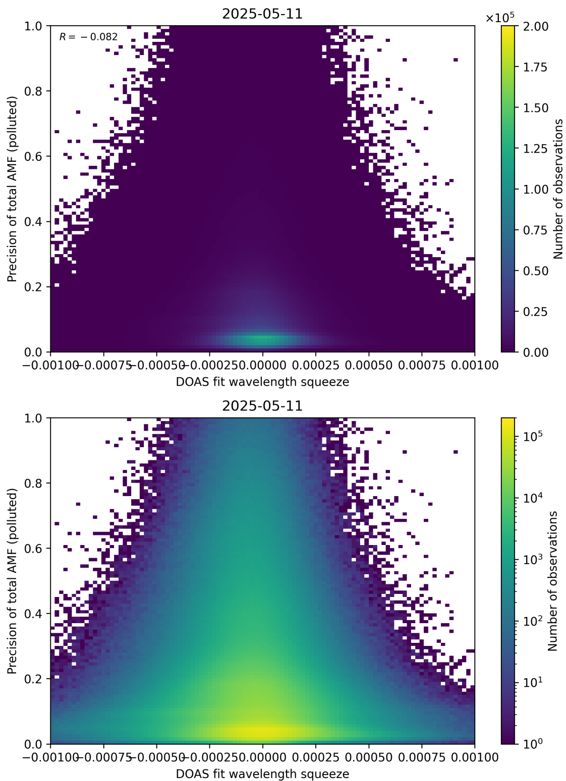
Figure 146: Scatter density plot of “DOAS fit wavelength squeeze” against “Precision of total AMF (polluted)” for 2025-05-10 to 2025-05-12.
