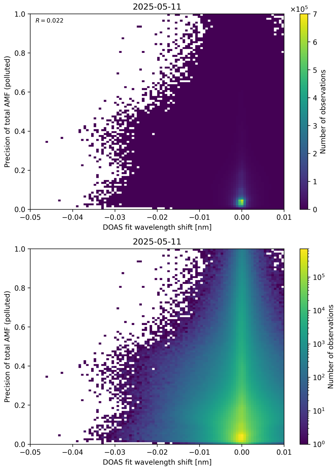
Figure 142: Scatter density plot of “DOAS fit wavelength shift” against “Precision of total AMF (polluted)” for 2025-05-10 to 2025-05-12.
