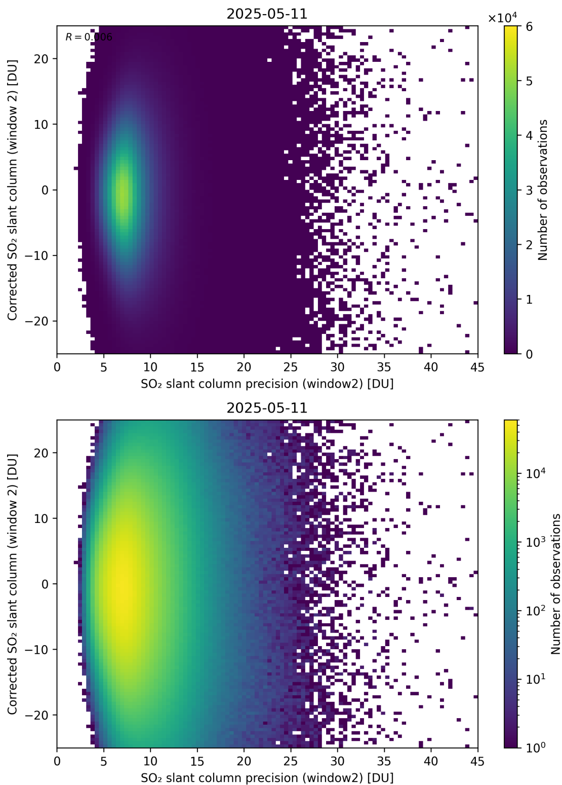
Figure 297: Scatter density plot of “SO 2 slant column precision (window2)” against “Corrected SO 2 slant column (window 2)” for 2025-05-10 to 2025-05-12.
