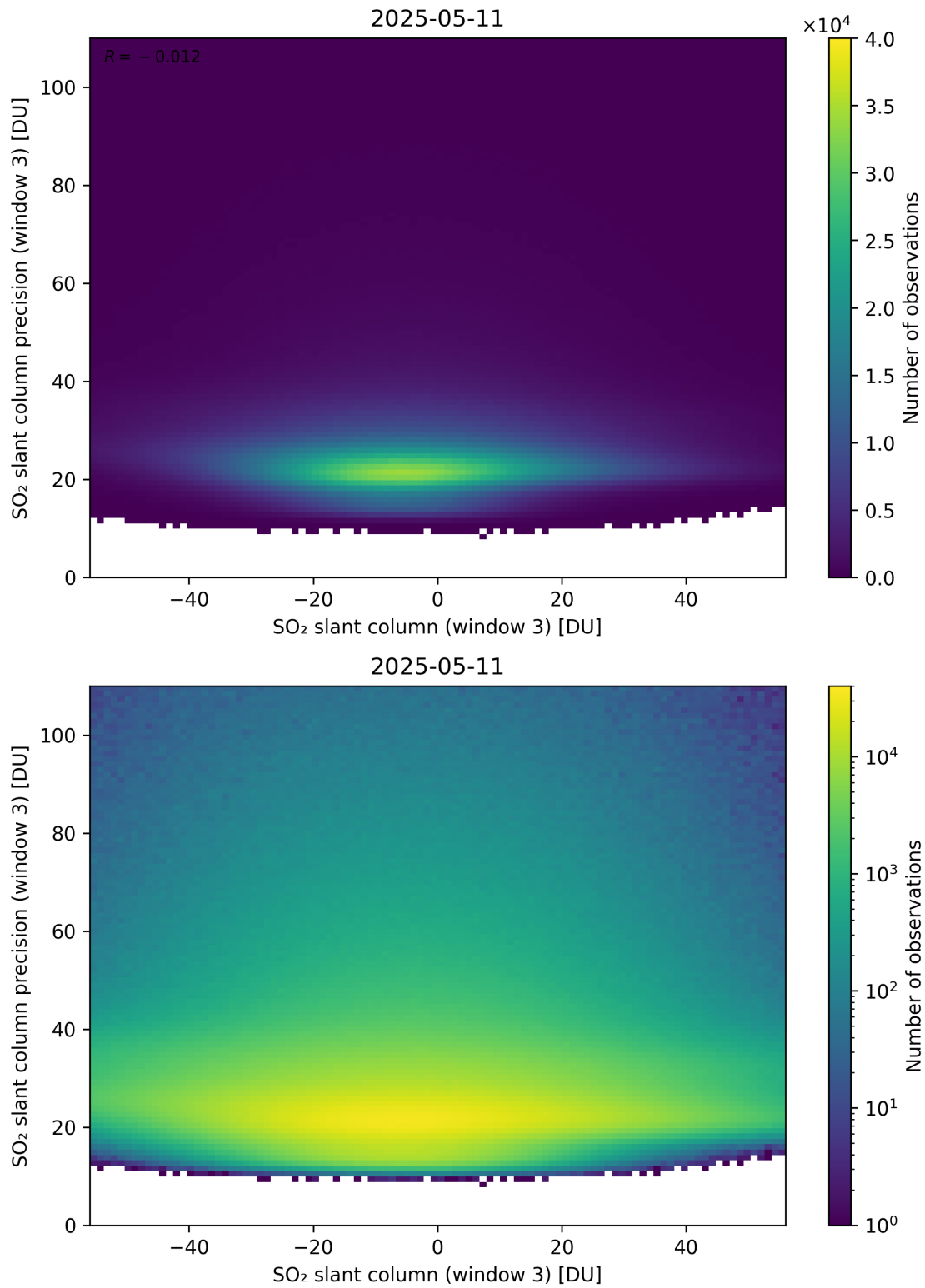
Figure 317: Scatter density plot of “SO 2 slant column (window 3)” against “SO 2 slant column precision (window 3)” for 2025-05-10 to 2025-05-12.
