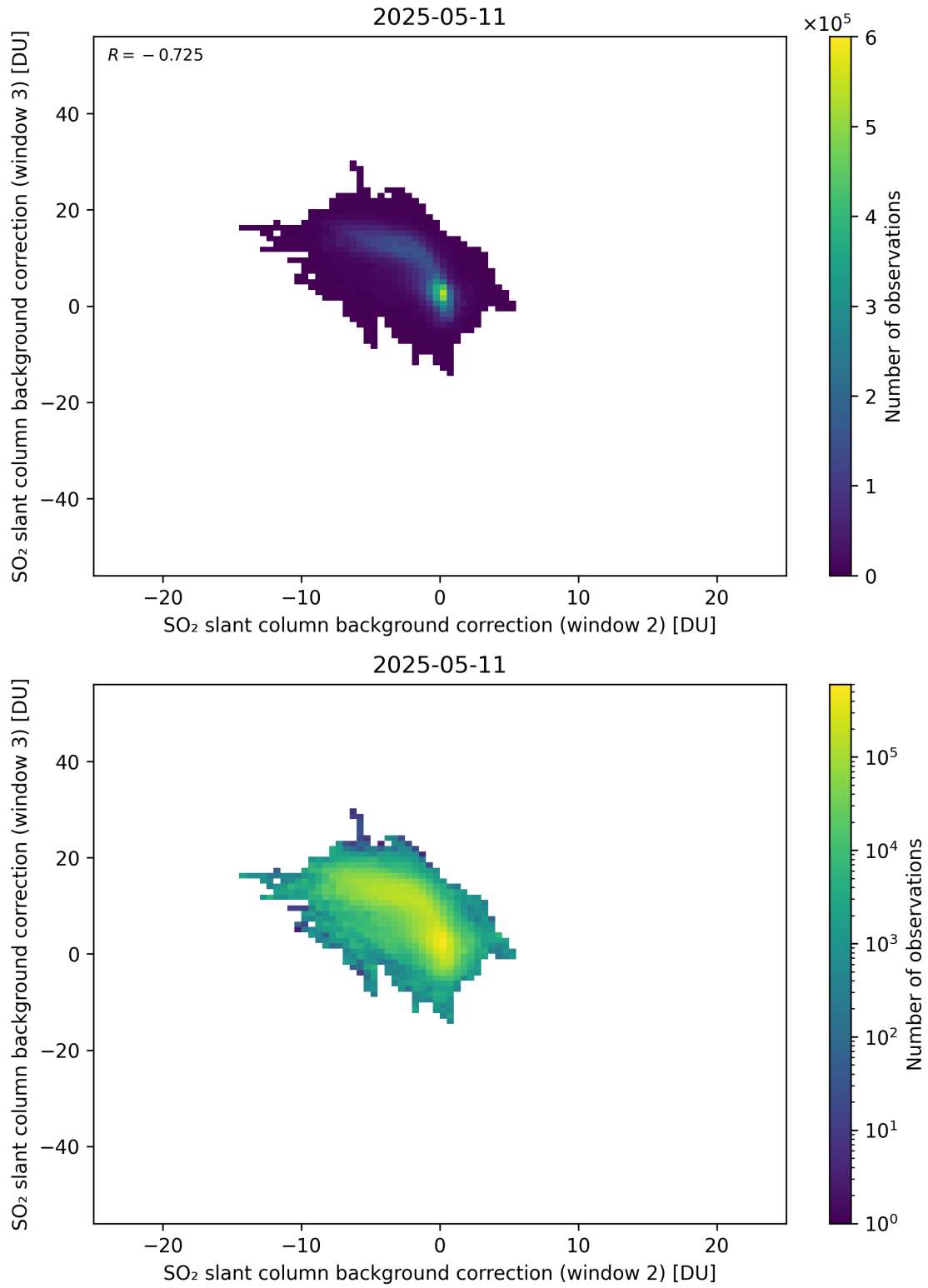
Figure 122: Scatter density plot of “SO 2 slant column background correction (window 2)” against “SO 2 slant column background correction (window 3)” for 2025-05-10 to 2025-05-12.
