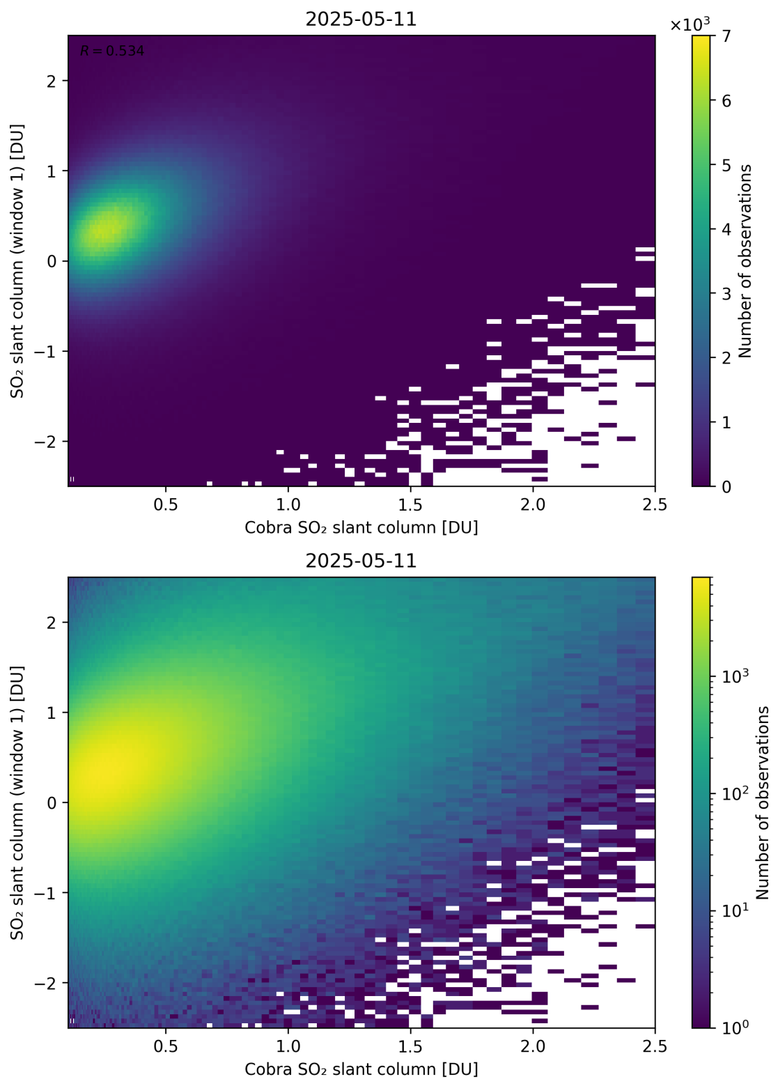
Figure 219: Scatter density plot of “Cobra SO 2 slant column” against “SO 2 slant column (window 1)” for 2025-05-10 to 2025-05-12.
