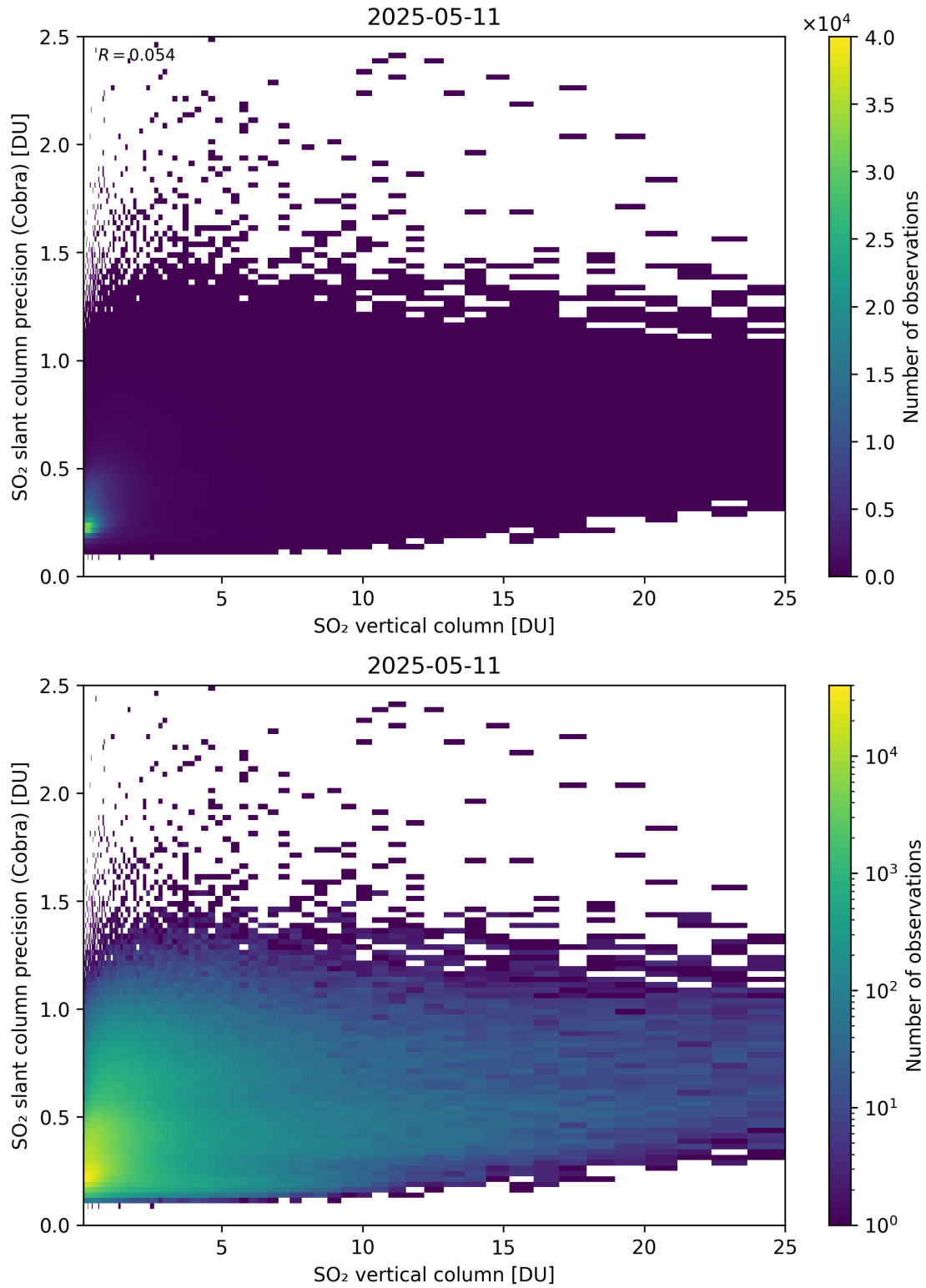
Figure 350: Scatter density plot of “SO 2 vertical column” against “SO 2 slant column precision (Cobra)” for 2025-05-10 to 2025-05-12.
