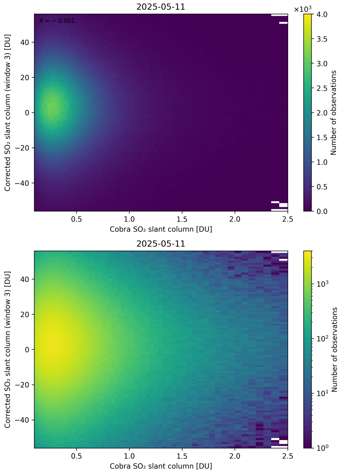
Figure 218: Scatter density plot of “Cobra SO 2 slant column” against “Corrected SO 2 slant column (window 3)” for 2025-05-10 to 2025-05-12.
