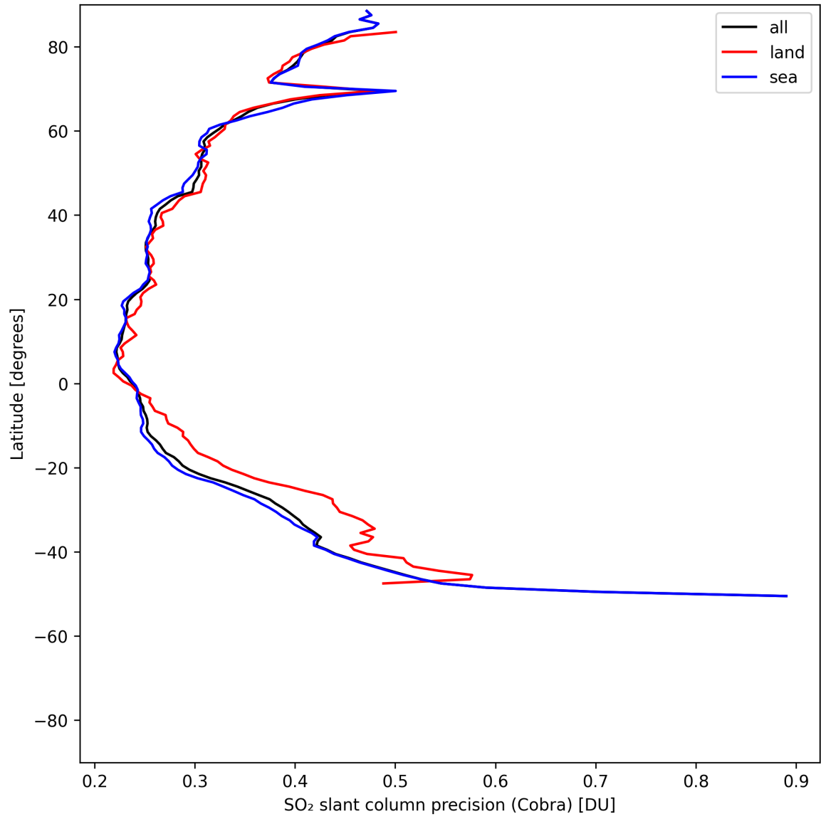
Figure 36: Zonal average of “SO 2 slant column precision (Cobra)” for 2025-05-10 to 2025-05-12.
