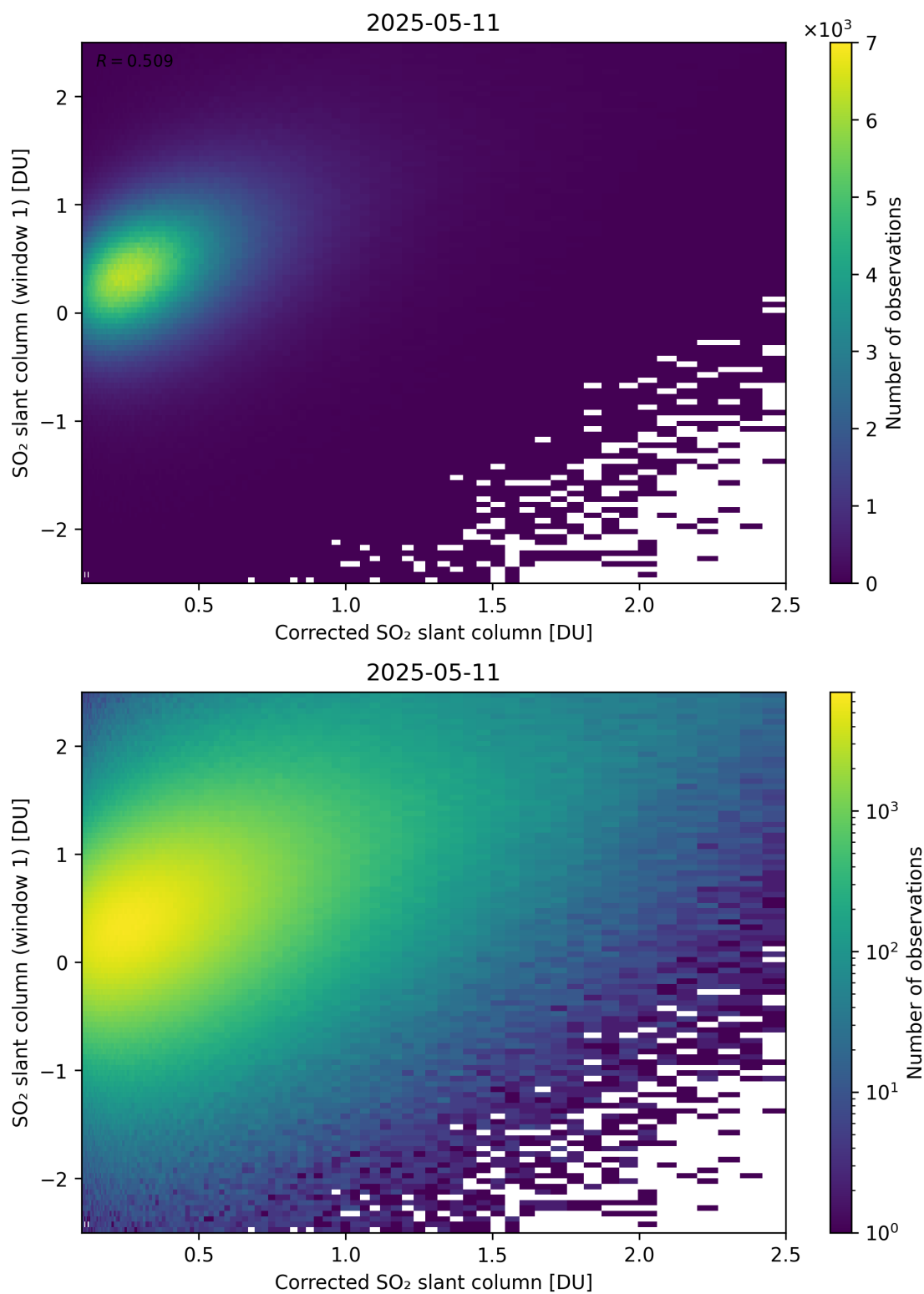
Figure 237: Scatter density plot of “Corrected SO 2 slant column” against “SO 2 slant column (window 1)” for 2025-05-10 to 2025-05-12.
