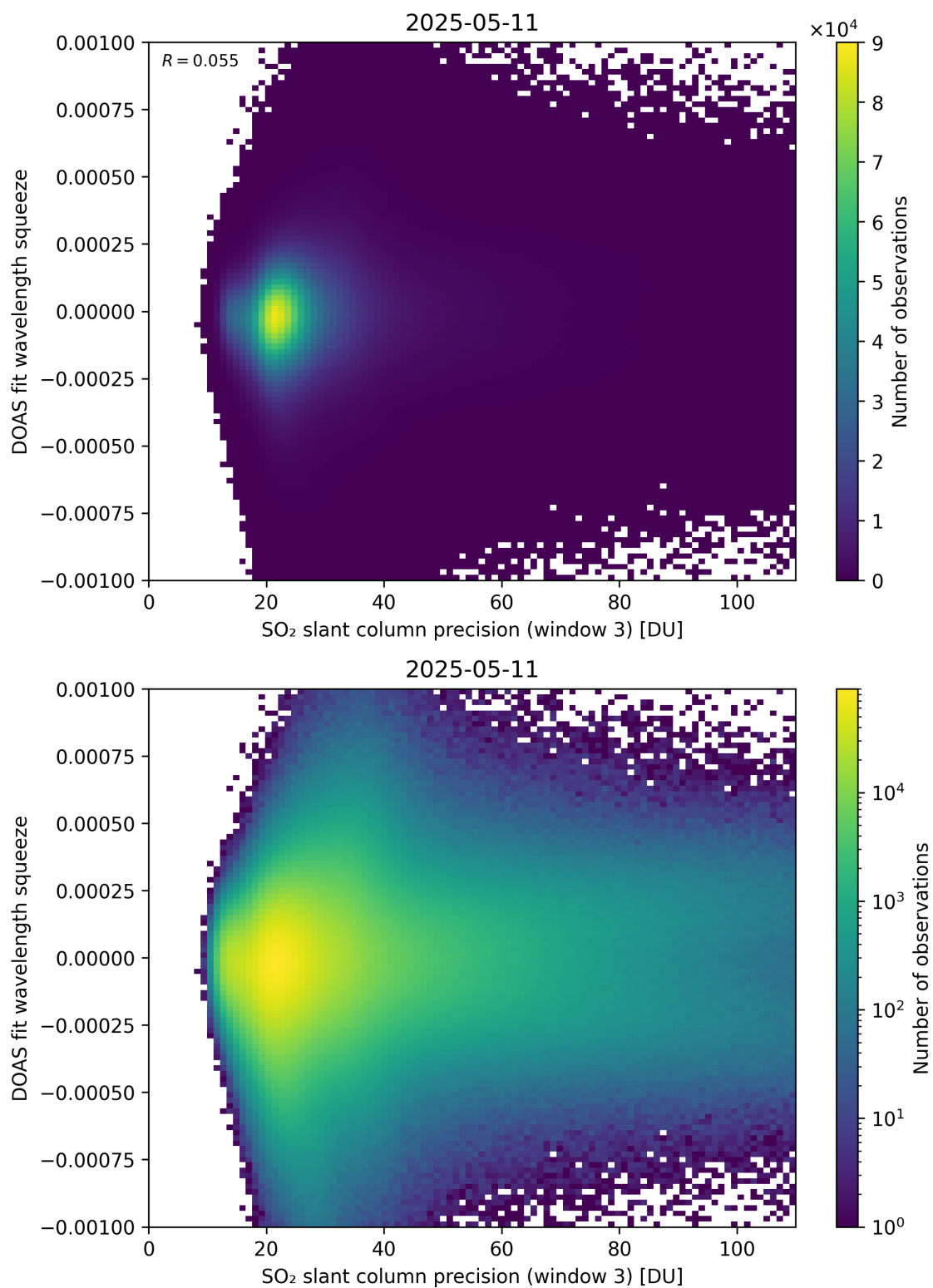
Figure 309: Scatter density plot of “SO 2 slant column precision (window 3)” against “DOAS fit wavelength squeeze” for 2025-05-10 to 2025-05-12.
