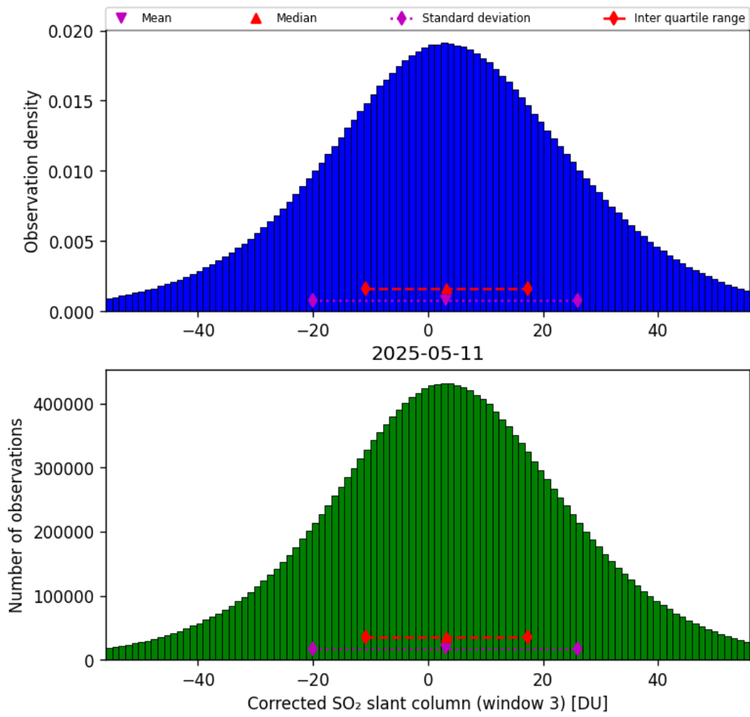
Figure 73: Histogram of “Corrected SO 2 slant column (window 3)” for 2025-05-10 to 2025-05-12
