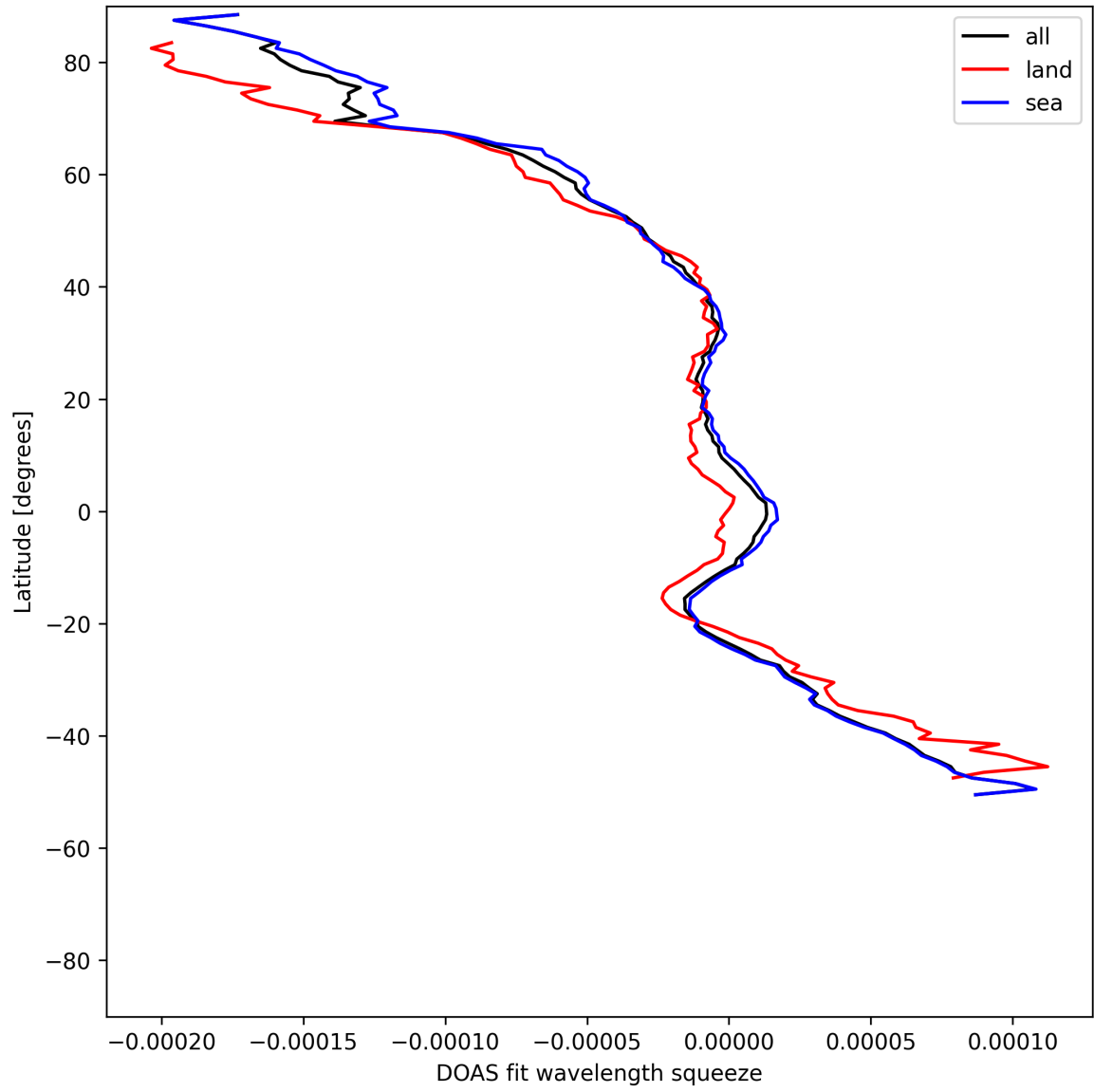
Figure 51: Zonal average of “DOAS fit wavelength squeeze” for 2025-05-10 to 2025-05-12.
