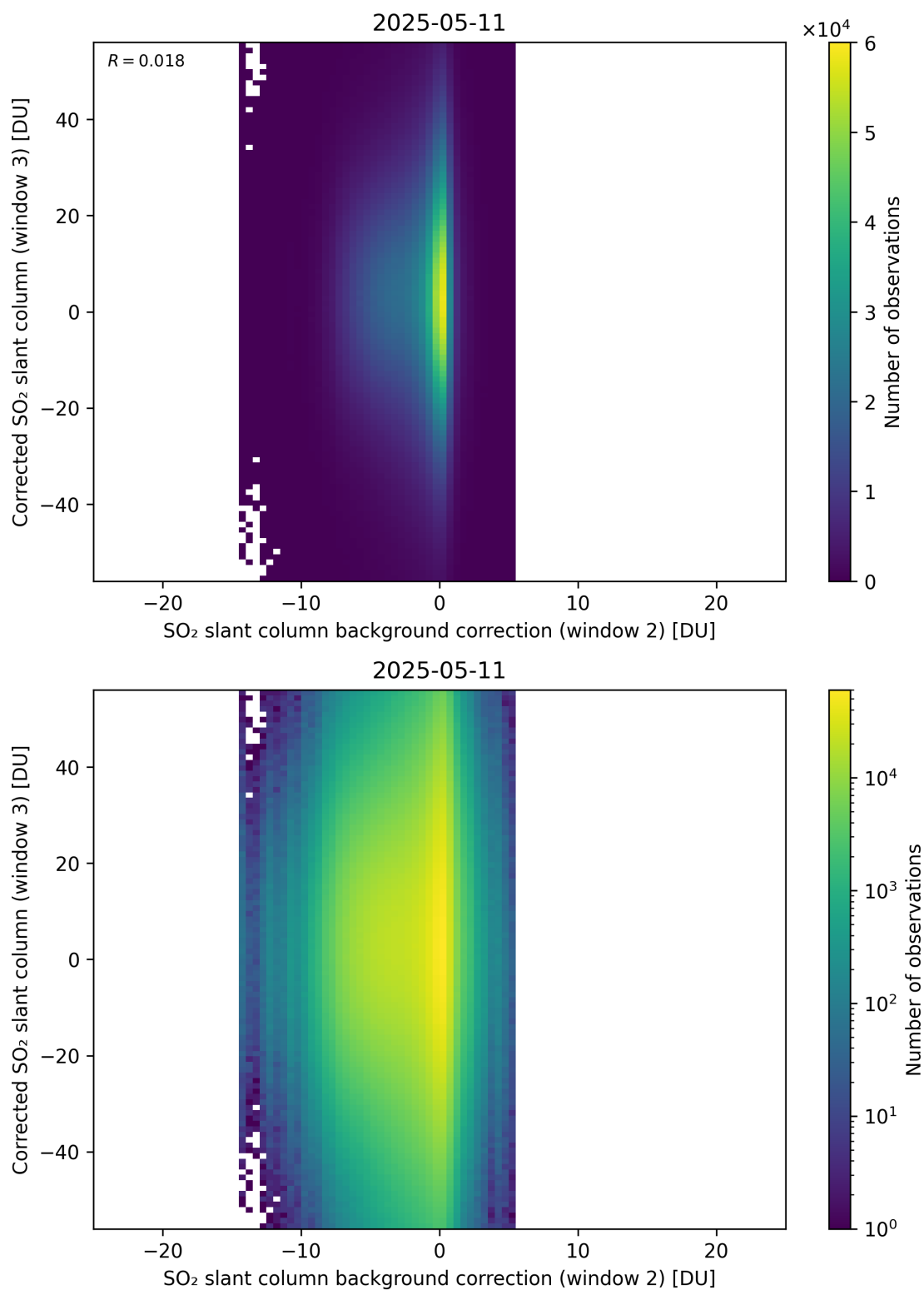
Figure 127: Scatter density plot of “SO 2 slant column background correction (window 2)” against “Corrected SO 2 slant column (window 3)” for 2025-05-10 to 2025-05-12.
