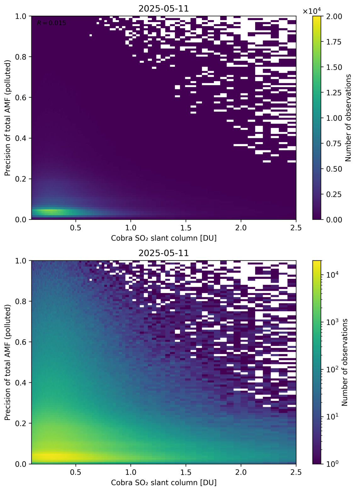
Figure 225: Scatter density plot of “Cobra SO 2 slant column” against “Precision of total AMF (polluted)” for 2025-05-10 to 2025-05-12.
