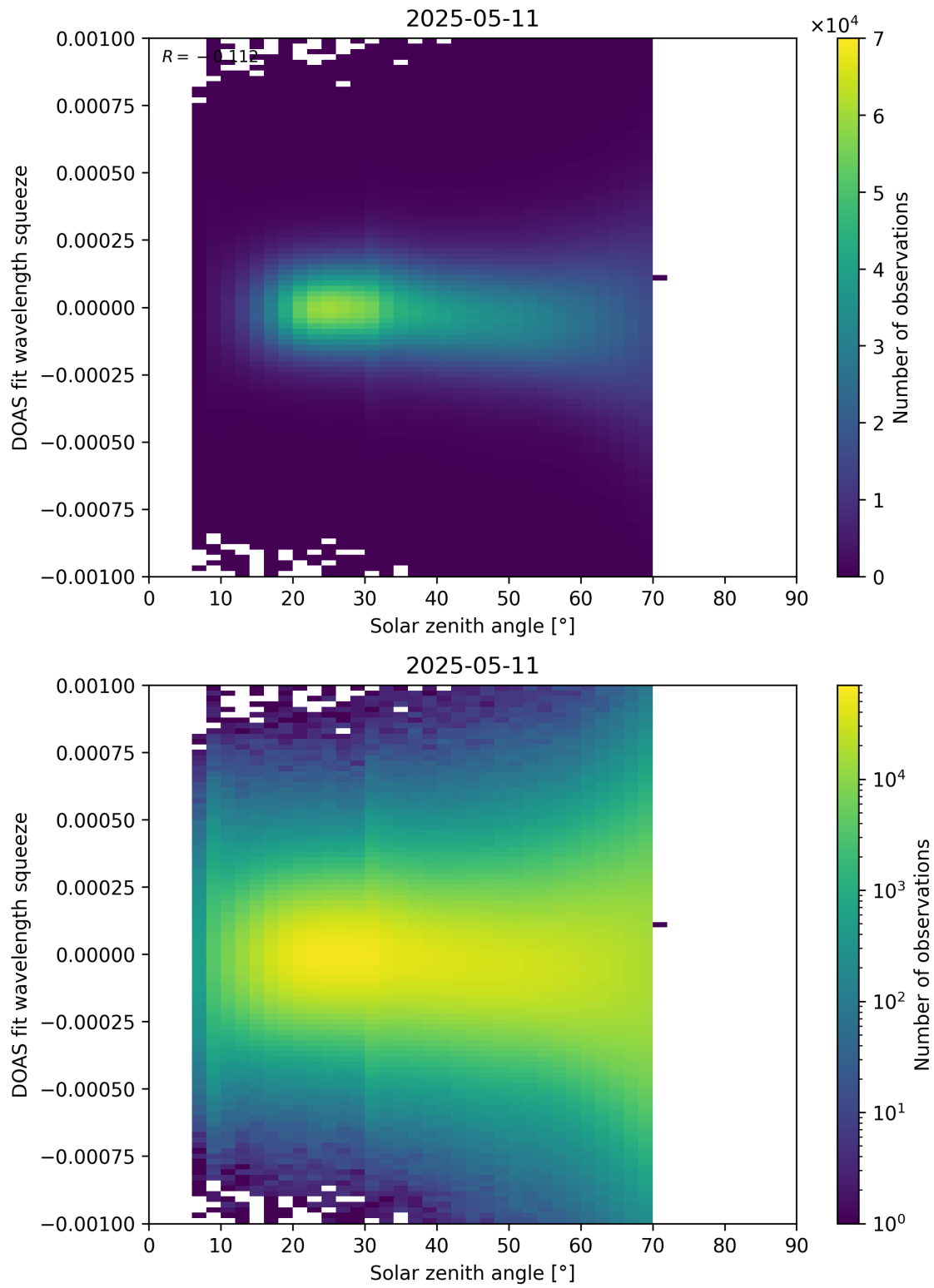
Figure 175: Scatter density plot of “Solar zenith angle” against “DOAS fit wavelength squeeze” for 2025-05-10 to 2025-05-12.
