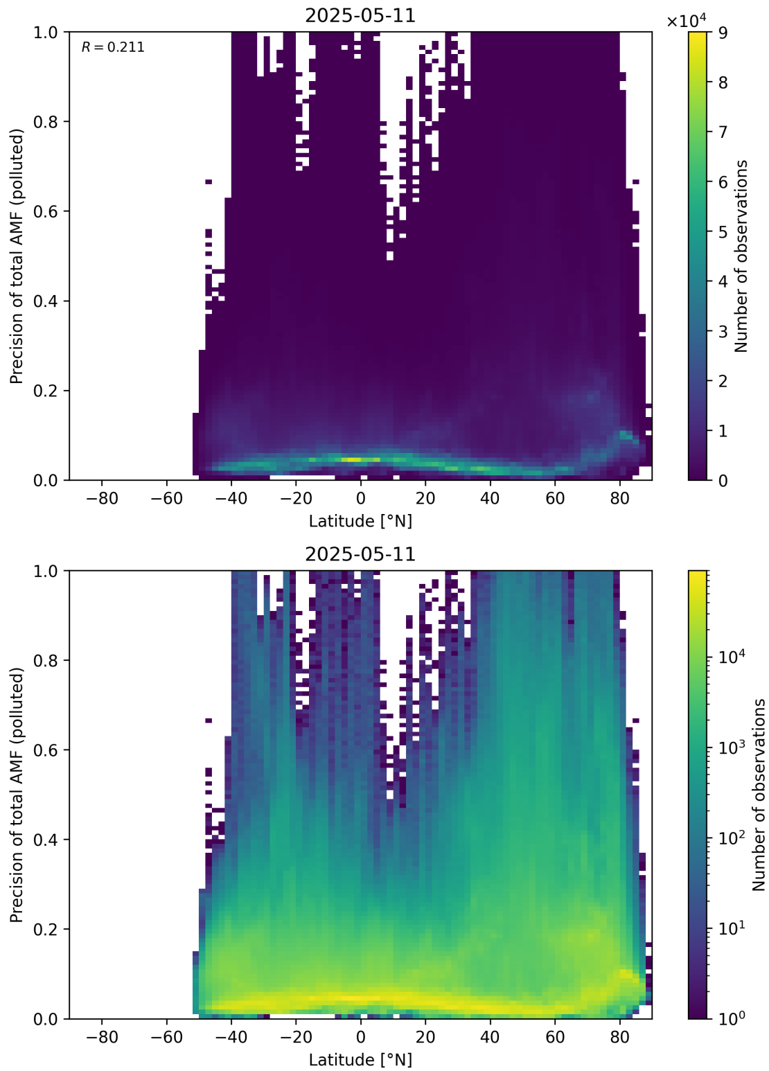
Figure 168: Scatter density plot of “Latitude” against “Precision of total AMF (polluted)” for 2025-05-10 to 2025-05-12.
