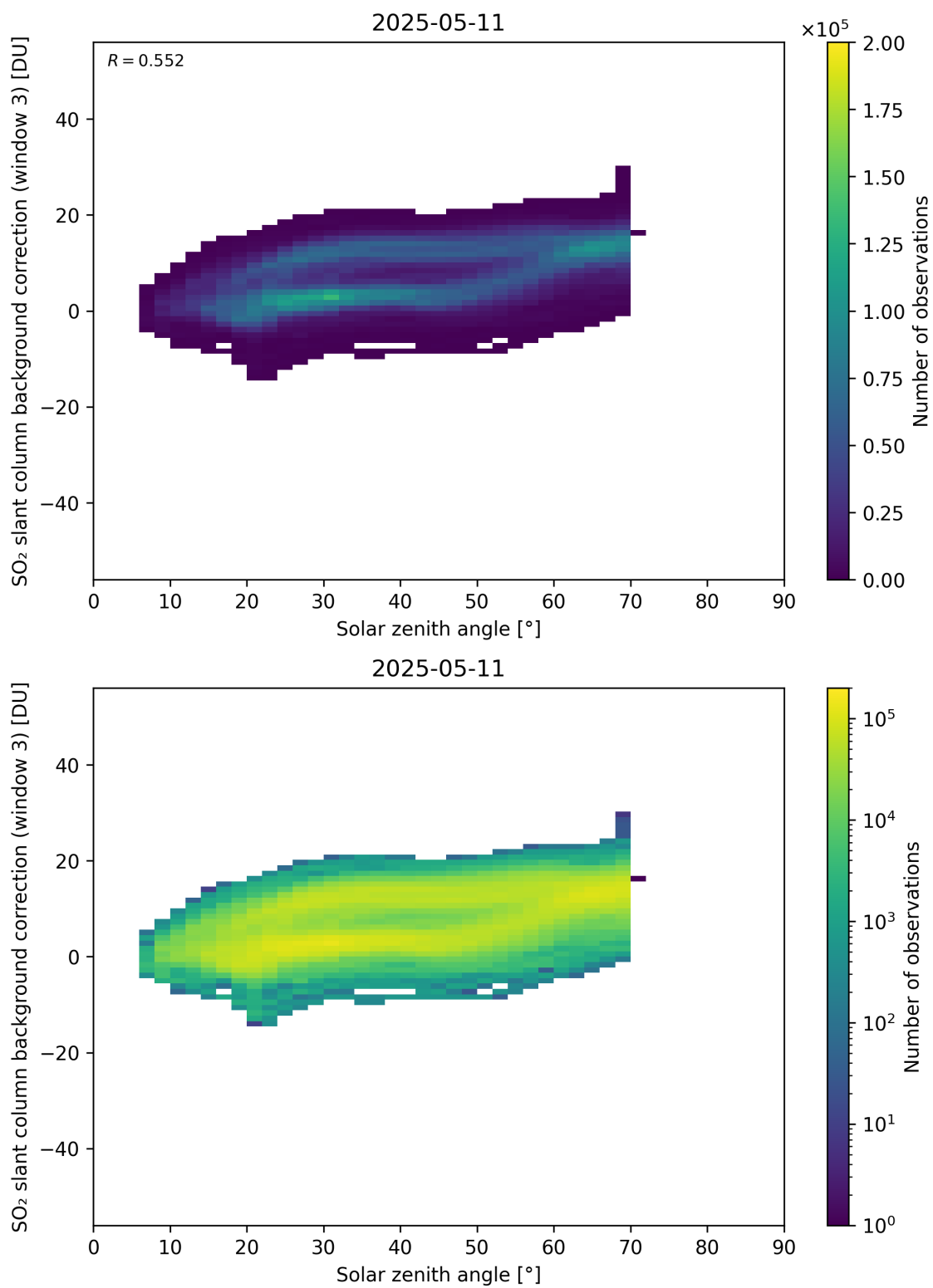
Figure 173: Scatter density plot of “Solar zenith angle” against “SO 2 slant column background correction (window 3)” for 2025-05-10 to 2025-05-12.
