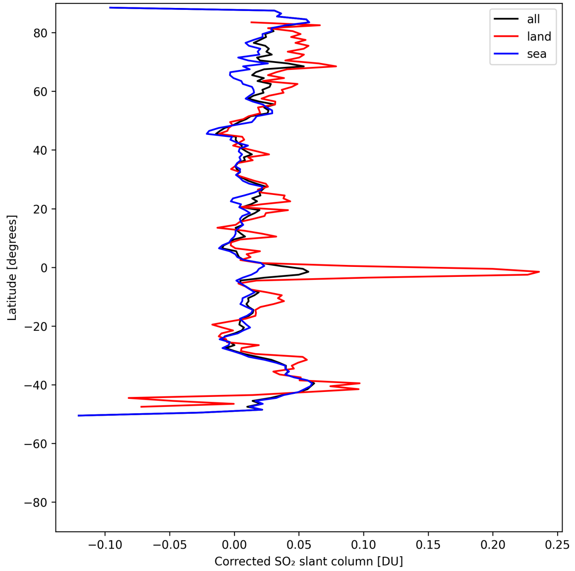
Figure 34: Zonal average of “Corrected SO 2 slant column” for 2025-05-10 to 2025-05-12.
