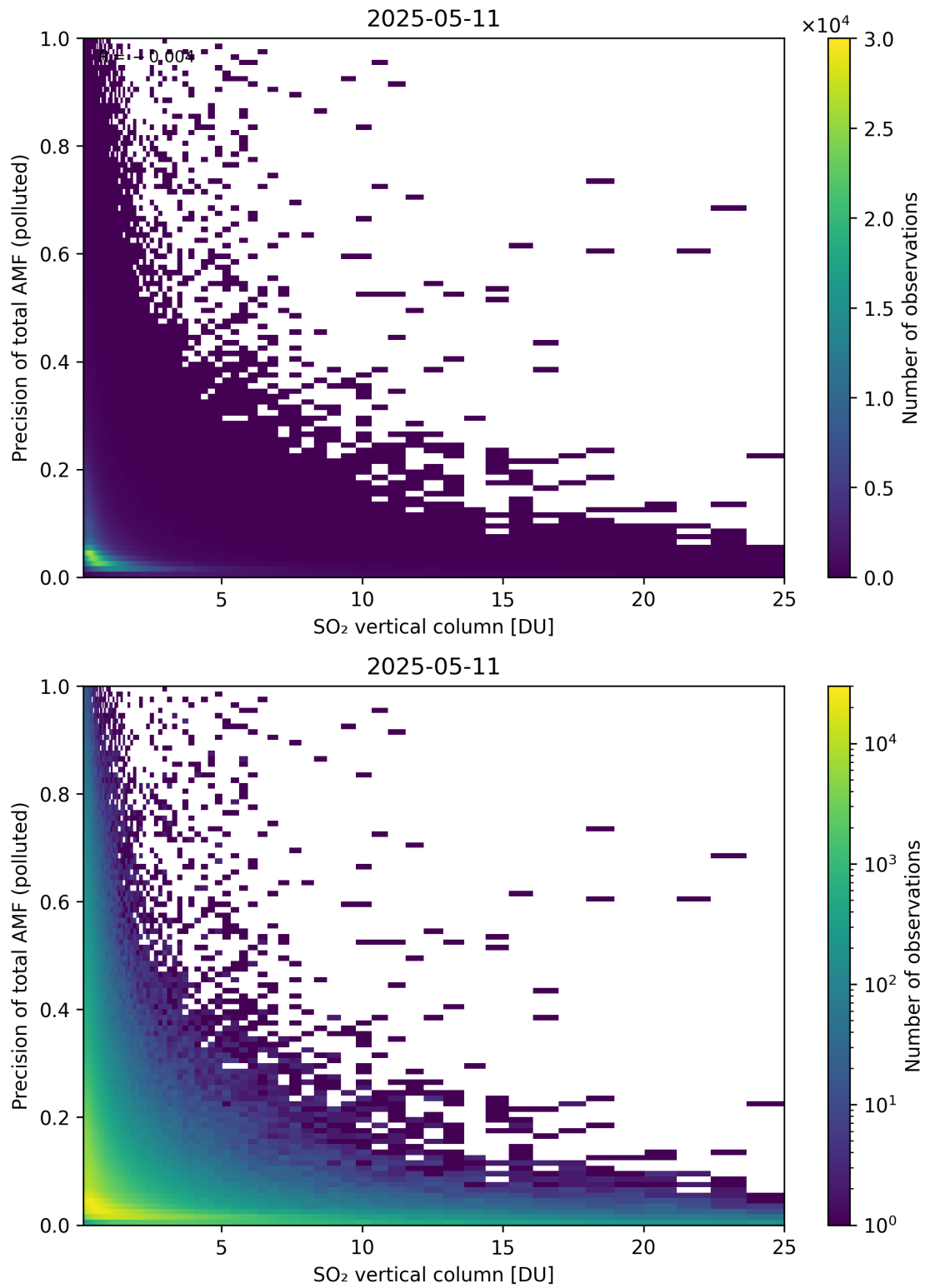
Figure 360: Scatter density plot of “SO 2 vertical column” against “Precision of total AMF (polluted)” for 2025-05-10 to 2025-05-12.
