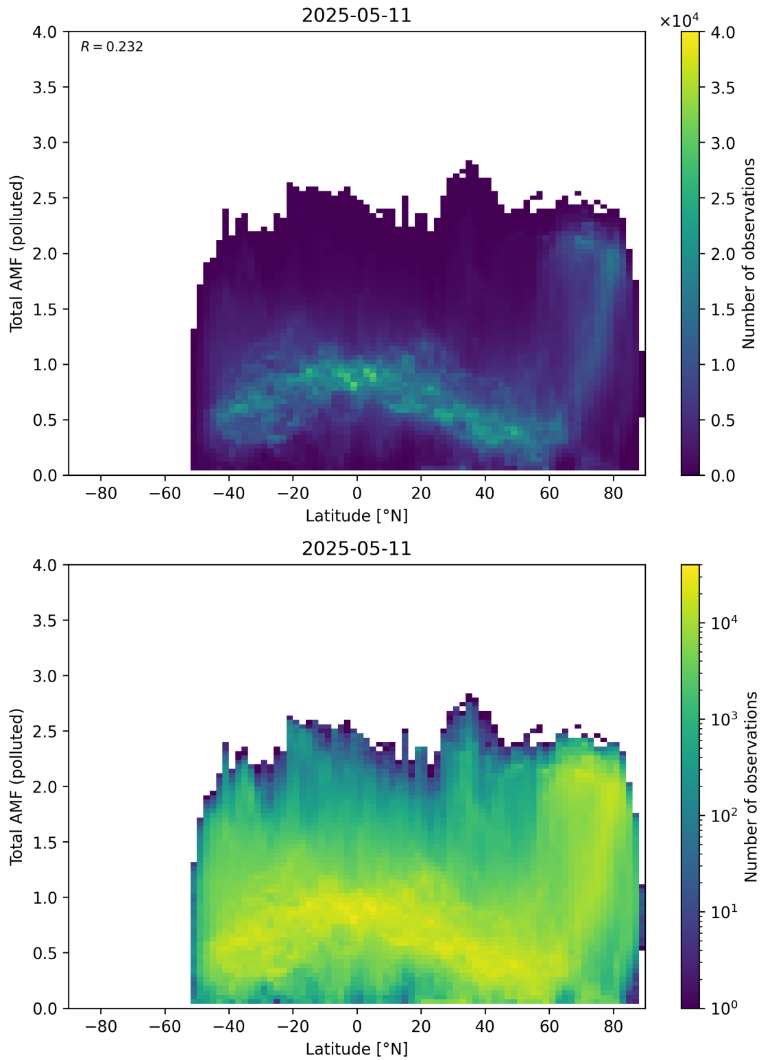
Figure 167: Scatter density plot of “Latitude” against “Total AMF (polluted)” for 2025-05-10 to 2025-05-12.
