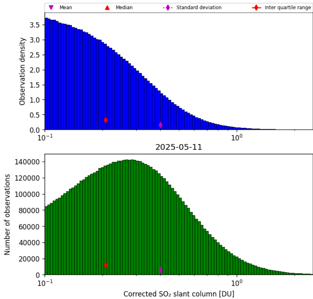
Figure 60: Histogram of “Corrected SO 2 slant column” for 2025-05-10 to 2025-05-12
