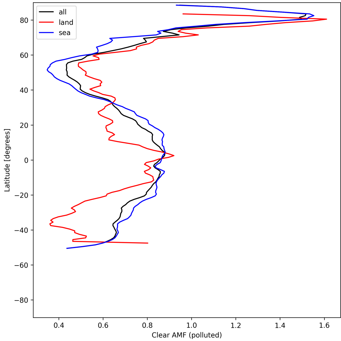
Figure 55: Zonal average of “Clear AMF (polluted)” for 2025-05-10 to 2025-05-12.
