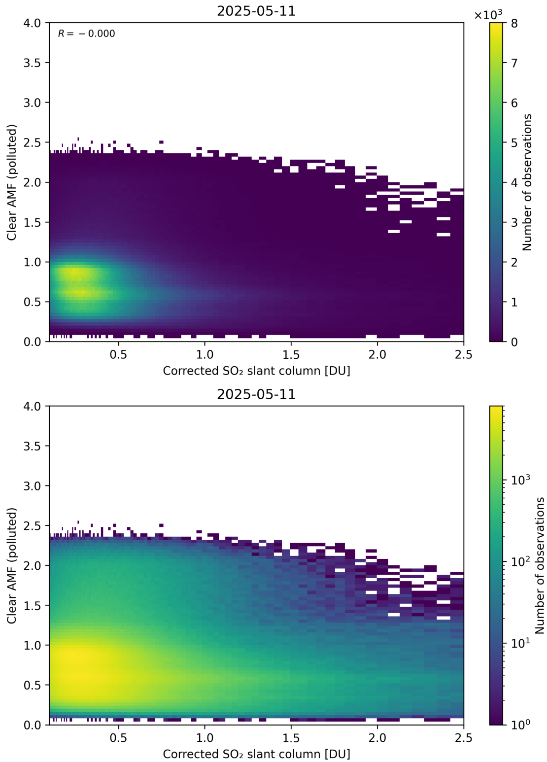
Figure 232: Scatter density plot of “Corrected SO 2 slant column” against “Clear AMF (polluted)” for 2025-05-10 to 2025-05-12.
