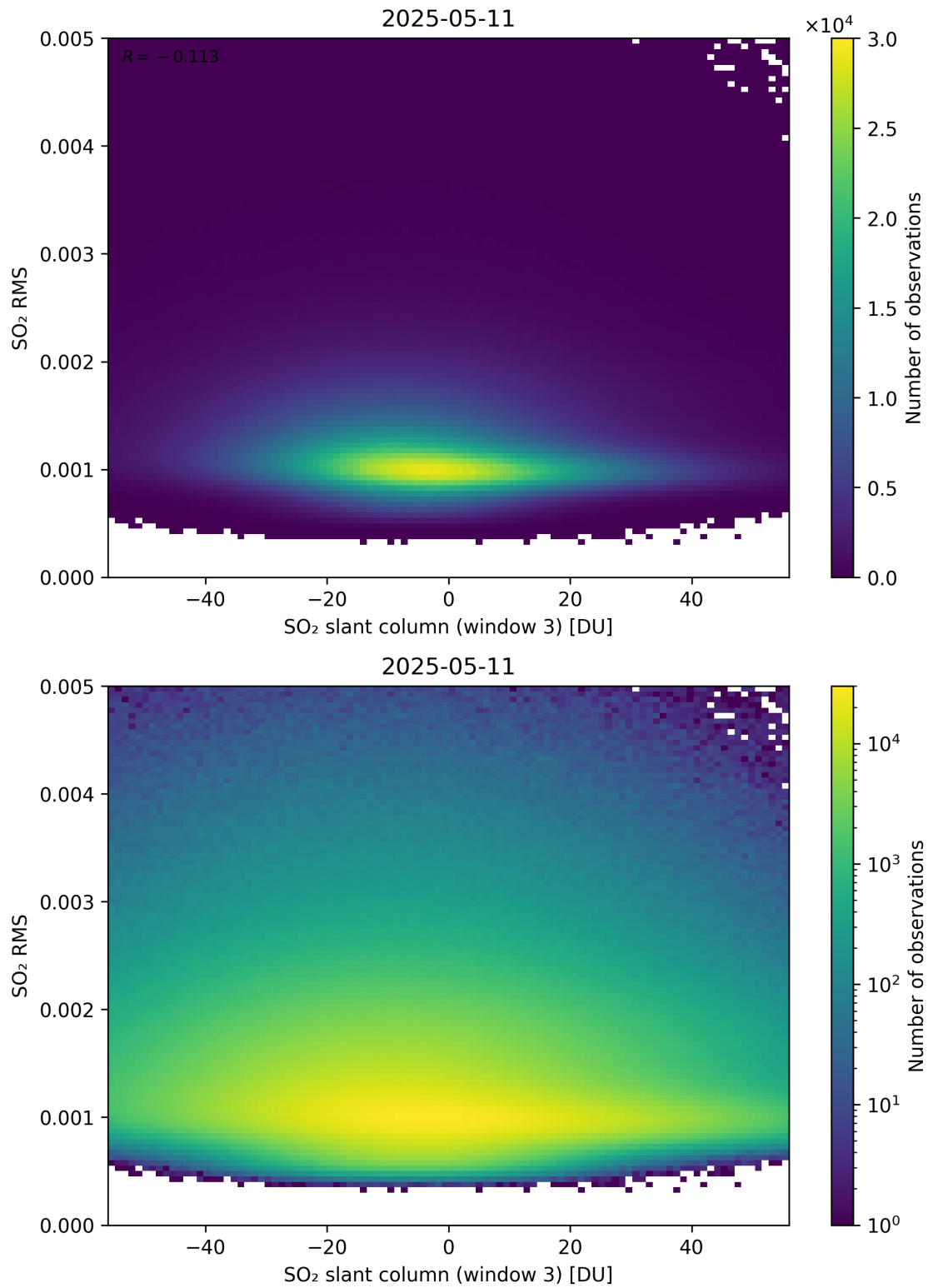
Figure 306: Scatter density plot of “SO 2 slant column (window 3)” against “SO 2 RMS” for 2025-05-10 to 2025-05-12.
