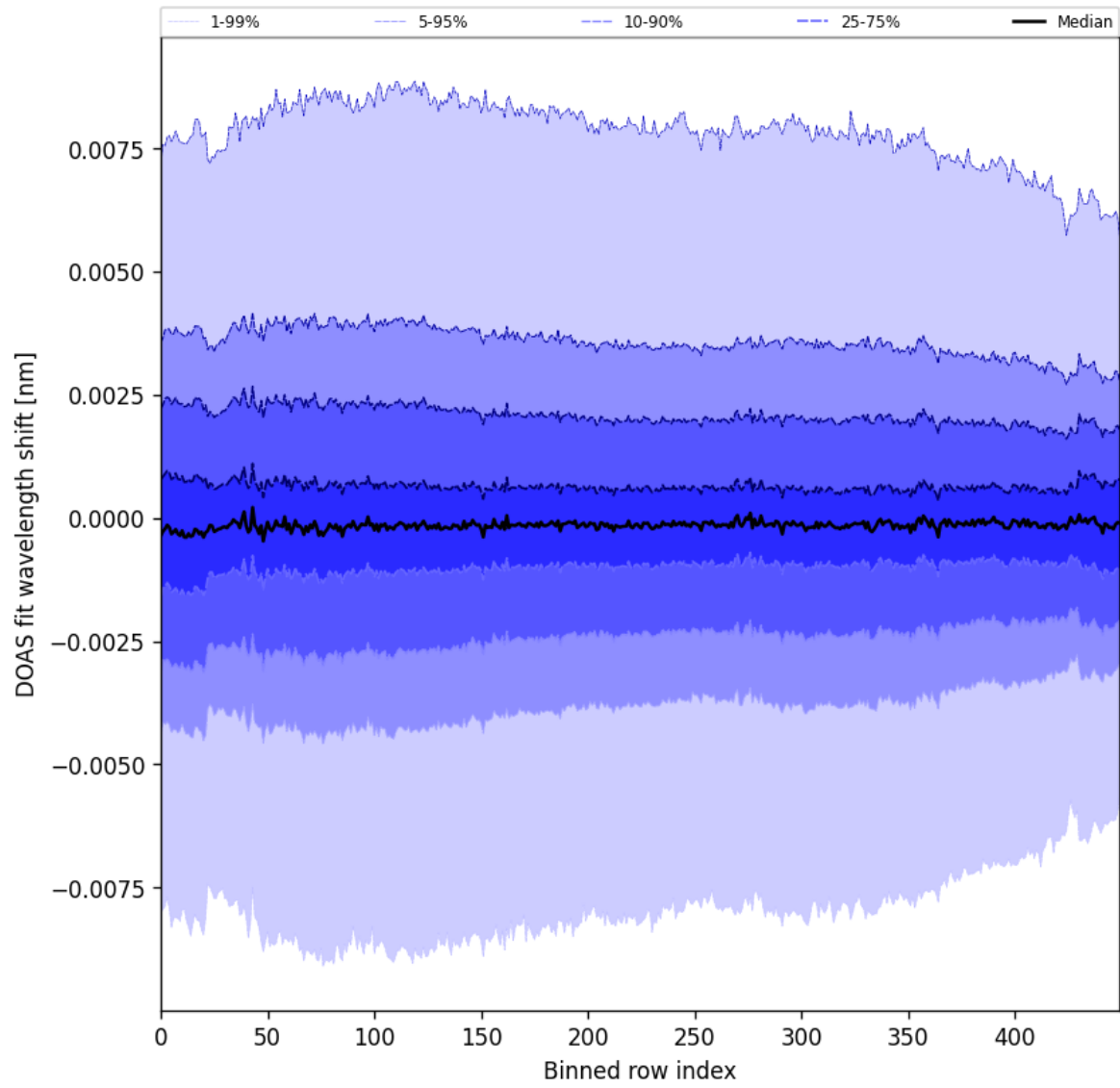
Figure 102: Along track statistics of “DOAS fit wavelength shift” for 2025-05-10 to 2025-05-12
