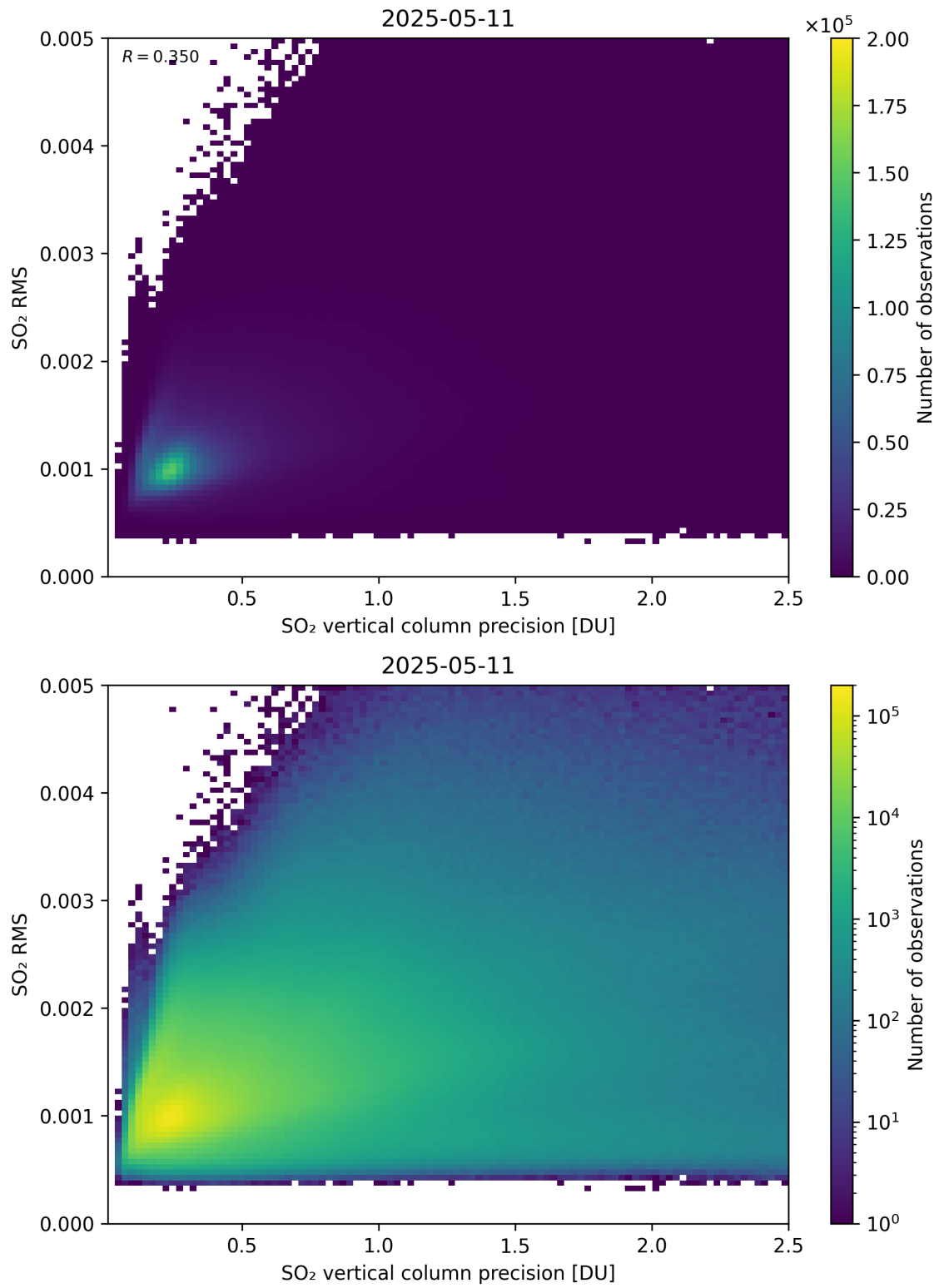
Figure 334: Scatter density plot of “SO 2 vertical column precision” against “SO 2 RMS” for 2025-05-10 to 2025-05-12.
