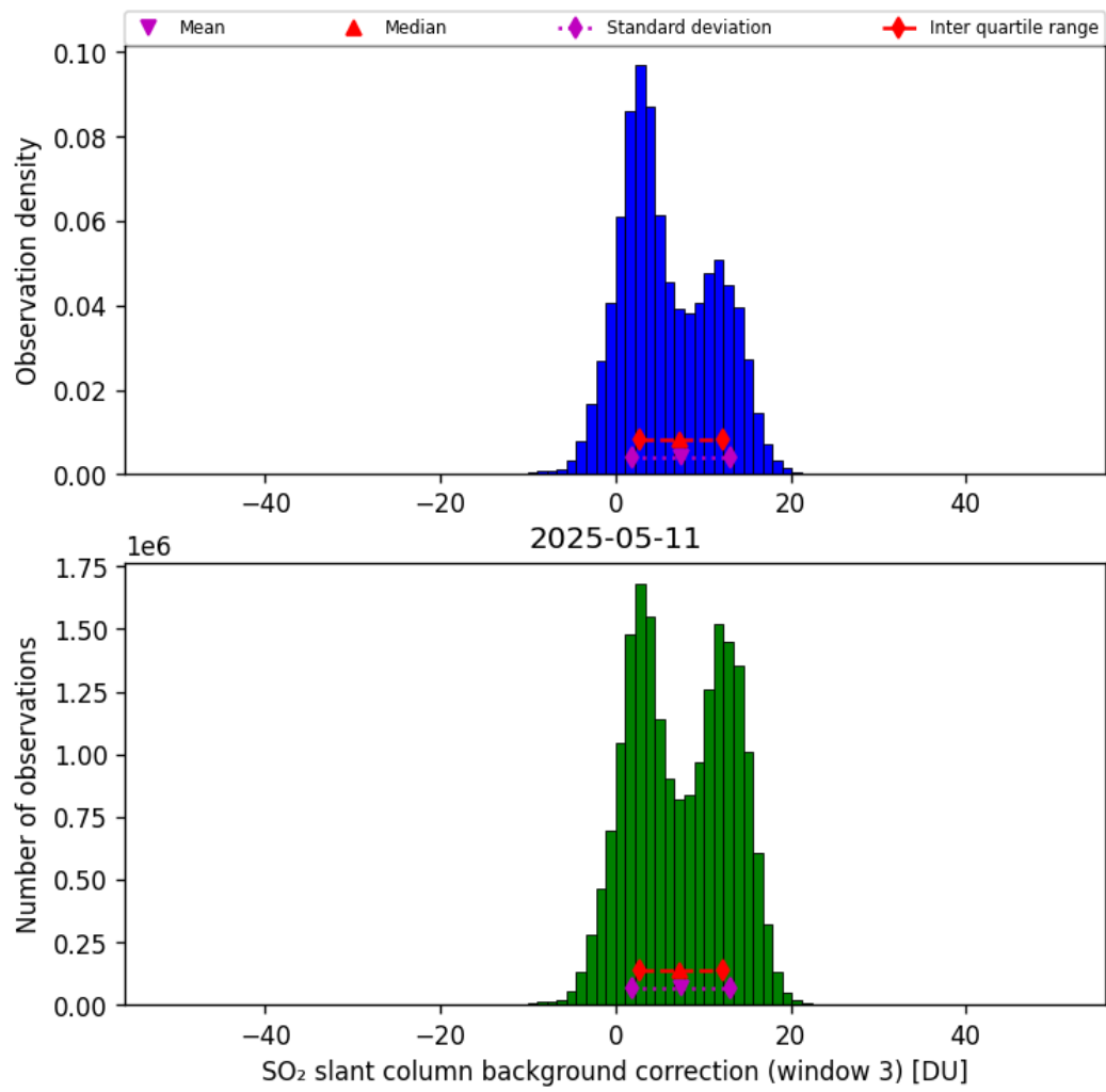
Figure 74: Histogram of “SO 2 slant column background correction (window 3)” for 2025-05-10 to 2025-05-12
