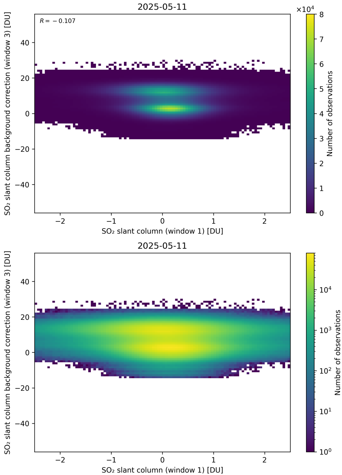
Figure 264: Scatter density plot of “SO 2 slant column (window 1)” against “SO 2 slant column background correction (window 3)” for 2025-05-10 to 2025-05-12.
