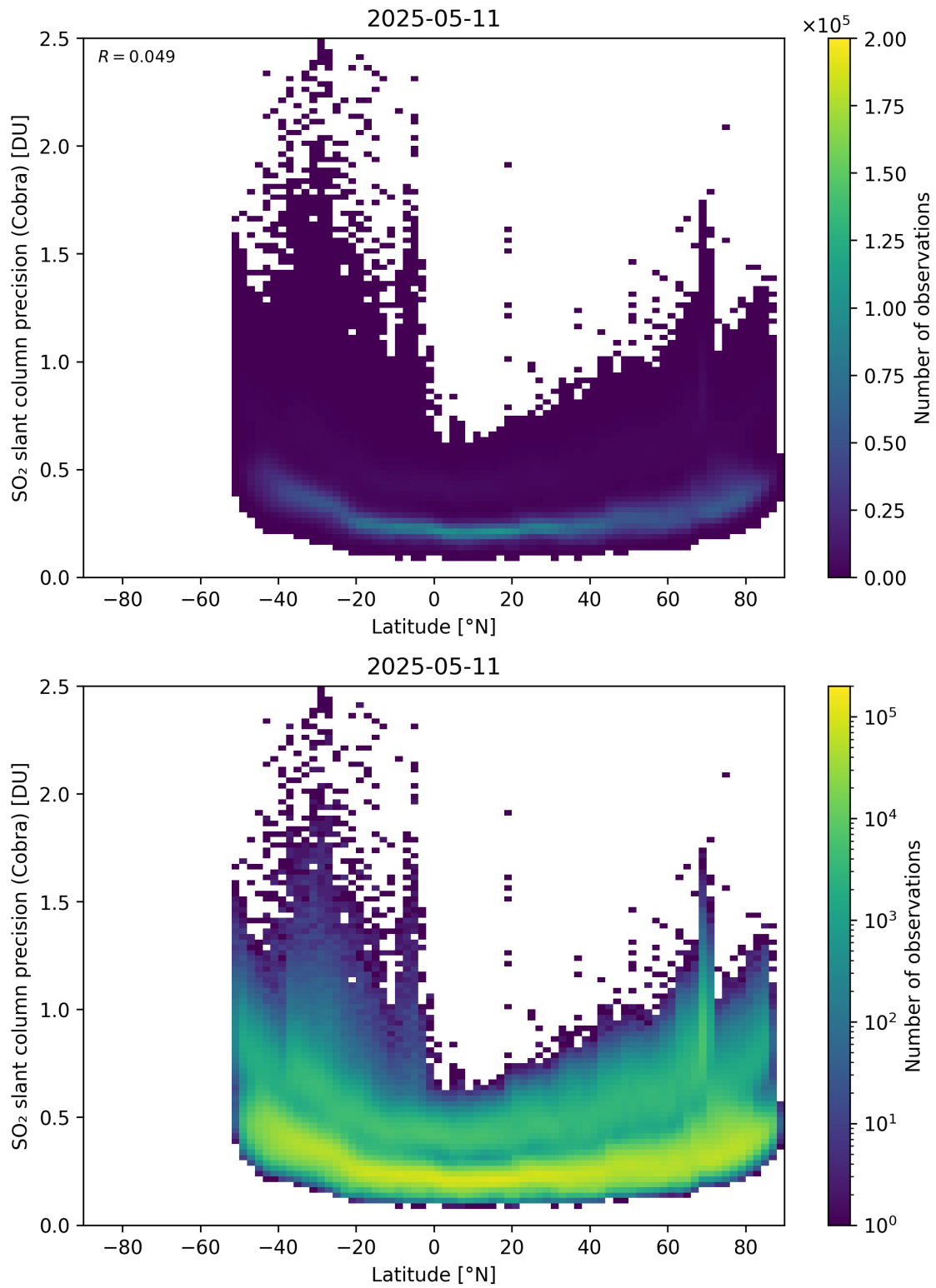
Figure 158: Scatter density plot of “Latitude” against “SO 2 slant column precision (Cobra)” for 2025-05-10 to 2025-05-12.
