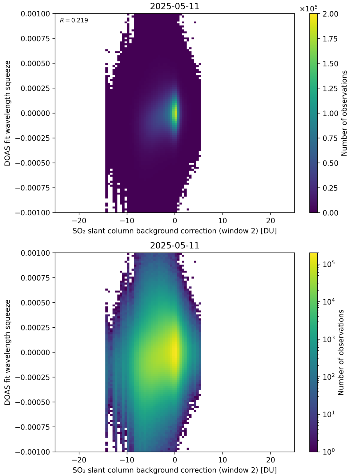
Figure 124: Scatter density plot of “SO 2 slant column background correction (window 2)” against “DOAS fit wavelength squeeze” for 2025-05-10 to 2025-05-12.
