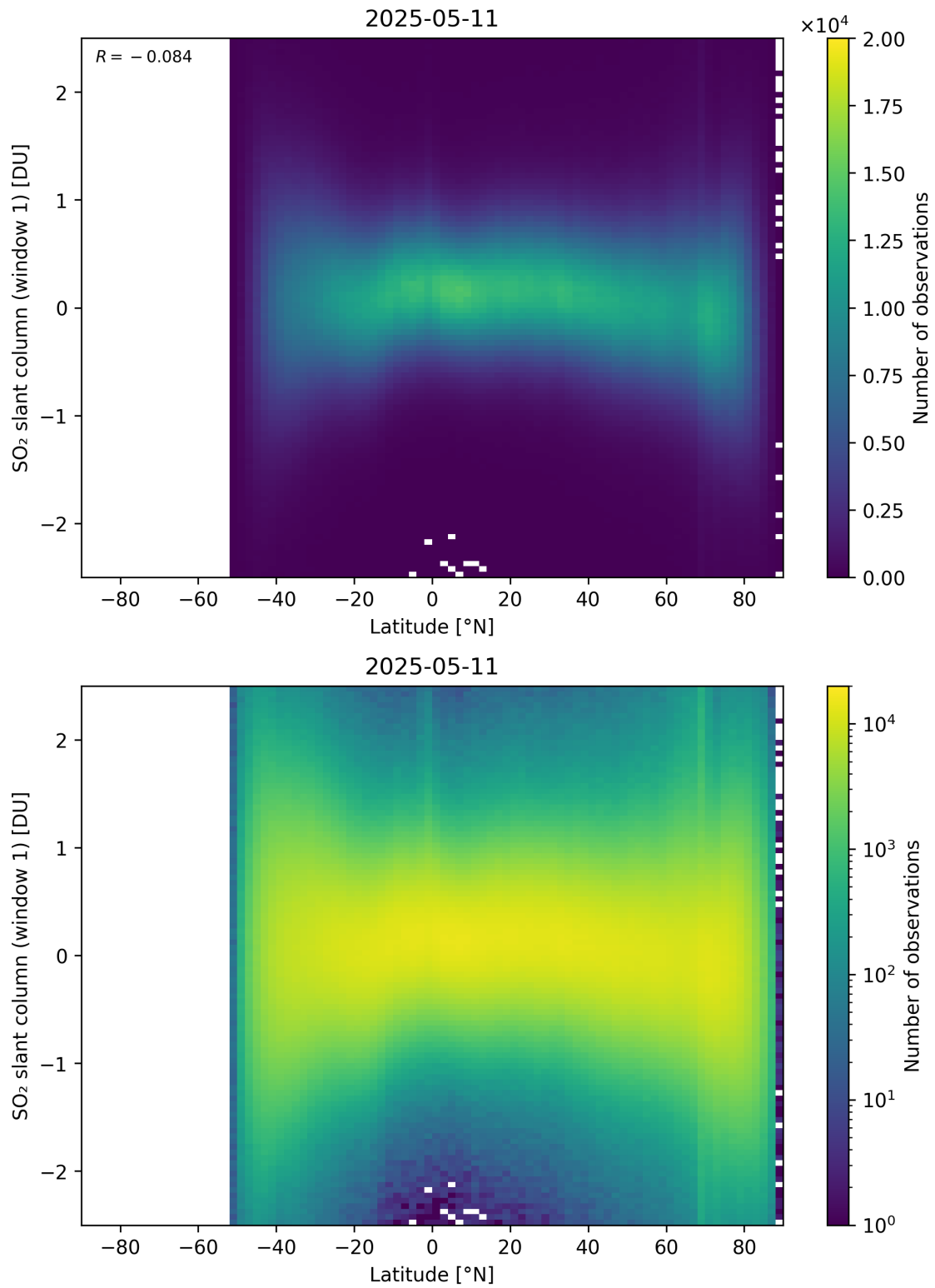
Figure 162: Scatter density plot of “Latitude” against “SO 2 slant column (window 1)” for 2025-05-10 to 2025-05-12.
