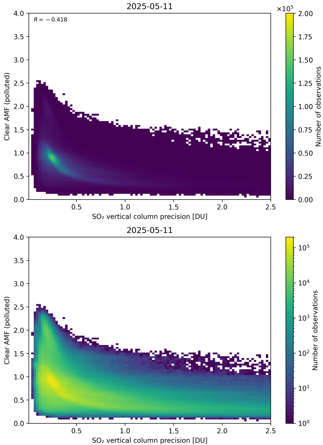
Figure 335: Scatter density plot of “SO 2 vertical column precision” against “Clear AMF (polluted)” for 2025-05-10 to 2025-05-12.
