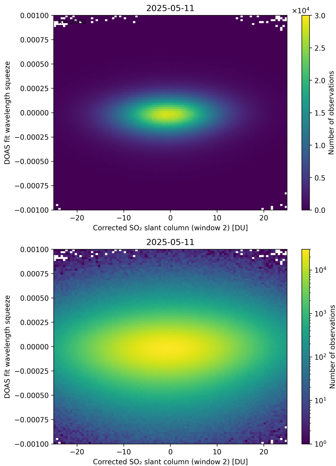
Figure 247: Scatter density plot of “Corrected SO 2 slant column (window 2)” against “DOAS fit wavelength squeeze” for 2025-05-10 to 2025-05-12.
