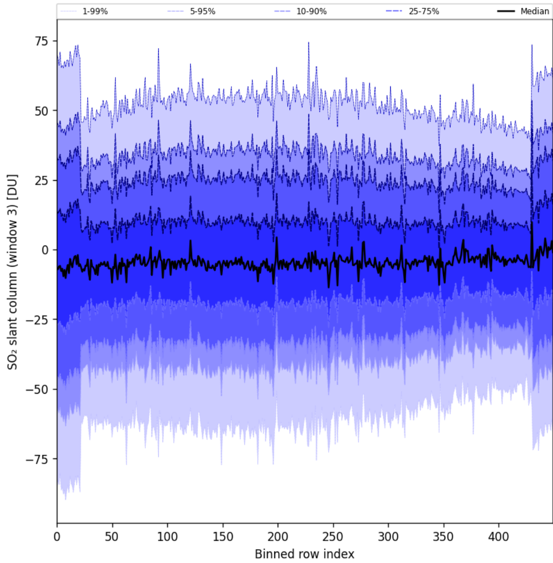
Figure 97: Along track statistics of “SO 2 slant column (window 3)” for 2025-05-10 to 2025-05-12
