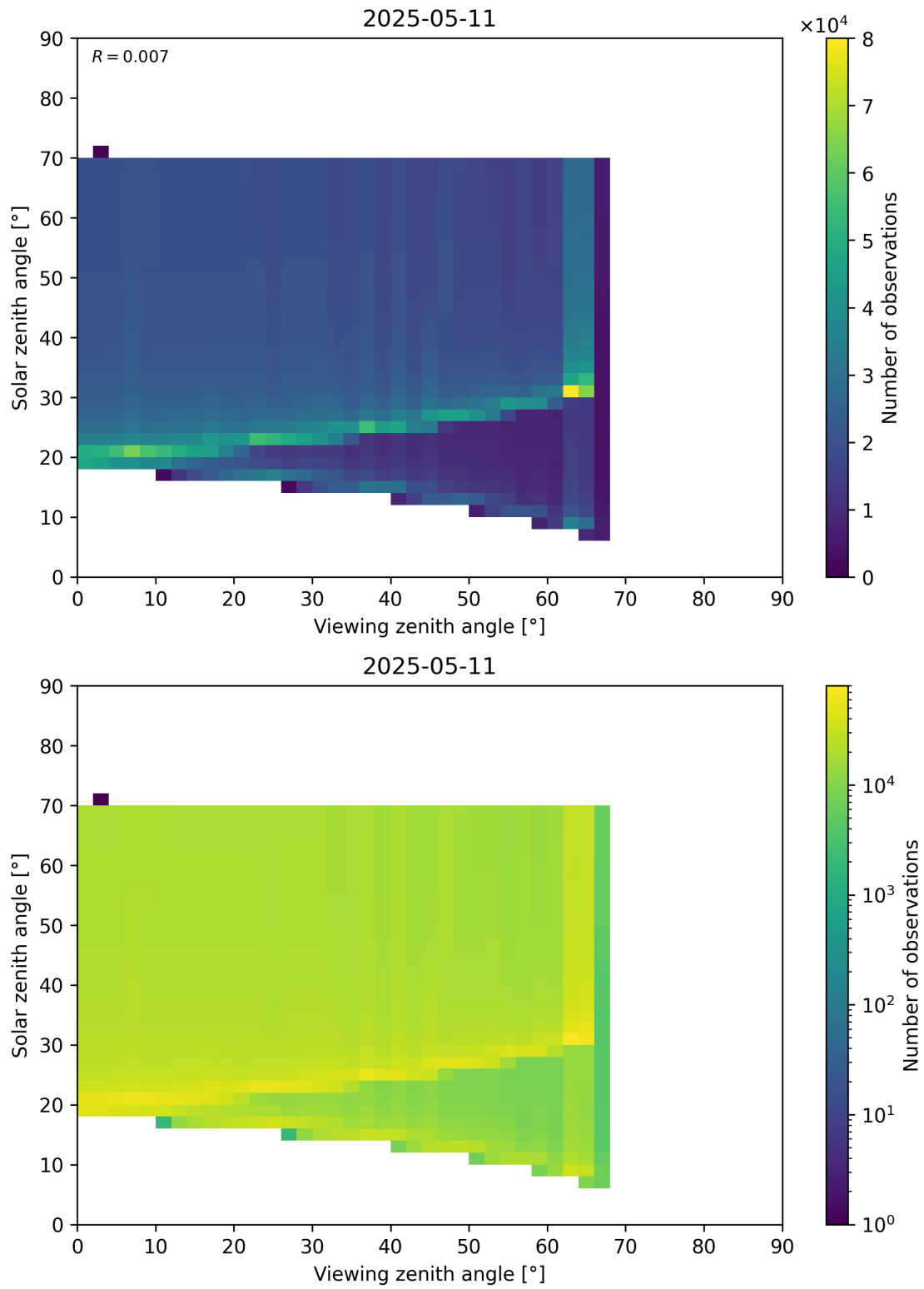
Figure 369: Scatter density plot of “Viewing zenith angle” against “Solar zenith angle” for 2025-05-10 to 2025-05-12.
