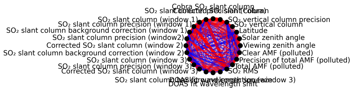
Figure 1: Map of correlation graph for 2025-05-11 to 2025-05-13.
