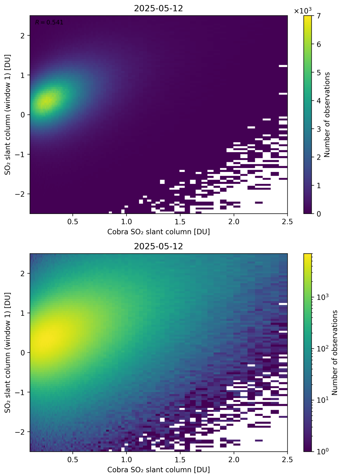
Figure 219: Scatter density plot of “Cobra SO 2 slant column” against “SO 2 slant column (window 1)” for 2025-05-11 to 2025-05-13.
