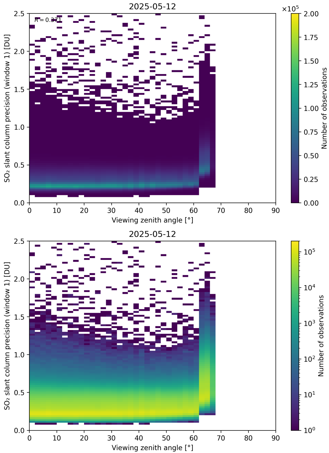
Figure 377: Scatter density plot of “Viewing zenith angle” against “SO 2 slant column precision (window 1)” for 2025-05-11 to 2025-05-13.
