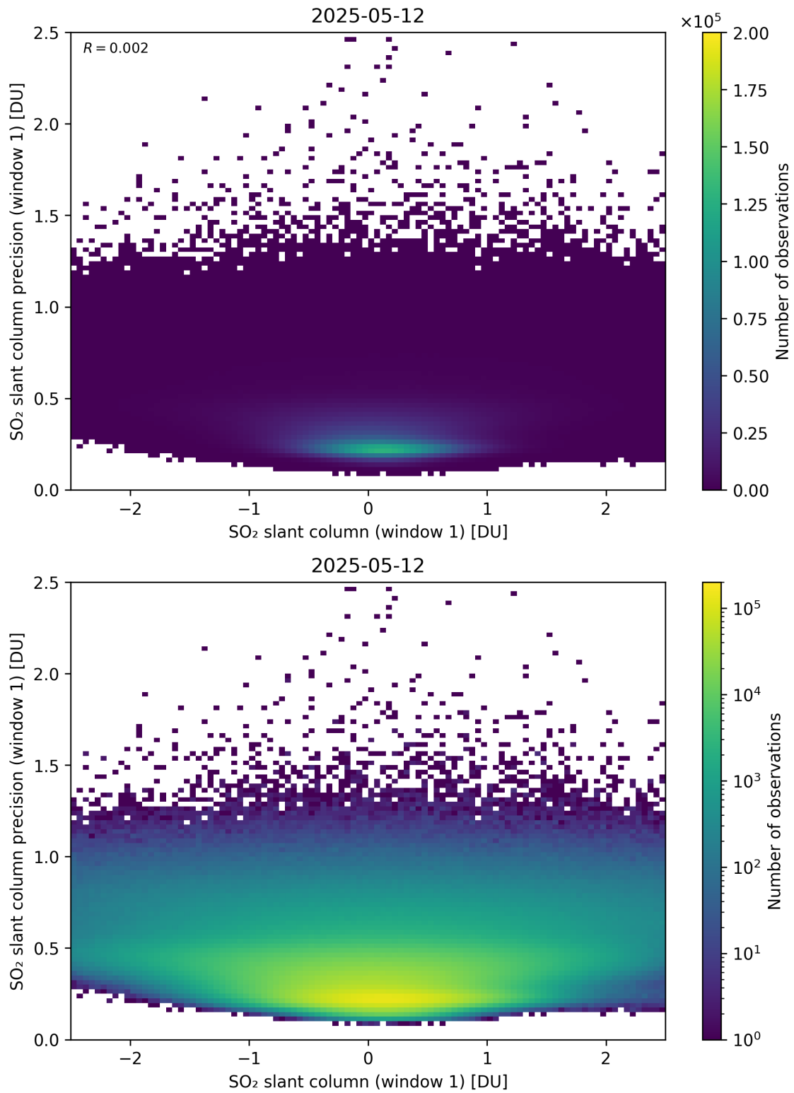
Figure 285: Scatter density plot of “SO 2 slant column (window 1)” against “SO 2 slant column precision (window 1)” for 2025-05-11 to 2025-05-13.
