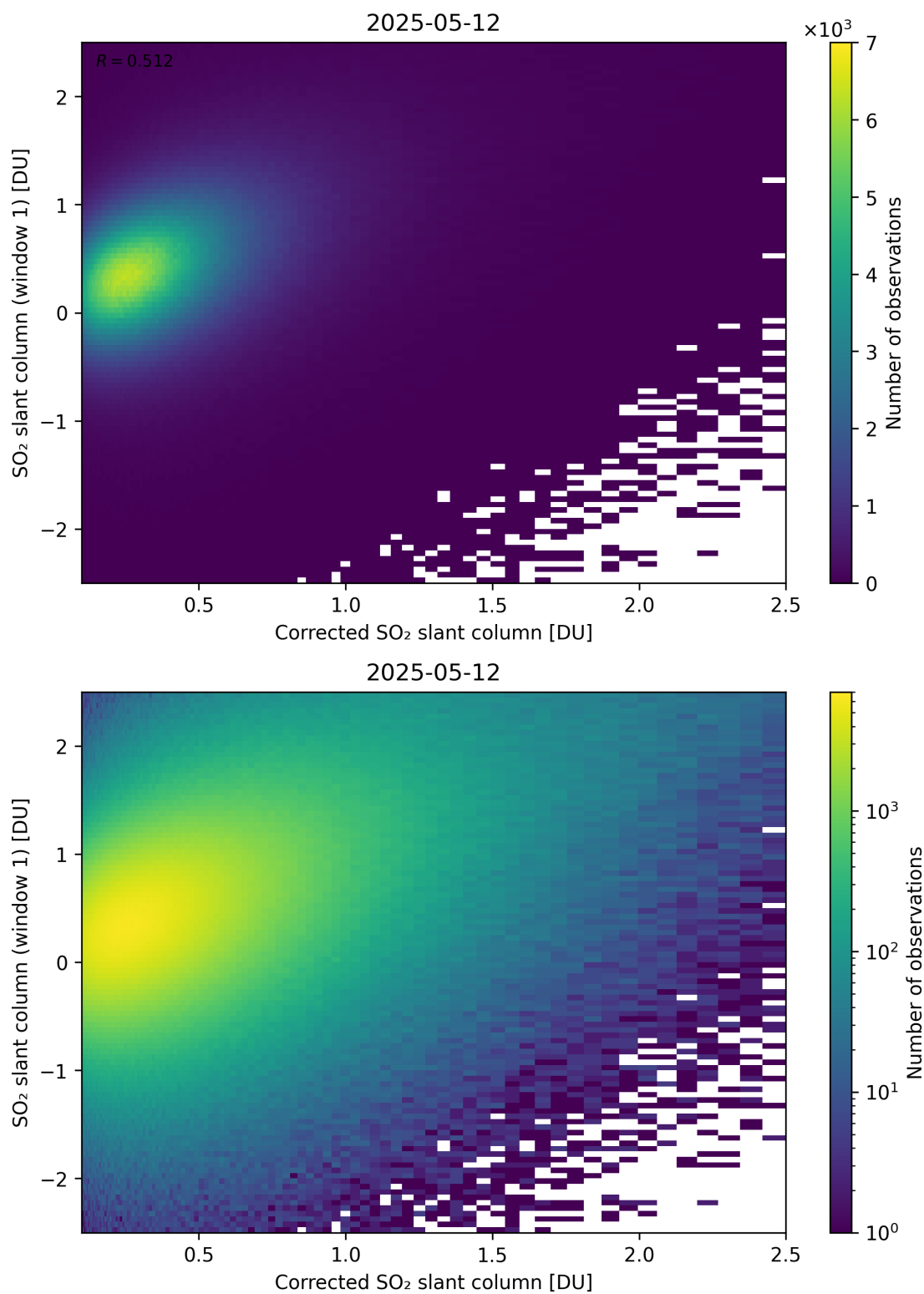
Figure 237: Scatter density plot of “Corrected SO 2 slant column” against “SO 2 slant column (window 1)” for 2025-05-11 to 2025-05-13.
