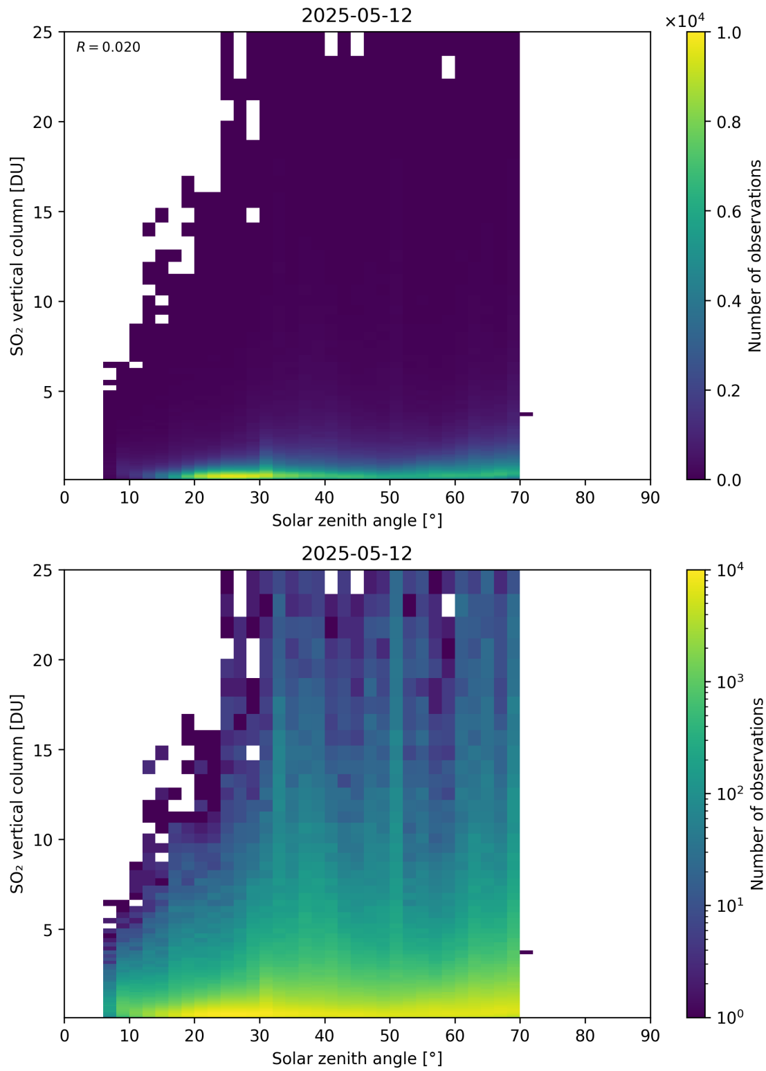
Figure 191: Scatter density plot of “Solar zenith angle” against “SO 2 vertical column” for 2025-05-11 to 2025-05-13.
