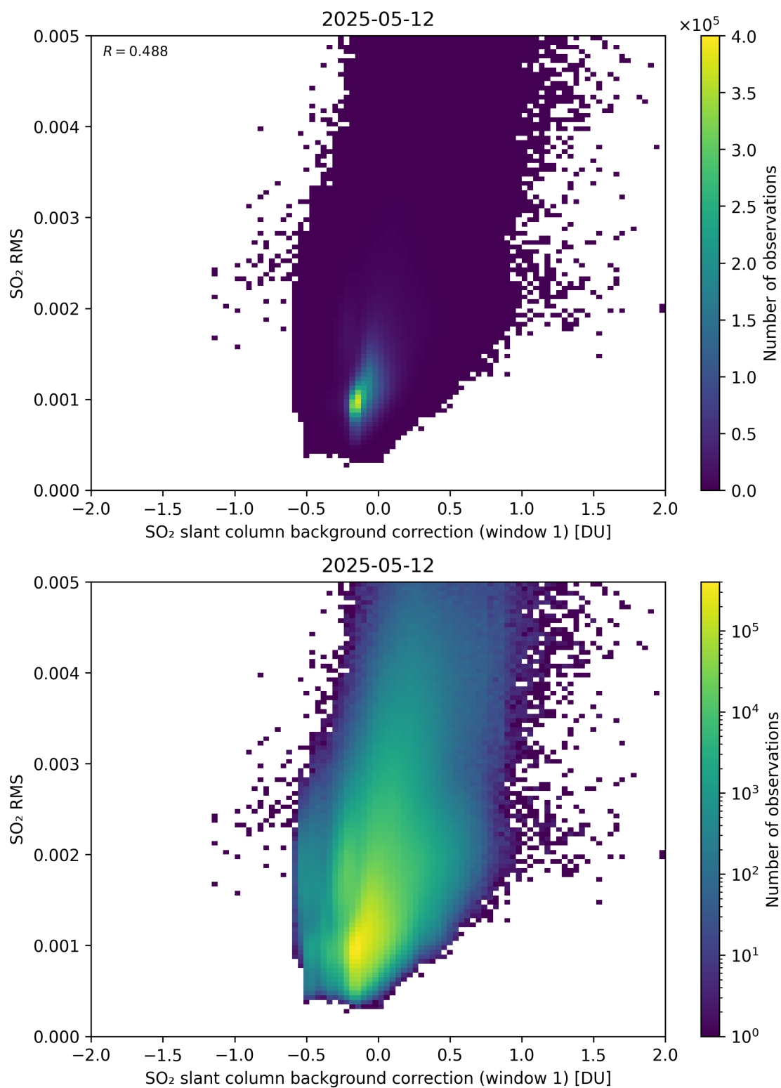
Figure 113: Scatter density plot of “SO 2 slant column background correction (window 1)” against “SO 2 RMS” for 2025-05-11 to 2025-05-13.
