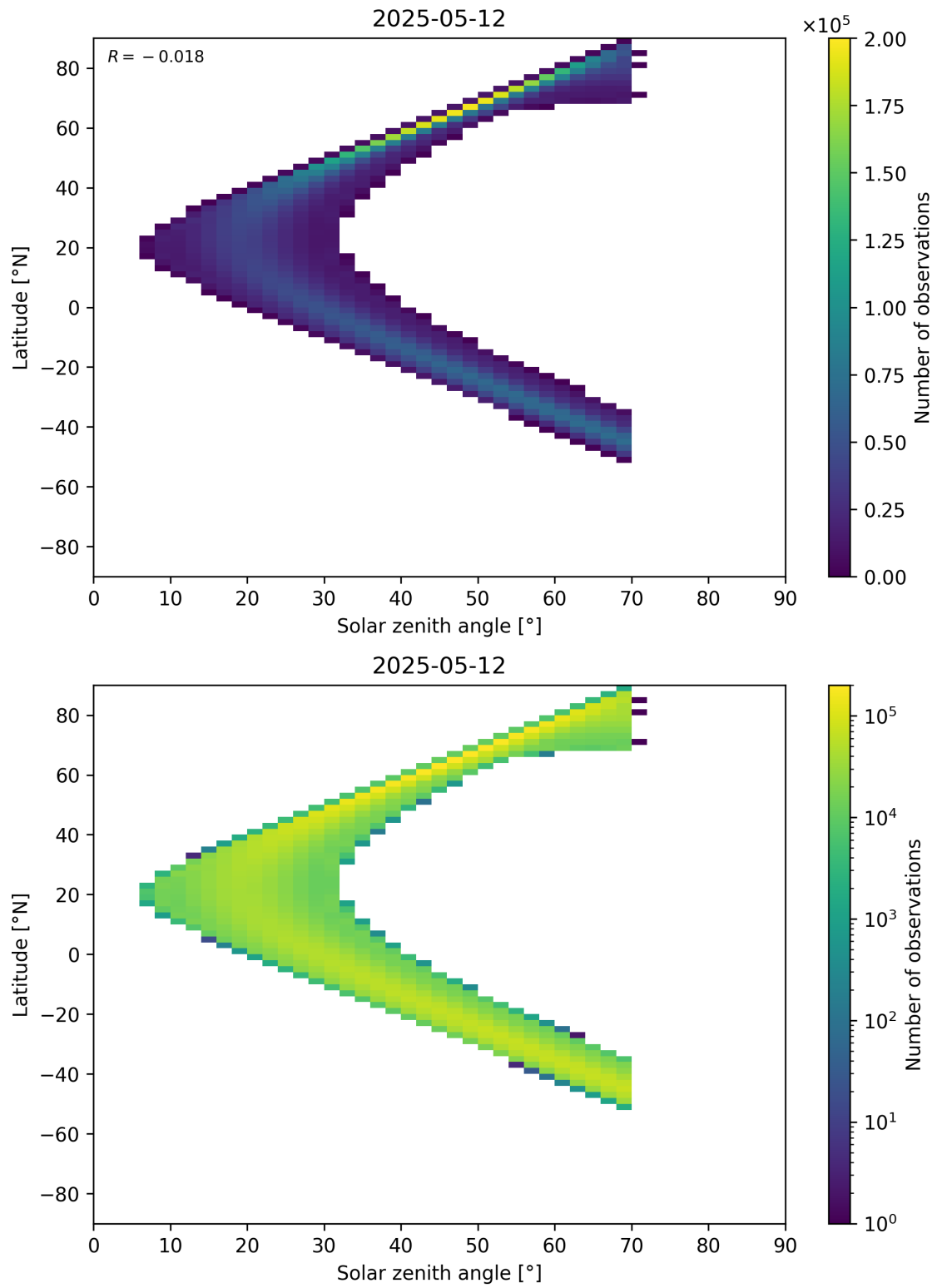
Figure 177: Scatter density plot of “Solar zenith angle” against “Latitude” for 2025-05-11 to 2025-05-13.
