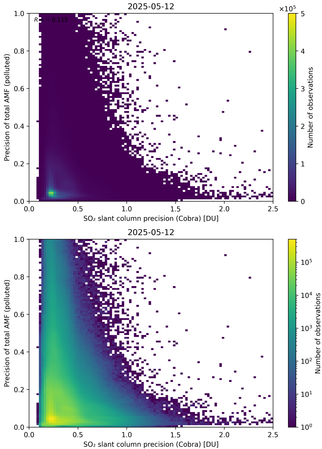
Figure 214: Scatter density plot of “SO 2 slant column precision (Cobra)” against “Precision of total AMF (polluted)” for 2025-05-11 to 2025-05-13.
