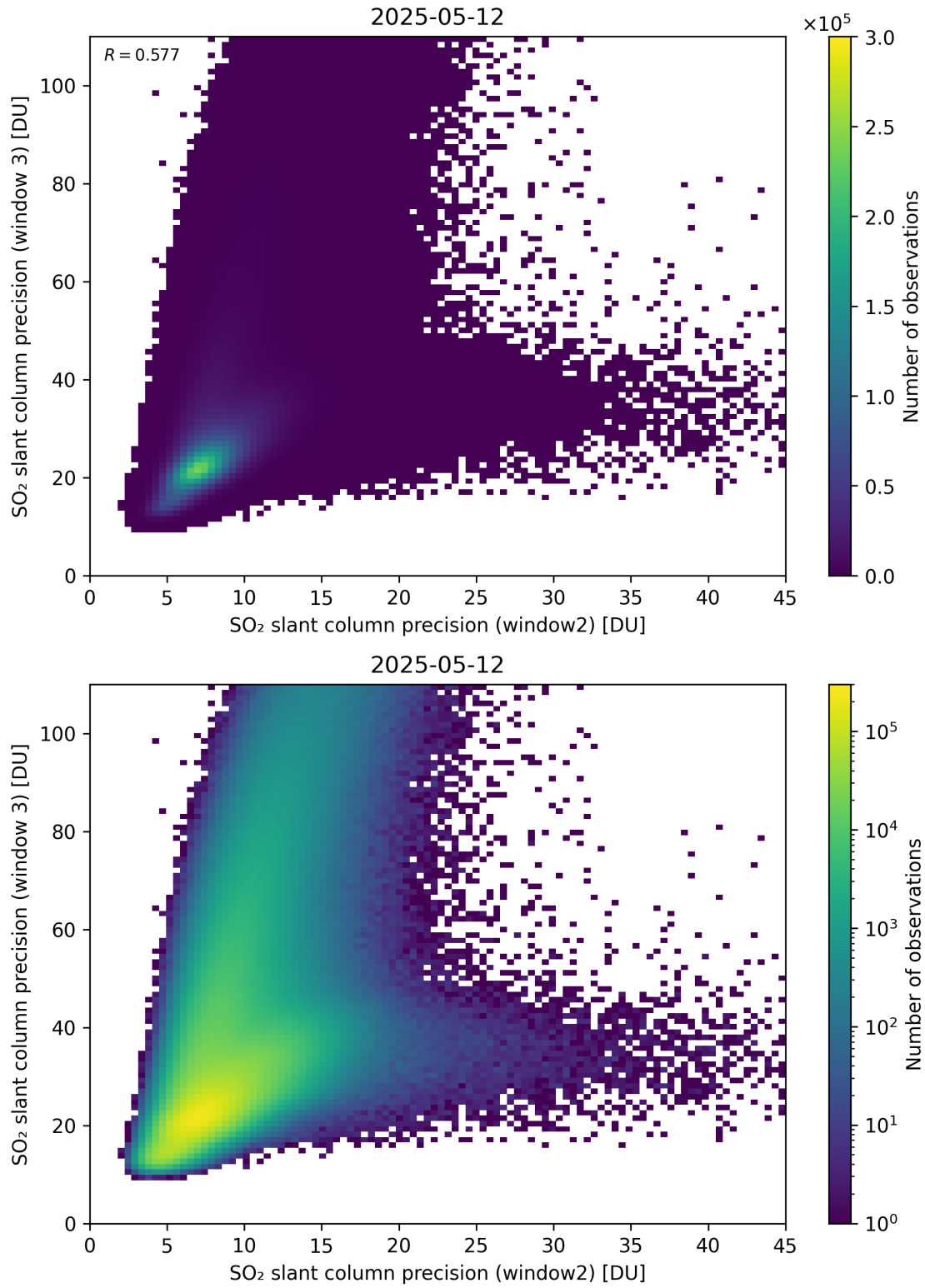
Figure 300: Scatter density plot of “SO 2 slant column precision (window2)” against “SO 2 slant column precision (window 3)” for 2025-05-11 to 2025-05-13.
