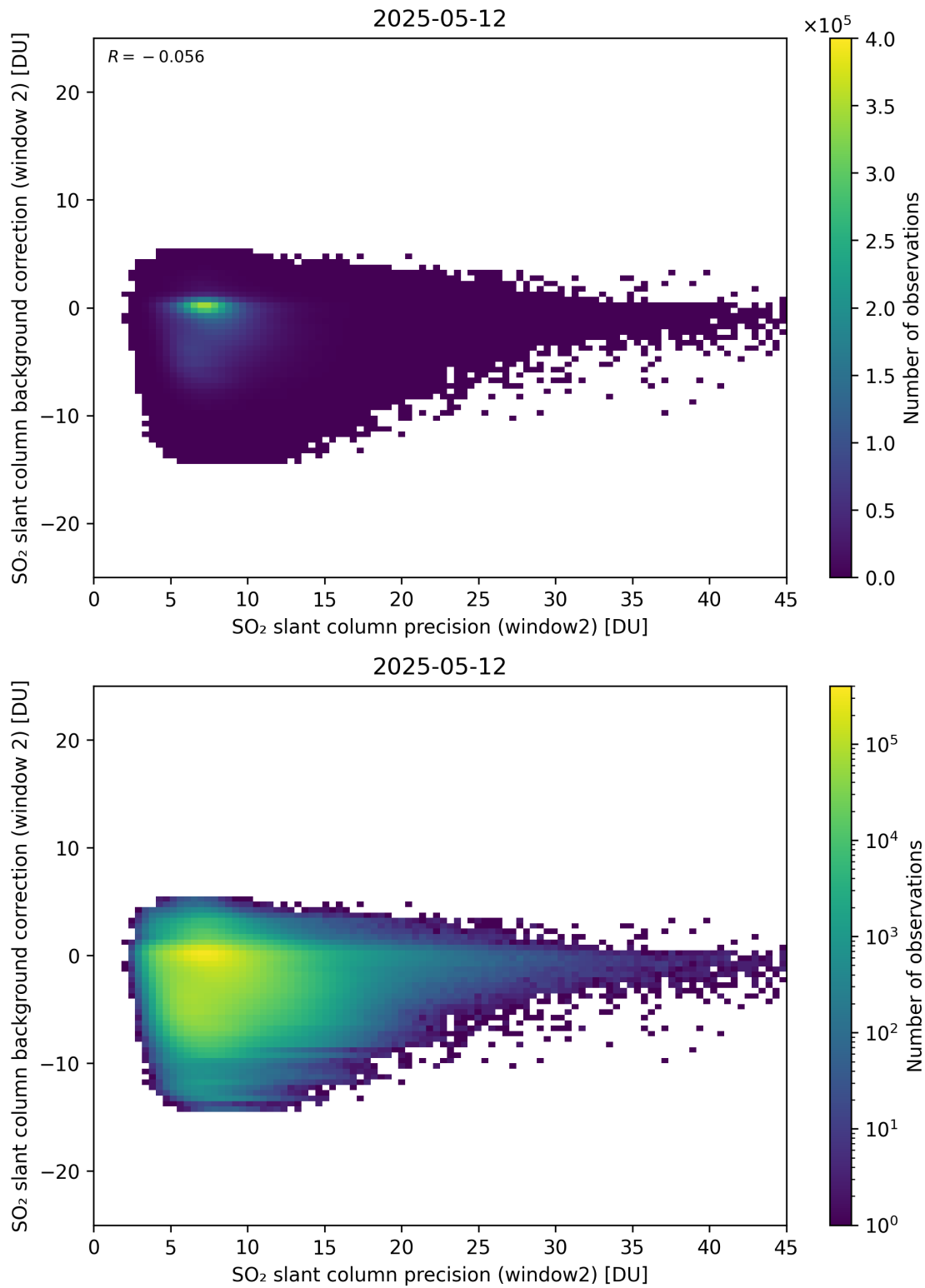
Figure 291: Scatter density plot of “SO 2 slant column precision (window2)” against “SO 2 slant column background correction (window 2)” for 2025-05-11 to 2025-05-13.
