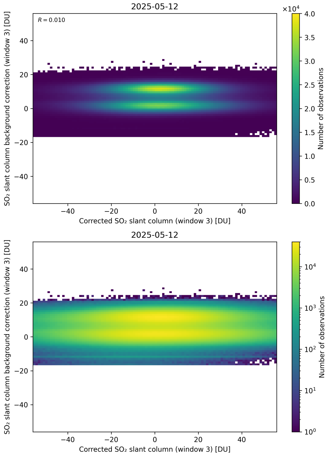
Figure 255: Scatter density plot of “Corrected SO 2 slant column (window 3)” against “SO 2 slant column background correction (window 3)” for 2025-05-11 to 2025-05-13.
