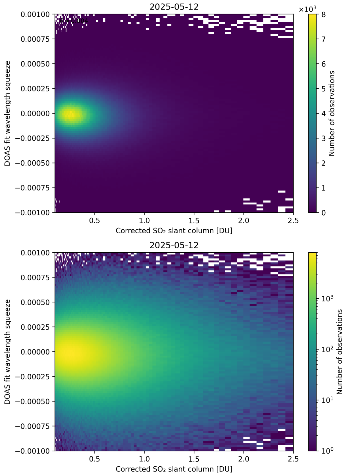
Figure 230: Scatter density plot of “Corrected SO 2 slant column” against “DOAS fit wavelength squeeze” for 2025-05-11 to 2025-05-13.
