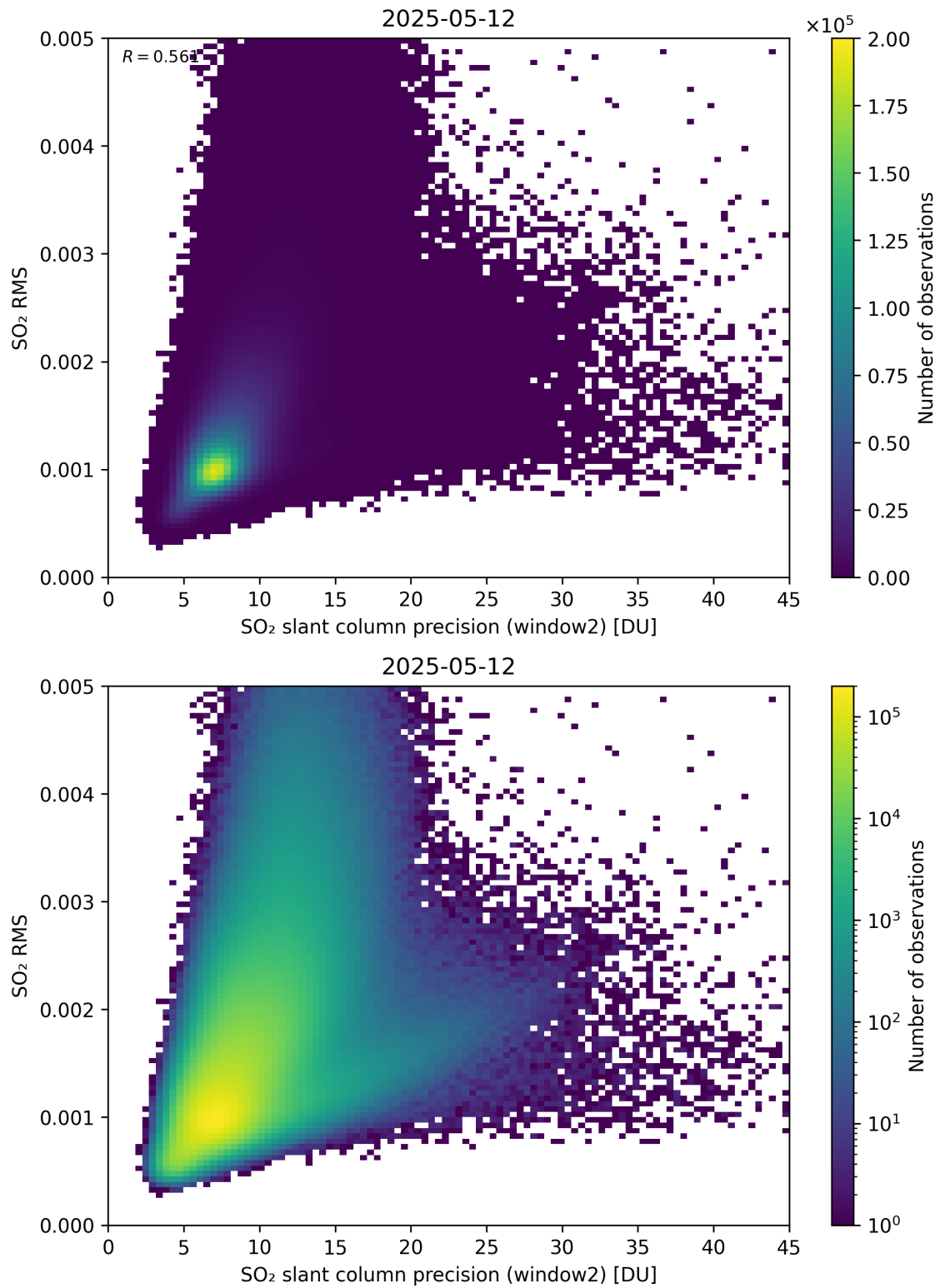
Figure 295: Scatter density plot of “SO 2 slant column precision (window2)” against “SO 2 RMS” for 2025-05-11 to 2025-05-13.
