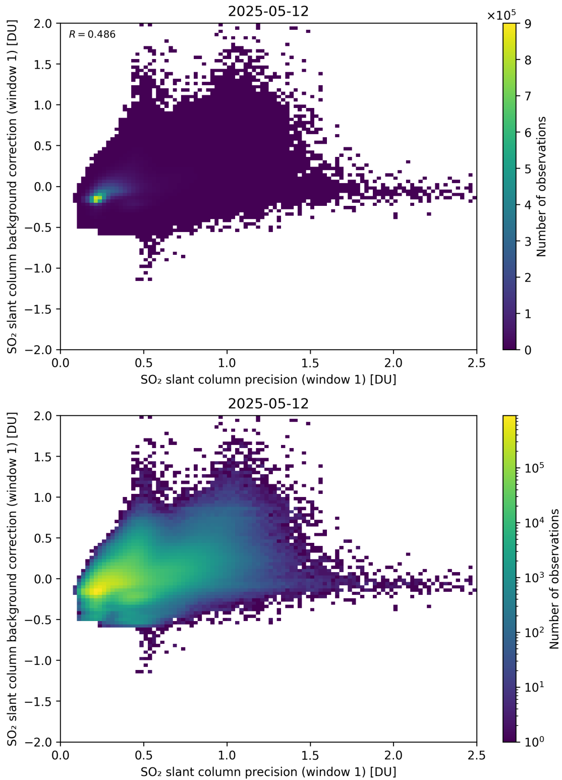
Figure 268: Scatter density plot of “SO 2 slant column precision (window 1)” against “SO 2 slant column background correction (window 1)” for 2025-05-11 to 2025-05-13.
