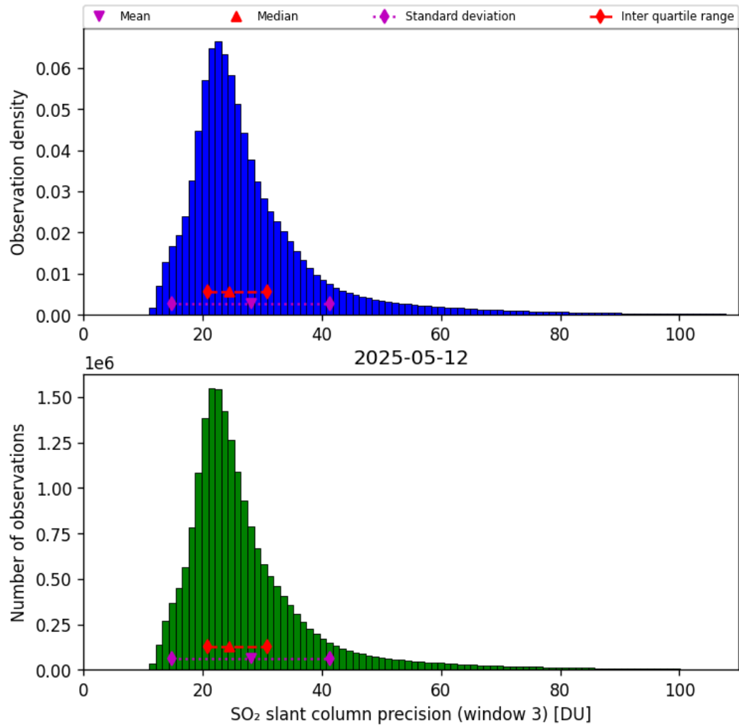
Figure 72: Histogram of “SO 2 slant column precision (window 3)” for 2025-05-11 to 2025-05-13
