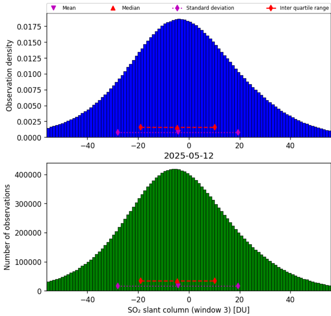
Figure 71: Histogram of “SO 2 slant column (window 3)” for 2025-05-11 to 2025-05-13
