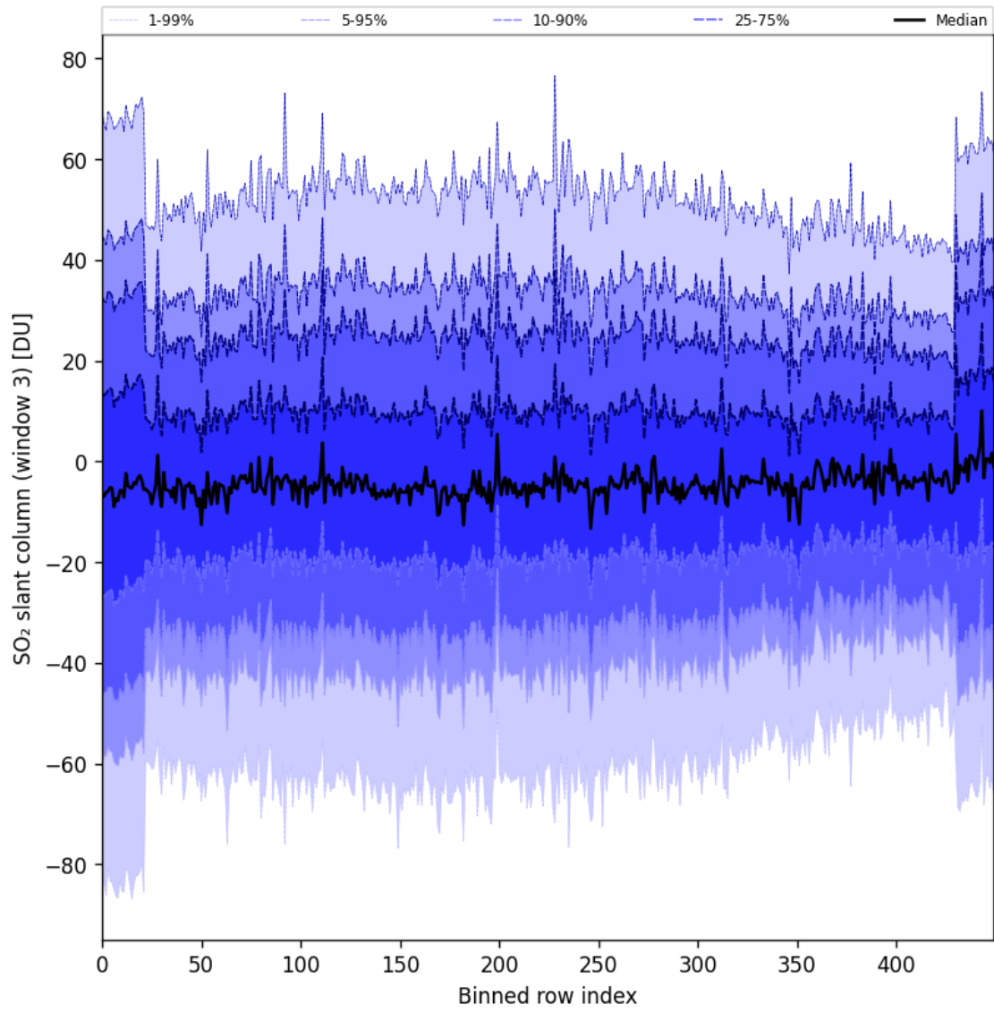
Figure 97: Along track statistics of “SO 2 slant column (window 3)” for 2025-05-11 to 2025-05-13
