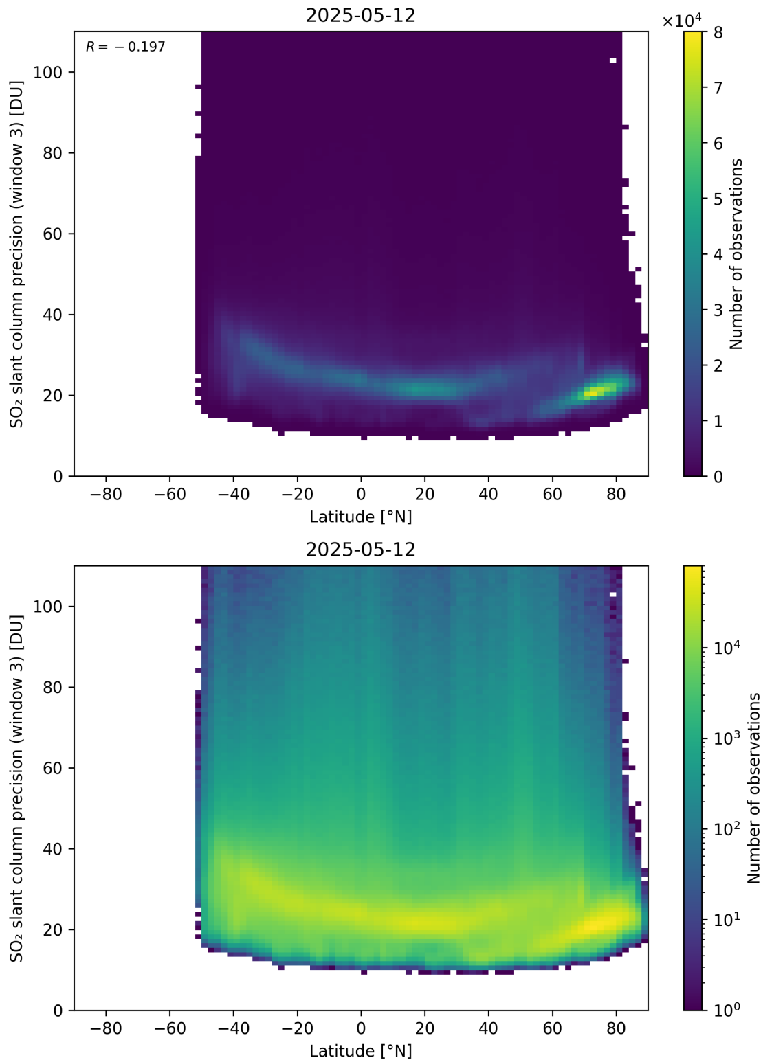
Figure 166: Scatter density plot of “Latitude” against “SO 2 slant column precision (window 3)” for 2025-05-11 to 2025-05-13.
