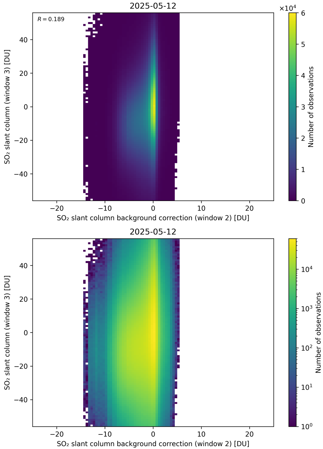
Figure 128: Scatter density plot of “SO 2 slant column background correction (window 2)” against “SO 2 slant column (window 3)” for 2025-05-11 to 2025-05-13.
