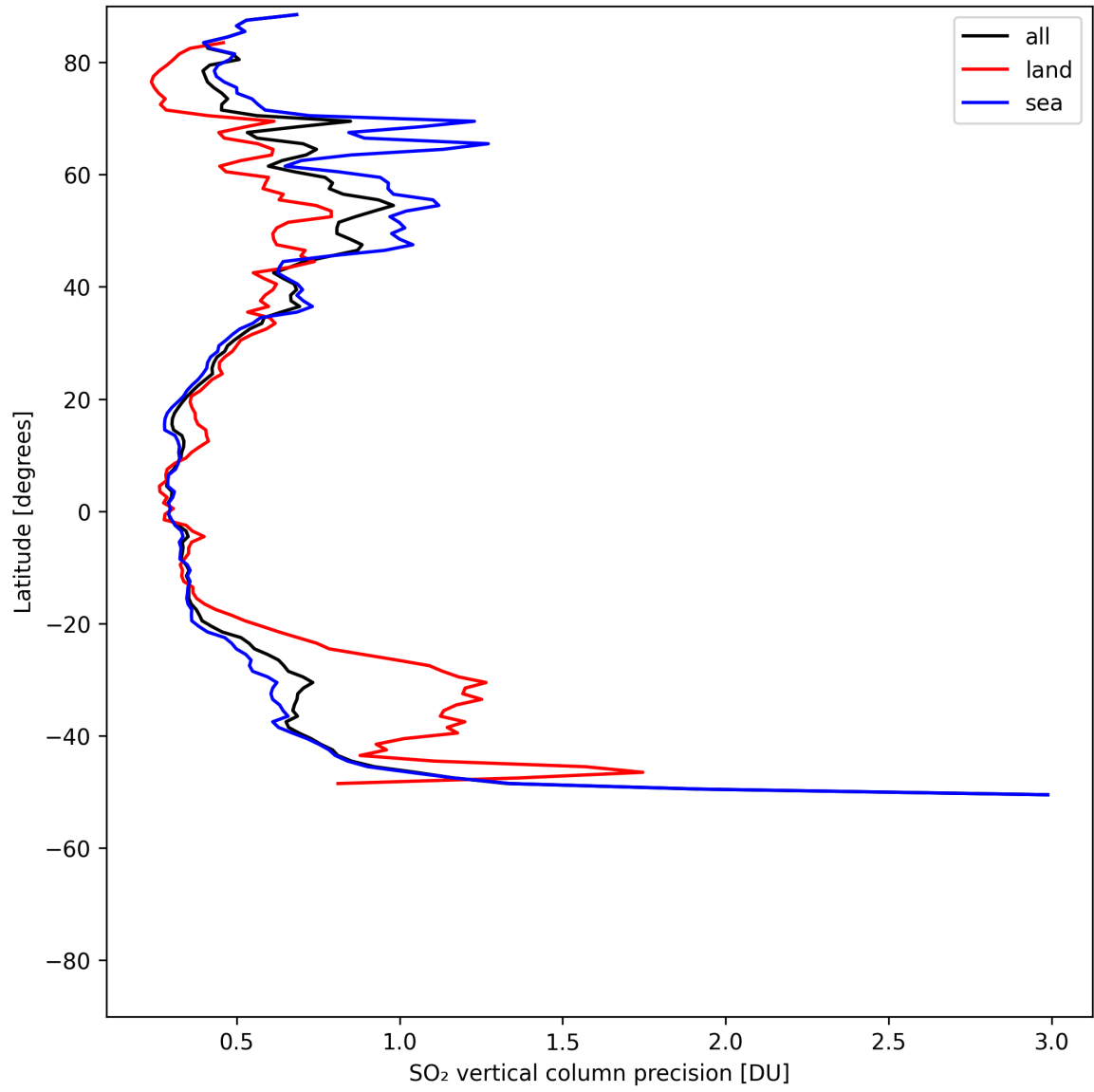
Figure 33: Zonal average of “SO 2 vertical column precision” for 2025-05-11 to 2025-05-13.
