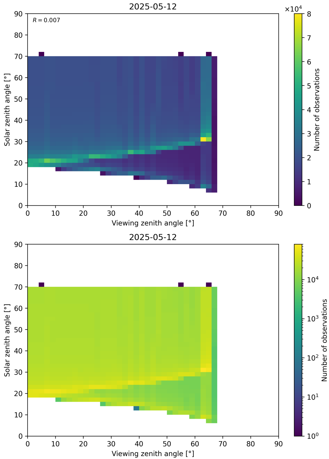
Figure 369: Scatter density plot of “Viewing zenith angle” against “Solar zenith angle” for 2025-05-11 to 2025-05-13.
