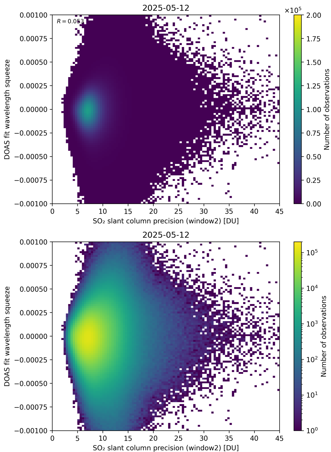
Figure 294: Scatter density plot of “SO 2 slant column precision (window2)” against “DOAS fit wavelength squeeze” for 2025-05-11 to 2025-05-13.
