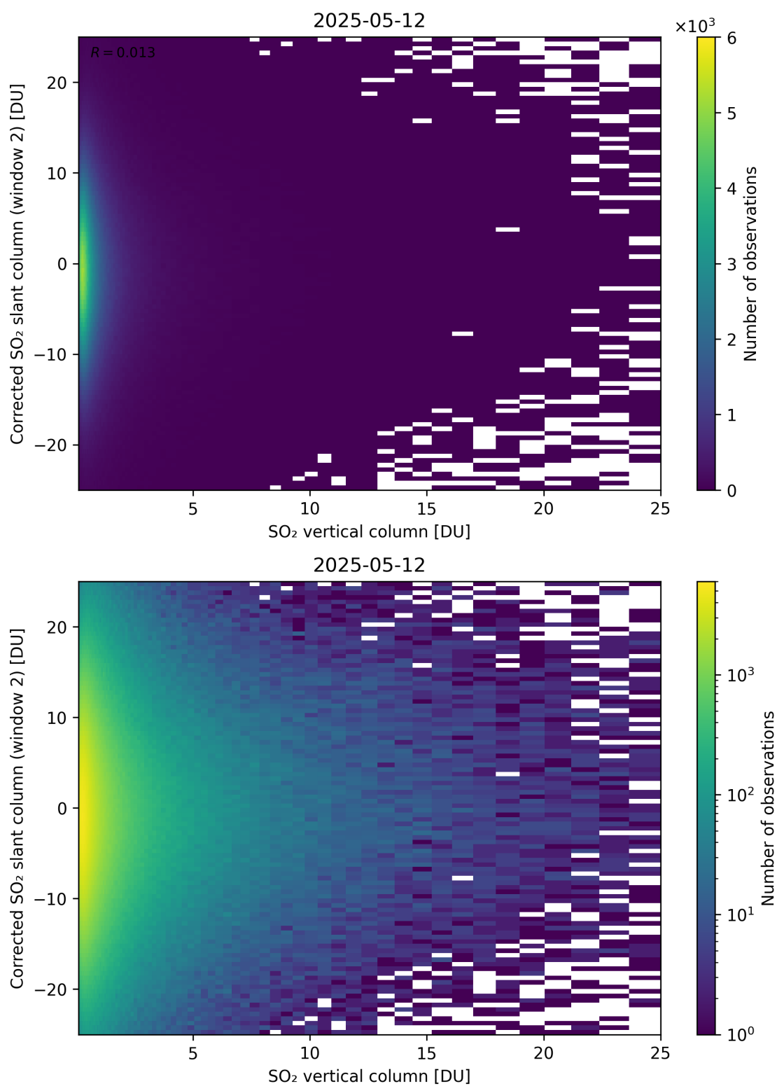
Figure 352: Scatter density plot of “SO 2 vertical column” against “Corrected SO 2 slant column (window 2)” for 2025-05-11 to 2025-05-13.
