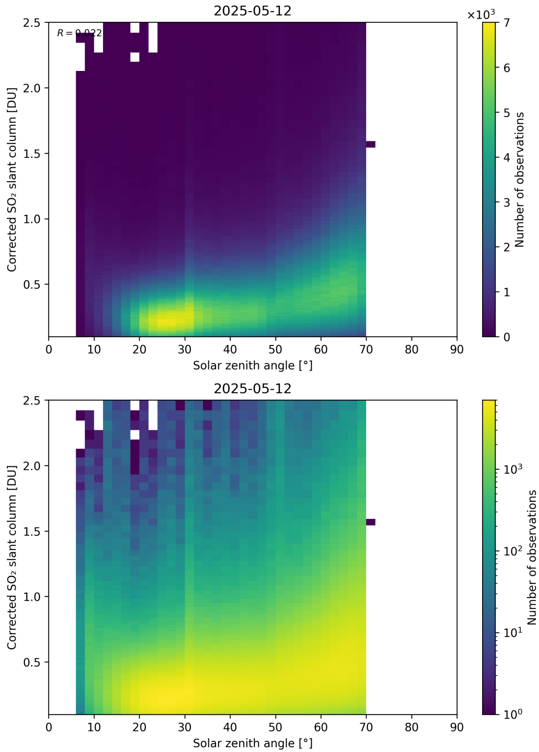
Figure 181: Scatter density plot of “Solar zenith angle” against “Corrected SO 2 slant column” for 2025-05-11 to 2025-05-13.
