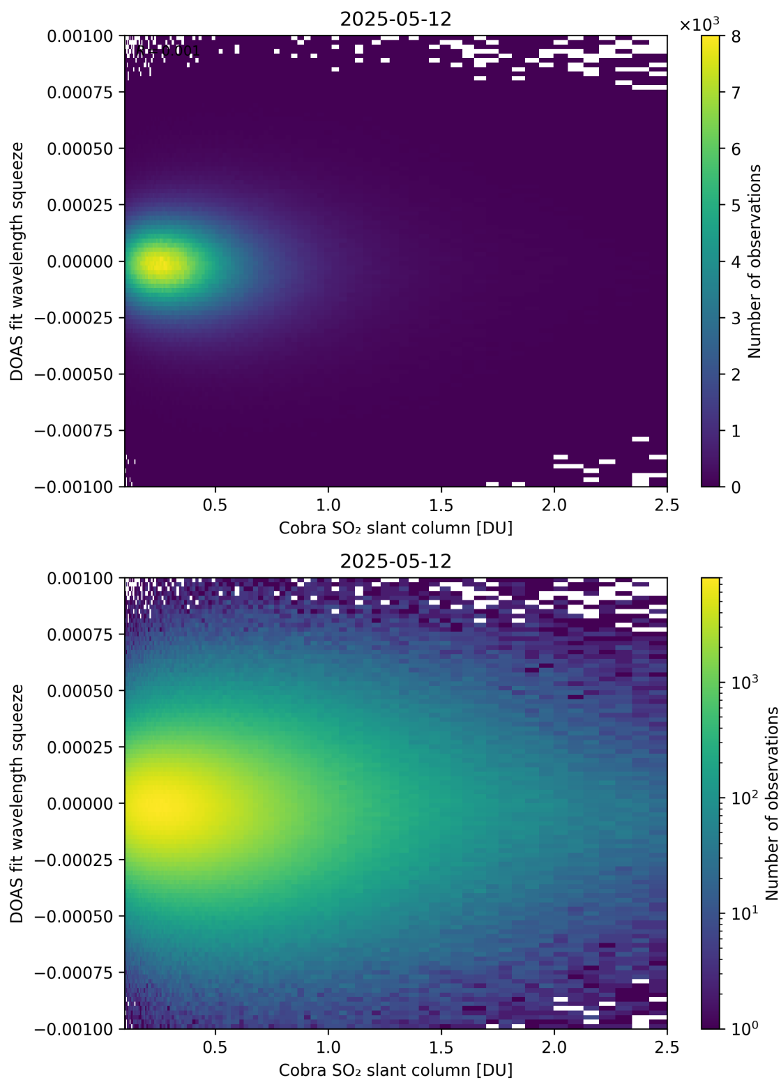
Figure 197: Scatter density plot of “Cobra SO 2 slant column” against “DOAS fit wavelength squeeze” for 2025-05-11 to 2025-05-13.
