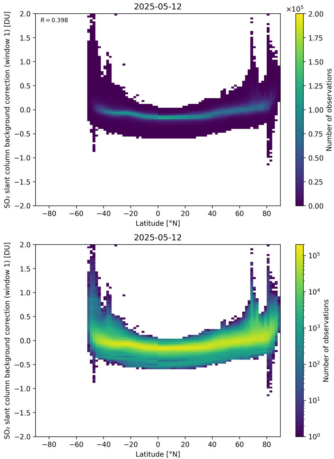
Figure 150: Scatter density plot of “Latitude” against “SO 2 slant column background correction (window 1)” for 2025-05-11 to 2025-05-13.
