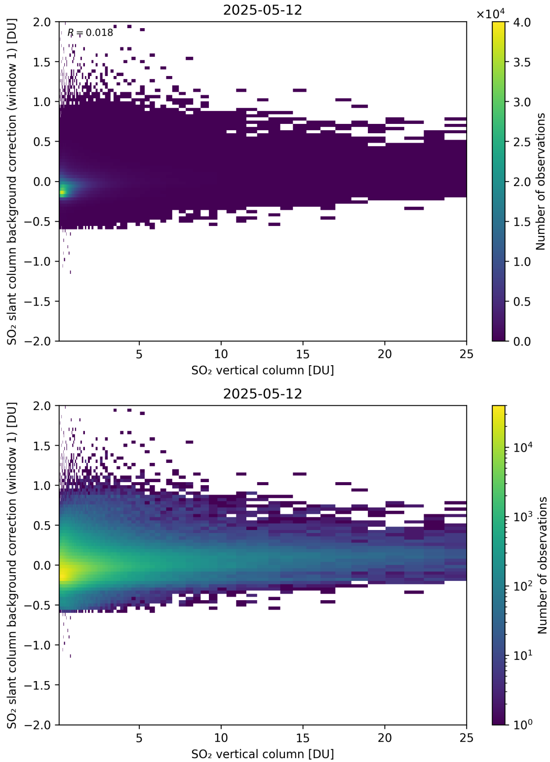
Figure 323: Scatter density plot of “SO 2 vertical column” against “SO 2 slant column background correction (window 1)” for 2025-05-11 to 2025-05-13.
