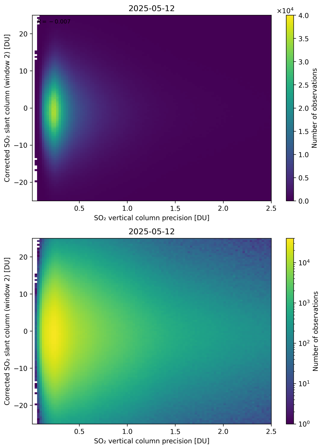
Figure 339: Scatter density plot of “SO 2 vertical column precision” against “Corrected SO 2 slant column (window 2)” for 2025-05-11 to 2025-05-13.
