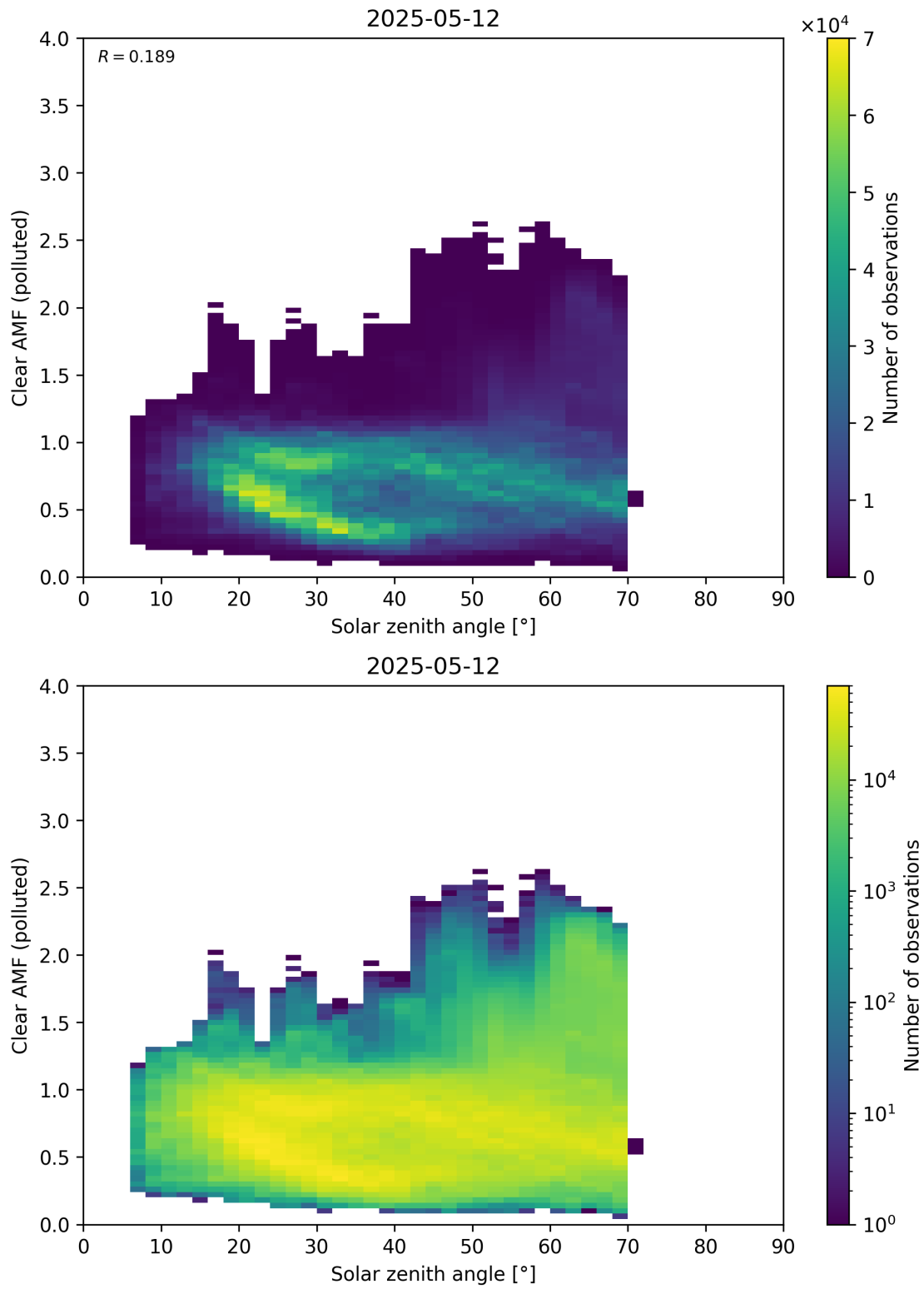
Figure 178: Scatter density plot of “Solar zenith angle” against “Clear AMF (polluted)” for 2025-05-11 to 2025-05-13.
