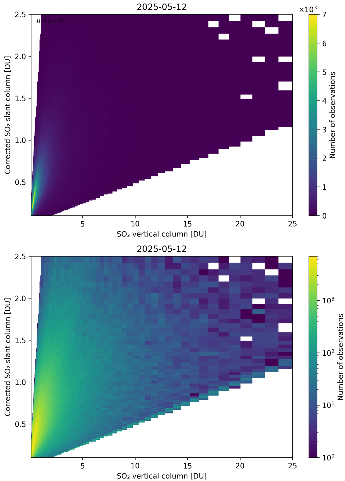
Figure 351: Scatter density plot of “SO 2 vertical column” against “Corrected SO 2 slant column” for 2025-05-11 to 2025-05-13.
