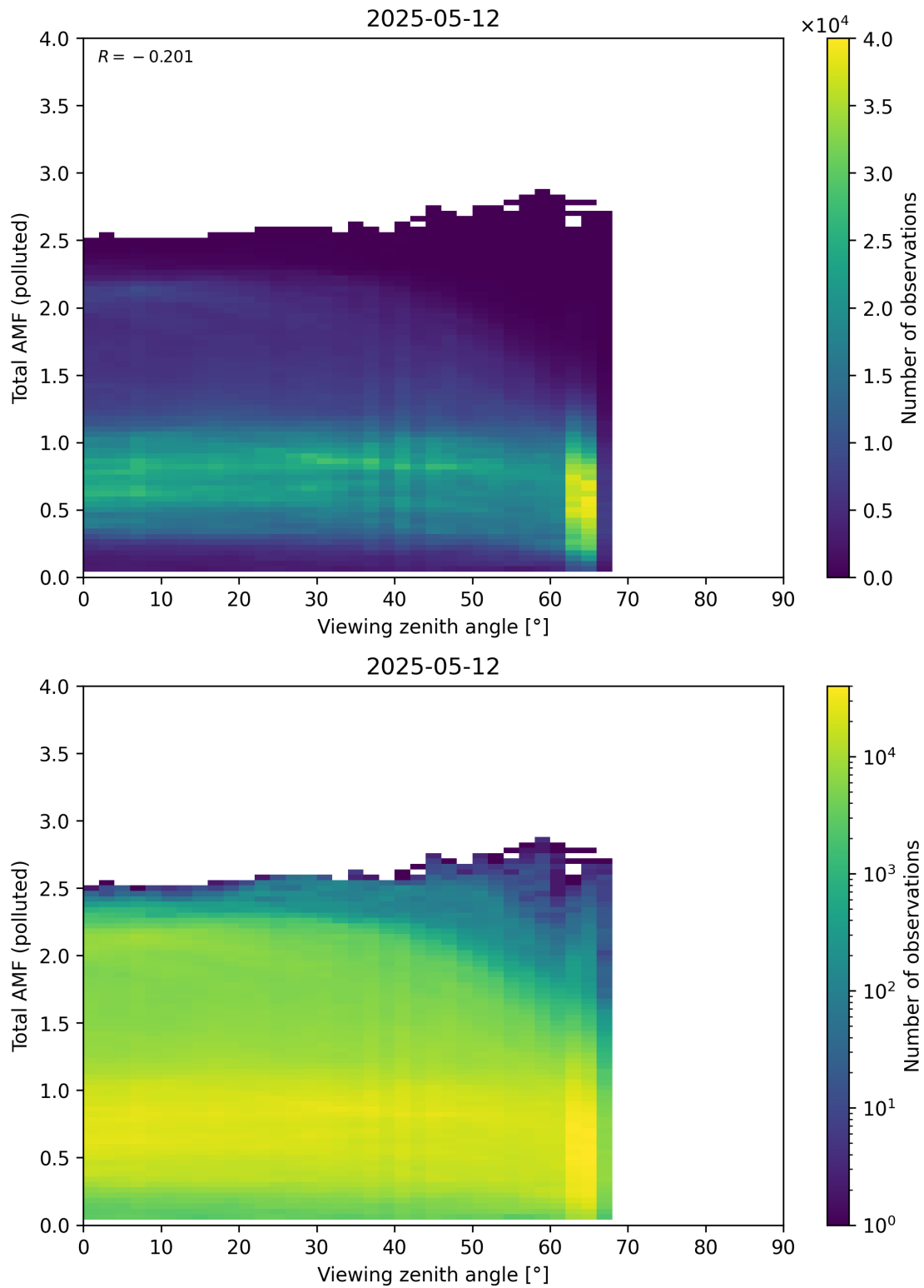
Figure 381: Scatter density plot of “Viewing zenith angle” against “Total AMF (polluted)” for 2025-05-11 to 2025-05-13.
