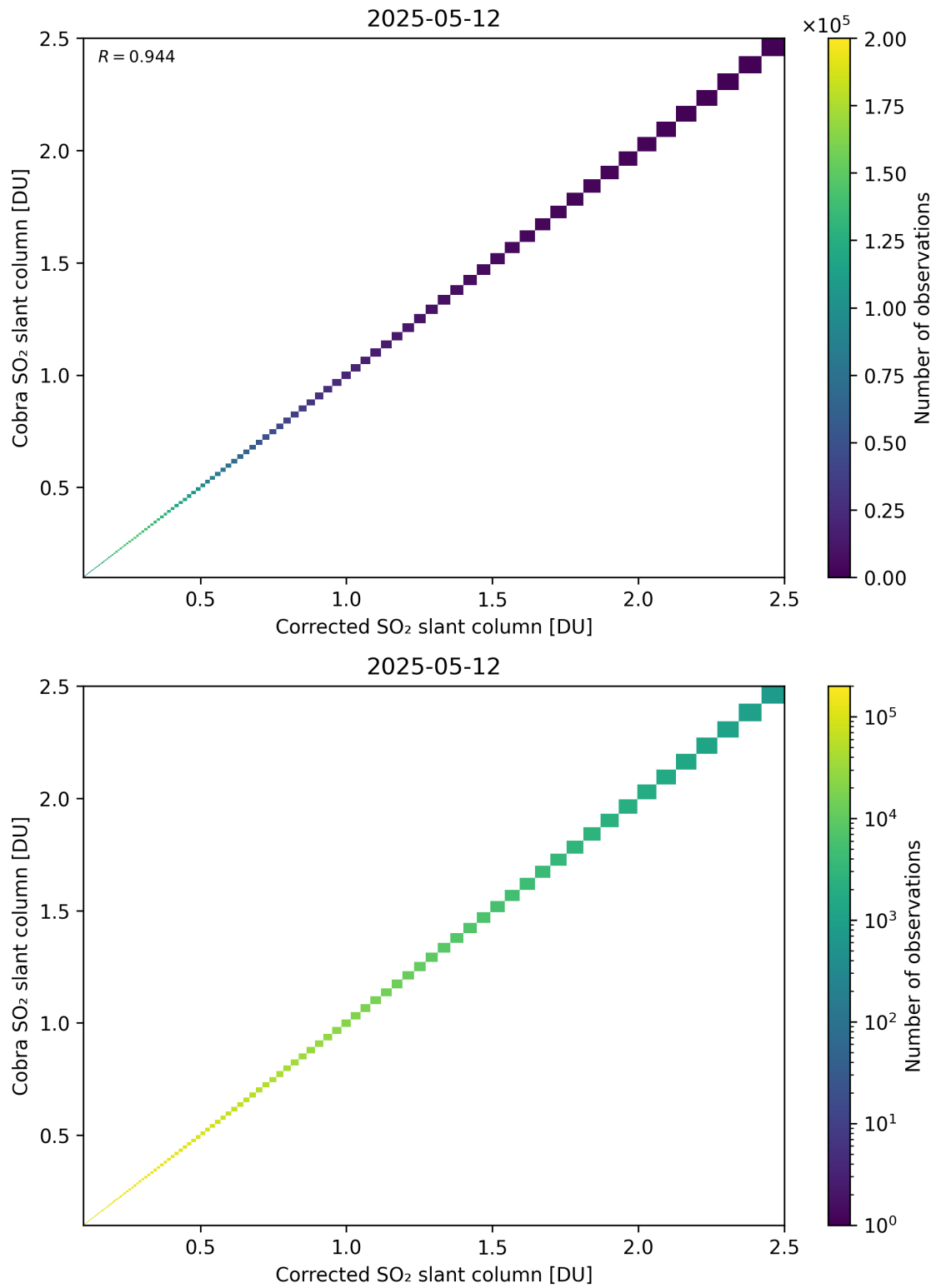
Figure 233: Scatter density plot of “Corrected SO 2 slant column” against “Cobra SO 2 slant column” for 2025-05-11 to 2025-05-13.
