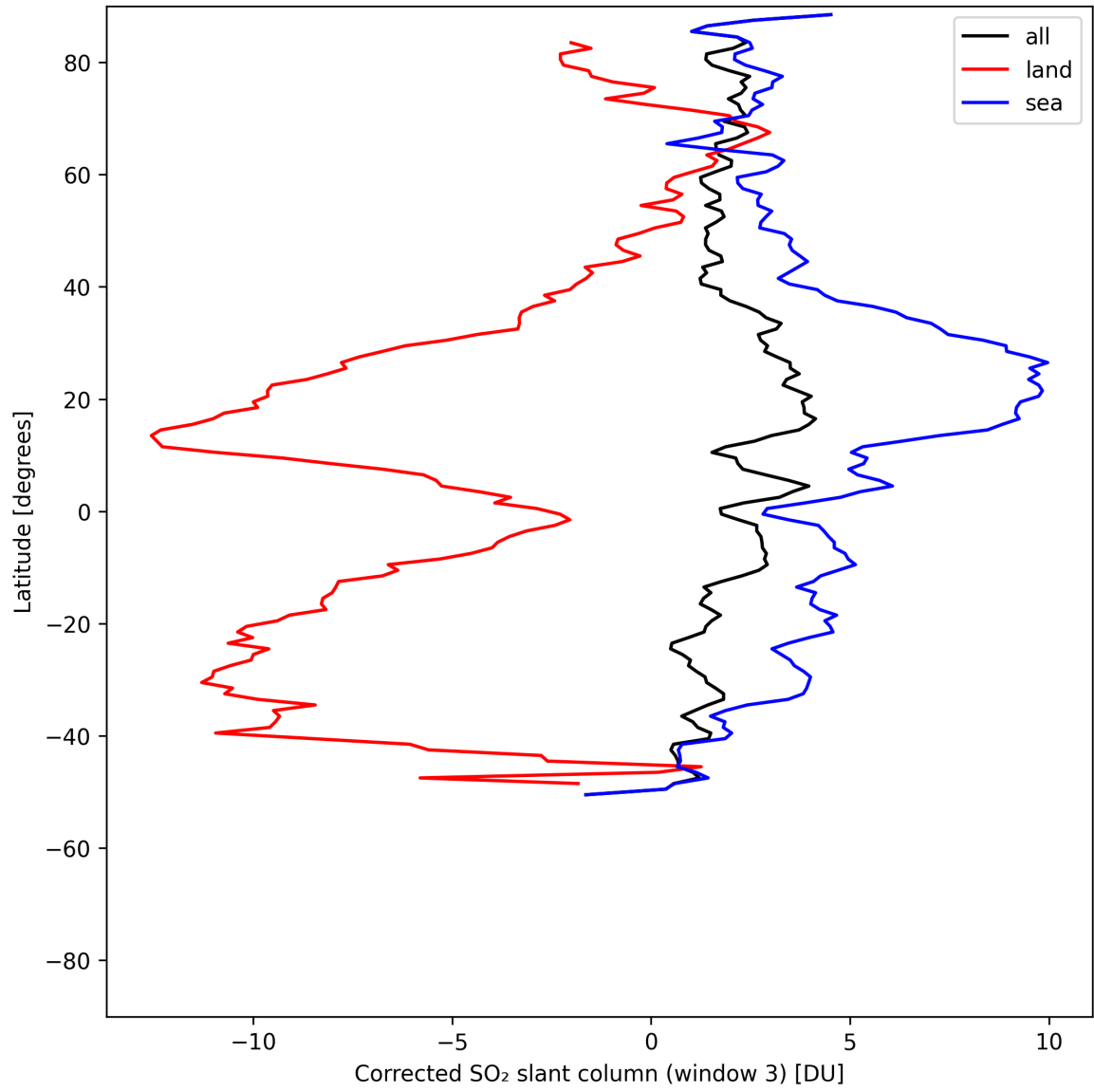
Figure 47: Zonal average of “Corrected SO 2 slant column (window 3)” for 2025-05-11 to 2025-05-13.
