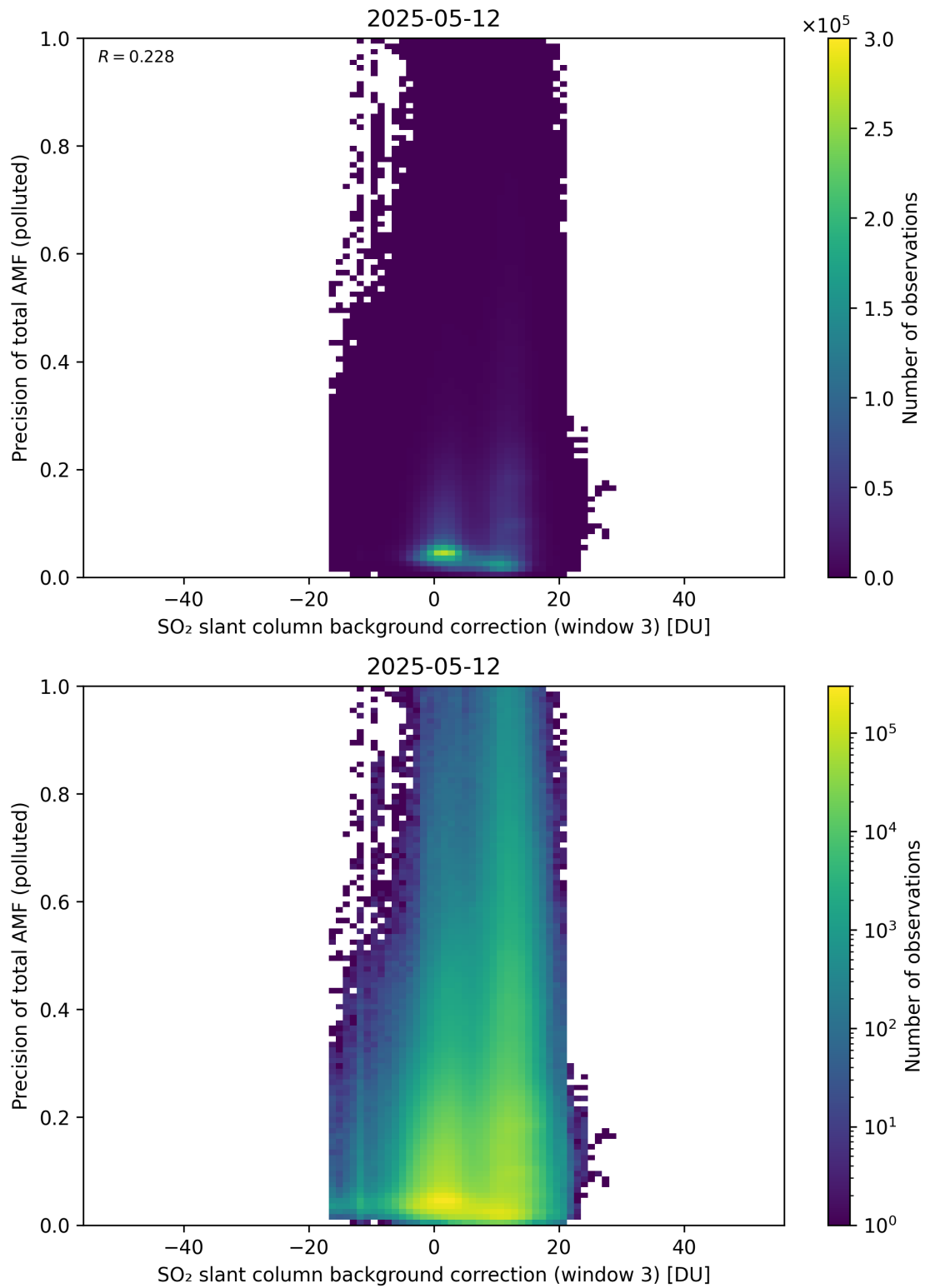
Figure 137: Scatter density plot of “SO 2 slant column background correction (window 3)” against “Precision of total AMF (polluted)” for 2025-05-11 to 2025-05-13.
