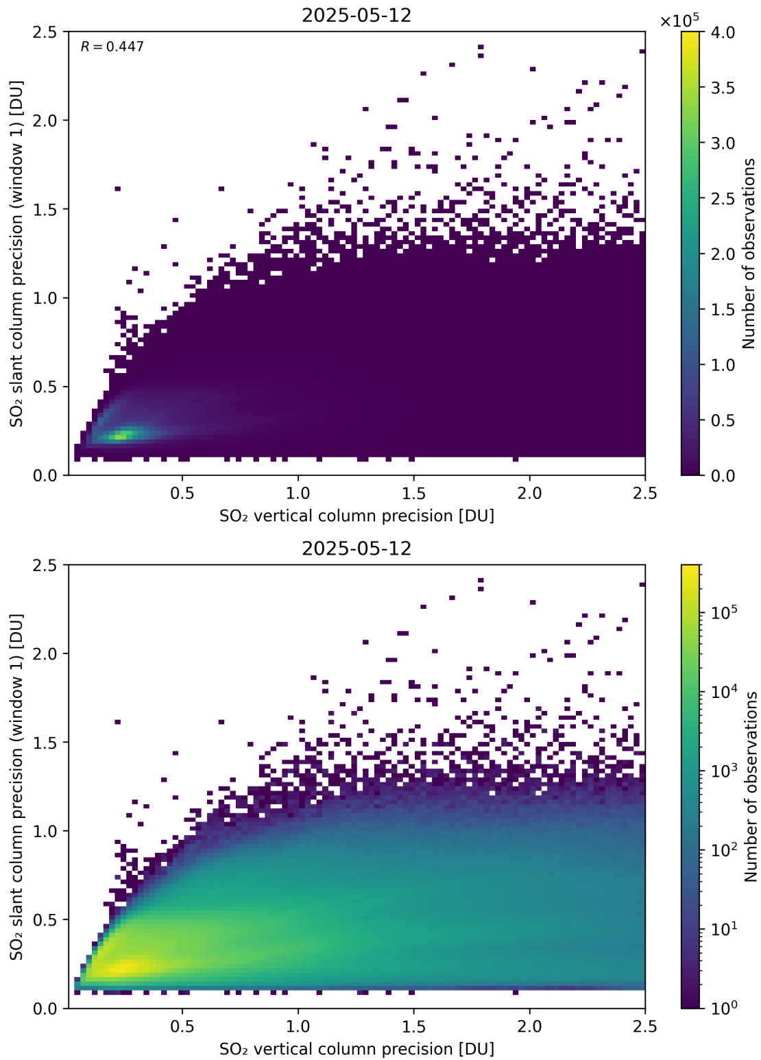
Figure 342: Scatter density plot of “SO 2 vertical column precision” against “SO 2 slant column precision (window 1)” for 2025-05-11 to 2025-05-13.
