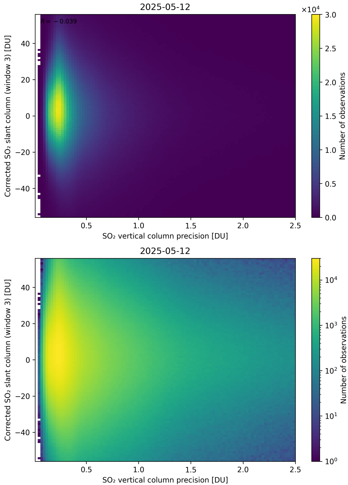
Figure 340: Scatter density plot of “SO 2 vertical column precision” against “Corrected SO 2 slant column (window 3)” for 2025-05-11 to 2025-05-13.
