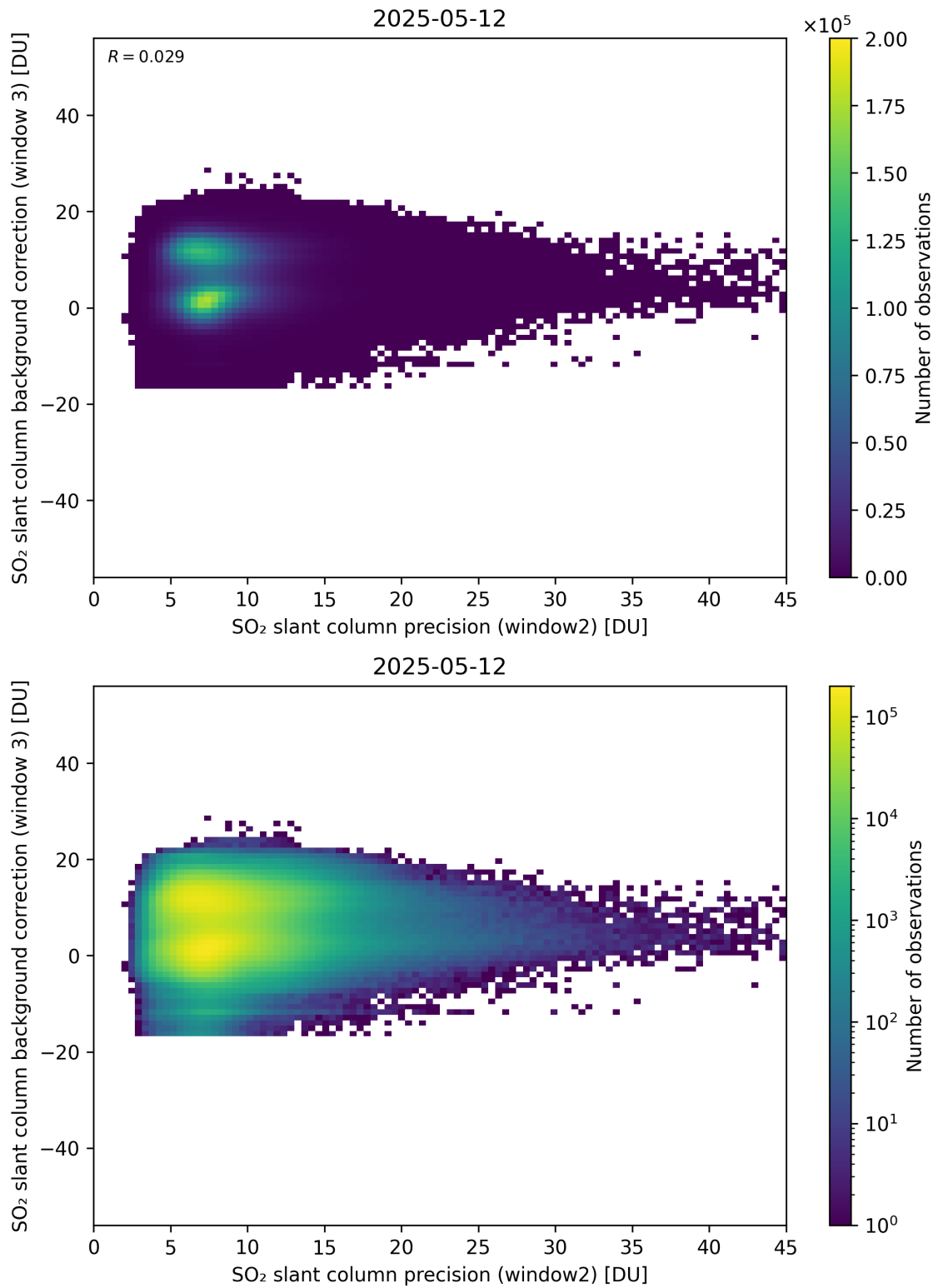
Figure 292: Scatter density plot of “SO 2 slant column precision (window2)” against “SO 2 slant column background correction (window 3)” for 2025-05-11 to 2025-05-13.
