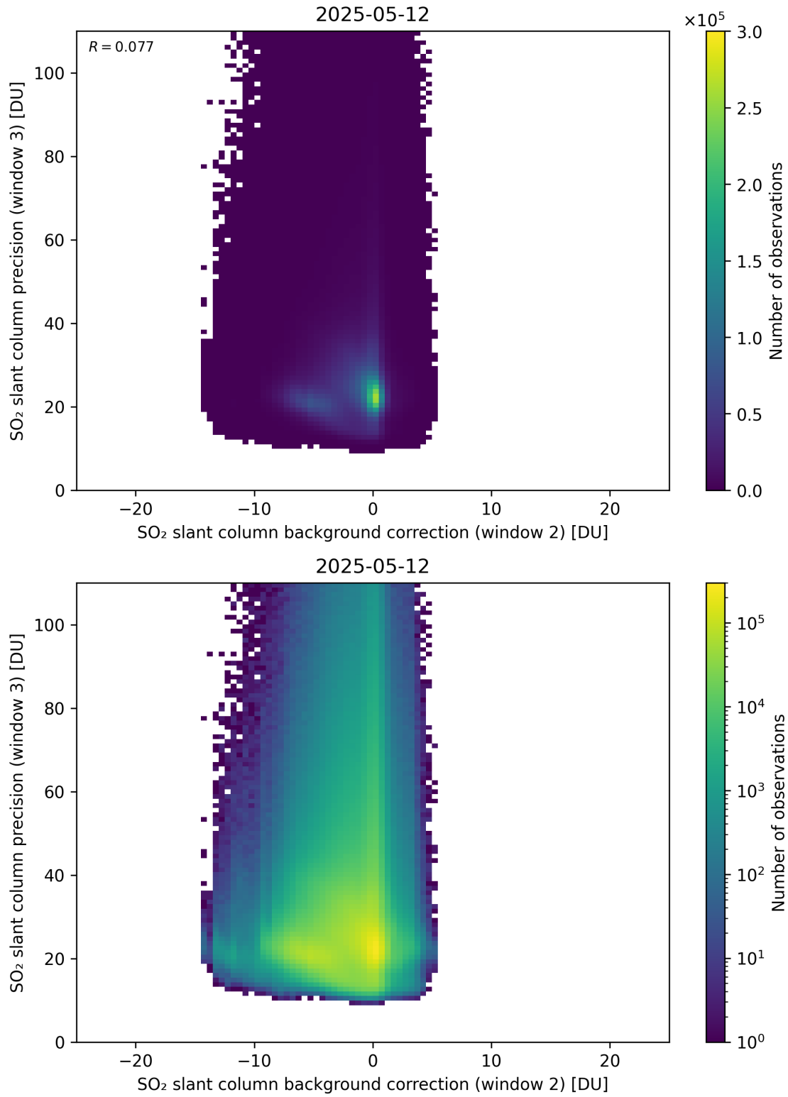
Figure 129: Scatter density plot of “SO 2 slant column background correction (window 2)” against “SO 2 slant column precision (window 3)” for 2025-05-11 to 2025-05-13.
