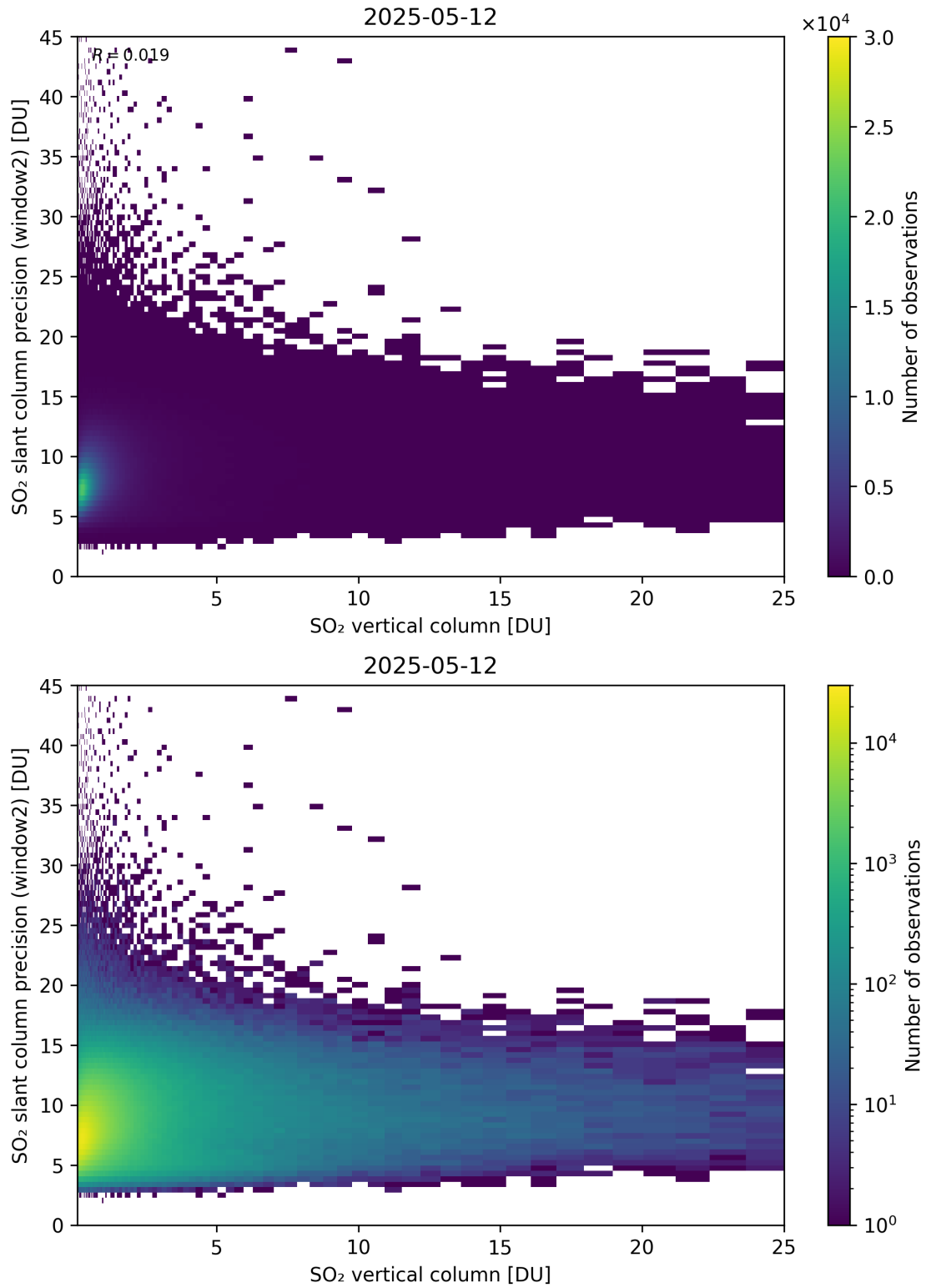
Figure 356: Scatter density plot of “SO 2 vertical column” against “SO 2 slant column precision (window2)” for 2025-05-11 to 2025-05-13.
