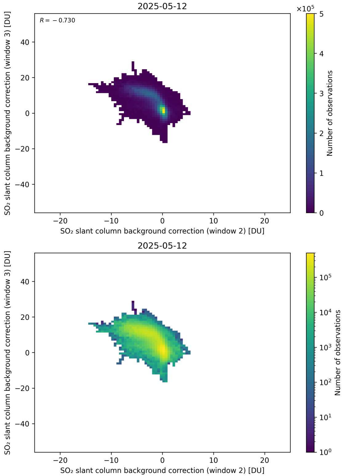
Figure 122: Scatter density plot of “SO 2 slant column background correction (window 2)” against “SO 2 slant column background correction (window 3)” for 2025-05-11 to 2025-05-13.
