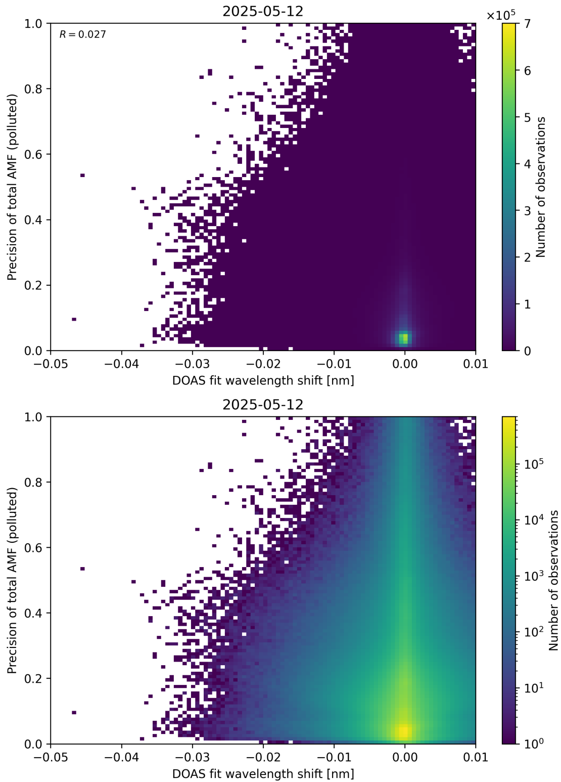
Figure 142: Scatter density plot of “DOAS fit wavelength shift” against “Precision of total AMF (polluted)” for 2025-05-11 to 2025-05-13.
