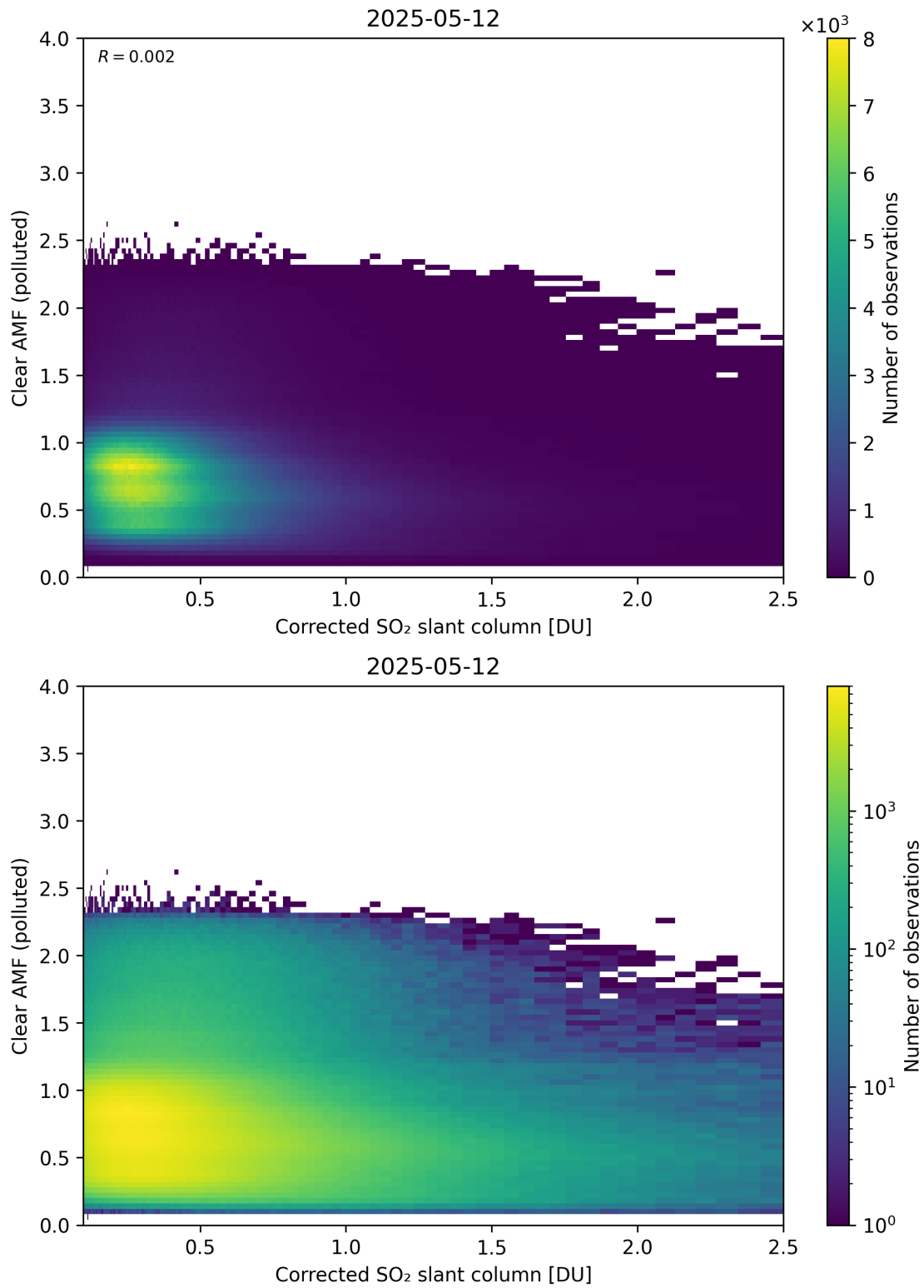
Figure 232: Scatter density plot of “Corrected SO 2 slant column” against “Clear AMF (polluted)” for 2025-05-11 to 2025-05-13.
