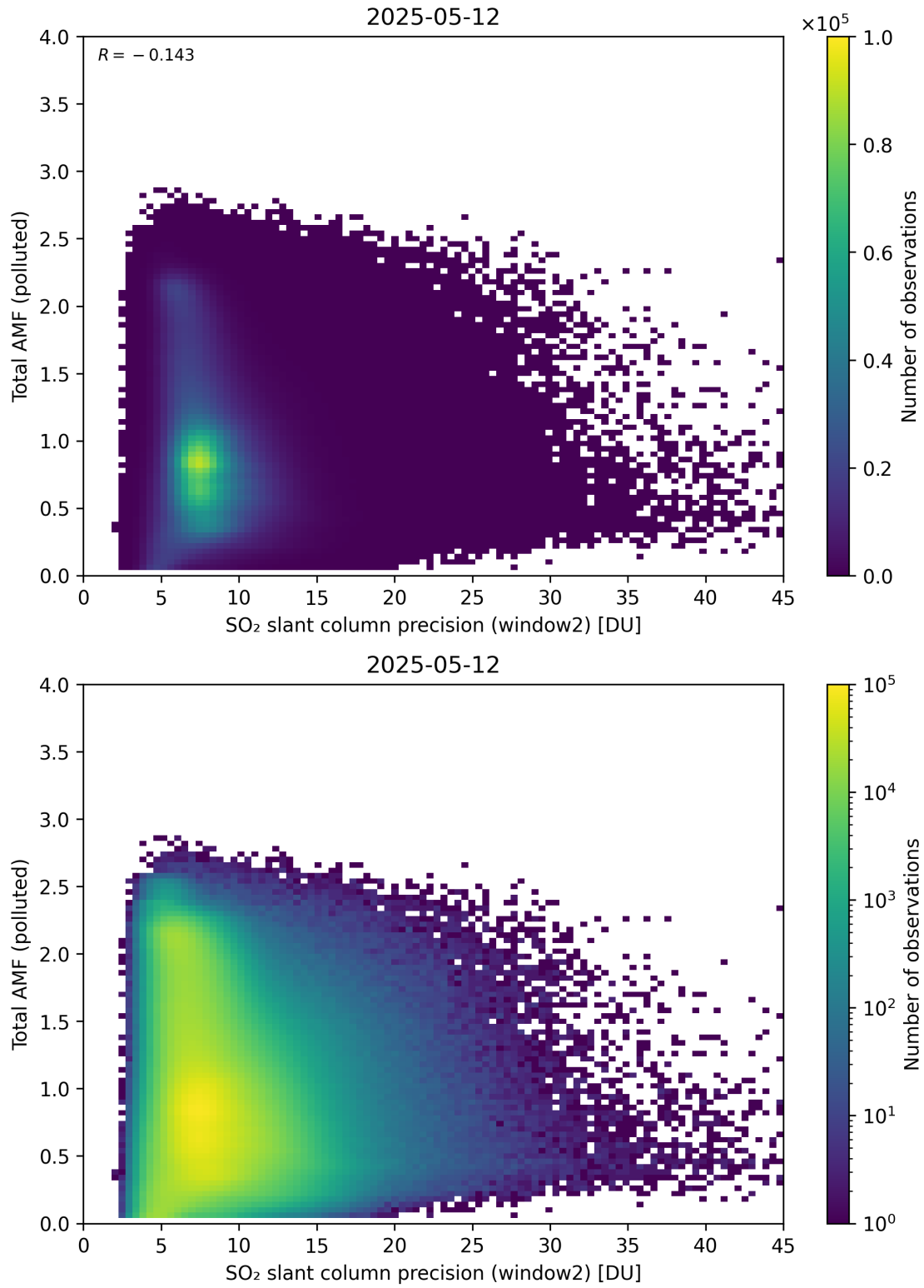
Figure 301: Scatter density plot of “SO 2 slant column precision (window2)” against “Total AMF (polluted)” for 2025-05-11 to 2025-05-13.
