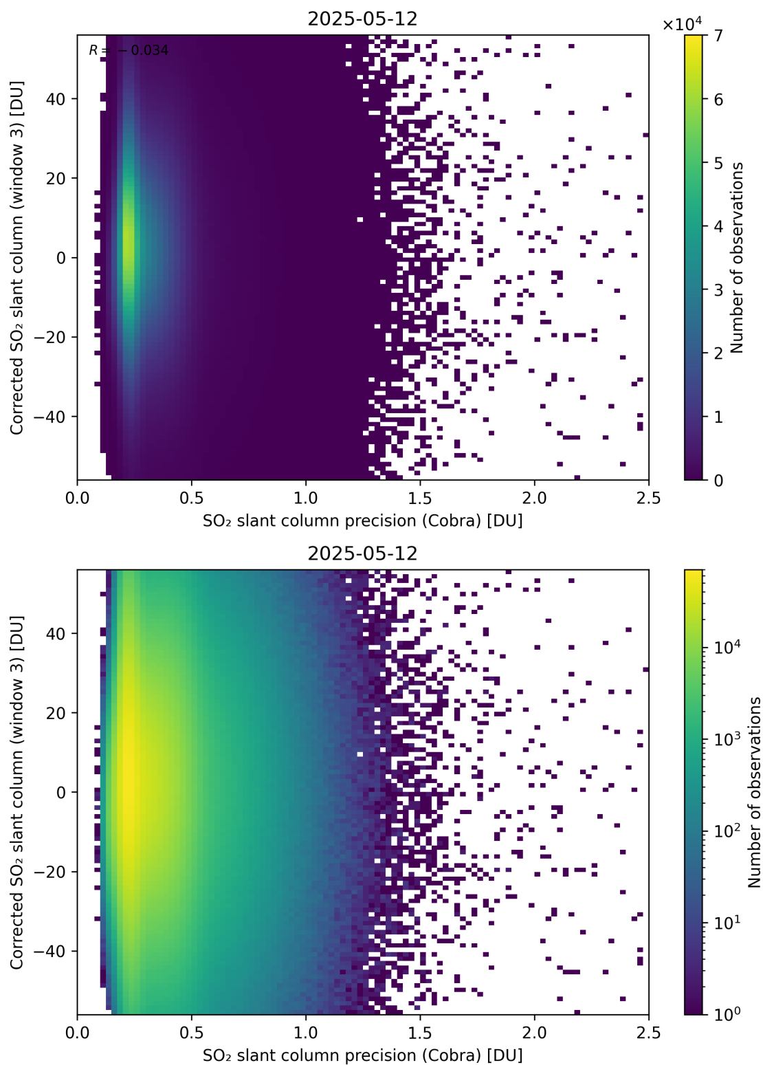
Figure 207: Scatter density plot of “SO 2 slant column precision (Cobra)” against “Corrected SO 2 slant column (window 3)” for 2025-05-11 to 2025-05-13.
