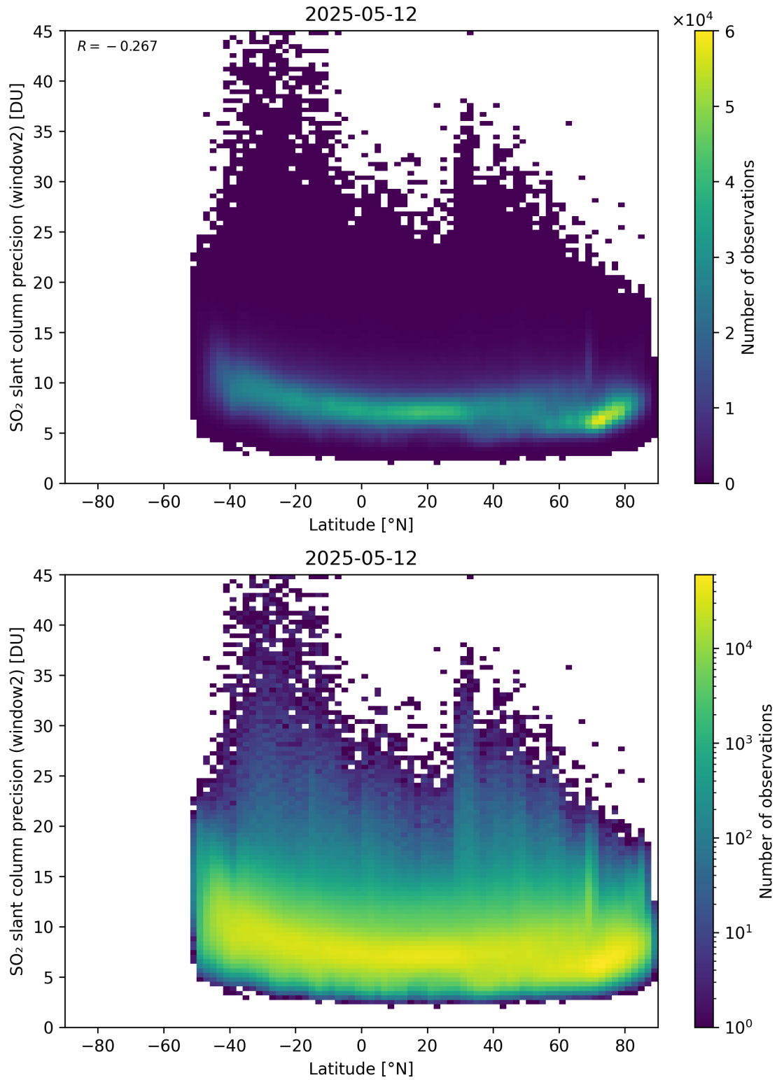
Figure 164: Scatter density plot of “Latitude” against “SO 2 slant column precision (window2)” for 2025-05-11 to 2025-05-13.
