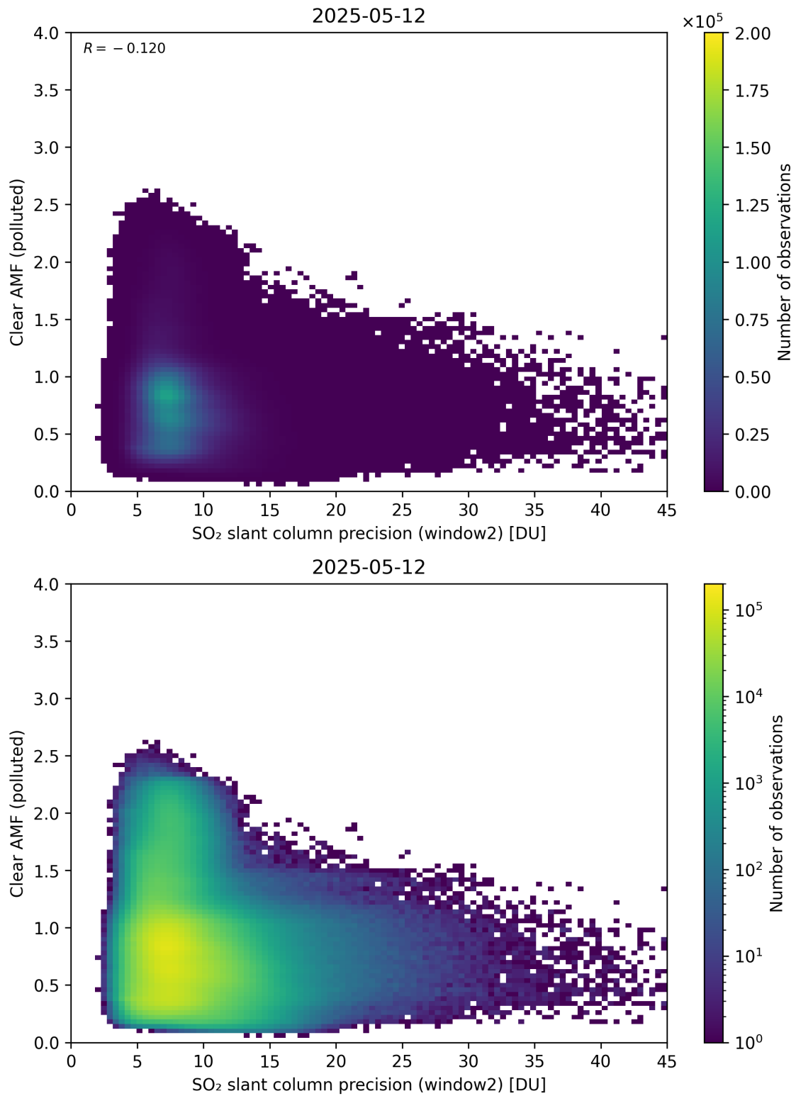
Figure 296: Scatter density plot of “SO 2 slant column precision (window2)” against “Clear AMF (polluted)” for 2025-05-11 to 2025-05-13.
