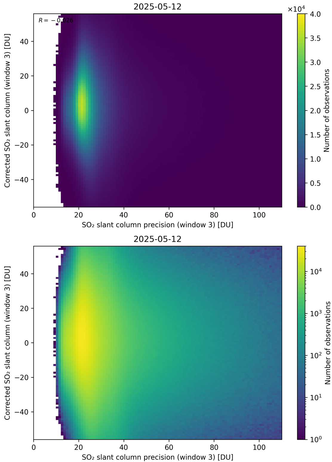
Figure 312: Scatter density plot of “SO 2 slant column precision (window 3)” against “Corrected SO 2 slant column (window 3)” for 2025-05-11 to 2025-05-13.
