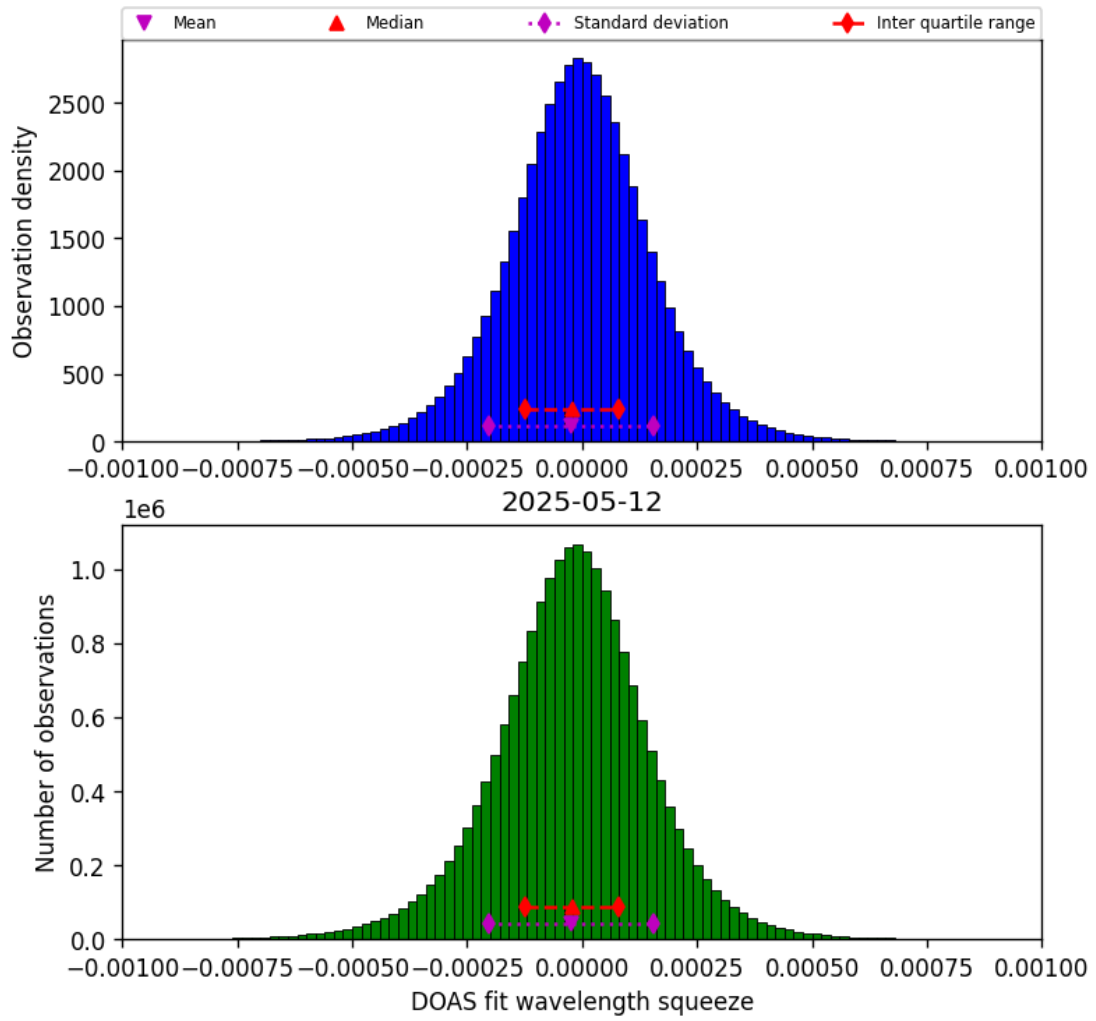
Figure 77: Histogram of “DOAS fit wavelength squeeze” for 2025-05-11 to 2025-05-13
