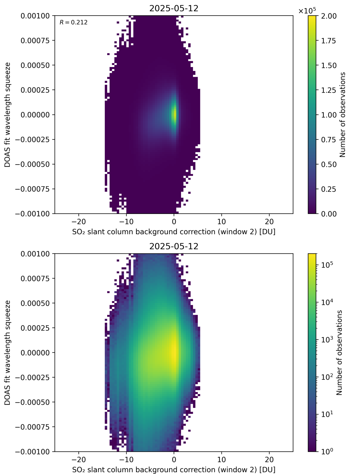
Figure 124: Scatter density plot of “SO 2 slant column background correction (window 2)” against “DOAS fit wavelength squeeze” for 2025-05-11 to 2025-05-13.
