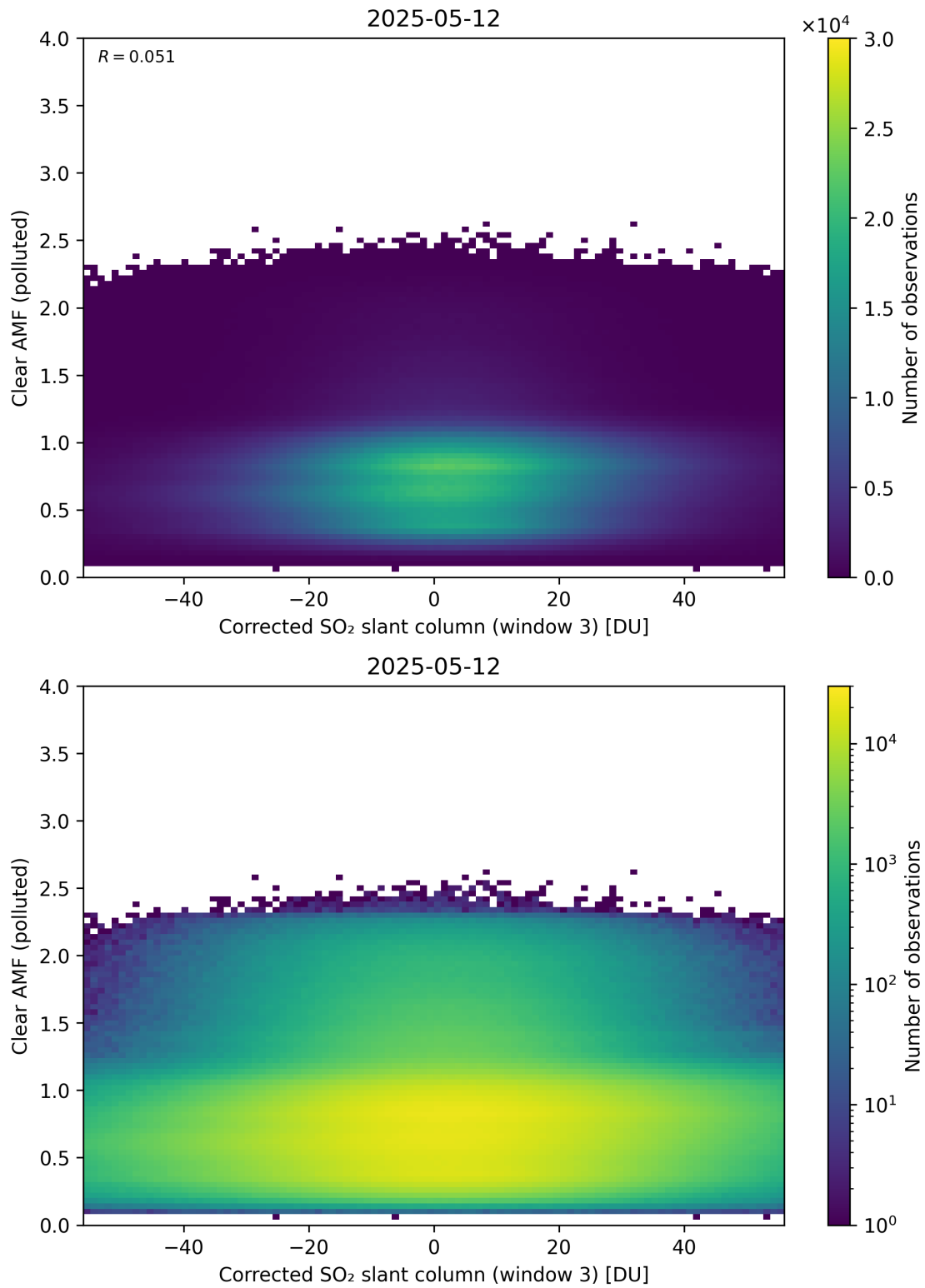
Figure 259: Scatter density plot of “Corrected SO 2 slant column (window 3)” against “Clear AMF (polluted)” for 2025-05-11 to 2025-05-13.
