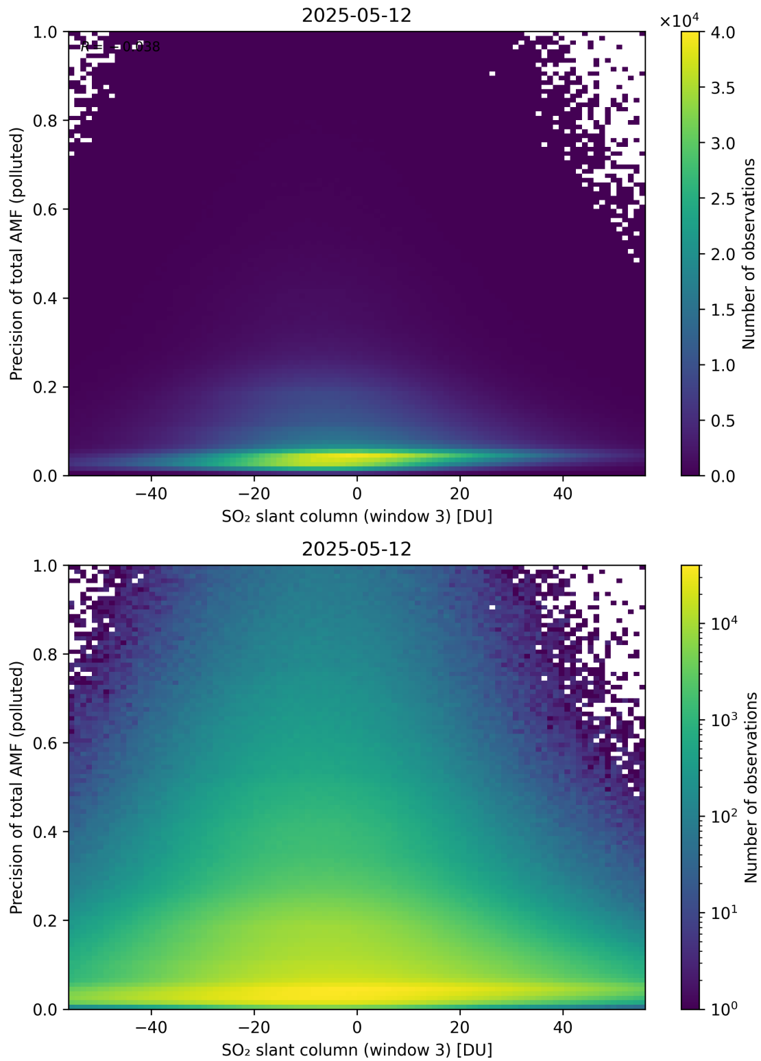
Figure 319: Scatter density plot of “SO 2 slant column (window 3)” against “Precision of total AMF (polluted)” for 2025-05-11 to 2025-05-13.
