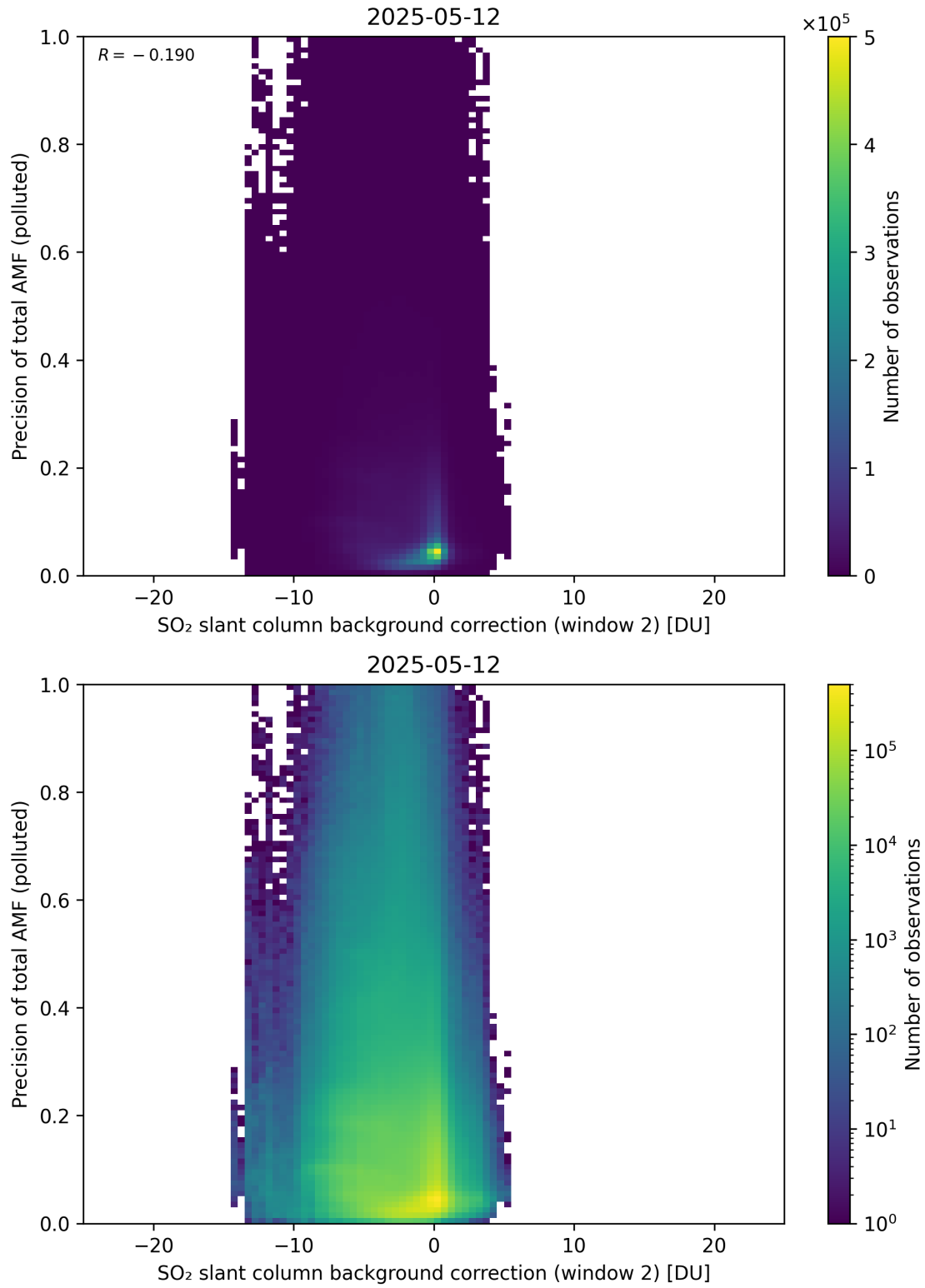
Figure 131: Scatter density plot of “SO 2 slant column background correction (window 2)” against “Precision of total AMF (polluted)” for 2025-05-11 to 2025-05-13.
