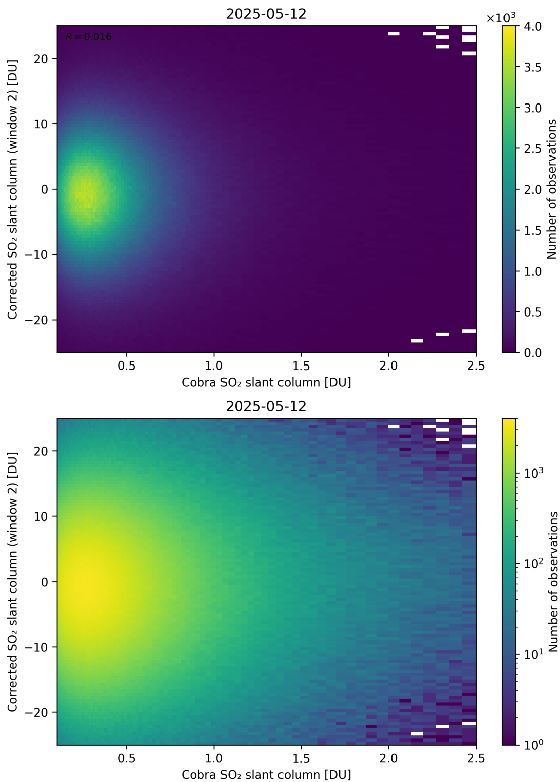
Figure 217: Scatter density plot of “Cobra SO 2 slant column” against “Corrected SO 2 slant column (window 2)” for 2025-05-11 to 2025-05-13.
