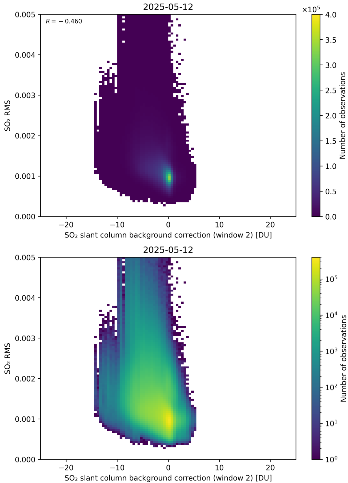
Figure 125: Scatter density plot of “SO 2 slant column background correction (window 2)” against “SO 2 RMS” for 2025-05-11 to 2025-05-13.
