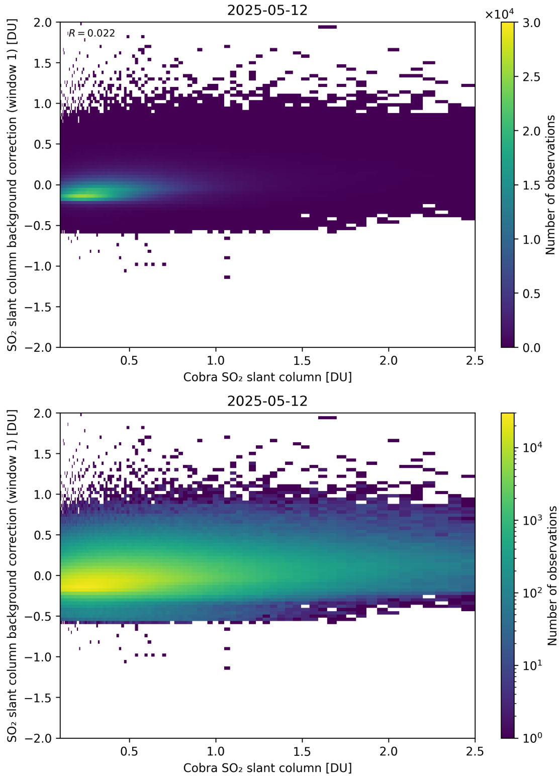
Figure 193: Scatter density plot of “Cobra SO 2 slant column” against “SO 2 slant column background correction (window 1)” for 2025-05-11 to 2025-05-13.
