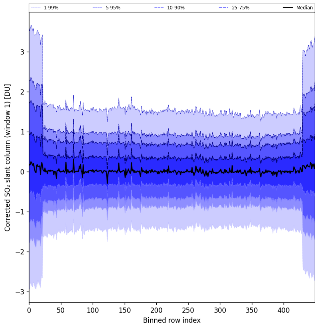
Figure 91: Along track statistics of “Corrected SO 2 slant column (window 1)” for 2025-05-11 to 2025-05-13
