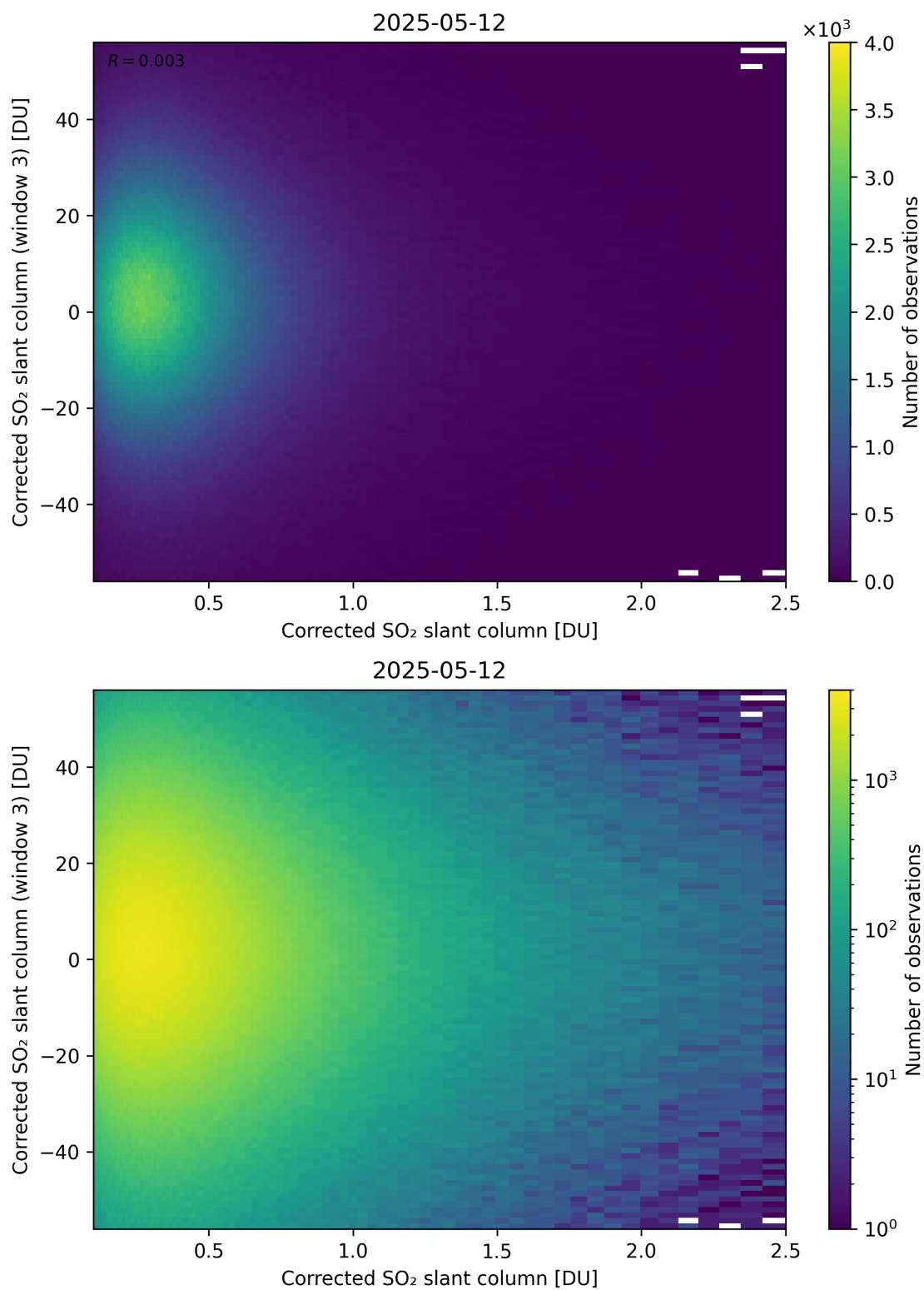
Figure 236: Scatter density plot of “Corrected SO 2 slant column” against “Corrected SO 2 slant column (window 3)” for 2025-05-11 to 2025-05-13.
