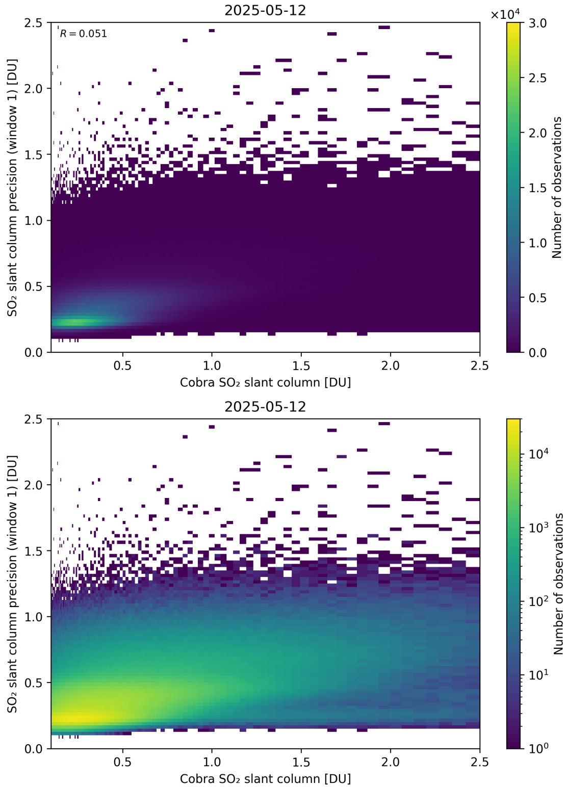
Figure 220: Scatter density plot of “Cobra SO 2 slant column” against “SO 2 slant column precision (window 1)” for 2025-05-11 to 2025-05-13.
