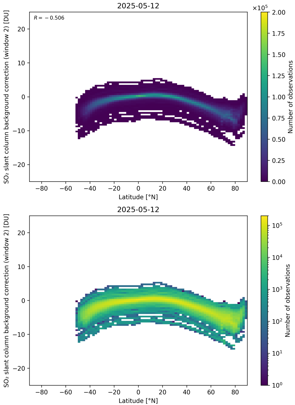
Figure 151: Scatter density plot of “Latitude” against “SO 2 slant column background correction (window 2)” for 2025-05-11 to 2025-05-13.
