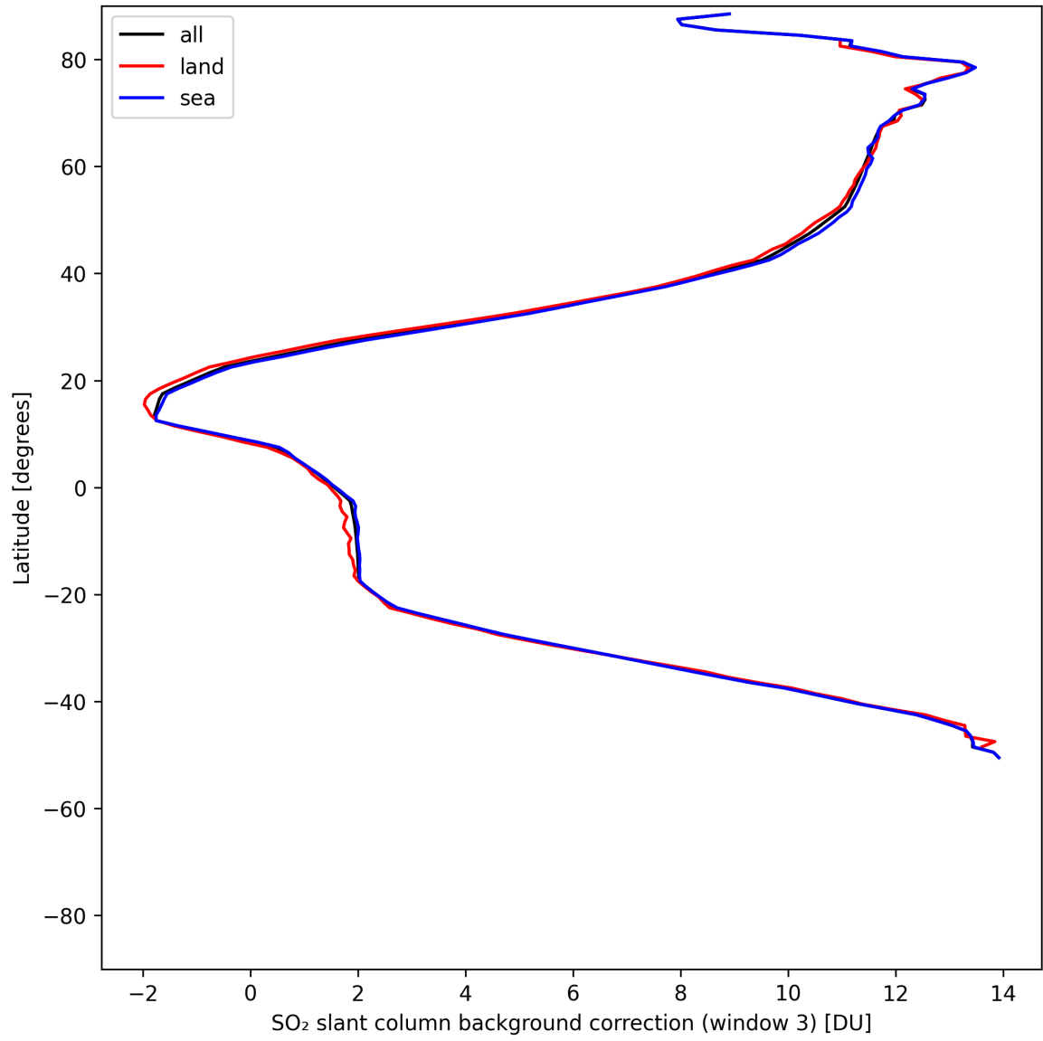
Figure 48: Zonal average of “SO 2 slant column background correction (window 3)” for 2025-05-11 to 2025-05-13.
