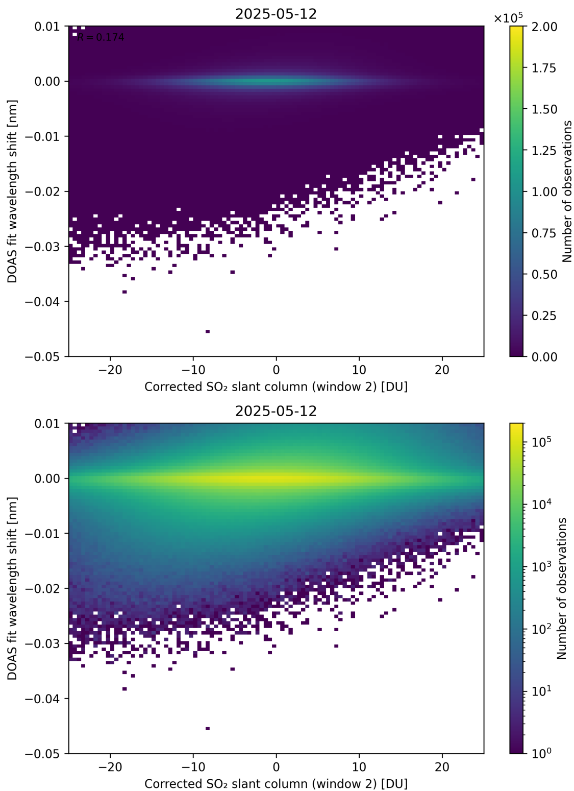
Figure 246: Scatter density plot of “Corrected SO 2 slant column (window 2)” against “DOAS fit wavelength shift” for 2025-05-11 to 2025-05-13.
