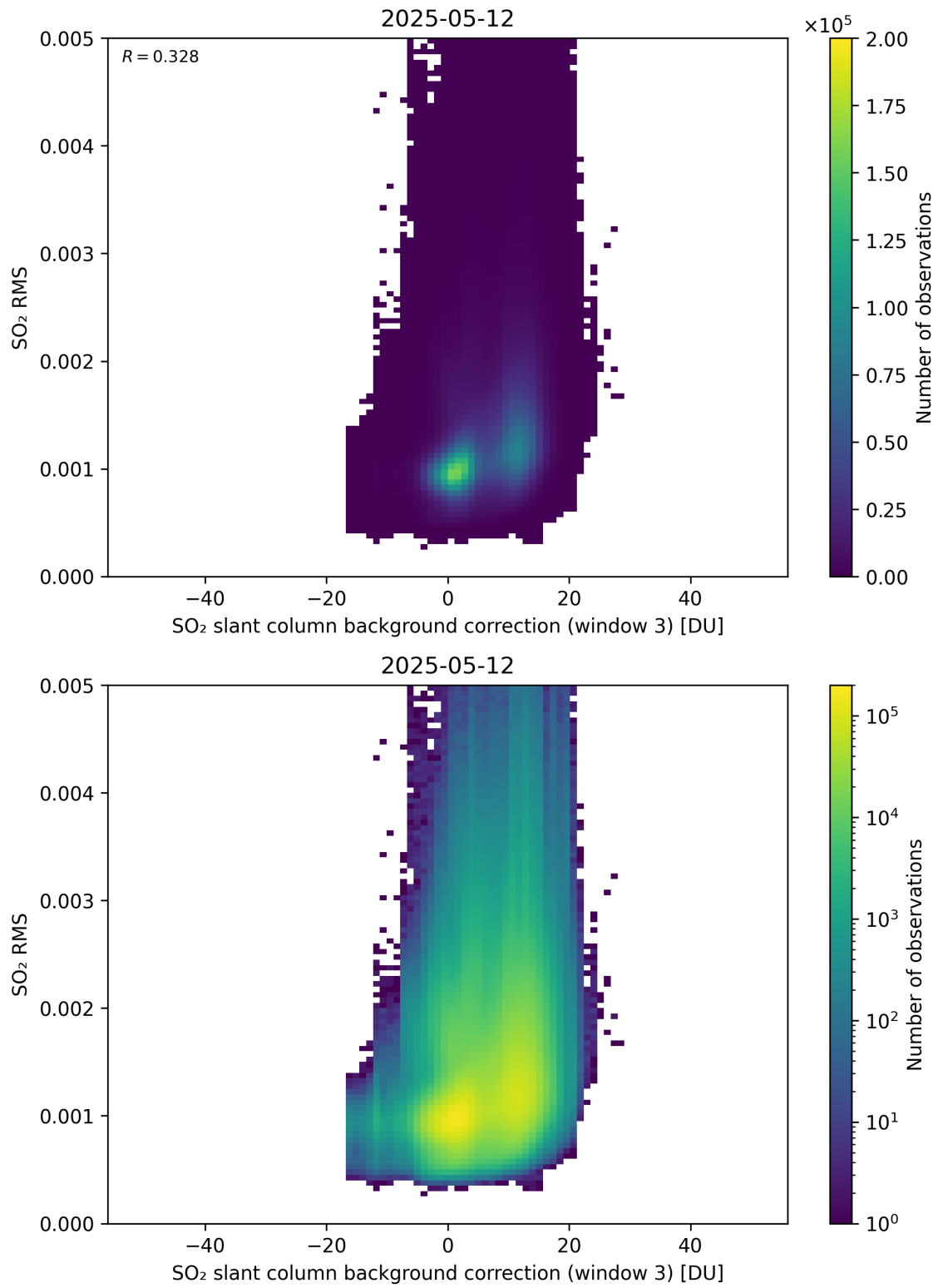
Figure 134: Scatter density plot of “SO 2 slant column background correction (window 3)” against “SO 2 RMS” for 2025-05-11 to 2025-05-13.
