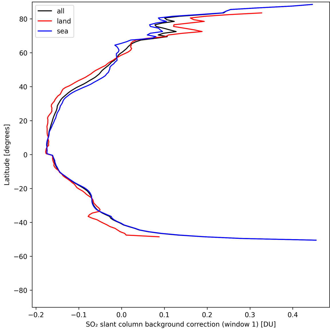
Figure 40: Zonal average of “SO 2 slant column background correction (window 1)” for 2025-05-11 to 2025-05-13.
