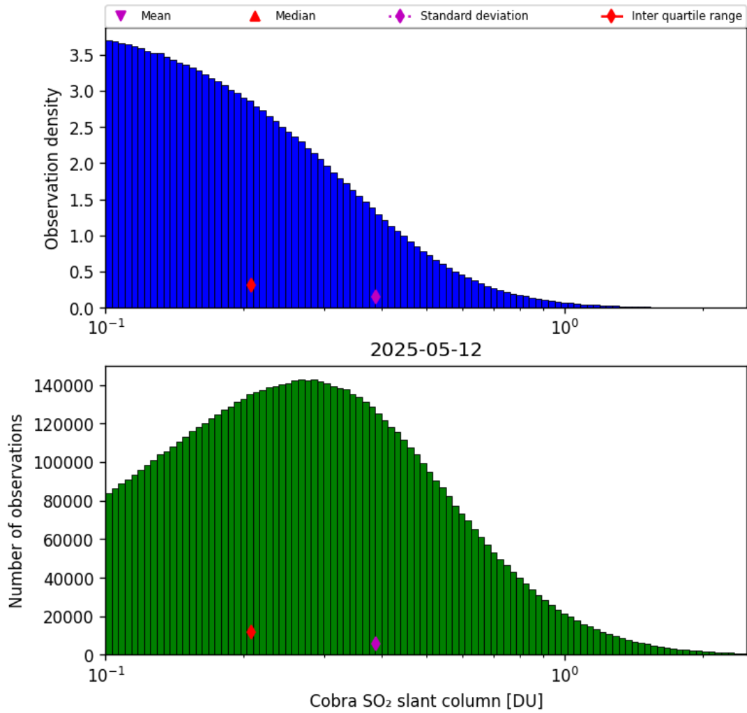
Figure 61: Histogram of “Cobra SO 2 slant column” for 2025-05-11 to 2025-05-13
