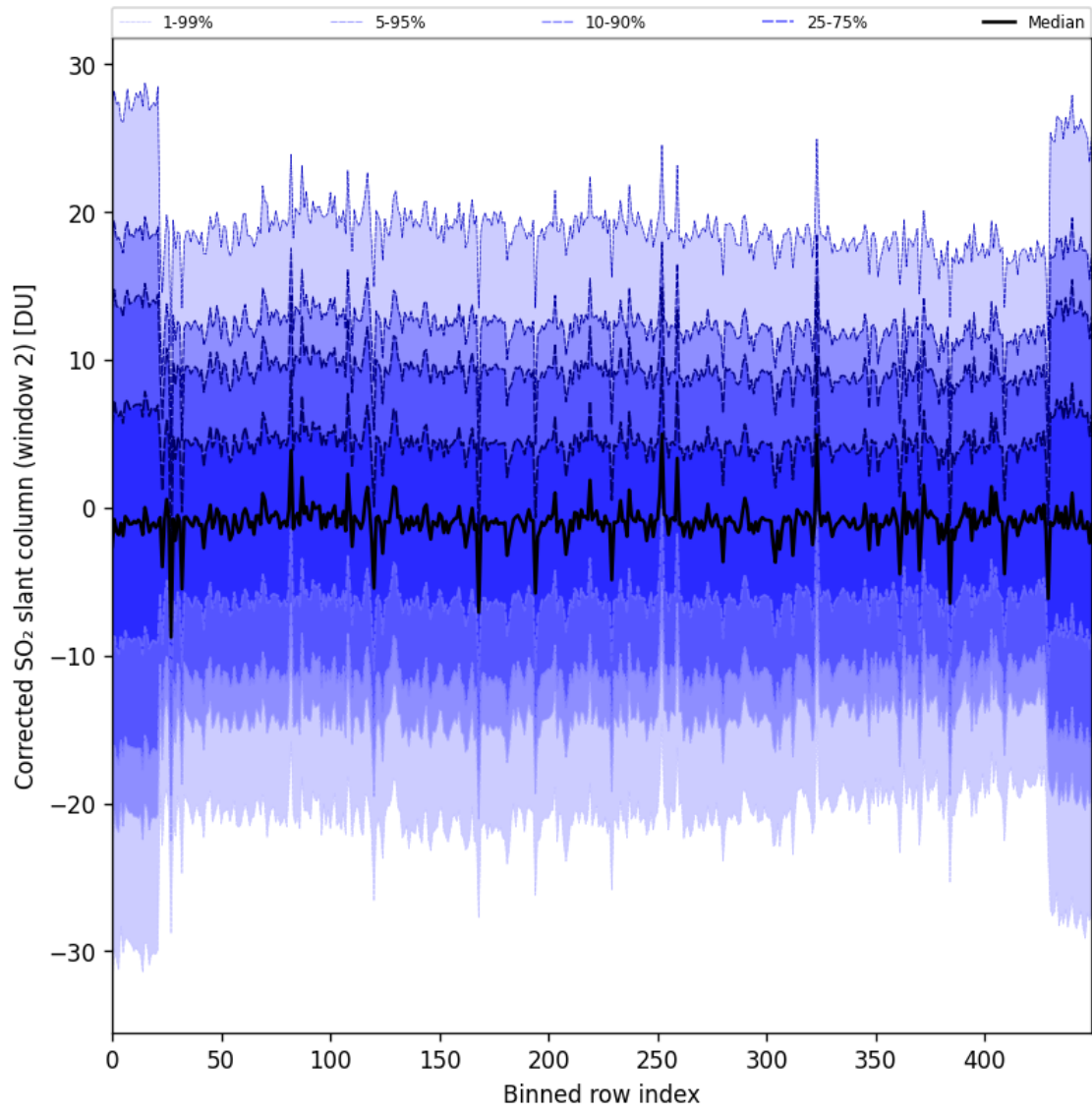
Figure 95: Along track statistics of “Corrected SO 2 slant column (window 2)” for 2025-05-11 to 2025-05-13
