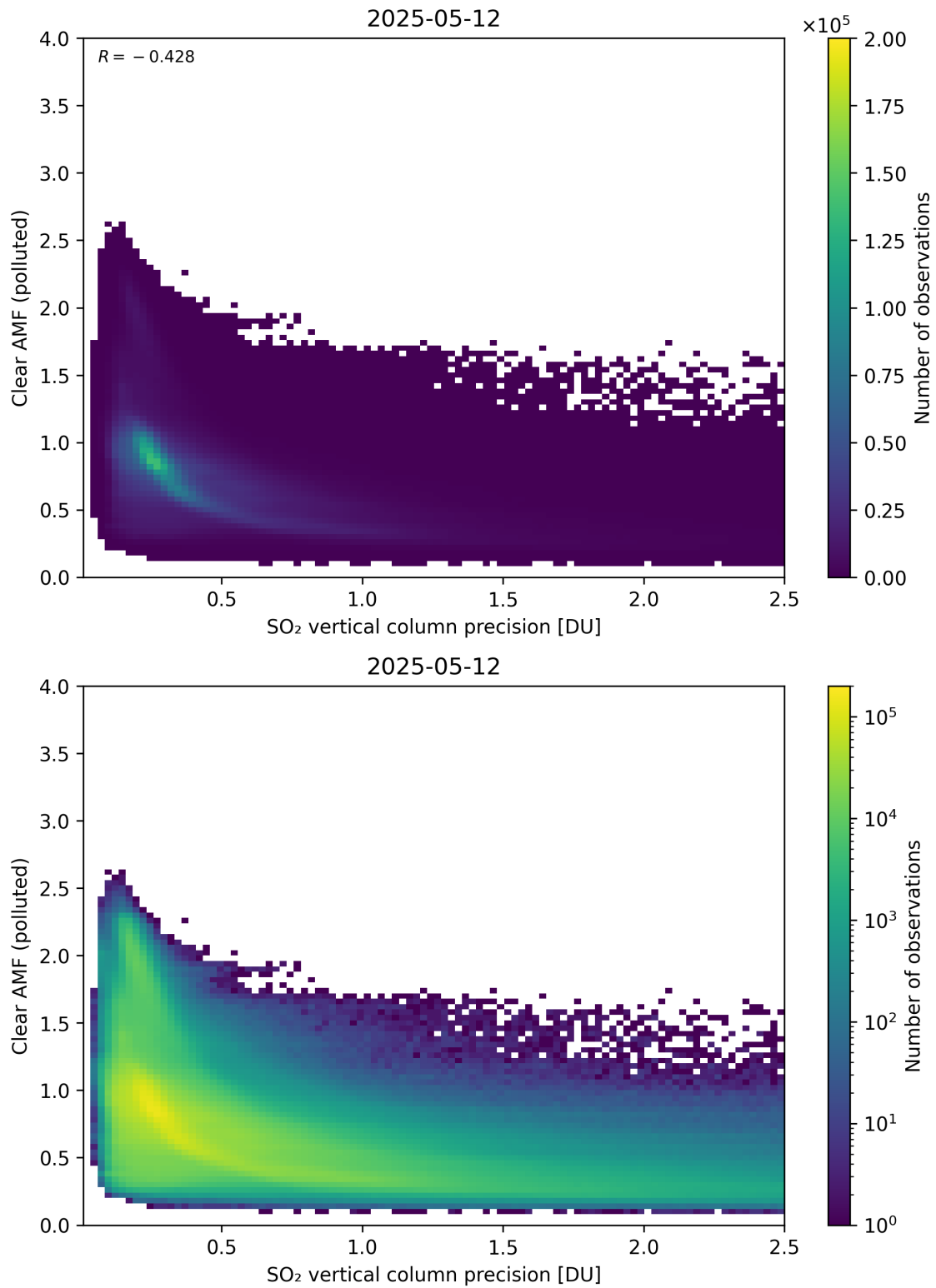
Figure 335: Scatter density plot of “SO 2 vertical column precision” against “Clear AMF (polluted)” for 2025-05-11 to 2025-05-13.
