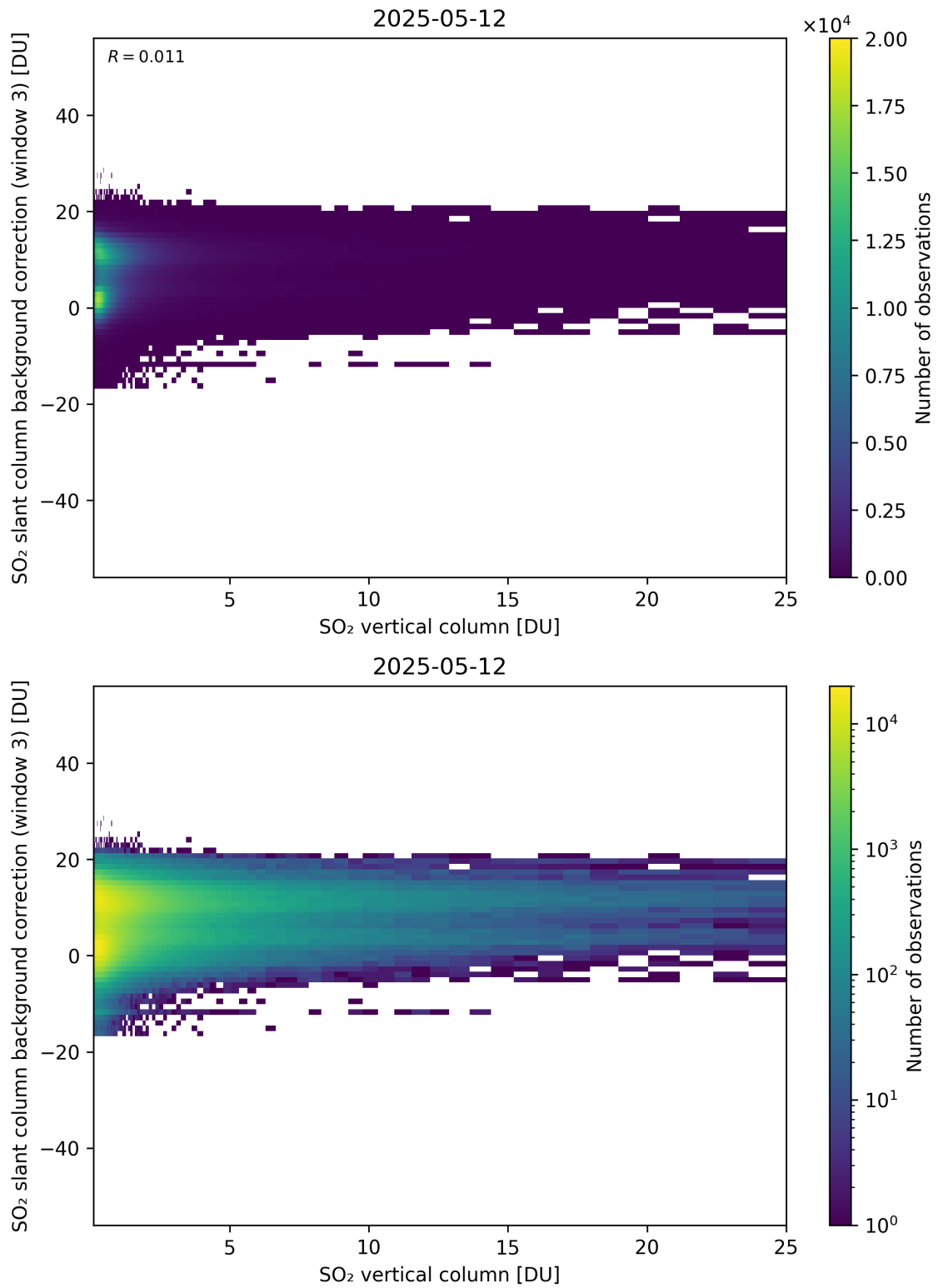
Figure 325: Scatter density plot of “SO 2 vertical column” against “SO 2 slant column background correction (window 3)” for 2025-05-11 to 2025-05-13.
