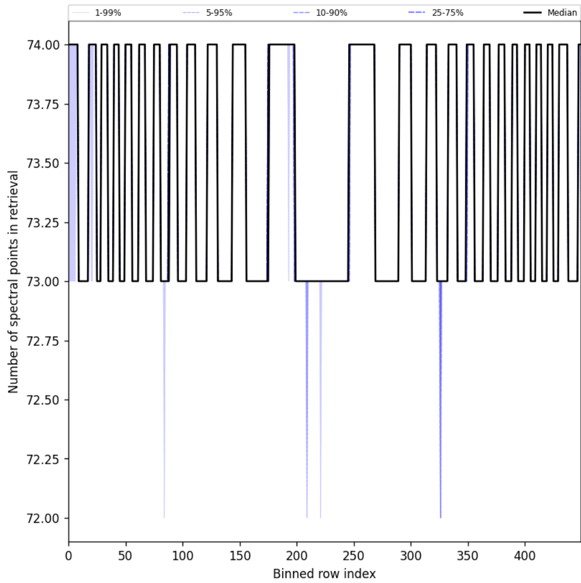
Figure 108: Along track statistics of “Number of spectral points in retrieval” for 2025-05-11 to 2025-05-13
