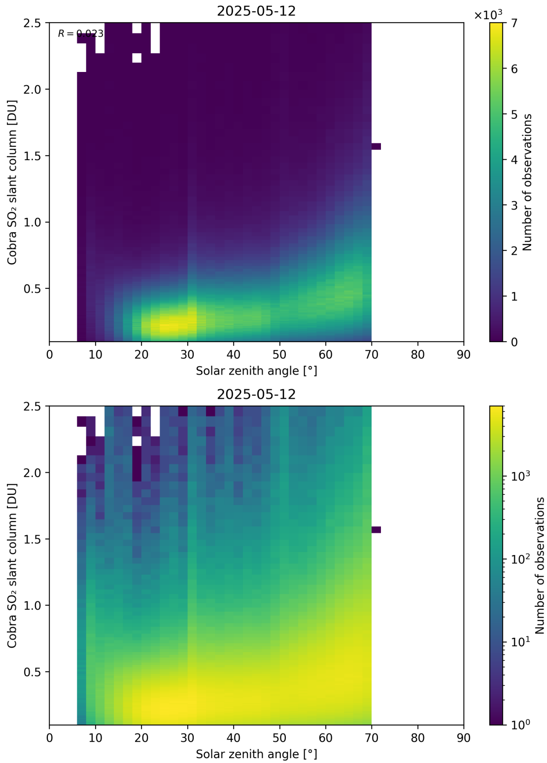
Figure 179: Scatter density plot of “Solar zenith angle” against “Cobra SO 2 slant column” for 2025-05-11 to 2025-05-13.
