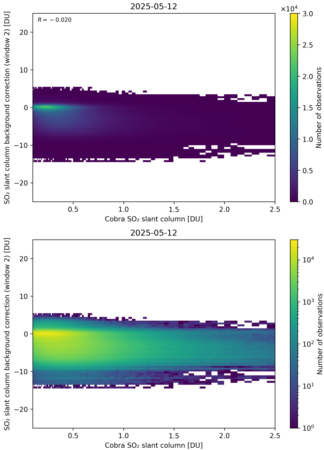
Figure 194: Scatter density plot of “Cobra SO 2 slant column” against “SO 2 slant column background correction (window 2)” for 2025-05-11 to 2025-05-13.
