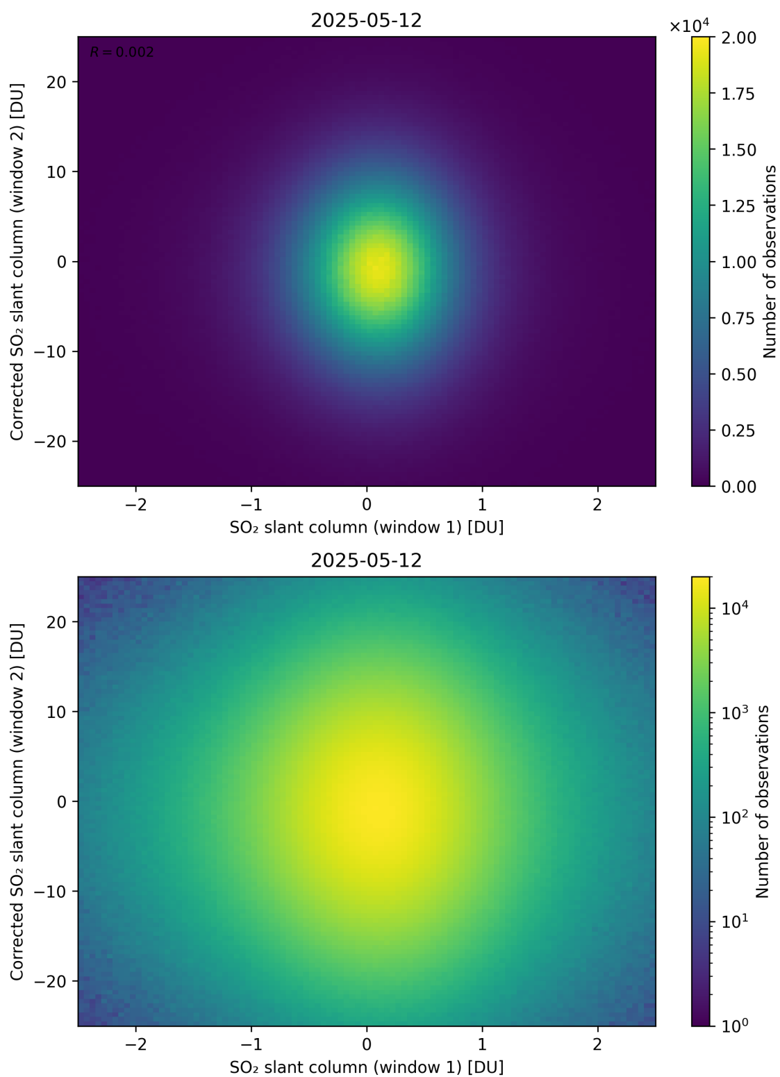
Figure 283: Scatter density plot of “SO 2 slant column (window 1)” against “Corrected SO 2 slant column (window 2)” for 2025-05-11 to 2025-05-13.
