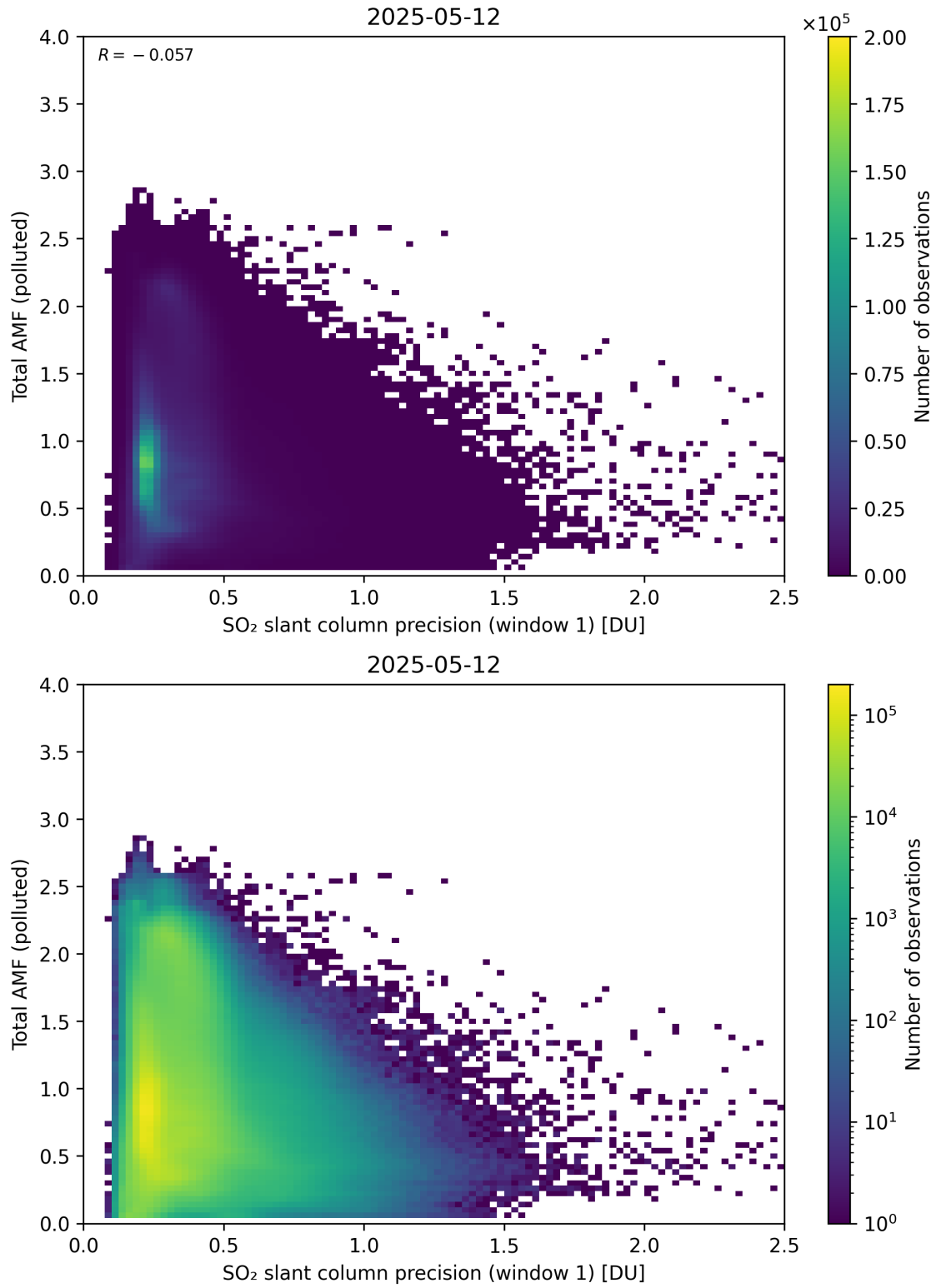
Figure 280: Scatter density plot of “SO 2 slant column precision (window 1)” against “Total AMF (polluted)” for 2025-05-11 to 2025-05-13.
