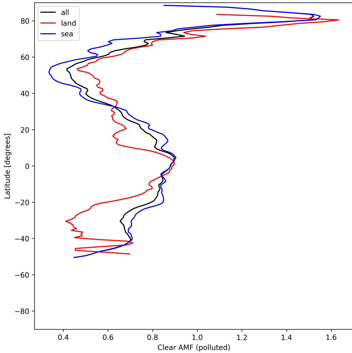
Figure 55: Zonal average of “Clear AMF (polluted)” for 2025-05-11 to 2025-05-13.
