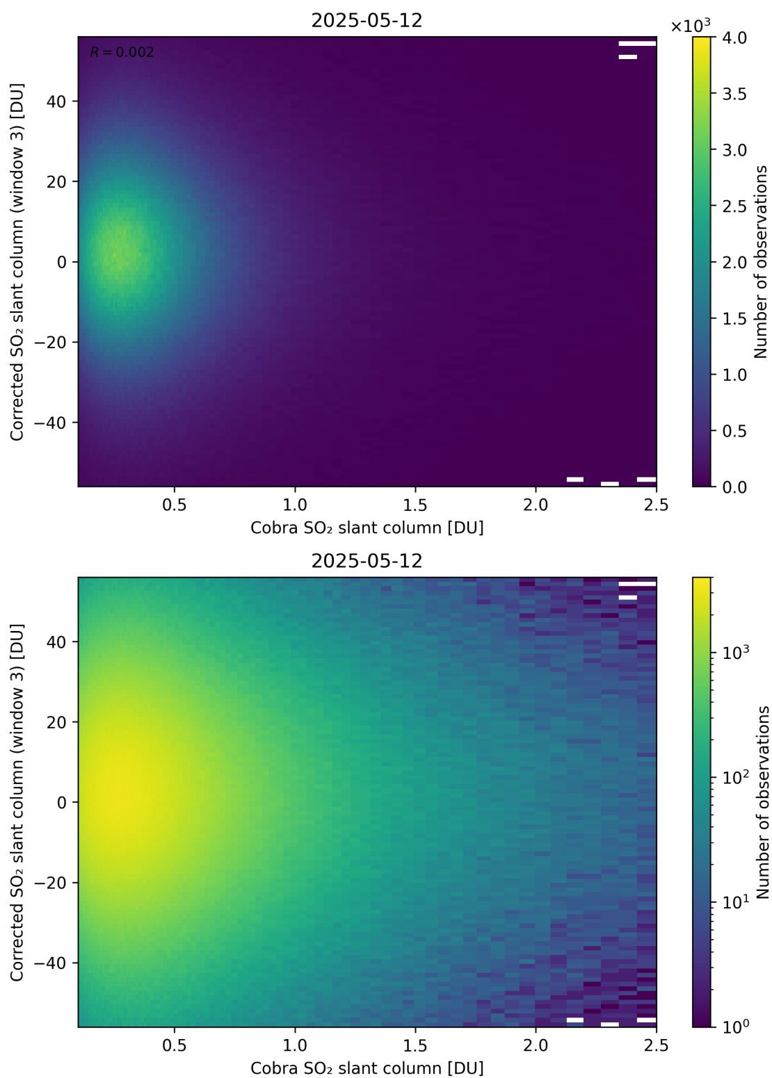
Figure 218: Scatter density plot of “Cobra SO 2 slant column” against “Corrected SO 2 slant column (window 3)” for 2025-05-11 to 2025-05-13.
