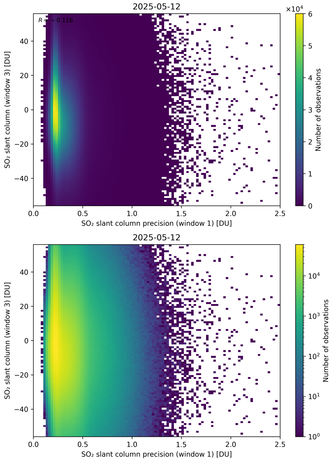
Figure 278: Scatter density plot of “SO 2 slant column precision (window 1)” against “SO 2 slant column (window 3)” for 2025-05-11 to 2025-05-13.
