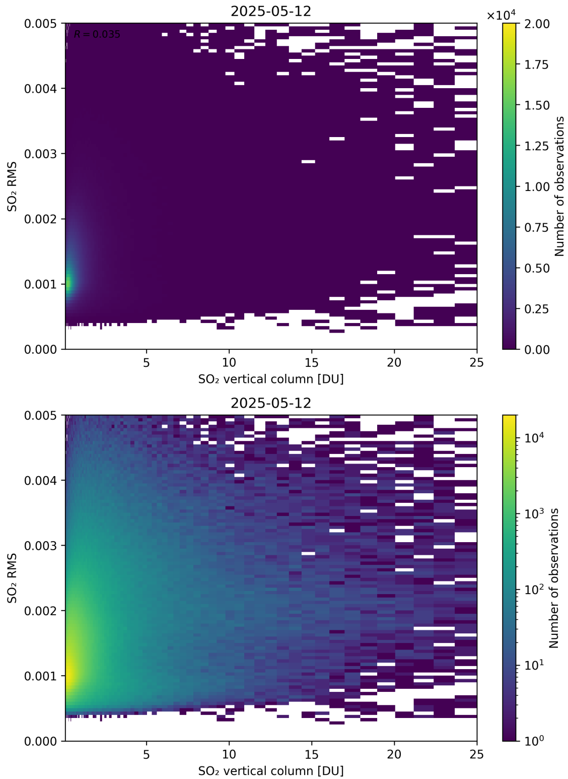
Figure 328: Scatter density plot of “SO 2 vertical column” against “SO 2 RMS” for 2025-05-11 to 2025-05-13.
