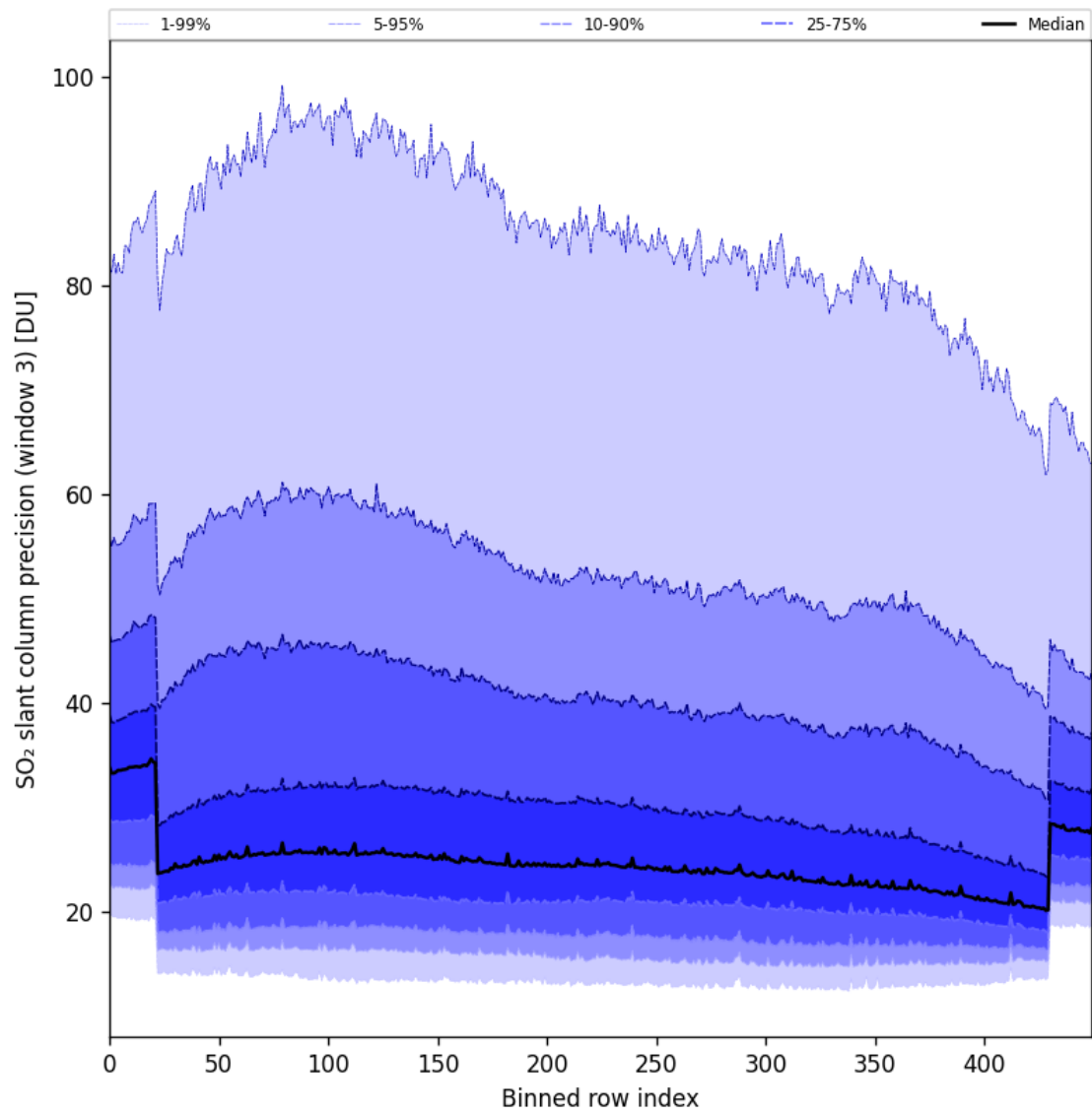
Figure 98: Along track statistics of “SO 2 slant column precision (window 3)” for 2025-05-11 to 2025-05-13
