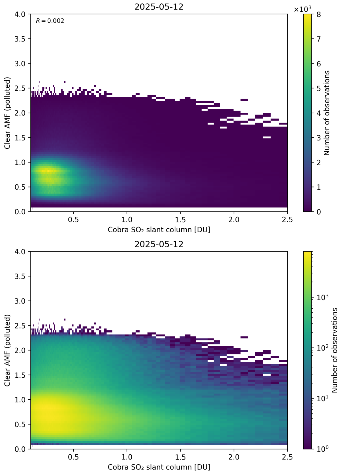
Figure 215: Scatter density plot of “Cobra SO 2 slant column” against “Clear AMF (polluted)” for 2025-05-11 to 2025-05-13.
