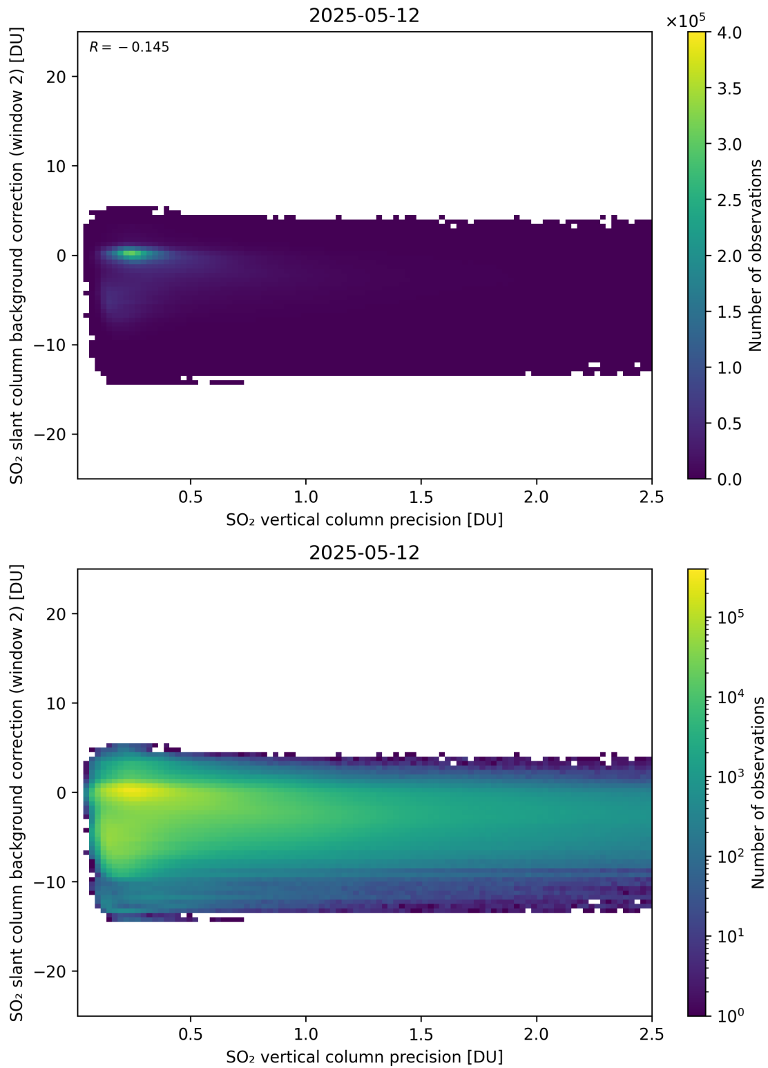
Figure 330: Scatter density plot of “SO 2 vertical column precision” against “SO 2 slant column background correction (window 2)” for 2025-05-11 to 2025-05-13.
