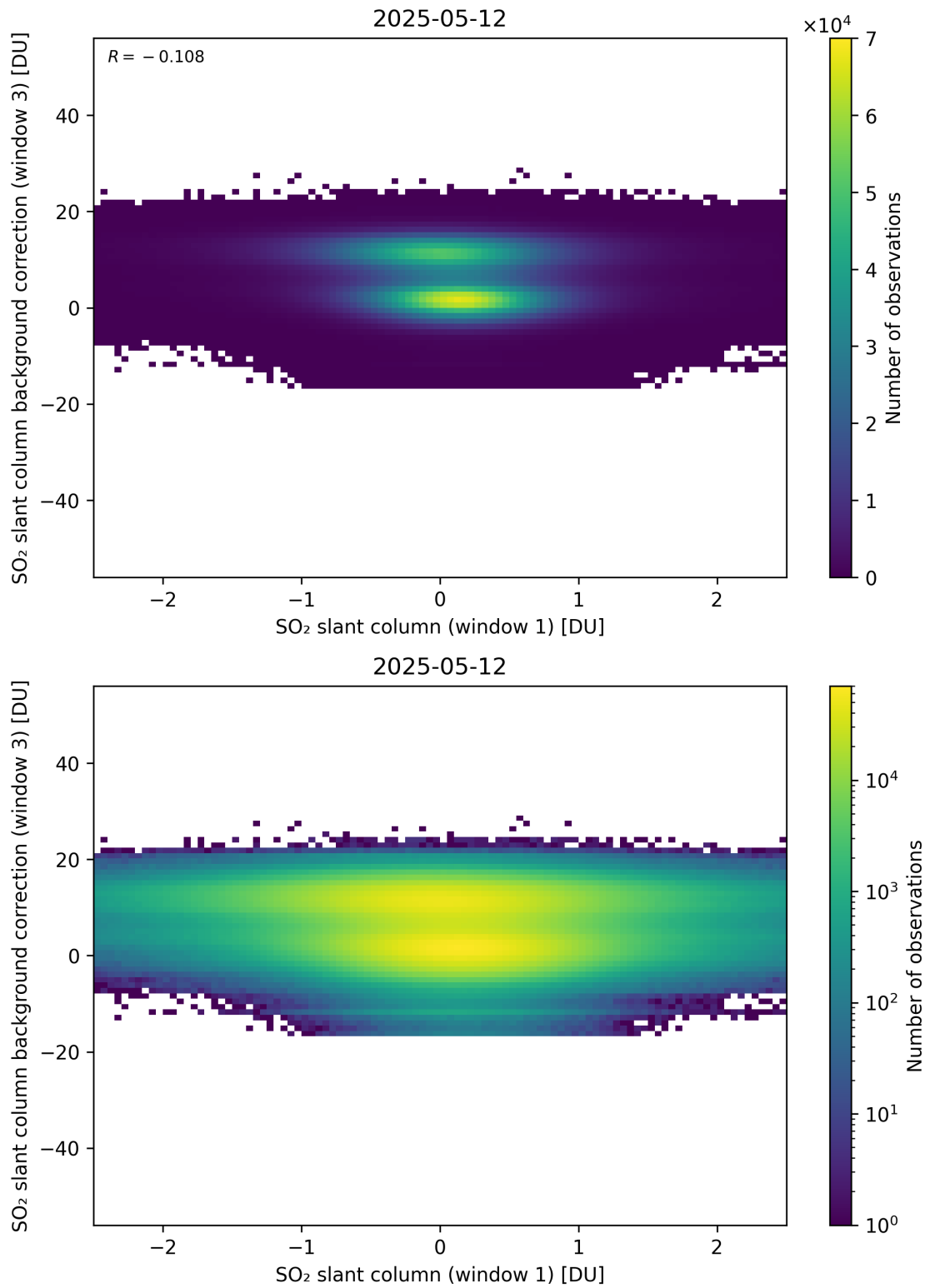
Figure 264: Scatter density plot of “SO 2 slant column (window 1)” against “SO 2 slant column background correction (window 3)” for 2025-05-11 to 2025-05-13.
