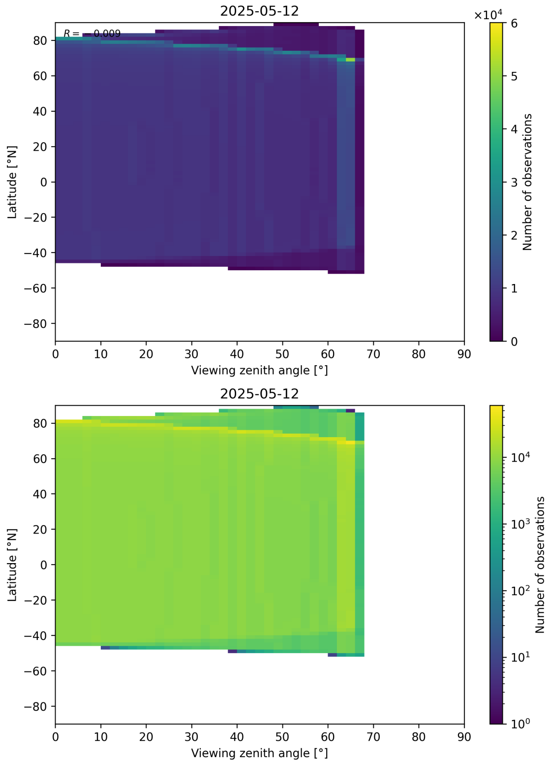
Figure 368: Scatter density plot of “Viewing zenith angle” against “Latitude” for 2025-05-11 to 2025-05-13.
