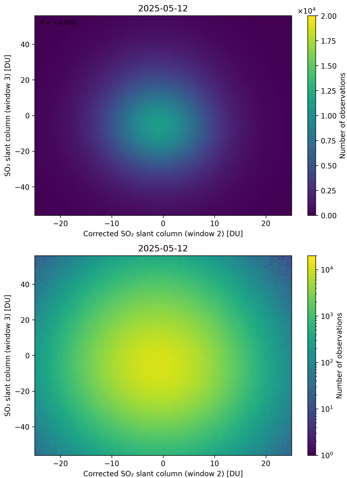
Figure 251: Scatter density plot of “Corrected SO 2 slant column (window 2)” against “SO 2 slant column (window 3)” for 2025-05-11 to 2025-05-13.
