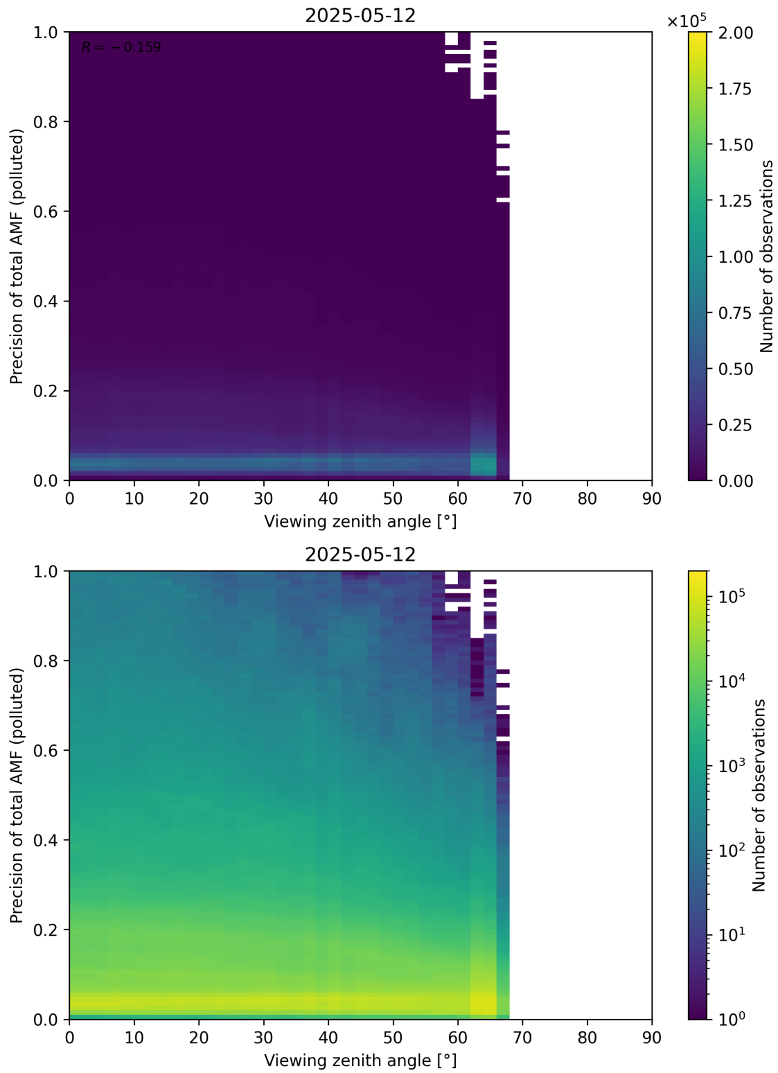
Figure 382: Scatter density plot of “Viewing zenith angle” against “Precision of total AMF (polluted)” for 2025-05-11 to 2025-05-13.
