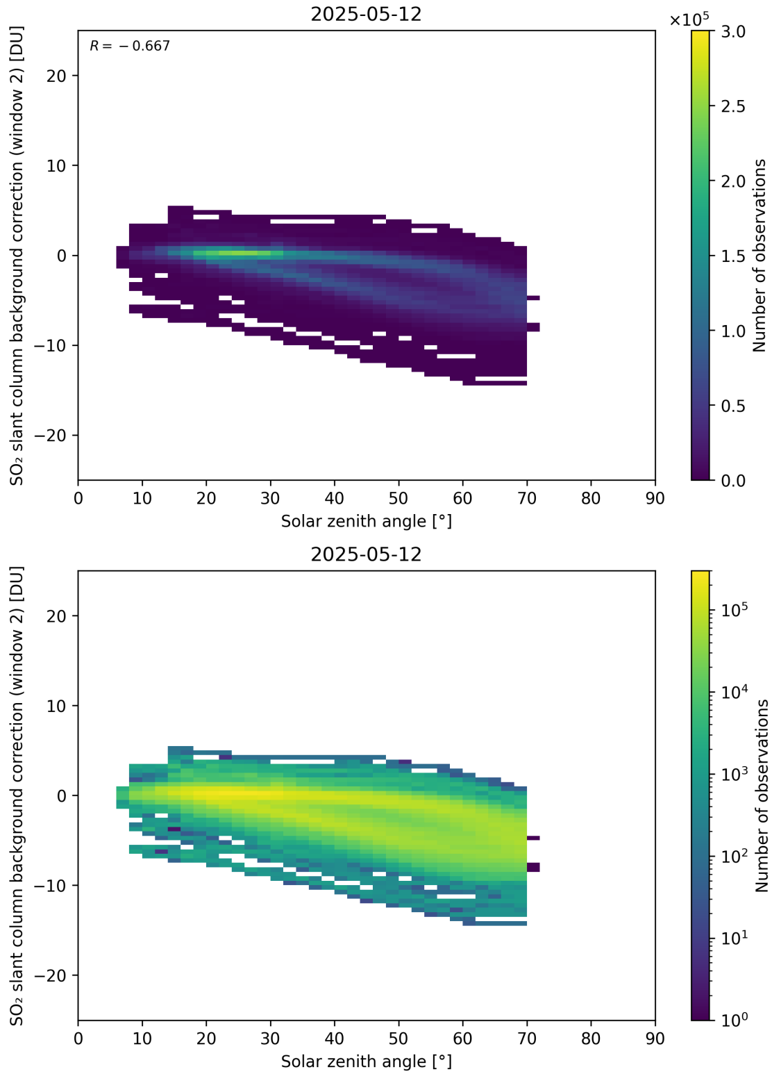
Figure 172: Scatter density plot of “Solar zenith angle” against “SO 2 slant column background correction (window 2)” for 2025-05-11 to 2025-05-13.
