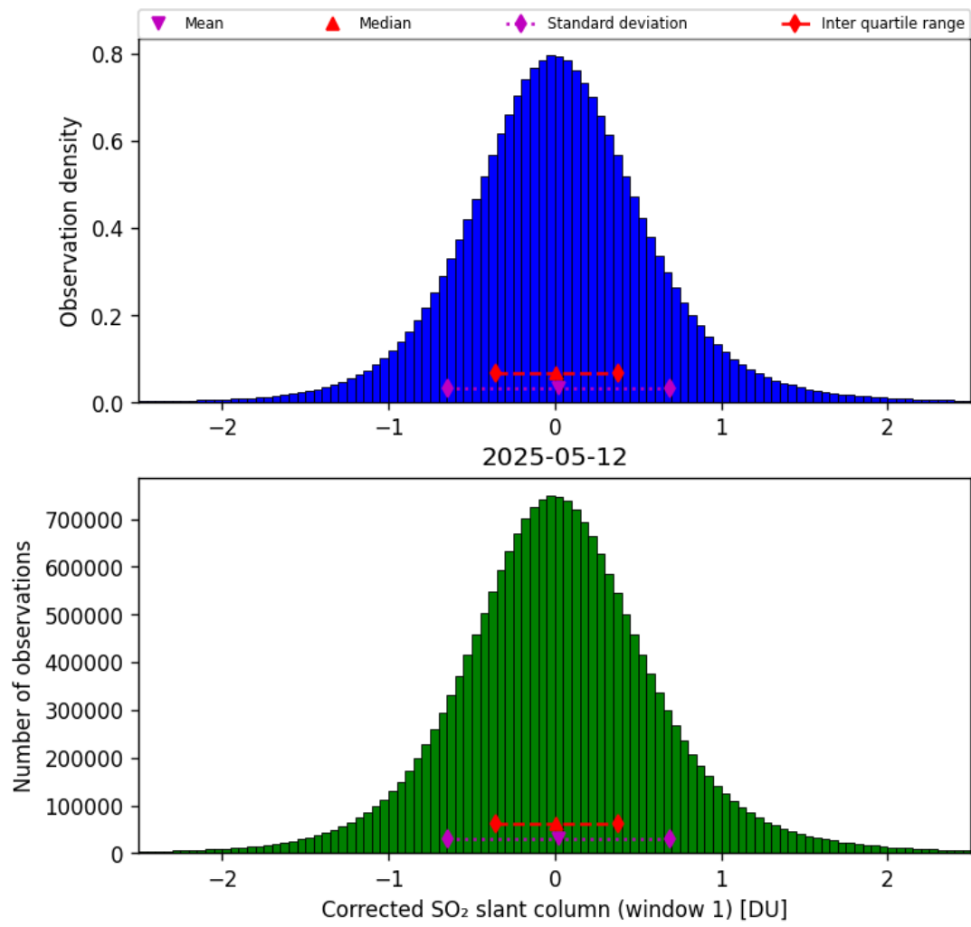
Figure 65: Histogram of “Corrected SO 2 slant column (window 1)” for 2025-05-11 to 2025-05-13
