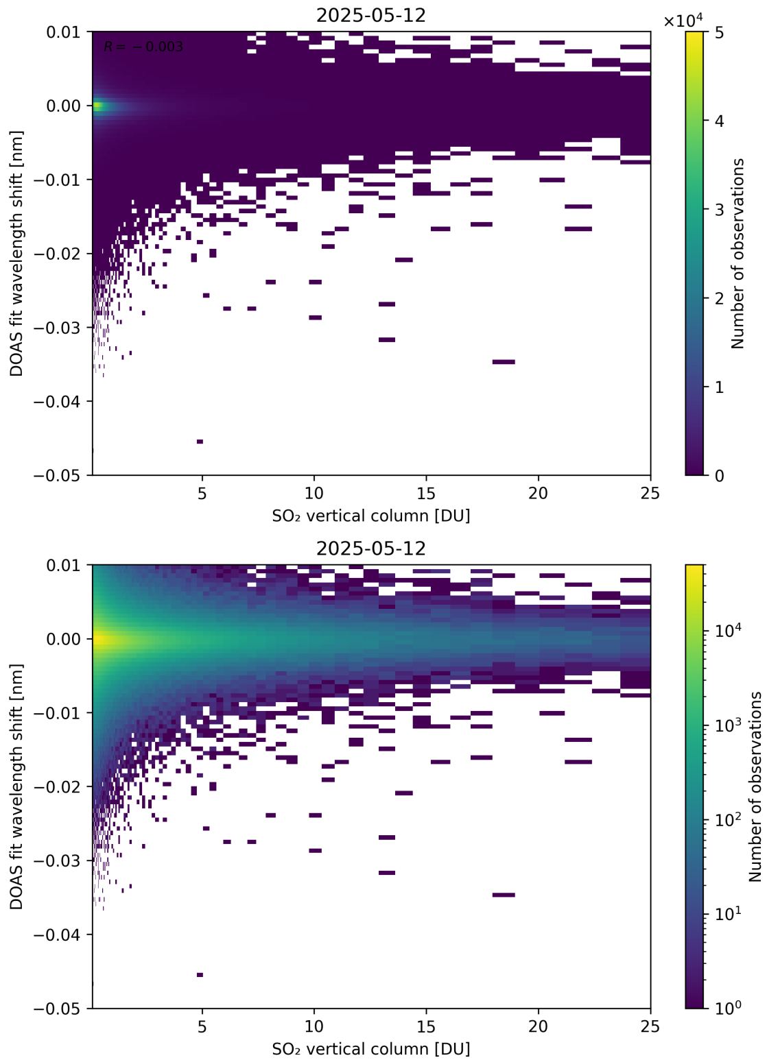
Figure 326: Scatter density plot of “SO 2 vertical column” against “DOAS fit wavelength shift” for 2025-05-11 to 2025-05-13.
