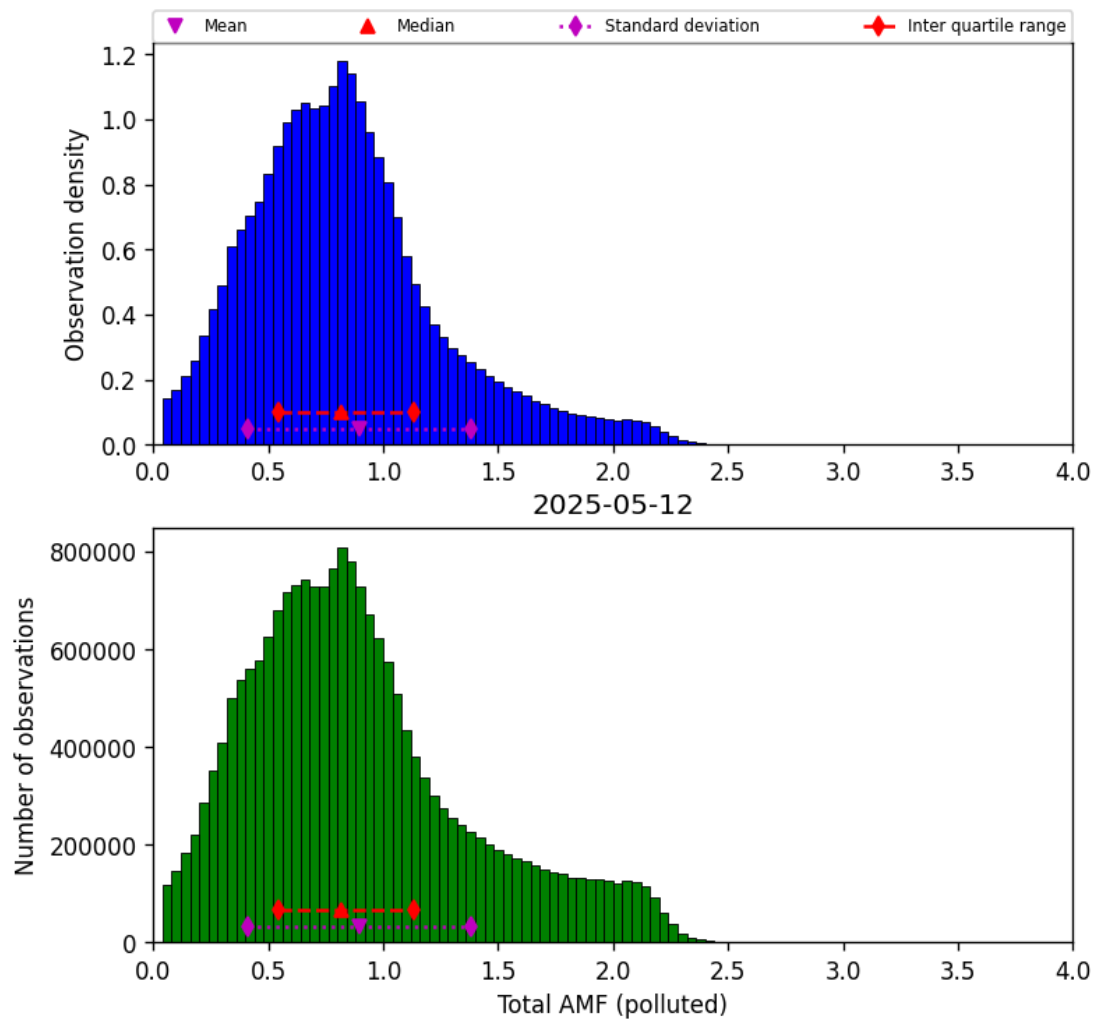
Figure 79: Histogram of “Total AMF (polluted)” for 2025-05-11 to 2025-05-13
