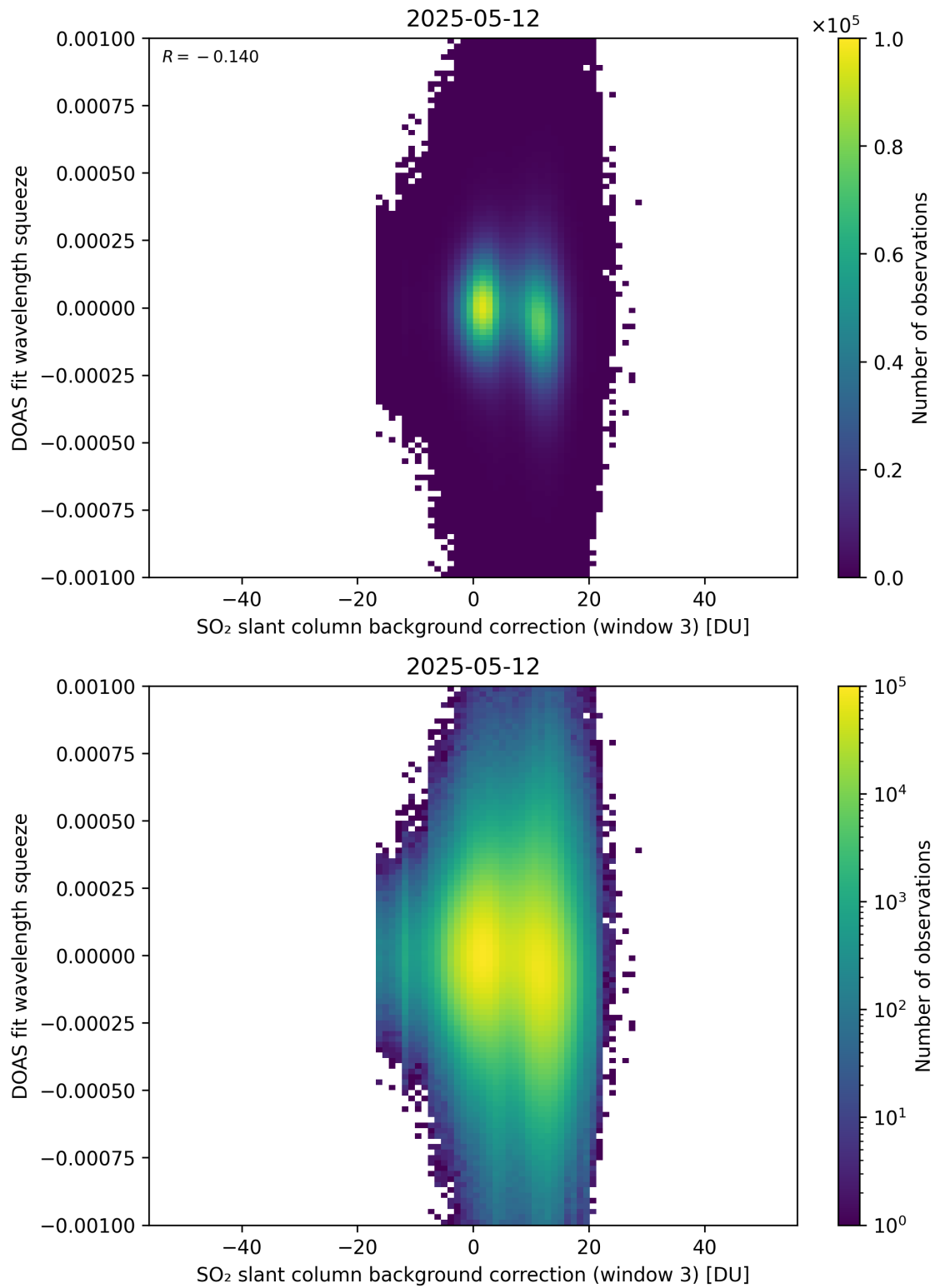
Figure 133: Scatter density plot of “SO 2 slant column background correction (window 3)” against “DOAS fit wavelength squeeze” for 2025-05-11 to 2025-05-13.
