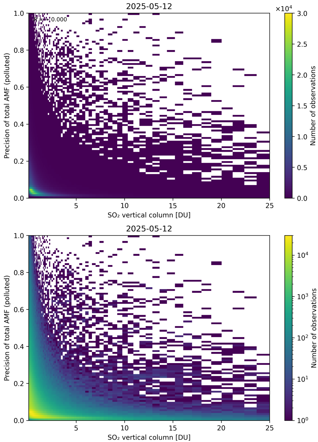
Figure 360: Scatter density plot of “SO 2 vertical column” against “Precision of total AMF (polluted)” for 2025-05-11 to 2025-05-13.
