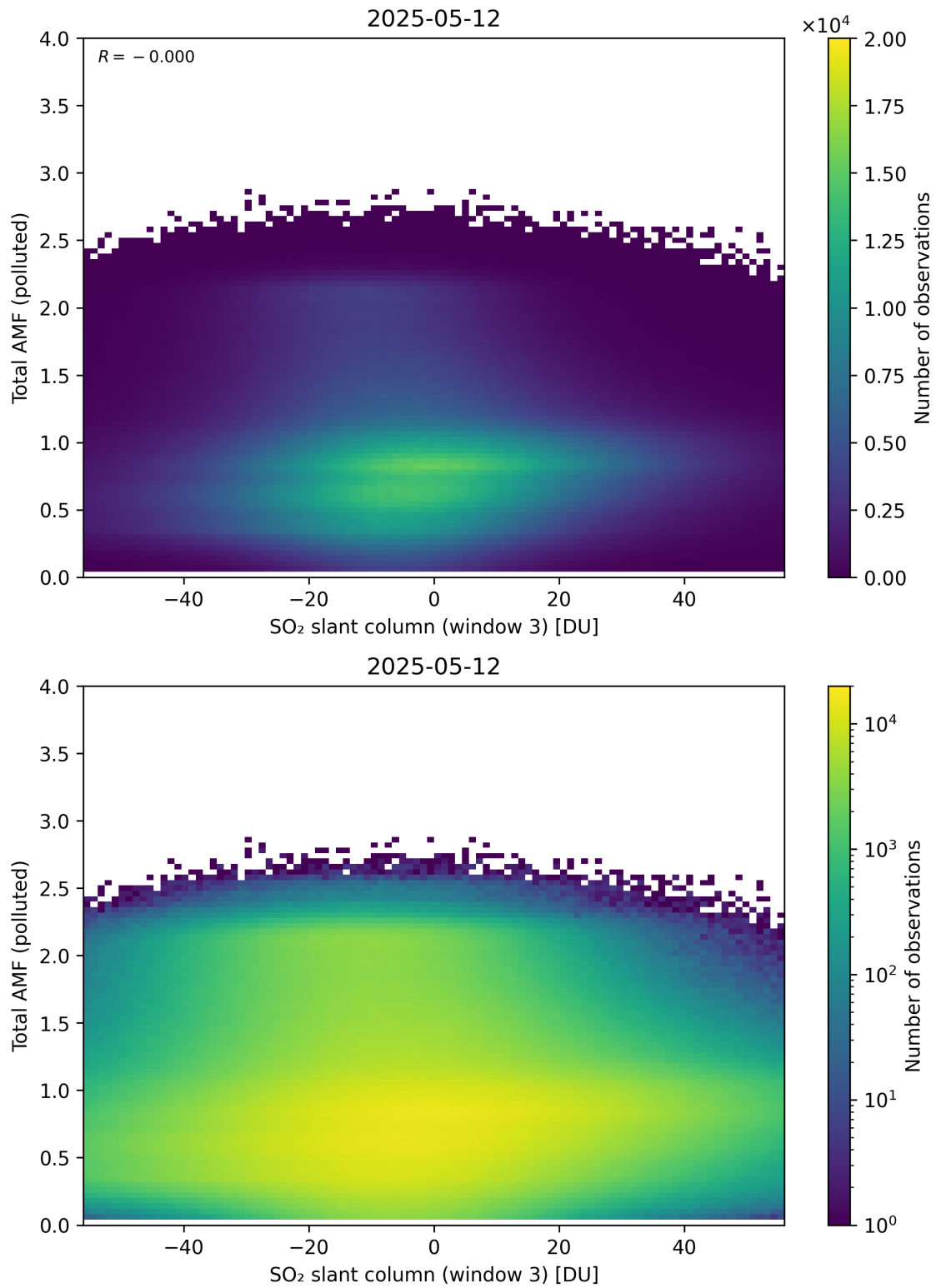
Figure 318: Scatter density plot of “SO 2 slant column (window 3)” against “Total AMF (polluted)” for 2025-05-11 to 2025-05-13.
