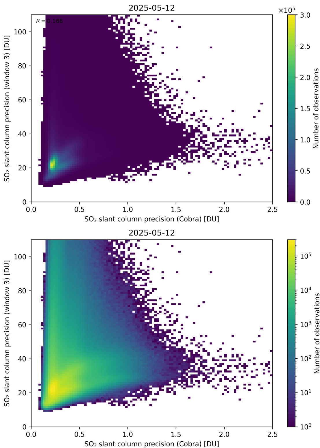
Figure 212: Scatter density plot of “SO 2 slant column precision (Cobra)” against “SO 2 slant column precision (window 3)” for 2025-05-11 to 2025-05-13.
