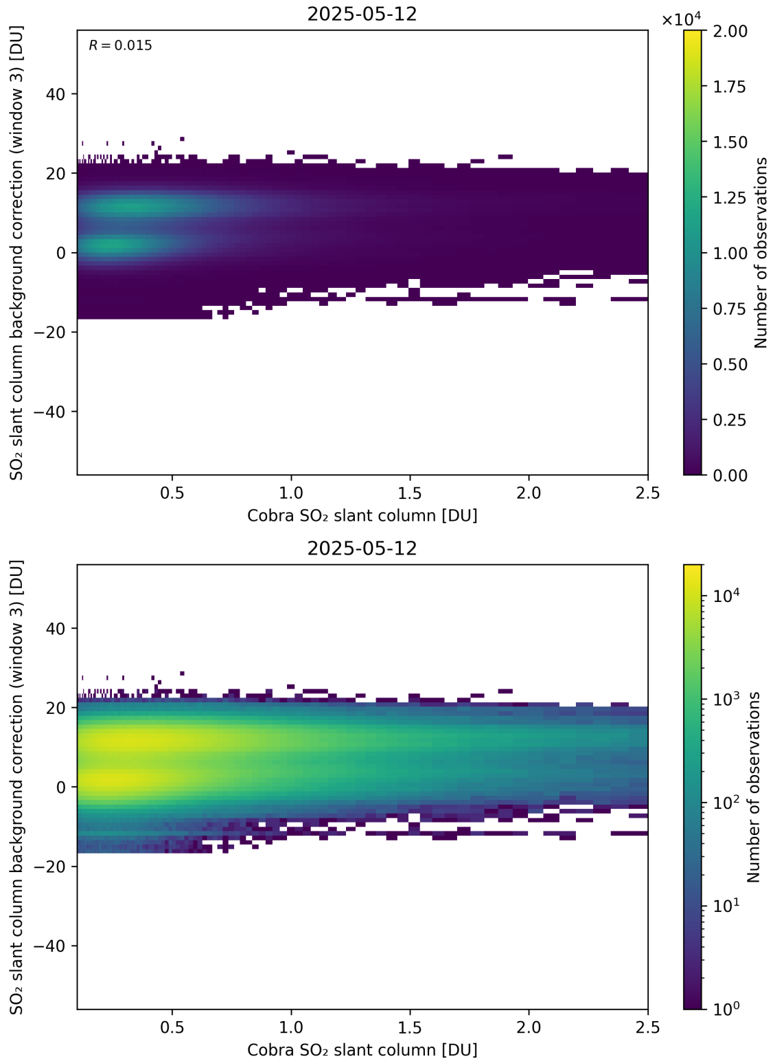
Figure 195: Scatter density plot of “Cobra SO 2 slant column” against “SO 2 slant column background correction (window 3)” for 2025-05-11 to 2025-05-13.
