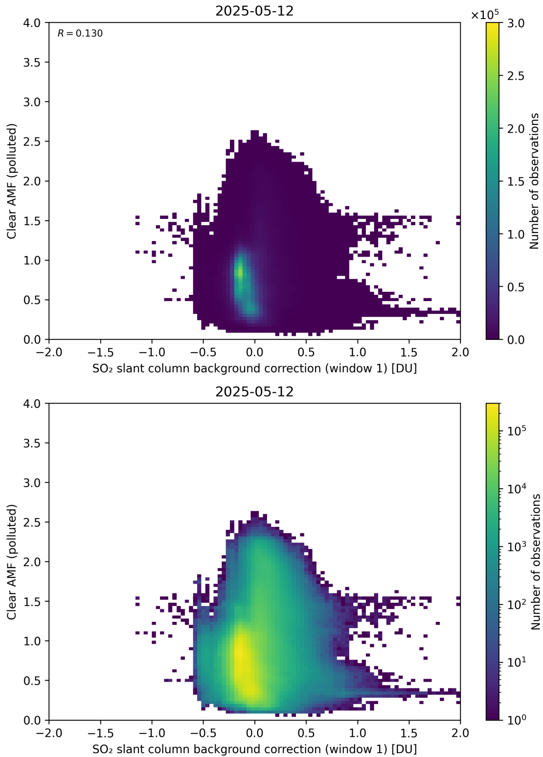
Figure 114: Scatter density plot of “SO 2 slant column background correction (window 1)” against “Clear AMF (polluted)” for 2025-05-11 to 2025-05-13.
