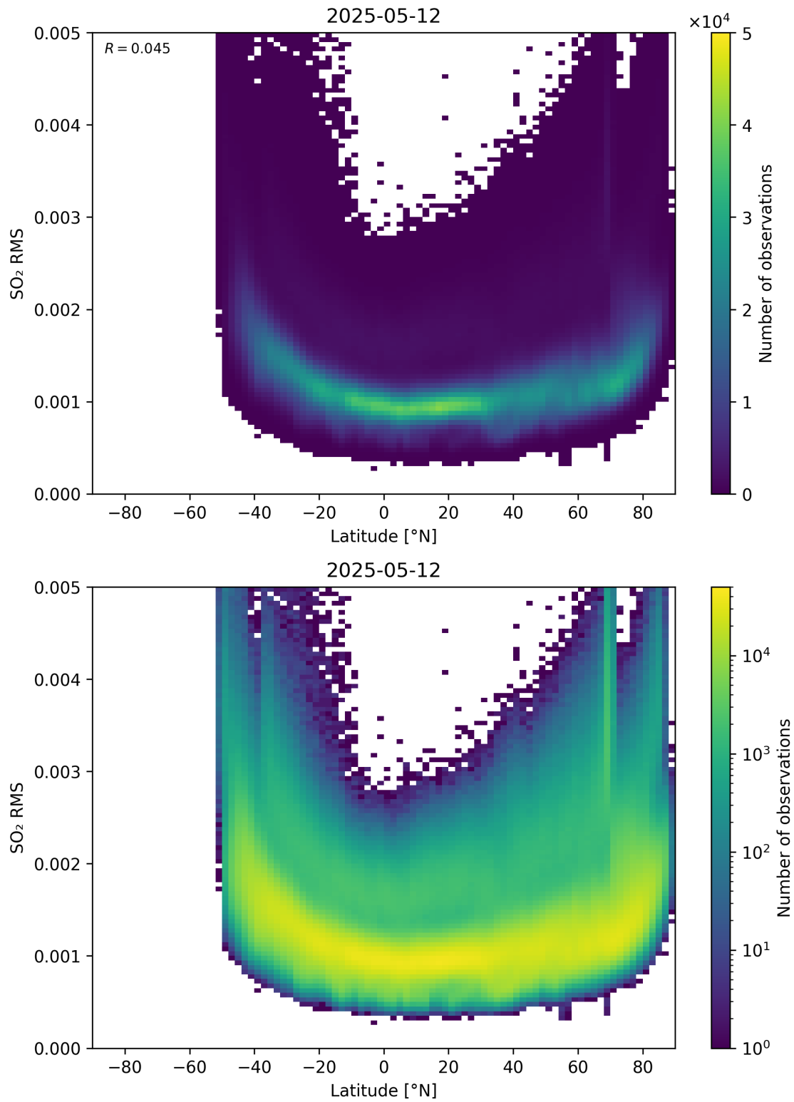
Figure 155: Scatter density plot of “Latitude” against “SO 2 RMS” for 2025-05-11 to 2025-05-13.
