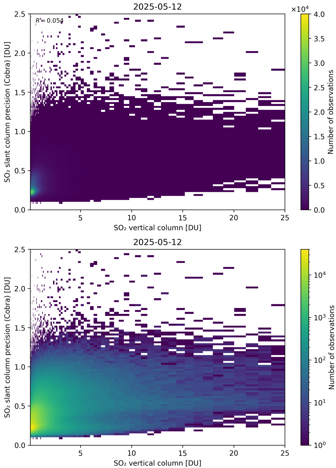
Figure 350: Scatter density plot of “SO 2 vertical column” against “SO 2 slant column precision (Cobra)” for 2025-05-11 to 2025-05-13.
