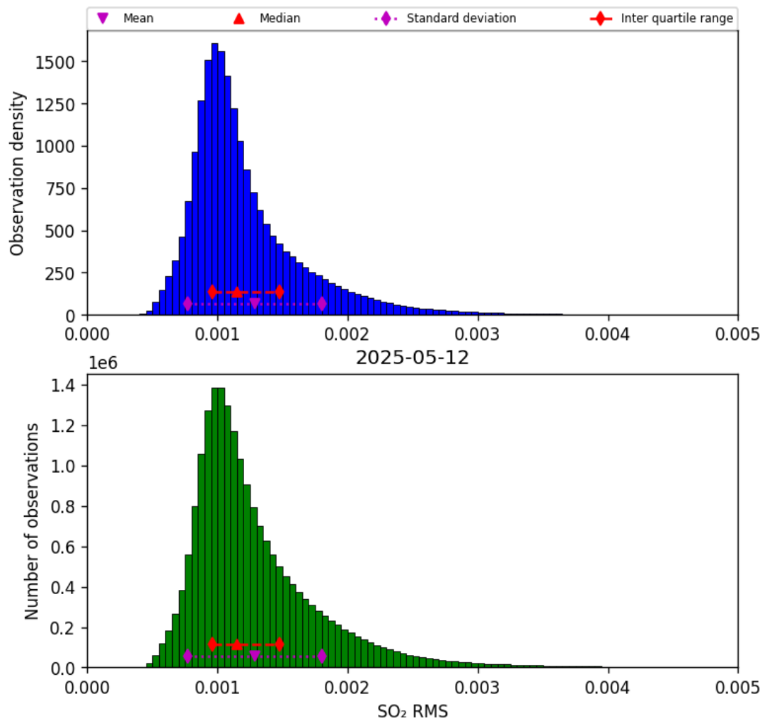
Figure 78: Histogram of “SO 2 RMS” for 2025-05-11 to 2025-05-13
