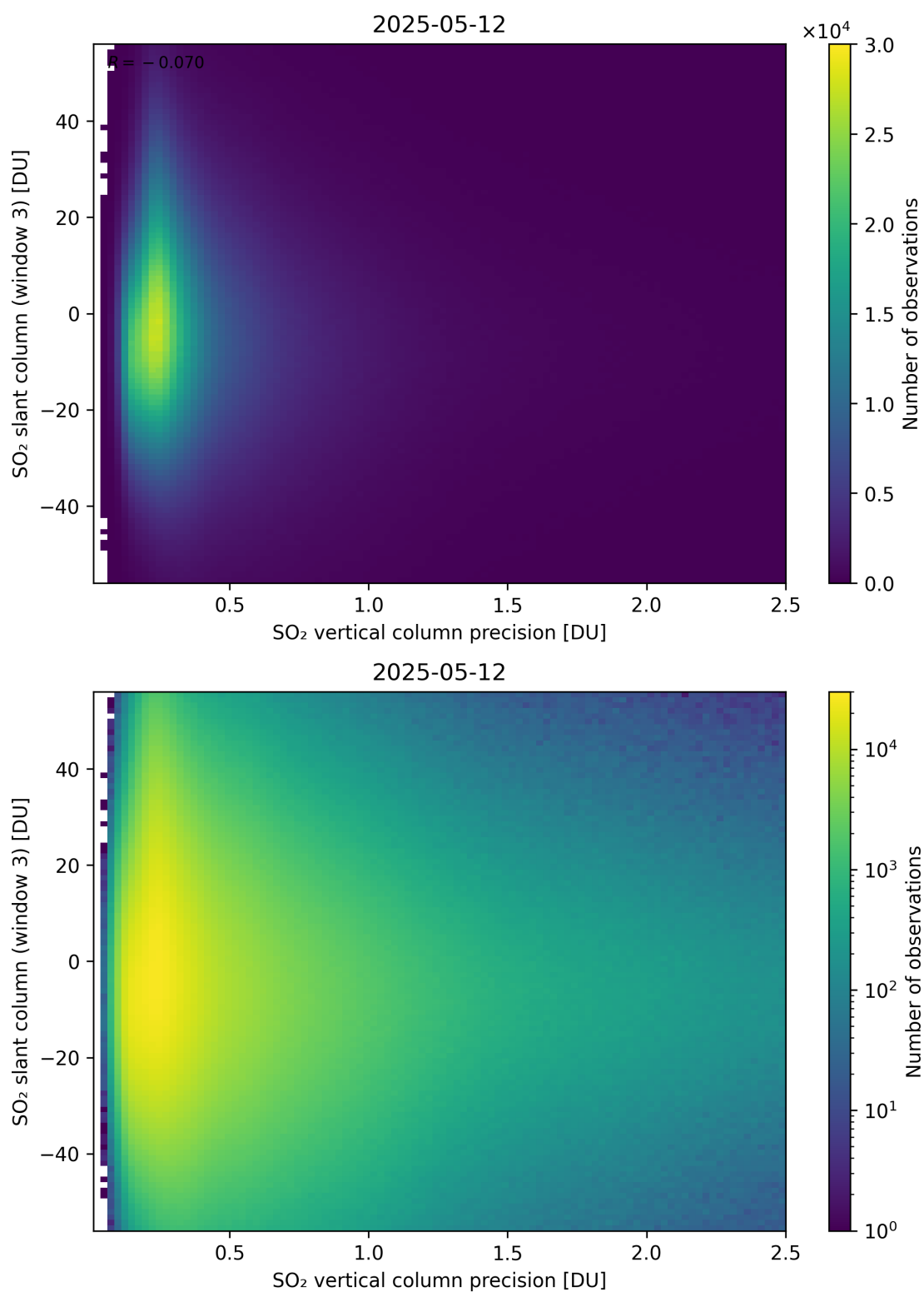
Figure 344: Scatter density plot of “SO 2 vertical column precision” against “SO 2 slant column (window 3)” for 2025-05-11 to 2025-05-13.
