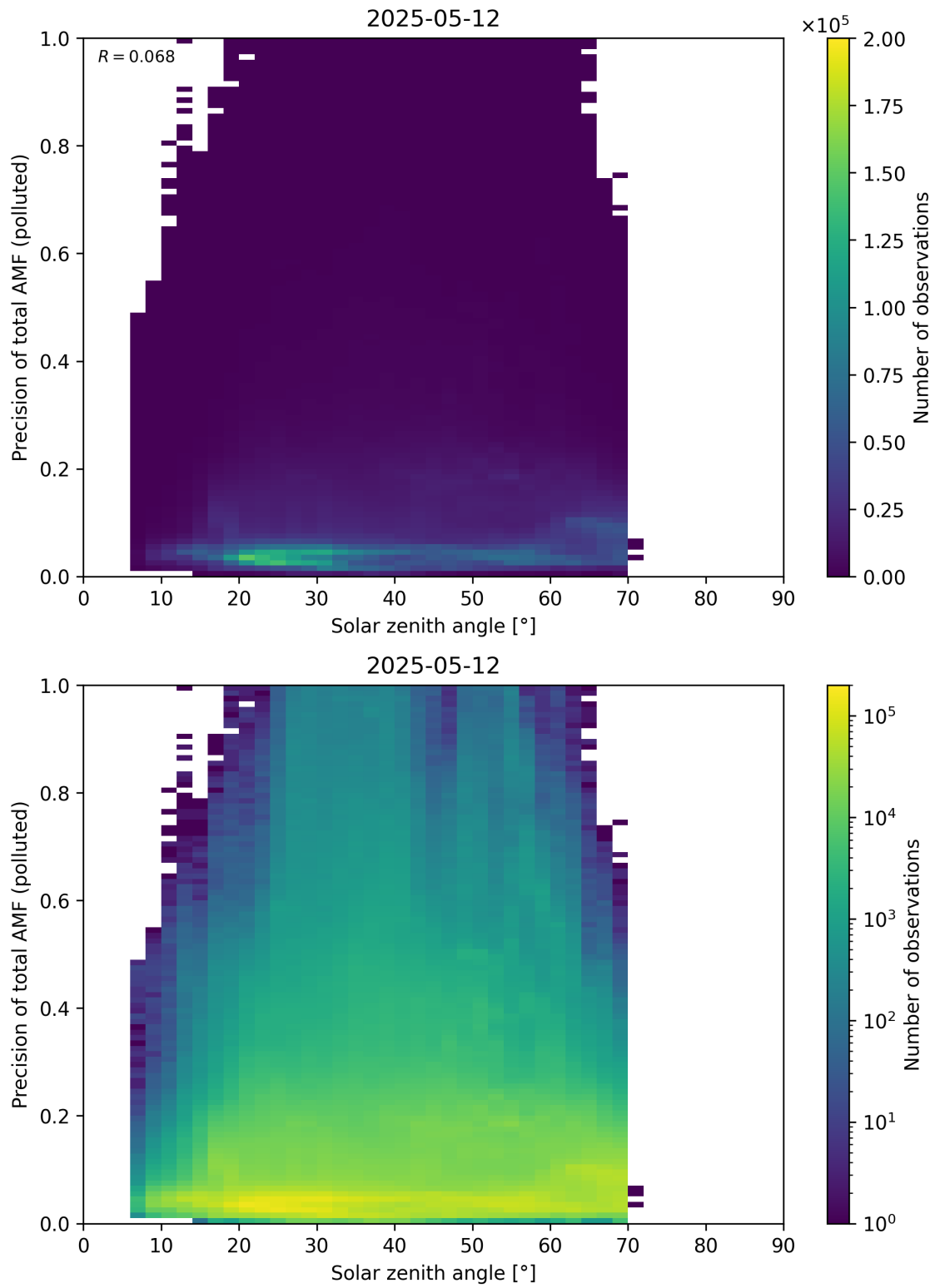
Figure 190: Scatter density plot of “Solar zenith angle” against “Precision of total AMF (polluted)” for 2025-05-11 to 2025-05-13.
