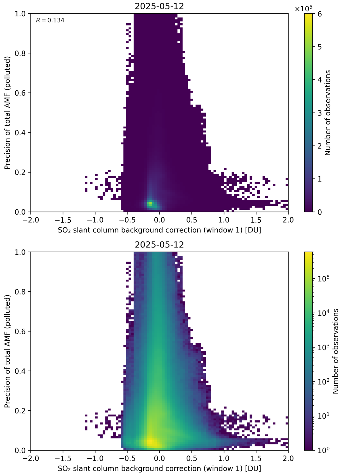
Figure 121: Scatter density plot of “SO 2 slant column background correction (window 1)” against “Precision of total AMF (polluted)” for 2025-05-11 to 2025-05-13.
