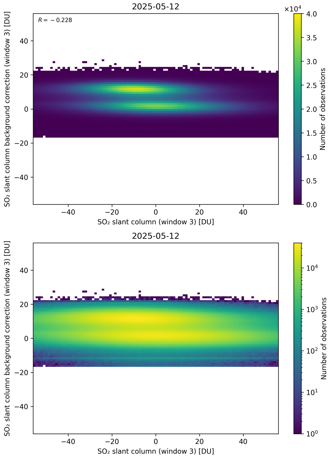
Figure 303: Scatter density plot of “SO 2 slant column (window 3)” against “SO 2 slant column background correction (window 3)” for 2025-05-11 to 2025-05-13.
