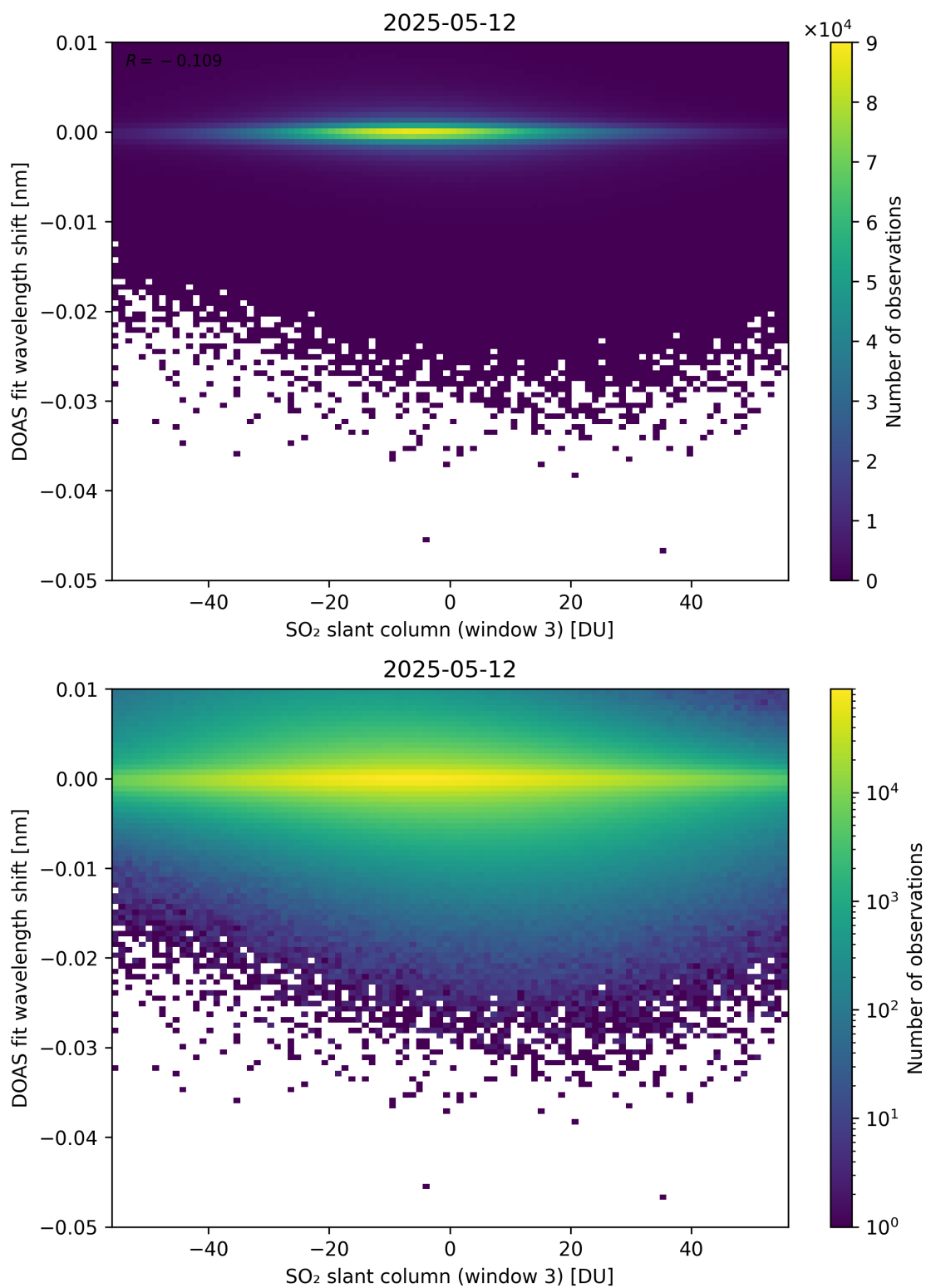
Figure 304: Scatter density plot of “SO 2 slant column (window 3)” against “DOAS fit wavelength shift” for 2025-05-11 to 2025-05-13.
