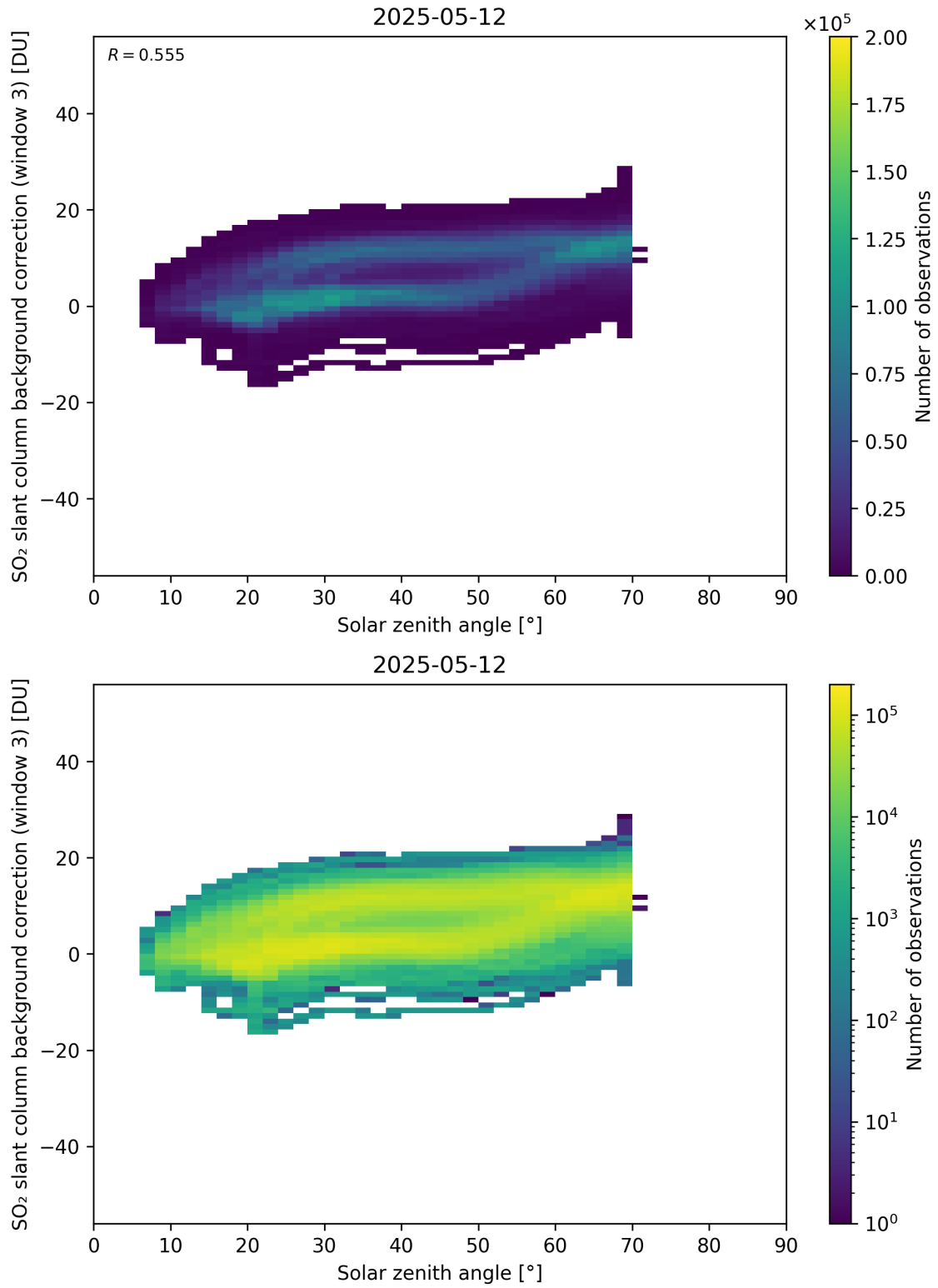
Figure 173: Scatter density plot of “Solar zenith angle” against “SO 2 slant column background correction (window 3)” for 2025-05-11 to 2025-05-13.
