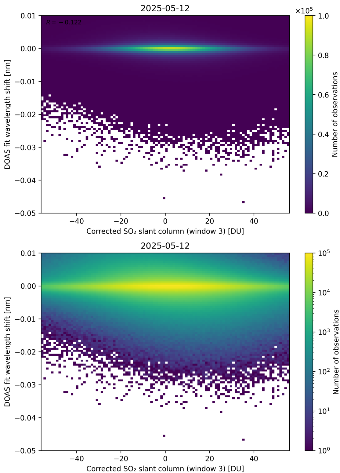
Figure 256: Scatter density plot of “Corrected SO 2 slant column (window 3)” against “DOAS fit wavelength shift” for 2025-05-11 to 2025-05-13.
