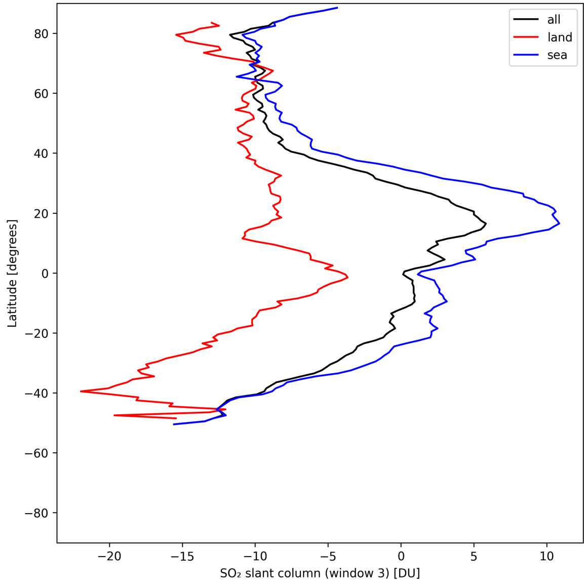
Figure 45: Zonal average of “SO 2 slant column (window 3)” for 2025-05-11 to 2025-05-13.
