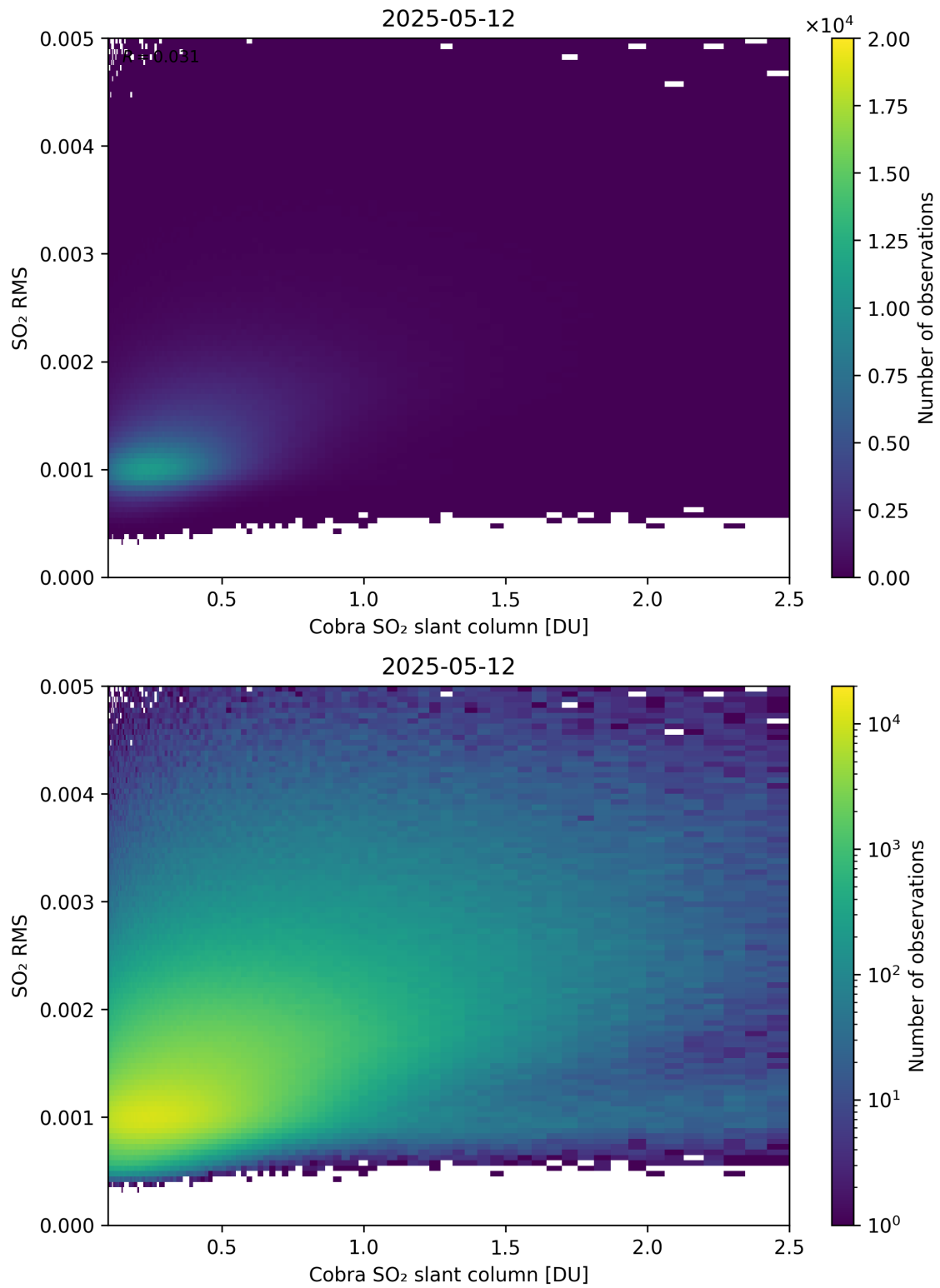
Figure 198: Scatter density plot of “Cobra SO 2 slant column” against “SO 2 RMS” for 2025-05-11 to 2025-05-13.
