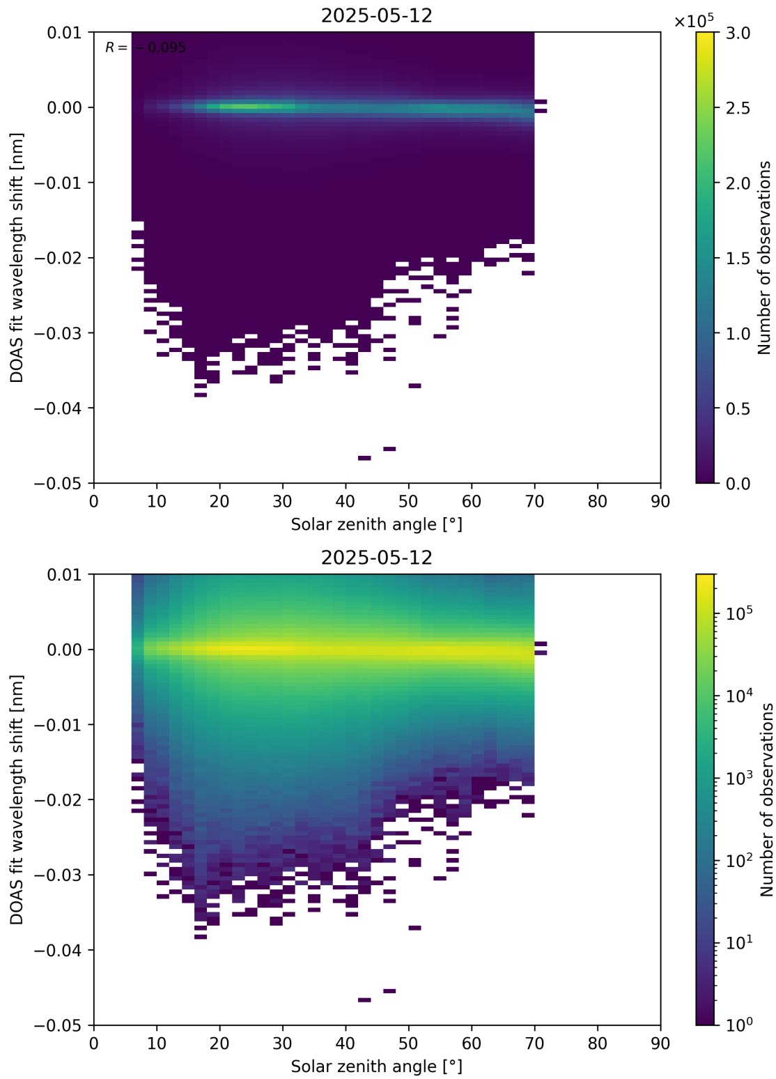
Figure 174: Scatter density plot of “Solar zenith angle” against “DOAS fit wavelength shift” for 2025-05-11 to 2025-05-13.
