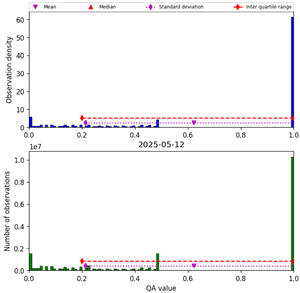
Figure 57: Histogram of “QA value” for 2025-05-11 to 2025-05-13
