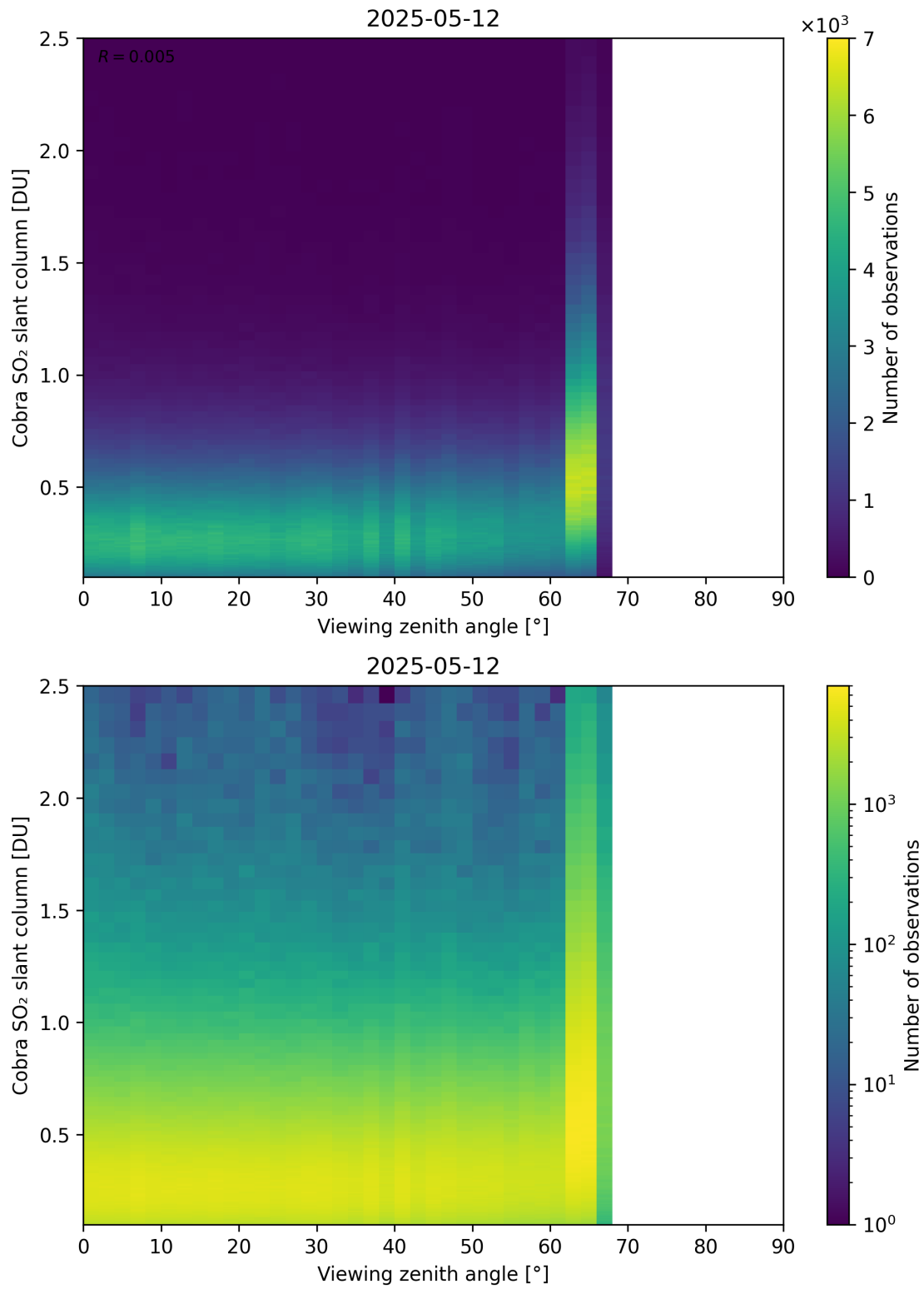
Figure 371: Scatter density plot of “Viewing zenith angle” against “Cobra SO 2 slant column” for 2025-05-11 to 2025-05-13.
