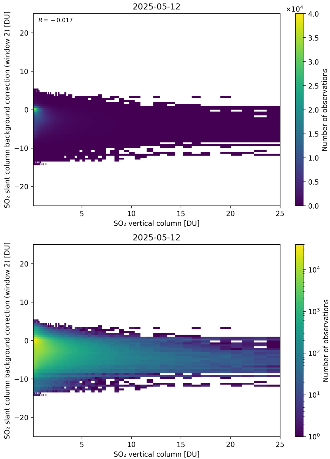
Figure 324: Scatter density plot of “SO 2 vertical column” against “SO 2 slant column background correction (window 2)” for 2025-05-11 to 2025-05-13.
