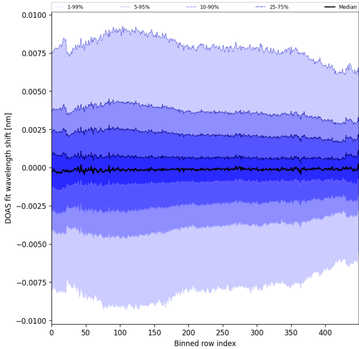
Figure 102: Along track statistics of “DOAS fit wavelength shift” for 2025-05-11 to 2025-05-13
