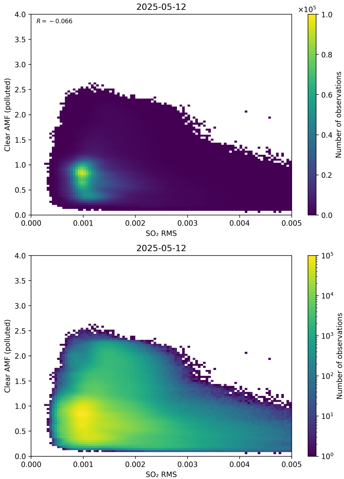
Figure 147: Scatter density plot of “SO 2 RMS” against “Clear AMF (polluted)” for 2025-05-11 to 2025-05-13.
