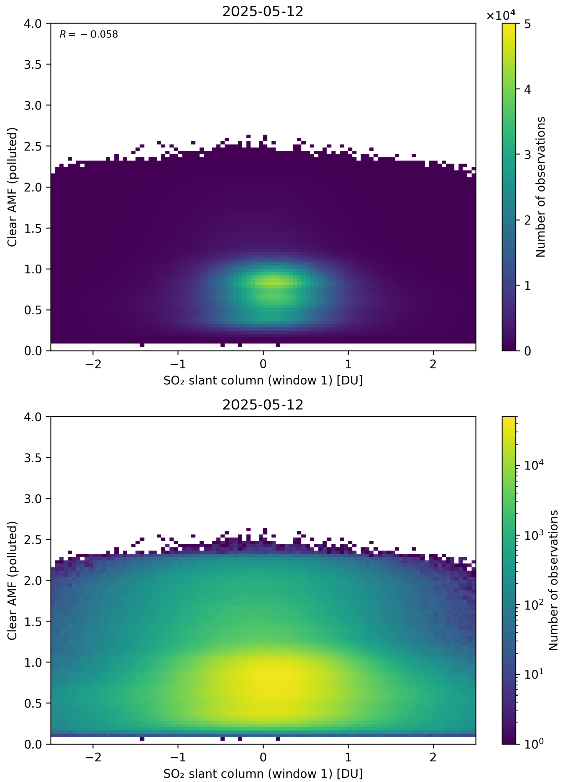
Figure 282: Scatter density plot of “SO 2 slant column (window 1)” against “Clear AMF (polluted)” for 2025-05-11 to 2025-05-13.
