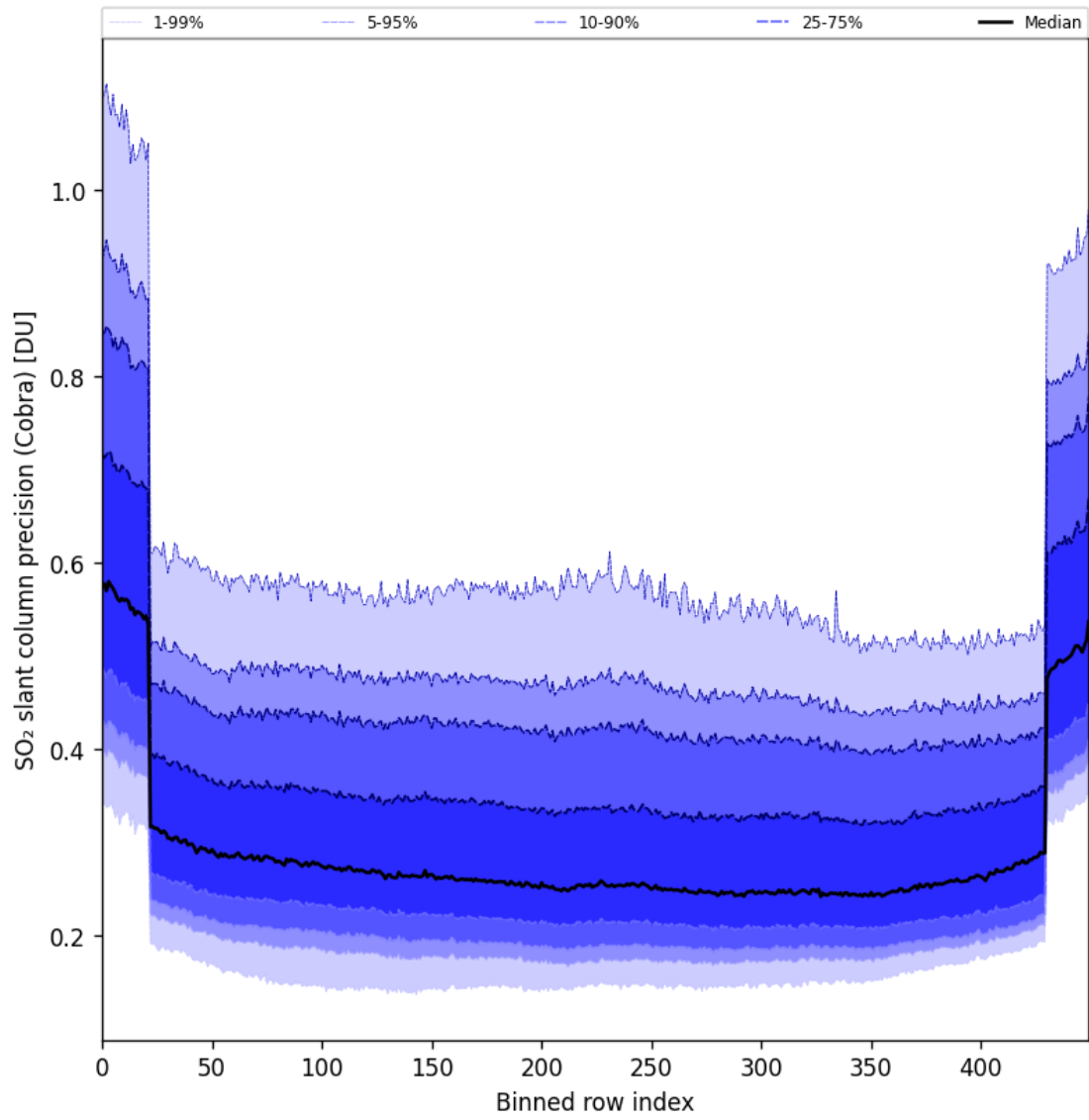
Figure 88: Along track statistics of “SO 2 slant column precision (Cobra)” for 2025-05-11 to 2025-05-13
