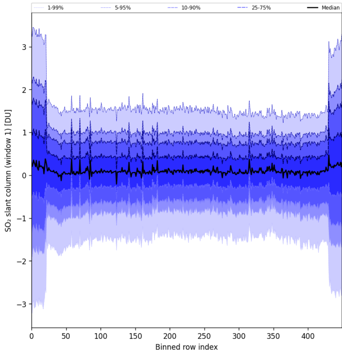
Figure 89: Along track statistics of “SO 2 slant column (window 1)” for 2025-05-11 to 2025-05-13
