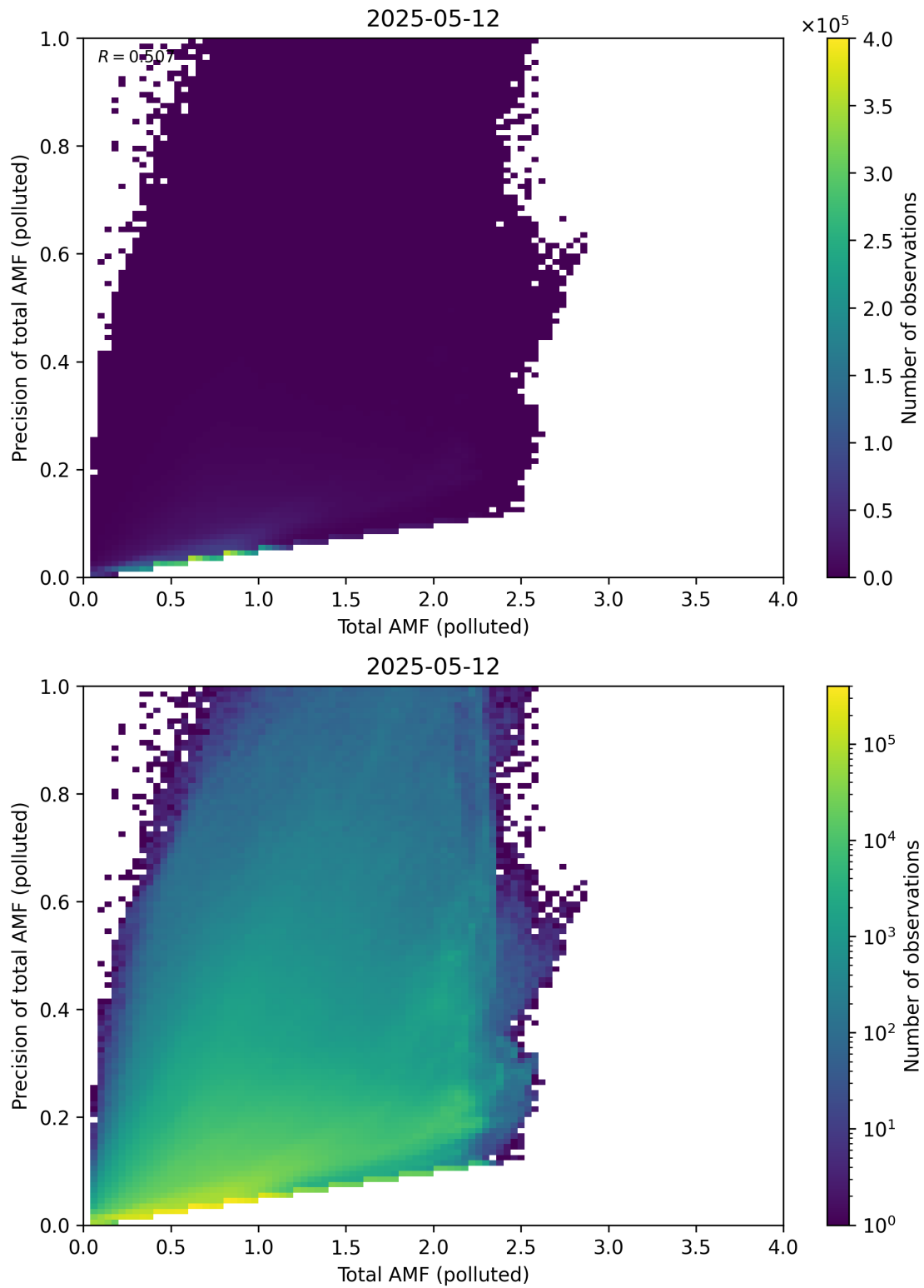
Figure 322: Scatter density plot of “Total AMF (polluted)” against “Precision of total AMF (polluted)” for 2025-05-11 to 2025-05-13.
