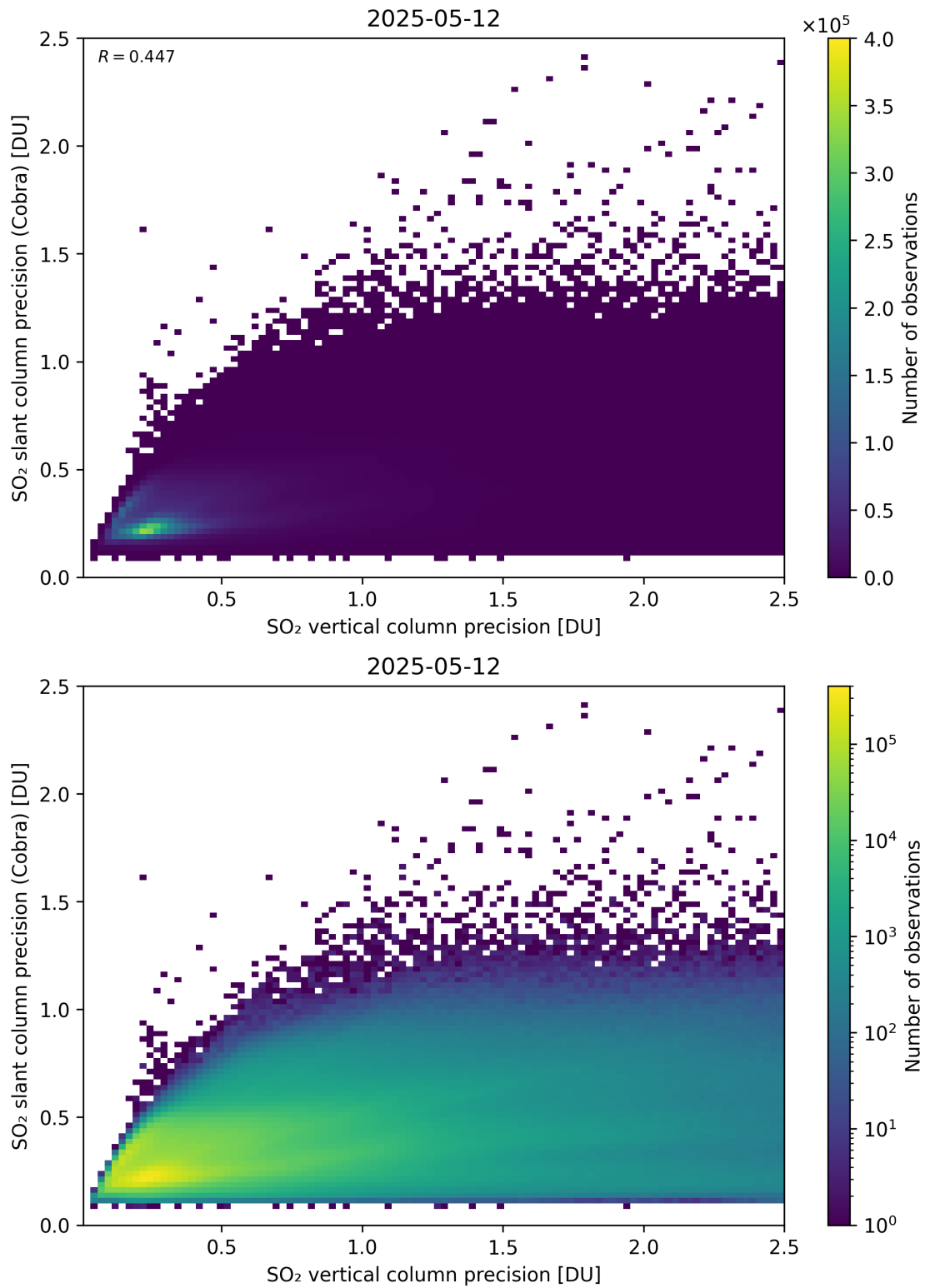
Figure 337: Scatter density plot of “SO 2 vertical column precision” against “SO 2 slant column precision (Cobra)” for 2025-05-11 to 2025-05-13.
