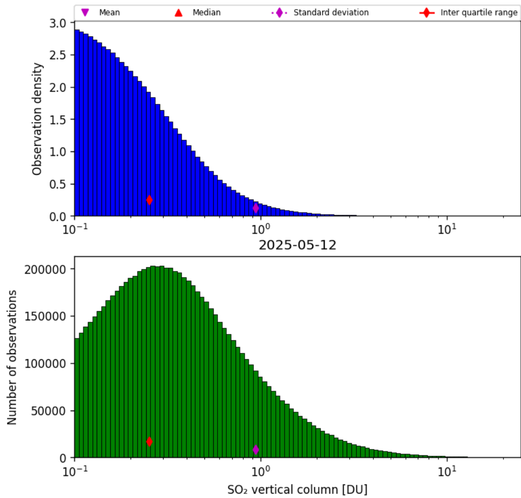
Figure 58: Histogram of “SO 2 vertical column” for 2025-05-11 to 2025-05-13
