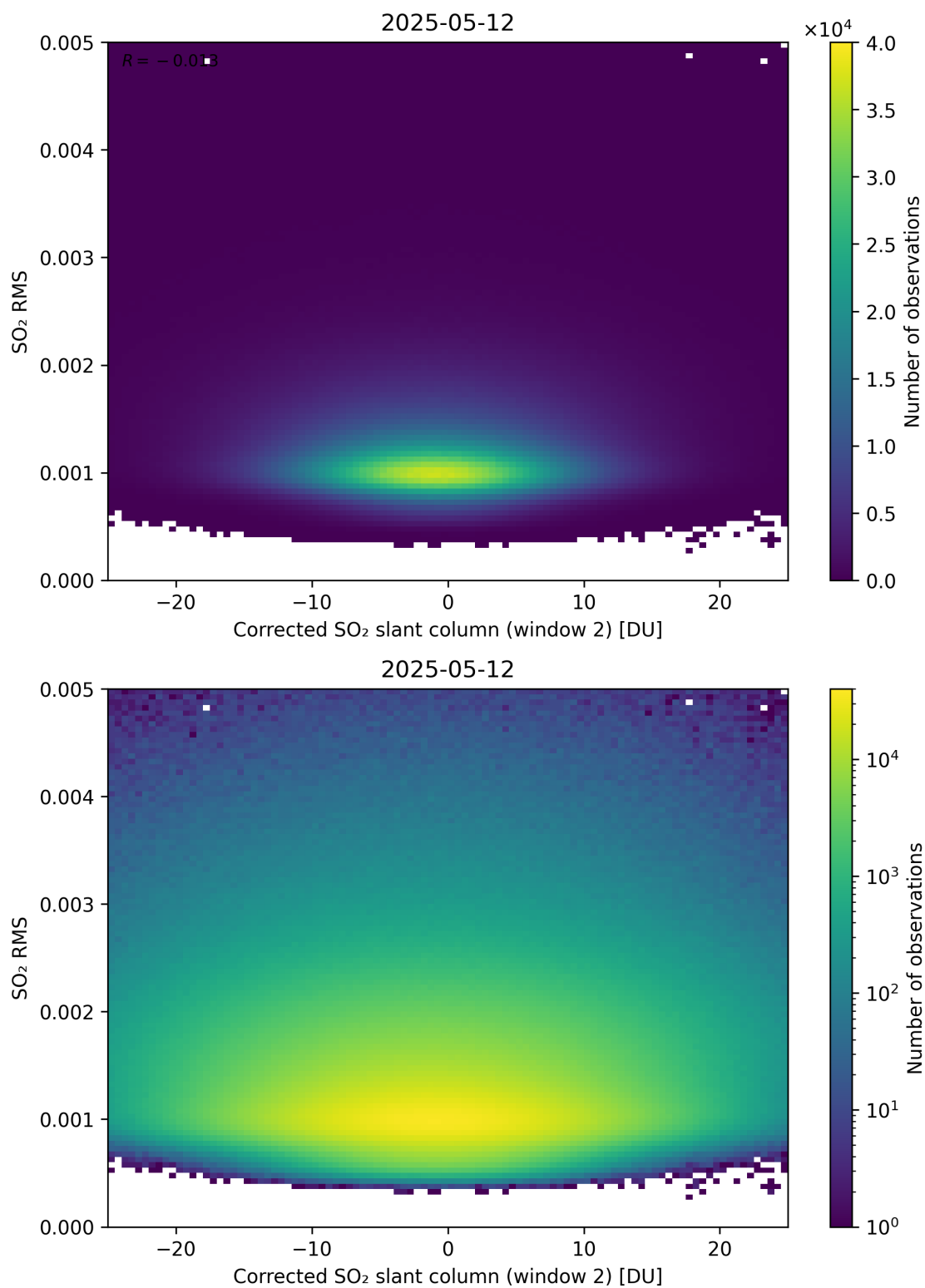
Figure 248: Scatter density plot of “Corrected SO 2 slant column (window 2)” against “SO 2 RMS” for 2025-05-11 to 2025-05-13.
