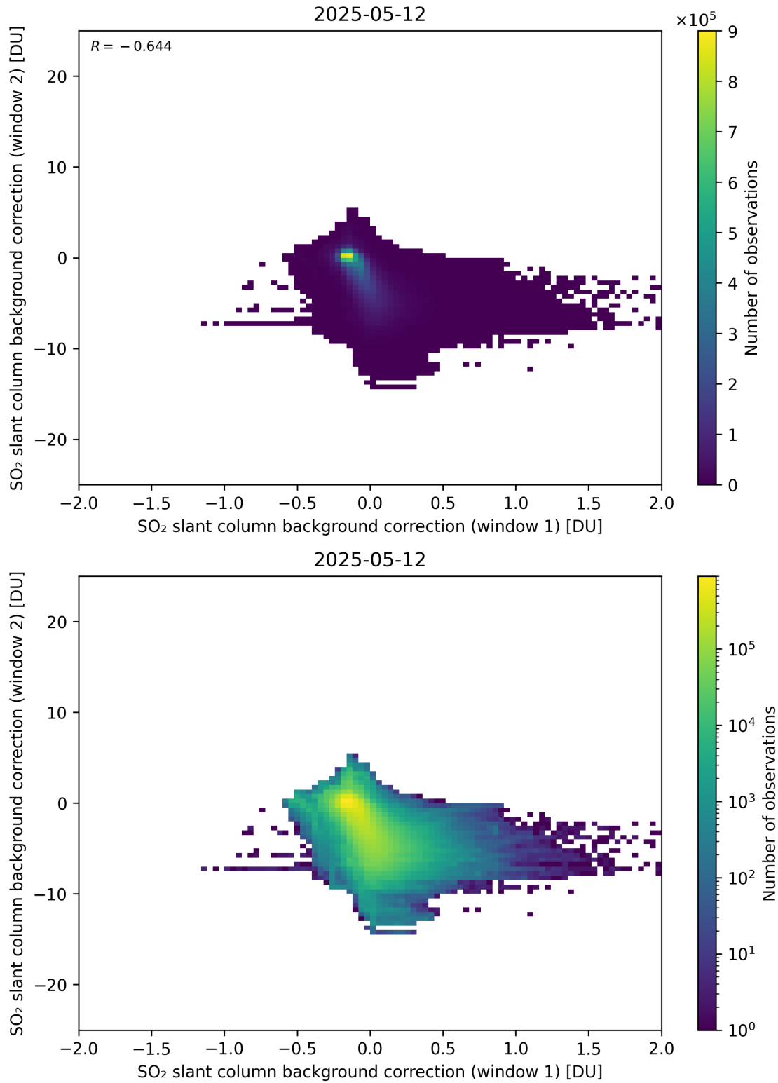
Figure 109: Scatter density plot of “SO 2 slant column background correction (window 1)” against “SO 2 slant column background correction (window 2)” for 2025-05-11 to 2025-05-13.
