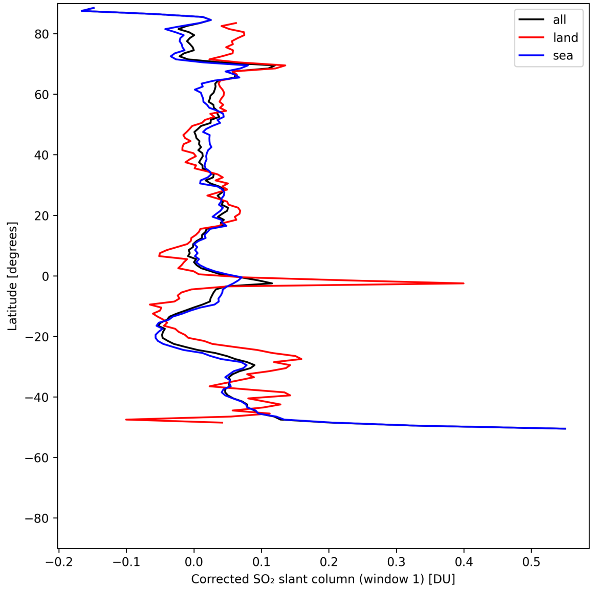
Figure 39: Zonal average of “Corrected SO 2 slant column (window 1)” for 2025-05-11 to 2025-05-13.
