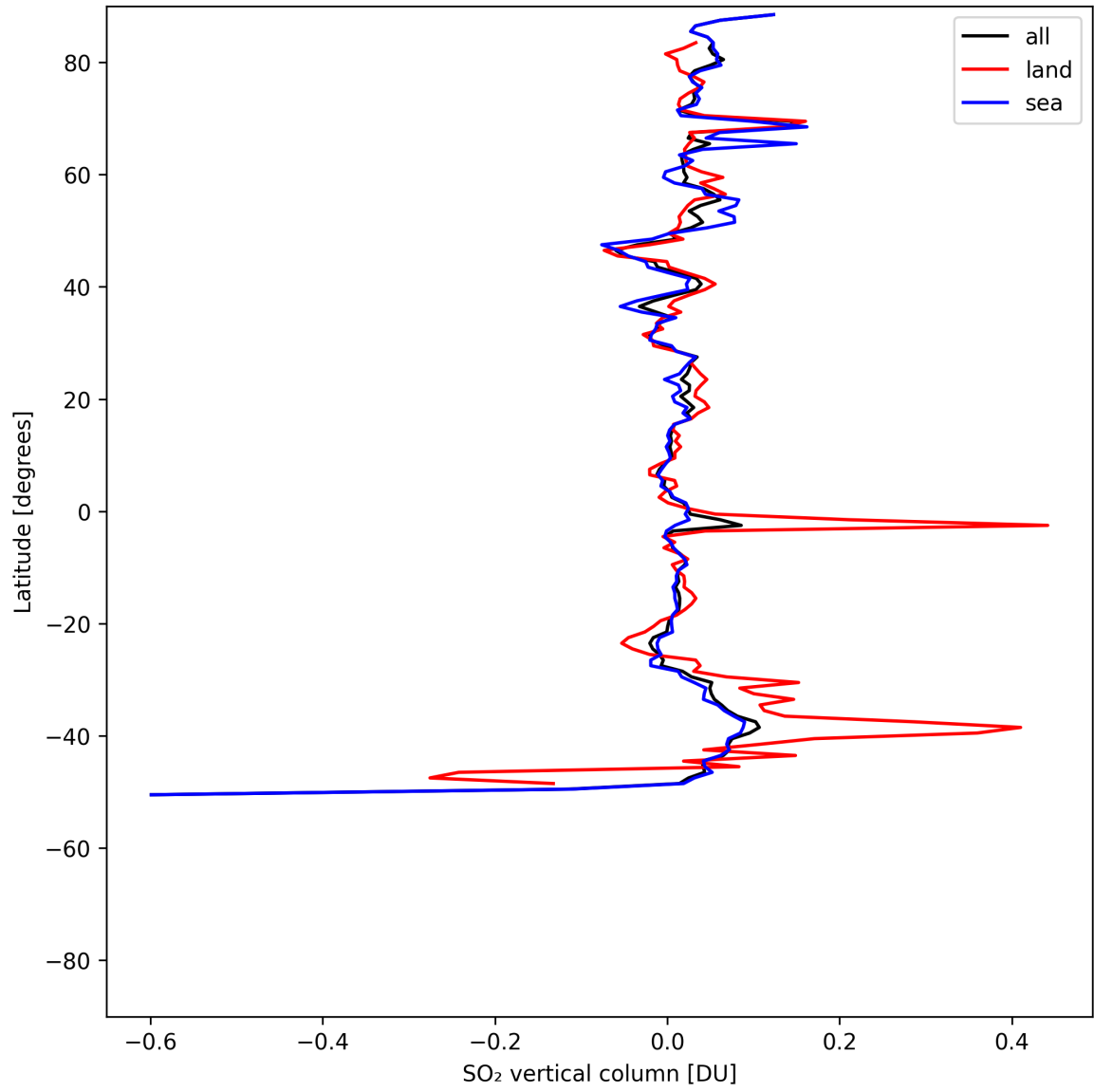
Figure 32: Zonal average of “SO 2 vertical column” for 2025-05-11 to 2025-05-13.
