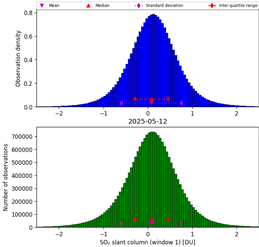
Figure 63: Histogram of “SO 2 slant column (window 1)” for 2025-05-11 to 2025-05-13
