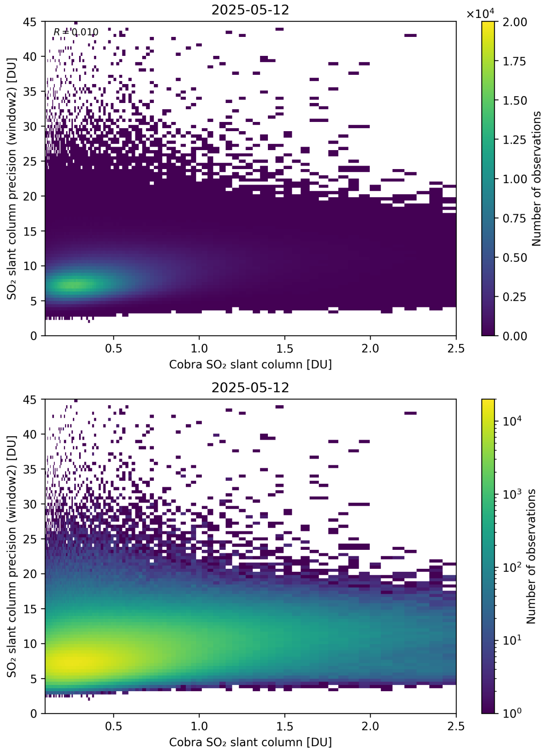
Figure 221: Scatter density plot of “Cobra SO 2 slant column” against “SO 2 slant column precision (window2)” for 2025-05-11 to 2025-05-13.
