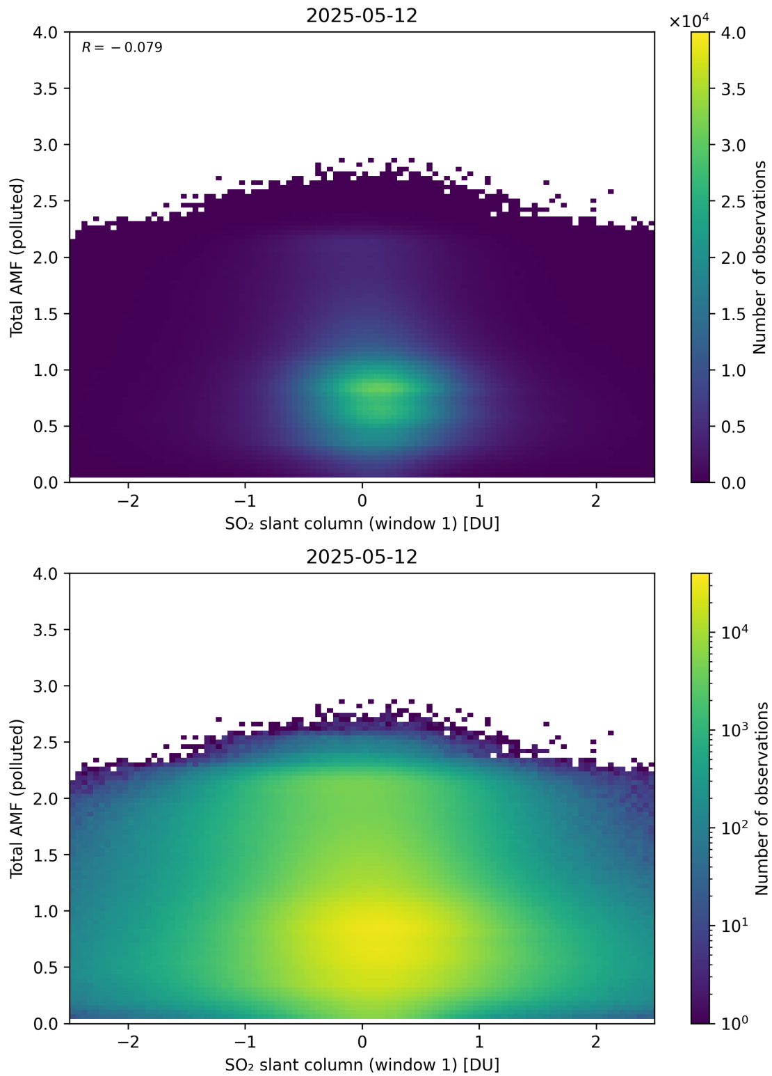
Figure 289: Scatter density plot of “SO 2 slant column (window 1)” against “Total AMF (polluted)” for 2025-05-11 to 2025-05-13.
