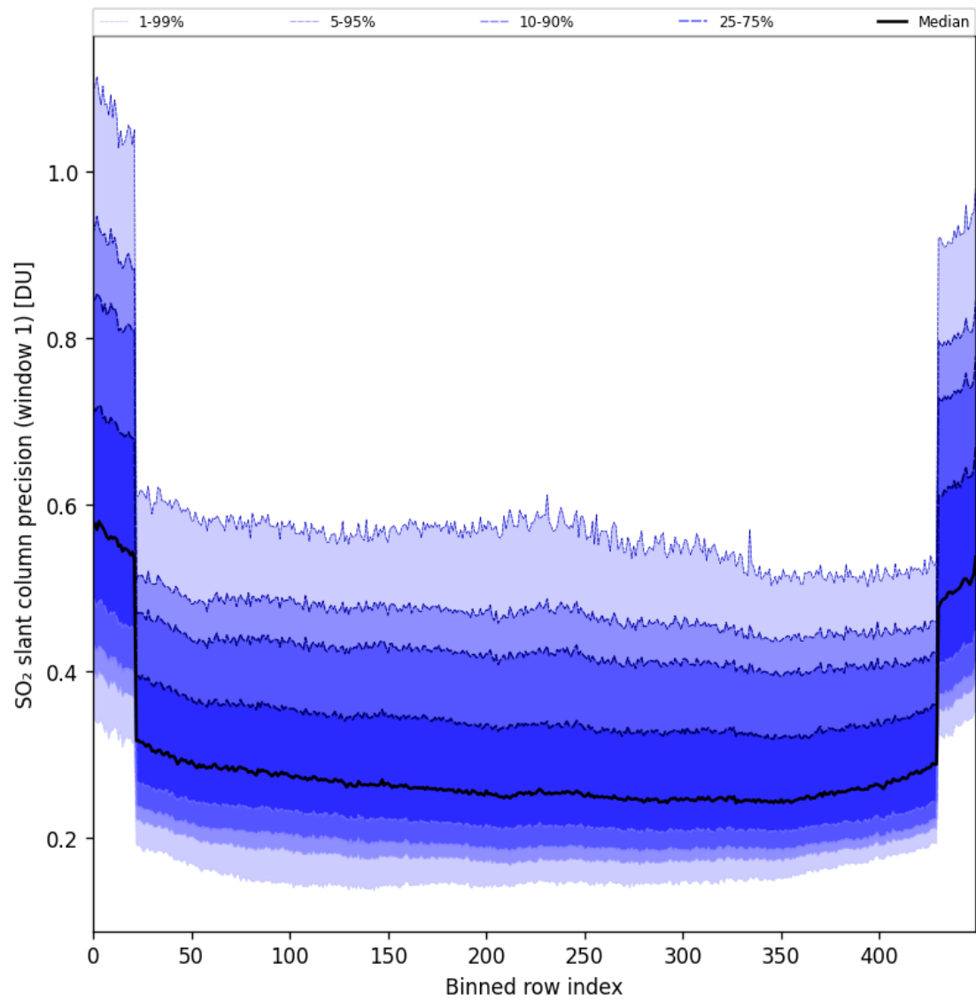
Figure 90: Along track statistics of “SO 2 slant column precision (window 1)” for 2025-05-11 to 2025-05-13
