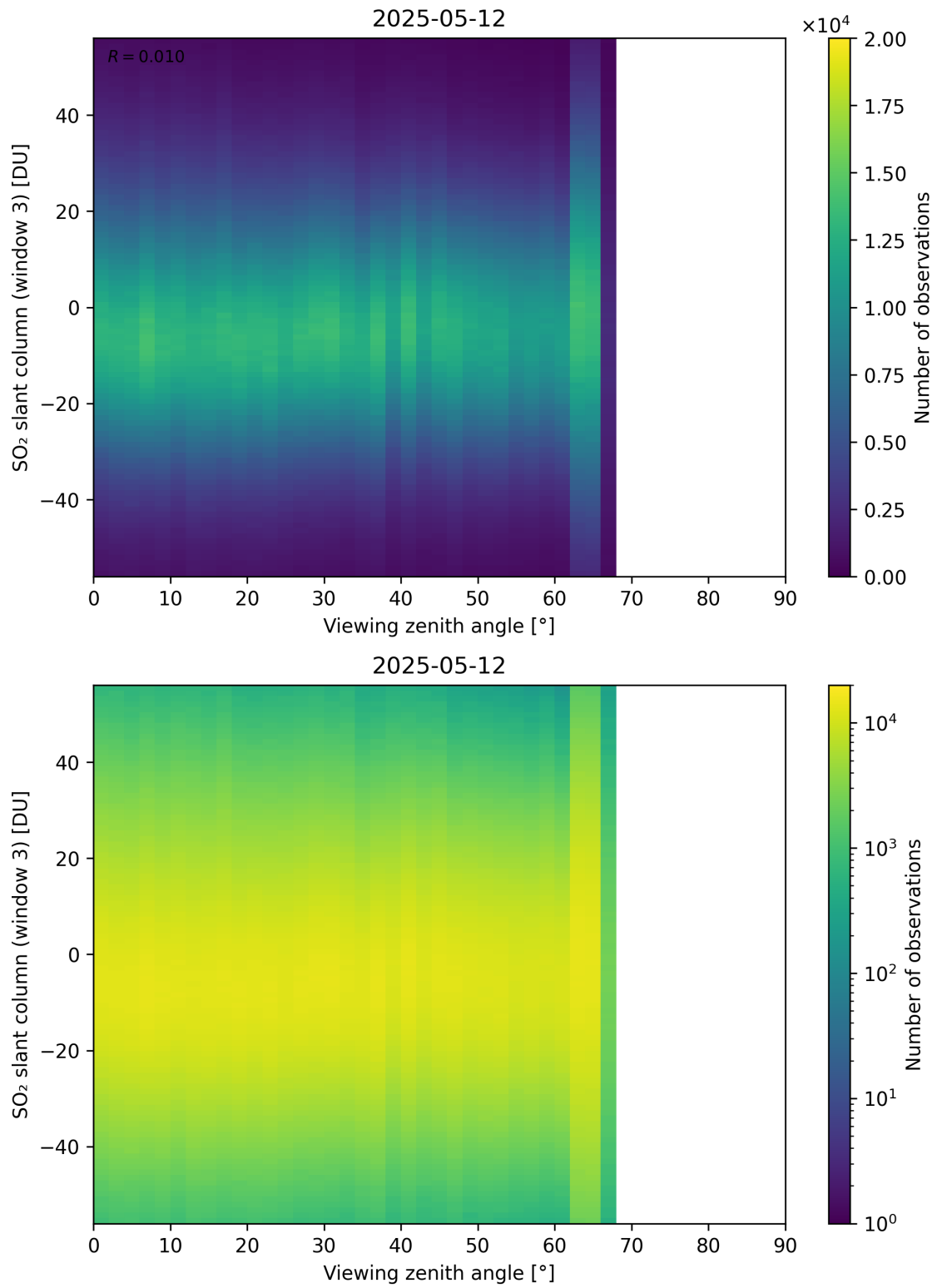
Figure 379: Scatter density plot of “Viewing zenith angle” against “SO 2 slant column (window 3)” for 2025-05-11 to 2025-05-13.
