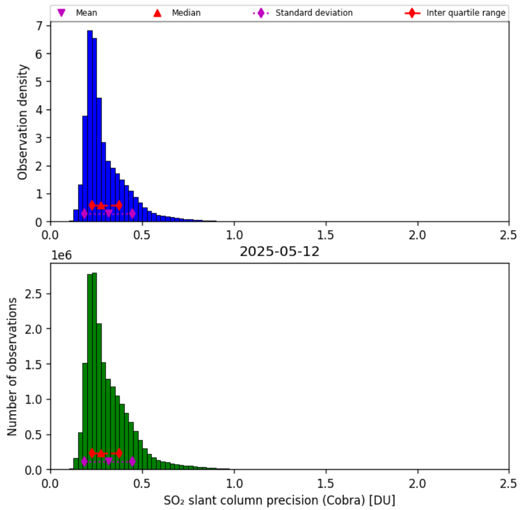
Figure 62: Histogram of “SO 2 slant column precision (Cobra)” for 2025-05-11 to 2025-05-13
