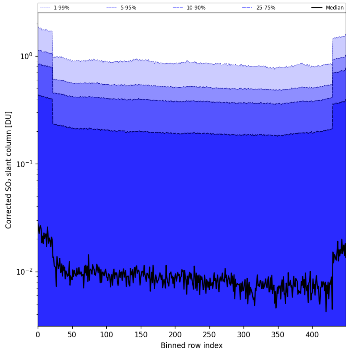
Figure 86: Along track statistics of "Corrected SO 2 slant column" for 2025-05-11 to 2025-05-13
