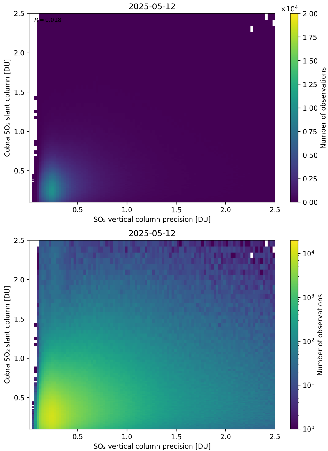
Figure 336: Scatter density plot of “SO 2 vertical column precision” against “Cobra SO 2 slant column” for 2025-05-11 to 2025-05-13.
