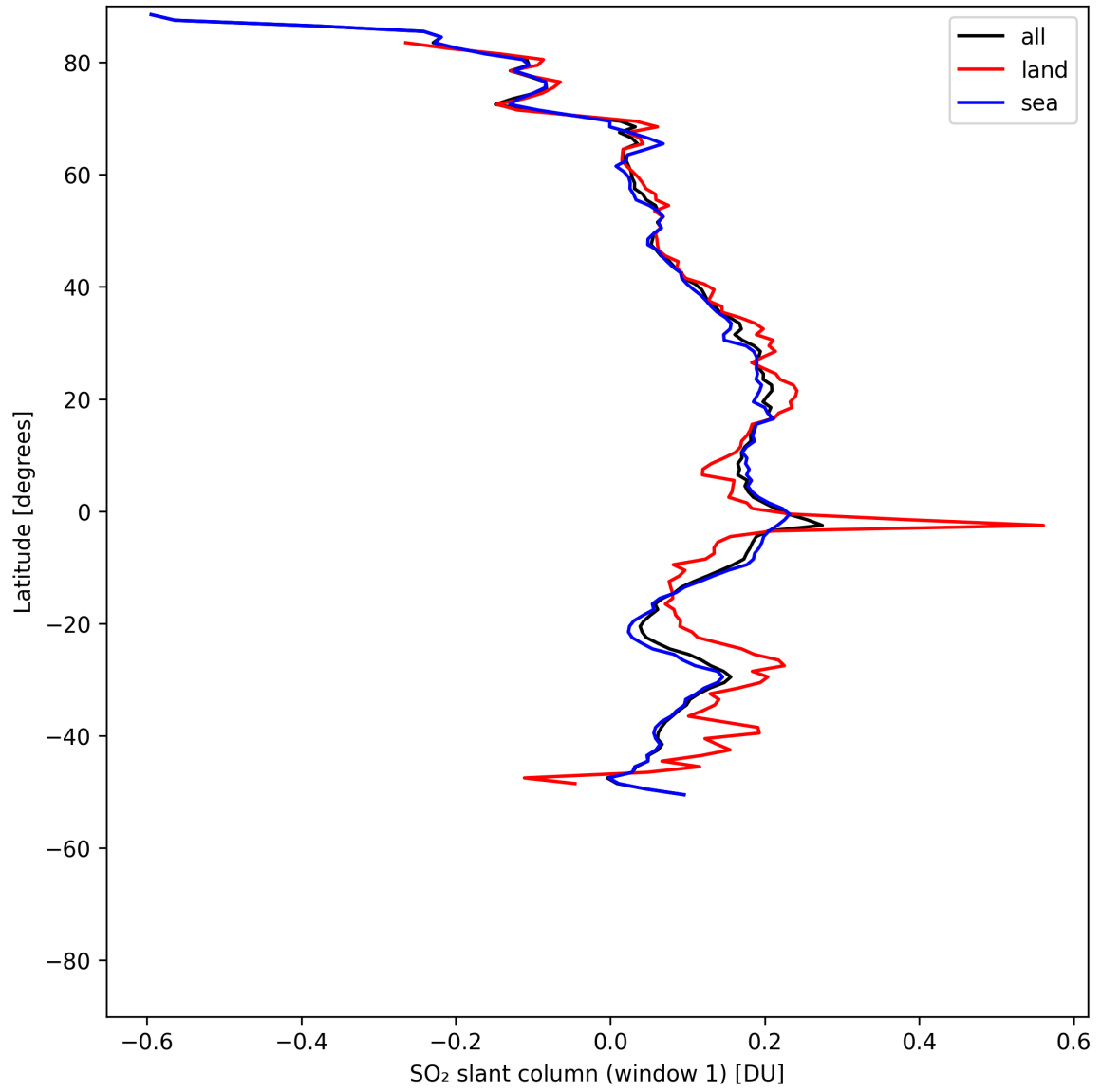
Figure 37: Zonal average of “SO 2 slant column (window 1)” for 2025-05-11 to 2025-05-13.
