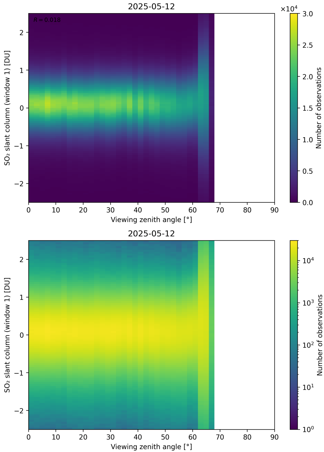
Figure 376: Scatter density plot of “Viewing zenith angle” against “SO 2 slant column (window 1)” for 2025-05-11 to 2025-05-13.
