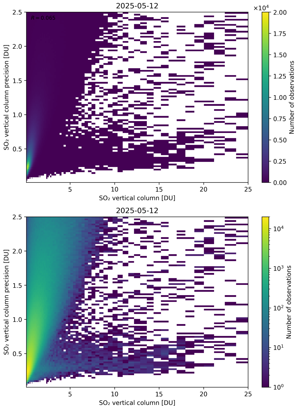
Figure 361: Scatter density plot of “SO 2 vertical column” against “SO 2 vertical column precision” for 2025-05-11 to 2025-05-13.
