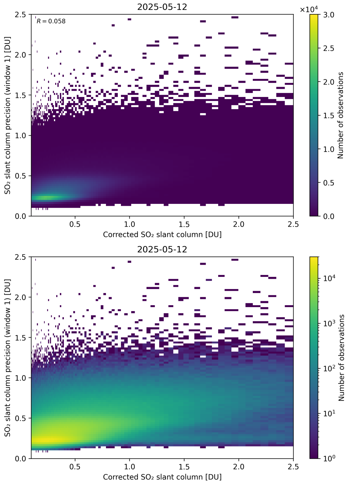
Figure 238: Scatter density plot of “Corrected SO 2 slant column” against “SO 2 slant column precision (window 1)” for 2025-05-11 to 2025-05-13.
