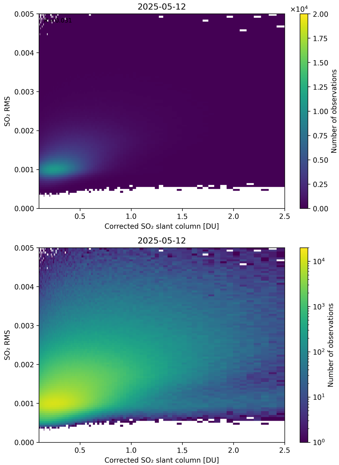
Figure 231: Scatter density plot of “Corrected SO 2 slant column” against “SO 2 RMS” for 2025-05-11 to 2025-05-13.
