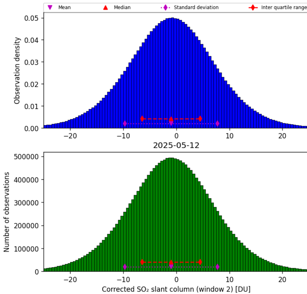
Figure 69: Histogram of “Corrected SO 2 slant column (window 2)” for 2025-05-11 to 2025-05-13
