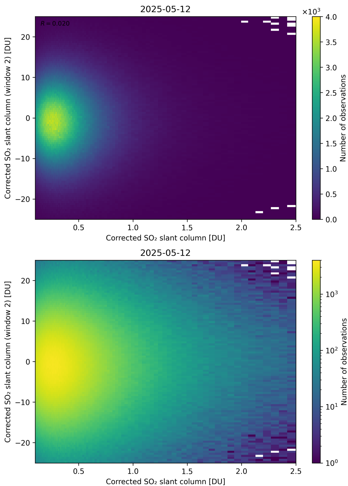
Figure 235: Scatter density plot of “Corrected SO 2 slant column” against “Corrected SO 2 slant column (window 2)” for 2025-05-11 to 2025-05-13.
