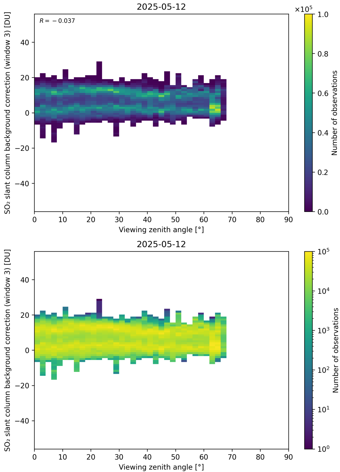
Figure 364: Scatter density plot of “Viewing zenith angle” against “SO 2 slant column background correction (window 3)” for 2025-05-11 to 2025-05-13.
