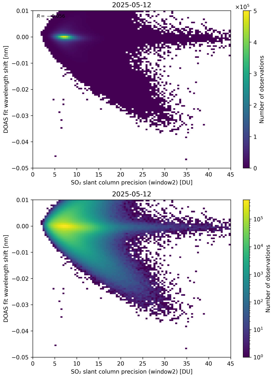
Figure 293: Scatter density plot of “SO 2 slant column precision (window2)” against “DOAS fit wavelength shift” for 2025-05-11 to 2025-05-13.
