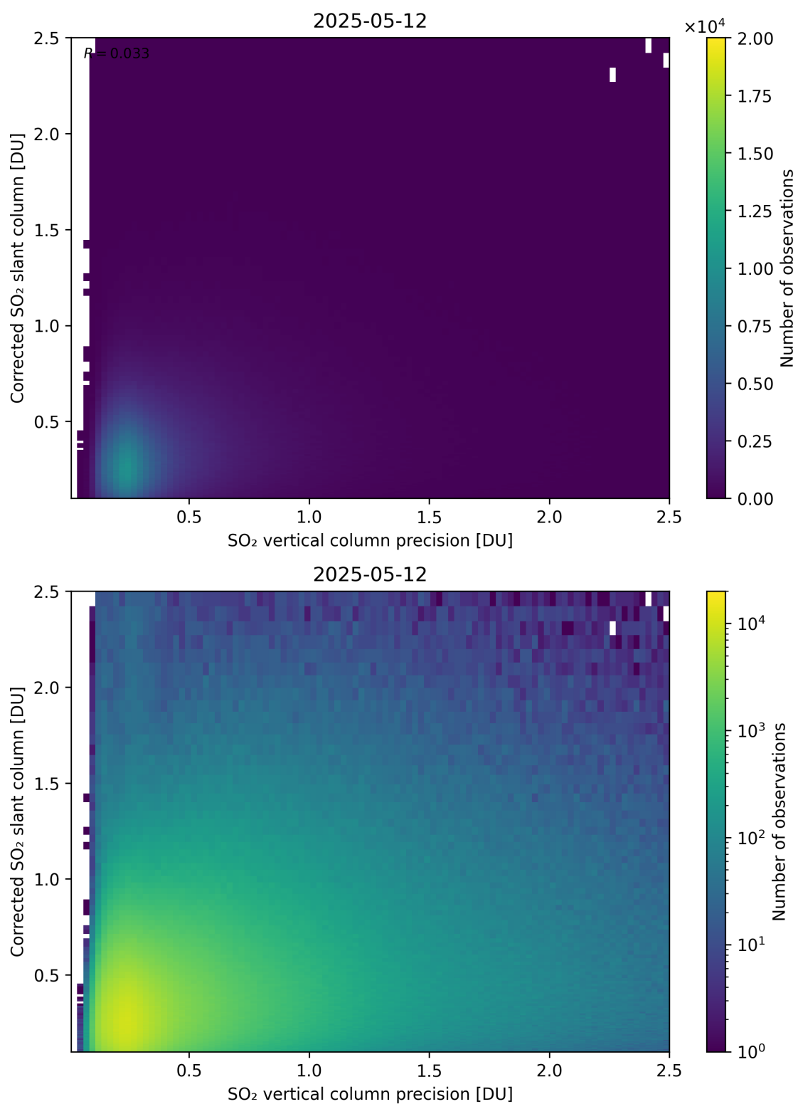
Figure 338: Scatter density plot of “SO 2 vertical column precision” against “Corrected SO 2 slant column” for 2025-05-11 to 2025-05-13.
