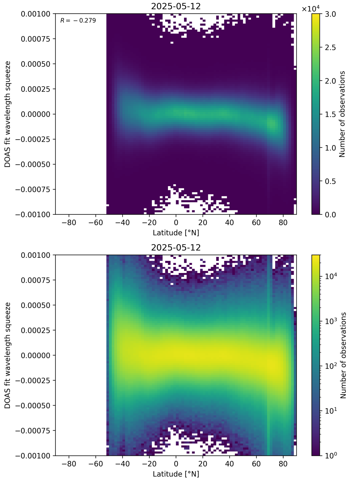
Figure 154: Scatter density plot of “Latitude” against “DOAS fit wavelength squeeze” for 2025-05-11 to 2025-05-13.
