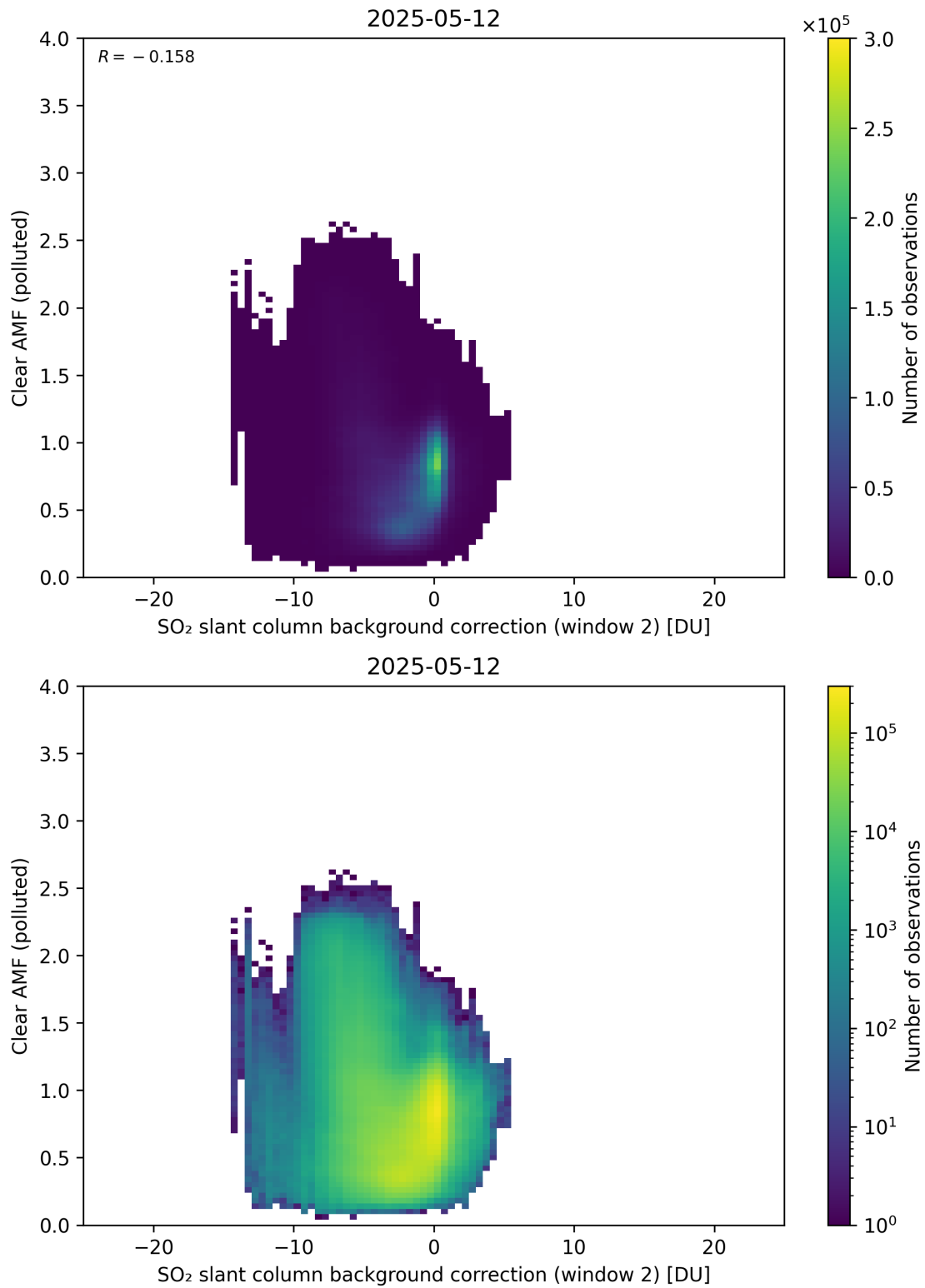
Figure 126: Scatter density plot of “SO 2 slant column background correction (window 2)” against “Clear AMF (polluted)” for 2025-05-11 to 2025-05-13.
