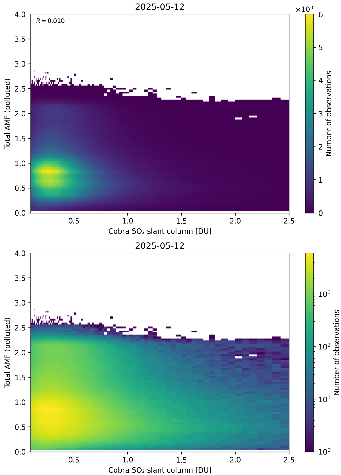
Figure 224: Scatter density plot of “Cobra SO 2 slant column” against “Total AMF (polluted)” for 2025-05-11 to 2025-05-13.
