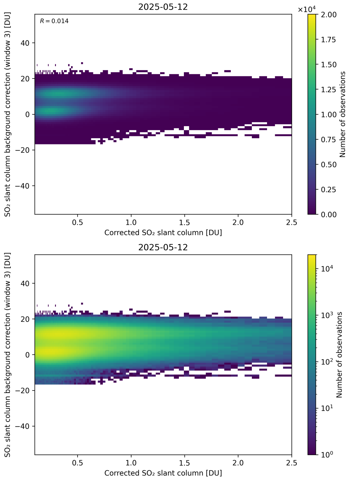
Figure 228: Scatter density plot of “Corrected SO 2 slant column” against “SO 2 slant column background correction (window 3)” for 2025-05-11 to 2025-05-13.
