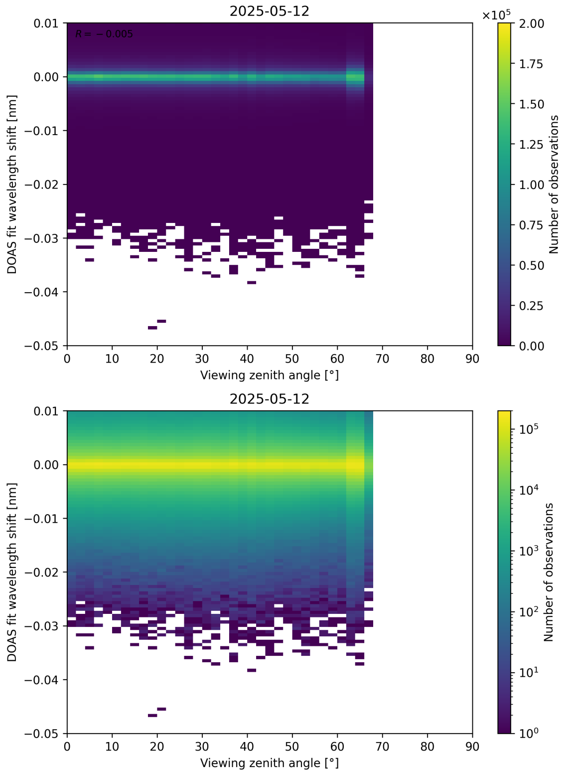
Figure 365: Scatter density plot of “Viewing zenith angle” against “DOAS fit wavelength shift” for 2025-05-11 to 2025-05-13.
