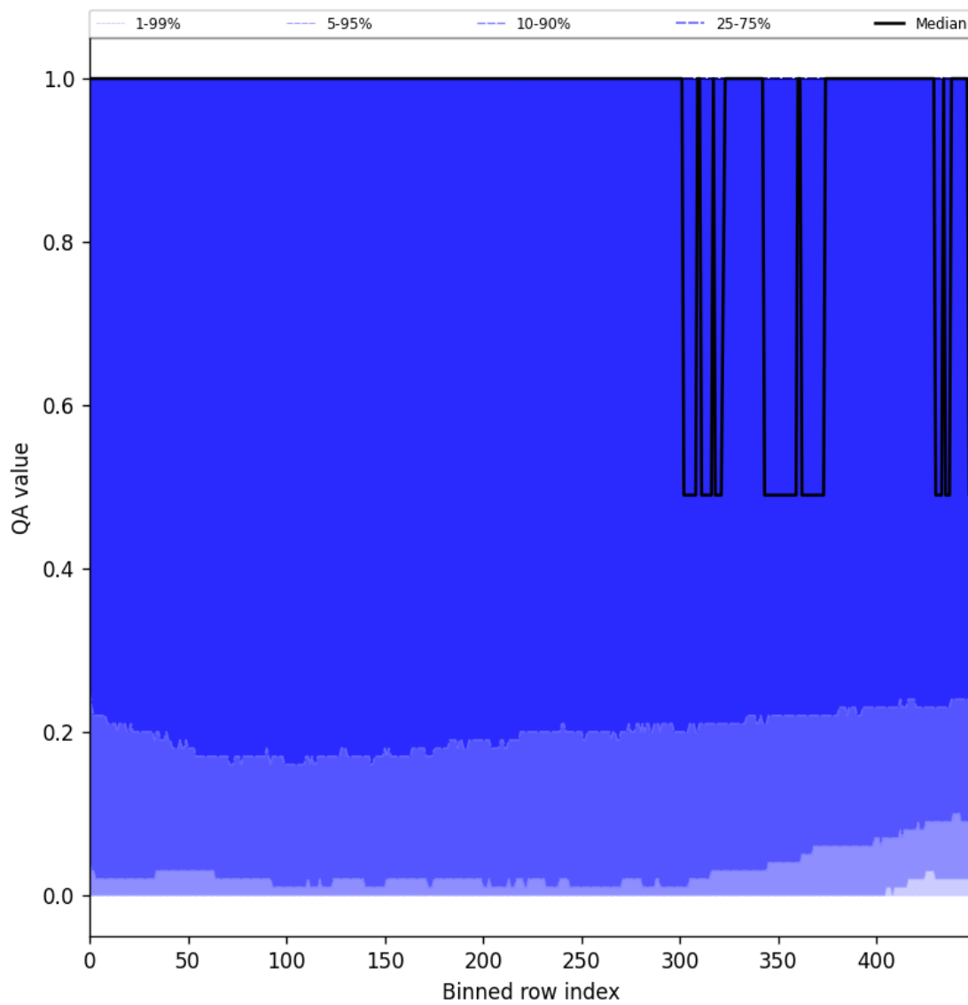
Figure 83: Along track statistics of “QA value” for 2025-05-11 to 2025-05-13
