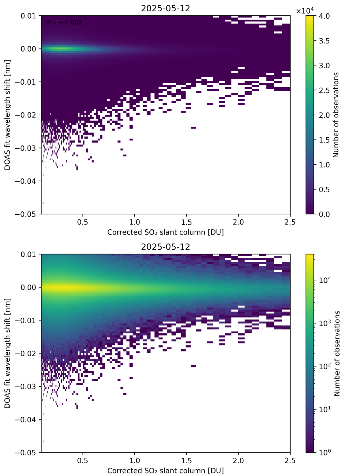
Figure 229: Scatter density plot of “Corrected SO 2 slant column” against “DOAS fit wavelength shift” for 2025-05-11 to 2025-05-13.
