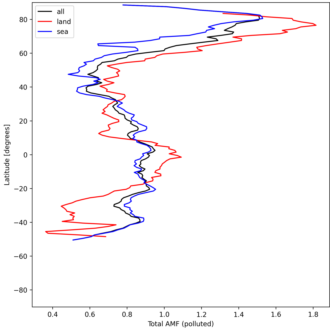
Figure 53: Zonal average of “Total AMF (polluted)” for 2025-05-11 to 2025-05-13.
