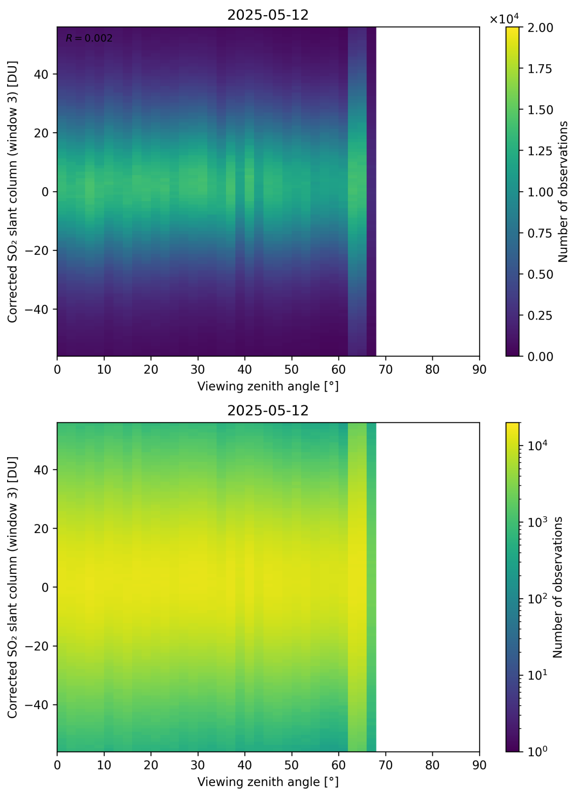
Figure 375: Scatter density plot of “Viewing zenith angle” against “Corrected SO 2 slant column (window 3)” for 2025-05-11 to 2025-05-13.
