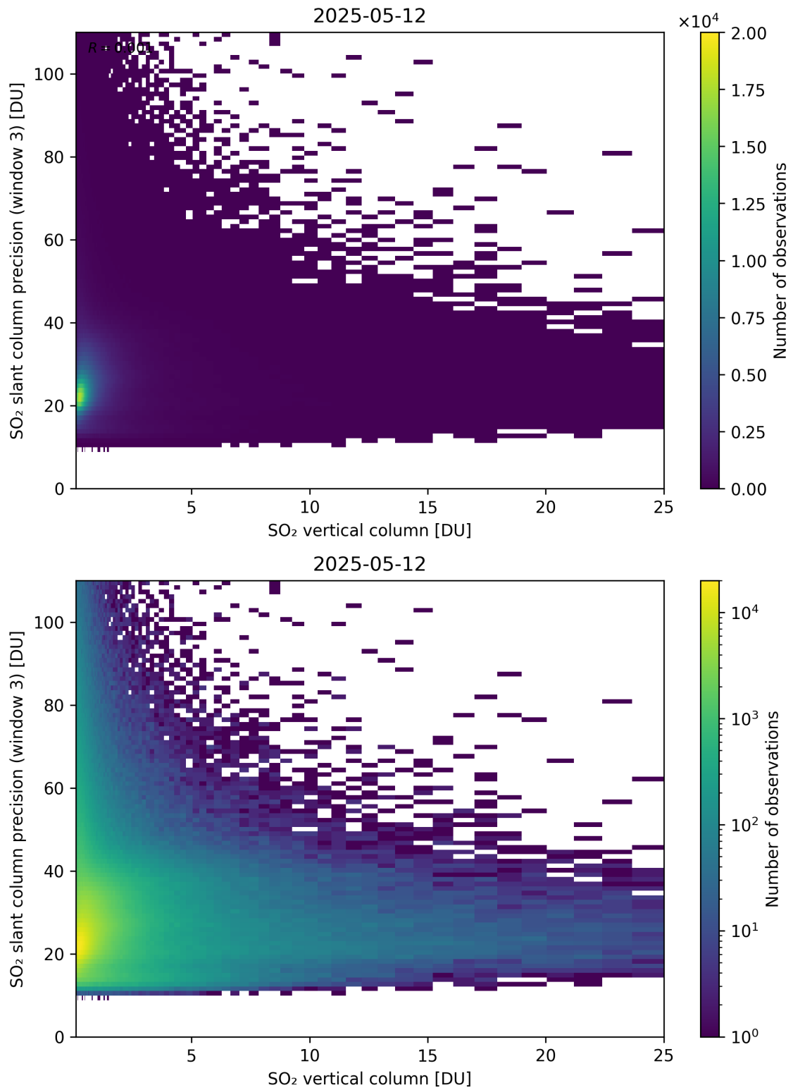
Figure 358: Scatter density plot of “SO 2 vertical column” against “SO 2 slant column precision (window 3)” for 2025-05-11 to 2025-05-13.
