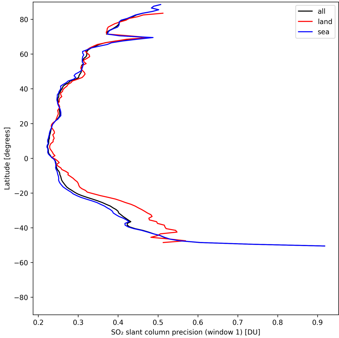
Figure 38: Zonal average of “SO 2 slant column precision (window 1)” for 2025-05-11 to 2025-05-13.
