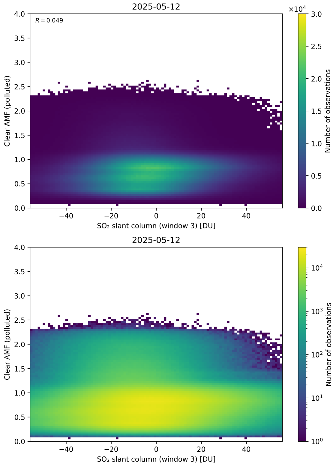
Figure 315: Scatter density plot of “SO 2 slant column (window 3)” against “Clear AMF (polluted)” for 2025-05-11 to 2025-05-13.
