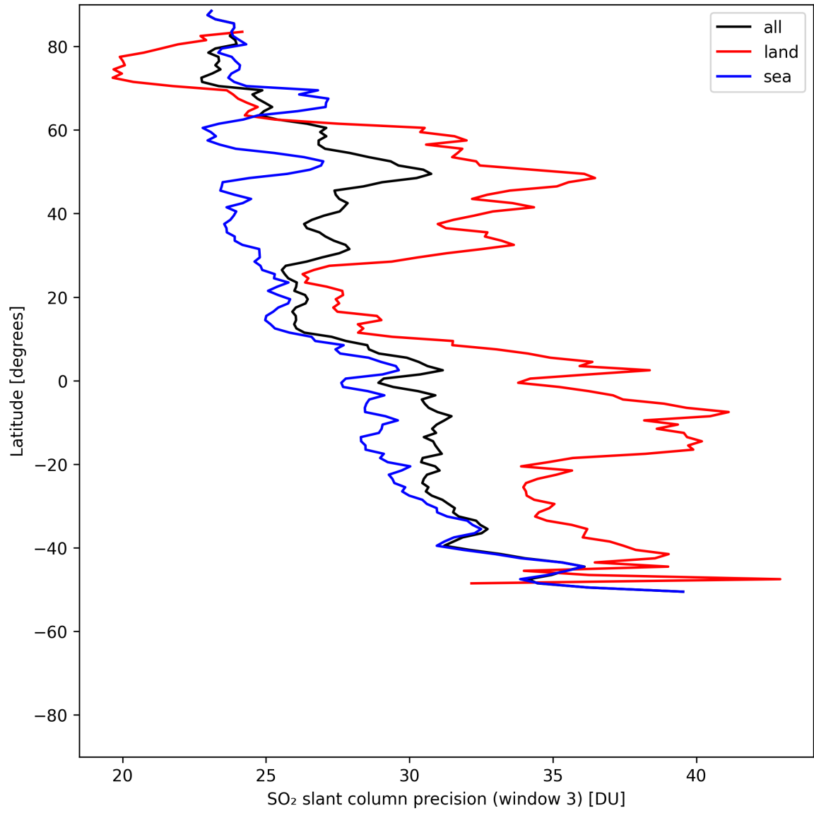
Figure 46: Zonal average of “SO 2 slant column precision (window 3)” for 2025-05-11 to 2025-05-13.
