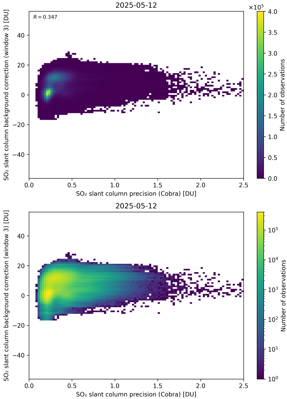
Figure 201: Scatter density plot of “SO 2 slant column precision (Cobra)” against “SO 2 slant column background correction (window 3)” for 2025-05-11 to 2025-05-13.
