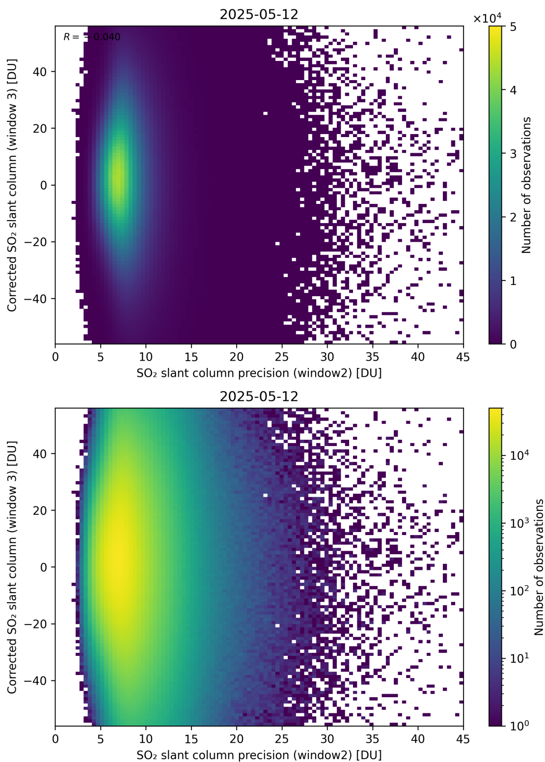
Figure 298: Scatter density plot of “SO 2 slant column precision (window2)” against “Corrected SO 2 slant column (window 3)” for 2025-05-11 to 2025-05-13.
