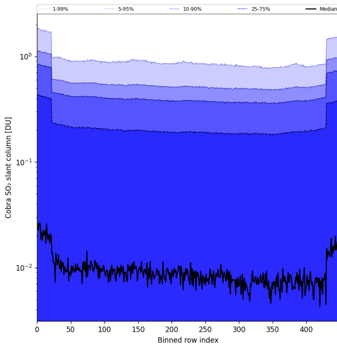
Figure 87: Along track statistics of "Cobra SO 2 slant column" for 2025-05-11 to 2025-05-13
