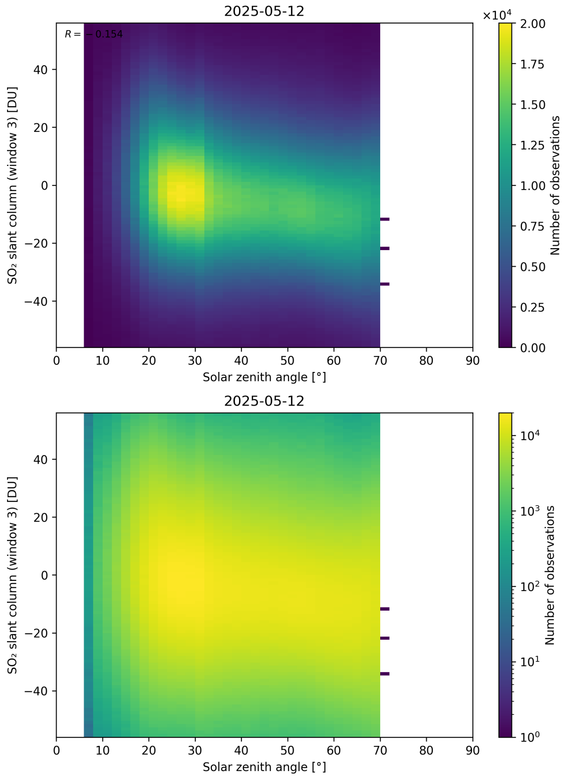
Figure 187: Scatter density plot of “Solar zenith angle” against “SO 2 slant column (window 3)” for 2025-05-11 to 2025-05-13.
