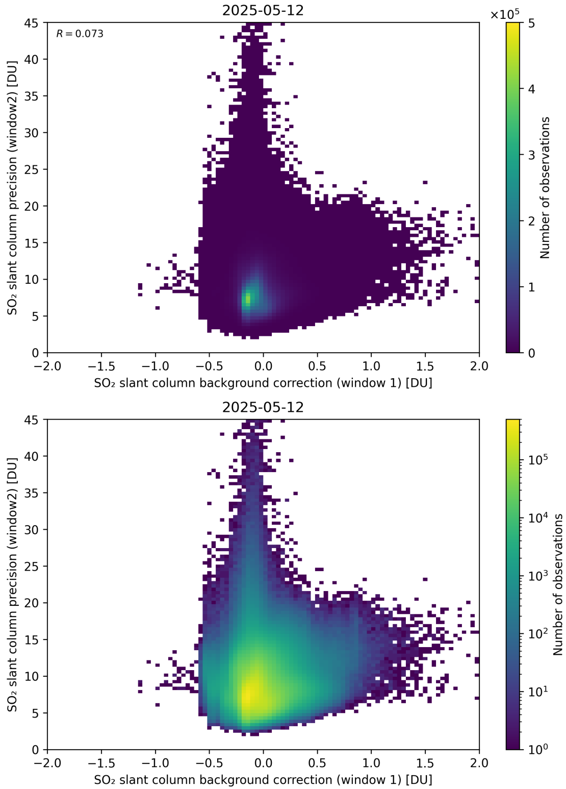
Figure 117: Scatter density plot of “SO 2 slant column background correction (window 1)” against “SO 2 slant column precision (window2)” for 2025-05-11 to 2025-05-13.
