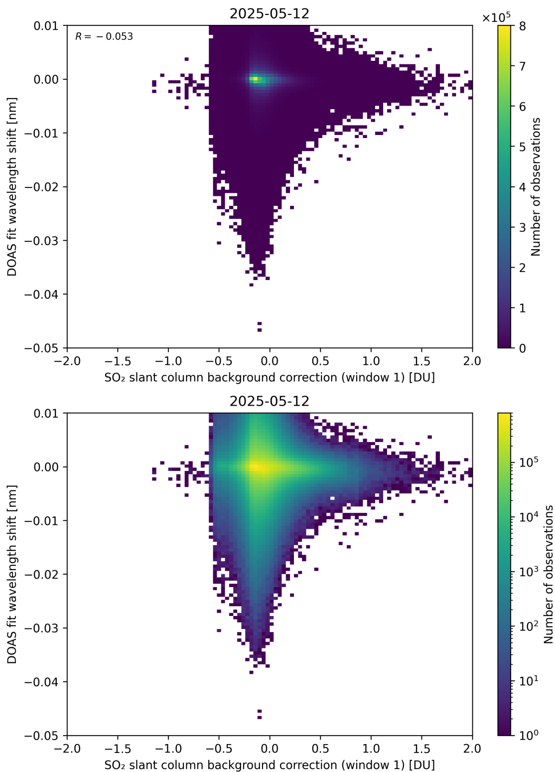
Figure 111: Scatter density plot of “SO 2 slant column background correction (window 1)” against “DOAS fit wavelength shift” for 2025-05-11 to 2025-05-13.
