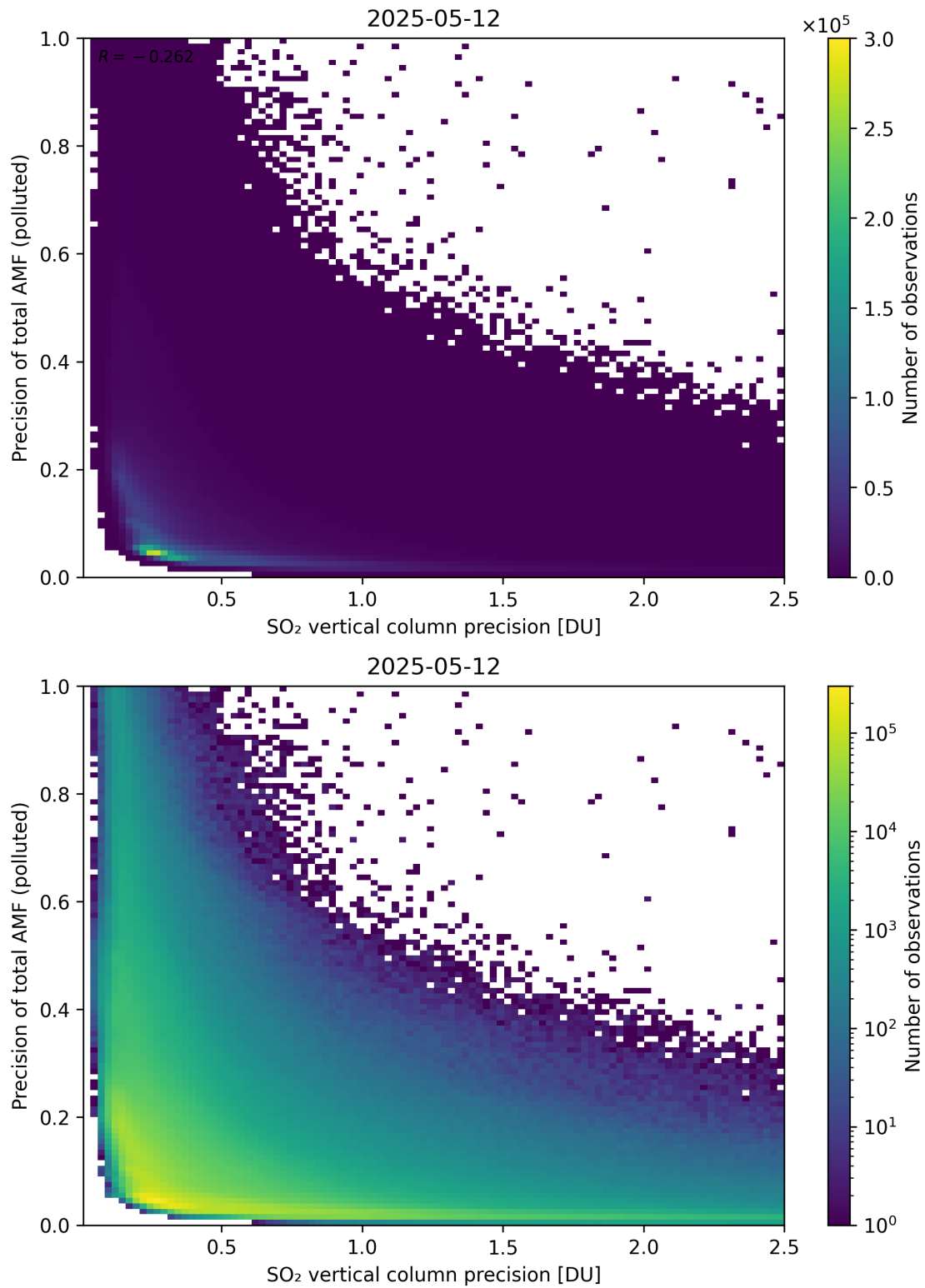
Figure 347: Scatter density plot of “SO 2 vertical column precision” against “Precision of total AMF (polluted)” for 2025-05-11 to 2025-05-13.
