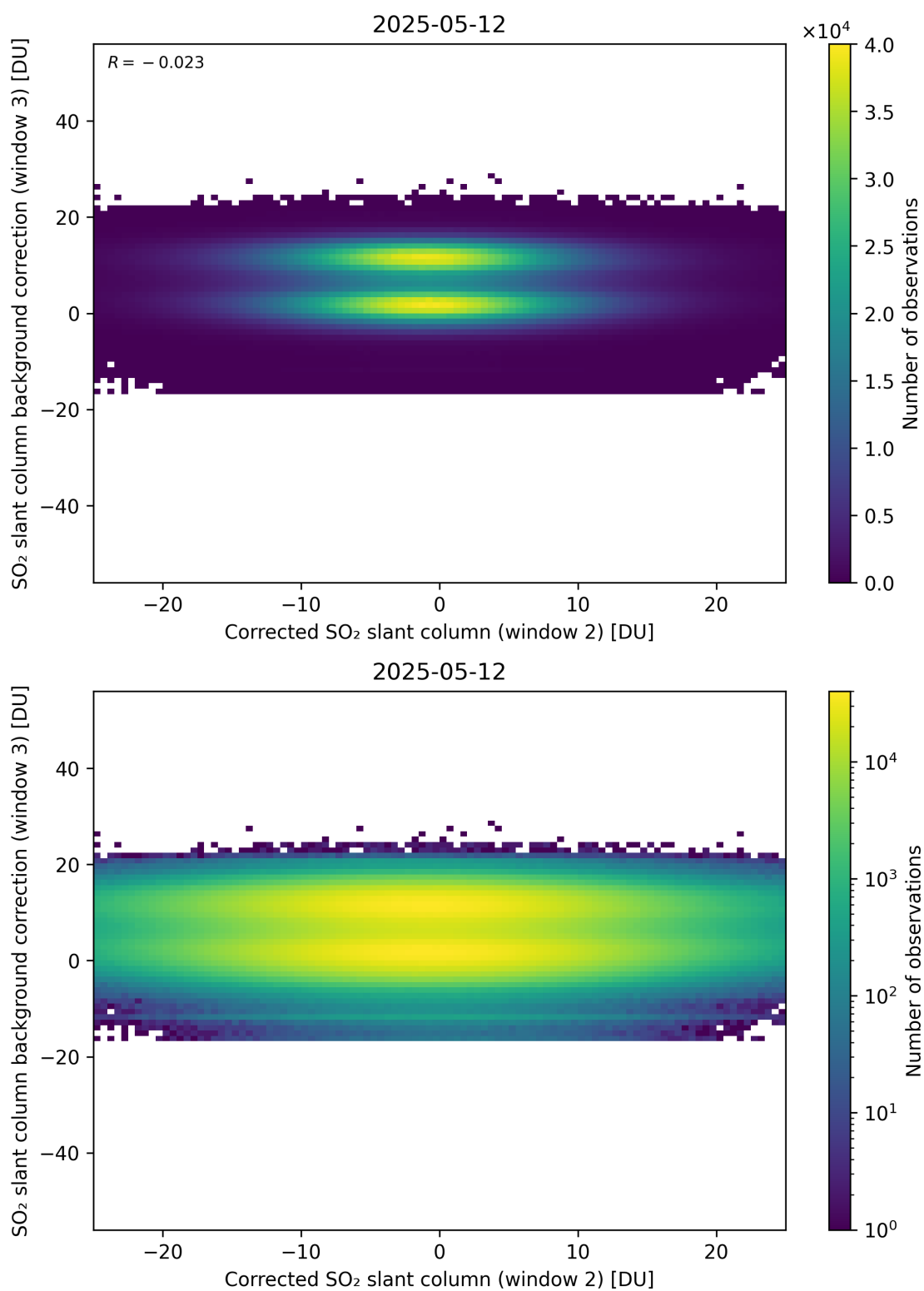
Figure 245: Scatter density plot of “Corrected SO 2 slant column (window 2)” against “SO 2 slant column background correction (window 3)” for 2025-05-11 to 2025-05-13.
