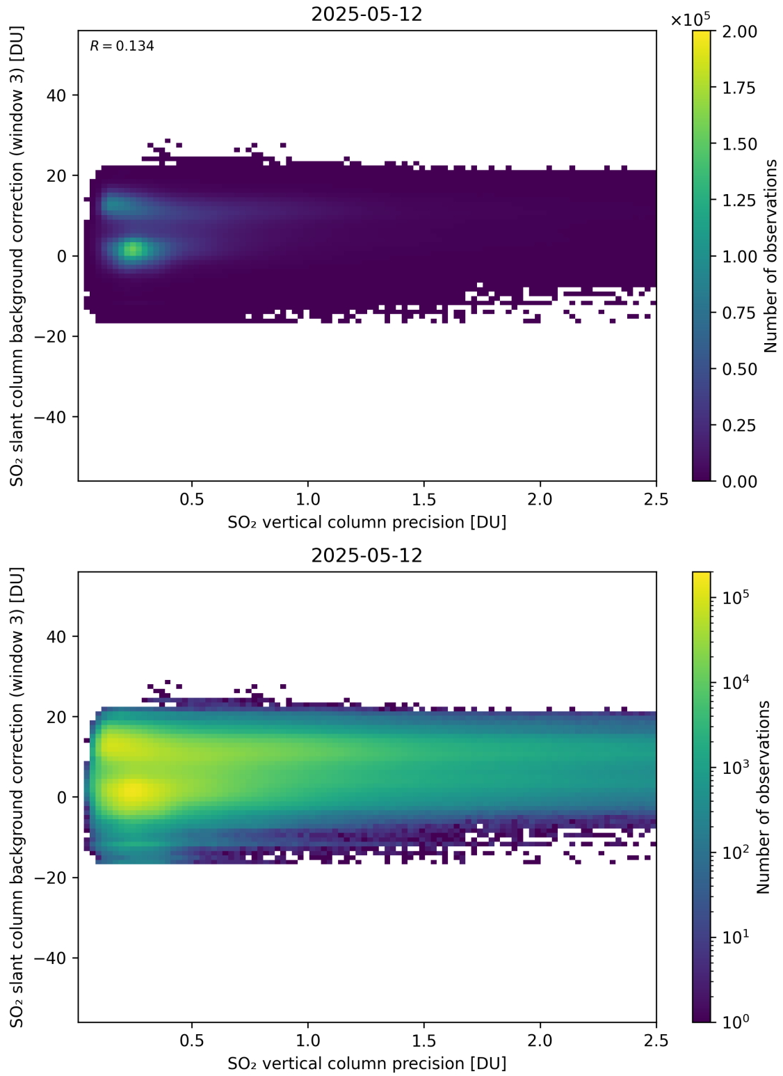
Figure 331: Scatter density plot of “SO 2 vertical column precision” against “SO 2 slant column background correction (window 3)” for 2025-05-11 to 2025-05-13.
