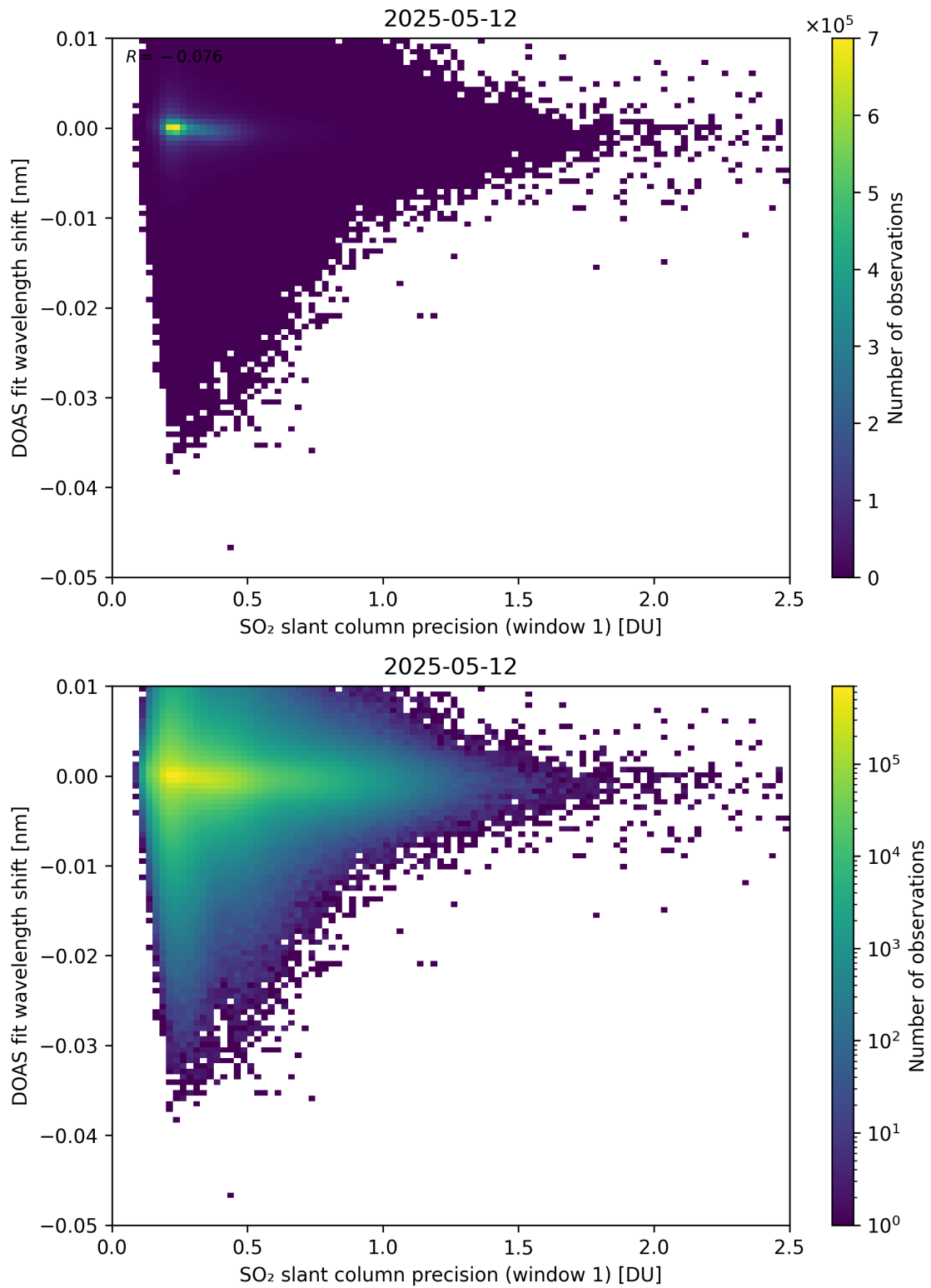
Figure 271: Scatter density plot of “SO 2 slant column precision (window 1)” against “DOAS fit wavelength shift” for 2025-05-11 to 2025-05-13.
