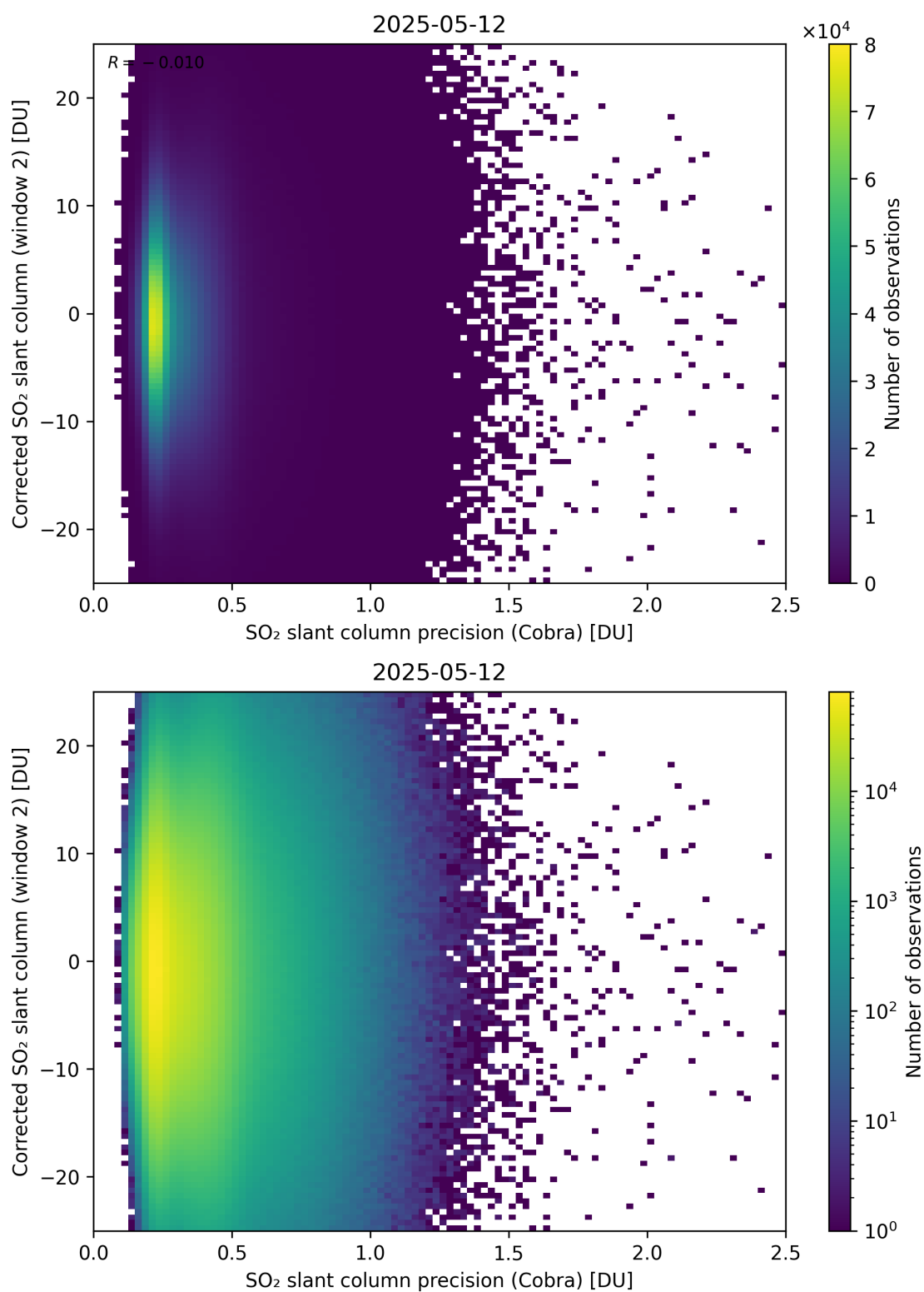
Figure 206: Scatter density plot of “SO 2 slant column precision (Cobra)” against “Corrected SO 2 slant column (window 2)” for 2025-05-11 to 2025-05-13.
