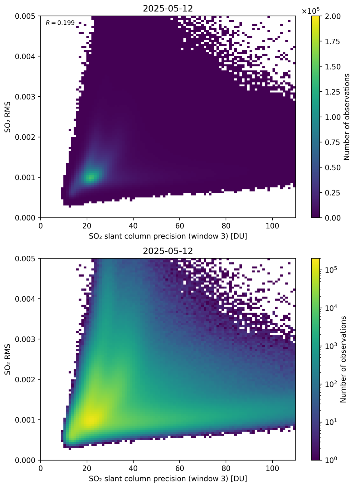
Figure 310: Scatter density plot of “SO 2 slant column precision (window 3)” against “SO 2 RMS” for 2025-05-11 to 2025-05-13.
