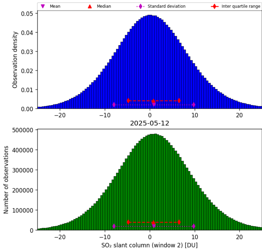
Figure 67: Histogram of “SO 2 slant column (window 2)” for 2025-05-11 to 2025-05-13
