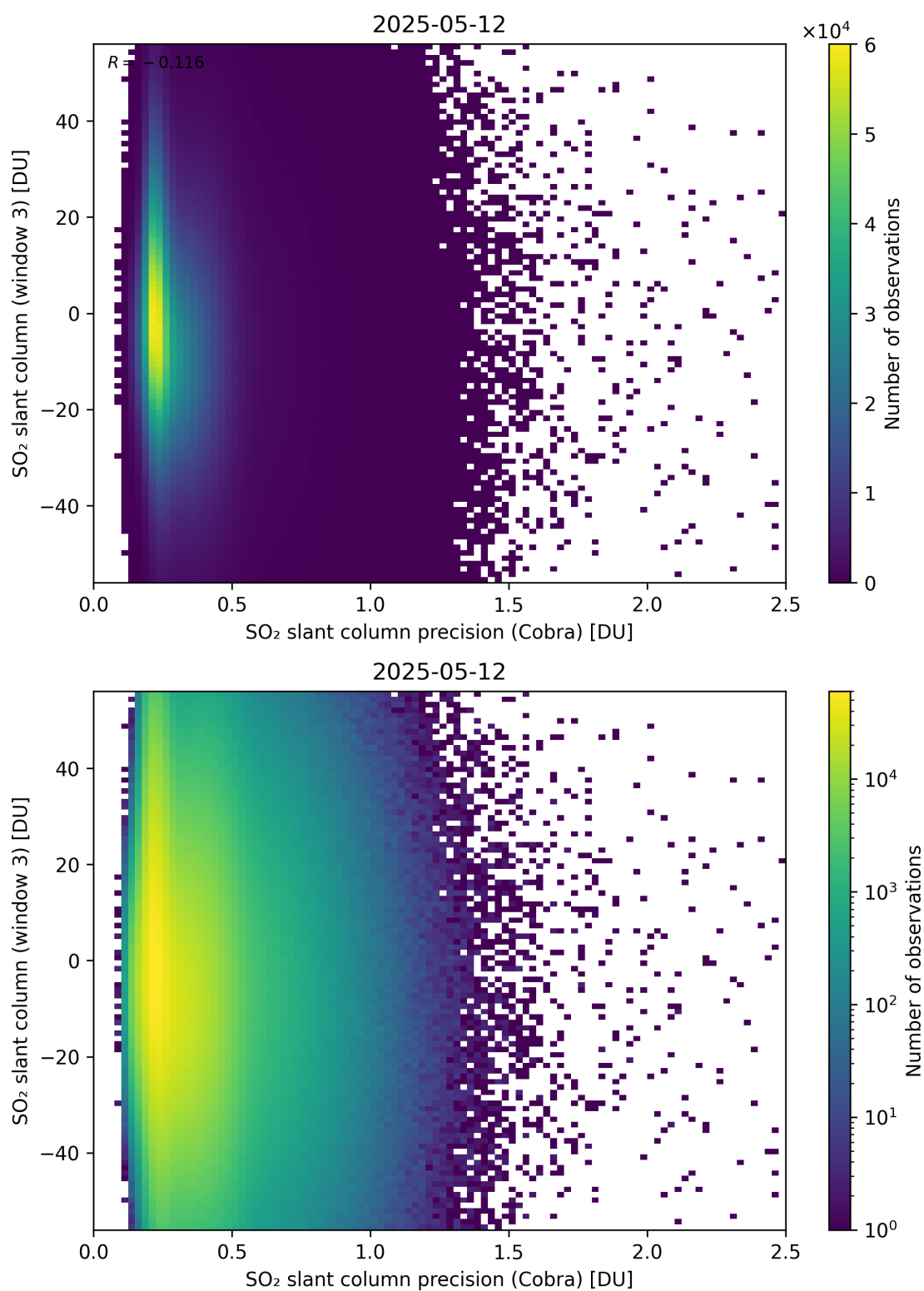
Figure 211: Scatter density plot of “SO 2 slant column precision (Cobra)” against “SO 2 slant column (window 3)” for 2025-05-11 to 2025-05-13.
