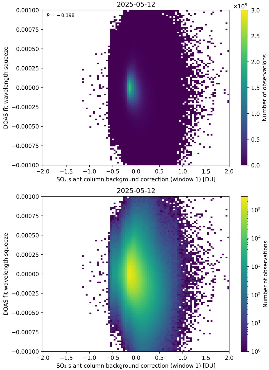
Figure 112: Scatter density plot of “SO 2 slant column background correction (window 1)” against “DOAS fit wavelength squeeze” for 2025-05-11 to 2025-05-13.
