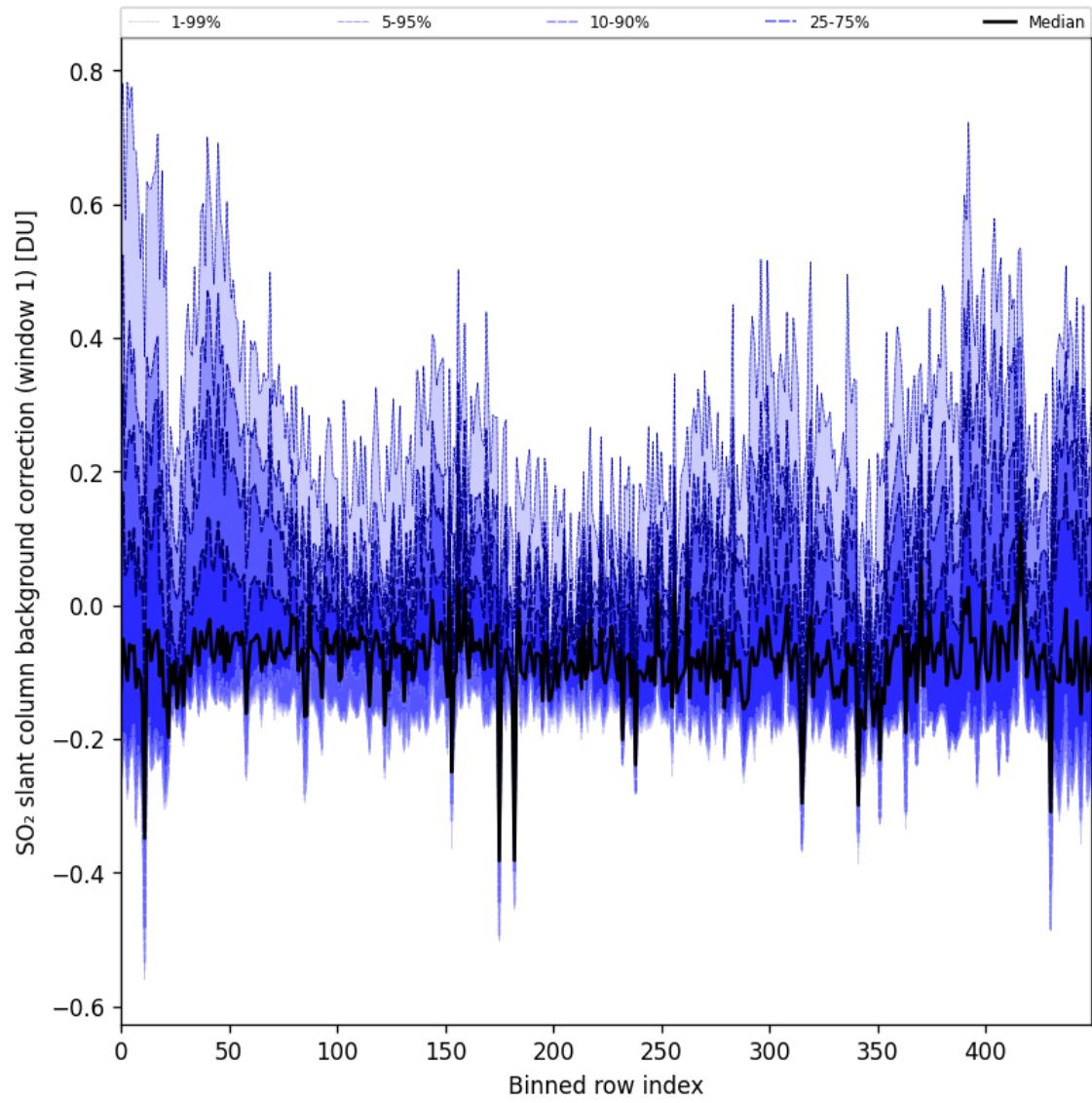
Figure 92: Along track statistics of “SO 2 slant column background correction (window 1)” for 2025-05-11 to 2025-05-13
