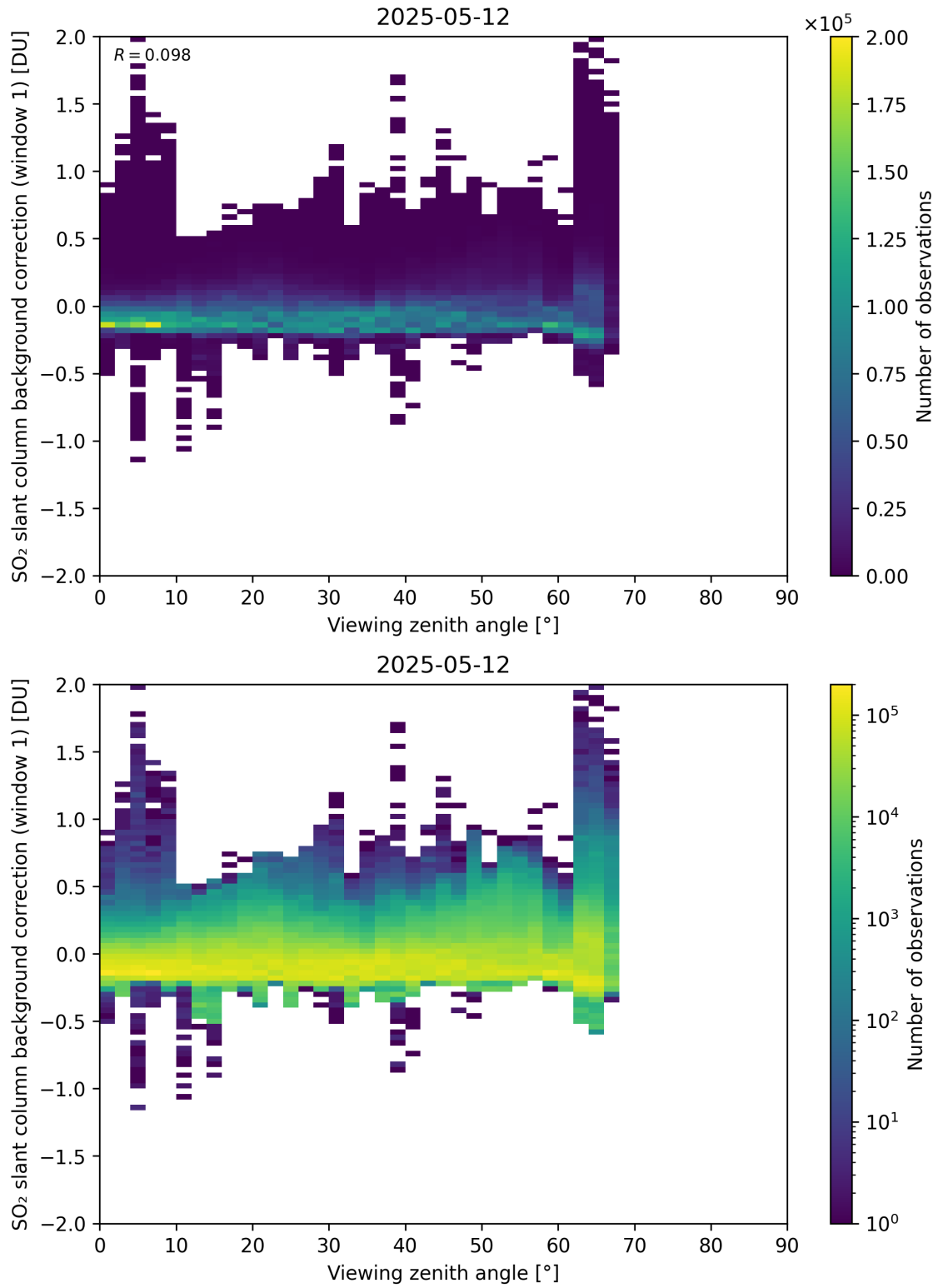
Figure 362: Scatter density plot of “Viewing zenith angle” against “SO 2 slant column background correction (window 1)” for 2025-05-11 to 2025-05-13.
