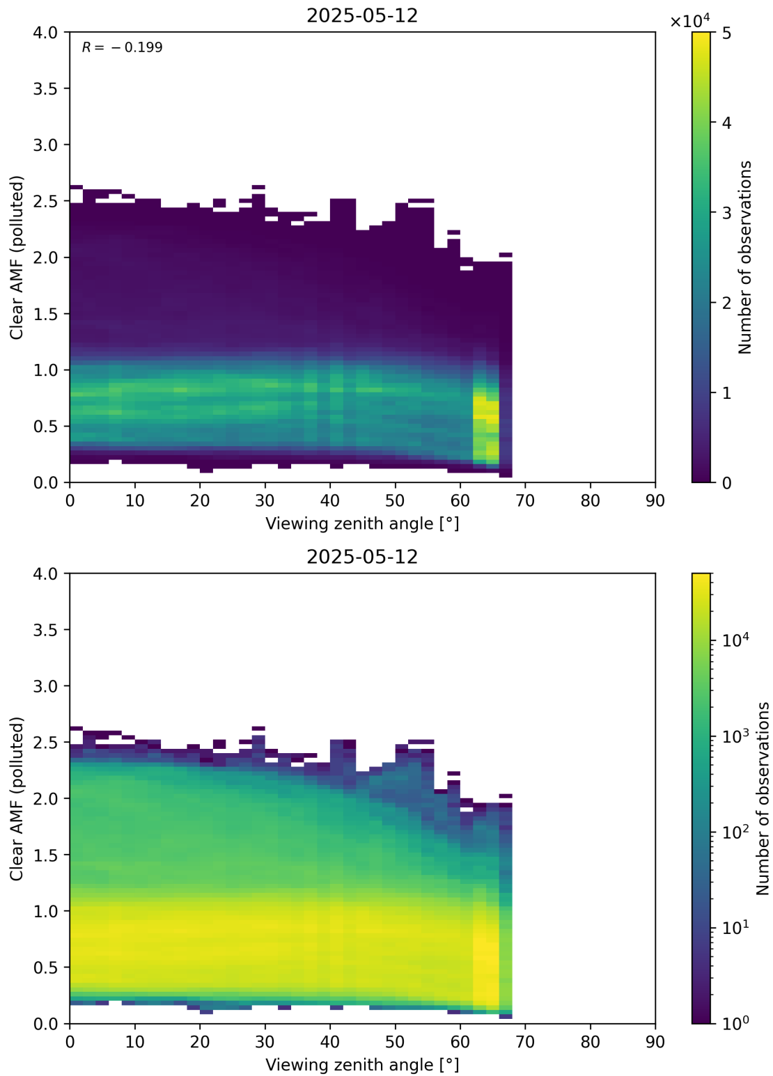
Figure 370: Scatter density plot of “Viewing zenith angle” against “Clear AMF (polluted)” for 2025-05-11 to 2025-05-13.
