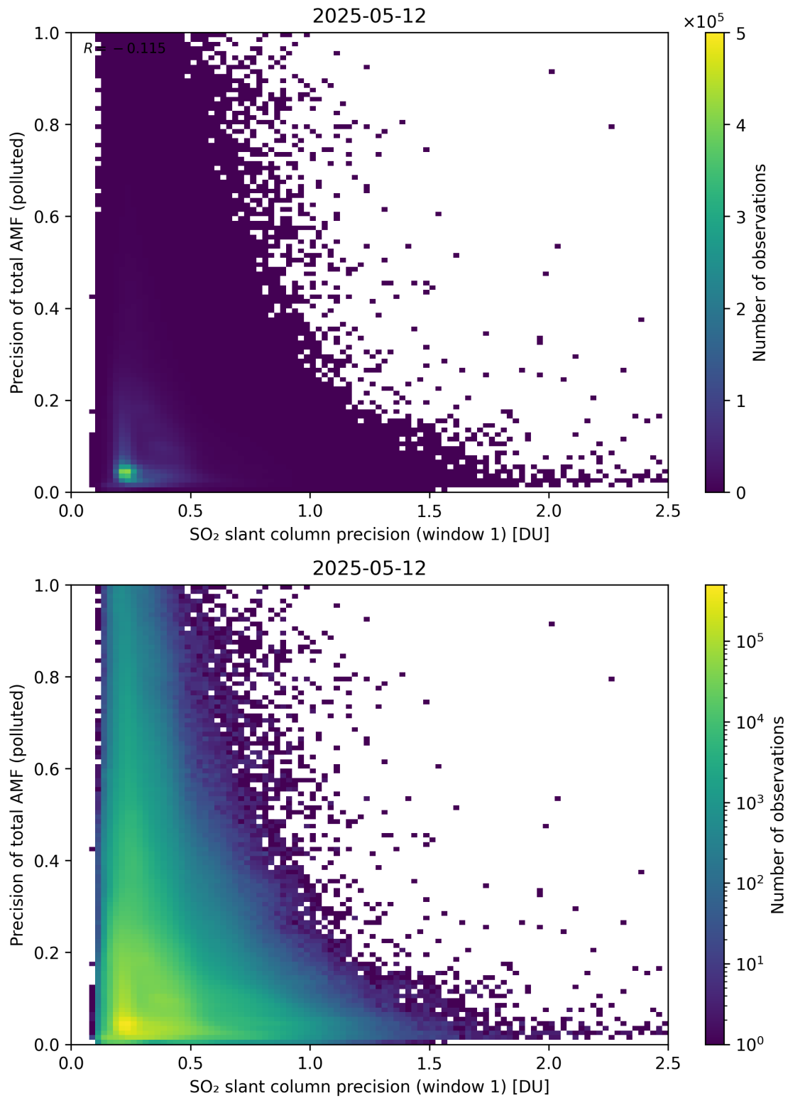
Figure 281: Scatter density plot of “SO 2 slant column precision (window 1)” against “Precision of total AMF (polluted)” for 2025-05-11 to 2025-05-13.
