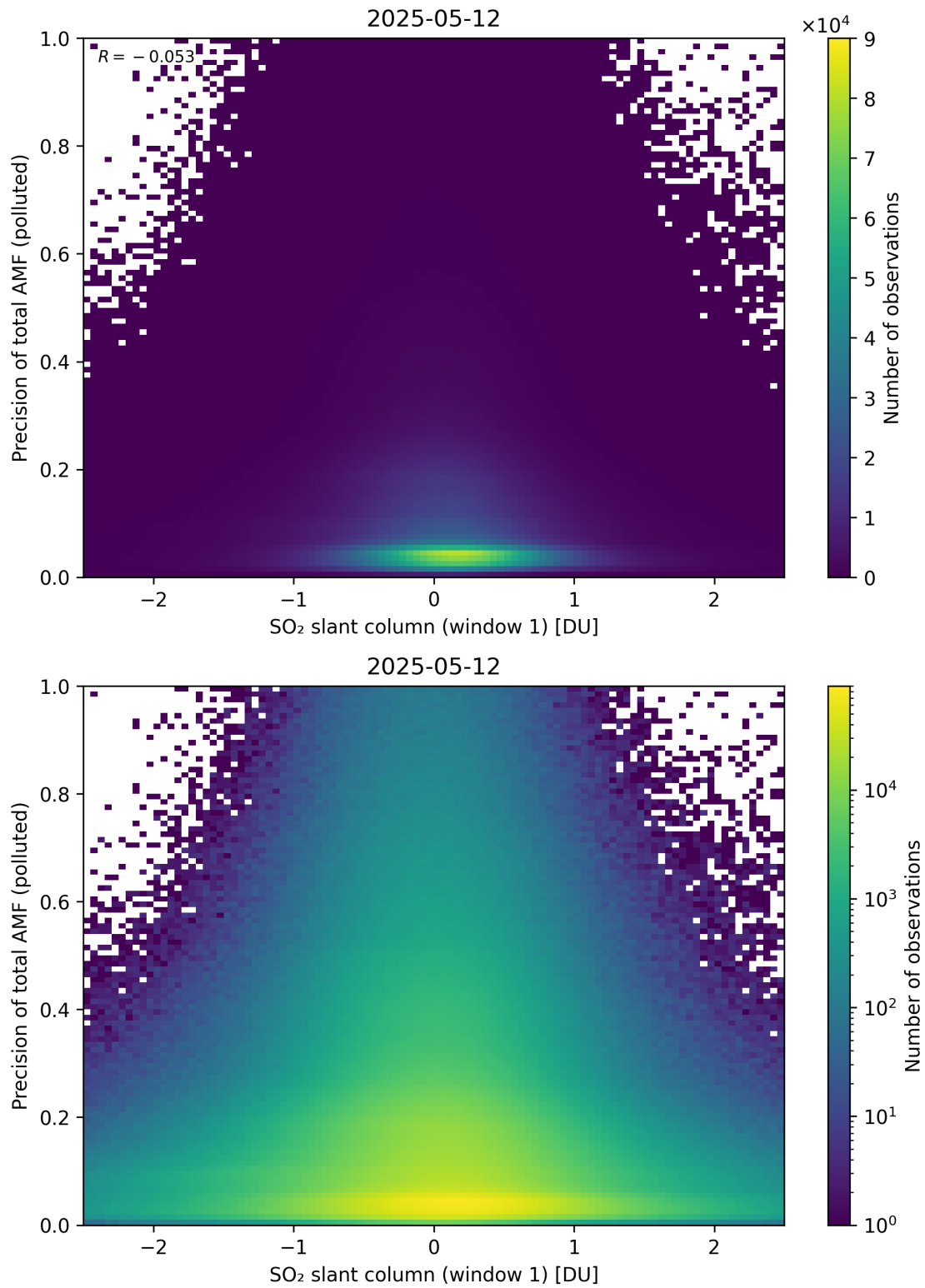
Figure 290: Scatter density plot of “SO 2 slant column (window 1)” against “Precision of total AMF (polluted)” for 2025-05-11 to 2025-05-13.
