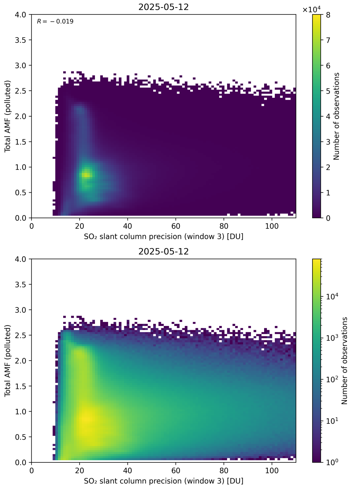
Figure 313: Scatter density plot of “SO 2 slant column precision (window 3)” against “Total AMF (polluted)” for 2025-05-11 to 2025-05-13.
