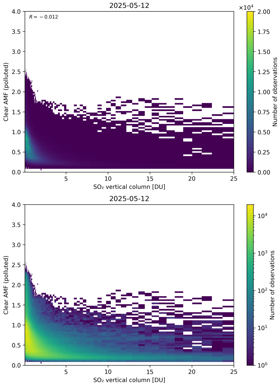
Figure 348: Scatter density plot of “SO 2 vertical column” against “Clear AMF (polluted)” for 2025-05-11 to 2025-05-13.
