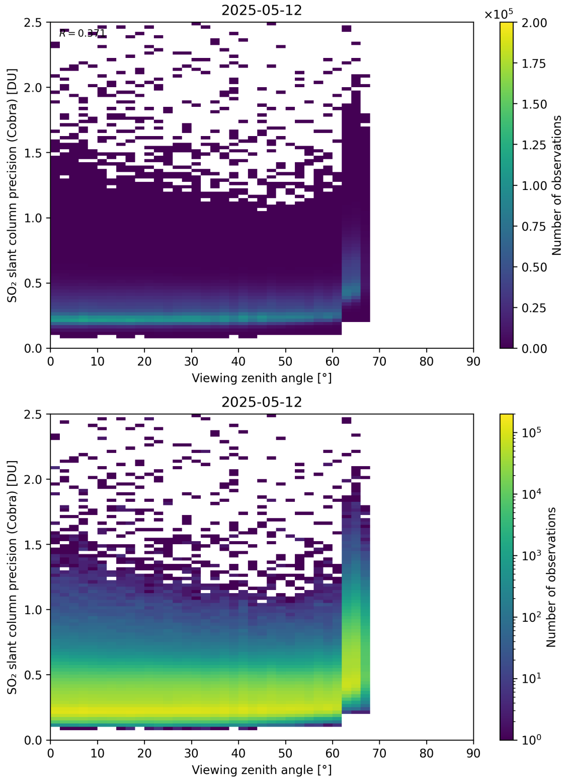
Figure 372: Scatter density plot of “Viewing zenith angle” against “SO 2 slant column precision (Cobra)” for 2025-05-11 to 2025-05-13.
