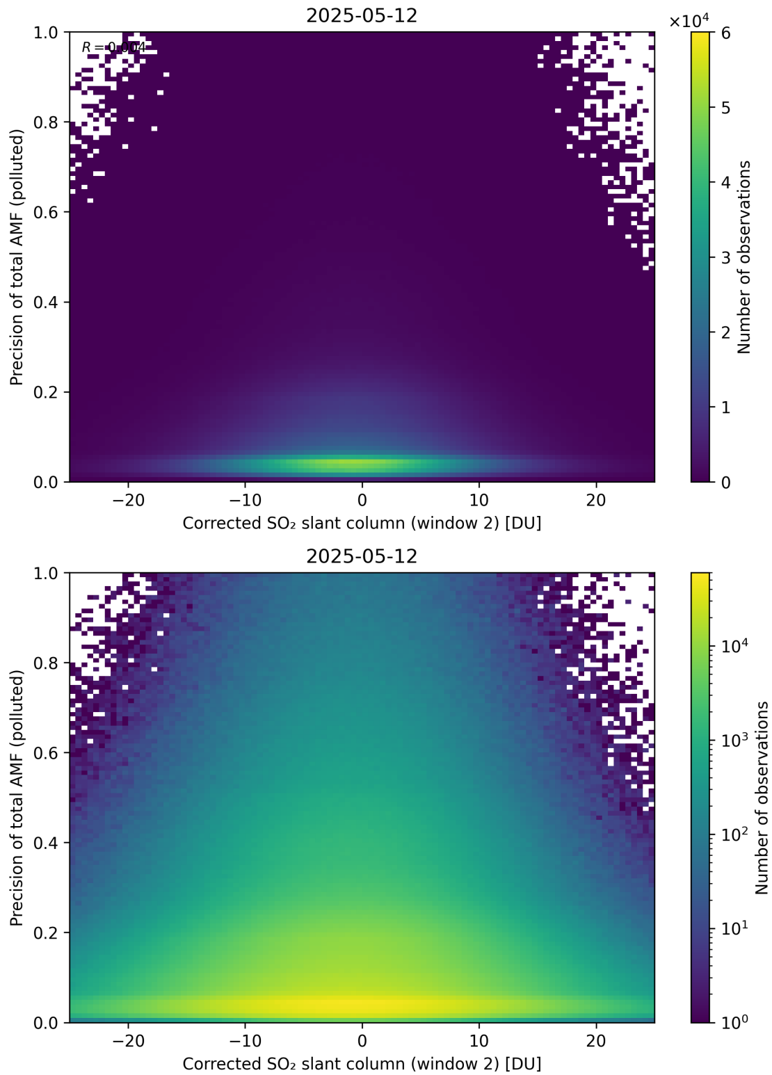
Figure 254: Scatter density plot of “Corrected SO 2 slant column (window 2)” against “Precision of total AMF (polluted)” for 2025-05-11 to 2025-05-13.
