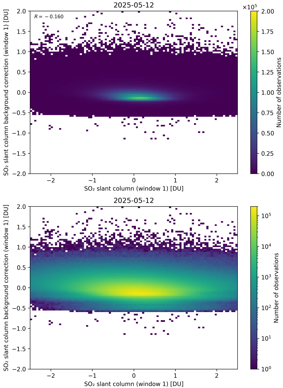
Figure 262: Scatter density plot of “SO 2 slant column (window 1)” against “SO 2 slant column background correction (window 1)” for 2025-05-11 to 2025-05-13.
