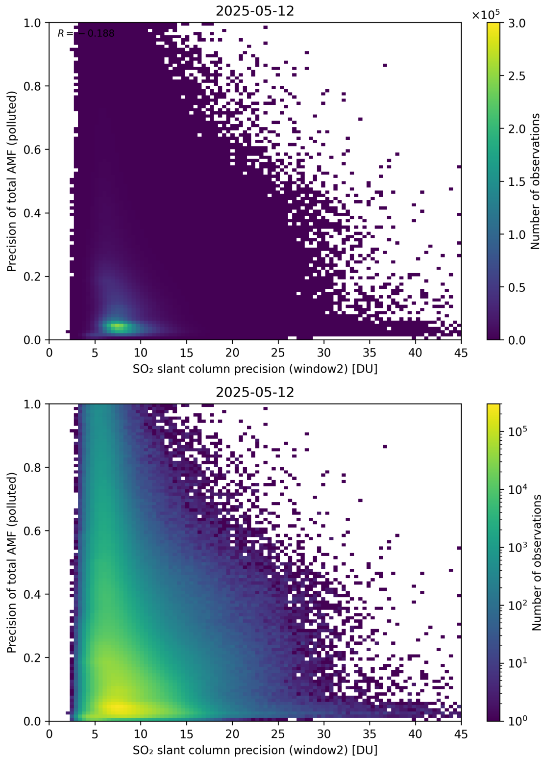
Figure 302: Scatter density plot of “SO 2 slant column precision (window2)” against “Precision of total AMF (polluted)” for 2025-05-11 to 2025-05-13.
