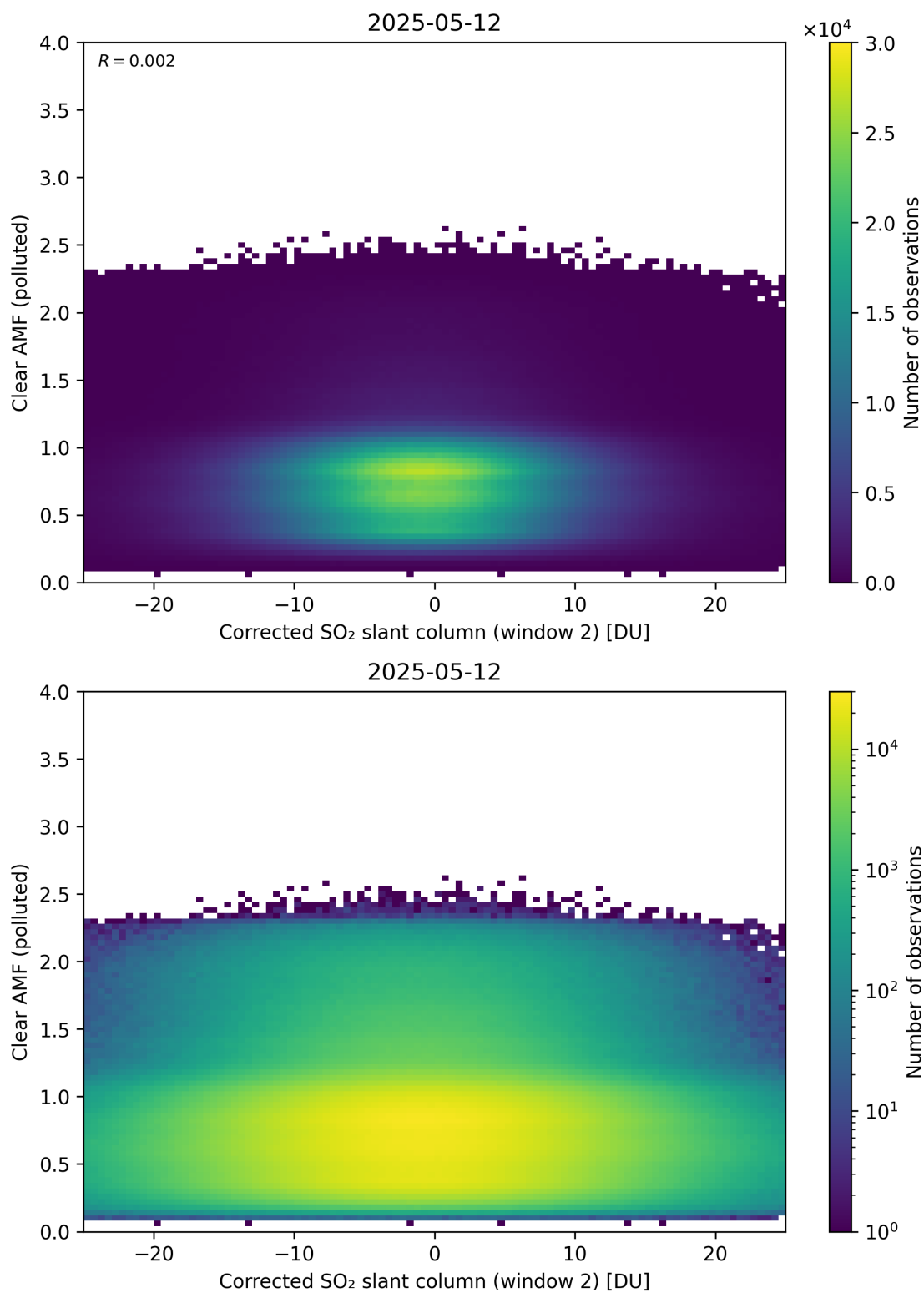
Figure 249: Scatter density plot of “Corrected SO 2 slant column (window 2)” against “Clear AMF (polluted)” for 2025-05-11 to 2025-05-13.
