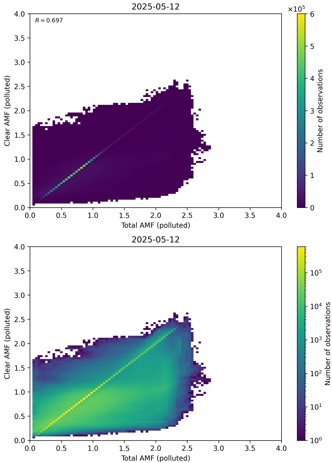
Figure 321: Scatter density plot of “Total AMF (polluted)” against “Clear AMF (polluted)” for 2025-05-11 to 2025-05-13.
