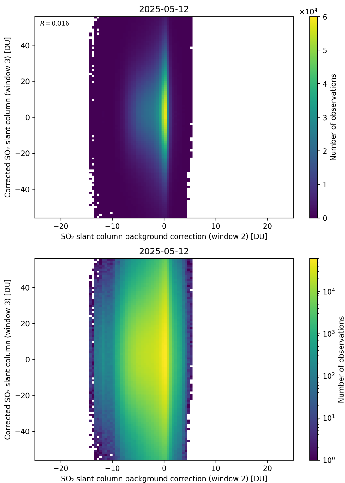
Figure 127: Scatter density plot of “SO 2 slant column background correction (window 2)” against “Corrected SO 2 slant column (window 3)” for 2025-05-11 to 2025-05-13.
