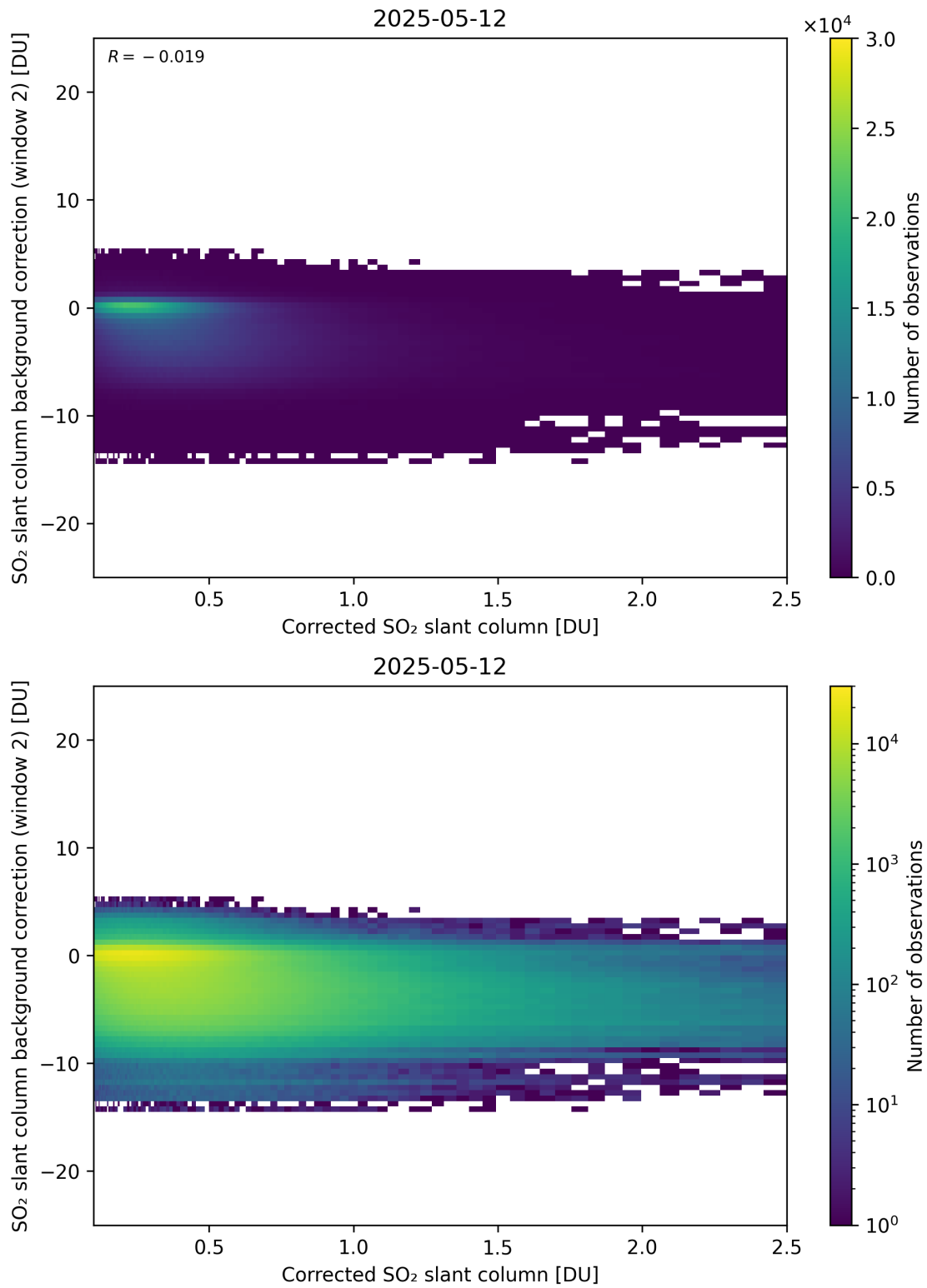
Figure 227: Scatter density plot of “Corrected SO 2 slant column” against “SO 2 slant column background correction (window 2)” for 2025-05-11 to 2025-05-13.
