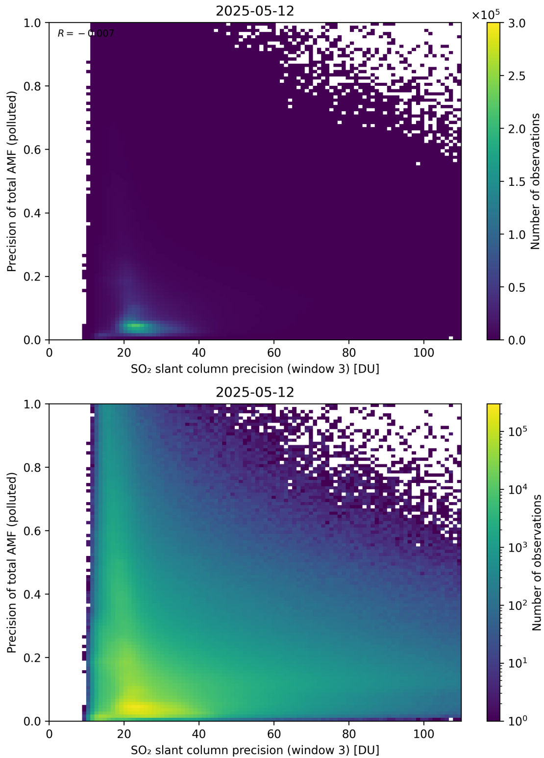
Figure 314: Scatter density plot of “SO 2 slant column precision (window 3)” against “Precision of total AMF (polluted)” for 2025-05-11 to 2025-05-13.
