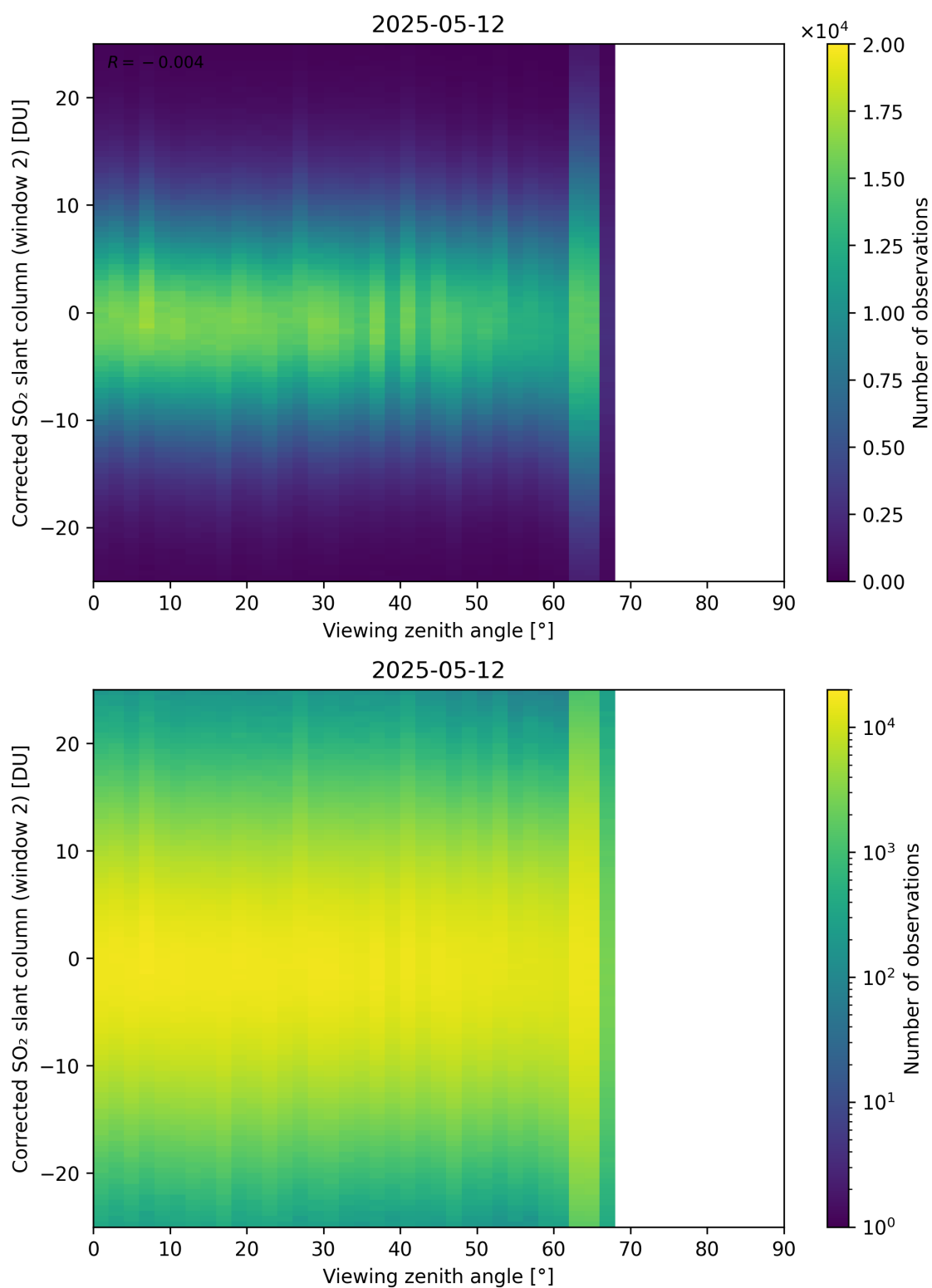
Figure 374: Scatter density plot of “Viewing zenith angle” against “Corrected SO 2 slant column (window 2)” for 2025-05-11 to 2025-05-13.
