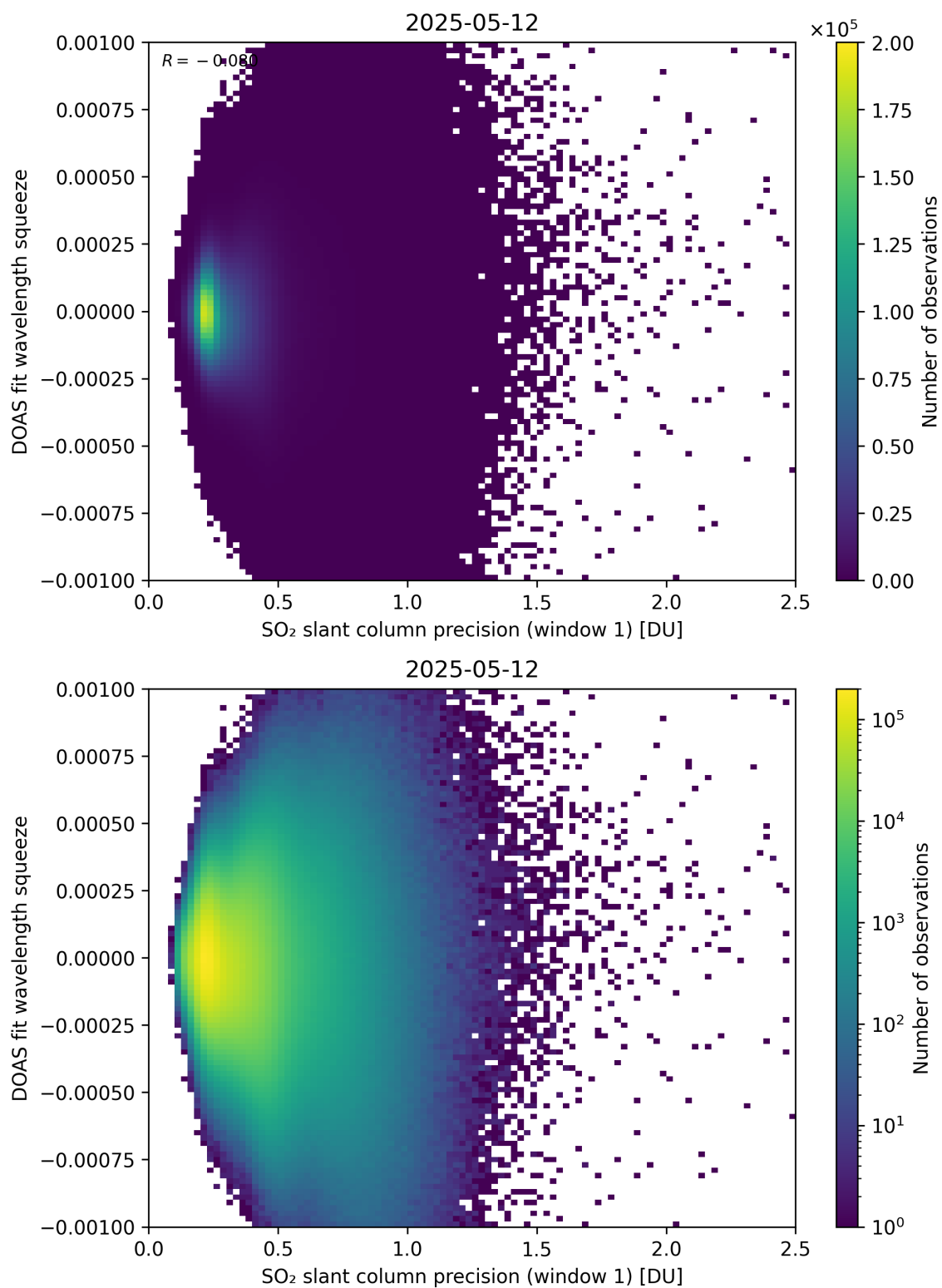
Figure 272: Scatter density plot of “SO 2 slant column precision (window 1)” against “DOAS fit wavelength squeeze” for 2025-05-11 to 2025-05-13.
