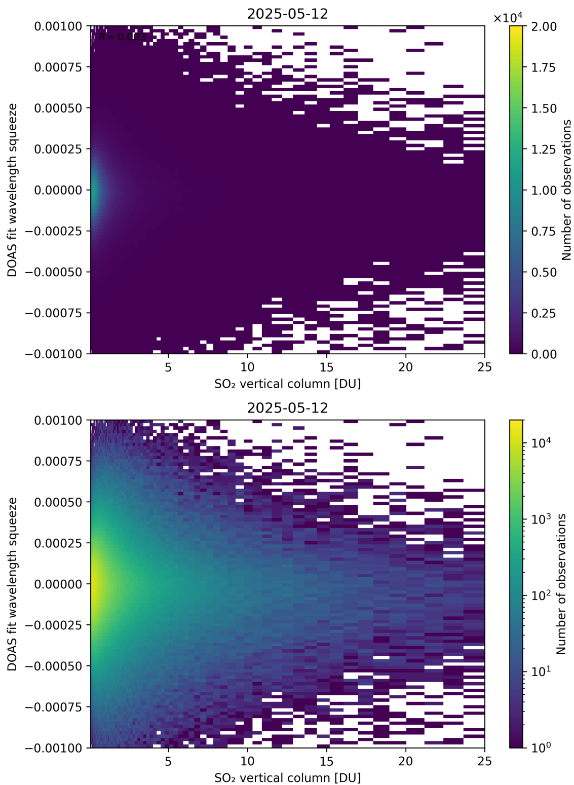
Figure 327: Scatter density plot of “SO 2 vertical column” against “DOAS fit wavelength squeeze” for 2025-05-11 to 2025-05-13.
