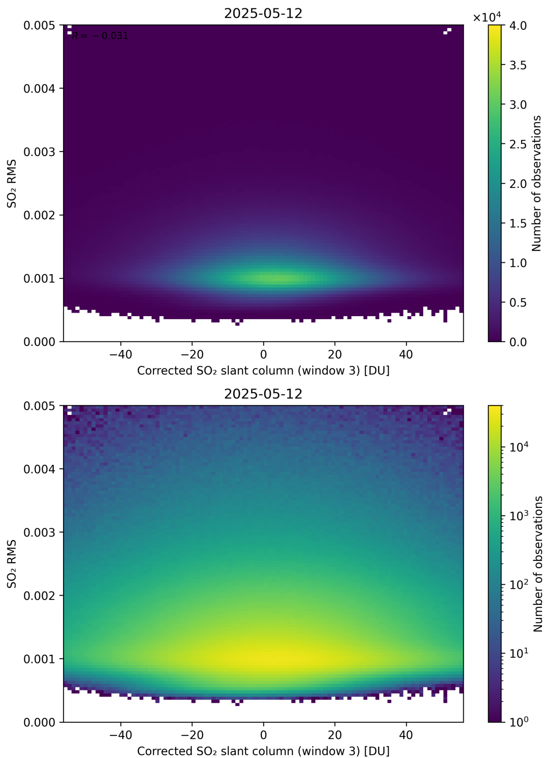
Figure 258: Scatter density plot of “Corrected SO 2 slant column (window 3)” against “SO 2 RMS” for 2025-05-11 to 2025-05-13.
