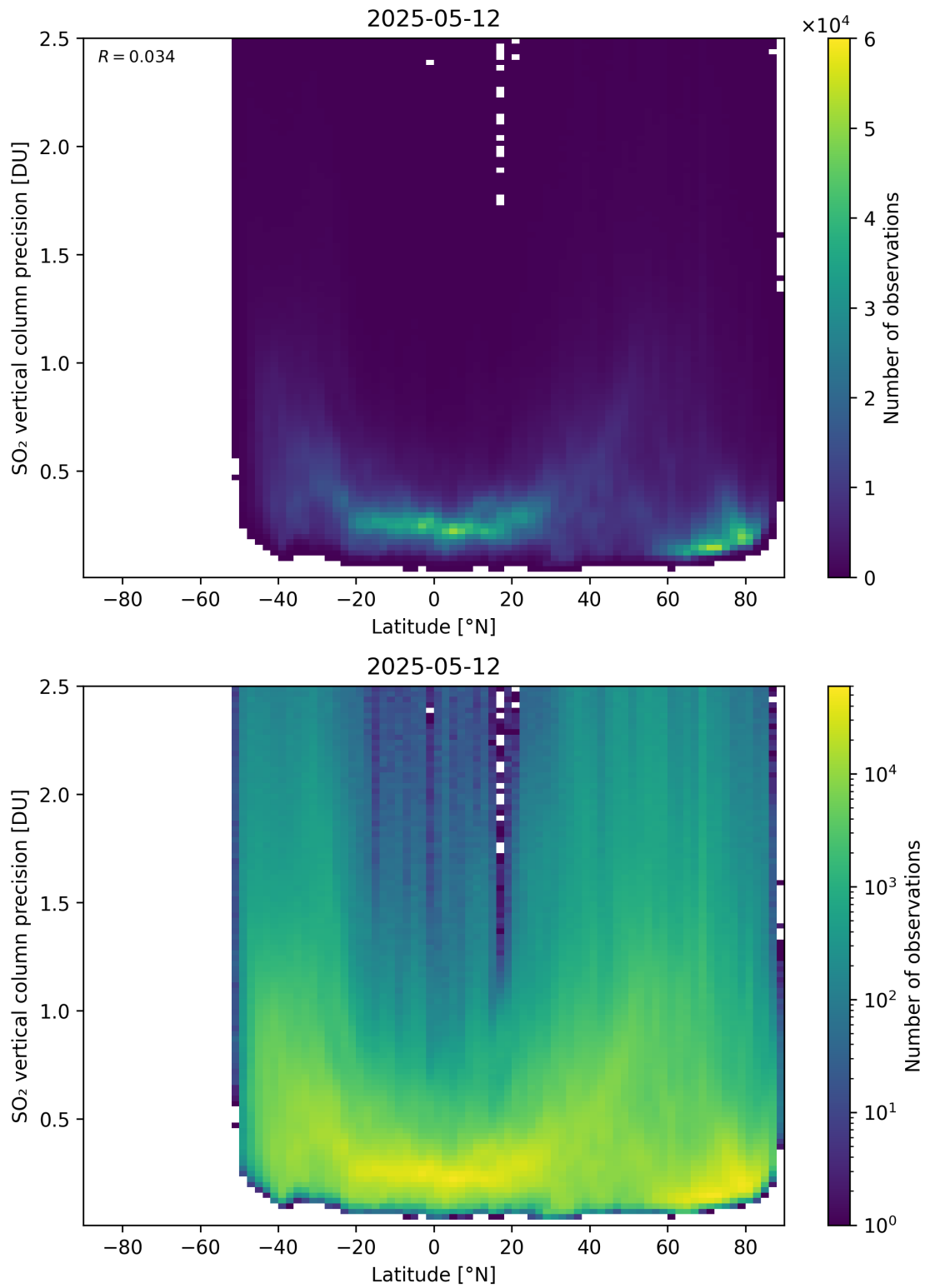
Figure 170: Scatter density plot of “Latitude” against “SO 2 vertical column precision” for 2025-05-11 to 2025-05-13.
