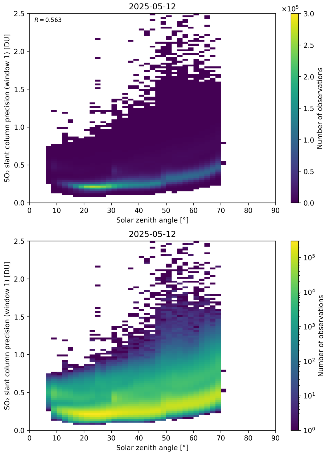
Figure 185: Scatter density plot of “Solar zenith angle” against “SO 2 slant column precision (window 1)” for 2025-05-11 to 2025-05-13.
