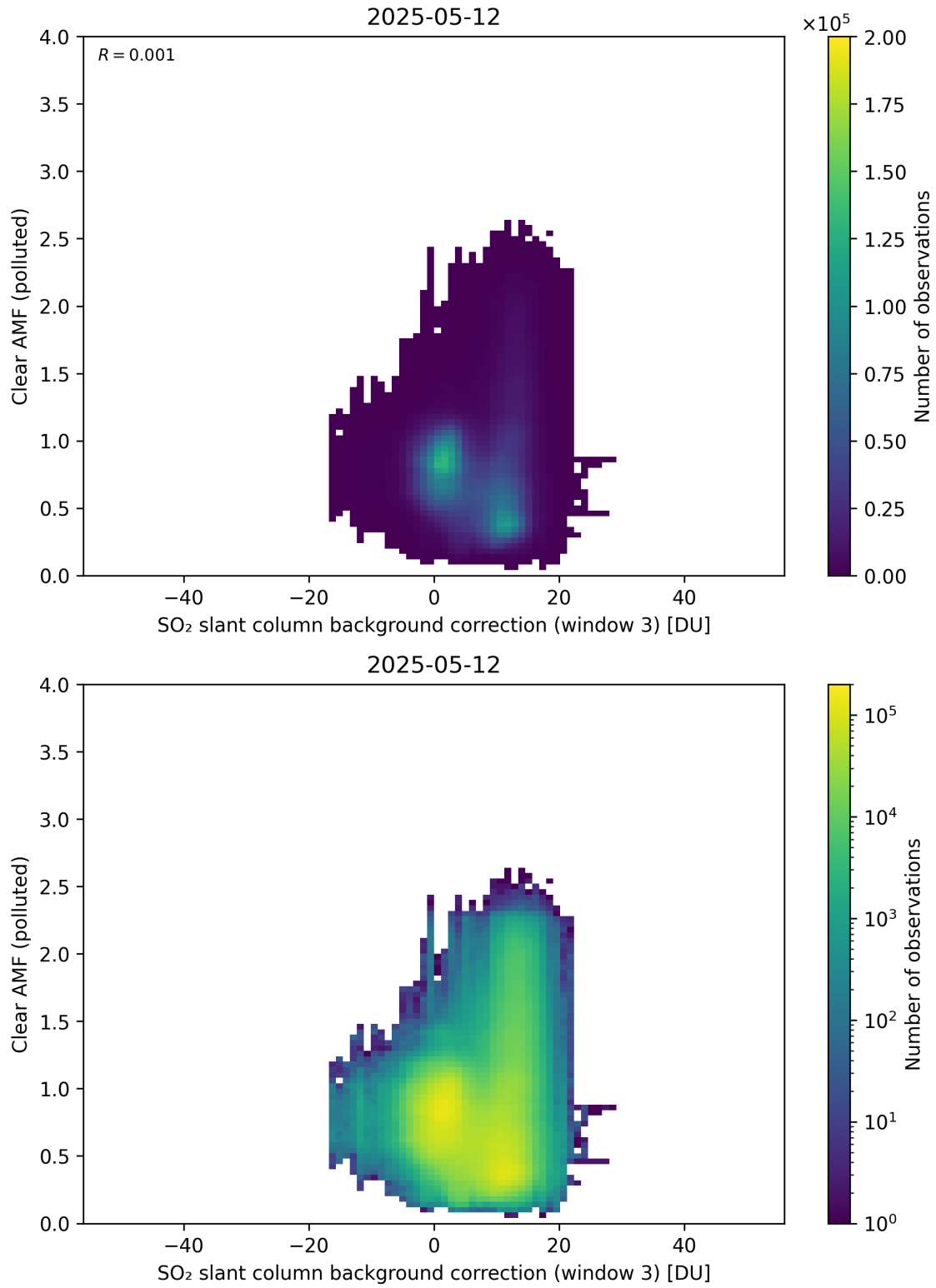
Figure 135: Scatter density plot of “SO 2 slant column background correction (window 3)” against “Clear AMF (polluted)” for 2025-05-11 to 2025-05-13.
