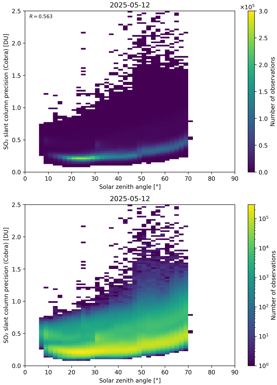
Figure 180: Scatter density plot of “Solar zenith angle” against “SO 2 slant column precision (Cobra)” for 2025-05-11 to 2025-05-13.
