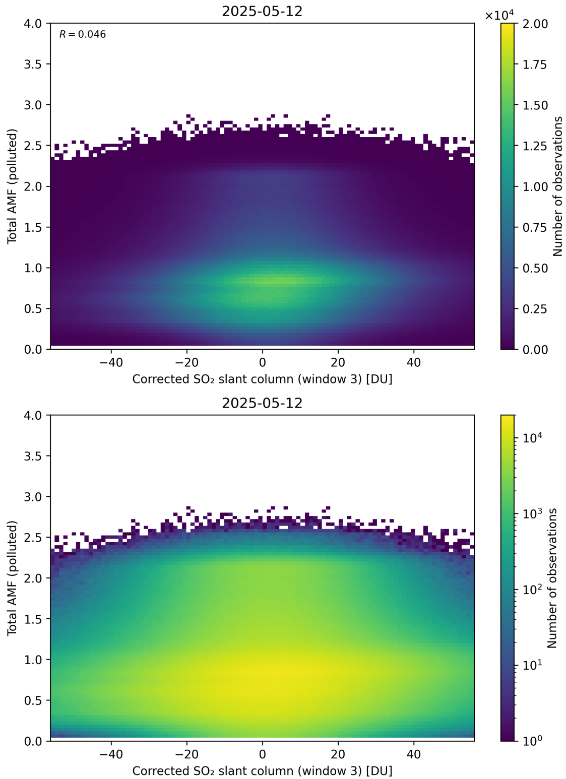
Figure 260: Scatter density plot of “Corrected SO 2 slant column (window 3)” against “Total AMF (polluted)” for 2025-05-11 to 2025-05-13.
