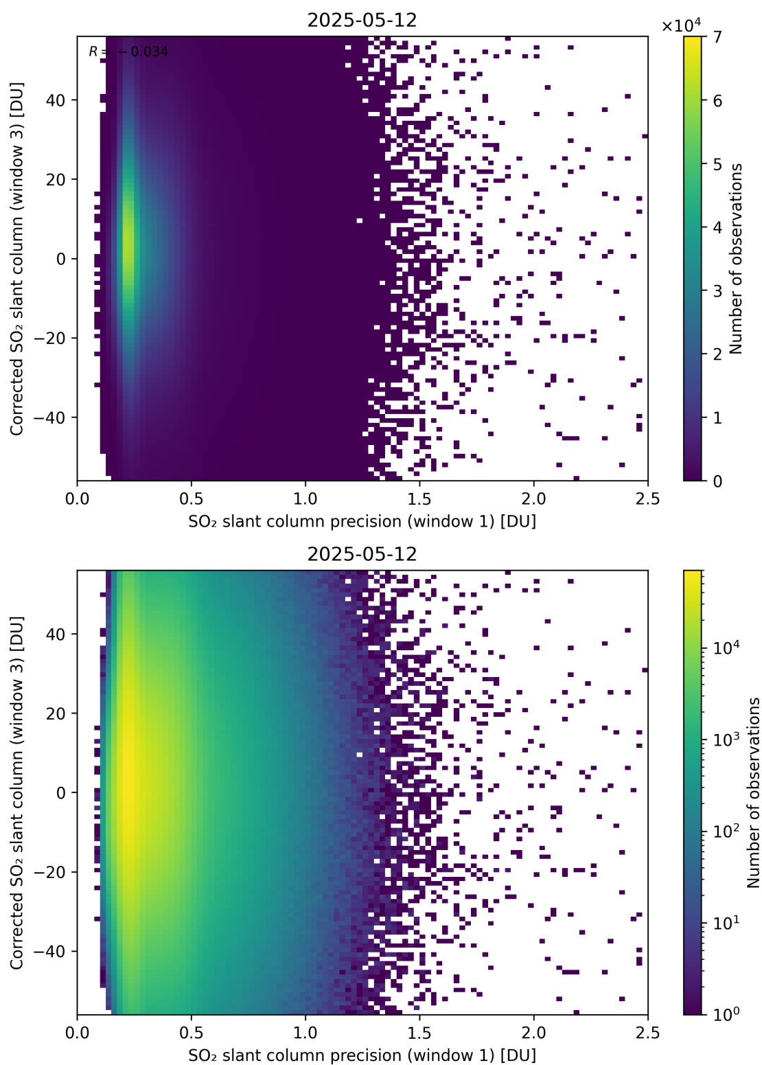
Figure 276: Scatter density plot of “SO 2 slant column precision (window 1)” against “Corrected SO 2 slant column (window 3)” for 2025-05-11 to 2025-05-13.
