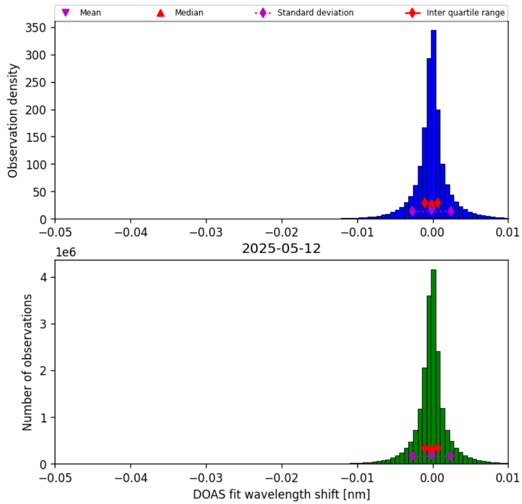
Figure 76: Histogram of “DOAS fit wavelength shift” for 2025-05-11 to 2025-05-13
