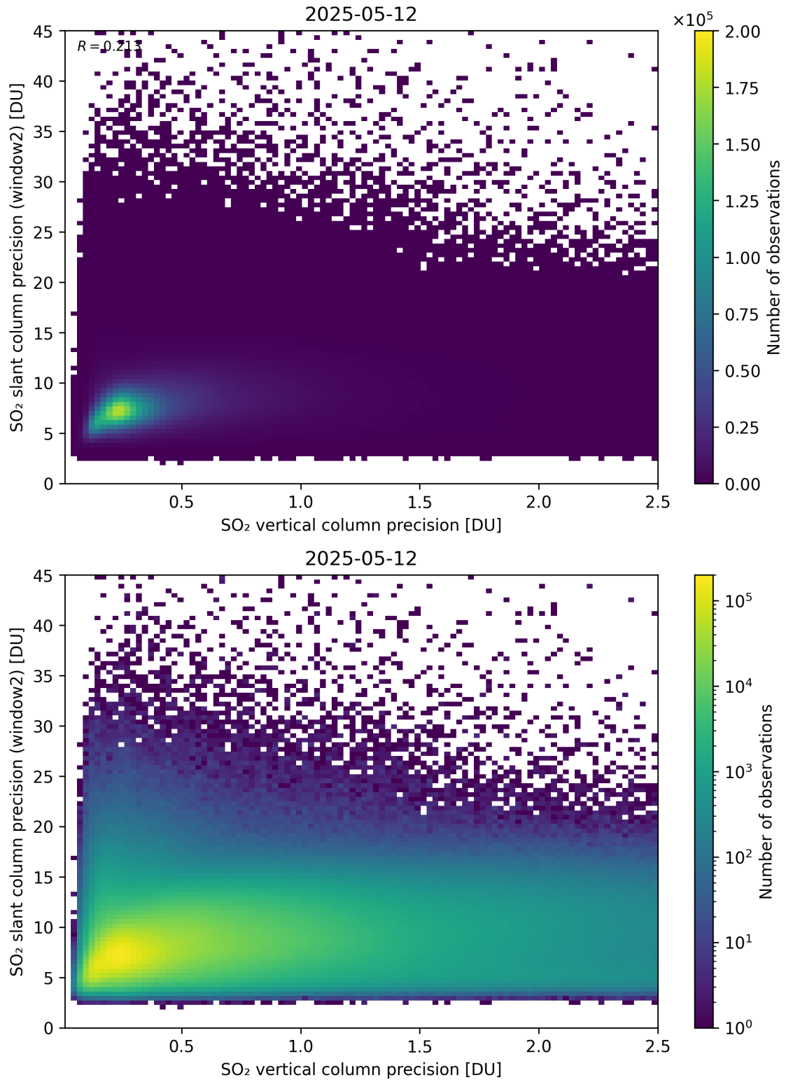
Figure 343: Scatter density plot of “SO 2 vertical column precision” against “SO 2 slant column precision (window2)” for 2025-05-11 to 2025-05-13.
