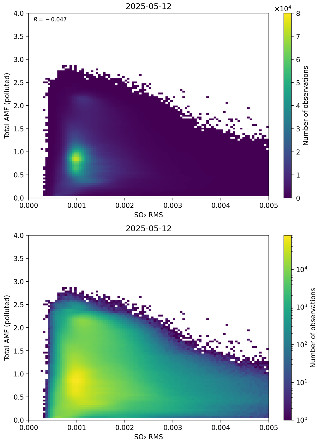
Figure 148: Scatter density plot of “SO 2 RMS” against “Total AMF (polluted)” for 2025-05-11 to 2025-05-13.
