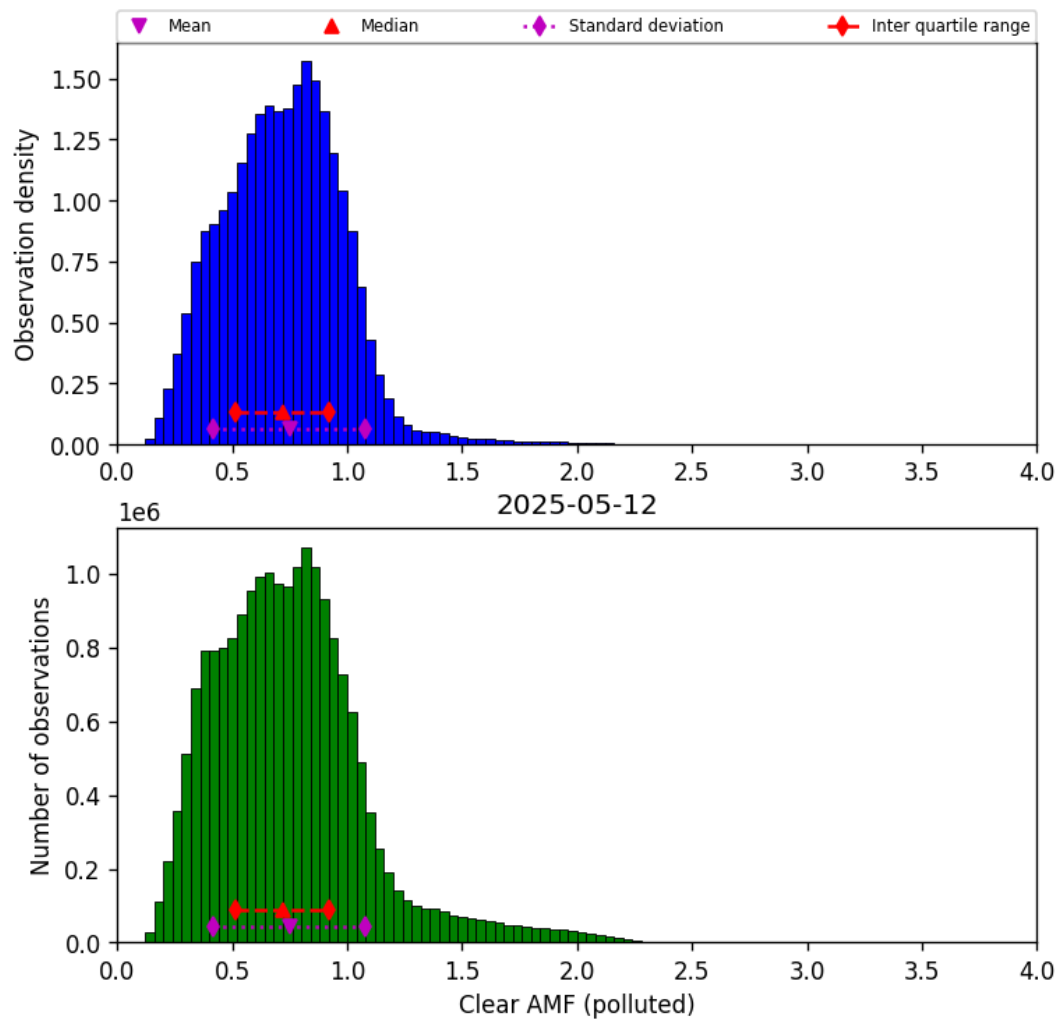
Figure 81: Histogram of “Clear AMF (polluted)” for 2025-05-11 to 2025-05-13
