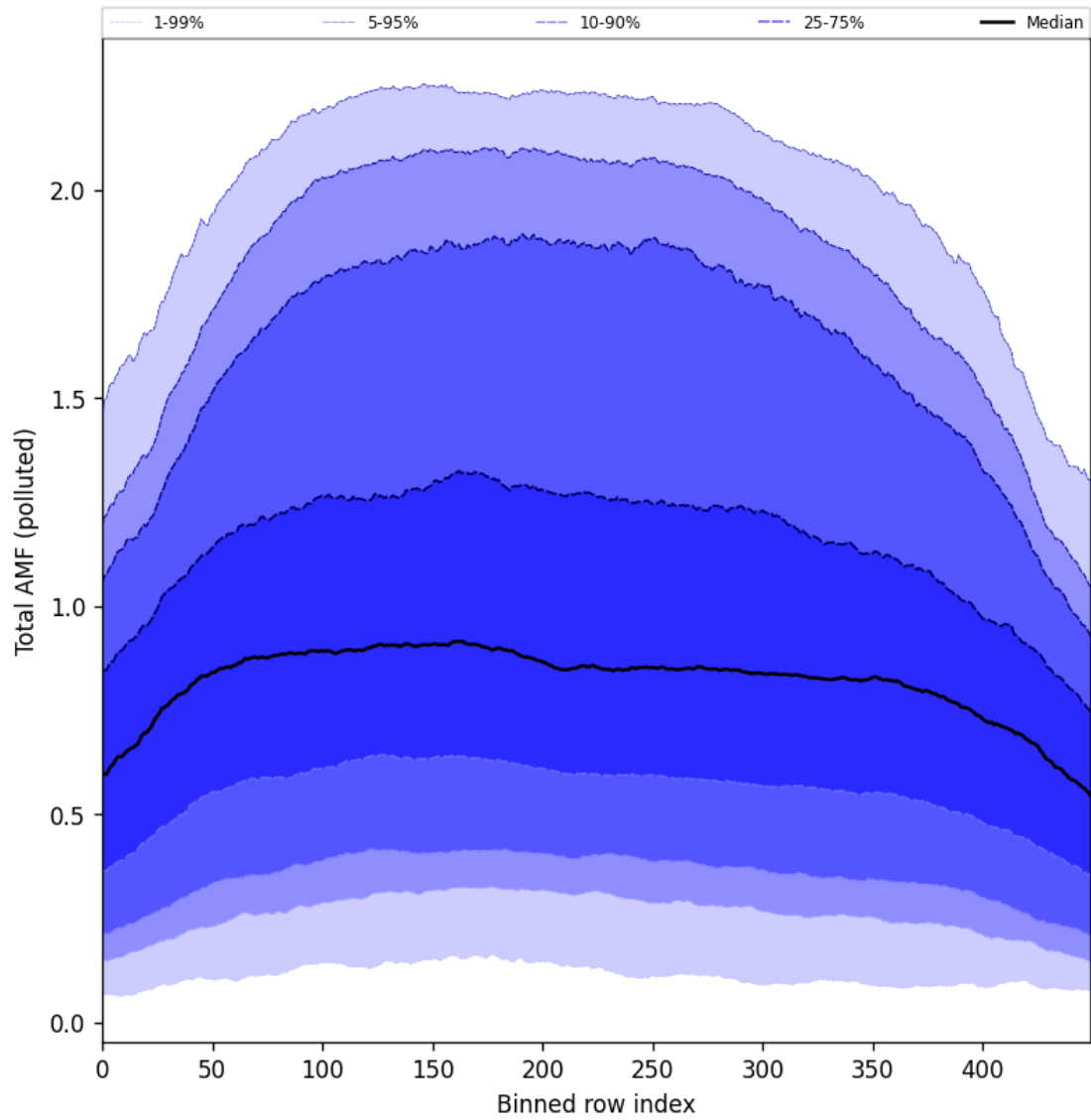
Figure 105: Along track statistics of “Total AMF (polluted)” for 2025-05-11 to 2025-05-13
