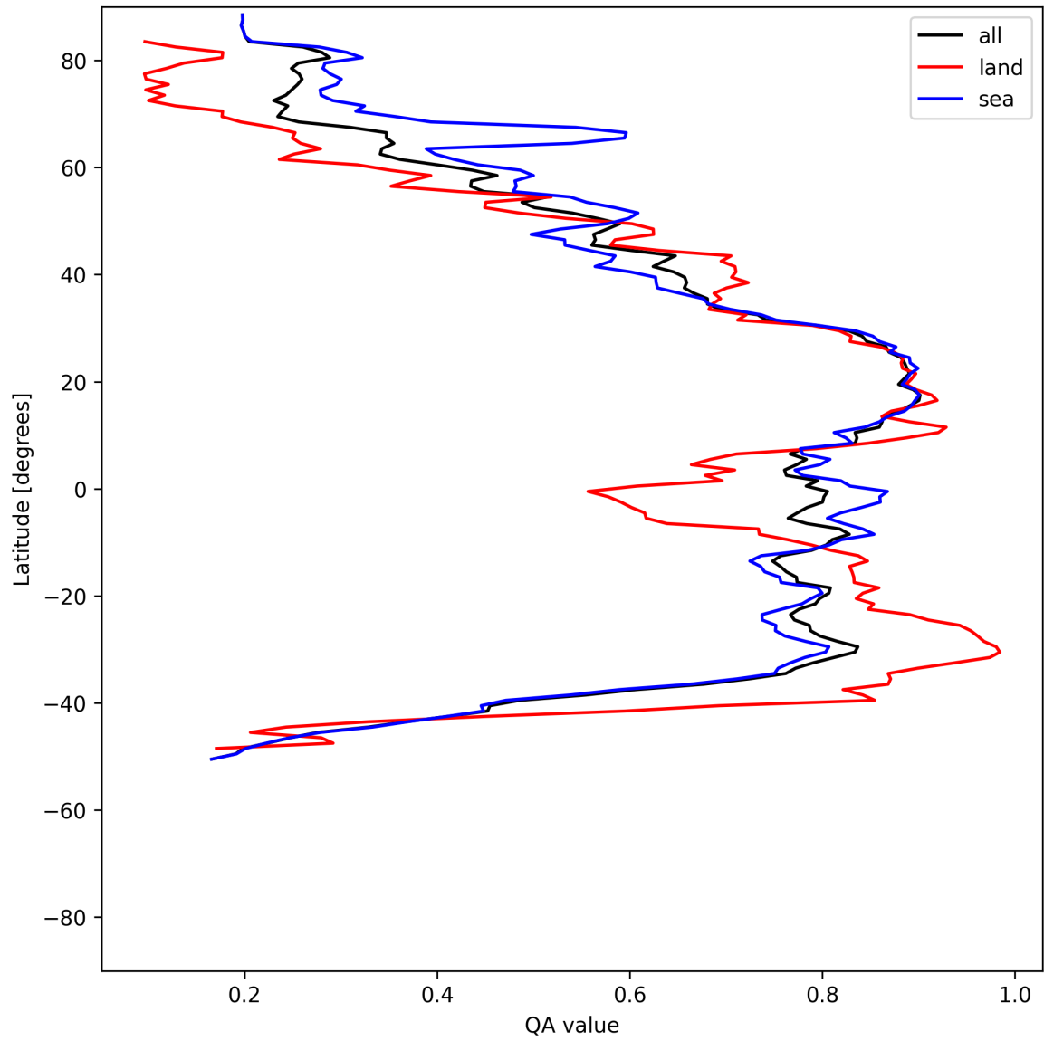
Figure 31: Zonal average of “QA value” for 2025-05-11 to 2025-05-13.
