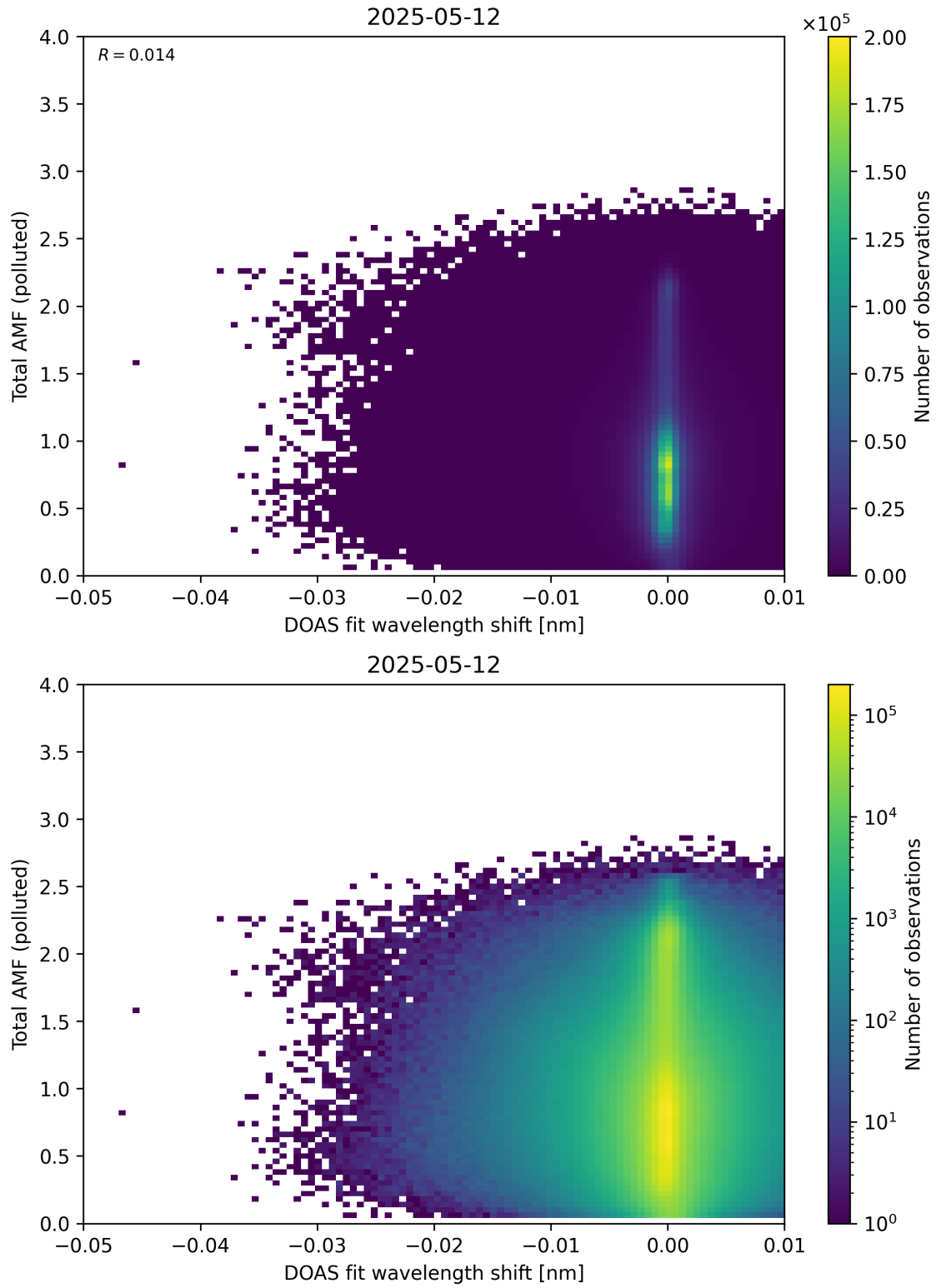
Figure 141: Scatter density plot of “DOAS fit wavelength shift” against “Total AMF (polluted)” for 2025-05-11 to 2025-05-13.
