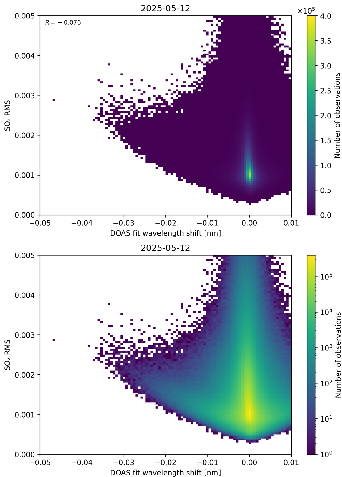
Figure 139: Scatter density plot of “DOAS fit wavelength shift” against “SO 2 RMS” for 2025-05-11 to 2025-05-13.
