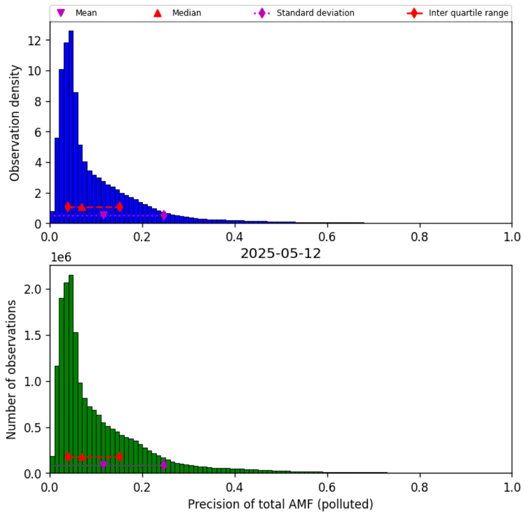
Figure 80: Histogram of “Precision of total AMF (polluted)” for 2025-05-11 to 2025-05-13
