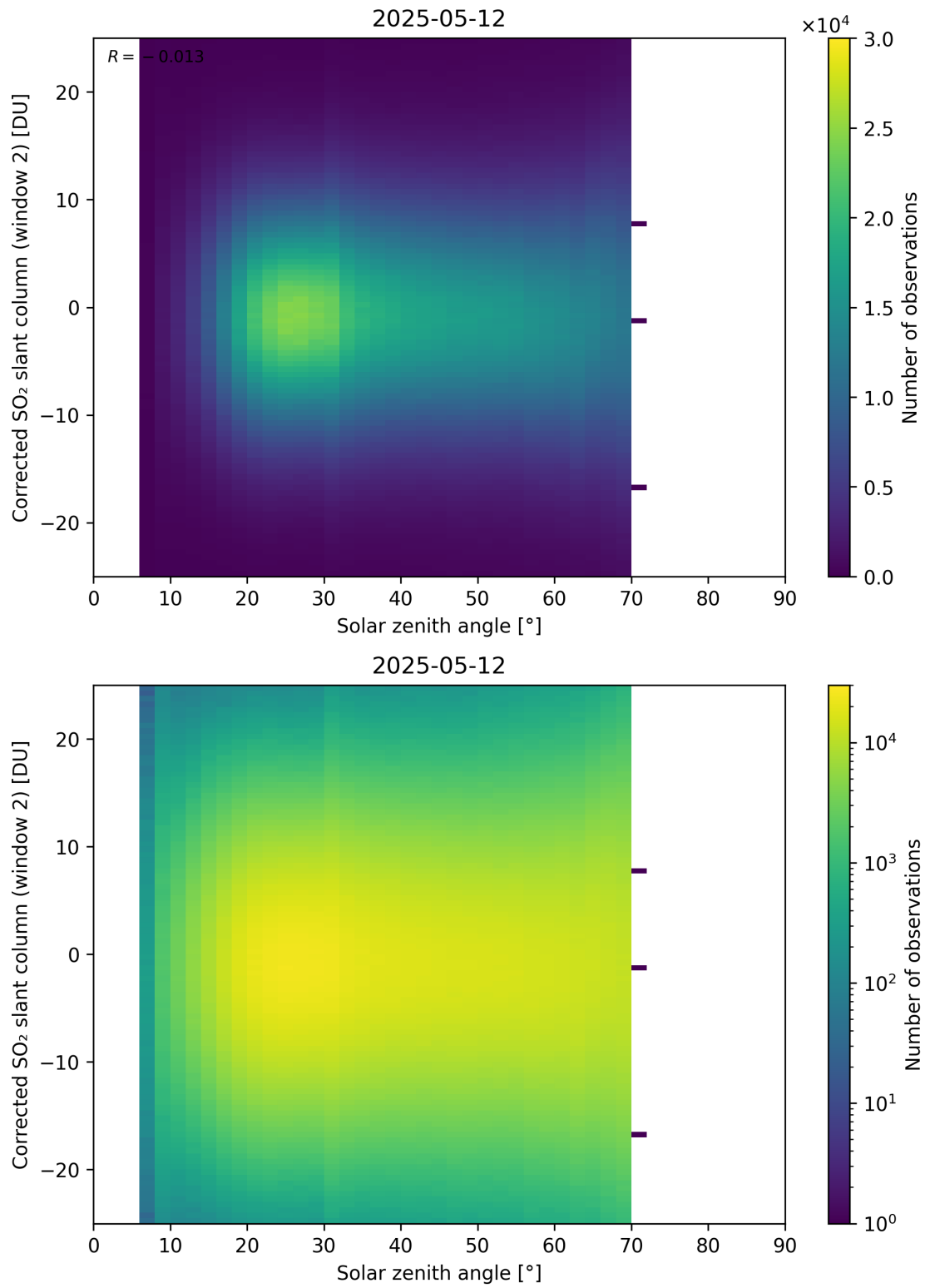
Figure 182: Scatter density plot of “Solar zenith angle” against “Corrected SO 2 slant column (window 2)” for 2025-05-11 to 2025-05-13.
