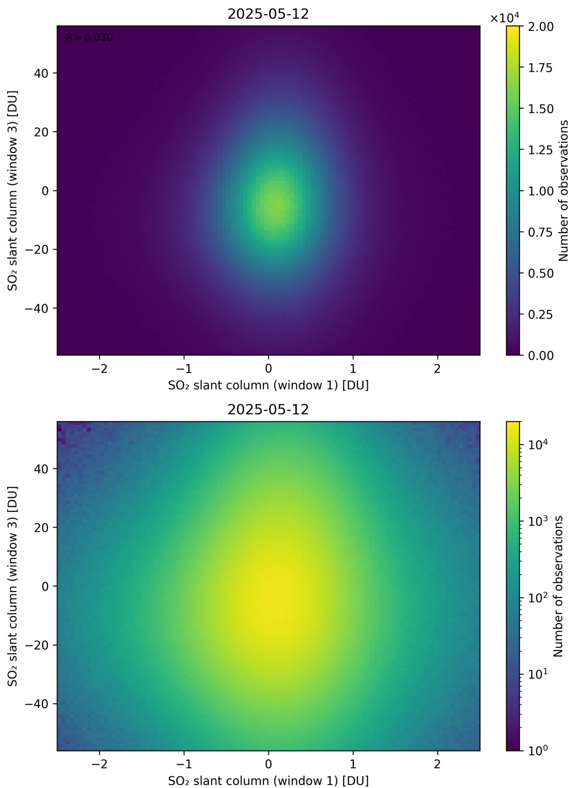
Figure 287: Scatter density plot of “SO 2 slant column (window 1)” against “SO 2 slant column (window 3)” for 2025-05-11 to 2025-05-13.
