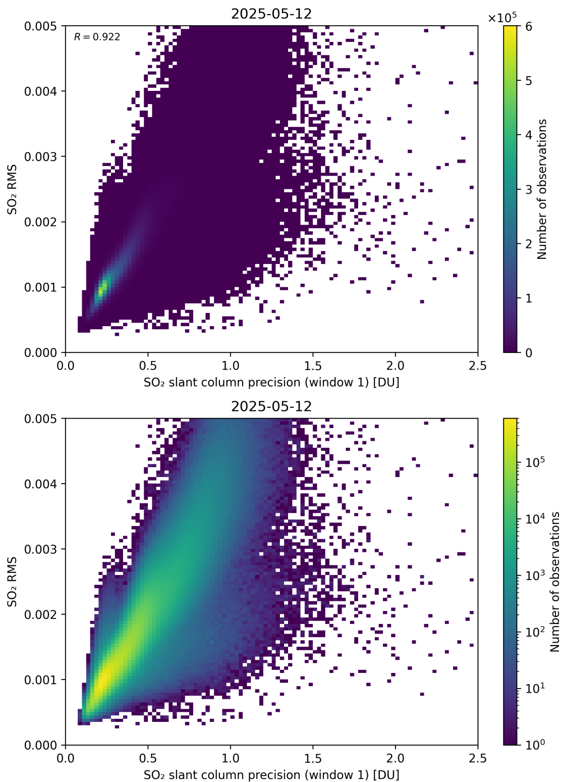
Figure 273: Scatter density plot of “SO 2 slant column precision (window 1)” against “SO 2 RMS” for 2025-05-11 to 2025-05-13.
