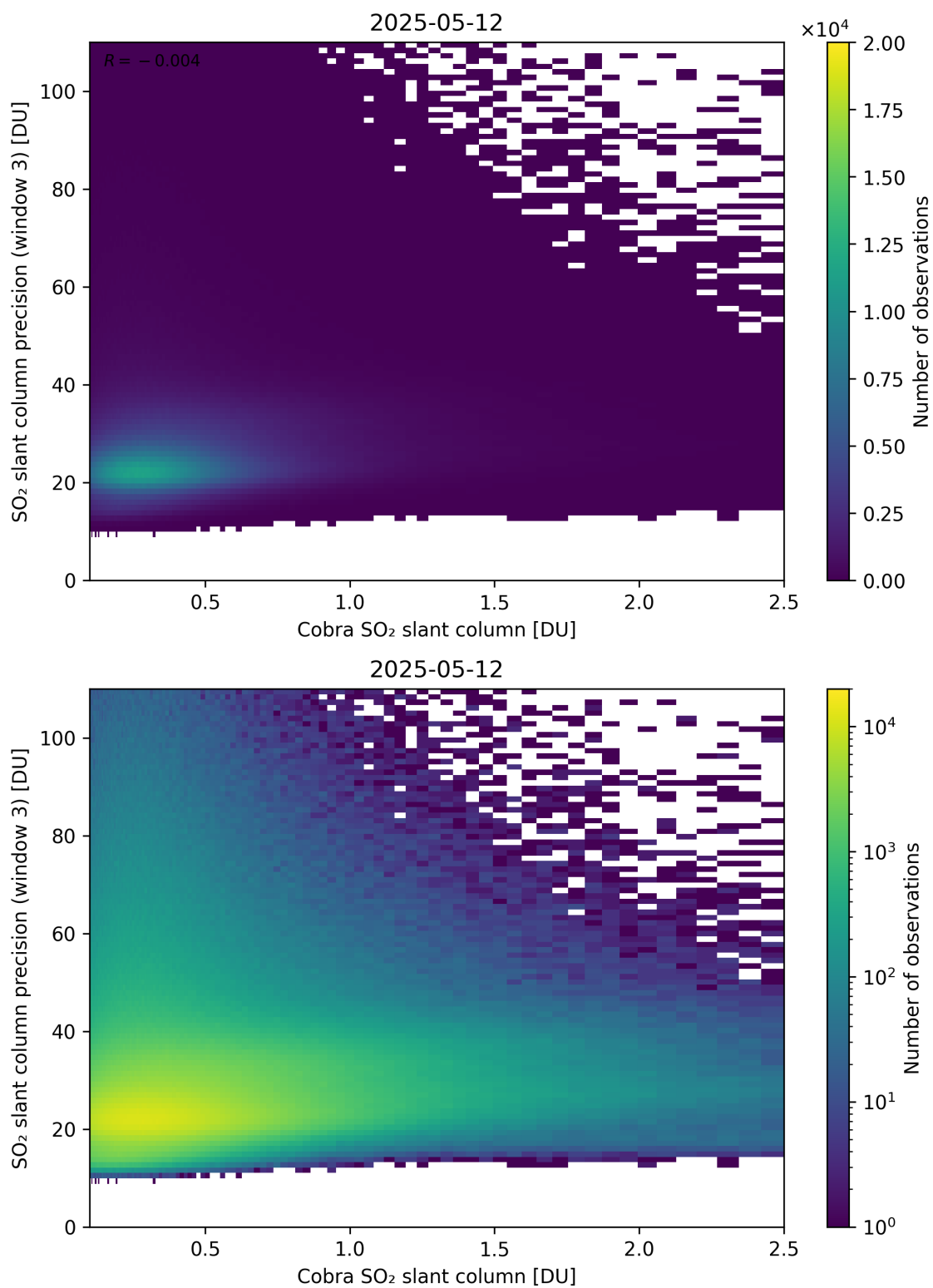
Figure 223: Scatter density plot of “Cobra SO 2 slant column” against “SO 2 slant column precision (window 3)” for 2025-05-11 to 2025-05-13.
