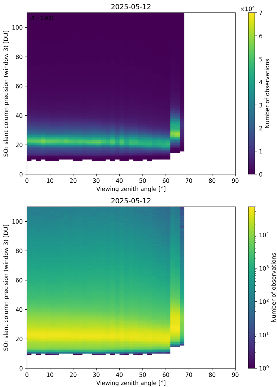
Figure 380: Scatter density plot of “Viewing zenith angle” against “SO 2 slant column precision (window 3)” for 2025-05-11 to 2025-05-13.
