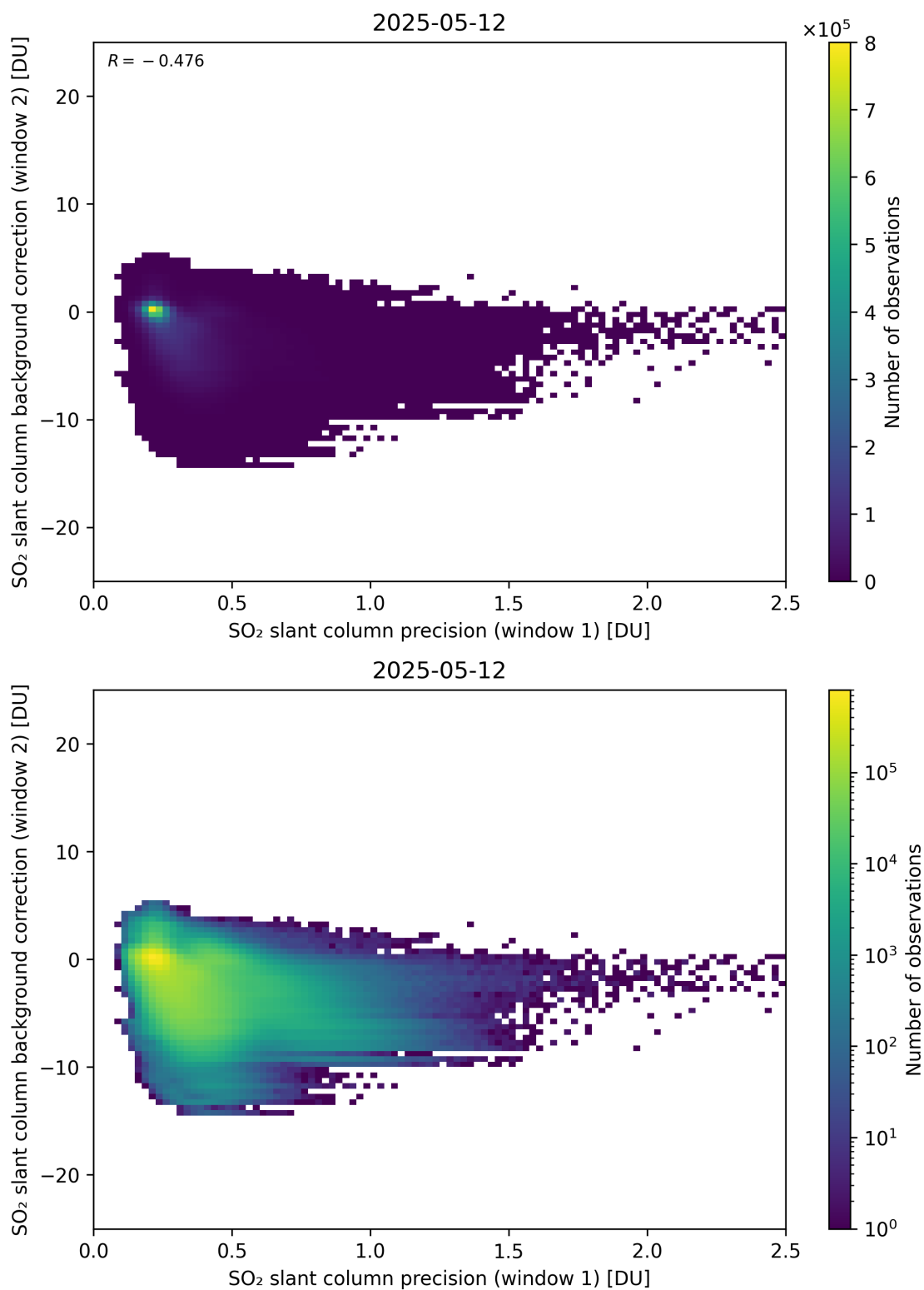
Figure 269: Scatter density plot of “SO 2 slant column precision (window 1)” against “SO 2 slant column background correction (window 2)” for 2025-05-11 to 2025-05-13.
