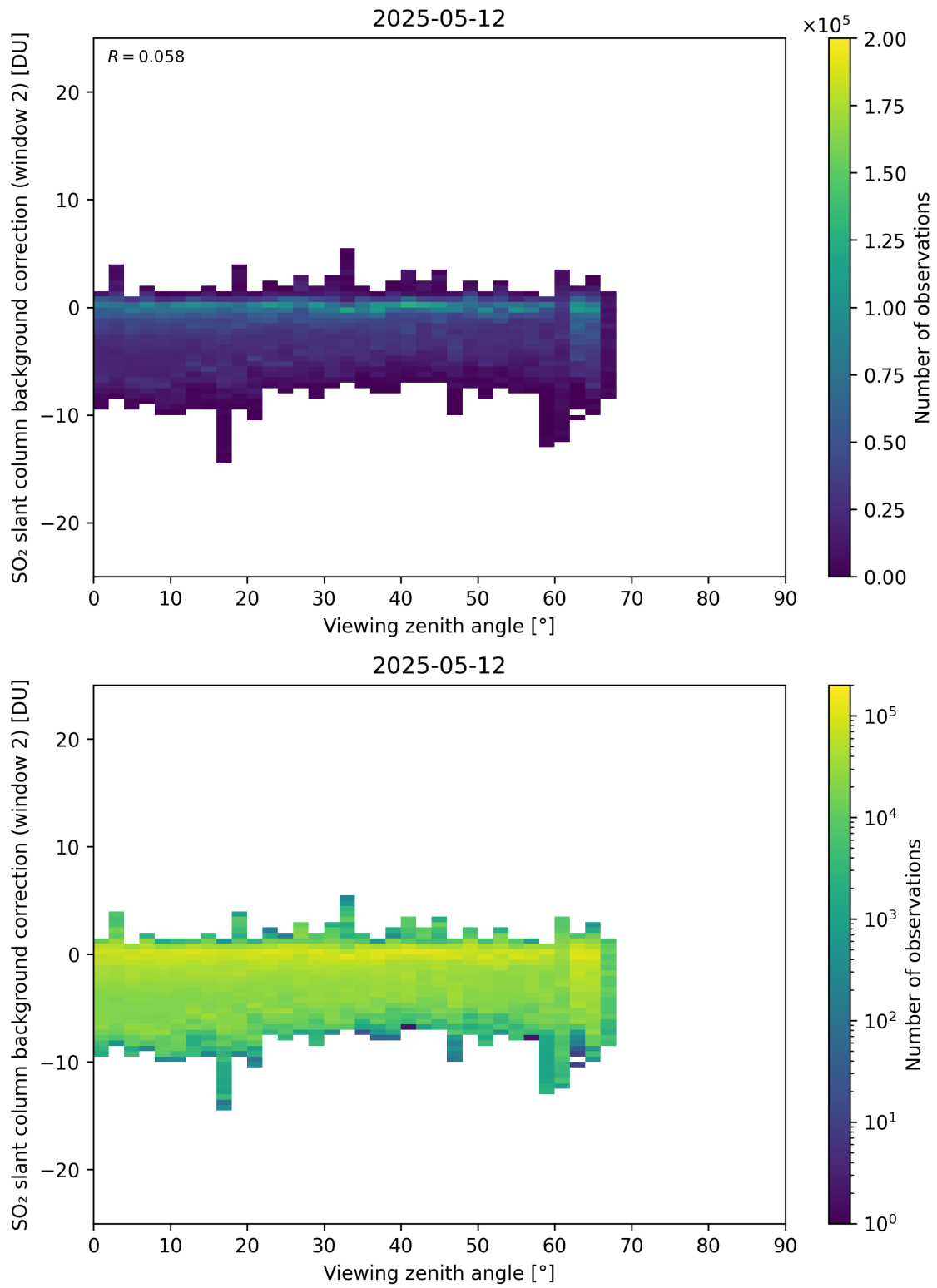
Figure 363: Scatter density plot of “Viewing zenith angle” against “SO 2 slant column background correction (window 2)” for 2025-05-11 to 2025-05-13.
