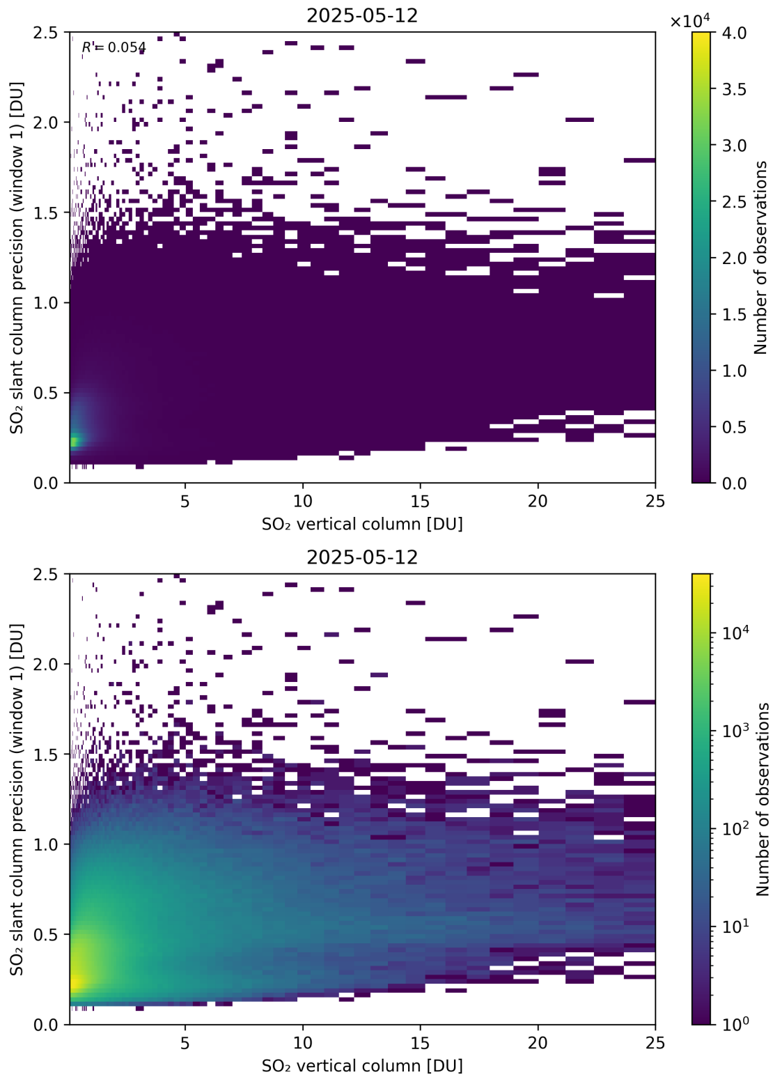
Figure 355: Scatter density plot of “SO 2 vertical column” against “SO 2 slant column precision (window 1)” for 2025-05-11 to 2025-05-13.
