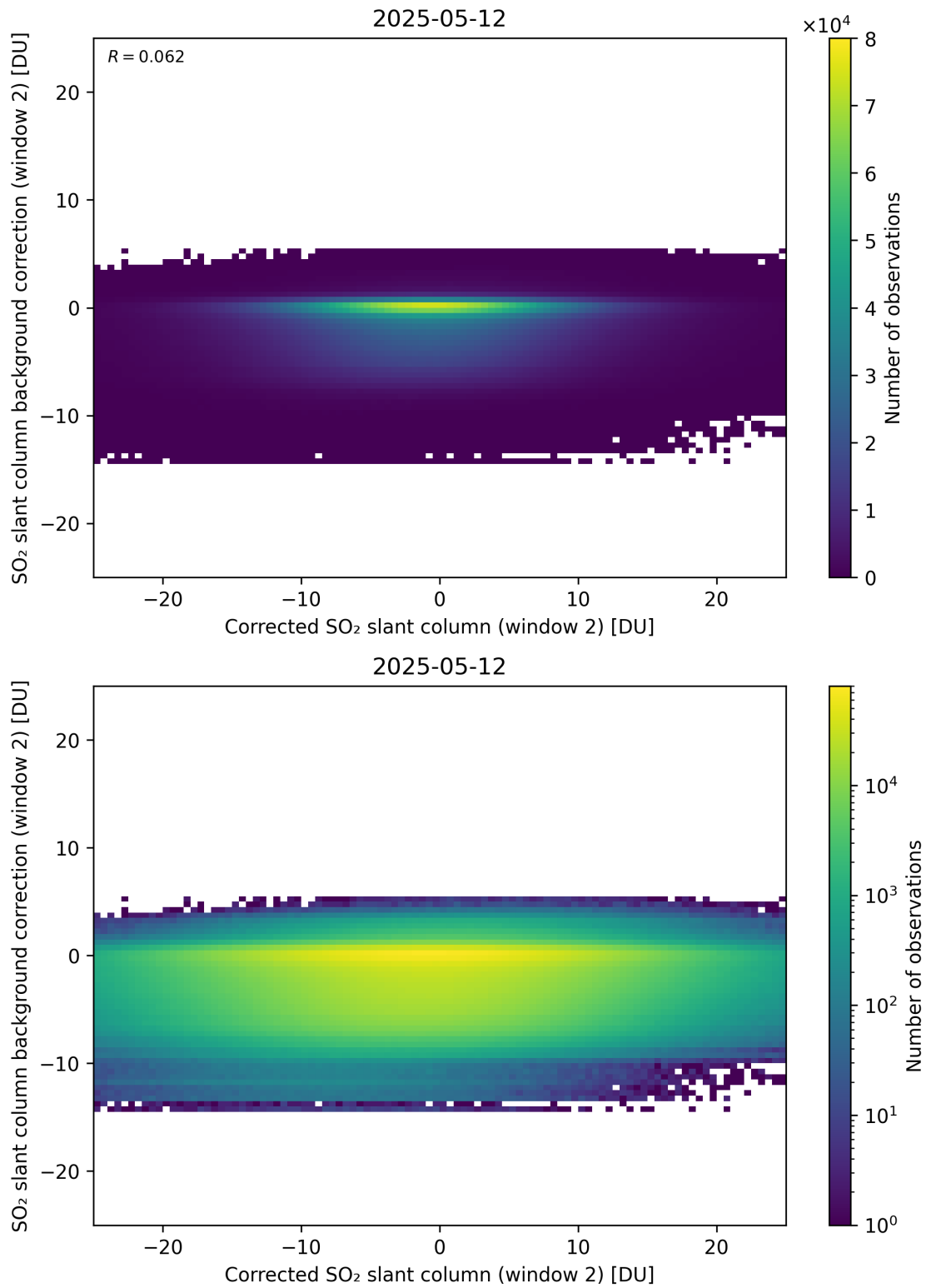
Figure 244: Scatter density plot of “Corrected SO 2 slant column (window 2)” against “SO 2 slant column background correction (window 2)” for 2025-05-11 to 2025-05-13.
