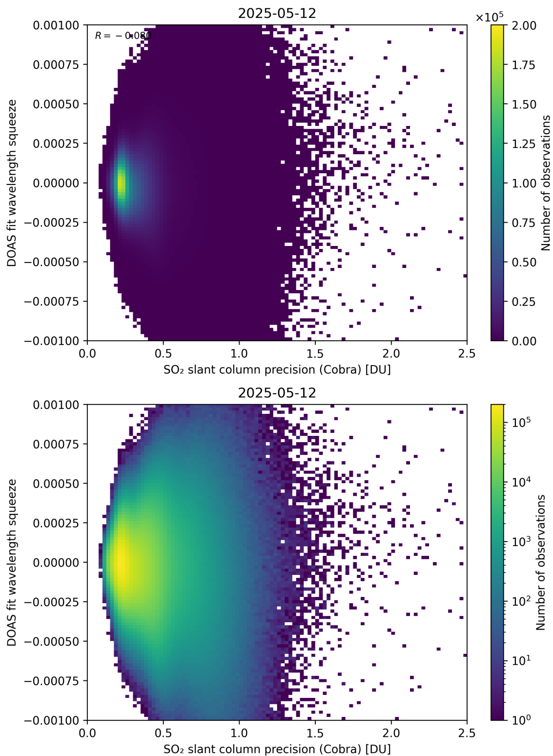
Figure 203: Scatter density plot of “SO 2 slant column precision (Cobra)” against “DOAS fit wavelength squeeze” for 2025-05-11 to 2025-05-13.
