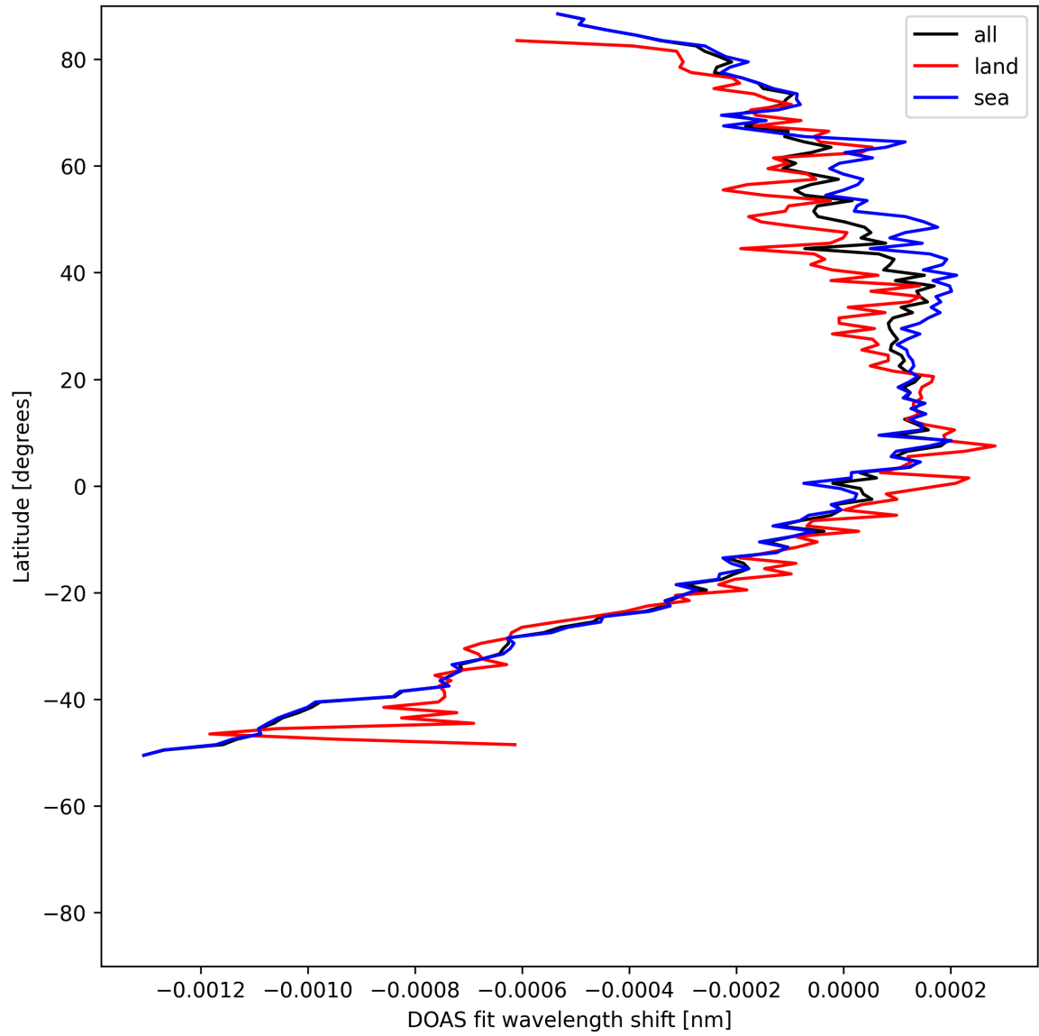
Figure 50: Zonal average of “DOAS fit wavelength shift” for 2025-05-11 to 2025-05-13.
