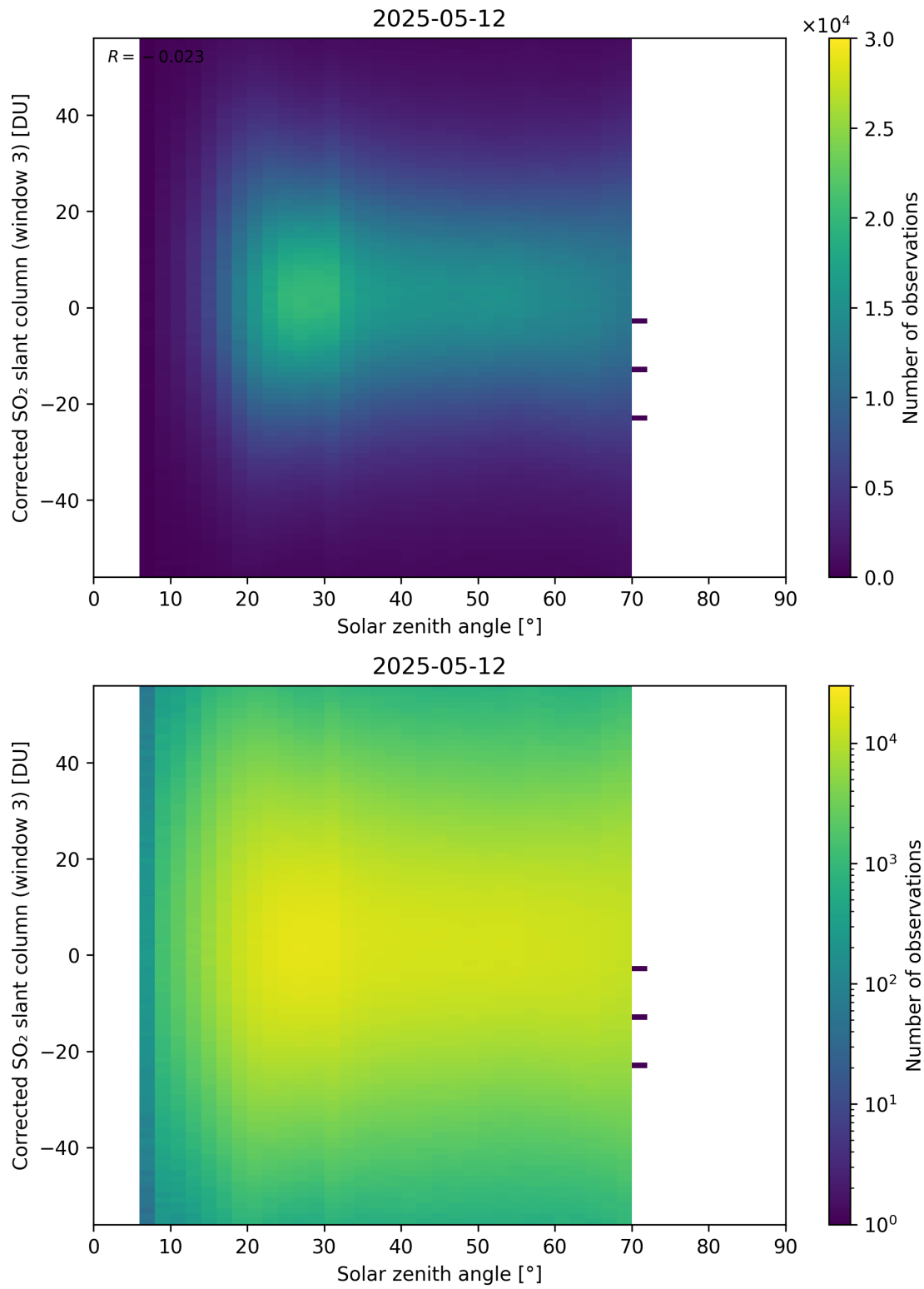
Figure 183: Scatter density plot of “Solar zenith angle” against “Corrected SO 2 slant column (window 3)” for 2025-05-11 to 2025-05-13.
