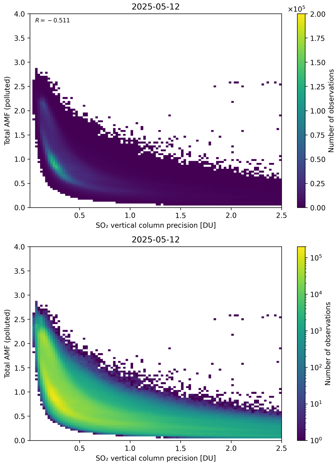
Figure 346: Scatter density plot of “SO 2 vertical column precision” against “Total AMF (polluted)” for 2025-05-11 to 2025-05-13.
