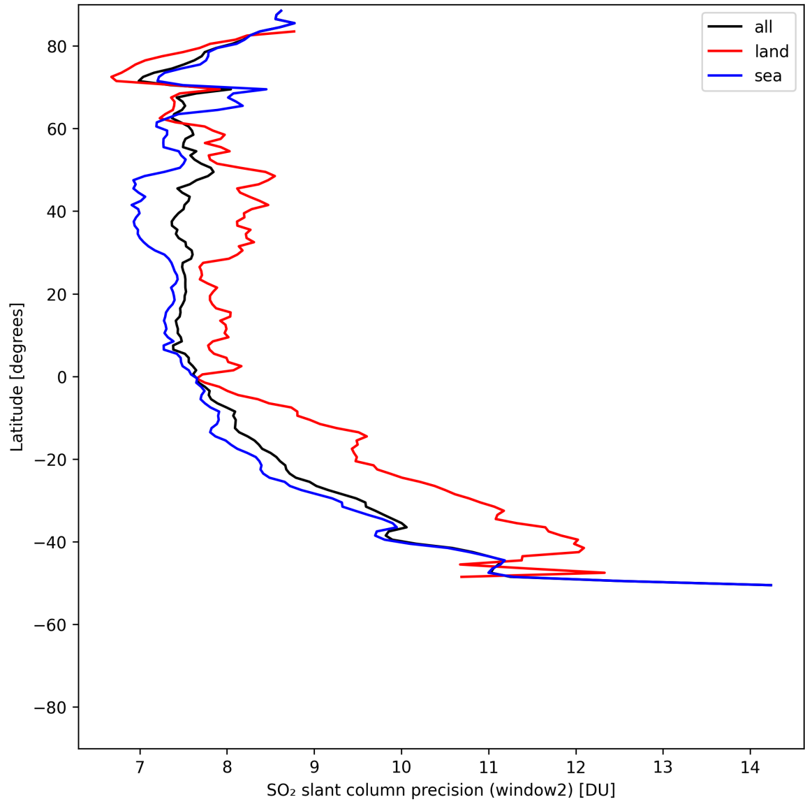
Figure 42: Zonal average of “SO 2 slant column precision (window2)” for 2025-05-11 to 2025-05-13.
