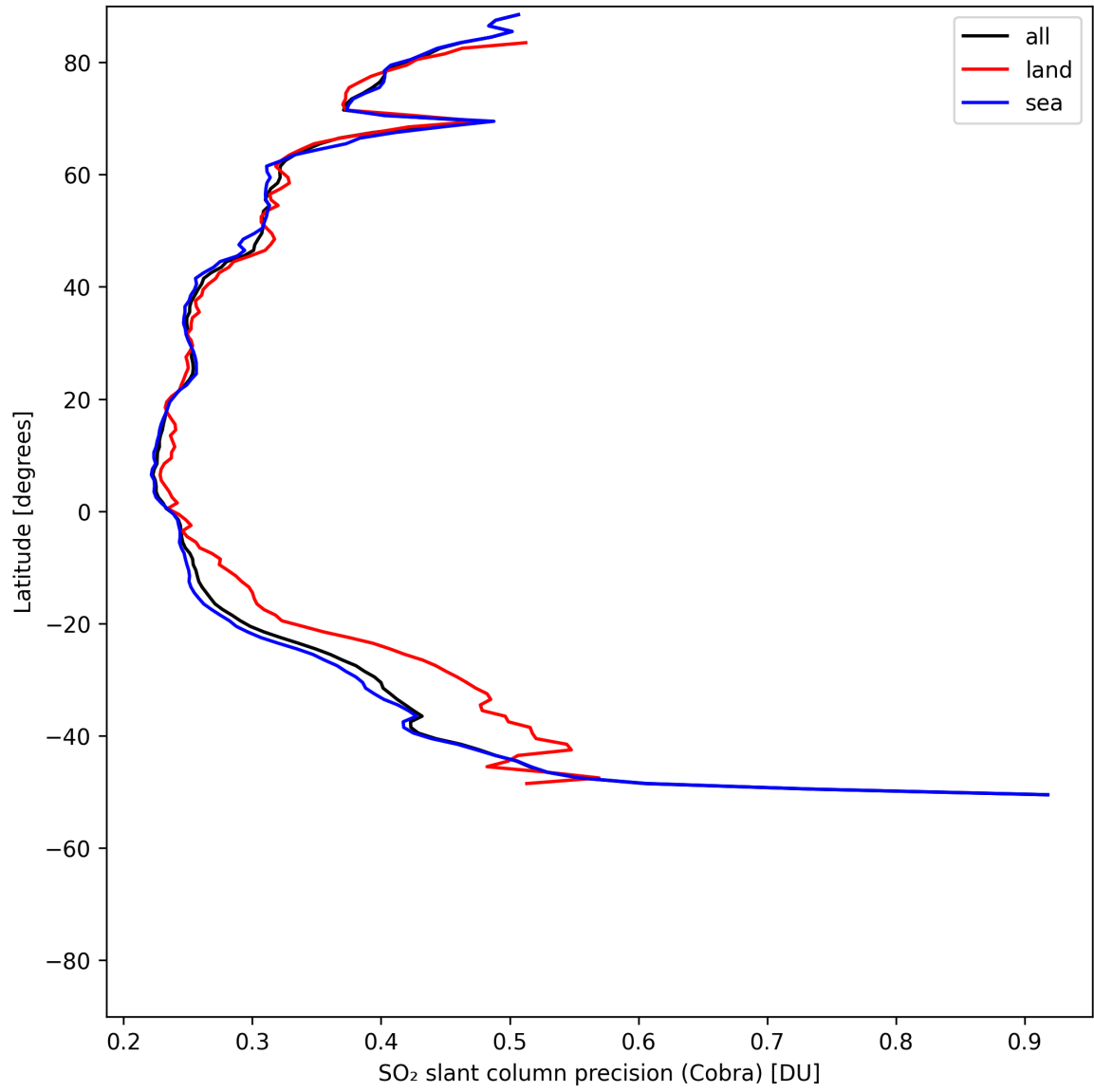
Figure 36: Zonal average of “SO 2 slant column precision (Cobra)” for 2025-05-11 to 2025-05-13.
