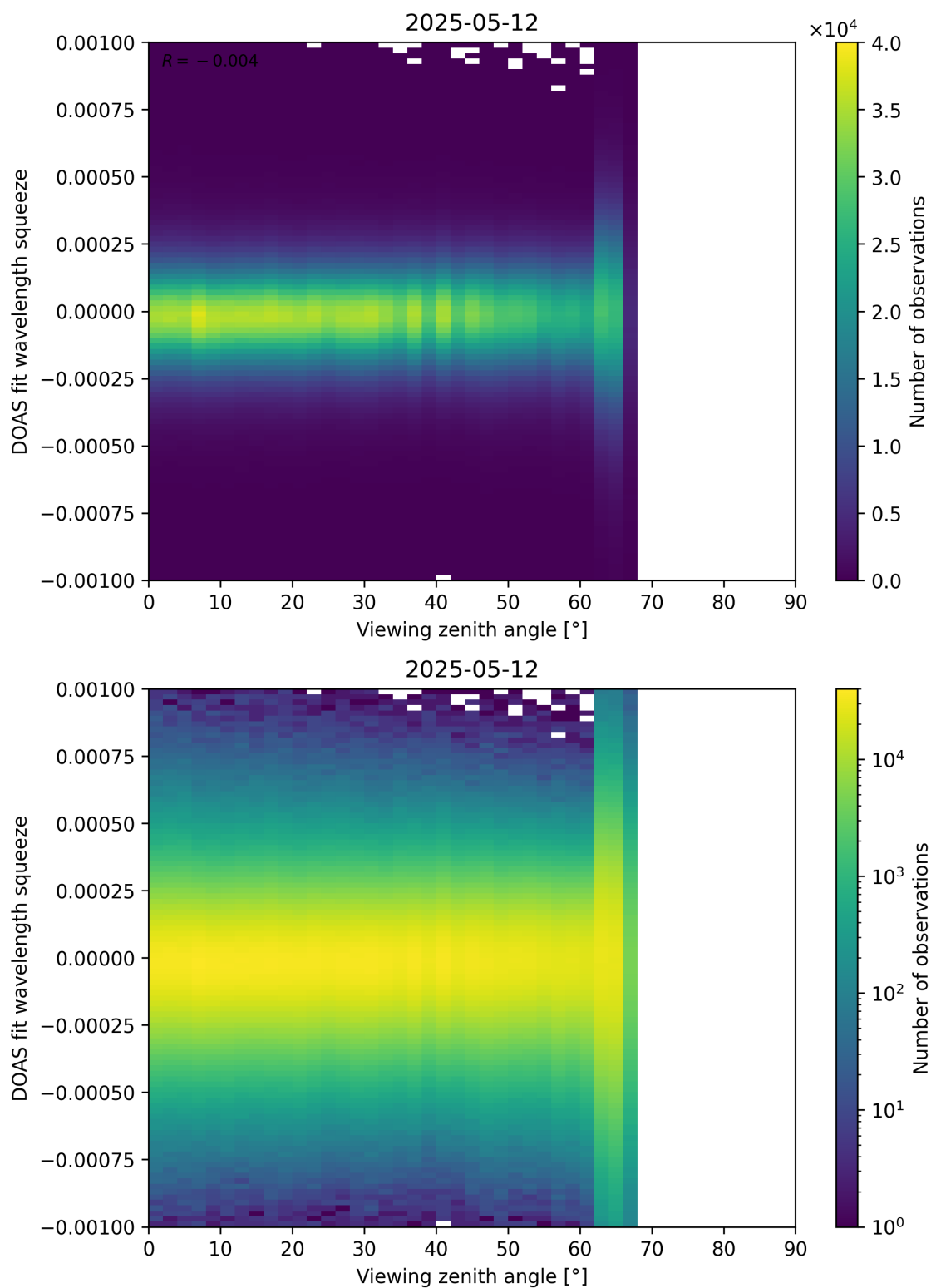
Figure 366: Scatter density plot of “Viewing zenith angle” against “DOAS fit wavelength squeeze” for 2025-05-11 to 2025-05-13.
