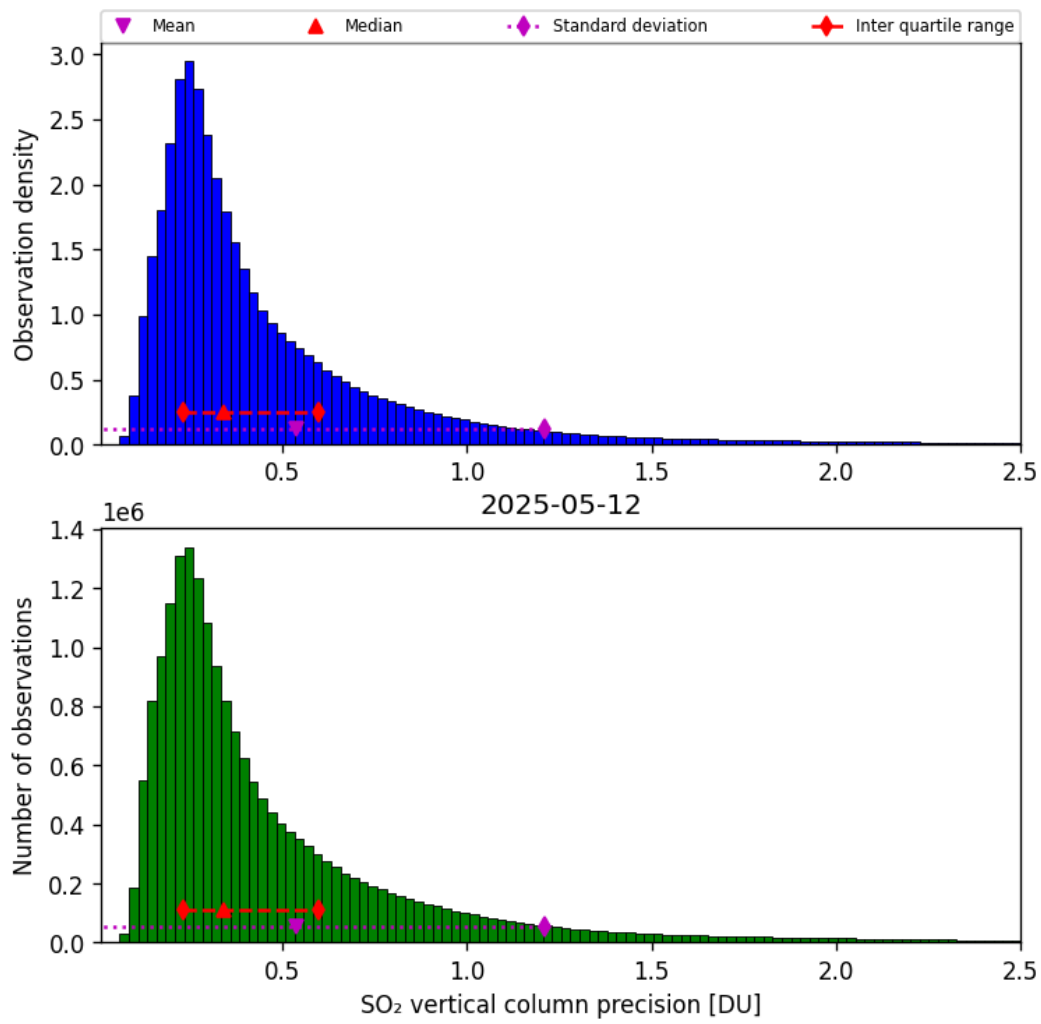
Figure 59: Histogram of “SO 2 vertical column precision” for 2025-05-11 to 2025-05-13
