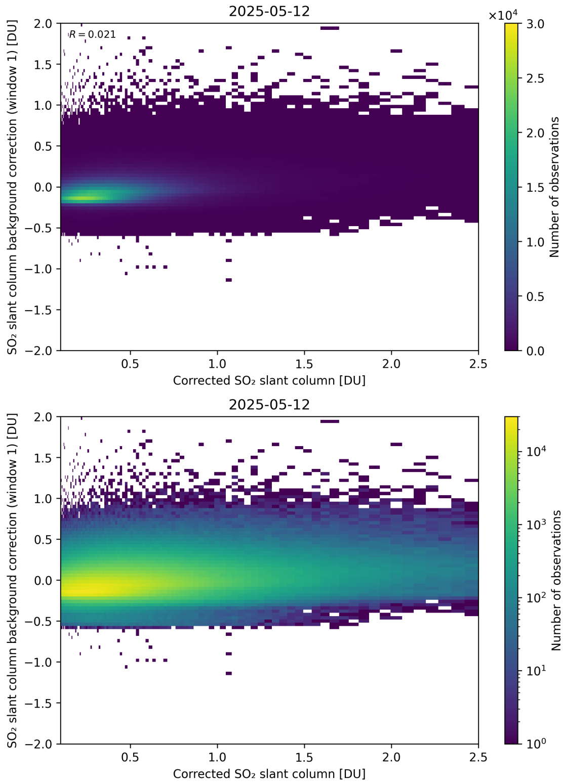
Figure 226: Scatter density plot of “Corrected SO 2 slant column” against “SO 2 slant column background correction (window 1)” for 2025-05-11 to 2025-05-13.
