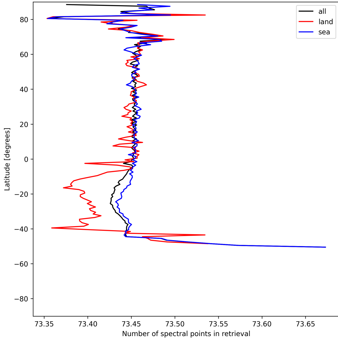
Figure 56: Zonal average of “Number of spectral points in retrieval” for 2025-05-11 to 2025-05-13.
