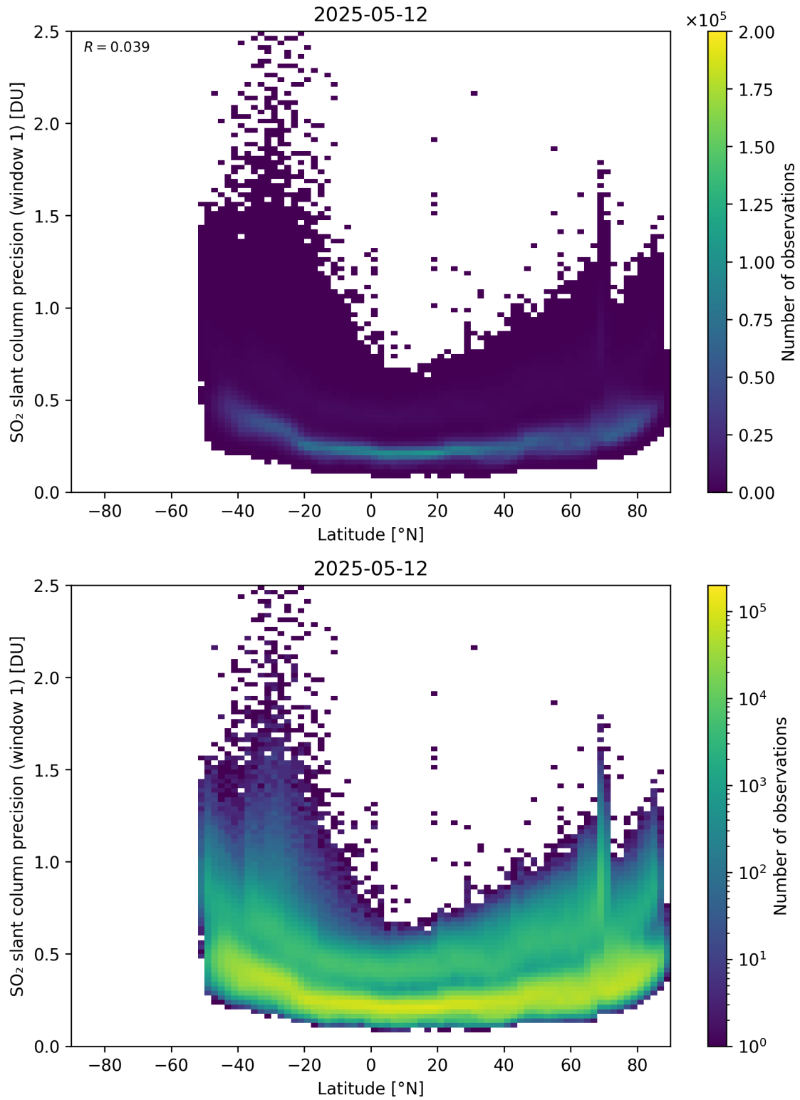
Figure 163: Scatter density plot of “Latitude” against “SO 2 slant column precision (window 1)” for 2025-05-11 to 2025-05-13.
