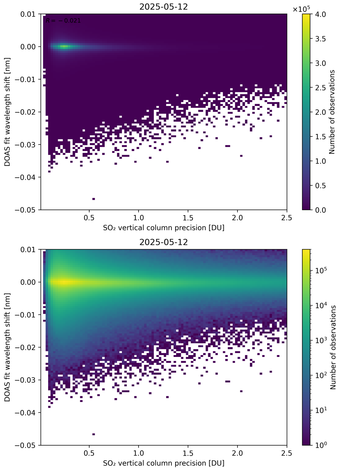
Figure 332: Scatter density plot of “SO 2 vertical column precision” against “DOAS fit wavelength shift” for 2025-05-11 to 2025-05-13.
