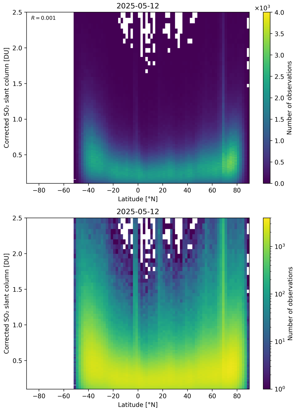
Figure 159: Scatter density plot of “Latitude” against “Corrected SO 2 slant column” for 2025-05-11 to 2025-05-13.
