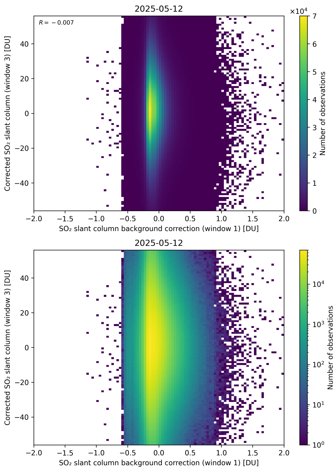
Figure 116: Scatter density plot of “SO 2 slant column background correction (window 1)” against “Corrected SO 2 slant column (window 3)” for 2025-05-11 to 2025-05-13.
