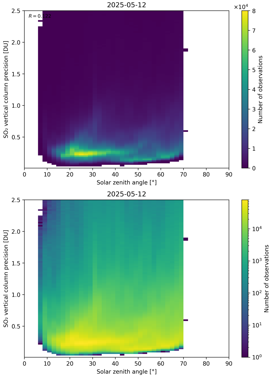
Figure 192: Scatter density plot of “Solar zenith angle” against “SO 2 vertical column precision” for 2025-05-11 to 2025-05-13.
