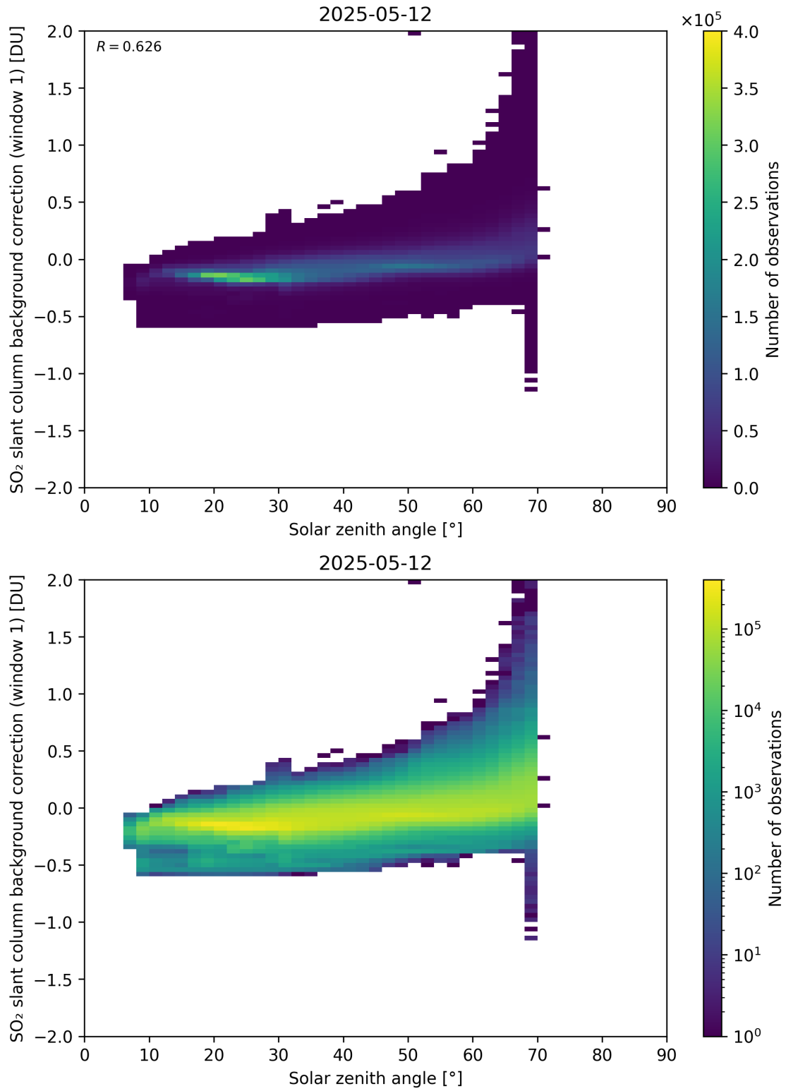
Figure 171: Scatter density plot of “Solar zenith angle” against “SO 2 slant column background correction (window 1)” for 2025-05-11 to 2025-05-13.
