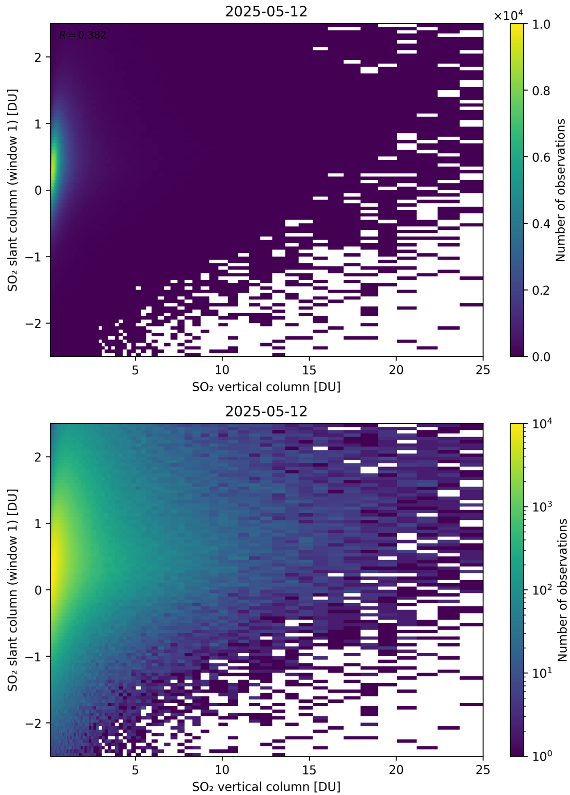
Figure 354: Scatter density plot of “SO 2 vertical column” against “SO 2 slant column (window 1)” for 2025-05-11 to 2025-05-13.
