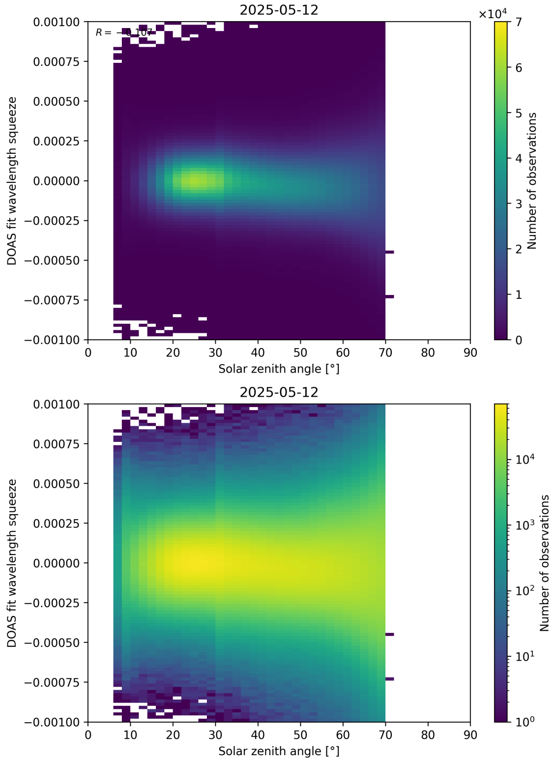
Figure 175: Scatter density plot of “Solar zenith angle” against “DOAS fit wavelength squeeze” for 2025-05-11 to 2025-05-13.
