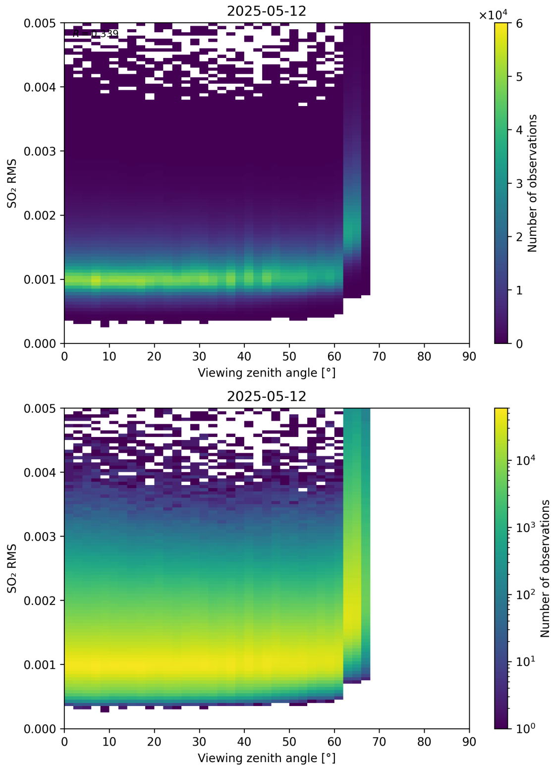
Figure 367: Scatter density plot of “Viewing zenith angle” against “SO 2 RMS” for 2025-05-11 to 2025-05-13.
