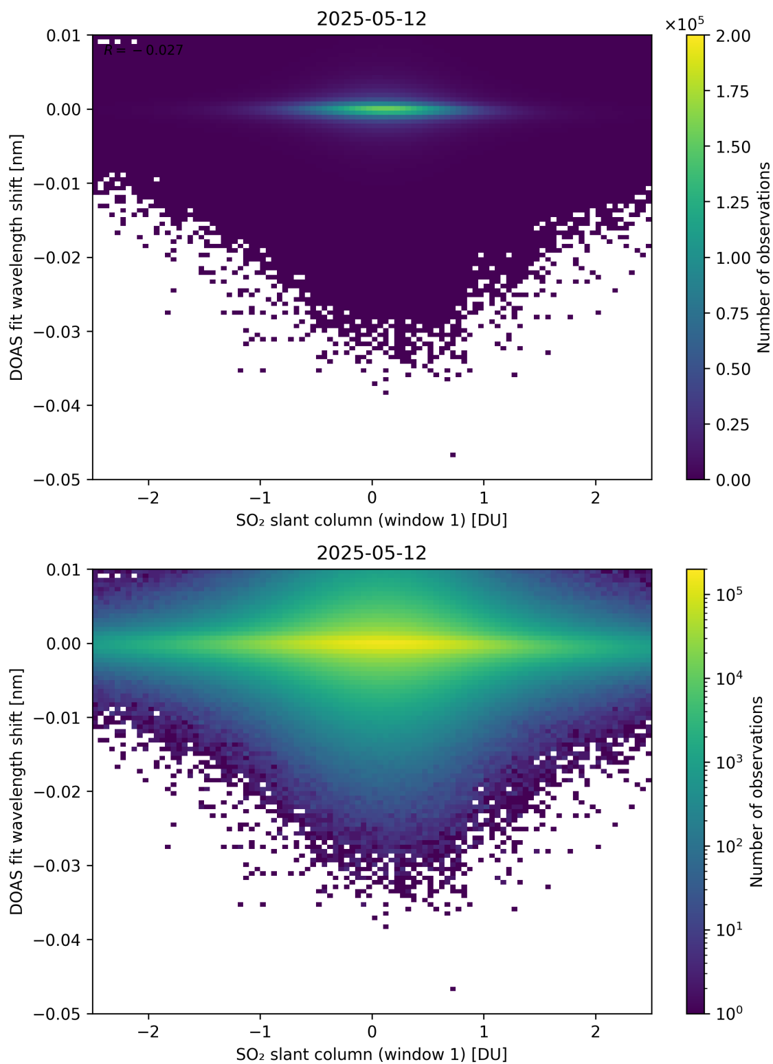
Figure 265: Scatter density plot of “SO 2 slant column (window 1)” against “DOAS fit wavelength shift” for 2025-05-11 to 2025-05-13.
