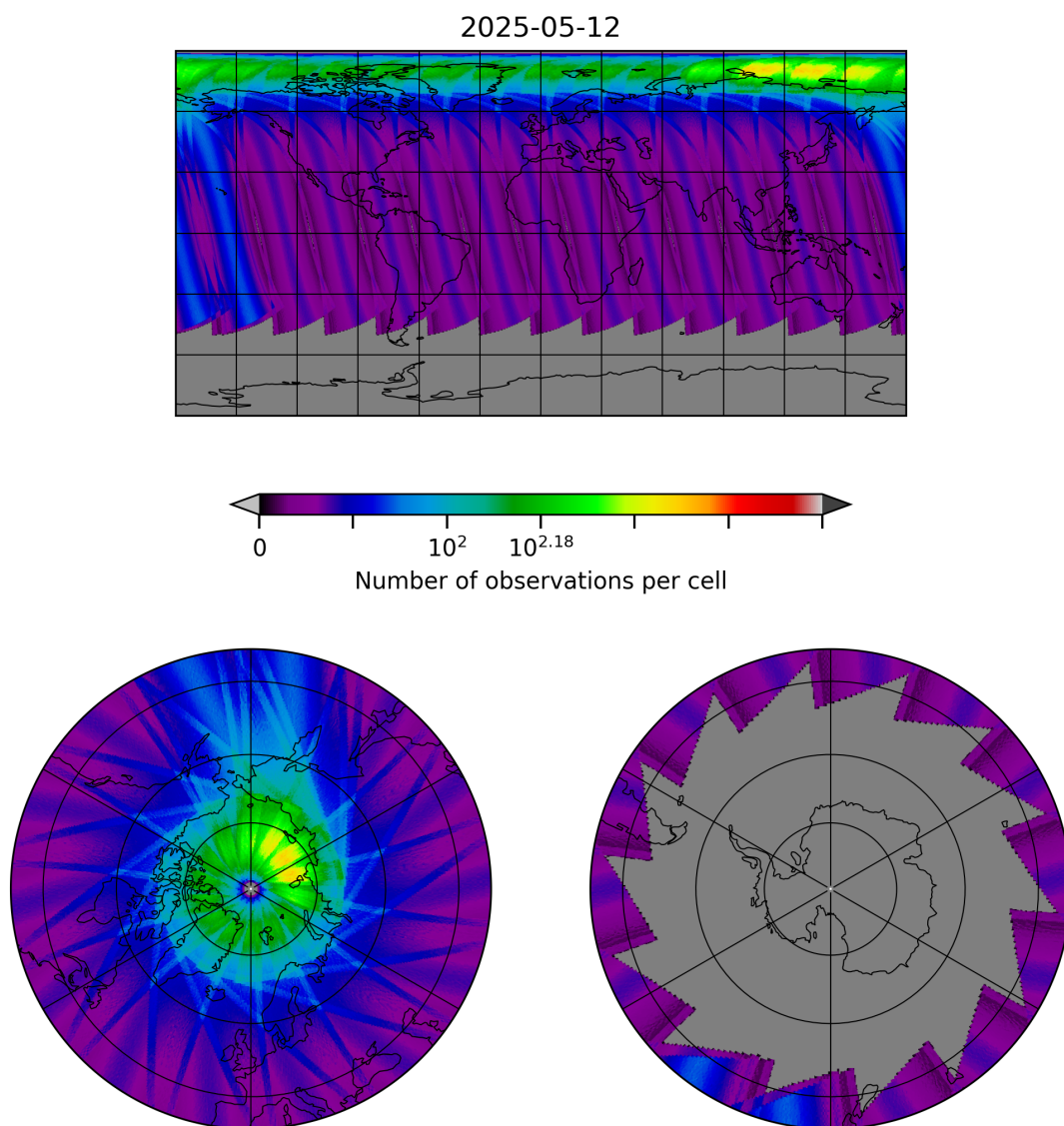
Figure 30: Map of the number of observations for 2025-05-11 to 2025-05-13
