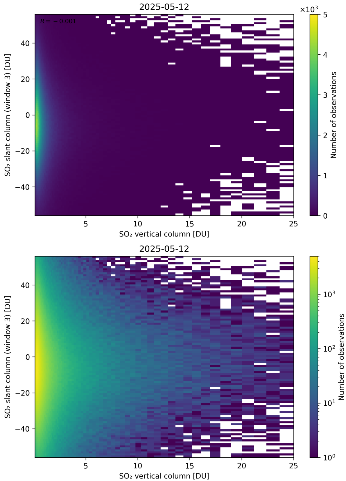
Figure 357: Scatter density plot of “SO 2 vertical column” against “SO 2 slant column (window 3)” for 2025-05-11 to 2025-05-13.
