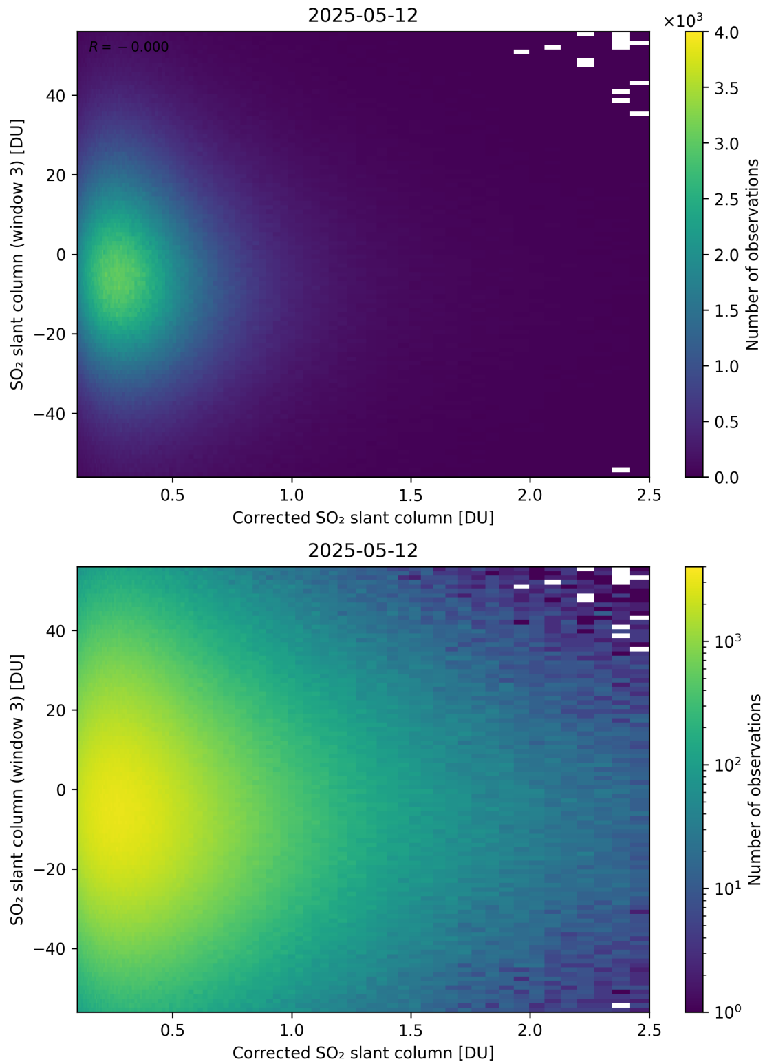
Figure 240: Scatter density plot of “Corrected SO 2 slant column” against “SO 2 slant column (window 3)” for 2025-05-11 to 2025-05-13.
