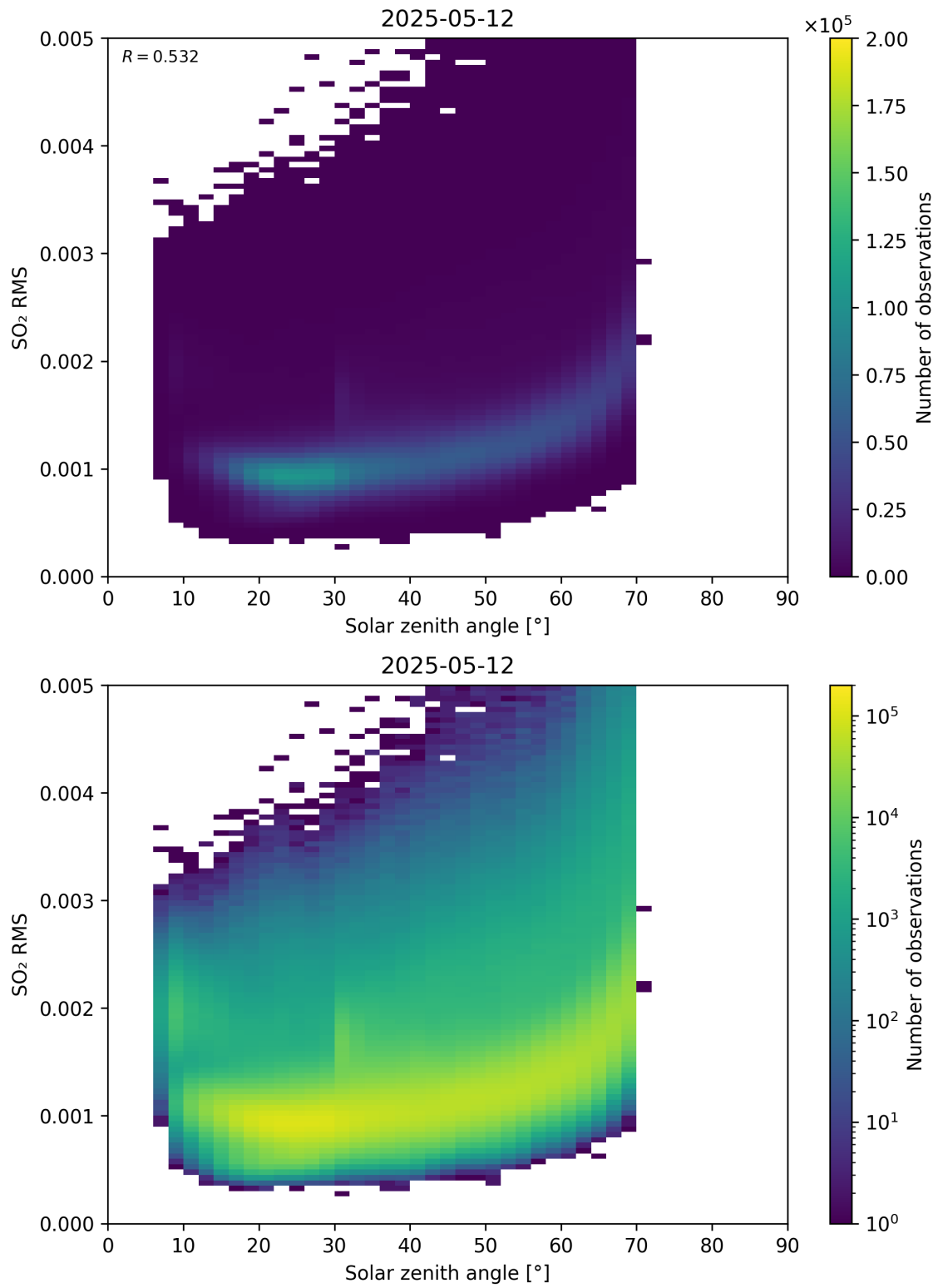
Figure 176: Scatter density plot of “Solar zenith angle” against “SO 2 RMS” for 2025-05-11 to 2025-05-13.
