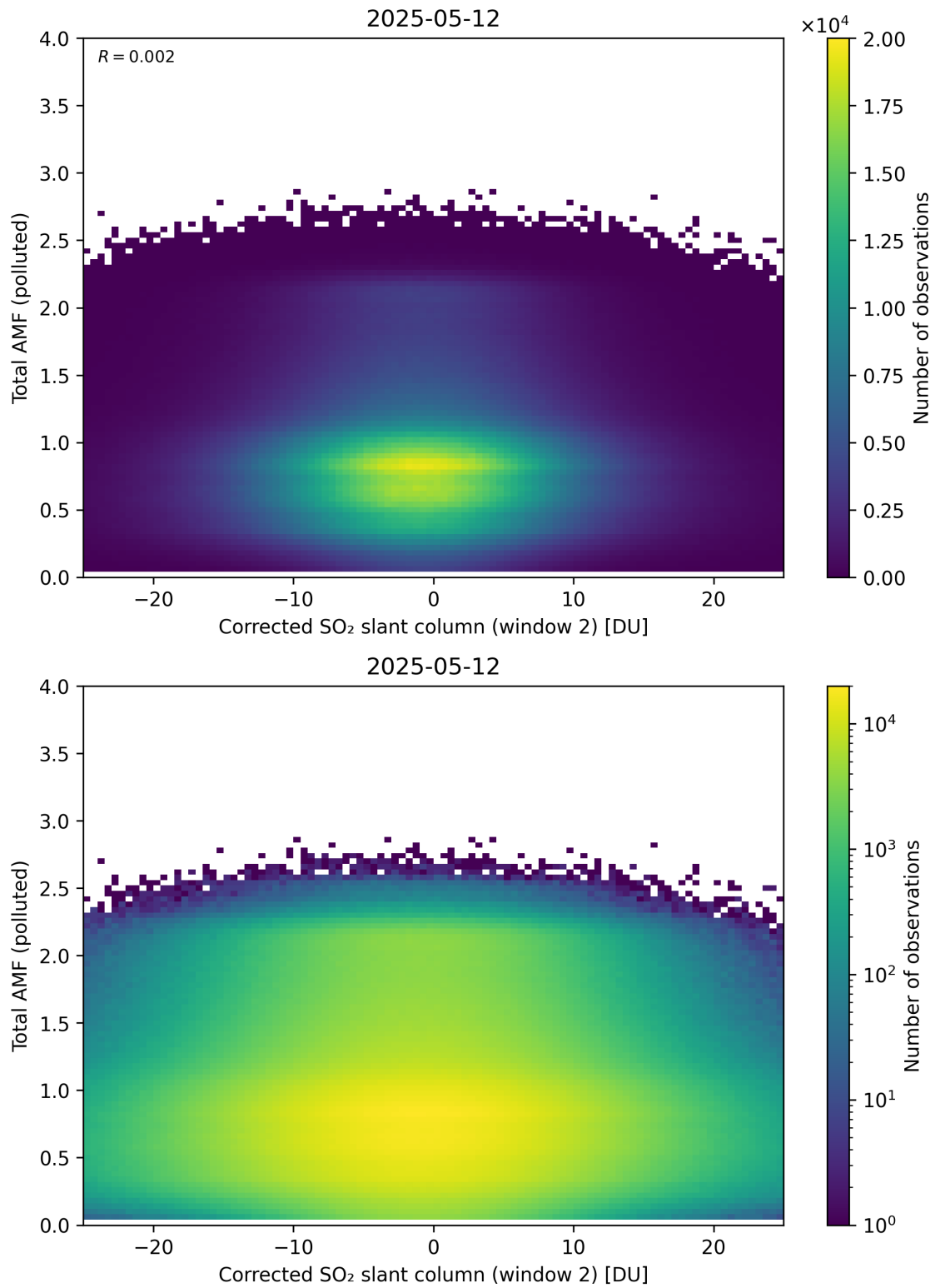
Figure 253: Scatter density plot of “Corrected SO 2 slant column (window 2)” against “Total AMF (polluted)” for 2025-05-11 to 2025-05-13.
