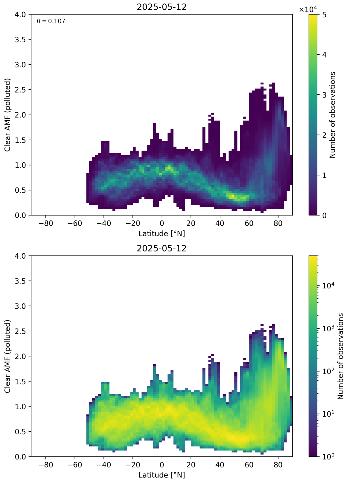
Figure 156: Scatter density plot of “Latitude” against “Clear AMF (polluted)” for 2025-05-11 to 2025-05-13.
