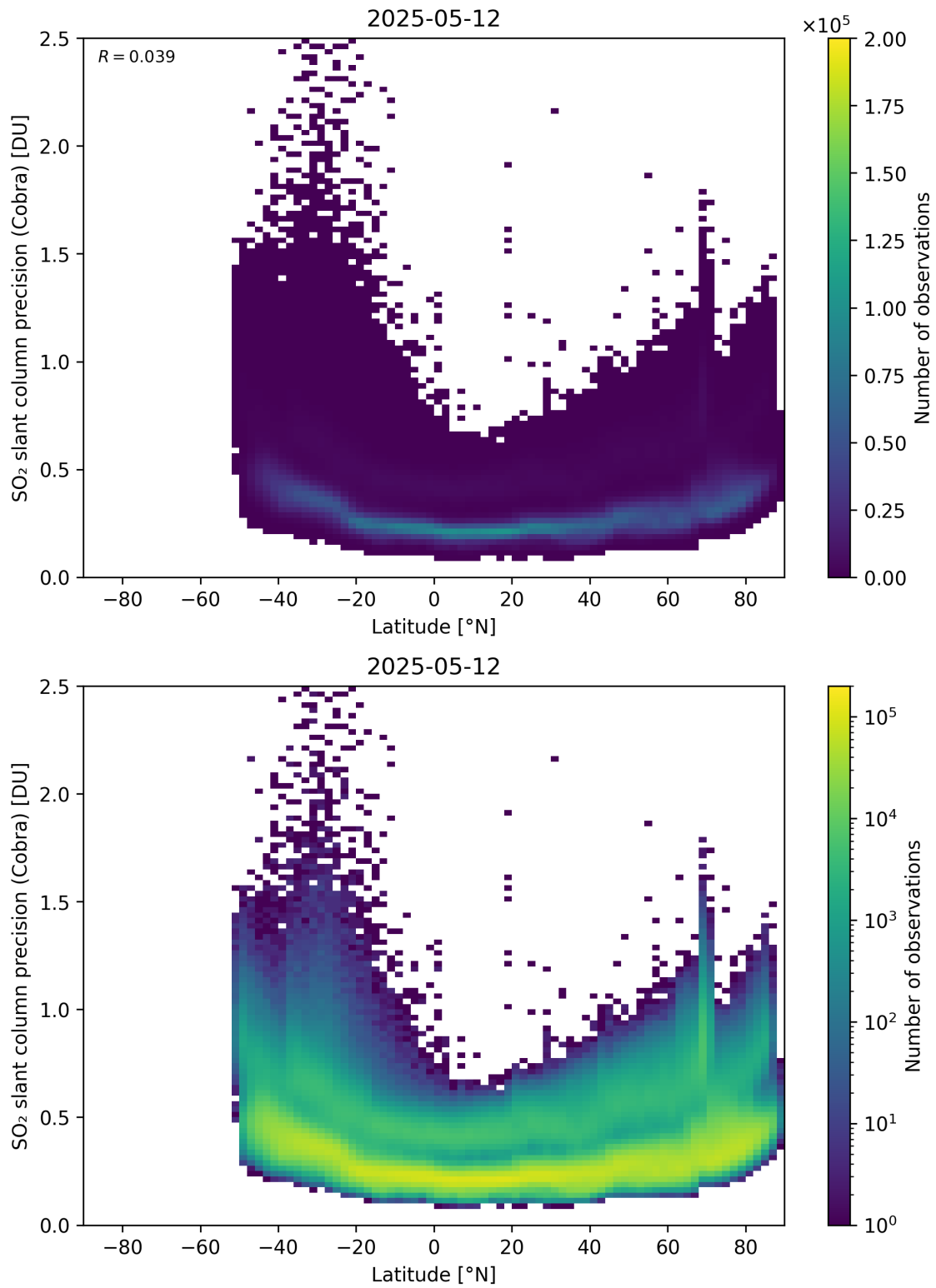
Figure 158: Scatter density plot of “Latitude” against “SO 2 slant column precision (Cobra)” for 2025-05-11 to 2025-05-13.
