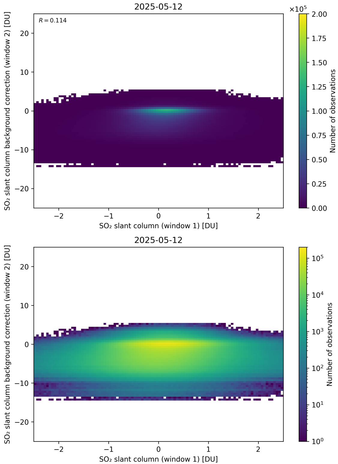
Figure 263: Scatter density plot of “SO 2 slant column (window 1)” against “SO 2 slant column background correction (window 2)” for 2025-05-11 to 2025-05-13.
