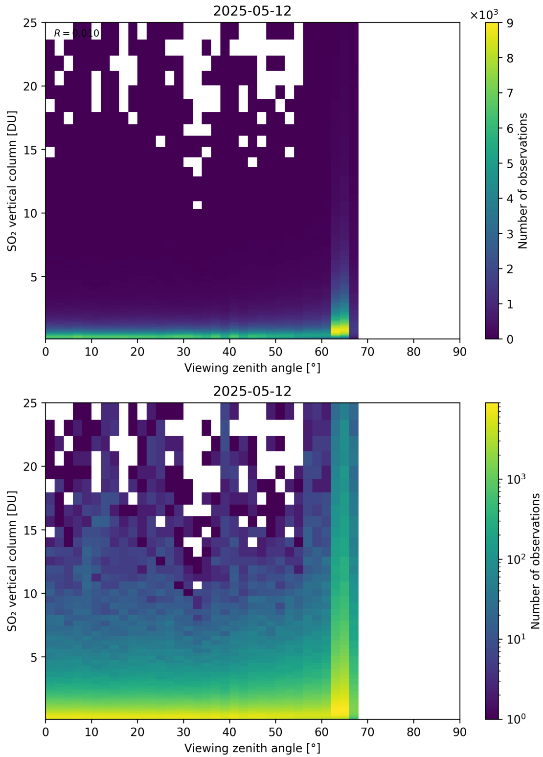
Figure 383: Scatter density plot of “Viewing zenith angle” against “SO 2 vertical column” for 2025-05-11 to 2025-05-13.
