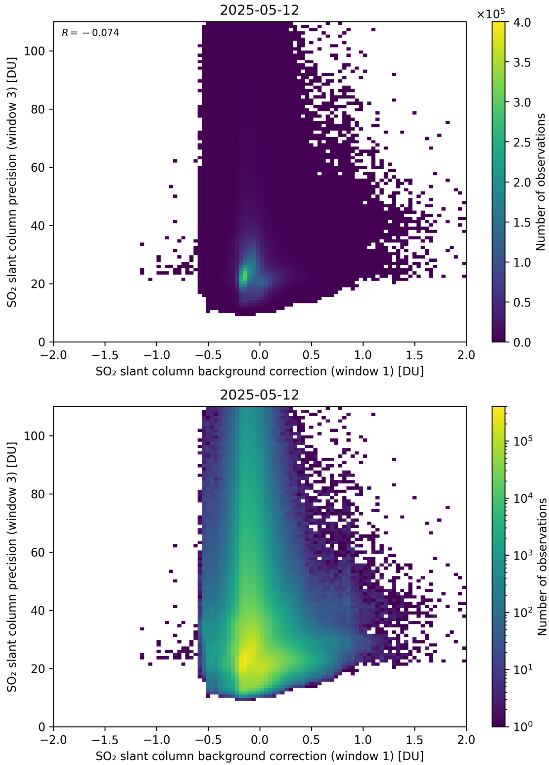
Figure 119: Scatter density plot of “SO 2 slant column background correction (window 1)” against “SO 2 slant column precision (window 3)” for 2025-05-11 to 2025-05-13.
