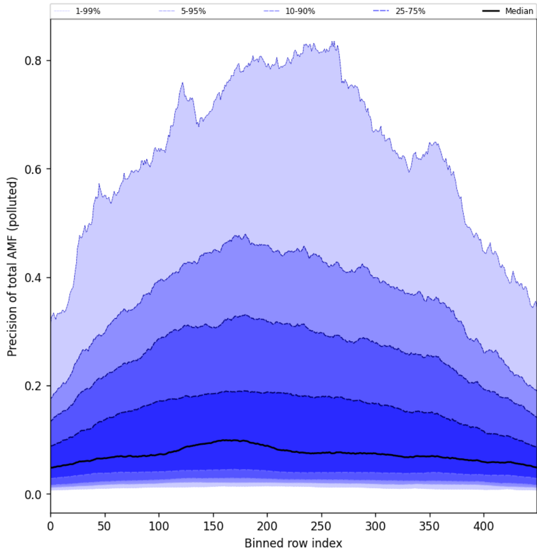
Figure 106: Along track statistics of “Precision of total AMF (polluted)” for 2025-05-11 to 2025-05-13
