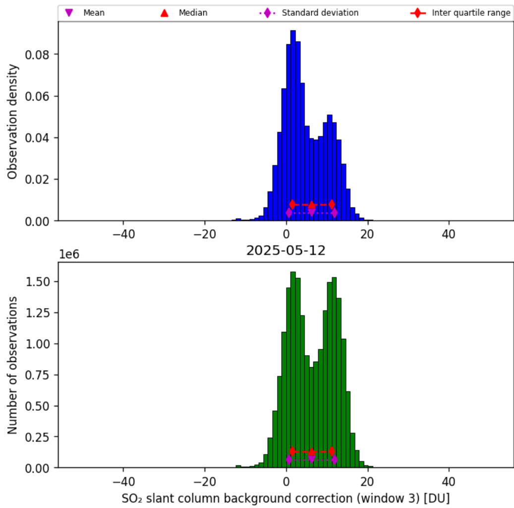
Figure 74: Histogram of “SO 2 slant column background correction (window 3)” for 2025-05-11 to 2025-05-13
