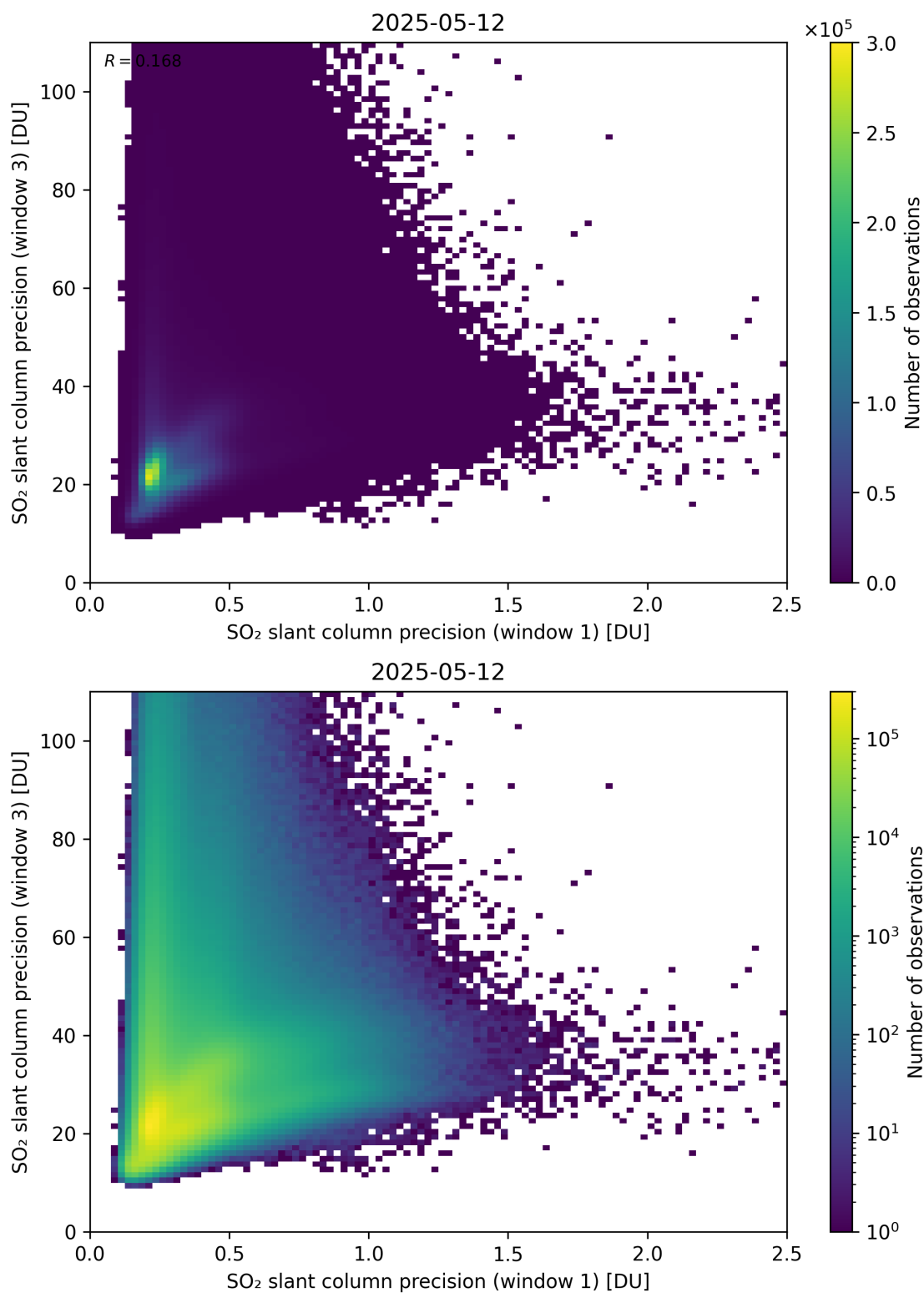
Figure 279: Scatter density plot of “SO 2 slant column precision (window 1)” against “SO 2 slant column precision (window 3)” for 2025-05-11 to 2025-05-13.
