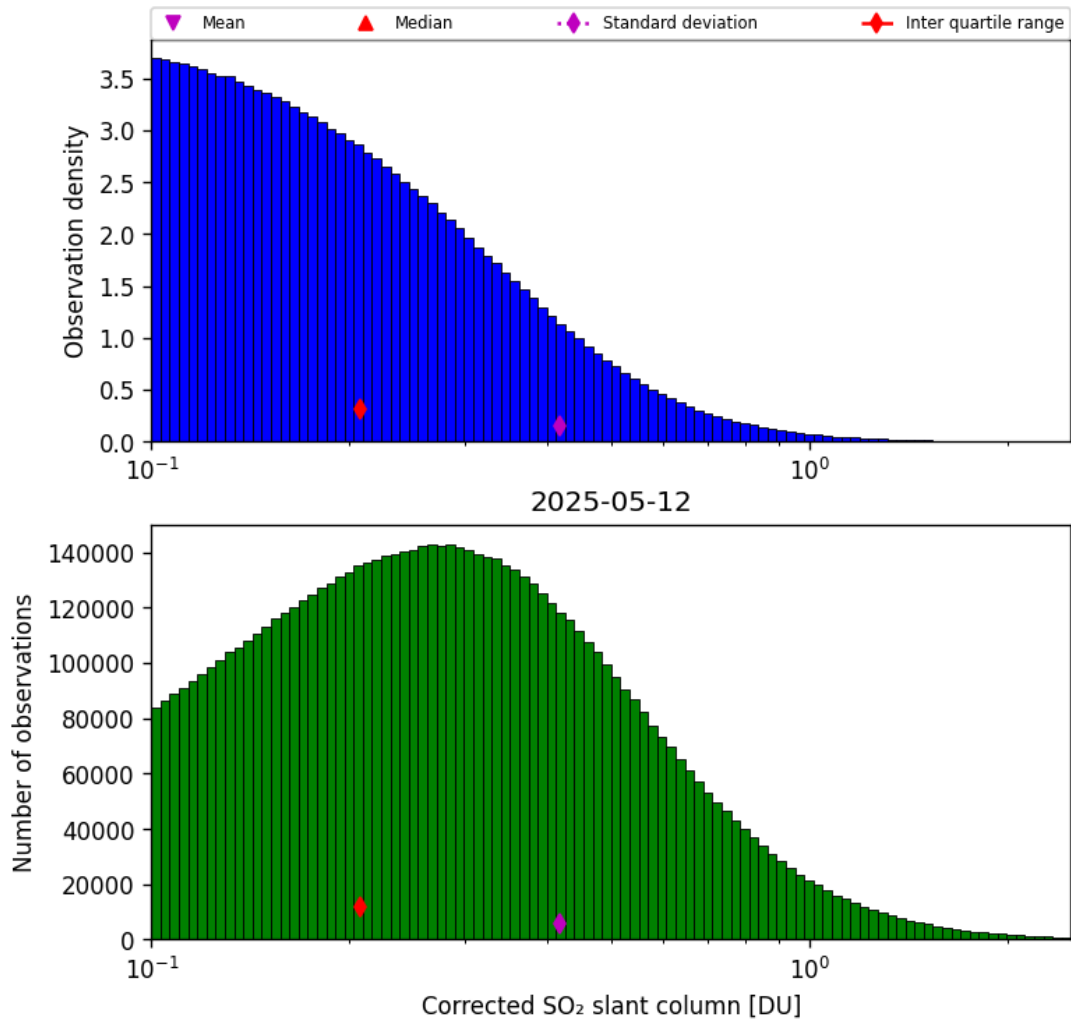
Figure 60: Histogram of “Corrected SO 2 slant column” for 2025-05-11 to 2025-05-13
