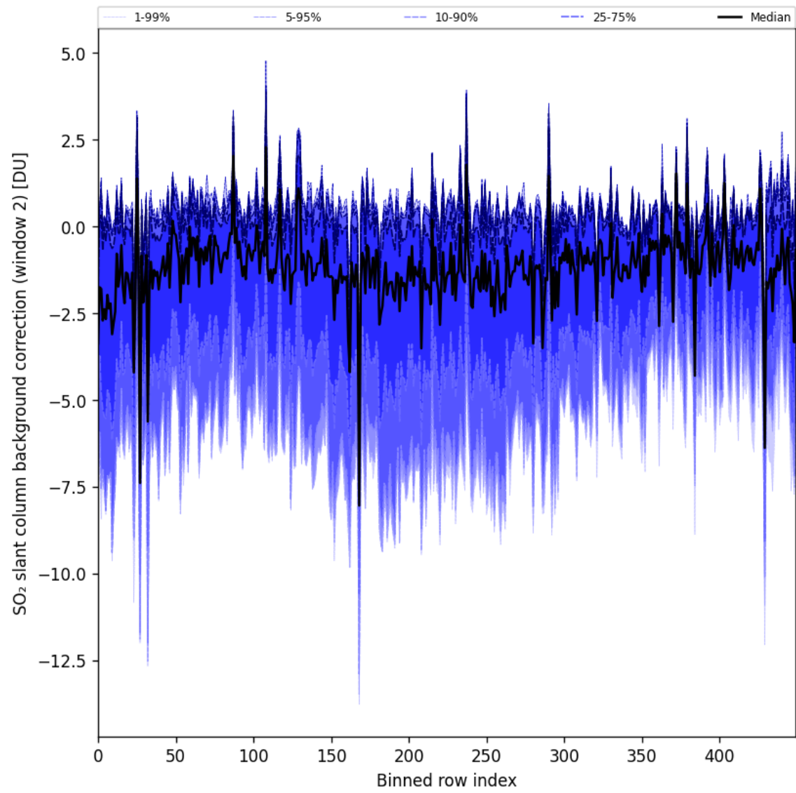
Figure 96: Along track statistics of “SO 2 slant column background correction (window 2)” for 2025-05-11 to 2025-05-13
