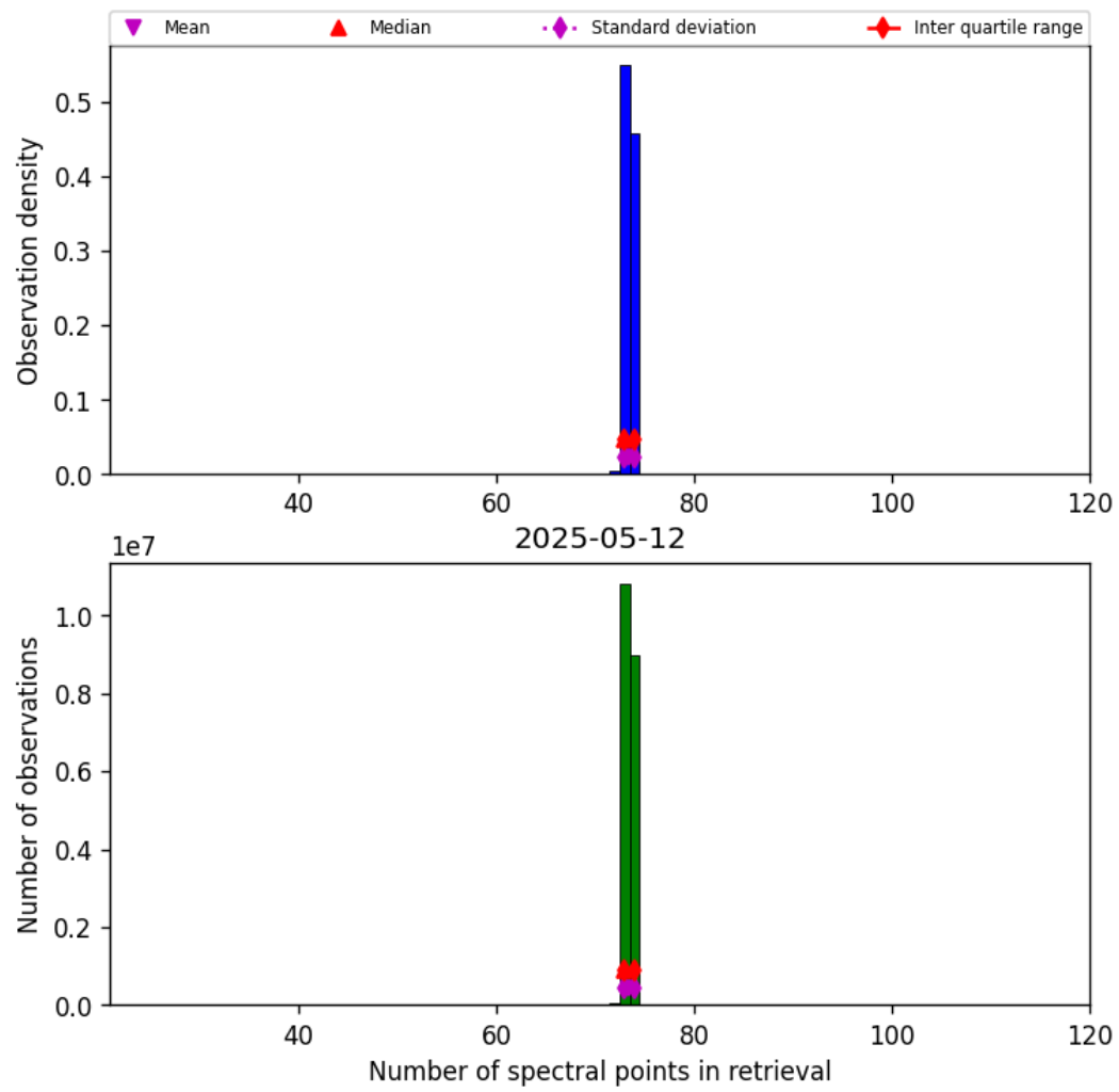
Figure 82: Histogram of “Number of spectral points in retrieval” for 2025-05-11 to 2025-05-13
