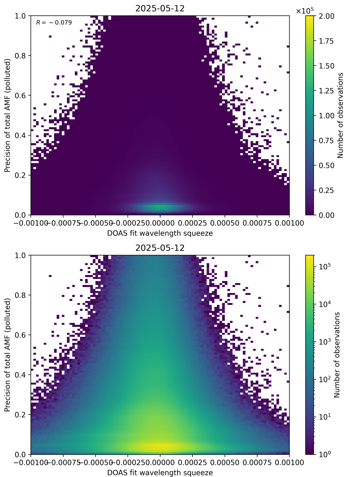
Figure 146: Scatter density plot of “DOAS fit wavelength squeeze” against “Precision of total AMF (polluted)” for 2025-05-11 to 2025-05-13.
