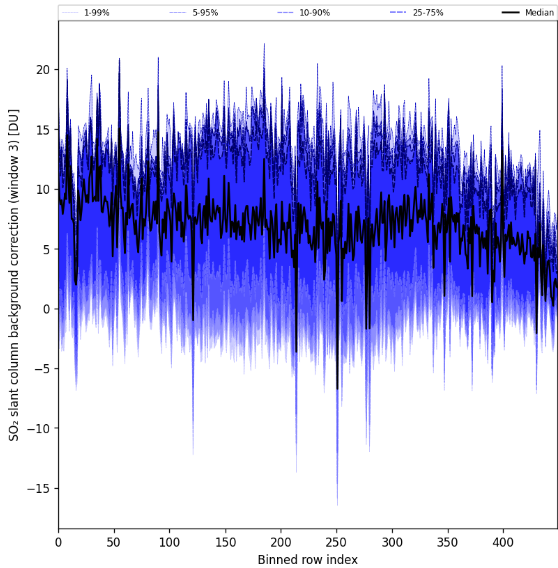
Figure 100: Along track statistics of “SO 2 slant column background correction (window 3)” for 2025-05-11 to 2025-05-13
