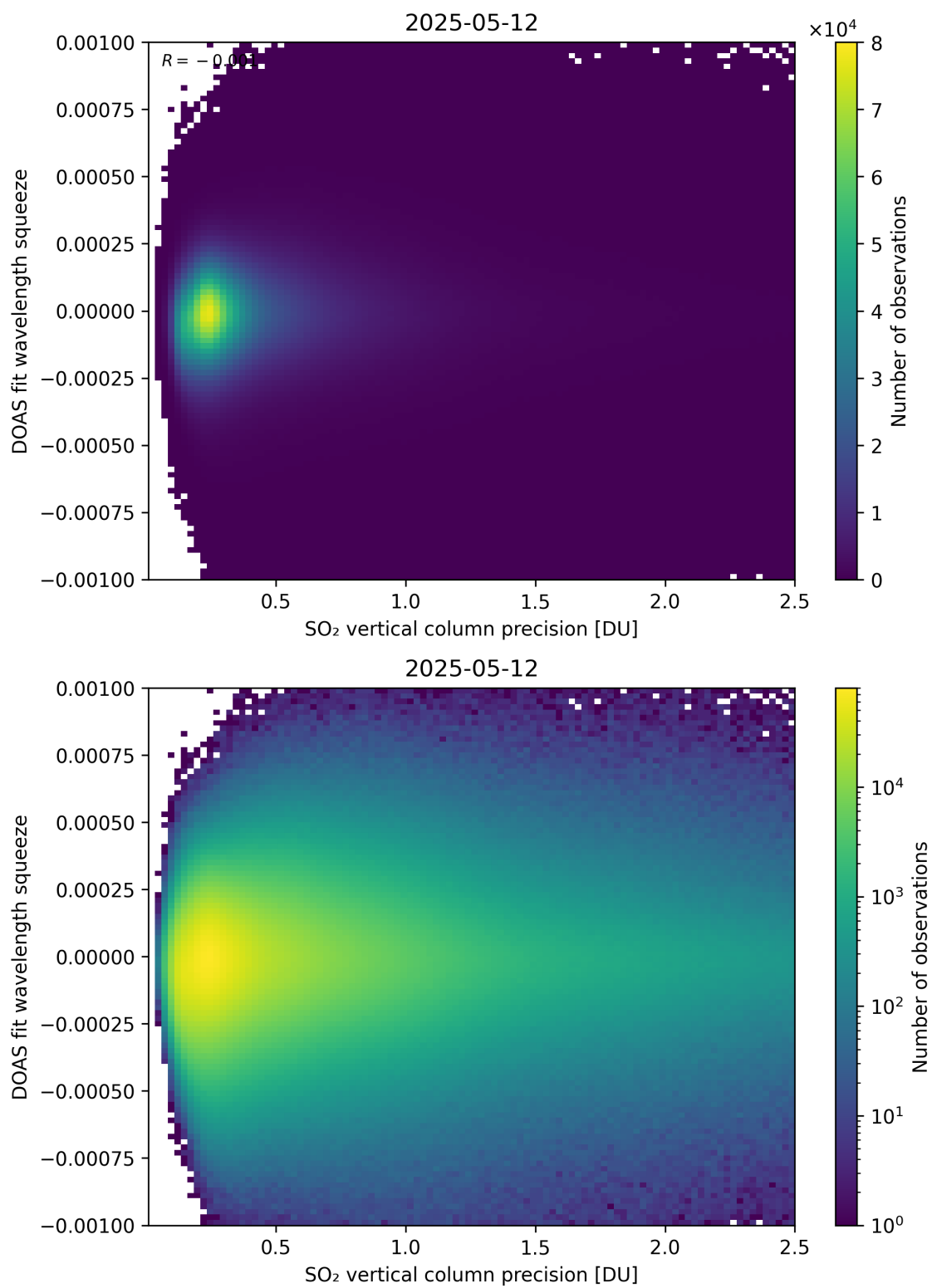
Figure 333: Scatter density plot of “SO 2 vertical column precision” against “DOAS fit wavelength squeeze” for 2025-05-11 to 2025-05-13.
