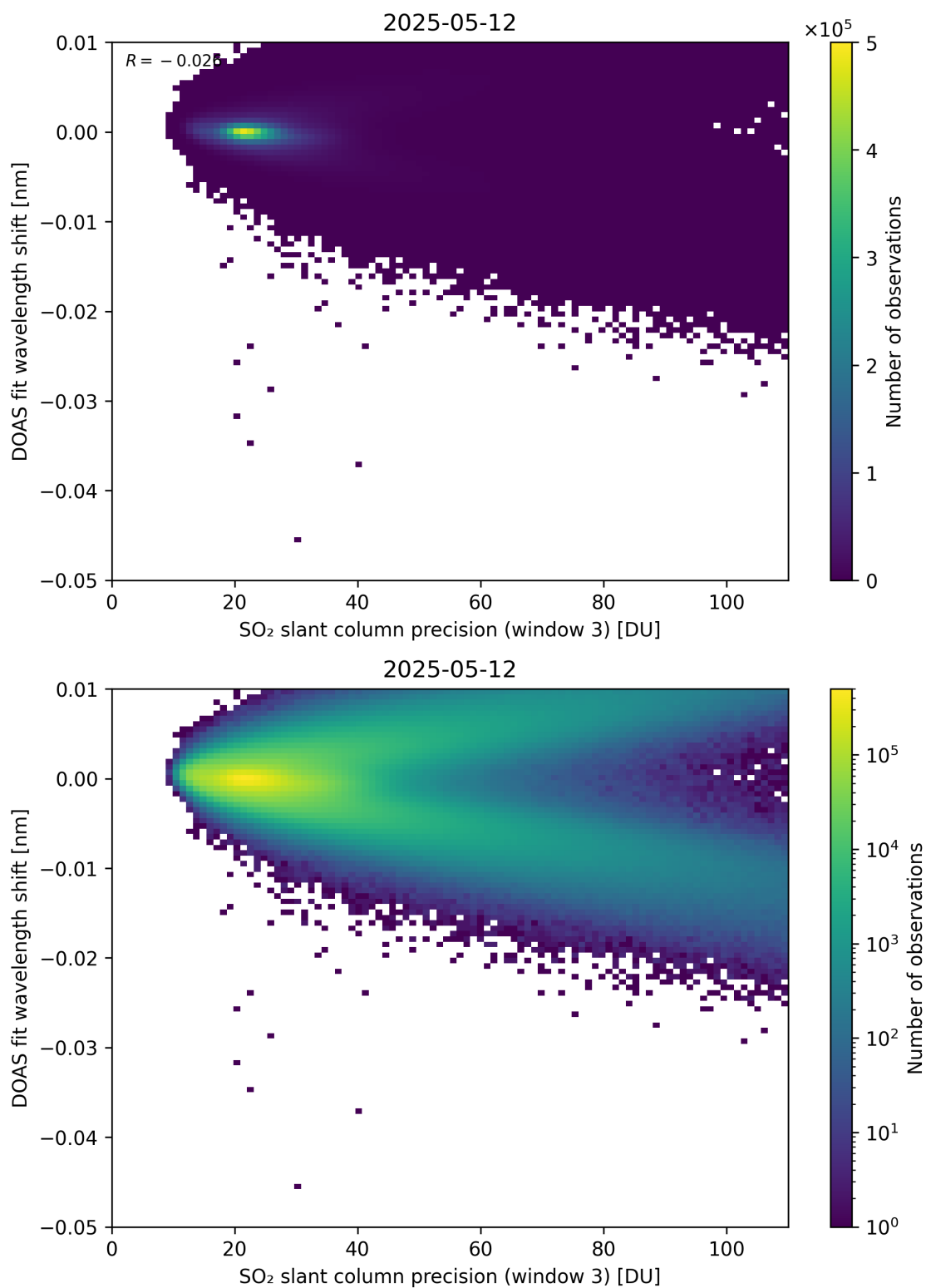
Figure 308: Scatter density plot of “SO 2 slant column precision (window 3)” against “DOAS fit wavelength shift” for 2025-05-11 to 2025-05-13.
