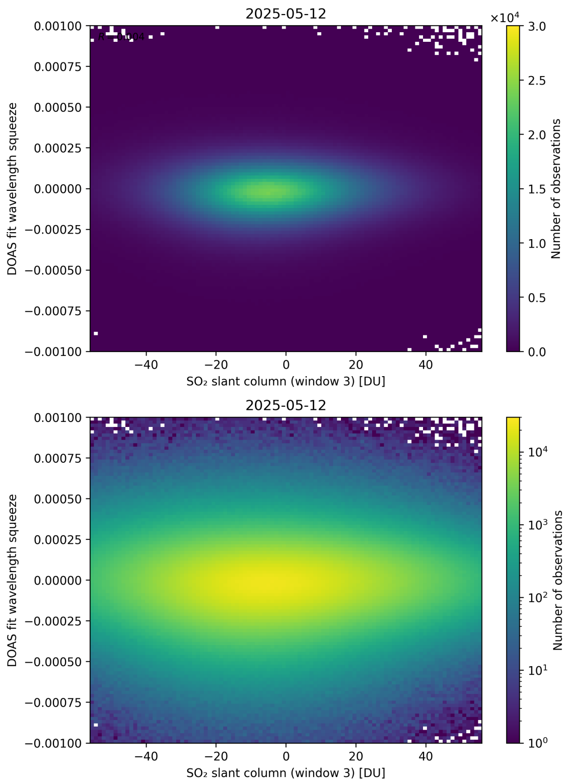
Figure 305: Scatter density plot of “SO 2 slant column (window 3)” against “DOAS fit wavelength squeeze” for 2025-05-11 to 2025-05-13.
