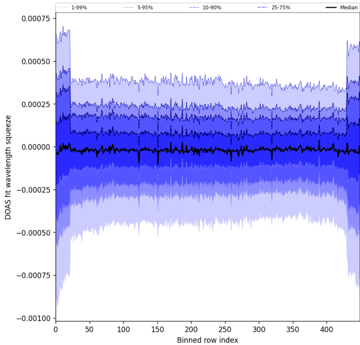
Figure 103: Along track statistics of “DOAS fit wavelength squeeze” for 2025-05-11 to 2025-05-13
