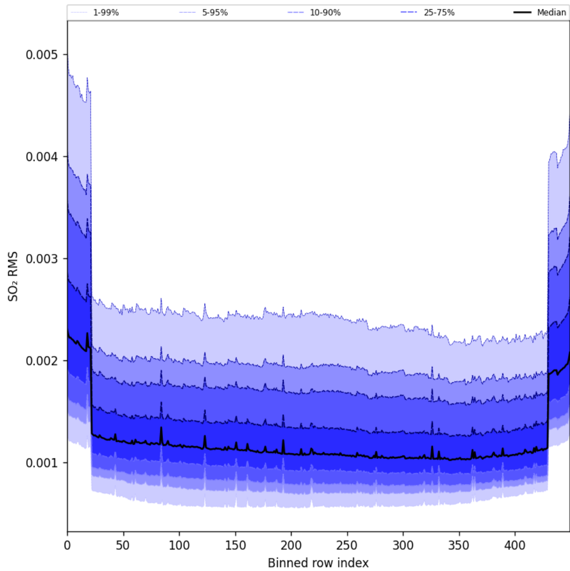
Figure 104: Along track statistics of “SO 2 RMS” for 2025-05-11 to 2025-05-13
