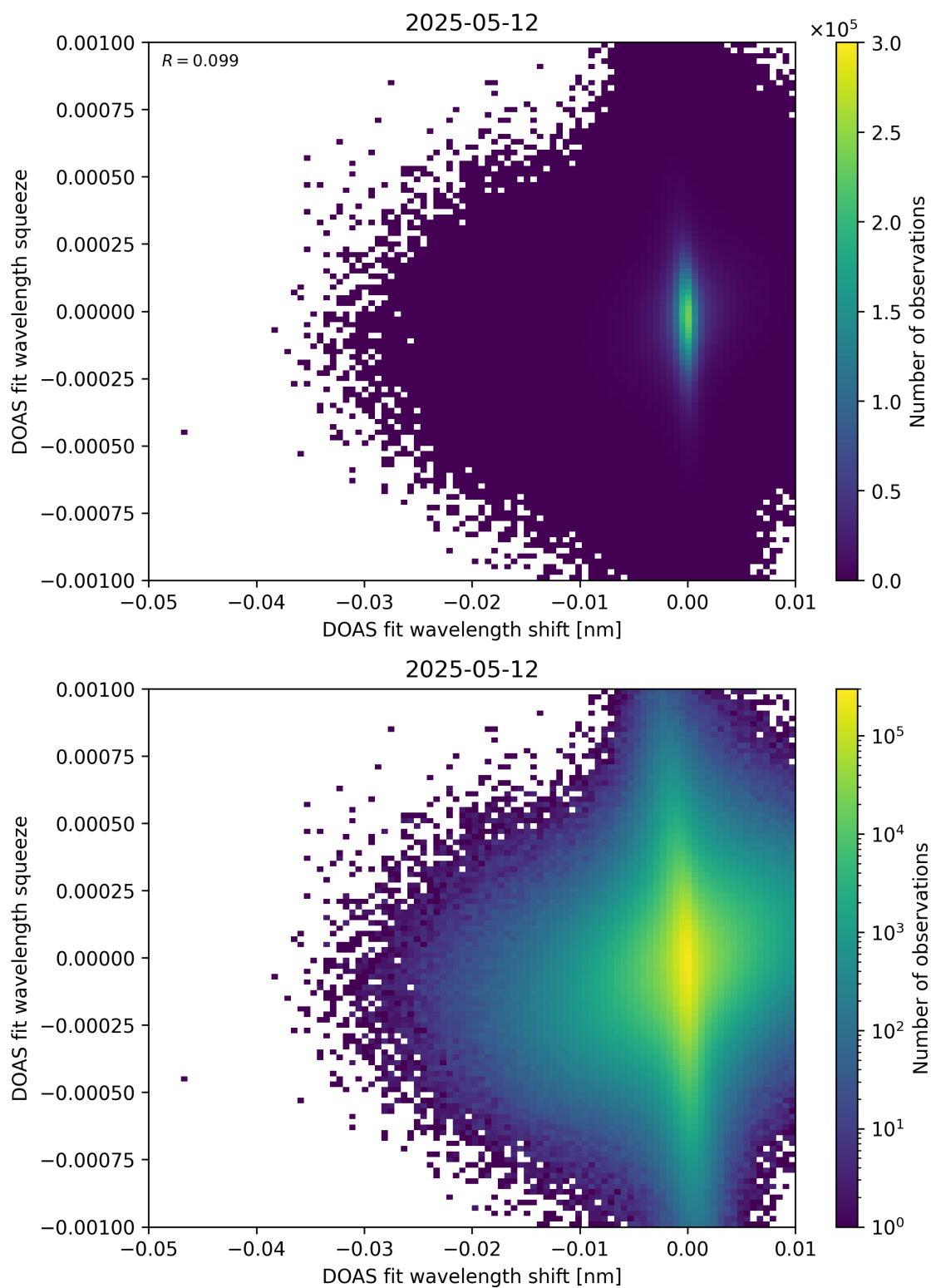
Figure 138: Scatter density plot of “DOAS fit wavelength shift” against “DOAS fit wavelength squeeze” for 2025-05-11 to 2025-05-13.
