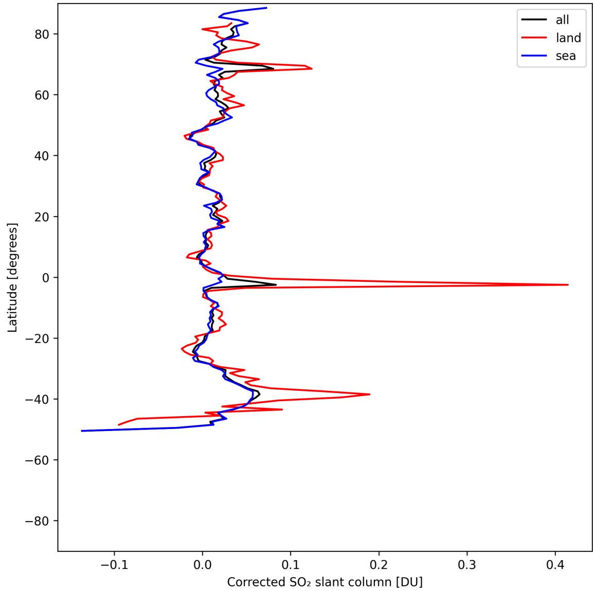
Figure 34: Zonal average of “Corrected SO 2 slant column” for 2025-05-11 to 2025-05-13.
