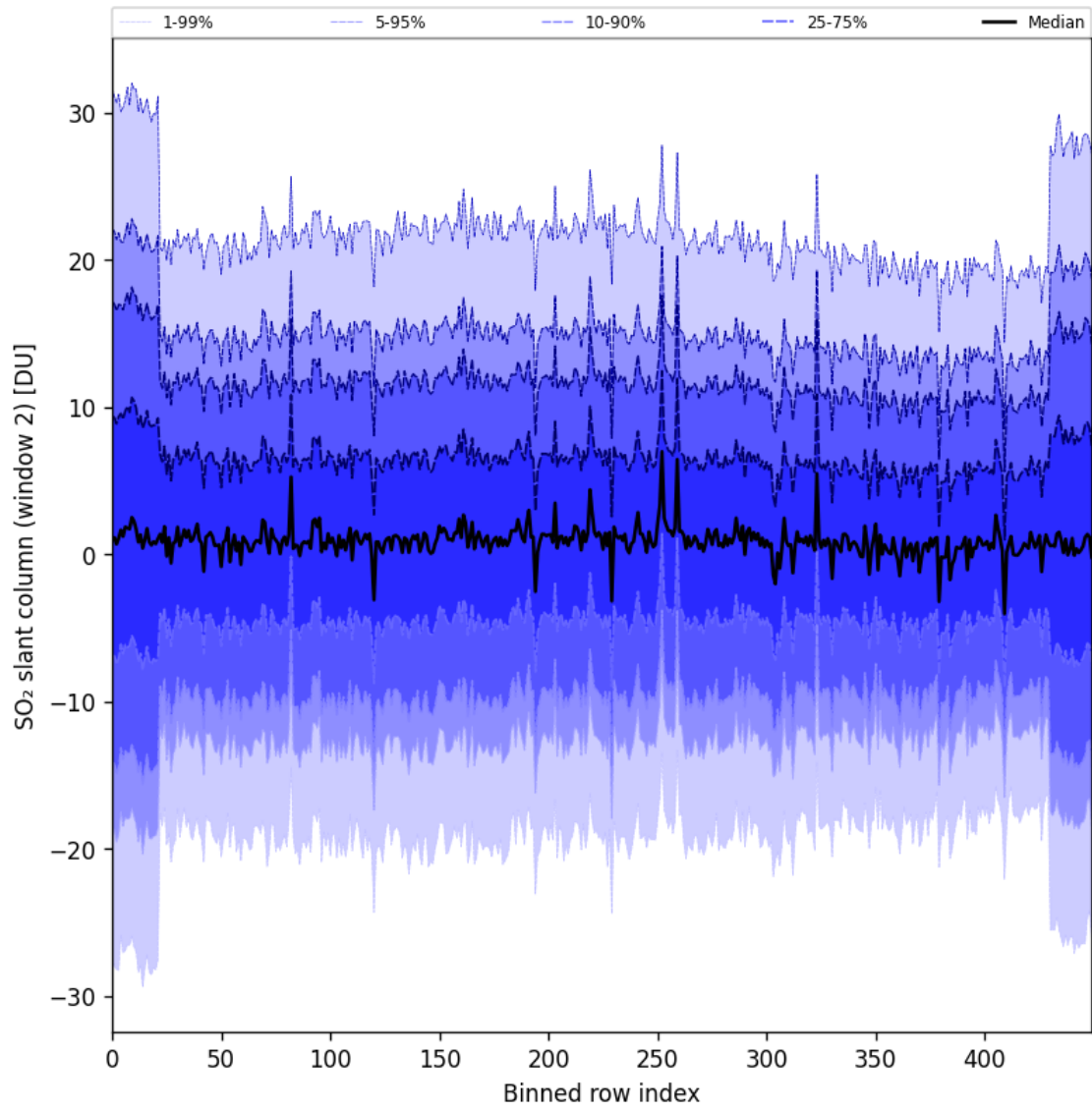
Figure 93: Along track statistics of “SO 2 slant column (window 2)” for 2025-05-11 to 2025-05-13
