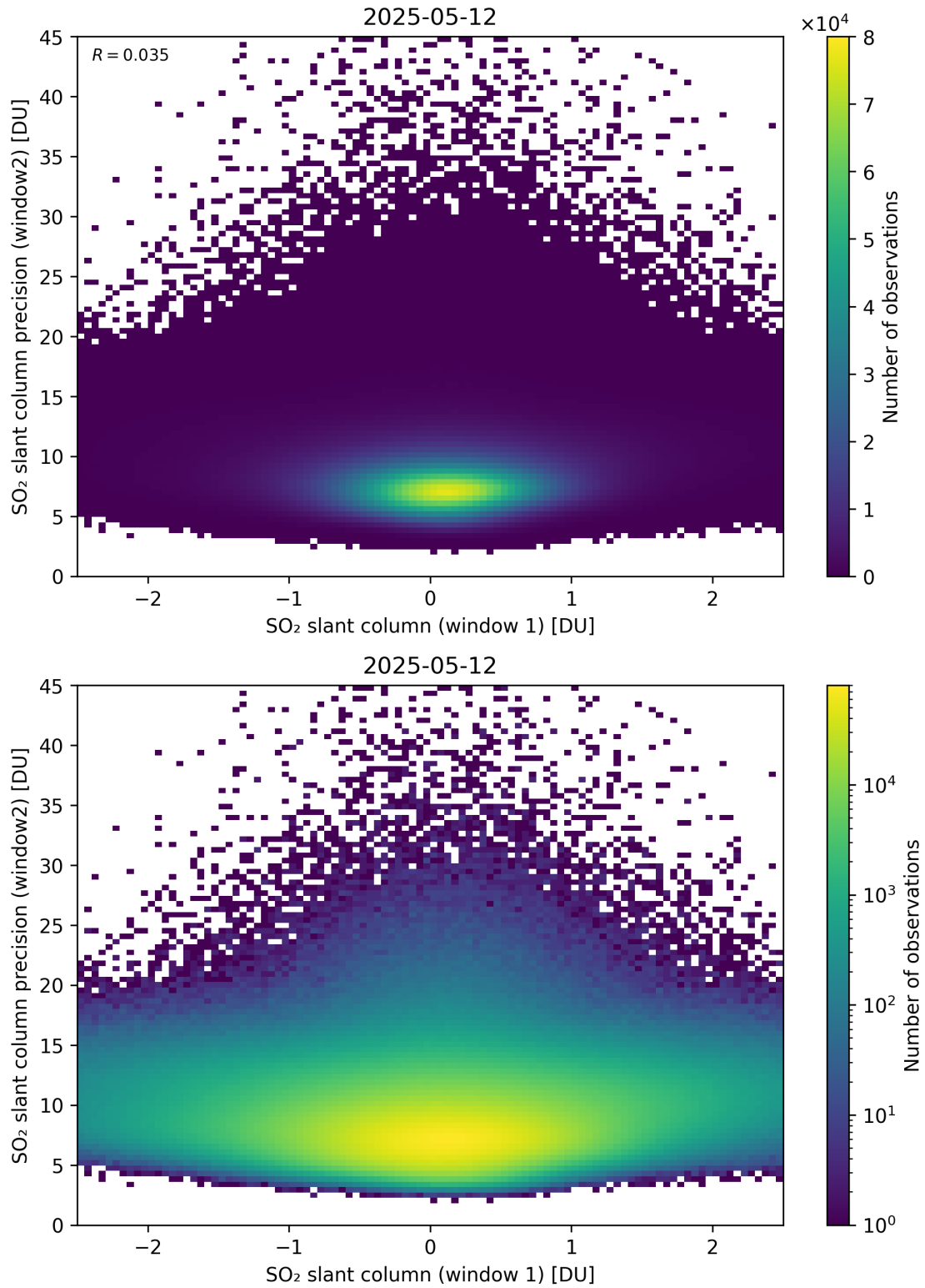
Figure 286: Scatter density plot of “SO 2 slant column (window 1)” against “SO 2 slant column precision (window2)” for 2025-05-11 to 2025-05-13.
