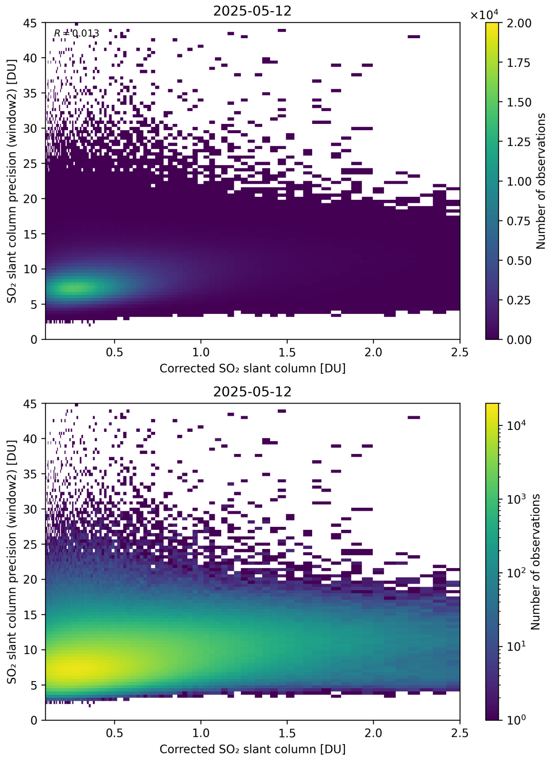
Figure 239: Scatter density plot of “Corrected SO 2 slant column” against “SO 2 slant column precision (window2)” for 2025-05-11 to 2025-05-13.
