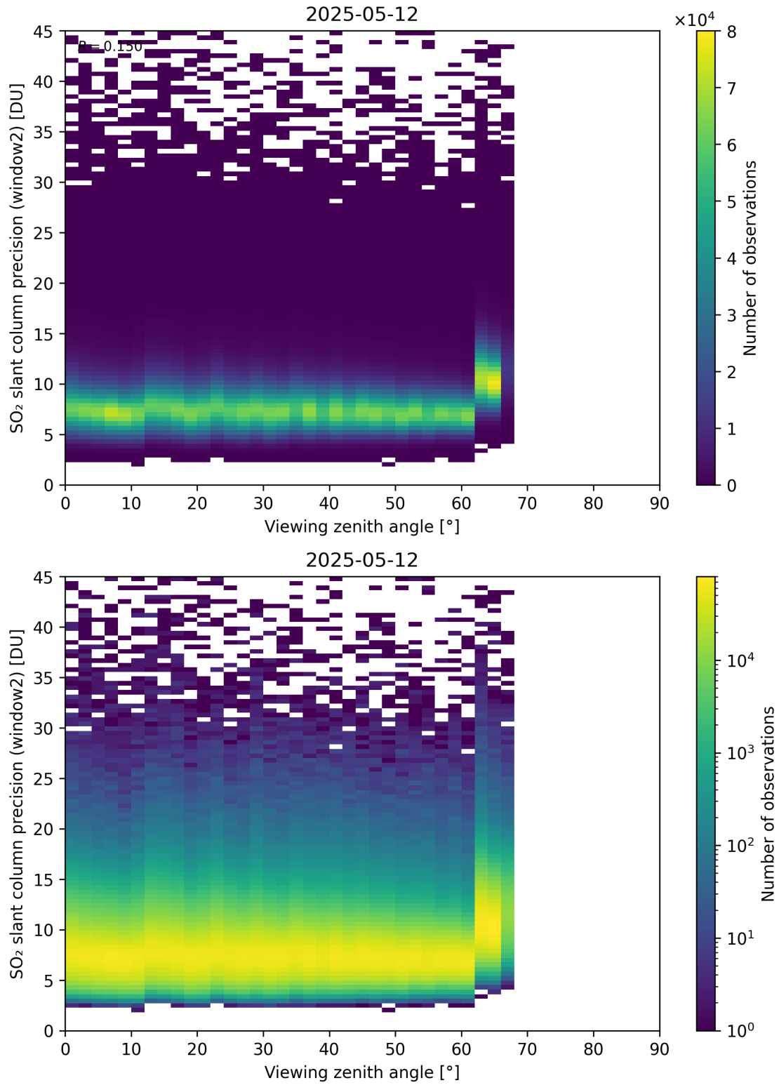
Figure 378: Scatter density plot of “Viewing zenith angle” against “SO 2 slant column precision (window2)” for 2025-05-11 to 2025-05-13.
