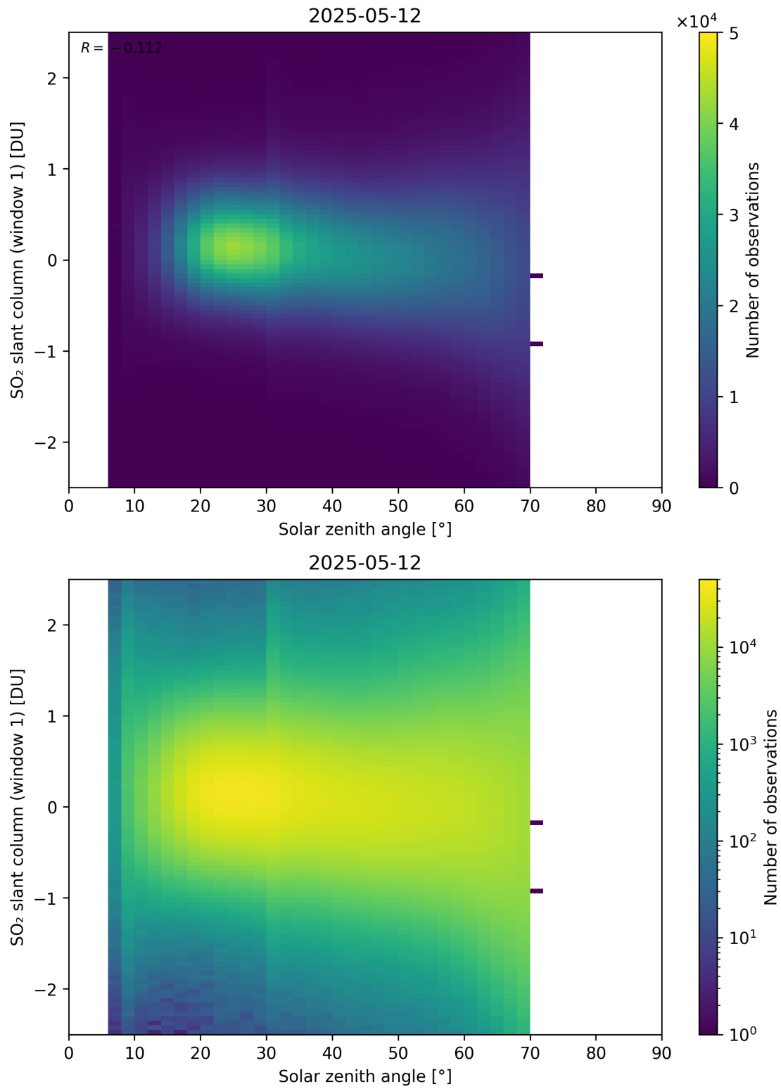
Figure 184: Scatter density plot of “Solar zenith angle” against “SO 2 slant column (window 1)” for 2025-05-11 to 2025-05-13.
