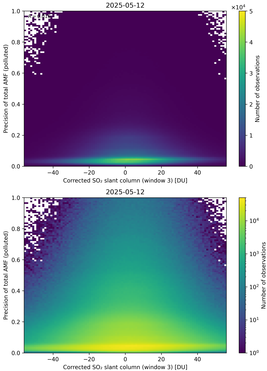
Figure 261: Scatter density plot of “Corrected SO 2 slant column (window 3)” against “Precision of total AMF (polluted)” for 2025-05-11 to 2025-05-13.
