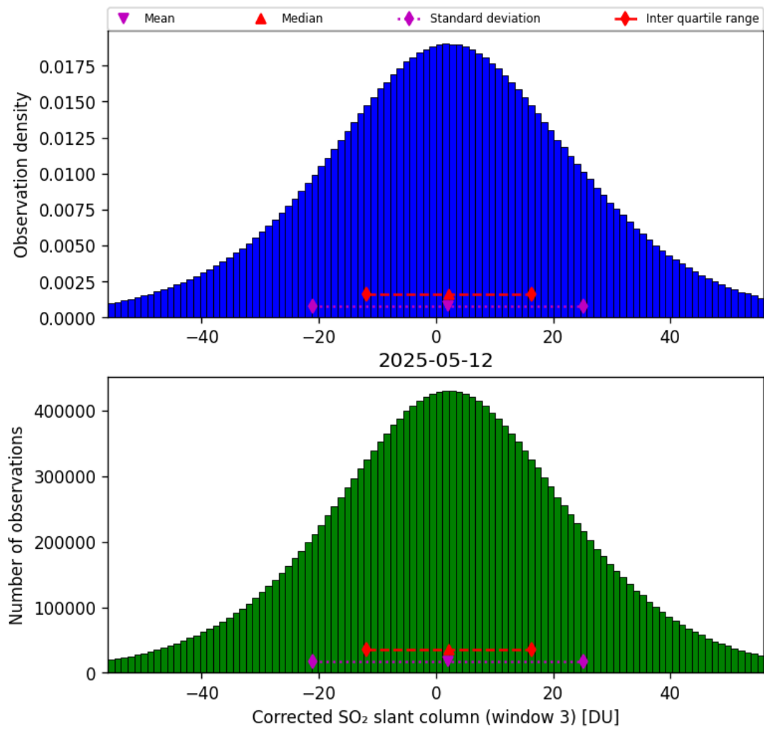
Figure 73: Histogram of “Corrected SO 2 slant column (window 3)” for 2025-05-11 to 2025-05-13
