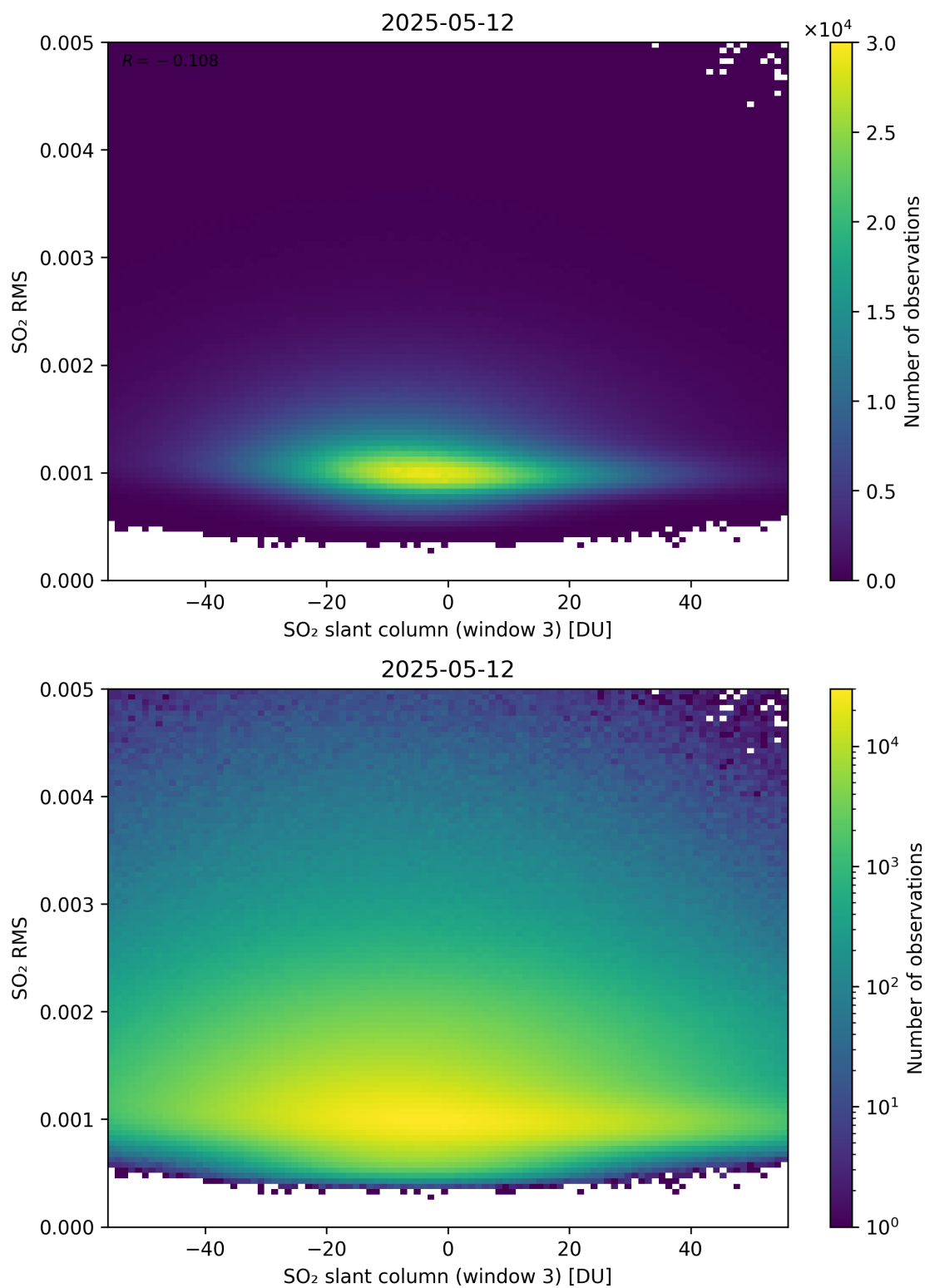
Figure 306: Scatter density plot of “SO 2 slant column (window 3)” against “SO 2 RMS” for 2025-05-11 to 2025-05-13.
