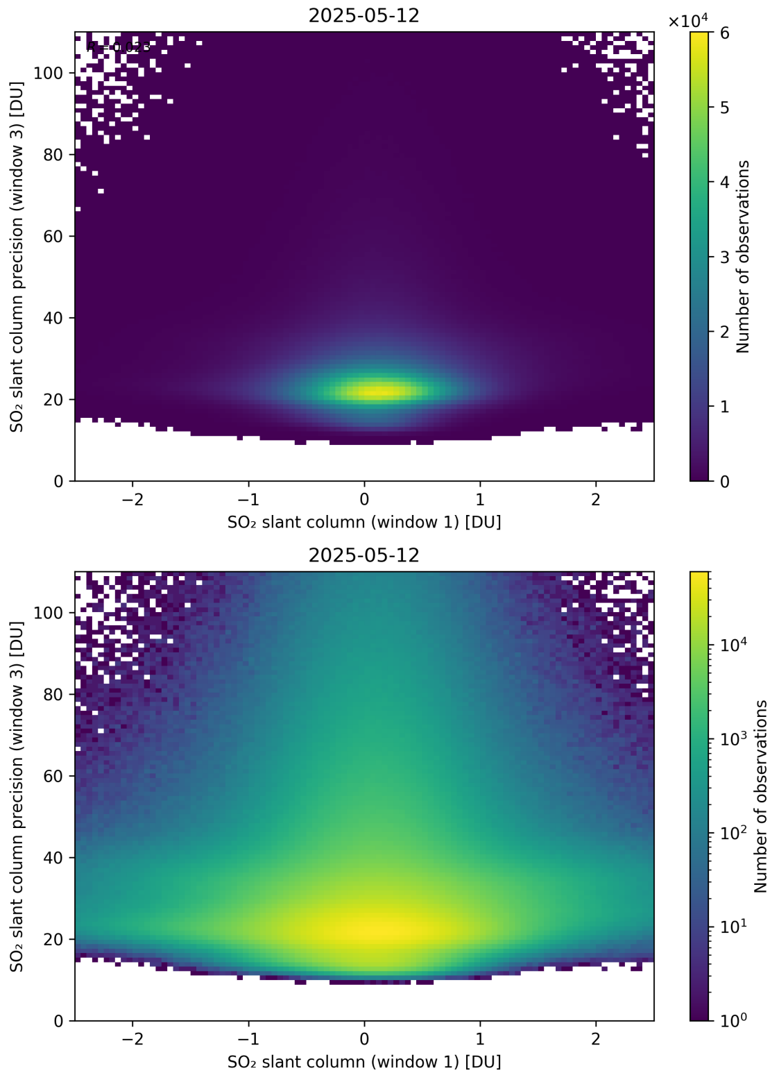
Figure 288: Scatter density plot of “SO 2 slant column (window 1)” against “SO 2 slant column precision (window 3)” for 2025-05-11 to 2025-05-13.
