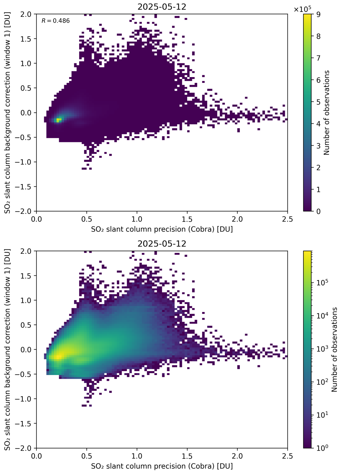
Figure 199: Scatter density plot of “SO 2 slant column precision (Cobra)” against “SO 2 slant column background correction (window 1)” for 2025-05-11 to 2025-05-13.
