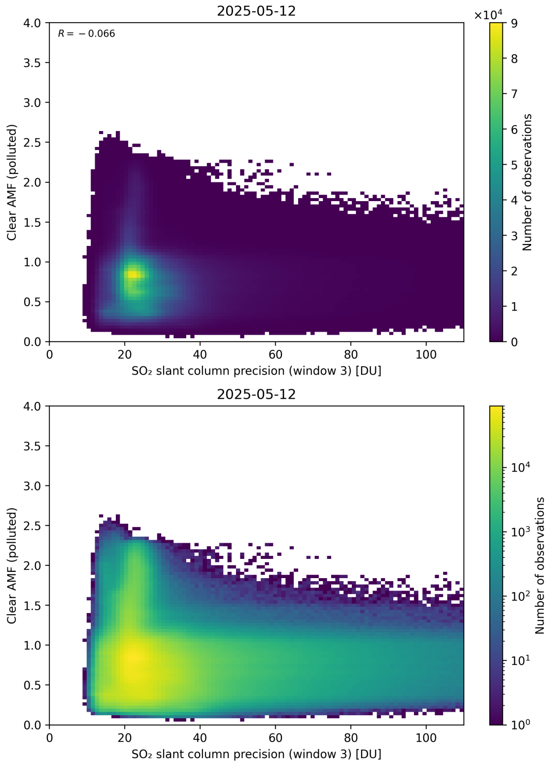
Figure 311: Scatter density plot of “SO 2 slant column precision (window 3)” against “Clear AMF (polluted)” for 2025-05-11 to 2025-05-13.
