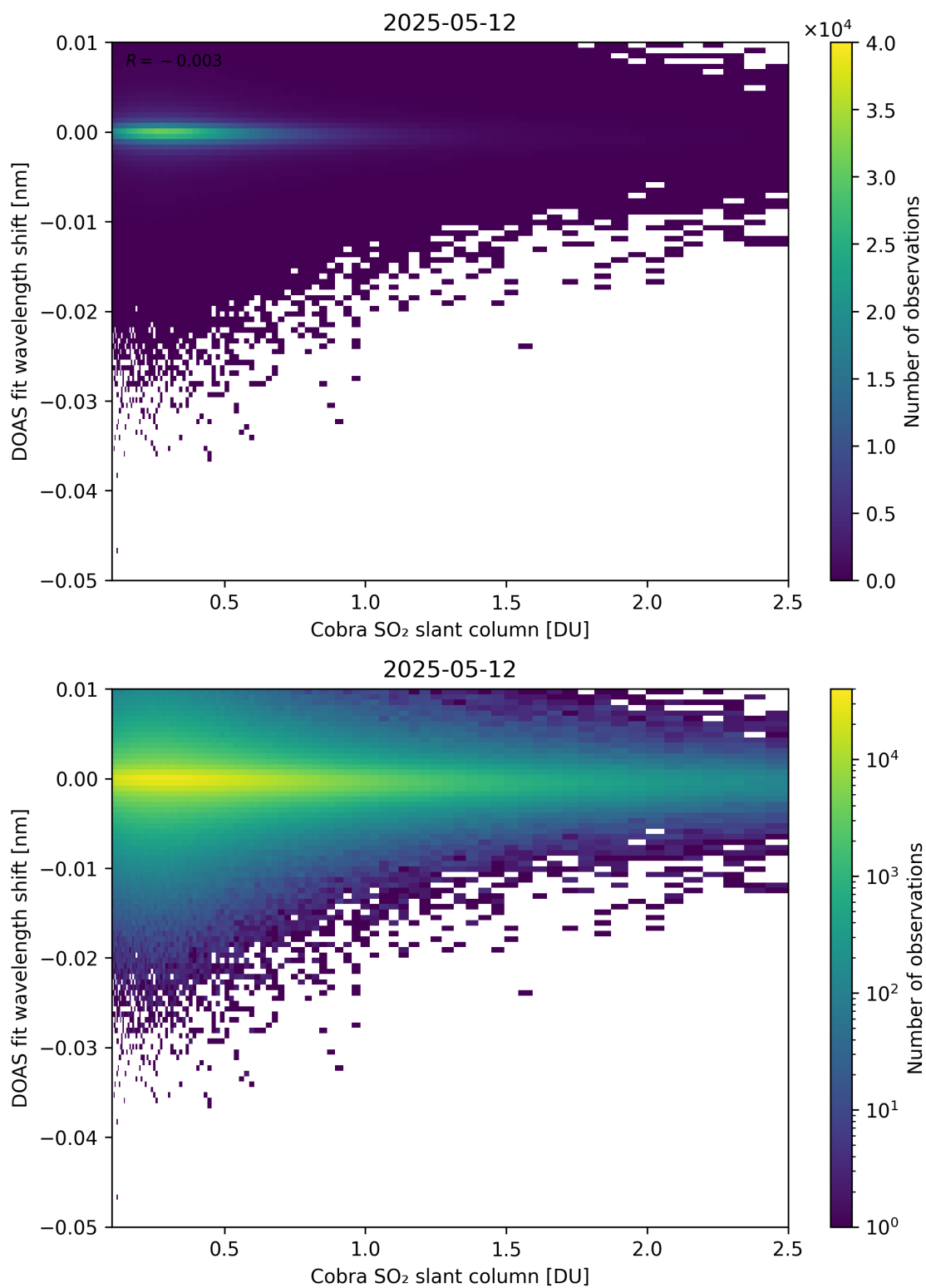
Figure 196: Scatter density plot of “Cobra SO 2 slant column” against “DOAS fit wavelength shift” for 2025-05-11 to 2025-05-13.
