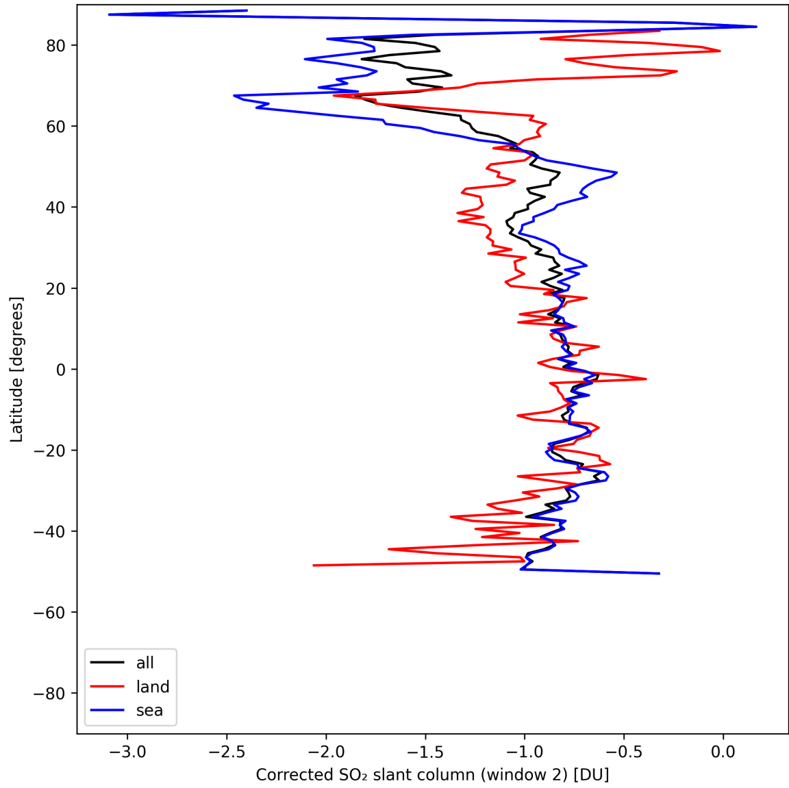
Figure 43: Zonal average of “Corrected SO 2 slant column (window 2)” for 2025-05-11 to 2025-05-13.
