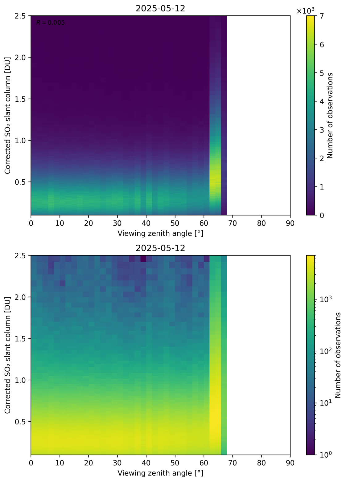
Figure 373: Scatter density plot of “Viewing zenith angle” against “Corrected SO 2 slant column” for 2025-05-11 to 2025-05-13.
