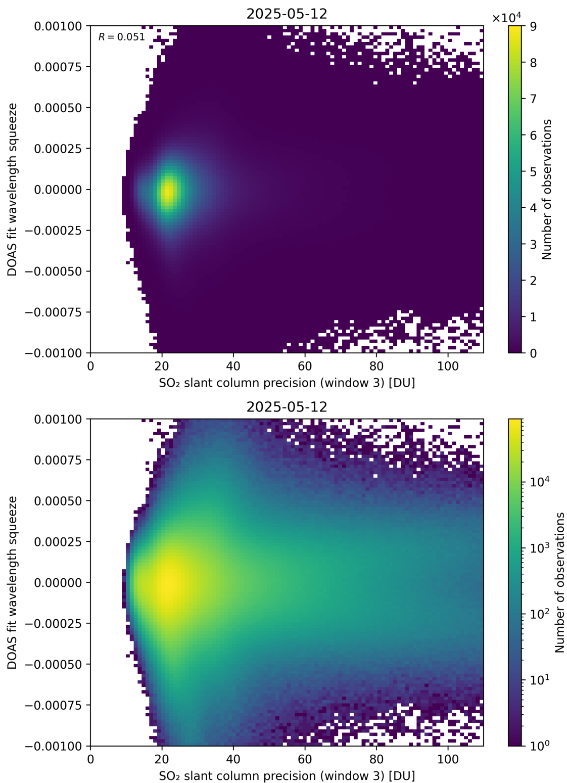
Figure 309: Scatter density plot of “SO 2 slant column precision (window 3)” against “DOAS fit wavelength squeeze” for 2025-05-11 to 2025-05-13.
