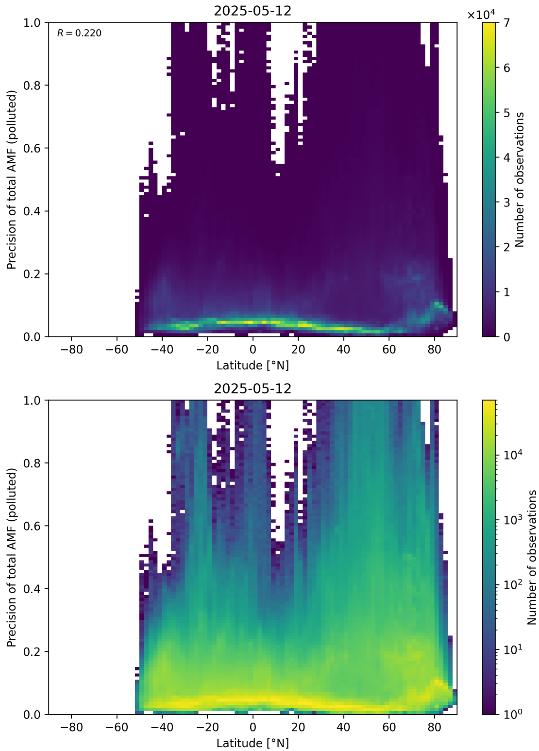
Figure 168: Scatter density plot of “Latitude” against “Precision of total AMF (polluted)” for 2025-05-11 to 2025-05-13.
