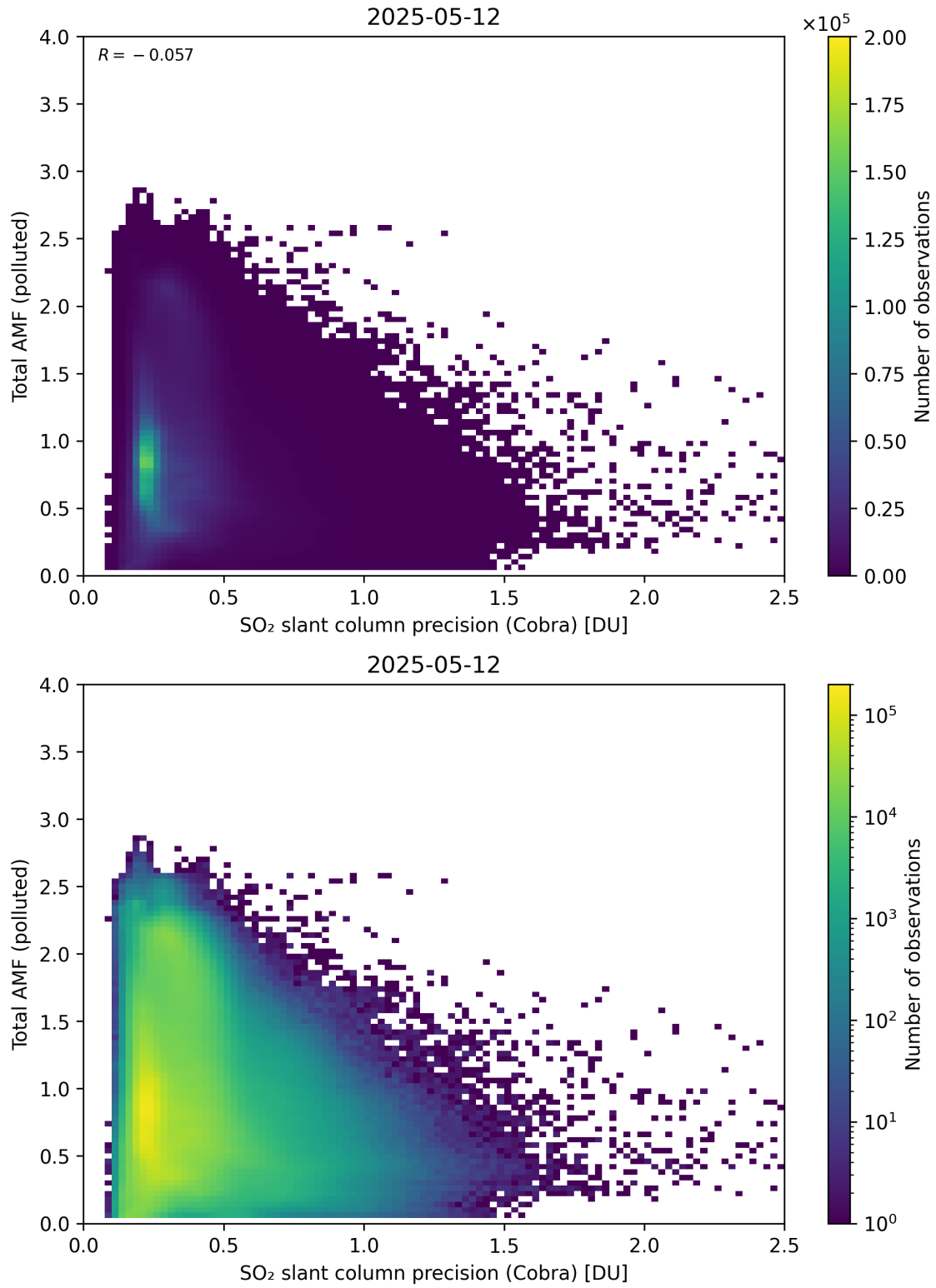
Figure 213: Scatter density plot of “SO 2 slant column precision (Cobra)” against “Total AMF (polluted)” for 2025-05-11 to 2025-05-13.
