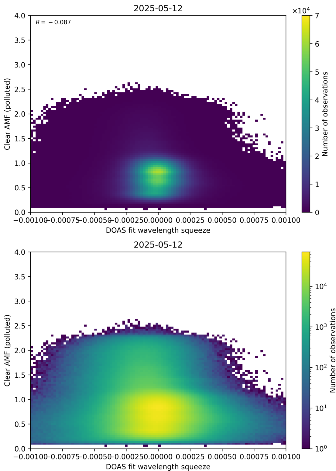
Figure 144: Scatter density plot of “DOAS fit wavelength squeeze” against “Clear AMF (polluted)” for 2025-05-11 to 2025-05-13.
