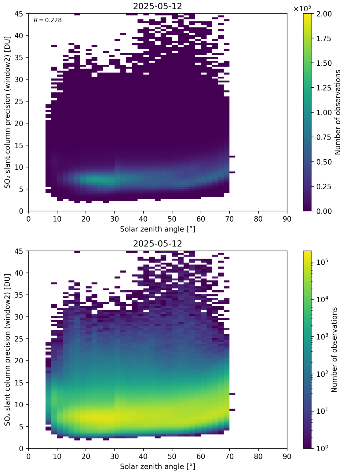
Figure 186: Scatter density plot of “Solar zenith angle” against “SO 2 slant column precision (window2)” for 2025-05-11 to 2025-05-13.
