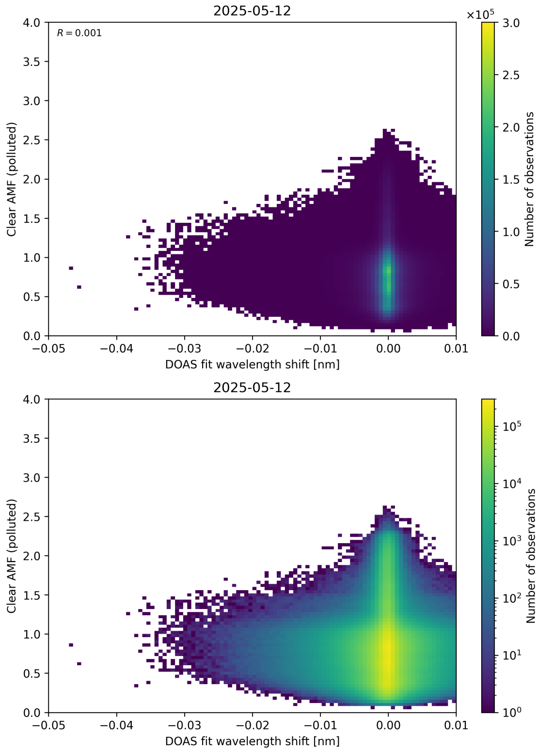
Figure 140: Scatter density plot of “DOAS fit wavelength shift” against “Clear AMF (polluted)” for 2025-05-11 to 2025-05-13.
