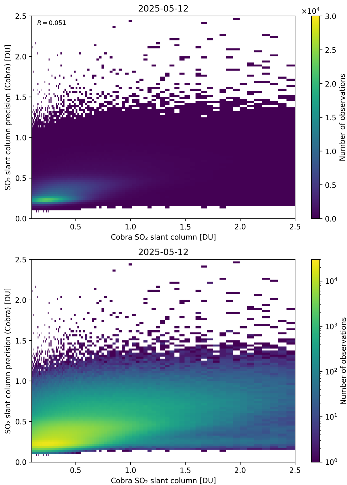
Figure 216: Scatter density plot of “Cobra SO 2 slant column” against “SO 2 slant column precision (Cobra)” for 2025-05-11 to 2025-05-13.
