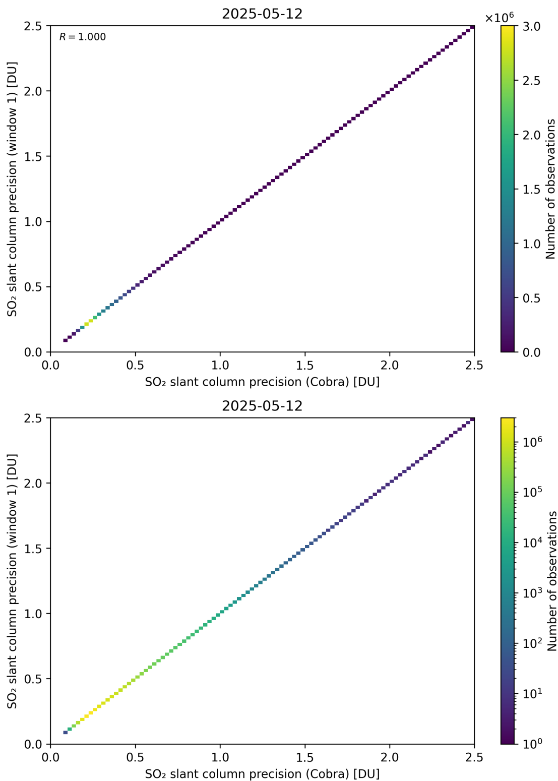
Figure 209: Scatter density plot of “SO 2 slant column precision (Cobra)” against “SO 2 slant column precision (window 1)” for 2025-05-11 to 2025-05-13.
