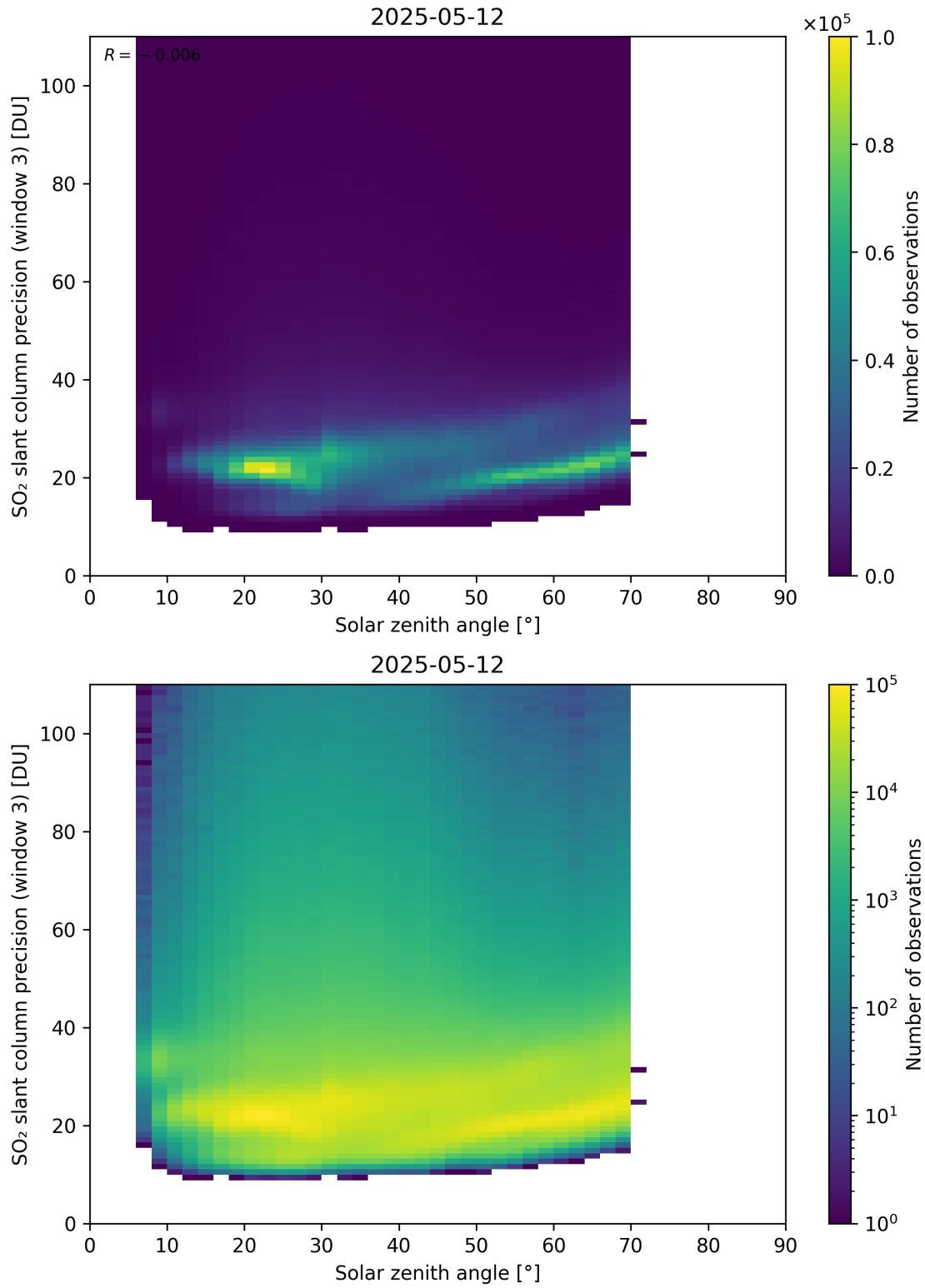
Figure 188: Scatter density plot of “Solar zenith angle” against “SO 2 slant column precision (window 3)” for 2025-05-11 to 2025-05-13.
