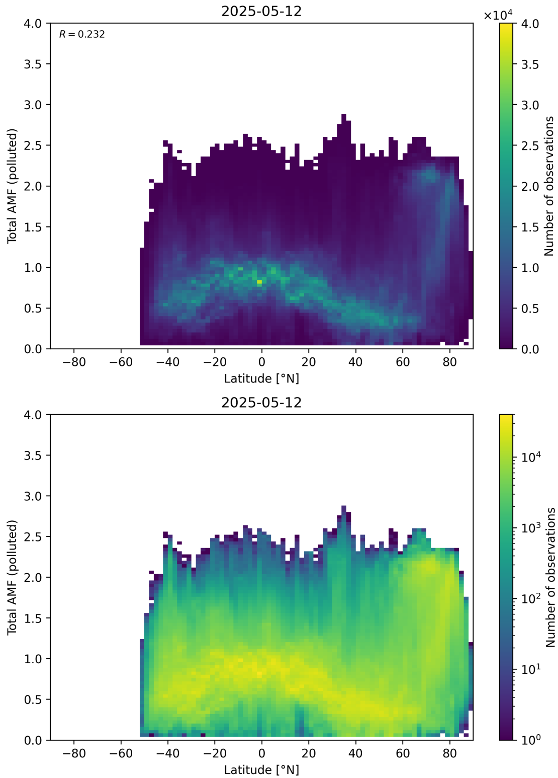
Figure 167: Scatter density plot of “Latitude” against “Total AMF (polluted)” for 2025-05-11 to 2025-05-13.
