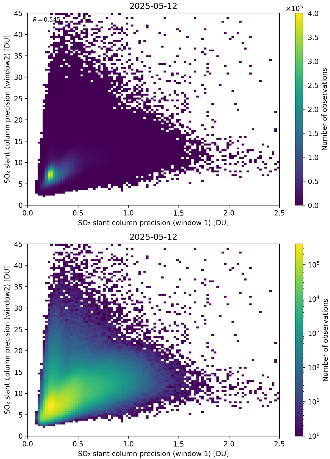
Figure 277: Scatter density plot of “SO 2 slant column precision (window 1)” against “SO 2 slant column precision (window2)” for 2025-05-11 to 2025-05-13.
