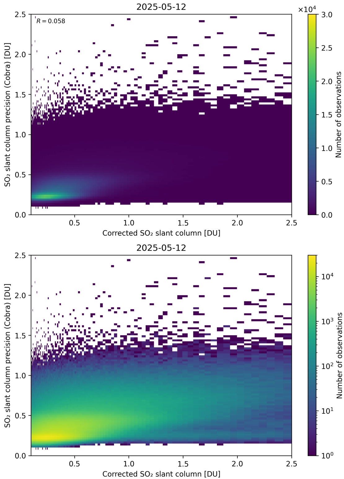
Figure 234: Scatter density plot of “Corrected SO 2 slant column” against “SO 2 slant column precision (Cobra)” for 2025-05-11 to 2025-05-13.
