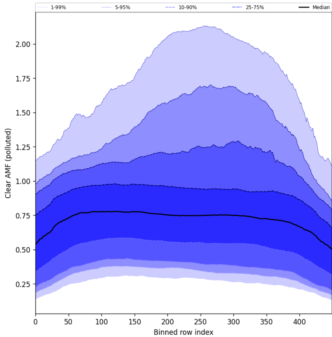
Figure 107: Along track statistics of “Clear AMF (polluted)” for 2025-05-11 to 2025-05-13
