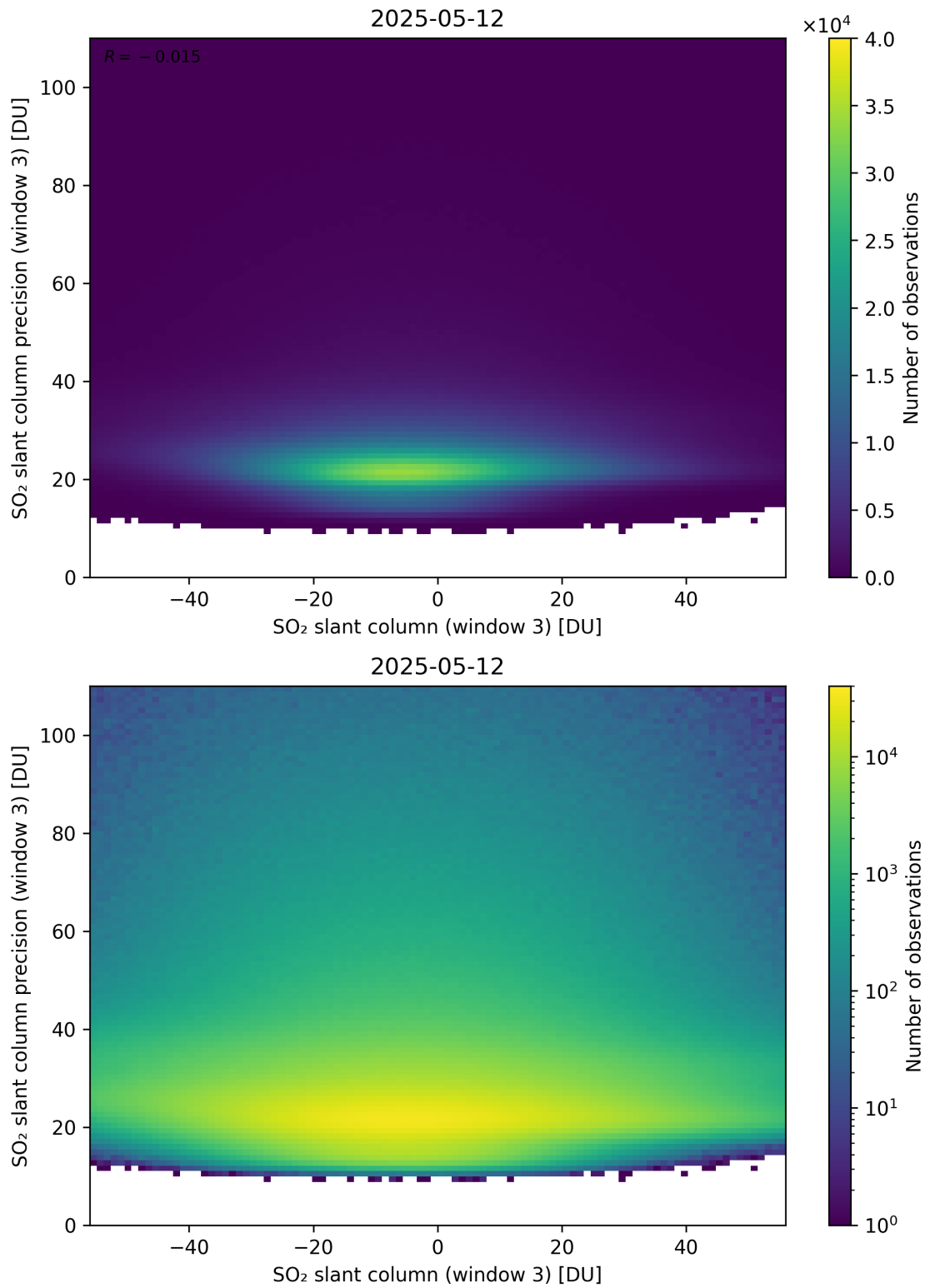
Figure 317: Scatter density plot of “SO 2 slant column (window 3)” against “SO 2 slant column precision (window 3)” for 2025-05-11 to 2025-05-13.
