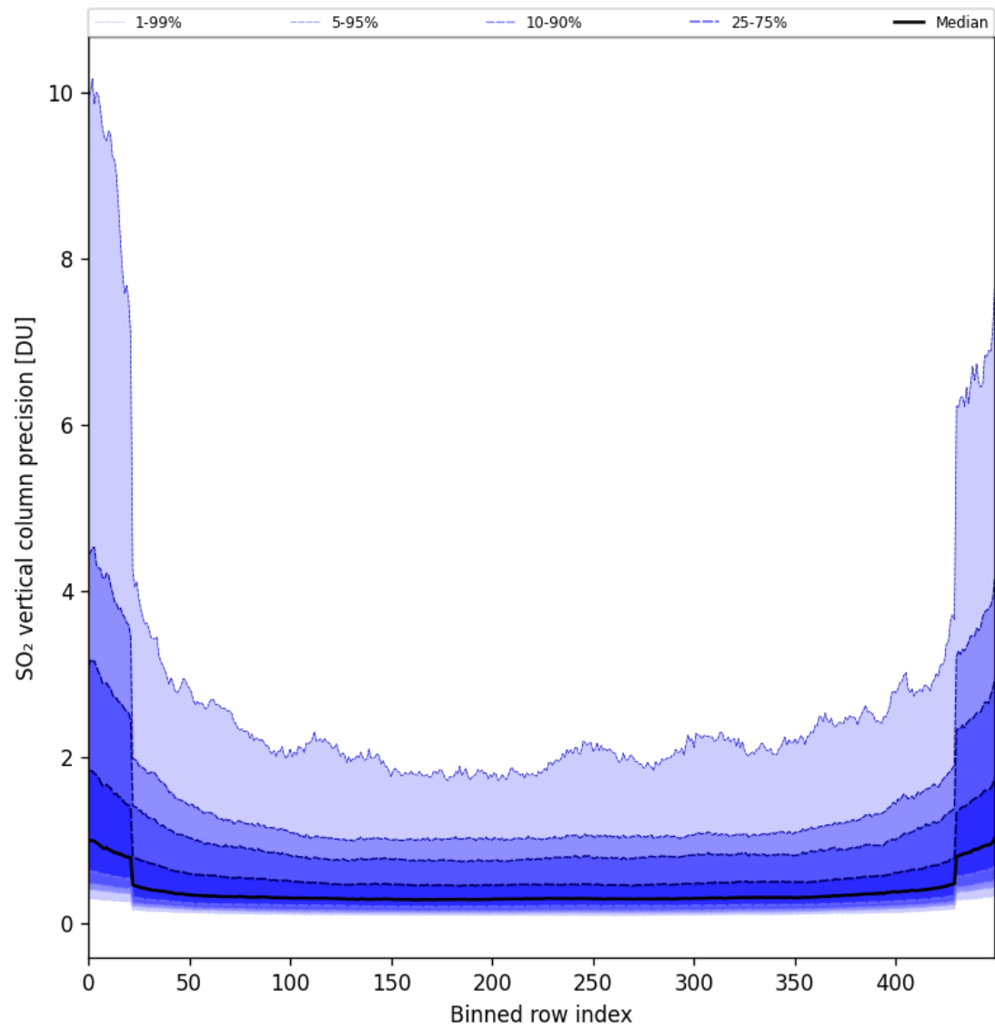
Figure 85: Along track statistics of “SO 2 vertical column precision” for 2025-05-11 to 2025-05-13
