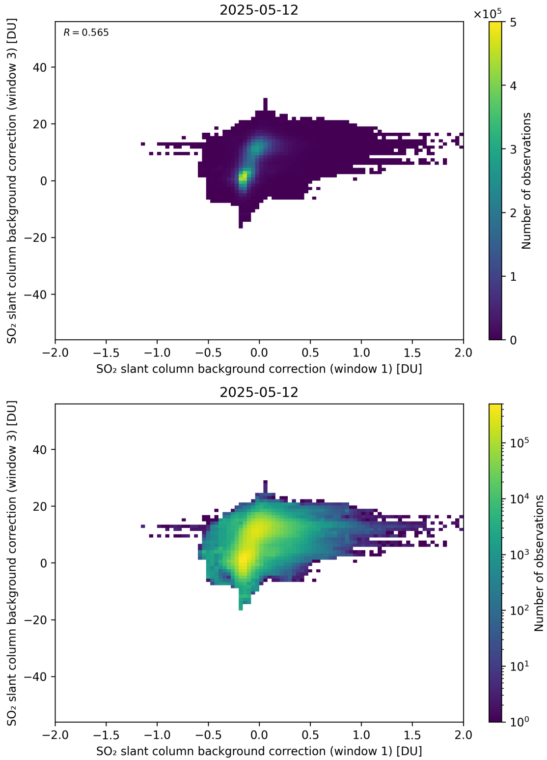
Figure 110: Scatter density plot of “SO 2 slant column background correction (window 1)” against “SO 2 slant column background correction (window 3)” for 2025-05-11 to 2025-05-13.
