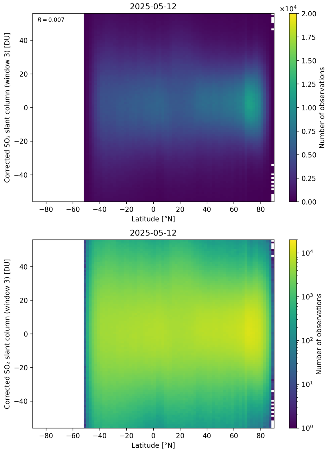
Figure 161: Scatter density plot of “Latitude” against “Corrected SO 2 slant column (window 3)” for 2025-05-11 to 2025-05-13.
