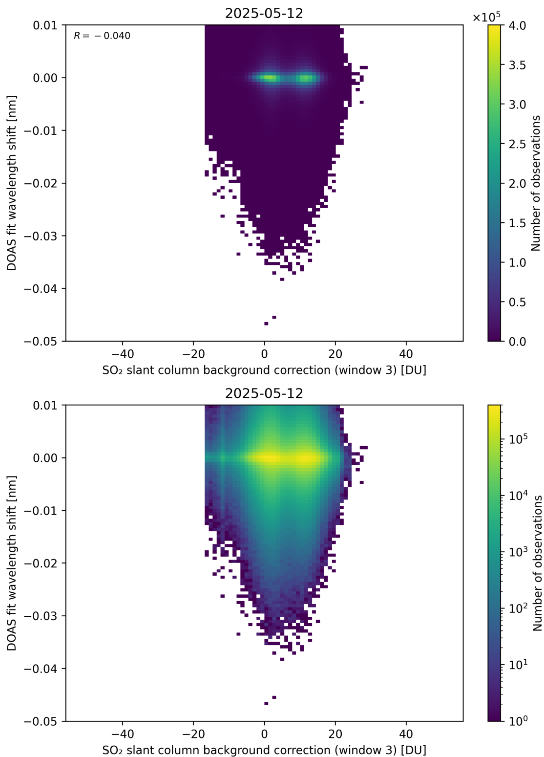
Figure 132: Scatter density plot of “SO 2 slant column background correction (window 3)” against “DOAS fit wavelength shift” for 2025-05-11 to 2025-05-13.
