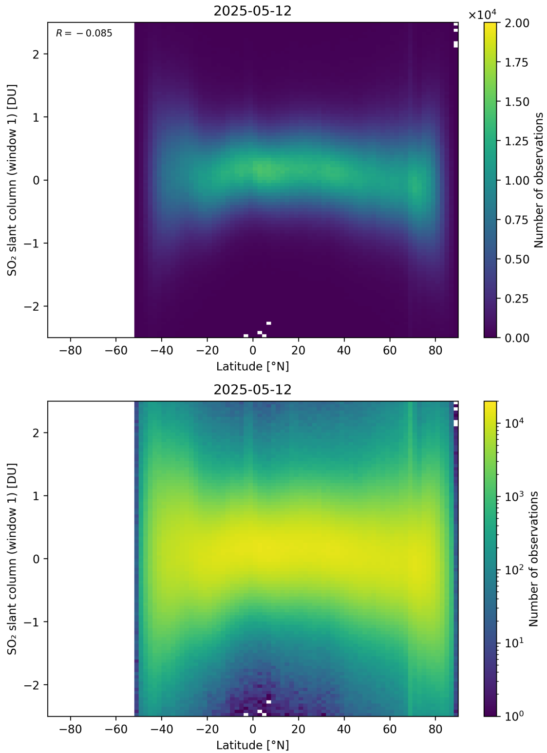
Figure 162: Scatter density plot of “Latitude” against “SO 2 slant column (window 1)” for 2025-05-11 to 2025-05-13.
