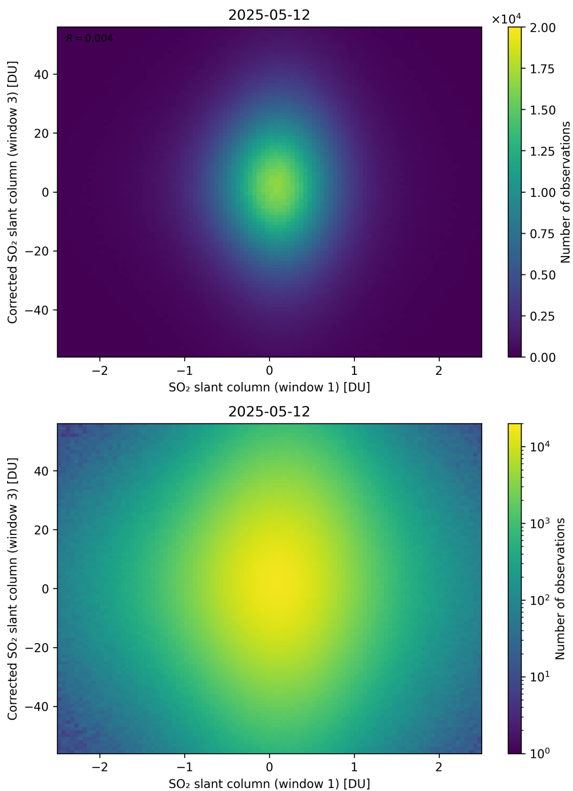
Figure 284: Scatter density plot of “SO 2 slant column (window 1)” against “Corrected SO 2 slant column (window 3)” for 2025-05-11 to 2025-05-13.
