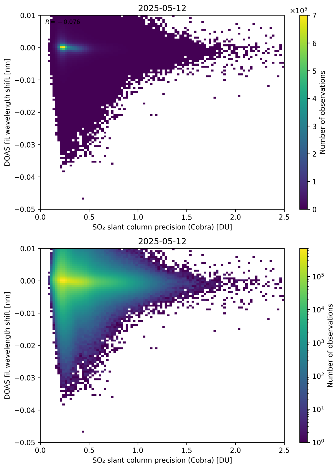
Figure 202: Scatter density plot of “SO 2 slant column precision (Cobra)” against “DOAS fit wavelength shift” for 2025-05-11 to 2025-05-13.
