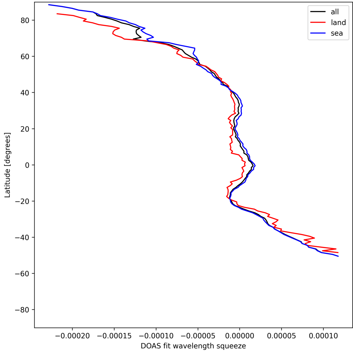
Figure 51: Zonal average of “DOAS fit wavelength squeeze” for 2025-05-11 to 2025-05-13.
