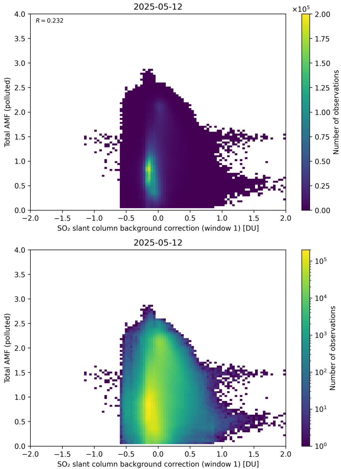
Figure 120: Scatter density plot of “SO 2 slant column background correction (window 1)” against “Total AMF (polluted)” for 2025-05-11 to 2025-05-13.
