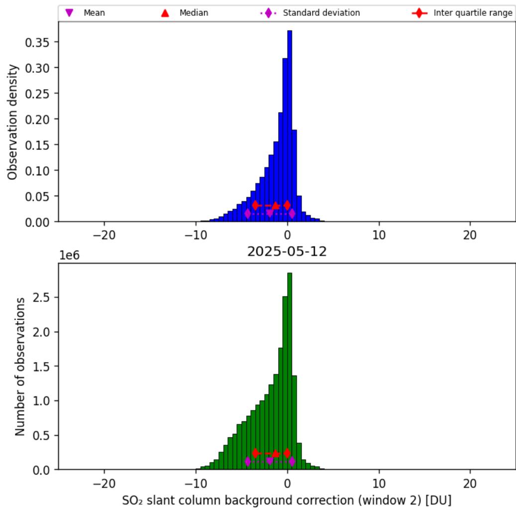
Figure 70: Histogram of “SO 2 slant column background correction (window 2)” for 2025-05-11 to 2025-05-13
