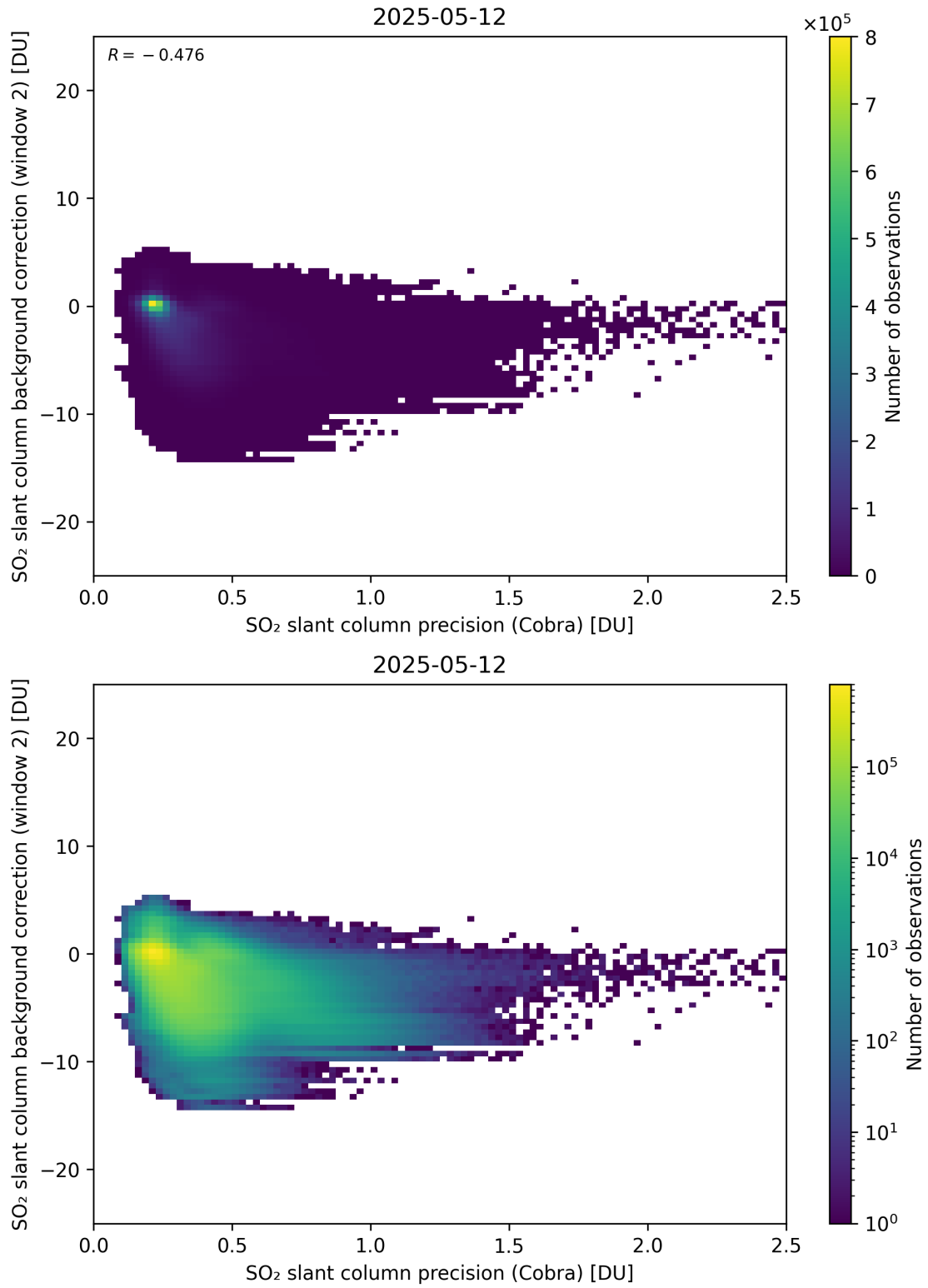
Figure 200: Scatter density plot of “SO 2 slant column precision (Cobra)” against “SO 2 slant column background correction (window 2)” for 2025-05-11 to 2025-05-13.
