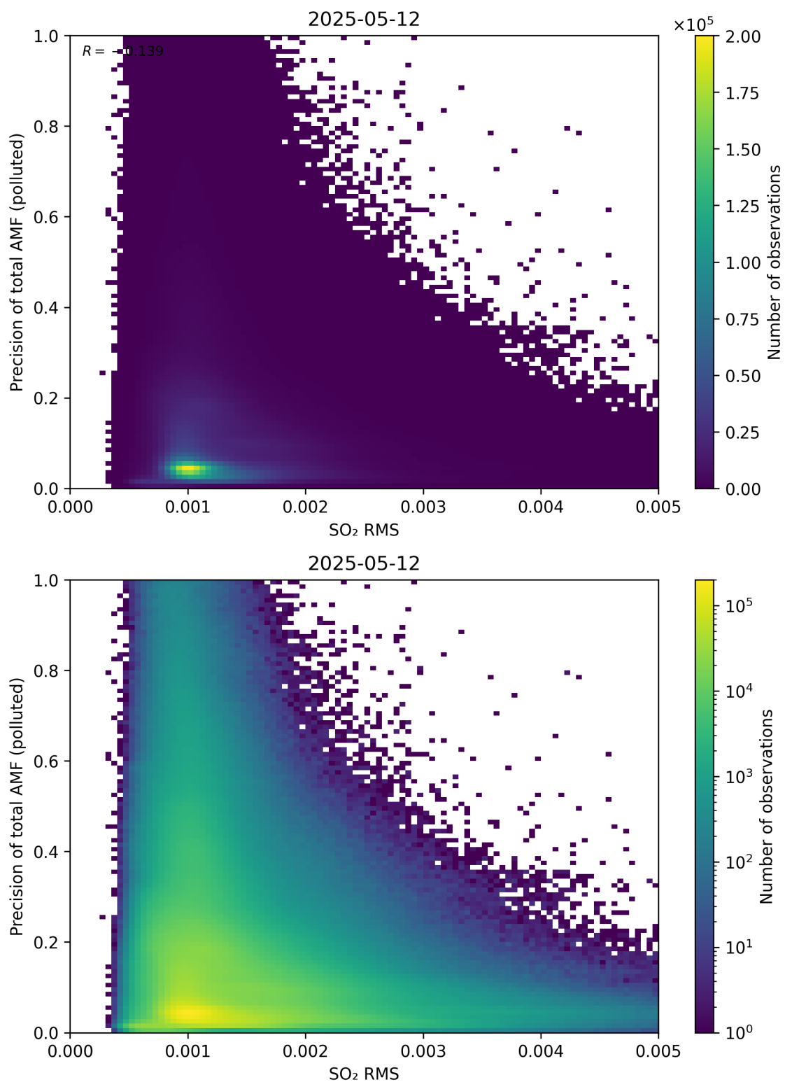
Figure 149: Scatter density plot of “SO 2 RMS” against “Precision of total AMF (polluted)” for 2025-05-11 to 2025-05-13.
