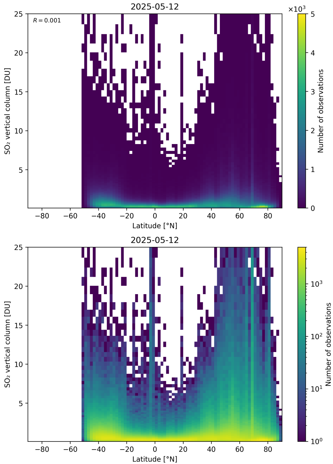
Figure 169: Scatter density plot of “Latitude” against “SO 2 vertical column” for 2025-05-11 to 2025-05-13.
