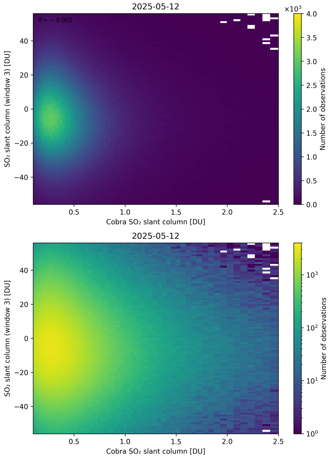
Figure 222: Scatter density plot of “Cobra SO 2 slant column” against “SO 2 slant column (window 3)” for 2025-05-11 to 2025-05-13.
