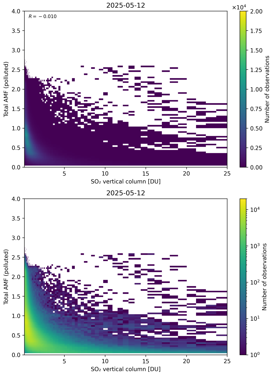
Figure 359: Scatter density plot of “SO 2 vertical column” against “Total AMF (polluted)” for 2025-05-11 to 2025-05-13.
