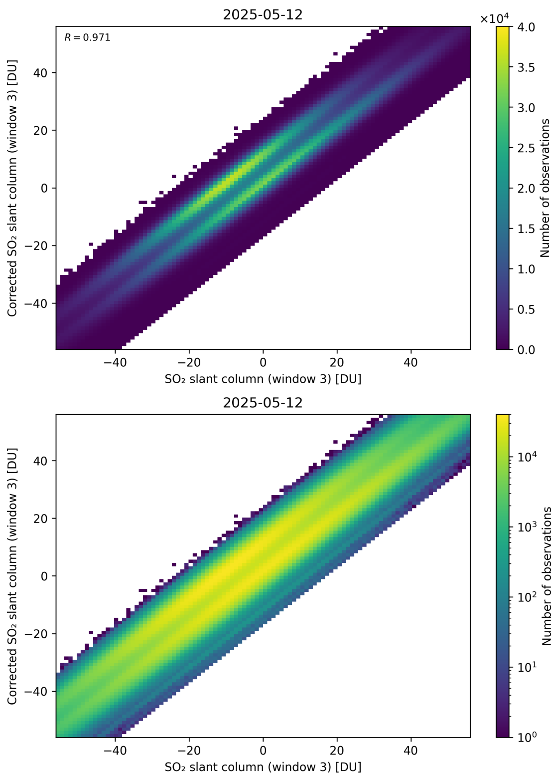
Figure 316: Scatter density plot of “SO 2 slant column (window 3)” against “Corrected SO 2 slant column (window 3)” for 2025-05-11 to 2025-05-13.
