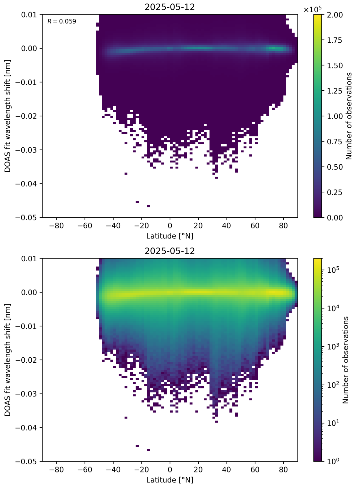
Figure 153: Scatter density plot of “Latitude” against “DOAS fit wavelength shift” for 2025-05-11 to 2025-05-13.
