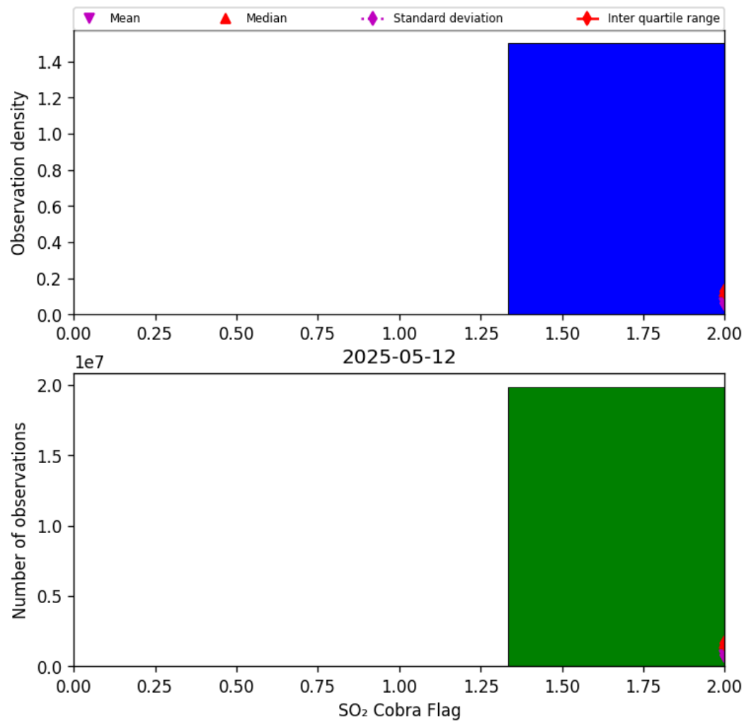
Figure 75: Histogram of “SO 2 Cobra Flag” for 2025-05-11 to 2025-05-13
