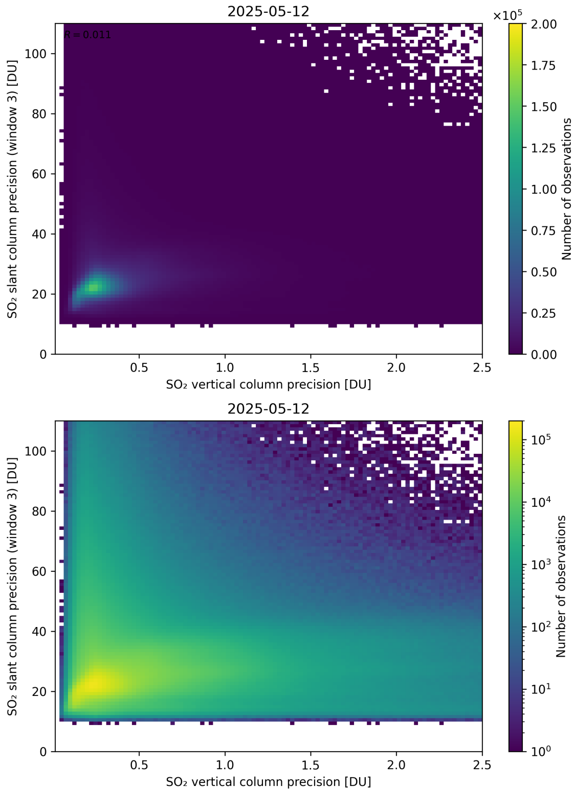
Figure 345: Scatter density plot of “SO 2 vertical column precision” against “SO 2 slant column precision (window 3)” for 2025-05-11 to 2025-05-13.
