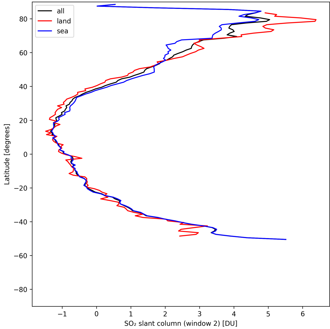
Figure 41: Zonal average of “SO 2 slant column (window 2)” for 2025-05-11 to 2025-05-13.
