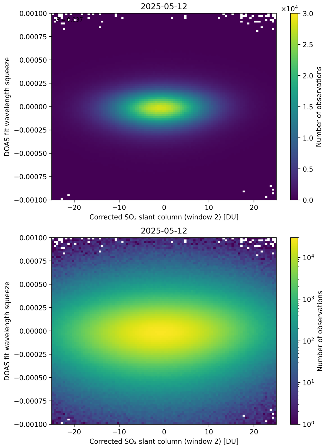
Figure 247: Scatter density plot of “Corrected SO 2 slant column (window 2)” against “DOAS fit wavelength squeeze” for 2025-05-11 to 2025-05-13.
