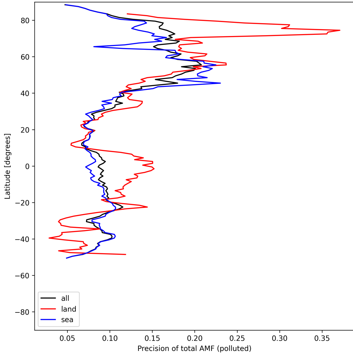
Figure 54: Zonal average of “Precision of total AMF (polluted)” for 2025-05-11 to 2025-05-13.
