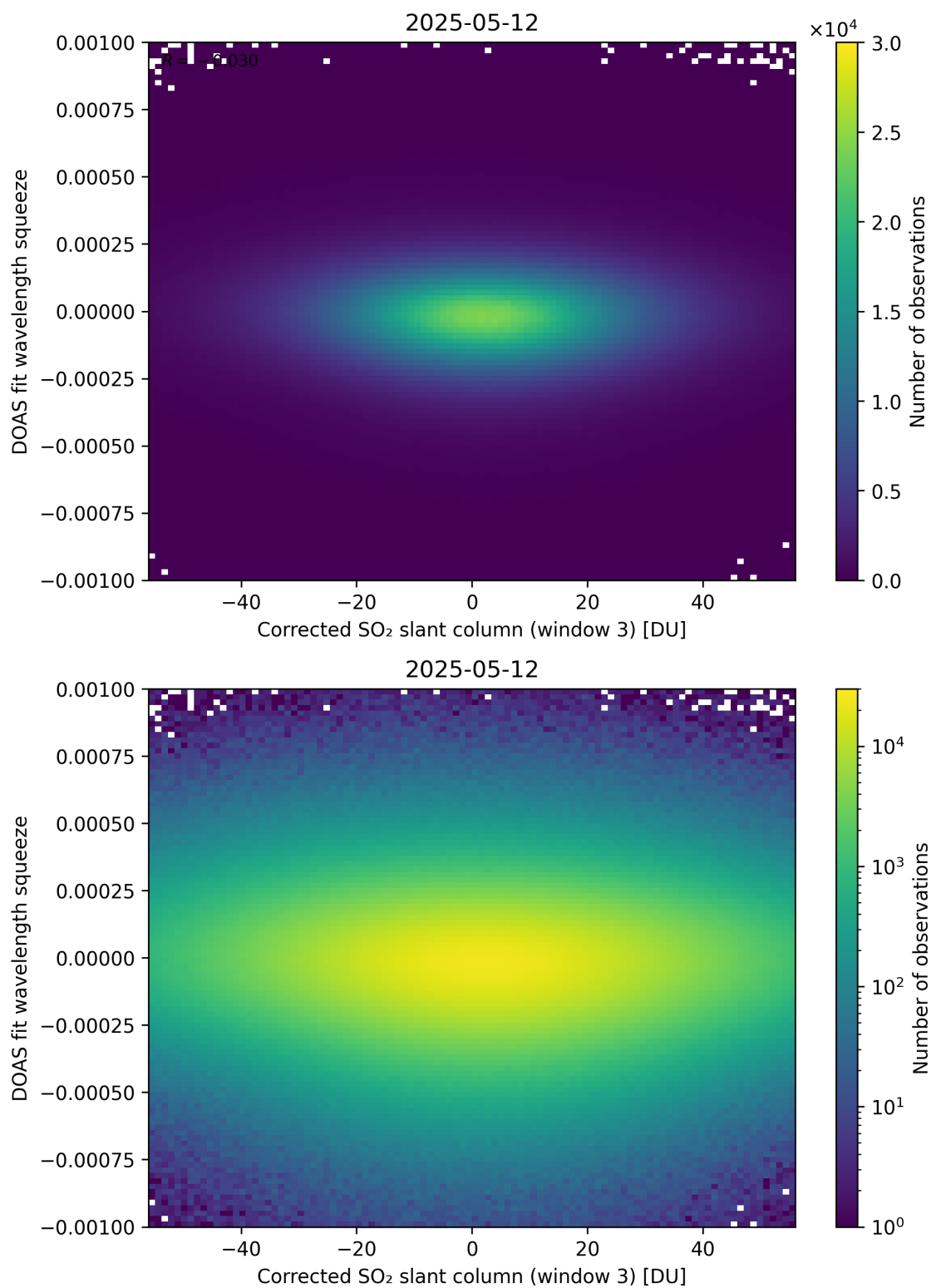
Figure 257: Scatter density plot of “Corrected SO 2 slant column (window 3)” against “DOAS fit wavelength squeeze” for 2025-05-11 to 2025-05-13.
