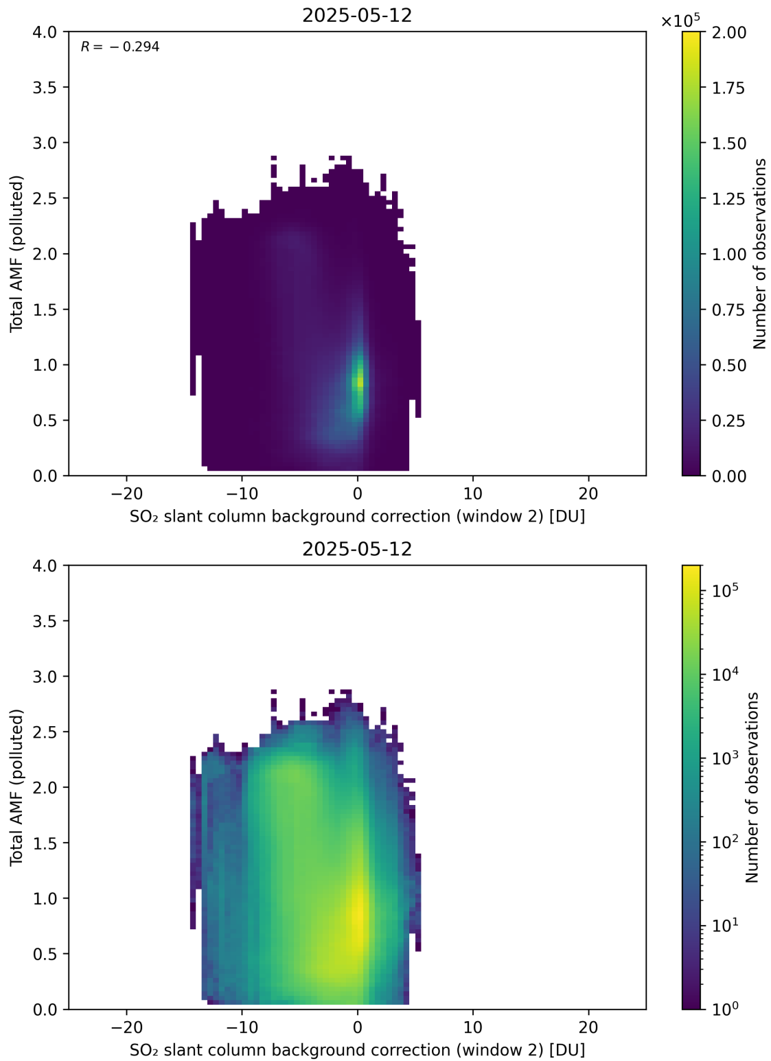
Figure 130: Scatter density plot of “SO 2 slant column background correction (window 2)” against “Total AMF (polluted)” for 2025-05-11 to 2025-05-13.
