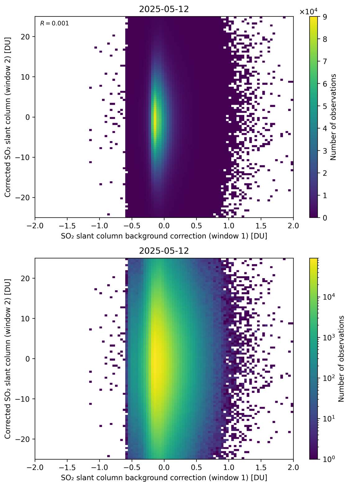
Figure 115: Scatter density plot of “SO 2 slant column background correction (window 1)” against “Corrected SO 2 slant column (window 2)” for 2025-05-11 to 2025-05-13.
