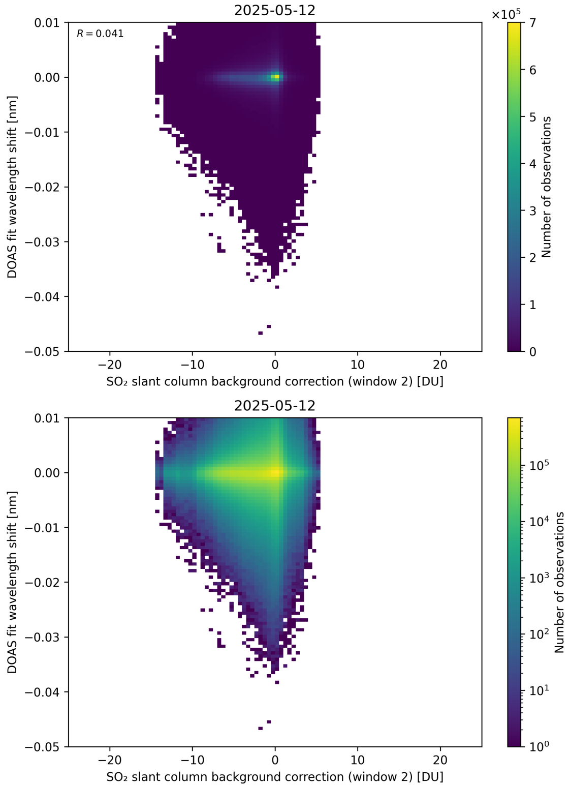
Figure 123: Scatter density plot of “SO 2 slant column background correction (window 2)” against “DOAS fit wavelength shift” for 2025-05-11 to 2025-05-13.
