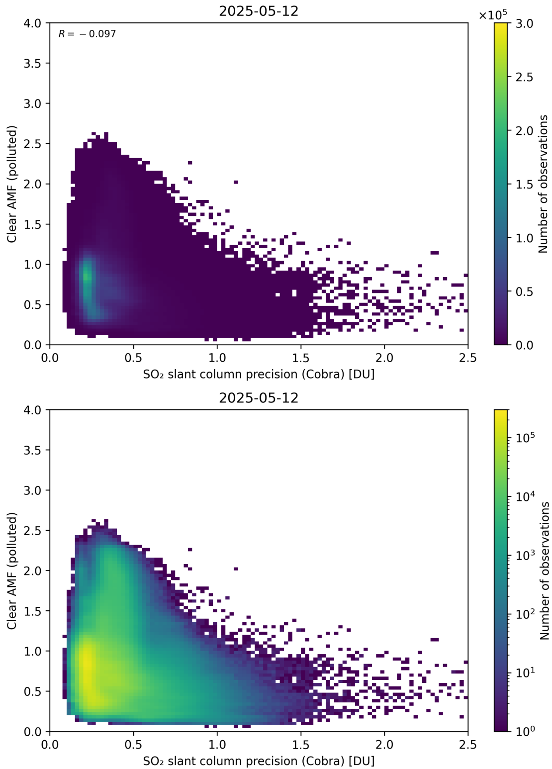
Figure 205: Scatter density plot of “SO 2 slant column precision (Cobra)” against “Clear AMF (polluted)” for 2025-05-11 to 2025-05-13.
