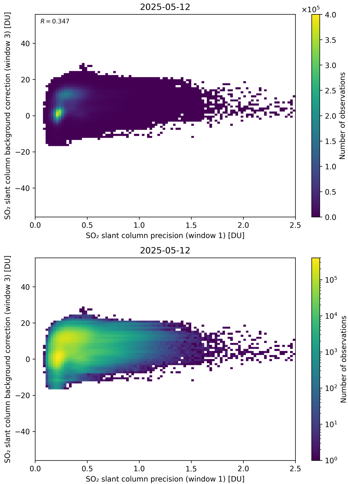
Figure 270: Scatter density plot of “SO 2 slant column precision (window 1)” against “SO 2 slant column background correction (window 3)” for 2025-05-11 to 2025-05-13.
