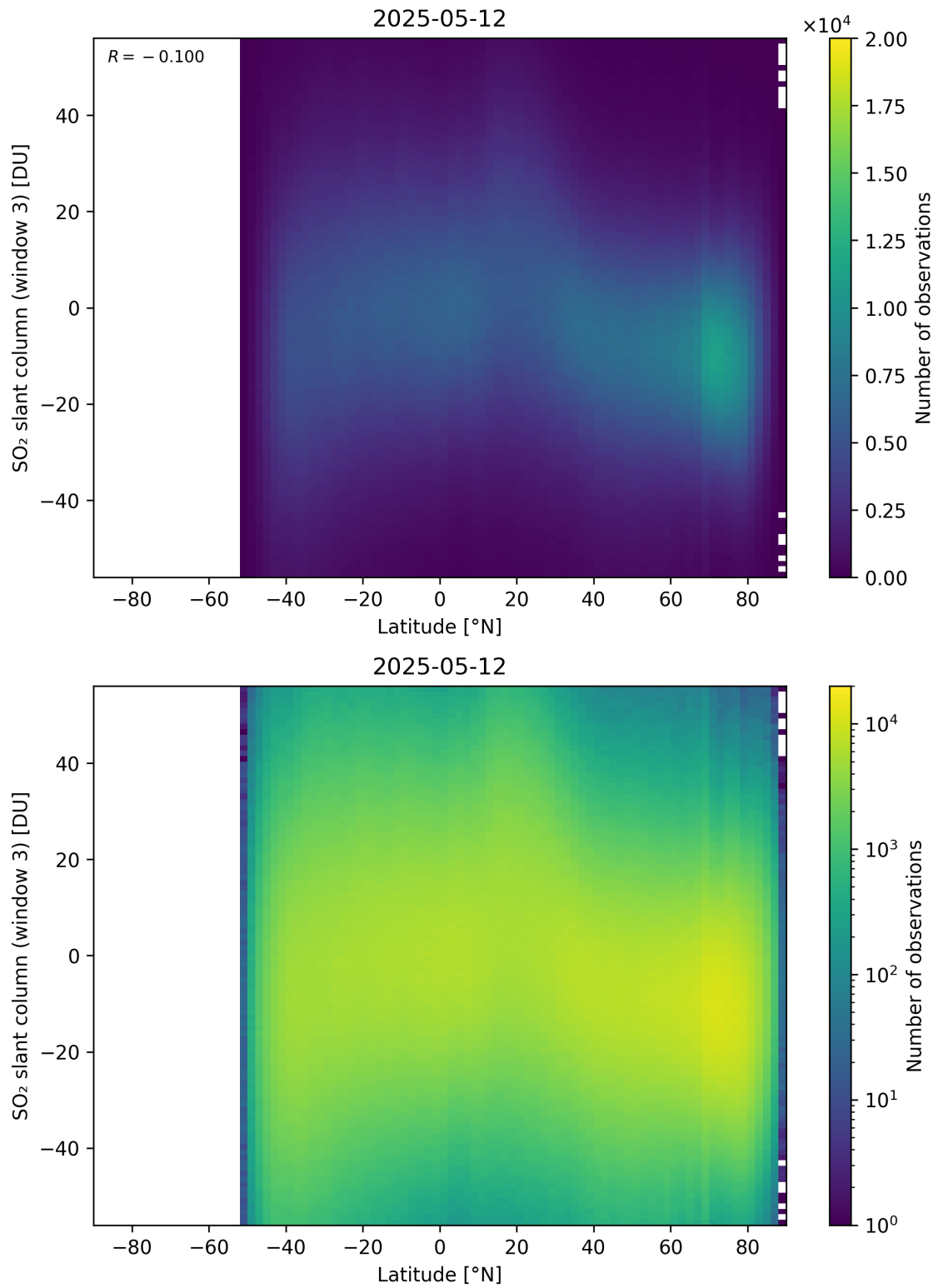
Figure 165: Scatter density plot of “Latitude” against “SO 2 slant column (window 3)” for 2025-05-11 to 2025-05-13.
