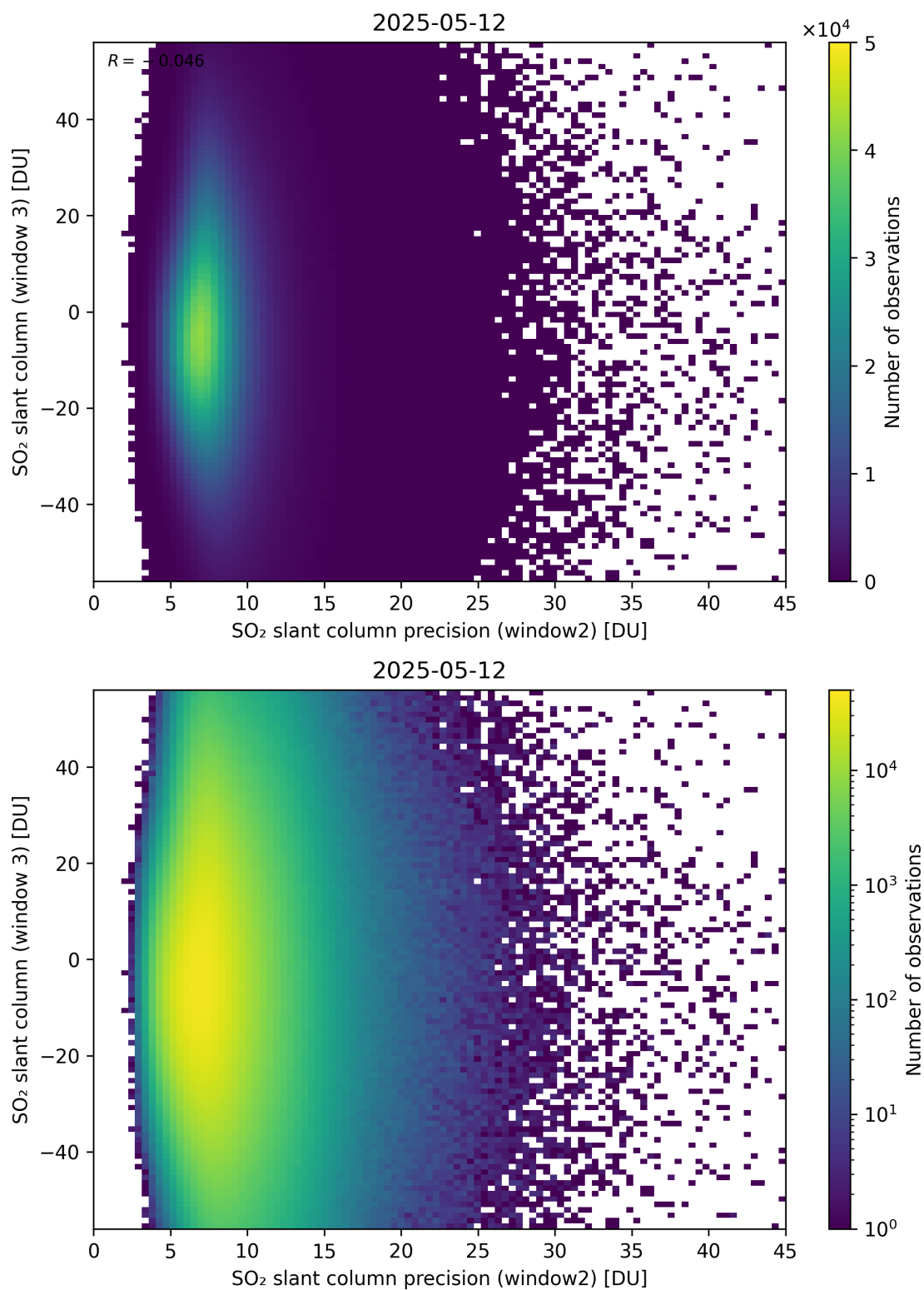
Figure 299: Scatter density plot of “SO 2 slant column precision (window2)” against “SO 2 slant column (window 3)” for 2025-05-11 to 2025-05-13.
