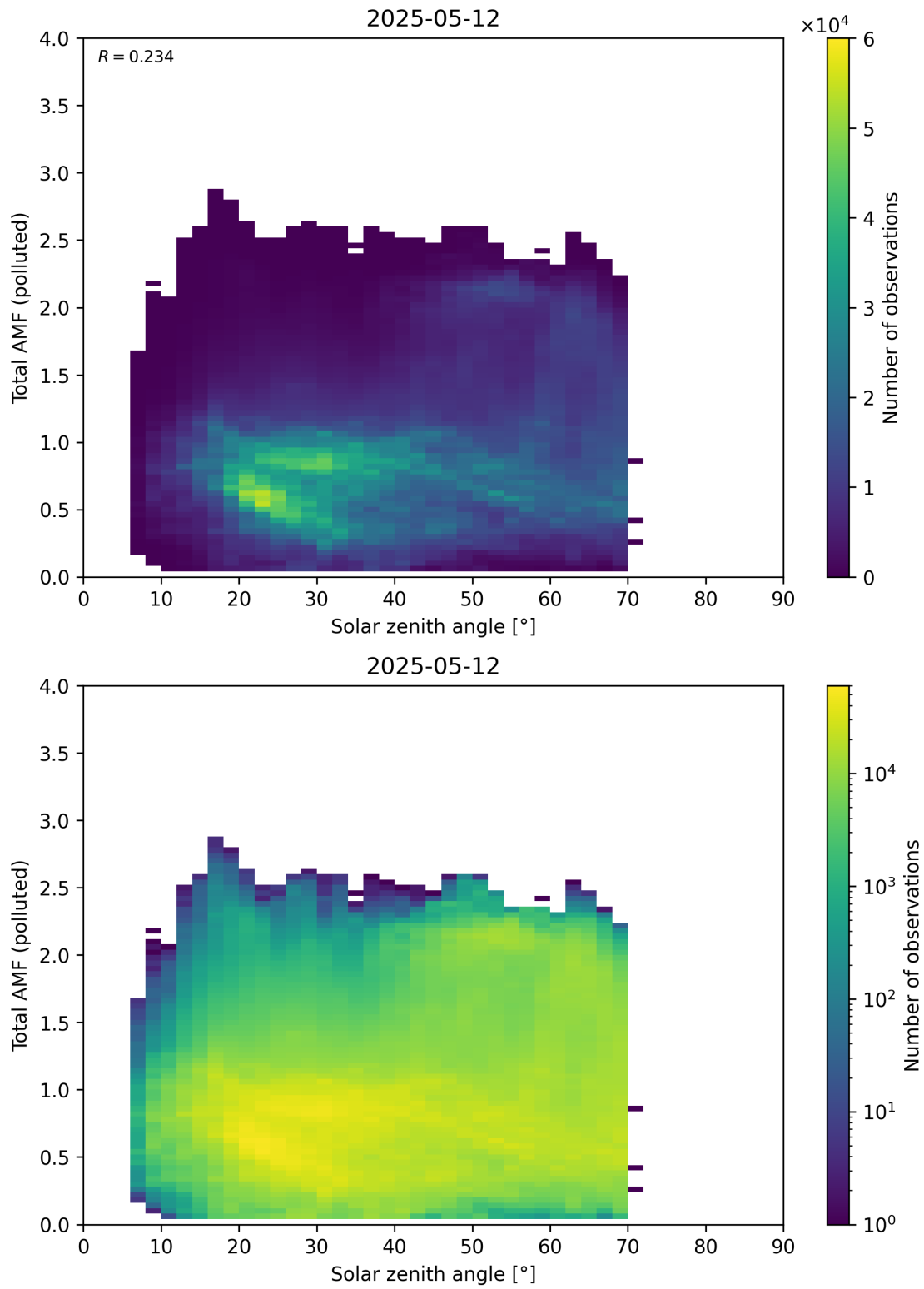
Figure 189: Scatter density plot of “Solar zenith angle” against “Total AMF (polluted)” for 2025-05-11 to 2025-05-13.
