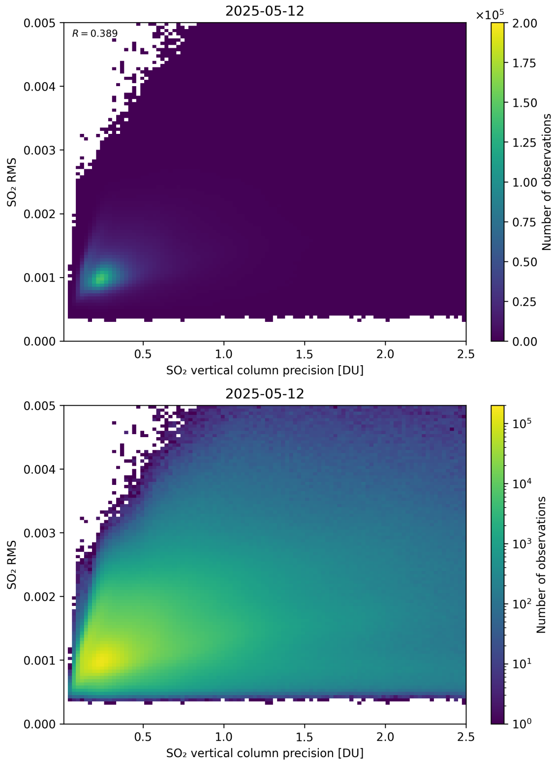
Figure 334: Scatter density plot of “SO 2 vertical column precision” against “SO 2 RMS” for 2025-05-11 to 2025-05-13.
