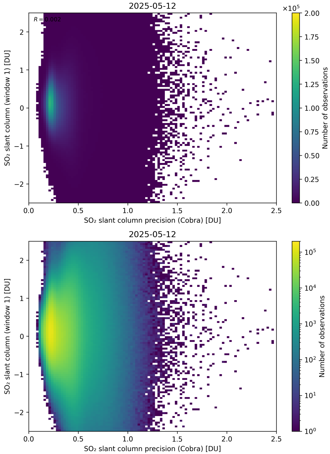
Figure 208: Scatter density plot of “SO 2 slant column precision (Cobra)” against “SO 2 slant column (window 1)” for 2025-05-11 to 2025-05-13.
