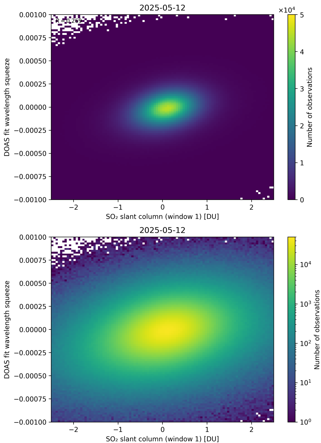
Figure 266: Scatter density plot of “SO 2 slant column (window 1)” against “DOAS fit wavelength squeeze” for 2025-05-11 to 2025-05-13.
