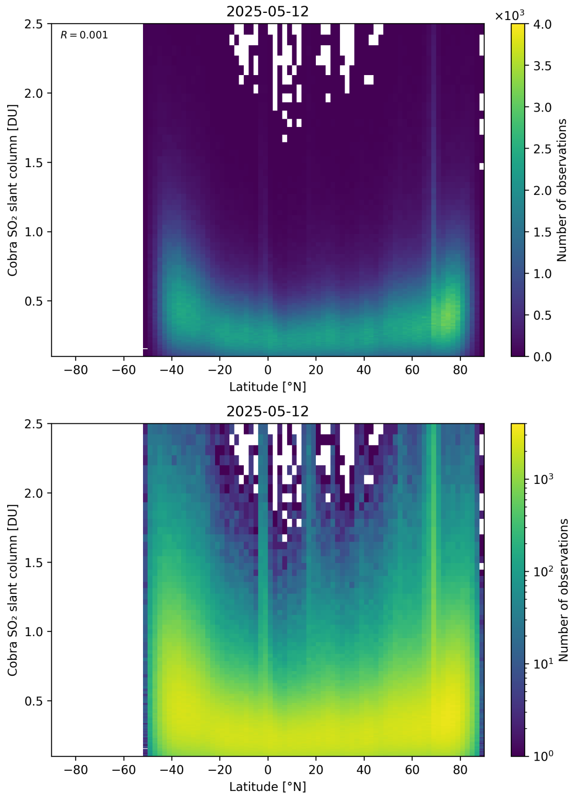
Figure 157: Scatter density plot of “Latitude” against “Cobra SO 2 slant column” for 2025-05-11 to 2025-05-13.
