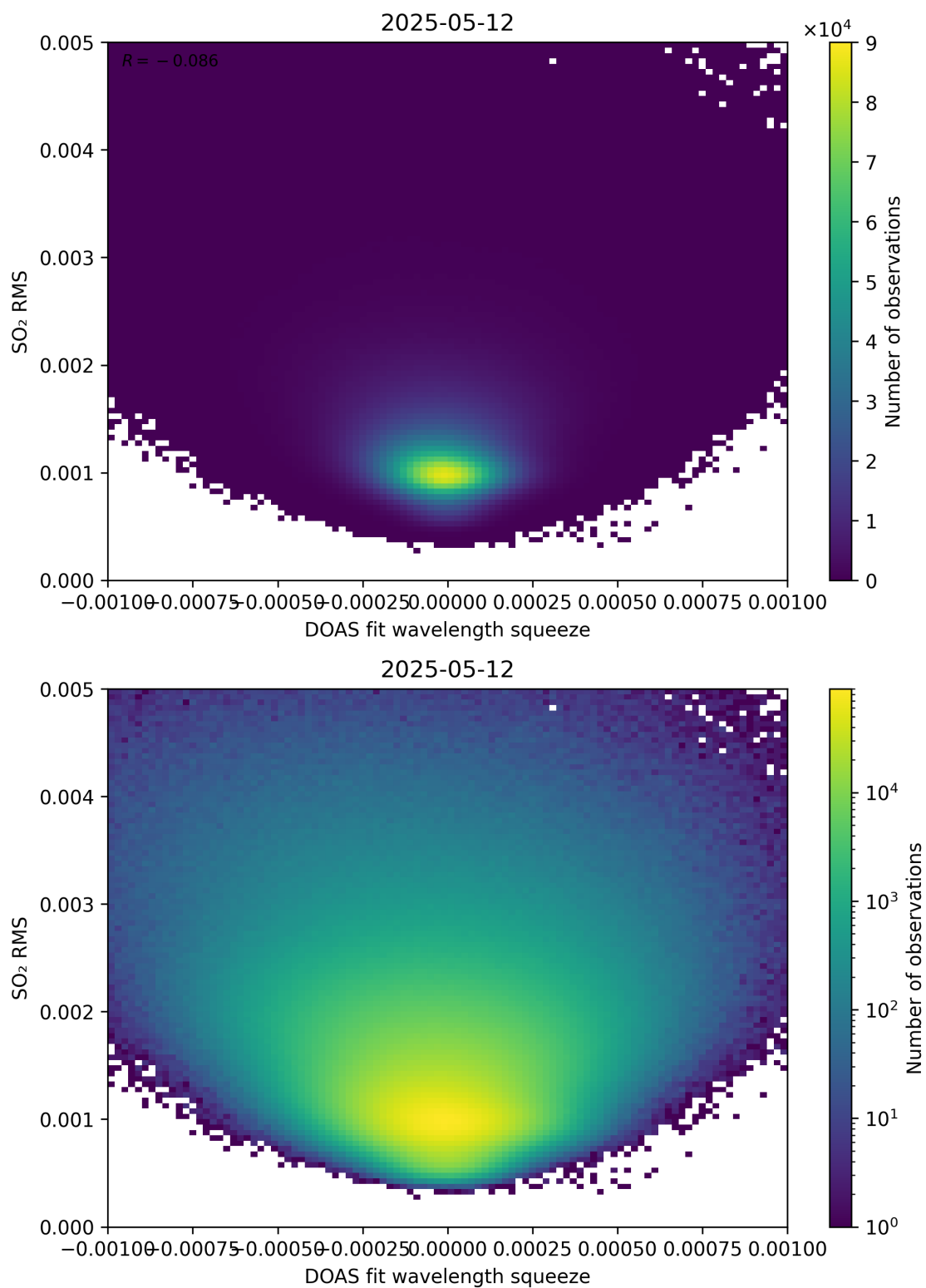
Figure 143: Scatter density plot of “DOAS fit wavelength squeeze” against “SO 2 RMS” for 2025-05-11 to 2025-05-13.
