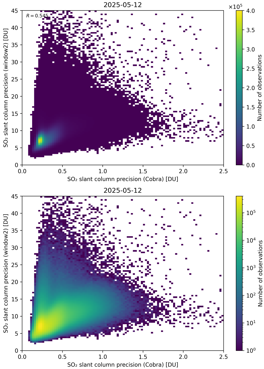
Figure 210: Scatter density plot of “SO 2 slant column precision (Cobra)” against “SO 2 slant column precision (window2)” for 2025-05-11 to 2025-05-13.
