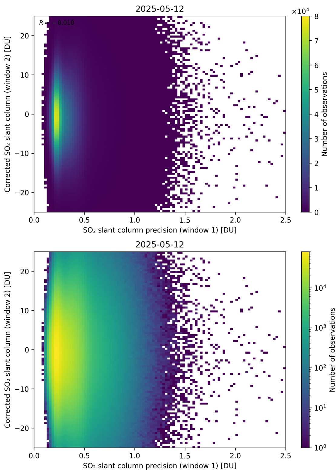
Figure 275: Scatter density plot of “SO 2 slant column precision (window 1)” against “Corrected SO 2 slant column (window 2)” for 2025-05-11 to 2025-05-13.
