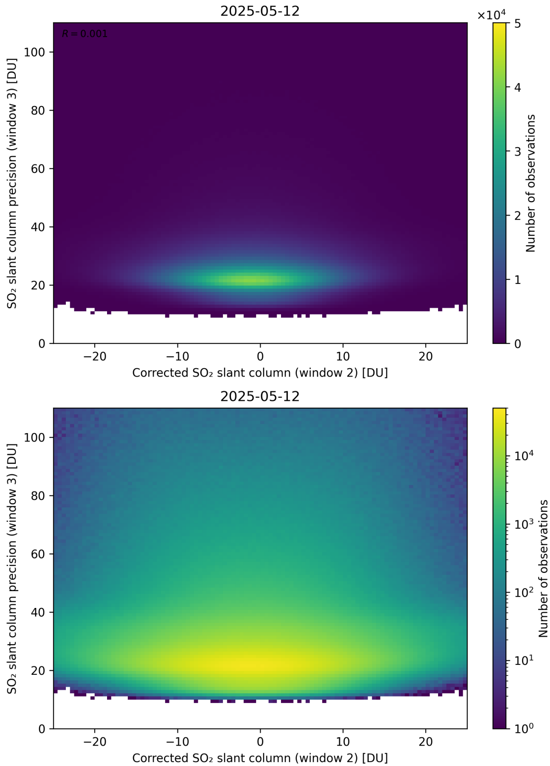
Figure 252: Scatter density plot of “Corrected SO 2 slant column (window 2)” against “SO 2 slant column precision (window 3)” for 2025-05-11 to 2025-05-13.
