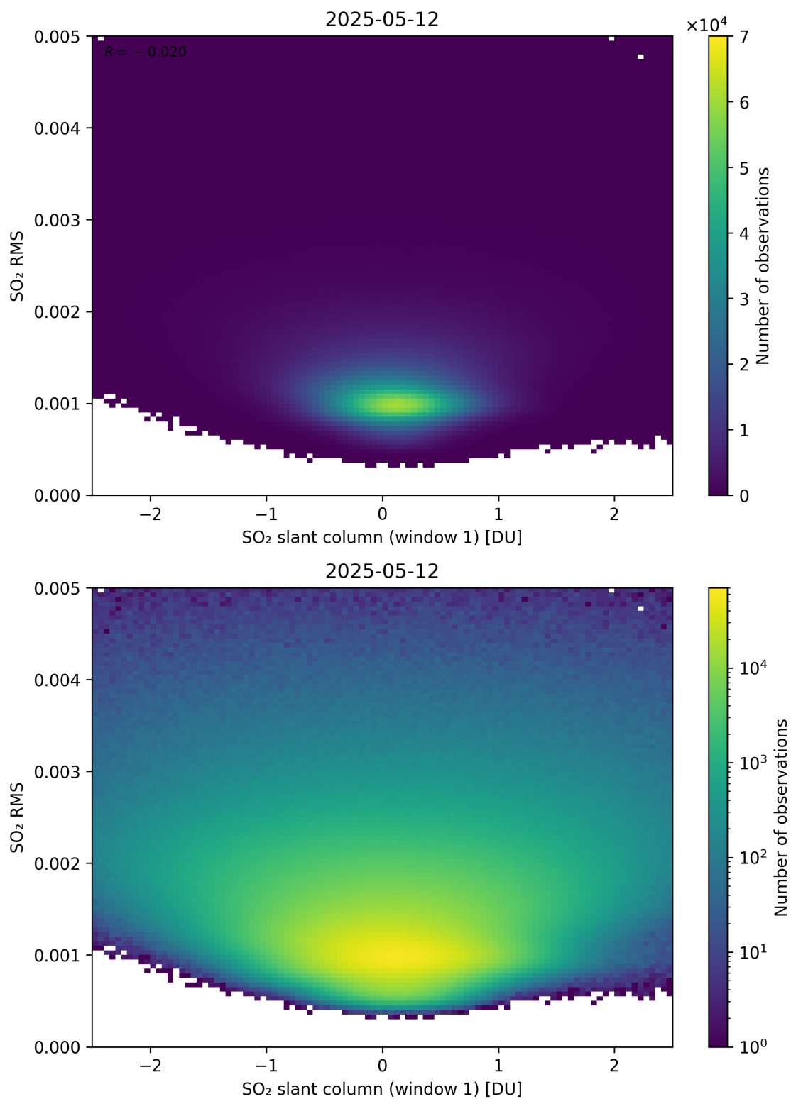
Figure 267: Scatter density plot of “SO 2 slant column (window 1)” against “SO 2 RMS” for 2025-05-11 to 2025-05-13.
