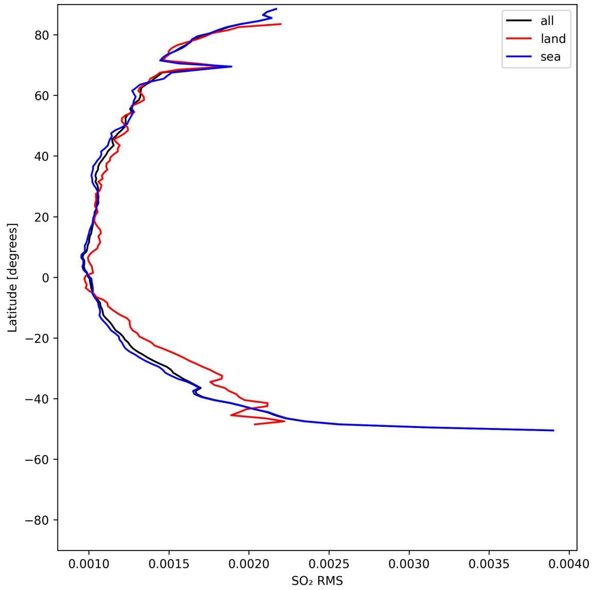
Figure 52: Zonal average of “SO 2 RMS” for 2025-05-11 to 2025-05-13.
