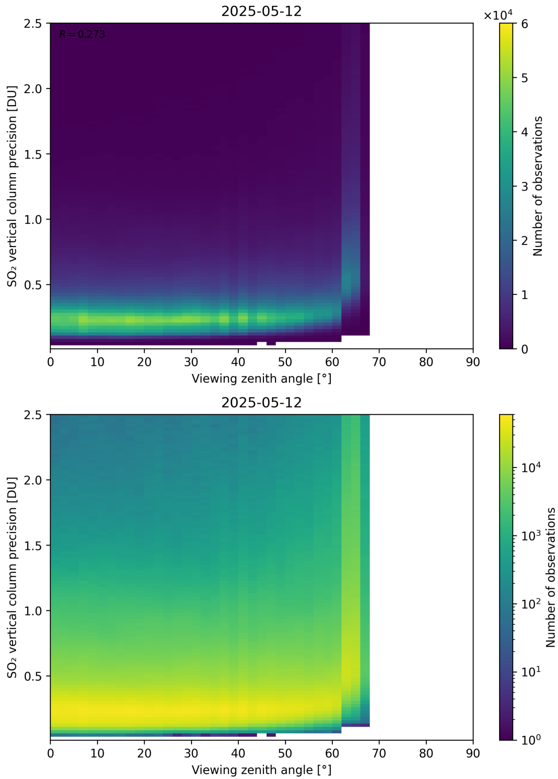
Figure 384: Scatter density plot of “Viewing zenith angle” against “SO 2 vertical column precision” for 2025-05-11 to 2025-05-13.
