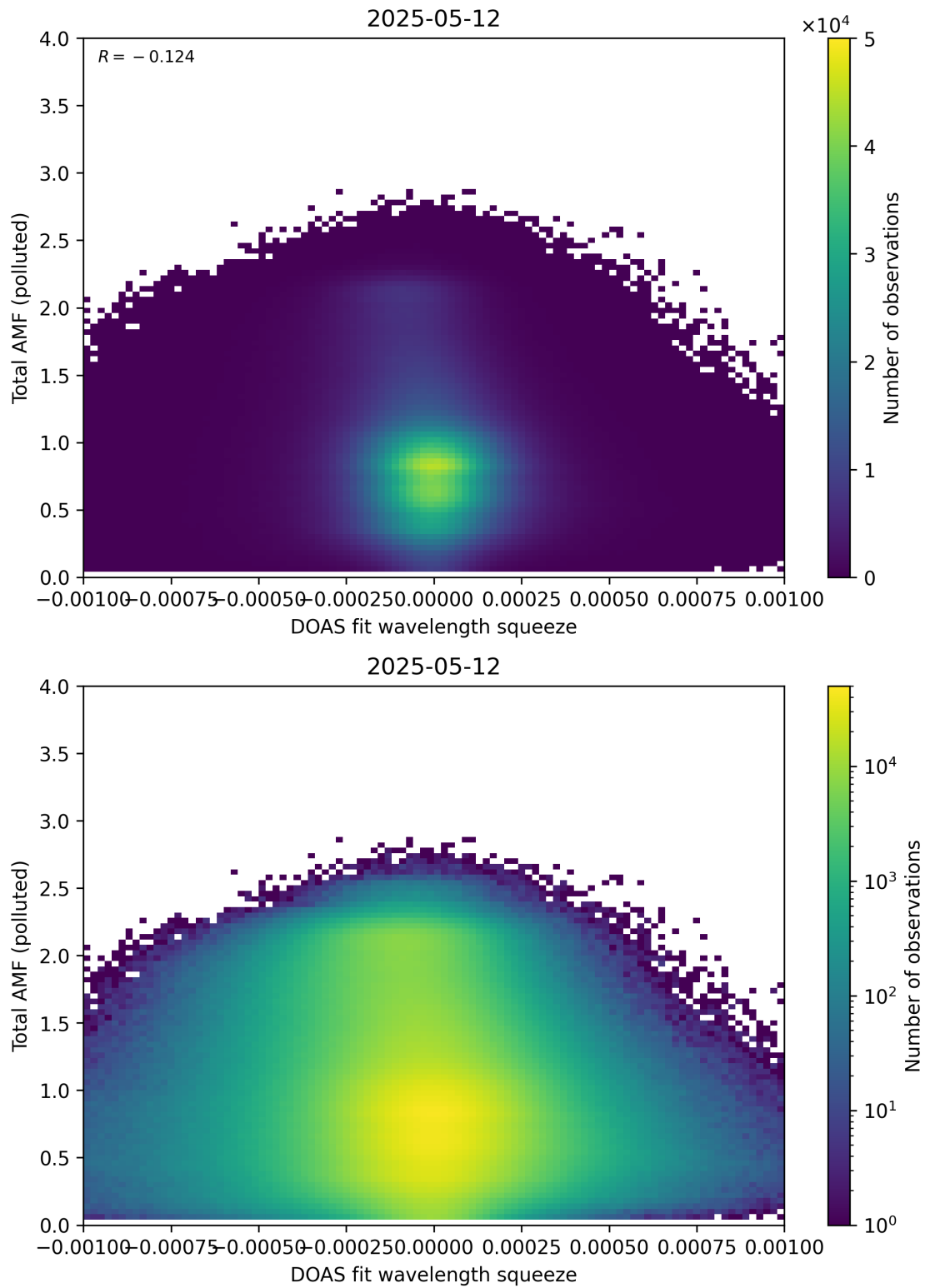
Figure 145: Scatter density plot of “DOAS fit wavelength squeeze” against “Total AMF (polluted)” for 2025-05-11 to 2025-05-13.
