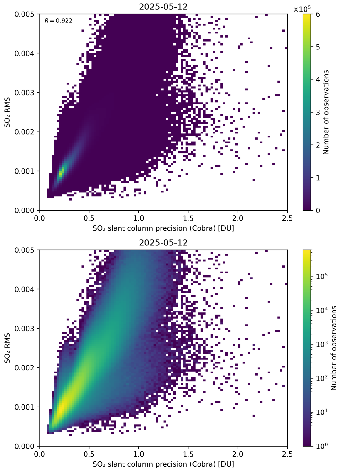
Figure 204: Scatter density plot of “SO 2 slant column precision (Cobra)” against “SO 2 RMS” for 2025-05-11 to 2025-05-13.
