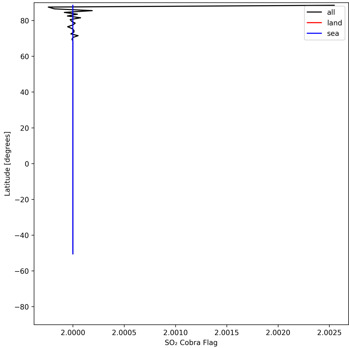
Figure 49: Zonal average of “SO 2 Cobra Flag” for 2025-05-11 to 2025-05-13.
