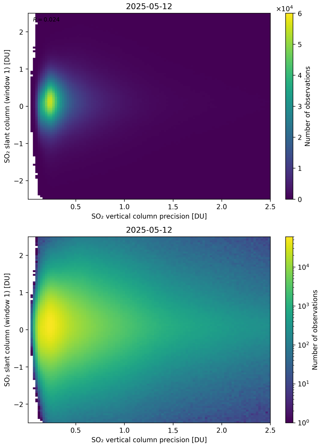
Figure 341: Scatter density plot of “SO 2 vertical column precision” against “SO 2 slant column (window 1)” for 2025-05-11 to 2025-05-13.
