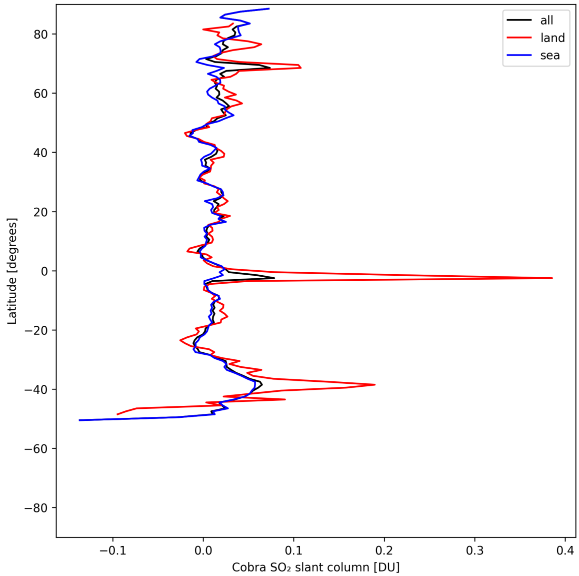
Figure 35: Zonal average of “Cobra SO 2 slant column” for 2025-05-11 to 2025-05-13.
