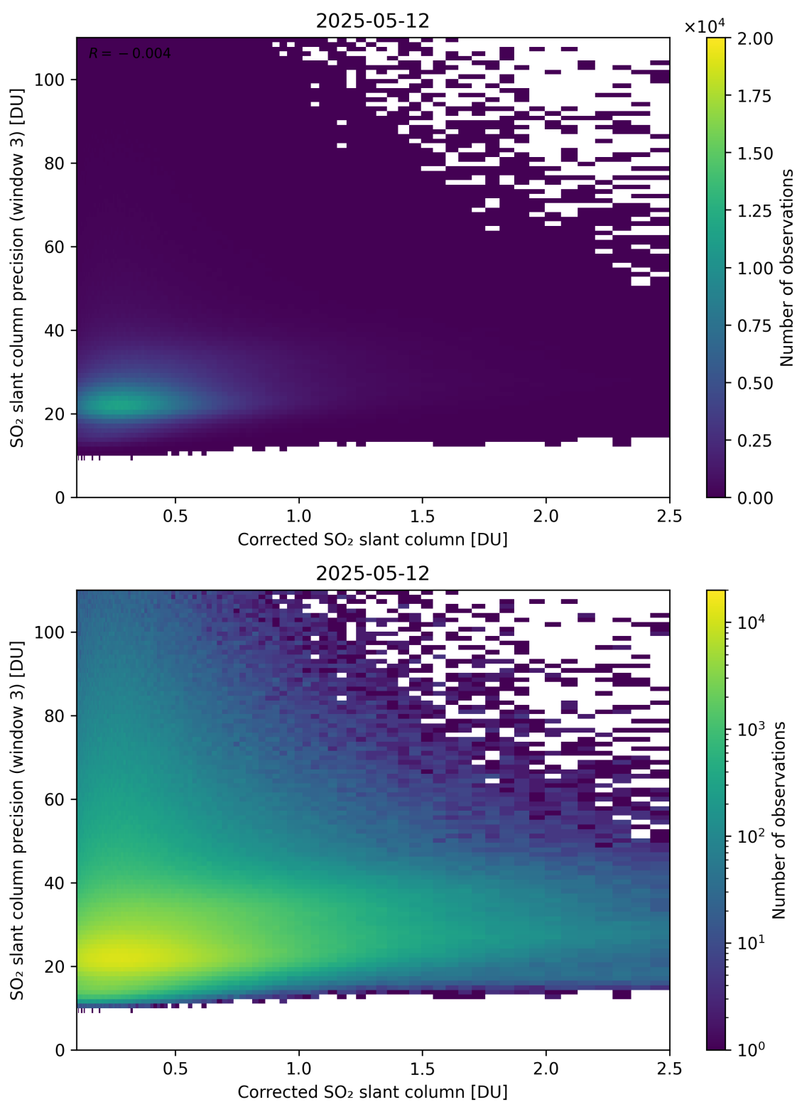
Figure 241: Scatter density plot of “Corrected SO 2 slant column” against “SO 2 slant column precision (window 3)” for 2025-05-11 to 2025-05-13.
