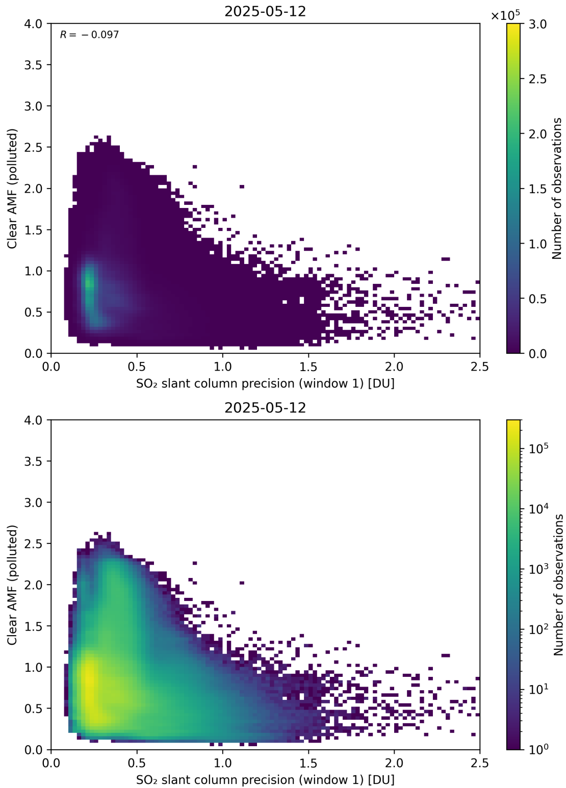
Figure 274: Scatter density plot of “SO 2 slant column precision (window 1)” against “Clear AMF (polluted)” for 2025-05-11 to 2025-05-13.
