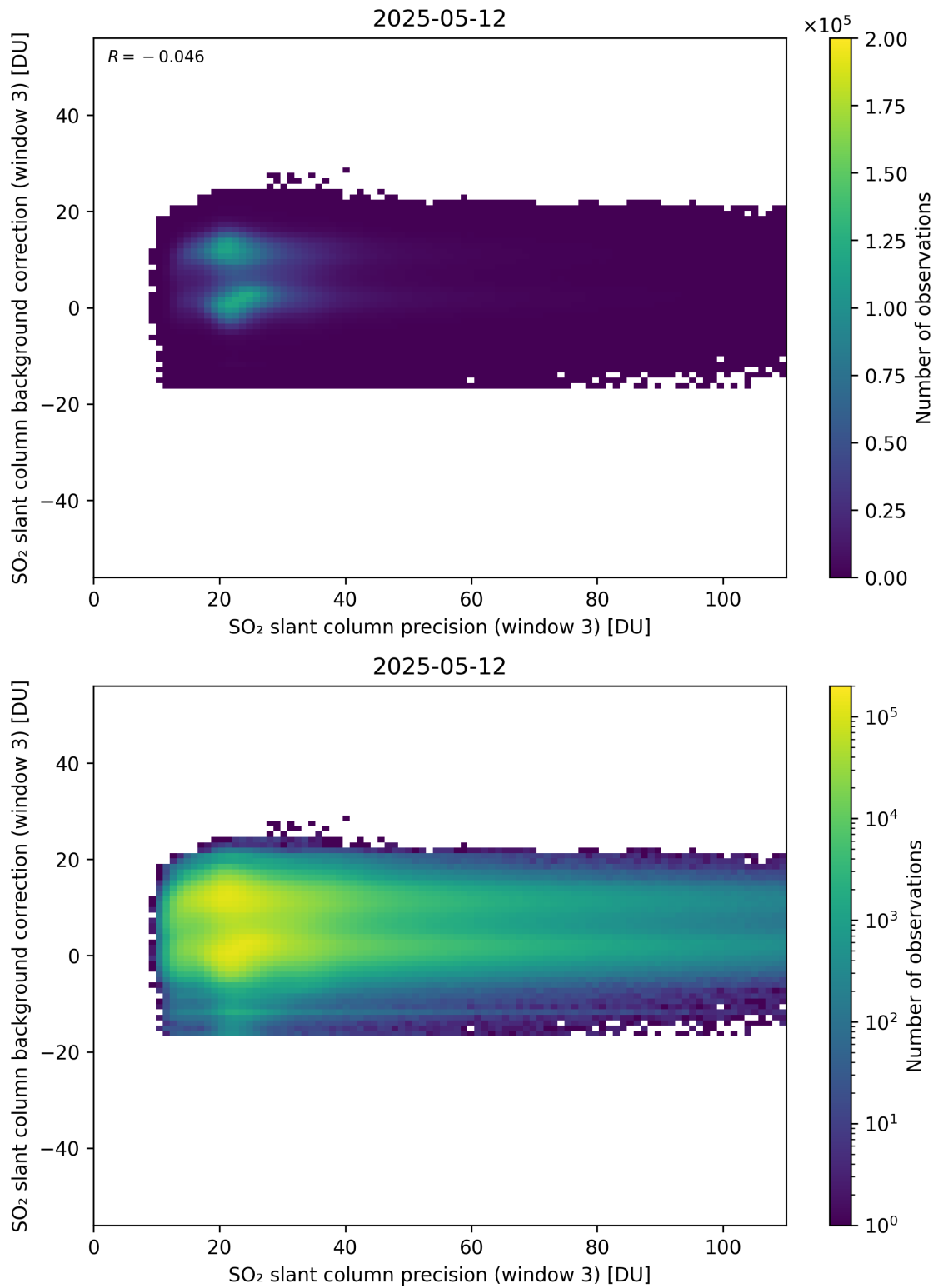
Figure 307: Scatter density plot of “SO 2 slant column precision (window 3)” against “SO 2 slant column background correction (window 3)” for 2025-05-11 to 2025-05-13.
