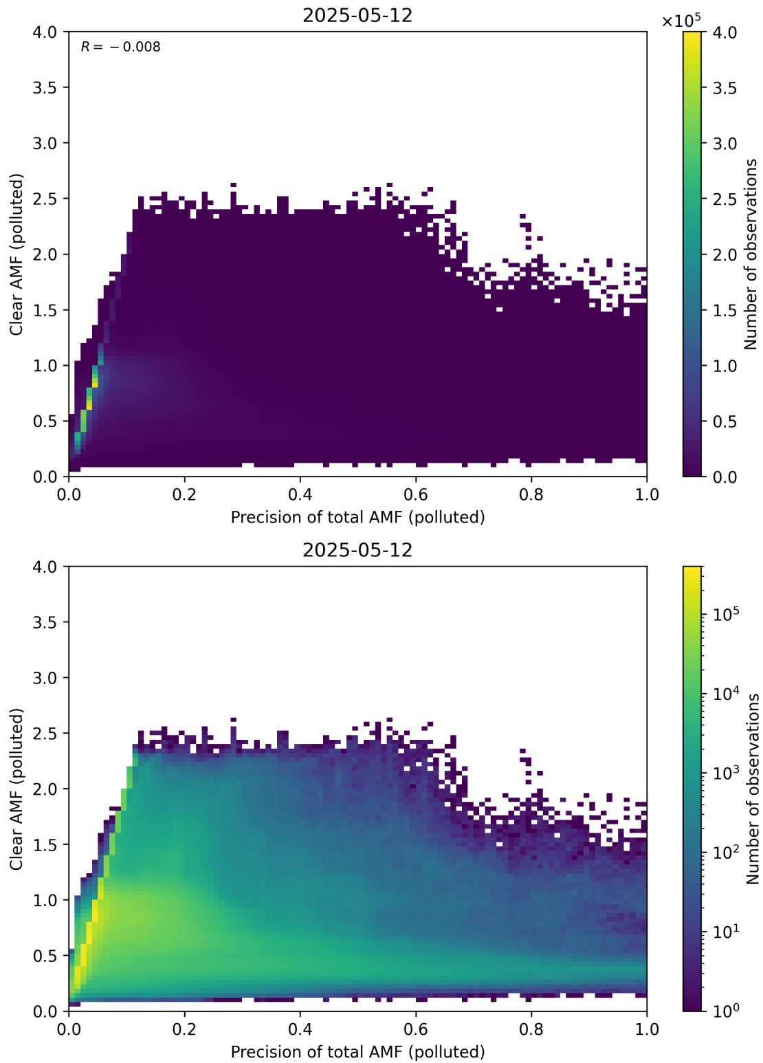
Figure 320: Scatter density plot of “Precision of total AMF (polluted)” against “Clear AMF (polluted)” for 2025-05-11 to 2025-05-13.
