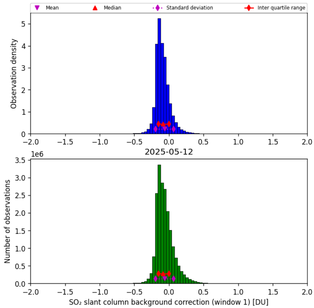
Figure 66: Histogram of “SO 2 slant column background correction (window 1)” for 2025-05-11 to 2025-05-13
