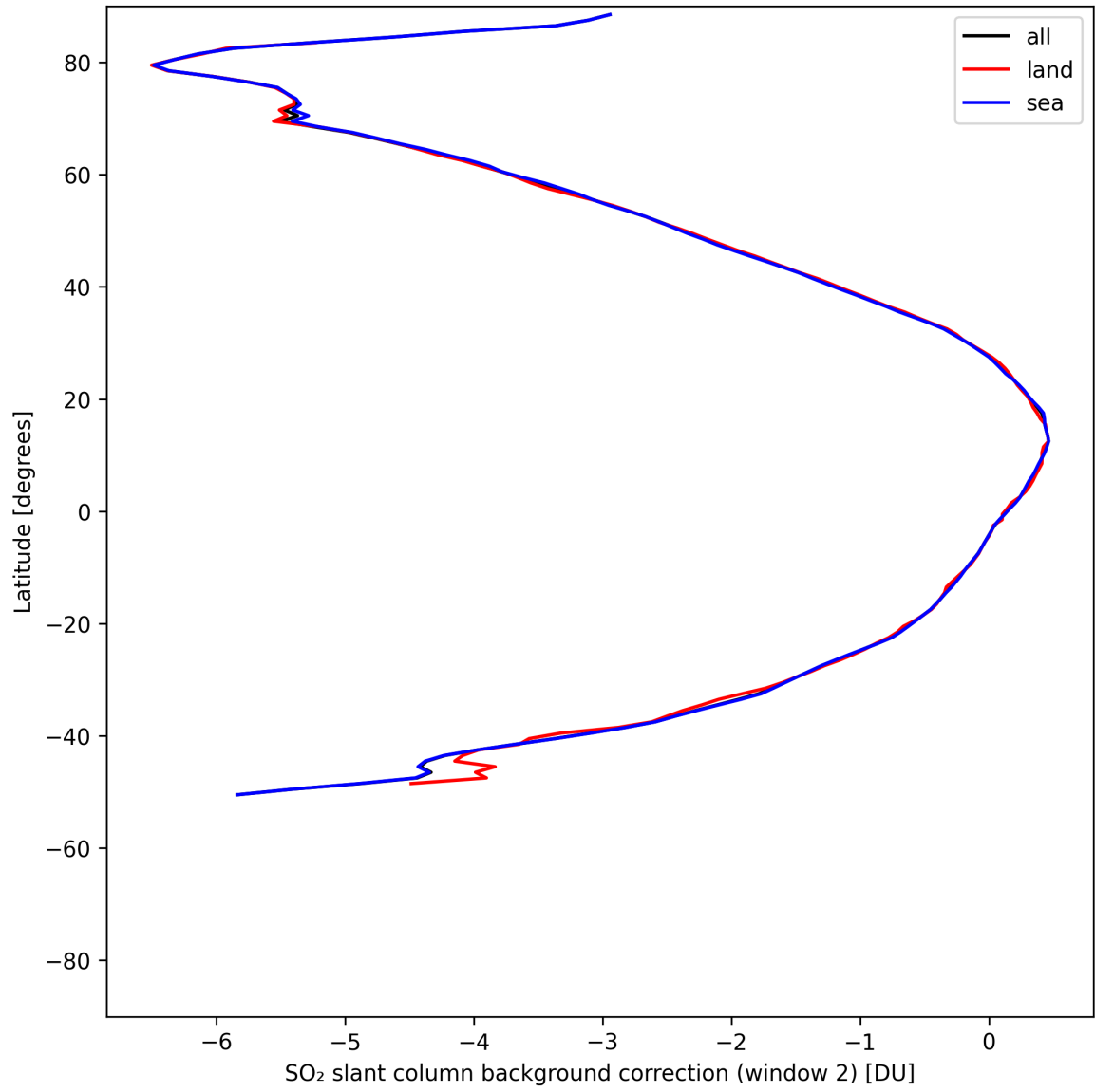
Figure 44: Zonal average of “SO 2 slant column background correction (window 2)” for 2025-05-11 to 2025-05-13.
