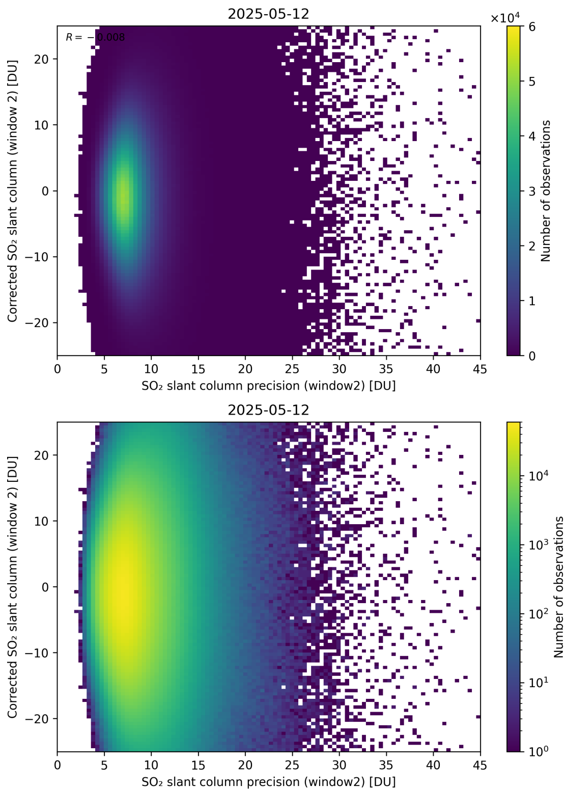
Figure 297: Scatter density plot of “SO 2 slant column precision (window2)” against “Corrected SO 2 slant column (window 2)” for 2025-05-11 to 2025-05-13.
