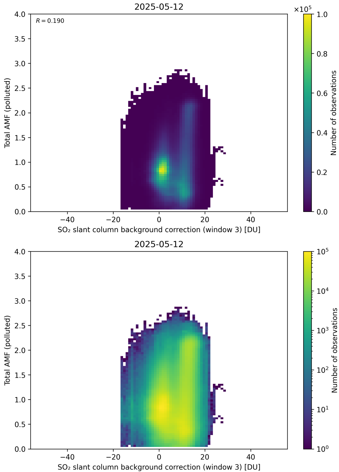
Figure 136: Scatter density plot of “SO 2 slant column background correction (window 3)” against “Total AMF (polluted)” for 2025-05-11 to 2025-05-13.
