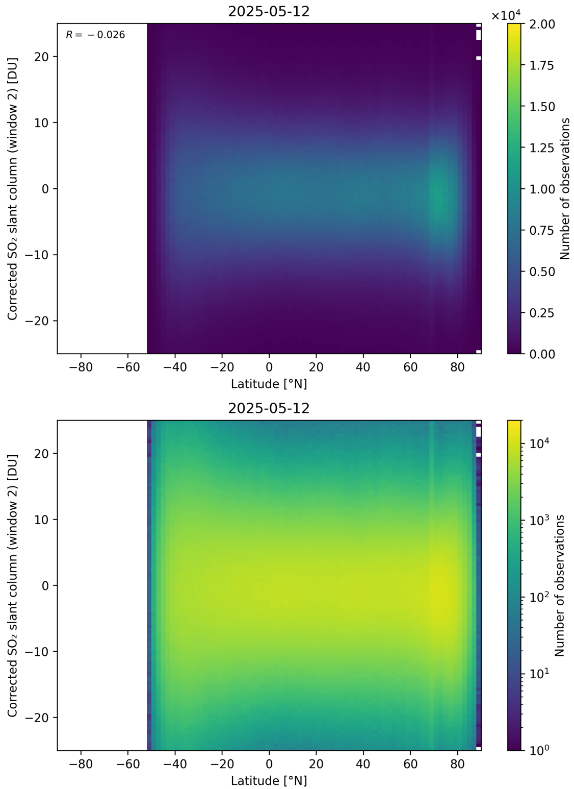
Figure 160: Scatter density plot of “Latitude” against “Corrected SO 2 slant column (window 2)” for 2025-05-11 to 2025-05-13.
