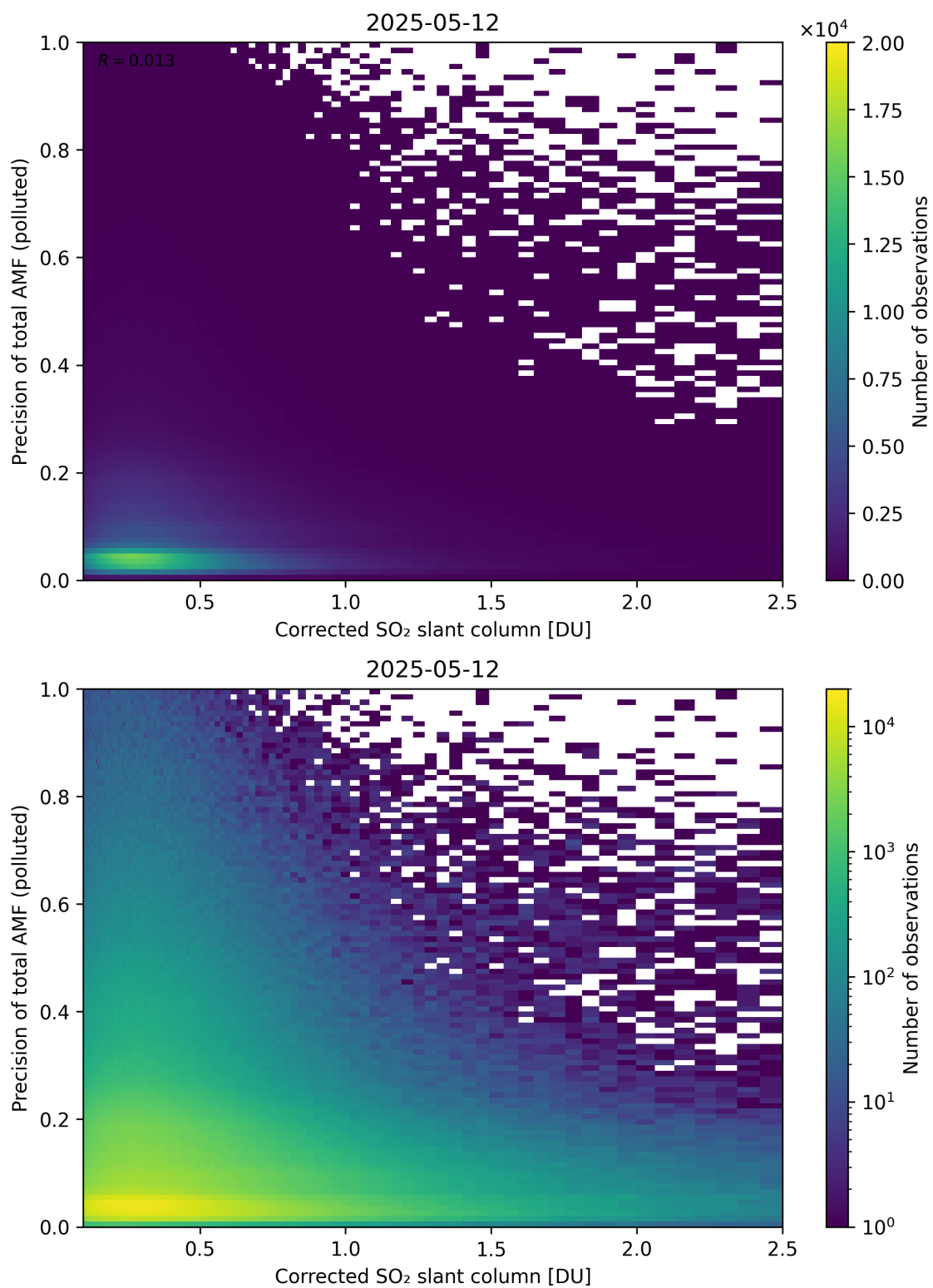
Figure 243: Scatter density plot of “Corrected SO 2 slant column” against “Precision of total AMF (polluted)” for 2025-05-11 to 2025-05-13.
