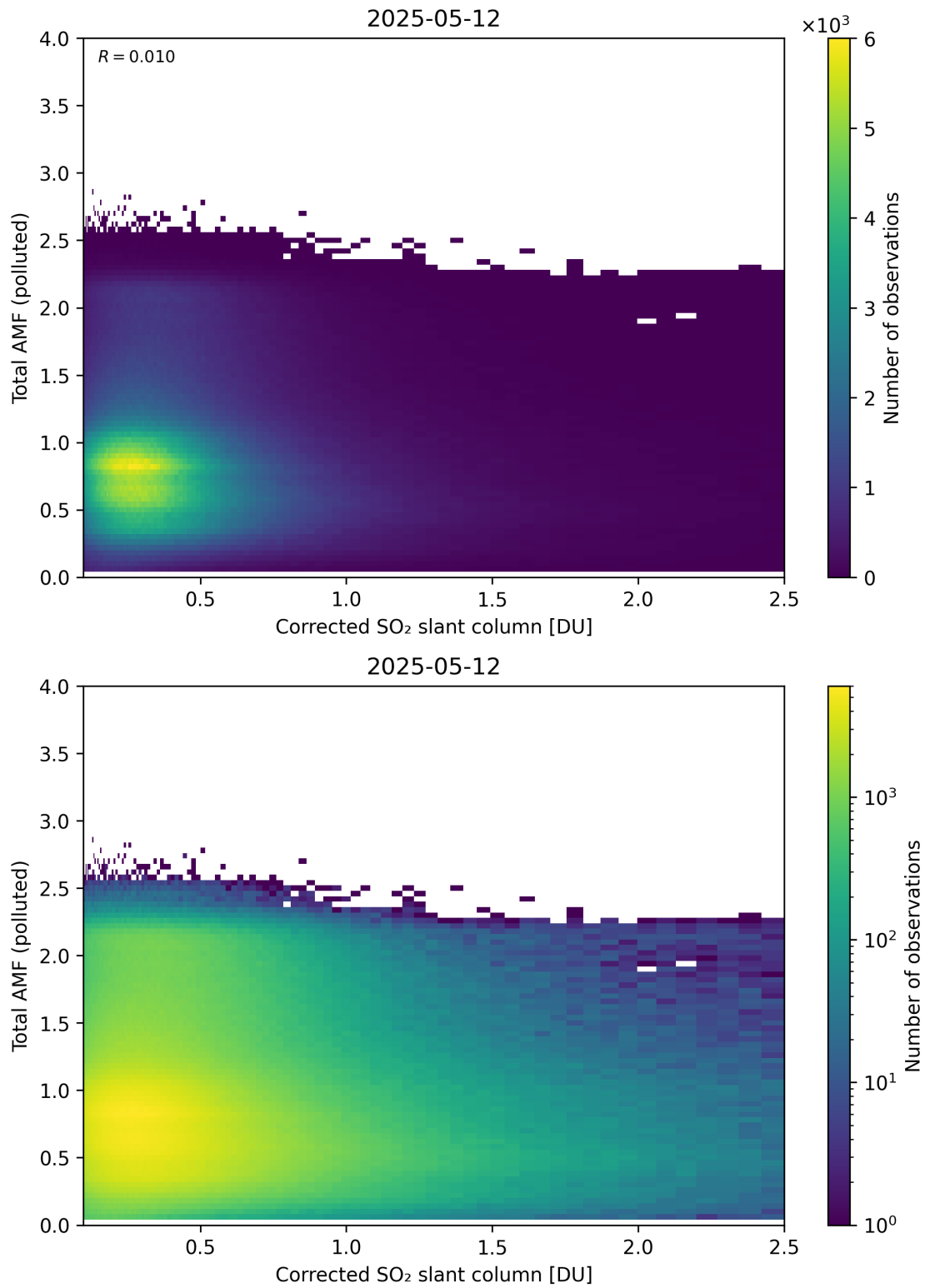
Figure 242: Scatter density plot of “Corrected SO 2 slant column” against “Total AMF (polluted)” for 2025-05-11 to 2025-05-13.
