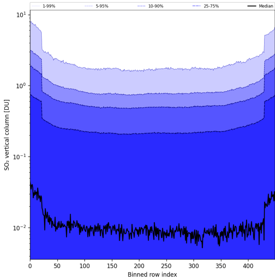
Figure 84: Along track statistics of “SO 2 vertical column” for 2025-05-11 to 2025-05-13
