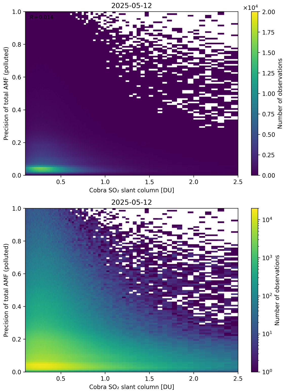
Figure 225: Scatter density plot of “Cobra SO 2 slant column” against “Precision of total AMF (polluted)” for 2025-05-11 to 2025-05-13.
