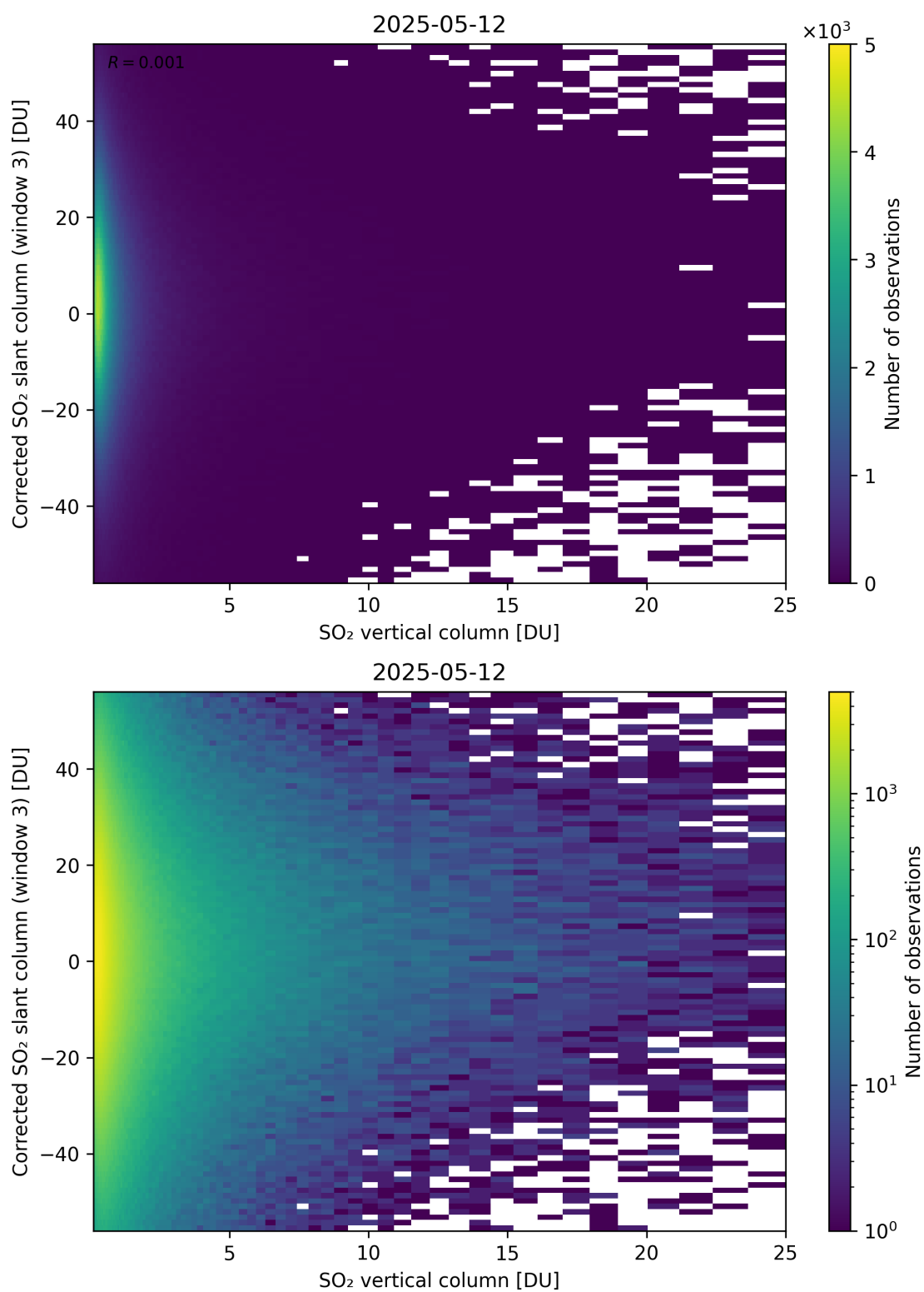
Figure 353: Scatter density plot of “SO 2 vertical column” against “Corrected SO 2 slant column (window 3)” for 2025-05-11 to 2025-05-13.
