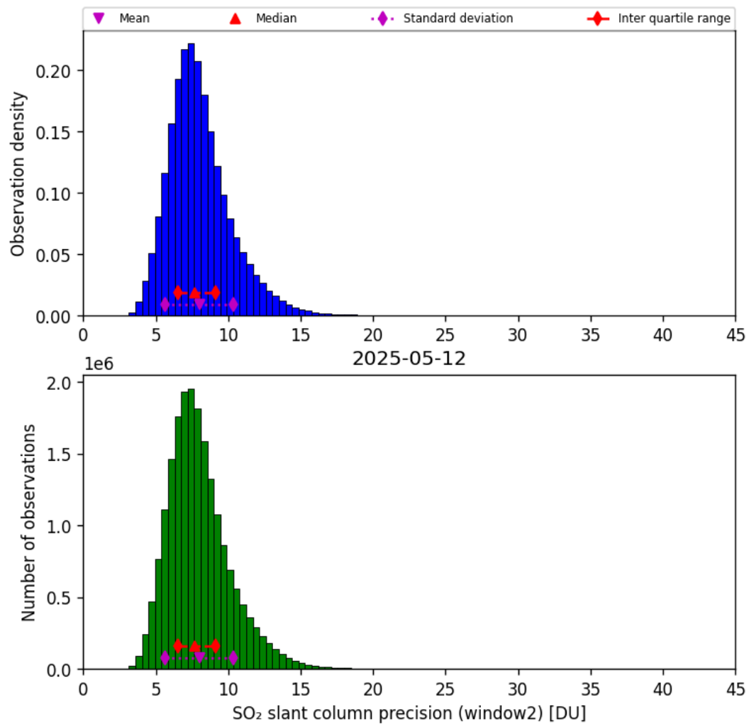
Figure 68: Histogram of “SO 2 slant column precision (window2)” for 2025-05-11 to 2025-05-13
