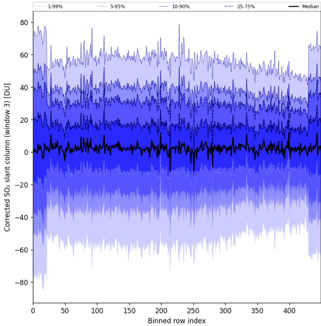
Figure 99: Along track statistics of “Corrected SO 2 slant column (window 3)” for 2025-05-11 to 2025-05-13
