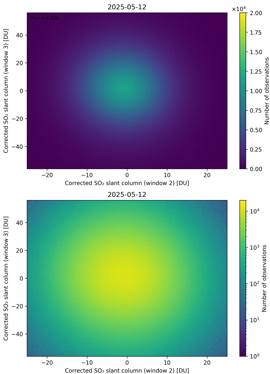
Figure 250: Scatter density plot of “Corrected SO 2 slant column (window 2)” against “Corrected SO 2 slant column (window 3)” for 2025-05-11 to 2025-05-13.
