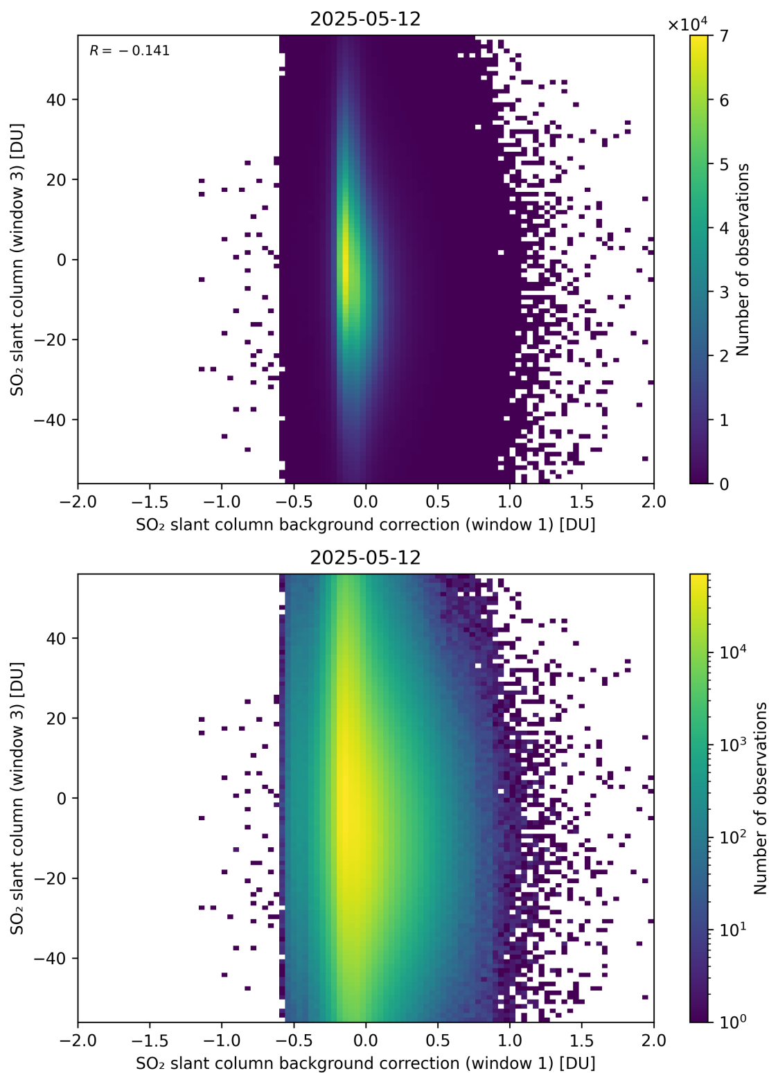
Figure 118: Scatter density plot of “SO 2 slant column background correction (window 1)” against “SO 2 slant column (window 3)” for 2025-05-11 to 2025-05-13.
