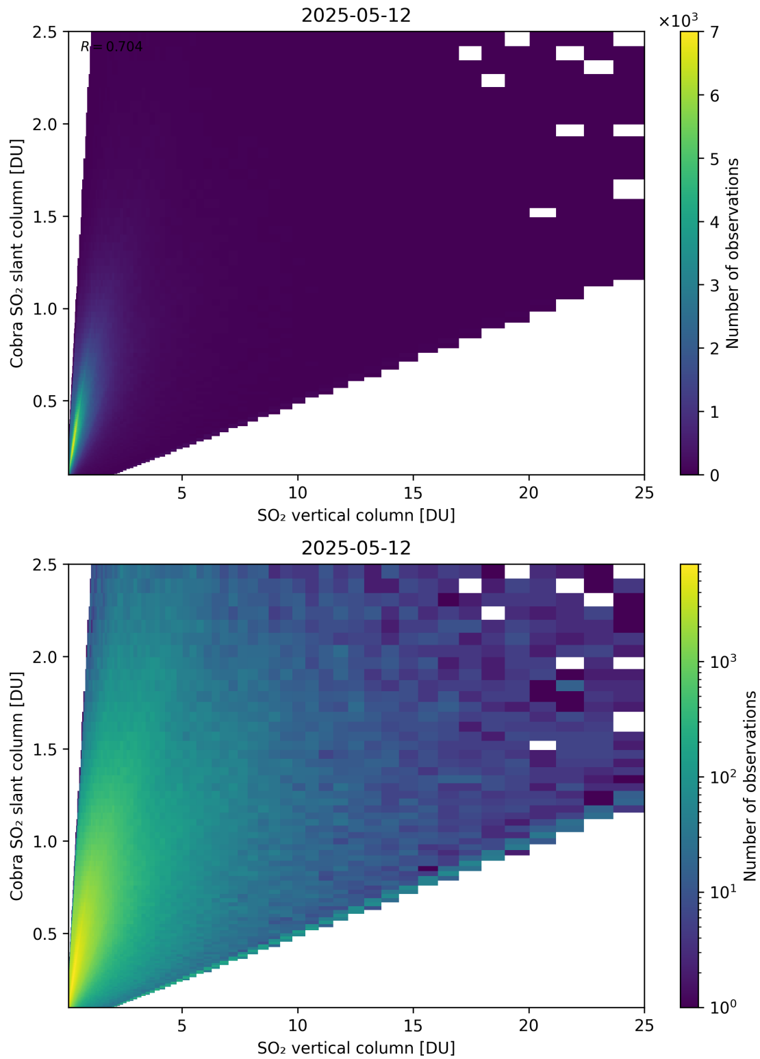
Figure 349: Scatter density plot of “SO 2 vertical column” against “Cobra SO 2 slant column” for 2025-05-11 to 2025-05-13.
