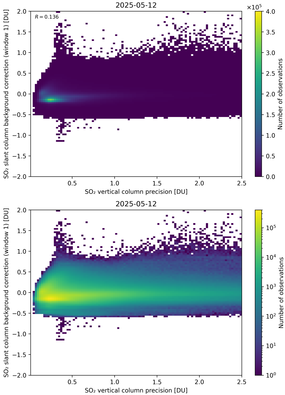
Figure 329: Scatter density plot of “SO 2 vertical column precision” against “SO 2 slant column background correction (window 1)” for 2025-05-11 to 2025-05-13.
