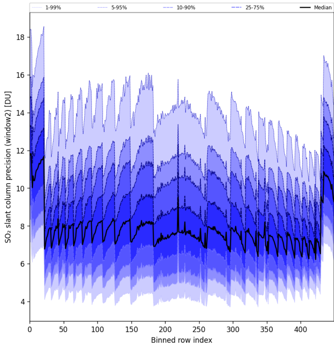
Figure 94: Along track statistics of “SO 2 slant column precision (window2)” for 2025-05-11 to 2025-05-13
