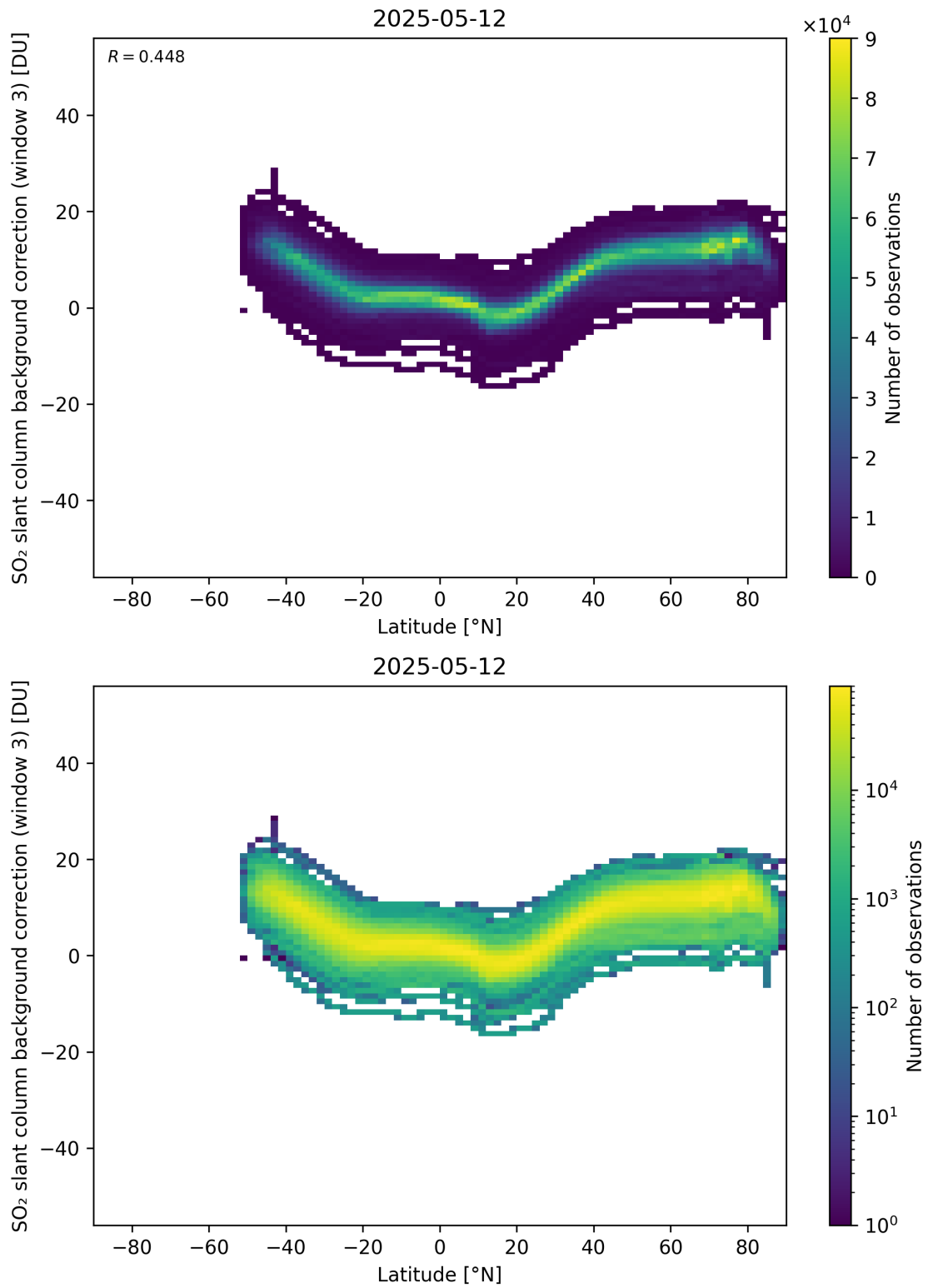
Figure 152: Scatter density plot of “Latitude” against “SO 2 slant column background correction (window 3)” for 2025-05-11 to 2025-05-13.
