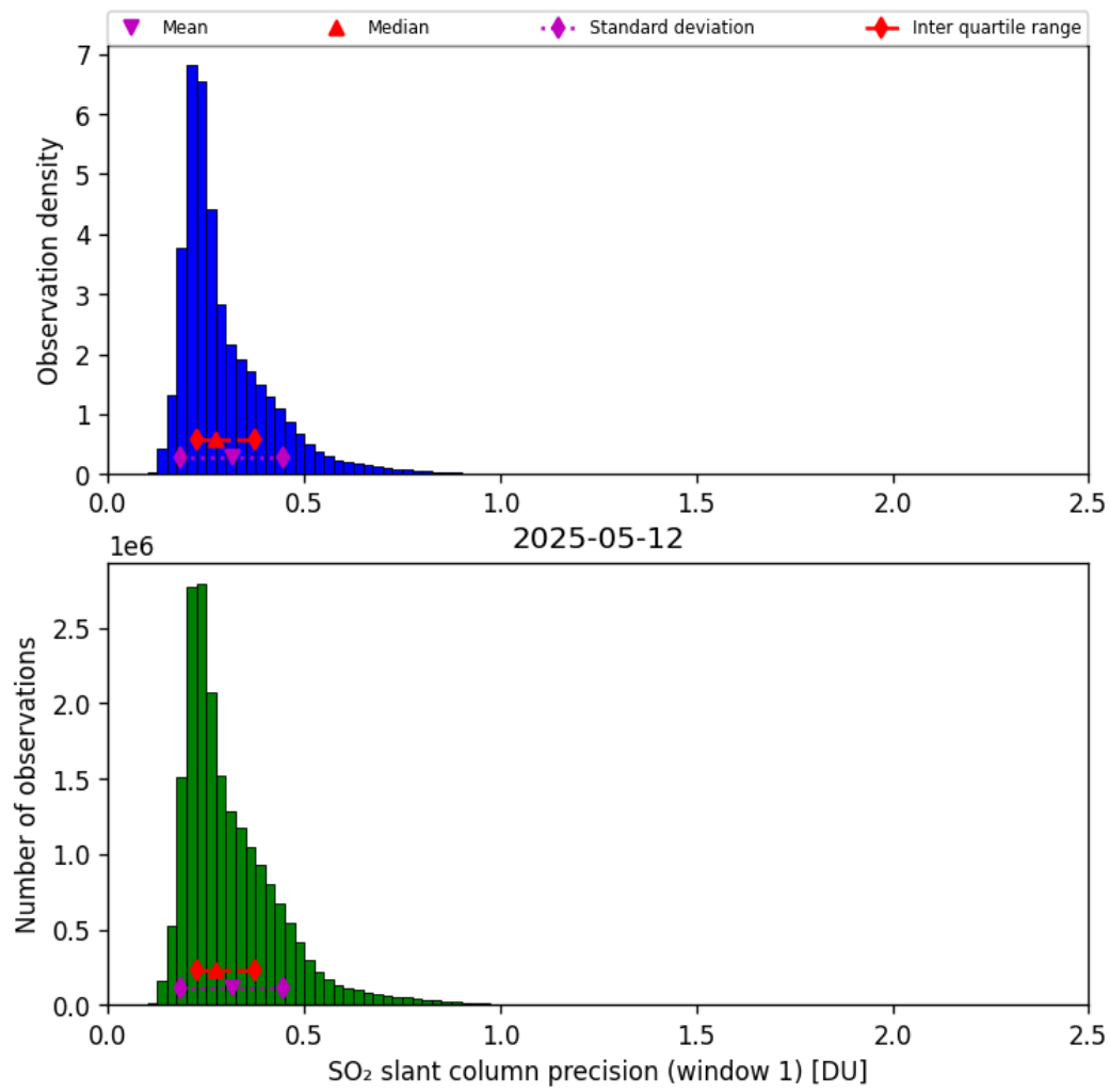
Figure 64: Histogram of “SO 2 slant column precision (window 1)” for 2025-05-11 to 2025-05-13
