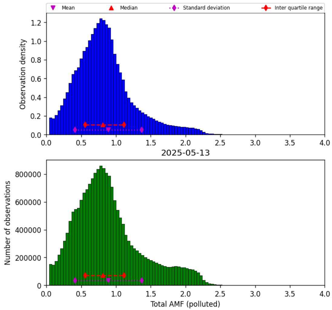
Figure 79: Histogram of “Total AMF (polluted)” for 2025-05-12 to 2025-05-14
