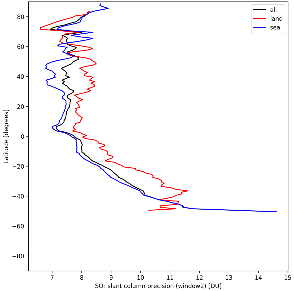
Figure 42: Zonal average of “SO 2 slant column precision (window2)” for 2025-05-12 to 2025-05-14.
