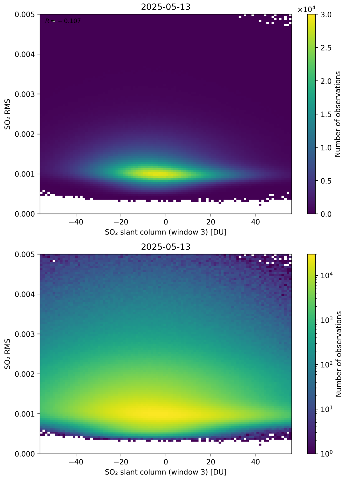
Figure 306: Scatter density plot of “SO 2 slant column (window 3)” against “SO 2 RMS” for 2025-05-12 to 2025-05-14.
