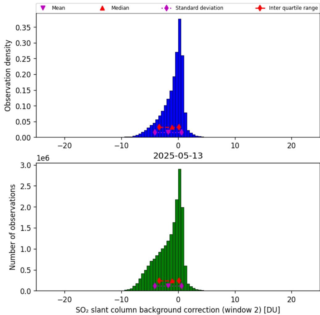
Figure 70: Histogram of “SO 2 slant column background correction (window 2)” for 2025-05-12 to 2025-05-14
