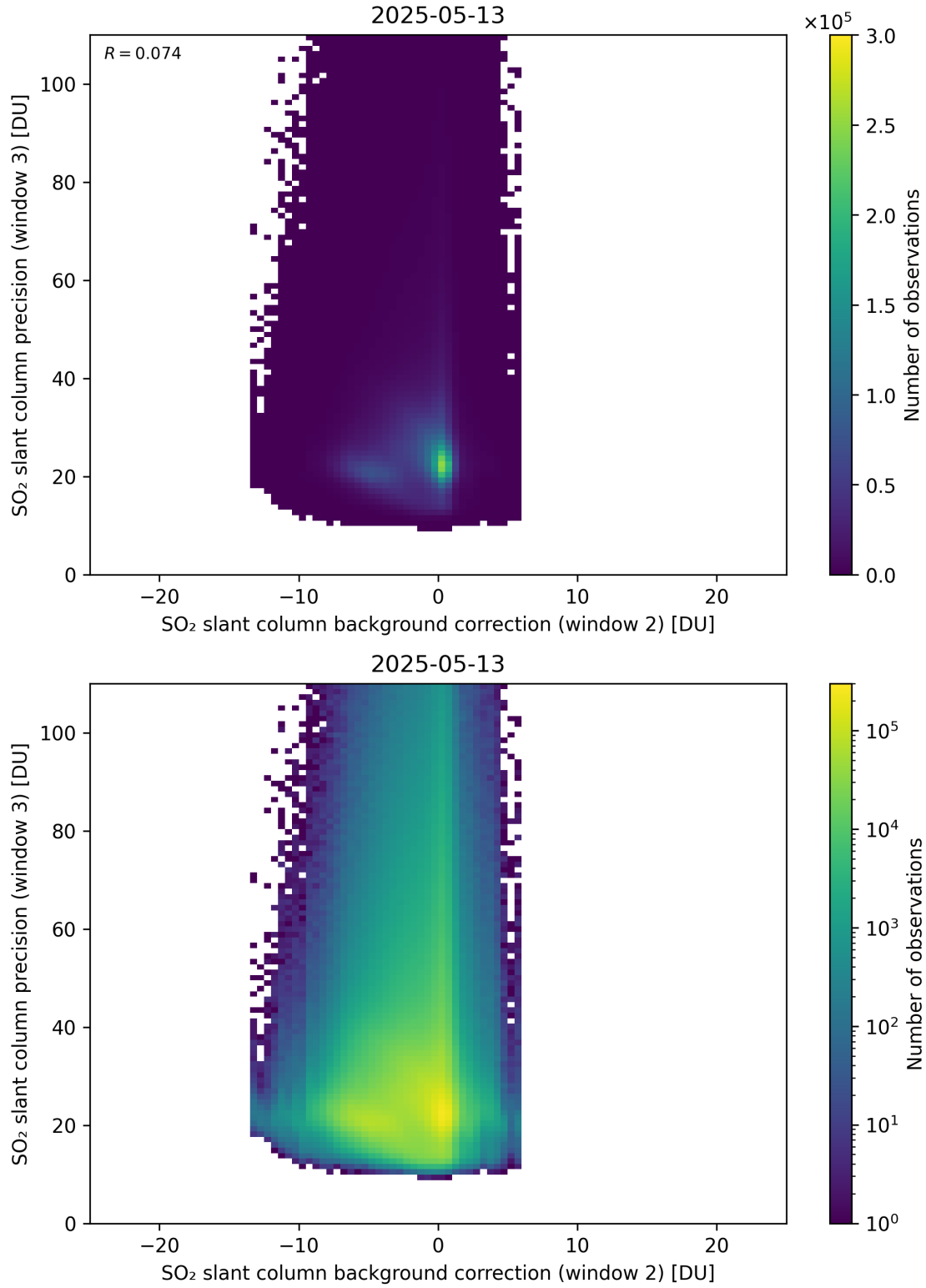
Figure 129: Scatter density plot of “SO 2 slant column background correction (window 2)” against “SO 2 slant column precision (window 3)” for 2025-05-12 to 2025-05-14.
