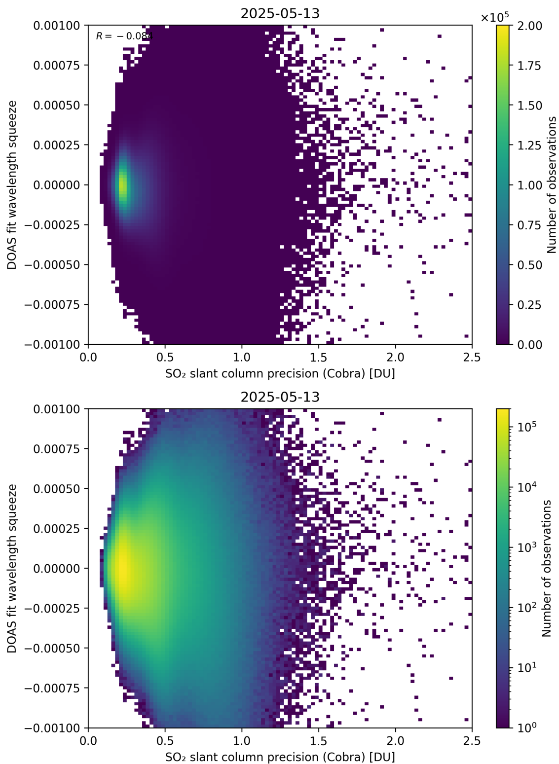
Figure 203: Scatter density plot of “SO 2 slant column precision (Cobra)” against “DOAS fit wavelength squeeze” for 2025-05-12 to 2025-05-14.
