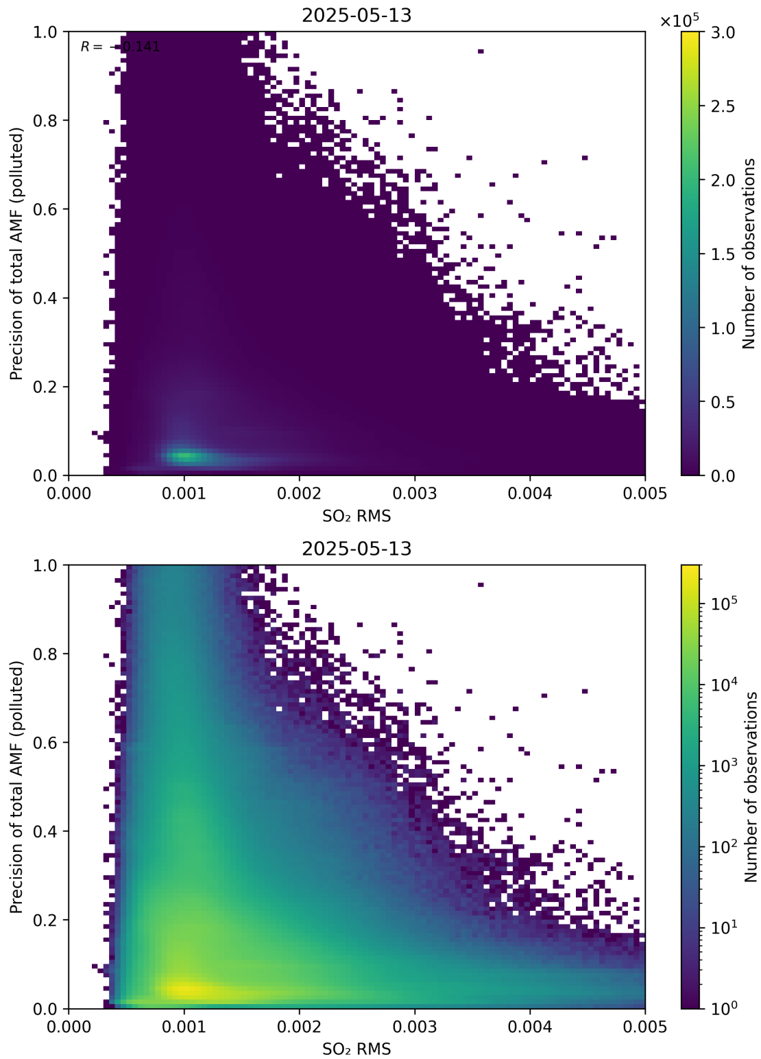
Figure 149: Scatter density plot of “SO 2 RMS” against “Precision of total AMF (polluted)” for 2025-05-12 to 2025-05-14.
