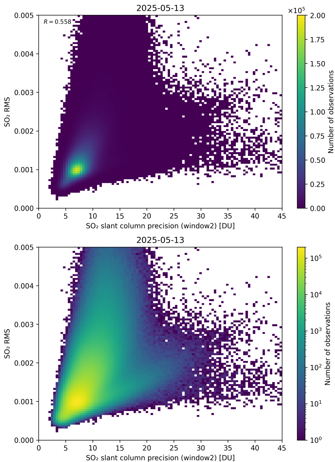
Figure 295: Scatter density plot of “SO 2 slant column precision (window2)” against “SO 2 RMS” for 2025-05-12 to 2025-05-14.
