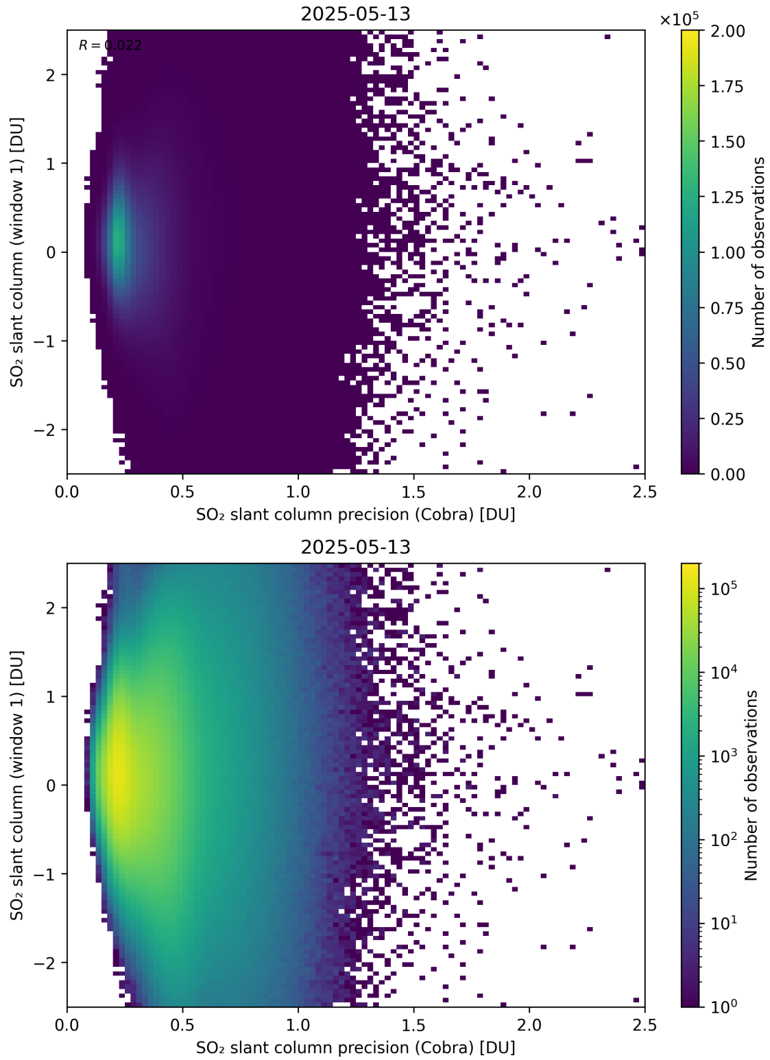
Figure 208: Scatter density plot of “SO 2 slant column precision (Cobra)” against “SO 2 slant column (window 1)” for 2025-05-12 to 2025-05-14.
