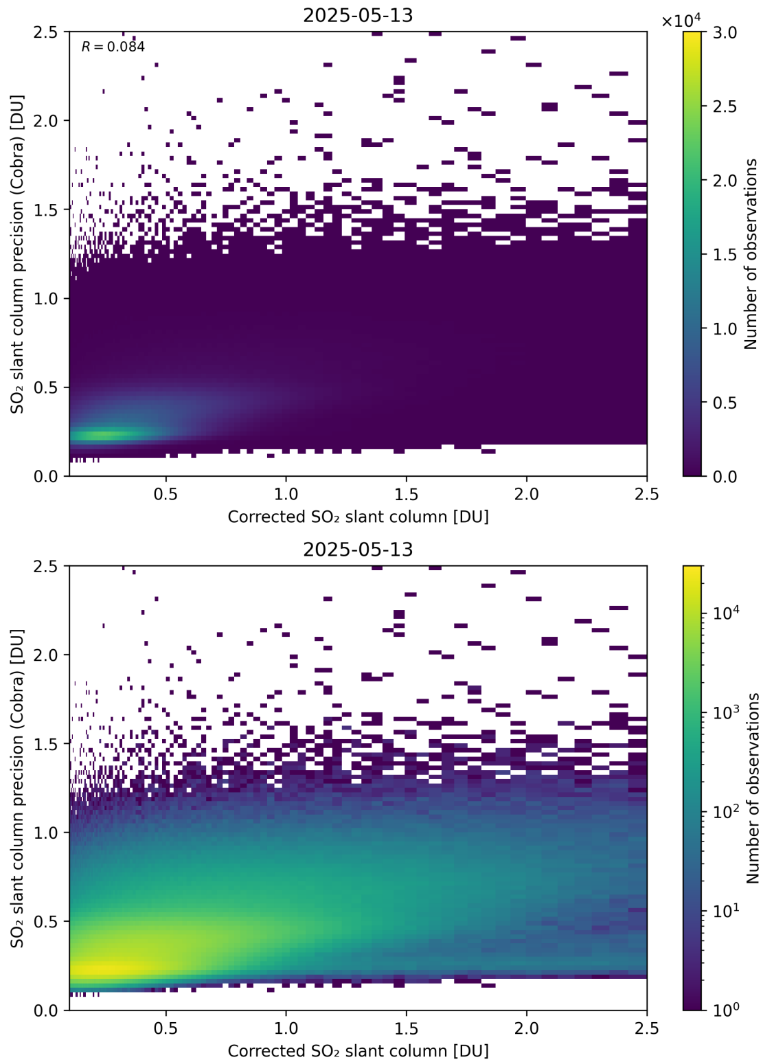
Figure 234: Scatter density plot of “Corrected SO 2 slant column” against “SO 2 slant column precision (Cobra)” for 2025-05-12 to 2025-05-14.
