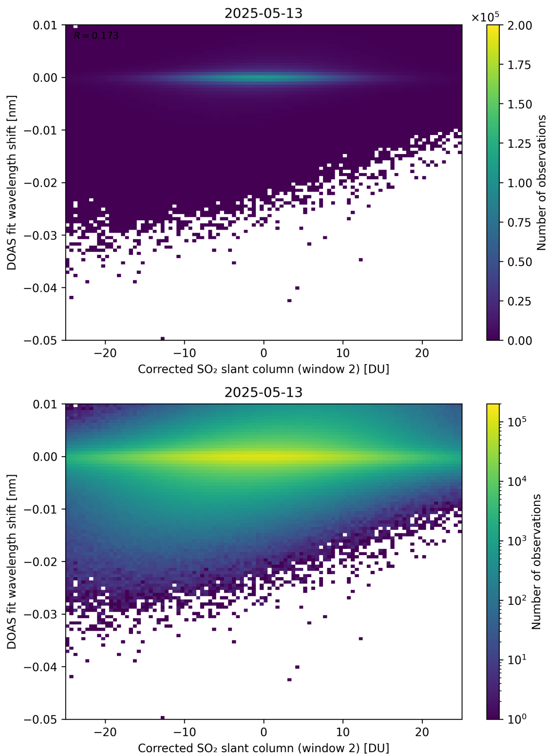
Figure 246: Scatter density plot of “Corrected SO 2 slant column (window 2)” against “DOAS fit wavelength shift” for 2025-05-12 to 2025-05-14.
