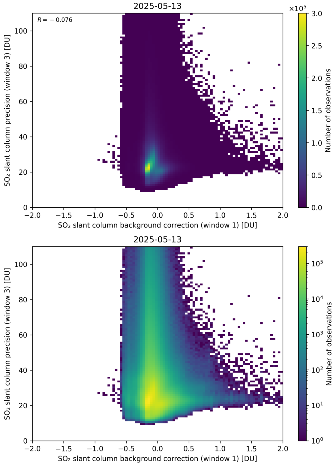
Figure 119: Scatter density plot of “SO 2 slant column background correction (window 1)” against “SO 2 slant column precision (window 3)” for 2025-05-12 to 2025-05-14.
