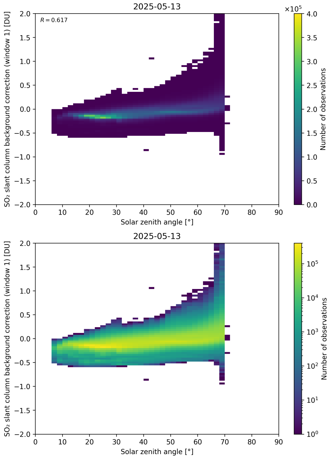
Figure 171: Scatter density plot of “Solar zenith angle” against “SO 2 slant column background correction (window 1)” for 2025-05-12 to 2025-05-14.
