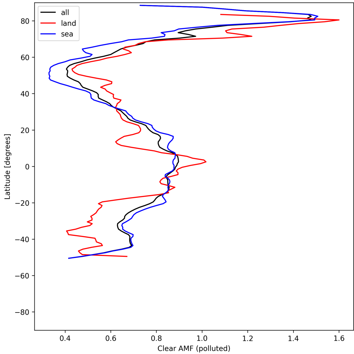
Figure 55: Zonal average of “Clear AMF (polluted)” for 2025-05-12 to 2025-05-14.
