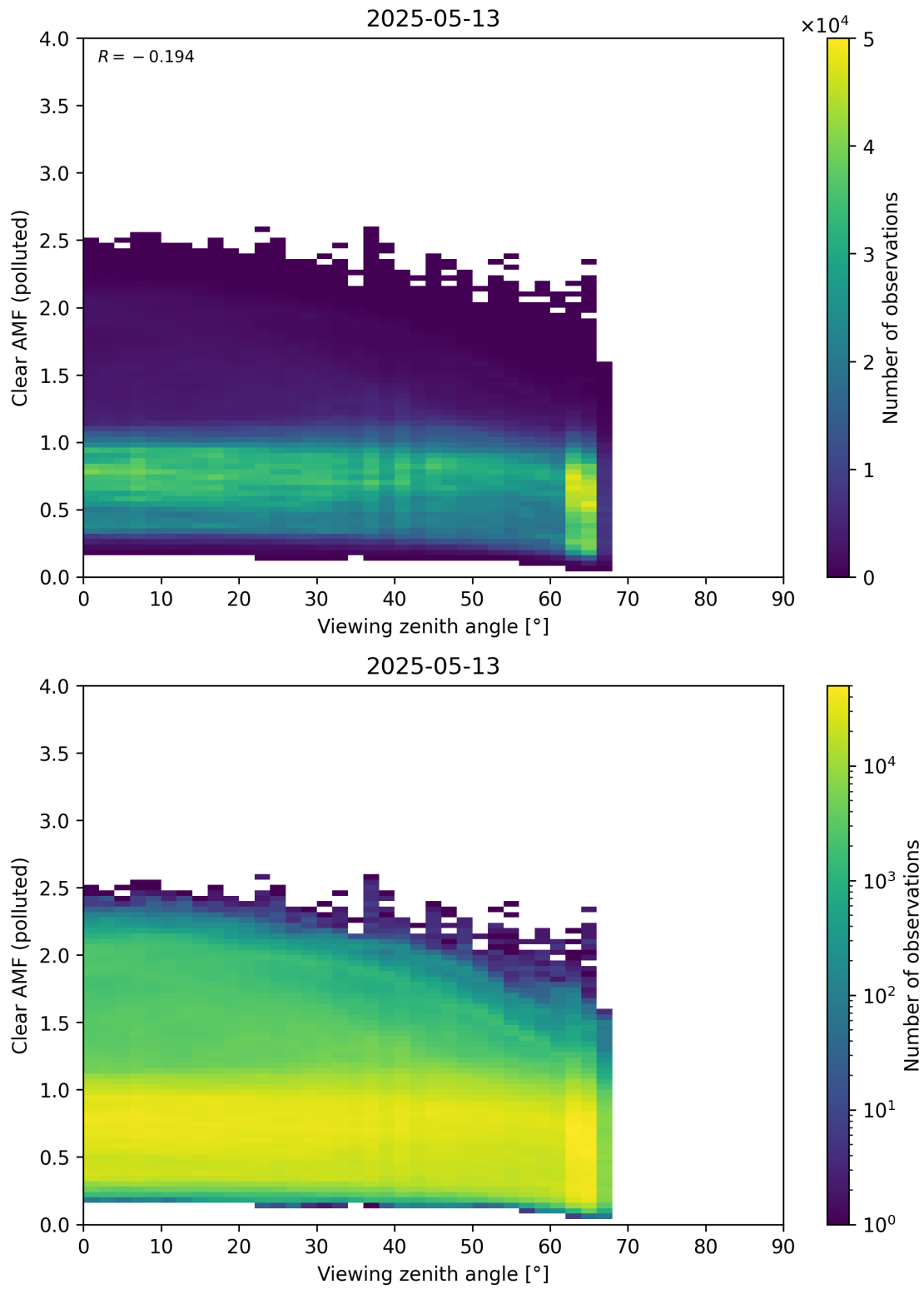
Figure 370: Scatter density plot of “Viewing zenith angle” against “Clear AMF (polluted)” for 2025-05-12 to 2025-05-14.
