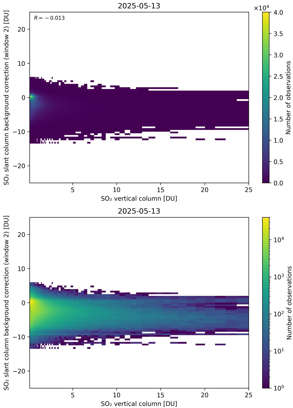
Figure 324: Scatter density plot of “SO 2 vertical column” against “SO 2 slant column background correction (window 2)” for 2025-05-12 to 2025-05-14.
