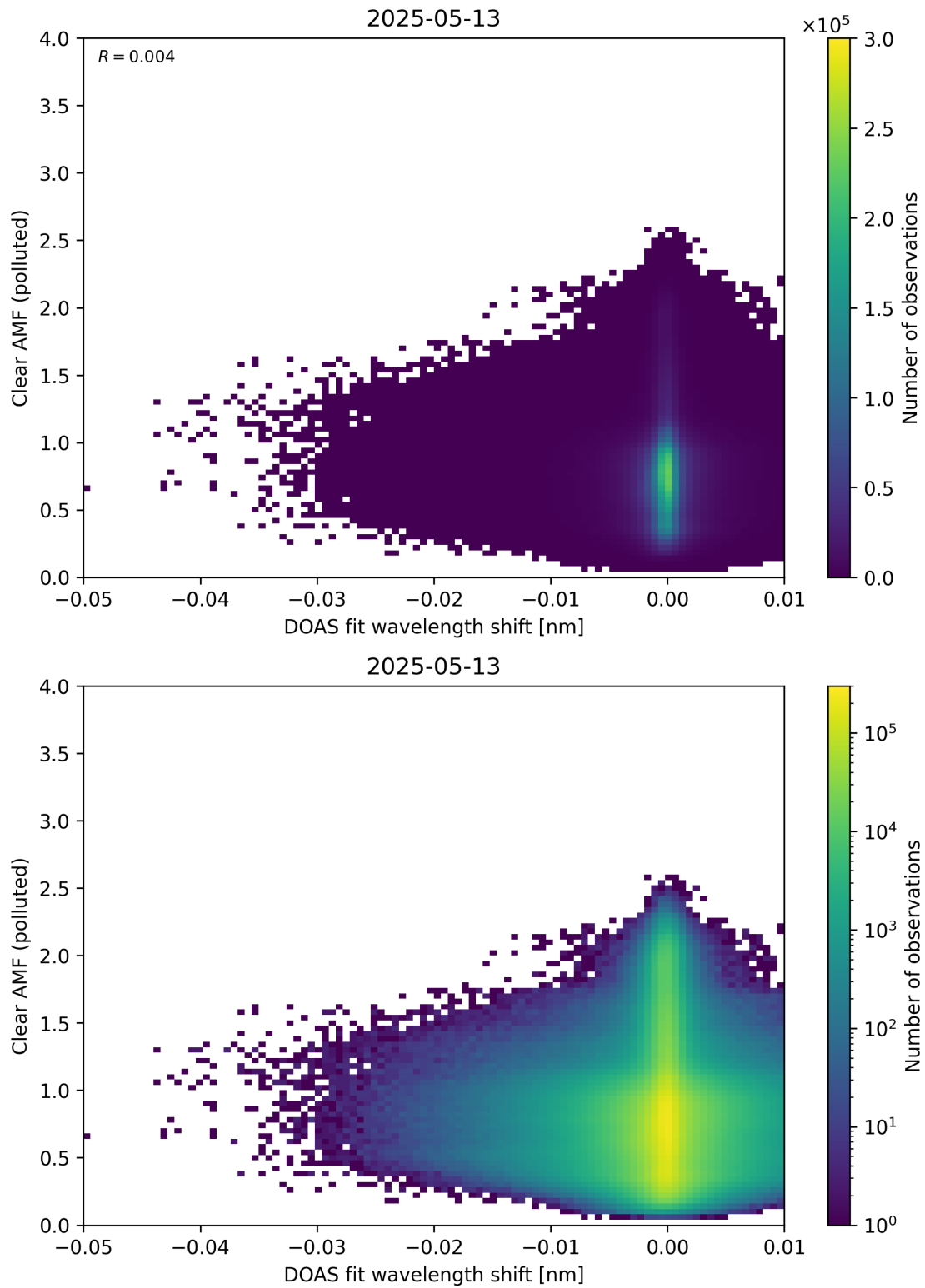
Figure 140: Scatter density plot of “DOAS fit wavelength shift” against “Clear AMF (polluted)” for 2025-05-12 to 2025-05-14.
