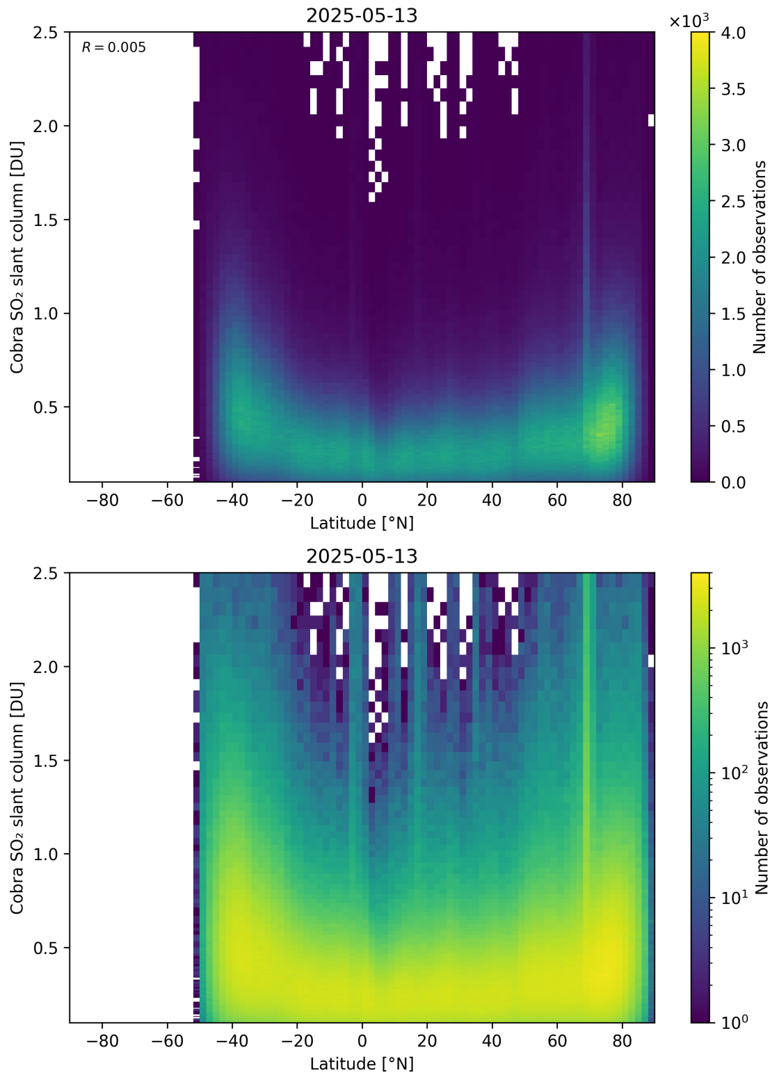
Figure 157: Scatter density plot of “Latitude” against “Cobra SO 2 slant column” for 2025-05-12 to 2025-05-14.
