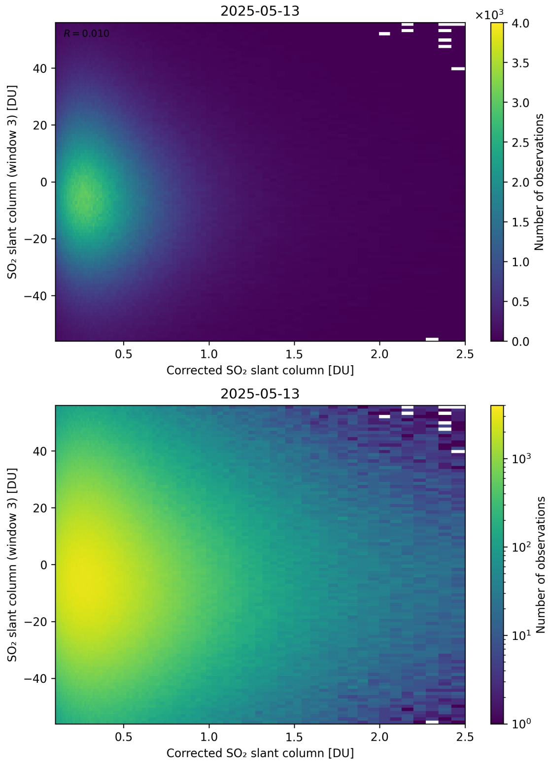
Figure 240: Scatter density plot of “Corrected SO 2 slant column” against “SO 2 slant column (window 3)” for 2025-05-12 to 2025-05-14.
