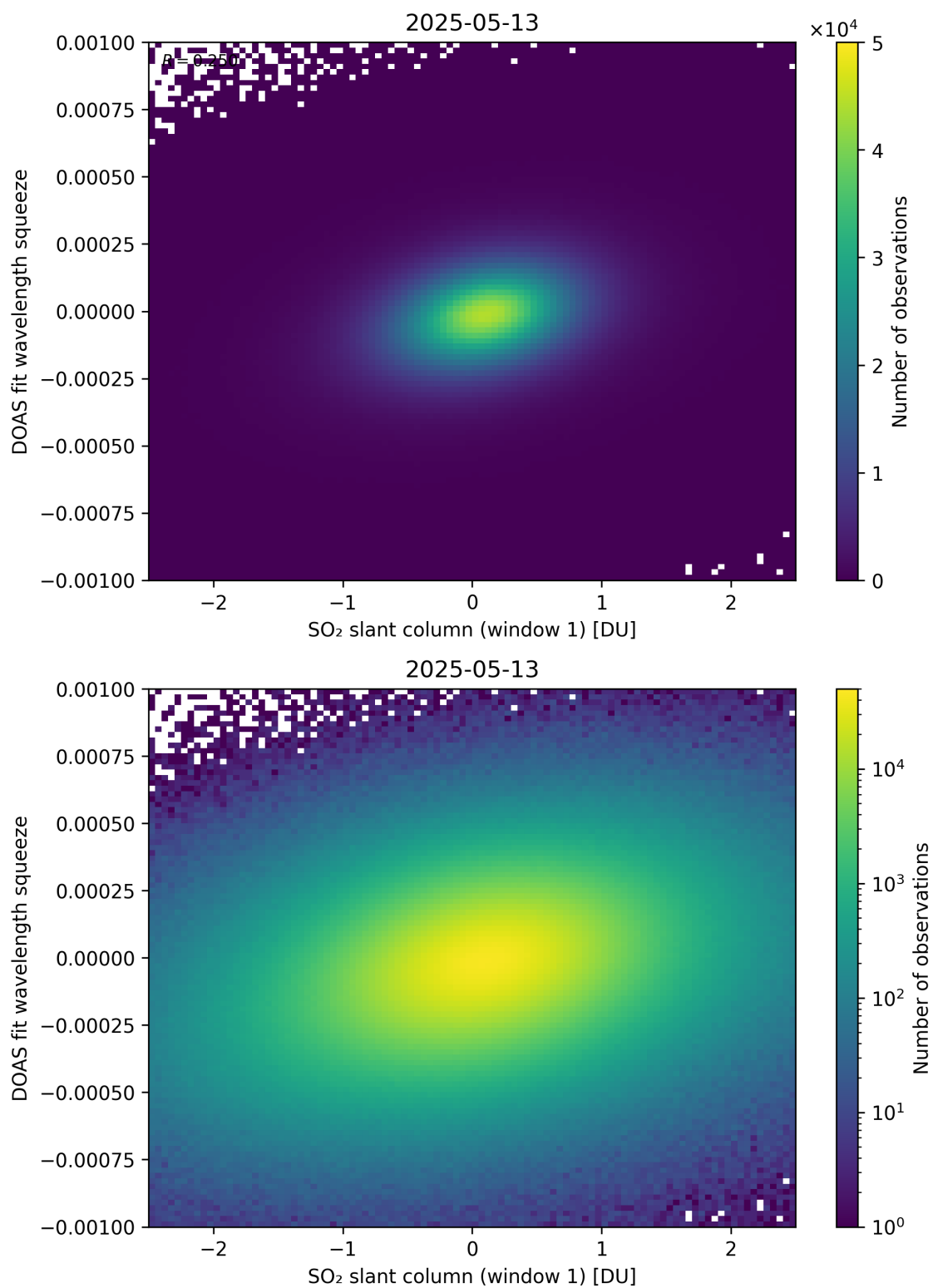
Figure 266: Scatter density plot of “SO 2 slant column (window 1)” against “DOAS fit wavelength squeeze” for 2025-05-12 to 2025-05-14.
