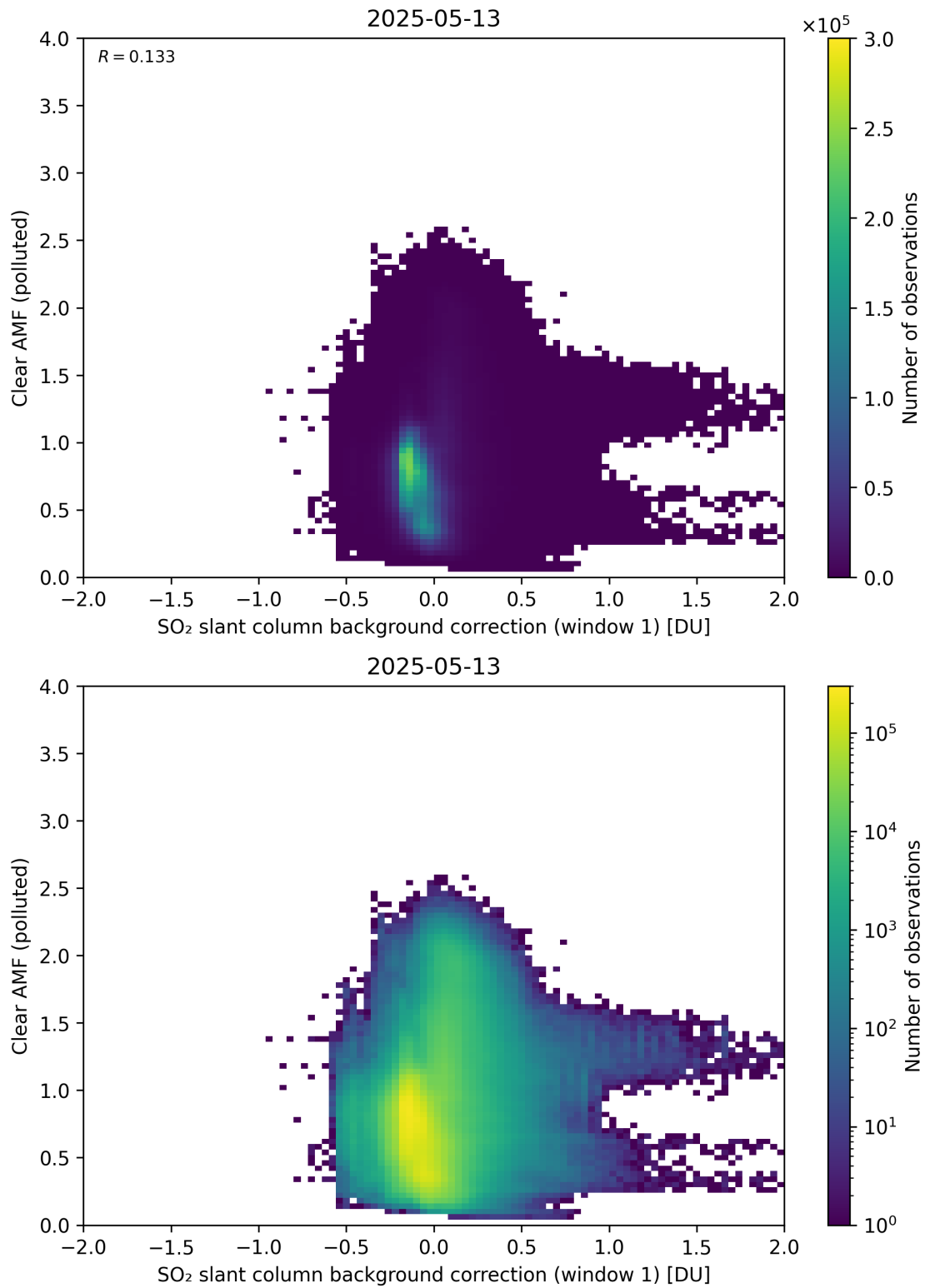
Figure 114: Scatter density plot of “SO 2 slant column background correction (window 1)” against “Clear AMF (polluted)” for 2025-05-12 to 2025-05-14.
