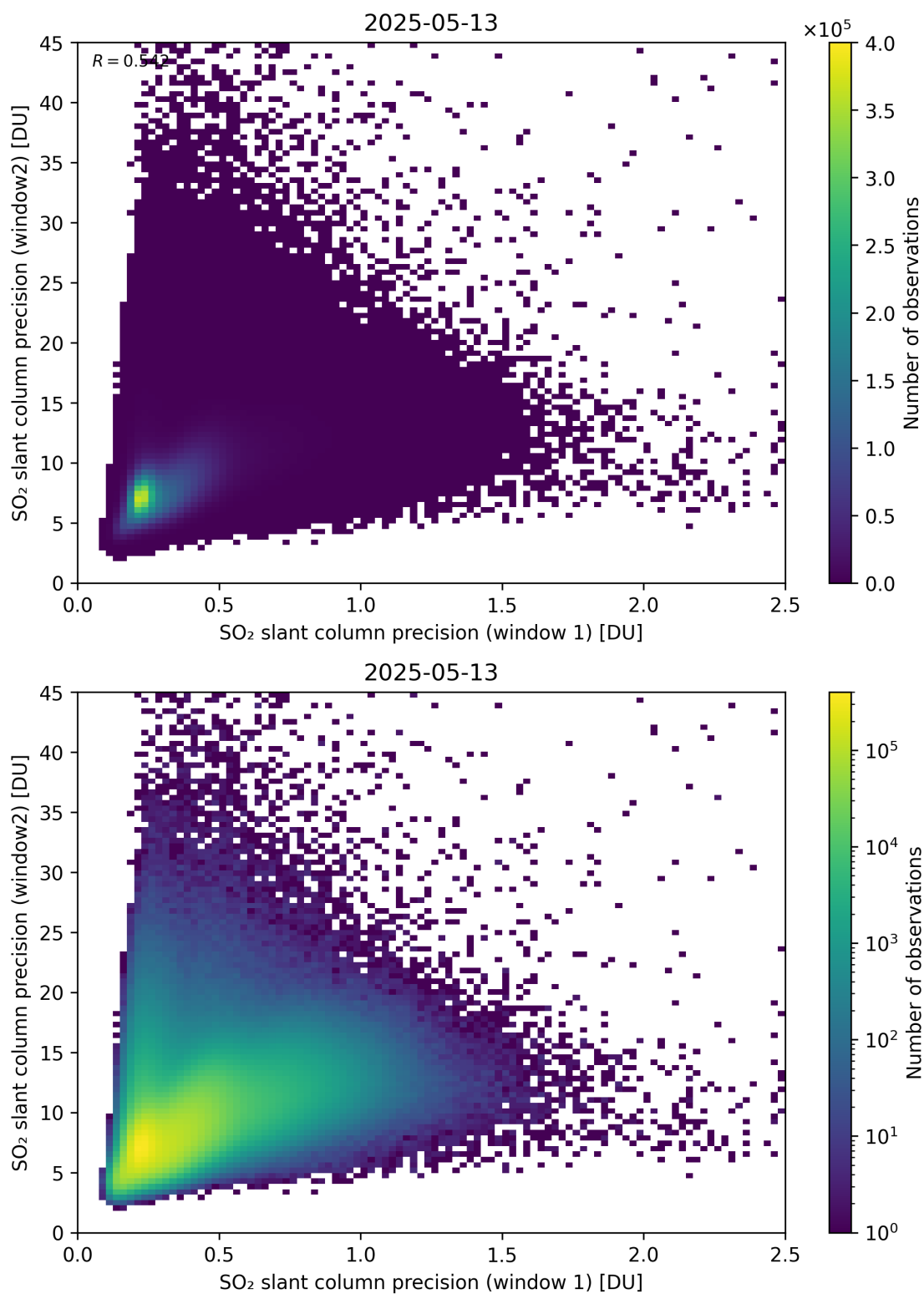
Figure 277: Scatter density plot of “SO 2 slant column precision (window 1)” against “SO 2 slant column precision (window2)” for 2025-05-12 to 2025-05-14.
