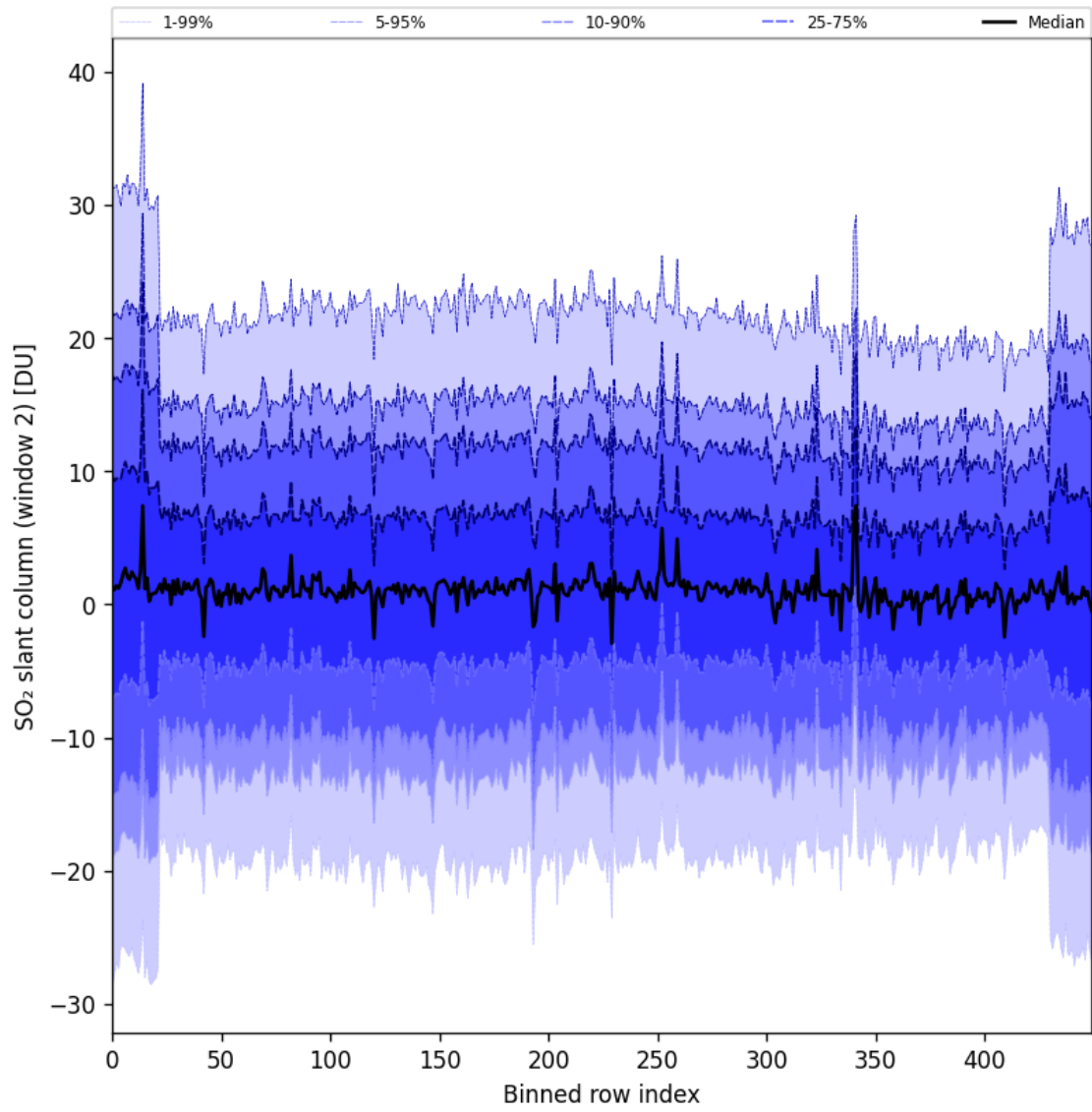
Figure 93: Along track statistics of "SO 2 slant column (window 2)" for 2025-05-12 to 2025-05-14
