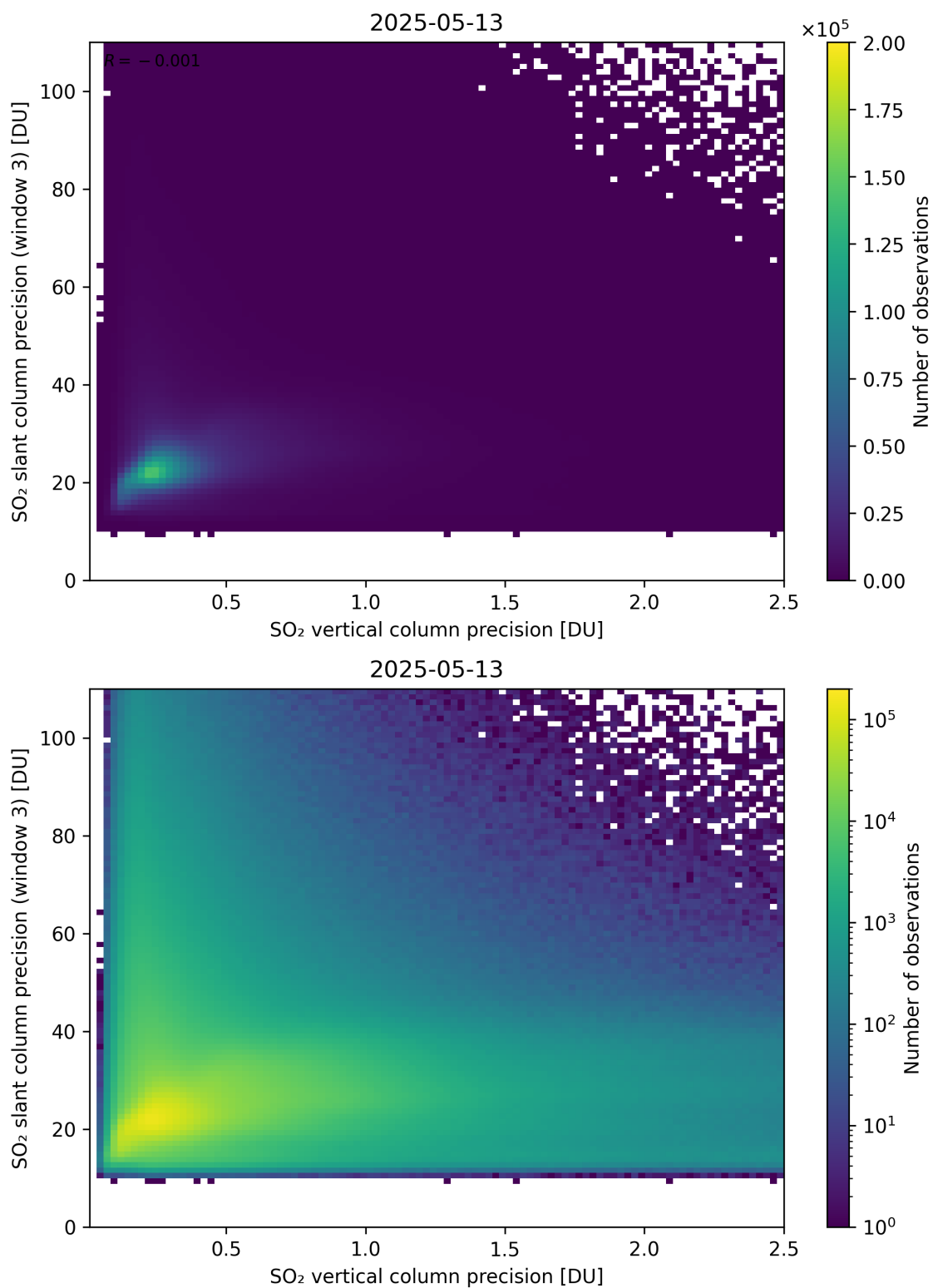
Figure 345: Scatter density plot of “SO 2 vertical column precision” against “SO 2 slant column precision (window 3)” for 2025-05-12 to 2025-05-14.
