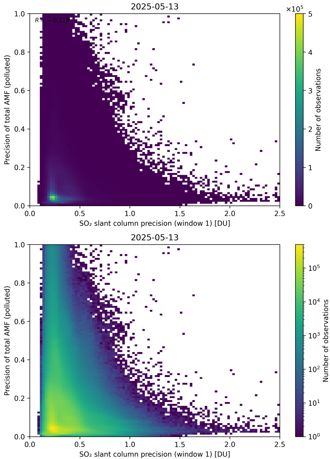
Figure 281: Scatter density plot of “SO 2 slant column precision (window 1)” against “Precision of total AMF (polluted)” for 2025-05-12 to 2025-05-14.
