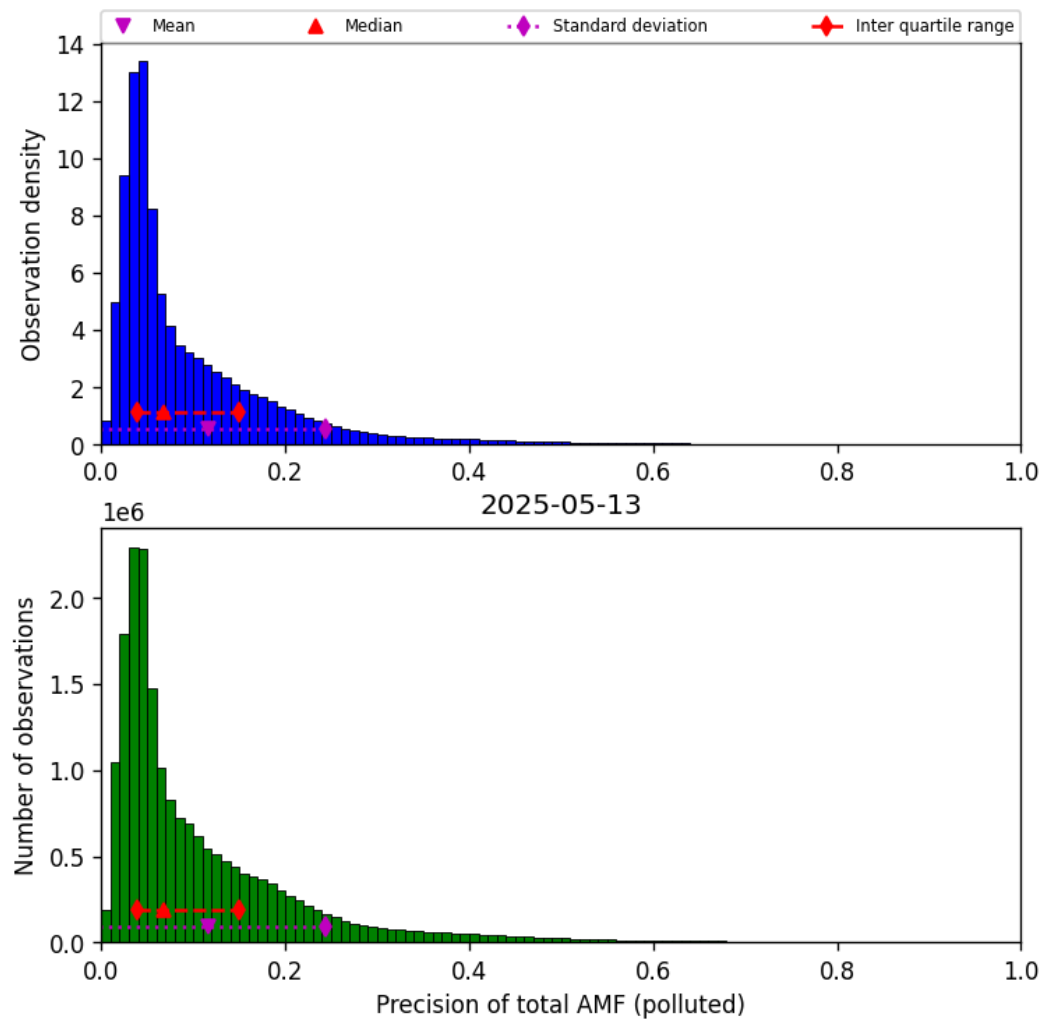
Figure 80: Histogram of “Precision of total AMF (polluted)” for 2025-05-12 to 2025-05-14
