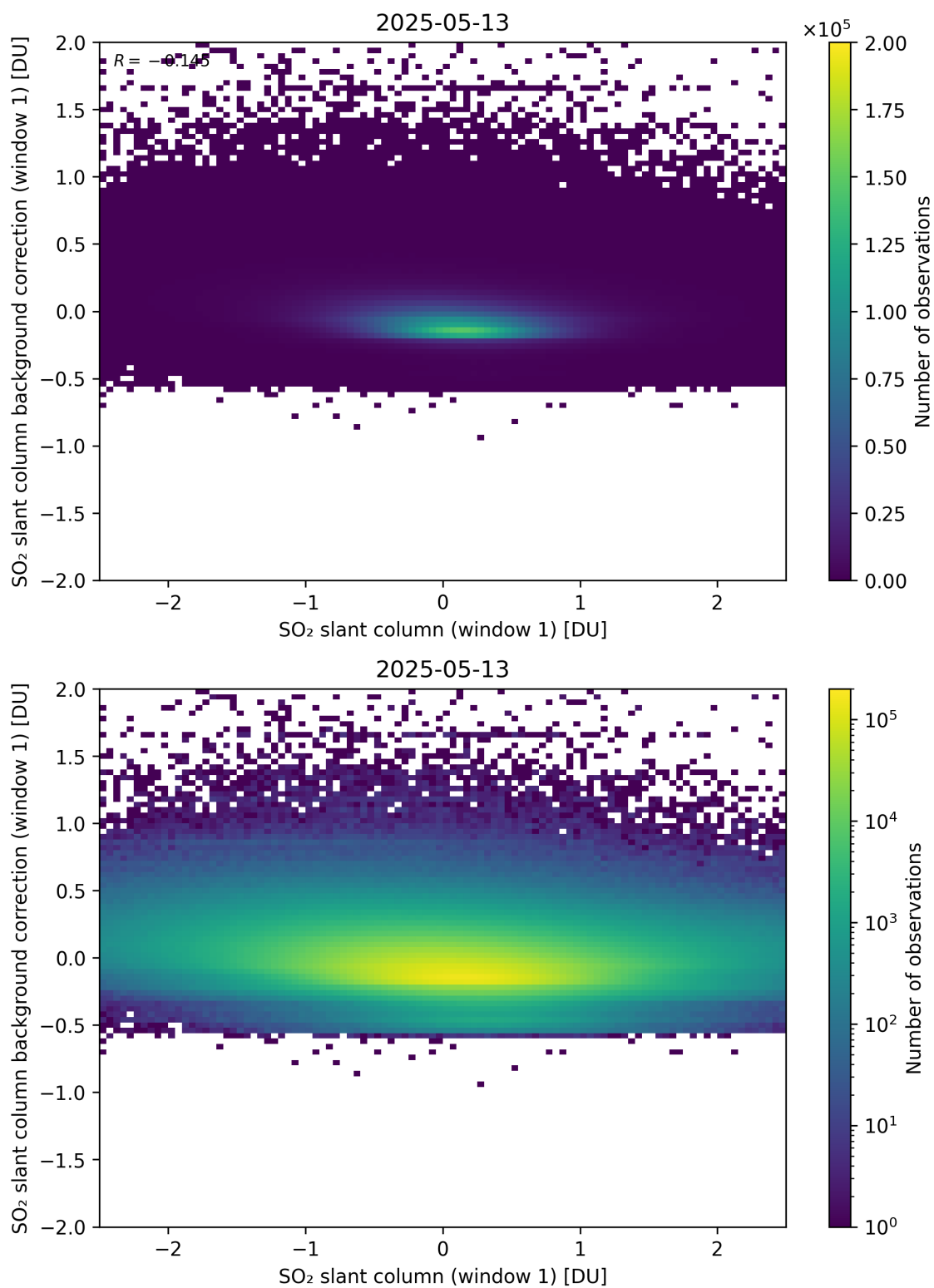
Figure 262: Scatter density plot of “SO 2 slant column (window 1)” against “SO 2 slant column background correction (window 1)” for 2025-05-12 to 2025-05-14.
