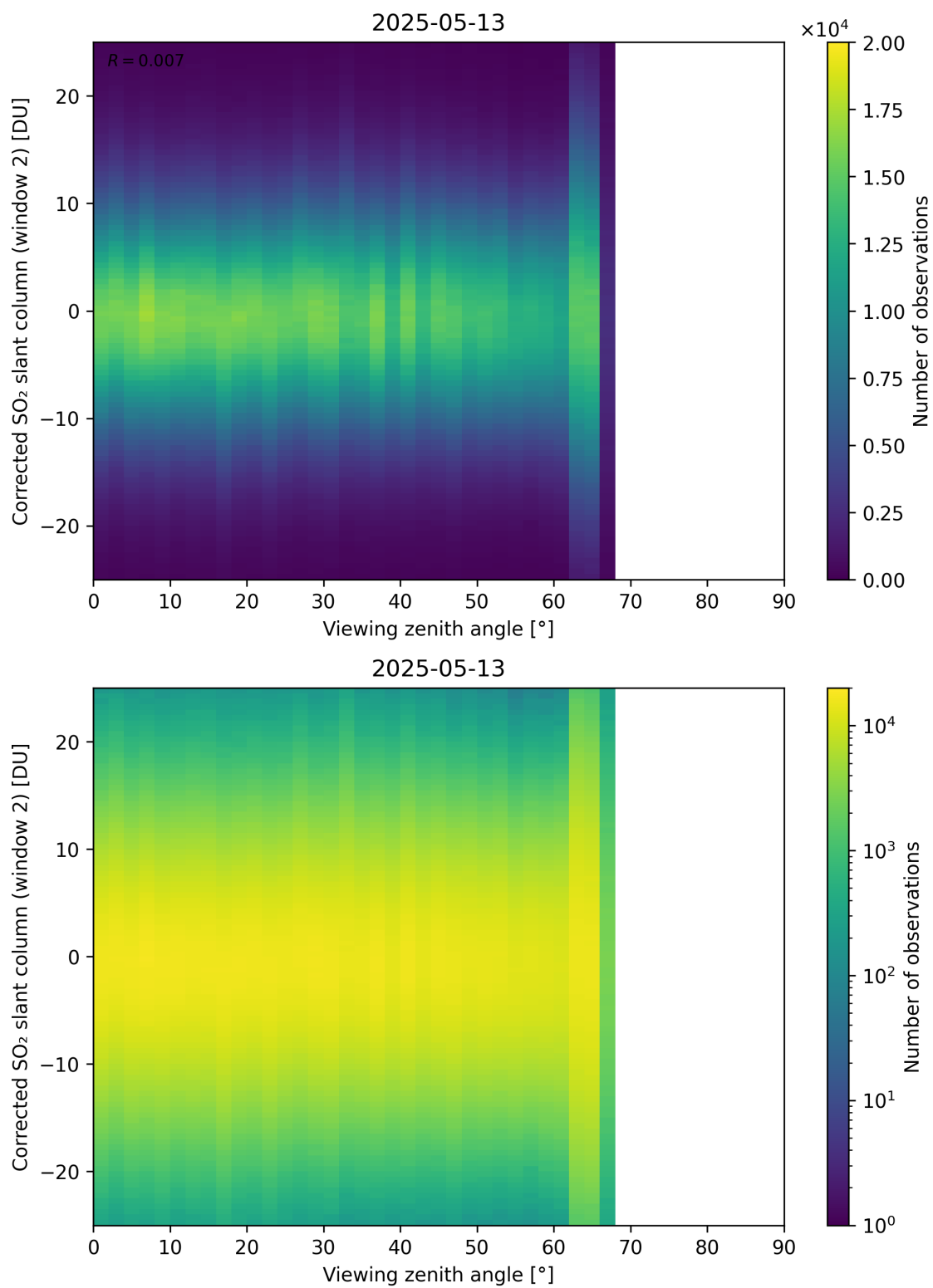
Figure 374: Scatter density plot of “Viewing zenith angle” against “Corrected SO 2 slant column (window 2)” for 2025-05-12 to 2025-05-14.
