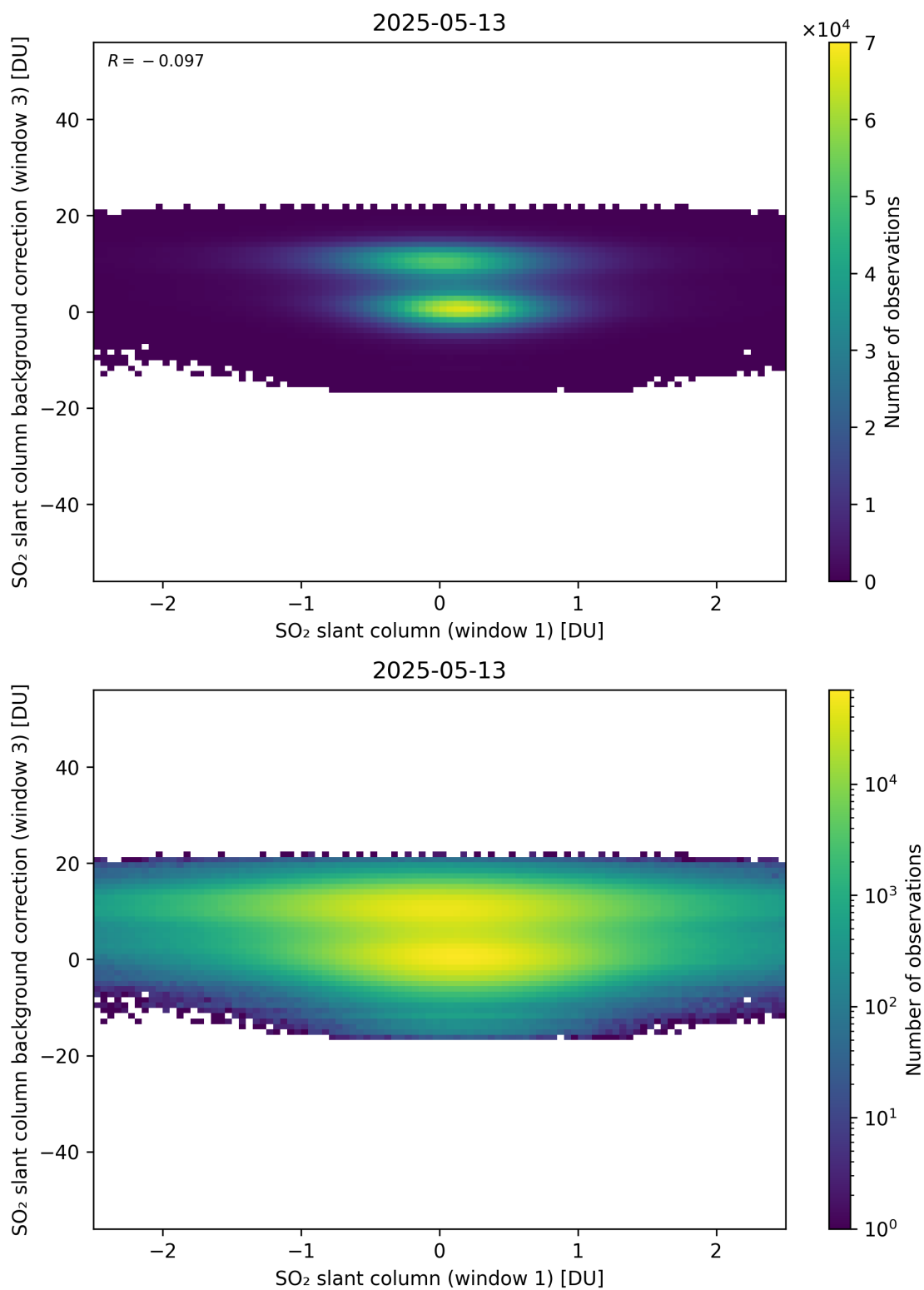
Figure 264: Scatter density plot of “SO 2 slant column (window 1)” against “SO 2 slant column background correction (window 3)” for 2025-05-12 to 2025-05-14.
