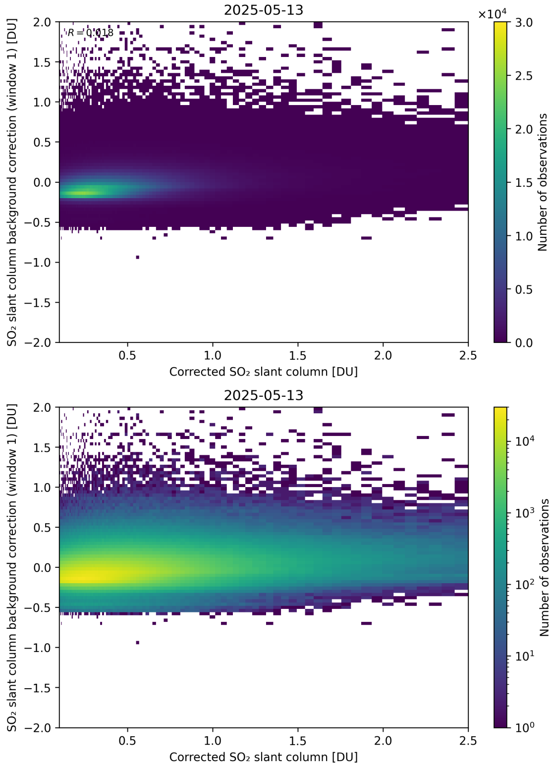
Figure 226: Scatter density plot of “Corrected SO 2 slant column” against “SO 2 slant column background correction (window 1)” for 2025-05-12 to 2025-05-14.
