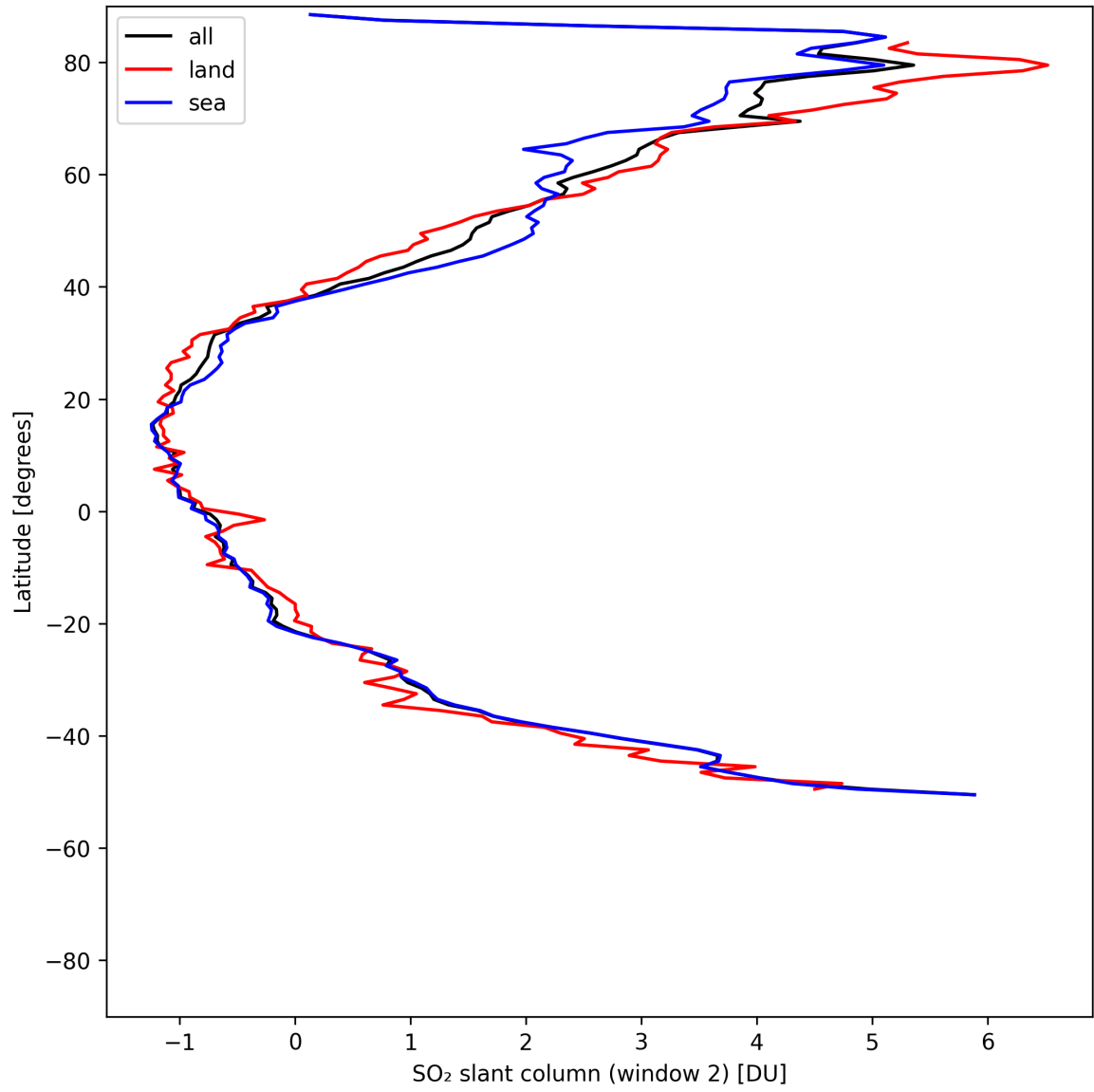
Figure 41: Zonal average of “SO 2 slant column (window 2)” for 2025-05-12 to 2025-05-14.
