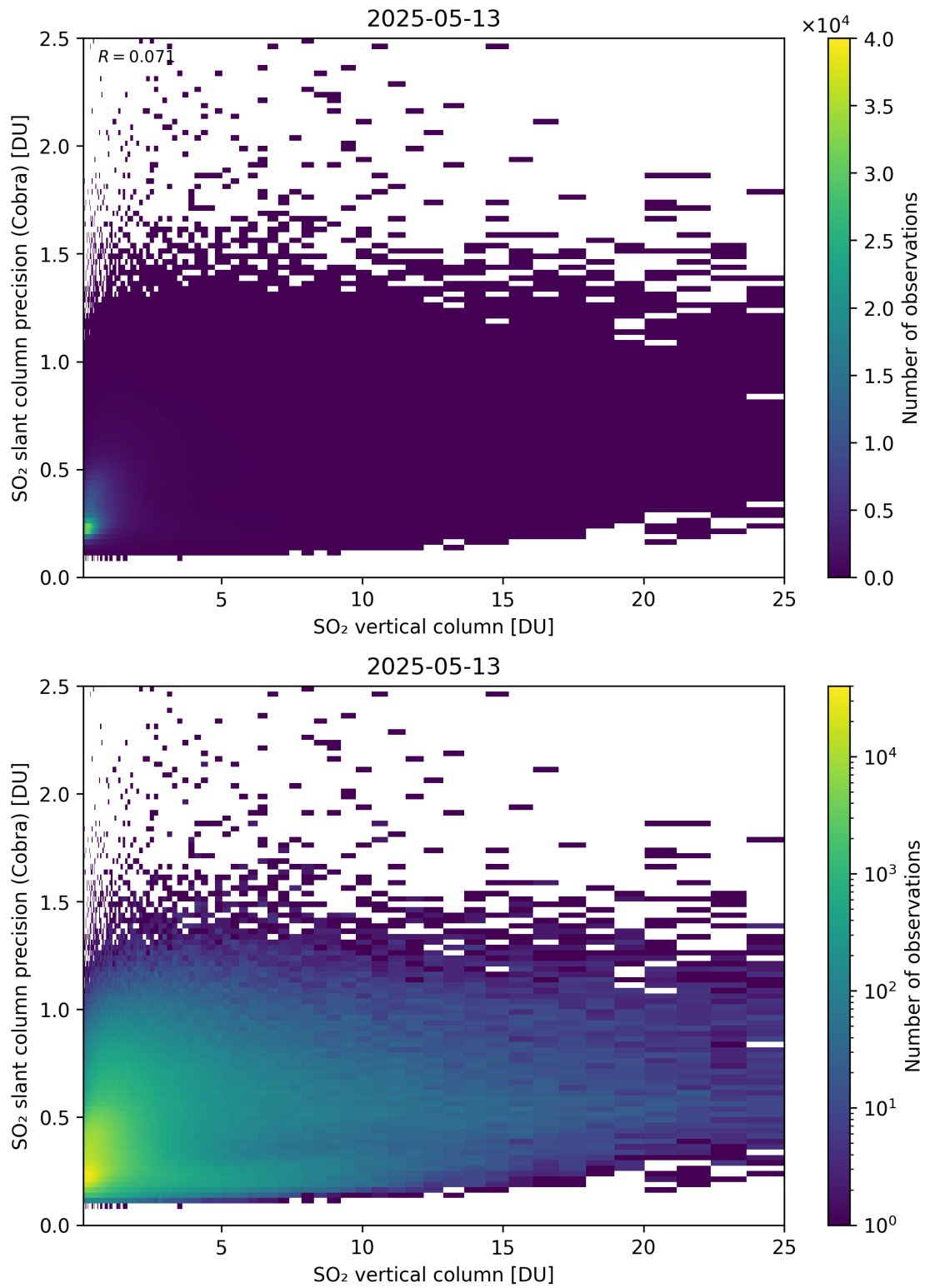
Figure 350: Scatter density plot of “SO 2 vertical column” against “SO 2 slant column precision (Cobra)” for 2025-05-12 to 2025-05-14.
