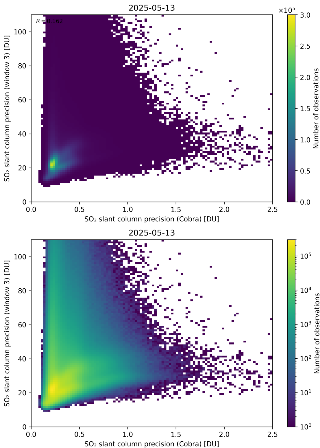
Figure 212: Scatter density plot of “SO 2 slant column precision (Cobra)” against “SO 2 slant column precision (window 3)” for 2025-05-12 to 2025-05-14.
