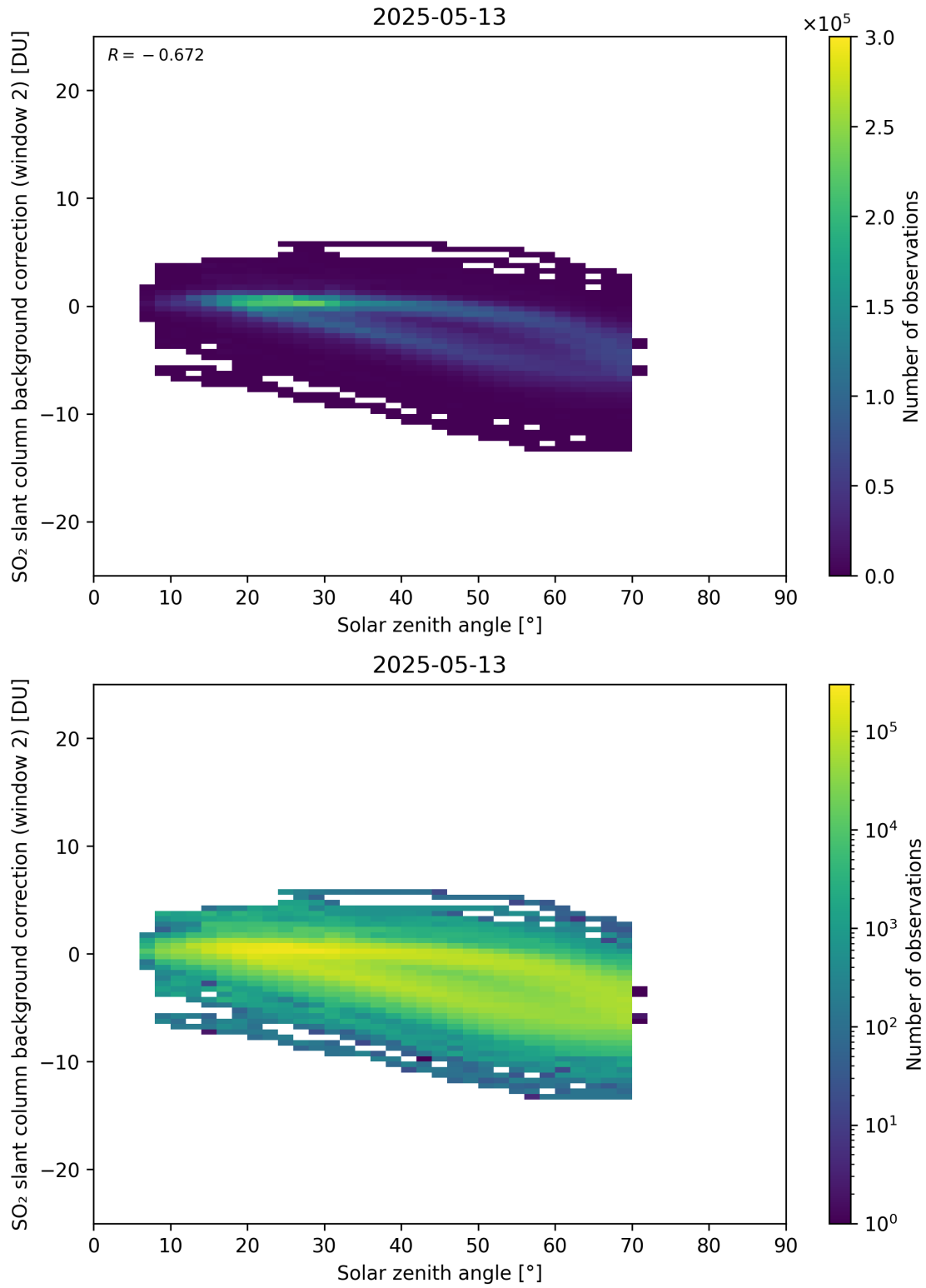
Figure 172: Scatter density plot of “Solar zenith angle” against “SO 2 slant column background correction (window 2)” for 2025-05-12 to 2025-05-14.
