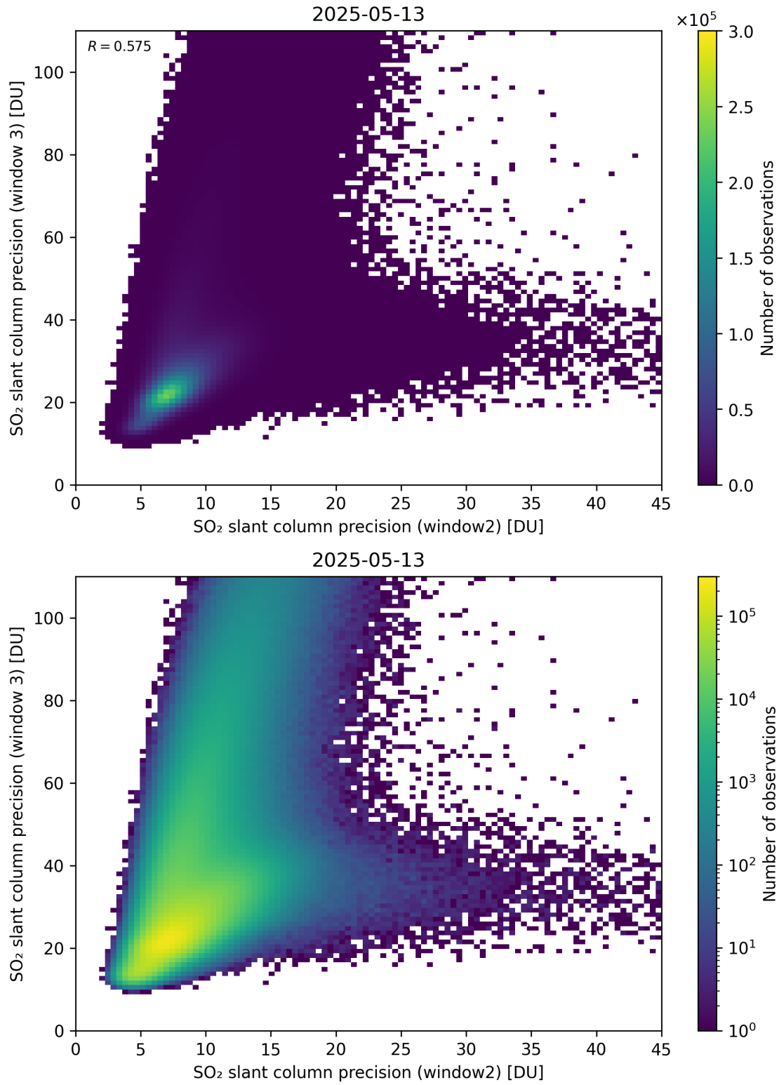
Figure 300: Scatter density plot of “SO 2 slant column precision (window2)” against “SO 2 slant column precision (window 3)” for 2025-05-12 to 2025-05-14.
