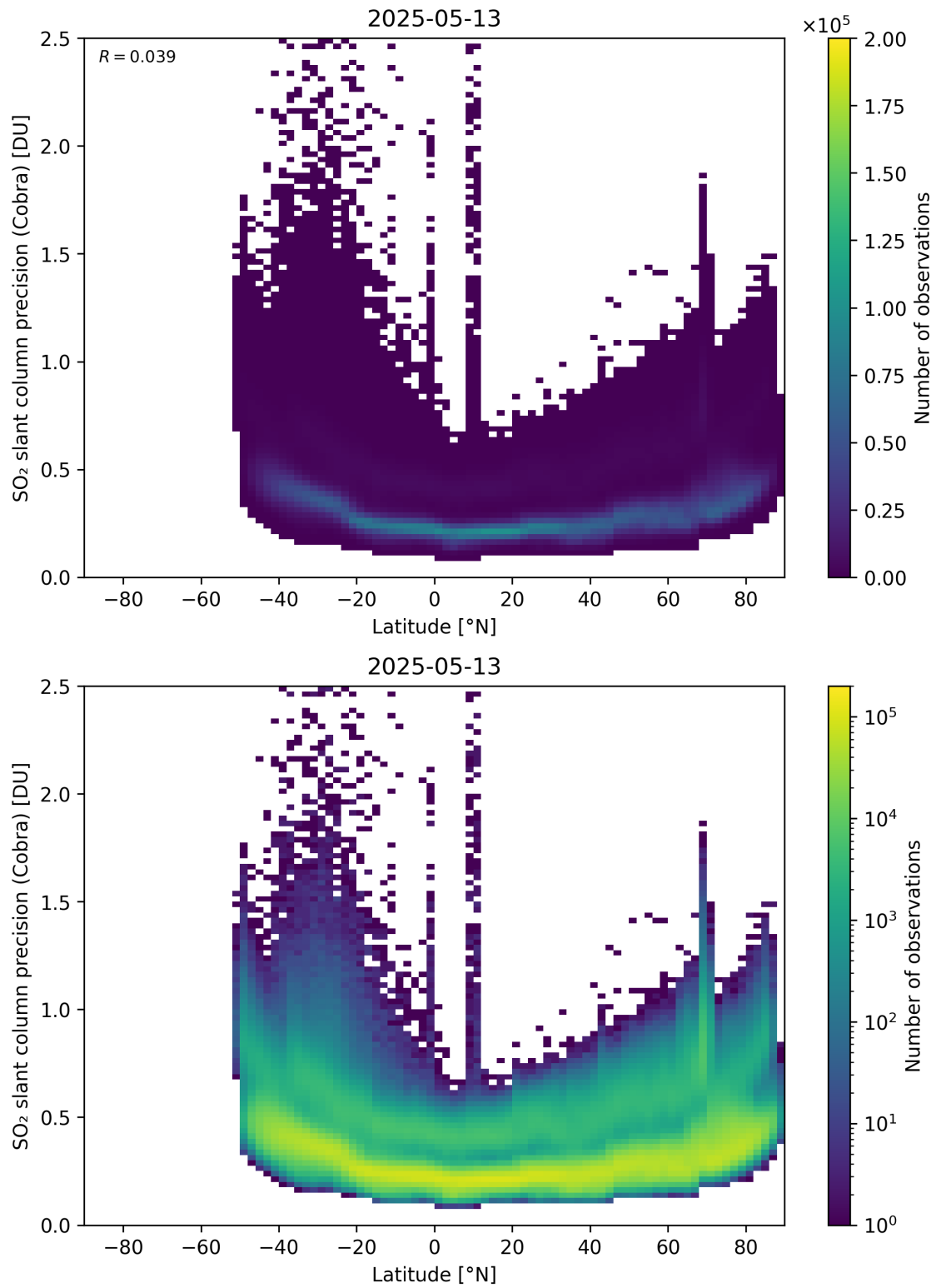
Figure 158: Scatter density plot of “Latitude” against “SO 2 slant column precision (Cobra)” for 2025-05-12 to 2025-05-14.
