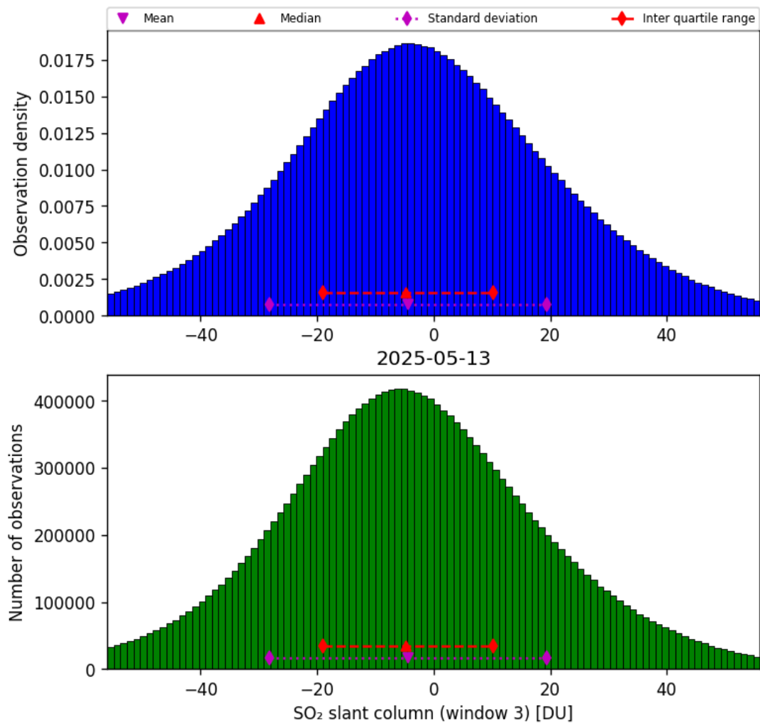
Figure 71: Histogram of “SO 2 slant column (window 3)” for 2025-05-12 to 2025-05-14
