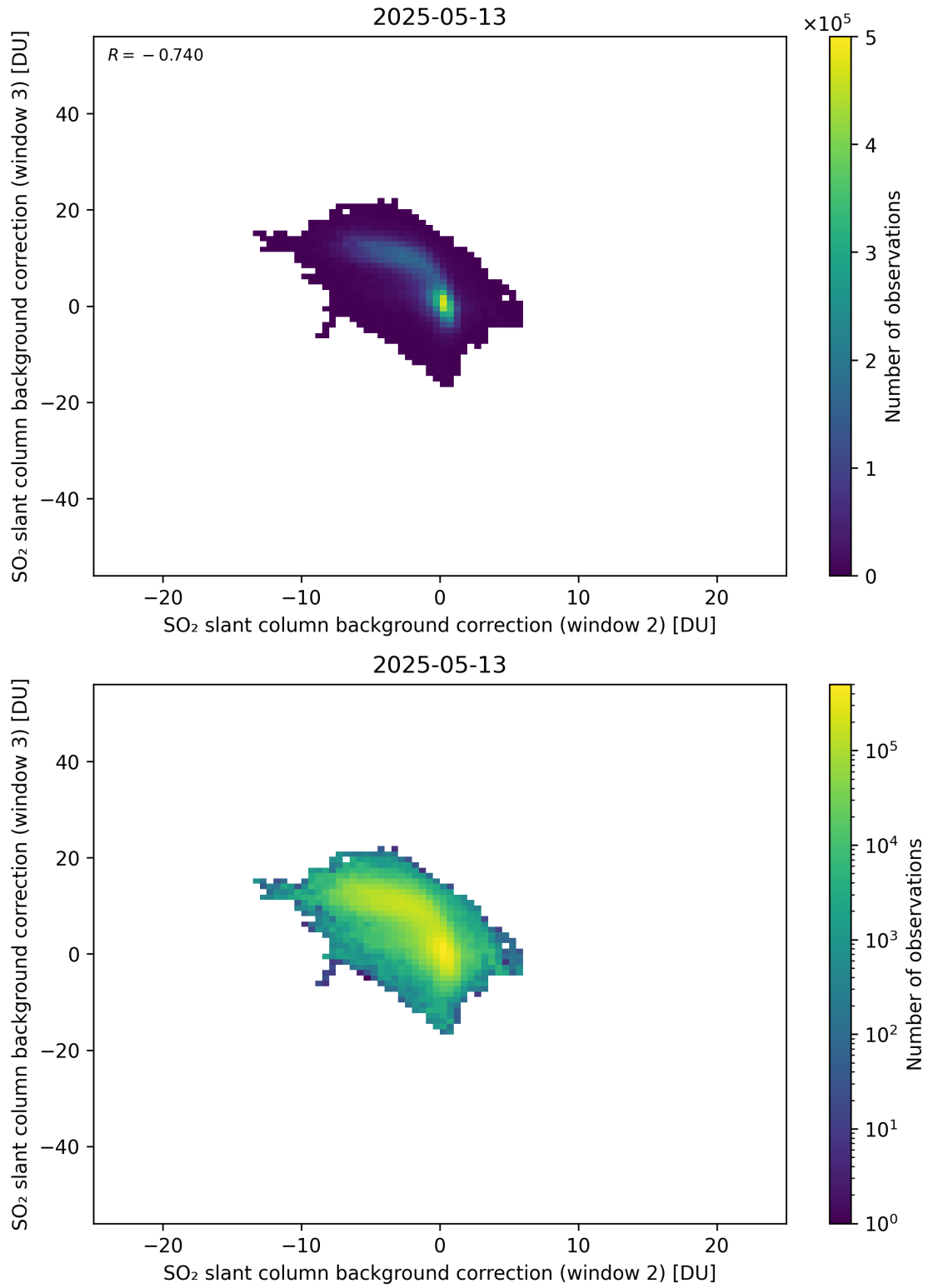
Figure 122: Scatter density plot of “SO 2 slant column background correction (window 2)” against “SO 2 slant column background correction (window 3)” for 2025-05-12 to 2025-05-14.
