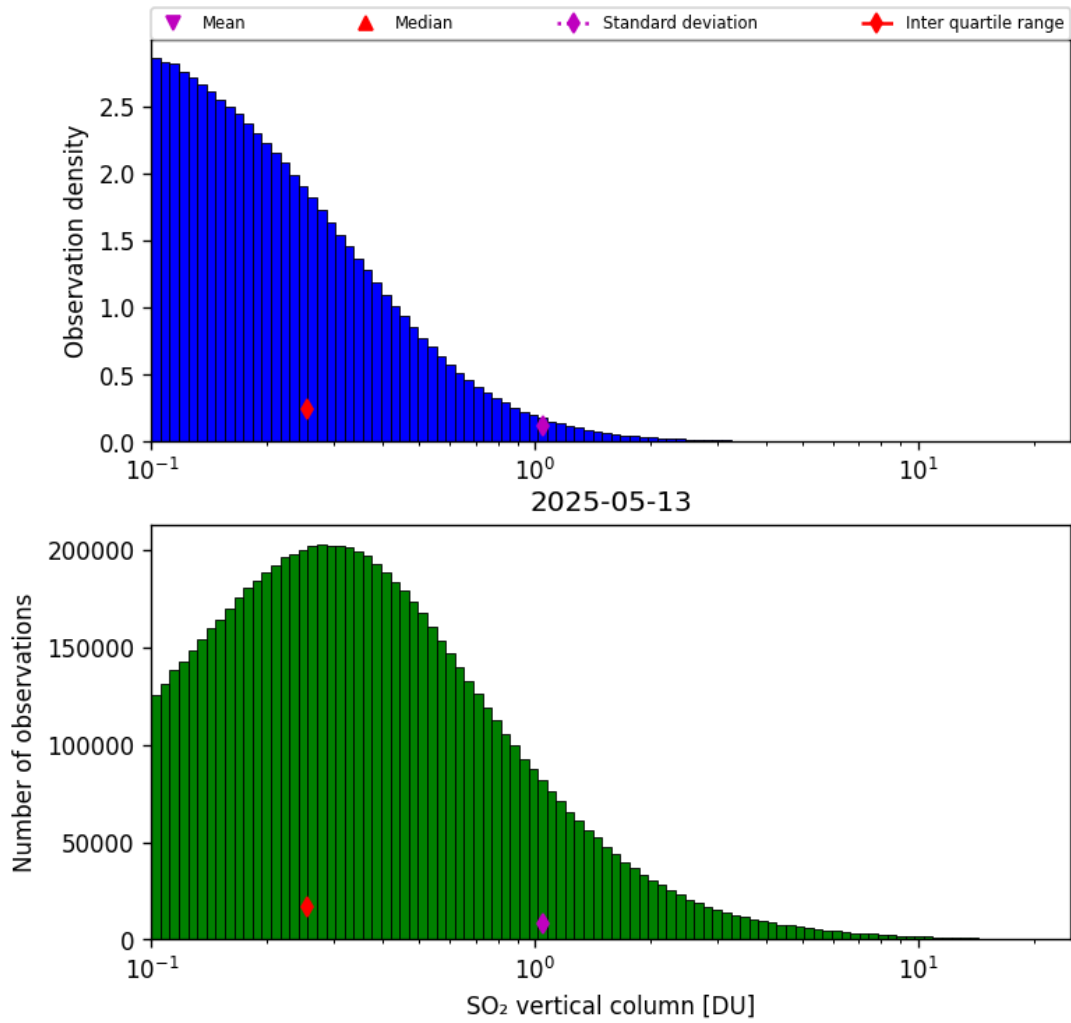
Figure 58: Histogram of “SO 2 vertical column” for 2025-05-12 to 2025-05-14
