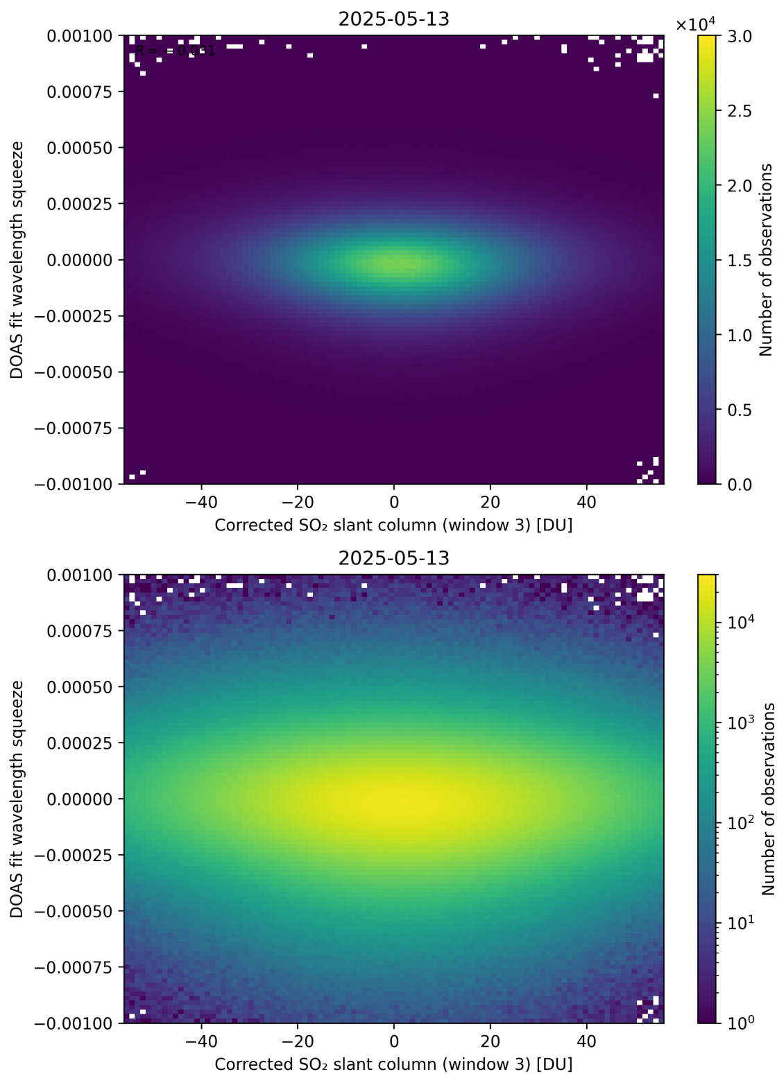
Figure 257: Scatter density plot of “Corrected SO 2 slant column (window 3)” against “DOAS fit wavelength squeeze” for 2025-05-12 to 2025-05-14.
