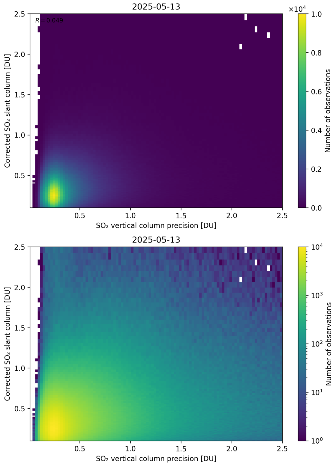
Figure 338: Scatter density plot of “SO 2 vertical column precision” against “Corrected SO 2 slant column” for 2025-05-12 to 2025-05-14.
