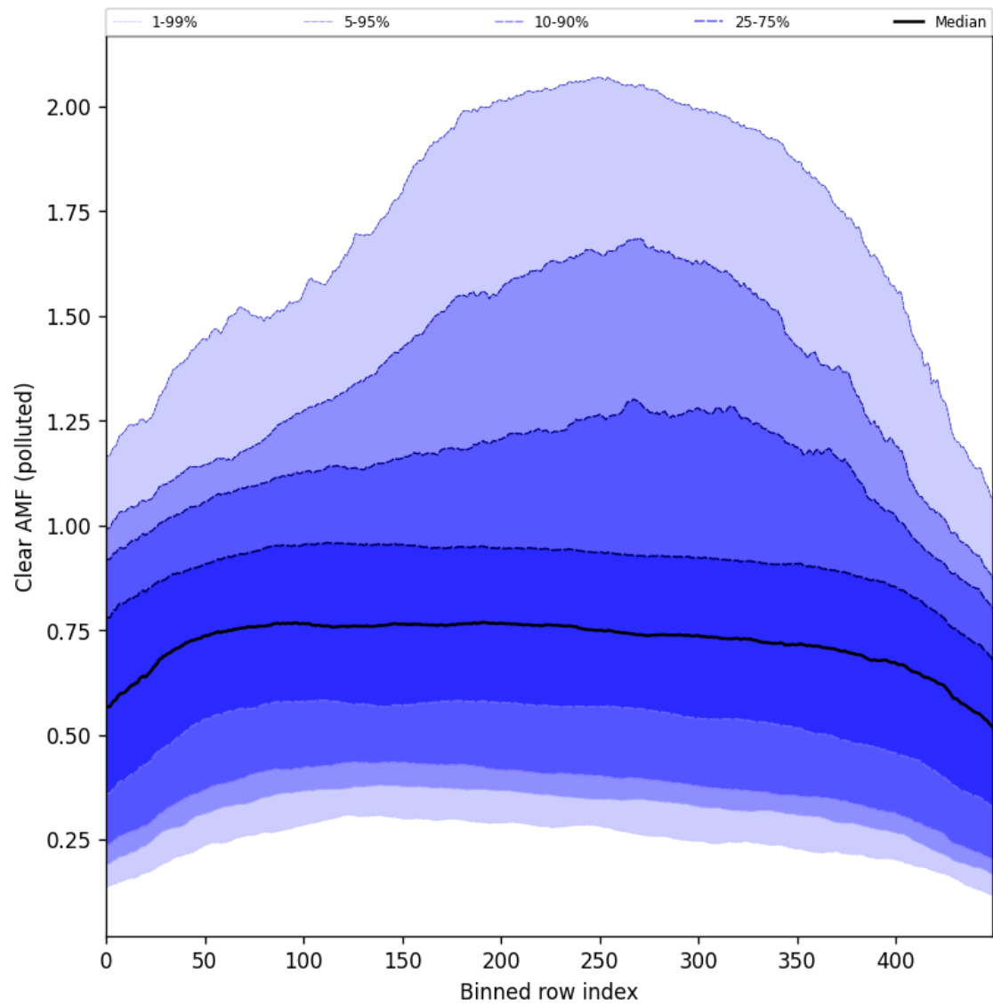
Figure 107: Along track statistics of “Clear AMF (polluted)” for 2025-05-12 to 2025-05-14
