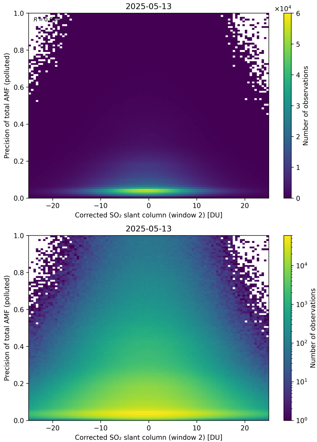
Figure 254: Scatter density plot of “Corrected SO 2 slant column (window 2)” against “Precision of total AMF (polluted)” for 2025-05-12 to 2025-05-14.
