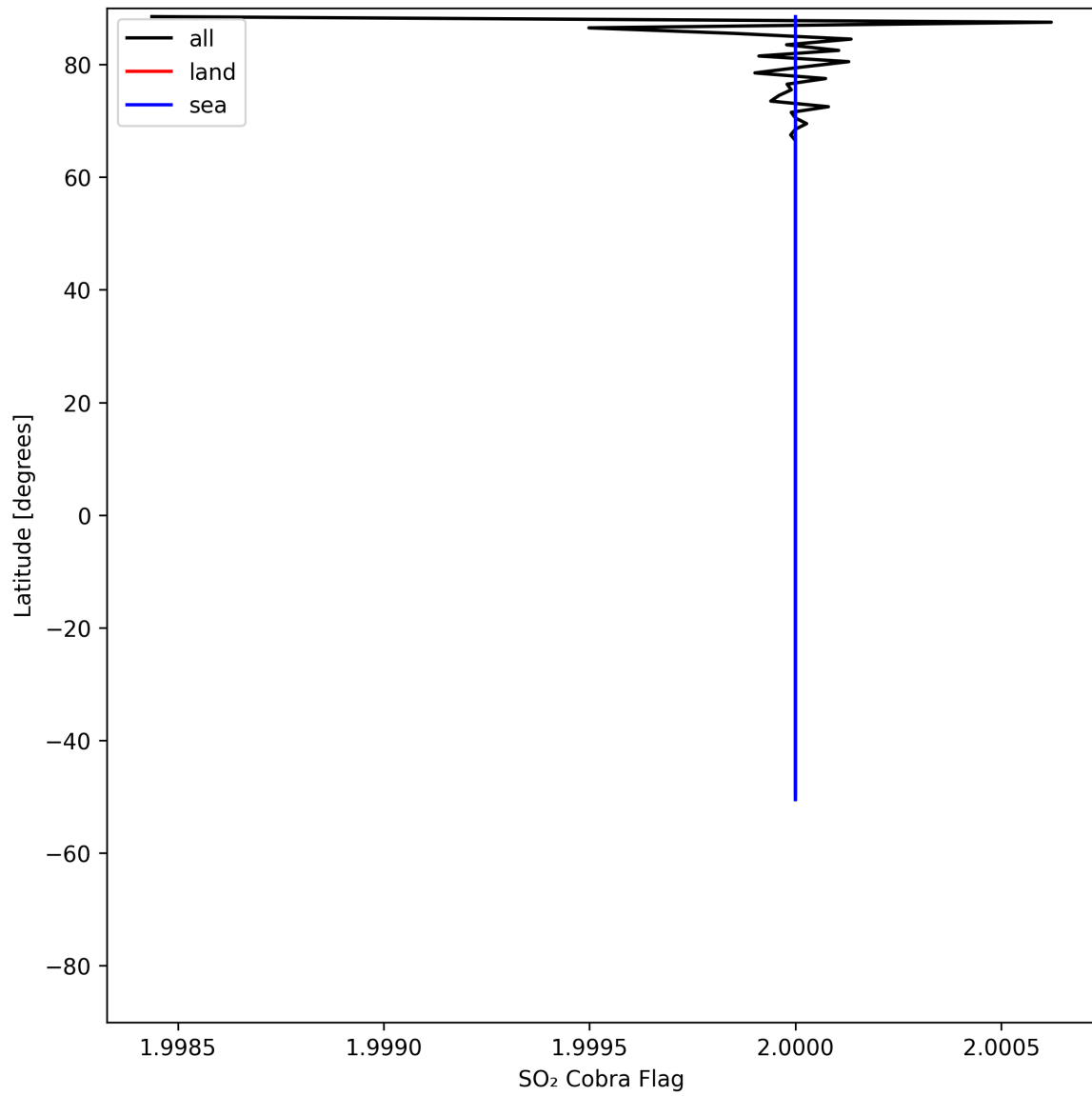
Figure 49: Zonal average of “SO 2 Cobra Flag” for 2025-05-12 to 2025-05-14.
