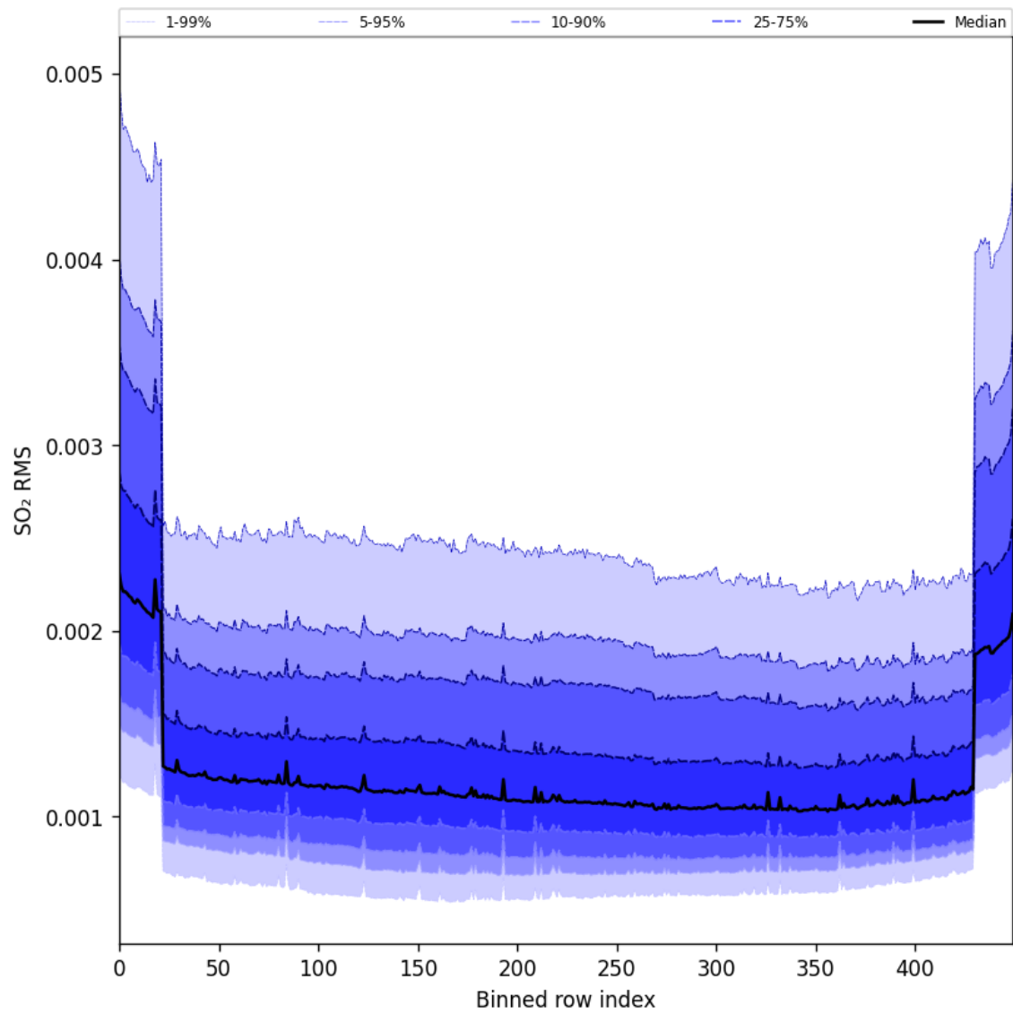
Figure 104: Along track statistics of “SO 2 RMS” for 2025-05-12 to 2025-05-14
