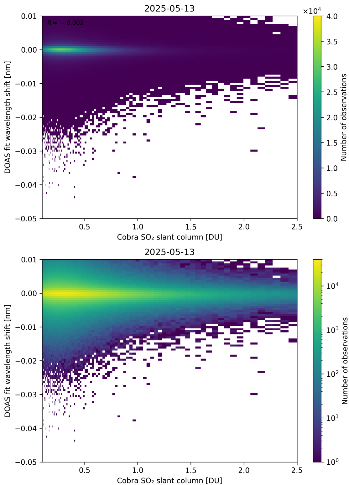
Figure 196: Scatter density plot of “Cobra SO 2 slant column” against “DOAS fit wavelength shift” for 2025-05-12 to 2025-05-14.
