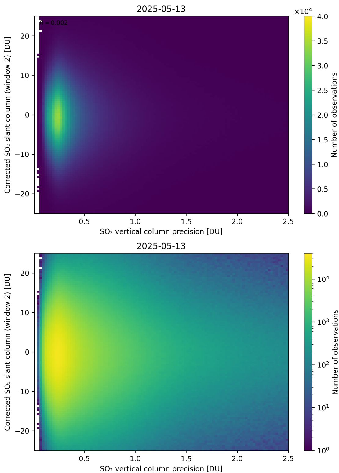
Figure 339: Scatter density plot of “SO 2 vertical column precision” against “Corrected SO 2 slant column (window 2)” for 2025-05-12 to 2025-05-14.
