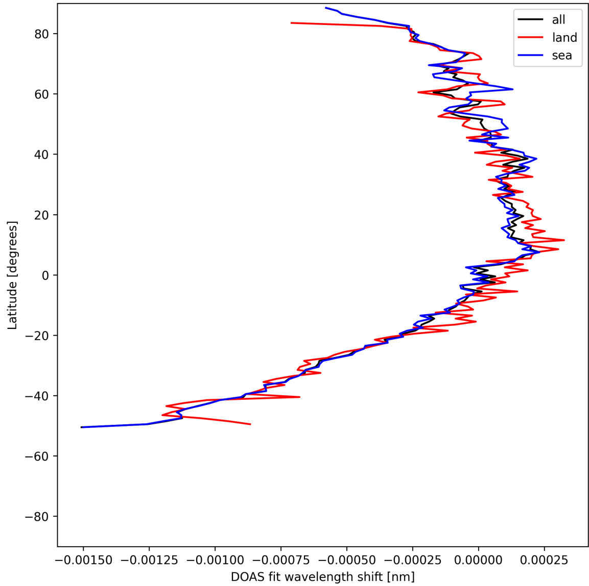
Figure 50: Zonal average of “DOAS fit wavelength shift” for 2025-05-12 to 2025-05-14.
