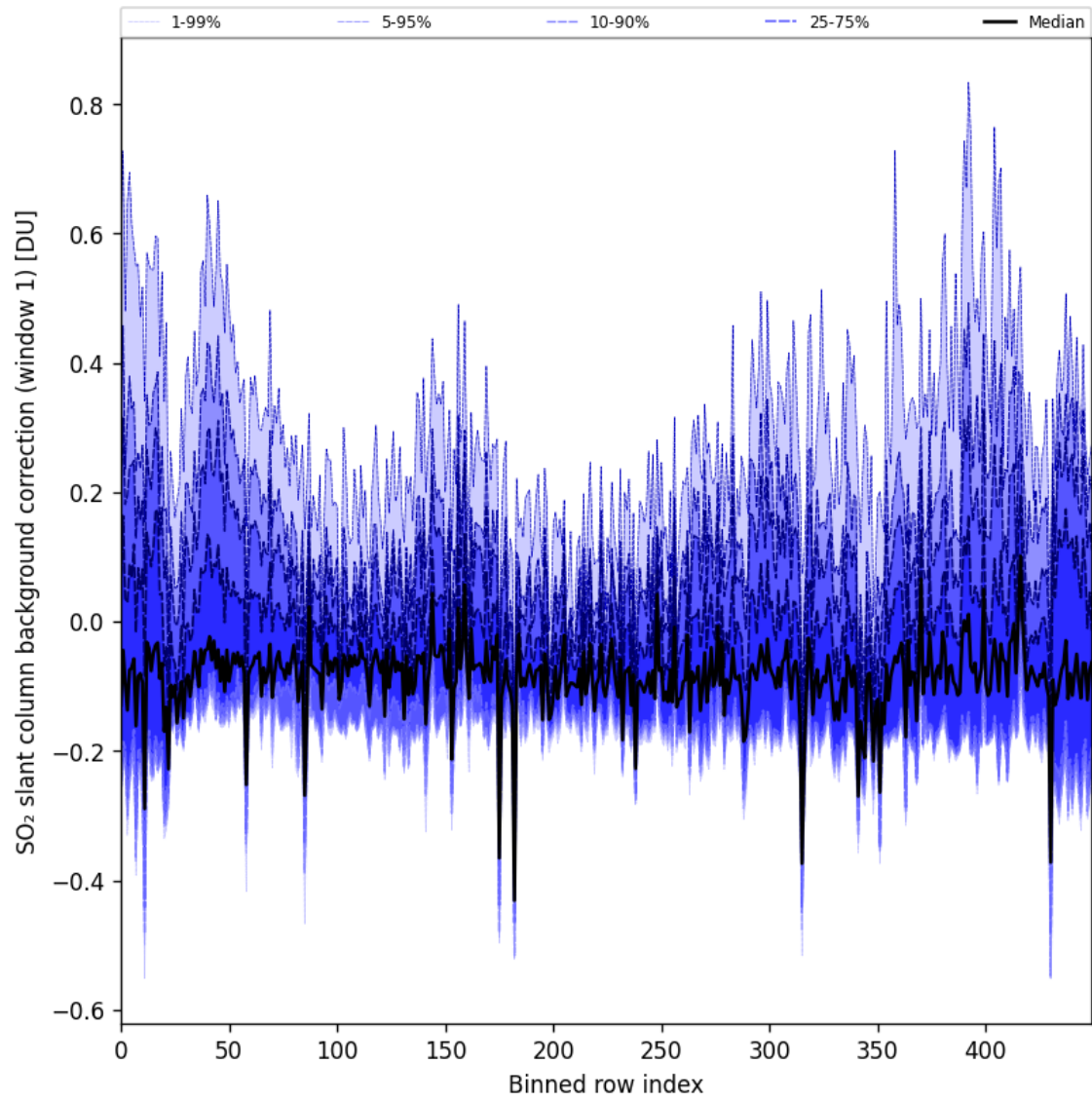
Figure 92: Along track statistics of “SO 2 slant column background correction (window 1)” for 2025-05-12 to 2025-05-14
