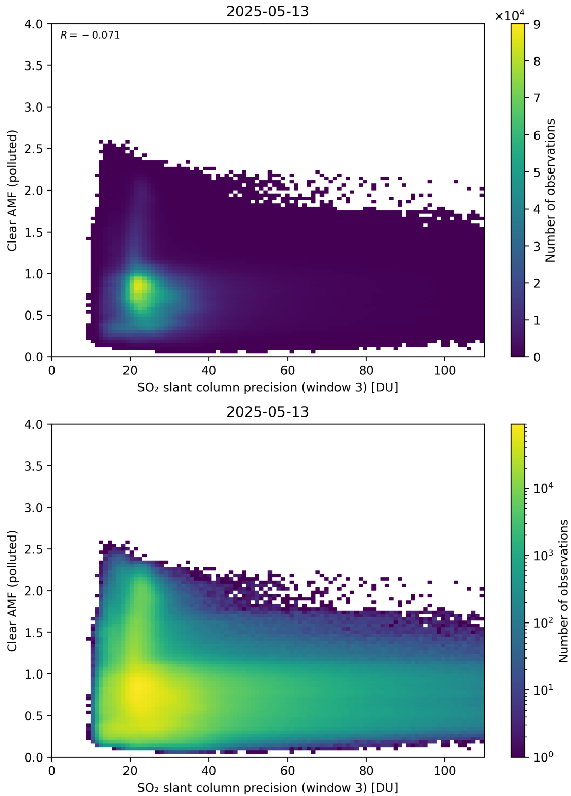
Figure 311: Scatter density plot of “SO 2 slant column precision (window 3)” against “Clear AMF (polluted)” for 2025-05-12 to 2025-05-14.
