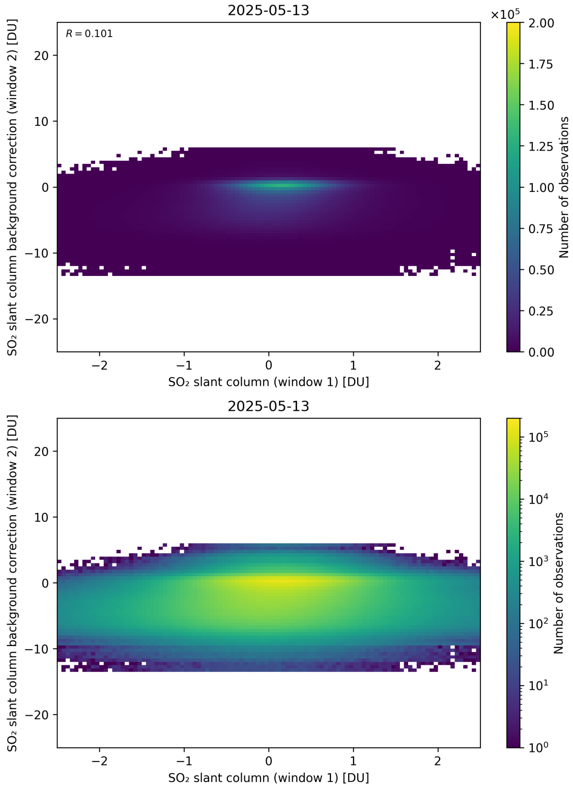
Figure 263: Scatter density plot of “SO 2 slant column (window 1)” against “SO 2 slant column background correction (window 2)” for 2025-05-12 to 2025-05-14.
