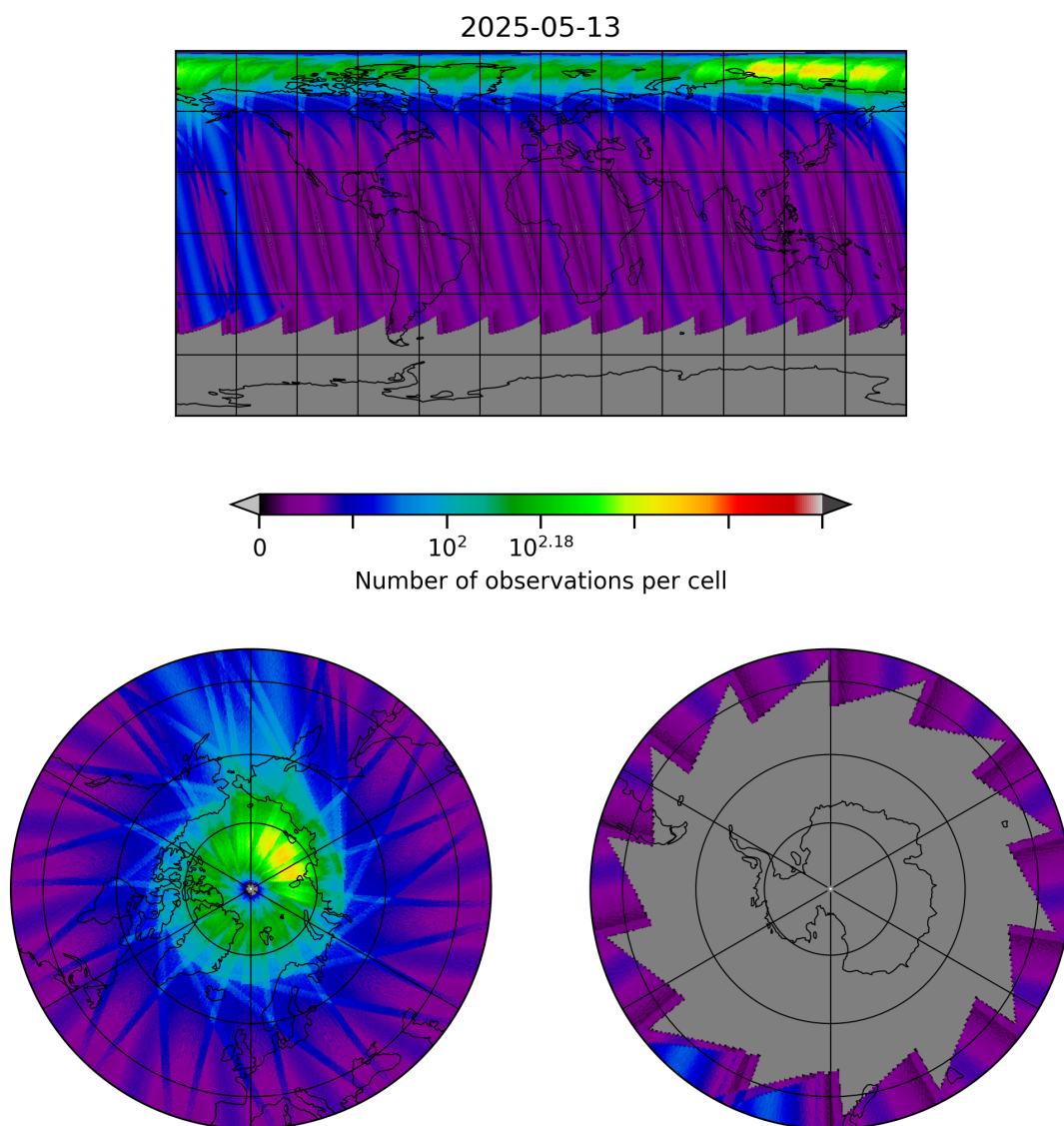
Figure 30: Map of the number of observations for 2025-05-12 to 2025-05-14
