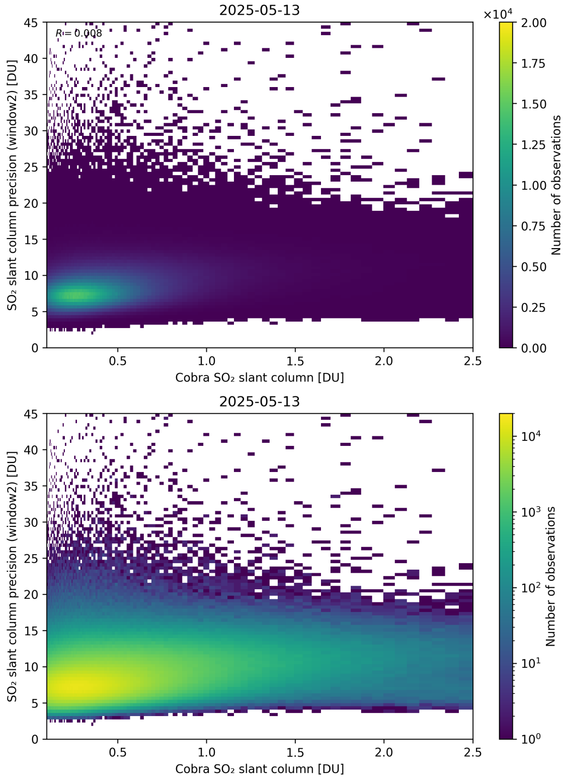
Figure 221: Scatter density plot of “Cobra SO 2 slant column” against “SO 2 slant column precision (window2)” for 2025-05-12 to 2025-05-14.
