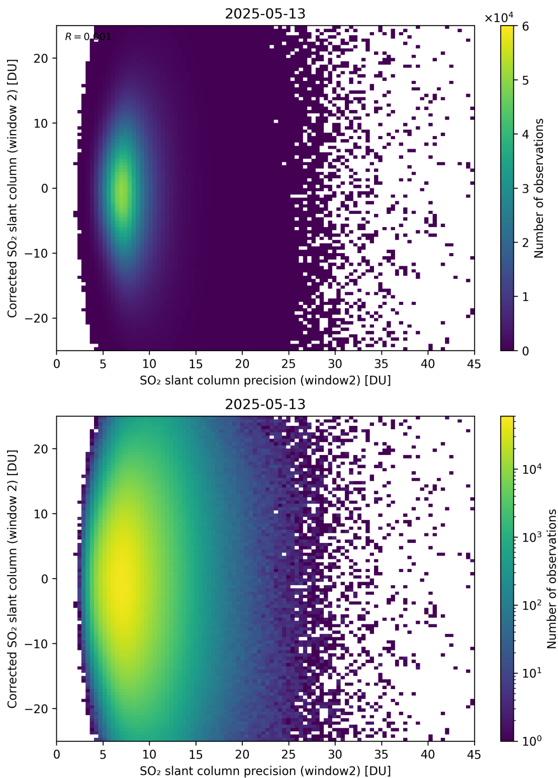
Figure 297: Scatter density plot of “SO 2 slant column precision (window2)” against “Corrected SO 2 slant column (window 2)” for 2025-05-12 to 2025-05-14.
