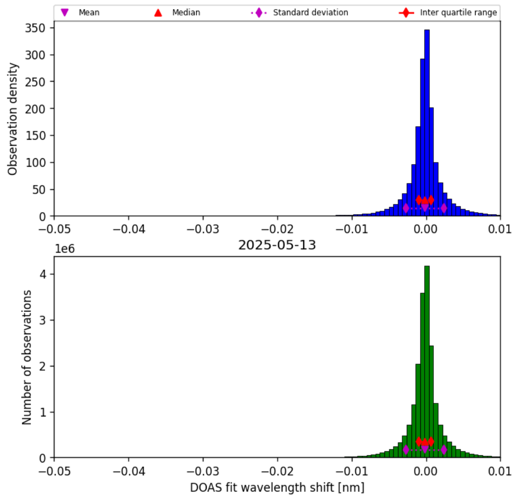
Figure 76: Histogram of “DOAS fit wavelength shift” for 2025-05-12 to 2025-05-14
