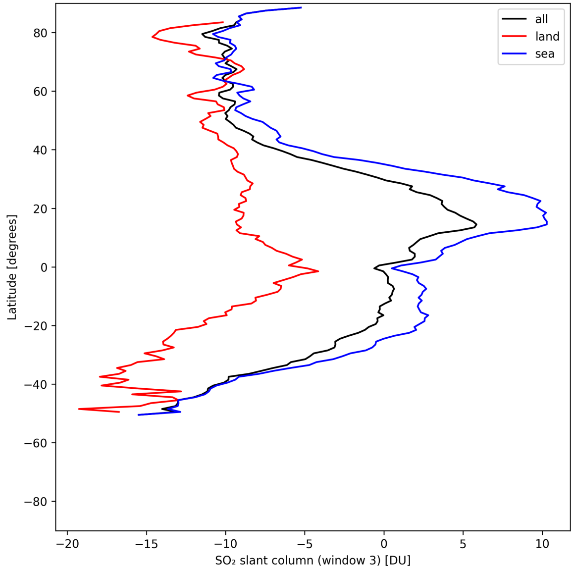
Figure 45: Zonal average of “SO 2 slant column (window 3)” for 2025-05-12 to 2025-05-14.
