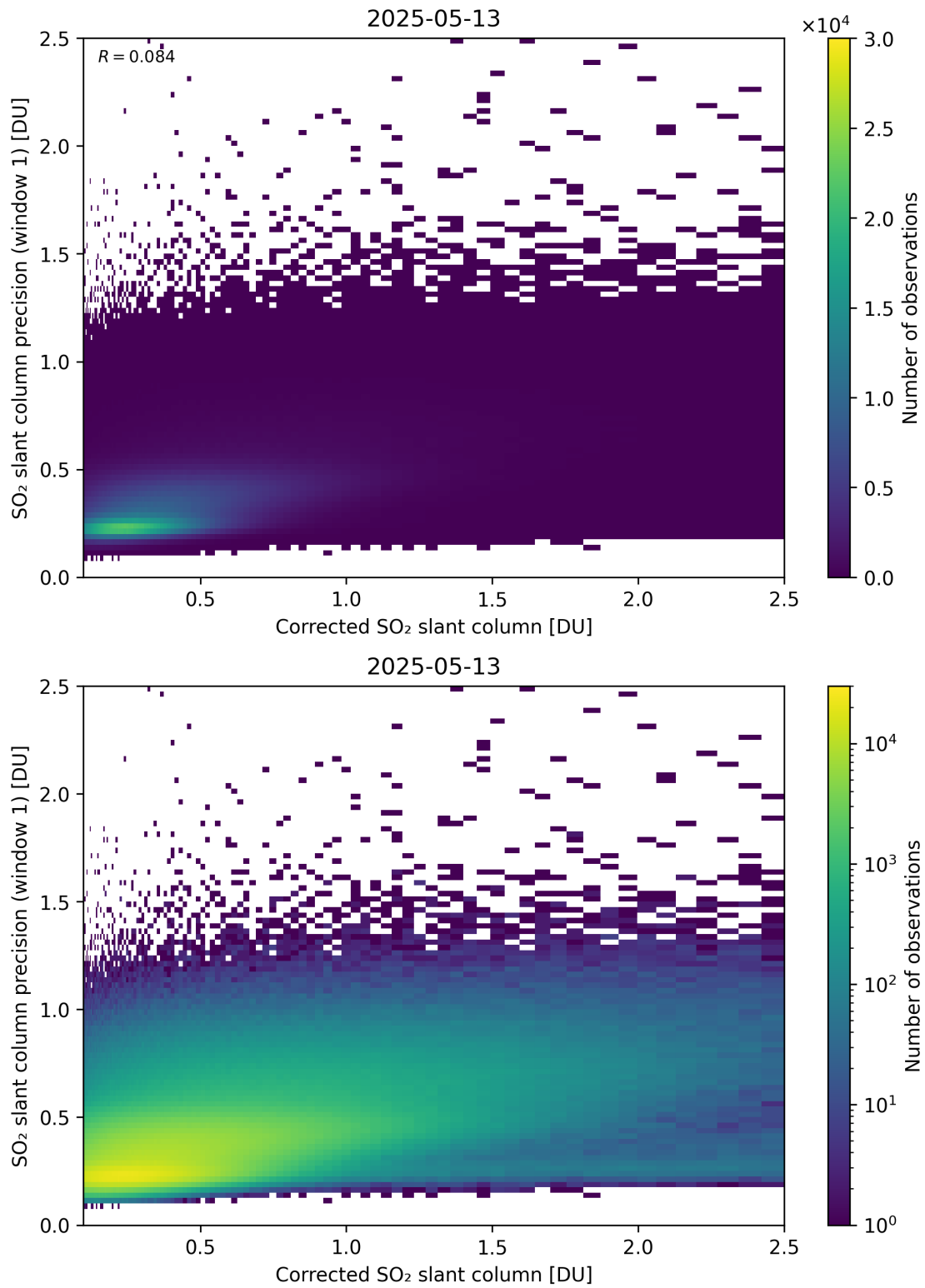
Figure 238: Scatter density plot of “Corrected SO 2 slant column” against “SO 2 slant column precision (window 1)” for 2025-05-12 to 2025-05-14.
