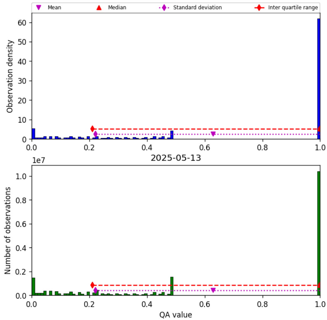
Figure 57: Histogram of “QA value” for 2025-05-12 to 2025-05-14
