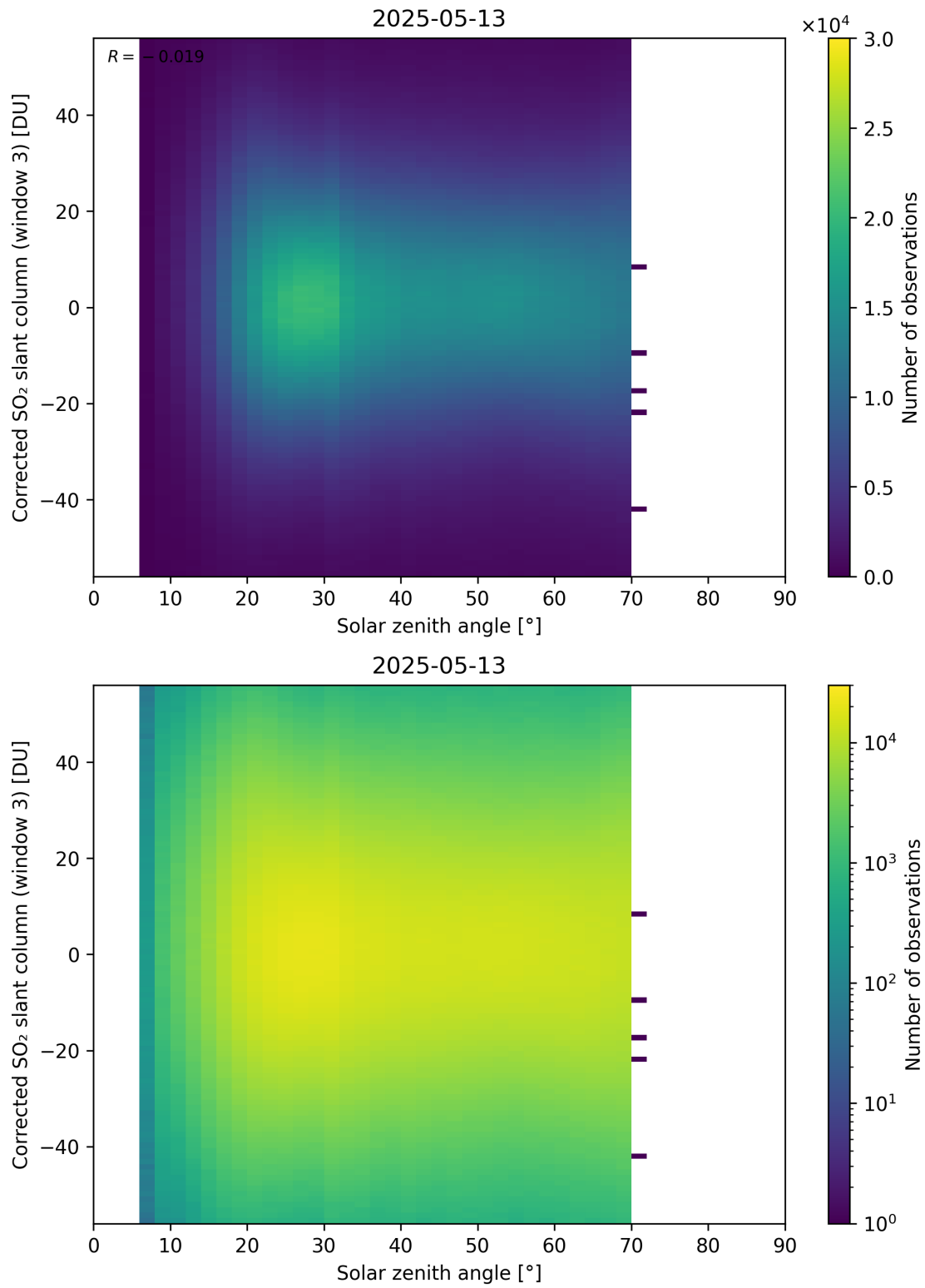
Figure 183: Scatter density plot of “Solar zenith angle” against “Corrected SO 2 slant column (window 3)” for 2025-05-12 to 2025-05-14.
