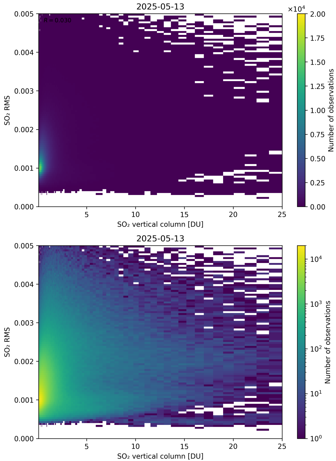
Figure 328: Scatter density plot of “SO 2 vertical column” against “SO 2 RMS” for 2025-05-12 to 2025-05-14.
