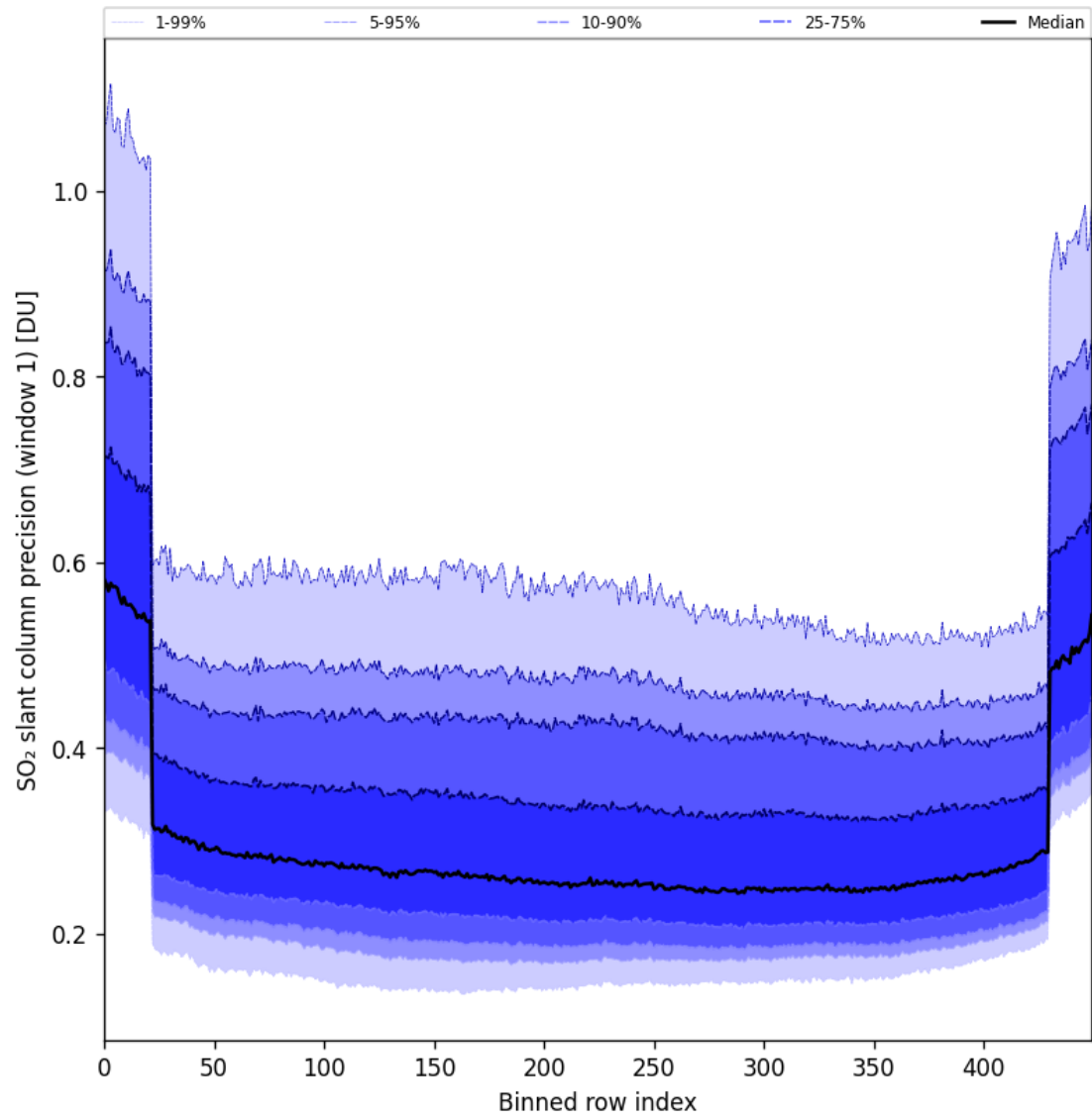
Figure 90: Along track statistics of “SO 2 slant column precision (window 1)” for 2025-05-12 to 2025-05-14
