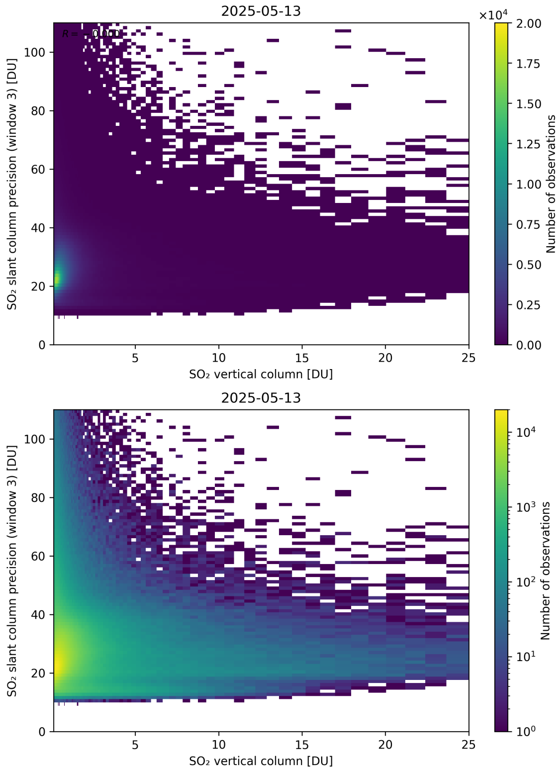
Figure 358: Scatter density plot of “SO 2 vertical column” against “SO 2 slant column precision (window 3)” for 2025-05-12 to 2025-05-14.
