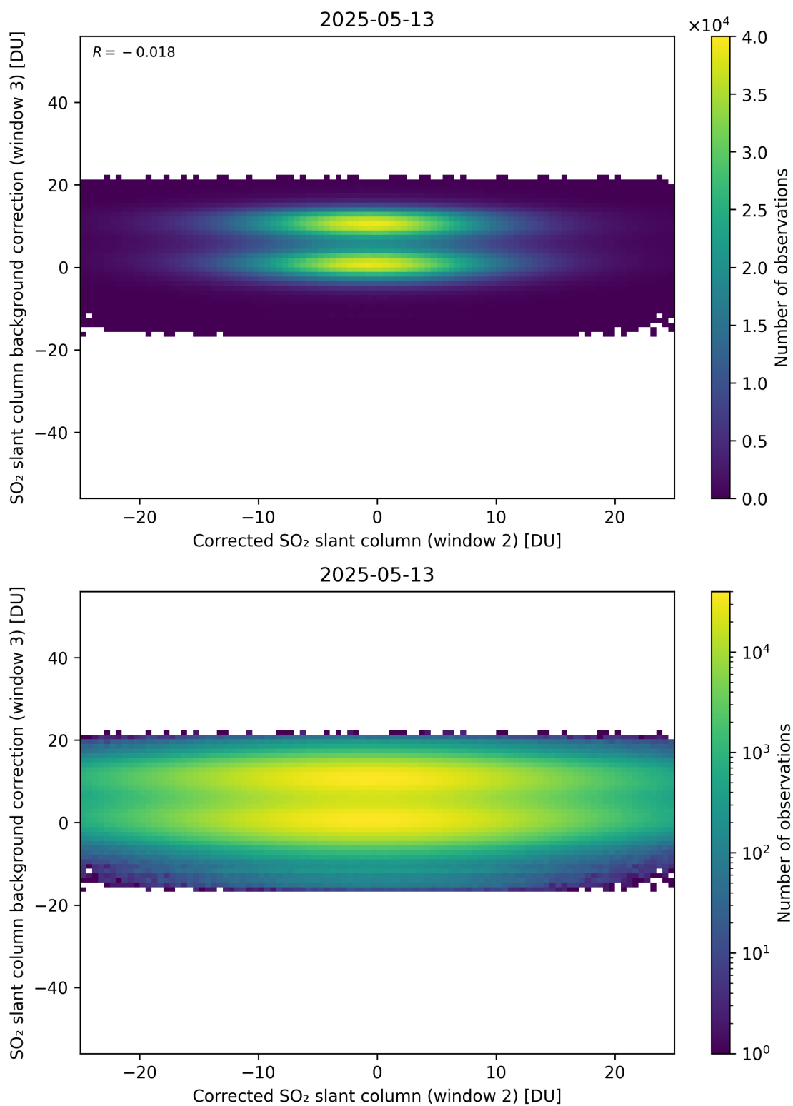
Figure 245: Scatter density plot of “Corrected SO 2 slant column (window 2)” against “SO 2 slant column background correction (window 3)” for 2025-05-12 to 2025-05-14.
