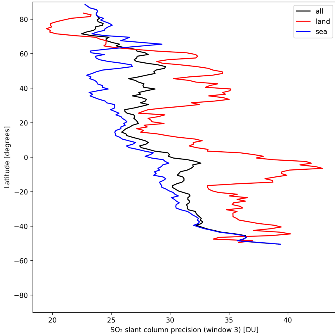
Figure 46: Zonal average of “SO 2 slant column precision (window 3)” for 2025-05-12 to 2025-05-14.
