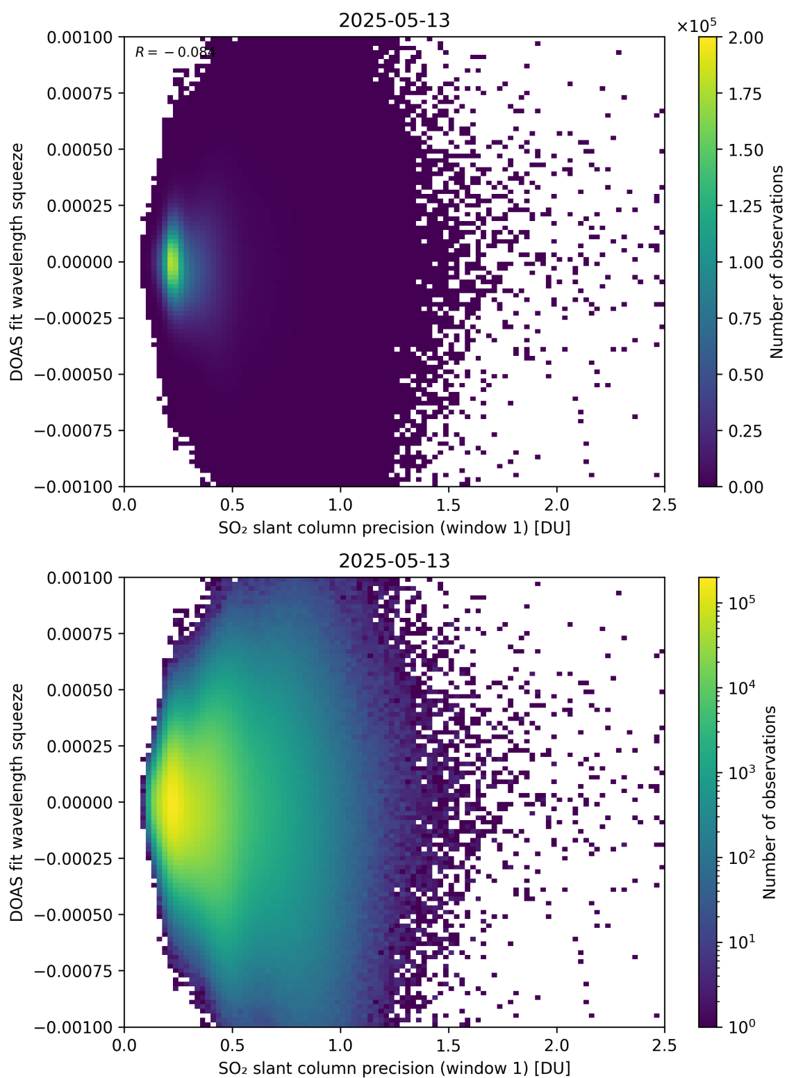
Figure 272: Scatter density plot of “SO 2 slant column precision (window 1)” against “DOAS fit wavelength squeeze” for 2025-05-12 to 2025-05-14.
