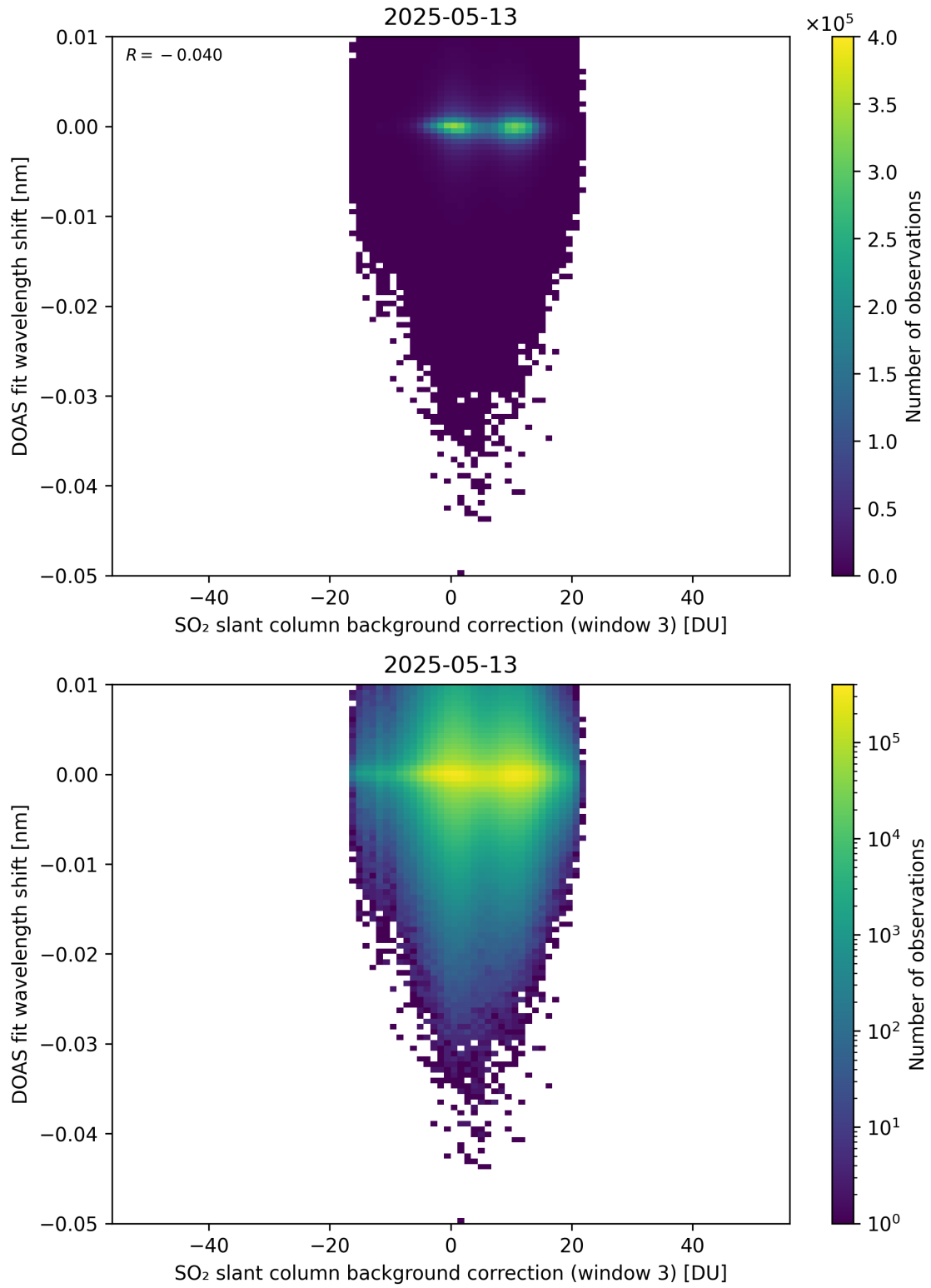
Figure 132: Scatter density plot of “SO 2 slant column background correction (window 3)” against “DOAS fit wavelength shift” for 2025-05-12 to 2025-05-14.
