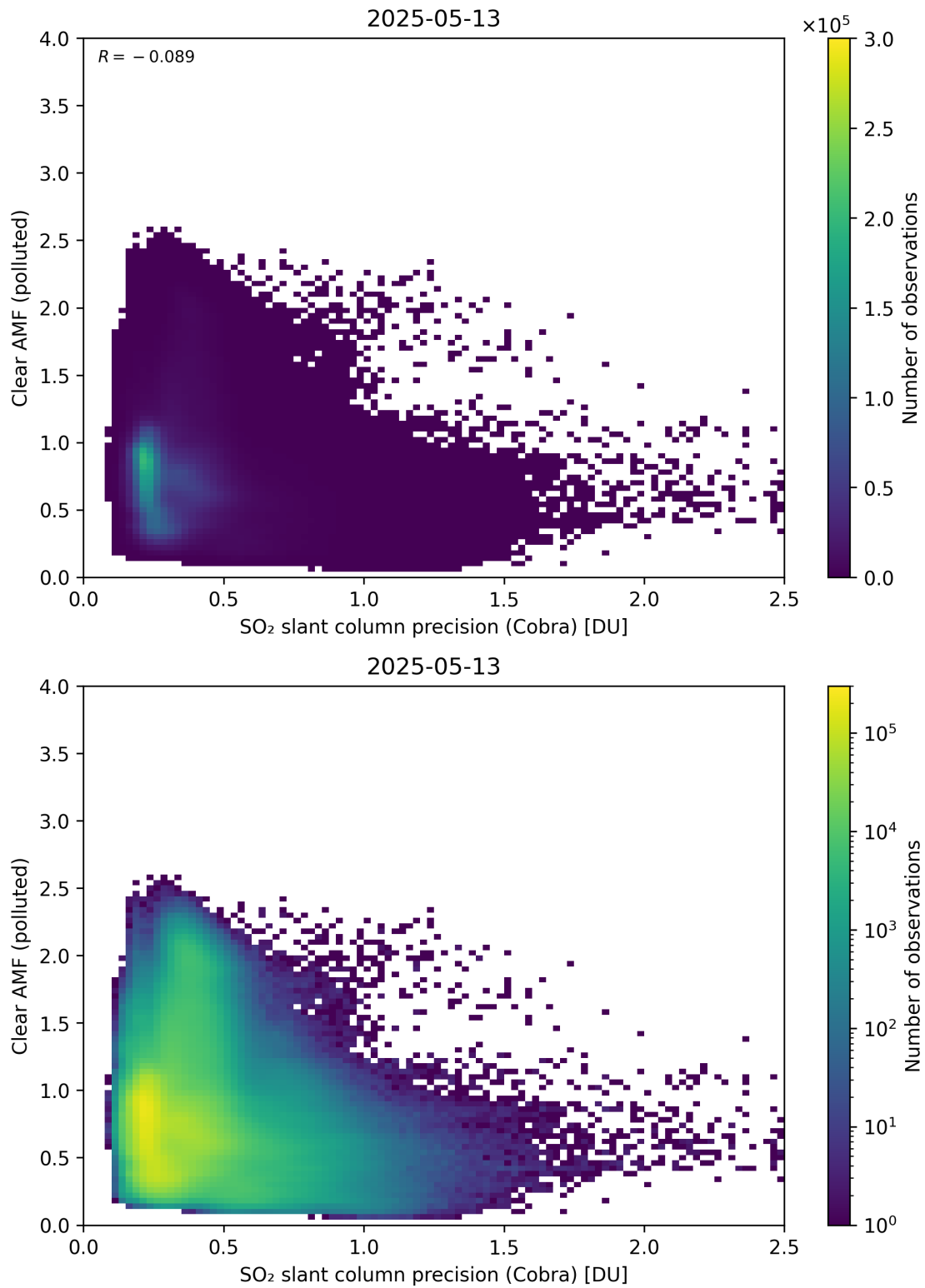
Figure 205: Scatter density plot of “SO 2 slant column precision (Cobra)” against “Clear AMF (polluted)” for 2025-05-12 to 2025-05-14.
