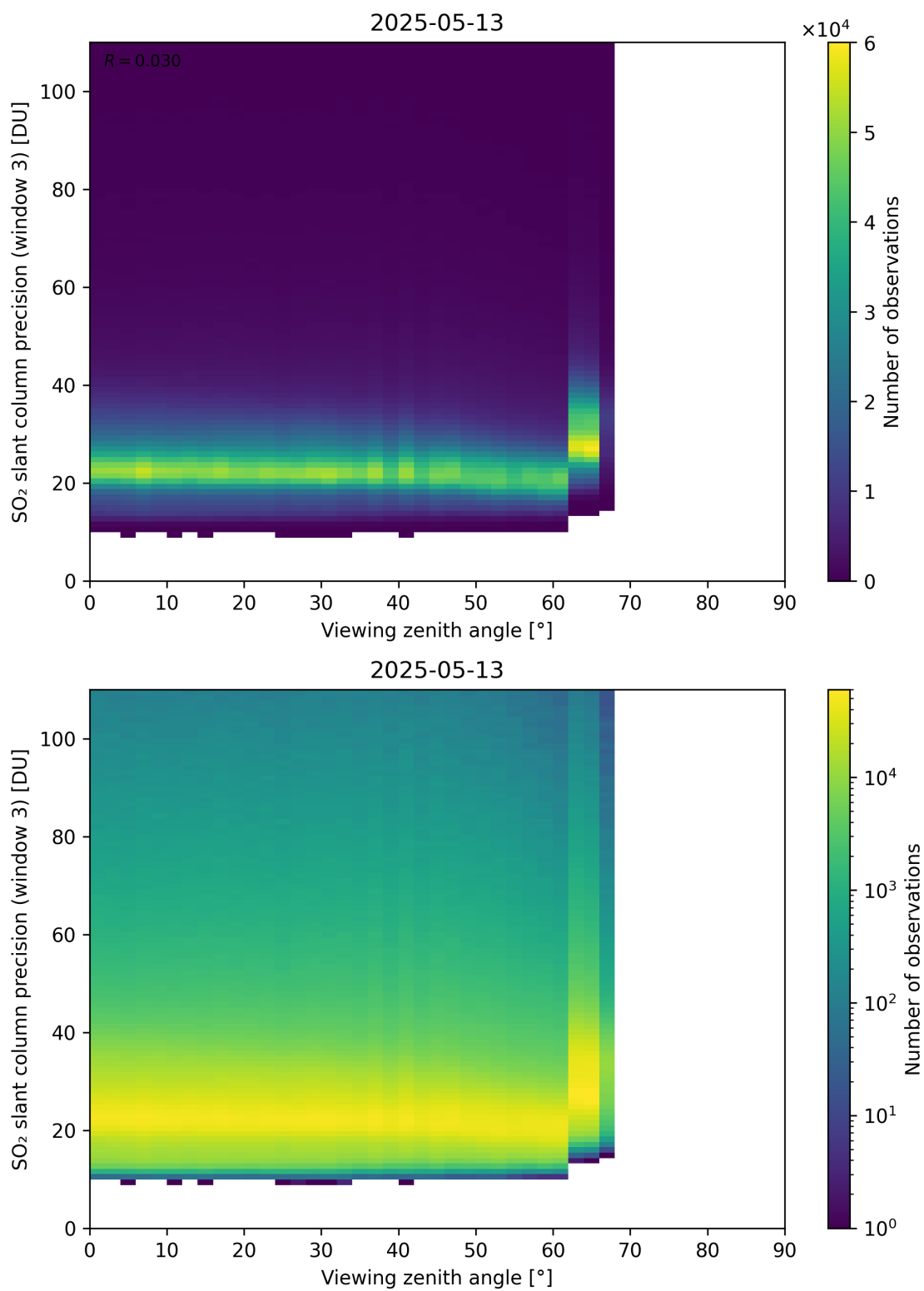
Figure 380: Scatter density plot of “Viewing zenith angle” against “SO 2 slant column precision (window 3)” for 2025-05-12 to 2025-05-14.
