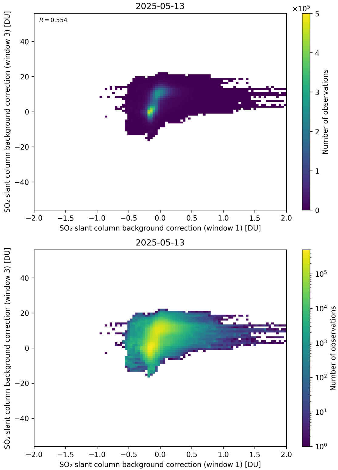
Figure 110: Scatter density plot of “SO 2 slant column background correction (window 1)” against “SO 2 slant column background correction (window 3)” for 2025-05-12 to 2025-05-14.
