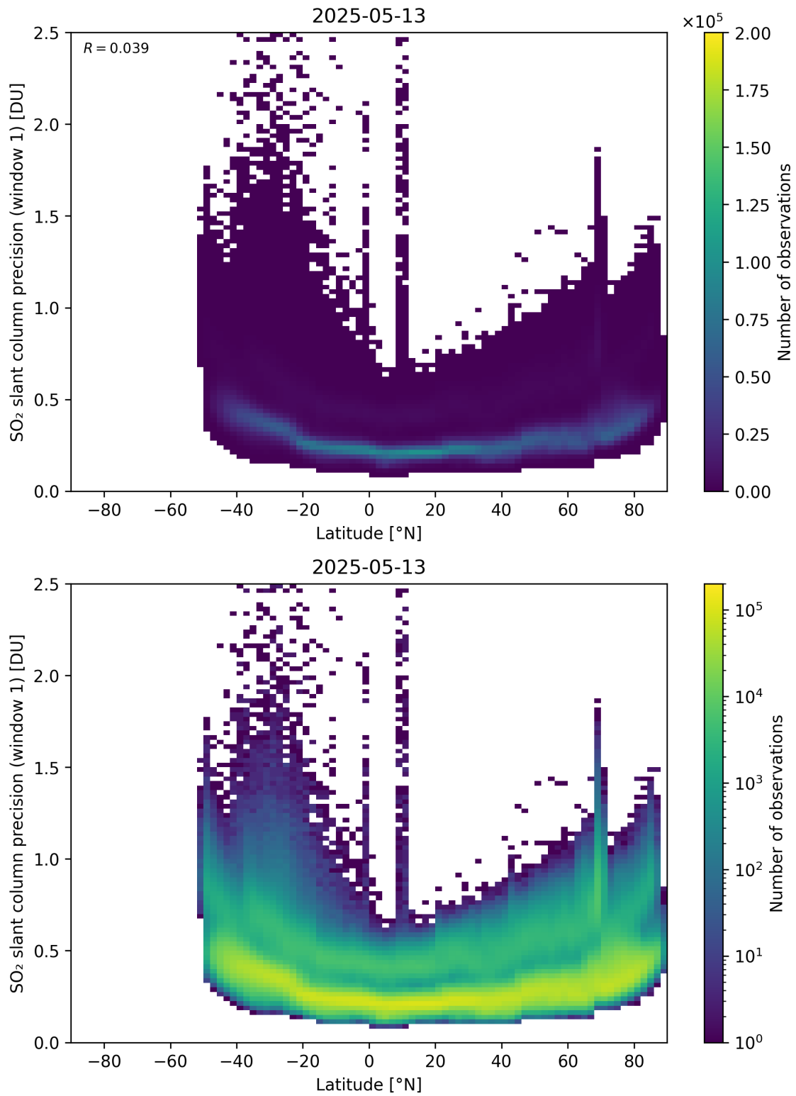
Figure 163: Scatter density plot of “Latitude” against “SO 2 slant column precision (window 1)” for 2025-05-12 to 2025-05-14.
