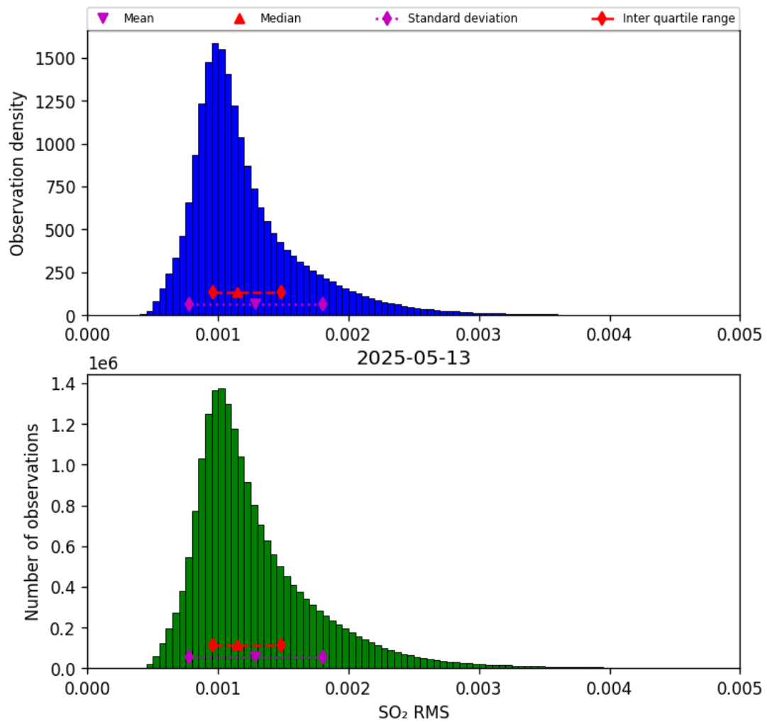
Figure 78: Histogram of “SO 2 RMS” for 2025-05-12 to 2025-05-14
