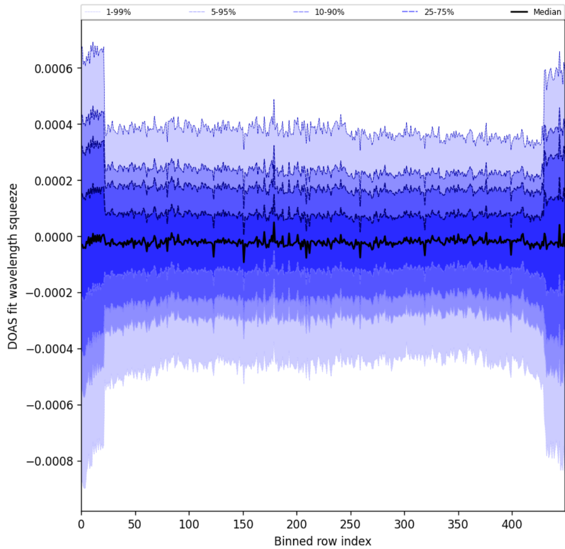
Figure 103: Along track statistics of “DOAS fit wavelength squeeze” for 2025-05-12 to 2025-05-14
