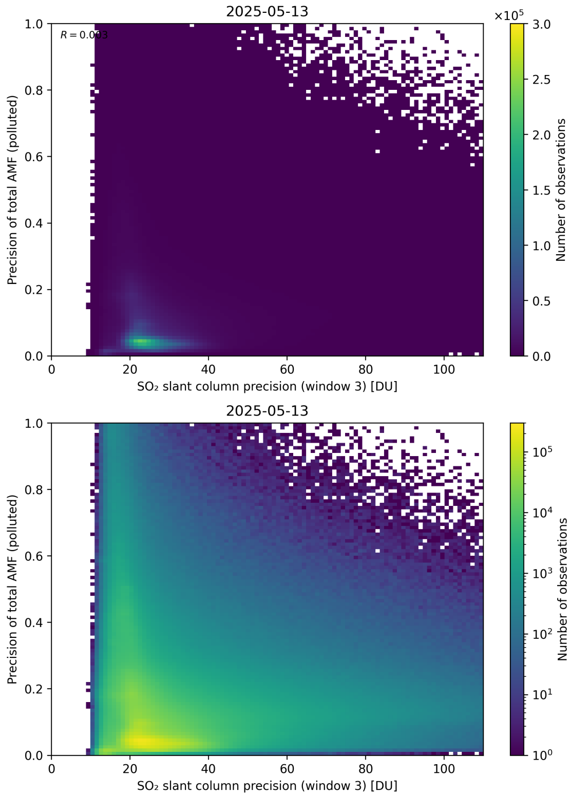
Figure 314: Scatter density plot of “SO 2 slant column precision (window 3)” against “Precision of total AMF (polluted)” for 2025-05-12 to 2025-05-14.
