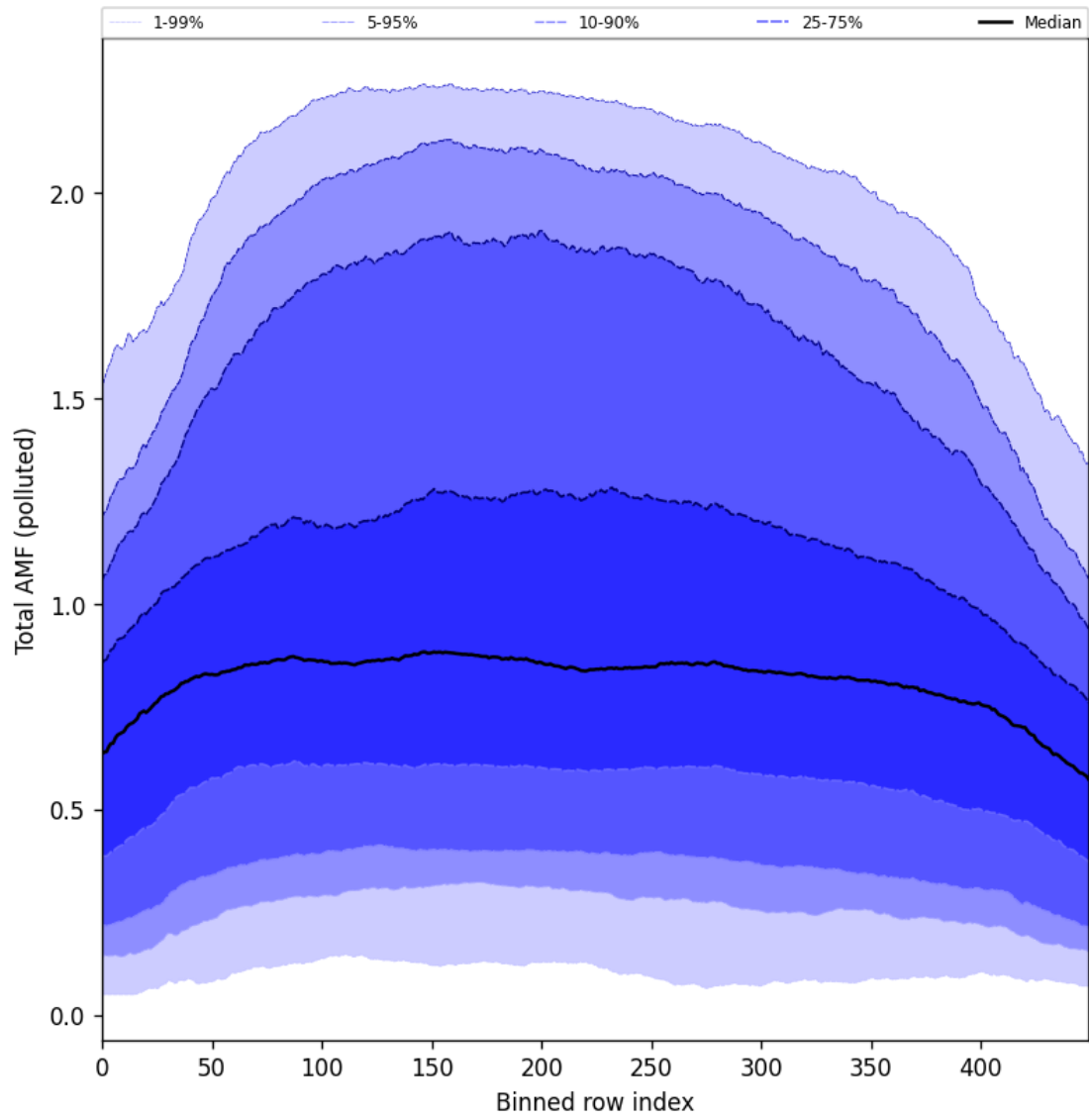
Figure 105: Along track statistics of “Total AMF (polluted)” for 2025-05-12 to 2025-05-14
