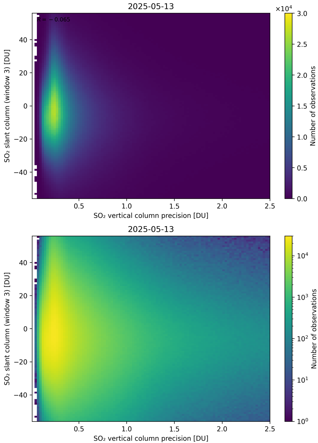
Figure 344: Scatter density plot of “SO 2 vertical column precision” against “SO 2 slant column (window 3)” for 2025-05-12 to 2025-05-14.
