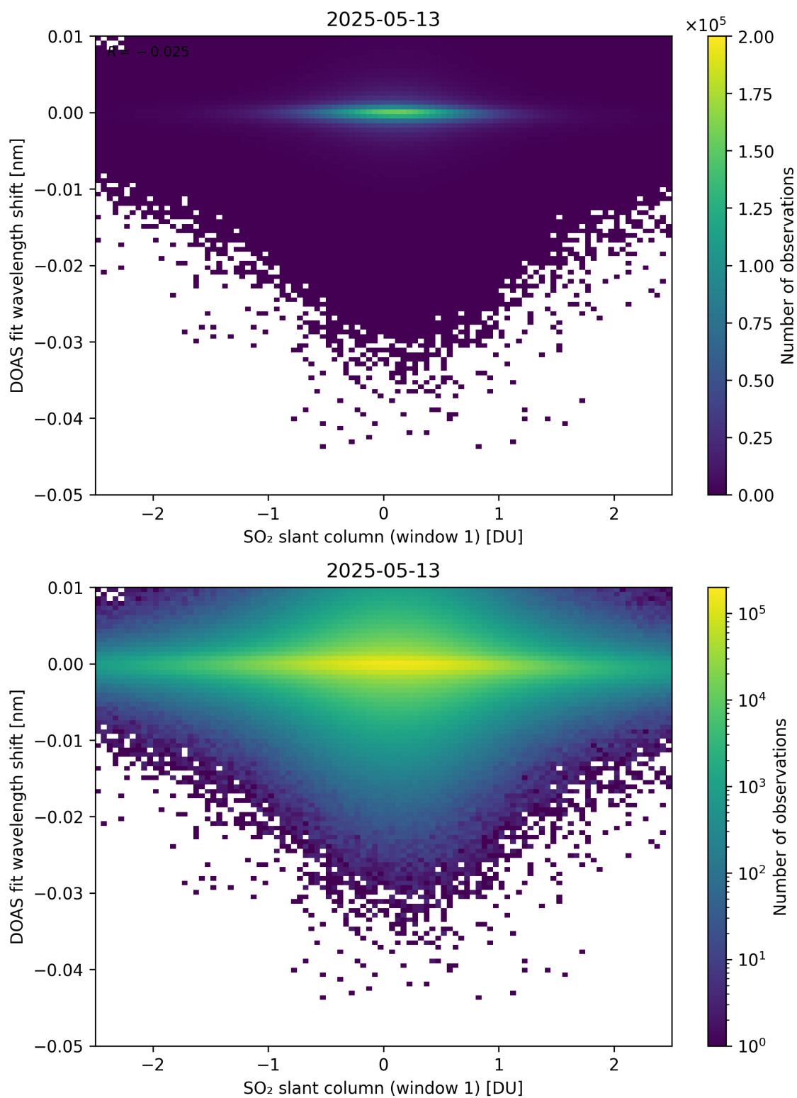
Figure 265: Scatter density plot of “SO 2 slant column (window 1)” against “DOAS fit wavelength shift” for 2025-05-12 to 2025-05-14.
