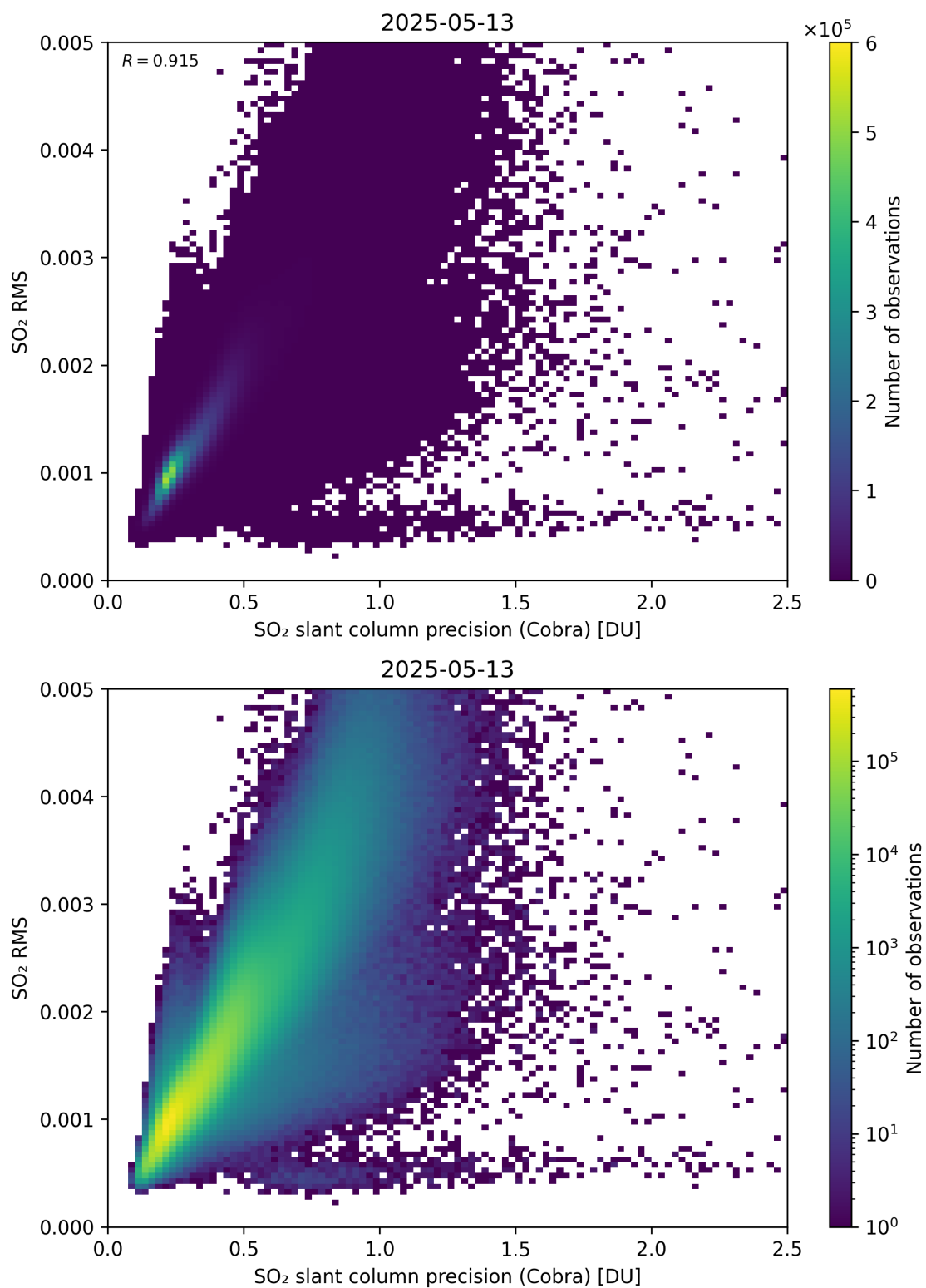
Figure 204: Scatter density plot of “SO 2 slant column precision (Cobra)” against “SO 2 RMS” for 2025-05-12 to 2025-05-14.
