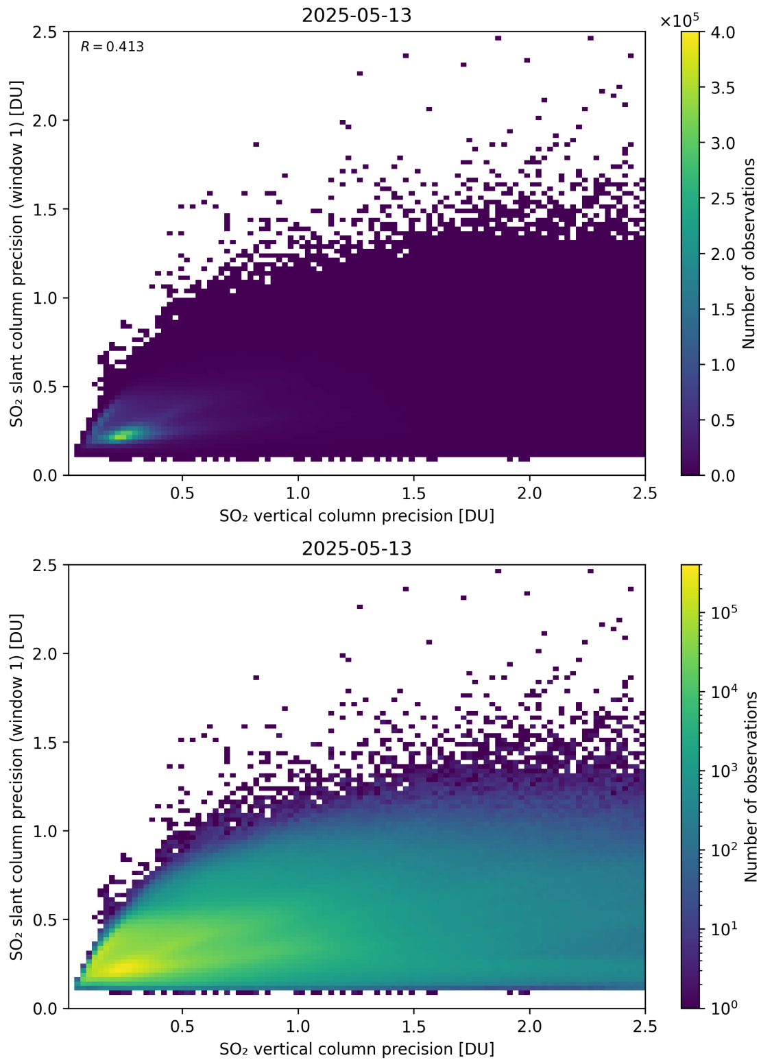
Figure 342: Scatter density plot of “SO 2 vertical column precision” against “SO 2 slant column precision (window 1)” for 2025-05-12 to 2025-05-14.
