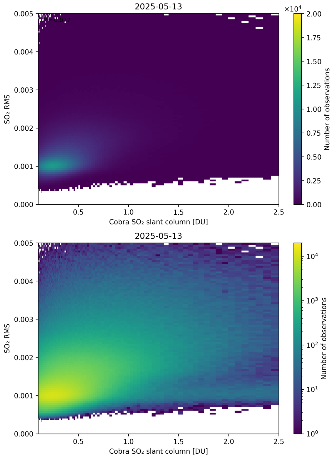
Figure 198: Scatter density plot of “Cobra SO 2 slant column” against “SO 2 RMS” for 2025-05-12 to 2025-05-14.
