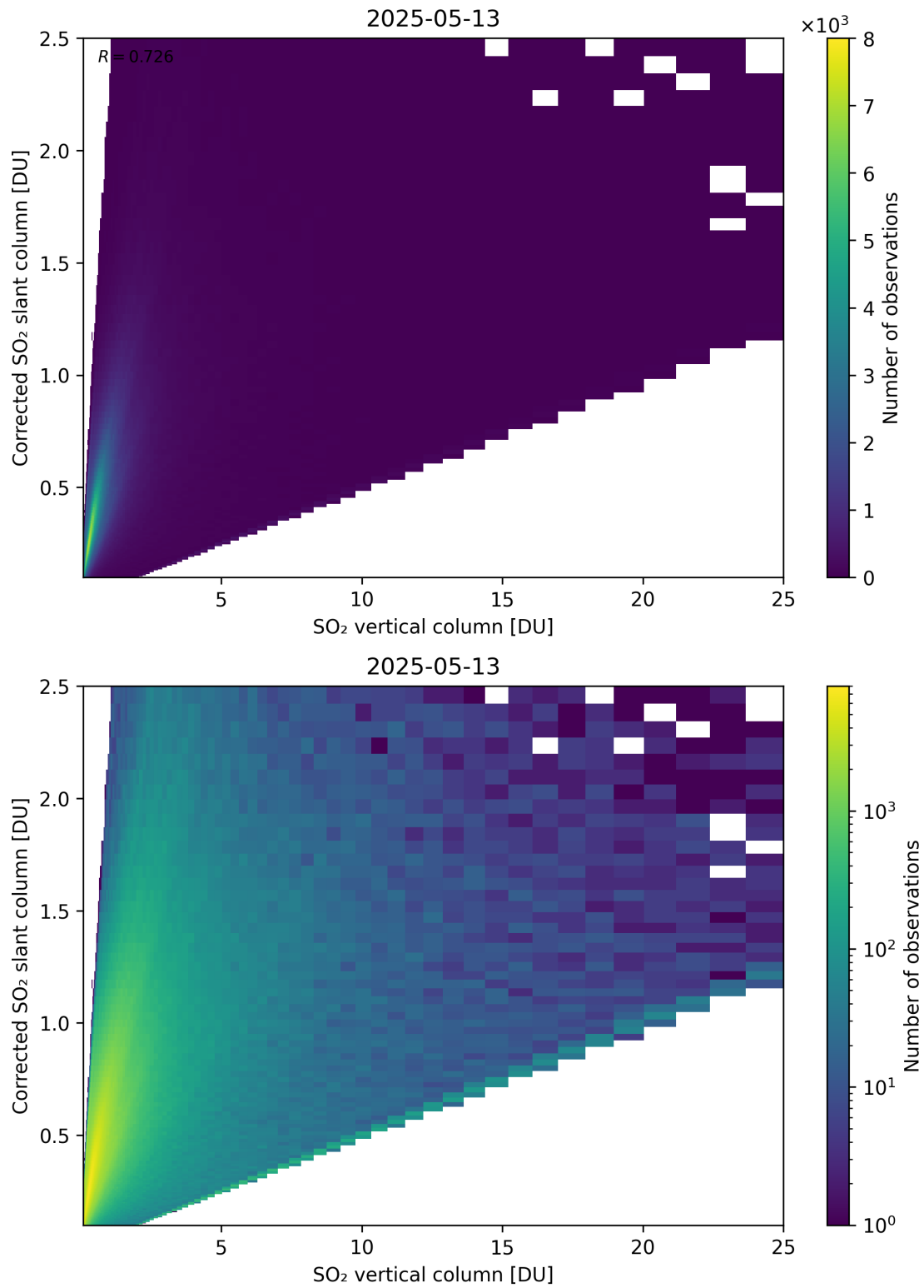
Figure 351: Scatter density plot of “SO 2 vertical column” against “Corrected SO 2 slant column” for 2025-05-12 to 2025-05-14.
