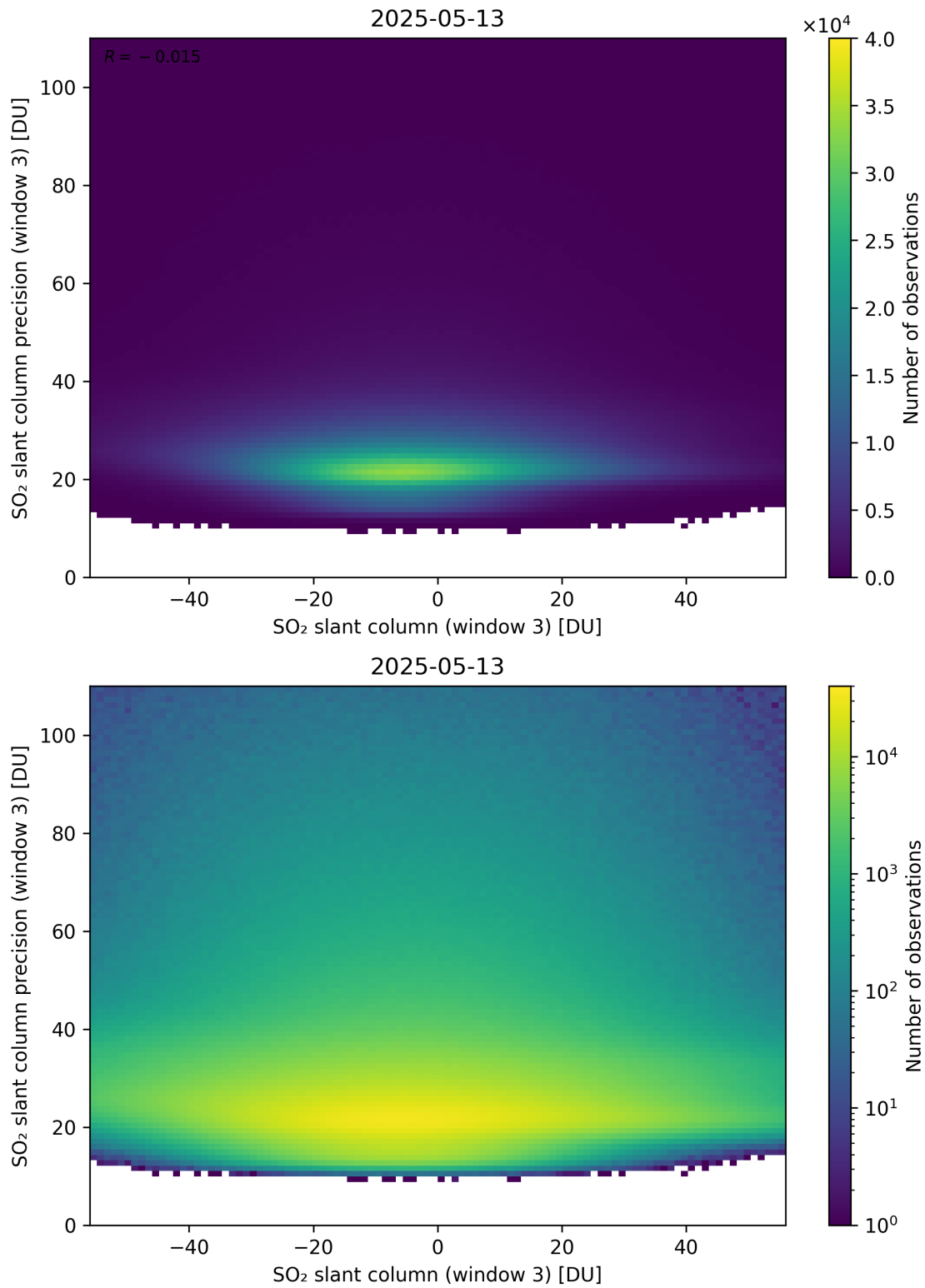
Figure 317: Scatter density plot of “SO 2 slant column (window 3)” against “SO 2 slant column precision (window 3)” for 2025-05-12 to 2025-05-14.
