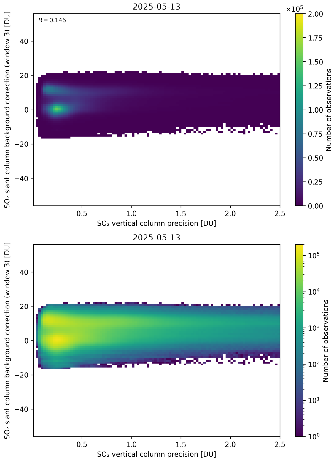
Figure 331: Scatter density plot of “SO 2 vertical column precision” against “SO 2 slant column background correction (window 3)” for 2025-05-12 to 2025-05-14.
