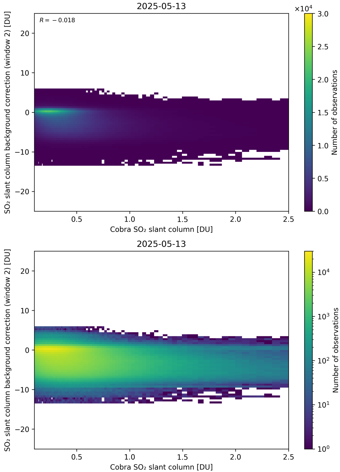
Figure 194: Scatter density plot of “Cobra SO 2 slant column” against “SO 2 slant column background correction (window 2)” for 2025-05-12 to 2025-05-14.
