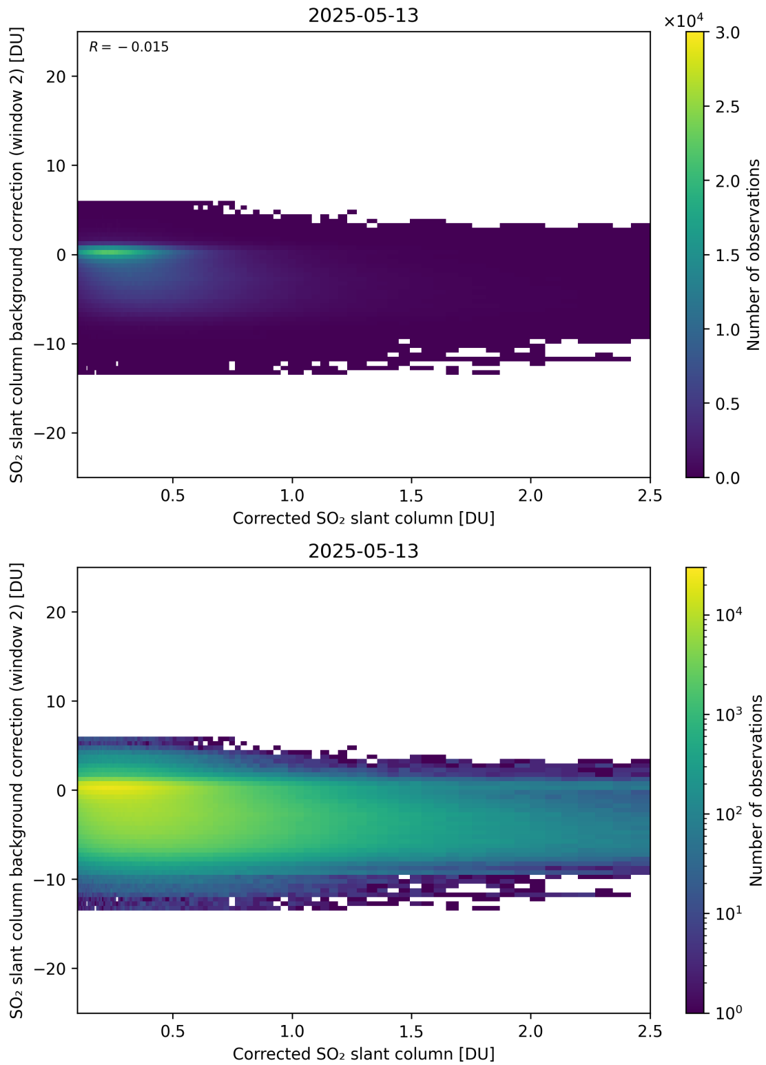
Figure 227: Scatter density plot of “Corrected SO 2 slant column” against “SO 2 slant column background correction (window 2)” for 2025-05-12 to 2025-05-14.
