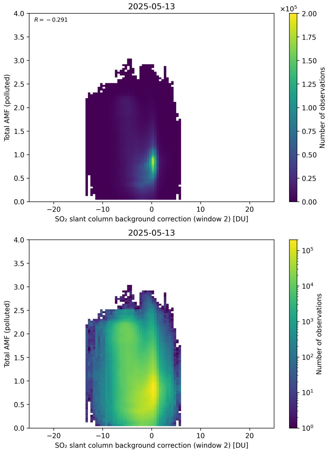
Figure 130: Scatter density plot of “SO 2 slant column background correction (window 2)” against “Total AMF (polluted)” for 2025-05-12 to 2025-05-14.
