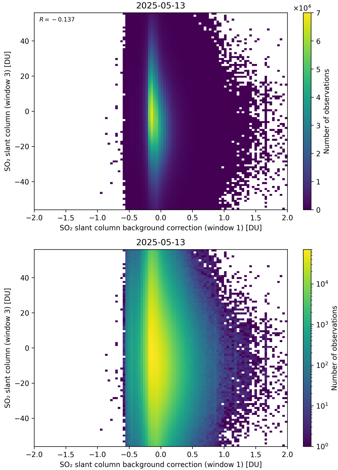
Figure 118: Scatter density plot of “SO 2 slant column background correction (window 1)” against “SO 2 slant column (window 3)” for 2025-05-12 to 2025-05-14.
