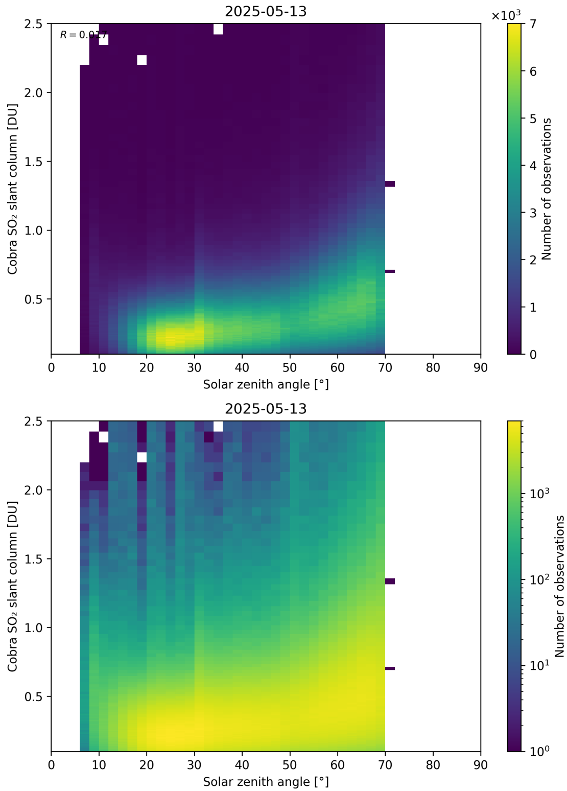
Figure 179: Scatter density plot of “Solar zenith angle” against “Cobra SO 2 slant column” for 2025-05-12 to 2025-05-14.
