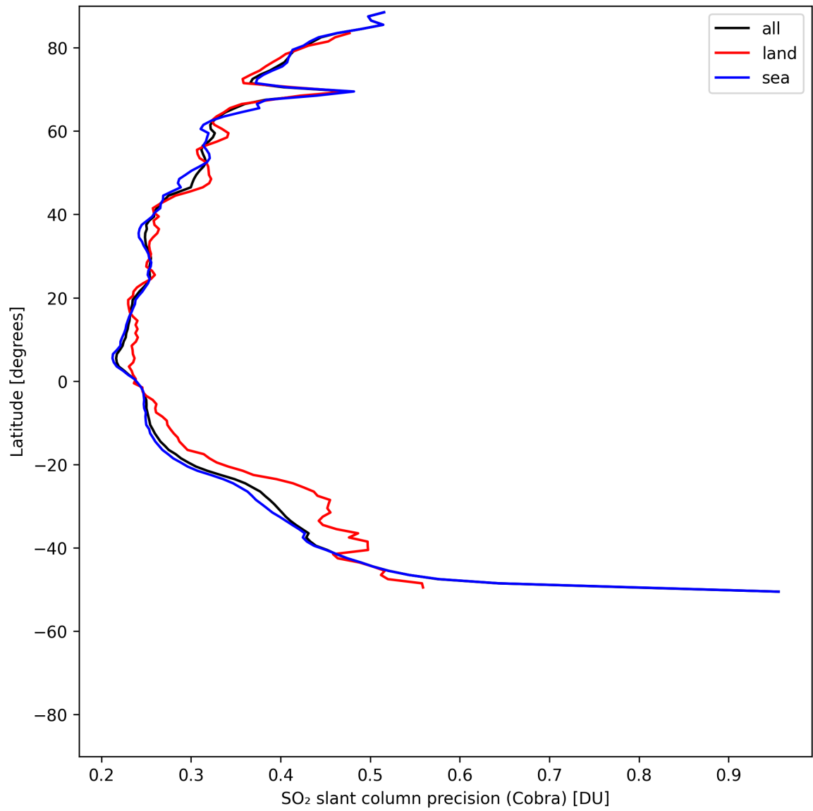
Figure 36: Zonal average of “SO 2 slant column precision (Cobra)” for 2025-05-12 to 2025-05-14.
