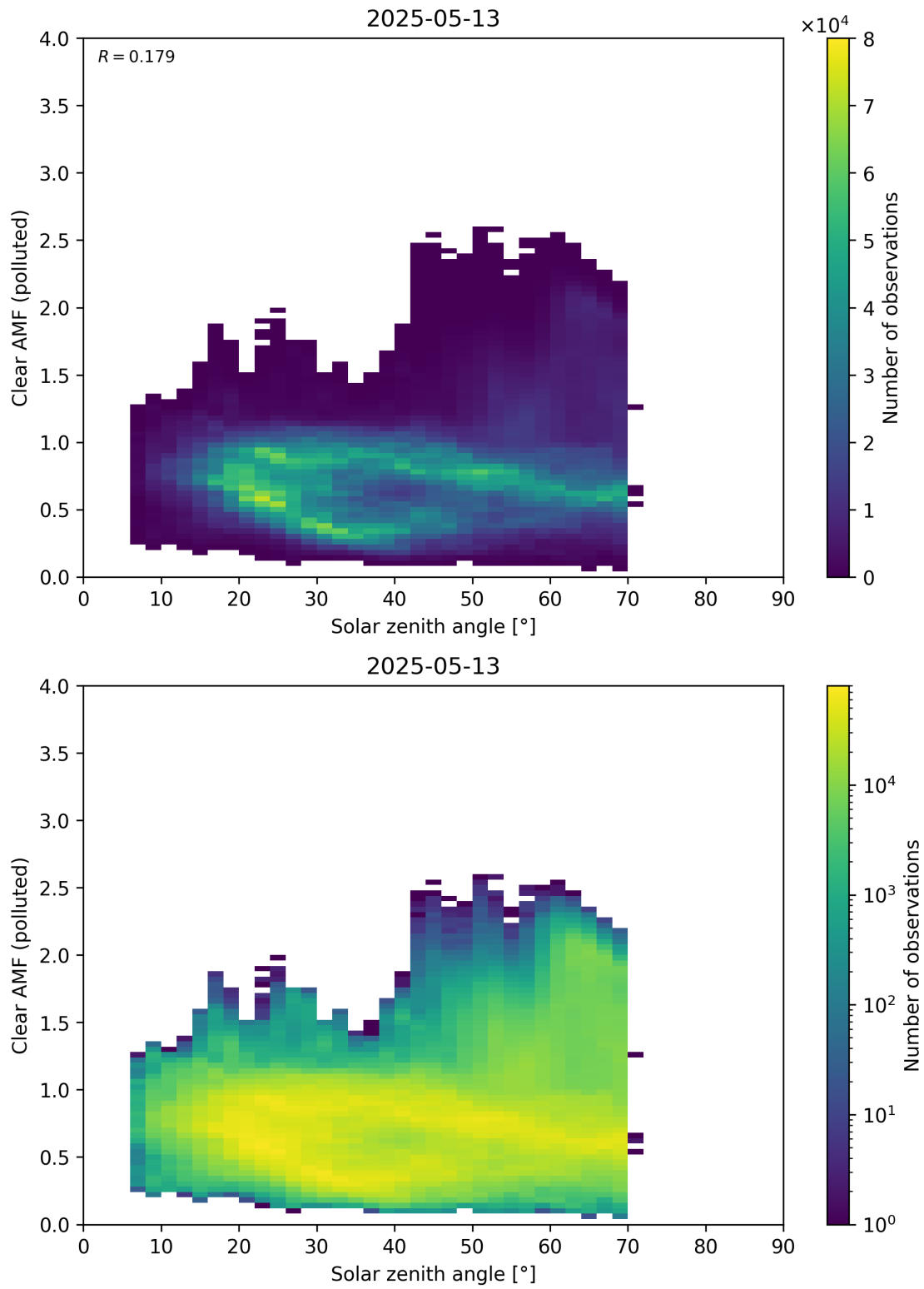
Figure 178: Scatter density plot of “Solar zenith angle” against “Clear AMF (polluted)” for 2025-05-12 to 2025-05-14.
