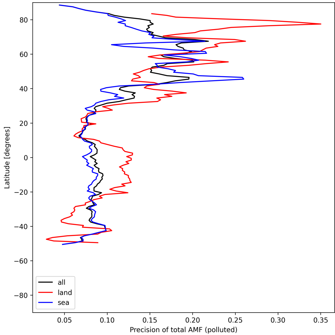
Figure 54: Zonal average of "Precision of total AMF (polluted)" for 2025-05-12 to 2025-05-14.
