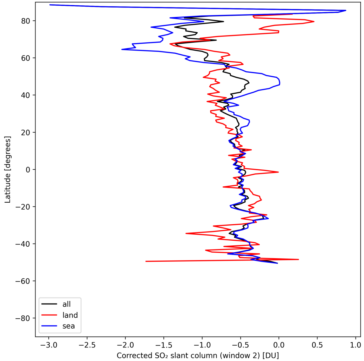
Figure 43: Zonal average of “Corrected SO 2 slant column (window 2)” for 2025-05-12 to 2025-05-14.
