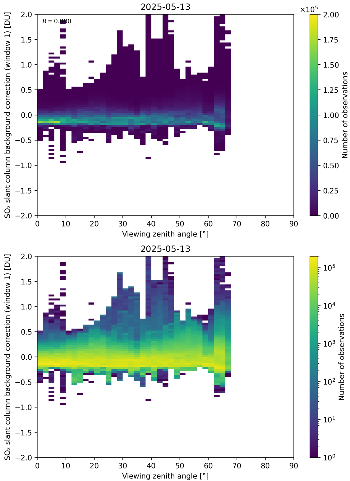
Figure 362: Scatter density plot of “Viewing zenith angle” against “SO 2 slant column background correction (window 1)” for 2025-05-12 to 2025-05-14.
