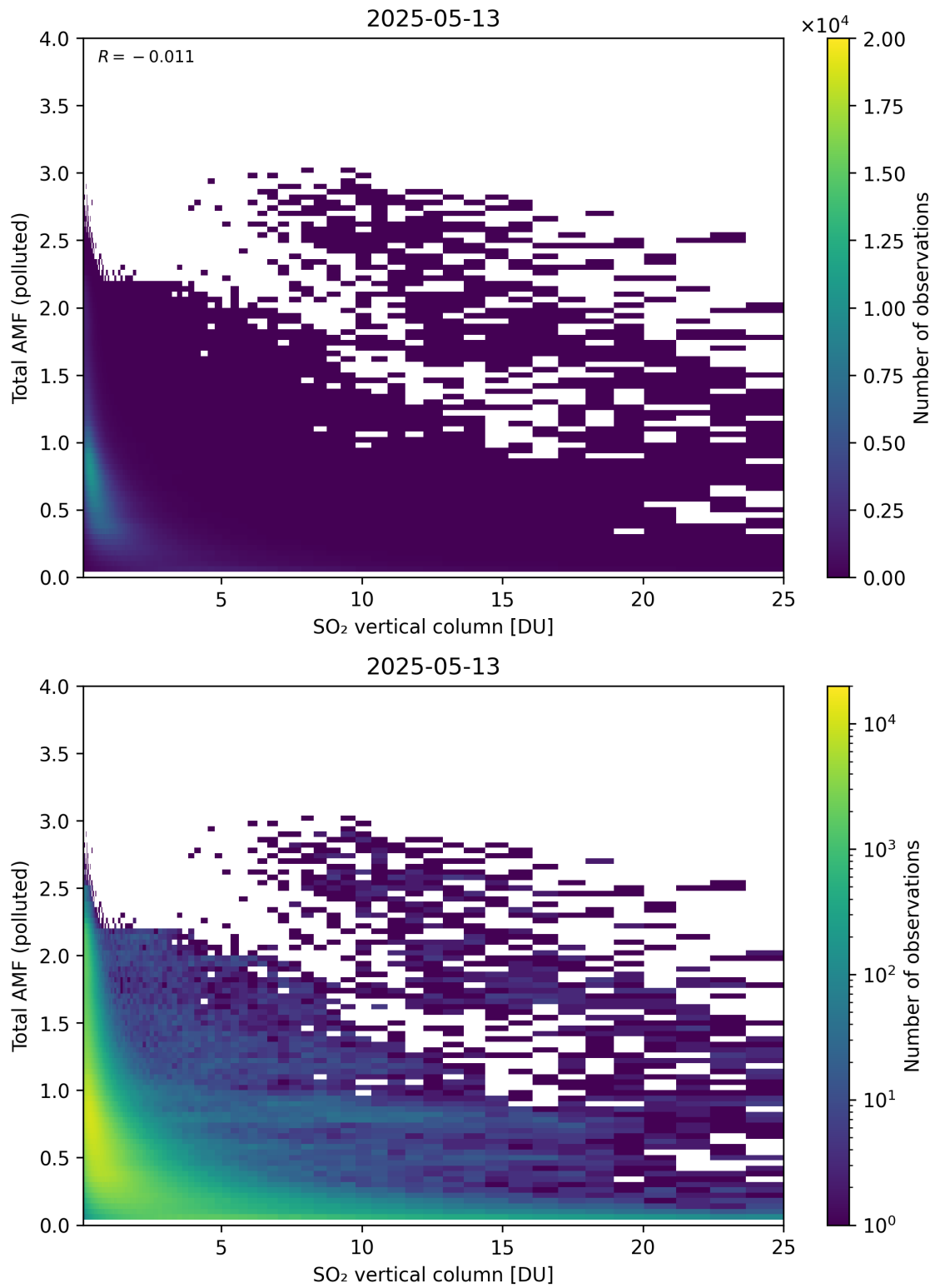
Figure 359: Scatter density plot of “SO 2 vertical column” against “Total AMF (polluted)” for 2025-05-12 to 2025-05-14.
