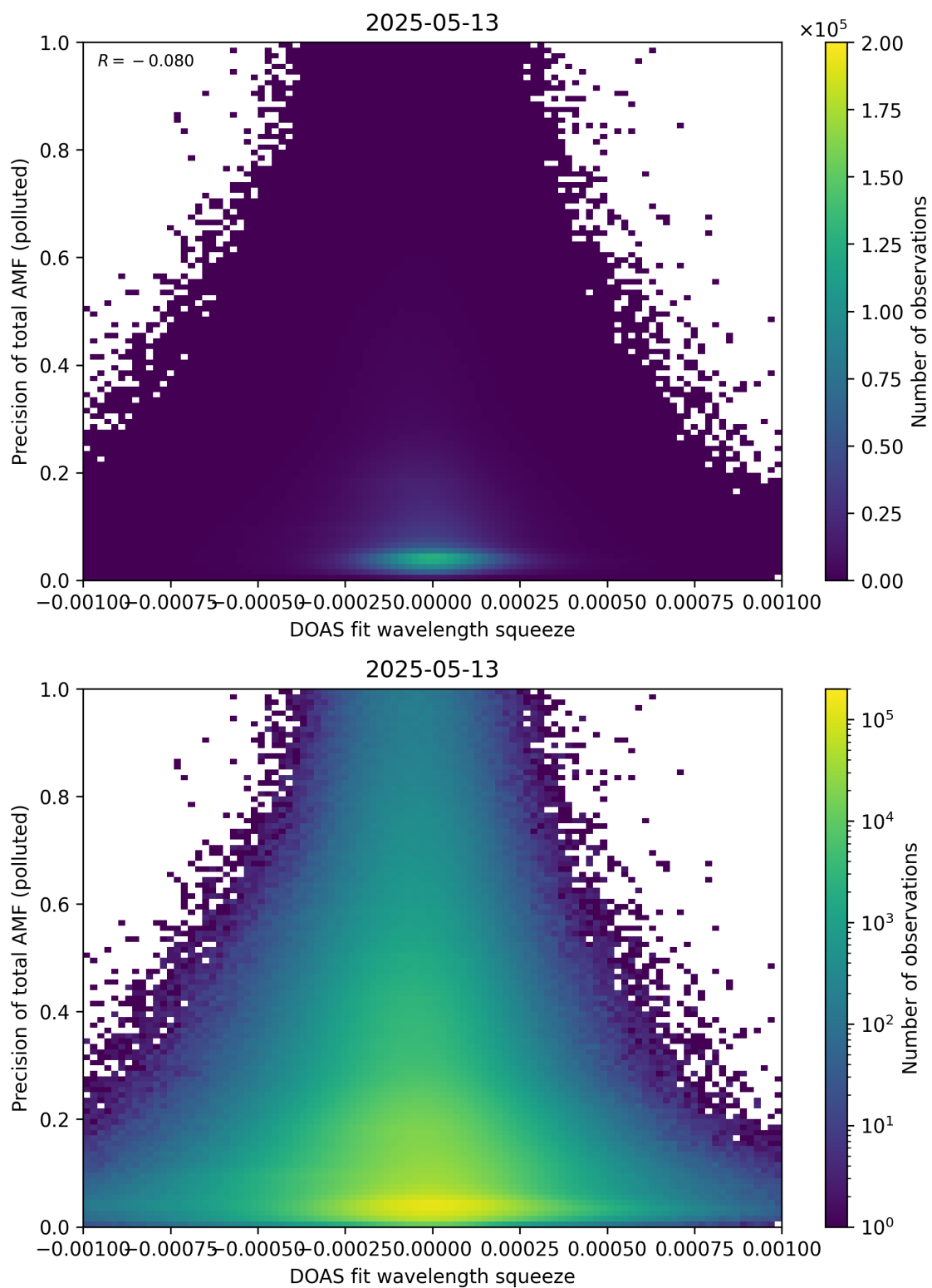
Figure 146: Scatter density plot of “DOAS fit wavelength squeeze” against “Precision of total AMF (polluted)” for 2025-05-12 to 2025-05-14.
