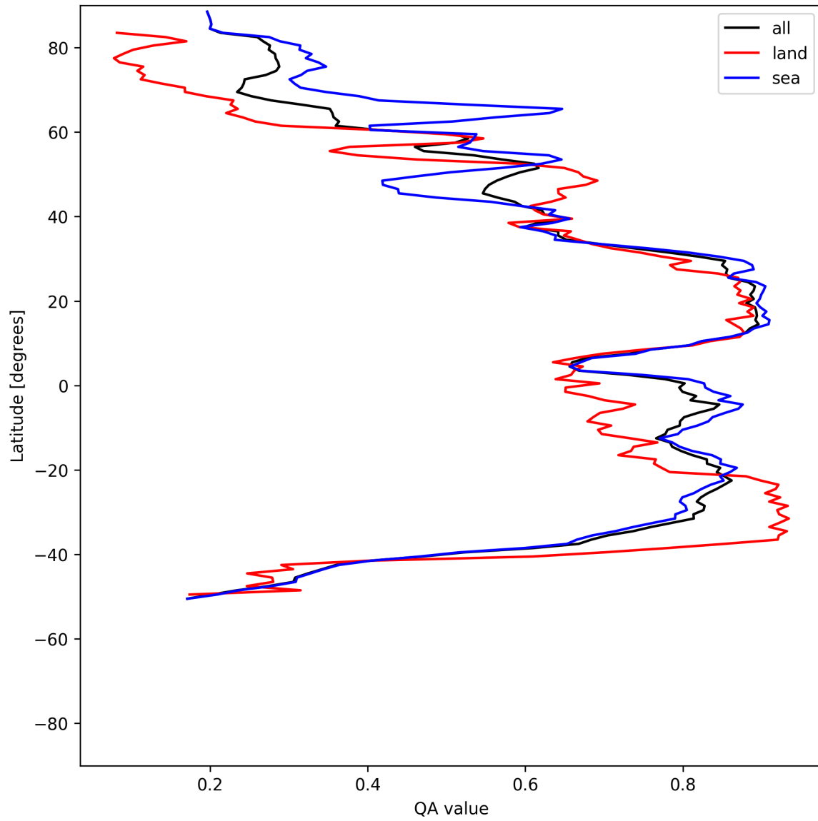
Figure 31: Zonal average of “QA value” for 2025-05-12 to 2025-05-14.
