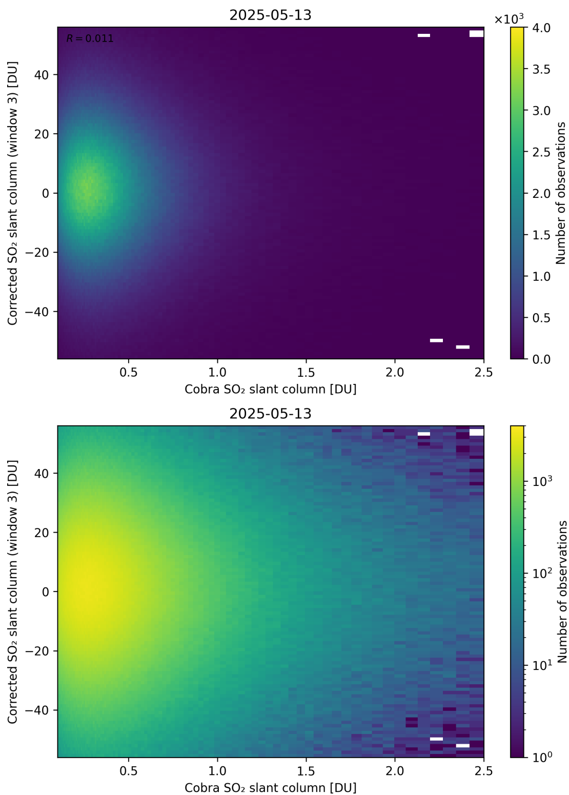
Figure 218: Scatter density plot of “Cobra SO 2 slant column” against “Corrected SO 2 slant column (window 3)” for 2025-05-12 to 2025-05-14.
