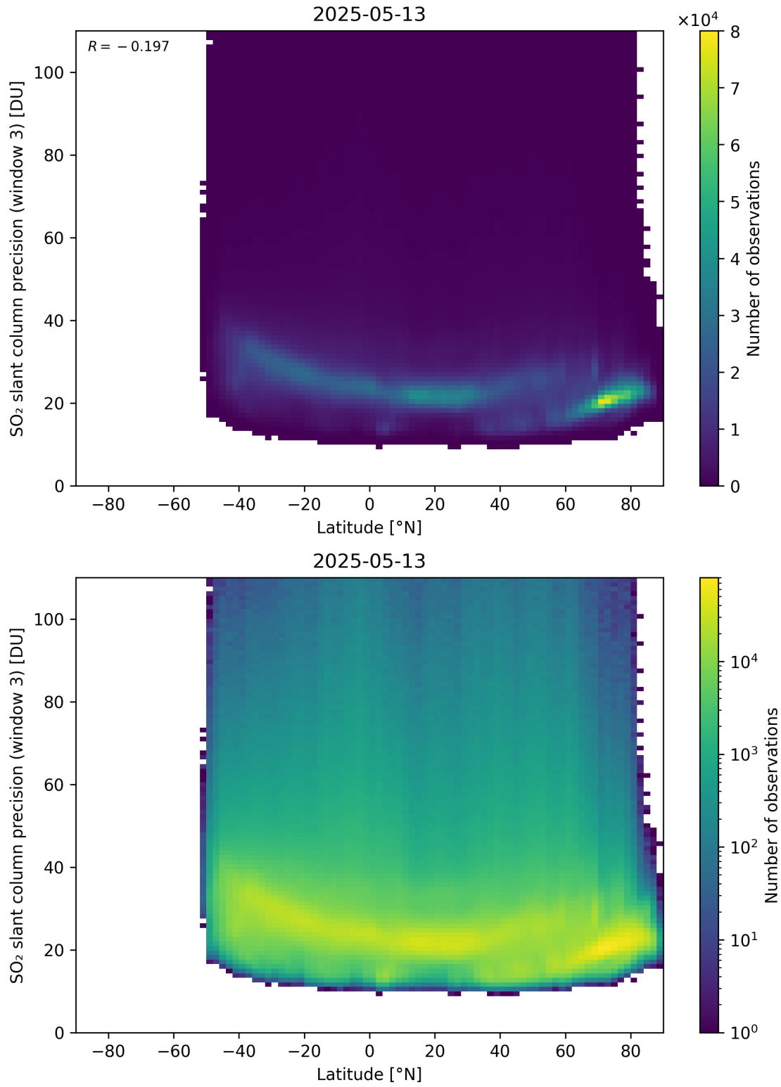
Figure 166: Scatter density plot of “Latitude” against “SO 2 slant column precision (window 3)” for 2025-05-12 to 2025-05-14.
