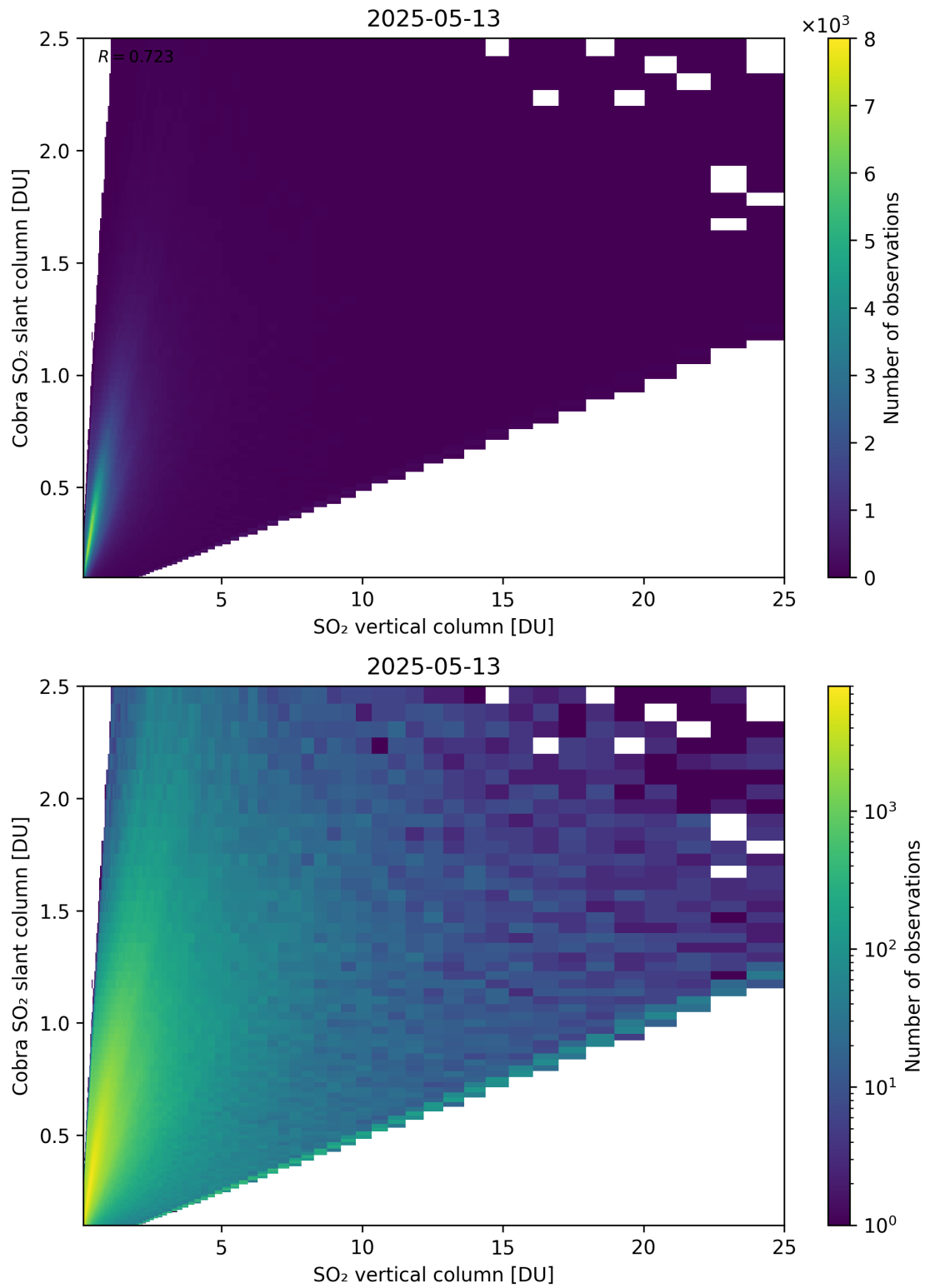
Figure 349: Scatter density plot of “SO 2 vertical column” against “Cobra SO 2 slant column” for 2025-05-12 to 2025-05-14.
