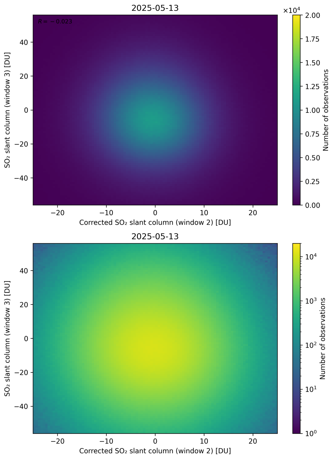
Figure 251: Scatter density plot of “Corrected SO 2 slant column (window 2)” against “SO 2 slant column (window 3)” for 2025-05-12 to 2025-05-14.
