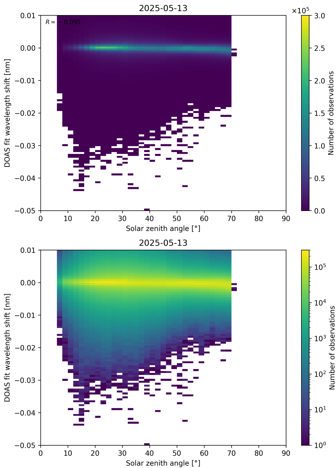
Figure 174: Scatter density plot of “Solar zenith angle” against “DOAS fit wavelength shift” for 2025-05-12 to 2025-05-14.
