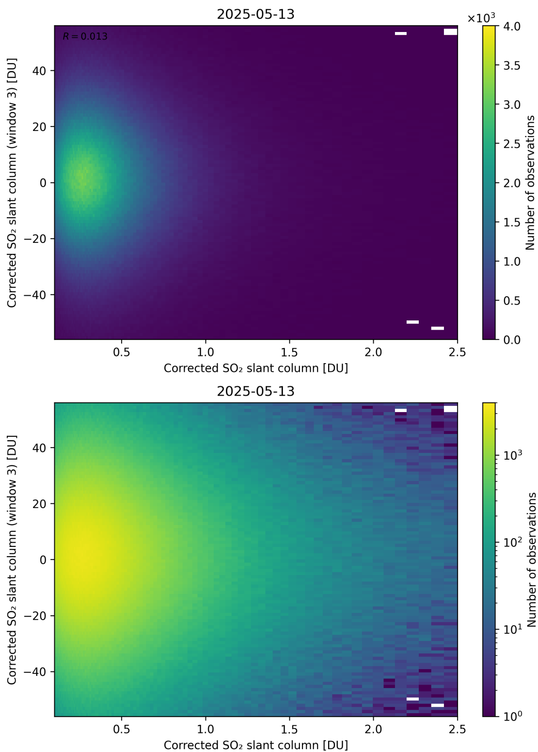
Figure 236: Scatter density plot of “Corrected SO 2 slant column” against “Corrected SO 2 slant column (window 3)” for 2025-05-12 to 2025-05-14.
