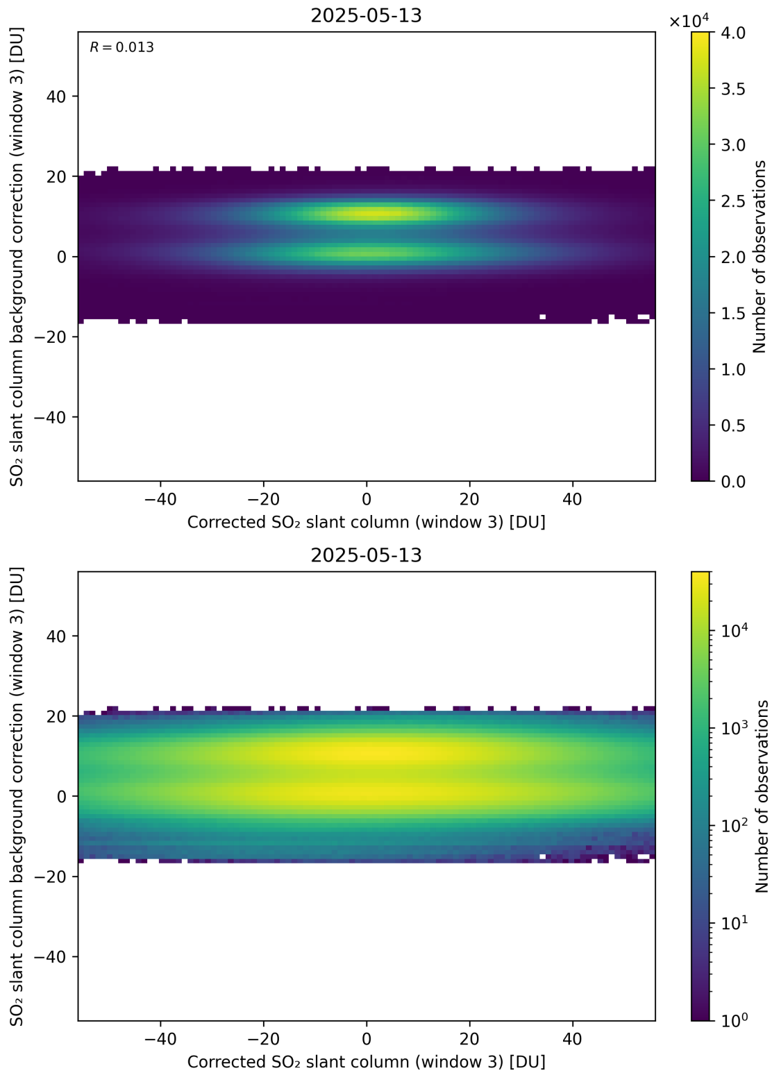
Figure 255: Scatter density plot of “Corrected SO 2 slant column (window 3)” against “SO 2 slant column background correction (window 3)” for 2025-05-12 to 2025-05-14.
