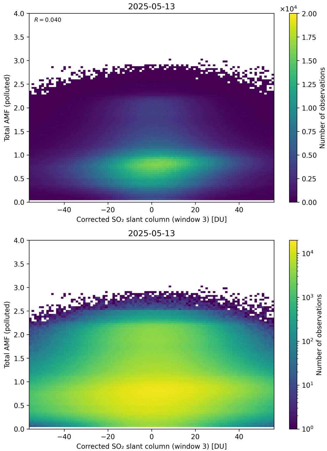
Figure 260: Scatter density plot of “Corrected SO 2 slant column (window 3)” against “Total AMF (polluted)” for 2025-05-12 to 2025-05-14.
