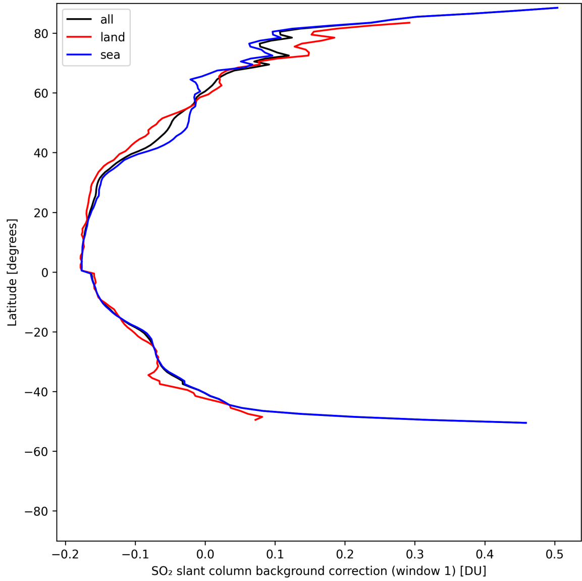
Figure 40: Zonal average of "SO 2 slant column background correction (window 1)" for 2025-05-12 to 2025-05-14.
