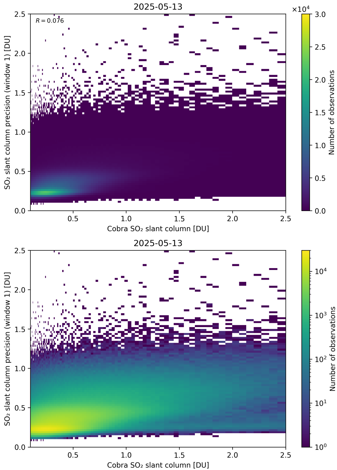
Figure 220: Scatter density plot of “Cobra SO 2 slant column” against “SO 2 slant column precision (window 1)” for 2025-05-12 to 2025-05-14.
