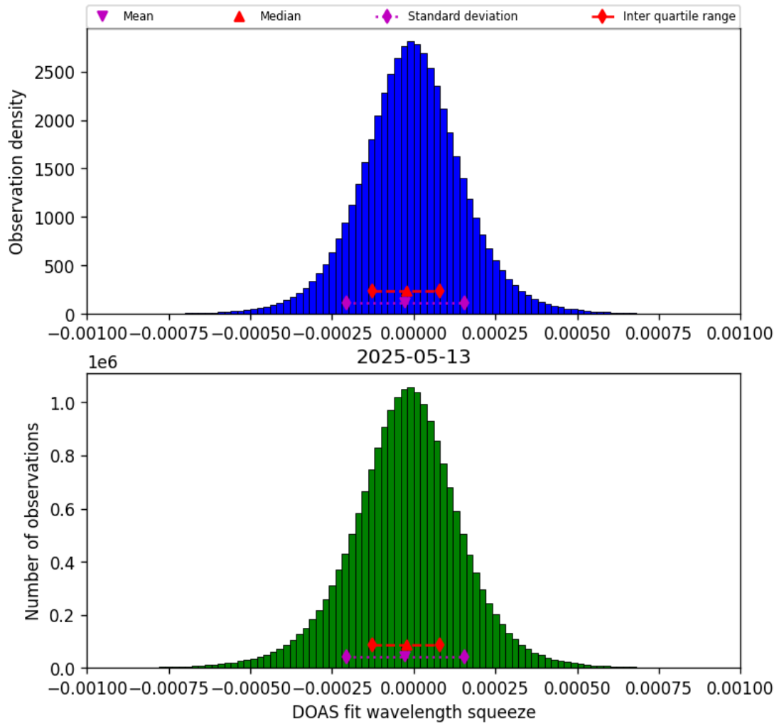
Figure 77: Histogram of “DOAS fit wavelength squeeze” for 2025-05-12 to 2025-05-14
