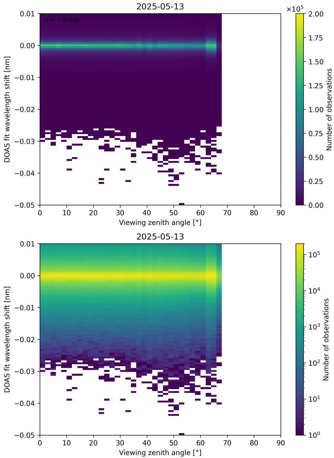
Figure 365: Scatter density plot of “Viewing zenith angle” against “DOAS fit wavelength shift” for 2025-05-12 to 2025-05-14.
