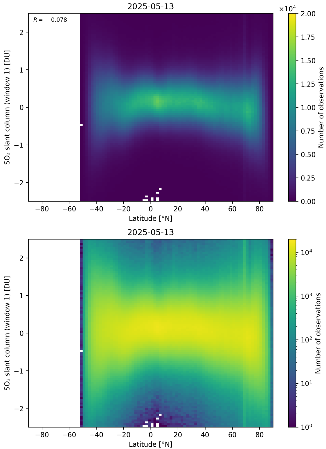
Figure 162: Scatter density plot of “Latitude” against “SO 2 slant column (window 1)” for 2025-05-12 to 2025-05-14.
