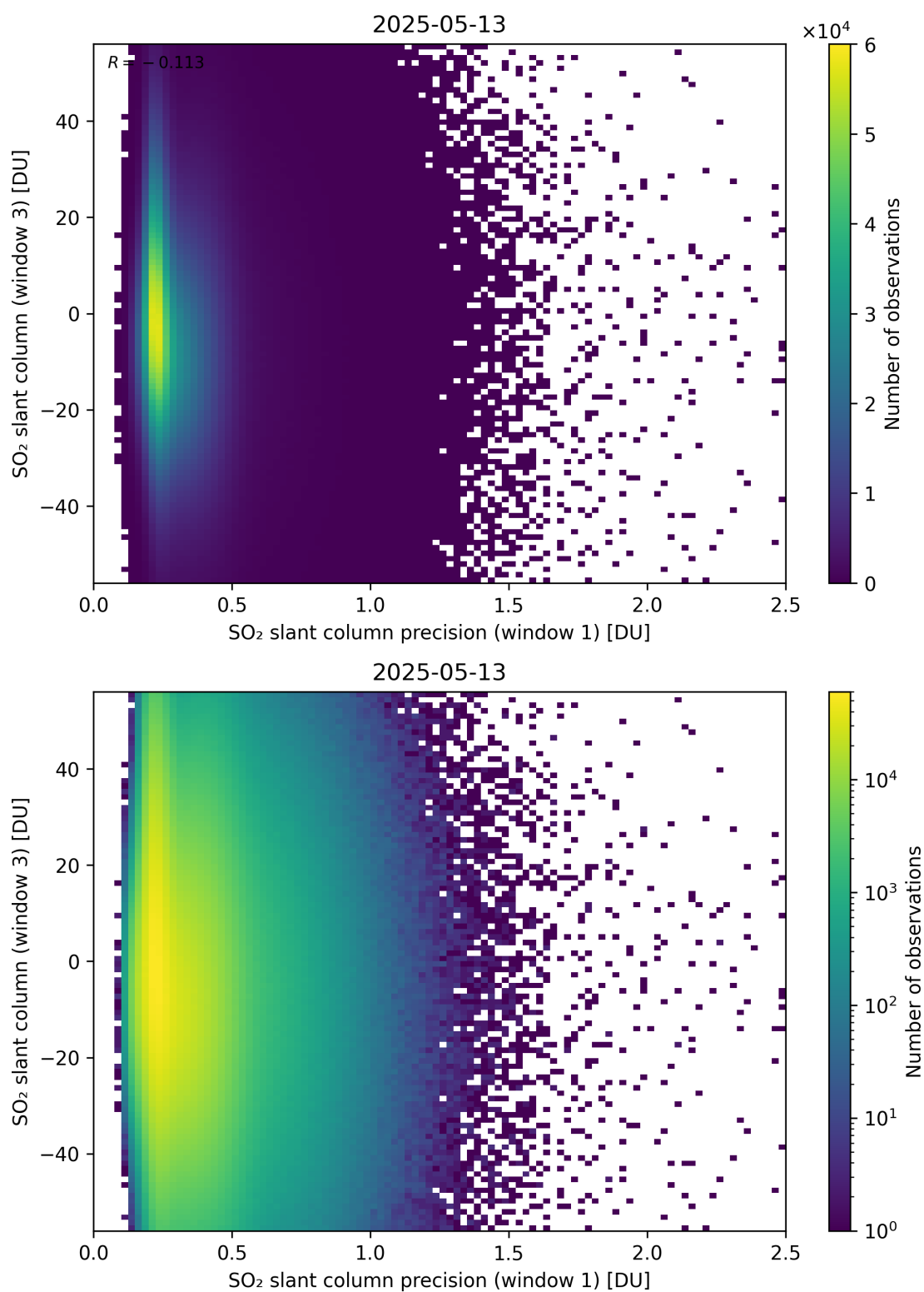
Figure 278: Scatter density plot of “SO 2 slant column precision (window 1)” against “SO 2 slant column (window 3)” for 2025-05-12 to 2025-05-14.
