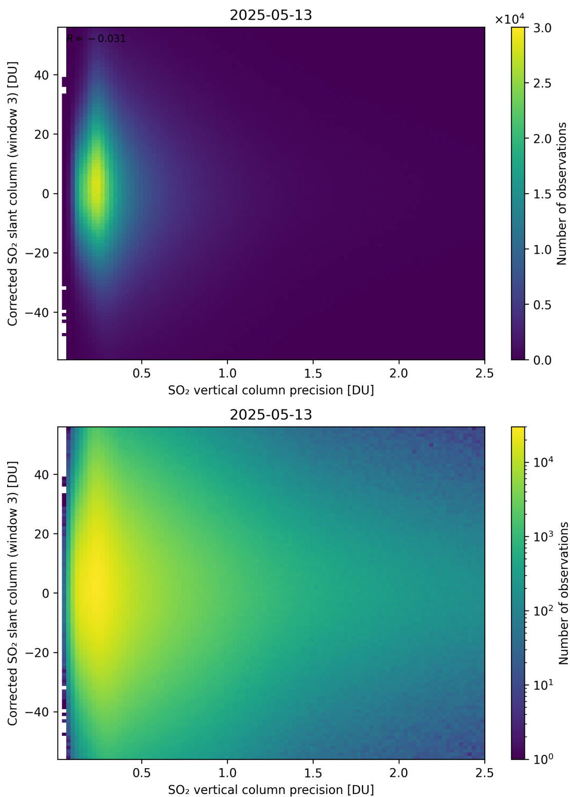
Figure 340: Scatter density plot of “SO 2 vertical column precision” against “Corrected SO 2 slant column (window 3)” for 2025-05-12 to 2025-05-14.
