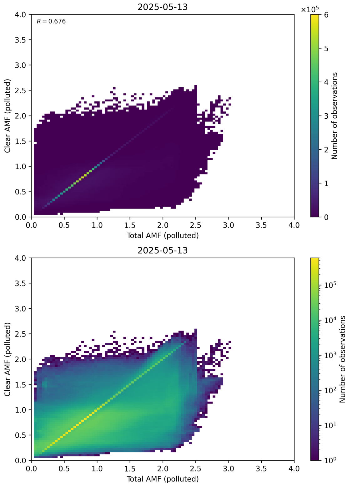
Figure 321: Scatter density plot of “Total AMF (polluted)” against “Clear AMF (polluted)” for 2025-05-12 to 2025-05-14.
