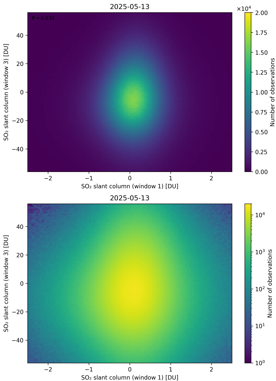
Figure 287: Scatter density plot of “SO 2 slant column (window 1)” against “SO 2 slant column (window 3)” for 2025-05-12 to 2025-05-14.
