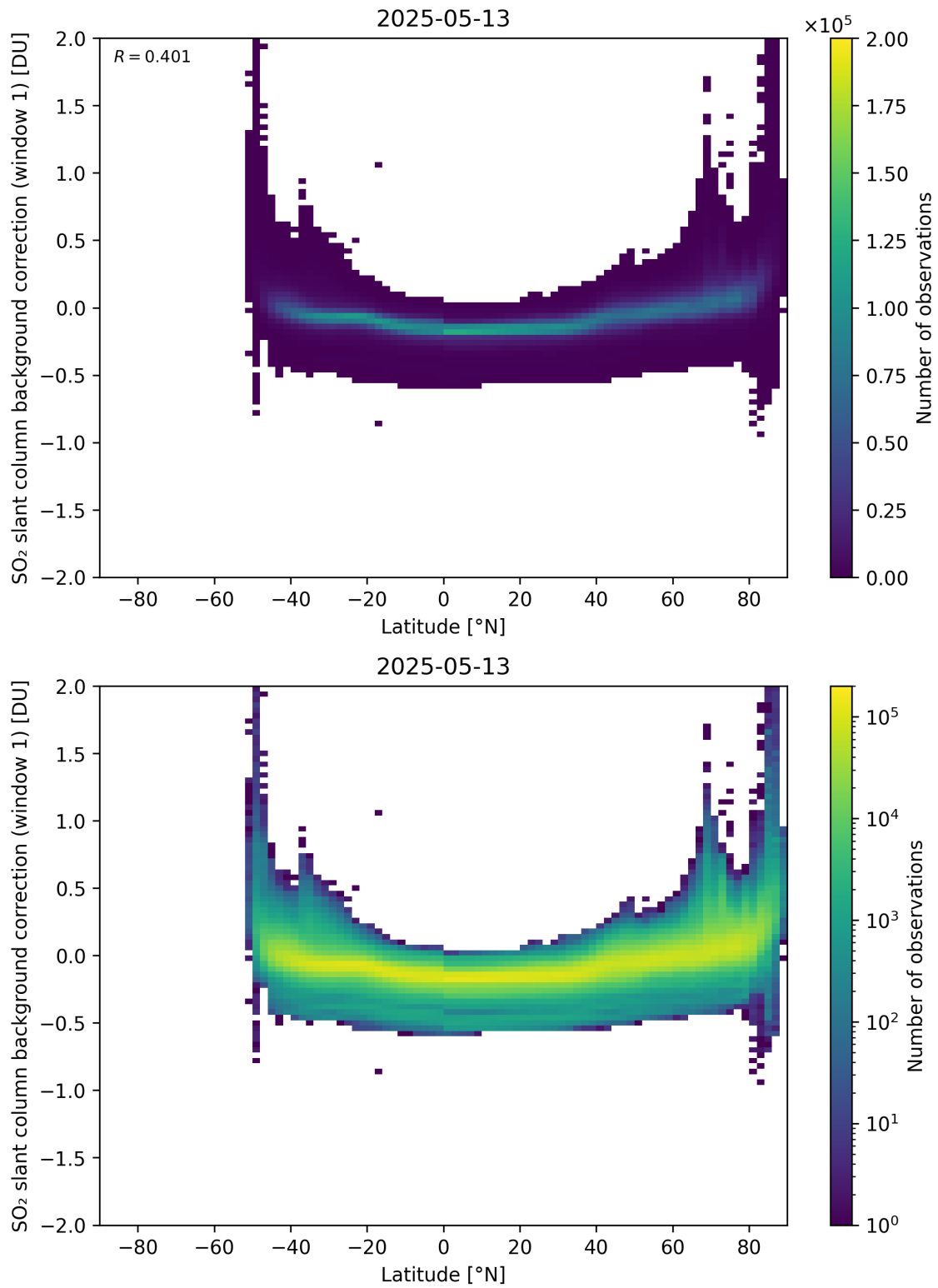
Figure 150: Scatter density plot of “Latitude” against “SO 2 slant column background correction (window 1)” for 2025-05-12 to 2025-05-14.
