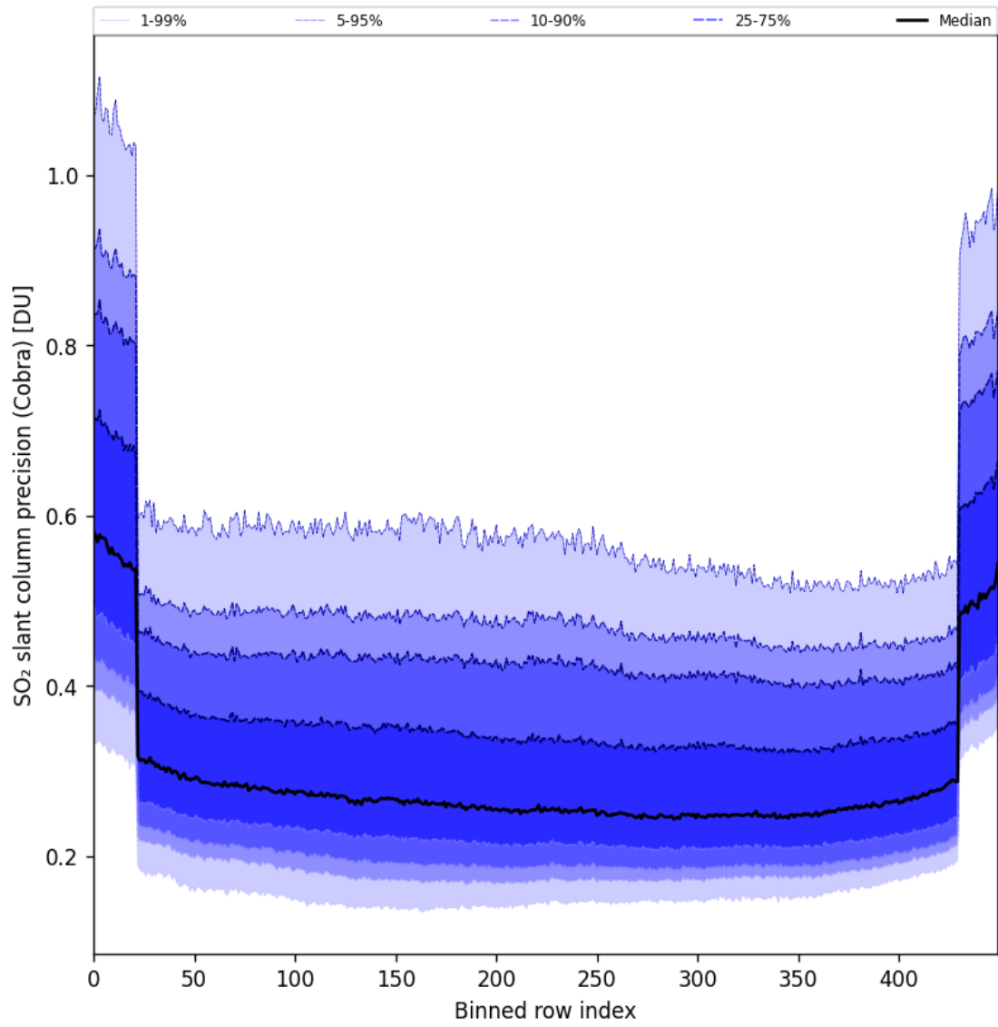
Figure 88: Along track statistics of “SO 2 slant column precision (Cobra)” for 2025-05-12 to 2025-05-14
