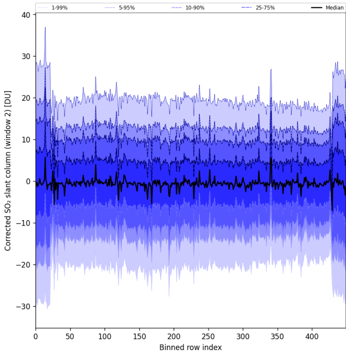
Figure 95: Along track statistics of “Corrected SO 2 slant column (window 2)” for 2025-05-12 to 2025-05-14
