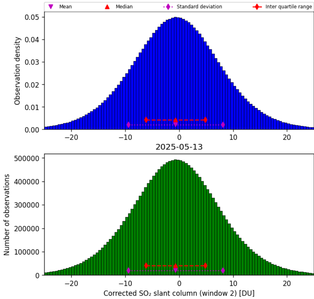
Figure 69: Histogram of “Corrected SO 2 slant column (window 2)” for 2025-05-12 to 2025-05-14
