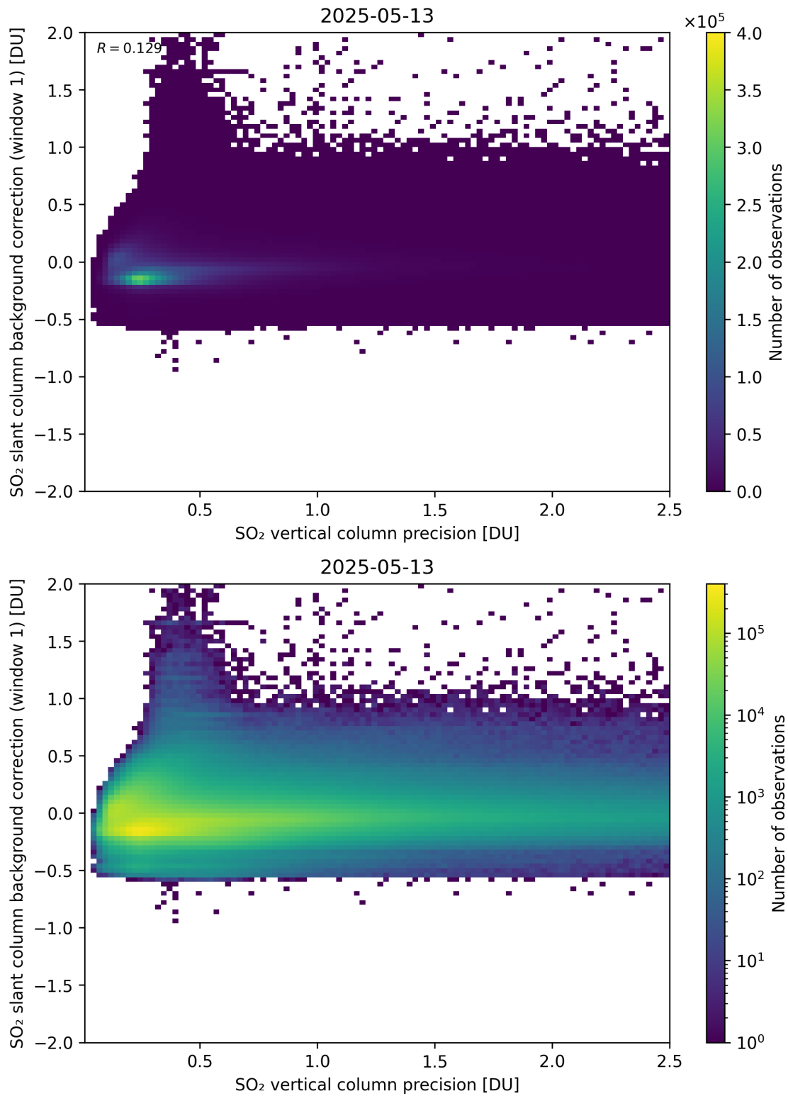
Figure 329: Scatter density plot of “SO 2 vertical column precision” against “SO 2 slant column background correction (window 1)” for 2025-05-12 to 2025-05-14.
