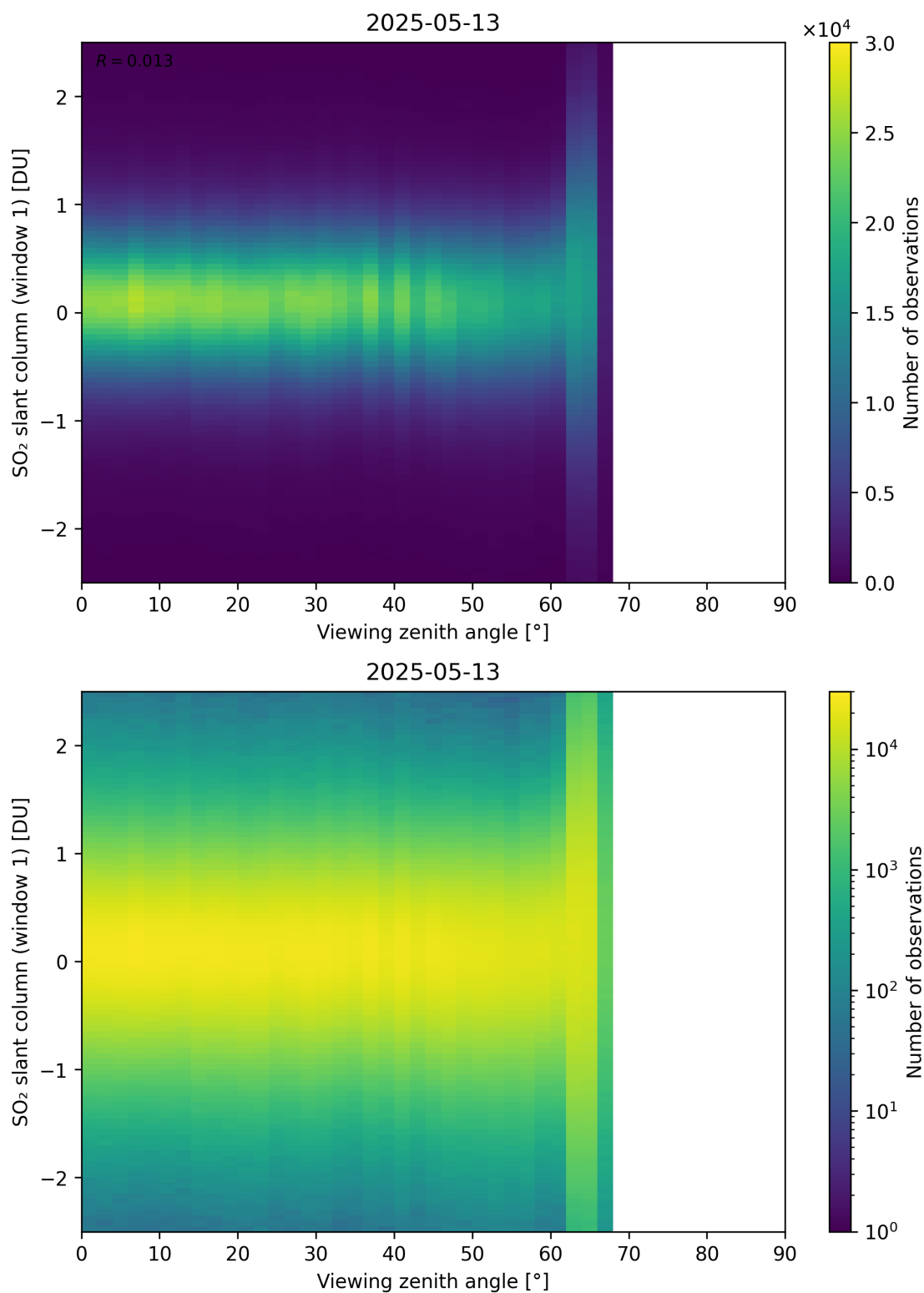
Figure 376: Scatter density plot of “Viewing zenith angle” against “SO 2 slant column (window 1)” for 2025-05-12 to 2025-05-14.
