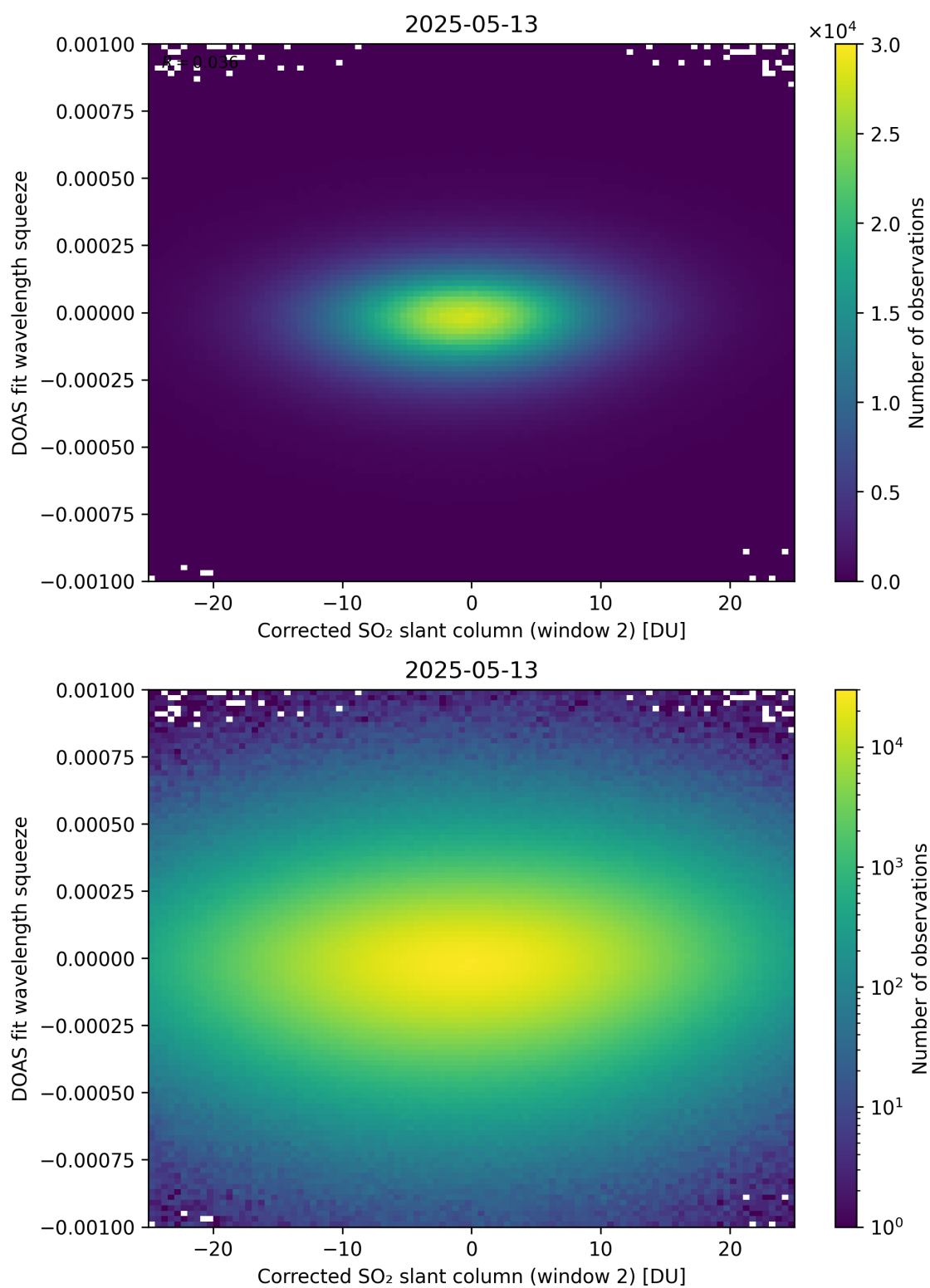
Figure 247: Scatter density plot of “Corrected SO 2 slant column (window 2)” against “DOAS fit wavelength squeeze” for 2025-05-12 to 2025-05-14.
