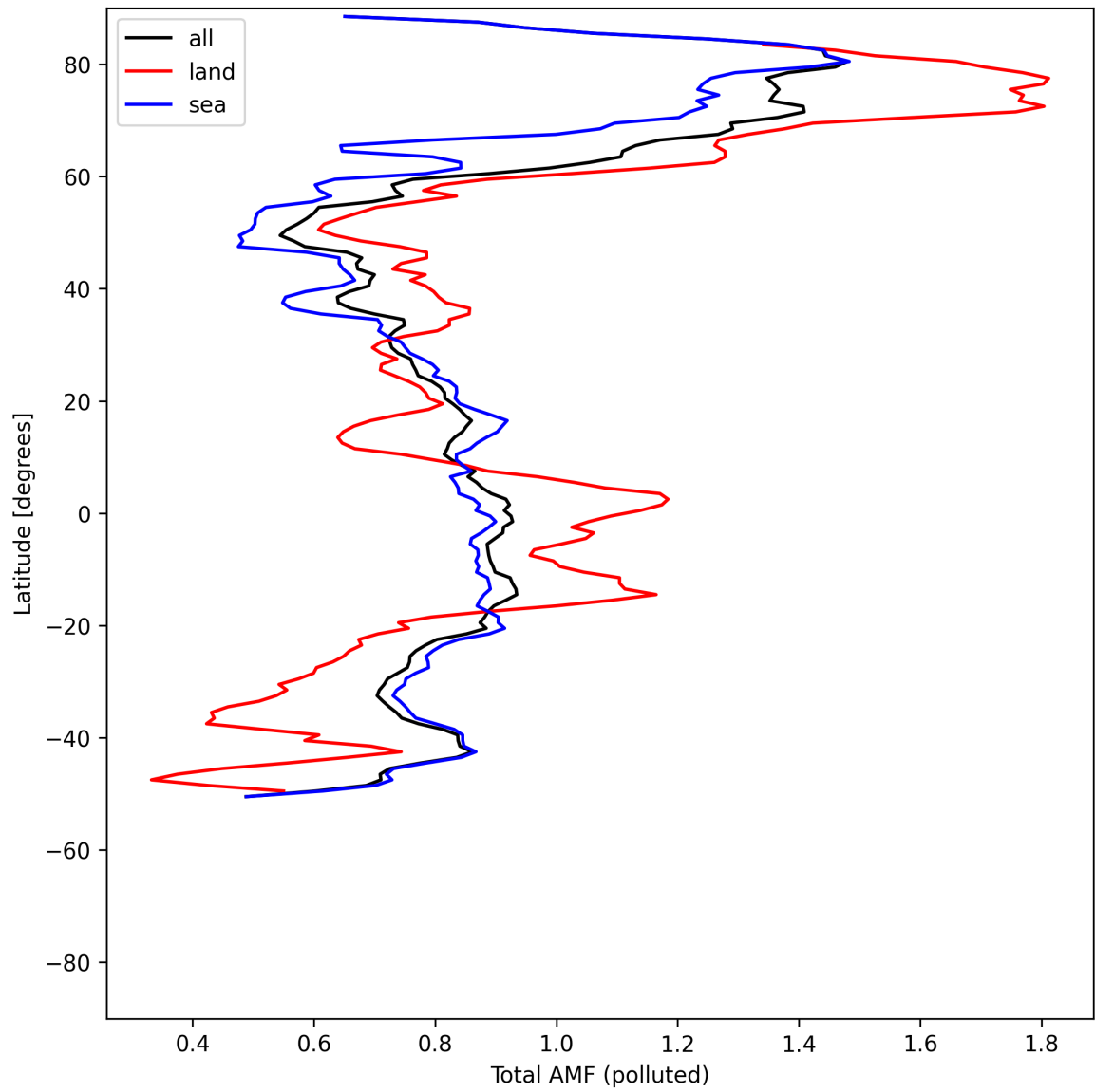
Figure 53: Zonal average of “Total AMF (polluted)” for 2025-05-12 to 2025-05-14.
