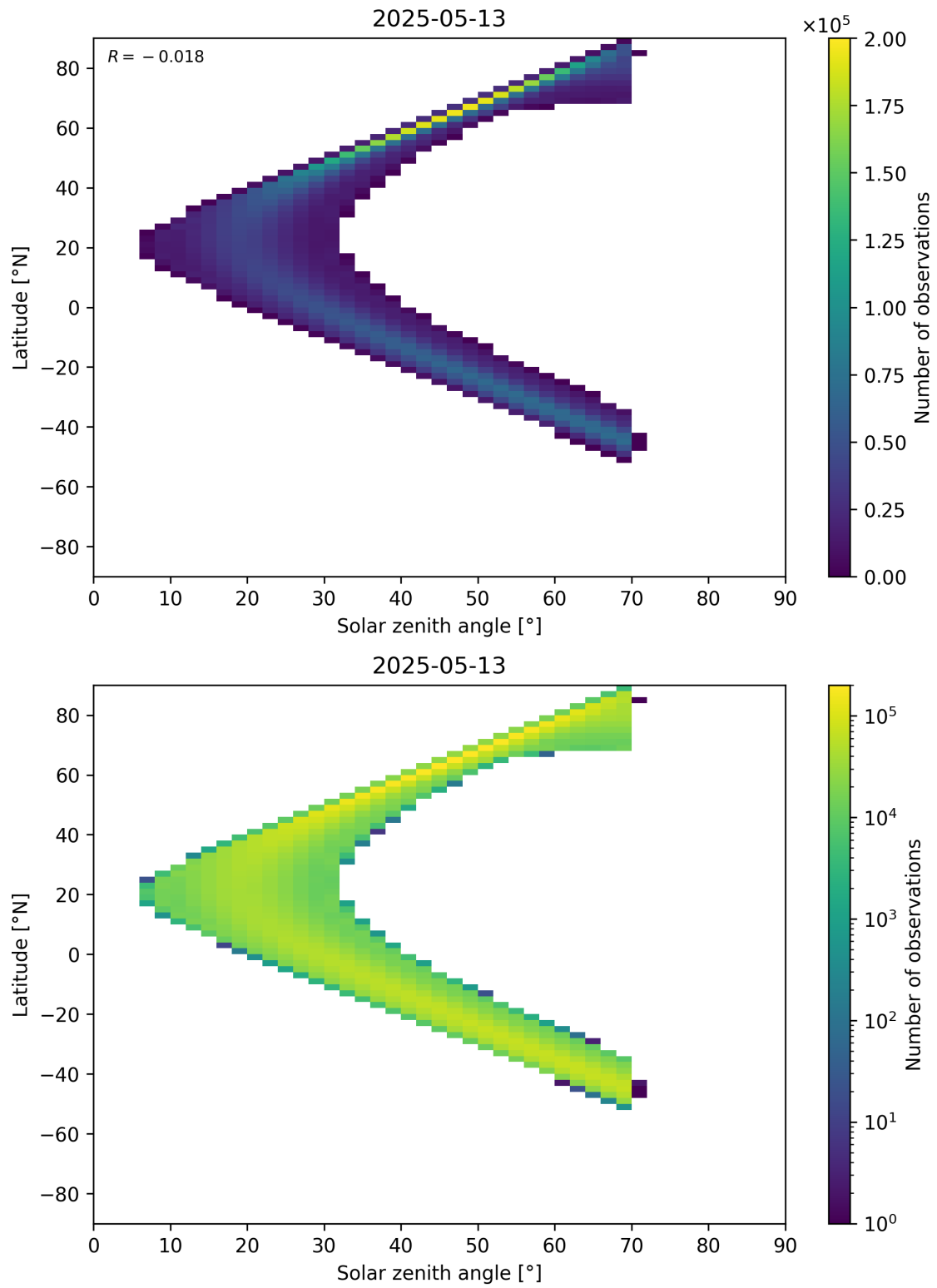
Figure 177: Scatter density plot of “Solar zenith angle” against “Latitude” for 2025-05-12 to 2025-05-14.
