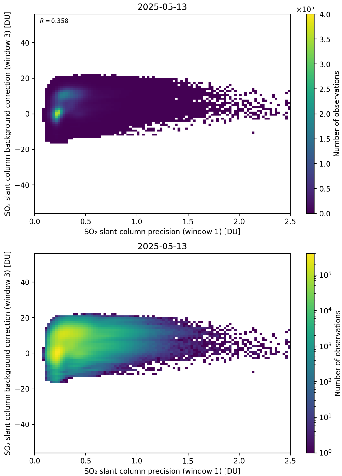
Figure 270: Scatter density plot of “SO 2 slant column precision (window 1)” against “SO 2 slant column background correction (window 3)” for 2025-05-12 to 2025-05-14.
