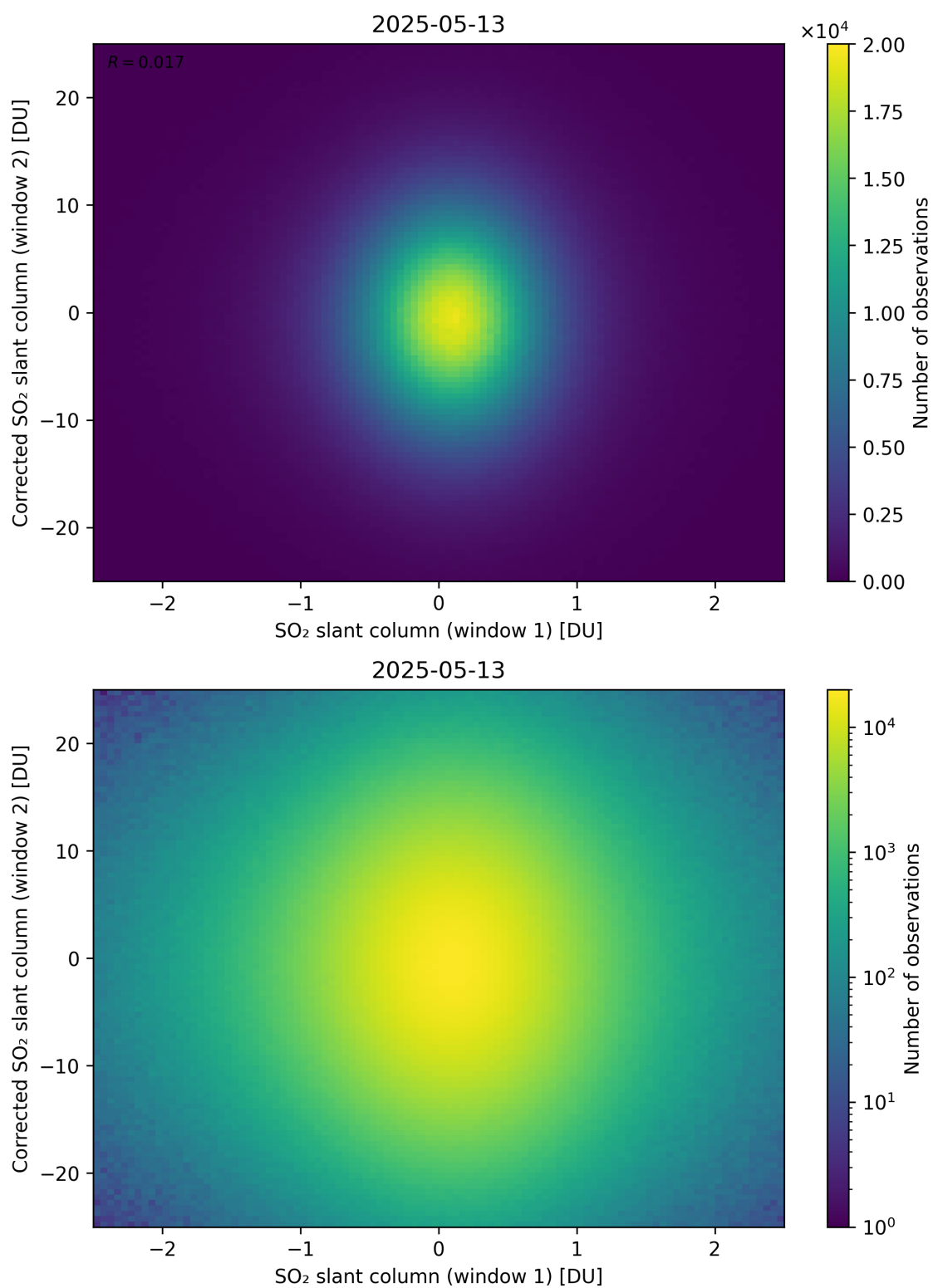
Figure 283: Scatter density plot of “SO 2 slant column (window 1)” against “Corrected SO 2 slant column (window 2)” for 2025-05-12 to 2025-05-14.
