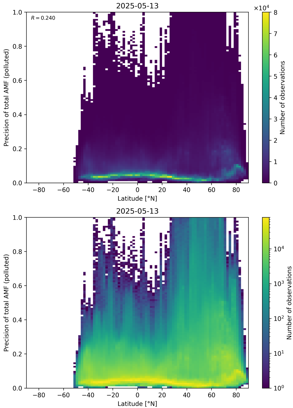
Figure 168: Scatter density plot of “Latitude” against “Precision of total AMF (polluted)” for 2025-05-12 to 2025-05-14.
