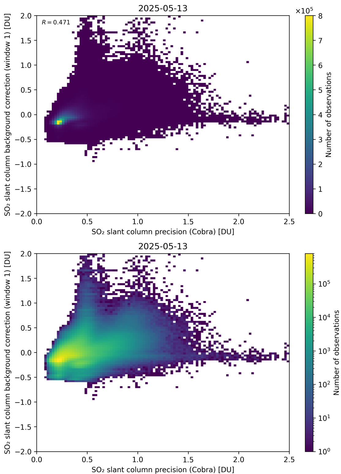
Figure 199: Scatter density plot of “SO 2 slant column precision (Cobra)” against “SO 2 slant column background correction (window 1)” for 2025-05-12 to 2025-05-14.
