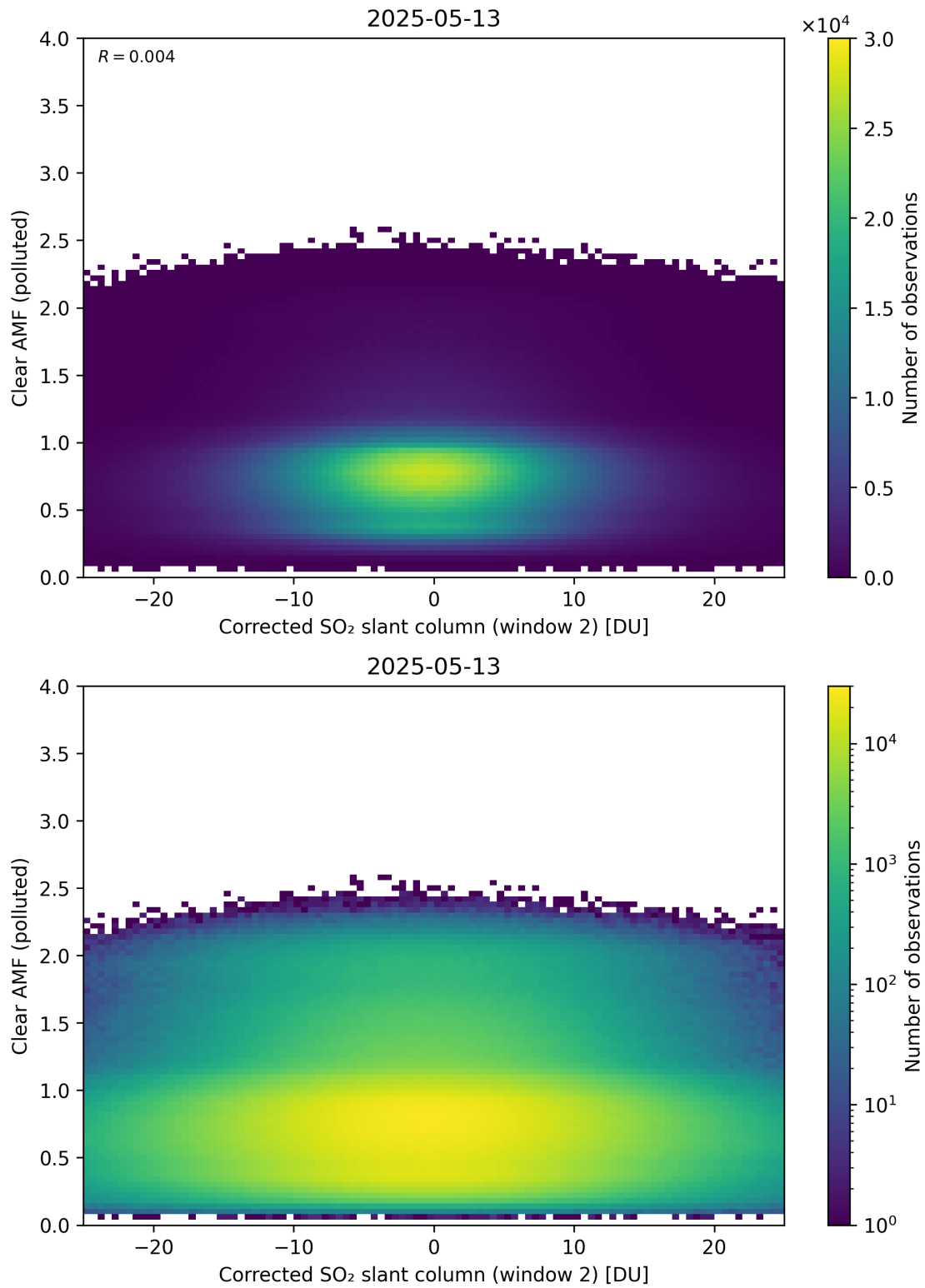
Figure 249: Scatter density plot of “Corrected SO 2 slant column (window 2)” against “Clear AMF (polluted)” for 2025-05-12 to 2025-05-14.
