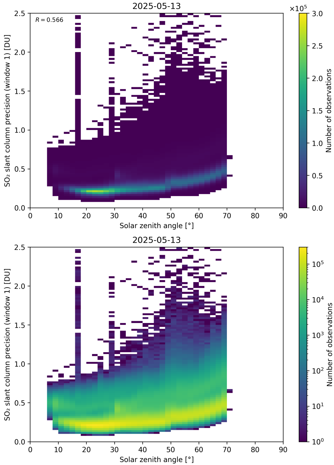
Figure 185: Scatter density plot of “Solar zenith angle” against “SO 2 slant column precision (window 1)” for 2025-05-12 to 2025-05-14.
