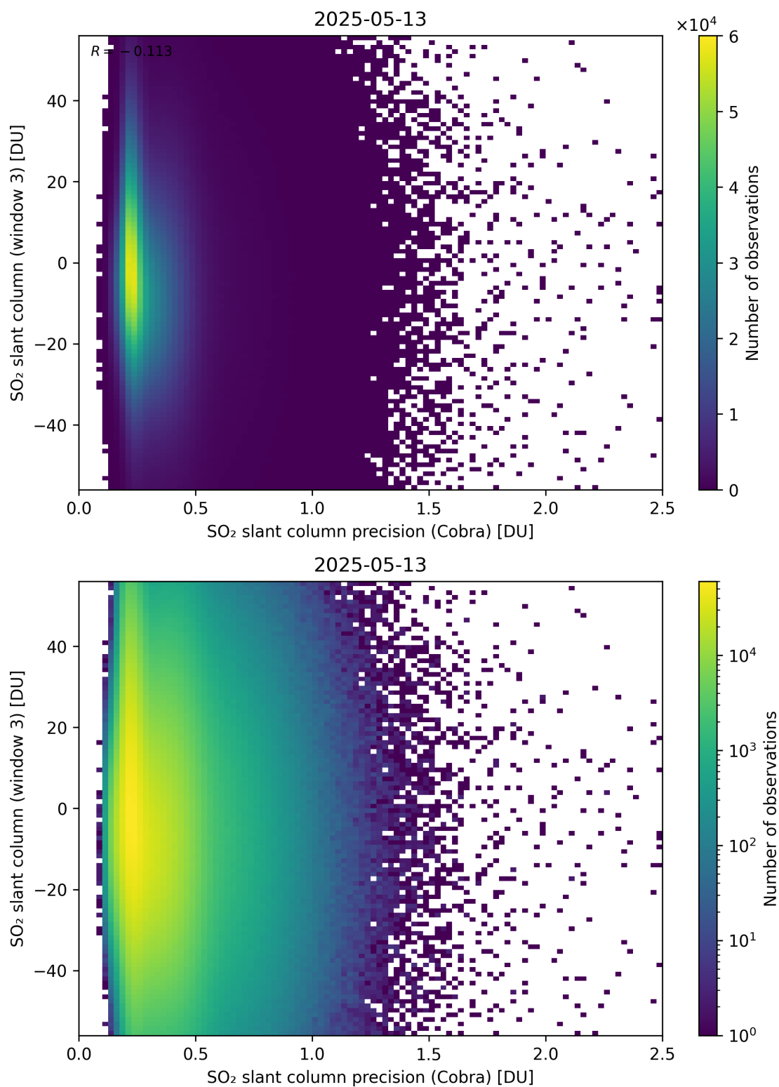
Figure 211: Scatter density plot of “SO 2 slant column precision (Cobra)” against “SO 2 slant column (window 3)” for 2025-05-12 to 2025-05-14.
