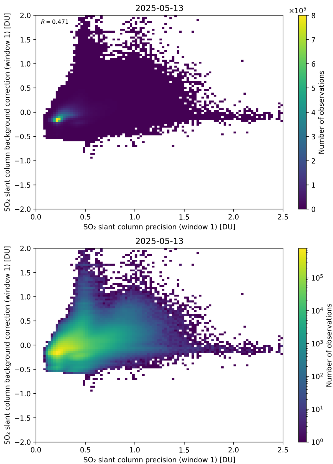
Figure 268: Scatter density plot of “SO 2 slant column precision (window 1)” against “SO 2 slant column background correction (window 1)” for 2025-05-12 to 2025-05-14.
