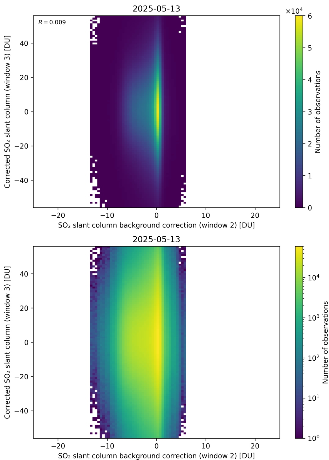
Figure 127: Scatter density plot of “SO 2 slant column background correction (window 2)” against “Corrected SO 2 slant column (window 3)” for 2025-05-12 to 2025-05-14.
