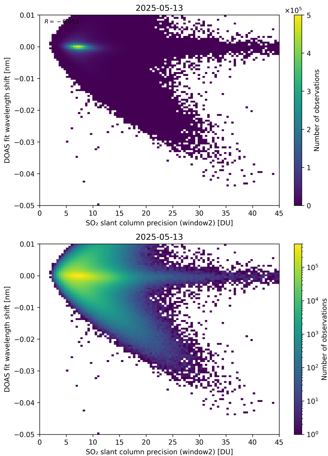
Figure 293: Scatter density plot of “SO 2 slant column precision (window2)” against “DOAS fit wavelength shift” for 2025-05-12 to 2025-05-14.
