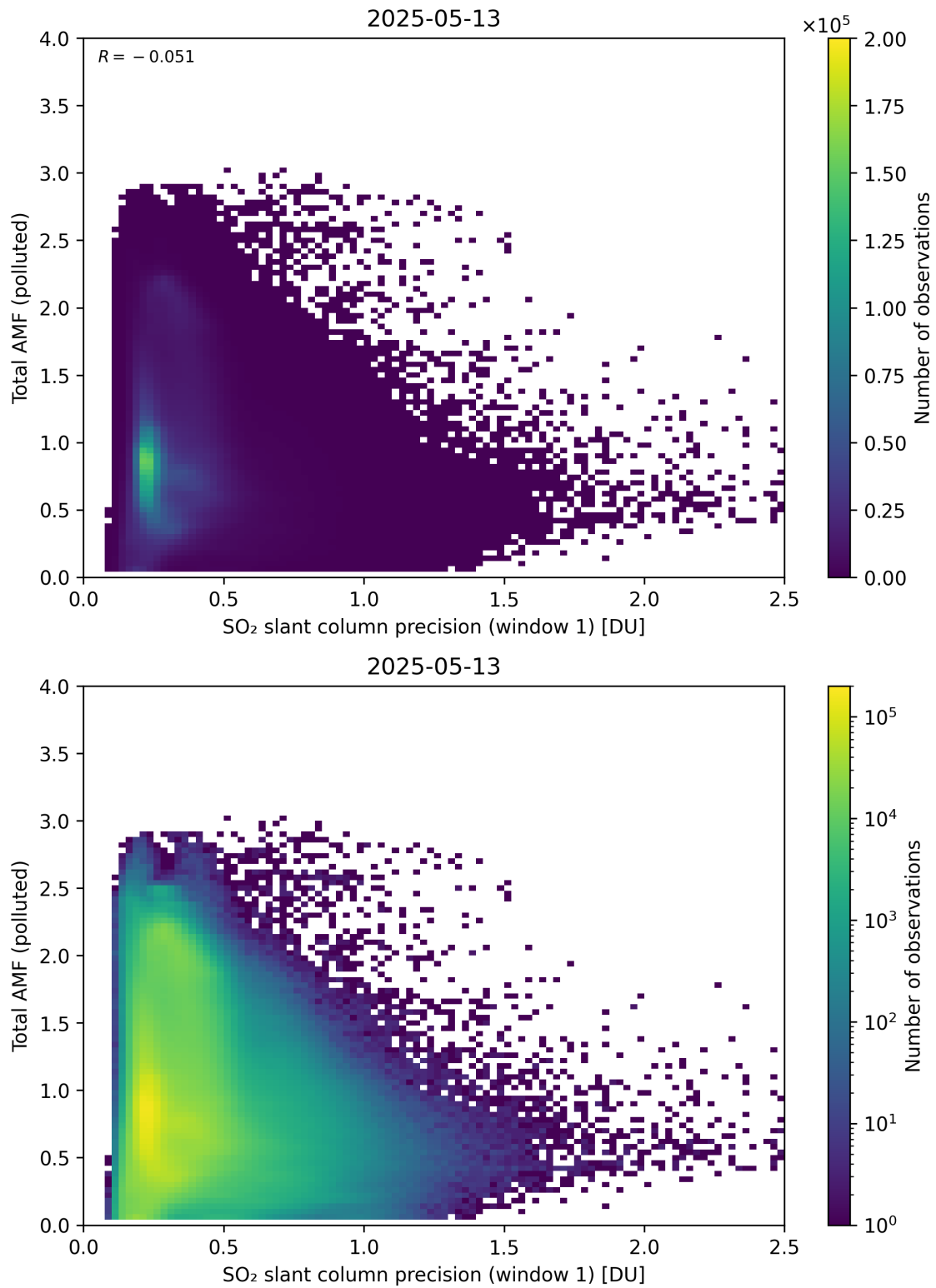
Figure 280: Scatter density plot of “SO 2 slant column precision (window 1)” against “Total AMF (polluted)” for 2025-05-12 to 2025-05-14.
