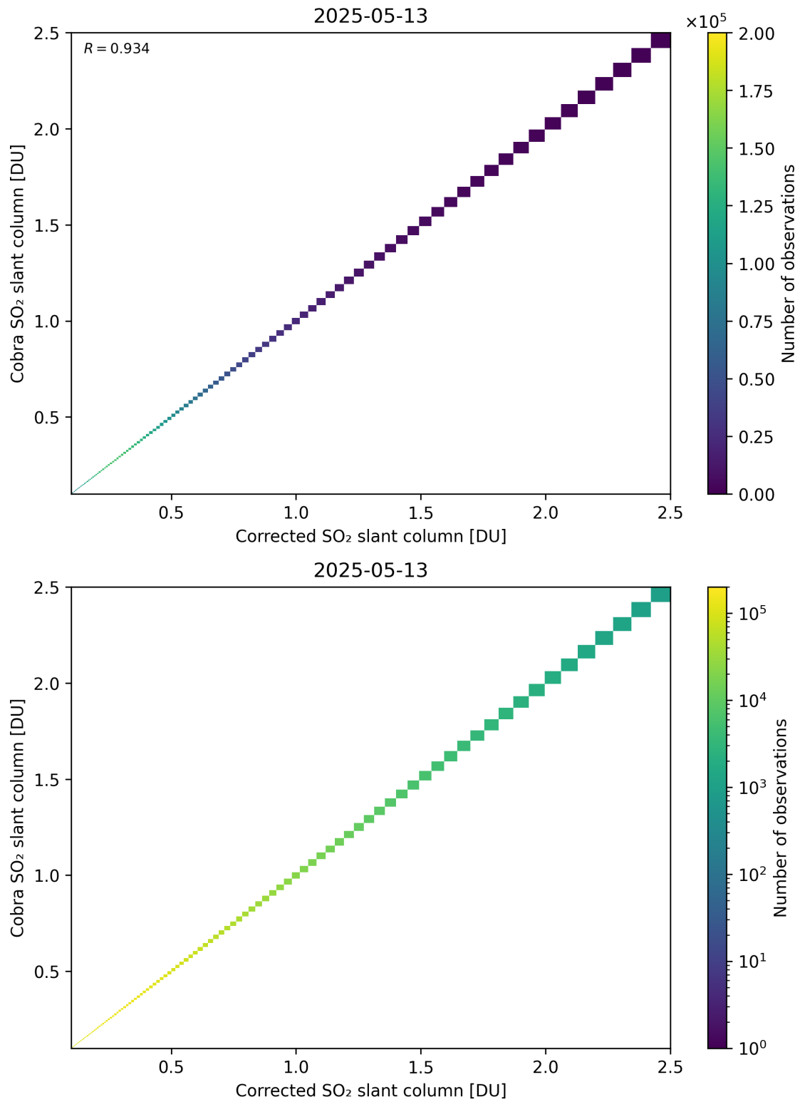
Figure 233: Scatter density plot of “Corrected SO 2 slant column” against “Cobra SO 2 slant column” for 2025-05-12 to 2025-05-14.
