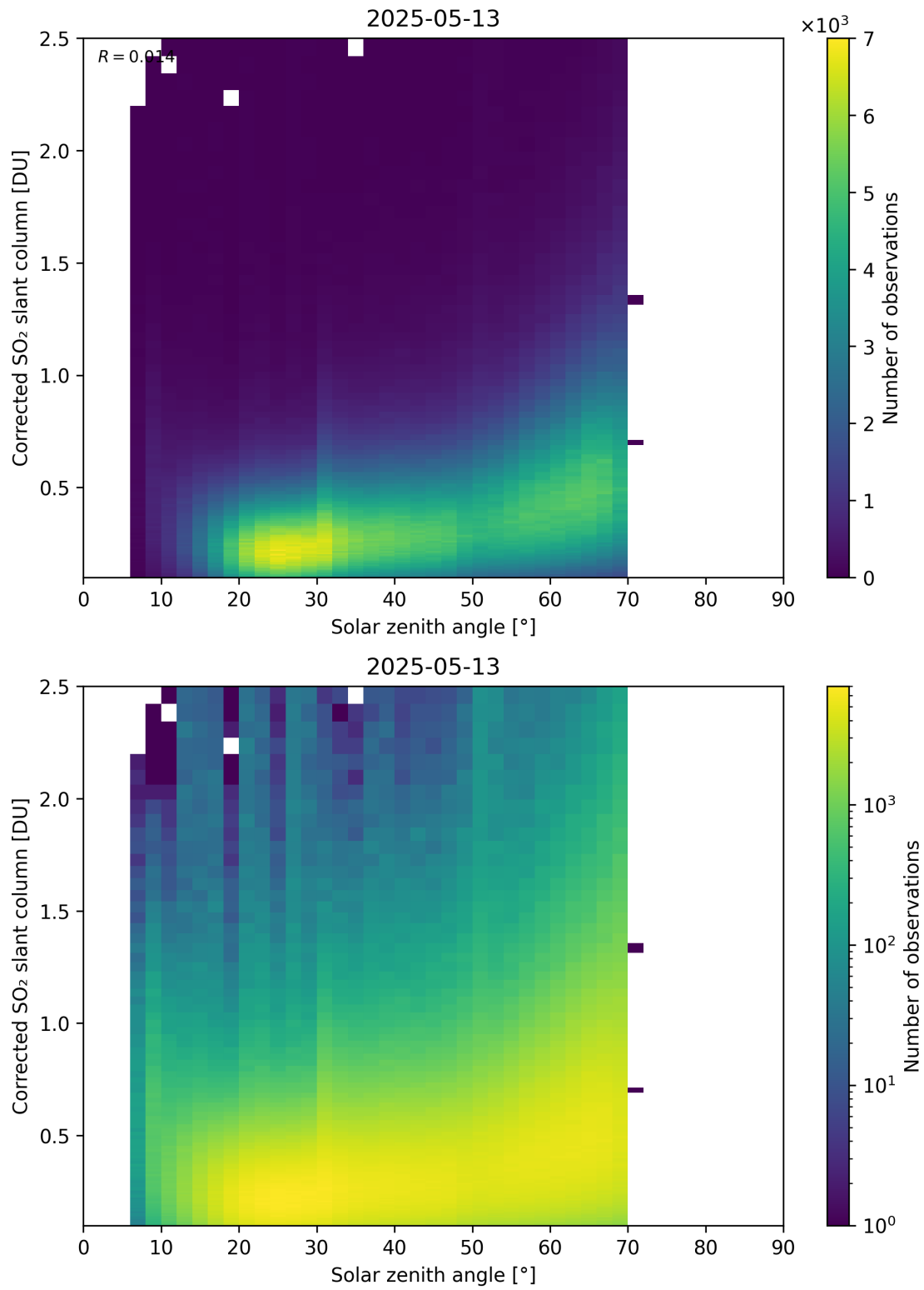
Figure 181: Scatter density plot of “Solar zenith angle” against “Corrected SO 2 slant column” for 2025-05-12 to 2025-05-14.
