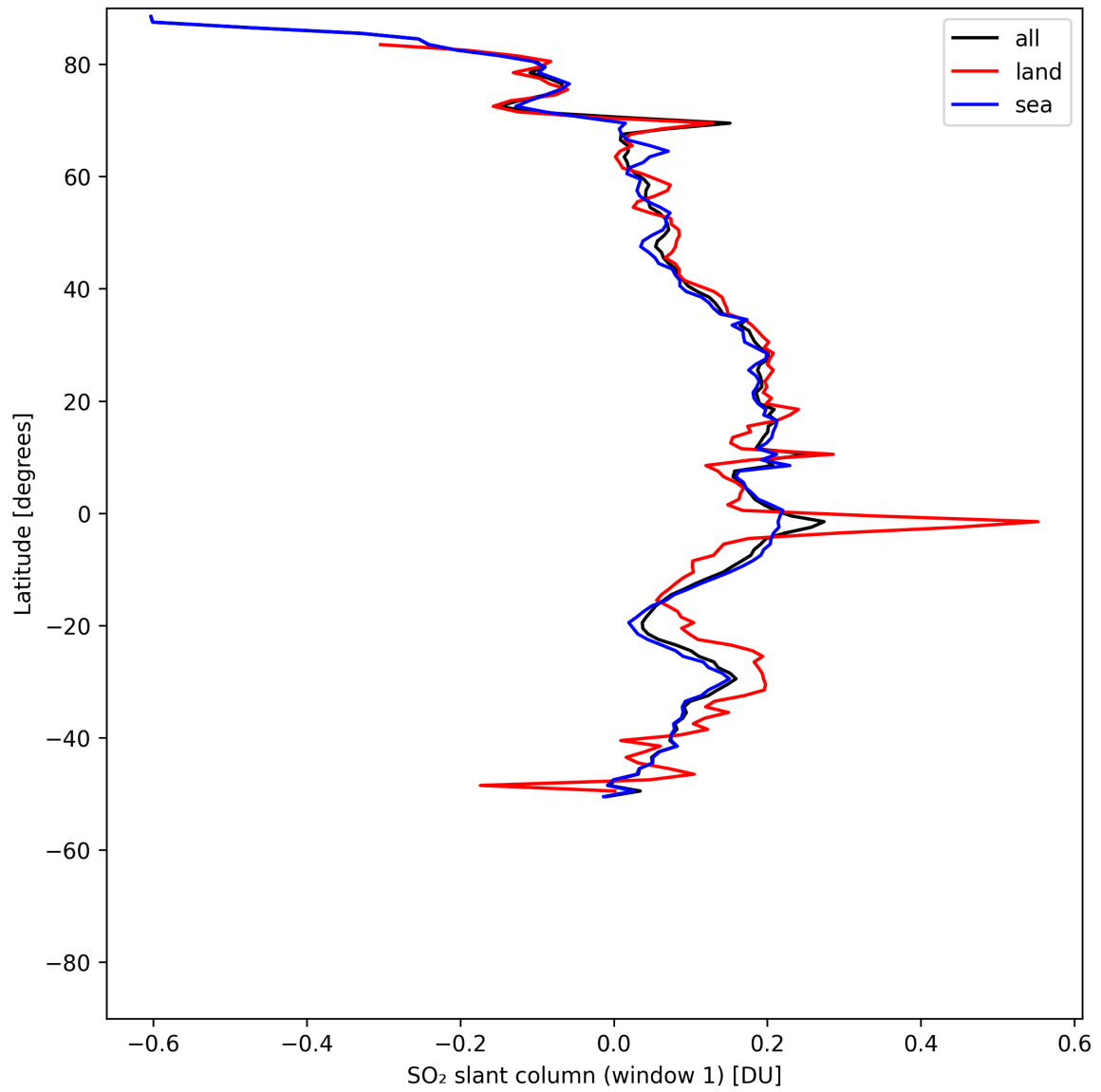
Figure 37: Zonal average of “SO 2 slant column (window 1)” for 2025-05-12 to 2025-05-14.
