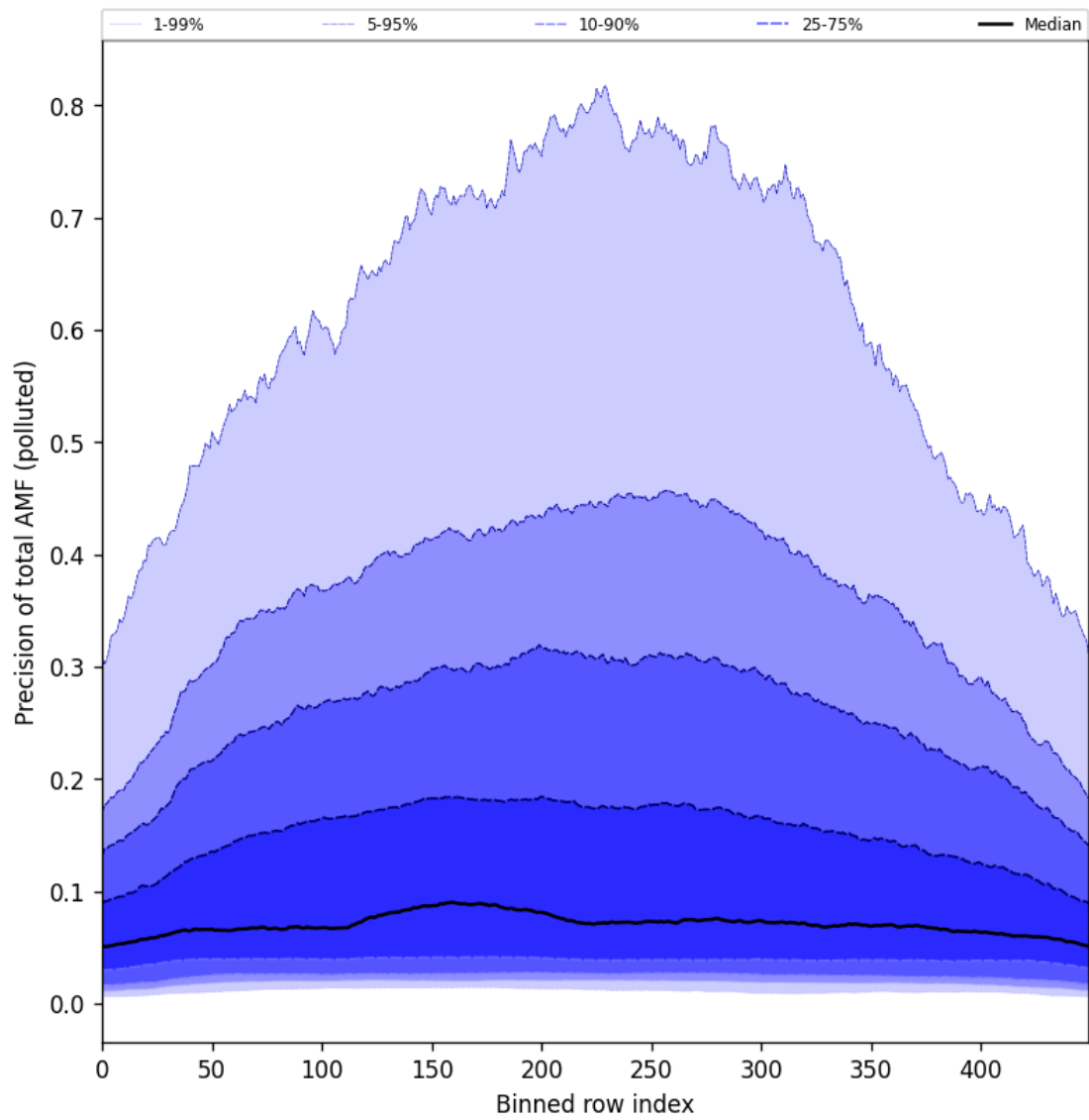
Figure 106: Along track statistics of “Precision of total AMF (polluted)” for 2025-05-12 to 2025-05-14
