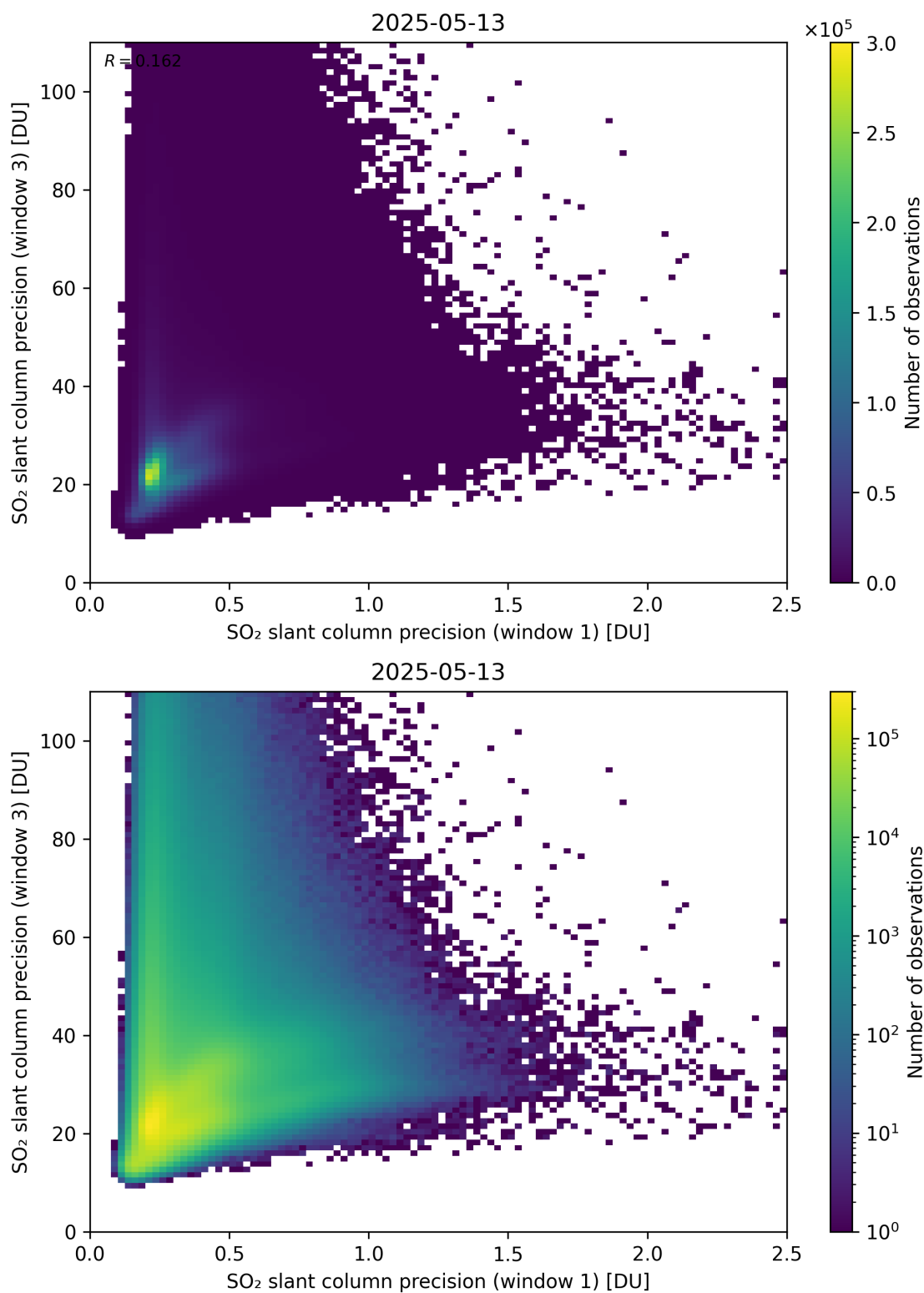
Figure 279: Scatter density plot of “SO 2 slant column precision (window 1)” against “SO 2 slant column precision (window 3)” for 2025-05-12 to 2025-05-14.
