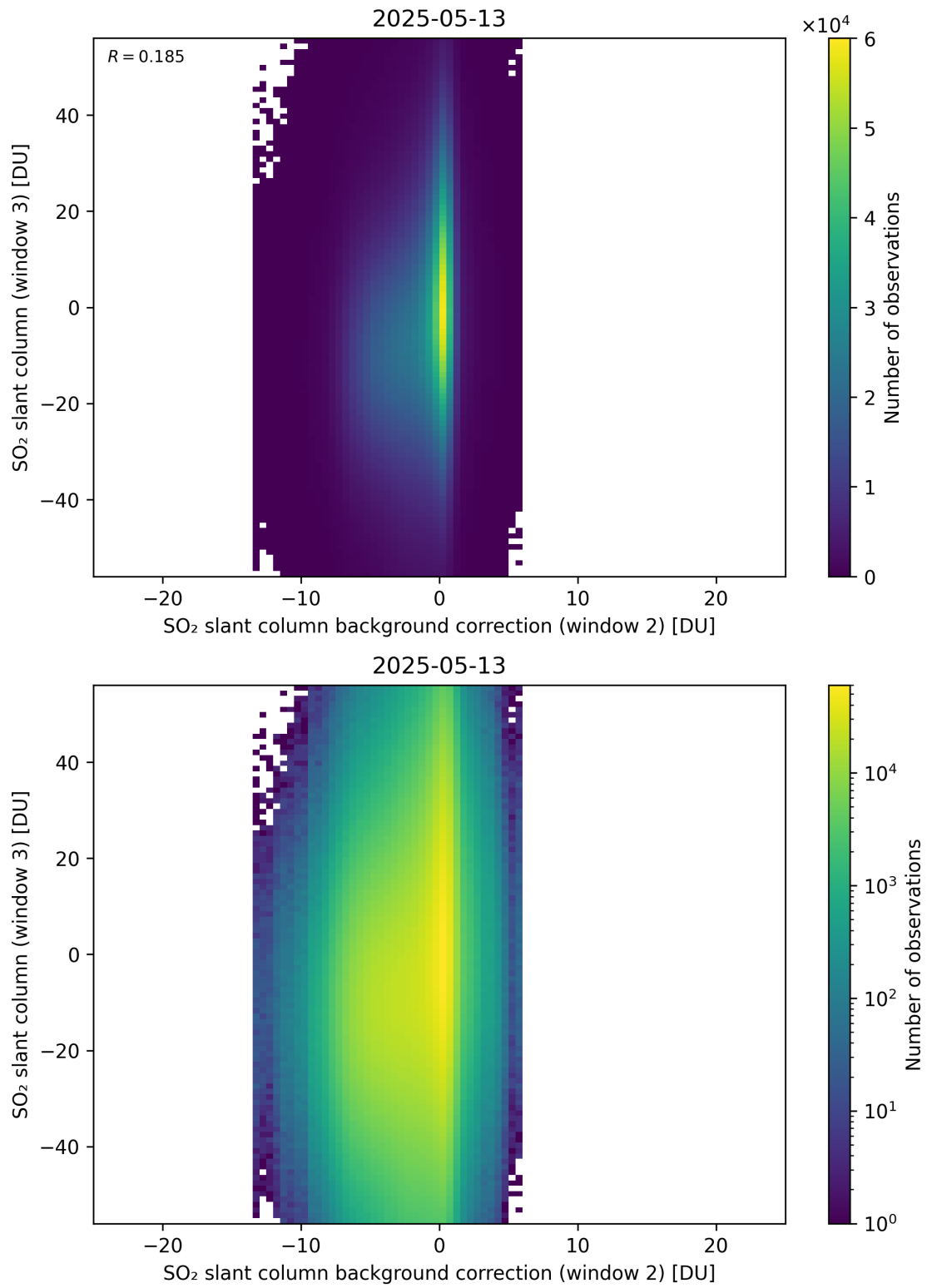
Figure 128: Scatter density plot of “SO 2 slant column background correction (window 2)” against “SO 2 slant column (window 3)” for 2025-05-12 to 2025-05-14.
