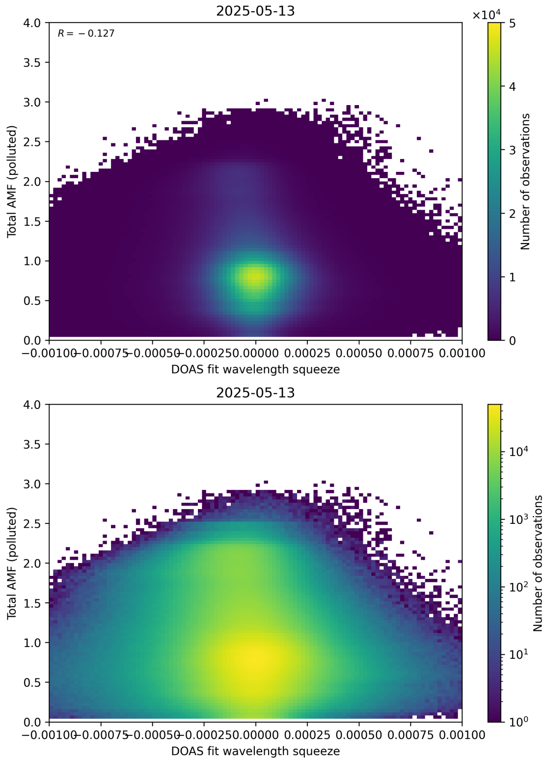
Figure 145: Scatter density plot of “DOAS fit wavelength squeeze” against “Total AMF (polluted)” for 2025-05-12 to 2025-05-14.
