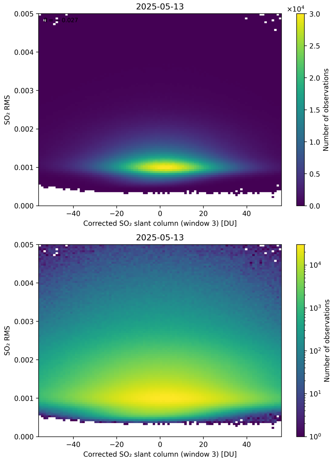
Figure 258: Scatter density plot of “Corrected SO 2 slant column (window 3)” against “SO 2 RMS” for 2025-05-12 to 2025-05-14.
