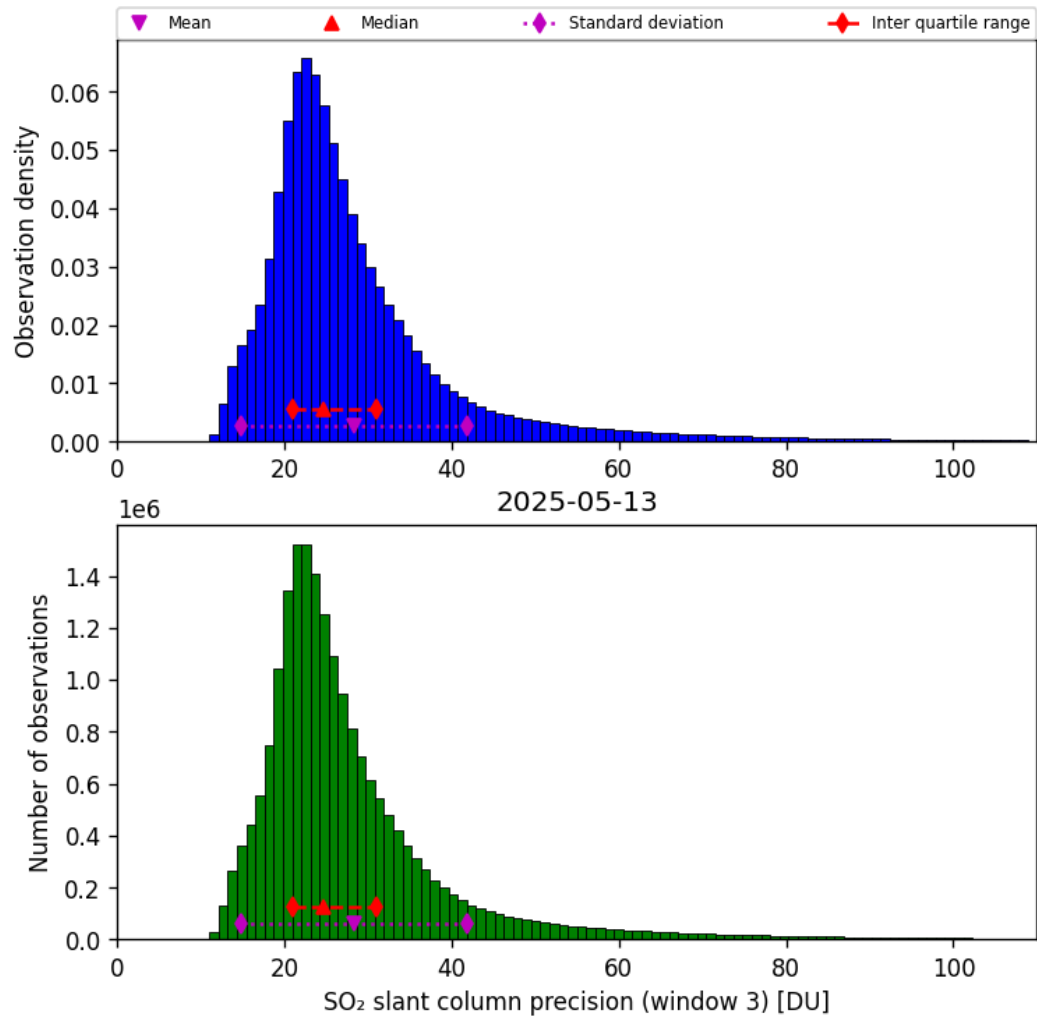
Figure 72: Histogram of “SO 2 slant column precision (window 3)” for 2025-05-12 to 2025-05-14
