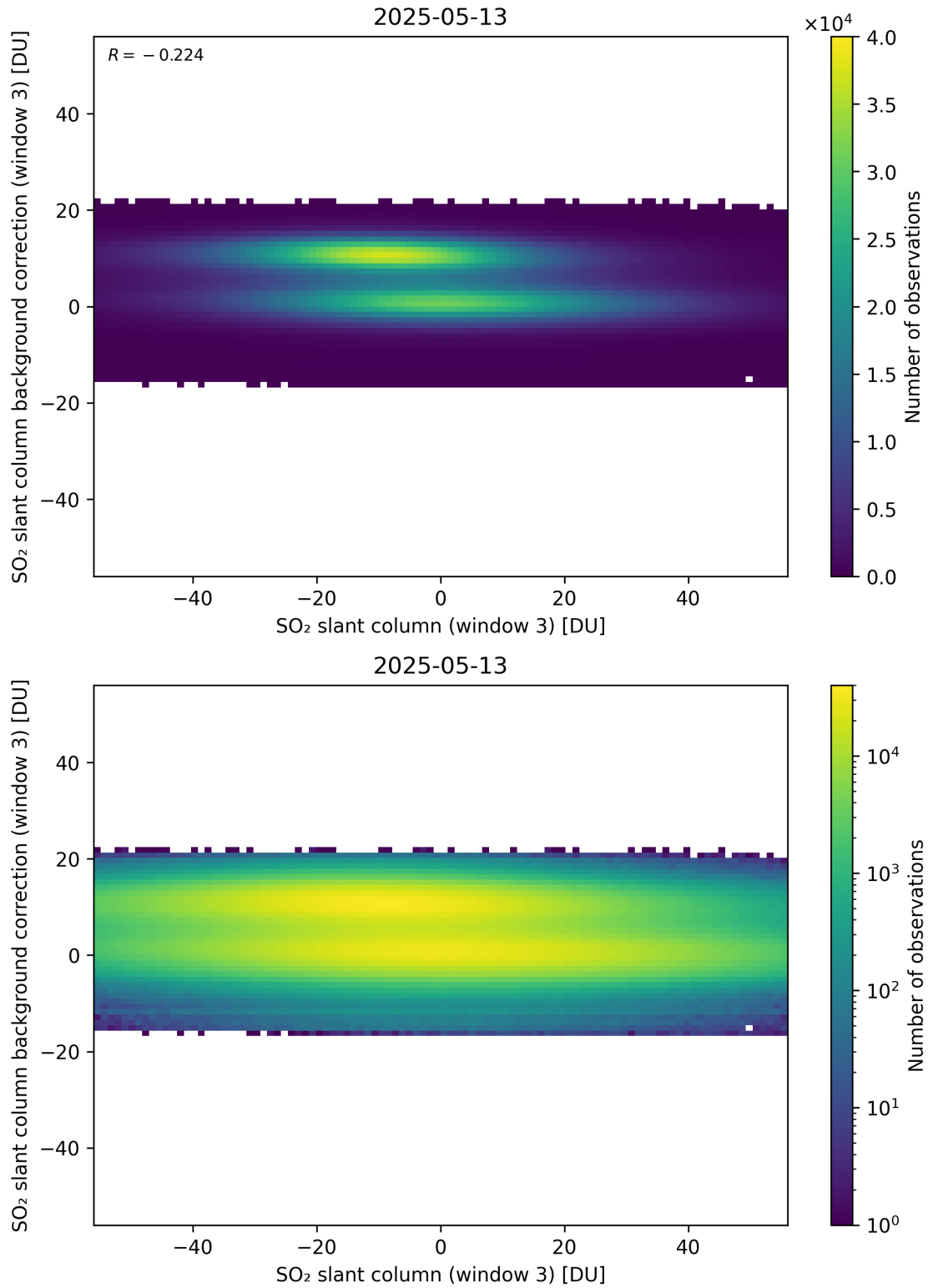
Figure 303: Scatter density plot of “SO 2 slant column (window 3)” against “SO 2 slant column background correction (window 3)” for 2025-05-12 to 2025-05-14.
