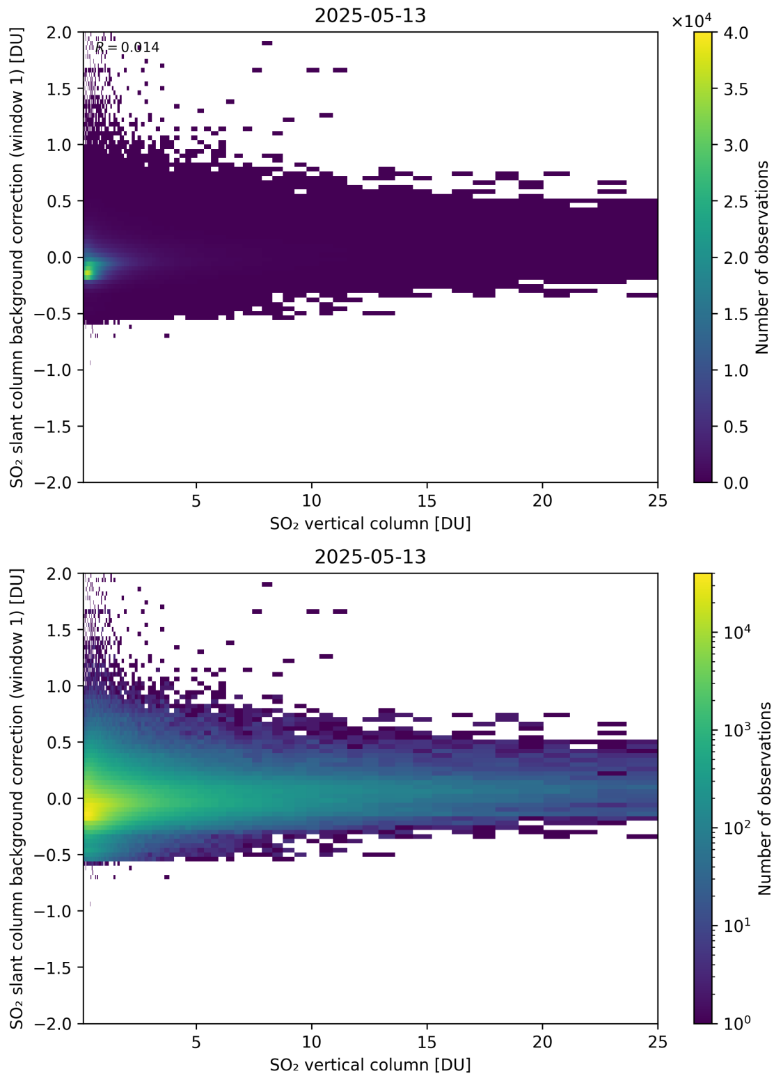
Figure 323: Scatter density plot of “SO 2 vertical column” against “SO 2 slant column background correction (window 1)” for 2025-05-12 to 2025-05-14.
