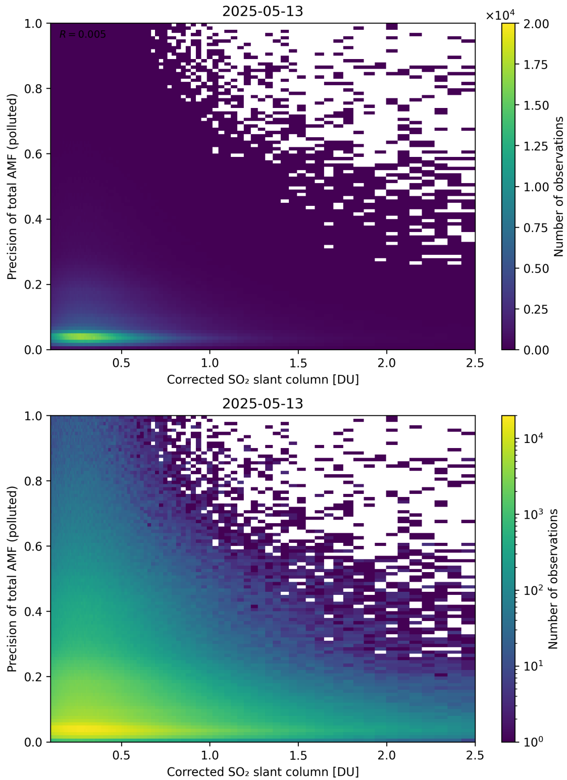
Figure 243: Scatter density plot of “Corrected SO 2 slant column” against “Precision of total AMF (polluted)” for 2025-05-12 to 2025-05-14.
