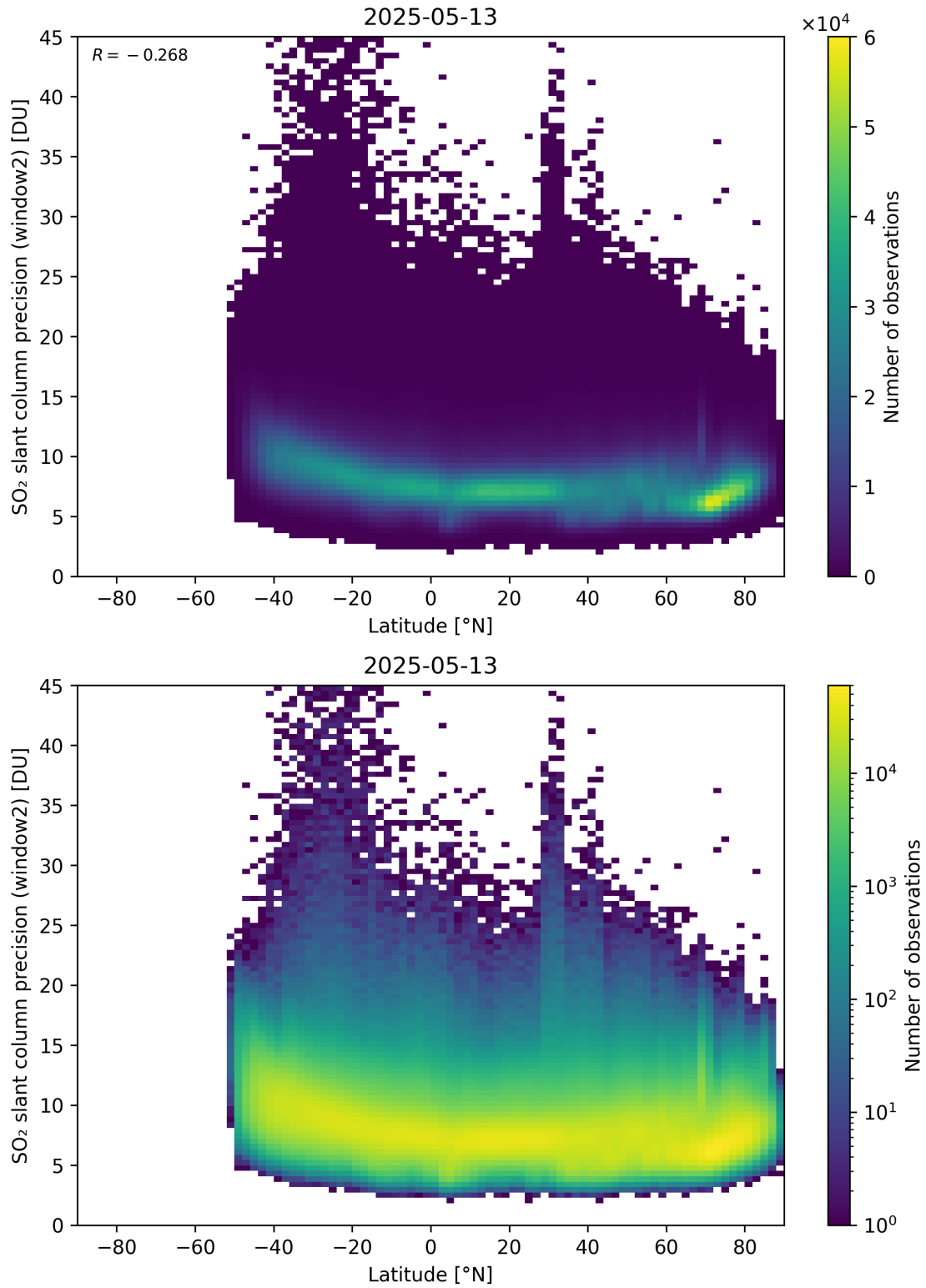
Figure 164: Scatter density plot of “Latitude” against “SO 2 slant column precision (window2)” for 2025-05-12 to 2025-05-14.
