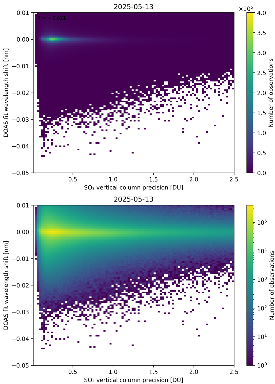
Figure 332: Scatter density plot of “SO 2 vertical column precision” against “DOAS fit wavelength shift” for 2025-05-12 to 2025-05-14.
