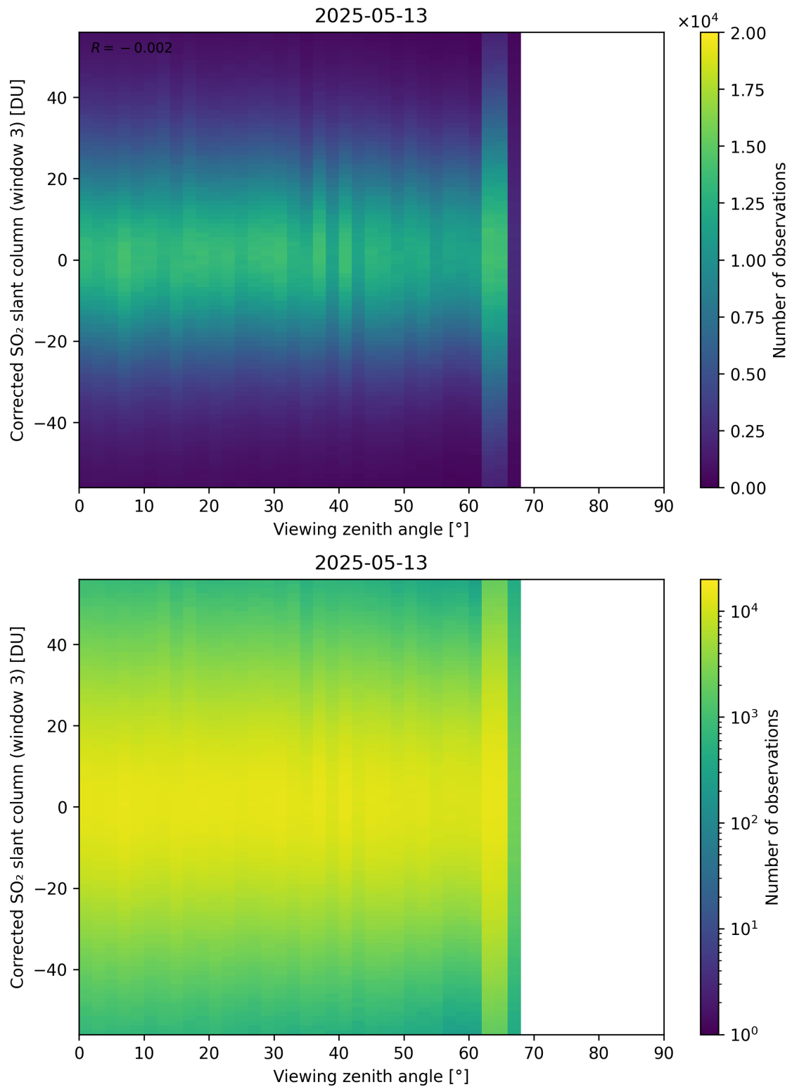
Figure 375: Scatter density plot of “Viewing zenith angle” against “Corrected SO 2 slant column (window 3)” for 2025-05-12 to 2025-05-14.
