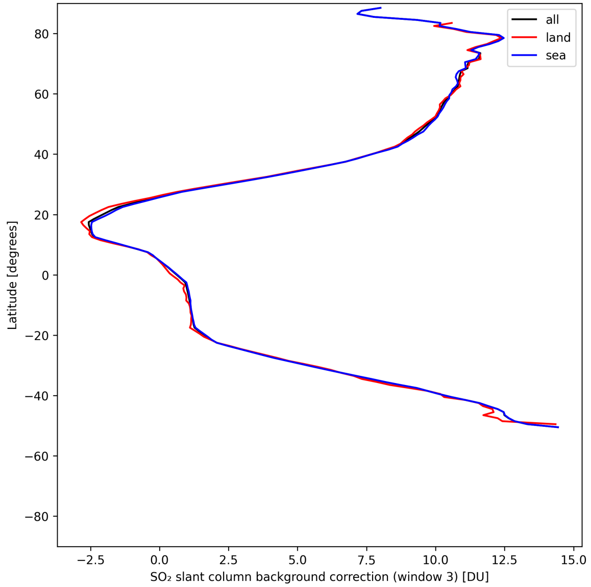
Figure 48: Zonal average of “SO 2 slant column background correction (window 3)” for 2025-05-12 to 2025-05-14.
