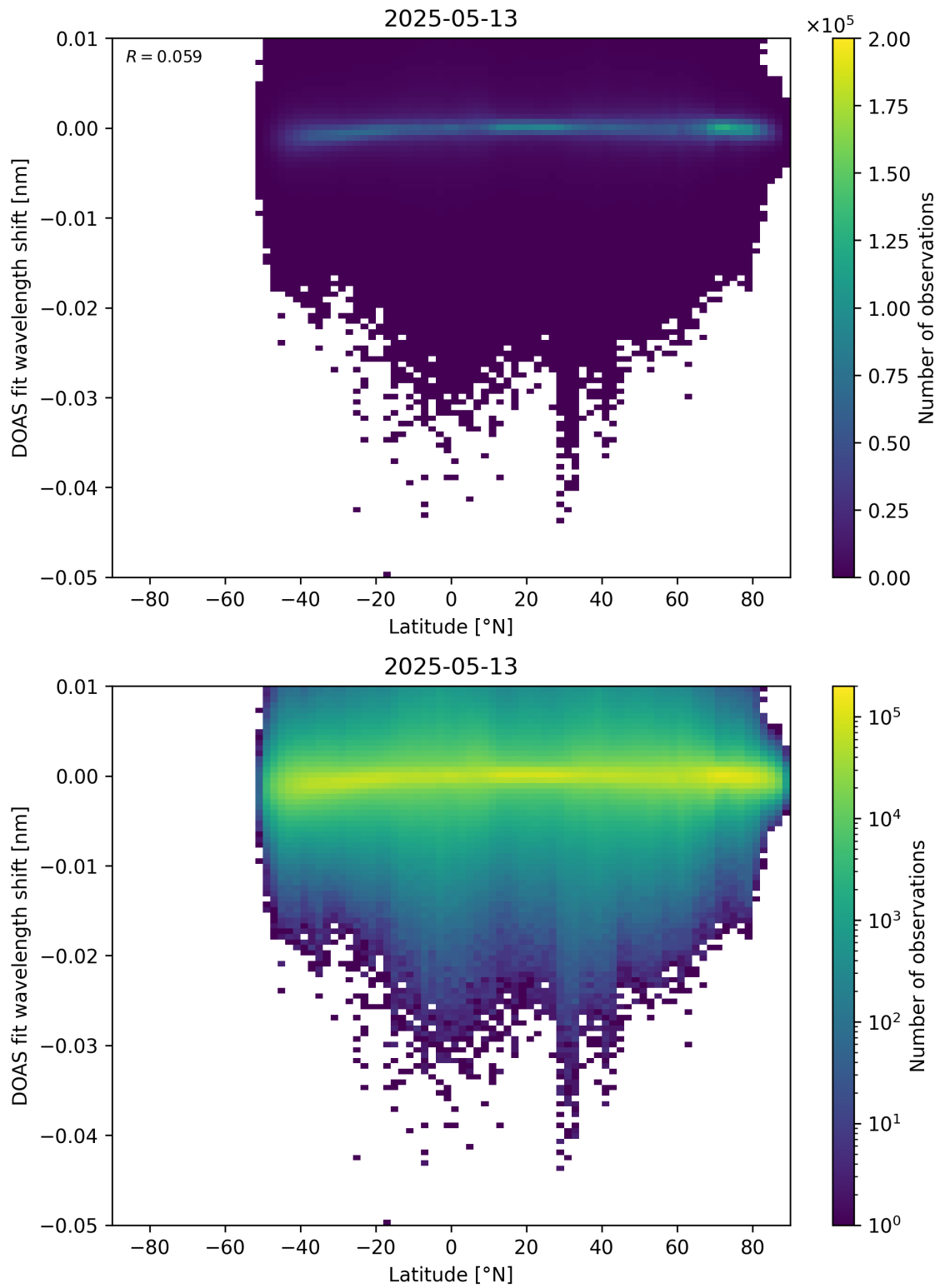
Figure 153: Scatter density plot of “Latitude” against “DOAS fit wavelength shift” for 2025-05-12 to 2025-05-14.
