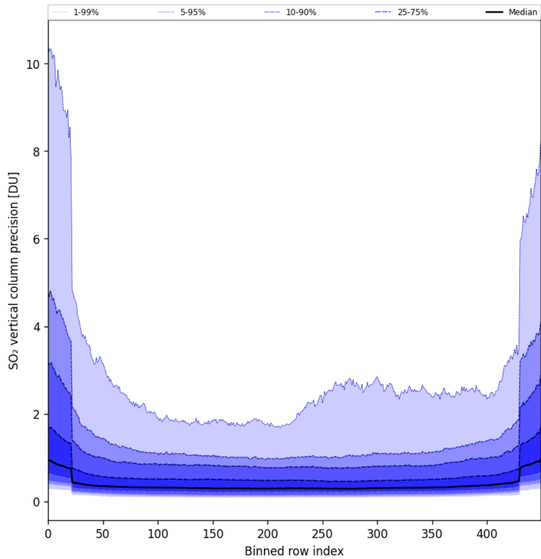
Figure 85: Along track statistics of “SO 2 vertical column precision” for 2025-05-12 to 2025-05-14
