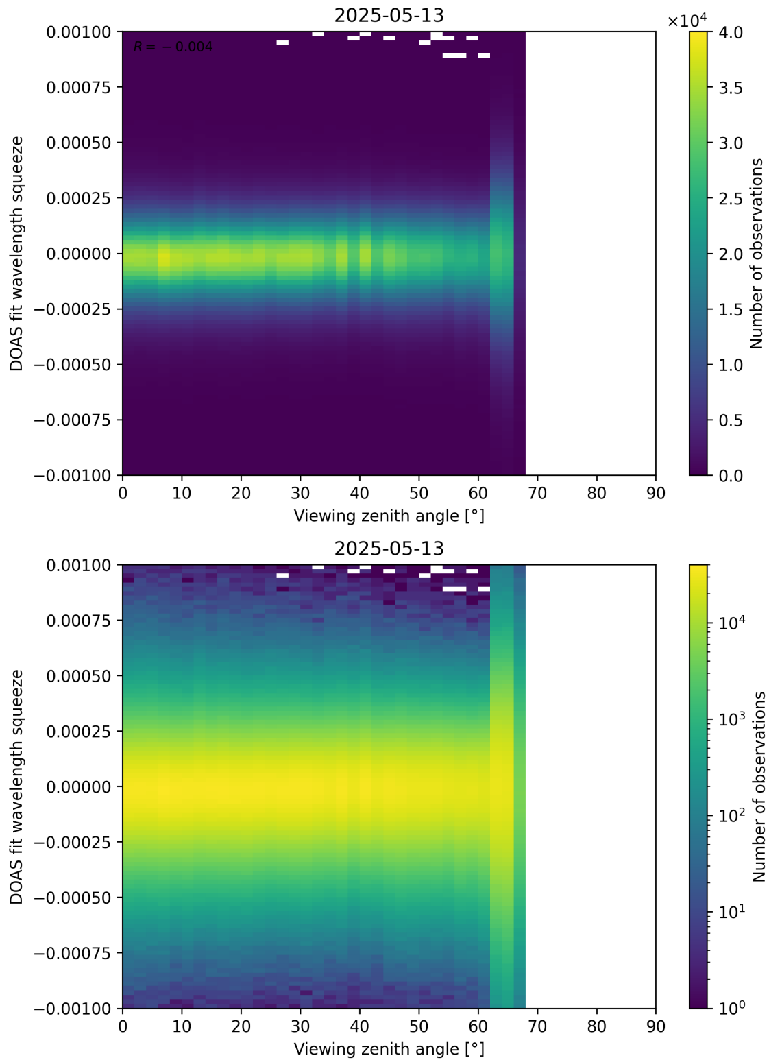
Figure 366: Scatter density plot of “Viewing zenith angle” against “DOAS fit wavelength squeeze” for 2025-05-12 to 2025-05-14.
