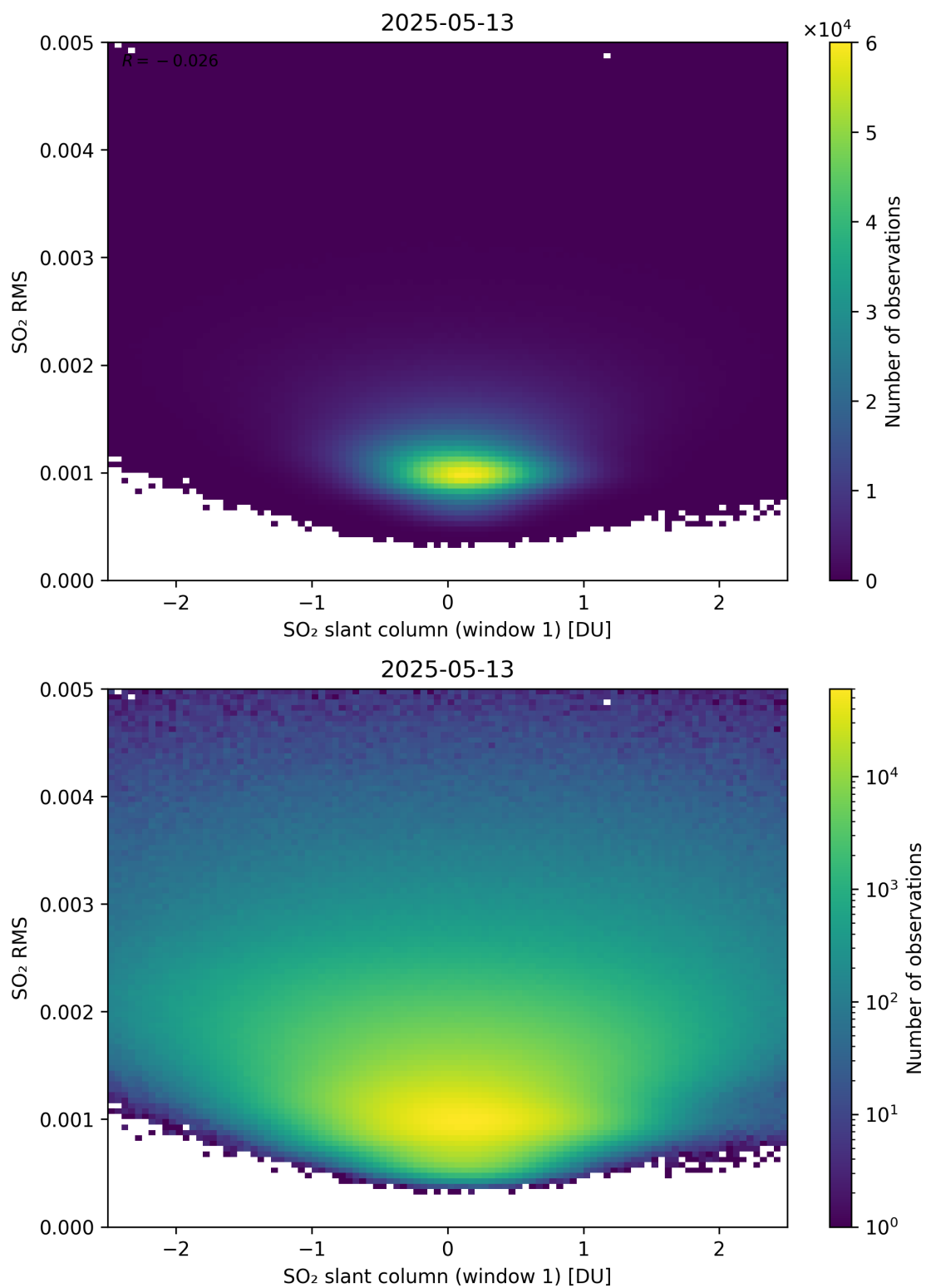
Figure 267: Scatter density plot of “SO 2 slant column (window 1)” against “SO 2 RMS” for 2025-05-12 to 2025-05-14.
