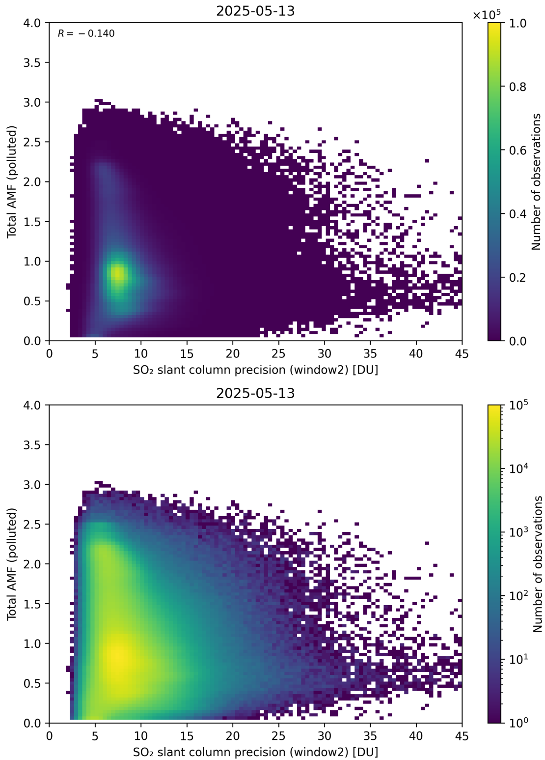
Figure 301: Scatter density plot of “SO 2 slant column precision (window2)” against “Total AMF (polluted)” for 2025-05-12 to 2025-05-14.
