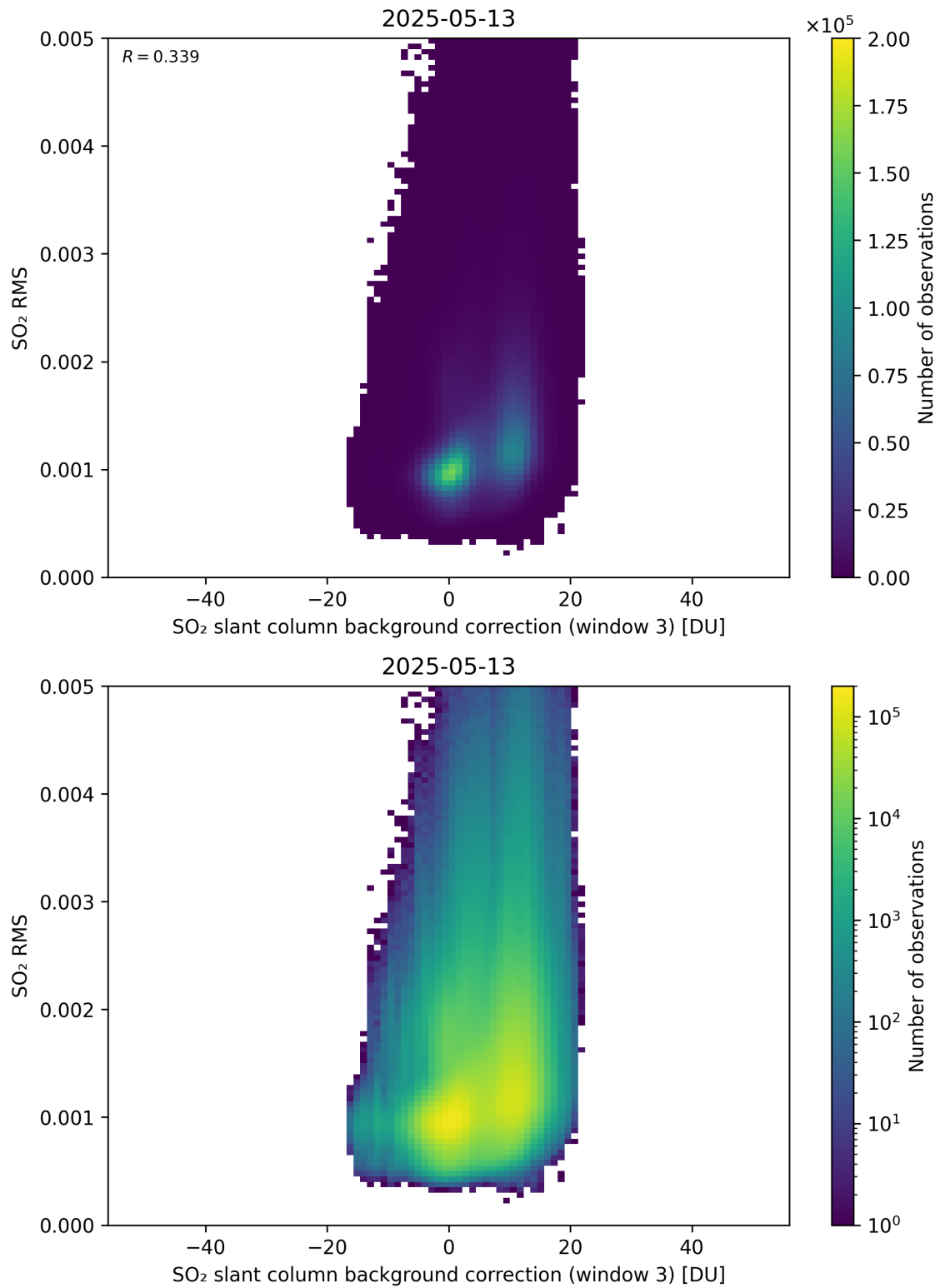
Figure 134: Scatter density plot of “SO 2 slant column background correction (window 3)” against “SO 2 RMS” for 2025-05-12 to 2025-05-14.
