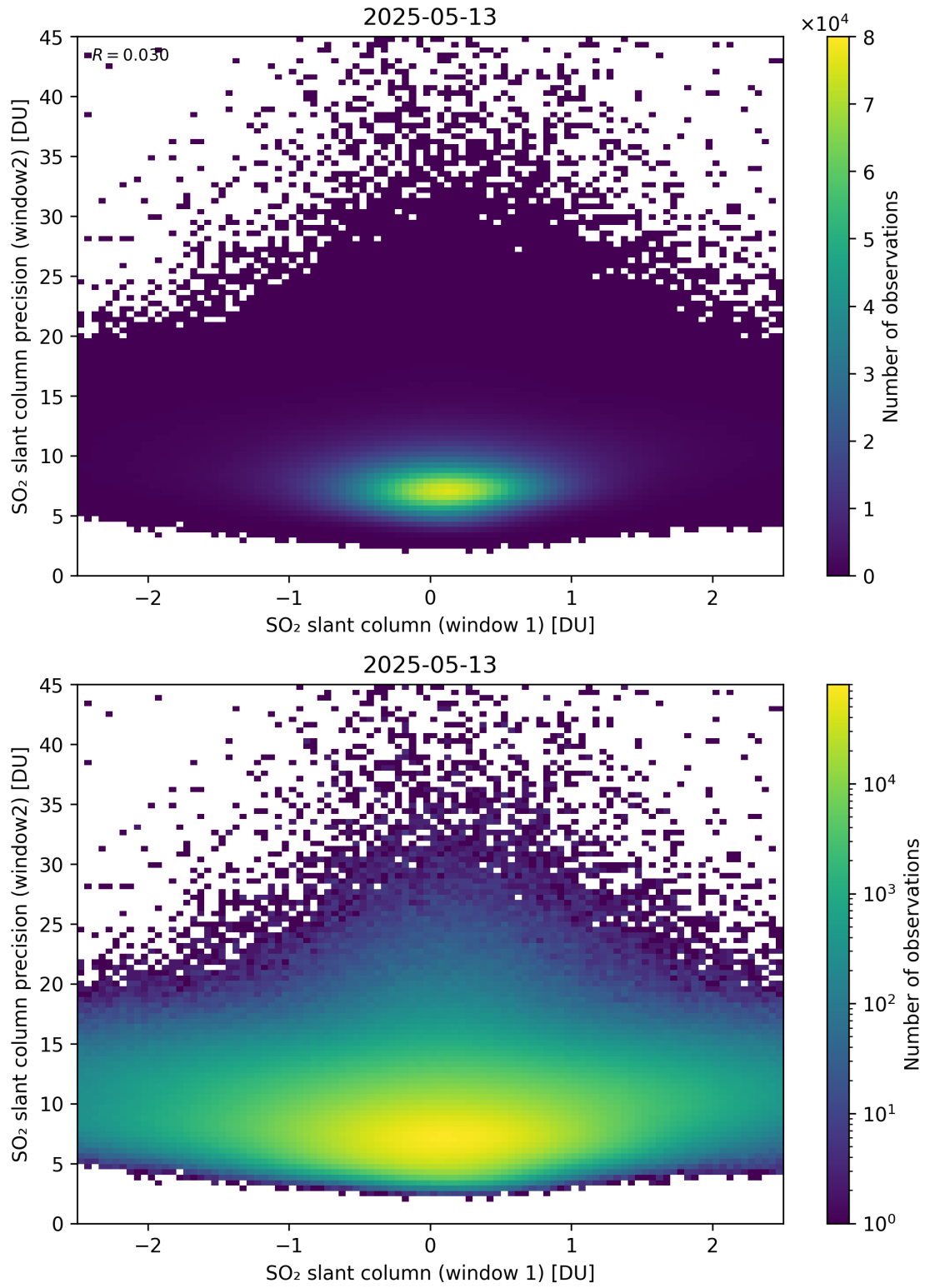
Figure 286: Scatter density plot of “SO 2 slant column (window 1)” against “SO 2 slant column precision (window2)” for 2025-05-12 to 2025-05-14.
