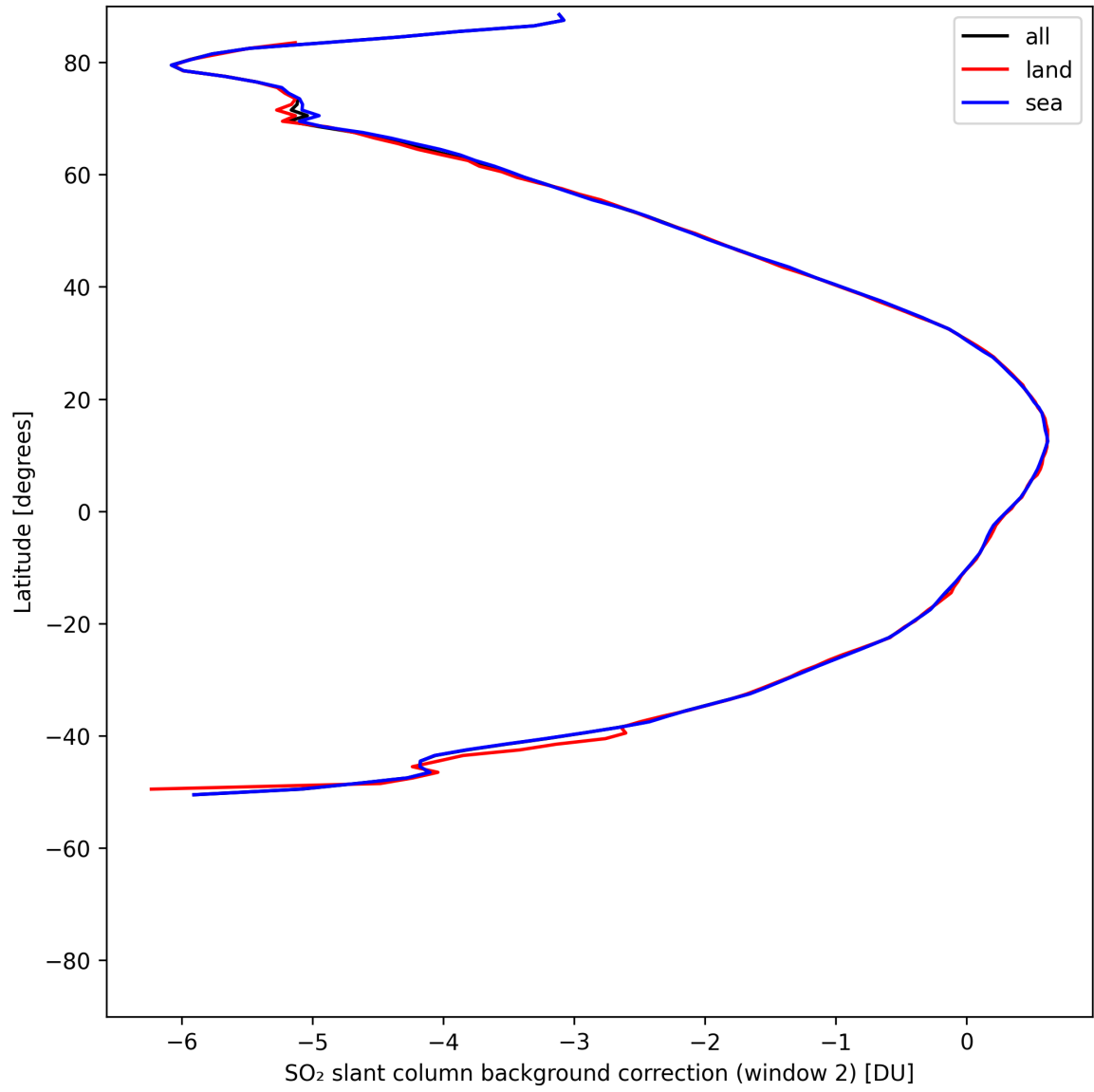
Figure 44: Zonal average of “SO 2 slant column background correction (window 2)” for 2025-05-12 to 2025-05-14.
