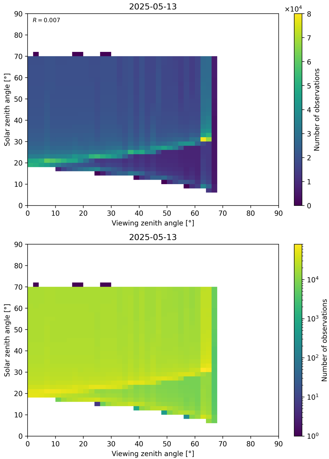
Figure 369: Scatter density plot of “Viewing zenith angle” against “Solar zenith angle” for 2025-05-12 to 2025-05-14.
