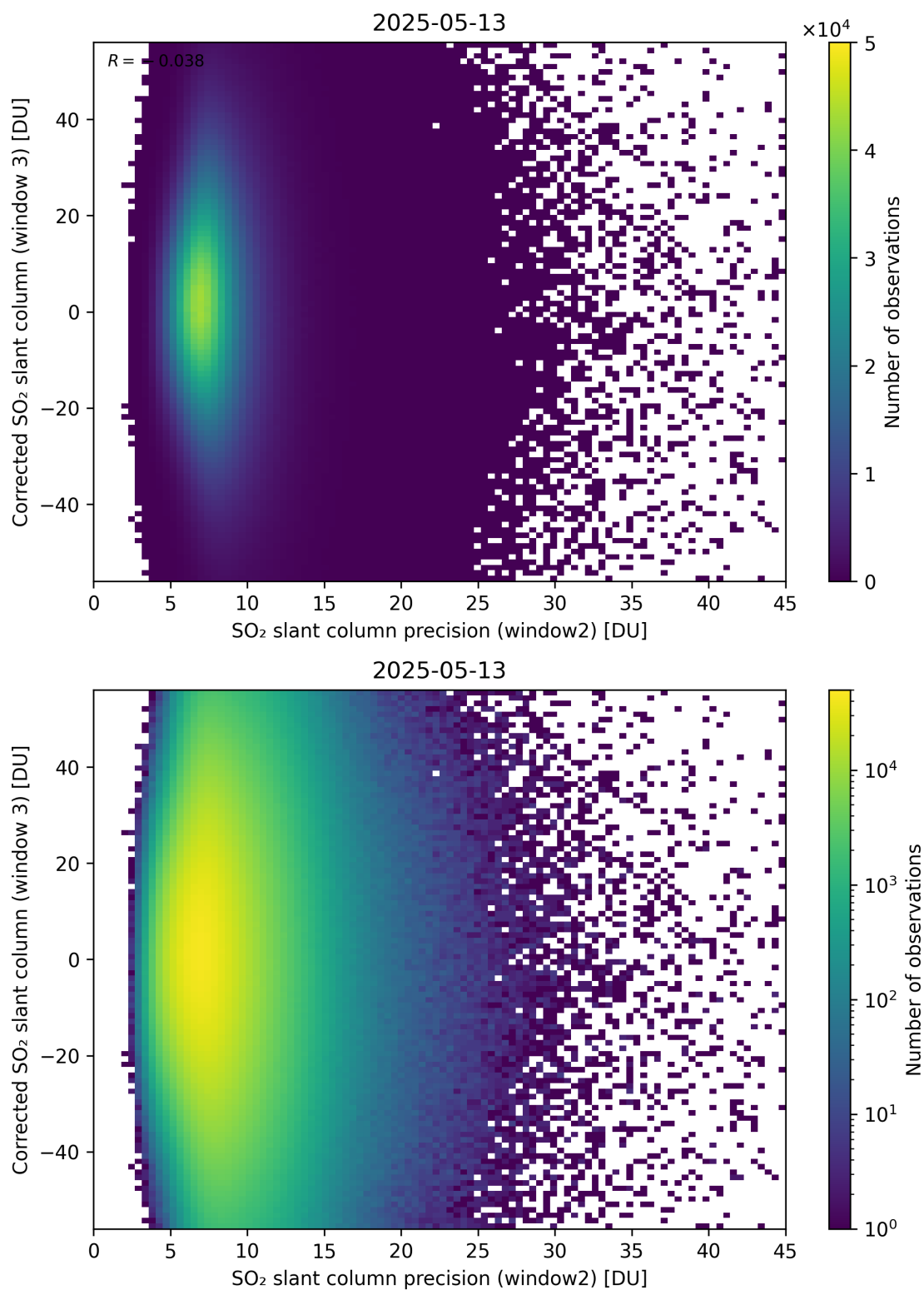
Figure 298: Scatter density plot of “SO 2 slant column precision (window2)” against “Corrected SO 2 slant column (window 3)” for 2025-05-12 to 2025-05-14.
