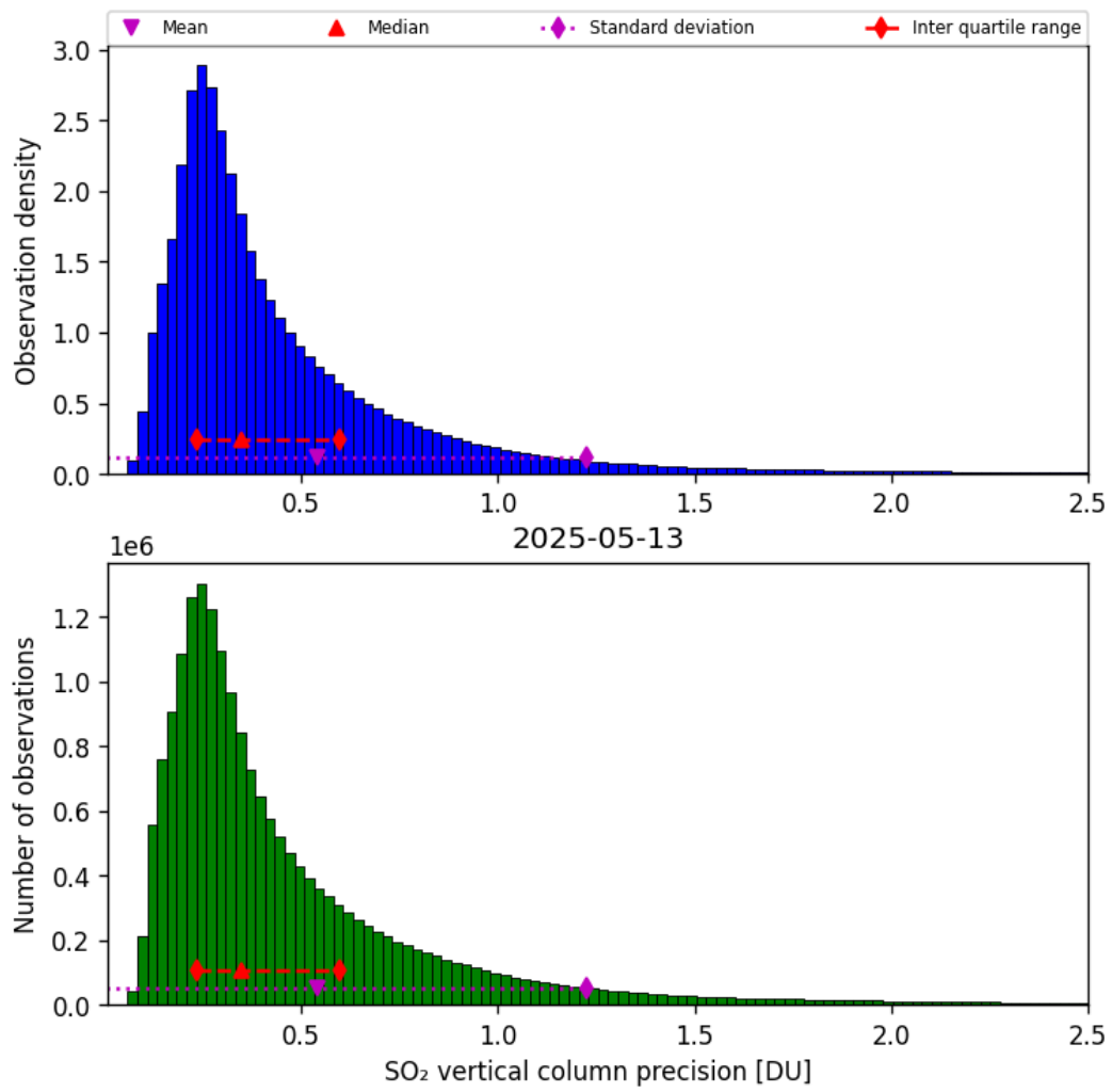
Figure 59: Histogram of “SO 2 vertical column precision” for 2025-05-12 to 2025-05-14
