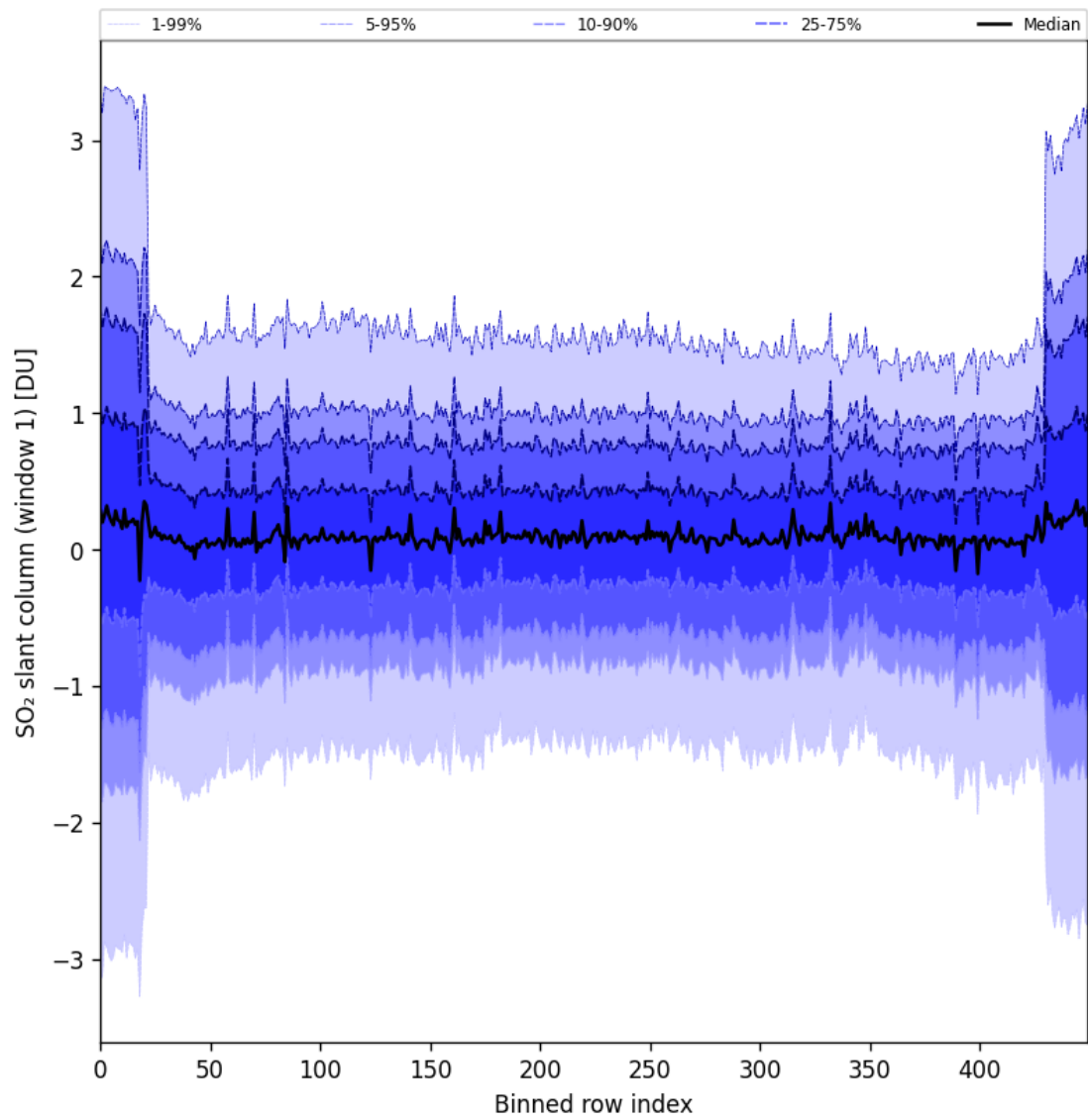
Figure 89: Along track statistics of “SO 2 slant column (window 1)” for 2025-05-12 to 2025-05-14
