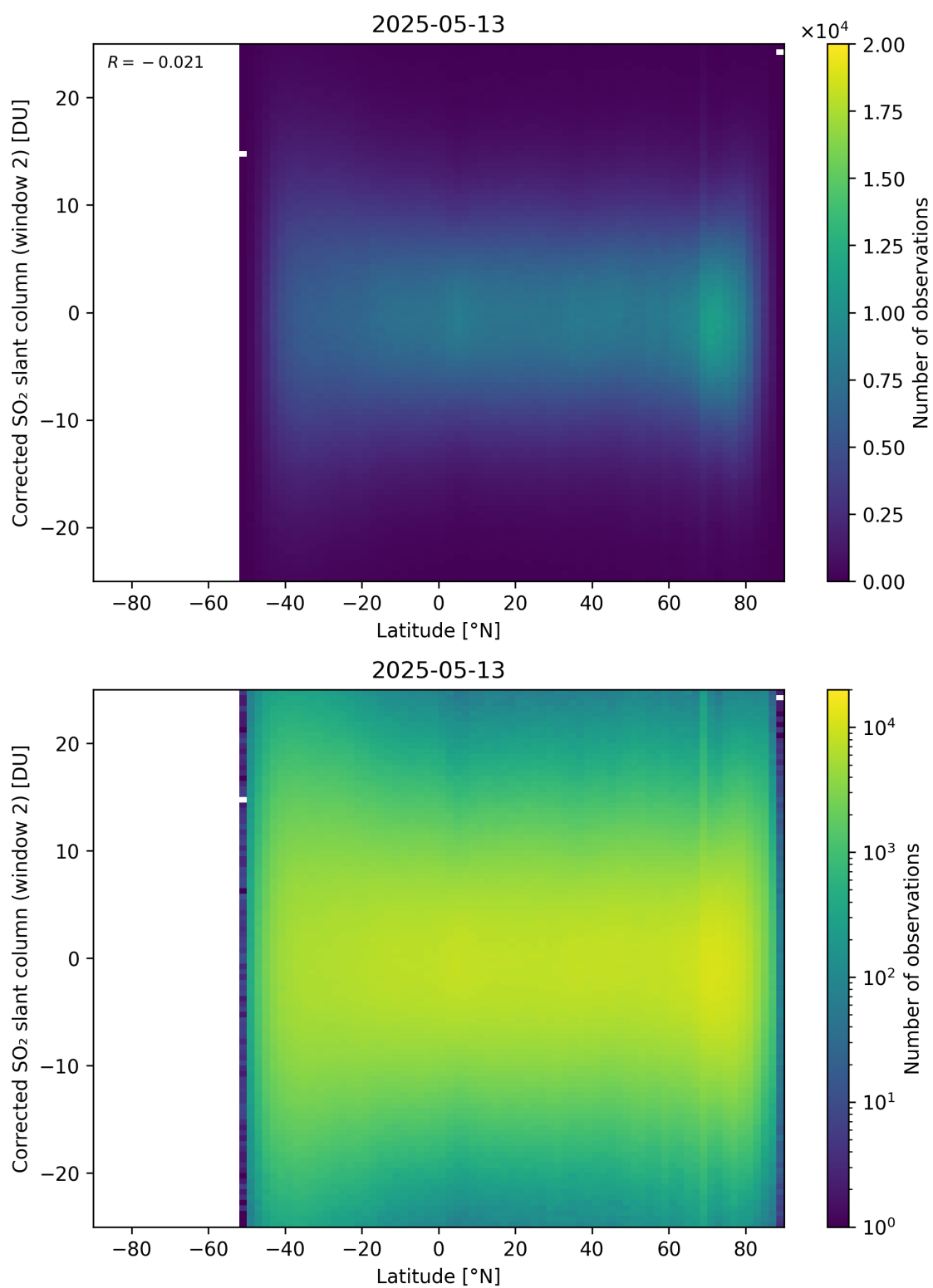
Figure 160: Scatter density plot of “Latitude” against “Corrected SO 2 slant column (window 2)” for 2025-05-12 to 2025-05-14.
