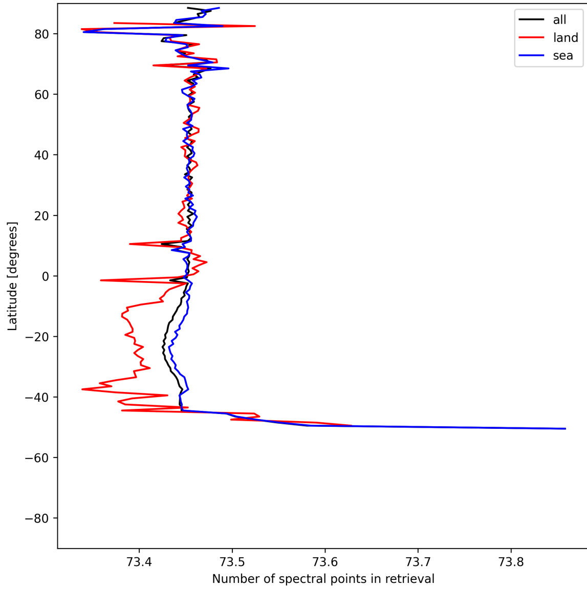
Figure 56: Zonal average of “Number of spectral points in retrieval” for 2025-05-12 to 2025-05-14.
