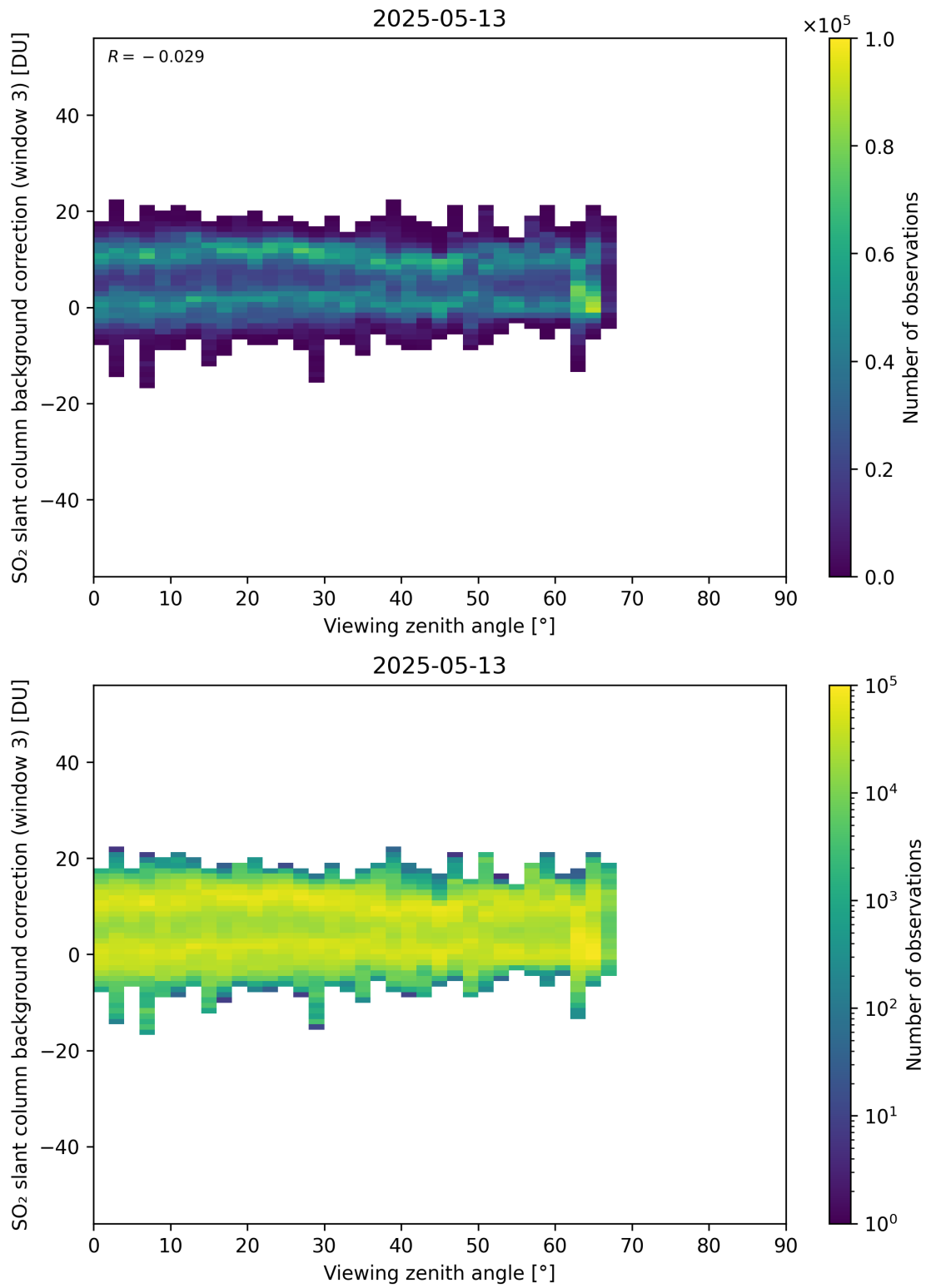
Figure 364: Scatter density plot of “Viewing zenith angle” against “SO 2 slant column background correction (window 3)” for 2025-05-12 to 2025-05-14.
