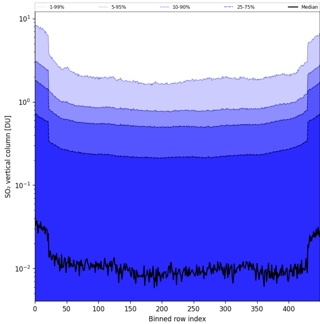
Figure 84: Along track statistics of “SO 2 vertical column” for 2025-05-12 to 2025-05-14
