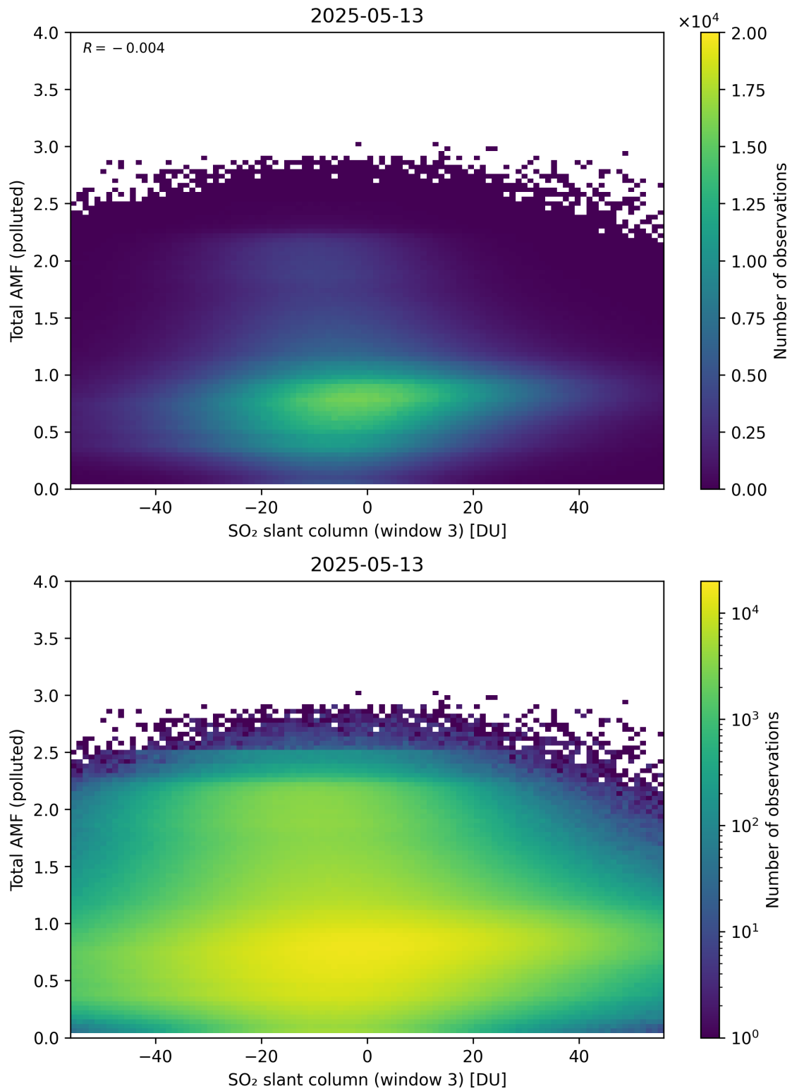
Figure 318: Scatter density plot of “SO 2 slant column (window 3)” against “Total AMF (polluted)” for 2025-05-12 to 2025-05-14.
