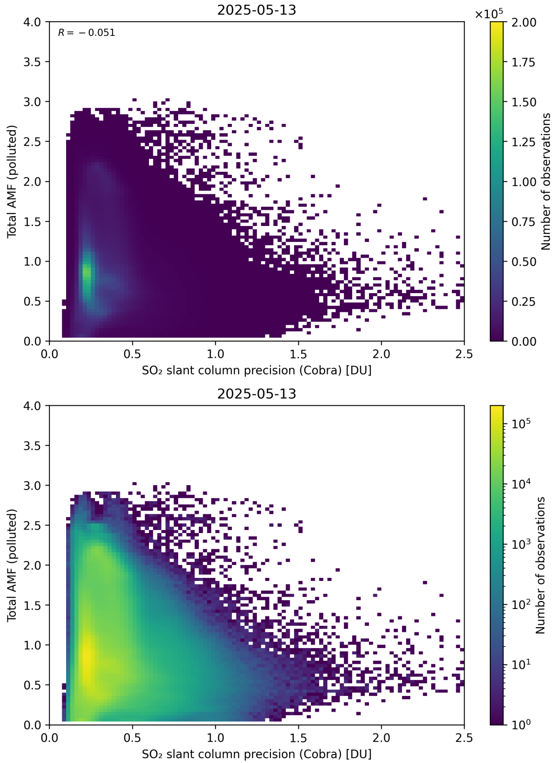
Figure 213: Scatter density plot of “SO 2 slant column precision (Cobra)” against “Total AMF (polluted)” for 2025-05-12 to 2025-05-14.
