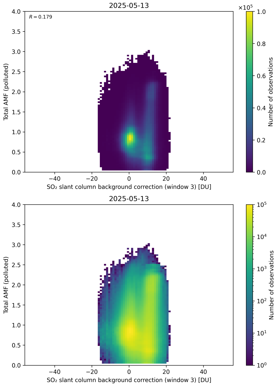
Figure 136: Scatter density plot of “SO 2 slant column background correction (window 3)” against “Total AMF (polluted)” for 2025-05-12 to 2025-05-14.
