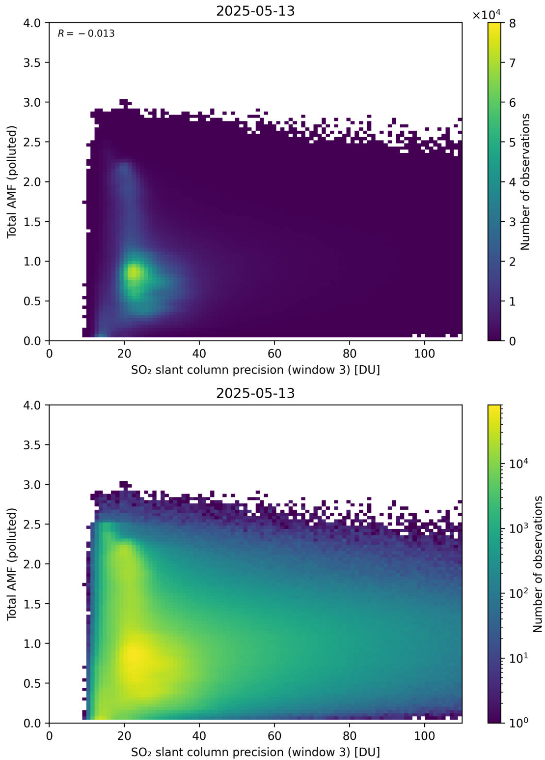
Figure 313: Scatter density plot of “SO 2 slant column precision (window 3)” against “Total AMF (polluted)” for 2025-05-12 to 2025-05-14.
