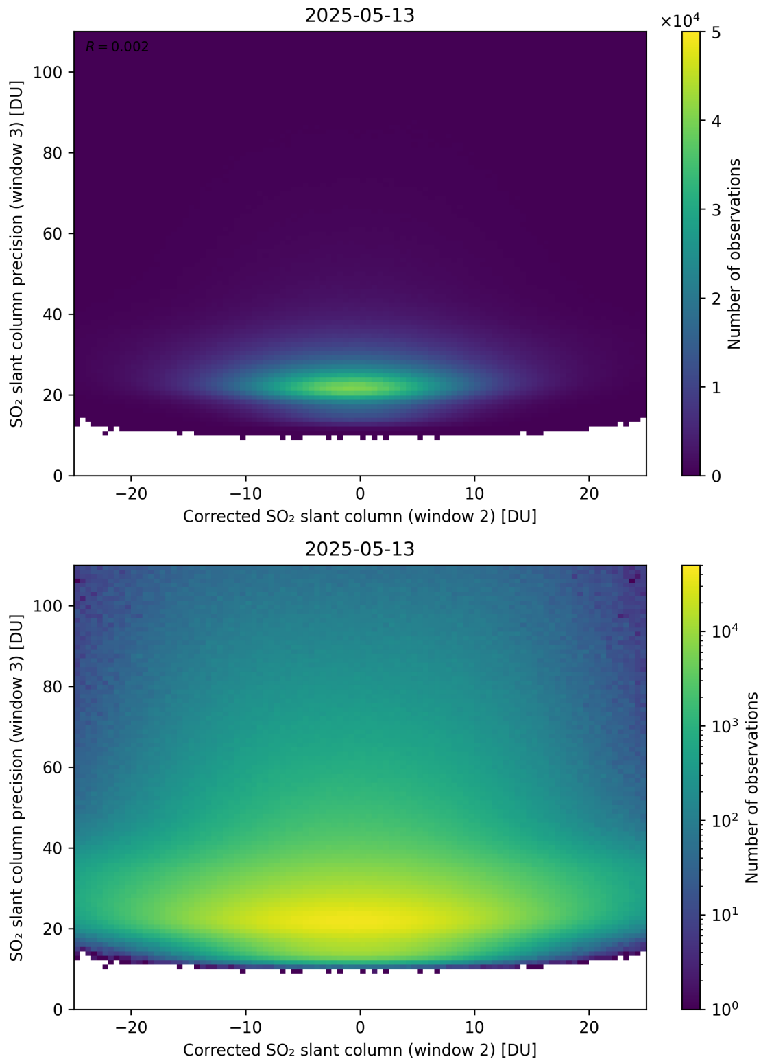
Figure 252: Scatter density plot of “Corrected SO 2 slant column (window 2)” against “SO 2 slant column precision (window 3)” for 2025-05-12 to 2025-05-14.
