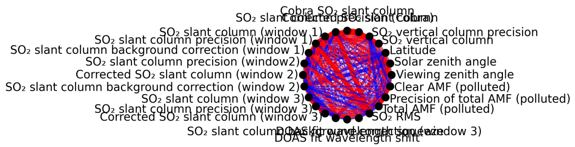
Figure 1: Map of correlation graph for 2025-05-12 to 2025-05-14.
