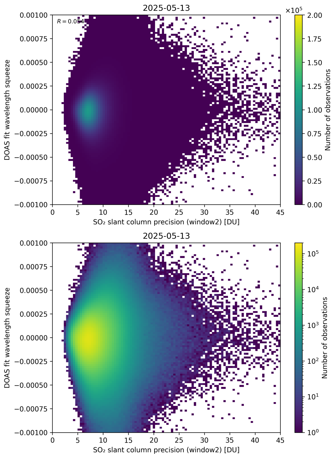
Figure 294: Scatter density plot of “SO 2 slant column precision (window2)” against “DOAS fit wavelength squeeze” for 2025-05-12 to 2025-05-14.
