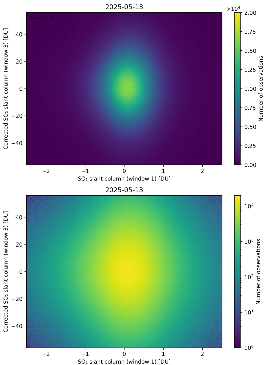
Figure 284: Scatter density plot of “SO 2 slant column (window 1)” against “Corrected SO 2 slant column (window 3)” for 2025-05-12 to 2025-05-14.
