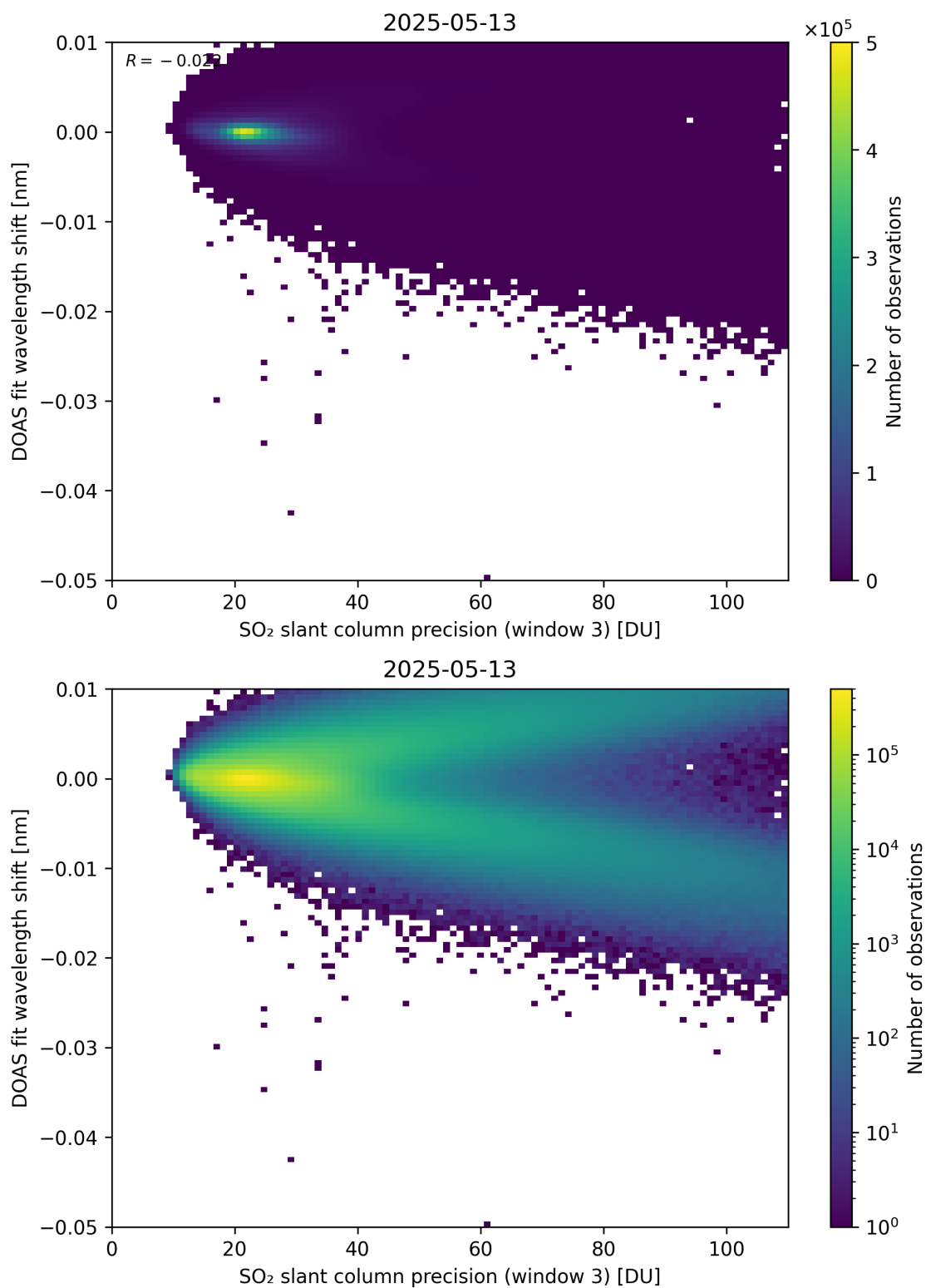
Figure 308: Scatter density plot of “SO 2 slant column precision (window 3)” against “DOAS fit wavelength shift” for 2025-05-12 to 2025-05-14.
