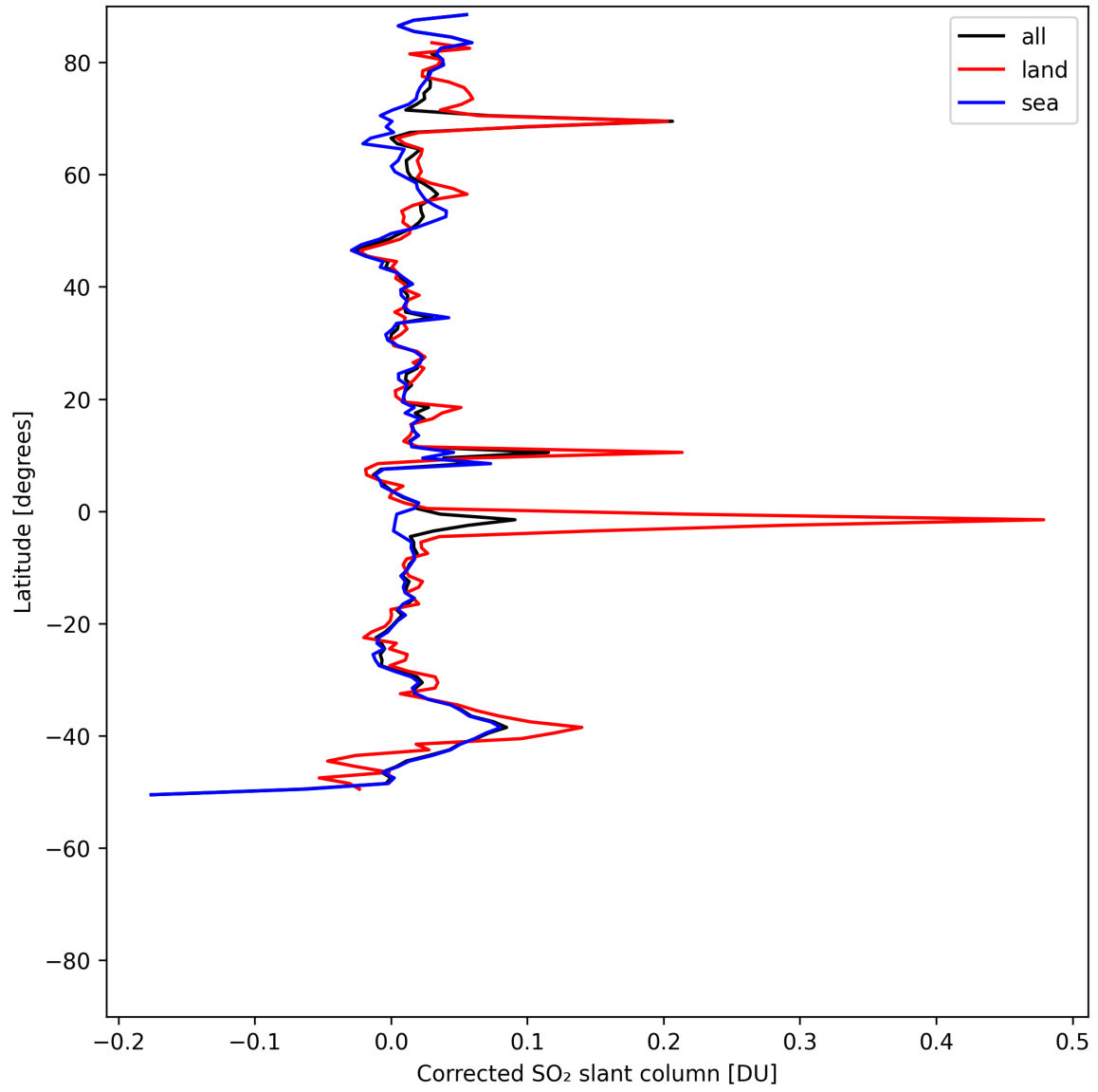
Figure 34: Zonal average of “Corrected SO 2 slant column” for 2025-05-12 to 2025-05-14.
