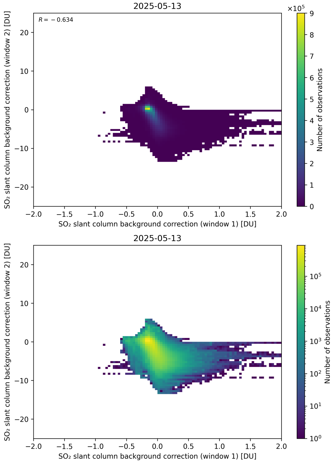
Figure 109: Scatter density plot of “SO 2 slant column background correction (window 1)” against “SO 2 slant column background correction (window 2)” for 2025-05-12 to 2025-05-14.
