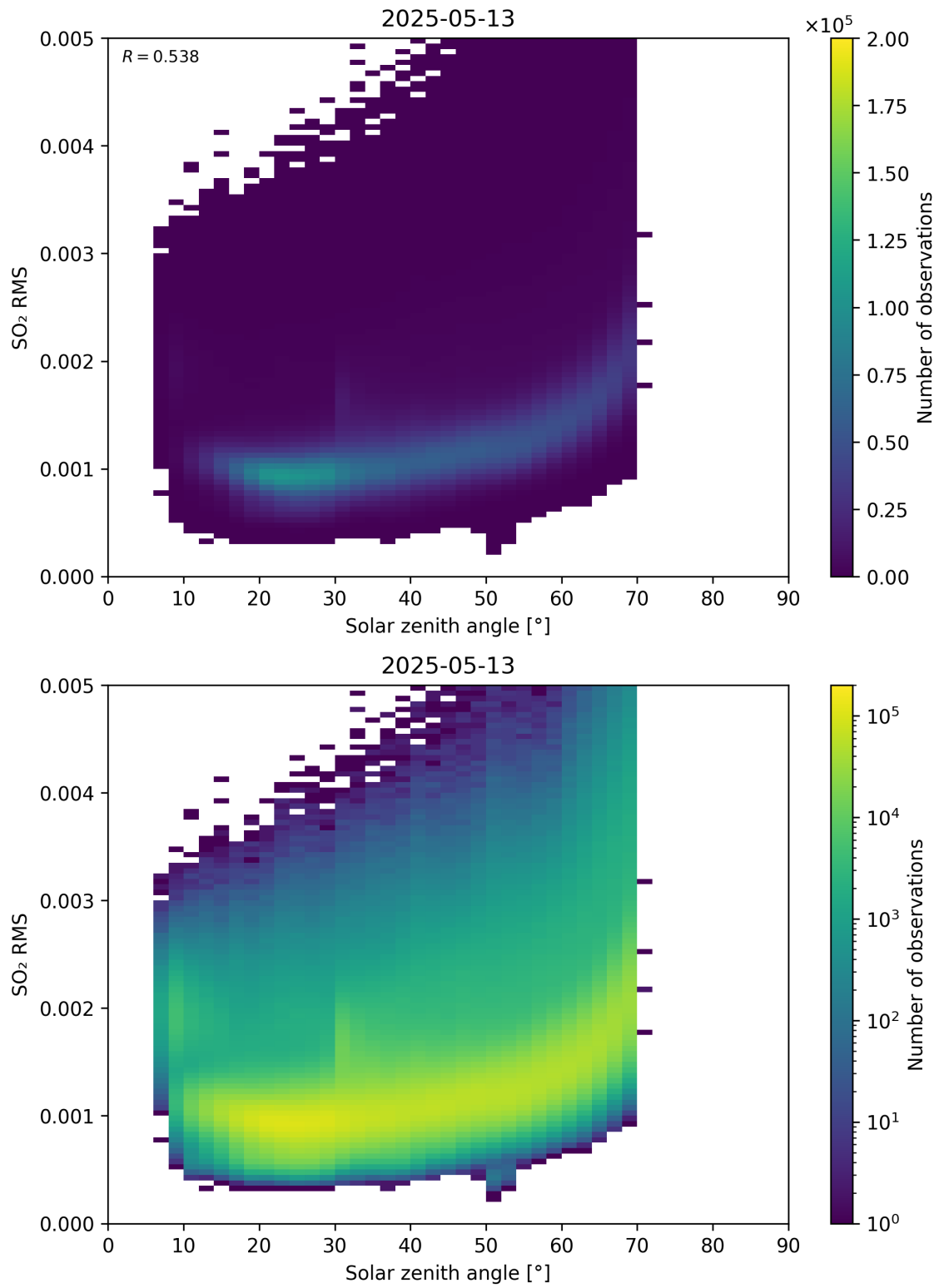
Figure 176: Scatter density plot of “Solar zenith angle” against “SO 2 RMS” for 2025-05-12 to 2025-05-14.
