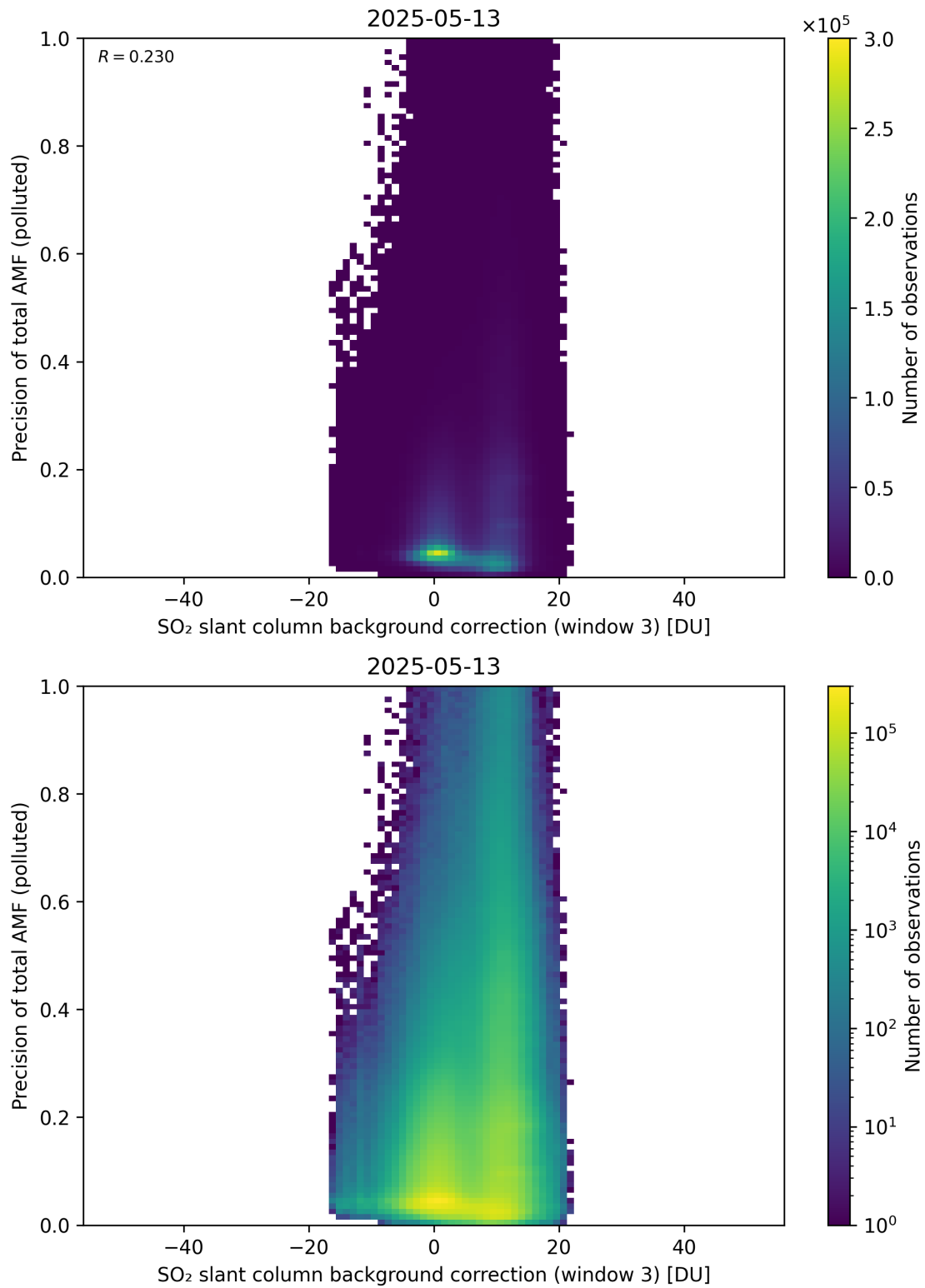
Figure 137: Scatter density plot of “SO 2 slant column background correction (window 3)” against “Precision of total AMF (polluted)” for 2025-05-12 to 2025-05-14.
