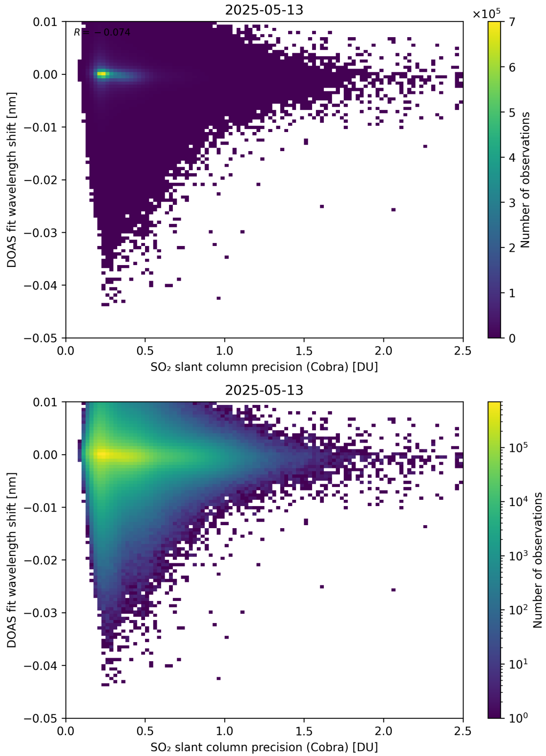
Figure 202: Scatter density plot of “SO 2 slant column precision (Cobra)” against “DOAS fit wavelength shift” for 2025-05-12 to 2025-05-14.
