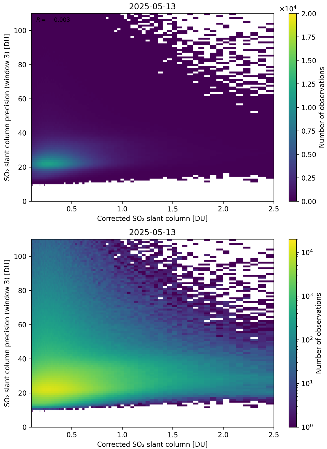
Figure 241: Scatter density plot of “Corrected SO 2 slant column” against “SO 2 slant column precision (window 3)” for 2025-05-12 to 2025-05-14.
