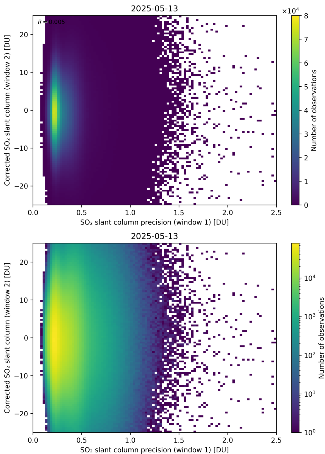
Figure 275: Scatter density plot of “SO 2 slant column precision (window 1)” against “Corrected SO 2 slant column (window 2)” for 2025-05-12 to 2025-05-14.
