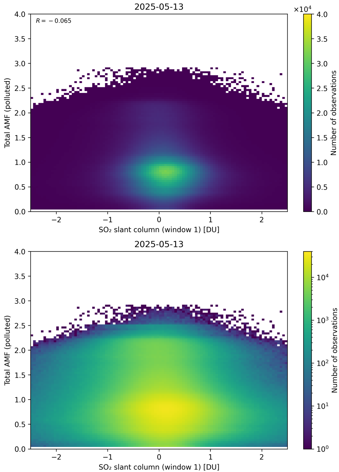
Figure 289: Scatter density plot of “SO 2 slant column (window 1)” against “Total AMF (polluted)” for 2025-05-12 to 2025-05-14.
