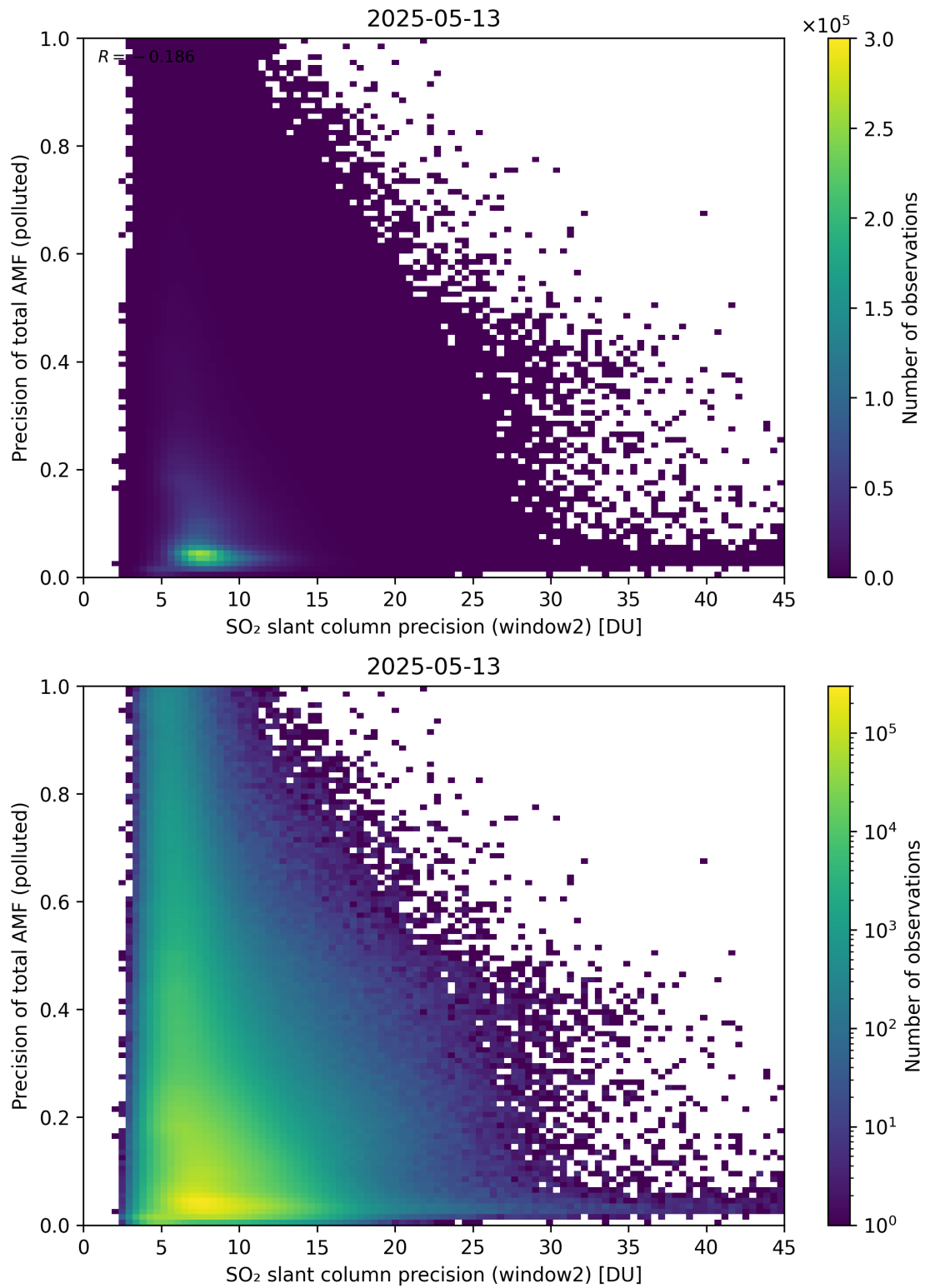
Figure 302: Scatter density plot of “SO 2 slant column precision (window2)” against “Precision of total AMF (polluted)” for 2025-05-12 to 2025-05-14.
