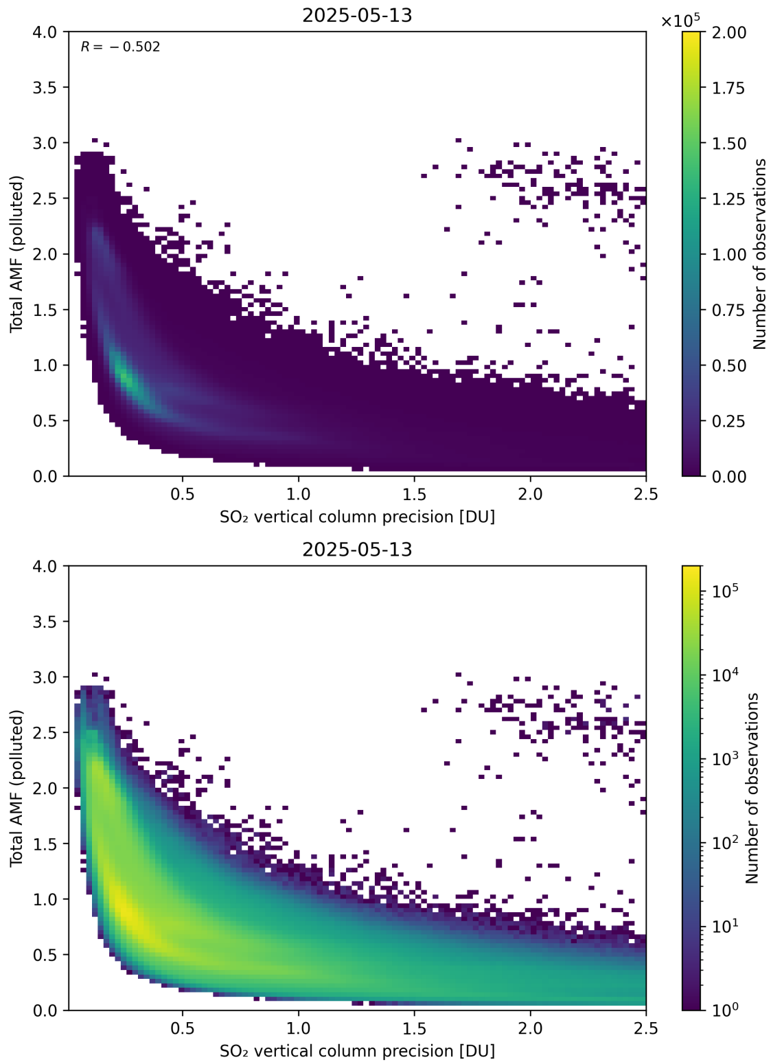
Figure 346: Scatter density plot of “SO 2 vertical column precision” against “Total AMF (polluted)” for 2025-05-12 to 2025-05-14.
