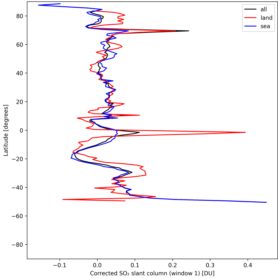
Figure 39: Zonal average of “Corrected SO 2 slant column (window 1)” for 2025-05-12 to 2025-05-14.
