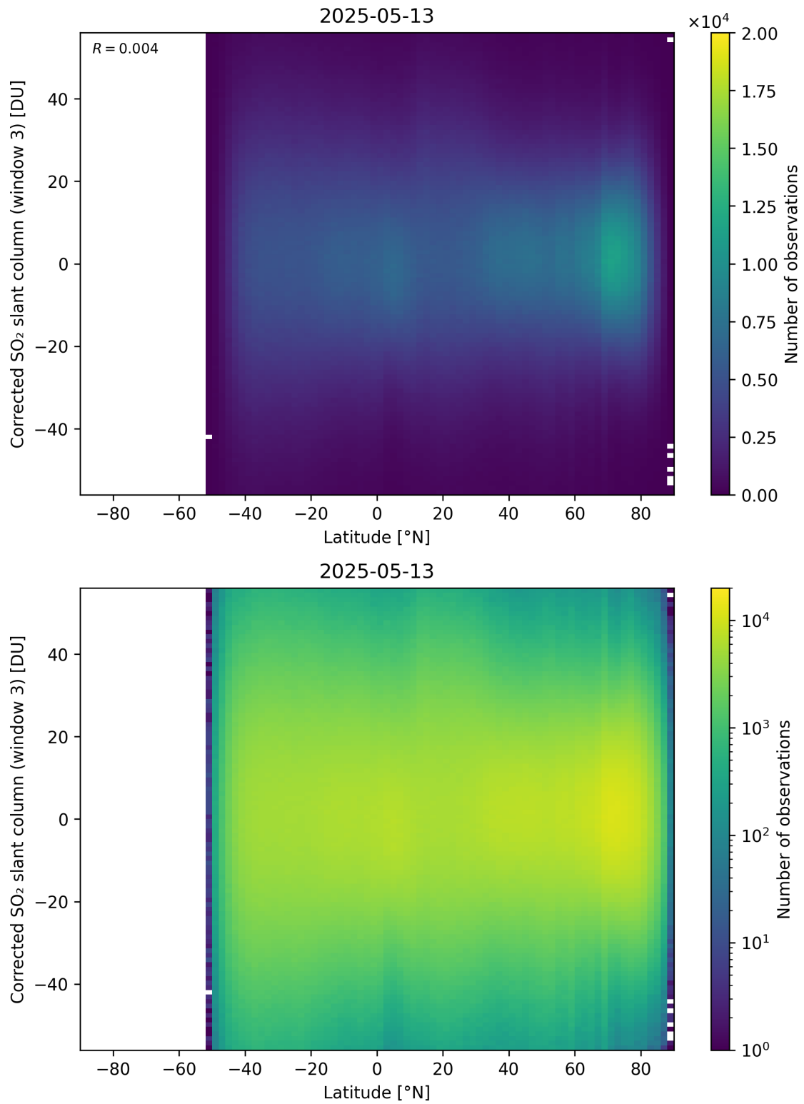
Figure 161: Scatter density plot of “Latitude” against “Corrected SO 2 slant column (window 3)” for 2025-05-12 to 2025-05-14.
