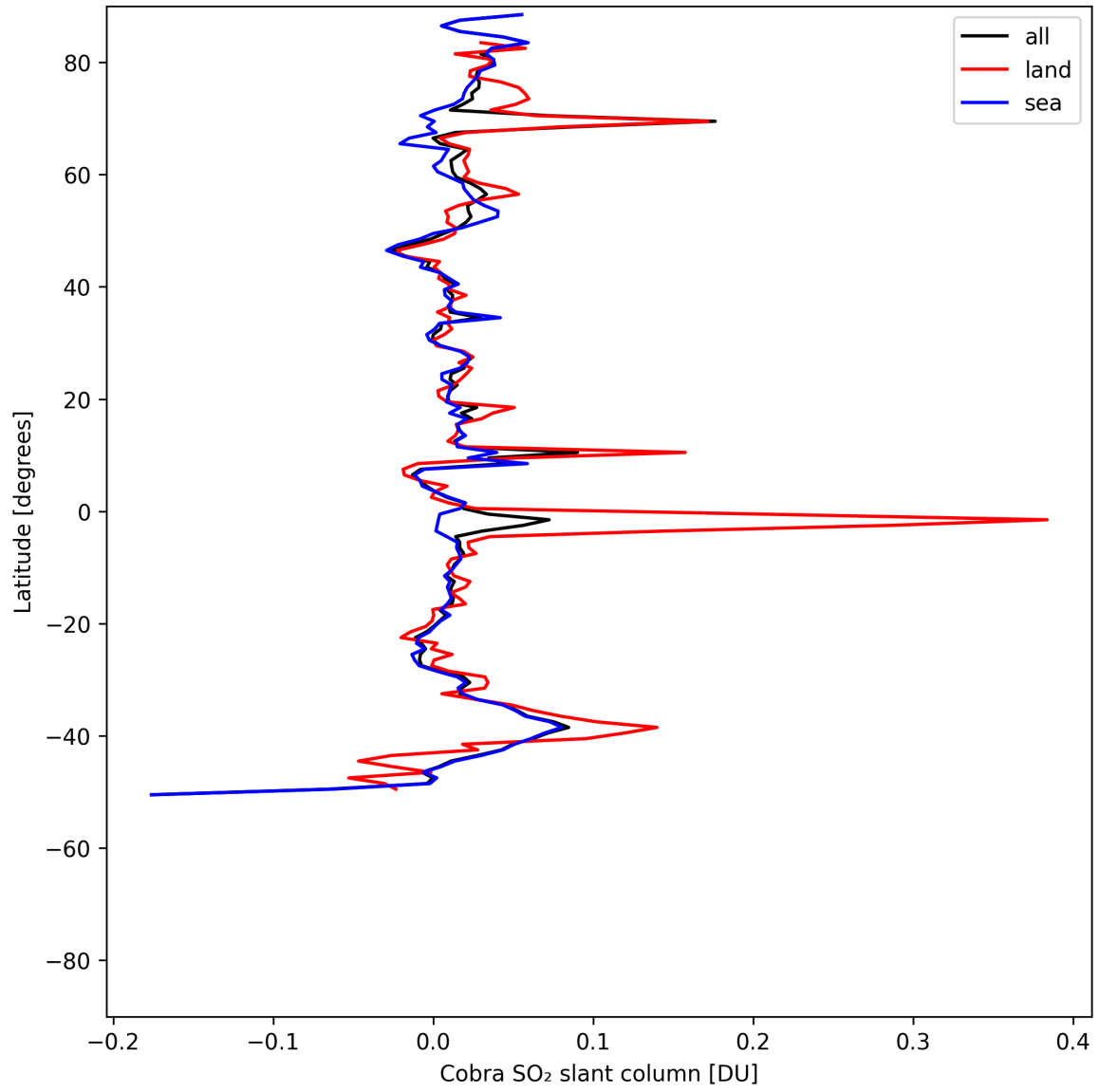
Figure 35: Zonal average of “Cobra SO 2 slant column” for 2025-05-12 to 2025-05-14.
