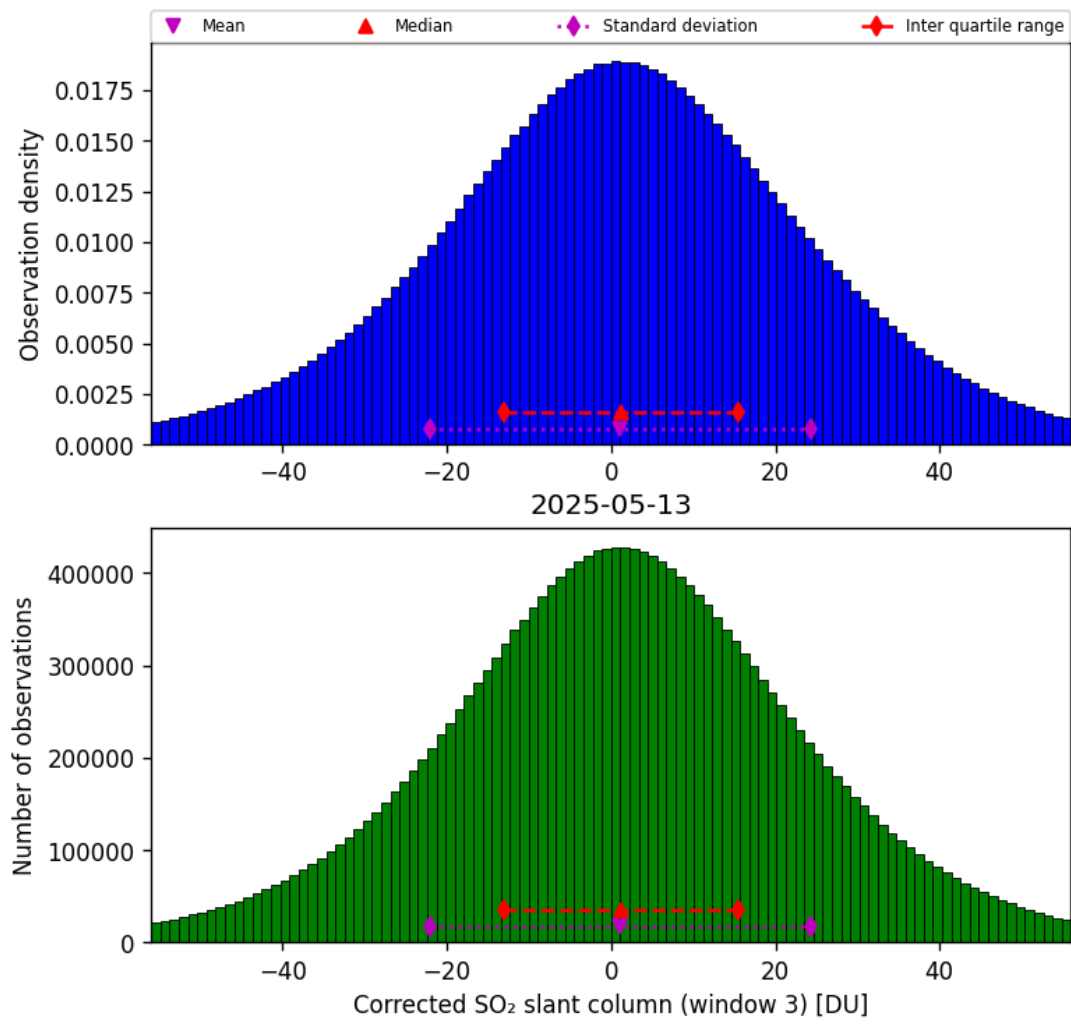
Figure 73: Histogram of “Corrected SO 2 slant column (window 3)” for 2025-05-12 to 2025-05-14
