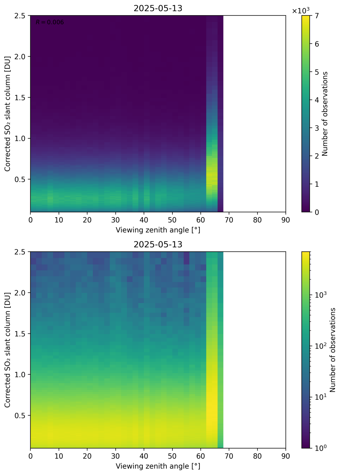
Figure 373: Scatter density plot of “Viewing zenith angle” against “Corrected SO 2 slant column” for 2025-05-12 to 2025-05-14.
