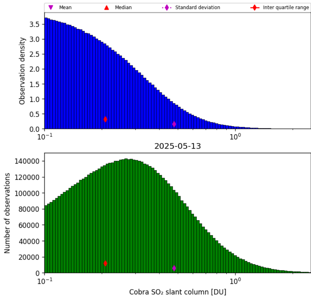
Figure 61: Histogram of “Cobra SO 2 slant column” for 2025-05-12 to 2025-05-14
