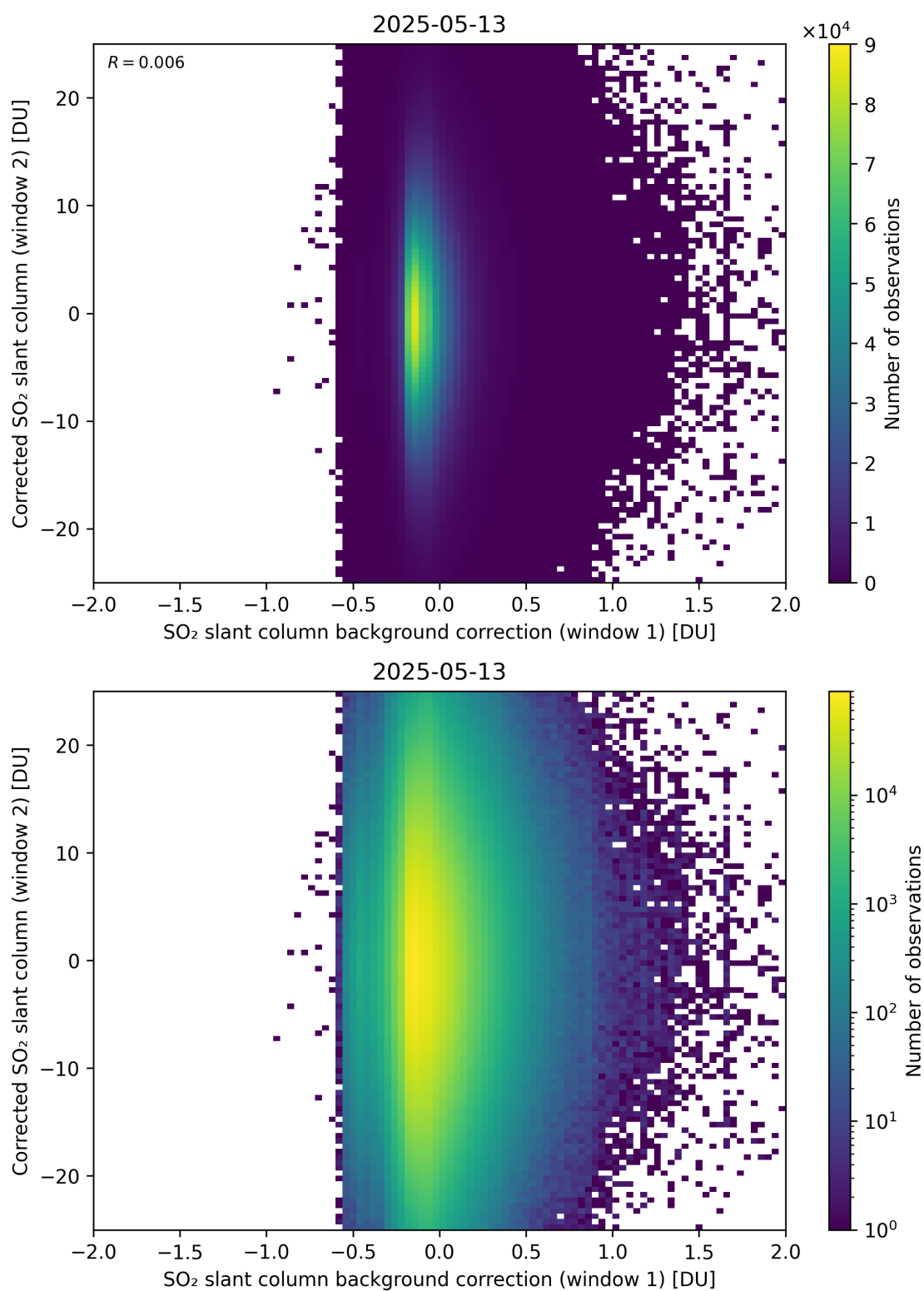
Figure 115: Scatter density plot of “SO 2 slant column background correction (window 1)” against “Corrected SO 2 slant column (window 2)” for 2025-05-12 to 2025-05-14.
