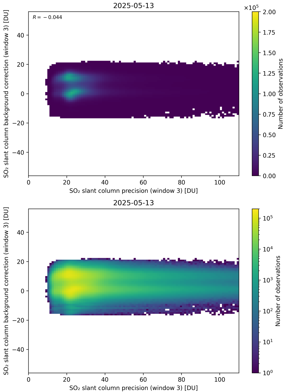
Figure 307: Scatter density plot of “SO 2 slant column precision (window 3)” against “SO 2 slant column background correction (window 3)” for 2025-05-12 to 2025-05-14.
