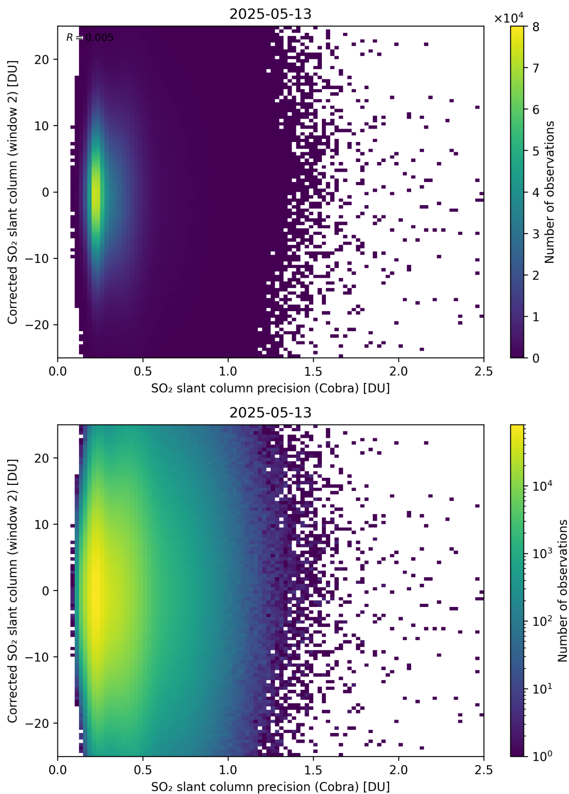
Figure 206: Scatter density plot of “SO 2 slant column precision (Cobra)” against “Corrected SO 2 slant column (window 2)” for 2025-05-12 to 2025-05-14.
