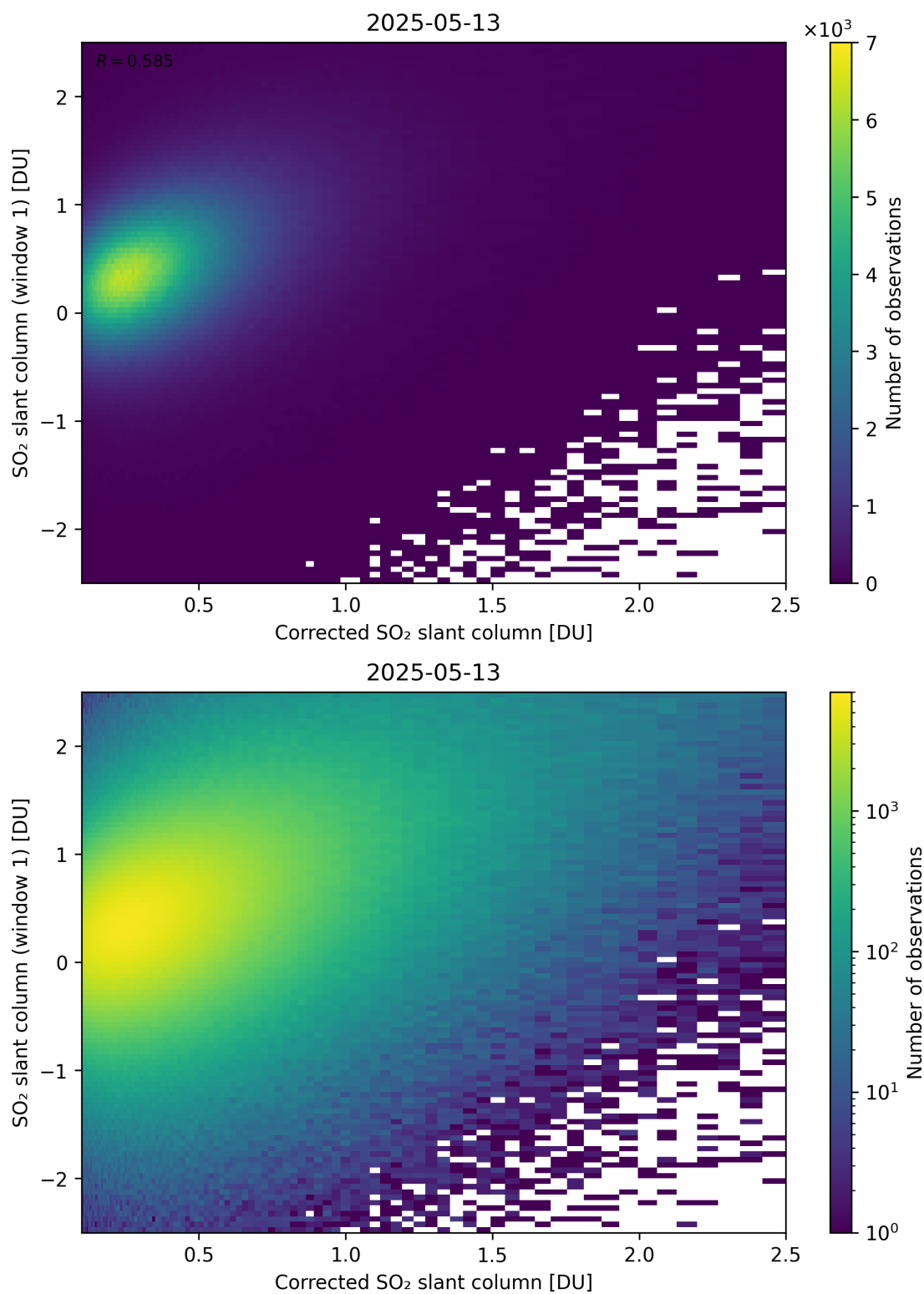
Figure 237: Scatter density plot of “Corrected SO 2 slant column” against “SO 2 slant column (window 1)” for 2025-05-12 to 2025-05-14.
