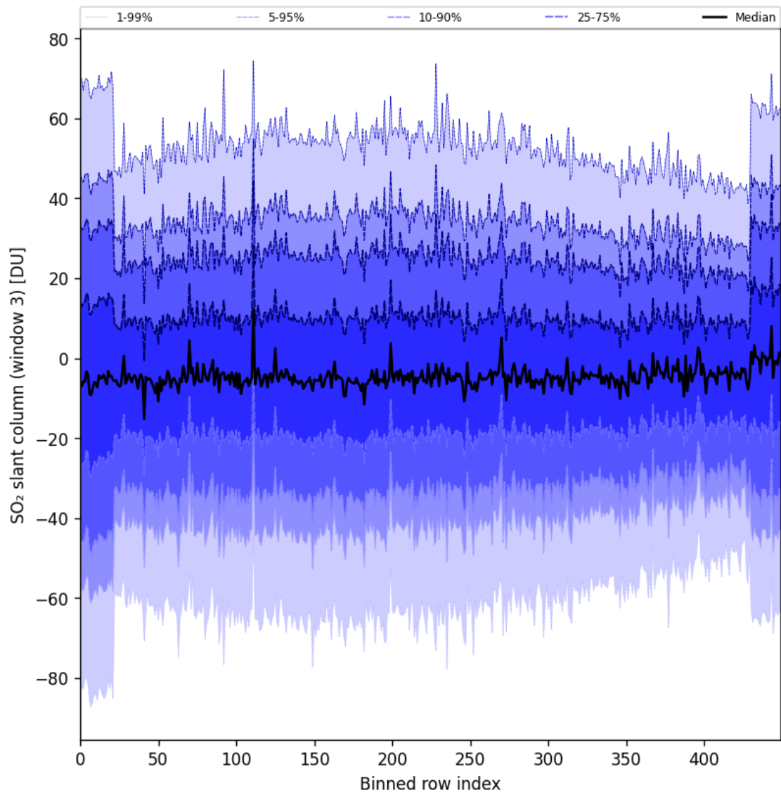
Figure 97: Along track statistics of “SO 2 slant column (window 3)” for 2025-05-12 to 2025-05-14
