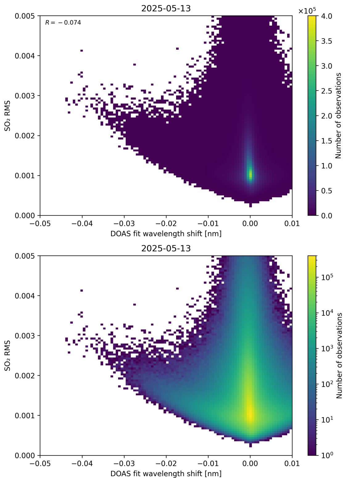
Figure 139: Scatter density plot of “DOAS fit wavelength shift” against “SO 2 RMS” for 2025-05-12 to 2025-05-14.
