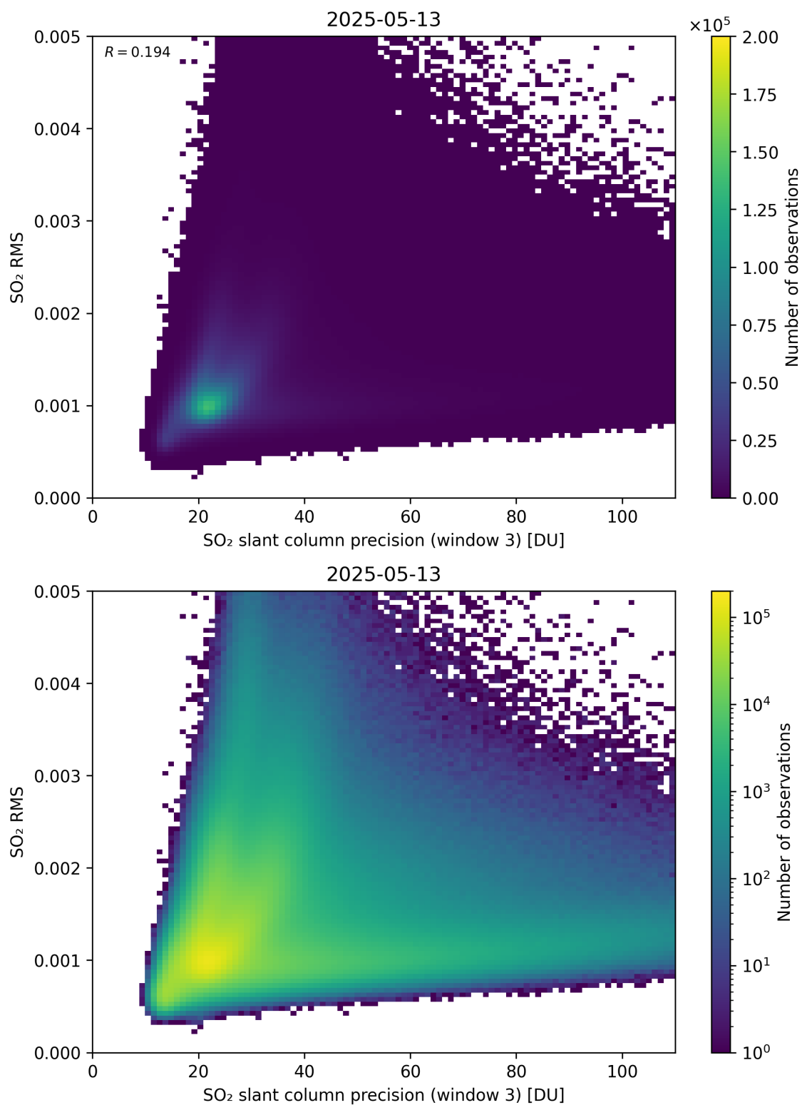
Figure 310: Scatter density plot of “SO 2 slant column precision (window 3)” against “SO 2 RMS” for 2025-05-12 to 2025-05-14.
