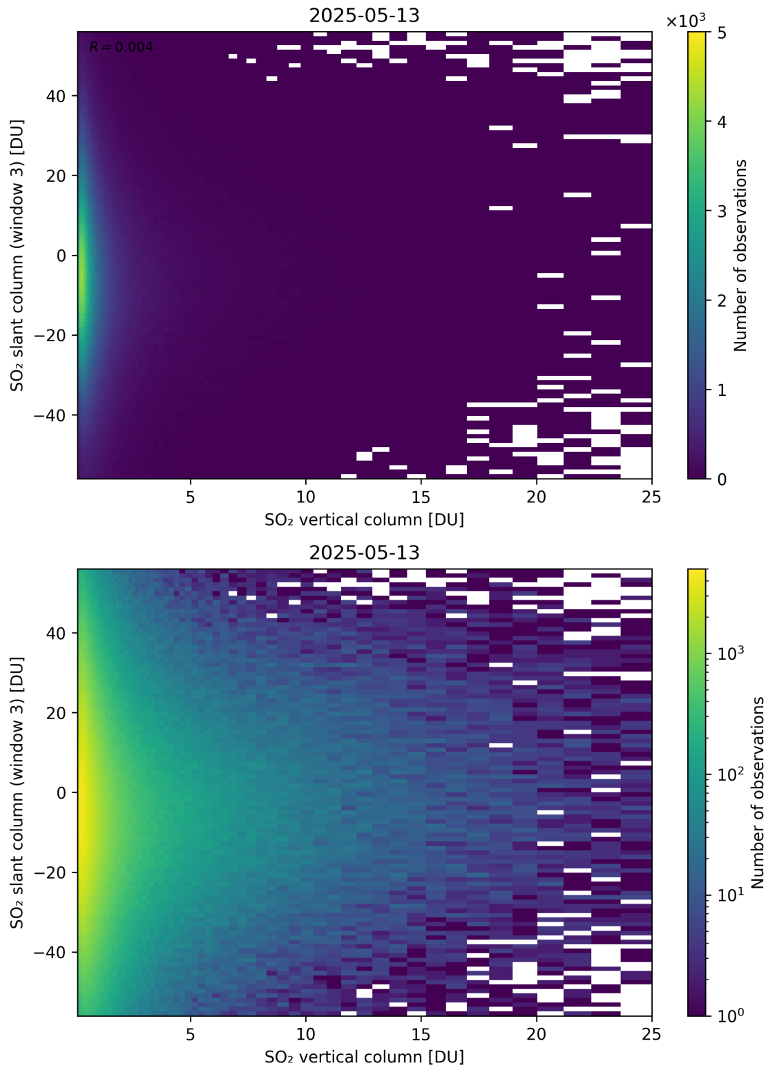
Figure 357: Scatter density plot of “SO 2 vertical column” against “SO 2 slant column (window 3)” for 2025-05-12 to 2025-05-14.
