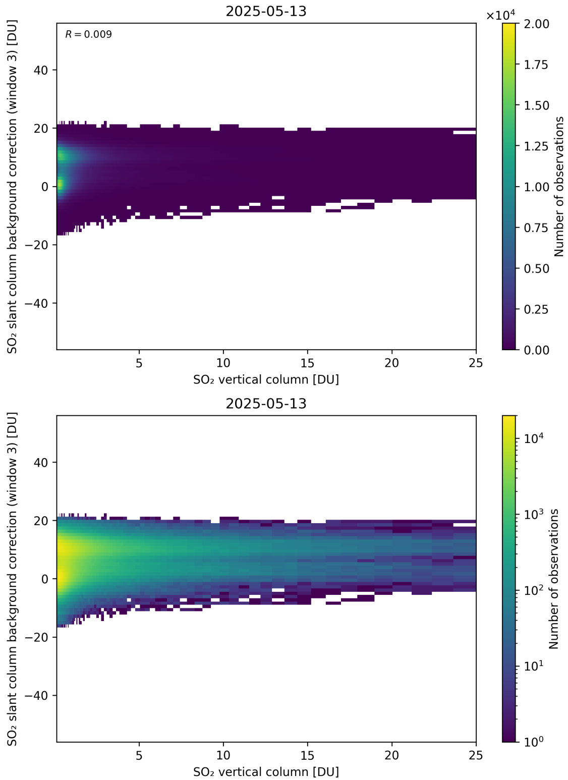
Figure 325: Scatter density plot of “SO 2 vertical column” against “SO 2 slant column background correction (window 3)” for 2025-05-12 to 2025-05-14.
