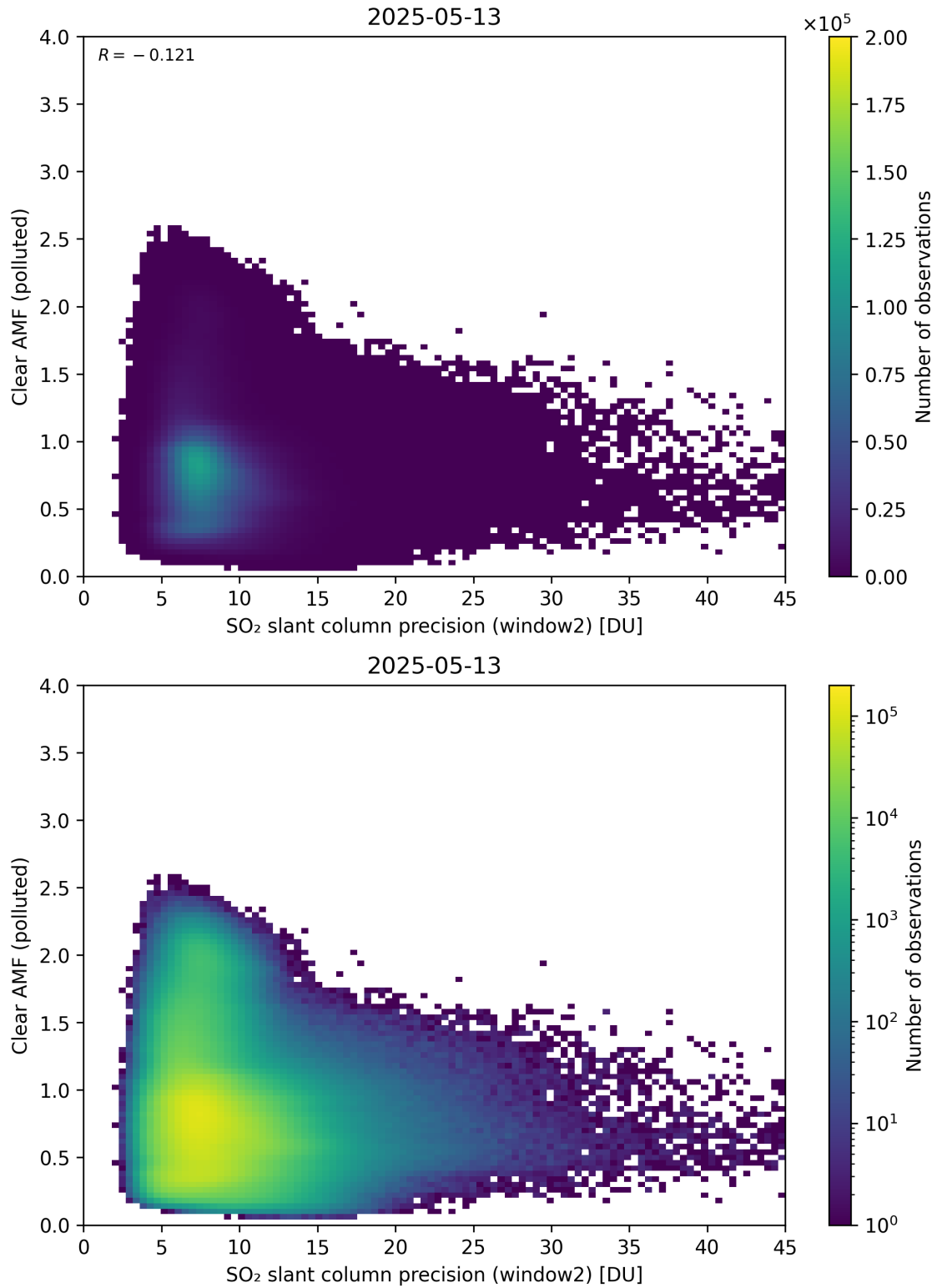
Figure 296: Scatter density plot of “SO 2 slant column precision (window2)” against “Clear AMF (polluted)” for 2025-05-12 to 2025-05-14.
