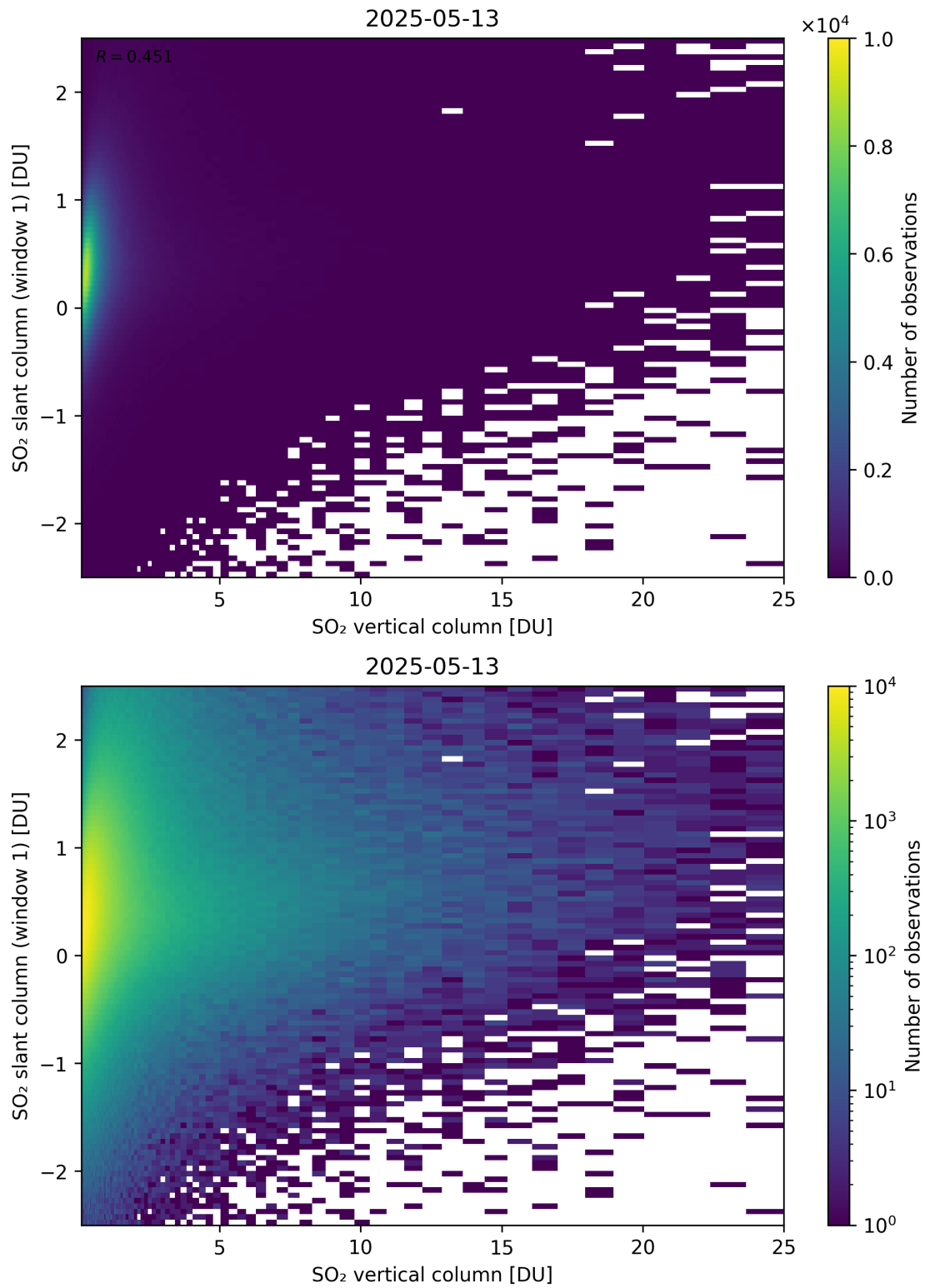
Figure 354: Scatter density plot of “SO 2 vertical column” against “SO 2 slant column (window 1)” for 2025-05-12 to 2025-05-14.
