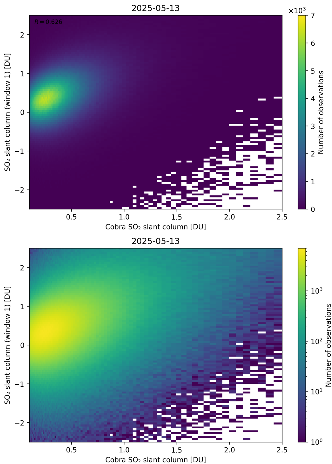
Figure 219: Scatter density plot of “Cobra SO 2 slant column” against “SO 2 slant column (window 1)” for 2025-05-12 to 2025-05-14.
