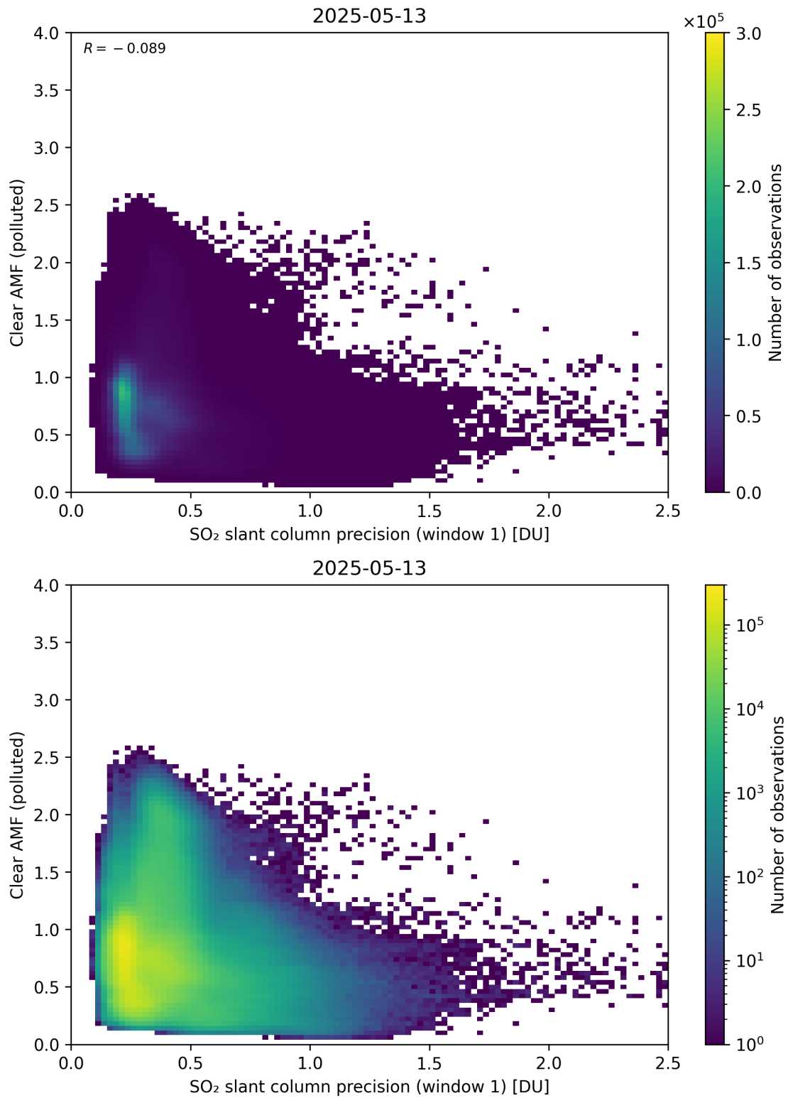
Figure 274: Scatter density plot of “SO 2 slant column precision (window 1)” against “Clear AMF (polluted)” for 2025-05-12 to 2025-05-14.
