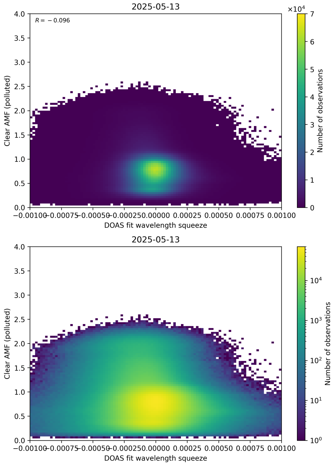
Figure 144: Scatter density plot of “DOAS fit wavelength squeeze” against “Clear AMF (polluted)” for 2025-05-12 to 2025-05-14.
