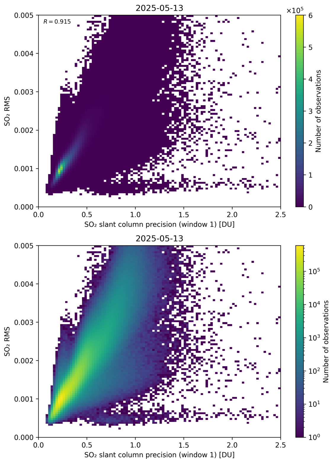
Figure 273: Scatter density plot of “SO 2 slant column precision (window 1)” against “SO 2 RMS” for 2025-05-12 to 2025-05-14.
