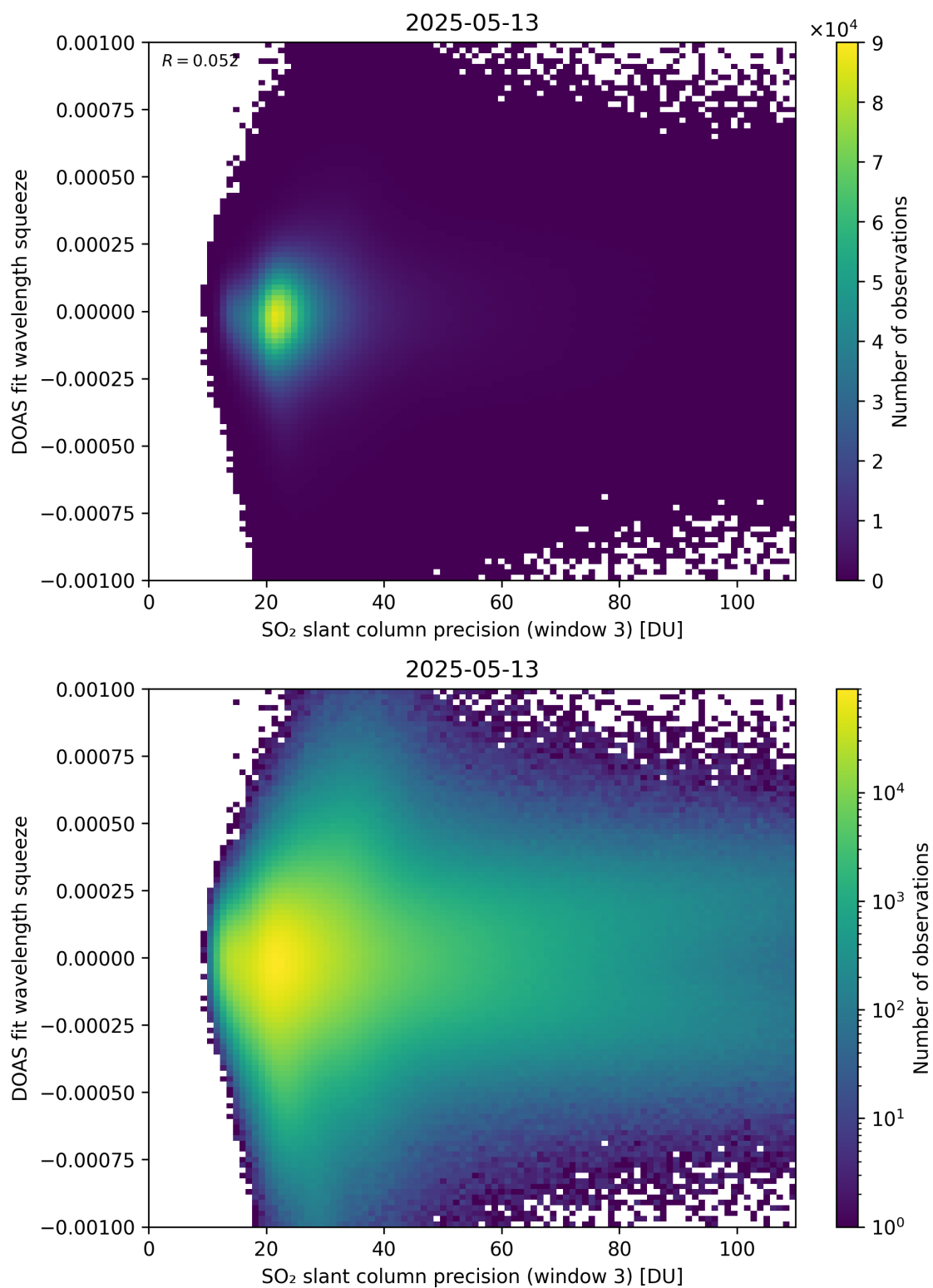
Figure 309: Scatter density plot of “SO 2 slant column precision (window 3)” against “DOAS fit wavelength squeeze” for 2025-05-12 to 2025-05-14.
