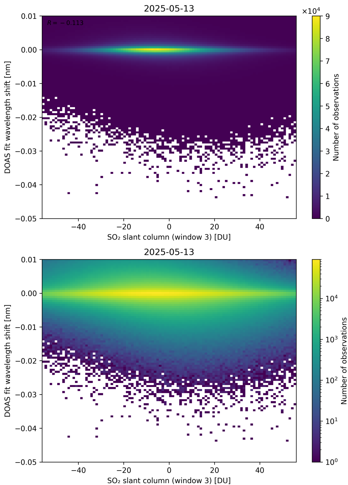
Figure 304: Scatter density plot of “SO 2 slant column (window 3)” against “DOAS fit wavelength shift” for 2025-05-12 to 2025-05-14.
