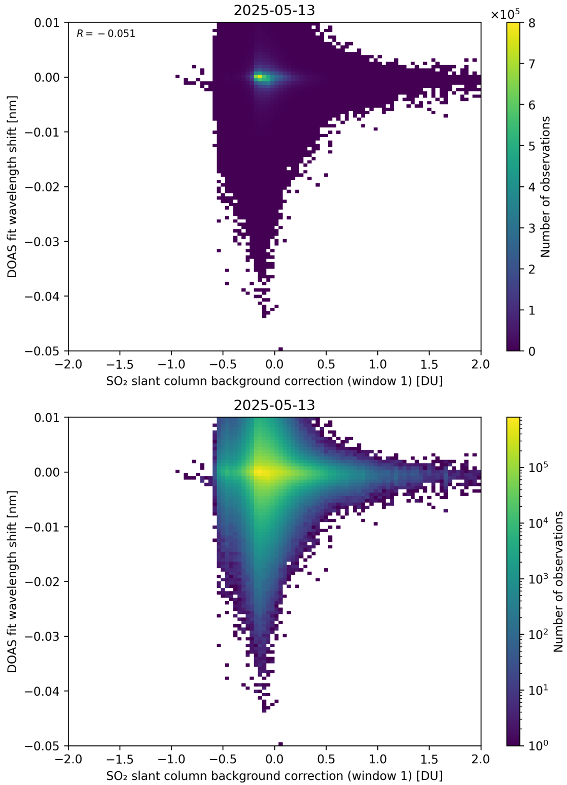
Figure 111: Scatter density plot of “SO 2 slant column background correction (window 1)” against “DOAS fit wavelength shift” for 2025-05-12 to 2025-05-14.
