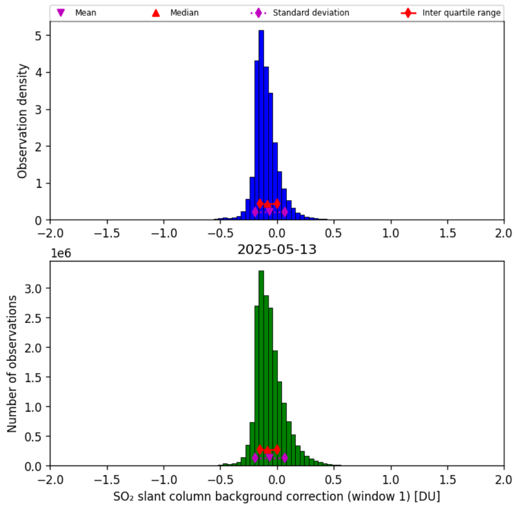
Figure 66: Histogram of “SO 2 slant column background correction (window 1)” for 2025-05-12 to 2025-05-14
