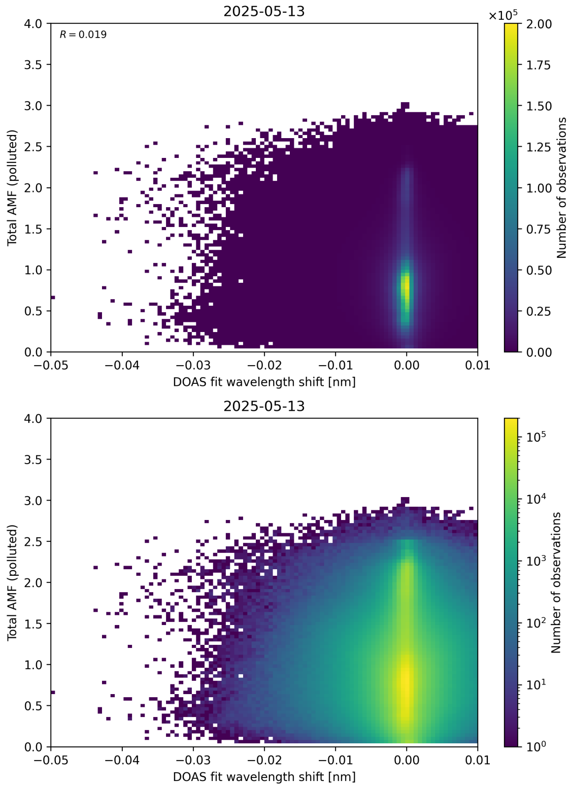
Figure 141: Scatter density plot of “DOAS fit wavelength shift” against “Total AMF (polluted)” for 2025-05-12 to 2025-05-14.
