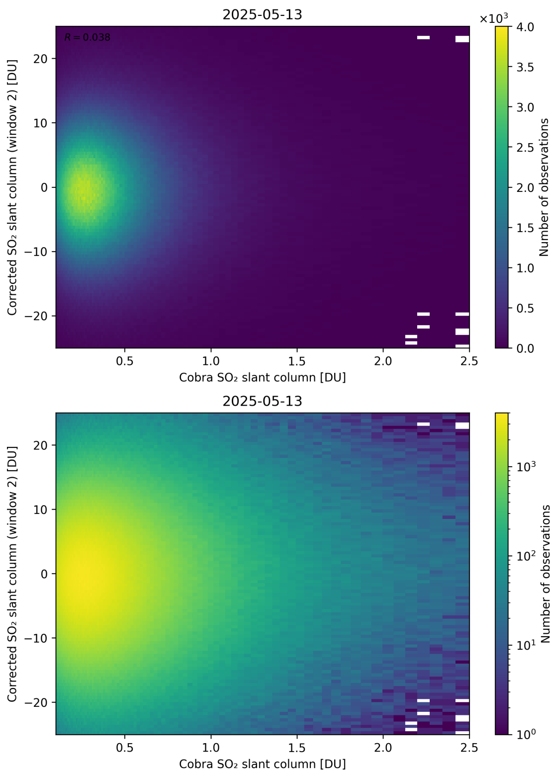
Figure 217: Scatter density plot of “Cobra SO 2 slant column” against “Corrected SO 2 slant column (window 2)” for 2025-05-12 to 2025-05-14.
