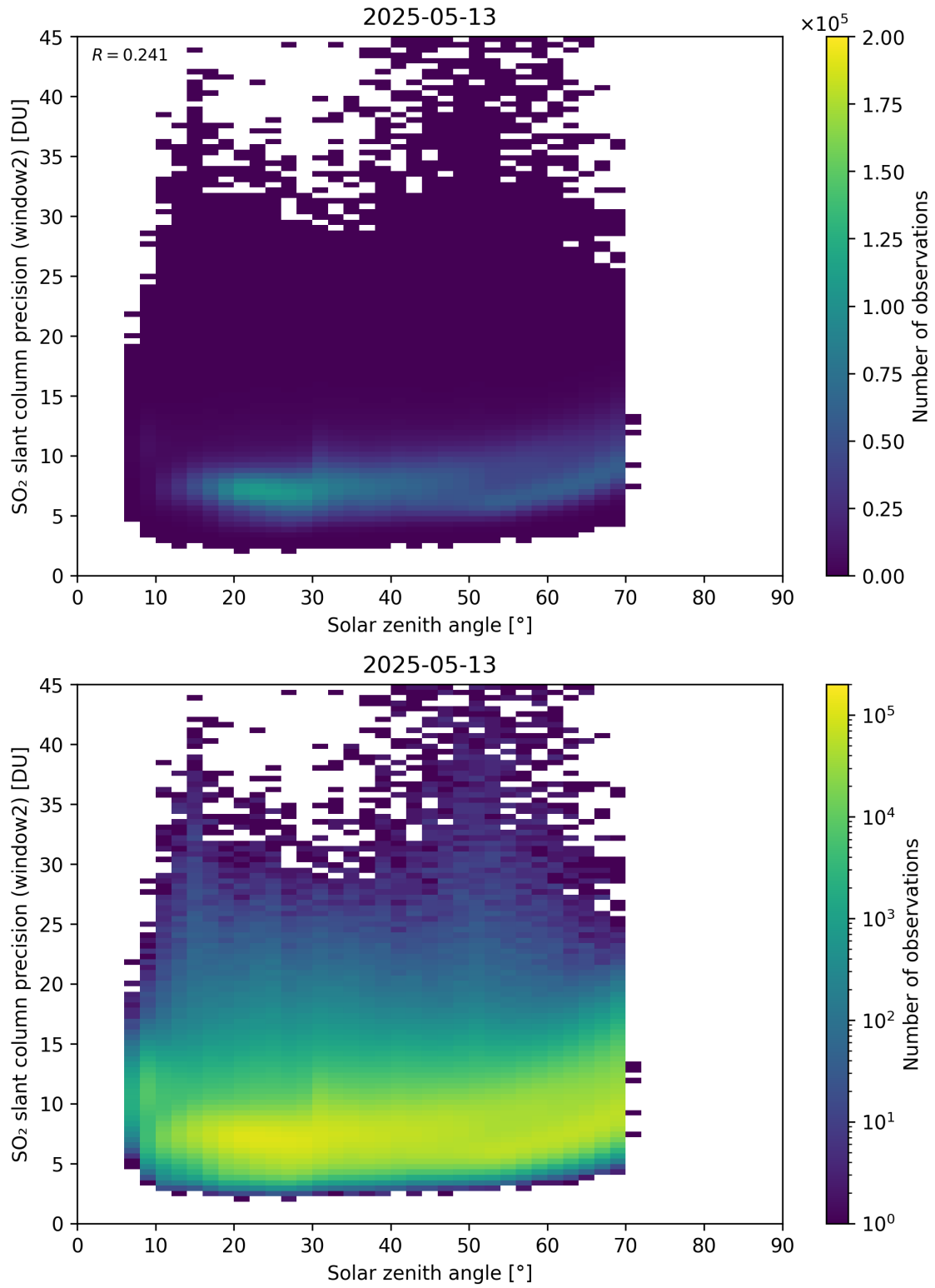
Figure 186: Scatter density plot of “Solar zenith angle” against “SO 2 slant column precision (window2)” for 2025-05-12 to 2025-05-14.
