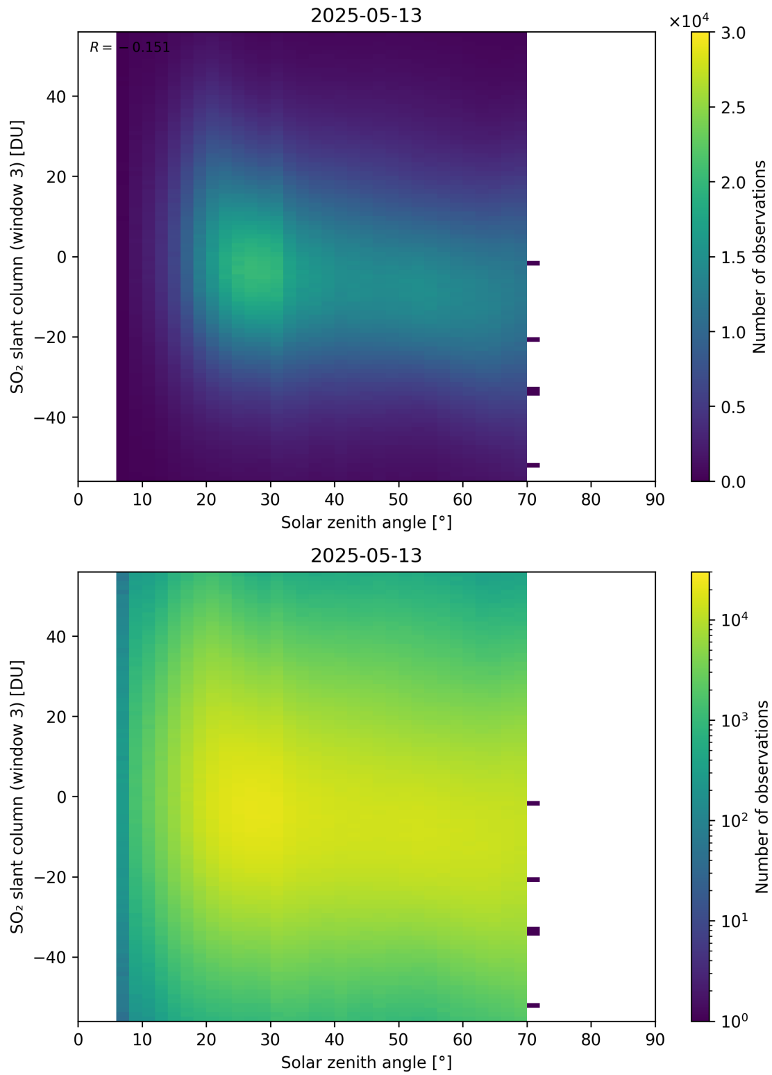
Figure 187: Scatter density plot of “Solar zenith angle” against “SO 2 slant column (window 3)” for 2025-05-12 to 2025-05-14.
