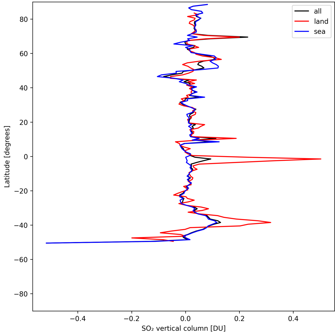
Figure 32: Zonal average of “SO 2 vertical column” for 2025-05-12 to 2025-05-14.
