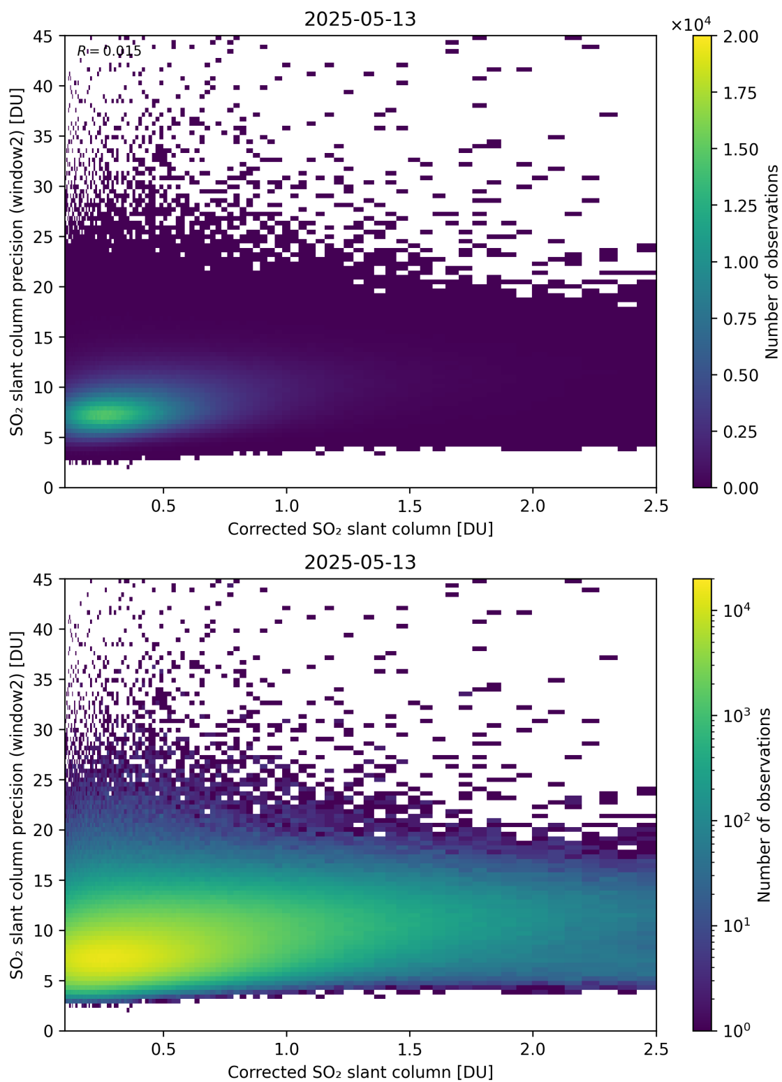
Figure 239: Scatter density plot of “Corrected SO 2 slant column” against “SO 2 slant column precision (window2)” for 2025-05-12 to 2025-05-14.
