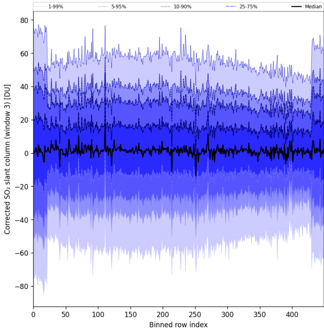
Figure 99: Along track statistics of “Corrected SO 2 slant column (window 3)” for 2025-05-12 to 2025-05-14
