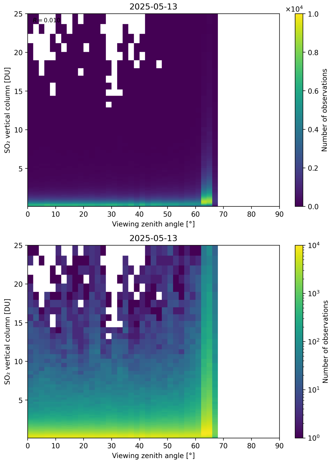
Figure 383: Scatter density plot of “Viewing zenith angle” against “SO 2 vertical column” for 2025-05-12 to 2025-05-14.
