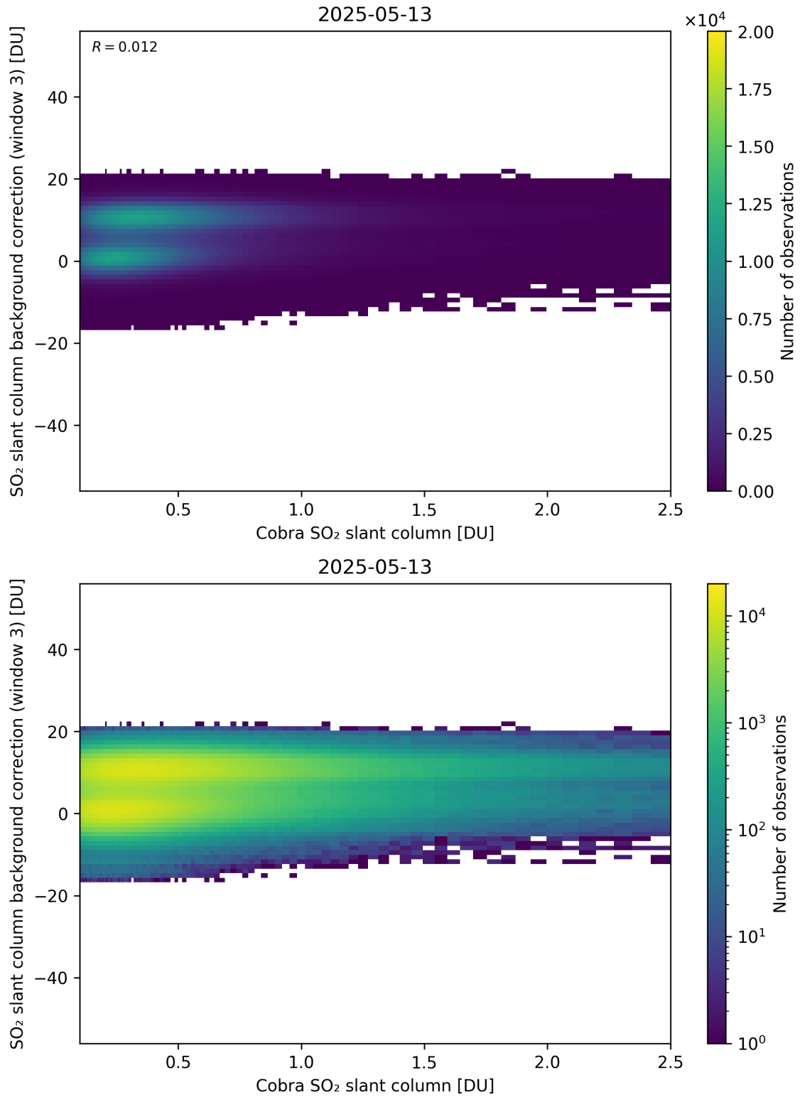
Figure 195: Scatter density plot of “Cobra SO 2 slant column” against “SO 2 slant column background correction (window 3)” for 2025-05-12 to 2025-05-14.
