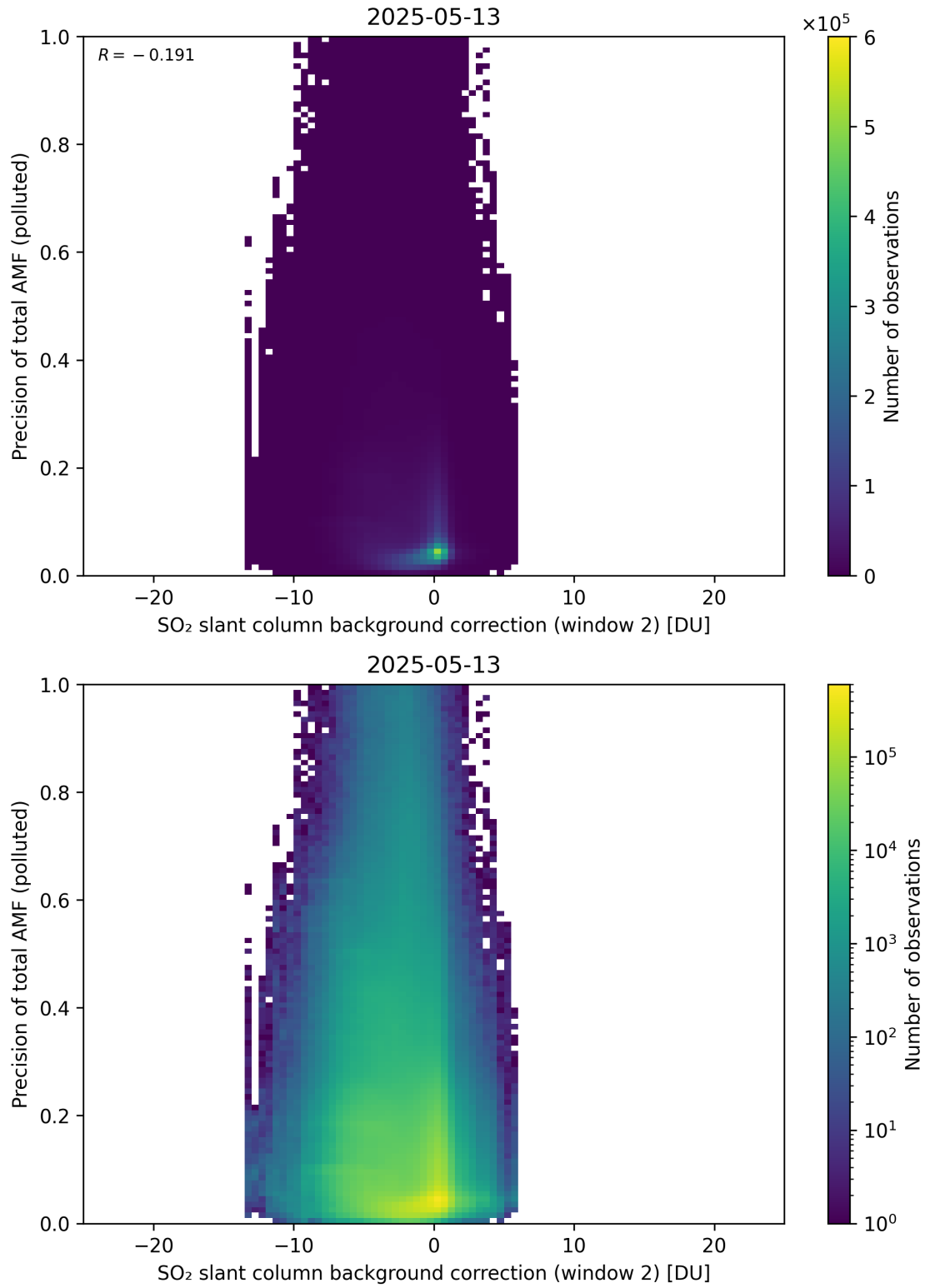
Figure 131: Scatter density plot of “SO 2 slant column background correction (window 2)” against “Precision of total AMF (polluted)” for 2025-05-12 to 2025-05-14.
