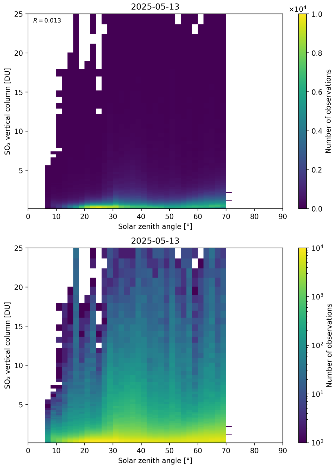
Figure 191: Scatter density plot of “Solar zenith angle” against “SO 2 vertical column” for 2025-05-12 to 2025-05-14.
