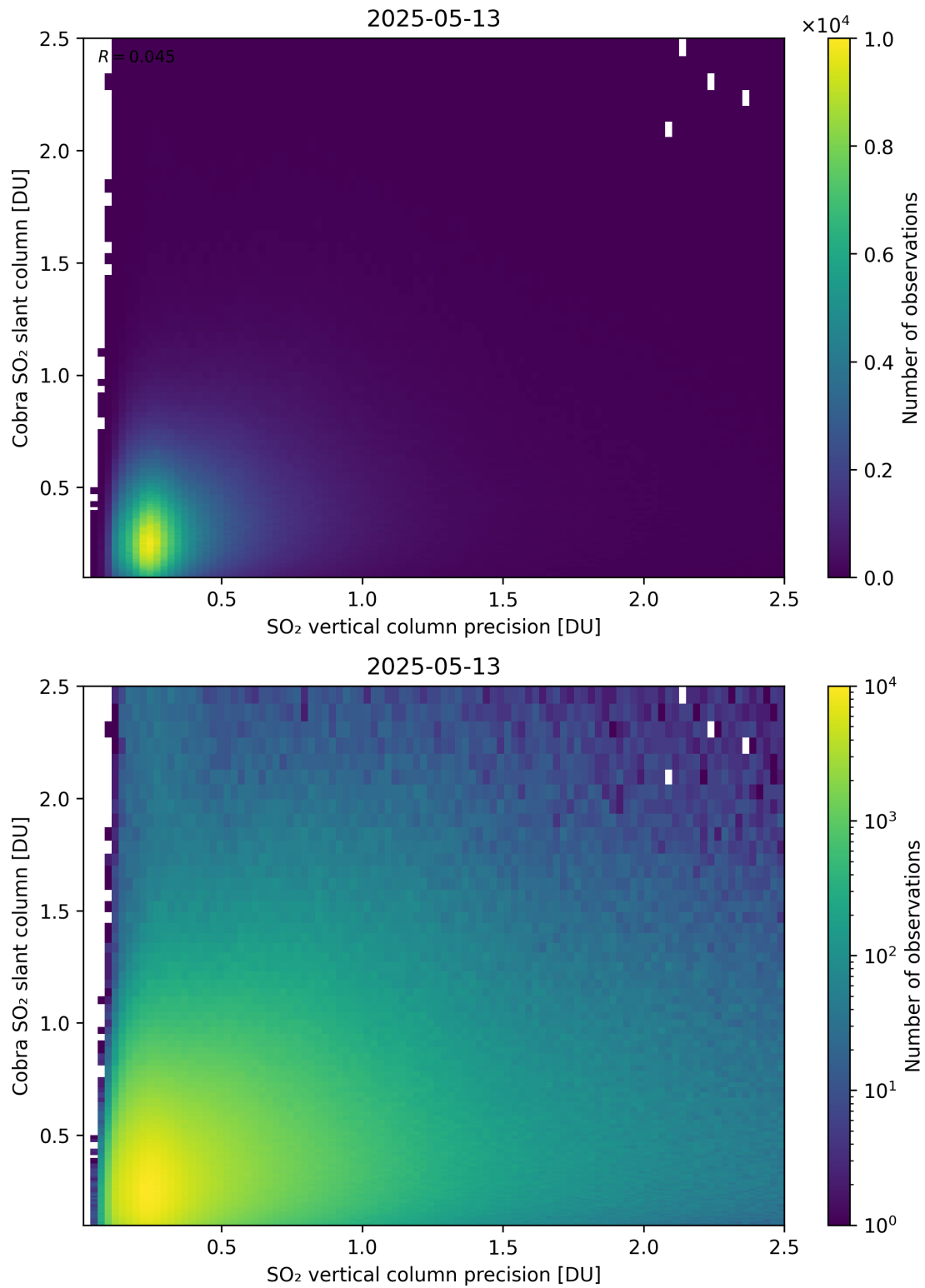
Figure 336: Scatter density plot of “SO 2 vertical column precision” against “Cobra SO 2 slant column” for 2025-05-12 to 2025-05-14.
