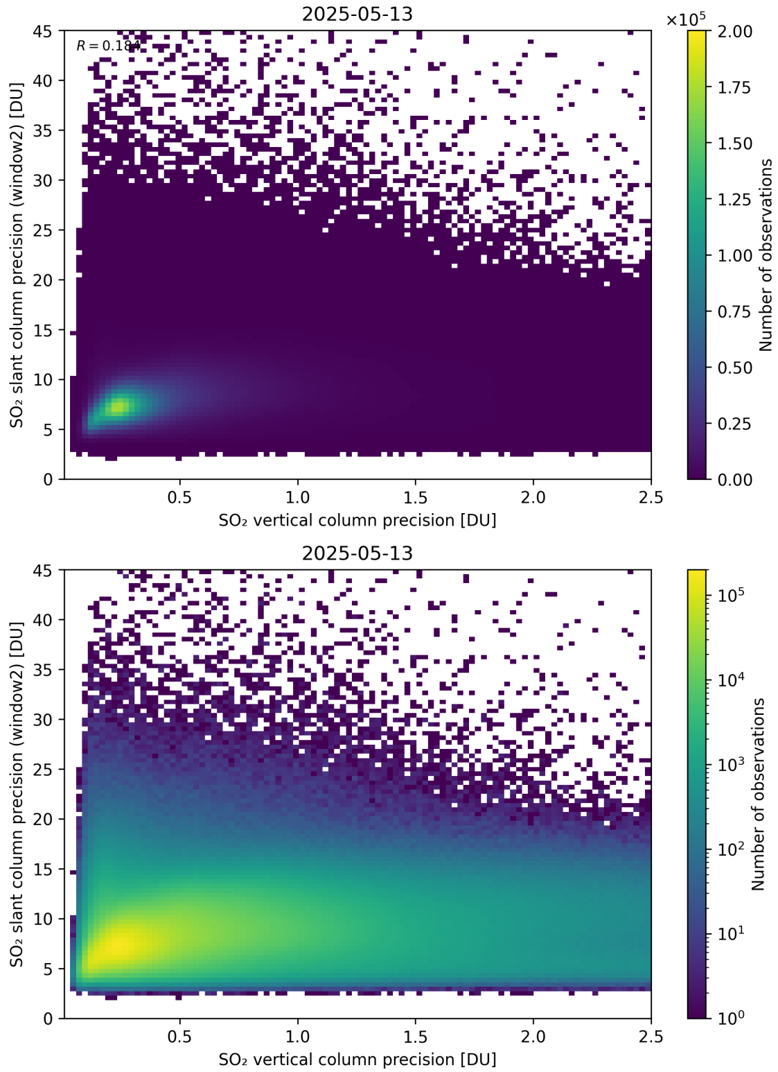
Figure 343: Scatter density plot of “SO 2 vertical column precision” against “SO 2 slant column precision (window2)” for 2025-05-12 to 2025-05-14.
