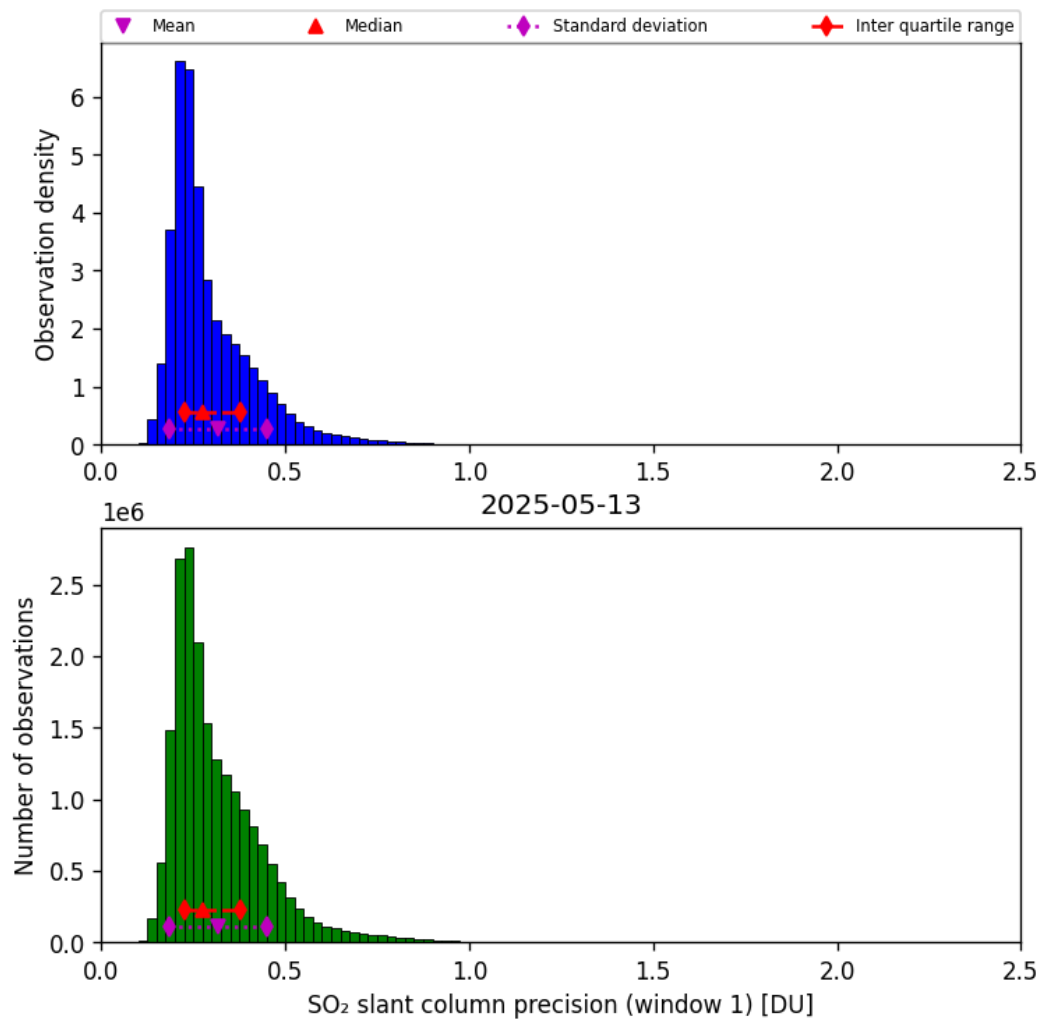
Figure 64: Histogram of “SO 2 slant column precision (window 1)” for 2025-05-12 to 2025-05-14
