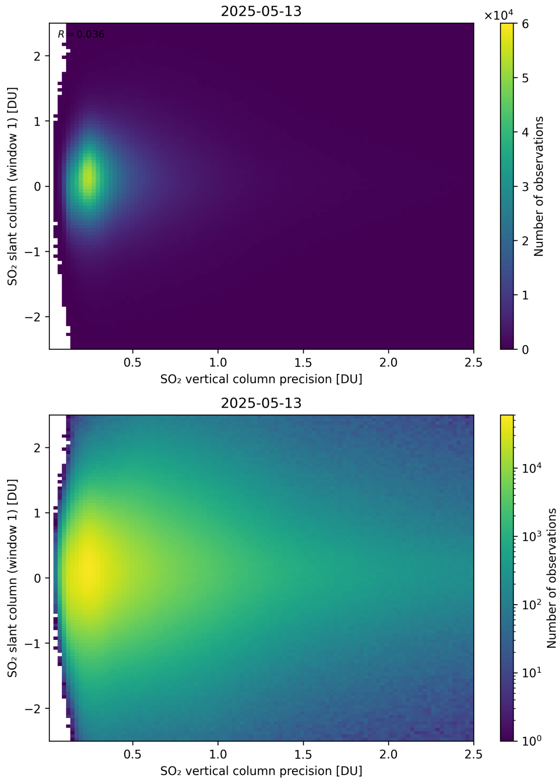
Figure 341: Scatter density plot of “SO 2 vertical column precision” against “SO 2 slant column (window 1)” for 2025-05-12 to 2025-05-14.
