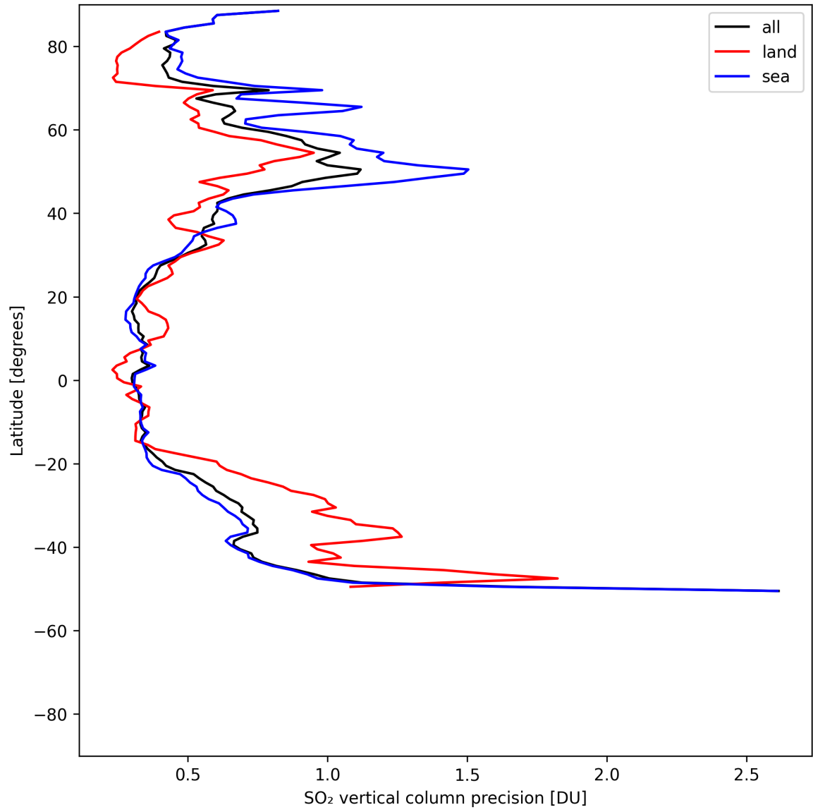
Figure 33: Zonal average of “SO 2 vertical column precision” for 2025-05-12 to 2025-05-14.
