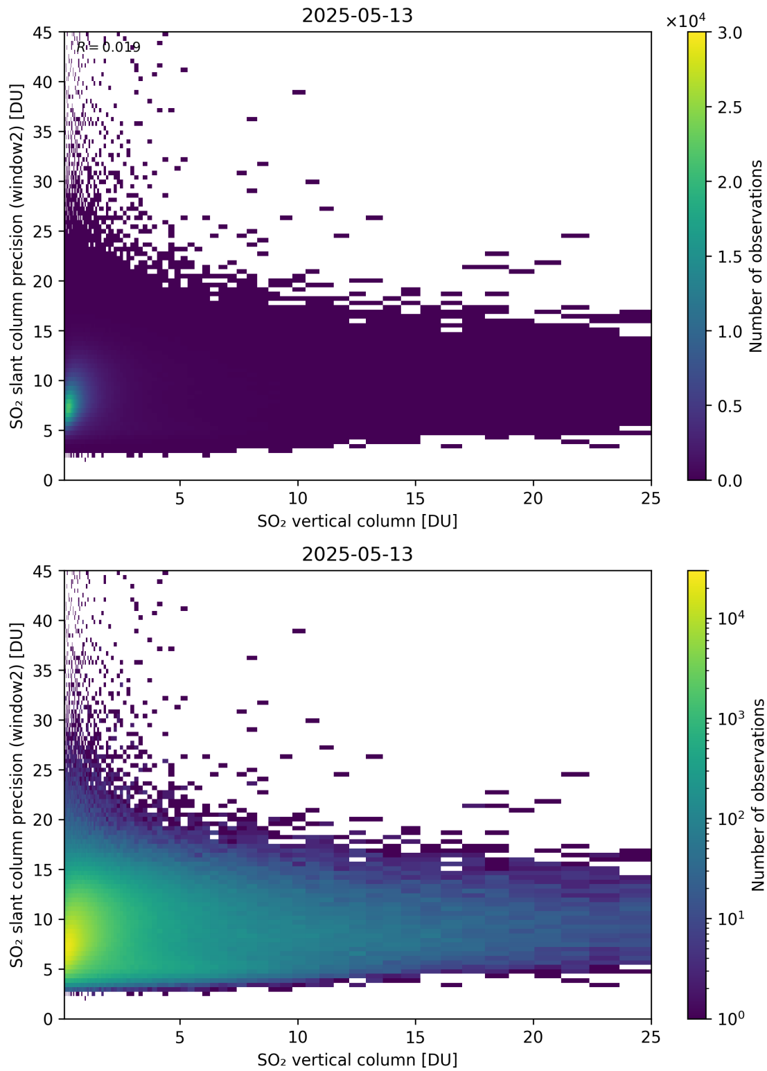
Figure 356: Scatter density plot of “SO 2 vertical column” against “SO 2 slant column precision (window2)” for 2025-05-12 to 2025-05-14.
