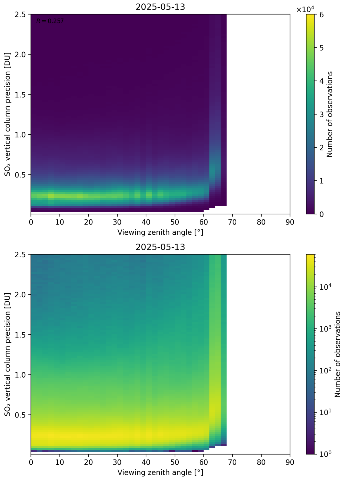
Figure 384: Scatter density plot of “Viewing zenith angle” against “SO 2 vertical column precision” for 2025-05-12 to 2025-05-14.
