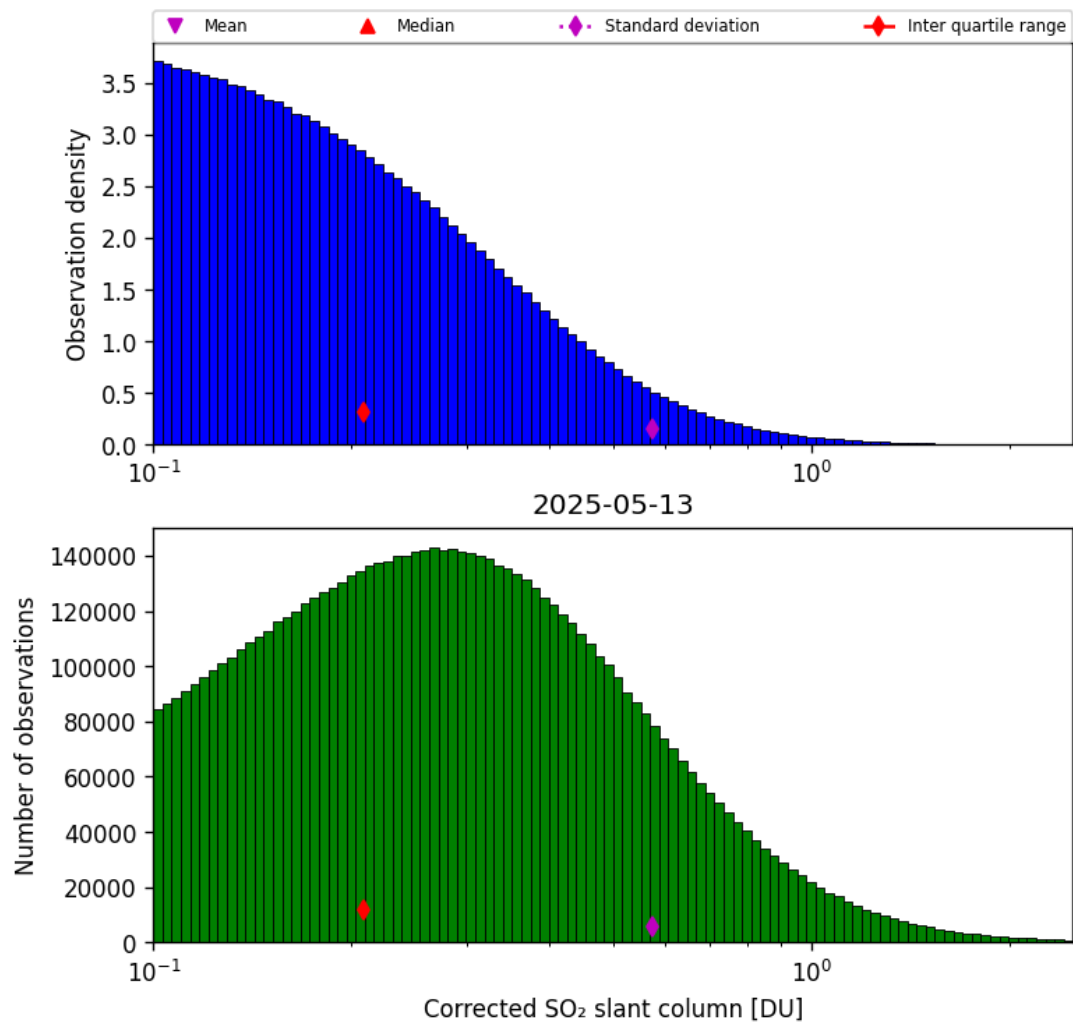
Figure 60: Histogram of “Corrected SO 2 slant column” for 2025-05-12 to 2025-05-14
