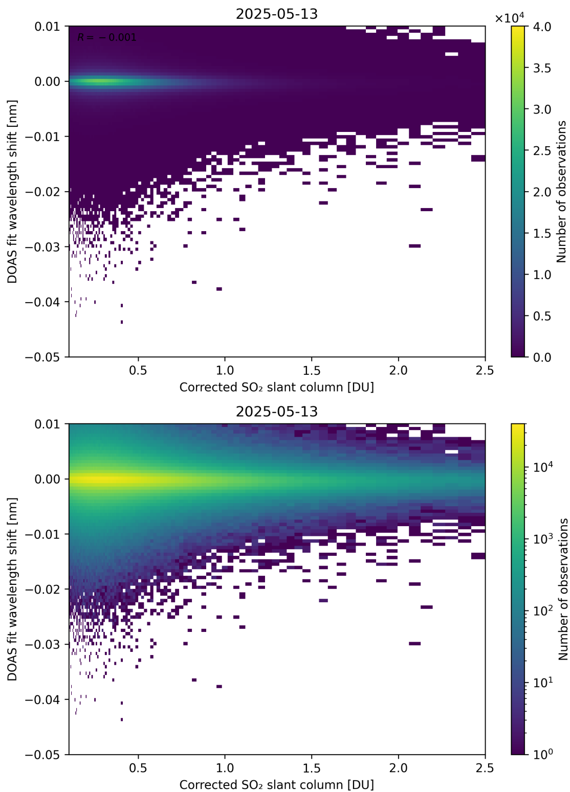
Figure 229: Scatter density plot of “Corrected SO 2 slant column” against “DOAS fit wavelength shift” for 2025-05-12 to 2025-05-14.
