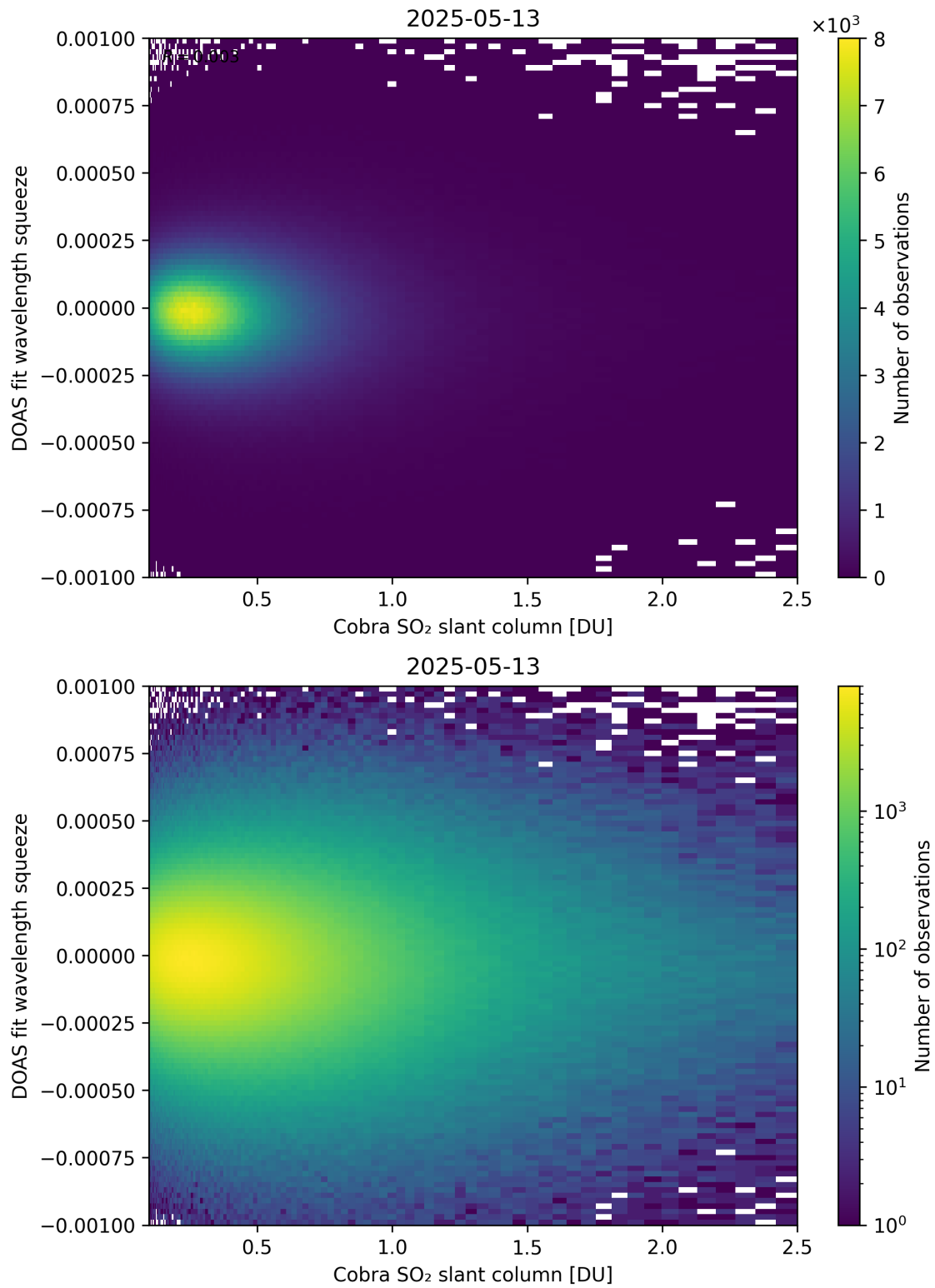
Figure 197: Scatter density plot of “Cobra SO 2 slant column” against “DOAS fit wavelength squeeze” for 2025-05-12 to 2025-05-14.
