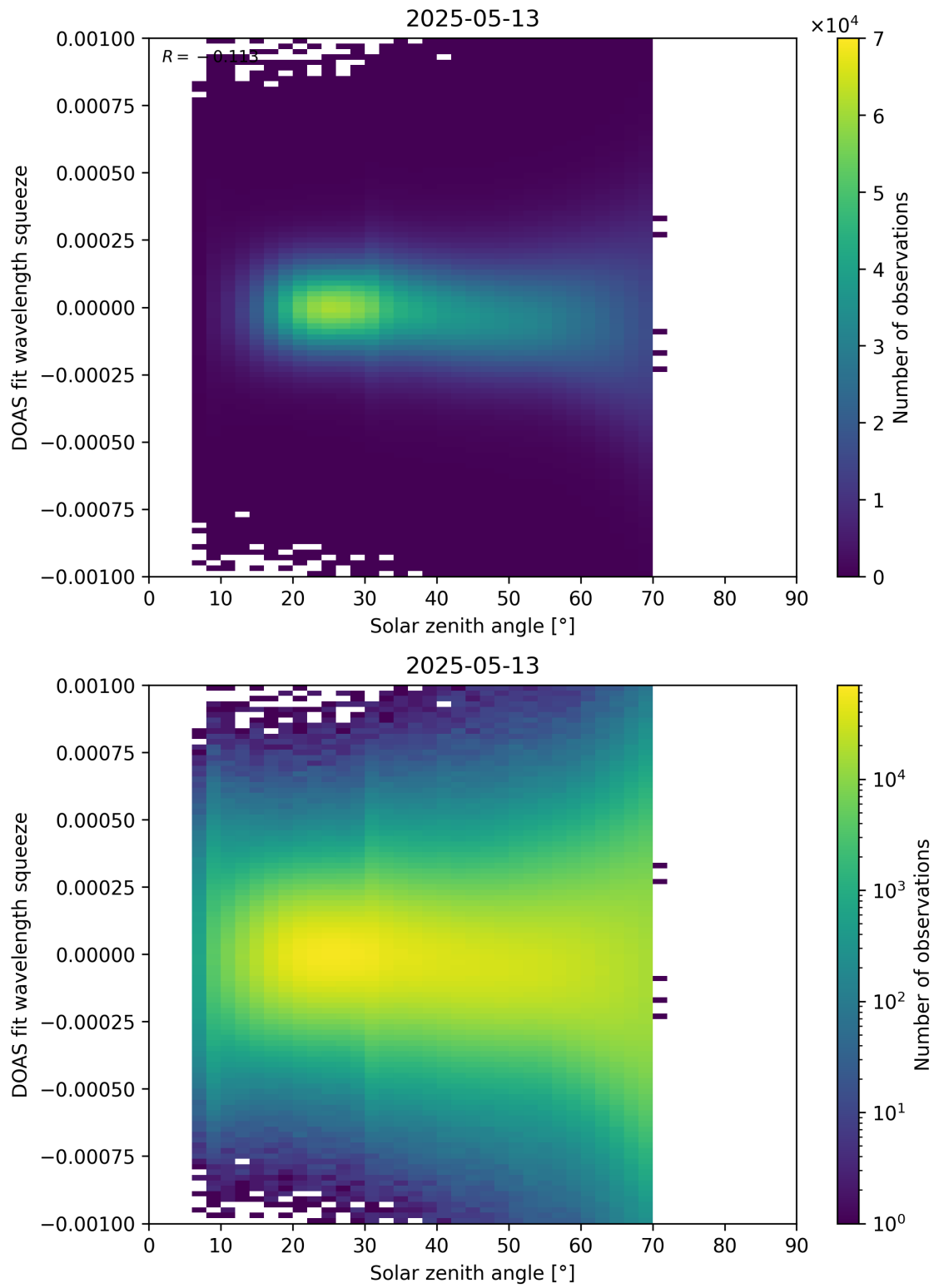
Figure 175: Scatter density plot of “Solar zenith angle” against “DOAS fit wavelength squeeze” for 2025-05-12 to 2025-05-14.
