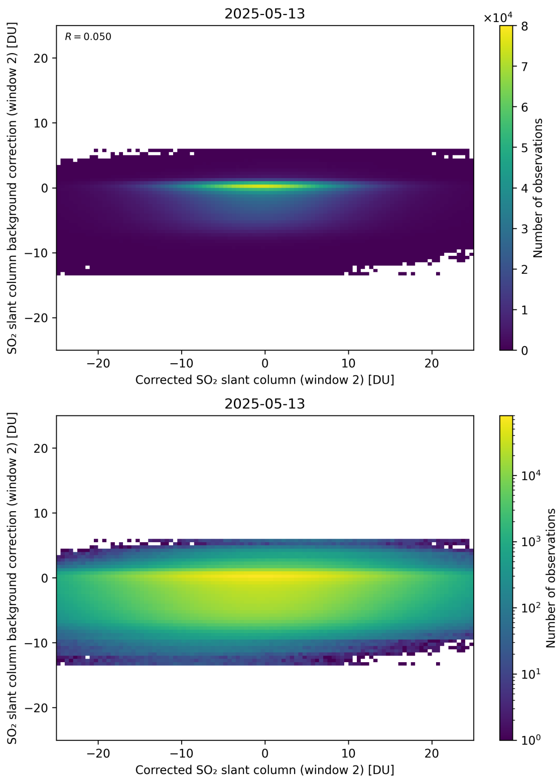
Figure 244: Scatter density plot of “Corrected SO 2 slant column (window 2)” against “SO 2 slant column background correction (window 2)” for 2025-05-12 to 2025-05-14.
