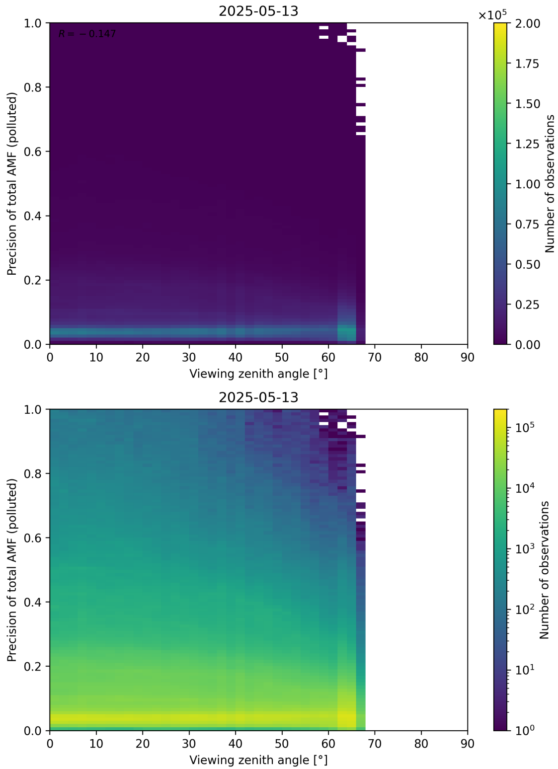
Figure 382: Scatter density plot of “Viewing zenith angle” against “Precision of total AMF (polluted)” for 2025-05-12 to 2025-05-14.
