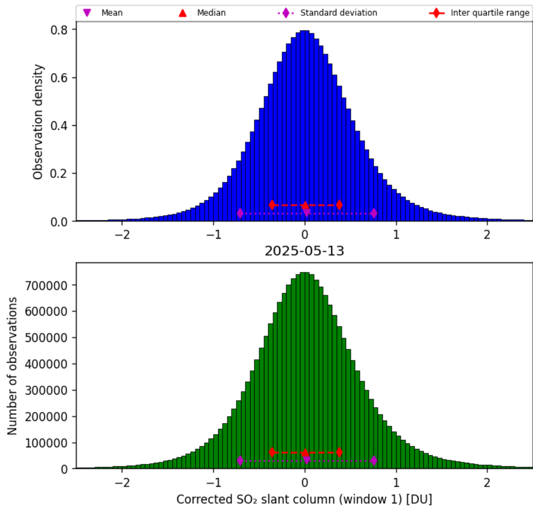
Figure 65: Histogram of “Corrected SO 2 slant column (window 1)” for 2025-05-12 to 2025-05-14
