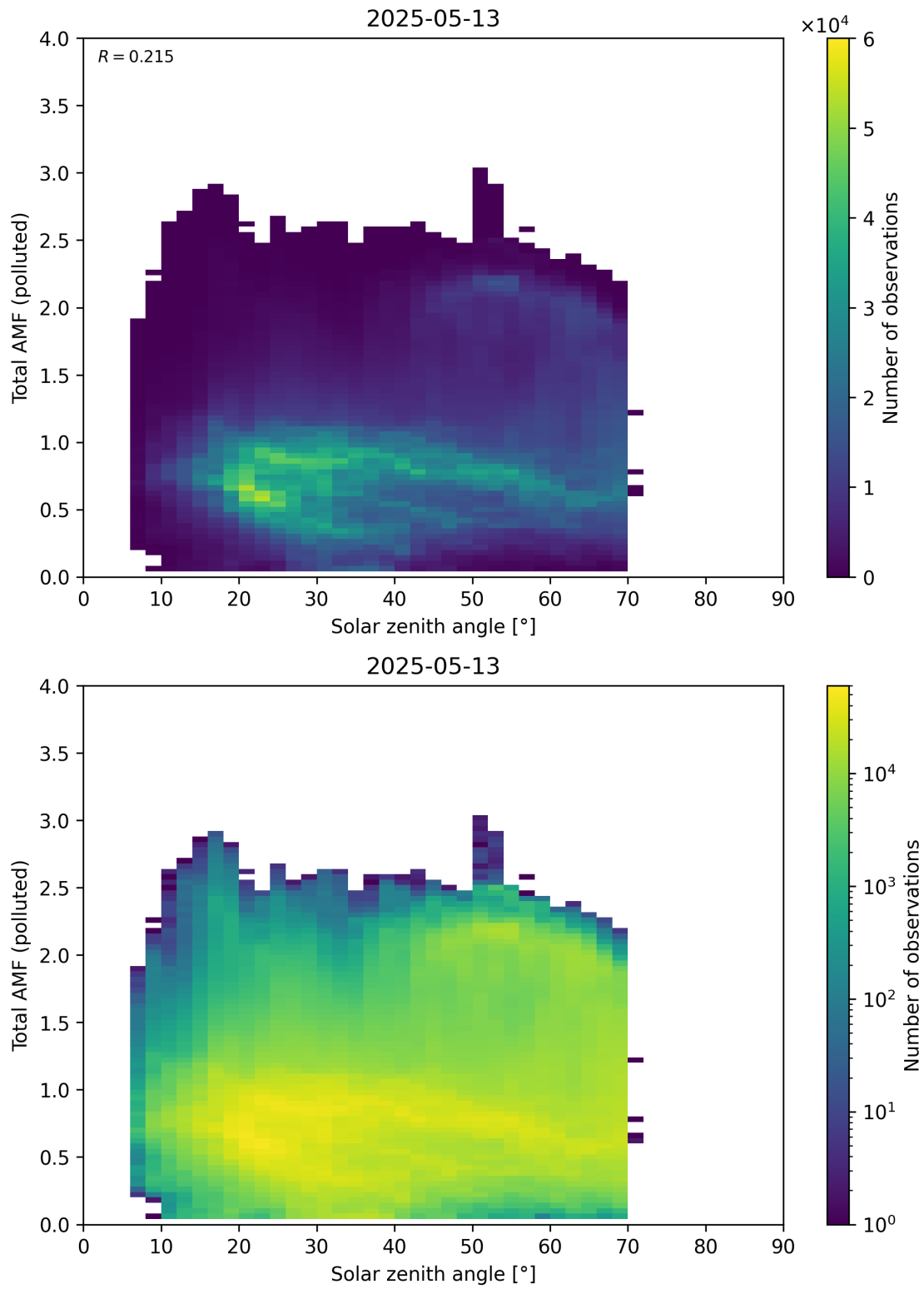
Figure 189: Scatter density plot of “Solar zenith angle” against “Total AMF (polluted)” for 2025-05-12 to 2025-05-14.
