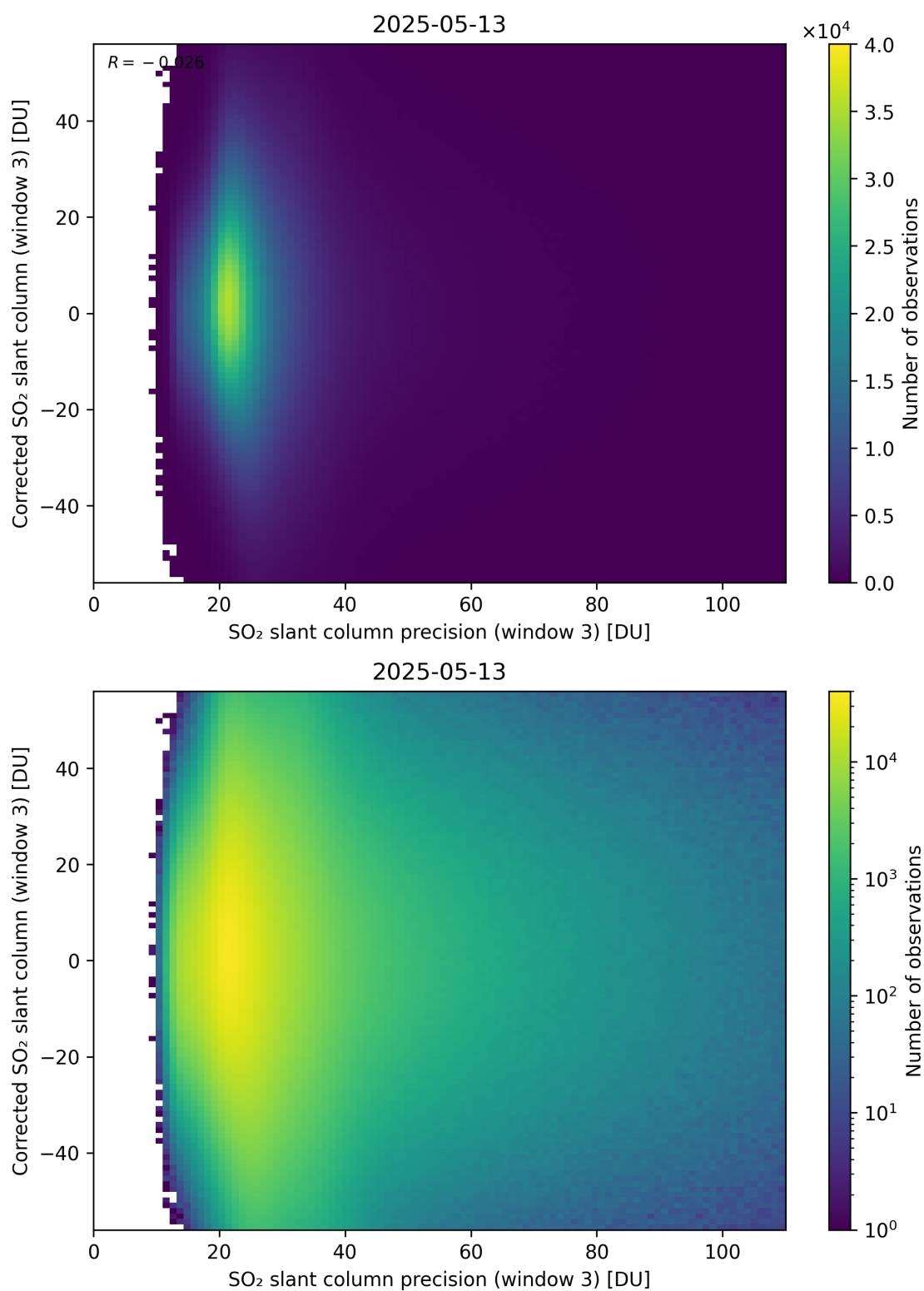
Figure 312: Scatter density plot of “SO 2 slant column precision (window 3)” against “Corrected SO 2 slant column (window 3)” for 2025-05-12 to 2025-05-14.
