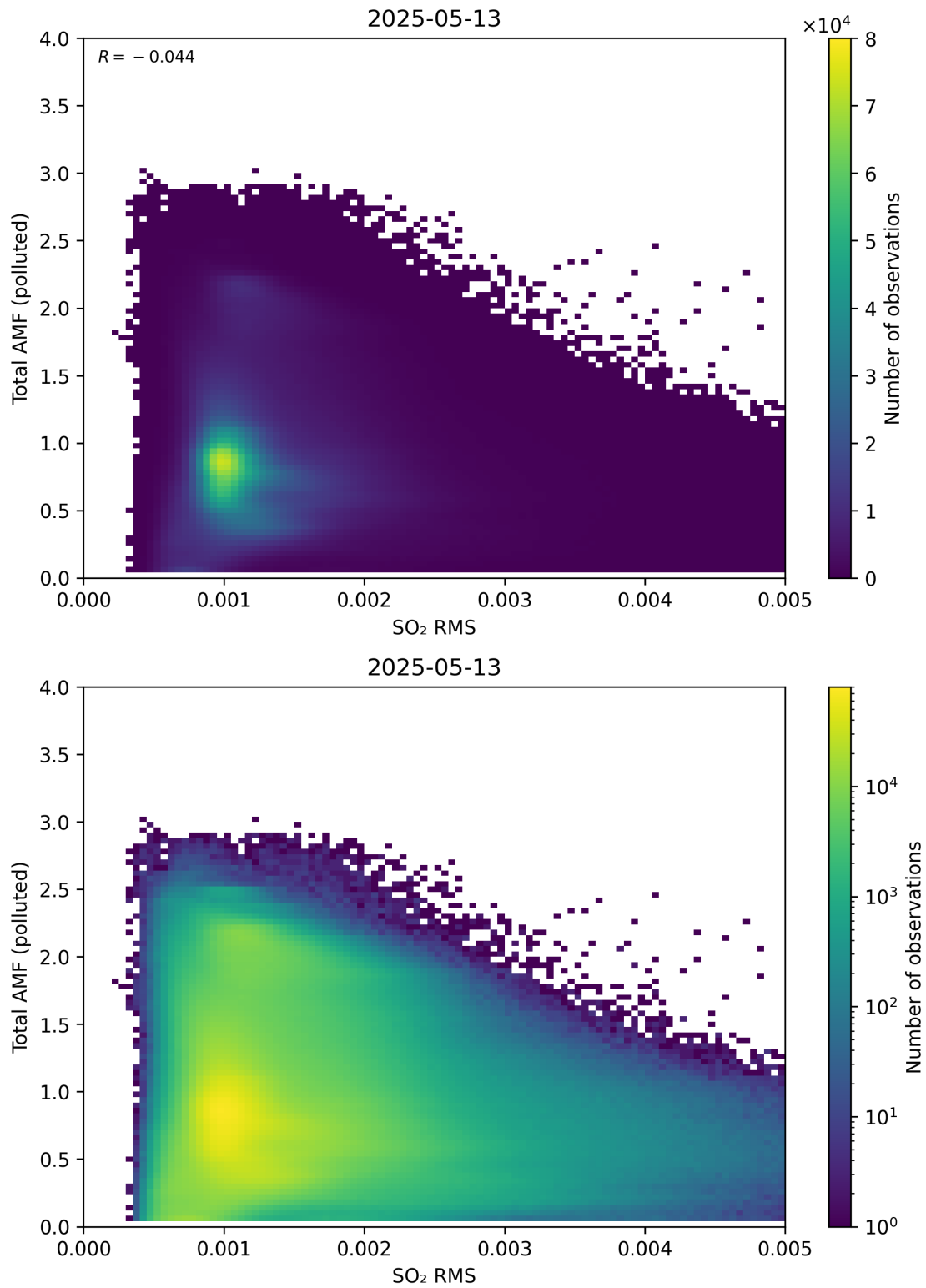
Figure 148: Scatter density plot of “SO 2 RMS” against “Total AMF (polluted)” for 2025-05-12 to 2025-05-14.
