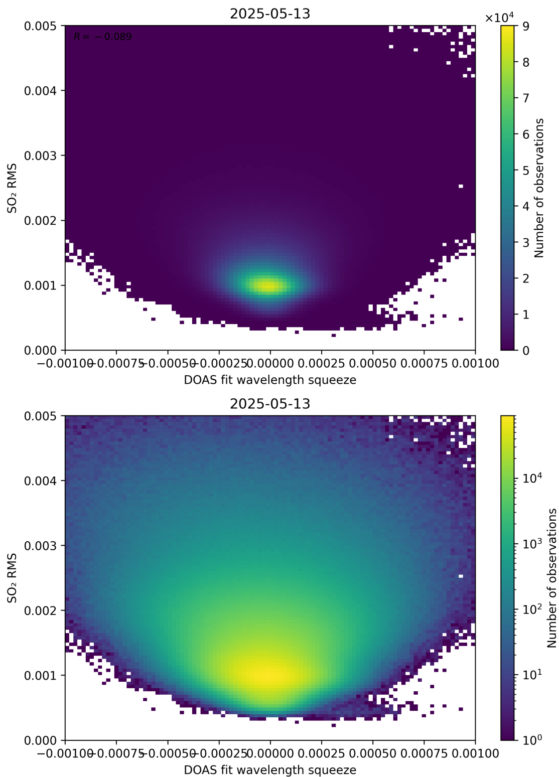
Figure 143: Scatter density plot of “DOAS fit wavelength squeeze” against “SO 2 RMS” for 2025-05-12 to 2025-05-14.
