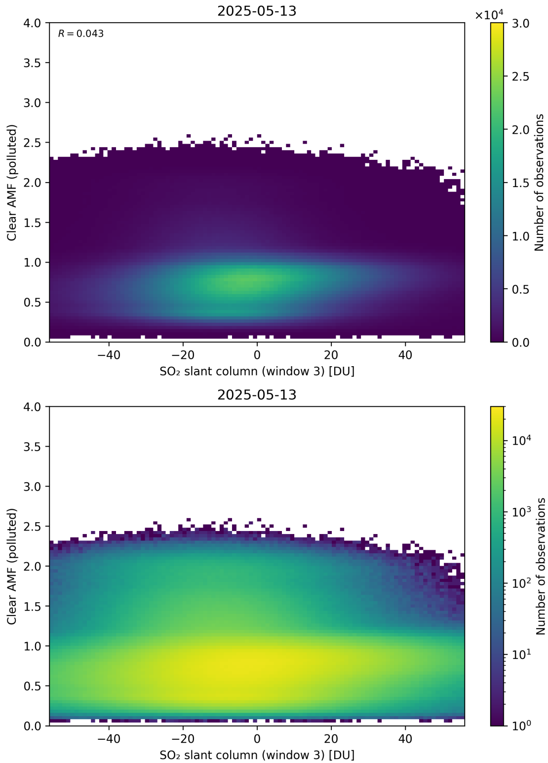
Figure 315: Scatter density plot of “SO 2 slant column (window 3)” against “Clear AMF (polluted)” for 2025-05-12 to 2025-05-14.
