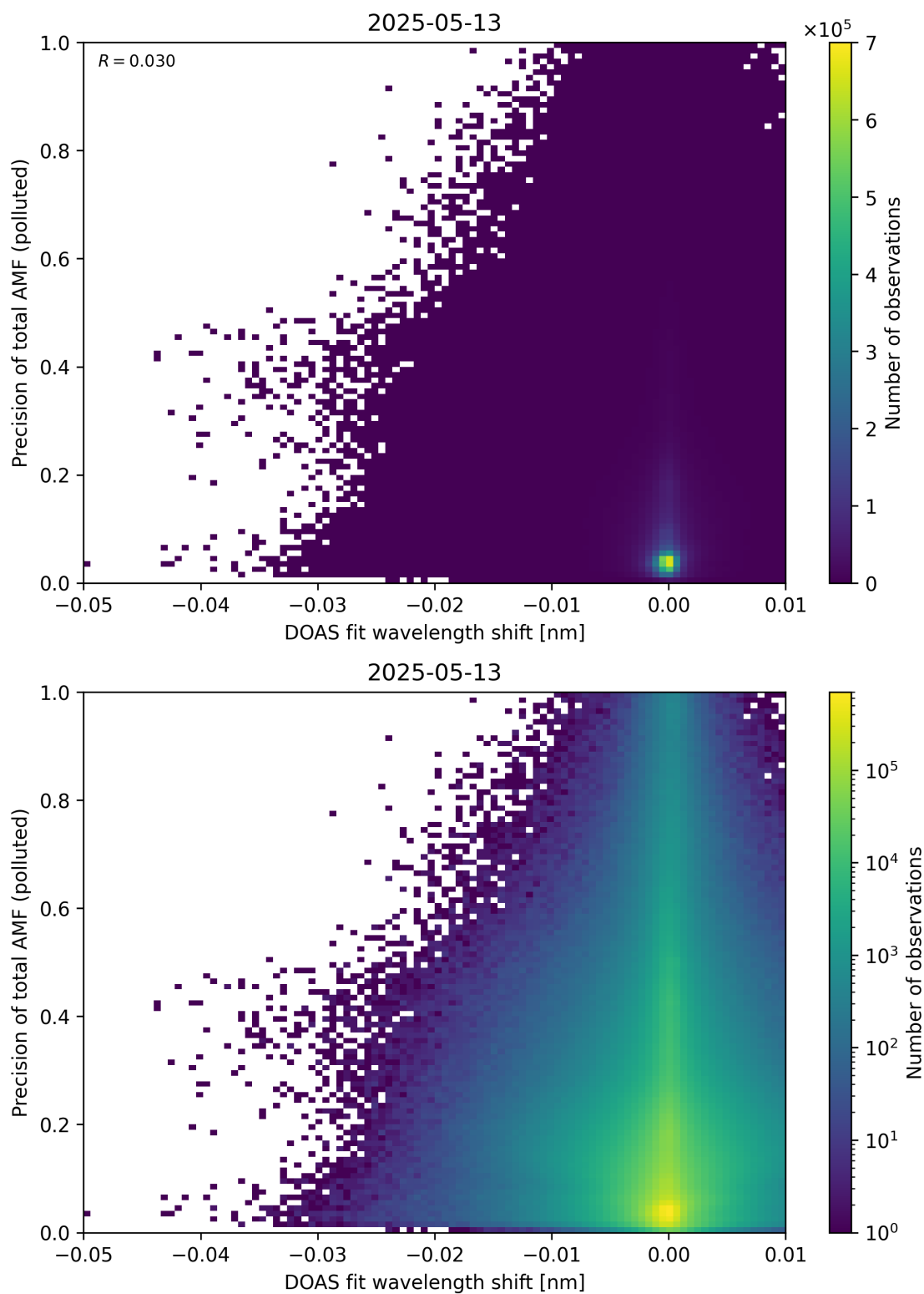
Figure 142: Scatter density plot of “DOAS fit wavelength shift” against “Precision of total AMF (polluted)” for 2025-05-12 to 2025-05-14.
