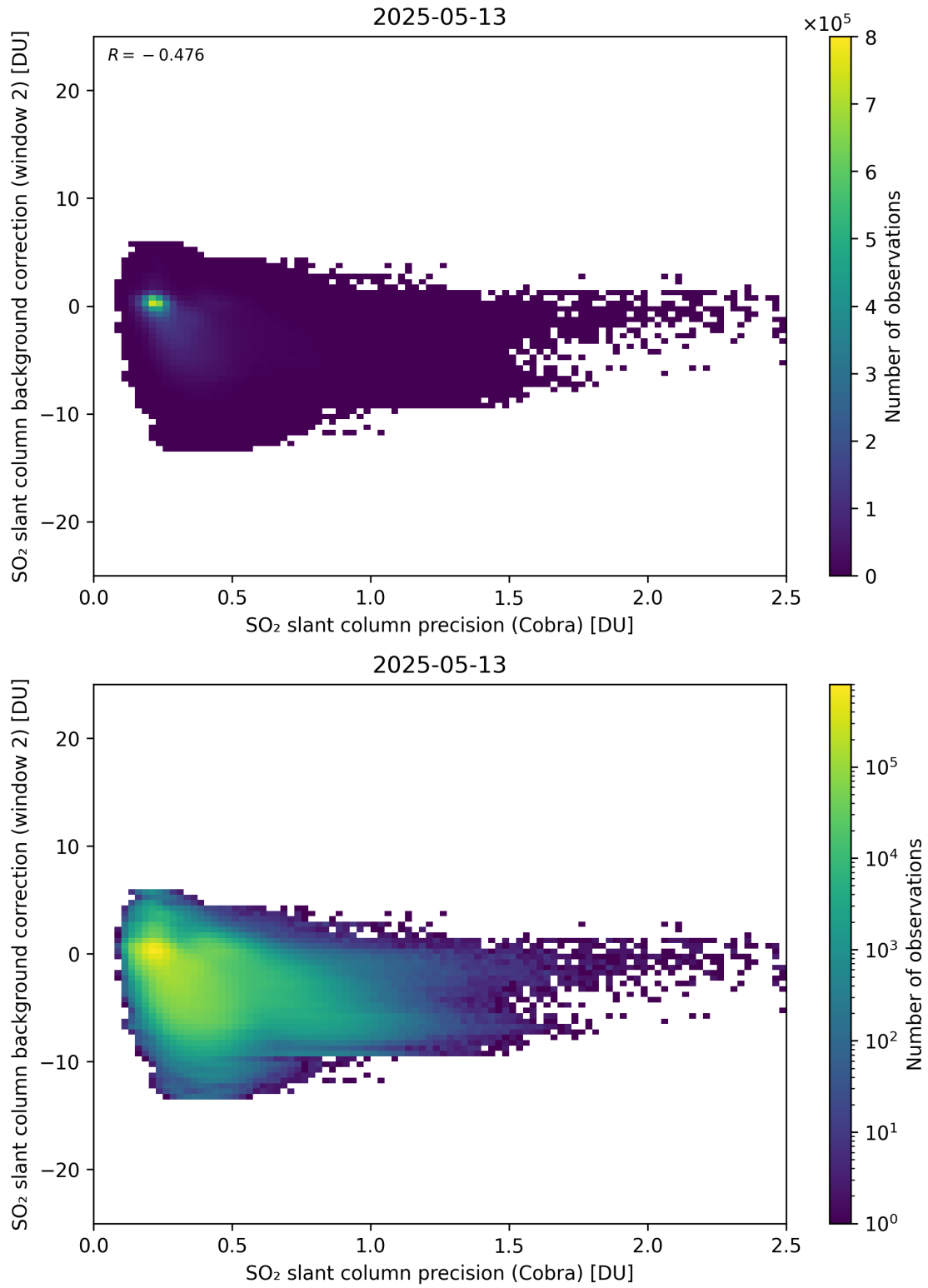
Figure 200: Scatter density plot of “SO 2 slant column precision (Cobra)” against “SO 2 slant column background correction (window 2)” for 2025-05-12 to 2025-05-14.
