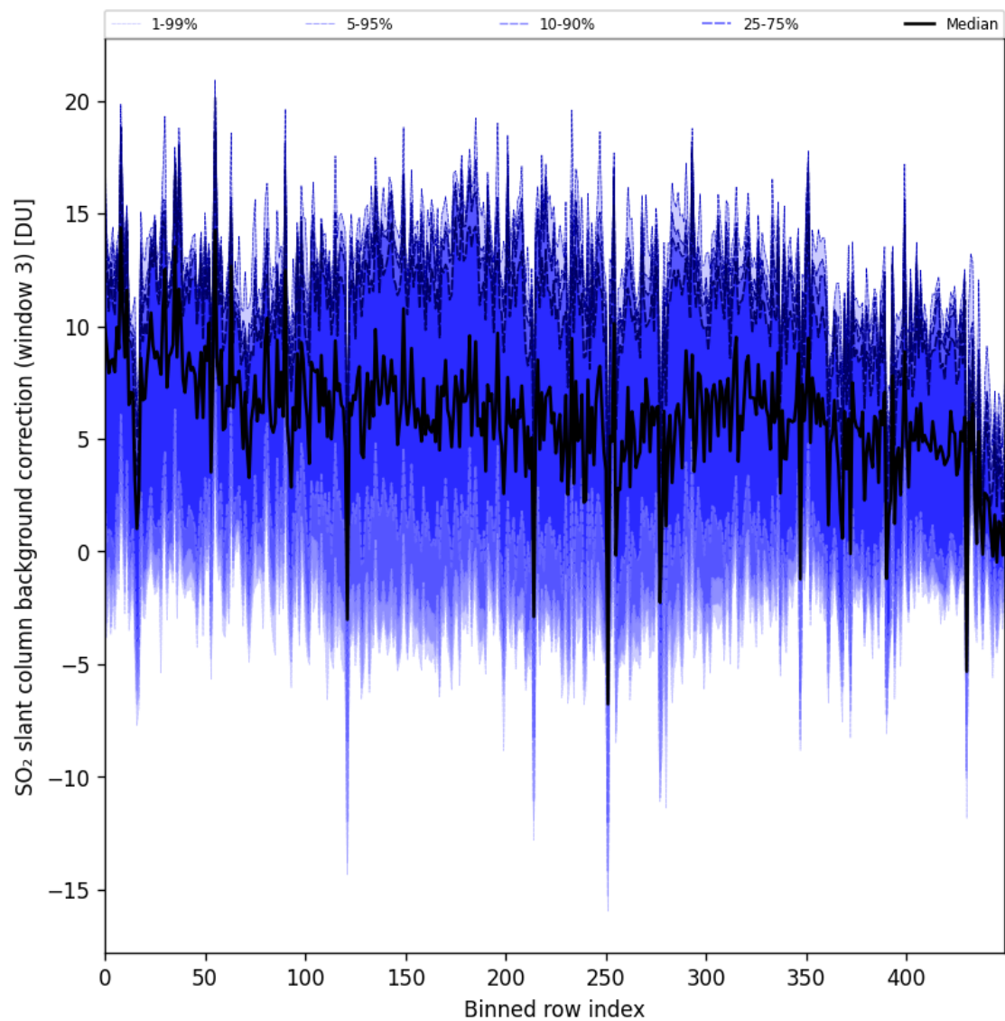
Figure 100: Along track statistics of “SO 2 slant column background correction (window 3)” for 2025-05-12 to 2025-05-14
