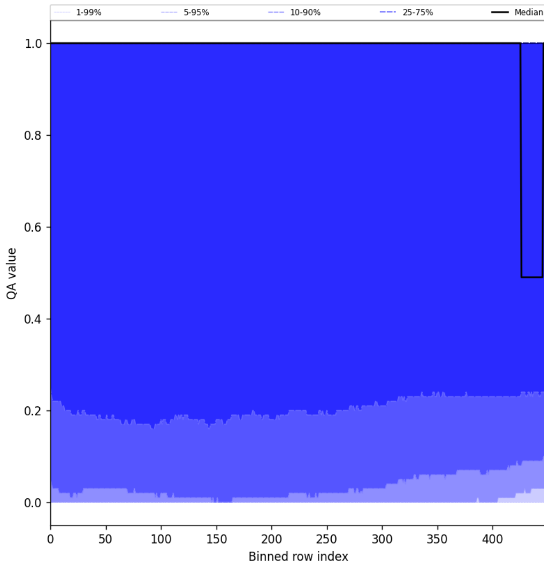
Figure 83: Along track statistics of “QA value” for 2025-05-12 to 2025-05-14
