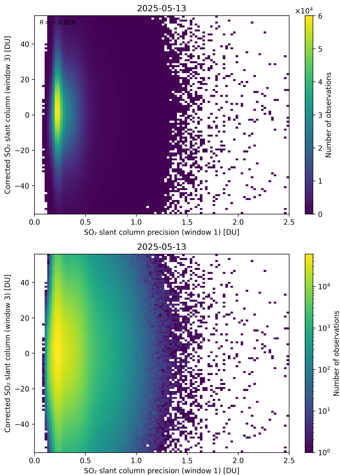
Figure 276: Scatter density plot of “SO 2 slant column precision (window 1)” against “Corrected SO 2 slant column (window 3)” for 2025-05-12 to 2025-05-14.
