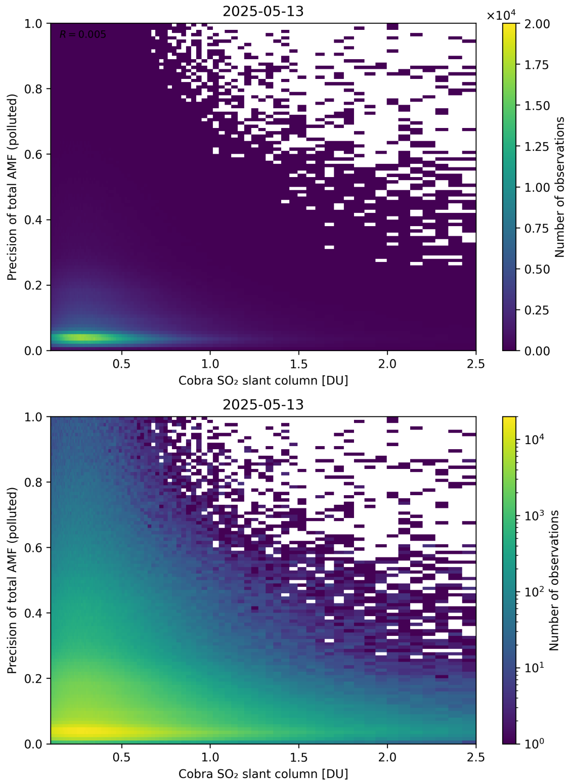
Figure 225: Scatter density plot of “Cobra SO 2 slant column” against “Precision of total AMF (polluted)” for 2025-05-12 to 2025-05-14.
