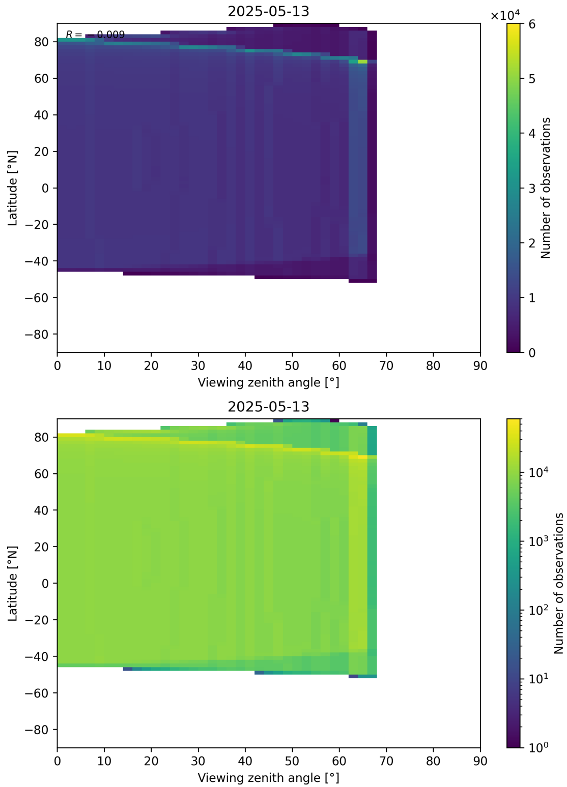
Figure 368: Scatter density plot of “Viewing zenith angle” against “Latitude” for 2025-05-12 to 2025-05-14.
