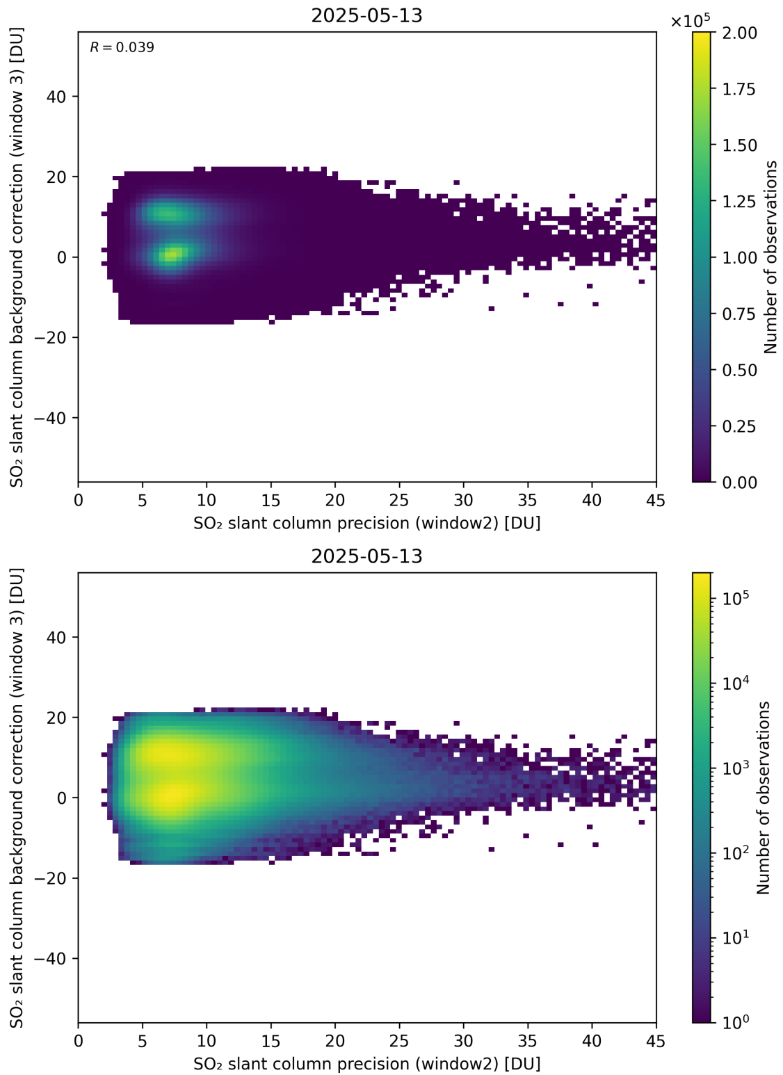
Figure 292: Scatter density plot of “SO 2 slant column precision (window2)” against “SO 2 slant column background correction (window 3)” for 2025-05-12 to 2025-05-14.
