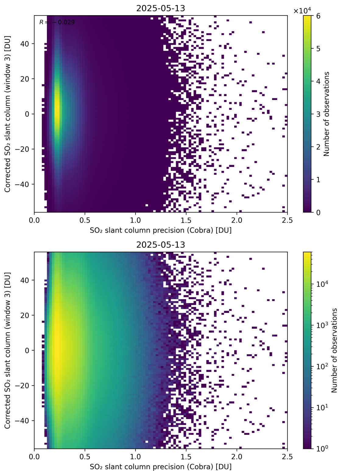
Figure 207: Scatter density plot of “SO 2 slant column precision (Cobra)” against “Corrected SO 2 slant column (window 3)” for 2025-05-12 to 2025-05-14.
