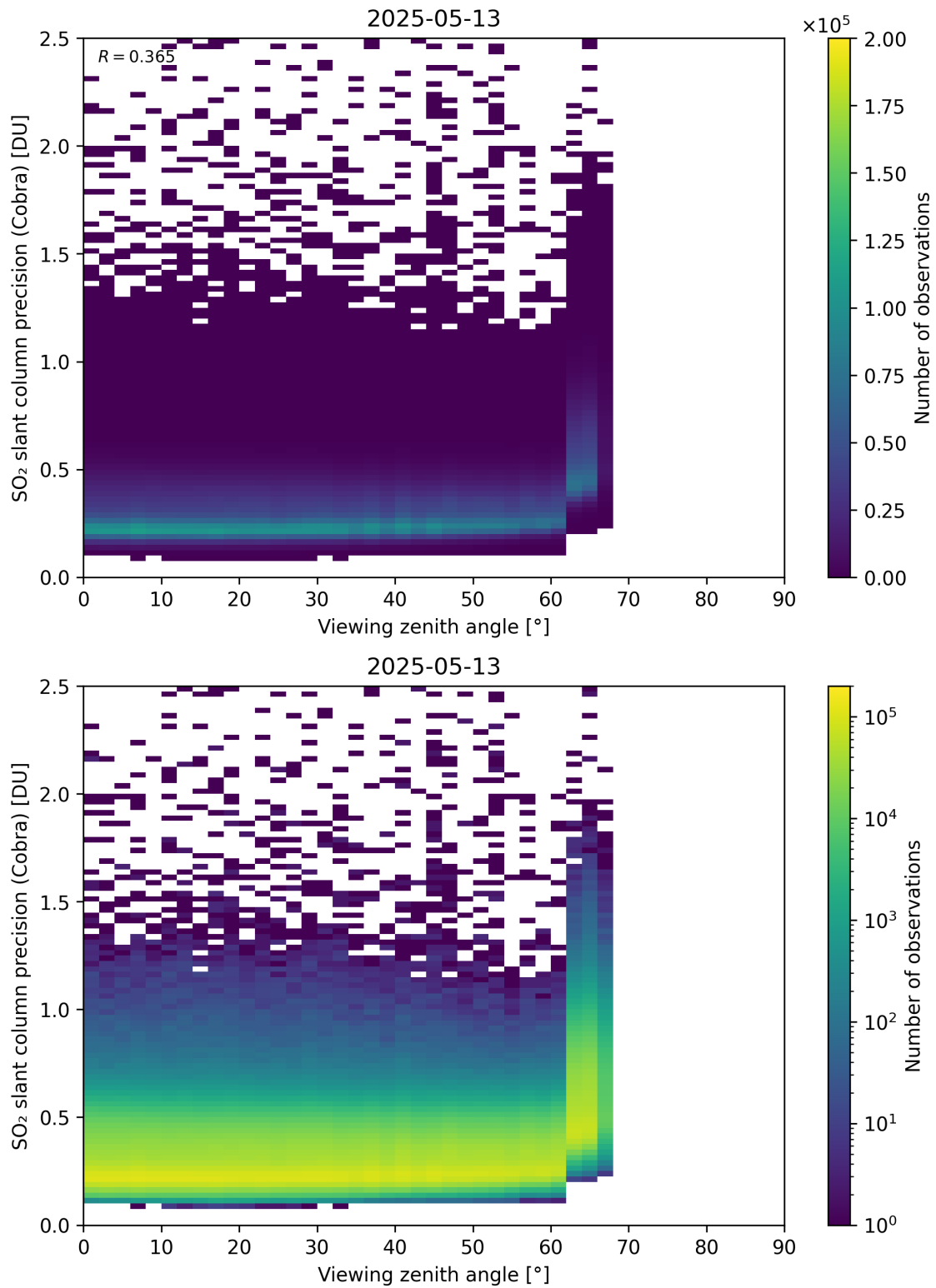
Figure 372: Scatter density plot of “Viewing zenith angle” against “SO 2 slant column precision (Cobra)” for 2025-05-12 to 2025-05-14.
