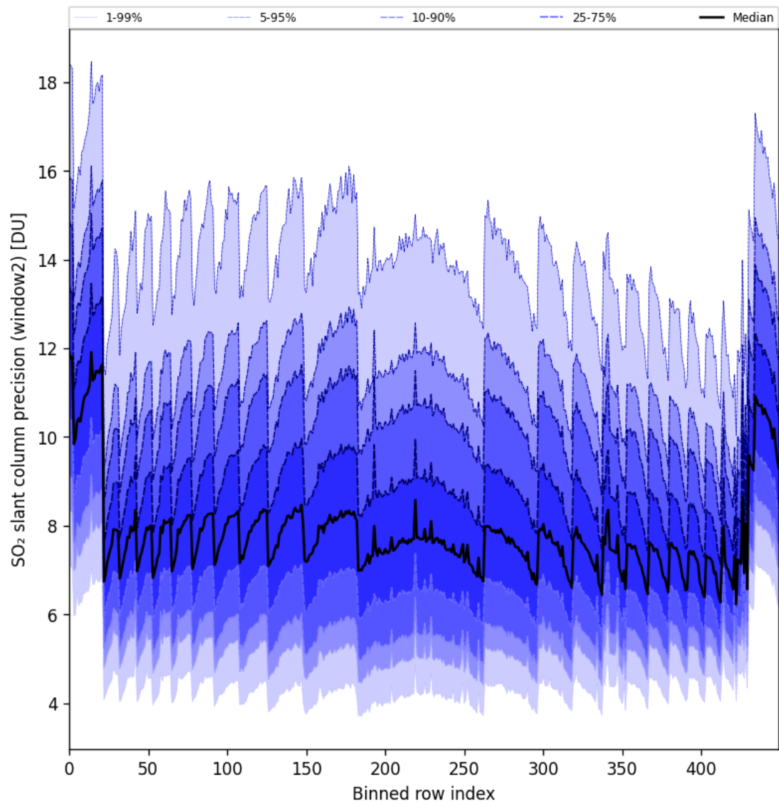
Figure 94: Along track statistics of “SO 2 slant column precision (window2)” for 2025-05-12 to 2025-05-14
