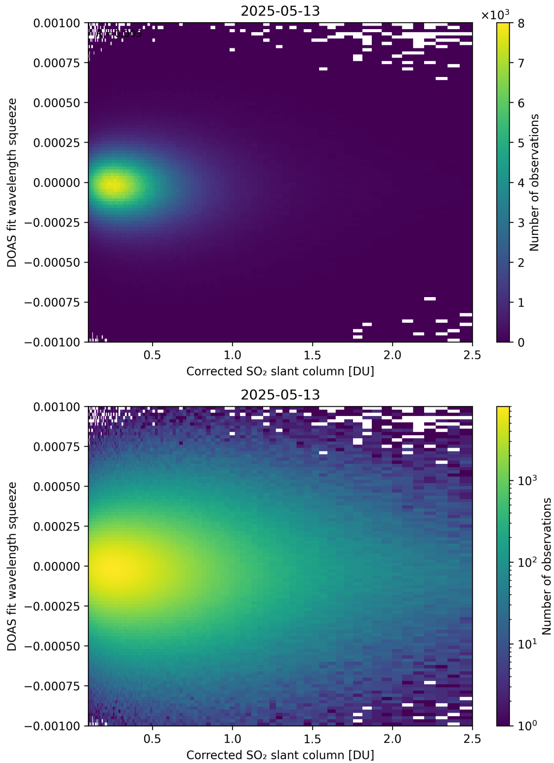
Figure 230: Scatter density plot of “Corrected SO 2 slant column” against “DOAS fit wavelength squeeze” for 2025-05-12 to 2025-05-14.
