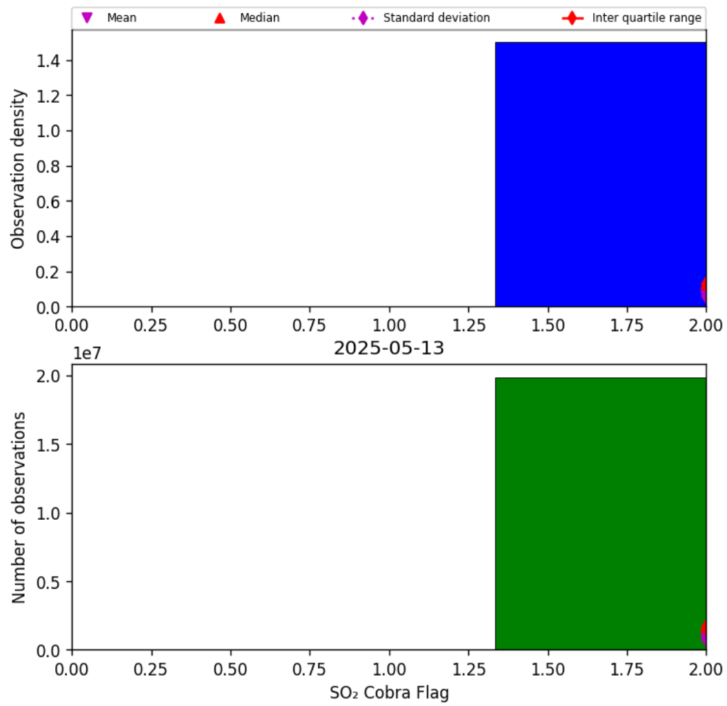
Figure 75: Histogram of “SO 2 Cobra Flag” for 2025-05-12 to 2025-05-14
