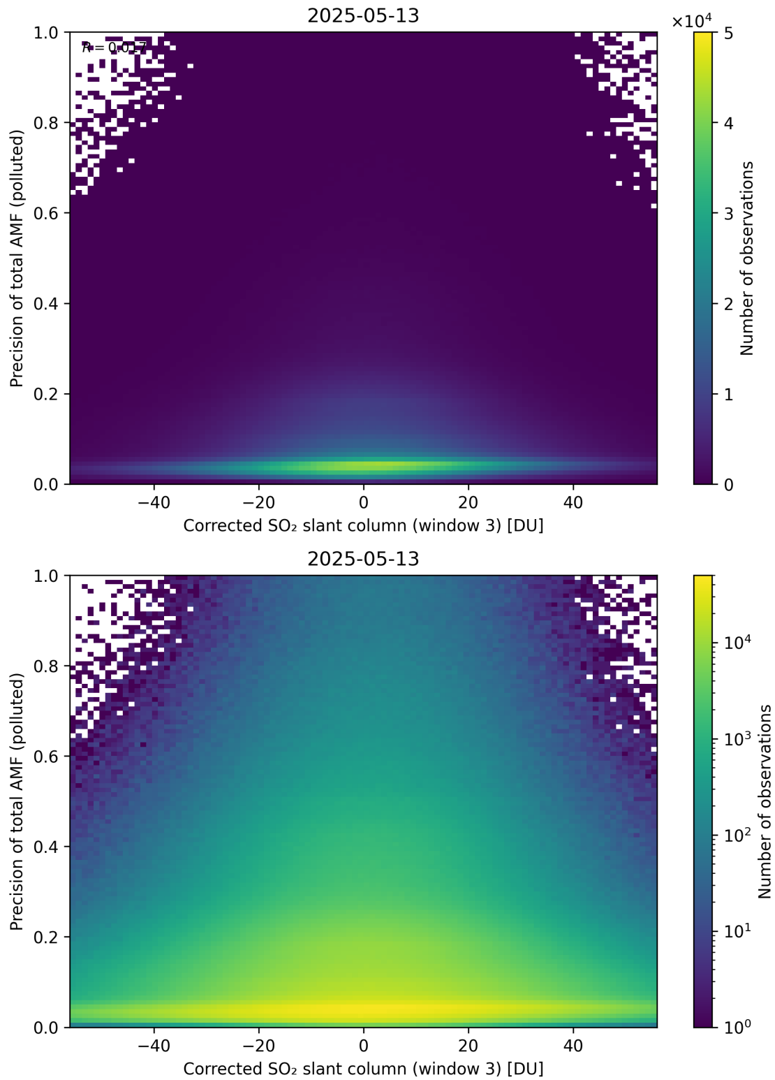
Figure 261: Scatter density plot of “Corrected SO 2 slant column (window 3)” against “Precision of total AMF (polluted)” for 2025-05-12 to 2025-05-14.
