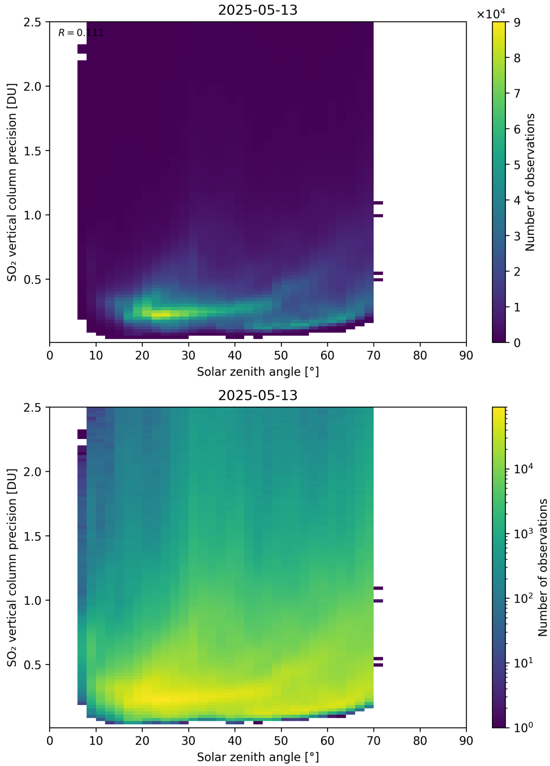
Figure 192: Scatter density plot of “Solar zenith angle” against “SO 2 vertical column precision” for 2025-05-12 to 2025-05-14.
