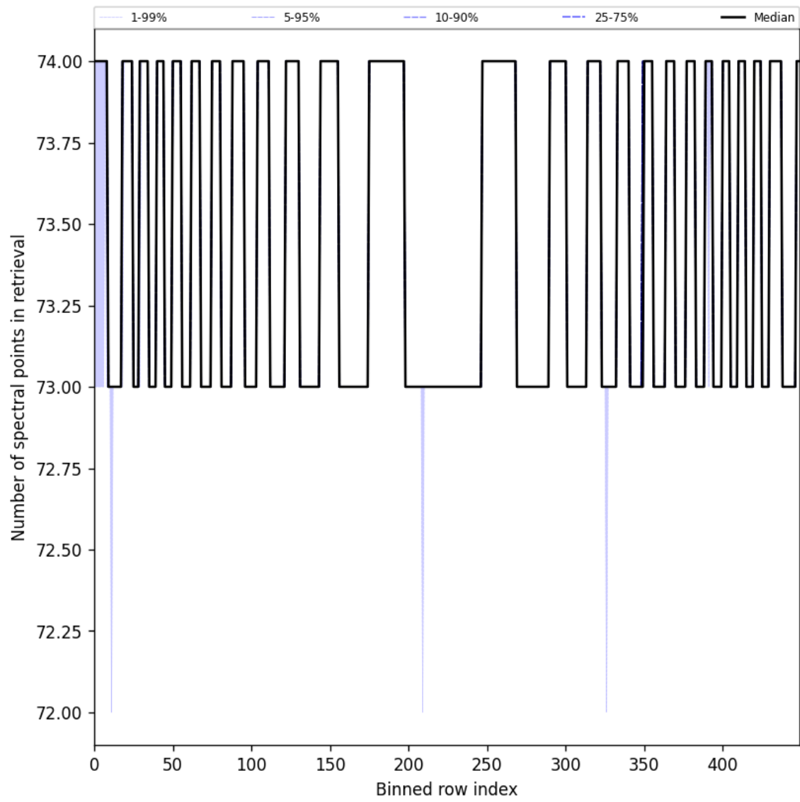
Figure 108: Along track statistics of “Number of spectral points in retrieval” for 2025-05-12 to 2025-05-14
