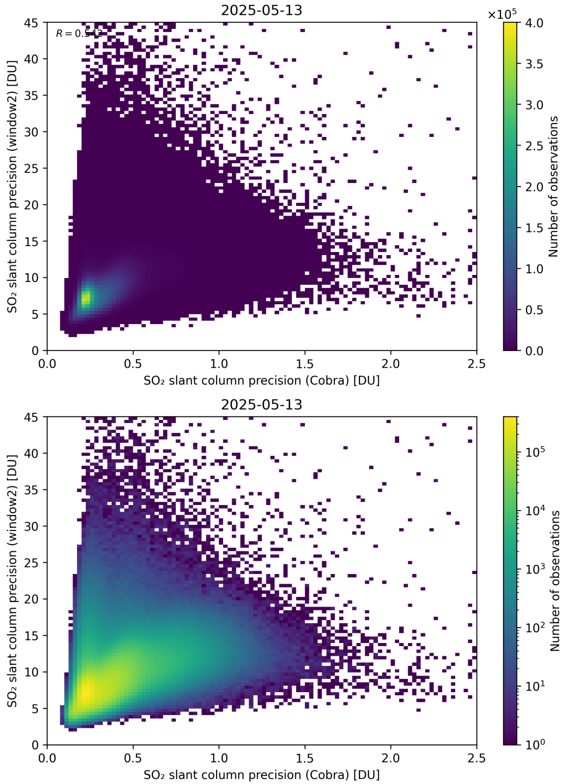
Figure 210: Scatter density plot of “SO 2 slant column precision (Cobra)” against “SO 2 slant column precision (window2)” for 2025-05-12 to 2025-05-14.
