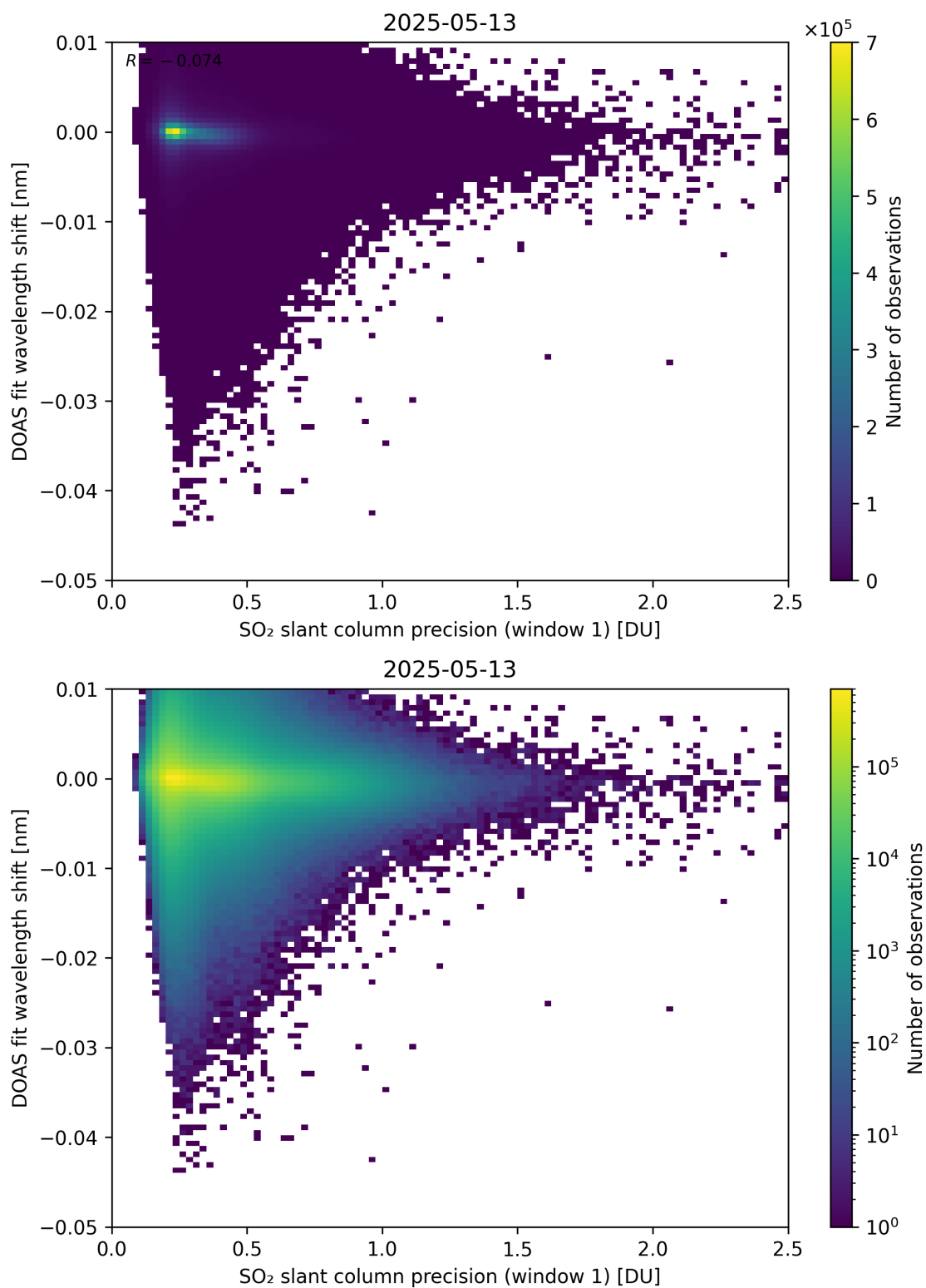
Figure 271: Scatter density plot of “SO 2 slant column precision (window 1)” against “DOAS fit wavelength shift” for 2025-05-12 to 2025-05-14.
