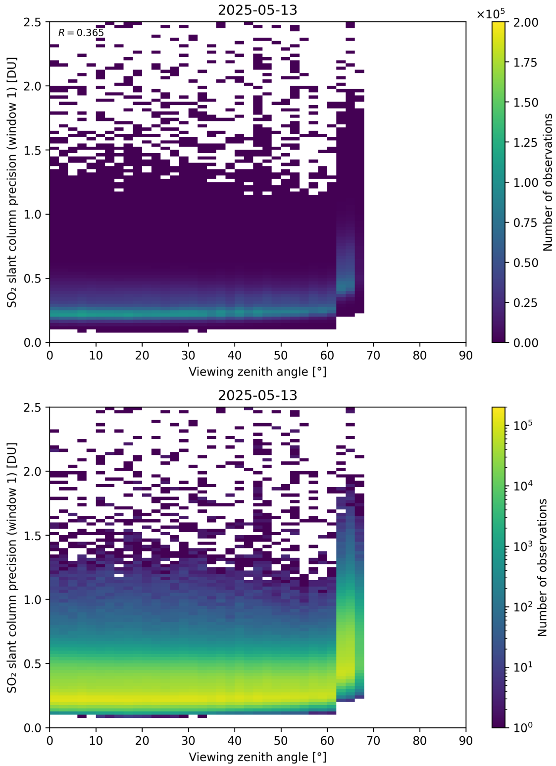
Figure 377: Scatter density plot of “Viewing zenith angle” against “SO 2 slant column precision (window 1)” for 2025-05-12 to 2025-05-14.
