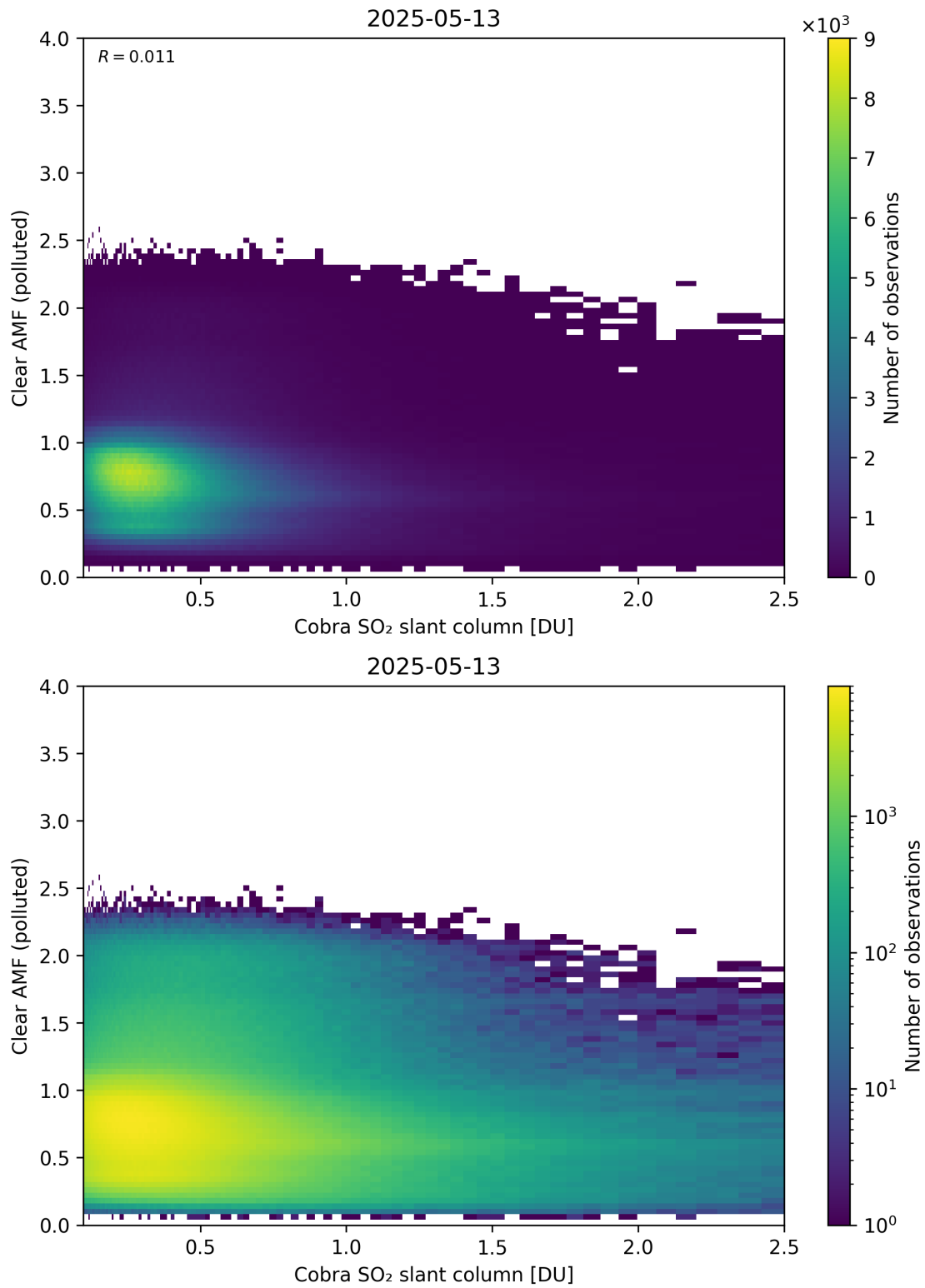
Figure 215: Scatter density plot of “Cobra SO 2 slant column” against “Clear AMF (polluted)” for 2025-05-12 to 2025-05-14.
