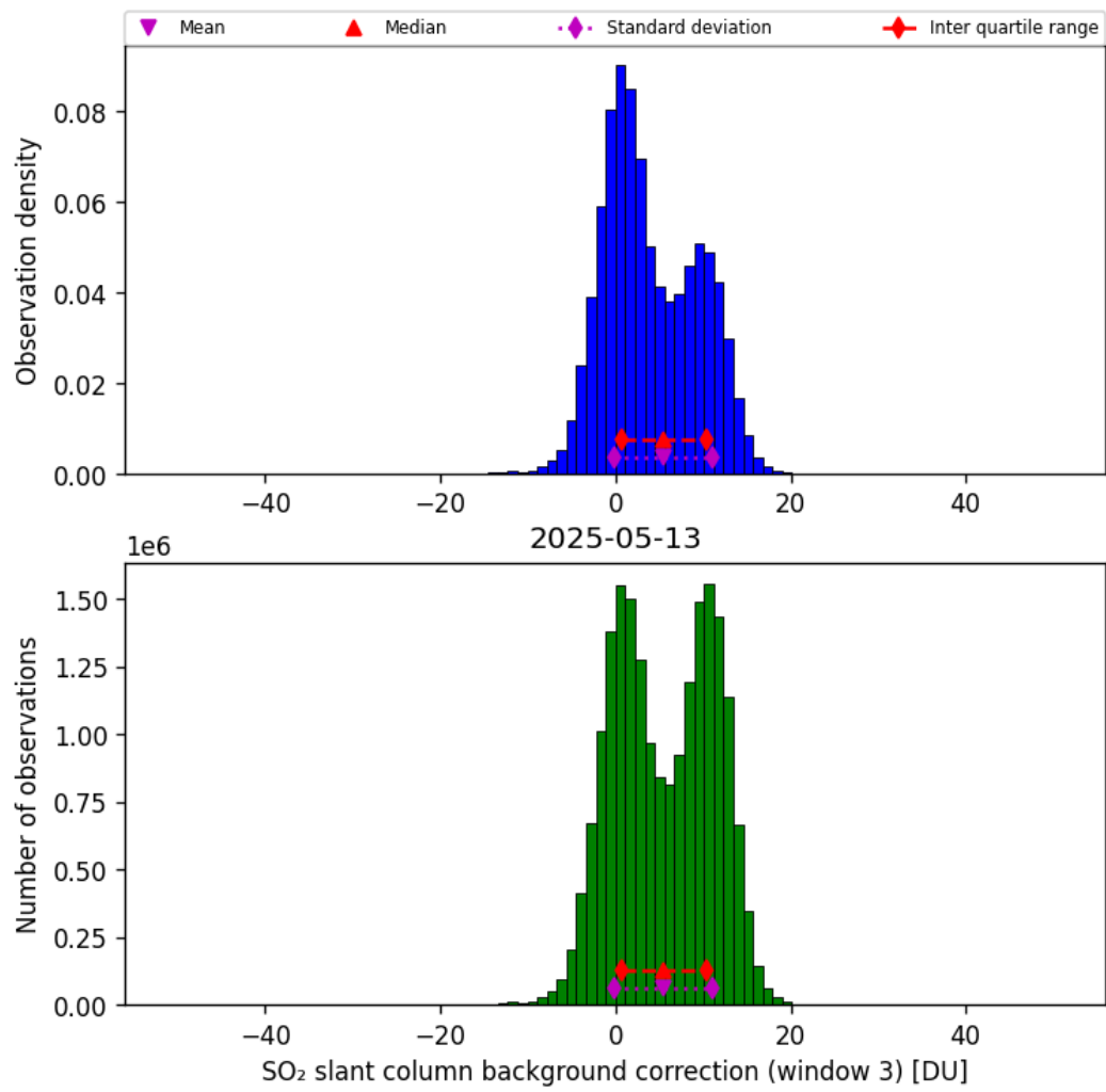
Figure 74: Histogram of “SO 2 slant column background correction (window 3)” for 2025-05-12 to 2025-05-14
