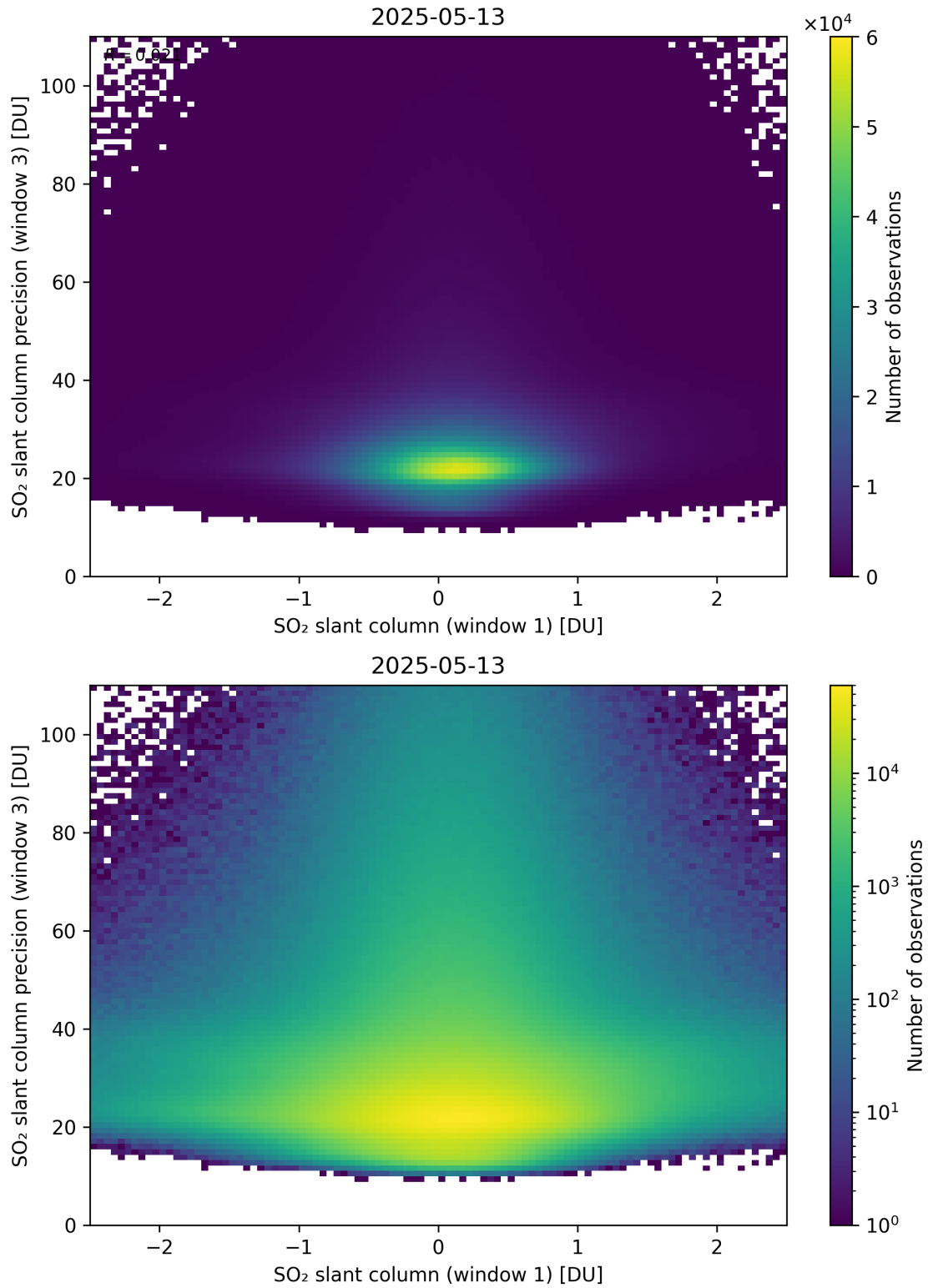
Figure 288: Scatter density plot of “SO 2 slant column (window 1)” against “SO 2 slant column precision (window 3)” for 2025-05-12 to 2025-05-14.
