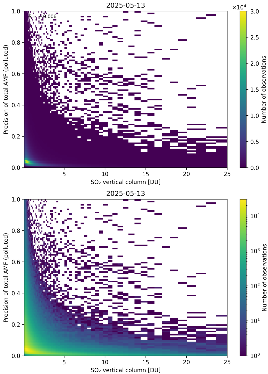
Figure 360: Scatter density plot of “SO 2 vertical column” against “Precision of total AMF (polluted)” for 2025-05-12 to 2025-05-14.
