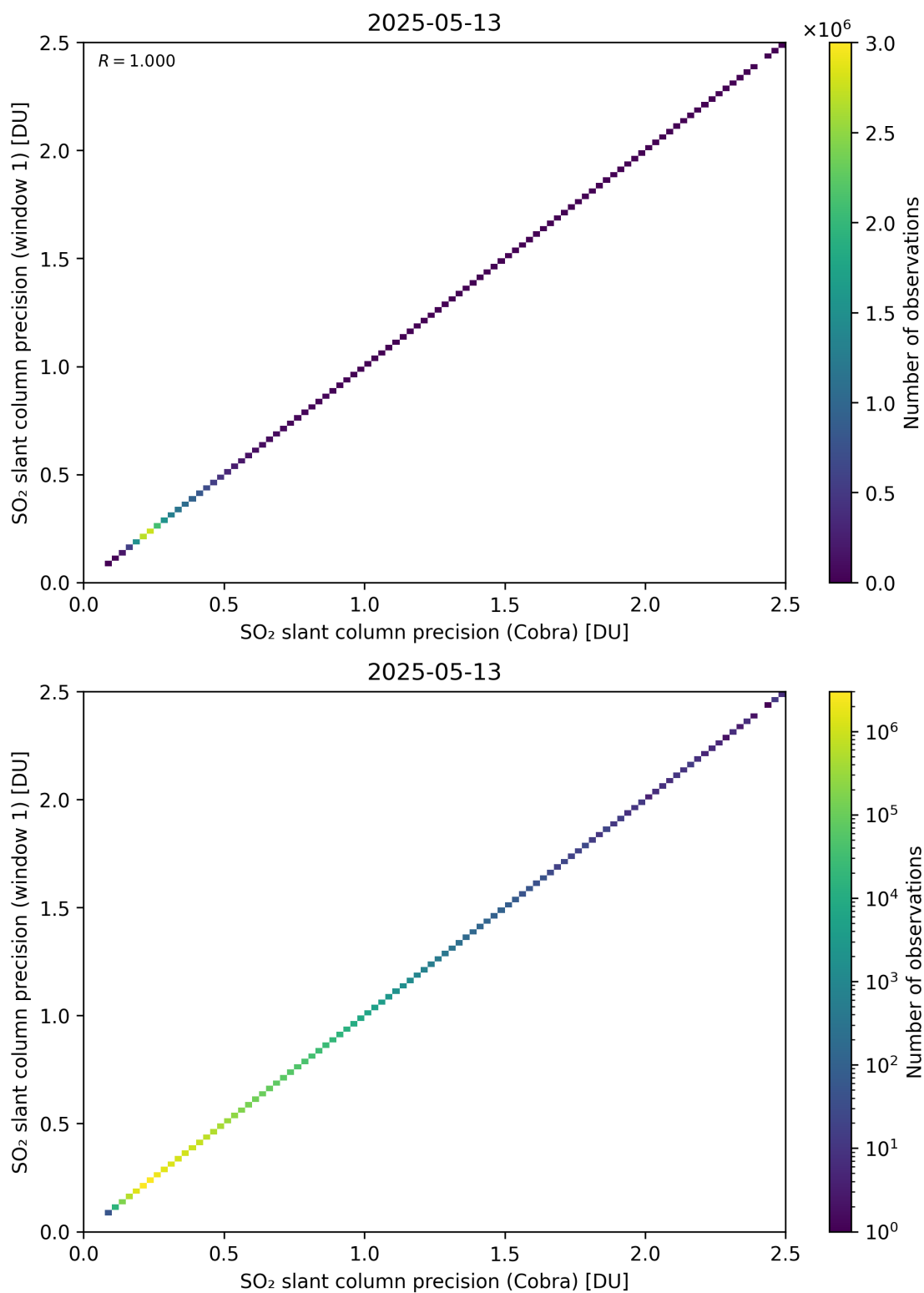
Figure 209: Scatter density plot of “SO 2 slant column precision (Cobra)” against “SO 2 slant column precision (window 1)” for 2025-05-12 to 2025-05-14.
