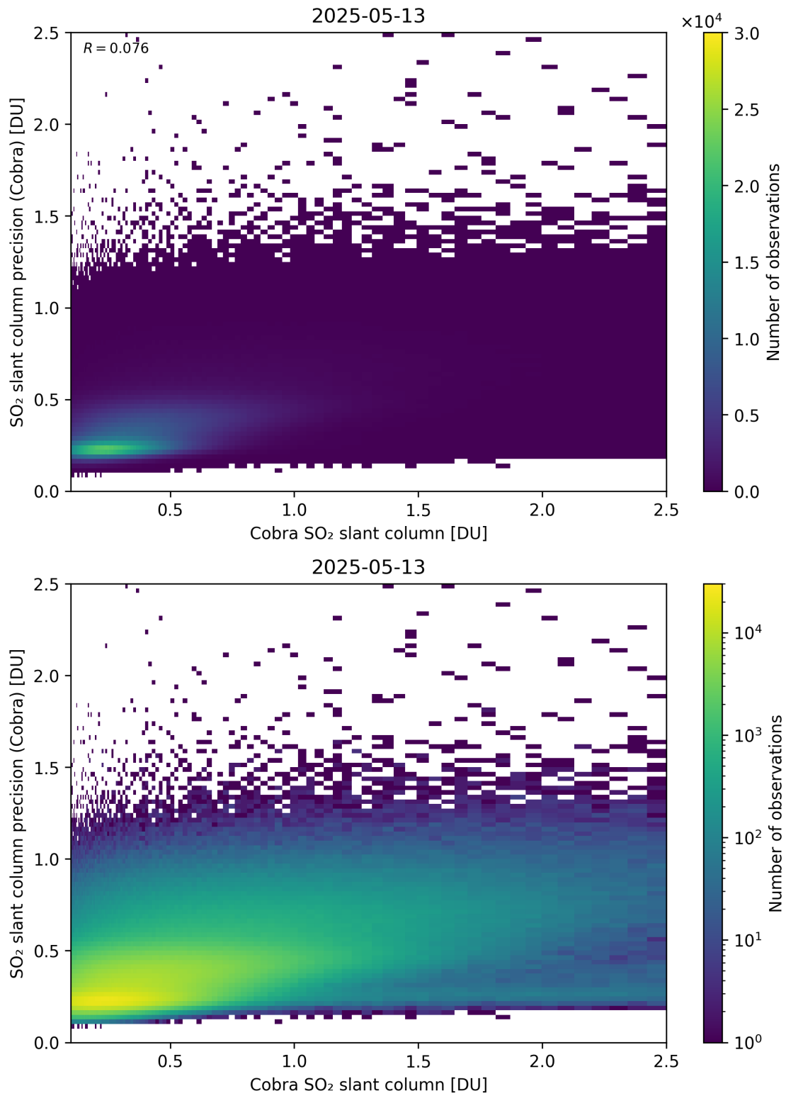
Figure 216: Scatter density plot of “Cobra SO 2 slant column” against “SO 2 slant column precision (Cobra)” for 2025-05-12 to 2025-05-14.
