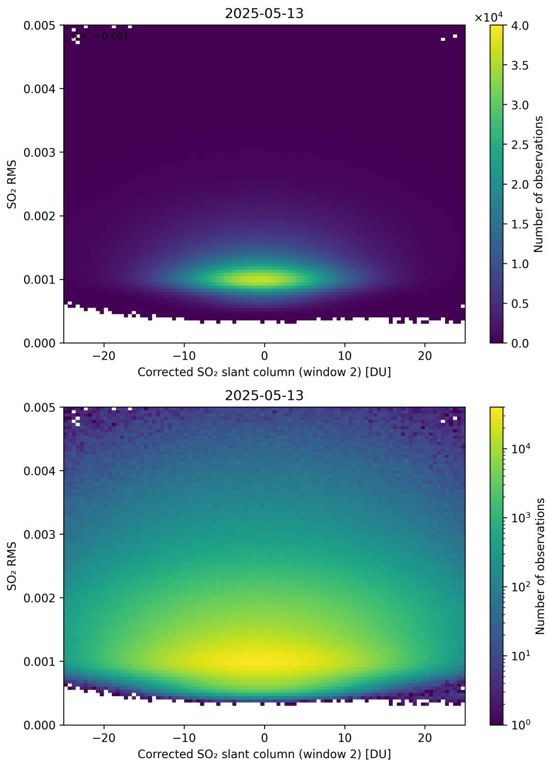
Figure 248: Scatter density plot of “Corrected SO 2 slant column (window 2)” against “SO 2 RMS” for 2025-05-12 to 2025-05-14.
