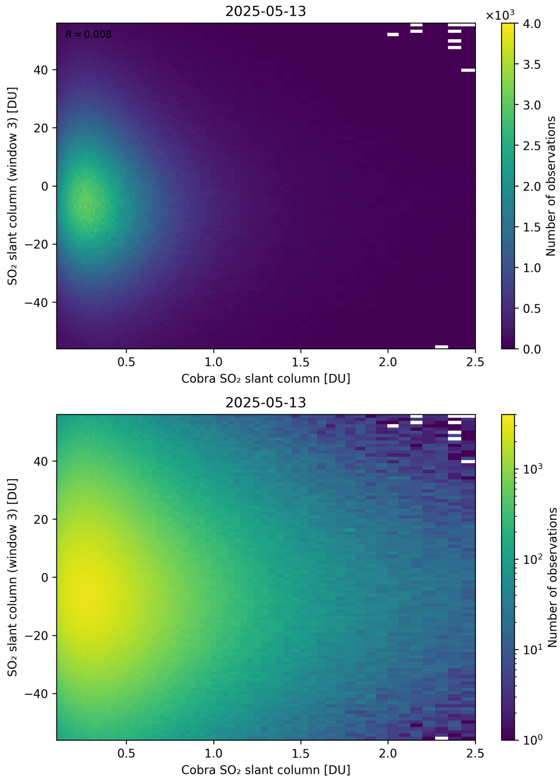
Figure 222: Scatter density plot of “Cobra SO 2 slant column” against “SO 2 slant column (window 3)” for 2025-05-12 to 2025-05-14.
