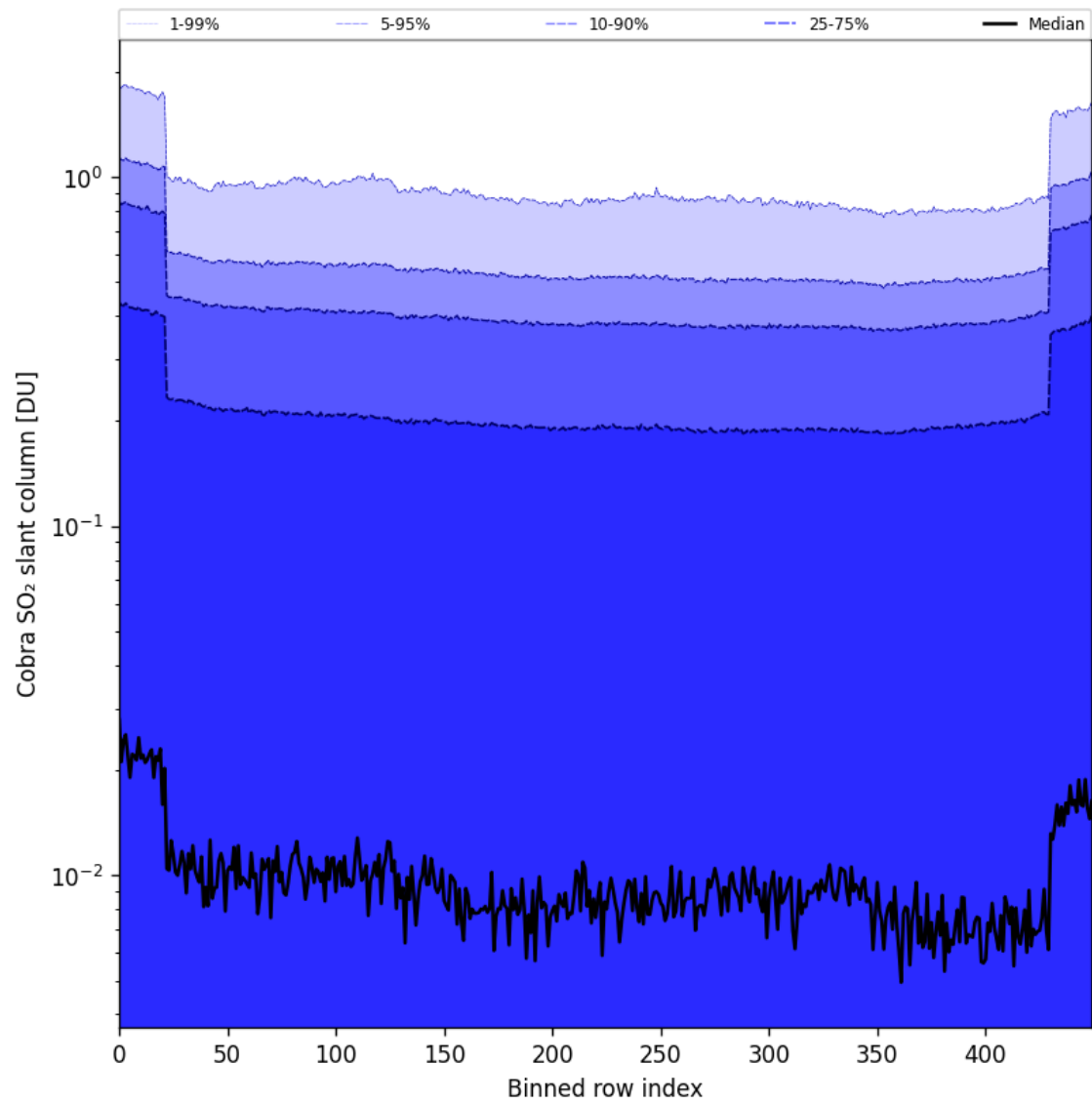
Figure 87: Along track statistics of “Cobra SO 2 slant column” for 2025-05-12 to 2025-05-14
