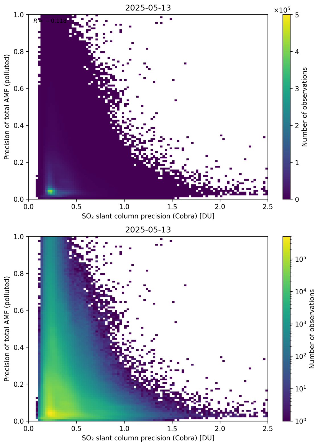
Figure 214: Scatter density plot of “SO 2 slant column precision (Cobra)” against “Precision of total AMF (polluted)” for 2025-05-12 to 2025-05-14.
