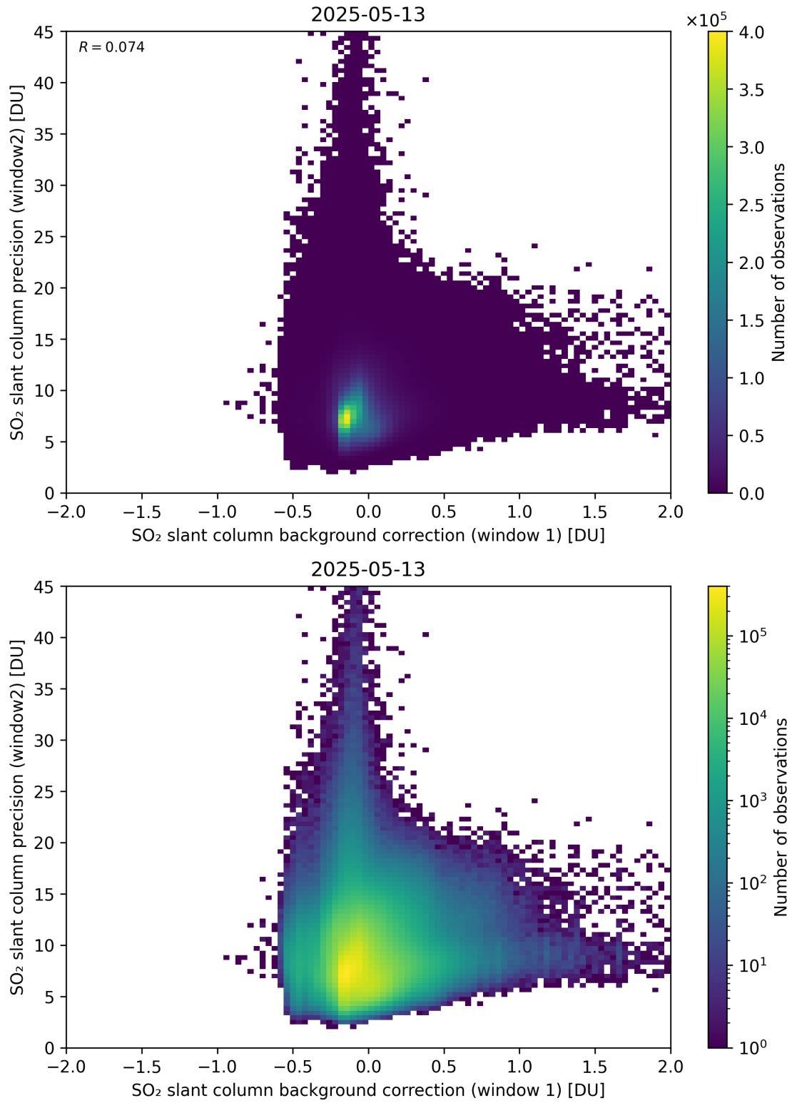
Figure 117: Scatter density plot of “SO 2 slant column background correction (window 1)” against “SO 2 slant column precision (window2)” for 2025-05-12 to 2025-05-14.
