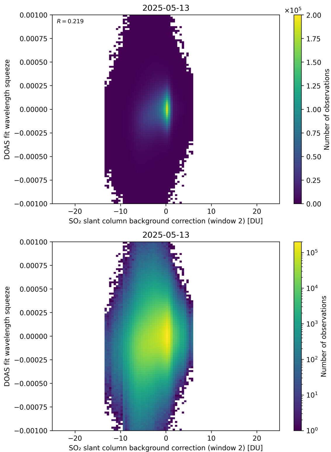
Figure 124: Scatter density plot of “SO 2 slant column background correction (window 2)” against “DOAS fit wavelength squeeze” for 2025-05-12 to 2025-05-14.
