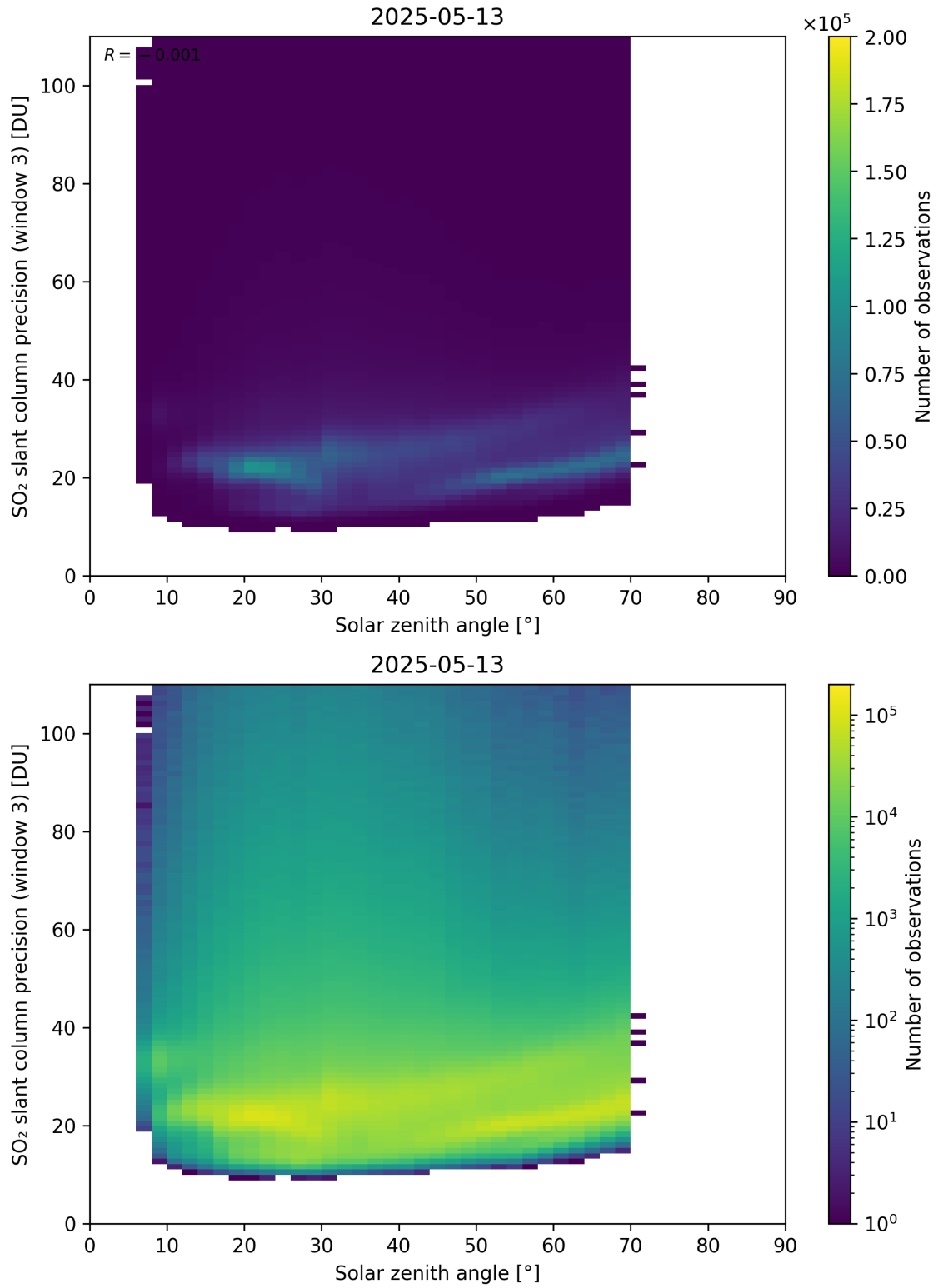
Figure 188: Scatter density plot of “Solar zenith angle” against “SO 2 slant column precision (window 3)” for 2025-05-12 to 2025-05-14.
