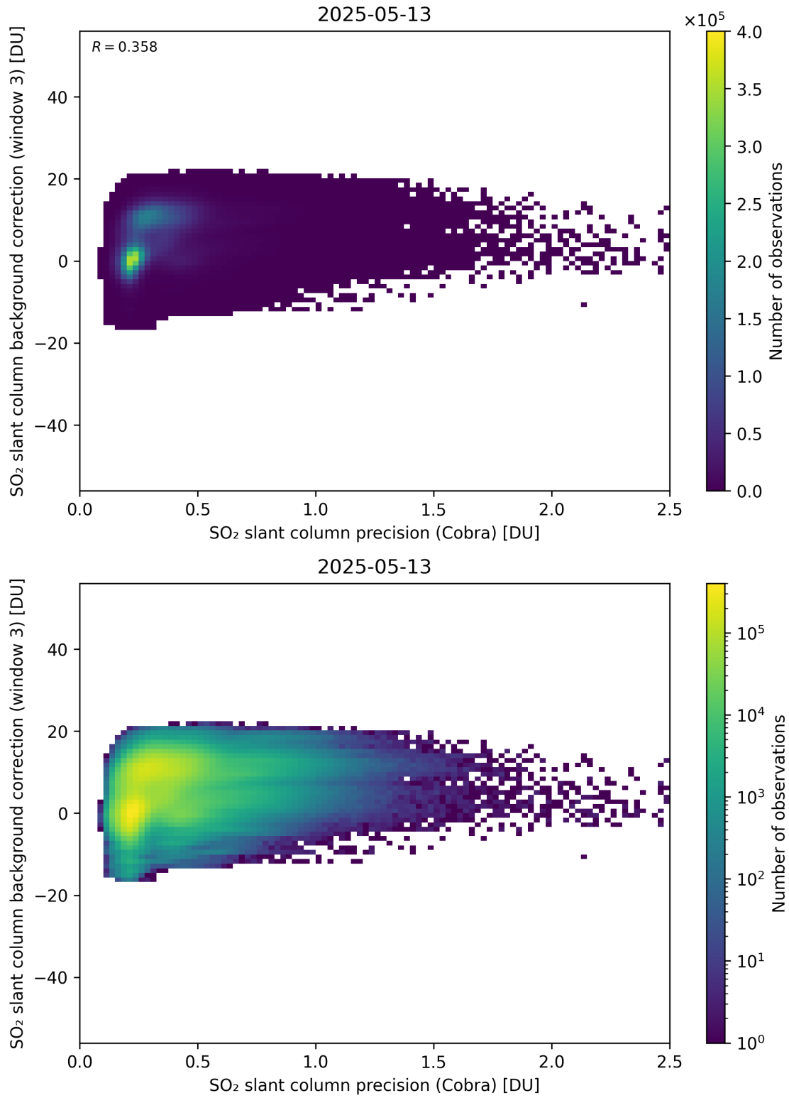
Figure 201: Scatter density plot of “SO 2 slant column precision (Cobra)” against “SO 2 slant column background correction (window 3)” for 2025-05-12 to 2025-05-14.
