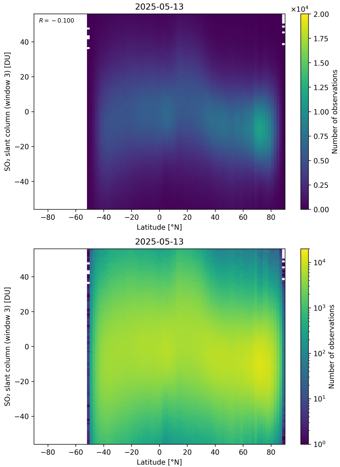
Figure 165: Scatter density plot of “Latitude” against “SO 2 slant column (window 3)” for 2025-05-12 to 2025-05-14.
