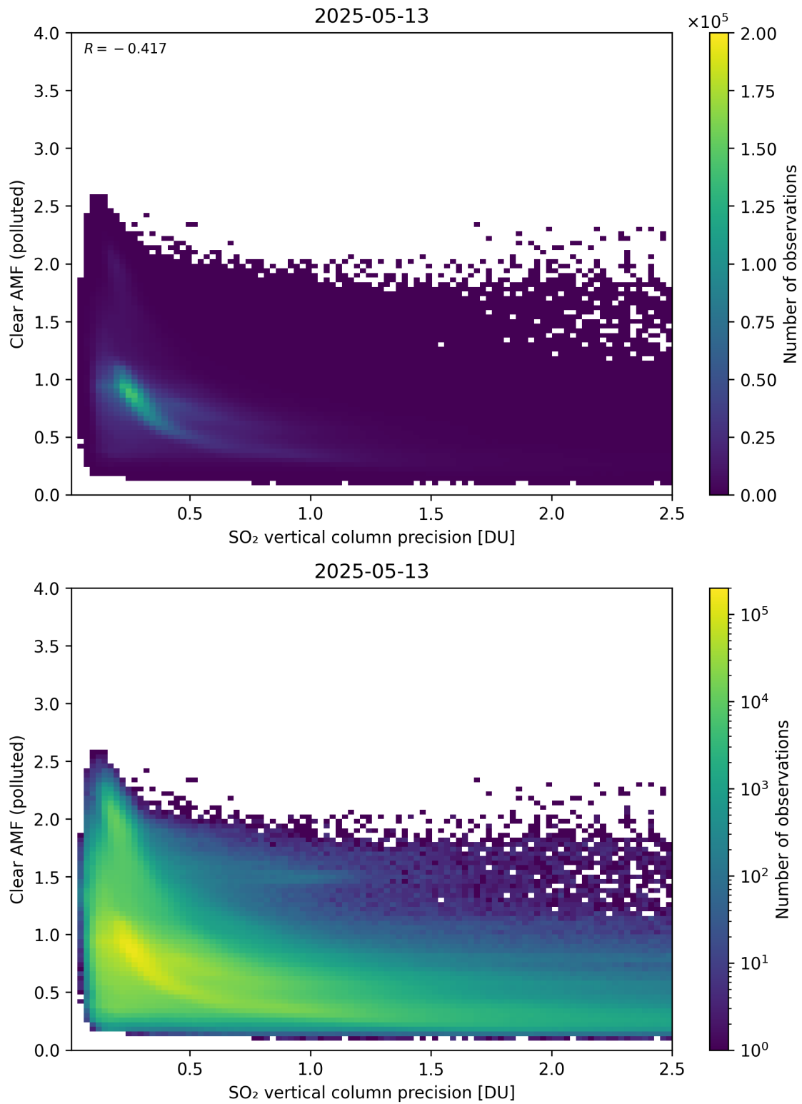
Figure 335: Scatter density plot of “SO 2 vertical column precision” against “Clear AMF (polluted)” for 2025-05-12 to 2025-05-14.
