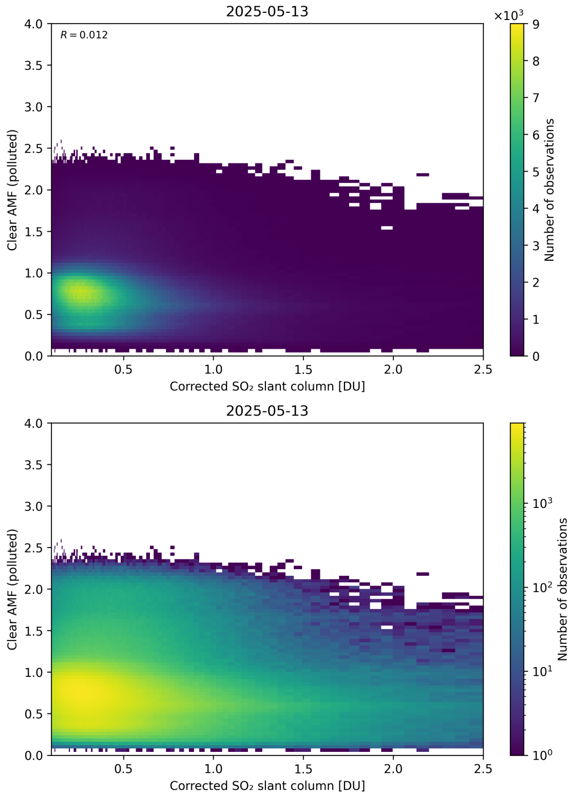
Figure 232: Scatter density plot of “Corrected SO 2 slant column” against “Clear AMF (polluted)” for 2025-05-12 to 2025-05-14.
