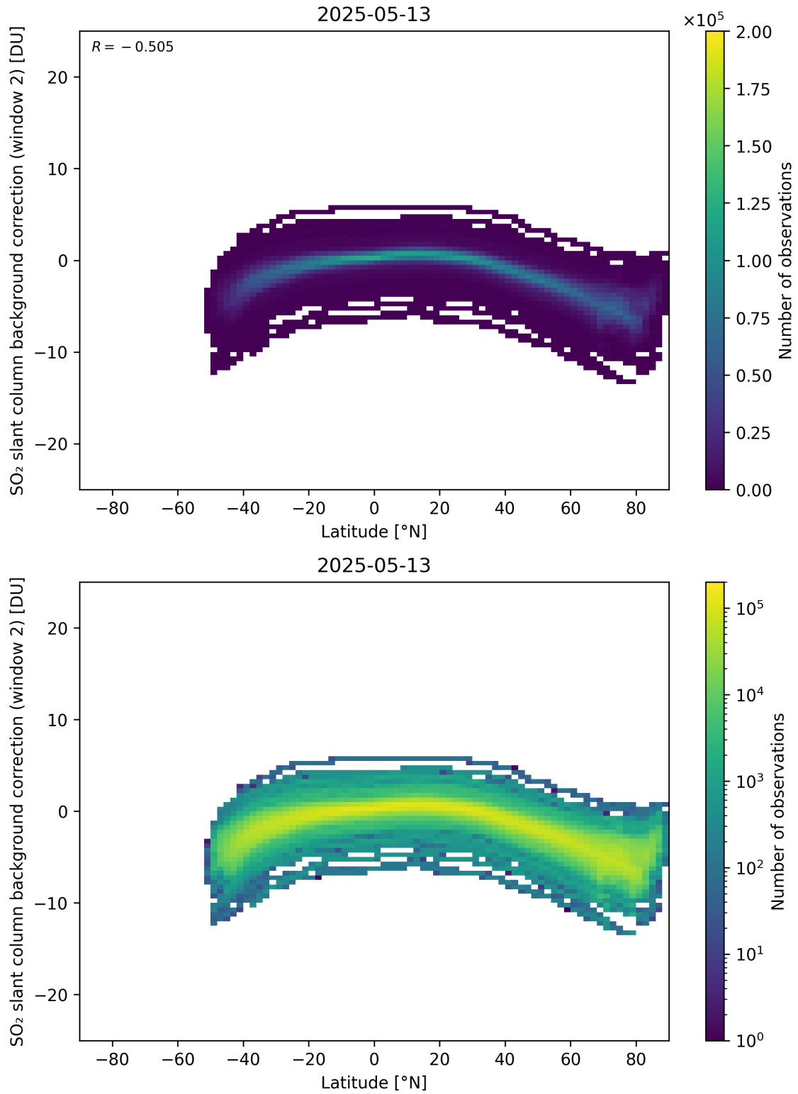
Figure 151: Scatter density plot of “Latitude” against “SO 2 slant column background correction (window 2)” for 2025-05-12 to 2025-05-14.
