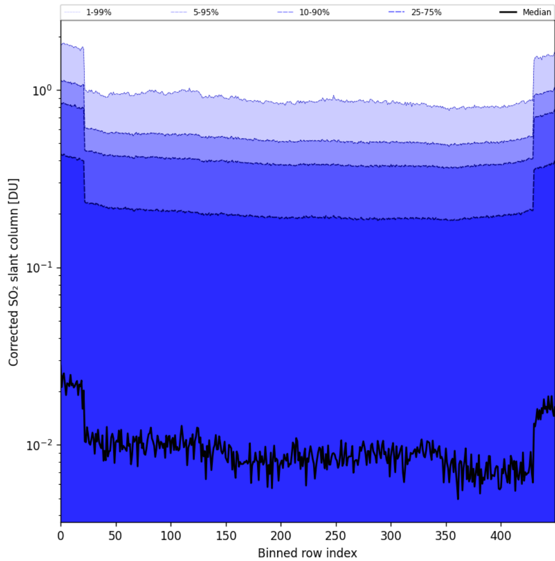
Figure 86: Along track statistics of “Corrected SO 2 slant column” for 2025-05-12 to 2025-05-14
