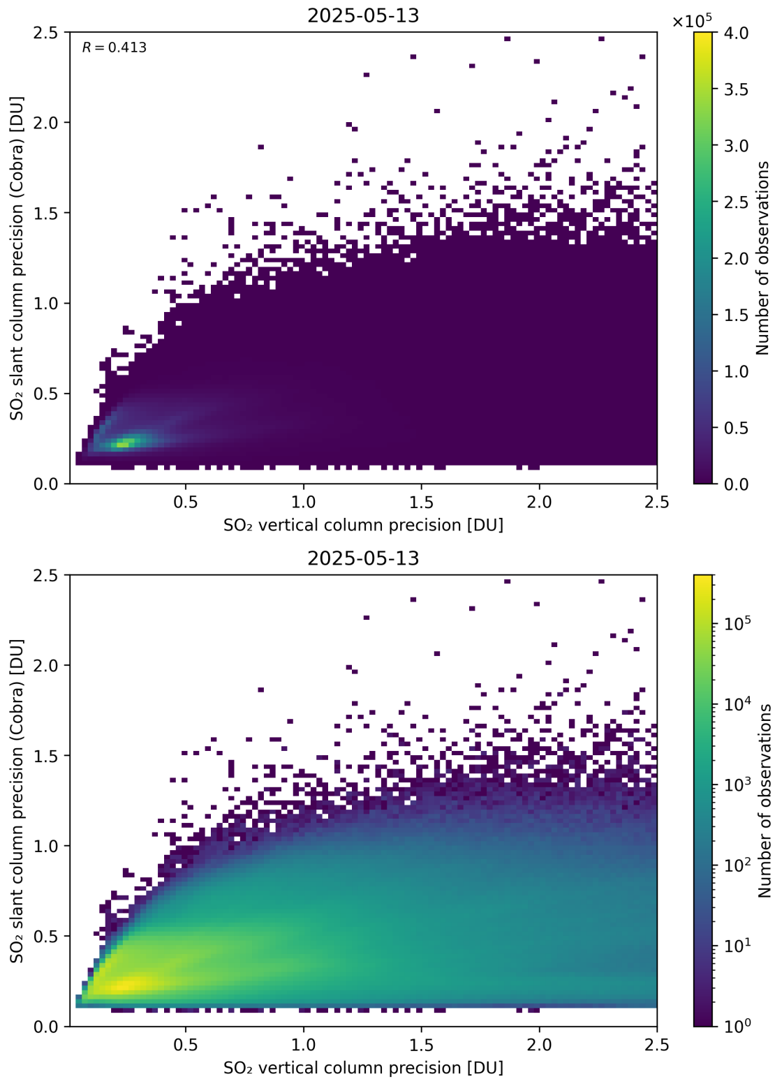
Figure 337: Scatter density plot of “SO 2 vertical column precision” against “SO 2 slant column precision (Cobra)” for 2025-05-12 to 2025-05-14.
