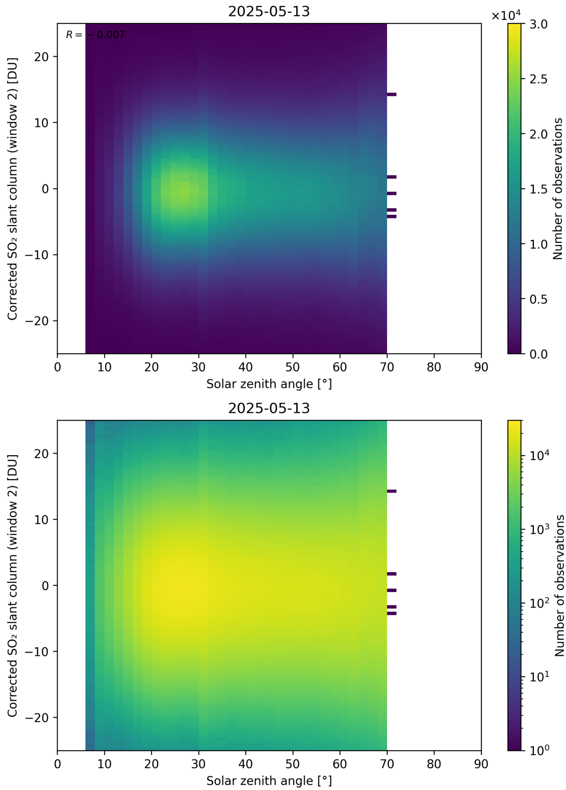
Figure 182: Scatter density plot of “Solar zenith angle” against “Corrected SO 2 slant column (window 2)” for 2025-05-12 to 2025-05-14.
