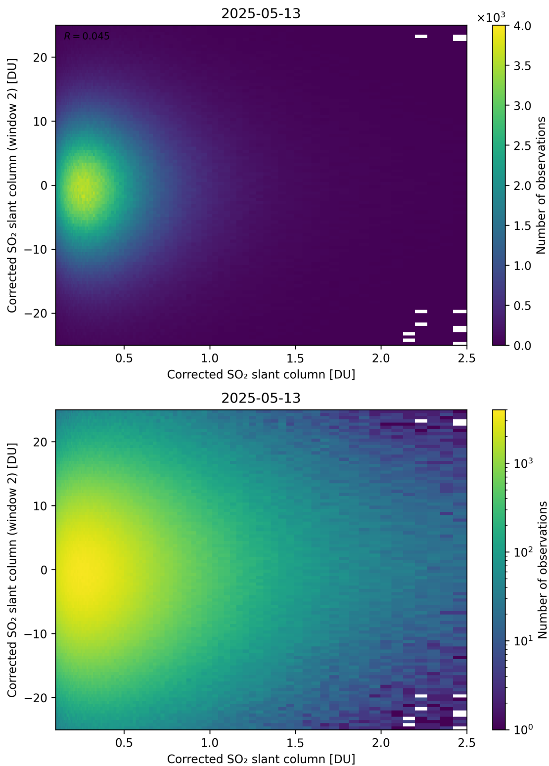
Figure 235: Scatter density plot of “Corrected SO 2 slant column” against “Corrected SO 2 slant column (window 2)” for 2025-05-12 to 2025-05-14.
