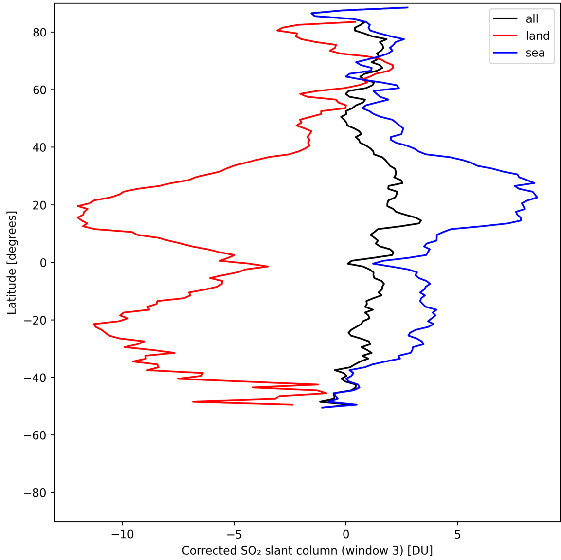
Figure 47: Zonal average of “Corrected SO 2 slant column (window 3)” for 2025-05-12 to 2025-05-14.
