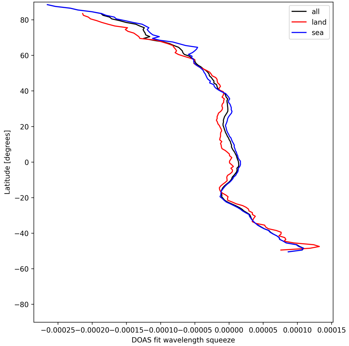
Figure 51: Zonal average of “DOAS fit wavelength squeeze” for 2025-05-12 to 2025-05-14.
