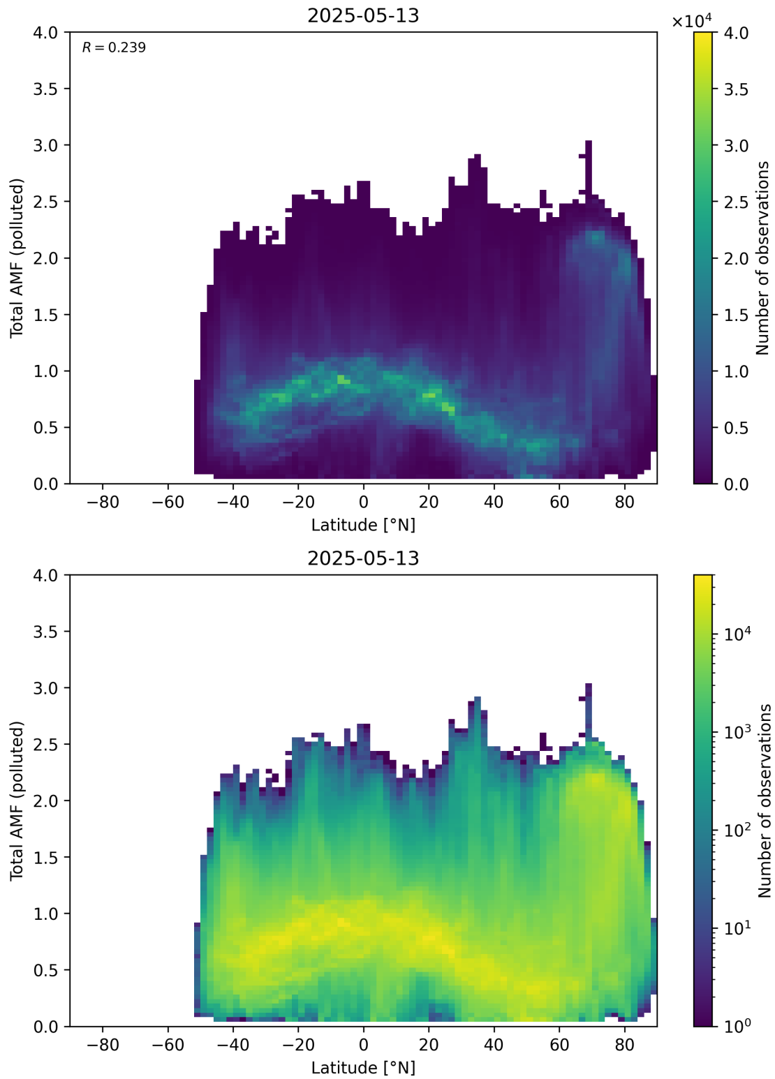
Figure 167: Scatter density plot of “Latitude” against “Total AMF (polluted)” for 2025-05-12 to 2025-05-14.
