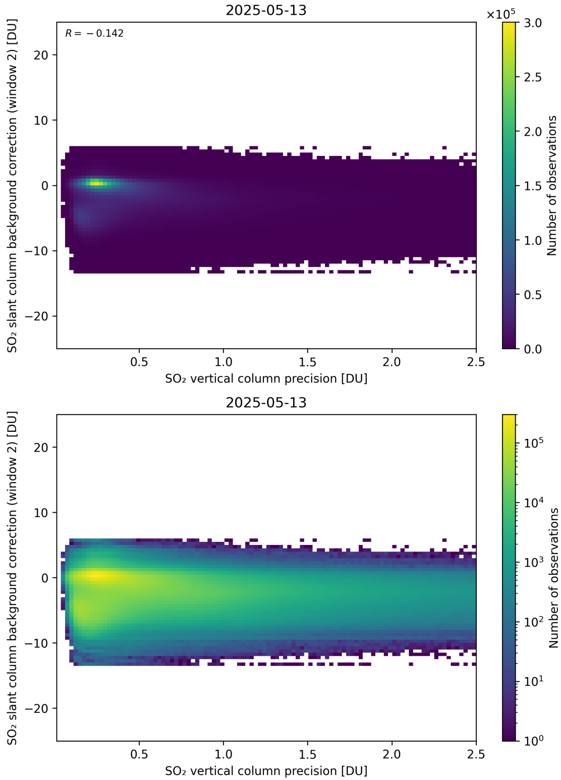
Figure 330: Scatter density plot of “SO 2 vertical column precision” against “SO 2 slant column background correction (window 2)” for 2025-05-12 to 2025-05-14.
