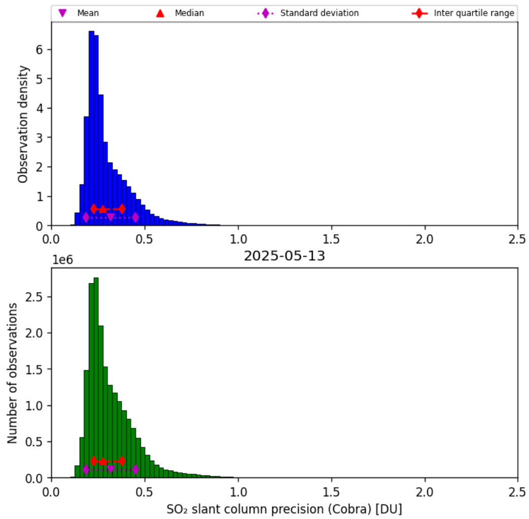
Figure 62: Histogram of “SO 2 slant column precision (Cobra)” for 2025-05-12 to 2025-05-14
