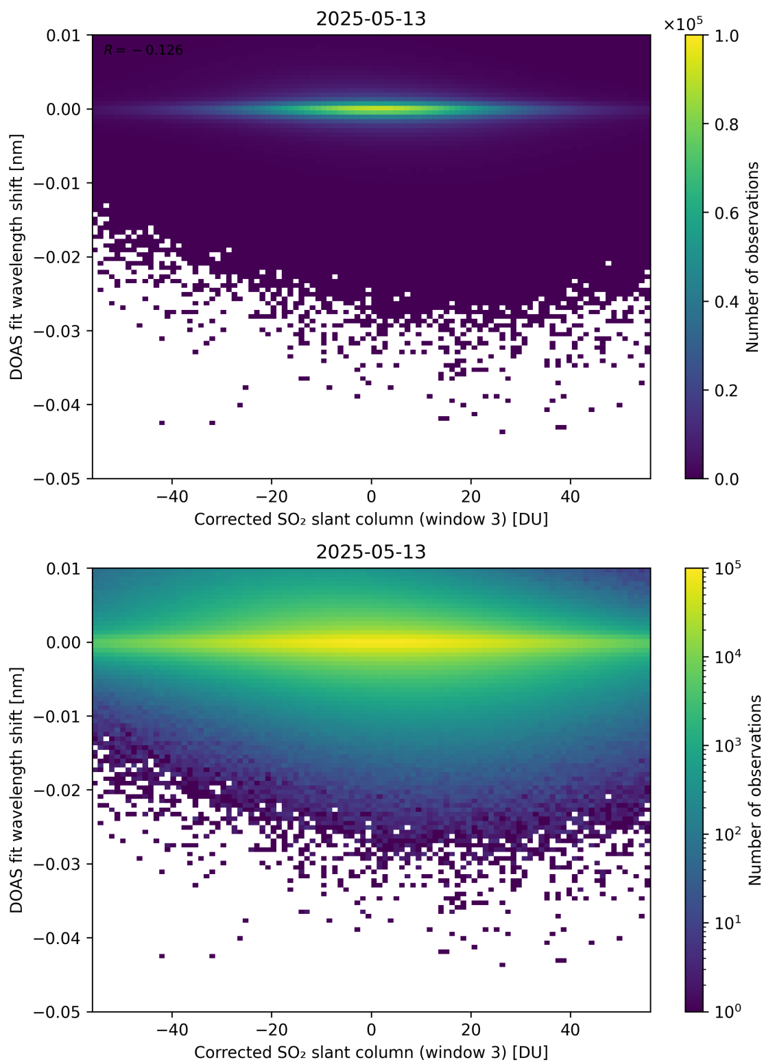
Figure 256: Scatter density plot of “Corrected SO 2 slant column (window 3)” against “DOAS fit wavelength shift” for 2025-05-12 to 2025-05-14.
