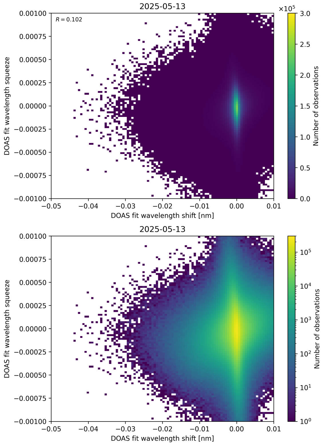
Figure 138: Scatter density plot of “DOAS fit wavelength shift” against “DOAS fit wavelength squeeze” for 2025-05-12 to 2025-05-14.
