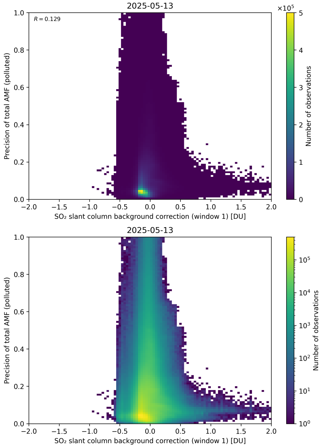
Figure 121: Scatter density plot of “SO 2 slant column background correction (window 1)” against “Precision of total AMF (polluted)” for 2025-05-12 to 2025-05-14.
