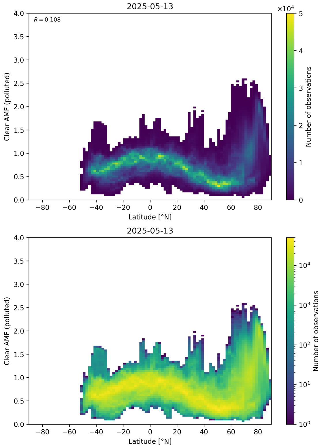
Figure 156: Scatter density plot of “Latitude” against “Clear AMF (polluted)” for 2025-05-12 to 2025-05-14.
