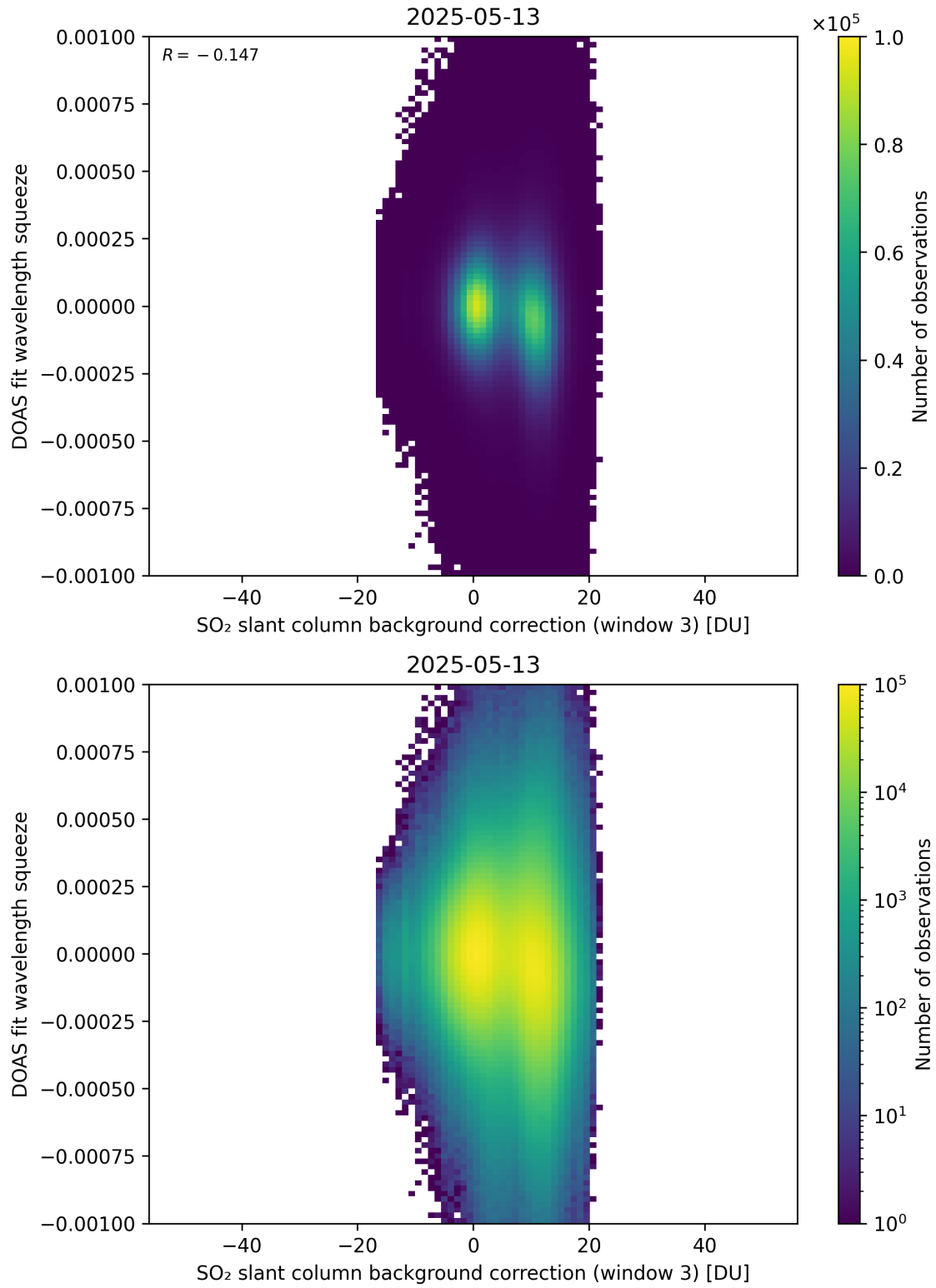
Figure 133: Scatter density plot of “SO 2 slant column background correction (window 3)” against “DOAS fit wavelength squeeze” for 2025-05-12 to 2025-05-14.
