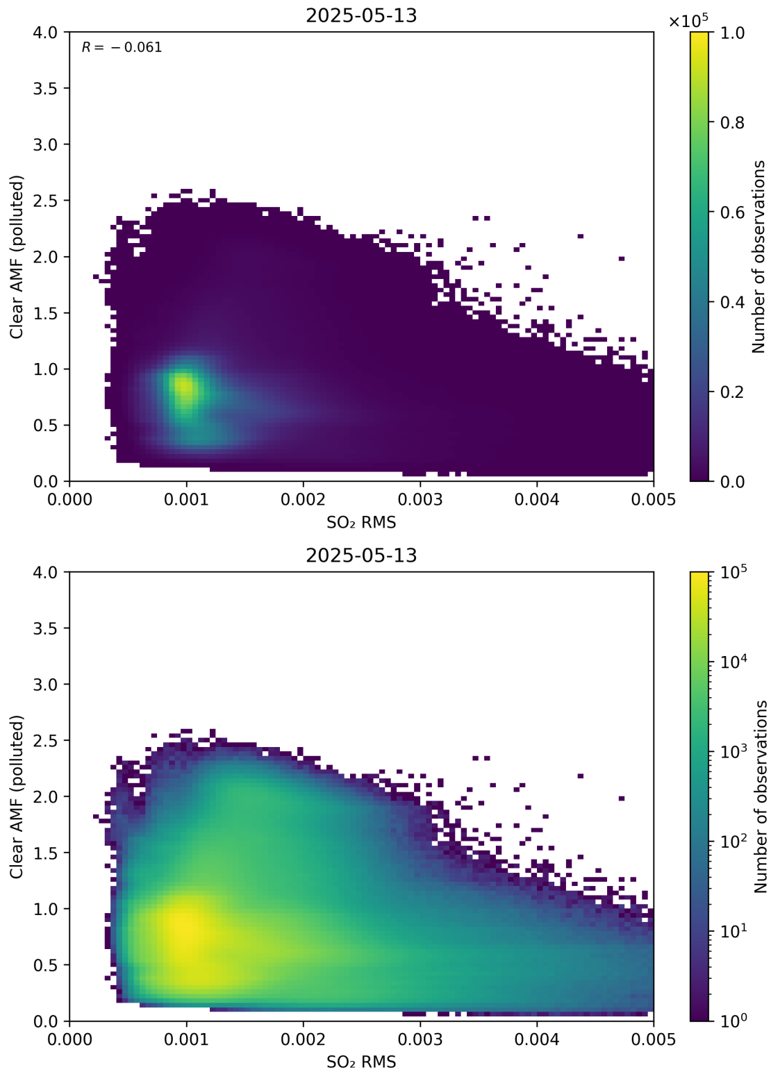
Figure 147: Scatter density plot of “SO 2 RMS” against “Clear AMF (polluted)” for 2025-05-12 to 2025-05-14.
