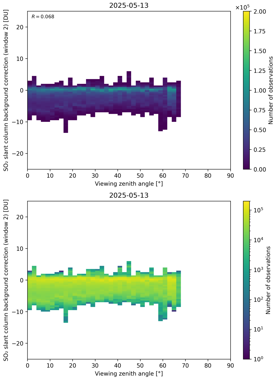
Figure 363: Scatter density plot of “Viewing zenith angle” against “SO 2 slant column background correction (window 2)” for 2025-05-12 to 2025-05-14.
