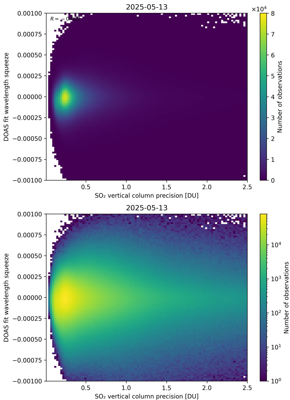
Figure 333: Scatter density plot of “SO 2 vertical column precision” against “DOAS fit wavelength squeeze” for 2025-05-12 to 2025-05-14.
