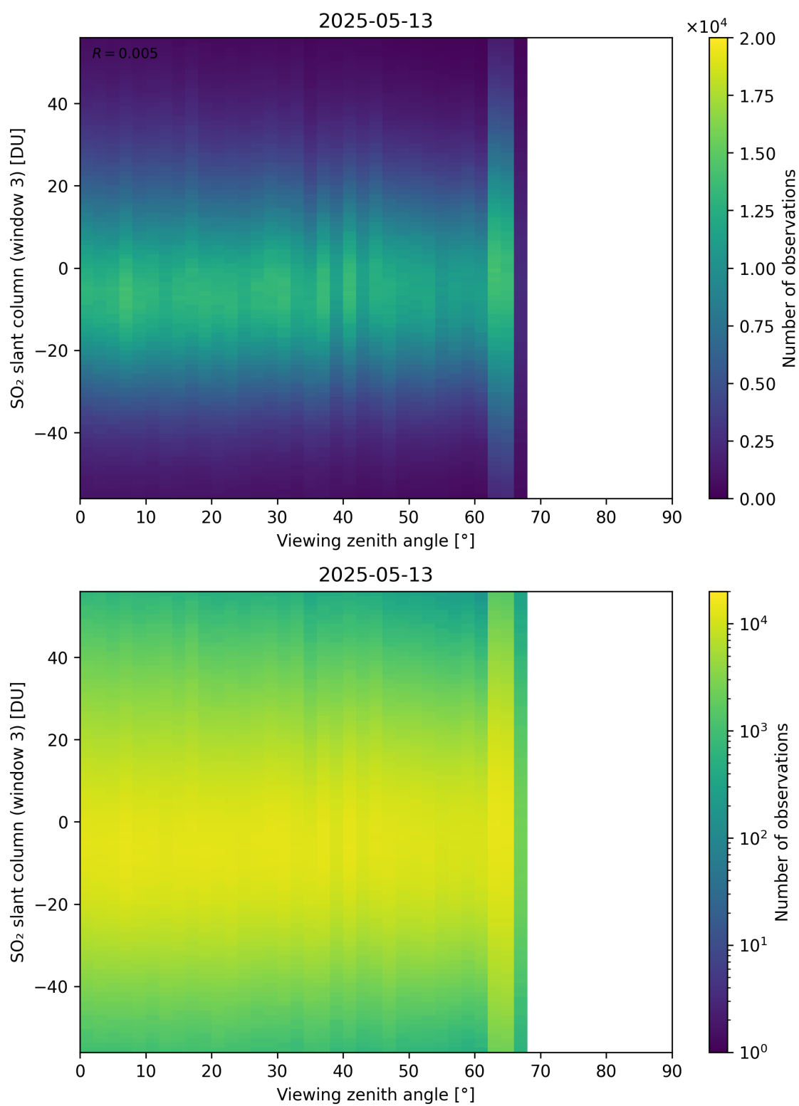
Figure 379: Scatter density plot of “Viewing zenith angle” against “SO 2 slant column (window 3)” for 2025-05-12 to 2025-05-14.
