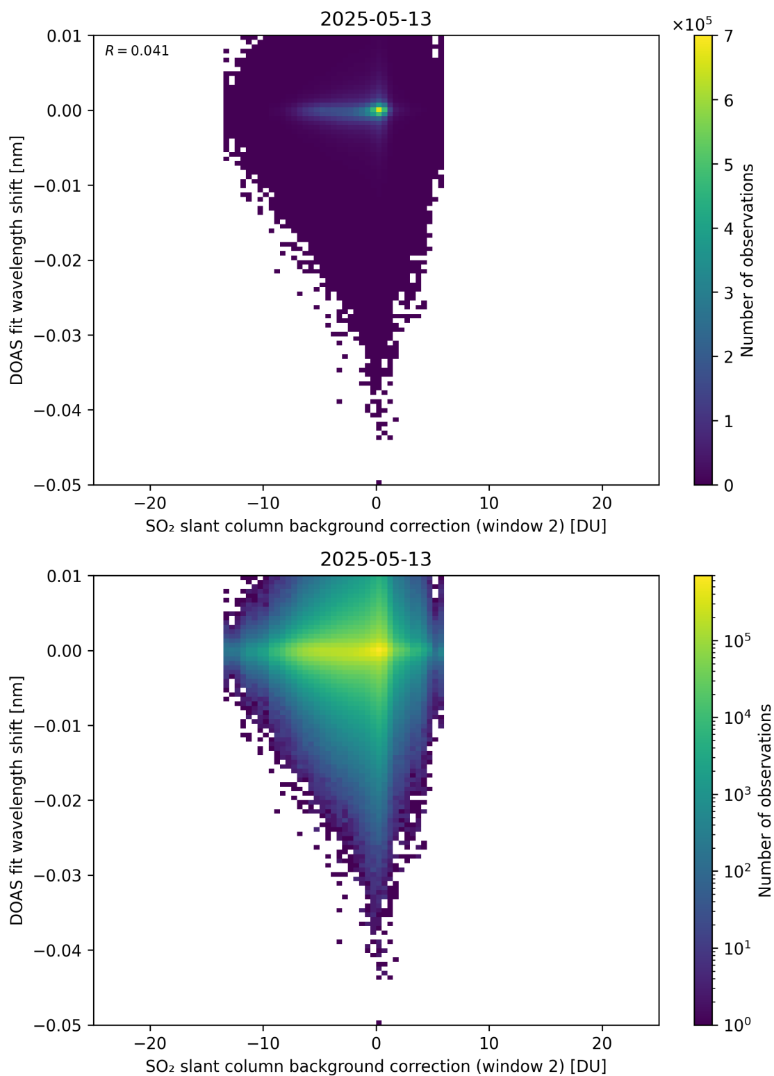
Figure 123: Scatter density plot of “SO 2 slant column background correction (window 2)” against “DOAS fit wavelength shift” for 2025-05-12 to 2025-05-14.
