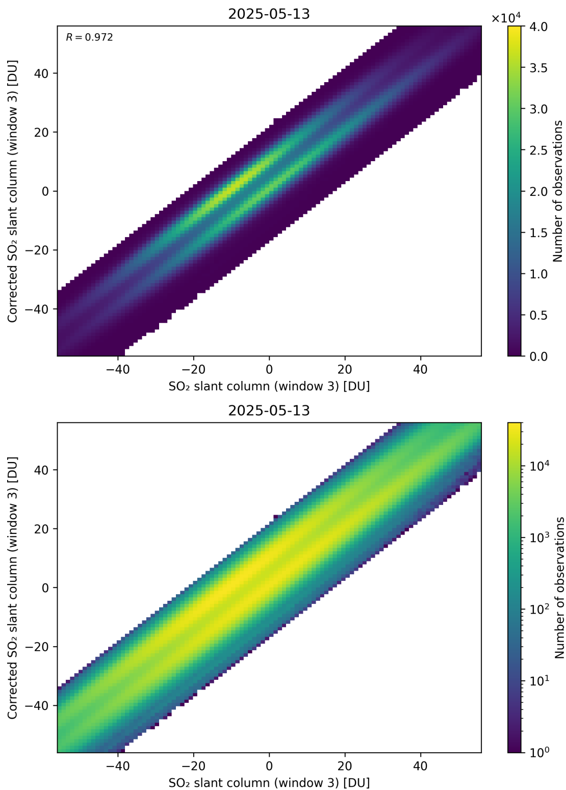
Figure 316: Scatter density plot of “SO 2 slant column (window 3)” against “Corrected SO 2 slant column (window 3)” for 2025-05-12 to 2025-05-14.
