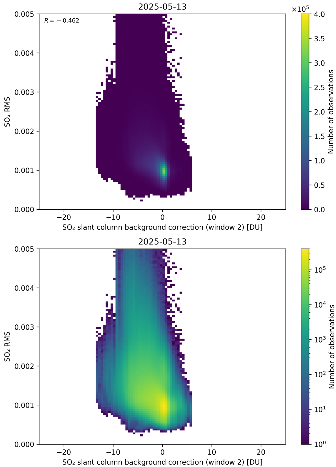
Figure 125: Scatter density plot of “SO 2 slant column background correction (window 2)” against “SO 2 RMS” for 2025-05-12 to 2025-05-14.
