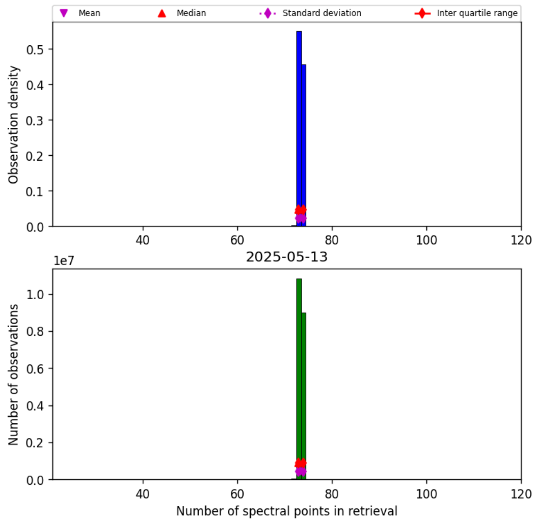
Figure 82: Histogram of “Number of spectral points in retrieval” for 2025-05-12 to 2025-05-14
