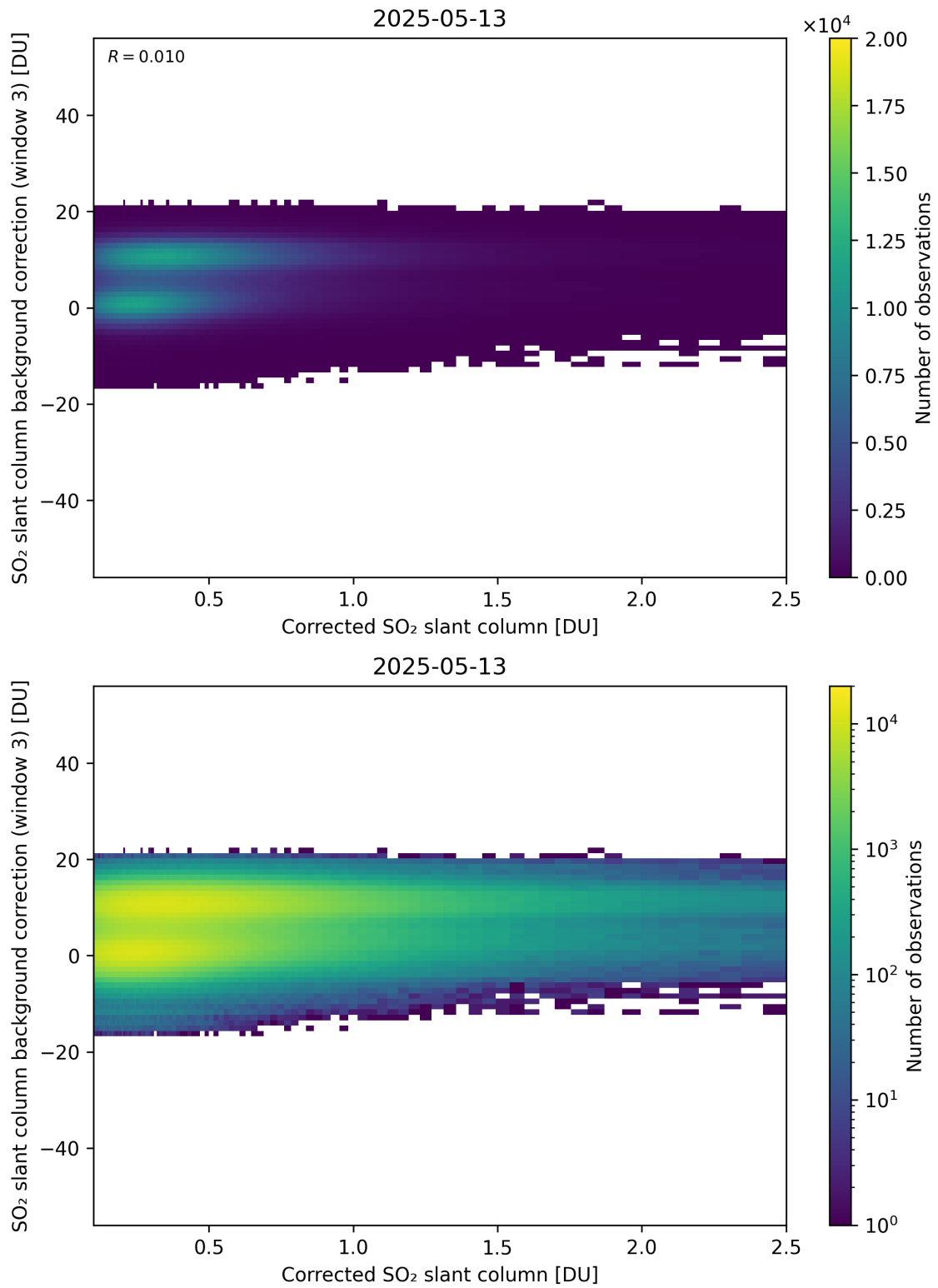
Figure 228: Scatter density plot of “Corrected SO 2 slant column” against “SO 2 slant column background correction (window 3)” for 2025-05-12 to 2025-05-14.
