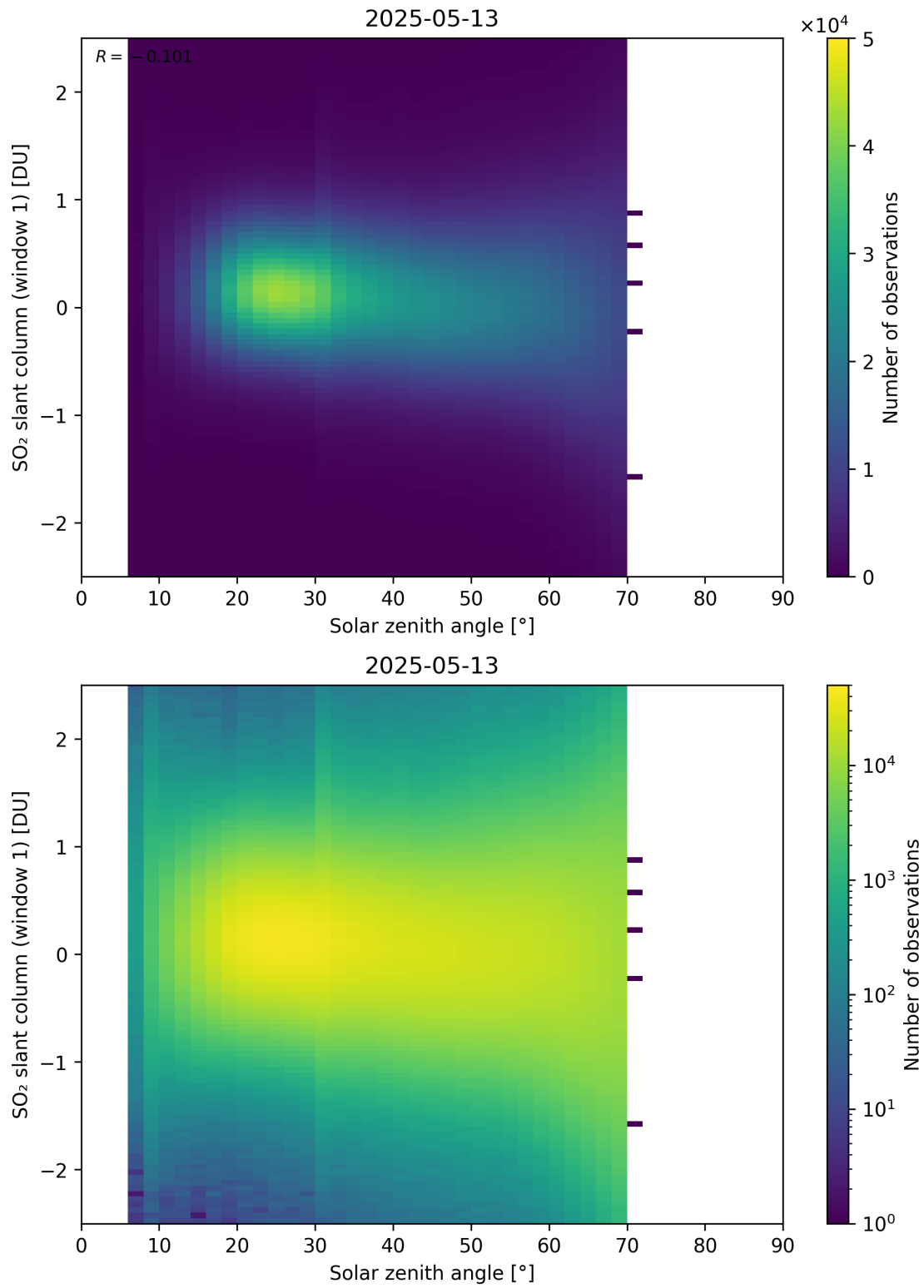
Figure 184: Scatter density plot of “Solar zenith angle” against “SO 2 slant column (window 1)” for 2025-05-12 to 2025-05-14.
