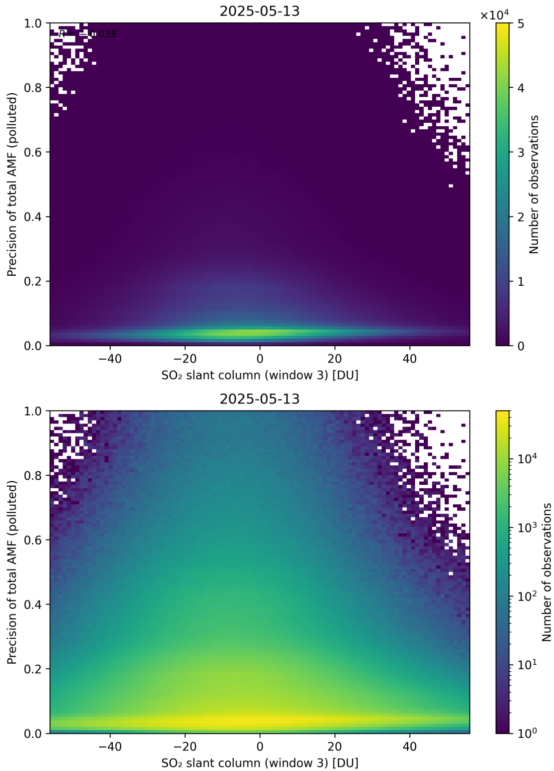
Figure 319: Scatter density plot of “SO 2 slant column (window 3)” against “Precision of total AMF (polluted)” for 2025-05-12 to 2025-05-14.
