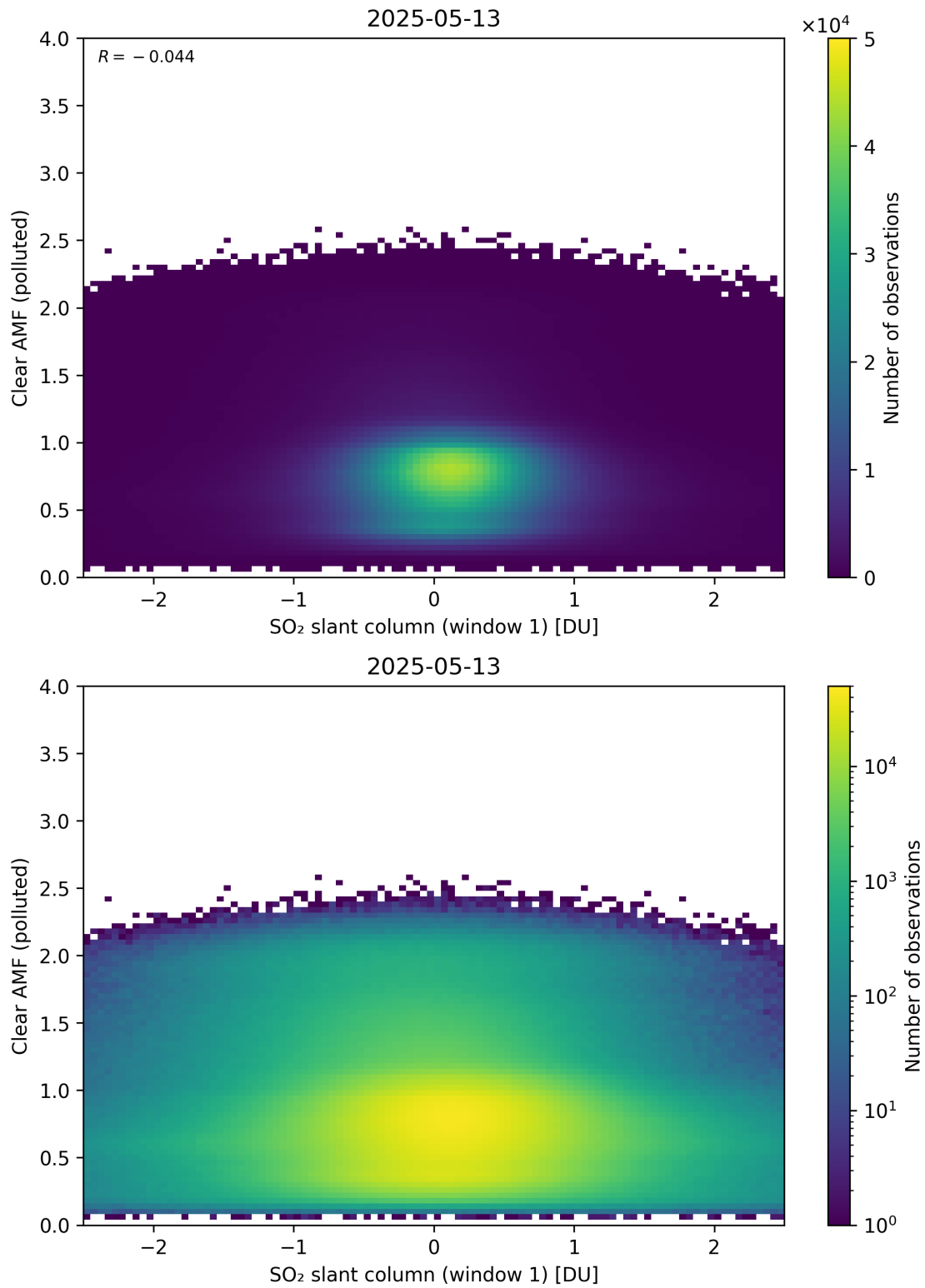
Figure 282: Scatter density plot of “SO 2 slant column (window 1)” against “Clear AMF (polluted)” for 2025-05-12 to 2025-05-14.
