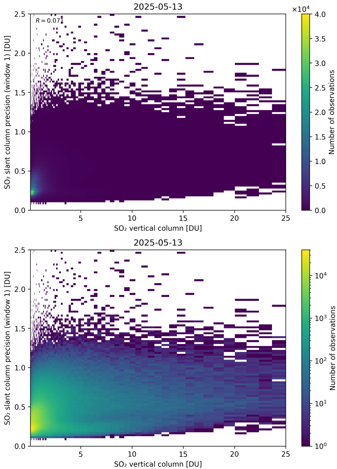
Figure 355: Scatter density plot of “SO 2 vertical column” against “SO 2 slant column precision (window 1)” for 2025-05-12 to 2025-05-14.
