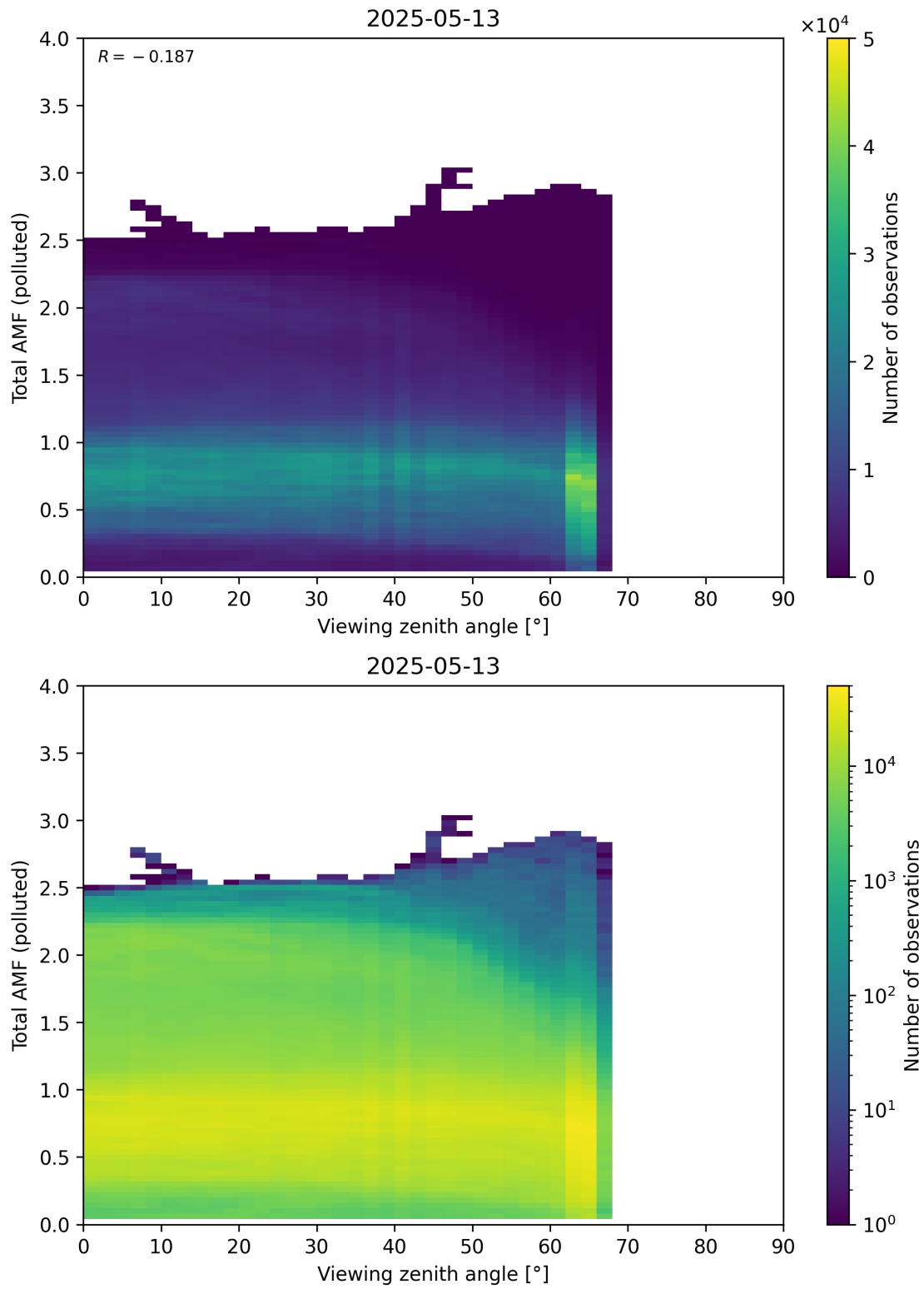
Figure 381: Scatter density plot of “Viewing zenith angle” against “Total AMF (polluted)” for 2025-05-12 to 2025-05-14.
