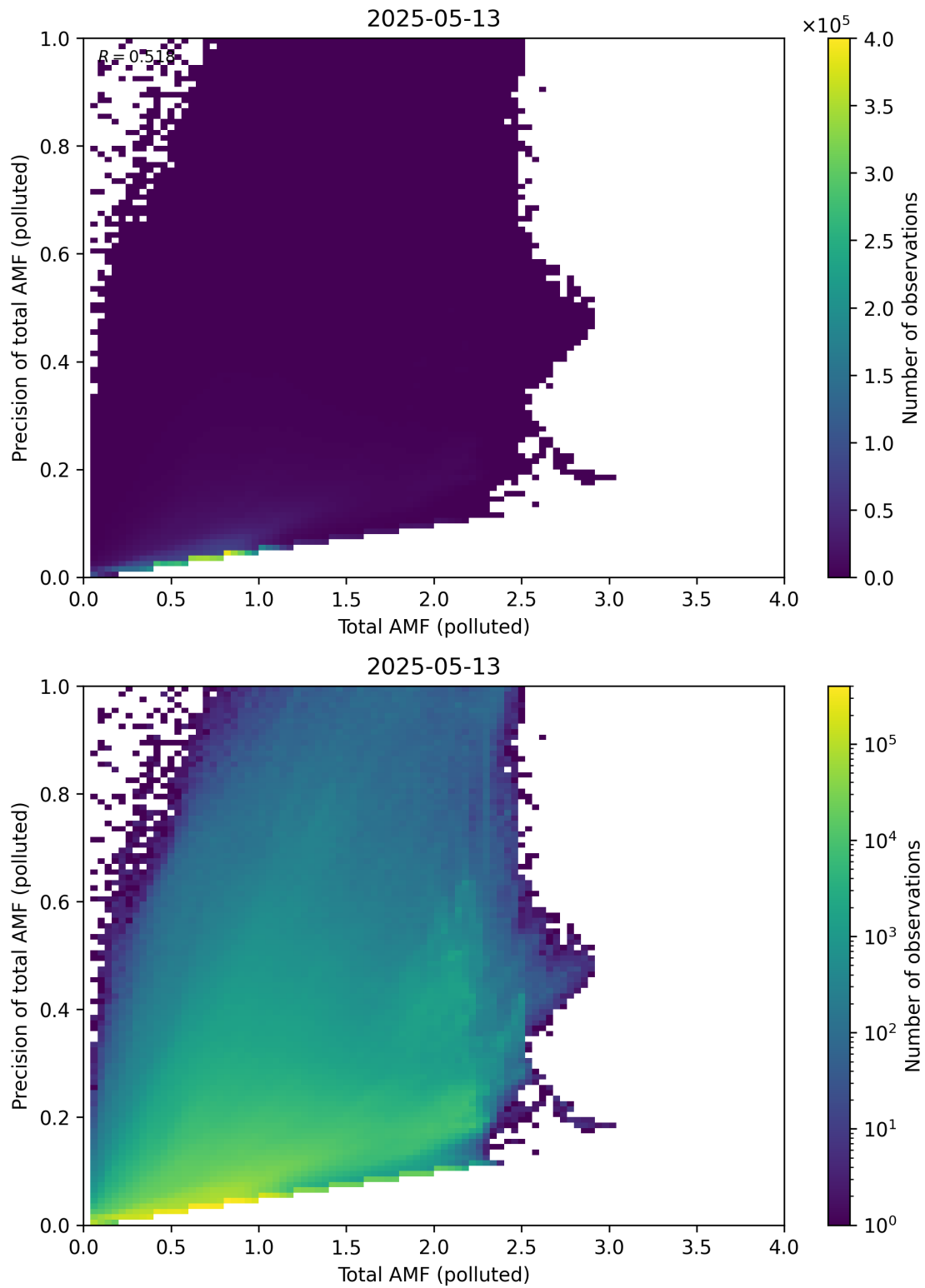
Figure 322: Scatter density plot of “Total AMF (polluted)” against “Precision of total AMF (polluted)” for 2025-05-12 to 2025-05-14.
