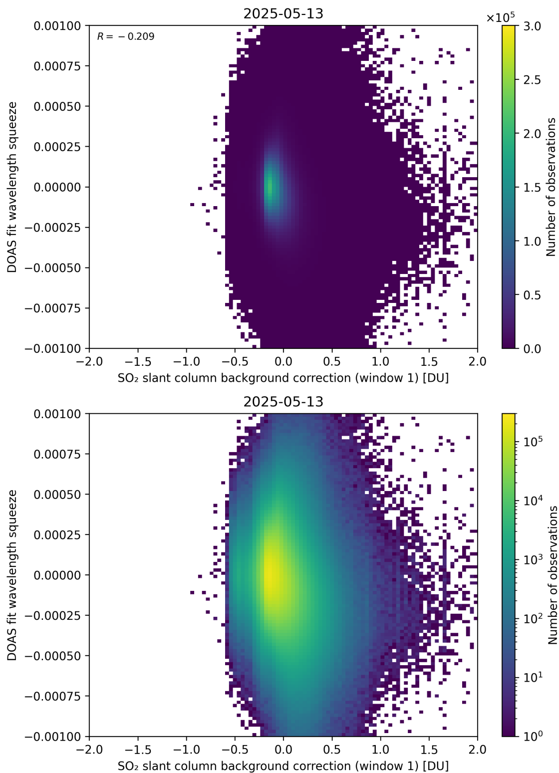
Figure 112: Scatter density plot of “SO 2 slant column background correction (window 1)” against “DOAS fit wavelength squeeze” for 2025-05-12 to 2025-05-14.
