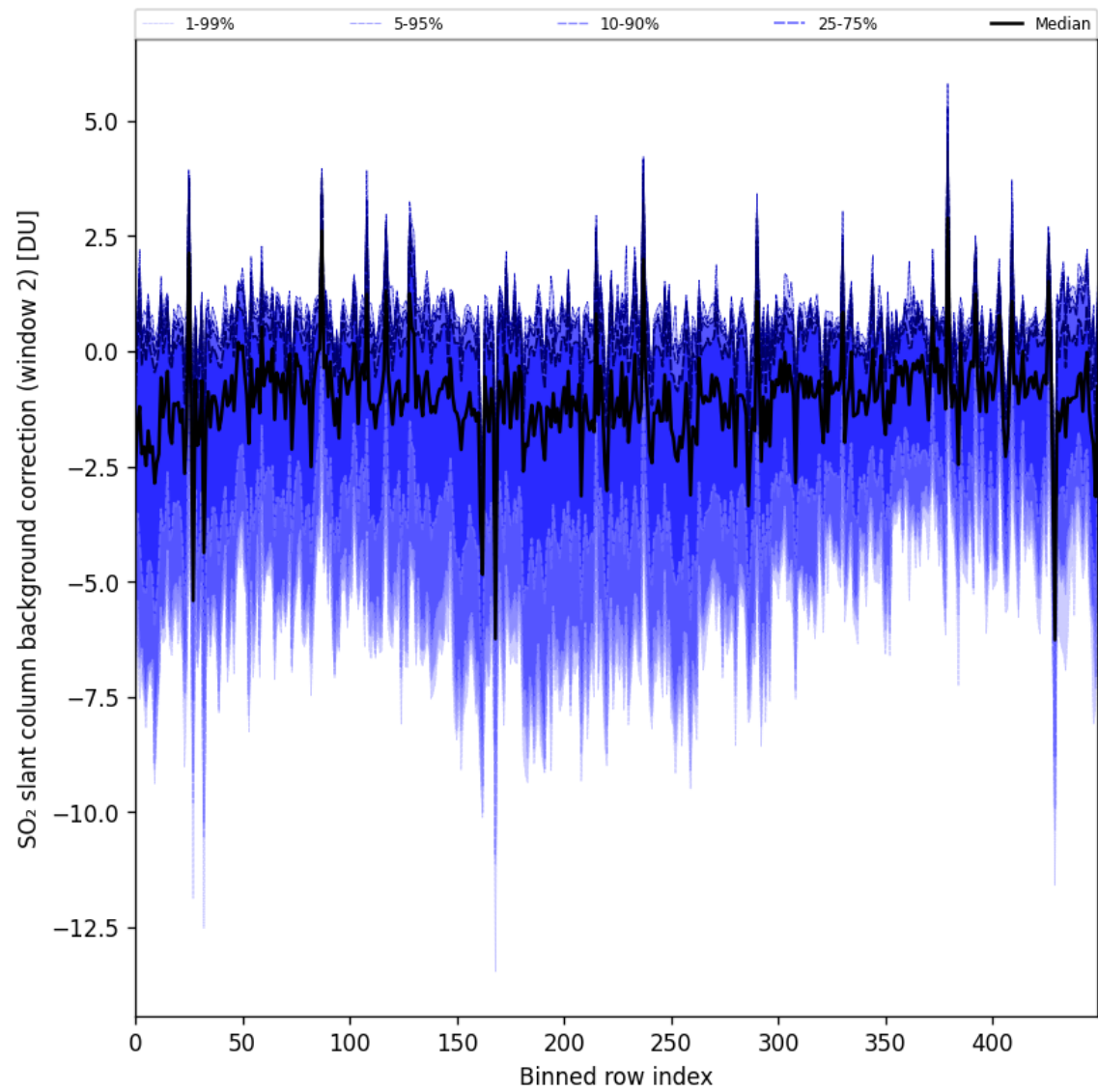
Figure 96: Along track statistics of “SO 2 slant column background correction (window 2)” for 2025-05-12 to 2025-05-14
