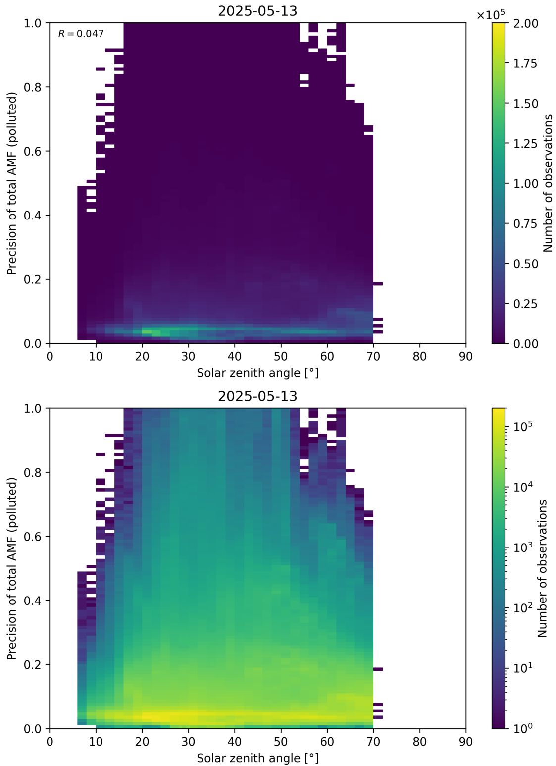
Figure 190: Scatter density plot of “Solar zenith angle” against “Precision of total AMF (polluted)” for 2025-05-12 to 2025-05-14.
