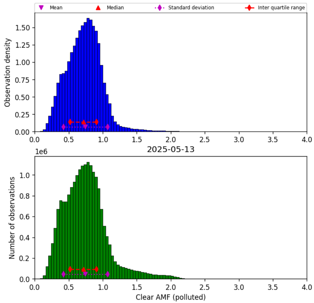
Figure 81: Histogram of “Clear AMF (polluted)” for 2025-05-12 to 2025-05-14
