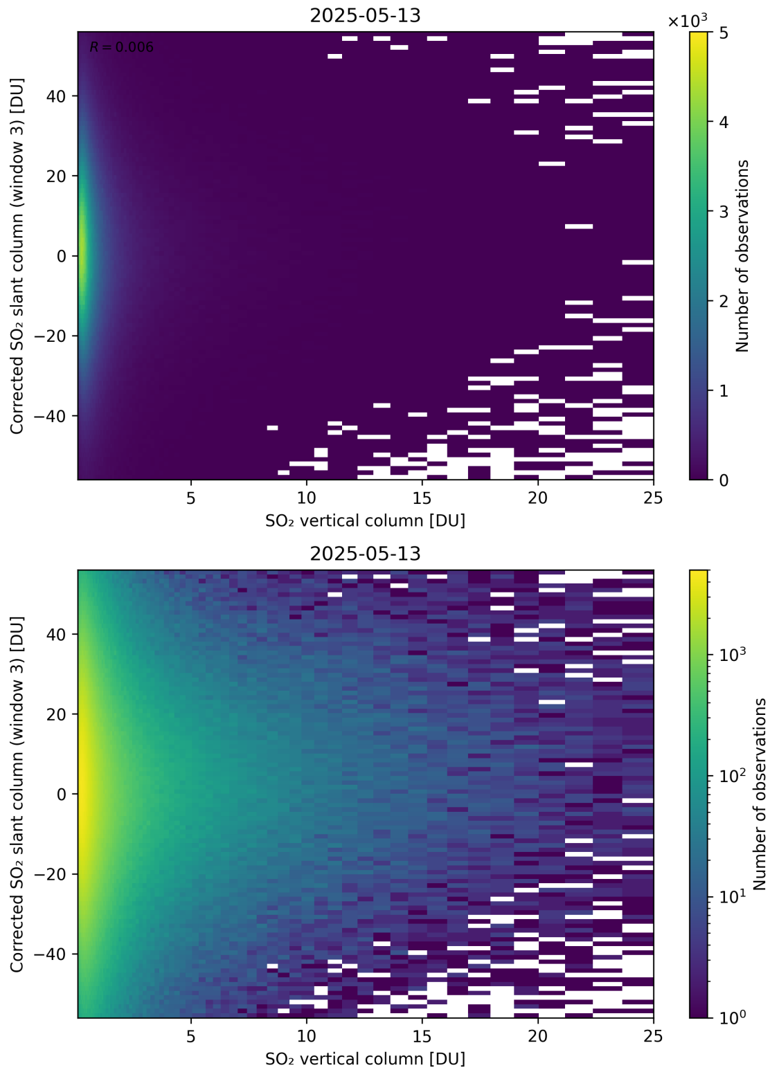
Figure 353: Scatter density plot of “SO 2 vertical column” against “Corrected SO 2 slant column (window 3)” for 2025-05-12 to 2025-05-14.
