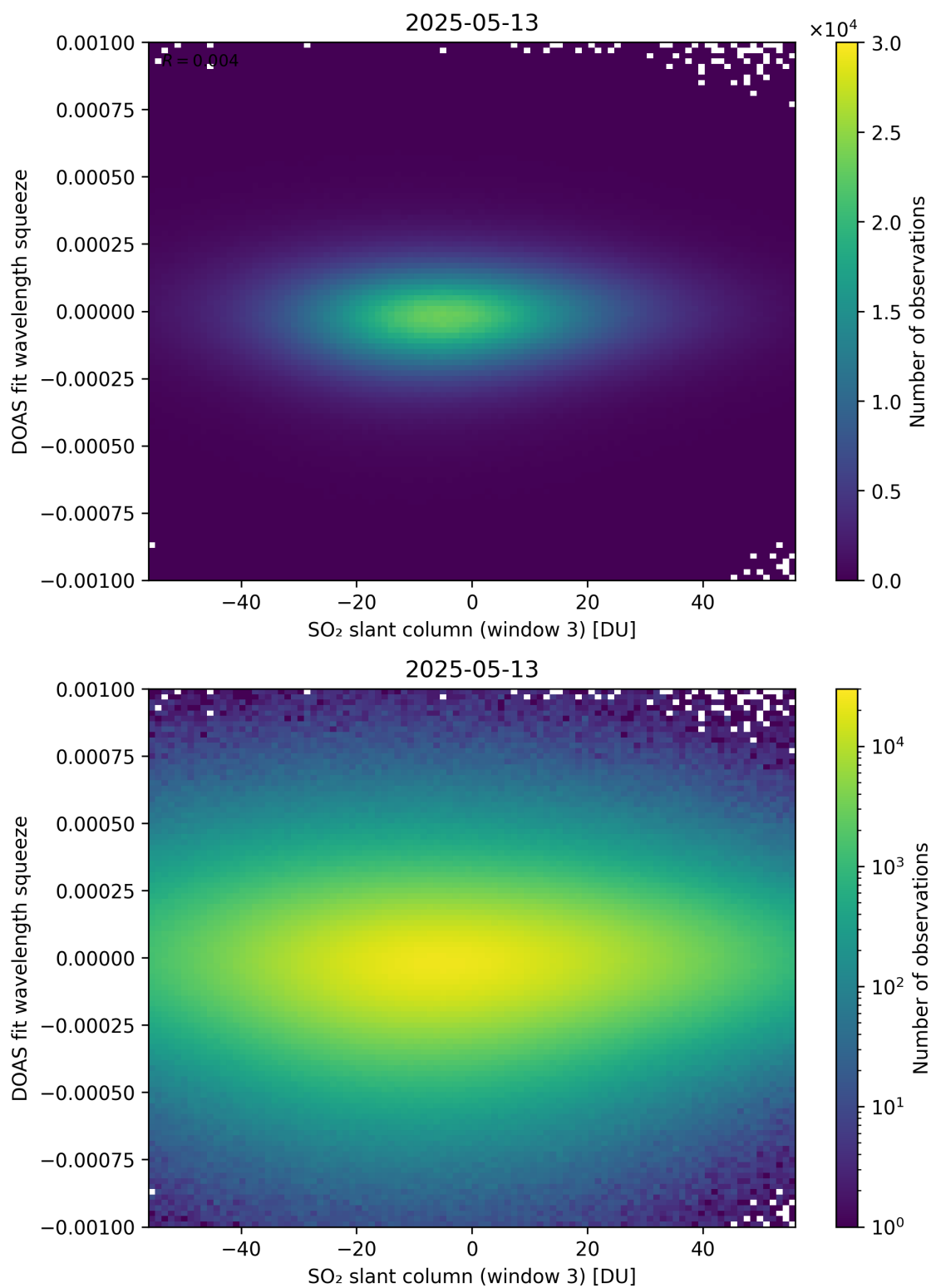
Figure 305: Scatter density plot of “SO 2 slant column (window 3)” against “DOAS fit wavelength squeeze” for 2025-05-12 to 2025-05-14.
