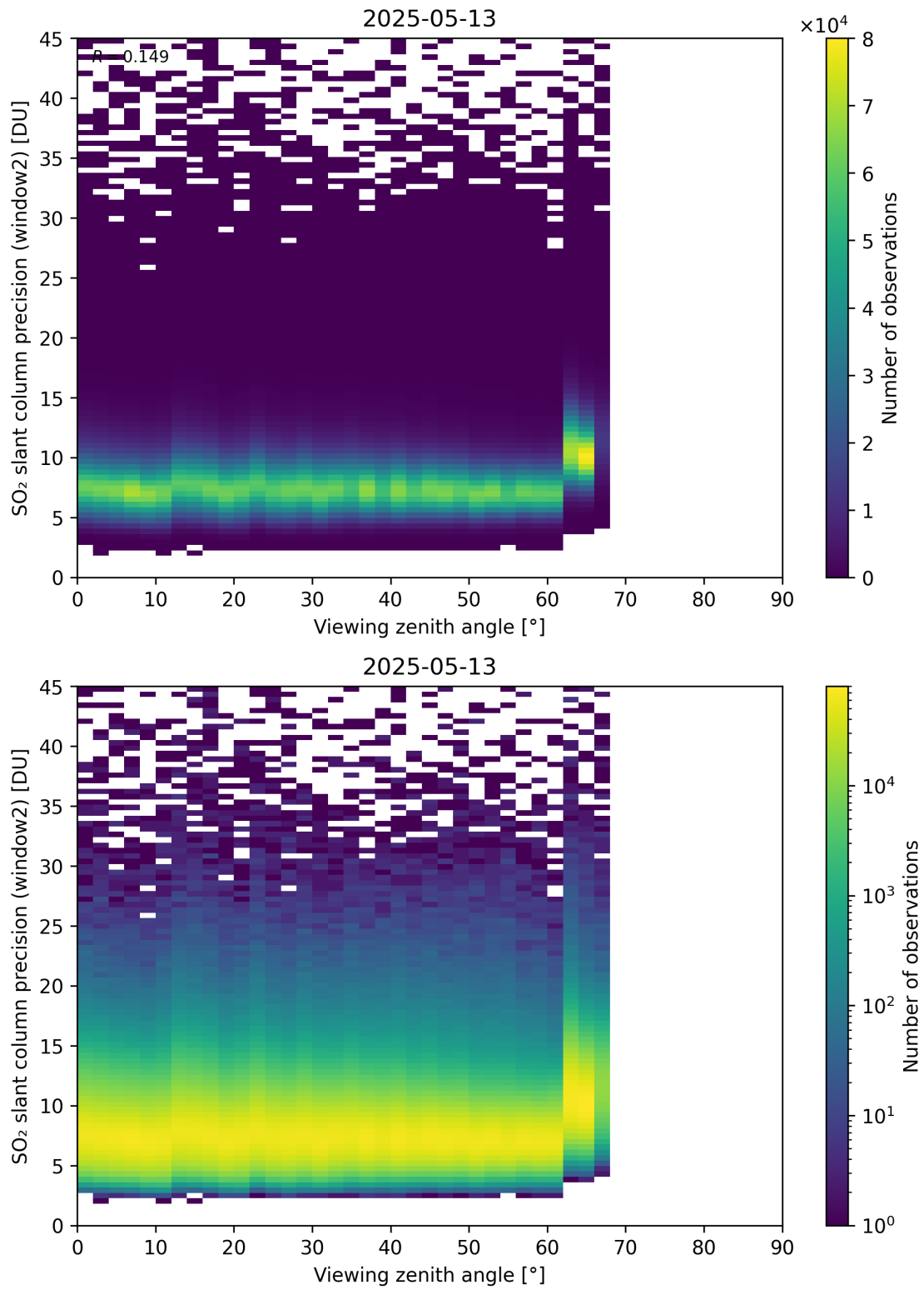
Figure 378: Scatter density plot of “Viewing zenith angle” against “SO 2 slant column precision (window2)” for 2025-05-12 to 2025-05-14.
