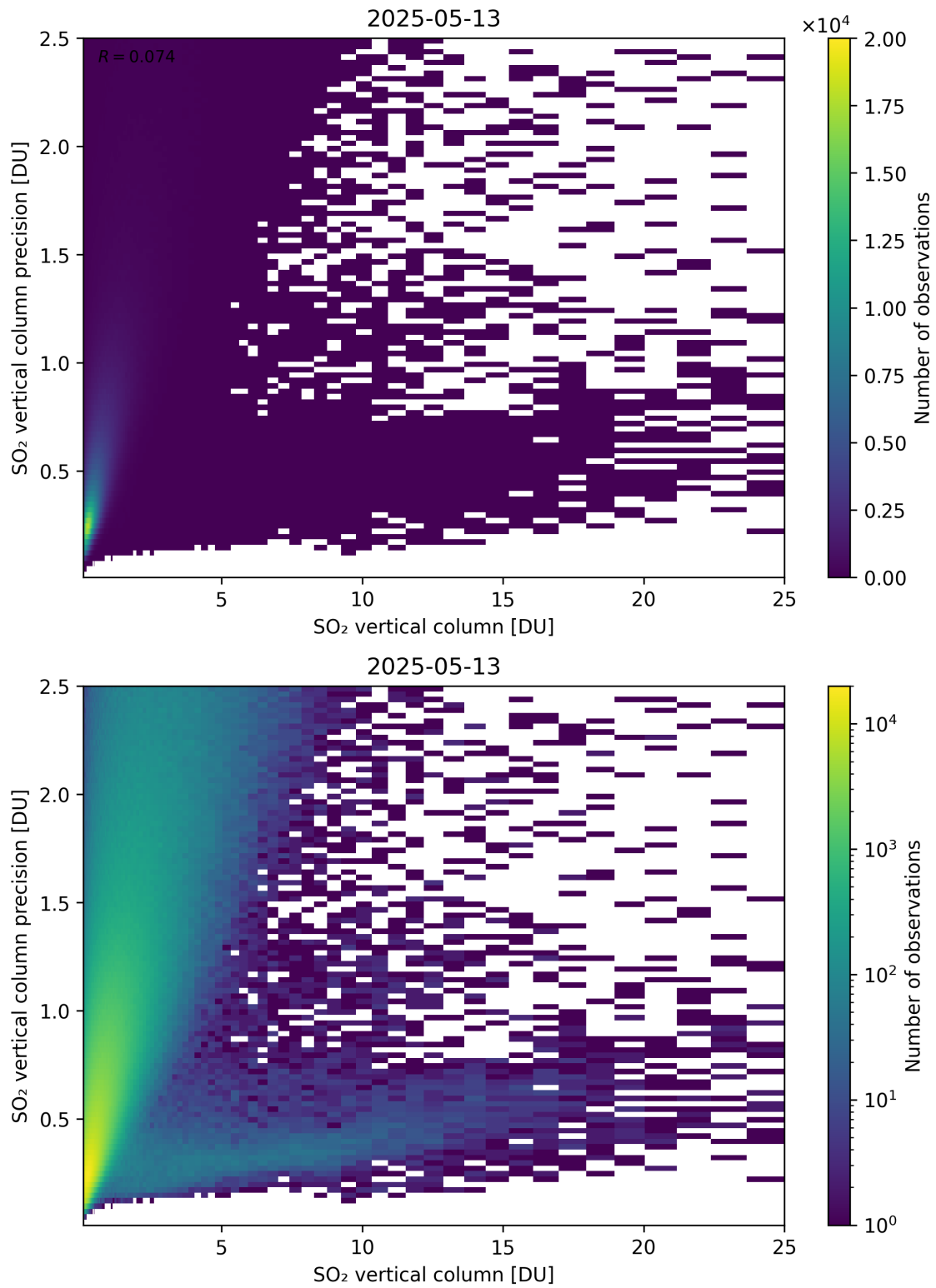
Figure 361: Scatter density plot of “SO 2 vertical column” against “SO 2 vertical column precision” for 2025-05-12 to 2025-05-14.
