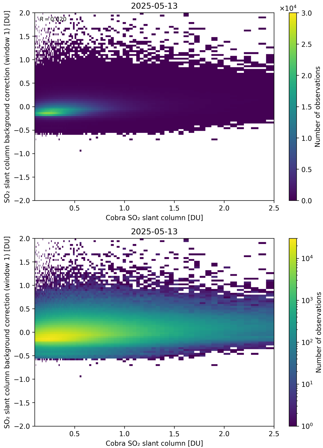
Figure 193: Scatter density plot of “Cobra SO 2 slant column” against “SO 2 slant column background correction (window 1)” for 2025-05-12 to 2025-05-14.
