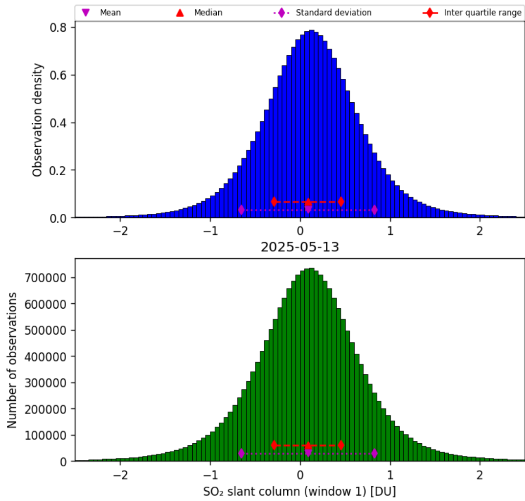
Figure 63: Histogram of “SO 2 slant column (window 1)” for 2025-05-12 to 2025-05-14
