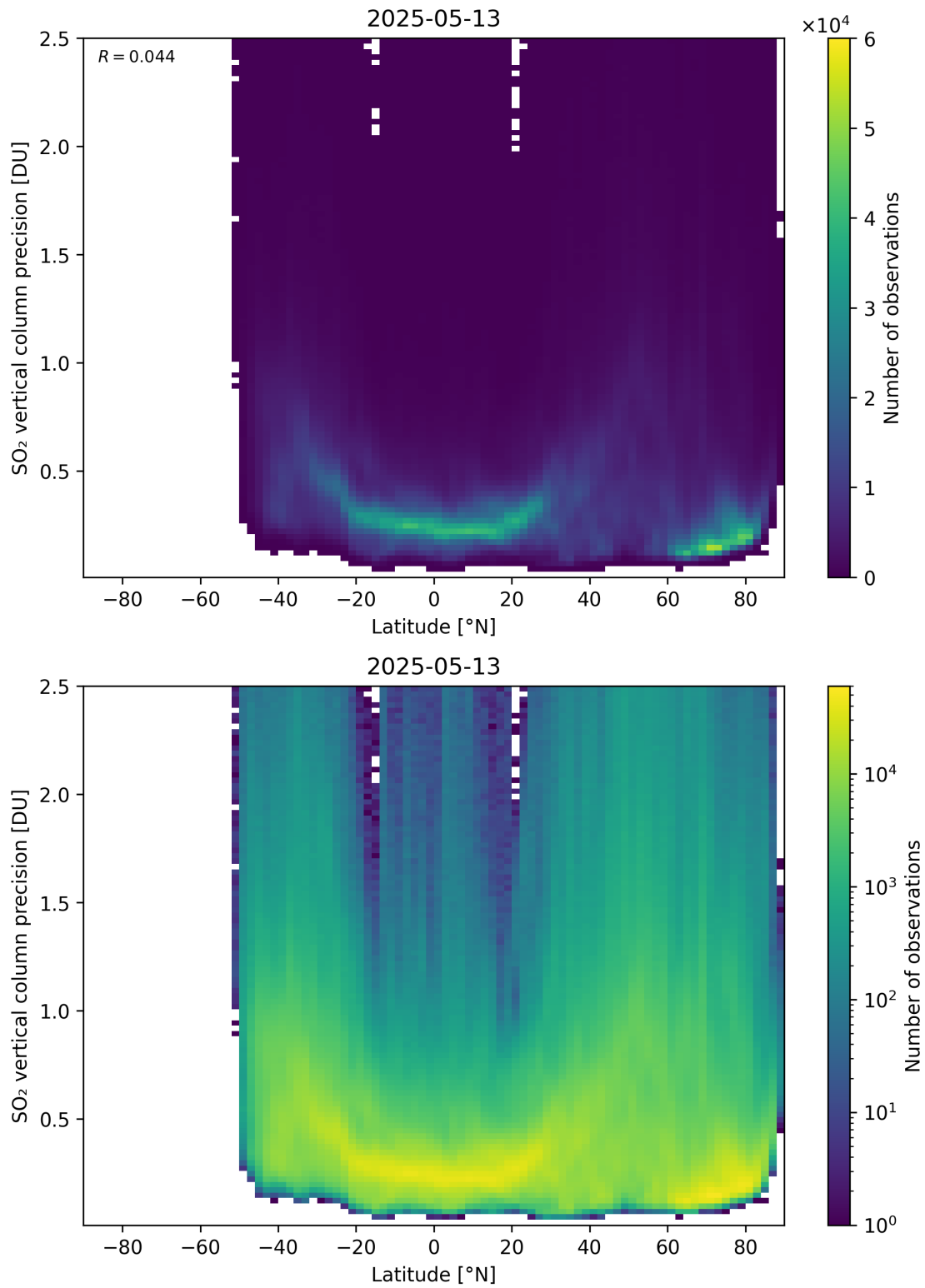
Figure 170: Scatter density plot of “Latitude” against “SO 2 vertical column precision” for 2025-05-12 to 2025-05-14.
