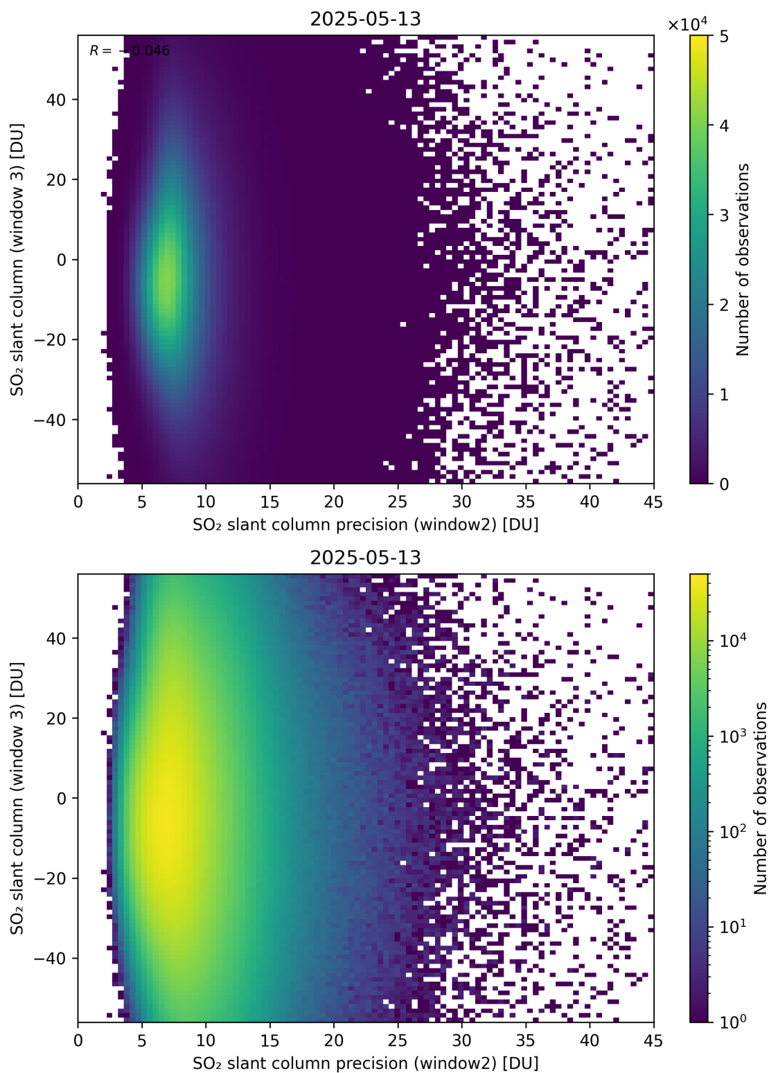
Figure 299: Scatter density plot of “SO 2 slant column precision (window2)” against “SO 2 slant column (window 3)” for 2025-05-12 to 2025-05-14.
