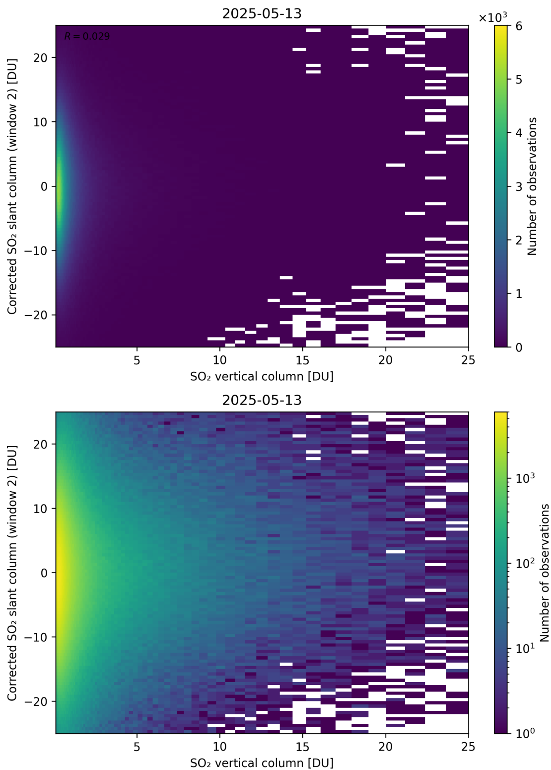
Figure 352: Scatter density plot of “SO 2 vertical column” against “Corrected SO 2 slant column (window 2)” for 2025-05-12 to 2025-05-14.
