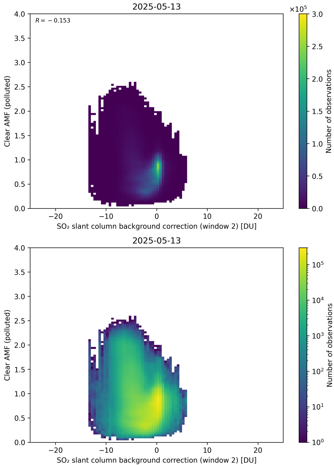
Figure 126: Scatter density plot of “SO 2 slant column background correction (window 2)” against “Clear AMF (polluted)” for 2025-05-12 to 2025-05-14.
