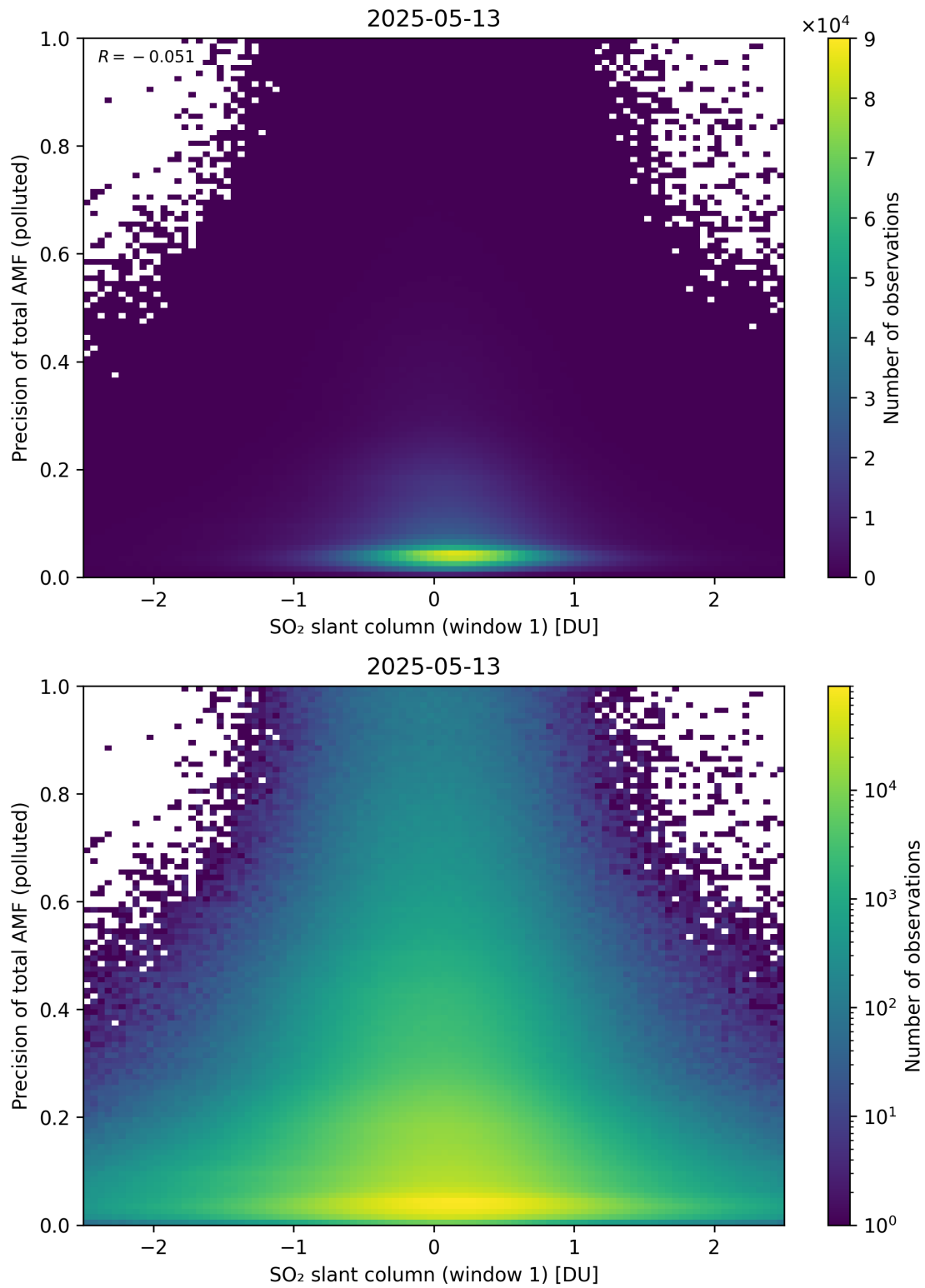
Figure 290: Scatter density plot of “SO 2 slant column (window 1)” against “Precision of total AMF (polluted)” for 2025-05-12 to 2025-05-14.
