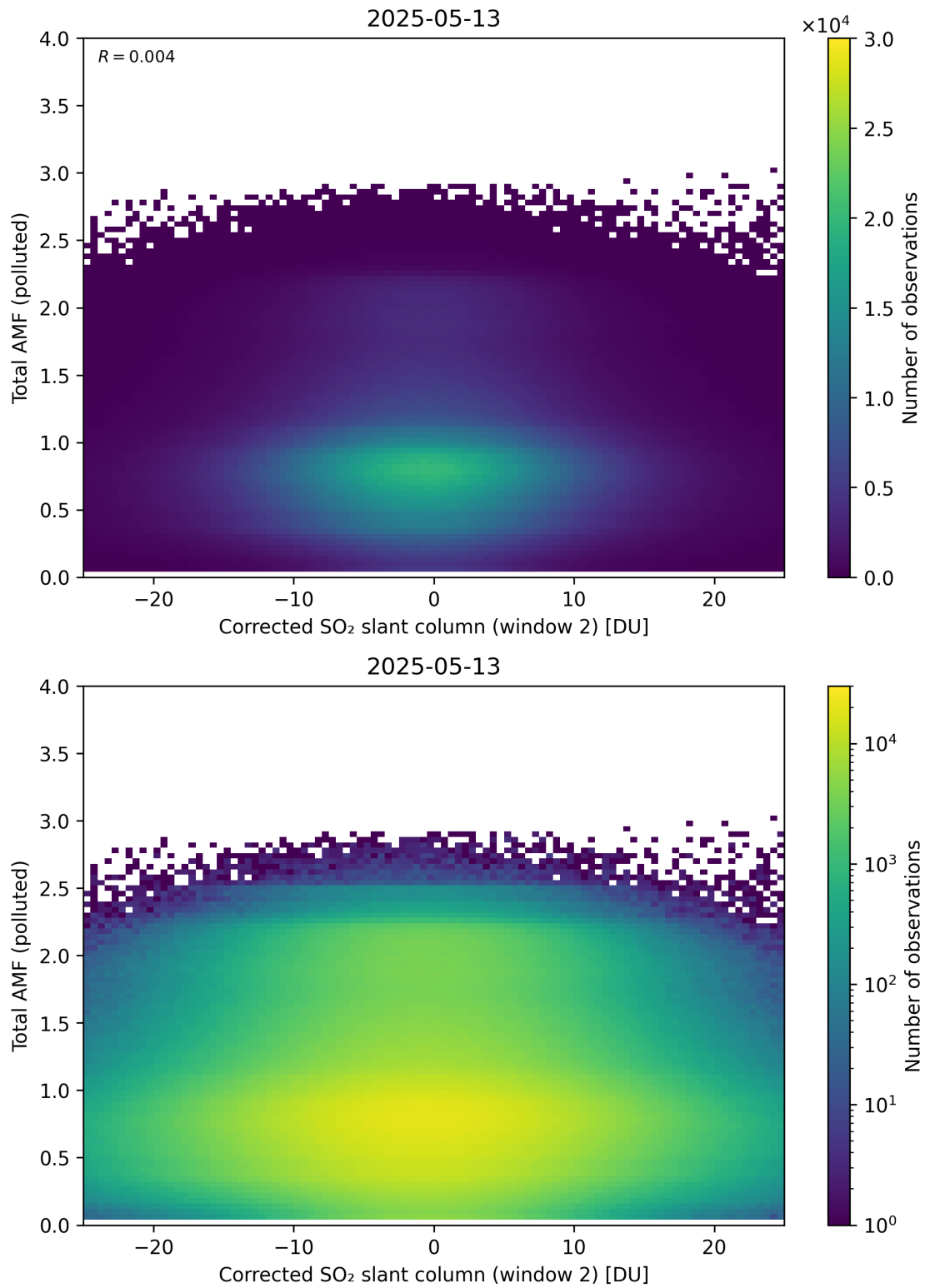
Figure 253: Scatter density plot of “Corrected SO 2 slant column (window 2)” against “Total AMF (polluted)” for 2025-05-12 to 2025-05-14.
