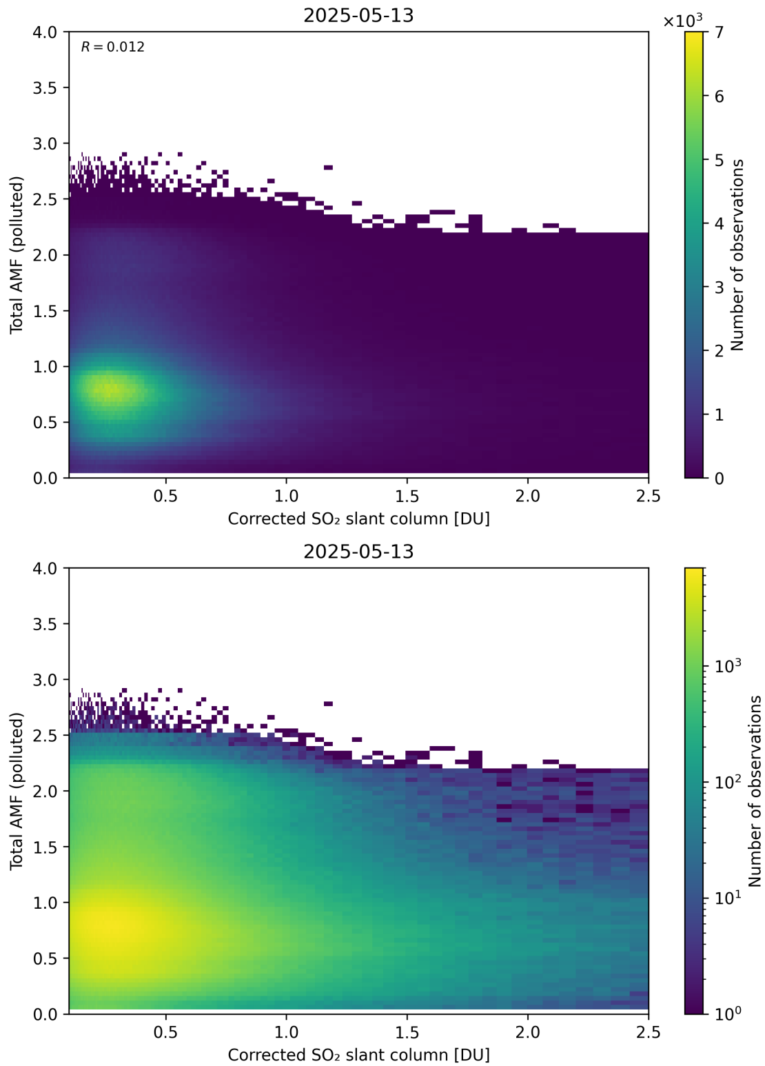
Figure 242: Scatter density plot of “Corrected SO 2 slant column” against “Total AMF (polluted)” for 2025-05-12 to 2025-05-14.
