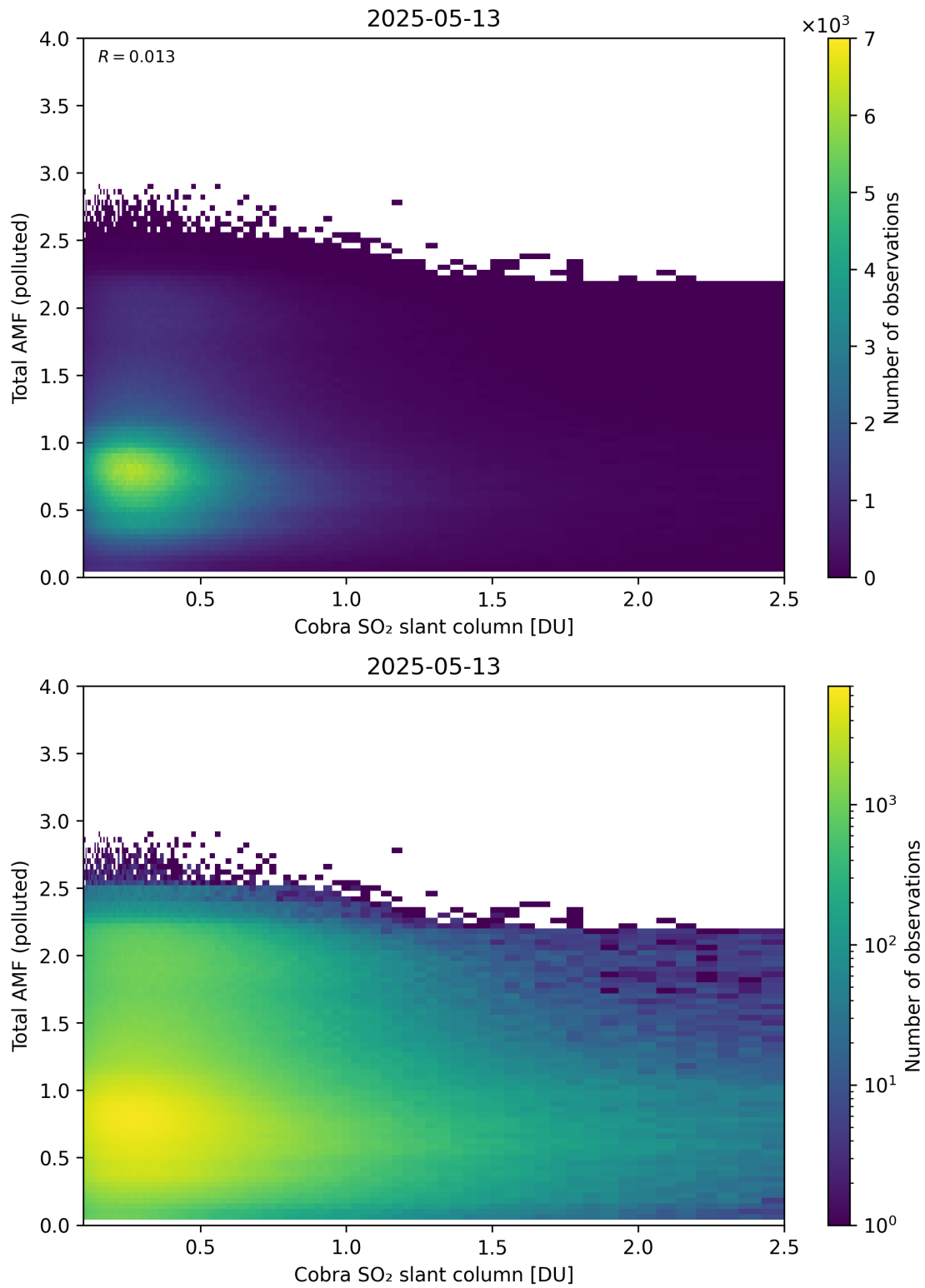
Figure 224: Scatter density plot of “Cobra SO 2 slant column” against “Total AMF (polluted)” for 2025-05-12 to 2025-05-14.
