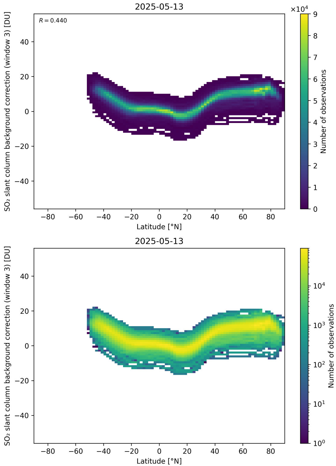
Figure 152: Scatter density plot of “Latitude” against “SO 2 slant column background correction (window 3)” for 2025-05-12 to 2025-05-14.
