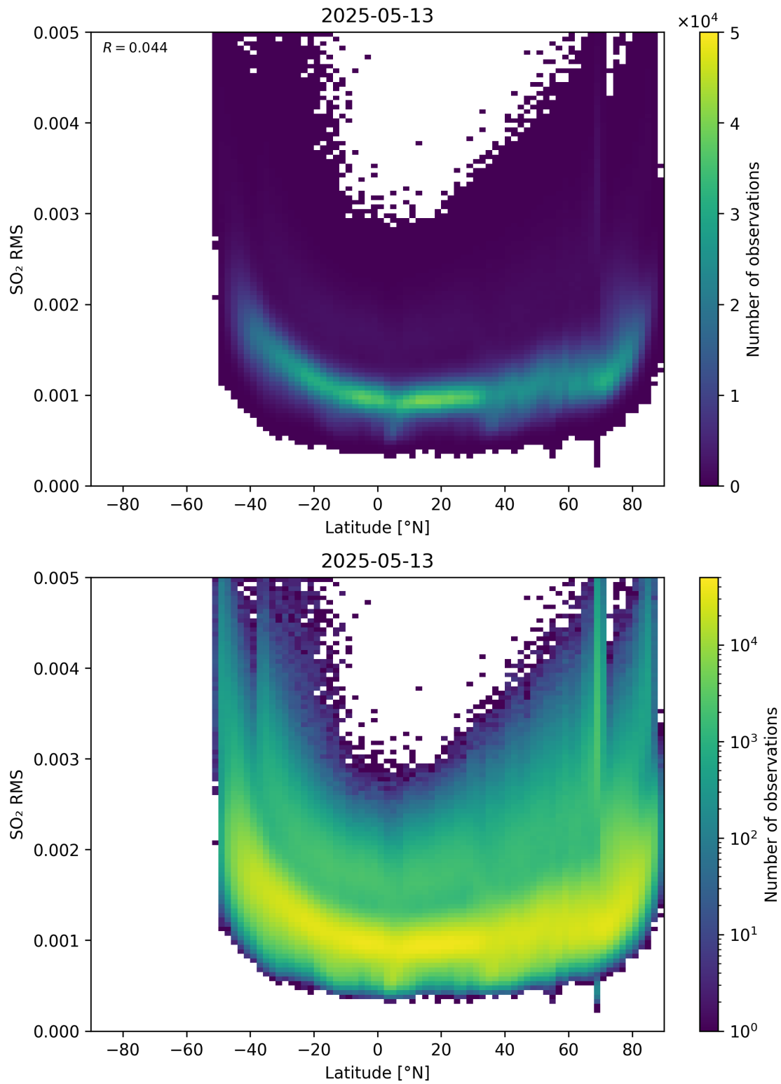
Figure 155: Scatter density plot of “Latitude” against “SO 2 RMS” for 2025-05-12 to 2025-05-14.
