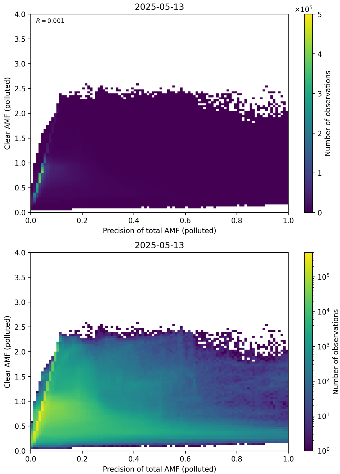
Figure 320: Scatter density plot of “Precision of total AMF (polluted)” against “Clear AMF (polluted)” for 2025-05-12 to 2025-05-14.
