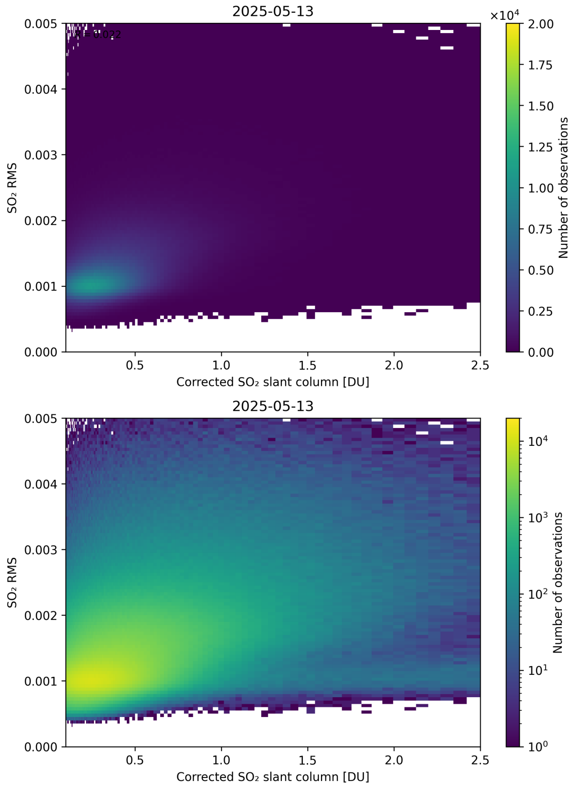
Figure 231: Scatter density plot of “Corrected SO 2 slant column” against “SO 2 RMS” for 2025-05-12 to 2025-05-14.
