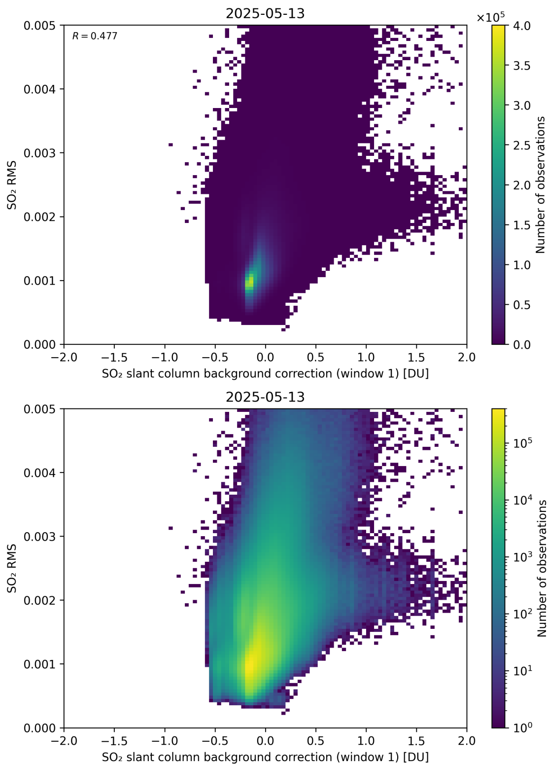
Figure 113: Scatter density plot of “SO 2 slant column background correction (window 1)” against “SO 2 RMS” for 2025-05-12 to 2025-05-14.
