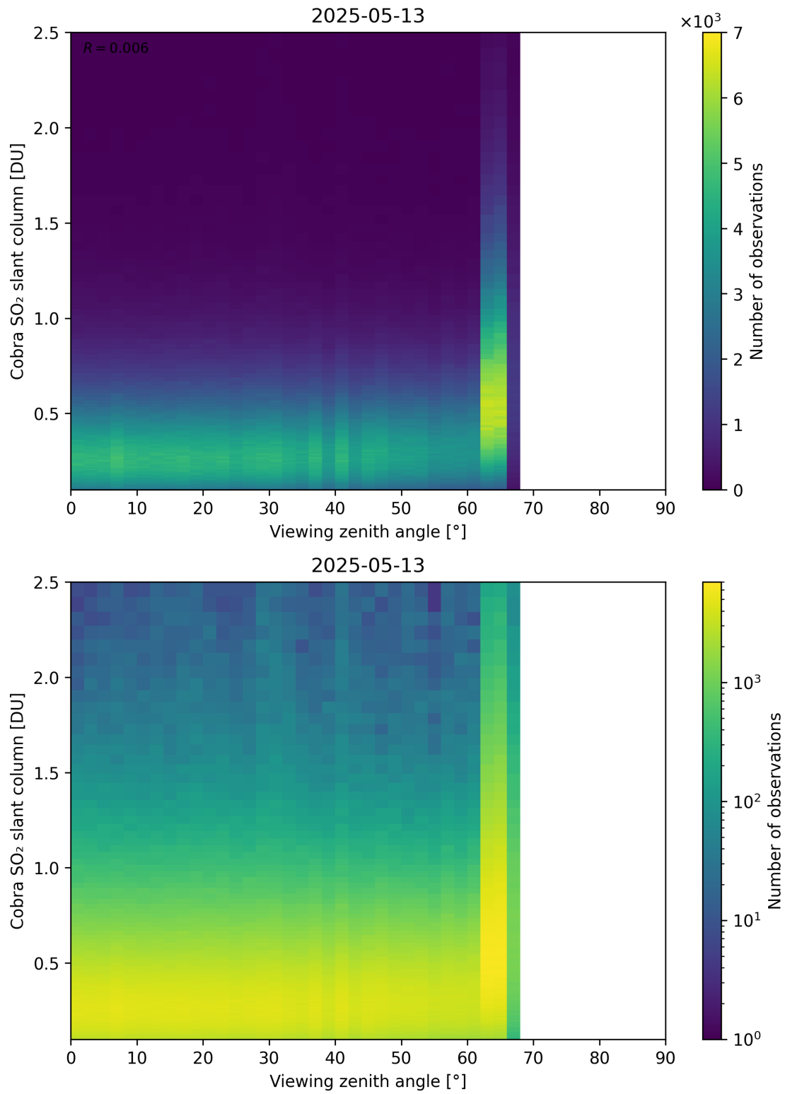
Figure 371: Scatter density plot of “Viewing zenith angle” against “Cobra SO 2 slant column” for 2025-05-12 to 2025-05-14.
