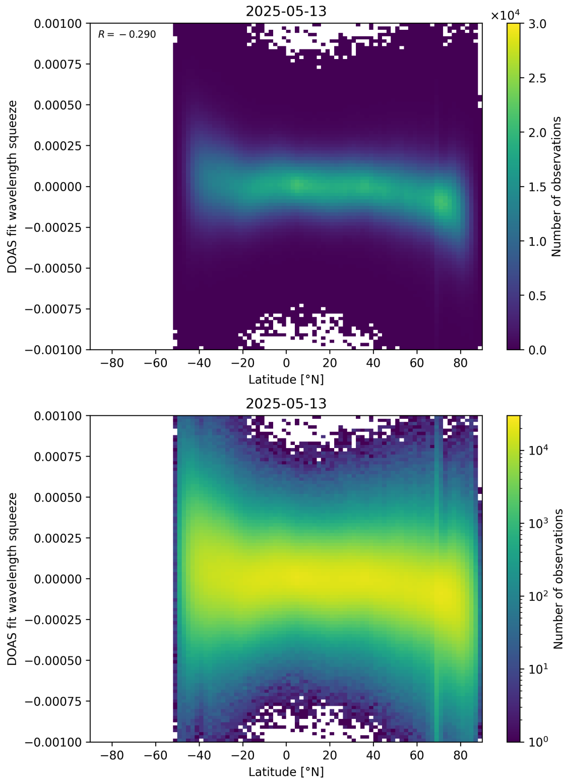
Figure 154: Scatter density plot of “Latitude” against “DOAS fit wavelength squeeze” for 2025-05-12 to 2025-05-14.
