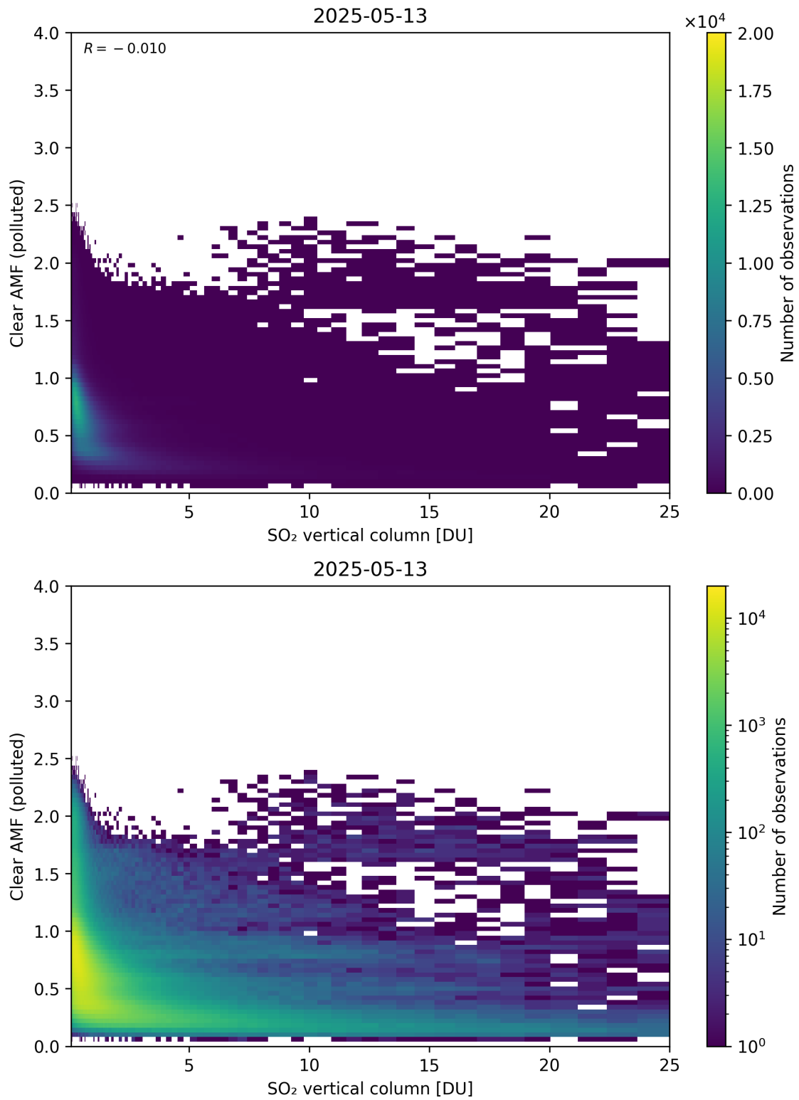
Figure 348: Scatter density plot of “SO 2 vertical column” against “Clear AMF (polluted)” for 2025-05-12 to 2025-05-14.
