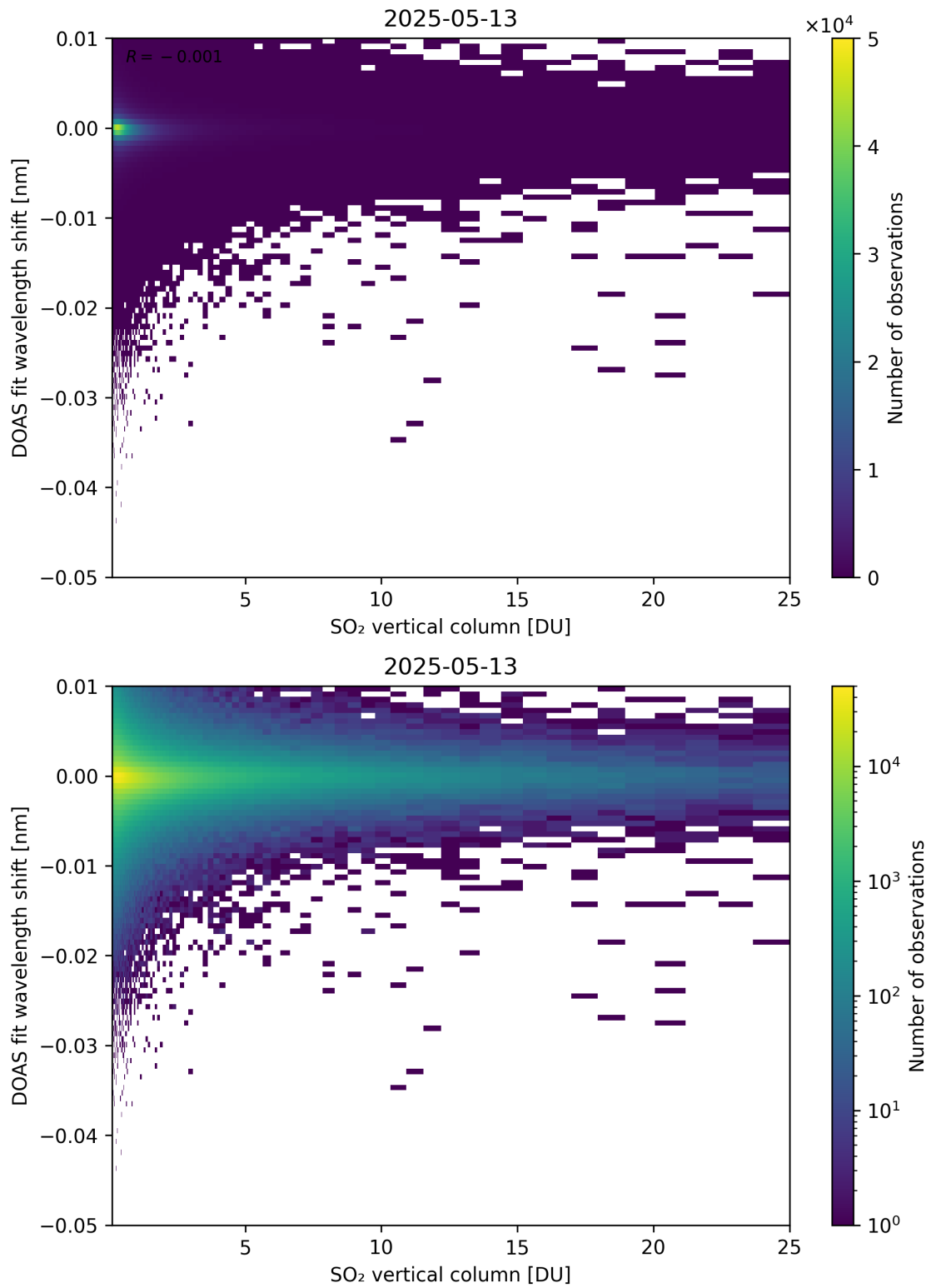
Figure 326: Scatter density plot of “SO 2 vertical column” against “DOAS fit wavelength shift” for 2025-05-12 to 2025-05-14.
