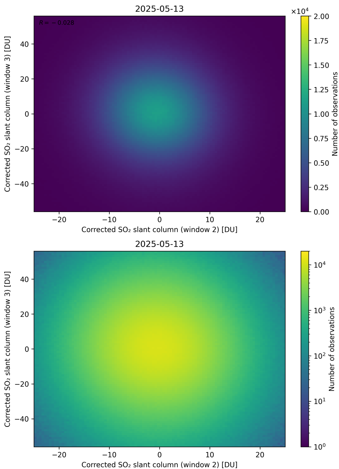
Figure 250: Scatter density plot of “Corrected SO 2 slant column (window 2)” against “Corrected SO 2 slant column (window 3)” for 2025-05-12 to 2025-05-14.
