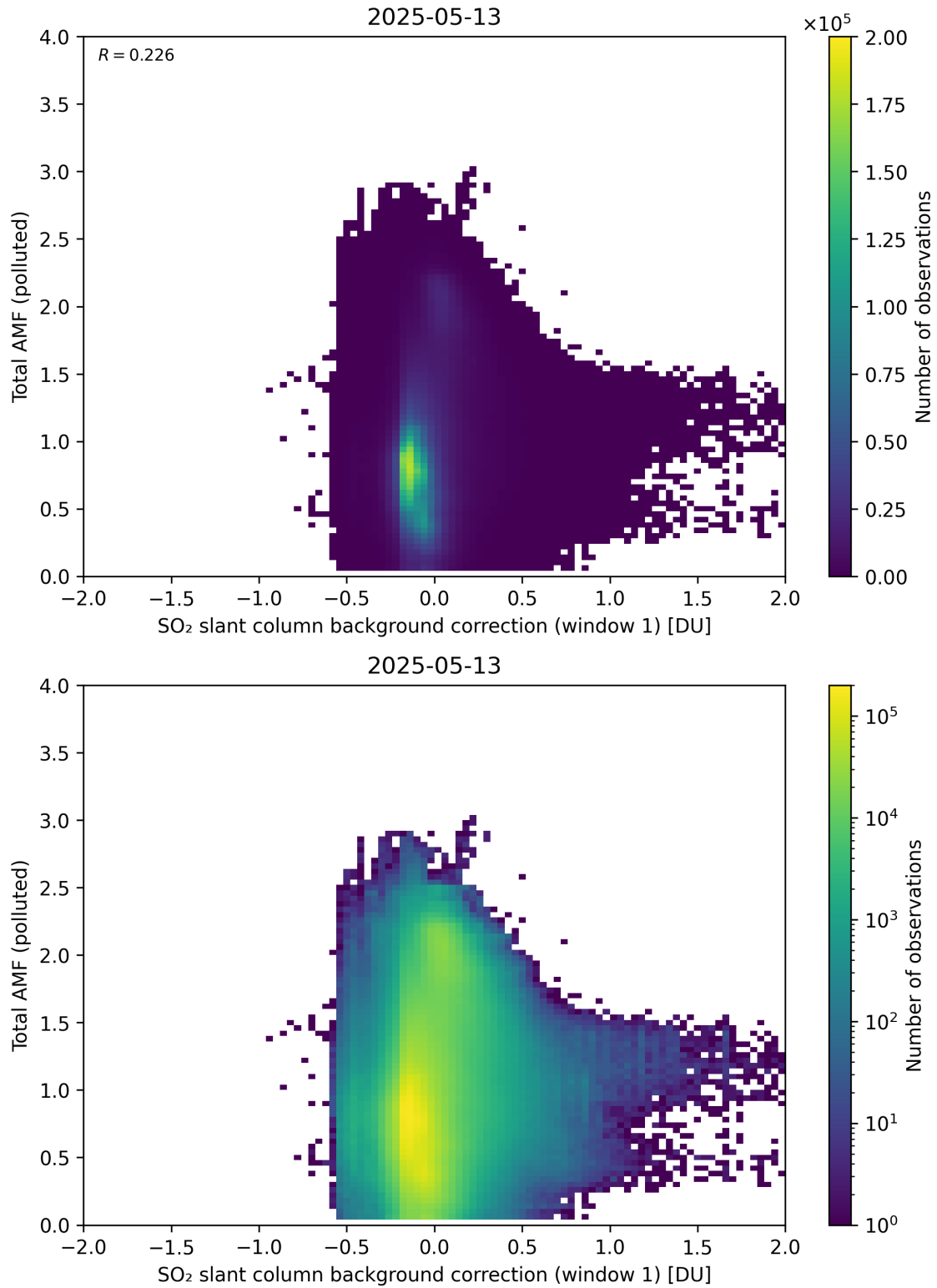
Figure 120: Scatter density plot of “SO 2 slant column background correction (window 1)” against “Total AMF (polluted)” for 2025-05-12 to 2025-05-14.
