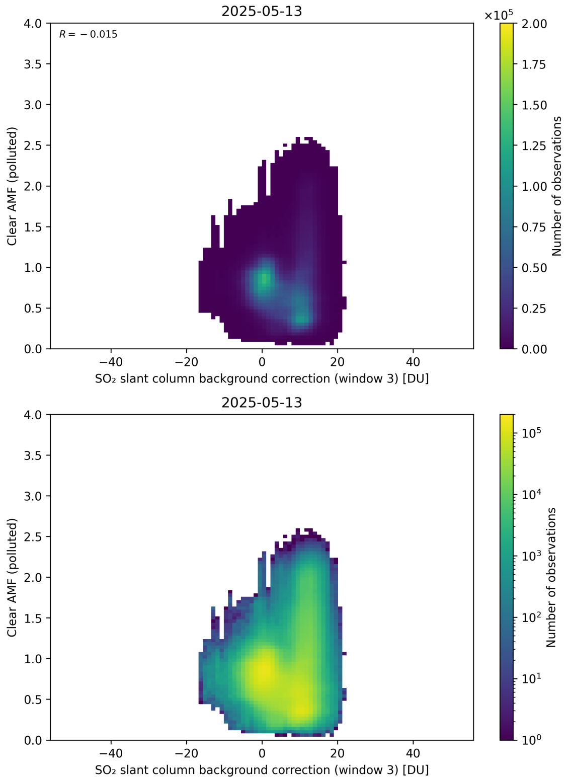
Figure 135: Scatter density plot of “SO 2 slant column background correction (window 3)” against “Clear AMF (polluted)” for 2025-05-12 to 2025-05-14.
