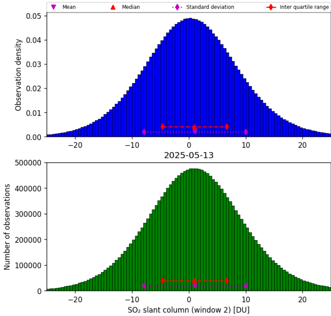
Figure 67: Histogram of “SO 2 slant column (window 2)” for 2025-05-12 to 2025-05-14
