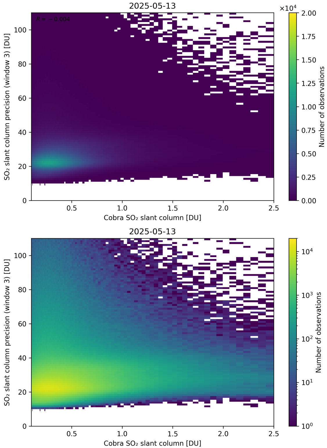
Figure 223: Scatter density plot of “Cobra SO 2 slant column” against “SO 2 slant column precision (window 3)” for 2025-05-12 to 2025-05-14.
