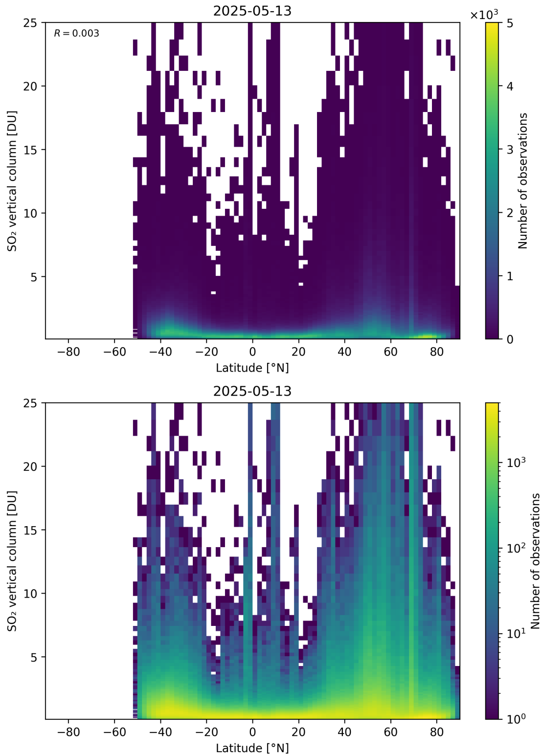
Figure 169: Scatter density plot of “Latitude” against “SO 2 vertical column” for 2025-05-12 to 2025-05-14.
