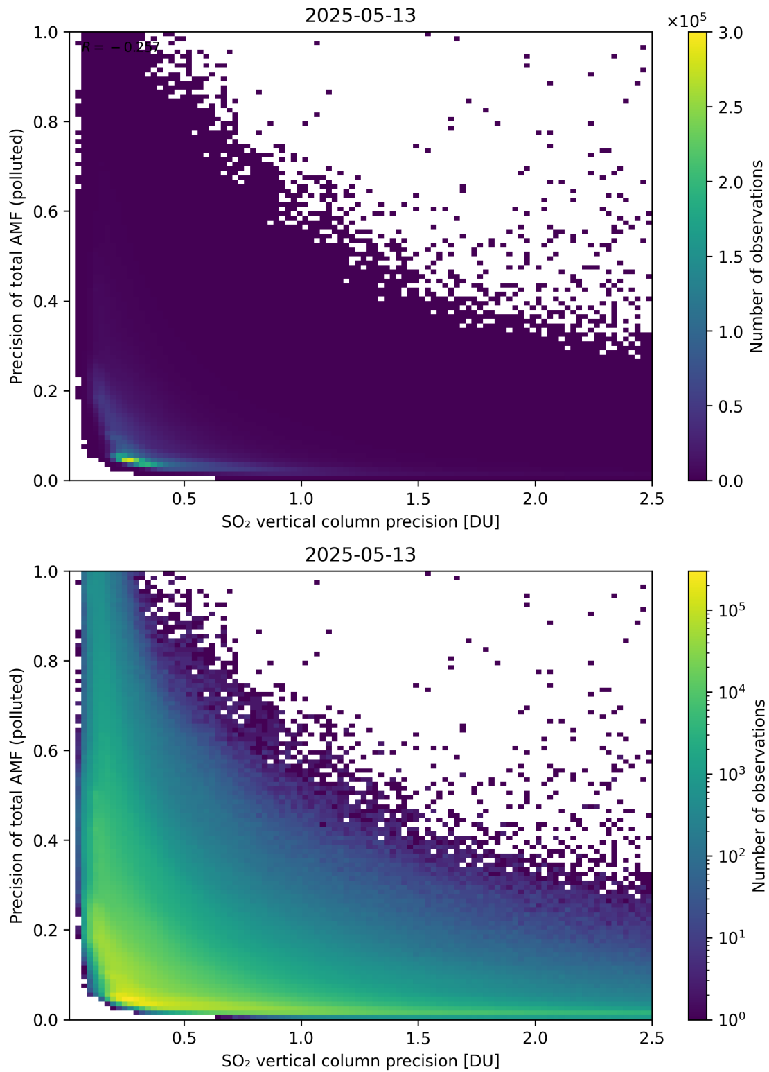
Figure 347: Scatter density plot of “SO 2 vertical column precision” against “Precision of total AMF (polluted)” for 2025-05-12 to 2025-05-14.
