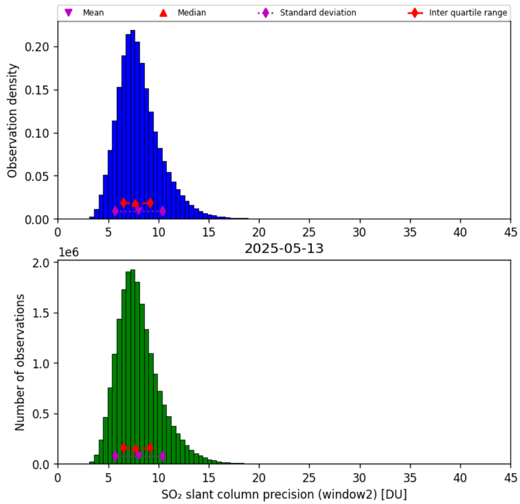
Figure 68: Histogram of “SO 2 slant column precision (window2)” for 2025-05-12 to 2025-05-14
