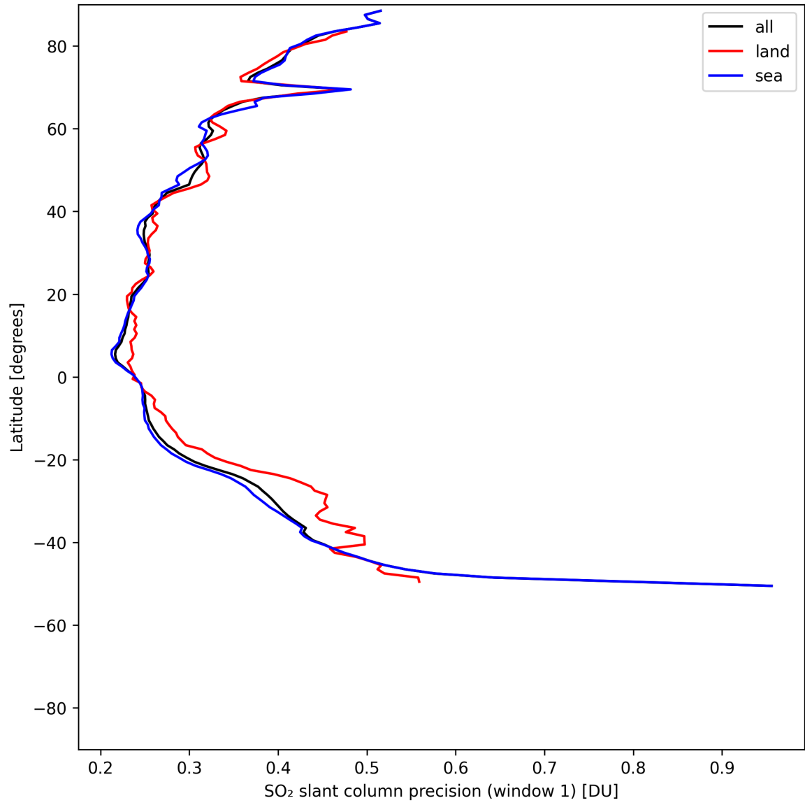
Figure 38: Zonal average of “SO 2 slant column precision (window 1)” for 2025-05-12 to 2025-05-14.
