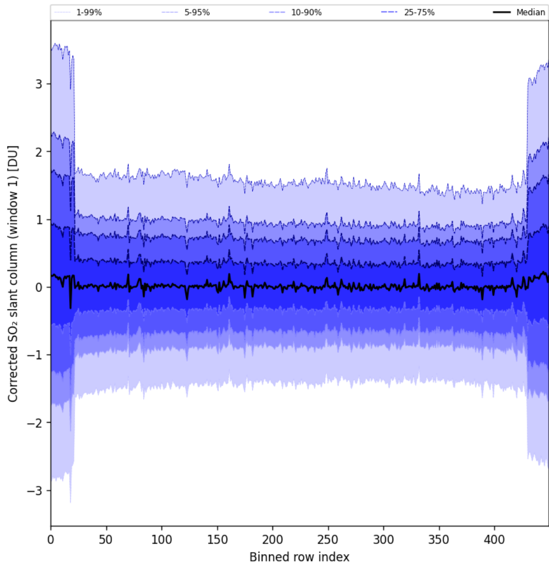
Figure 91: Along track statistics of “Corrected SO 2 slant column (window 1)” for 2025-05-12 to 2025-05-14
