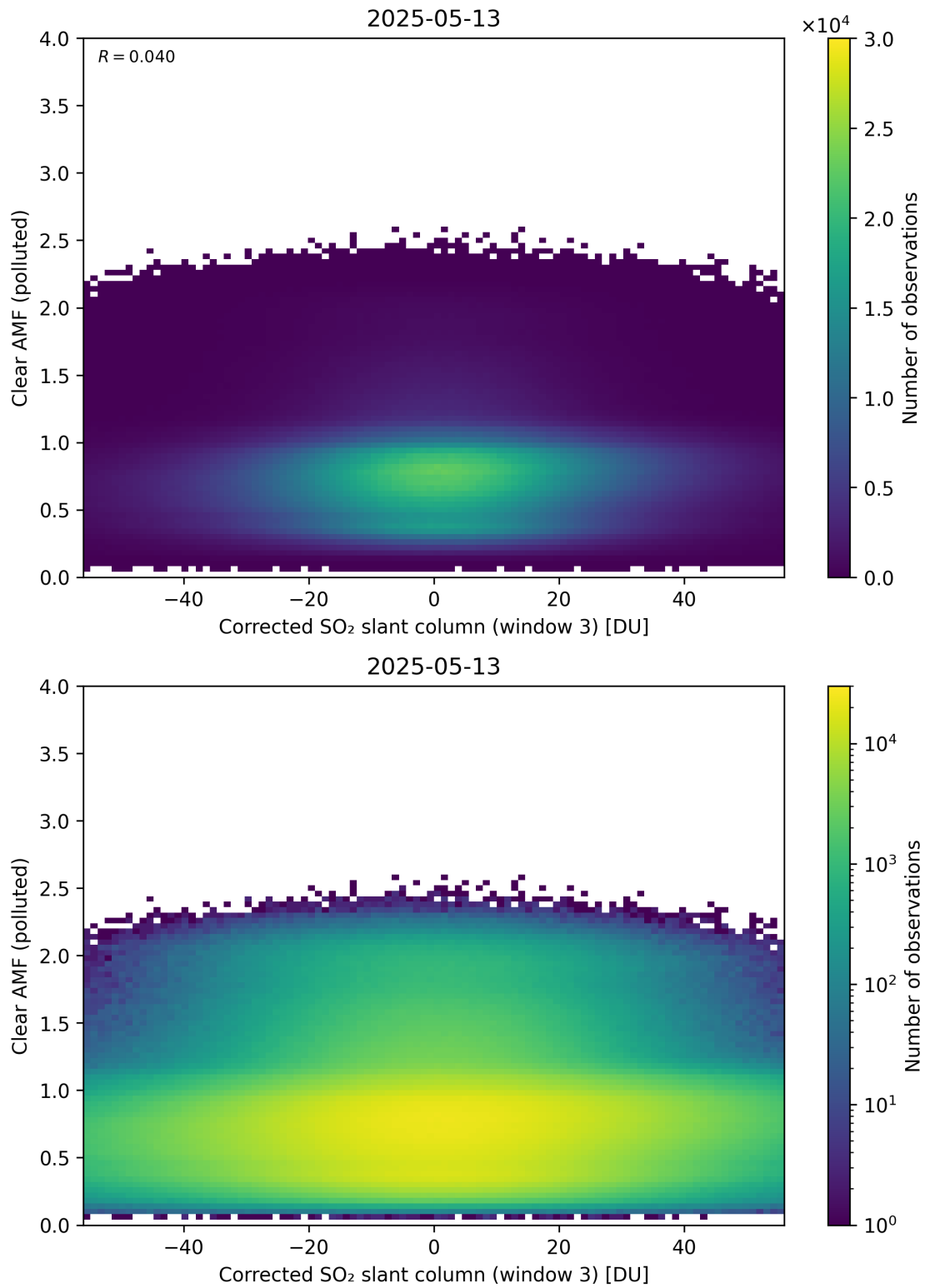
Figure 259: Scatter density plot of “Corrected SO 2 slant column (window 3)” against “Clear AMF (polluted)” for 2025-05-12 to 2025-05-14.
