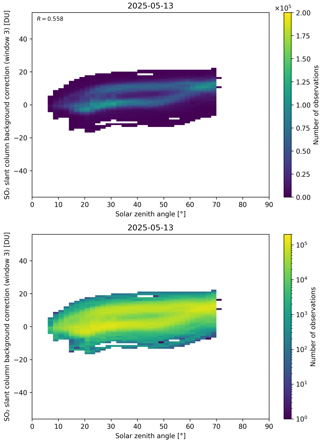
Figure 173: Scatter density plot of “Solar zenith angle” against “SO 2 slant column background correction (window 3)” for 2025-05-12 to 2025-05-14.
