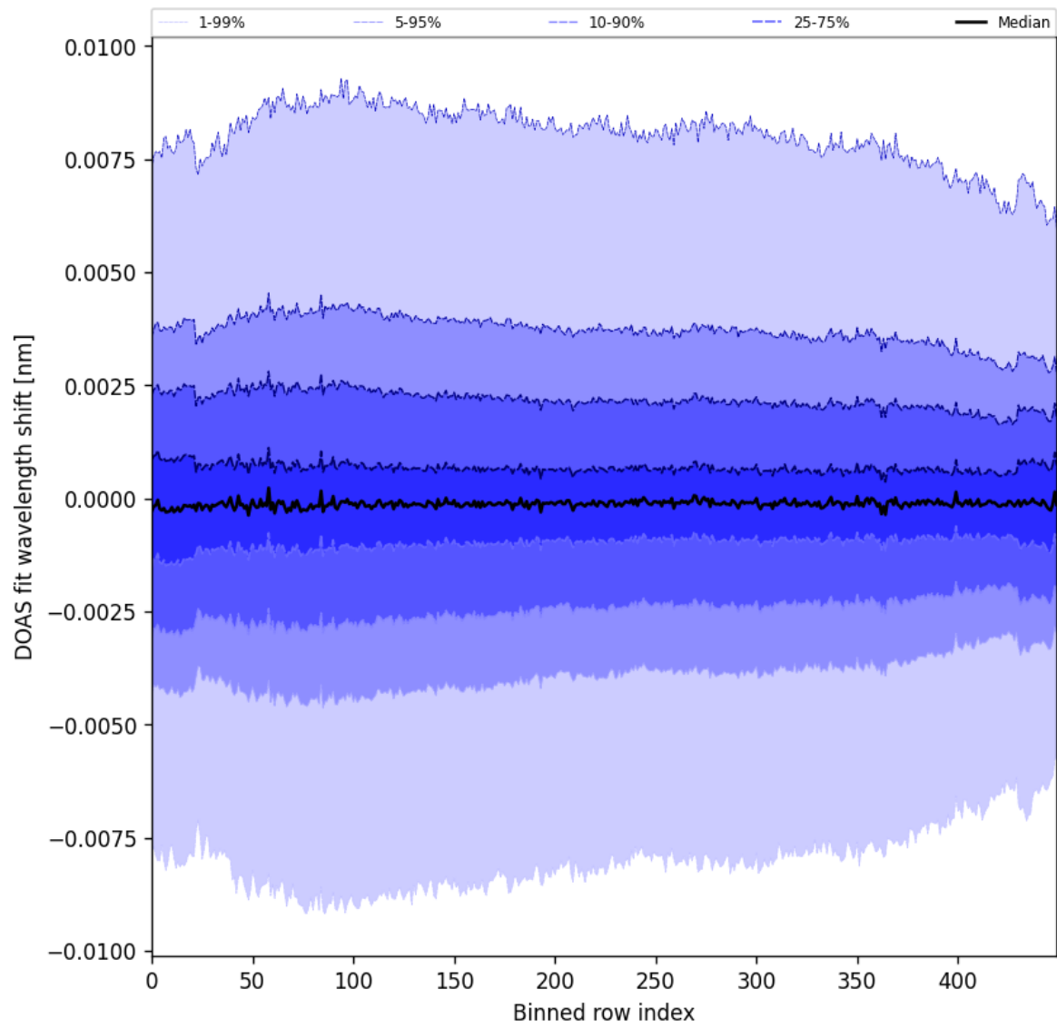
Figure 102: Along track statistics of “DOAS fit wavelength shift” for 2025-05-12 to 2025-05-14
