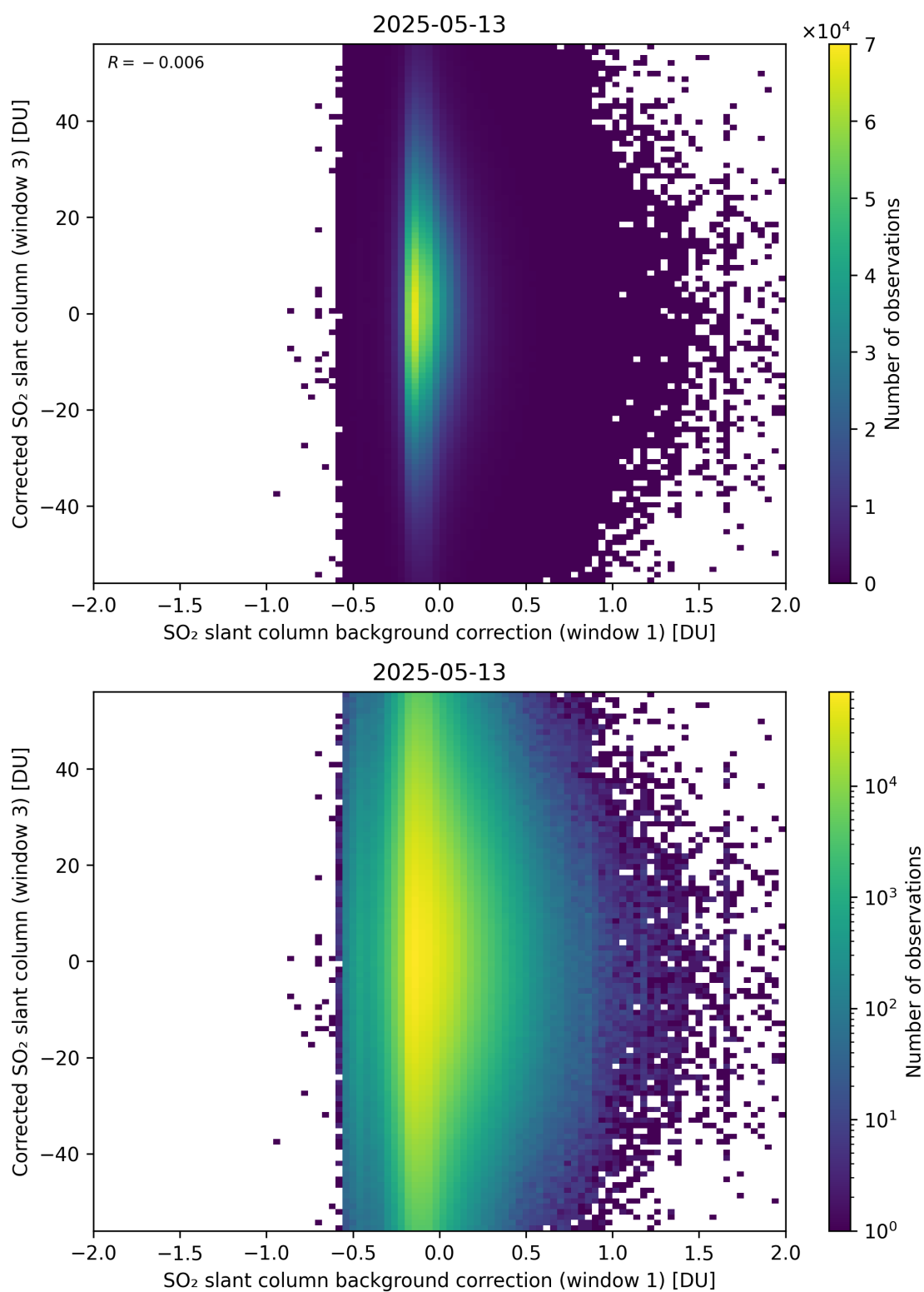
Figure 116: Scatter density plot of “SO 2 slant column background correction (window 1)” against “Corrected SO 2 slant column (window 3)” for 2025-05-12 to 2025-05-14.
