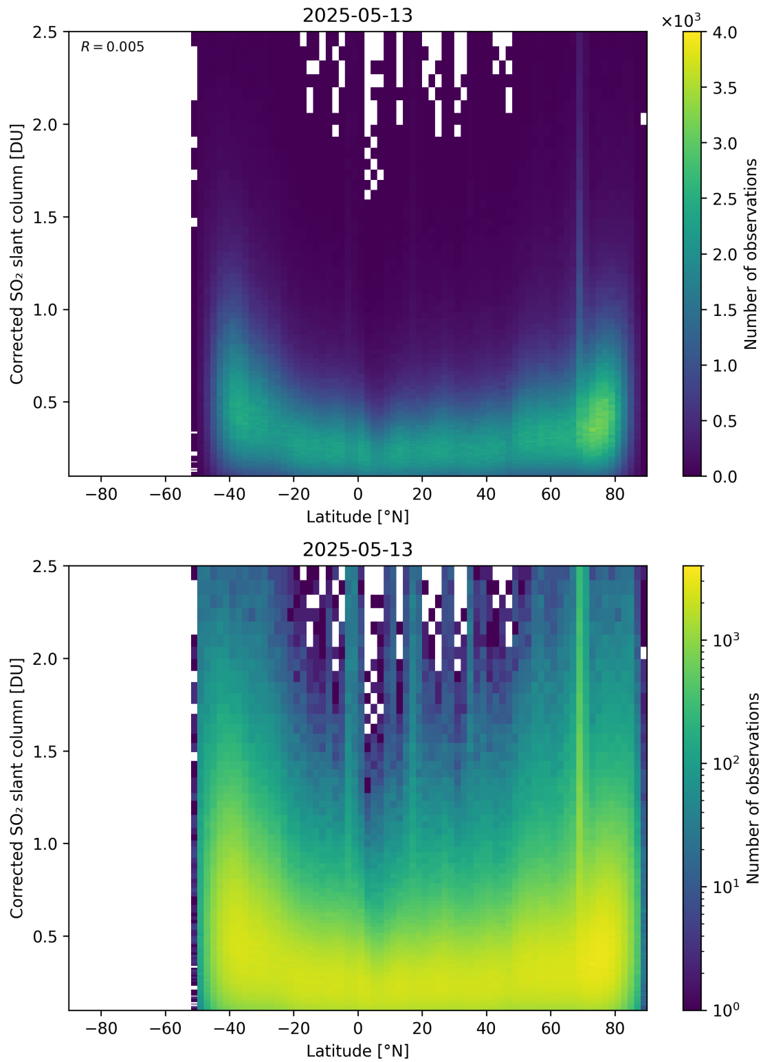
Figure 159: Scatter density plot of “Latitude” against “Corrected SO 2 slant column” for 2025-05-12 to 2025-05-14.
