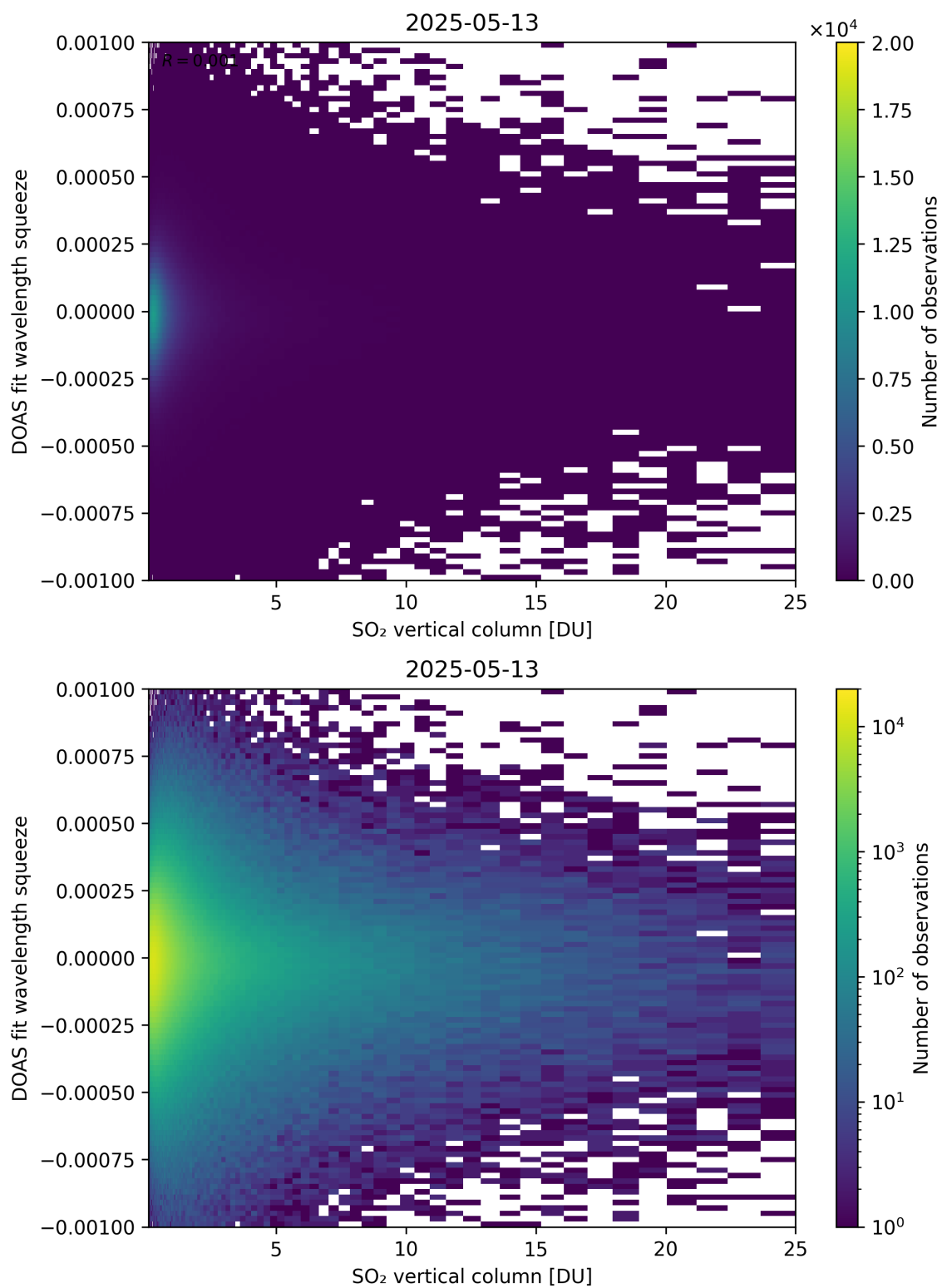
Figure 327: Scatter density plot of “SO 2 vertical column” against “DOAS fit wavelength squeeze” for 2025-05-12 to 2025-05-14.
