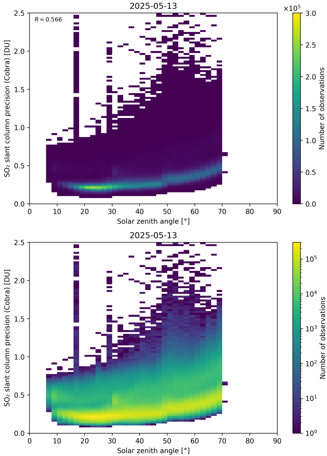
Figure 180: Scatter density plot of “Solar zenith angle” against “SO 2 slant column precision (Cobra)” for 2025-05-12 to 2025-05-14.
