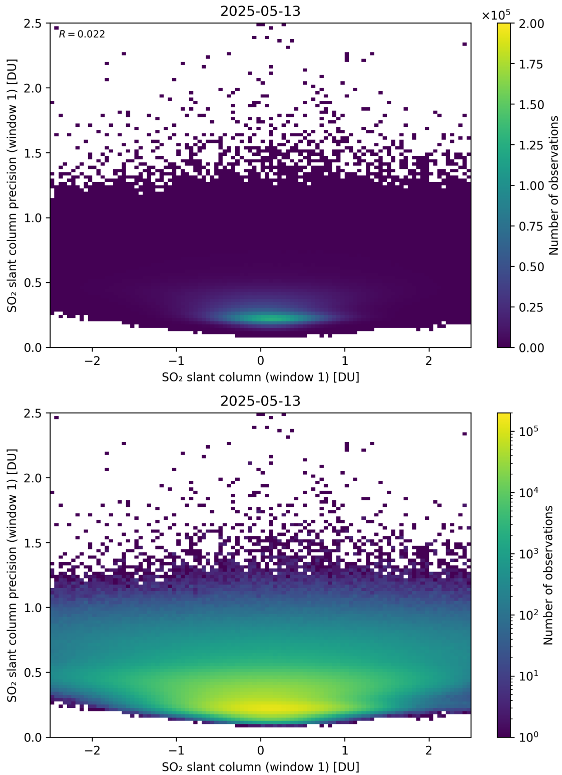
Figure 285: Scatter density plot of “SO 2 slant column (window 1)” against “SO 2 slant column precision (window 1)” for 2025-05-12 to 2025-05-14.
