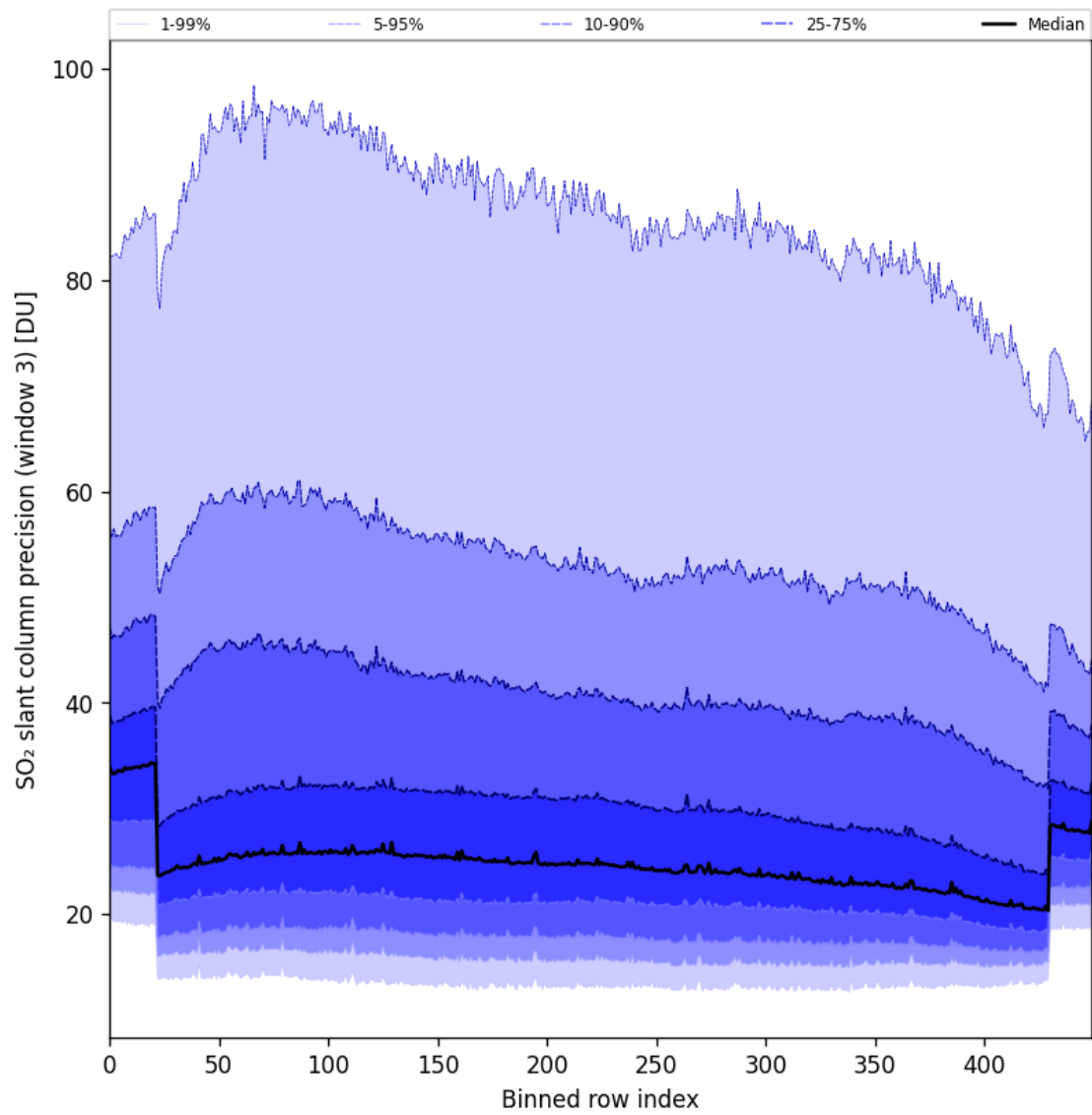
Figure 98: Along track statistics of “SO 2 slant column precision (window 3)” for 2025-05-12 to 2025-05-14
