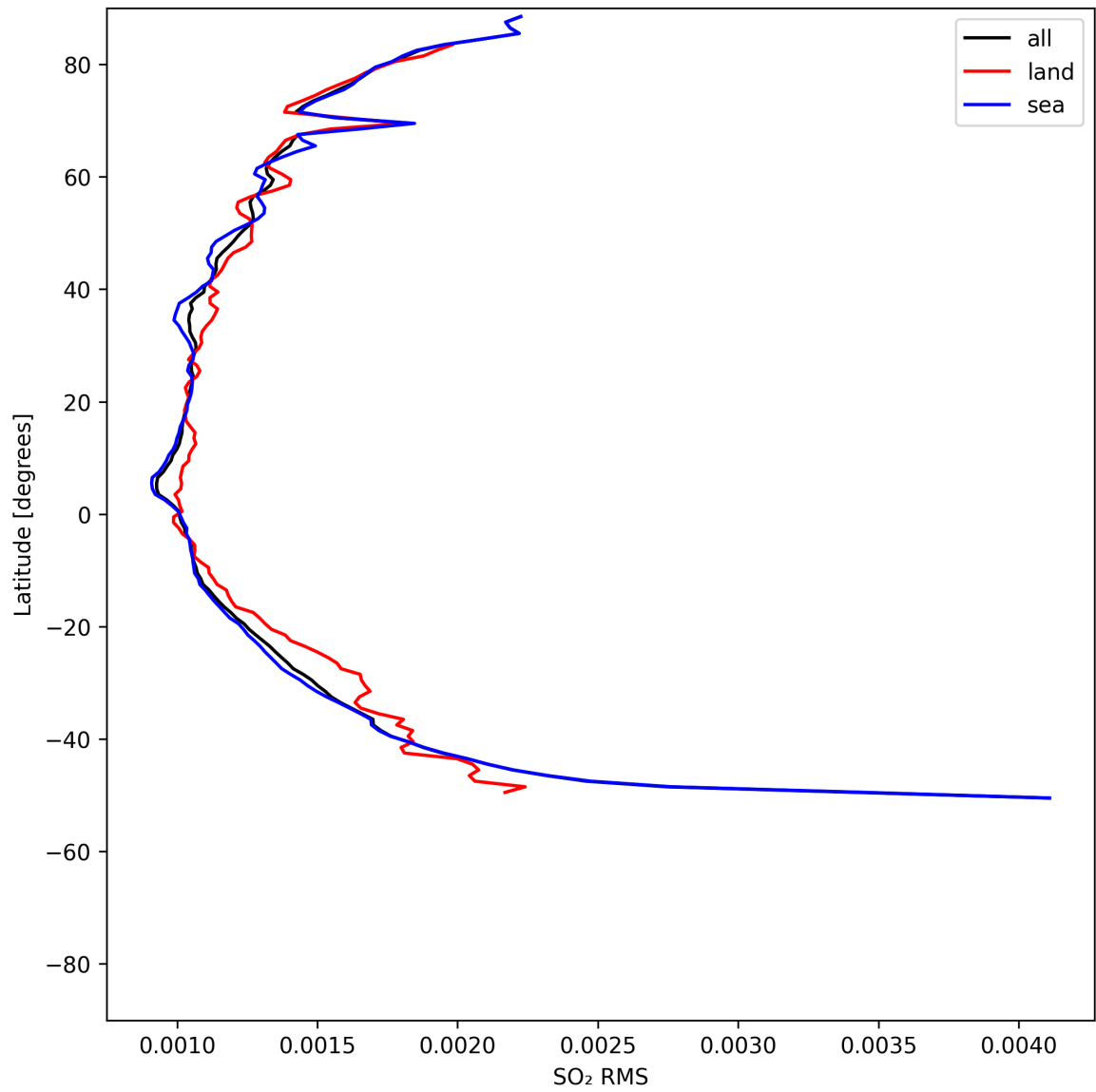
Figure 52: Zonal average of “SO 2 RMS” for 2025-05-12 to 2025-05-14.
