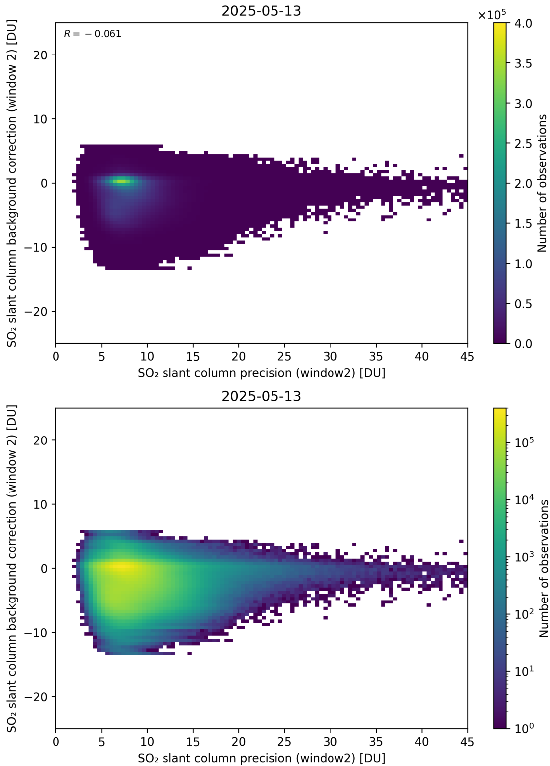
Figure 291: Scatter density plot of “SO 2 slant column precision (window2)” against “SO 2 slant column background correction (window 2)” for 2025-05-12 to 2025-05-14.
