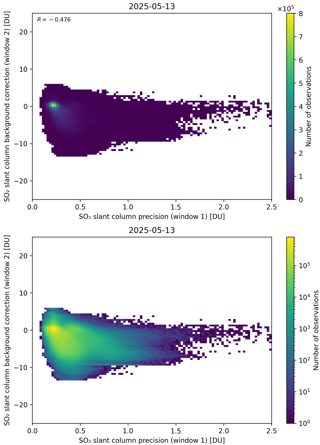
Figure 269: Scatter density plot of “SO 2 slant column precision (window 1)” against “SO 2 slant column background correction (window 2)” for 2025-05-12 to 2025-05-14.
