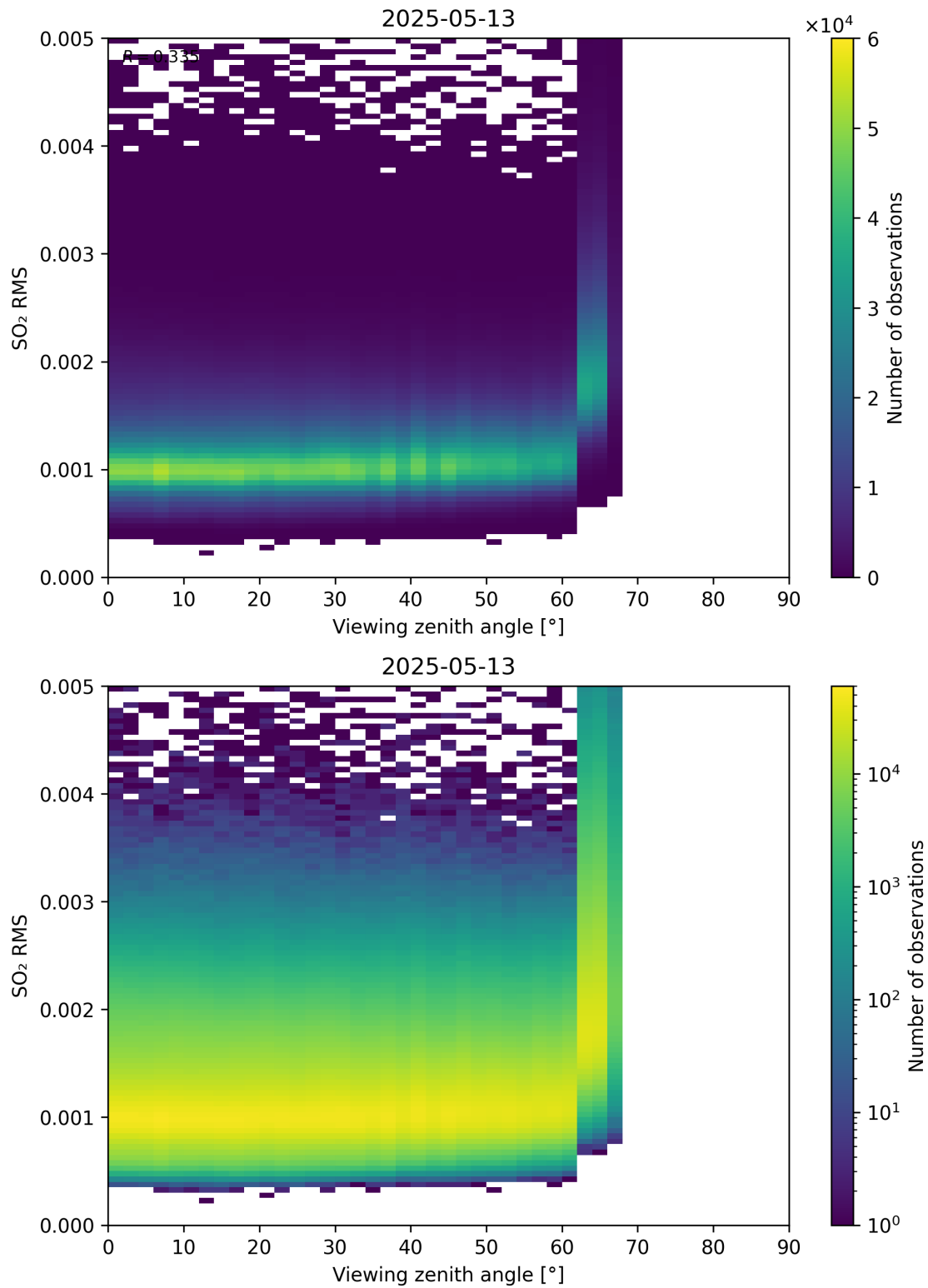
Figure 367: Scatter density plot of “Viewing zenith angle” against “SO 2 RMS” for 2025-05-12 to 2025-05-14.
