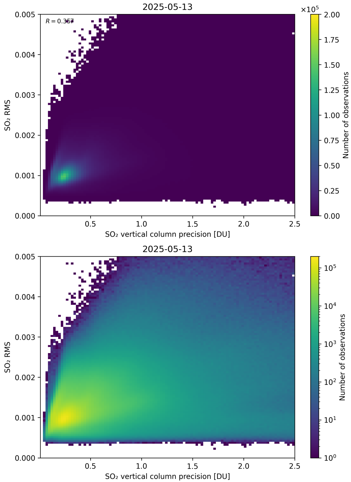
Figure 334: Scatter density plot of “SO 2 vertical column precision” against “SO 2 RMS” for 2025-05-12 to 2025-05-14.
