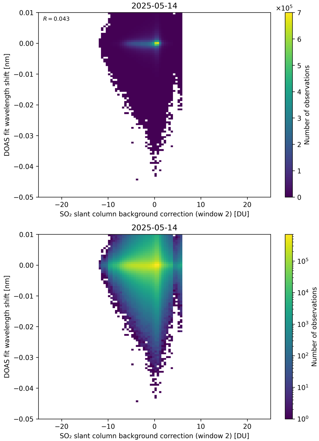
Figure 123: Scatter density plot of “SO 2 slant column background correction (window 2)” against “DOAS fit wavelength shift” for 2025-05-13 to 2025-05-15.
