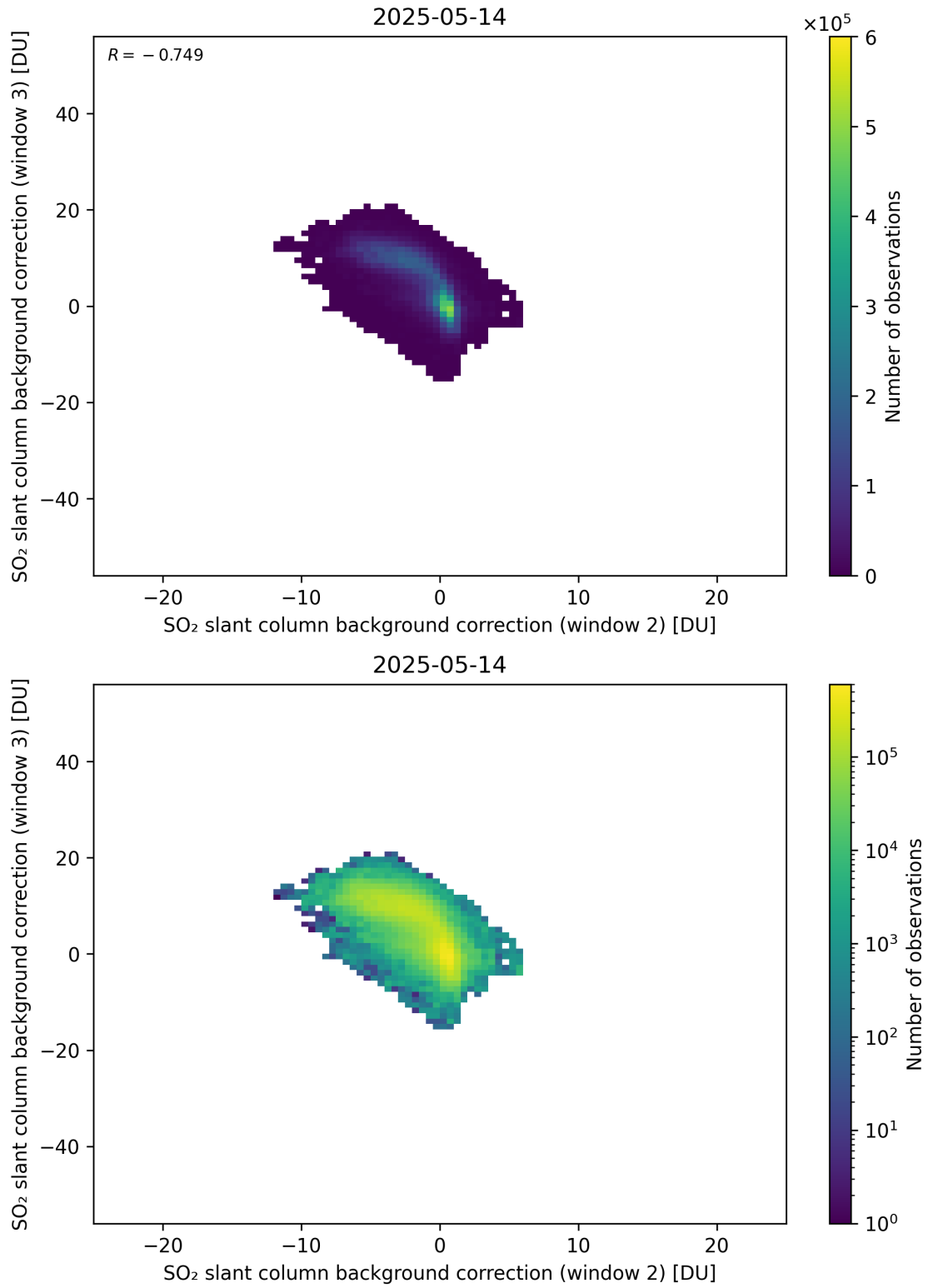
Figure 122: Scatter density plot of “SO 2 slant column background correction (window 2)” against “SO 2 slant column background correction (window 3)” for 2025-05-13 to 2025-05-15.
