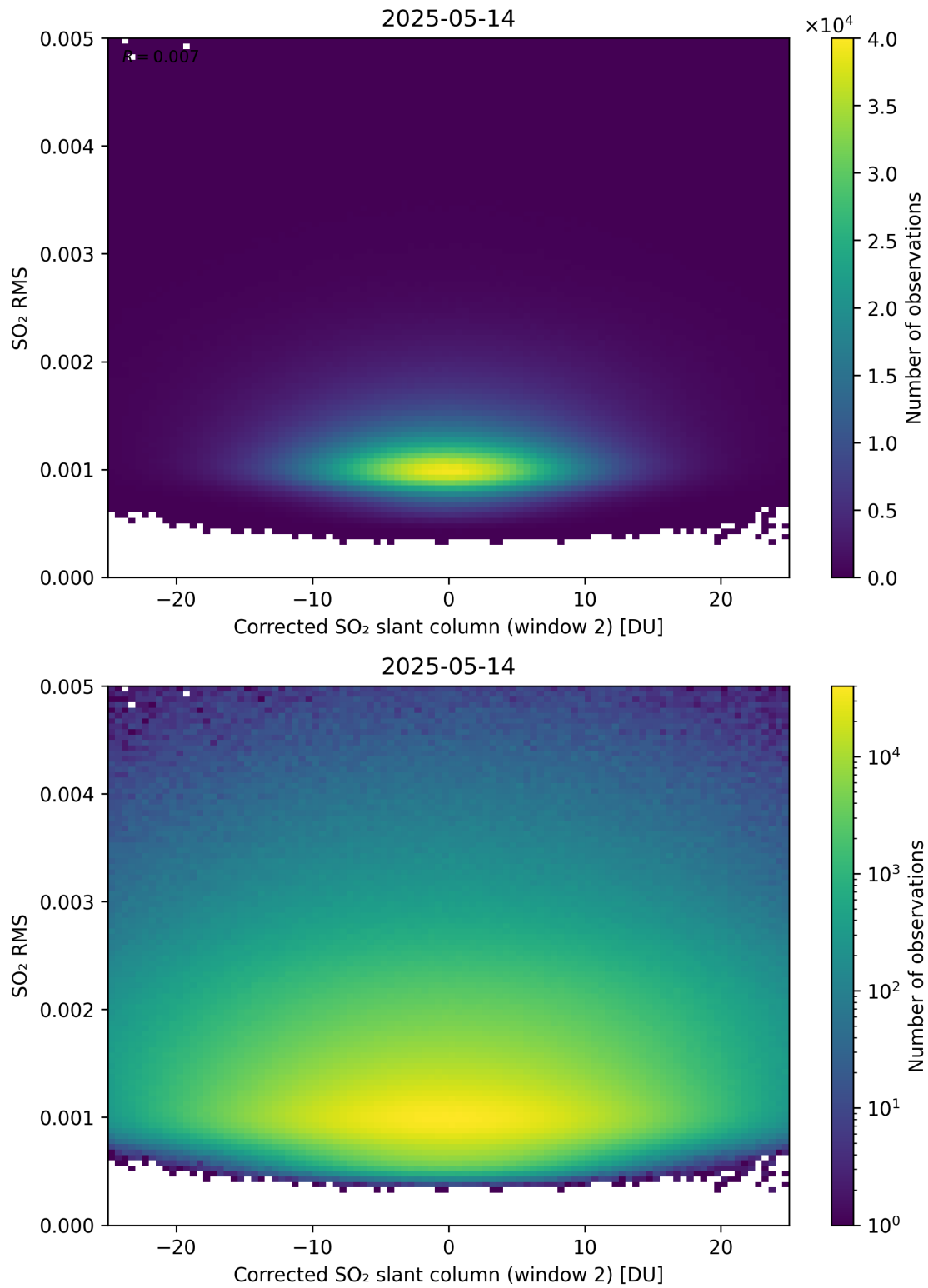
Figure 248: Scatter density plot of “Corrected SO 2 slant column (window 2)” against “SO 2 RMS” for 2025-05-13 to 2025-05-15.
