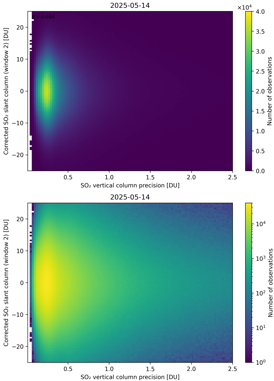
Figure 339: Scatter density plot of “SO 2 vertical column precision” against “Corrected SO 2 slant column (window 2)” for 2025-05-13 to 2025-05-15.
