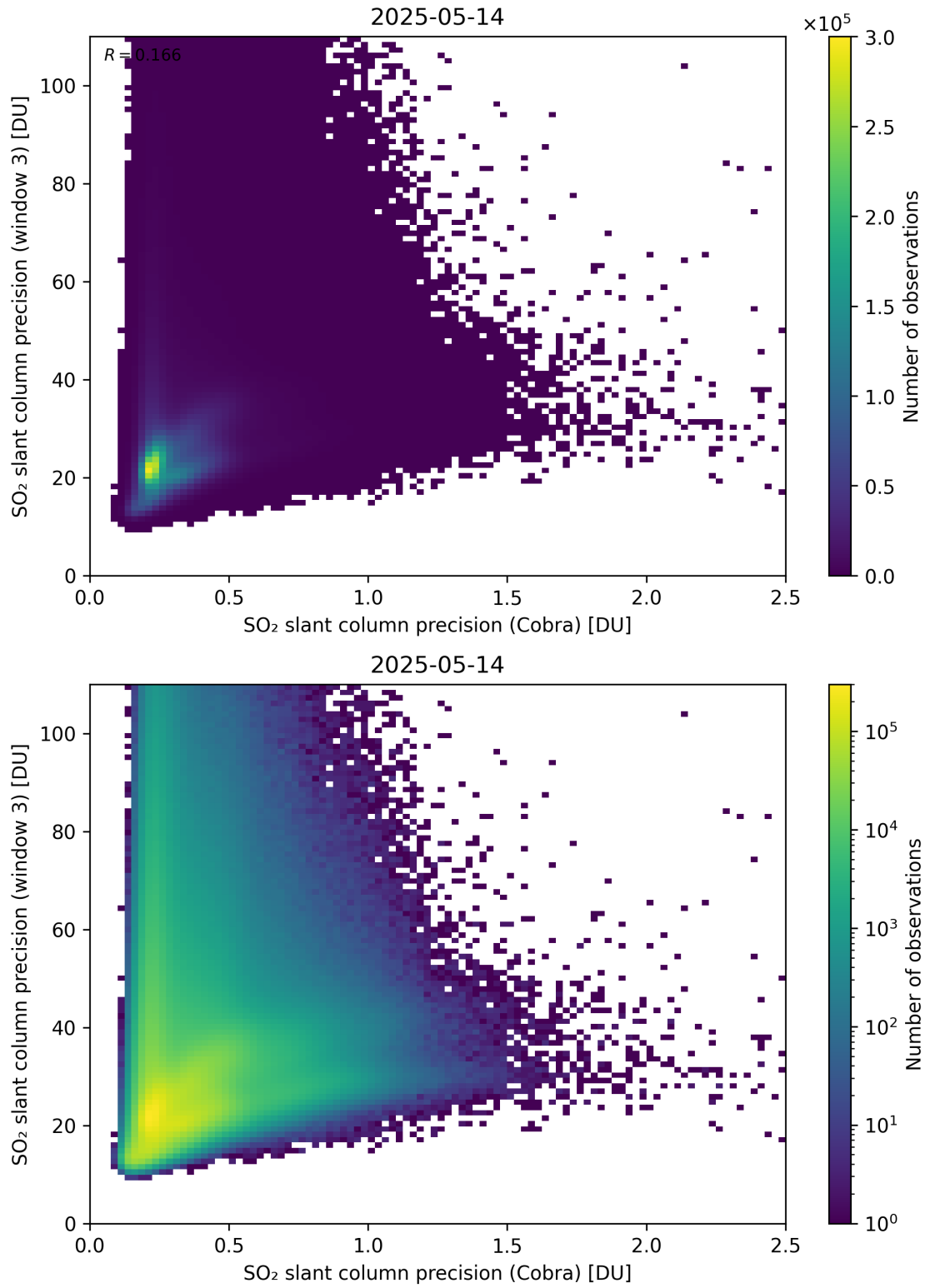
Figure 212: Scatter density plot of “SO 2 slant column precision (Cobra)” against “SO 2 slant column precision (window 3)” for 2025-05-13 to 2025-05-15.
