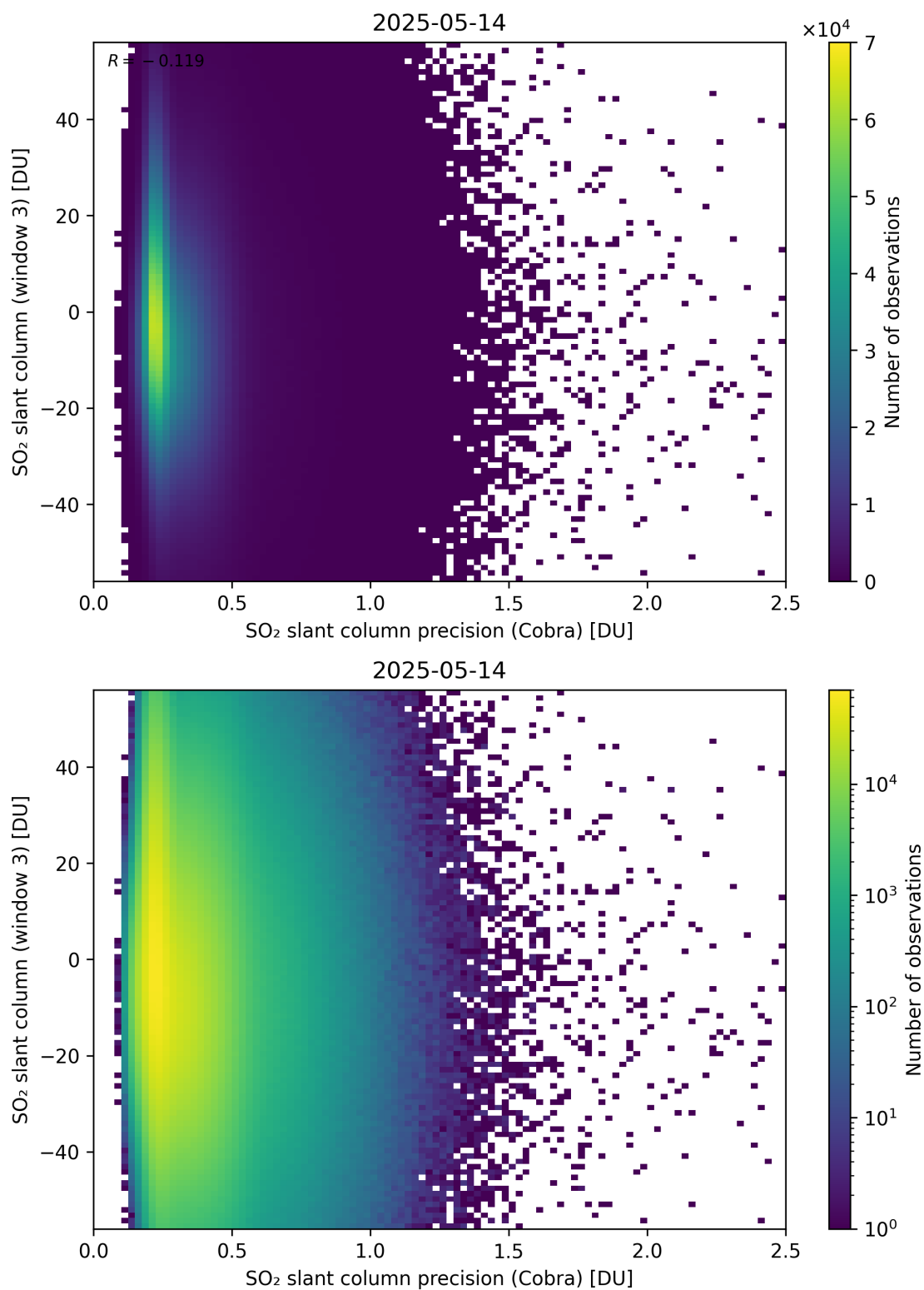
Figure 211: Scatter density plot of “SO 2 slant column precision (Cobra)” against “SO 2 slant column (window 3)” for 2025-05-13 to 2025-05-15.
