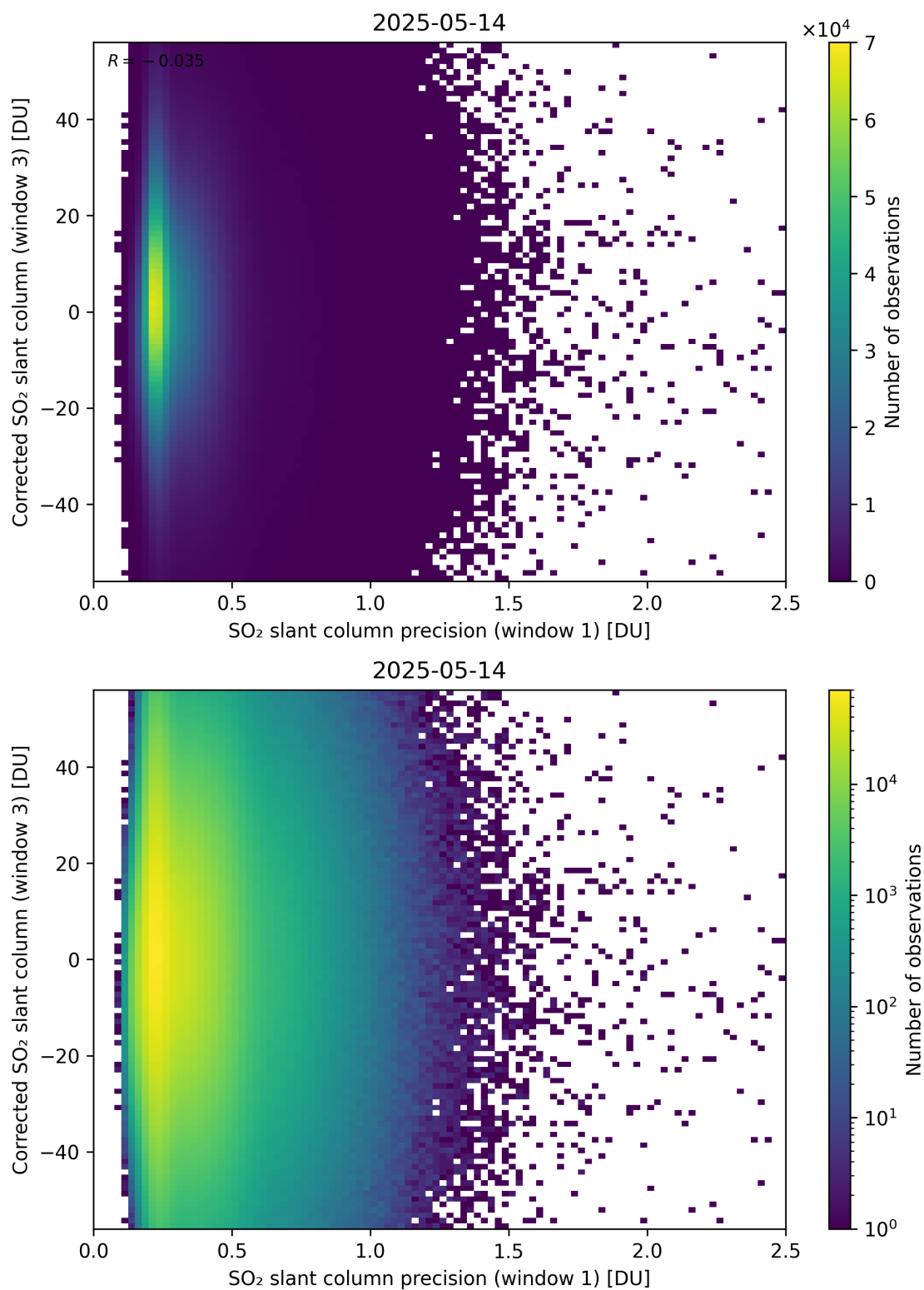
Figure 276: Scatter density plot of “SO 2 slant column precision (window 1)” against “Corrected SO 2 slant column (window 3)” for 2025-05-13 to 2025-05-15.
