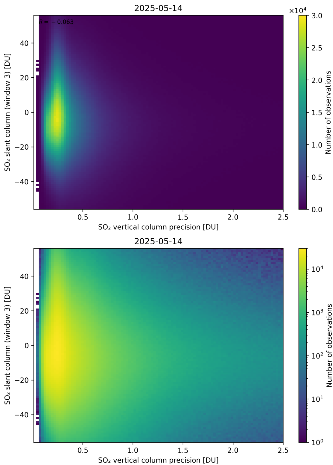
Figure 344: Scatter density plot of “SO 2 vertical column precision” against “SO 2 slant column (window 3)” for 2025-05-13 to 2025-05-15.
