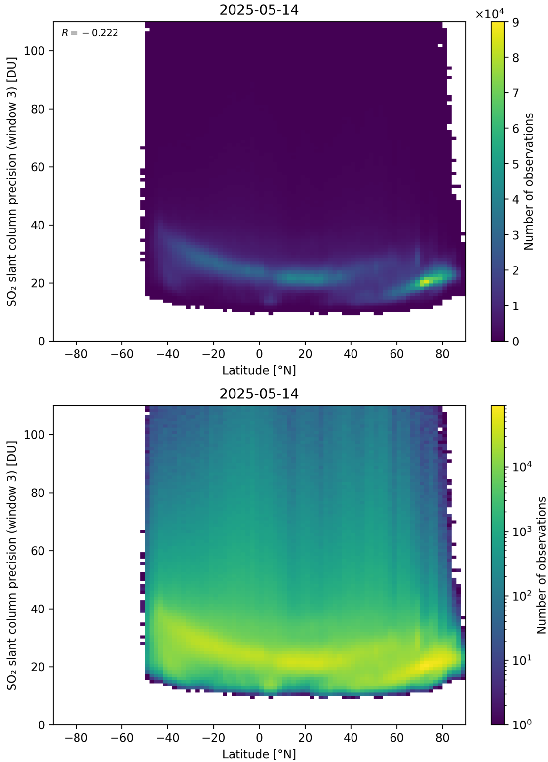
Figure 166: Scatter density plot of “Latitude” against “SO 2 slant column precision (window 3)” for 2025-05-13 to 2025-05-15.
