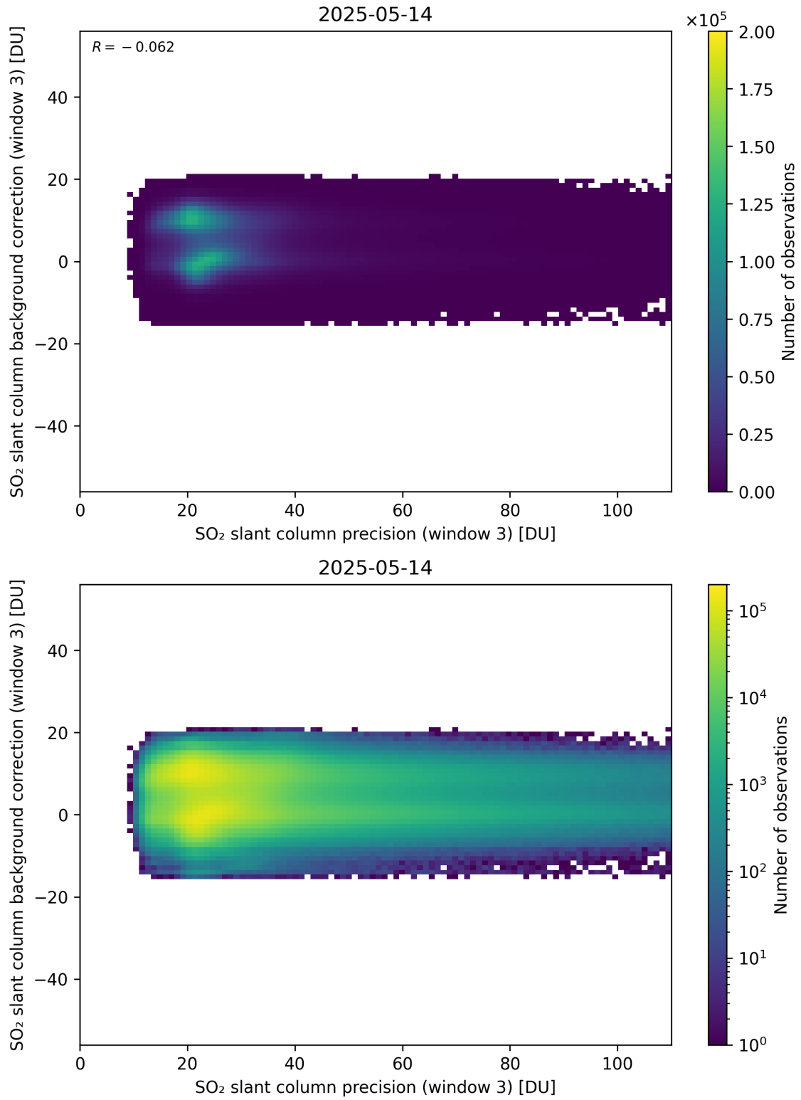
Figure 307: Scatter density plot of “SO 2 slant column precision (window 3)” against “SO 2 slant column background correction (window 3)” for 2025-05-13 to 2025-05-15.
