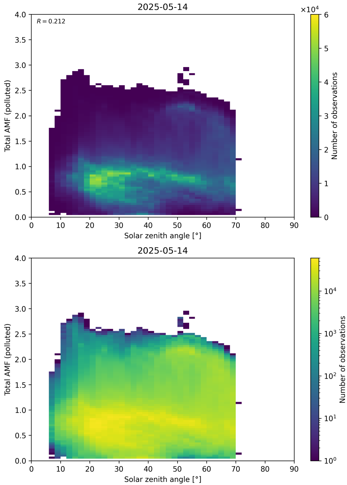
Figure 189: Scatter density plot of “Solar zenith angle” against “Total AMF (polluted)” for 2025-05-13 to 2025-05-15.
