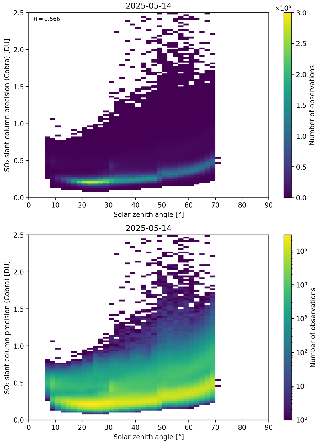
Figure 180: Scatter density plot of “Solar zenith angle” against “SO 2 slant column precision (Cobra)” for 2025-05-13 to 2025-05-15.
