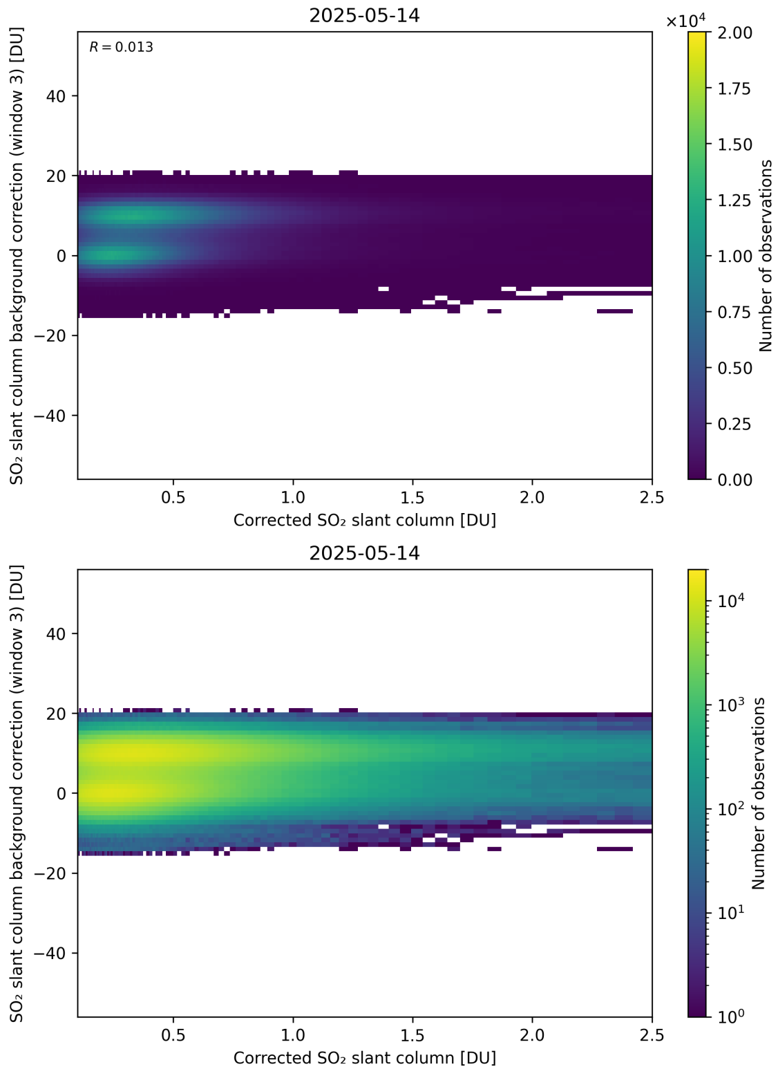
Figure 228: Scatter density plot of “Corrected SO 2 slant column” against “SO 2 slant column background correction (window 3)” for 2025-05-13 to 2025-05-15.
