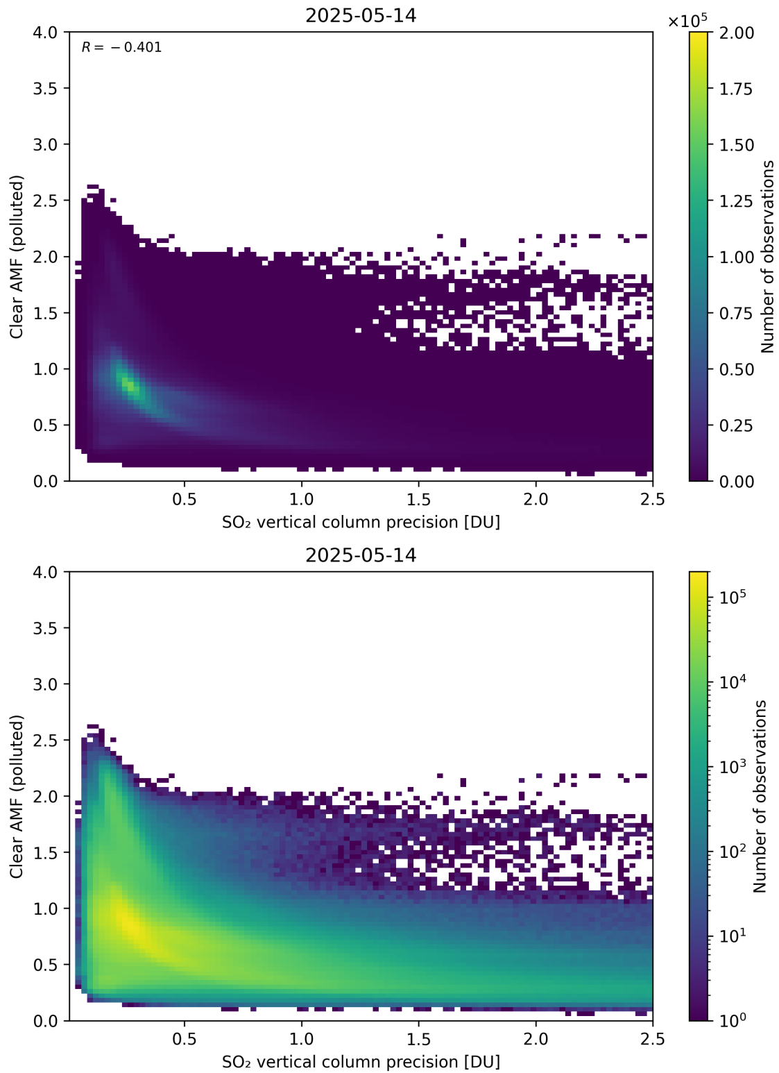
Figure 335: Scatter density plot of “SO 2 vertical column precision” against “Clear AMF (polluted)” for 2025-05-13 to 2025-05-15.
