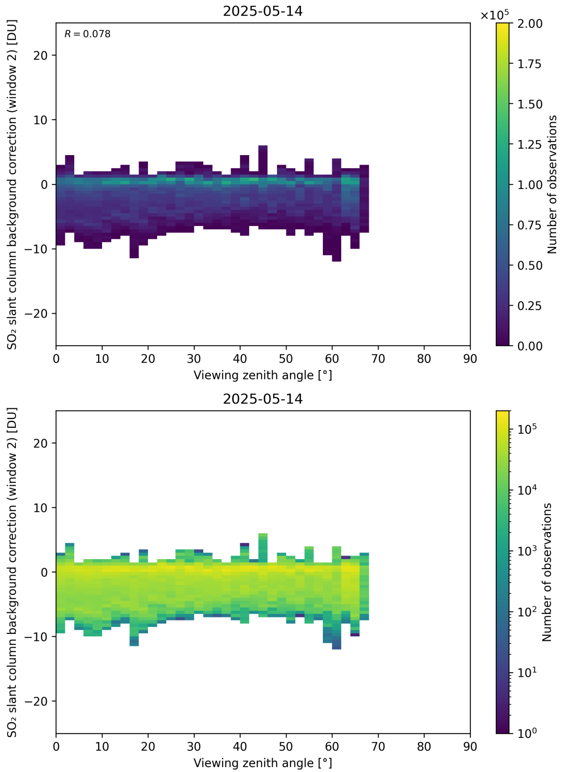
Figure 363: Scatter density plot of “Viewing zenith angle” against “SO 2 slant column background correction (window 2)” for 2025-05-13 to 2025-05-15.
