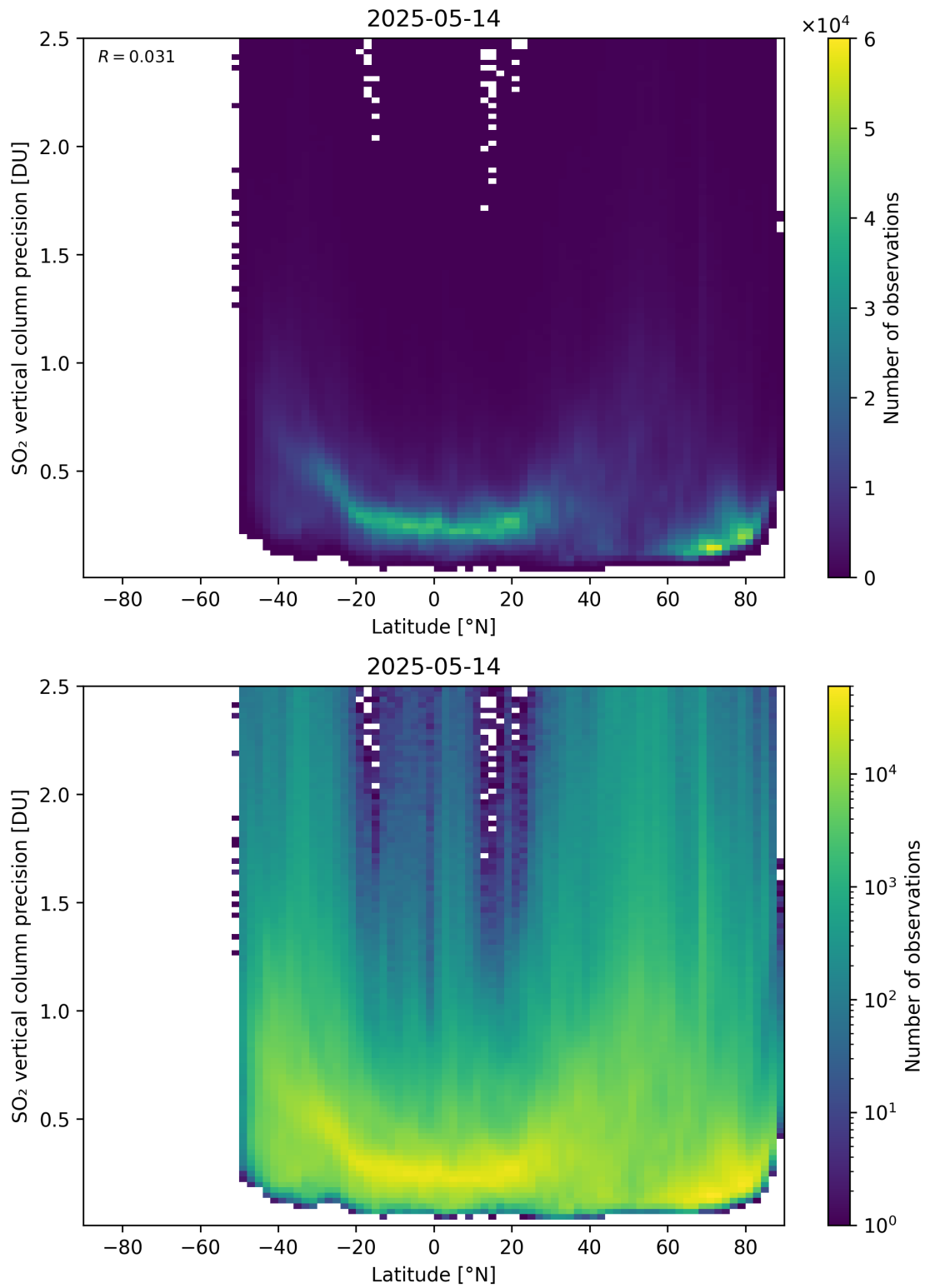
Figure 170: Scatter density plot of “Latitude” against “SO 2 vertical column precision” for 2025-05-13 to 2025-05-15.
