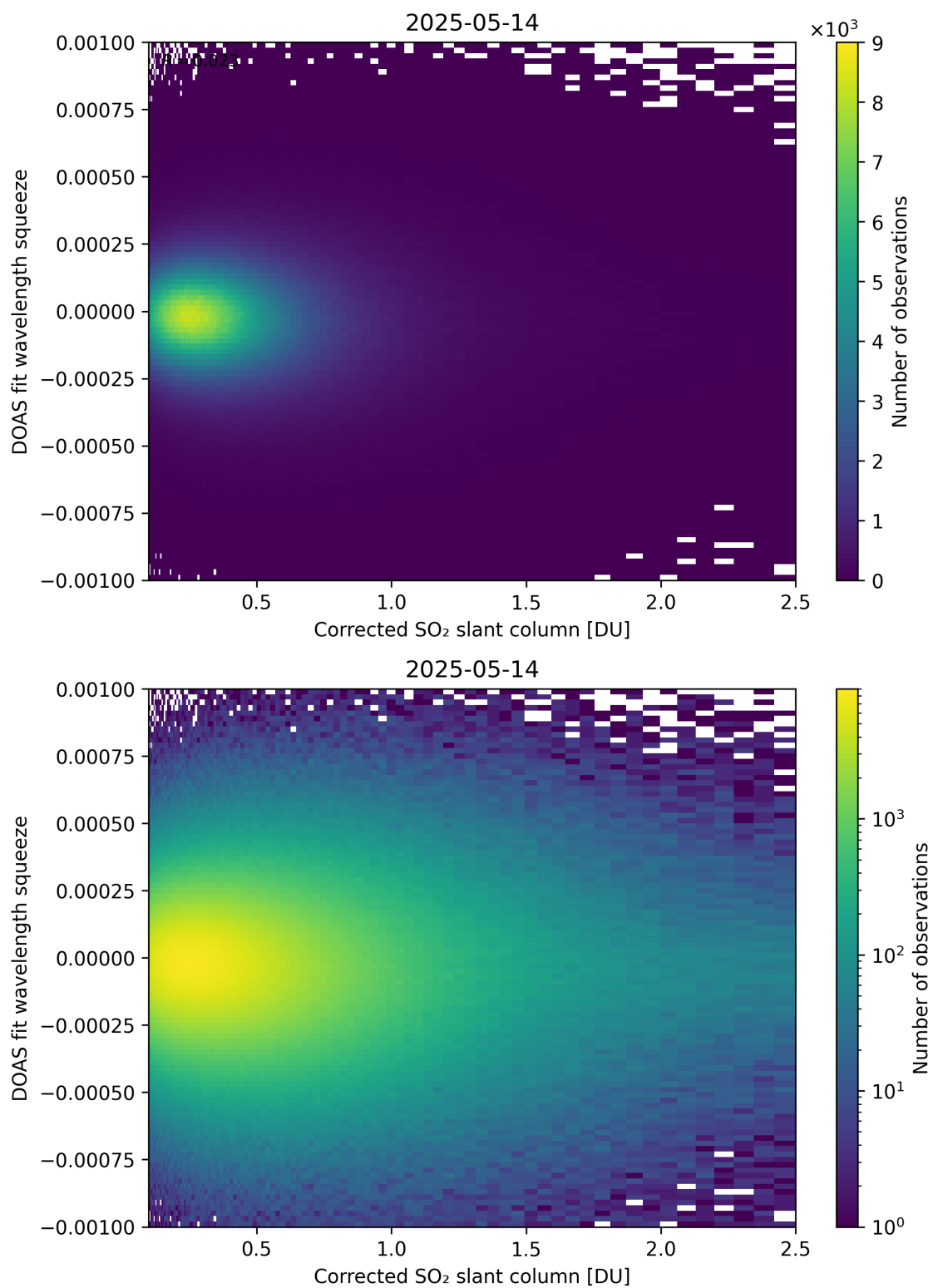
Figure 230: Scatter density plot of “Corrected SO 2 slant column” against “DOAS fit wavelength squeeze” for 2025-05-13 to 2025-05-15.
