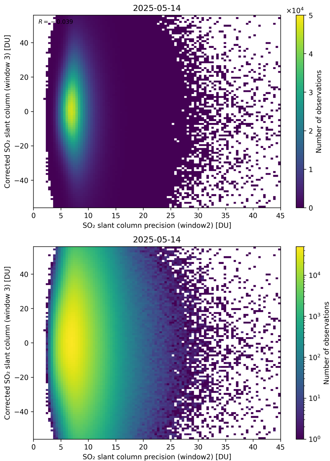
Figure 298: Scatter density plot of “SO 2 slant column precision (window2)” against “Corrected SO 2 slant column (window 3)” for 2025-05-13 to 2025-05-15.
