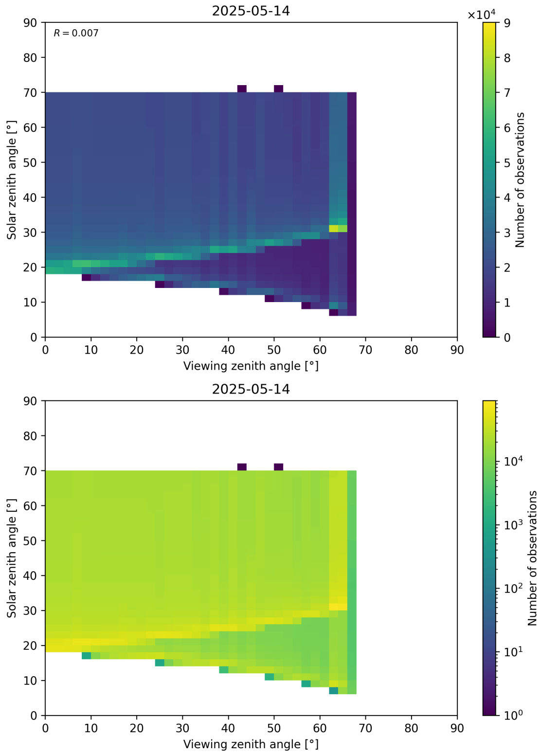
Figure 369: Scatter density plot of “Viewing zenith angle” against “Solar zenith angle” for 2025-05-13 to 2025-05-15.
