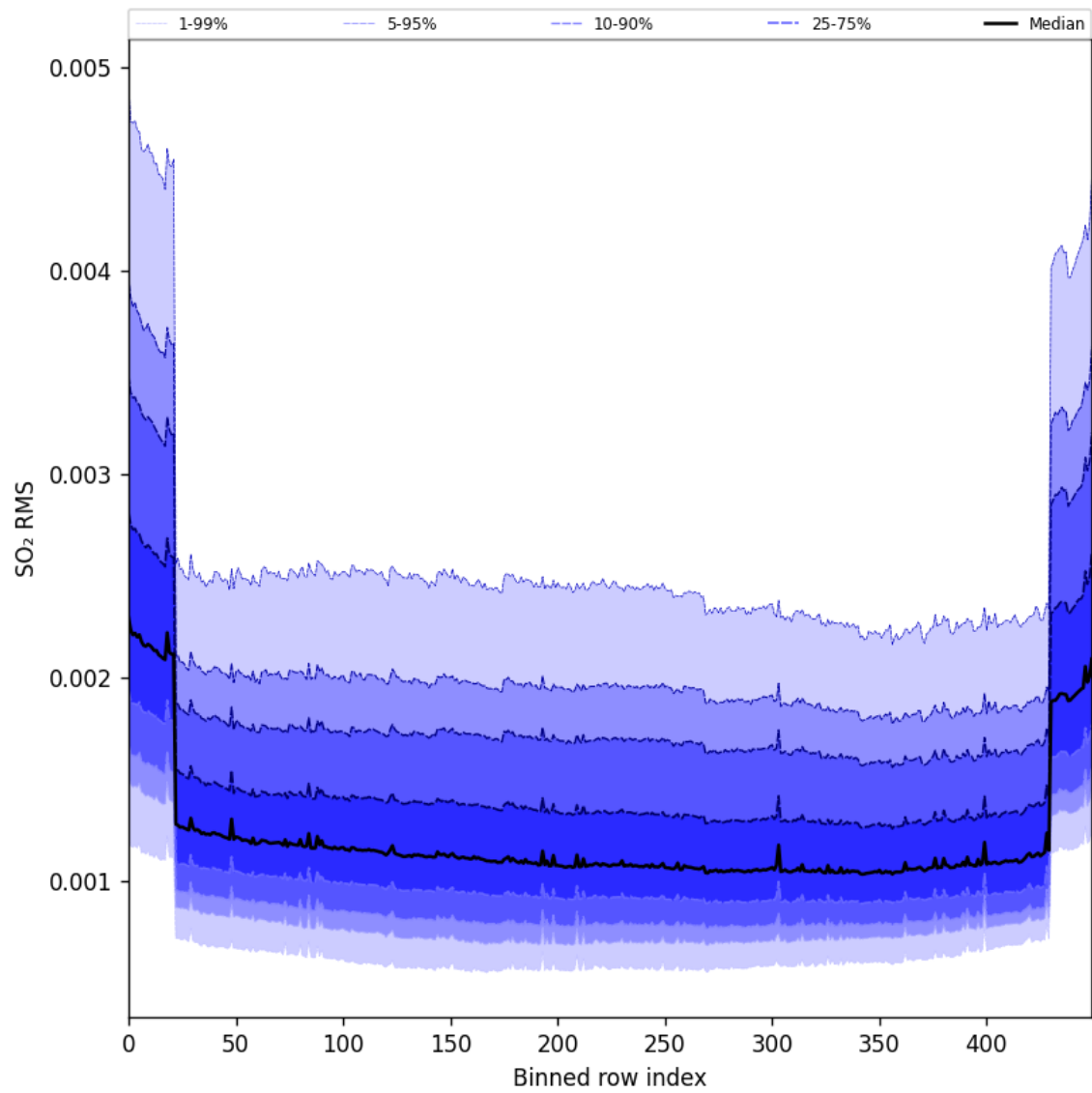
Figure 104: Along track statistics of “SO 2 RMS” for 2025-05-13 to 2025-05-15
