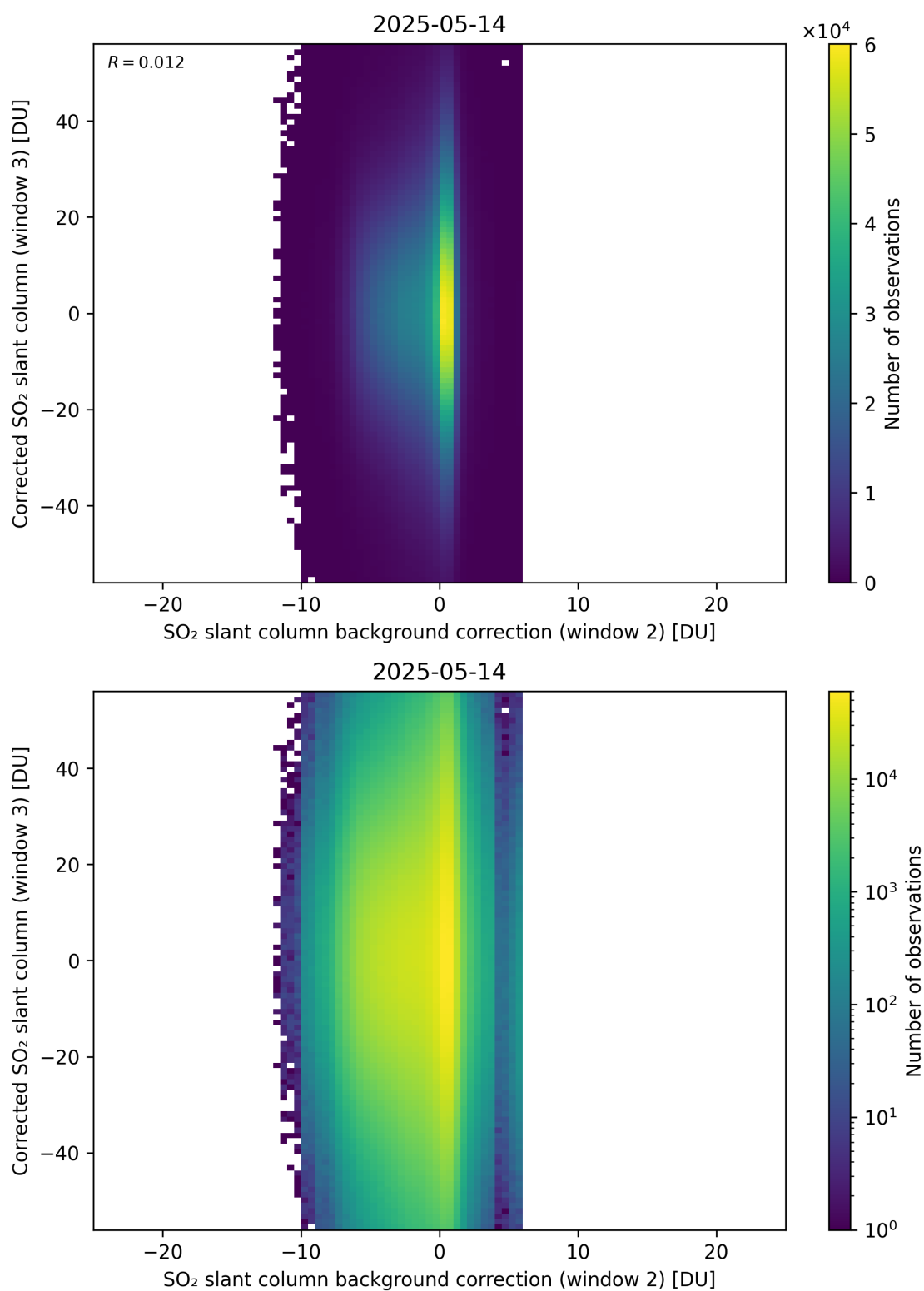
Figure 127: Scatter density plot of “SO 2 slant column background correction (window 2)” against “Corrected SO 2 slant column (window 3)” for 2025-05-13 to 2025-05-15.
