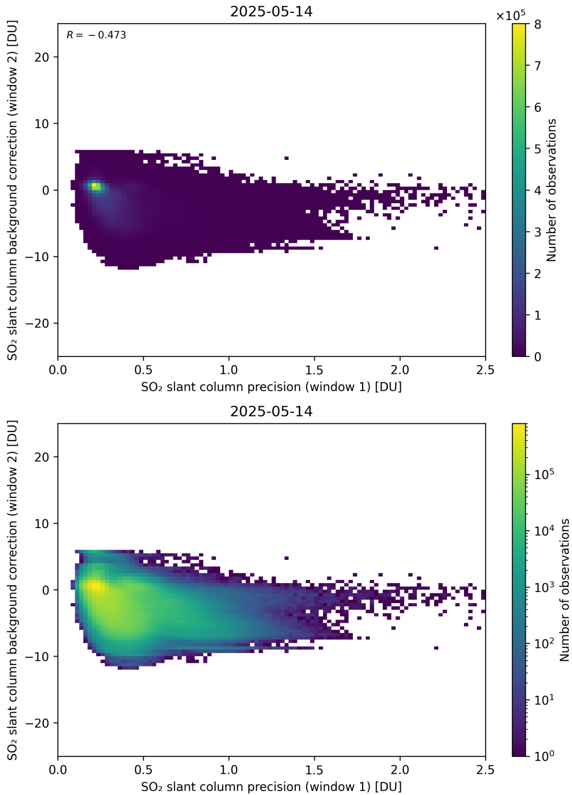
Figure 269: Scatter density plot of “SO 2 slant column precision (window 1)” against “SO 2 slant column background correction (window 2)” for 2025-05-13 to 2025-05-15.
