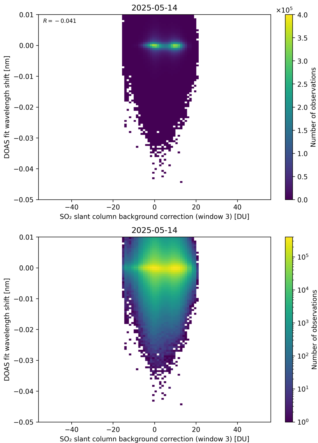
Figure 132: Scatter density plot of “SO 2 slant column background correction (window 3)” against “DOAS fit wavelength shift” for 2025-05-13 to 2025-05-15.
