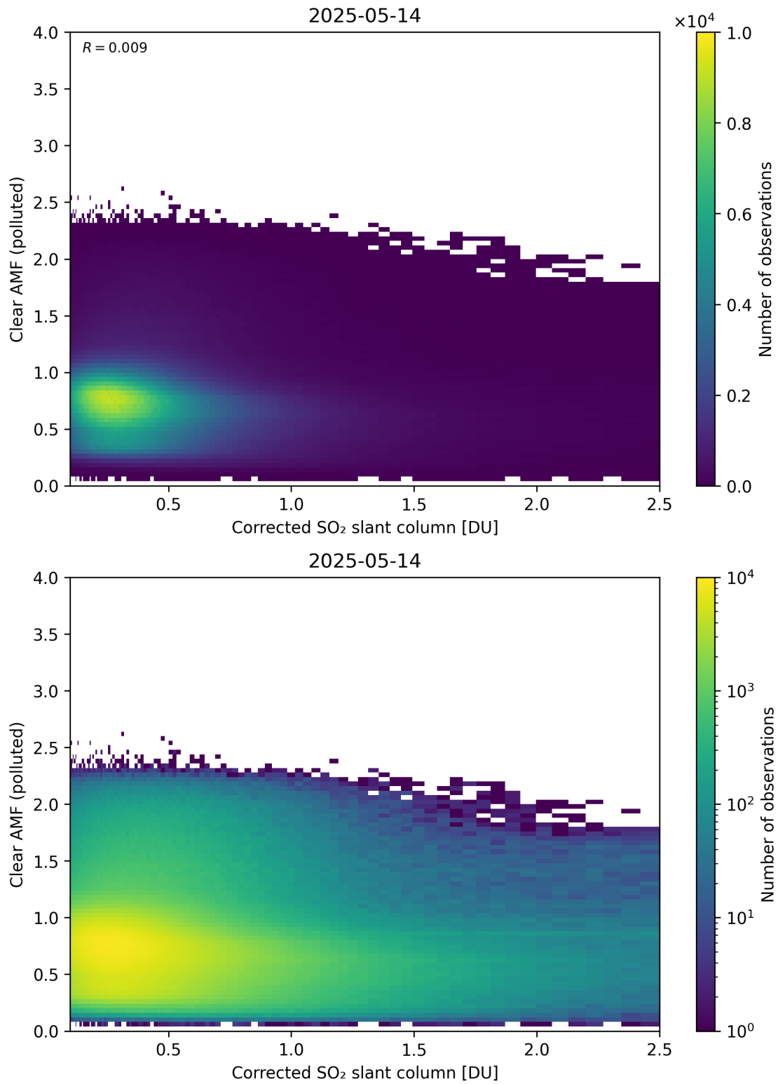
Figure 232: Scatter density plot of “Corrected SO 2 slant column” against “Clear AMF (polluted)” for 2025-05-13 to 2025-05-15.
