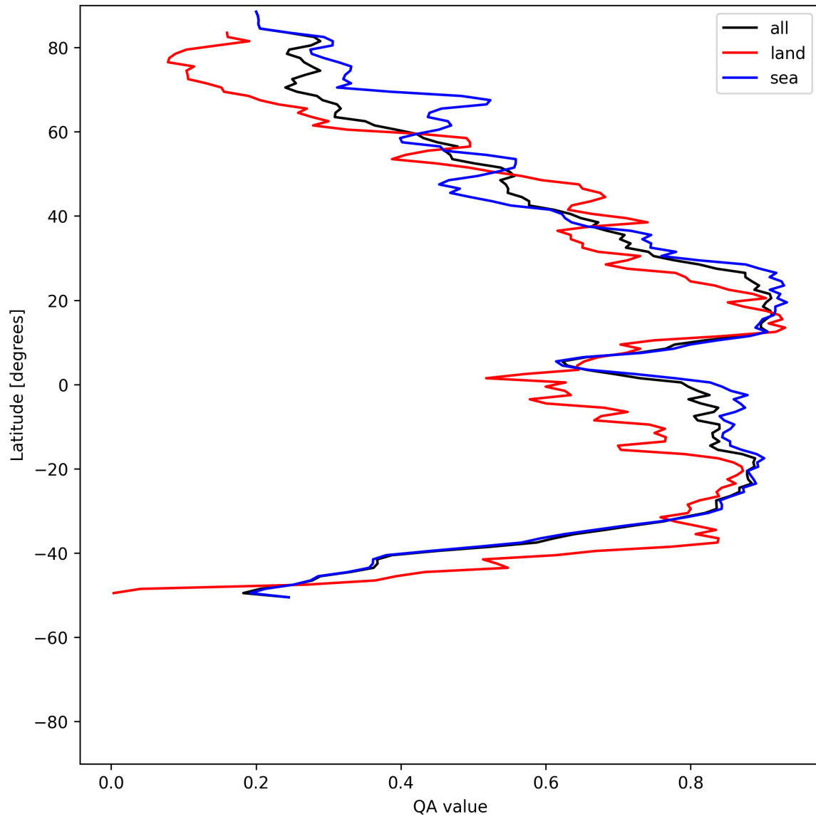
Figure 31: Zonal average of “QA value” for 2025-05-13 to 2025-05-15.
