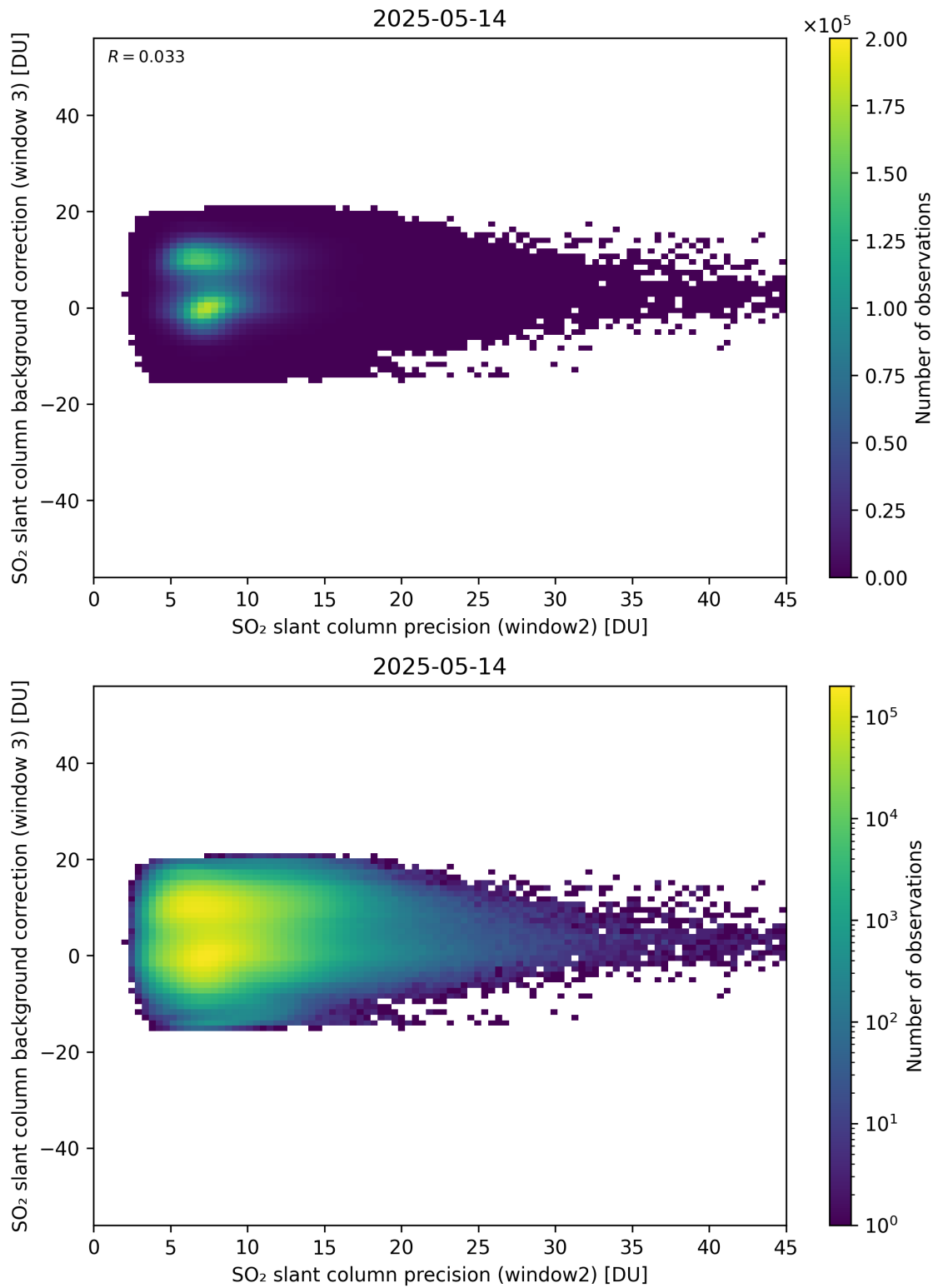
Figure 292: Scatter density plot of “SO 2 slant column precision (window2)” against “SO 2 slant column background correction (window 3)” for 2025-05-13 to 2025-05-15.
