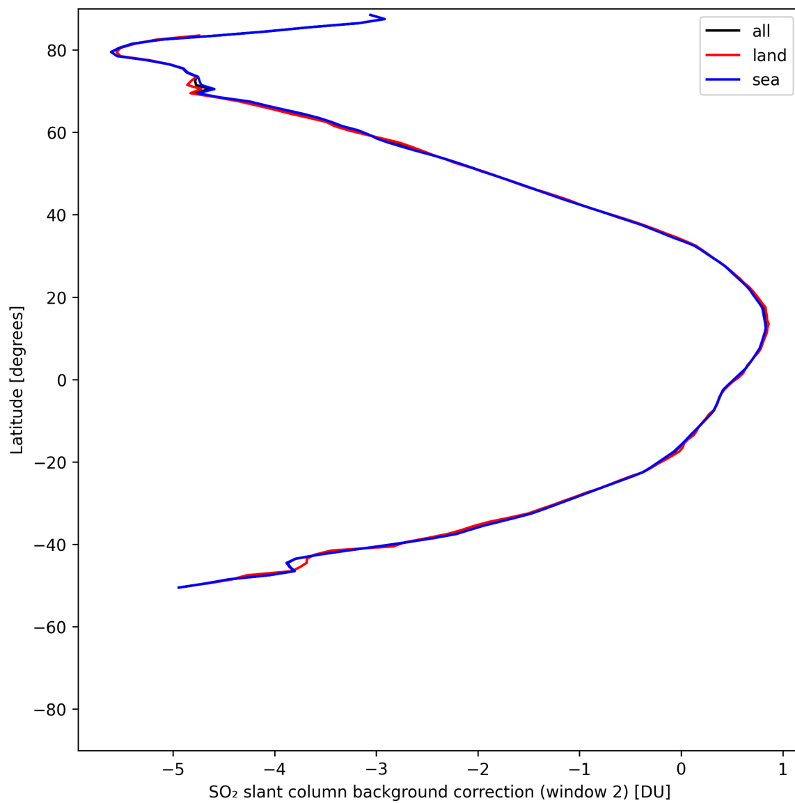
Figure 44: Zonal average of “SO 2 slant column background correction (window 2)” for 2025-05-13 to 2025-05-15.
