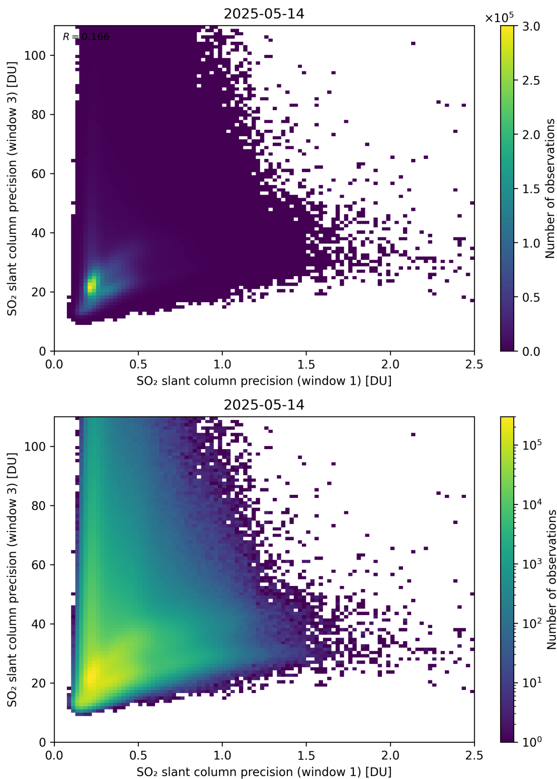
Figure 279: Scatter density plot of “SO 2 slant column precision (window 1)” against “SO 2 slant column precision (window 3)” for 2025-05-13 to 2025-05-15.
