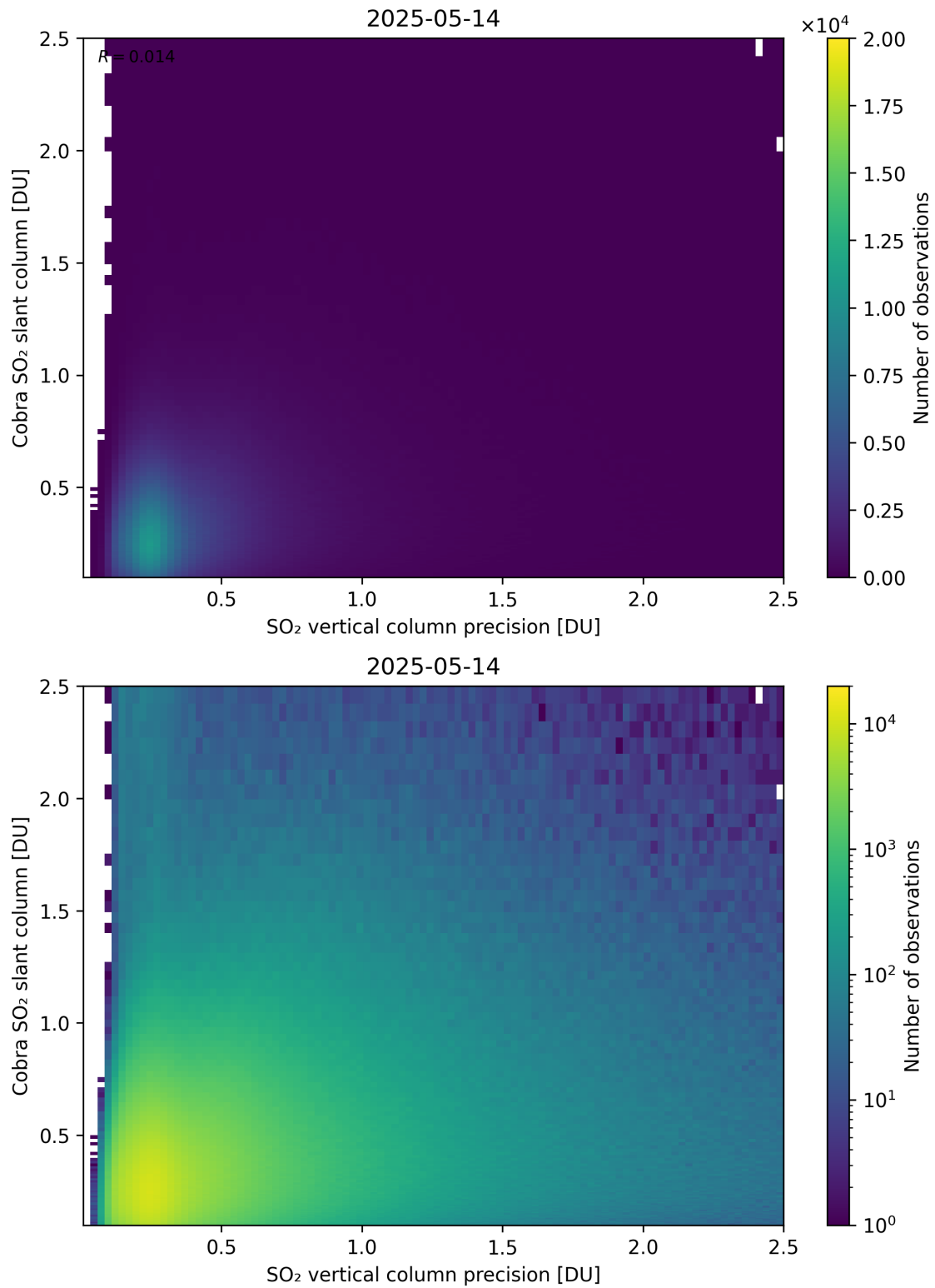
Figure 336: Scatter density plot of “SO 2 vertical column precision” against “Cobra SO 2 slant column” for 2025-05-13 to 2025-05-15.
