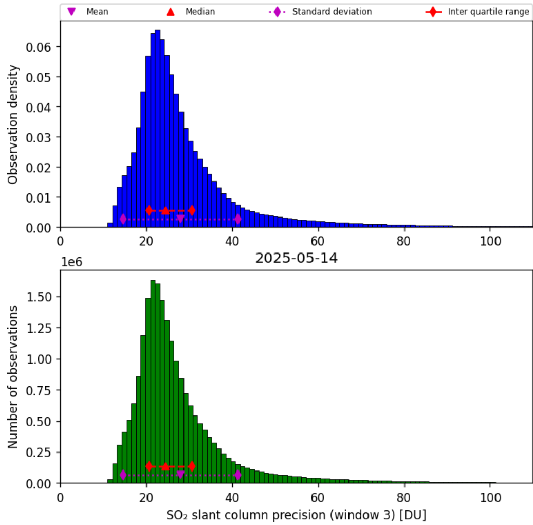
Figure 72: Histogram of “SO 2 slant column precision (window 3)” for 2025-05-13 to 2025-05-15
