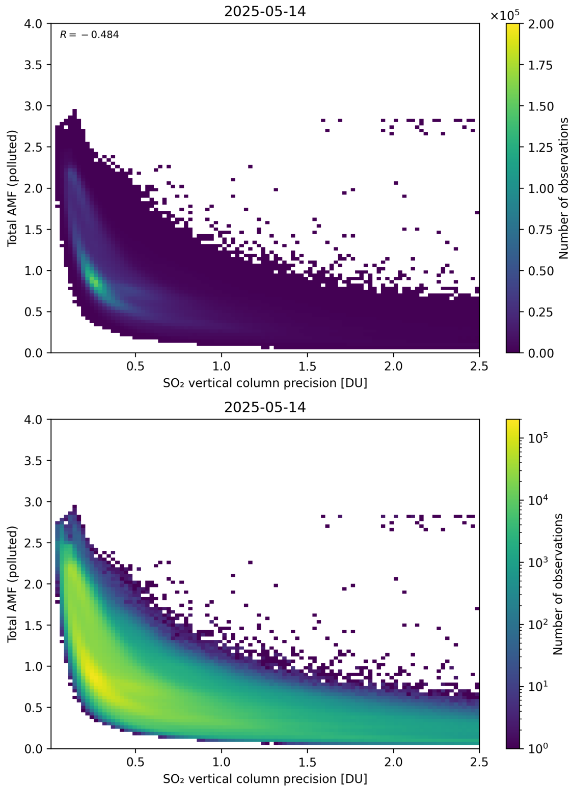
Figure 346: Scatter density plot of “SO 2 vertical column precision” against “Total AMF (polluted)” for 2025-05-13 to 2025-05-15.
