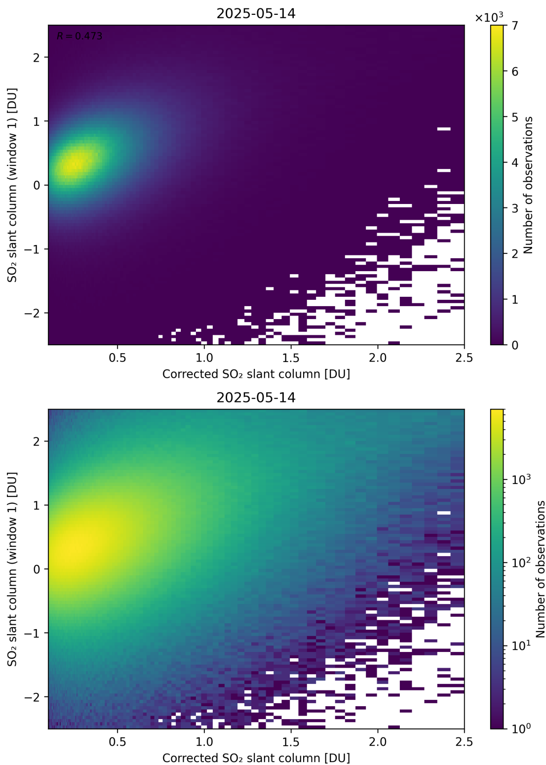
Figure 237: Scatter density plot of “Corrected SO 2 slant column” against “SO 2 slant column (window 1)” for 2025-05-13 to 2025-05-15.
