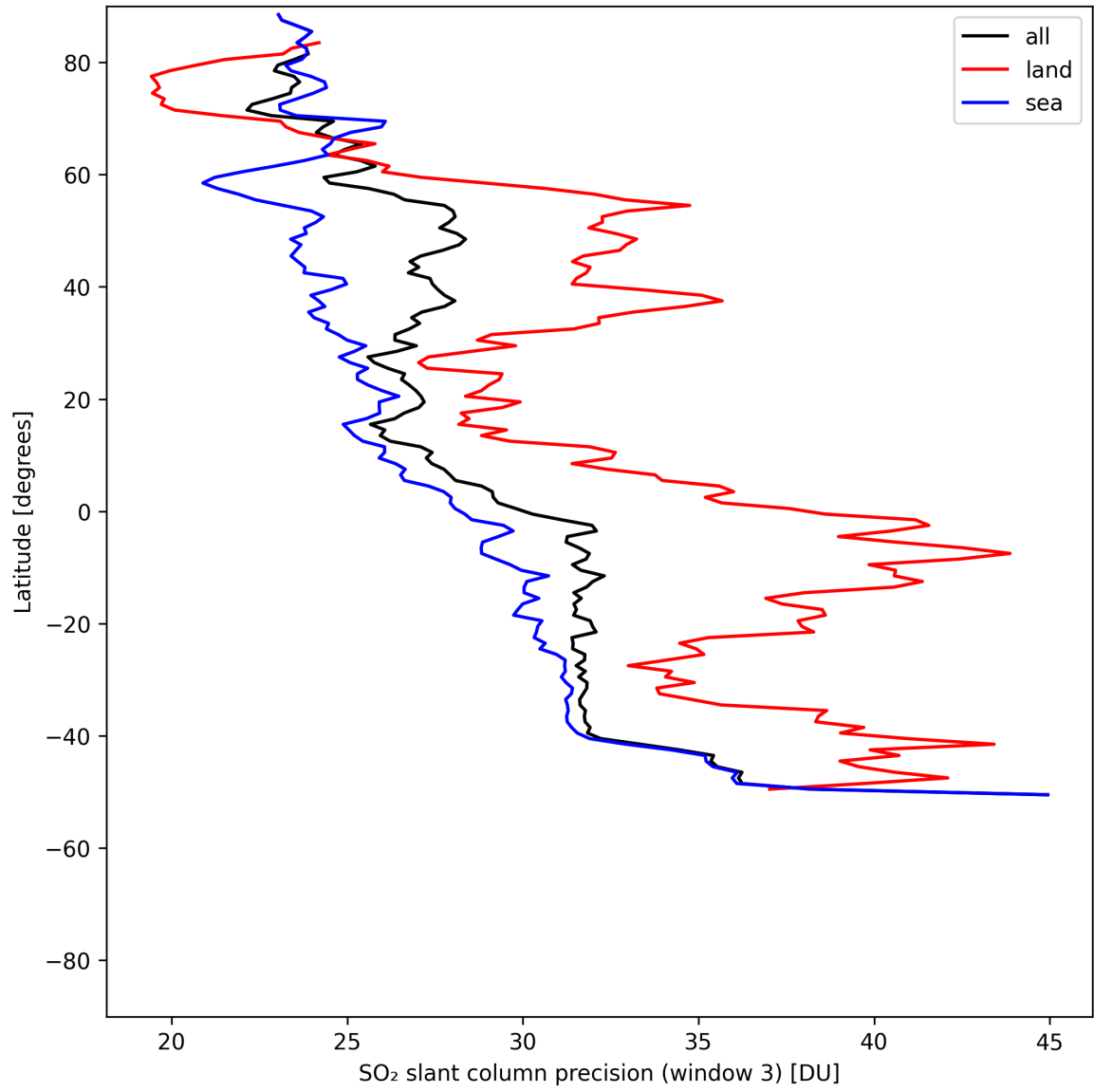
Figure 46: Zonal average of “SO 2 slant column precision (window 3)” for 2025-05-13 to 2025-05-15.
