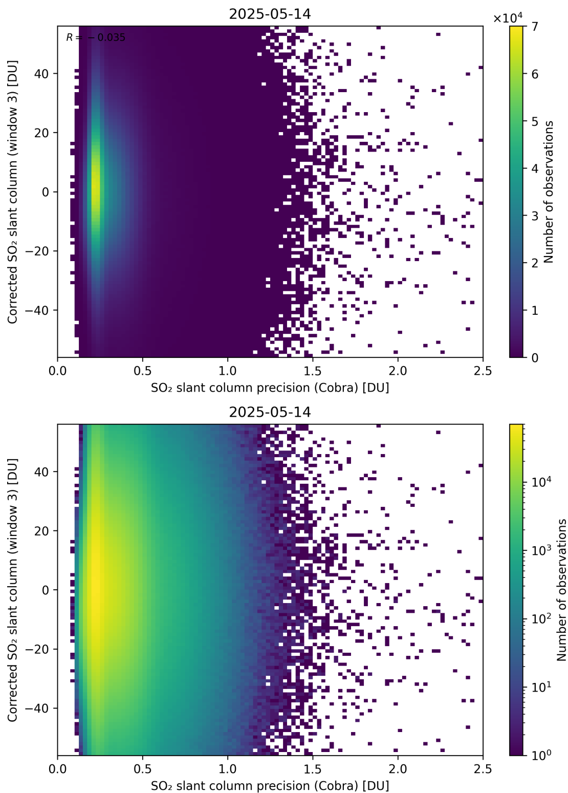
Figure 207: Scatter density plot of “SO 2 slant column precision (Cobra)” against “Corrected SO 2 slant column (window 3)” for 2025-05-13 to 2025-05-15.
