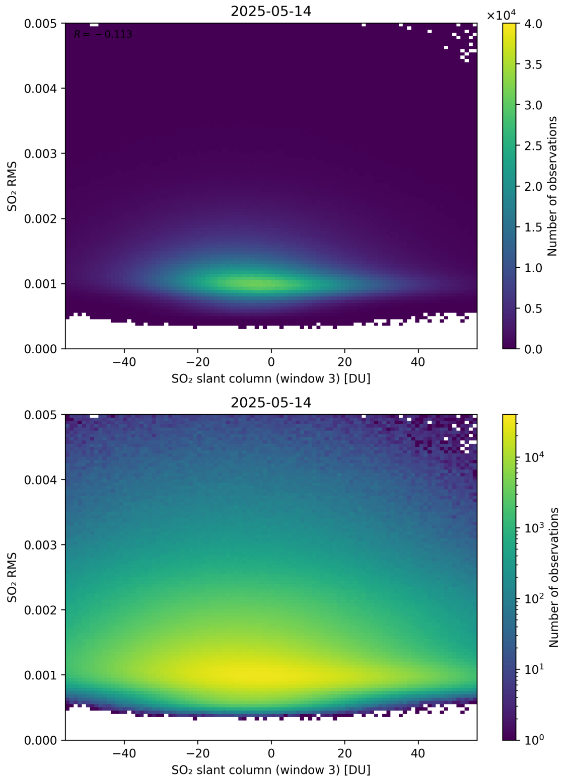
Figure 306: Scatter density plot of “SO 2 slant column (window 3)” against “SO 2 RMS” for 2025-05-13 to 2025-05-15.
