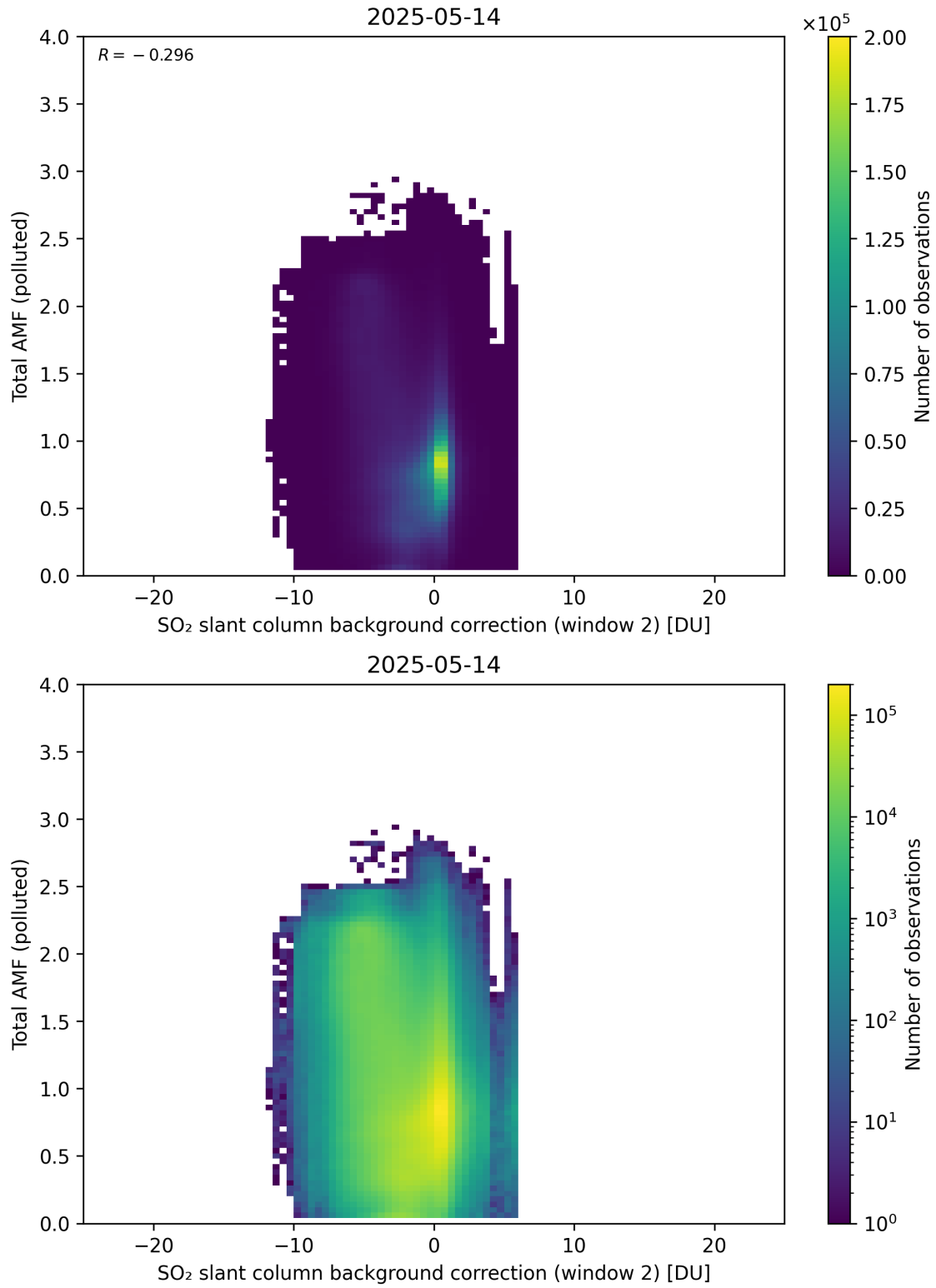
Figure 130: Scatter density plot of “SO 2 slant column background correction (window 2)” against “Total AMF (polluted)” for 2025-05-13 to 2025-05-15.
