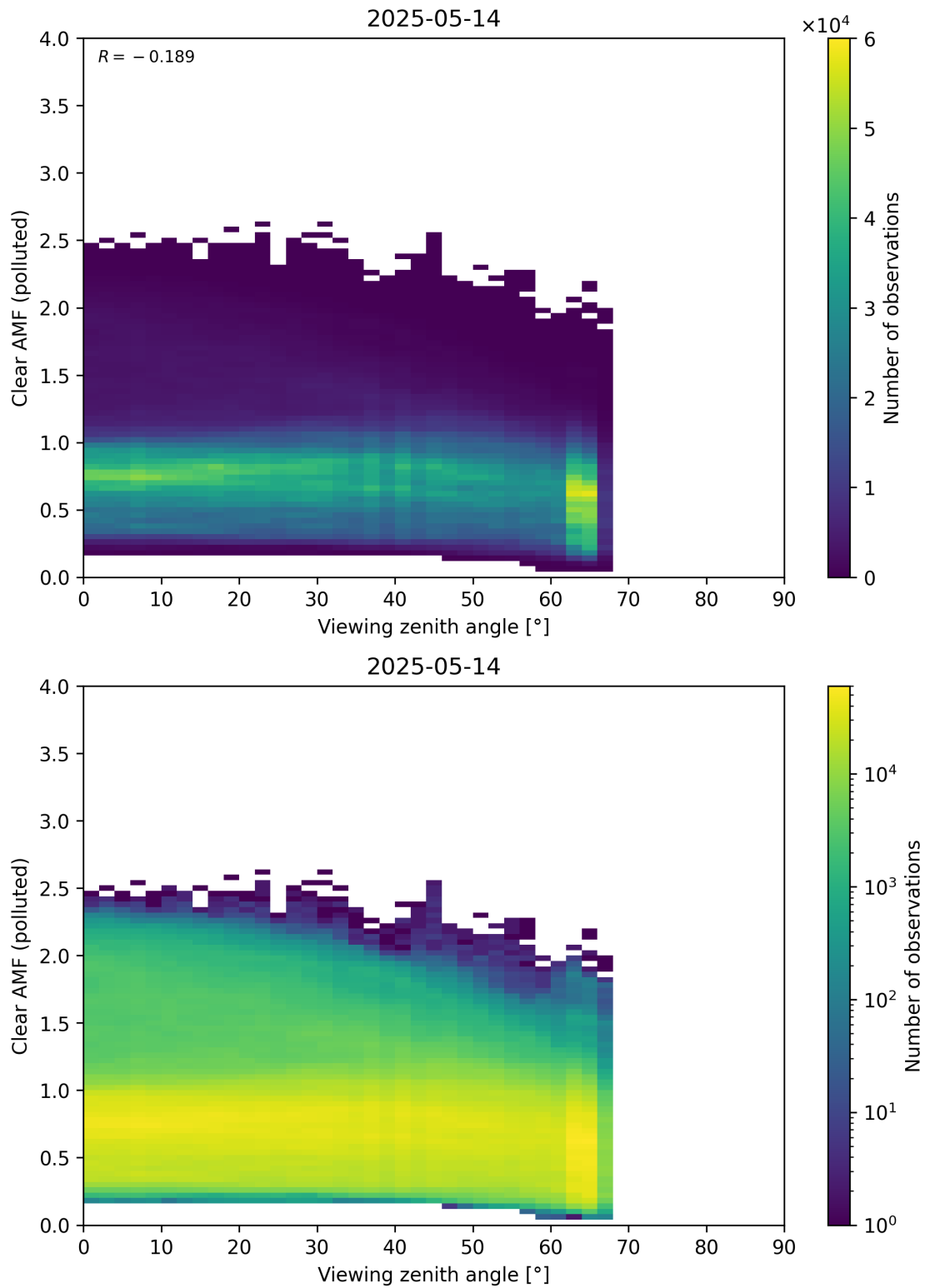
Figure 370: Scatter density plot of “Viewing zenith angle” against “Clear AMF (polluted)” for 2025-05-13 to 2025-05-15.
