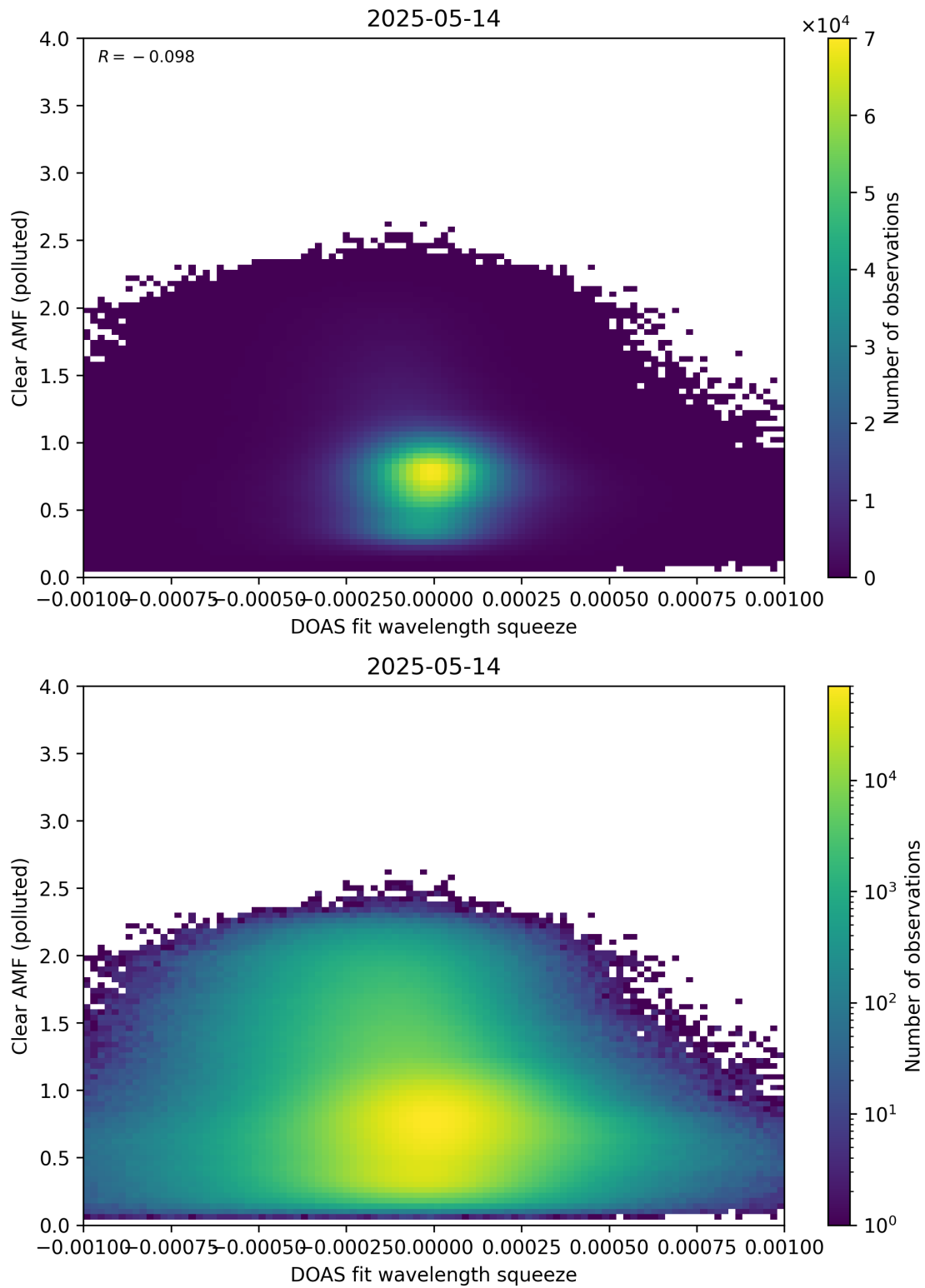
Figure 144: Scatter density plot of “DOAS fit wavelength squeeze” against “Clear AMF (polluted)” for 2025-05-13 to 2025-05-15.
