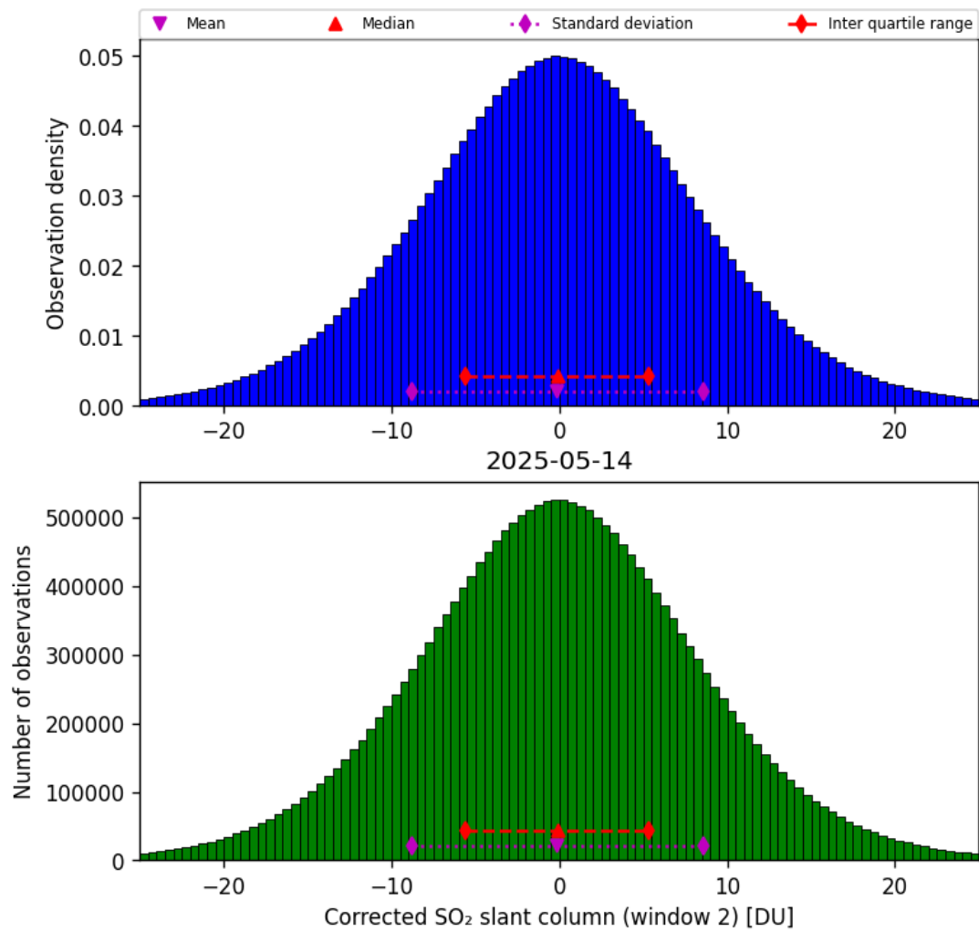
Figure 69: Histogram of “Corrected SO 2 slant column (window 2)” for 2025-05-13 to 2025-05-15
