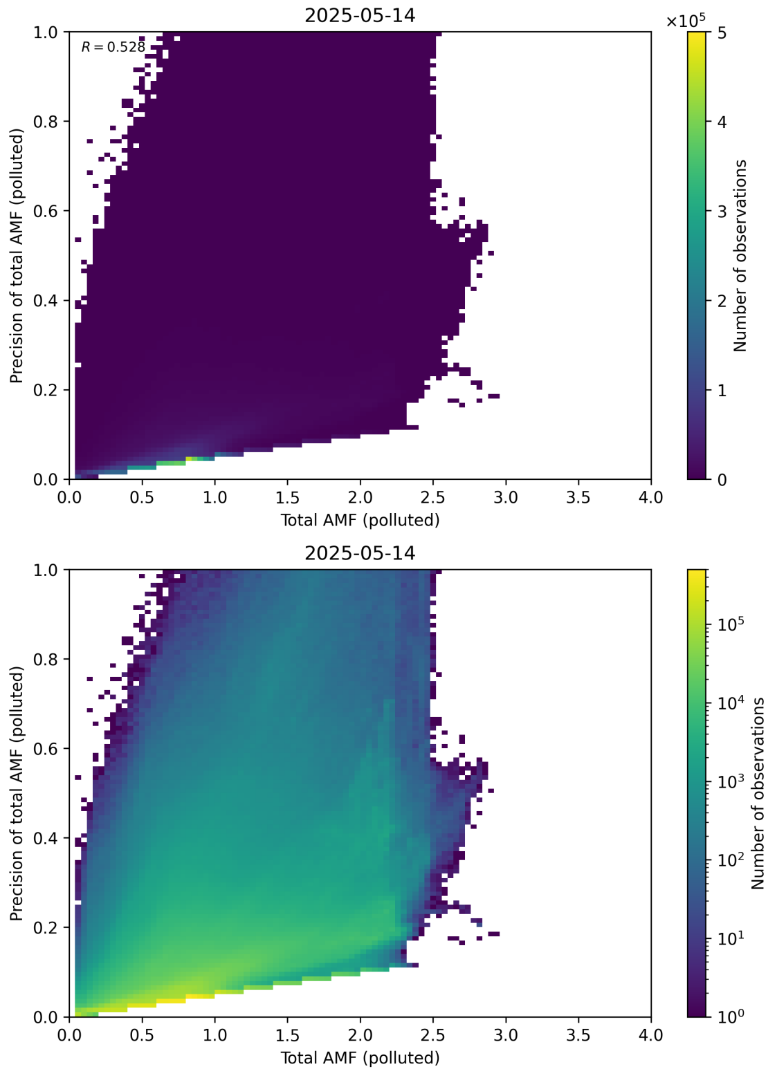
Figure 322: Scatter density plot of “Total AMF (polluted)” against “Precision of total AMF (polluted)” for 2025-05-13 to 2025-05-15.
