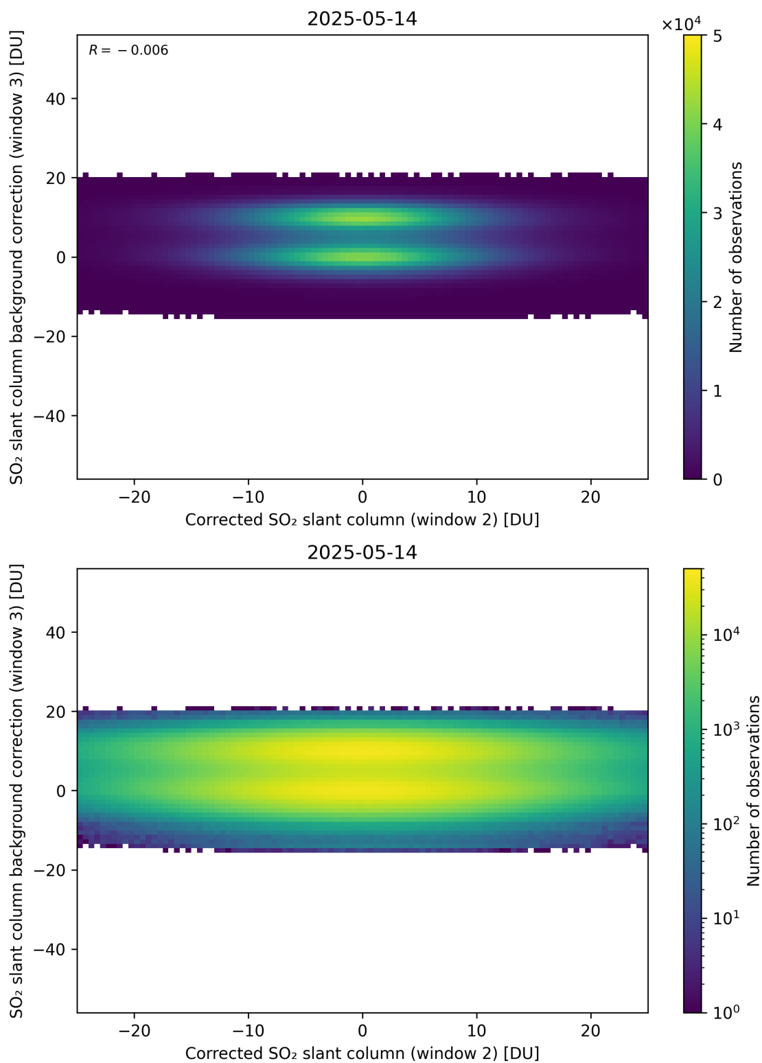
Figure 245: Scatter density plot of “Corrected SO 2 slant column (window 2)” against “SO 2 slant column background correction (window 3)” for 2025-05-13 to 2025-05-15.
