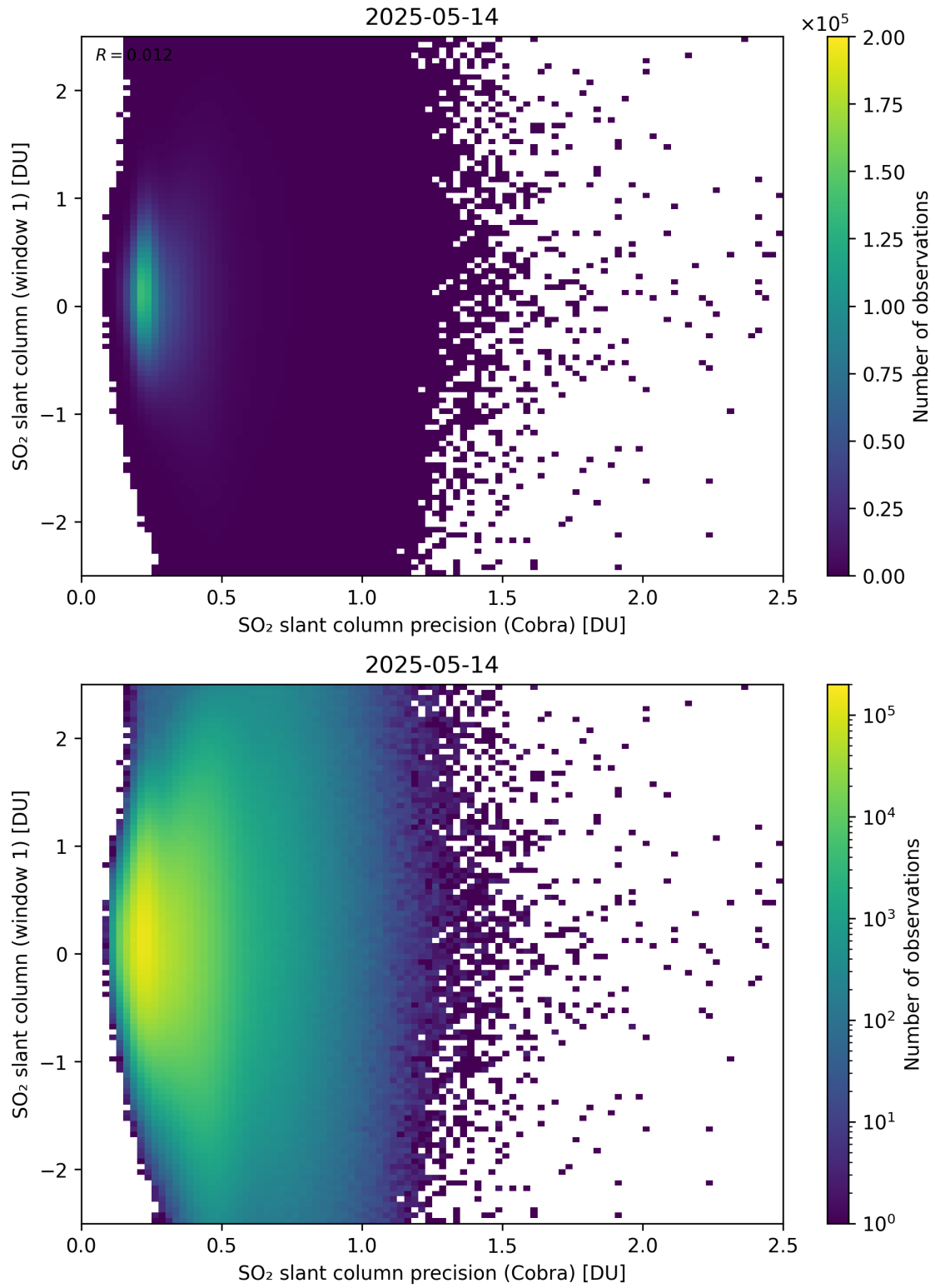
Figure 208: Scatter density plot of “SO 2 slant column precision (Cobra)” against “SO 2 slant column (window 1)” for 2025-05-13 to 2025-05-15.
