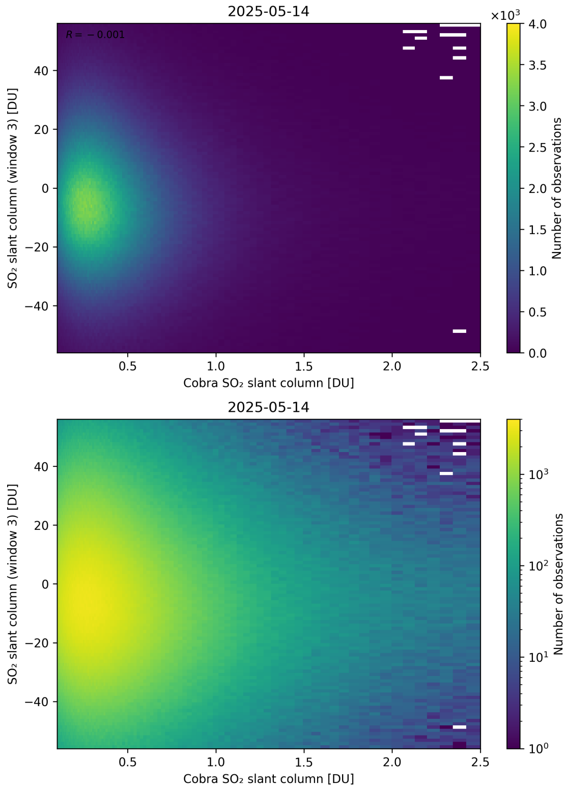
Figure 222: Scatter density plot of “Cobra SO 2 slant column” against “SO 2 slant column (window 3)” for 2025-05-13 to 2025-05-15.
