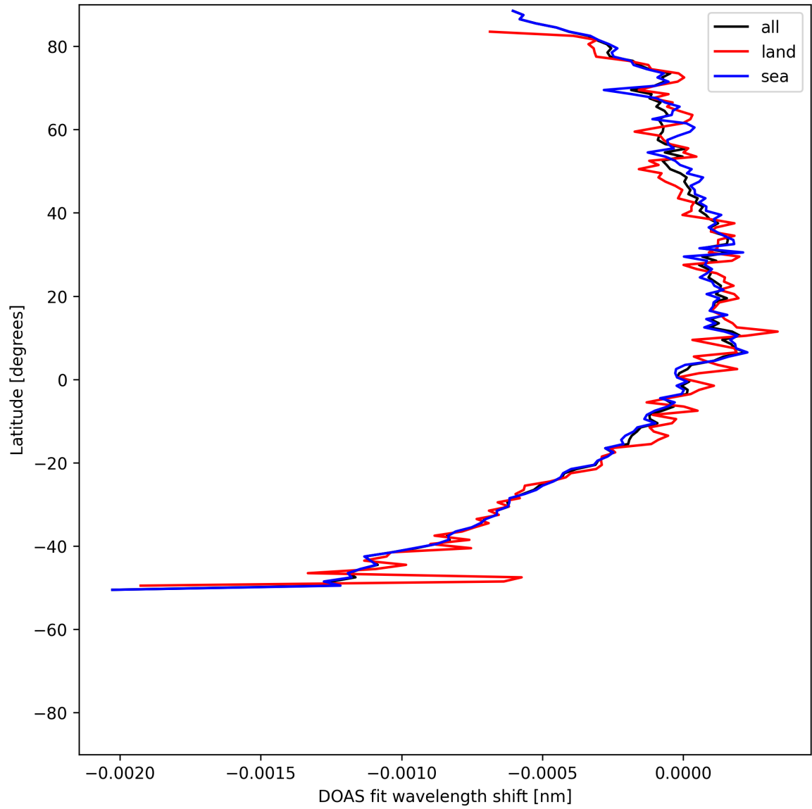
Figure 50: Zonal average of “DOAS fit wavelength shift” for 2025-05-13 to 2025-05-15.
