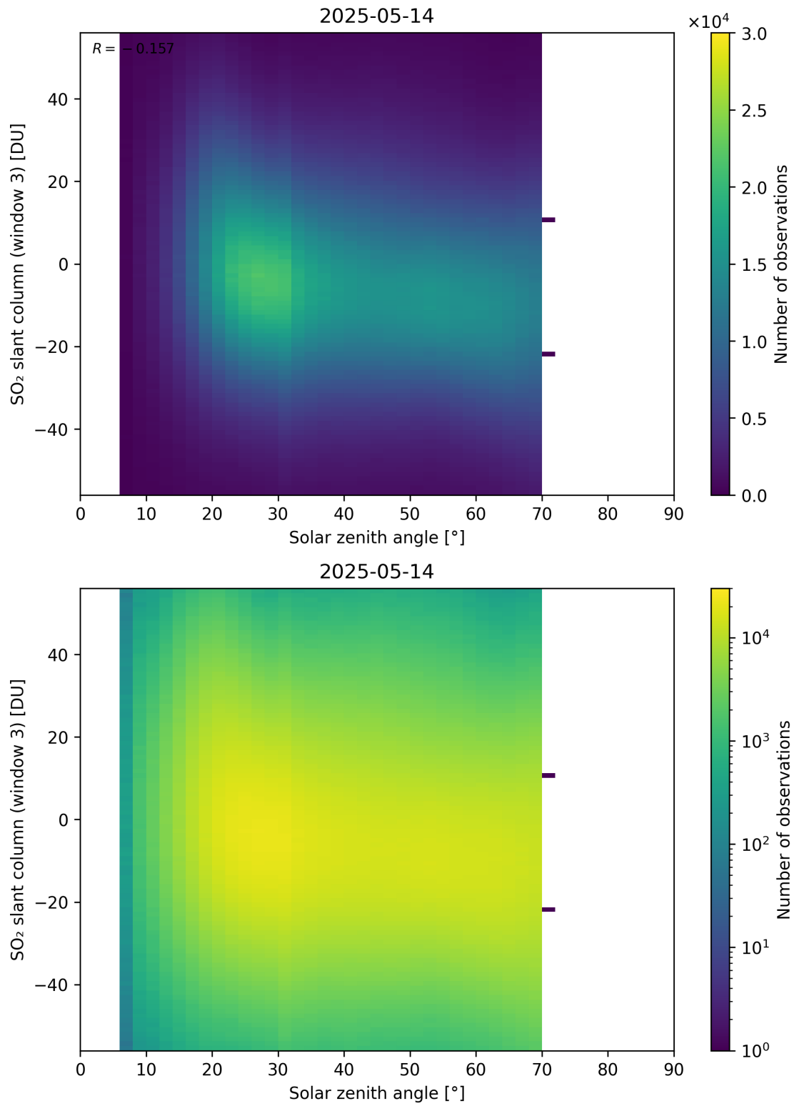
Figure 187: Scatter density plot of “Solar zenith angle” against “SO 2 slant column (window 3)” for 2025-05-13 to 2025-05-15.
