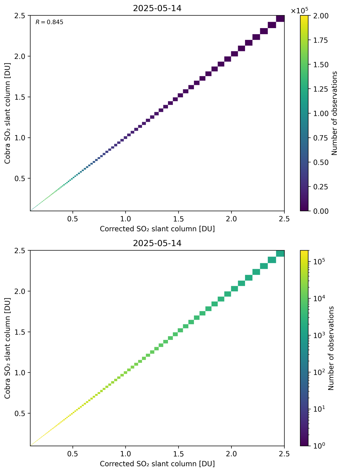
Figure 233: Scatter density plot of “Corrected SO 2 slant column” against “Cobra SO 2 slant column” for 2025-05-13 to 2025-05-15.
