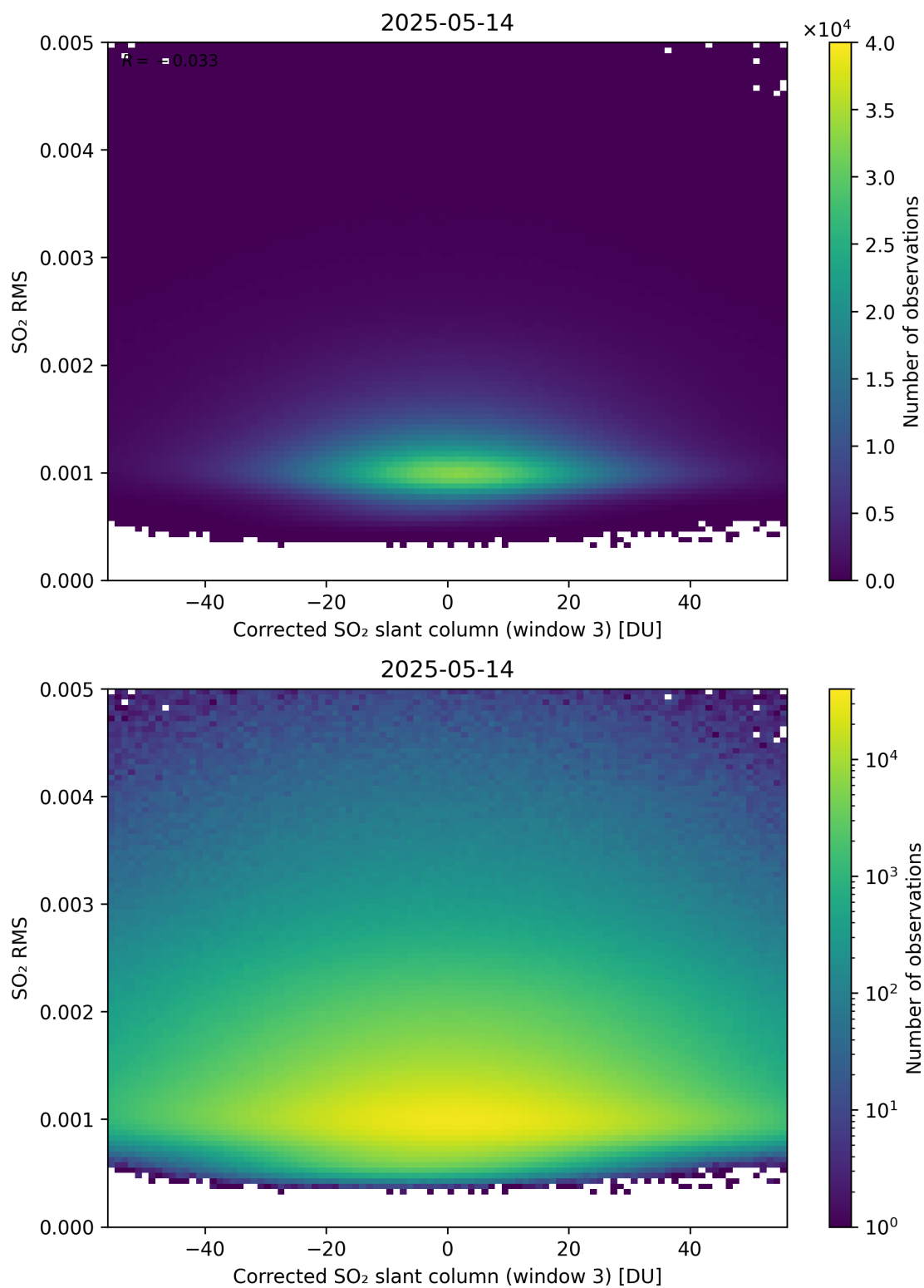
Figure 258: Scatter density plot of “Corrected SO 2 slant column (window 3)” against “SO 2 RMS” for 2025-05-13 to 2025-05-15.
