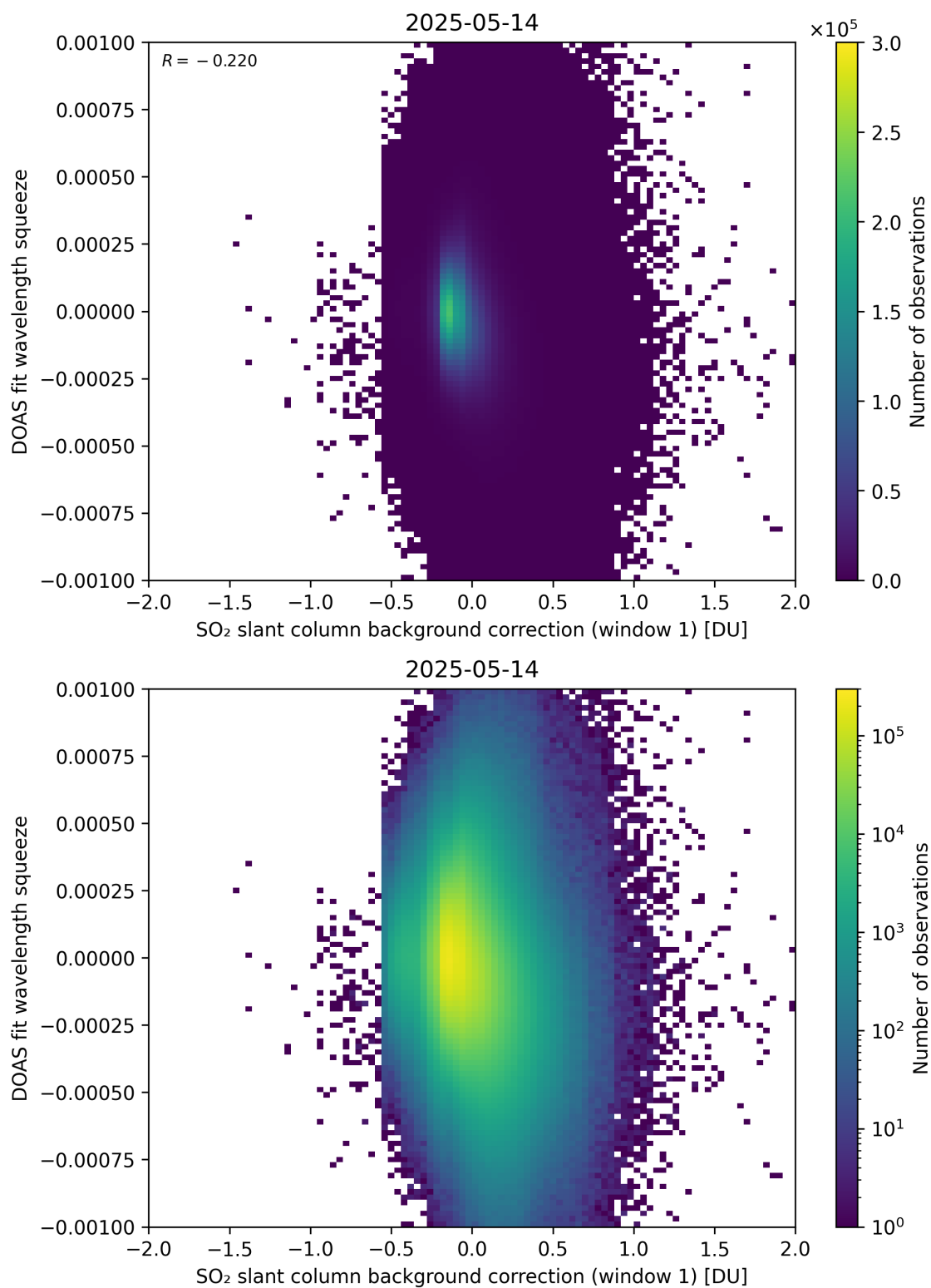
Figure 112: Scatter density plot of “SO 2 slant column background correction (window 1)” against “DOAS fit wavelength squeeze” for 2025-05-13 to 2025-05-15.
