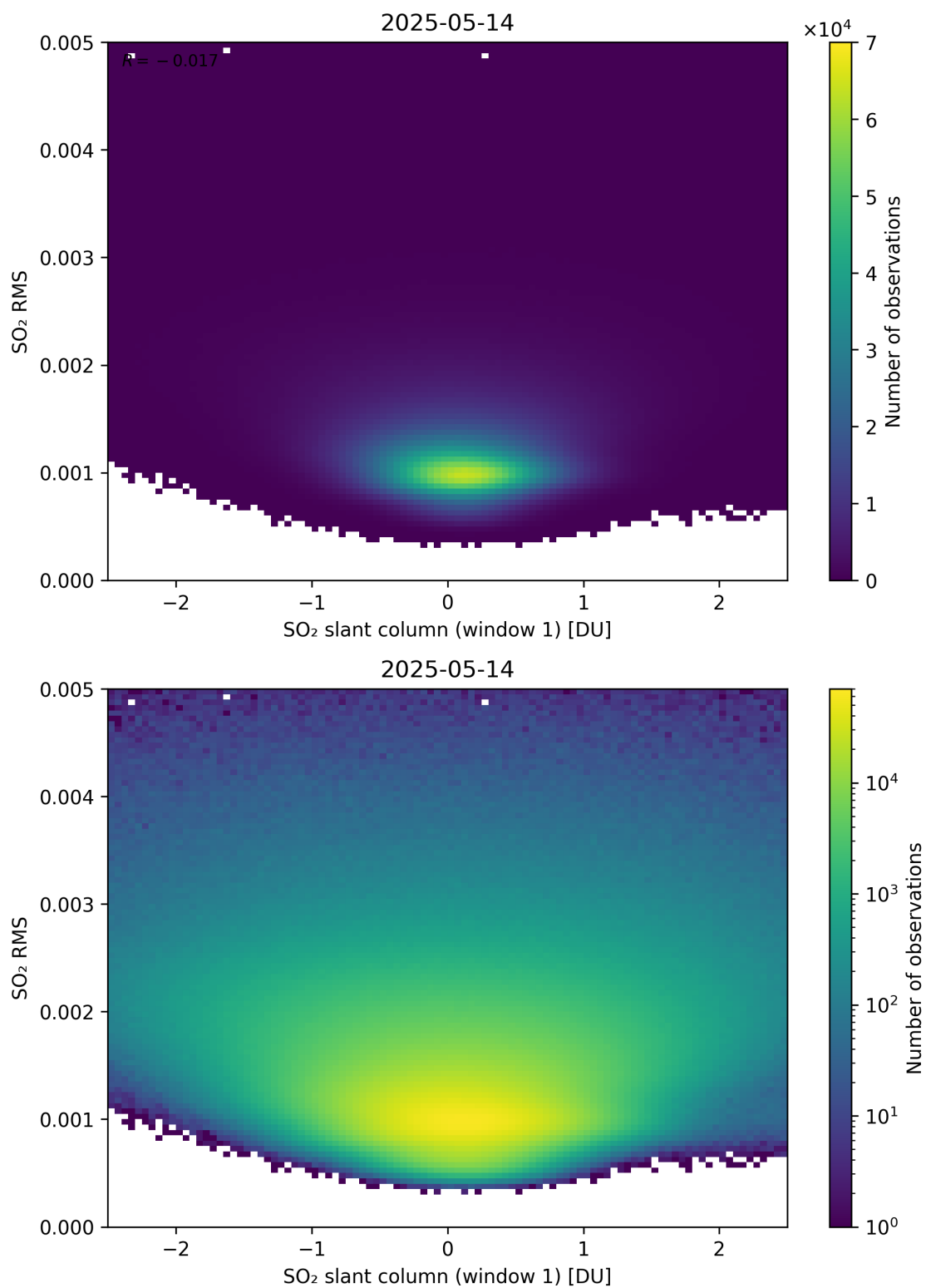
Figure 267: Scatter density plot of “SO 2 slant column (window 1)” against “SO 2 RMS” for 2025-05-13 to 2025-05-15.
