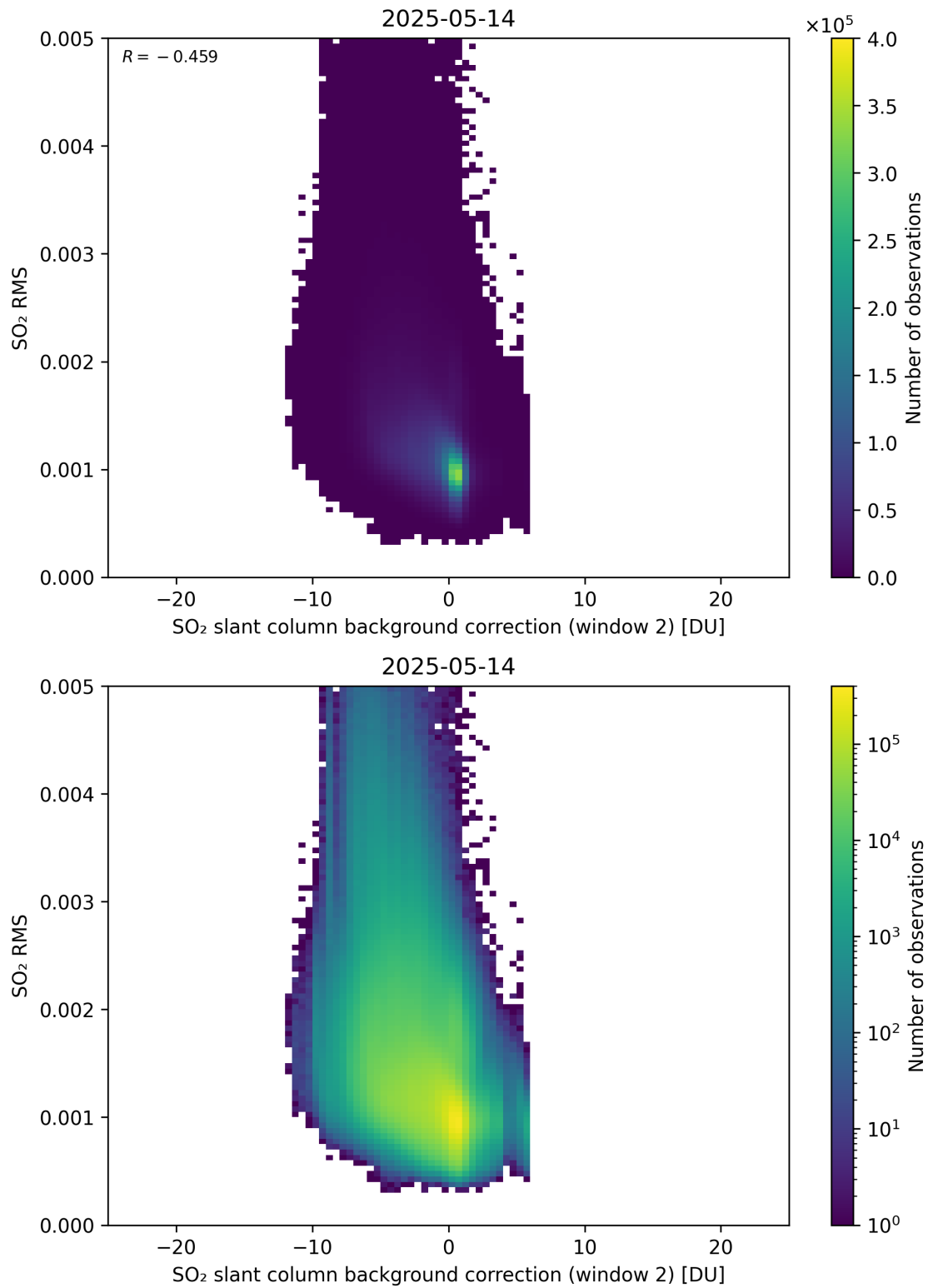
Figure 125: Scatter density plot of “SO 2 slant column background correction (window 2)” against “SO 2 RMS” for 2025-05-13 to 2025-05-15.
