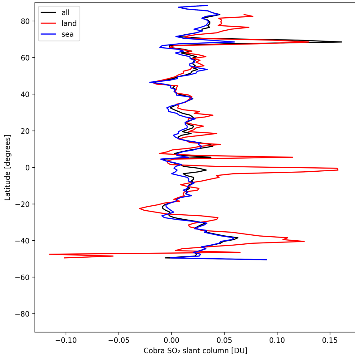
Figure 35: Zonal average of “Cobra SO 2 slant column” for 2025-05-13 to 2025-05-15.
