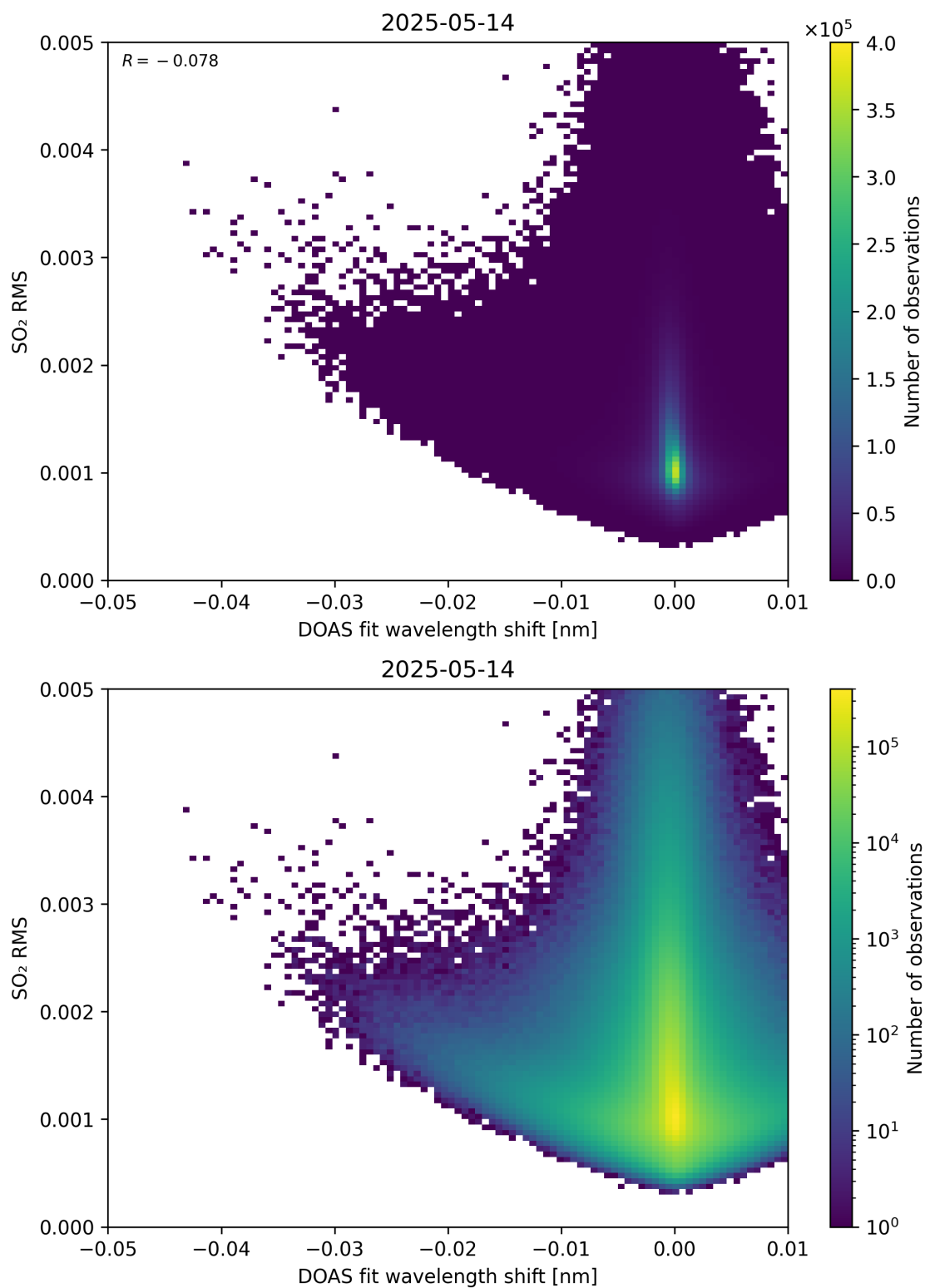
Figure 139: Scatter density plot of “DOAS fit wavelength shift” against “SO 2 RMS” for 2025-05-13 to 2025-05-15.
