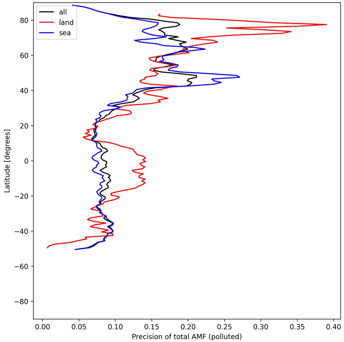
Figure 54: Zonal average of “Precision of total AMF (polluted)” for 2025-05-13 to 2025-05-15.
