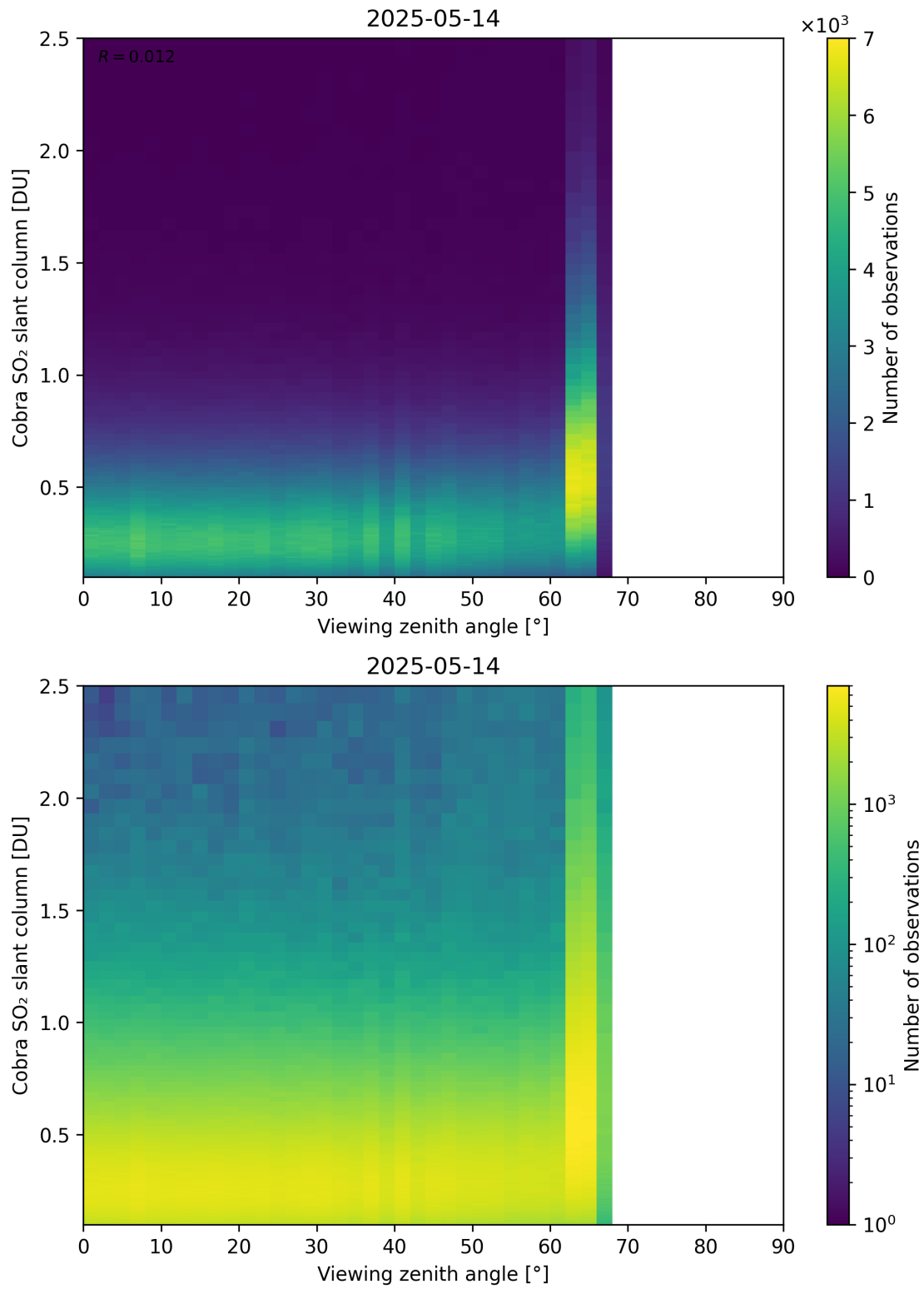
Figure 371: Scatter density plot of “Viewing zenith angle” against “Cobra SO 2 slant column” for 2025-05-13 to 2025-05-15.
