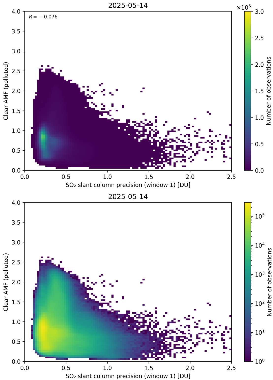
Figure 274: Scatter density plot of “SO 2 slant column precision (window 1)” against “Clear AMF (polluted)” for 2025-05-13 to 2025-05-15.
