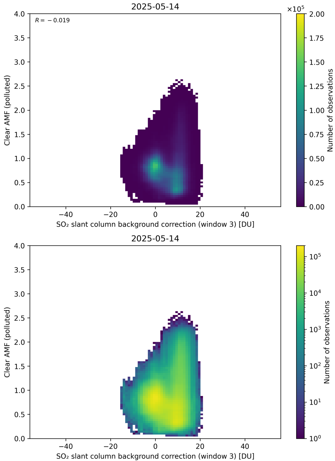
Figure 135: Scatter density plot of “SO 2 slant column background correction (window 3)” against “Clear AMF (polluted)” for 2025-05-13 to 2025-05-15.
