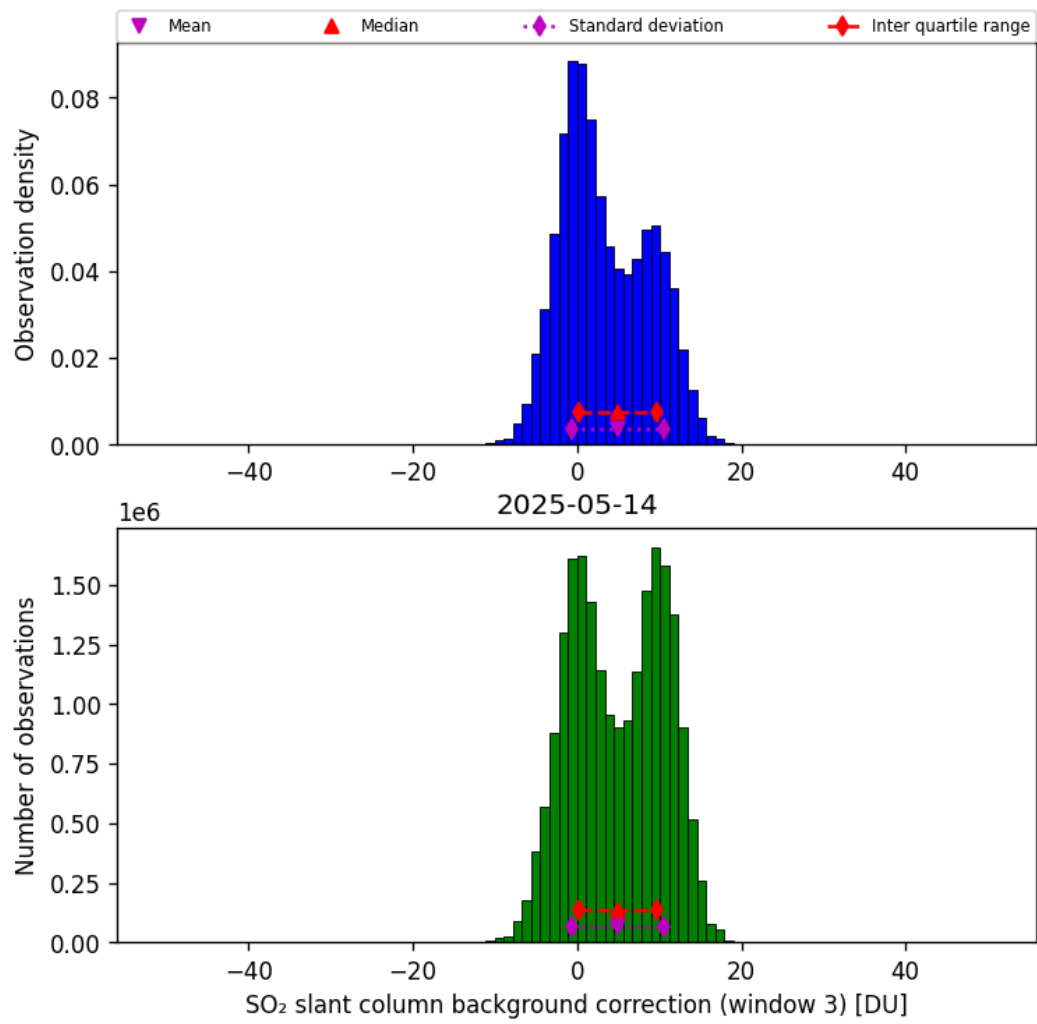
Figure 74: Histogram of “SO 2 slant column background correction (window 3)” for 2025-05-13 to 2025-05-15
