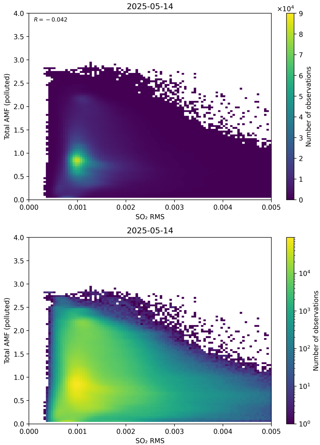
Figure 148: Scatter density plot of “SO 2 RMS” against “Total AMF (polluted)” for 2025-05-13 to 2025-05-15.
