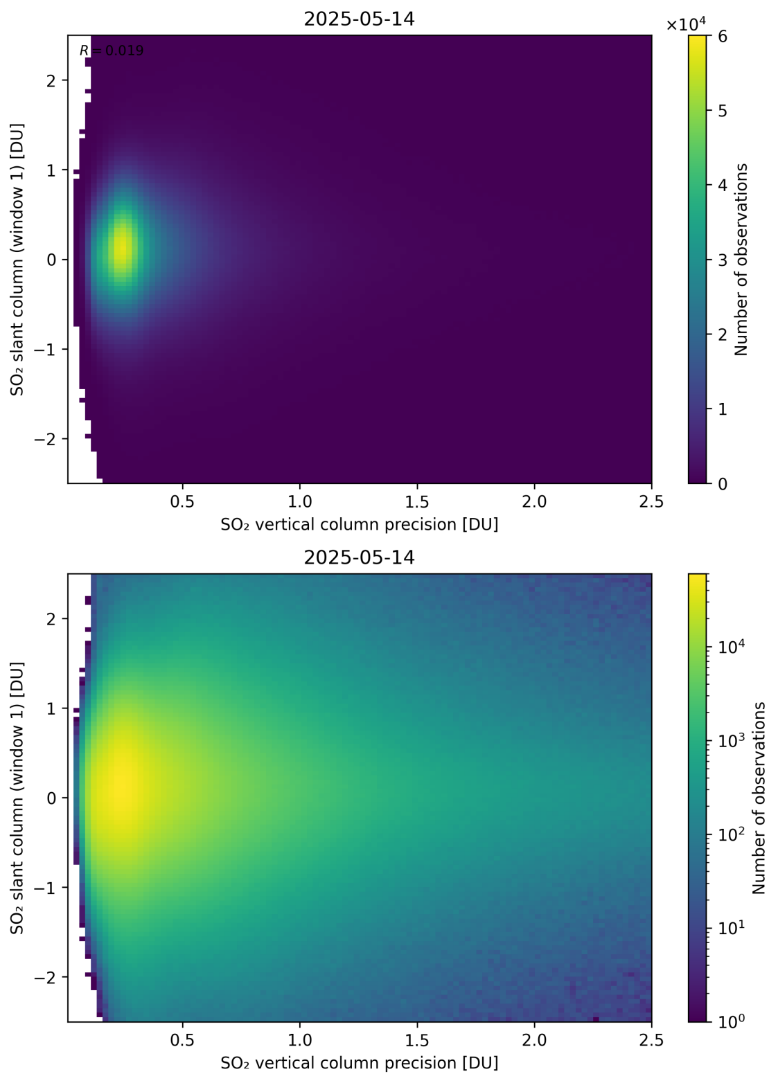
Figure 341: Scatter density plot of “SO 2 vertical column precision” against “SO 2 slant column (window 1)” for 2025-05-13 to 2025-05-15.
