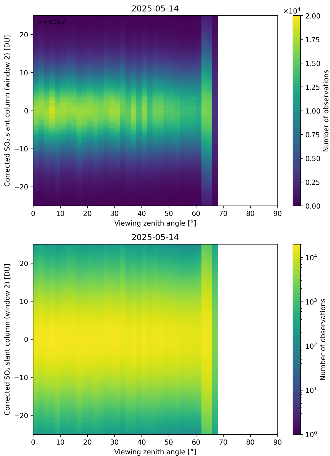
Figure 374: Scatter density plot of “Viewing zenith angle” against “Corrected SO 2 slant column (window 2)” for 2025-05-13 to 2025-05-15.
