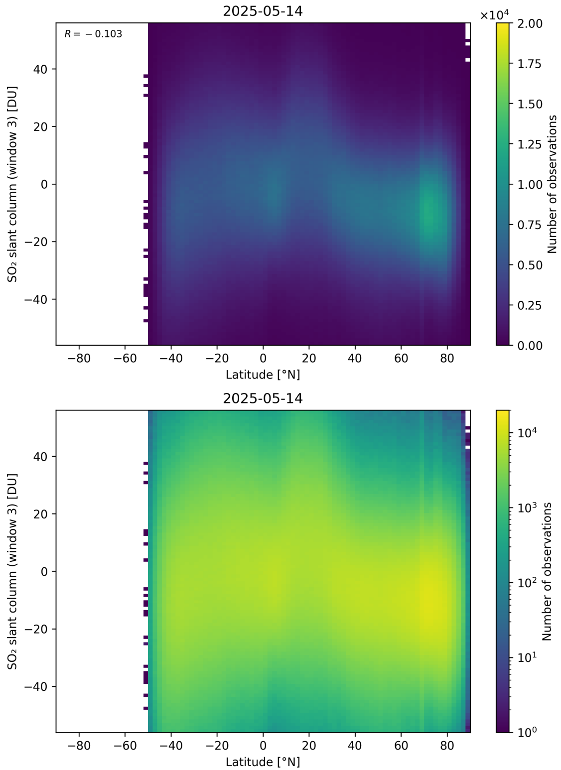
Figure 165: Scatter density plot of “Latitude” against “SO 2 slant column (window 3)” for 2025-05-13 to 2025-05-15.
