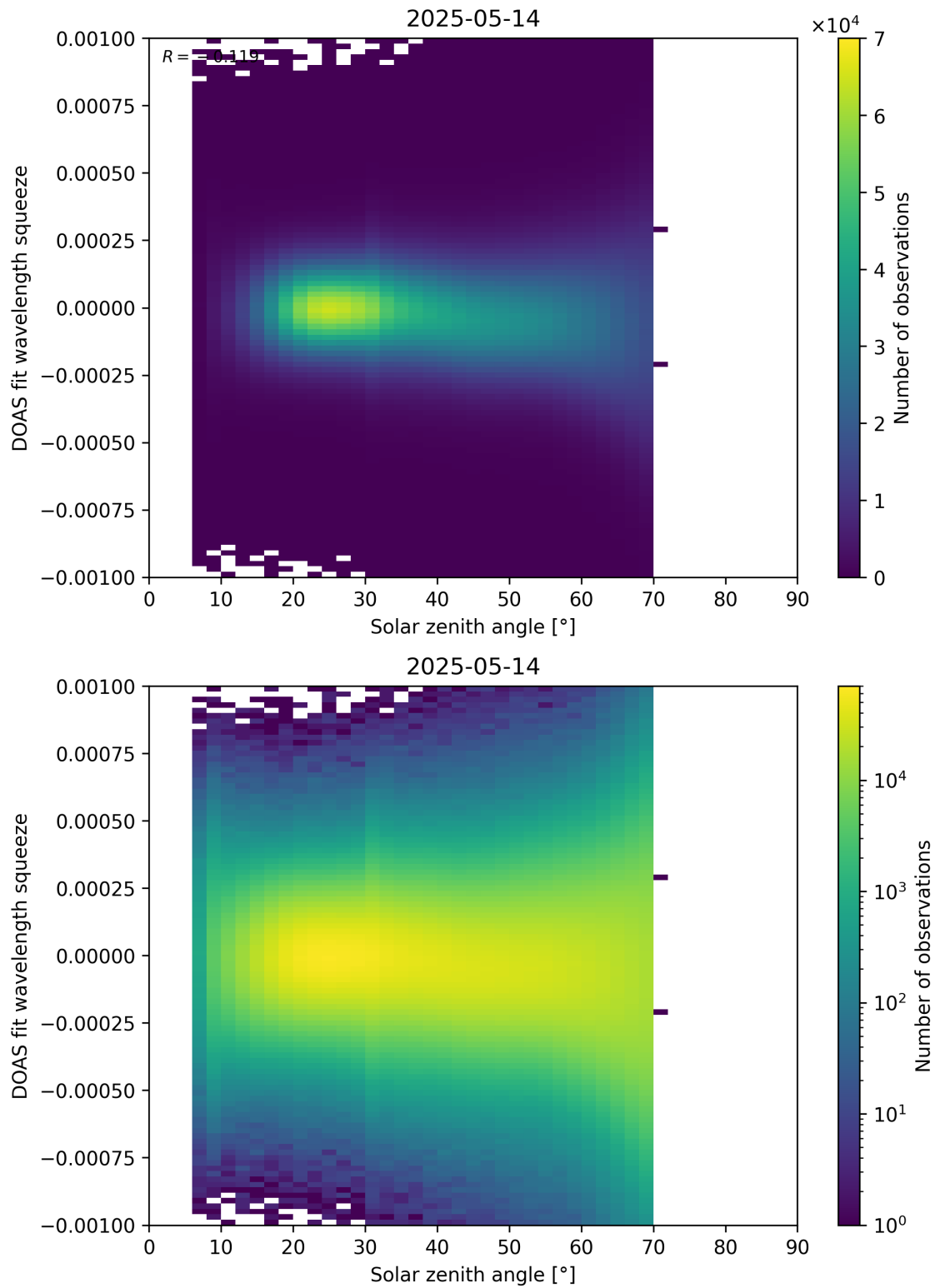
Figure 175: Scatter density plot of “Solar zenith angle” against “DOAS fit wavelength squeeze” for 2025-05-13 to 2025-05-15.
