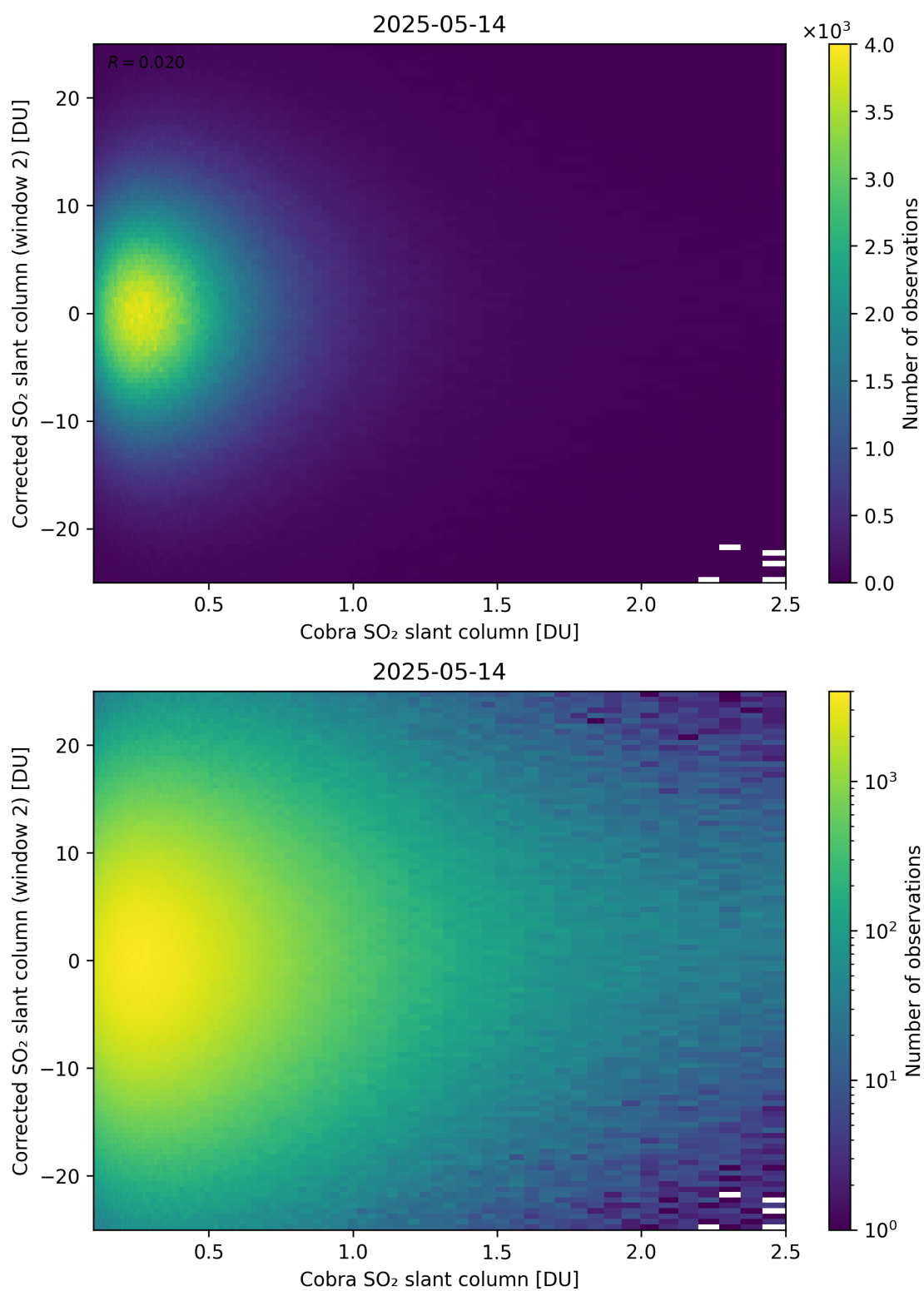
Figure 217: Scatter density plot of “Cobra SO 2 slant column” against “Corrected SO 2 slant column (window 2)” for 2025-05-13 to 2025-05-15.
