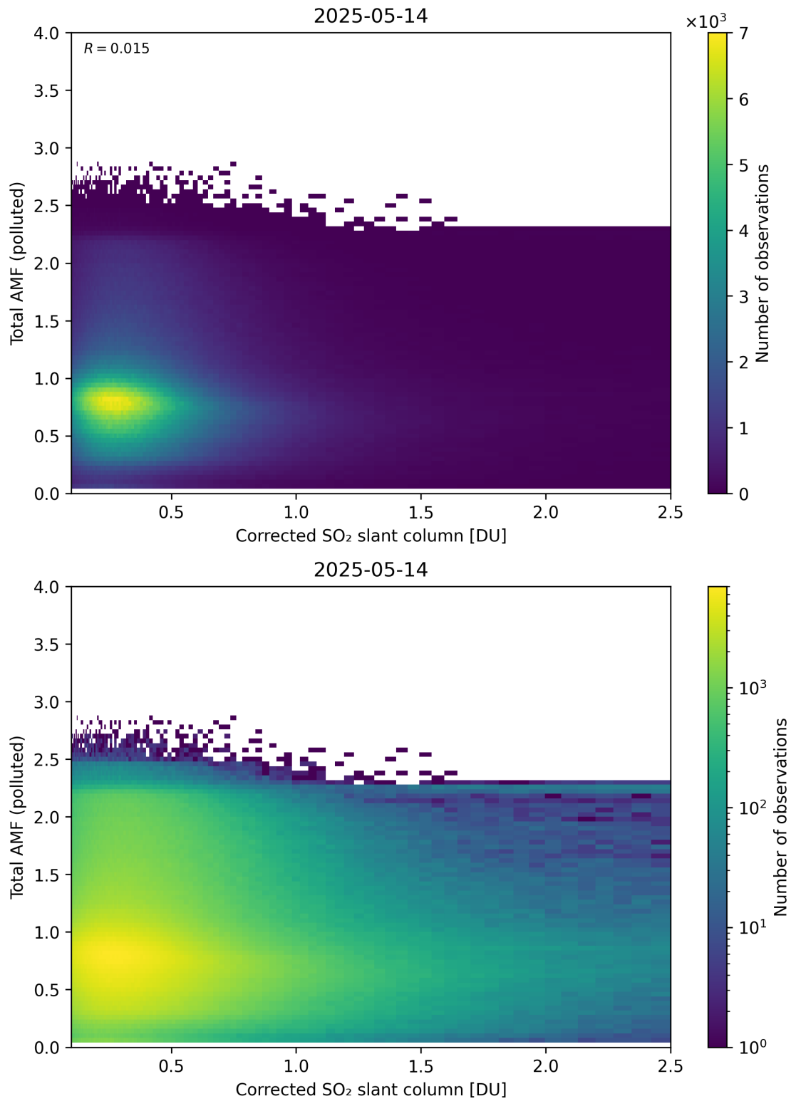
Figure 242: Scatter density plot of “Corrected SO 2 slant column” against “Total AMF (polluted)” for 2025-05-13 to 2025-05-15.
