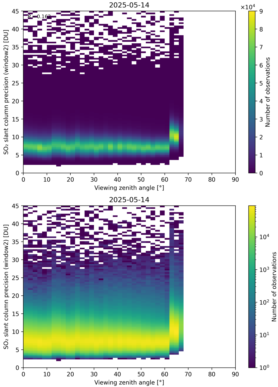
Figure 378: Scatter density plot of “Viewing zenith angle” against “SO 2 slant column precision (window2)” for 2025-05-13 to 2025-05-15.
