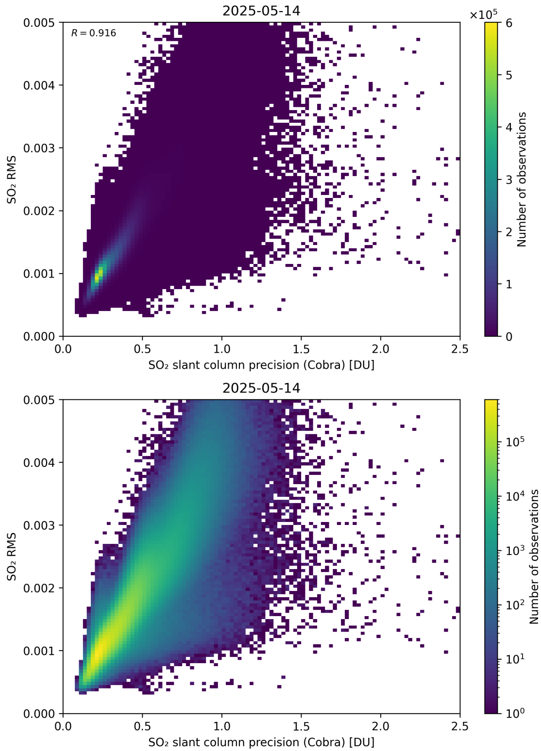
Figure 204: Scatter density plot of “SO 2 slant column precision (Cobra)” against “SO 2 RMS” for 2025-05-13 to 2025-05-15.
