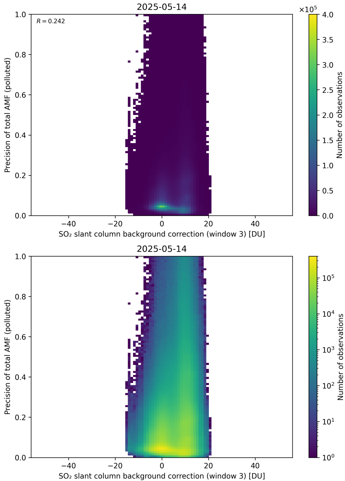
Figure 137: Scatter density plot of “SO 2 slant column background correction (window 3)” against “Precision of total AMF (polluted)” for 2025-05-13 to 2025-05-15.
