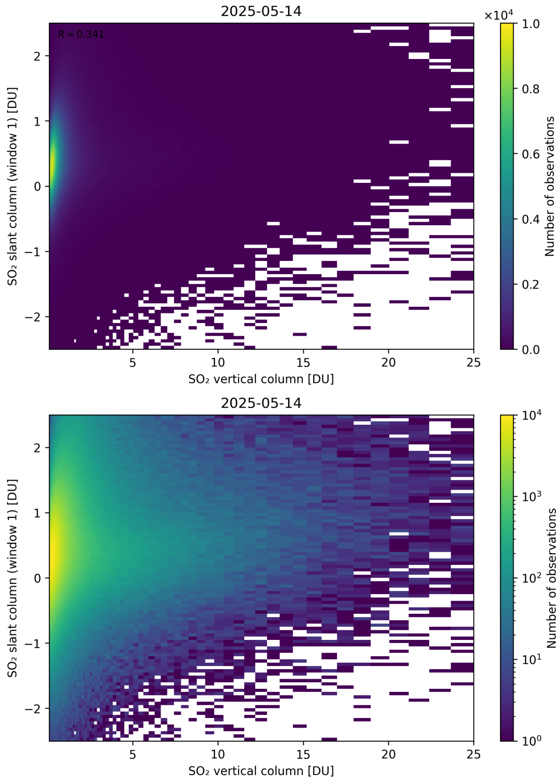
Figure 354: Scatter density plot of “SO 2 vertical column” against “SO 2 slant column (window 1)” for 2025-05-13 to 2025-05-15.
