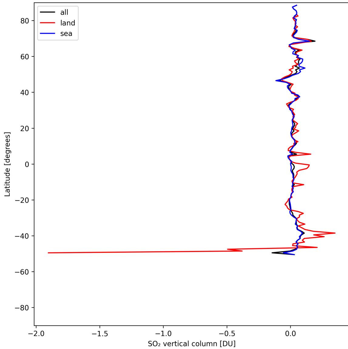
Figure 32: Zonal average of “SO 2 vertical column” for 2025-05-13 to 2025-05-15.
