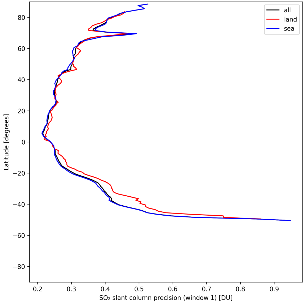
Figure 38: Zonal average of “SO 2 slant column precision (window 1)” for 2025-05-13 to 2025-05-15.
