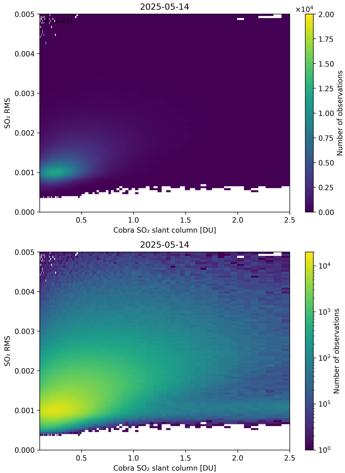
Figure 198: Scatter density plot of “Cobra SO 2 slant column” against “SO 2 RMS” for 2025-05-13 to 2025-05-15.
