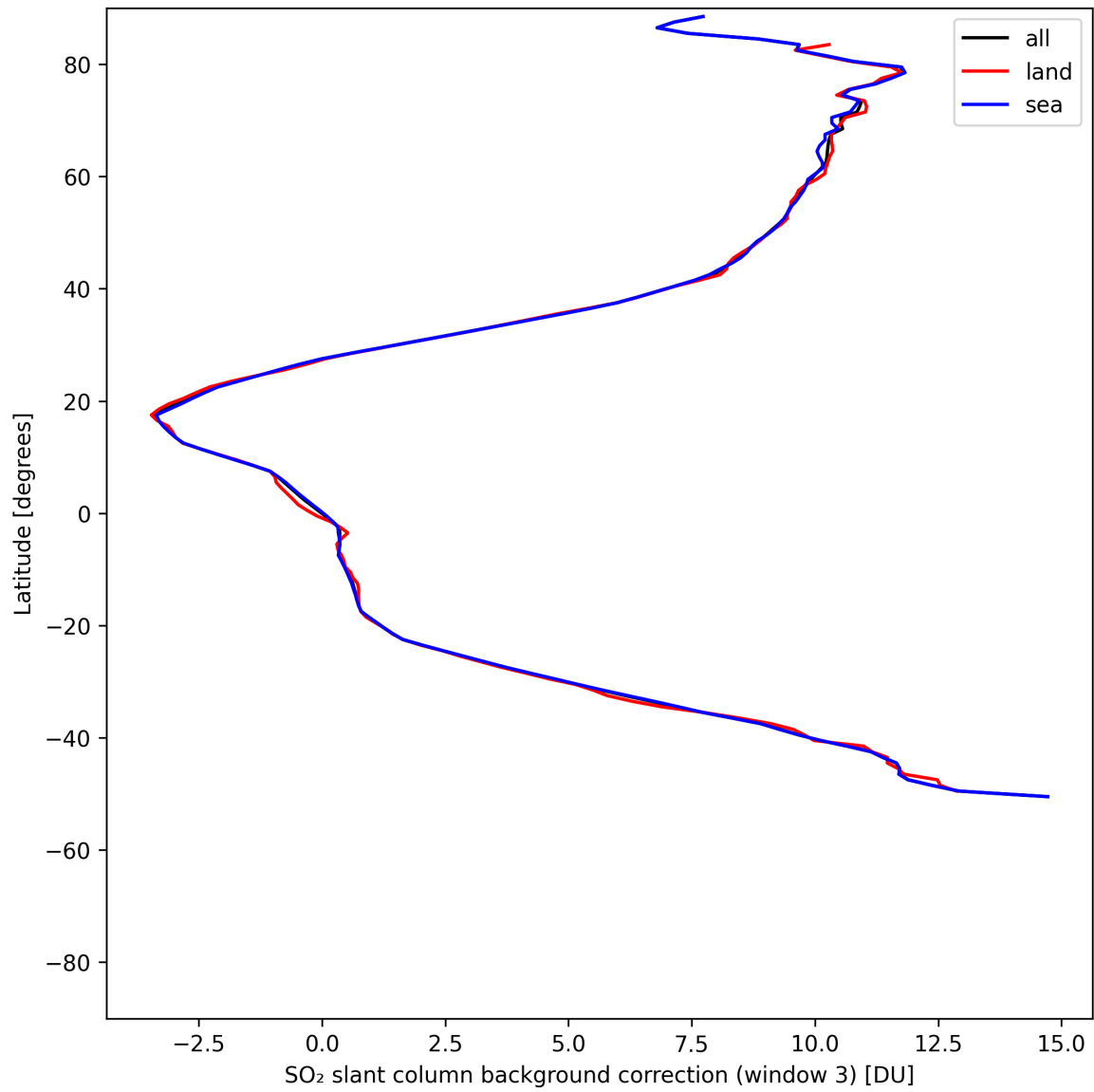
Figure 48: Zonal average of “SO 2 slant column background correction (window 3)” for 2025-05-13 to 2025-05-15.
