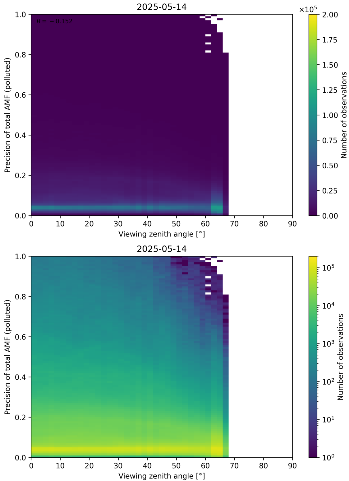
Figure 382: Scatter density plot of “Viewing zenith angle” against “Precision of total AMF (polluted)” for 2025-05-13 to 2025-05-15.
