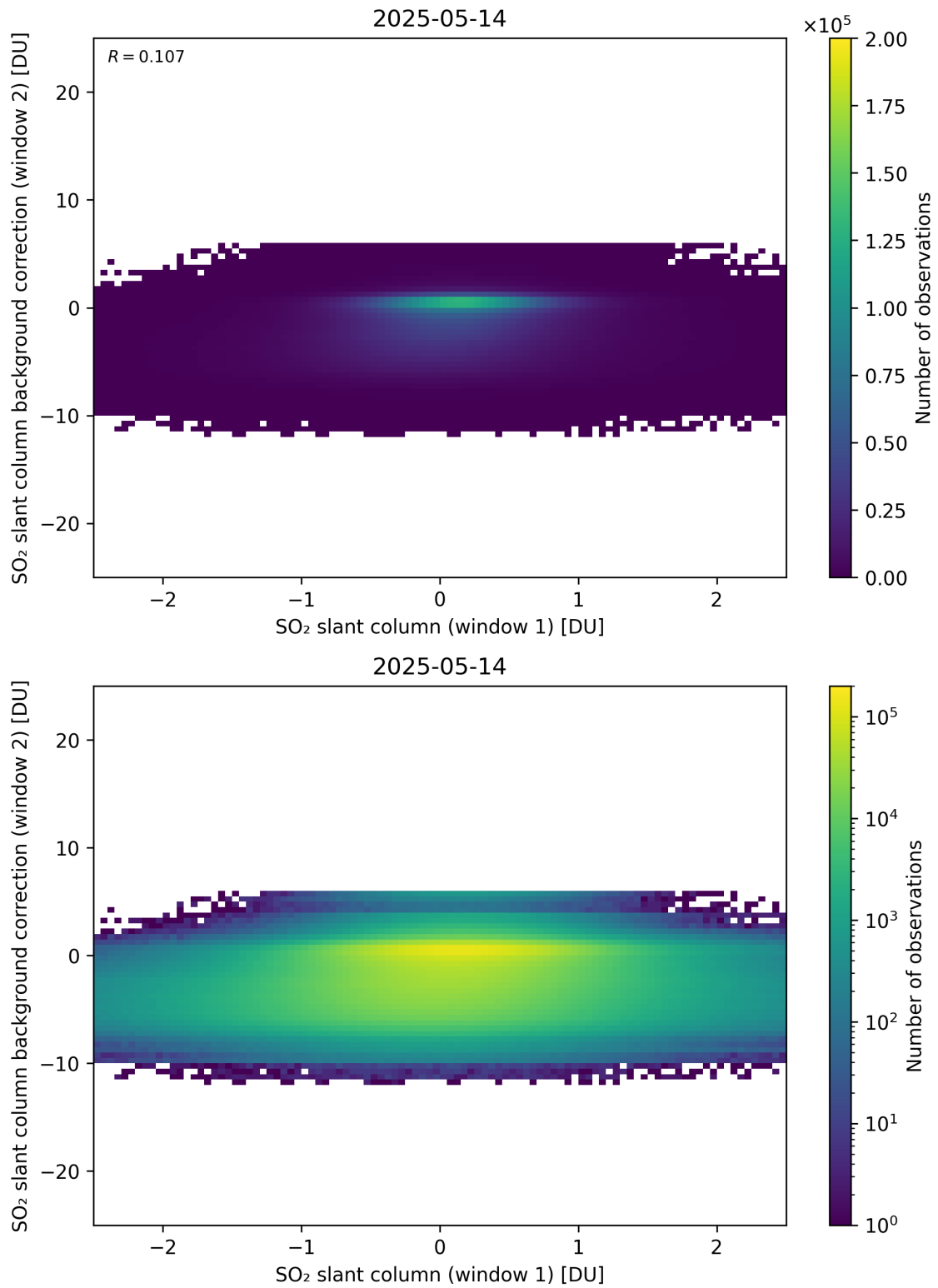
Figure 263: Scatter density plot of “SO 2 slant column (window 1)” against “SO 2 slant column background correction (window 2)” for 2025-05-13 to 2025-05-15.
