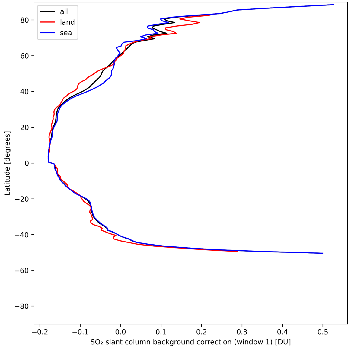
Figure 40: Zonal average of "SO 2 slant column background correction (window 1)" for 2025-05-13 to 2025-05-15.
