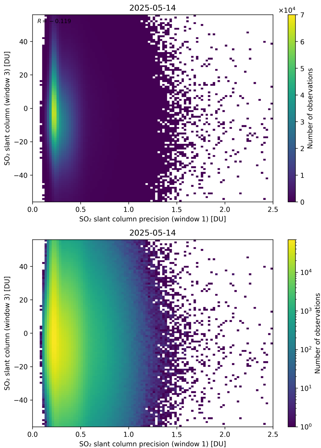
Figure 278: Scatter density plot of “SO 2 slant column precision (window 1)” against “SO 2 slant column (window 3)” for 2025-05-13 to 2025-05-15.
