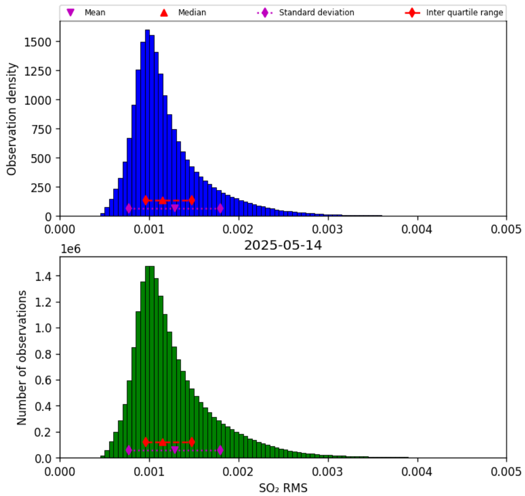
Figure 78: Histogram of “SO 2 RMS” for 2025-05-13 to 2025-05-15
