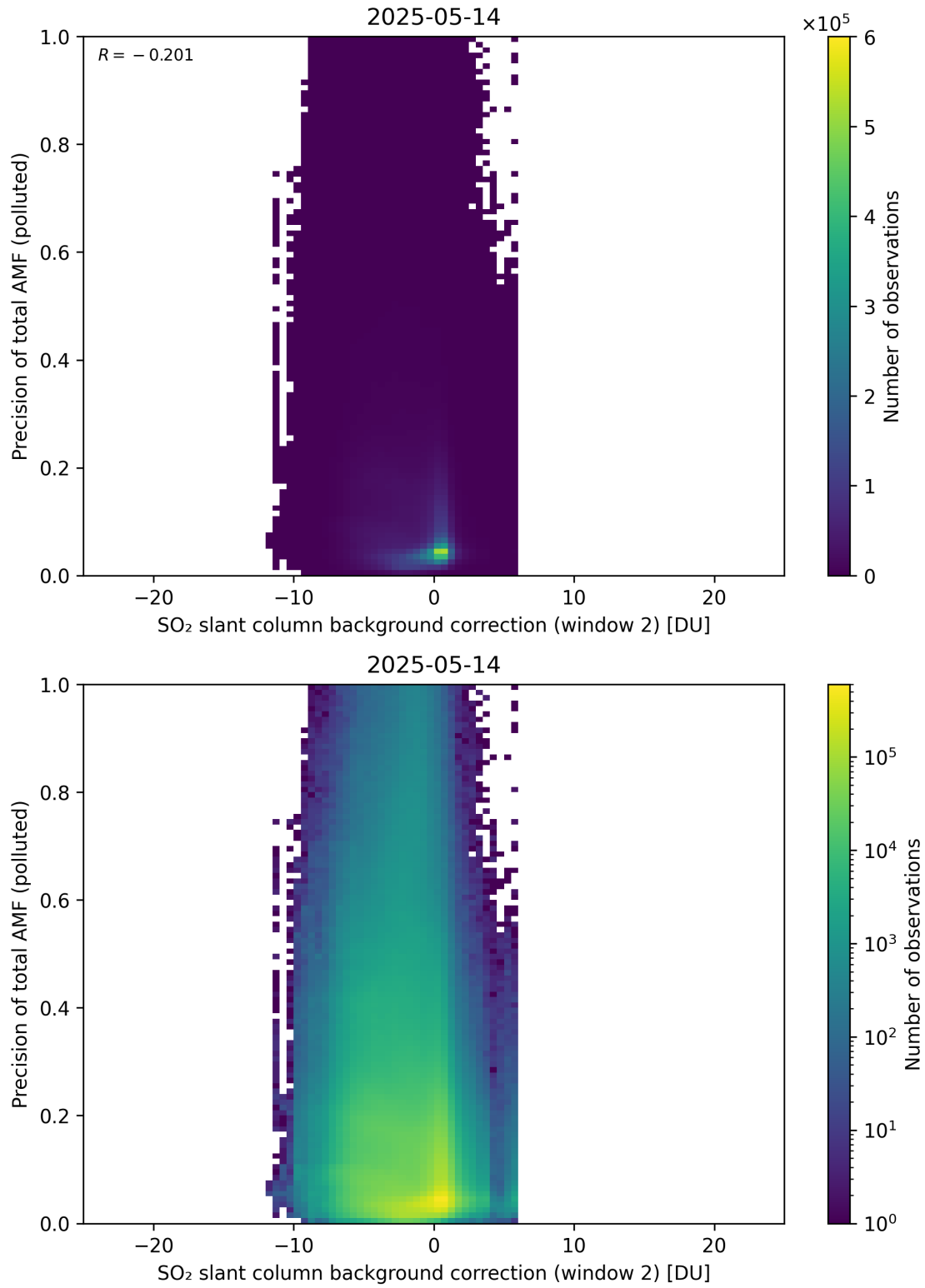
Figure 131: Scatter density plot of “SO 2 slant column background correction (window 2)” against “Precision of total AMF (polluted)” for 2025-05-13 to 2025-05-15.
