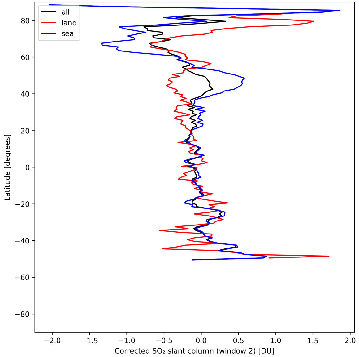
Figure 43: Zonal average of “Corrected SO 2 slant column (window 2)” for 2025-05-13 to 2025-05-15.
