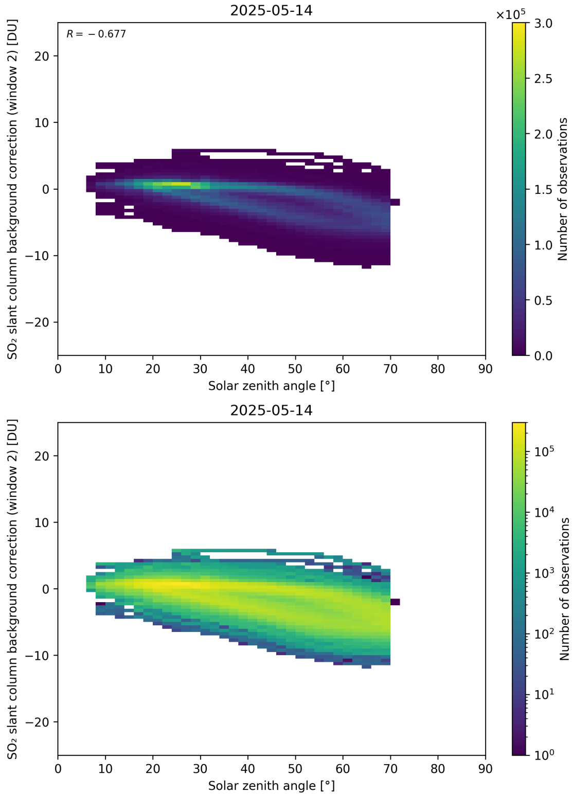
Figure 172: Scatter density plot of “Solar zenith angle” against “SO 2 slant column background correction (window 2)” for 2025-05-13 to 2025-05-15.
