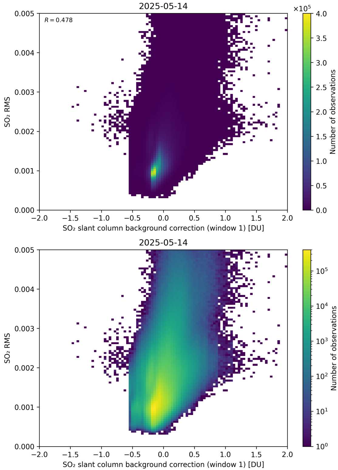
Figure 113: Scatter density plot of “SO 2 slant column background correction (window 1)” against “SO 2 RMS” for 2025-05-13 to 2025-05-15.
