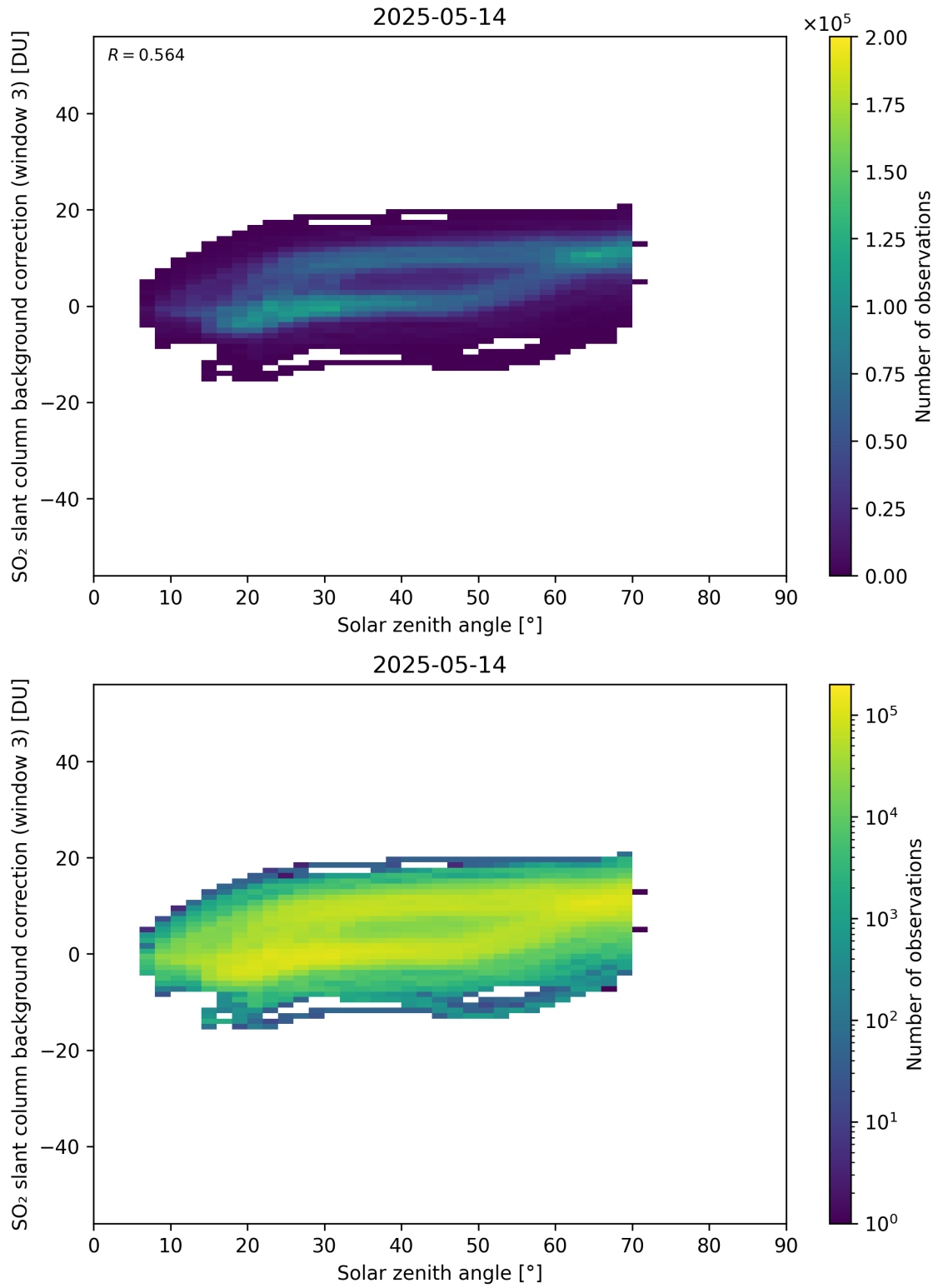
Figure 173: Scatter density plot of “Solar zenith angle” against “SO 2 slant column background correction (window 3)” for 2025-05-13 to 2025-05-15.
