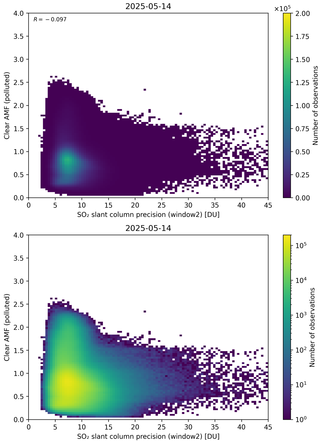
Figure 296: Scatter density plot of “SO 2 slant column precision (window2)” against “Clear AMF (polluted)” for 2025-05-13 to 2025-05-15.
