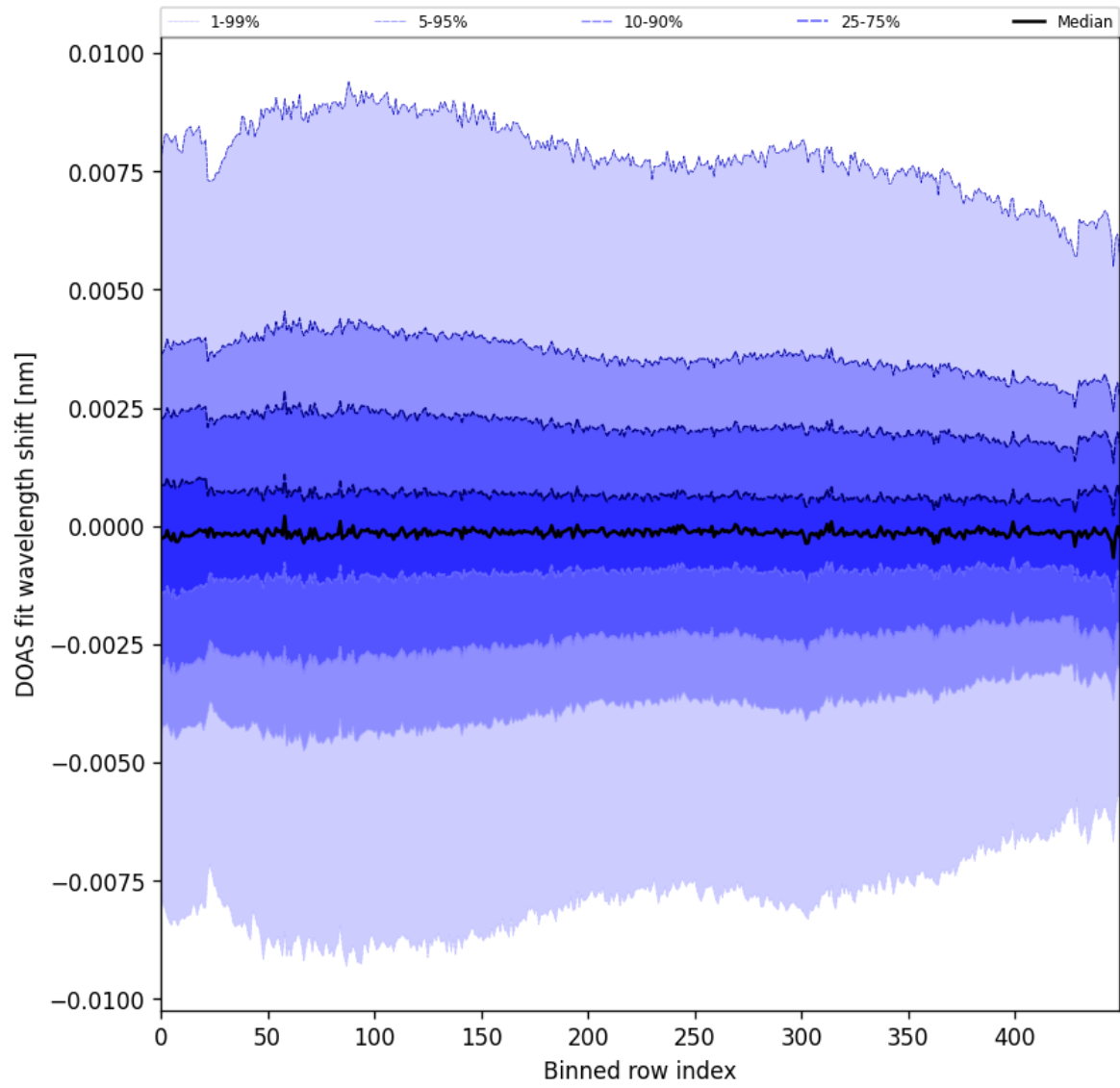
Figure 102: Along track statistics of “DOAS fit wavelength shift” for 2025-05-13 to 2025-05-15
