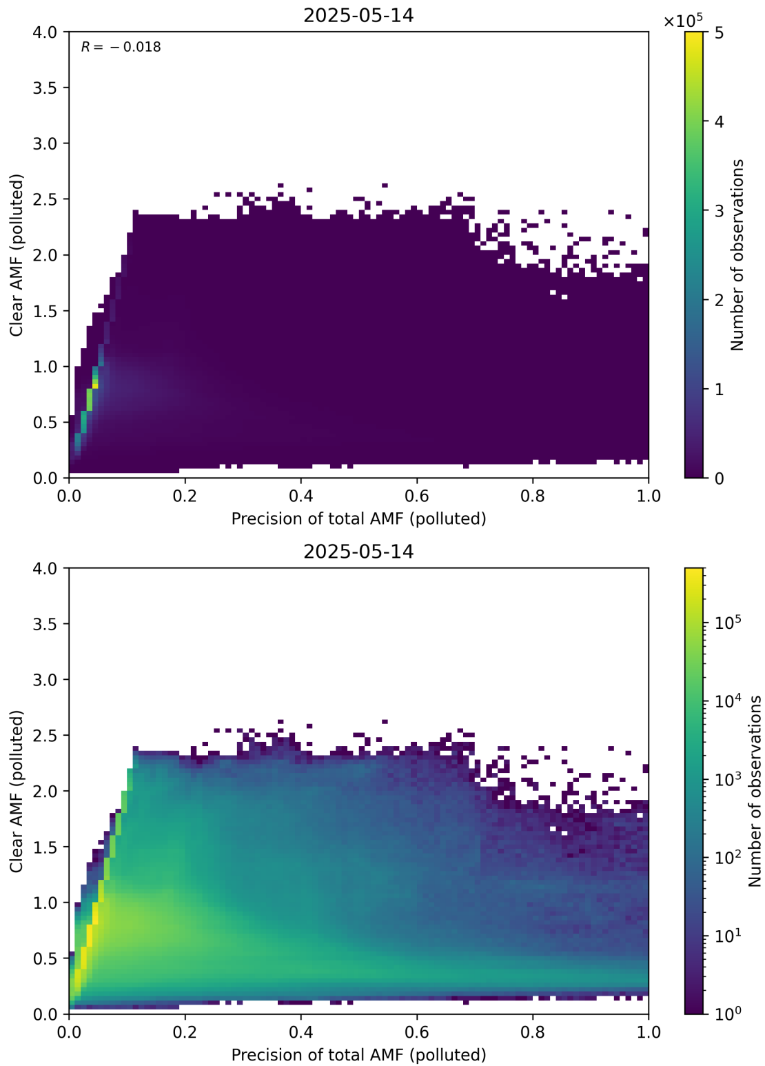
Figure 320: Scatter density plot of “Precision of total AMF (polluted)” against “Clear AMF (polluted)” for 2025-05-13 to 2025-05-15.
