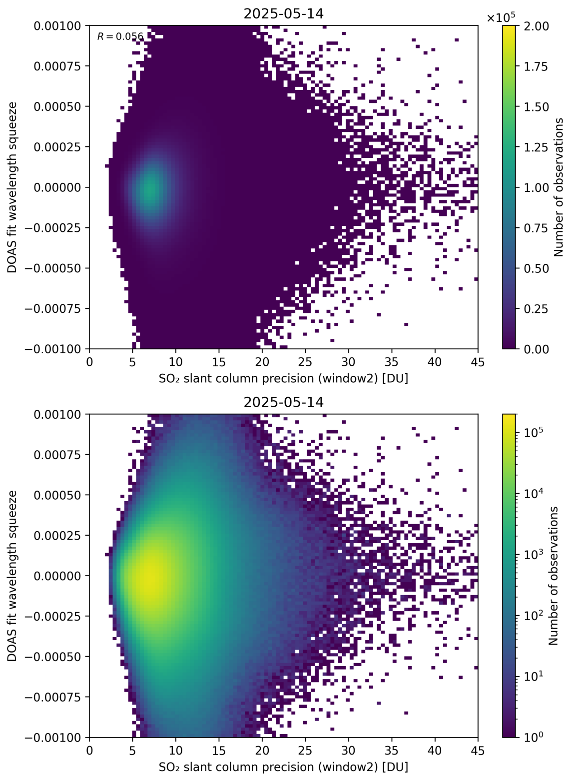
Figure 294: Scatter density plot of “SO 2 slant column precision (window2)” against “DOAS fit wavelength squeeze” for 2025-05-13 to 2025-05-15.
