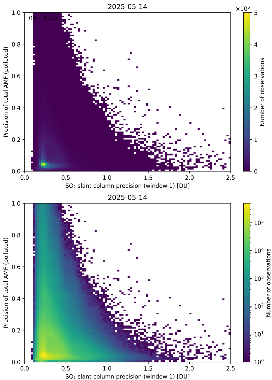
Figure 281: Scatter density plot of “SO 2 slant column precision (window 1)” against “Precision of total AMF (polluted)” for 2025-05-13 to 2025-05-15.
