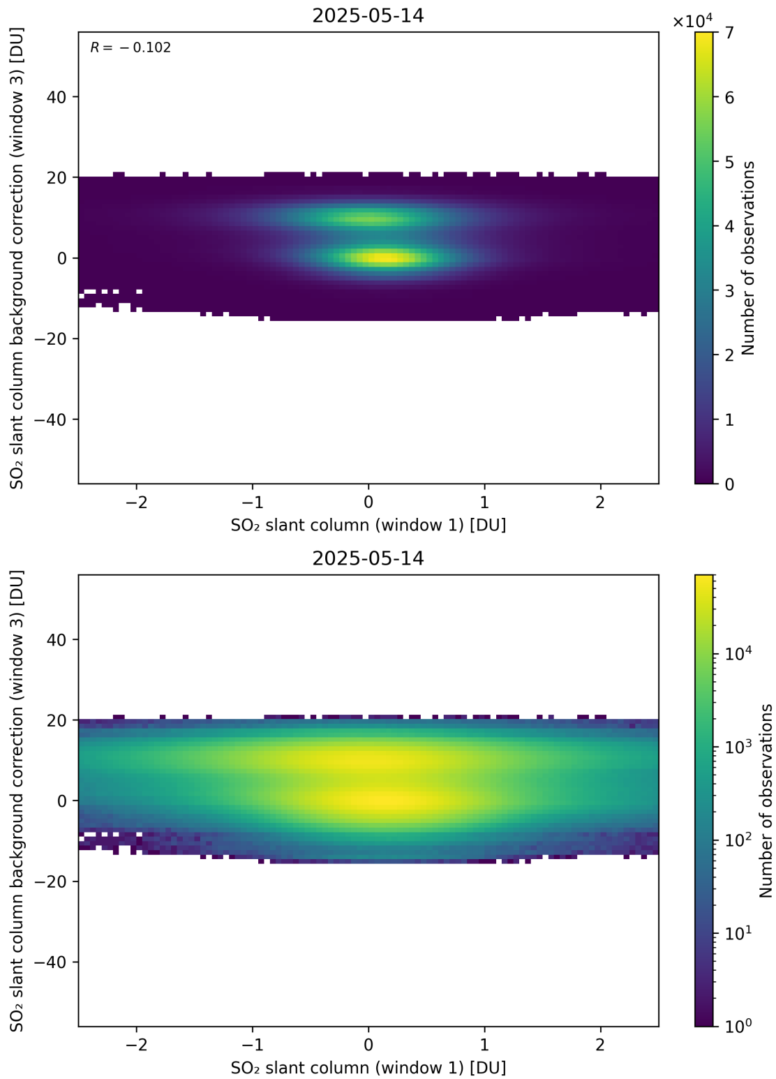
Figure 264: Scatter density plot of “SO 2 slant column (window 1)” against “SO 2 slant column background correction (window 3)” for 2025-05-13 to 2025-05-15.
