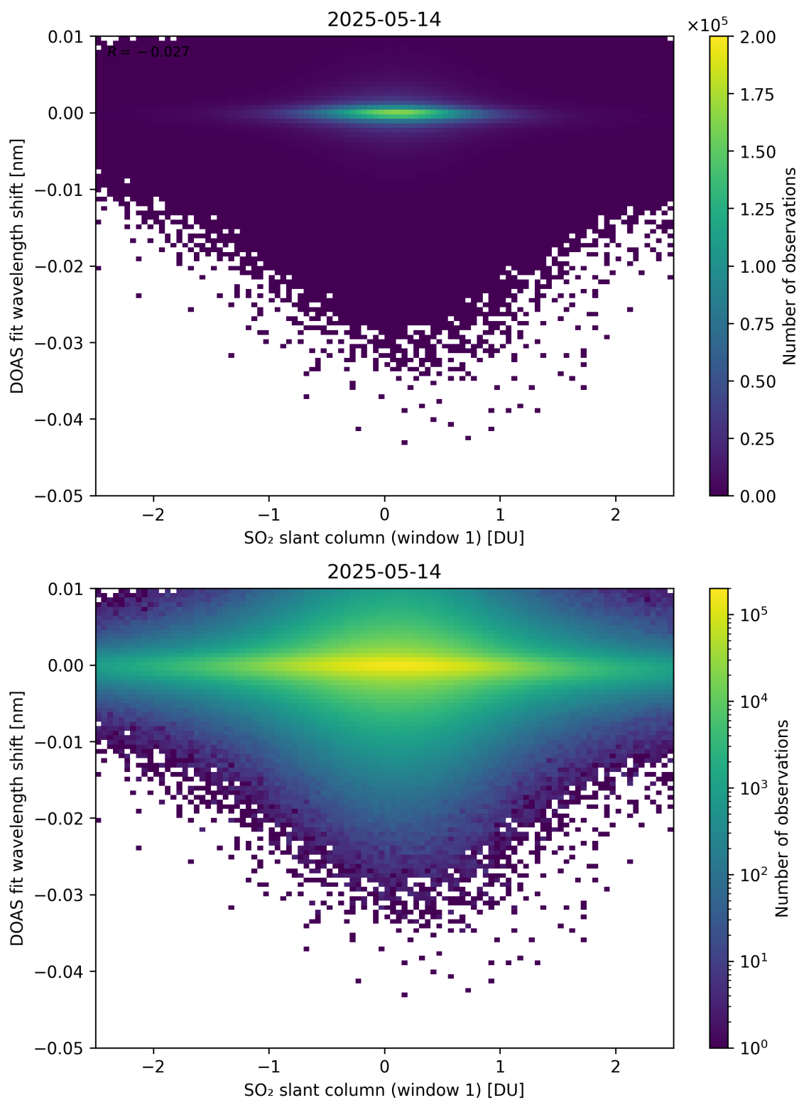
Figure 265: Scatter density plot of “SO 2 slant column (window 1)” against “DOAS fit wavelength shift” for 2025-05-13 to 2025-05-15.
