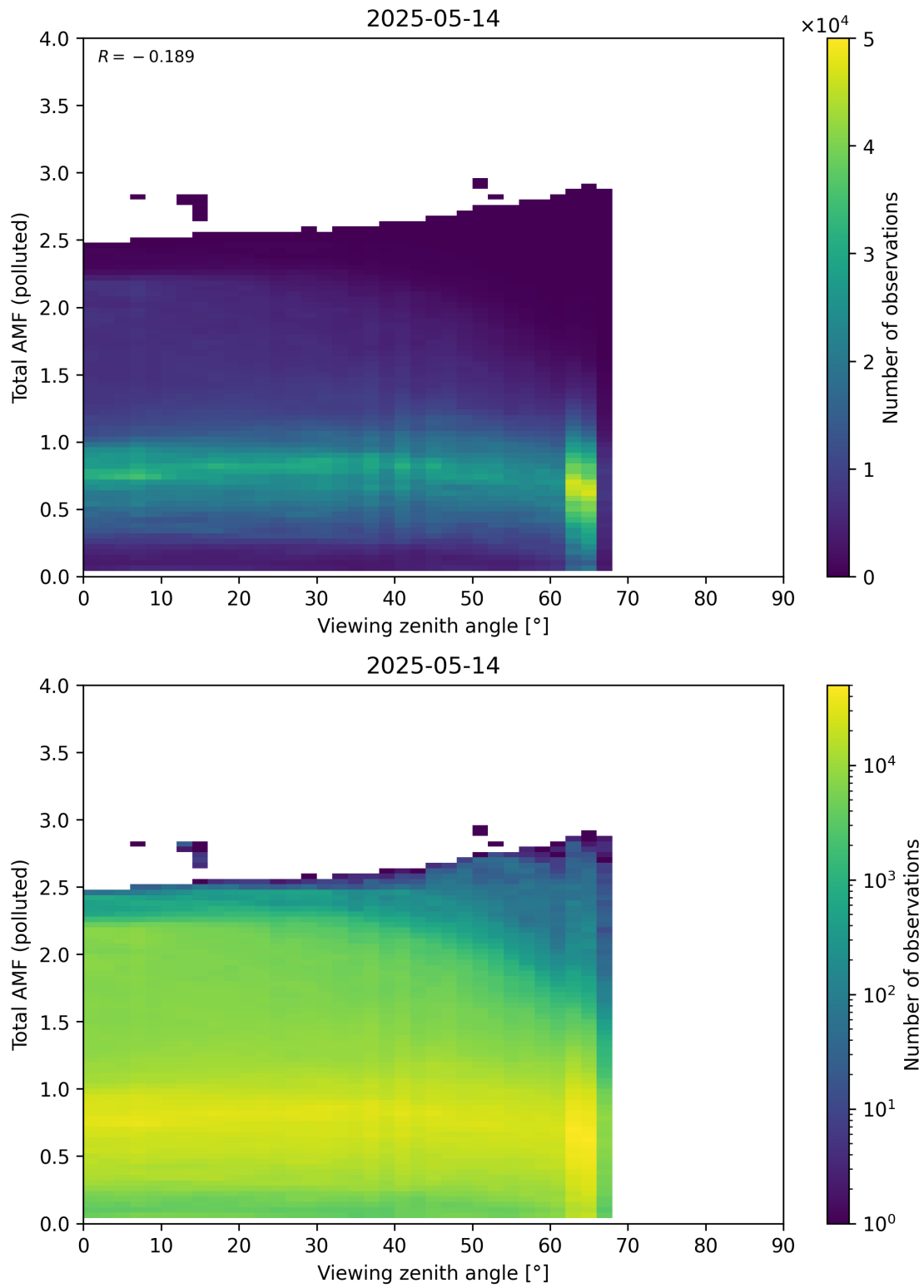
Figure 381: Scatter density plot of “Viewing zenith angle” against “Total AMF (polluted)” for 2025-05-13 to 2025-05-15.
