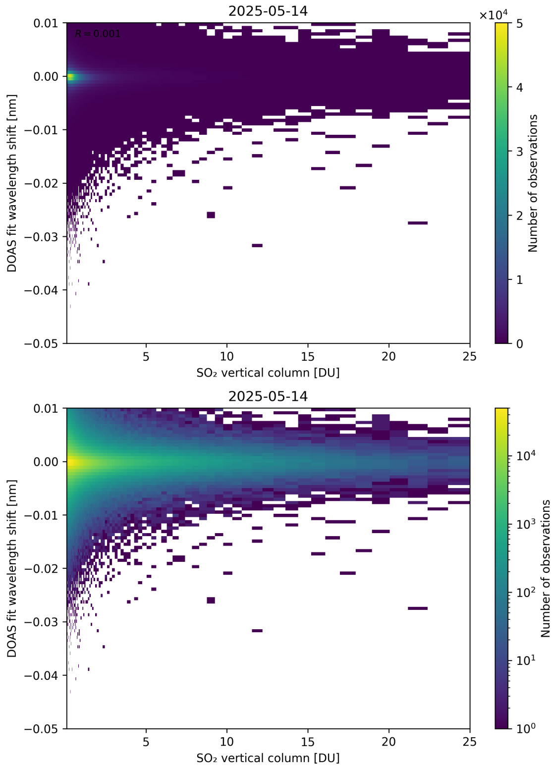
Figure 326: Scatter density plot of “SO 2 vertical column” against “DOAS fit wavelength shift” for 2025-05-13 to 2025-05-15.
