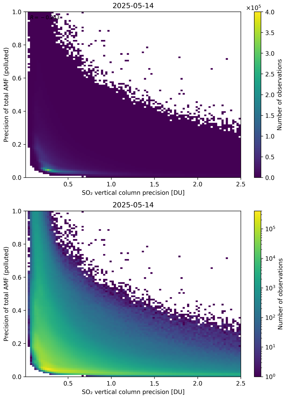
Figure 347: Scatter density plot of “SO 2 vertical column precision” against “Precision of total AMF (polluted)” for 2025-05-13 to 2025-05-15.
