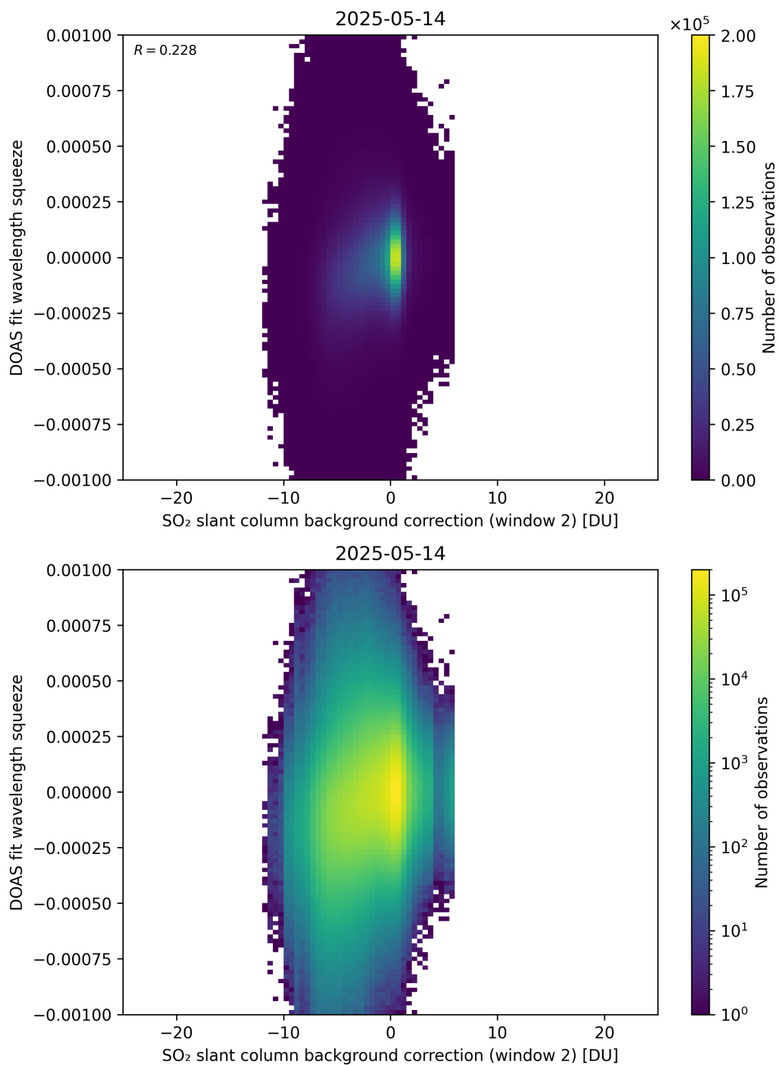
Figure 124: Scatter density plot of “SO 2 slant column background correction (window 2)” against “DOAS fit wavelength squeeze” for 2025-05-13 to 2025-05-15.
