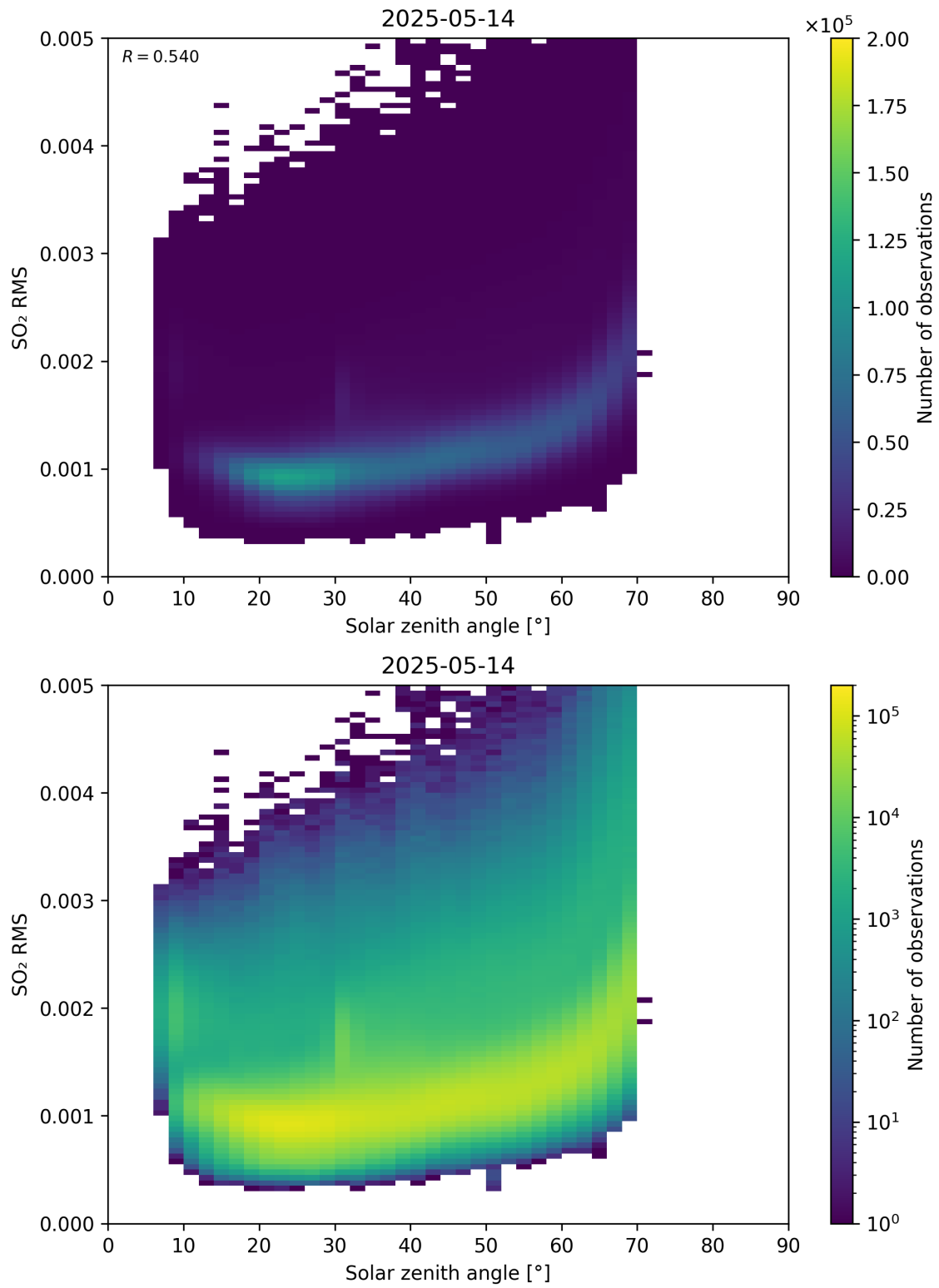
Figure 176: Scatter density plot of “Solar zenith angle” against “SO 2 RMS” for 2025-05-13 to 2025-05-15.
