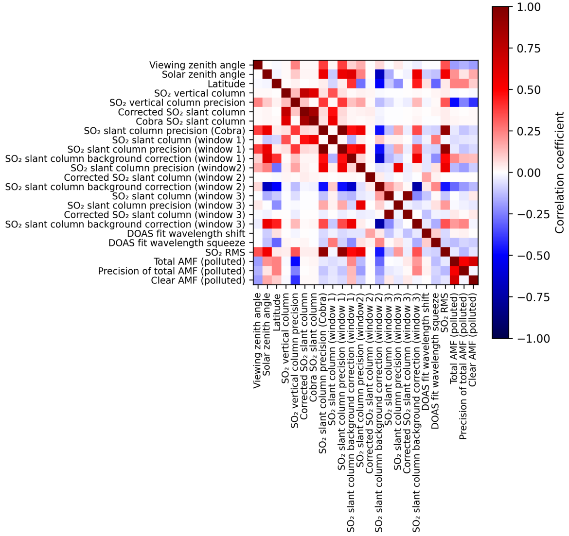
Figure 2: Map of correlation matrix for 2025-05-13 to 2025-05-15.
