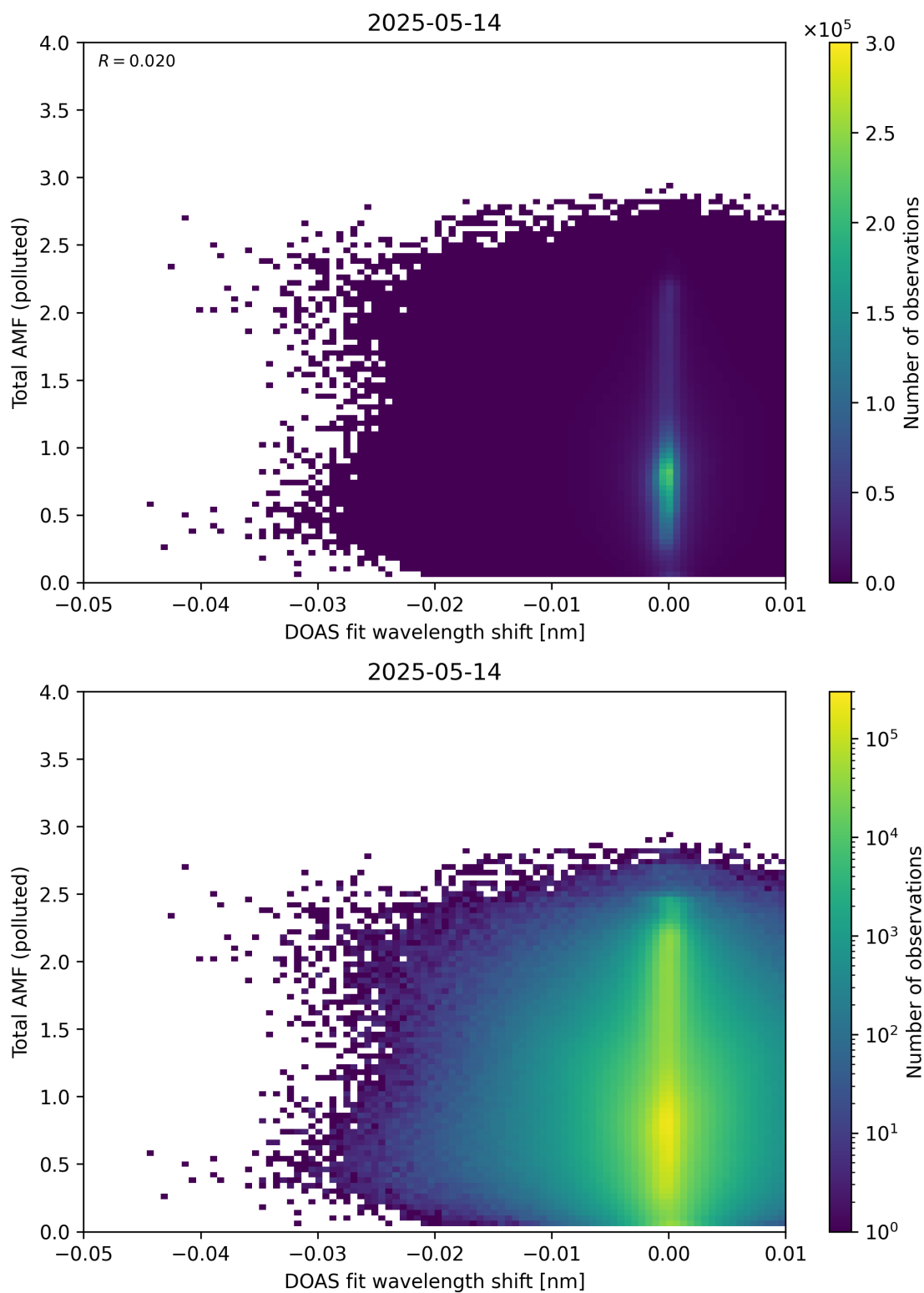
Figure 141: Scatter density plot of “DOAS fit wavelength shift” against “Total AMF (polluted)” for 2025-05-13 to 2025-05-15.
