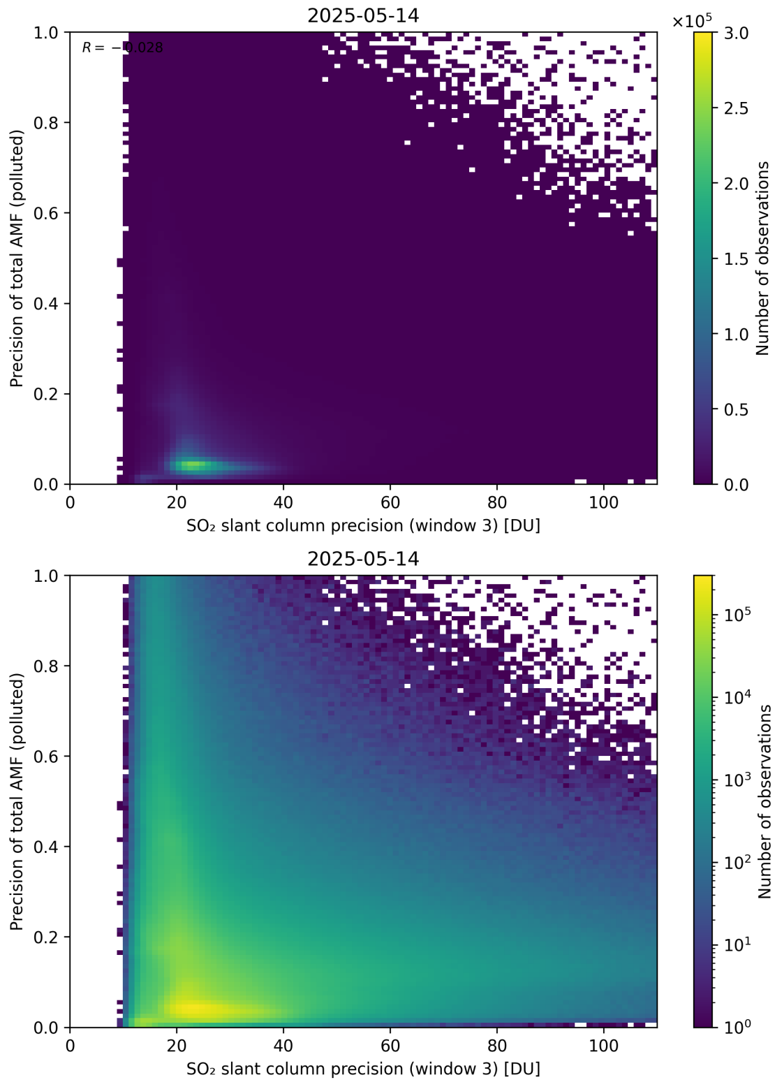
Figure 314: Scatter density plot of “SO 2 slant column precision (window 3)” against “Precision of total AMF (polluted)” for 2025-05-13 to 2025-05-15.
