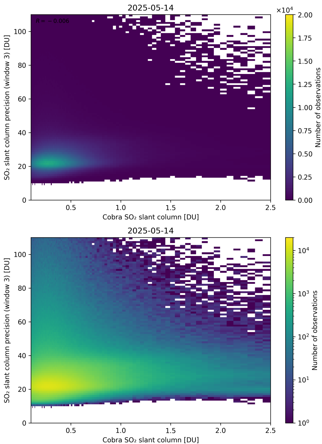
Figure 223: Scatter density plot of “Cobra SO 2 slant column” against “SO 2 slant column precision (window 3)” for 2025-05-13 to 2025-05-15.
