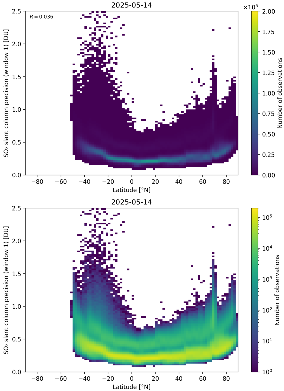
Figure 163: Scatter density plot of “Latitude” against “SO 2 slant column precision (window 1)” for 2025-05-13 to 2025-05-15.
