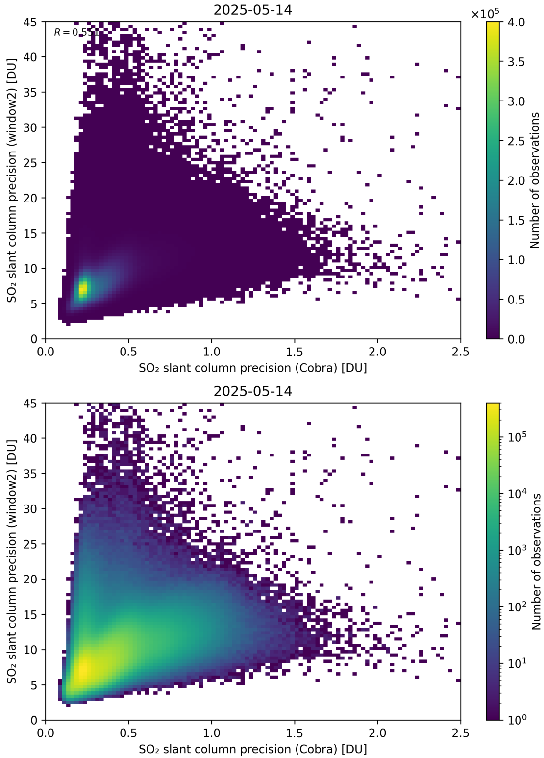
Figure 210: Scatter density plot of “SO 2 slant column precision (Cobra)” against “SO 2 slant column precision (window2)” for 2025-05-13 to 2025-05-15.
