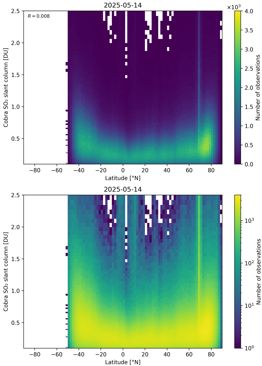
Figure 157: Scatter density plot of “Latitude” against “Cobra SO 2 slant column” for 2025-05-13 to 2025-05-15.
