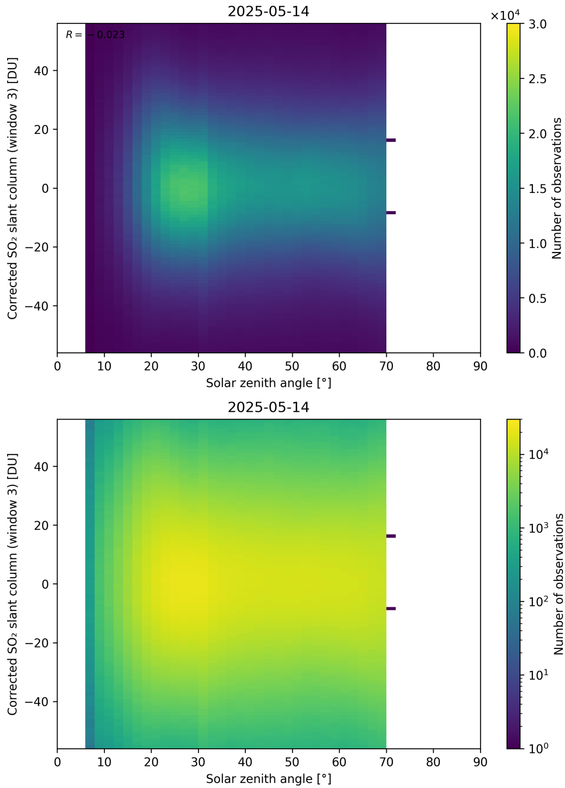
Figure 183: Scatter density plot of “Solar zenith angle” against “Corrected SO 2 slant column (window 3)” for 2025-05-13 to 2025-05-15.
