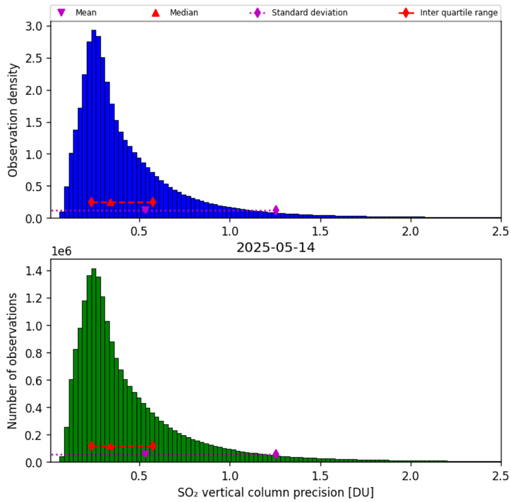
Figure 59: Histogram of “SO 2 vertical column precision” for 2025-05-13 to 2025-05-15
