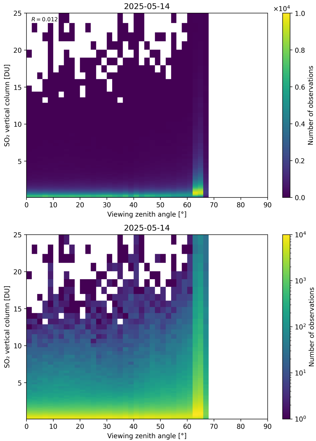
Figure 383: Scatter density plot of “Viewing zenith angle” against “SO 2 vertical column” for 2025-05-13 to 2025-05-15.
