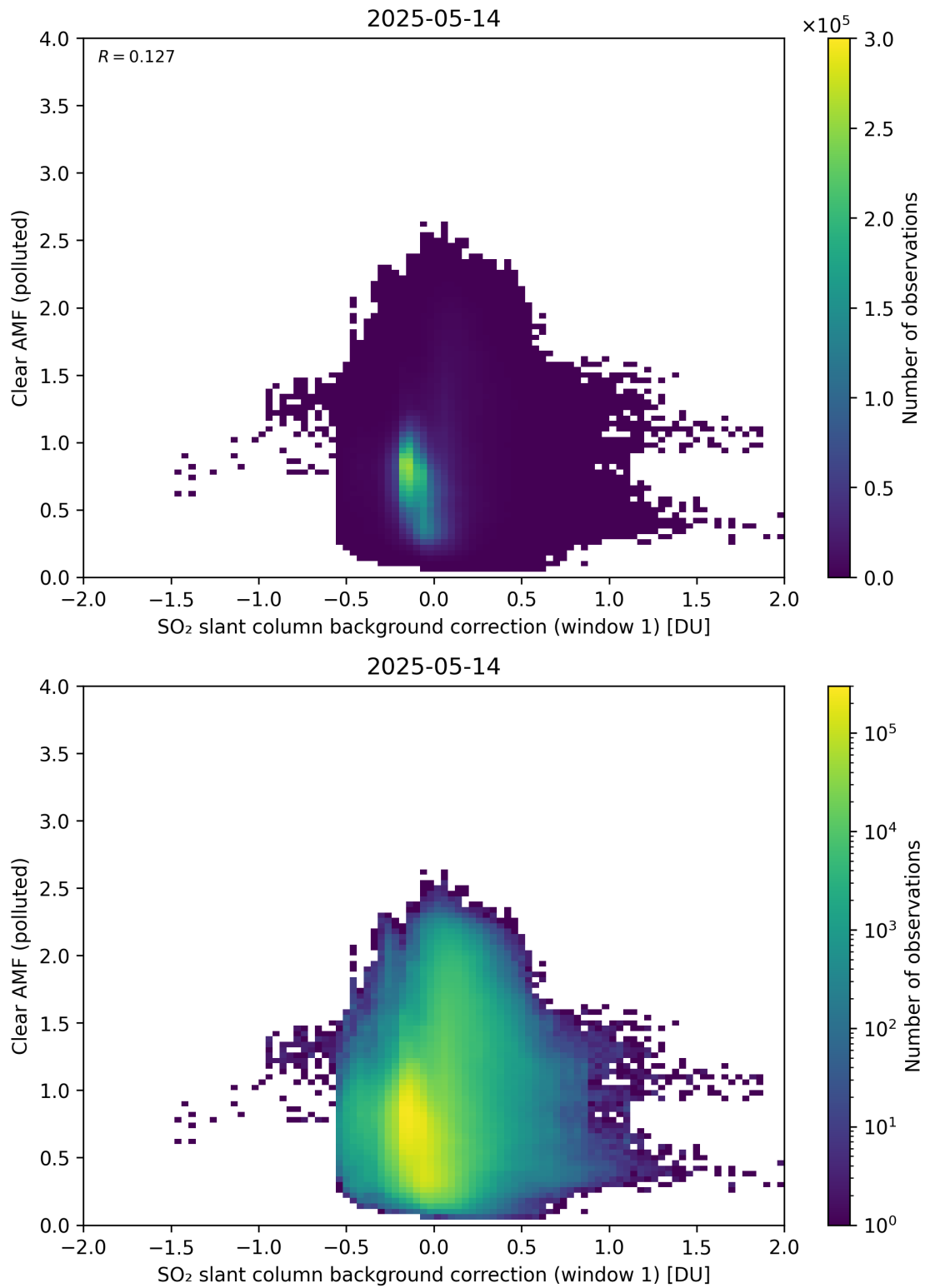
Figure 114: Scatter density plot of “SO 2 slant column background correction (window 1)” against “Clear AMF (polluted)” for 2025-05-13 to 2025-05-15.
