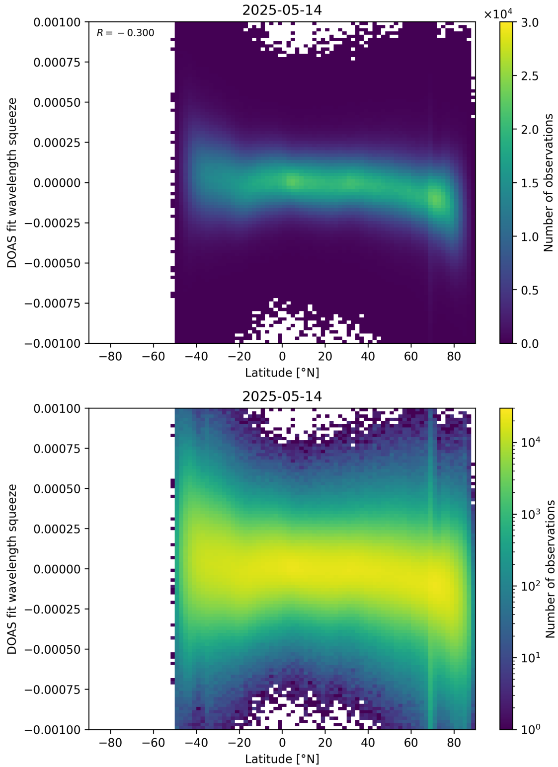
Figure 154: Scatter density plot of “Latitude” against “DOAS fit wavelength squeeze” for 2025-05-13 to 2025-05-15.
