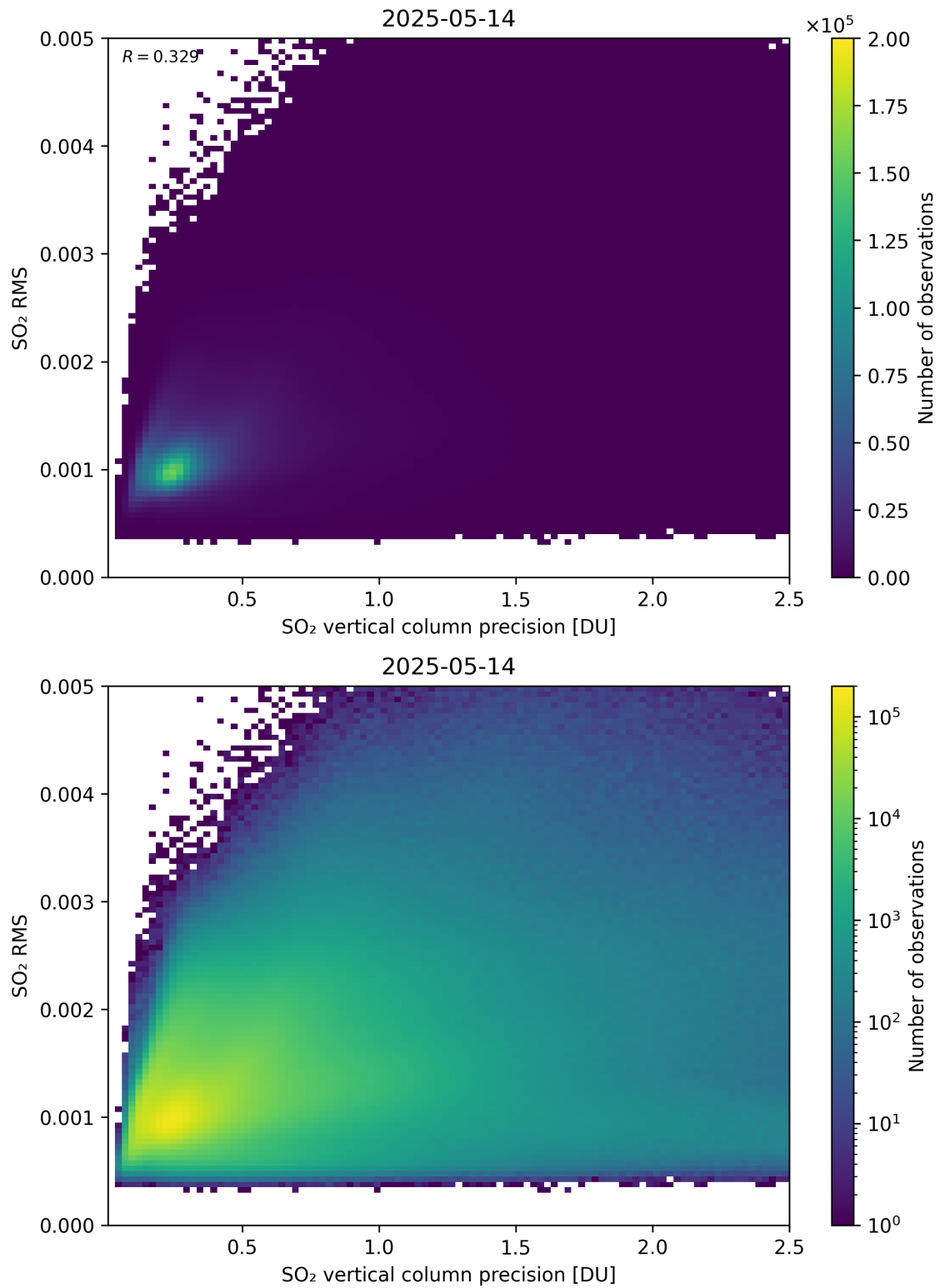
Figure 334: Scatter density plot of “SO 2 vertical column precision” against “SO 2 RMS” for 2025-05-13 to 2025-05-15.
