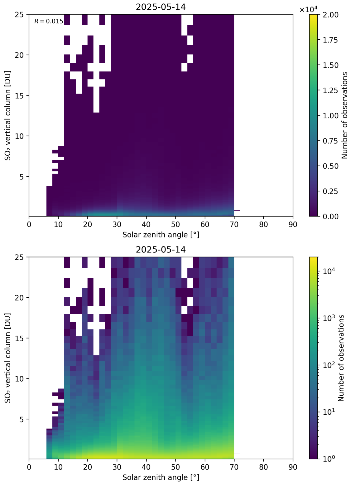
Figure 191: Scatter density plot of “Solar zenith angle” against “SO 2 vertical column” for 2025-05-13 to 2025-05-15.
