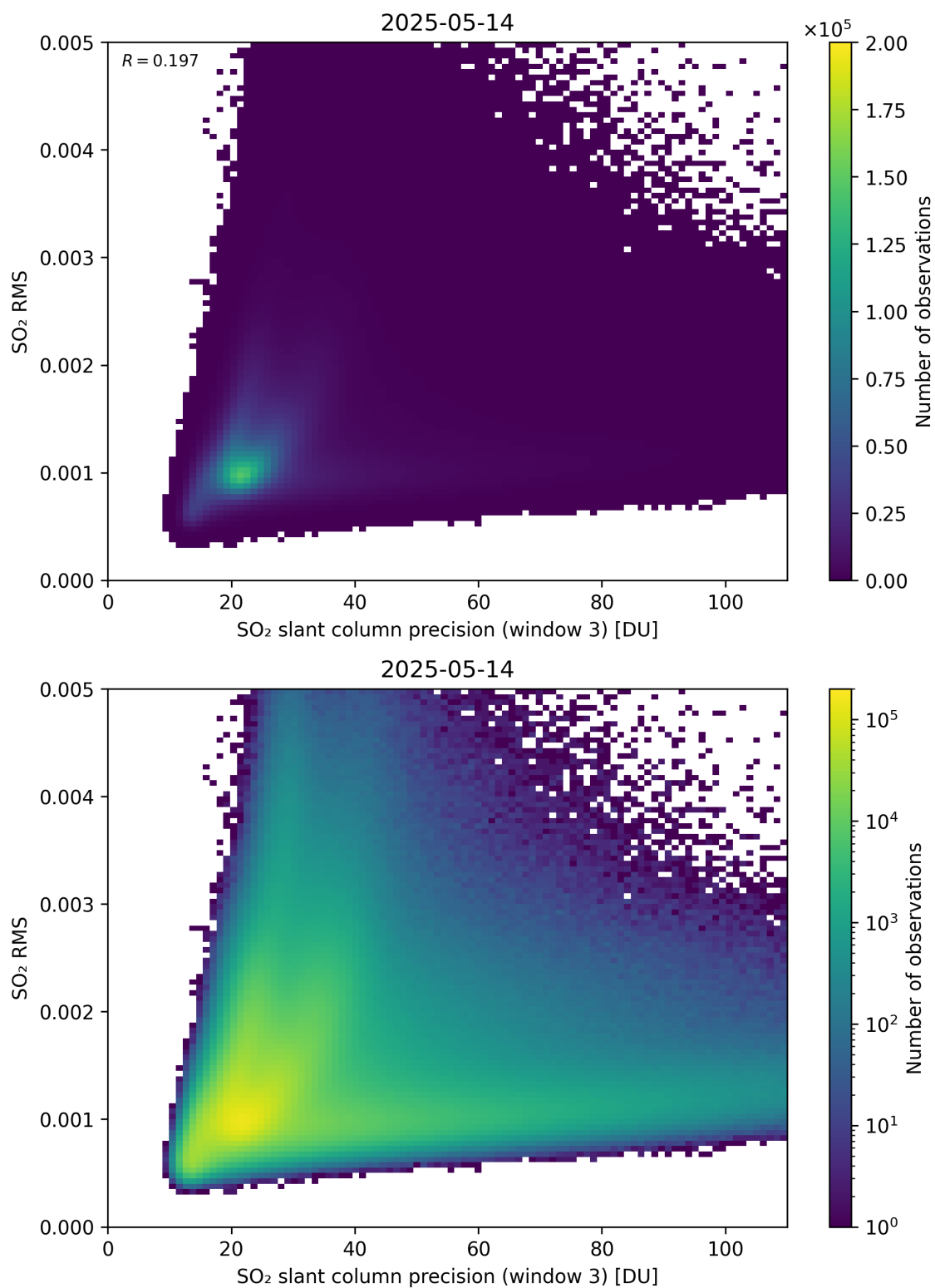
Figure 310: Scatter density plot of “SO 2 slant column precision (window 3)” against “SO 2 RMS” for 2025-05-13 to 2025-05-15.
