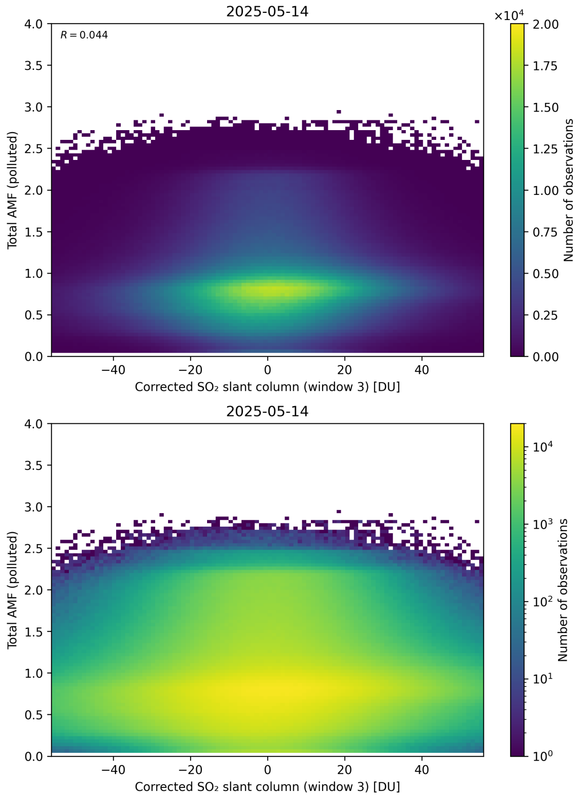
Figure 260: Scatter density plot of “Corrected SO 2 slant column (window 3)” against “Total AMF (polluted)” for 2025-05-13 to 2025-05-15.
