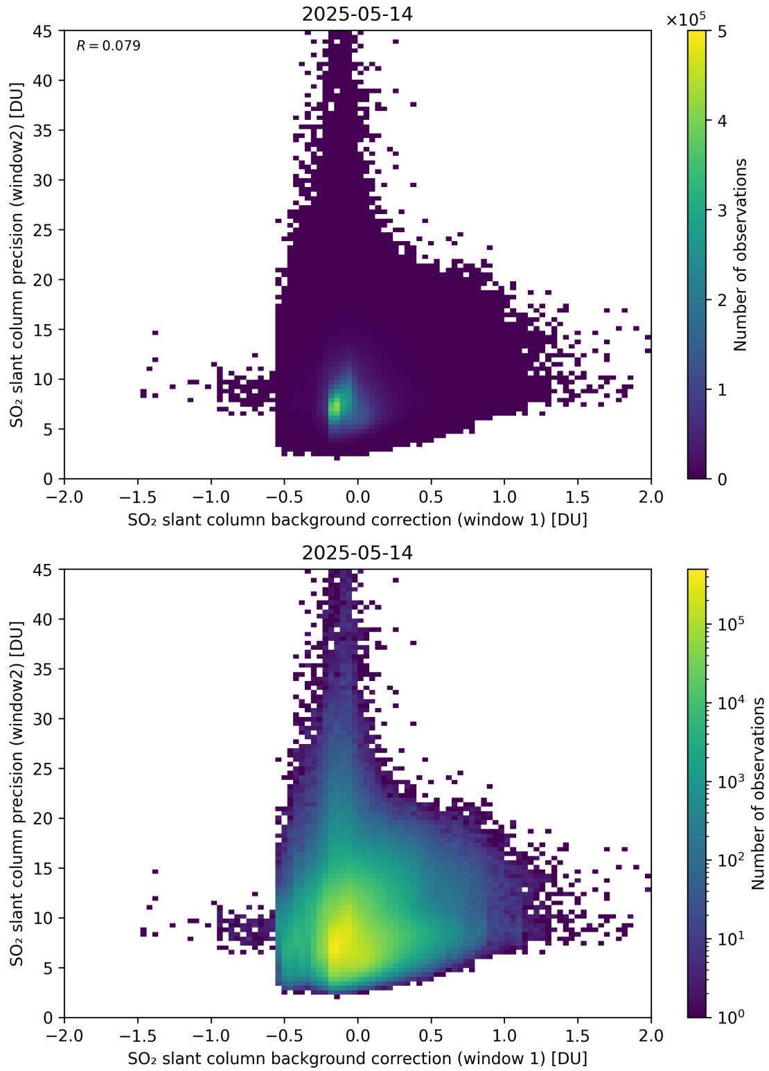
Figure 117: Scatter density plot of “SO 2 slant column background correction (window 1)” against “SO 2 slant column precision (window2)” for 2025-05-13 to 2025-05-15.
