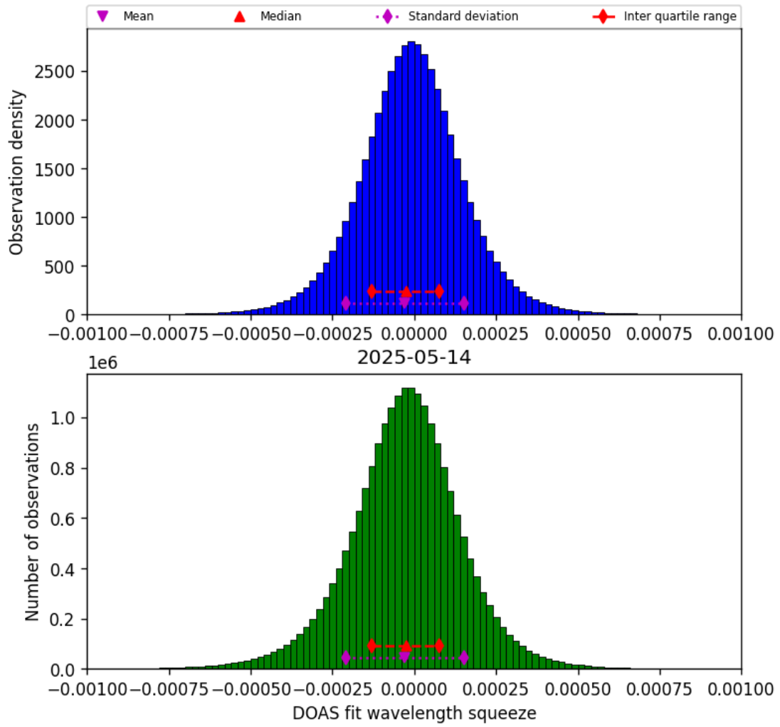
Figure 77: Histogram of "DOAS fit wavelength squeeze" for 2025-05-13 to 2025-05-15
