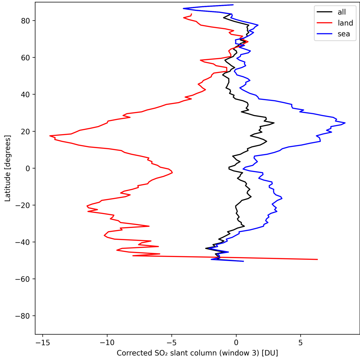
Figure 47: Zonal average of “Corrected SO 2 slant column (window 3)” for 2025-05-13 to 2025-05-15.
