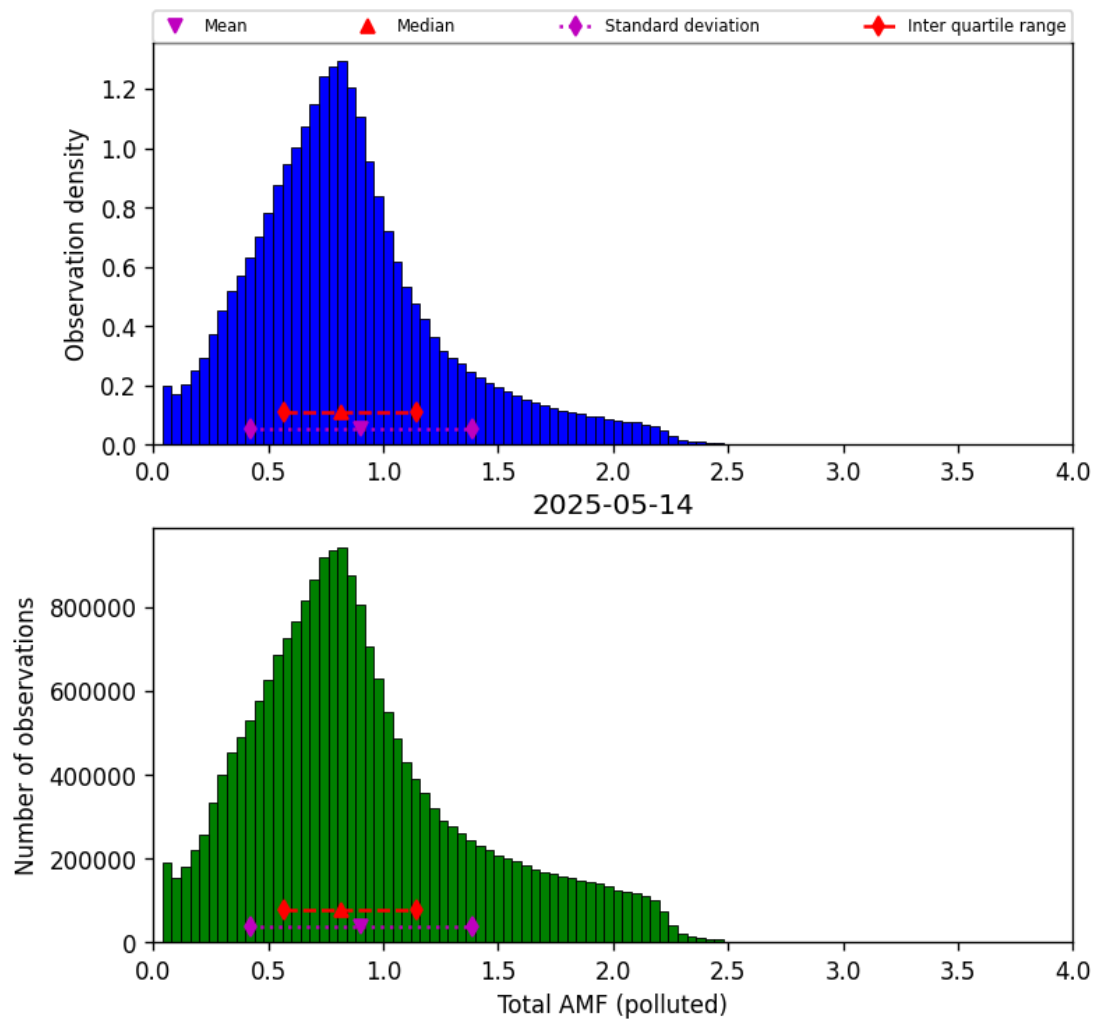
Figure 79: Histogram of “Total AMF (polluted)” for 2025-05-13 to 2025-05-15
