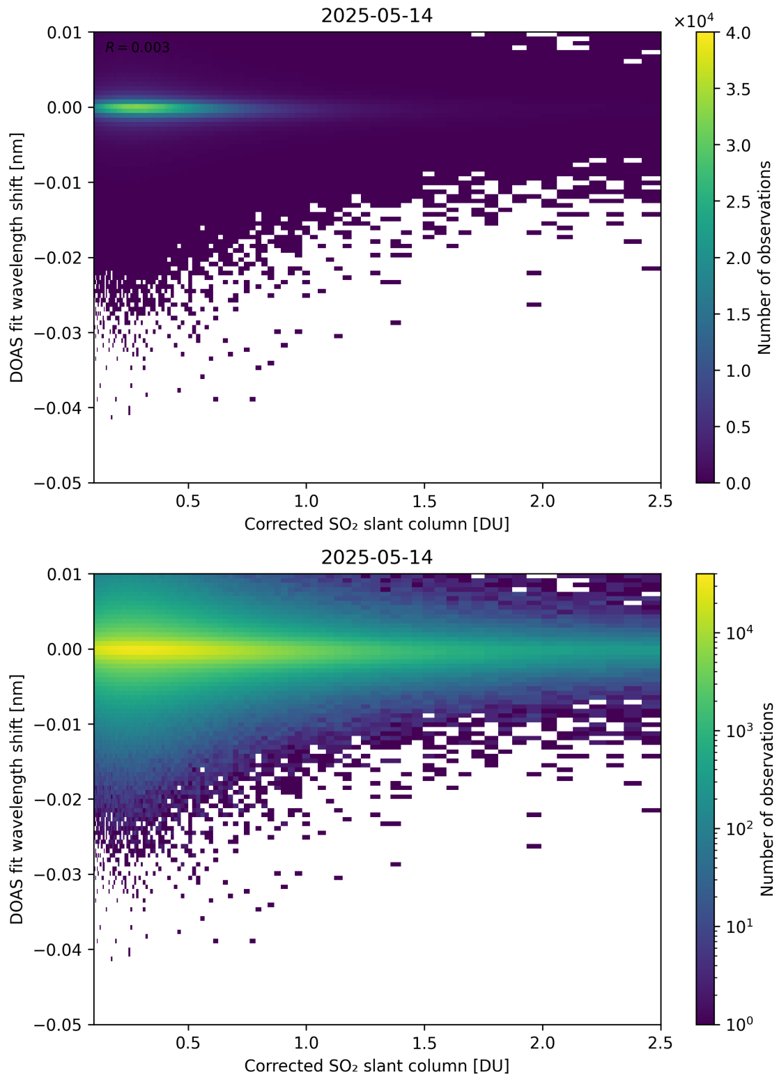
Figure 229: Scatter density plot of “Corrected SO 2 slant column” against “DOAS fit wavelength shift” for 2025-05-13 to 2025-05-15.
