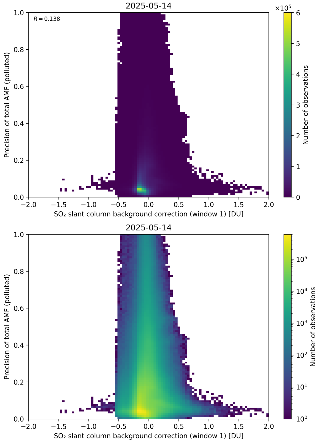
Figure 121: Scatter density plot of “SO 2 slant column background correction (window 1)” against “Precision of total AMF (polluted)” for 2025-05-13 to 2025-05-15.
