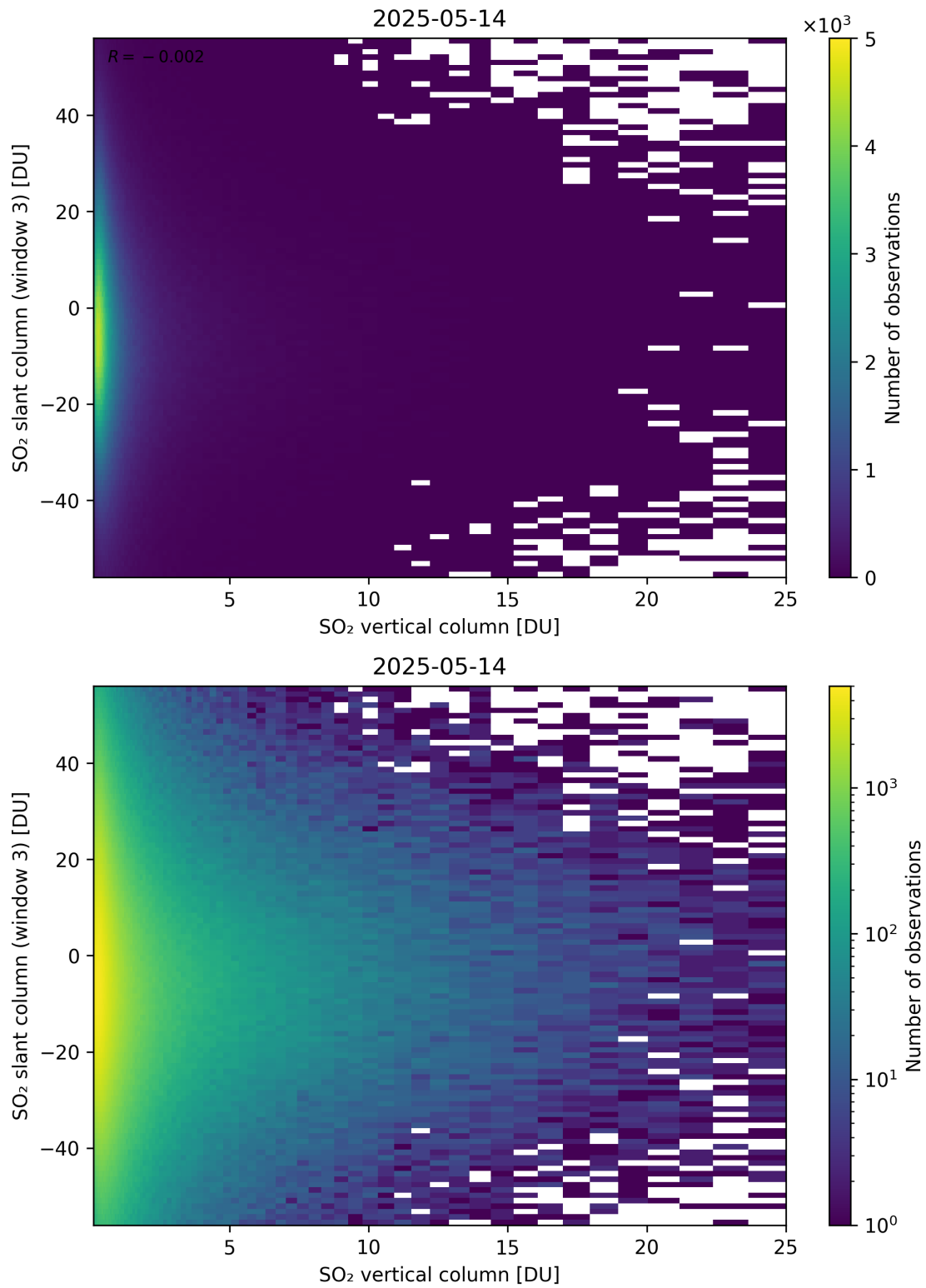
Figure 357: Scatter density plot of “SO 2 vertical column” against “SO 2 slant column (window 3)” for 2025-05-13 to 2025-05-15.
