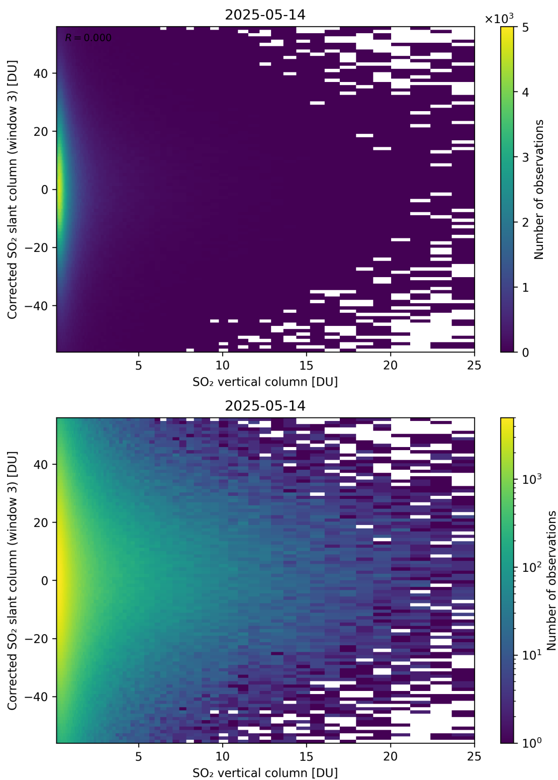
Figure 353: Scatter density plot of “SO 2 vertical column” against “Corrected SO 2 slant column (window 3)” for 2025-05-13 to 2025-05-15.
