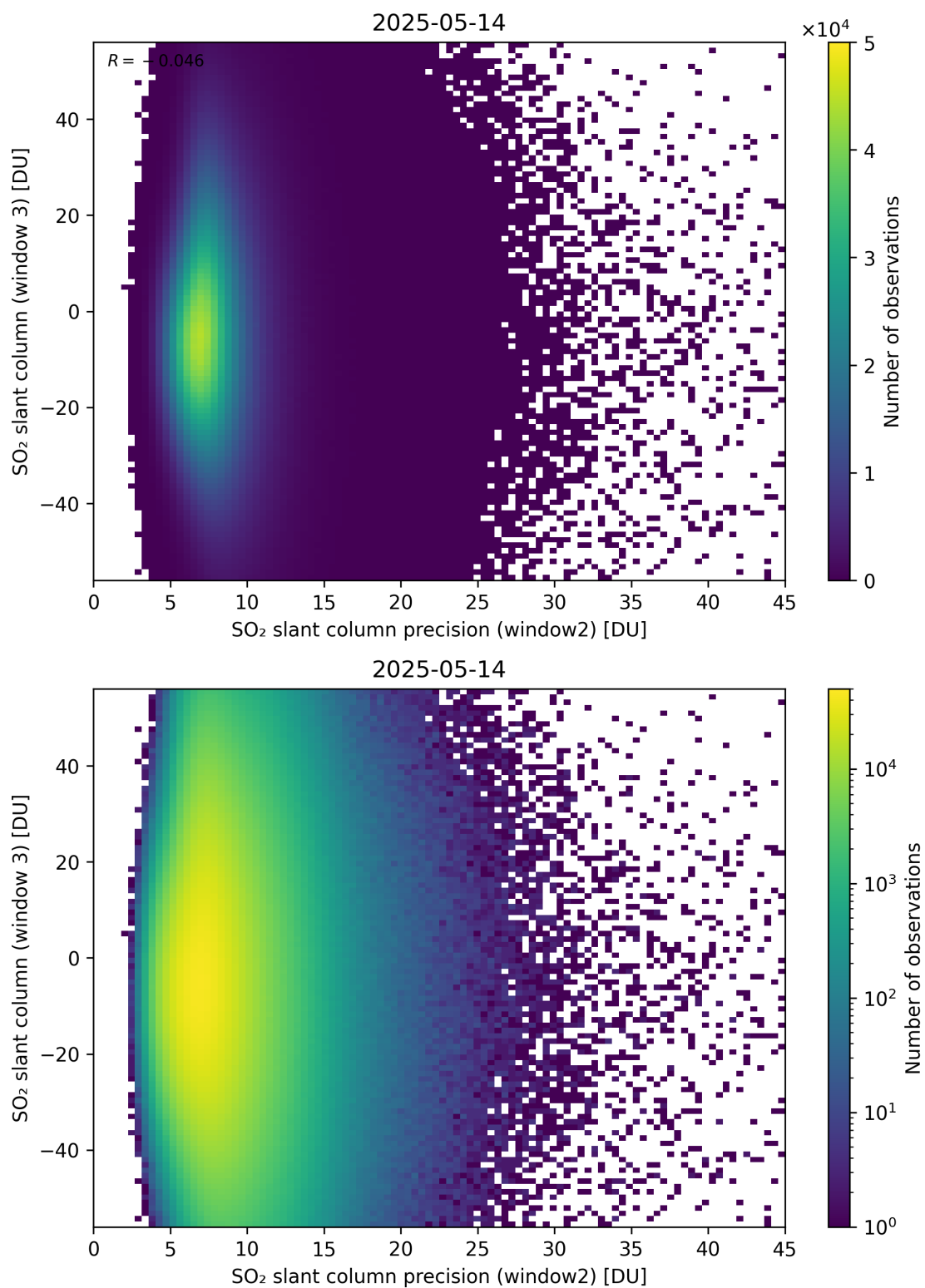
Figure 299: Scatter density plot of “SO 2 slant column precision (window2)” against “SO 2 slant column (window 3)” for 2025-05-13 to 2025-05-15.
