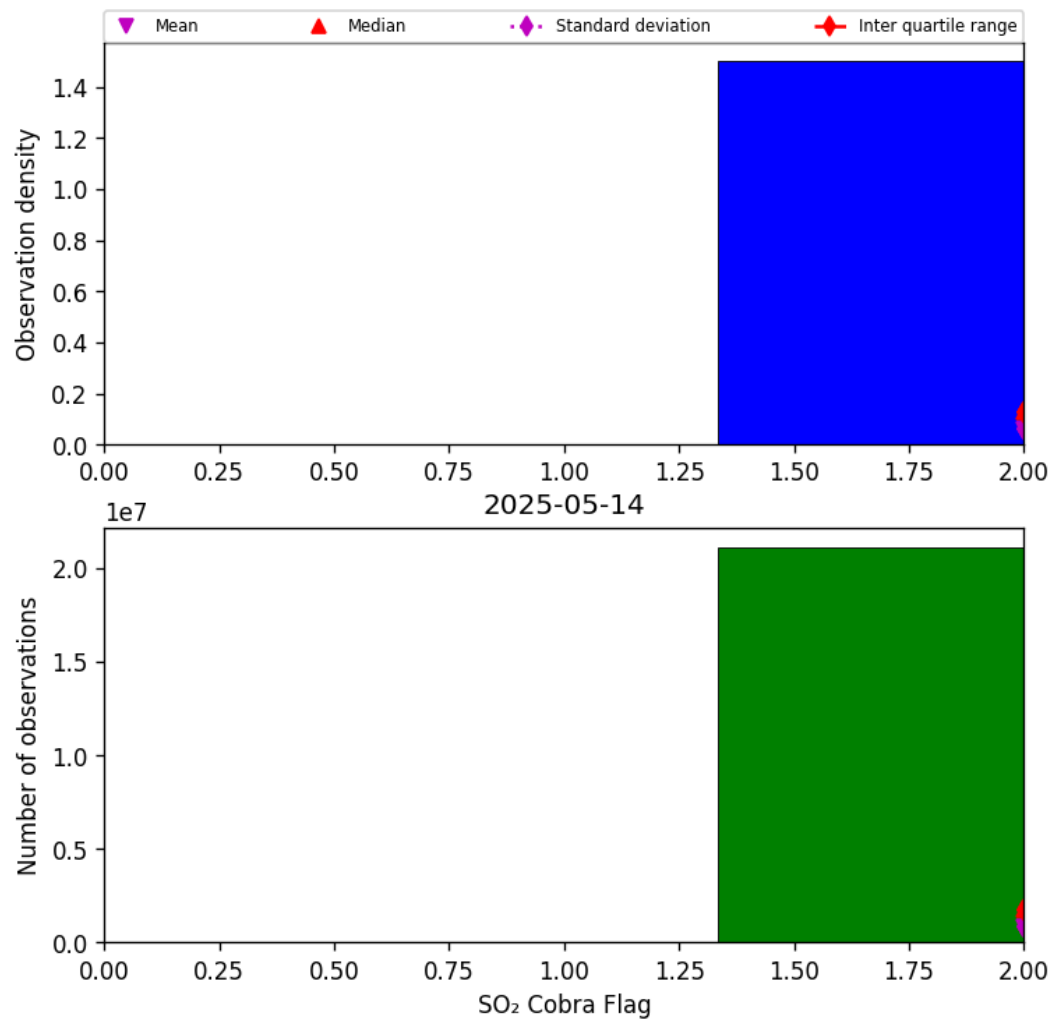
Figure 75: Histogram of “SO 2 Cobra Flag” for 2025-05-13 to 2025-05-15
