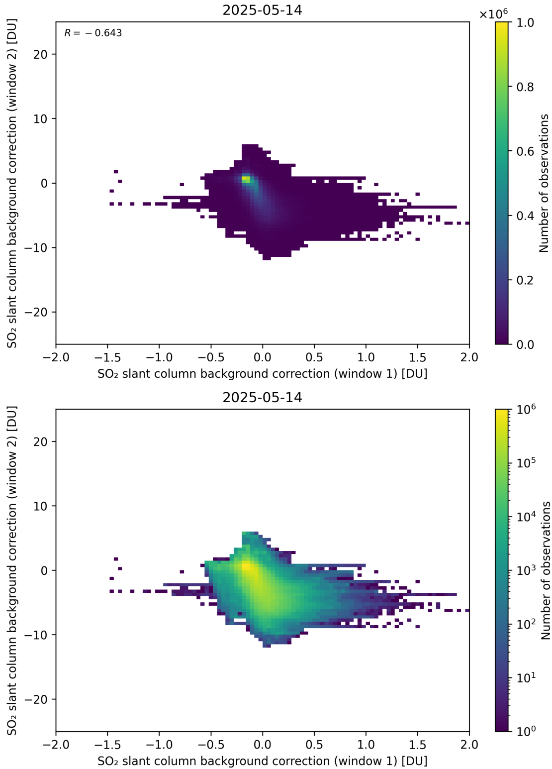
Figure 109: Scatter density plot of “SO 2 slant column background correction (window 1)” against “SO 2 slant column background correction (window 2)” for 2025-05-13 to 2025-05-15.
