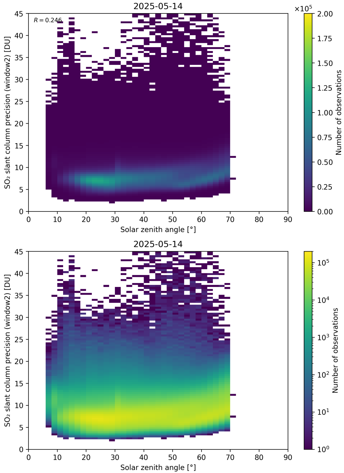
Figure 186: Scatter density plot of “Solar zenith angle” against “SO 2 slant column precision (window2)” for 2025-05-13 to 2025-05-15.
