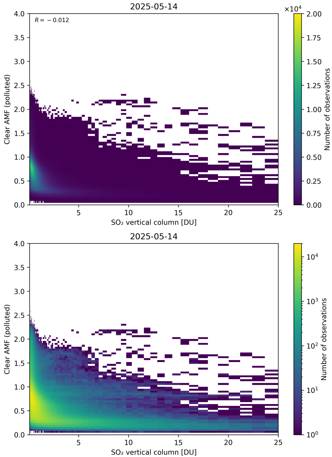
Figure 348: Scatter density plot of “SO 2 vertical column” against “Clear AMF (polluted)” for 2025-05-13 to 2025-05-15.
