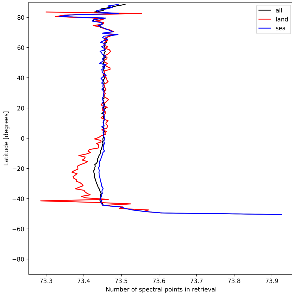
Figure 56: Zonal average of “Number of spectral points in retrieval” for 2025-05-13 to 2025-05-15.
