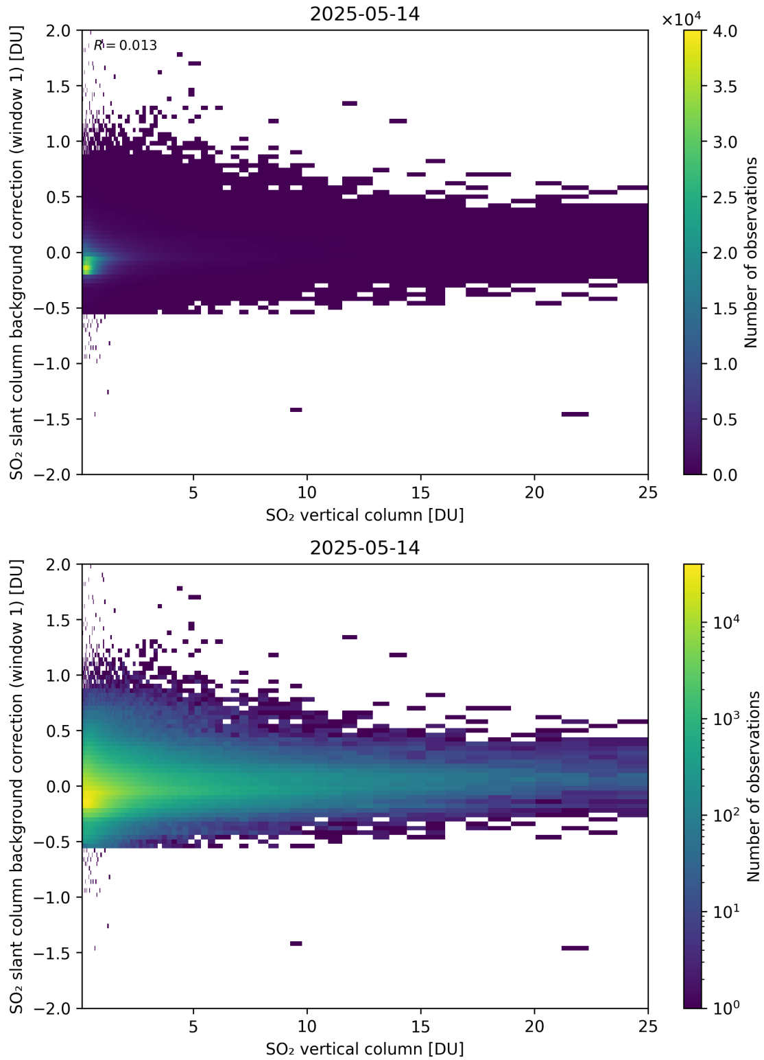
Figure 323: Scatter density plot of “SO 2 vertical column” against “SO 2 slant column background correction (window 1)” for 2025-05-13 to 2025-05-15.
