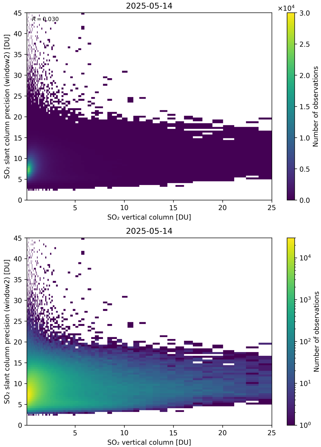
Figure 356: Scatter density plot of “SO 2 vertical column” against “SO 2 slant column precision (window2)” for 2025-05-13 to 2025-05-15.
