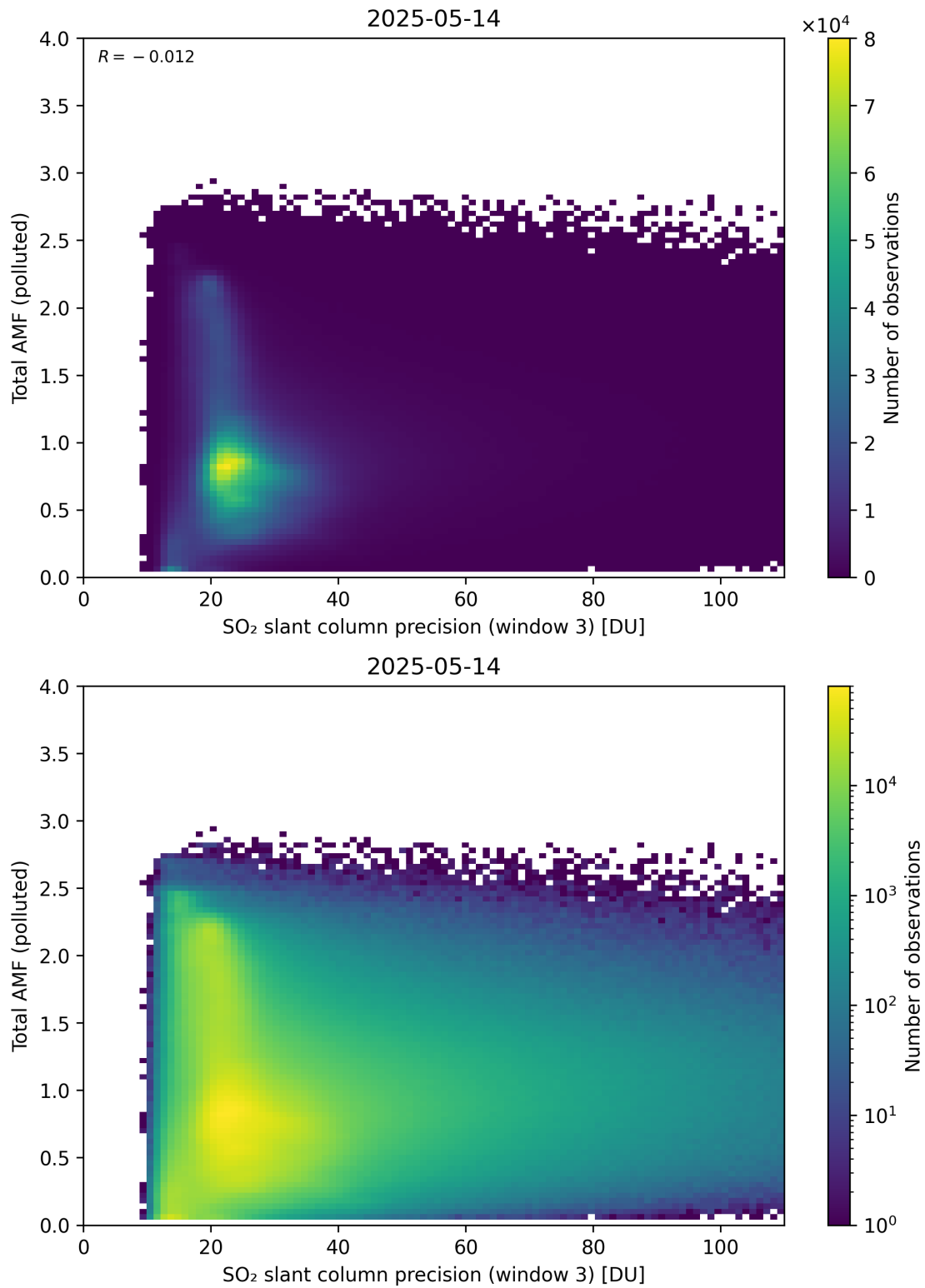
Figure 313: Scatter density plot of “SO 2 slant column precision (window 3)” against “Total AMF (polluted)” for 2025-05-13 to 2025-05-15.
