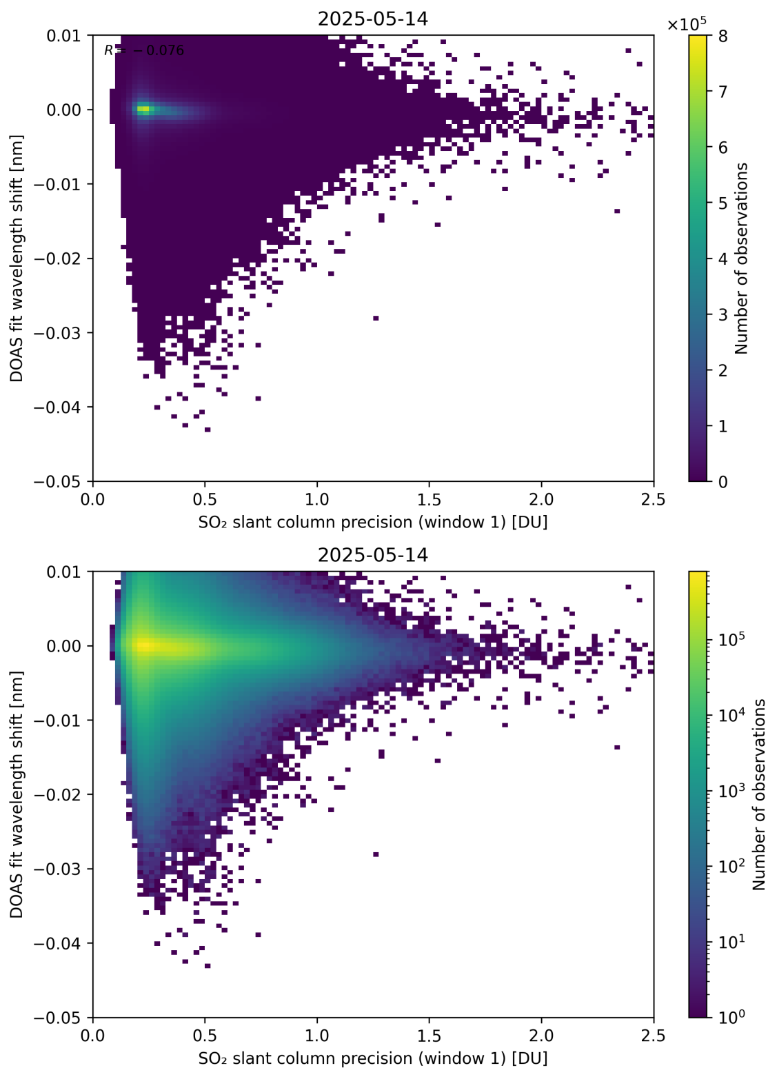
Figure 271: Scatter density plot of “SO 2 slant column precision (window 1)” against “DOAS fit wavelength shift” for 2025-05-13 to 2025-05-15.
