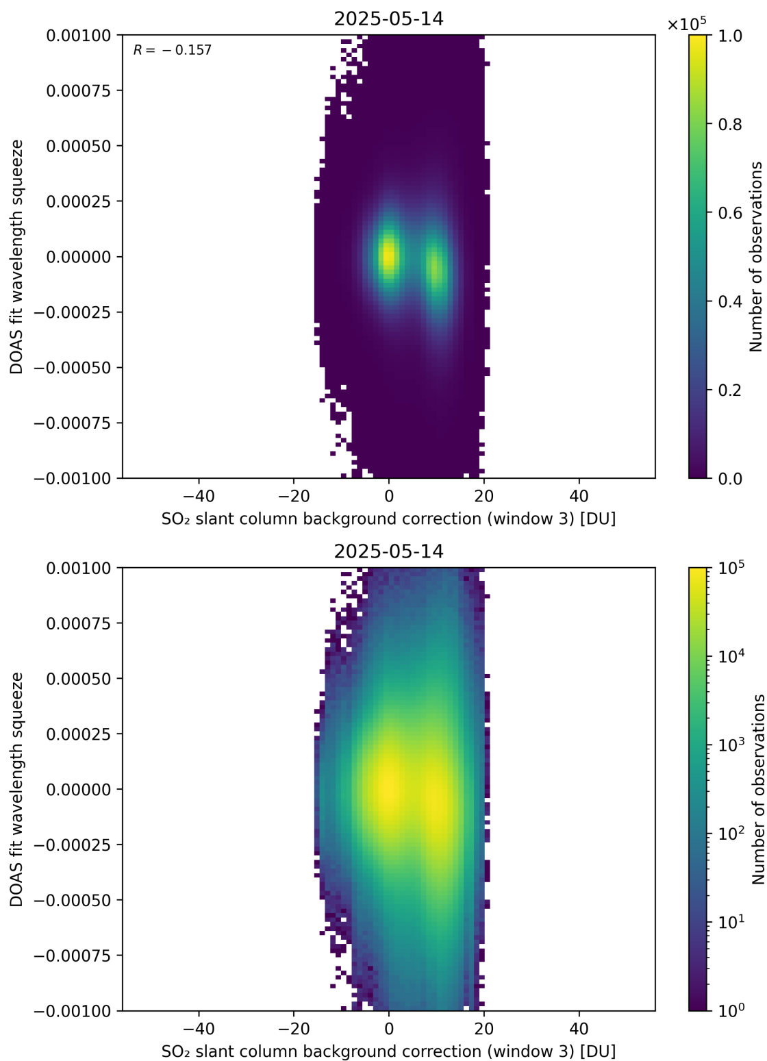
Figure 133: Scatter density plot of “SO 2 slant column background correction (window 3)” against “DOAS fit wavelength squeeze” for 2025-05-13 to 2025-05-15.
