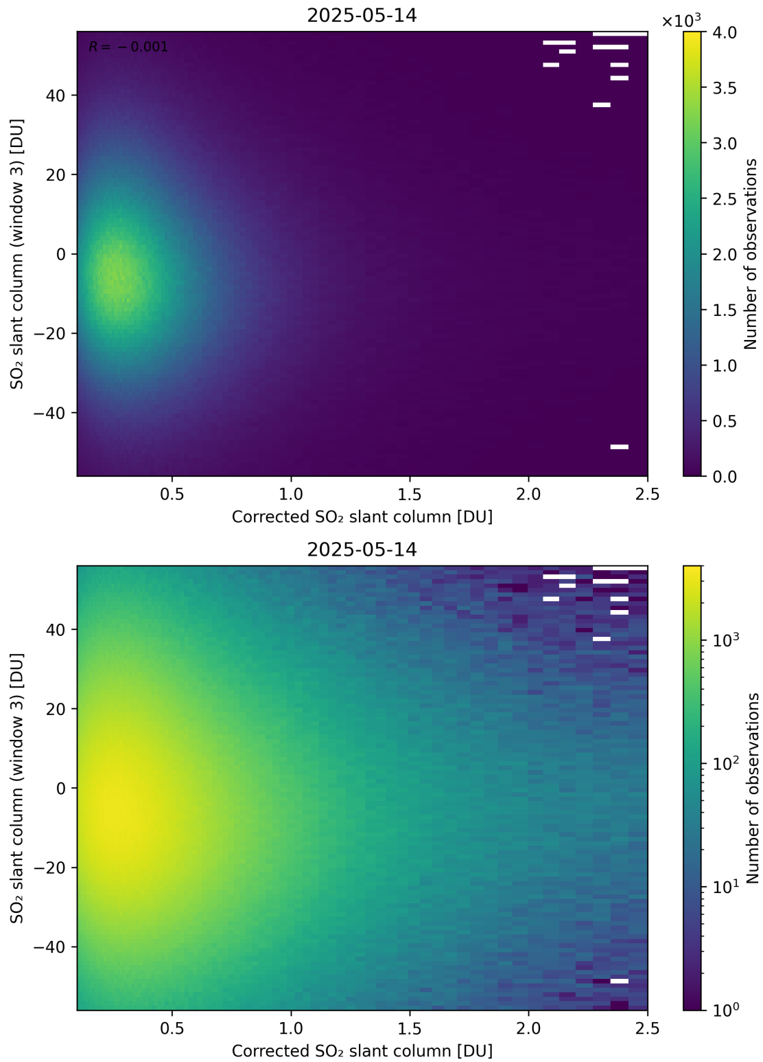
Figure 240: Scatter density plot of “Corrected SO 2 slant column” against “SO 2 slant column (window 3)” for 2025-05-13 to 2025-05-15.
