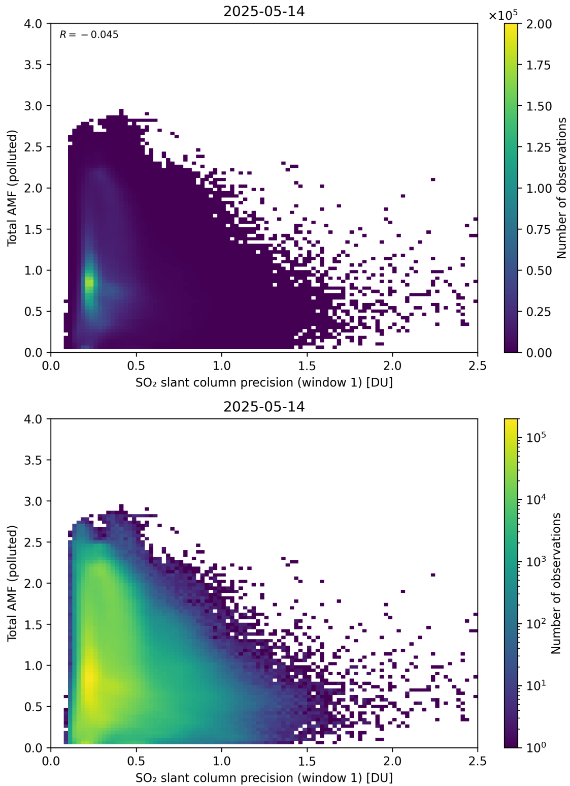
Figure 280: Scatter density plot of “SO 2 slant column precision (window 1)” against “Total AMF (polluted)” for 2025-05-13 to 2025-05-15.
