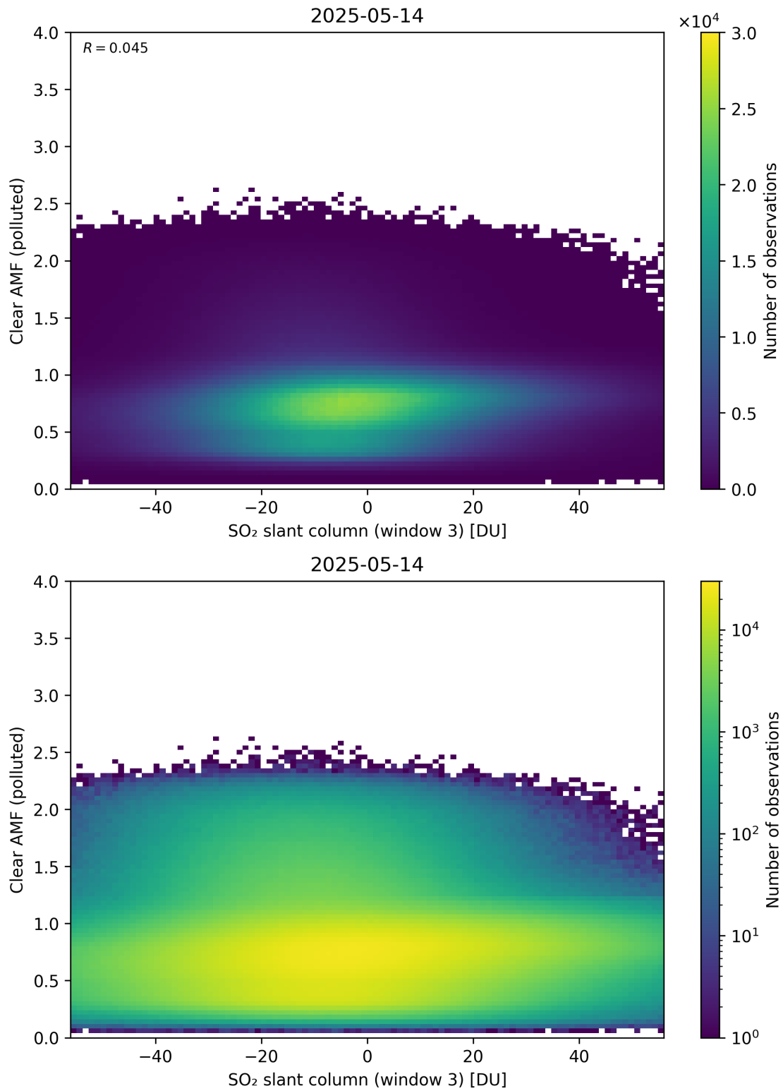
Figure 315: Scatter density plot of “SO 2 slant column (window 3)” against “Clear AMF (polluted)” for 2025-05-13 to 2025-05-15.
