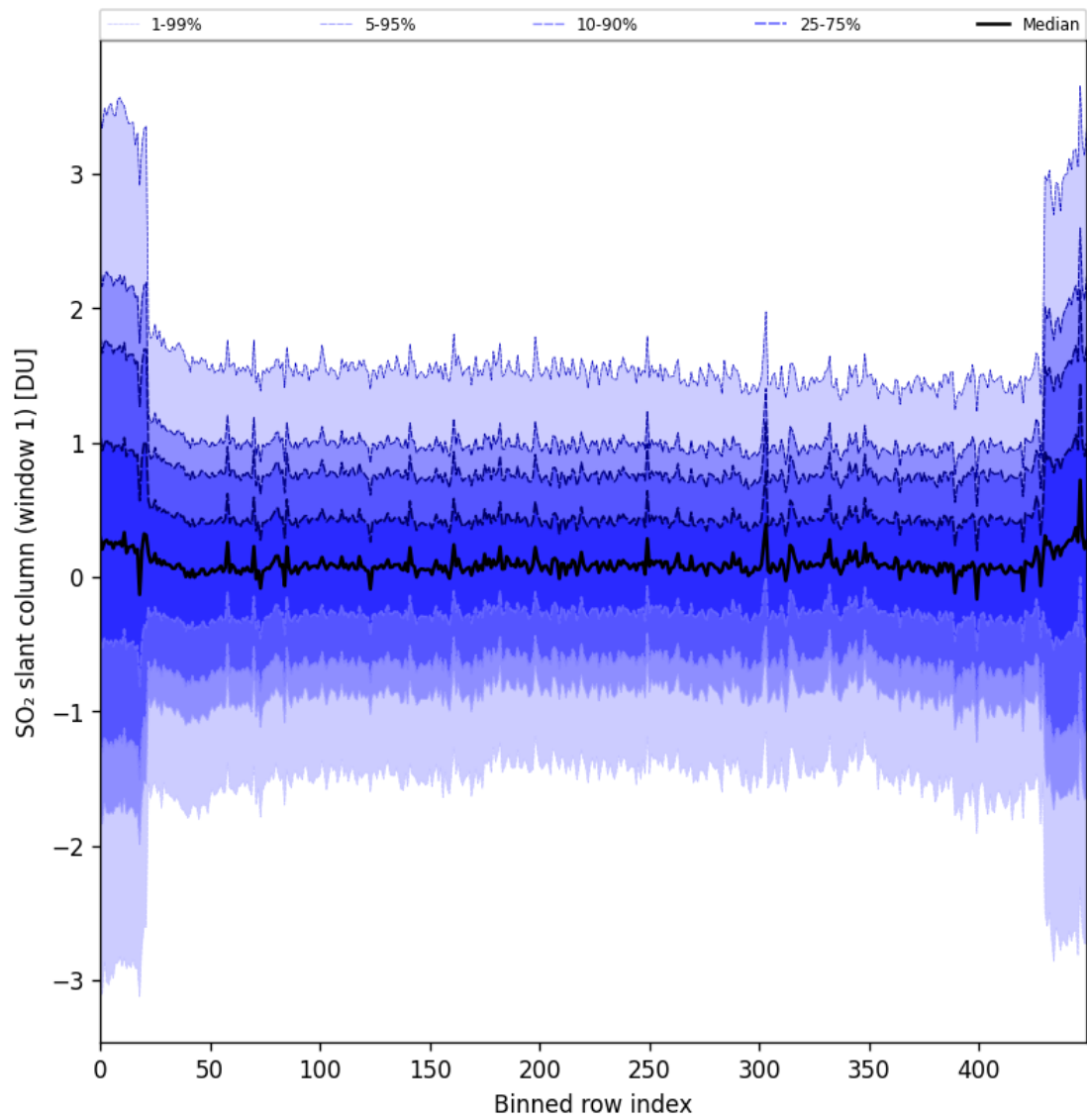
Figure 89: Along track statistics of “SO 2 slant column (window 1)” for 2025-05-13 to 2025-05-15
