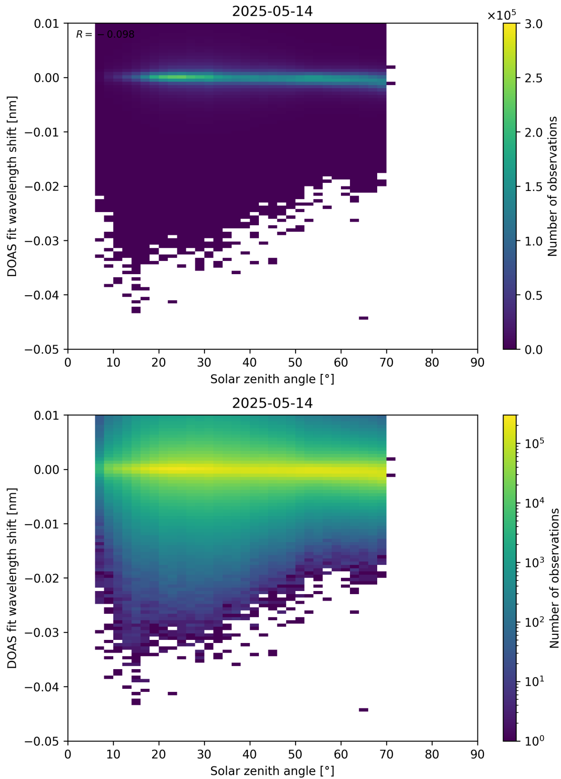
Figure 174: Scatter density plot of “Solar zenith angle” against “DOAS fit wavelength shift” for 2025-05-13 to 2025-05-15.
