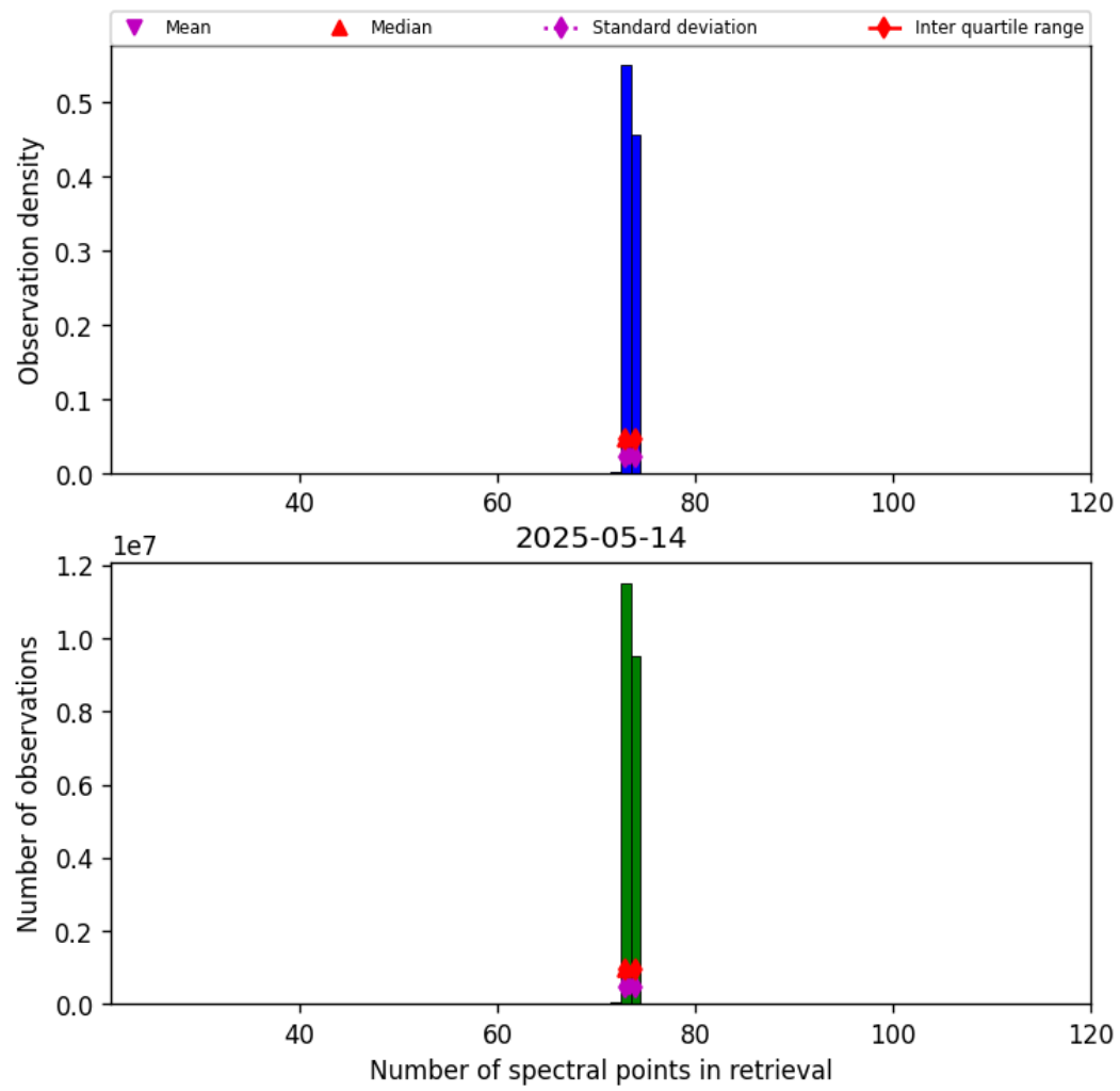
Figure 82: Histogram of “Number of spectral points in retrieval” for 2025-05-13 to 2025-05-15
