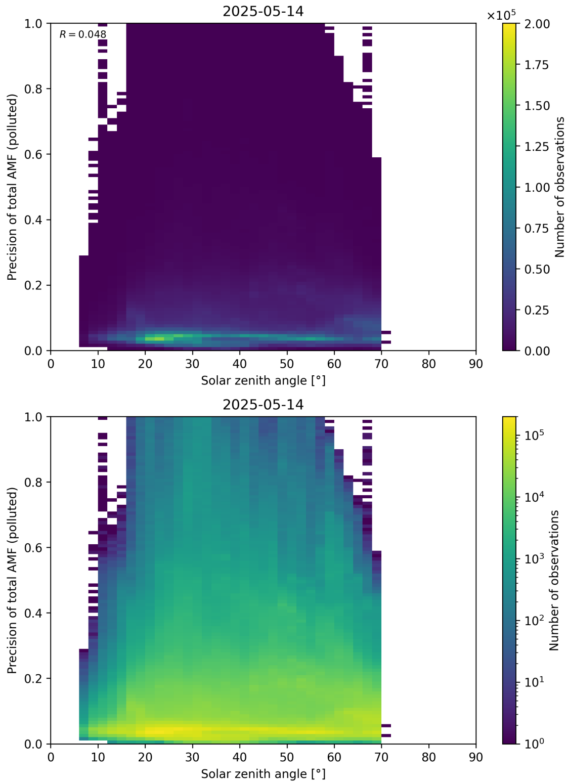
Figure 190: Scatter density plot of “Solar zenith angle” against “Precision of total AMF (polluted)” for 2025-05-13 to 2025-05-15.
