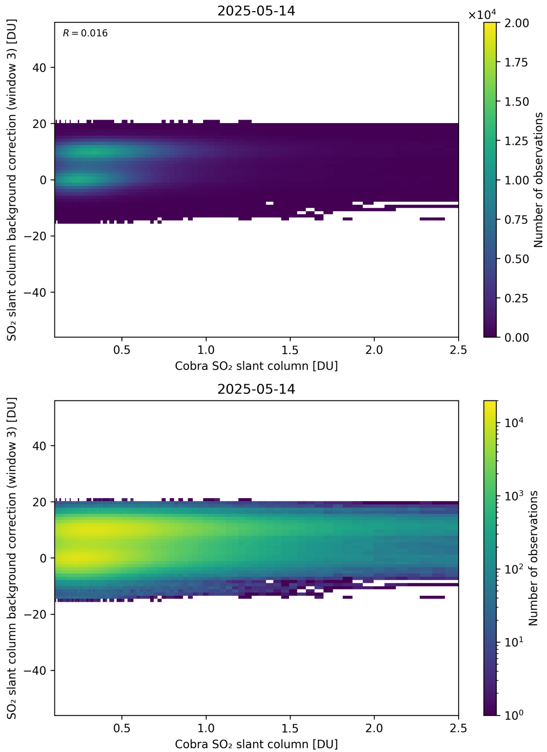
Figure 195: Scatter density plot of “Cobra SO 2 slant column” against “SO 2 slant column background correction (window 3)” for 2025-05-13 to 2025-05-15.
