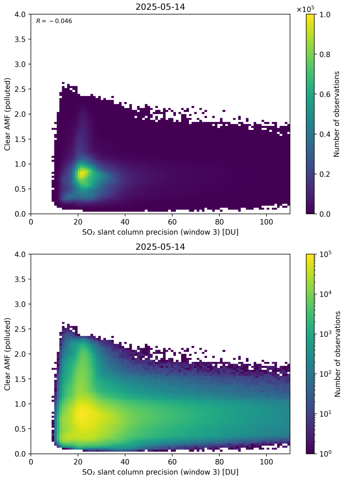
Figure 311: Scatter density plot of “SO 2 slant column precision (window 3)” against “Clear AMF (polluted)” for 2025-05-13 to 2025-05-15.
