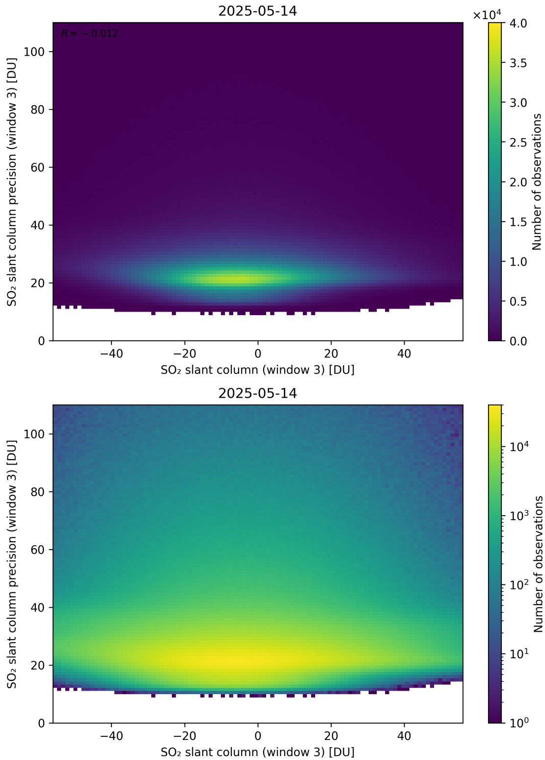
Figure 317: Scatter density plot of “SO 2 slant column (window 3)” against “SO 2 slant column precision (window 3)” for 2025-05-13 to 2025-05-15.
