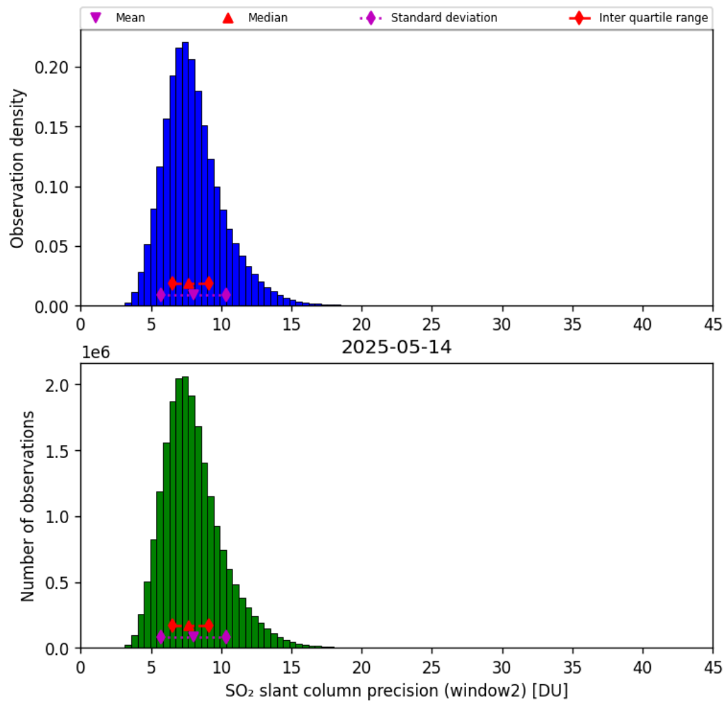
Figure 68: Histogram of “SO 2 slant column precision (window2)” for 2025-05-13 to 2025-05-15
