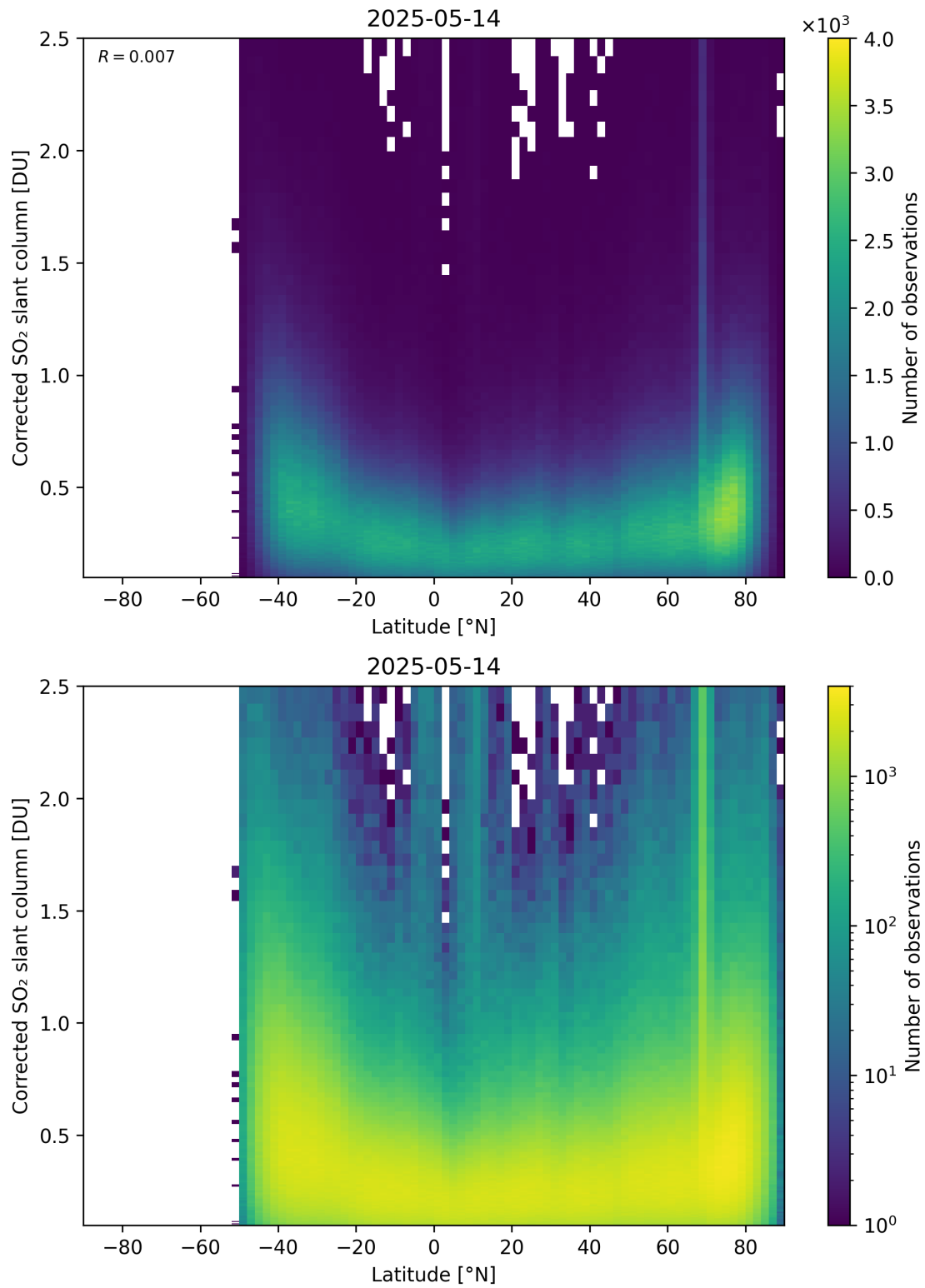
Figure 159: Scatter density plot of “Latitude” against “Corrected SO 2 slant column” for 2025-05-13 to 2025-05-15.
