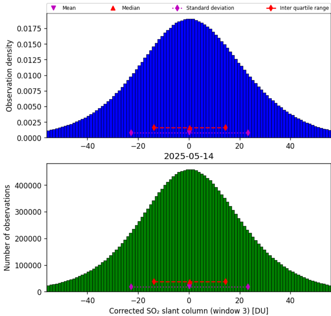
Figure 73: Histogram of “Corrected SO 2 slant column (window 3)” for 2025-05-13 to 2025-05-15
