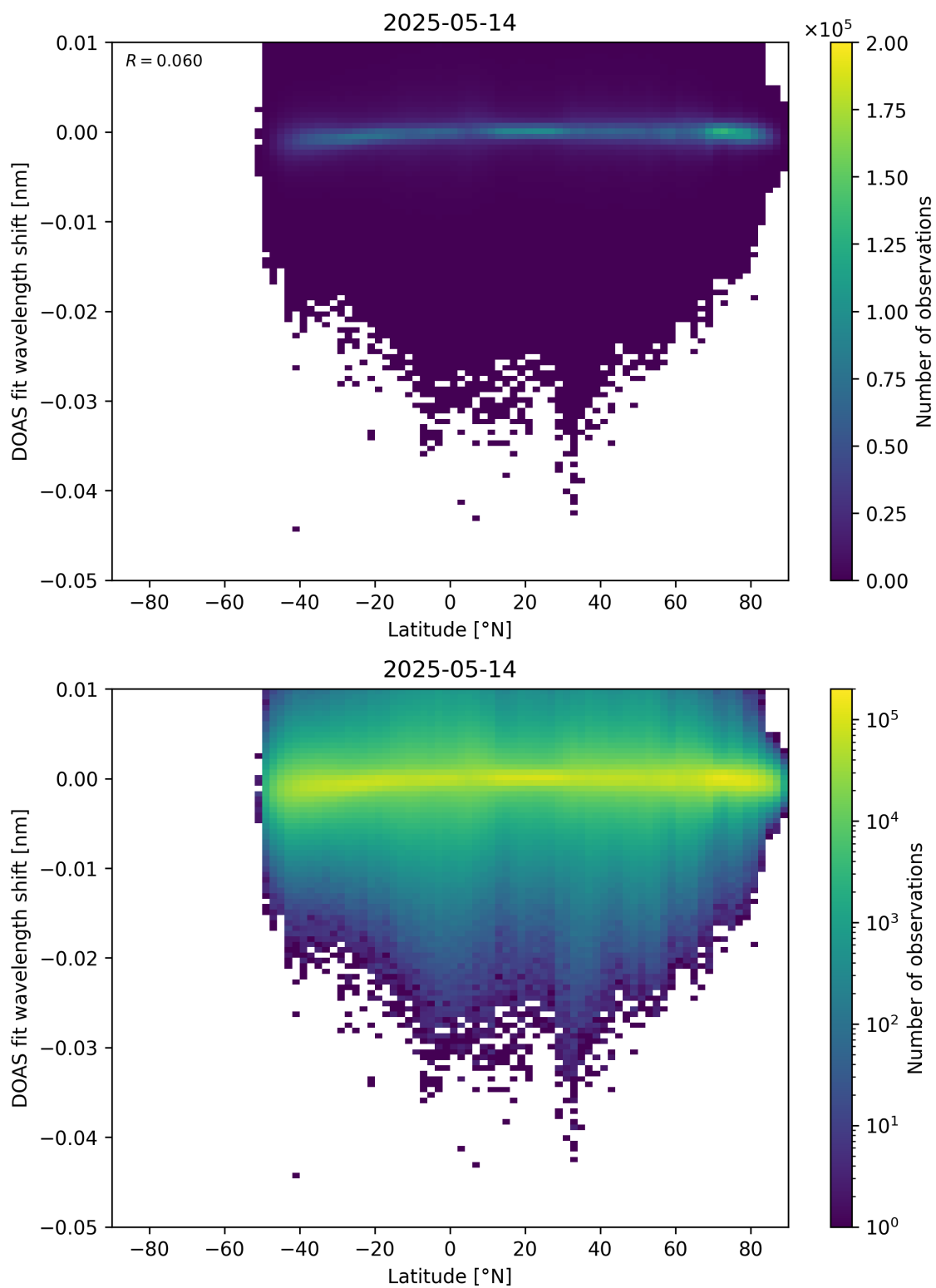
Figure 153: Scatter density plot of “Latitude” against “DOAS fit wavelength shift” for 2025-05-13 to 2025-05-15.
