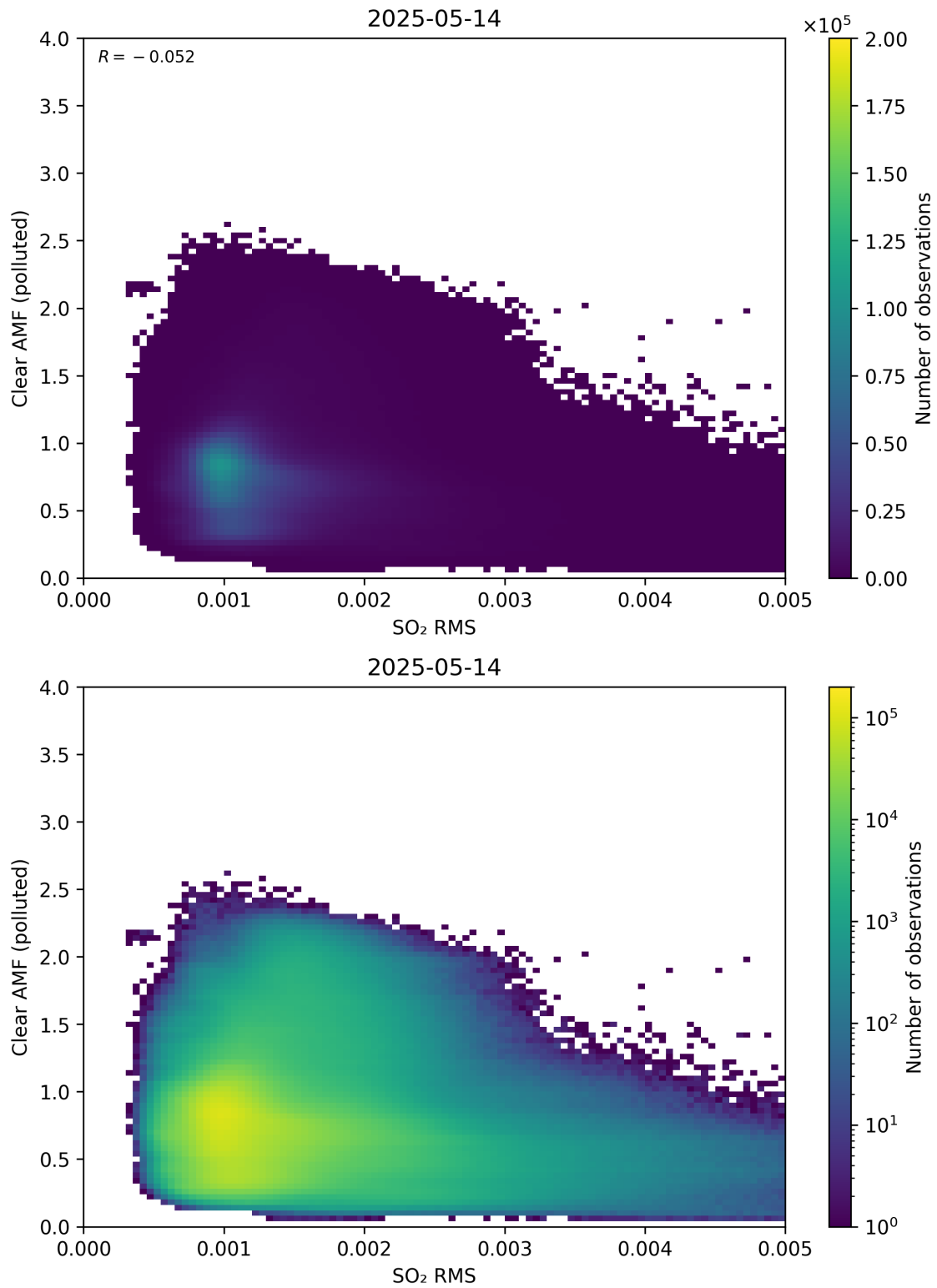
Figure 147: Scatter density plot of “SO 2 RMS” against “Clear AMF (polluted)” for 2025-05-13 to 2025-05-15.
