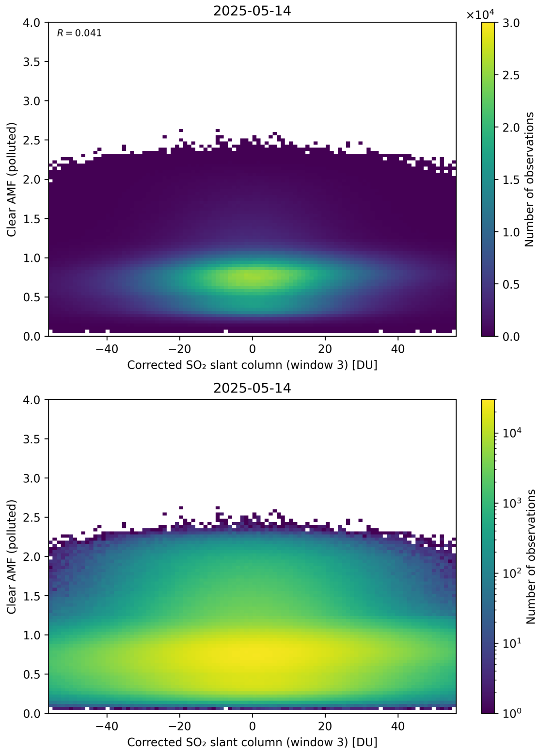
Figure 259: Scatter density plot of “Corrected SO 2 slant column (window 3)” against “Clear AMF (polluted)” for 2025-05-13 to 2025-05-15.
