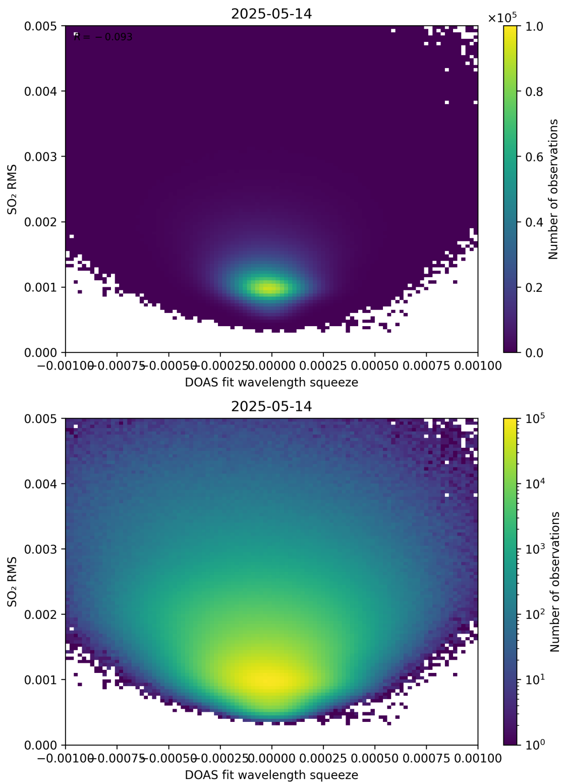
Figure 143: Scatter density plot of “DOAS fit wavelength squeeze” against “SO 2 RMS” for 2025-05-13 to 2025-05-15.
