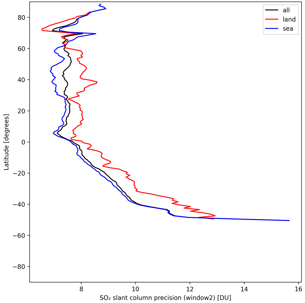
Figure 42: Zonal average of “SO 2 slant column precision (window2)” for 2025-05-13 to 2025-05-15.
