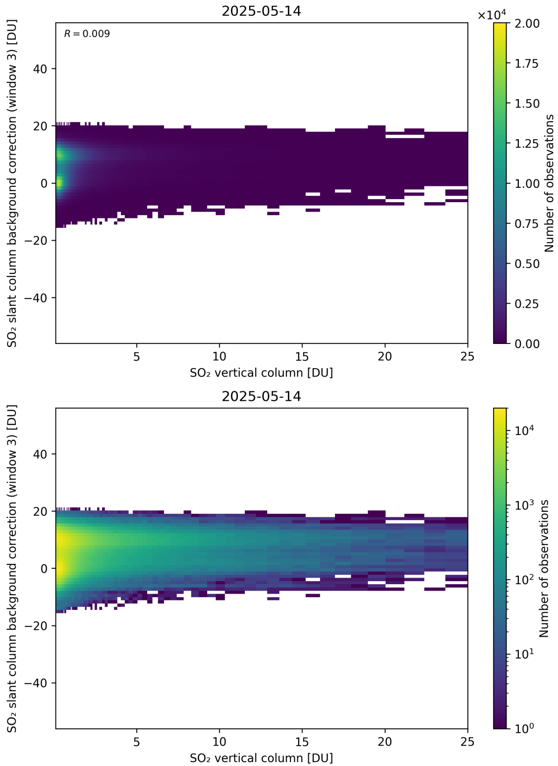
Figure 325: Scatter density plot of “SO 2 vertical column” against “SO 2 slant column background correction (window 3)” for 2025-05-13 to 2025-05-15.
