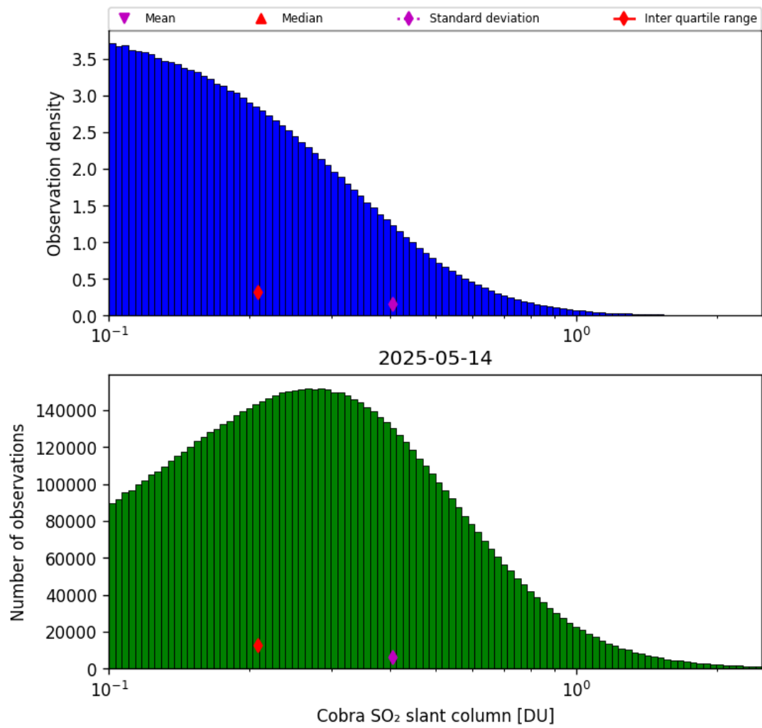
Figure 61: Histogram of “Cobra SO 2 slant column” for 2025-05-13 to 2025-05-15
