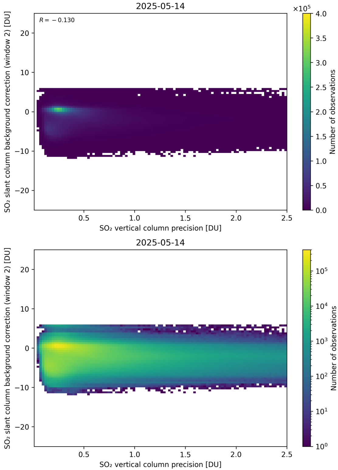
Figure 330: Scatter density plot of “SO 2 vertical column precision” against “SO 2 slant column background correction (window 2)” for 2025-05-13 to 2025-05-15.
