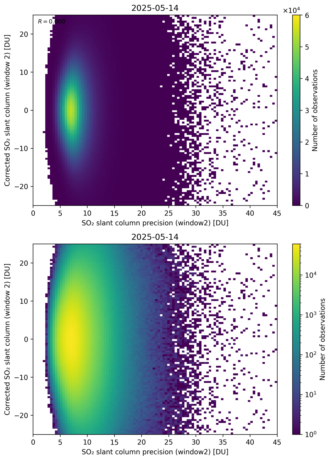
Figure 297: Scatter density plot of “SO 2 slant column precision (window2)” against “Corrected SO 2 slant column (window 2)” for 2025-05-13 to 2025-05-15.
