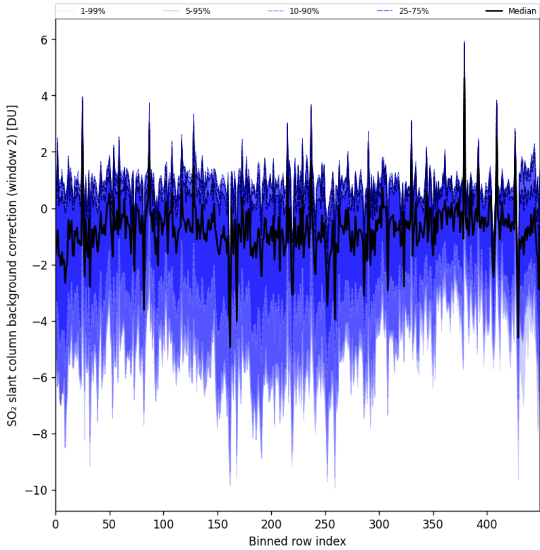
Figure 96: Along track statistics of “SO 2 slant column background correction (window 2)” for 2025-05-13 to 2025-05-15
