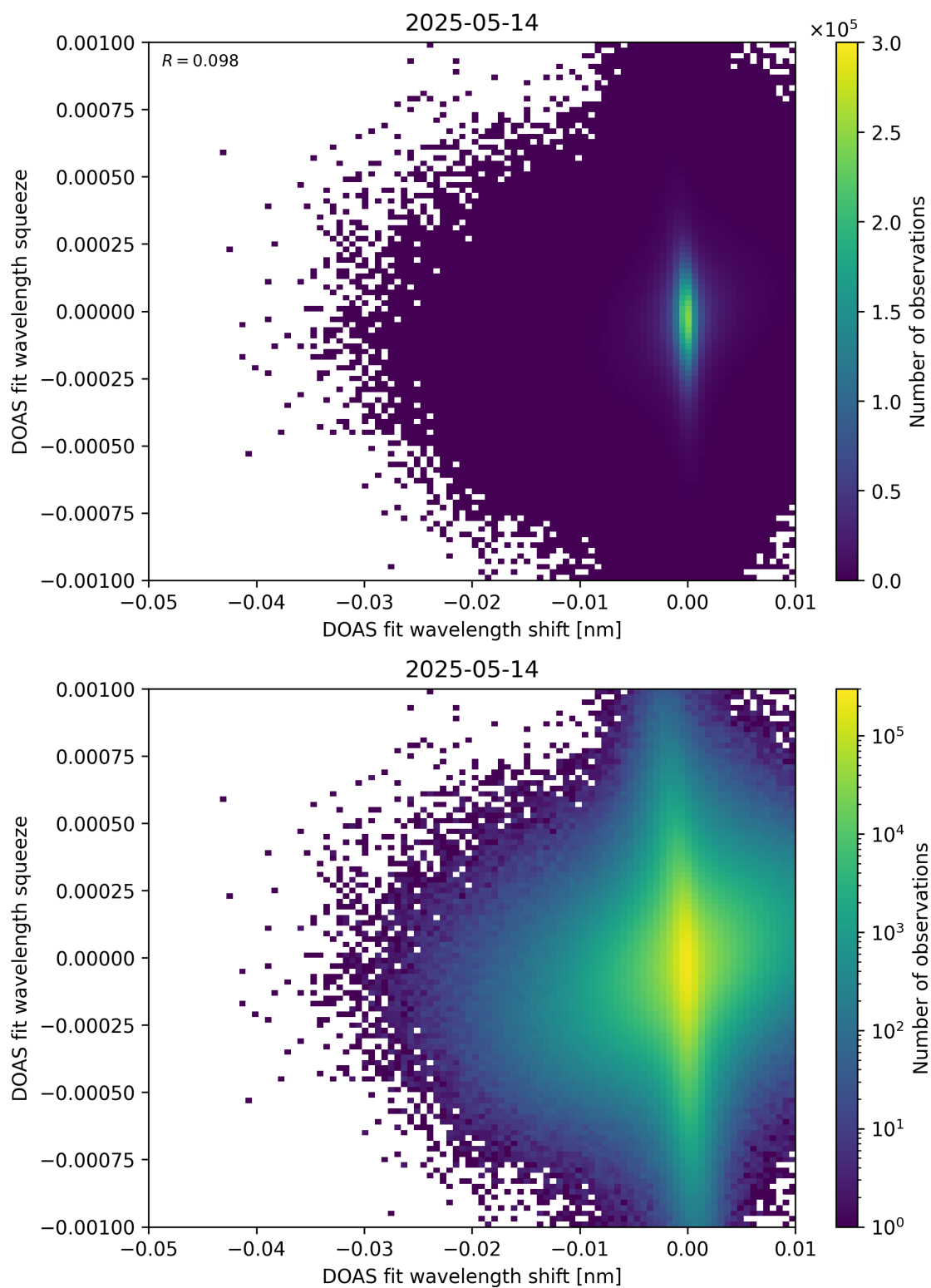
Figure 138: Scatter density plot of “DOAS fit wavelength shift” against “DOAS fit wavelength squeeze” for 2025-05-13 to 2025-05-15.
