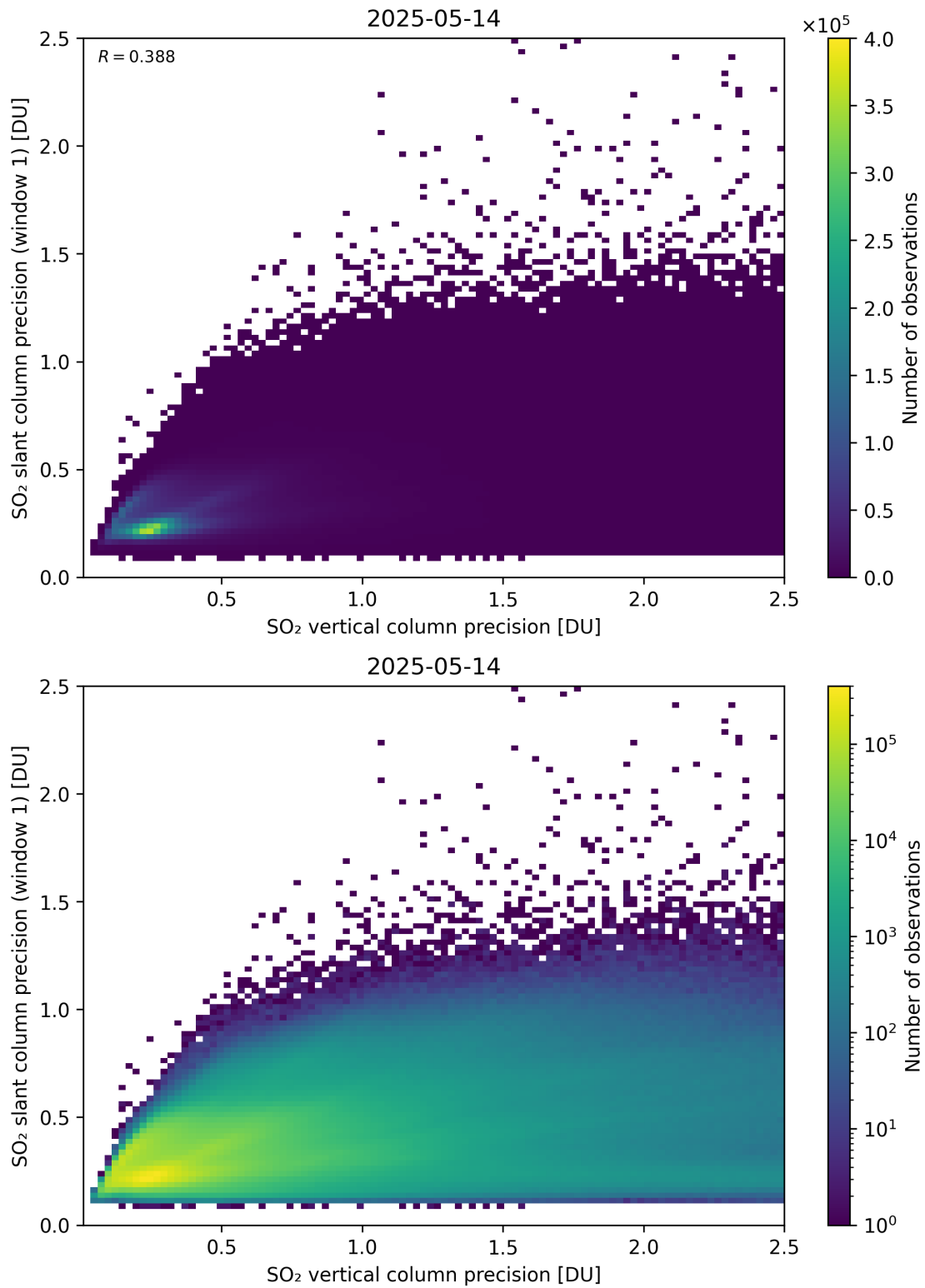
Figure 342: Scatter density plot of “SO 2 vertical column precision” against “SO 2 slant column precision (window 1)” for 2025-05-13 to 2025-05-15.
