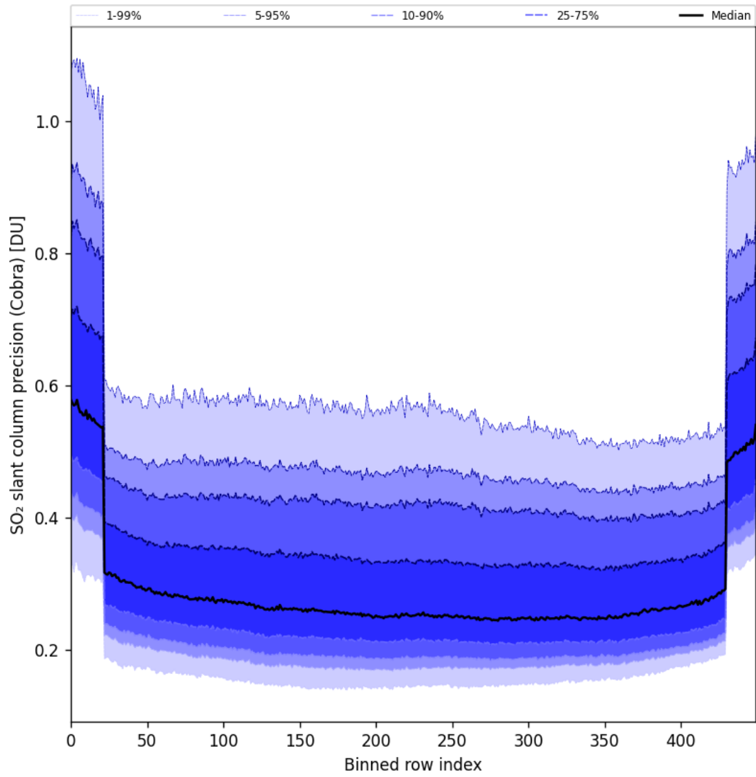
Figure 88: Along track statistics of “SO 2 slant column precision (Cobra)” for 2025-05-13 to 2025-05-15
