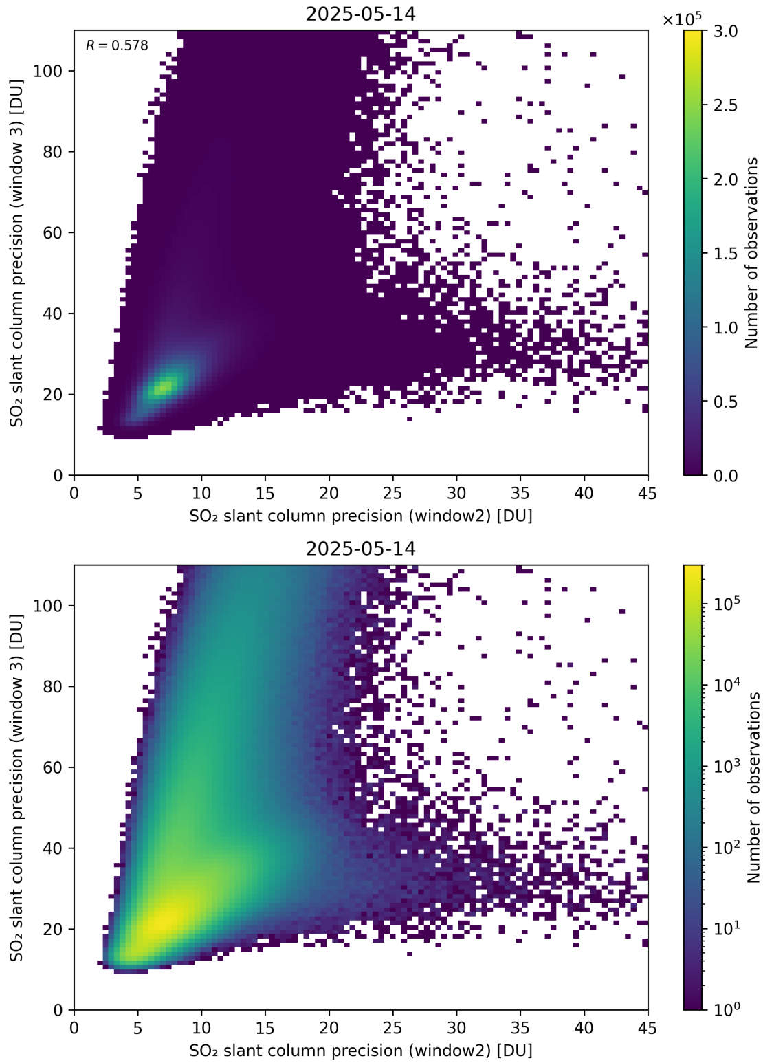
Figure 300: Scatter density plot of “SO 2 slant column precision (window2)” against “SO 2 slant column precision (window 3)” for 2025-05-13 to 2025-05-15.
