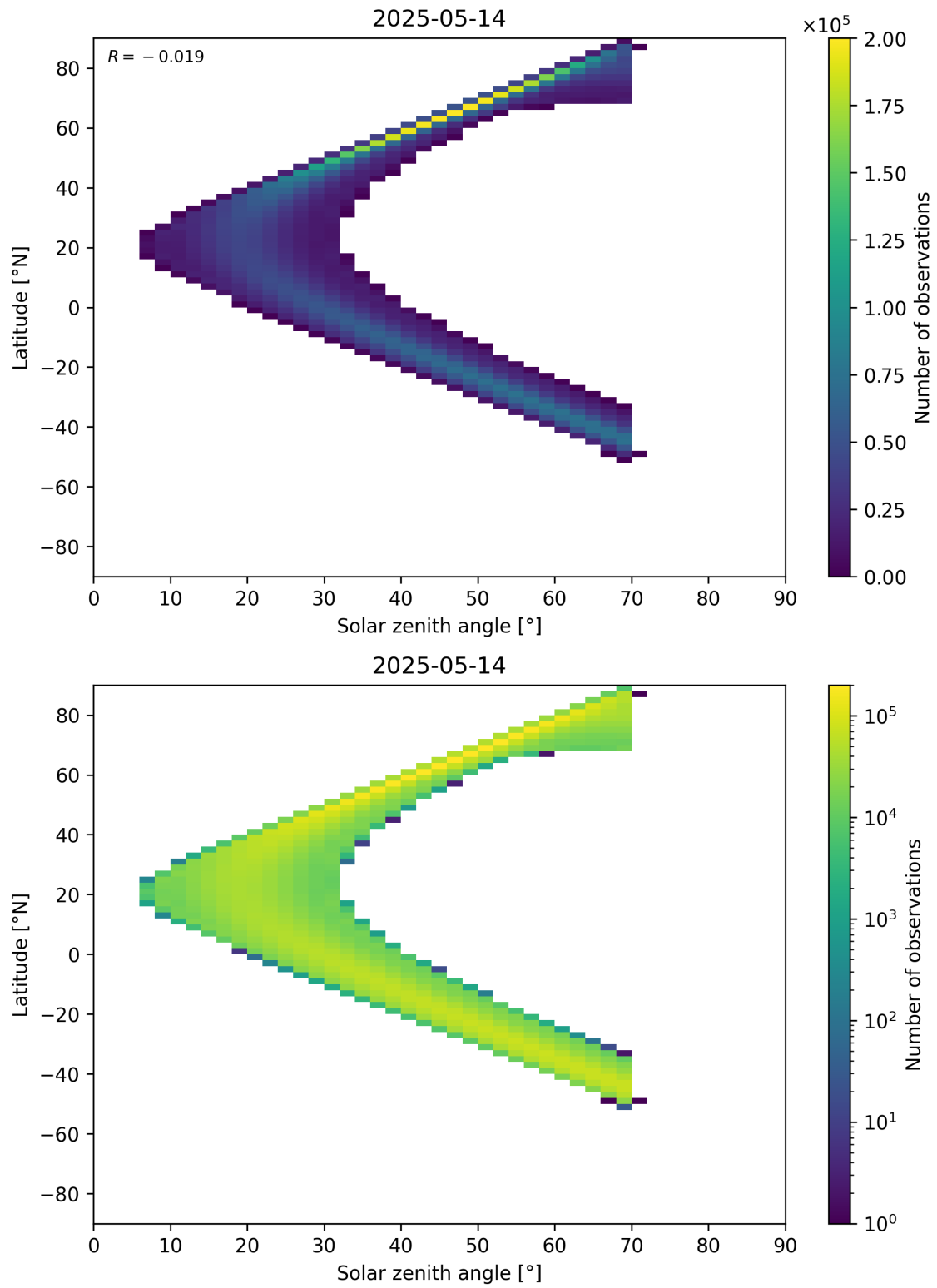
Figure 177: Scatter density plot of “Solar zenith angle” against “Latitude” for 2025-05-13 to 2025-05-15.
