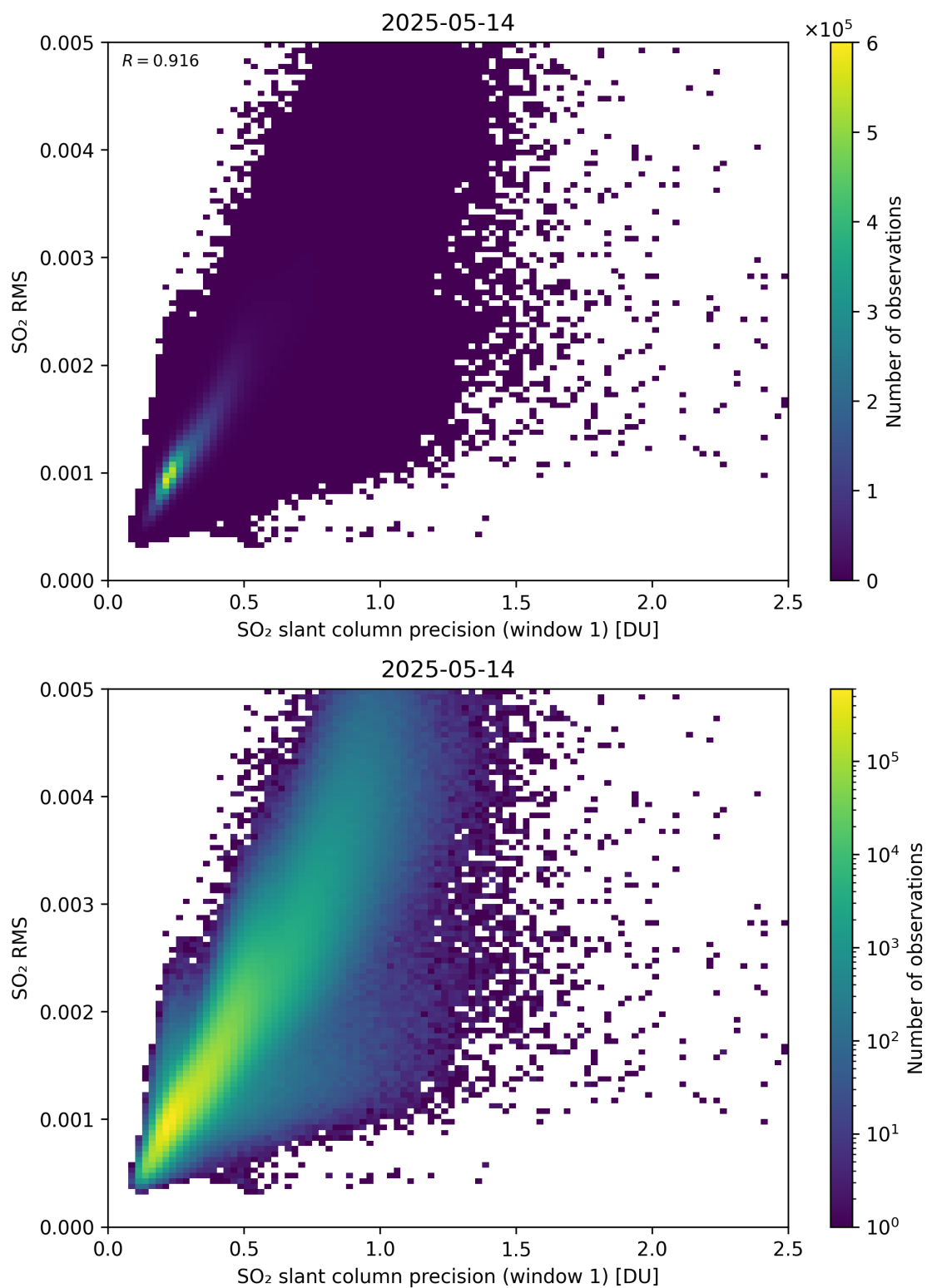
Figure 273: Scatter density plot of “SO 2 slant column precision (window 1)” against “SO 2 RMS” for 2025-05-13 to 2025-05-15.
