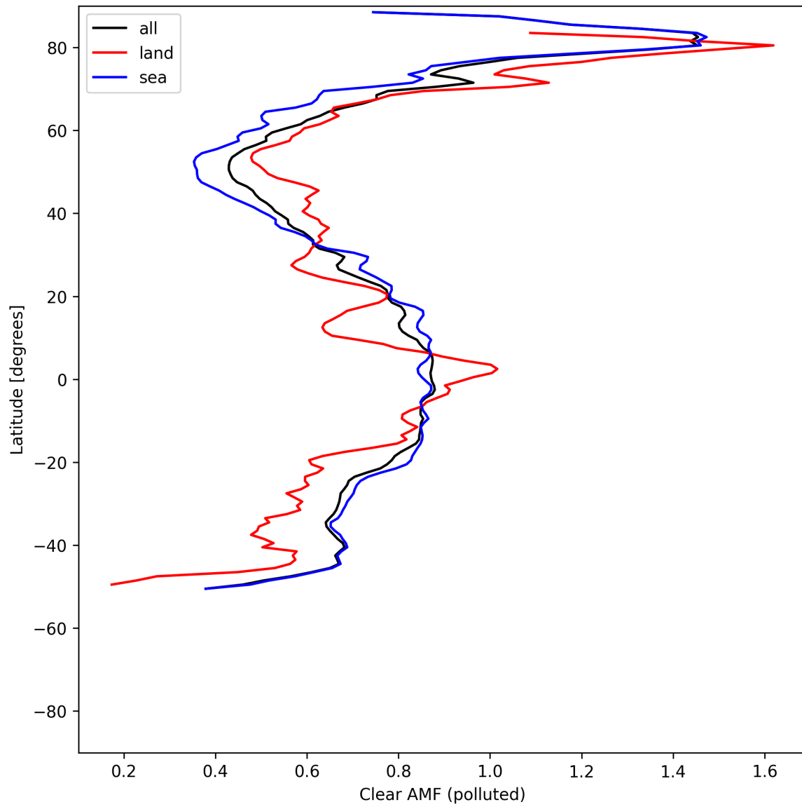
Figure 55: Zonal average of “Clear AMF (polluted)” for 2025-05-13 to 2025-05-15.
