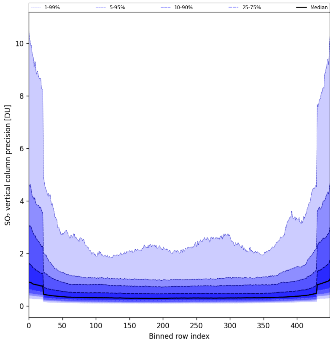
Figure 85: Along track statistics of “SO 2 vertical column precision” for 2025-05-13 to 2025-05-15
