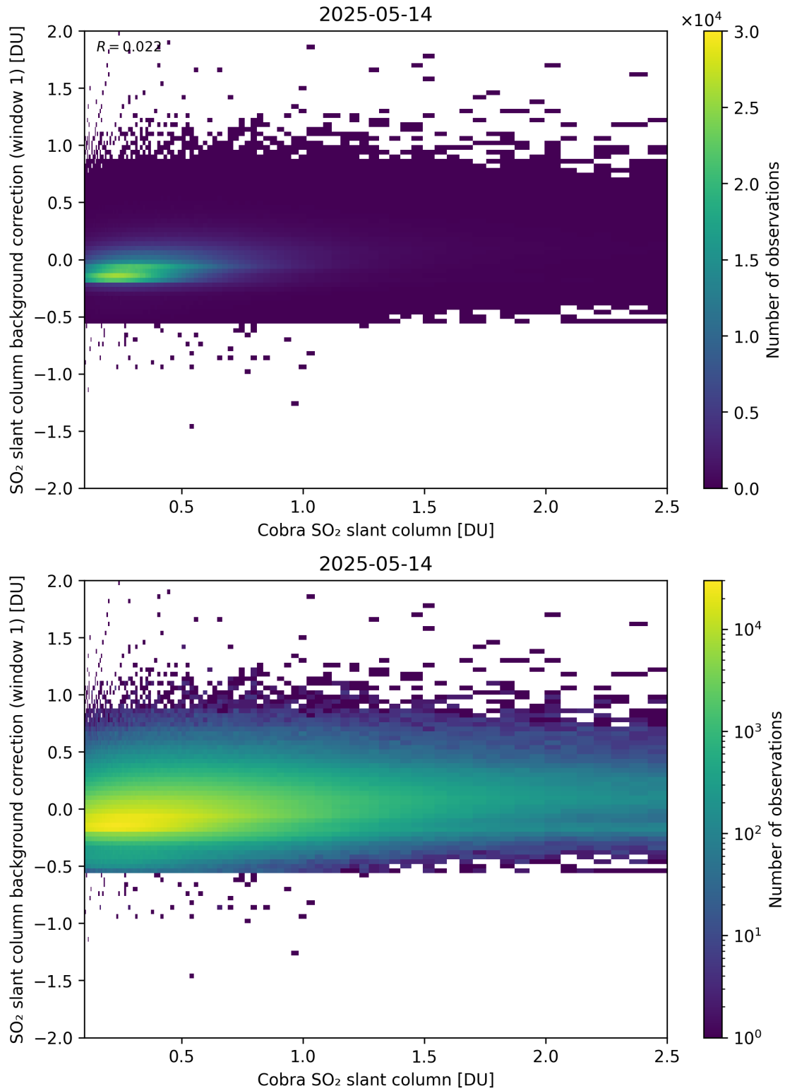
Figure 193: Scatter density plot of “Cobra SO 2 slant column” against “SO 2 slant column background correction (window 1)” for 2025-05-13 to 2025-05-15.
