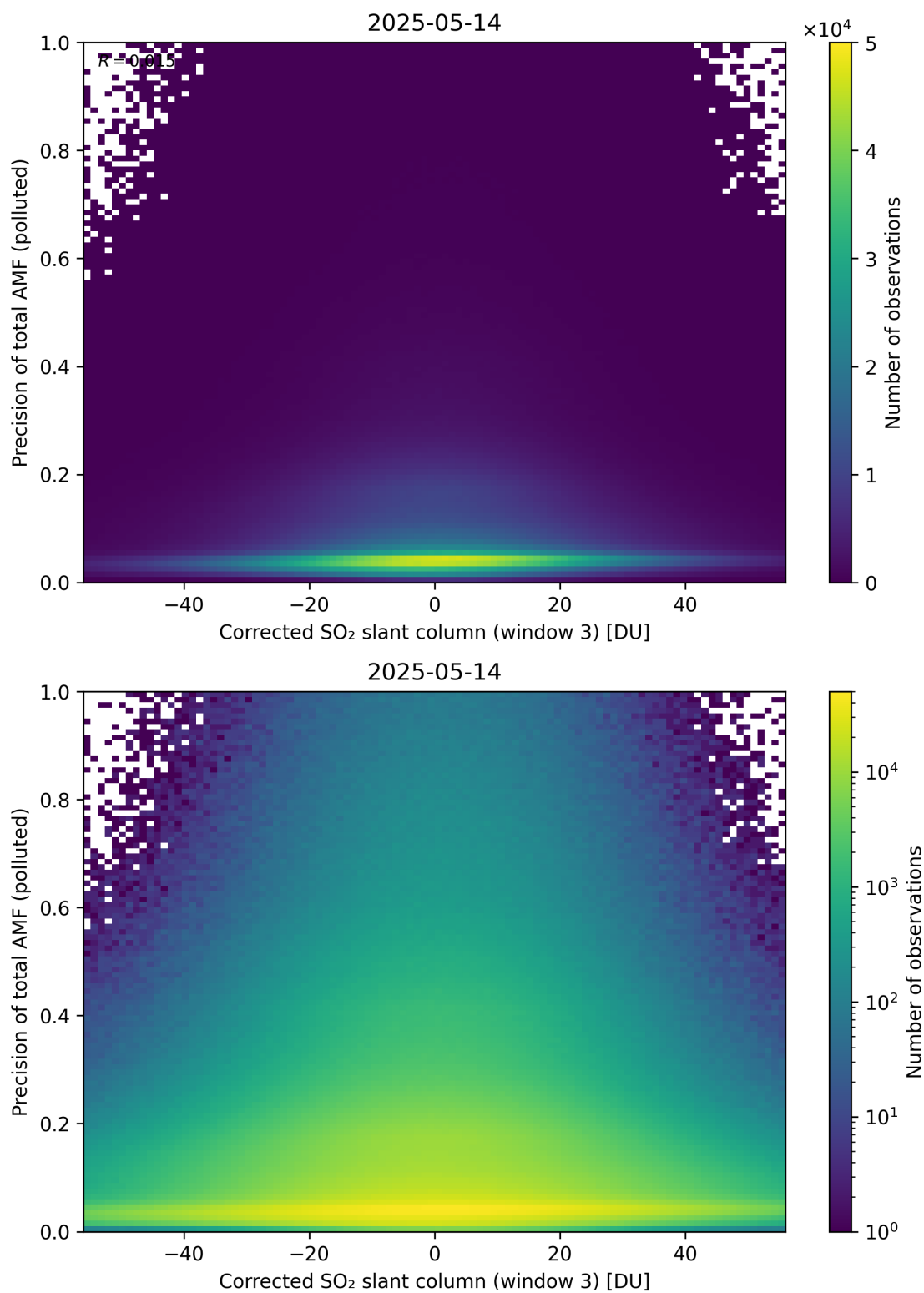
Figure 261: Scatter density plot of “Corrected SO 2 slant column (window 3)” against “Precision of total AMF (polluted)” for 2025-05-13 to 2025-05-15.
