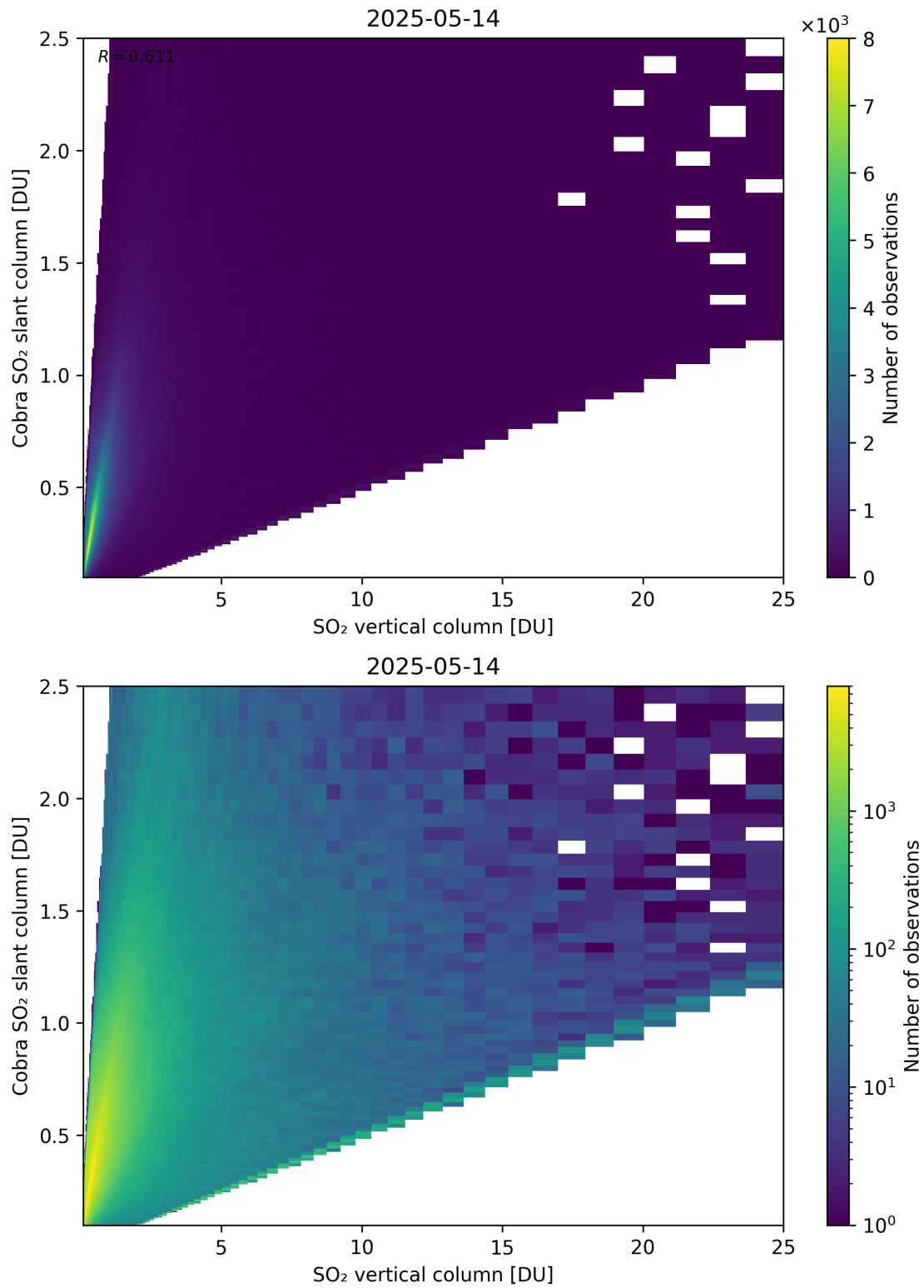
Figure 349: Scatter density plot of “SO 2 vertical column” against “Cobra SO 2 slant column” for 2025-05-13 to 2025-05-15.
