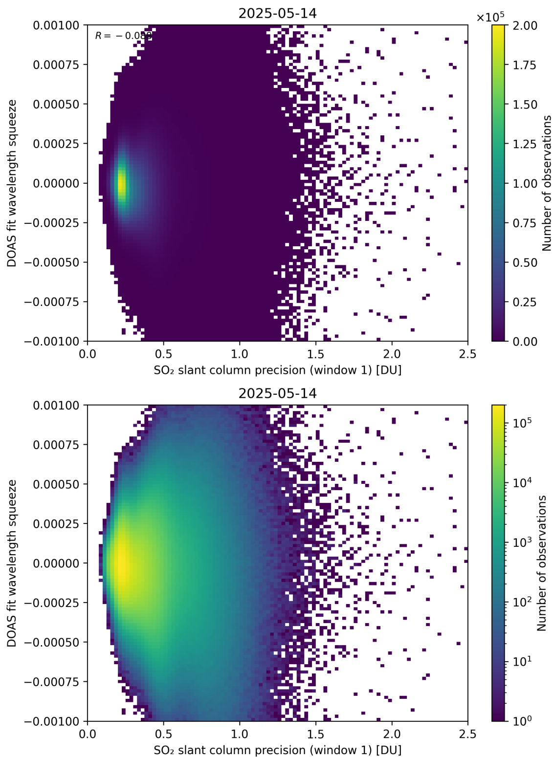
Figure 272: Scatter density plot of “SO 2 slant column precision (window 1)” against “DOAS fit wavelength squeeze” for 2025-05-13 to 2025-05-15.
