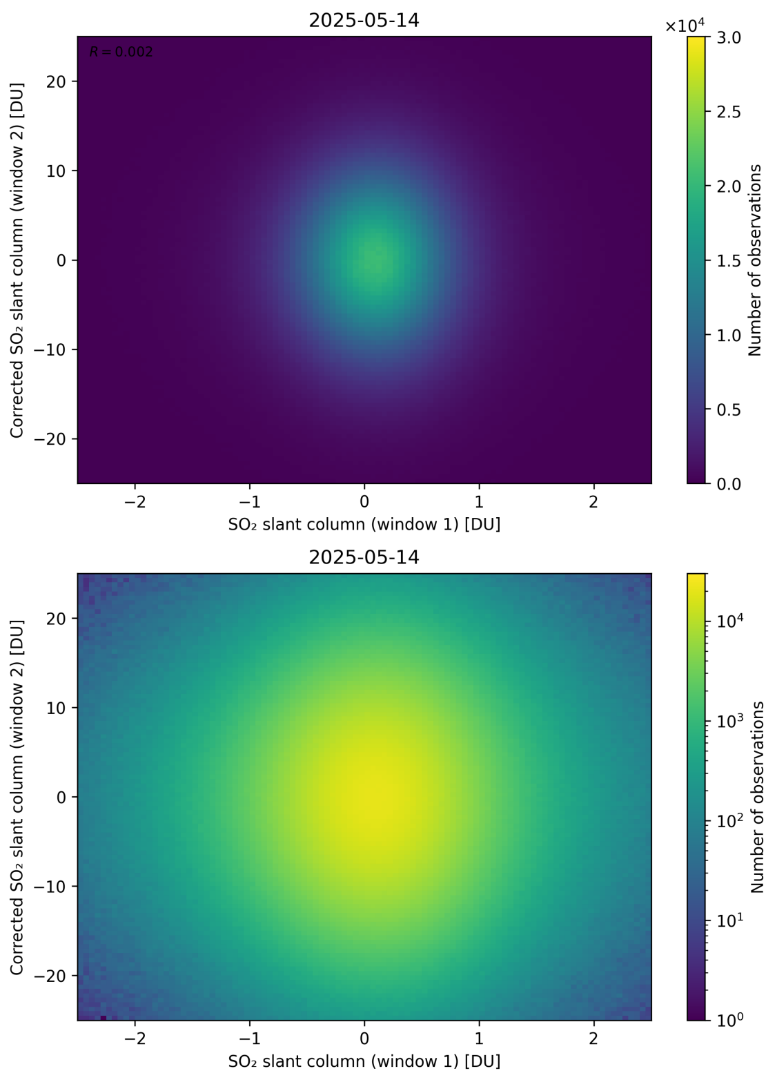
Figure 283: Scatter density plot of “SO 2 slant column (window 1)” against “Corrected SO 2 slant column (window 2)” for 2025-05-13 to 2025-05-15.
