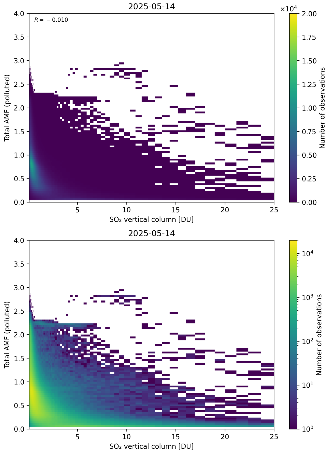
Figure 359: Scatter density plot of “SO 2 vertical column” against “Total AMF (polluted)” for 2025-05-13 to 2025-05-15.
