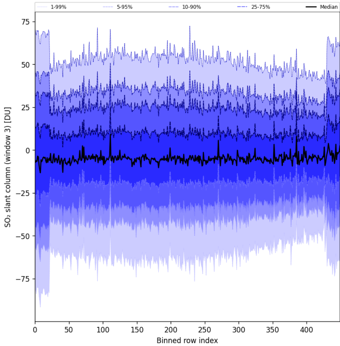
Figure 97: Along track statistics of “SO 2 slant column (window 3)” for 2025-05-13 to 2025-05-15
