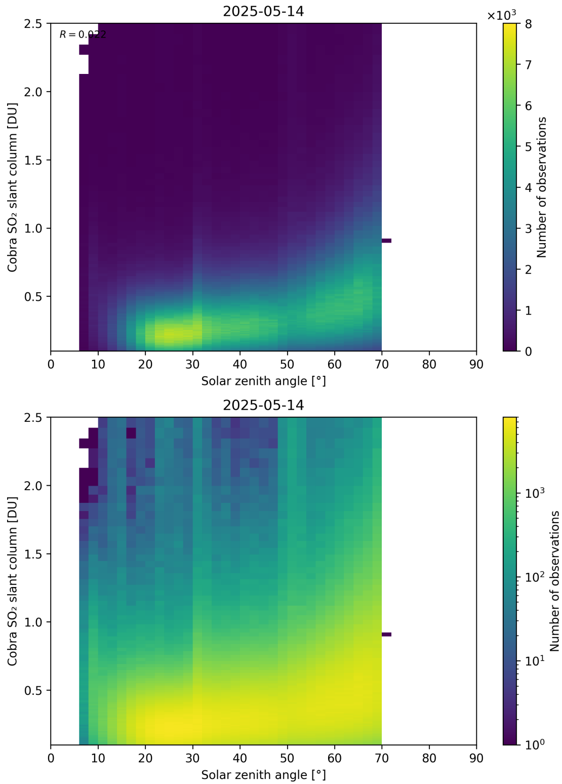
Figure 179: Scatter density plot of “Solar zenith angle” against “Cobra SO 2 slant column” for 2025-05-13 to 2025-05-15.
