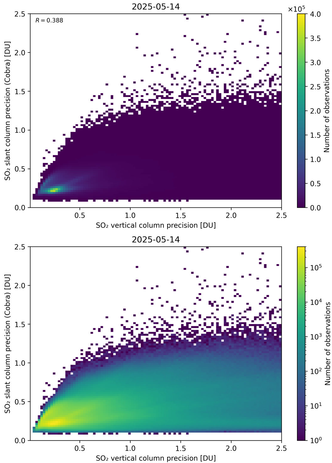
Figure 337: Scatter density plot of “SO 2 vertical column precision” against “SO 2 slant column precision (Cobra)” for 2025-05-13 to 2025-05-15.
