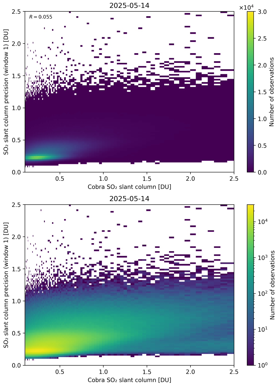
Figure 220: Scatter density plot of “Cobra SO 2 slant column” against “SO 2 slant column precision (window 1)” for 2025-05-13 to 2025-05-15.
