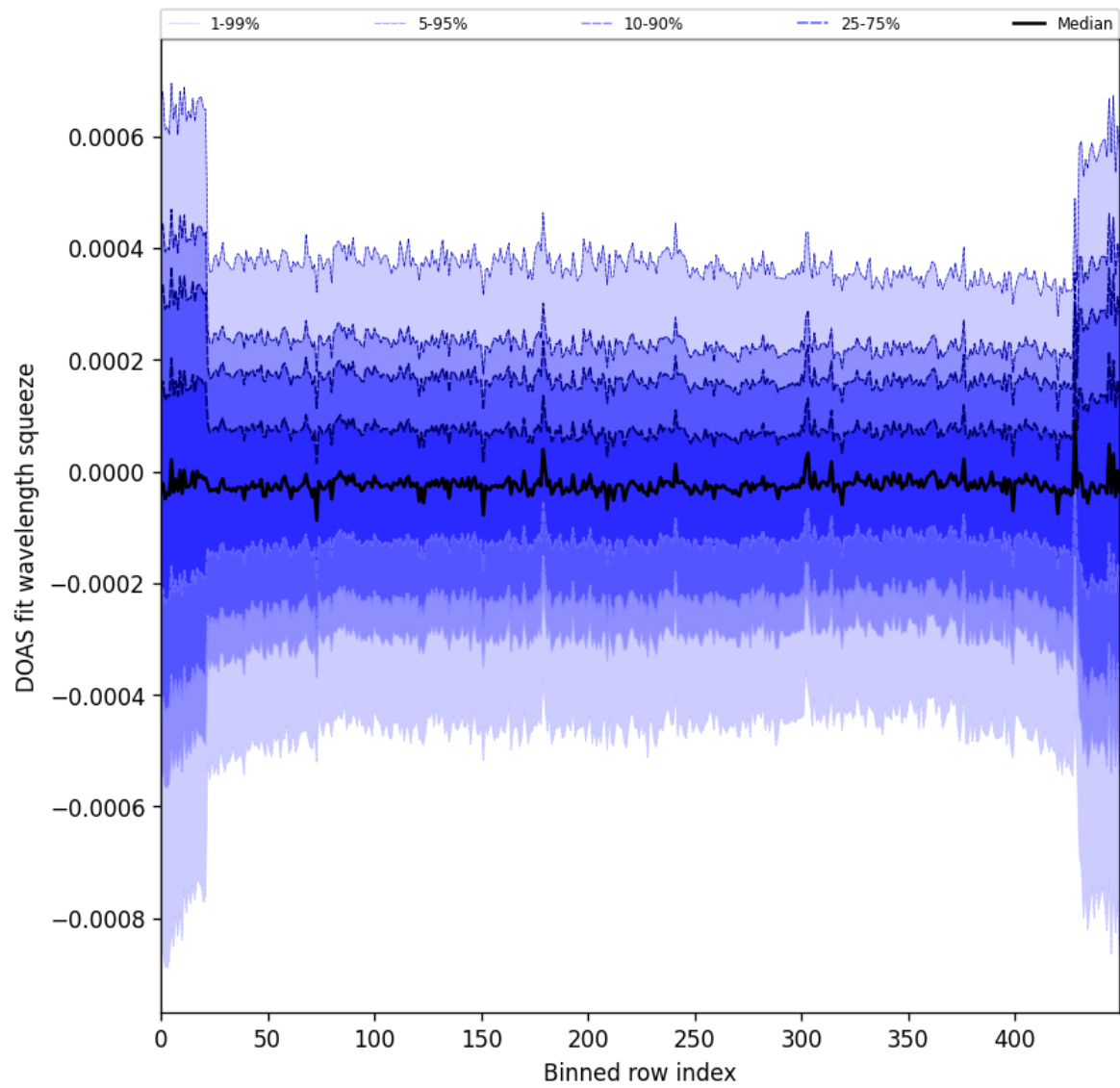
Figure 103: Along track statistics of “DOAS fit wavelength squeeze” for 2025-05-13 to 2025-05-15
