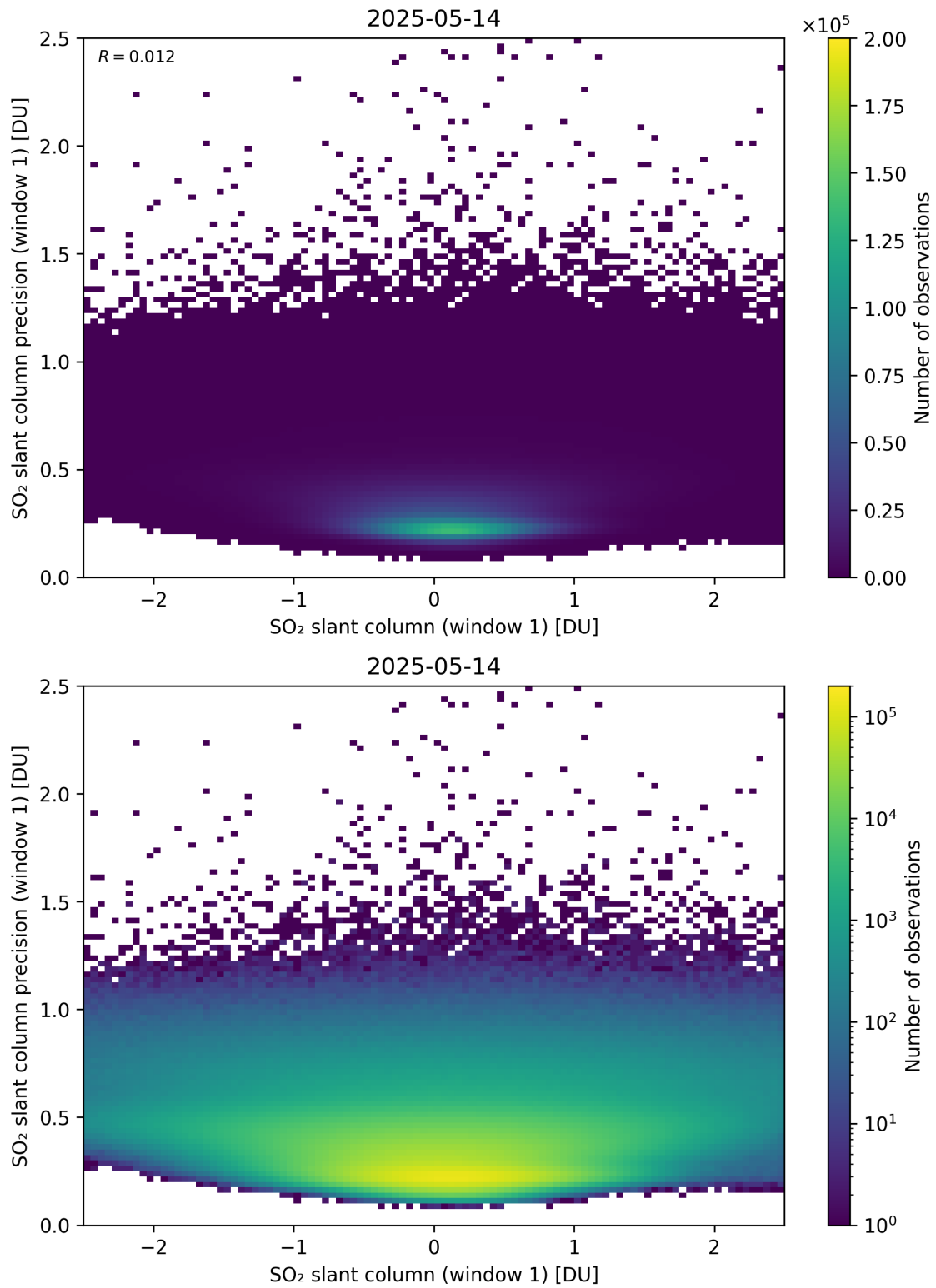
Figure 285: Scatter density plot of “SO 2 slant column (window 1)” against “SO 2 slant column precision (window 1)” for 2025-05-13 to 2025-05-15.
