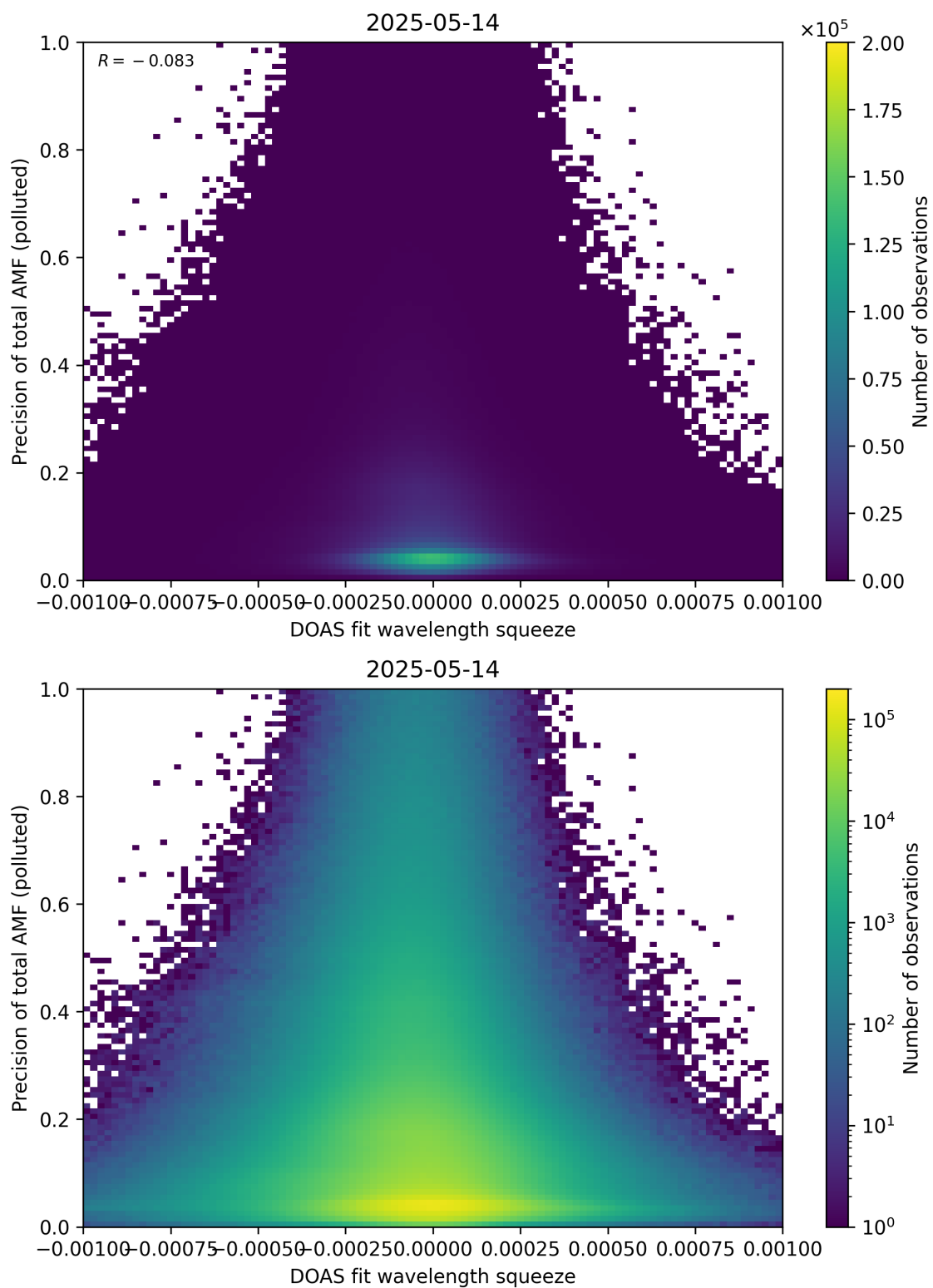
Figure 146: Scatter density plot of “DOAS fit wavelength squeeze” against “Precision of total AMF (polluted)” for 2025-05-13 to 2025-05-15.
