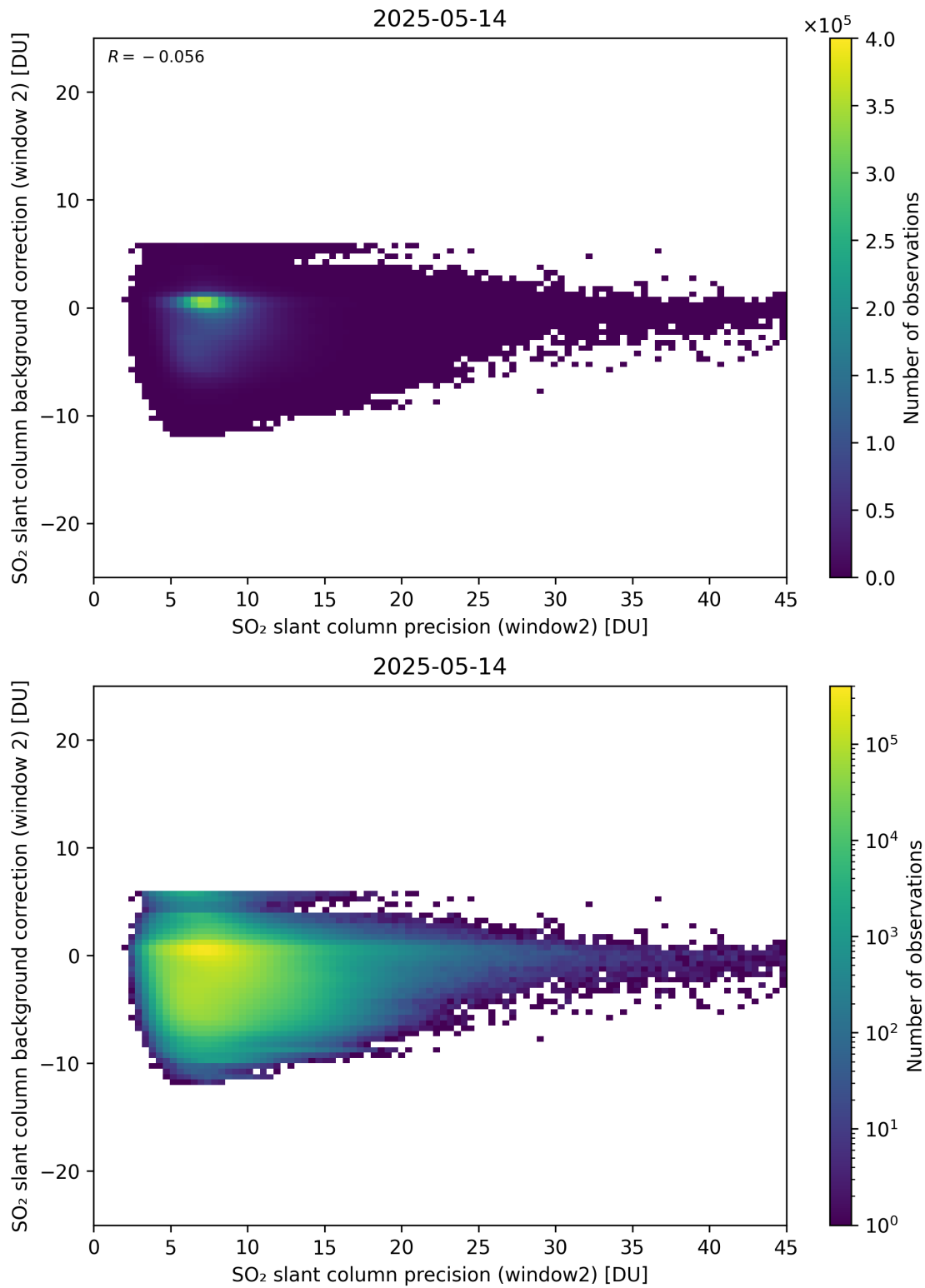
Figure 291: Scatter density plot of “SO 2 slant column precision (window2)” against “SO 2 slant column background correction (window 2)” for 2025-05-13 to 2025-05-15.
