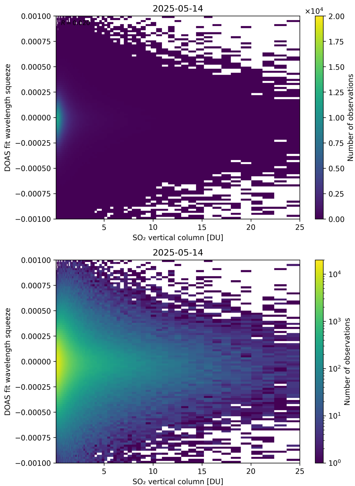
Figure 327: Scatter density plot of “SO 2 vertical column” against “DOAS fit wavelength squeeze” for 2025-05-13 to 2025-05-15.
