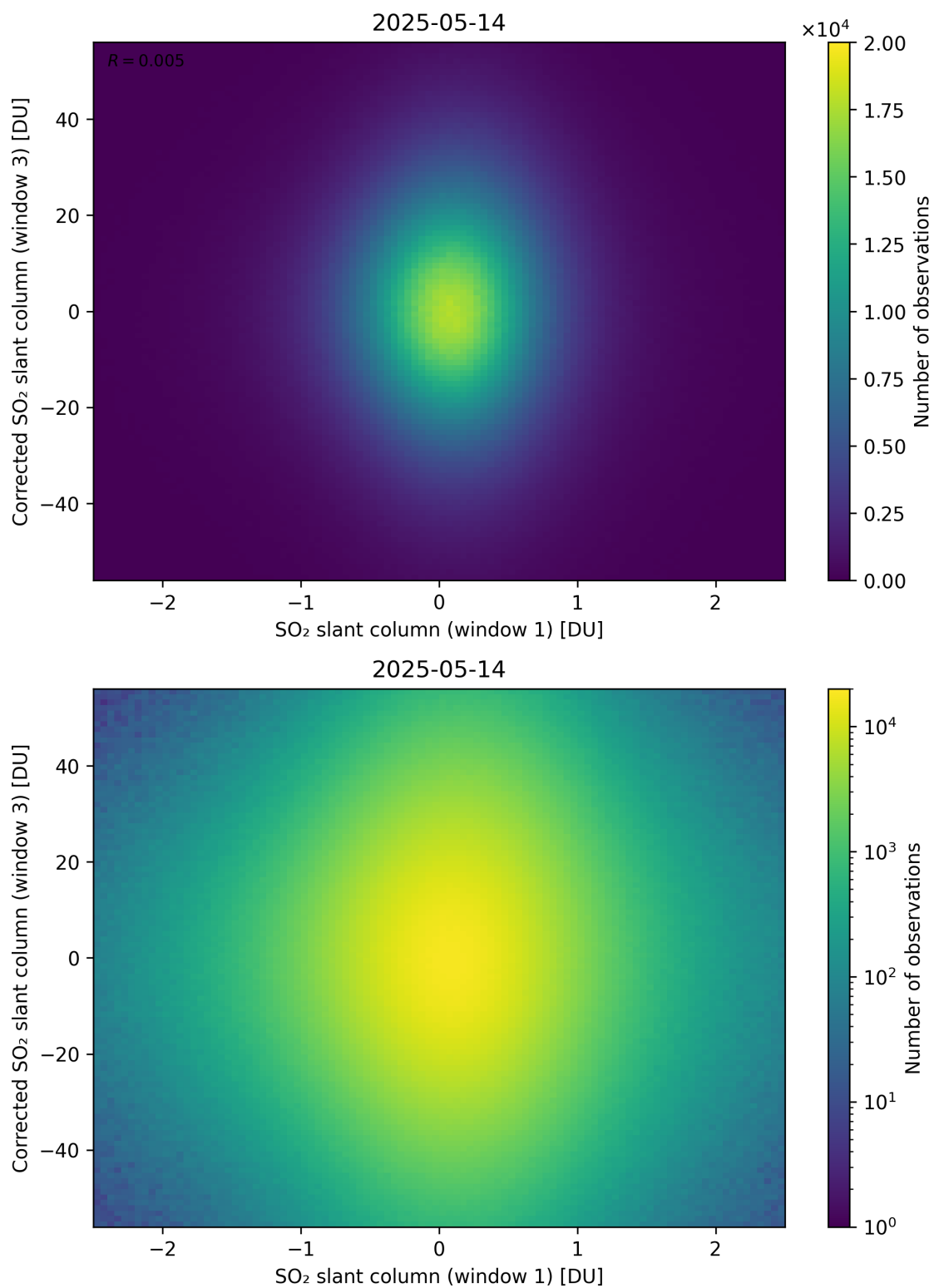
Figure 284: Scatter density plot of “SO 2 slant column (window 1)” against “Corrected SO 2 slant column (window 3)” for 2025-05-13 to 2025-05-15.
