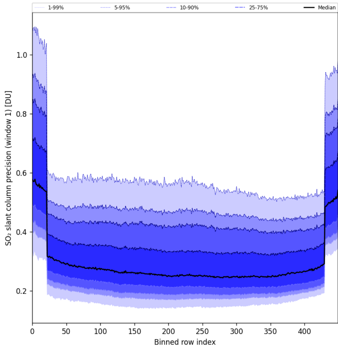
Figure 90: Along track statistics of “SO 2 slant column precision (window 1)” for 2025-05-13 to 2025-05-15
