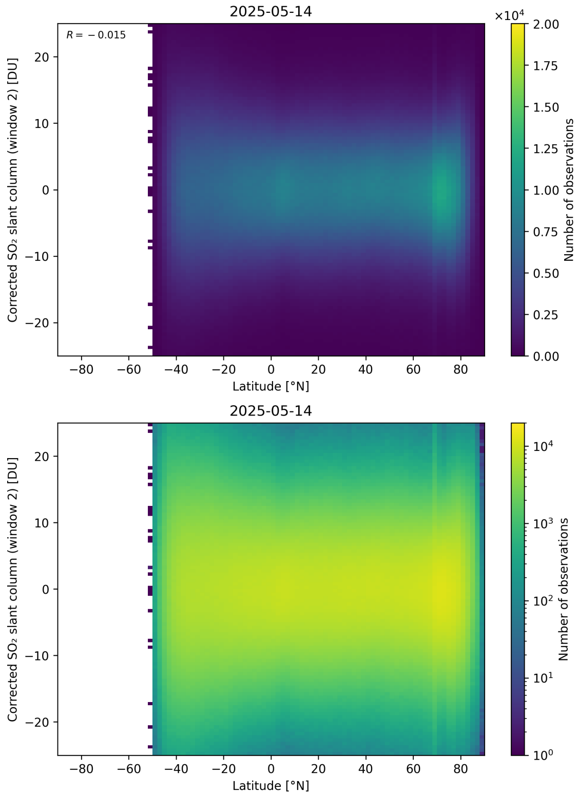
Figure 160: Scatter density plot of “Latitude” against “Corrected SO 2 slant column (window 2)” for 2025-05-13 to 2025-05-15.
