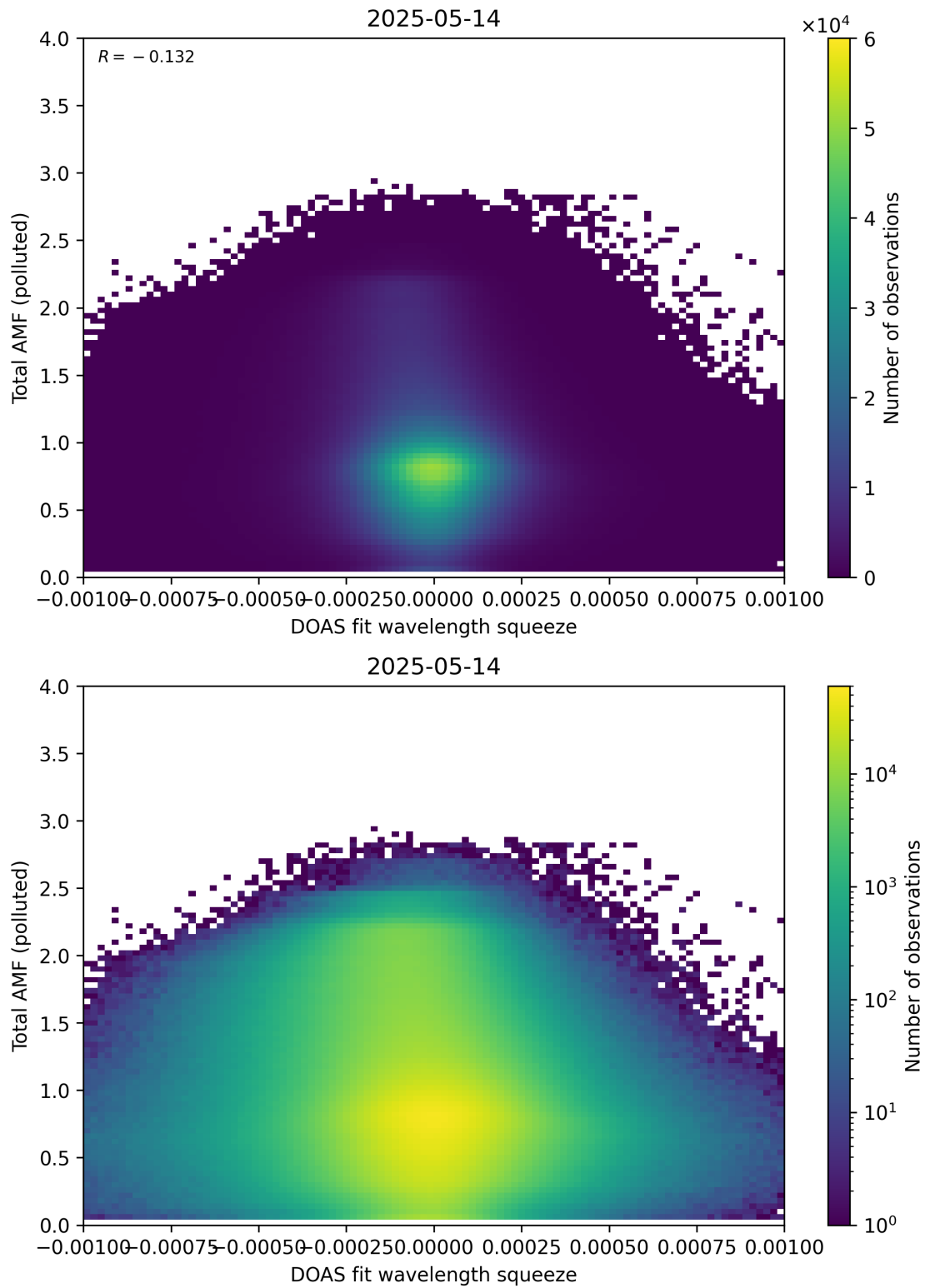
Figure 145: Scatter density plot of “DOAS fit wavelength squeeze” against “Total AMF (polluted)” for 2025-05-13 to 2025-05-15.
