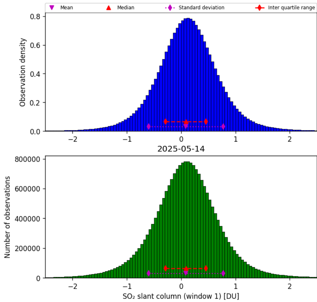
Figure 63: Histogram of “SO 2 slant column (window 1)” for 2025-05-13 to 2025-05-15
