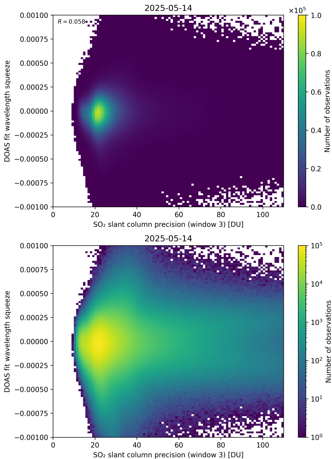
Figure 309: Scatter density plot of “SO 2 slant column precision (window 3)” against “DOAS fit wavelength squeeze” for 2025-05-13 to 2025-05-15.
