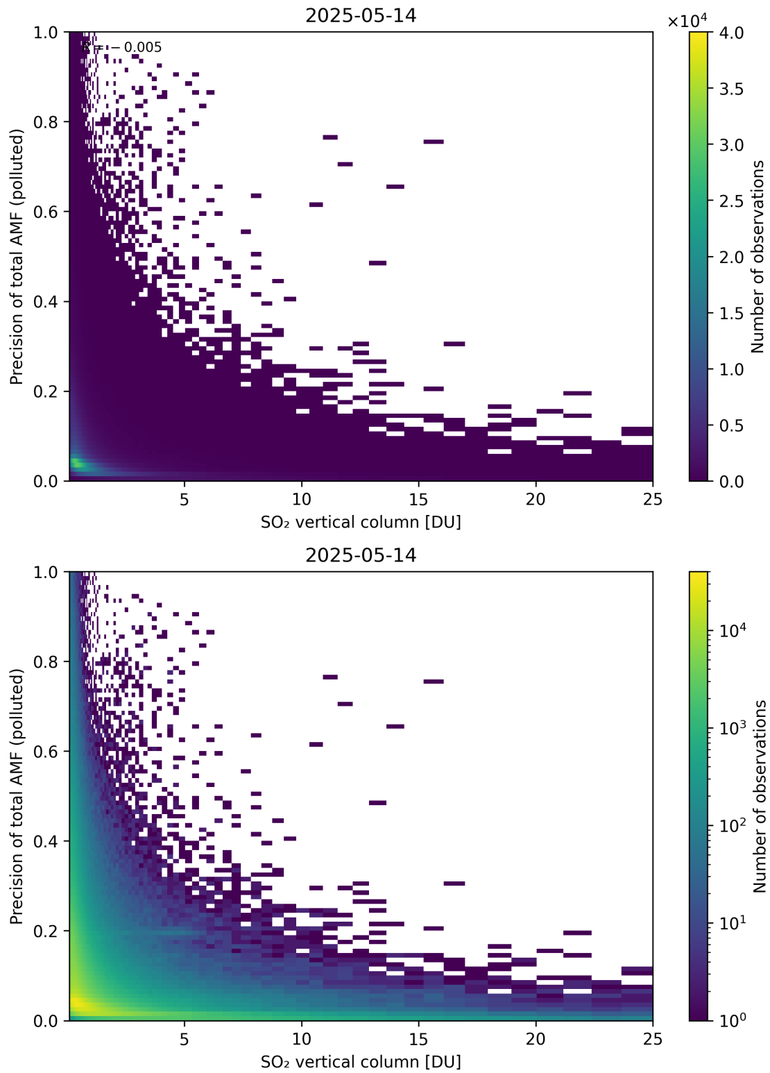
Figure 360: Scatter density plot of “SO 2 vertical column” against “Precision of total AMF (polluted)” for 2025-05-13 to 2025-05-15.
