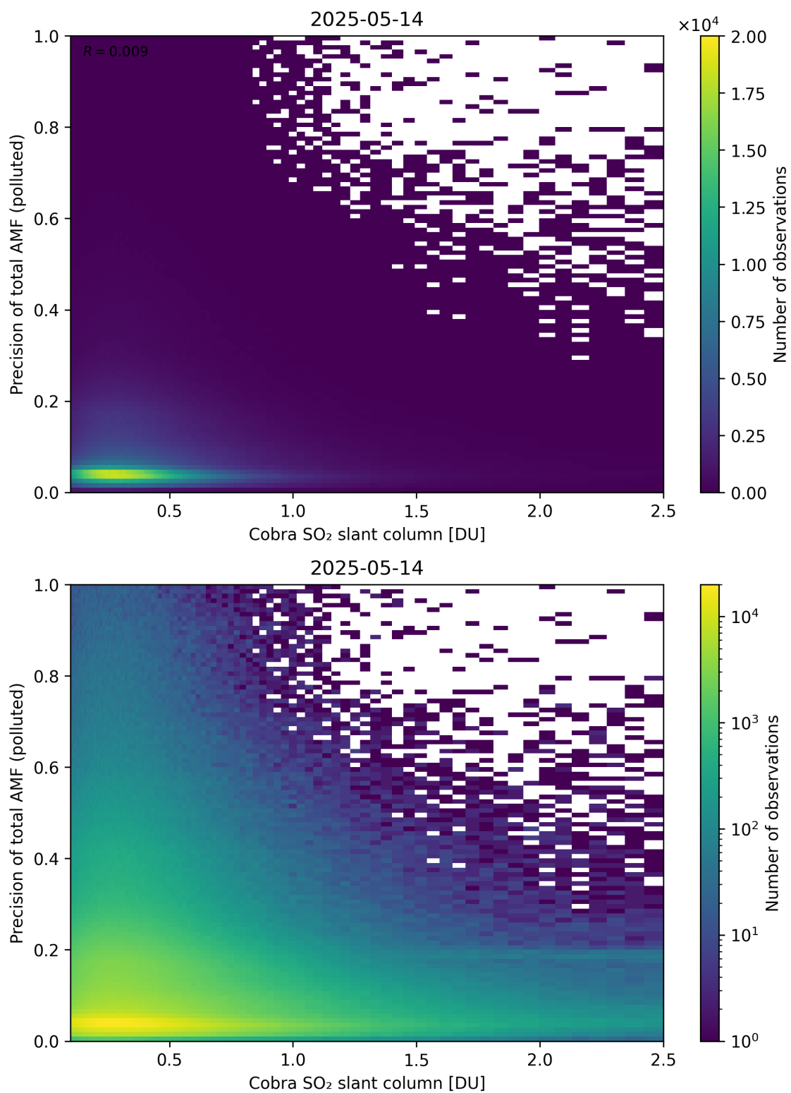
Figure 225: Scatter density plot of “Cobra SO 2 slant column” against “Precision of total AMF (polluted)” for 2025-05-13 to 2025-05-15.
