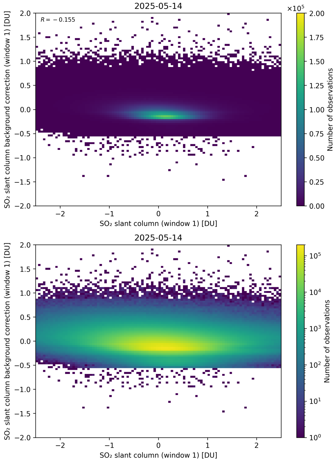
Figure 262: Scatter density plot of “SO 2 slant column (window 1)” against “SO 2 slant column background correction (window 1)” for 2025-05-13 to 2025-05-15.
