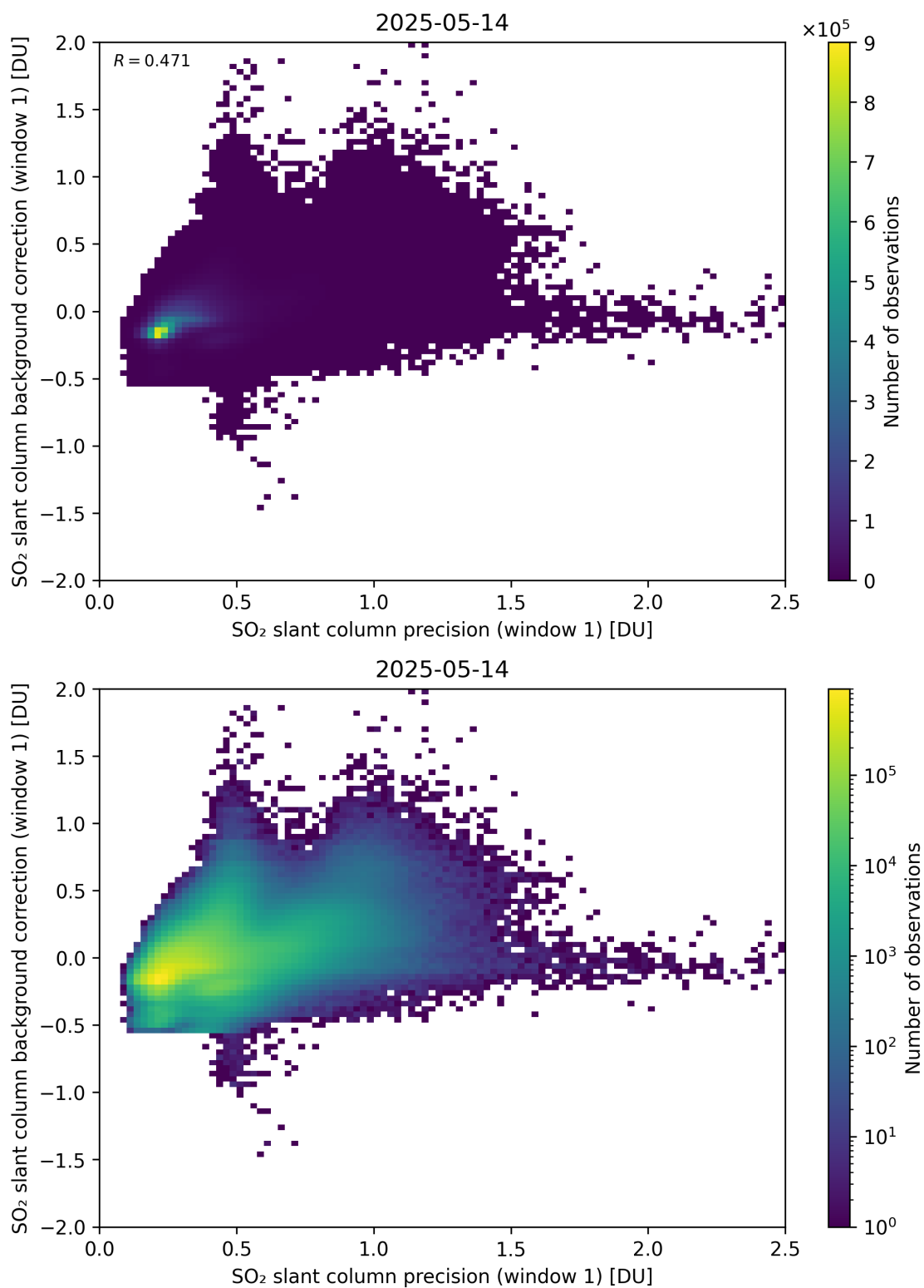
Figure 268: Scatter density plot of “SO 2 slant column precision (window 1)” against “SO 2 slant column background correction (window 1)” for 2025-05-13 to 2025-05-15.
