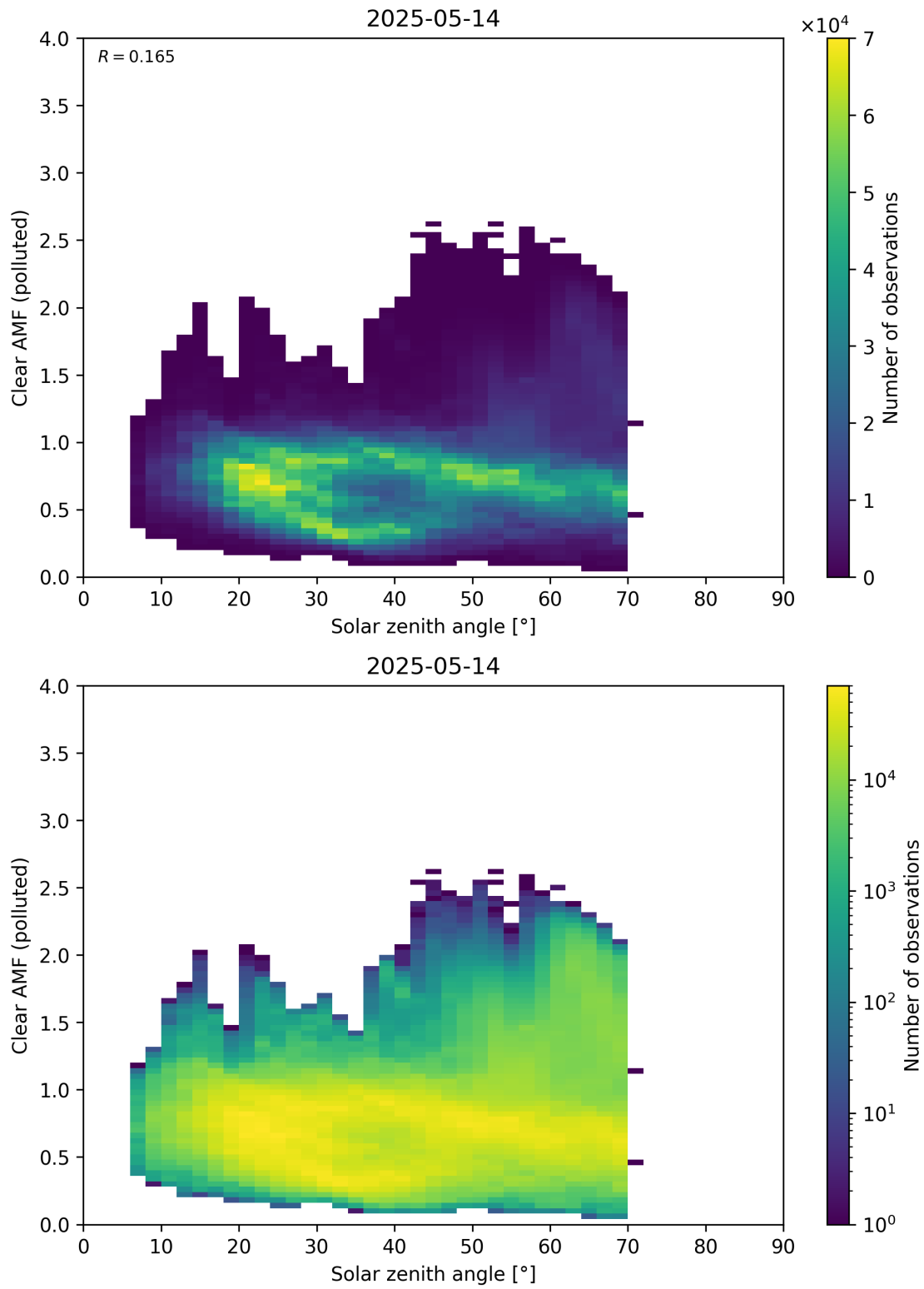
Figure 178: Scatter density plot of “Solar zenith angle” against “Clear AMF (polluted)” for 2025-05-13 to 2025-05-15.
