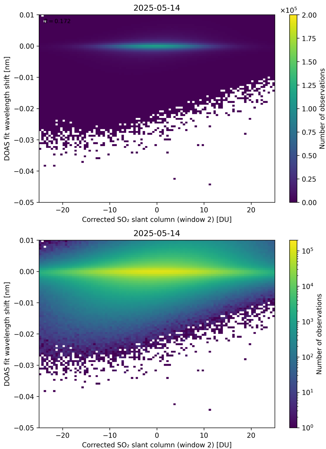
Figure 246: Scatter density plot of “Corrected SO 2 slant column (window 2)” against “DOAS fit wavelength shift” for 2025-05-13 to 2025-05-15.
