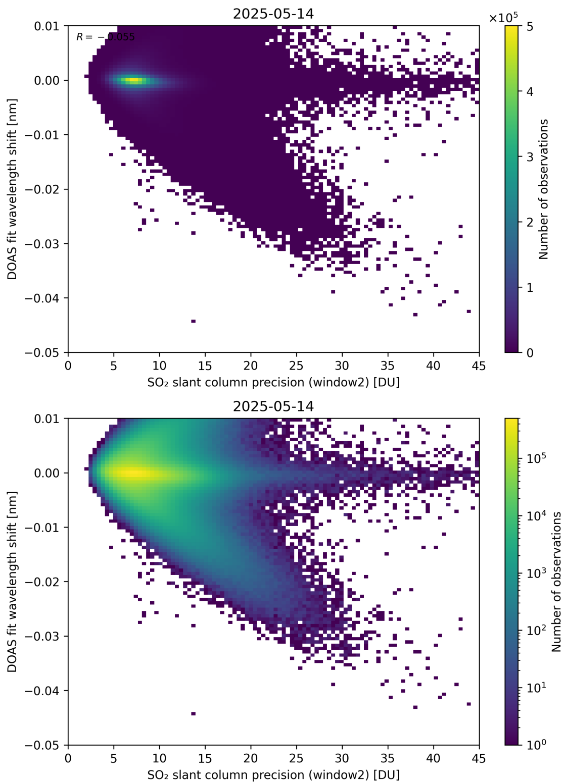
Figure 293: Scatter density plot of “SO 2 slant column precision (window2)” against “DOAS fit wavelength shift” for 2025-05-13 to 2025-05-15.
