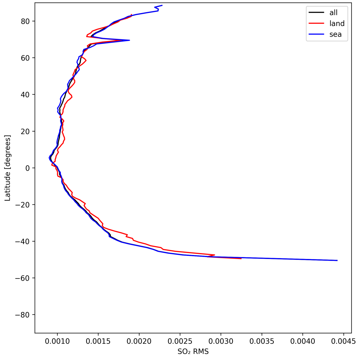
Figure 52: Zonal average of “SO 2 RMS” for 2025-05-13 to 2025-05-15.
