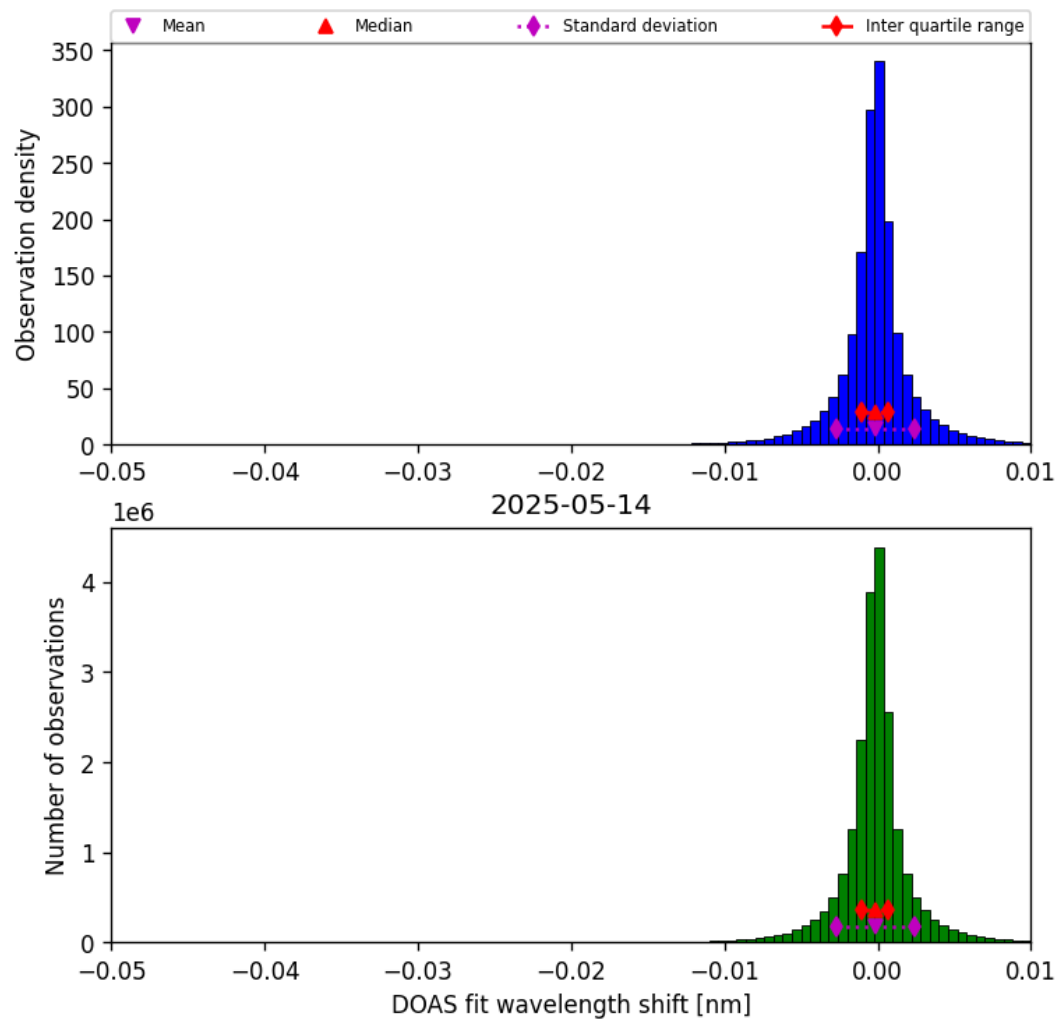
Figure 76: Histogram of “DOAS fit wavelength shift” for 2025-05-13 to 2025-05-15
