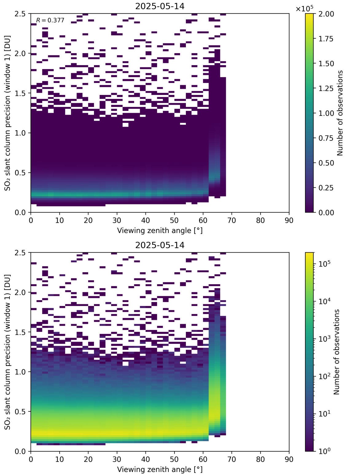
Figure 377: Scatter density plot of “Viewing zenith angle” against “SO 2 slant column precision (window 1)” for 2025-05-13 to 2025-05-15.
