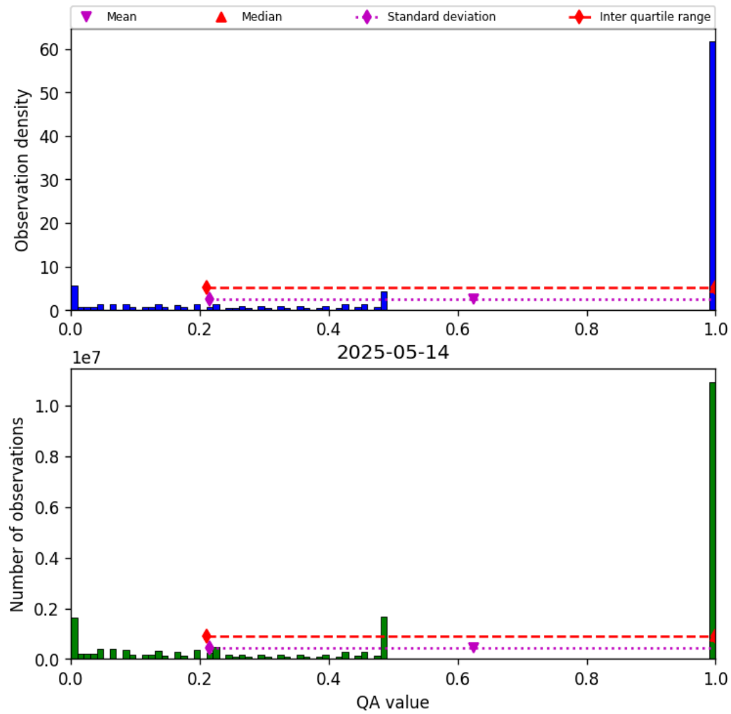
Figure 57: Histogram of “QA value” for 2025-05-13 to 2025-05-15
