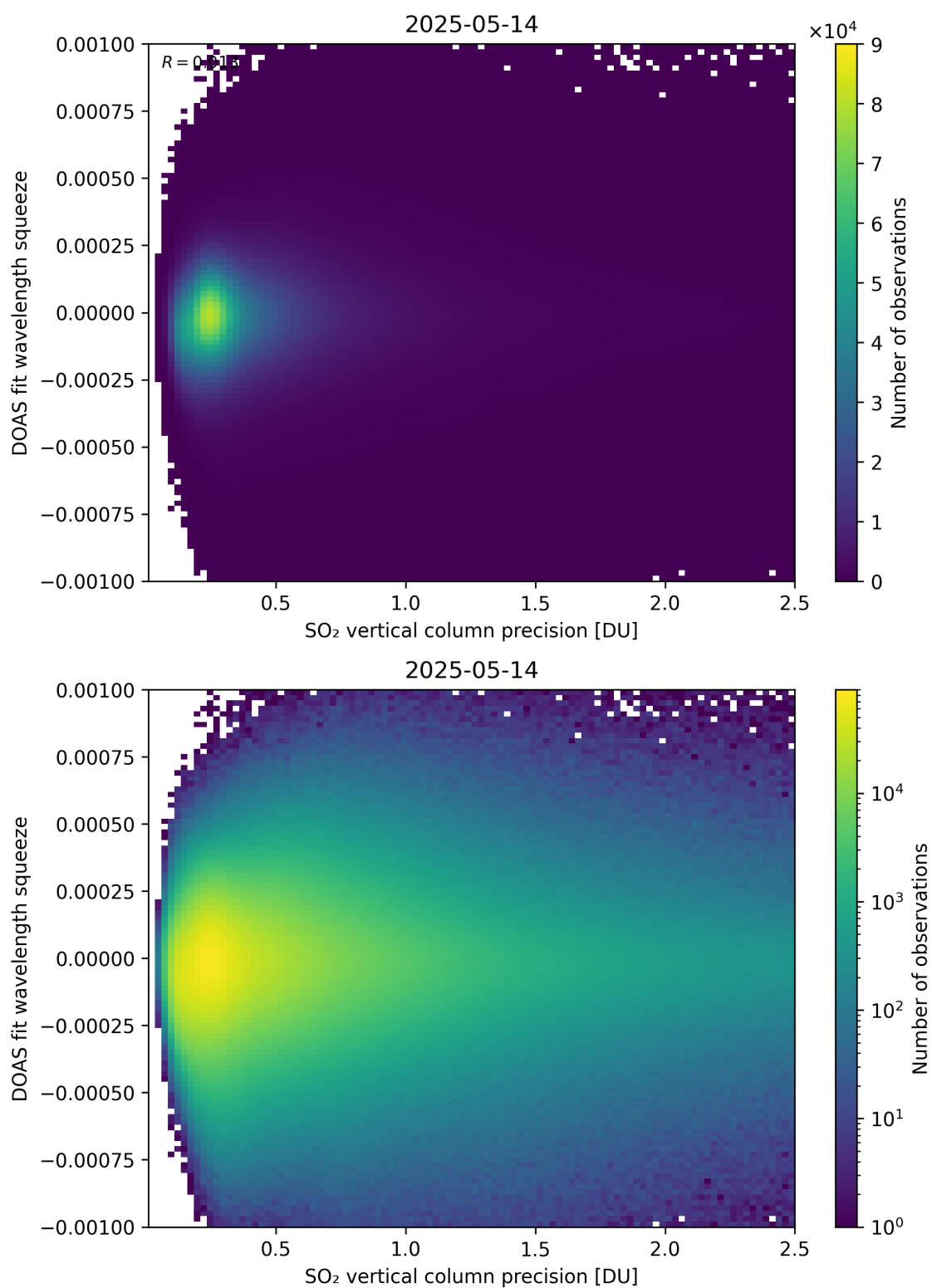
Figure 333: Scatter density plot of “SO 2 vertical column precision” against “DOAS fit wavelength squeeze” for 2025-05-13 to 2025-05-15.
