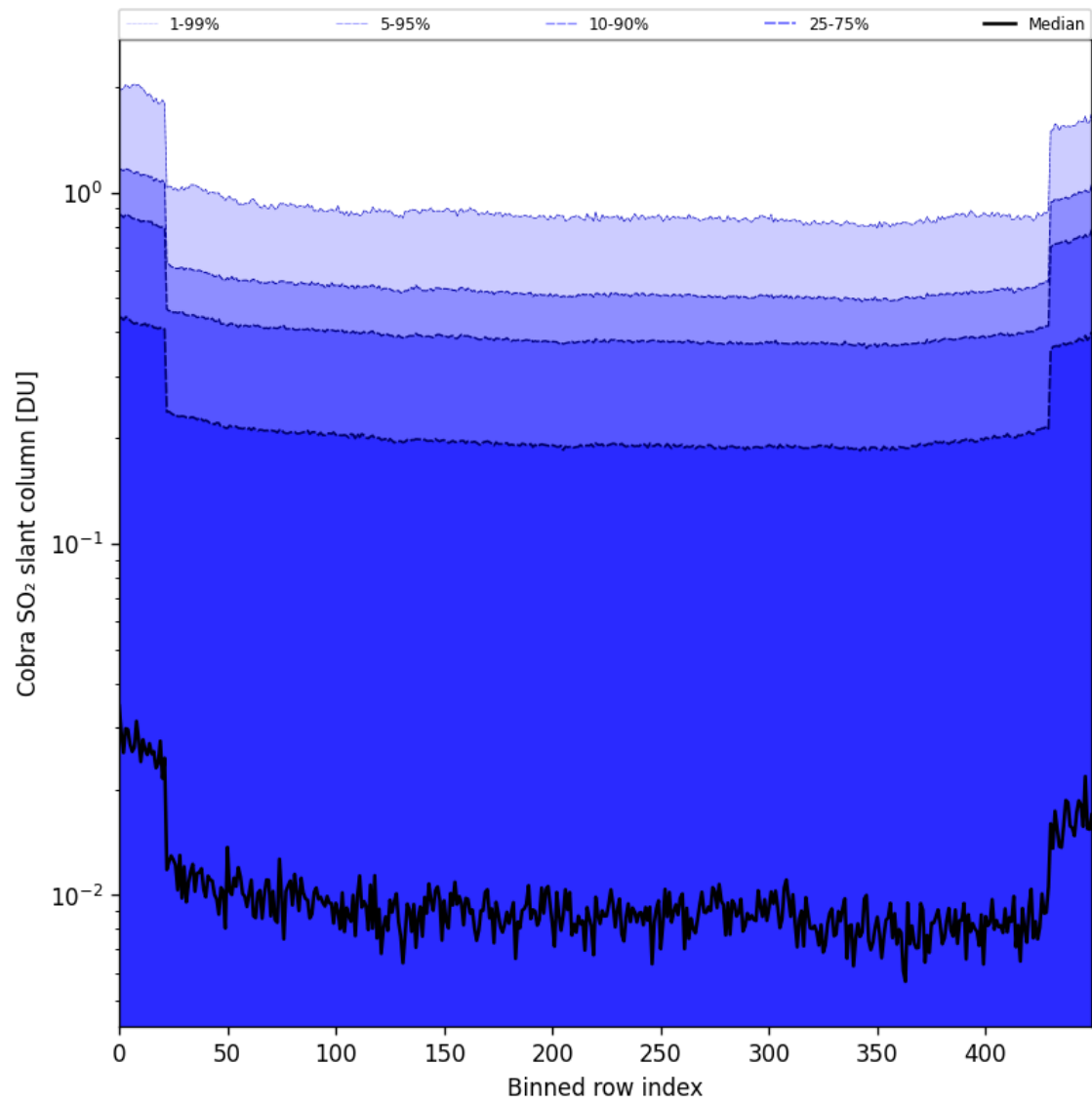
Figure 87: Along track statistics of “Cobra SO 2 slant column” for 2025-05-13 to 2025-05-15
