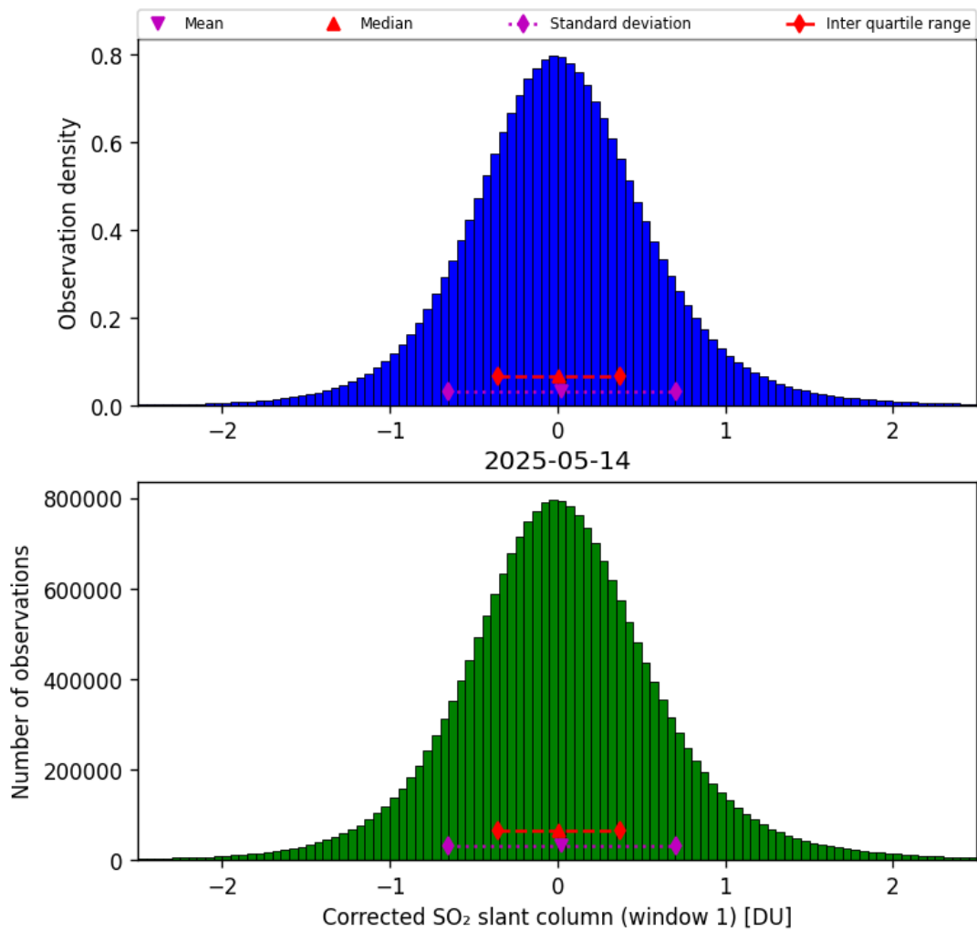
Figure 65: Histogram of “Corrected SO 2 slant column (window 1)” for 2025-05-13 to 2025-05-15
