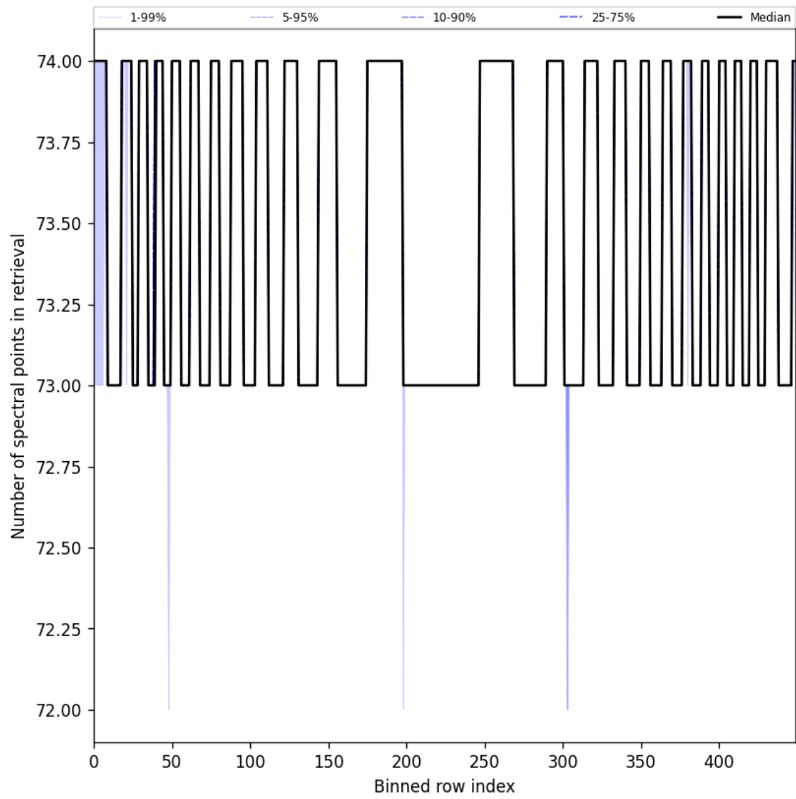
Figure 108: Along track statistics of “Number of spectral points in retrieval” for 2025-05-13 to 2025-05-15
