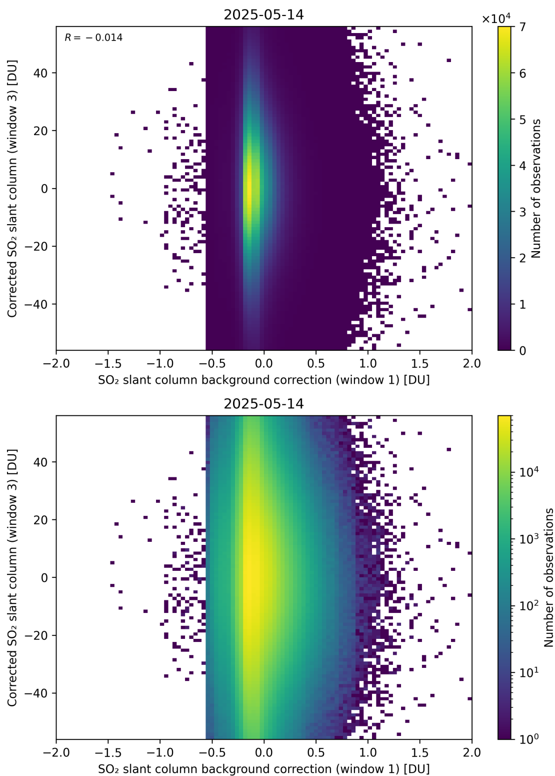
Figure 116: Scatter density plot of “SO 2 slant column background correction (window 1)” against “Corrected SO 2 slant column (window 3)” for 2025-05-13 to 2025-05-15.
