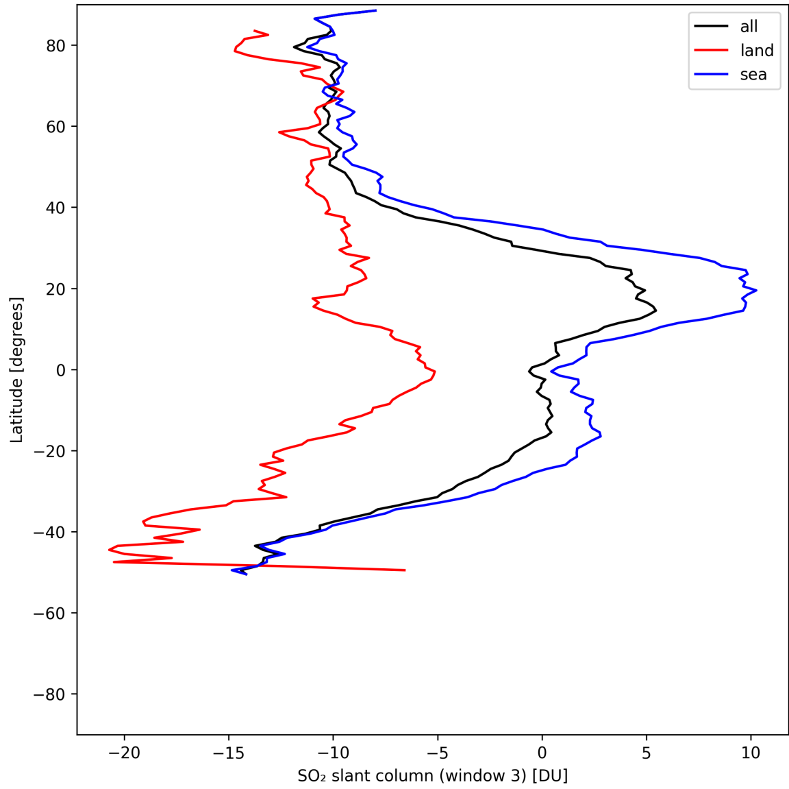
Figure 45: Zonal average of “SO 2 slant column (window 3)” for 2025-05-13 to 2025-05-15.
