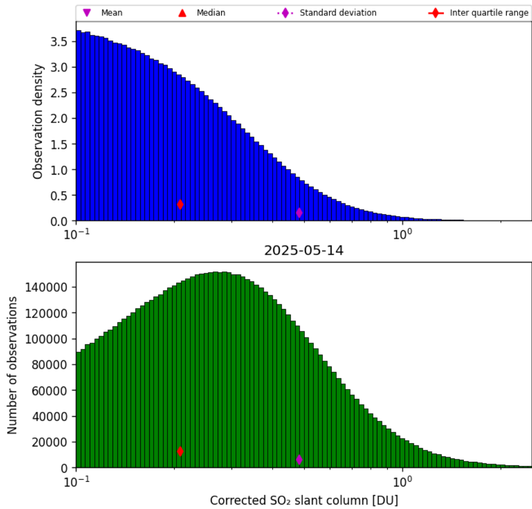
Figure 60: Histogram of "Corrected SO 2 slant column" for 2025-05-13 to 2025-05-15
