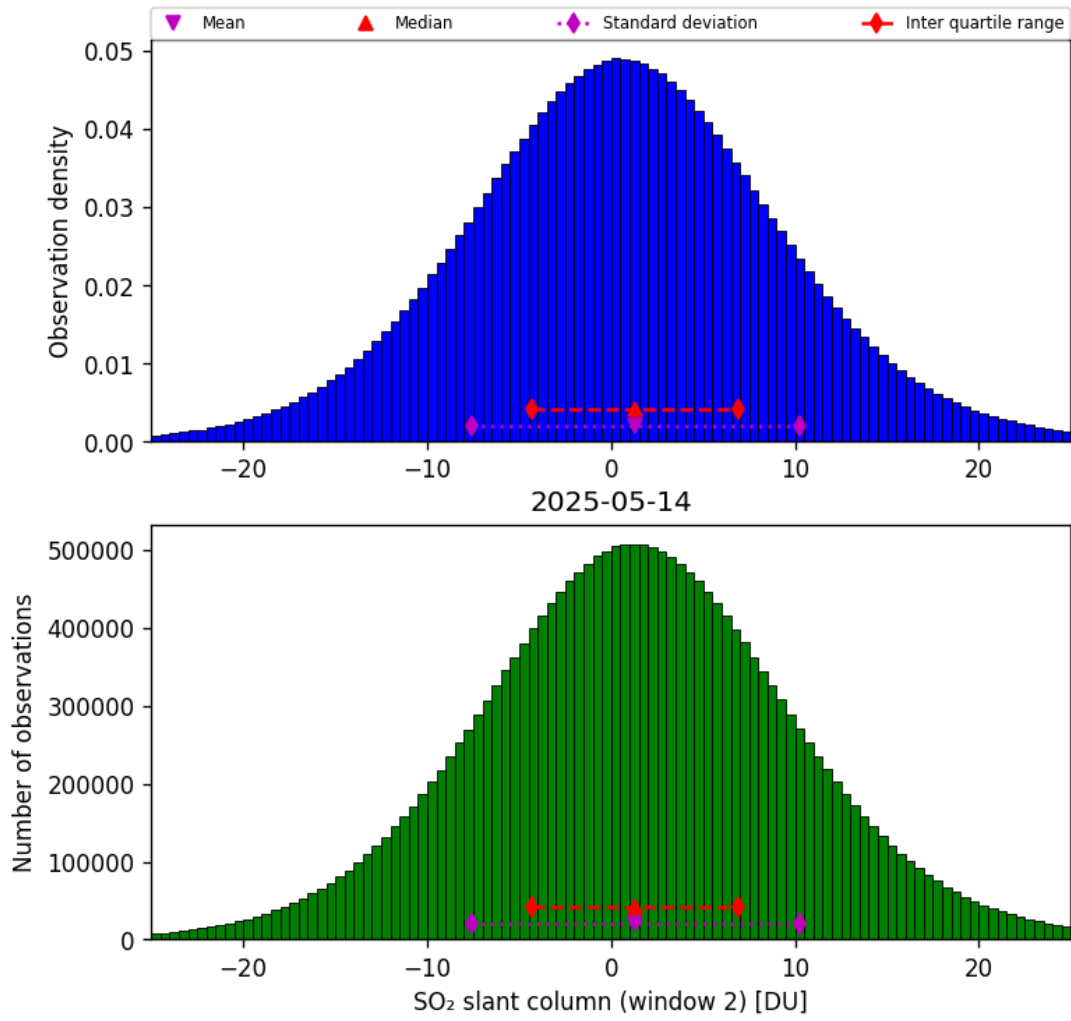
Figure 67: Histogram of “SO 2 slant column (window 2)” for 2025-05-13 to 2025-05-15
