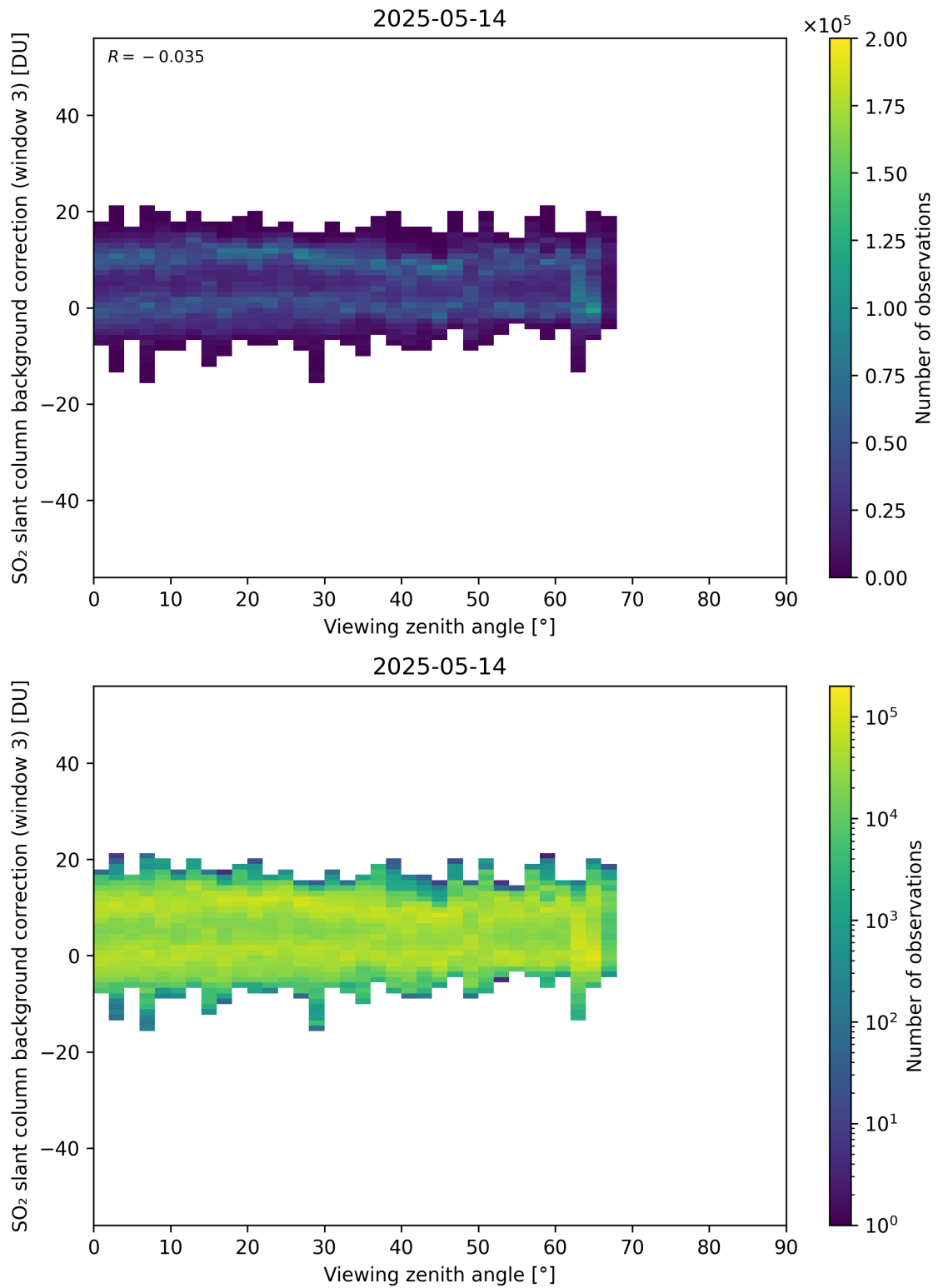
Figure 364: Scatter density plot of “Viewing zenith angle” against “SO 2 slant column background correction (window 3)” for 2025-05-13 to 2025-05-15.
