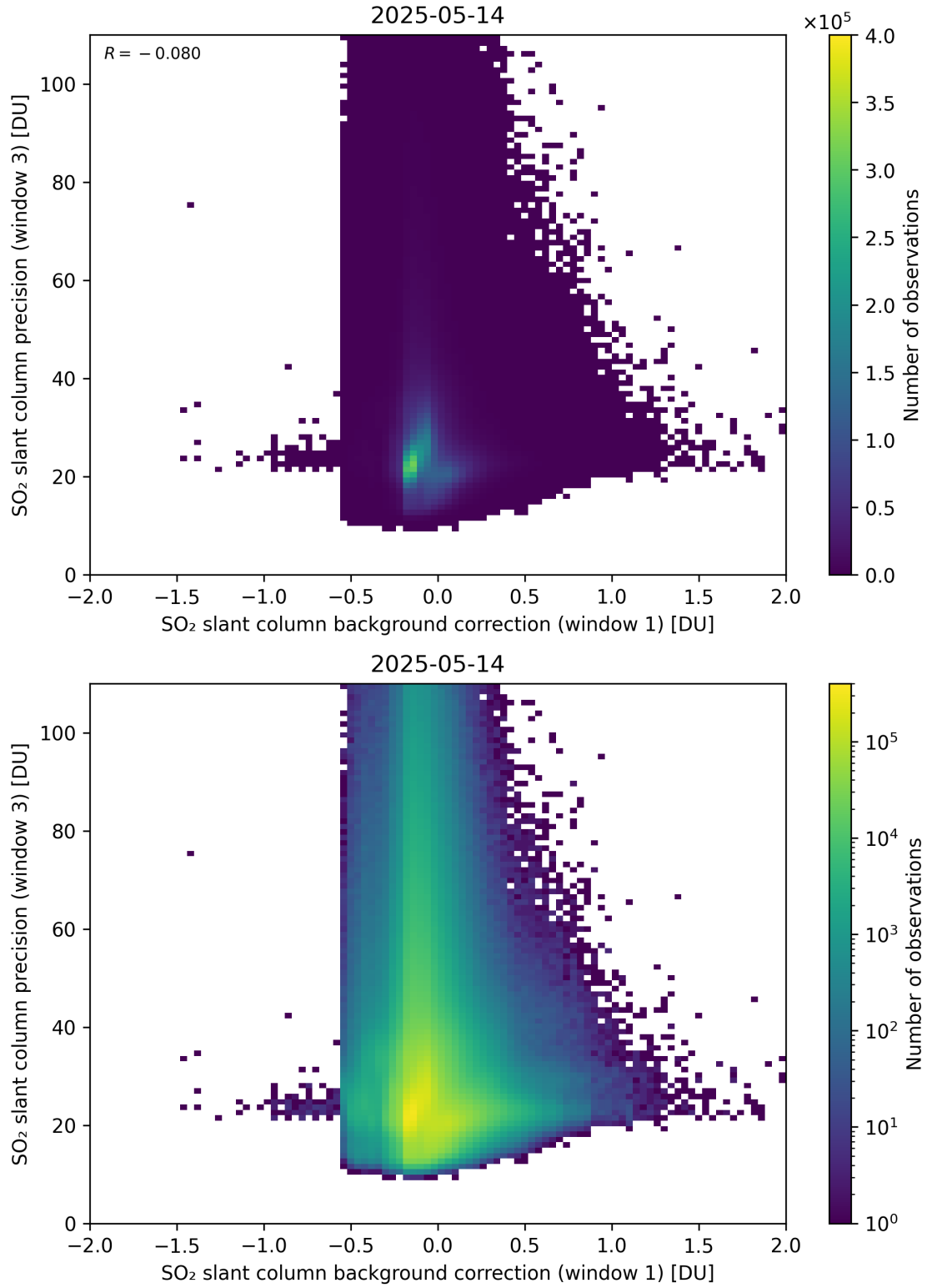
Figure 119: Scatter density plot of “SO 2 slant column background correction (window 1)” against “SO 2 slant column precision (window 3)” for 2025-05-13 to 2025-05-15.
