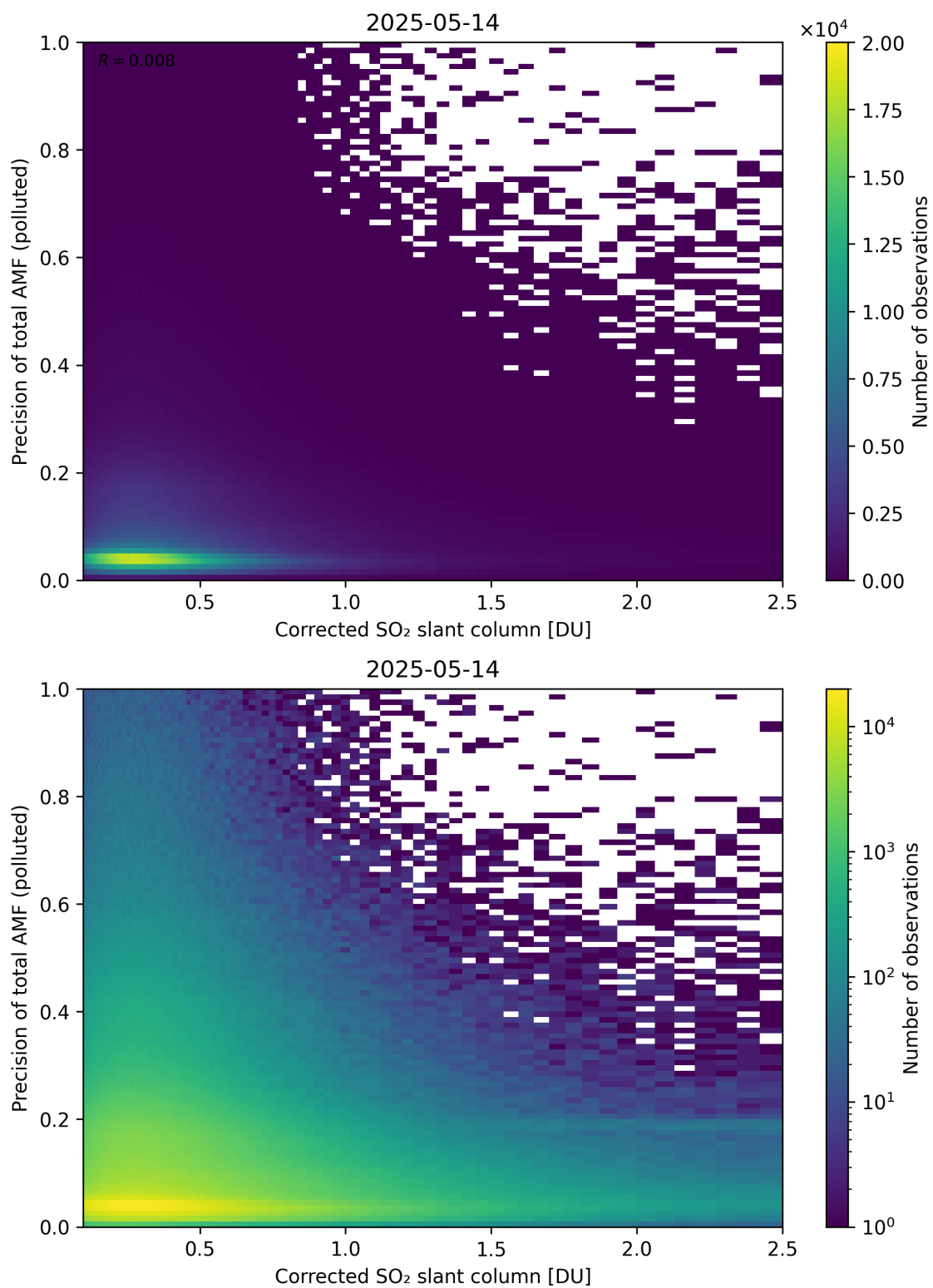
Figure 243: Scatter density plot of “Corrected SO 2 slant column” against “Precision of total AMF (polluted)” for 2025-05-13 to 2025-05-15.
