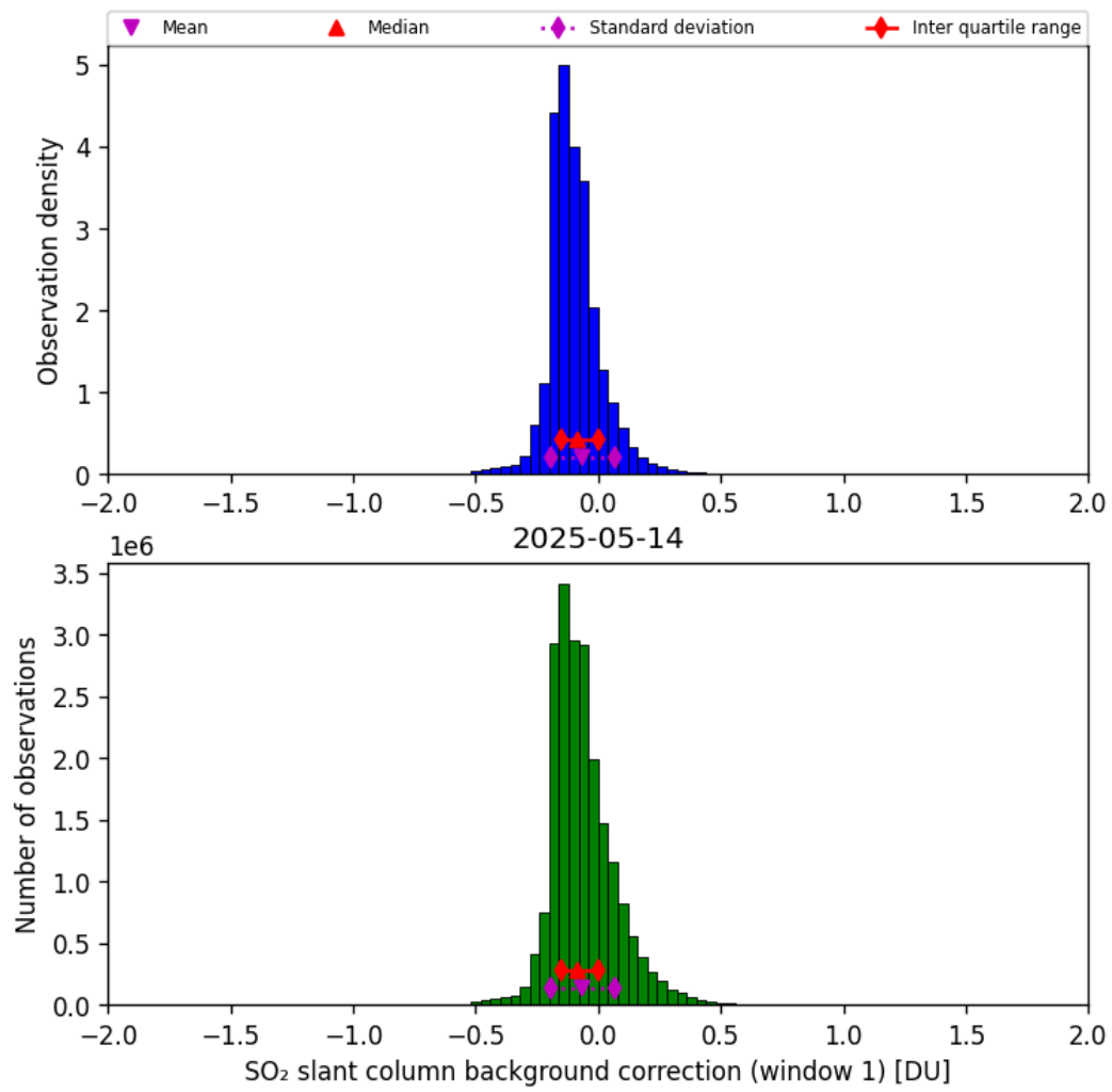
Figure 66: Histogram of “SO 2 slant column background correction (window 1)” for 2025-05-13 to 2025-05-15
