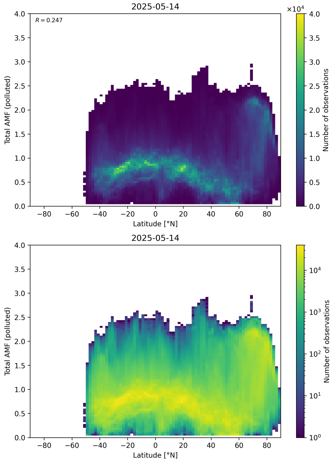
Figure 167: Scatter density plot of “Latitude” against “Total AMF (polluted)” for 2025-05-13 to 2025-05-15.
