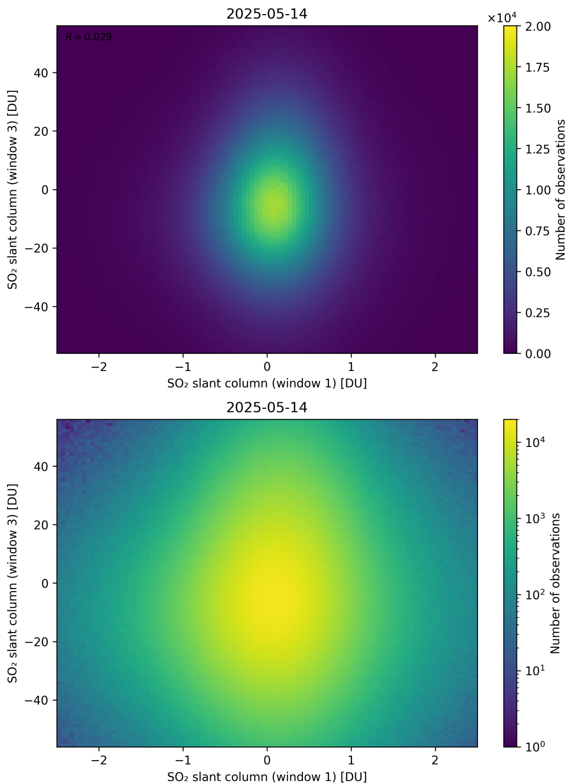
Figure 287: Scatter density plot of “SO 2 slant column (window 1)” against “SO 2 slant column (window 3)” for 2025-05-13 to 2025-05-15.
