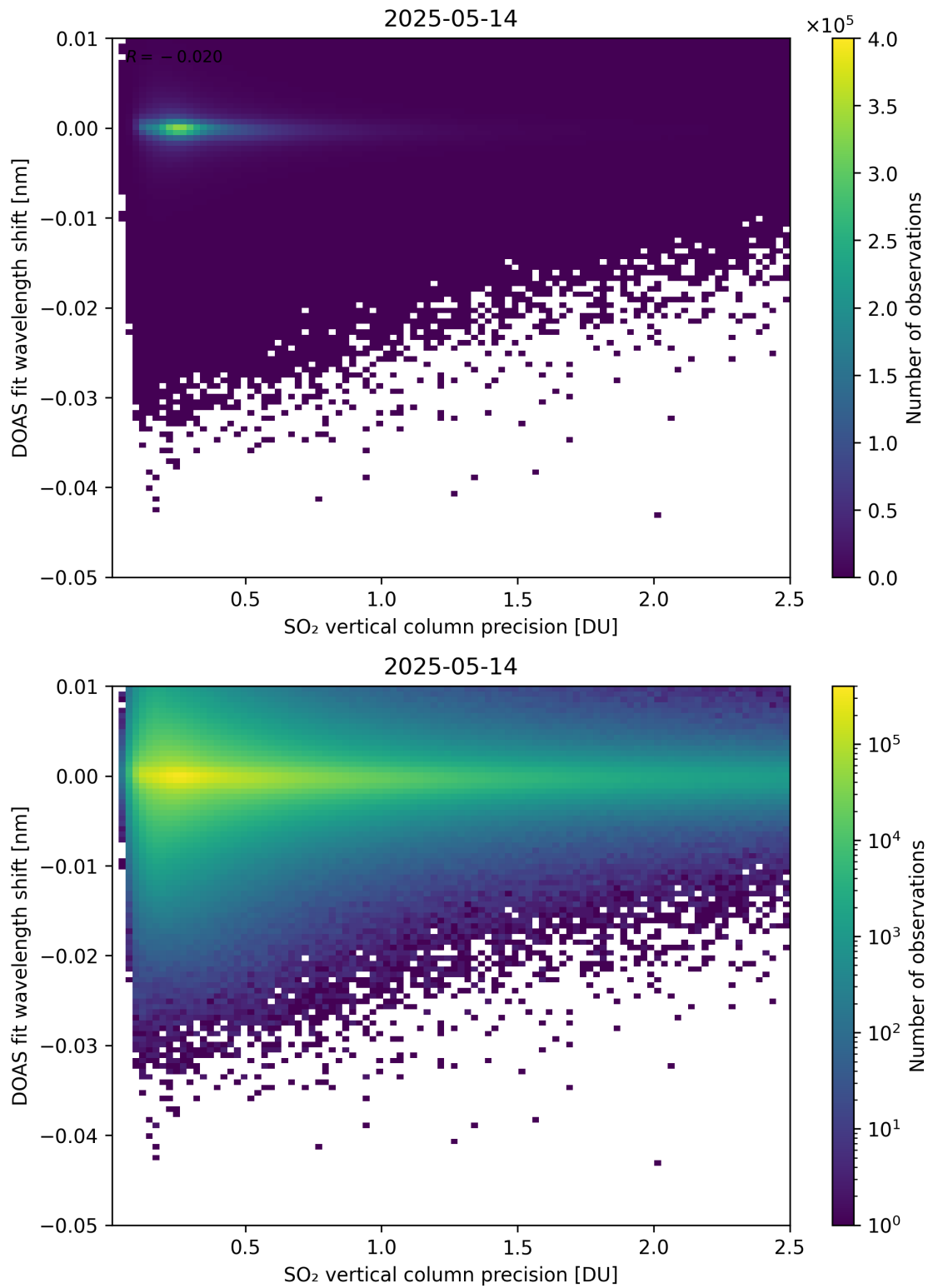
Figure 332: Scatter density plot of “SO 2 vertical column precision” against “DOAS fit wavelength shift” for 2025-05-13 to 2025-05-15.
