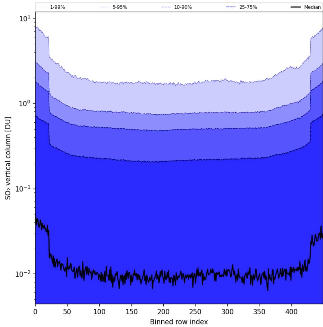
Figure 84: Along track statistics of "SO 2 vertical column" for 2025-05-13 to 2025-05-15
