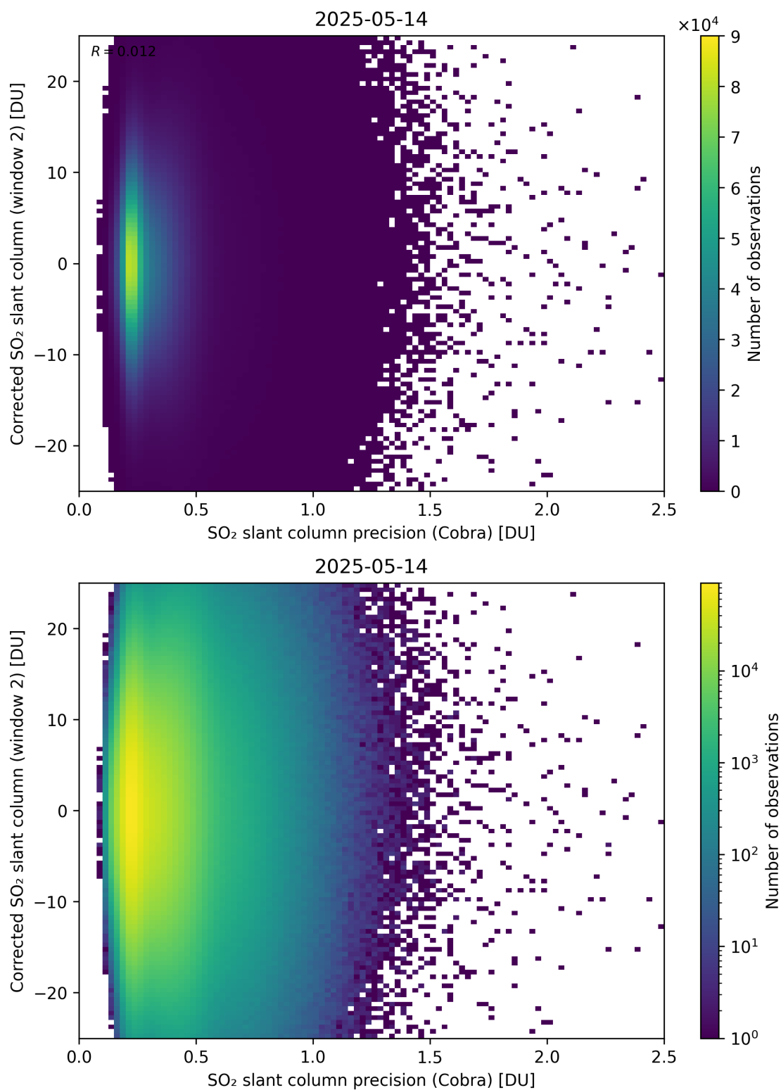
Figure 206: Scatter density plot of “SO 2 slant column precision (Cobra)” against “Corrected SO 2 slant column (window 2)” for 2025-05-13 to 2025-05-15.
