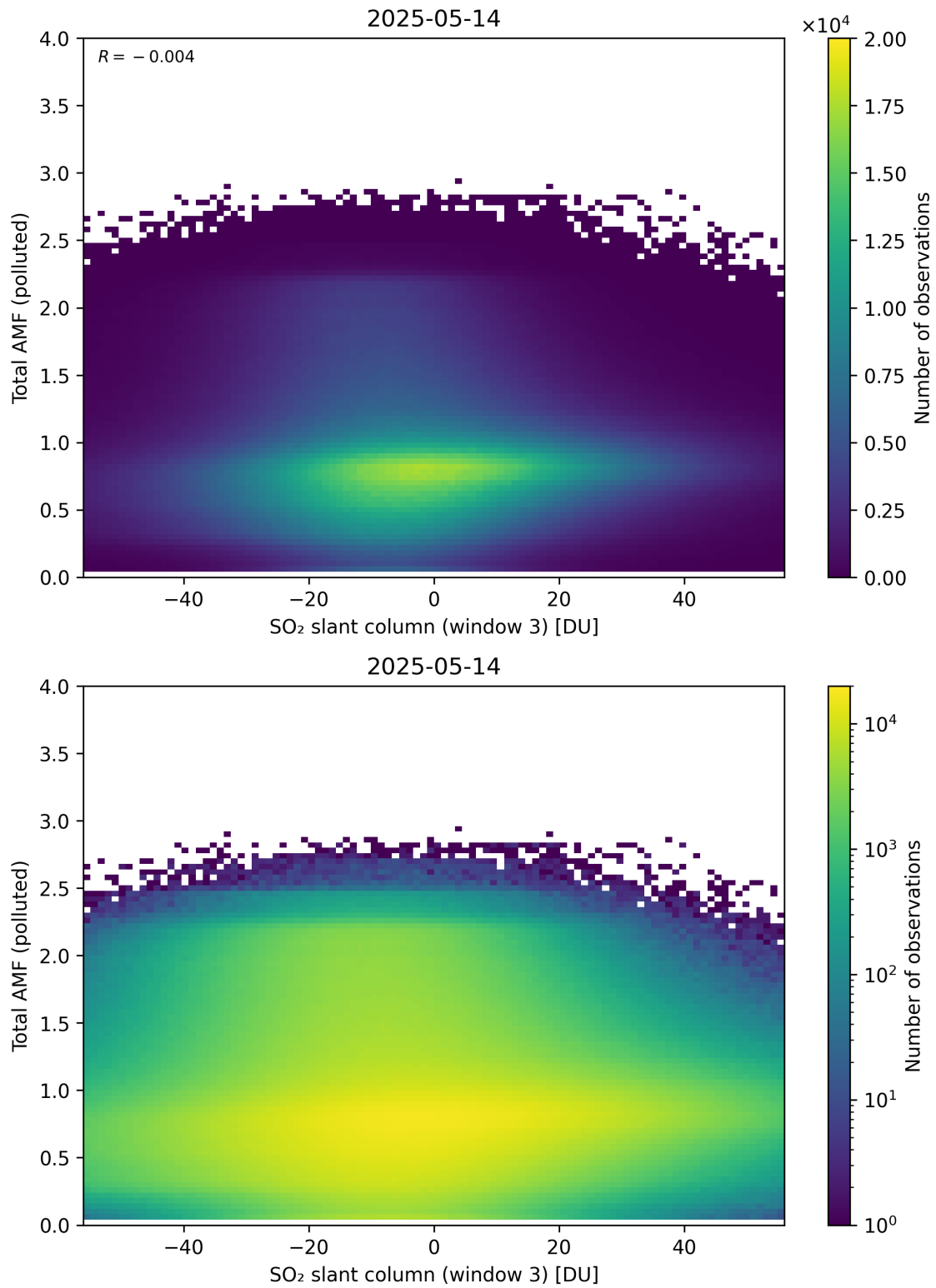
Figure 318: Scatter density plot of “SO 2 slant column (window 3)” against “Total AMF (polluted)” for 2025-05-13 to 2025-05-15.
