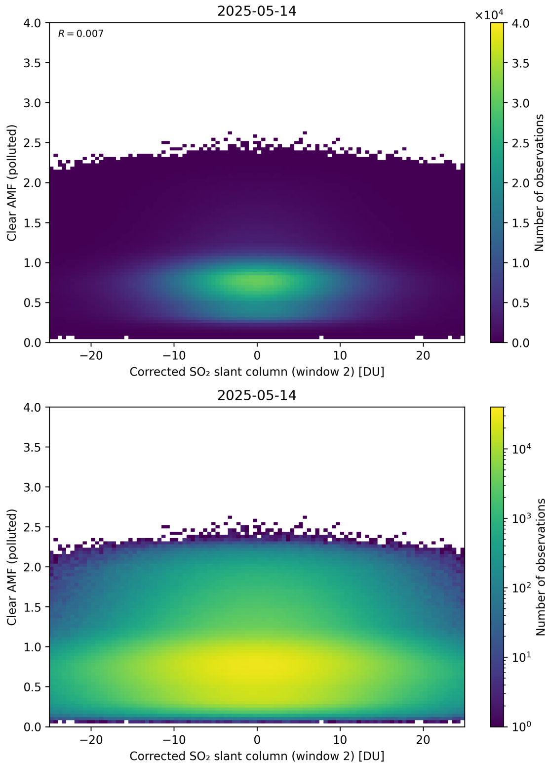
Figure 249: Scatter density plot of “Corrected SO 2 slant column (window 2)” against “Clear AMF (polluted)” for 2025-05-13 to 2025-05-15.
