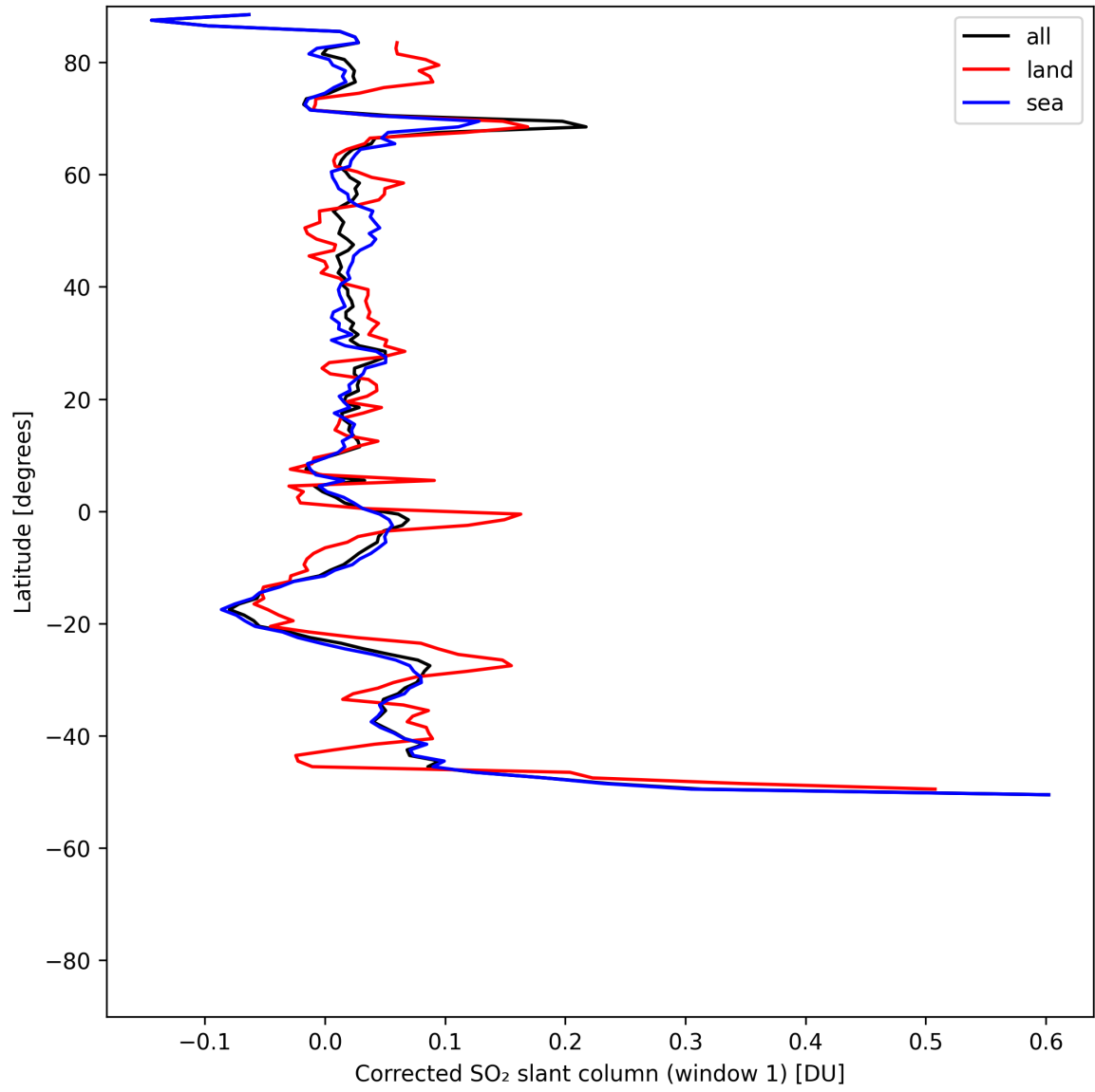
Figure 39: Zonal average of “Corrected SO 2 slant column (window 1)” for 2025-05-13 to 2025-05-15.
