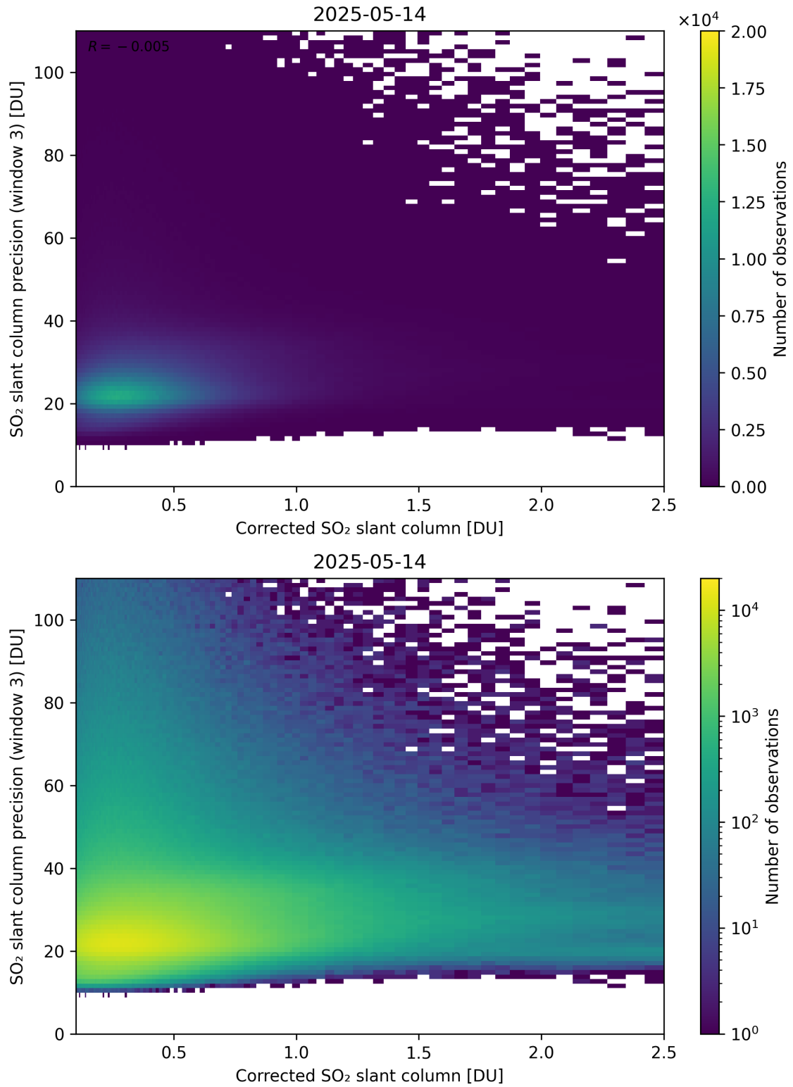
Figure 241: Scatter density plot of “Corrected SO 2 slant column” against “SO 2 slant column precision (window 3)” for 2025-05-13 to 2025-05-15.
