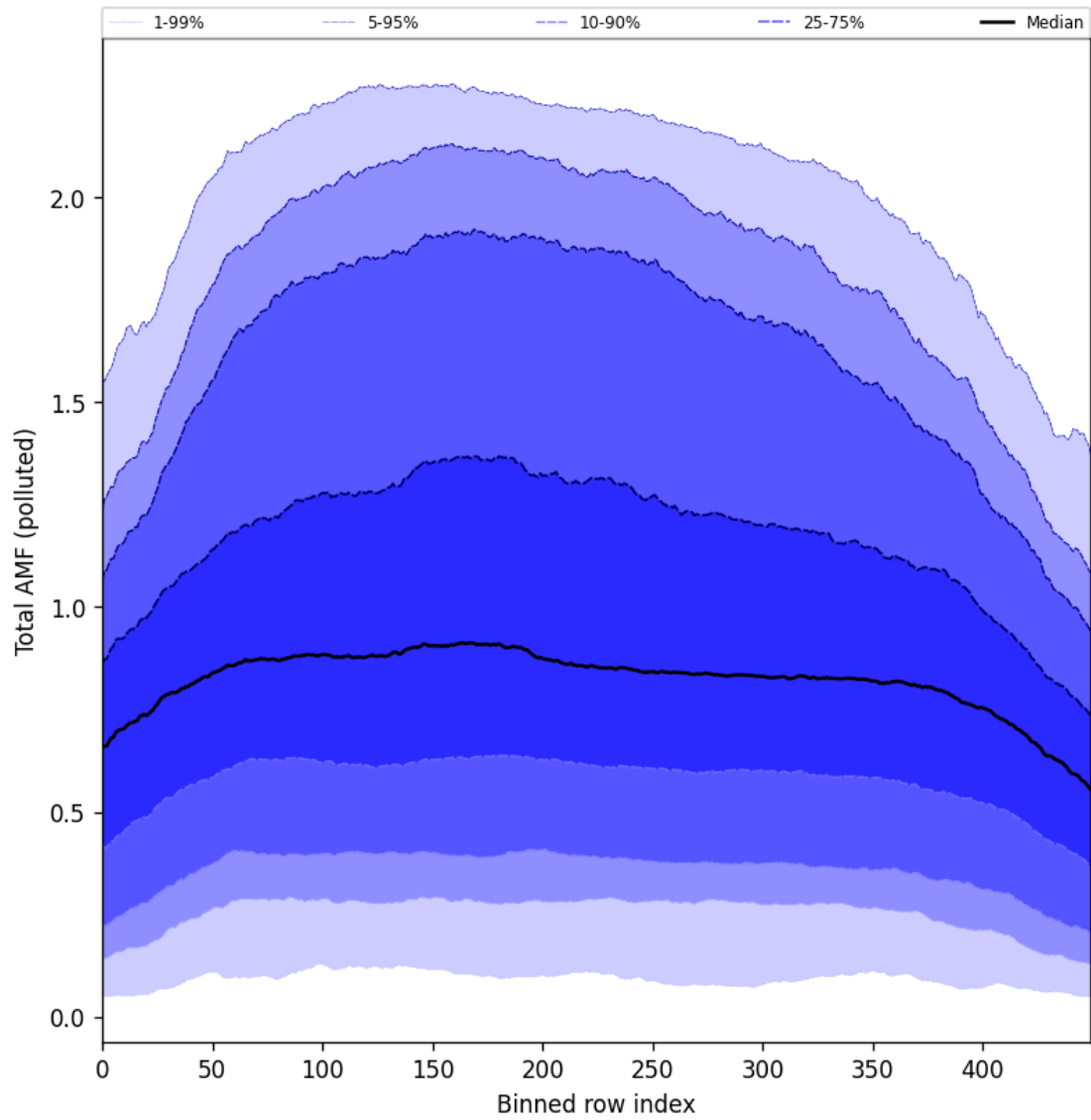
Figure 105: Along track statistics of “Total AMF (polluted)” for 2025-05-13 to 2025-05-15
