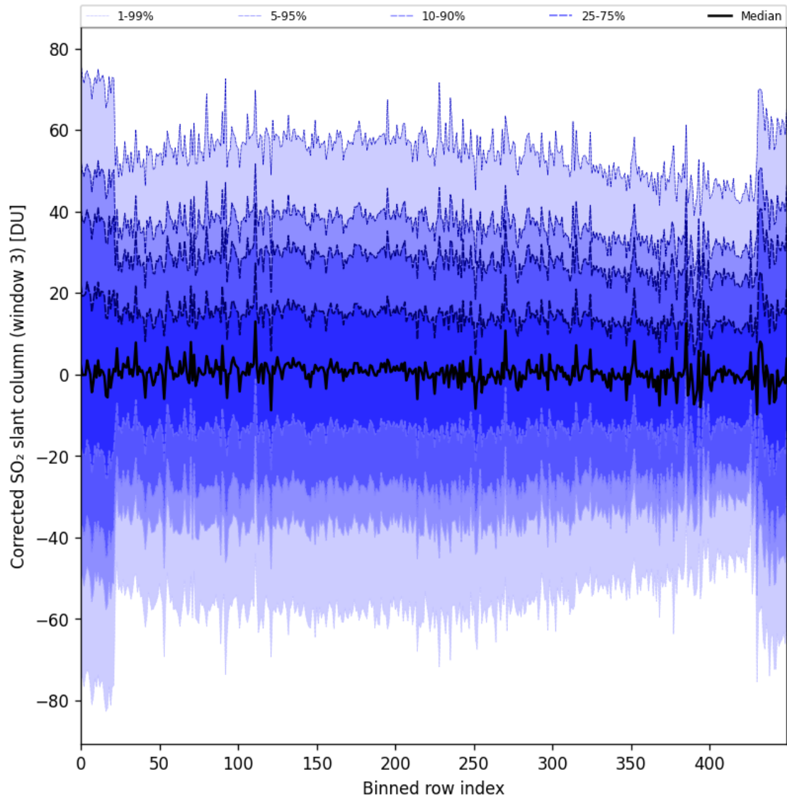
Figure 99: Along track statistics of “Corrected SO 2 slant column (window 3)” for 2025-05-13 to 2025-05-15
