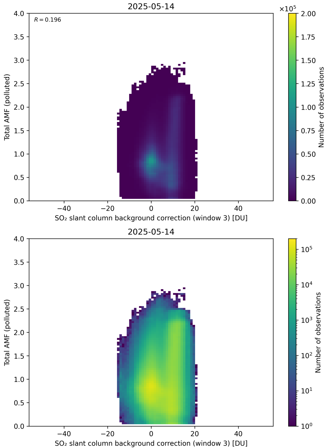
Figure 136: Scatter density plot of “SO 2 slant column background correction (window 3)” against “Total AMF (polluted)” for 2025-05-13 to 2025-05-15.
