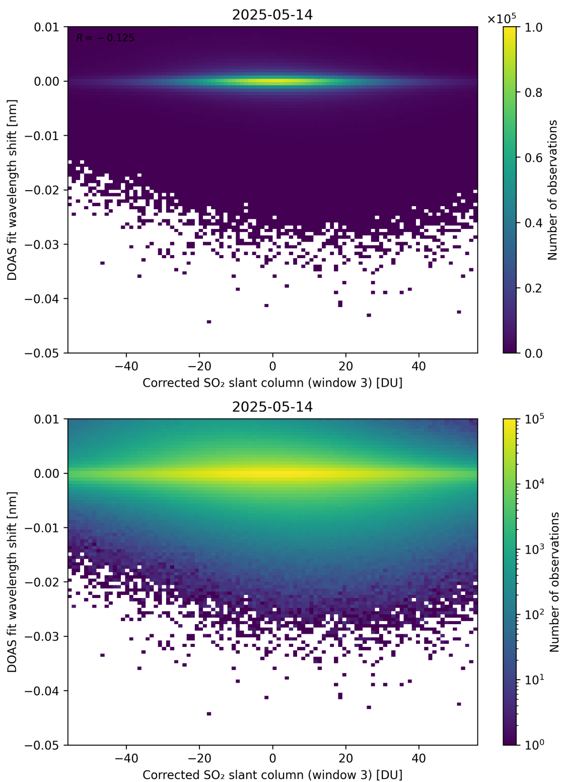
Figure 256: Scatter density plot of “Corrected SO 2 slant column (window 3)” against “DOAS fit wavelength shift” for 2025-05-13 to 2025-05-15.
