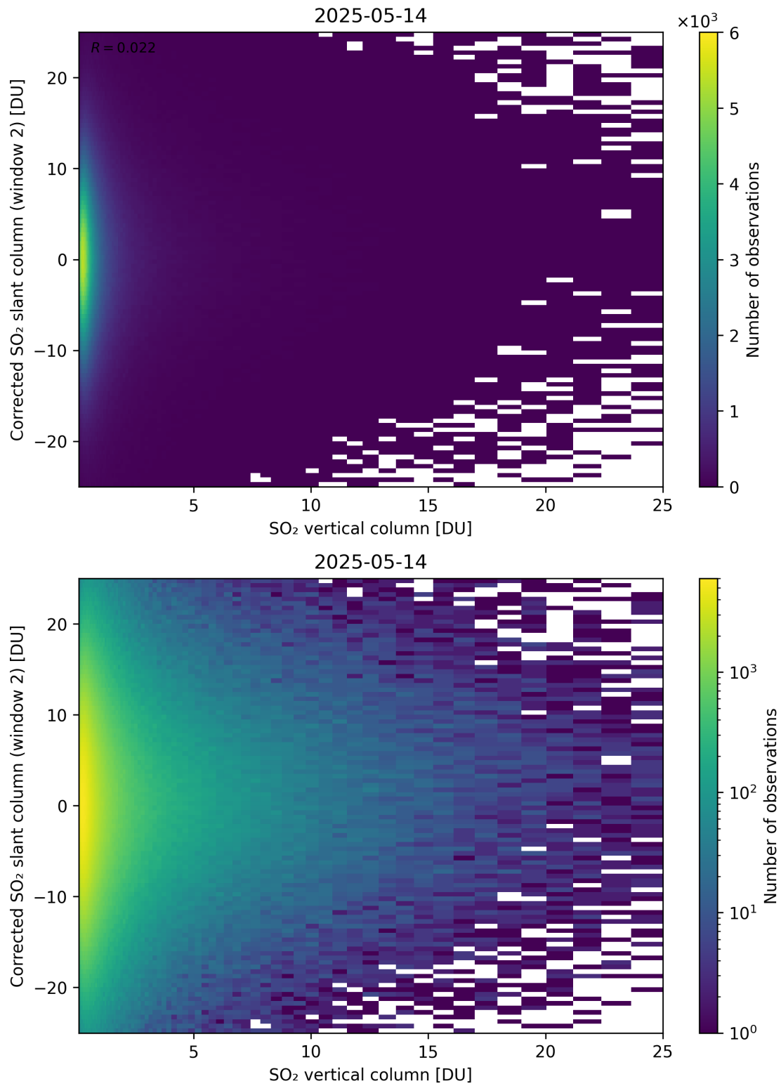
Figure 352: Scatter density plot of “SO 2 vertical column” against “Corrected SO 2 slant column (window 2)” for 2025-05-13 to 2025-05-15.
