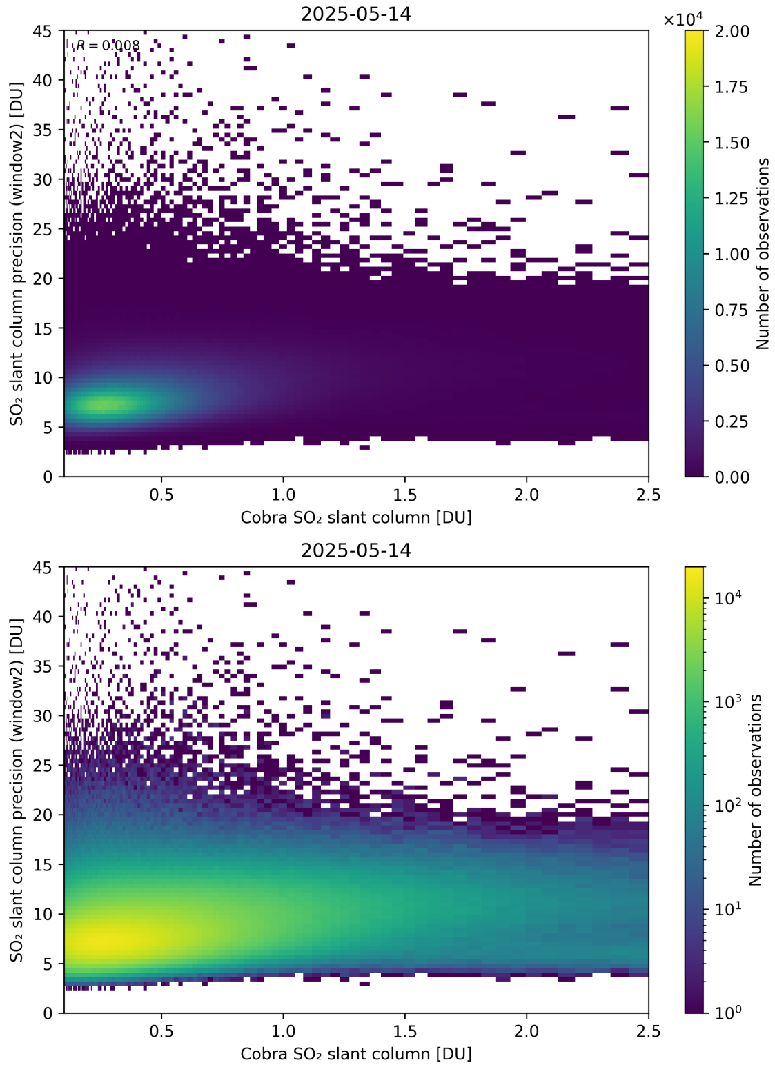
Figure 221: Scatter density plot of “Cobra SO 2 slant column” against “SO 2 slant column precision (window2)” for 2025-05-13 to 2025-05-15.
