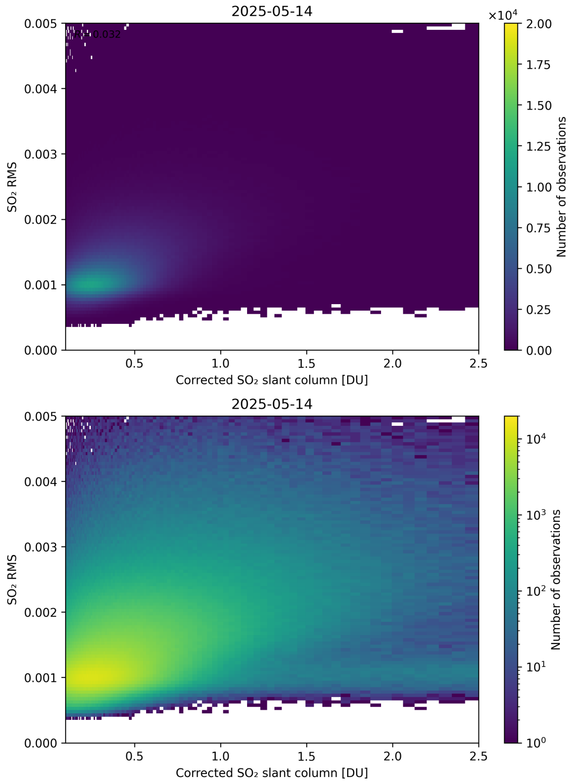
Figure 231: Scatter density plot of “Corrected SO 2 slant column” against “SO 2 RMS” for 2025-05-13 to 2025-05-15.
