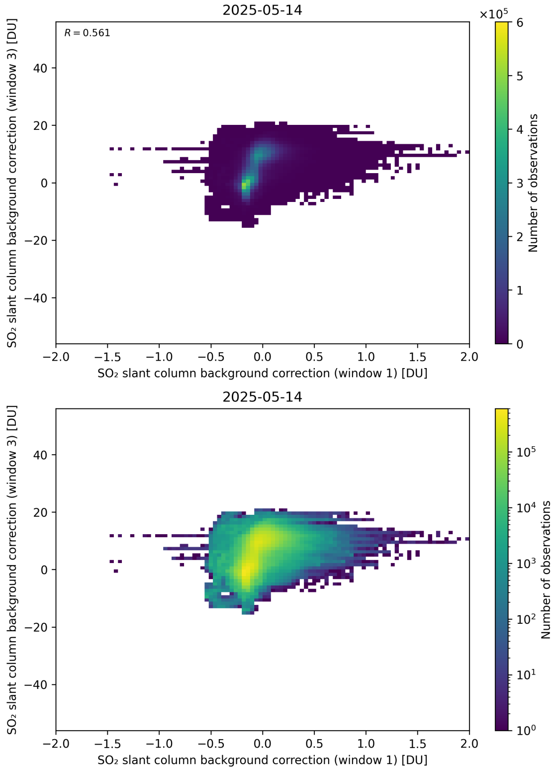
Figure 110: Scatter density plot of “SO 2 slant column background correction (window 1)” against “SO 2 slant column background correction (window 3)” for 2025-05-13 to 2025-05-15.
