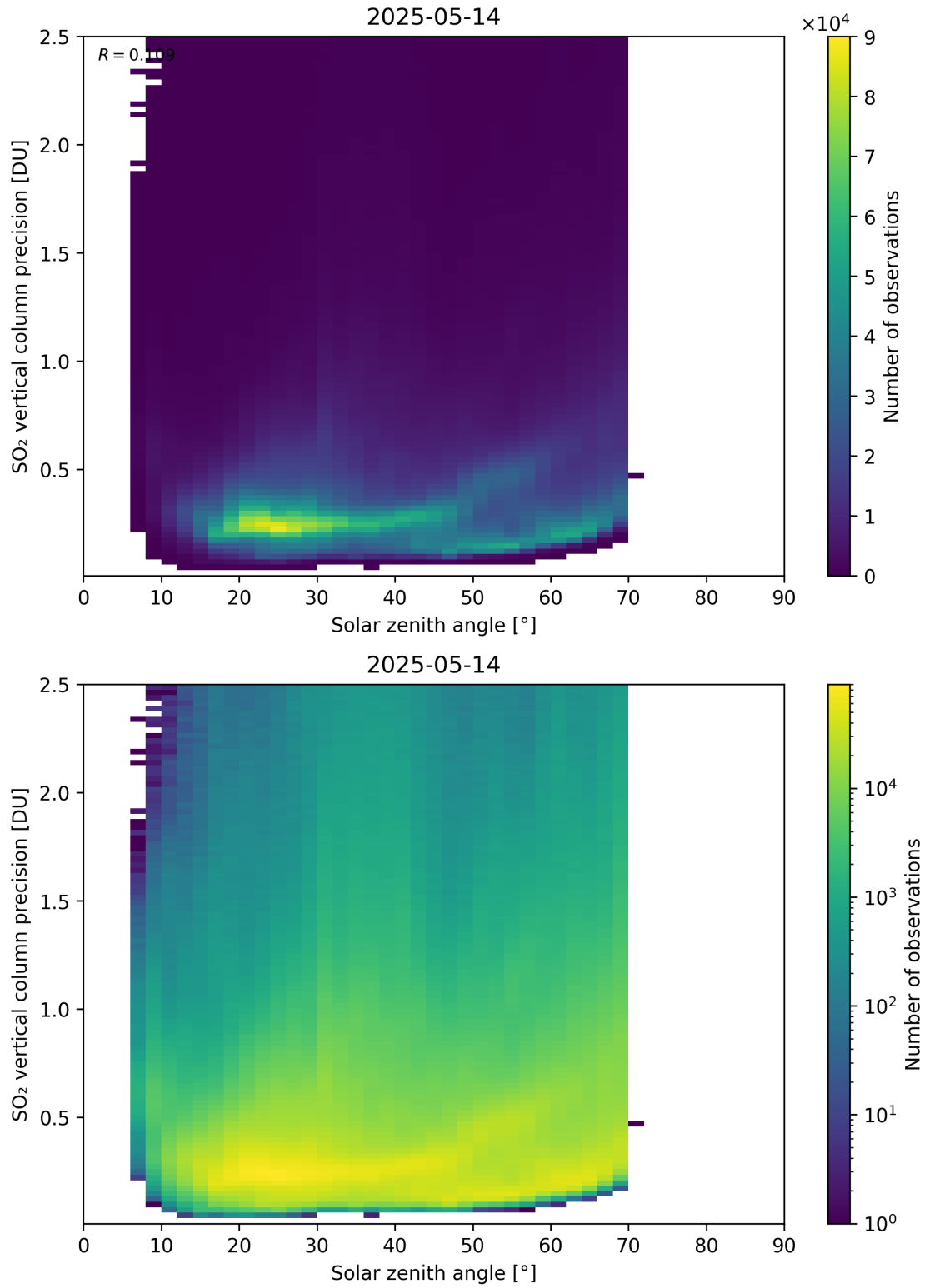
Figure 192: Scatter density plot of “Solar zenith angle” against “SO 2 vertical column precision” for 2025-05-13 to 2025-05-15.
