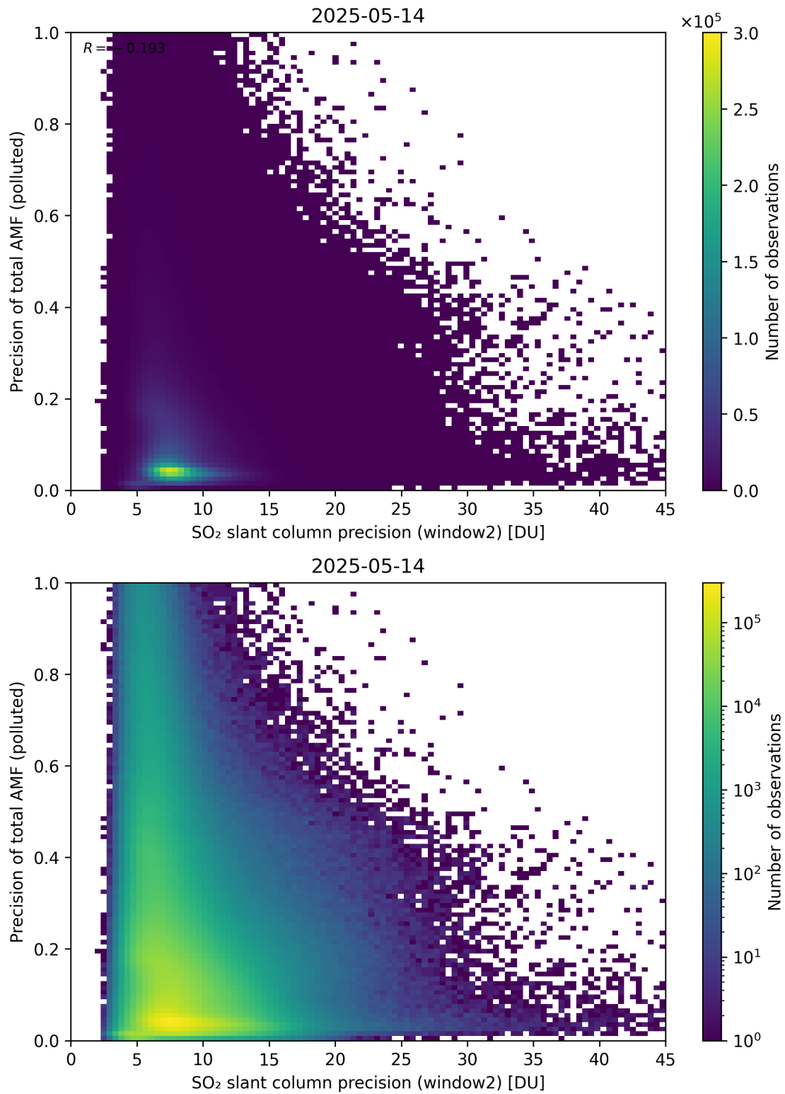
Figure 302: Scatter density plot of “SO 2 slant column precision (window2)” against “Precision of total AMF (polluted)” for 2025-05-13 to 2025-05-15.
