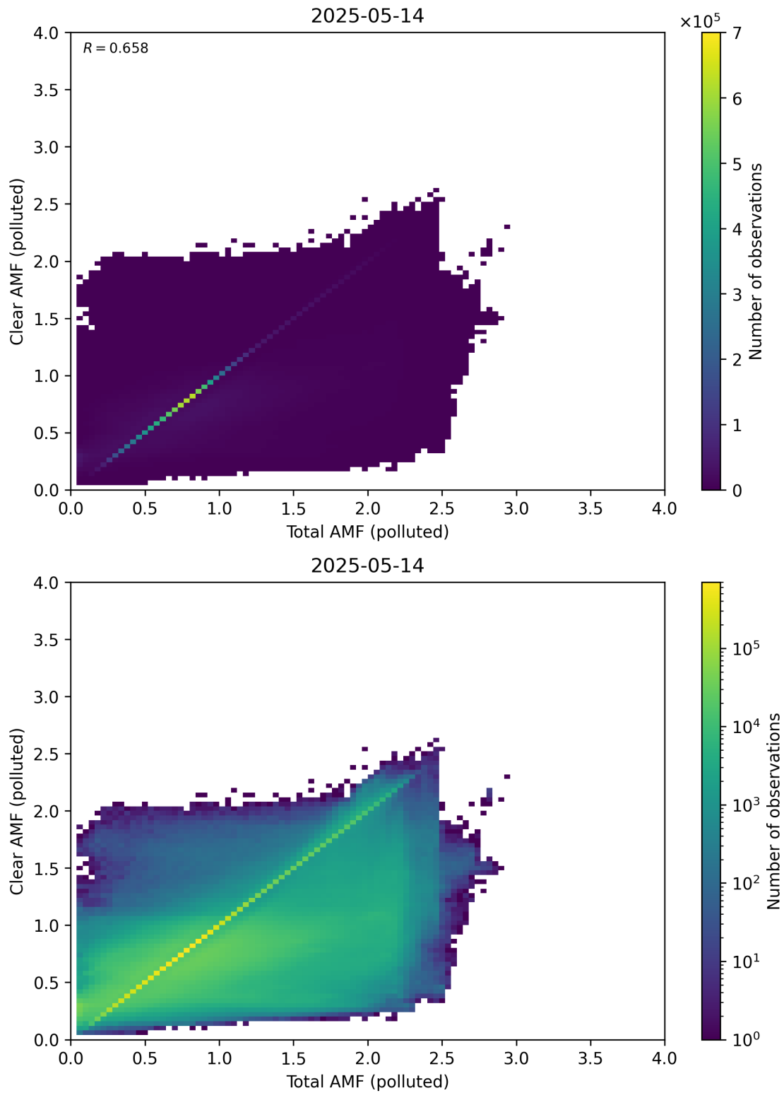
Figure 321: Scatter density plot of “Total AMF (polluted)” against “Clear AMF (polluted)” for 2025-05-13 to 2025-05-15.
