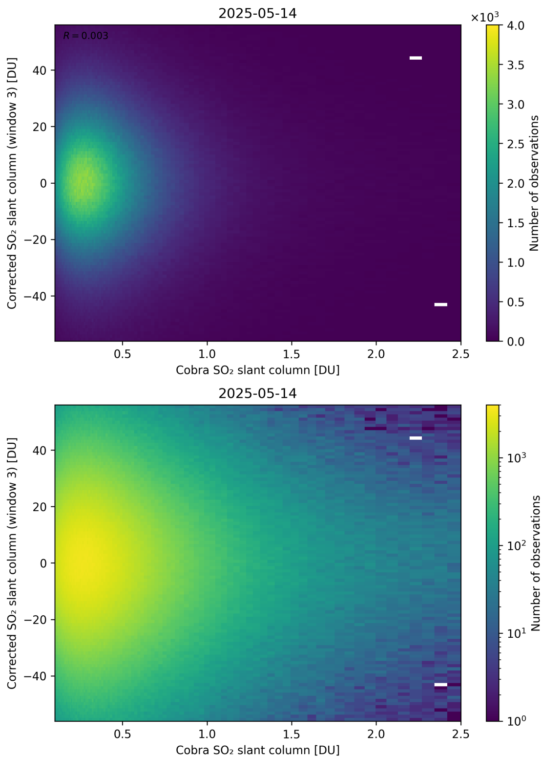
Figure 218: Scatter density plot of “Cobra SO 2 slant column” against “Corrected SO 2 slant column (window 3)” for 2025-05-13 to 2025-05-15.
