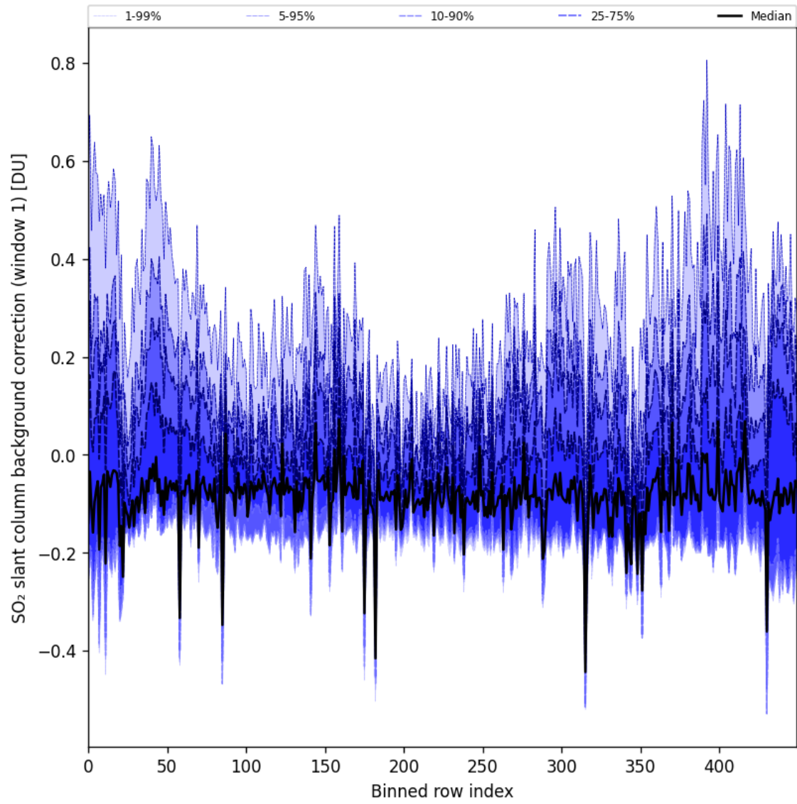
Figure 92: Along track statistics of “SO 2 slant column background correction (window 1)” for 2025-05-13 to 2025-05-15
