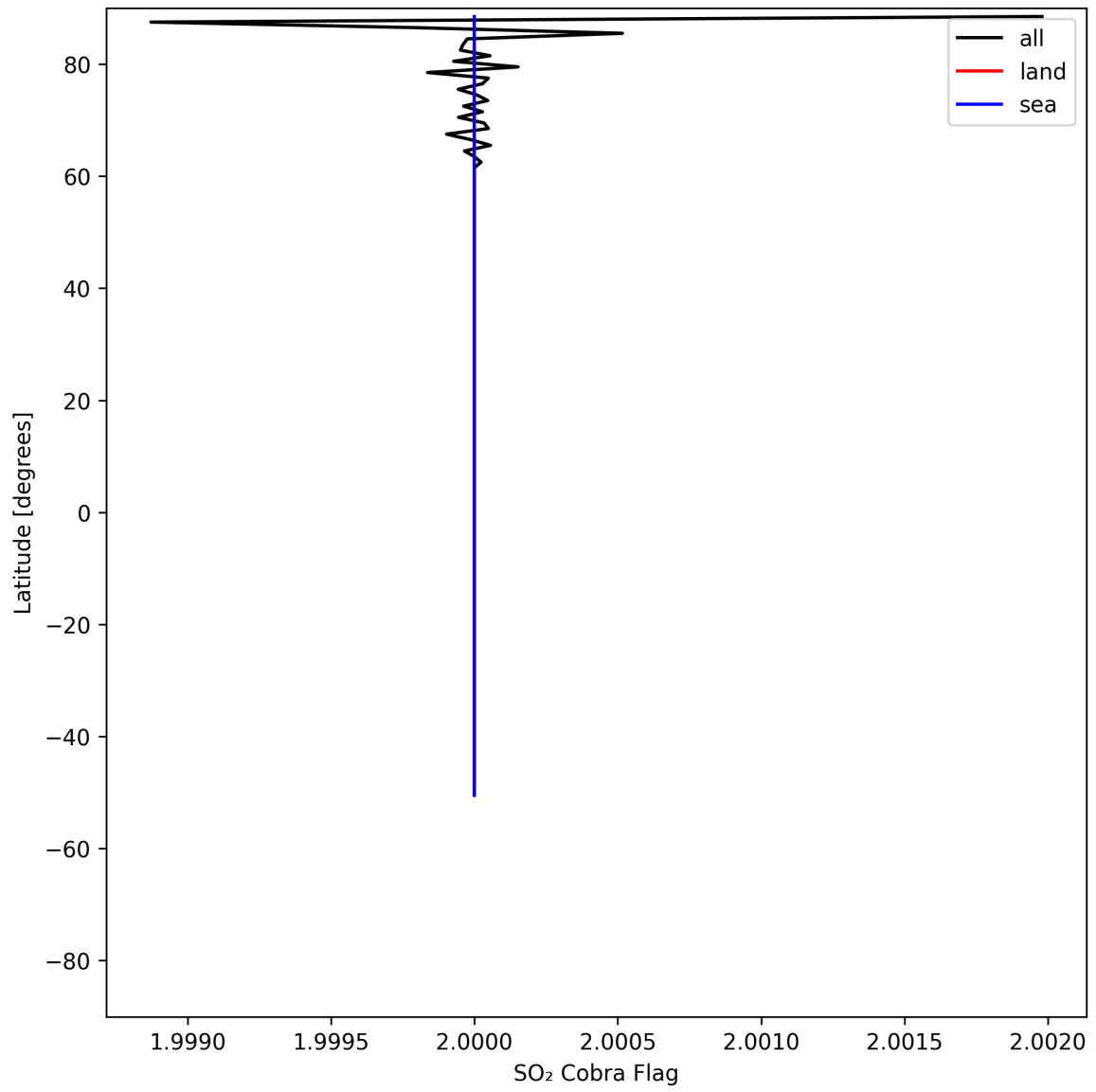
Figure 49: Zonal average of "SO 2 Cobra Flag" for 2025-05-13 to 2025-05-15.
