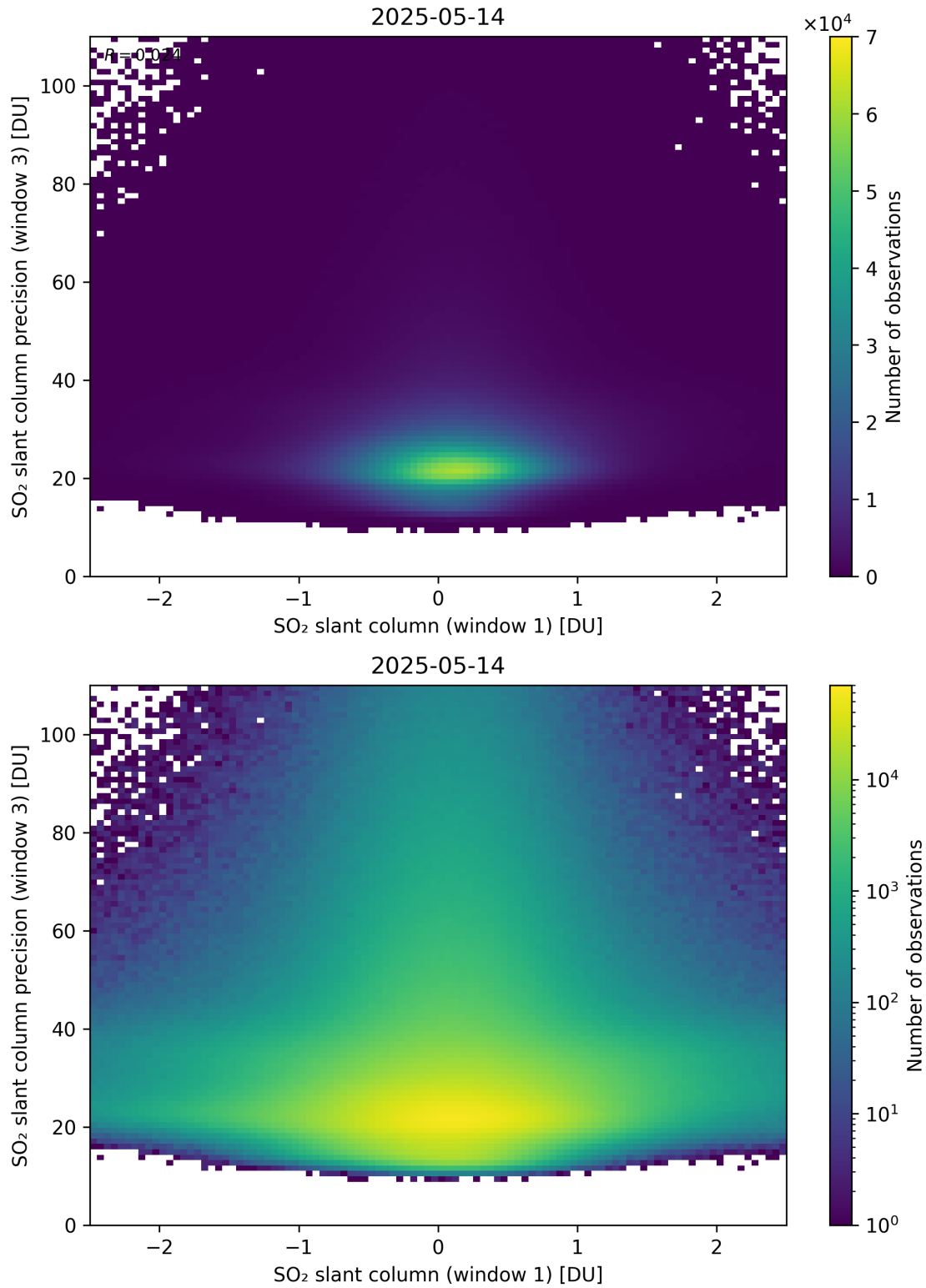
Figure 288: Scatter density plot of “SO 2 slant column (window 1)” against “SO 2 slant column precision (window 3)” for 2025-05-13 to 2025-05-15.
