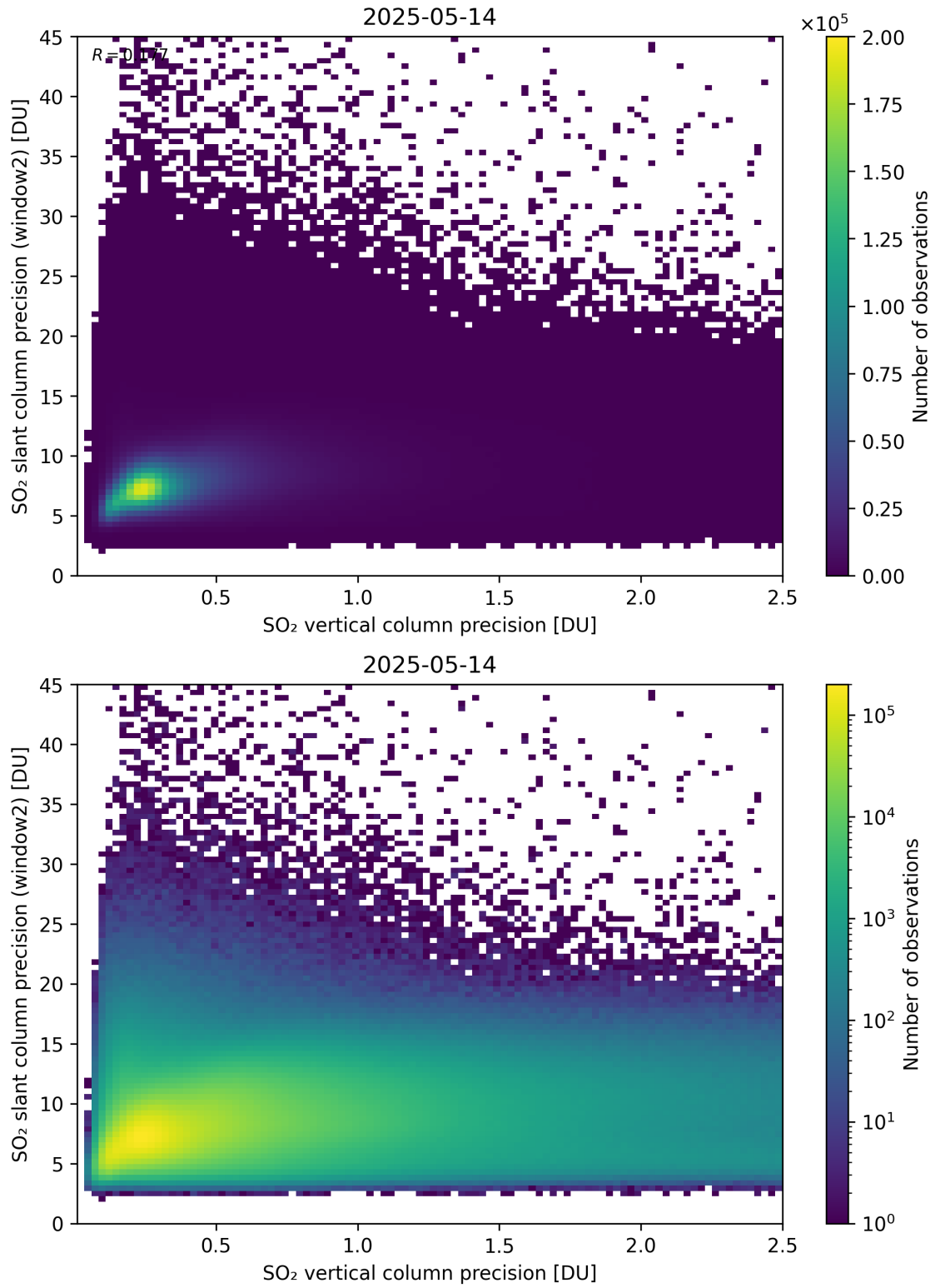
Figure 343: Scatter density plot of “SO 2 vertical column precision” against “SO 2 slant column precision (window2)” for 2025-05-13 to 2025-05-15.
