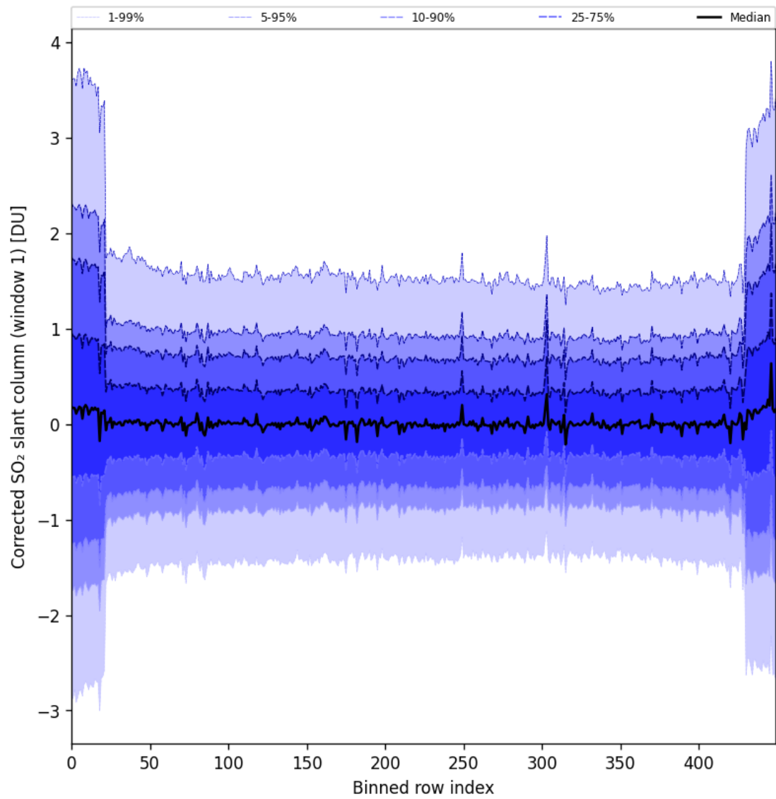
Figure 91: Along track statistics of "Corrected SO 2 slant column (window 1)" for 2025-05-13 to 2025-05-15
