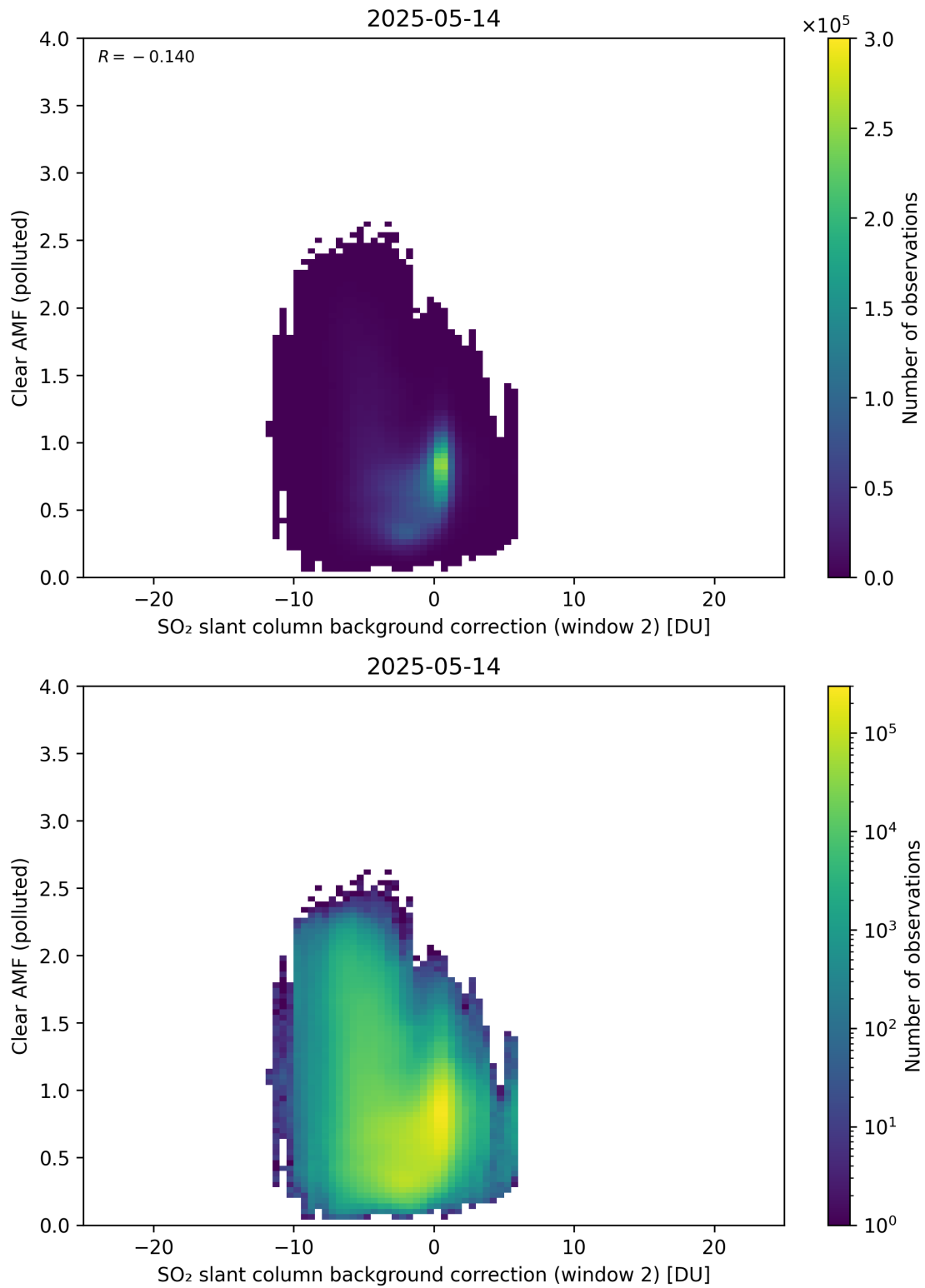
Figure 126: Scatter density plot of “SO 2 slant column background correction (window 2)” against “Clear AMF (polluted)” for 2025-05-13 to 2025-05-15.
