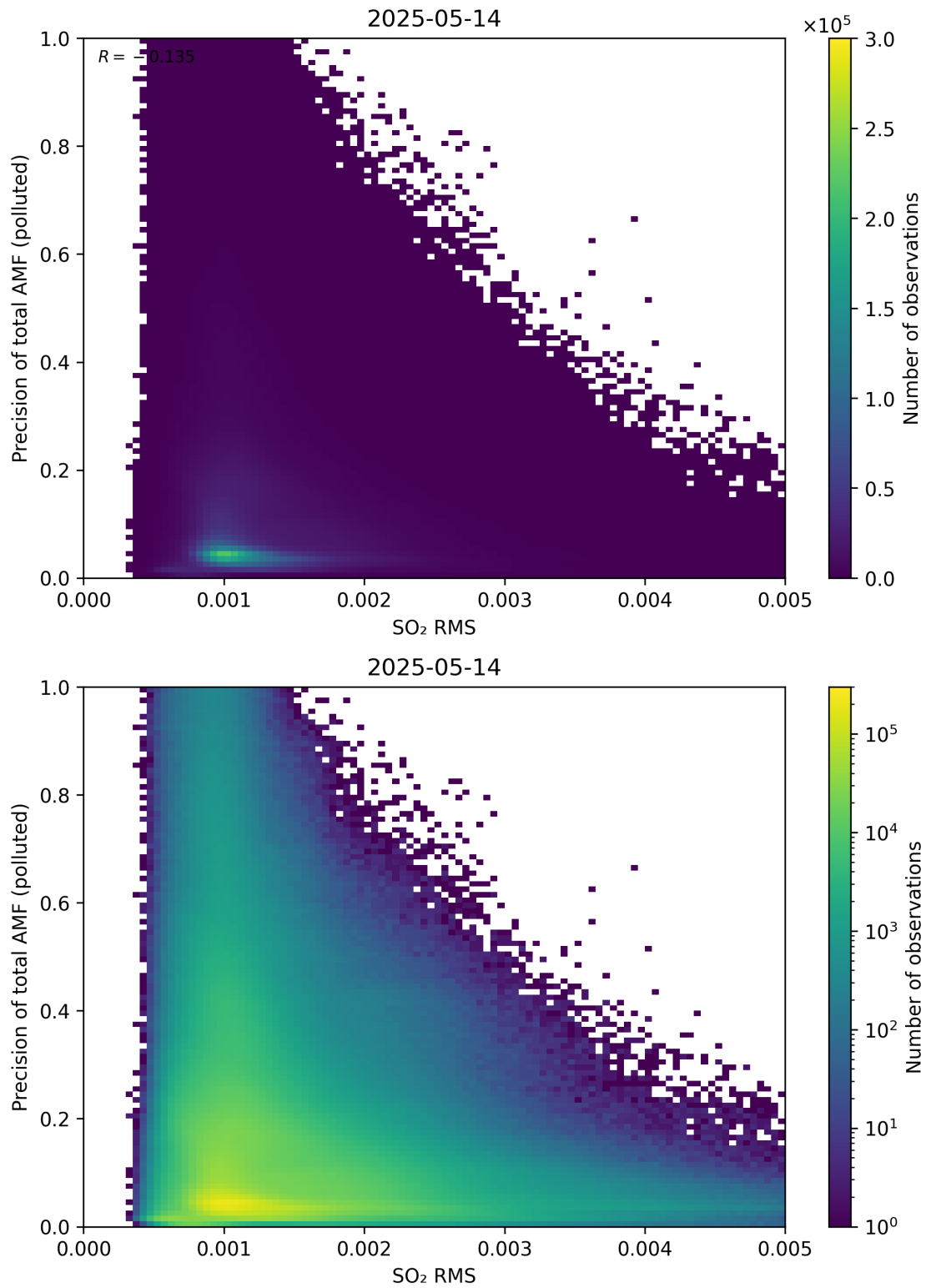
Figure 149: Scatter density plot of “SO 2 RMS” against “Precision of total AMF (polluted)” for 2025-05-13 to 2025-05-15.
