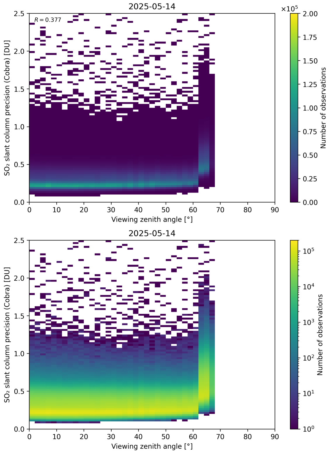
Figure 372: Scatter density plot of “Viewing zenith angle” against “SO 2 slant column precision (Cobra)” for 2025-05-13 to 2025-05-15.
