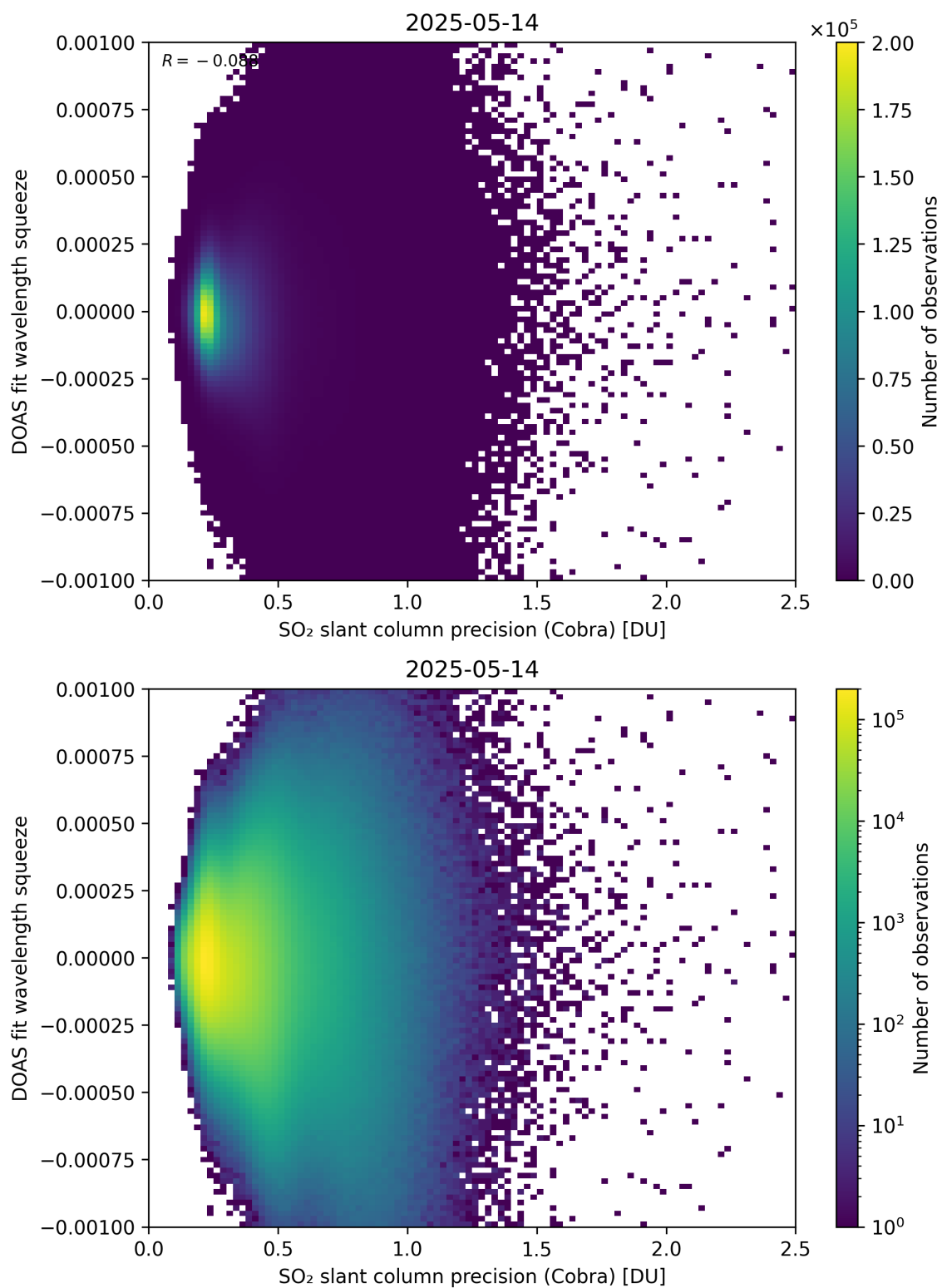
Figure 203: Scatter density plot of “SO 2 slant column precision (Cobra)” against “DOAS fit wavelength squeeze” for 2025-05-13 to 2025-05-15.
