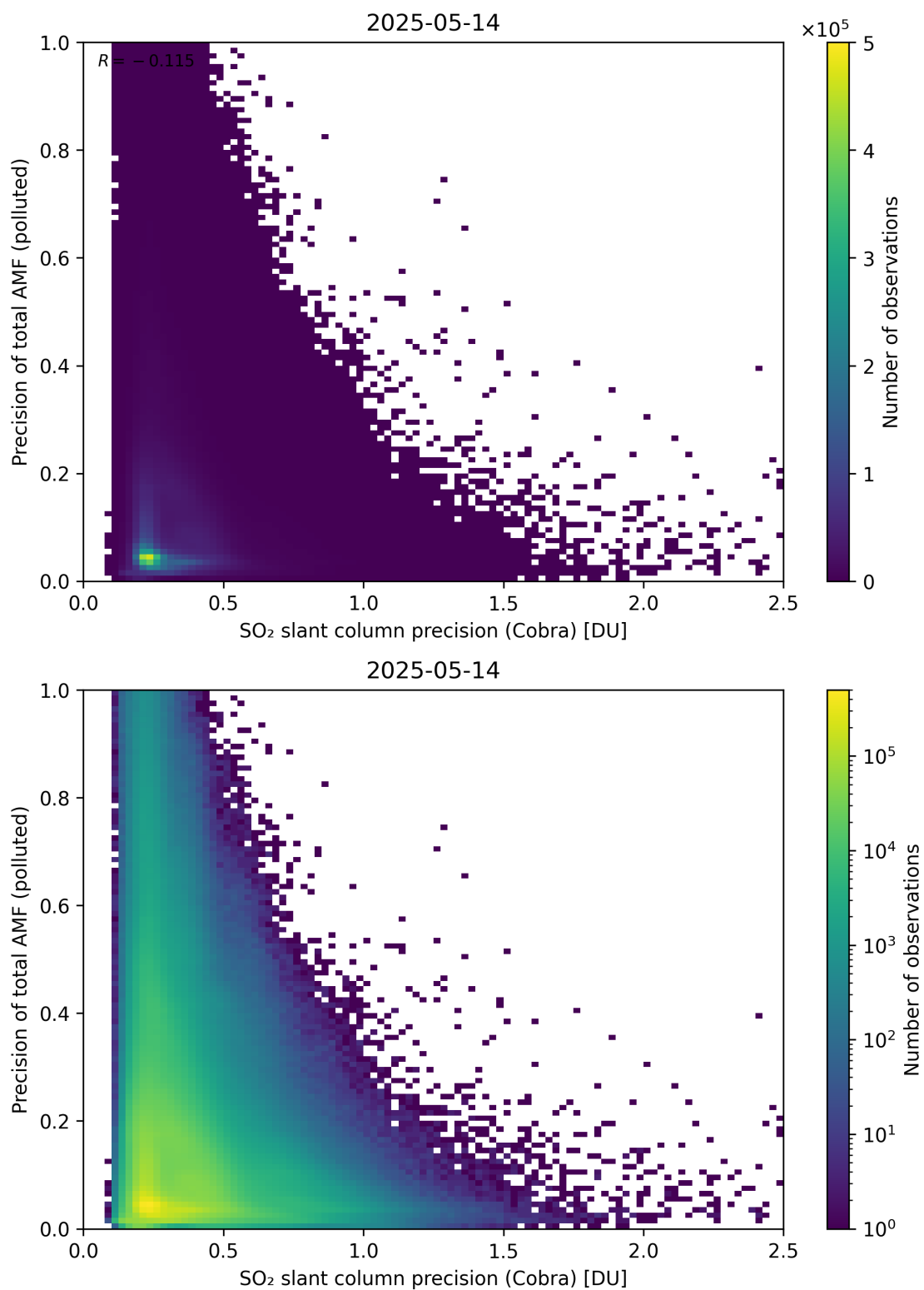
Figure 214: Scatter density plot of “SO 2 slant column precision (Cobra)” against “Precision of total AMF (polluted)” for 2025-05-13 to 2025-05-15.
