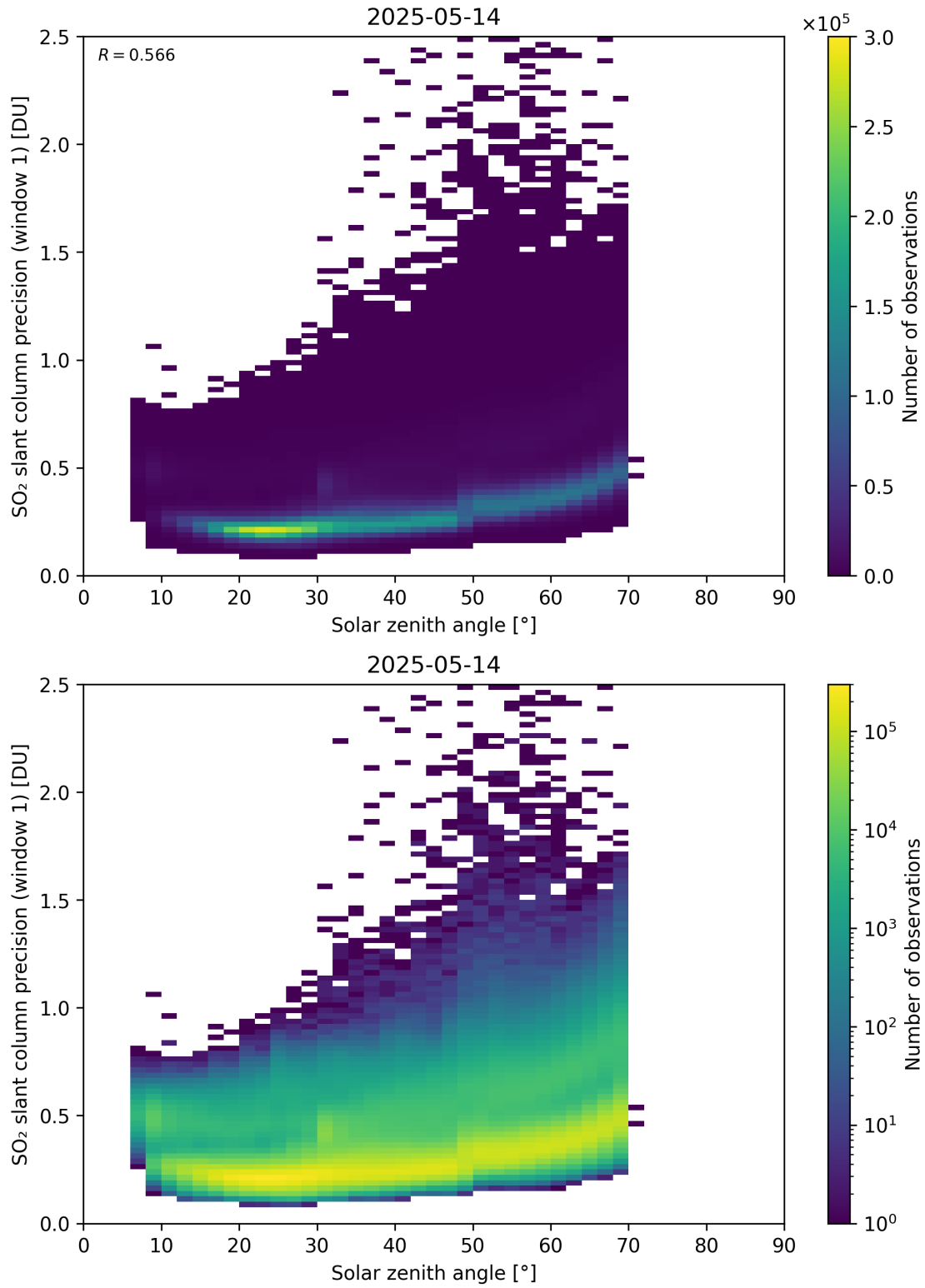
Figure 185: Scatter density plot of “Solar zenith angle” against “SO 2 slant column precision (window 1)” for 2025-05-13 to 2025-05-15.
