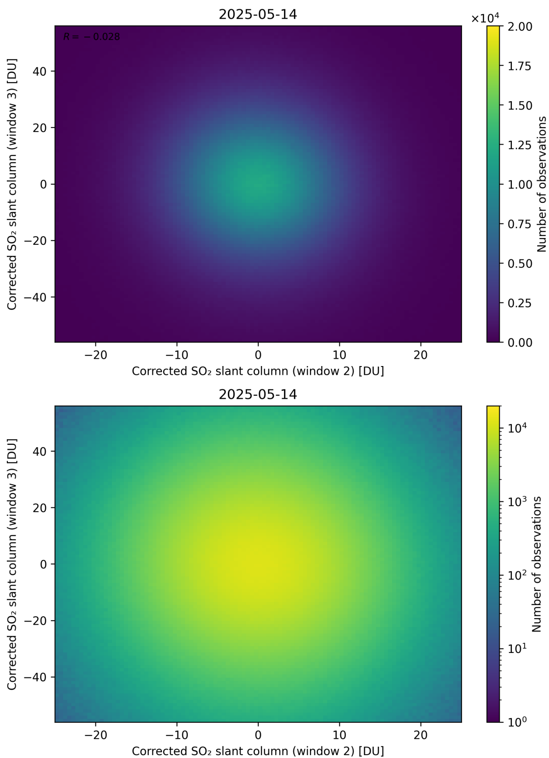
Figure 250: Scatter density plot of “Corrected SO 2 slant column (window 2)” against “Corrected SO 2 slant column (window 3)” for 2025-05-13 to 2025-05-15.
