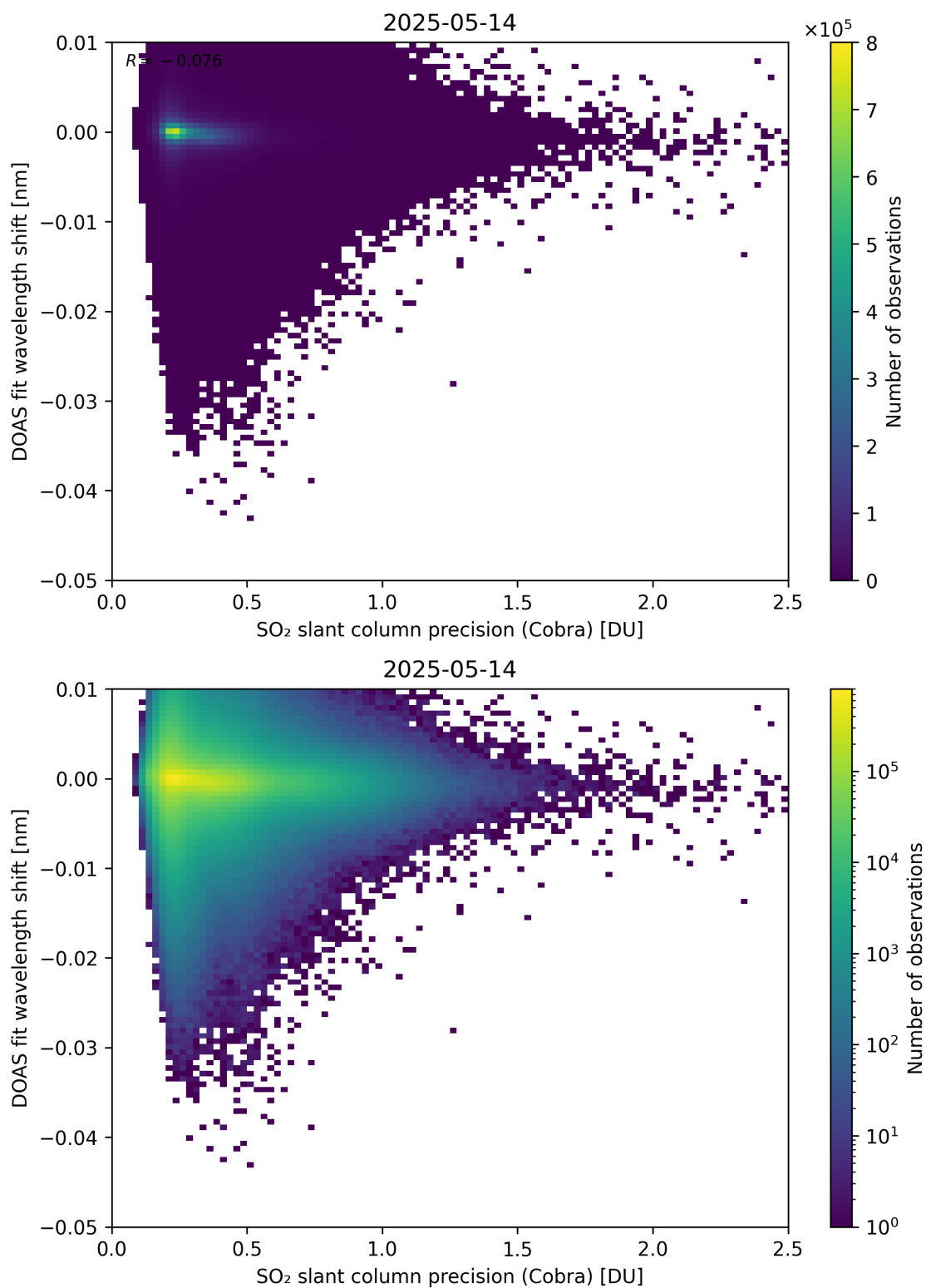
Figure 202: Scatter density plot of “SO 2 slant column precision (Cobra)” against “DOAS fit wavelength shift” for 2025-05-13 to 2025-05-15.
