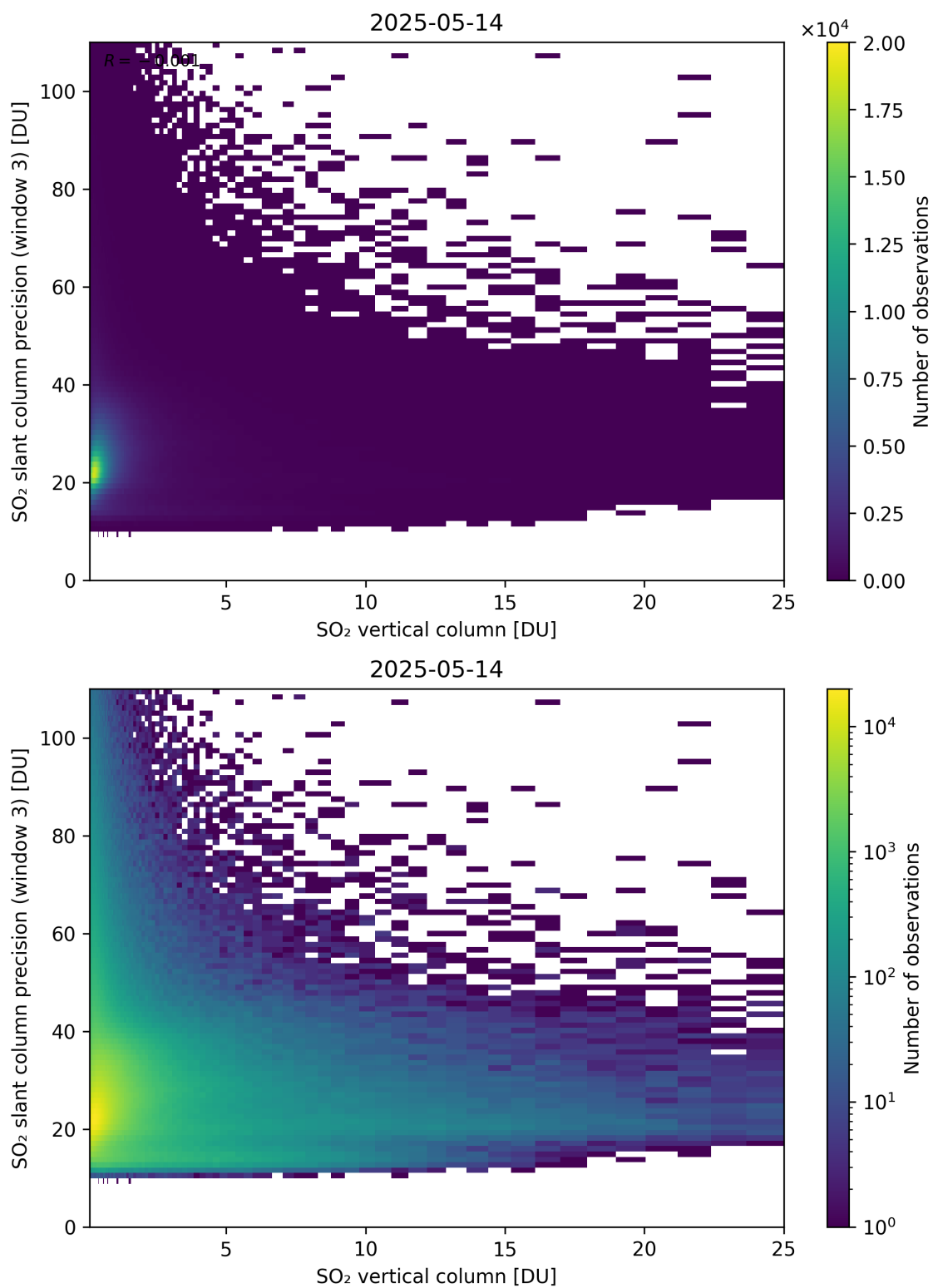
Figure 358: Scatter density plot of “SO 2 vertical column” against “SO 2 slant column precision (window 3)” for 2025-05-13 to 2025-05-15.
