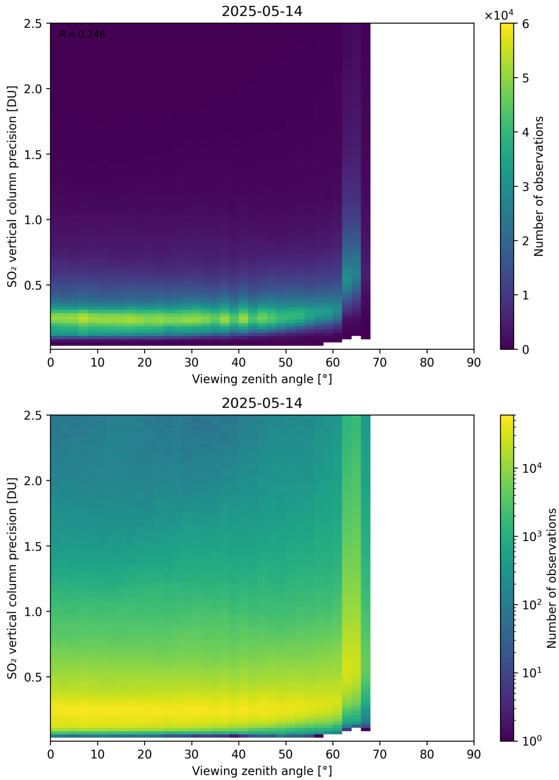
Figure 384: Scatter density plot of “Viewing zenith angle” against “SO 2 vertical column precision” for 2025-05-13 to 2025-05-15.
