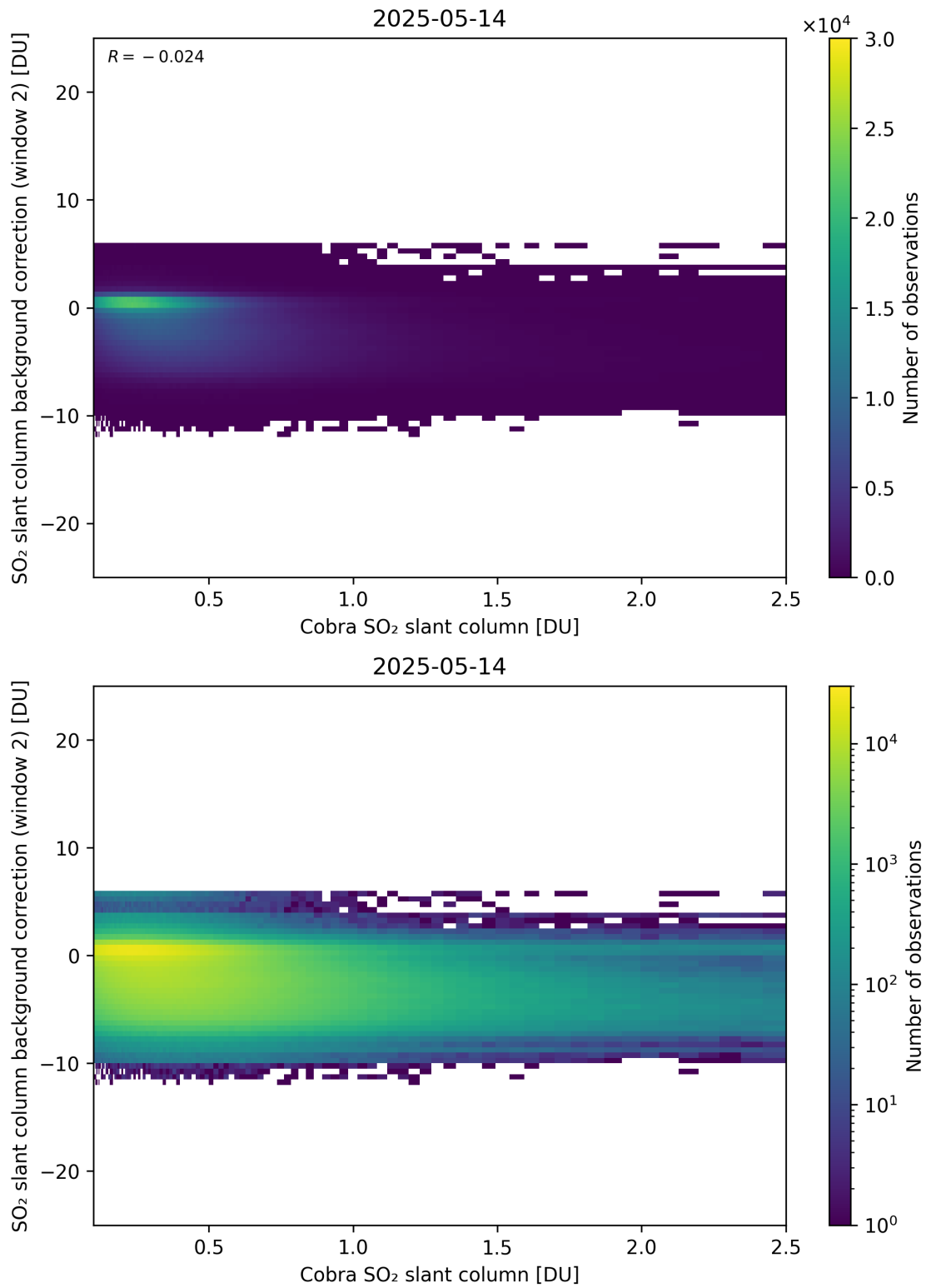
Figure 194: Scatter density plot of “Cobra SO 2 slant column” against “SO 2 slant column background correction (window 2)” for 2025-05-13 to 2025-05-15.
