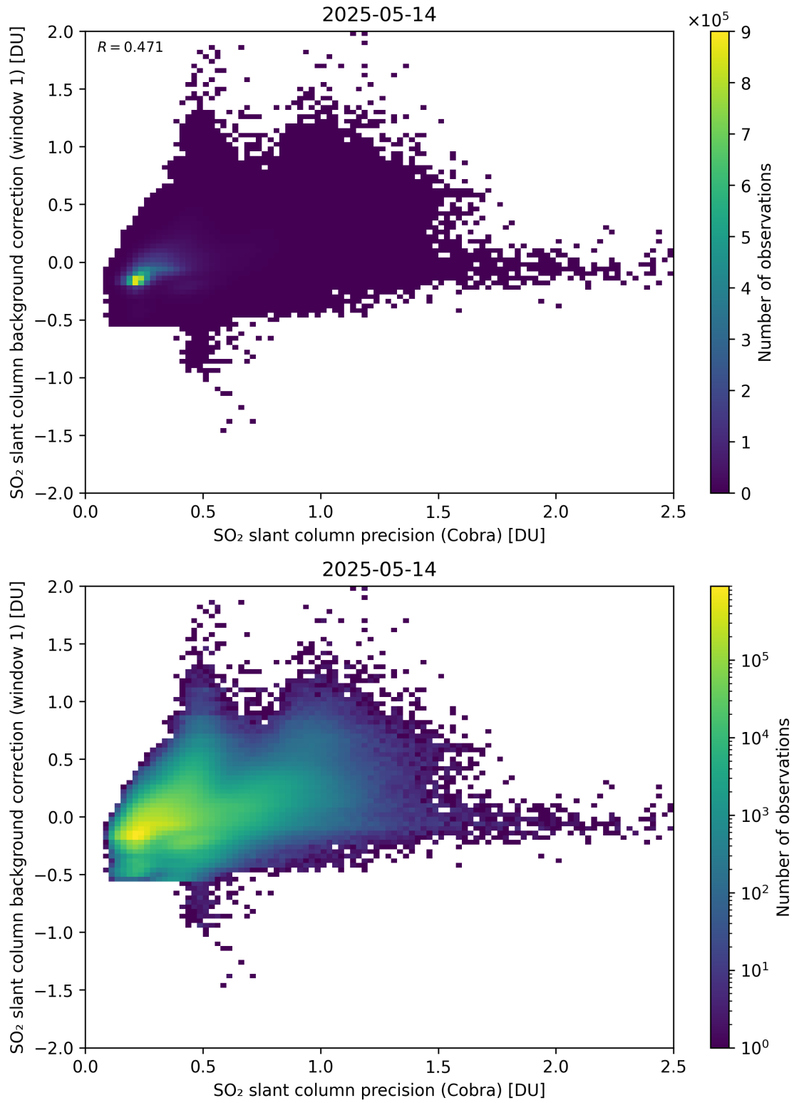
Figure 199: Scatter density plot of “SO 2 slant column precision (Cobra)” against “SO 2 slant column background correction (window 1)” for 2025-05-13 to 2025-05-15.
