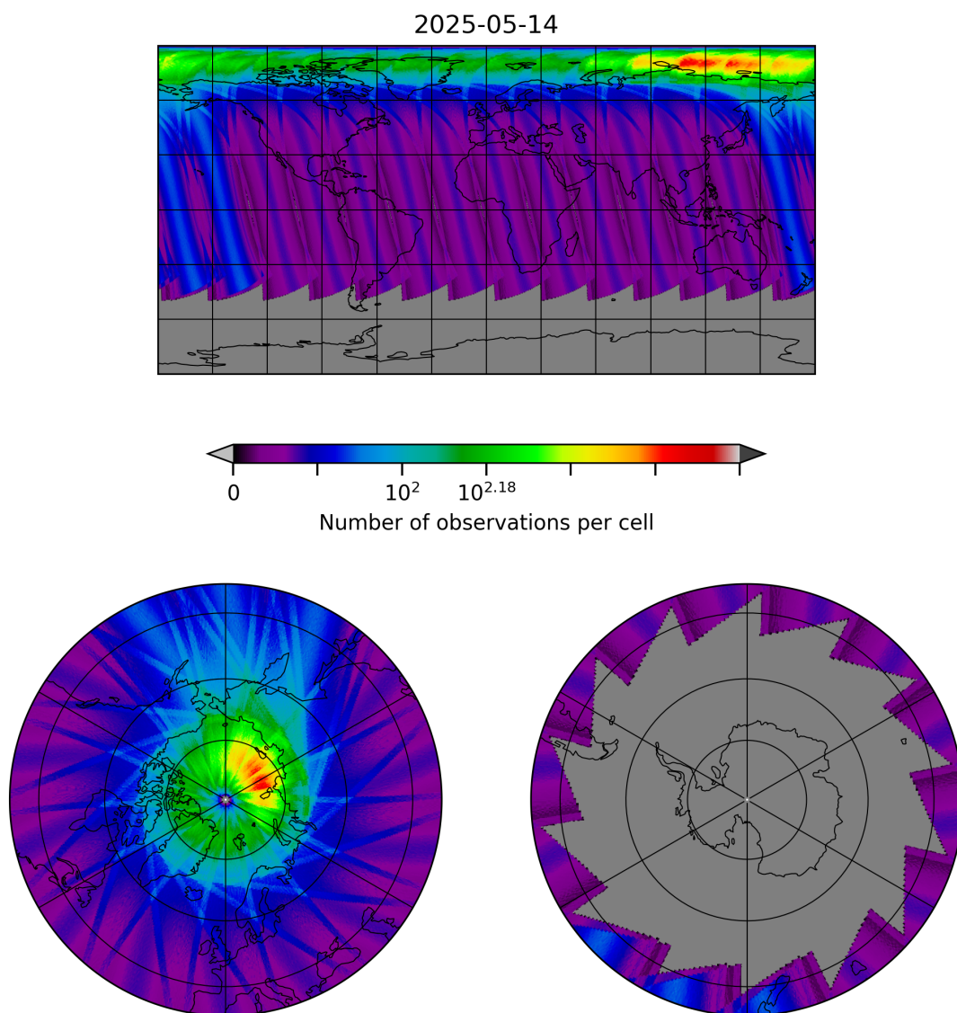
Figure 30: Map of the number of observations for 2025-05-13 to 2025-05-15
