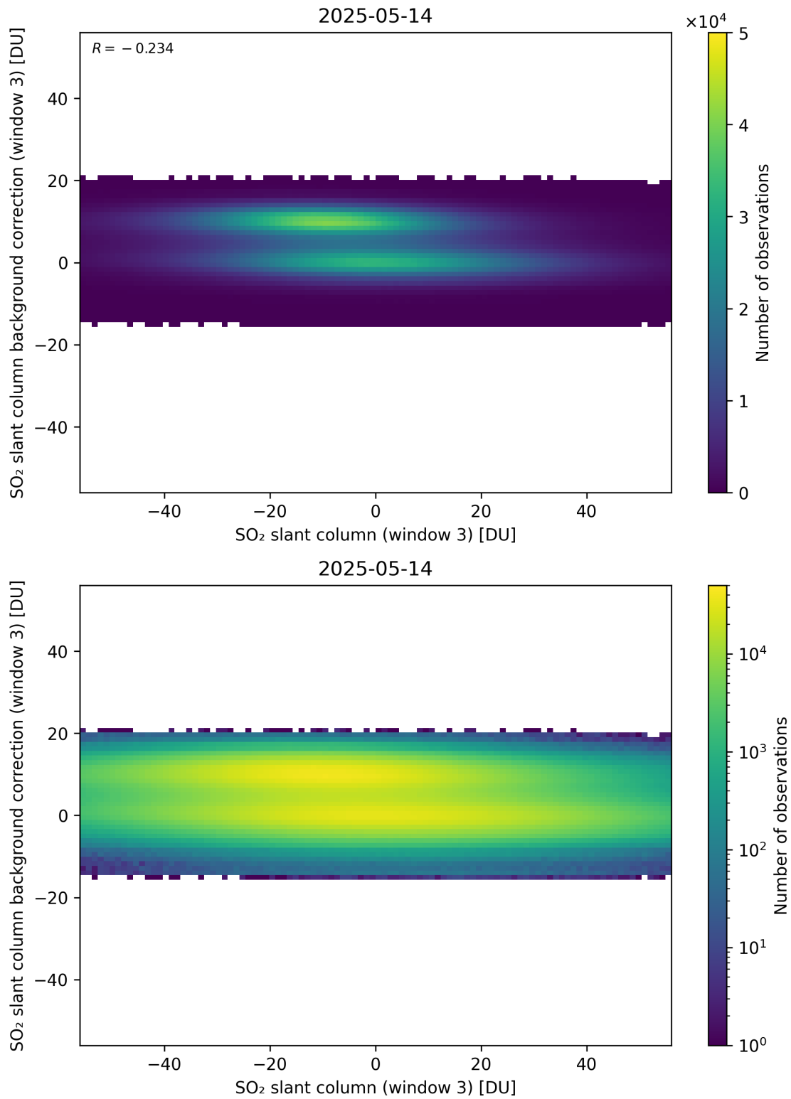
Figure 303: Scatter density plot of “SO 2 slant column (window 3)” against “SO 2 slant column background correction (window 3)” for 2025-05-13 to 2025-05-15.
