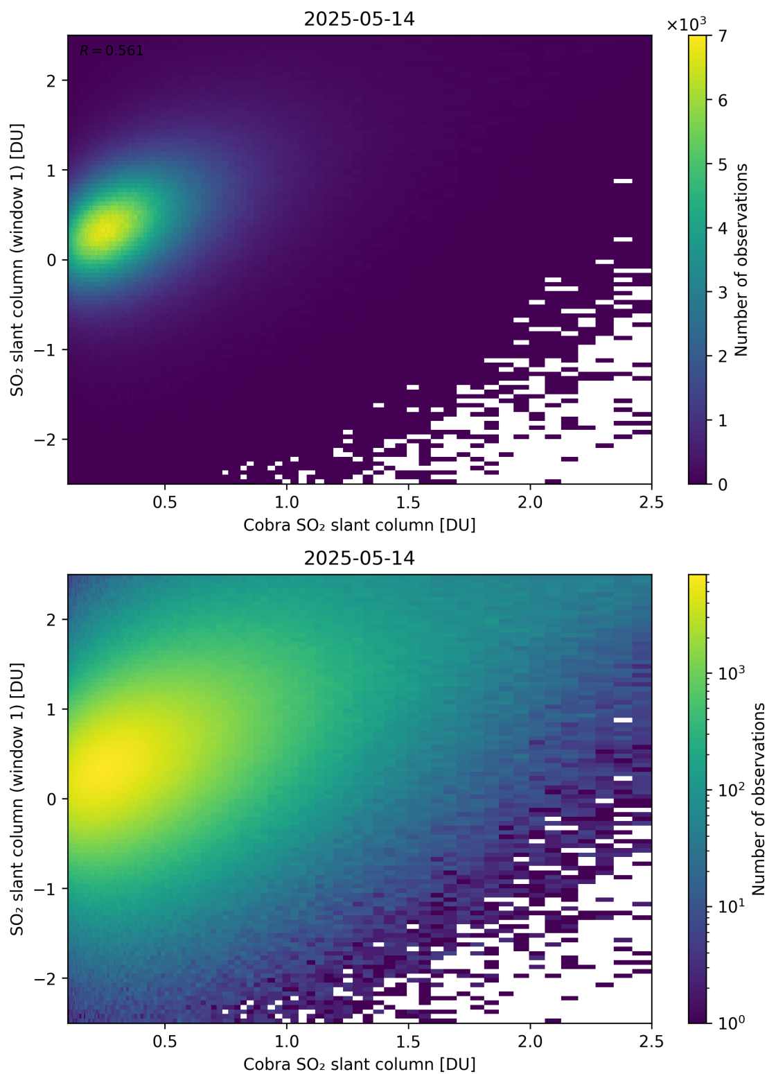
Figure 219: Scatter density plot of “Cobra SO 2 slant column” against “SO 2 slant column (window 1)” for 2025-05-13 to 2025-05-15.
