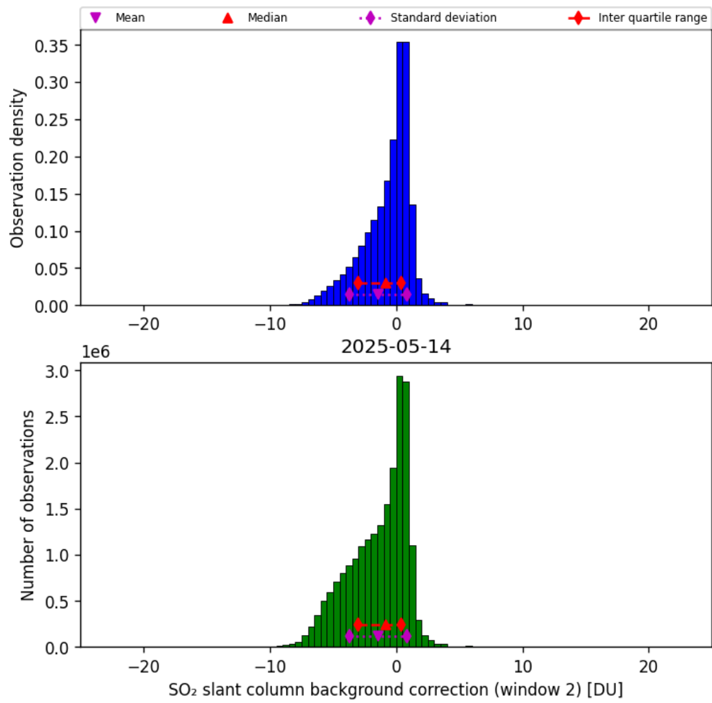
Figure 70: Histogram of “SO 2 slant column background correction (window 2)” for 2025-05-13 to 2025-05-15
