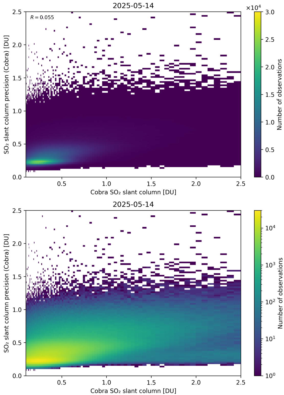
Figure 216: Scatter density plot of “Cobra SO 2 slant column” against “SO 2 slant column precision (Cobra)” for 2025-05-13 to 2025-05-15.
