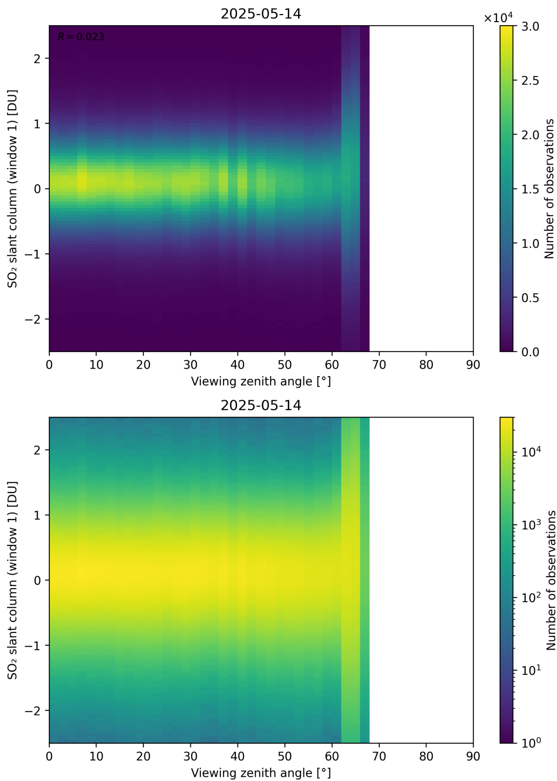
Figure 376: Scatter density plot of “Viewing zenith angle” against “SO 2 slant column (window 1)” for 2025-05-13 to 2025-05-15.
