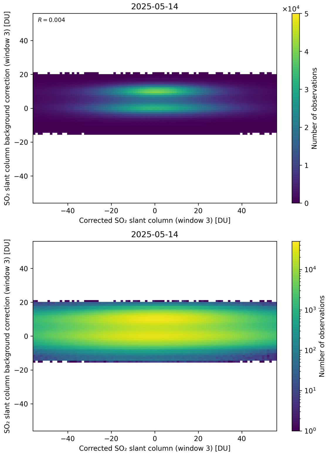
Figure 255: Scatter density plot of “Corrected SO 2 slant column (window 3)” against “SO 2 slant column background correction (window 3)” for 2025-05-13 to 2025-05-15.
