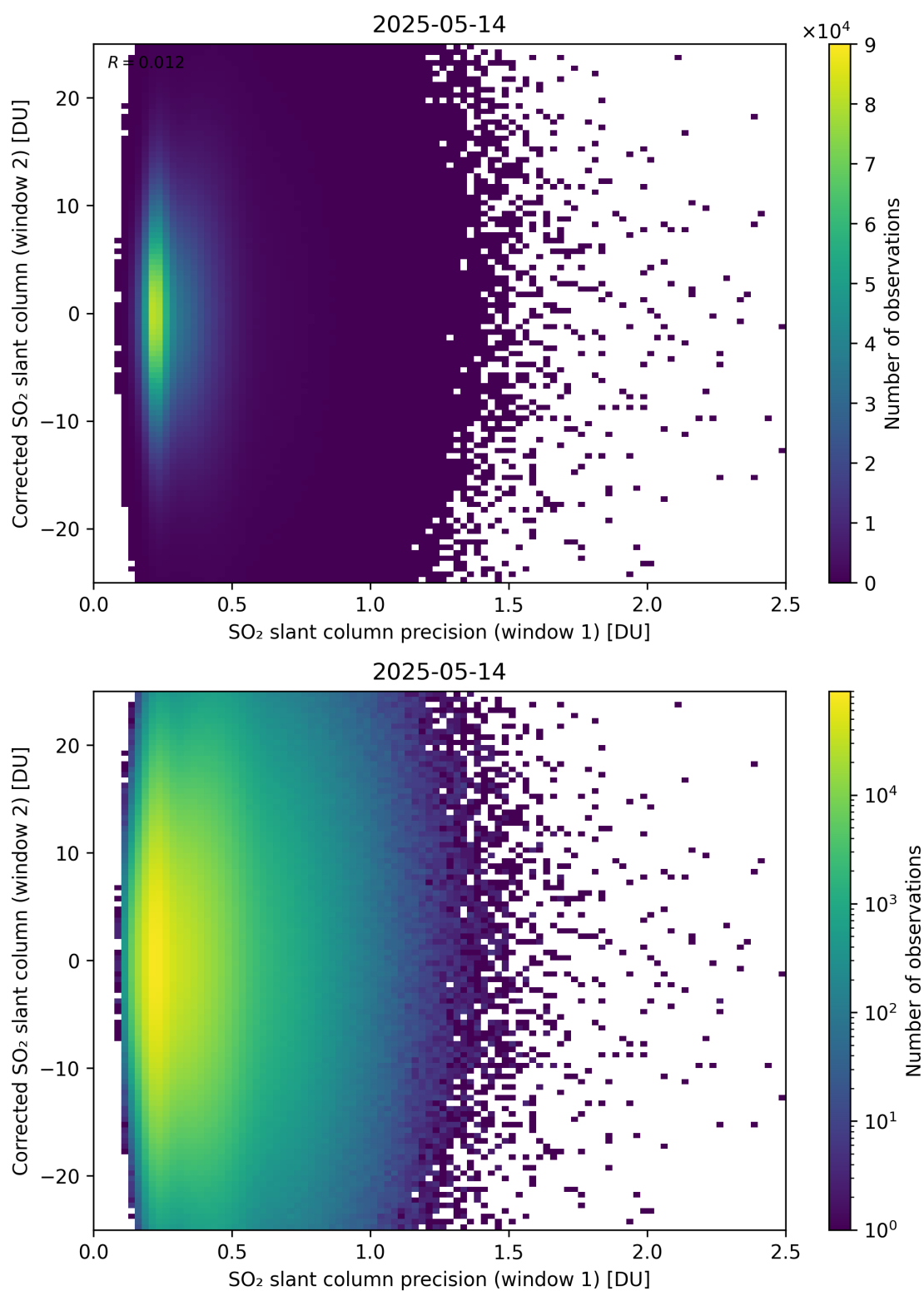
Figure 275: Scatter density plot of “SO 2 slant column precision (window 1)” against “Corrected SO 2 slant column (window 2)” for 2025-05-13 to 2025-05-15.
