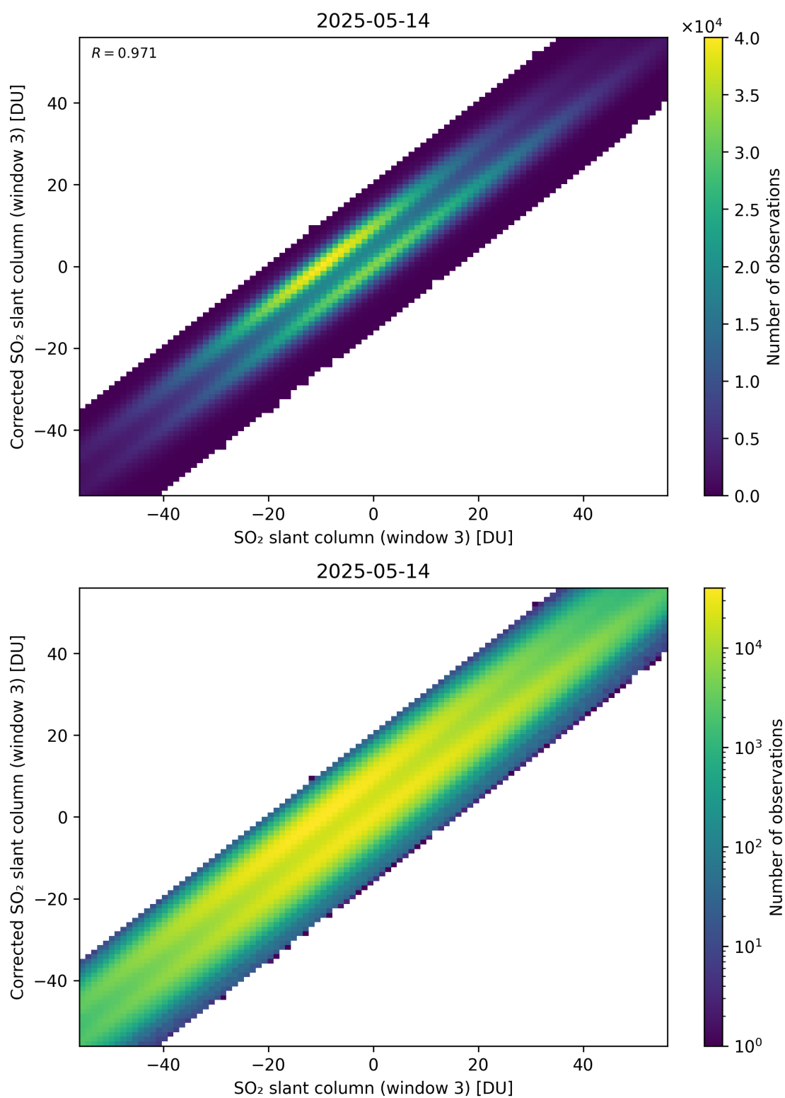
Figure 316: Scatter density plot of “SO 2 slant column (window 3)” against “Corrected SO 2 slant column (window 3)” for 2025-05-13 to 2025-05-15.
