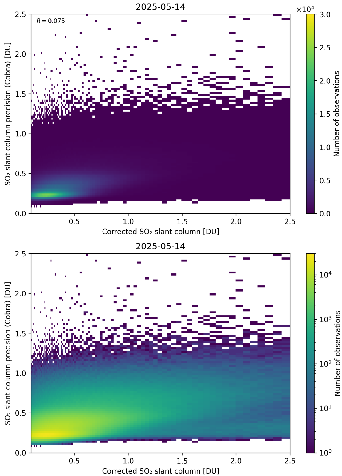
Figure 234: Scatter density plot of “Corrected SO 2 slant column” against “SO 2 slant column precision (Cobra)” for 2025-05-13 to 2025-05-15.
