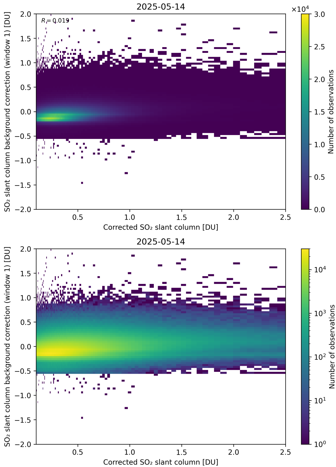
Figure 226: Scatter density plot of “Corrected SO 2 slant column” against “SO 2 slant column background correction (window 1)” for 2025-05-13 to 2025-05-15.
