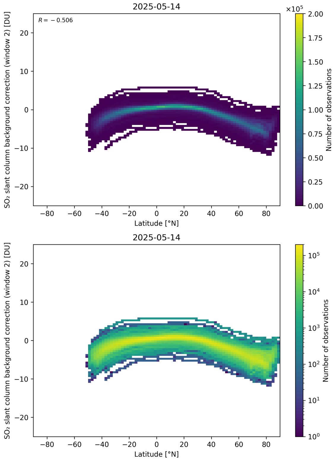
Figure 151: Scatter density plot of “Latitude” against “SO 2 slant column background correction (window 2)” for 2025-05-13 to 2025-05-15.
