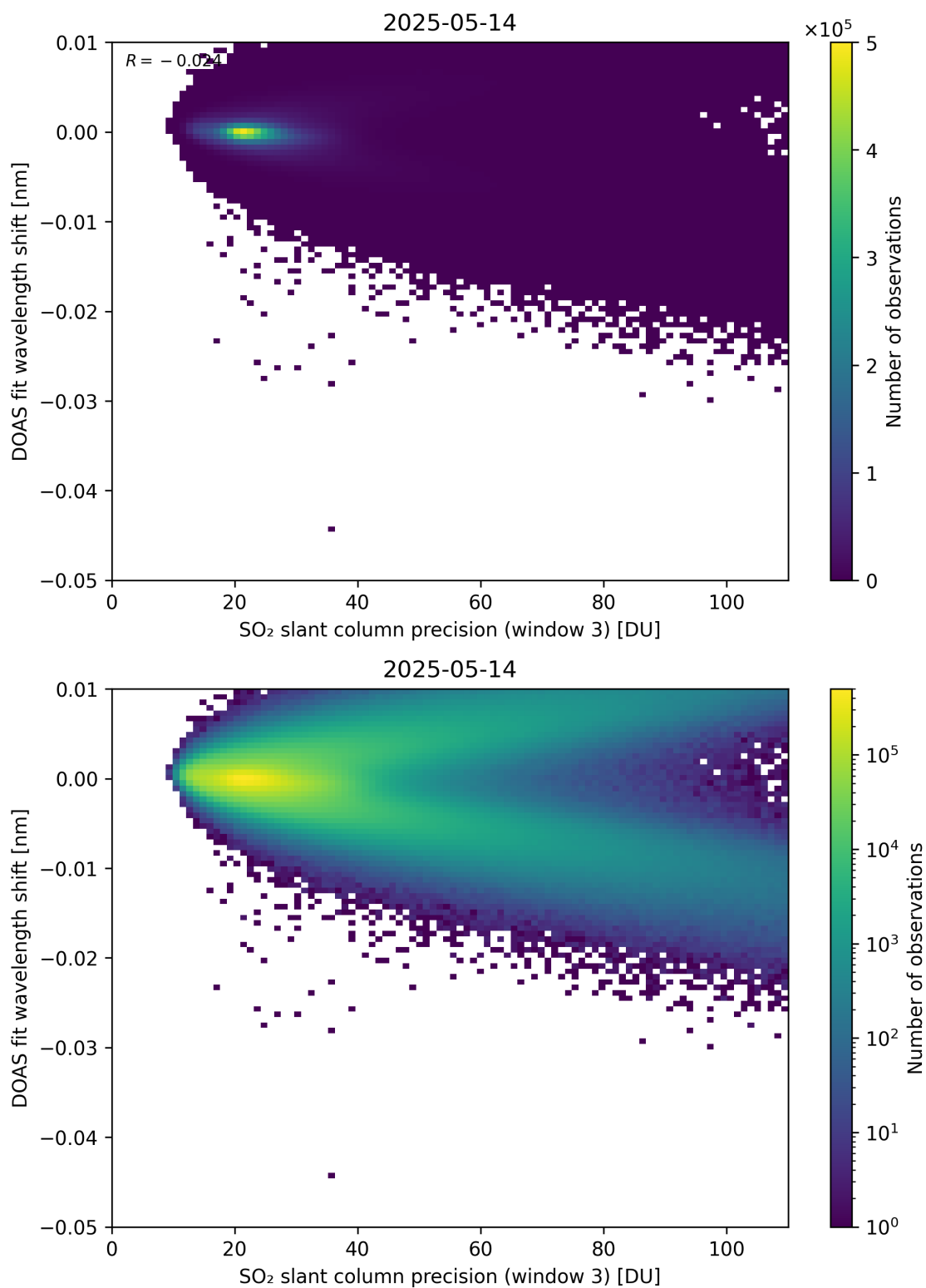
Figure 308: Scatter density plot of “SO 2 slant column precision (window 3)” against “DOAS fit wavelength shift” for 2025-05-13 to 2025-05-15.
