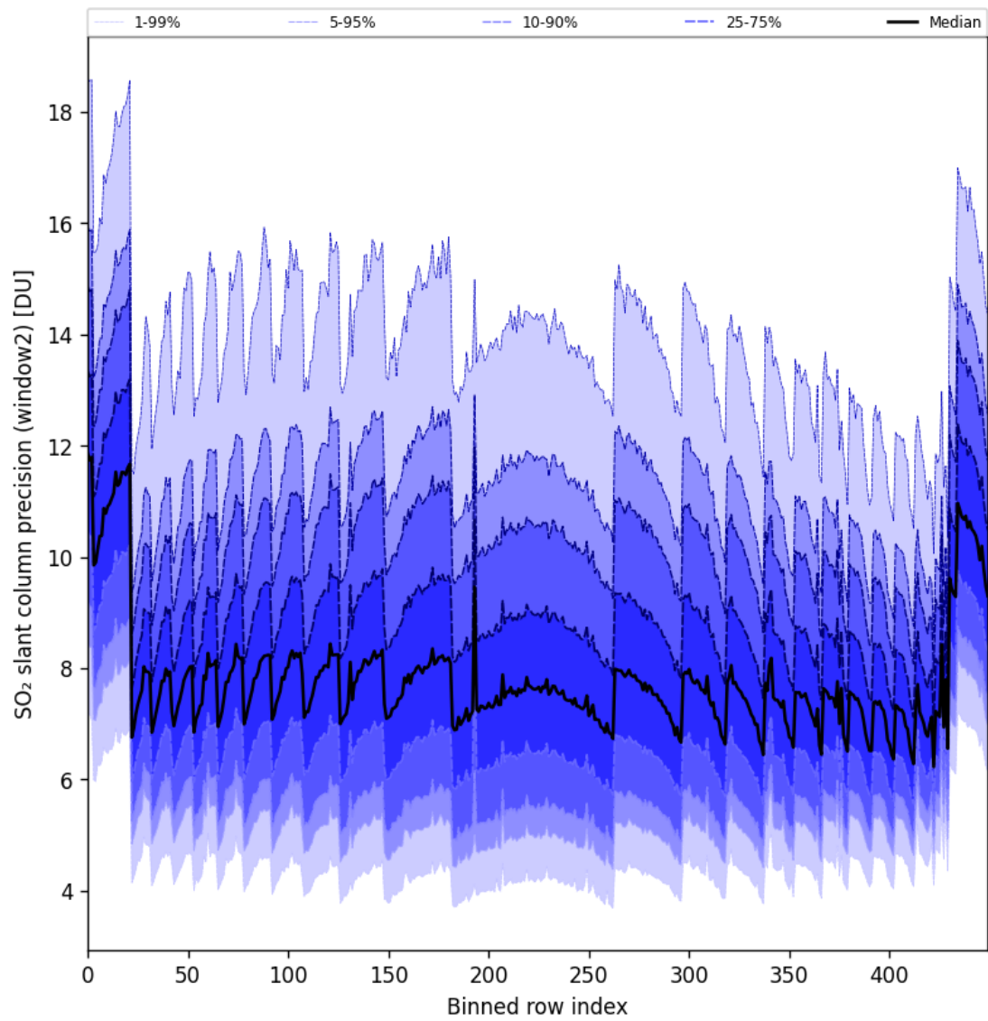
Figure 94: Along track statistics of “SO 2 slant column precision (window2)” for 2025-05-13 to 2025-05-15
