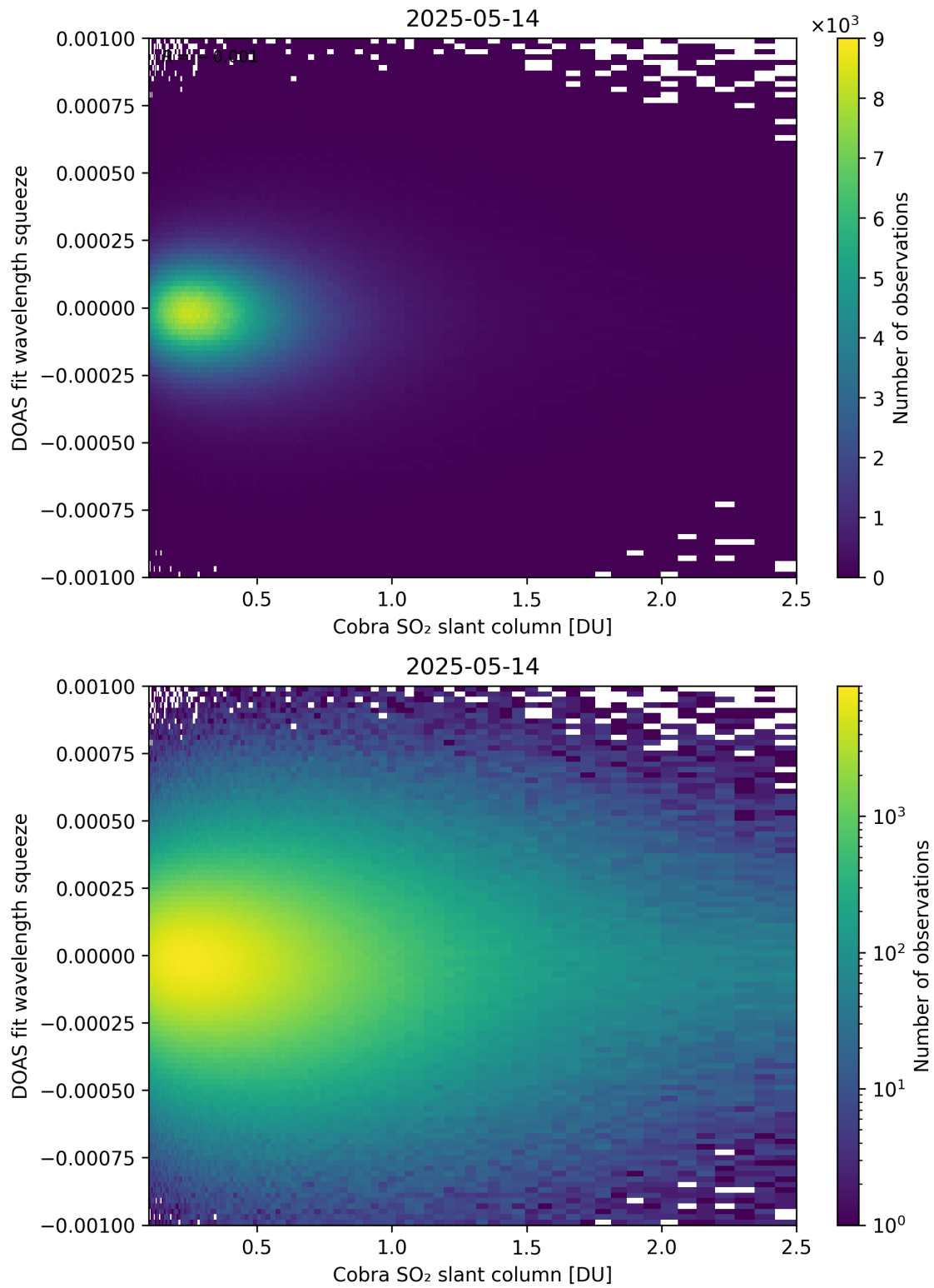
Figure 197: Scatter density plot of “Cobra SO 2 slant column” against “DOAS fit wavelength squeeze” for 2025-05-13 to 2025-05-15.
