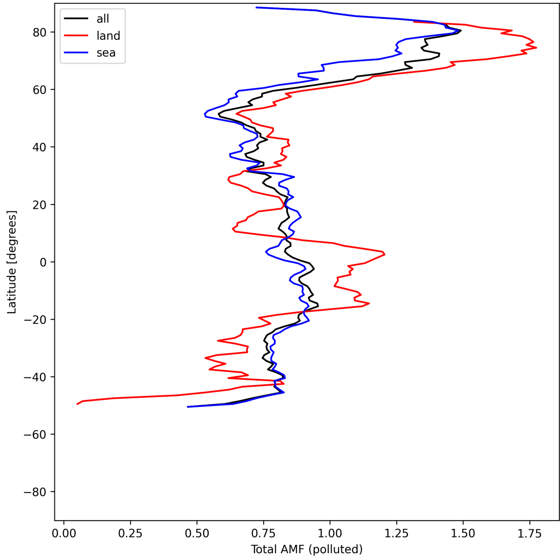
Figure 53: Zonal average of “Total AMF (polluted)” for 2025-05-13 to 2025-05-15.
