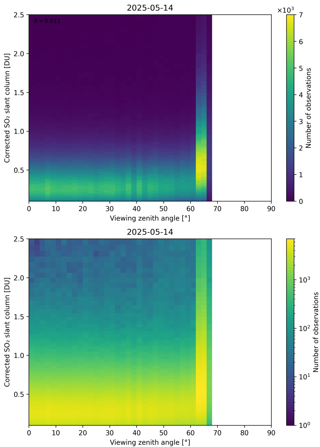
Figure 373: Scatter density plot of “Viewing zenith angle” against “Corrected SO 2 slant column” for 2025-05-13 to 2025-05-15.
