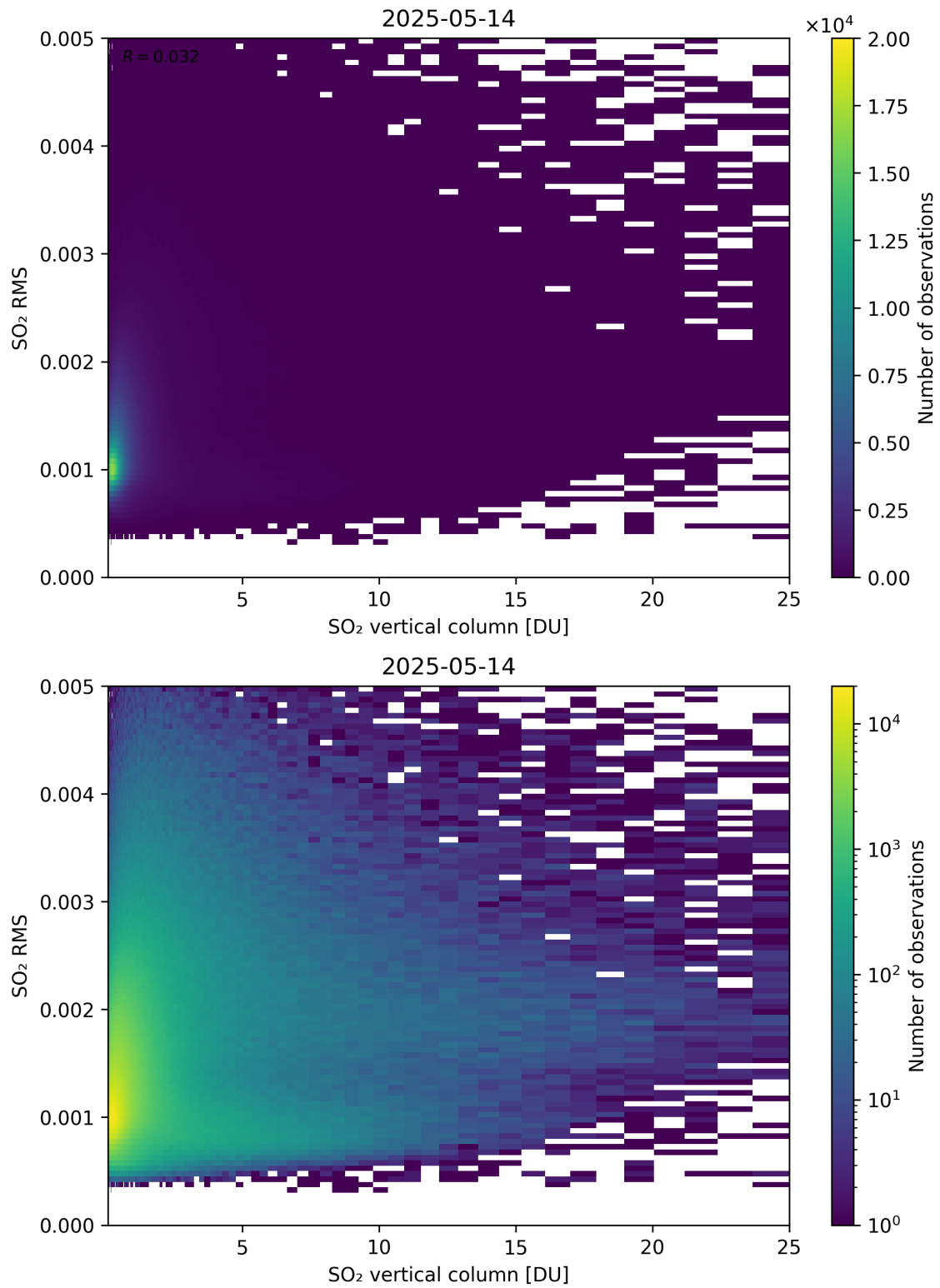
Figure 328: Scatter density plot of “SO 2 vertical column” against “SO 2 RMS” for 2025-05-13 to 2025-05-15.
