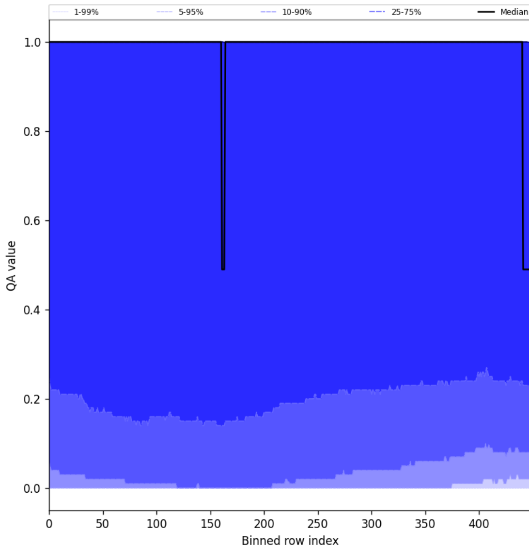
Figure 83: Along track statistics of “QA value” for 2025-05-13 to 2025-05-15
