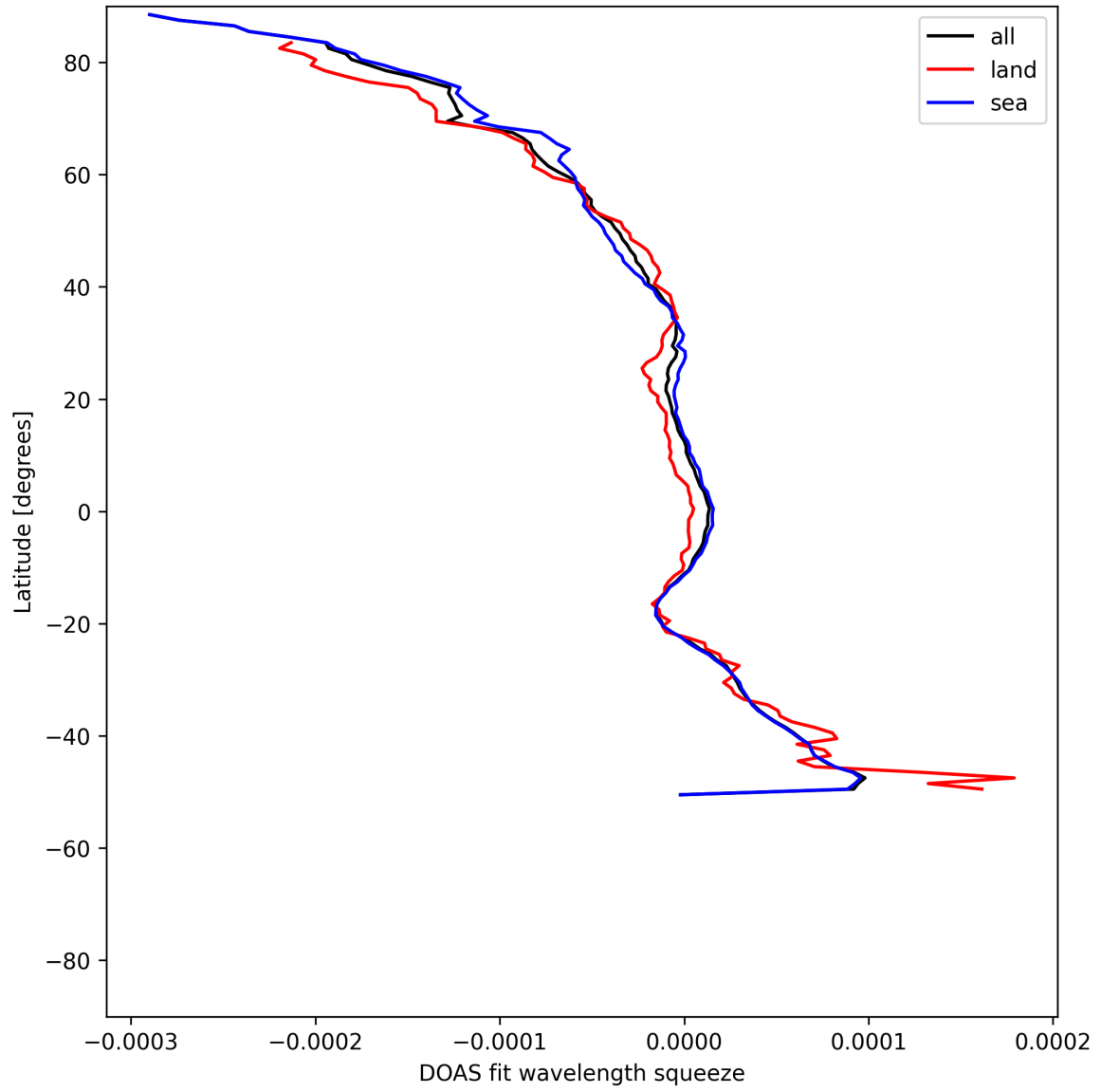
Figure 51: Zonal average of “DOAS fit wavelength squeeze” for 2025-05-13 to 2025-05-15.
