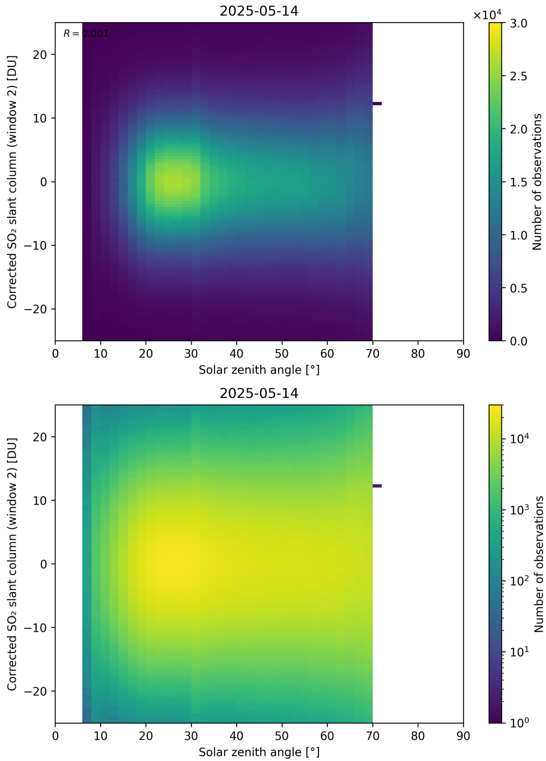
Figure 182: Scatter density plot of “Solar zenith angle” against “Corrected SO 2 slant column (window 2)” for 2025-05-13 to 2025-05-15.
