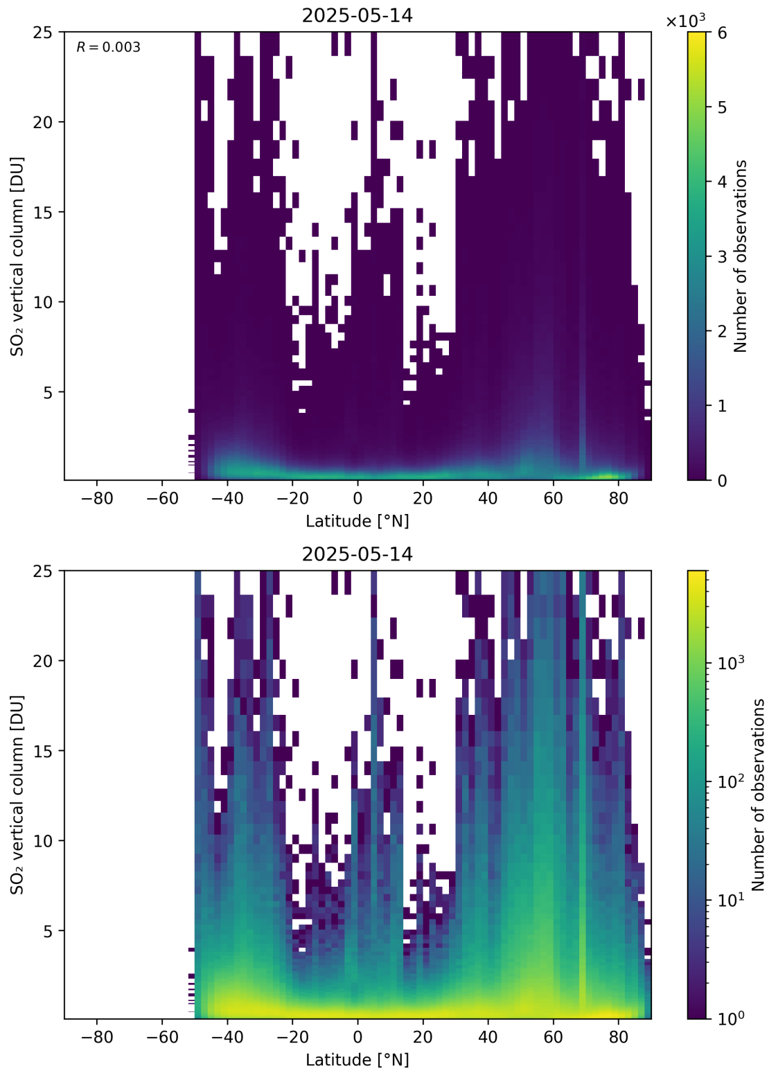
Figure 169: Scatter density plot of “Latitude” against “SO 2 vertical column” for 2025-05-13 to 2025-05-15.
