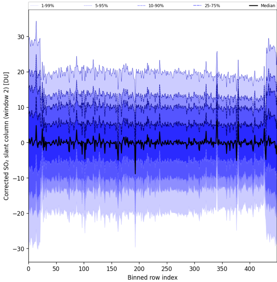
Figure 95: Along track statistics of “Corrected SO 2 slant column (window 2)” for 2025-05-13 to 2025-05-15
