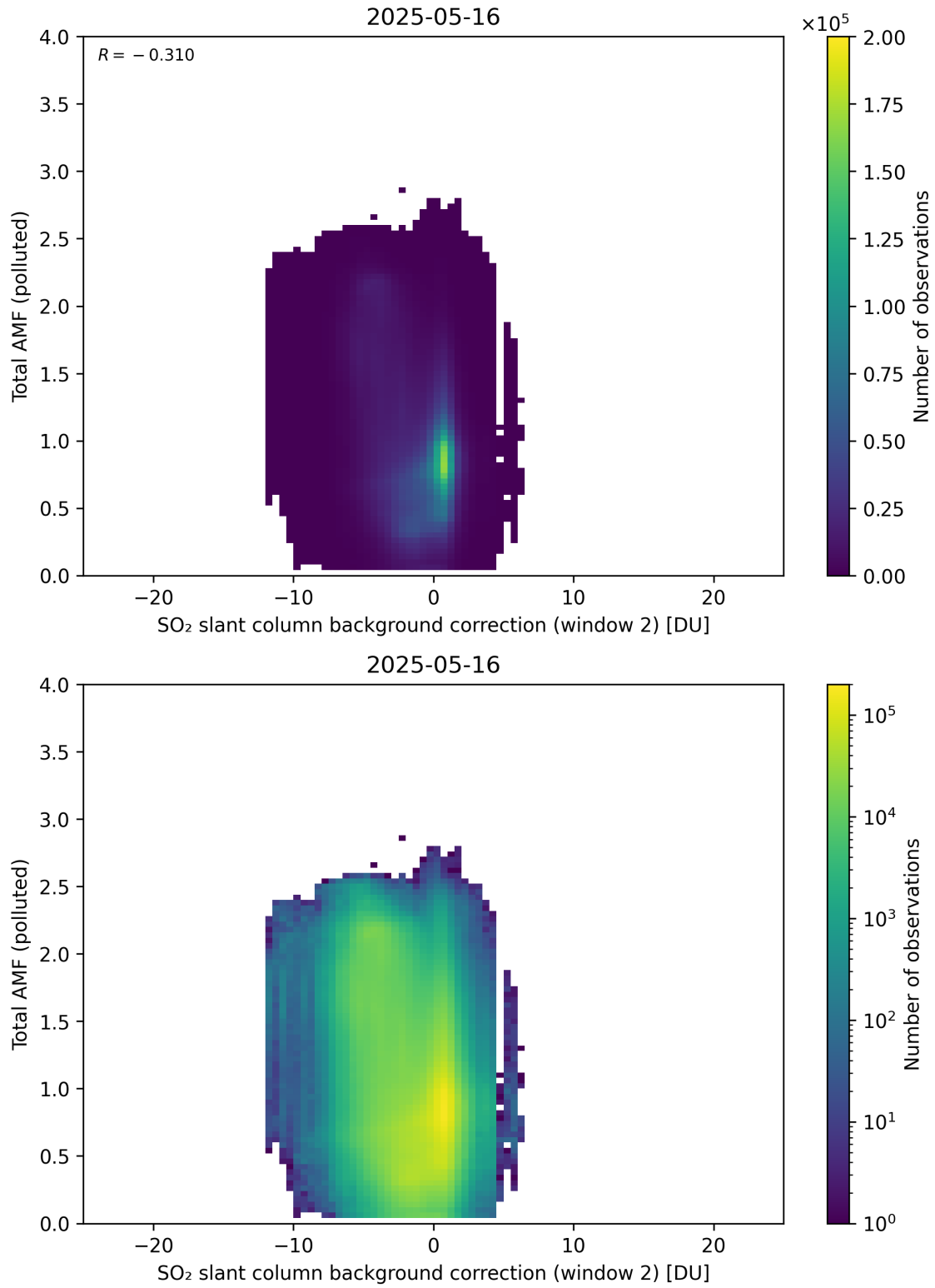
Figure 130: Scatter density plot of “SO 2 slant column background correction (window 2)” against “Total AMF (polluted)” for 2025-05-15 to 2025-05-17.
