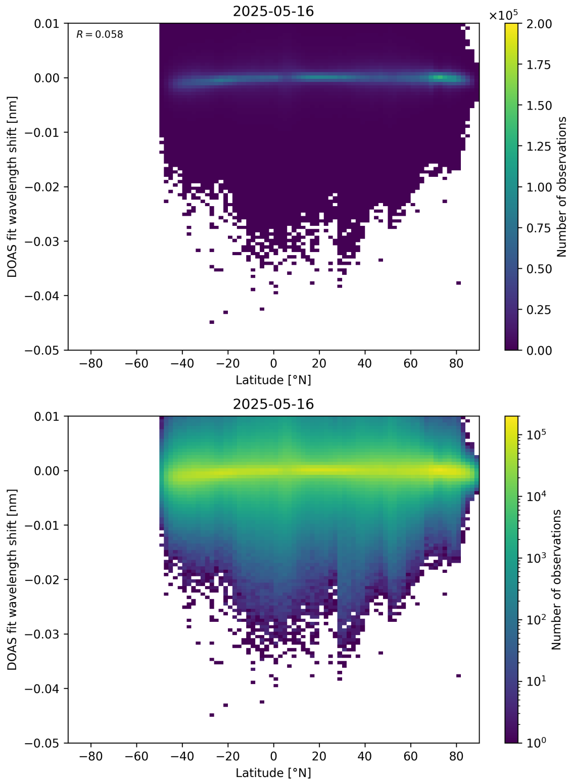
Figure 153: Scatter density plot of “Latitude” against “DOAS fit wavelength shift” for 2025-05-15 to 2025-05-17.
