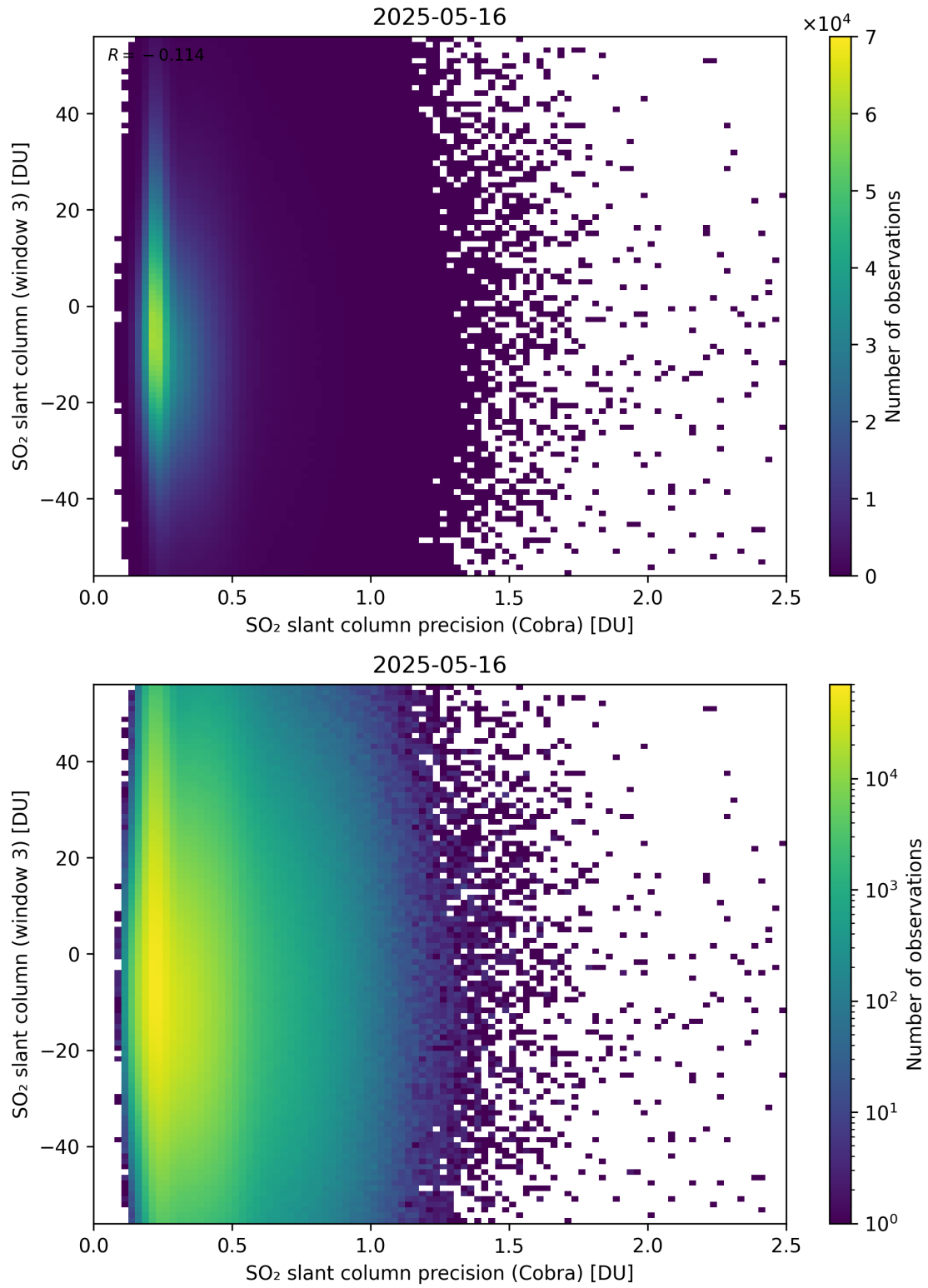
Figure 211: Scatter density plot of “SO 2 slant column precision (Cobra)” against “SO 2 slant column (window 3)” for 2025-05-15 to 2025-05-17.
