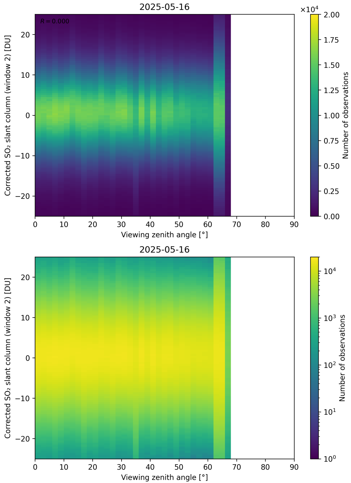
Figure 374: Scatter density plot of “Viewing zenith angle” against “Corrected SO 2 slant column (window 2)” for 2025-05-15 to 2025-05-17.
