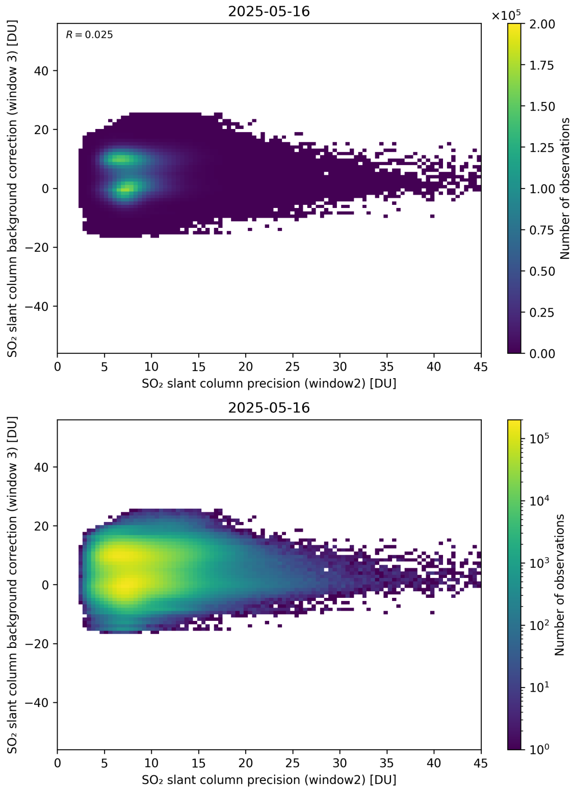
Figure 292: Scatter density plot of “SO 2 slant column precision (window2)” against “SO 2 slant column background correction (window 3)” for 2025-05-15 to 2025-05-17.
