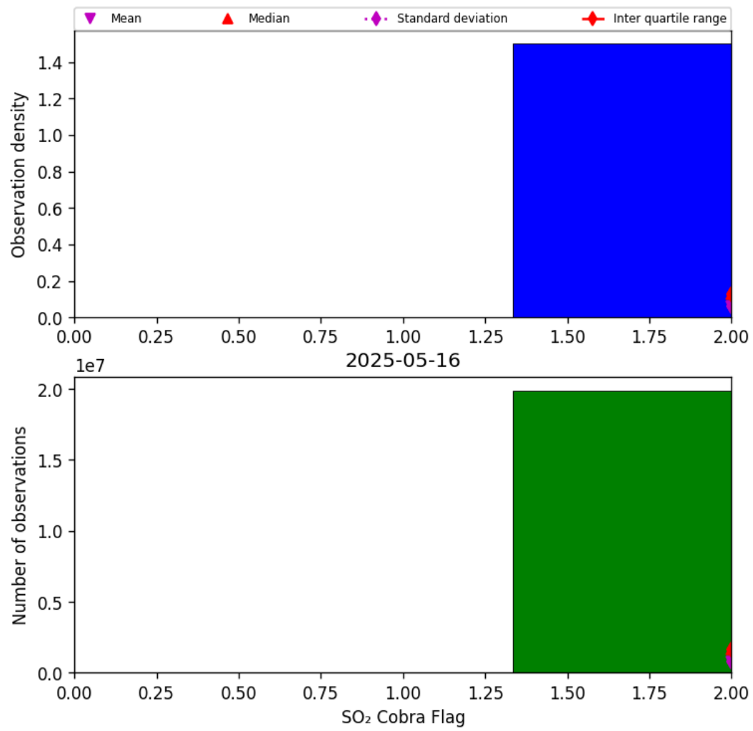
Figure 75: Histogram of “SO 2 Cobra Flag” for 2025-05-15 to 2025-05-17
