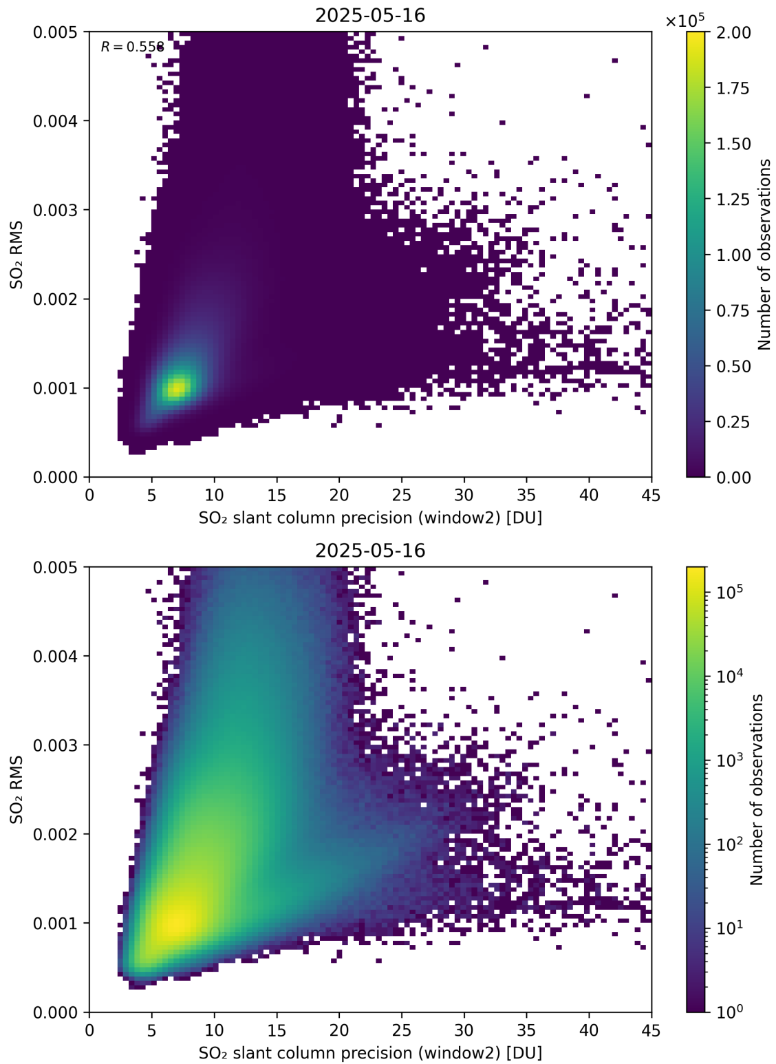
Figure 295: Scatter density plot of “SO 2 slant column precision (window2)” against “SO 2 RMS” for 2025-05-15 to 2025-05-17.
