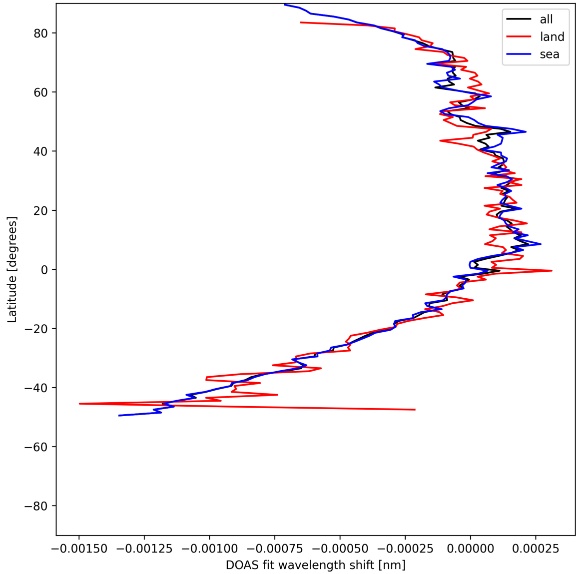
Figure 50: Zonal average of “DOAS fit wavelength shift” for 2025-05-15 to 2025-05-17.
