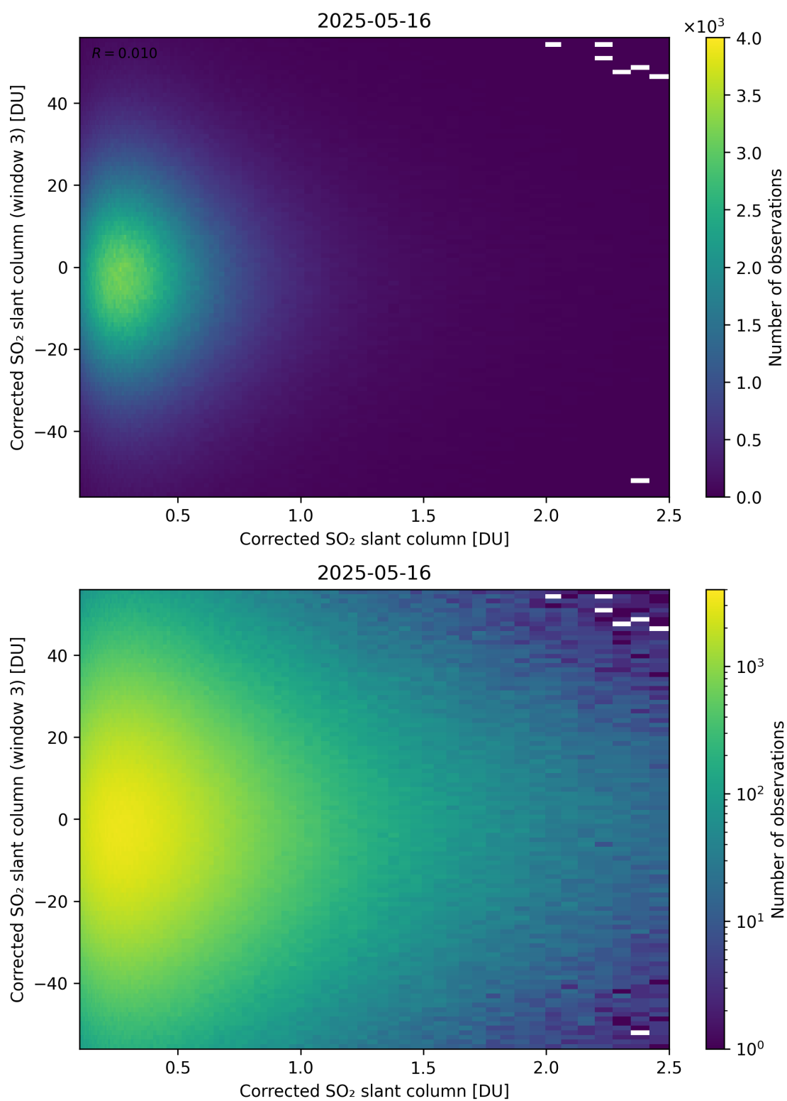
Figure 236: Scatter density plot of “Corrected SO 2 slant column” against “Corrected SO 2 slant column (window 3)” for 2025-05-15 to 2025-05-17.
