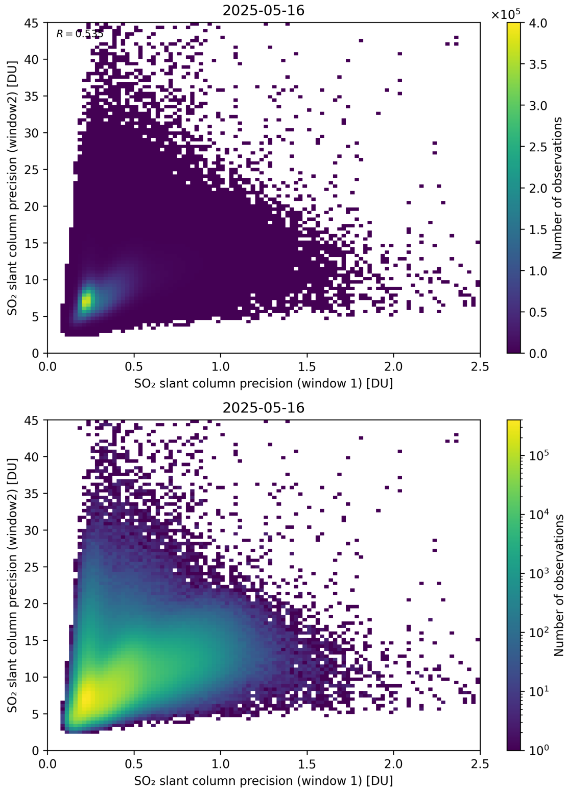
Figure 277: Scatter density plot of “SO 2 slant column precision (window 1)” against “SO 2 slant column precision (window2)” for 2025-05-15 to 2025-05-17.
