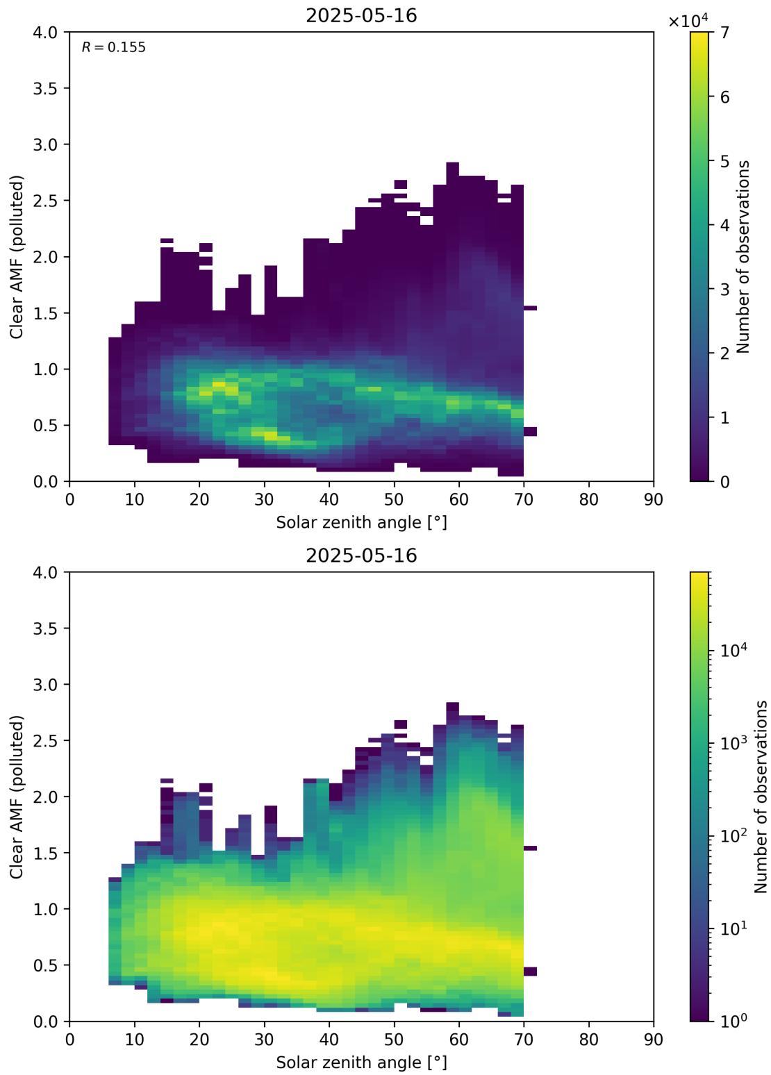
Figure 178: Scatter density plot of “Solar zenith angle” against “Clear AMF (polluted)” for 2025-05-15 to 2025-05-17.
