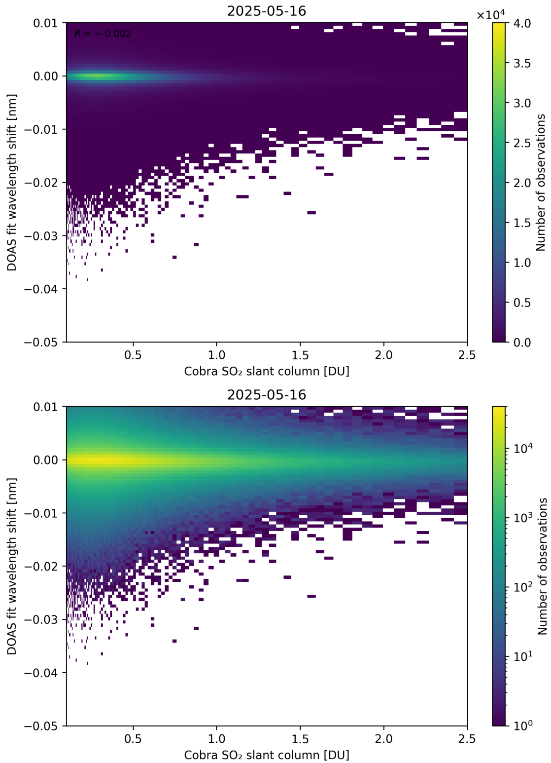
Figure 196: Scatter density plot of “Cobra SO 2 slant column” against “DOAS fit wavelength shift” for 2025-05-15 to 2025-05-17.
