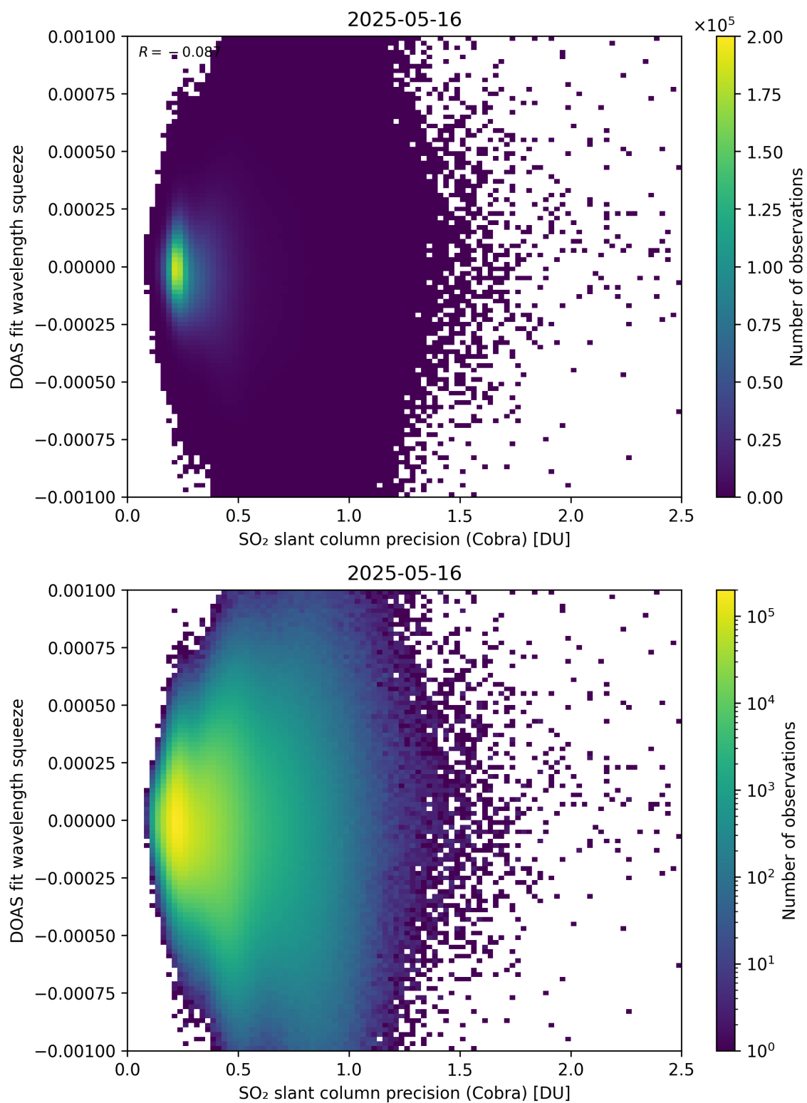
Figure 203: Scatter density plot of “SO 2 slant column precision (Cobra)” against “DOAS fit wavelength squeeze” for 2025-05-15 to 2025-05-17.
