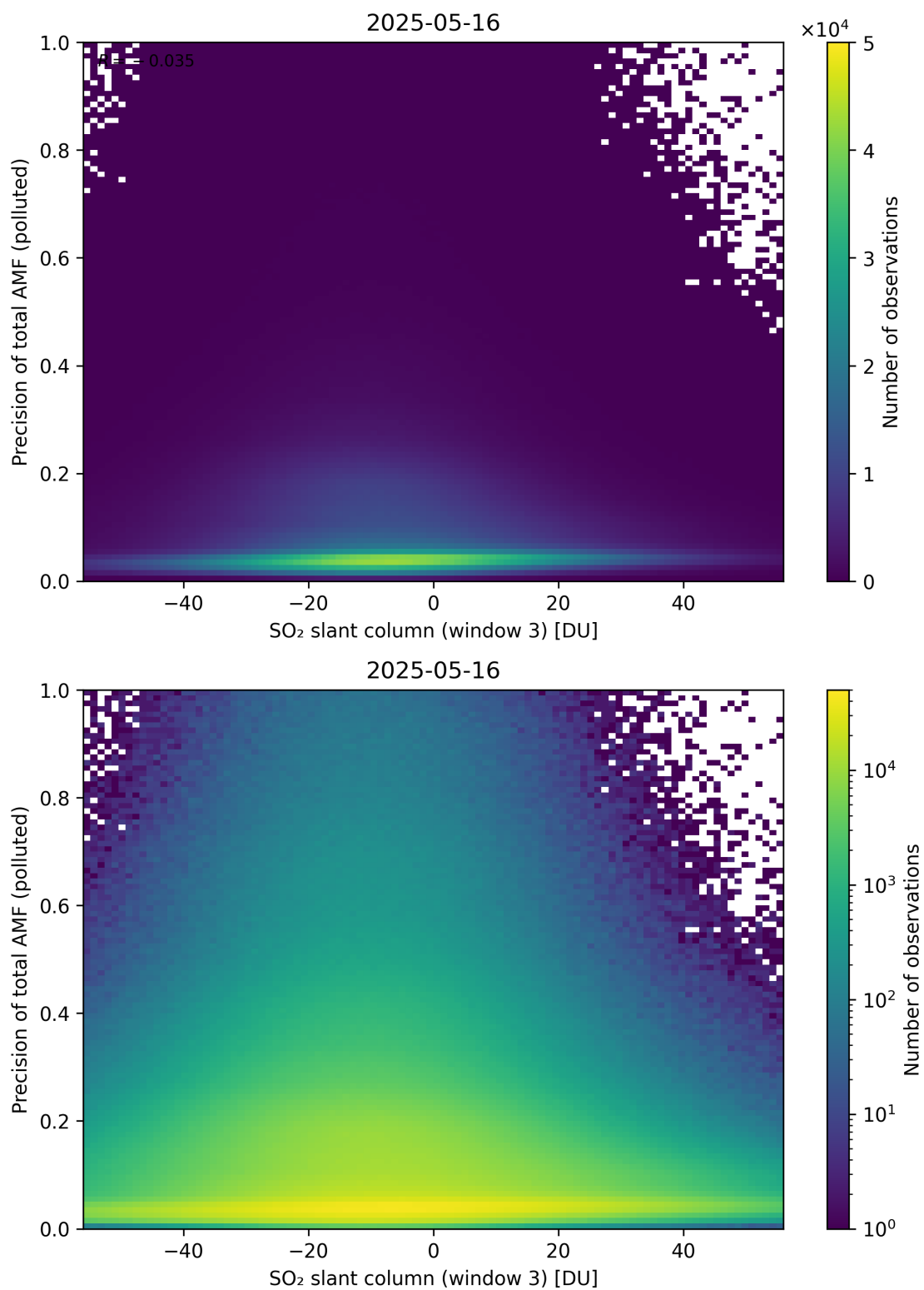
Figure 319: Scatter density plot of “SO 2 slant column (window 3)” against “Precision of total AMF (polluted)” for 2025-05-15 to 2025-05-17.
