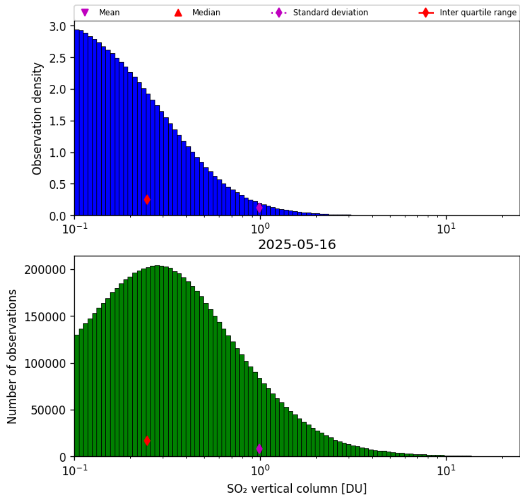
Figure 58: Histogram of “SO 2 vertical column” for 2025-05-15 to 2025-05-17
