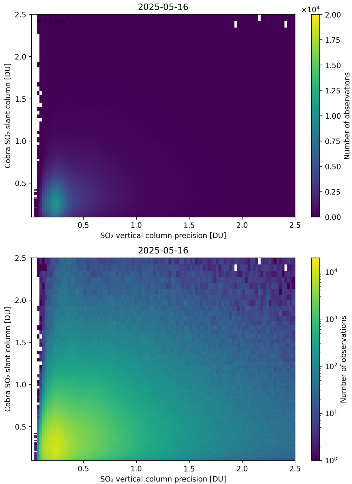
Figure 336: Scatter density plot of “SO 2 vertical column precision” against “Cobra SO 2 slant column” for 2025-05-15 to 2025-05-17.
