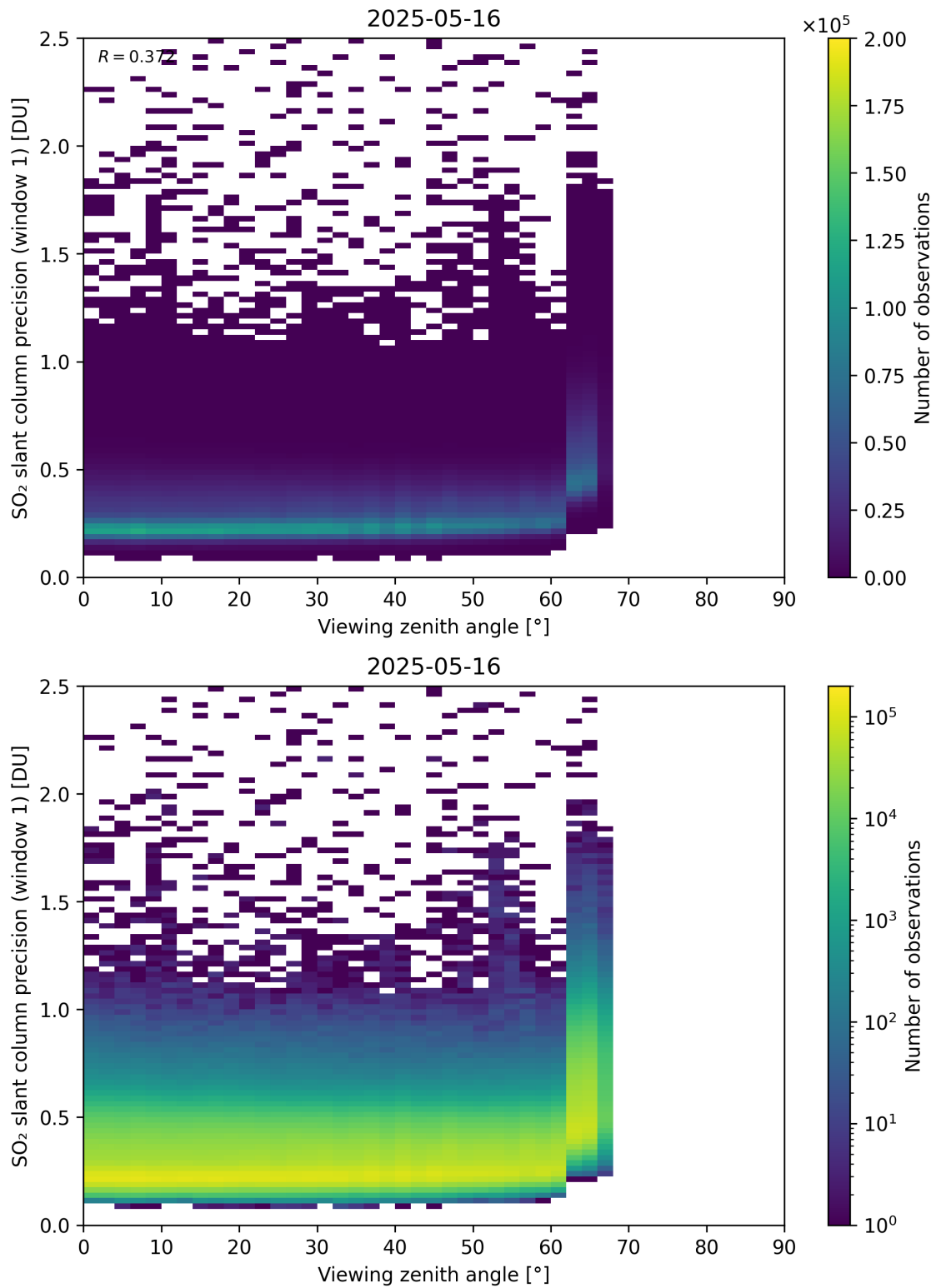
Figure 377: Scatter density plot of “Viewing zenith angle” against “SO 2 slant column precision (window 1)” for 2025-05-15 to 2025-05-17.
