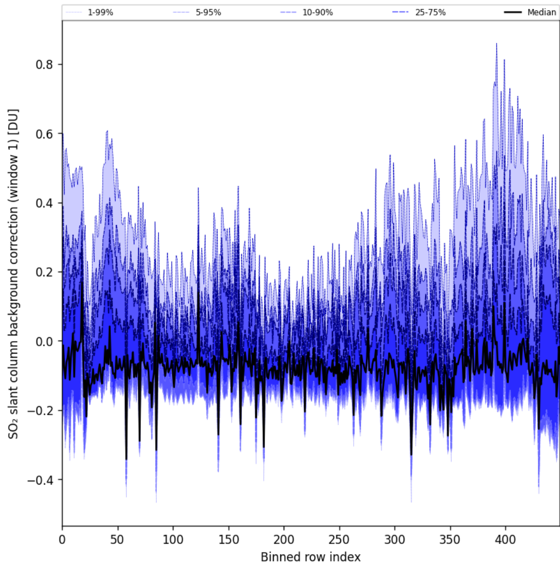
Figure 92: Along track statistics of “SO 2 slant column background correction (window 1)” for 2025-05-15 to 2025-05-17
