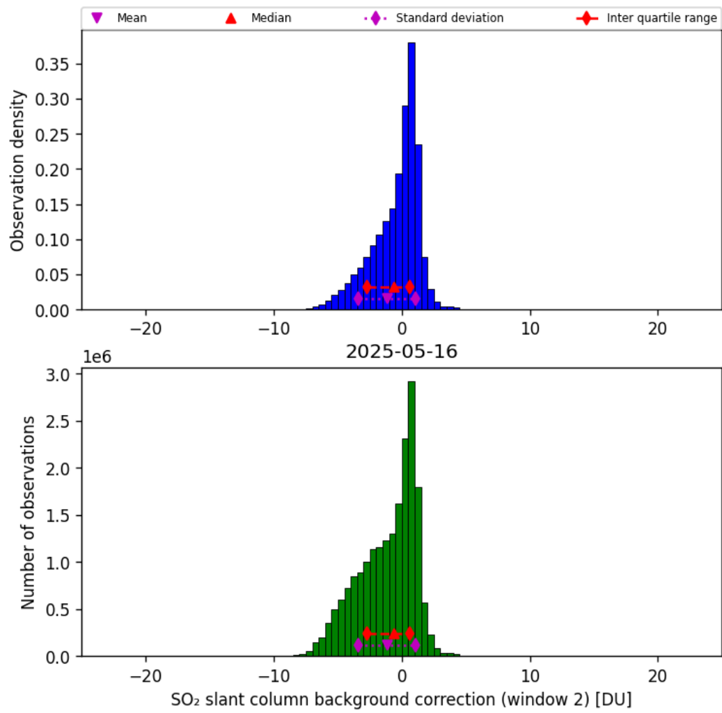
Figure 70: Histogram of “SO 2 slant column background correction (window 2)” for 2025-05-15 to 2025-05-17
