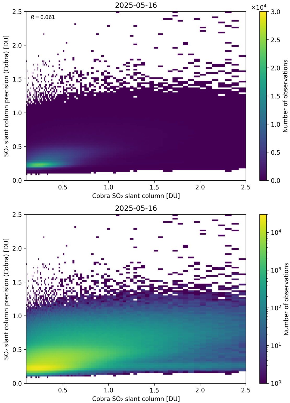
Figure 216: Scatter density plot of “Cobra SO 2 slant column” against “SO 2 slant column precision (Cobra)” for 2025-05-15 to 2025-05-17.
