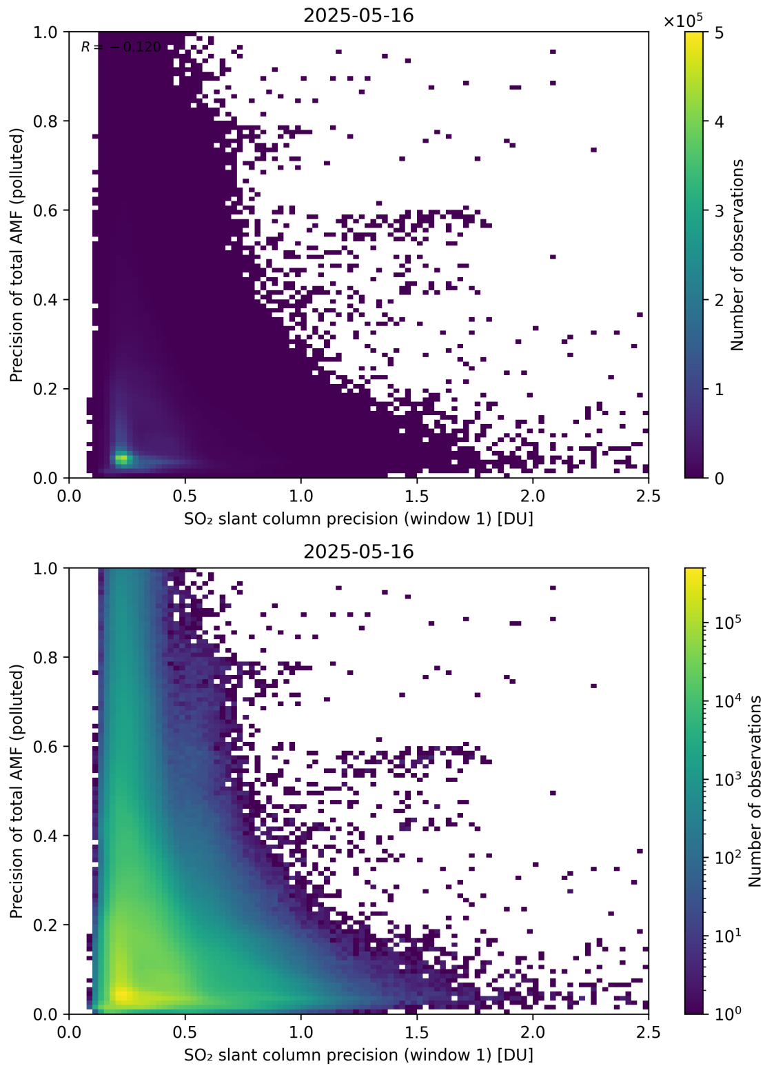
Figure 281: Scatter density plot of “SO 2 slant column precision (window 1)” against “Precision of total AMF (polluted)” for 2025-05-15 to 2025-05-17.
