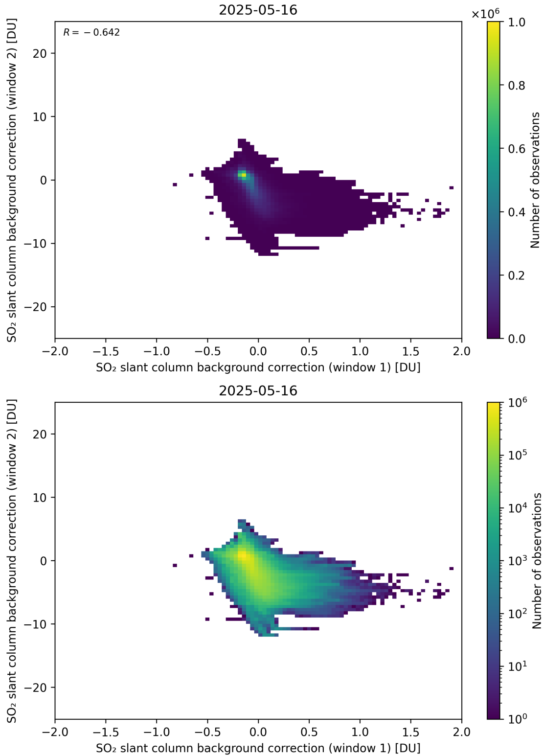
Figure 109: Scatter density plot of “SO 2 slant column background correction (window 1)” against “SO 2 slant column background correction (window 2)” for 2025-05-15 to 2025-05-17.
