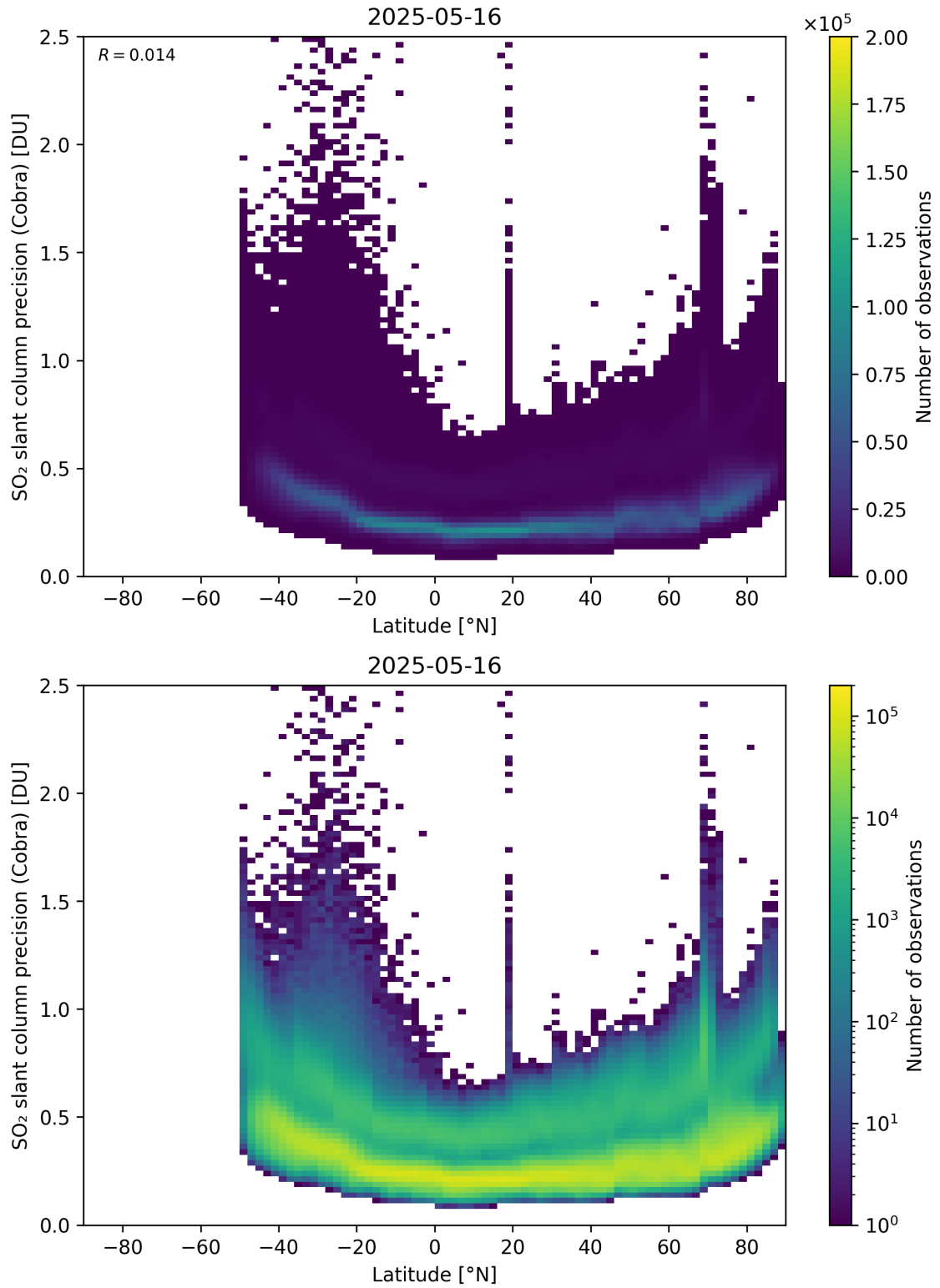
Figure 158: Scatter density plot of “Latitude” against “SO 2 slant column precision (Cobra)” for 2025-05-15 to 2025-05-17.
