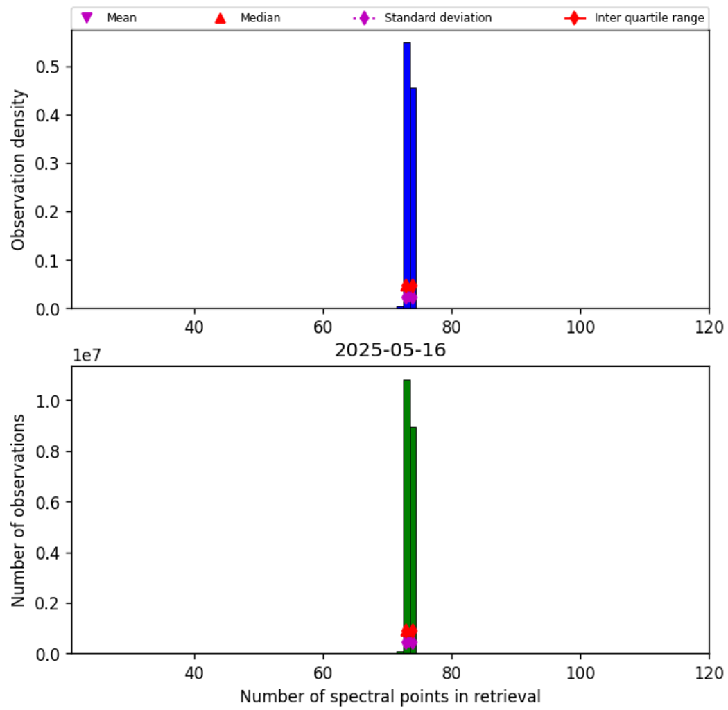
Figure 82: Histogram of “Number of spectral points in retrieval” for 2025-05-15 to 2025-05-17
