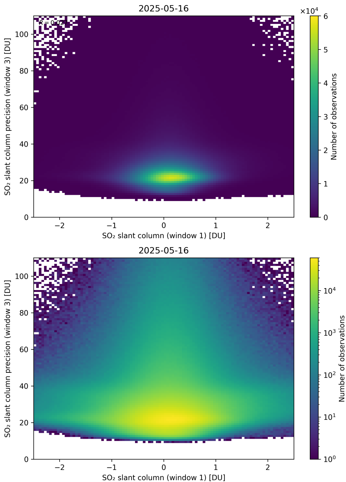
Figure 288: Scatter density plot of “SO 2 slant column (window 1)” against “SO 2 slant column precision (window 3)” for 2025-05-15 to 2025-05-17.
