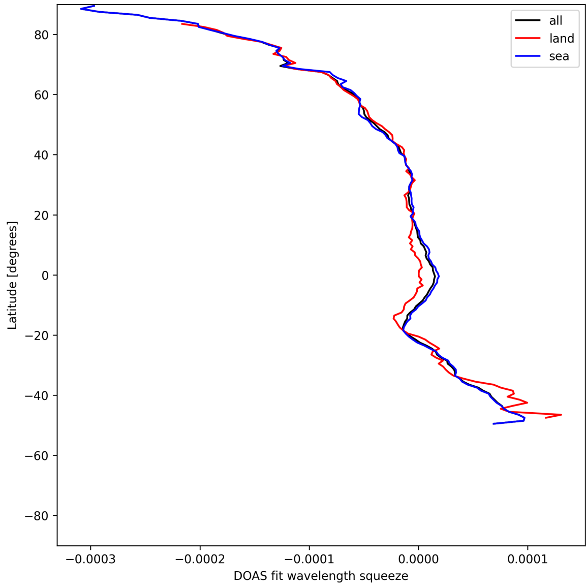
Figure 51: Zonal average of “DOAS fit wavelength squeeze” for 2025-05-15 to 2025-05-17.
