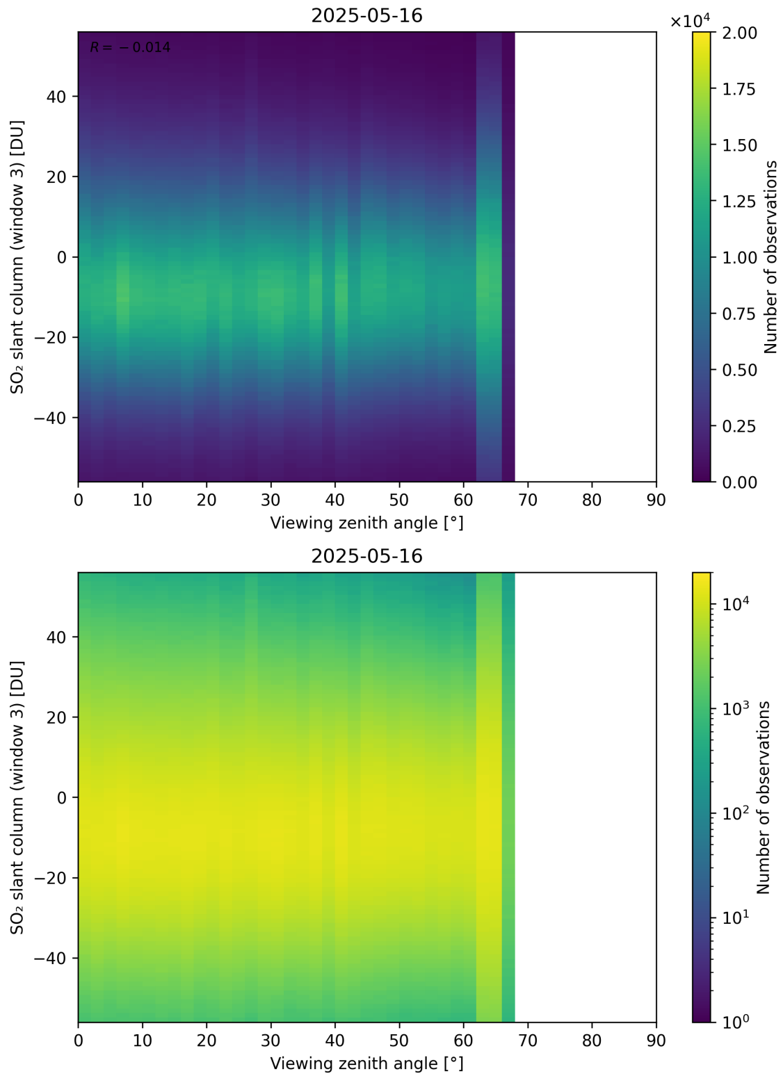
Figure 379: Scatter density plot of “Viewing zenith angle” against “SO 2 slant column (window 3)” for 2025-05-15 to 2025-05-17.
