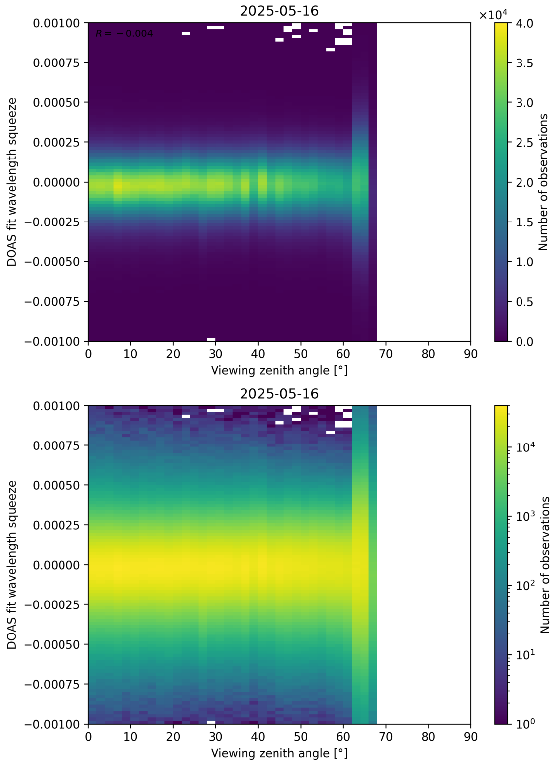
Figure 366: Scatter density plot of “Viewing zenith angle” against “DOAS fit wavelength squeeze” for 2025-05-15 to 2025-05-17.
