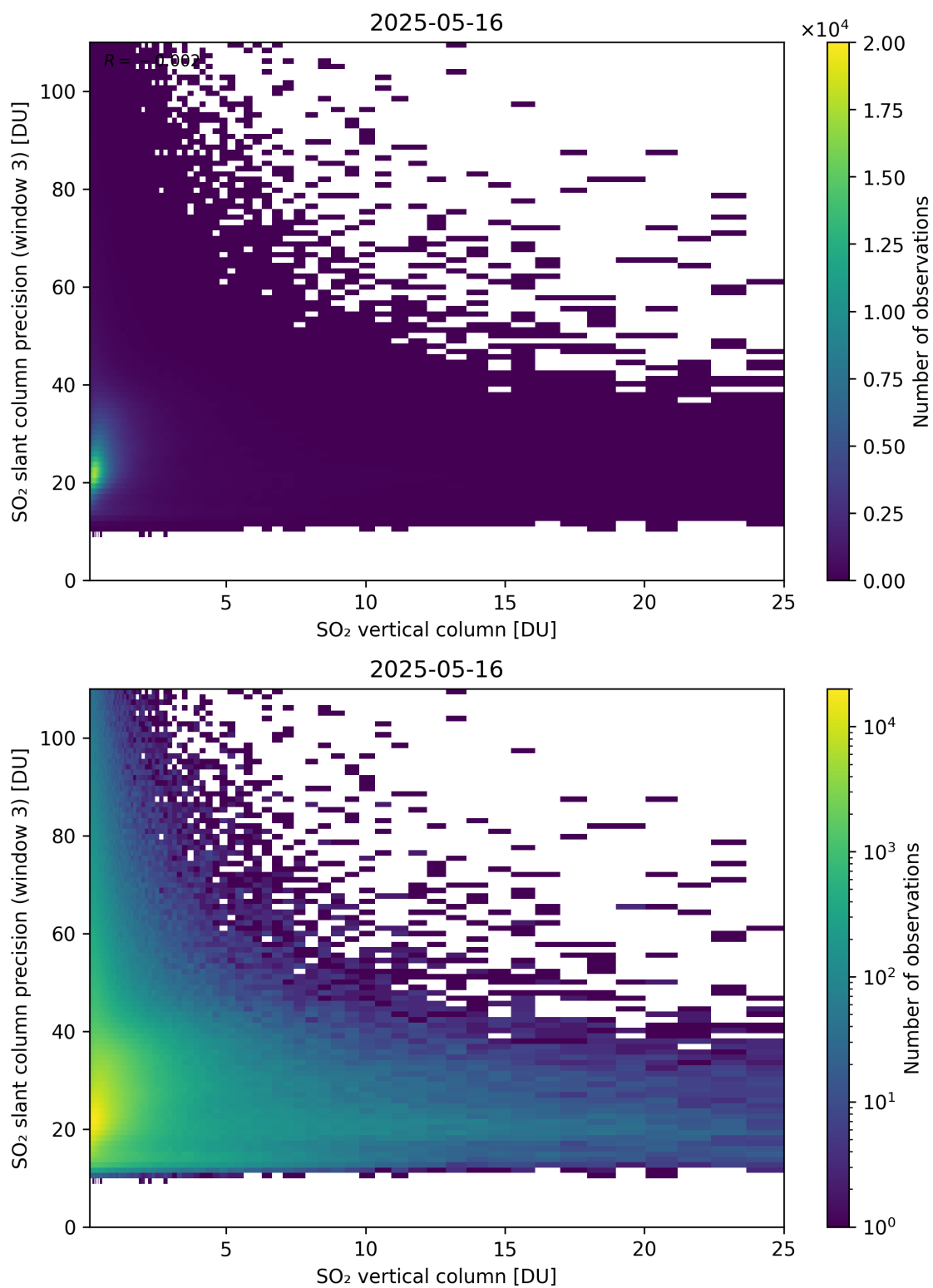
Figure 358: Scatter density plot of “SO 2 vertical column” against “SO 2 slant column precision (window 3)” for 2025-05-15 to 2025-05-17.
