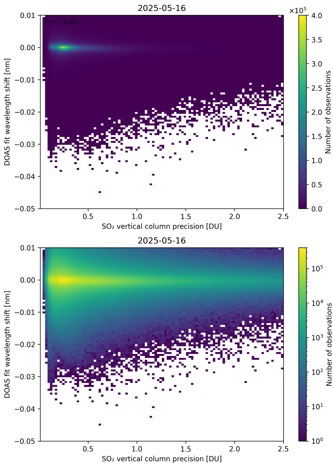
Figure 332: Scatter density plot of “SO 2 vertical column precision” against “DOAS fit wavelength shift” for 2025-05-15 to 2025-05-17.
