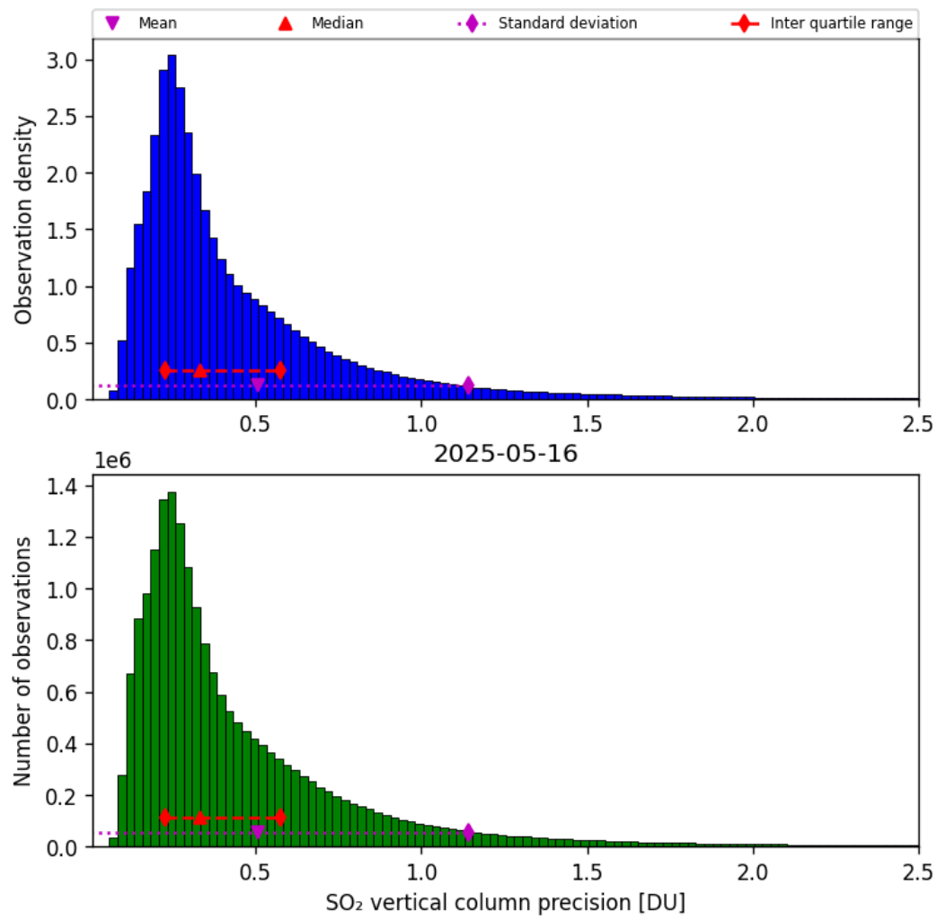
Figure 59: Histogram of “SO 2 vertical column precision” for 2025-05-15 to 2025-05-17
