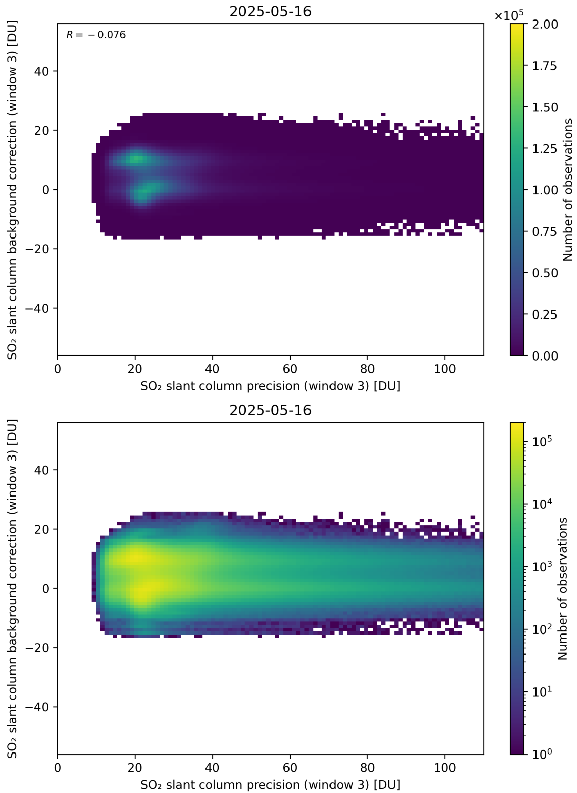
Figure 307: Scatter density plot of “SO 2 slant column precision (window 3)” against “SO 2 slant column background correction (window 3)” for 2025-05-15 to 2025-05-17.
