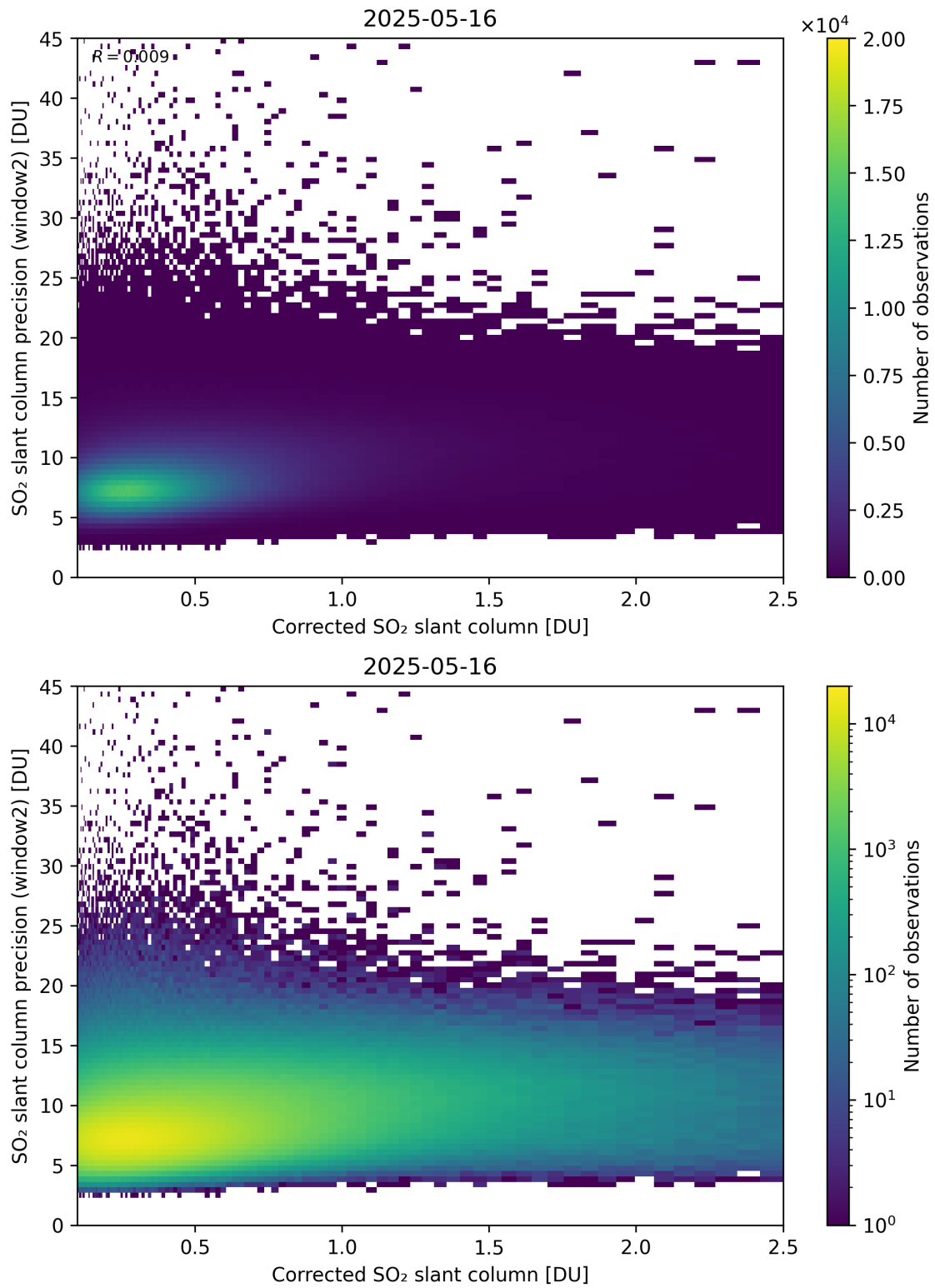
Figure 239: Scatter density plot of “Corrected SO 2 slant column” against “SO 2 slant column precision (window2)” for 2025-05-15 to 2025-05-17.
