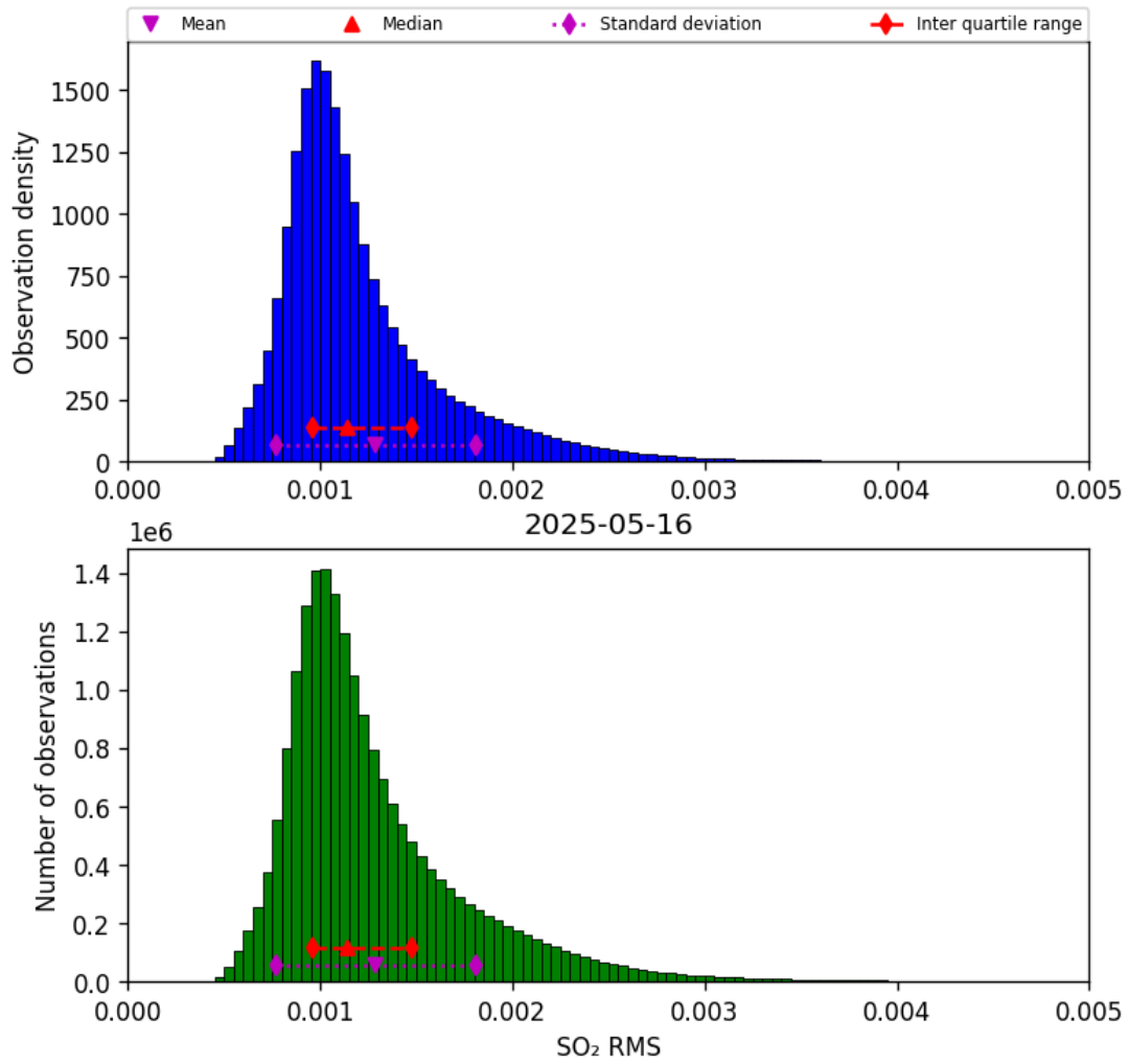
Figure 78: Histogram of “SO 2 RMS” for 2025-05-15 to 2025-05-17
