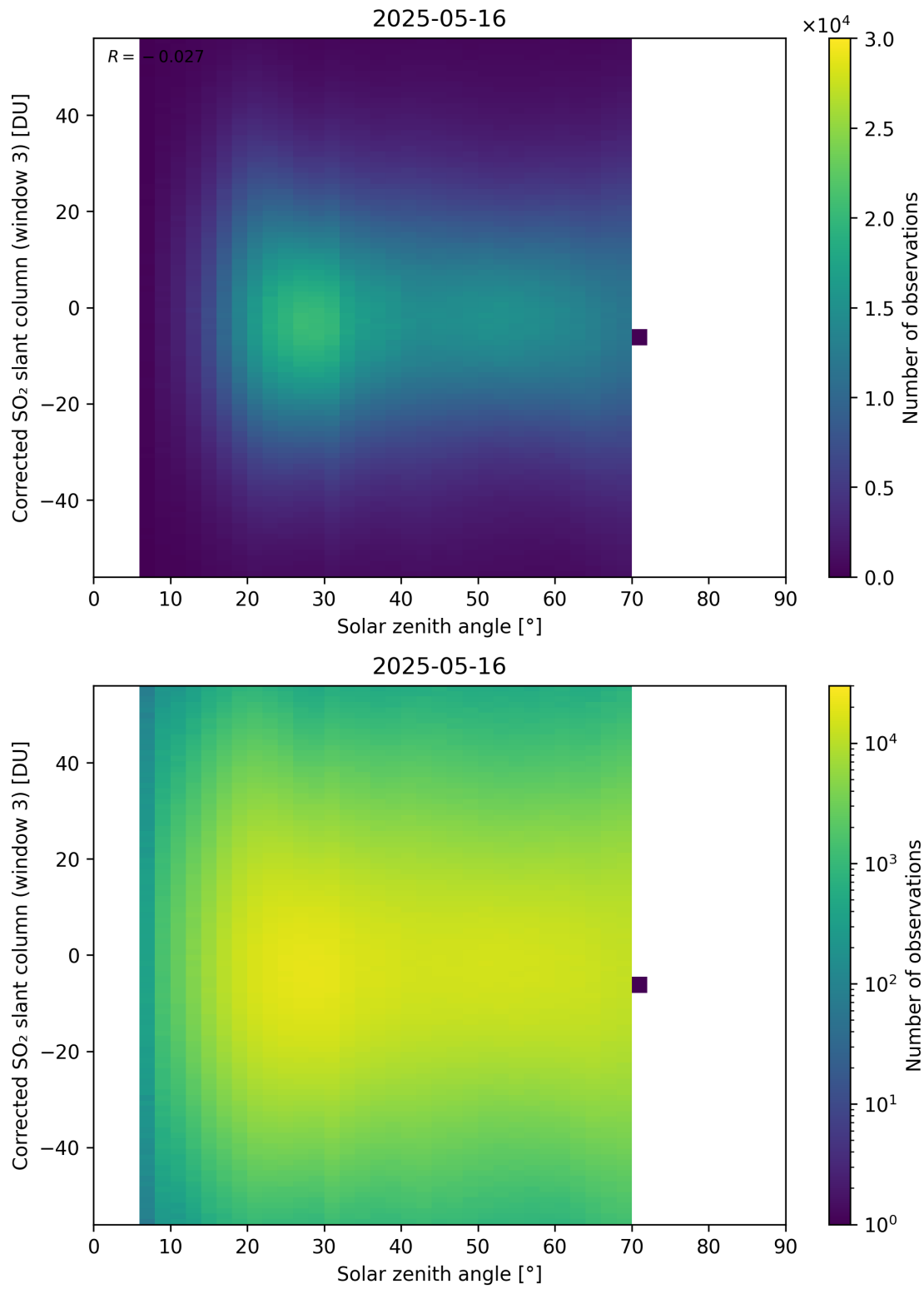
Figure 183: Scatter density plot of “Solar zenith angle” against “Corrected SO 2 slant column (window 3)” for 2025-05-15 to 2025-05-17.
