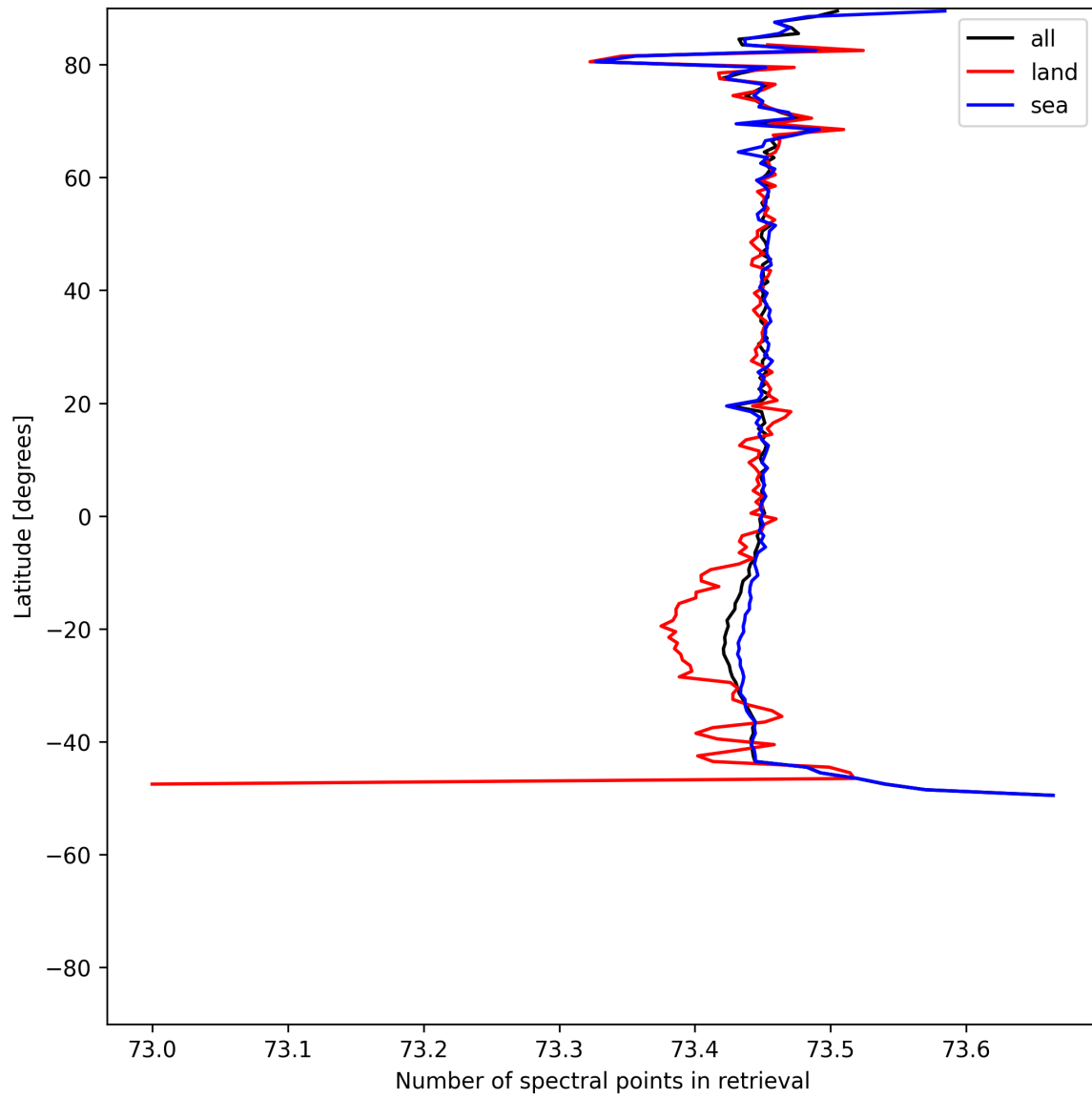
Figure 56: Zonal average of “Number of spectral points in retrieval” for 2025-05-15 to 2025-05-17.
