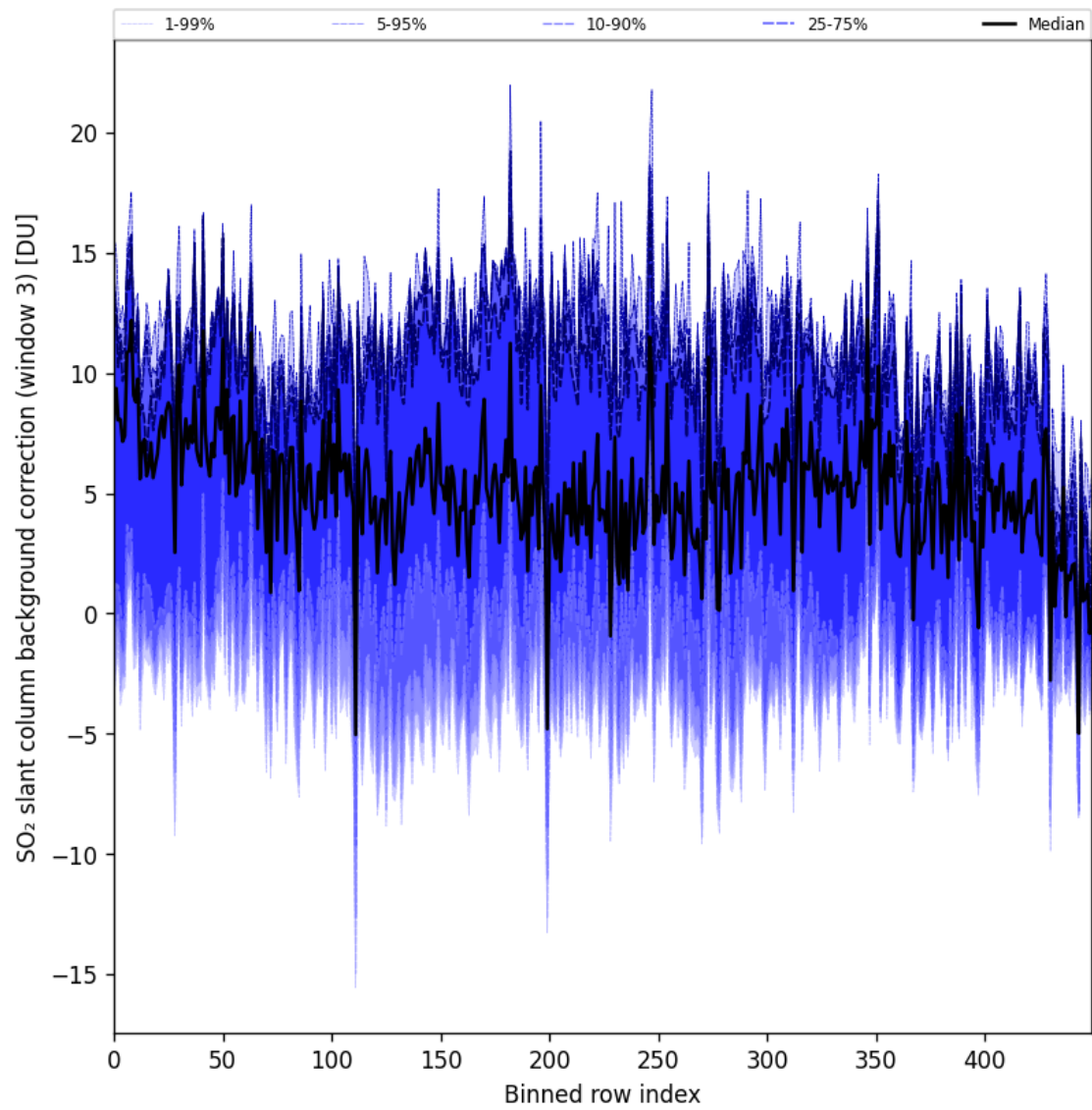
Figure 100: Along track statistics of “SO 2 slant column background correction (window 3)” for 2025-05-15 to 2025-05-17
