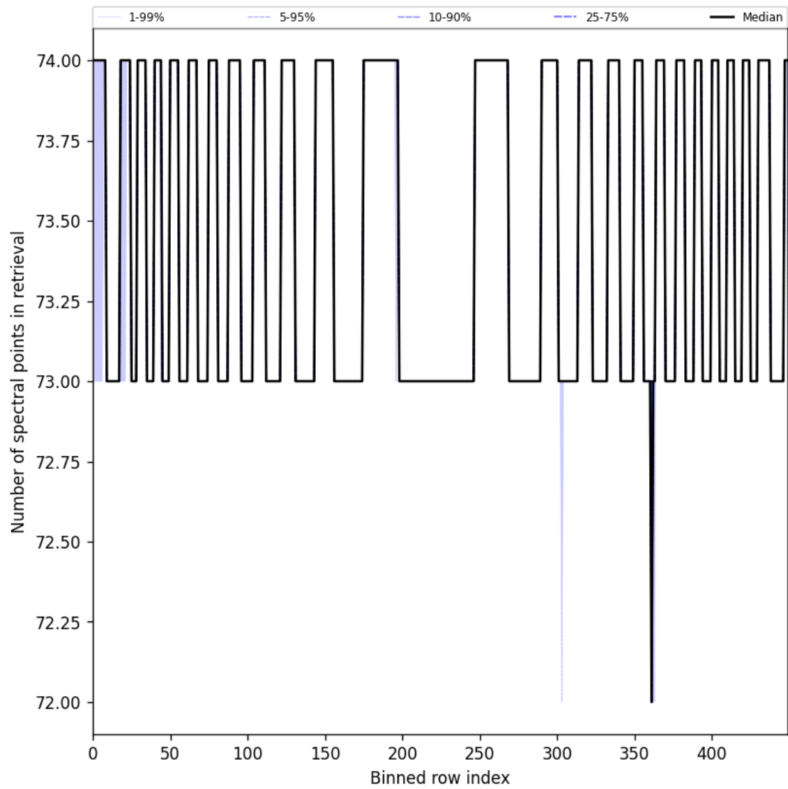
Figure 108: Along track statistics of “Number of spectral points in retrieval” for 2025-05-15 to 2025-05-17
