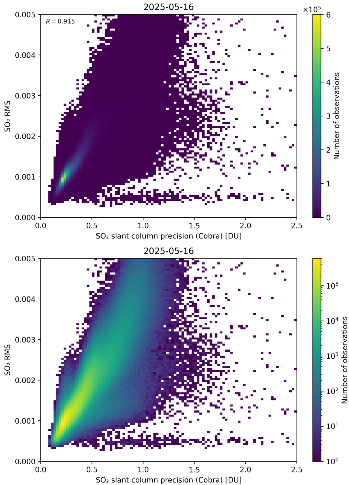
Figure 204: Scatter density plot of “SO 2 slant column precision (Cobra)” against “SO 2 RMS” for 2025-05-15 to 2025-05-17.
