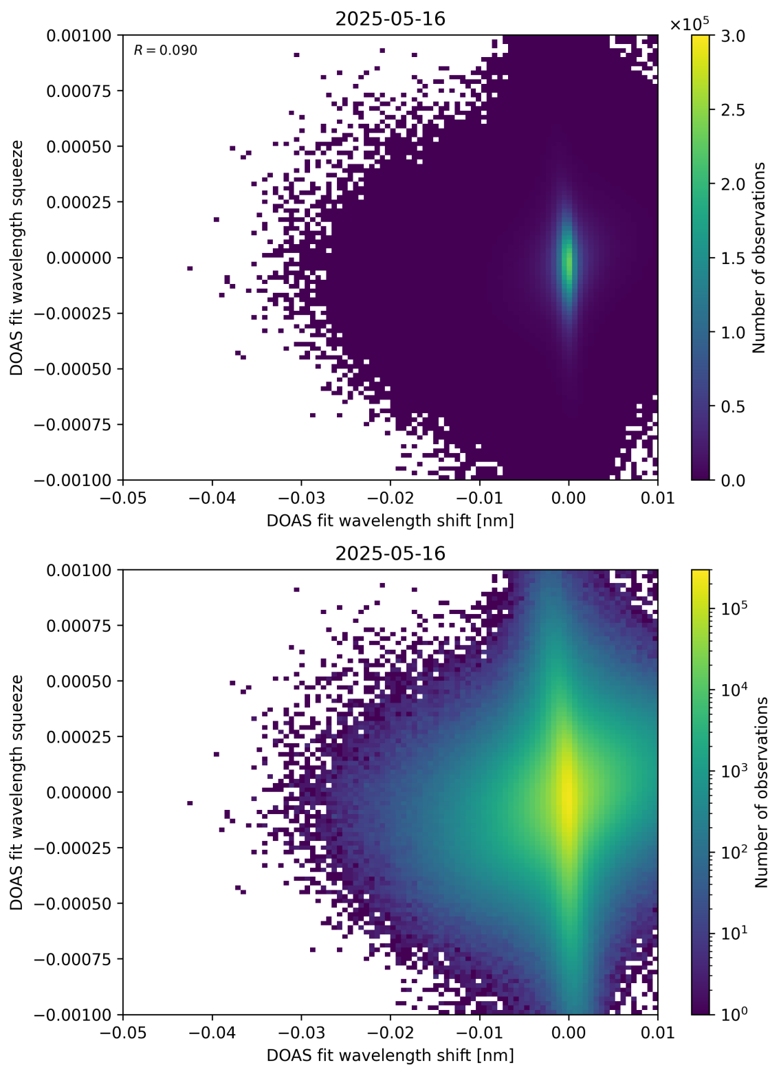
Figure 138: Scatter density plot of “DOAS fit wavelength shift” against “DOAS fit wavelength squeeze” for 2025-05-15 to 2025-05-17.
