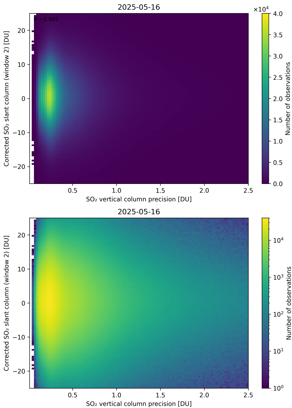
Figure 339: Scatter density plot of “SO 2 vertical column precision” against “Corrected SO 2 slant column (window 2)” for 2025-05-15 to 2025-05-17.
