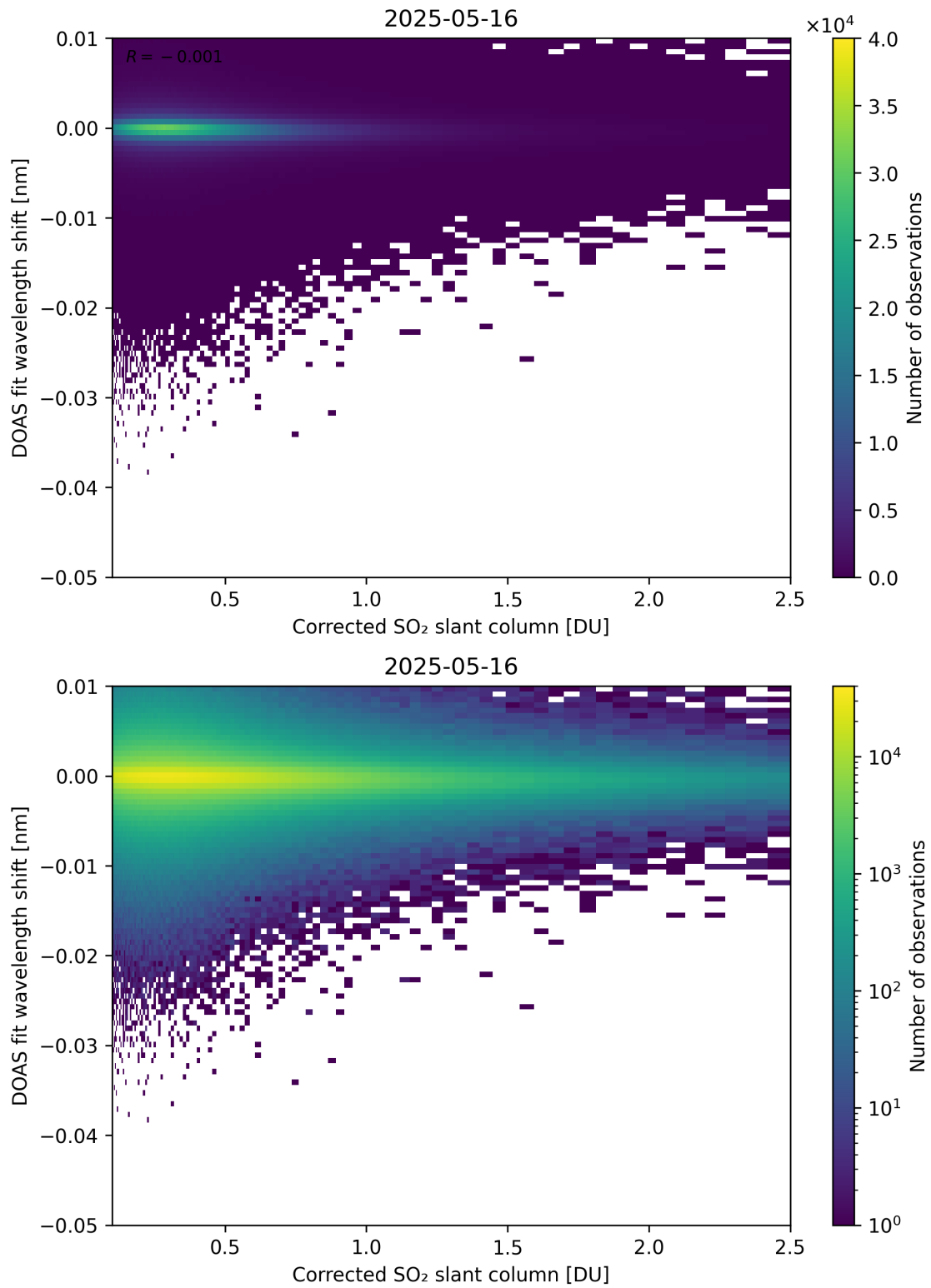
Figure 229: Scatter density plot of “Corrected SO 2 slant column” against “DOAS fit wavelength shift” for 2025-05-15 to 2025-05-17.
