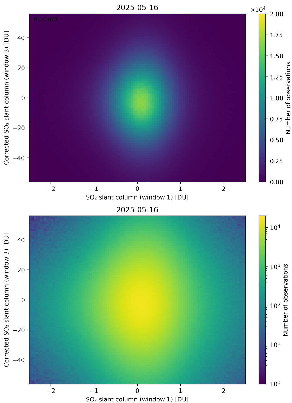
Figure 284: Scatter density plot of “SO 2 slant column (window 1)” against “Corrected SO 2 slant column (window 3)” for 2025-05-15 to 2025-05-17.
