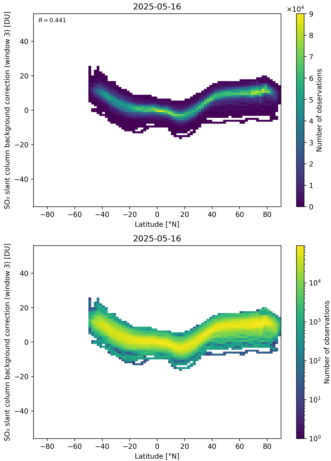
Figure 152: Scatter density plot of “Latitude” against “SO 2 slant column background correction (window 3)” for 2025-05-15 to 2025-05-17.
