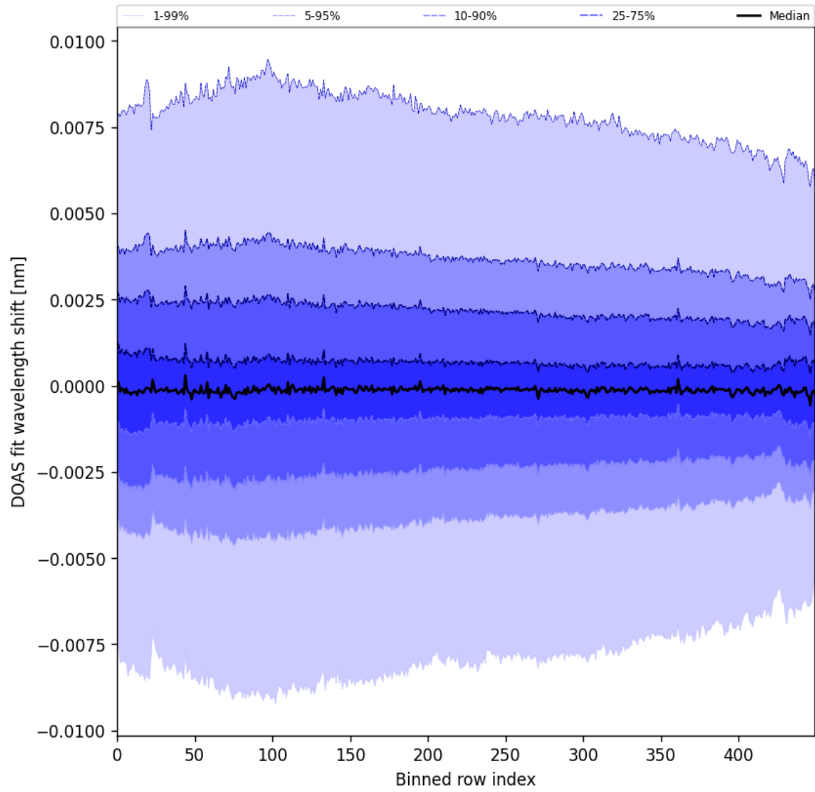
Figure 102: Along track statistics of “DOAS fit wavelength shift” for 2025-05-15 to 2025-05-17
