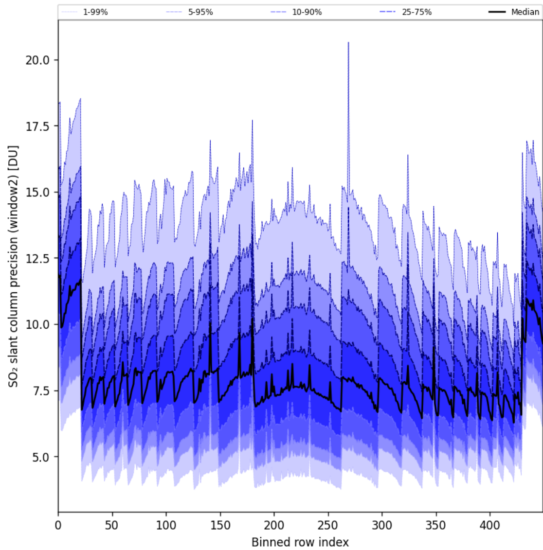
Figure 94: Along track statistics of “SO 2 slant column precision (window2)” for 2025-05-15 to 2025-05-17
