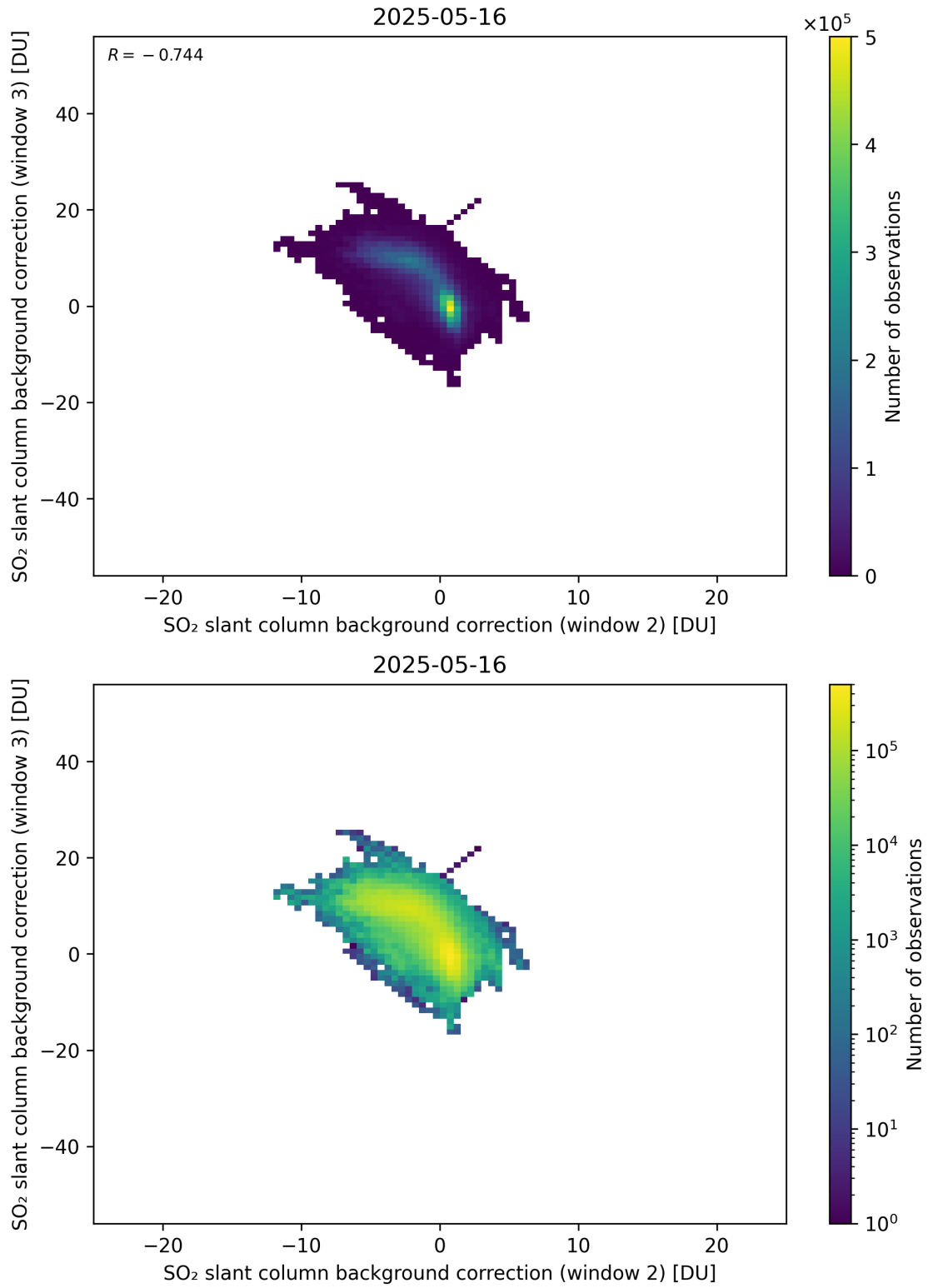
Figure 122: Scatter density plot of “SO 2 slant column background correction (window 2)” against “SO 2 slant column background correction (window 3)” for 2025-05-15 to 2025-05-17.
