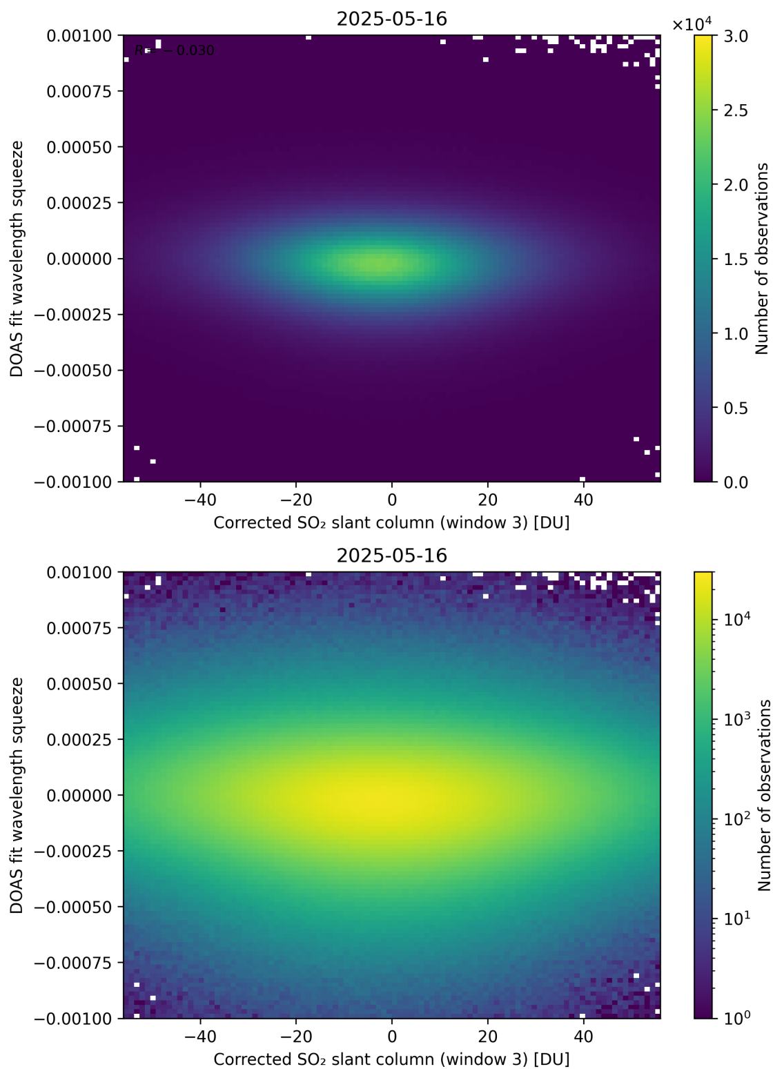
Figure 257: Scatter density plot of “Corrected SO 2 slant column (window 3)” against “DOAS fit wavelength squeeze” for 2025-05-15 to 2025-05-17.
