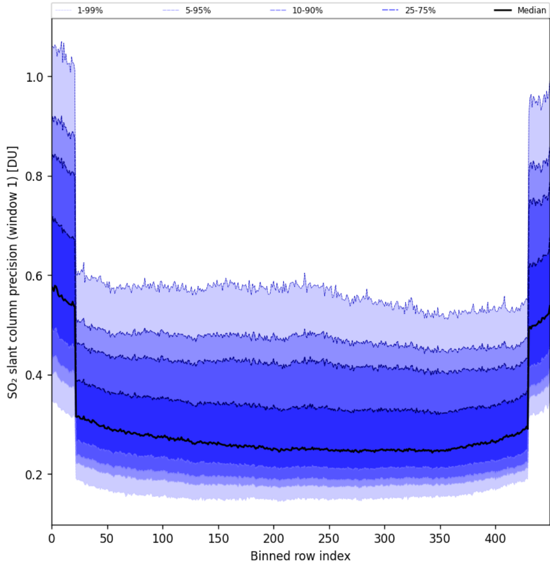
Figure 90: Along track statistics of “SO 2 slant column precision (window 1)” for 2025-05-15 to 2025-05-17
