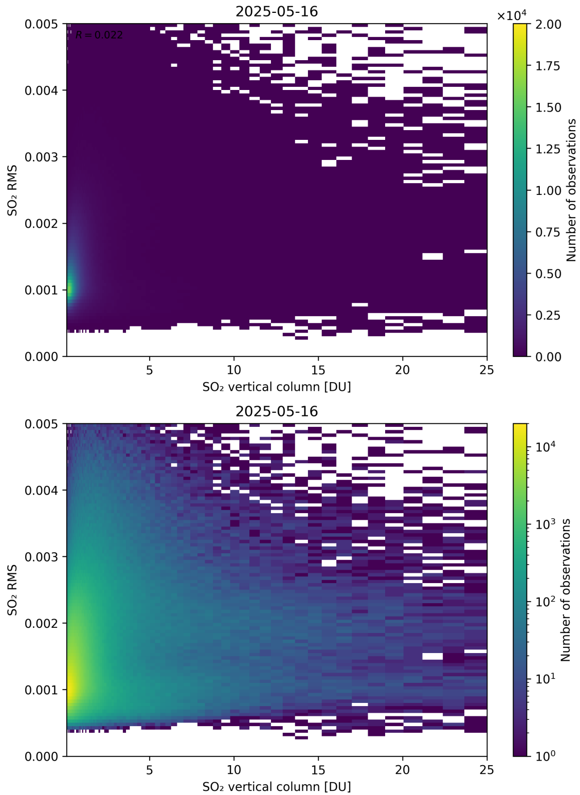
Figure 328: Scatter density plot of “SO 2 vertical column” against “SO 2 RMS” for 2025-05-15 to 2025-05-17.
