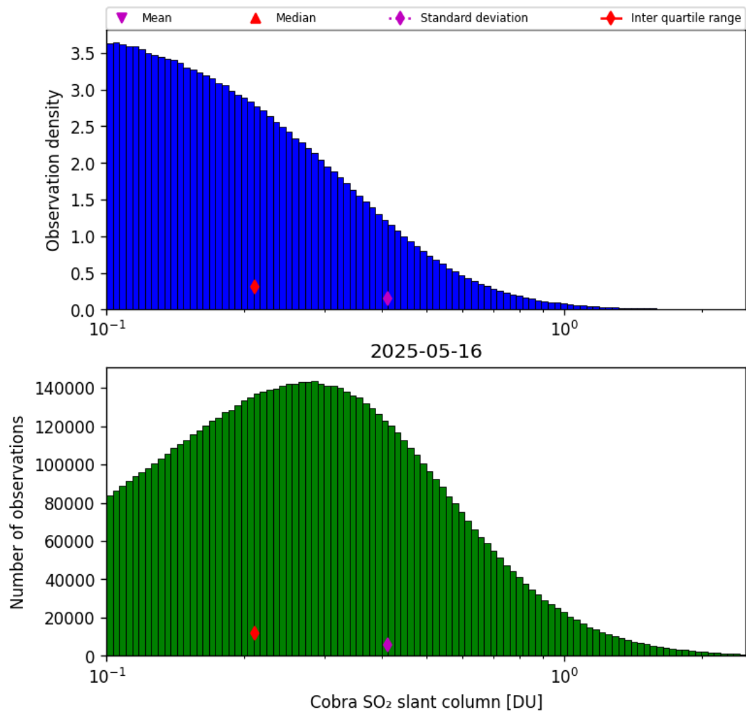
Figure 61: Histogram of “Cobra SO 2 slant column” for 2025-05-15 to 2025-05-17
