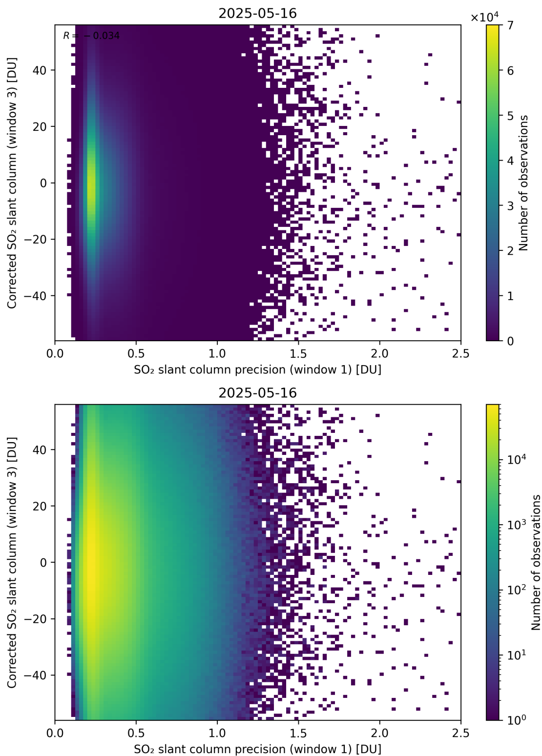
Figure 276: Scatter density plot of “SO 2 slant column precision (window 1)” against “Corrected SO 2 slant column (window 3)” for 2025-05-15 to 2025-05-17.
