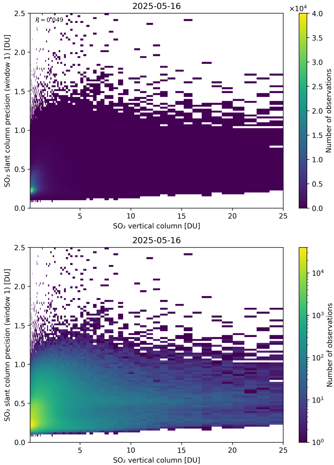
Figure 355: Scatter density plot of “SO 2 vertical column” against “SO 2 slant column precision (window 1)” for 2025-05-15 to 2025-05-17.
