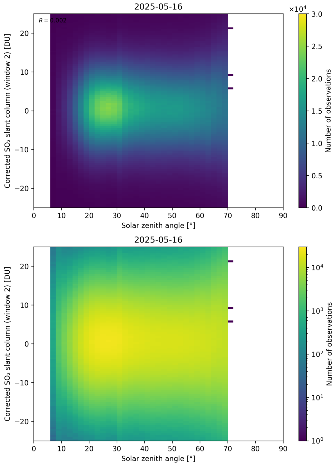
Figure 182: Scatter density plot of “Solar zenith angle” against “Corrected SO 2 slant column (window 2)” for 2025-05-15 to 2025-05-17.
