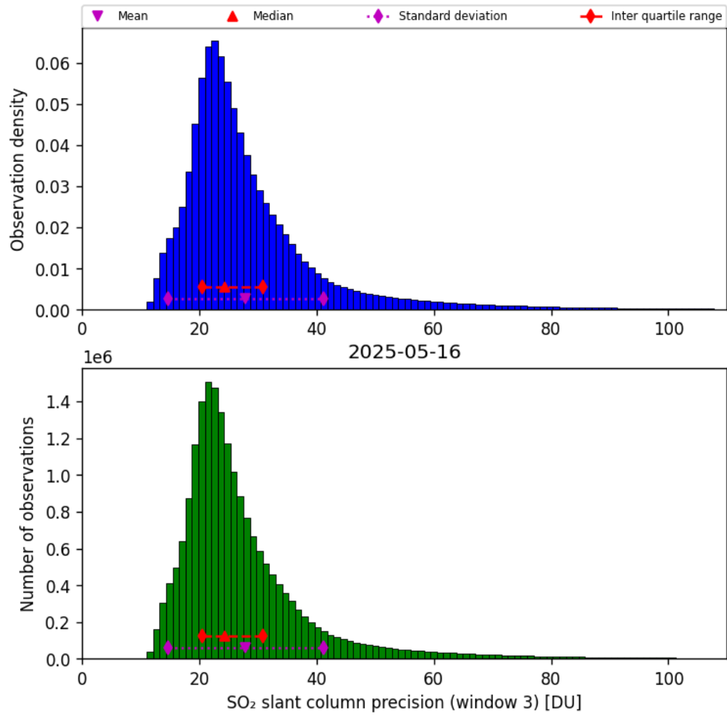
Figure 72: Histogram of “SO 2 slant column precision (window 3)” for 2025-05-15 to 2025-05-17
