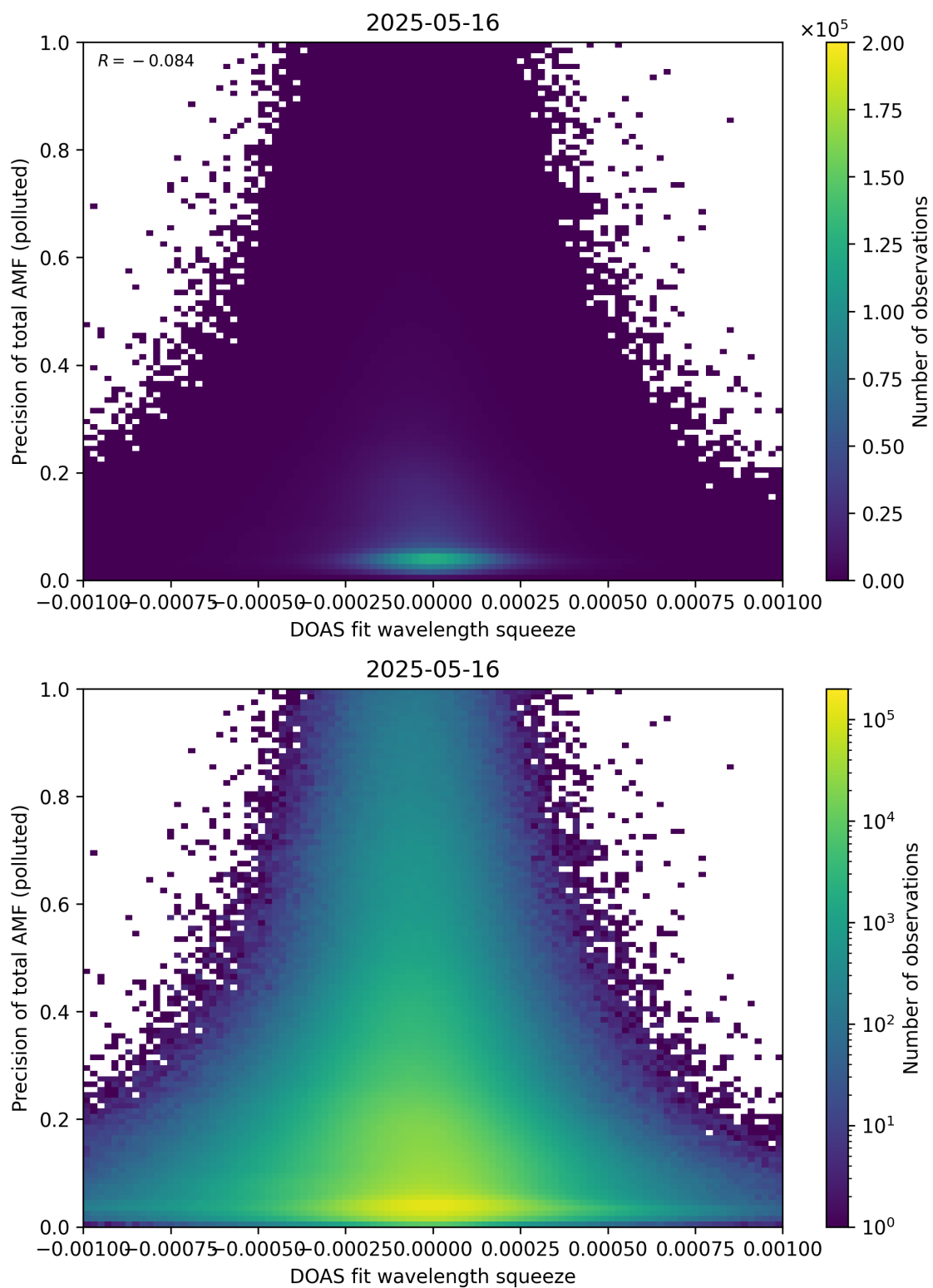
Figure 146: Scatter density plot of “DOAS fit wavelength squeeze” against “Precision of total AMF (polluted)” for 2025-05-15 to 2025-05-17.
