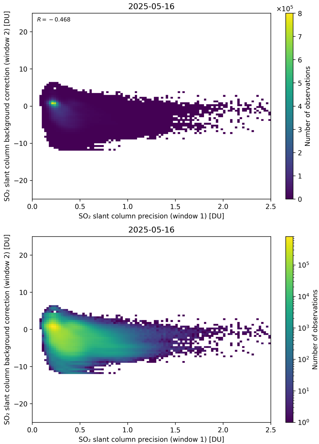
Figure 269: Scatter density plot of “SO 2 slant column precision (window 1)” against “SO 2 slant column background correction (window 2)” for 2025-05-15 to 2025-05-17.
