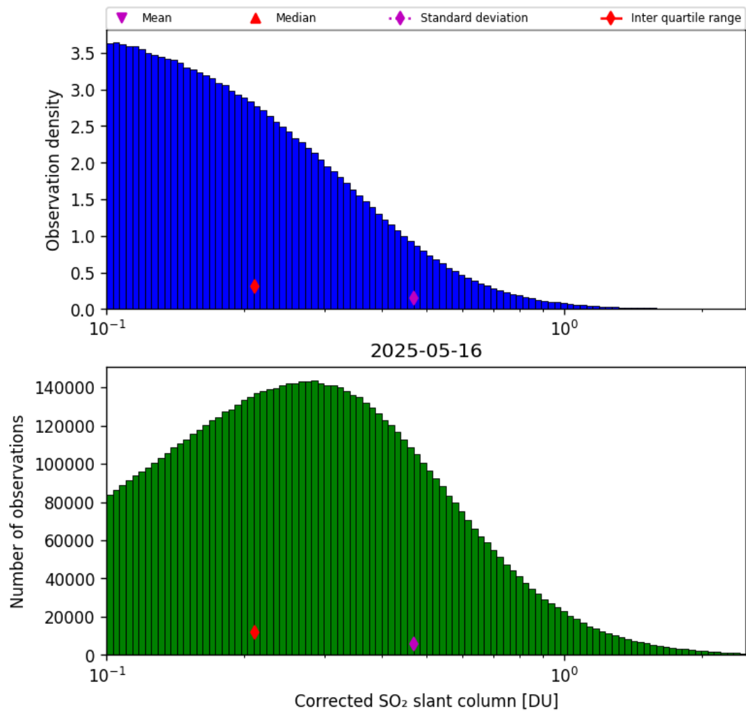
Figure 60: Histogram of “Corrected SO 2 slant column” for 2025-05-15 to 2025-05-17
