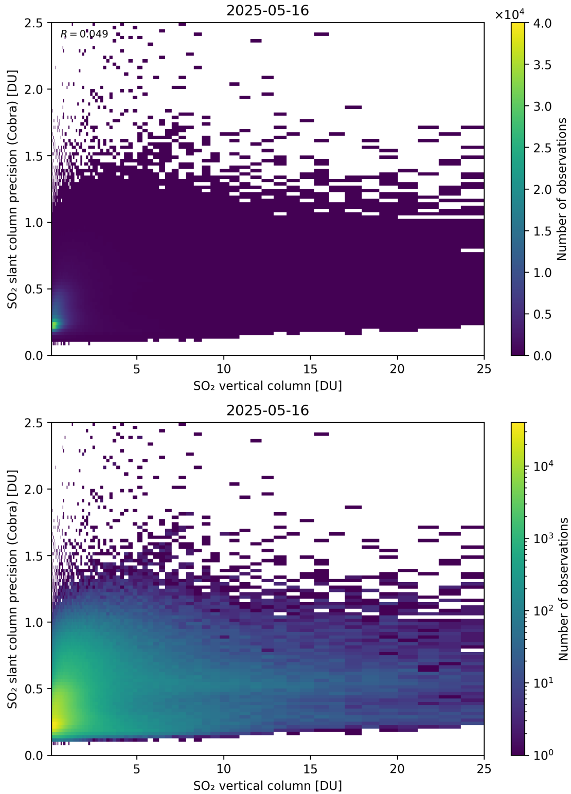
Figure 350: Scatter density plot of “SO 2 vertical column” against “SO 2 slant column precision (Cobra)” for 2025-05-15 to 2025-05-17.
