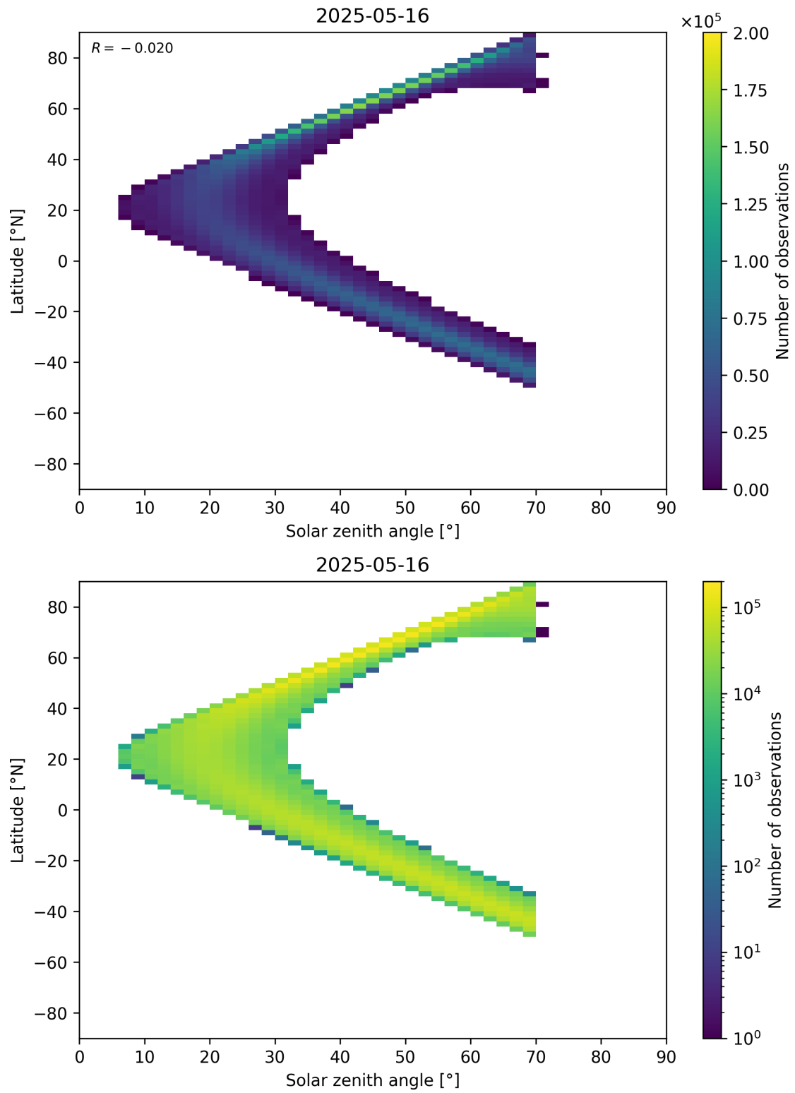
Figure 177: Scatter density plot of “Solar zenith angle” against “Latitude” for 2025-05-15 to 2025-05-17.
