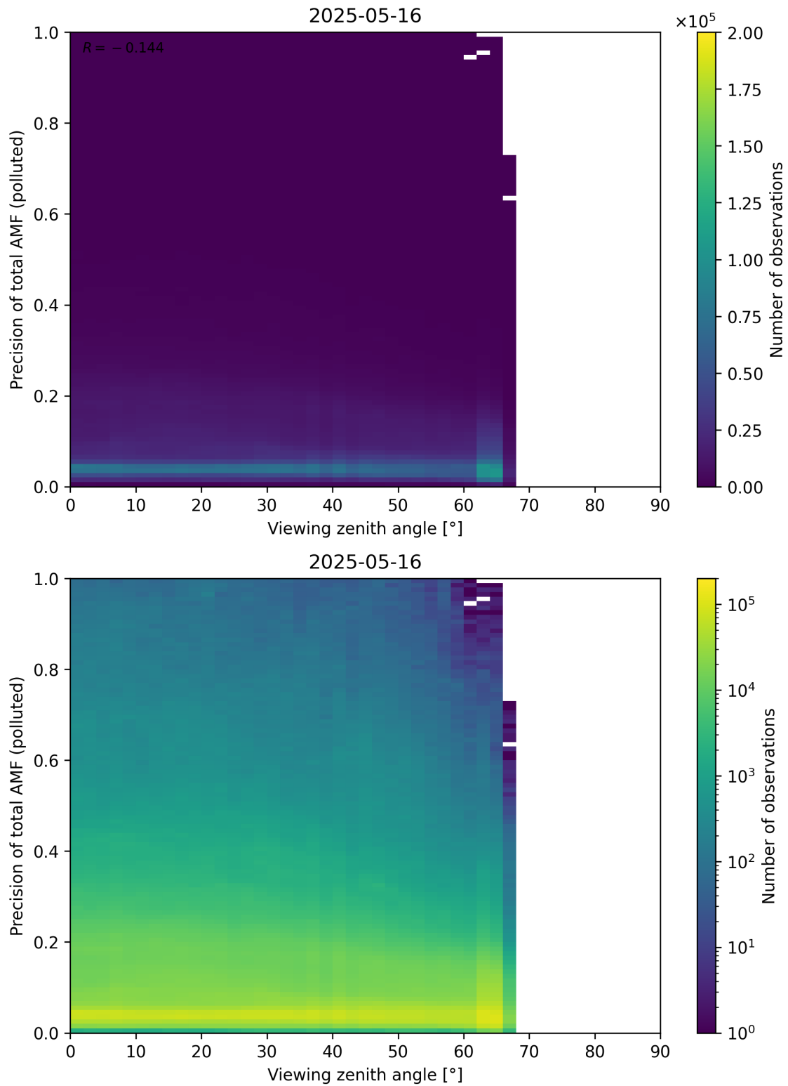
Figure 382: Scatter density plot of “Viewing zenith angle” against “Precision of total AMF (polluted)” for 2025-05-15 to 2025-05-17.
