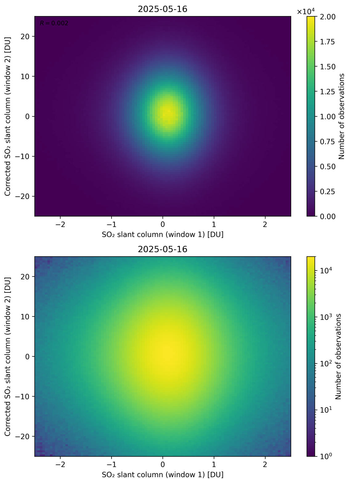
Figure 283: Scatter density plot of “SO 2 slant column (window 1)” against “Corrected SO 2 slant column (window 2)” for 2025-05-15 to 2025-05-17.
