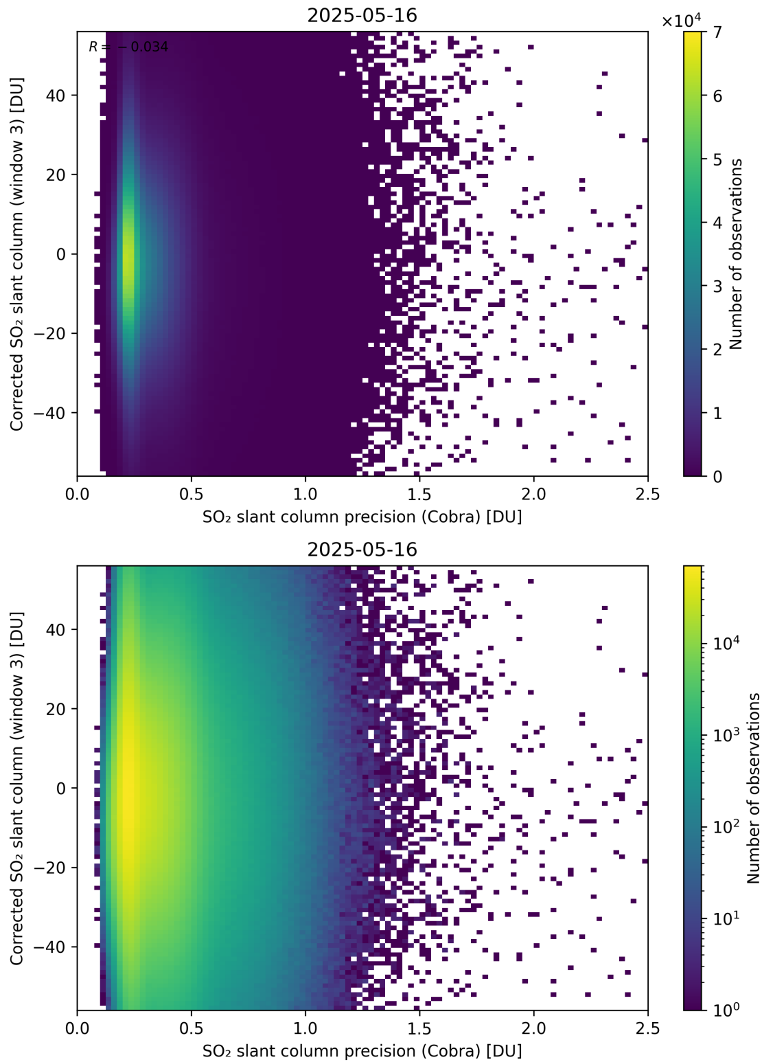
Figure 207: Scatter density plot of “SO 2 slant column precision (Cobra)” against “Corrected SO 2 slant column (window 3)” for 2025-05-15 to 2025-05-17.
