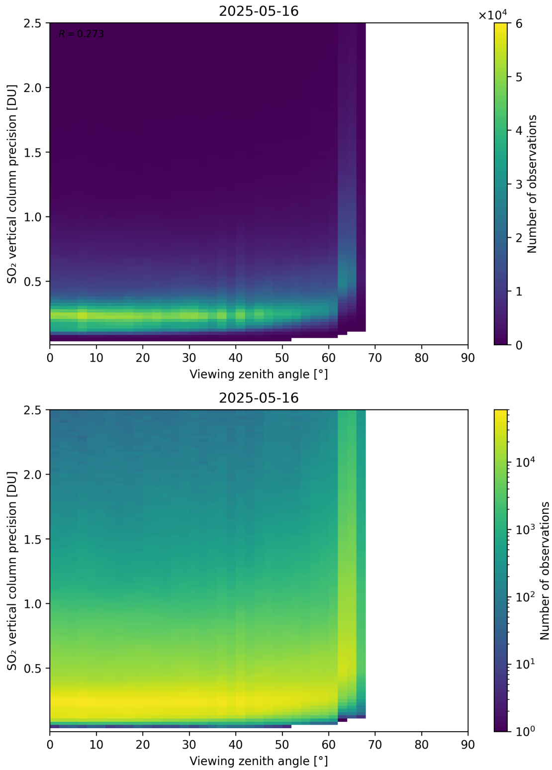
Figure 384: Scatter density plot of “Viewing zenith angle” against “SO 2 vertical column precision” for 2025-05-15 to 2025-05-17.
