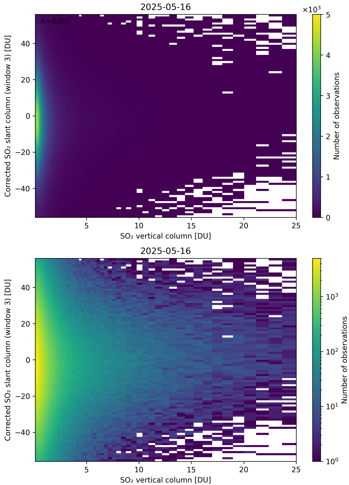
Figure 353: Scatter density plot of “SO 2 vertical column” against “Corrected SO 2 slant column (window 3)” for 2025-05-15 to 2025-05-17.
