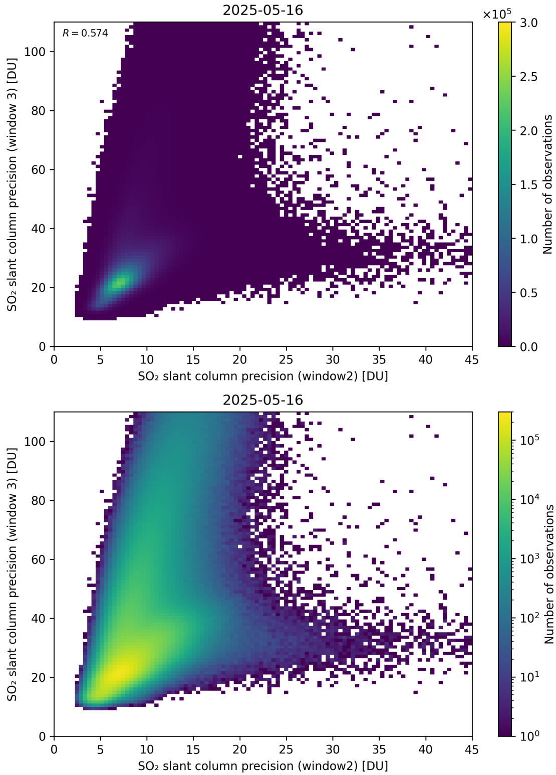
Figure 300: Scatter density plot of “SO 2 slant column precision (window2)” against “SO 2 slant column precision (window 3)” for 2025-05-15 to 2025-05-17.
