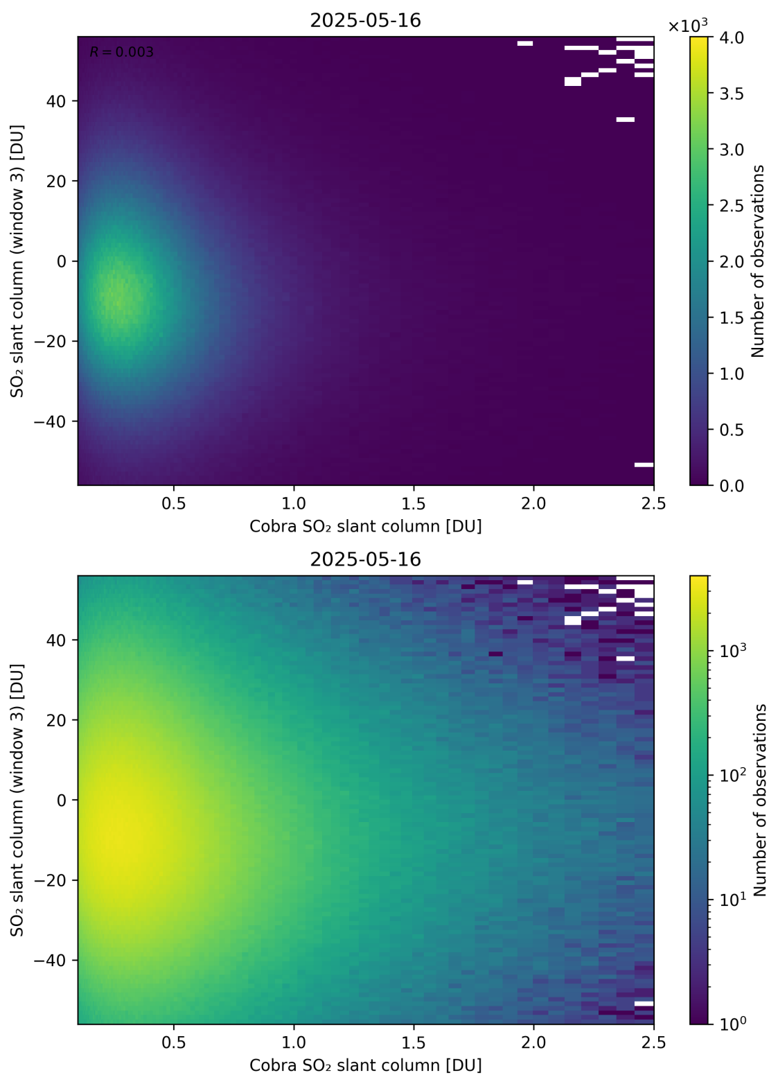
Figure 222: Scatter density plot of “Cobra SO 2 slant column” against “SO 2 slant column (window 3)” for 2025-05-15 to 2025-05-17.
