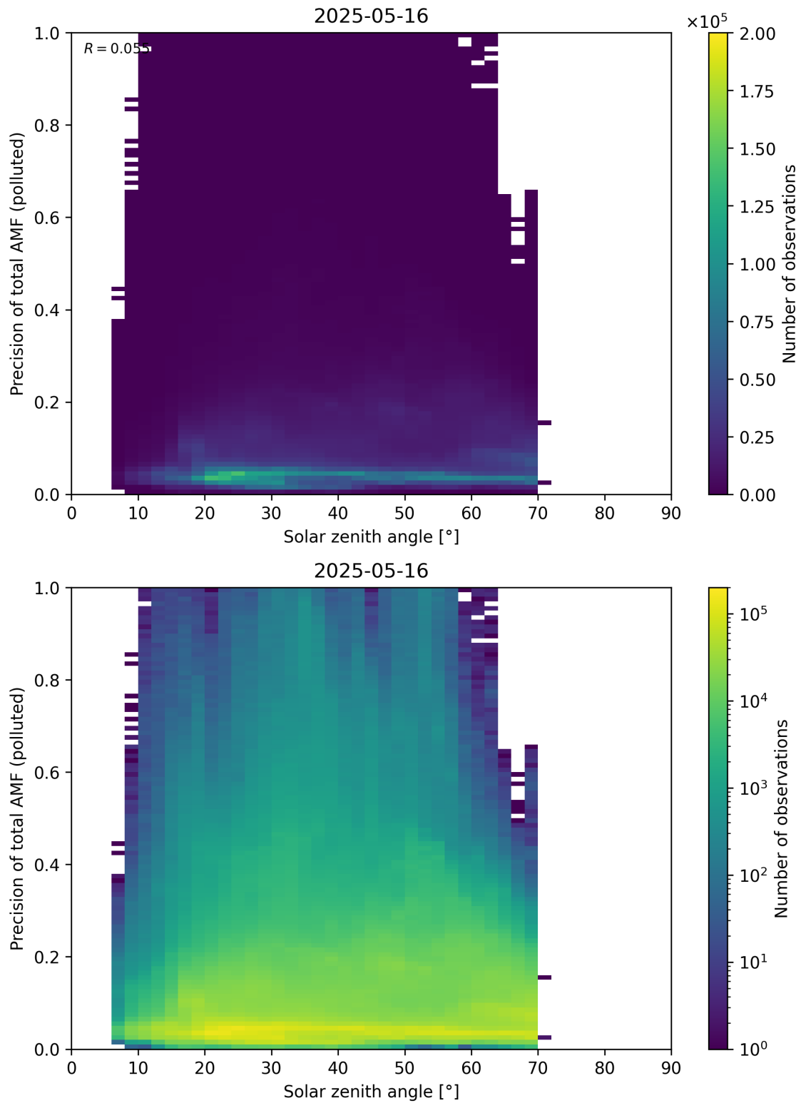
Figure 190: Scatter density plot of “Solar zenith angle” against “Precision of total AMF (polluted)” for 2025-05-15 to 2025-05-17.
