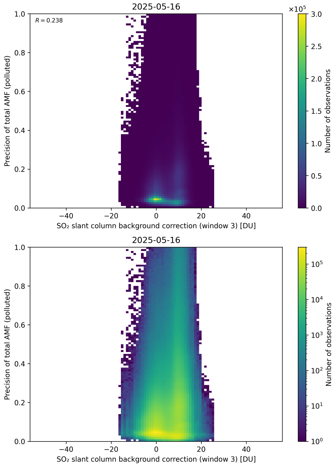
Figure 137: Scatter density plot of “SO 2 slant column background correction (window 3)” against “Precision of total AMF (polluted)” for 2025-05-15 to 2025-05-17.
