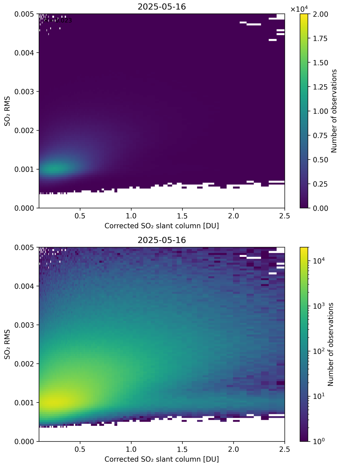
Figure 231: Scatter density plot of “Corrected SO 2 slant column” against “SO 2 RMS” for 2025-05-15 to 2025-05-17.
