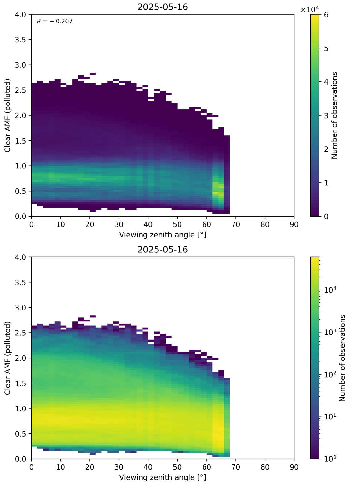
Figure 370: Scatter density plot of “Viewing zenith angle” against “Clear AMF (polluted)” for 2025-05-15 to 2025-05-17.
