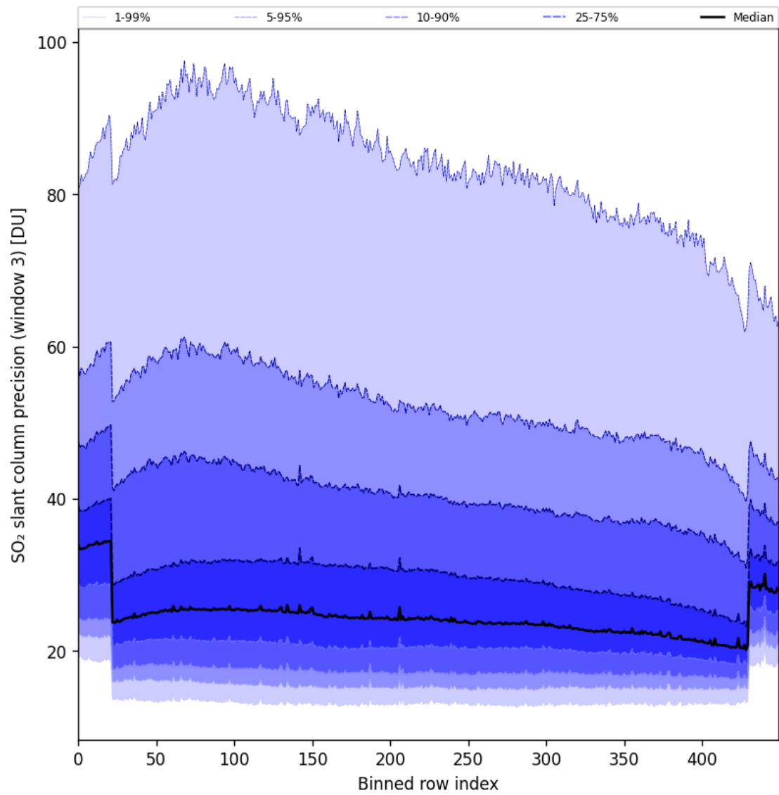
Figure 98: Along track statistics of “SO 2 slant column precision (window 3)” for 2025-05-15 to 2025-05-17
