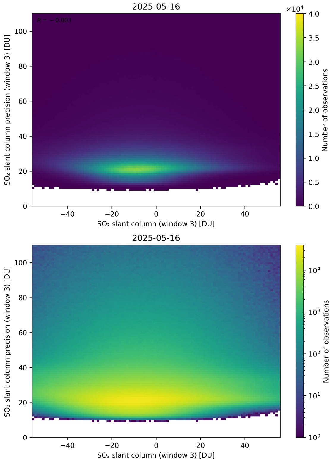
Figure 317: Scatter density plot of “SO 2 slant column (window 3)” against “SO 2 slant column precision (window 3)” for 2025-05-15 to 2025-05-17.
