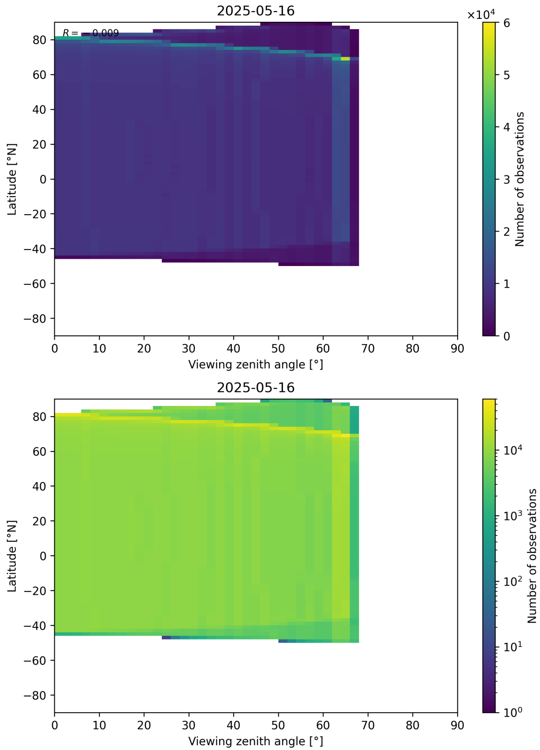
Figure 368: Scatter density plot of “Viewing zenith angle” against “Latitude” for 2025-05-15 to 2025-05-17.
