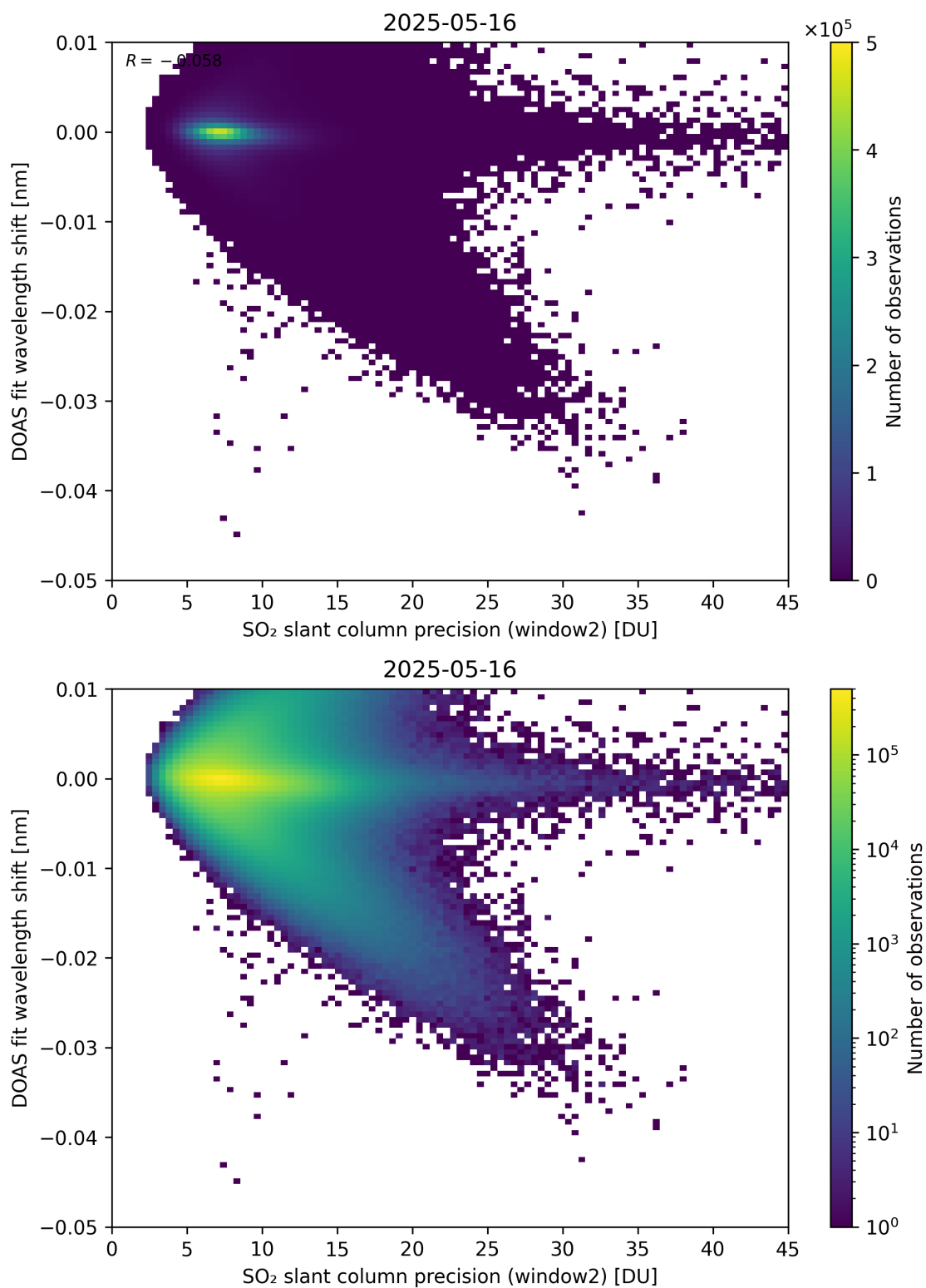
Figure 293: Scatter density plot of “SO 2 slant column precision (window2)” against “DOAS fit wavelength shift” for 2025-05-15 to 2025-05-17.
