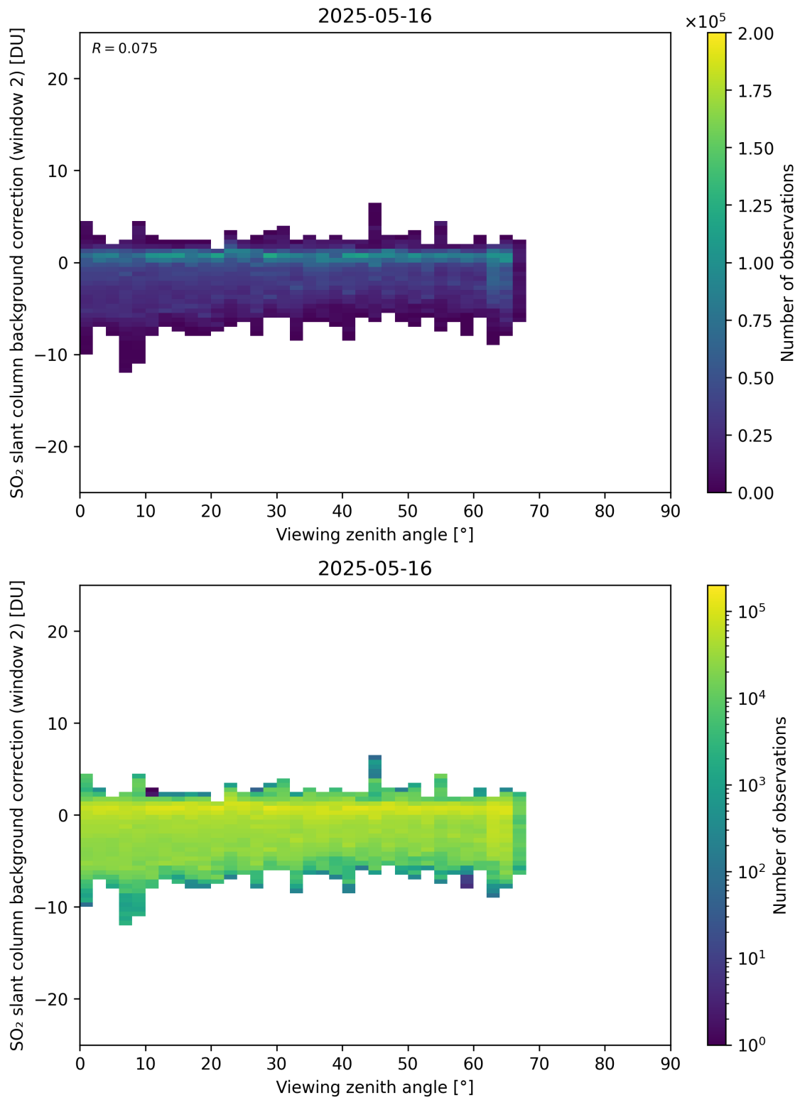
Figure 363: Scatter density plot of “Viewing zenith angle” against “SO 2 slant column background correction (window 2)” for 2025-05-15 to 2025-05-17.
