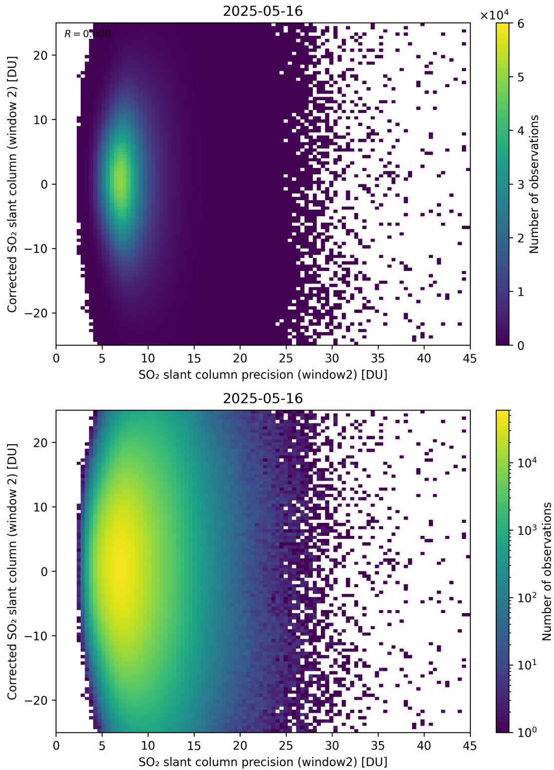
Figure 297: Scatter density plot of “SO 2 slant column precision (window2)” against “Corrected SO 2 slant column (window 2)” for 2025-05-15 to 2025-05-17.
