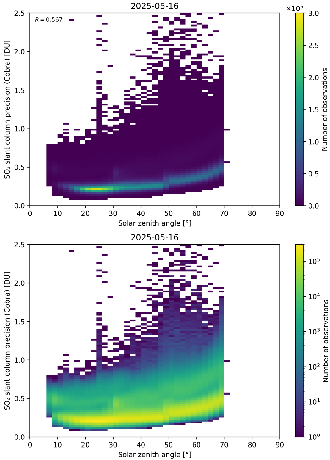
Figure 180: Scatter density plot of “Solar zenith angle” against “SO 2 slant column precision (Cobra)” for 2025-05-15 to 2025-05-17.
