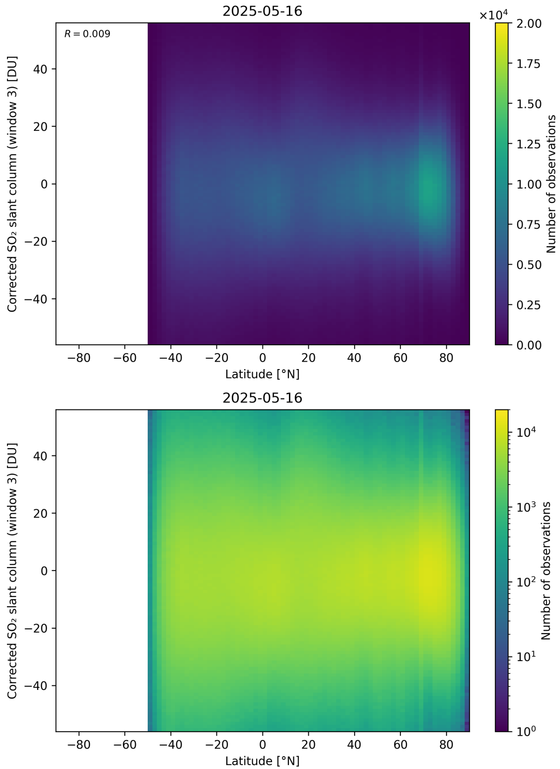
Figure 161: Scatter density plot of “Latitude” against “Corrected SO 2 slant column (window 3)” for 2025-05-15 to 2025-05-17.
