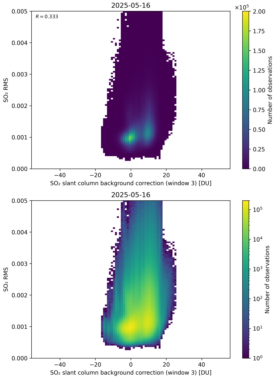
Figure 134: Scatter density plot of “SO 2 slant column background correction (window 3)” against “SO 2 RMS” for 2025-05-15 to 2025-05-17.
