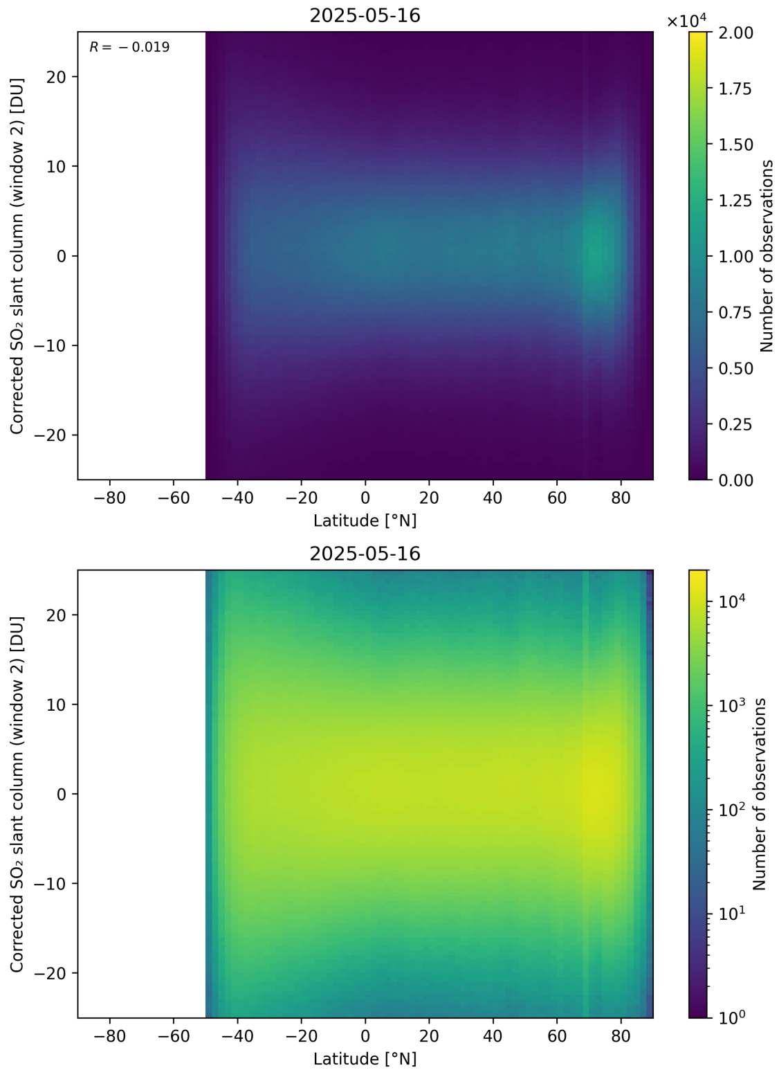
Figure 160: Scatter density plot of “Latitude” against “Corrected SO 2 slant column (window 2)” for 2025-05-15 to 2025-05-17.
