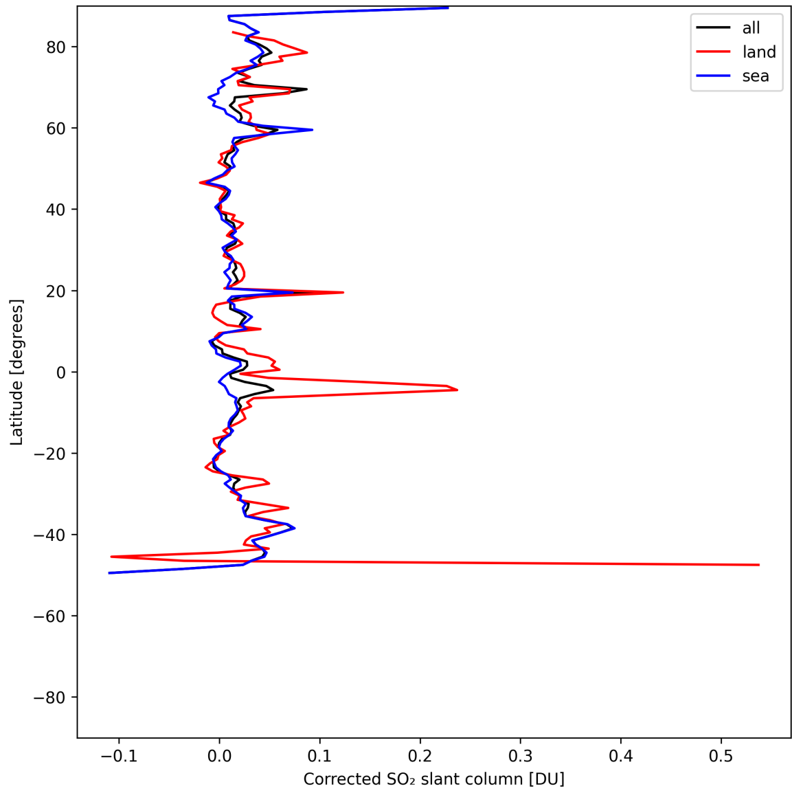
Figure 34: Zonal average of “Corrected SO 2 slant column” for 2025-05-15 to 2025-05-17.
