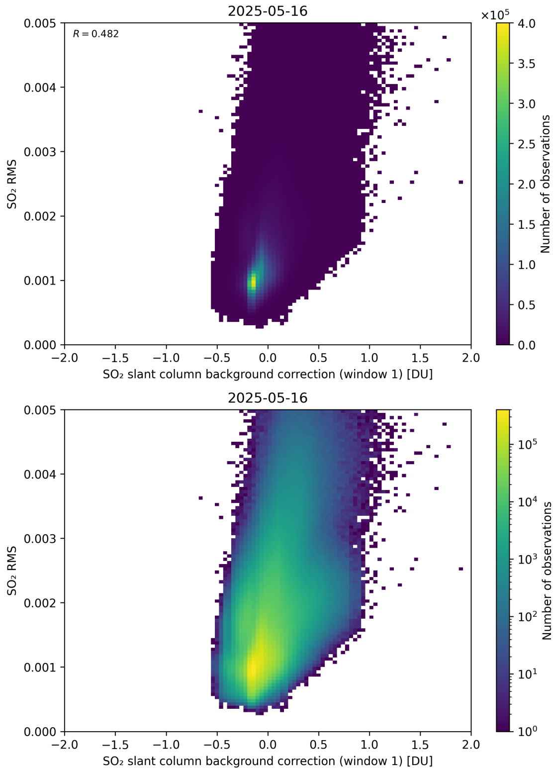
Figure 113: Scatter density plot of “SO 2 slant column background correction (window 1)” against “SO 2 RMS” for 2025-05-15 to 2025-05-17.
