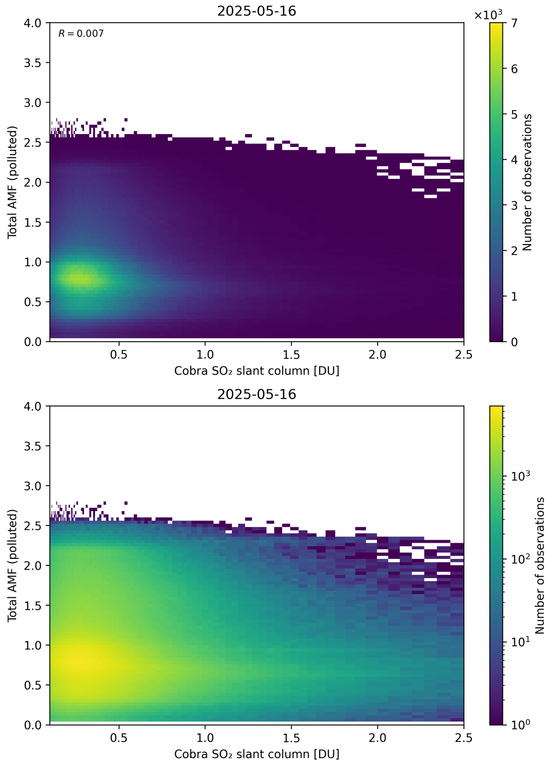
Figure 224: Scatter density plot of “Cobra SO 2 slant column” against “Total AMF (polluted)” for 2025-05-15 to 2025-05-17.
