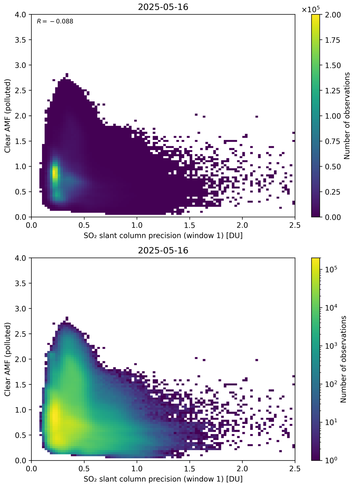
Figure 274: Scatter density plot of “SO 2 slant column precision (window 1)” against “Clear AMF (polluted)” for 2025-05-15 to 2025-05-17.
