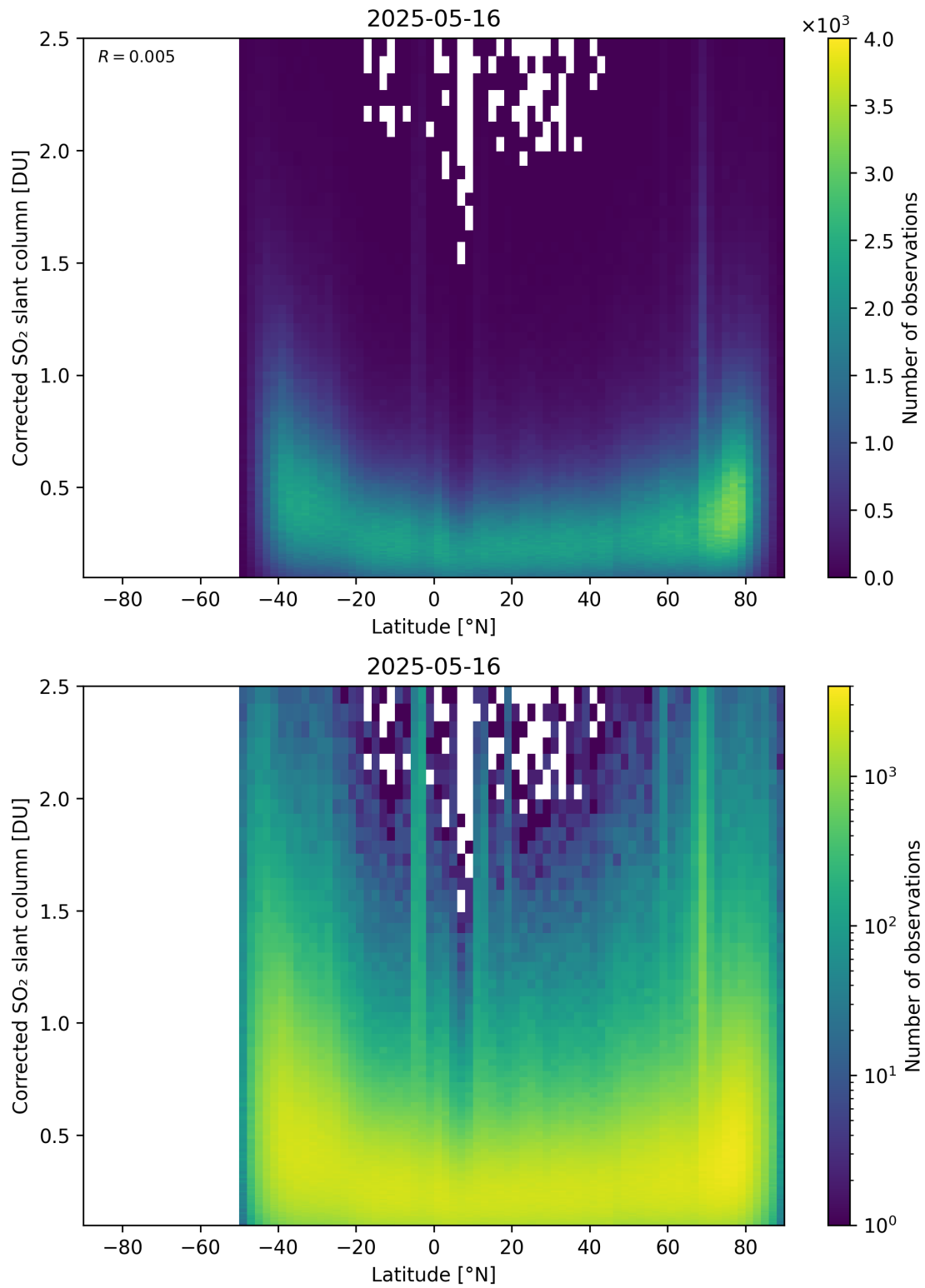
Figure 159: Scatter density plot of “Latitude” against “Corrected SO 2 slant column” for 2025-05-15 to 2025-05-17.
