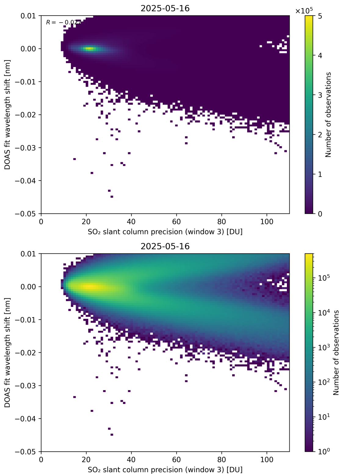
Figure 308: Scatter density plot of “SO 2 slant column precision (window 3)” against “DOAS fit wavelength shift” for 2025-05-15 to 2025-05-17.
