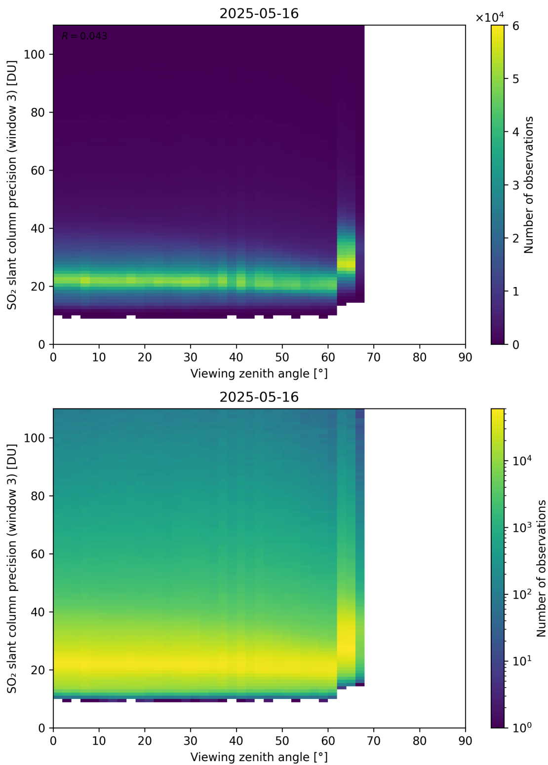
Figure 380: Scatter density plot of “Viewing zenith angle” against “SO 2 slant column precision (window 3)” for 2025-05-15 to 2025-05-17.
