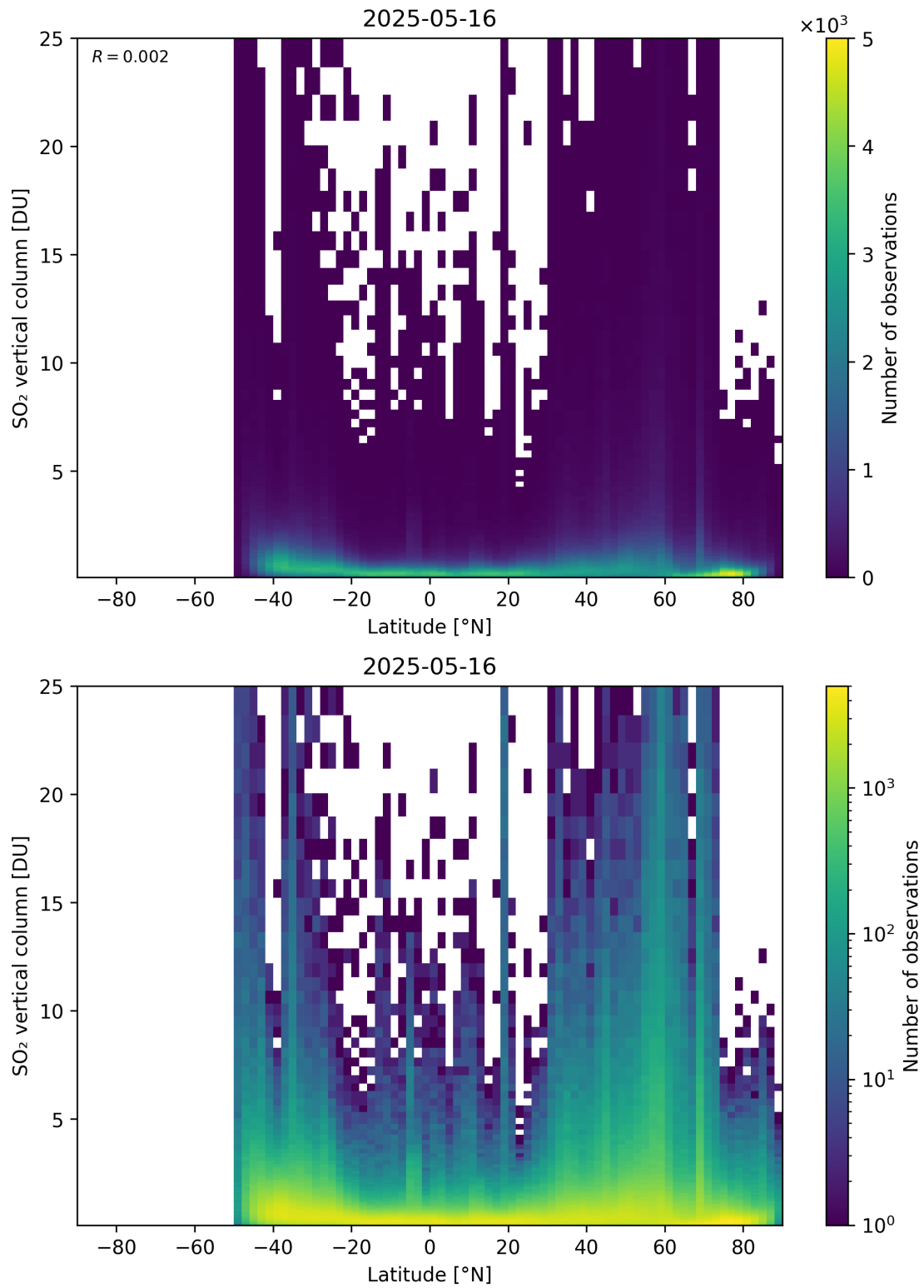
Figure 169: Scatter density plot of “Latitude” against “SO 2 vertical column” for 2025-05-15 to 2025-05-17.
