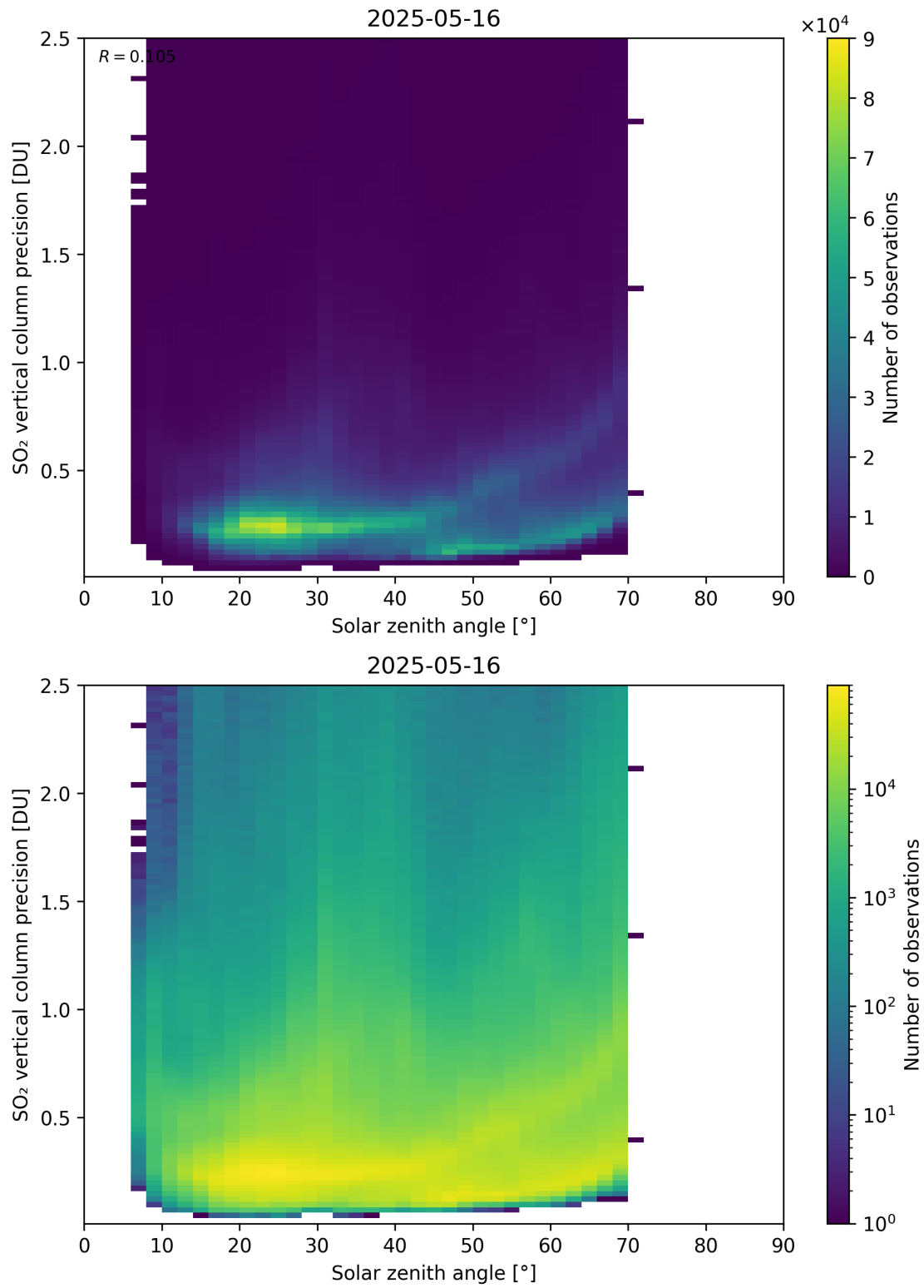
Figure 192: Scatter density plot of “Solar zenith angle” against “SO 2 vertical column precision” for 2025-05-15 to 2025-05-17.
