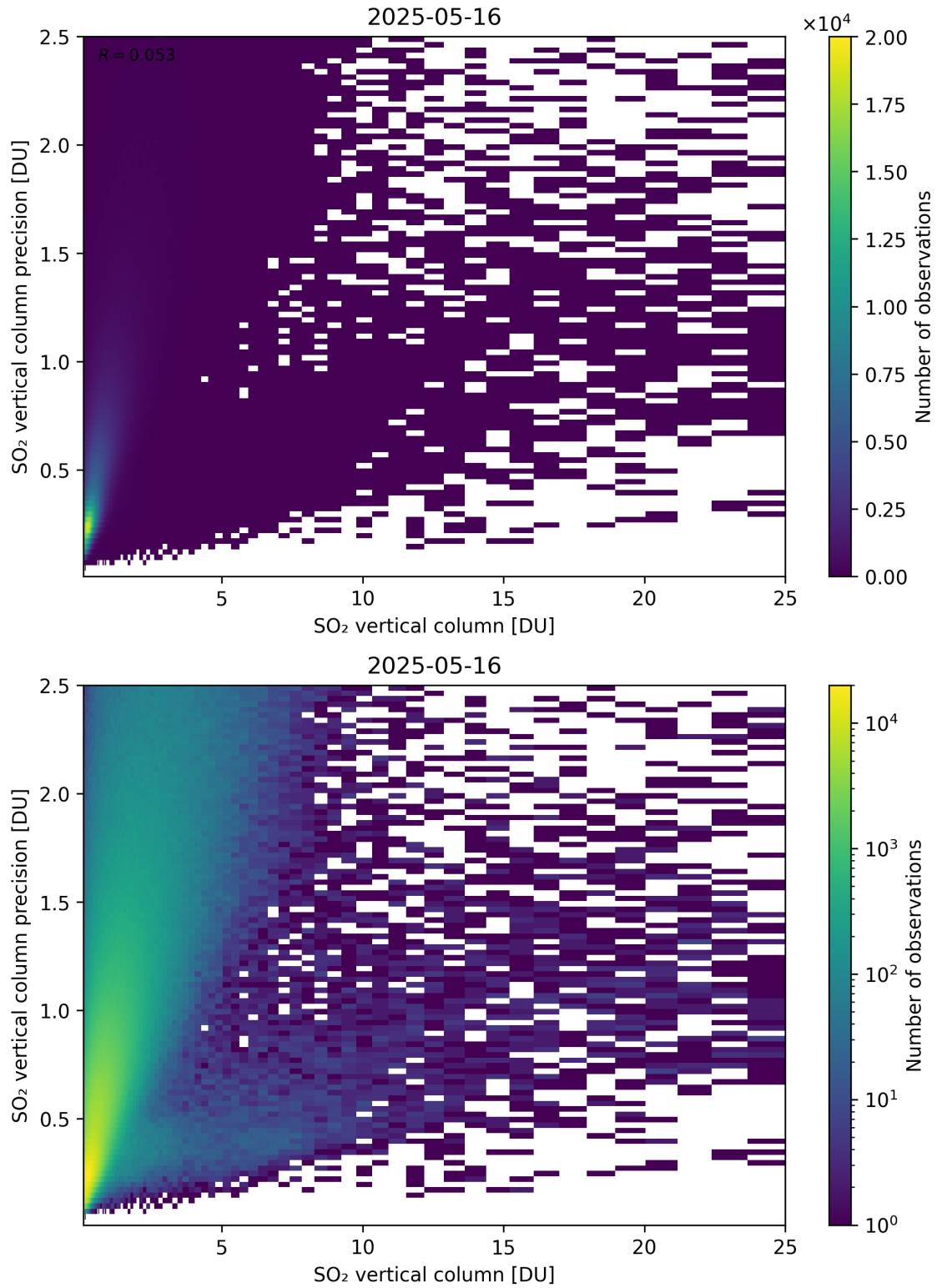
Figure 361: Scatter density plot of “SO 2 vertical column” against “SO 2 vertical column precision” for 2025-05-15 to 2025-05-17.
