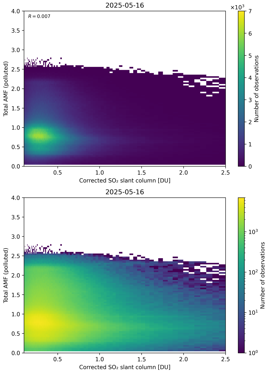
Figure 242: Scatter density plot of “Corrected SO 2 slant column” against “Total AMF (polluted)” for 2025-05-15 to 2025-05-17.
