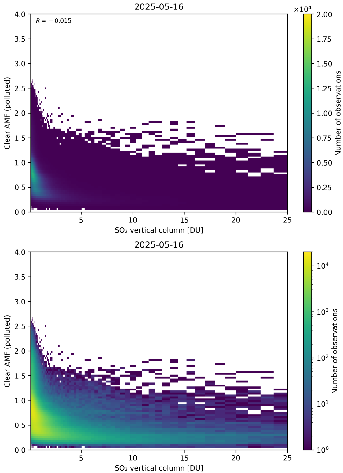
Figure 348: Scatter density plot of “SO 2 vertical column” against “Clear AMF (polluted)” for 2025-05-15 to 2025-05-17.
