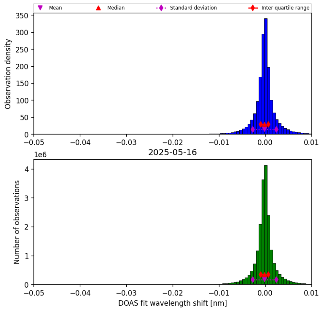
Figure 76: Histogram of “DOAS fit wavelength shift” for 2025-05-15 to 2025-05-17
