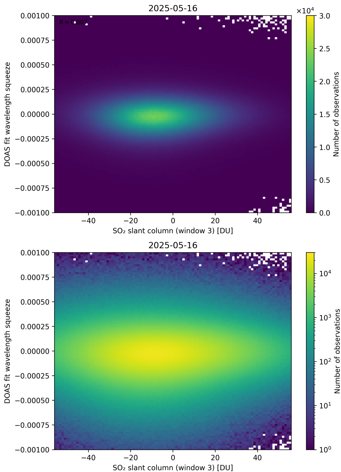
Figure 305: Scatter density plot of “SO 2 slant column (window 3)” against “DOAS fit wavelength squeeze” for 2025-05-15 to 2025-05-17.
