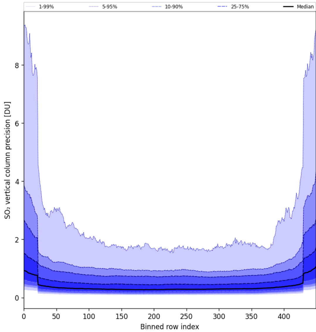
Figure 85: Along track statistics of “SO 2 vertical column precision” for 2025-05-15 to 2025-05-17
