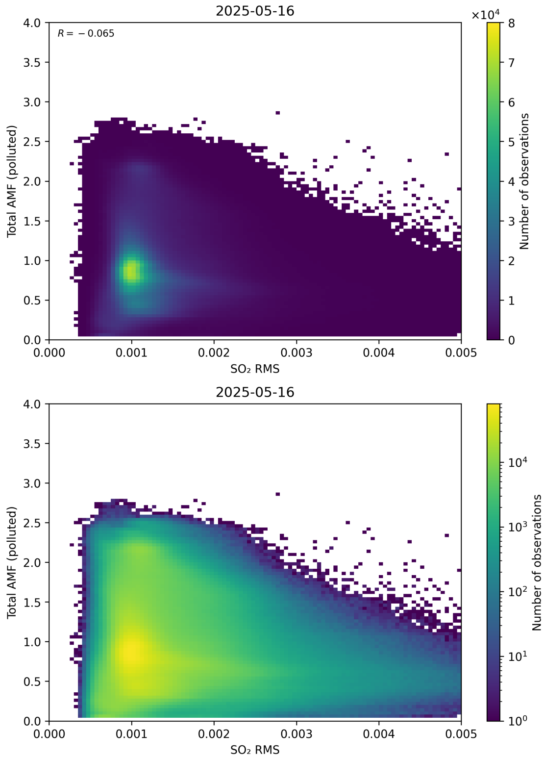
Figure 148: Scatter density plot of “SO 2 RMS” against “Total AMF (polluted)” for 2025-05-15 to 2025-05-17.
