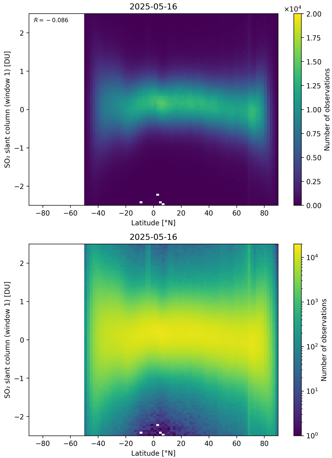
Figure 162: Scatter density plot of “Latitude” against “SO 2 slant column (window 1)” for 2025-05-15 to 2025-05-17.
