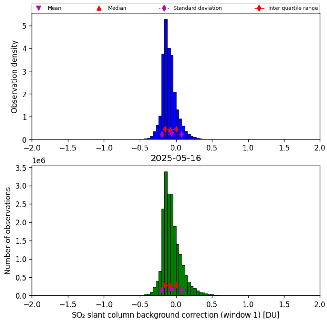
Figure 66: Histogram of “SO 2 slant column background correction (window 1)” for 2025-05-15 to 2025-05-17
