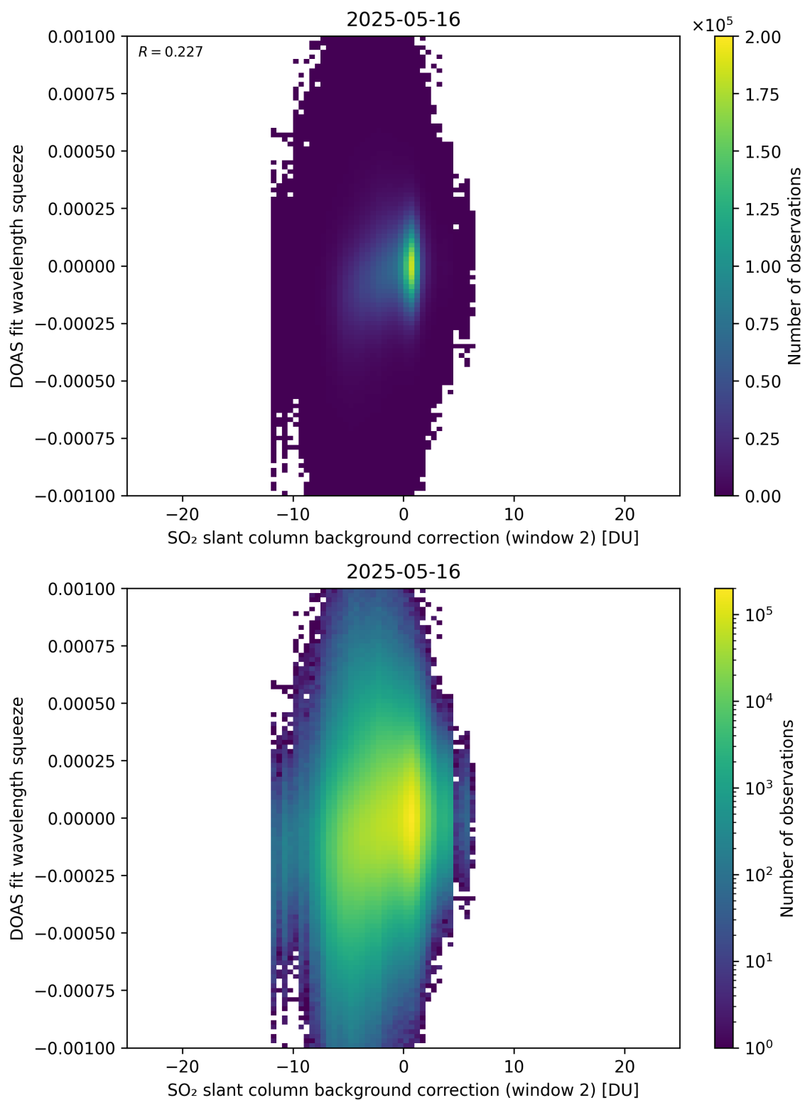
Figure 124: Scatter density plot of “SO 2 slant column background correction (window 2)” against “DOAS fit wavelength squeeze” for 2025-05-15 to 2025-05-17.
