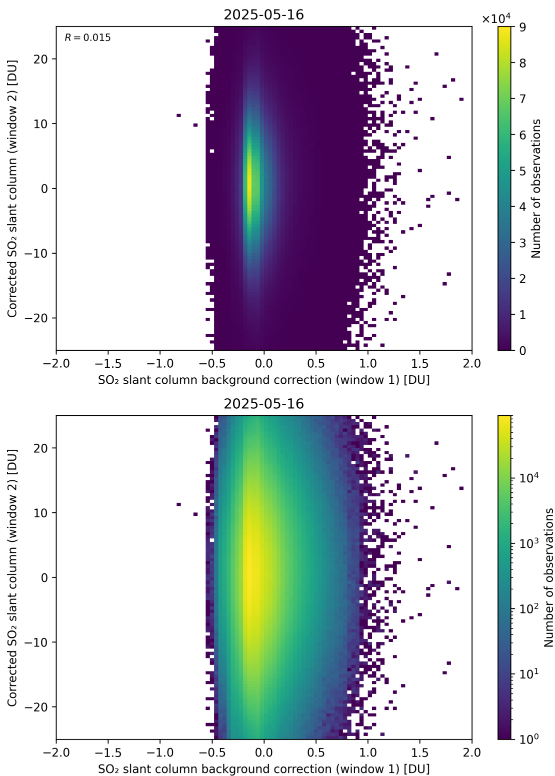
Figure 115: Scatter density plot of “SO 2 slant column background correction (window 1)” against “Corrected SO 2 slant column (window 2)” for 2025-05-15 to 2025-05-17.
