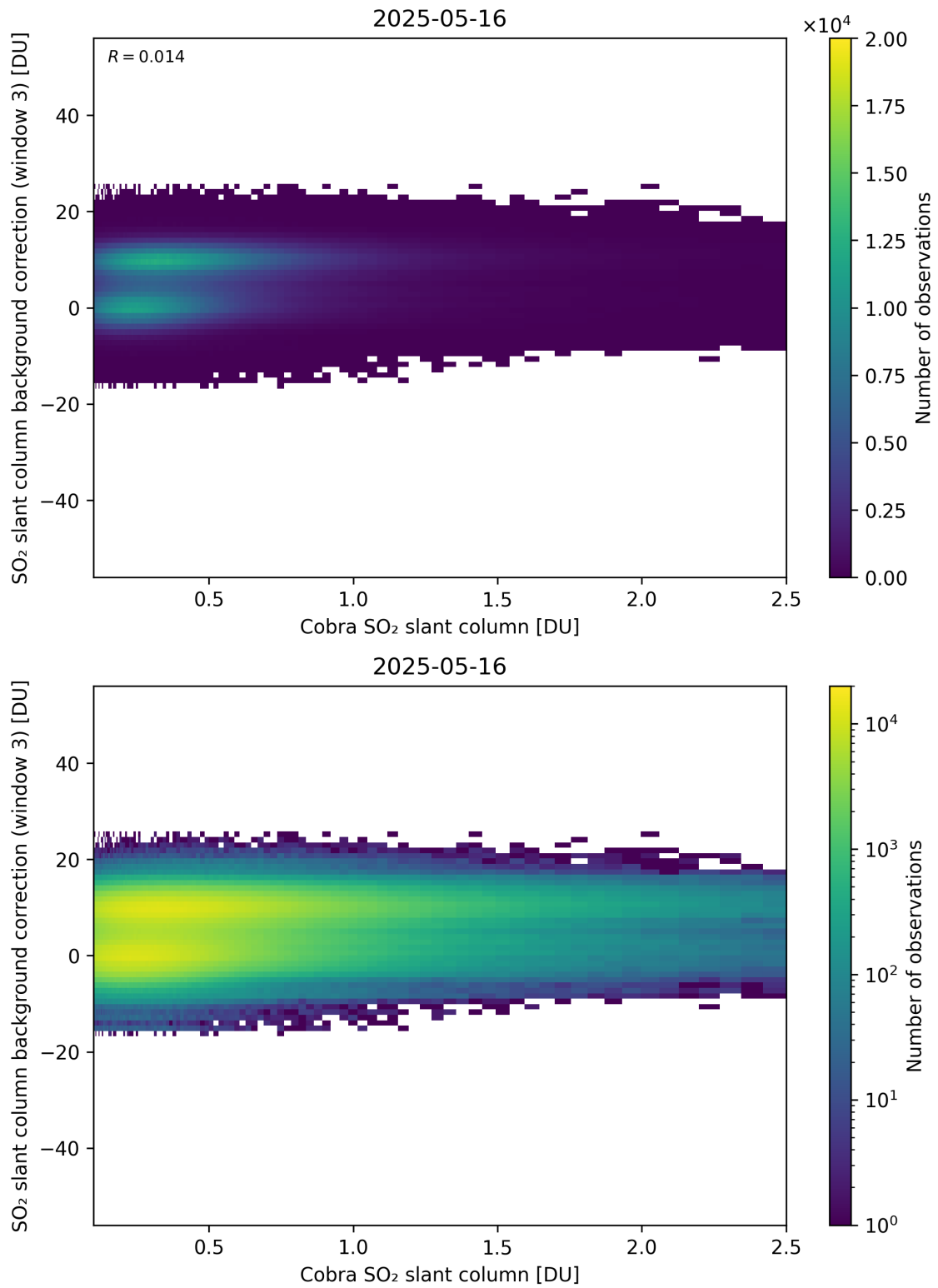
Figure 195: Scatter density plot of “Cobra SO 2 slant column” against “SO 2 slant column background correction (window 3)” for 2025-05-15 to 2025-05-17.
