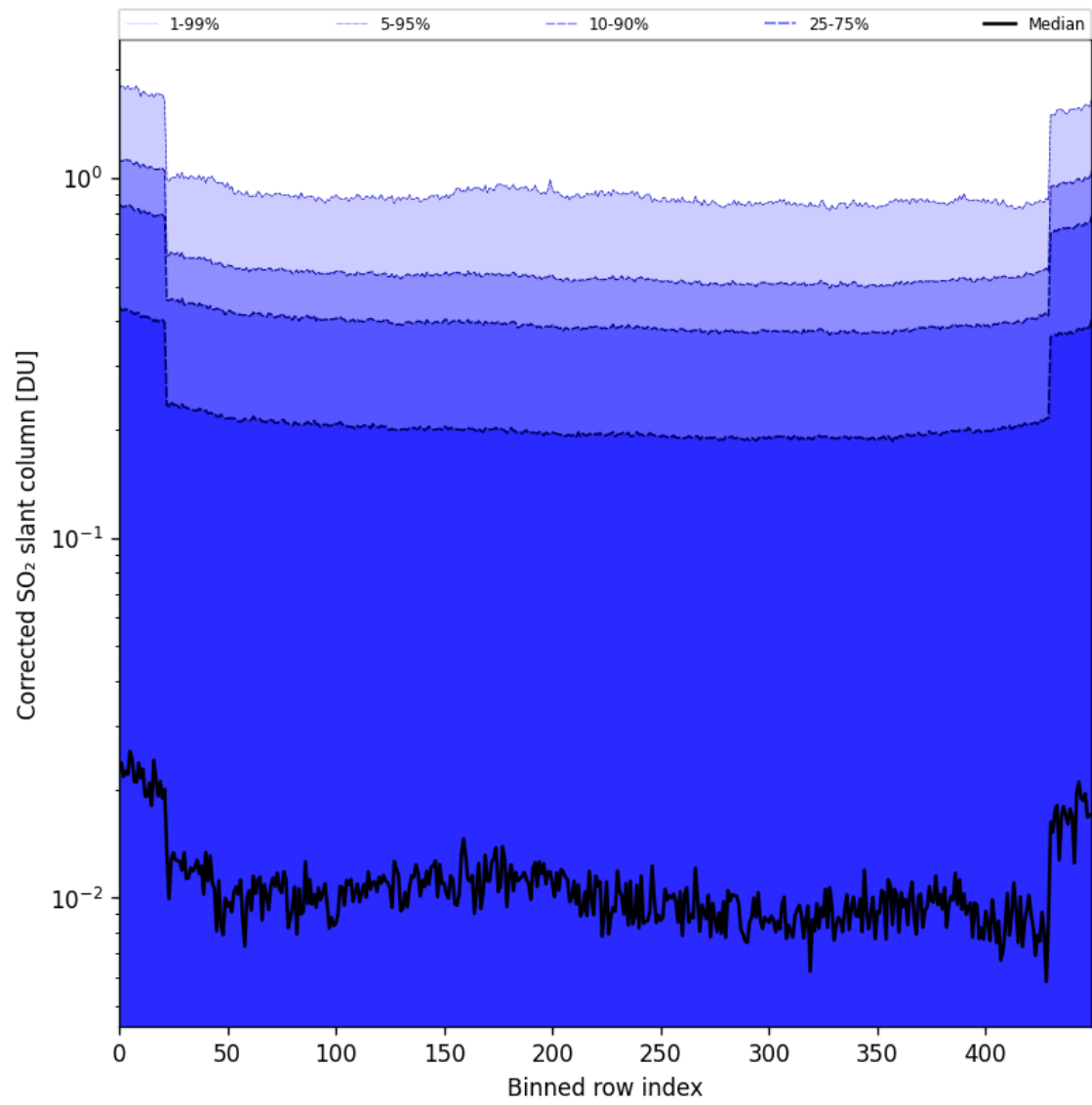
Figure 86: Along track statistics of “Corrected SO 2 slant column” for 2025-05-15 to 2025-05-17
