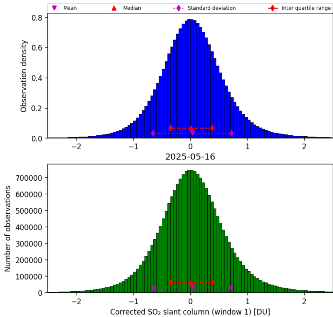
Figure 65: Histogram of “Corrected SO 2 slant column (window 1)” for 2025-05-15 to 2025-05-17
