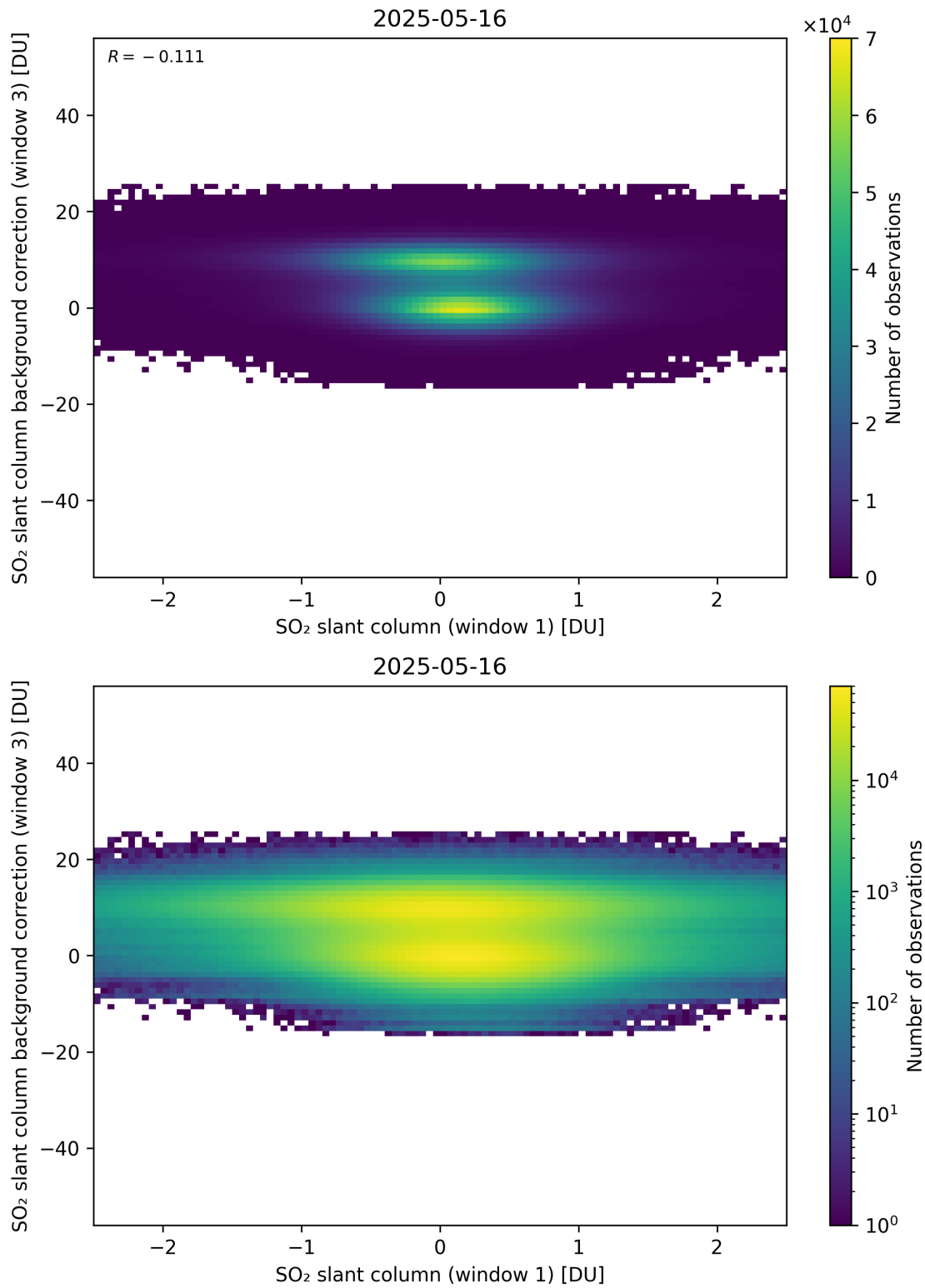
Figure 264: Scatter density plot of “SO 2 slant column (window 1)” against “SO 2 slant column background correction (window 3)” for 2025-05-15 to 2025-05-17.
