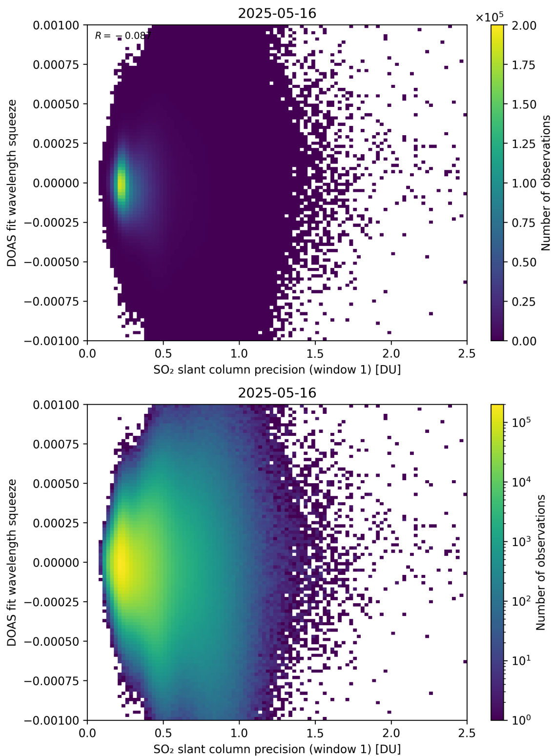
Figure 272: Scatter density plot of “SO 2 slant column precision (window 1)” against “DOAS fit wavelength squeeze” for 2025-05-15 to 2025-05-17.
