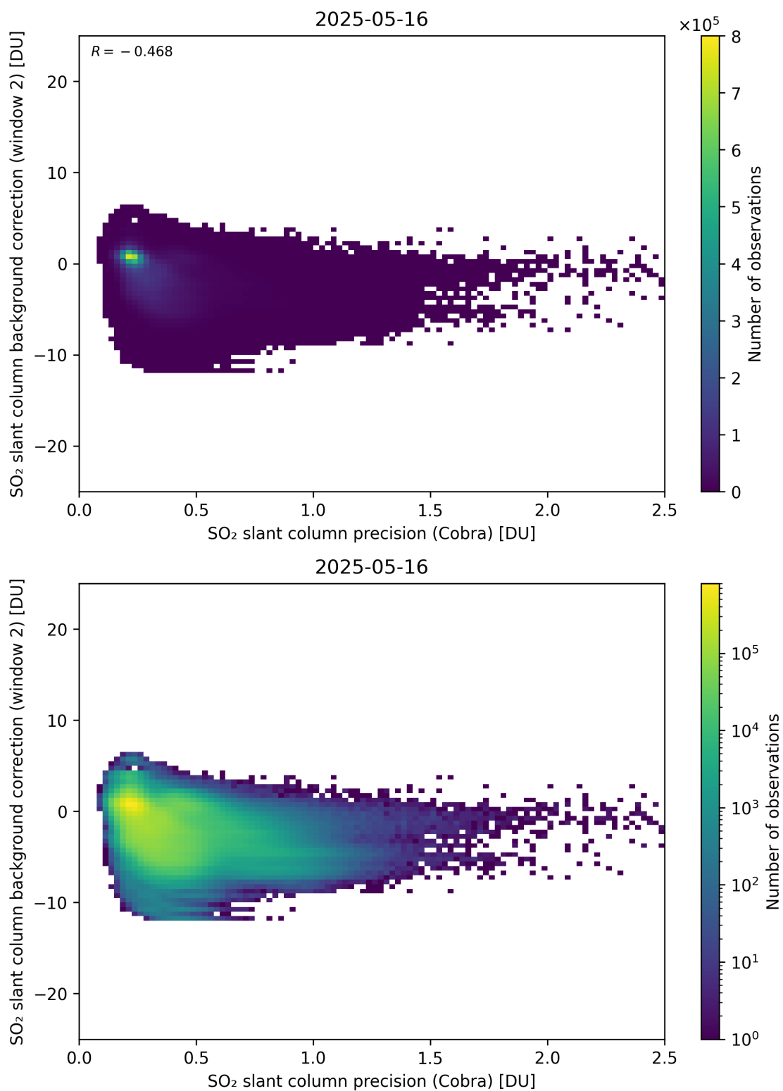
Figure 200: Scatter density plot of “SO 2 slant column precision (Cobra)” against “SO 2 slant column background correction (window 2)” for 2025-05-15 to 2025-05-17.
