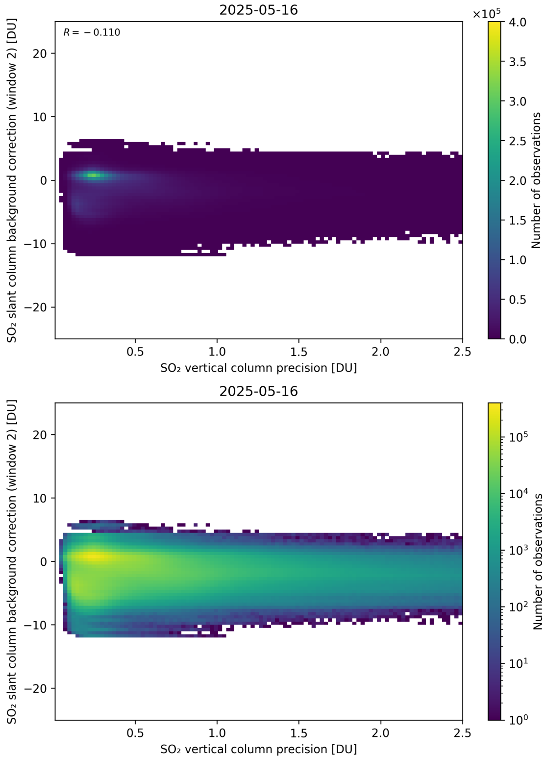
Figure 330: Scatter density plot of “SO 2 vertical column precision” against “SO 2 slant column background correction (window 2)” for 2025-05-15 to 2025-05-17.
