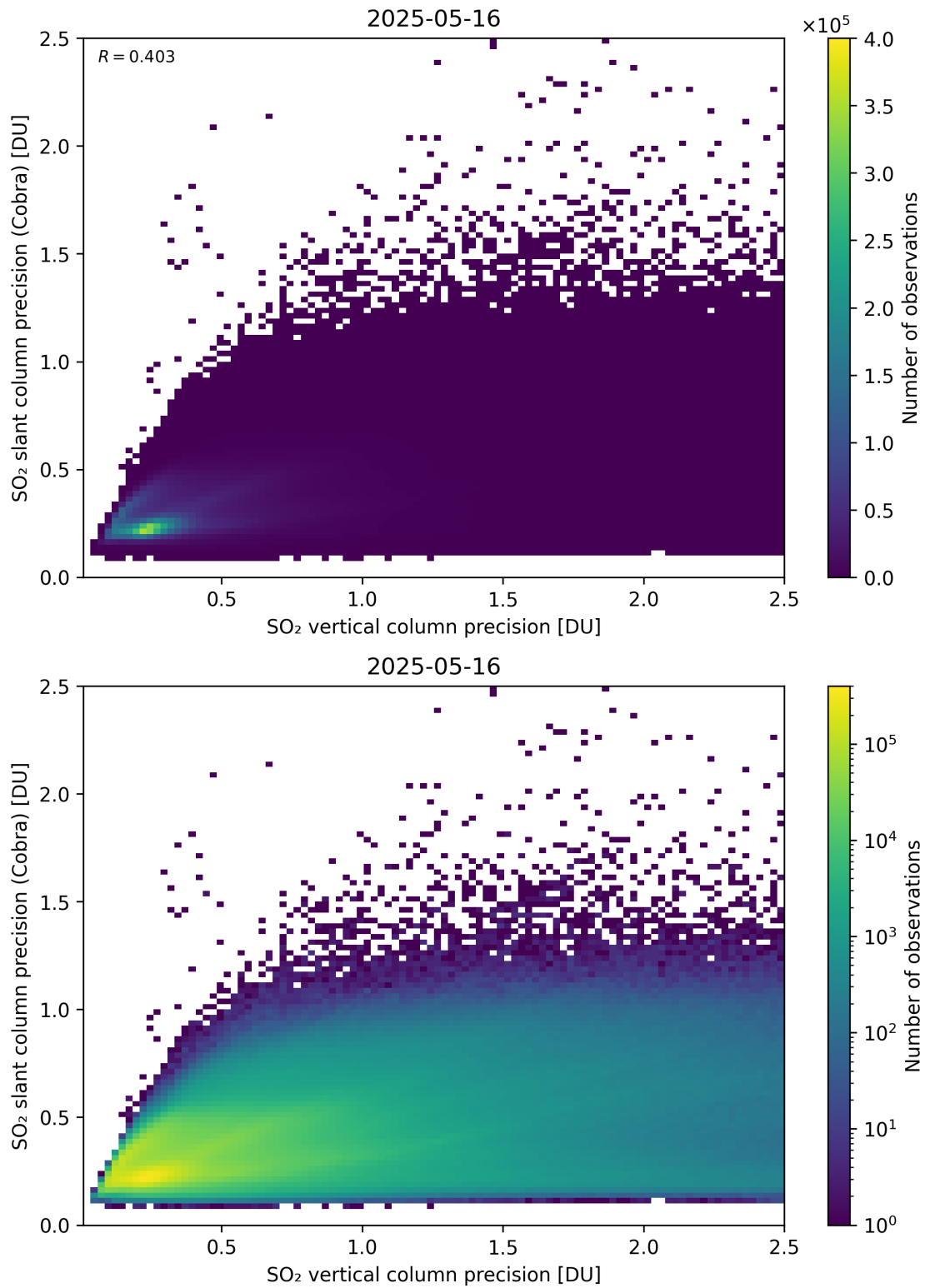
Figure 337: Scatter density plot of “SO 2 vertical column precision” against “SO 2 slant column precision (Cobra)” for 2025-05-15 to 2025-05-17.
