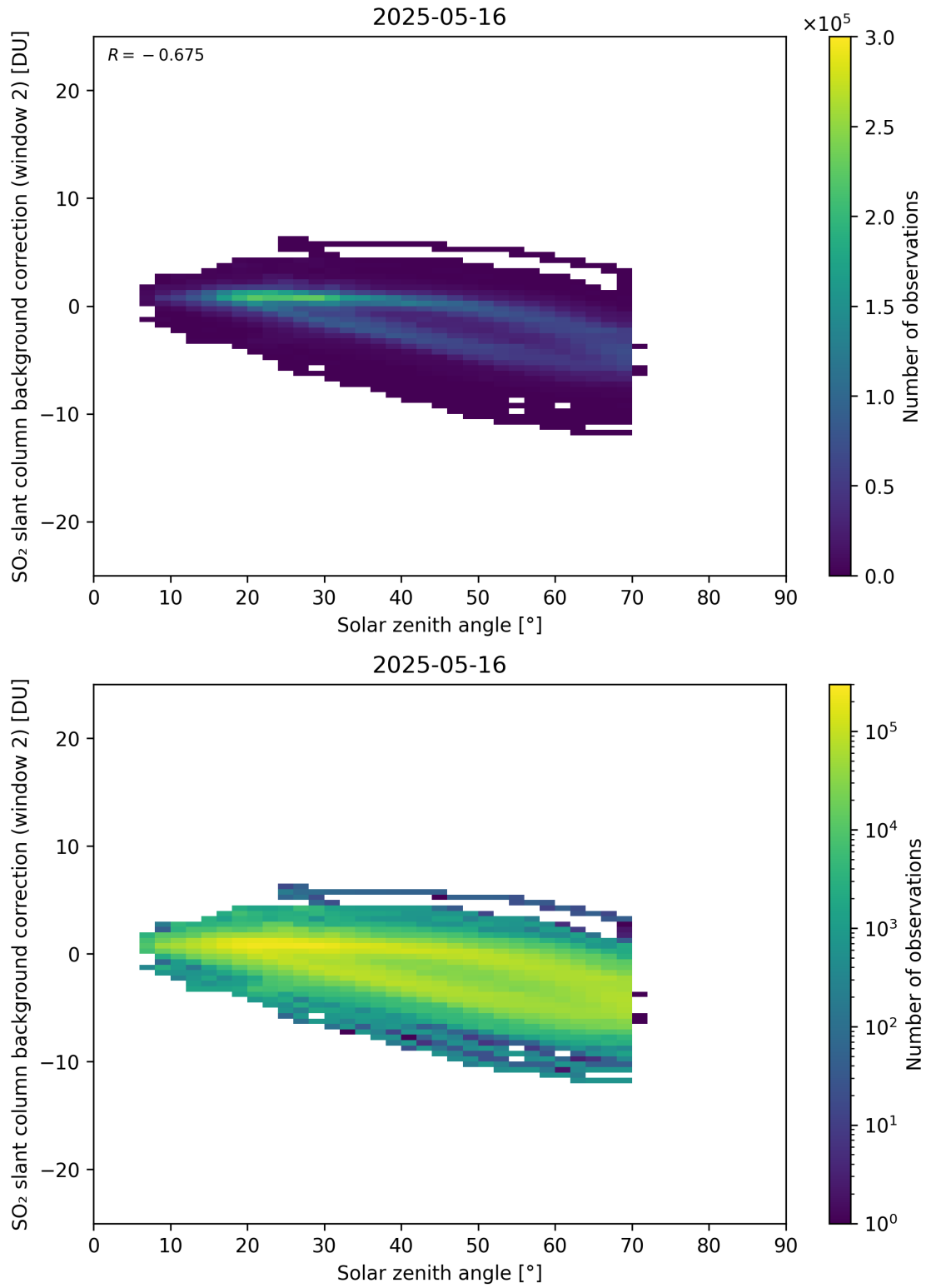
Figure 172: Scatter density plot of “Solar zenith angle” against “SO 2 slant column background correction (window 2)” for 2025-05-15 to 2025-05-17.
