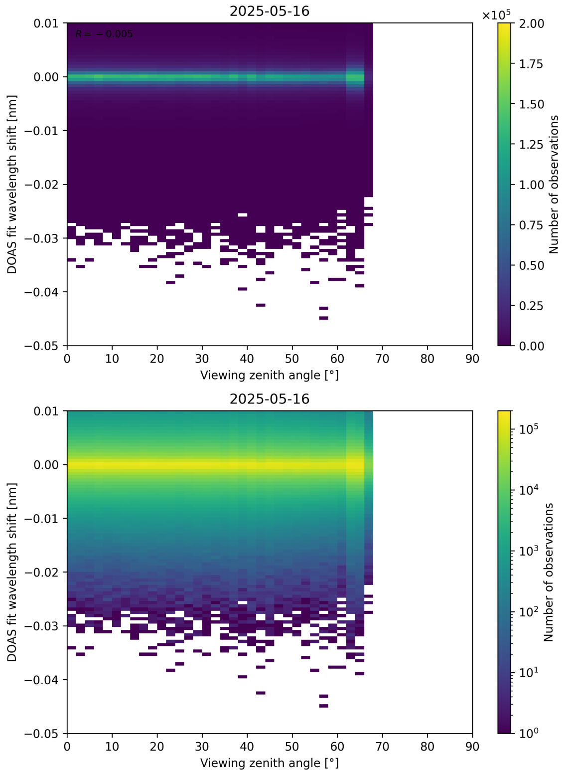
Figure 365: Scatter density plot of “Viewing zenith angle” against “DOAS fit wavelength shift” for 2025-05-15 to 2025-05-17.
