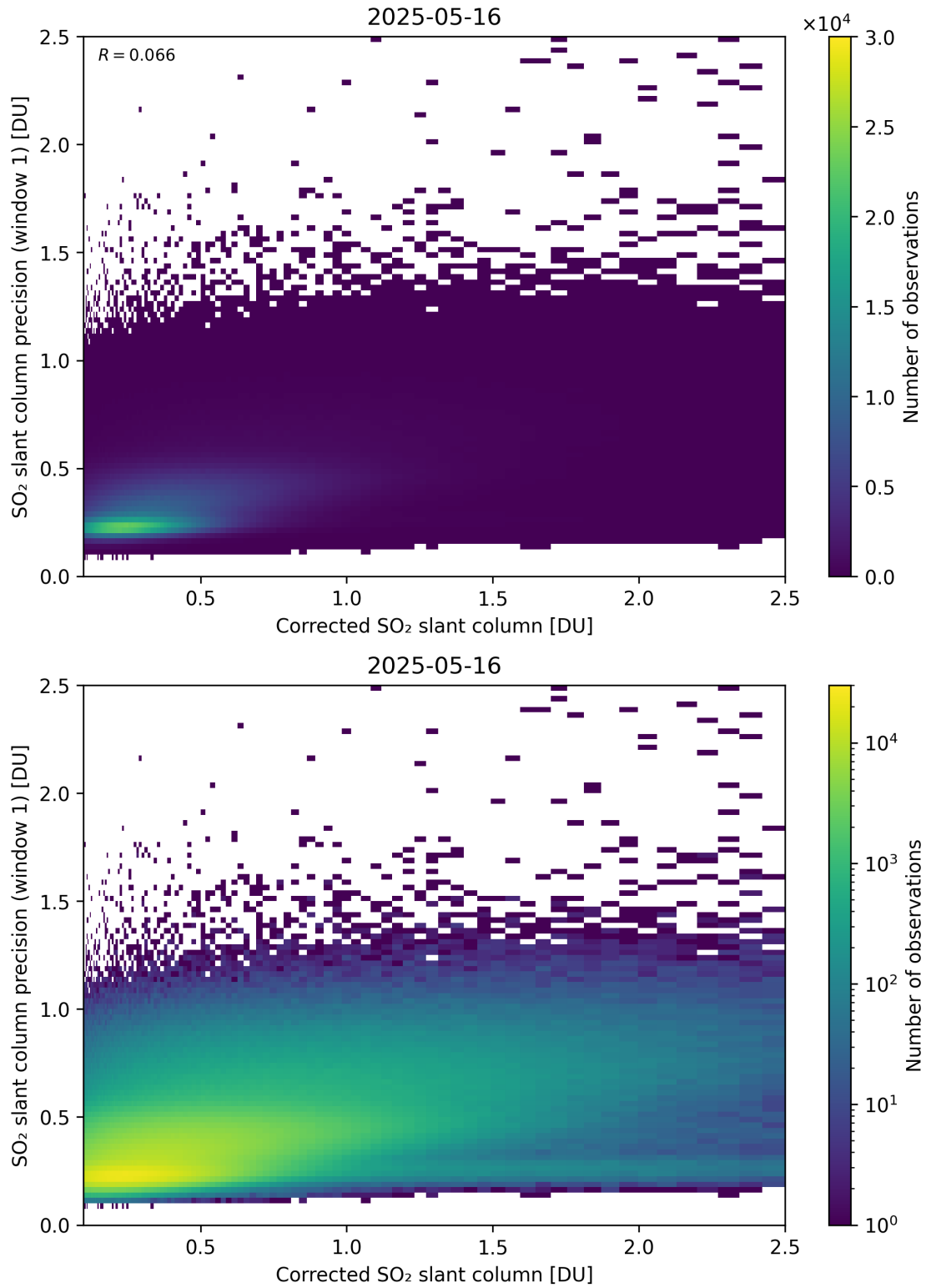
Figure 238: Scatter density plot of “Corrected SO 2 slant column” against “SO 2 slant column precision (window 1)” for 2025-05-15 to 2025-05-17.
