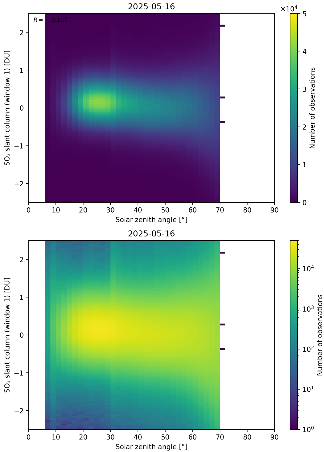
Figure 184: Scatter density plot of “Solar zenith angle” against “SO 2 slant column (window 1)” for 2025-05-15 to 2025-05-17.
