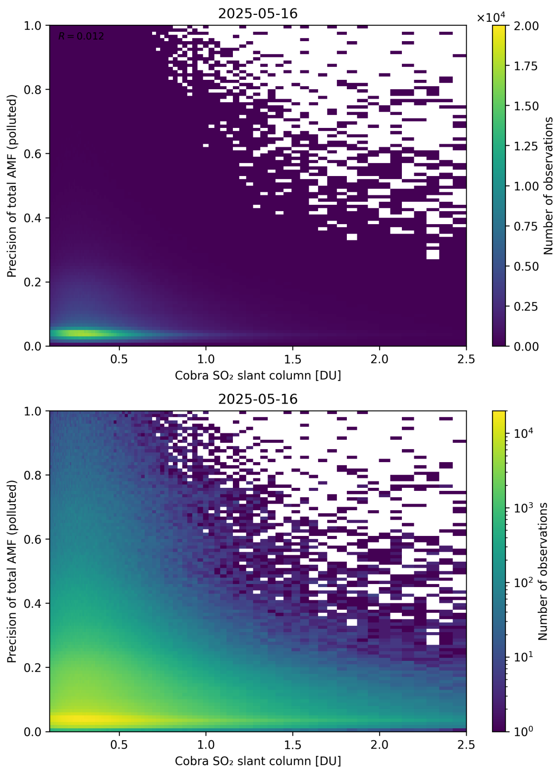
Figure 225: Scatter density plot of “Cobra SO 2 slant column” against “Precision of total AMF (polluted)” for 2025-05-15 to 2025-05-17.
