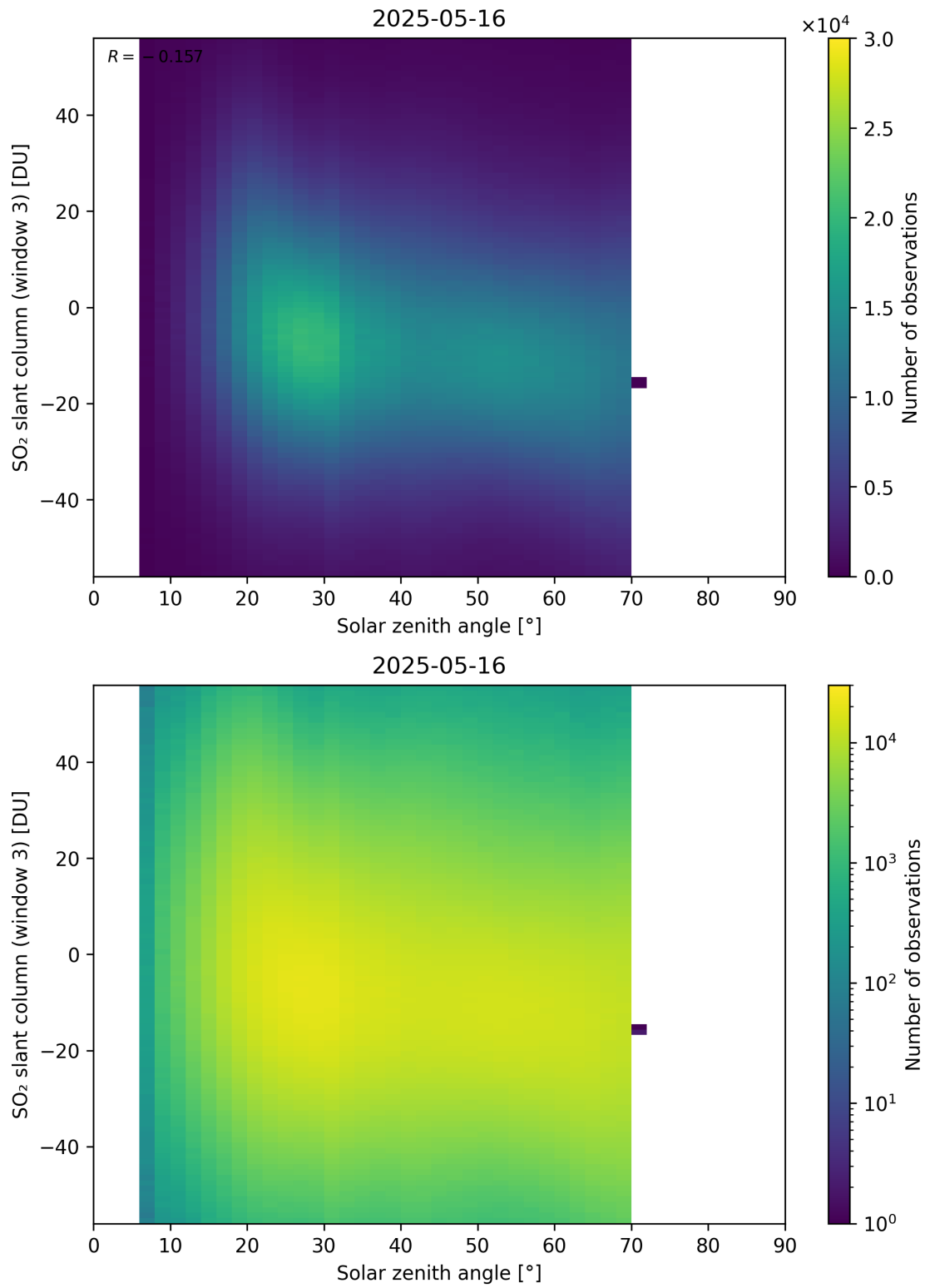
Figure 187: Scatter density plot of “Solar zenith angle” against “SO 2 slant column (window 3)” for 2025-05-15 to 2025-05-17.
