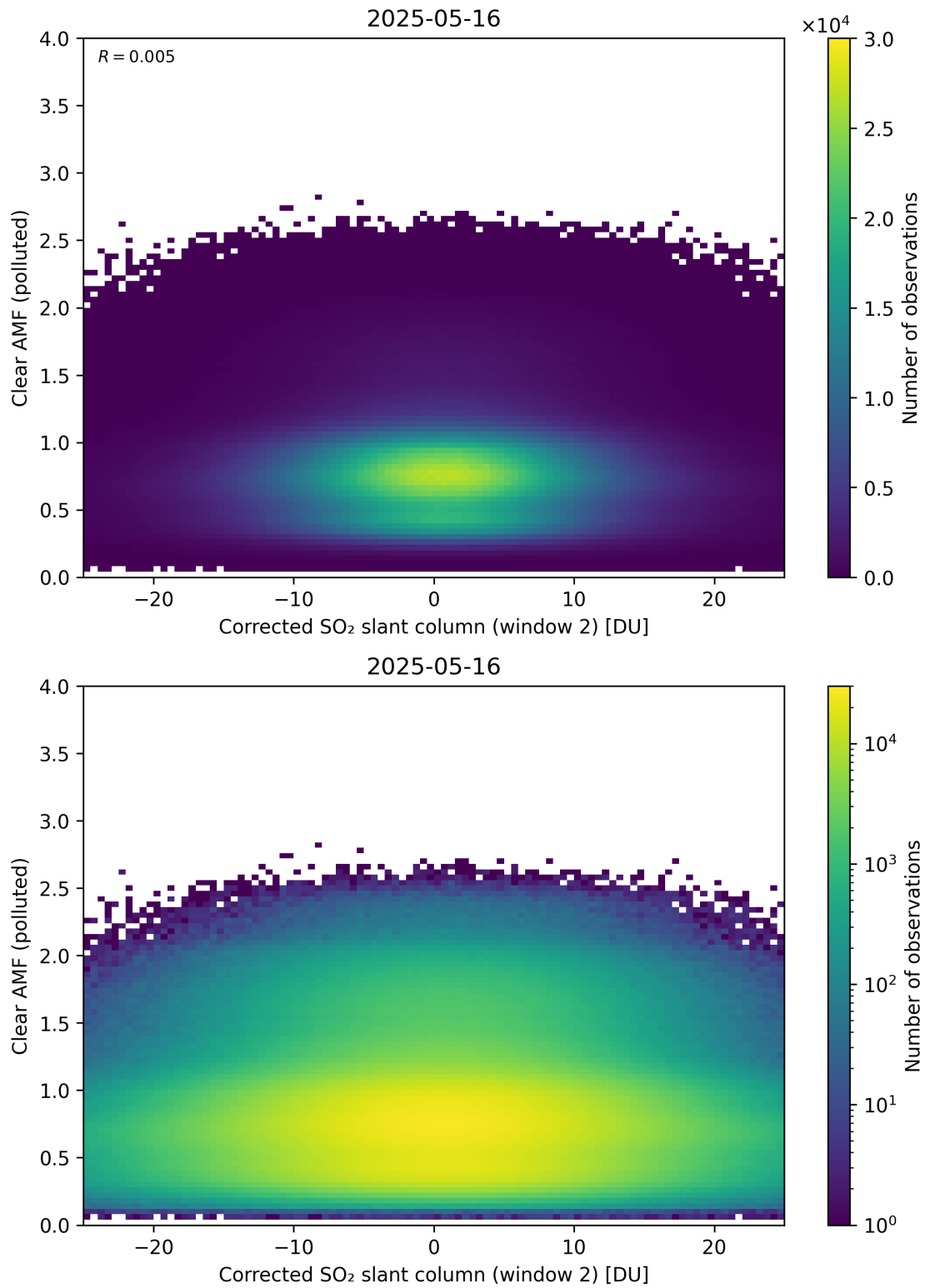
Figure 249: Scatter density plot of “Corrected SO 2 slant column (window 2)” against “Clear AMF (polluted)” for 2025-05-15 to 2025-05-17.
