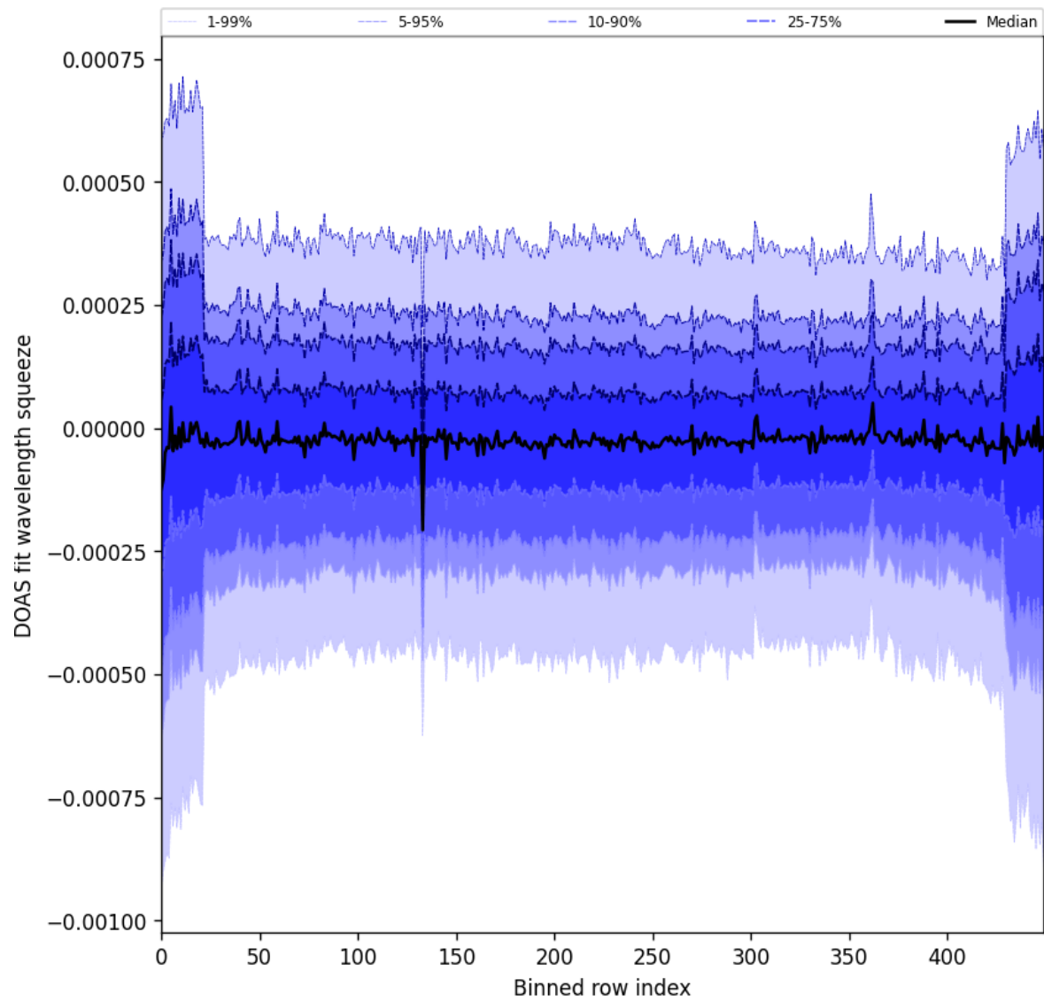
Figure 103: Along track statistics of “DOAS fit wavelength squeeze” for 2025-05-15 to 2025-05-17
