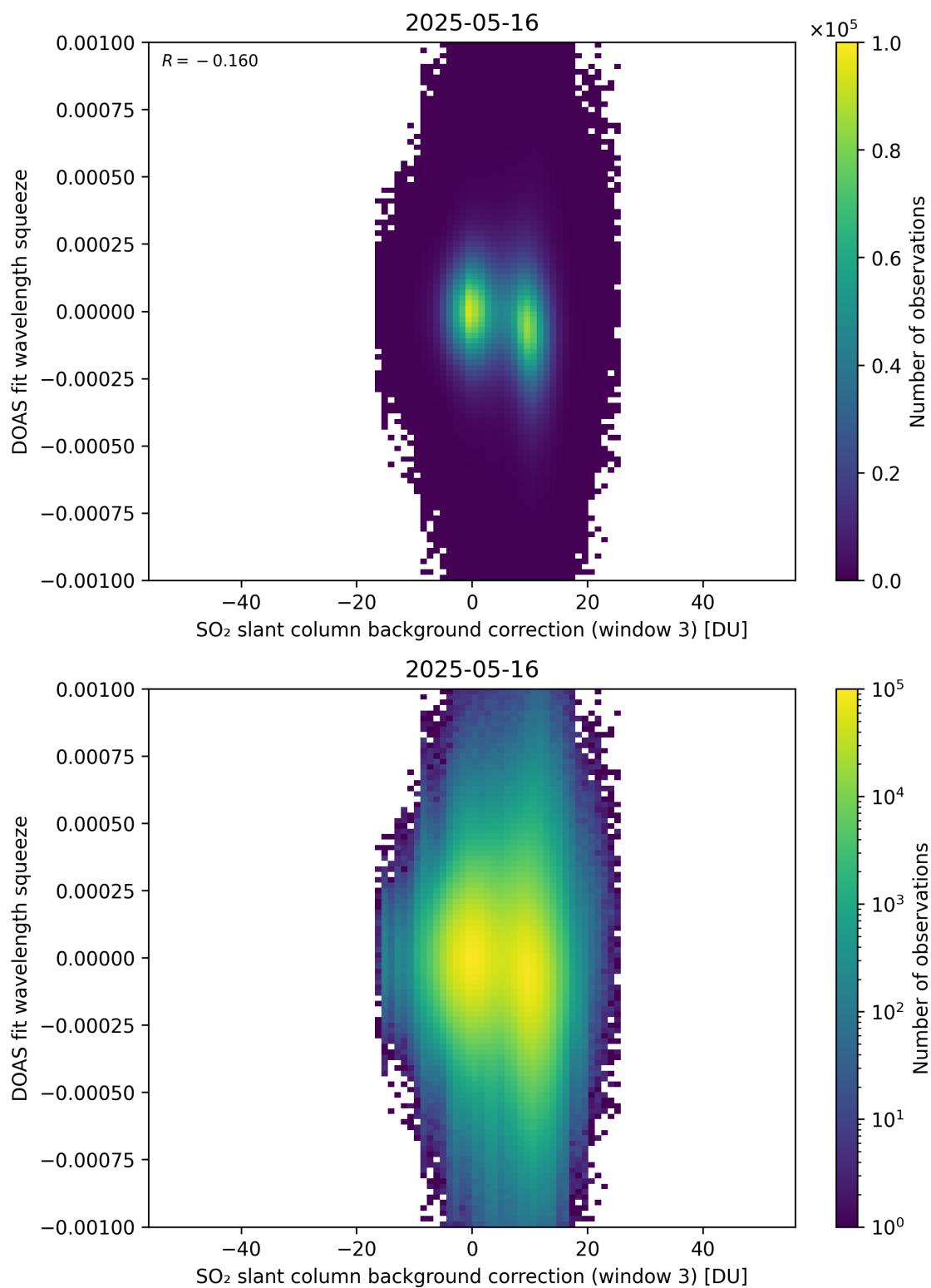
Figure 133: Scatter density plot of “SO 2 slant column background correction (window 3)” against “DOAS fit wavelength squeeze” for 2025-05-15 to 2025-05-17.
