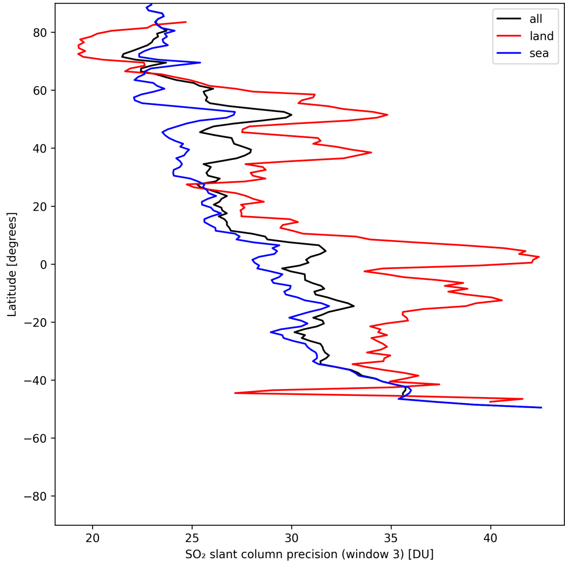
Figure 46: Zonal average of “SO 2 slant column precision (window 3)” for 2025-05-15 to 2025-05-17.
