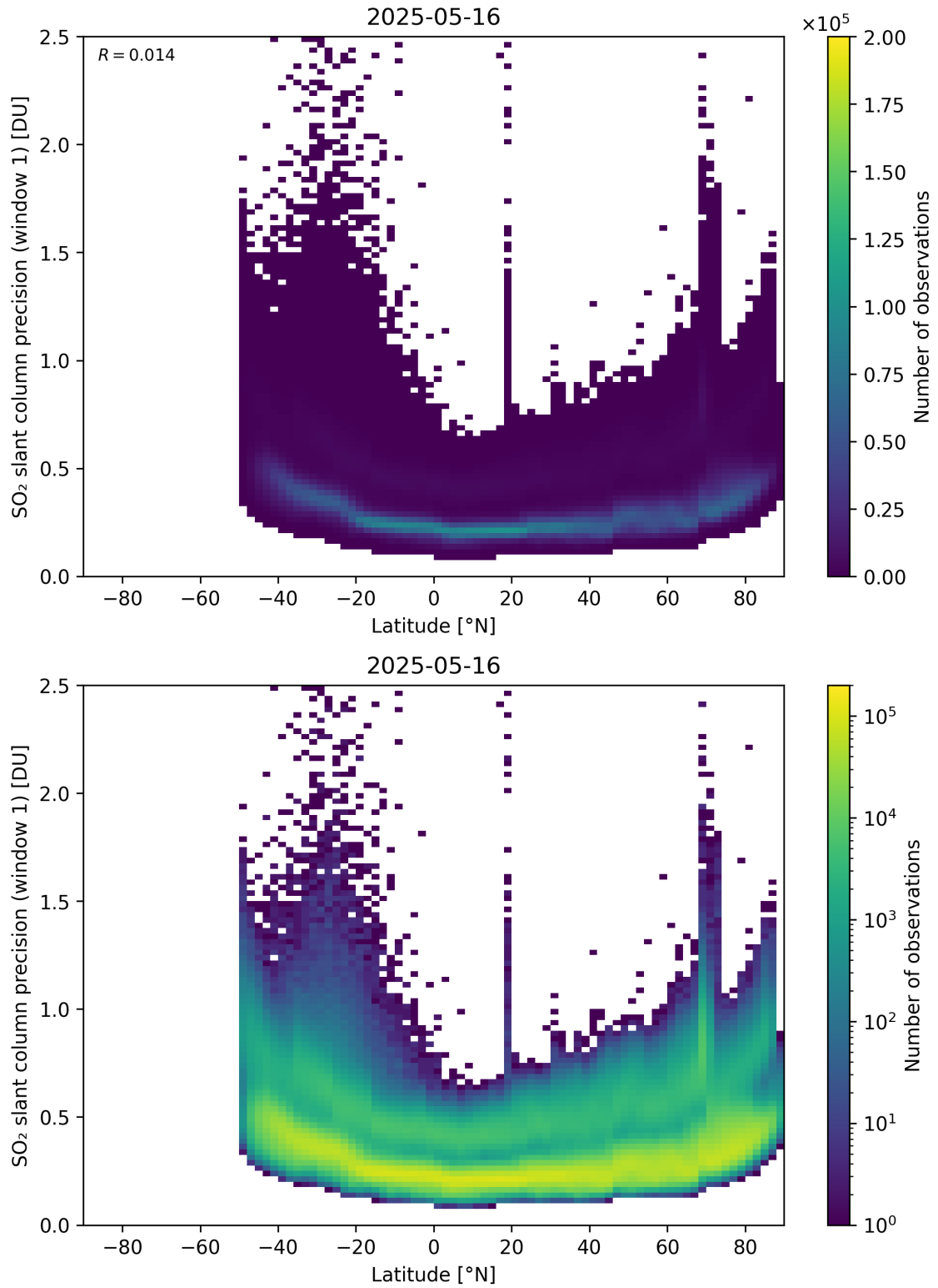
Figure 163: Scatter density plot of “Latitude” against “SO 2 slant column precision (window 1)” for 2025-05-15 to 2025-05-17.
