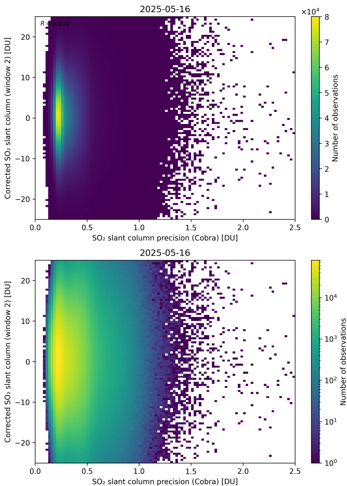
Figure 206: Scatter density plot of “SO 2 slant column precision (Cobra)” against “Corrected SO 2 slant column (window 2)” for 2025-05-15 to 2025-05-17.
