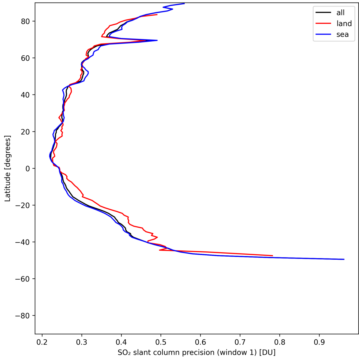
Figure 38: Zonal average of “SO 2 slant column precision (window 1)” for 2025-05-15 to 2025-05-17.
