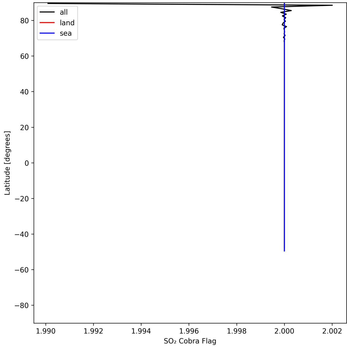
Figure 49: Zonal average of “SO 2 Cobra Flag” for 2025-05-15 to 2025-05-17.
