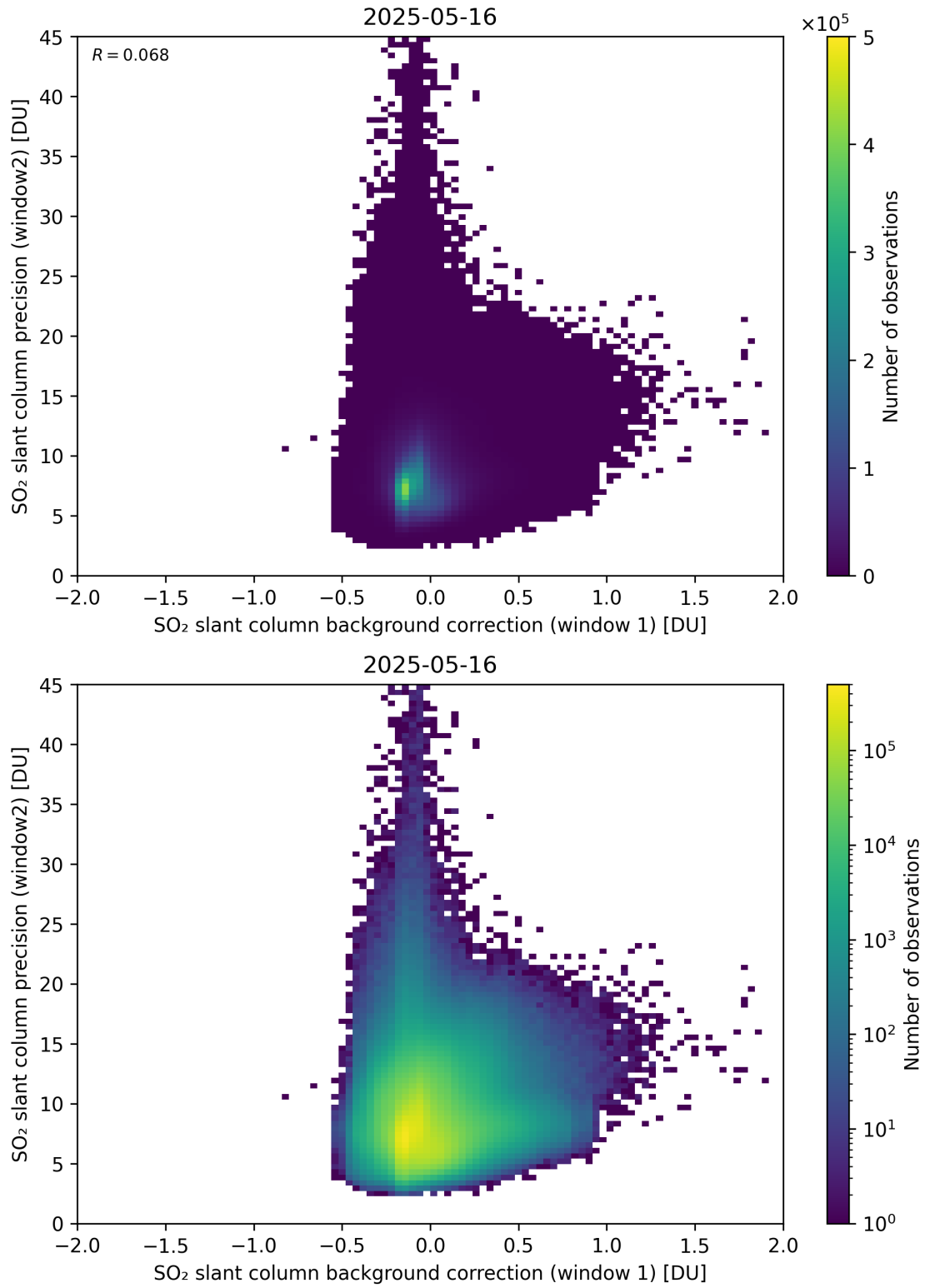
Figure 117: Scatter density plot of “SO 2 slant column background correction (window 1)” against “SO 2 slant column precision (window2)” for 2025-05-15 to 2025-05-17.
