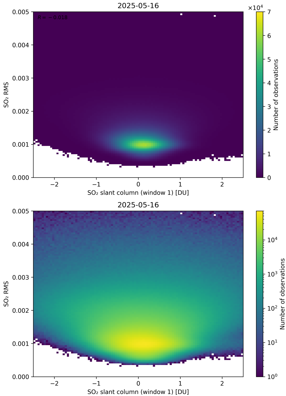
Figure 267: Scatter density plot of “SO 2 slant column (window 1)” against “SO 2 RMS” for 2025-05-15 to 2025-05-17.
