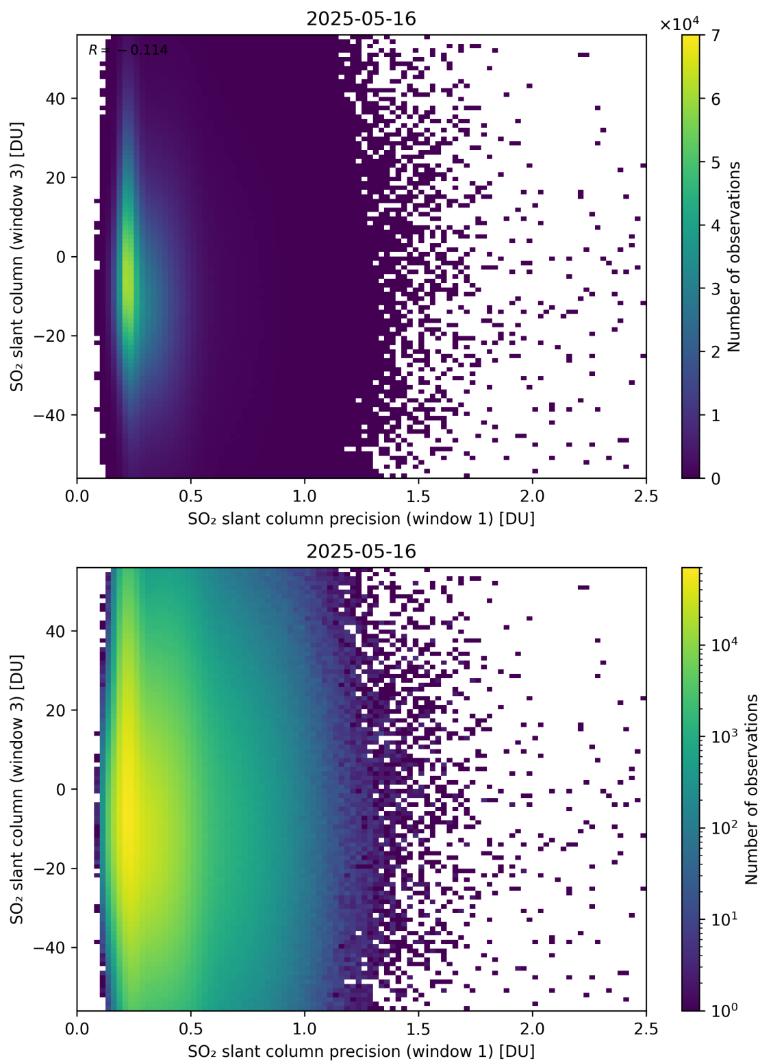
Figure 278: Scatter density plot of “SO 2 slant column precision (window 1)” against “SO 2 slant column (window 3)” for 2025-05-15 to 2025-05-17.
