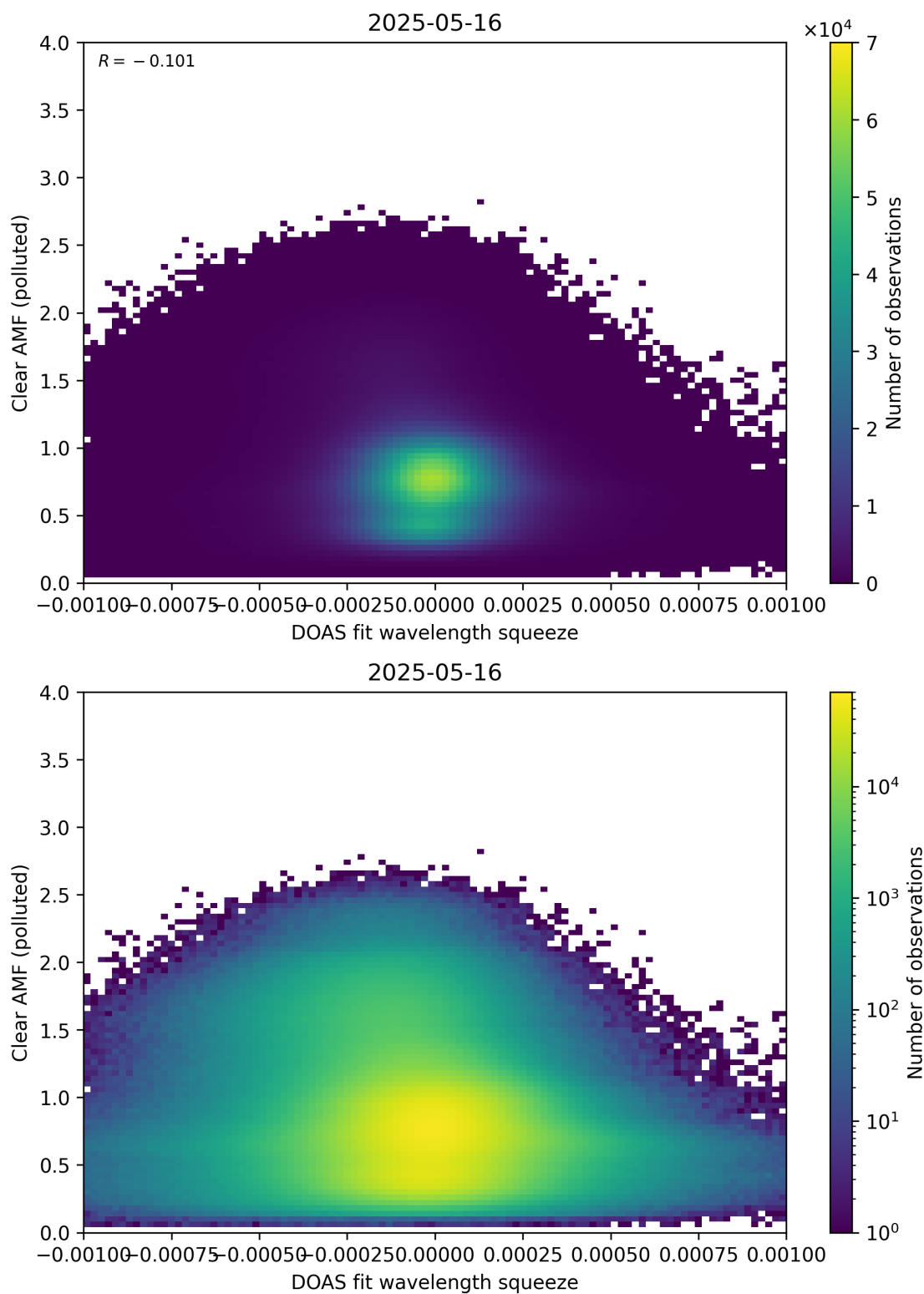
Figure 144: Scatter density plot of “DOAS fit wavelength squeeze” against “Clear AMF (polluted)” for 2025-05-15 to 2025-05-17.
