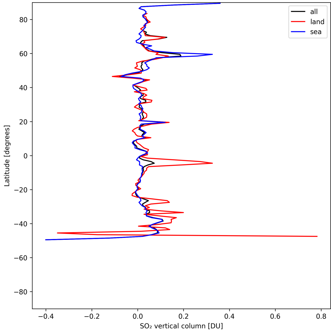
Figure 32: Zonal average of “SO 2 vertical column” for 2025-05-15 to 2025-05-17.
