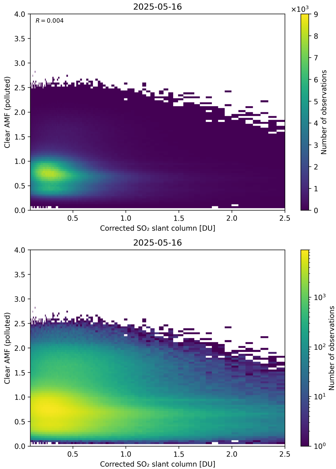
Figure 232: Scatter density plot of “Corrected SO 2 slant column” against “Clear AMF (polluted)” for 2025-05-15 to 2025-05-17.
