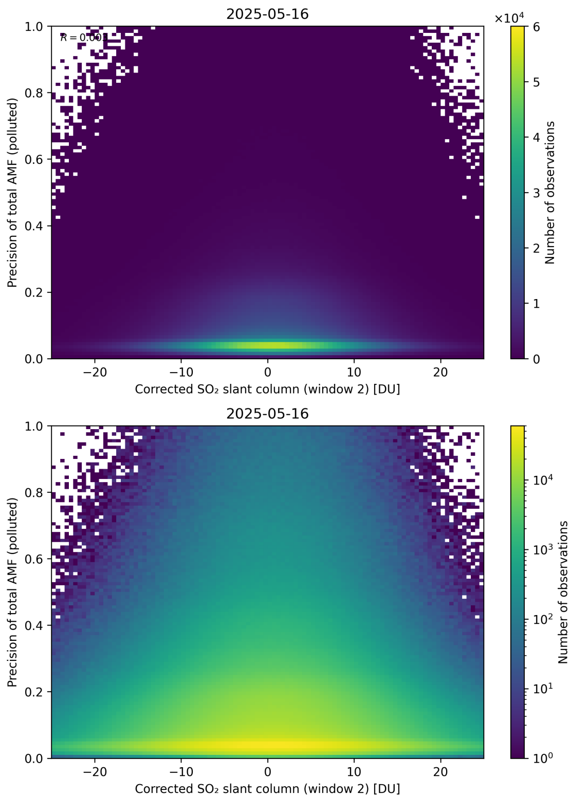
Figure 254: Scatter density plot of “Corrected SO 2 slant column (window 2)” against “Precision of total AMF (polluted)” for 2025-05-15 to 2025-05-17.
