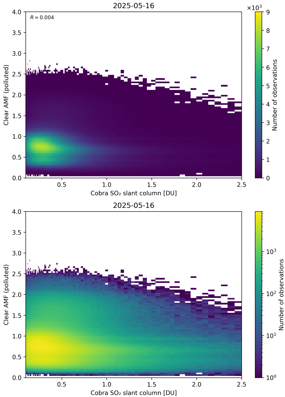
Figure 215: Scatter density plot of “Cobra SO 2 slant column” against “Clear AMF (polluted)” for 2025-05-15 to 2025-05-17.
