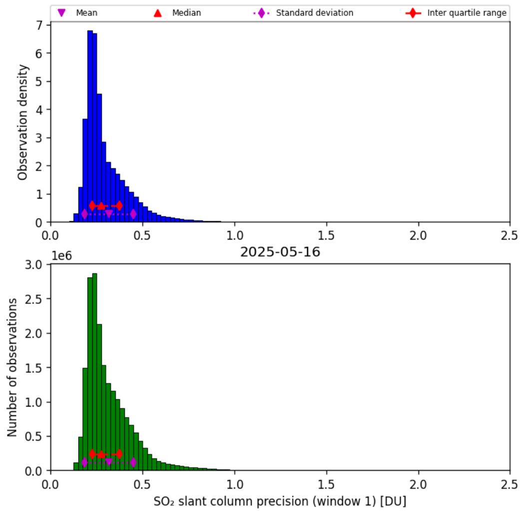
Figure 64: Histogram of “SO 2 slant column precision (window 1)” for 2025-05-15 to 2025-05-17
