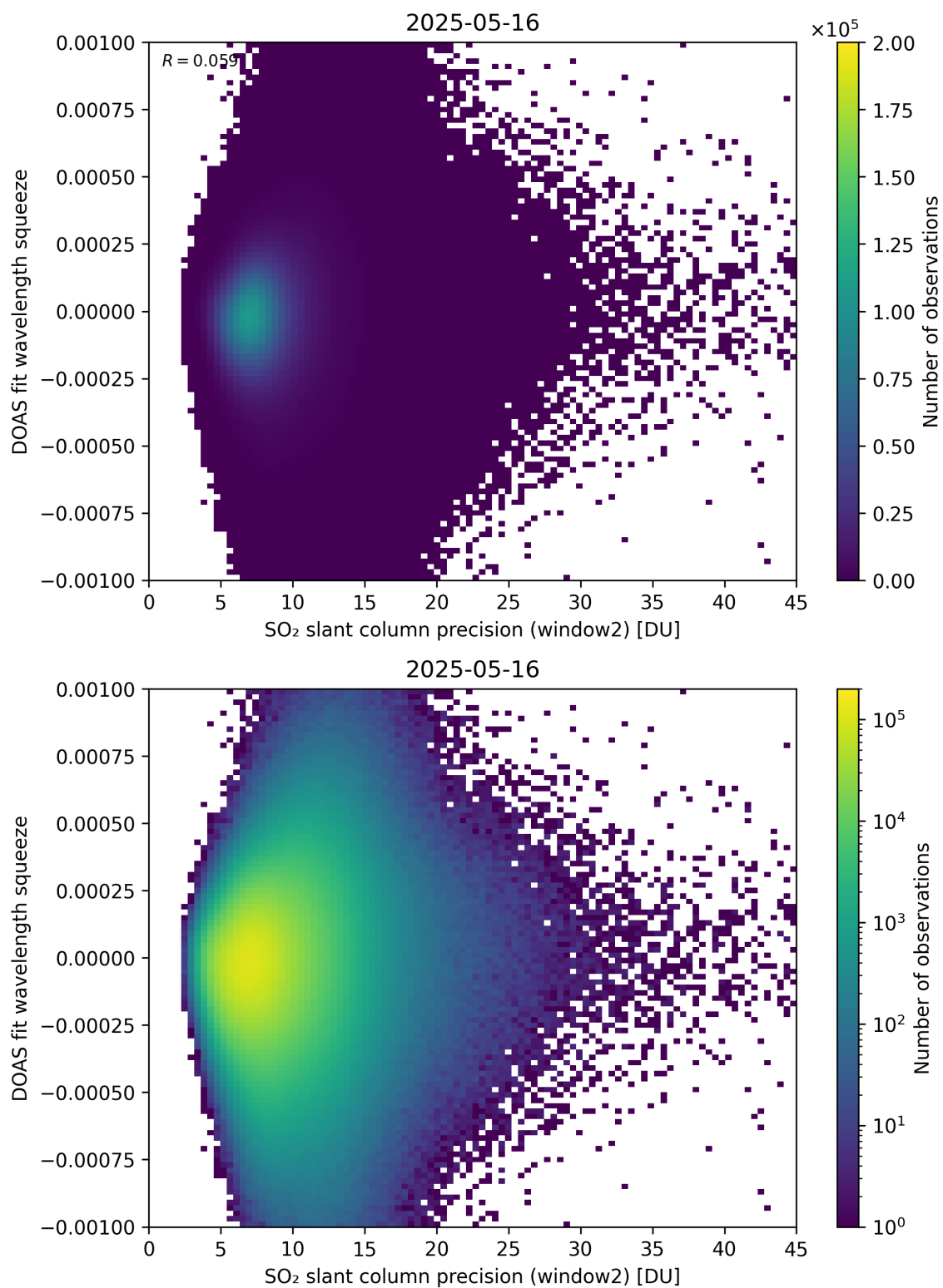
Figure 294: Scatter density plot of “SO 2 slant column precision (window2)” against “DOAS fit wavelength squeeze” for 2025-05-15 to 2025-05-17.
