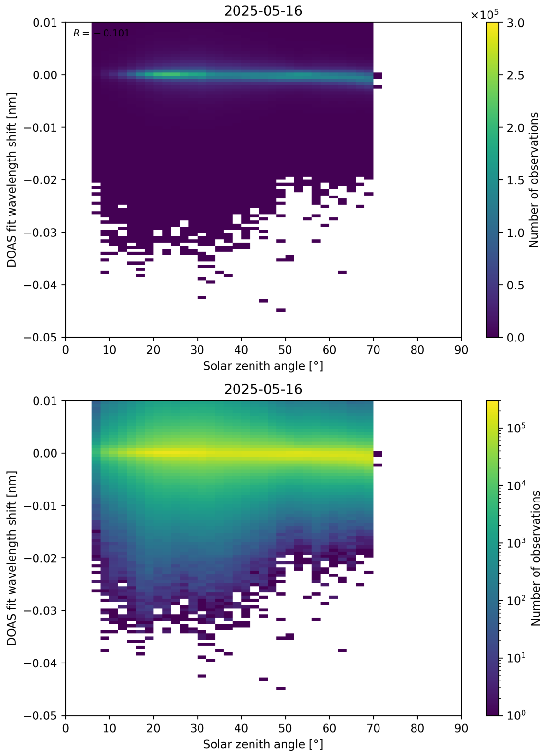
Figure 174: Scatter density plot of “Solar zenith angle” against “DOAS fit wavelength shift” for 2025-05-15 to 2025-05-17.
