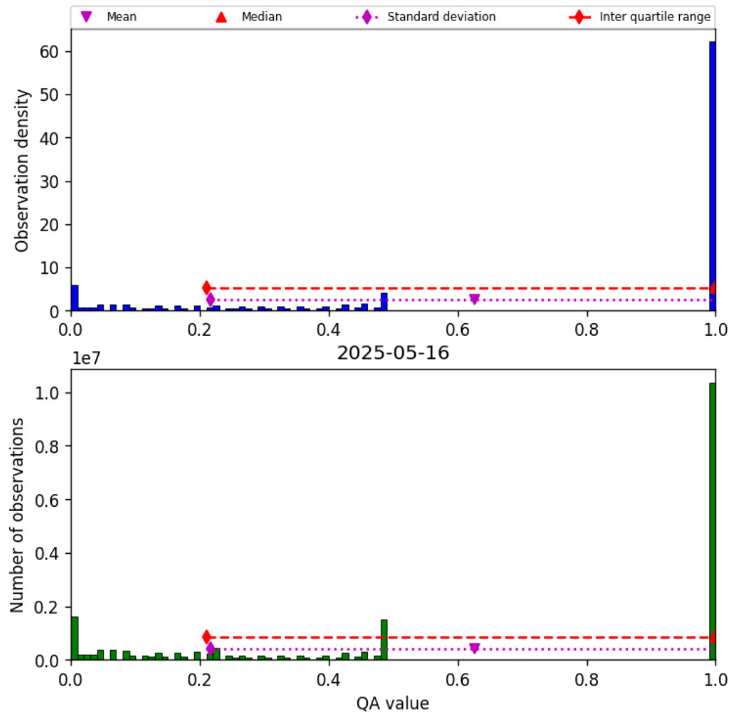
Figure 57: Histogram of “QA value” for 2025-05-15 to 2025-05-17
