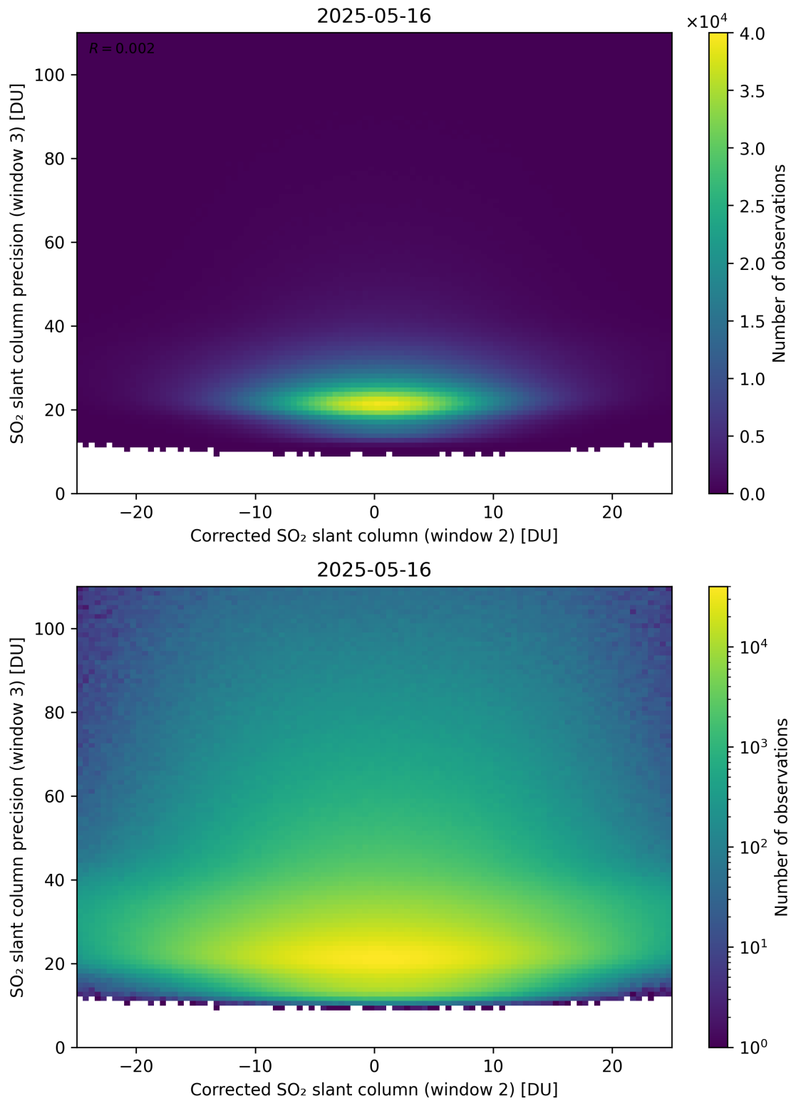
Figure 252: Scatter density plot of “Corrected SO 2 slant column (window 2)” against “SO 2 slant column precision (window 3)” for 2025-05-15 to 2025-05-17.
