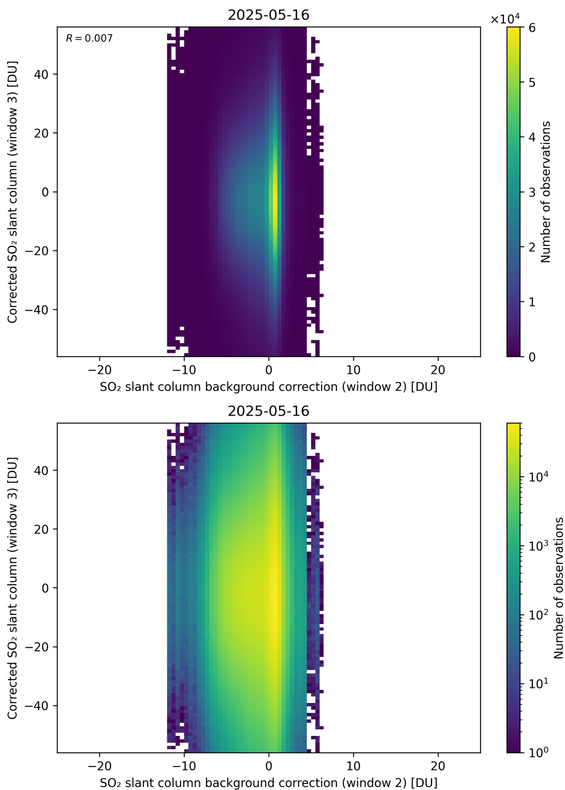
Figure 127: Scatter density plot of “SO 2 slant column background correction (window 2)” against “Corrected SO 2 slant column (window 3)” for 2025-05-15 to 2025-05-17.
