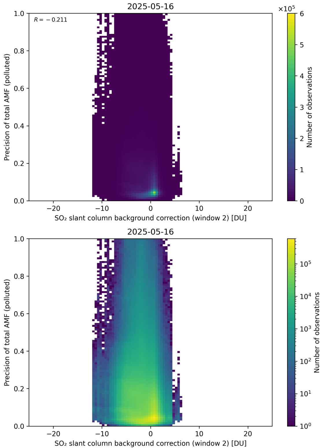
Figure 131: Scatter density plot of “SO 2 slant column background correction (window 2)” against “Precision of total AMF (polluted)” for 2025-05-15 to 2025-05-17.
