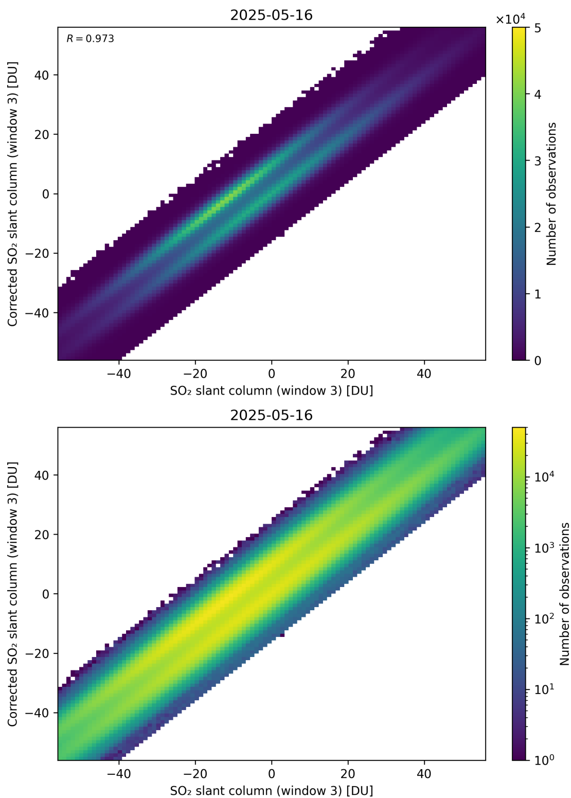
Figure 316: Scatter density plot of “SO 2 slant column (window 3)” against “Corrected SO 2 slant column (window 3)” for 2025-05-15 to 2025-05-17.
