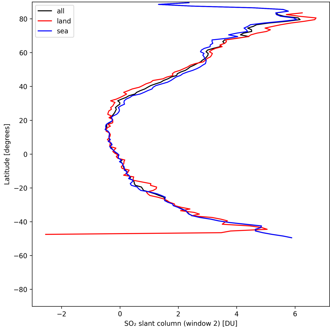
Figure 41: Zonal average of “SO 2 slant column (window 2)” for 2025-05-15 to 2025-05-17.
