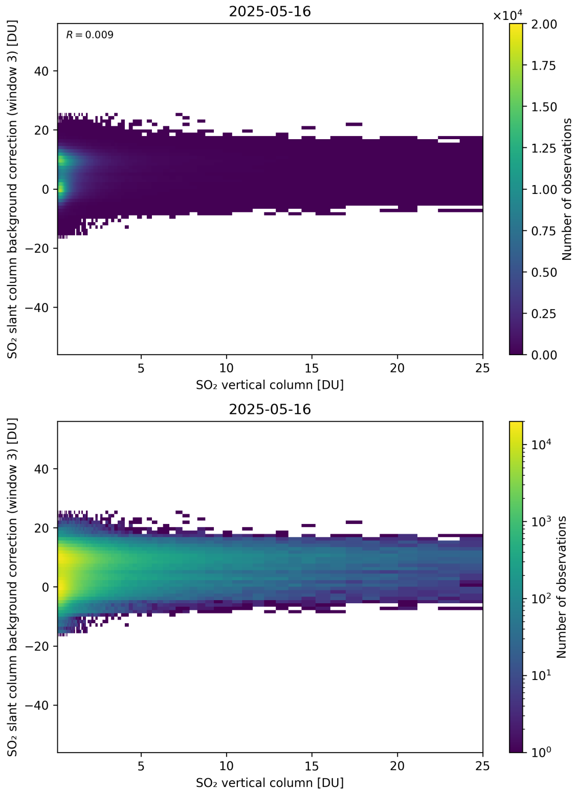
Figure 325: Scatter density plot of “SO 2 vertical column” against “SO 2 slant column background correction (window 3)” for 2025-05-15 to 2025-05-17.
