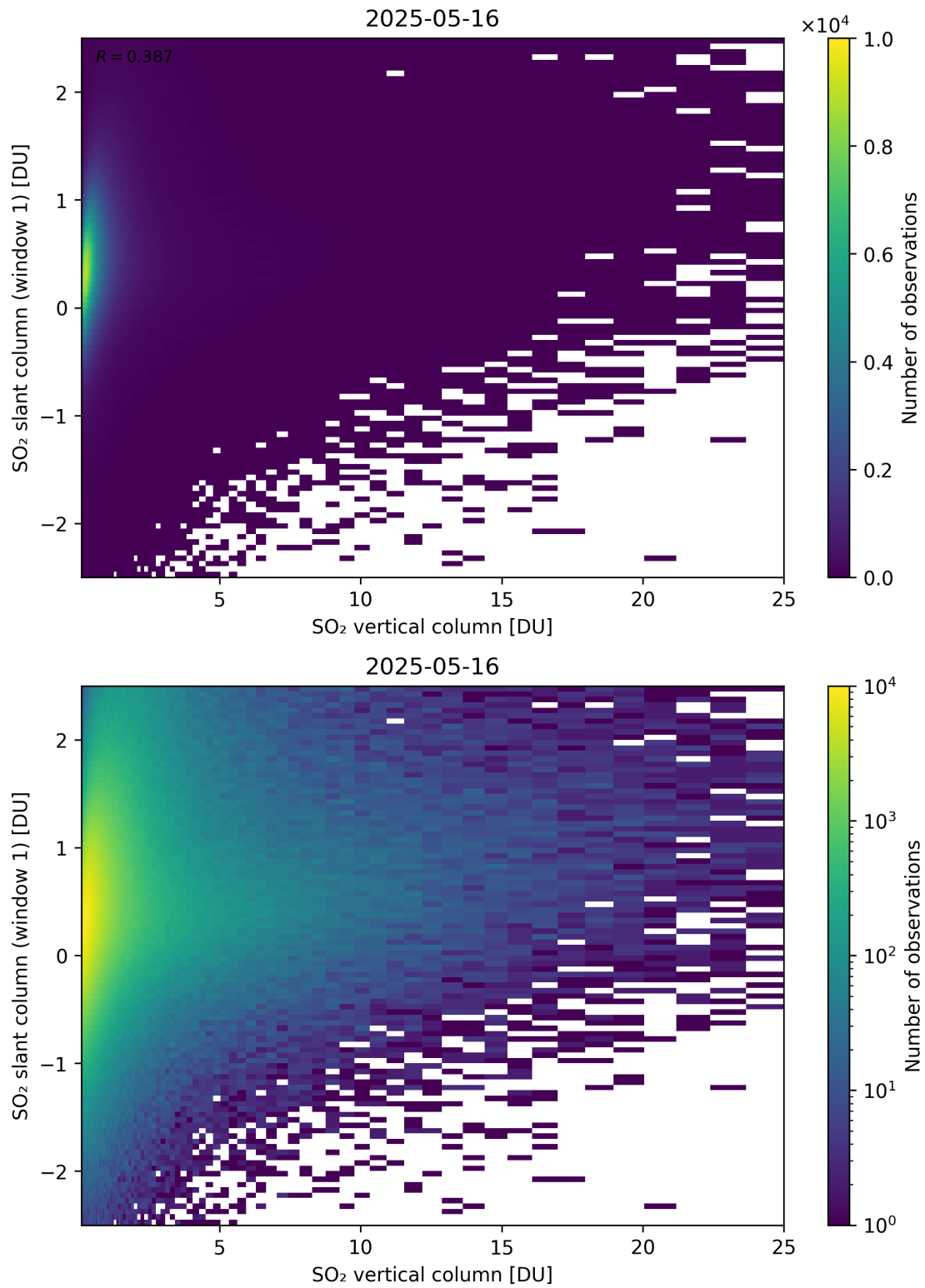
Figure 354: Scatter density plot of “SO 2 vertical column” against “SO 2 slant column (window 1)” for 2025-05-15 to 2025-05-17.
