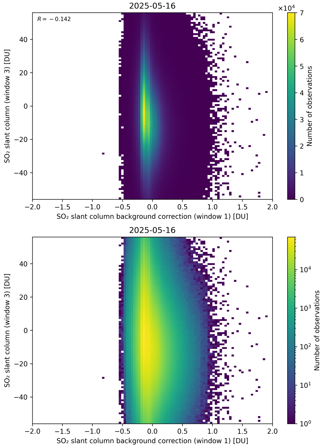
Figure 118: Scatter density plot of “SO 2 slant column background correction (window 1)” against “SO 2 slant column (window 3)” for 2025-05-15 to 2025-05-17.
