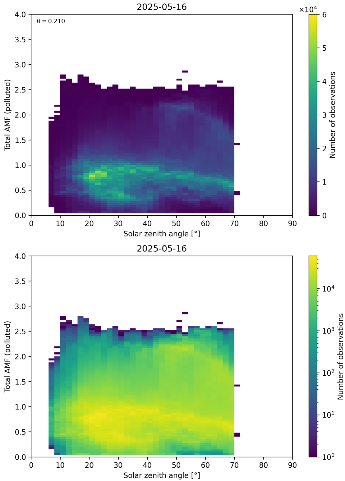
Figure 189: Scatter density plot of “Solar zenith angle” against “Total AMF (polluted)” for 2025-05-15 to 2025-05-17.
