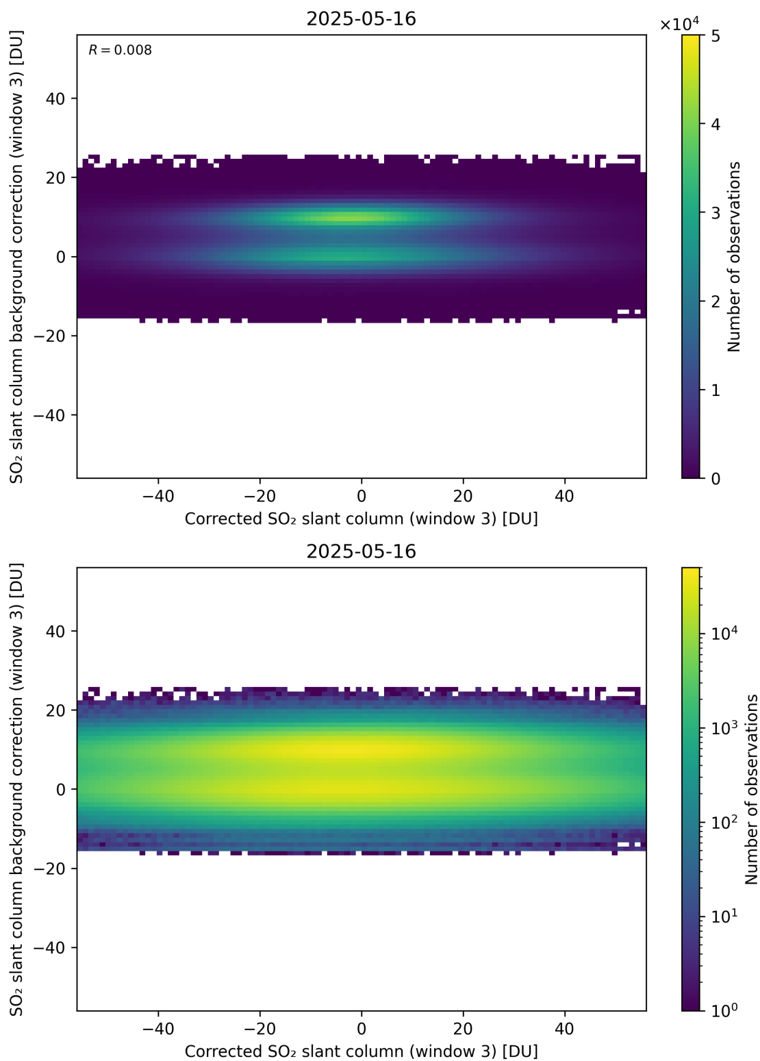
Figure 255: Scatter density plot of “Corrected SO 2 slant column (window 3)” against “SO 2 slant column background correction (window 3)” for 2025-05-15 to 2025-05-17.
