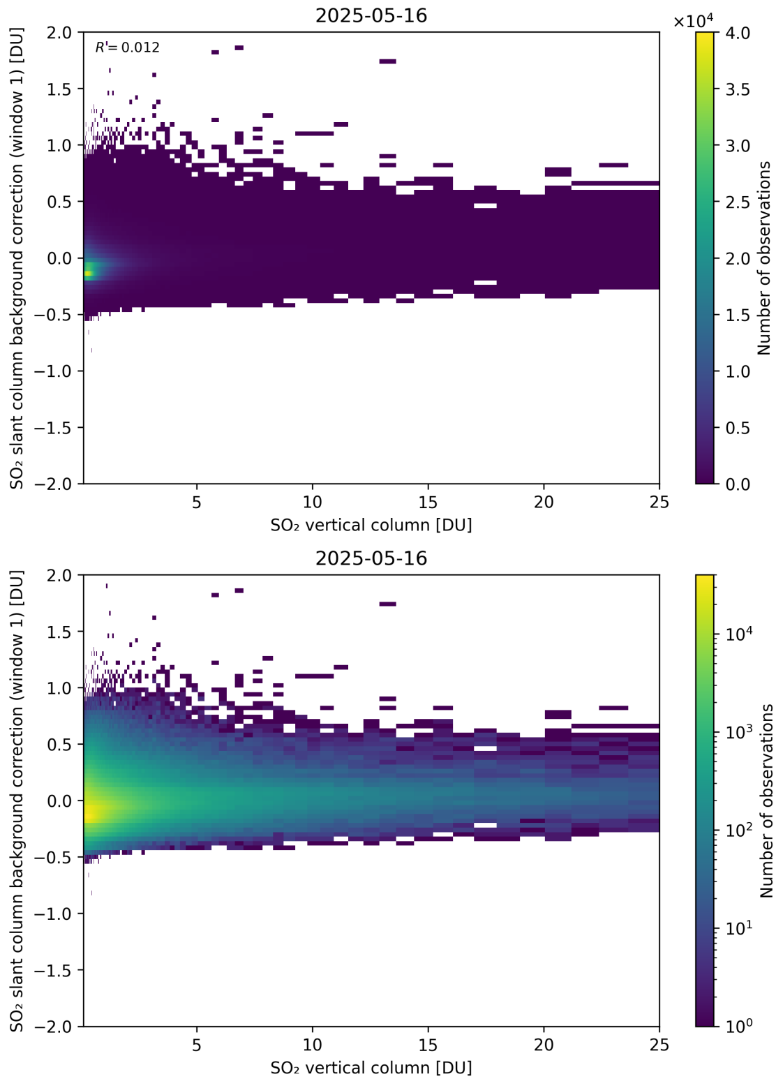
Figure 323: Scatter density plot of “SO 2 vertical column” against “SO 2 slant column background correction (window 1)” for 2025-05-15 to 2025-05-17.
