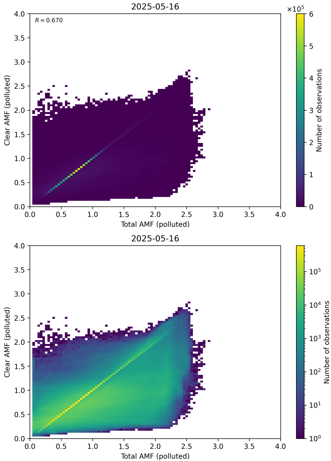
Figure 321: Scatter density plot of “Total AMF (polluted)” against “Clear AMF (polluted)” for 2025-05-15 to 2025-05-17.
