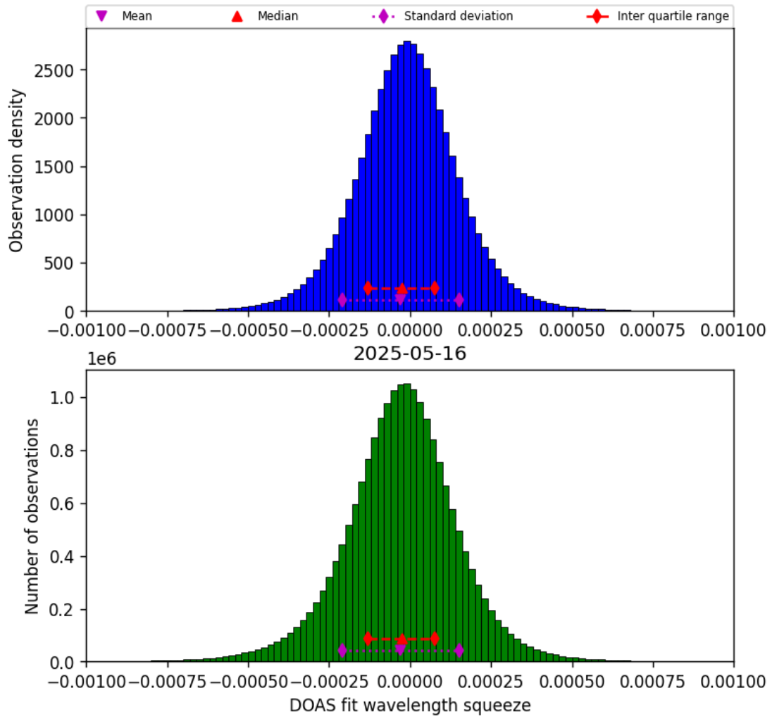
Figure 77: Histogram of “DOAS fit wavelength squeeze” for 2025-05-15 to 2025-05-17
