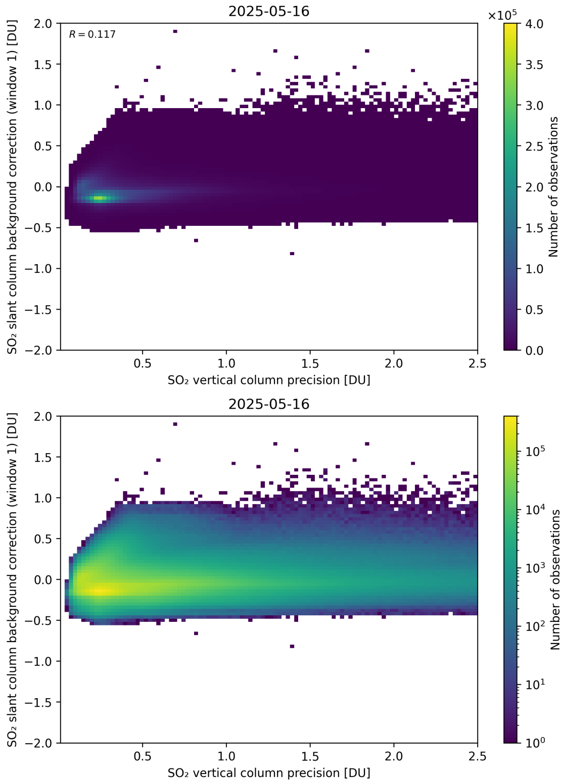
Figure 329: Scatter density plot of “SO 2 vertical column precision” against “SO 2 slant column background correction (window 1)” for 2025-05-15 to 2025-05-17.
