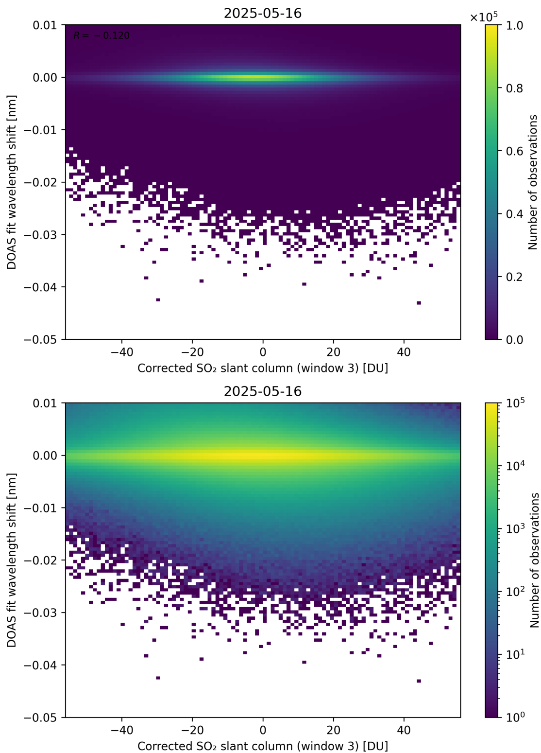
Figure 256: Scatter density plot of “Corrected SO 2 slant column (window 3)” against “DOAS fit wavelength shift” for 2025-05-15 to 2025-05-17.
