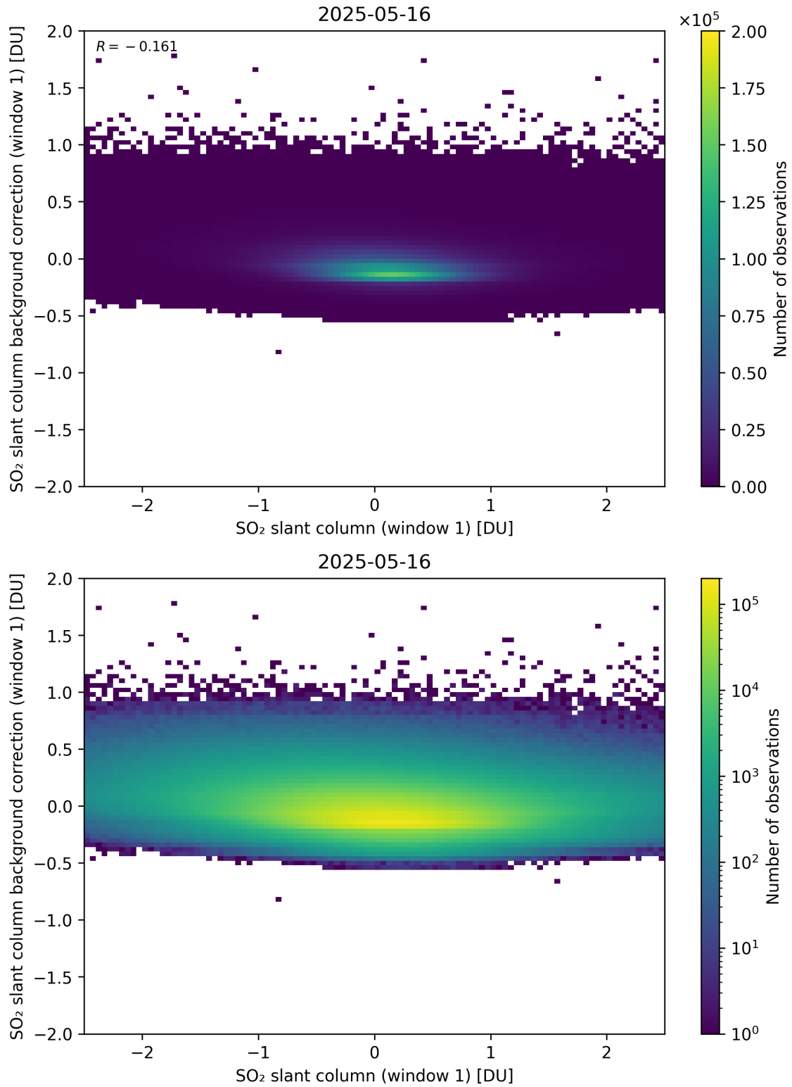
Figure 262: Scatter density plot of “SO 2 slant column (window 1)” against “SO 2 slant column background correction (window 1)” for 2025-05-15 to 2025-05-17.
