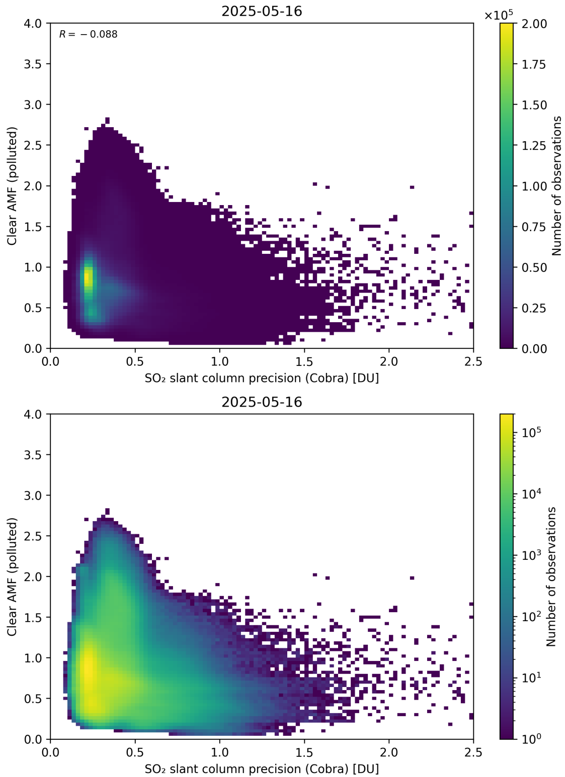
Figure 205: Scatter density plot of “SO 2 slant column precision (Cobra)” against “Clear AMF (polluted)” for 2025-05-15 to 2025-05-17.
