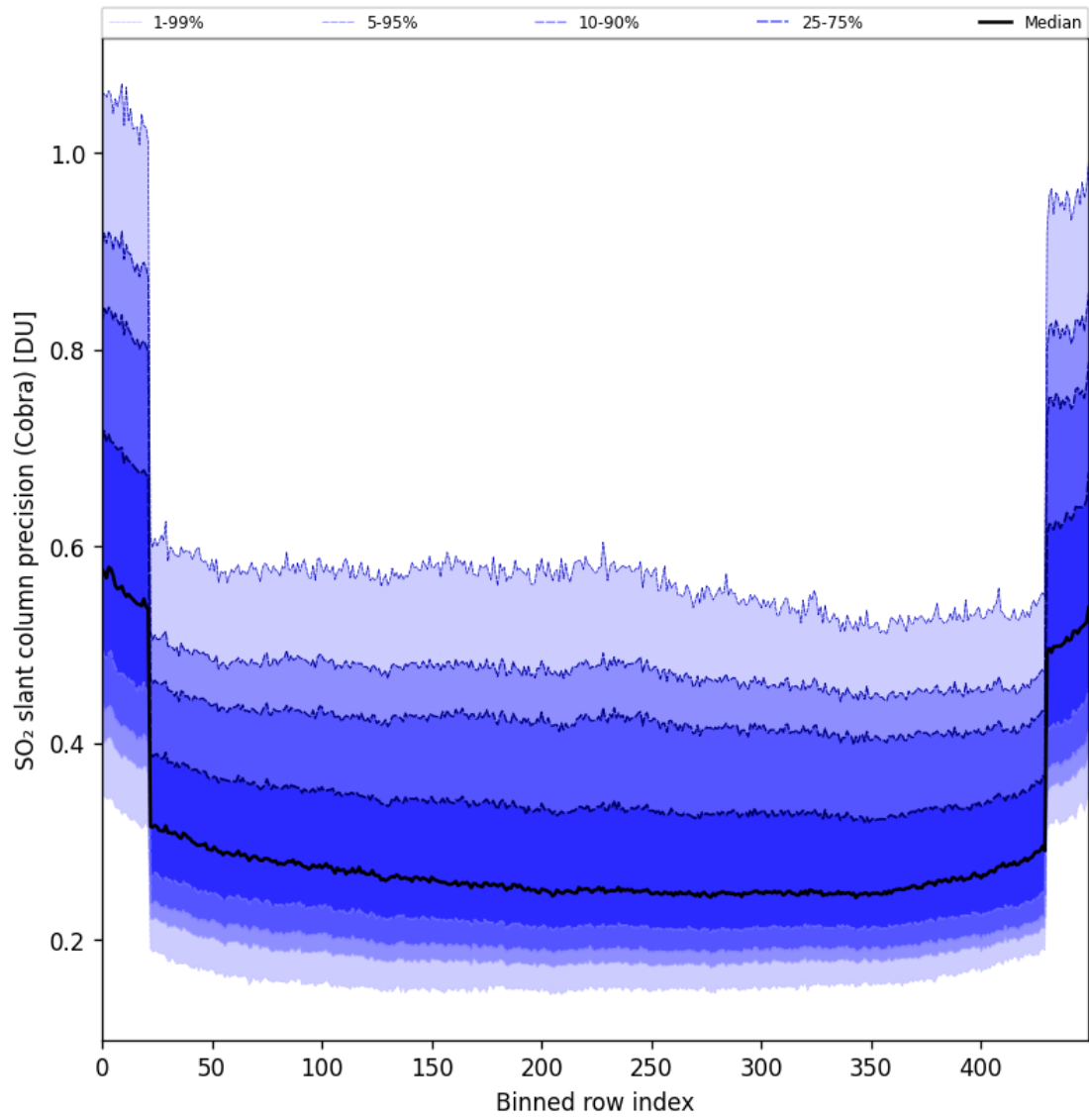
Figure 88: Along track statistics of “SO 2 slant column precision (Cobra)” for 2025-05-15 to 2025-05-17
