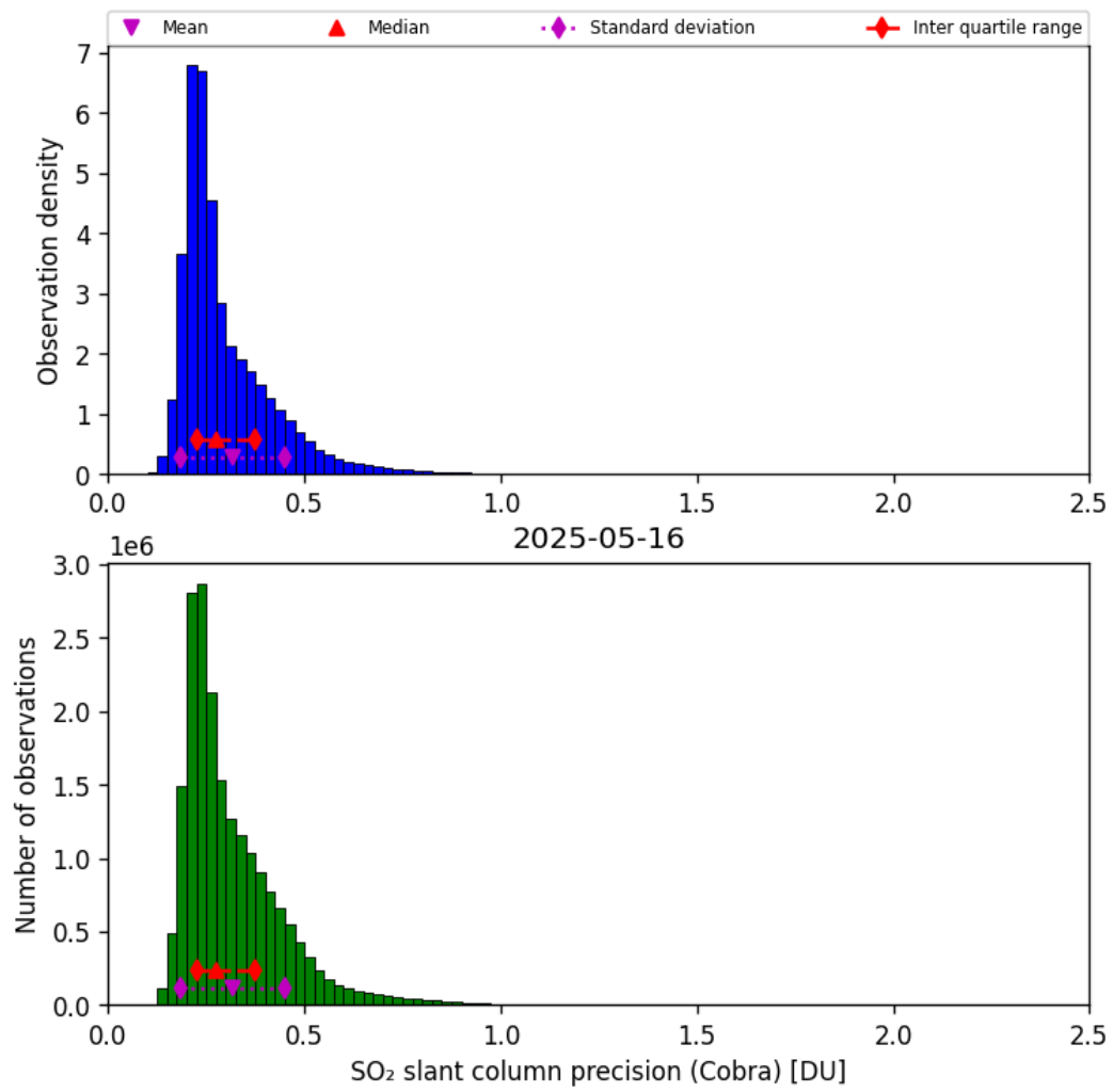
Figure 62: Histogram of “SO 2 slant column precision (Cobra)” for 2025-05-15 to 2025-05-17
