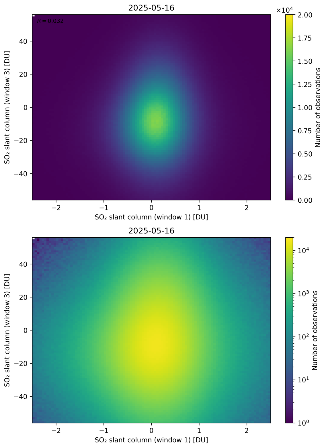
Figure 287: Scatter density plot of “SO 2 slant column (window 1)” against “SO 2 slant column (window 3)” for 2025-05-15 to 2025-05-17.
