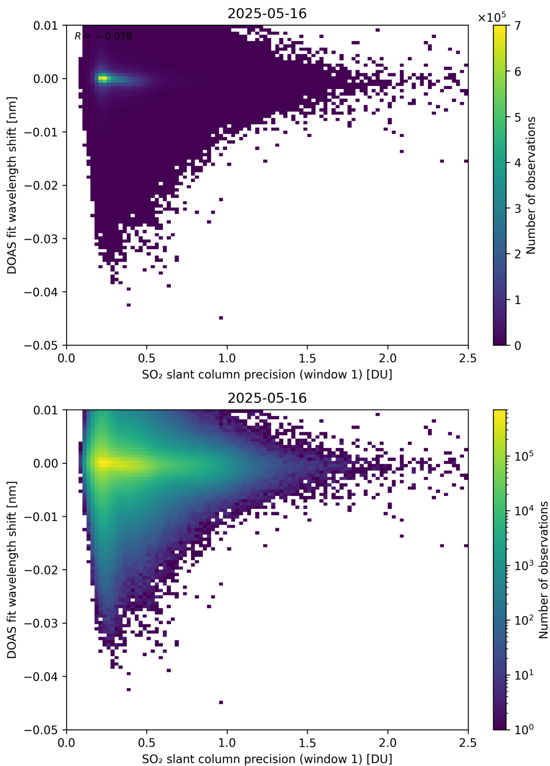
Figure 271: Scatter density plot of “SO 2 slant column precision (window 1)” against “DOAS fit wavelength shift” for 2025-05-15 to 2025-05-17.
