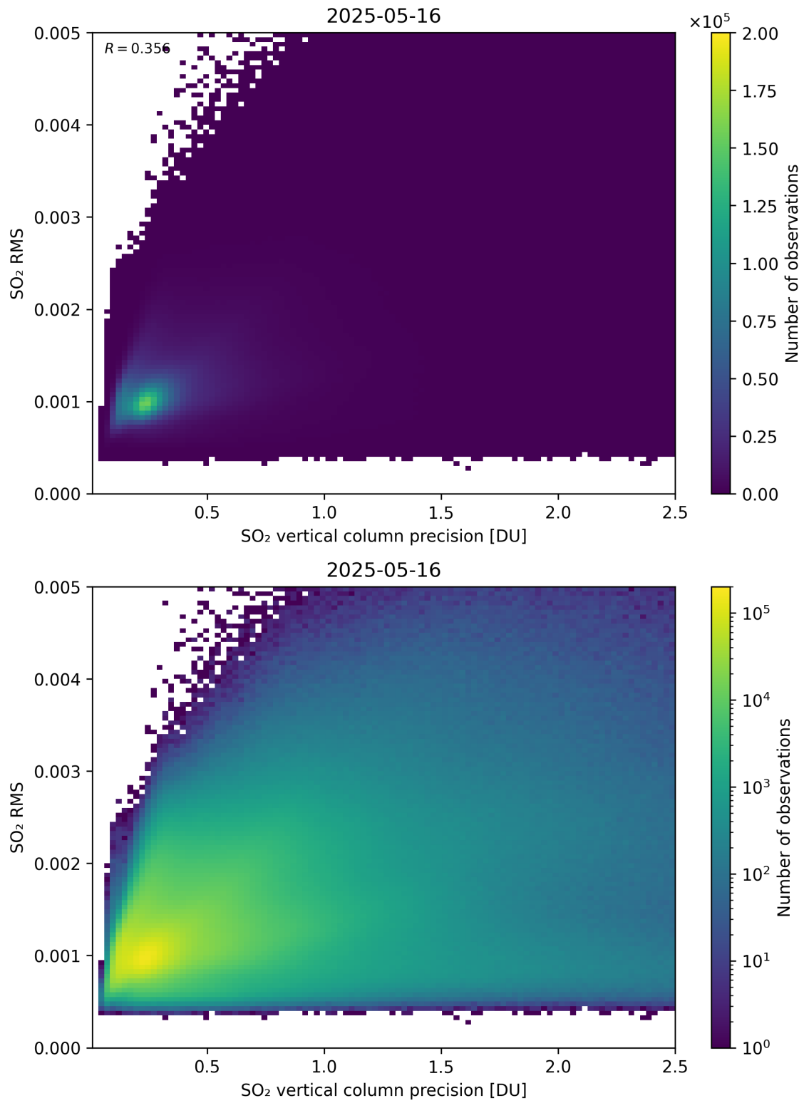
Figure 334: Scatter density plot of “SO 2 vertical column precision” against “SO 2 RMS” for 2025-05-15 to 2025-05-17.
