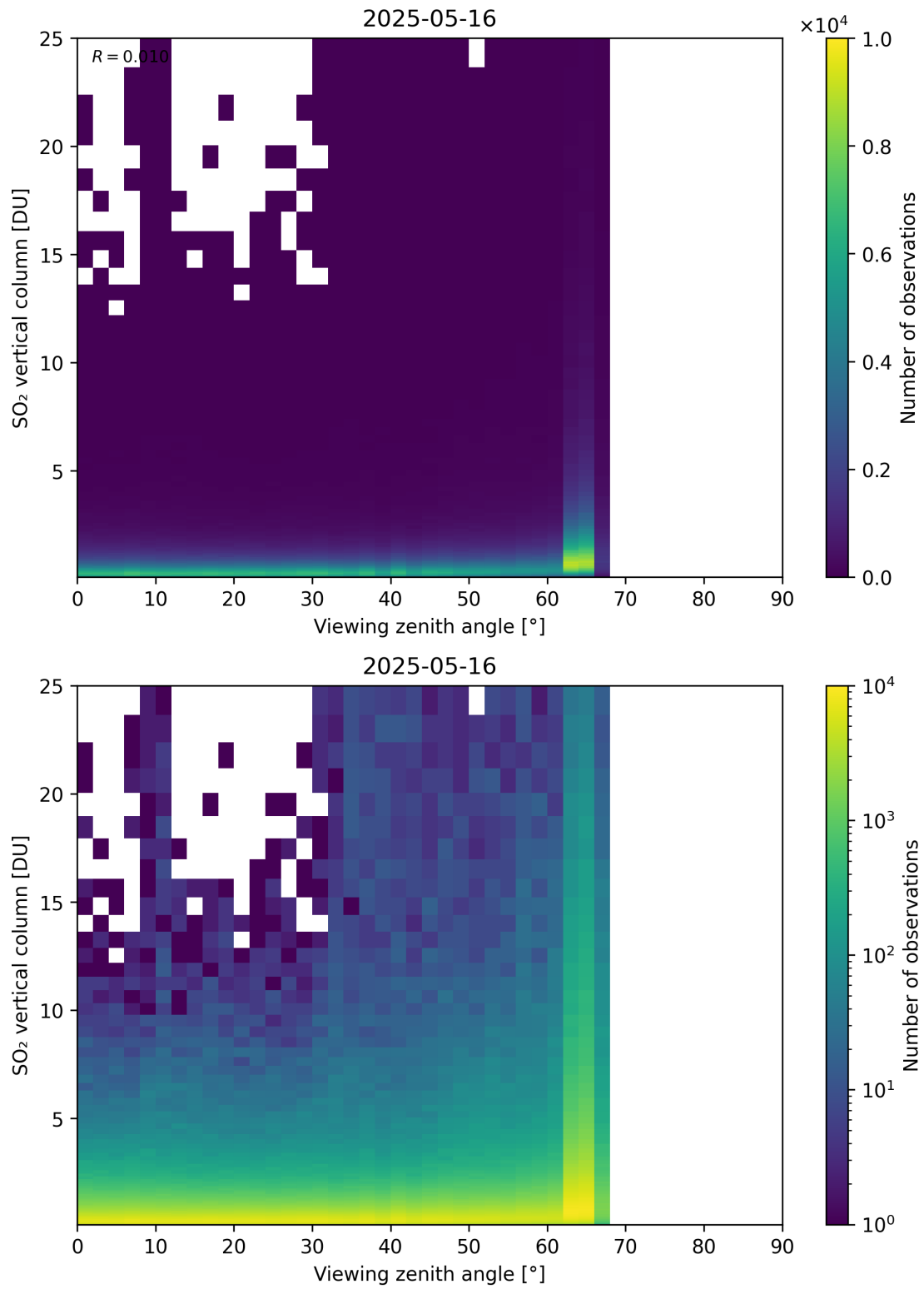
Figure 383: Scatter density plot of “Viewing zenith angle” against “SO 2 vertical column” for 2025-05-15 to 2025-05-17.
