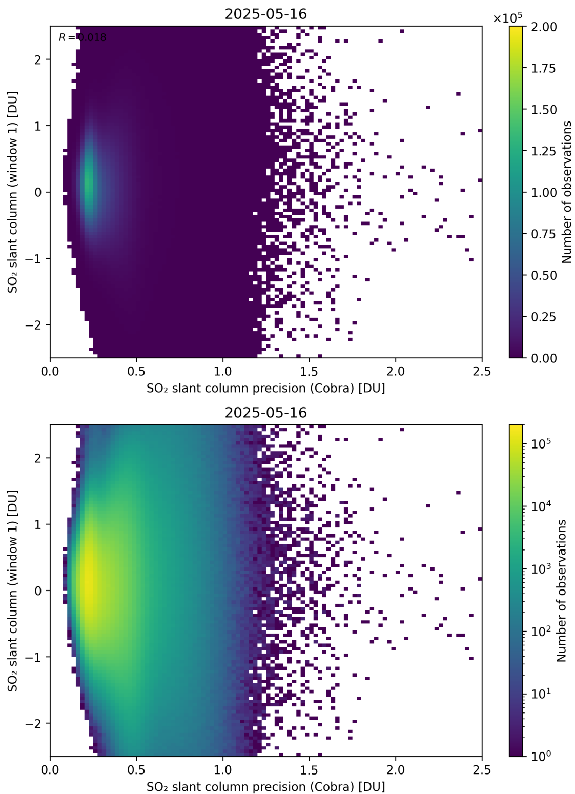
Figure 208: Scatter density plot of “SO 2 slant column precision (Cobra)” against “SO 2 slant column (window 1)” for 2025-05-15 to 2025-05-17.
