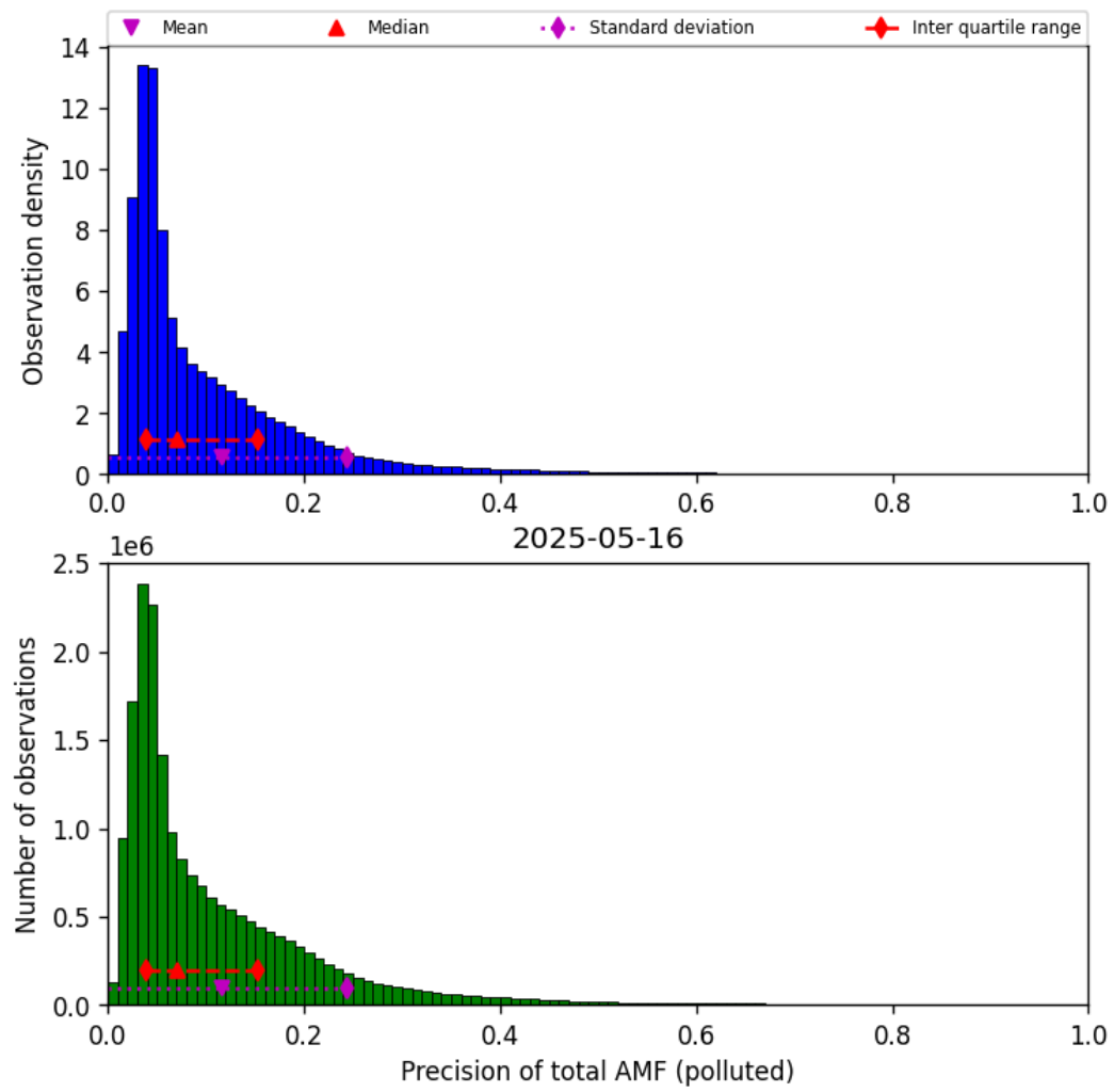
Figure 80: Histogram of “Precision of total AMF (polluted)” for 2025-05-15 to 2025-05-17
