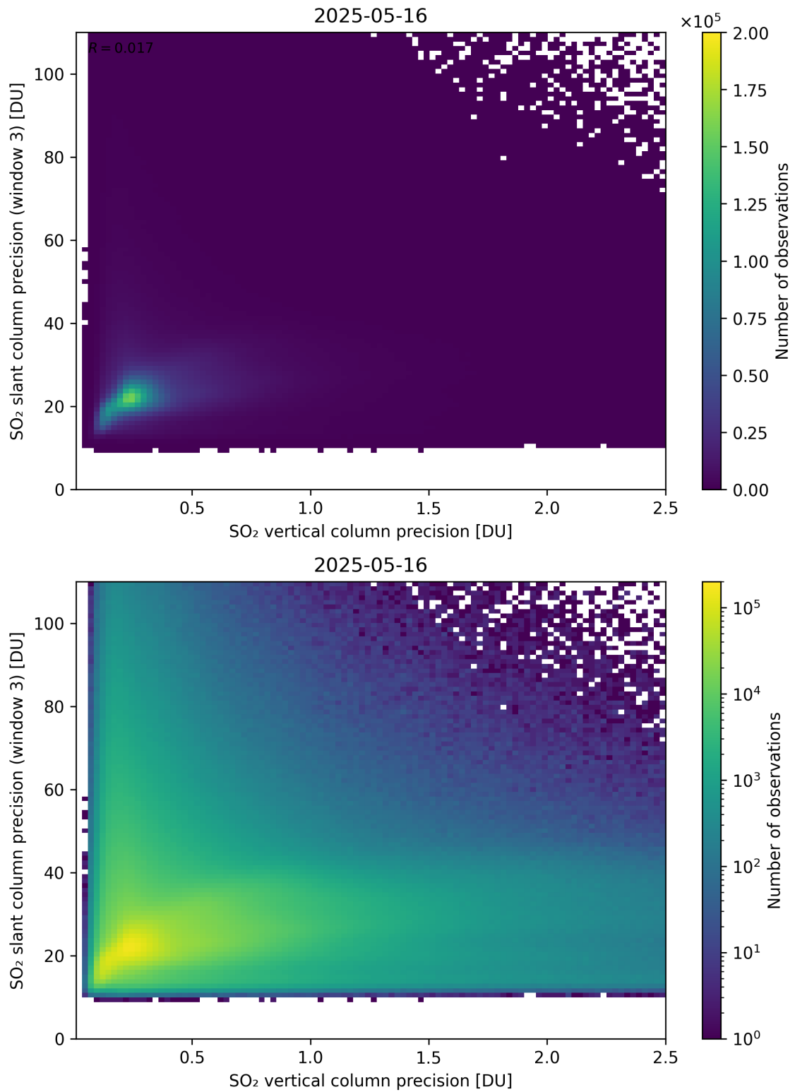
Figure 345: Scatter density plot of “SO 2 vertical column precision” against “SO 2 slant column precision (window 3)” for 2025-05-15 to 2025-05-17.
