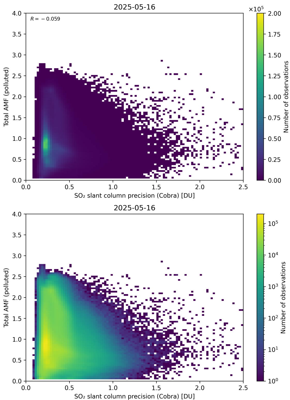
Figure 213: Scatter density plot of “SO 2 slant column precision (Cobra)” against “Total AMF (polluted)” for 2025-05-15 to 2025-05-17.
