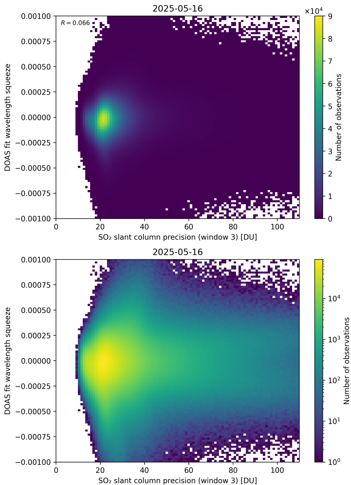
Figure 309: Scatter density plot of “SO 2 slant column precision (window 3)” against “DOAS fit wavelength squeeze” for 2025-05-15 to 2025-05-17.
