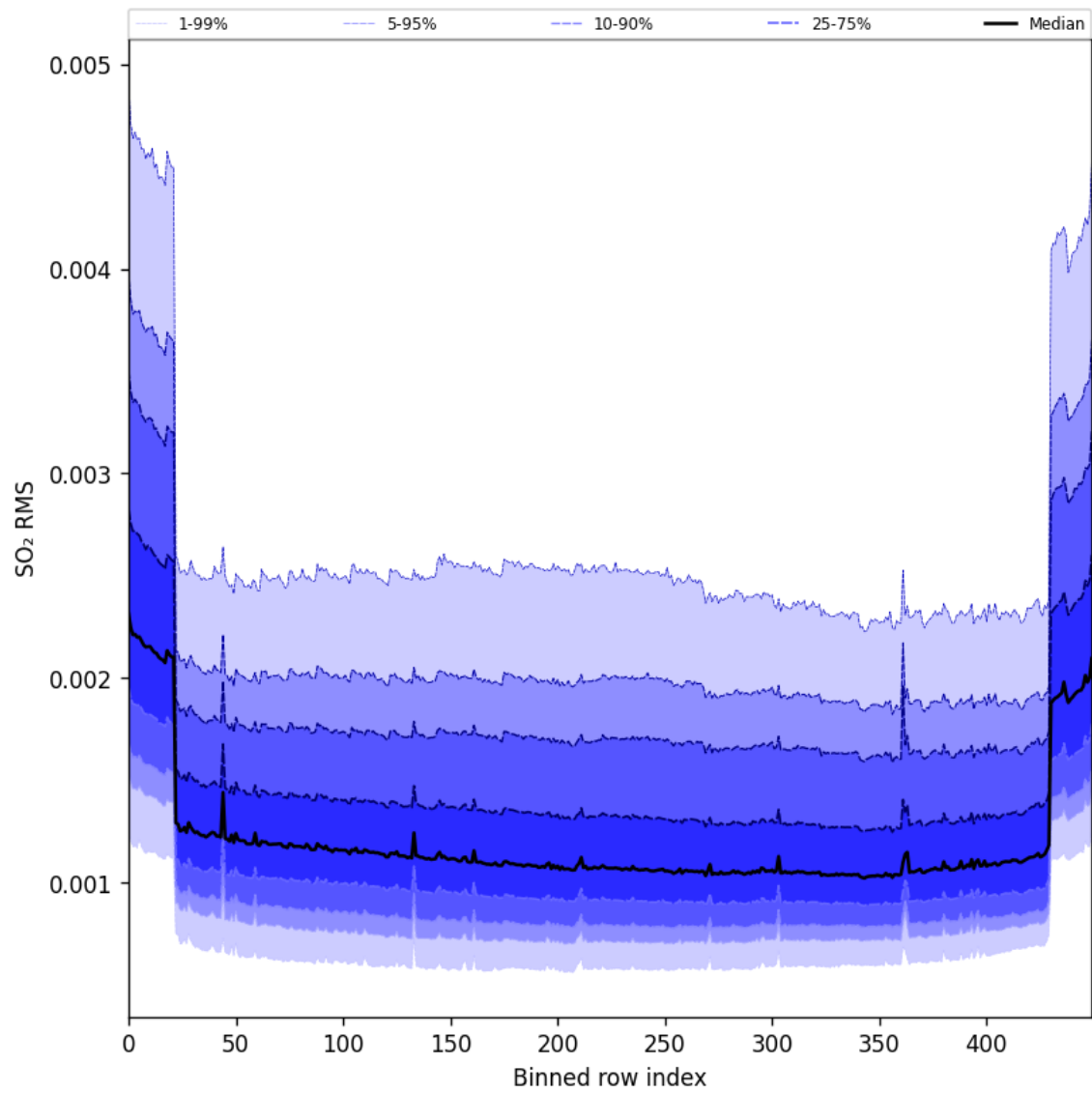
Figure 104: Along track statistics of “SO 2 RMS” for 2025-05-15 to 2025-05-17
