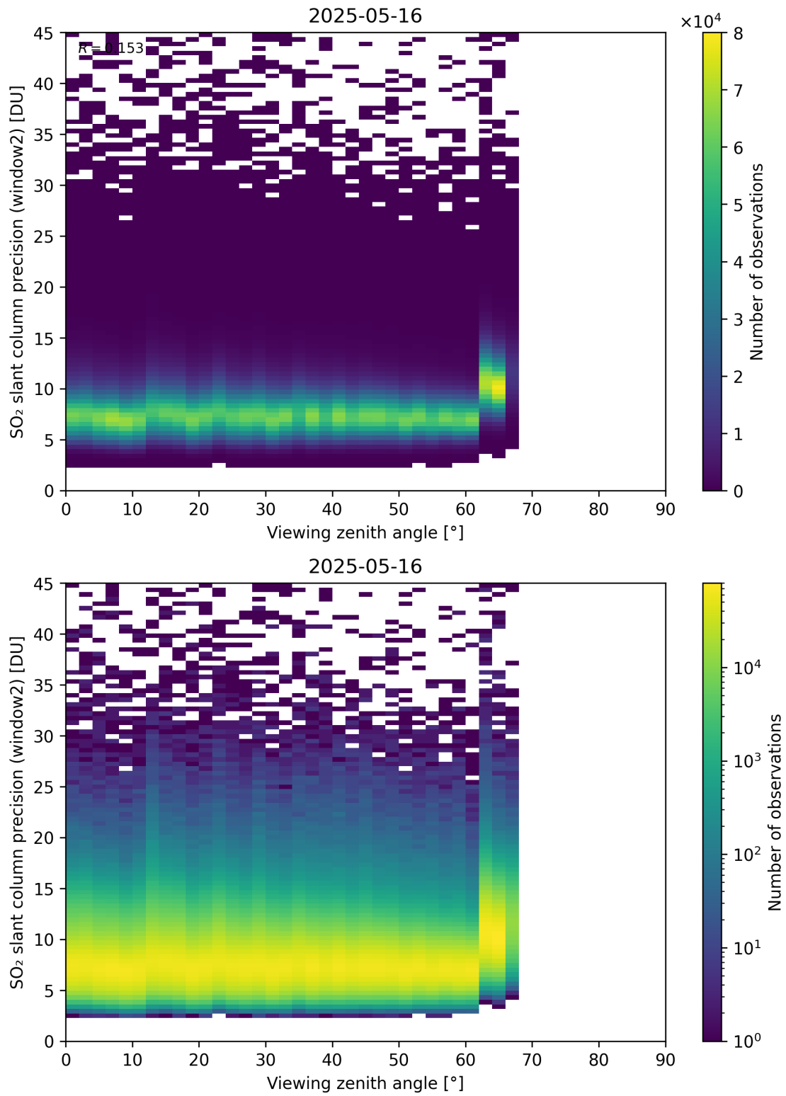
Figure 378: Scatter density plot of “Viewing zenith angle” against “SO 2 slant column precision (window2)” for 2025-05-15 to 2025-05-17.
