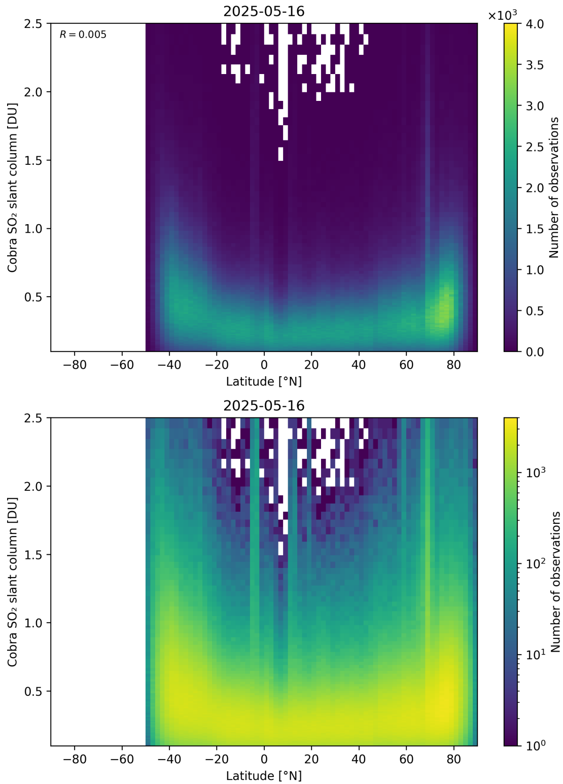
Figure 157: Scatter density plot of “Latitude” against “Cobra SO 2 slant column” for 2025-05-15 to 2025-05-17.
