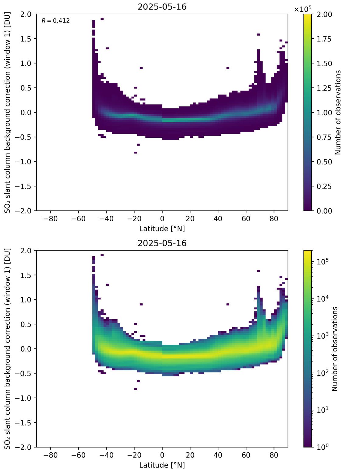
Figure 150: Scatter density plot of “Latitude” against “SO 2 slant column background correction (window 1)” for 2025-05-15 to 2025-05-17.
