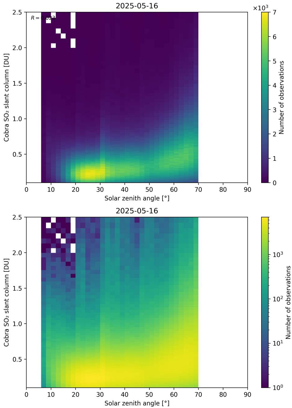
Figure 179: Scatter density plot of “Solar zenith angle” against “Cobra SO 2 slant column” for 2025-05-15 to 2025-05-17.
