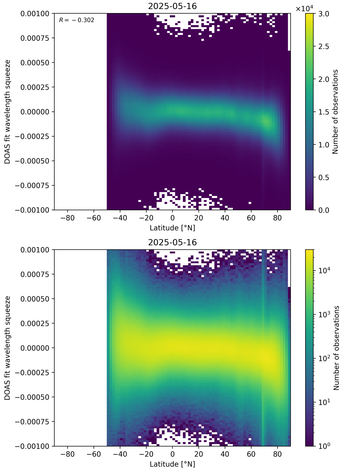
Figure 154: Scatter density plot of “Latitude” against “DOAS fit wavelength squeeze” for 2025-05-15 to 2025-05-17.
