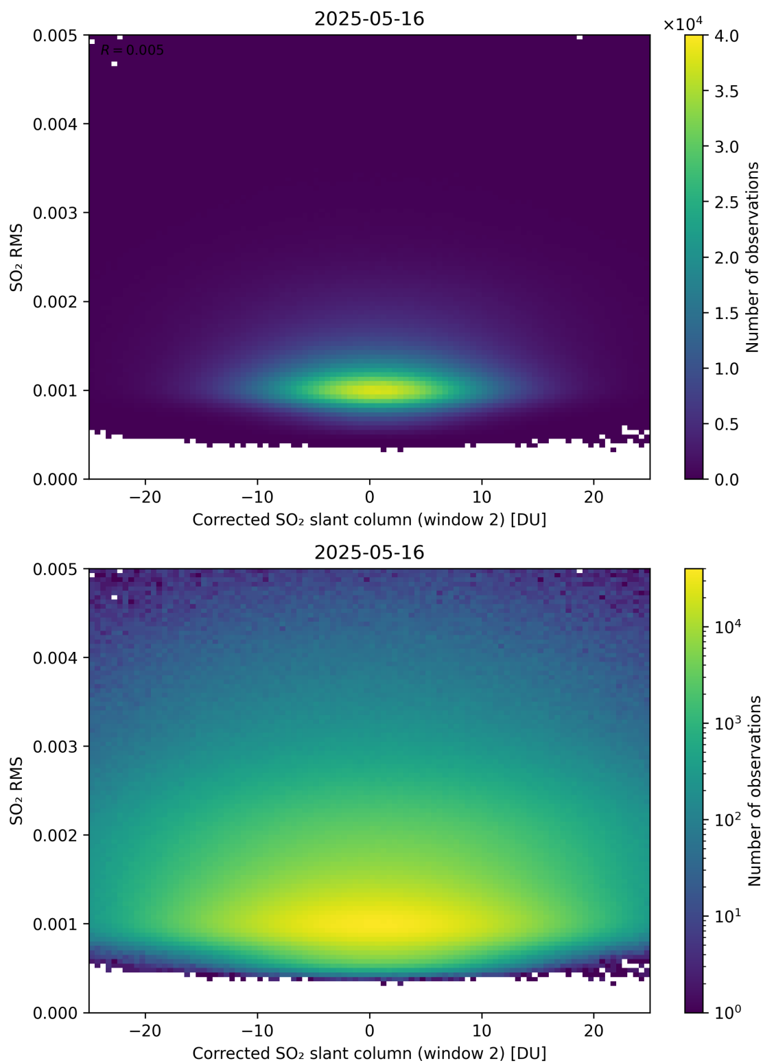
Figure 248: Scatter density plot of “Corrected SO 2 slant column (window 2)” against “SO 2 RMS” for 2025-05-15 to 2025-05-17.
