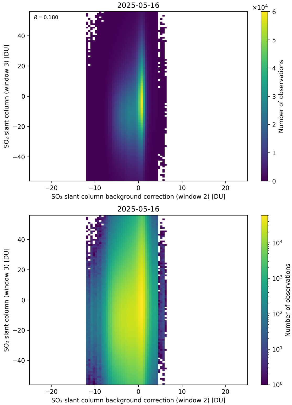
Figure 128: Scatter density plot of “SO 2 slant column background correction (window 2)” against “SO 2 slant column (window 3)” for 2025-05-15 to 2025-05-17.
