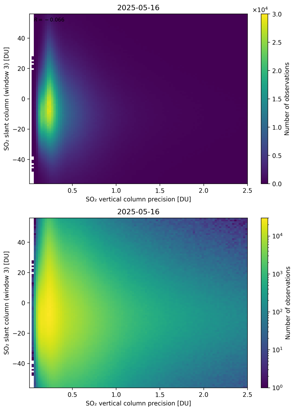
Figure 344: Scatter density plot of “SO 2 vertical column precision” against “SO 2 slant column (window 3)” for 2025-05-15 to 2025-05-17.
