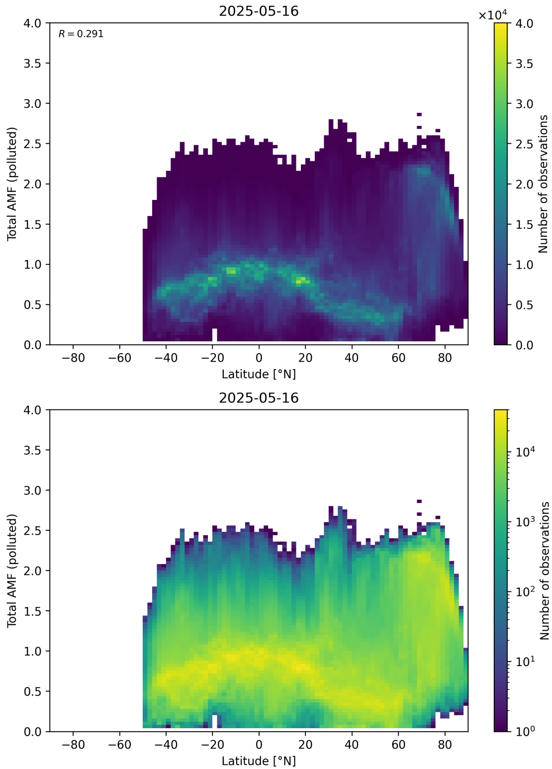
Figure 167: Scatter density plot of “Latitude” against “Total AMF (polluted)” for 2025-05-15 to 2025-05-17.
