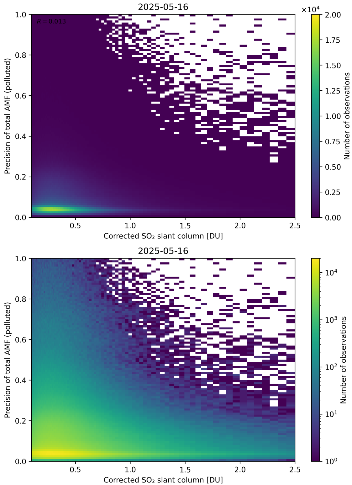
Figure 243: Scatter density plot of “Corrected SO 2 slant column” against “Precision of total AMF (polluted)” for 2025-05-15 to 2025-05-17.
