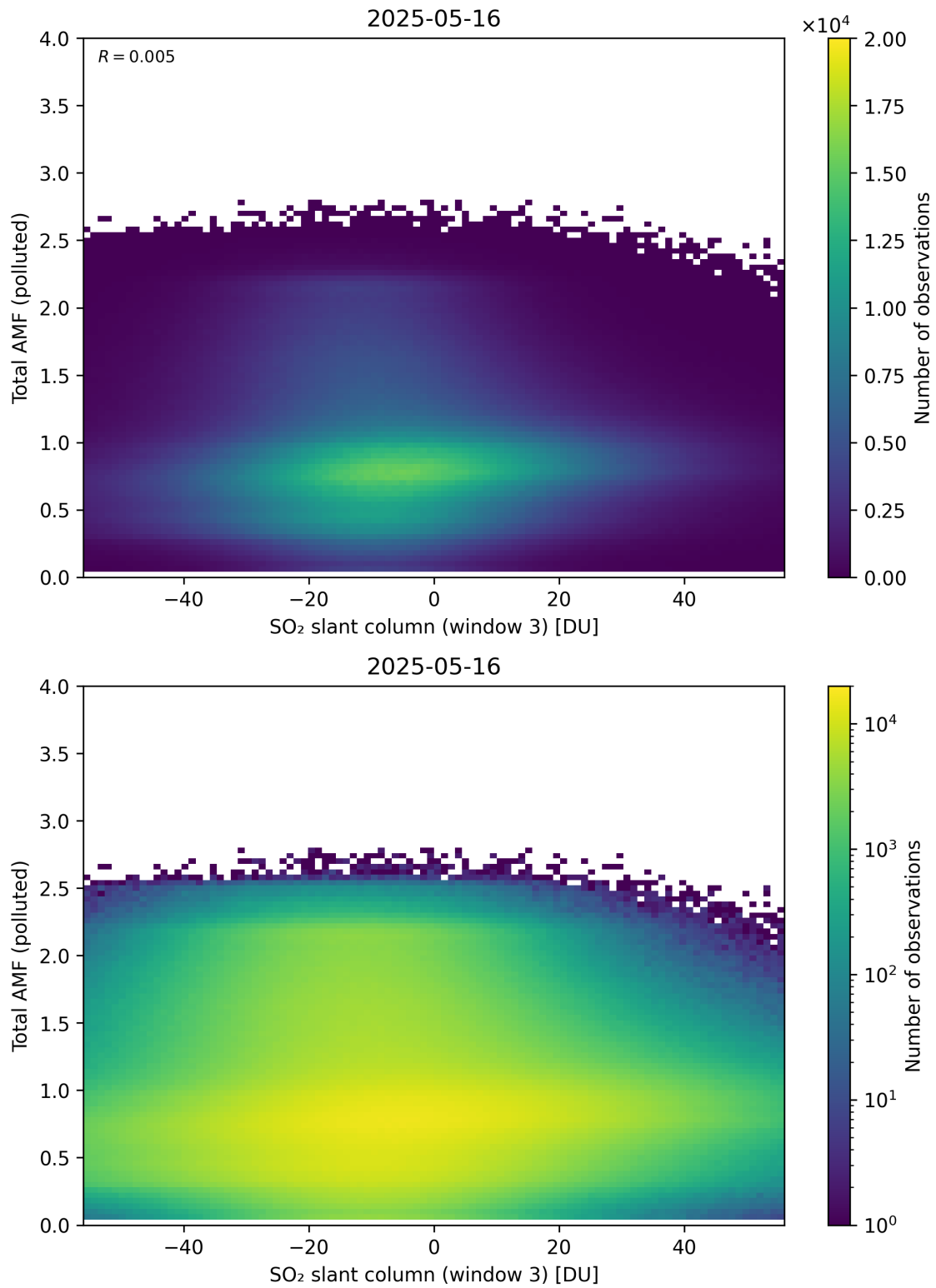
Figure 318: Scatter density plot of “SO 2 slant column (window 3)” against “Total AMF (polluted)” for 2025-05-15 to 2025-05-17.
