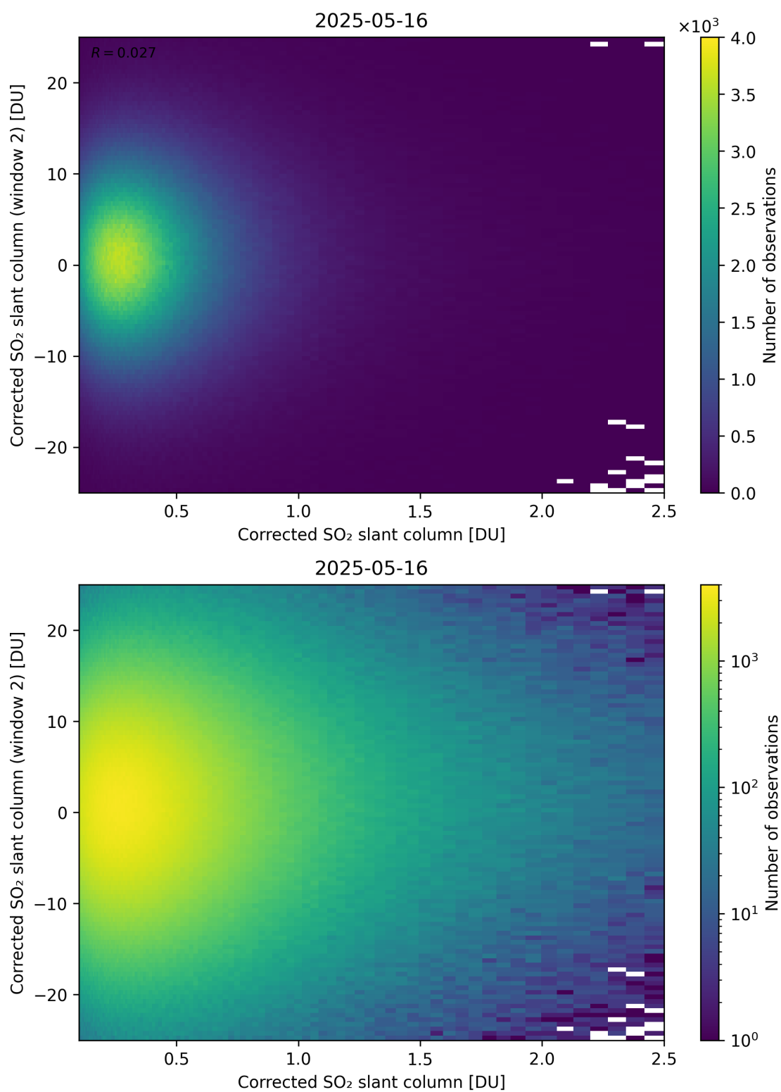
Figure 235: Scatter density plot of “Corrected SO 2 slant column” against “Corrected SO 2 slant column (window 2)” for 2025-05-15 to 2025-05-17.
