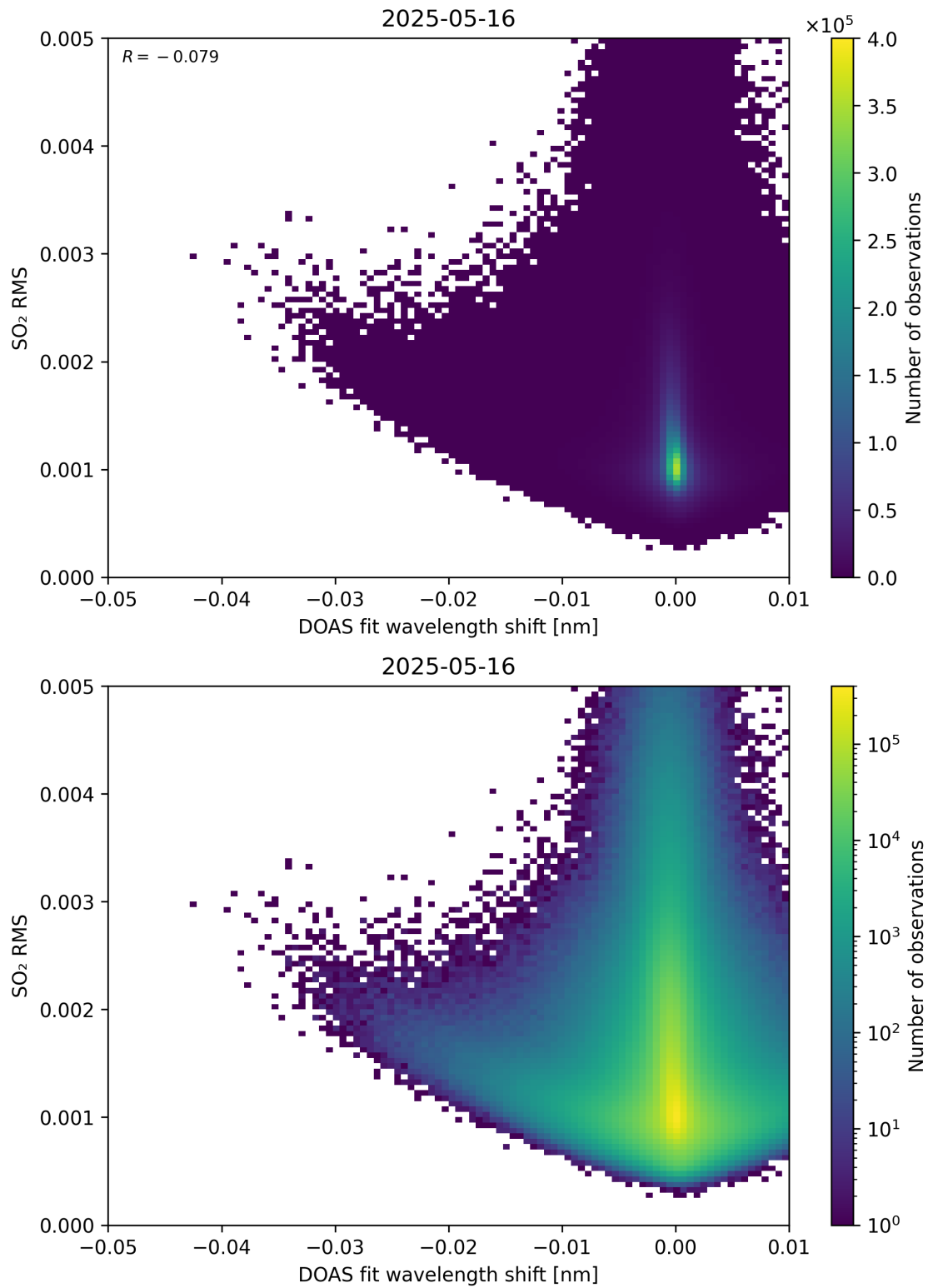
Figure 139: Scatter density plot of “DOAS fit wavelength shift” against “SO 2 RMS” for 2025-05-15 to 2025-05-17.
