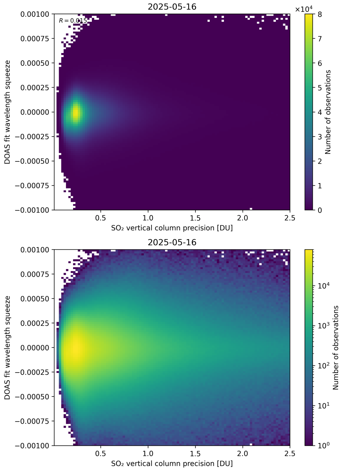
Figure 333: Scatter density plot of “SO 2 vertical column precision” against “DOAS fit wavelength squeeze” for 2025-05-15 to 2025-05-17.
