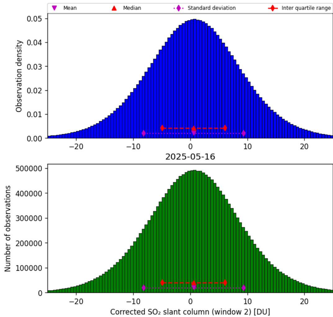
Figure 69: Histogram of “Corrected SO 2 slant column (window 2)” for 2025-05-15 to 2025-05-17
