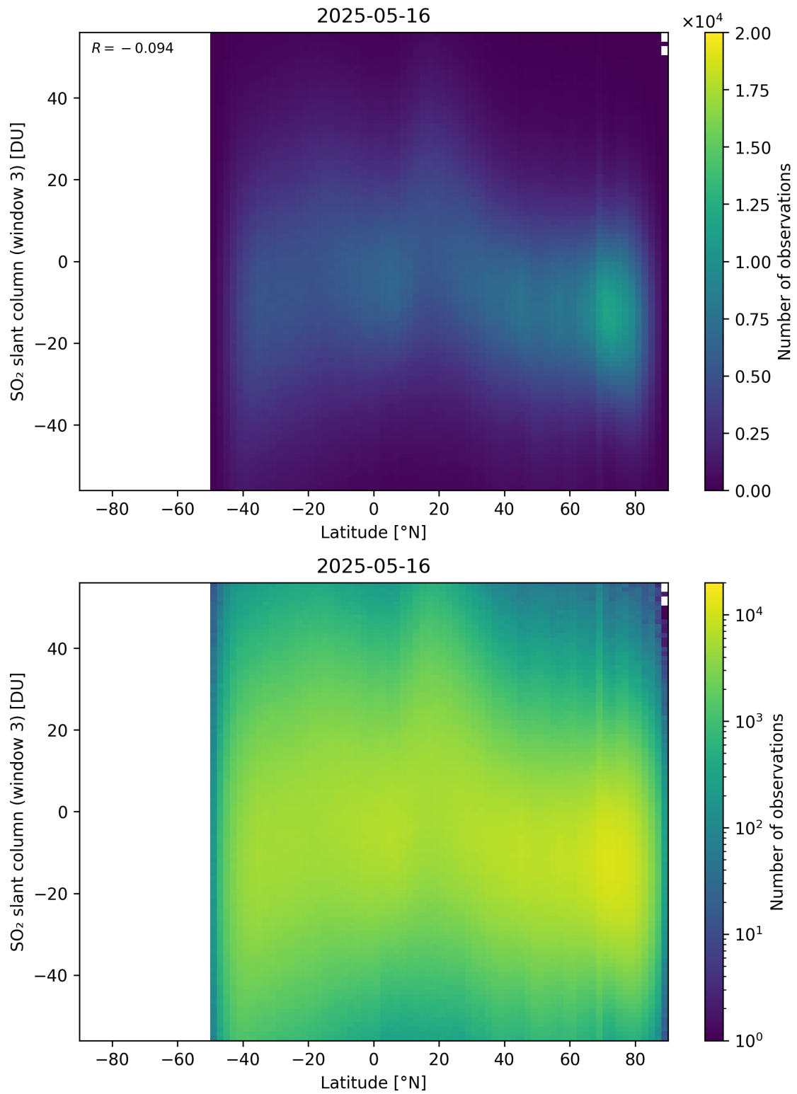
Figure 165: Scatter density plot of “Latitude” against “SO 2 slant column (window 3)” for 2025-05-15 to 2025-05-17.
