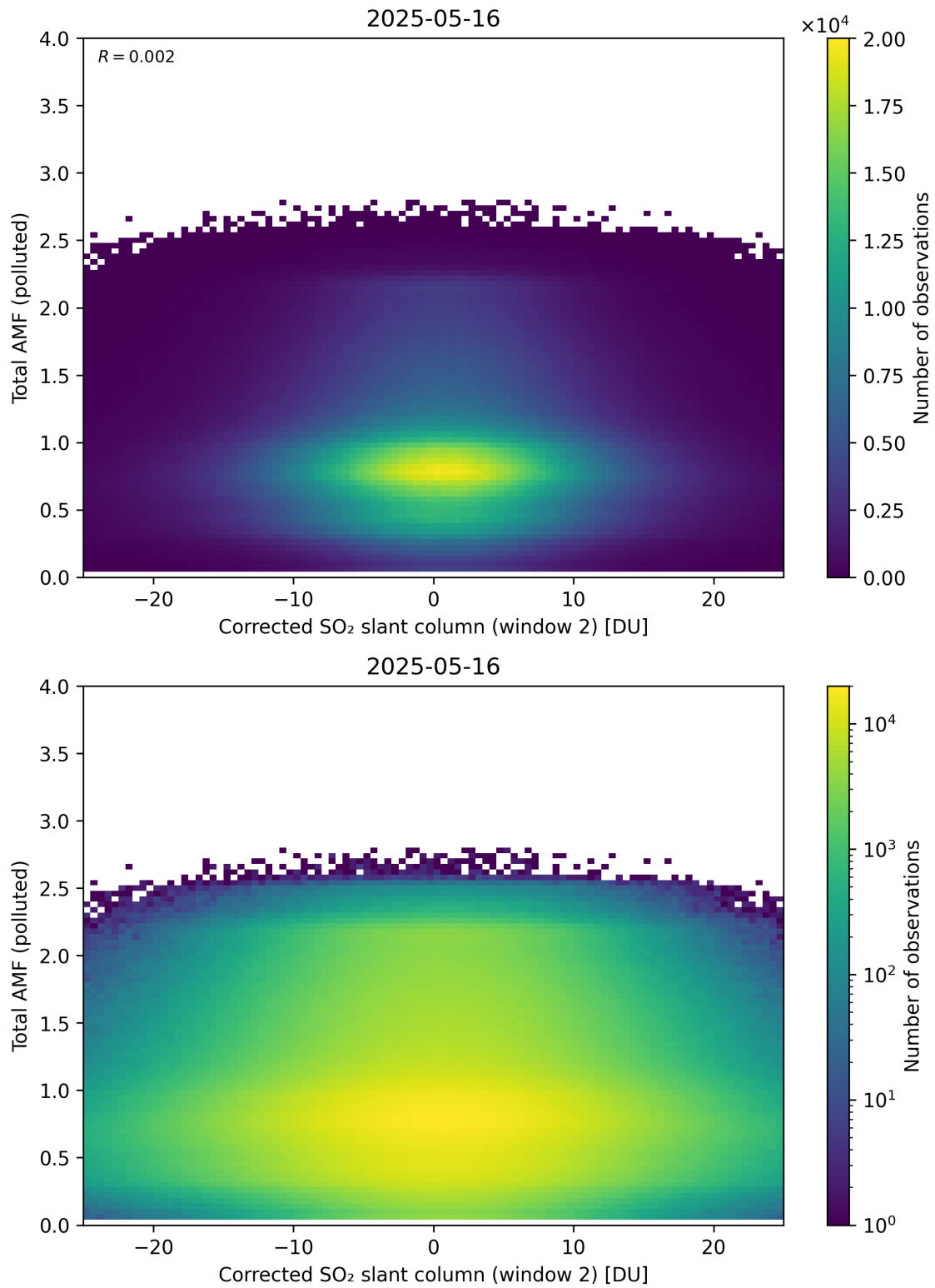
Figure 253: Scatter density plot of “Corrected SO 2 slant column (window 2)” against “Total AMF (polluted)” for 2025-05-15 to 2025-05-17.
