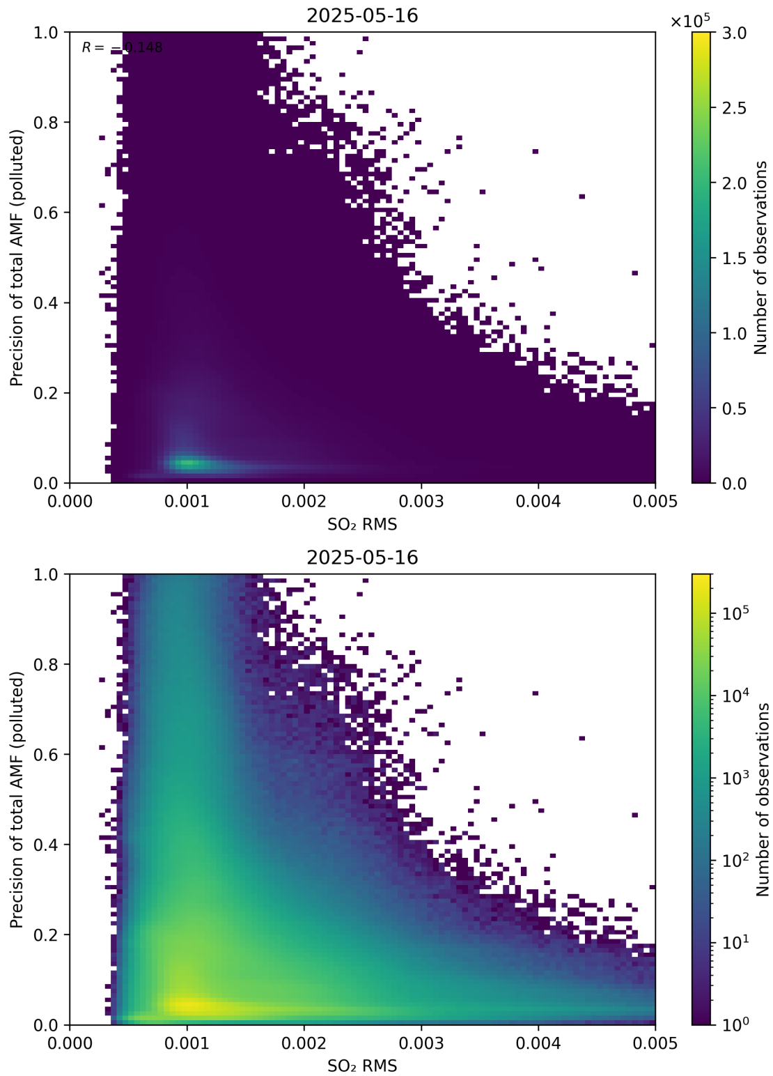
Figure 149: Scatter density plot of “SO 2 RMS” against “Precision of total AMF (polluted)” for 2025-05-15 to 2025-05-17.
