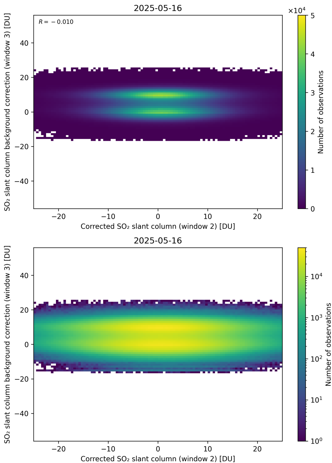
Figure 245: Scatter density plot of “Corrected SO 2 slant column (window 2)” against “SO 2 slant column background correction (window 3)” for 2025-05-15 to 2025-05-17.
