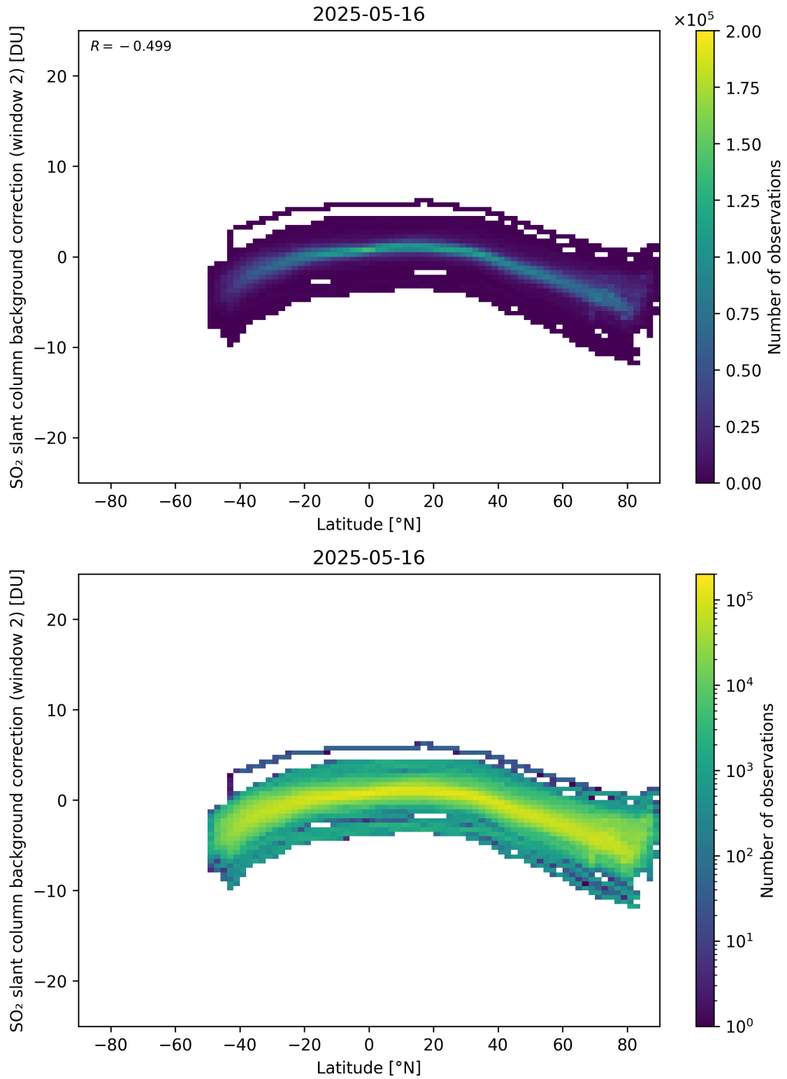
Figure 151: Scatter density plot of “Latitude” against “SO 2 slant column background correction (window 2)” for 2025-05-15 to 2025-05-17.
