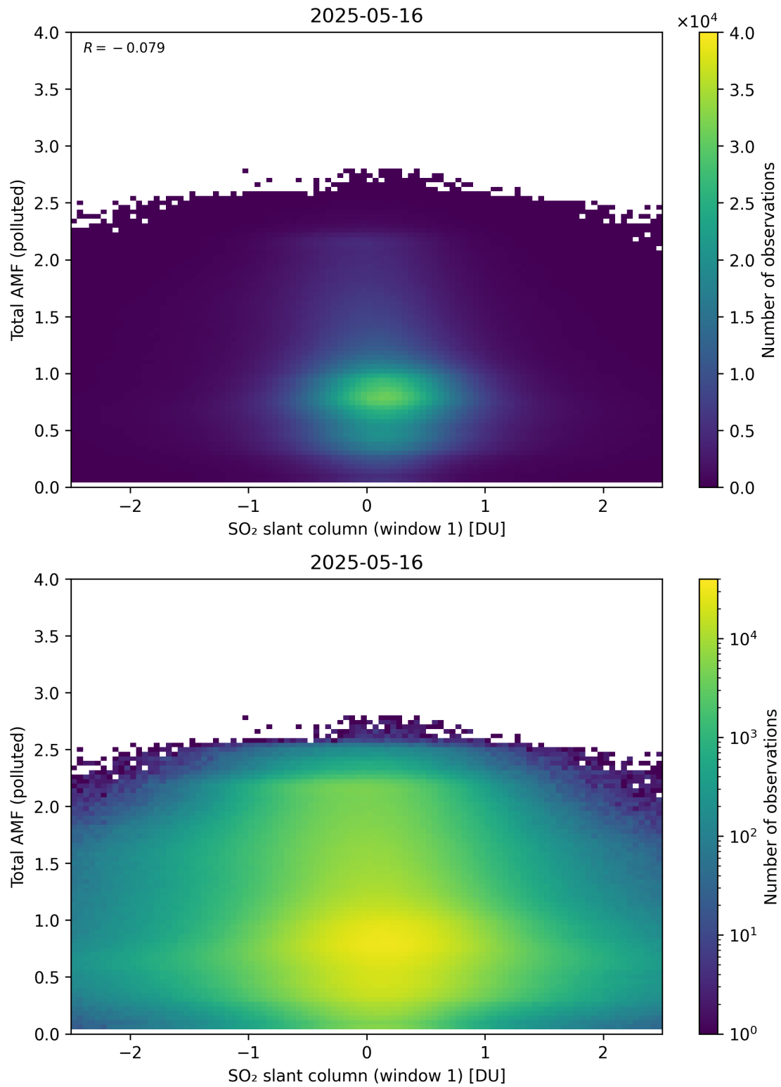
Figure 289: Scatter density plot of “SO 2 slant column (window 1)” against “Total AMF (polluted)” for 2025-05-15 to 2025-05-17.
