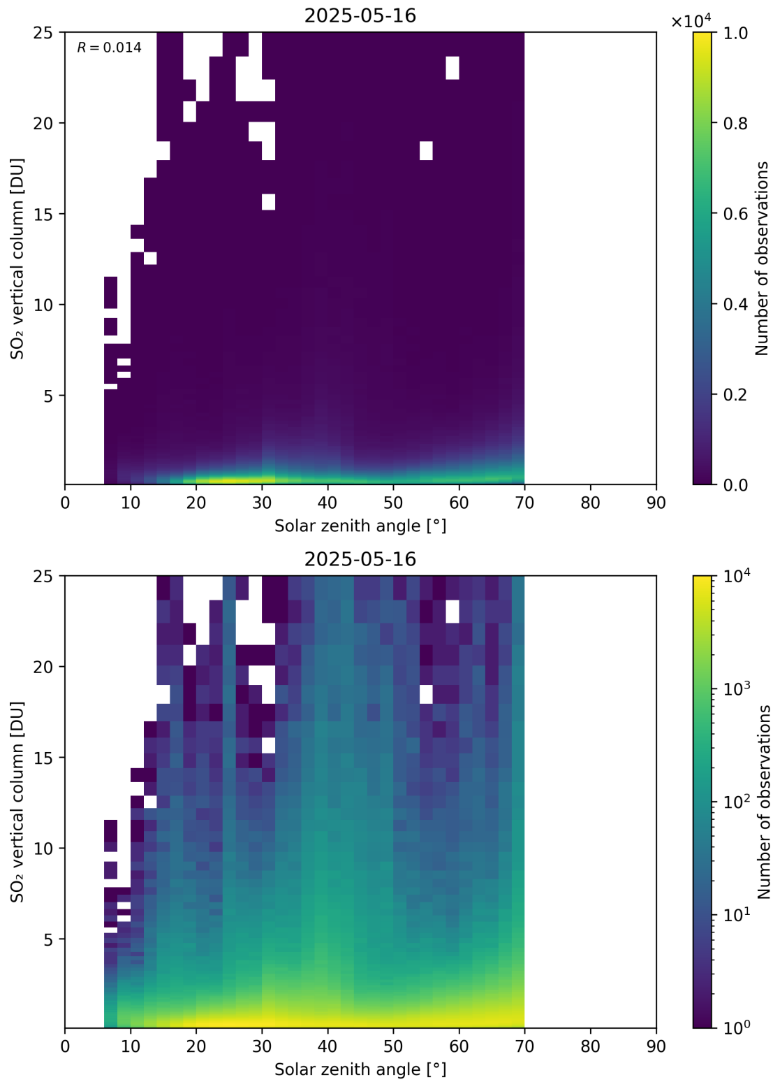
Figure 191: Scatter density plot of “Solar zenith angle” against “SO 2 vertical column” for 2025-05-15 to 2025-05-17.
