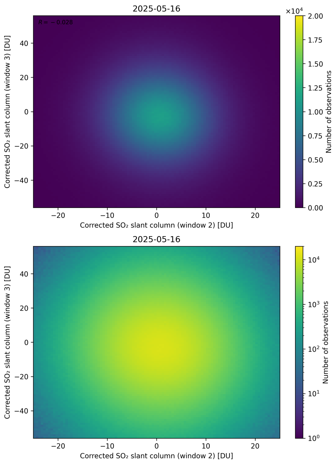
Figure 250: Scatter density plot of “Corrected SO 2 slant column (window 2)” against “Corrected SO 2 slant column (window 3)” for 2025-05-15 to 2025-05-17.
