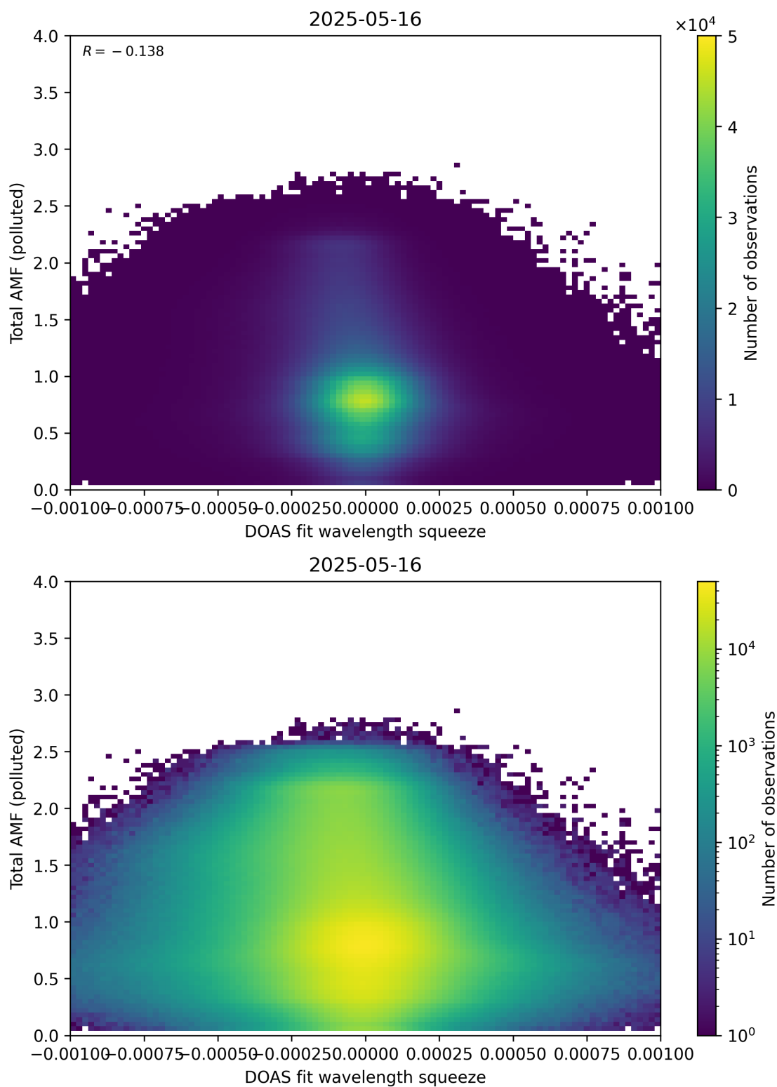
Figure 145: Scatter density plot of “DOAS fit wavelength squeeze” against “Total AMF (polluted)” for 2025-05-15 to 2025-05-17.
