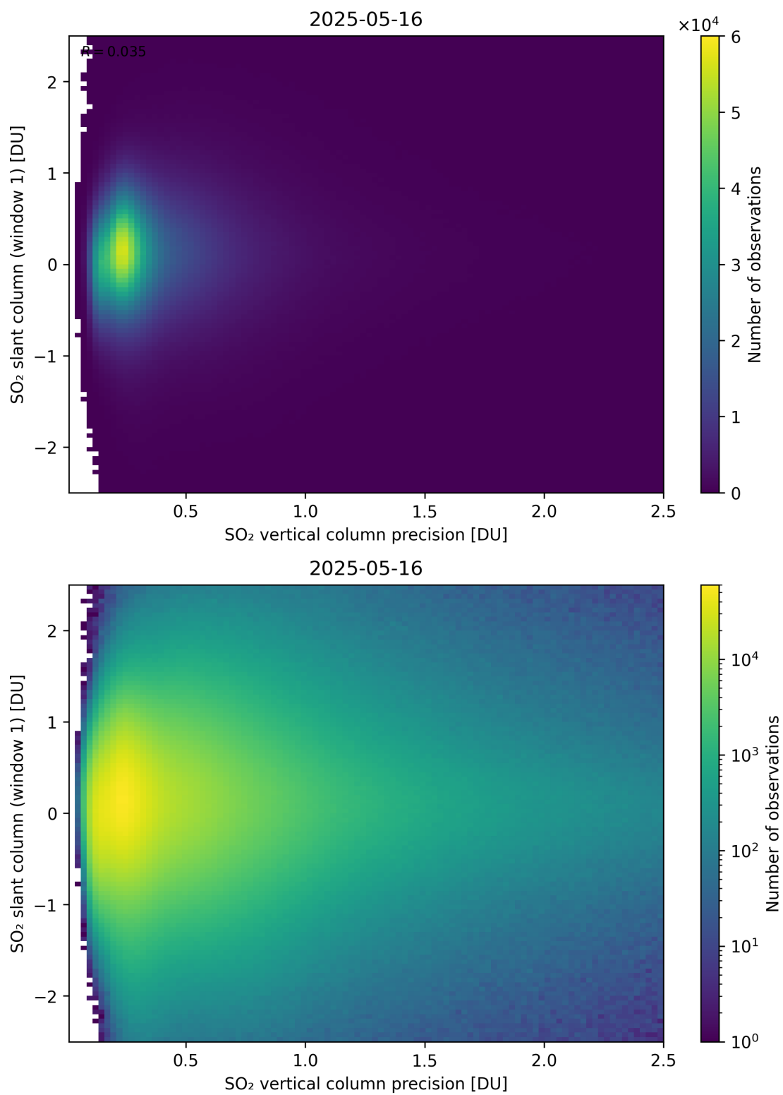
Figure 341: Scatter density plot of “SO 2 vertical column precision” against “SO 2 slant column (window 1)” for 2025-05-15 to 2025-05-17.
