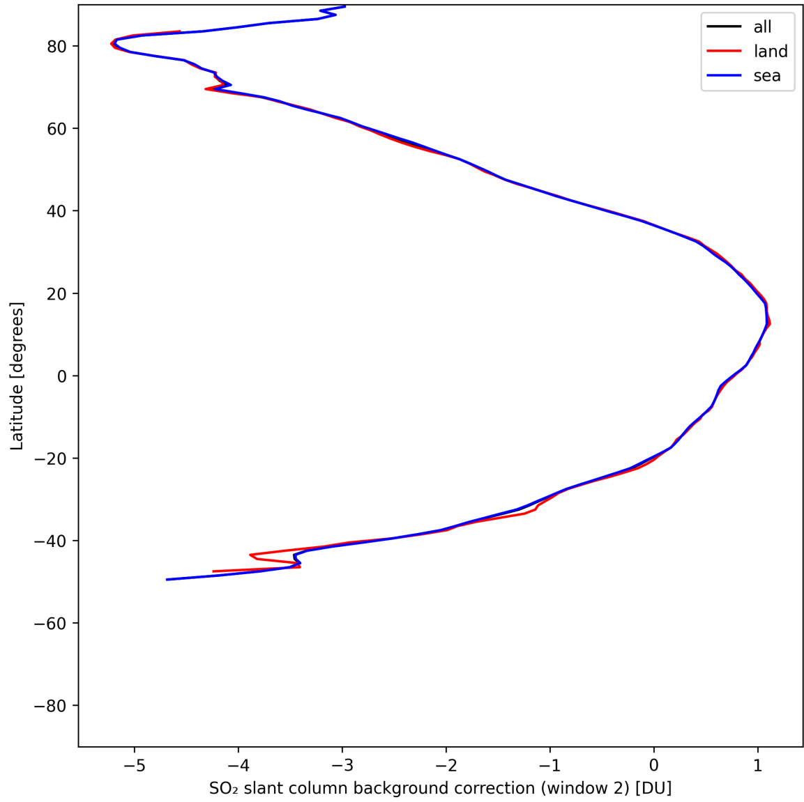
Figure 44: Zonal average of “SO 2 slant column background correction (window 2)” for 2025-05-15 to 2025-05-17.
