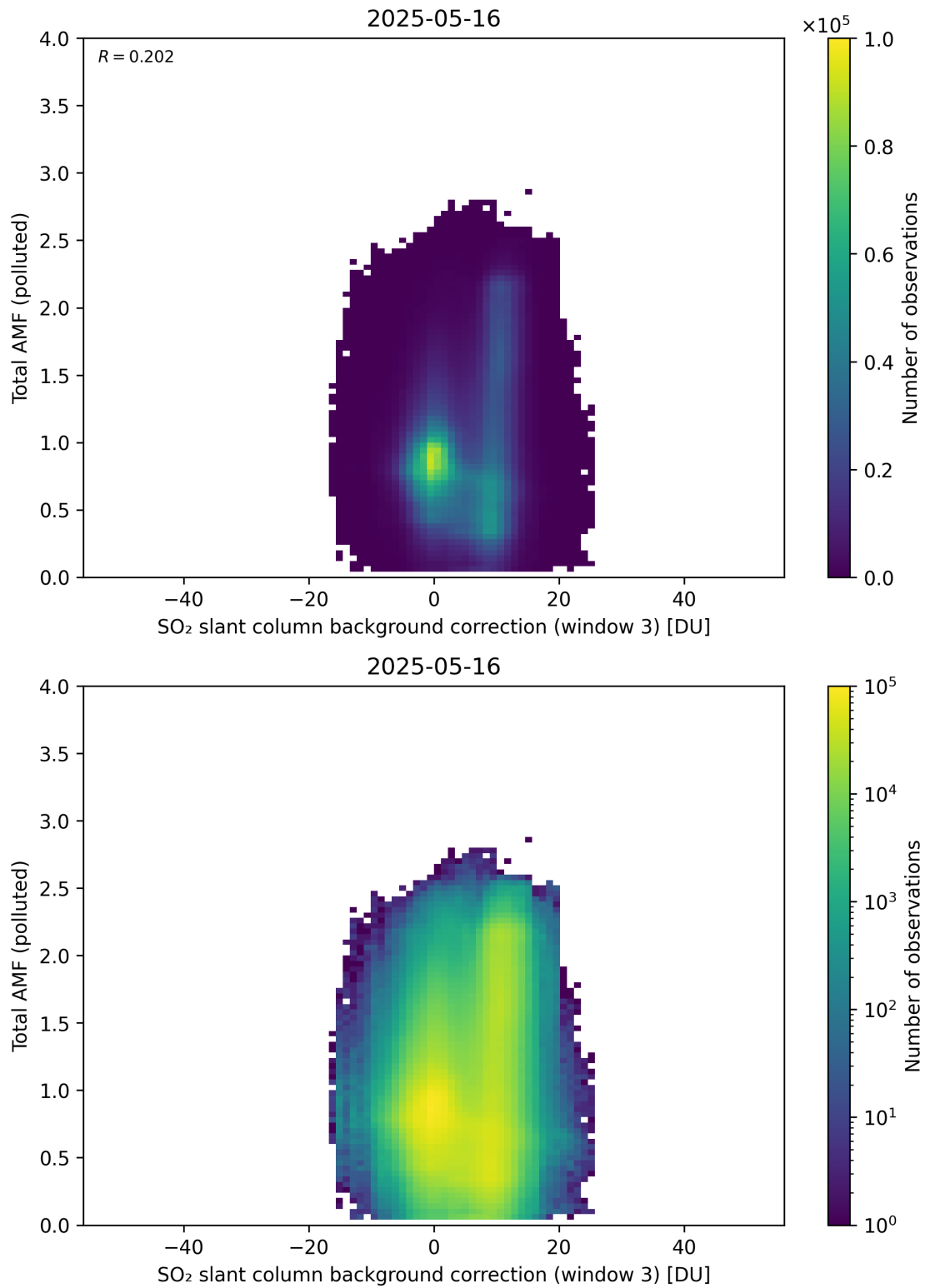
Figure 136: Scatter density plot of “SO 2 slant column background correction (window 3)” against “Total AMF (polluted)” for 2025-05-15 to 2025-05-17.
