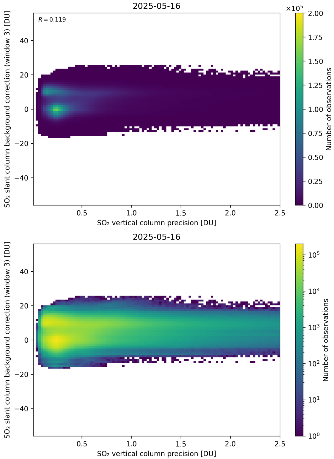
Figure 331: Scatter density plot of “SO 2 vertical column precision” against “SO 2 slant column background correction (window 3)” for 2025-05-15 to 2025-05-17.
