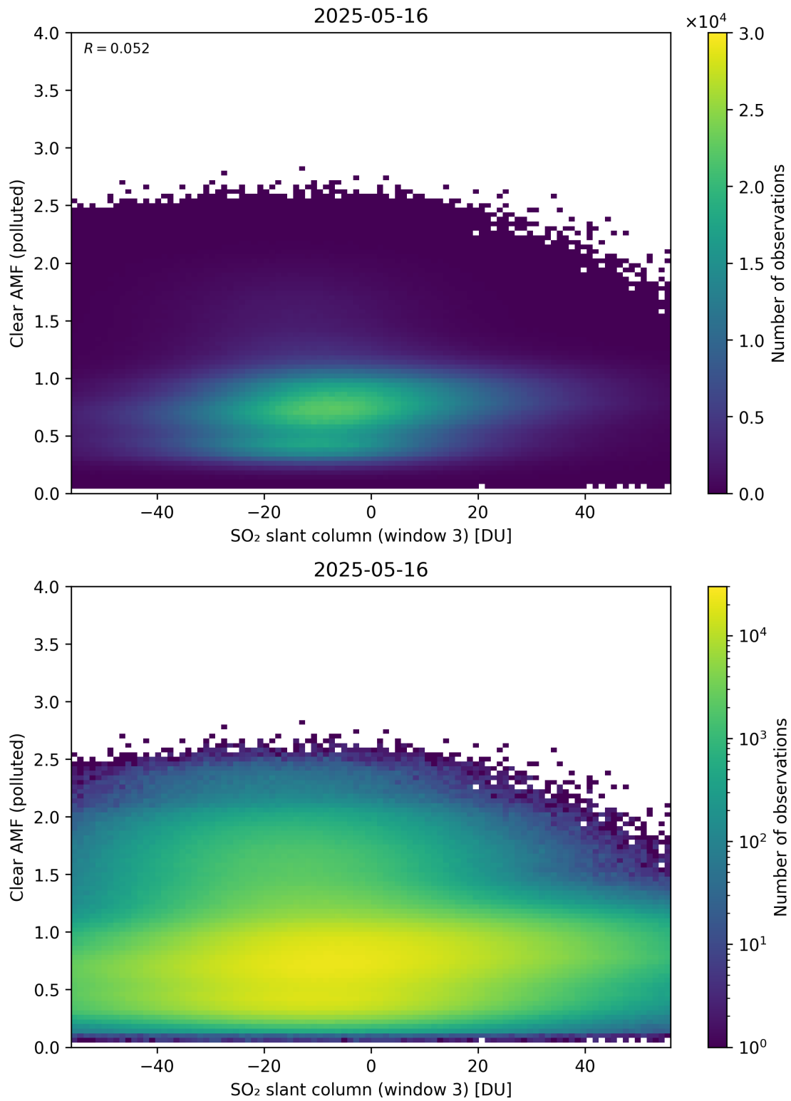
Figure 315: Scatter density plot of “SO 2 slant column (window 3)” against “Clear AMF (polluted)” for 2025-05-15 to 2025-05-17.
