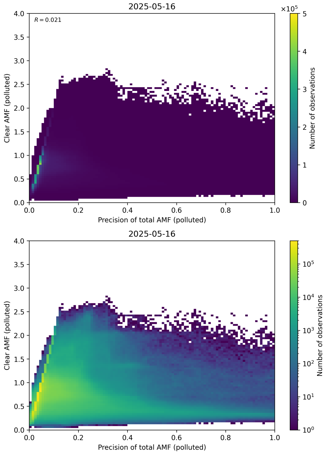
Figure 320: Scatter density plot of “Precision of total AMF (polluted)” against “Clear AMF (polluted)” for 2025-05-15 to 2025-05-17.
