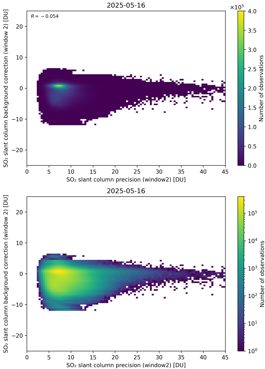
Figure 291: Scatter density plot of “SO 2 slant column precision (window2)” against “SO 2 slant column background correction (window 2)” for 2025-05-15 to 2025-05-17.
