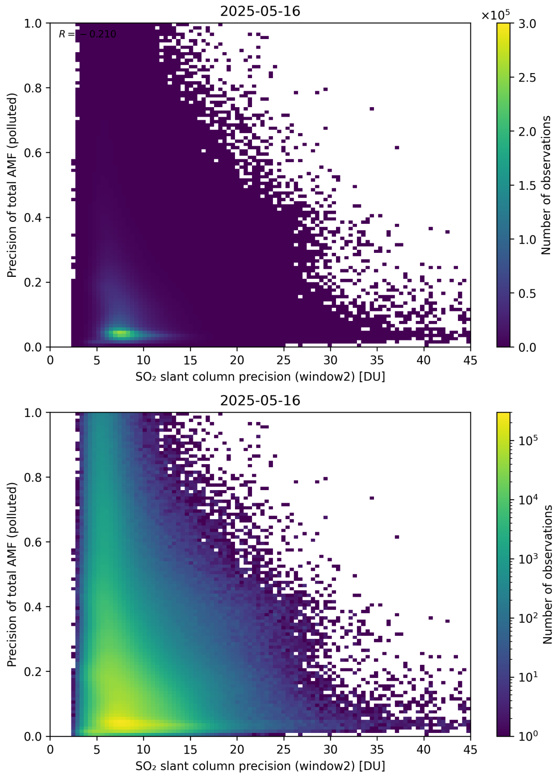
Figure 302: Scatter density plot of “SO 2 slant column precision (window2)” against “Precision of total AMF (polluted)” for 2025-05-15 to 2025-05-17.
