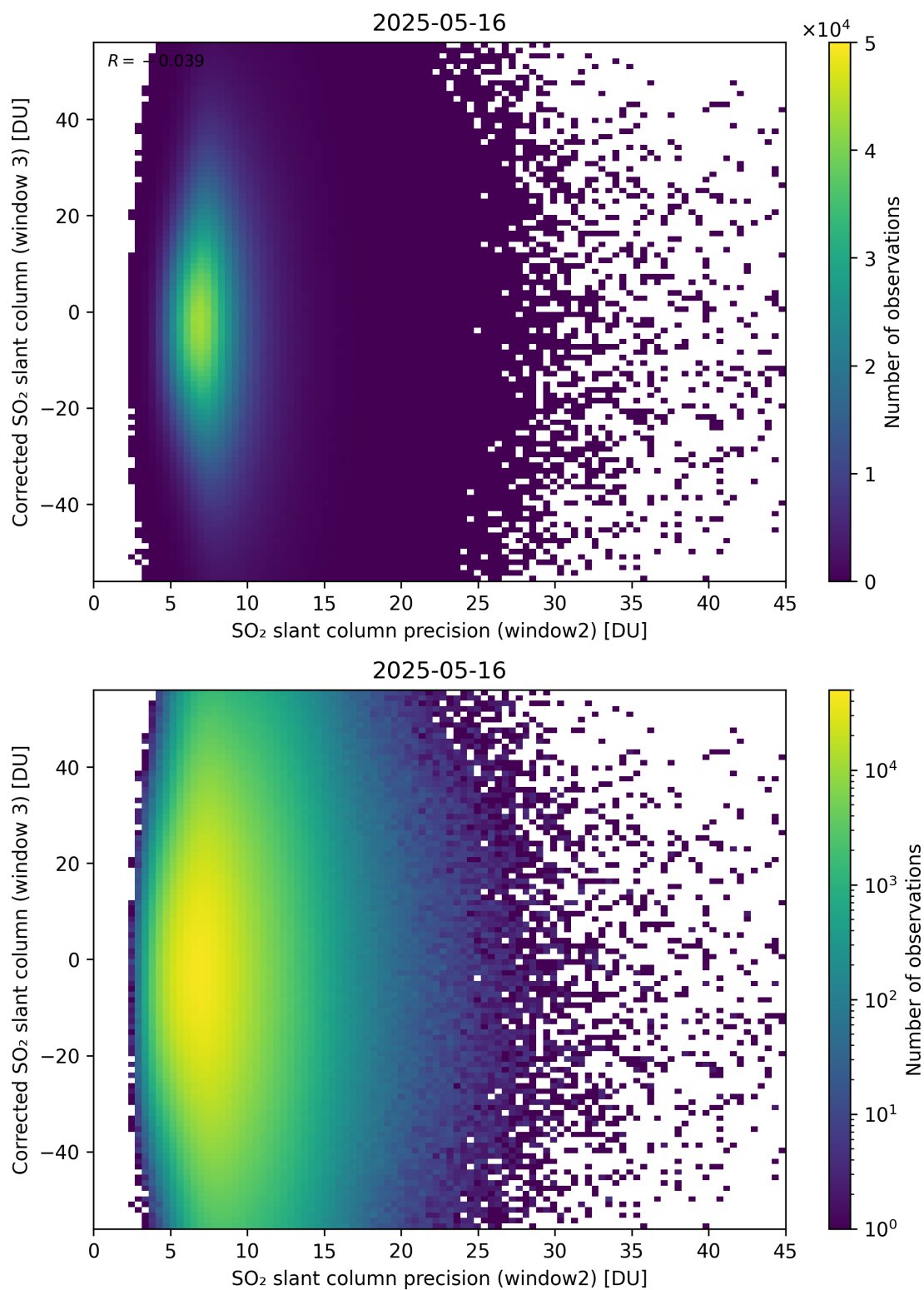
Figure 298: Scatter density plot of “SO 2 slant column precision (window2)” against “Corrected SO 2 slant column (window 3)” for 2025-05-15 to 2025-05-17.
