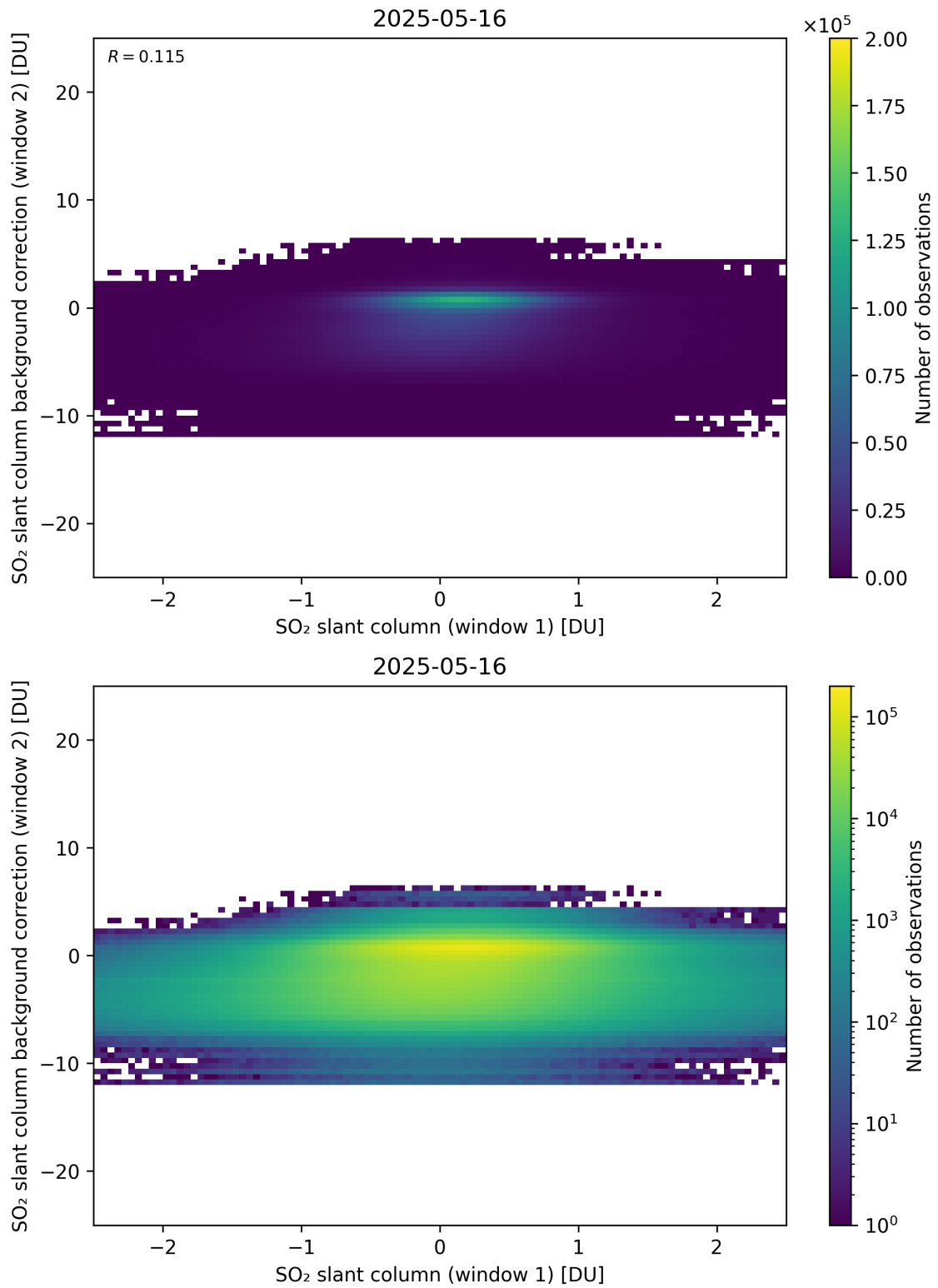
Figure 263: Scatter density plot of “SO 2 slant column (window 1)” against “SO 2 slant column background correction (window 2)” for 2025-05-15 to 2025-05-17.
