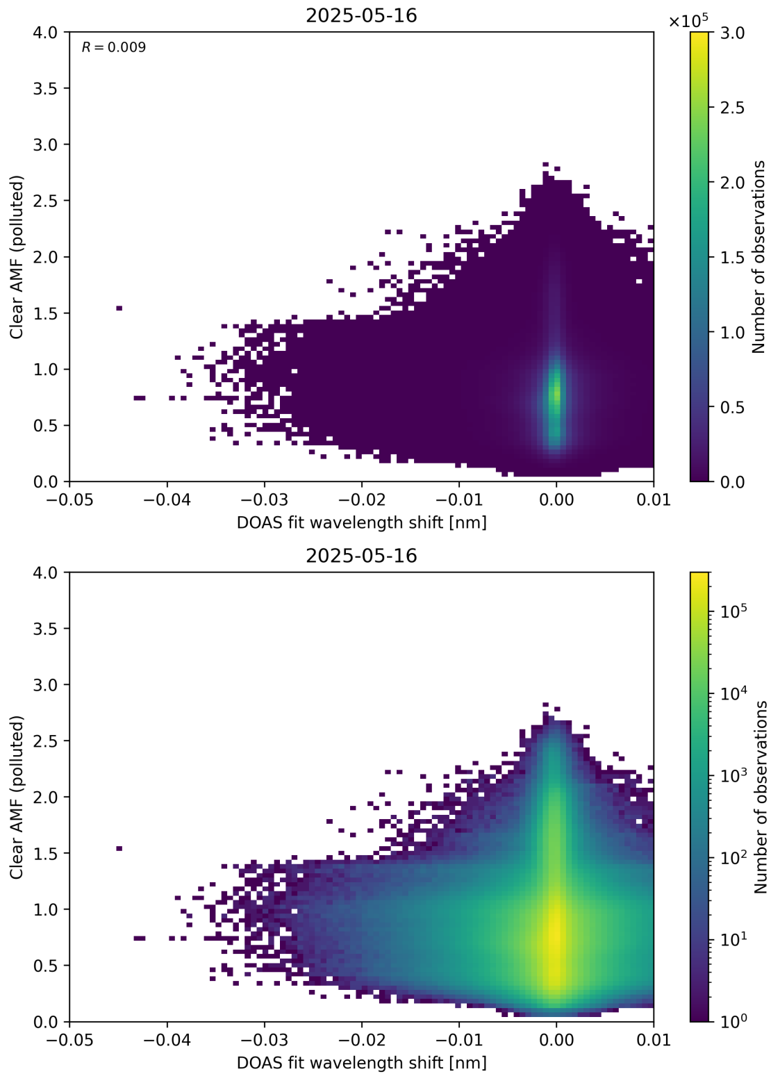
Figure 140: Scatter density plot of “DOAS fit wavelength shift” against “Clear AMF (polluted)” for 2025-05-15 to 2025-05-17.
