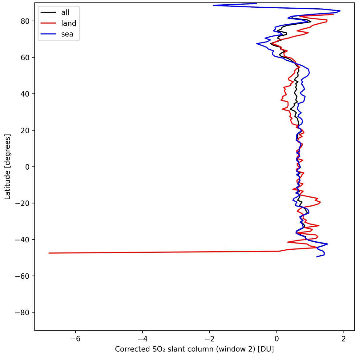
Figure 43: Zonal average of “Corrected SO 2 slant column (window 2)” for 2025-05-15 to 2025-05-17.
