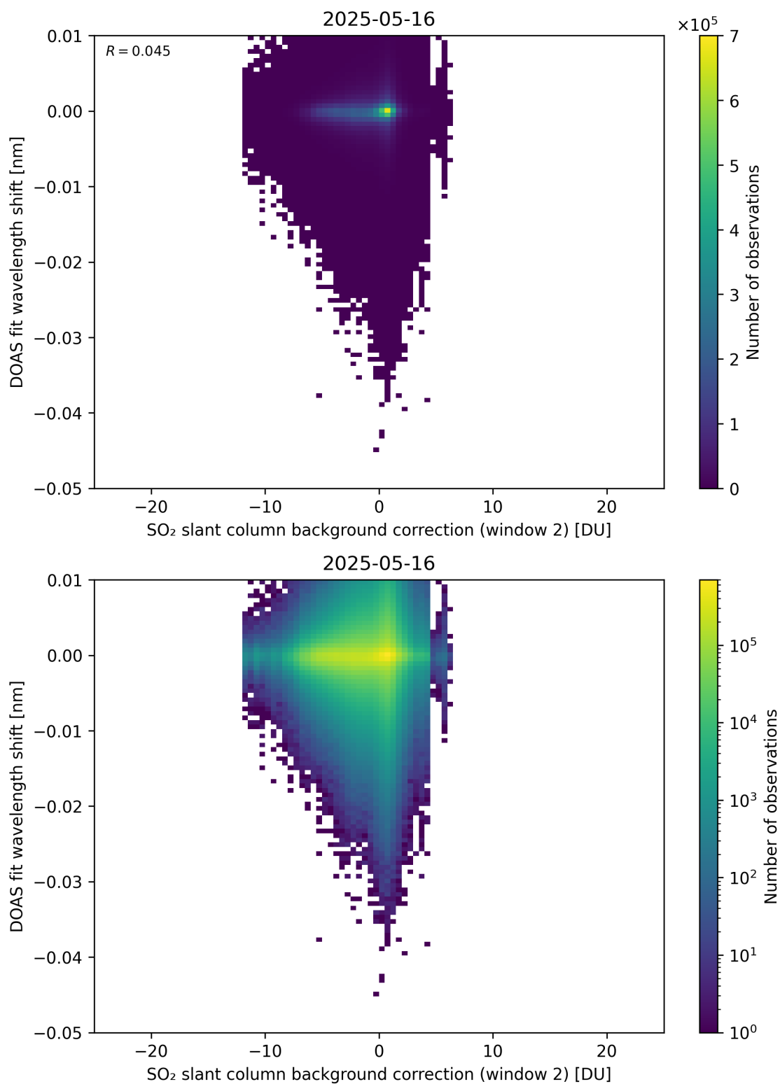
Figure 123: Scatter density plot of “SO 2 slant column background correction (window 2)” against “DOAS fit wavelength shift” for 2025-05-15 to 2025-05-17.
