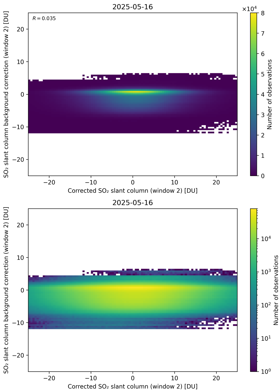
Figure 244: Scatter density plot of “Corrected SO 2 slant column (window 2)” against “SO 2 slant column background correction (window 2)” for 2025-05-15 to 2025-05-17.
