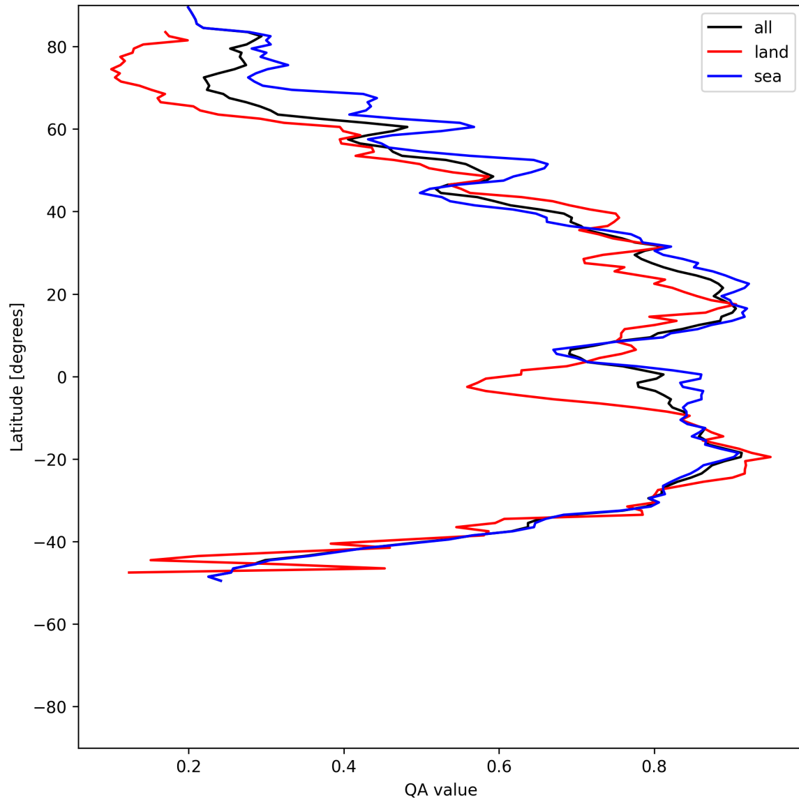
Figure 31: Zonal average of “QA value” for 2025-05-15 to 2025-05-17.
