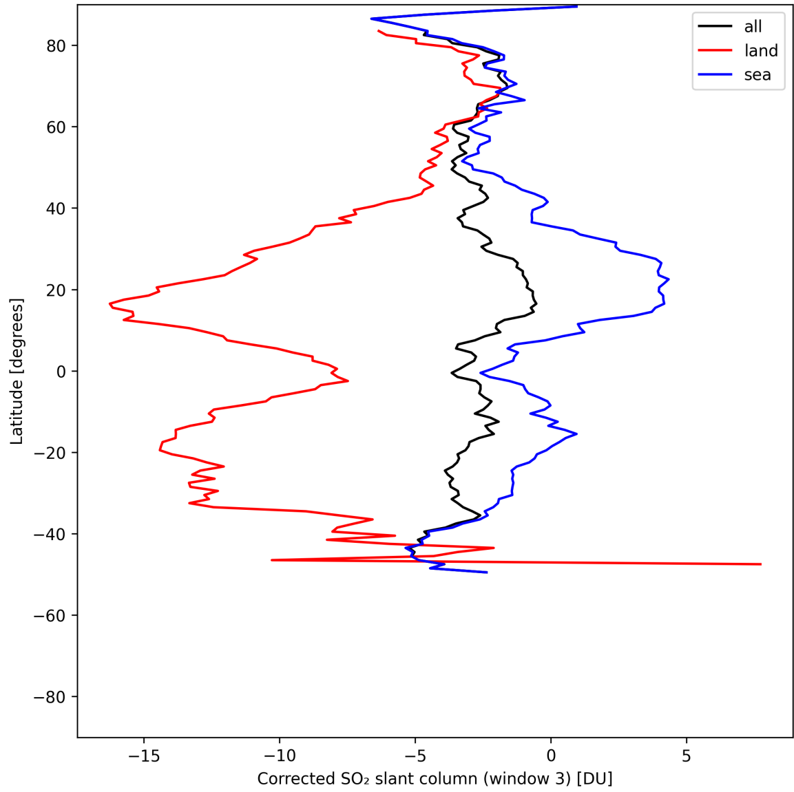
Figure 47: Zonal average of “Corrected SO 2 slant column (window 3)” for 2025-05-15 to 2025-05-17.
