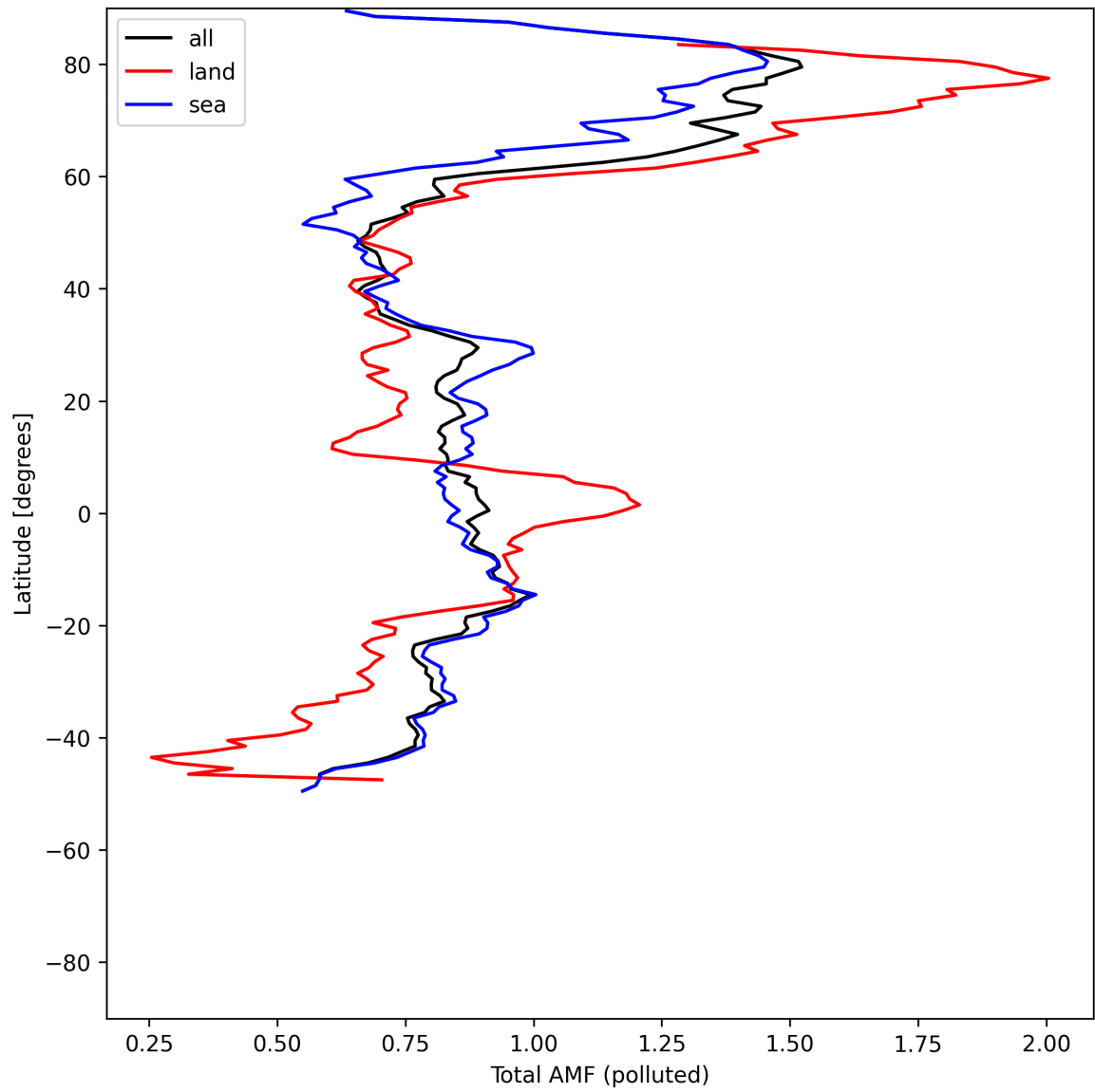
Figure 53: Zonal average of “Total AMF (polluted)” for 2025-05-15 to 2025-05-17.
