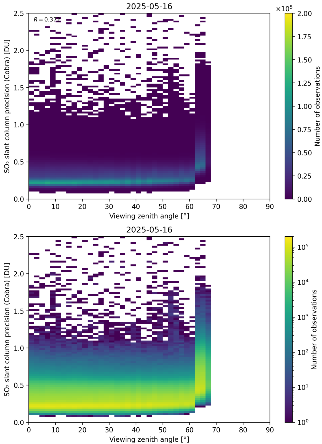
Figure 372: Scatter density plot of “Viewing zenith angle” against “SO 2 slant column precision (Cobra)” for 2025-05-15 to 2025-05-17.
