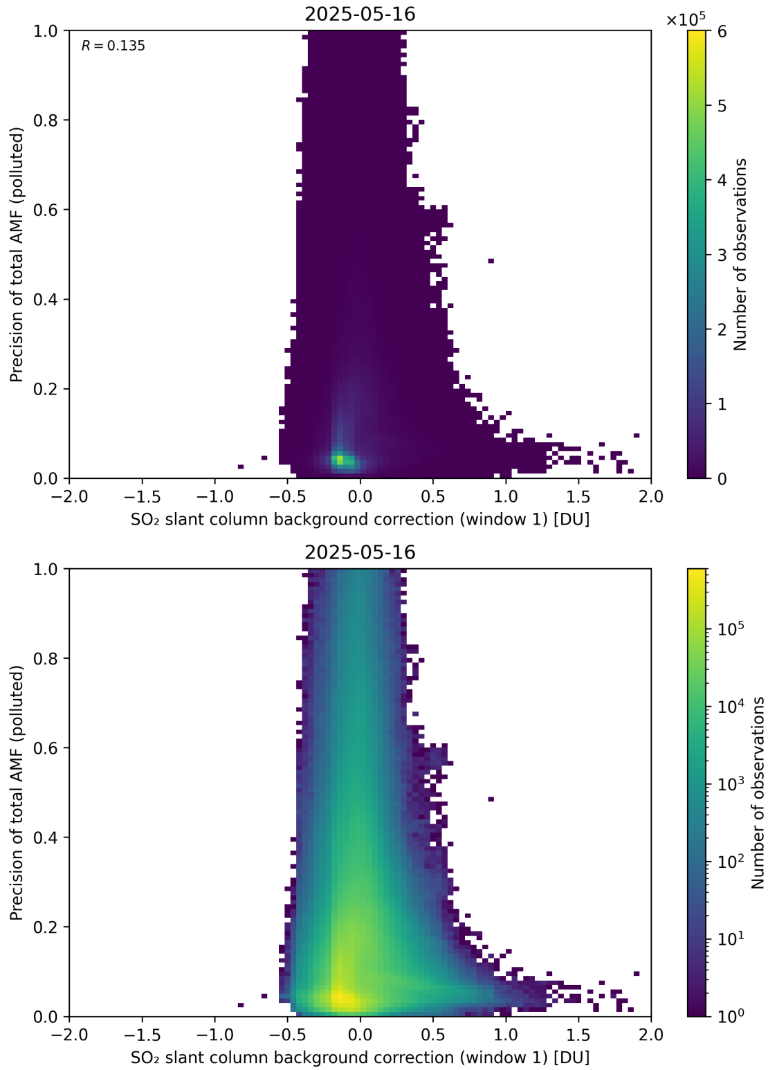
Figure 121: Scatter density plot of “SO 2 slant column background correction (window 1)” against “Precision of total AMF (polluted)” for 2025-05-15 to 2025-05-17.
