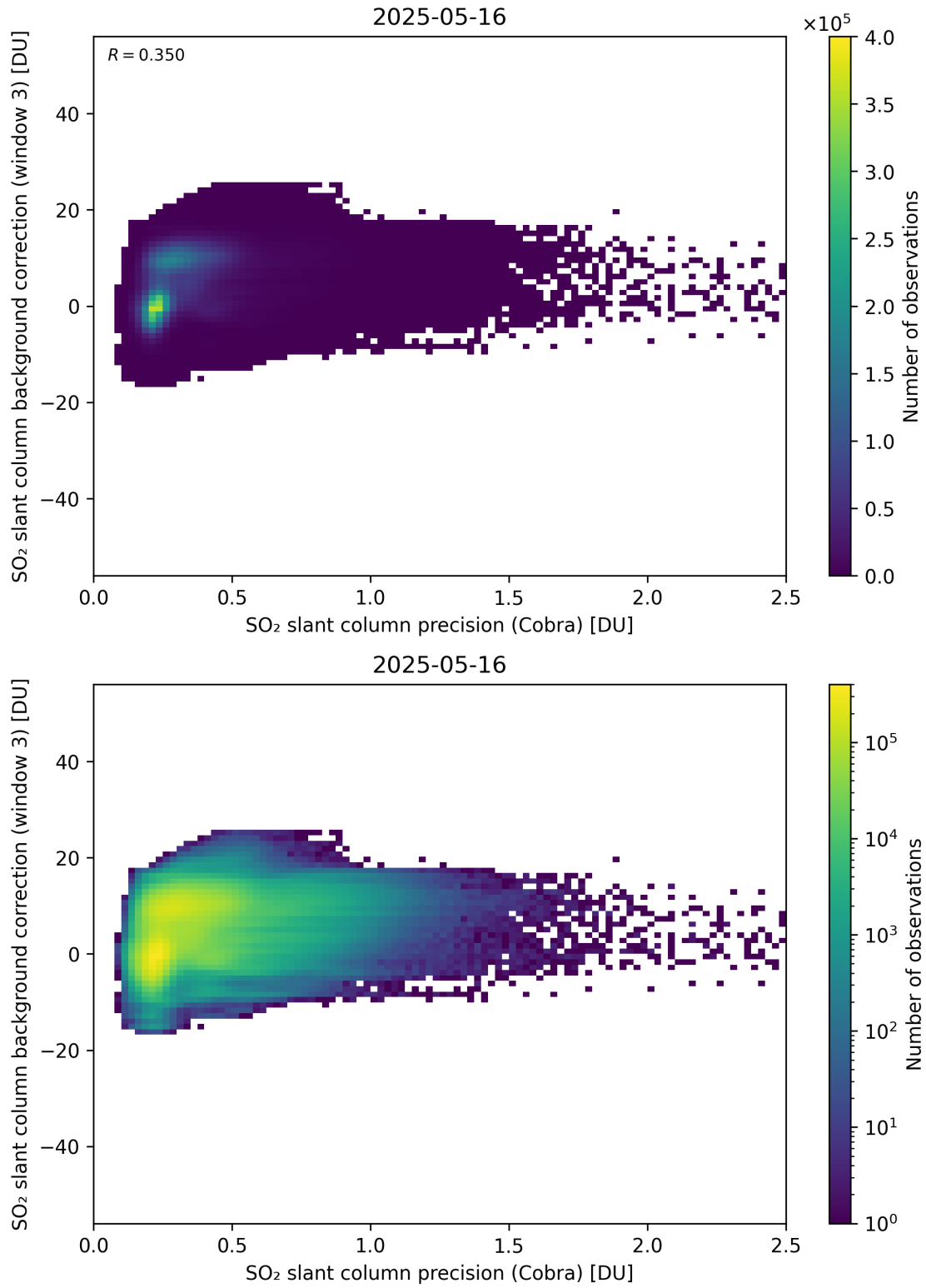
Figure 201: Scatter density plot of “SO 2 slant column precision (Cobra)” against “SO 2 slant column background correction (window 3)” for 2025-05-15 to 2025-05-17.
