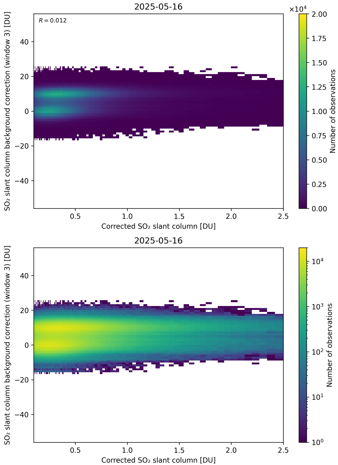
Figure 228: Scatter density plot of “Corrected SO 2 slant column” against “SO 2 slant column background correction (window 3)” for 2025-05-15 to 2025-05-17.
