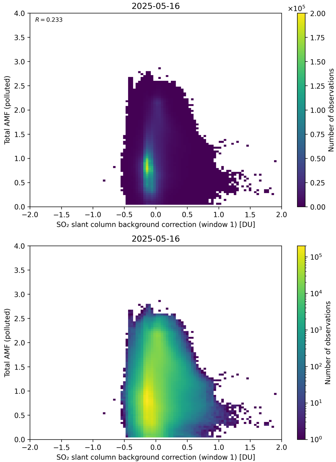
Figure 120: Scatter density plot of “SO 2 slant column background correction (window 1)” against “Total AMF (polluted)” for 2025-05-15 to 2025-05-17.
