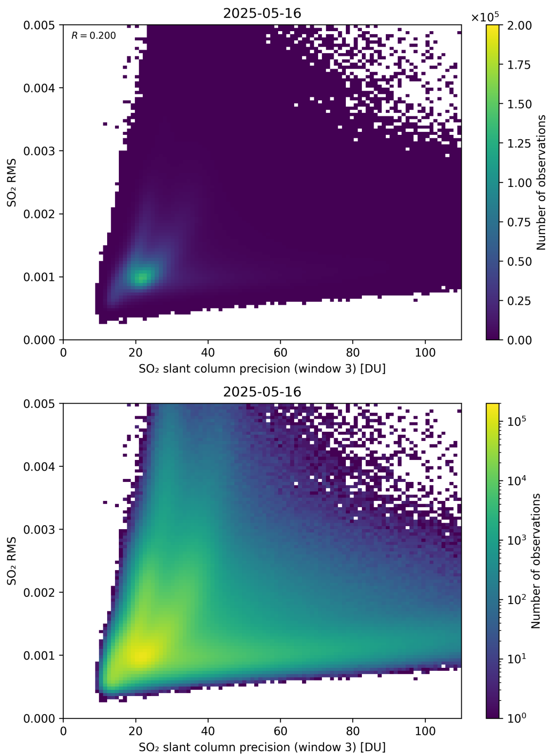
Figure 310: Scatter density plot of “SO 2 slant column precision (window 3)” against “SO 2 RMS” for 2025-05-15 to 2025-05-17.
