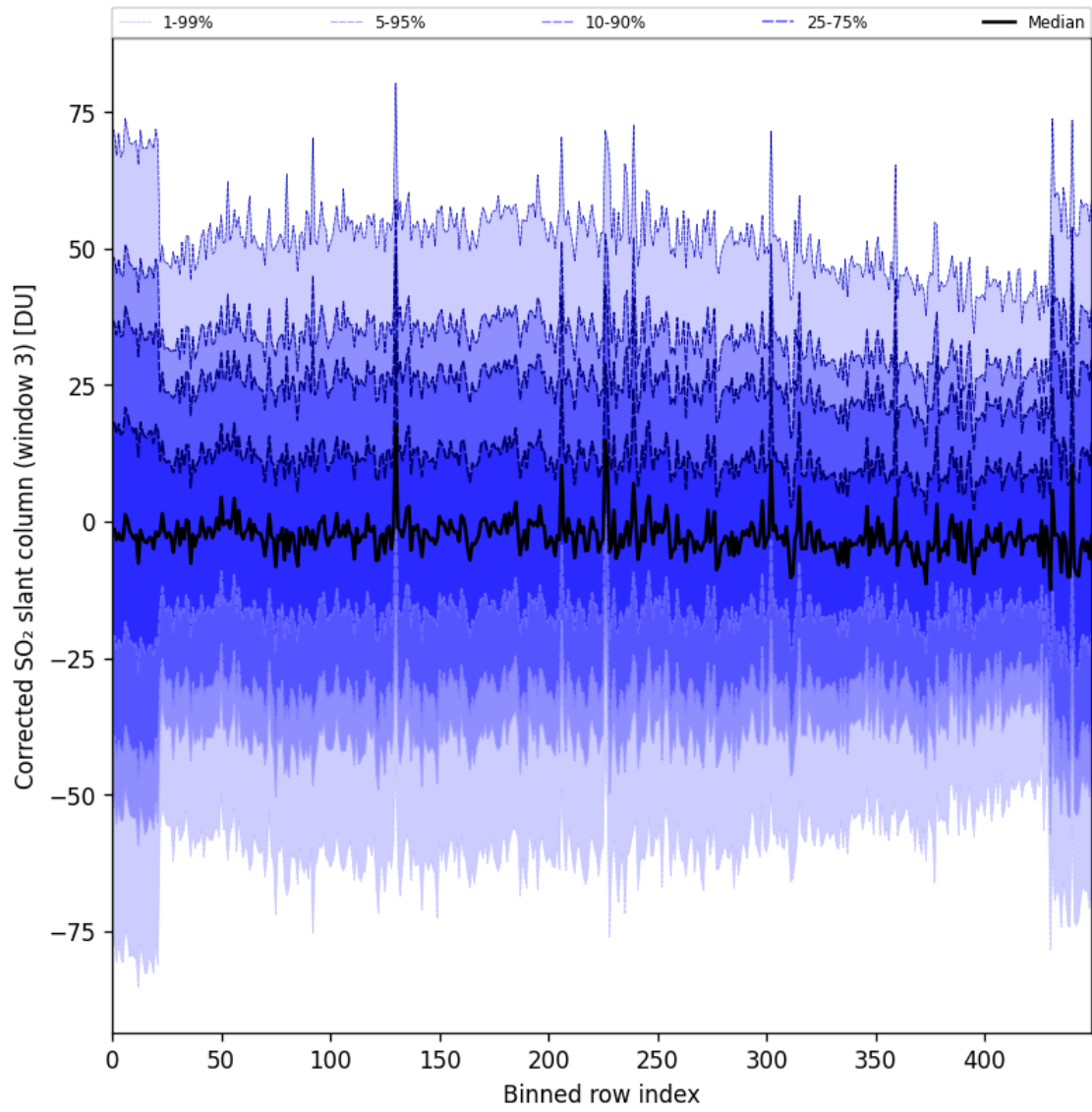
Figure 99: Along track statistics of “Corrected SO 2 slant column (window 3)” for 2025-05-15 to 2025-05-17
