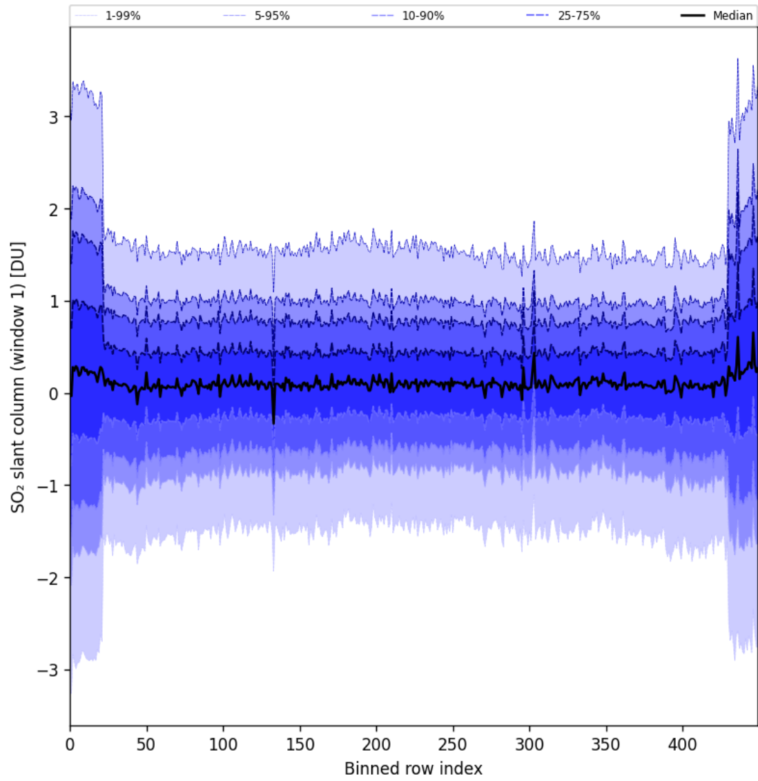
Figure 89: Along track statistics of “SO 2 slant column (window 1)” for 2025-05-15 to 2025-05-17
