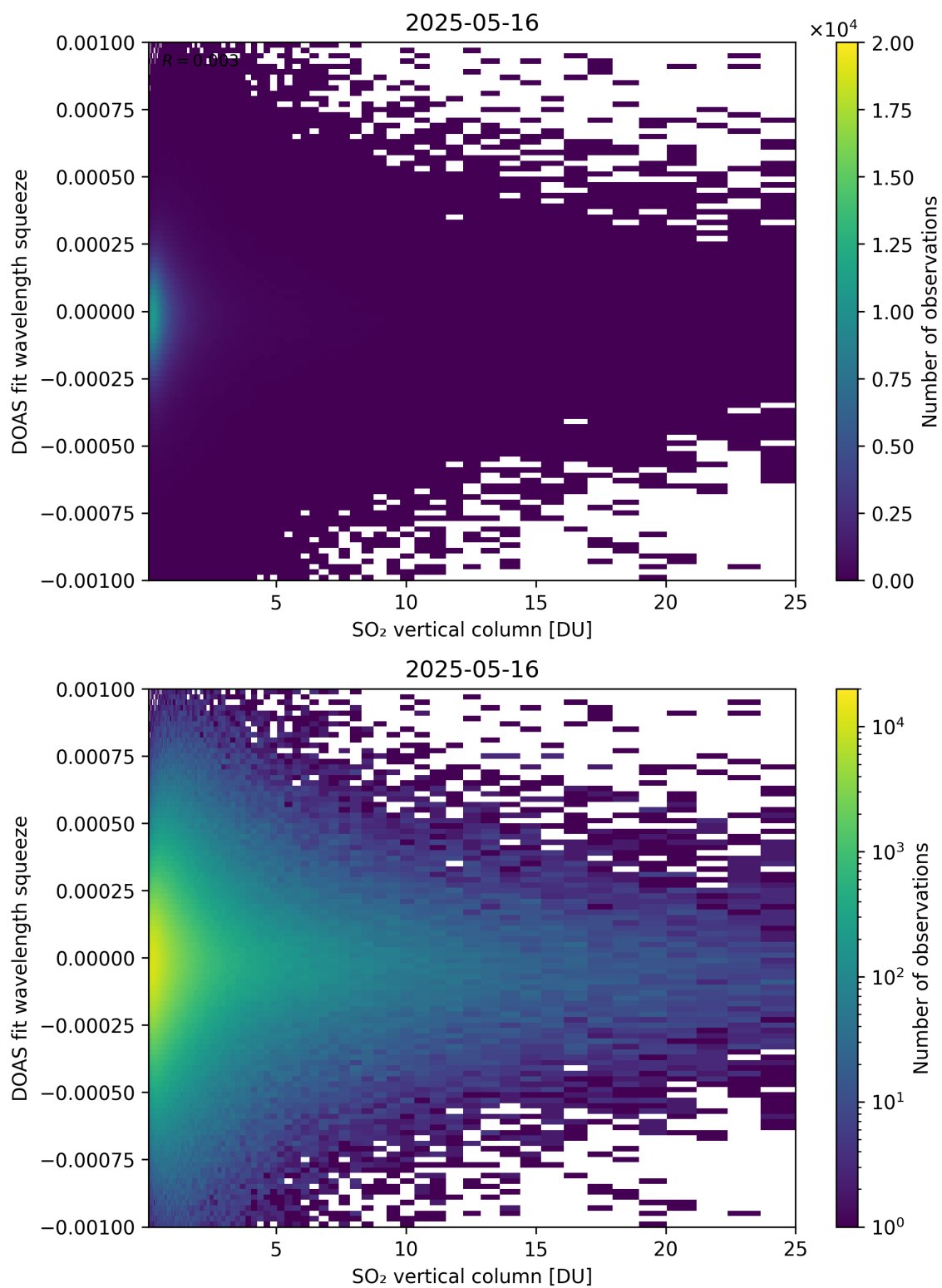
Figure 327: Scatter density plot of “SO 2 vertical column” against “DOAS fit wavelength squeeze” for 2025-05-15 to 2025-05-17.
