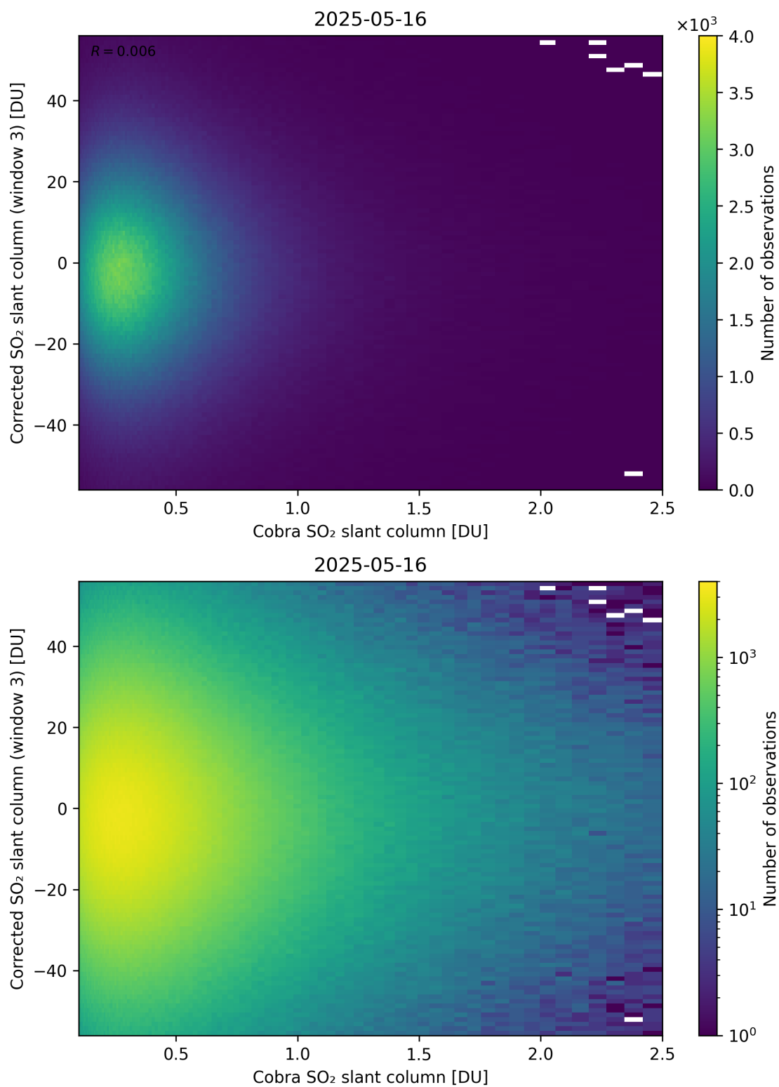
Figure 218: Scatter density plot of “Cobra SO 2 slant column” against “Corrected SO 2 slant column (window 3)” for 2025-05-15 to 2025-05-17.
