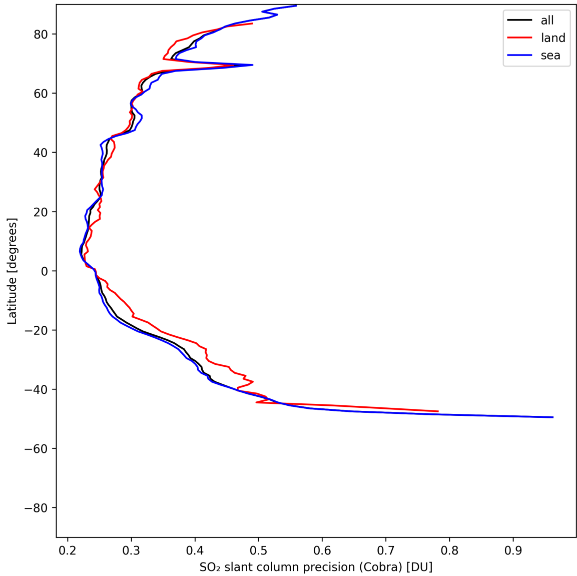
Figure 36: Zonal average of “SO 2 slant column precision (Cobra)” for 2025-05-15 to 2025-05-17.
