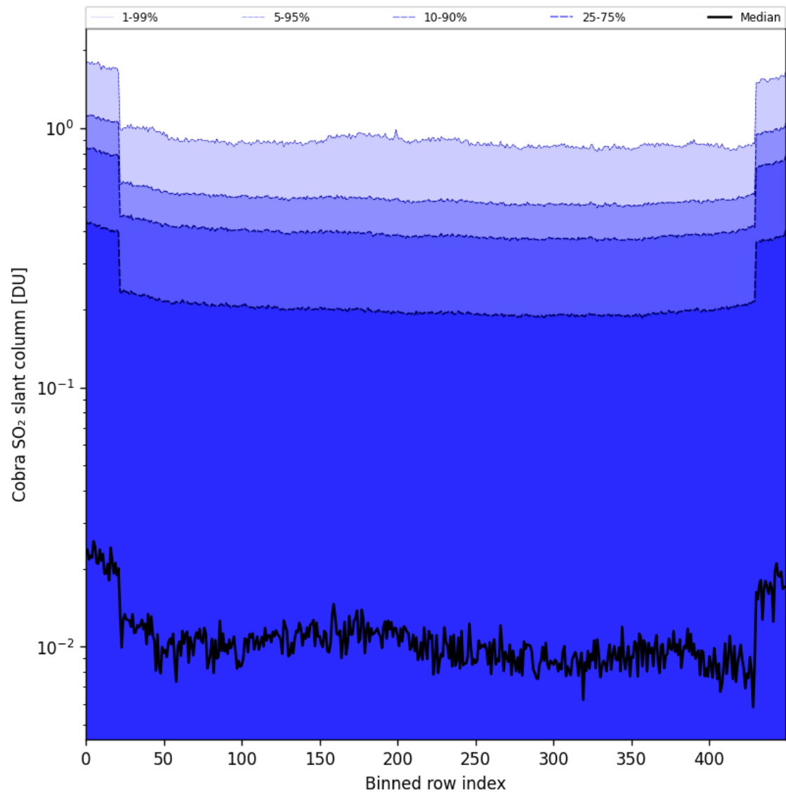
Figure 87: Along track statistics of “Cobra SO 2 slant column” for 2025-05-15 to 2025-05-17
