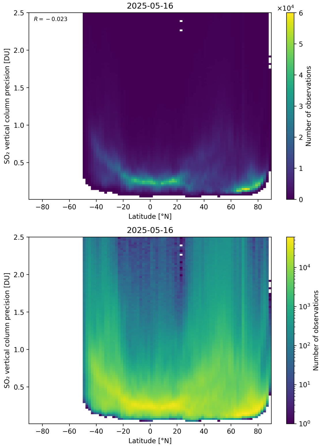
Figure 170: Scatter density plot of “Latitude” against “SO 2 vertical column precision” for 2025-05-15 to 2025-05-17.
