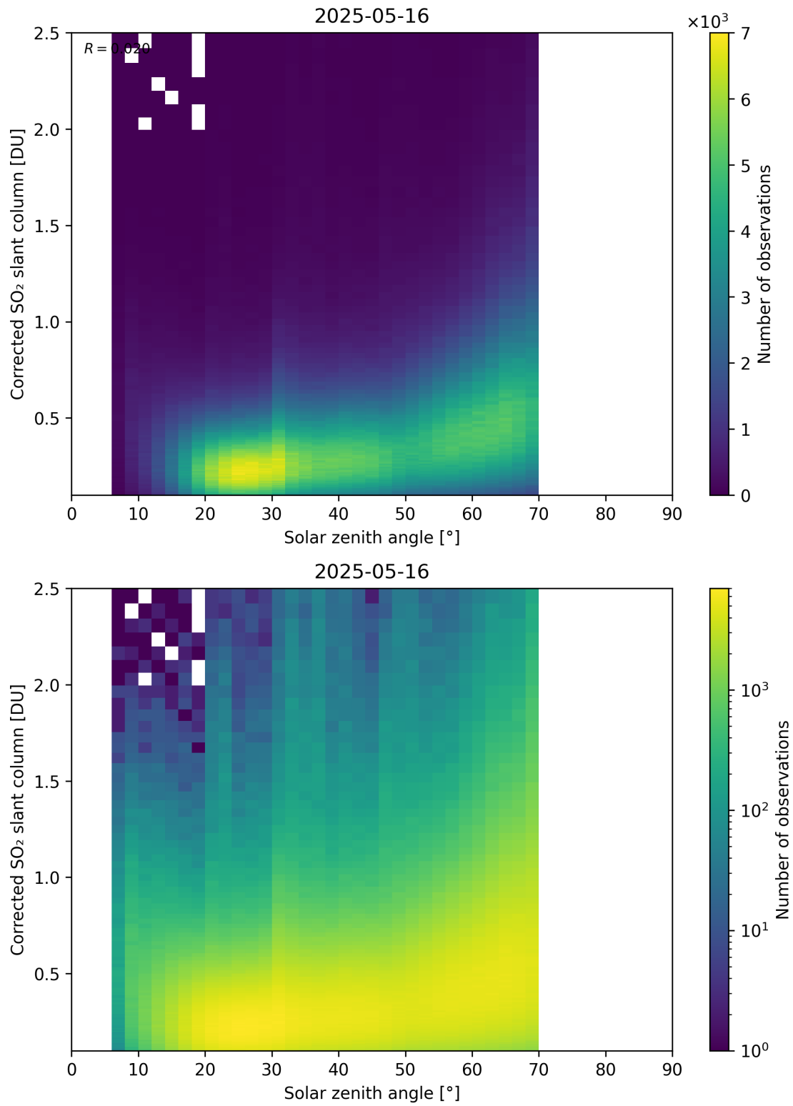
Figure 181: Scatter density plot of “Solar zenith angle” against “Corrected SO 2 slant column” for 2025-05-15 to 2025-05-17.
