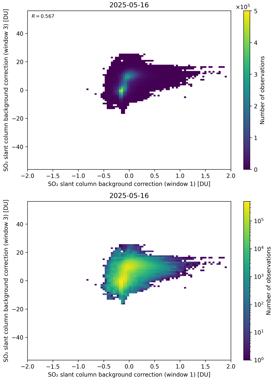
Figure 110: Scatter density plot of “SO 2 slant column background correction (window 1)” against “SO 2 slant column background correction (window 3)” for 2025-05-15 to 2025-05-17.
