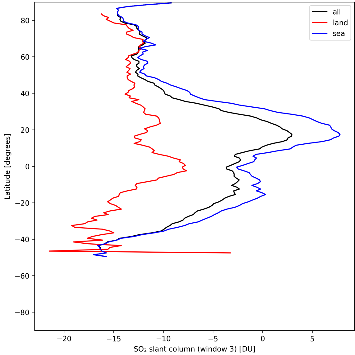
Figure 45: Zonal average of “SO 2 slant column (window 3)” for 2025-05-15 to 2025-05-17.
