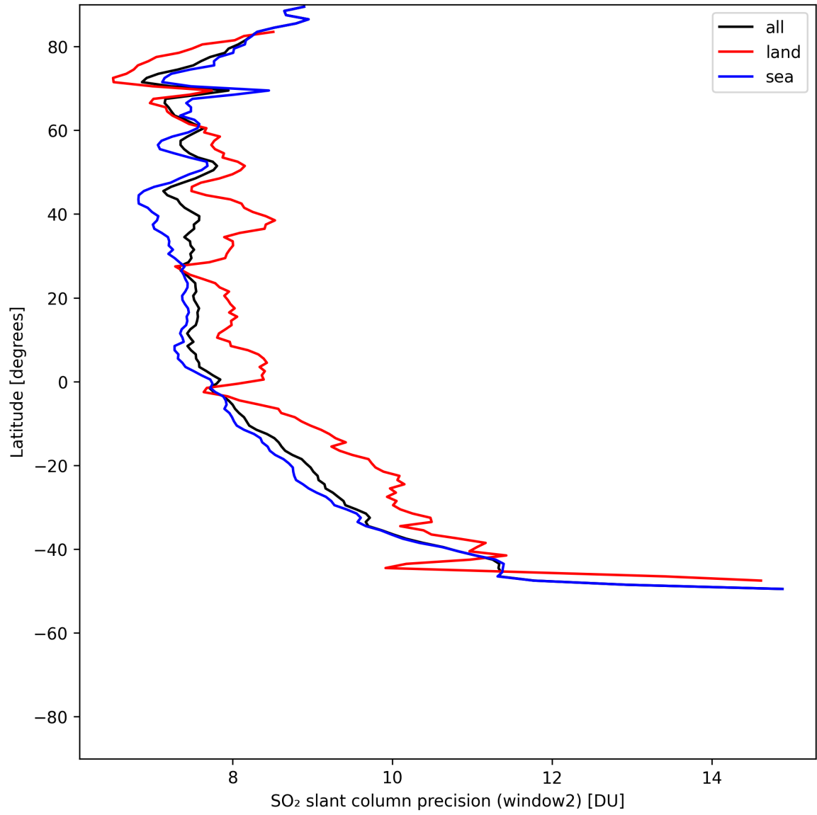
Figure 42: Zonal average of “SO 2 slant column precision (window2)” for 2025-05-15 to 2025-05-17.
