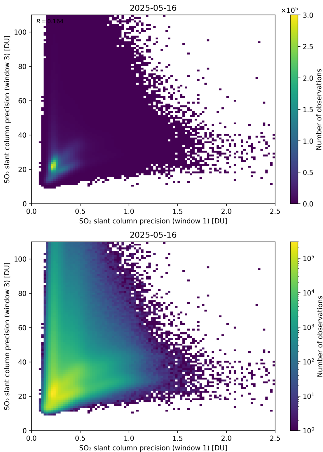
Figure 279: Scatter density plot of “SO 2 slant column precision (window 1)” against “SO 2 slant column precision (window 3)” for 2025-05-15 to 2025-05-17.
