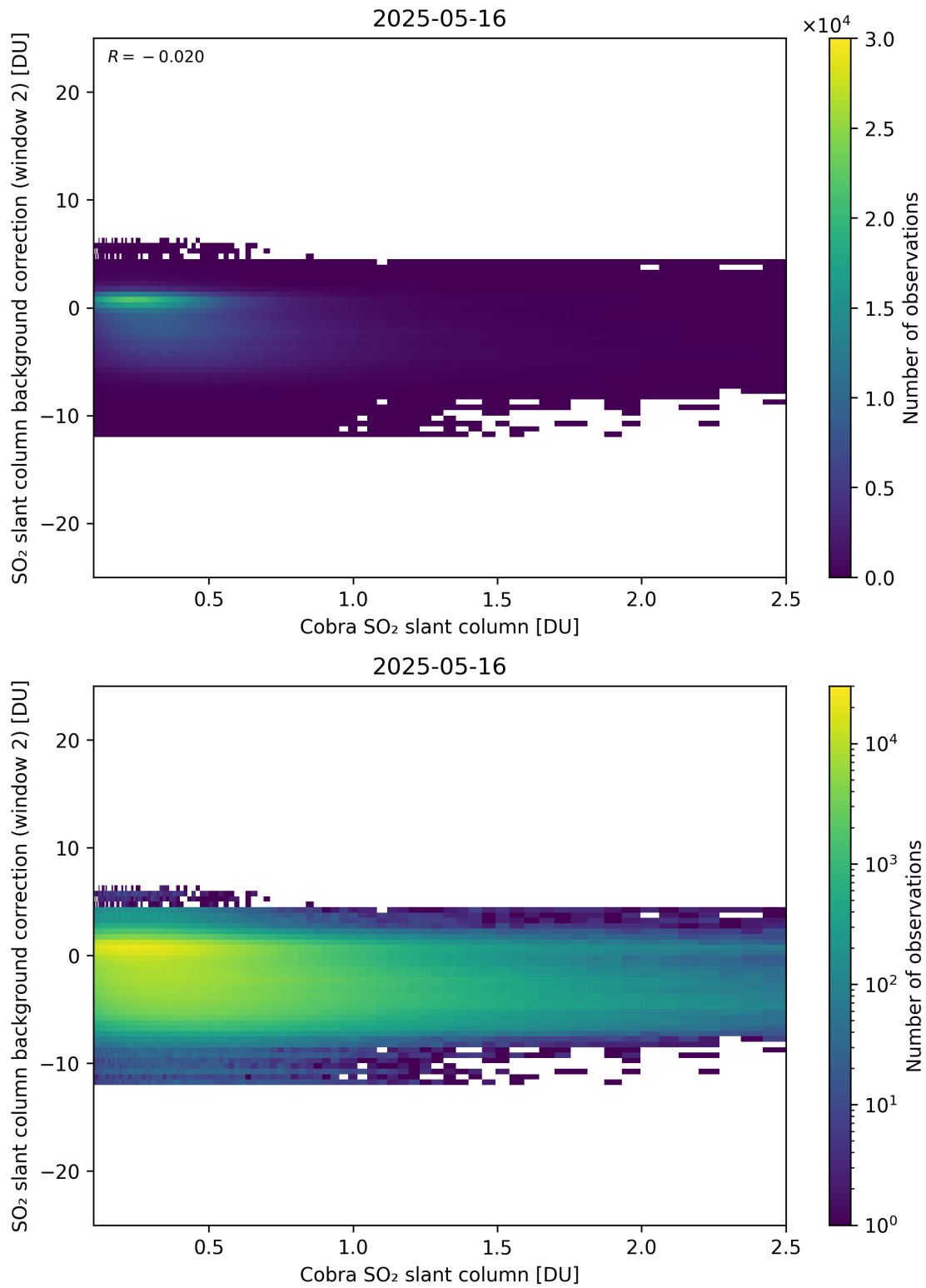
Figure 194: Scatter density plot of “Cobra SO 2 slant column” against “SO 2 slant column background correction (window 2)” for 2025-05-15 to 2025-05-17.
