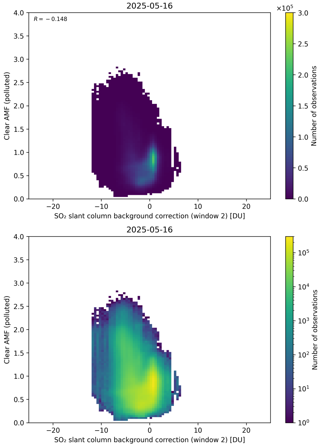
Figure 126: Scatter density plot of “SO 2 slant column background correction (window 2)” against “Clear AMF (polluted)” for 2025-05-15 to 2025-05-17.
