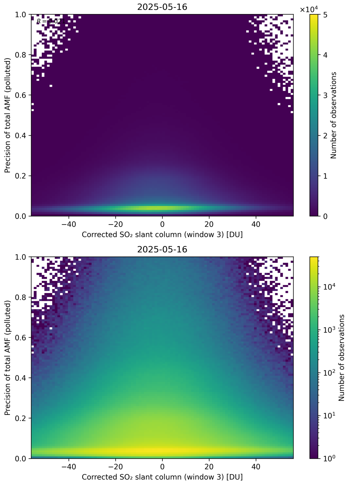
Figure 261: Scatter density plot of “Corrected SO 2 slant column (window 3)” against “Precision of total AMF (polluted)” for 2025-05-15 to 2025-05-17.
