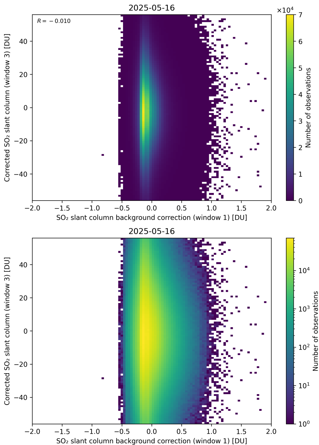
Figure 116: Scatter density plot of “SO 2 slant column background correction (window 1)” against “Corrected SO 2 slant column (window 3)” for 2025-05-15 to 2025-05-17.
