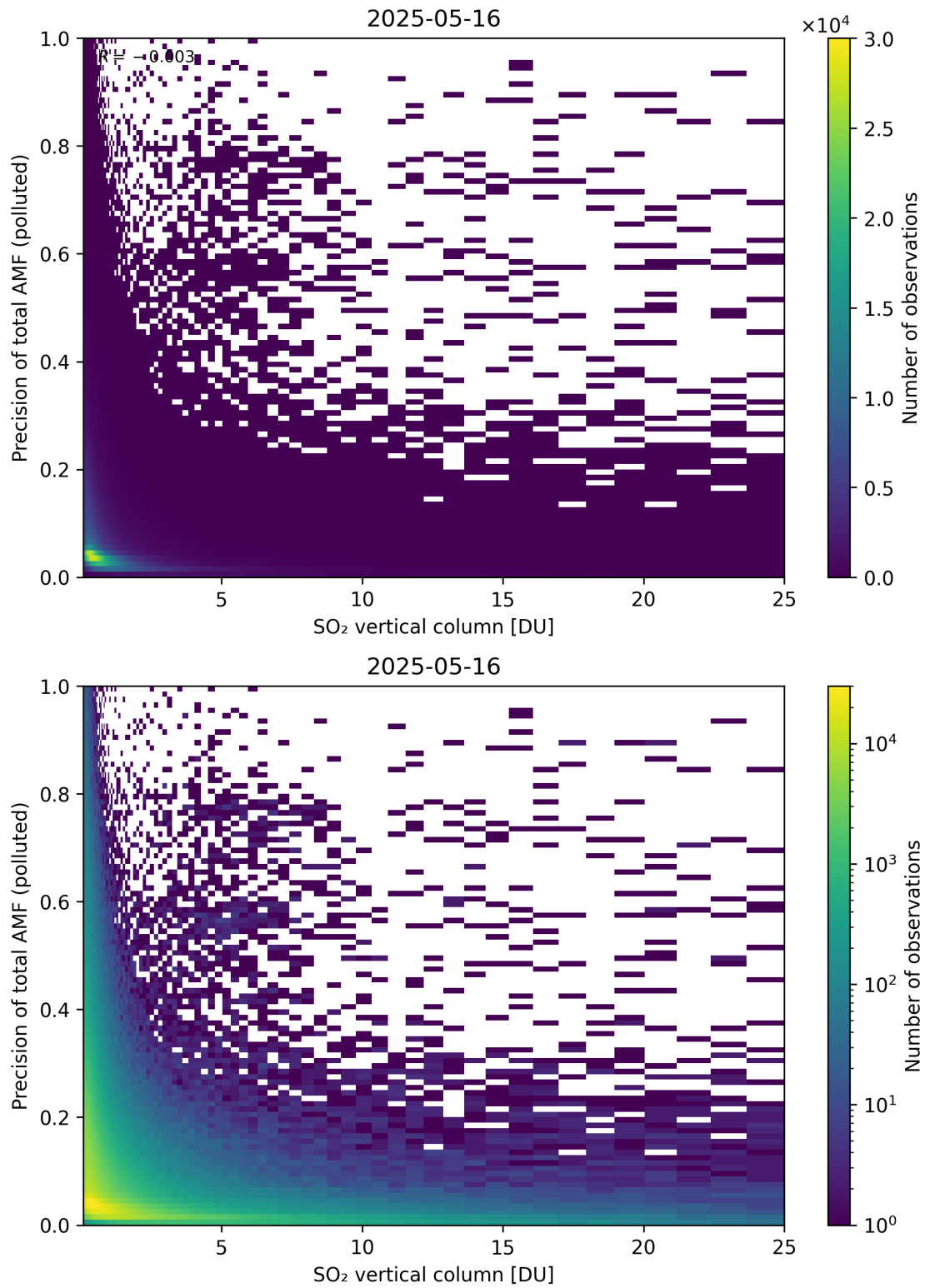
Figure 360: Scatter density plot of “SO 2 vertical column” against “Precision of total AMF (polluted)” for 2025-05-15 to 2025-05-17.
