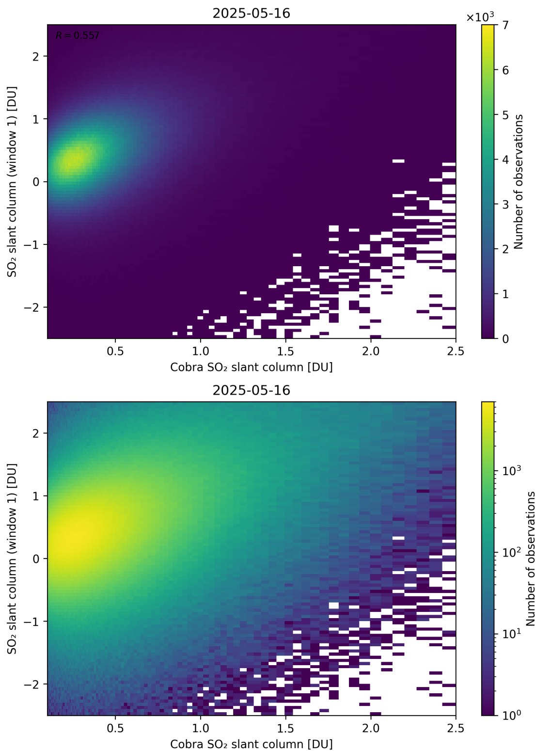
Figure 219: Scatter density plot of “Cobra SO 2 slant column” against “SO 2 slant column (window 1)” for 2025-05-15 to 2025-05-17.
