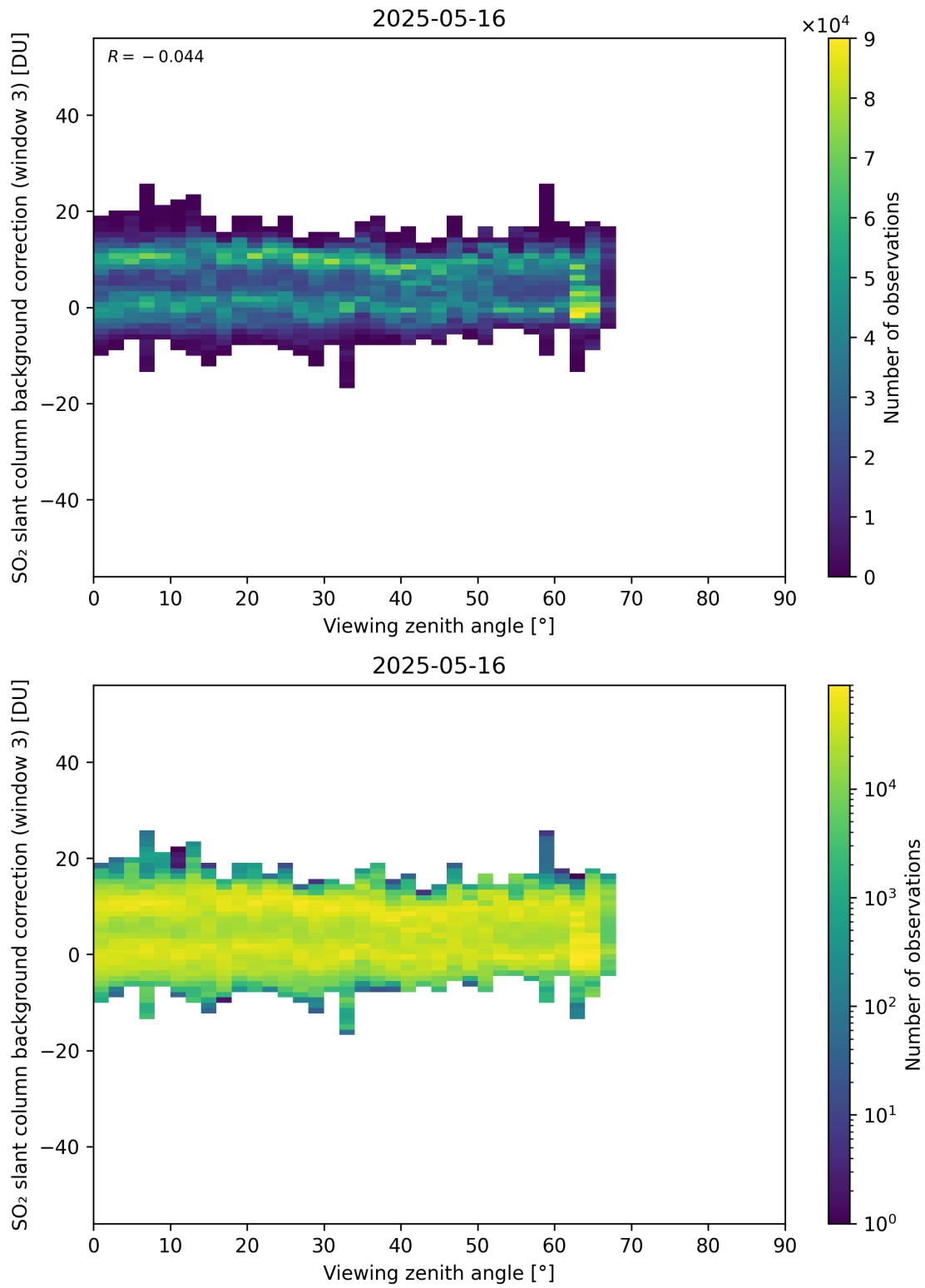
Figure 364: Scatter density plot of “Viewing zenith angle” against “SO 2 slant column background correction (window 3)” for 2025-05-15 to 2025-05-17.
