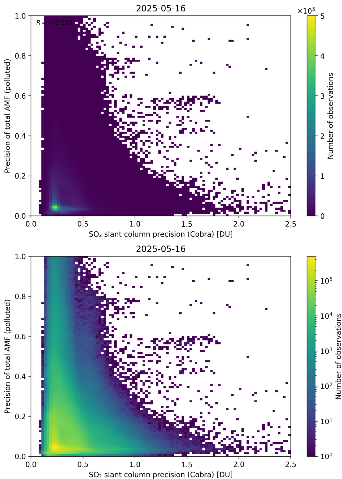
Figure 214: Scatter density plot of “SO 2 slant column precision (Cobra)” against “Precision of total AMF (polluted)” for 2025-05-15 to 2025-05-17.
