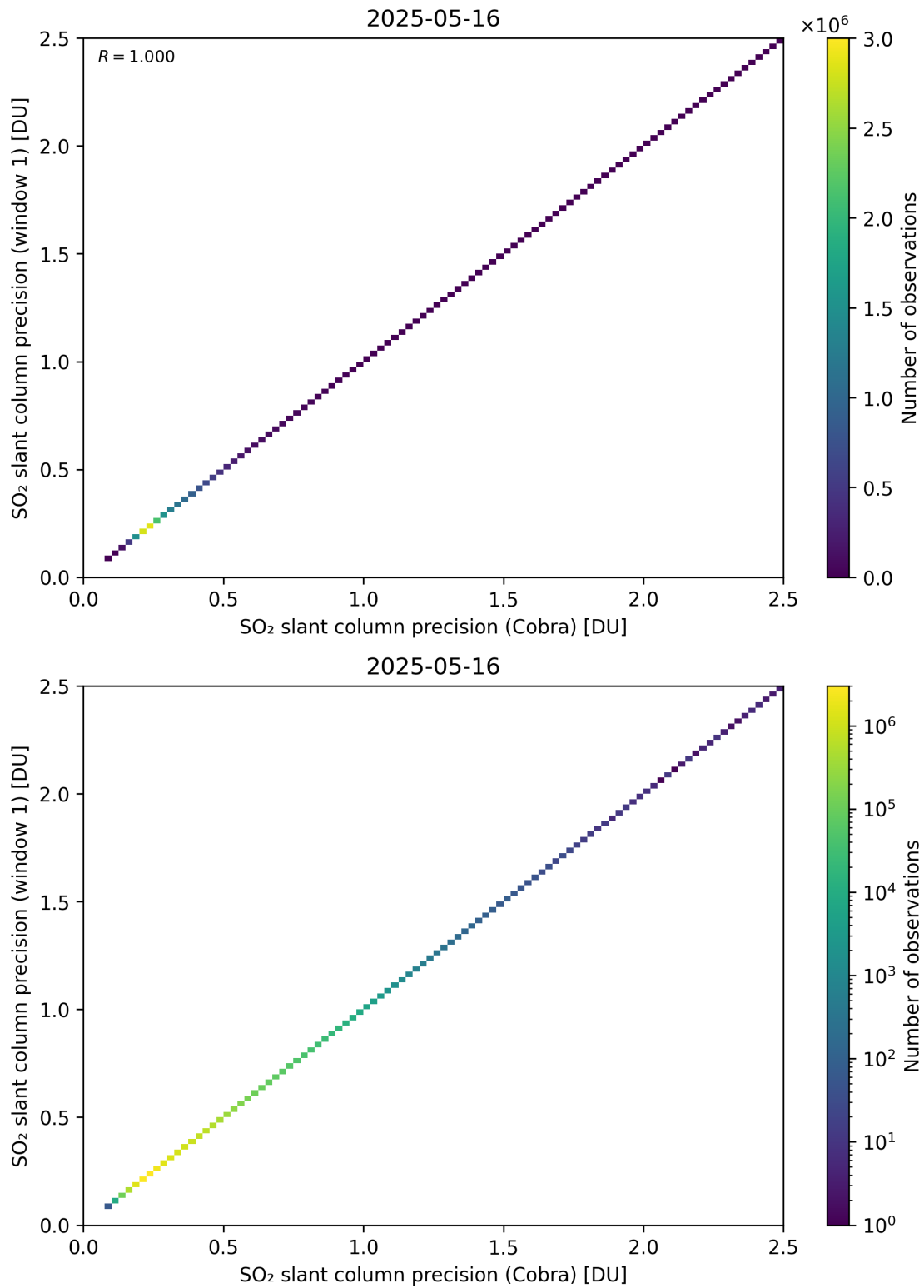
Figure 209: Scatter density plot of “SO 2 slant column precision (Cobra)” against “SO 2 slant column precision (window 1)” for 2025-05-15 to 2025-05-17.
