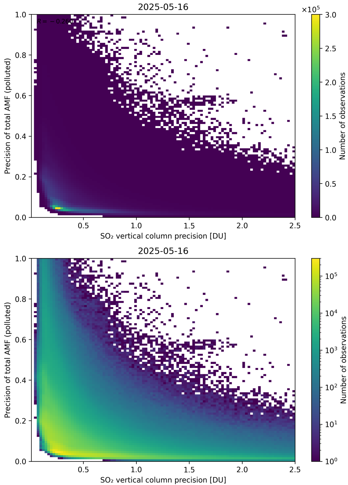
Figure 347: Scatter density plot of “SO 2 vertical column precision” against “Precision of total AMF (polluted)” for 2025-05-15 to 2025-05-17.
