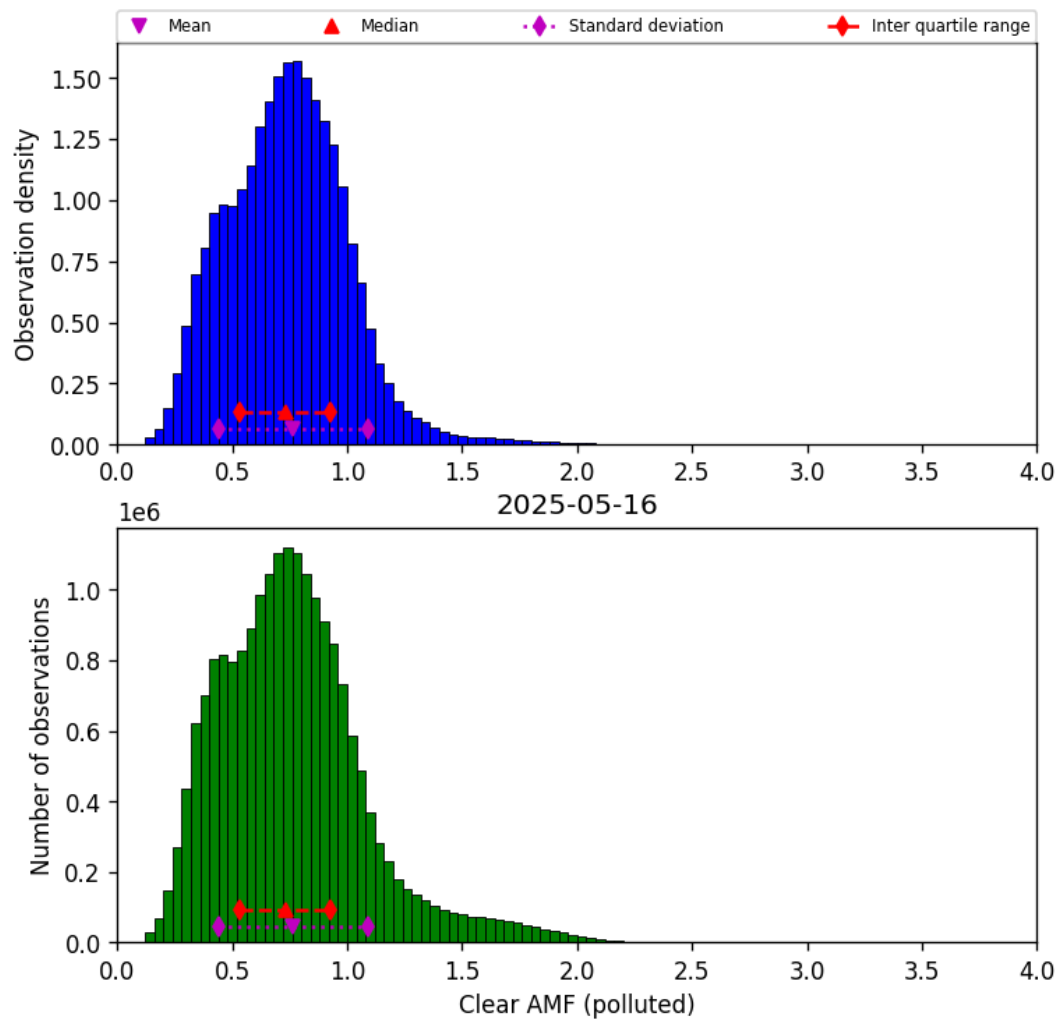
Figure 81: Histogram of “Clear AMF (polluted)” for 2025-05-15 to 2025-05-17
