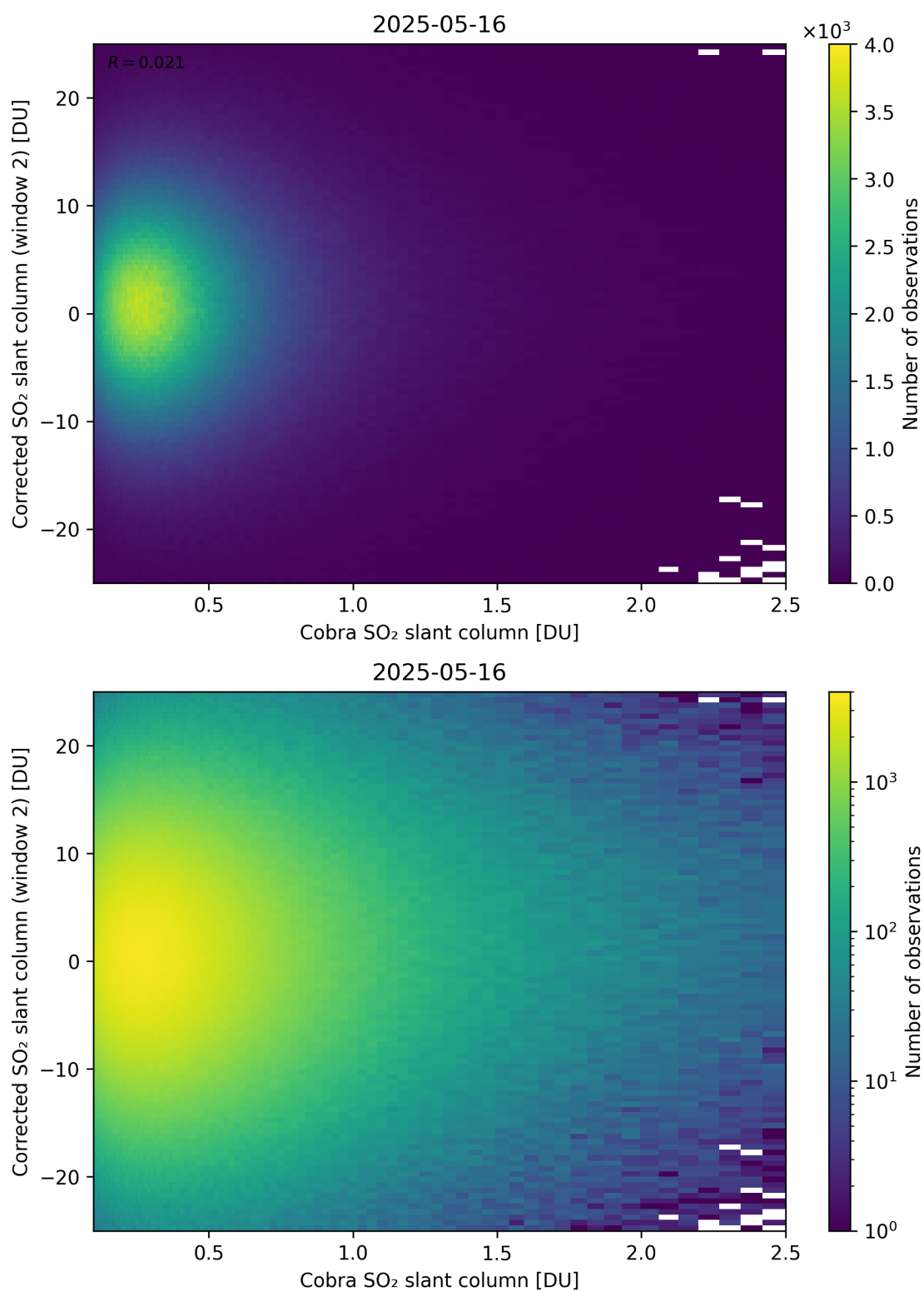
Figure 217: Scatter density plot of “Cobra SO 2 slant column” against “Corrected SO 2 slant column (window 2)” for 2025-05-15 to 2025-05-17.
