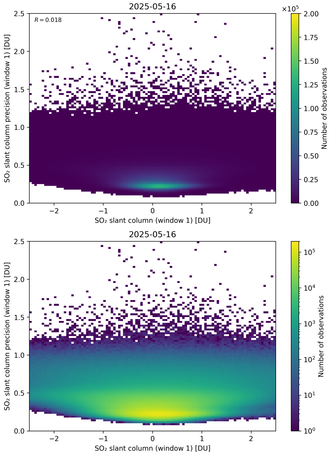
Figure 285: Scatter density plot of “SO 2 slant column (window 1)” against “SO 2 slant column precision (window 1)” for 2025-05-15 to 2025-05-17.
