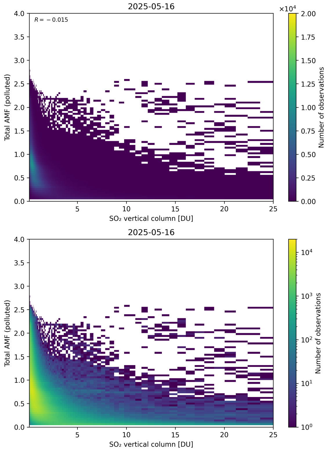
Figure 359: Scatter density plot of “SO 2 vertical column” against “Total AMF (polluted)” for 2025-05-15 to 2025-05-17.
