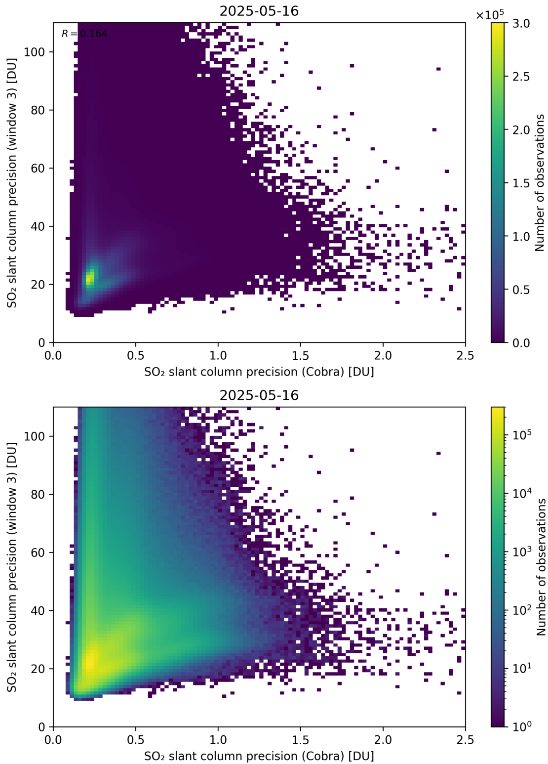
Figure 212: Scatter density plot of “SO 2 slant column precision (Cobra)” against “SO 2 slant column precision (window 3)” for 2025-05-15 to 2025-05-17.
