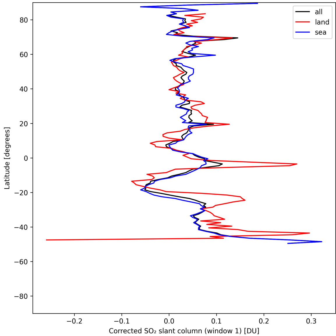
Figure 39: Zonal average of “Corrected SO 2 slant column (window 1)” for 2025-05-15 to 2025-05-17.
