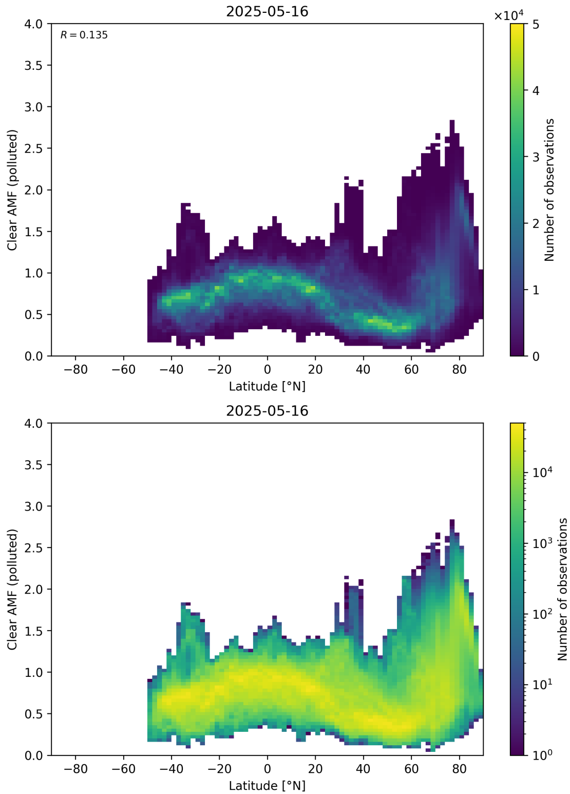
Figure 156: Scatter density plot of “Latitude” against “Clear AMF (polluted)” for 2025-05-15 to 2025-05-17.
