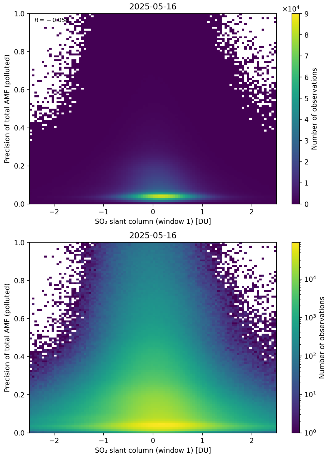
Figure 290: Scatter density plot of “SO 2 slant column (window 1)” against “Precision of total AMF (polluted)” for 2025-05-15 to 2025-05-17.
