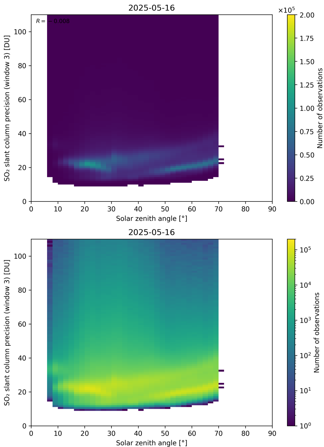
Figure 188: Scatter density plot of “Solar zenith angle” against “SO 2 slant column precision (window 3)” for 2025-05-15 to 2025-05-17.
