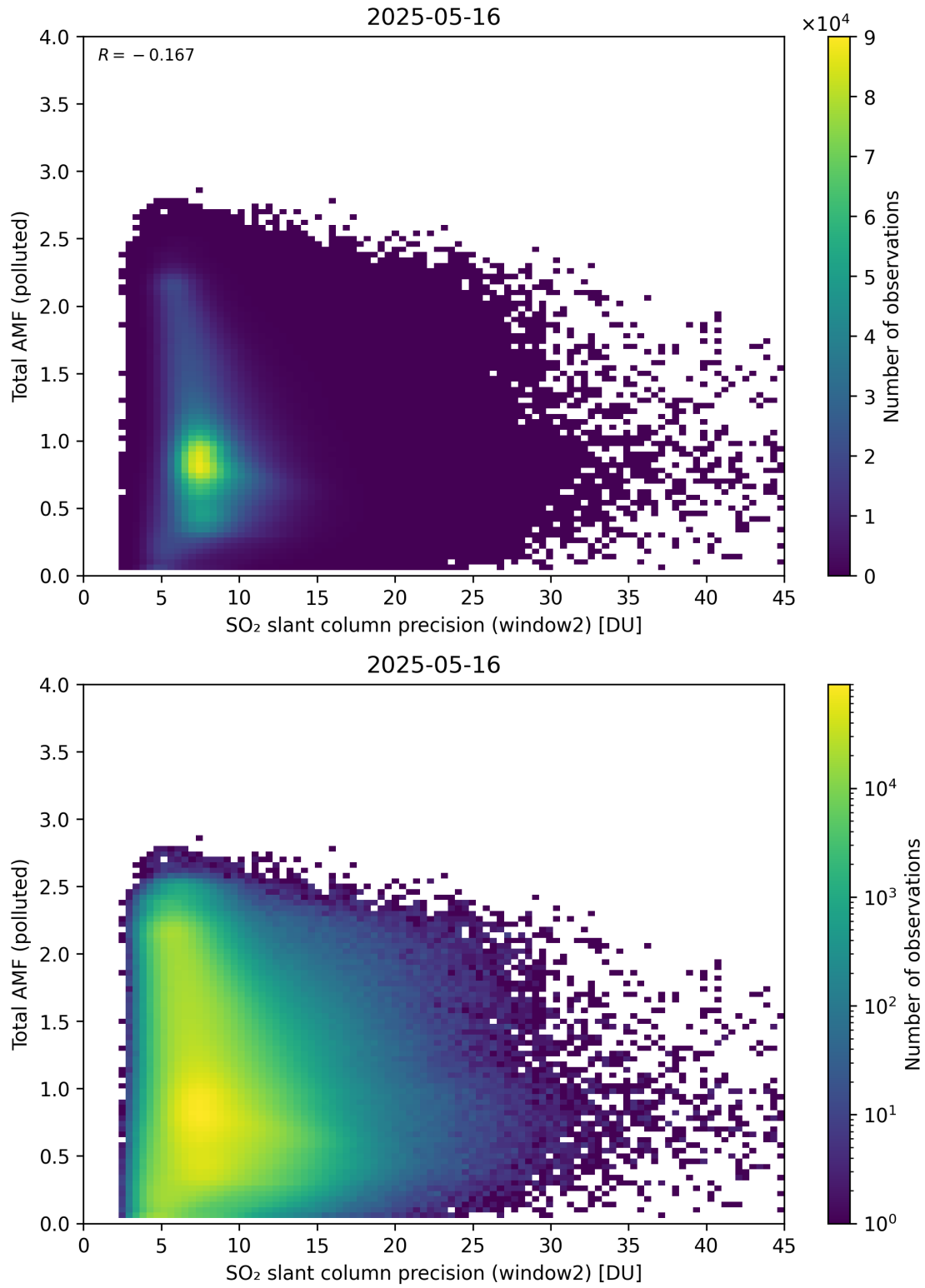
Figure 301: Scatter density plot of “SO 2 slant column precision (window2)” against “Total AMF (polluted)” for 2025-05-15 to 2025-05-17.
