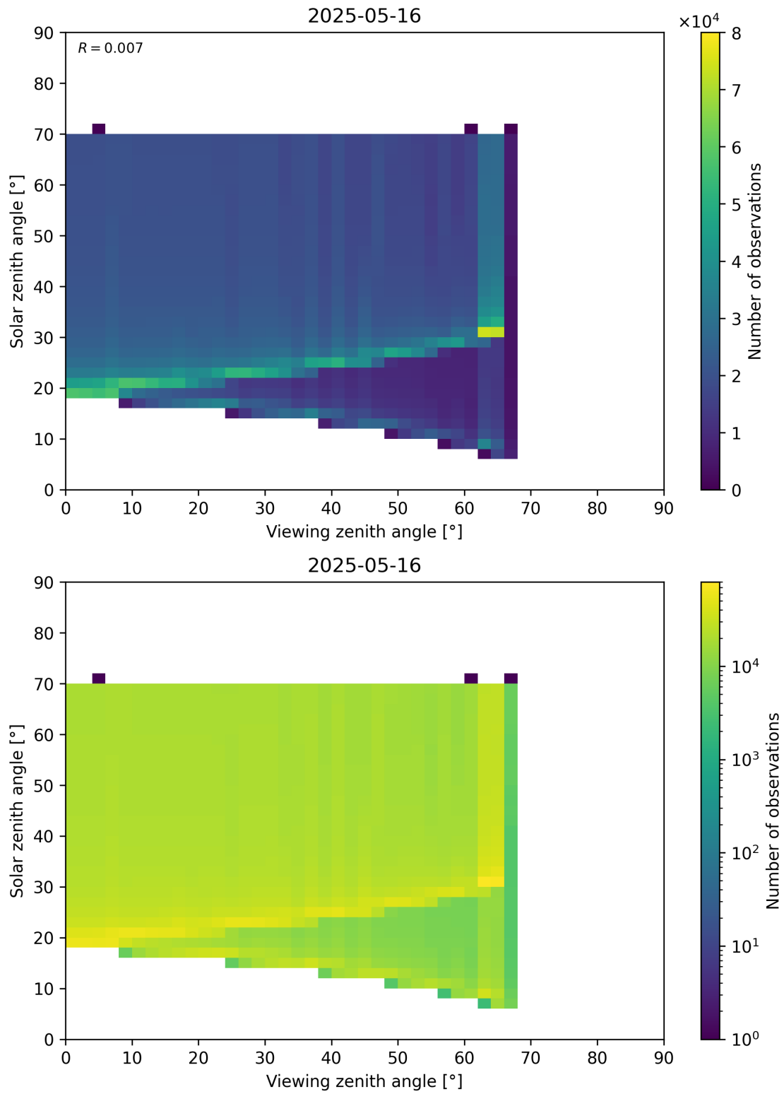
Figure 369: Scatter density plot of “Viewing zenith angle” against “Solar zenith angle” for 2025-05-15 to 2025-05-17.
