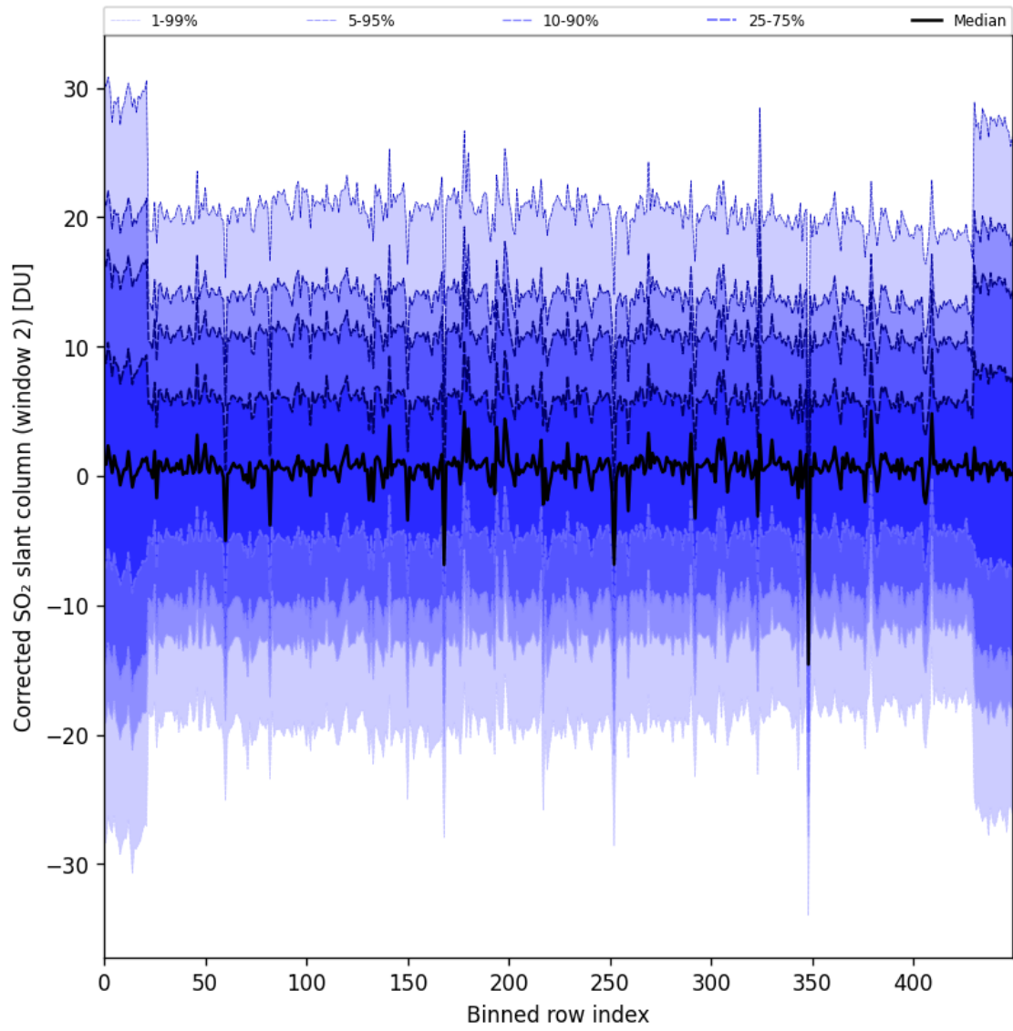
Figure 95: Along track statistics of “Corrected SO 2 slant column (window 2)” for 2025-05-15 to 2025-05-17
