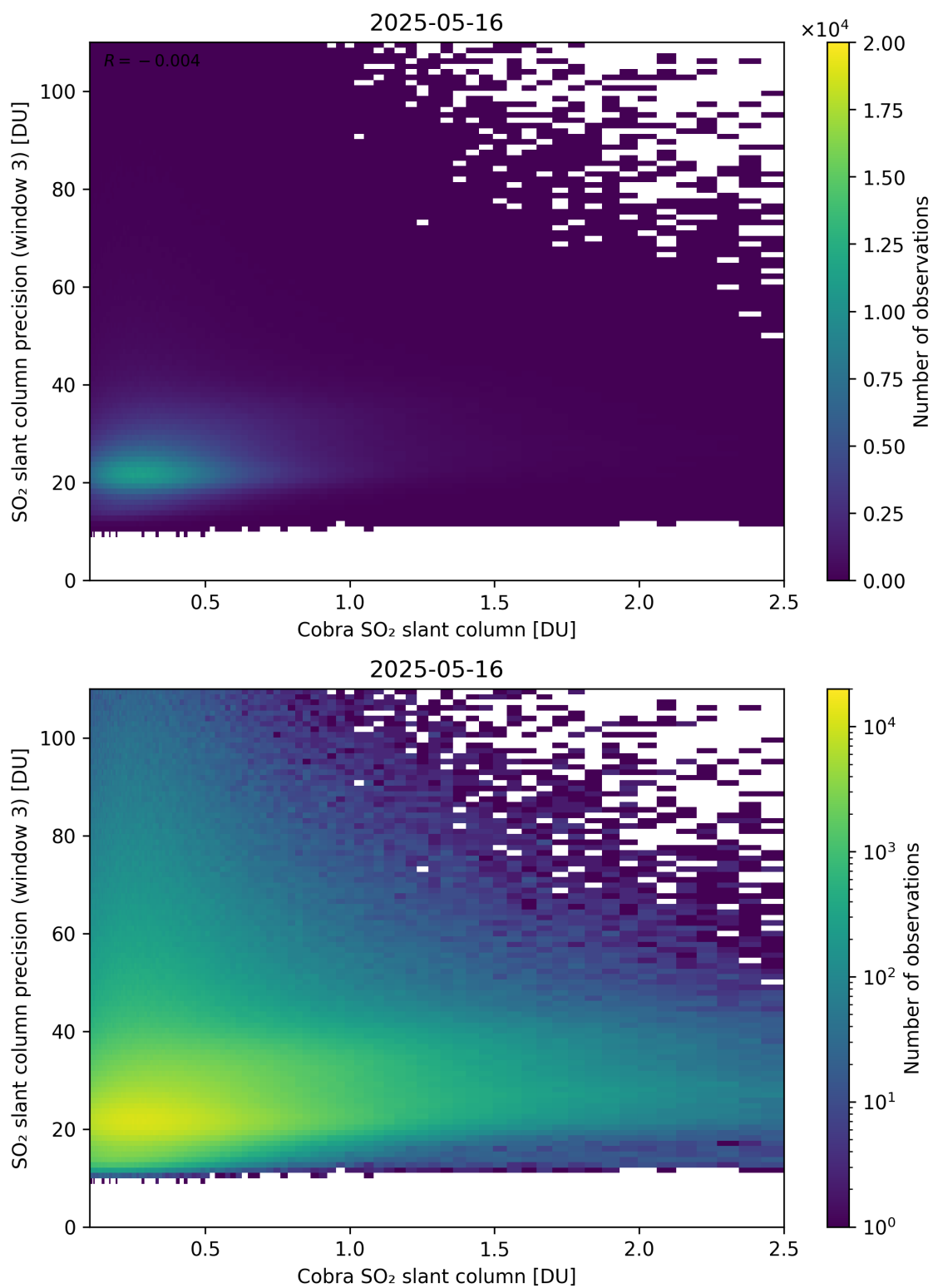
Figure 223: Scatter density plot of “Cobra SO 2 slant column” against “SO 2 slant column precision (window 3)” for 2025-05-15 to 2025-05-17.
