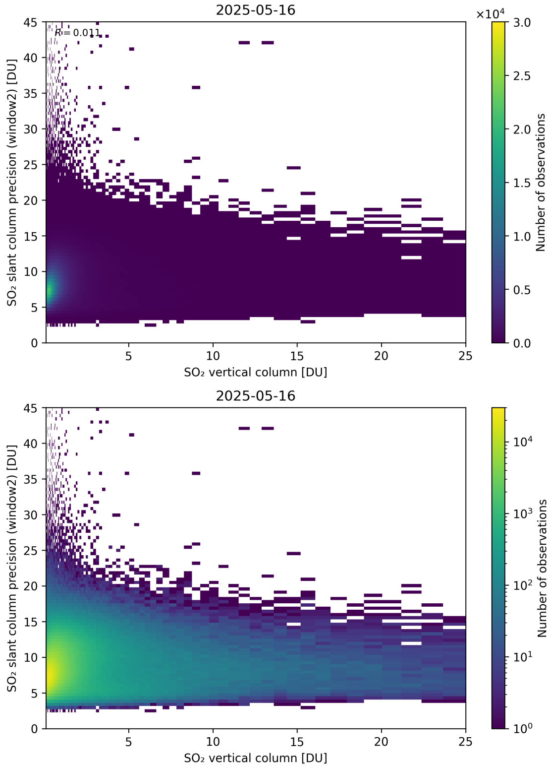
Figure 356: Scatter density plot of “SO 2 vertical column” against “SO 2 slant column precision (window2)” for 2025-05-15 to 2025-05-17.
