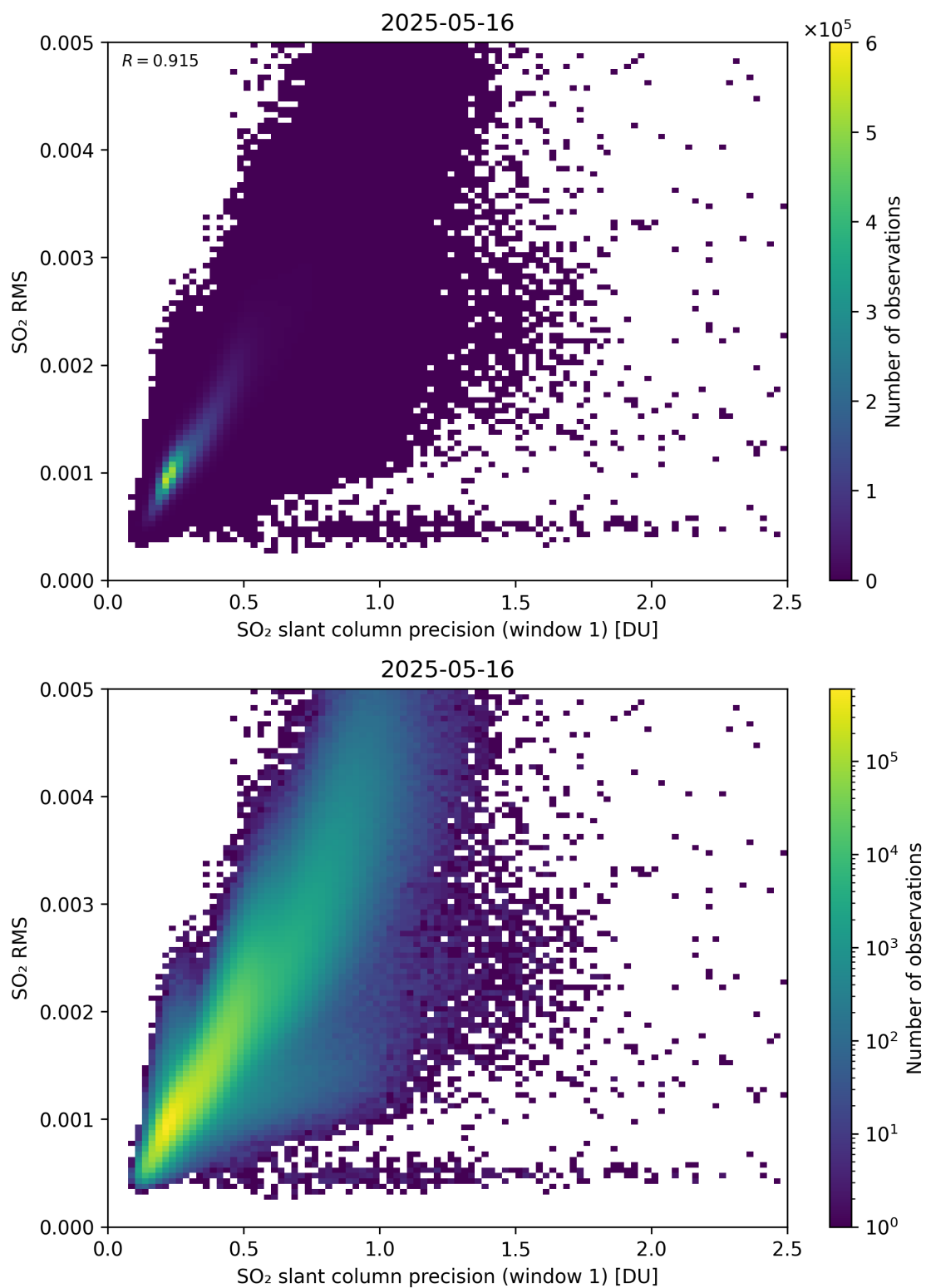
Figure 273: Scatter density plot of “SO 2 slant column precision (window 1)” against “SO 2 RMS” for 2025-05-15 to 2025-05-17.
