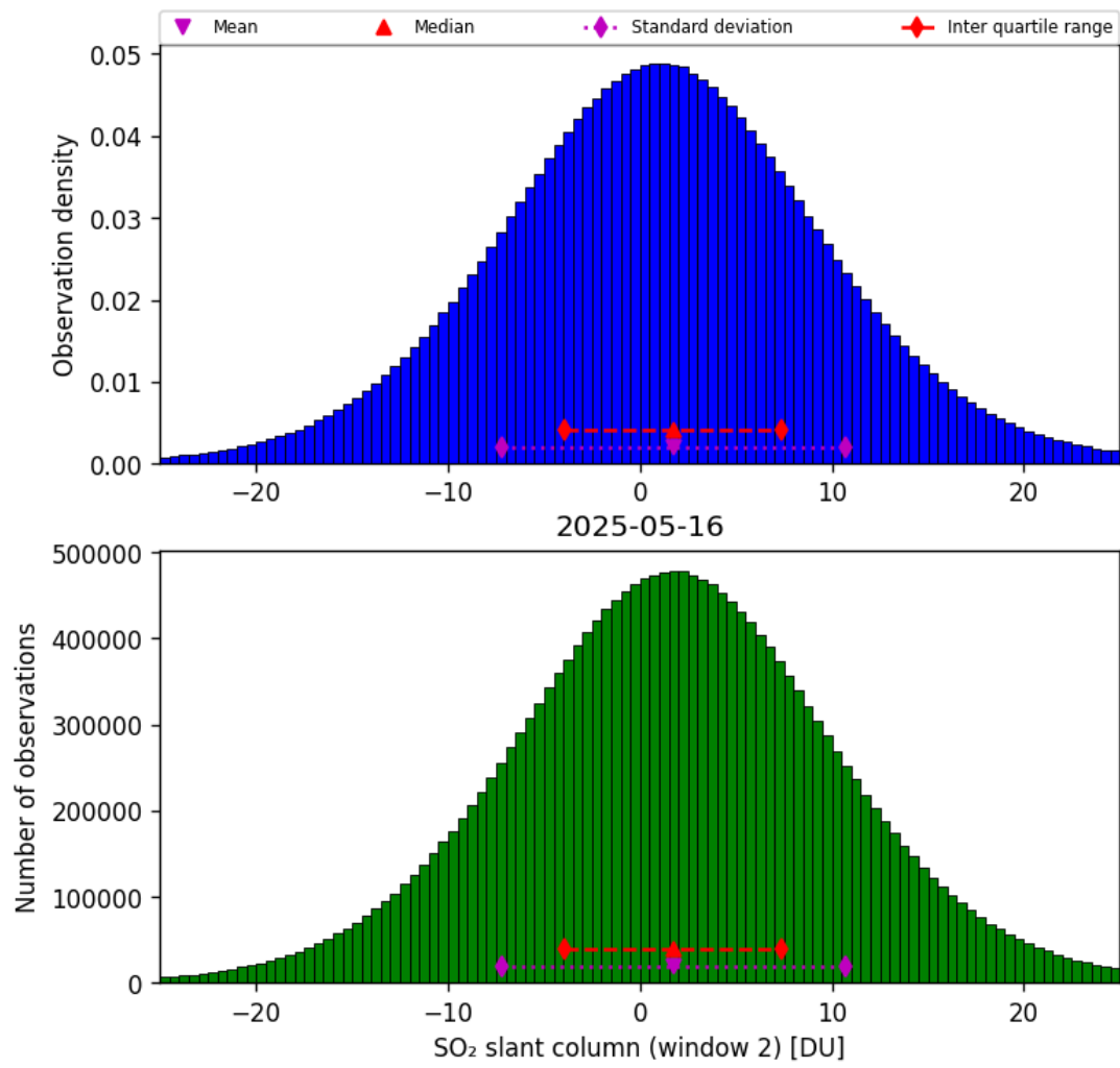
Figure 67: Histogram of “SO 2 slant column (window 2)” for 2025-05-15 to 2025-05-17
