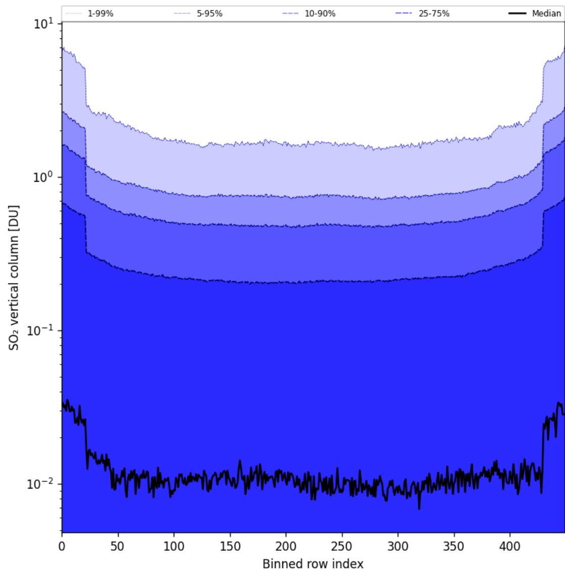
Figure 84: Along track statistics of “SO 2 vertical column” for 2025-05-15 to 2025-05-17
