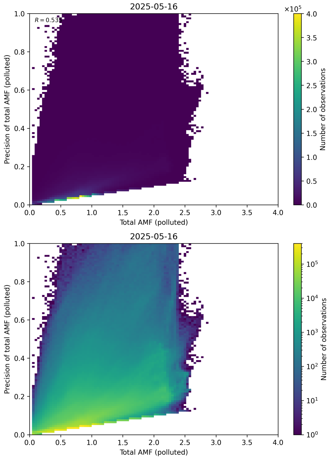
Figure 322: Scatter density plot of “Total AMF (polluted)” against “Precision of total AMF (polluted)” for 2025-05-15 to 2025-05-17.
