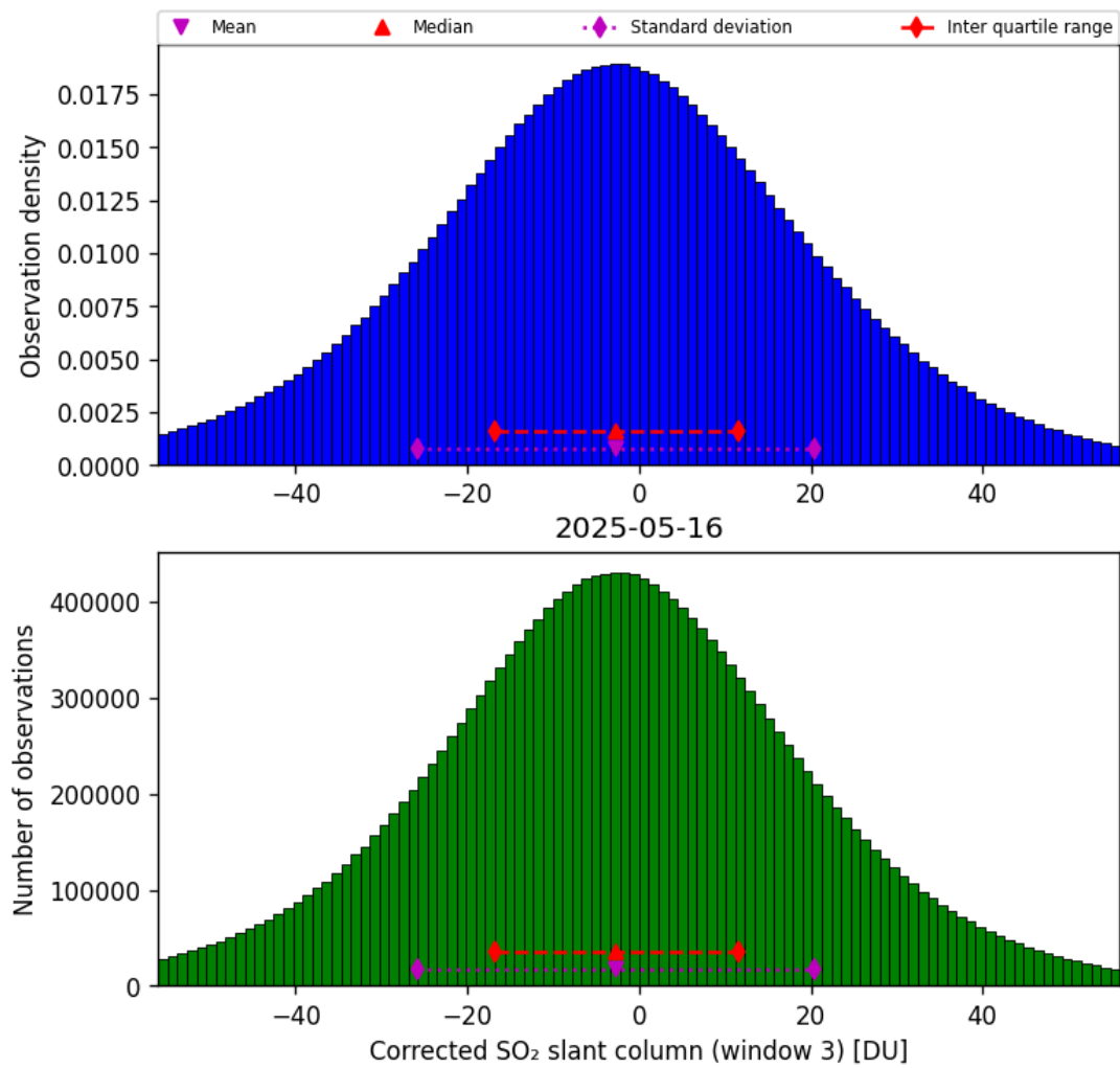
Figure 73: Histogram of “Corrected SO 2 slant column (window 3)” for 2025-05-15 to 2025-05-17
