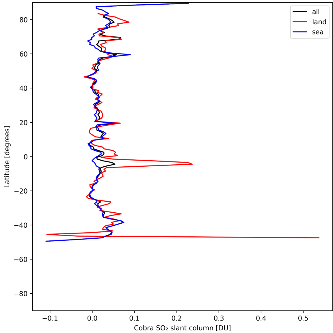
Figure 35: Zonal average of “Cobra SO 2 slant column” for 2025-05-15 to 2025-05-17.
