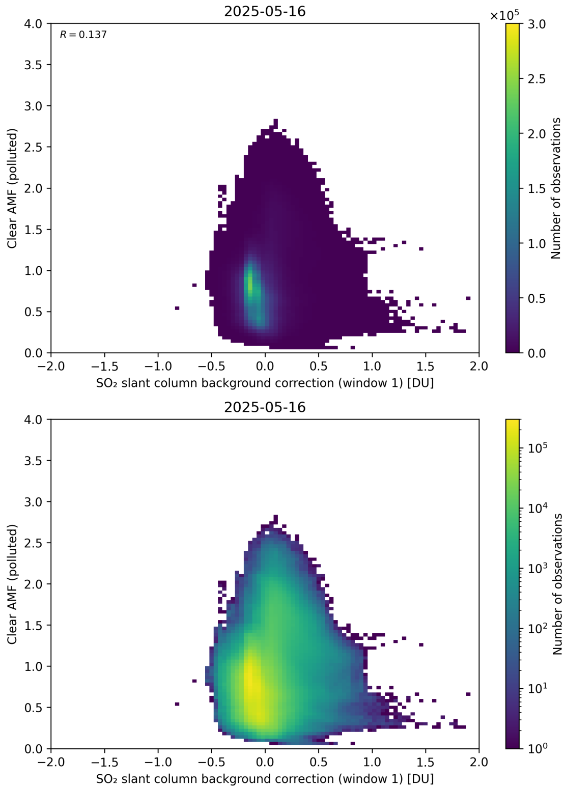
Figure 114: Scatter density plot of “SO 2 slant column background correction (window 1)” against “Clear AMF (polluted)” for 2025-05-15 to 2025-05-17.
