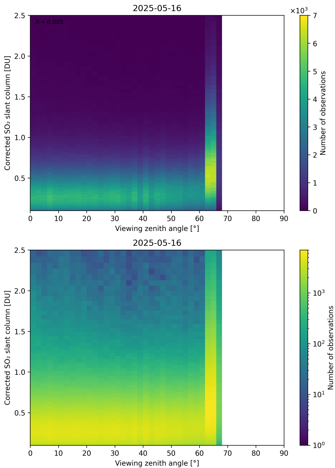
Figure 373: Scatter density plot of “Viewing zenith angle” against “Corrected SO 2 slant column” for 2025-05-15 to 2025-05-17.
