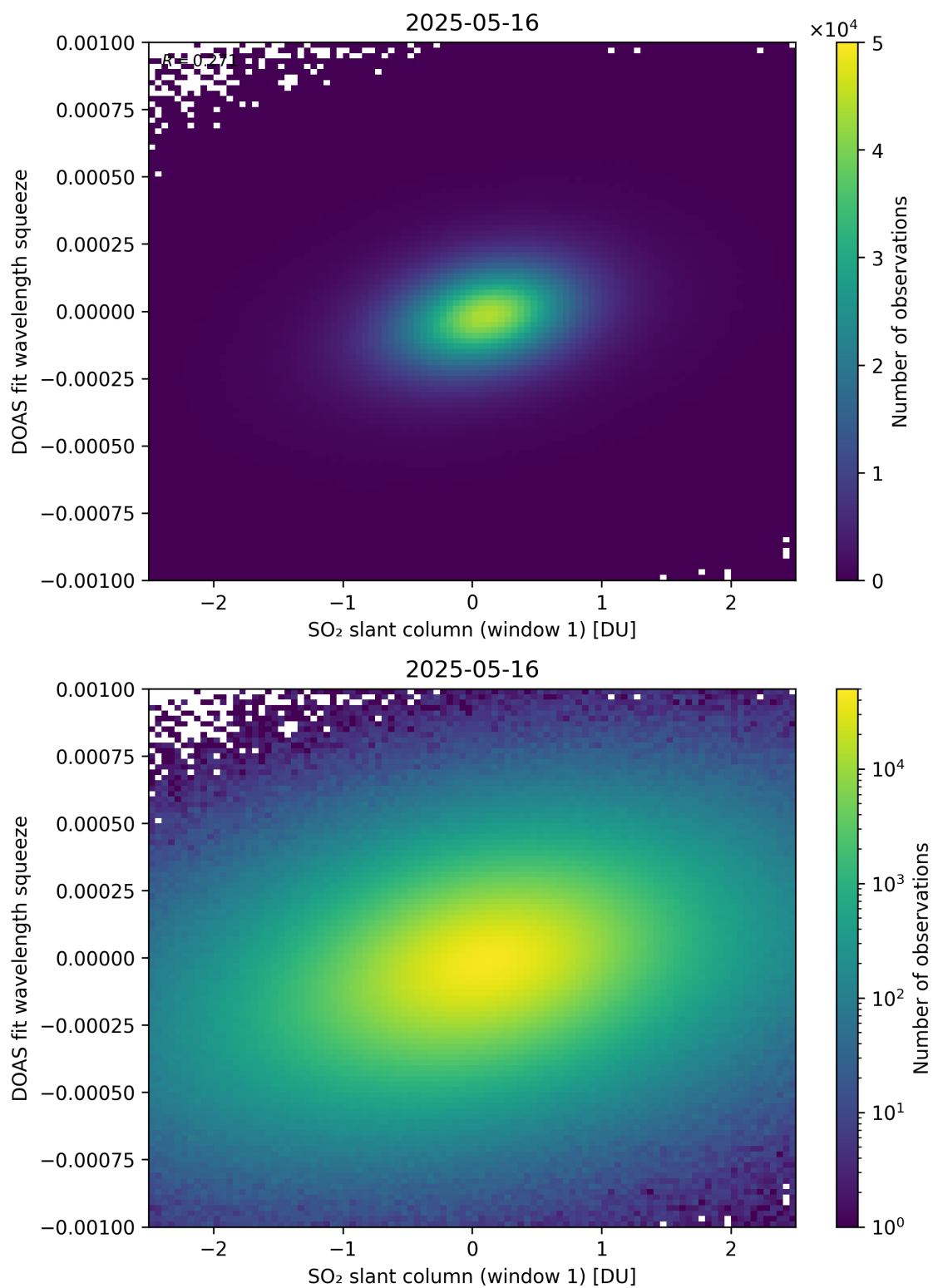
Figure 266: Scatter density plot of “SO 2 slant column (window 1)” against “DOAS fit wavelength squeeze” for 2025-05-15 to 2025-05-17.
