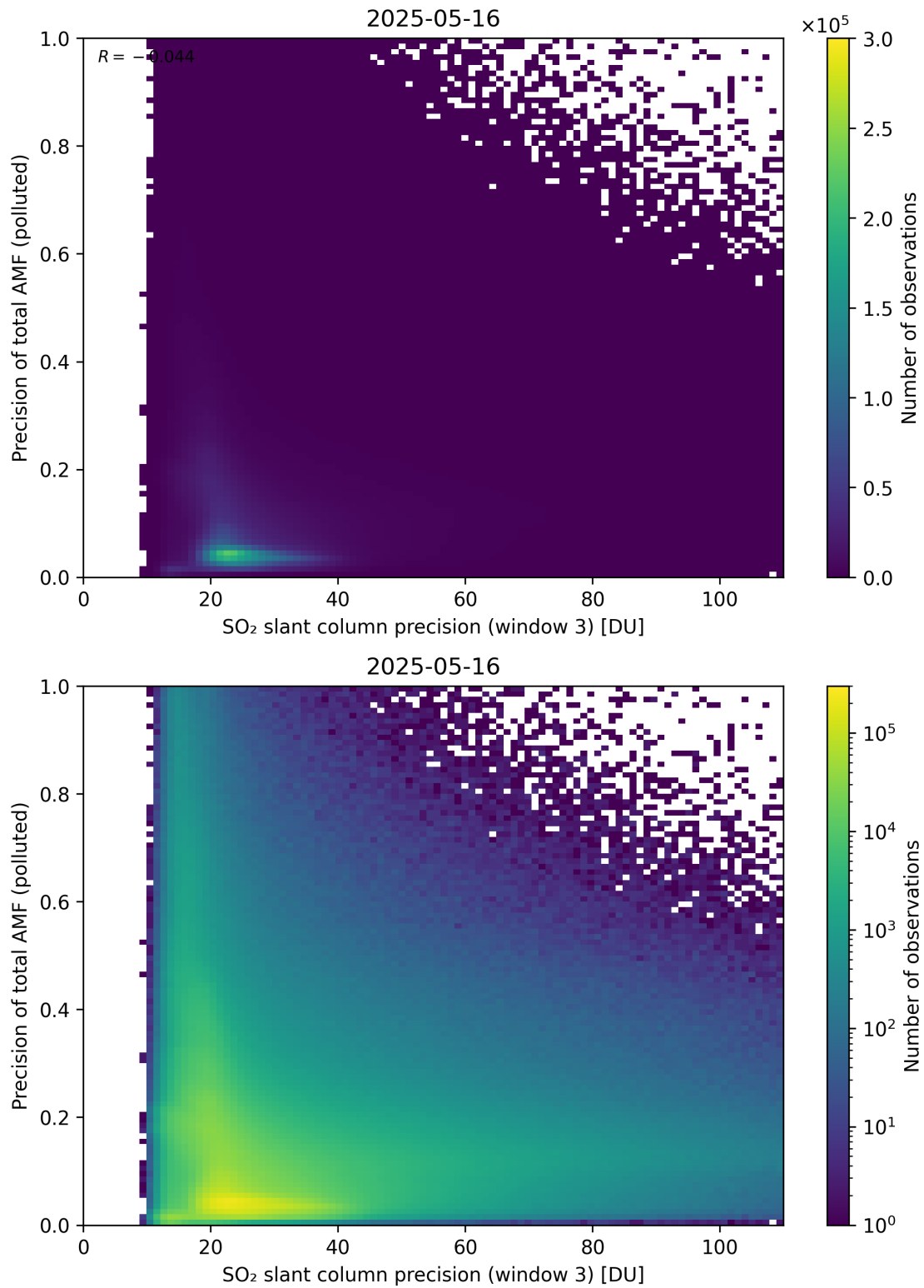
Figure 314: Scatter density plot of “SO 2 slant column precision (window 3)” against “Precision of total AMF (polluted)” for 2025-05-15 to 2025-05-17.
