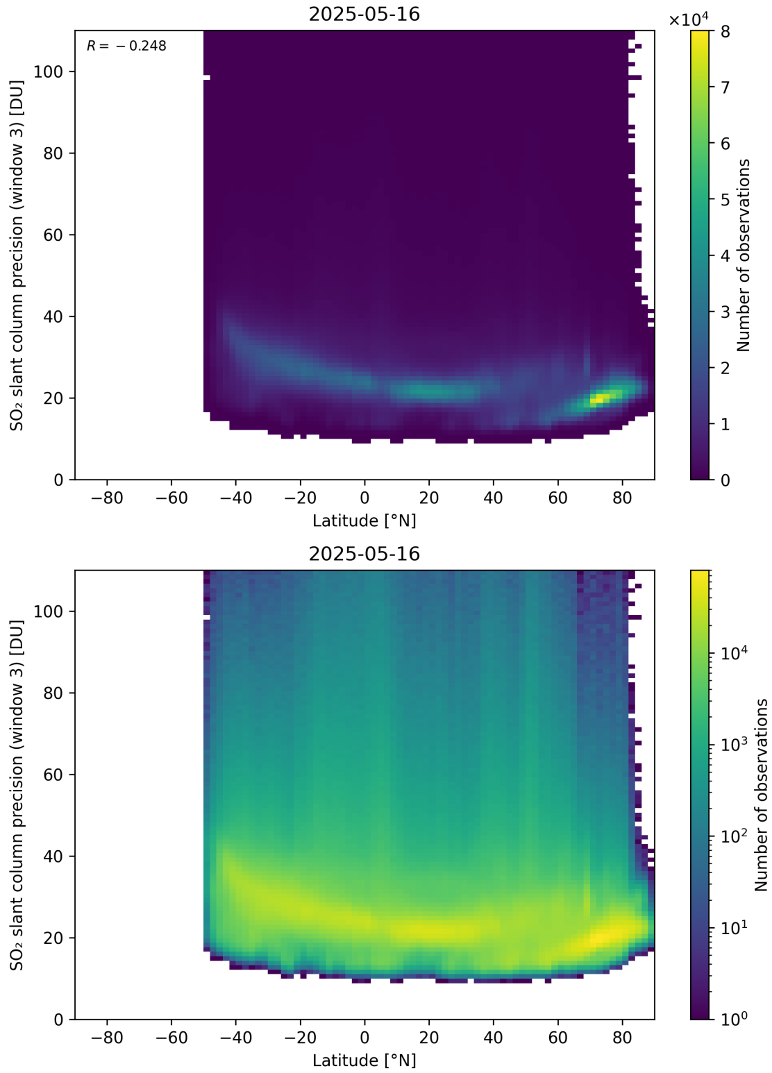
Figure 166: Scatter density plot of “Latitude” against “SO 2 slant column precision (window 3)” for 2025-05-15 to 2025-05-17.
