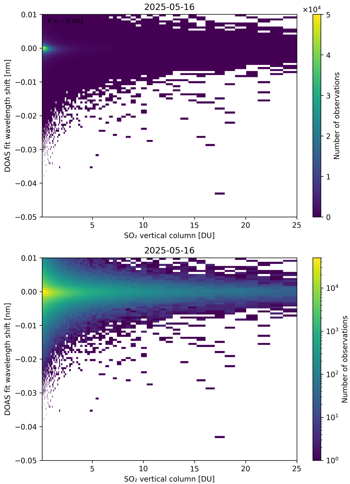
Figure 326: Scatter density plot of “SO 2 vertical column” against “DOAS fit wavelength shift” for 2025-05-15 to 2025-05-17.
