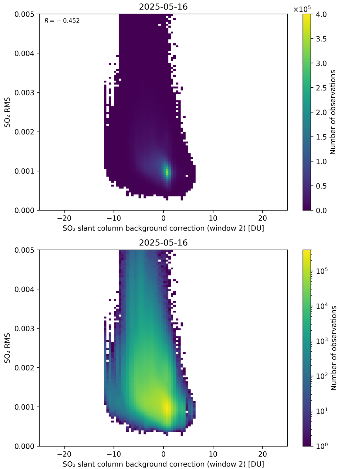
Figure 125: Scatter density plot of “SO 2 slant column background correction (window 2)” against “SO 2 RMS” for 2025-05-15 to 2025-05-17.
