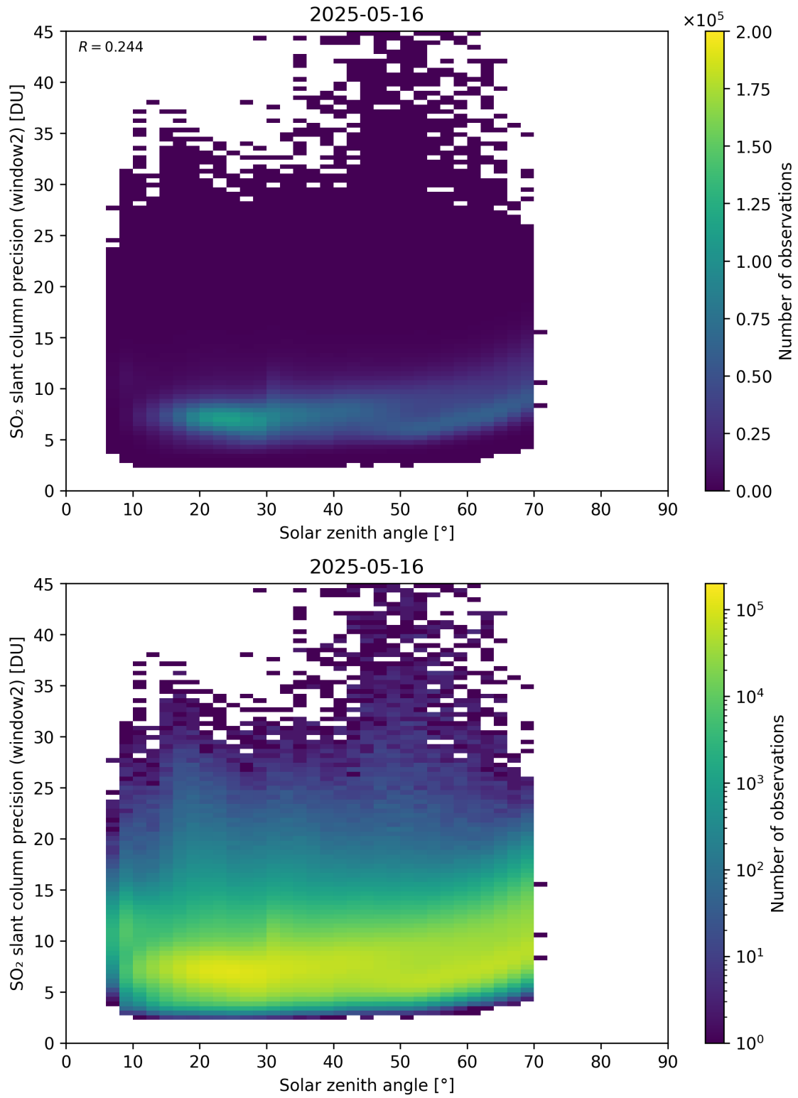
Figure 186: Scatter density plot of “Solar zenith angle” against “SO 2 slant column precision (window2)” for 2025-05-15 to 2025-05-17.
