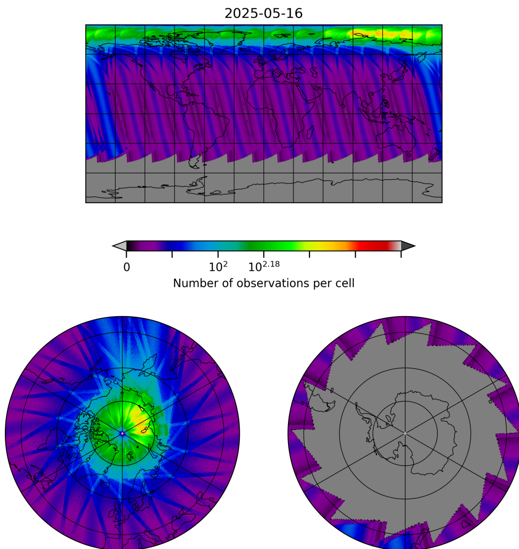
Figure 30: Map of the number of observations for 2025-05-15 to 2025-05-17
