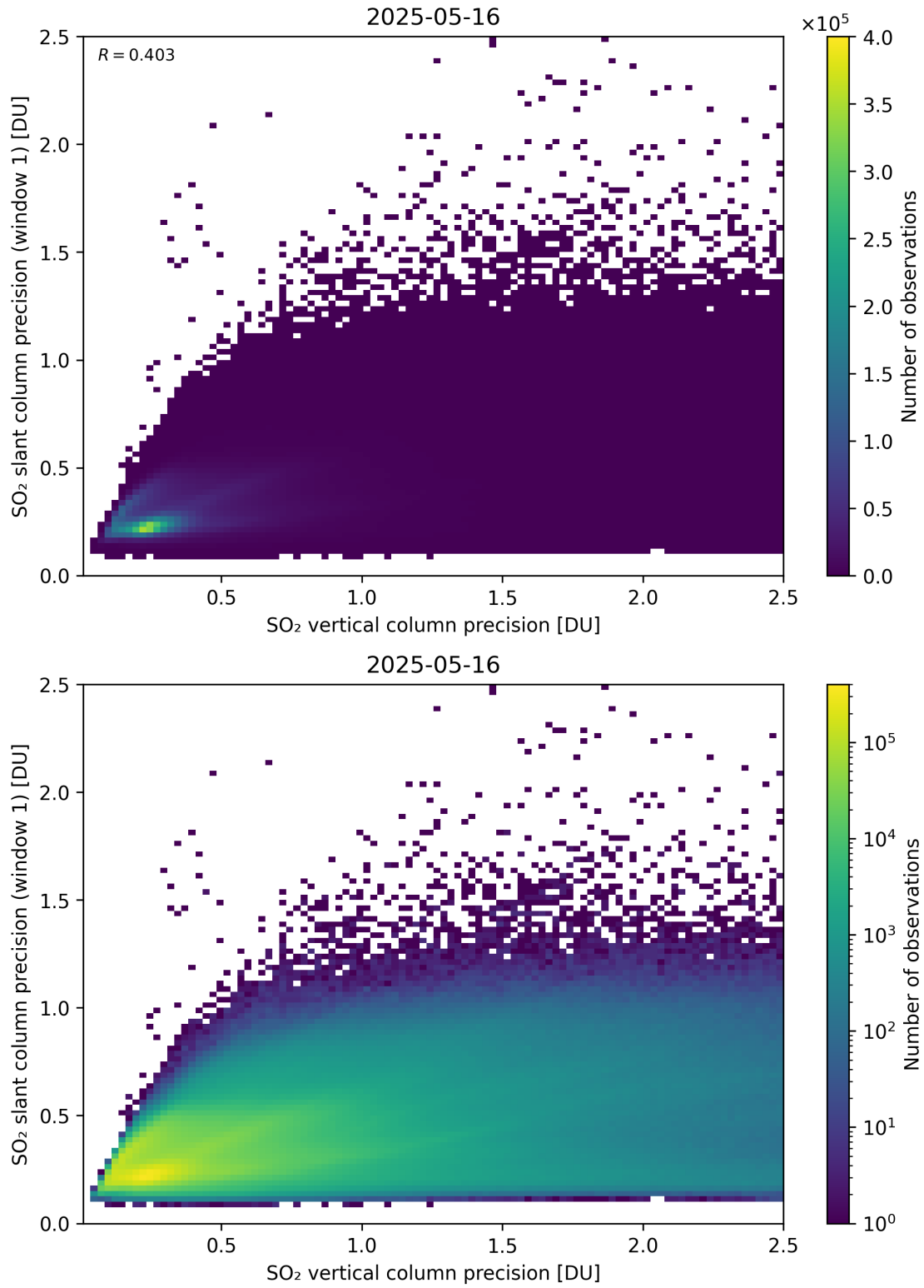
Figure 342: Scatter density plot of “SO 2 vertical column precision” against “SO 2 slant column precision (window 1)” for 2025-05-15 to 2025-05-17.
