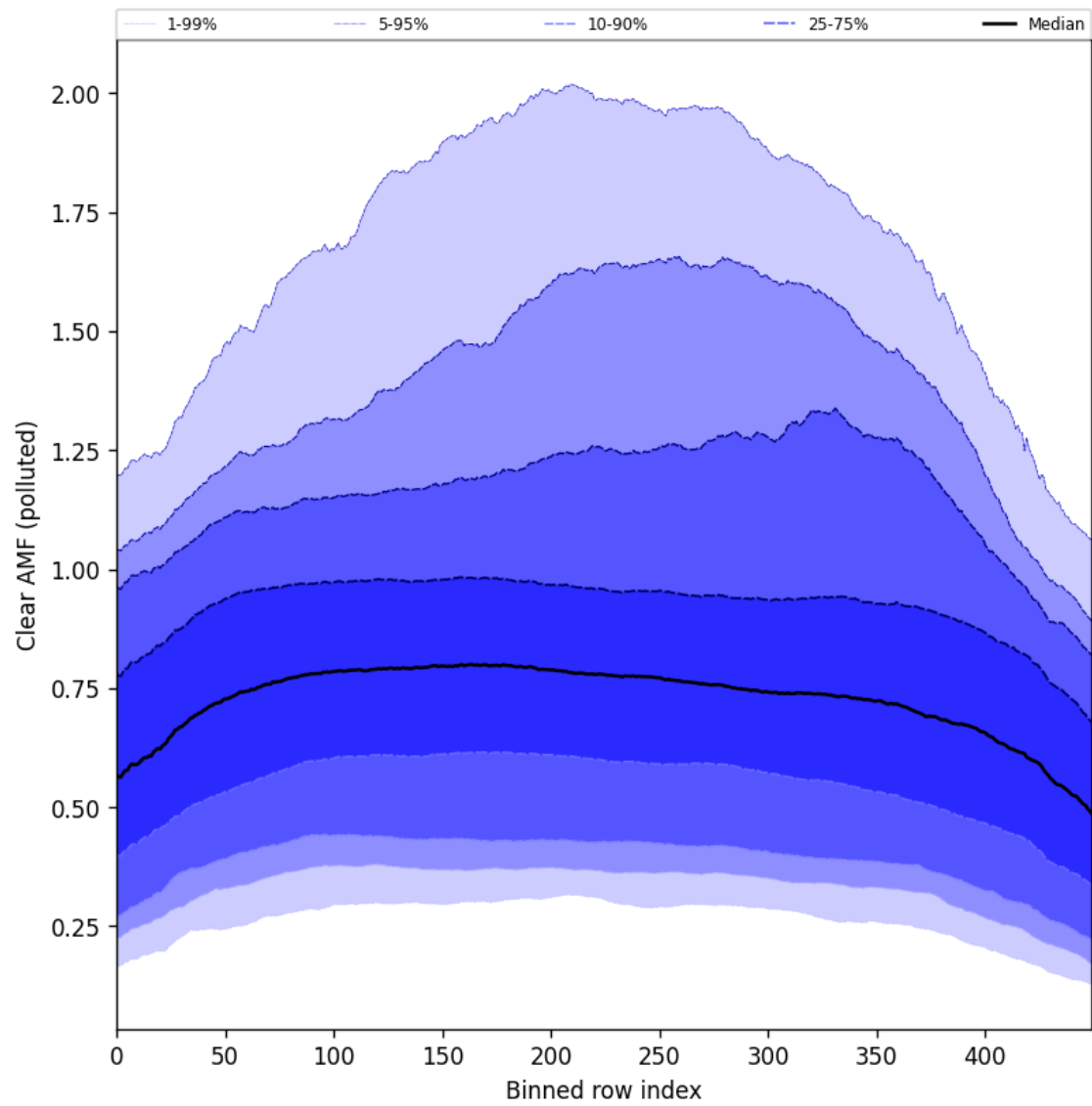
Figure 107: Along track statistics of “Clear AMF (polluted)” for 2025-05-15 to 2025-05-17
