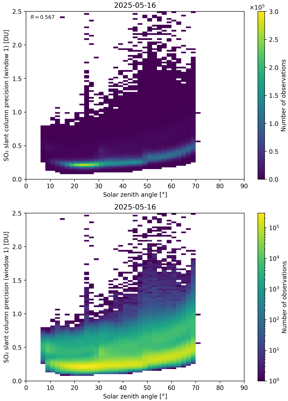
Figure 185: Scatter density plot of “Solar zenith angle” against “SO 2 slant column precision (window 1)” for 2025-05-15 to 2025-05-17.
