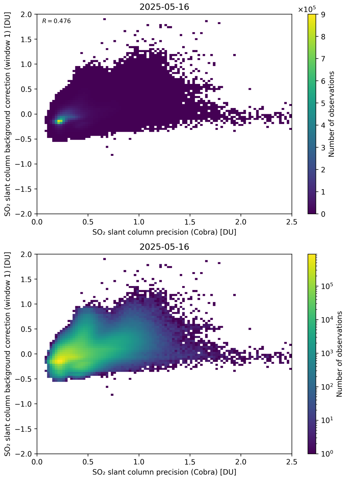
Figure 199: Scatter density plot of “SO 2 slant column precision (Cobra)” against “SO 2 slant column background correction (window 1)” for 2025-05-15 to 2025-05-17.
