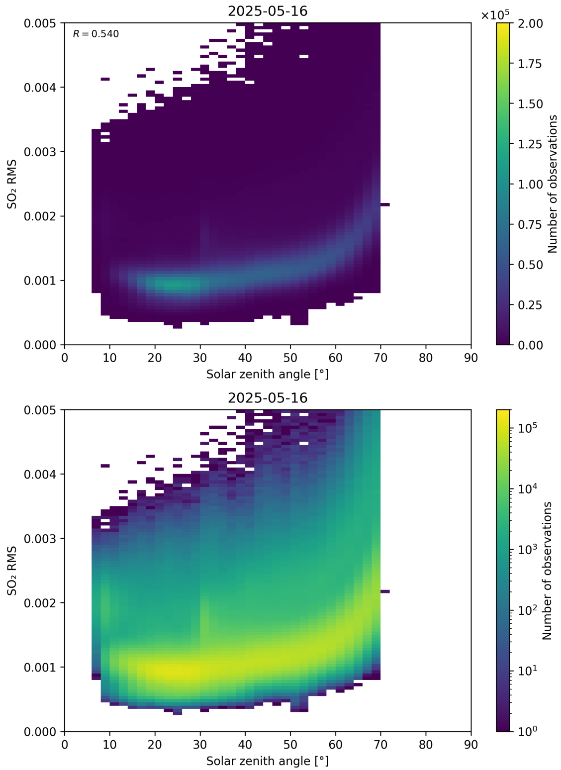
Figure 176: Scatter density plot of “Solar zenith angle” against “SO 2 RMS” for 2025-05-15 to 2025-05-17.
