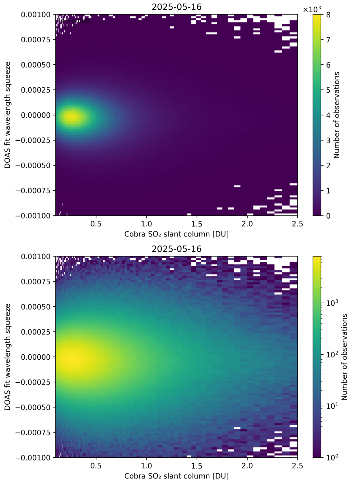
Figure 197: Scatter density plot of “Cobra SO 2 slant column” against “DOAS fit wavelength squeeze” for 2025-05-15 to 2025-05-17.
