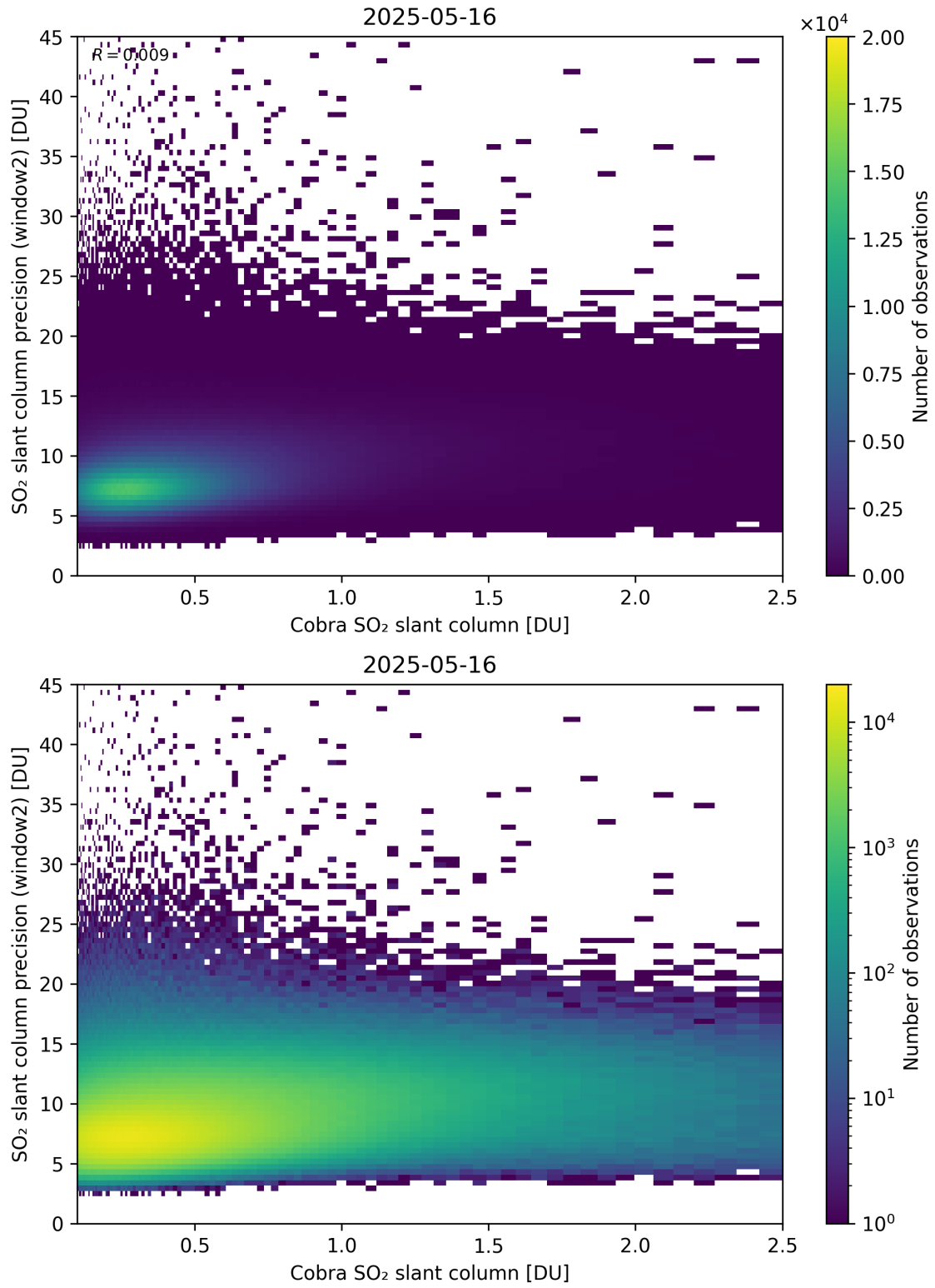
Figure 221: Scatter density plot of “Cobra SO 2 slant column” against “SO 2 slant column precision (window2)” for 2025-05-15 to 2025-05-17.
