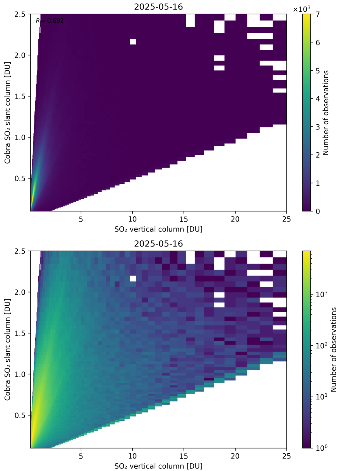
Figure 349: Scatter density plot of “SO 2 vertical column” against “Cobra SO 2 slant column” for 2025-05-15 to 2025-05-17.
