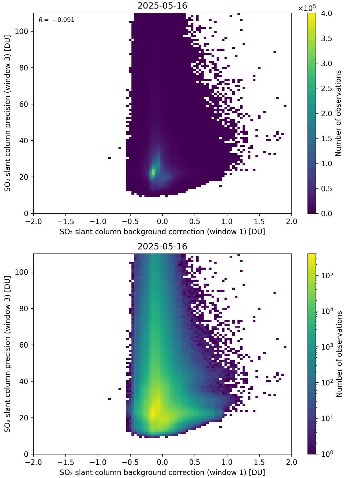
Figure 119: Scatter density plot of “SO 2 slant column background correction (window 1)” against “SO 2 slant column precision (window 3)” for 2025-05-15 to 2025-05-17.
