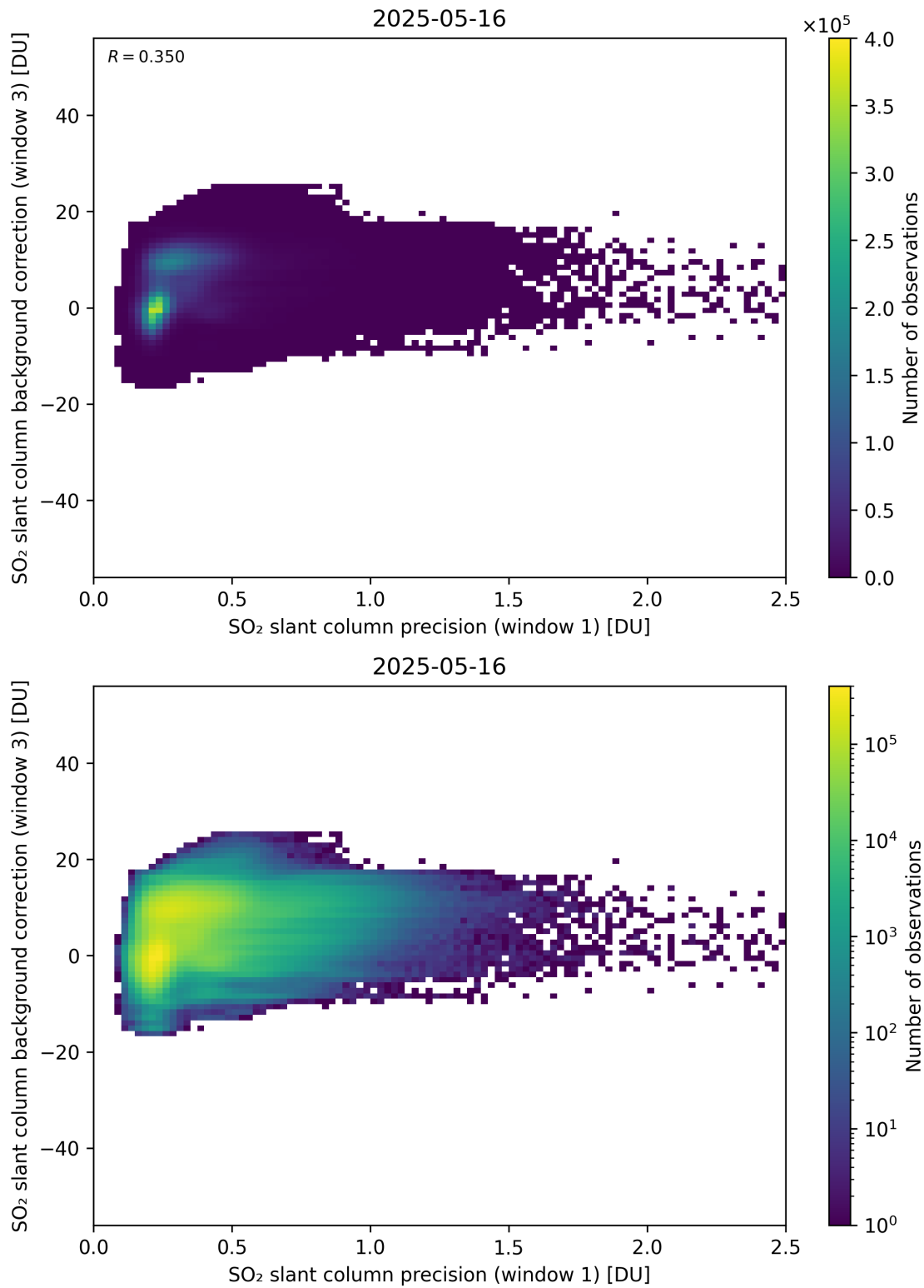
Figure 270: Scatter density plot of “SO 2 slant column precision (window 1)” against “SO 2 slant column background correction (window 3)” for 2025-05-15 to 2025-05-17.
