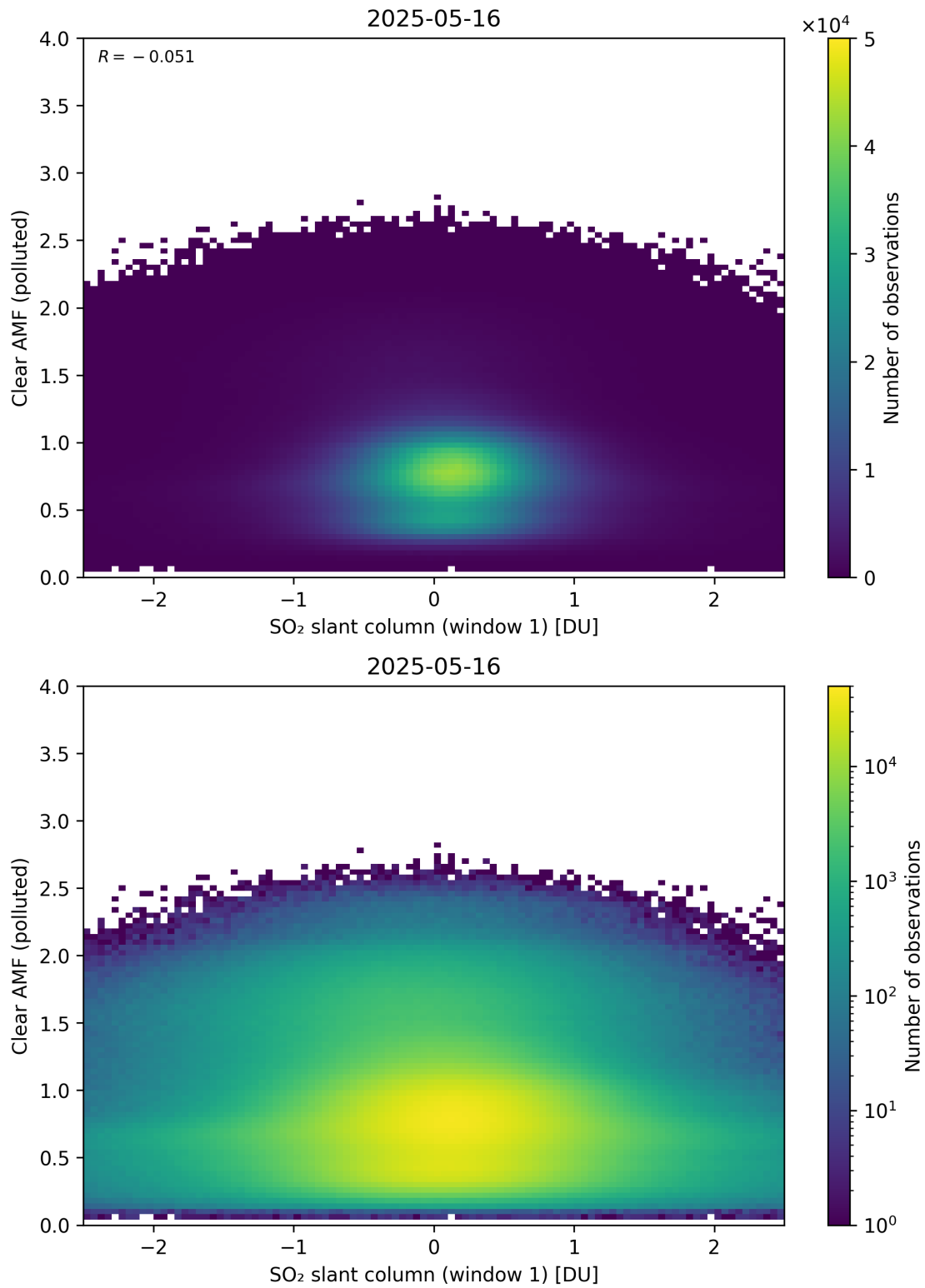
Figure 282: Scatter density plot of “SO 2 slant column (window 1)” against “Clear AMF (polluted)” for 2025-05-15 to 2025-05-17.
