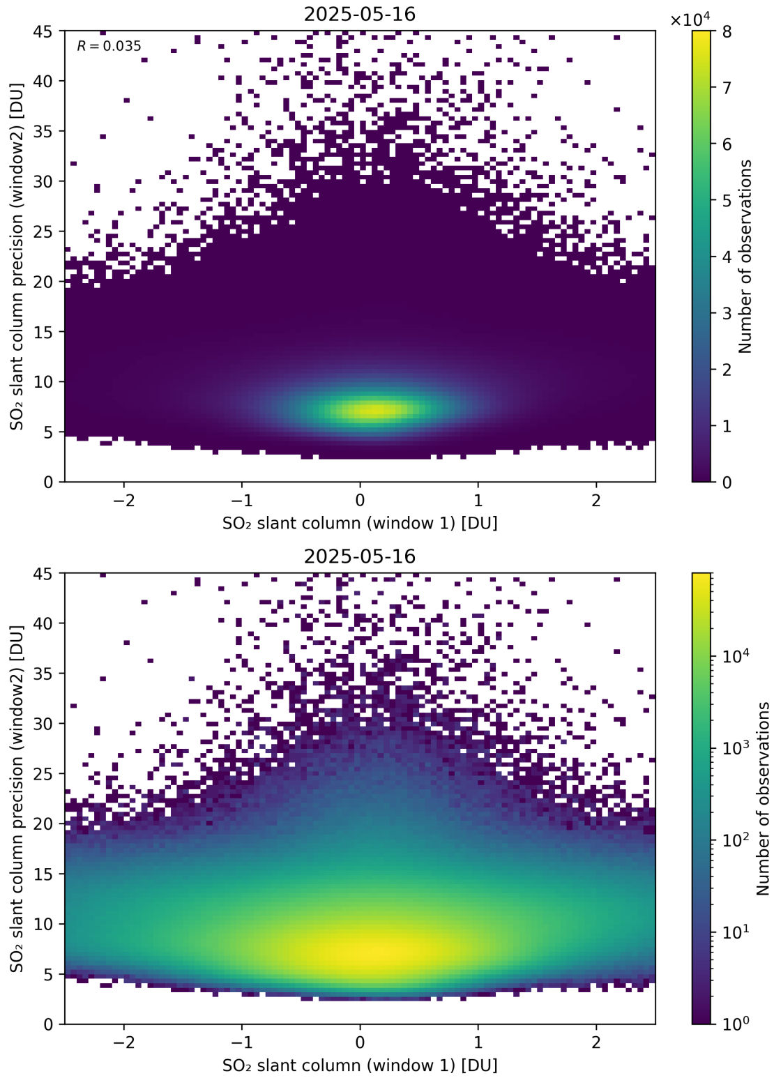
Figure 286: Scatter density plot of “SO 2 slant column (window 1)” against “SO 2 slant column precision (window2)” for 2025-05-15 to 2025-05-17.
