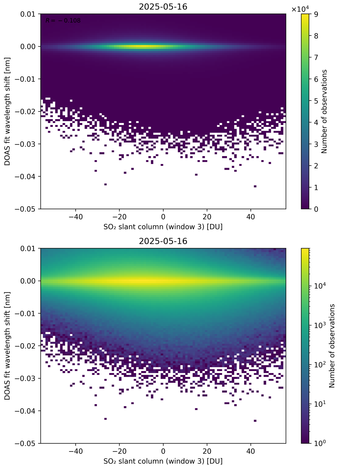
Figure 304: Scatter density plot of “SO 2 slant column (window 3)” against “DOAS fit wavelength shift” for 2025-05-15 to 2025-05-17.
