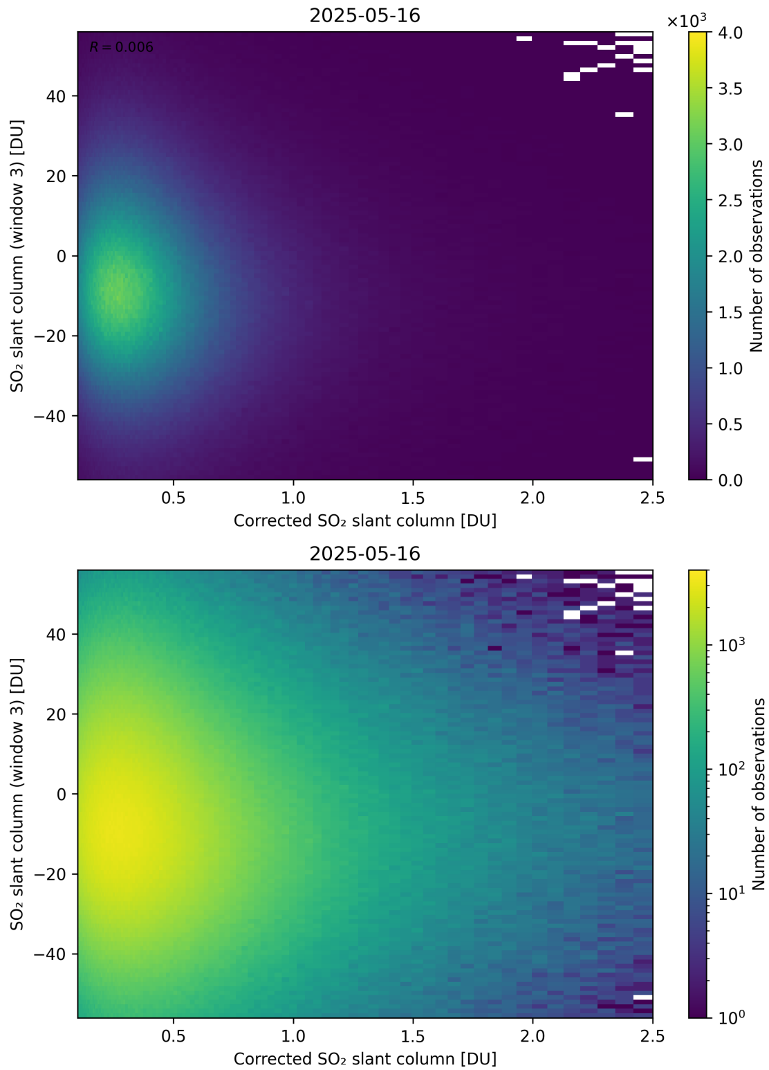
Figure 240: Scatter density plot of “Corrected SO 2 slant column” against “SO 2 slant column (window 3)” for 2025-05-15 to 2025-05-17.
