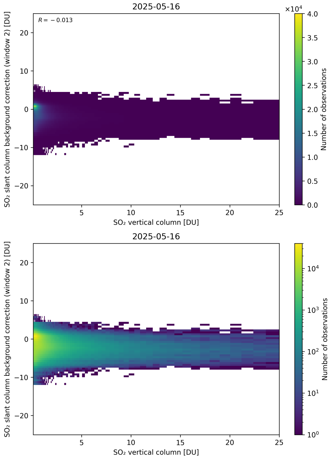
Figure 324: Scatter density plot of “SO 2 vertical column” against “SO 2 slant column background correction (window 2)” for 2025-05-15 to 2025-05-17.
