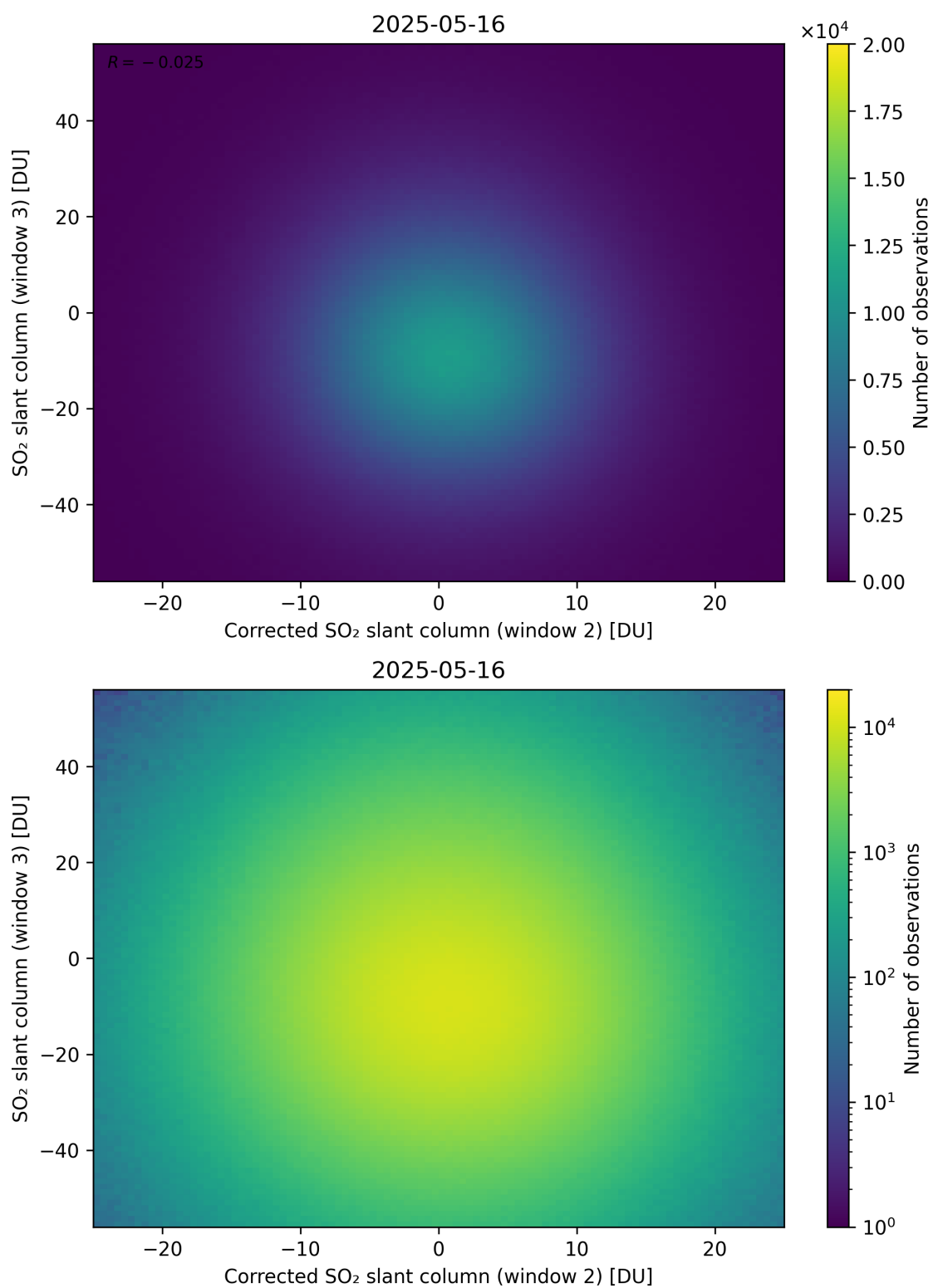
Figure 251: Scatter density plot of “Corrected SO 2 slant column (window 2)” against “SO 2 slant column (window 3)” for 2025-05-15 to 2025-05-17.
