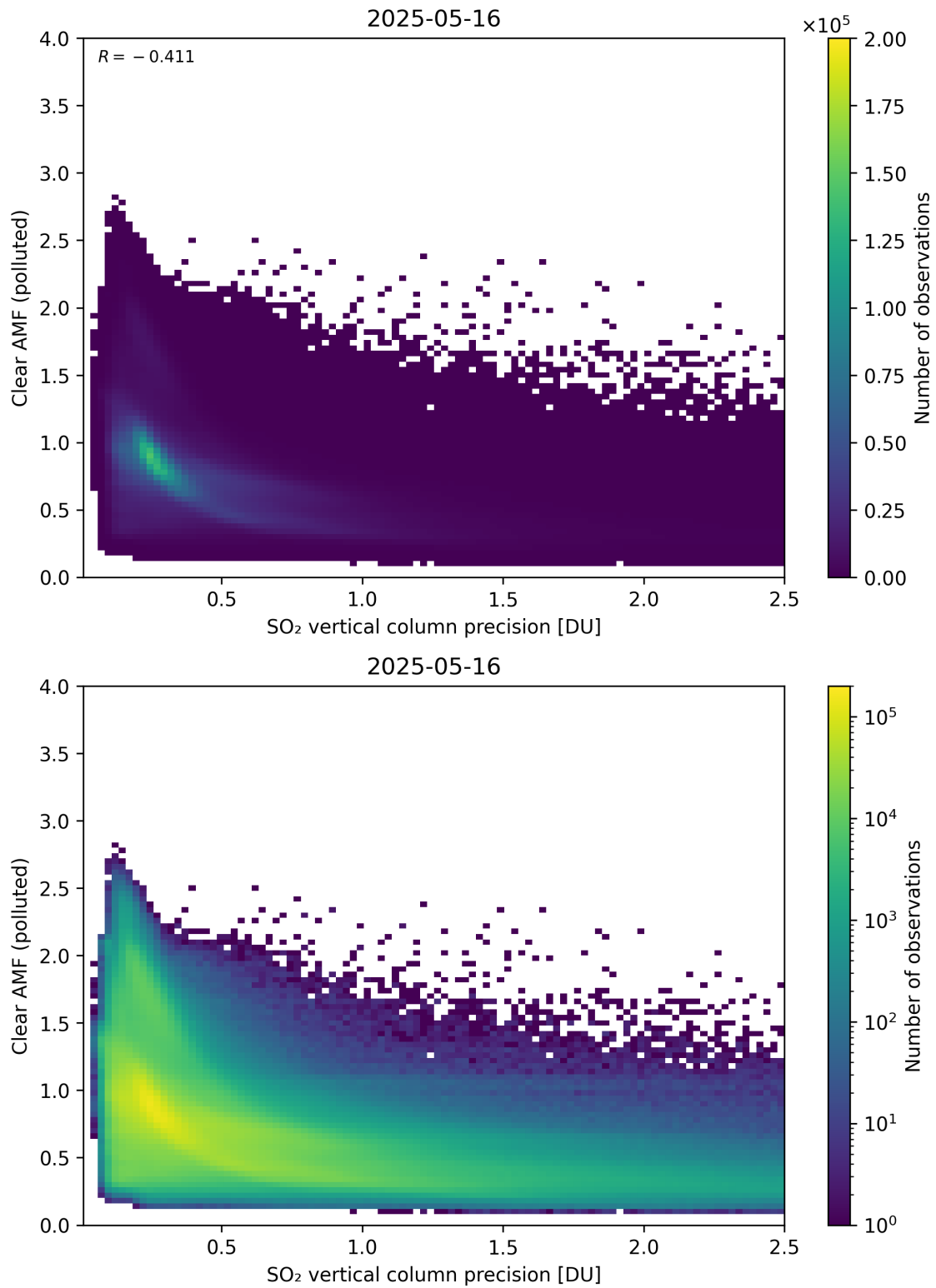
Figure 335: Scatter density plot of “SO 2 vertical column precision” against “Clear AMF (polluted)” for 2025-05-15 to 2025-05-17.
