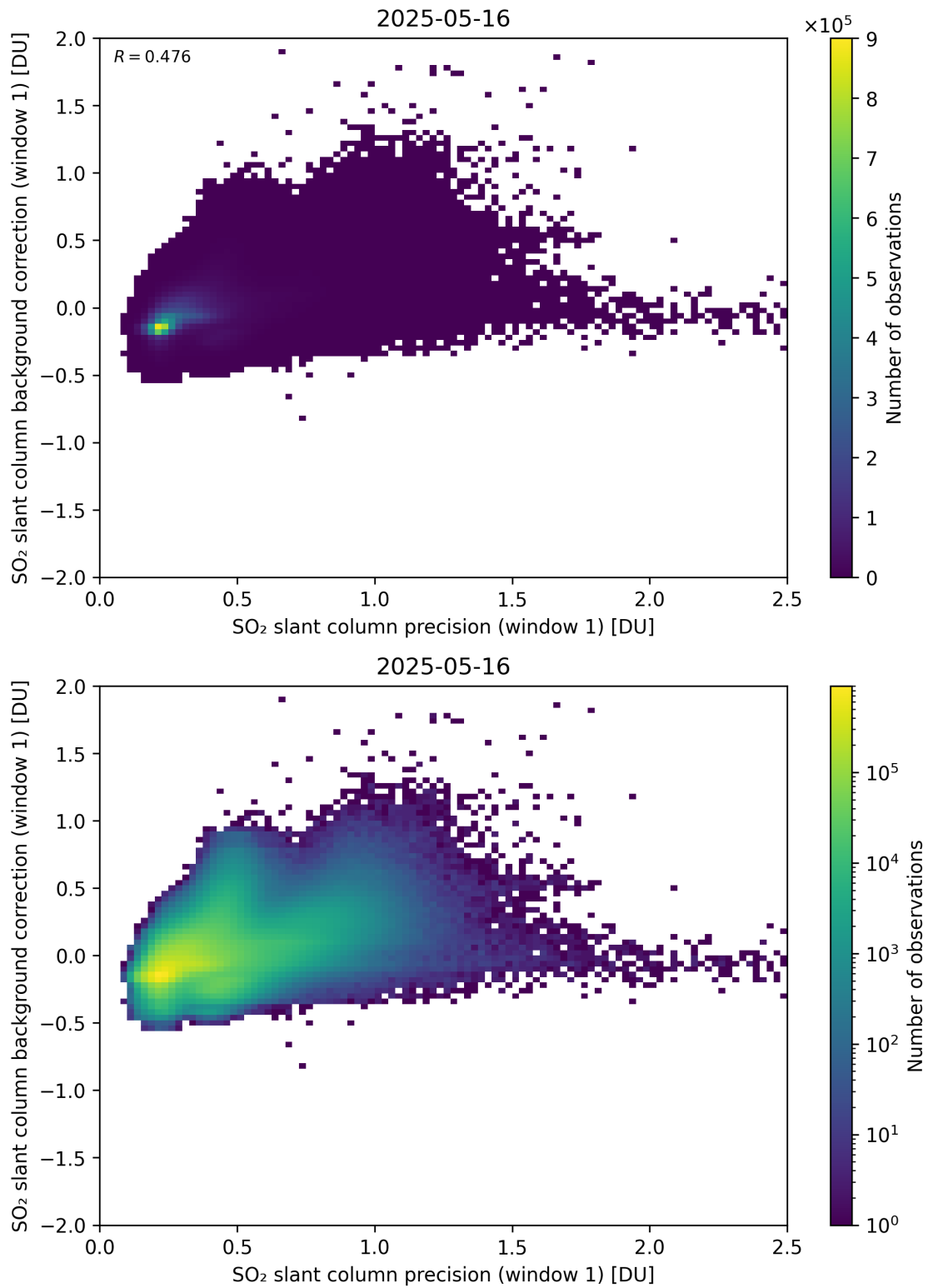
Figure 268: Scatter density plot of “SO 2 slant column precision (window 1)” against “SO 2 slant column background correction (window 1)” for 2025-05-15 to 2025-05-17.
