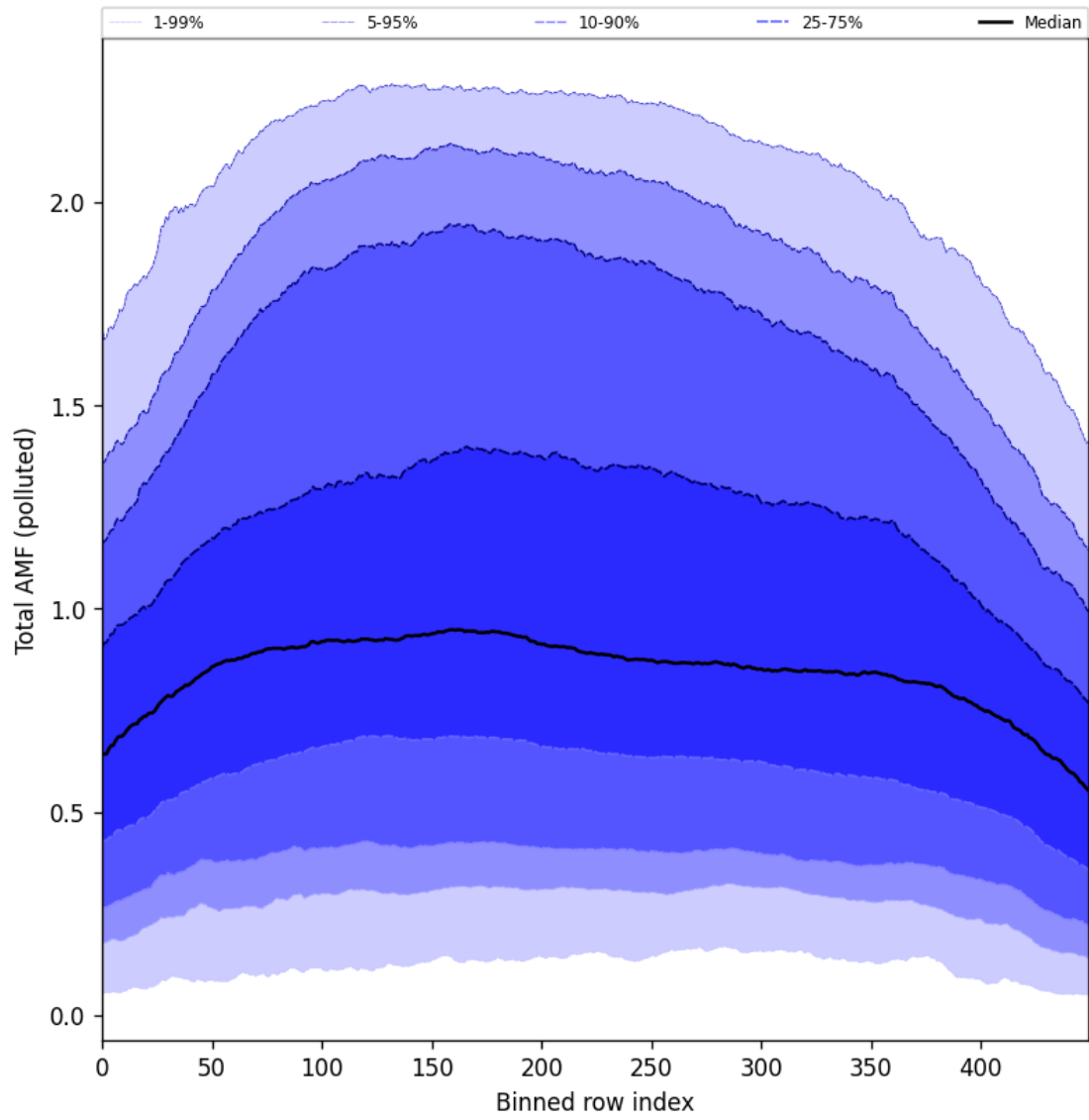
Figure 105: Along track statistics of “Total AMF (polluted)” for 2025-05-15 to 2025-05-17
