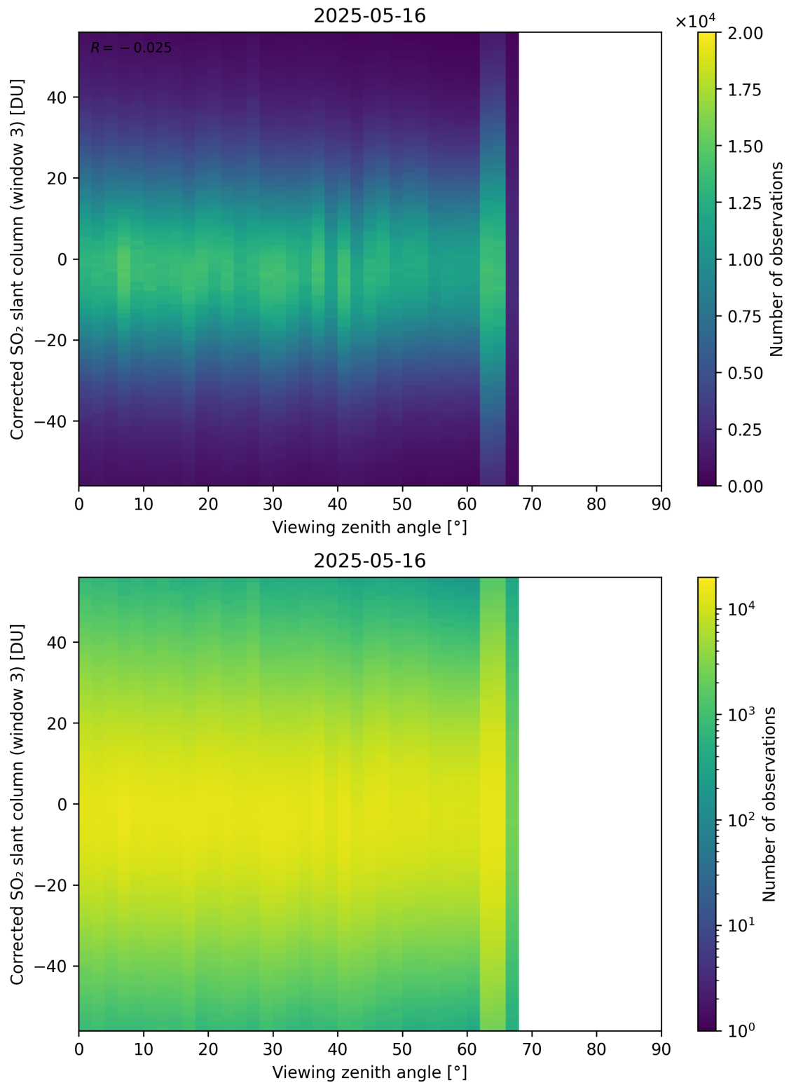
Figure 375: Scatter density plot of “Viewing zenith angle” against “Corrected SO 2 slant column (window 3)” for 2025-05-15 to 2025-05-17.
