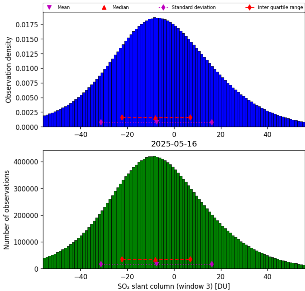
Figure 71: Histogram of “SO 2 slant column (window 3)” for 2025-05-15 to 2025-05-17
