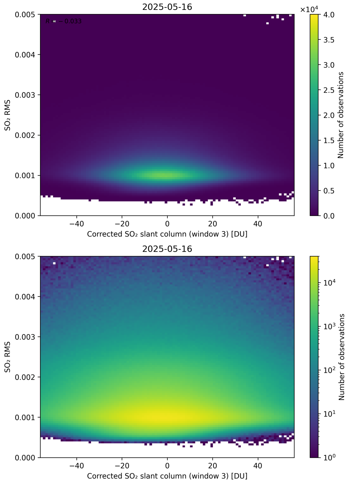
Figure 258: Scatter density plot of “Corrected SO 2 slant column (window 3)” against “SO 2 RMS” for 2025-05-15 to 2025-05-17.
