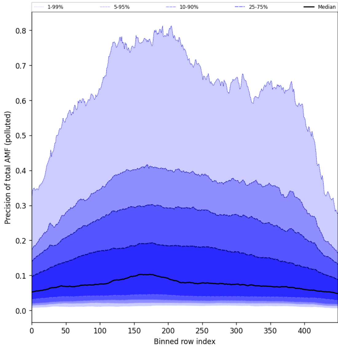
Figure 106: Along track statistics of “Precision of total AMF (polluted)” for 2025-05-15 to 2025-05-17
