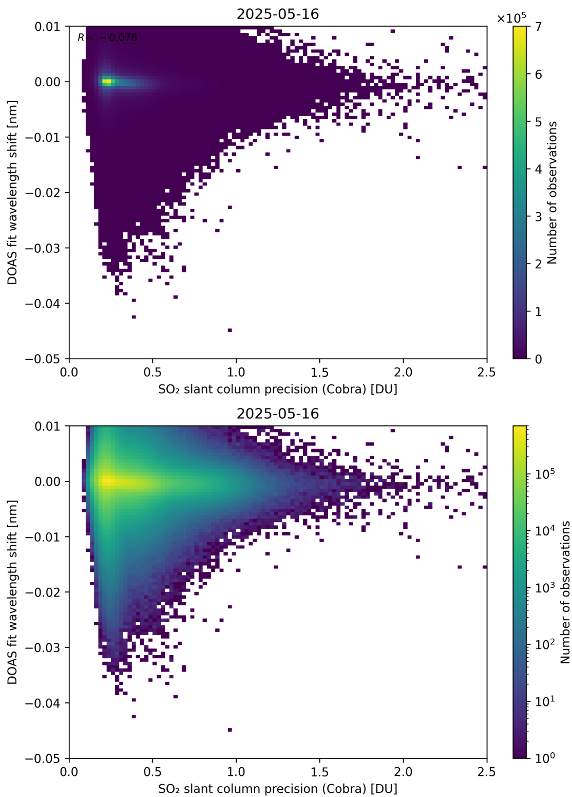
Figure 202: Scatter density plot of “SO 2 slant column precision (Cobra)” against “DOAS fit wavelength shift” for 2025-05-15 to 2025-05-17.
