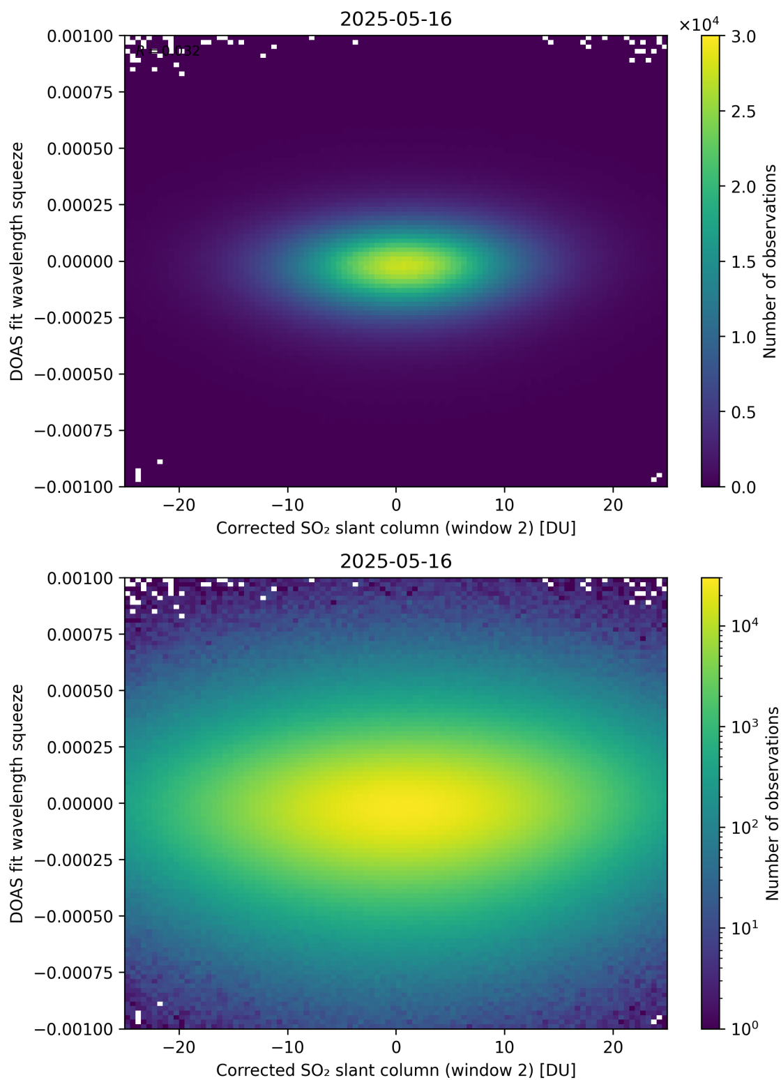
Figure 247: Scatter density plot of “Corrected SO 2 slant column (window 2)” against “DOAS fit wavelength squeeze” for 2025-05-15 to 2025-05-17.
