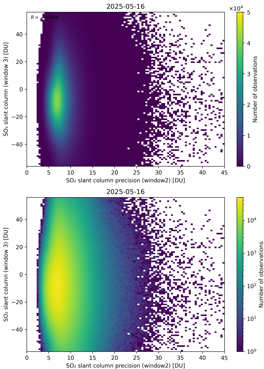
Figure 299: Scatter density plot of “SO 2 slant column precision (window2)” against “SO 2 slant column (window 3)” for 2025-05-15 to 2025-05-17.
