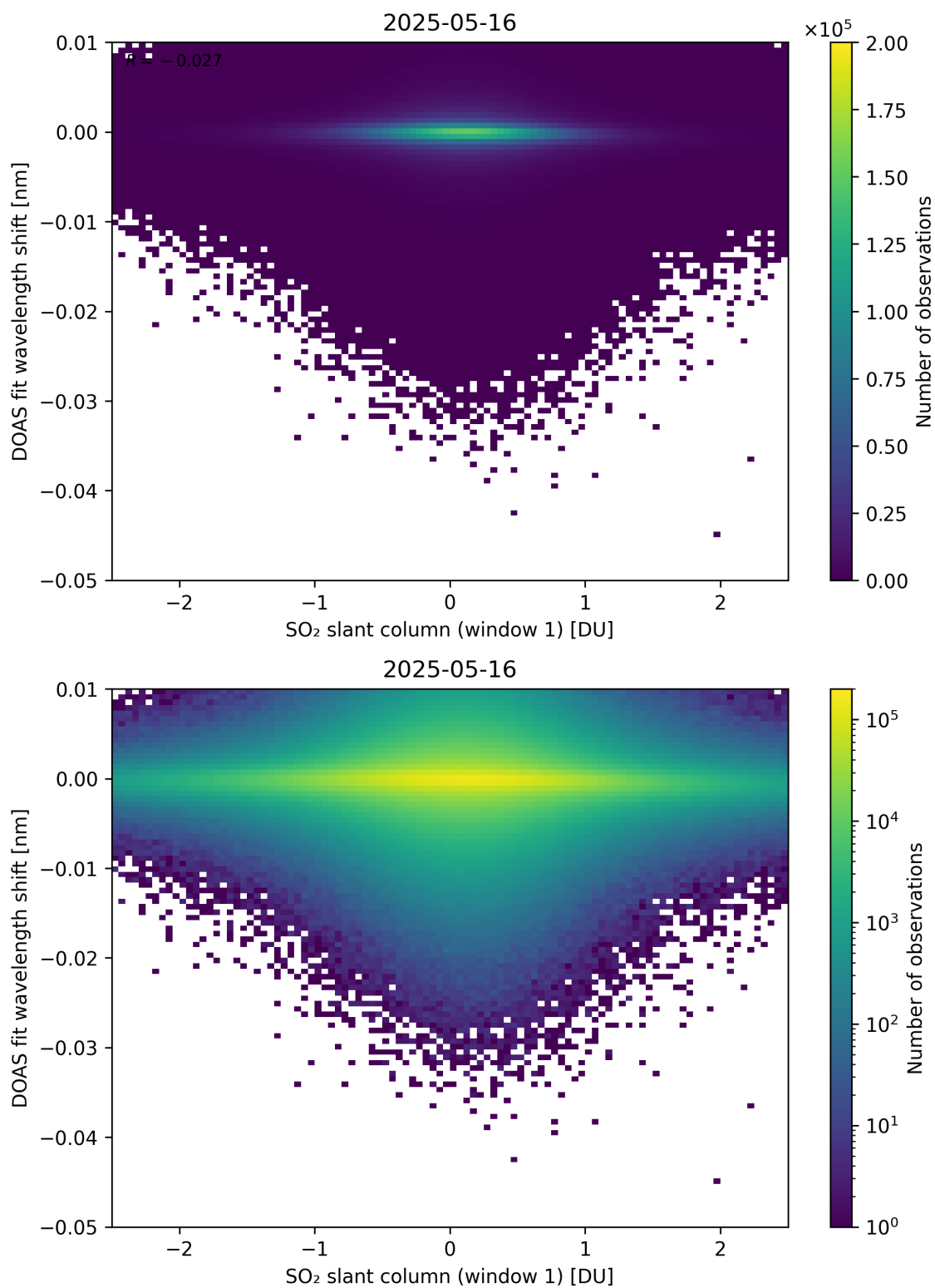
Figure 265: Scatter density plot of “SO 2 slant column (window 1)” against “DOAS fit wavelength shift” for 2025-05-15 to 2025-05-17.
