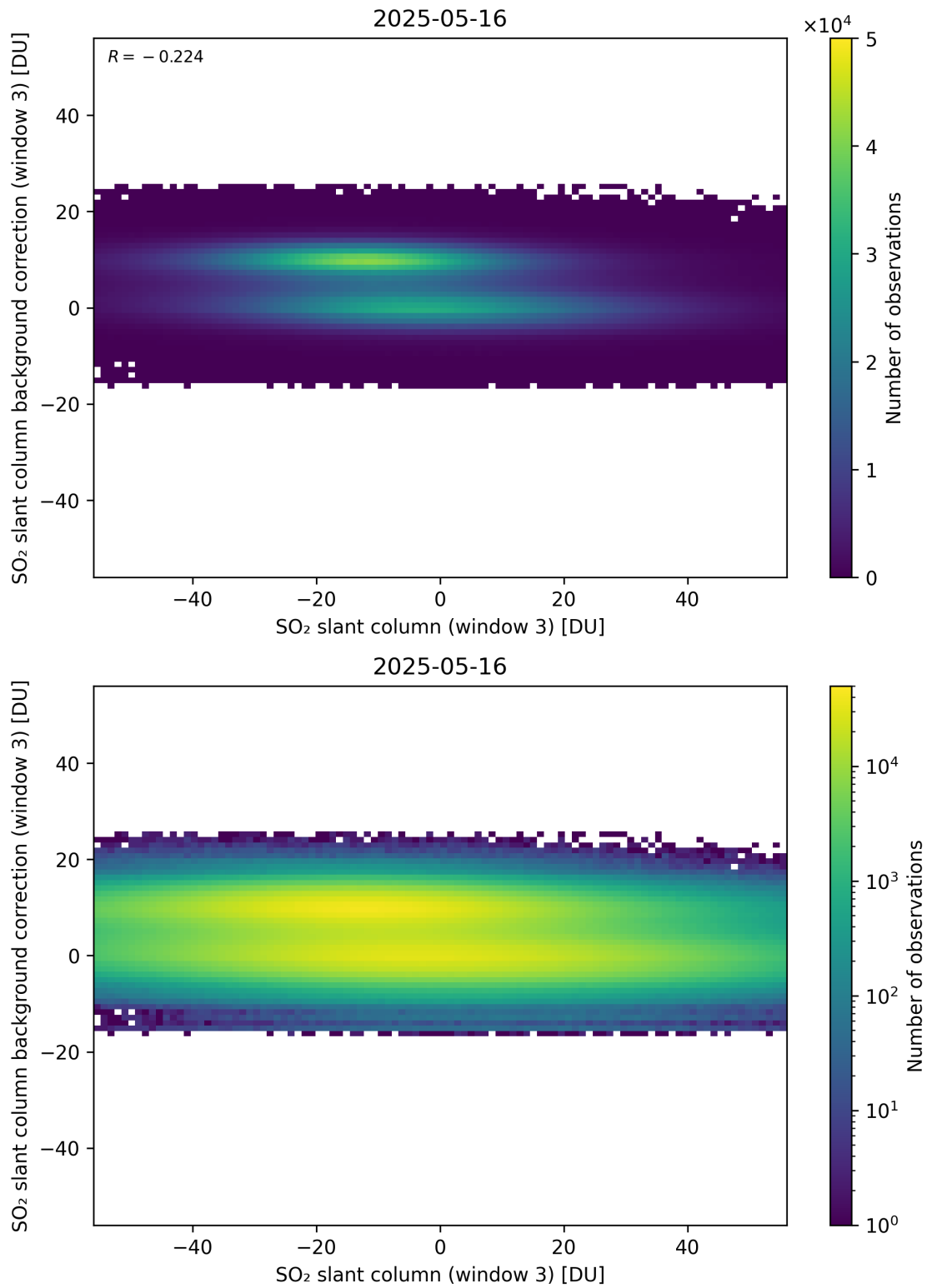
Figure 303: Scatter density plot of “SO 2 slant column (window 3)” against “SO 2 slant column background correction (window 3)” for 2025-05-15 to 2025-05-17.
