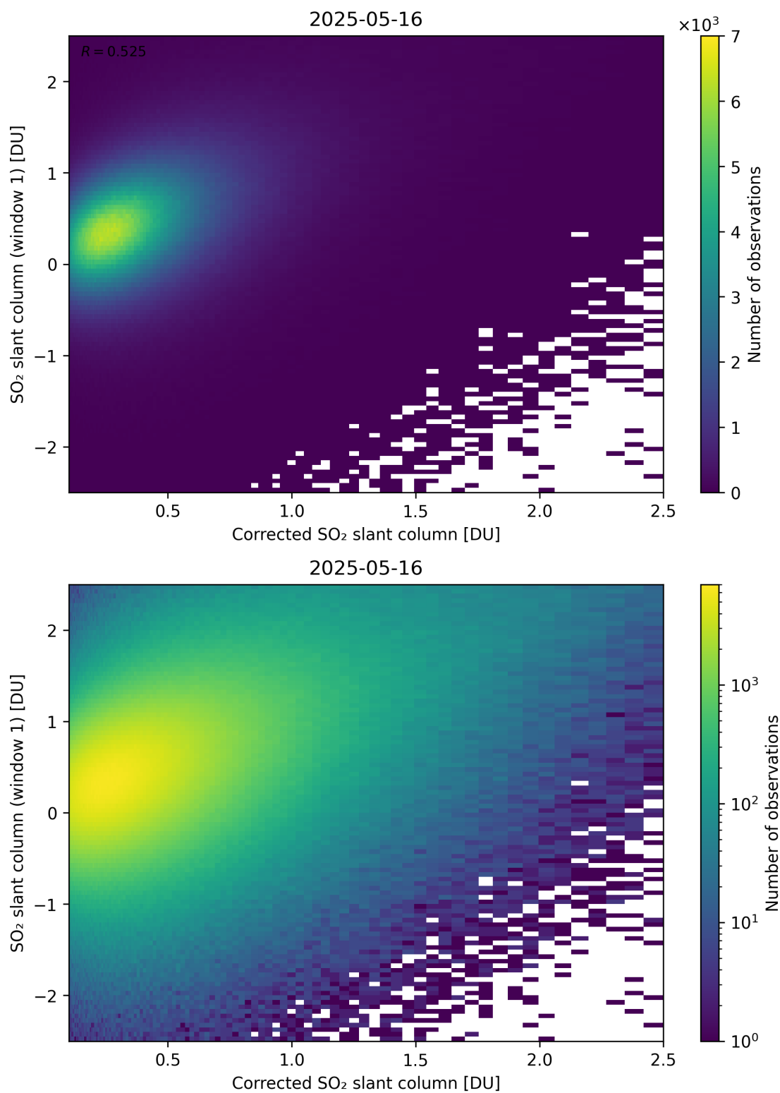
Figure 237: Scatter density plot of “Corrected SO 2 slant column” against “SO 2 slant column (window 1)” for 2025-05-15 to 2025-05-17.
