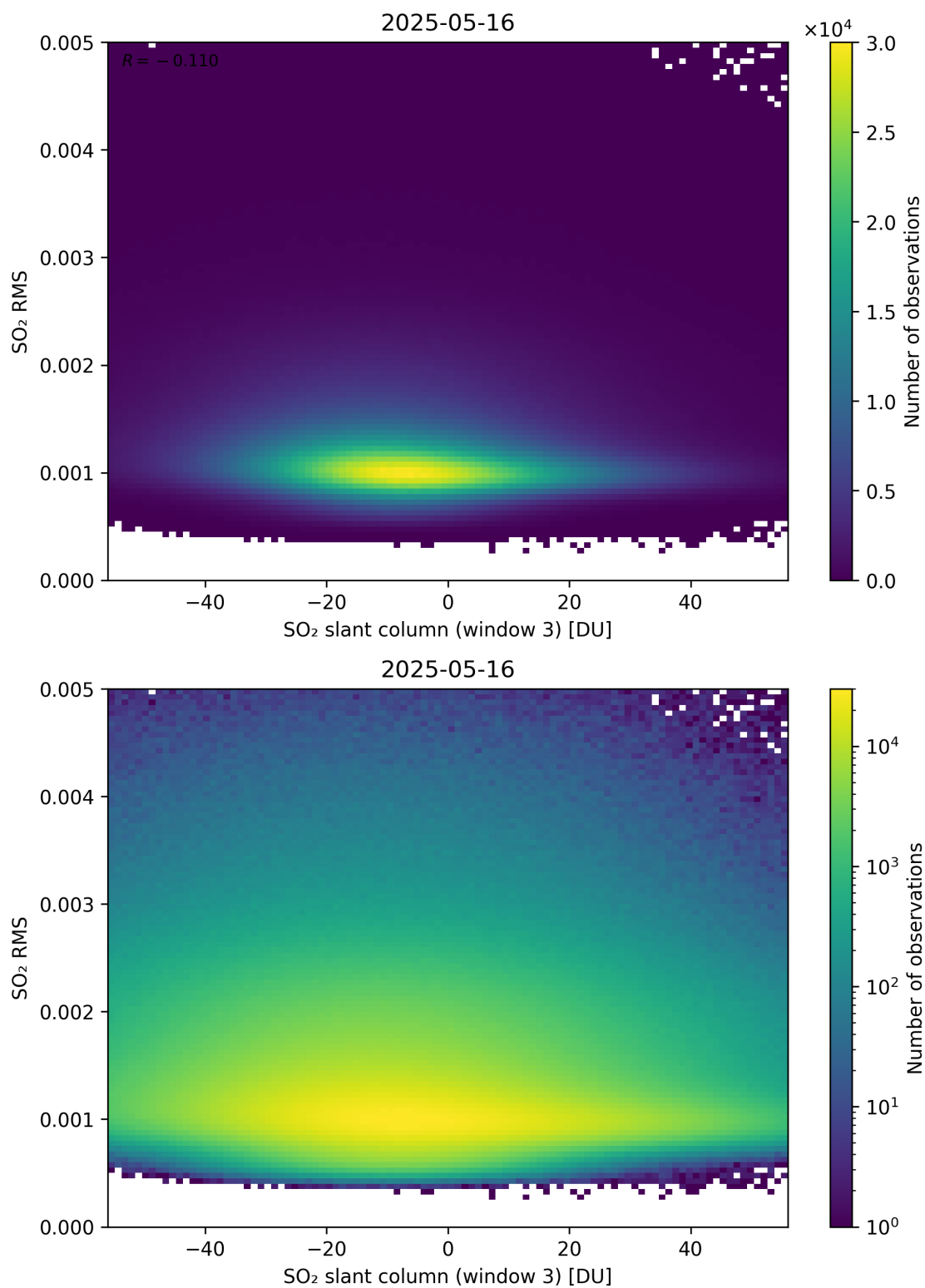
Figure 306: Scatter density plot of “SO 2 slant column (window 3)” against “SO 2 RMS” for 2025-05-15 to 2025-05-17.
