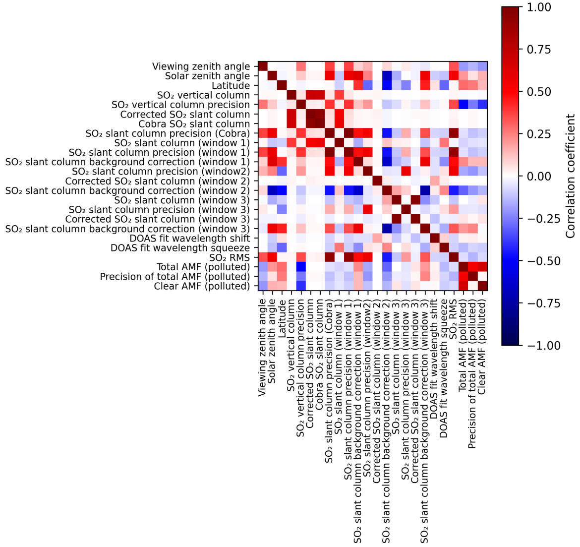
Figure 2: Map of correlation matrix for 2025-05-15 to 2025-05-17.
