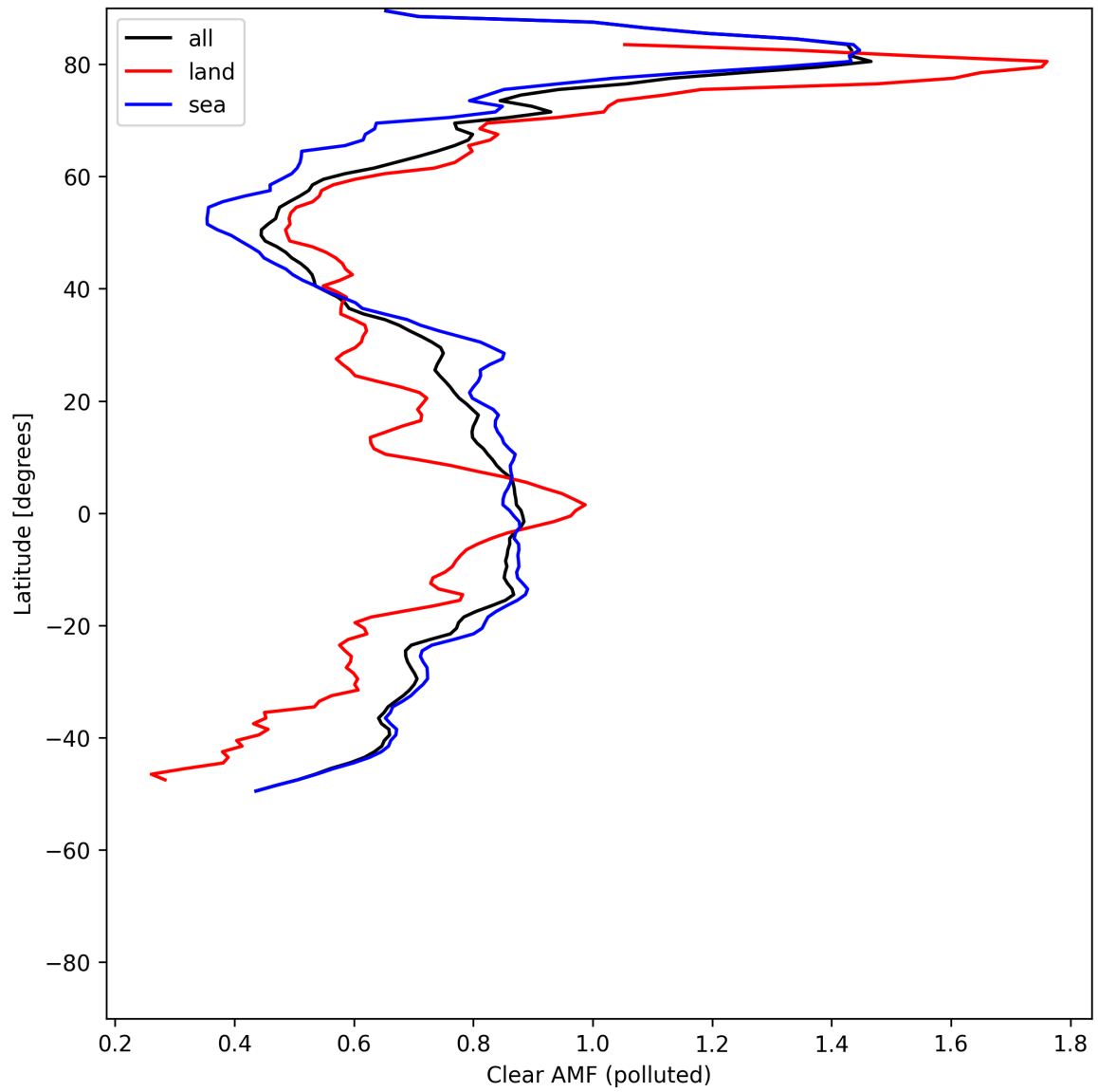
Figure 55: Zonal average of “Clear AMF (polluted)” for 2025-05-15 to 2025-05-17.
