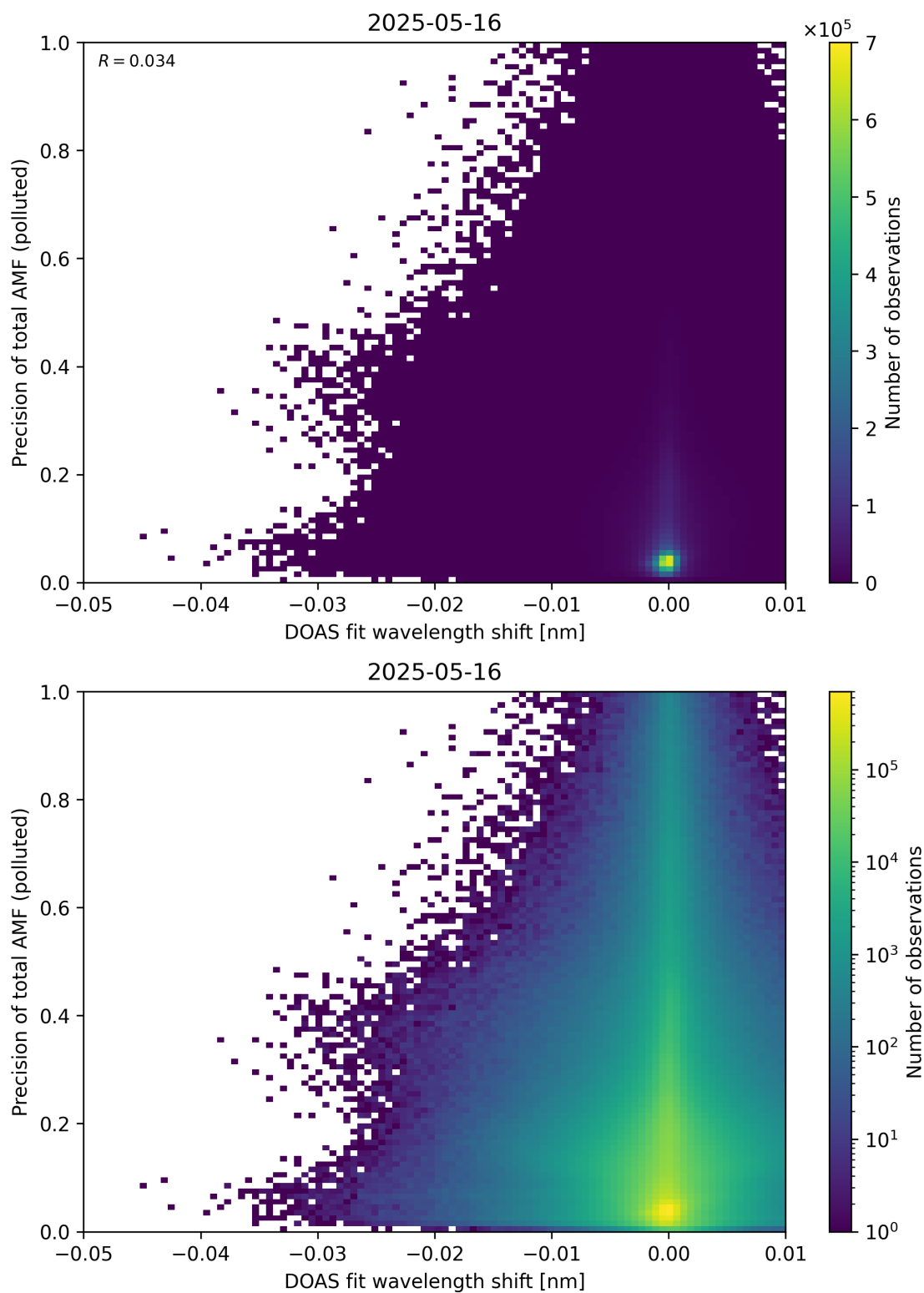
Figure 142: Scatter density plot of “DOAS fit wavelength shift” against “Precision of total AMF (polluted)” for 2025-05-15 to 2025-05-17.
