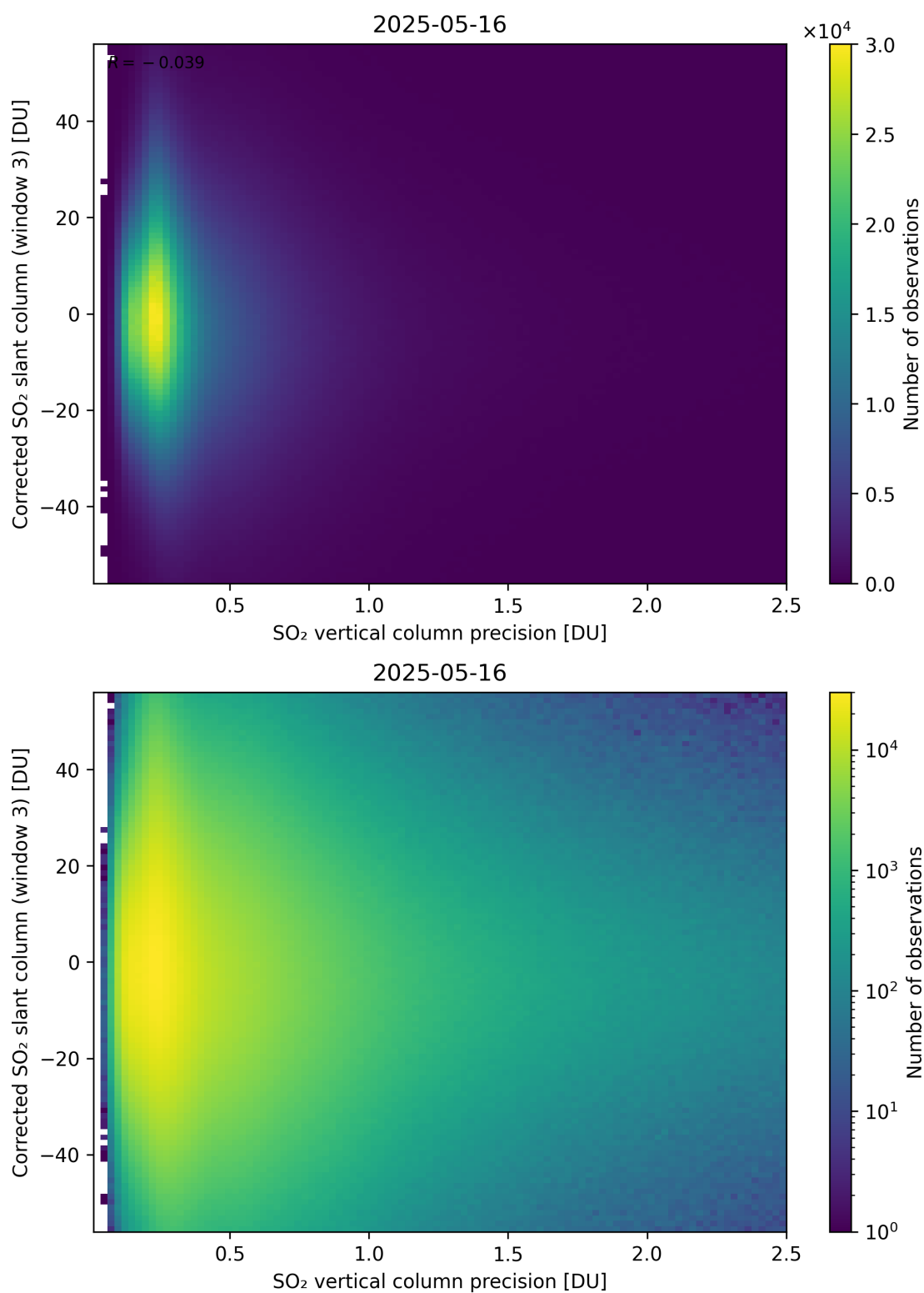
Figure 340: Scatter density plot of “SO 2 vertical column precision” against “Corrected SO 2 slant column (window 3)” for 2025-05-15 to 2025-05-17.
