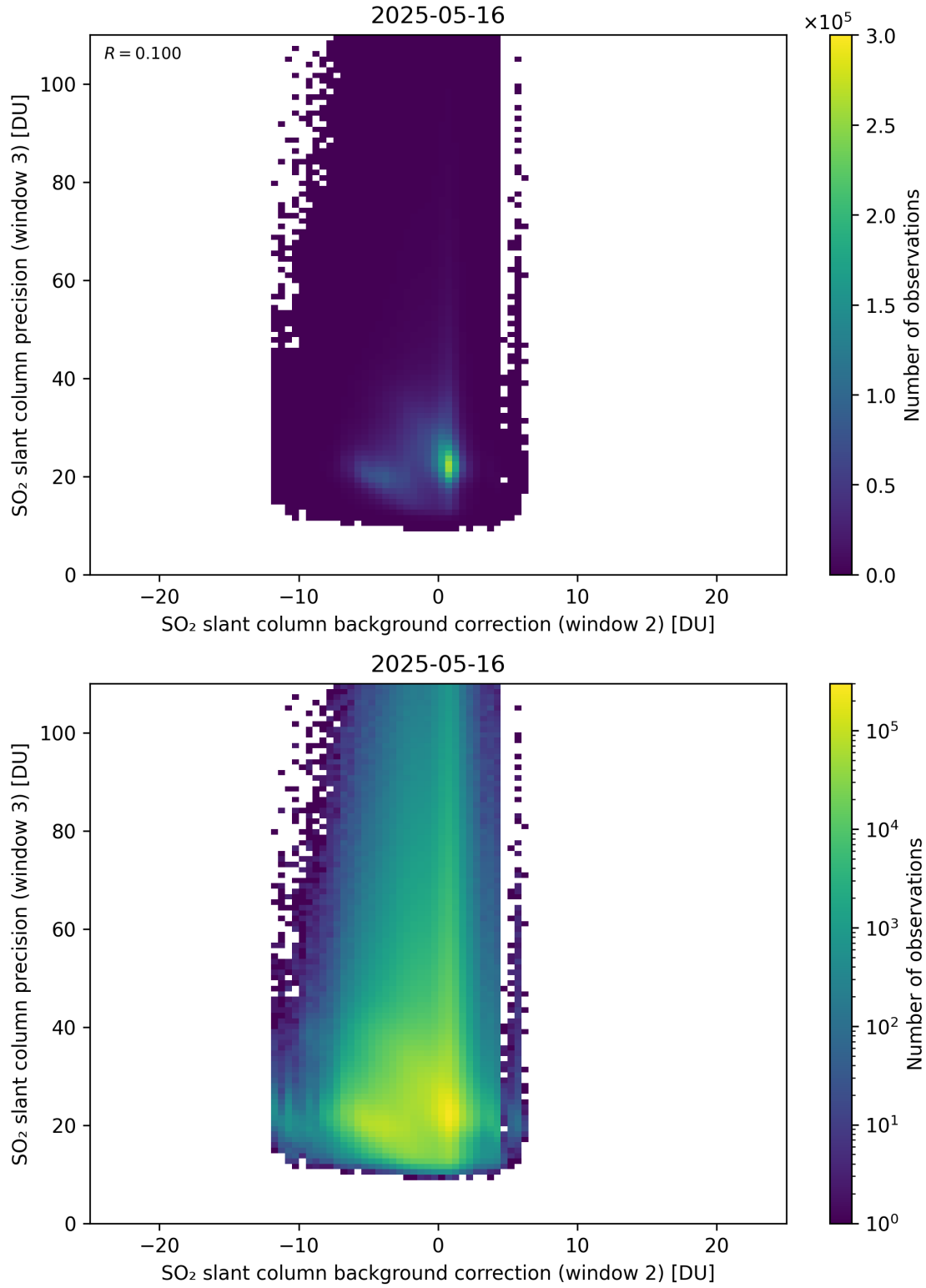
Figure 129: Scatter density plot of “SO 2 slant column background correction (window 2)” against “SO 2 slant column precision (window 3)” for 2025-05-15 to 2025-05-17.
