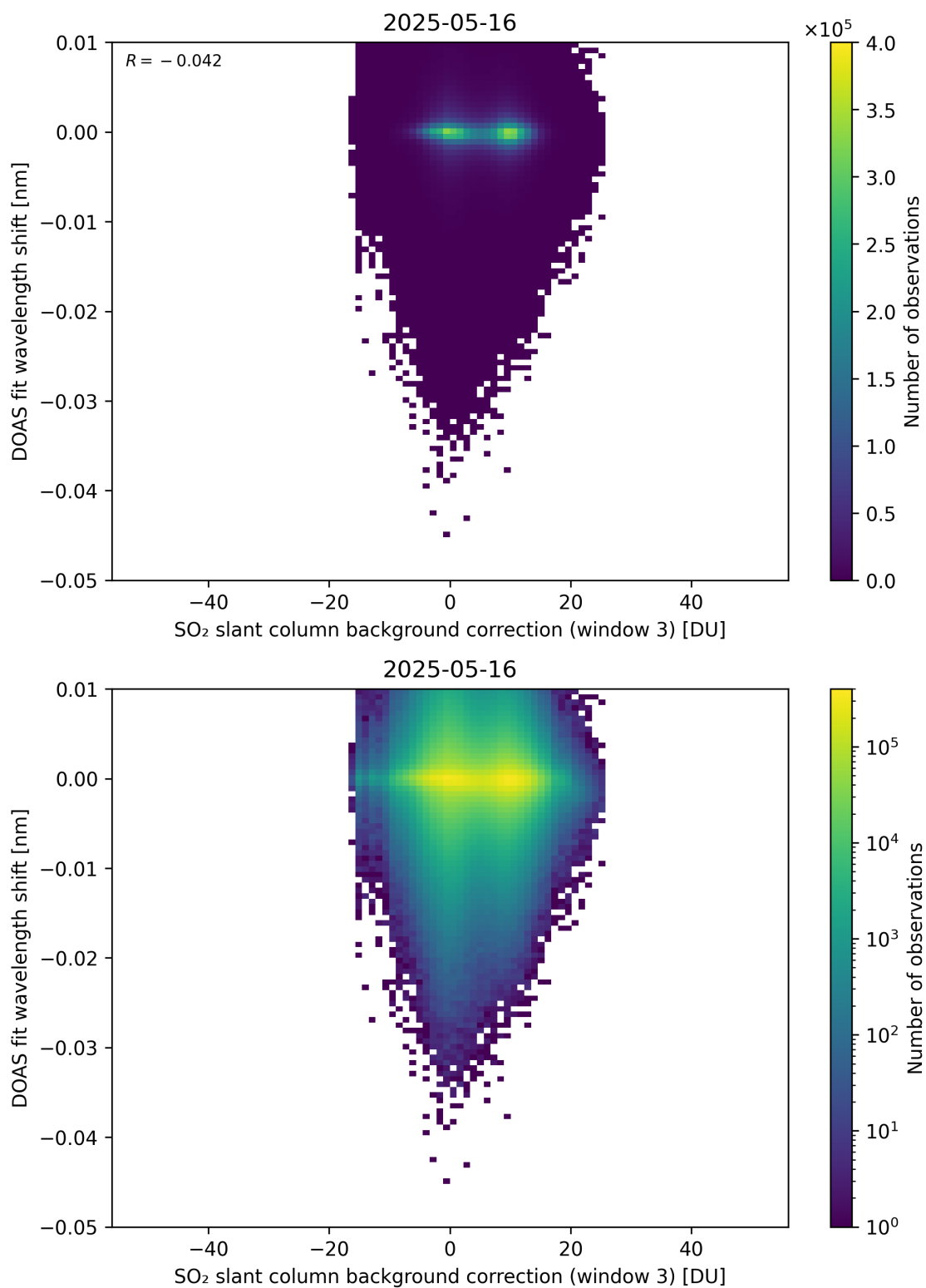
Figure 132: Scatter density plot of “SO 2 slant column background correction (window 3)” against “DOAS fit wavelength shift” for 2025-05-15 to 2025-05-17.
