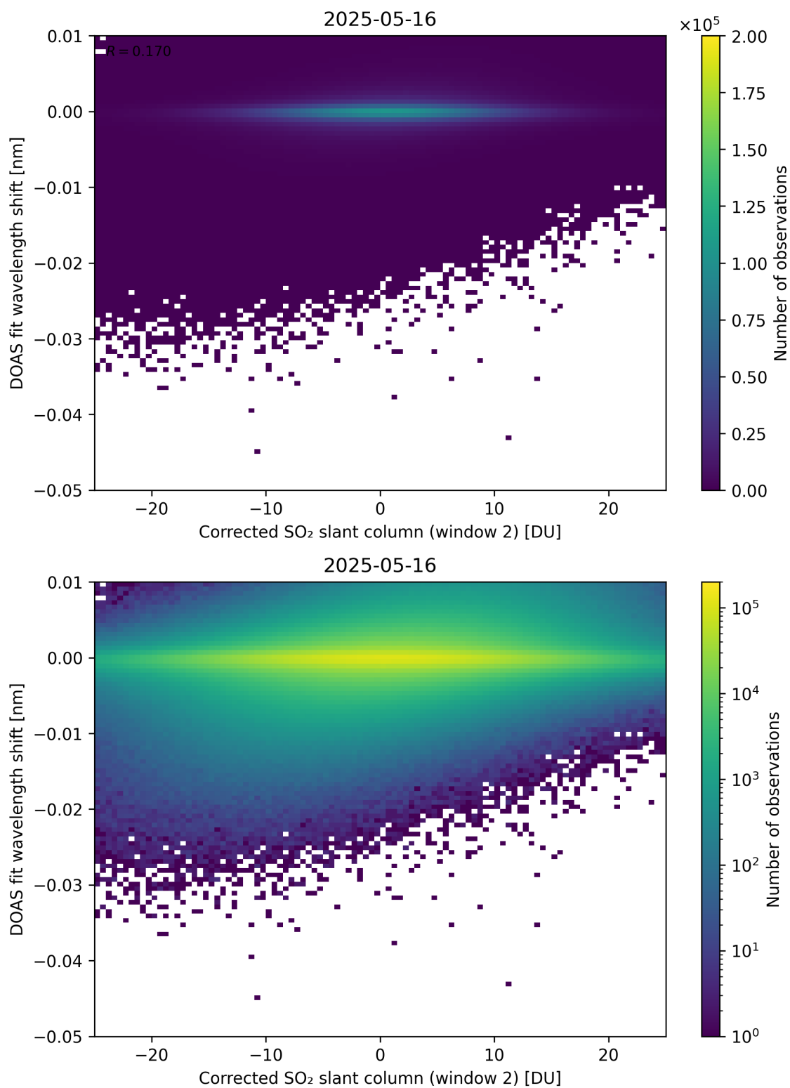
Figure 246: Scatter density plot of “Corrected SO 2 slant column (window 2)” against “DOAS fit wavelength shift” for 2025-05-15 to 2025-05-17.
