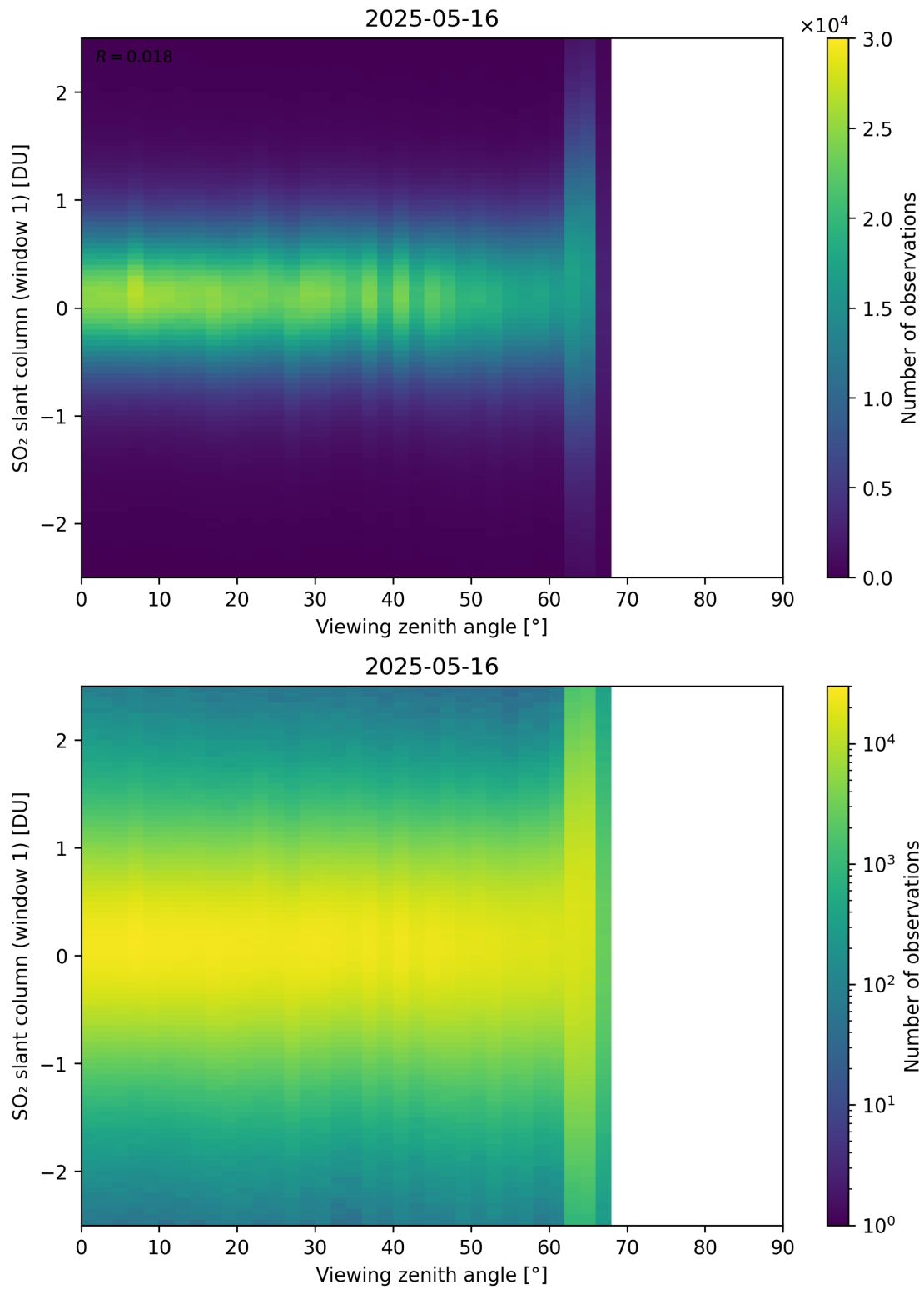
Figure 376: Scatter density plot of “Viewing zenith angle” against “SO 2 slant column (window 1)” for 2025-05-15 to 2025-05-17.
