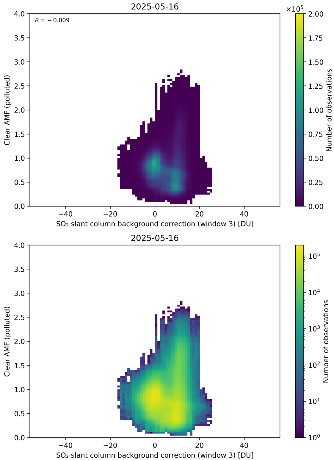
Figure 135: Scatter density plot of “SO 2 slant column background correction (window 3)” against “Clear AMF (polluted)” for 2025-05-15 to 2025-05-17.
