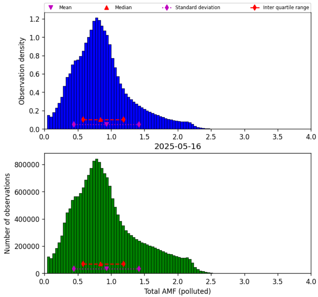
Figure 79: Histogram of “Total AMF (polluted)” for 2025-05-15 to 2025-05-17
