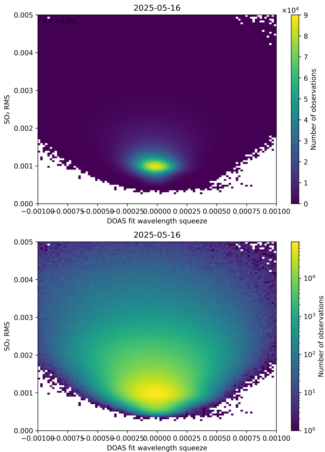
Figure 143: Scatter density plot of “DOAS fit wavelength squeeze” against “SO 2 RMS” for 2025-05-15 to 2025-05-17.
