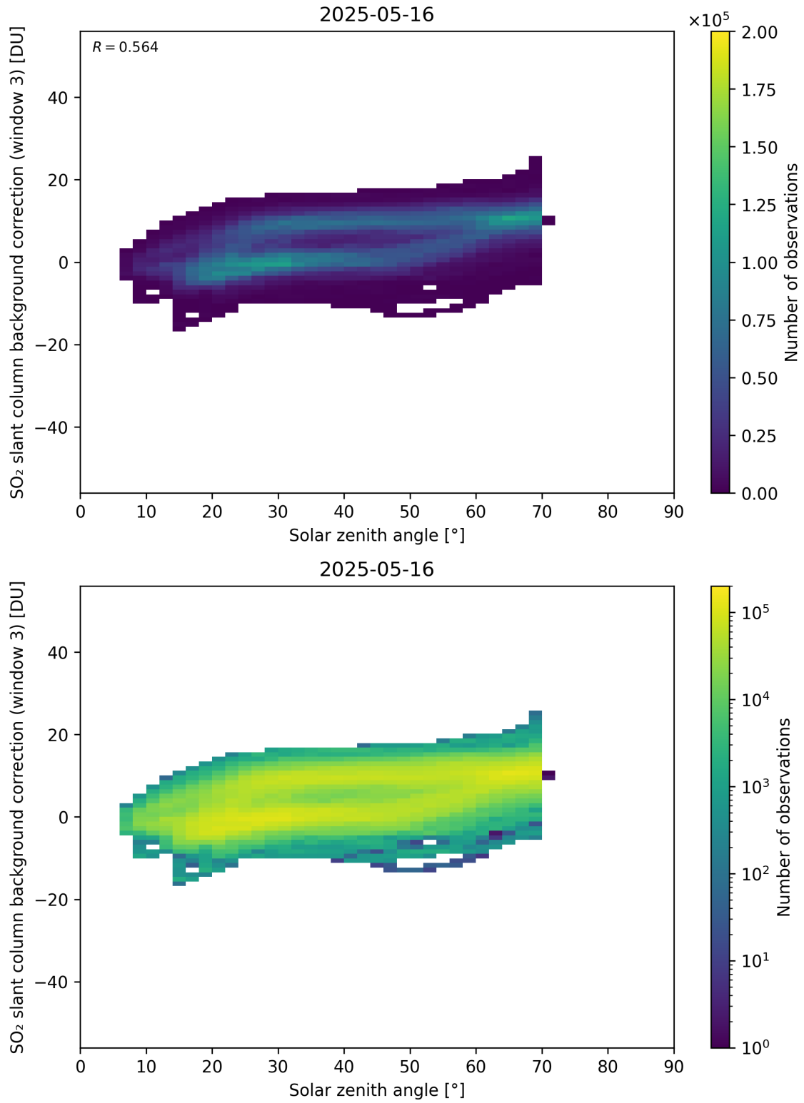
Figure 173: Scatter density plot of “Solar zenith angle” against “SO 2 slant column background correction (window 3)” for 2025-05-15 to 2025-05-17.
