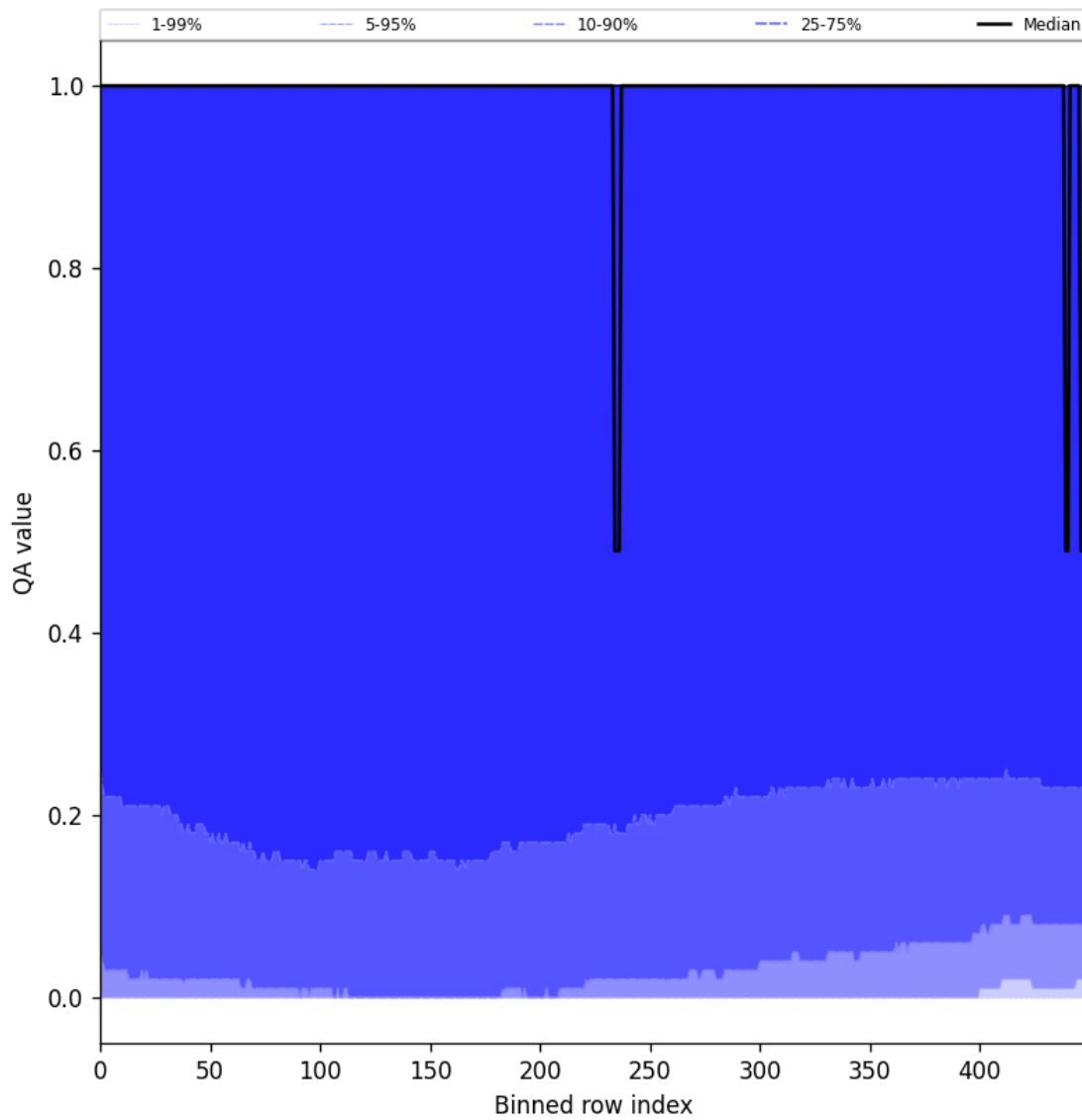
Figure 83: Along track statistics of “QA value” for 2025-05-15 to 2025-05-17
