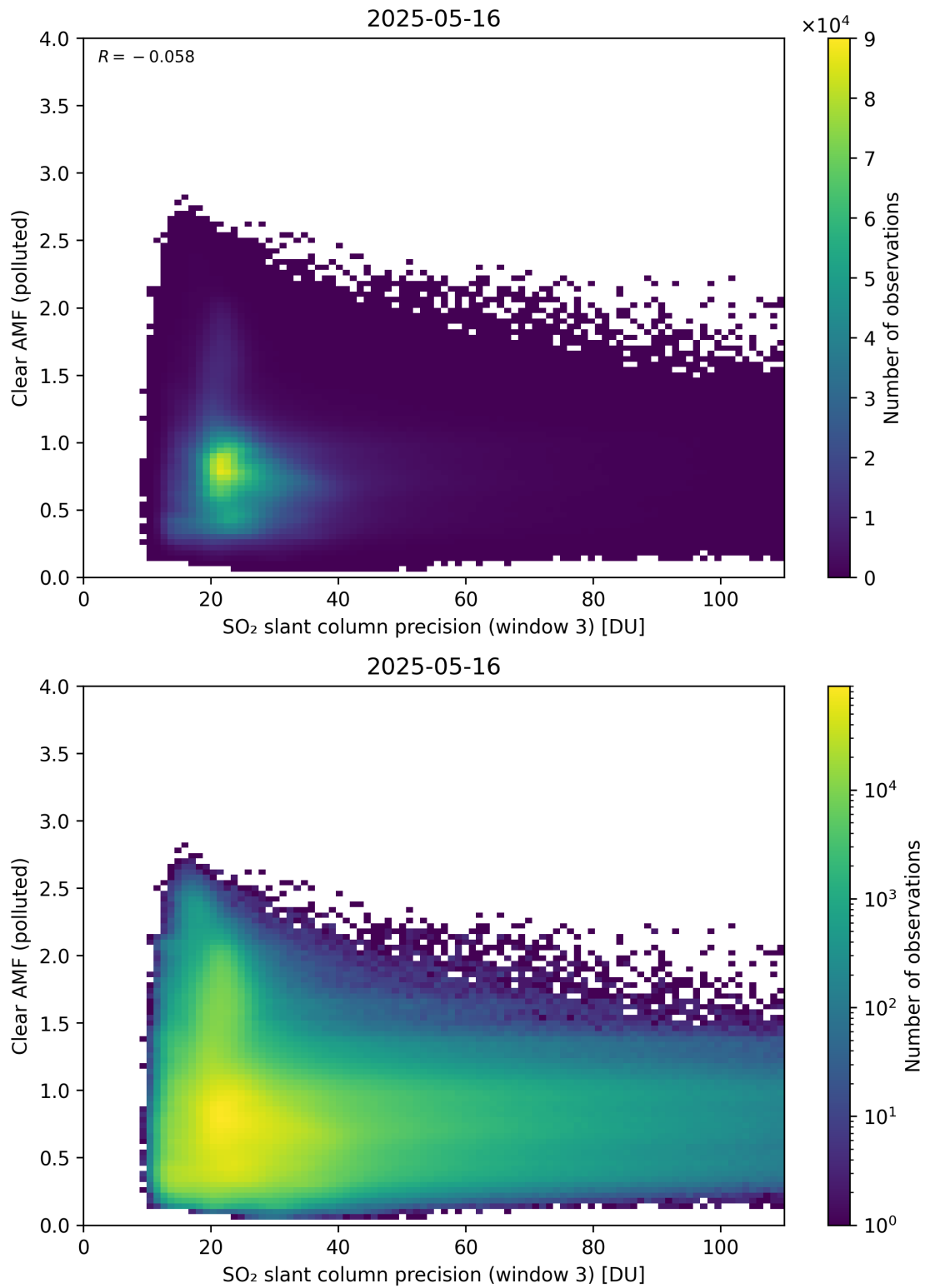
Figure 311: Scatter density plot of “SO 2 slant column precision (window 3)” against “Clear AMF (polluted)” for 2025-05-15 to 2025-05-17.
