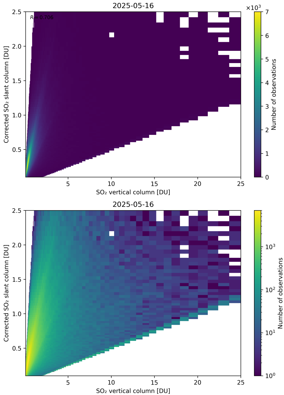
Figure 351: Scatter density plot of “SO 2 vertical column” against “Corrected SO 2 slant column” for 2025-05-15 to 2025-05-17.
