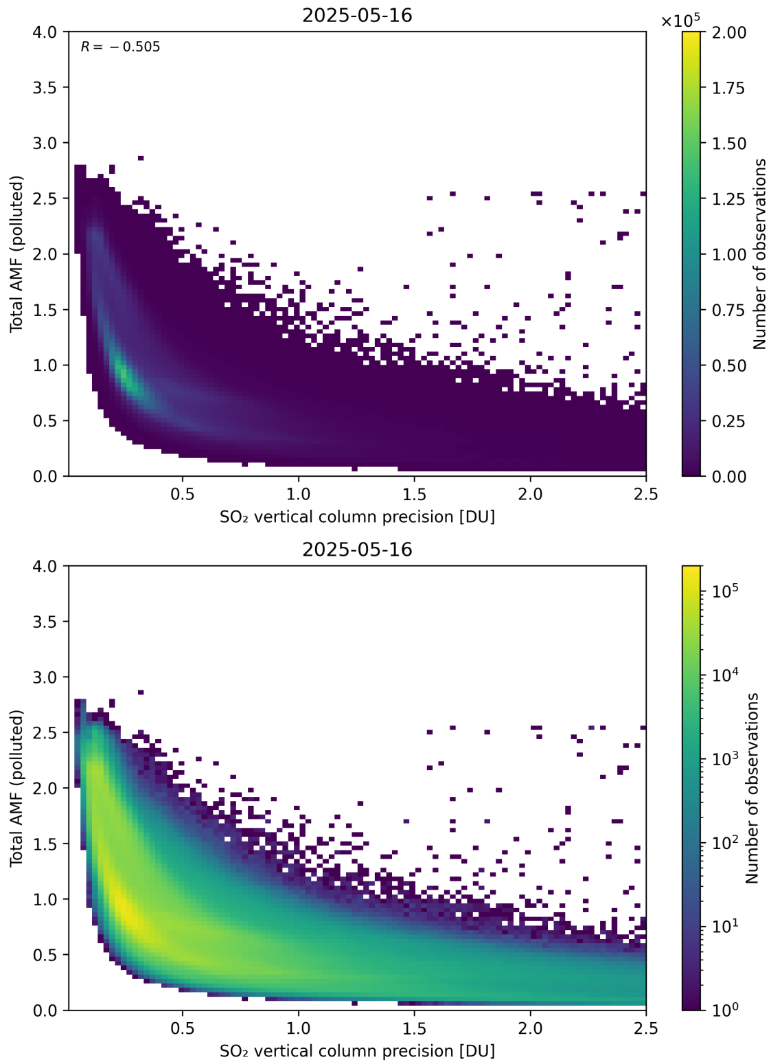
Figure 346: Scatter density plot of “SO 2 vertical column precision” against “Total AMF (polluted)” for 2025-05-15 to 2025-05-17.
