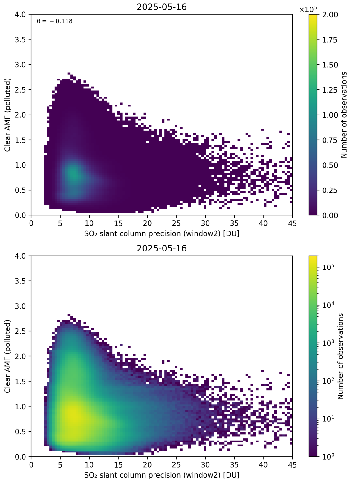
Figure 296: Scatter density plot of “SO 2 slant column precision (window2)” against “Clear AMF (polluted)” for 2025-05-15 to 2025-05-17.
