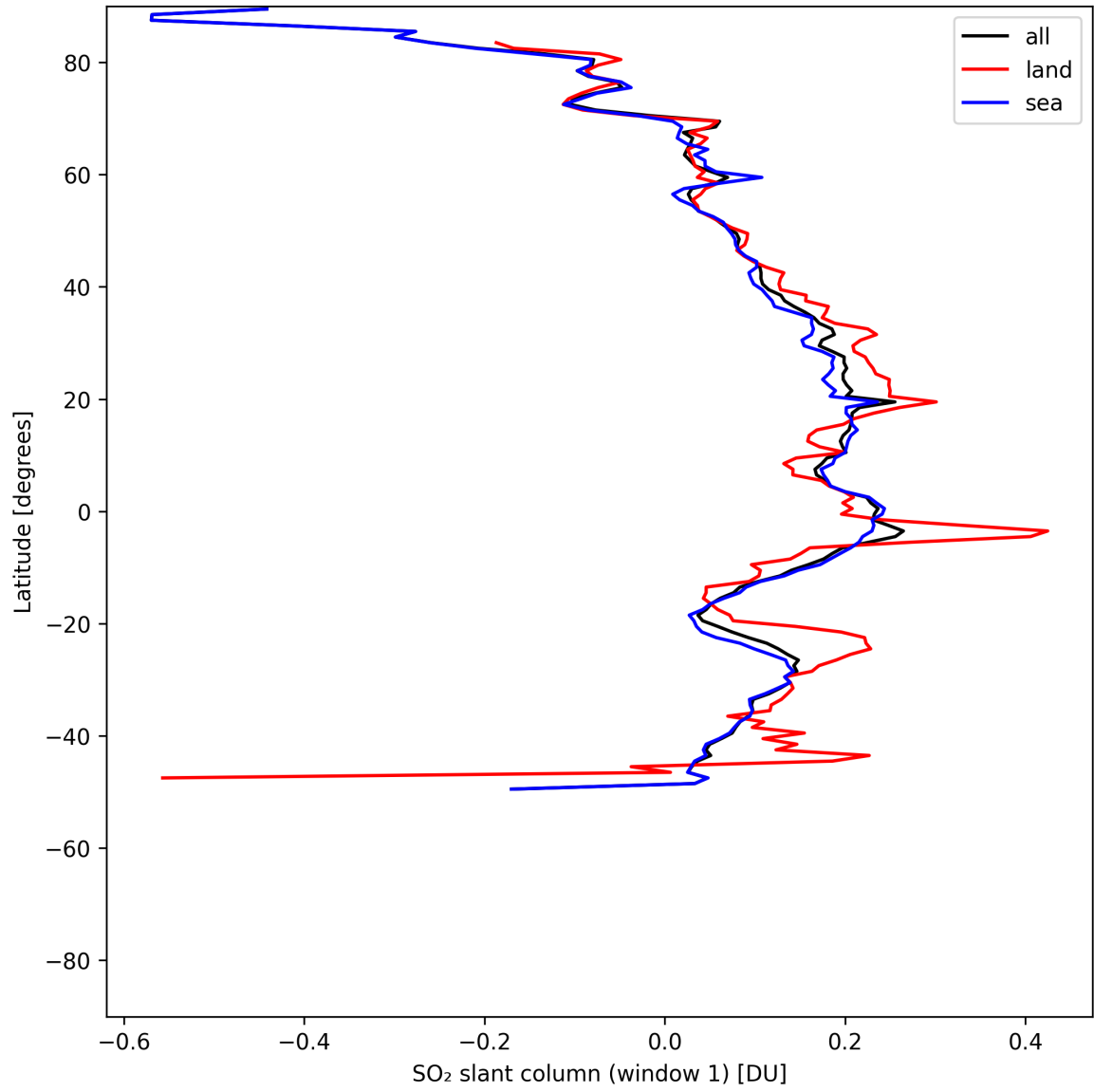
Figure 37: Zonal average of “SO 2 slant column (window 1)” for 2025-05-15 to 2025-05-17.
