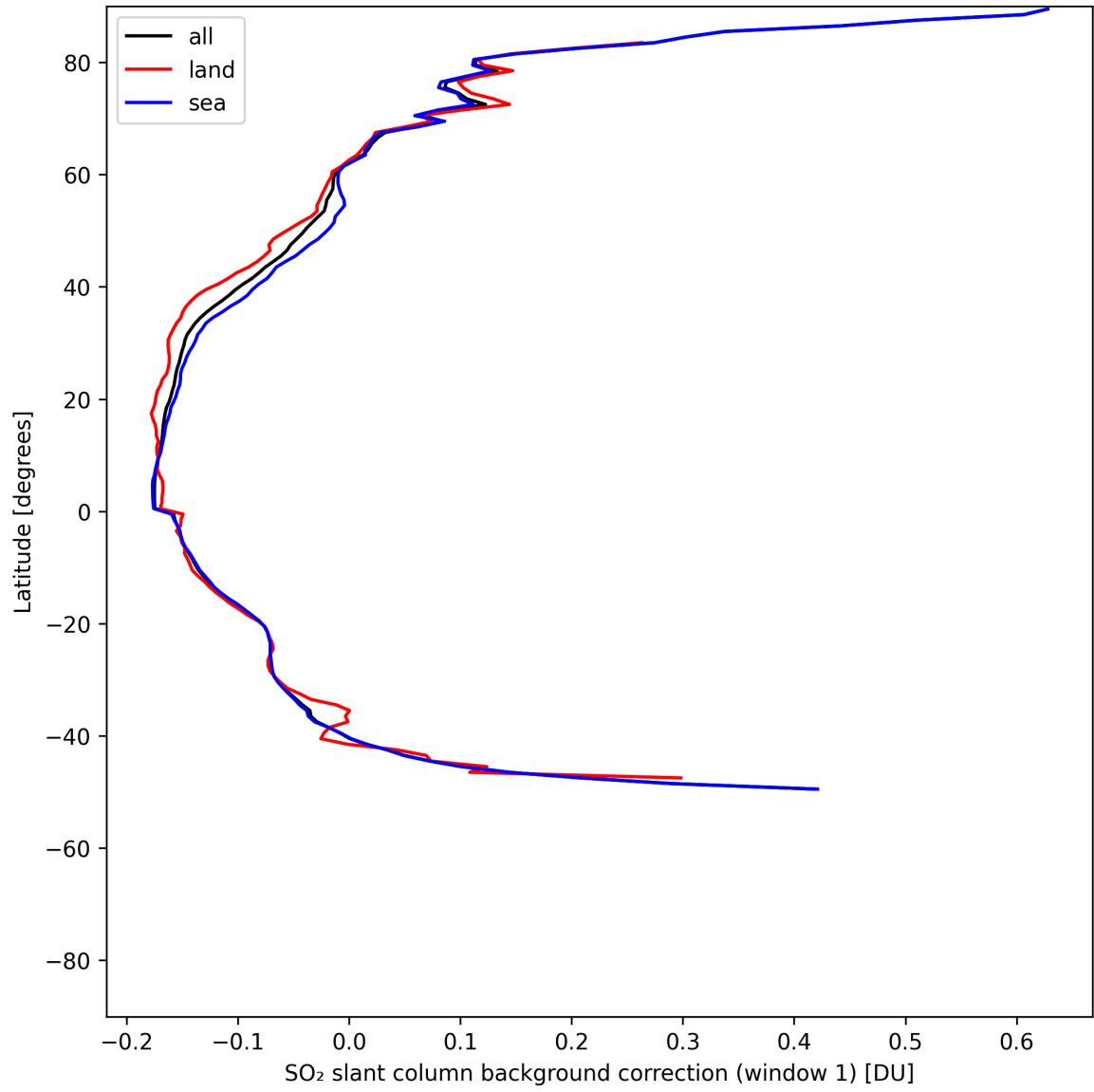
Figure 40: Zonal average of "SO 2 slant column background correction (window 1)" for 2025-05-15 to 2025-05-17.
