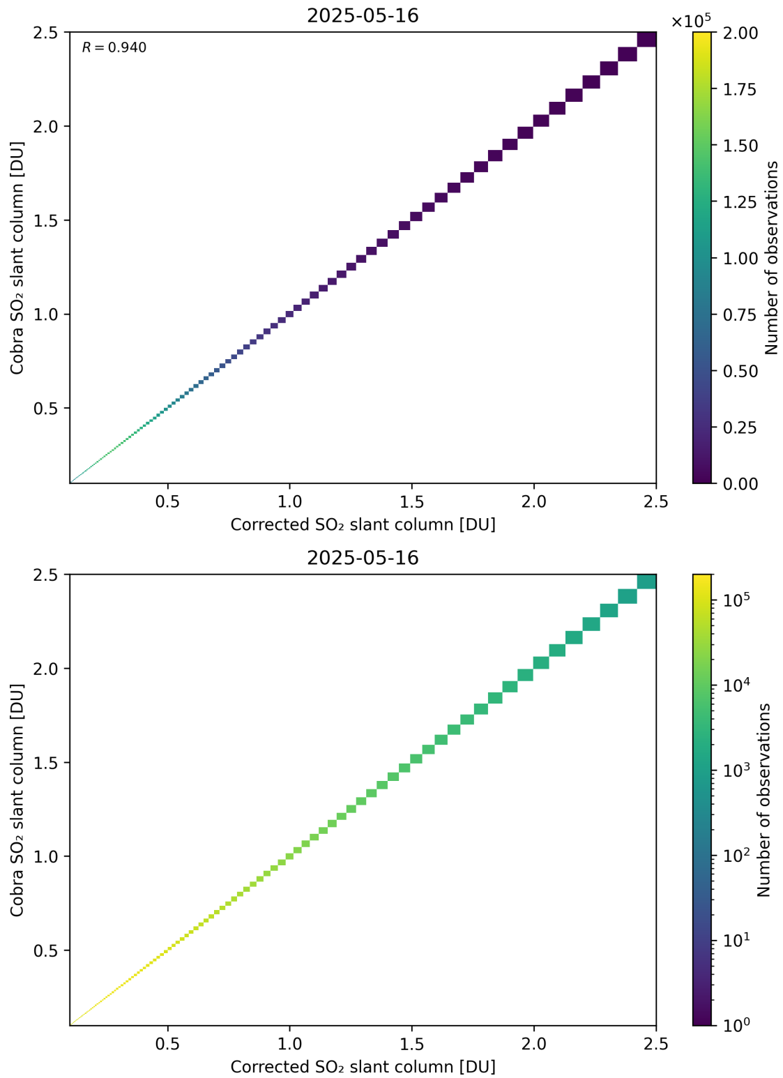
Figure 233: Scatter density plot of “Corrected SO 2 slant column” against “Cobra SO 2 slant column” for 2025-05-15 to 2025-05-17.
