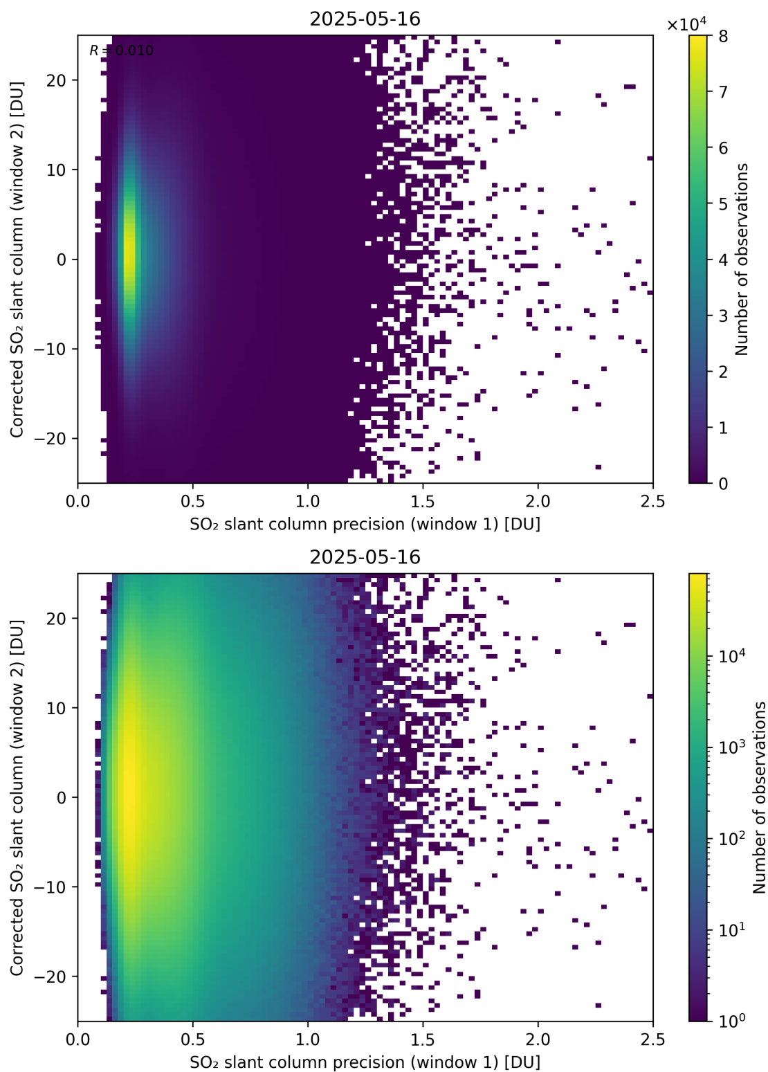
Figure 275: Scatter density plot of “SO 2 slant column precision (window 1)” against “Corrected SO 2 slant column (window 2)” for 2025-05-15 to 2025-05-17.
