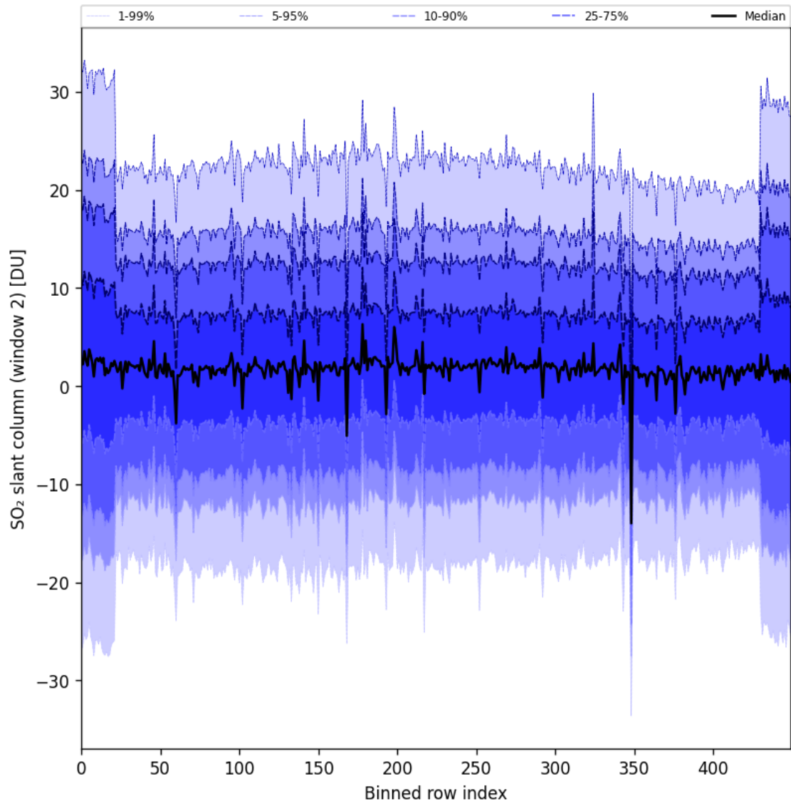
Figure 93: Along track statistics of “SO 2 slant column (window 2)” for 2025-05-15 to 2025-05-17
