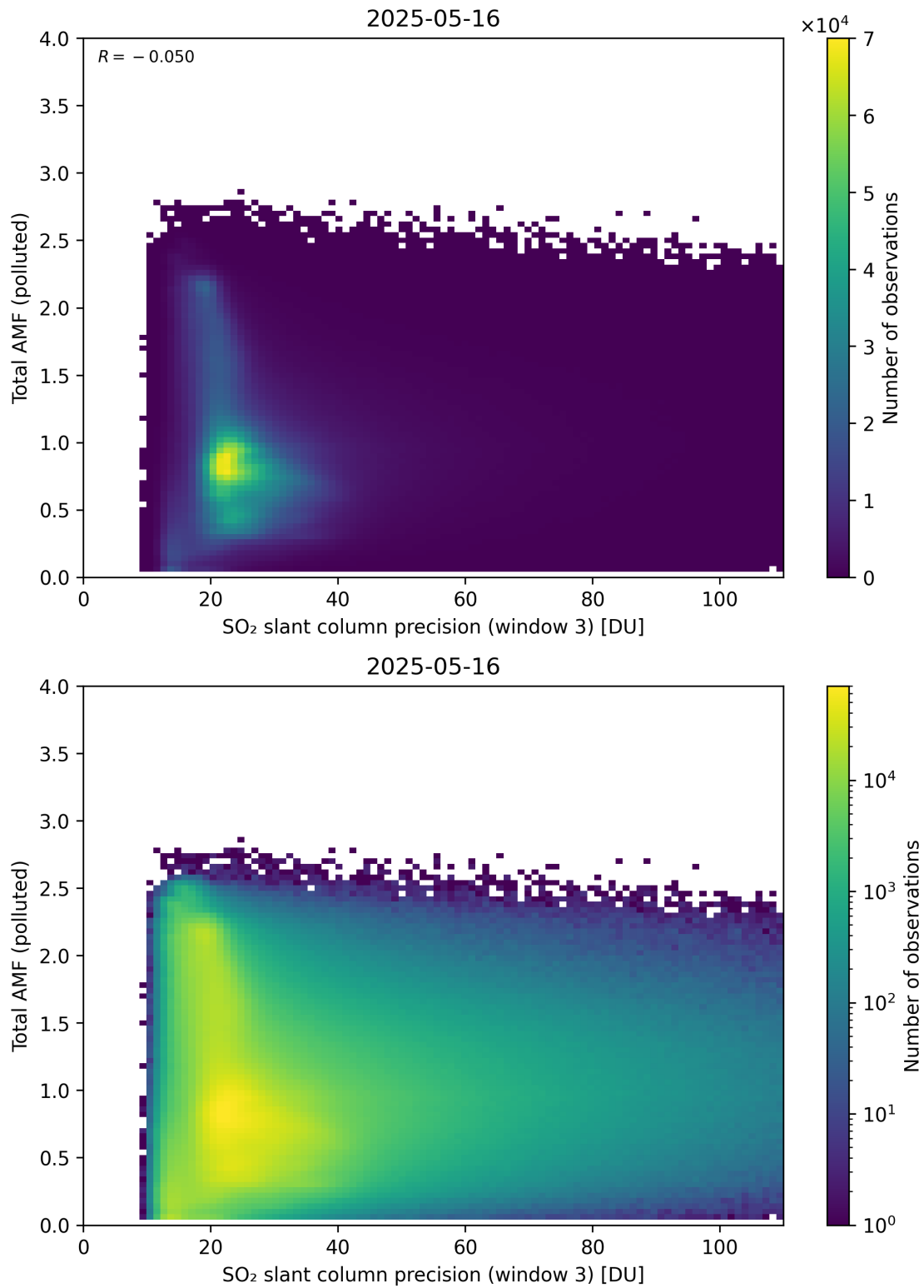
Figure 313: Scatter density plot of “SO 2 slant column precision (window 3)” against “Total AMF (polluted)” for 2025-05-15 to 2025-05-17.
