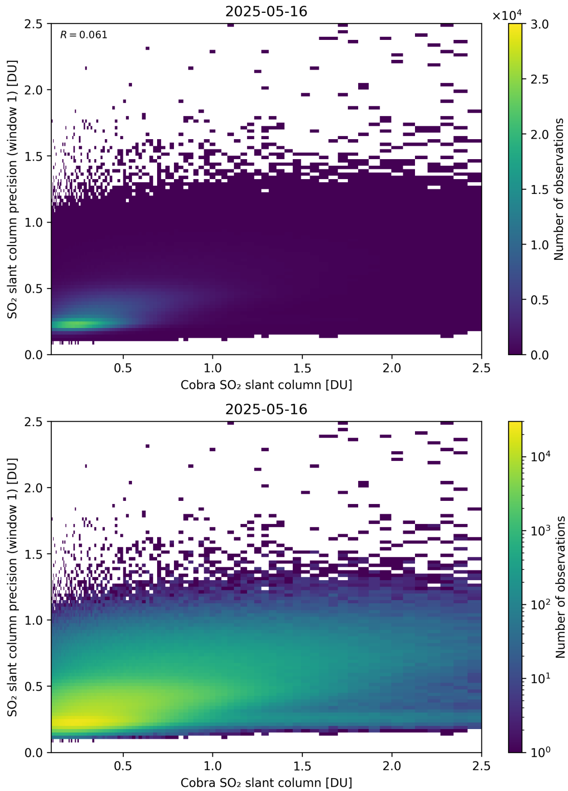
Figure 220: Scatter density plot of “Cobra SO 2 slant column” against “SO 2 slant column precision (window 1)” for 2025-05-15 to 2025-05-17.
