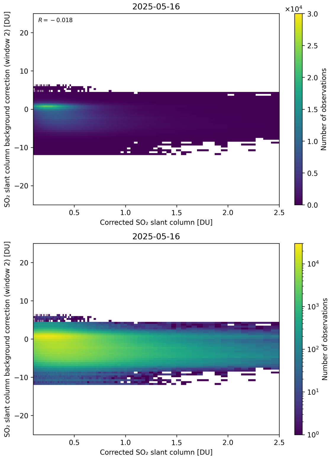
Figure 227: Scatter density plot of “Corrected SO 2 slant column” against “SO 2 slant column background correction (window 2)” for 2025-05-15 to 2025-05-17.
