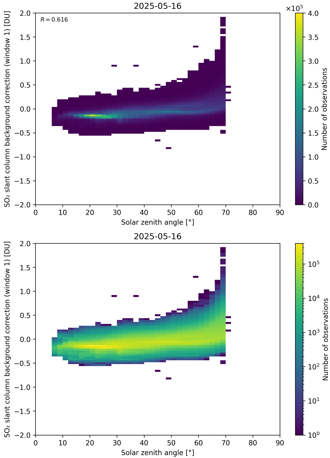
Figure 171: Scatter density plot of “Solar zenith angle” against “SO 2 slant column background correction (window 1)” for 2025-05-15 to 2025-05-17.
