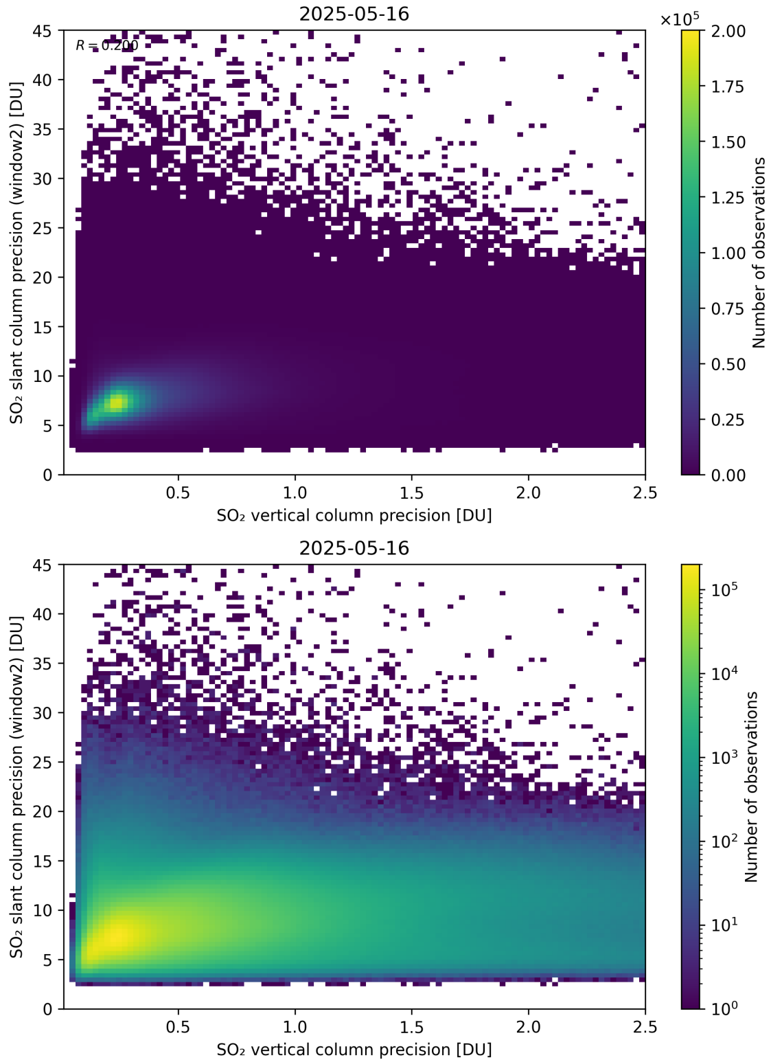
Figure 343: Scatter density plot of “SO 2 vertical column precision” against “SO 2 slant column precision (window2)” for 2025-05-15 to 2025-05-17.
