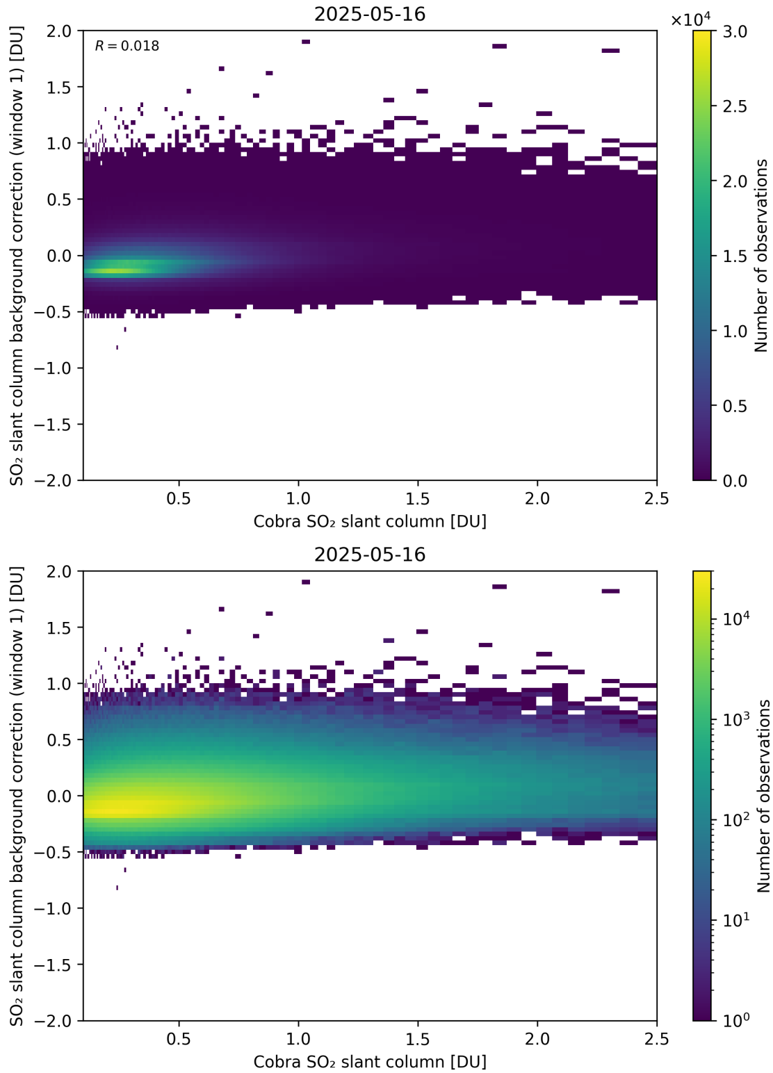
Figure 193: Scatter density plot of “Cobra SO 2 slant column” against “SO 2 slant column background correction (window 1)” for 2025-05-15 to 2025-05-17.
