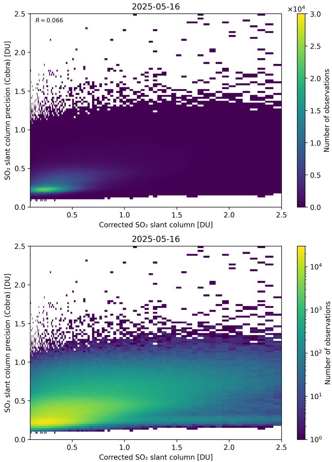
Figure 234: Scatter density plot of “Corrected SO 2 slant column” against “SO 2 slant column precision (Cobra)” for 2025-05-15 to 2025-05-17.
