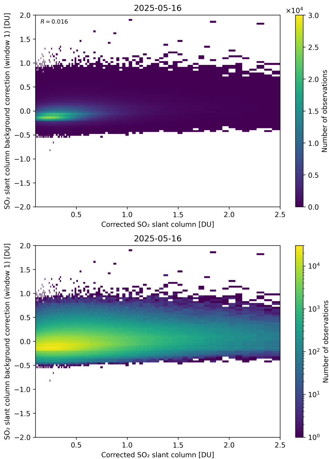
Figure 226: Scatter density plot of “Corrected SO 2 slant column” against “SO 2 slant column background correction (window 1)” for 2025-05-15 to 2025-05-17.
