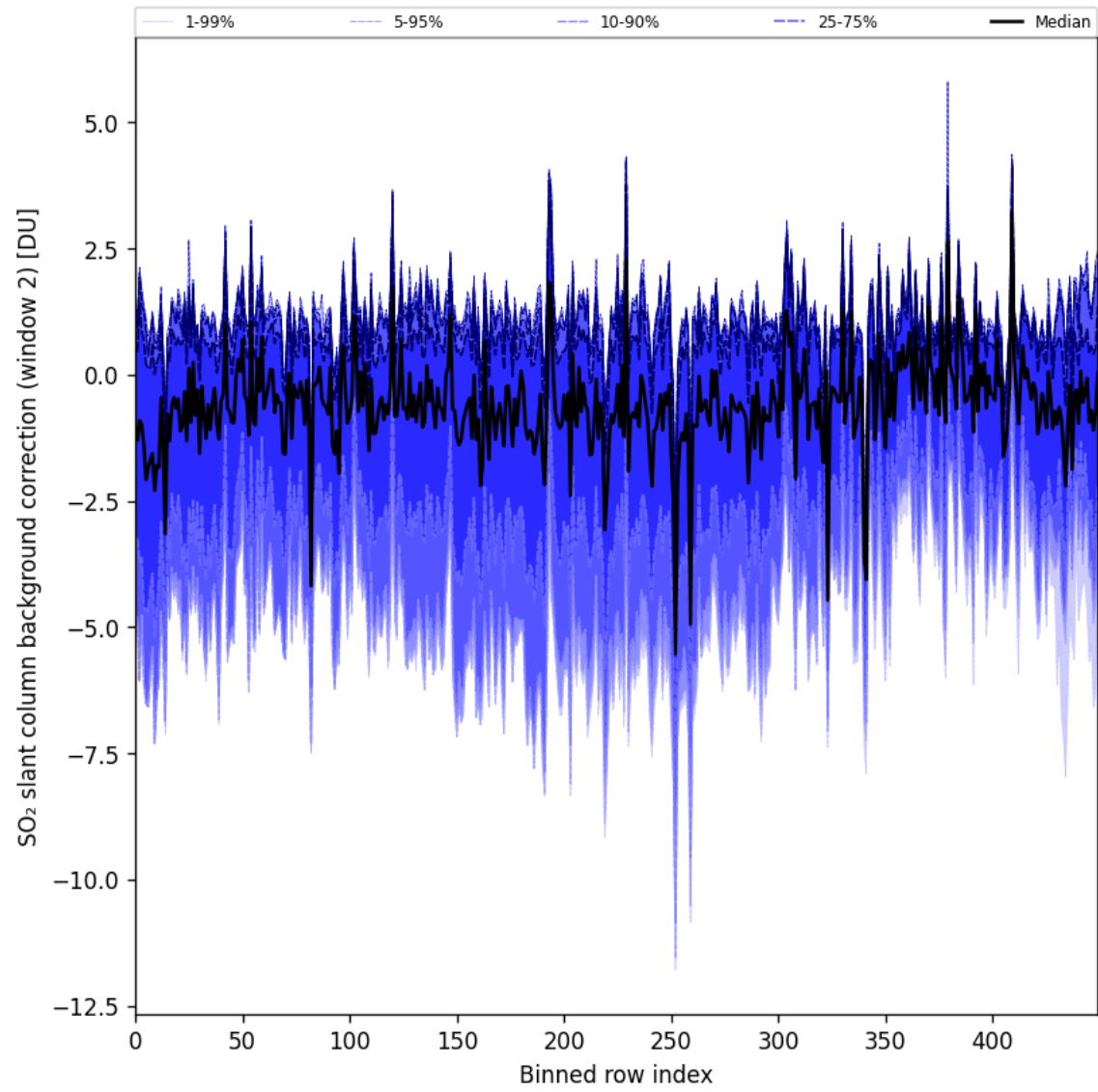
Figure 96: Along track statistics of “SO 2 slant column background correction (window 2)” for 2025-05-15 to 2025-05-17
