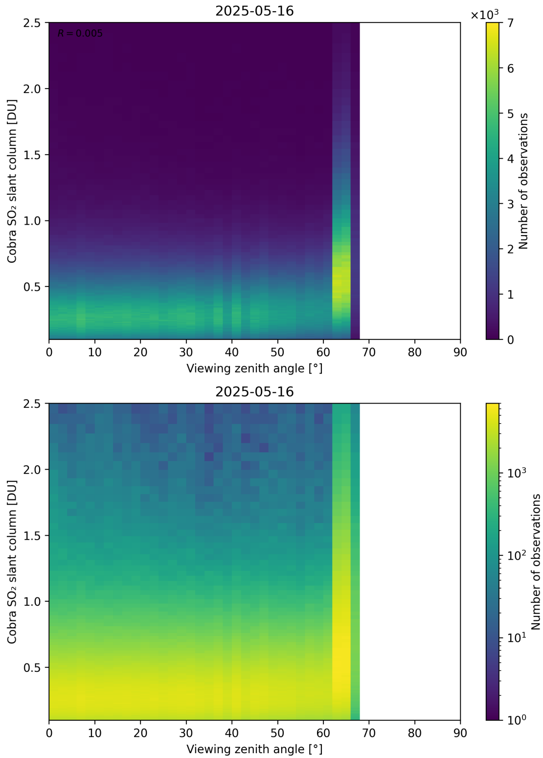
Figure 371: Scatter density plot of “Viewing zenith angle” against “Cobra SO 2 slant column” for 2025-05-15 to 2025-05-17.
