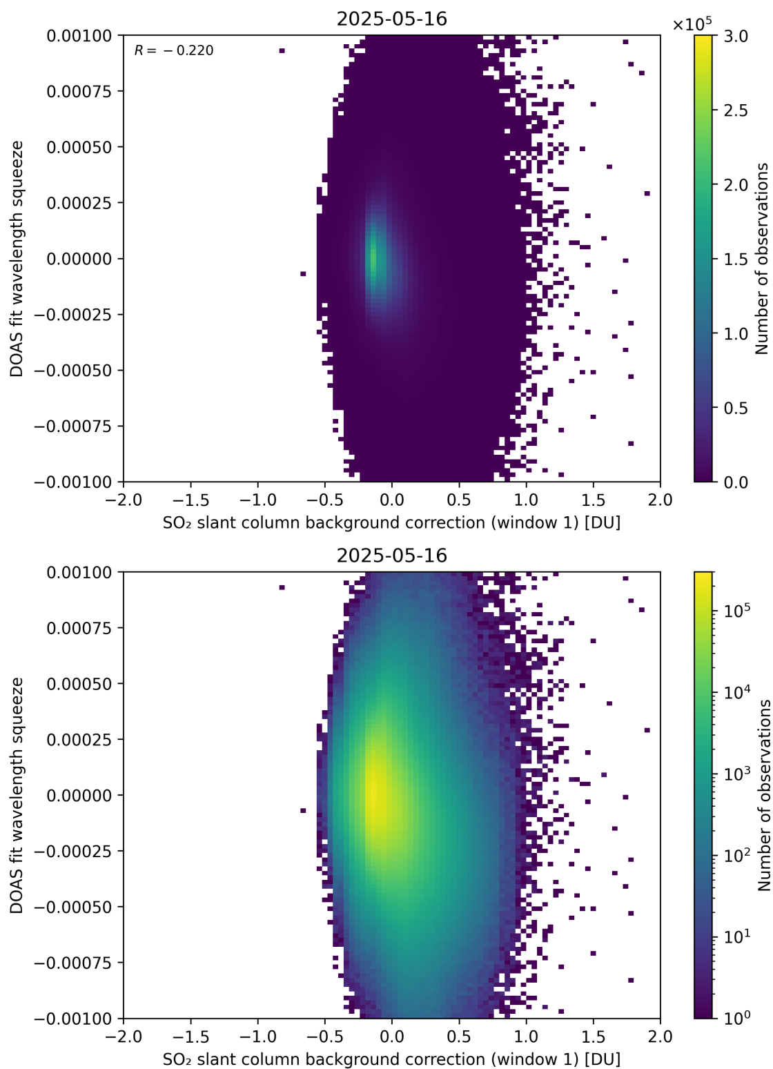
Figure 112: Scatter density plot of “SO 2 slant column background correction (window 1)” against “DOAS fit wavelength squeeze” for 2025-05-15 to 2025-05-17.
