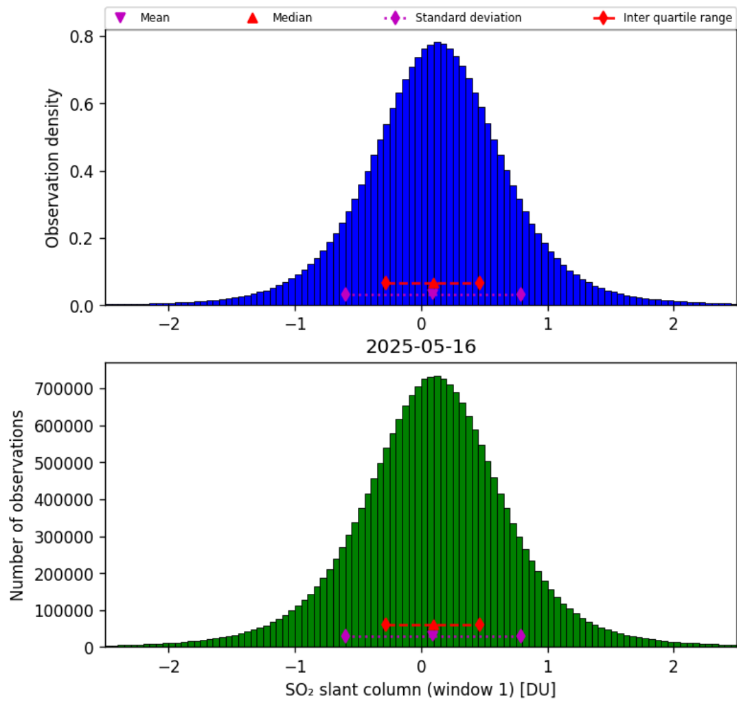
Figure 63: Histogram of “SO 2 slant column (window 1)” for 2025-05-15 to 2025-05-17
