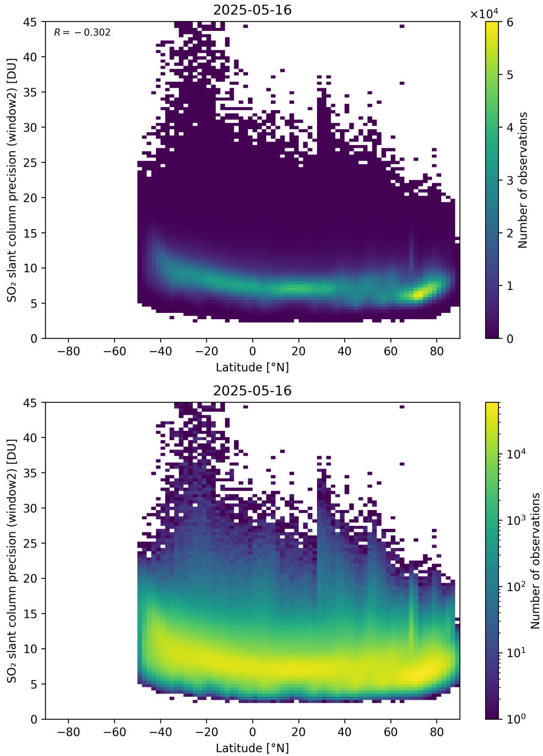
Figure 164: Scatter density plot of “Latitude” against “SO 2 slant column precision (window2)” for 2025-05-15 to 2025-05-17.
