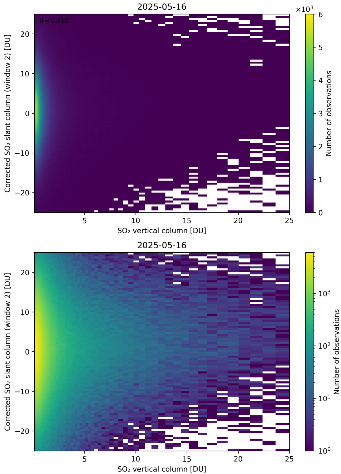
Figure 352: Scatter density plot of “SO 2 vertical column” against “Corrected SO 2 slant column (window 2)” for 2025-05-15 to 2025-05-17.
