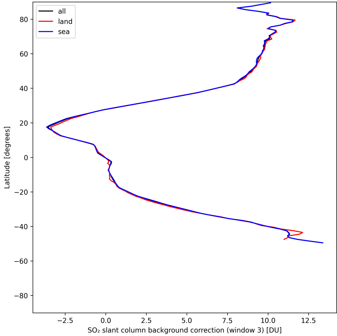
Figure 48: Zonal average of “SO 2 slant column background correction (window 3)” for 2025-05-15 to 2025-05-17.
