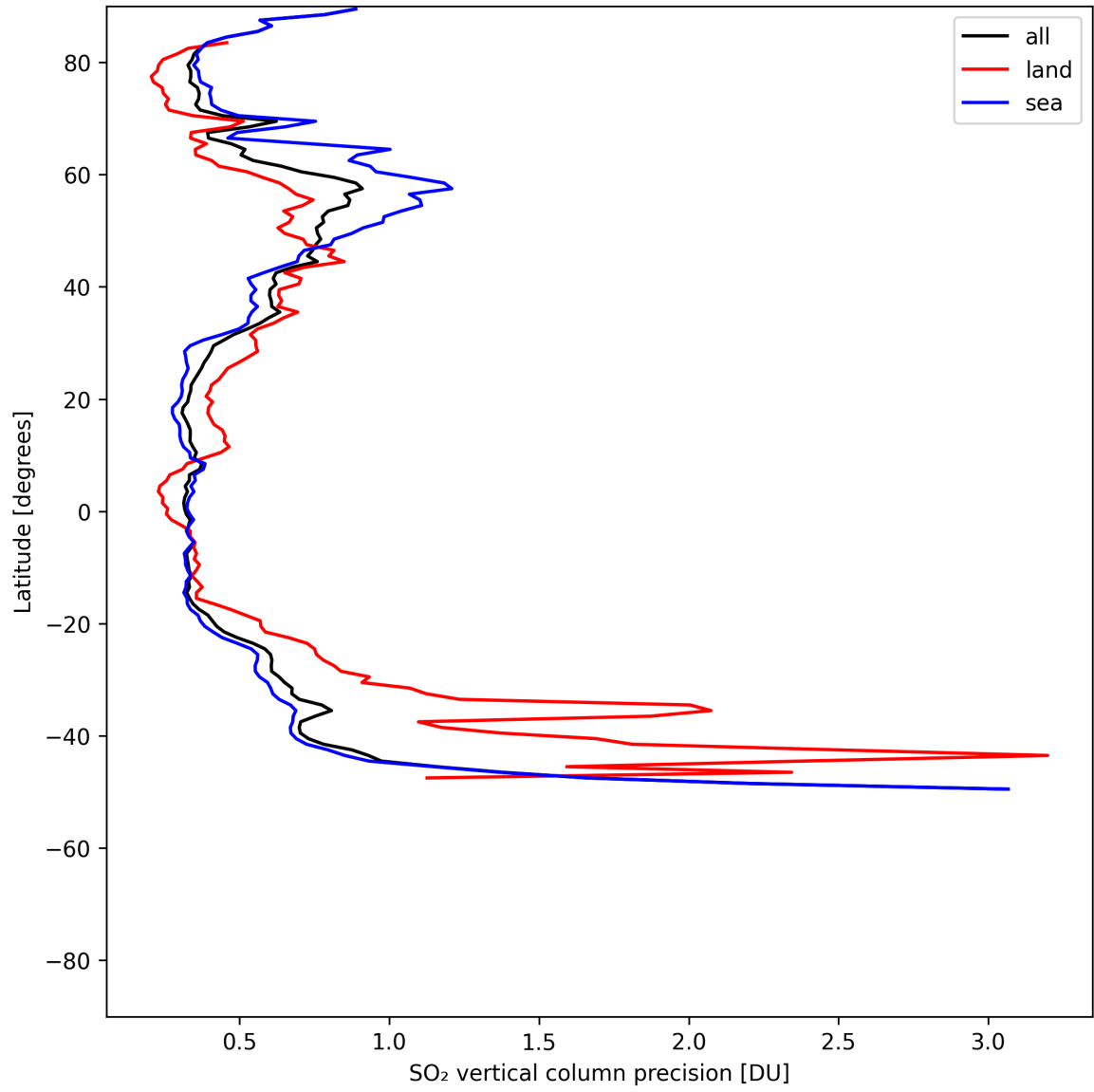
Figure 33: Zonal average of “SO 2 vertical column precision” for 2025-05-15 to 2025-05-17.
