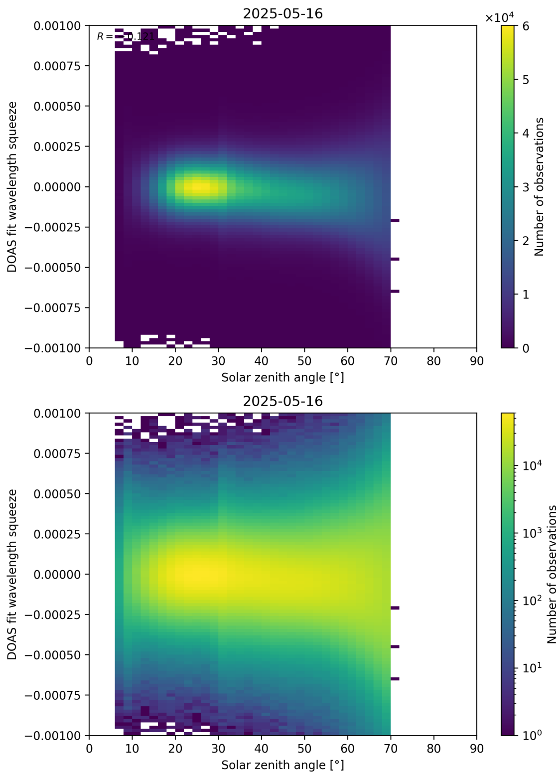
Figure 175: Scatter density plot of “Solar zenith angle” against “DOAS fit wavelength squeeze” for 2025-05-15 to 2025-05-17.
