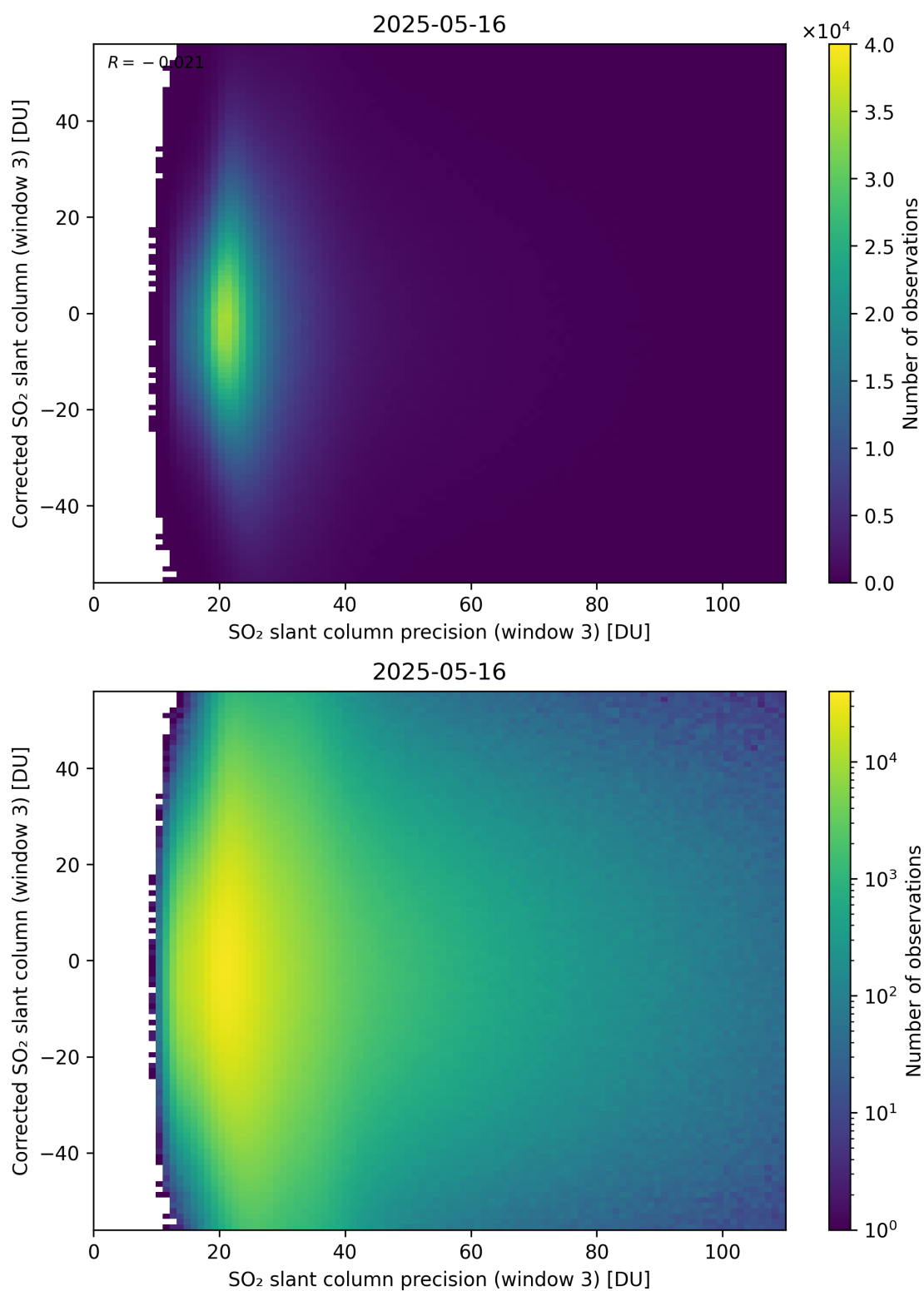
Figure 312: Scatter density plot of “SO 2 slant column precision (window 3)” against “Corrected SO 2 slant column (window 3)” for 2025-05-15 to 2025-05-17.
