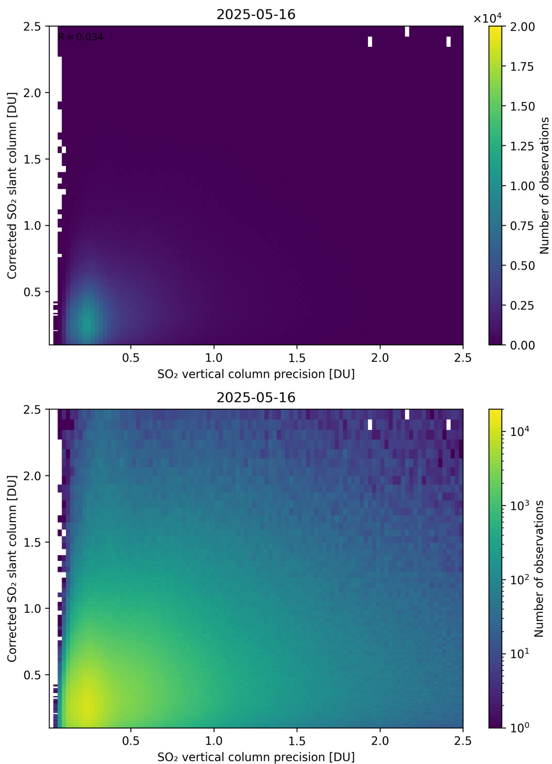
Figure 338: Scatter density plot of “SO 2 vertical column precision” against “Corrected SO 2 slant column” for 2025-05-15 to 2025-05-17.
