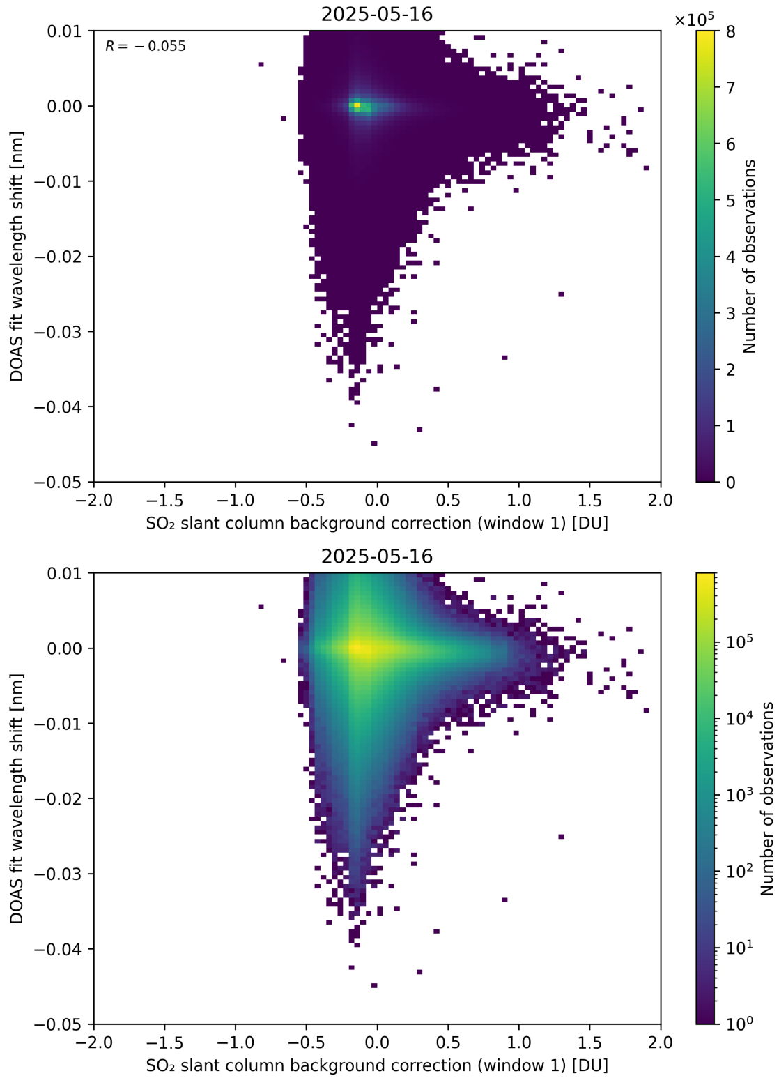
Figure 111: Scatter density plot of “SO 2 slant column background correction (window 1)” against “DOAS fit wavelength shift” for 2025-05-15 to 2025-05-17.
