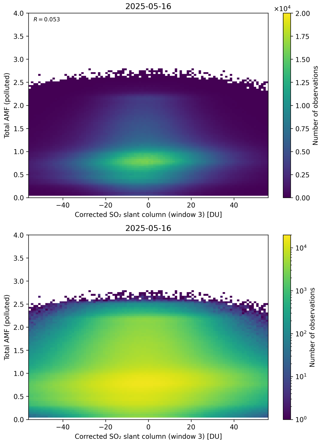
Figure 260: Scatter density plot of “Corrected SO 2 slant column (window 3)” against “Total AMF (polluted)” for 2025-05-15 to 2025-05-17.
