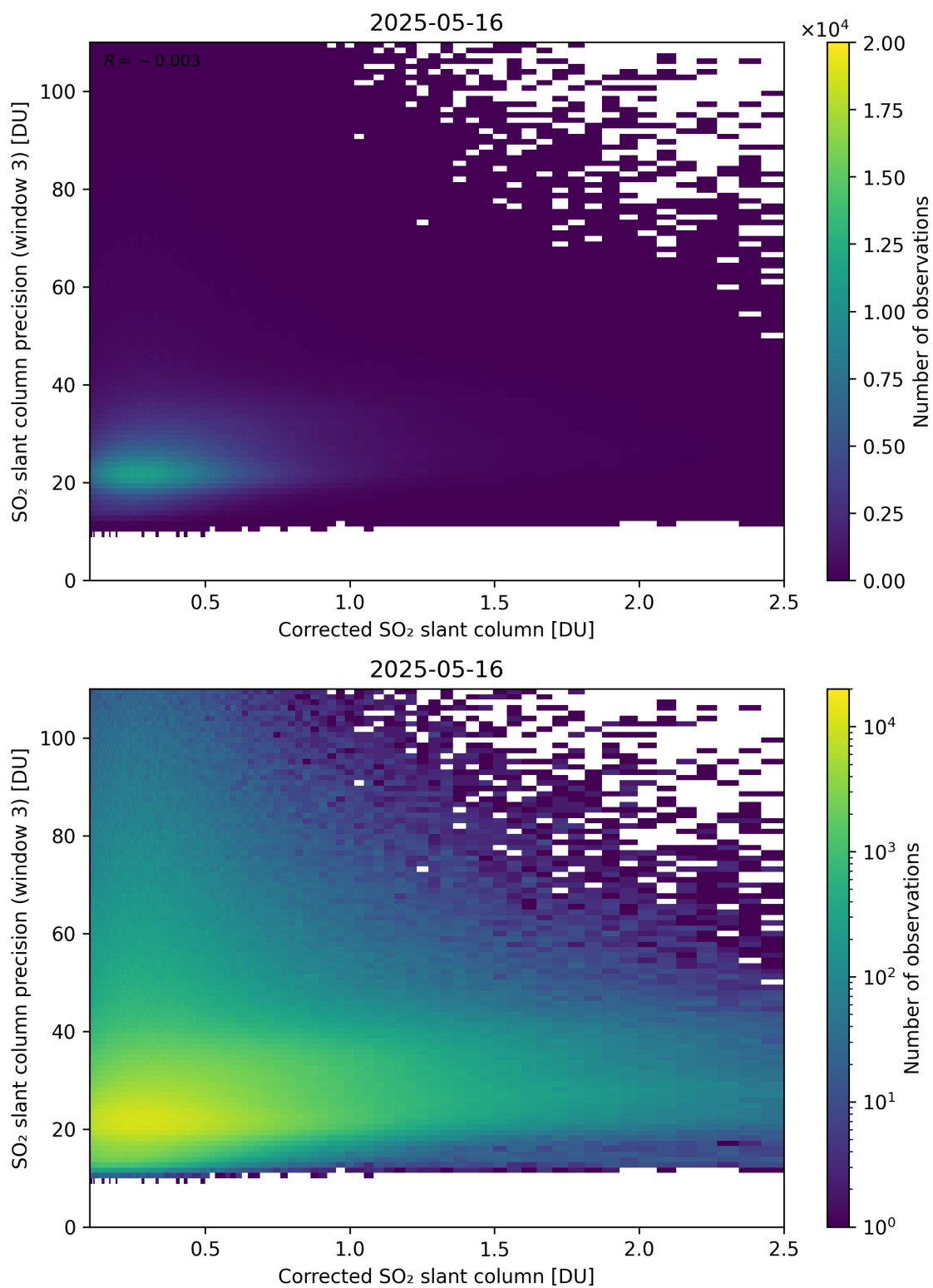
Figure 241: Scatter density plot of “Corrected SO 2 slant column” against “SO 2 slant column precision (window 3)” for 2025-05-15 to 2025-05-17.
