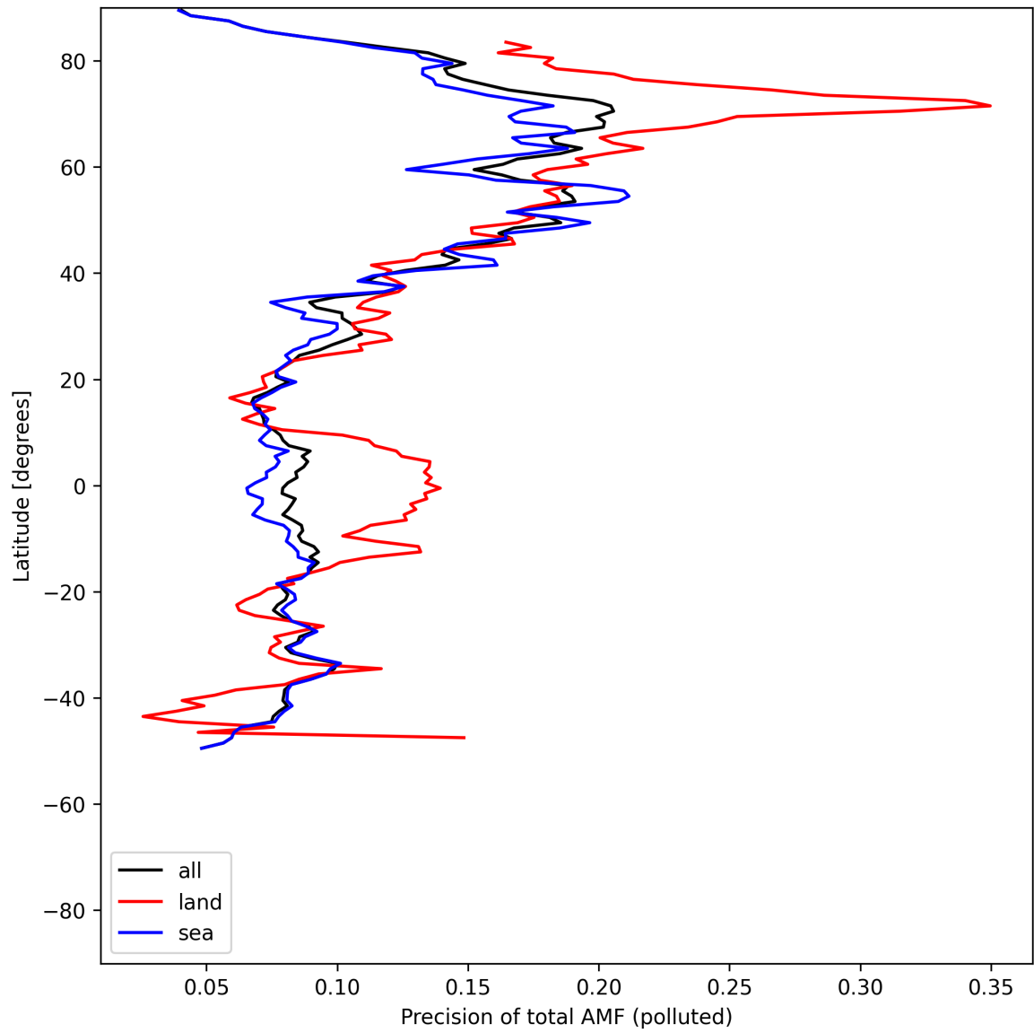
Figure 54: Zonal average of “Precision of total AMF (polluted)” for 2025-05-15 to 2025-05-17.
