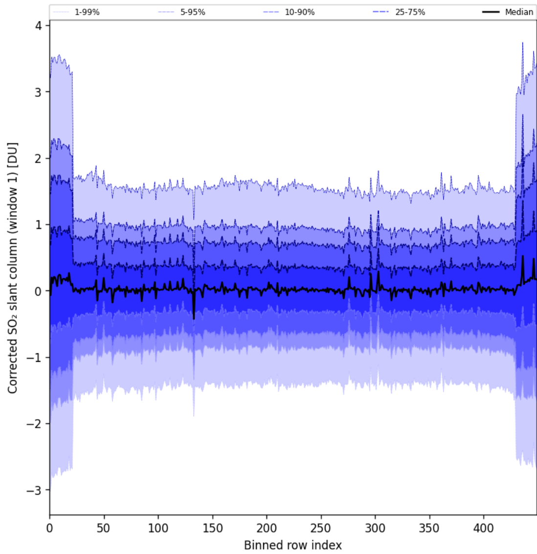
Figure 91: Along track statistics of “Corrected SO 2 slant column (window 1)” for 2025-05-15 to 2025-05-17
