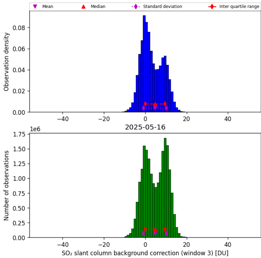
Figure 74: Histogram of “SO 2 slant column background correction (window 3)” for 2025-05-15 to 2025-05-17
