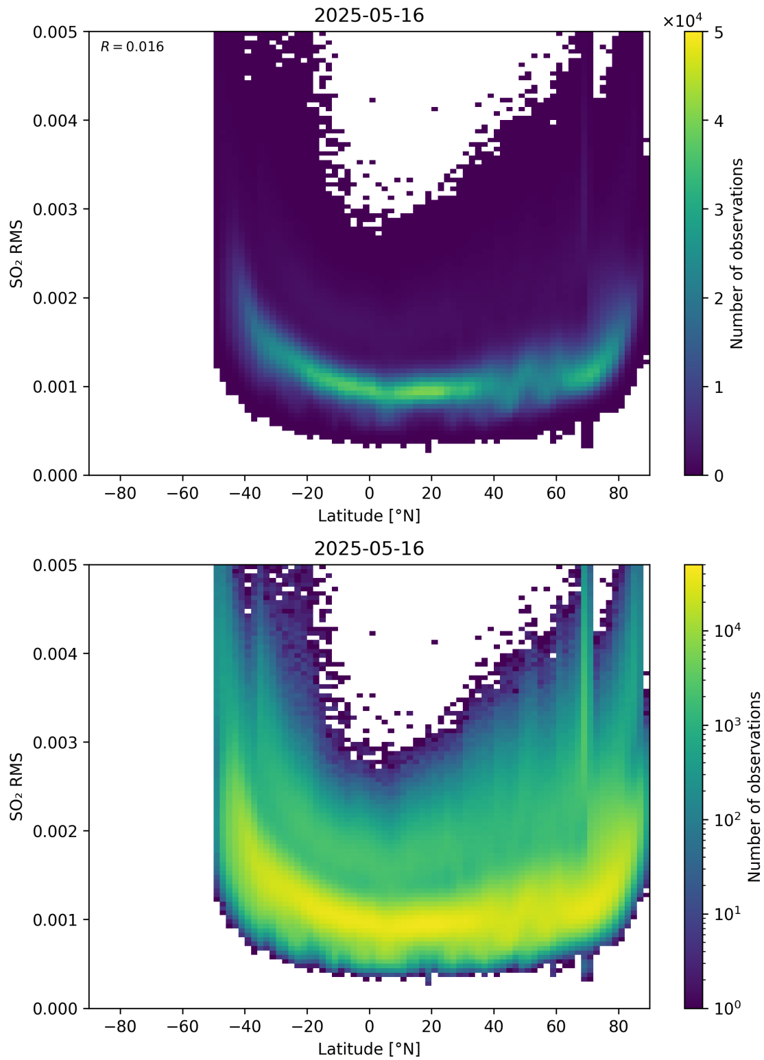
Figure 155: Scatter density plot of “Latitude” against “SO 2 RMS” for 2025-05-15 to 2025-05-17.
