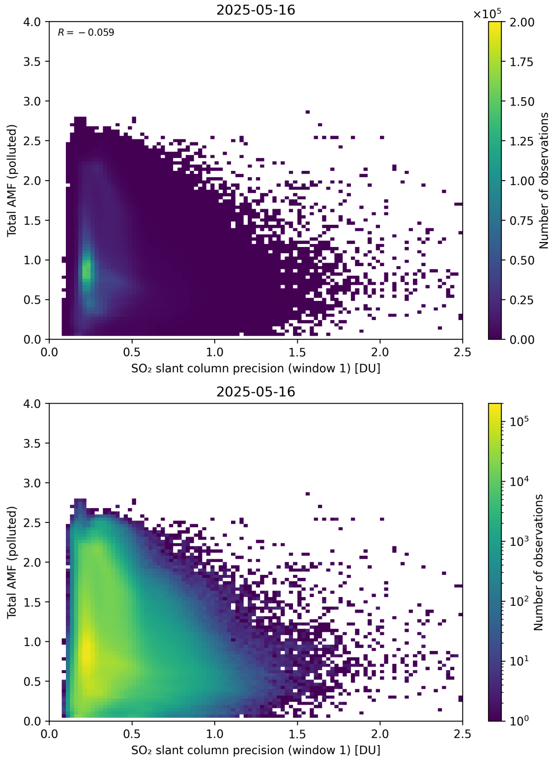
Figure 280: Scatter density plot of “SO 2 slant column precision (window 1)” against “Total AMF (polluted)” for 2025-05-15 to 2025-05-17.
