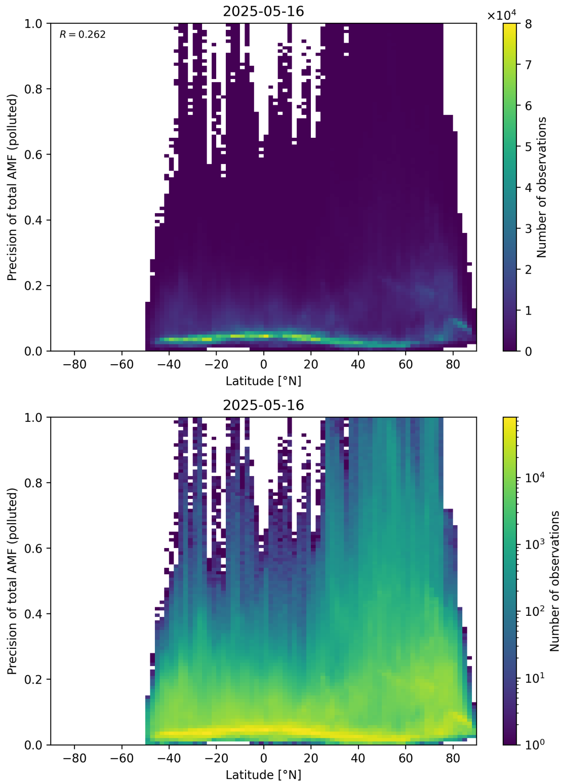
Figure 168: Scatter density plot of “Latitude” against “Precision of total AMF (polluted)” for 2025-05-15 to 2025-05-17.
