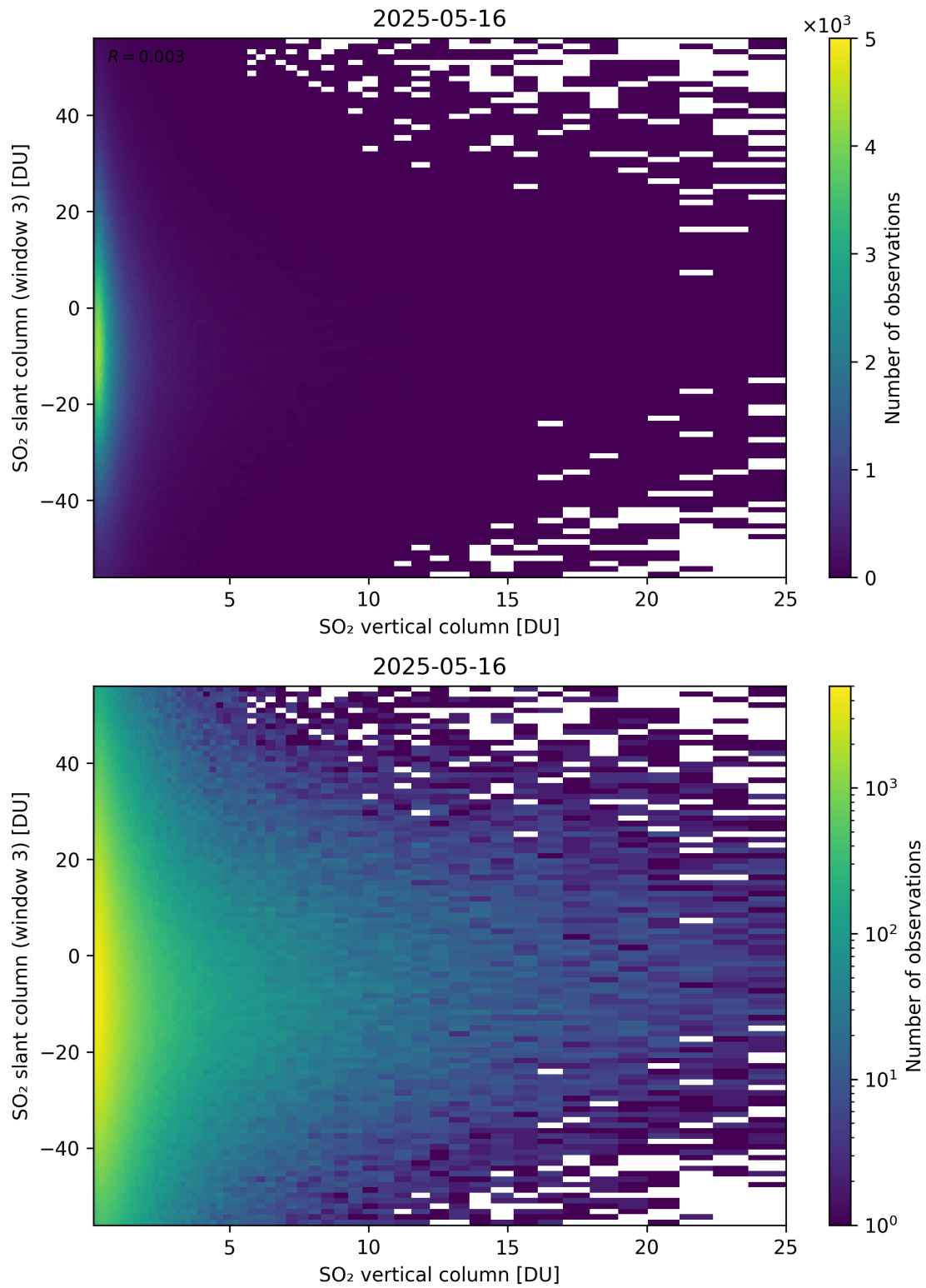
Figure 357: Scatter density plot of “SO 2 vertical column” against “SO 2 slant column (window 3)” for 2025-05-15 to 2025-05-17.
