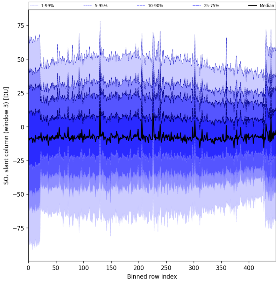
Figure 97: Along track statistics of “SO 2 slant column (window 3)” for 2025-05-15 to 2025-05-17
