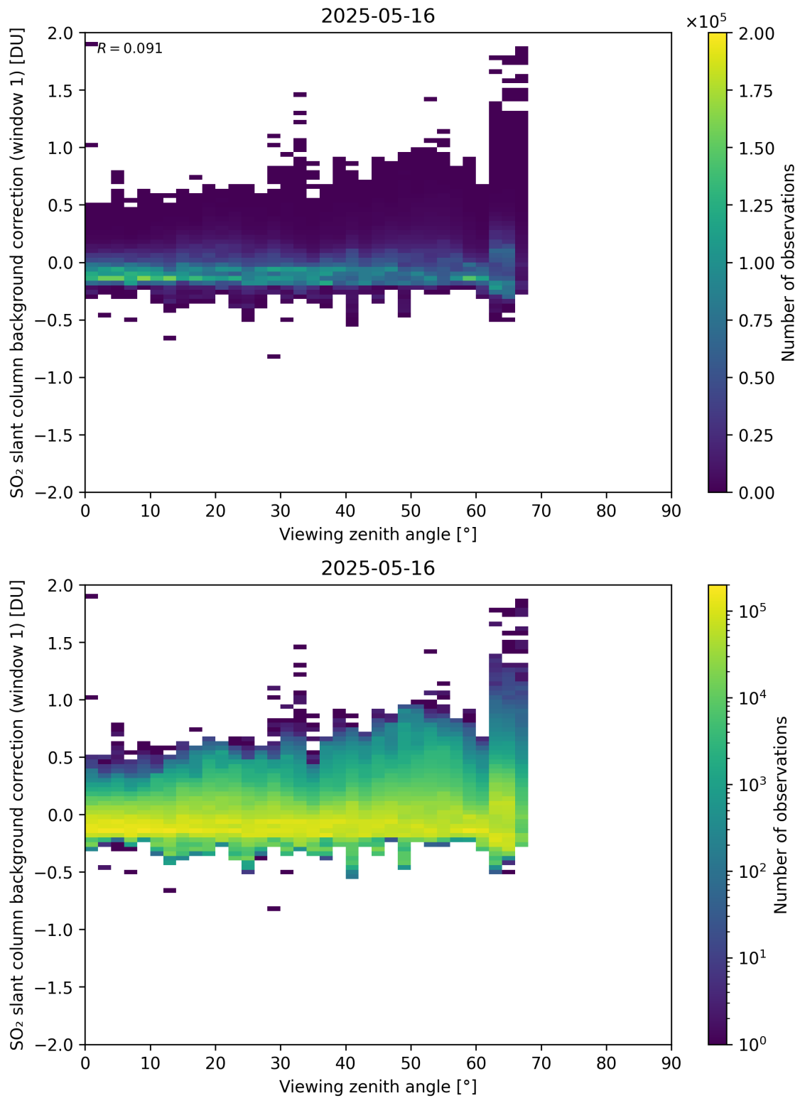
Figure 362: Scatter density plot of “Viewing zenith angle” against “SO 2 slant column background correction (window 1)” for 2025-05-15 to 2025-05-17.
