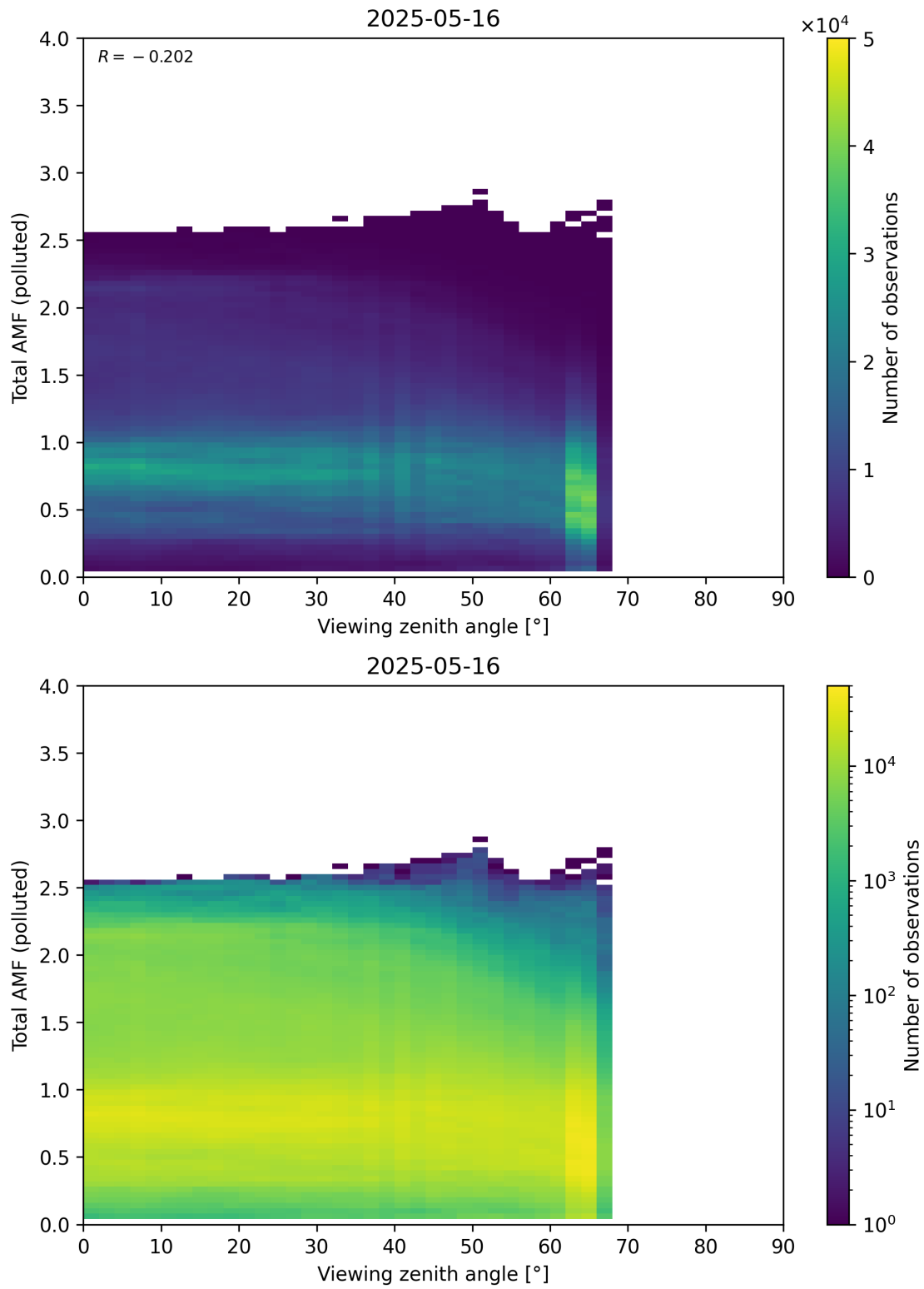
Figure 381: Scatter density plot of “Viewing zenith angle” against “Total AMF (polluted)” for 2025-05-15 to 2025-05-17.
