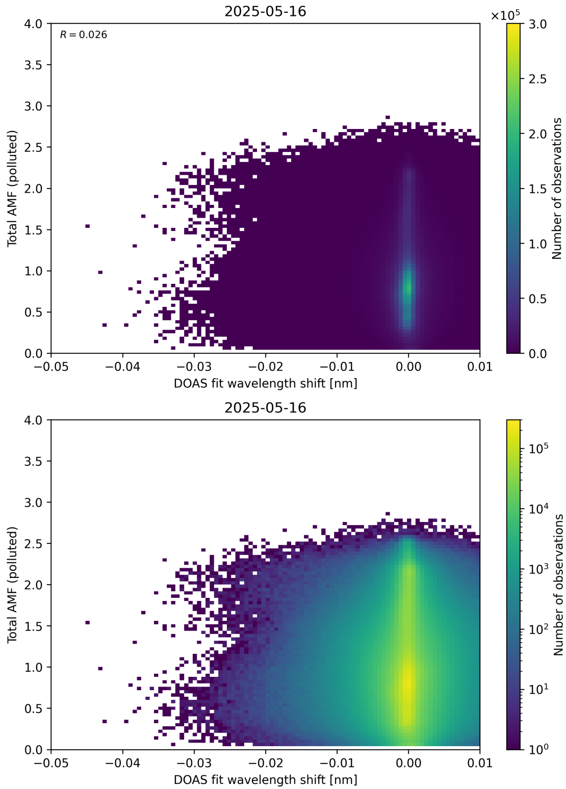
Figure 141: Scatter density plot of “DOAS fit wavelength shift” against “Total AMF (polluted)” for 2025-05-15 to 2025-05-17.
