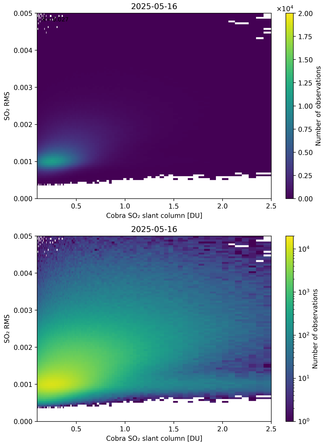
Figure 198: Scatter density plot of “Cobra SO 2 slant column” against “SO 2 RMS” for 2025-05-15 to 2025-05-17.
