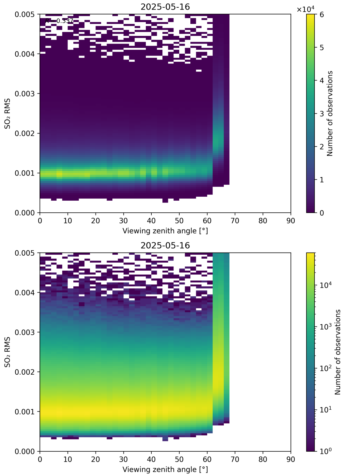
Figure 367: Scatter density plot of “Viewing zenith angle” against “SO 2 RMS” for 2025-05-15 to 2025-05-17.
