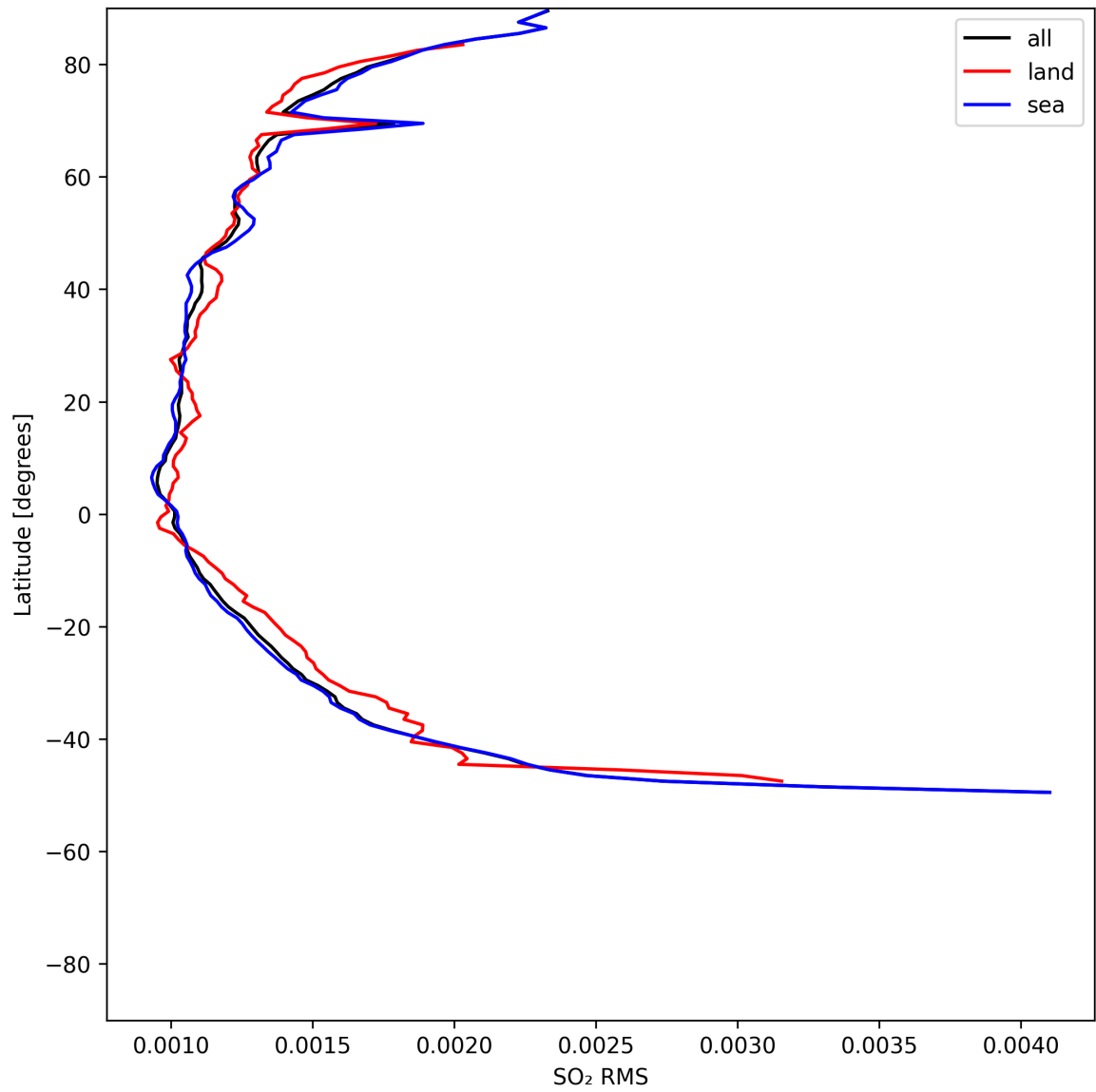
Figure 52: Zonal average of “SO 2 RMS” for 2025-05-15 to 2025-05-17.
