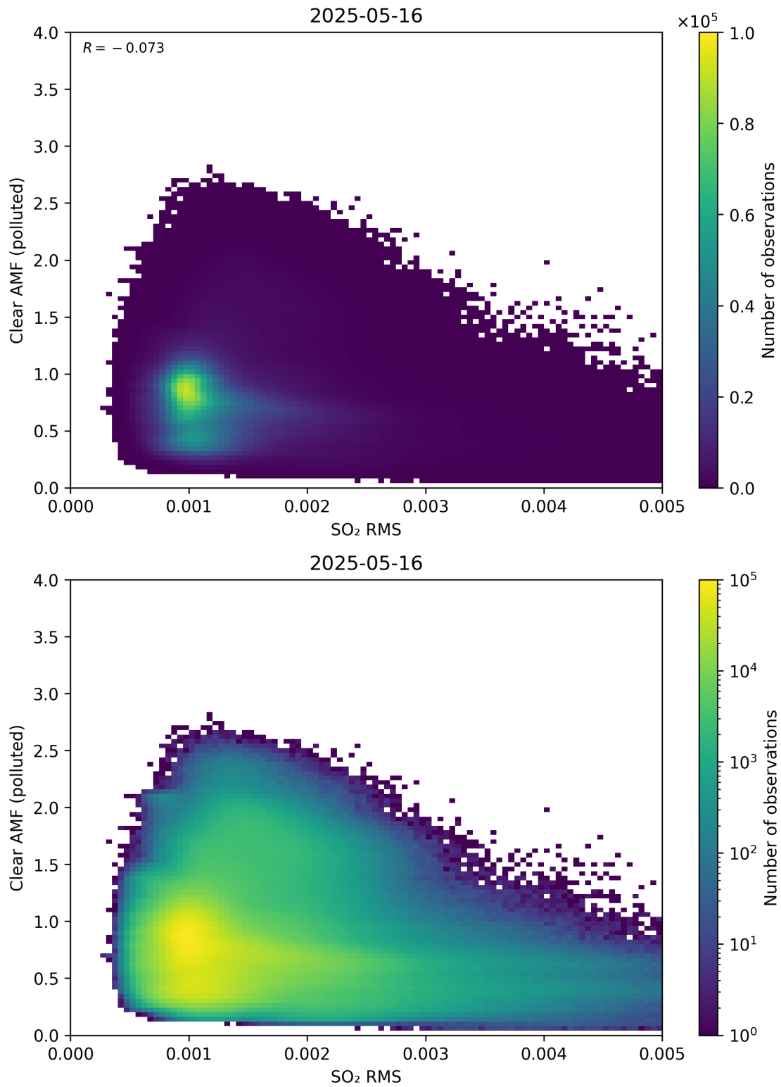
Figure 147: Scatter density plot of “SO 2 RMS” against “Clear AMF (polluted)” for 2025-05-15 to 2025-05-17.
