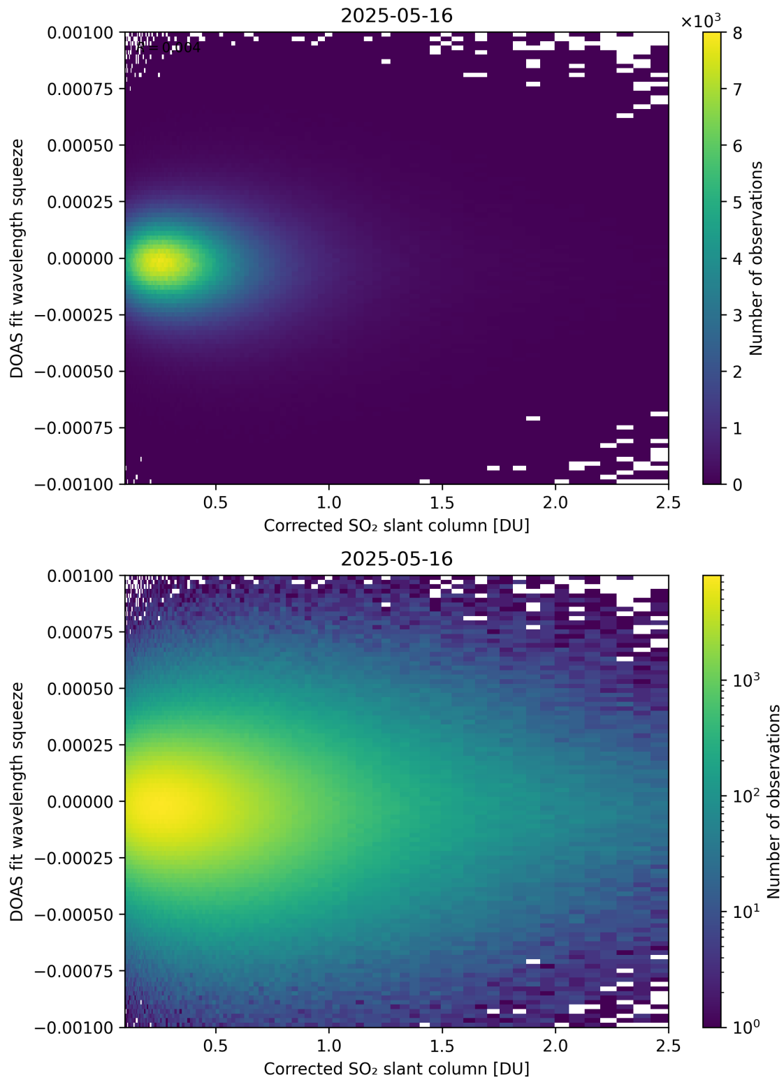
Figure 230: Scatter density plot of “Corrected SO 2 slant column” against “DOAS fit wavelength squeeze” for 2025-05-15 to 2025-05-17.
