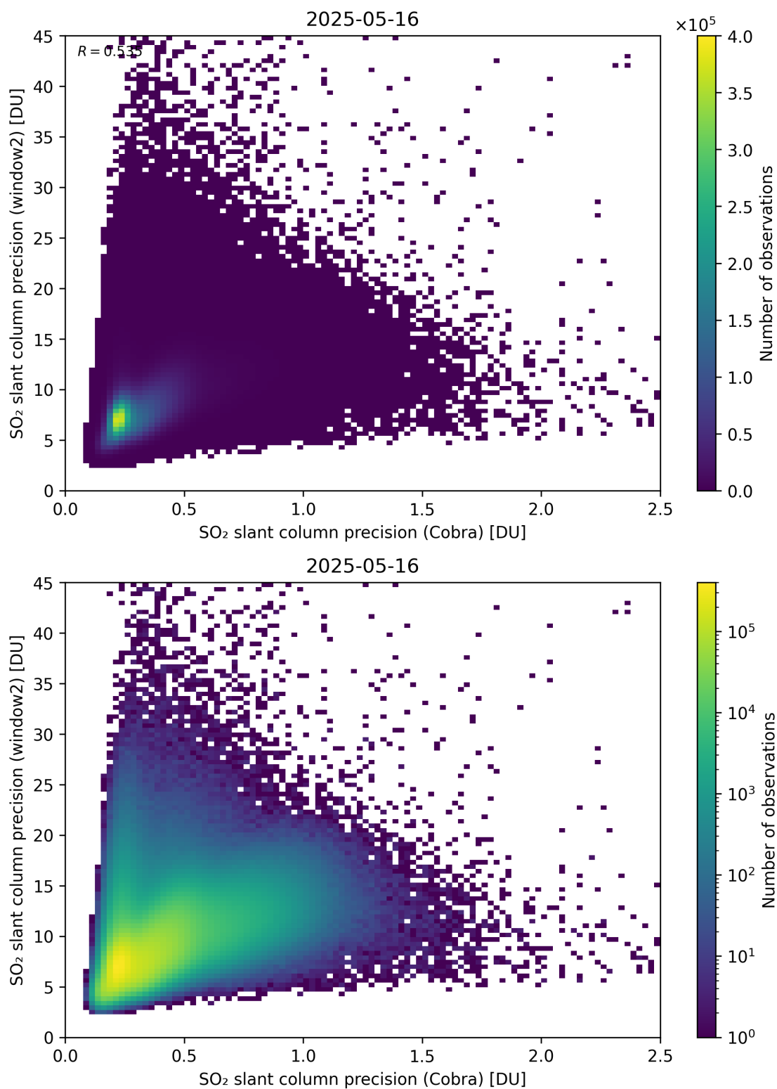
Figure 210: Scatter density plot of “SO 2 slant column precision (Cobra)” against “SO 2 slant column precision (window2)” for 2025-05-15 to 2025-05-17.
