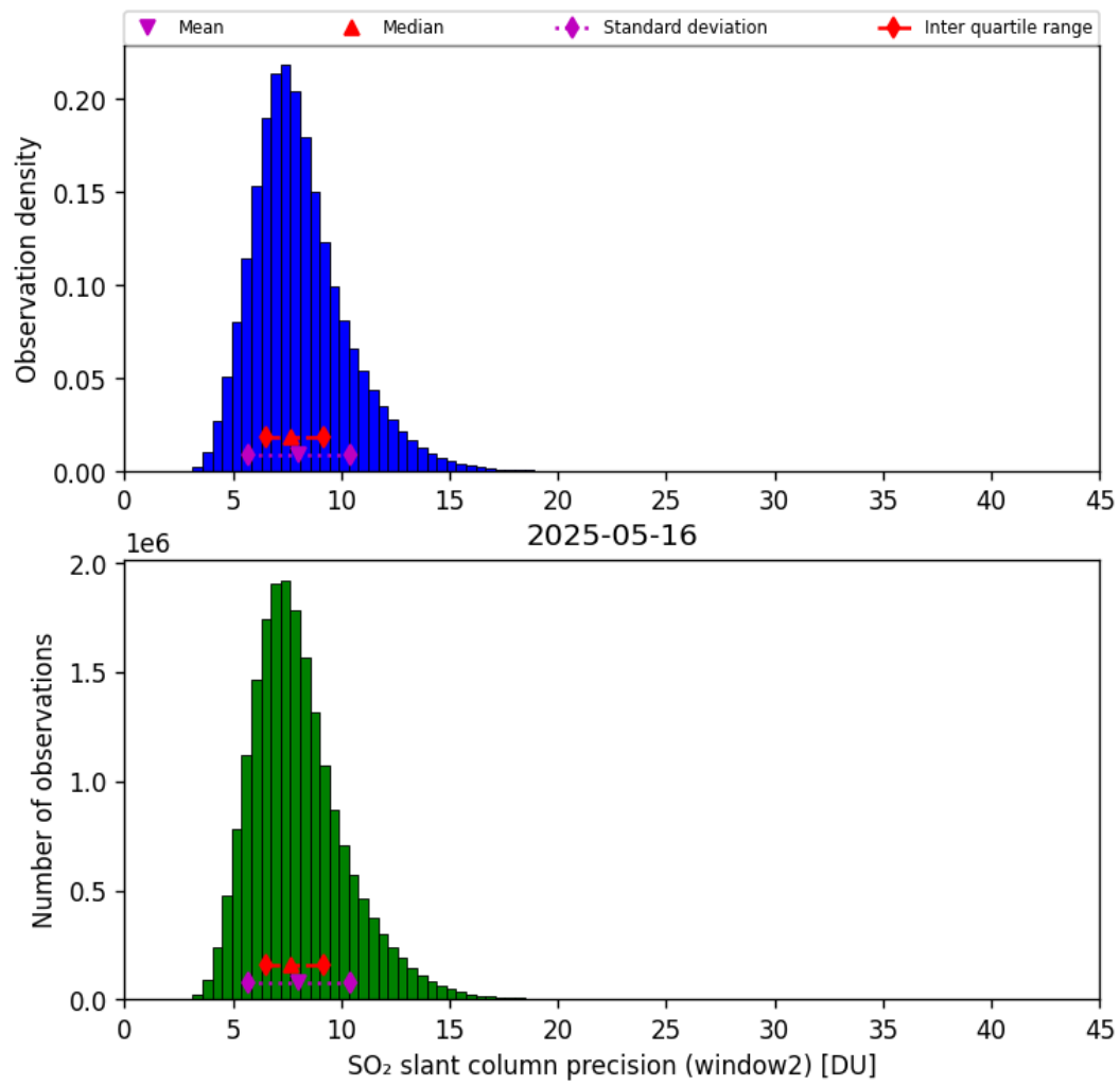
Figure 68: Histogram of “SO 2 slant column precision (window2)” for 2025-05-15 to 2025-05-17
