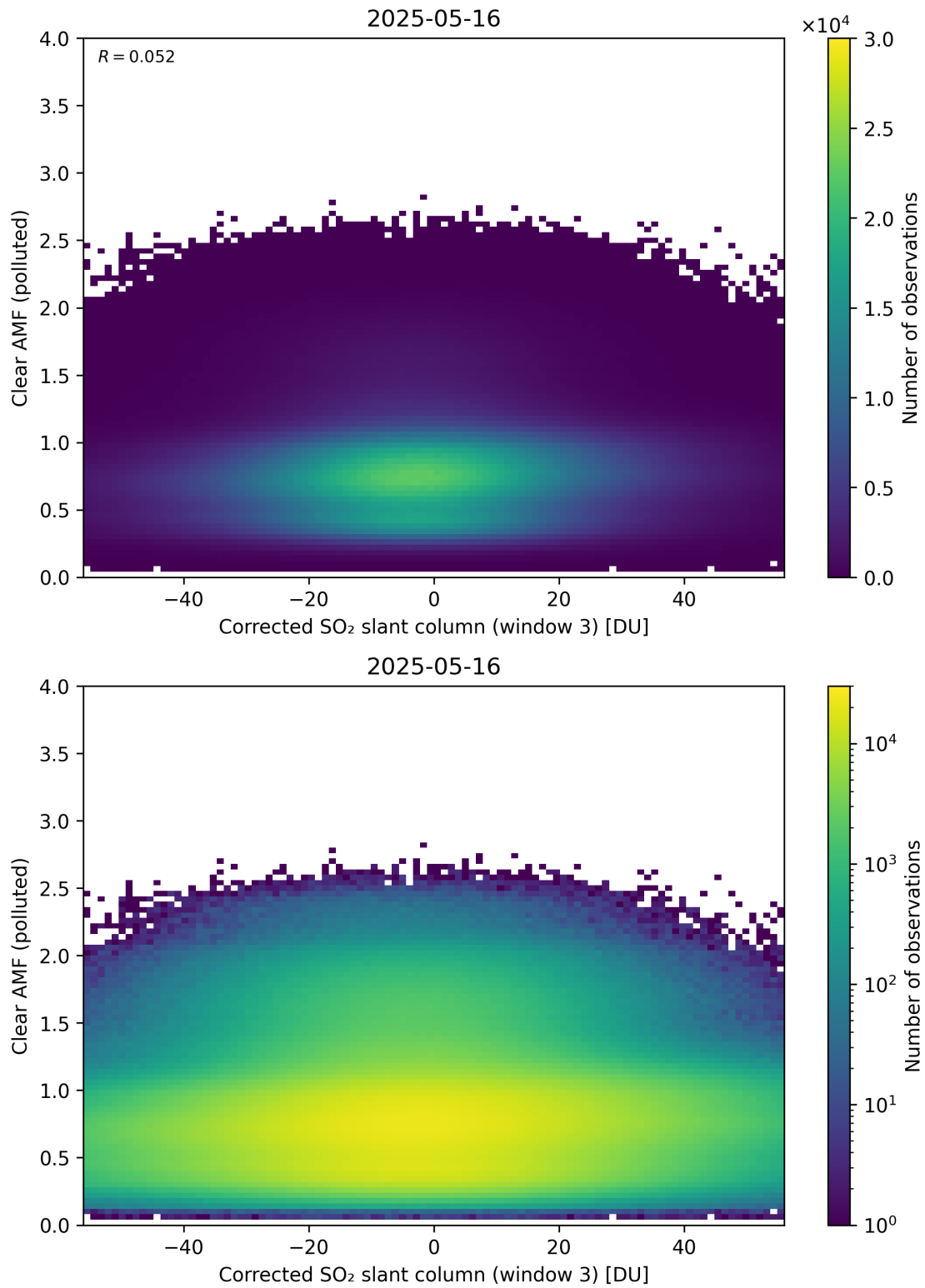
Figure 259: Scatter density plot of “Corrected SO 2 slant column (window 3)” against “Clear AMF (polluted)” for 2025-05-15 to 2025-05-17.
