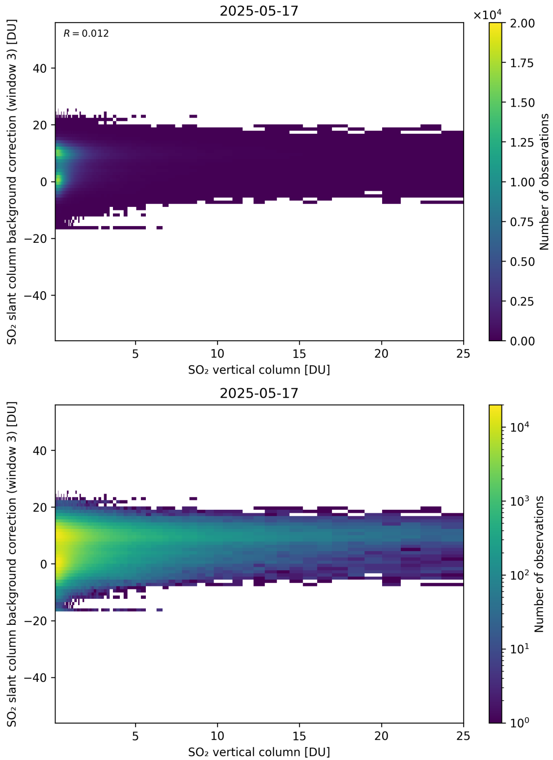
Figure 325: Scatter density plot of “SO 2 vertical column” against “SO 2 slant column background correction (window 3)” for 2025-05-16 to 2025-05-18.
