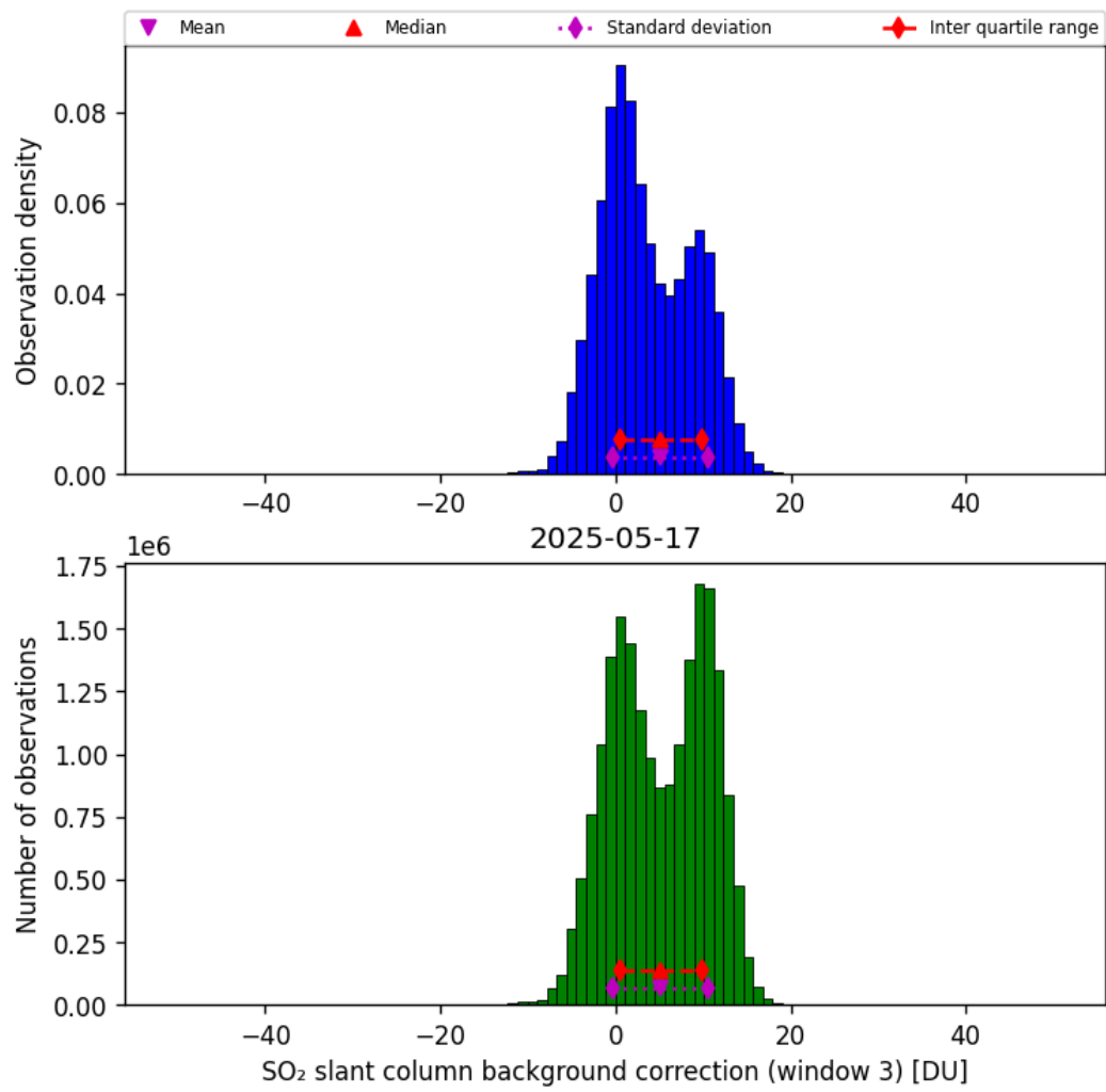
Figure 74: Histogram of “SO 2 slant column background correction (window 3)” for 2025-05-16 to 2025-05-18
