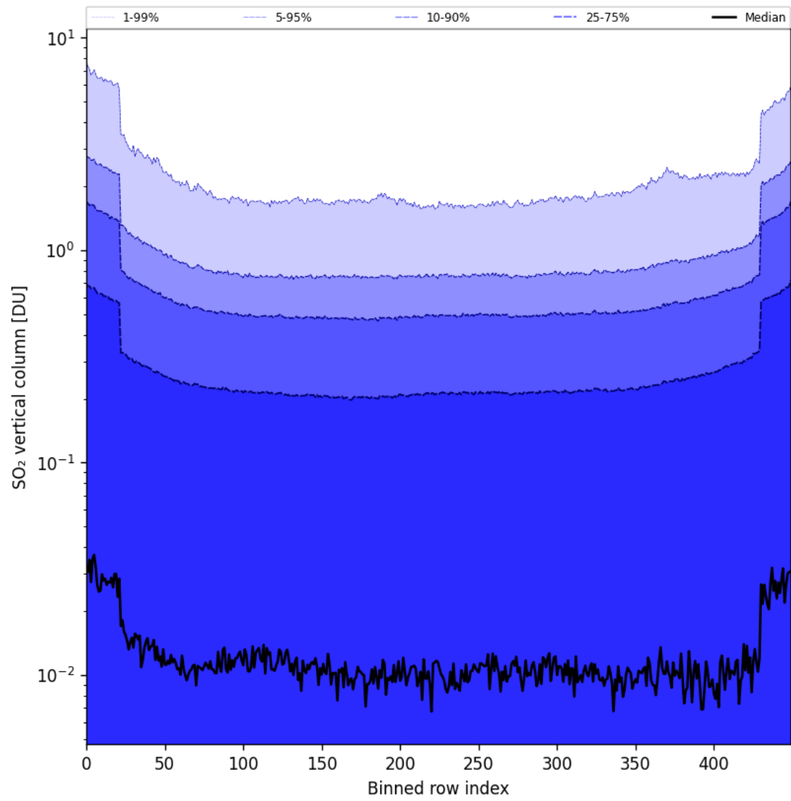
Figure 84: Along track statistics of “SO 2 vertical column” for 2025-05-16 to 2025-05-18
