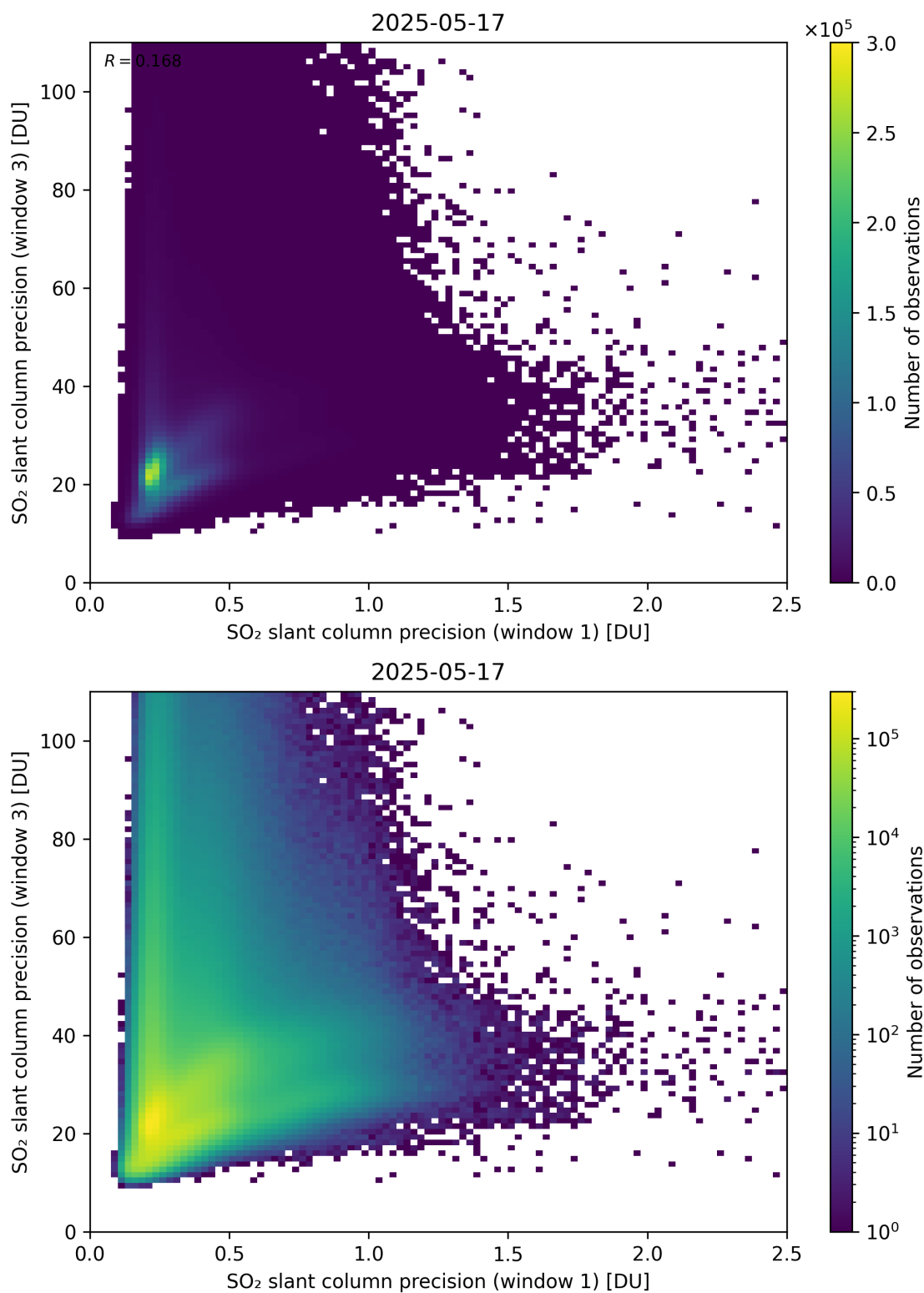
Figure 279: Scatter density plot of “SO 2 slant column precision (window 1)” against “SO 2 slant column precision (window 3)” for 2025-05-16 to 2025-05-18.
