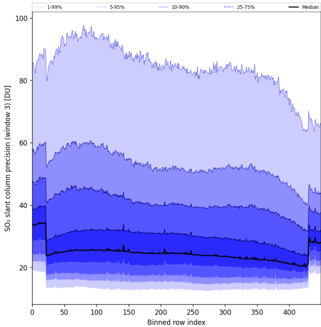
Figure 98: Along track statistics of “SO 2 slant column precision (window 3)” for 2025-05-16 to 2025-05-18
