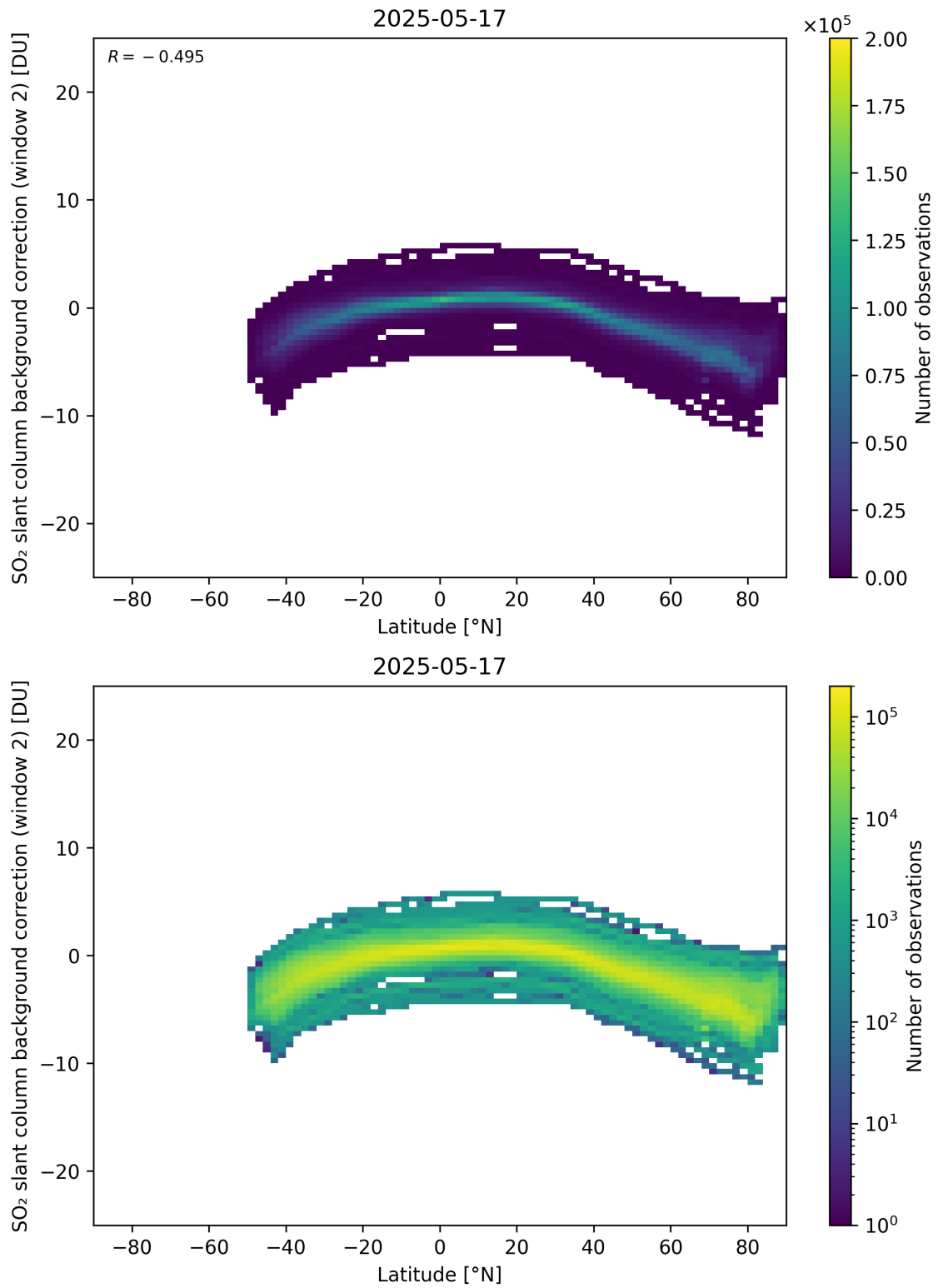
Figure 151: Scatter density plot of “Latitude” against “SO 2 slant column background correction (window 2)” for 2025-05-16 to 2025-05-18.
