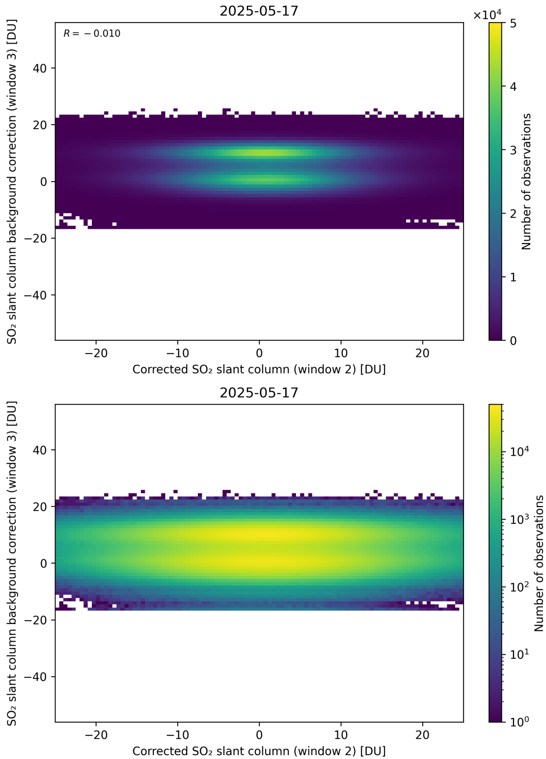
Figure 245: Scatter density plot of “Corrected SO 2 slant column (window 2)” against “SO 2 slant column background correction (window 3)” for 2025-05-16 to 2025-05-18.
