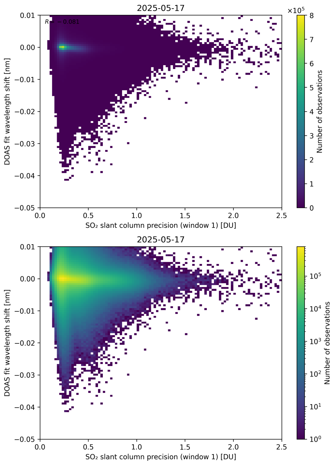
Figure 271: Scatter density plot of “SO 2 slant column precision (window 1)” against “DOAS fit wavelength shift” for 2025-05-16 to 2025-05-18.
