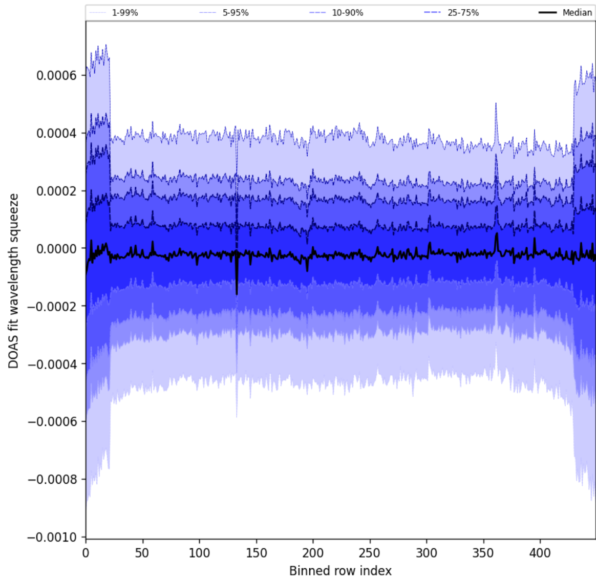
Figure 103: Along track statistics of “DOAS fit wavelength squeeze” for 2025-05-16 to 2025-05-18
