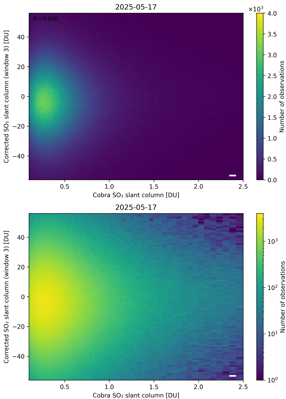
Figure 218: Scatter density plot of “Cobra SO 2 slant column” against “Corrected SO 2 slant column (window 3)” for 2025-05-16 to 2025-05-18.
