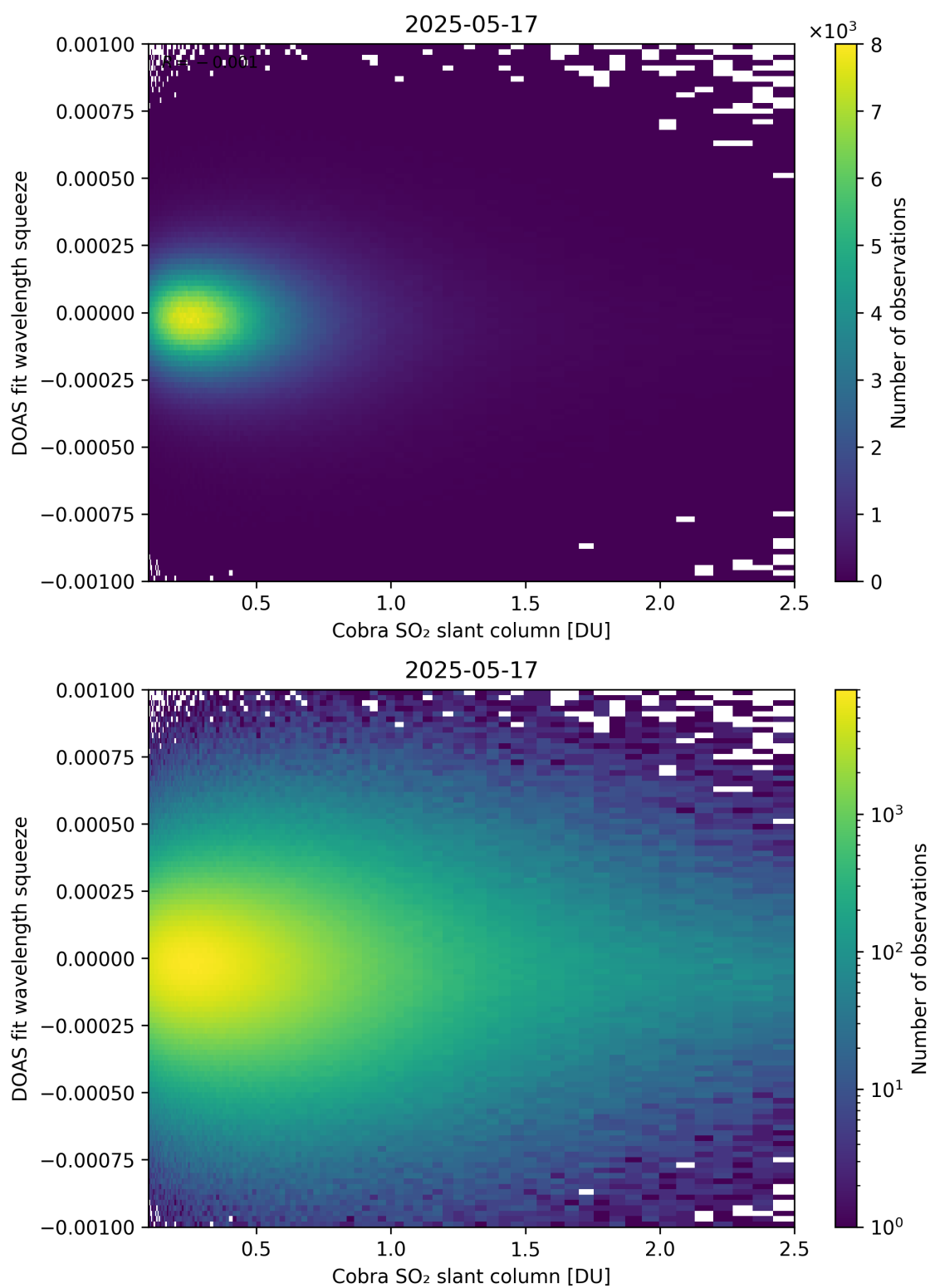
Figure 197: Scatter density plot of “Cobra SO 2 slant column” against “DOAS fit wavelength squeeze” for 2025-05-16 to 2025-05-18.
