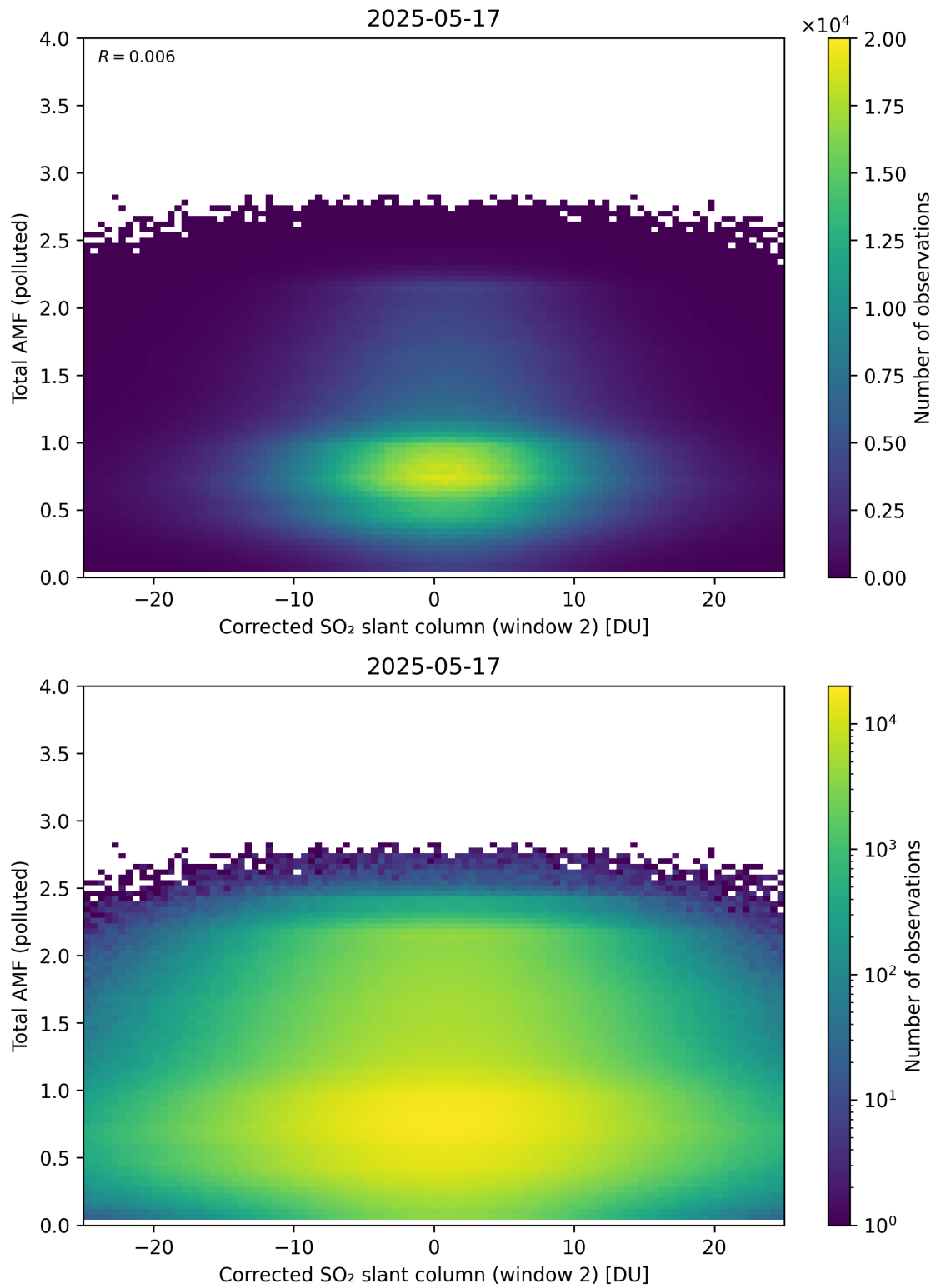
Figure 253: Scatter density plot of “Corrected SO 2 slant column (window 2)” against “Total AMF (polluted)” for 2025-05-16 to 2025-05-18.
