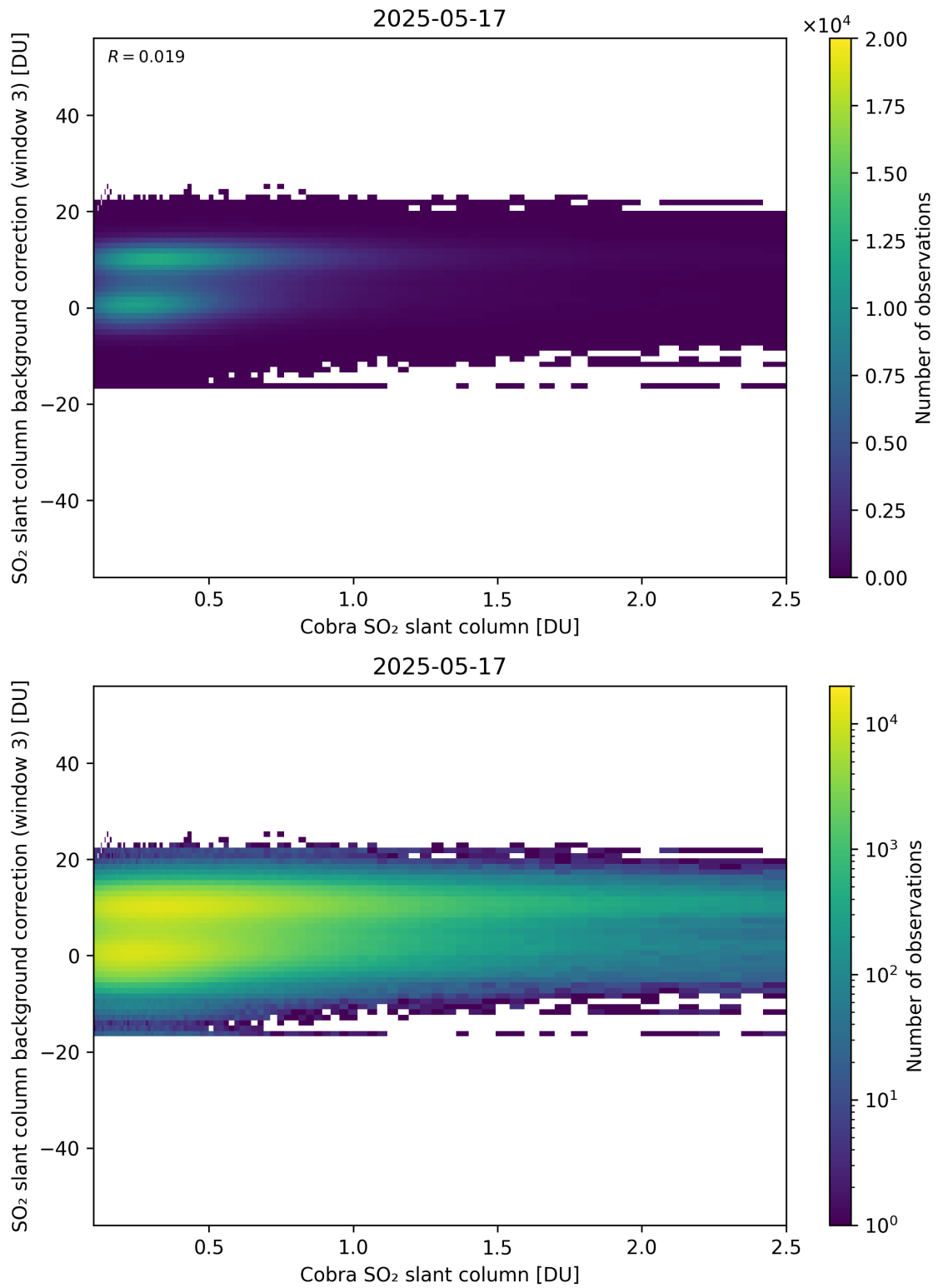
Figure 195: Scatter density plot of “Cobra SO 2 slant column” against “SO 2 slant column background correction (window 3)” for 2025-05-16 to 2025-05-18.
