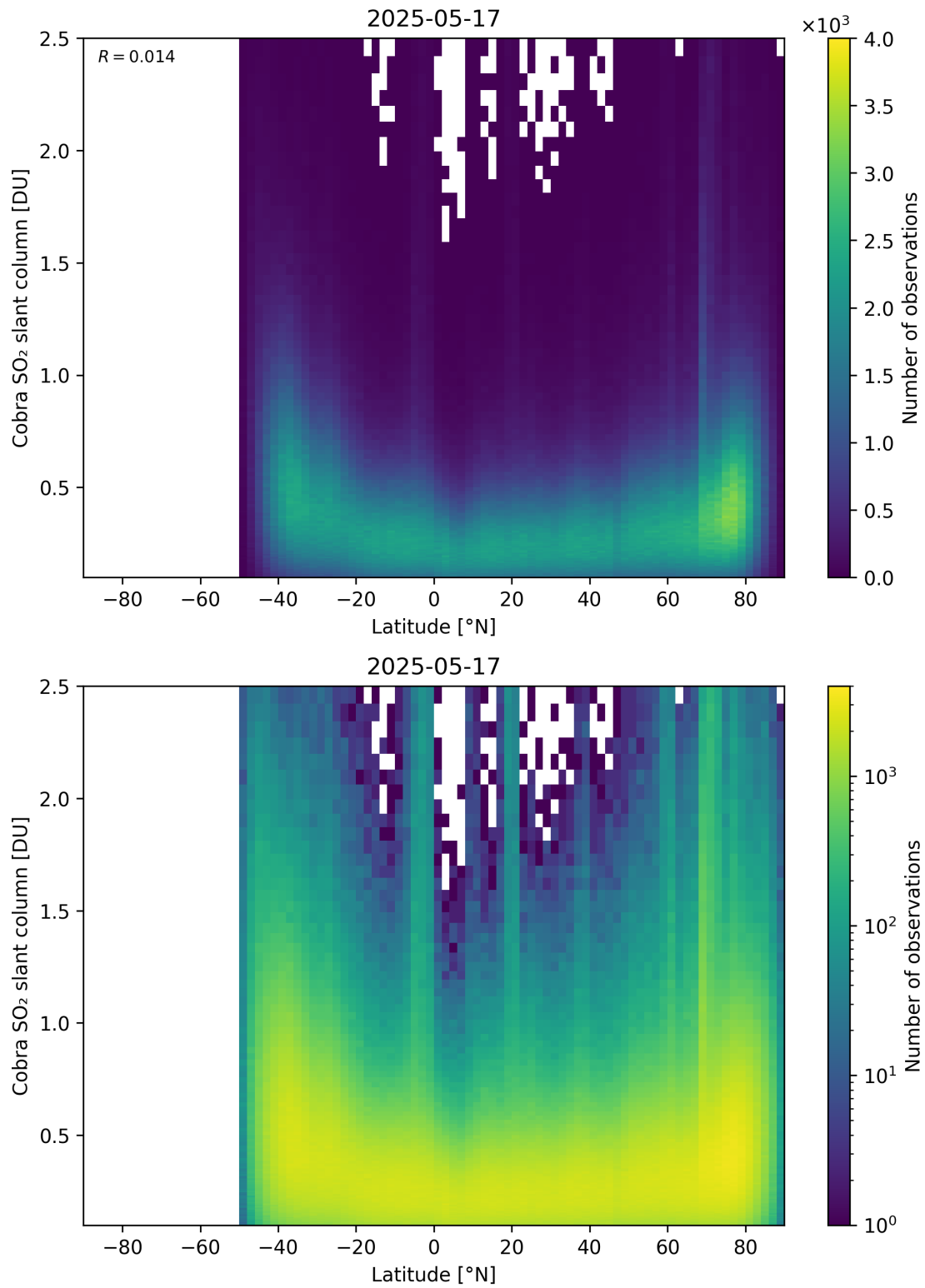
Figure 157: Scatter density plot of “Latitude” against “Cobra SO 2 slant column” for 2025-05-16 to 2025-05-18.
