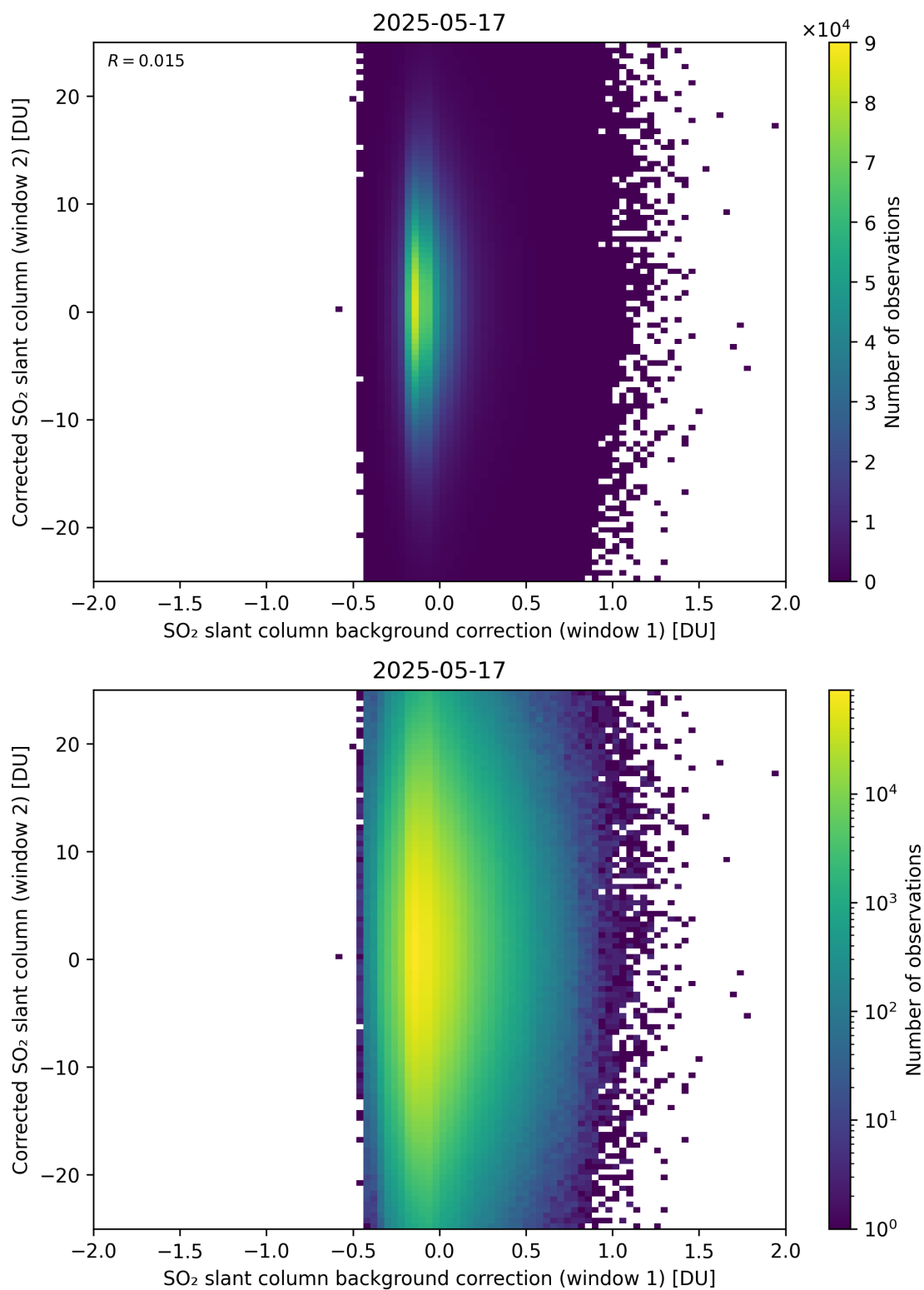
Figure 115: Scatter density plot of “SO 2 slant column background correction (window 1)” against “Corrected SO 2 slant column (window 2)” for 2025-05-16 to 2025-05-18.
