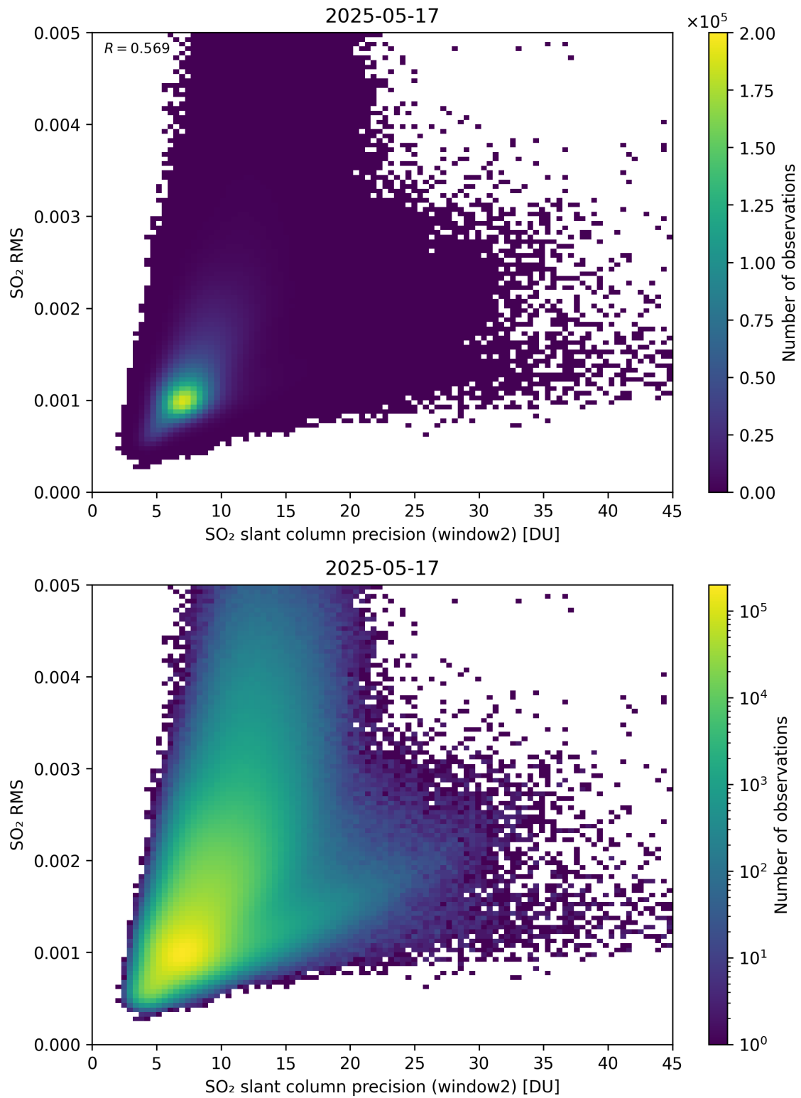
Figure 295: Scatter density plot of “SO 2 slant column precision (window2)” against “SO 2 RMS” for 2025-05-16 to 2025-05-18.
