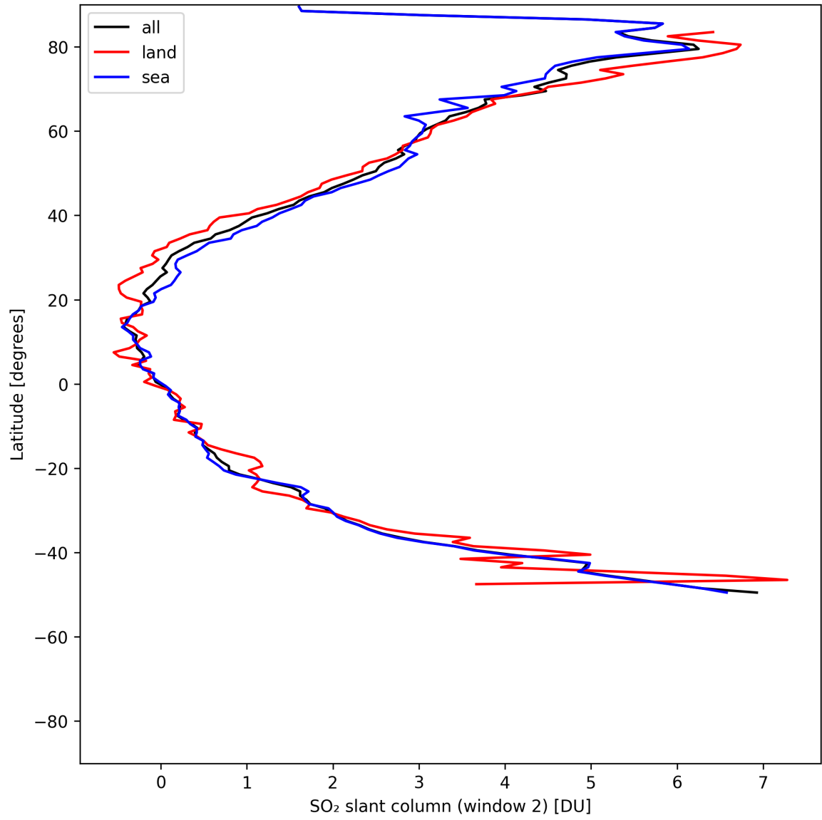
Figure 41: Zonal average of “SO 2 slant column (window 2)” for 2025-05-16 to 2025-05-18.
