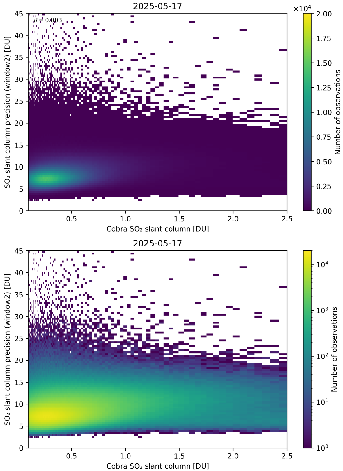
Figure 221: Scatter density plot of “Cobra SO 2 slant column” against “SO 2 slant column precision (window2)” for 2025-05-16 to 2025-05-18.
