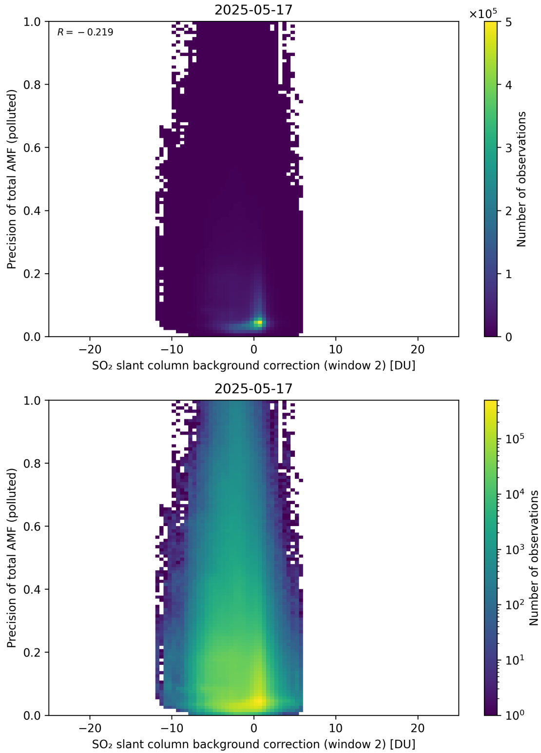
Figure 131: Scatter density plot of “SO 2 slant column background correction (window 2)” against “Precision of total AMF (polluted)” for 2025-05-16 to 2025-05-18.
