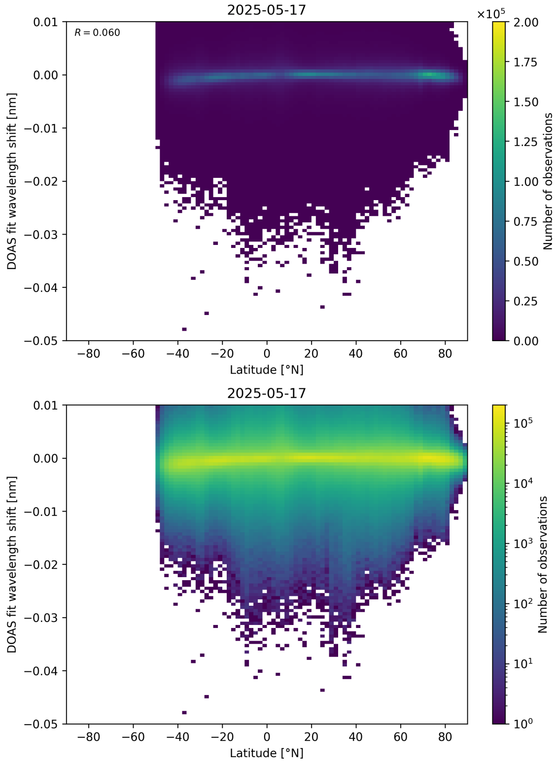
Figure 153: Scatter density plot of “Latitude” against “DOAS fit wavelength shift” for 2025-05-16 to 2025-05-18.
