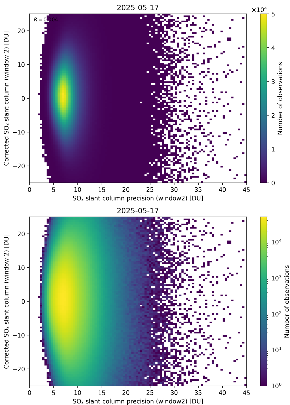
Figure 297: Scatter density plot of “SO 2 slant column precision (window2)” against “Corrected SO 2 slant column (window 2)” for 2025-05-16 to 2025-05-18.
