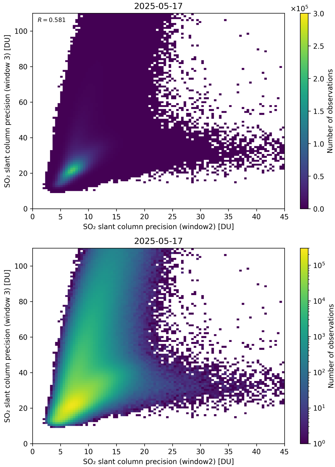
Figure 300: Scatter density plot of “SO 2 slant column precision (window2)” against “SO 2 slant column precision (window 3)” for 2025-05-16 to 2025-05-18.
