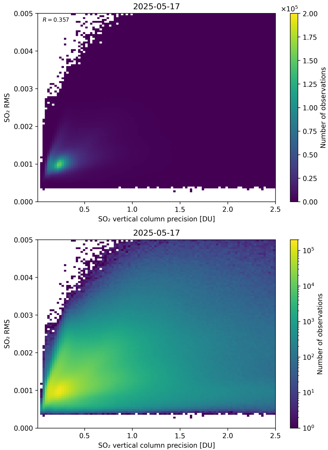
Figure 334: Scatter density plot of “SO 2 vertical column precision” against “SO 2 RMS” for 2025-05-16 to 2025-05-18.
