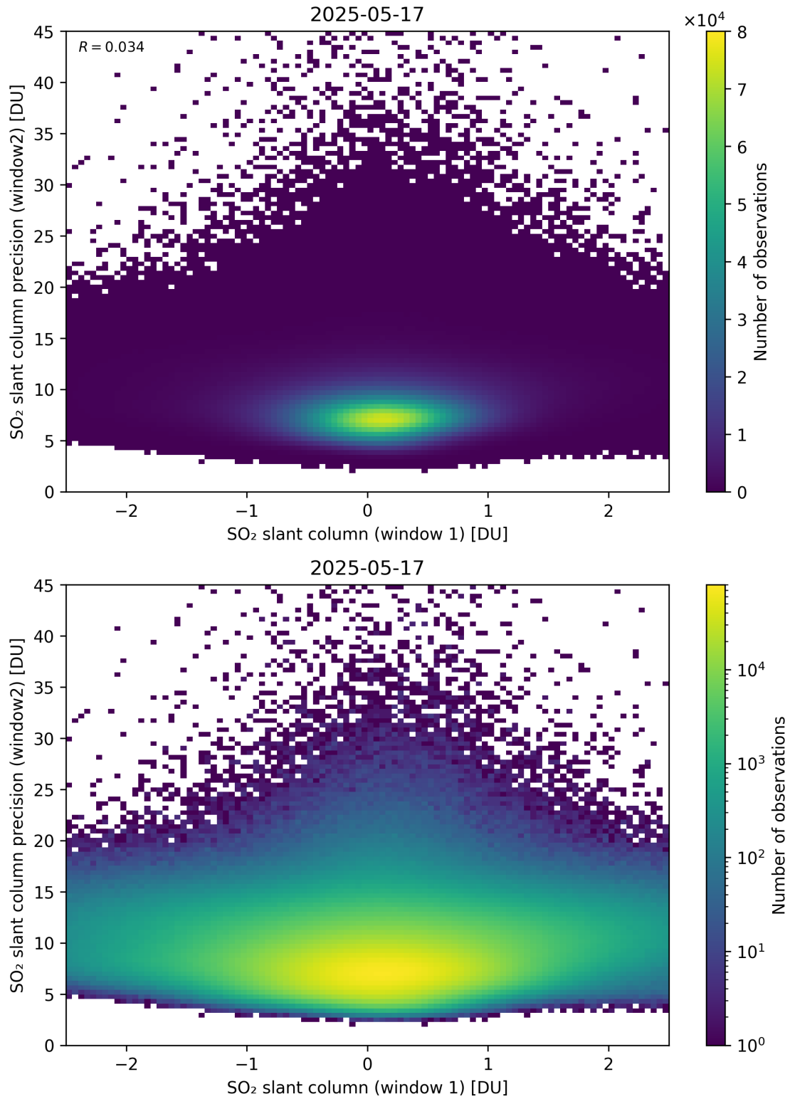
Figure 286: Scatter density plot of “SO 2 slant column (window 1)” against “SO 2 slant column precision (window2)” for 2025-05-16 to 2025-05-18.
