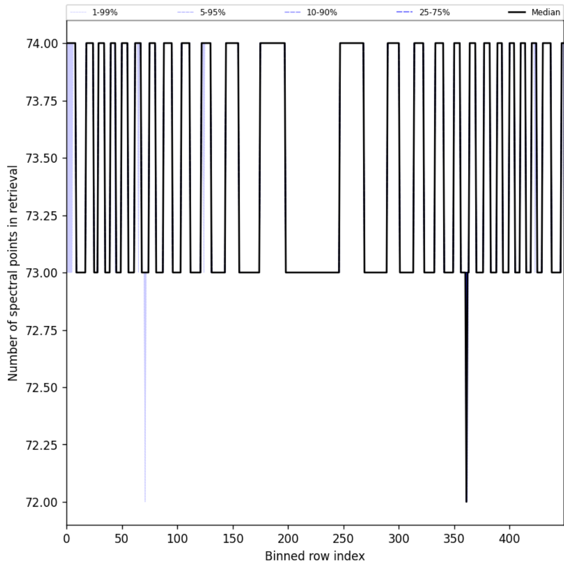
Figure 108: Along track statistics of “Number of spectral points in retrieval” for 2025-05-16 to 2025-05-18
