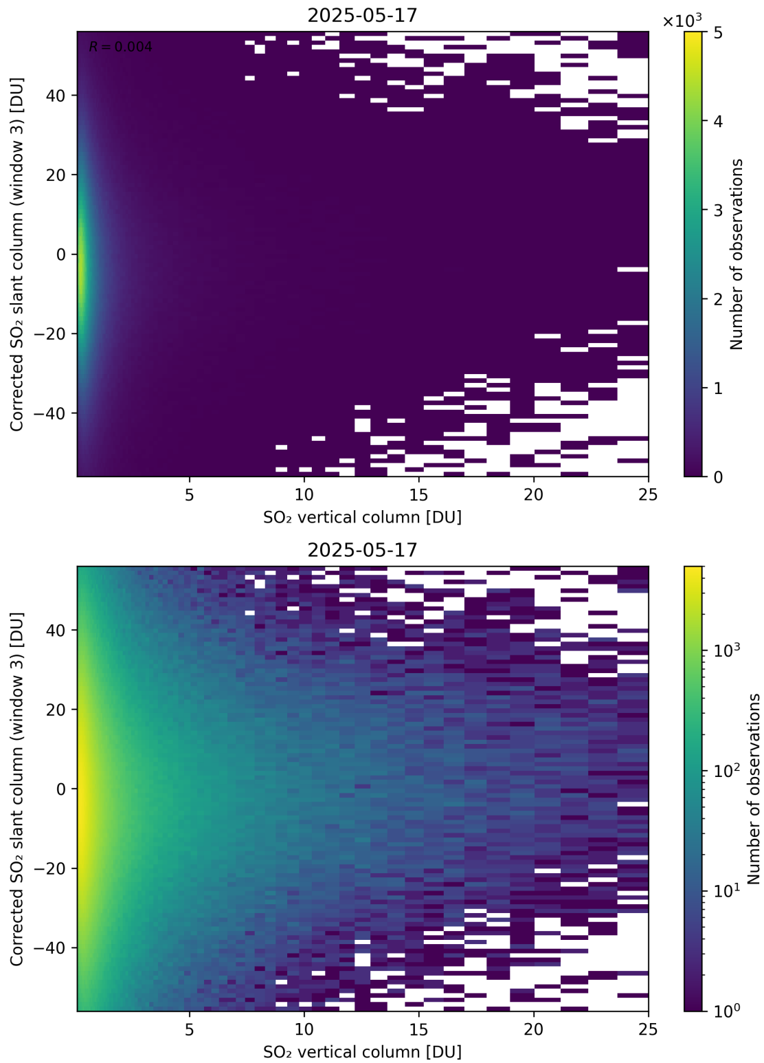
Figure 353: Scatter density plot of “SO 2 vertical column” against “Corrected SO 2 slant column (window 3)” for 2025-05-16 to 2025-05-18.
