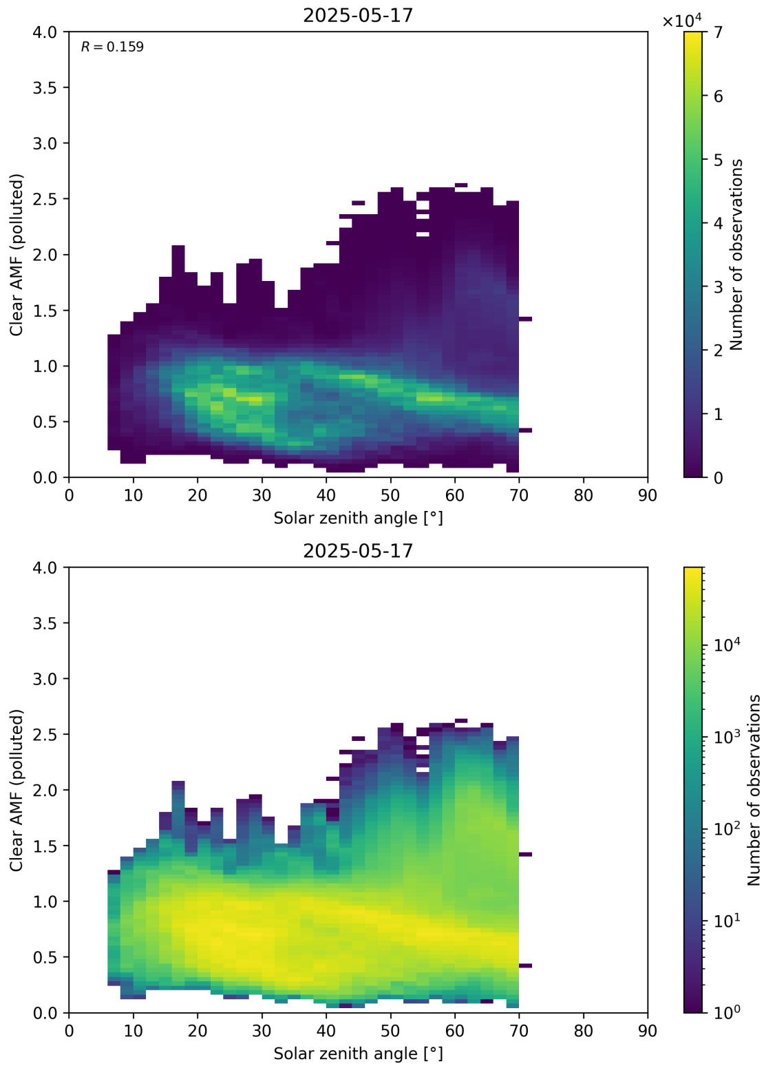
Figure 178: Scatter density plot of “Solar zenith angle” against “Clear AMF (polluted)” for 2025-05-16 to 2025-05-18.
