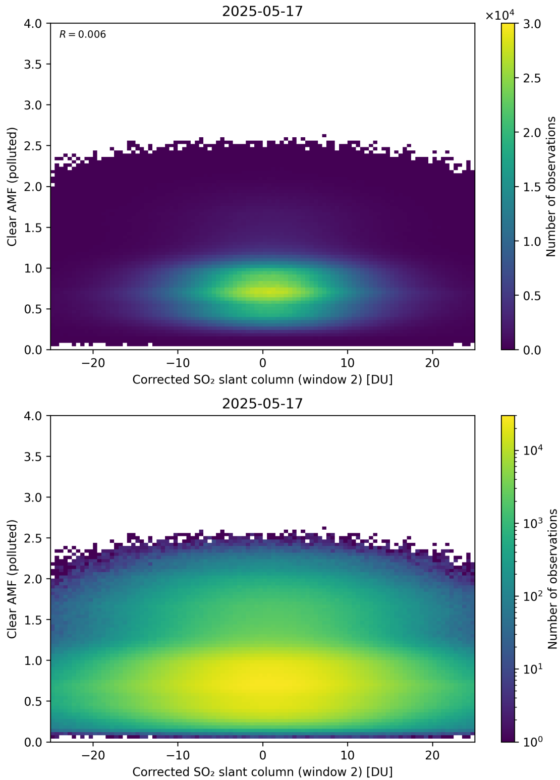
Figure 249: Scatter density plot of “Corrected SO 2 slant column (window 2)” against “Clear AMF (polluted)” for 2025-05-16 to 2025-05-18.
