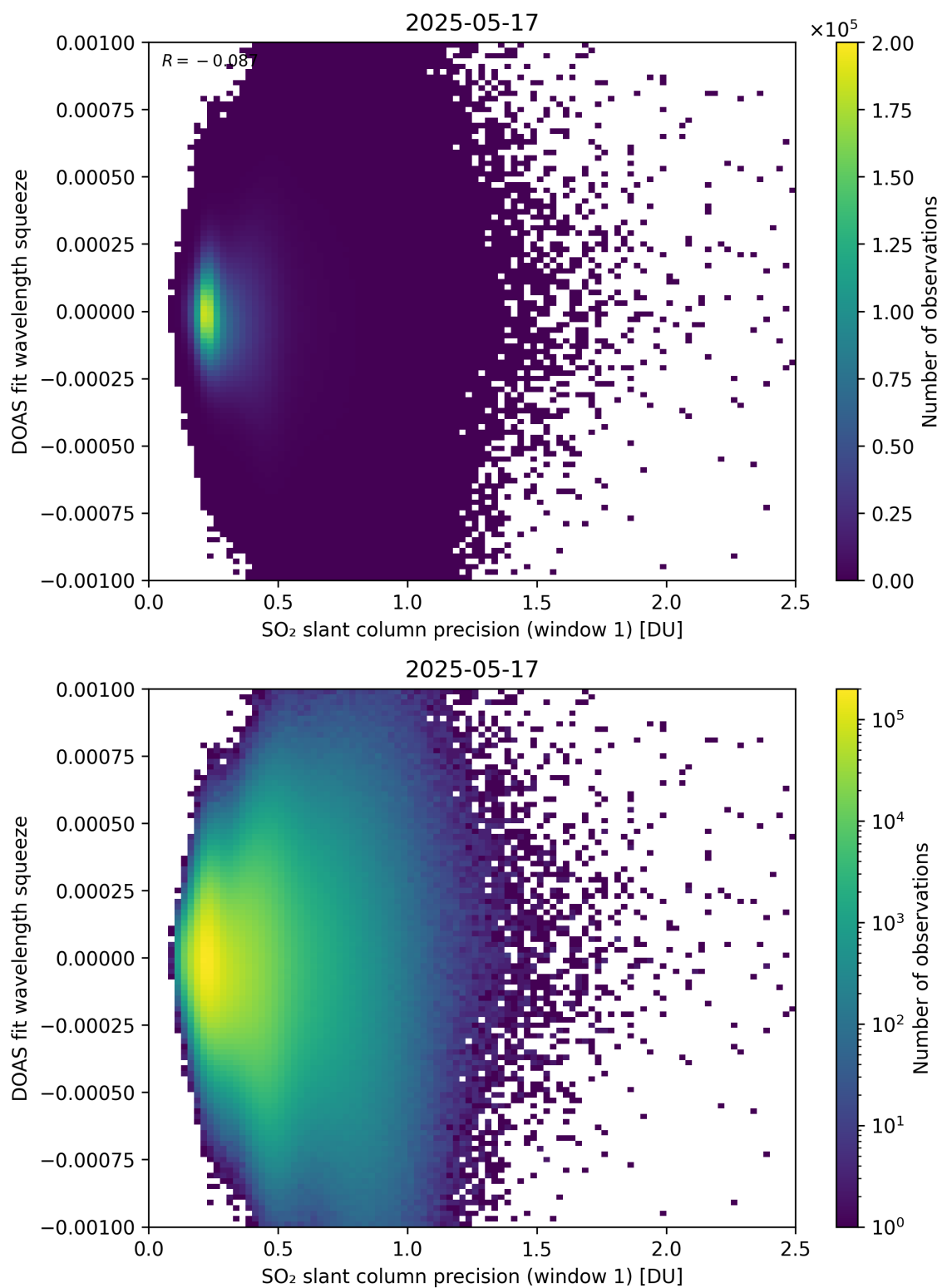
Figure 272: Scatter density plot of “SO 2 slant column precision (window 1)” against “DOAS fit wavelength squeeze” for 2025-05-16 to 2025-05-18.
