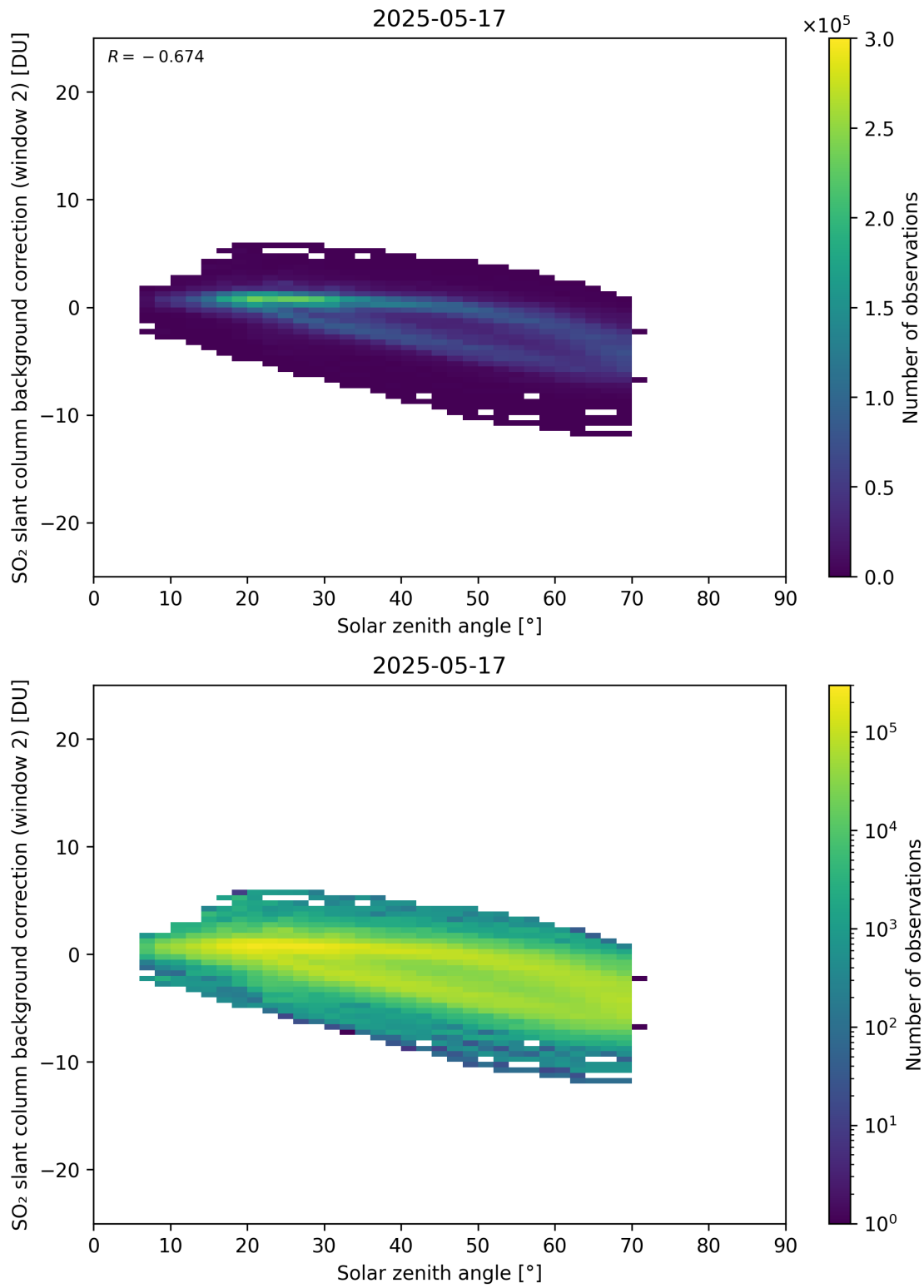
Figure 172: Scatter density plot of “Solar zenith angle” against “SO 2 slant column background correction (window 2)” for 2025-05-16 to 2025-05-18.
