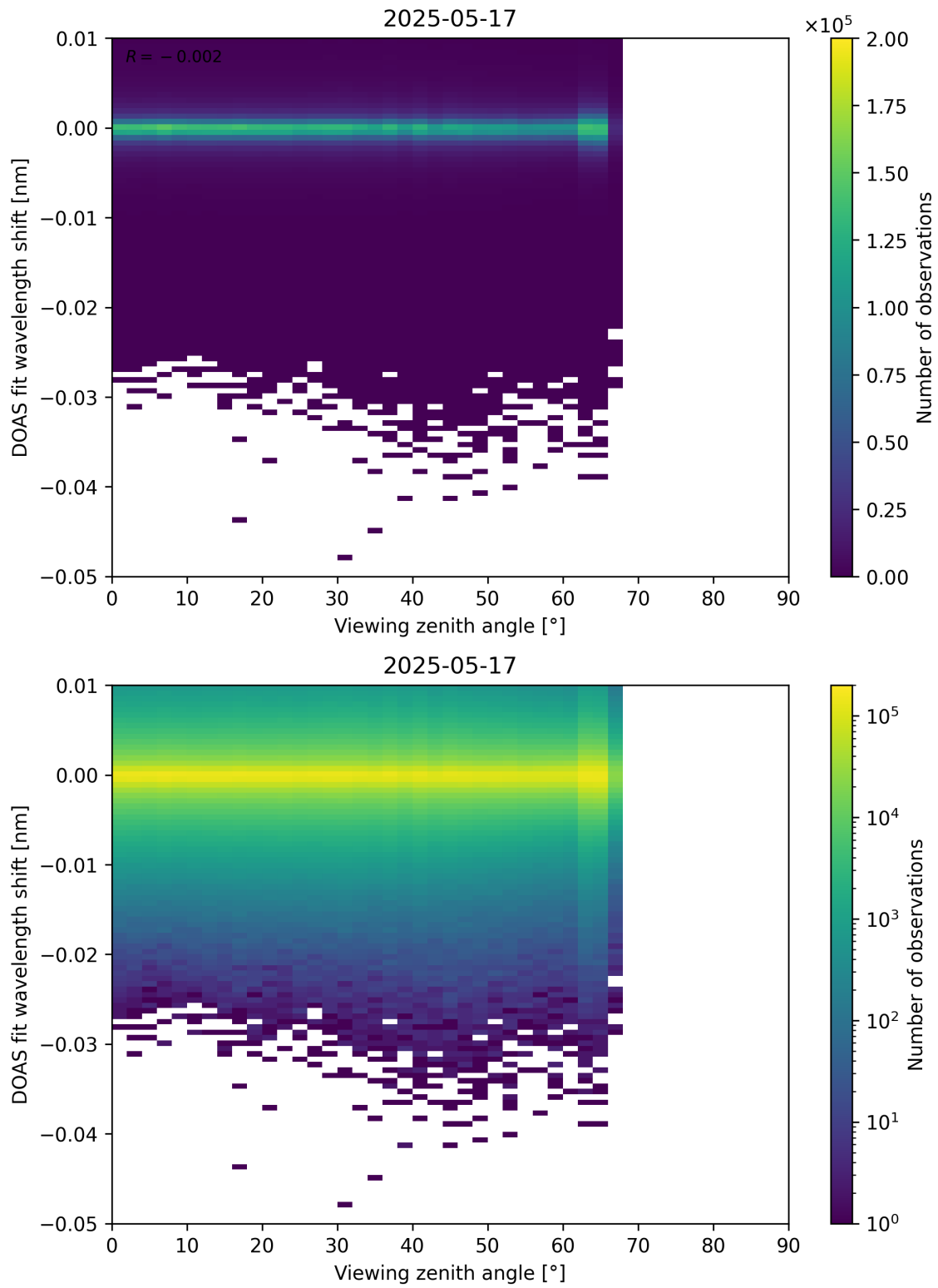
Figure 365: Scatter density plot of “Viewing zenith angle” against “DOAS fit wavelength shift” for 2025-05-16 to 2025-05-18.
