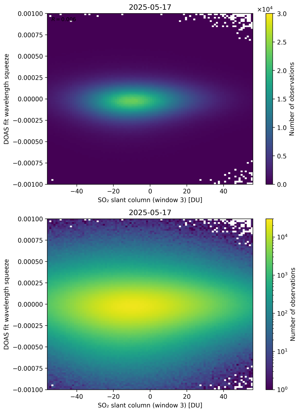
Figure 305: Scatter density plot of “SO 2 slant column (window 3)” against “DOAS fit wavelength squeeze” for 2025-05-16 to 2025-05-18.
