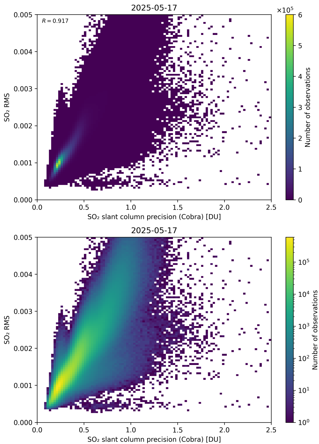
Figure 204: Scatter density plot of “SO 2 slant column precision (Cobra)” against “SO 2 RMS” for 2025-05-16 to 2025-05-18.
