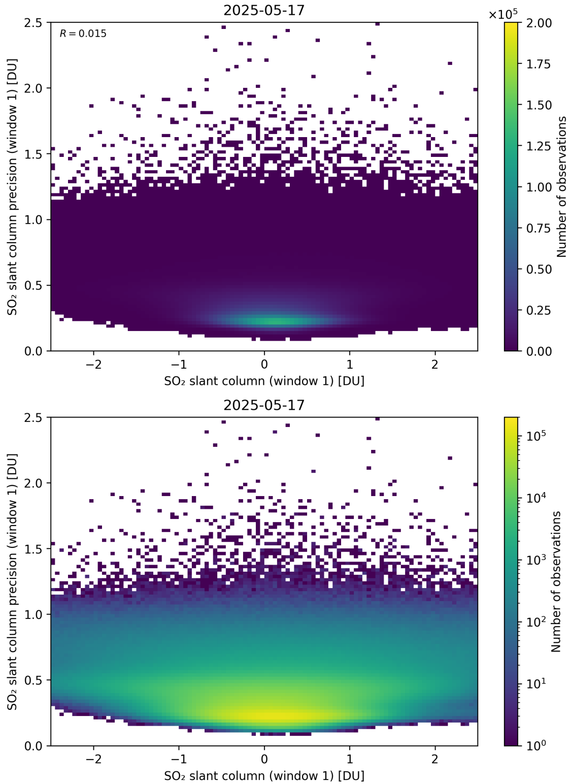
Figure 285: Scatter density plot of “SO 2 slant column (window 1)” against “SO 2 slant column precision (window 1)” for 2025-05-16 to 2025-05-18.
