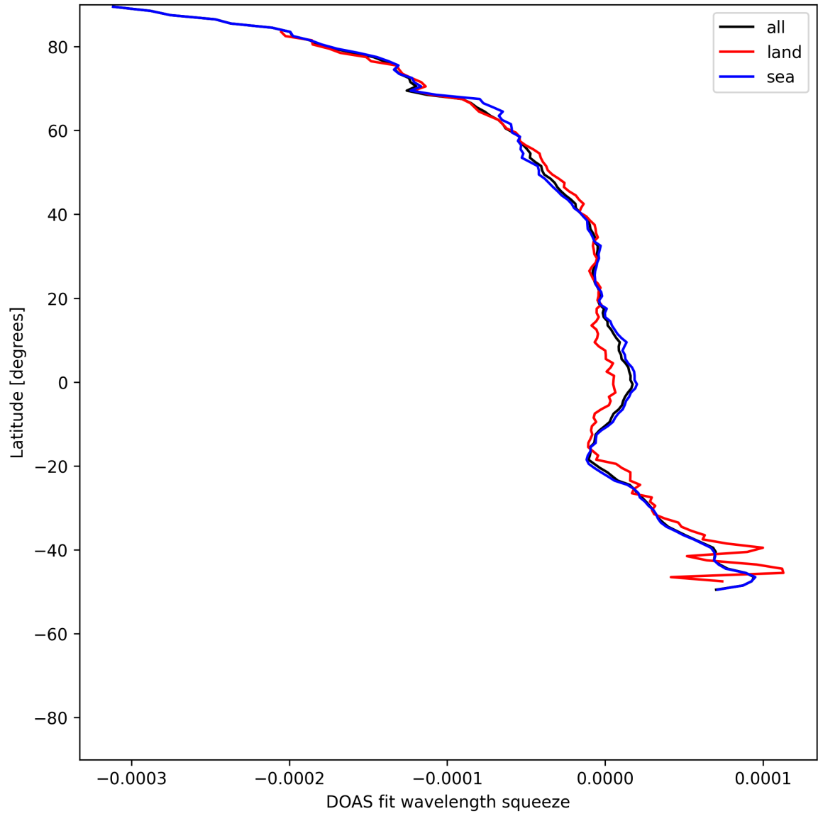
Figure 51: Zonal average of “DOAS fit wavelength squeeze” for 2025-05-16 to 2025-05-18.
