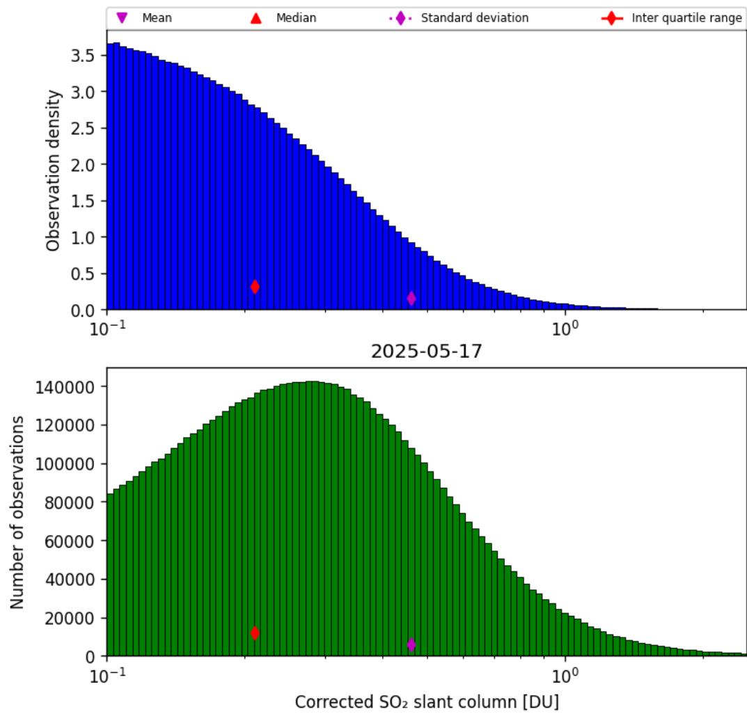
Figure 60: Histogram of “Corrected SO 2 slant column” for 2025-05-16 to 2025-05-18
