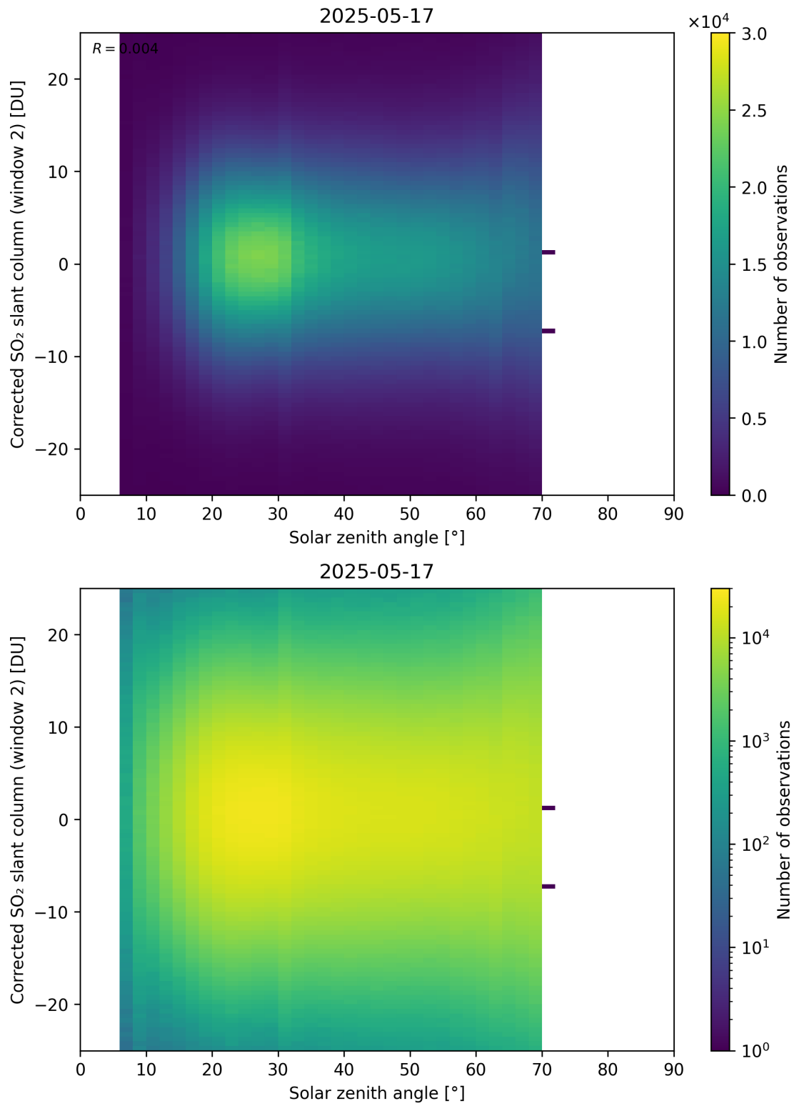
Figure 182: Scatter density plot of “Solar zenith angle” against “Corrected SO 2 slant column (window 2)” for 2025-05-16 to 2025-05-18.
