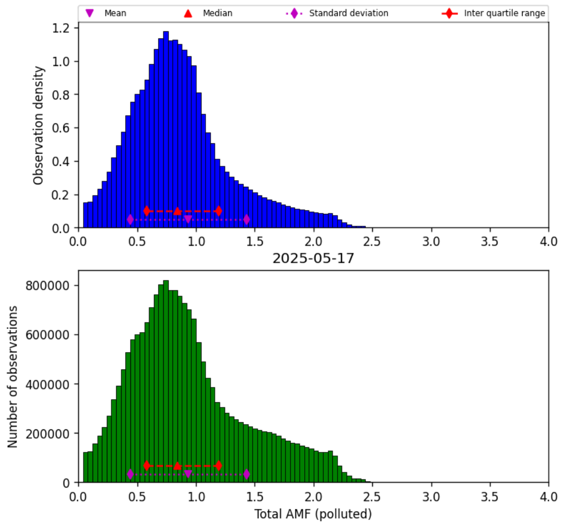
Figure 79: Histogram of “Total AMF (polluted)” for 2025-05-16 to 2025-05-18
