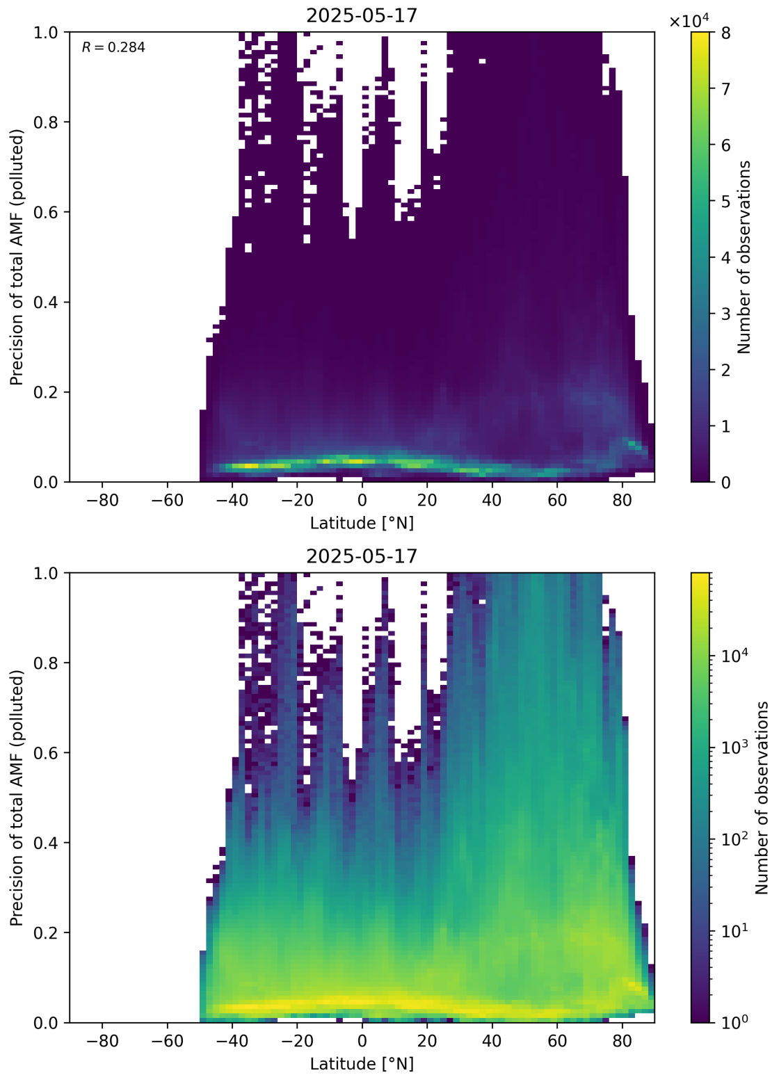
Figure 168: Scatter density plot of “Latitude” against “Precision of total AMF (polluted)” for 2025-05-16 to 2025-05-18.
