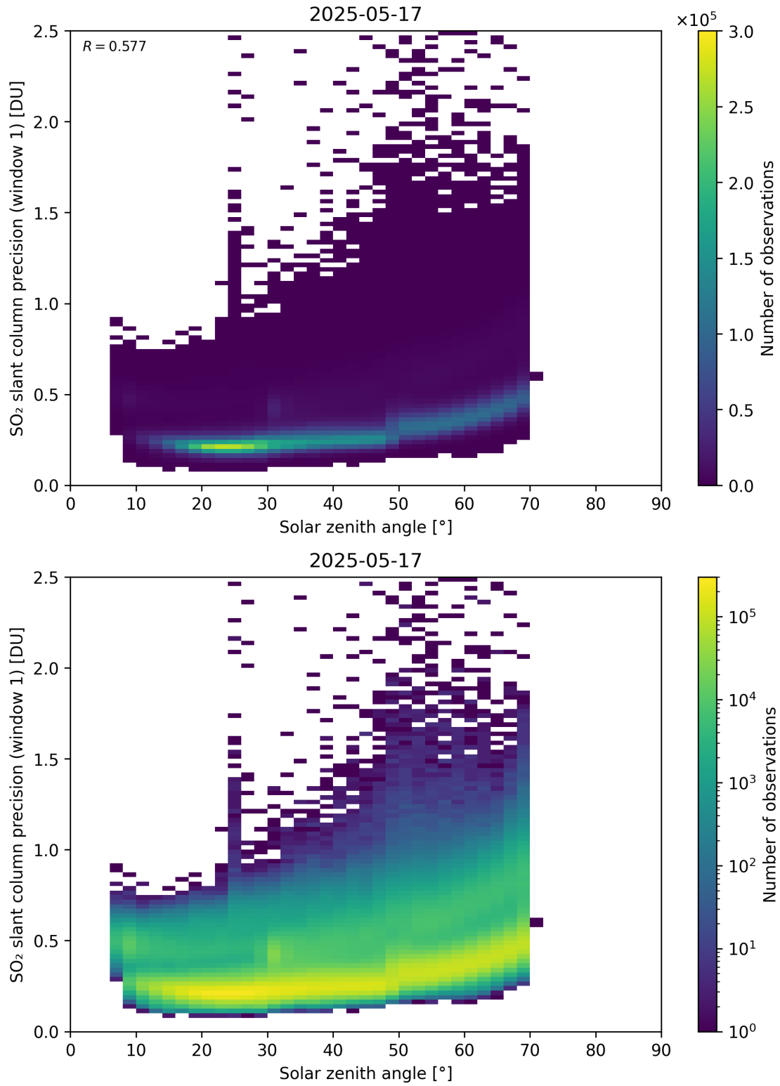
Figure 185: Scatter density plot of “Solar zenith angle” against “SO 2 slant column precision (window 1)” for 2025-05-16 to 2025-05-18.
