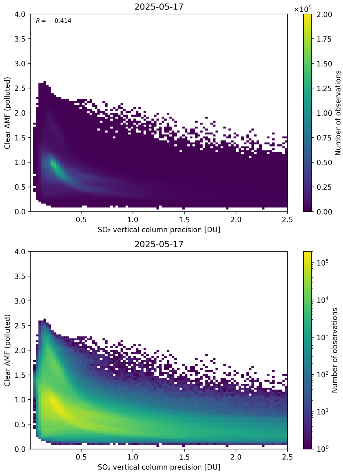
Figure 335: Scatter density plot of “SO 2 vertical column precision” against “Clear AMF (polluted)” for 2025-05-16 to 2025-05-18.
