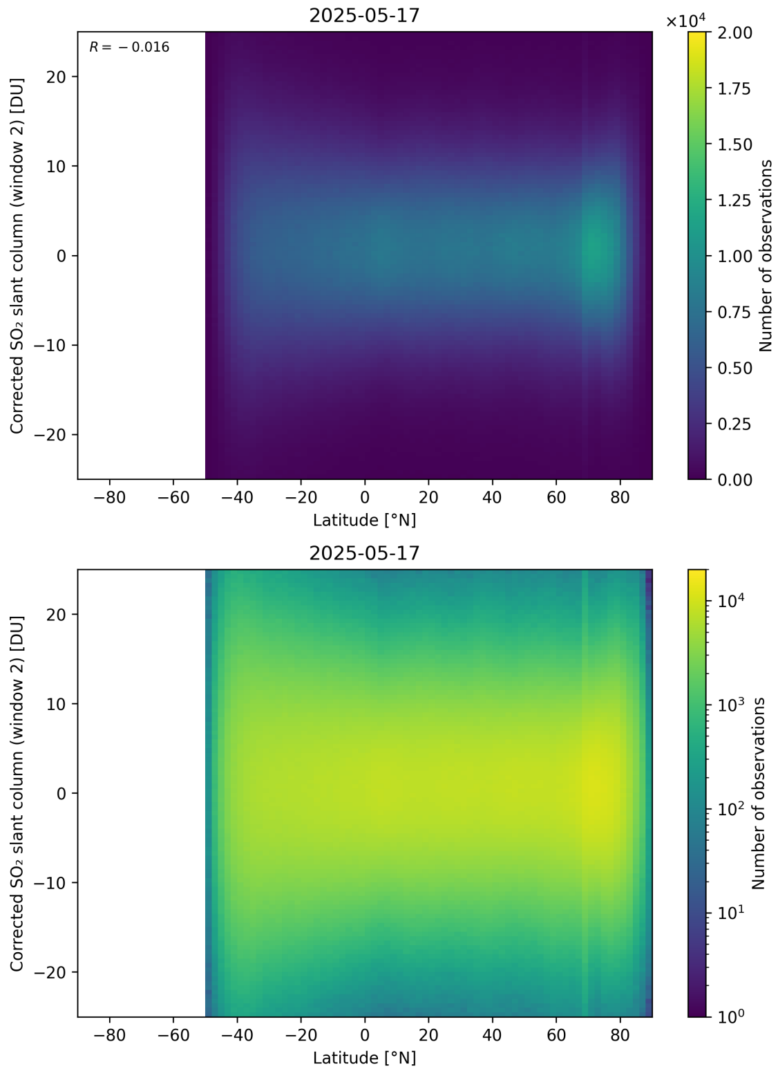
Figure 160: Scatter density plot of “Latitude” against “Corrected SO 2 slant column (window 2)” for 2025-05-16 to 2025-05-18.
