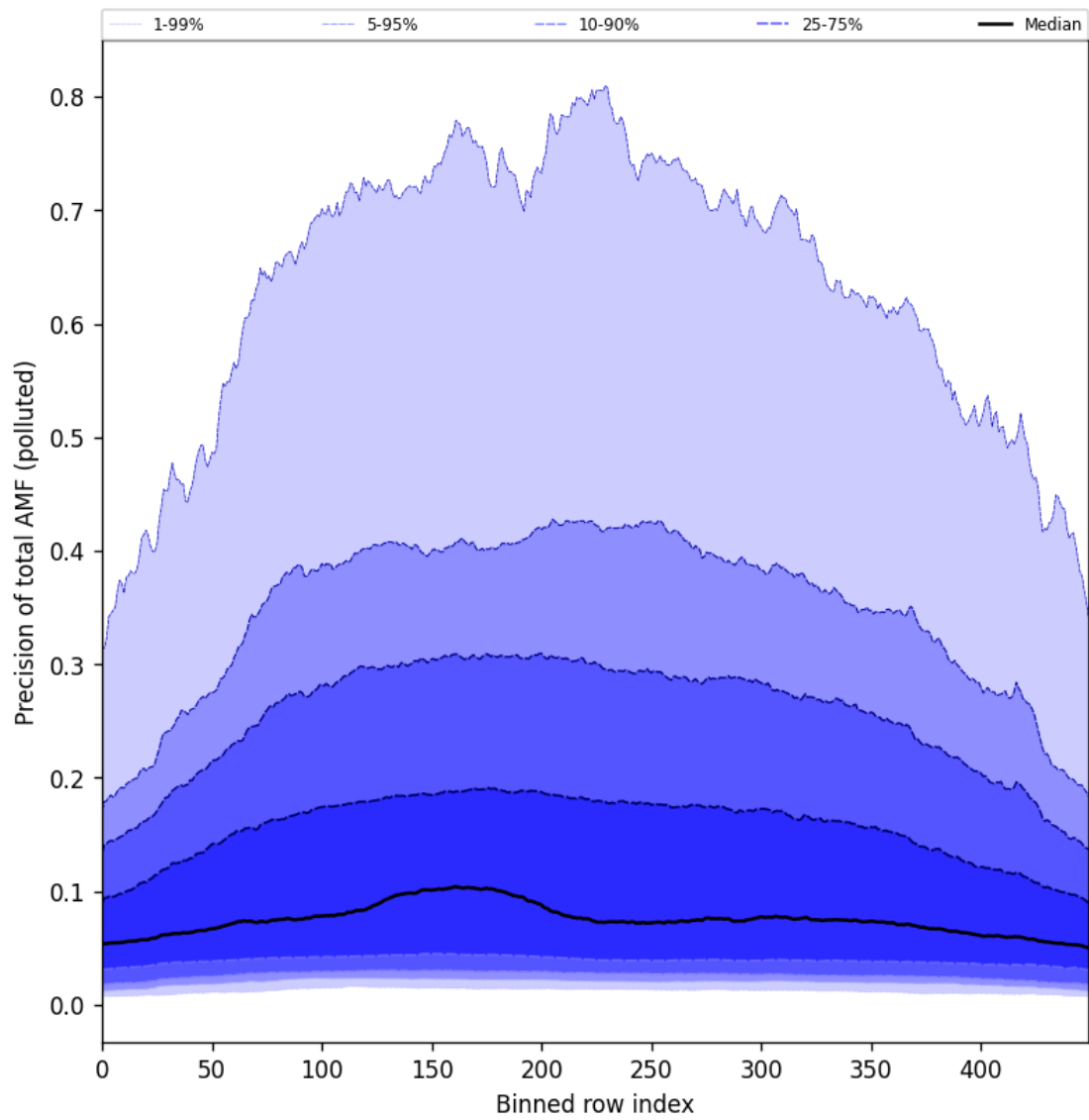
Figure 106: Along track statistics of “Precision of total AMF (polluted)” for 2025-05-16 to 2025-05-18
