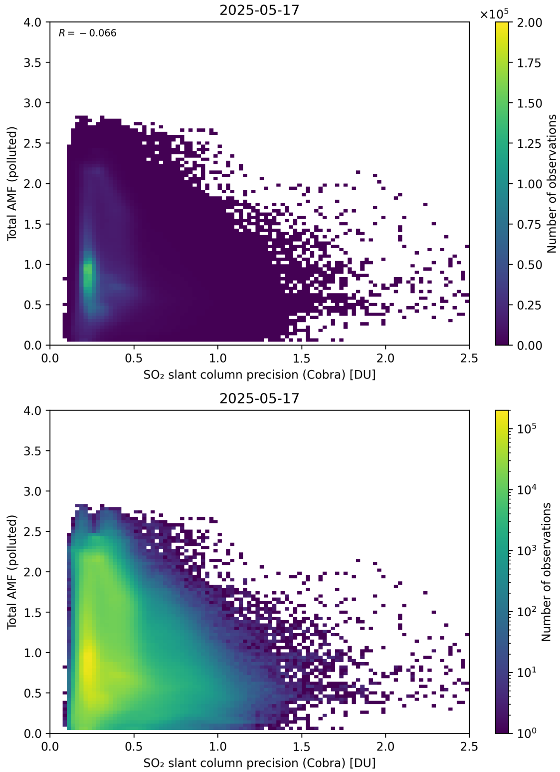
Figure 213: Scatter density plot of “SO 2 slant column precision (Cobra)” against “Total AMF (polluted)” for 2025-05-16 to 2025-05-18.
