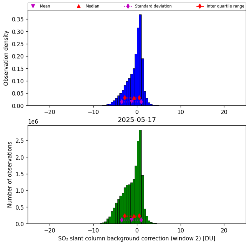
Figure 70: Histogram of “SO 2 slant column background correction (window 2)” for 2025-05-16 to 2025-05-18
