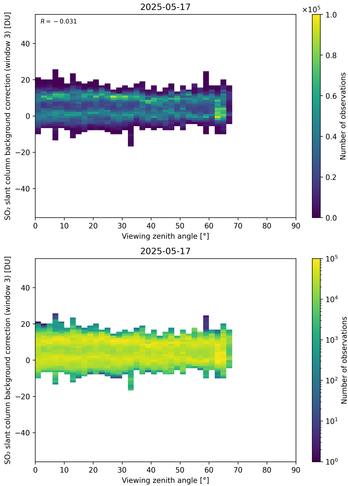
Figure 364: Scatter density plot of “Viewing zenith angle” against “SO 2 slant column background correction (window 3)” for 2025-05-16 to 2025-05-18.
