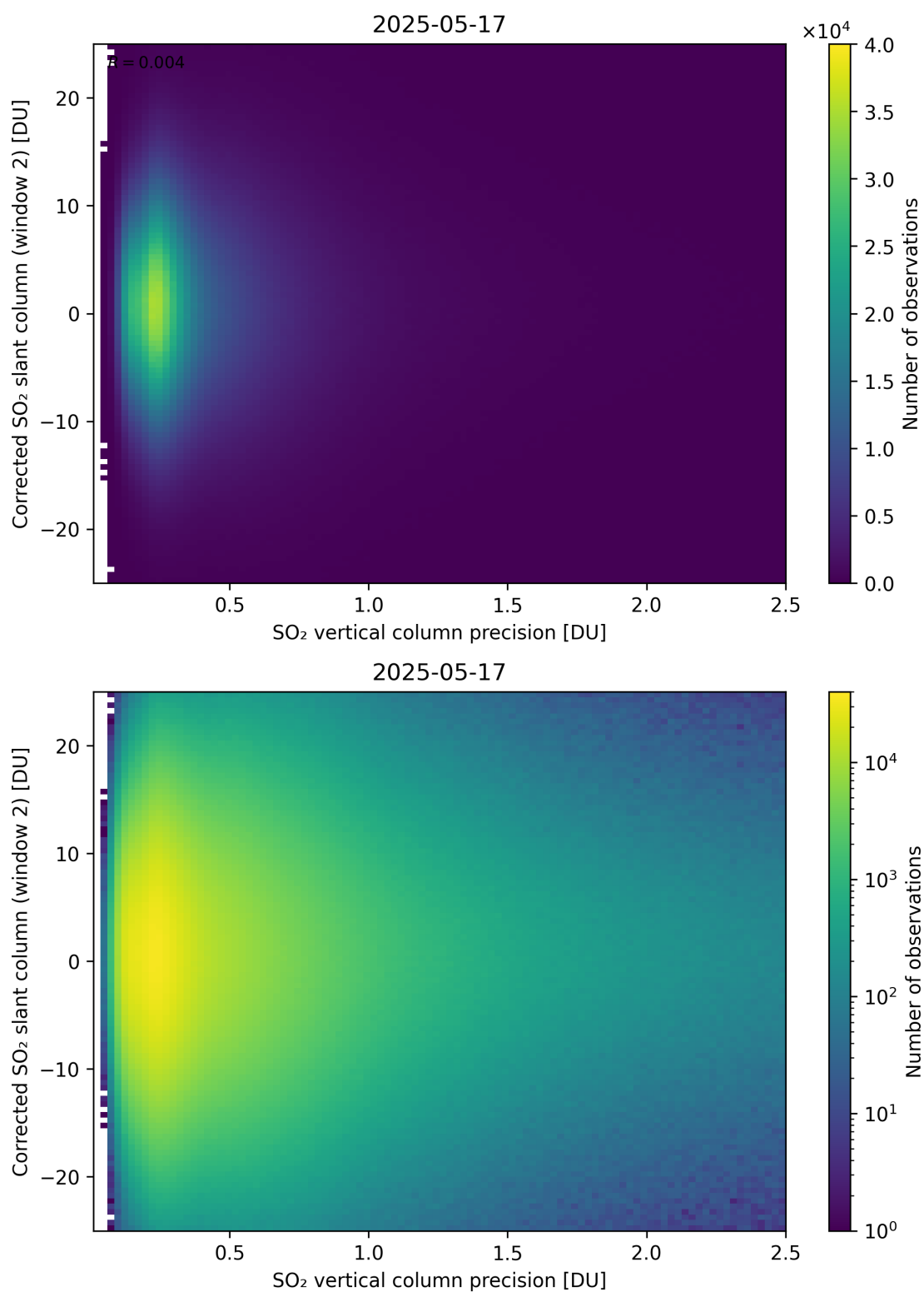
Figure 339: Scatter density plot of “SO 2 vertical column precision” against “Corrected SO 2 slant column (window 2)” for 2025-05-16 to 2025-05-18.
