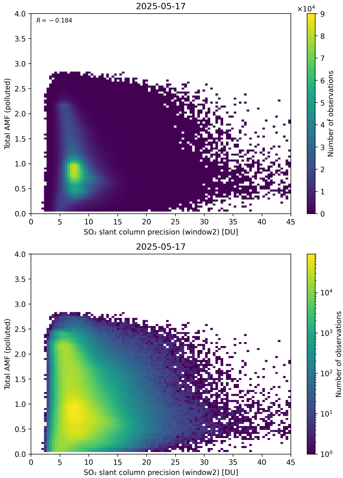
Figure 301: Scatter density plot of “SO 2 slant column precision (window2)” against “Total AMF (polluted)” for 2025-05-16 to 2025-05-18.
