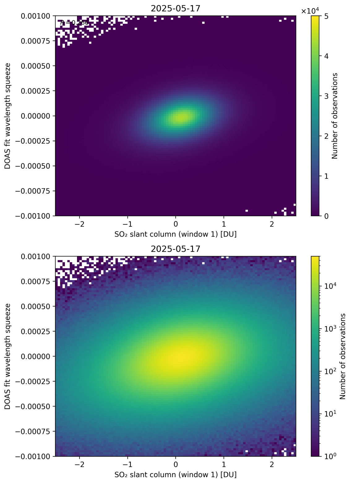
Figure 266: Scatter density plot of “SO 2 slant column (window 1)” against “DOAS fit wavelength squeeze” for 2025-05-16 to 2025-05-18.
