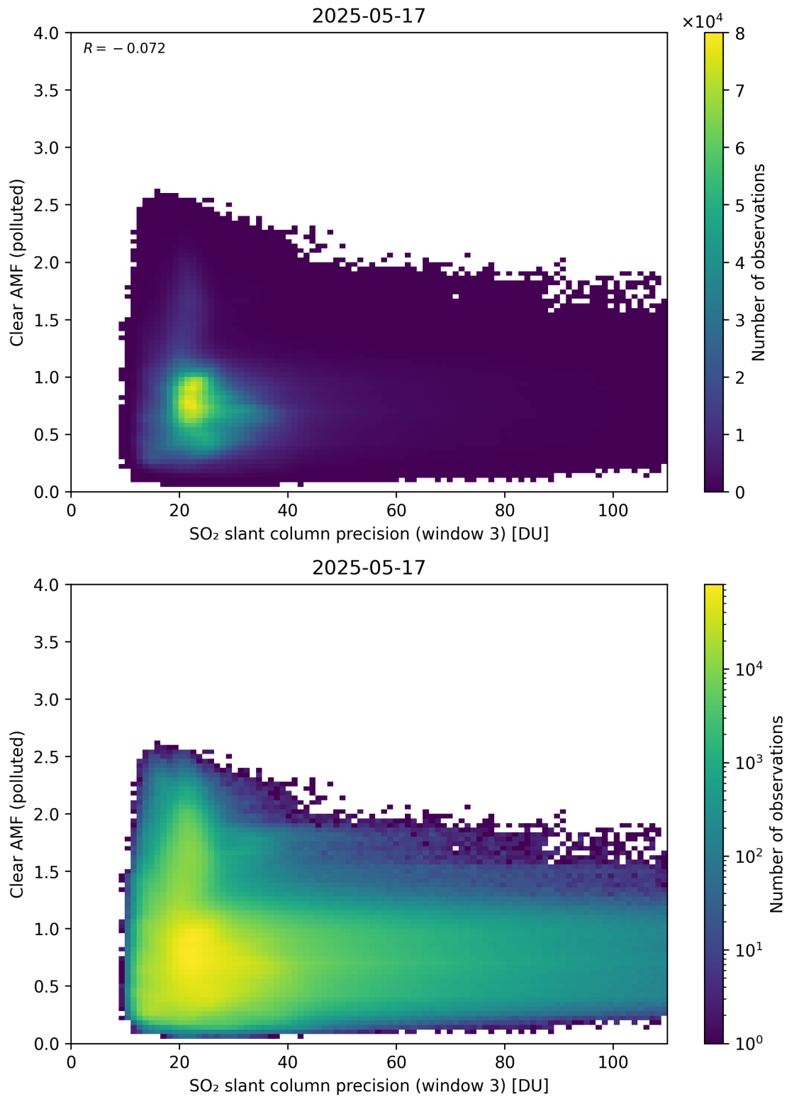
Figure 311: Scatter density plot of “SO 2 slant column precision (window 3)” against “Clear AMF (polluted)” for 2025-05-16 to 2025-05-18.
