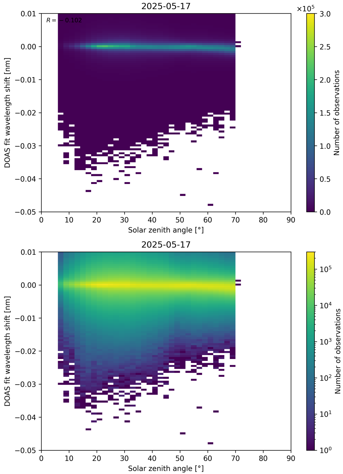
Figure 174: Scatter density plot of “Solar zenith angle” against “DOAS fit wavelength shift” for 2025-05-16 to 2025-05-18.
