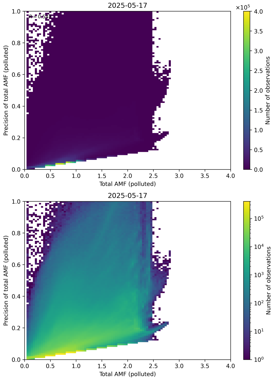
Figure 322: Scatter density plot of “Total AMF (polluted)” against “Precision of total AMF (polluted)” for 2025-05-16 to 2025-05-18.
