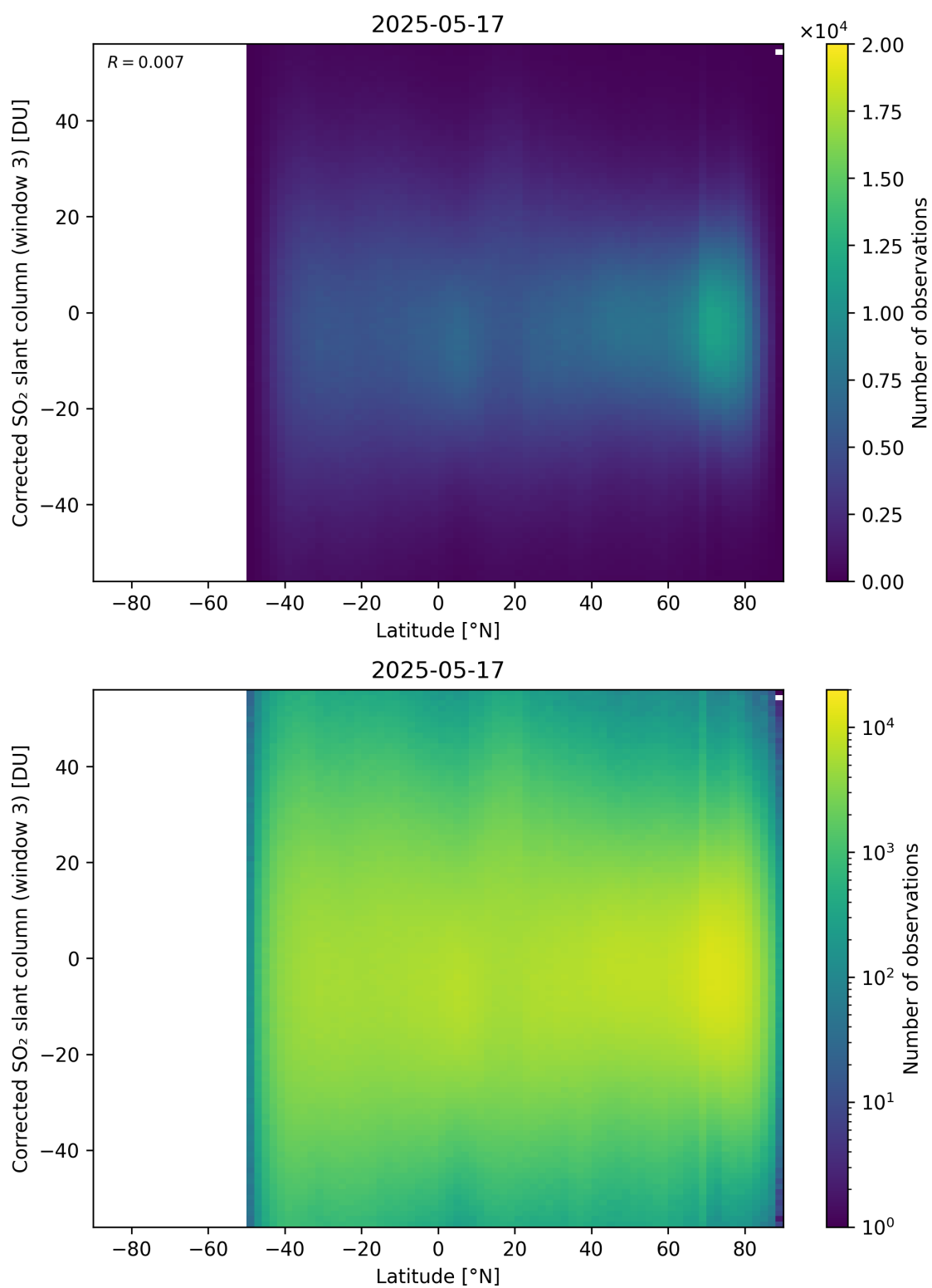
Figure 161: Scatter density plot of “Latitude” against “Corrected SO 2 slant column (window 3)” for 2025-05-16 to 2025-05-18.
