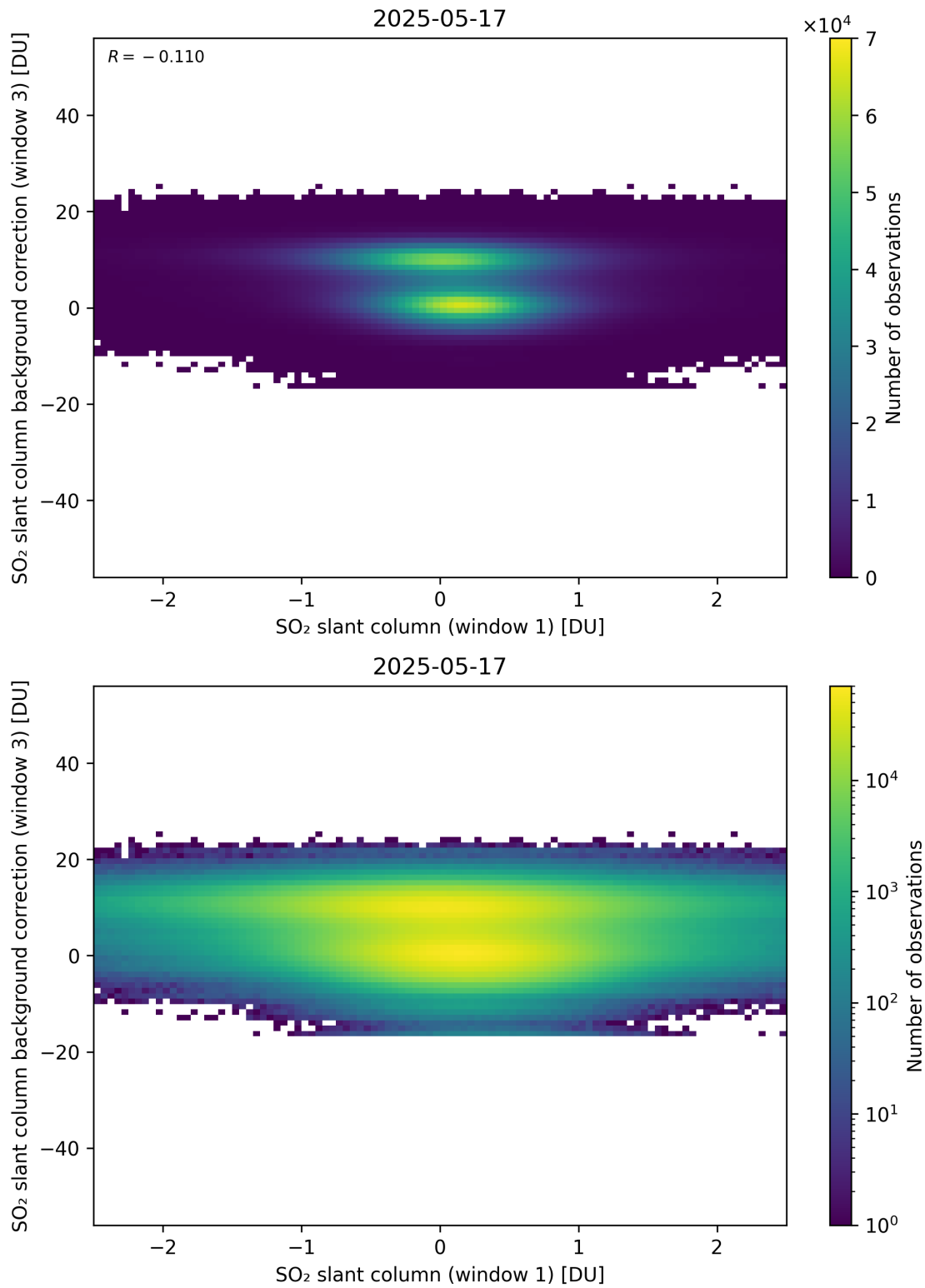
Figure 264: Scatter density plot of “SO 2 slant column (window 1)” against “SO 2 slant column background correction (window 3)” for 2025-05-16 to 2025-05-18.
