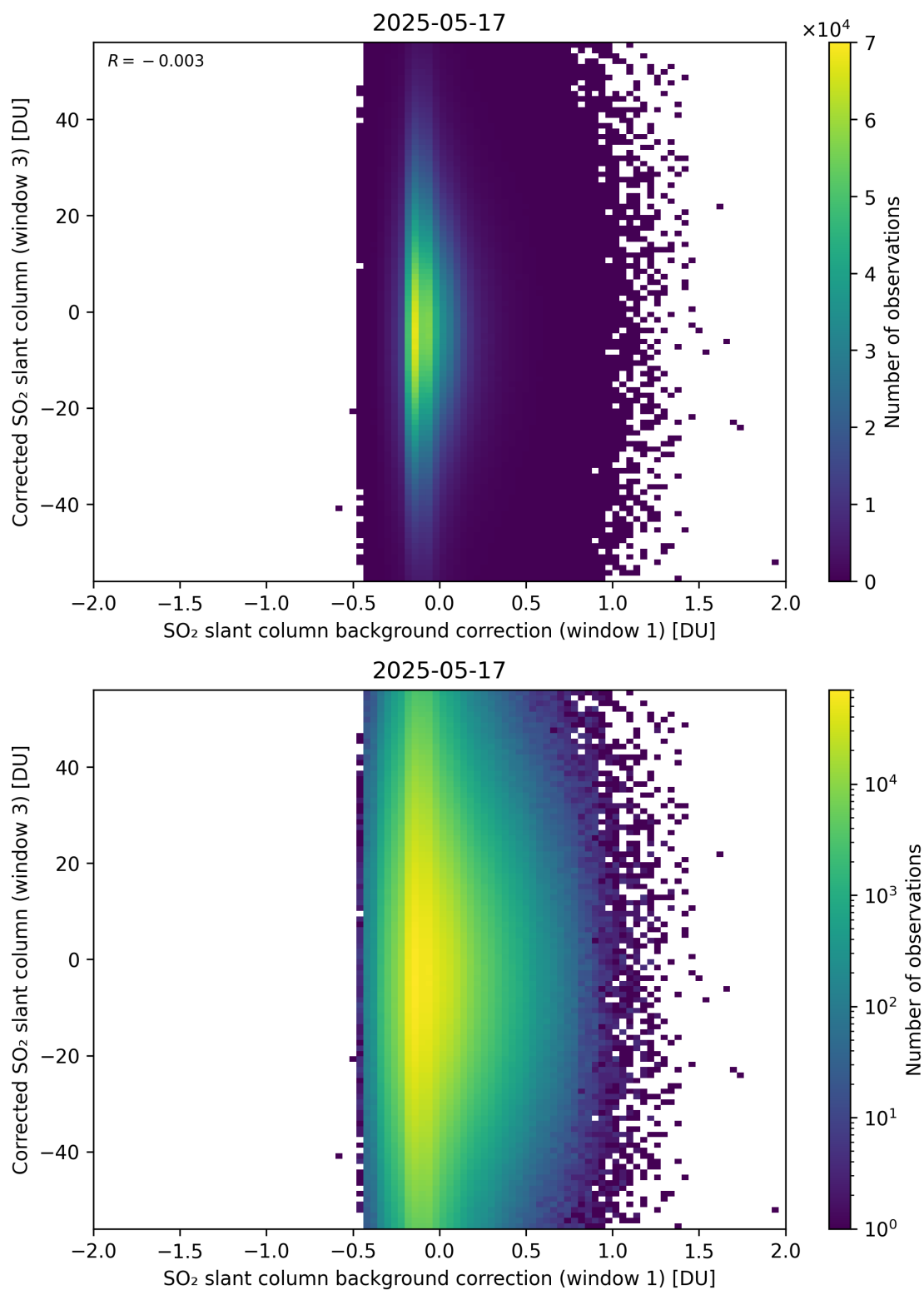
Figure 116: Scatter density plot of “SO 2 slant column background correction (window 1)” against “Corrected SO 2 slant column (window 3)” for 2025-05-16 to 2025-05-18.
