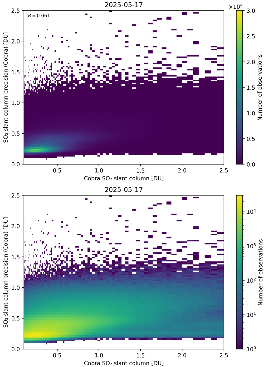
Figure 216: Scatter density plot of “Cobra SO 2 slant column” against “SO 2 slant column precision (Cobra)” for 2025-05-16 to 2025-05-18.
