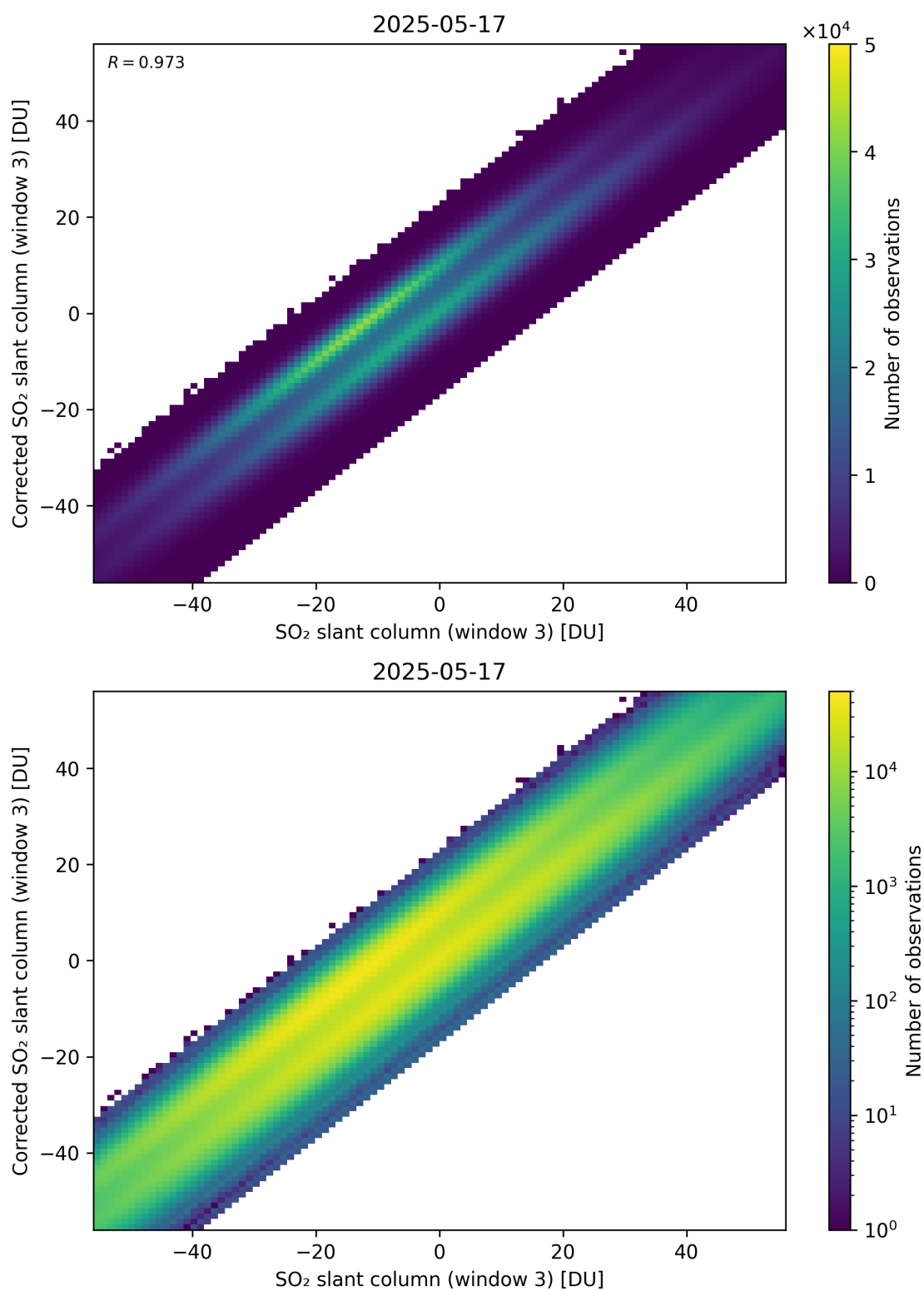
Figure 316: Scatter density plot of “SO 2 slant column (window 3)” against “Corrected SO 2 slant column (window 3)” for 2025-05-16 to 2025-05-18.
