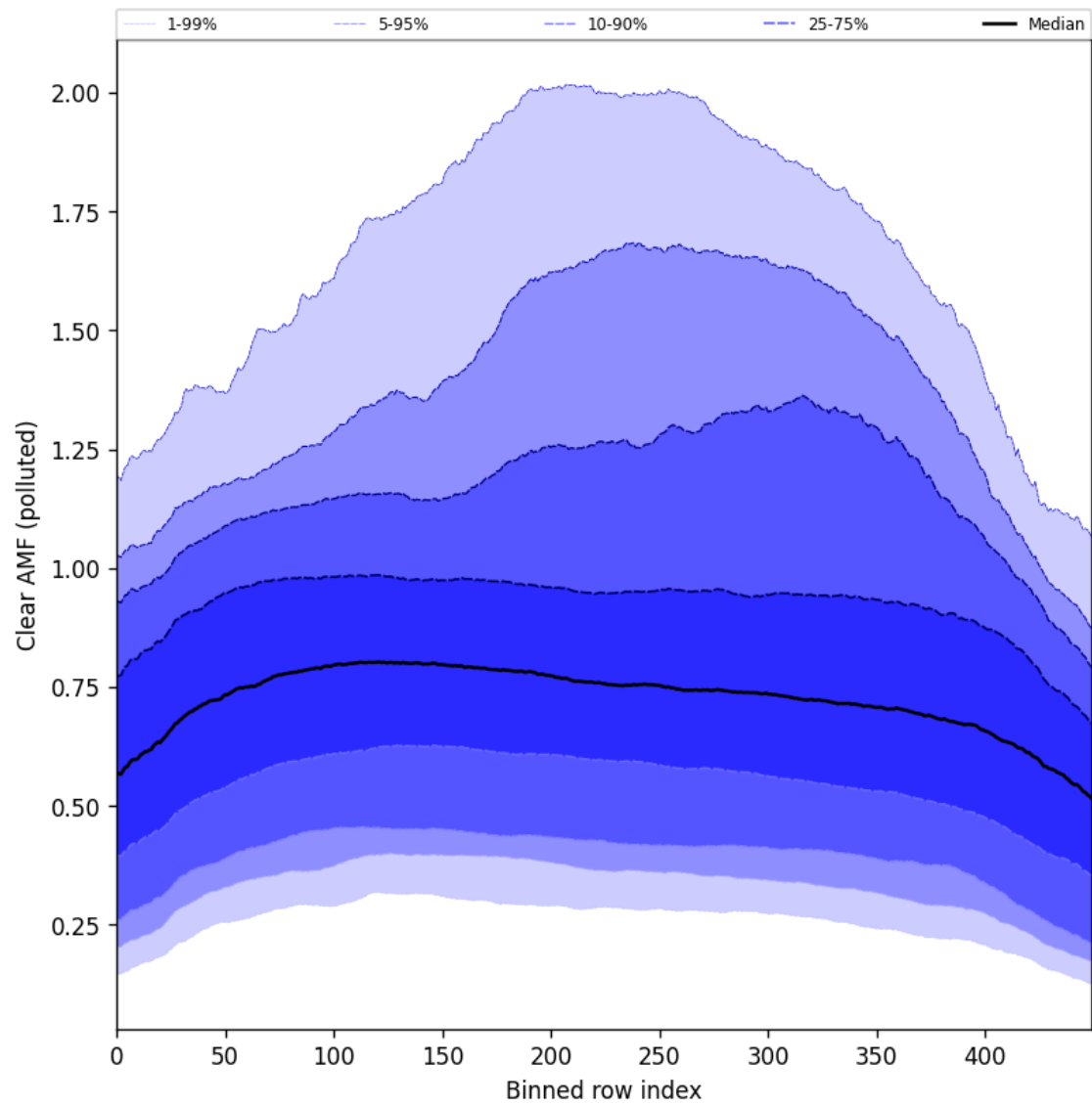
Figure 107: Along track statistics of “Clear AMF (polluted)” for 2025-05-16 to 2025-05-18
