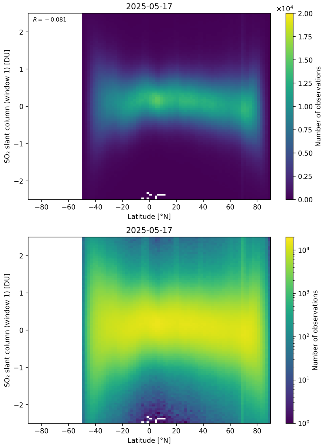
Figure 162: Scatter density plot of “Latitude” against “SO 2 slant column (window 1)” for 2025-05-16 to 2025-05-18.
