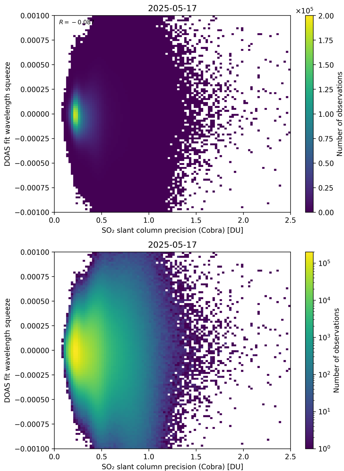
Figure 203: Scatter density plot of “SO 2 slant column precision (Cobra)” against “DOAS fit wavelength squeeze” for 2025-05-16 to 2025-05-18.
