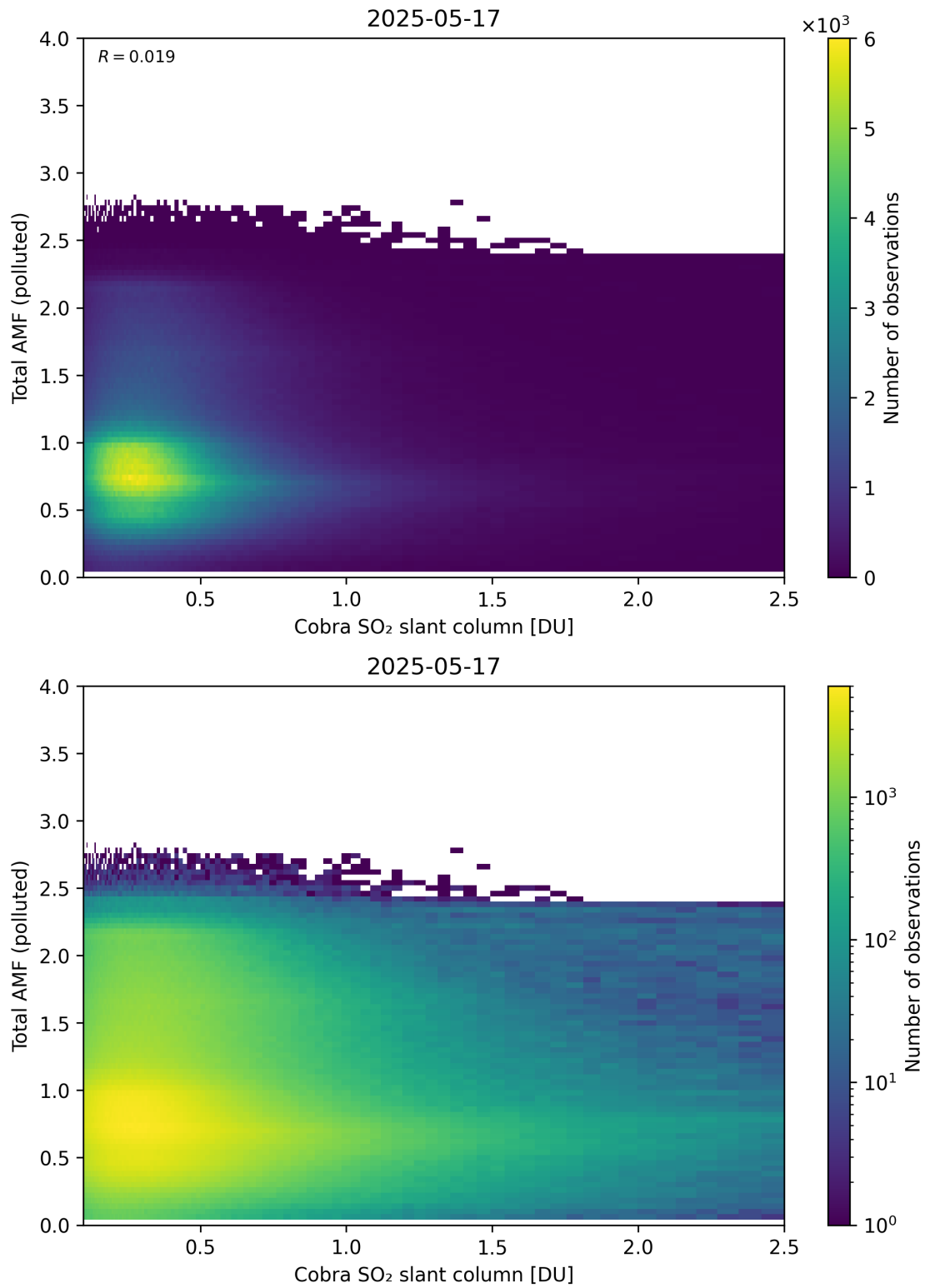
Figure 224: Scatter density plot of “Cobra SO 2 slant column” against “Total AMF (polluted)” for 2025-05-16 to 2025-05-18.
