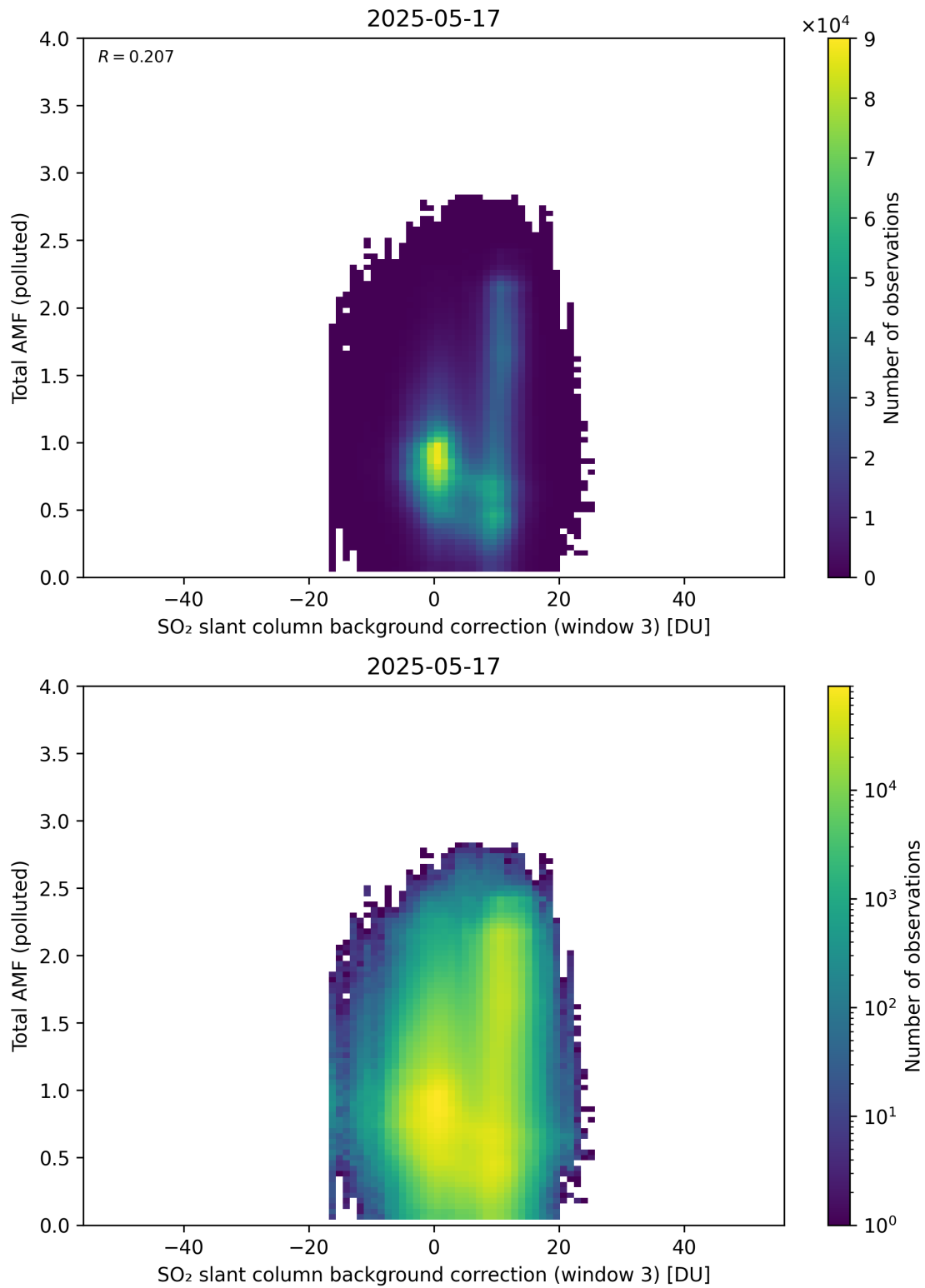
Figure 136: Scatter density plot of “SO 2 slant column background correction (window 3)” against “Total AMF (polluted)” for 2025-05-16 to 2025-05-18.
