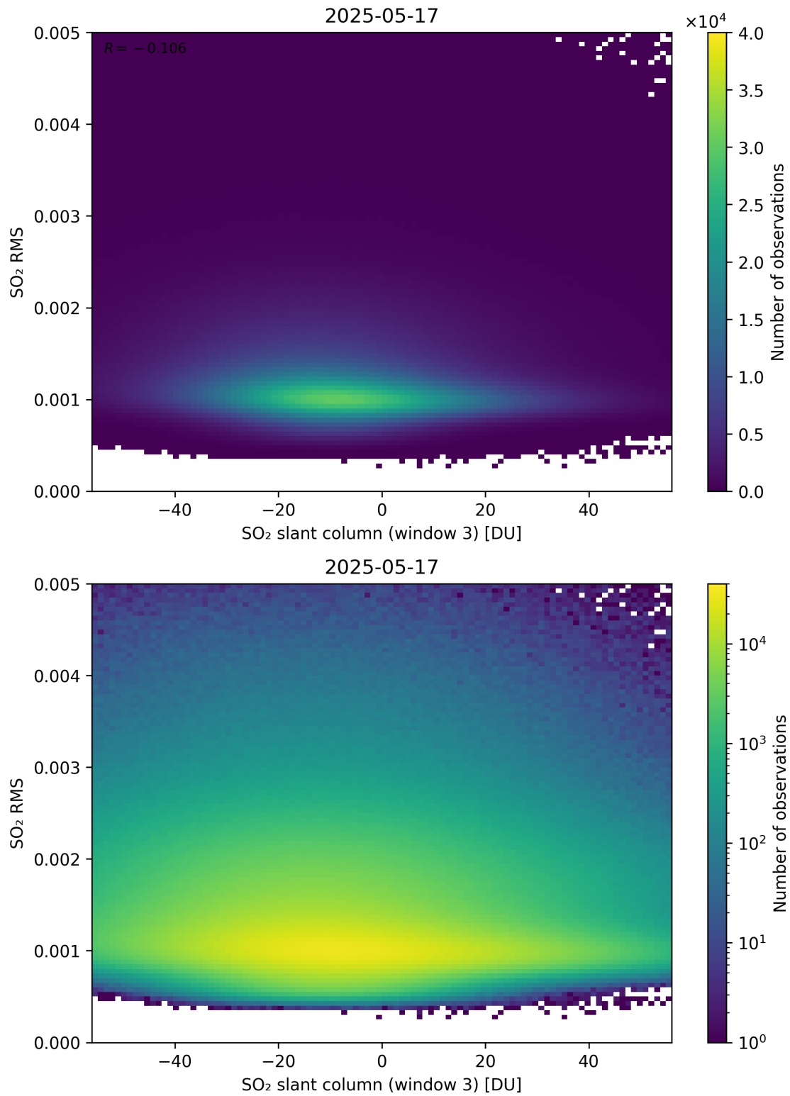
Figure 306: Scatter density plot of “SO 2 slant column (window 3)” against “SO 2 RMS” for 2025-05-16 to 2025-05-18.
