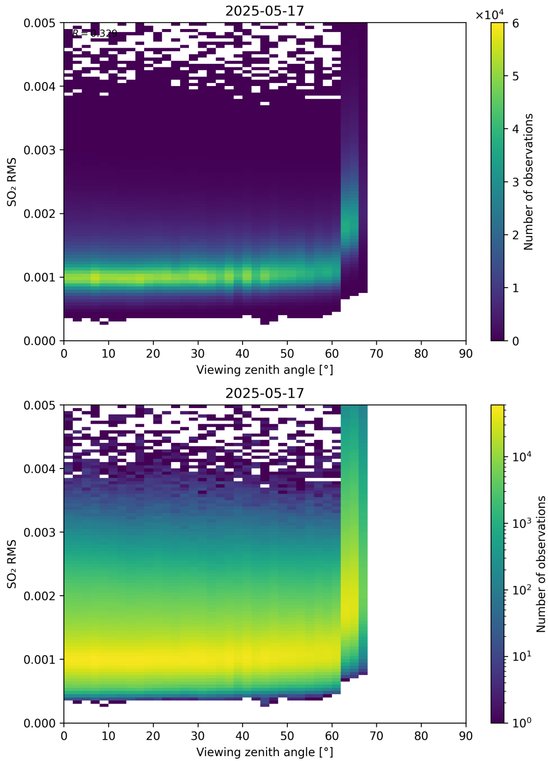
Figure 367: Scatter density plot of “Viewing zenith angle” against “SO 2 RMS” for 2025-05-16 to 2025-05-18.
