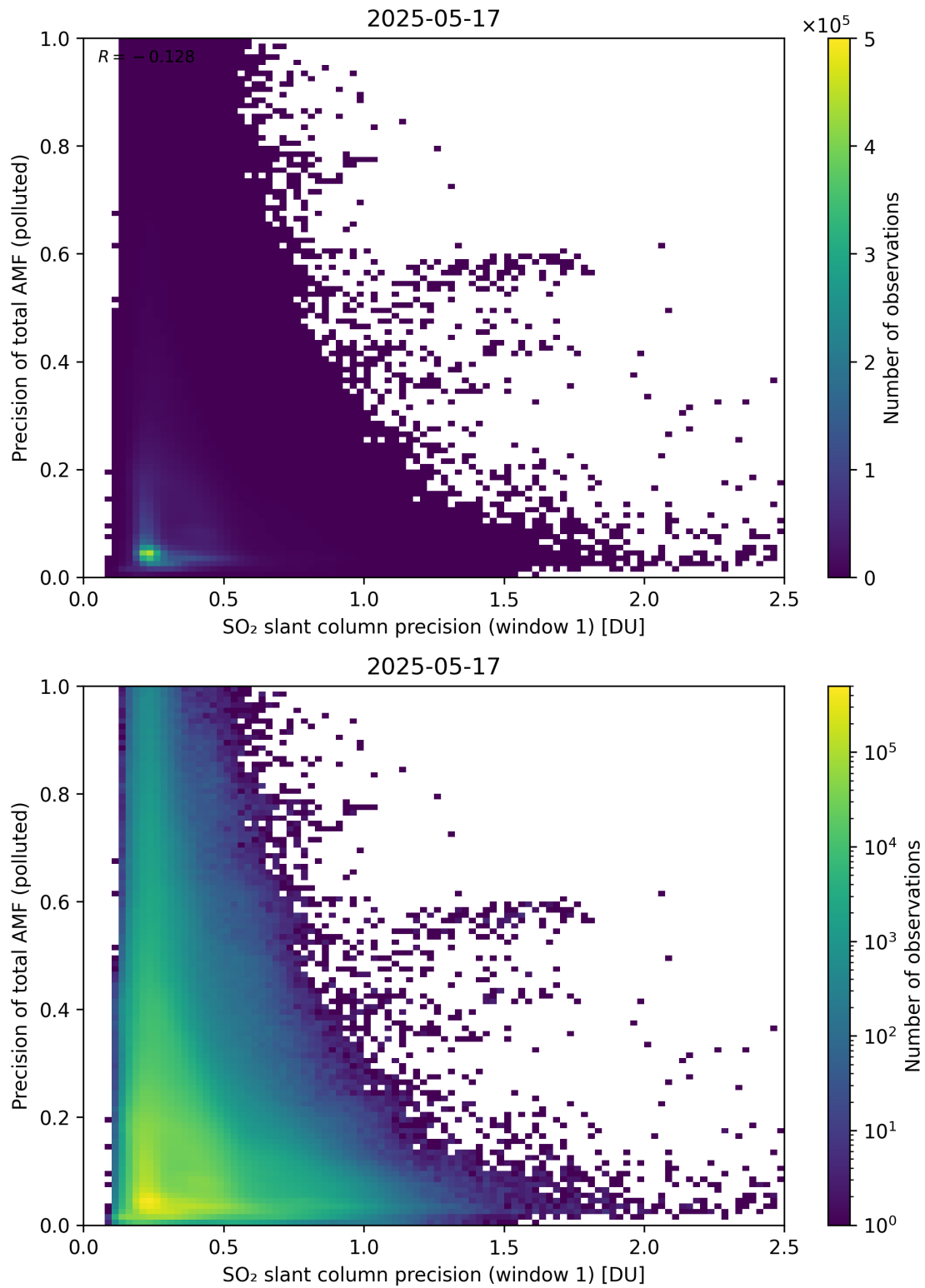
Figure 281: Scatter density plot of “SO 2 slant column precision (window 1)” against “Precision of total AMF (polluted)” for 2025-05-16 to 2025-05-18.
