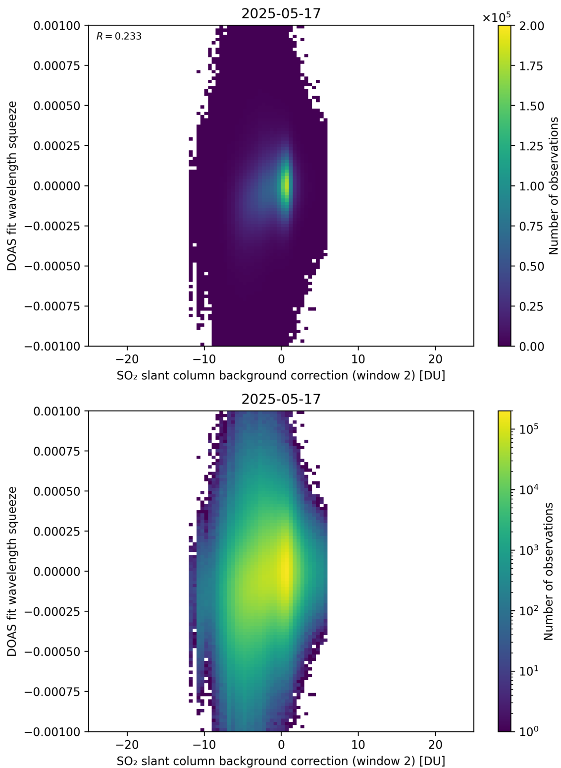
Figure 124: Scatter density plot of “SO 2 slant column background correction (window 2)” against “DOAS fit wavelength squeeze” for 2025-05-16 to 2025-05-18.
