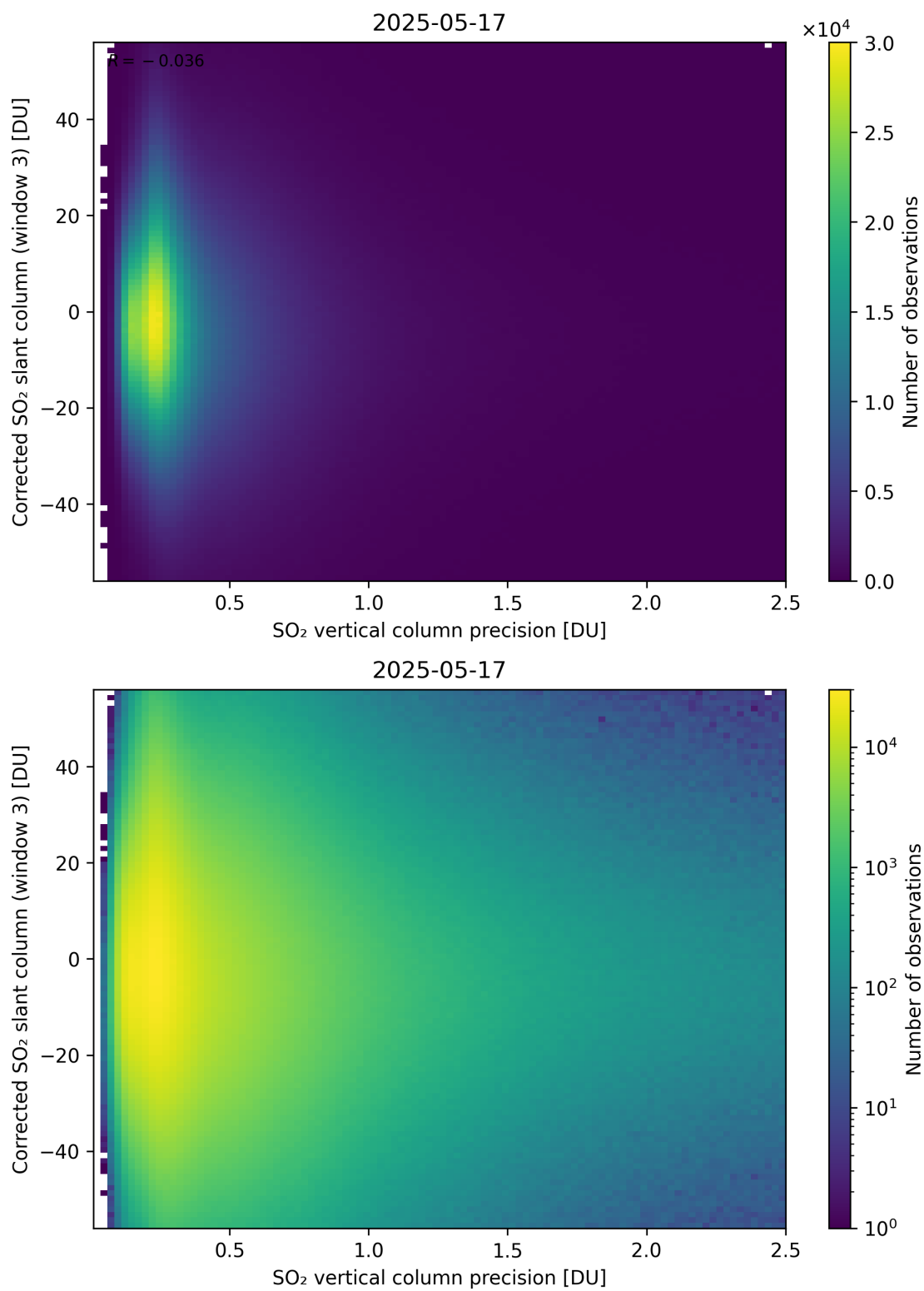
Figure 340: Scatter density plot of “SO 2 vertical column precision” against “Corrected SO 2 slant column (window 3)” for 2025-05-16 to 2025-05-18.
