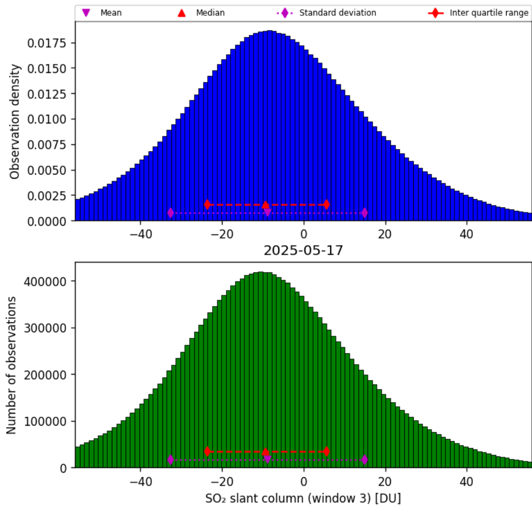
Figure 71: Histogram of “SO 2 slant column (window 3)” for 2025-05-16 to 2025-05-18
