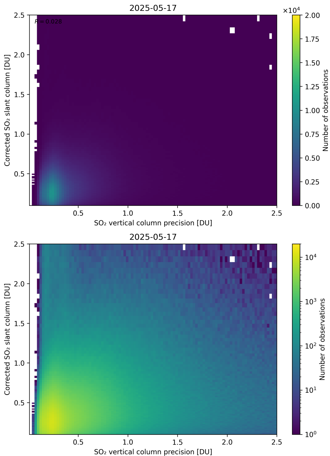
Figure 338: Scatter density plot of “SO 2 vertical column precision” against “Corrected SO 2 slant column” for 2025-05-16 to 2025-05-18.
