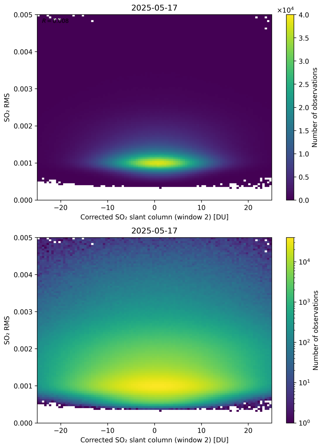
Figure 248: Scatter density plot of “Corrected SO 2 slant column (window 2)” against “SO 2 RMS” for 2025-05-16 to 2025-05-18.
