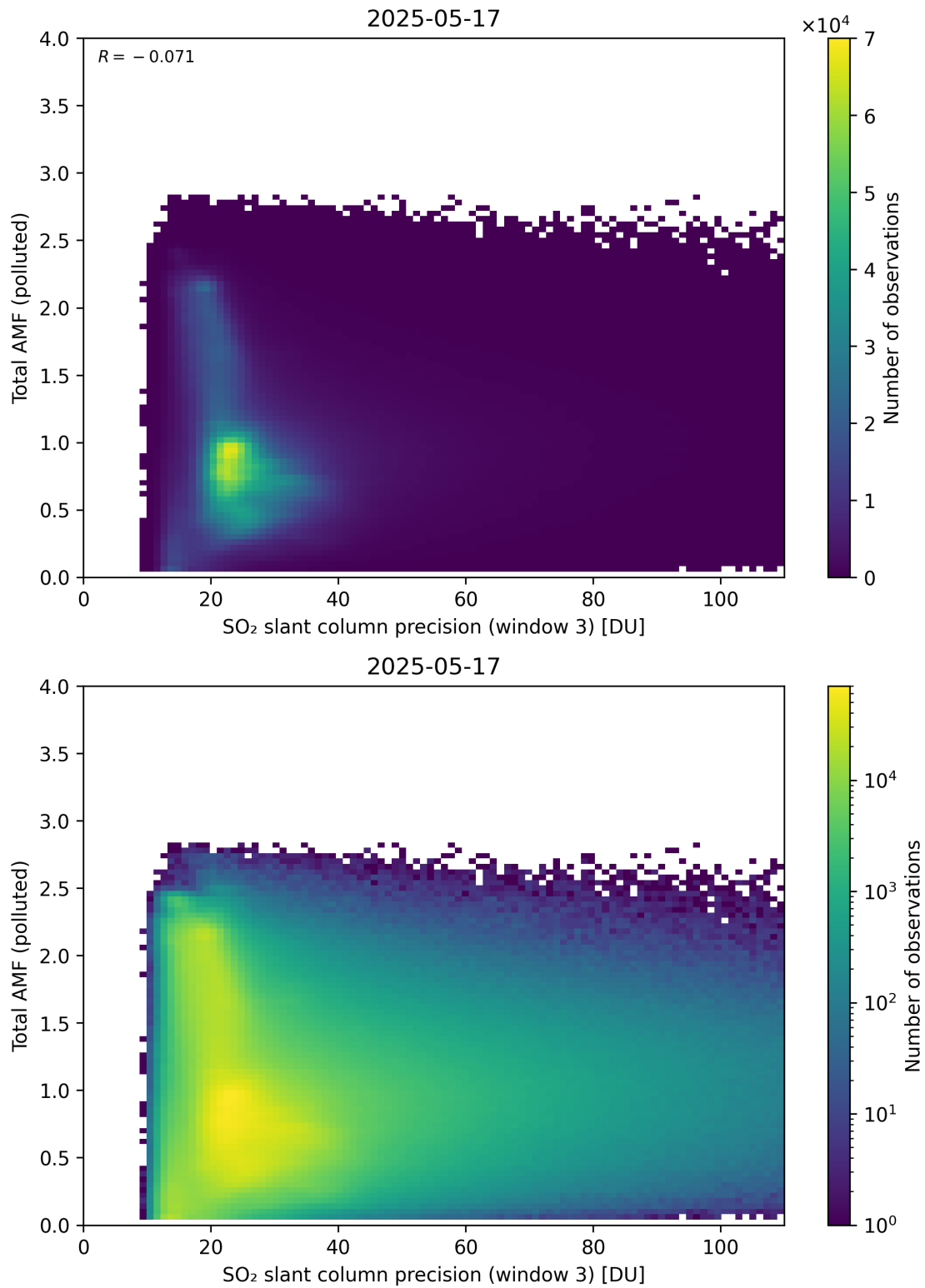
Figure 313: Scatter density plot of “SO 2 slant column precision (window 3)” against “Total AMF (polluted)” for 2025-05-16 to 2025-05-18.
