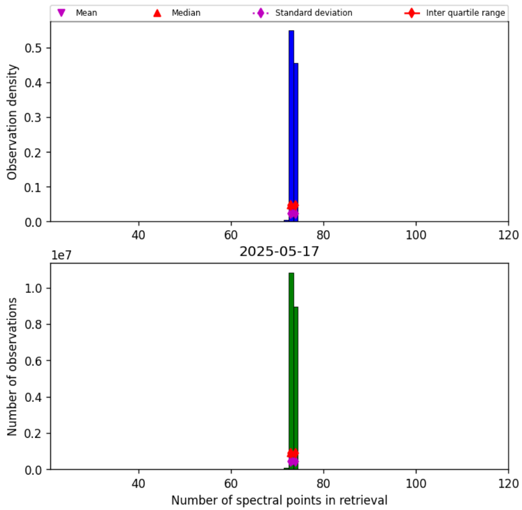
Figure 82: Histogram of “Number of spectral points in retrieval” for 2025-05-16 to 2025-05-18
