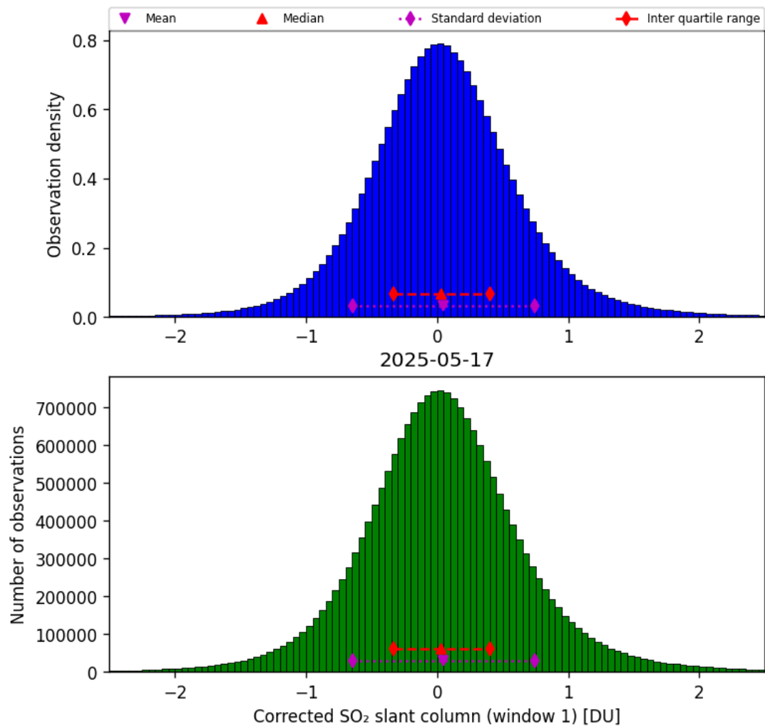
Figure 65: Histogram of “Corrected SO 2 slant column (window 1)” for 2025-05-16 to 2025-05-18
