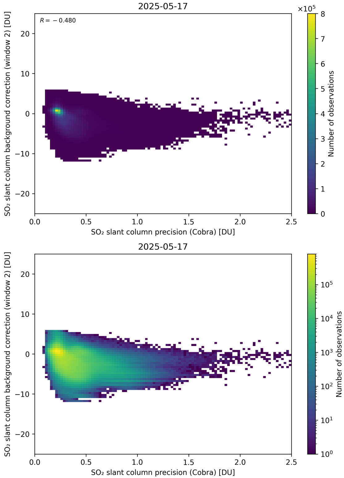
Figure 200: Scatter density plot of “SO 2 slant column precision (Cobra)” against “SO 2 slant column background correction (window 2)” for 2025-05-16 to 2025-05-18.
