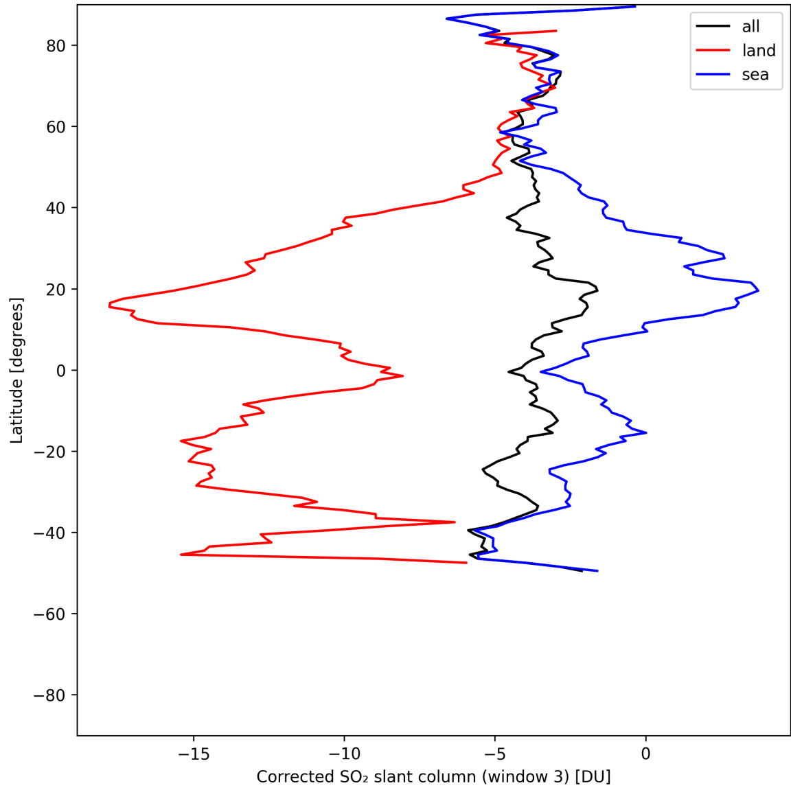
Figure 47: Zonal average of “Corrected SO 2 slant column (window 3)” for 2025-05-16 to 2025-05-18.
