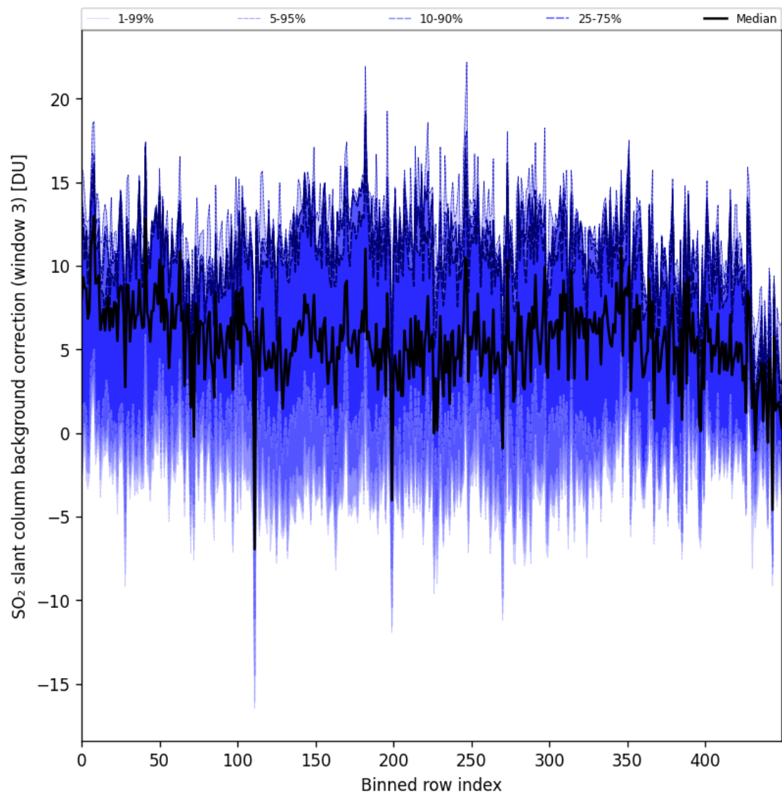
Figure 100: Along track statistics of “SO 2 slant column background correction (window 3)” for 2025-05-16 to 2025-05-18
