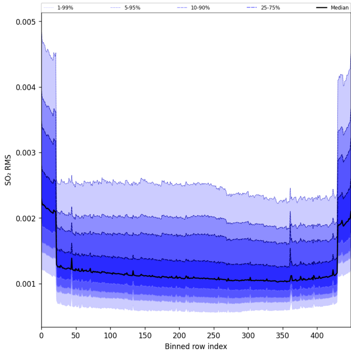
Figure 104: Along track statistics of “SO 2 RMS” for 2025-05-16 to 2025-05-18
