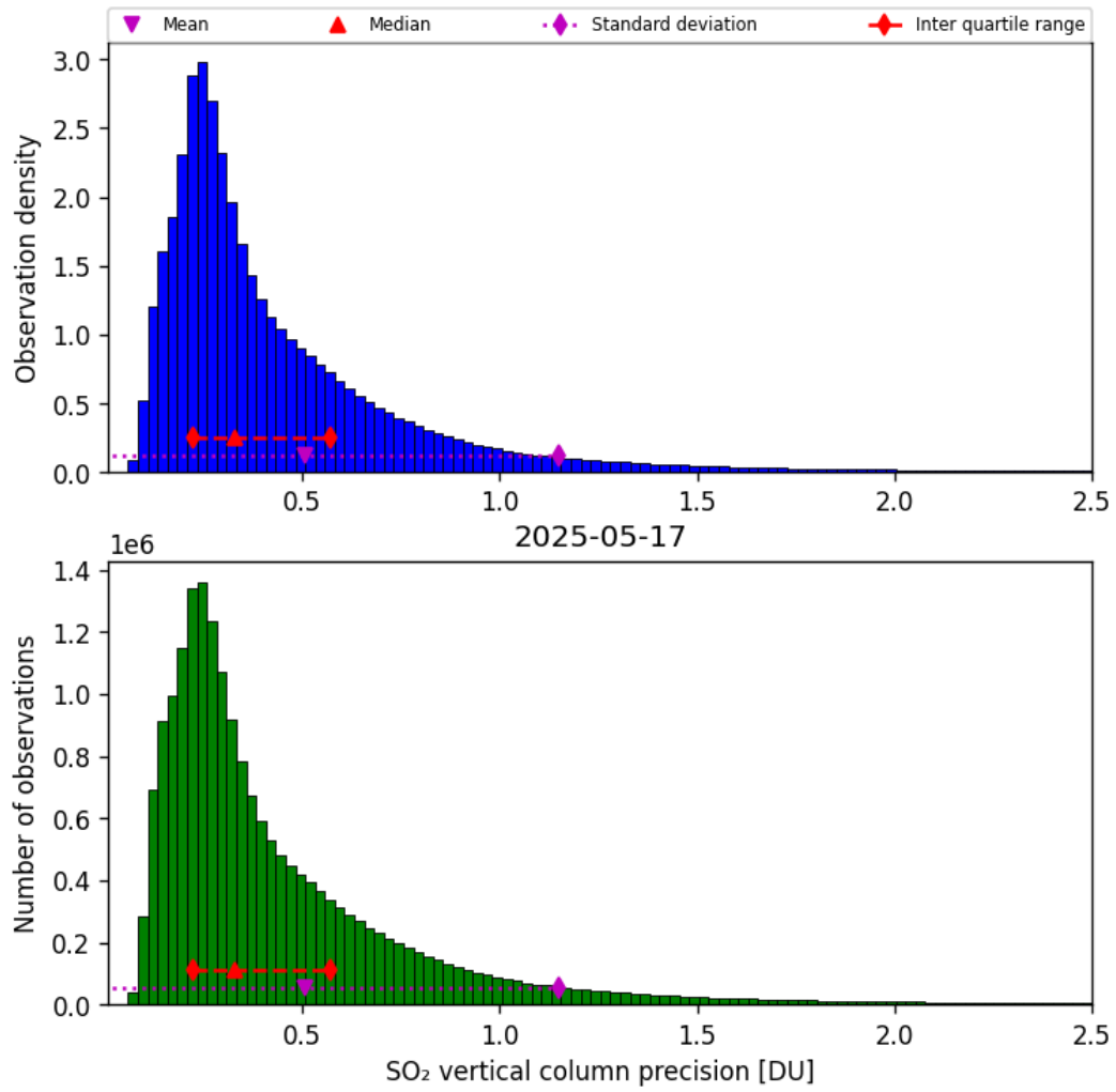
Figure 59: Histogram of “SO 2 vertical column precision” for 2025-05-16 to 2025-05-18
