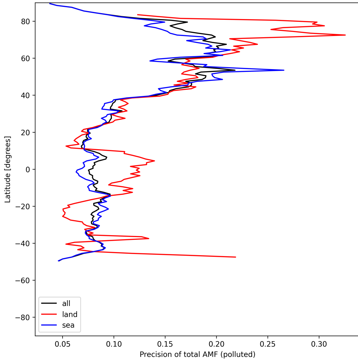
Figure 54: Zonal average of “Precision of total AMF (polluted)” for 2025-05-16 to 2025-05-18.
