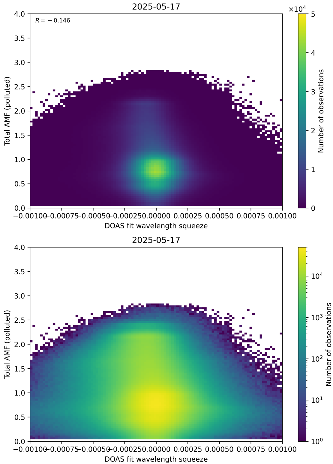
Figure 145: Scatter density plot of “DOAS fit wavelength squeeze” against “Total AMF (polluted)” for 2025-05-16 to 2025-05-18.
