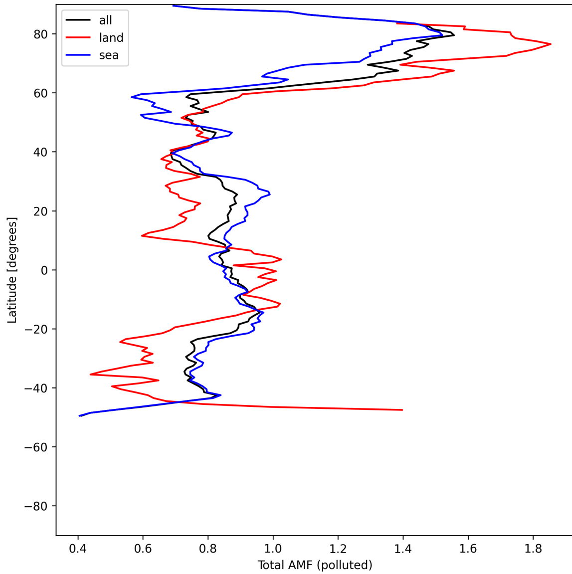
Figure 53: Zonal average of “Total AMF (polluted)” for 2025-05-16 to 2025-05-18.
