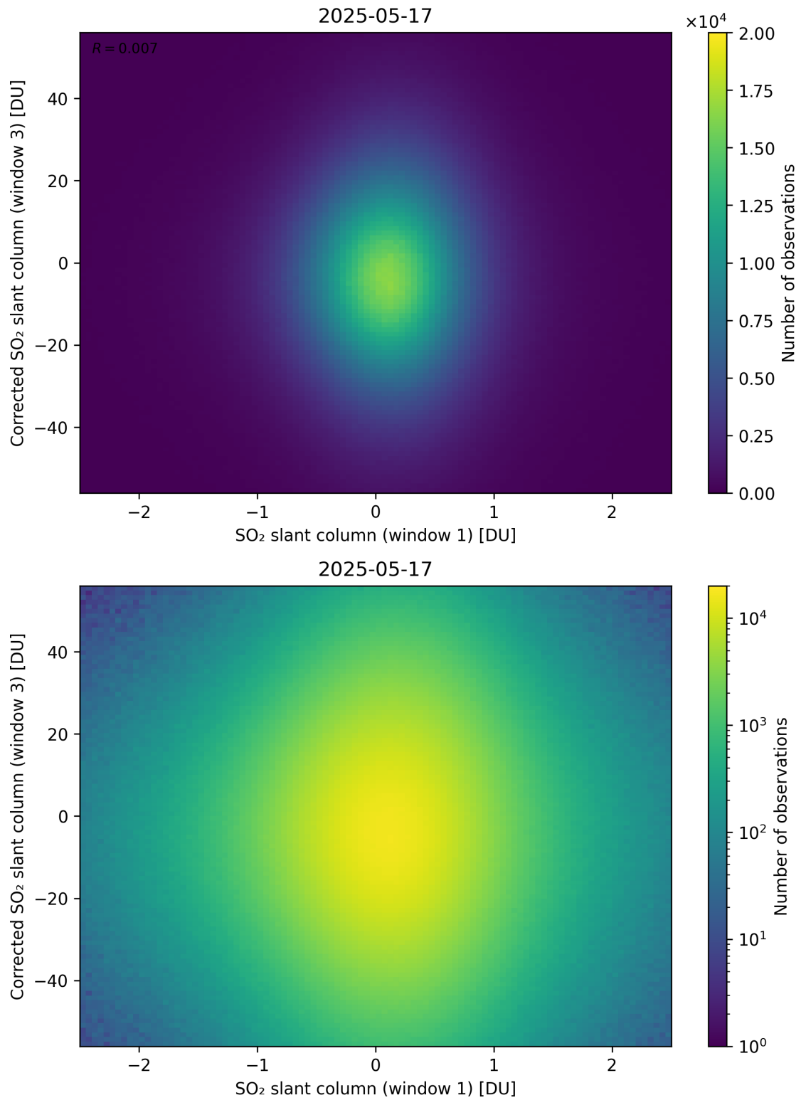
Figure 284: Scatter density plot of “SO 2 slant column (window 1)” against “Corrected SO 2 slant column (window 3)” for 2025-05-16 to 2025-05-18.
