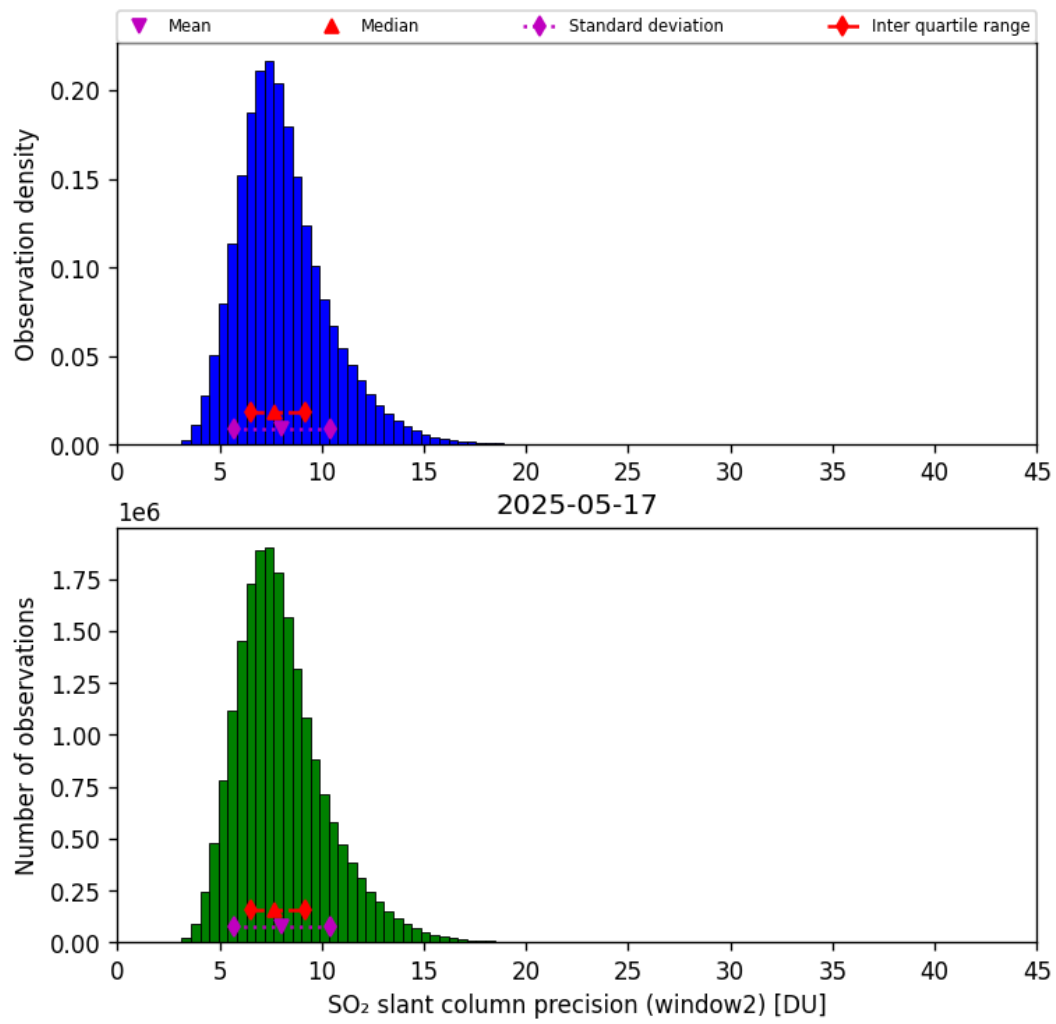
Figure 68: Histogram of “SO 2 slant column precision (window2)” for 2025-05-16 to 2025-05-18
