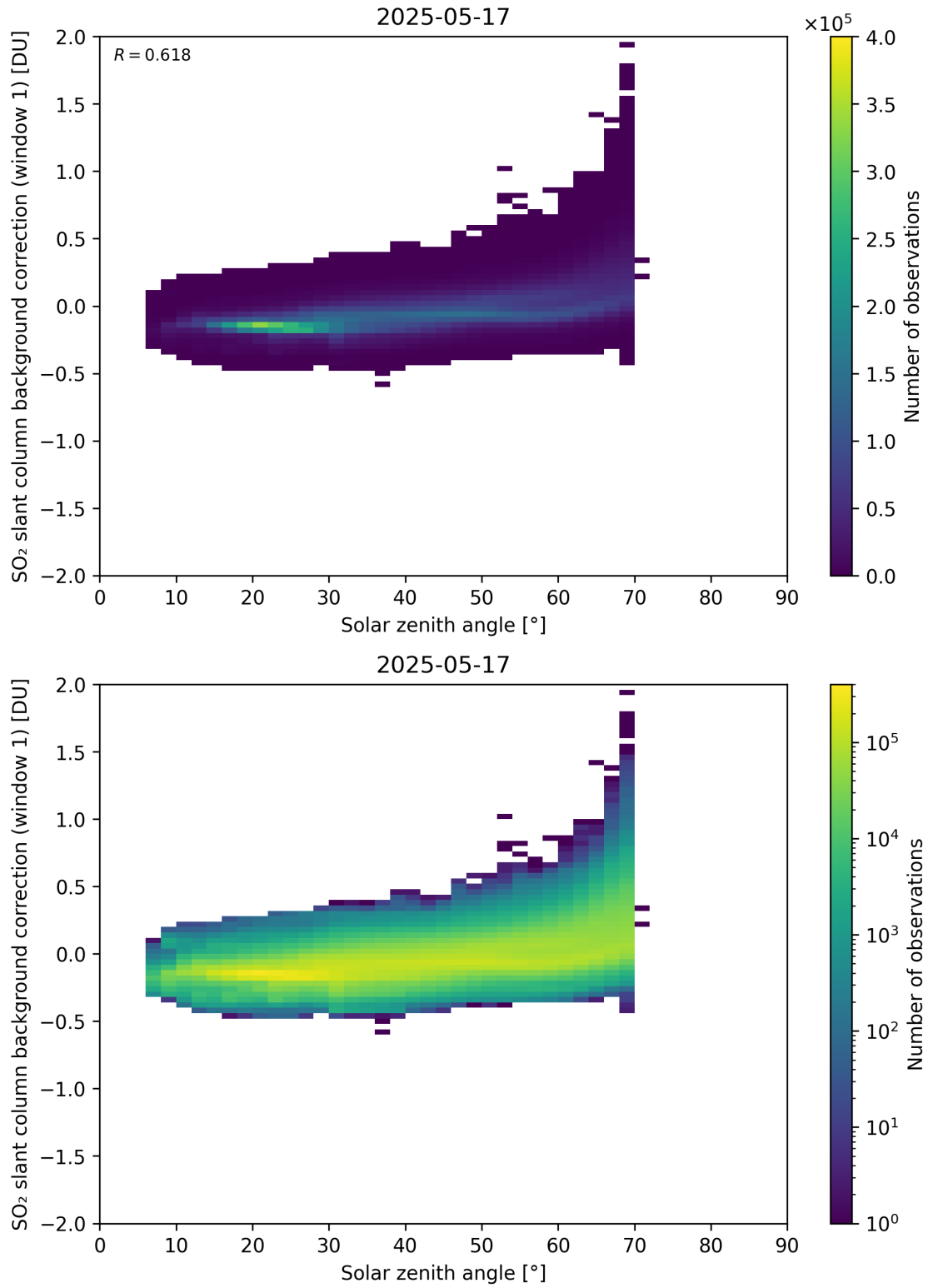
Figure 171: Scatter density plot of “Solar zenith angle” against “SO 2 slant column background correction (window 1)” for 2025-05-16 to 2025-05-18.
