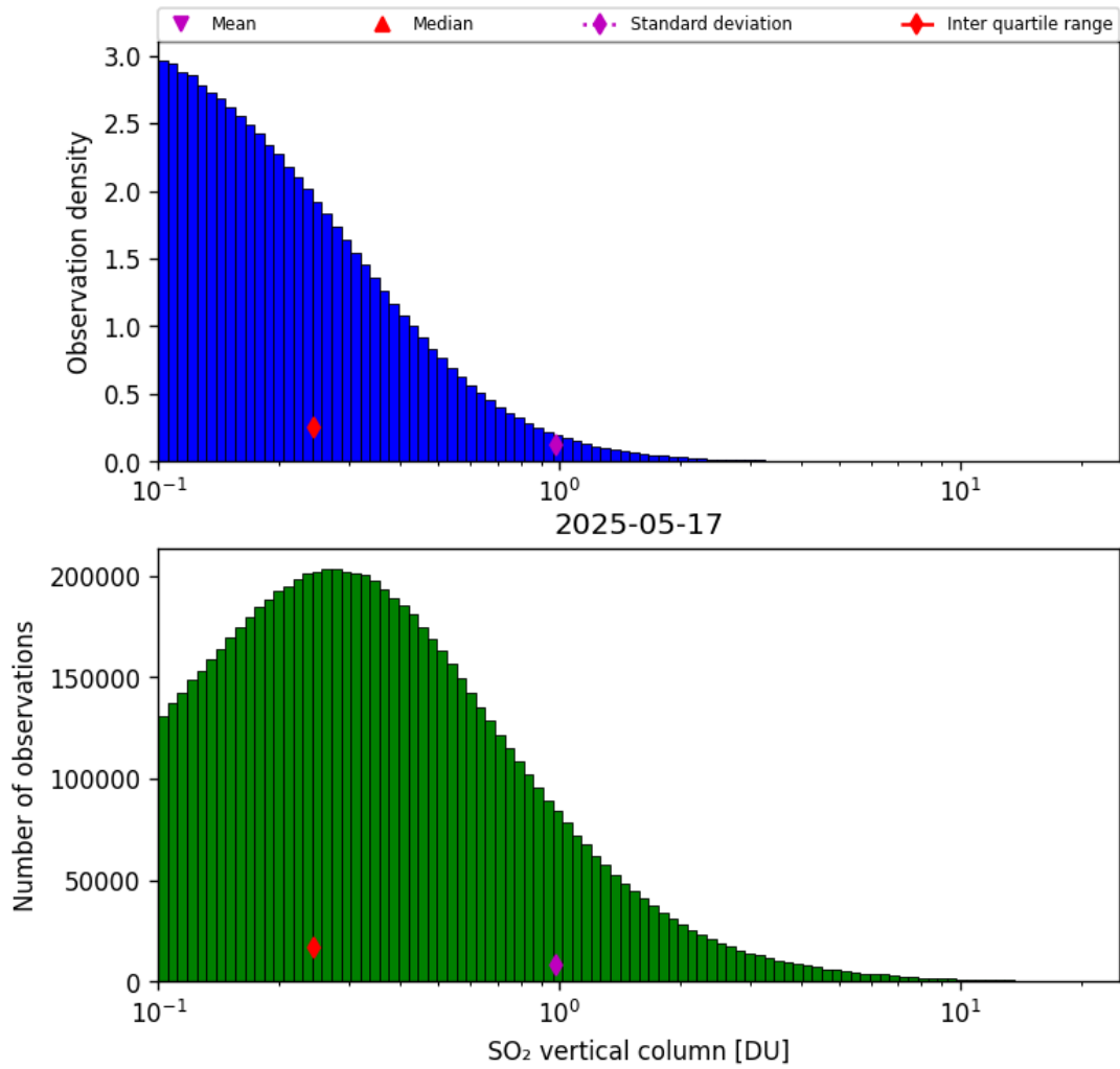
Figure 58: Histogram of “SO 2 vertical column” for 2025-05-16 to 2025-05-18
