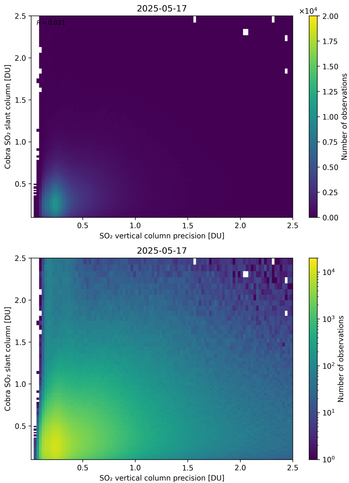
Figure 336: Scatter density plot of “SO 2 vertical column precision” against “Cobra SO 2 slant column” for 2025-05-16 to 2025-05-18.
