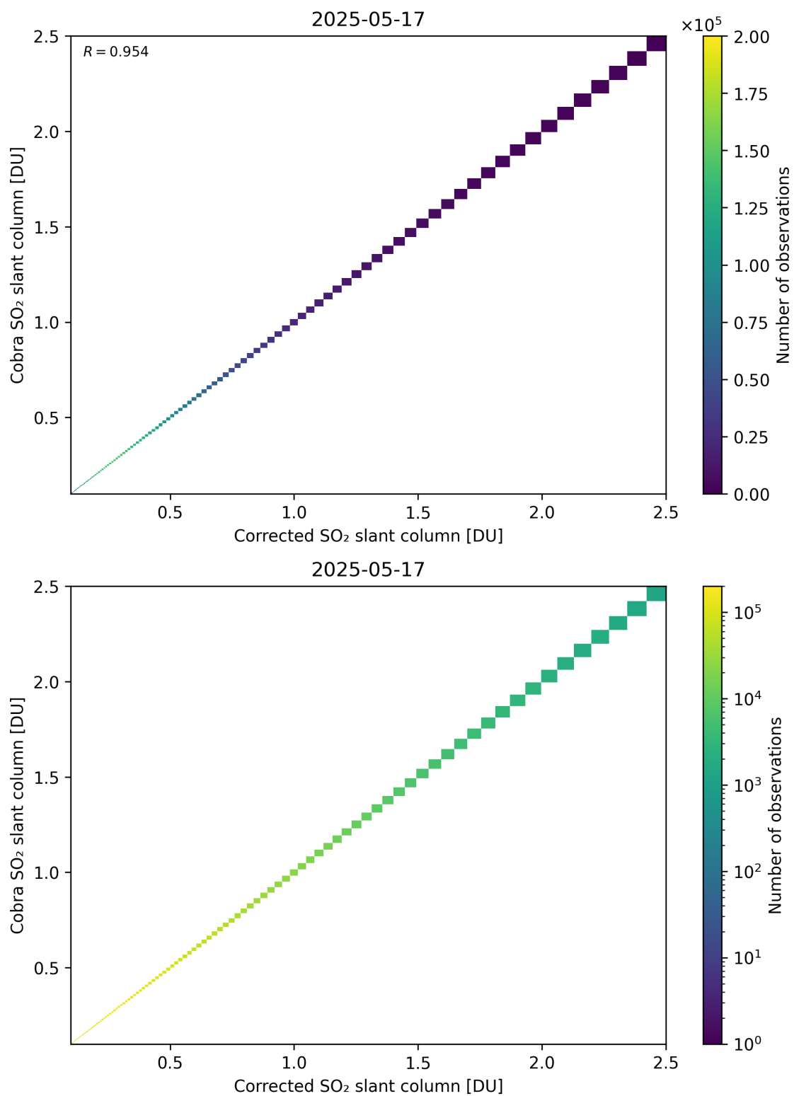
Figure 233: Scatter density plot of “Corrected SO 2 slant column” against “Cobra SO 2 slant column” for 2025-05-16 to 2025-05-18.
