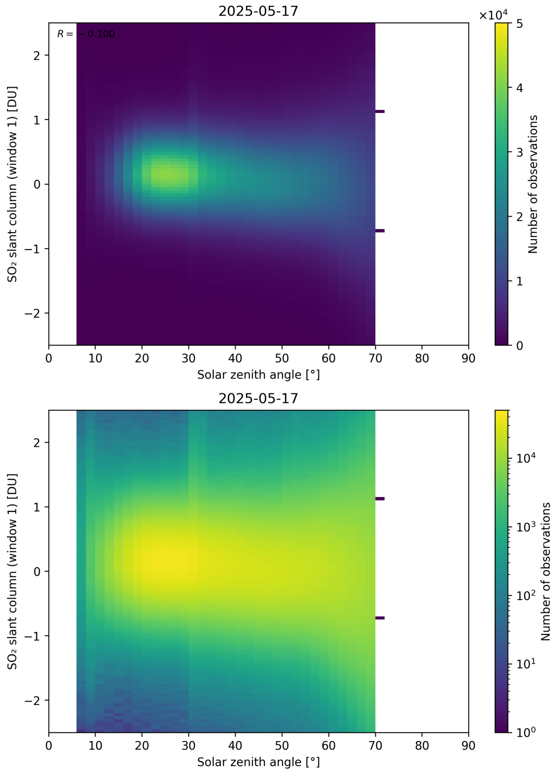
Figure 184: Scatter density plot of “Solar zenith angle” against “SO 2 slant column (window 1)” for 2025-05-16 to 2025-05-18.
