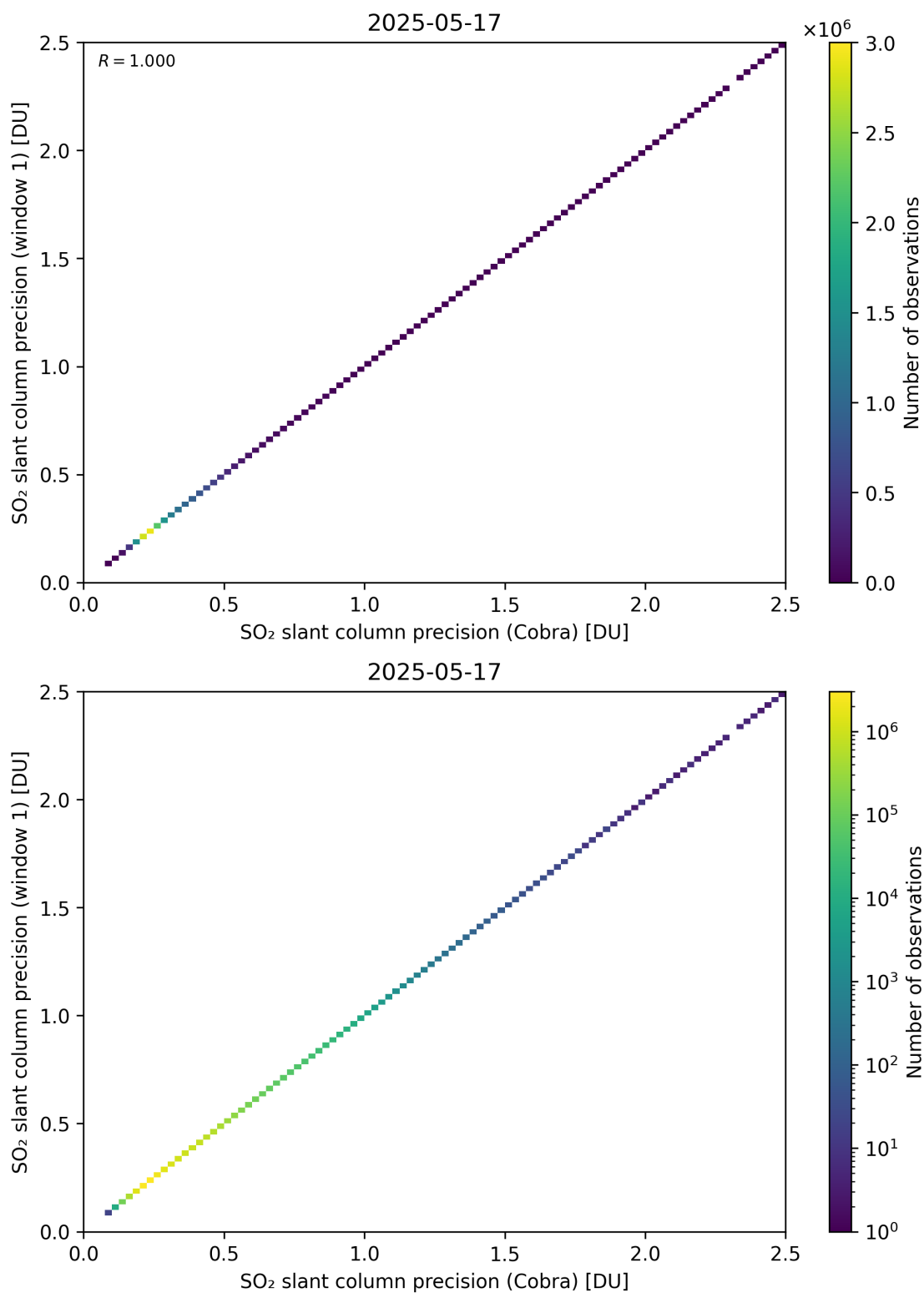
Figure 209: Scatter density plot of “SO 2 slant column precision (Cobra)” against “SO 2 slant column precision (window 1)” for 2025-05-16 to 2025-05-18.
