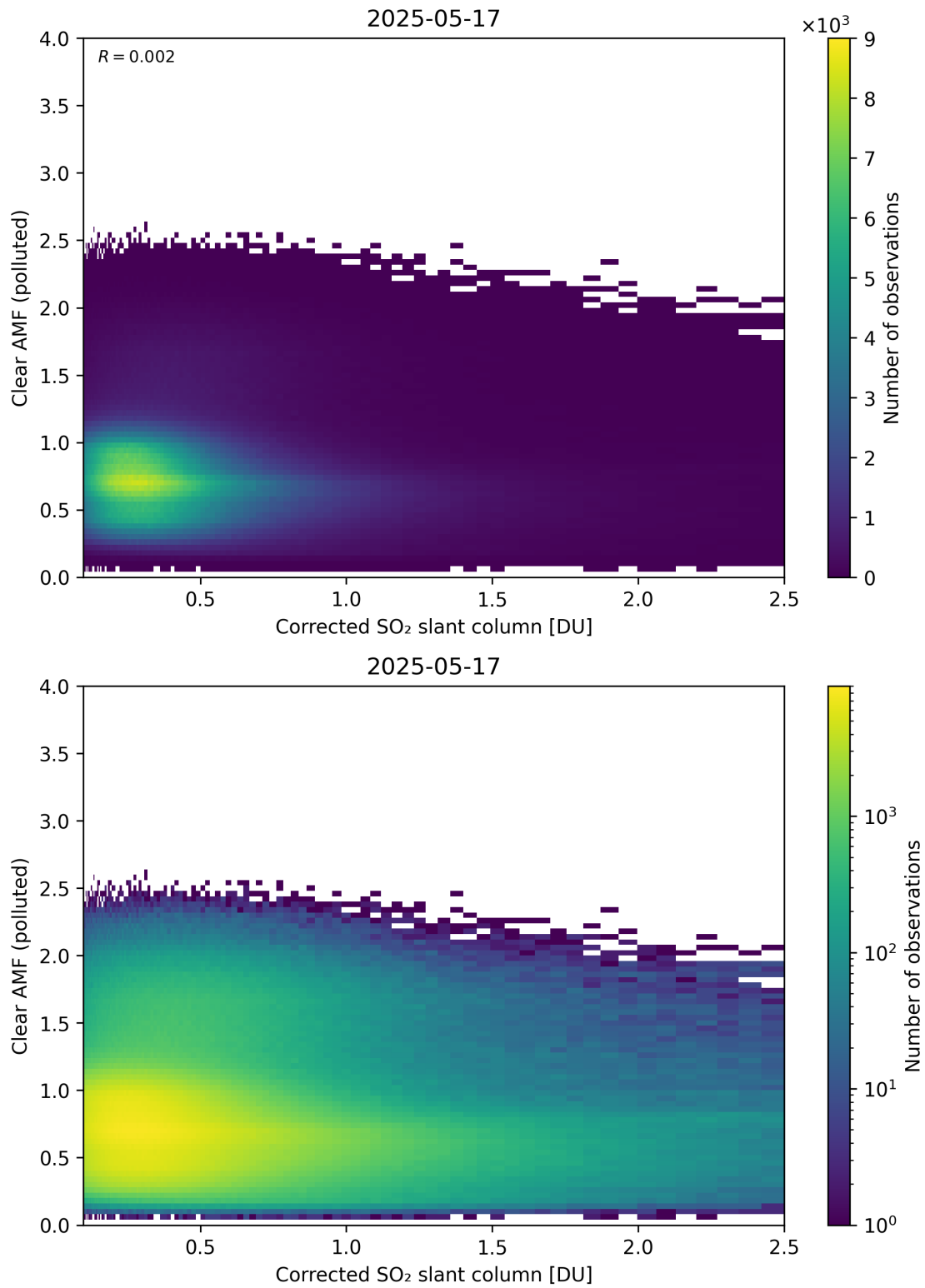
Figure 232: Scatter density plot of “Corrected SO 2 slant column” against “Clear AMF (polluted)” for 2025-05-16 to 2025-05-18.
