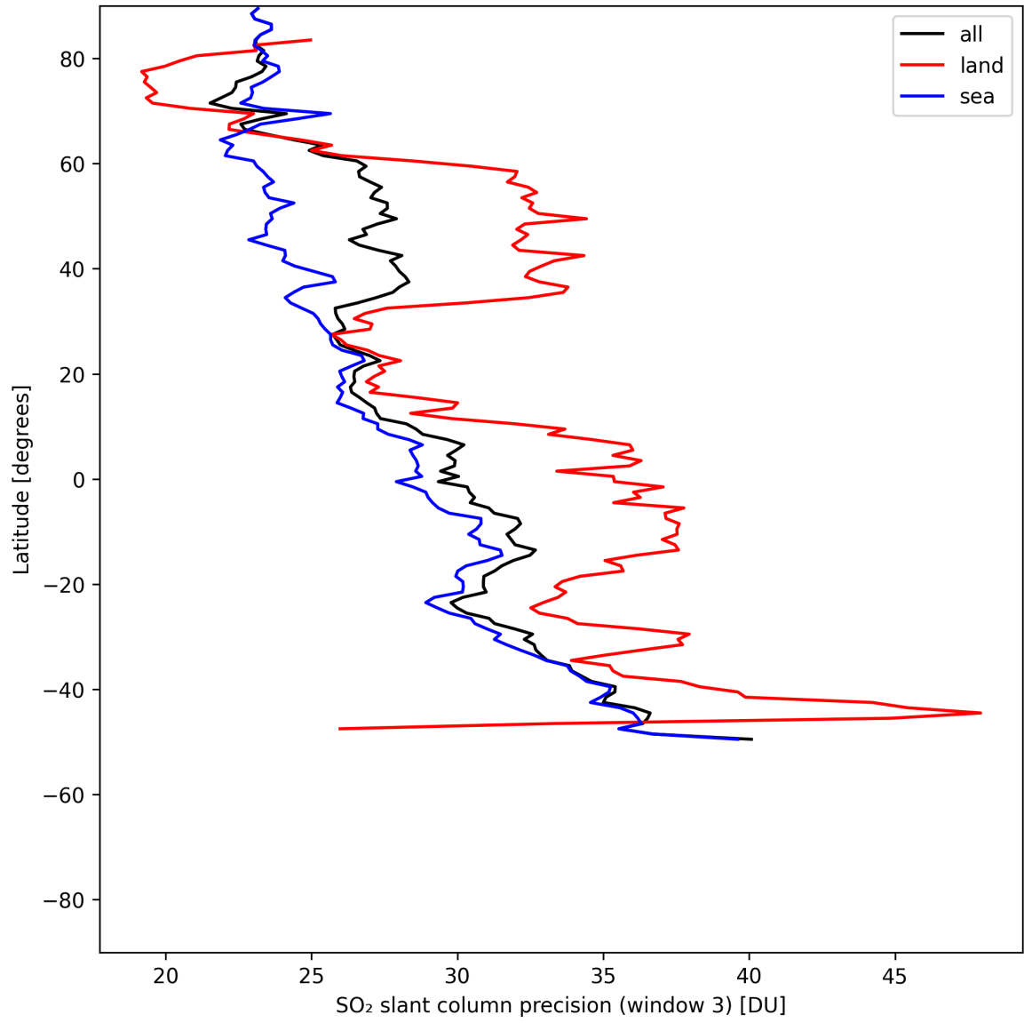
Figure 46: Zonal average of “SO 2 slant column precision (window 3)” for 2025-05-16 to 2025-05-18.
