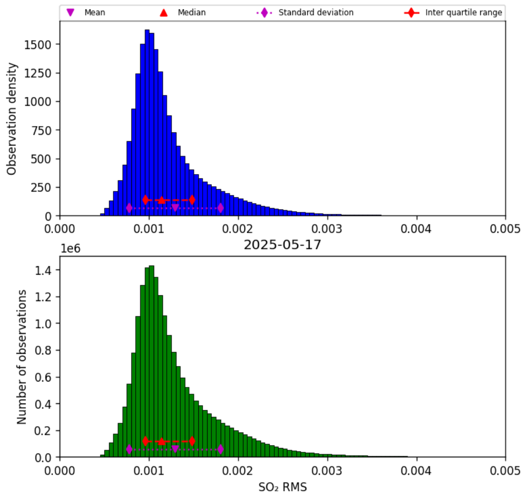
Figure 78: Histogram of “SO 2 RMS” for 2025-05-16 to 2025-05-18
