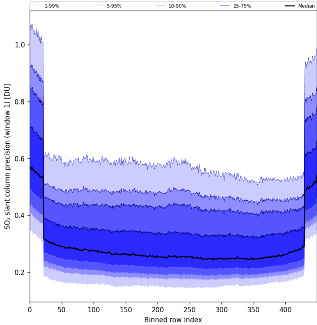
Figure 90: Along track statistics of “SO 2 slant column precision (window 1)” for 2025-05-16 to 2025-05-18
