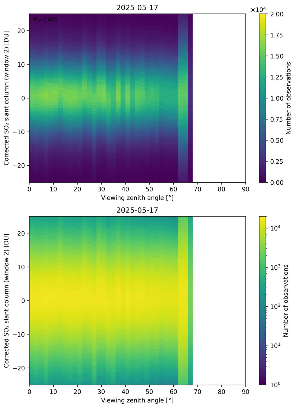
Figure 374: Scatter density plot of “Viewing zenith angle” against “Corrected SO 2 slant column (window 2)” for 2025-05-16 to 2025-05-18.
