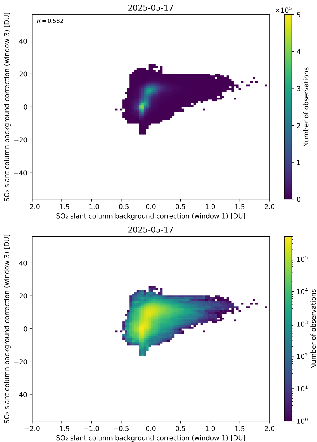
Figure 110: Scatter density plot of “SO 2 slant column background correction (window 1)” against “SO 2 slant column background correction (window 3)” for 2025-05-16 to 2025-05-18.
