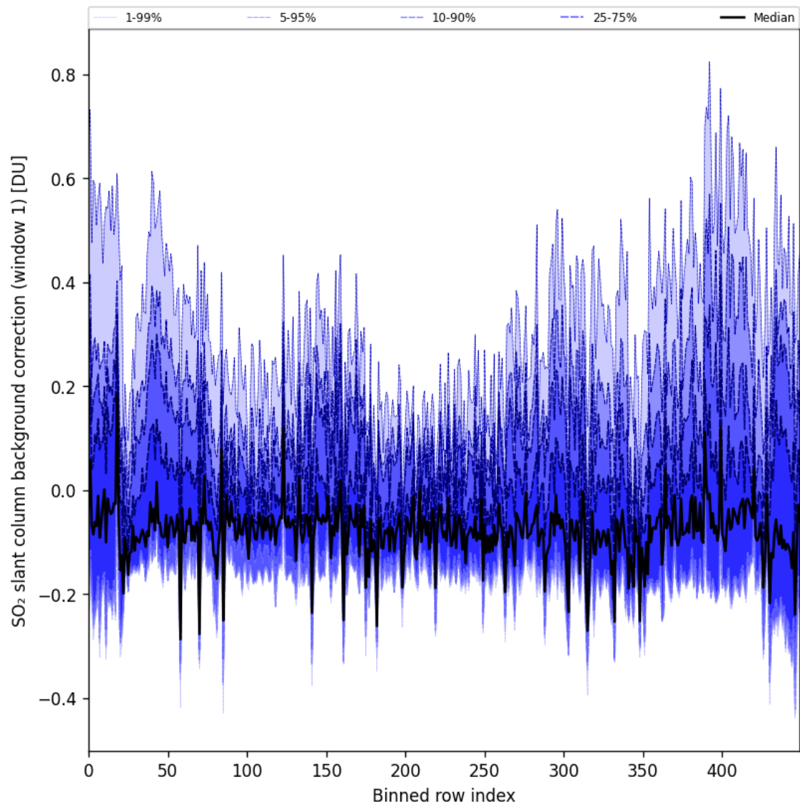
Figure 92: Along track statistics of “SO 2 slant column background correction (window 1)” for 2025-05-16 to 2025-05-18
