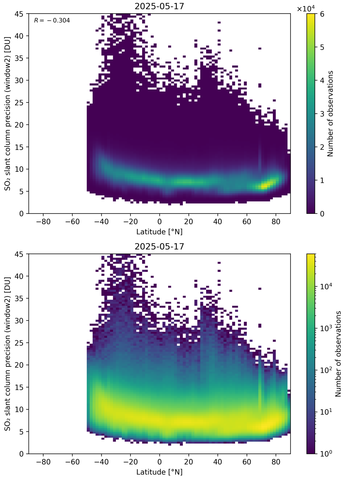
Figure 164: Scatter density plot of “Latitude” against “SO 2 slant column precision (window2)” for 2025-05-16 to 2025-05-18.
