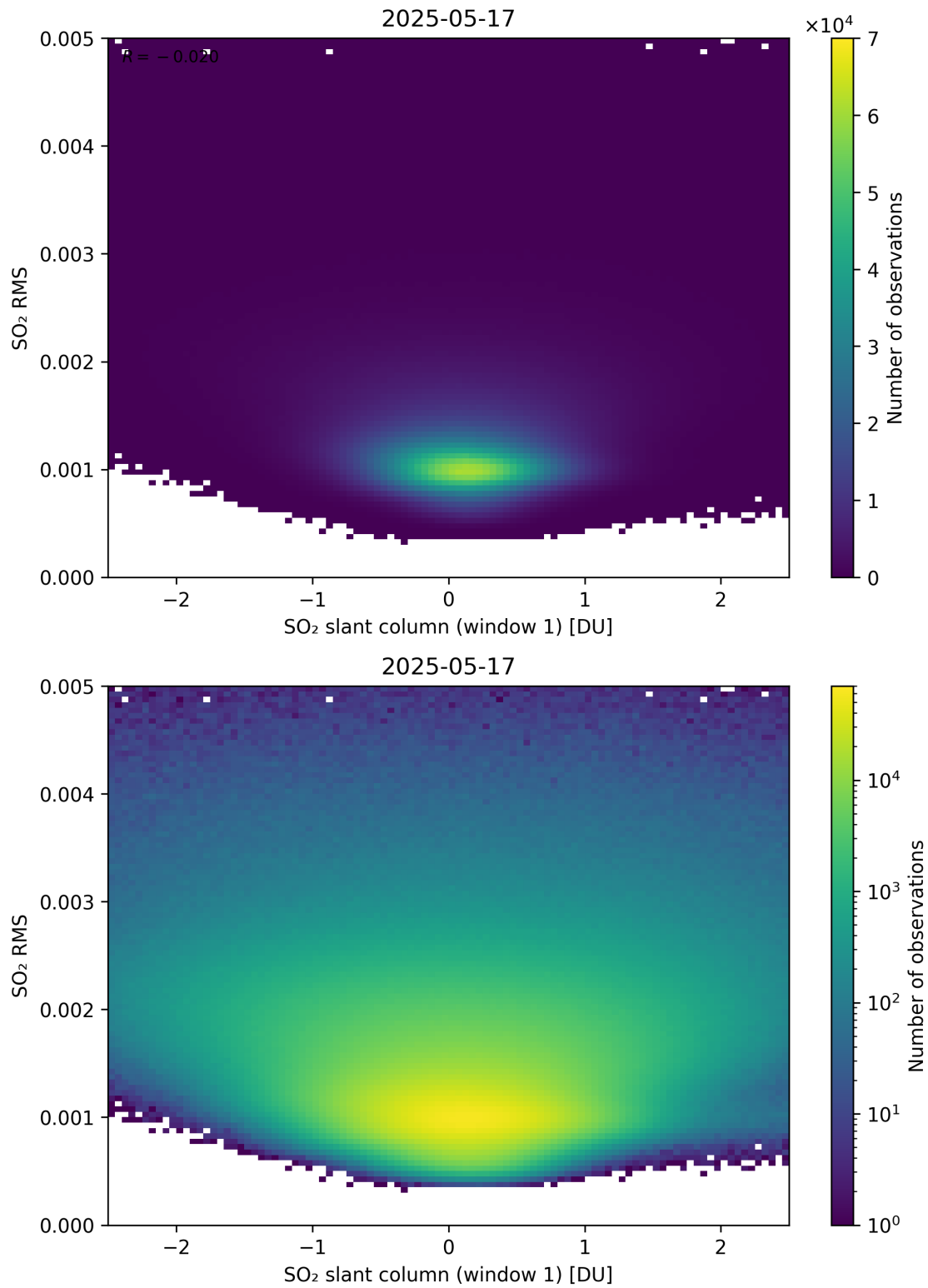
Figure 267: Scatter density plot of “SO 2 slant column (window 1)” against “SO 2 RMS” for 2025-05-16 to 2025-05-18.
