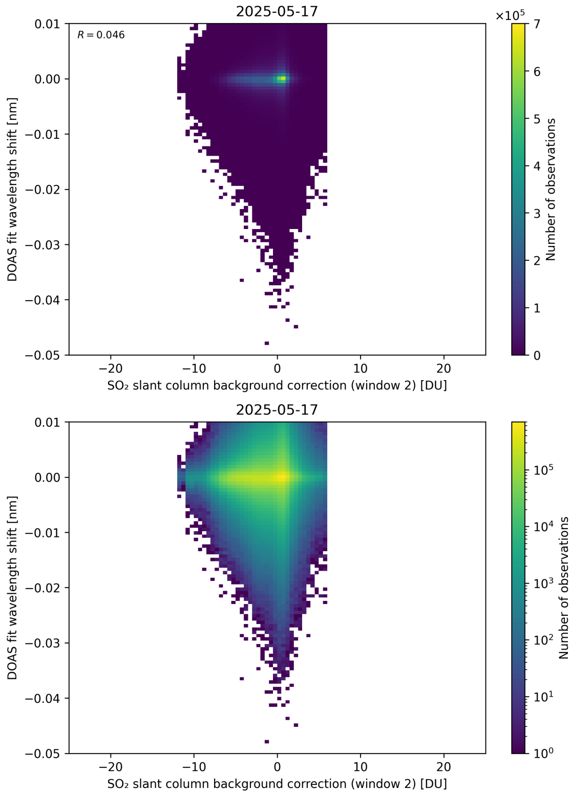
Figure 123: Scatter density plot of “SO 2 slant column background correction (window 2)” against “DOAS fit wavelength shift” for 2025-05-16 to 2025-05-18.
