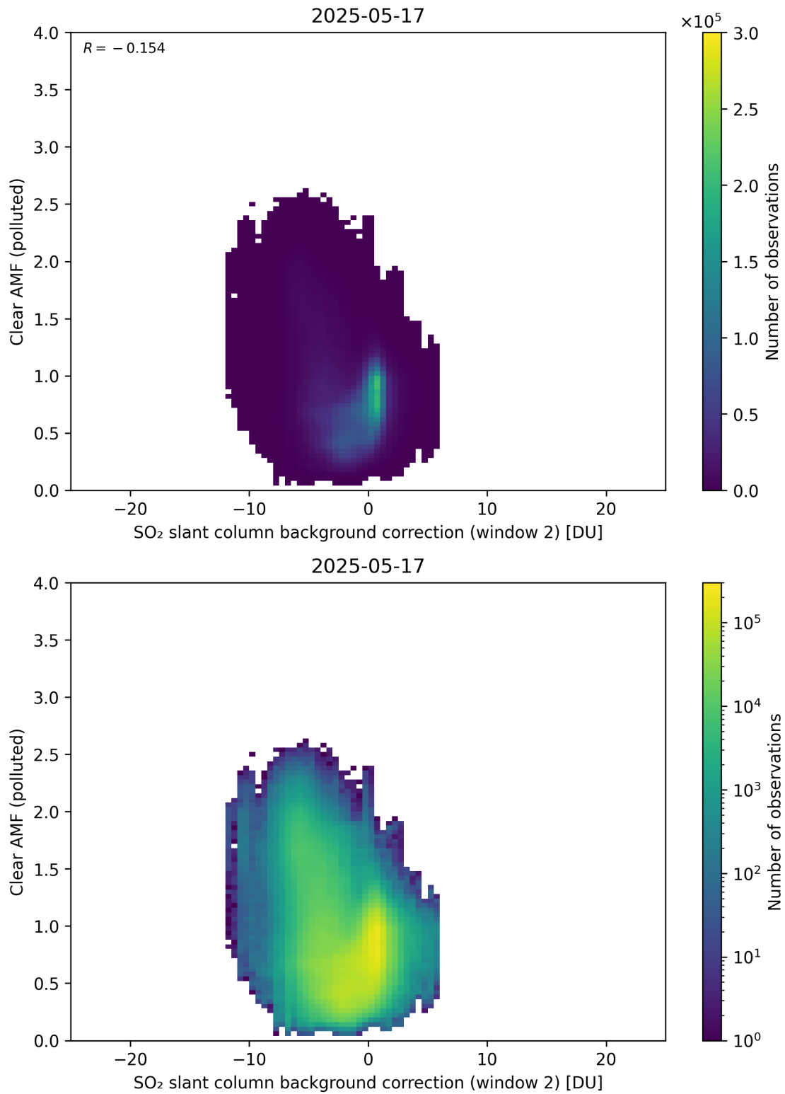
Figure 126: Scatter density plot of “SO 2 slant column background correction (window 2)” against “Clear AMF (polluted)” for 2025-05-16 to 2025-05-18.
