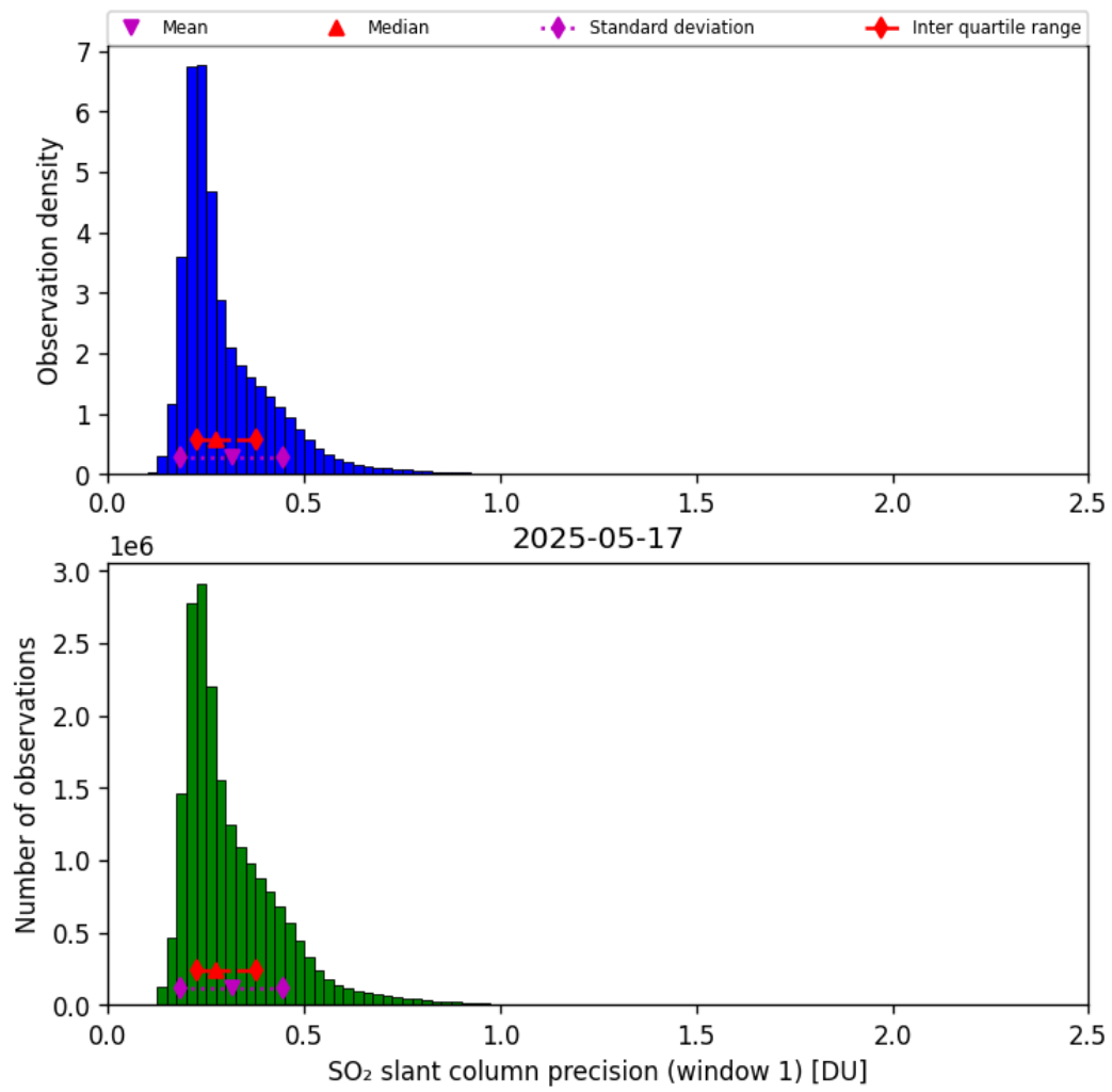
Figure 64: Histogram of “SO 2 slant column precision (window 1)” for 2025-05-16 to 2025-05-18
