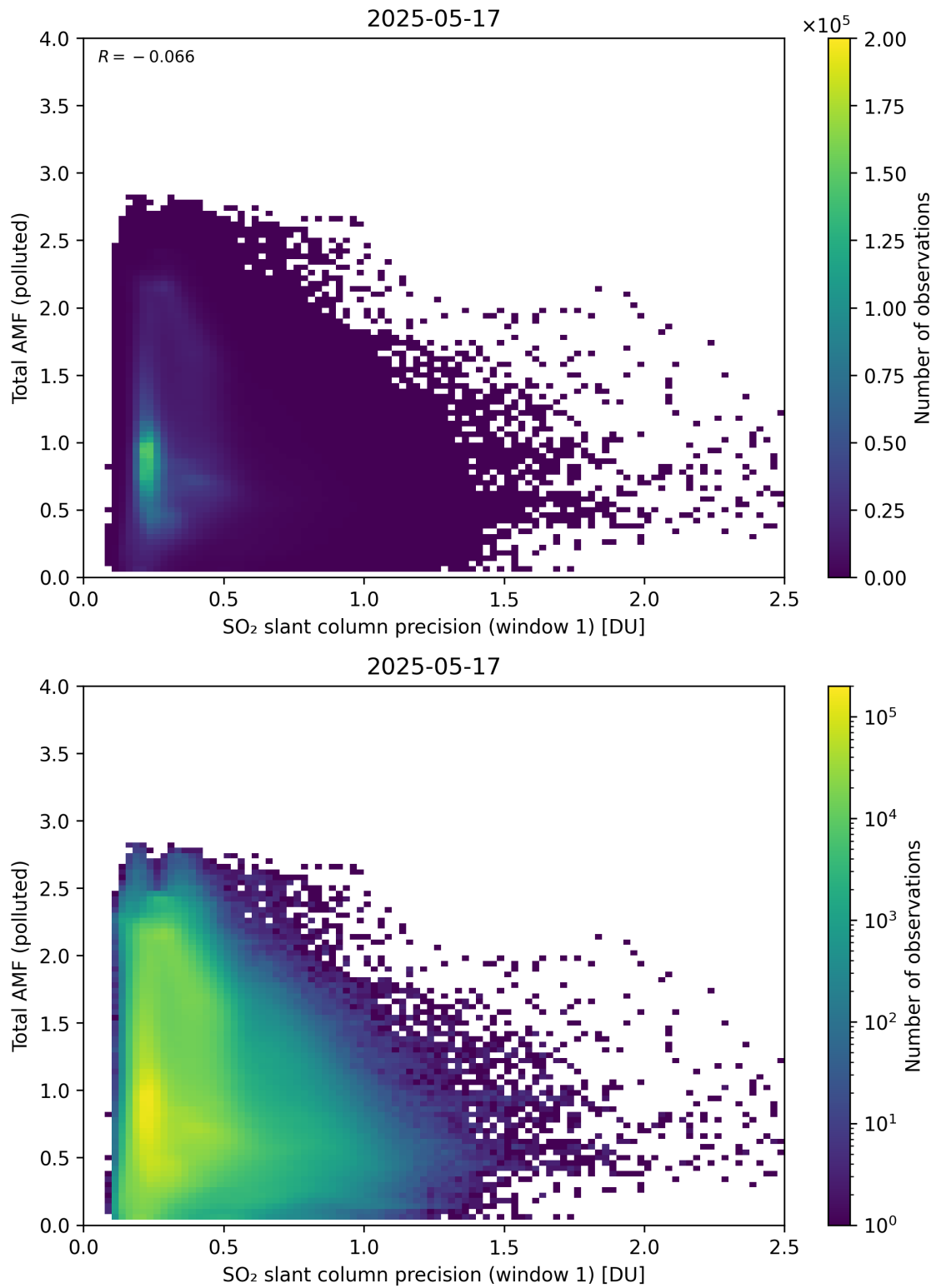
Figure 280: Scatter density plot of “SO 2 slant column precision (window 1)” against “Total AMF (polluted)” for 2025-05-16 to 2025-05-18.
