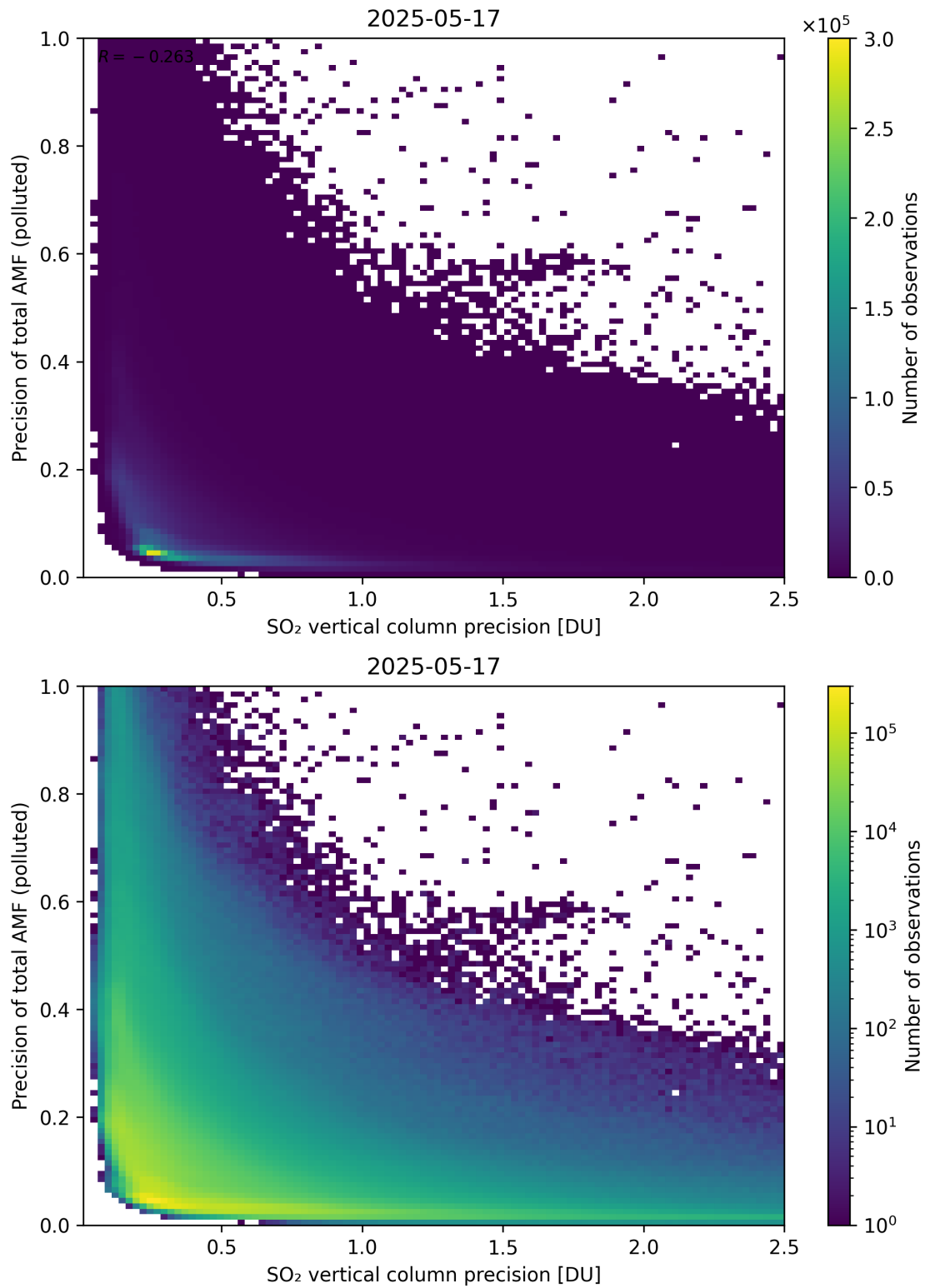
Figure 347: Scatter density plot of “SO 2 vertical column precision” against “Precision of total AMF (polluted)” for 2025-05-16 to 2025-05-18.
