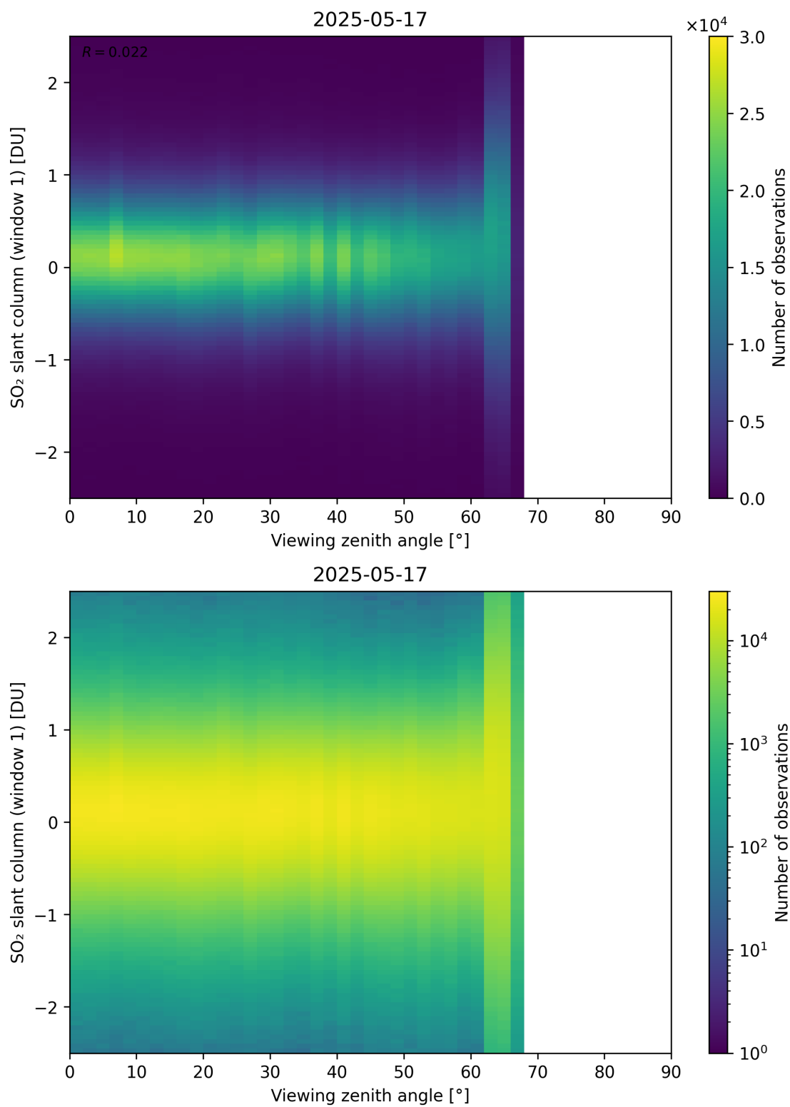
Figure 376: Scatter density plot of “Viewing zenith angle” against “SO 2 slant column (window 1)” for 2025-05-16 to 2025-05-18.
