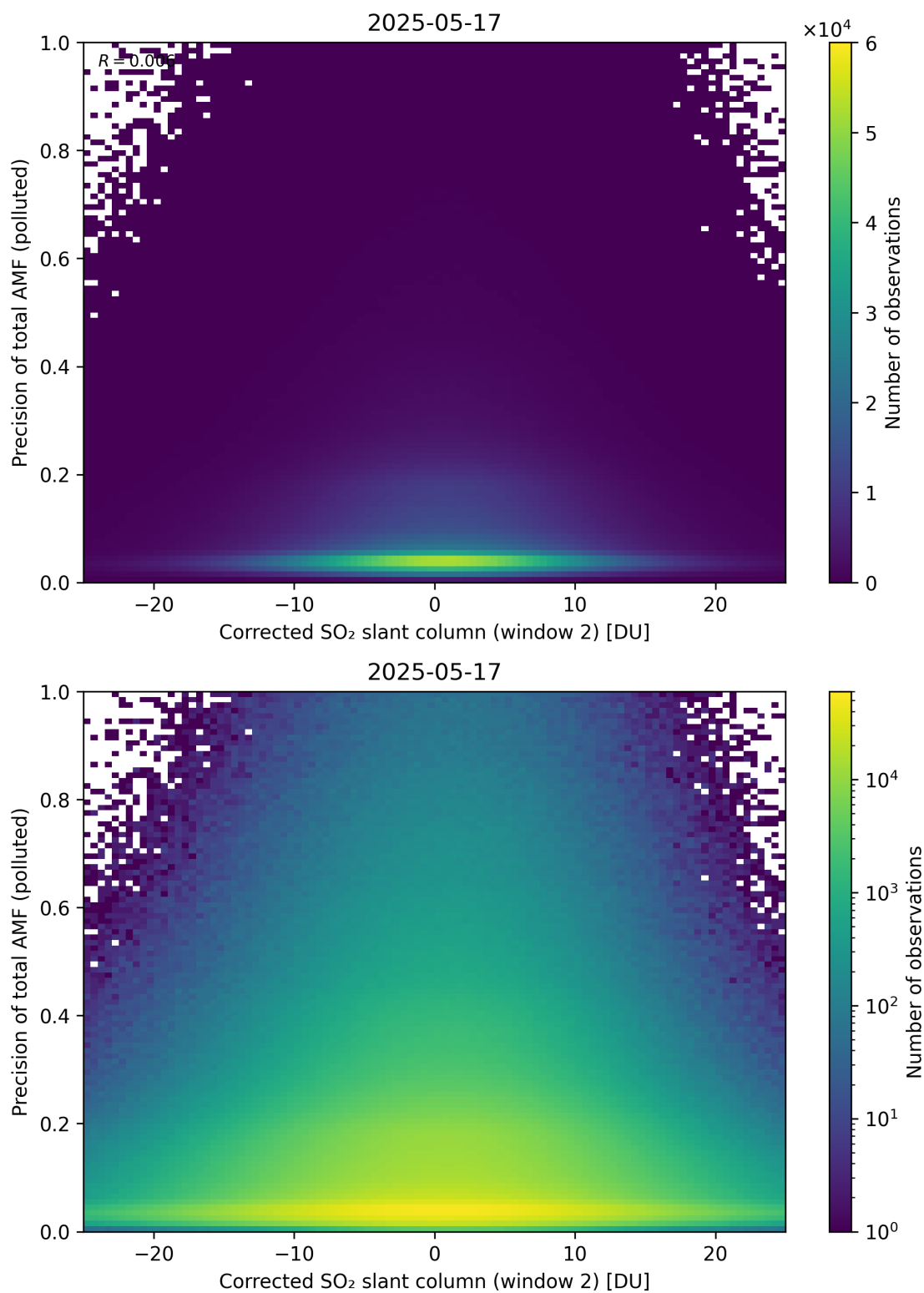
Figure 254: Scatter density plot of “Corrected SO 2 slant column (window 2)” against “Precision of total AMF (polluted)” for 2025-05-16 to 2025-05-18.
