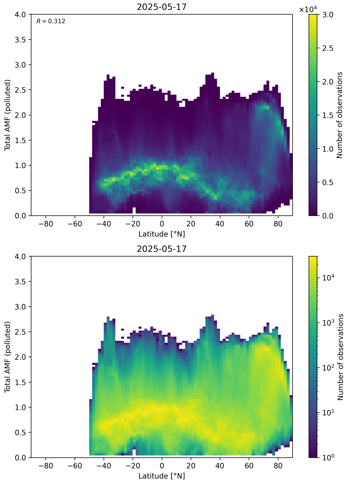
Figure 167: Scatter density plot of “Latitude” against “Total AMF (polluted)” for 2025-05-16 to 2025-05-18.
