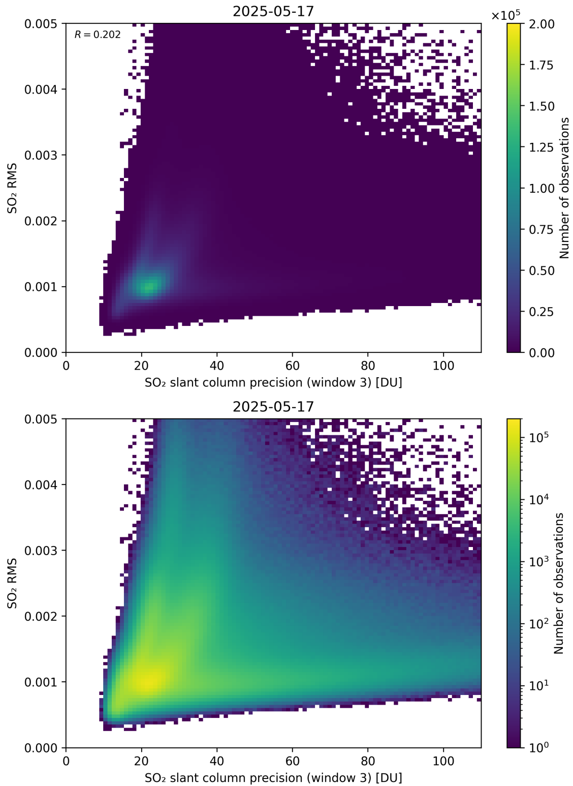
Figure 310: Scatter density plot of “SO 2 slant column precision (window 3)” against “SO 2 RMS” for 2025-05-16 to 2025-05-18.
