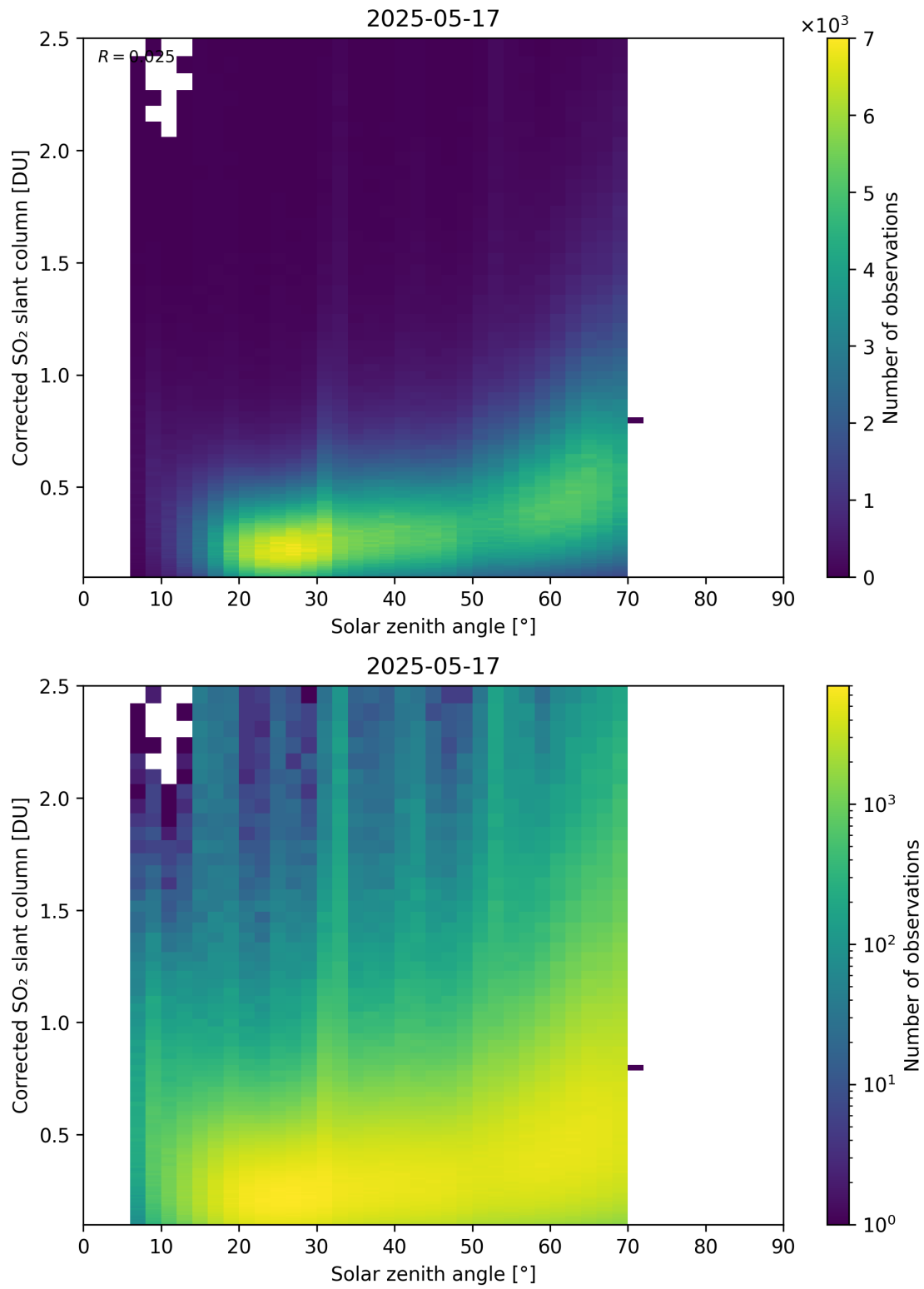
Figure 181: Scatter density plot of “Solar zenith angle” against “Corrected SO 2 slant column” for 2025-05-16 to 2025-05-18.
