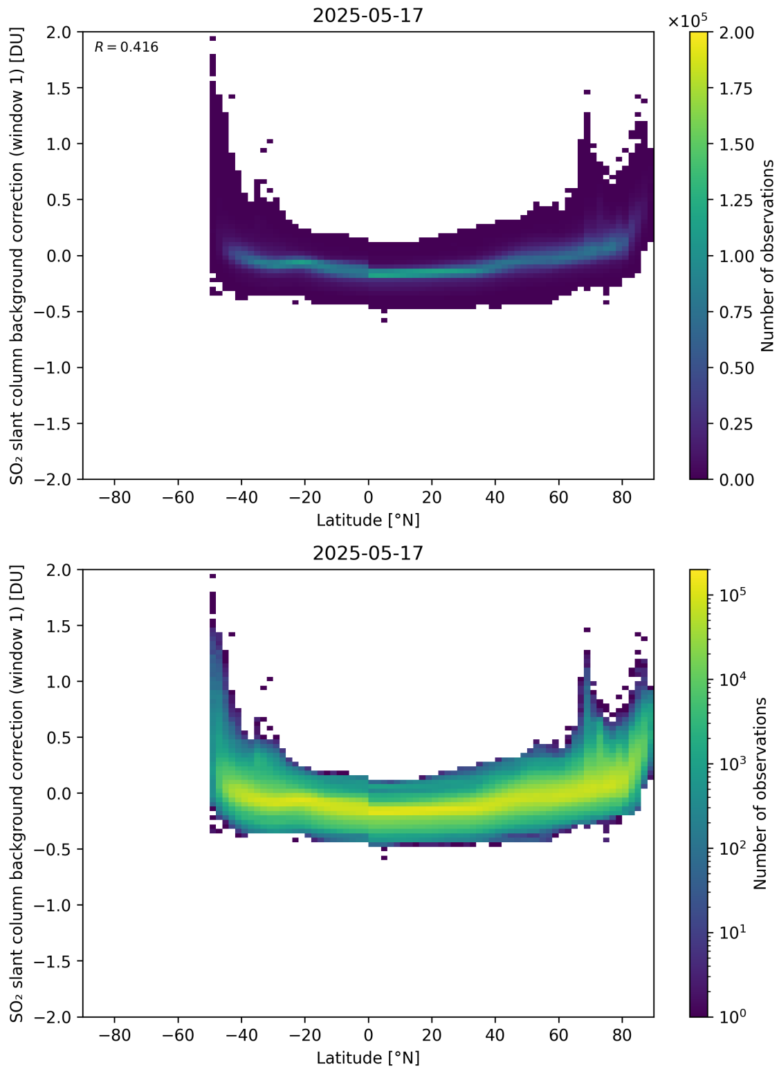
Figure 150: Scatter density plot of “Latitude” against “SO 2 slant column background correction (window 1)” for 2025-05-16 to 2025-05-18.
