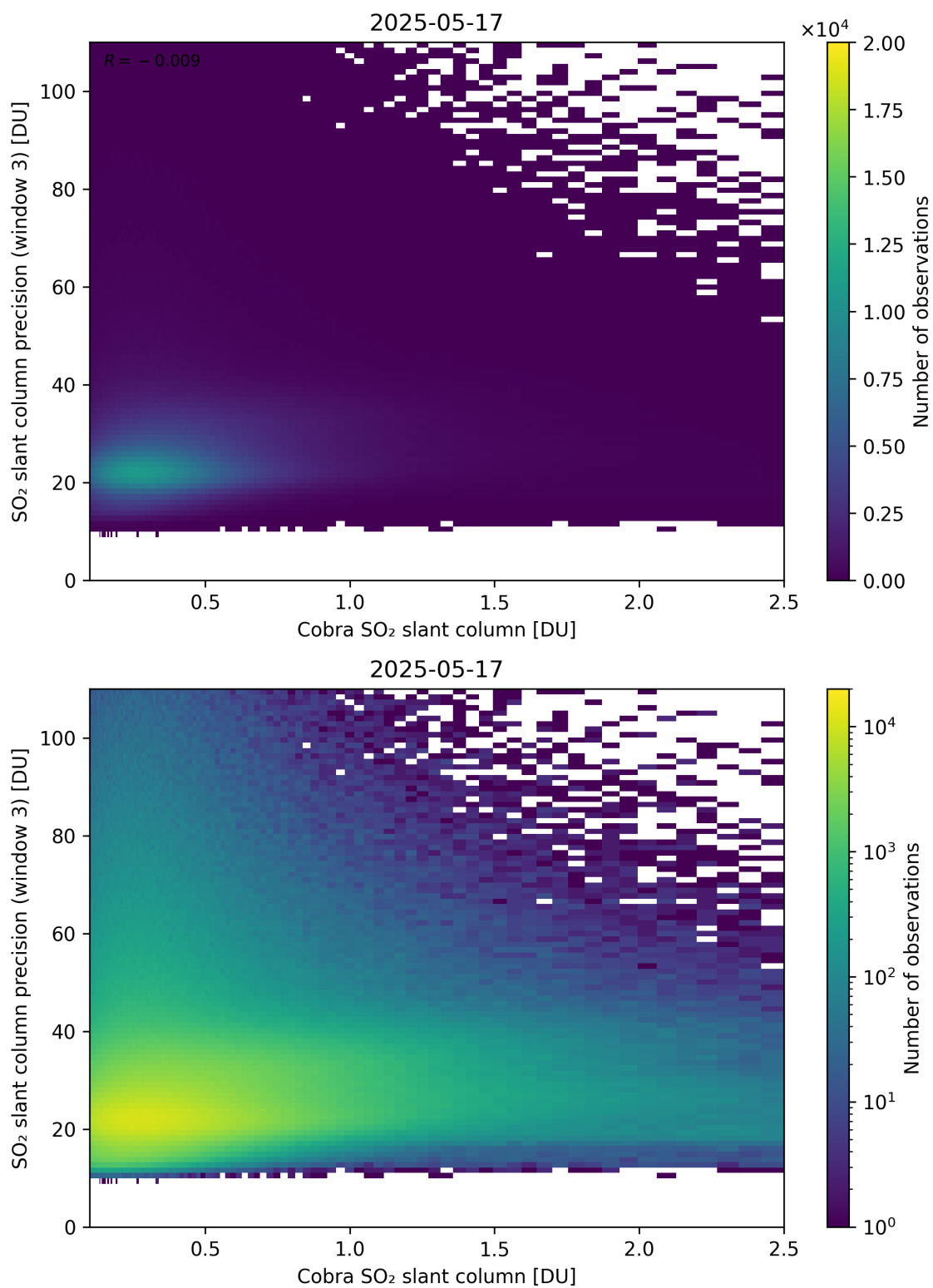
Figure 223: Scatter density plot of “Cobra SO 2 slant column” against “SO 2 slant column precision (window 3)” for 2025-05-16 to 2025-05-18.
