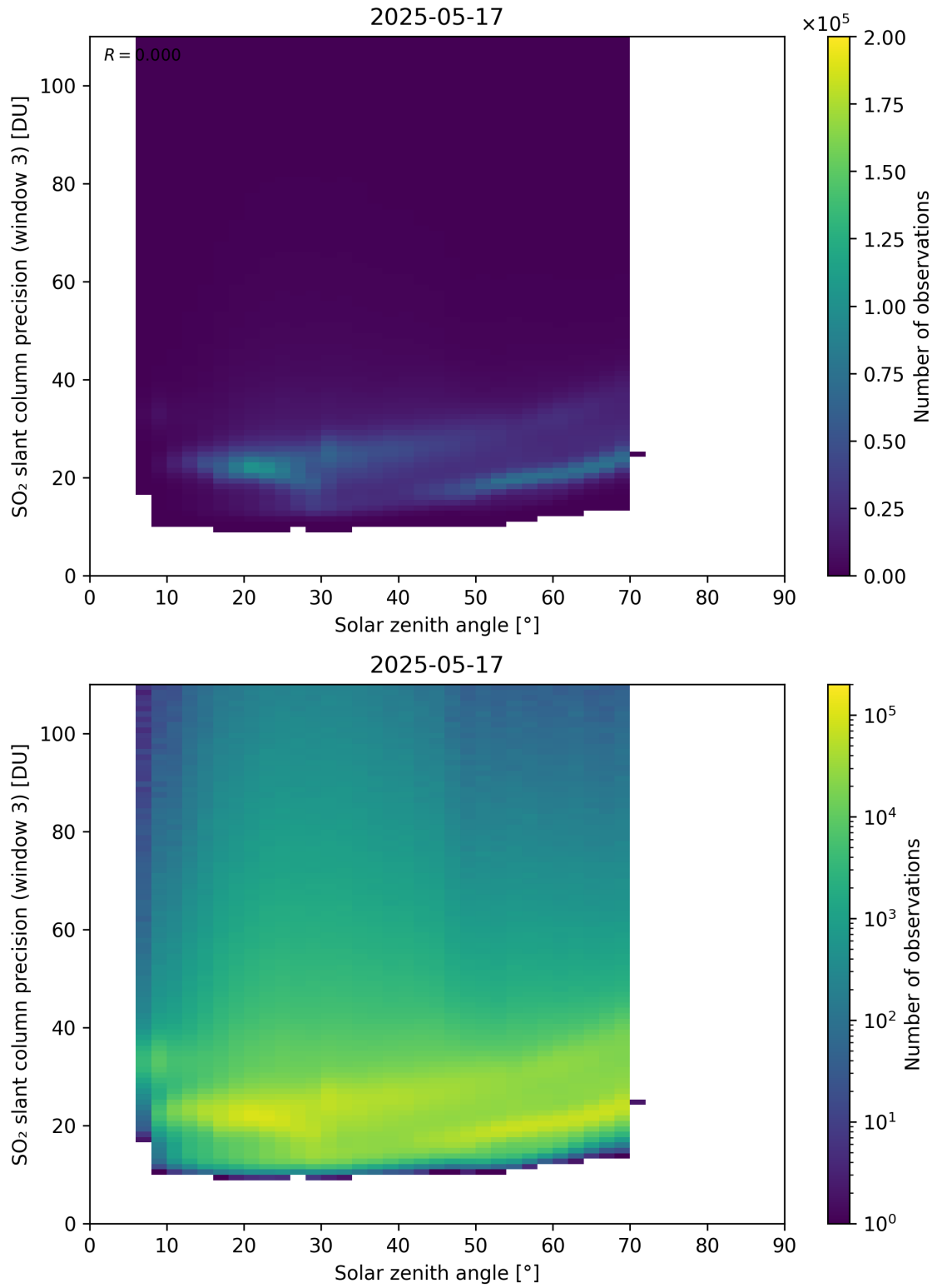
Figure 188: Scatter density plot of “Solar zenith angle” against “SO 2 slant column precision (window 3)” for 2025-05-16 to 2025-05-18.
