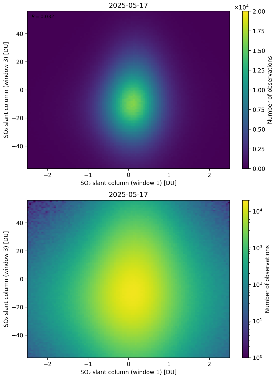
Figure 287: Scatter density plot of “SO 2 slant column (window 1)” against “SO 2 slant column (window 3)” for 2025-05-16 to 2025-05-18.
