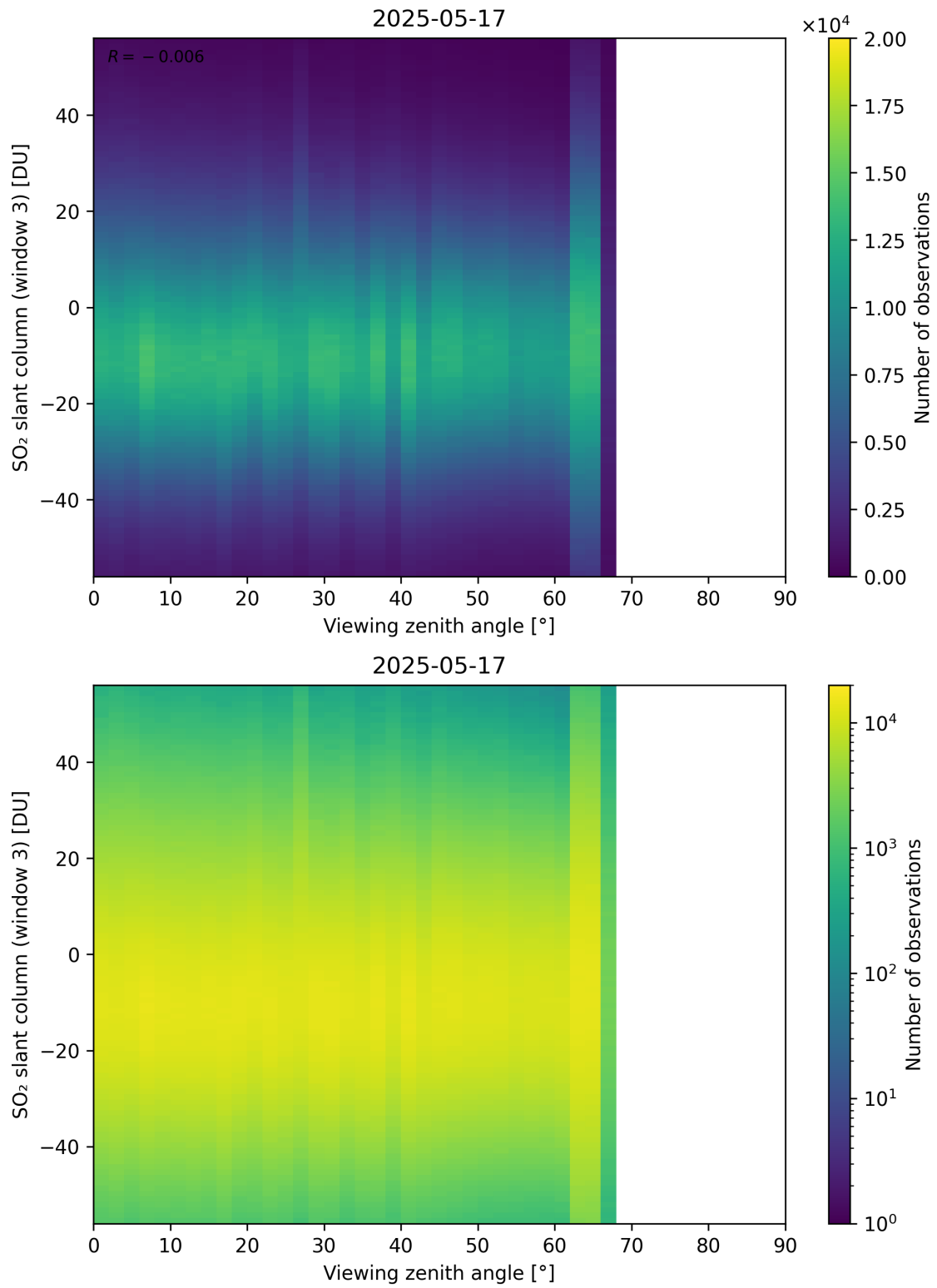
Figure 379: Scatter density plot of “Viewing zenith angle” against “SO 2 slant column (window 3)” for 2025-05-16 to 2025-05-18.
