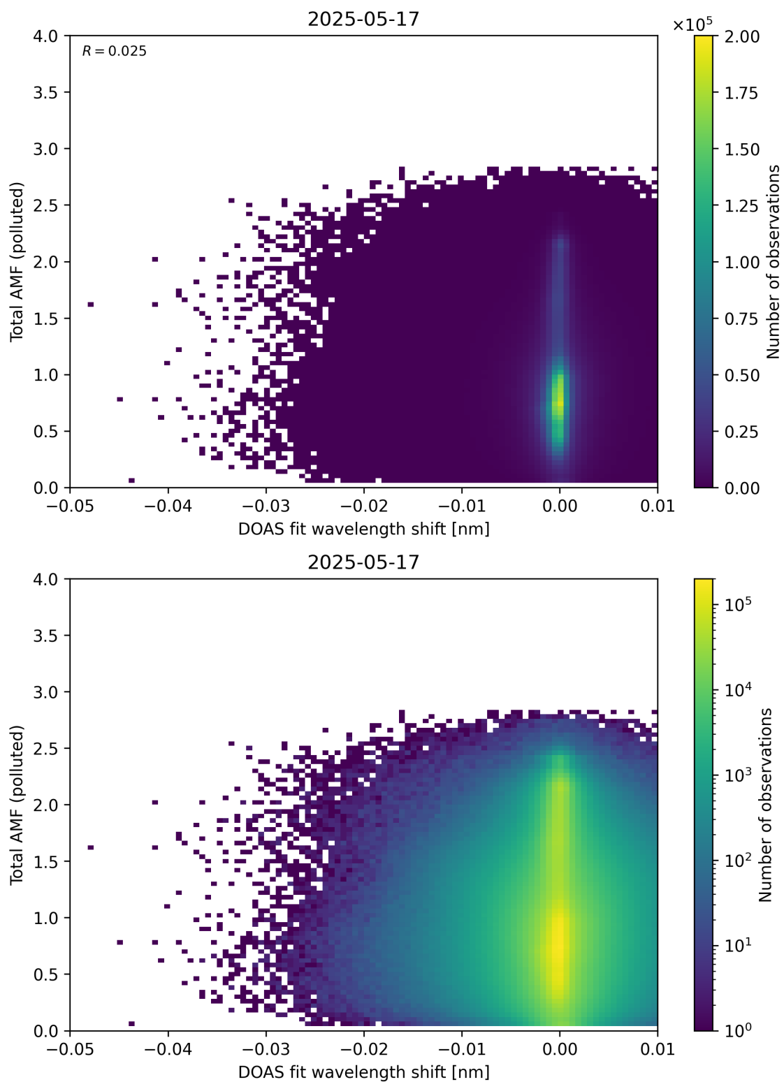
Figure 141: Scatter density plot of “DOAS fit wavelength shift” against “Total AMF (polluted)” for 2025-05-16 to 2025-05-18.
