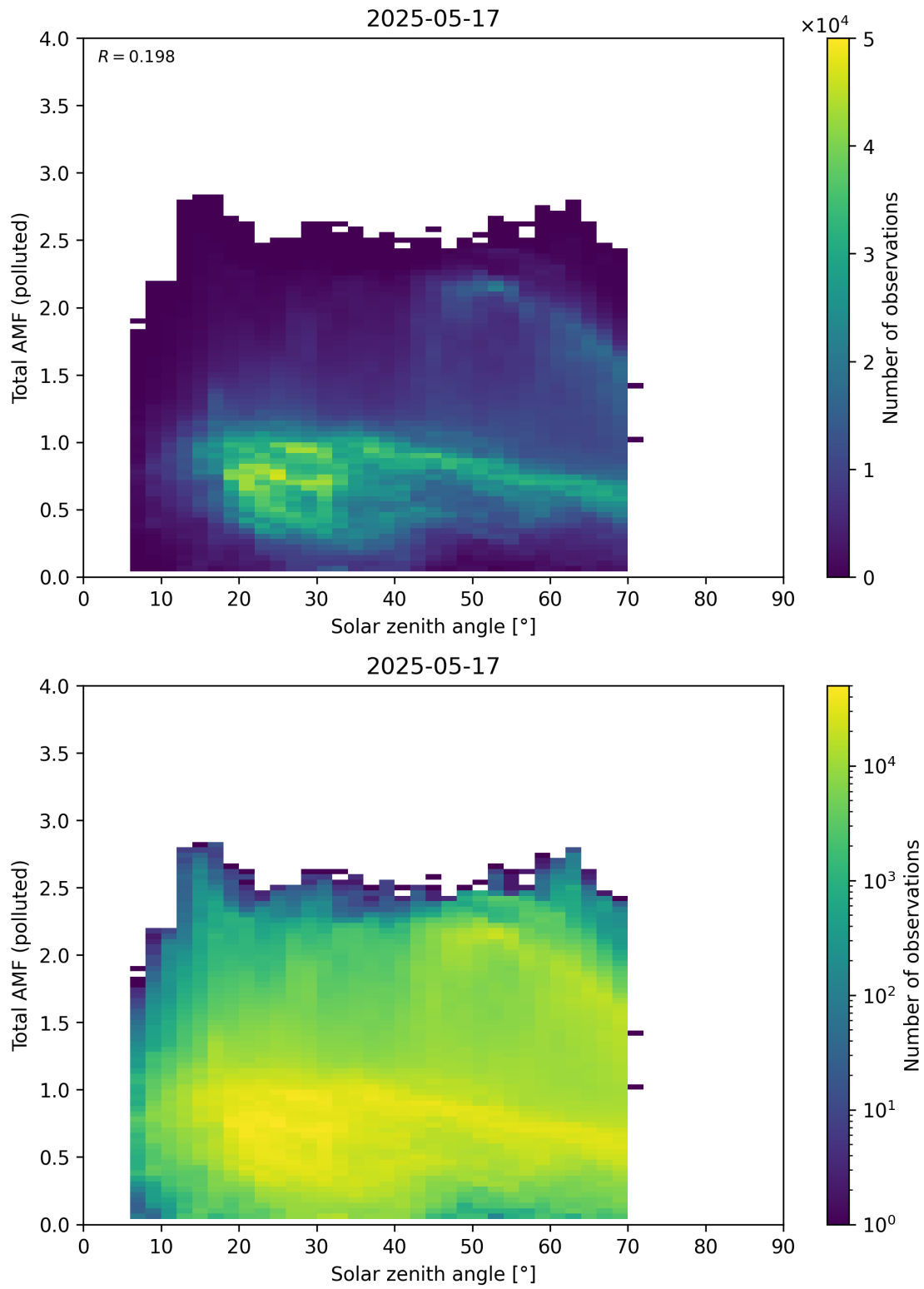
Figure 189: Scatter density plot of “Solar zenith angle” against “Total AMF (polluted)” for 2025-05-16 to 2025-05-18.
