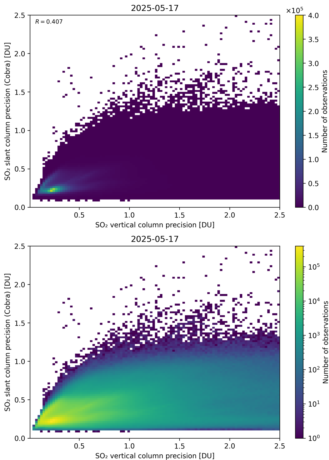
Figure 337: Scatter density plot of “SO 2 vertical column precision” against “SO 2 slant column precision (Cobra)” for 2025-05-16 to 2025-05-18.
