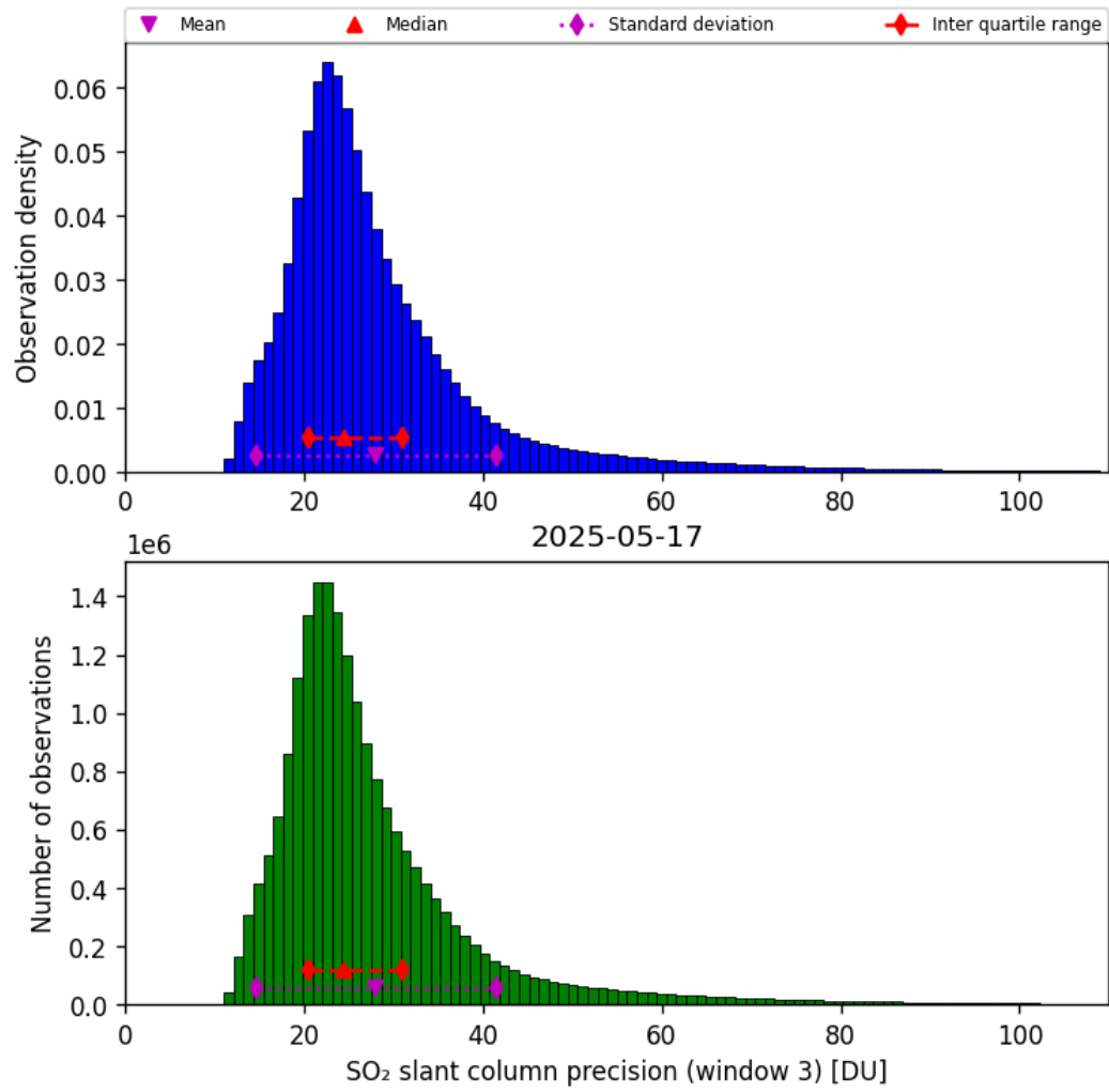
Figure 72: Histogram of “SO 2 slant column precision (window 3)” for 2025-05-16 to 2025-05-18
