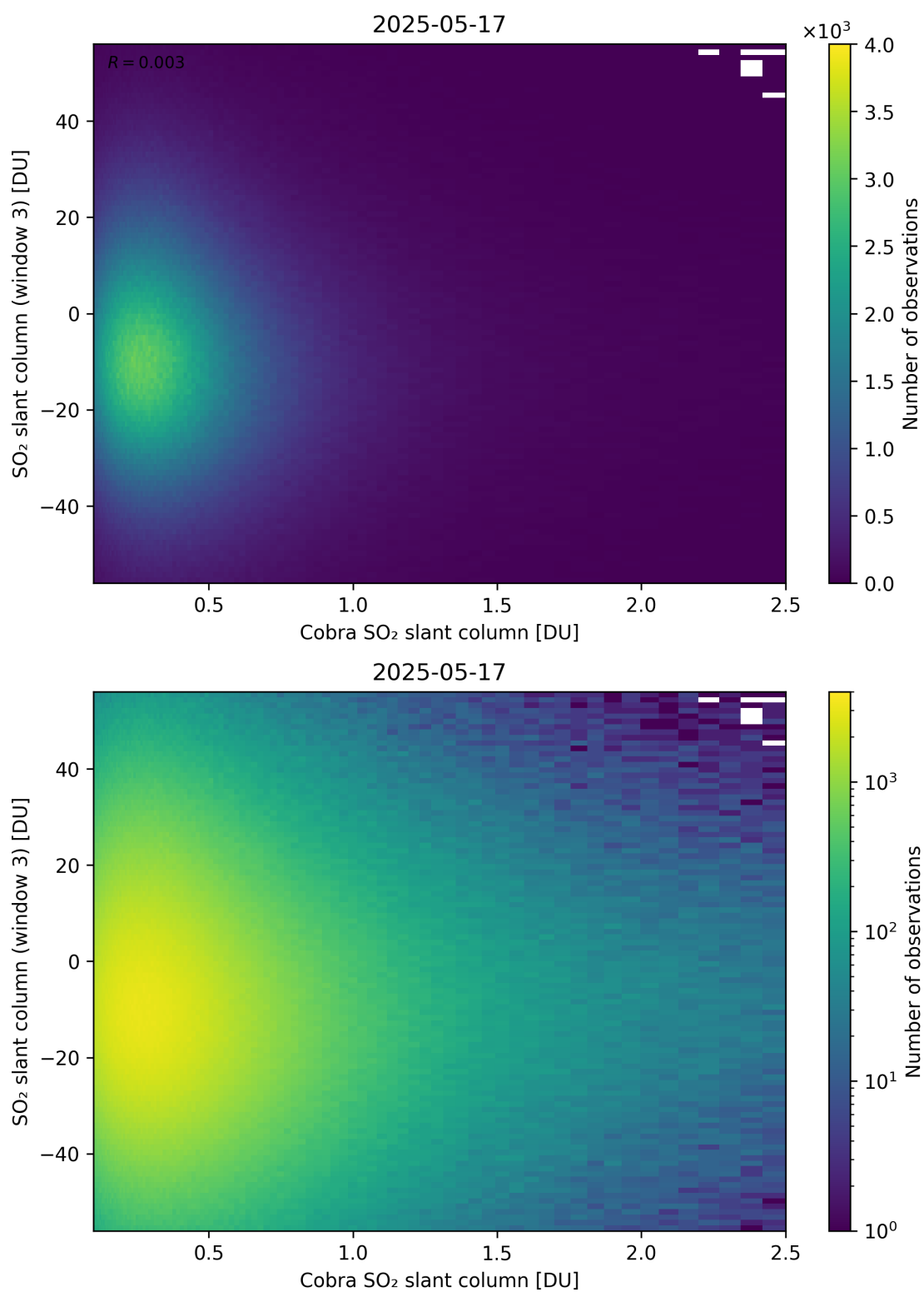
Figure 222: Scatter density plot of “Cobra SO 2 slant column” against “SO 2 slant column (window 3)” for 2025-05-16 to 2025-05-18.
