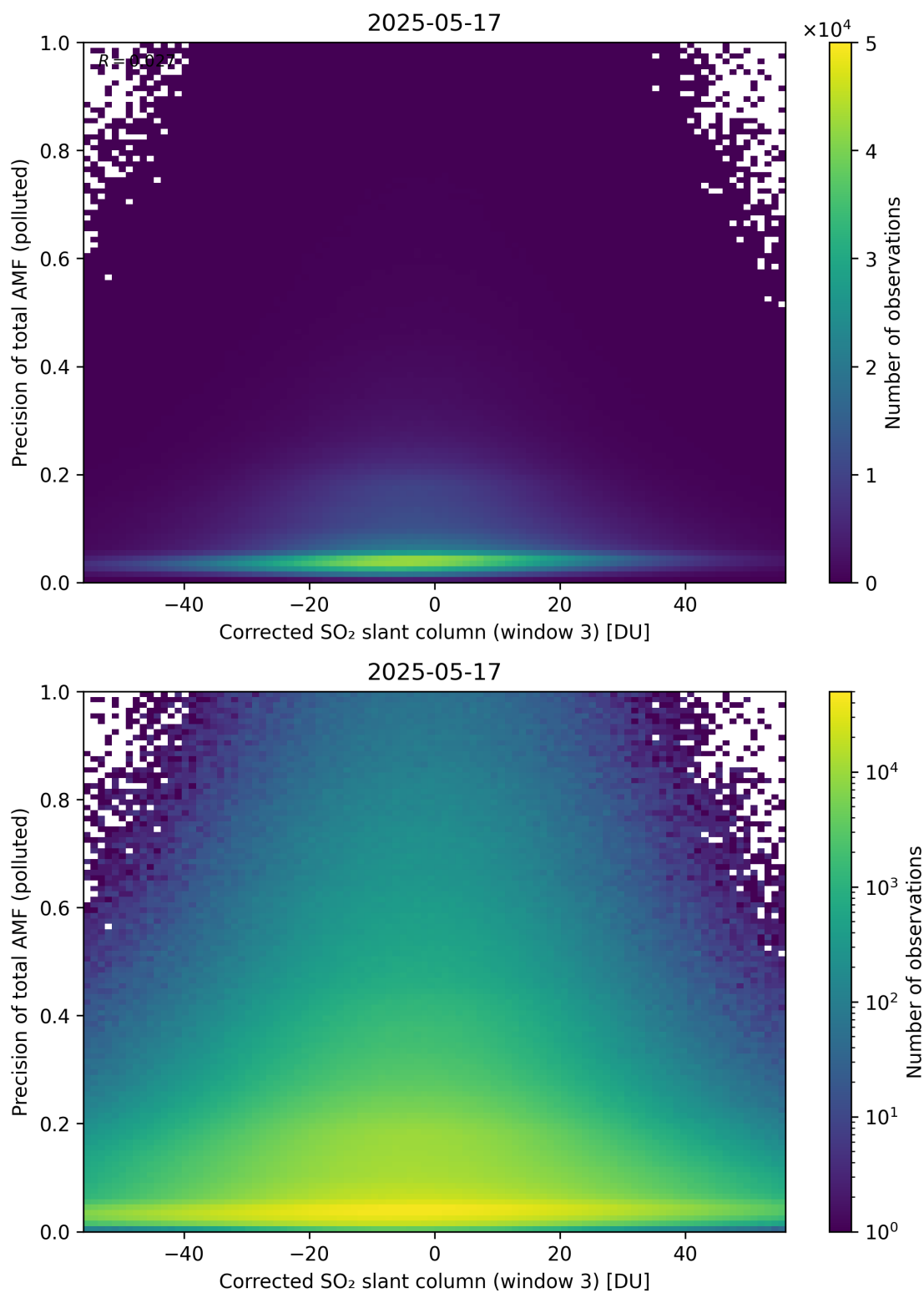
Figure 261: Scatter density plot of “Corrected SO 2 slant column (window 3)” against “Precision of total AMF (polluted)” for 2025-05-16 to 2025-05-18.
