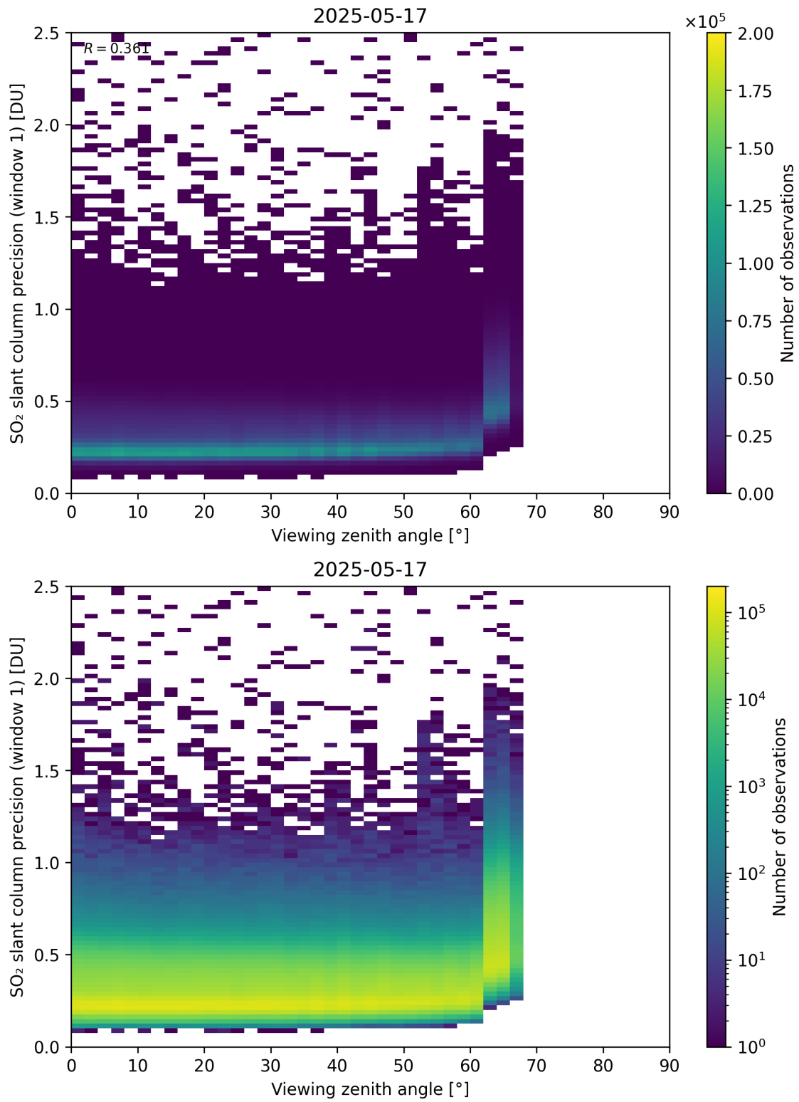
Figure 377: Scatter density plot of “Viewing zenith angle” against “SO 2 slant column precision (window 1)” for 2025-05-16 to 2025-05-18.
