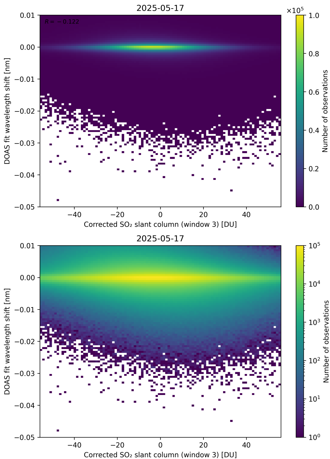
Figure 256: Scatter density plot of “Corrected SO 2 slant column (window 3)” against “DOAS fit wavelength shift” for 2025-05-16 to 2025-05-18.
