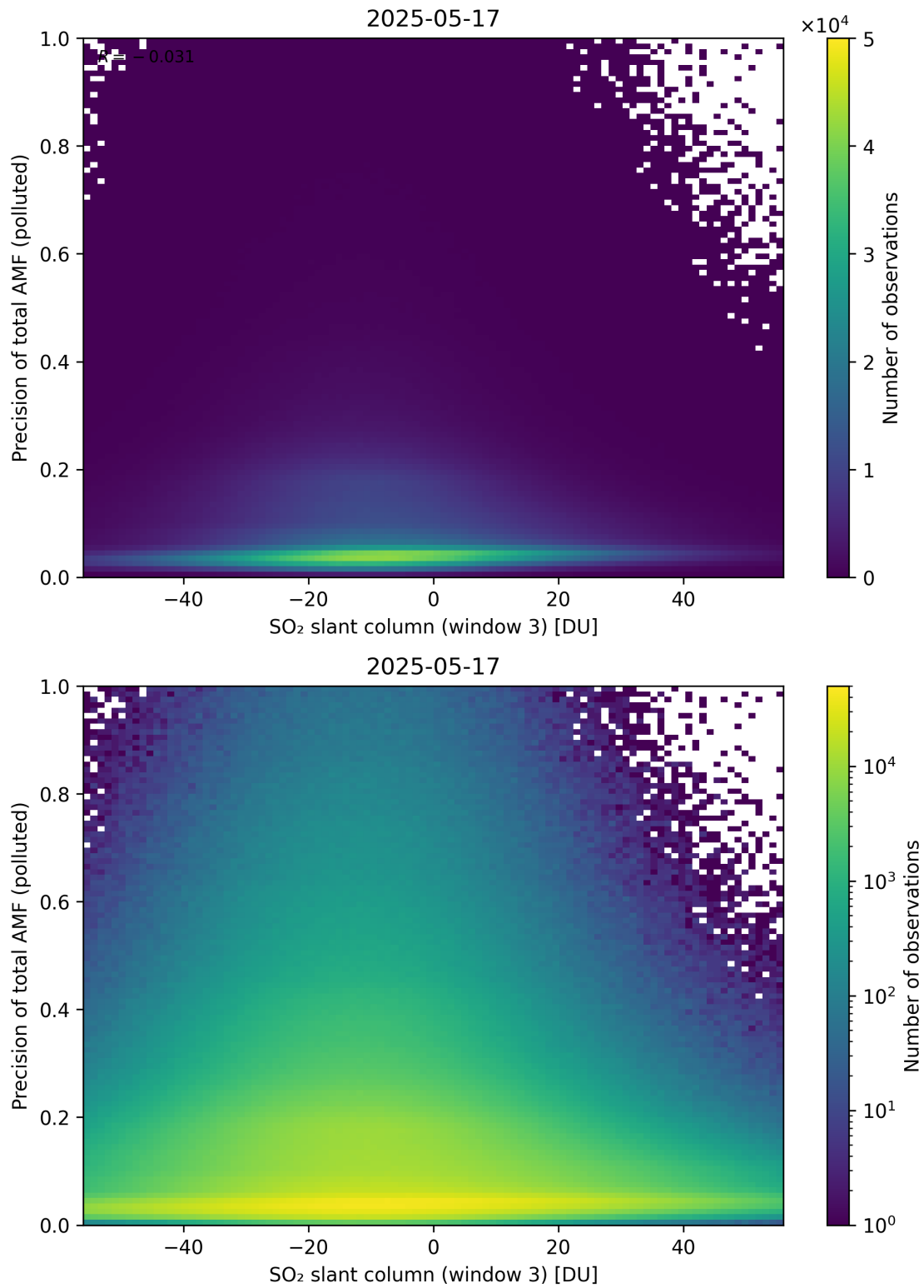
Figure 319: Scatter density plot of “SO 2 slant column (window 3)” against “Precision of total AMF (polluted)” for 2025-05-16 to 2025-05-18.
