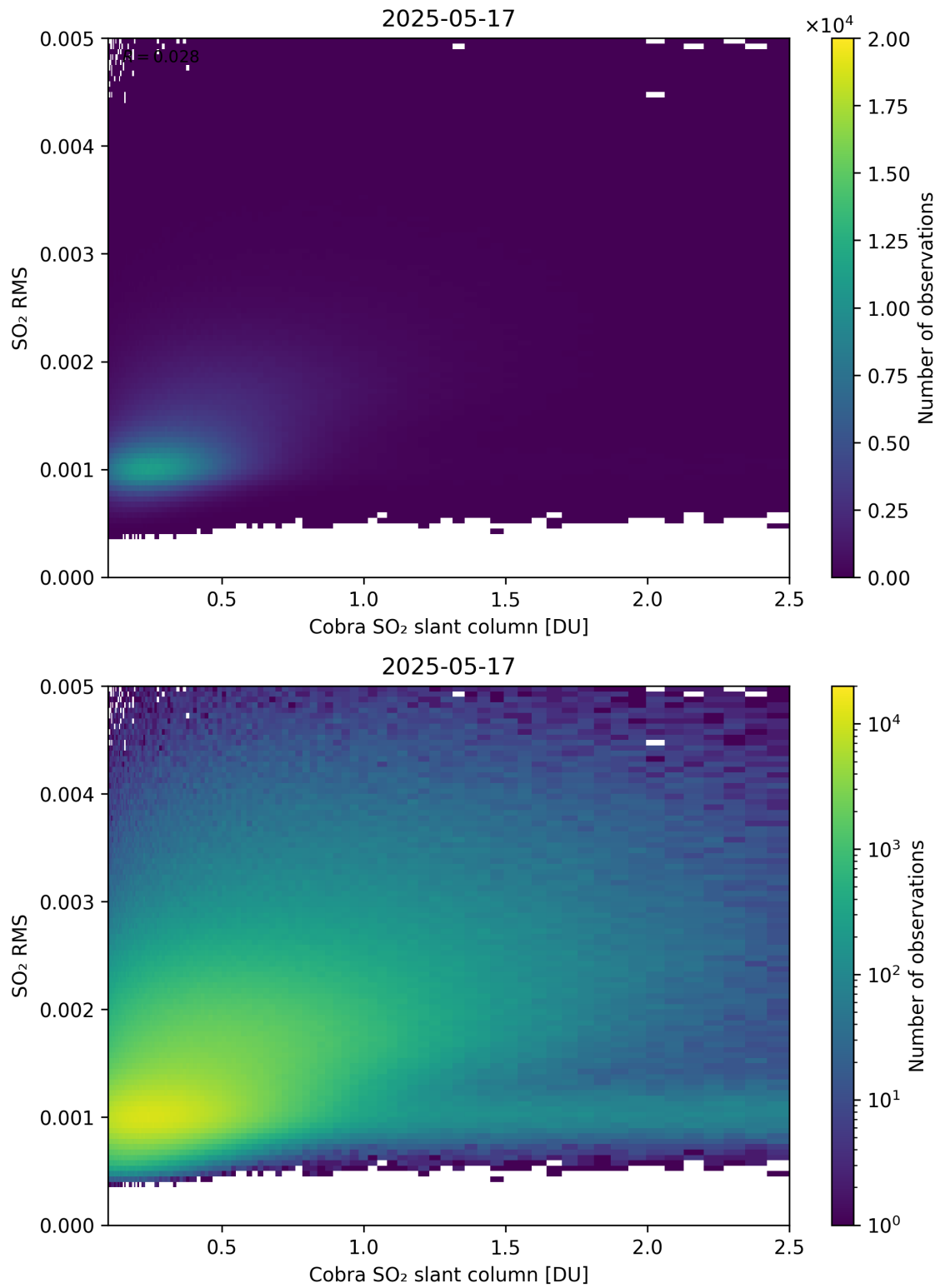
Figure 198: Scatter density plot of “Cobra SO 2 slant column” against “SO 2 RMS” for 2025-05-16 to 2025-05-18.
