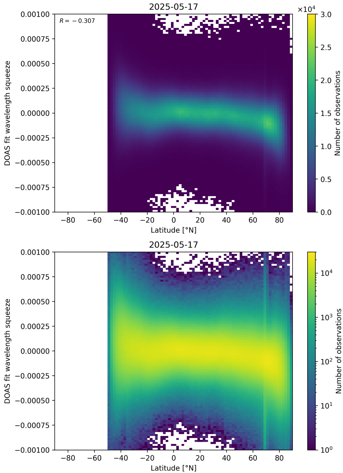
Figure 154: Scatter density plot of “Latitude” against “DOAS fit wavelength squeeze” for 2025-05-16 to 2025-05-18.
