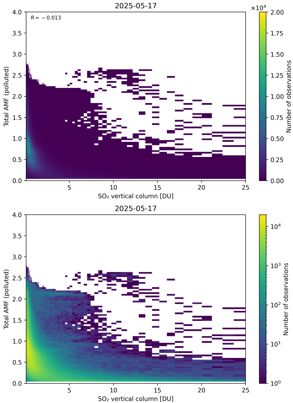
Figure 359: Scatter density plot of “SO 2 vertical column” against “Total AMF (polluted)” for 2025-05-16 to 2025-05-18.
