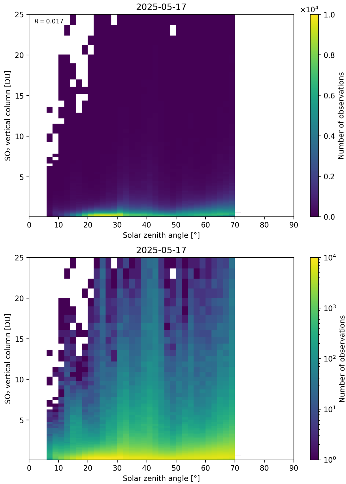
Figure 191: Scatter density plot of “Solar zenith angle” against “SO 2 vertical column” for 2025-05-16 to 2025-05-18.
