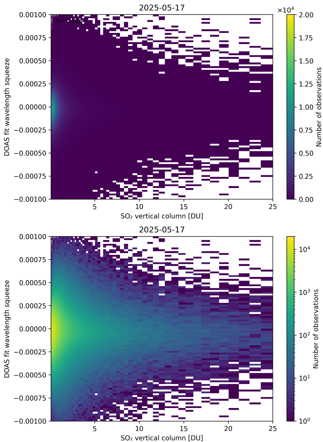
Figure 327: Scatter density plot of “SO 2 vertical column” against “DOAS fit wavelength squeeze” for 2025-05-16 to 2025-05-18.
