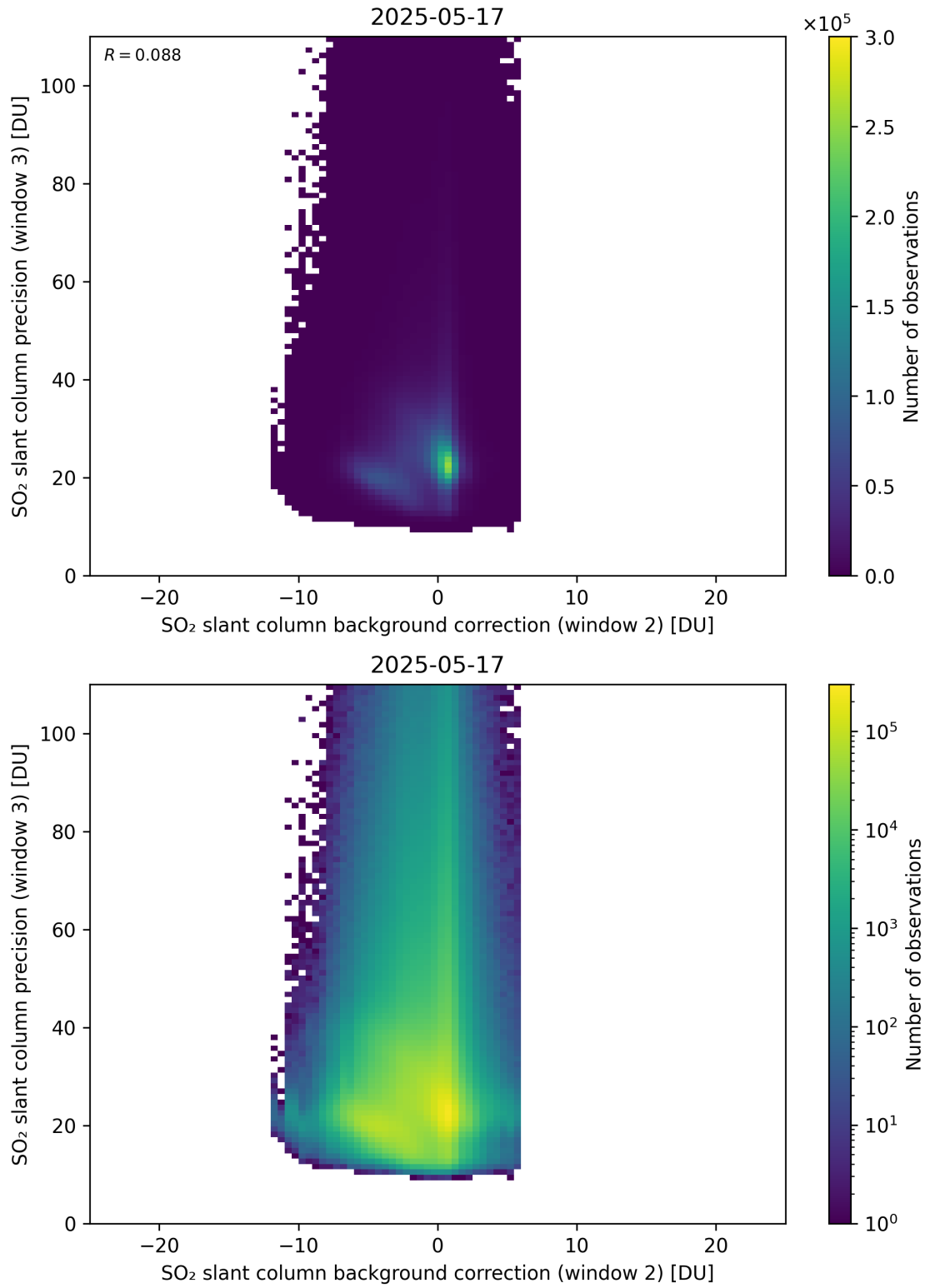
Figure 129: Scatter density plot of “SO 2 slant column background correction (window 2)” against “SO 2 slant column precision (window 3)” for 2025-05-16 to 2025-05-18.
