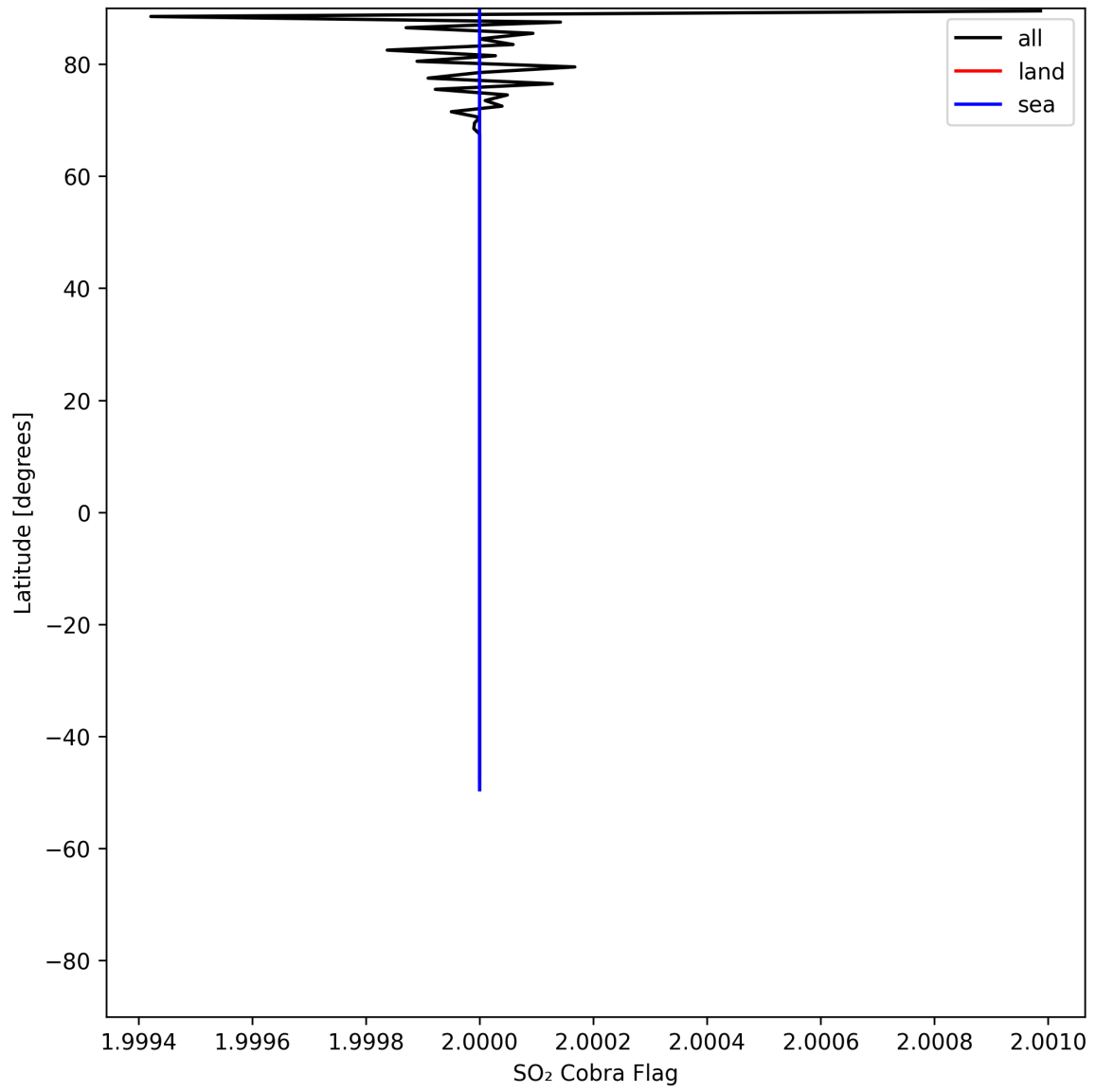
Figure 49: Zonal average of “SO 2 Cobra Flag” for 2025-05-16 to 2025-05-18.
