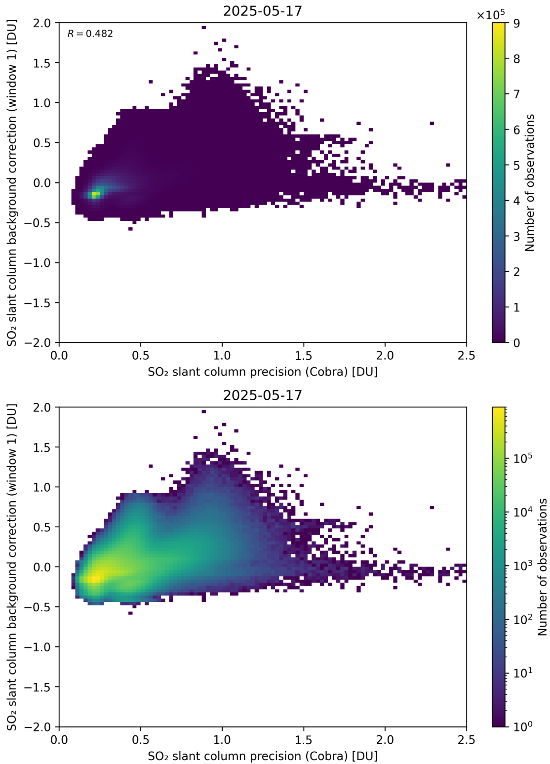
Figure 199: Scatter density plot of “SO 2 slant column precision (Cobra)” against “SO 2 slant column background correction (window 1)” for 2025-05-16 to 2025-05-18.
