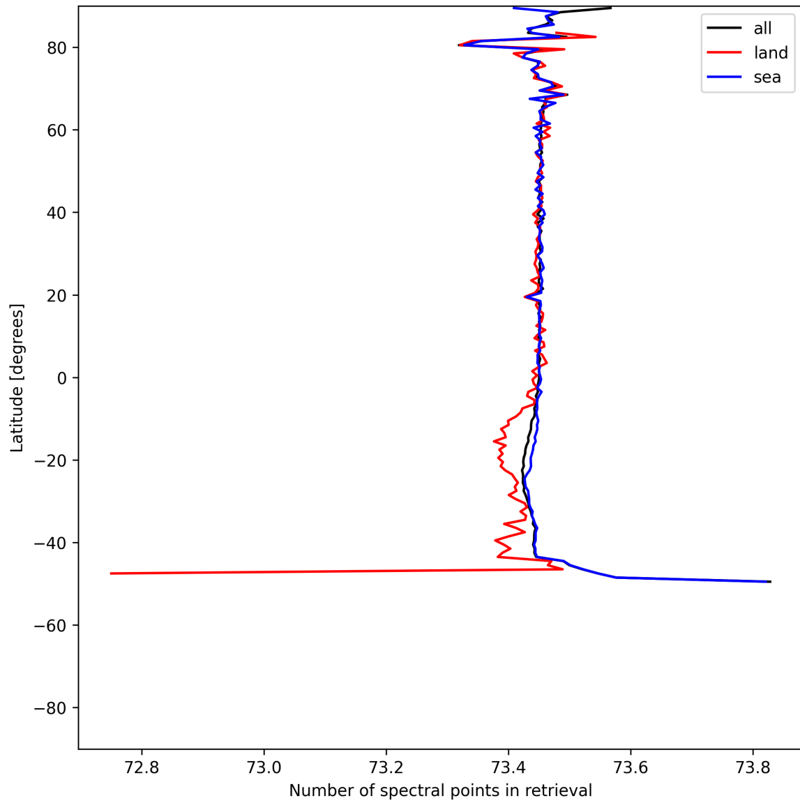
Figure 56: Zonal average of “Number of spectral points in retrieval” for 2025-05-16 to 2025-05-18.
