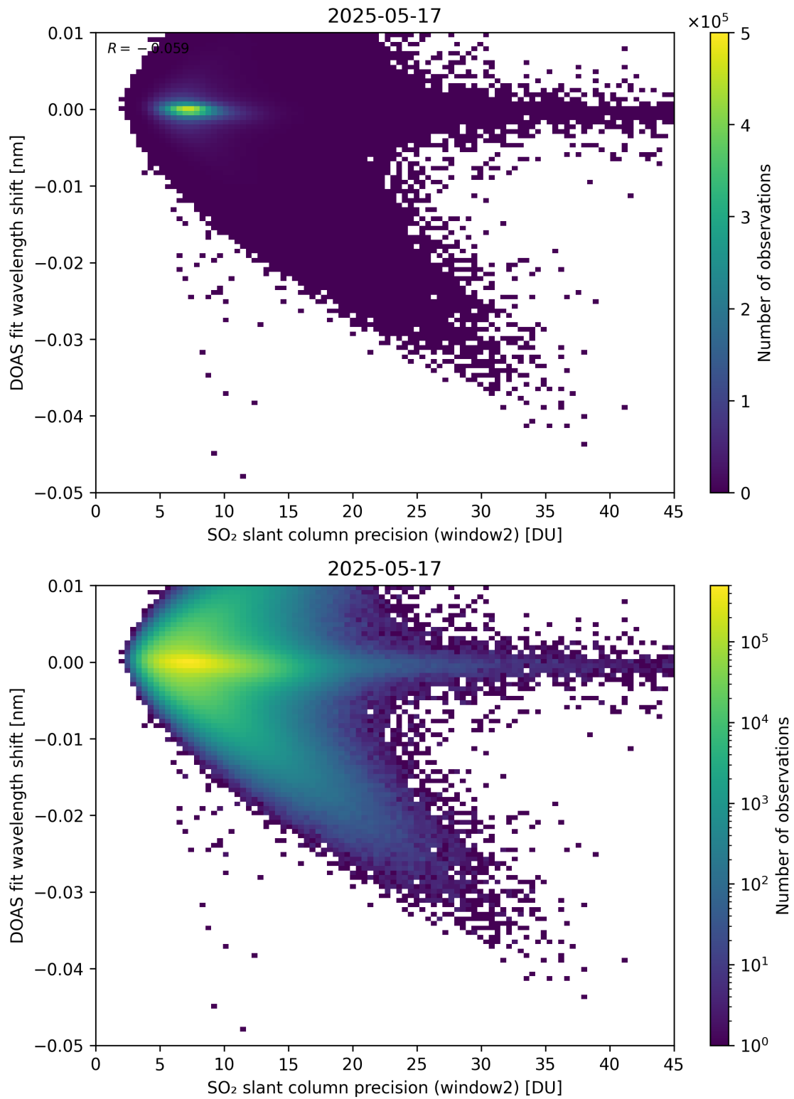
Figure 293: Scatter density plot of “SO 2 slant column precision (window2)” against “DOAS fit wavelength shift” for 2025-05-16 to 2025-05-18.
