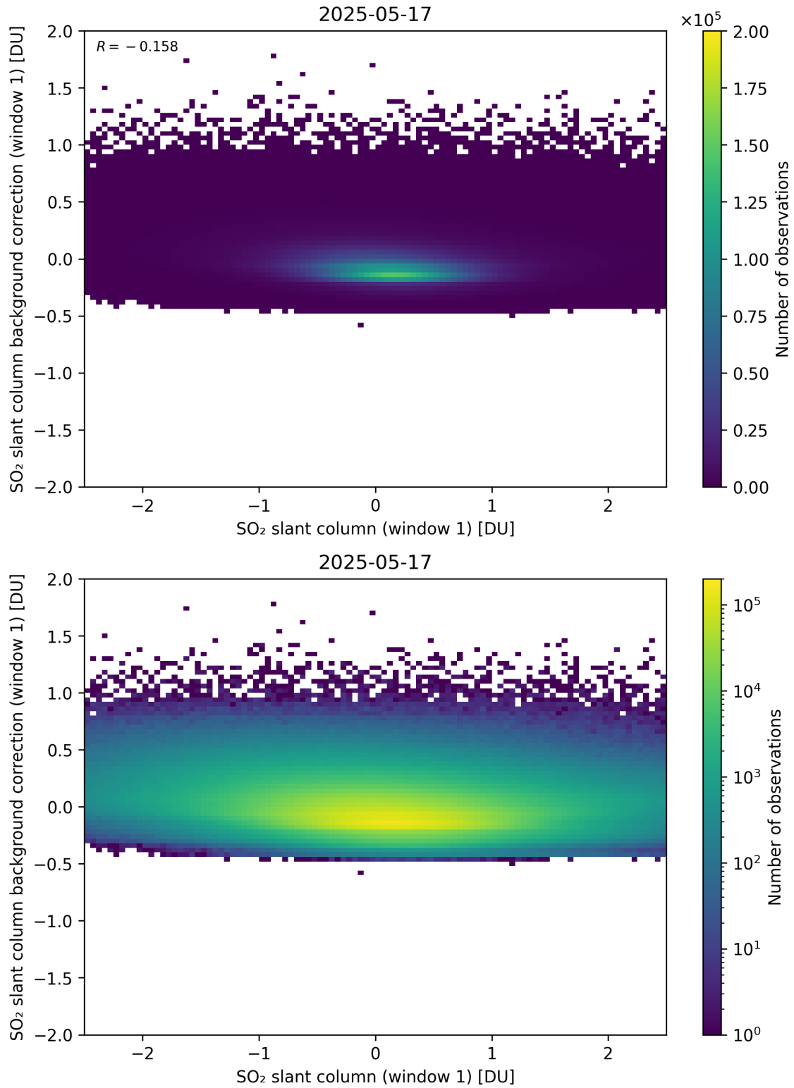
Figure 262: Scatter density plot of “SO 2 slant column (window 1)” against “SO 2 slant column background correction (window 1)” for 2025-05-16 to 2025-05-18.
