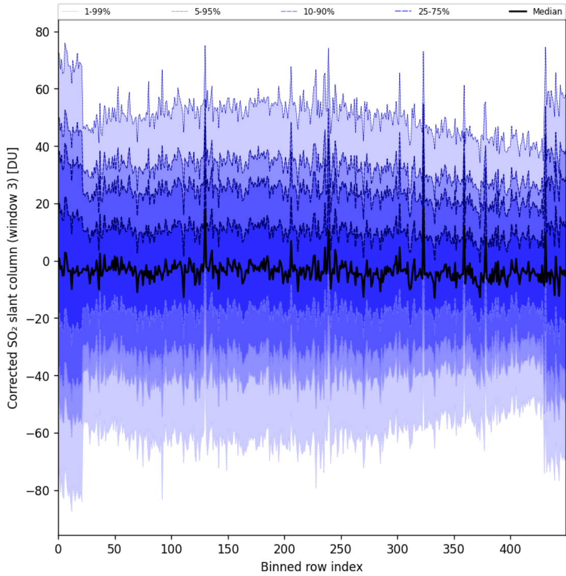
Figure 99: Along track statistics of “Corrected SO 2 slant column (window 3)” for 2025-05-16 to 2025-05-18
