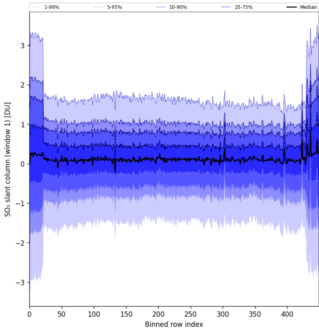
Figure 89: Along track statistics of “SO 2 slant column (window 1)” for 2025-05-16 to 2025-05-18
