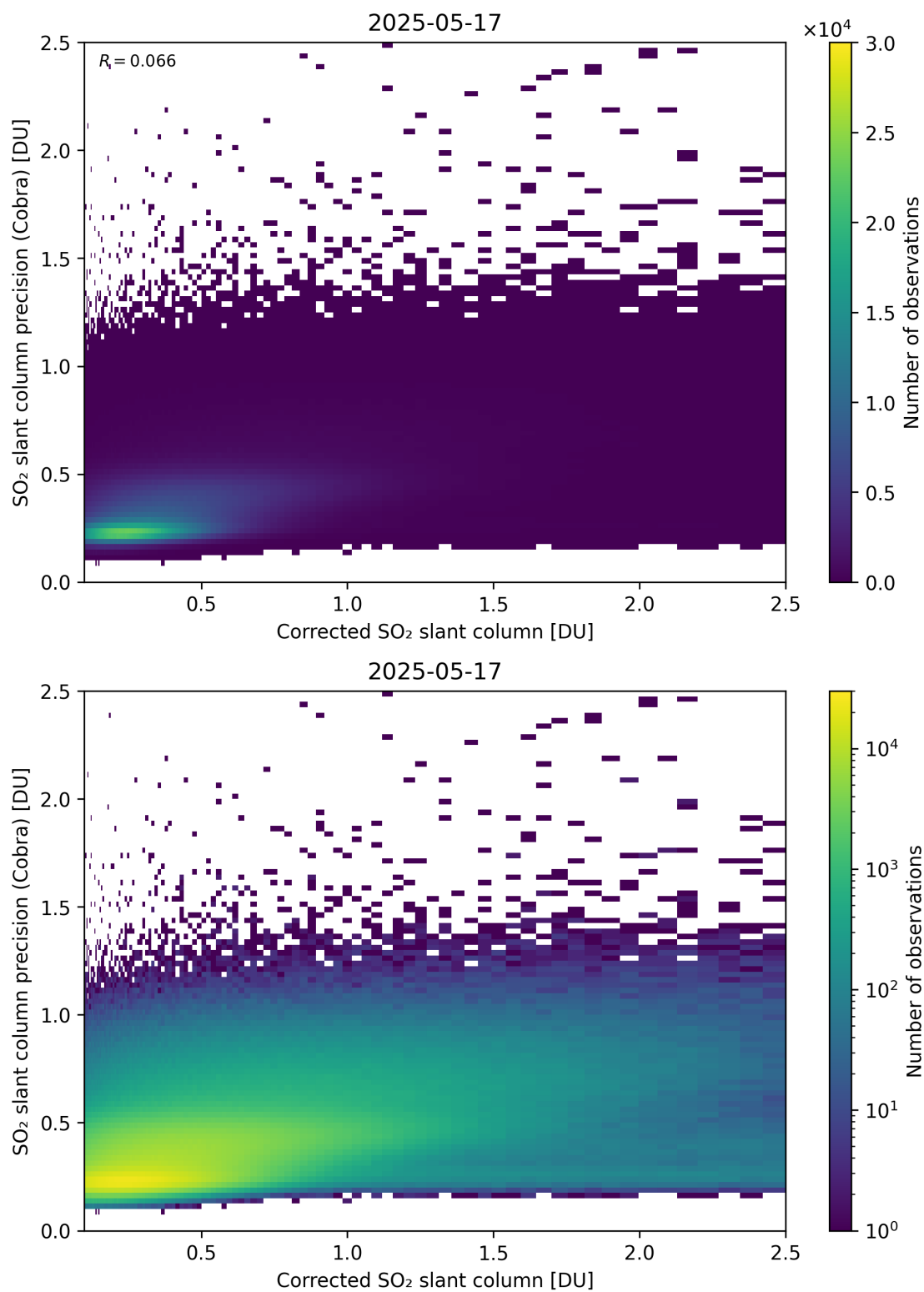
Figure 234: Scatter density plot of “Corrected SO 2 slant column” against “SO 2 slant column precision (Cobra)” for 2025-05-16 to 2025-05-18.
