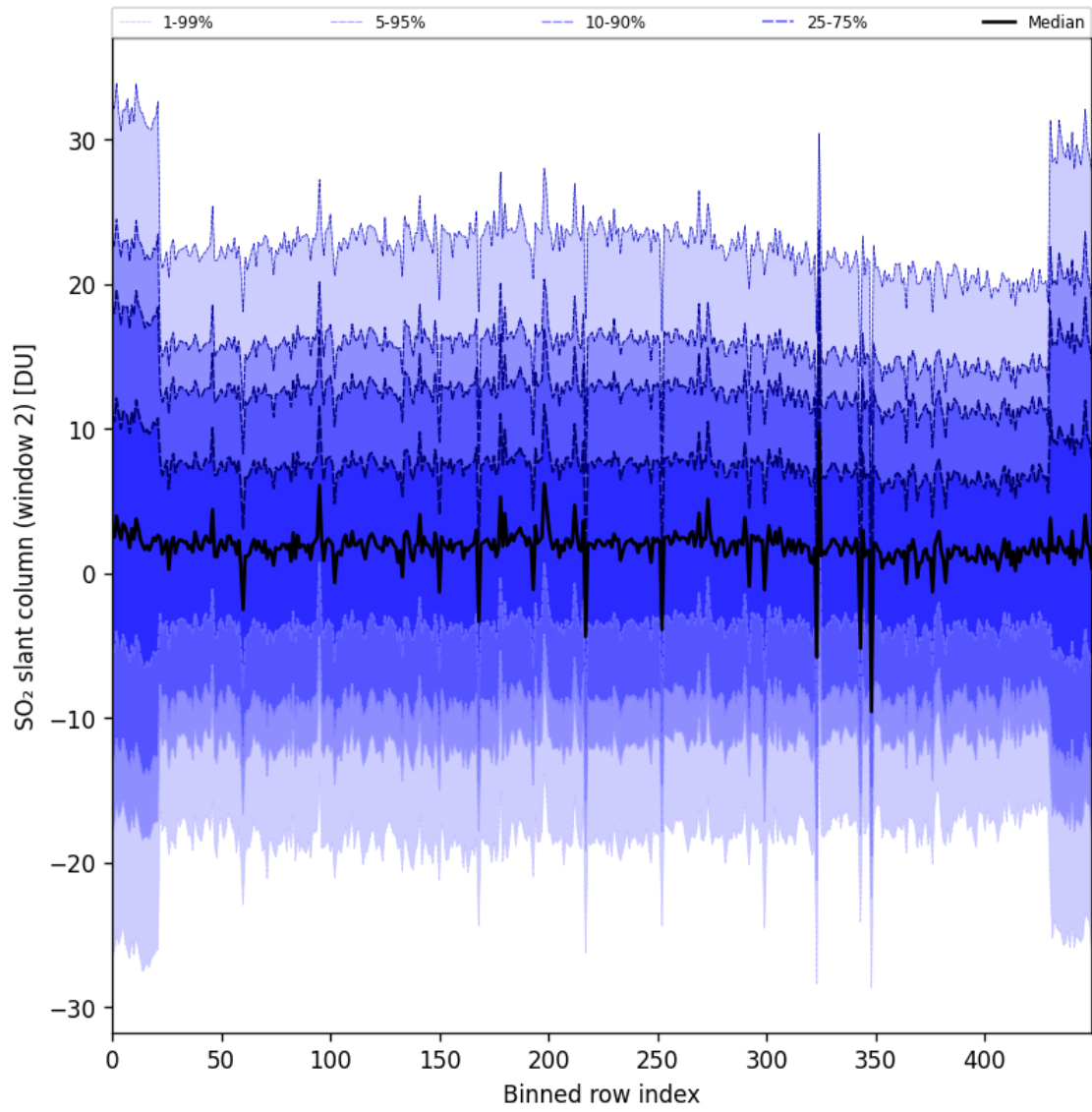
Figure 93: Along track statistics of “SO 2 slant column (window 2)” for 2025-05-16 to 2025-05-18
