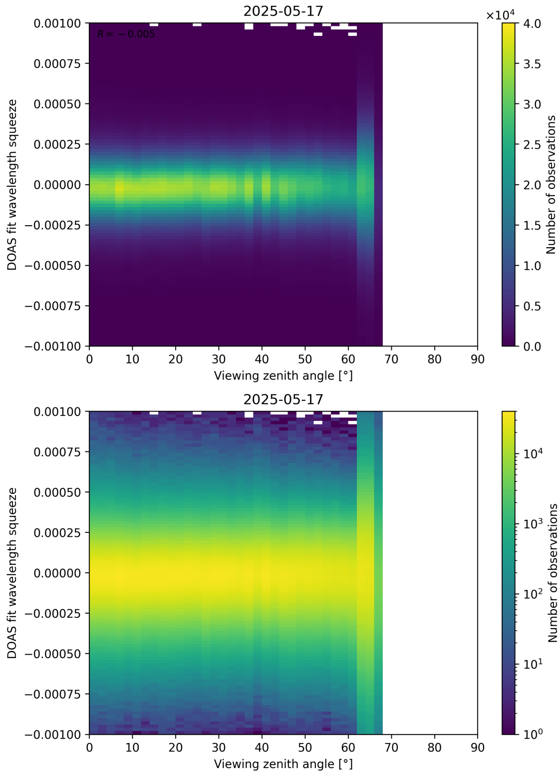
Figure 366: Scatter density plot of “Viewing zenith angle” against “DOAS fit wavelength squeeze” for 2025-05-16 to 2025-05-18.
