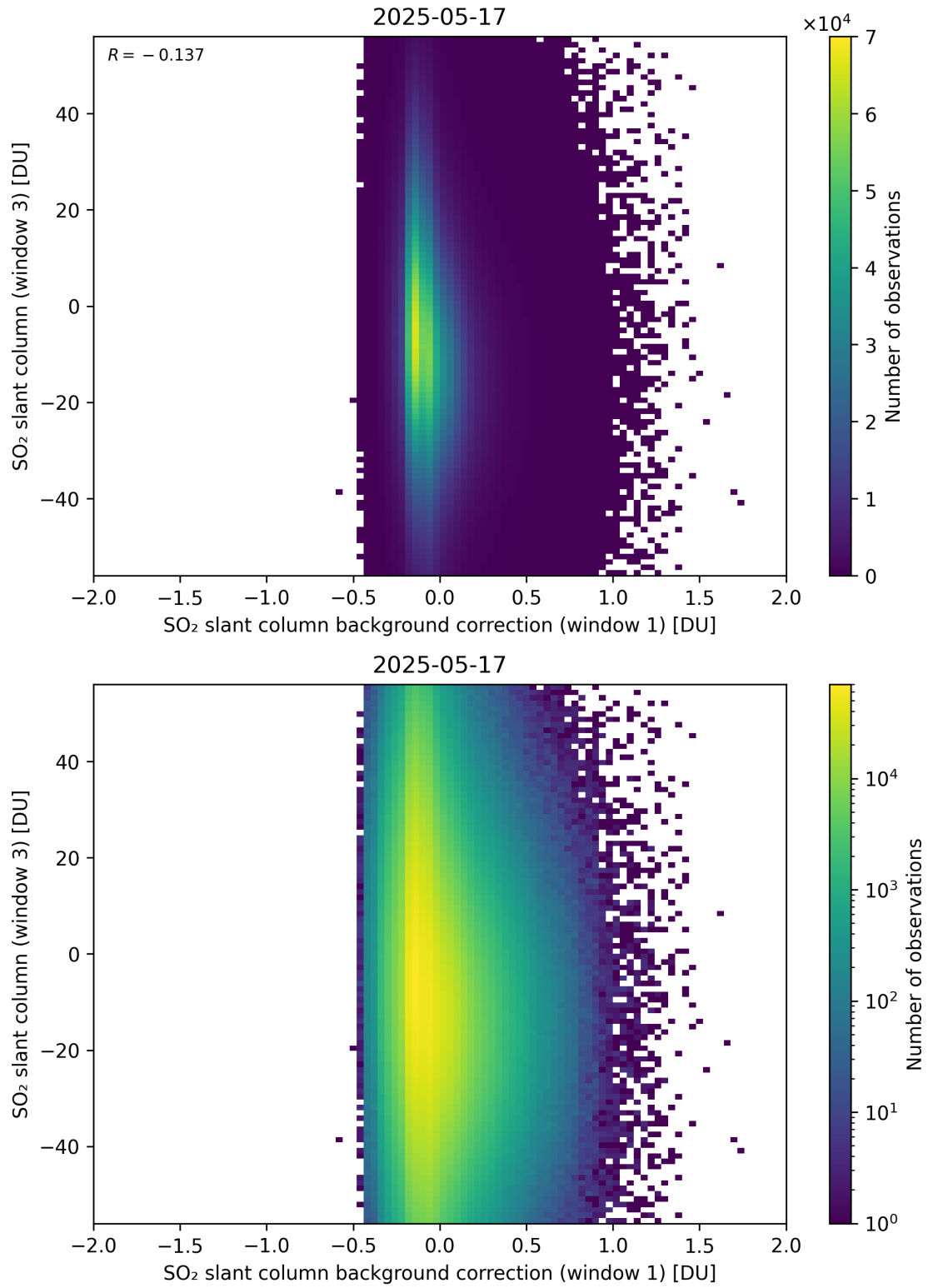
Figure 118: Scatter density plot of “SO 2 slant column background correction (window 1)” against “SO 2 slant column (window 3)” for 2025-05-16 to 2025-05-18.
