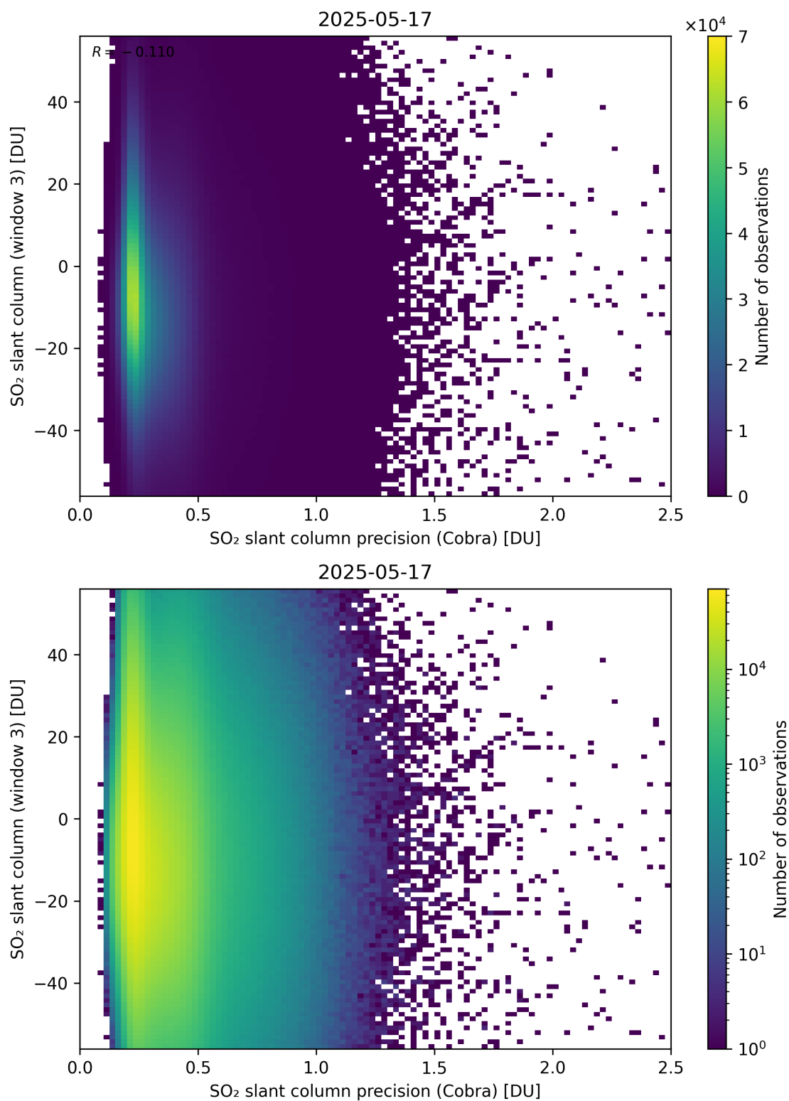
Figure 211: Scatter density plot of “SO 2 slant column precision (Cobra)” against “SO 2 slant column (window 3)” for 2025-05-16 to 2025-05-18.
