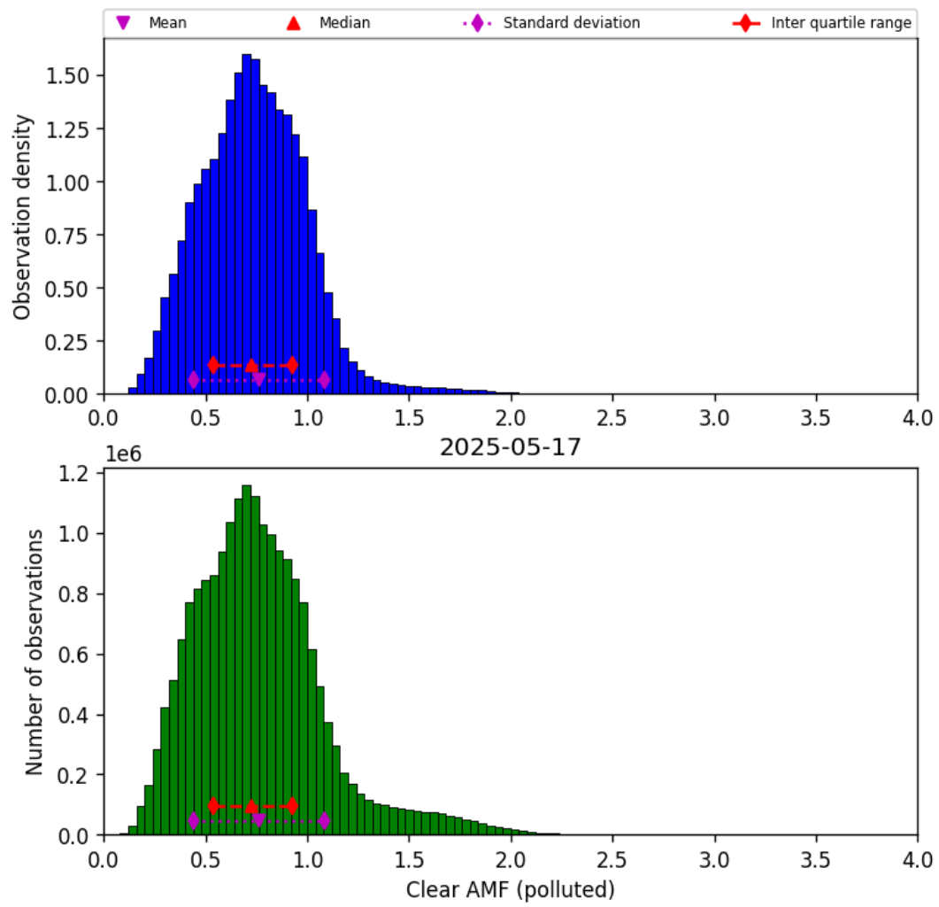
Figure 81: Histogram of “Clear AMF (polluted)” for 2025-05-16 to 2025-05-18
