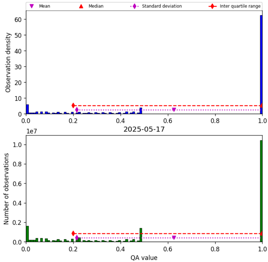
Figure 57: Histogram of “QA value” for 2025-05-16 to 2025-05-18
