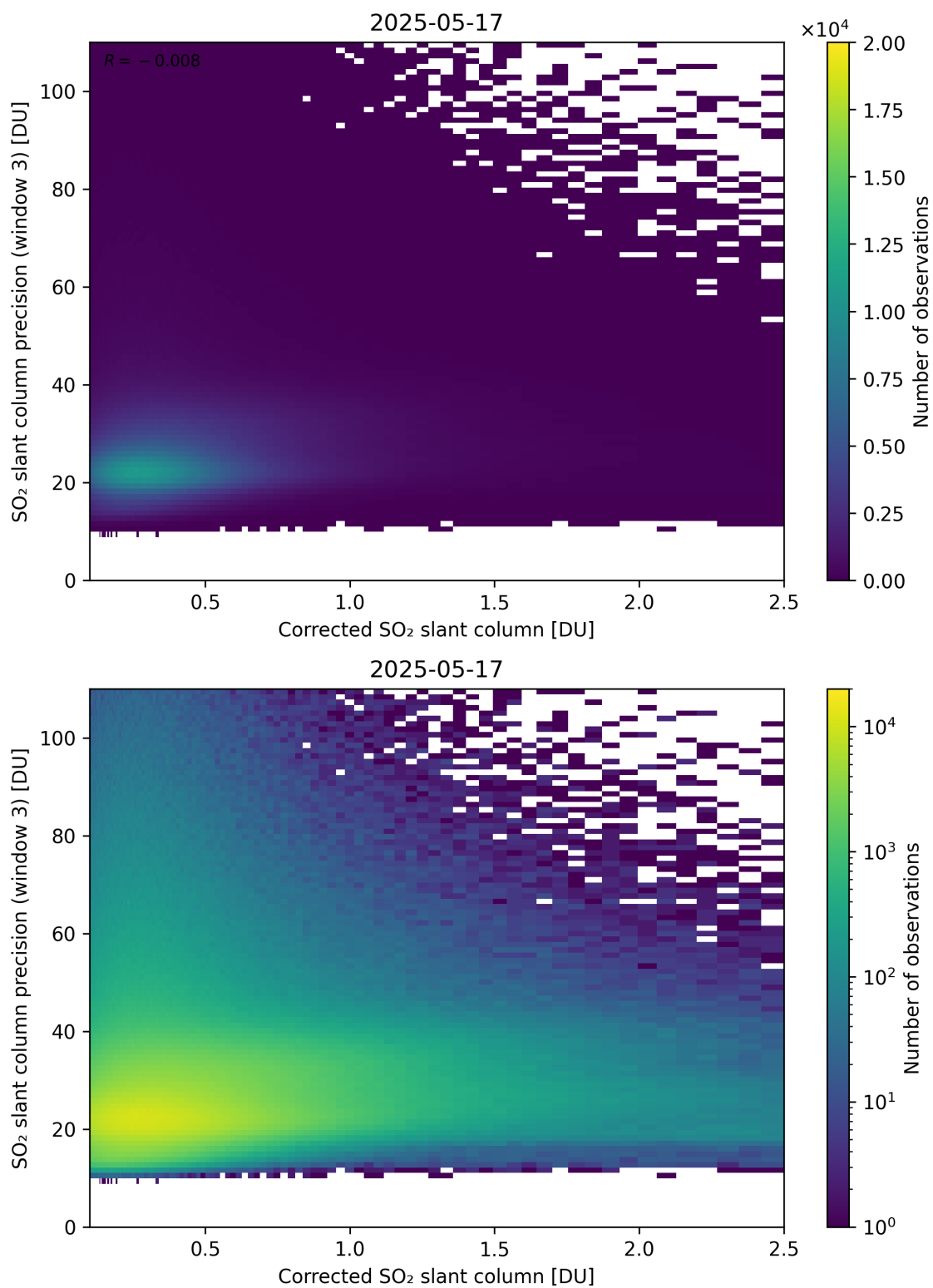
Figure 241: Scatter density plot of “Corrected SO 2 slant column” against “SO 2 slant column precision (window 3)” for 2025-05-16 to 2025-05-18.
