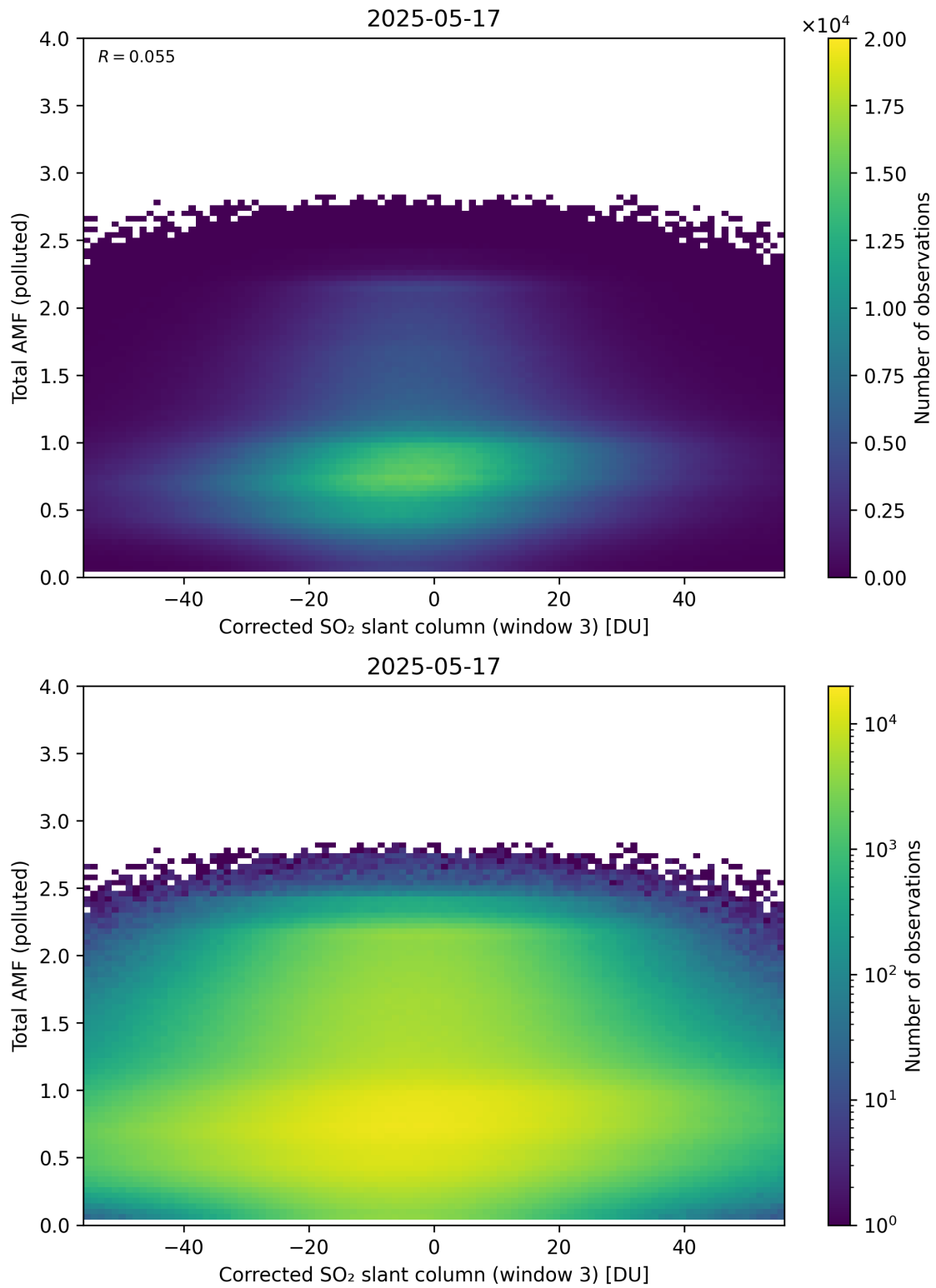
Figure 260: Scatter density plot of “Corrected SO 2 slant column (window 3)” against “Total AMF (polluted)” for 2025-05-16 to 2025-05-18.
