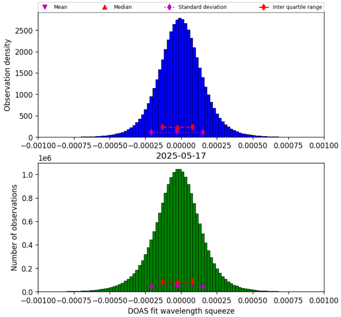
Figure 77: Histogram of “DOAS fit wavelength squeeze” for 2025-05-16 to 2025-05-18
