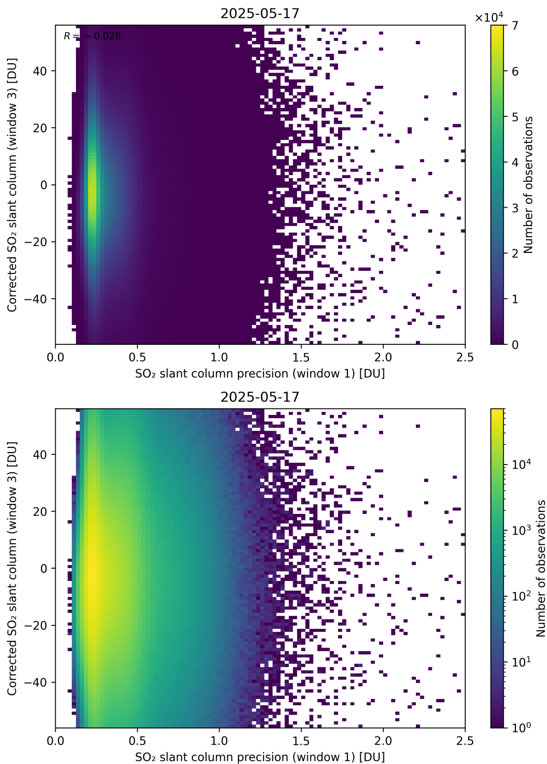
Figure 276: Scatter density plot of “SO 2 slant column precision (window 1)” against “Corrected SO 2 slant column (window 3)” for 2025-05-16 to 2025-05-18.
