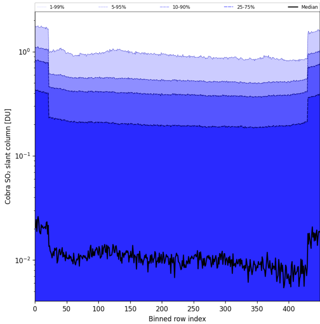
Figure 87: Along track statistics of “Cobra SO 2 slant column” for 2025-05-16 to 2025-05-18
