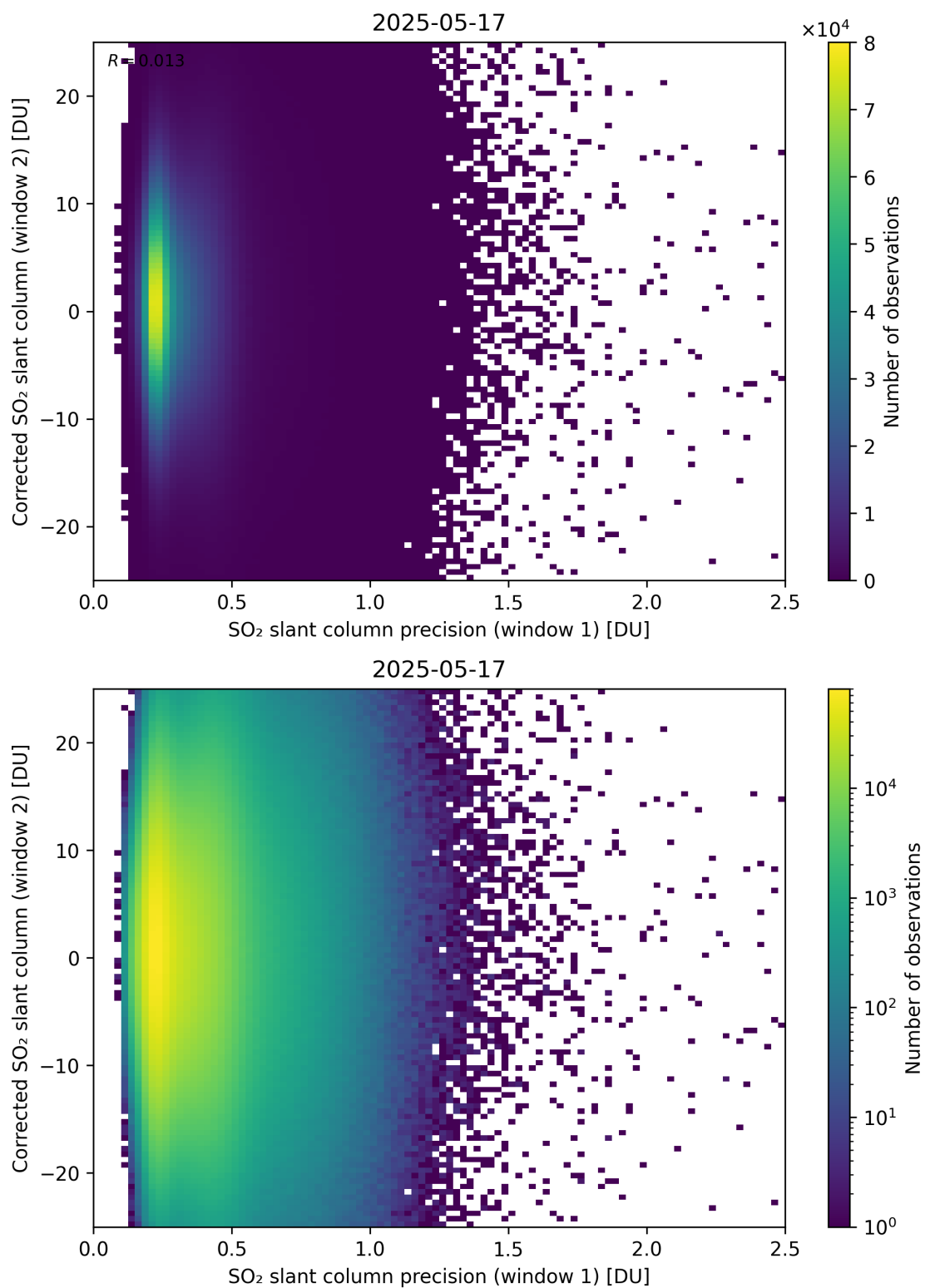
Figure 275: Scatter density plot of “SO 2 slant column precision (window 1)” against “Corrected SO 2 slant column (window 2)” for 2025-05-16 to 2025-05-18.
