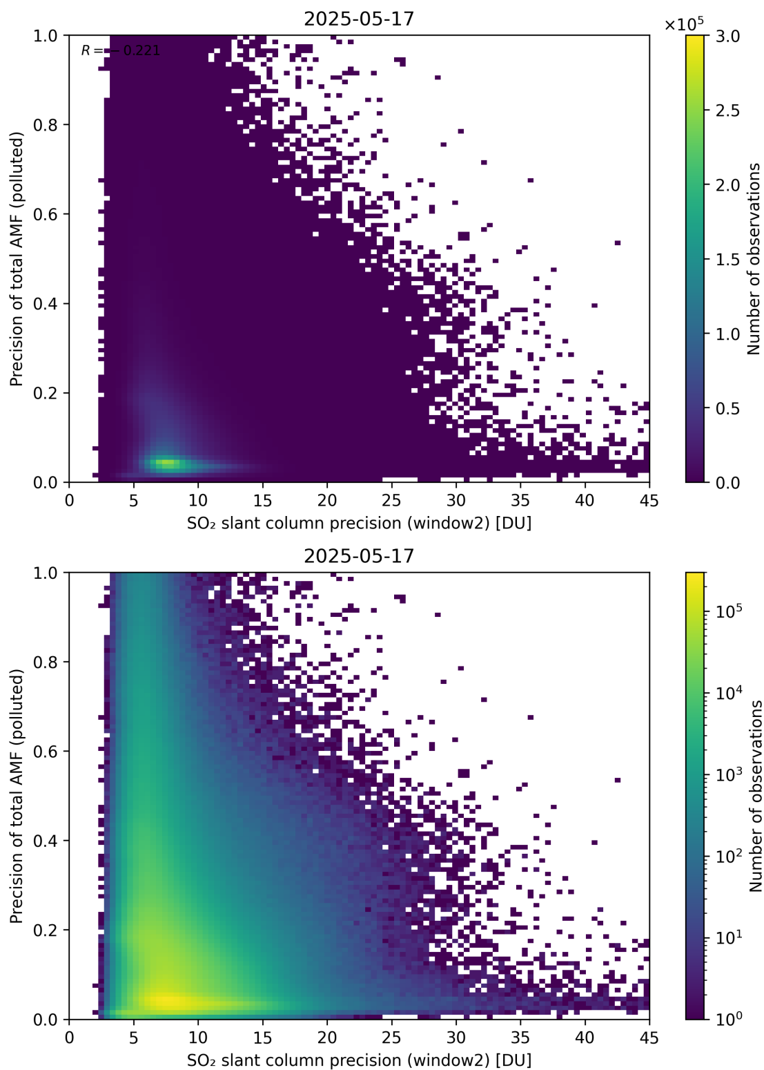
Figure 302: Scatter density plot of “SO 2 slant column precision (window2)” against “Precision of total AMF (polluted)” for 2025-05-16 to 2025-05-18.
