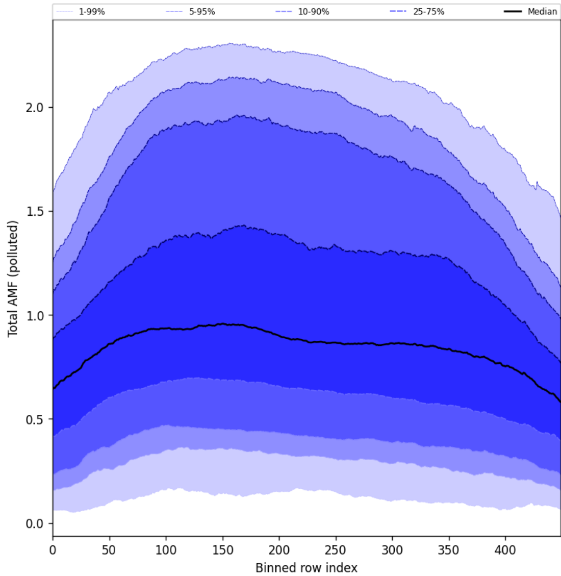
Figure 105: Along track statistics of “Total AMF (polluted)” for 2025-05-16 to 2025-05-18
