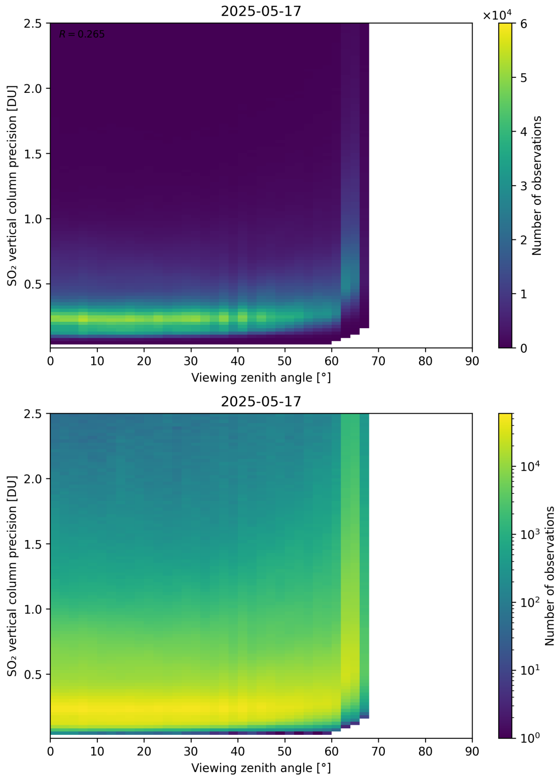
Figure 384: Scatter density plot of “Viewing zenith angle” against “SO 2 vertical column precision” for 2025-05-16 to 2025-05-18.
