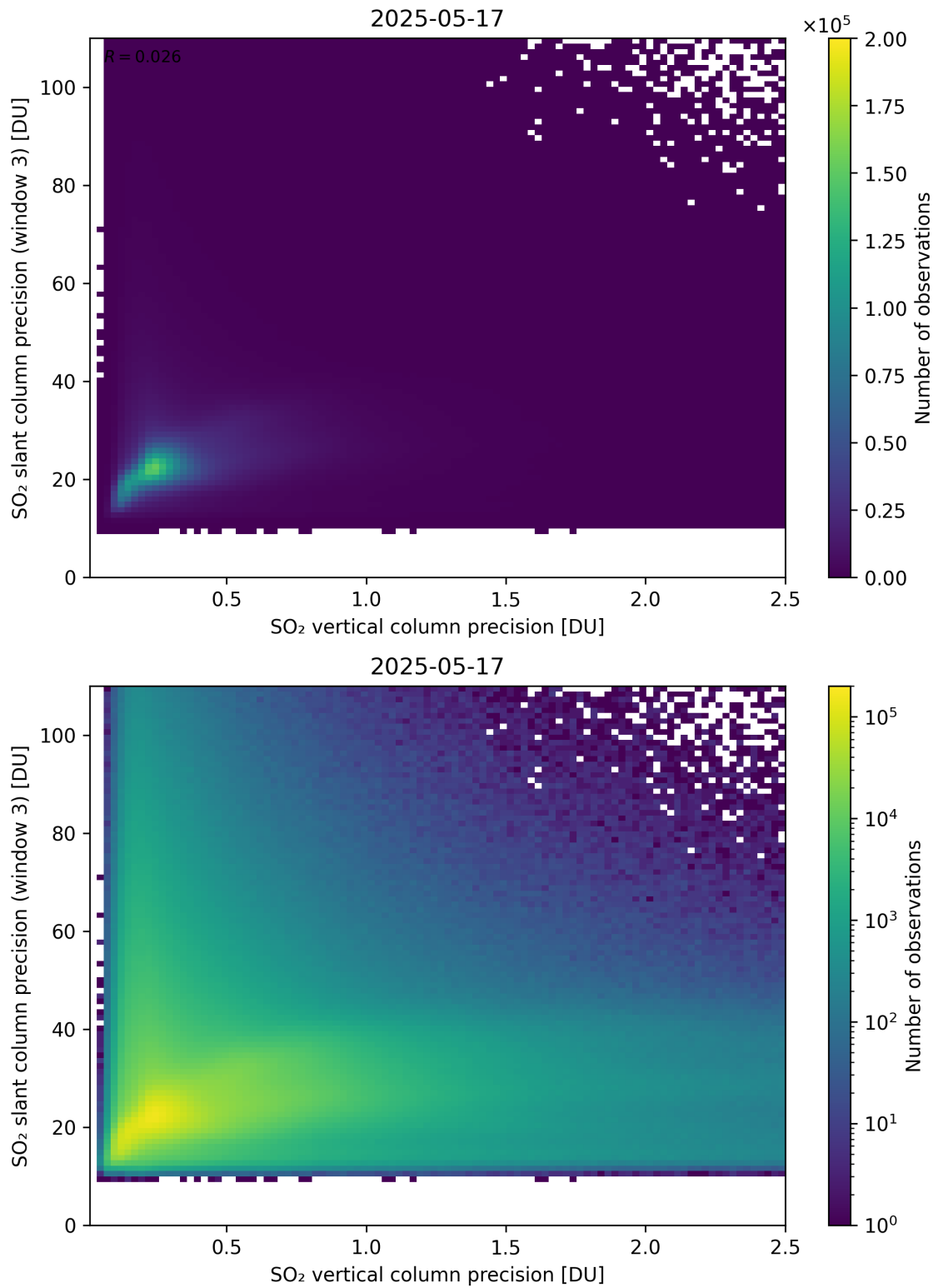
Figure 345: Scatter density plot of “SO 2 vertical column precision” against “SO 2 slant column precision (window 3)” for 2025-05-16 to 2025-05-18.
