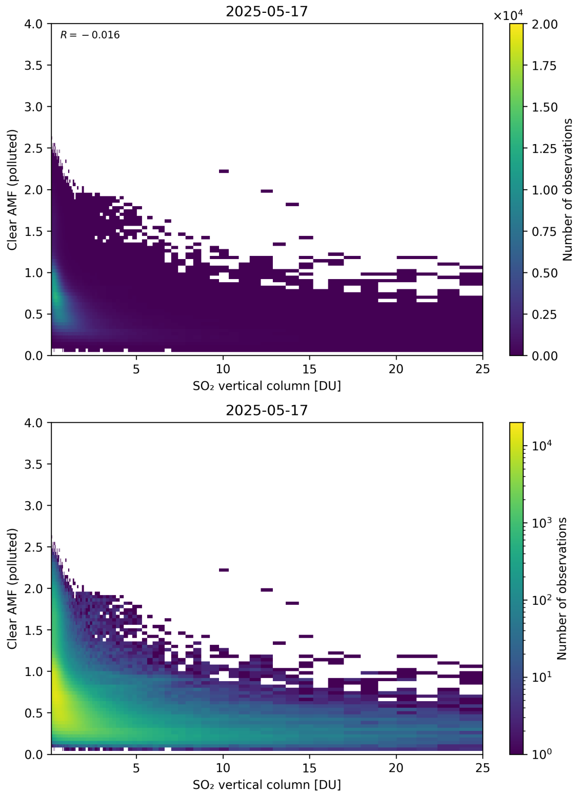
Figure 348: Scatter density plot of “SO 2 vertical column” against “Clear AMF (polluted)” for 2025-05-16 to 2025-05-18.
