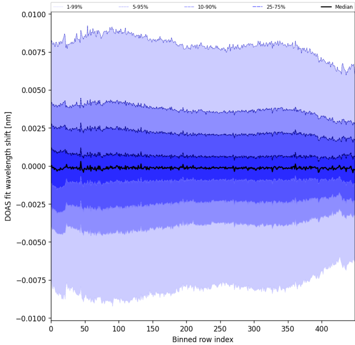
Figure 102: Along track statistics of “DOAS fit wavelength shift” for 2025-05-16 to 2025-05-18
