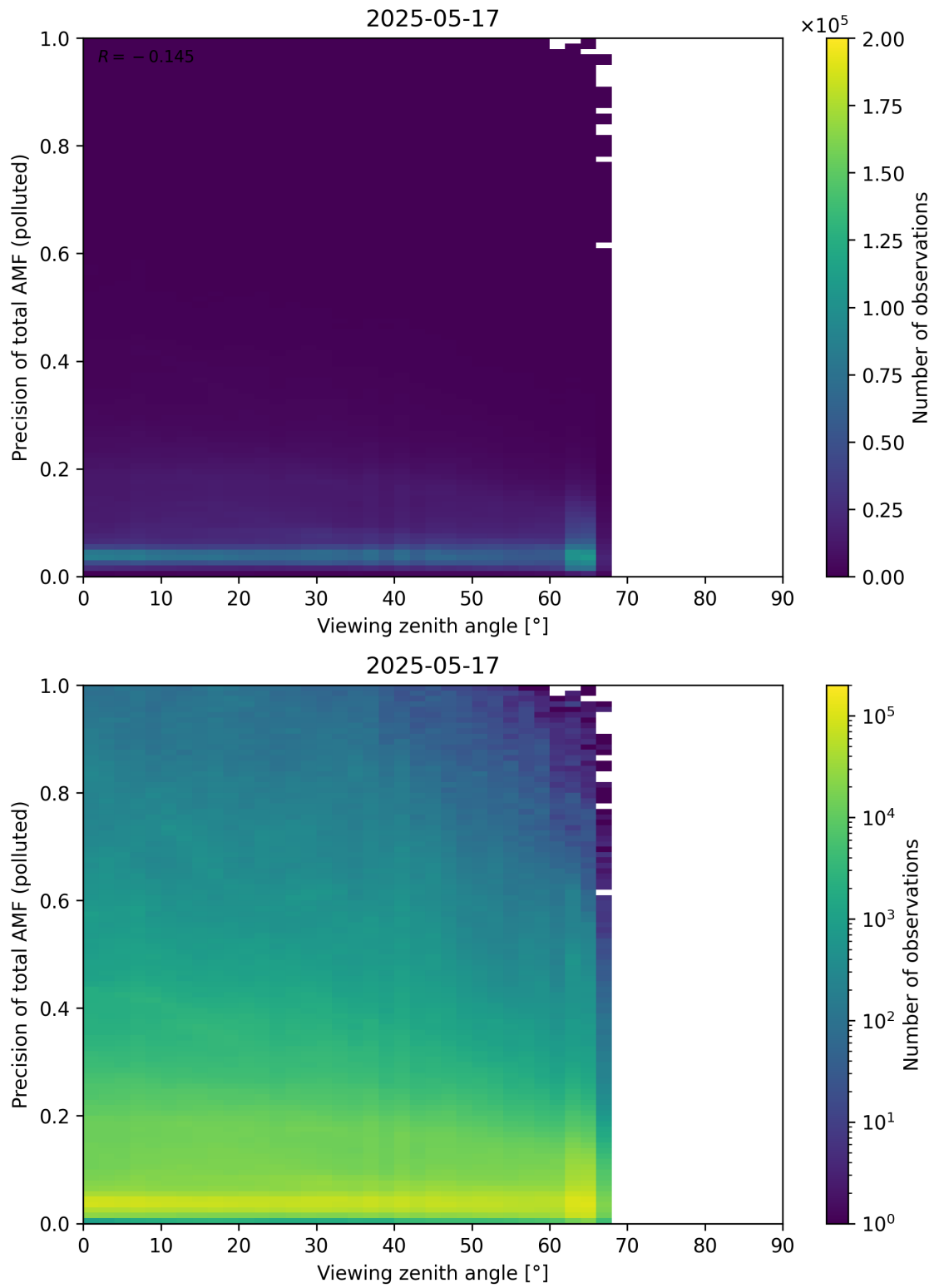
Figure 382: Scatter density plot of “Viewing zenith angle” against “Precision of total AMF (polluted)” for 2025-05-16 to 2025-05-18.
