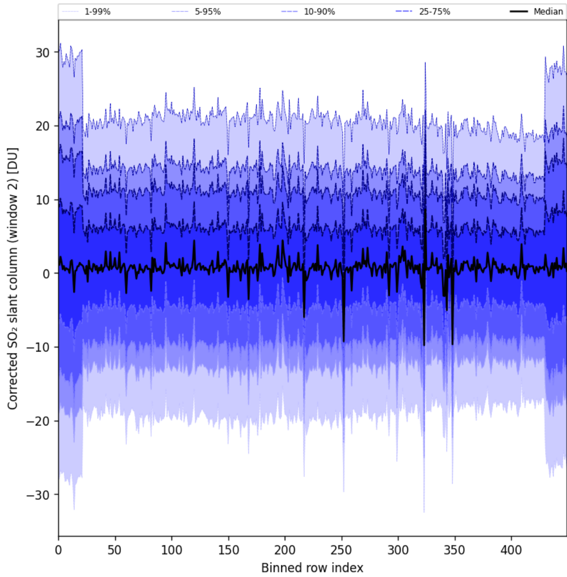
Figure 95: Along track statistics of “Corrected SO 2 slant column (window 2)” for 2025-05-16 to 2025-05-18
