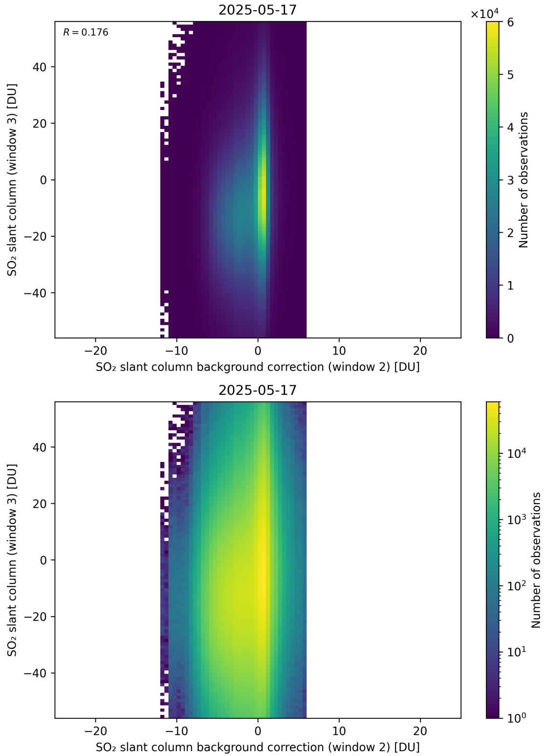
Figure 128: Scatter density plot of “SO 2 slant column background correction (window 2)” against “SO 2 slant column (window 3)” for 2025-05-16 to 2025-05-18.
