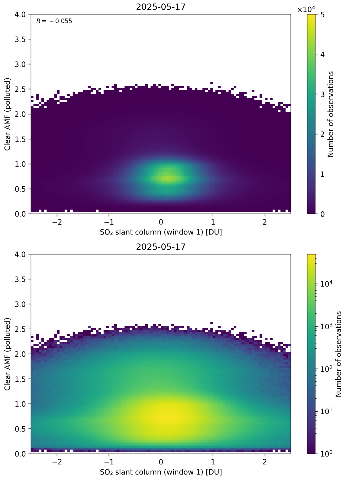
Figure 282: Scatter density plot of “SO 2 slant column (window 1)” against “Clear AMF (polluted)” for 2025-05-16 to 2025-05-18.
