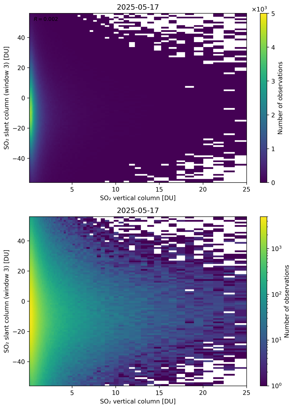
Figure 357: Scatter density plot of “SO 2 vertical column” against “SO 2 slant column (window 3)” for 2025-05-16 to 2025-05-18.
