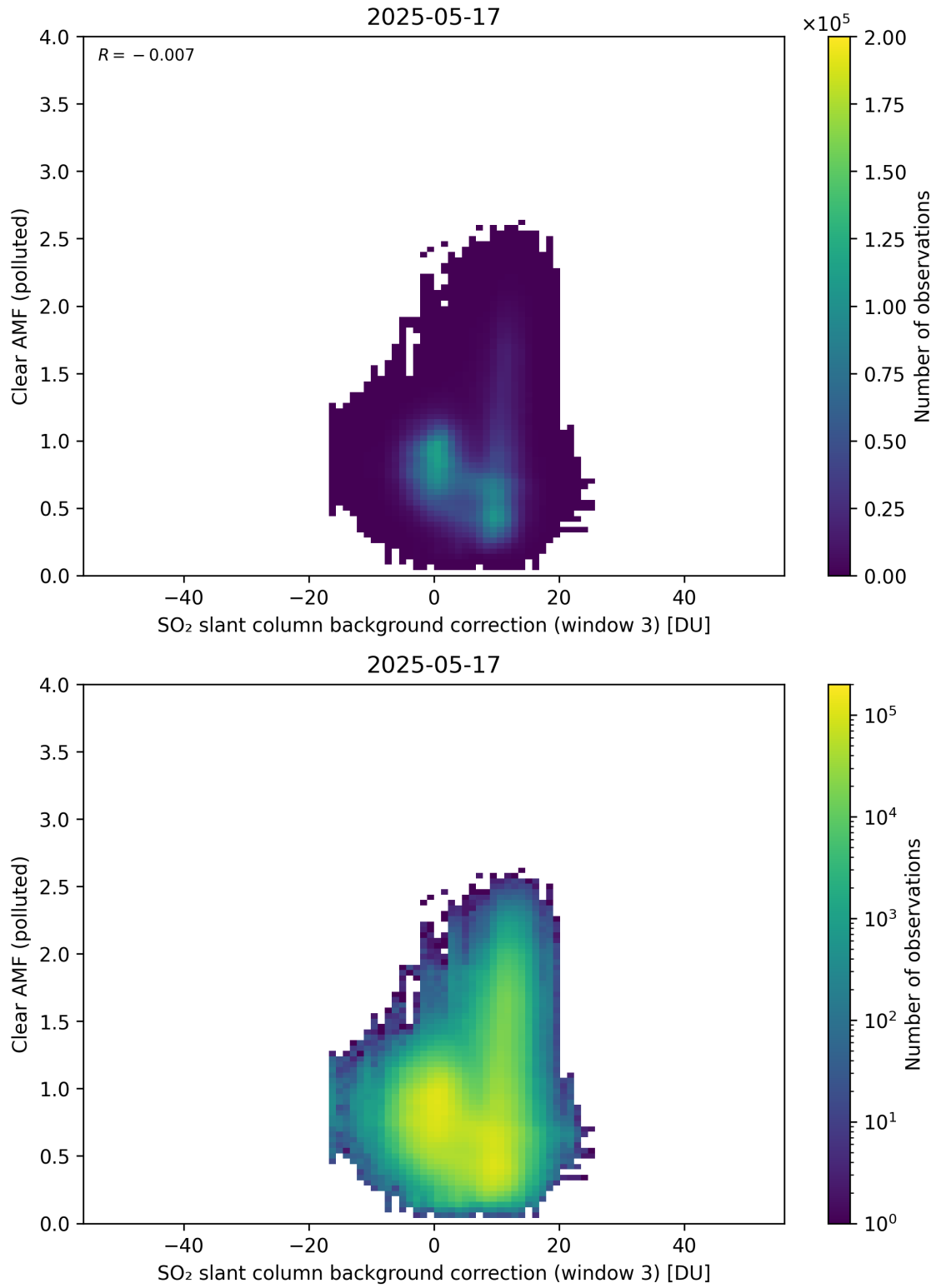
Figure 135: Scatter density plot of “SO 2 slant column background correction (window 3)” against “Clear AMF (polluted)” for 2025-05-16 to 2025-05-18.
