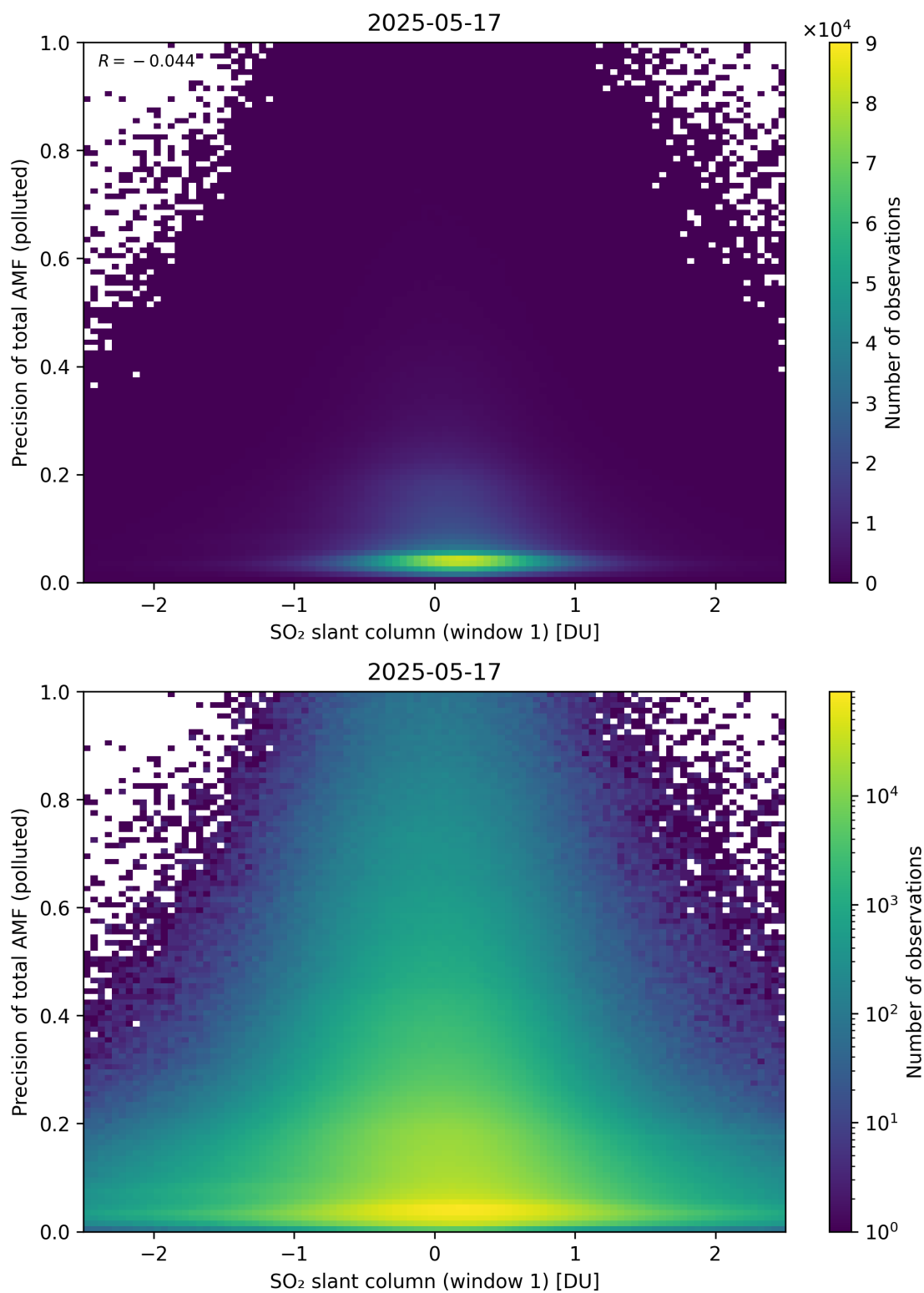
Figure 290: Scatter density plot of “SO 2 slant column (window 1)” against “Precision of total AMF (polluted)” for 2025-05-16 to 2025-05-18.
