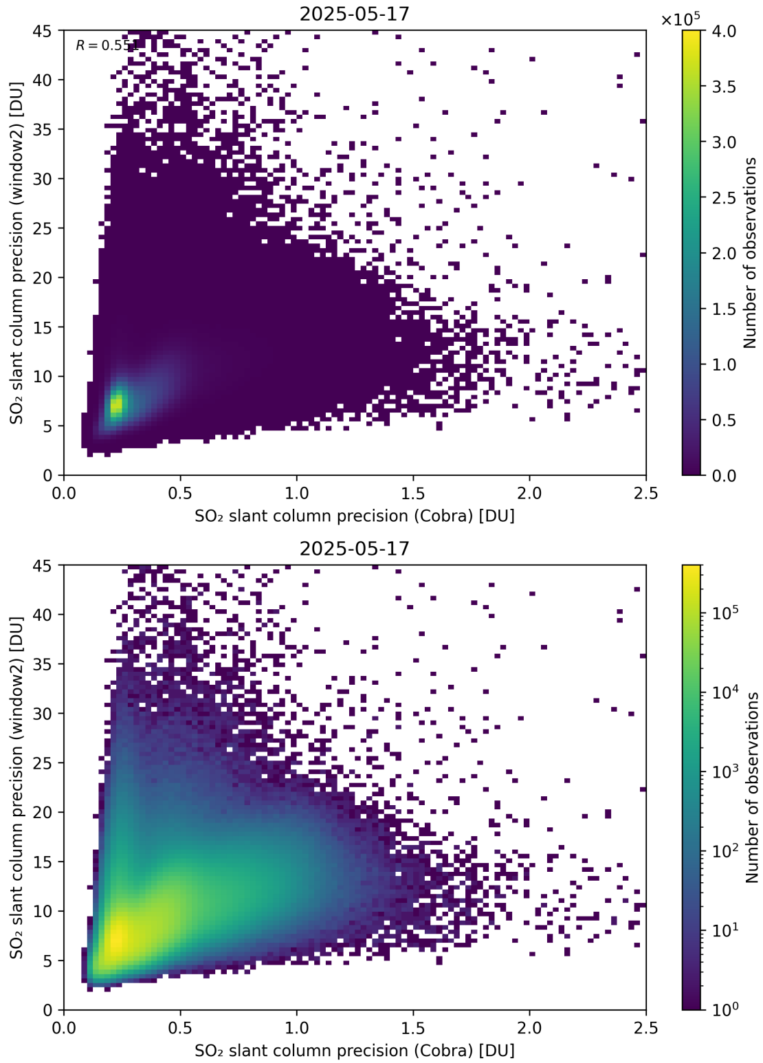
Figure 210: Scatter density plot of “SO 2 slant column precision (Cobra)” against “SO 2 slant column precision (window2)” for 2025-05-16 to 2025-05-18.
