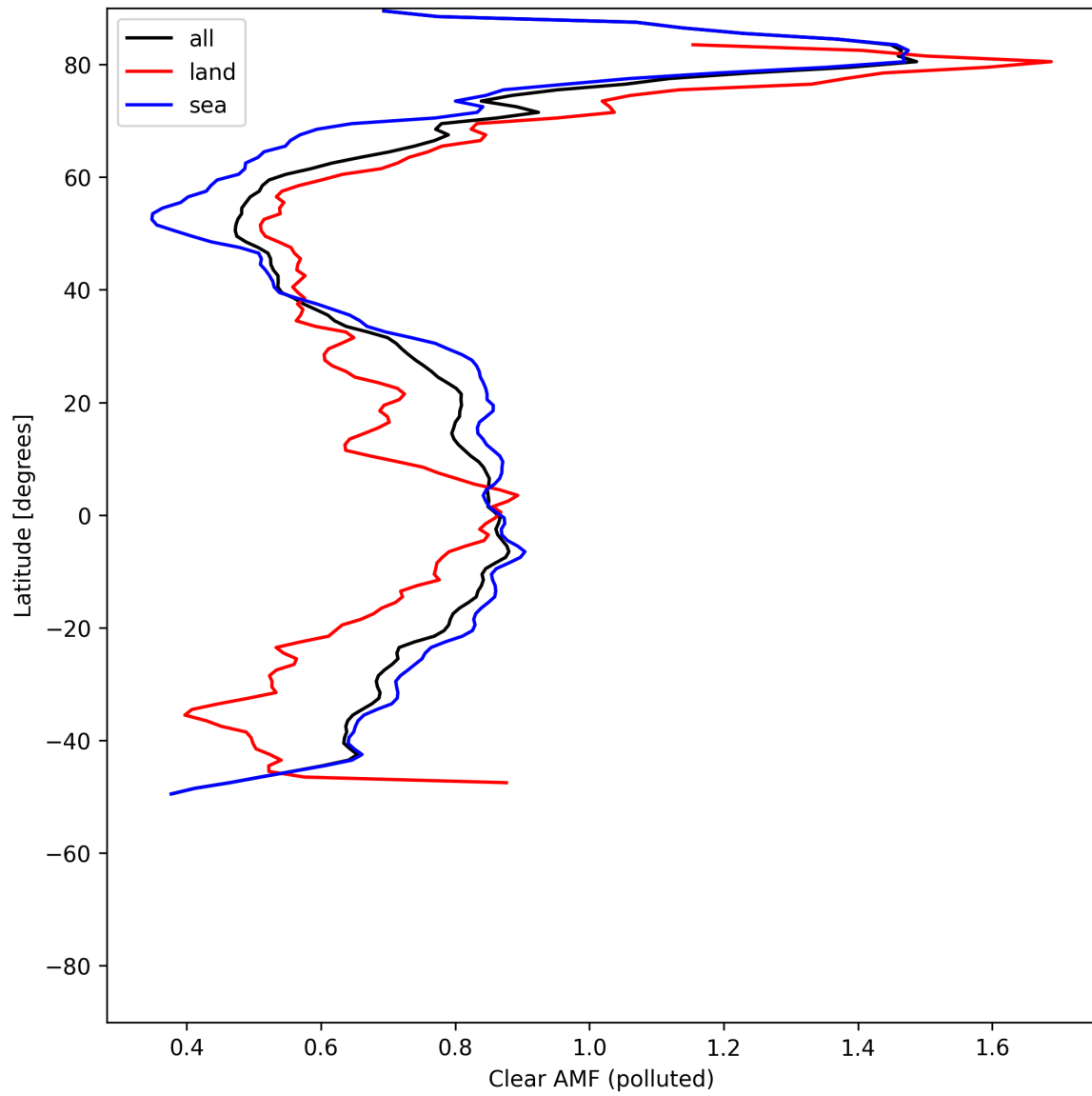
Figure 55: Zonal average of “Clear AMF (polluted)” for 2025-05-16 to 2025-05-18.
