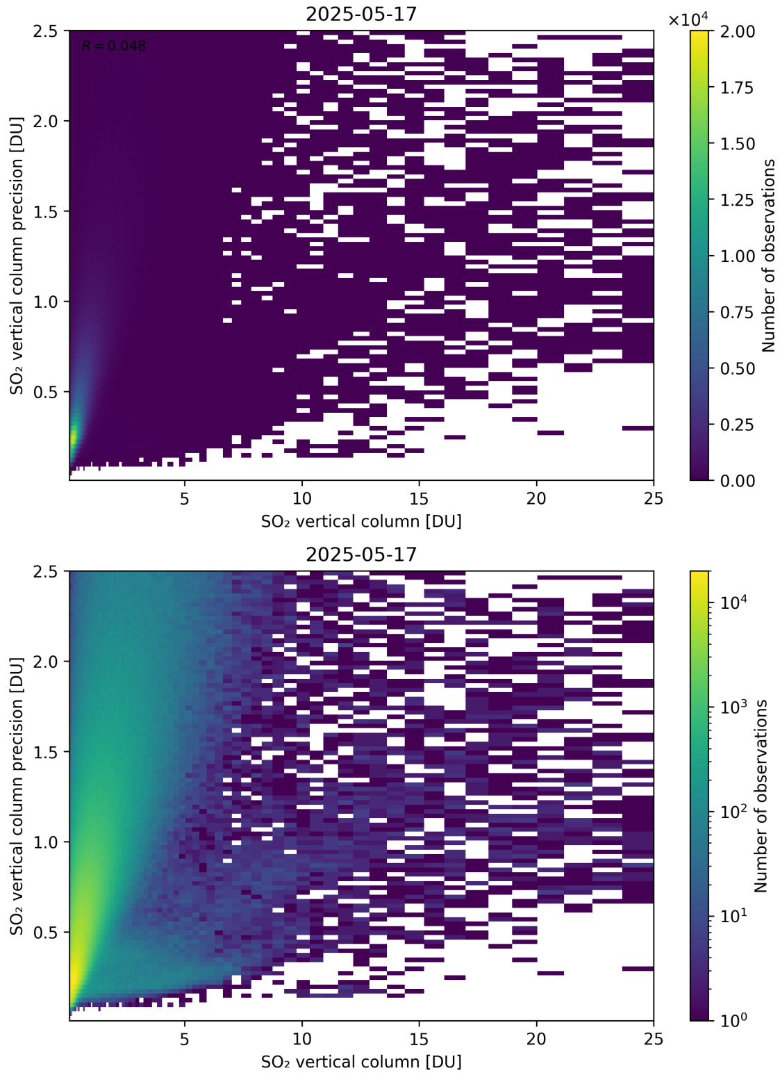
Figure 361: Scatter density plot of “SO 2 vertical column” against “SO 2 vertical column precision” for 2025-05-16 to 2025-05-18.
