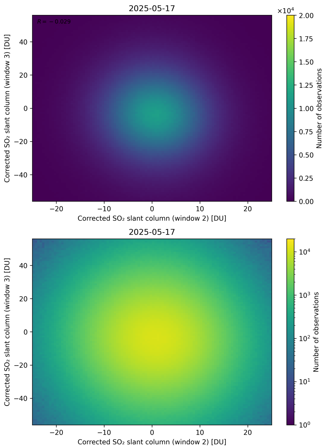
Figure 250: Scatter density plot of “Corrected SO 2 slant column (window 2)” against “Corrected SO 2 slant column (window 3)” for 2025-05-16 to 2025-05-18.
