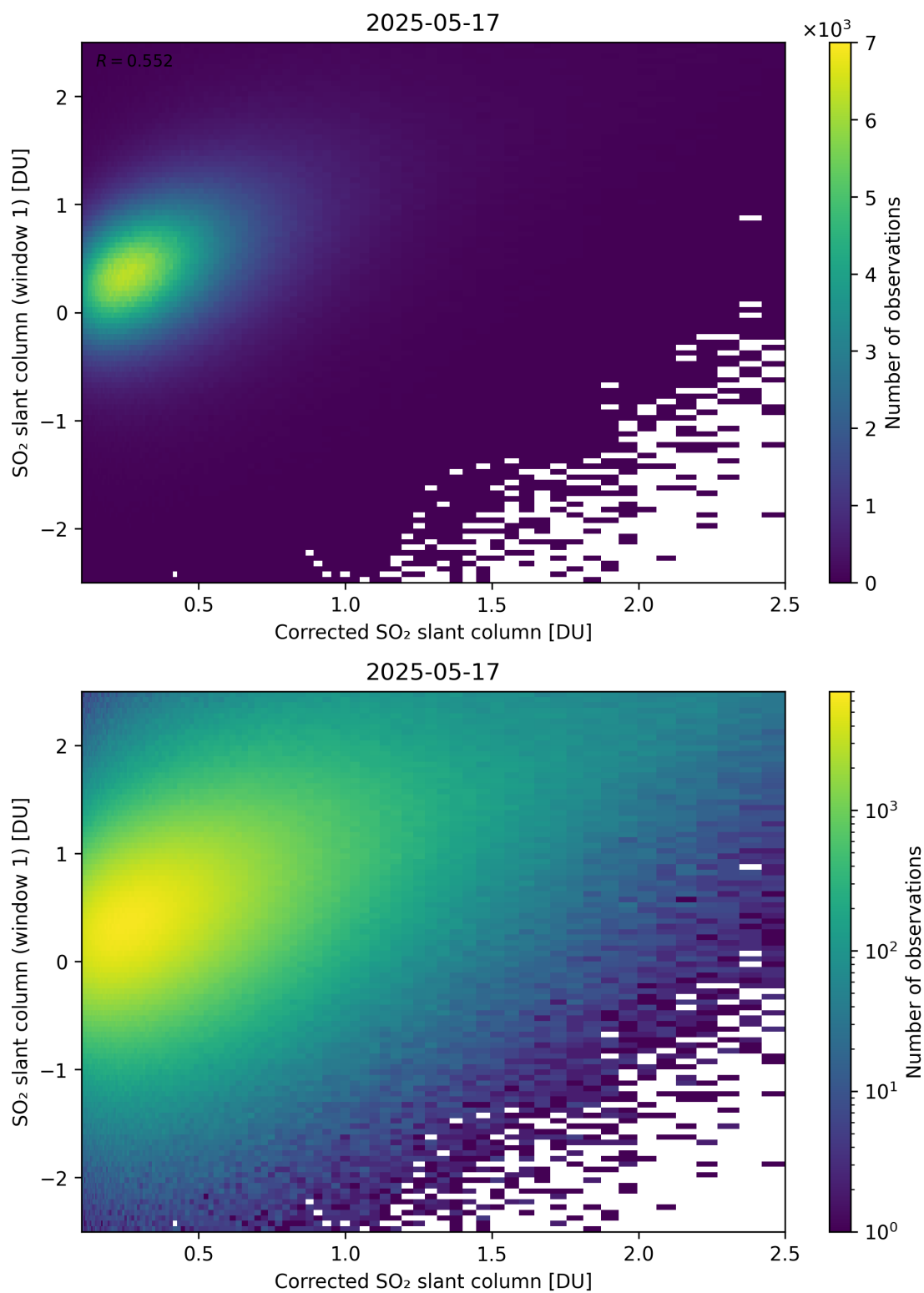
Figure 237: Scatter density plot of “Corrected SO 2 slant column” against “SO 2 slant column (window 1)” for 2025-05-16 to 2025-05-18.
