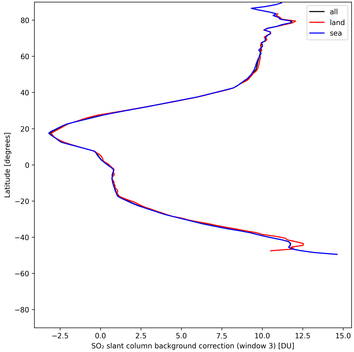
Figure 48: Zonal average of “SO 2 slant column background correction (window 3)” for 2025-05-16 to 2025-05-18.
