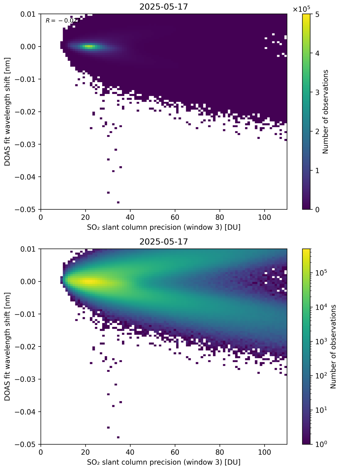
Figure 308: Scatter density plot of “SO 2 slant column precision (window 3)” against “DOAS fit wavelength shift” for 2025-05-16 to 2025-05-18.
