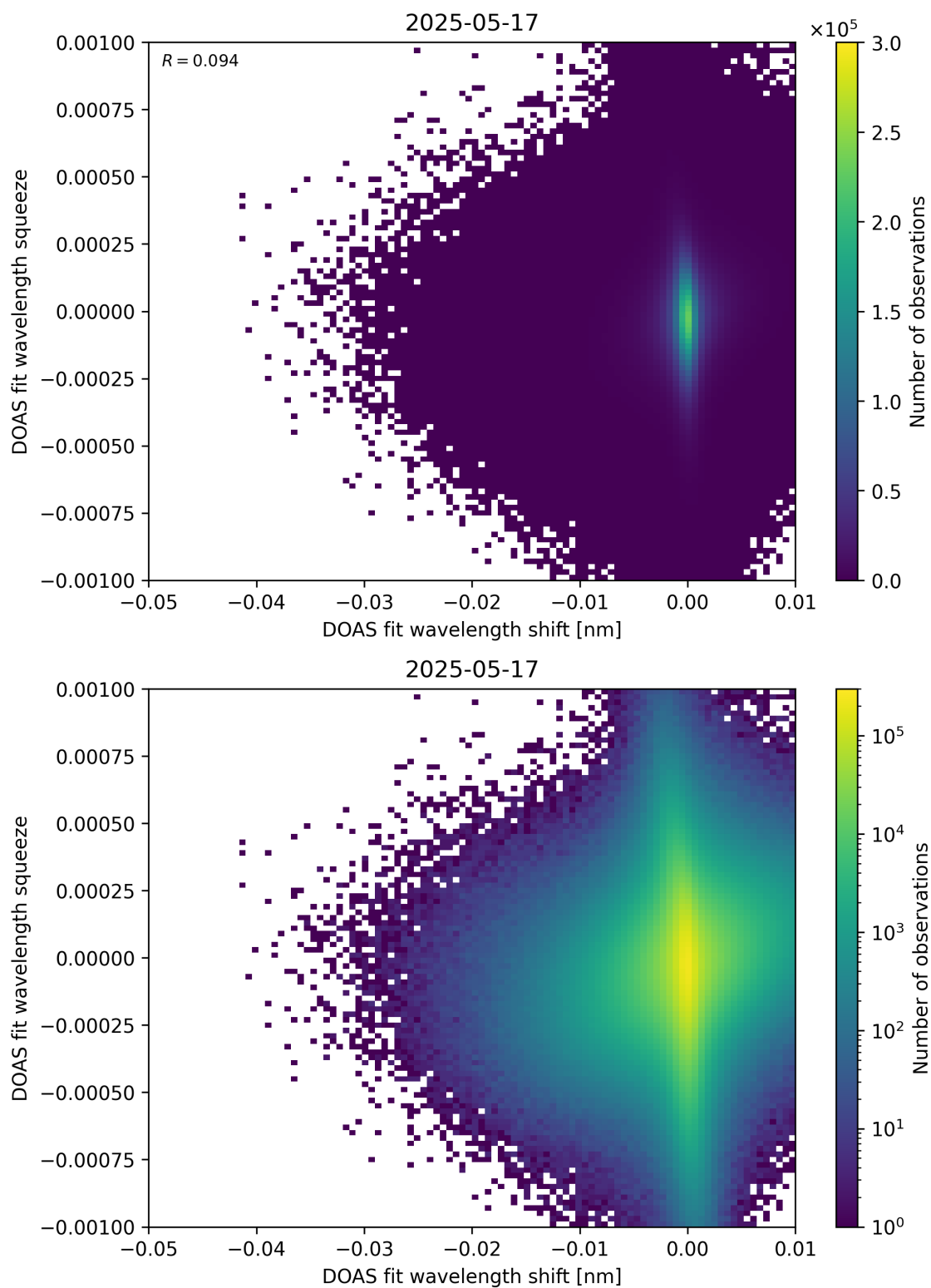
Figure 138: Scatter density plot of “DOAS fit wavelength shift” against “DOAS fit wavelength squeeze” for 2025-05-16 to 2025-05-18.
