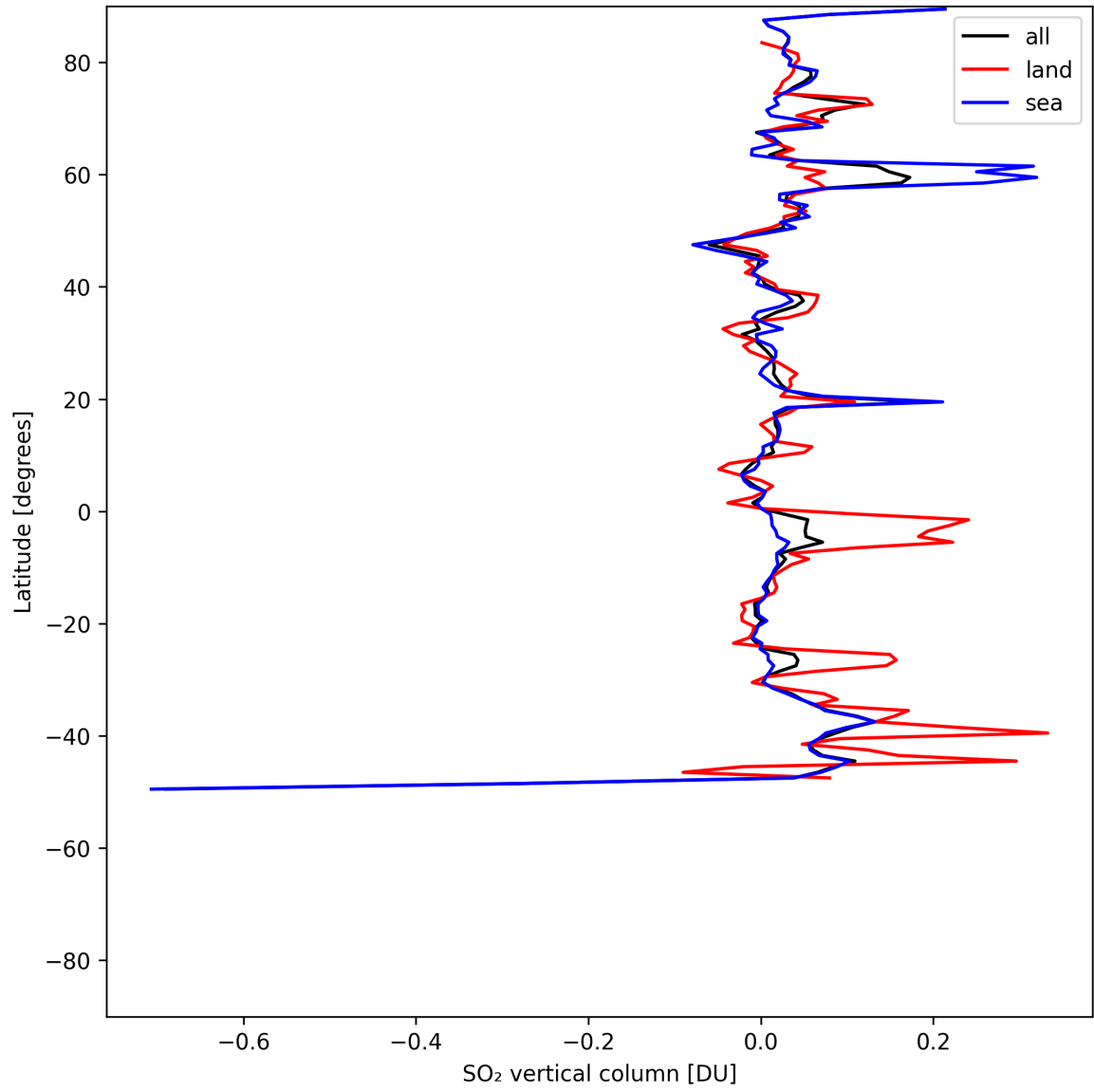
Figure 32: Zonal average of “SO 2 vertical column” for 2025-05-16 to 2025-05-18.
