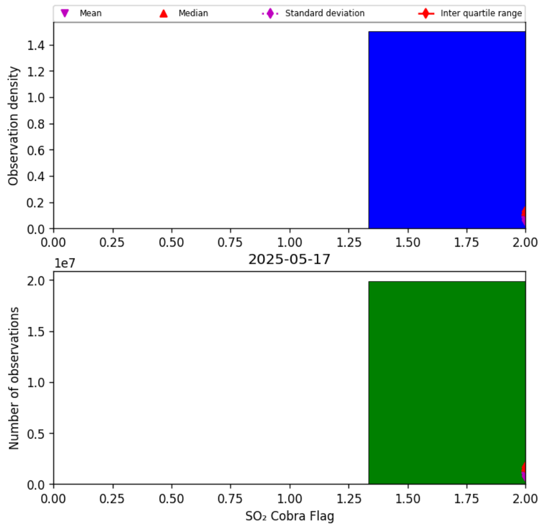
Figure 75: Histogram of “SO 2 Cobra Flag” for 2025-05-16 to 2025-05-18
