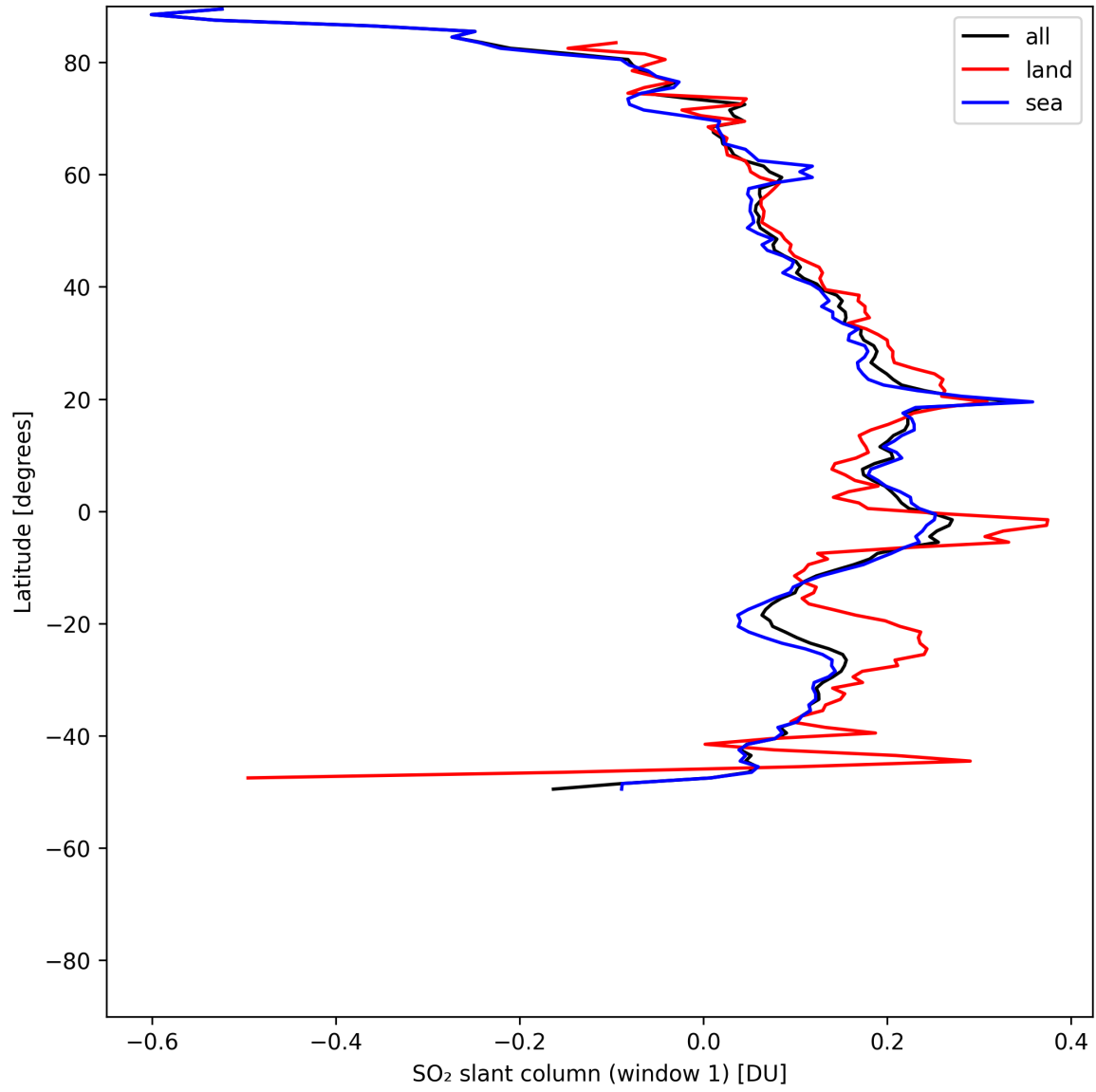
Figure 37: Zonal average of “SO 2 slant column (window 1)” for 2025-05-16 to 2025-05-18.
