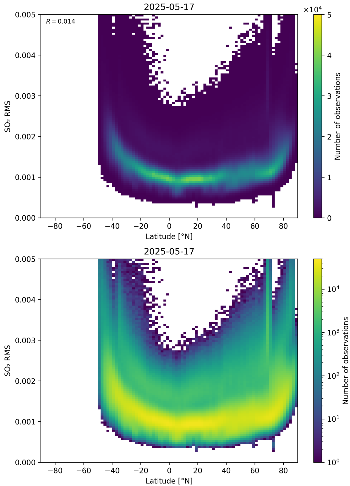
Figure 155: Scatter density plot of “Latitude” against “SO 2 RMS” for 2025-05-16 to 2025-05-18.
