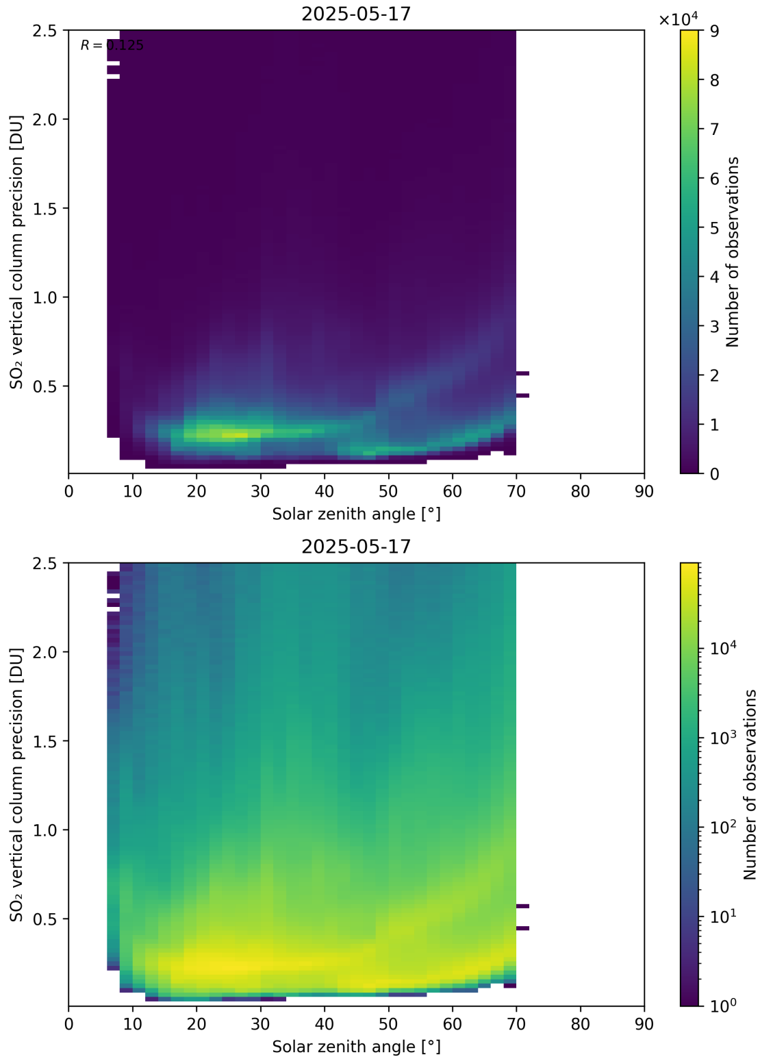
Figure 192: Scatter density plot of “Solar zenith angle” against “SO 2 vertical column precision” for 2025-05-16 to 2025-05-18.
