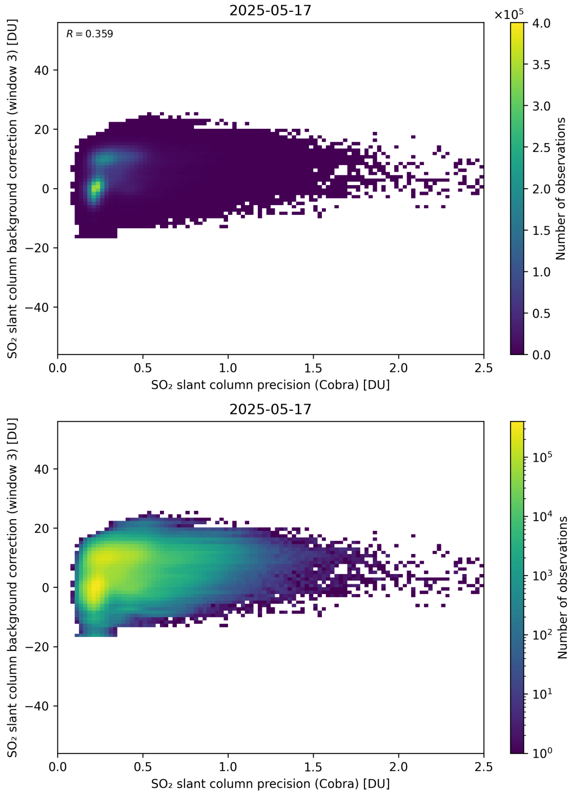
Figure 201: Scatter density plot of “SO 2 slant column precision (Cobra)” against “SO 2 slant column background correction (window 3)” for 2025-05-16 to 2025-05-18.
