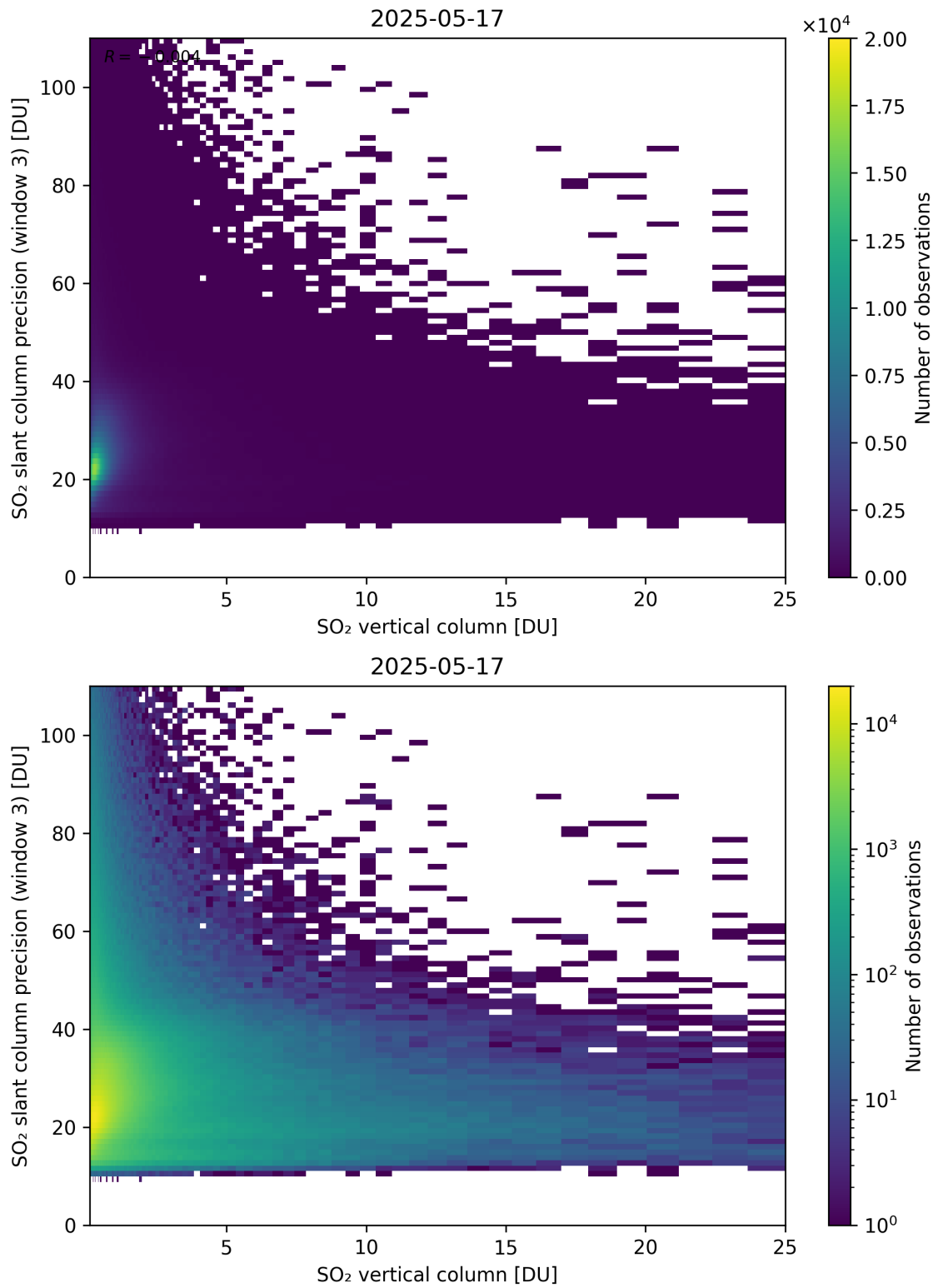
Figure 358: Scatter density plot of “SO 2 vertical column” against “SO 2 slant column precision (window 3)” for 2025-05-16 to 2025-05-18.
