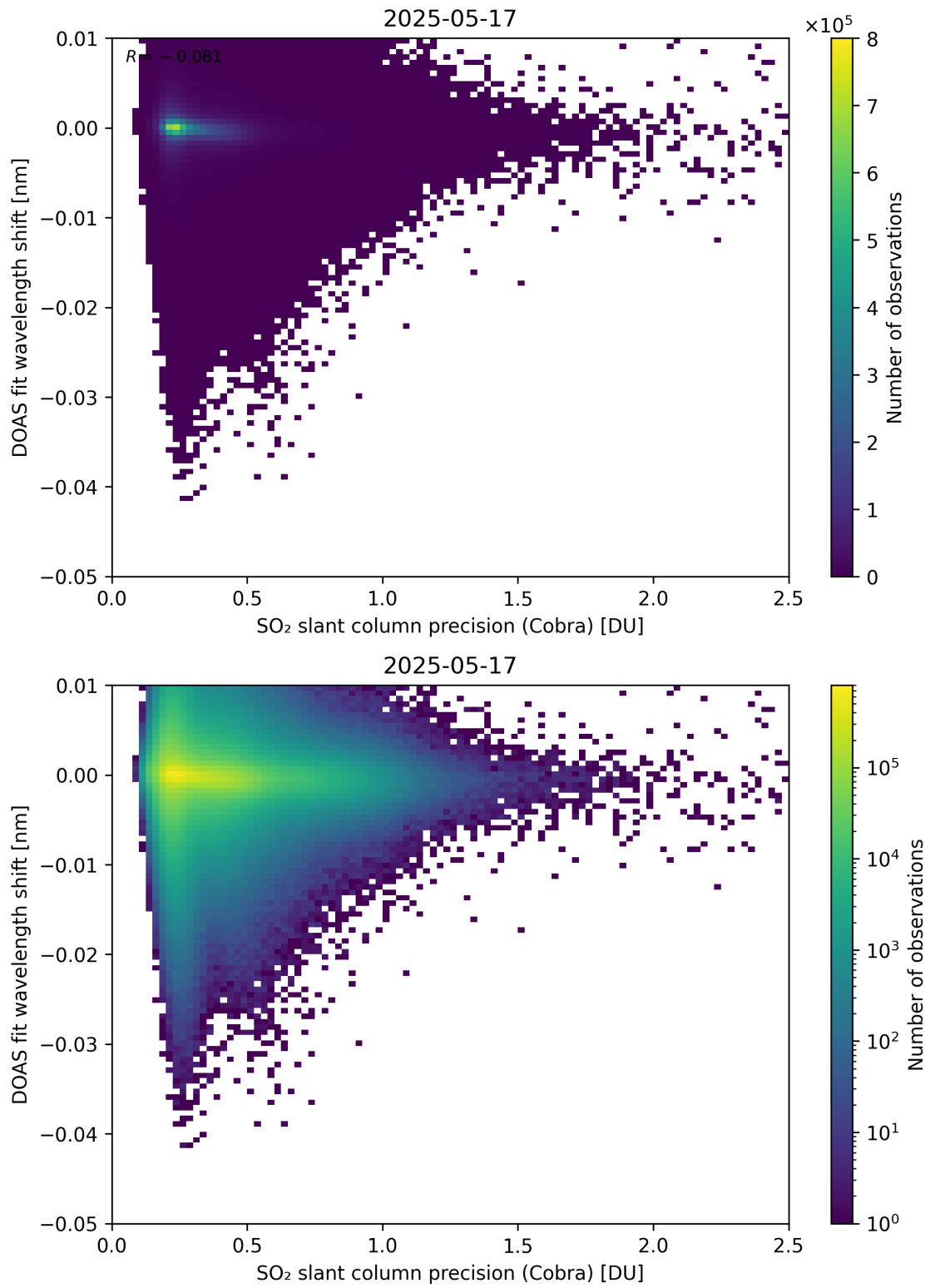
Figure 202: Scatter density plot of “SO 2 slant column precision (Cobra)” against “DOAS fit wavelength shift” for 2025-05-16 to 2025-05-18.
