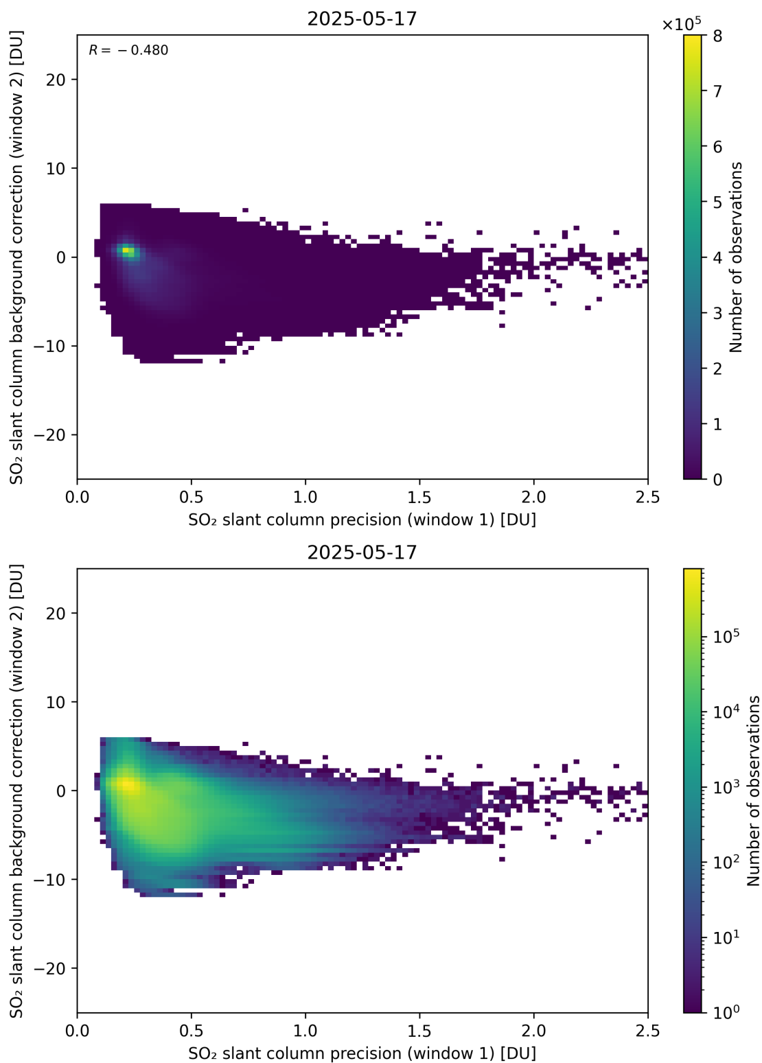
Figure 269: Scatter density plot of “SO 2 slant column precision (window 1)” against “SO 2 slant column background correction (window 2)” for 2025-05-16 to 2025-05-18.
