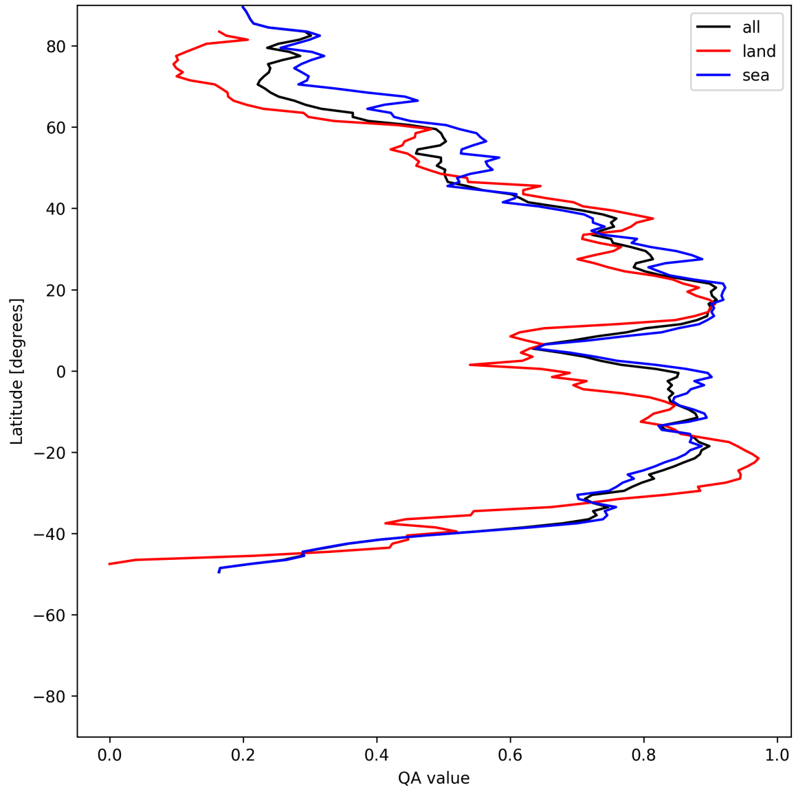
Figure 31: Zonal average of “QA value” for 2025-05-16 to 2025-05-18.
