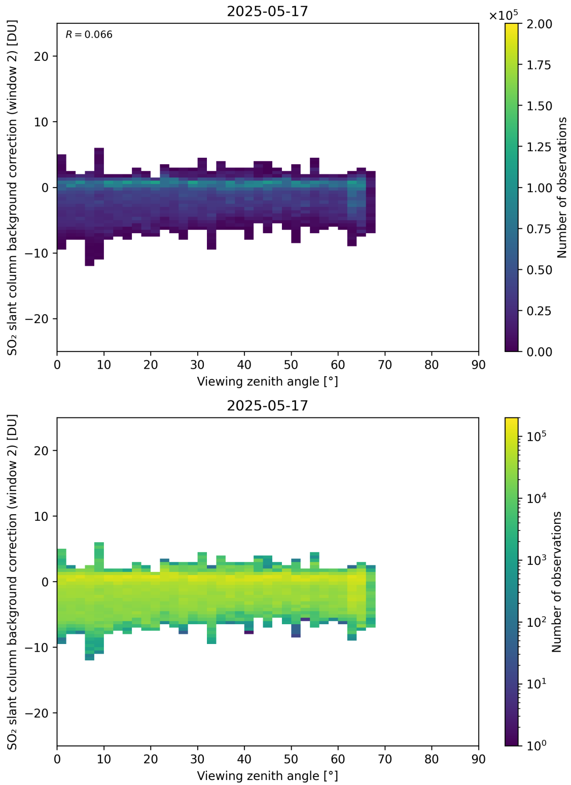
Figure 363: Scatter density plot of “Viewing zenith angle” against “SO 2 slant column background correction (window 2)” for 2025-05-16 to 2025-05-18.
