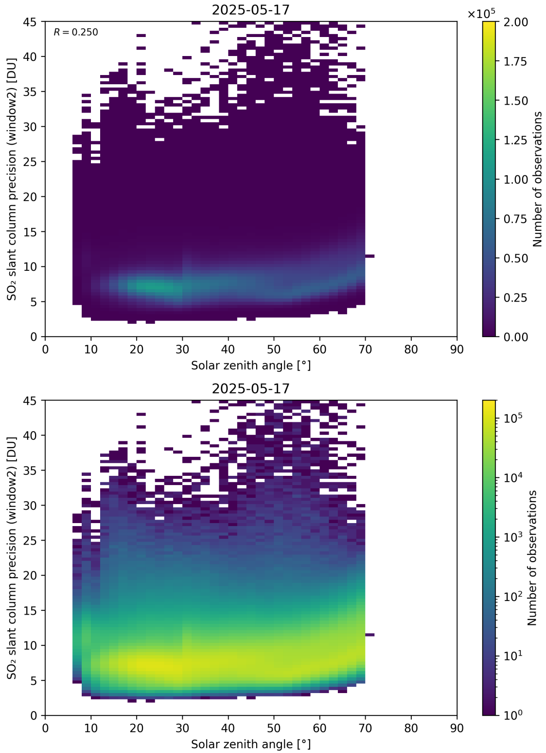
Figure 186: Scatter density plot of “Solar zenith angle” against “SO 2 slant column precision (window2)” for 2025-05-16 to 2025-05-18.
