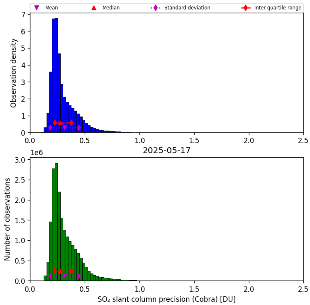
Figure 62: Histogram of “SO 2 slant column precision (Cobra)” for 2025-05-16 to 2025-05-18
