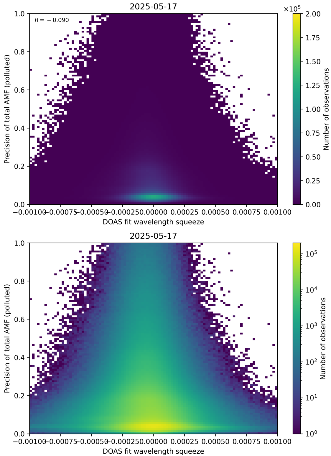
Figure 146: Scatter density plot of “DOAS fit wavelength squeeze” against “Precision of total AMF (polluted)” for 2025-05-16 to 2025-05-18.
