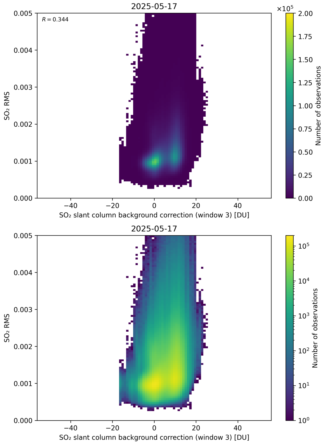
Figure 134: Scatter density plot of “SO 2 slant column background correction (window 3)” against “SO 2 RMS” for 2025-05-16 to 2025-05-18.
