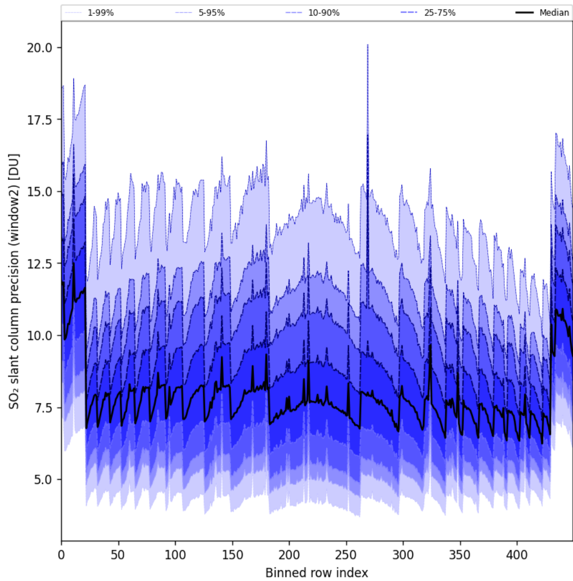
Figure 94: Along track statistics of “SO 2 slant column precision (window2)” for 2025-05-16 to 2025-05-18
