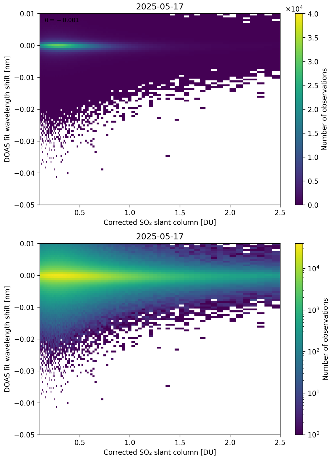
Figure 229: Scatter density plot of “Corrected SO 2 slant column” against “DOAS fit wavelength shift” for 2025-05-16 to 2025-05-18.
