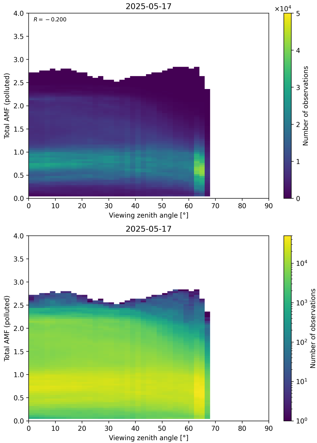
Figure 381: Scatter density plot of “Viewing zenith angle” against “Total AMF (polluted)” for 2025-05-16 to 2025-05-18.
