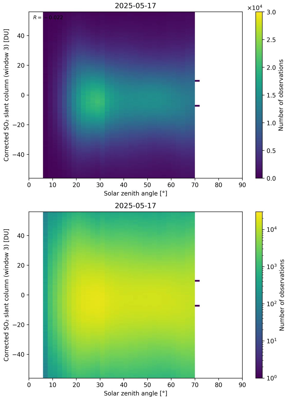
Figure 183: Scatter density plot of “Solar zenith angle” against “Corrected SO 2 slant column (window 3)” for 2025-05-16 to 2025-05-18.
