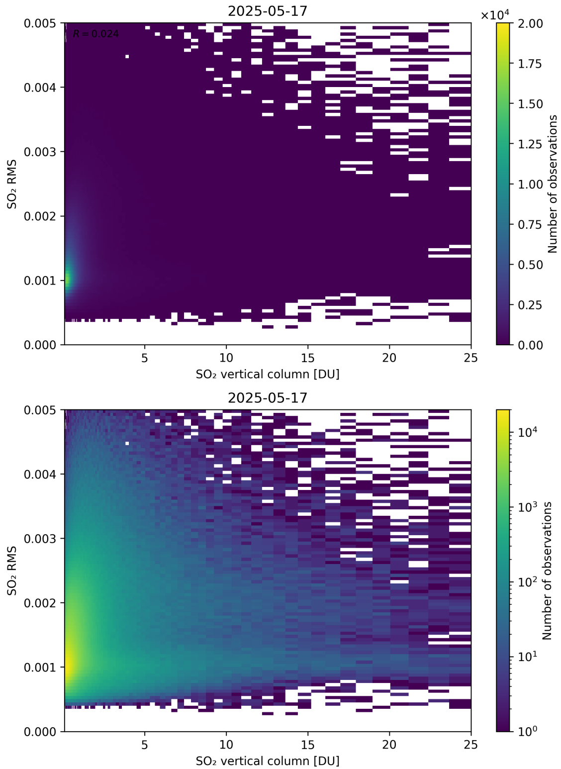
Figure 328: Scatter density plot of “SO 2 vertical column” against “SO 2 RMS” for 2025-05-16 to 2025-05-18.
