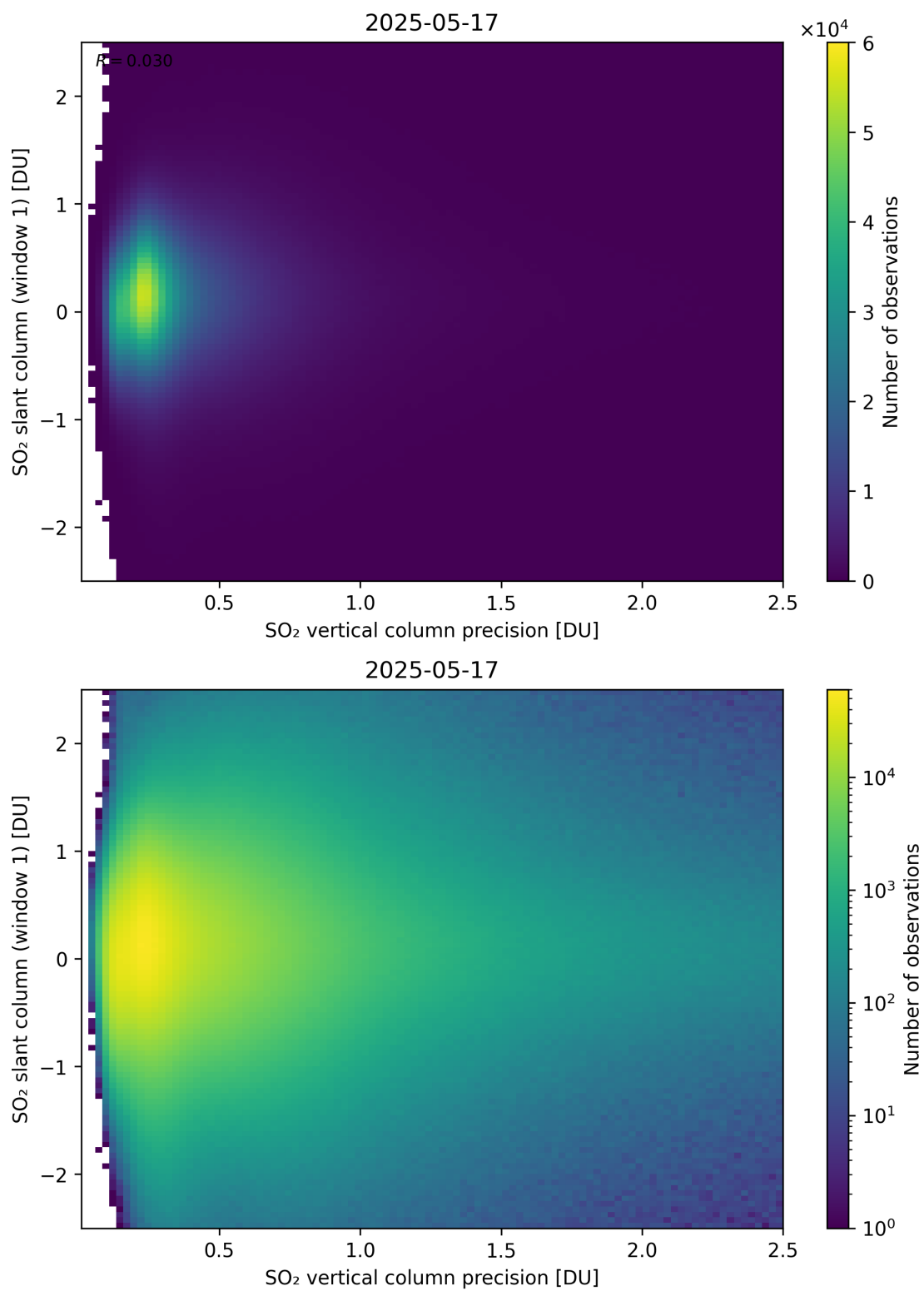
Figure 341: Scatter density plot of “SO 2 vertical column precision” against “SO 2 slant column (window 1)” for 2025-05-16 to 2025-05-18.
