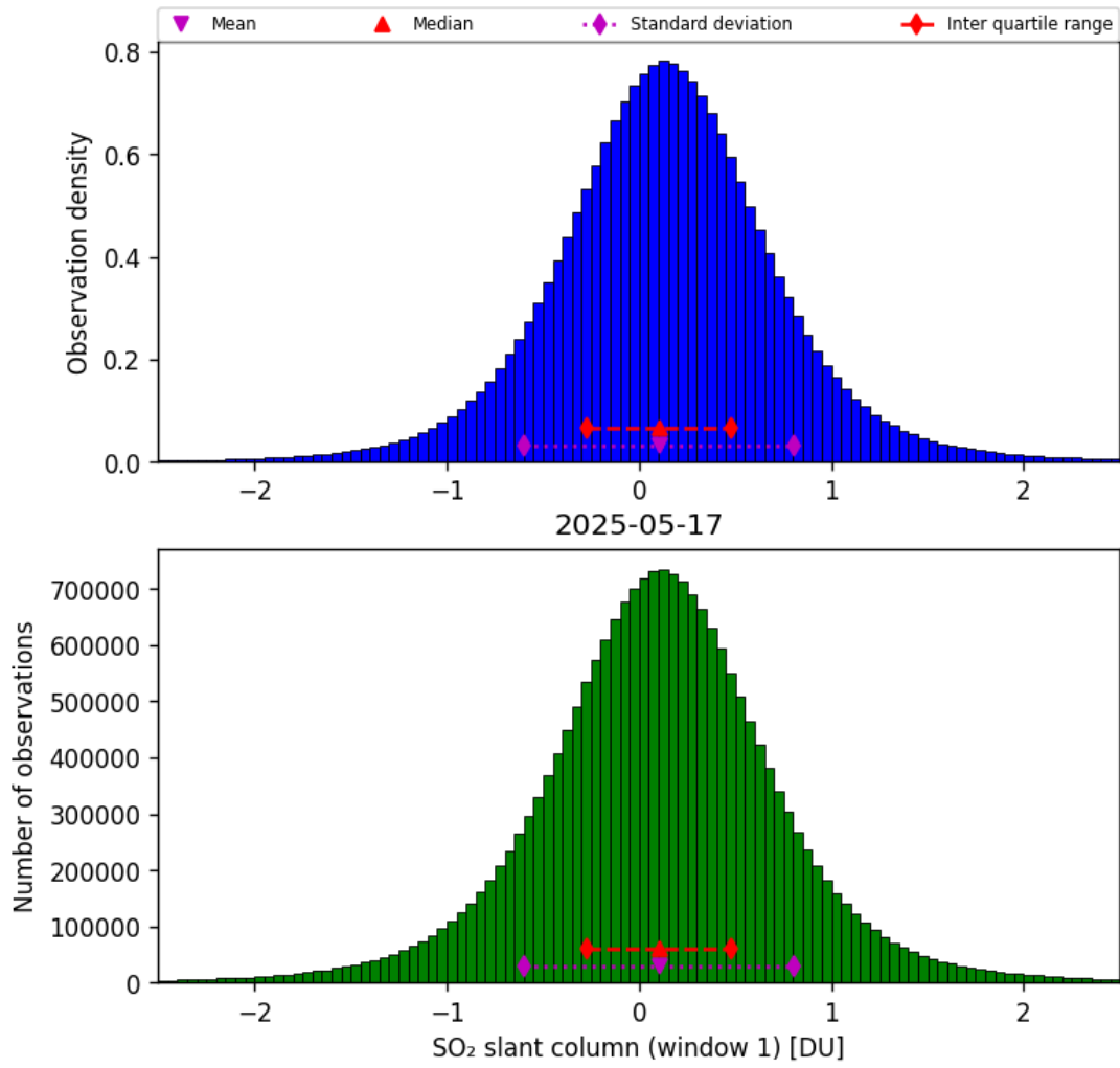
Figure 63: Histogram of “SO 2 slant column (window 1)” for 2025-05-16 to 2025-05-18
