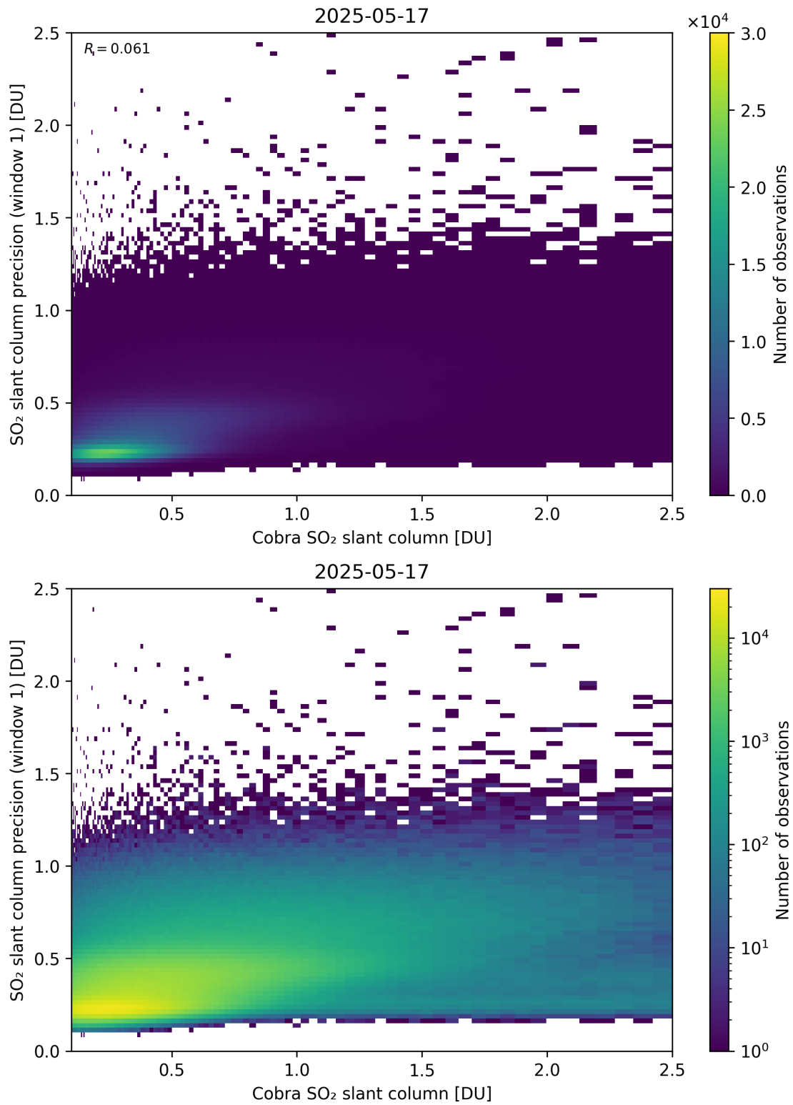
Figure 220: Scatter density plot of “Cobra SO 2 slant column” against “SO 2 slant column precision (window 1)” for 2025-05-16 to 2025-05-18.
