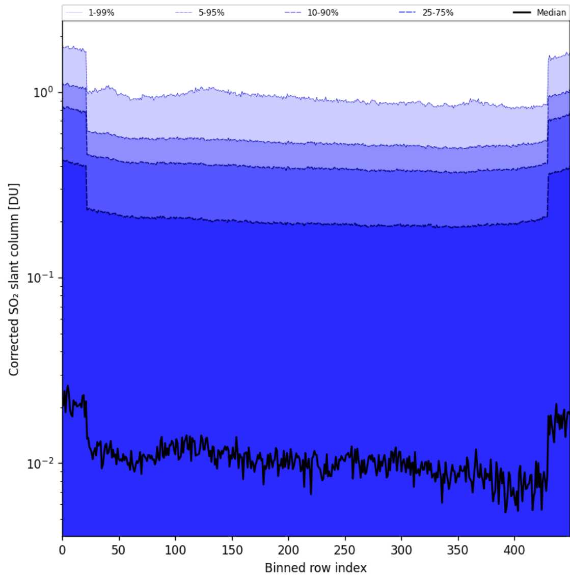
Figure 86: Along track statistics of “Corrected SO 2 slant column” for 2025-05-16 to 2025-05-18
