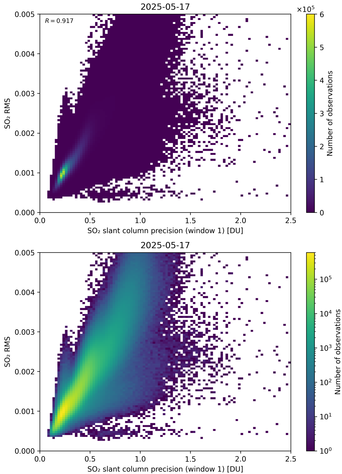
Figure 273: Scatter density plot of “SO 2 slant column precision (window 1)” against “SO 2 RMS” for 2025-05-16 to 2025-05-18.
