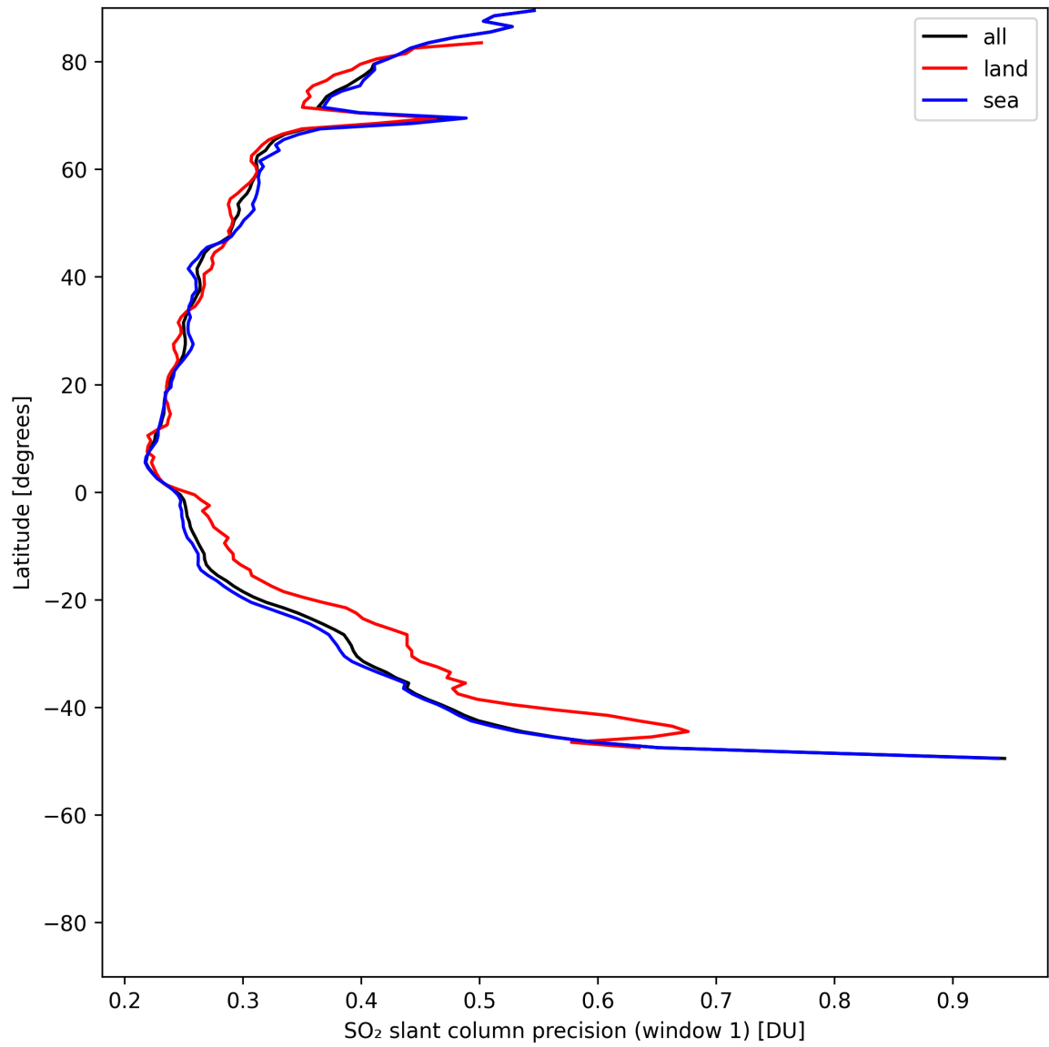
Figure 38: Zonal average of “SO 2 slant column precision (window 1)” for 2025-05-16 to 2025-05-18.
