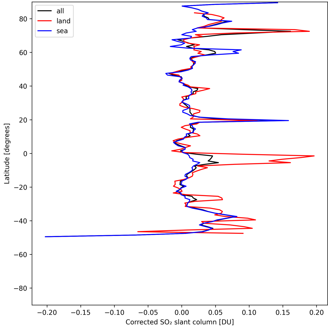
Figure 34: Zonal average of “Corrected SO 2 slant column” for 2025-05-16 to 2025-05-18.
