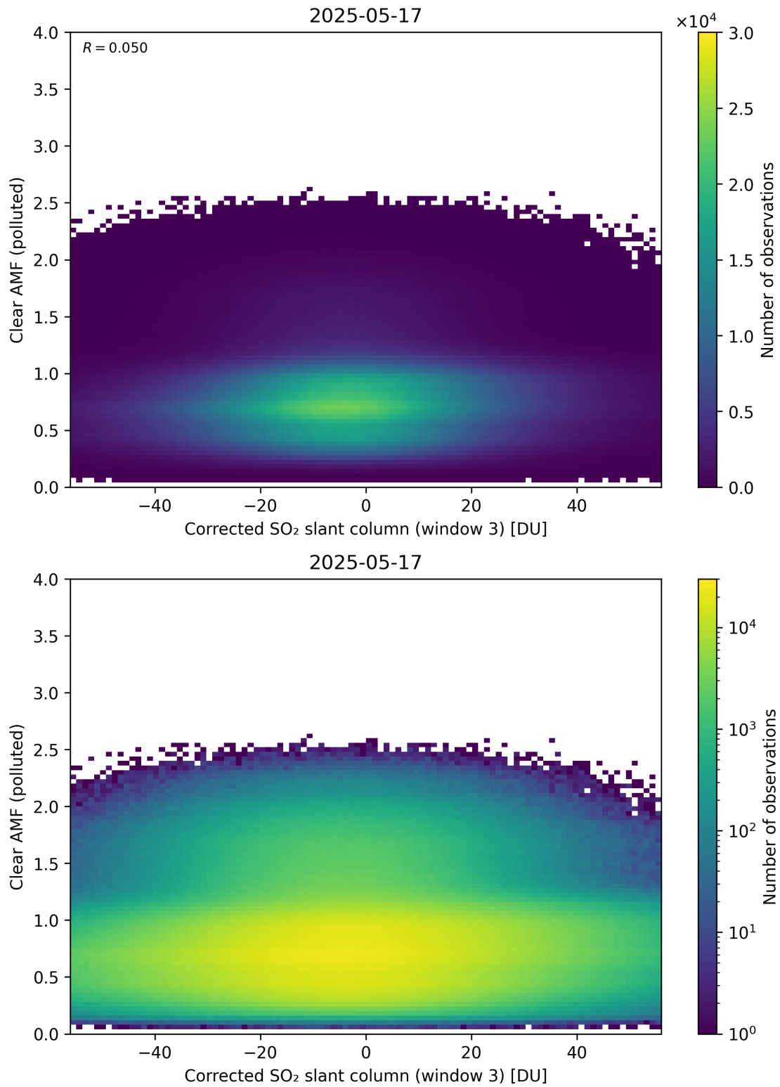
Figure 259: Scatter density plot of “Corrected SO 2 slant column (window 3)” against “Clear AMF (polluted)” for 2025-05-16 to 2025-05-18.
