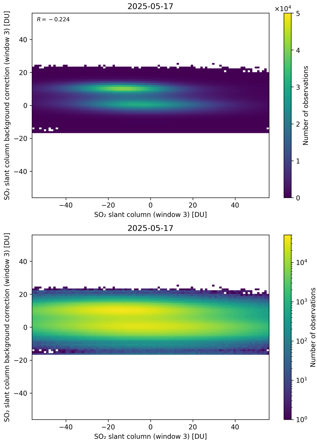
Figure 303: Scatter density plot of “SO 2 slant column (window 3)” against “SO 2 slant column background correction (window 3)” for 2025-05-16 to 2025-05-18.
