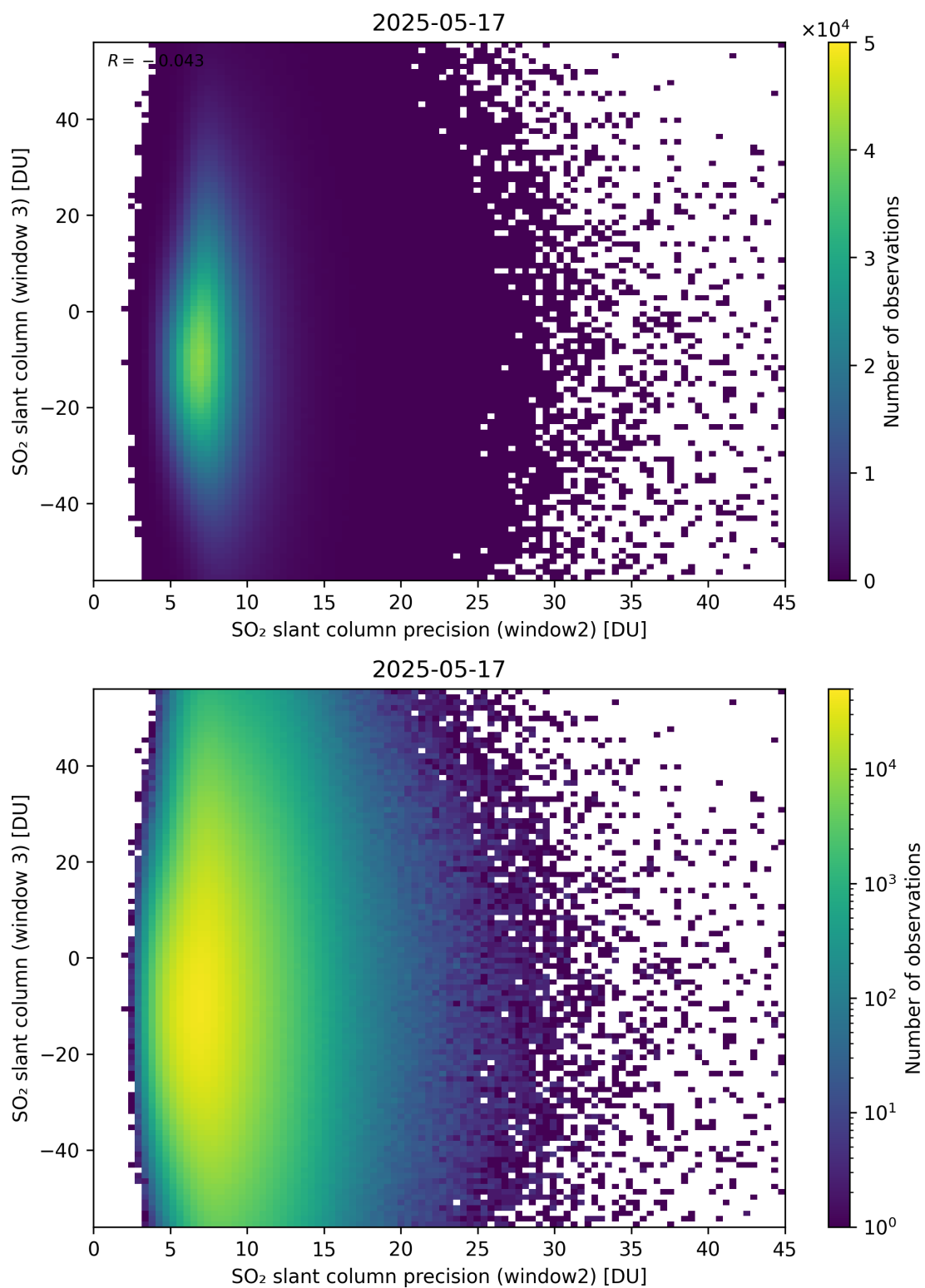
Figure 299: Scatter density plot of “SO 2 slant column precision (window2)” against “SO 2 slant column (window 3)” for 2025-05-16 to 2025-05-18.
