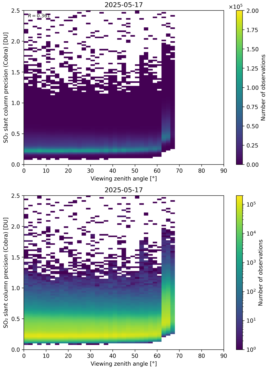
Figure 372: Scatter density plot of “Viewing zenith angle” against “SO 2 slant column precision (Cobra)” for 2025-05-16 to 2025-05-18.
