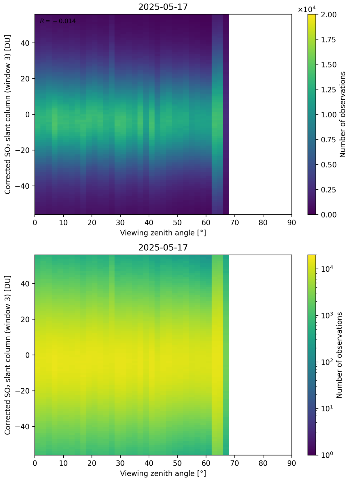
Figure 375: Scatter density plot of “Viewing zenith angle” against “Corrected SO 2 slant column (window 3)” for 2025-05-16 to 2025-05-18.
