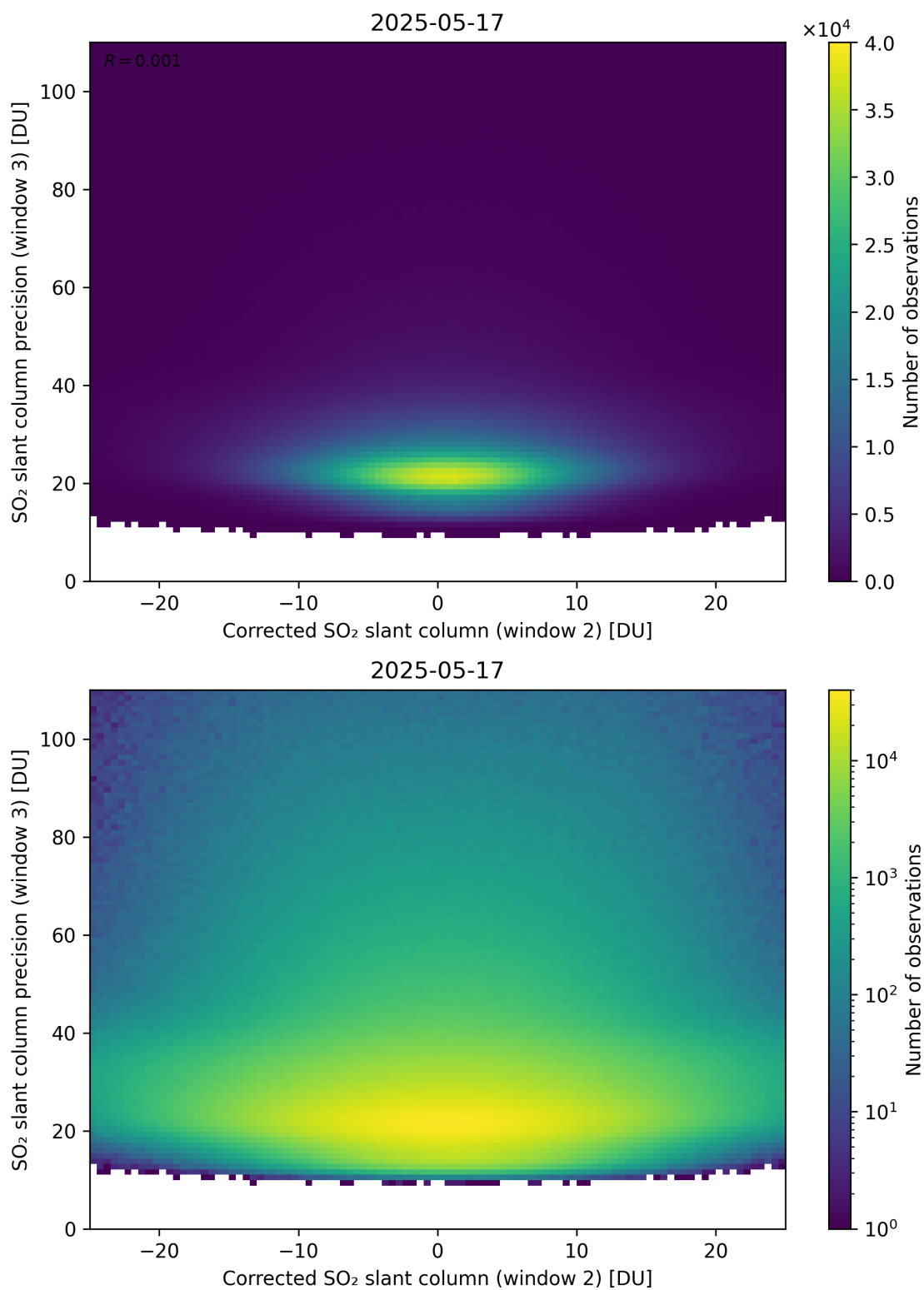
Figure 252: Scatter density plot of “Corrected SO 2 slant column (window 2)” against “SO 2 slant column precision (window 3)” for 2025-05-16 to 2025-05-18.
