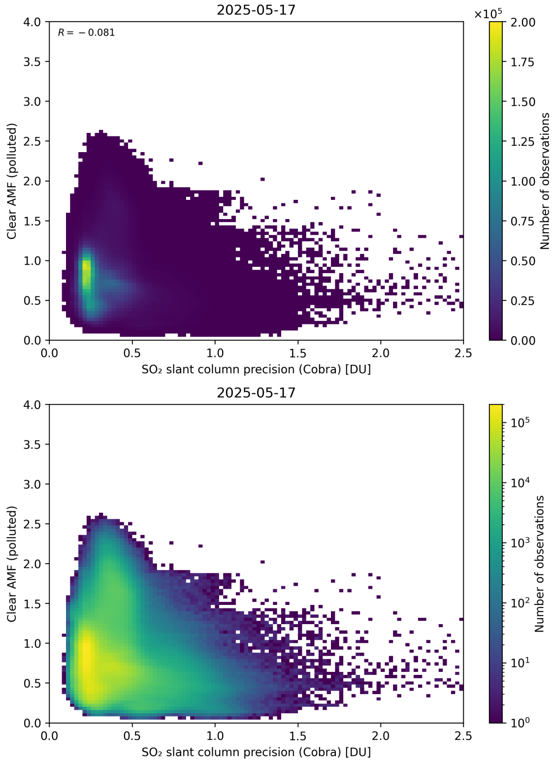
Figure 205: Scatter density plot of “SO 2 slant column precision (Cobra)” against “Clear AMF (polluted)” for 2025-05-16 to 2025-05-18.
