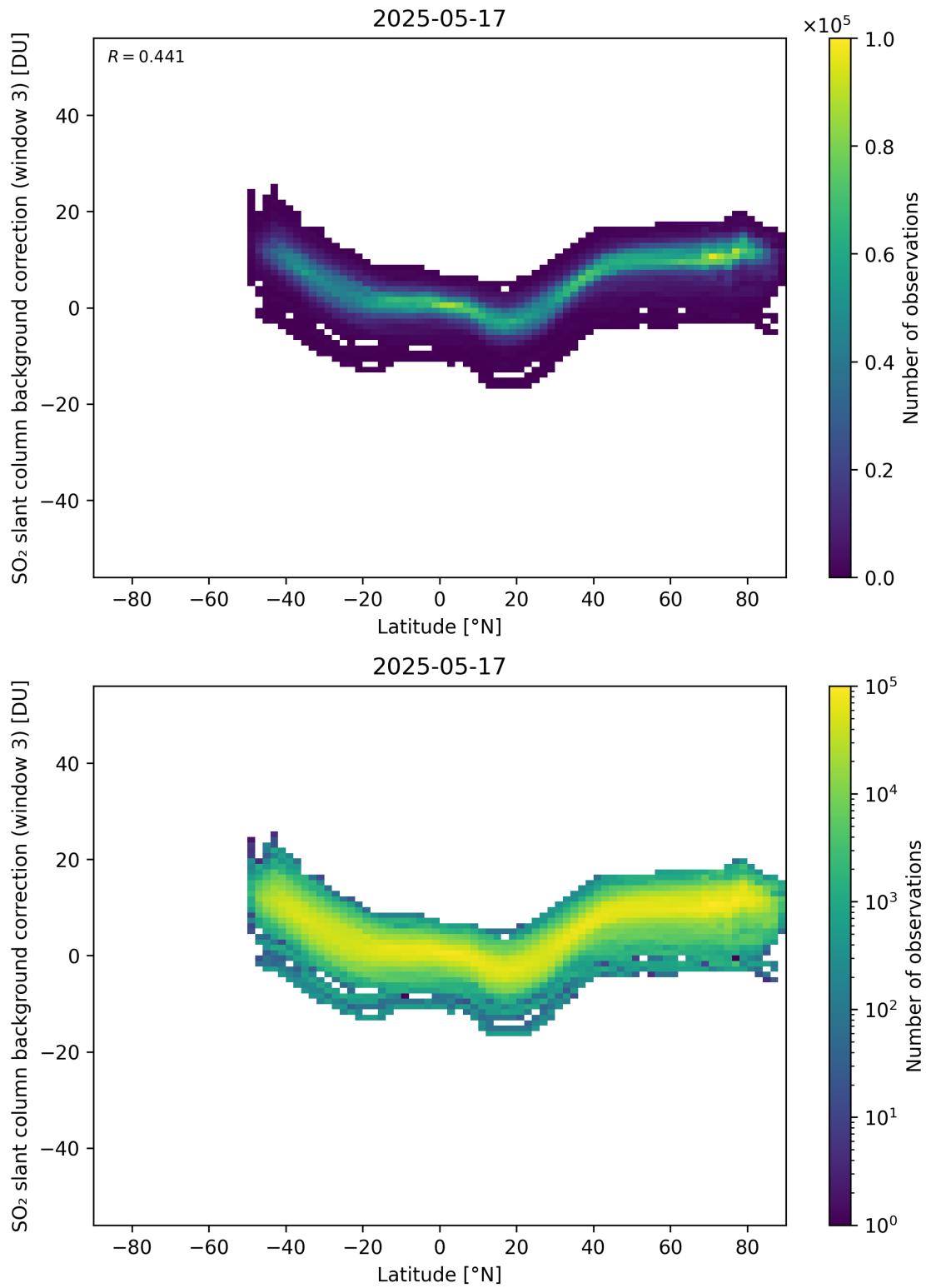
Figure 152: Scatter density plot of “Latitude” against “SO 2 slant column background correction (window 3)” for 2025-05-16 to 2025-05-18.
