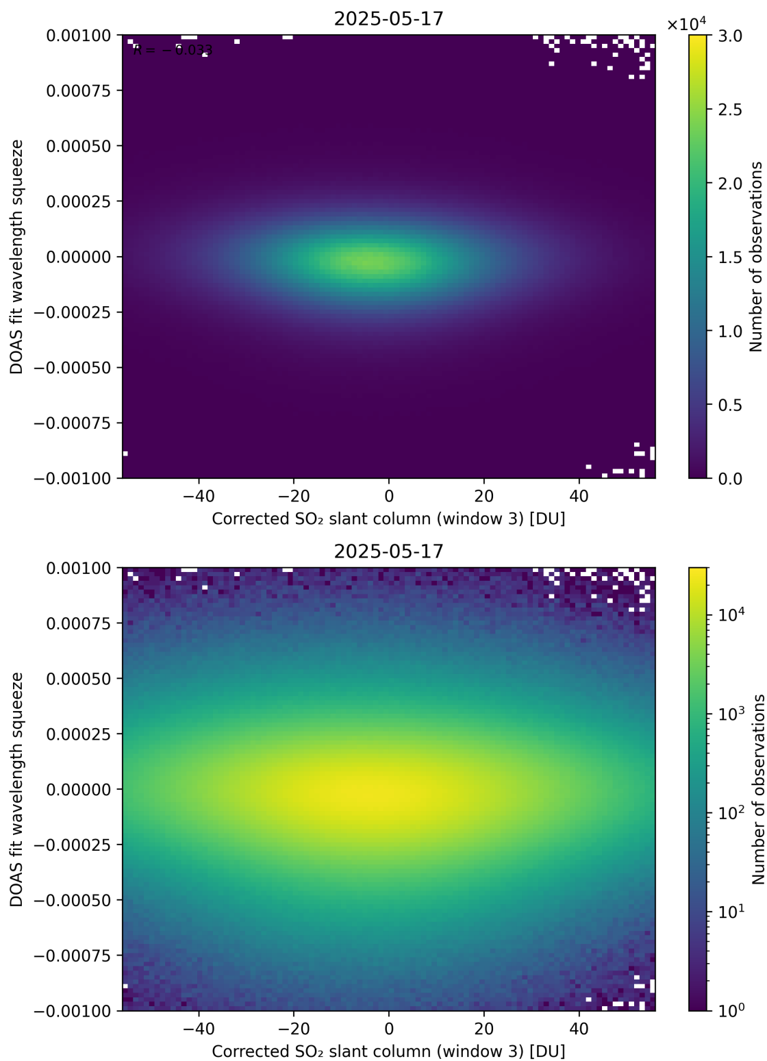
Figure 257: Scatter density plot of “Corrected SO 2 slant column (window 3)” against “DOAS fit wavelength squeeze” for 2025-05-16 to 2025-05-18.
