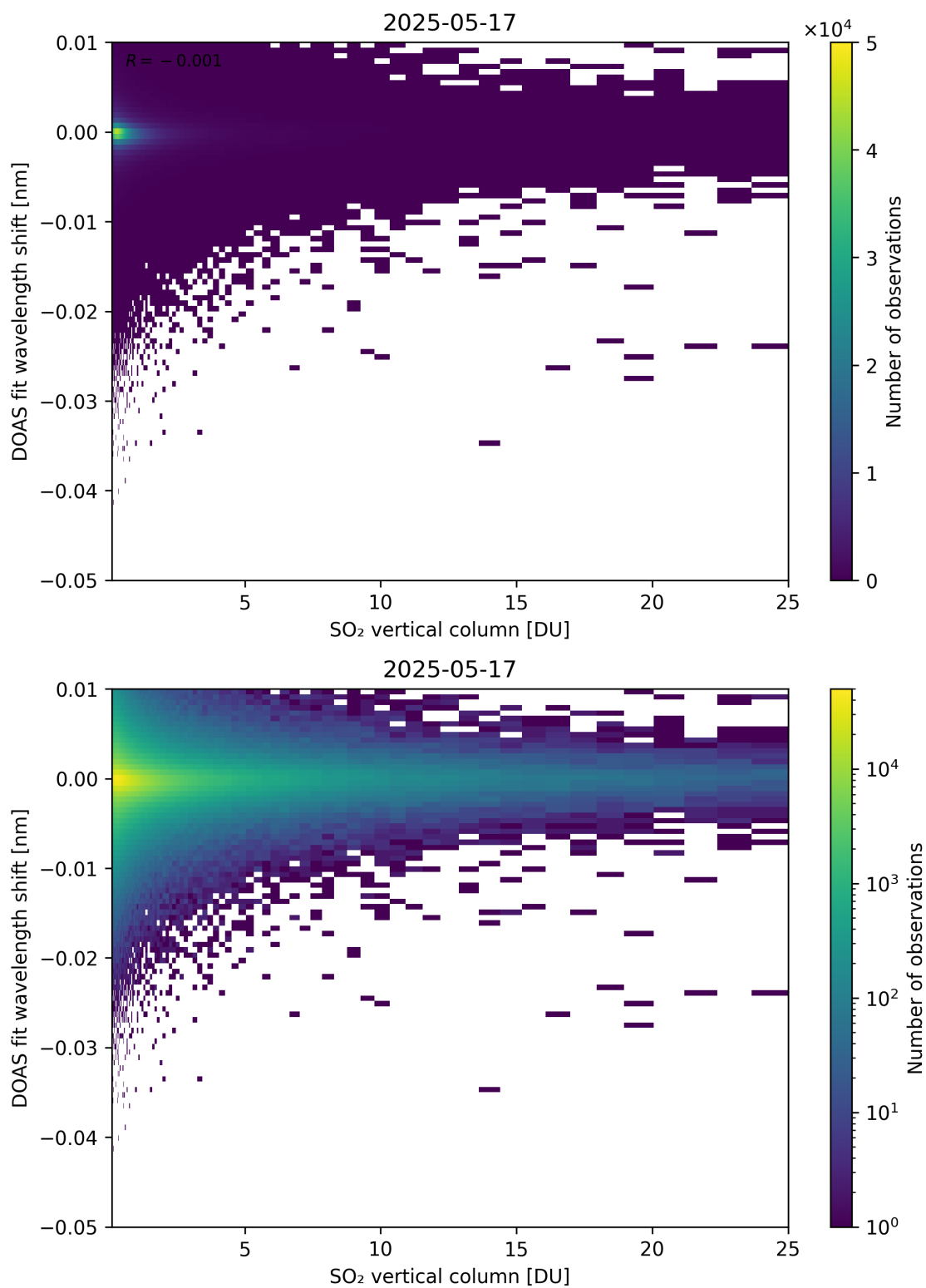
Figure 326: Scatter density plot of “SO 2 vertical column” against “DOAS fit wavelength shift” for 2025-05-16 to 2025-05-18.
