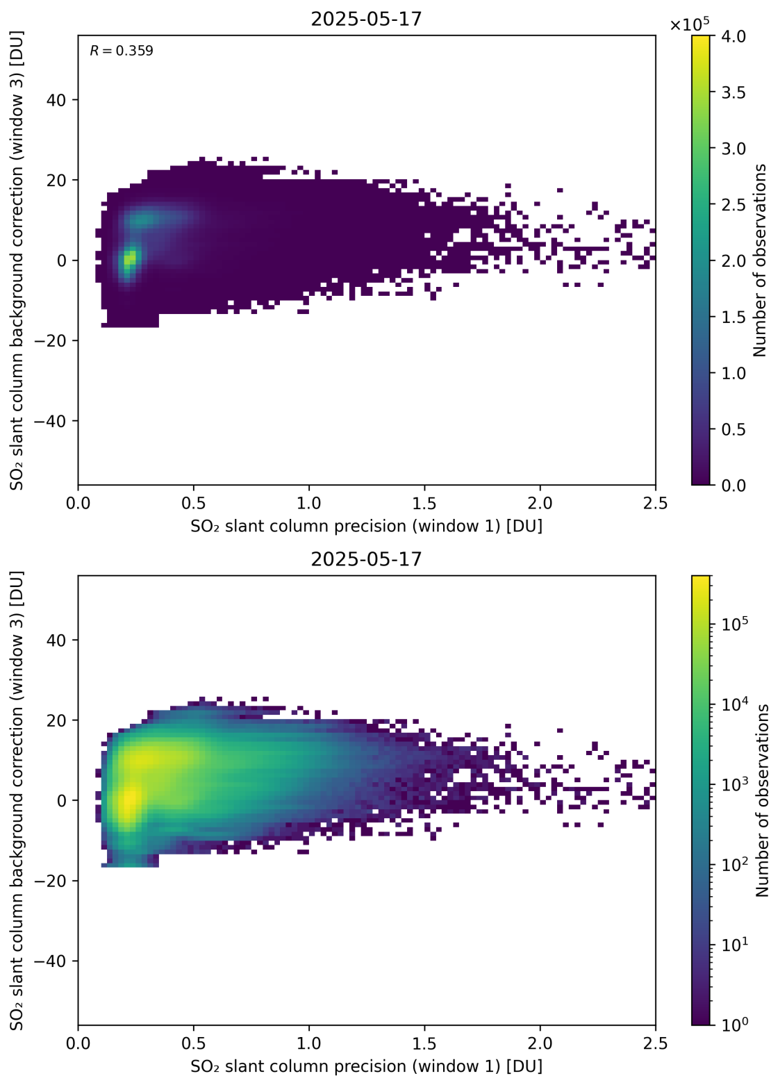
Figure 270: Scatter density plot of “SO 2 slant column precision (window 1)” against “SO 2 slant column background correction (window 3)” for 2025-05-16 to 2025-05-18.
