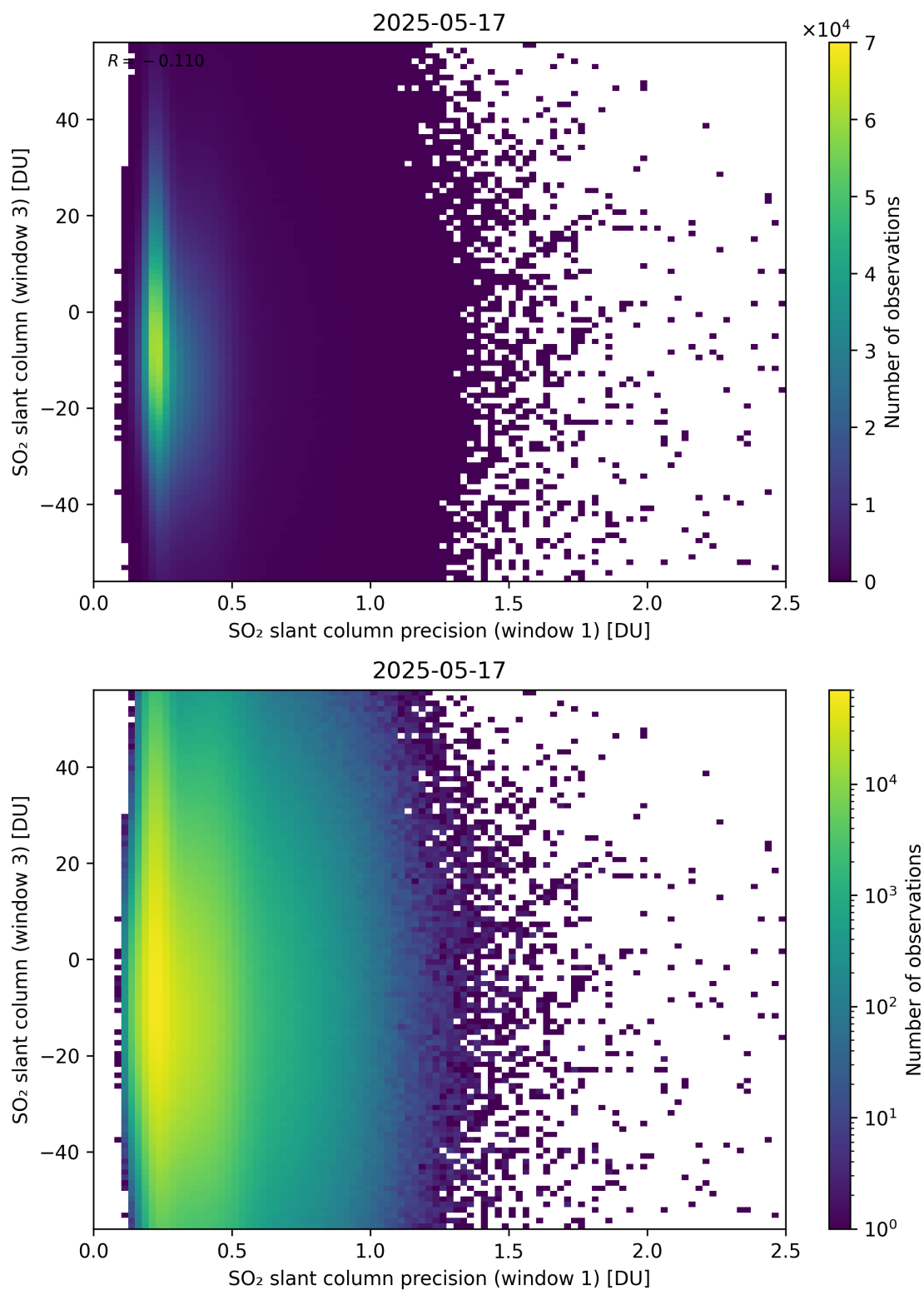
Figure 278: Scatter density plot of “SO 2 slant column precision (window 1)” against “SO 2 slant column (window 3)” for 2025-05-16 to 2025-05-18.
