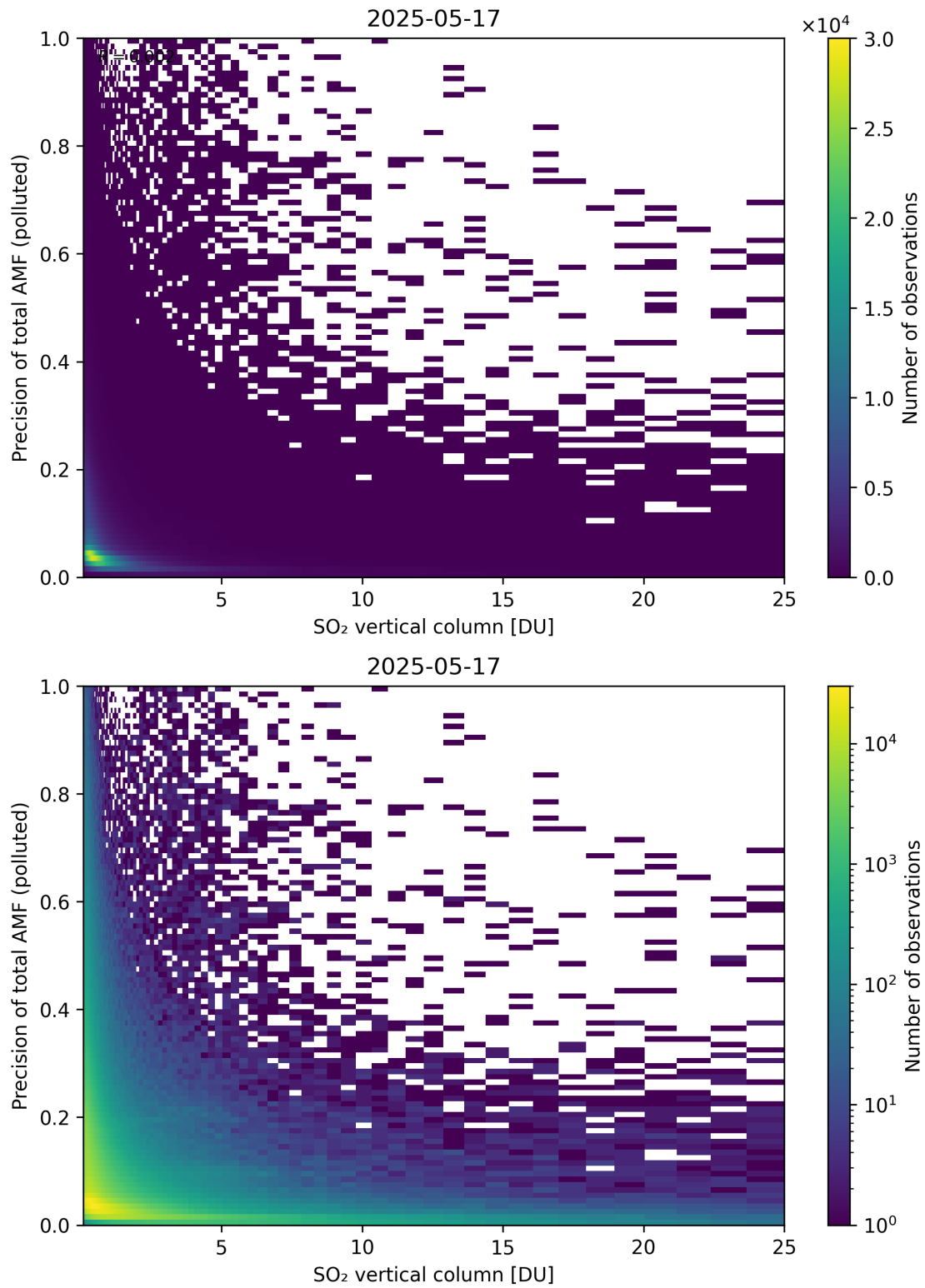
Figure 360: Scatter density plot of “SO 2 vertical column” against “Precision of total AMF (polluted)” for 2025-05-16 to 2025-05-18.
