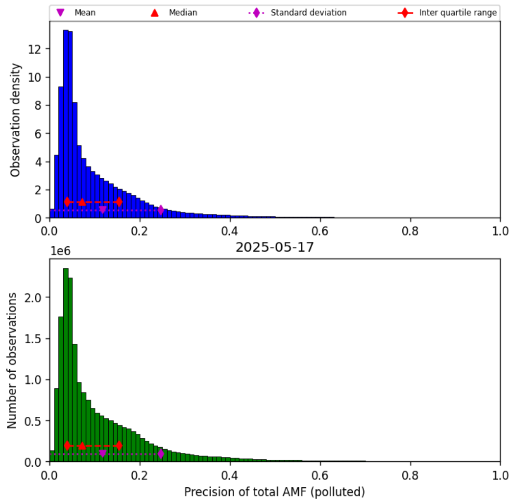
Figure 80: Histogram of “Precision of total AMF (polluted)” for 2025-05-16 to 2025-05-18
