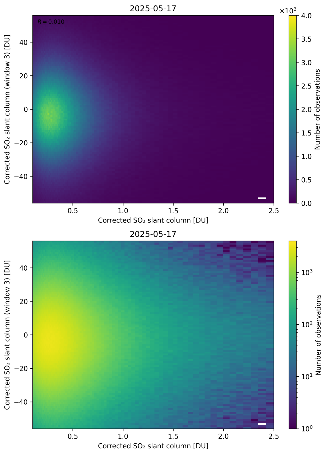
Figure 236: Scatter density plot of “Corrected SO 2 slant column” against “Corrected SO 2 slant column (window 3)” for 2025-05-16 to 2025-05-18.
