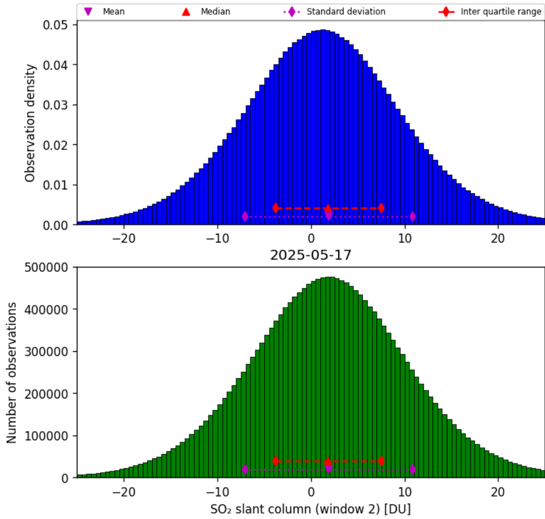
Figure 67: Histogram of “SO 2 slant column (window 2)” for 2025-05-16 to 2025-05-18
