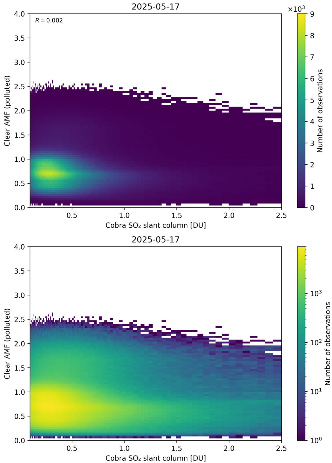
Figure 215: Scatter density plot of “Cobra SO 2 slant column” against “Clear AMF (polluted)” for 2025-05-16 to 2025-05-18.
