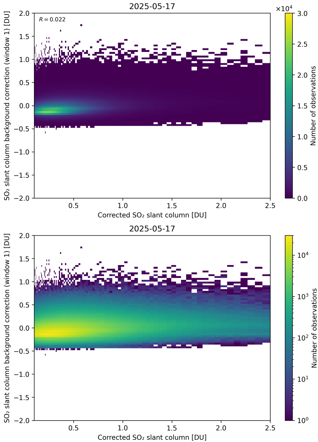
Figure 226: Scatter density plot of “Corrected SO 2 slant column” against “SO 2 slant column background correction (window 1)” for 2025-05-16 to 2025-05-18.
