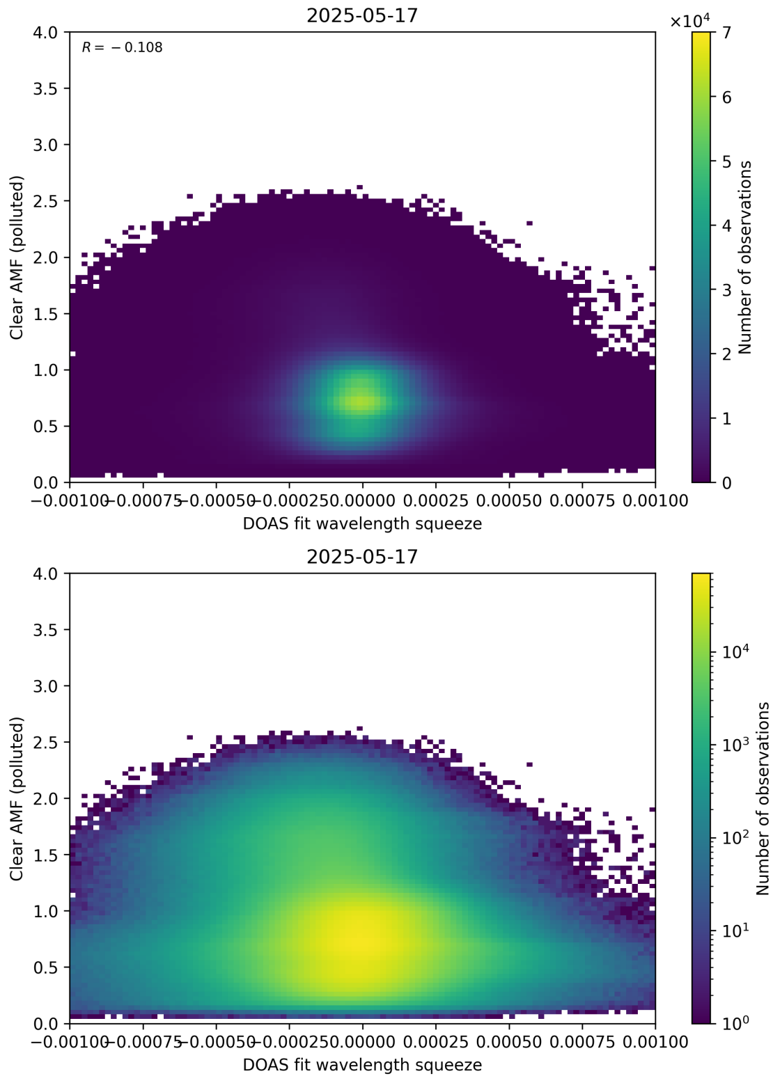
Figure 144: Scatter density plot of “DOAS fit wavelength squeeze” against “Clear AMF (polluted)” for 2025-05-16 to 2025-05-18.
