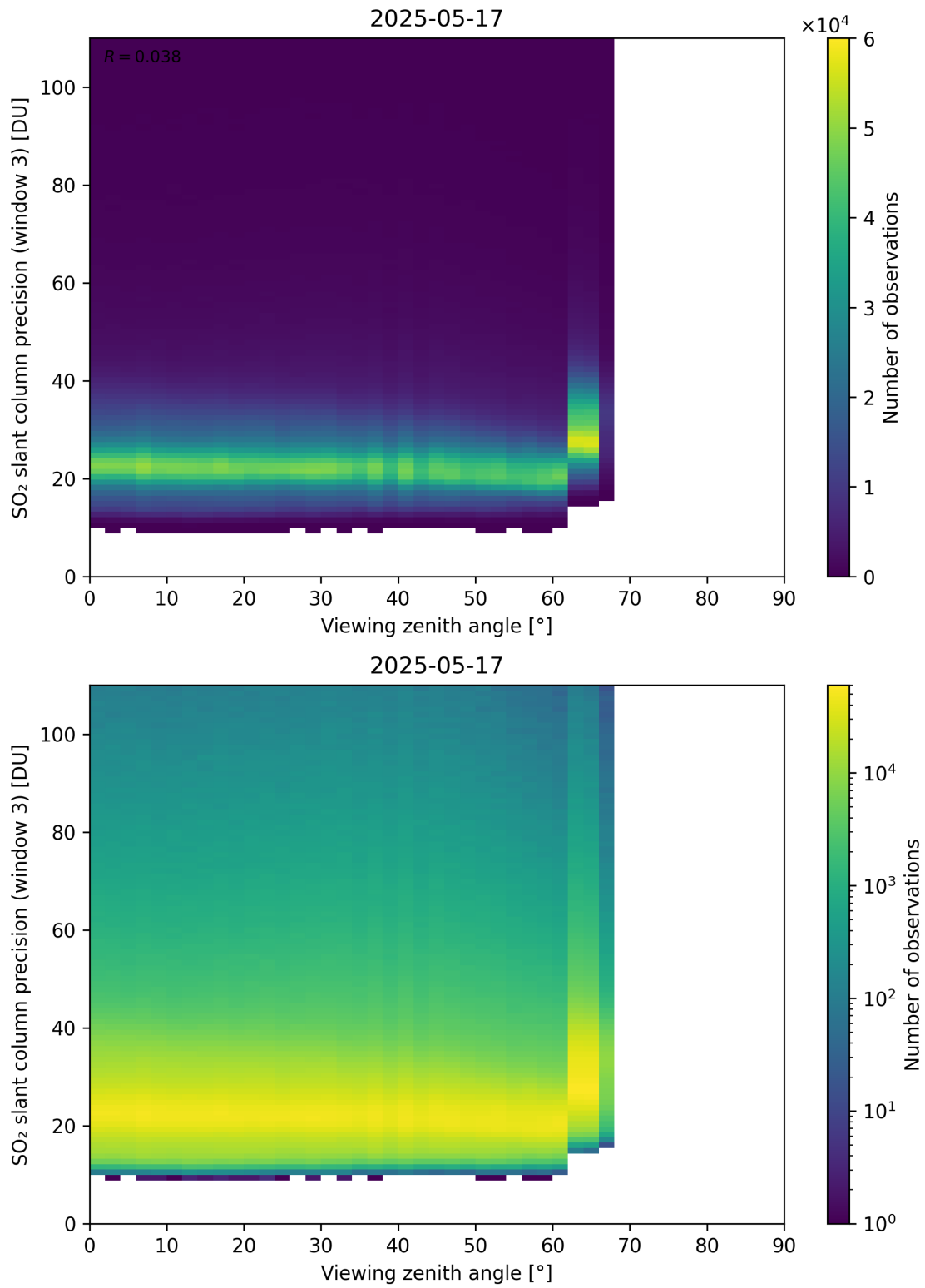
Figure 380: Scatter density plot of “Viewing zenith angle” against “SO 2 slant column precision (window 3)” for 2025-05-16 to 2025-05-18.
