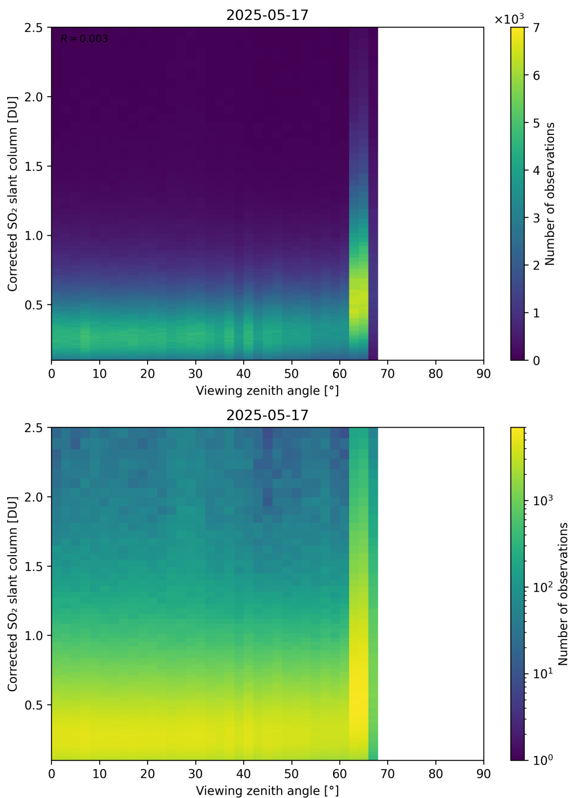
Figure 373: Scatter density plot of “Viewing zenith angle” against “Corrected SO 2 slant column” for 2025-05-16 to 2025-05-18.
