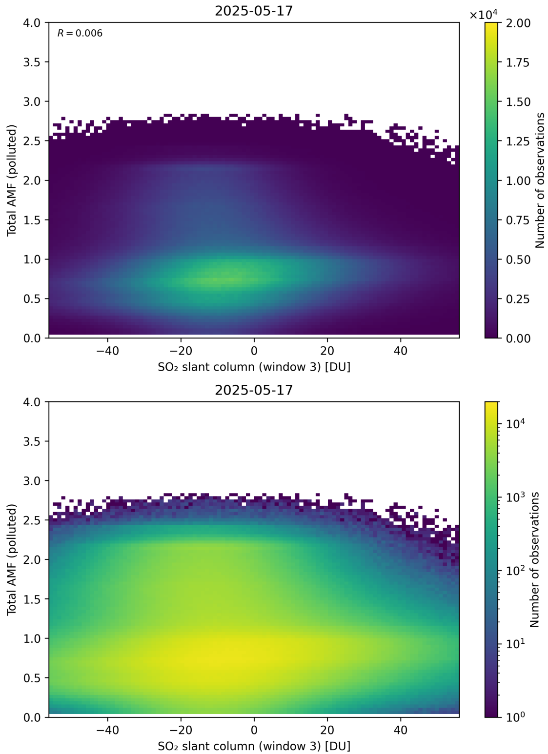
Figure 318: Scatter density plot of “SO 2 slant column (window 3)” against “Total AMF (polluted)” for 2025-05-16 to 2025-05-18.
