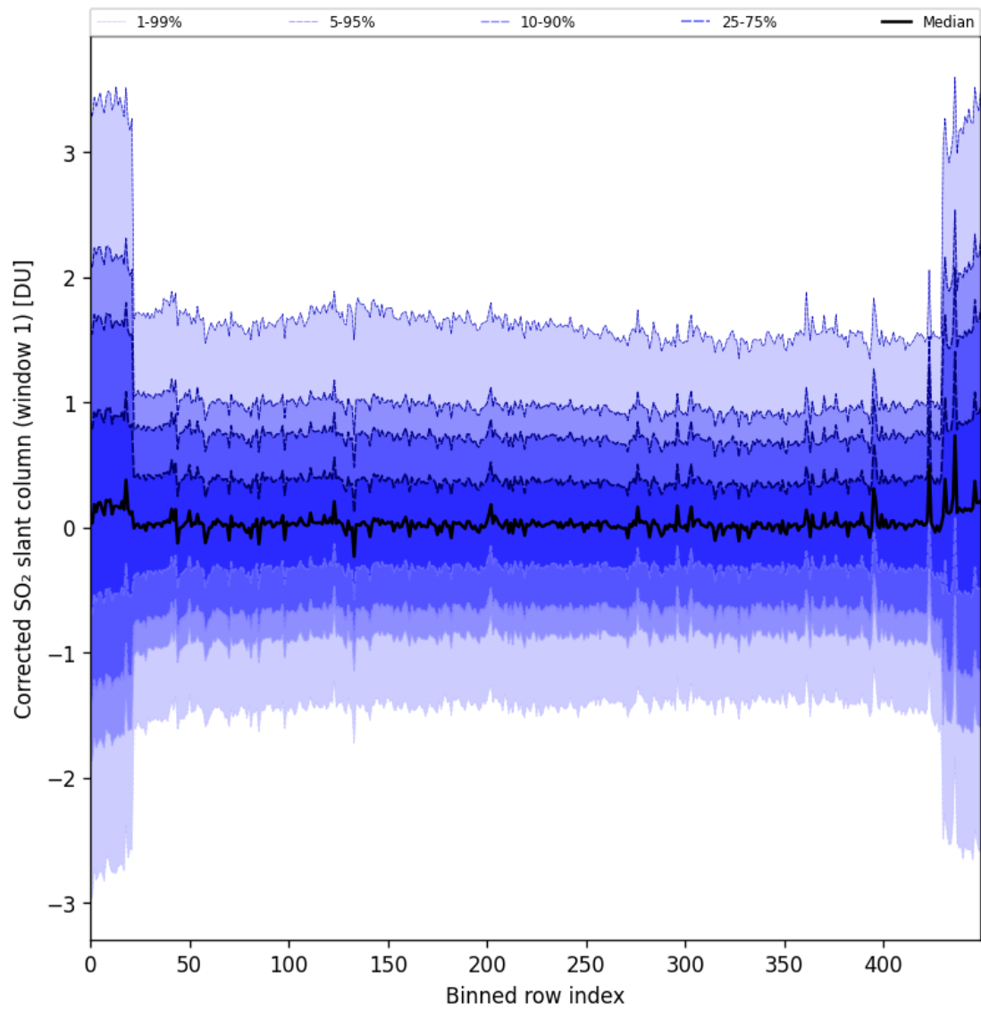
Figure 91: Along track statistics of “Corrected SO 2 slant column (window 1)” for 2025-05-16 to 2025-05-18
