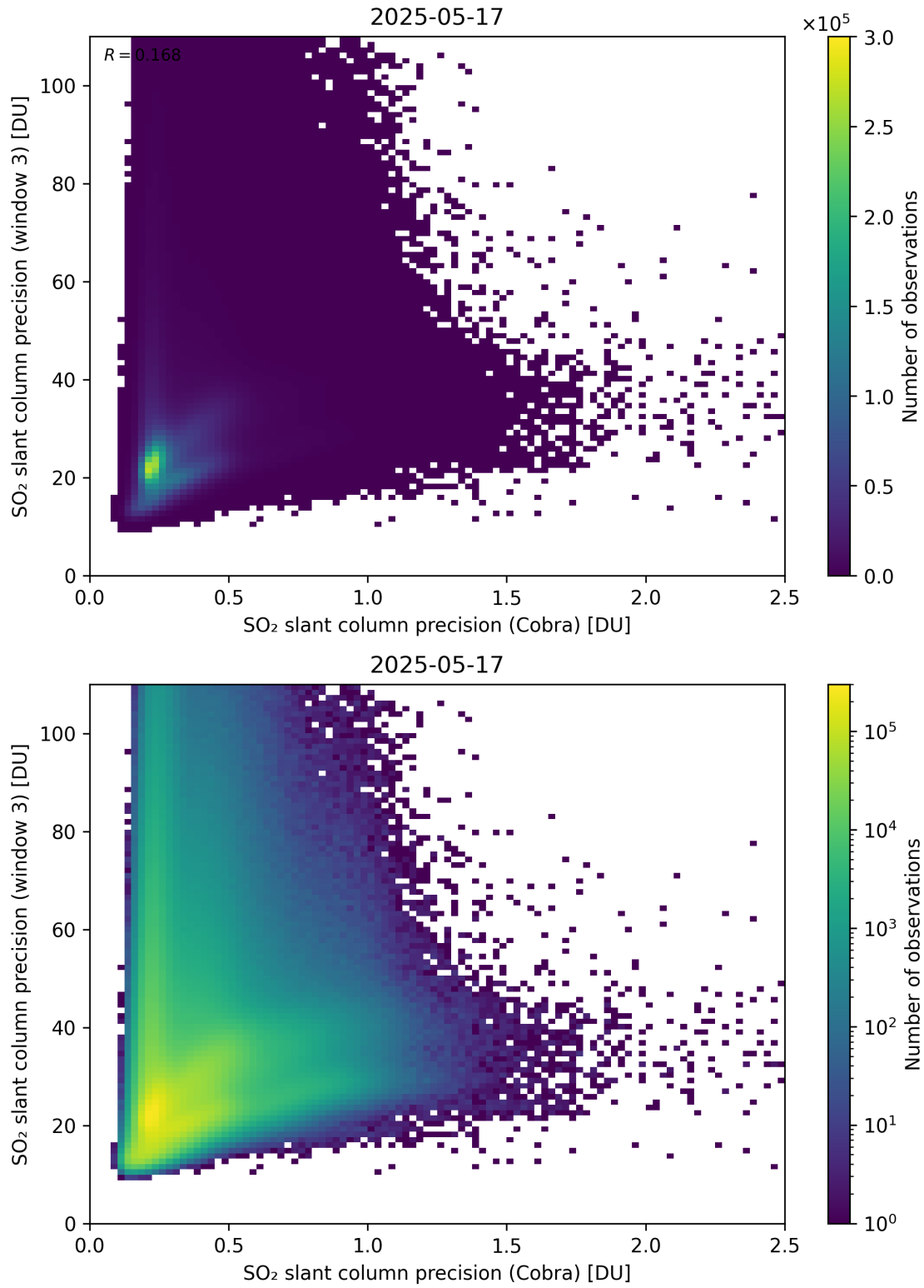
Figure 212: Scatter density plot of “SO 2 slant column precision (Cobra)” against “SO 2 slant column precision (window 3)” for 2025-05-16 to 2025-05-18.
