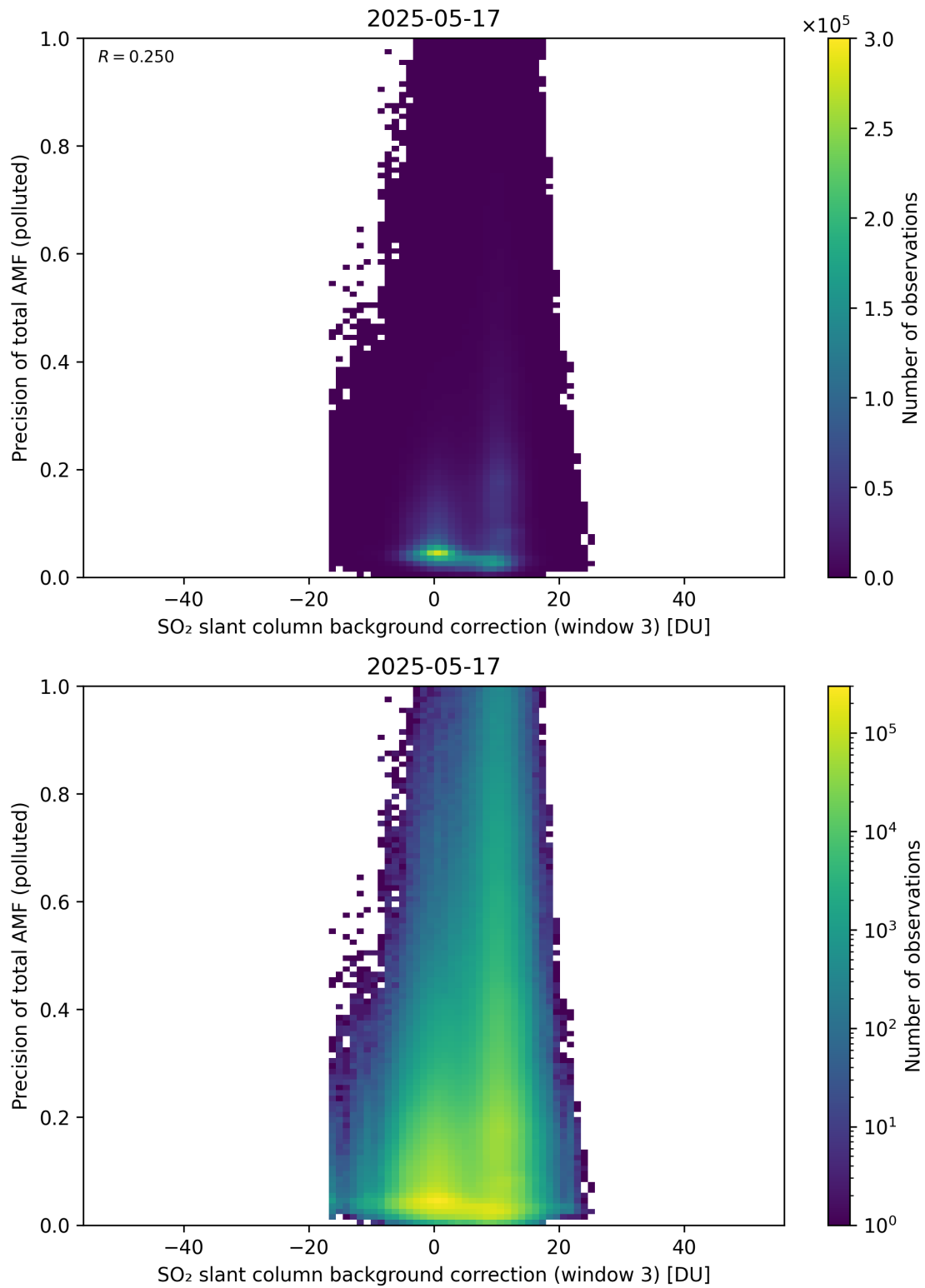
Figure 137: Scatter density plot of “SO 2 slant column background correction (window 3)” against “Precision of total AMF (polluted)” for 2025-05-16 to 2025-05-18.
