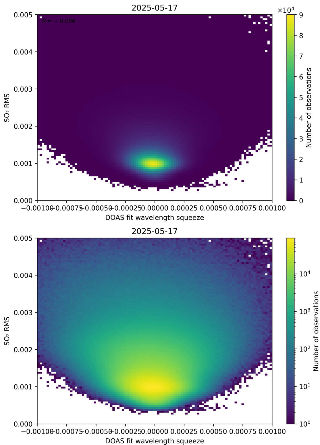
Figure 143: Scatter density plot of “DOAS fit wavelength squeeze” against “SO 2 RMS” for 2025-05-16 to 2025-05-18.
