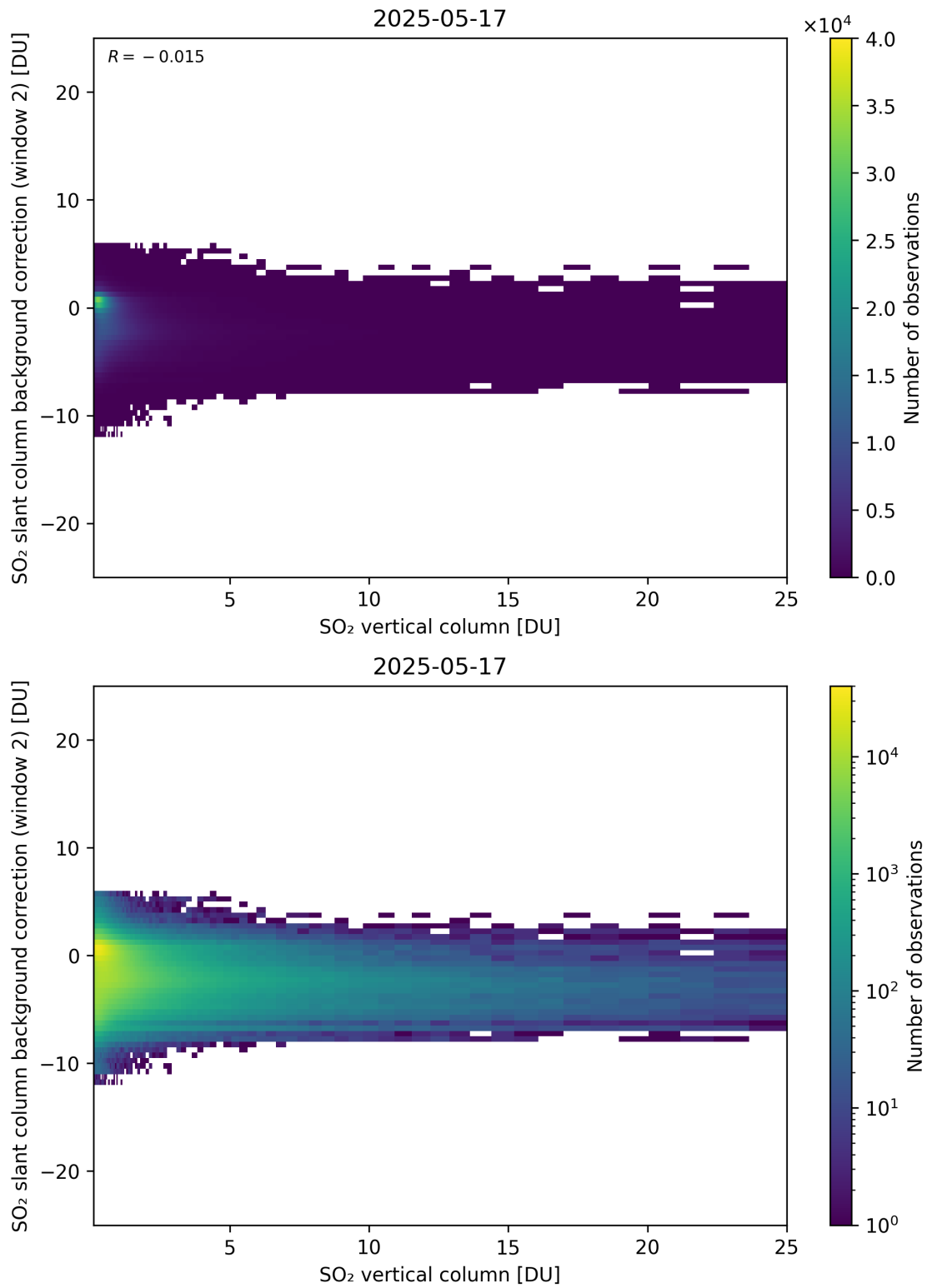
Figure 324: Scatter density plot of “SO 2 vertical column” against “SO 2 slant column background correction (window 2)” for 2025-05-16 to 2025-05-18.
