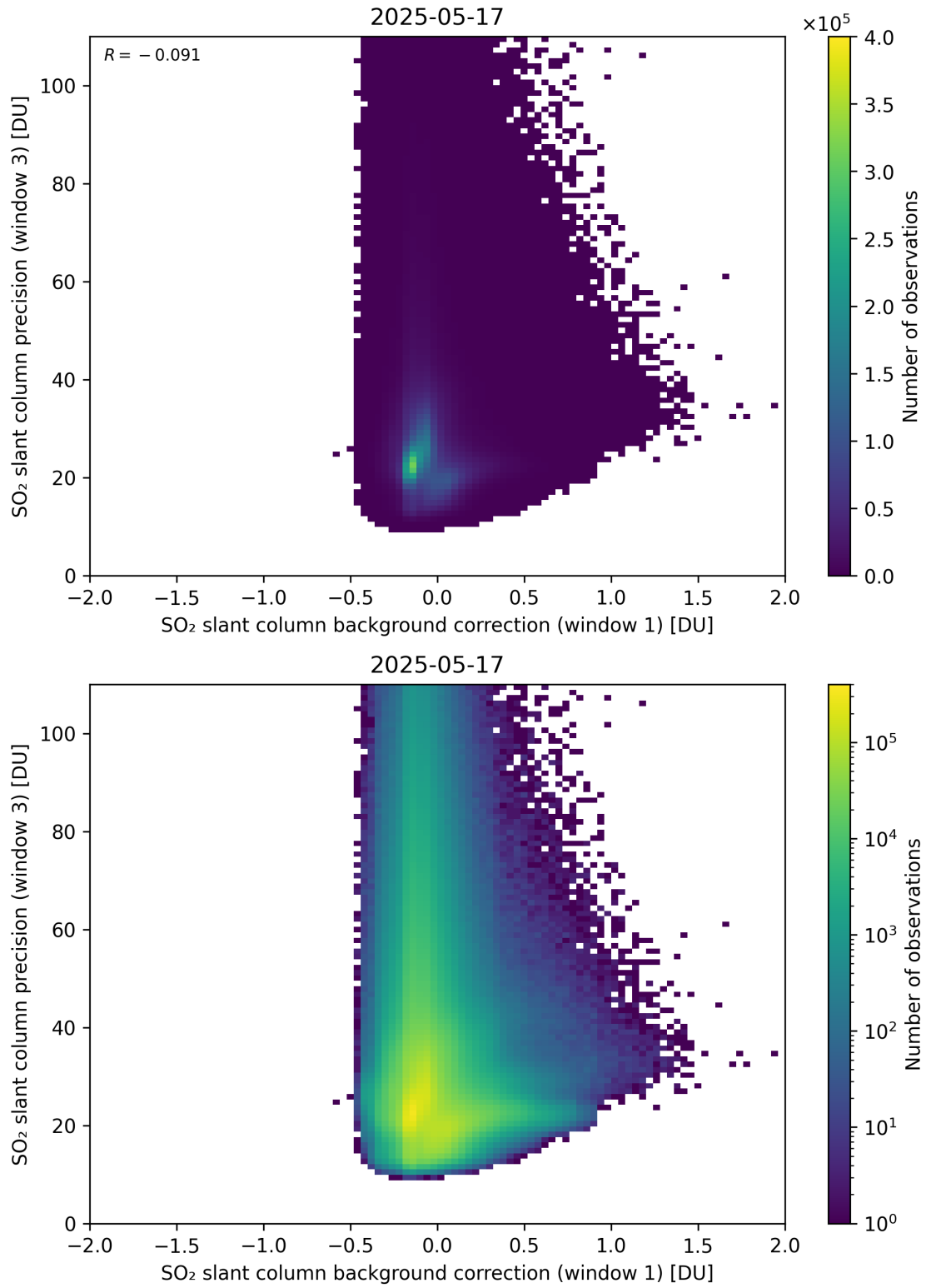
Figure 119: Scatter density plot of “SO 2 slant column background correction (window 1)” against “SO 2 slant column precision (window 3)” for 2025-05-16 to 2025-05-18.
