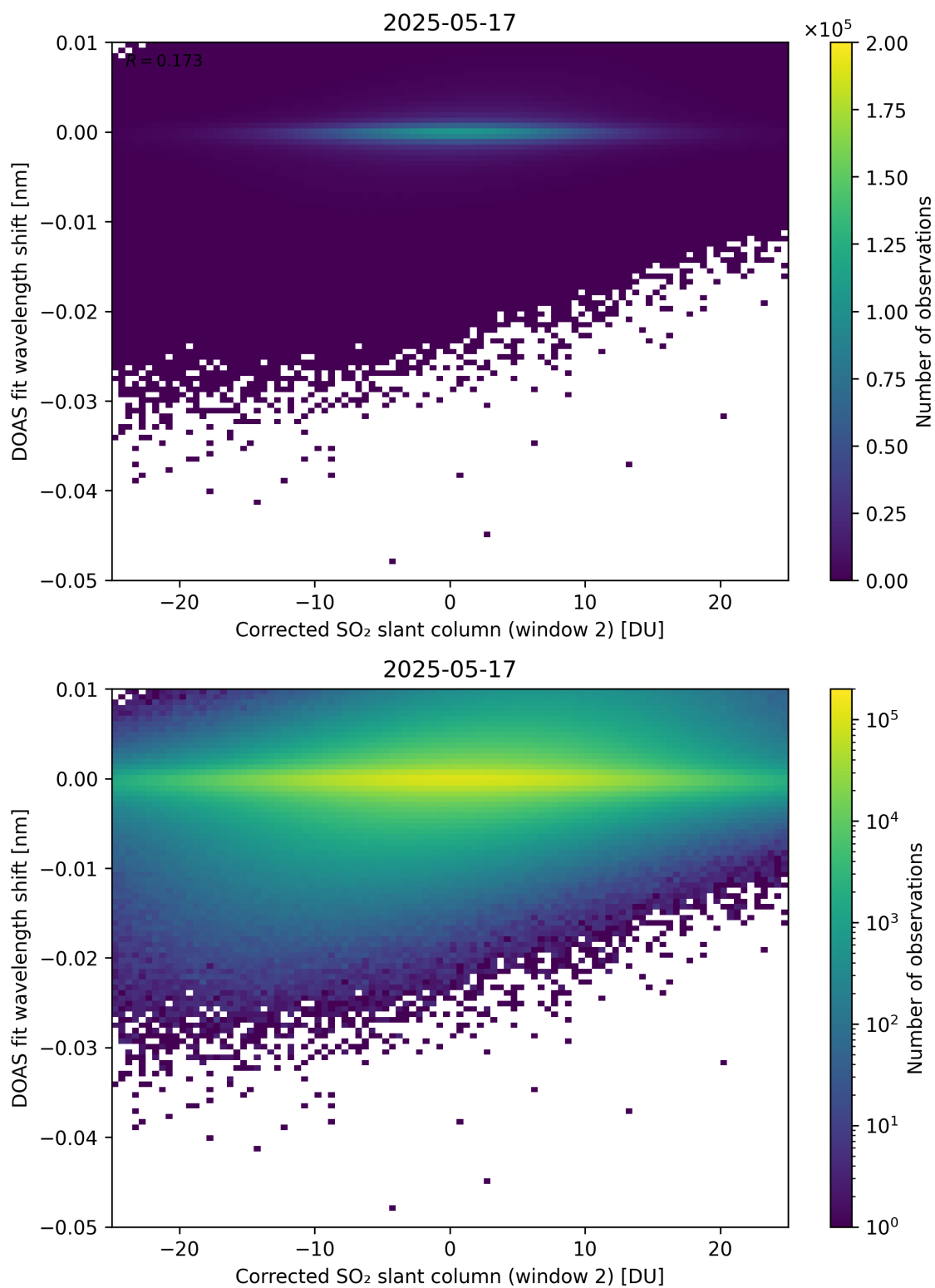
Figure 246: Scatter density plot of “Corrected SO 2 slant column (window 2)” against “DOAS fit wavelength shift” for 2025-05-16 to 2025-05-18.
