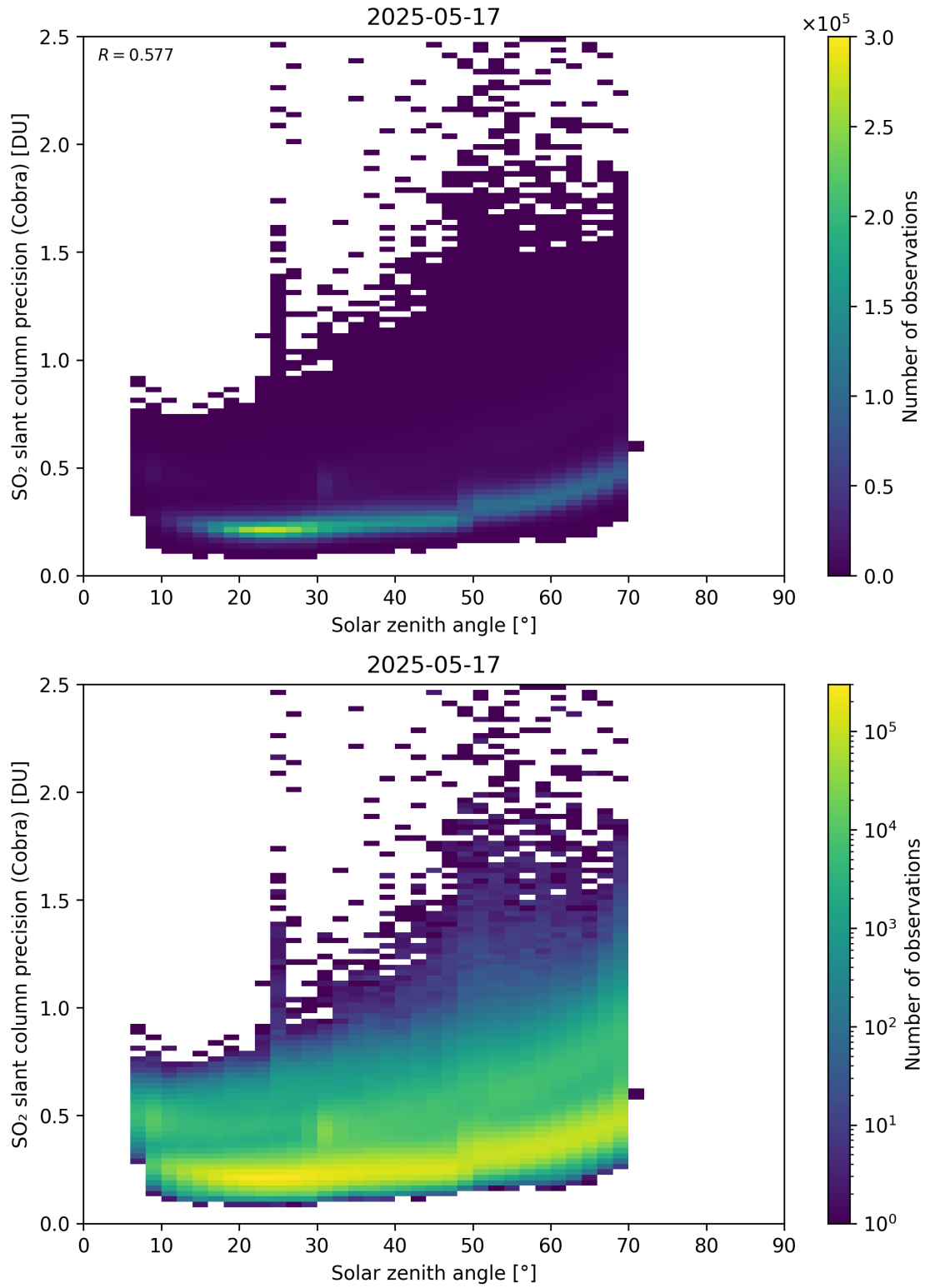
Figure 180: Scatter density plot of “Solar zenith angle” against “SO 2 slant column precision (Cobra)” for 2025-05-16 to 2025-05-18.
