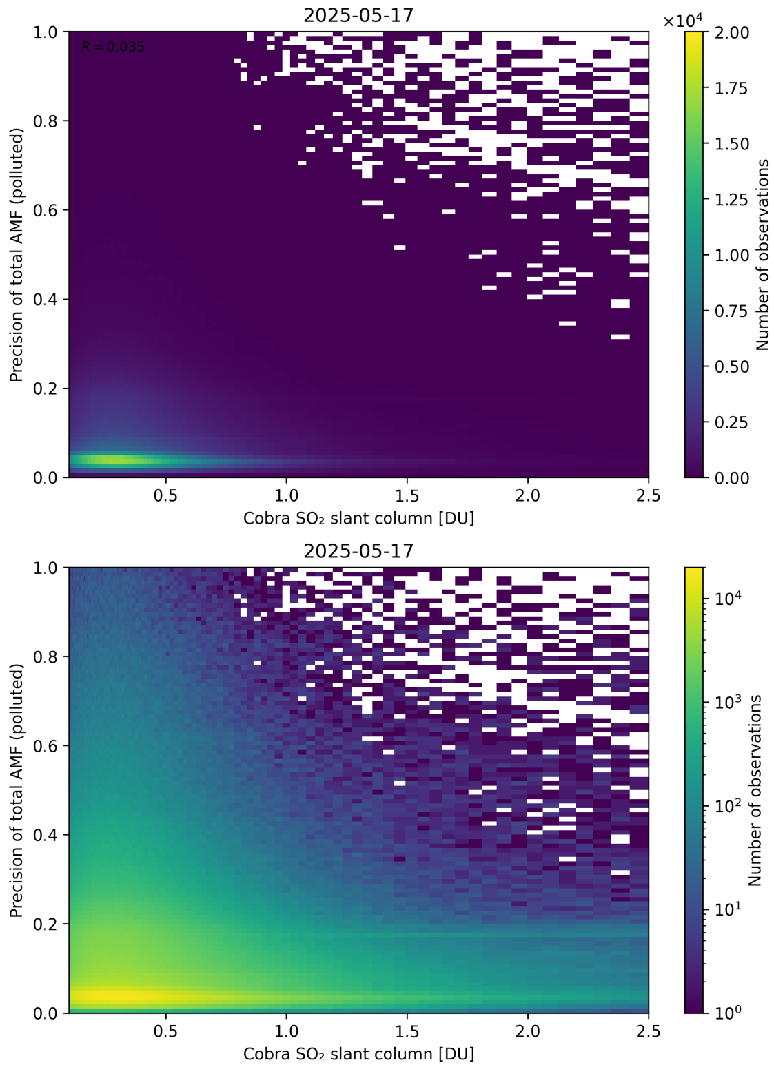
Figure 225: Scatter density plot of “Cobra SO 2 slant column” against “Precision of total AMF (polluted)” for 2025-05-16 to 2025-05-18.
