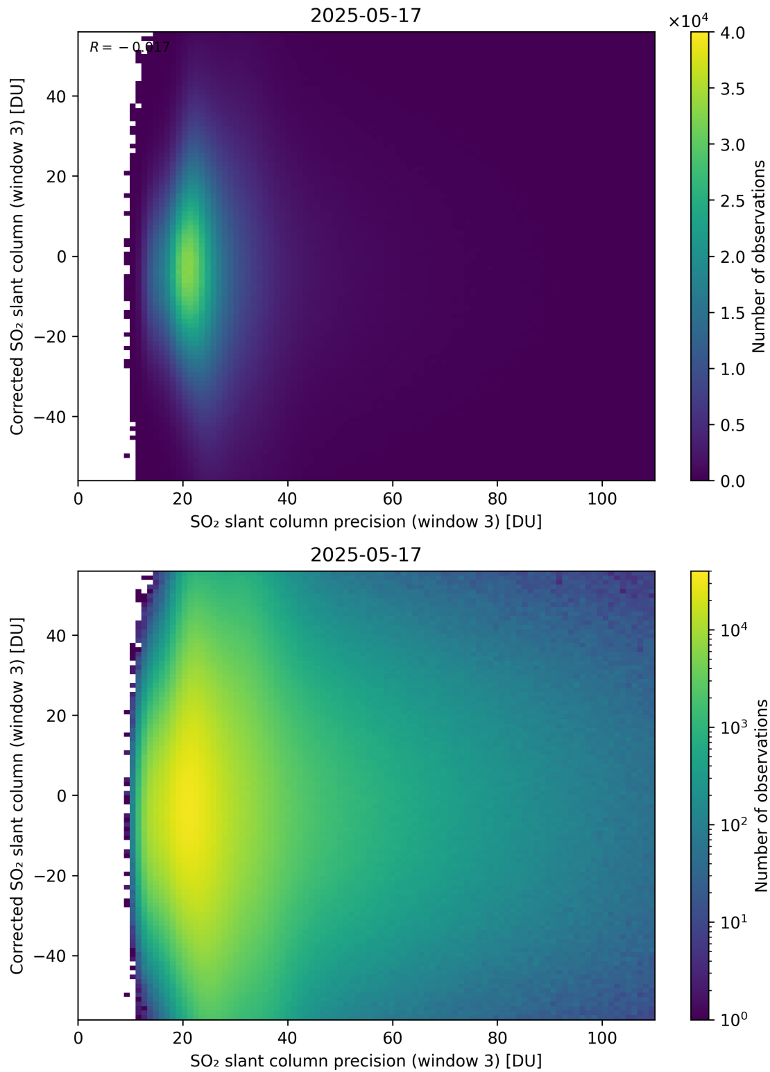
Figure 312: Scatter density plot of “SO 2 slant column precision (window 3)” against “Corrected SO 2 slant column (window 3)” for 2025-05-16 to 2025-05-18.
