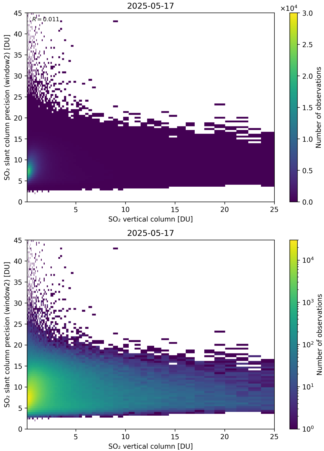
Figure 356: Scatter density plot of “SO 2 vertical column” against “SO 2 slant column precision (window2)” for 2025-05-16 to 2025-05-18.
