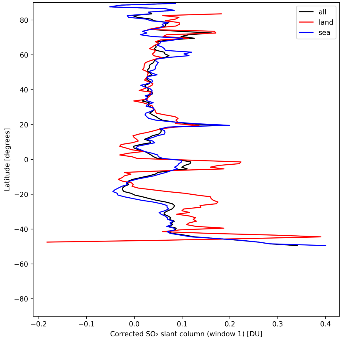
Figure 39: Zonal average of “Corrected SO 2 slant column (window 1)” for 2025-05-16 to 2025-05-18.
