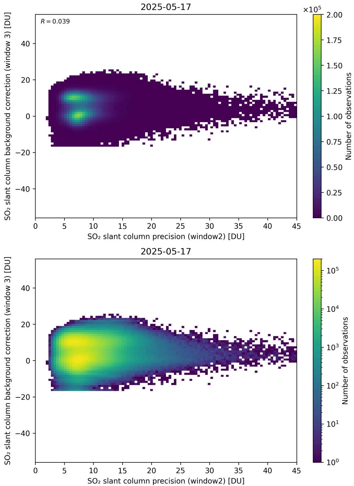
Figure 292: Scatter density plot of “SO 2 slant column precision (window2)” against “SO 2 slant column background correction (window 3)” for 2025-05-16 to 2025-05-18.
