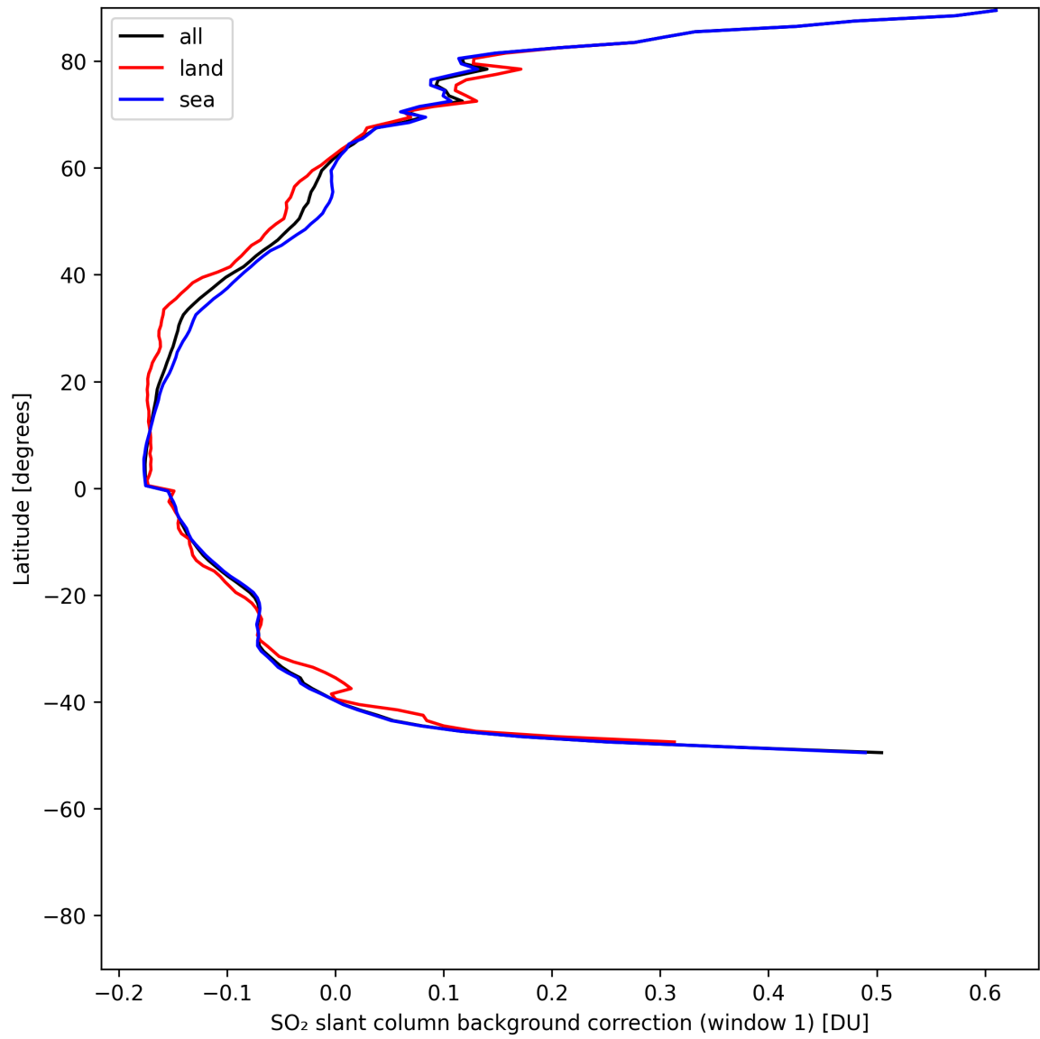
Figure 40: Zonal average of “SO 2 slant column background correction (window 1)” for 2025-05-16 to 2025-05-18.
