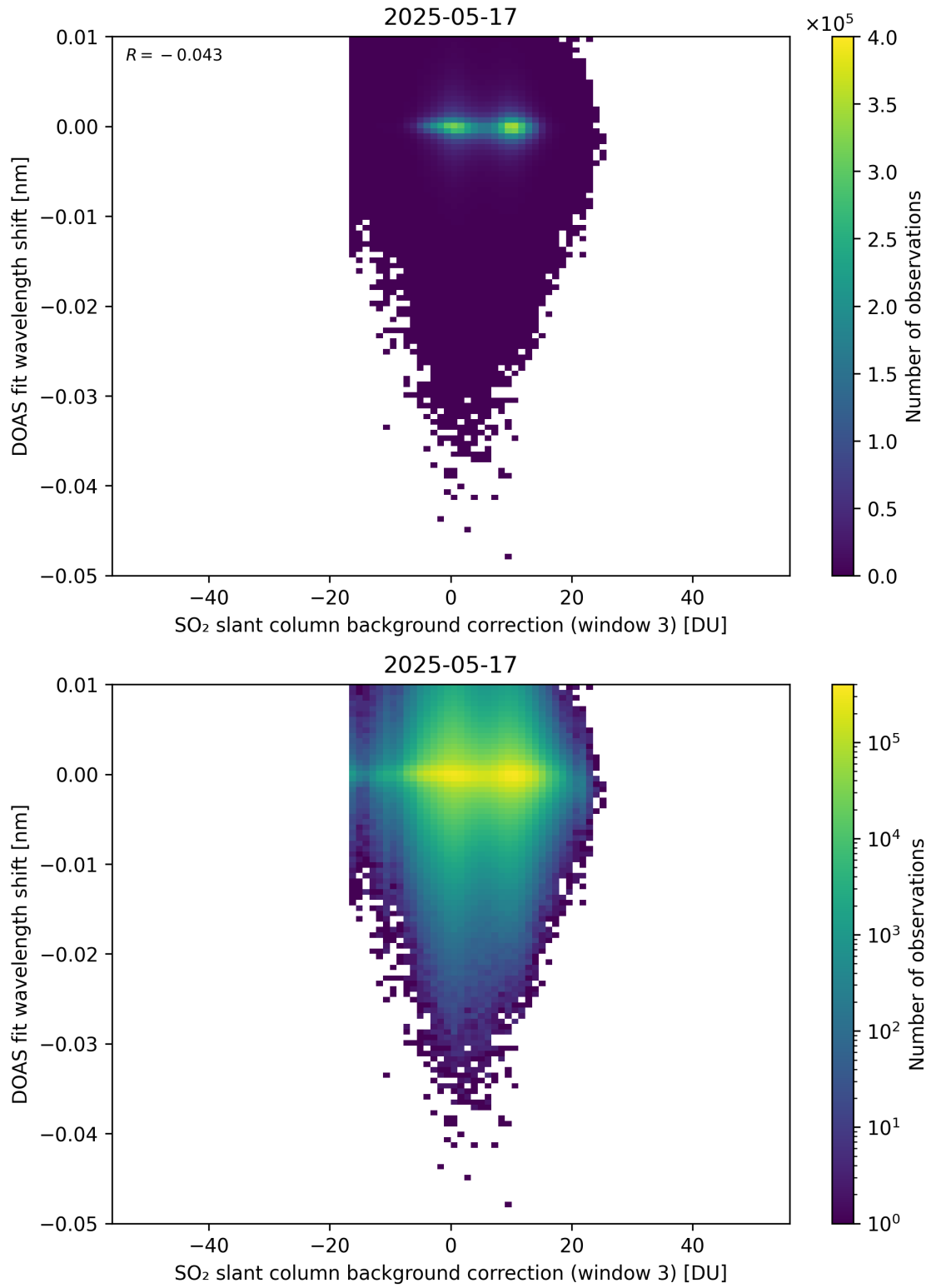
Figure 132: Scatter density plot of “SO 2 slant column background correction (window 3)” against “DOAS fit wavelength shift” for 2025-05-16 to 2025-05-18.
