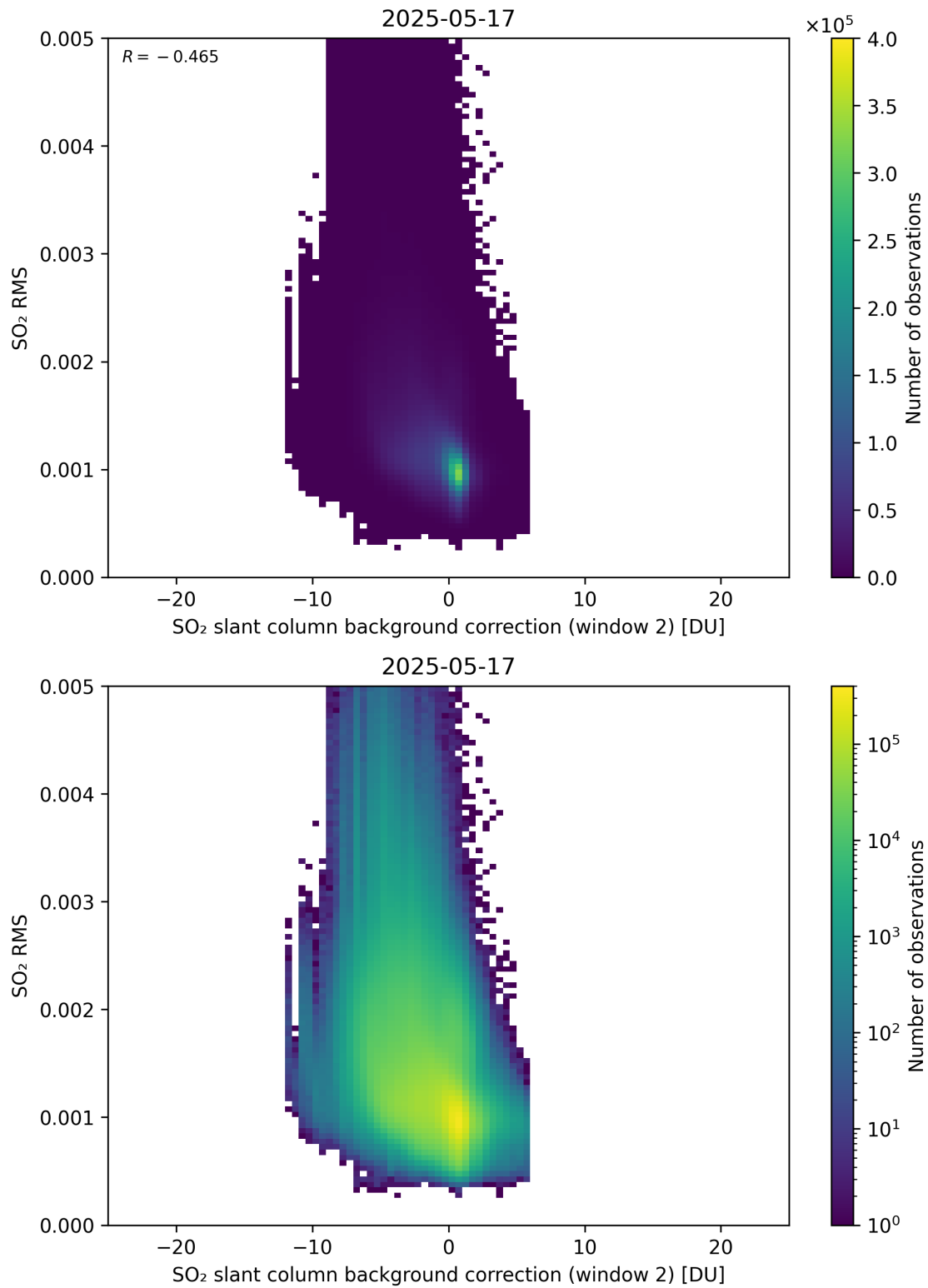
Figure 125: Scatter density plot of “SO 2 slant column background correction (window 2)” against “SO 2 RMS” for 2025-05-16 to 2025-05-18.
