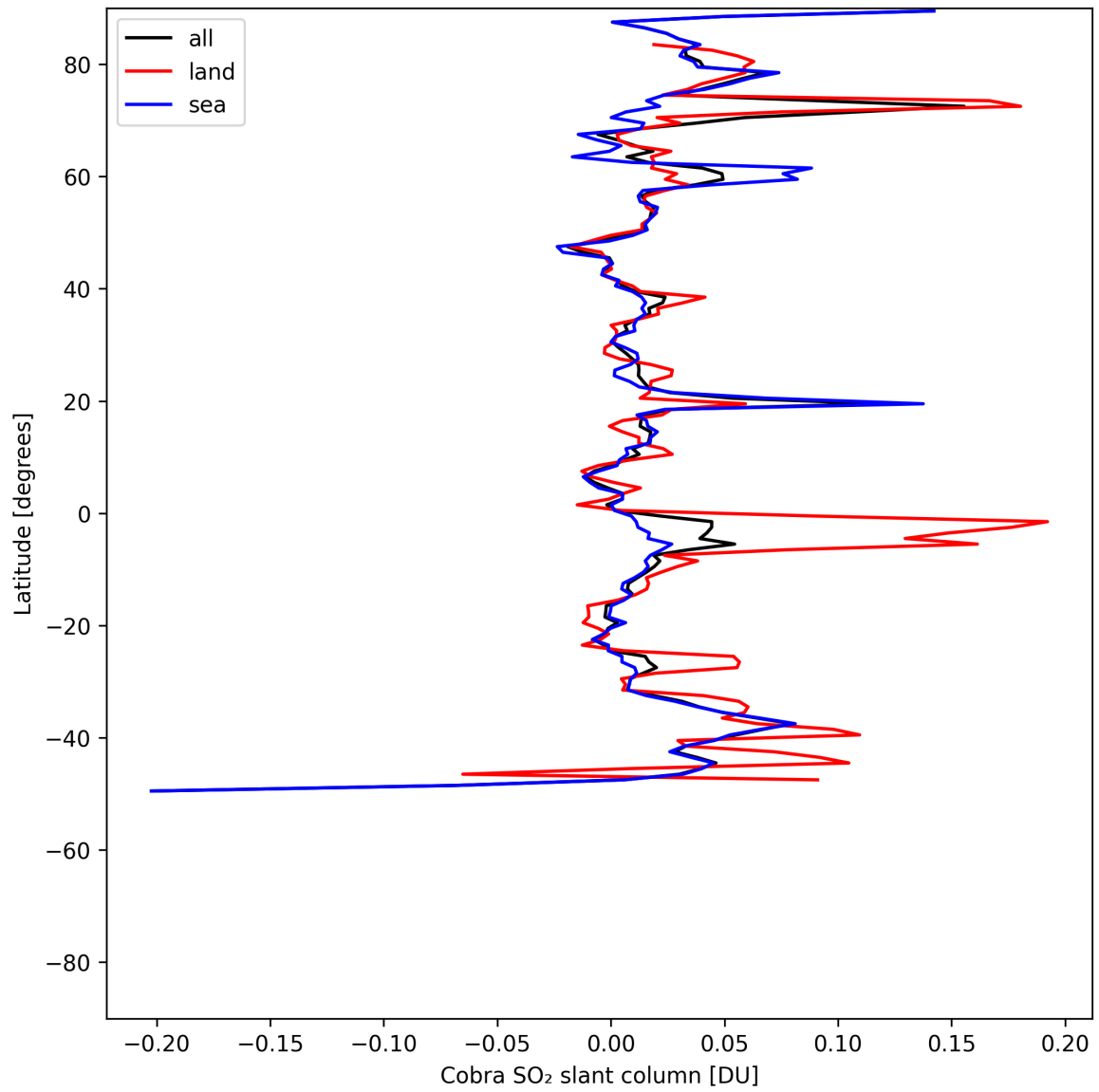
Figure 35: Zonal average of “Cobra SO 2 slant column” for 2025-05-16 to 2025-05-18.
