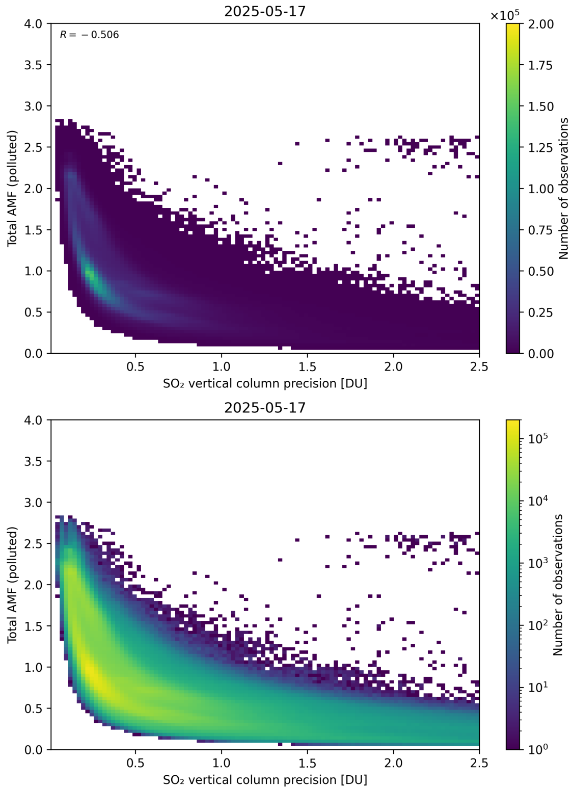
Figure 346: Scatter density plot of “SO 2 vertical column precision” against “Total AMF (polluted)” for 2025-05-16 to 2025-05-18.
