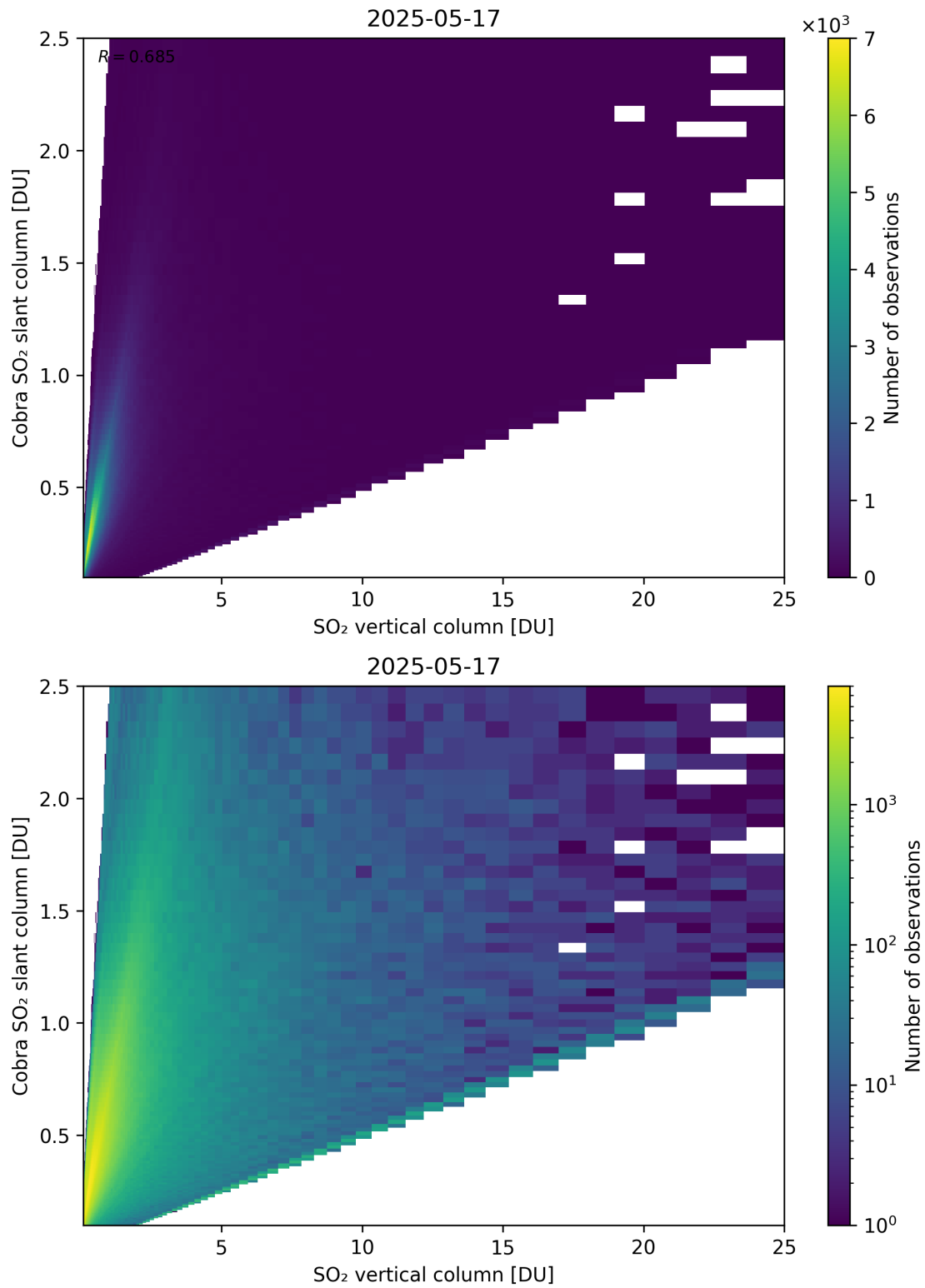
Figure 349: Scatter density plot of “SO 2 vertical column” against “Cobra SO 2 slant column” for 2025-05-16 to 2025-05-18.
