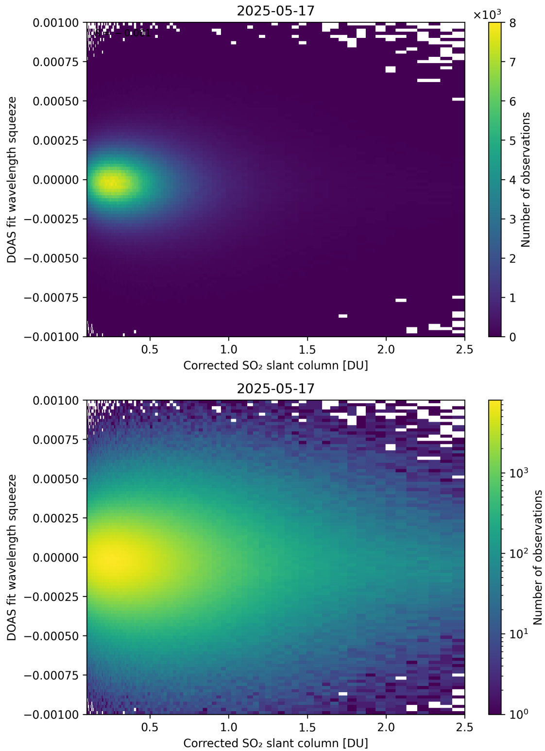
Figure 230: Scatter density plot of "Corrected SO 2 slant column" against "DOAS fit wavelength squeeze" for 2025-05-16 to 2025-05-18.
