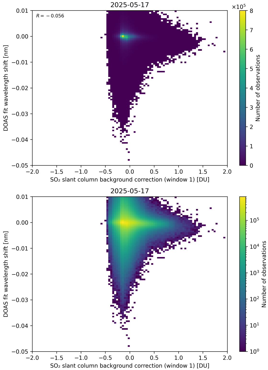
Figure 111: Scatter density plot of “SO 2 slant column background correction (window 1)” against “DOAS fit wavelength shift” for 2025-05-16 to 2025-05-18.
