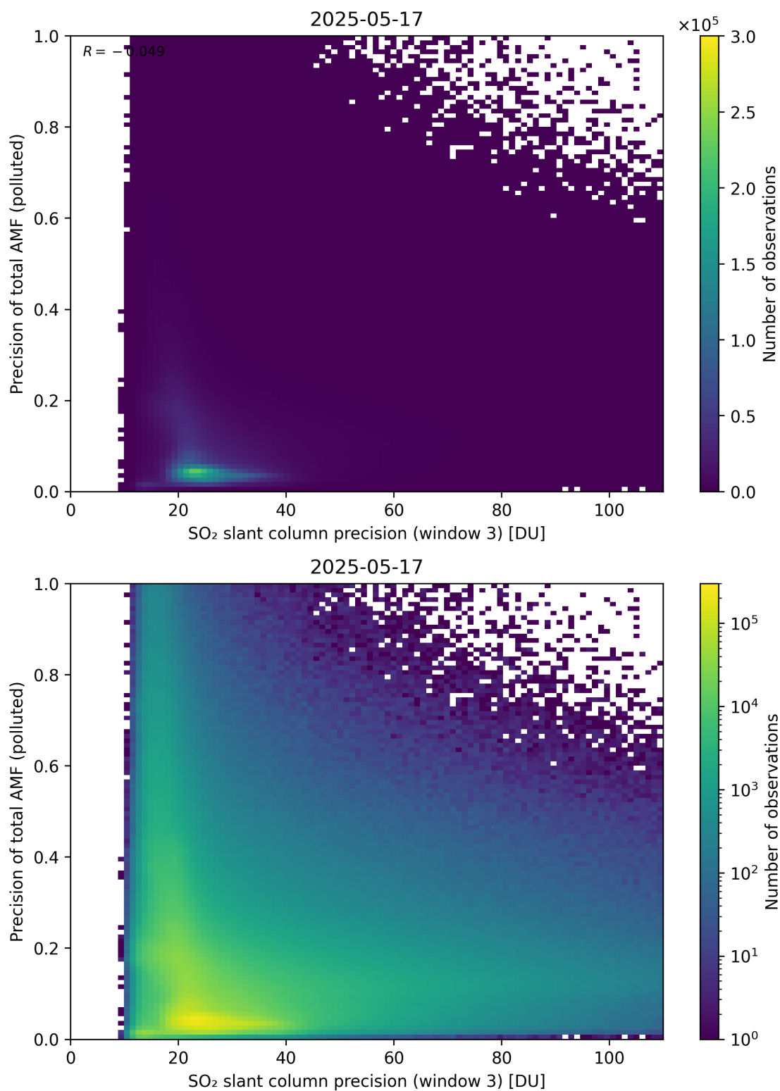
Figure 314: Scatter density plot of “SO 2 slant column precision (window 3)” against “Precision of total AMF (polluted)” for 2025-05-16 to 2025-05-18.
