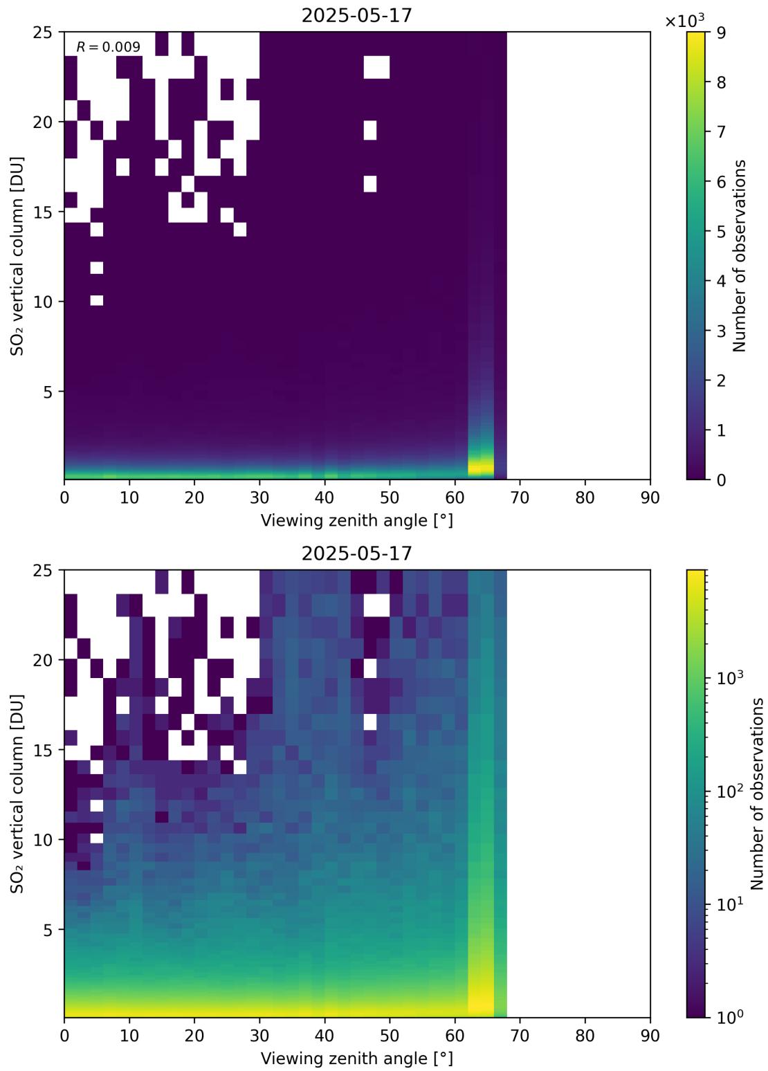
Figure 383: Scatter density plot of “Viewing zenith angle” against “SO 2 vertical column” for 2025-05-16 to 2025-05-18.
