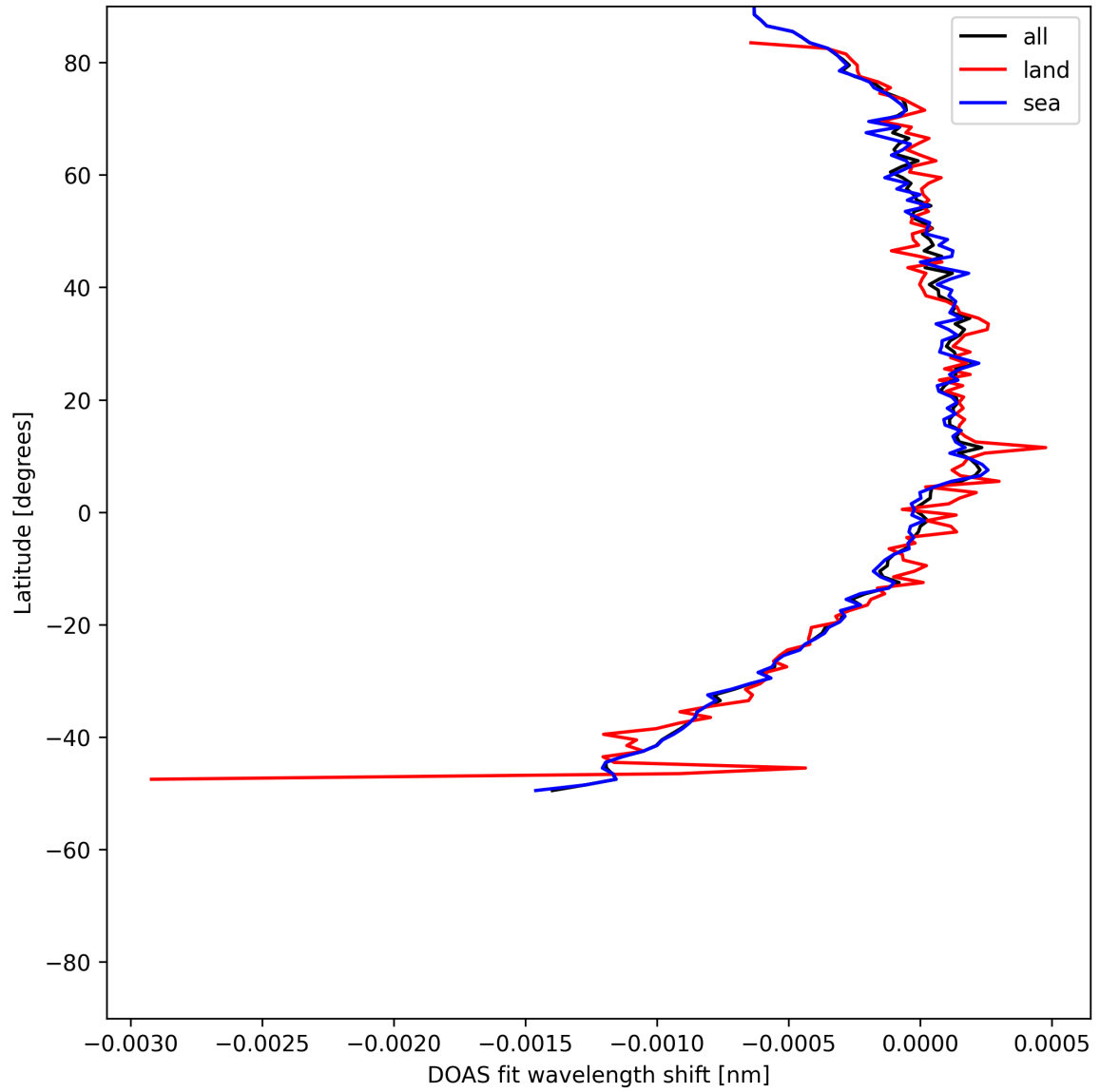
Figure 50: Zonal average of “DOAS fit wavelength shift” for 2025-05-16 to 2025-05-18.
