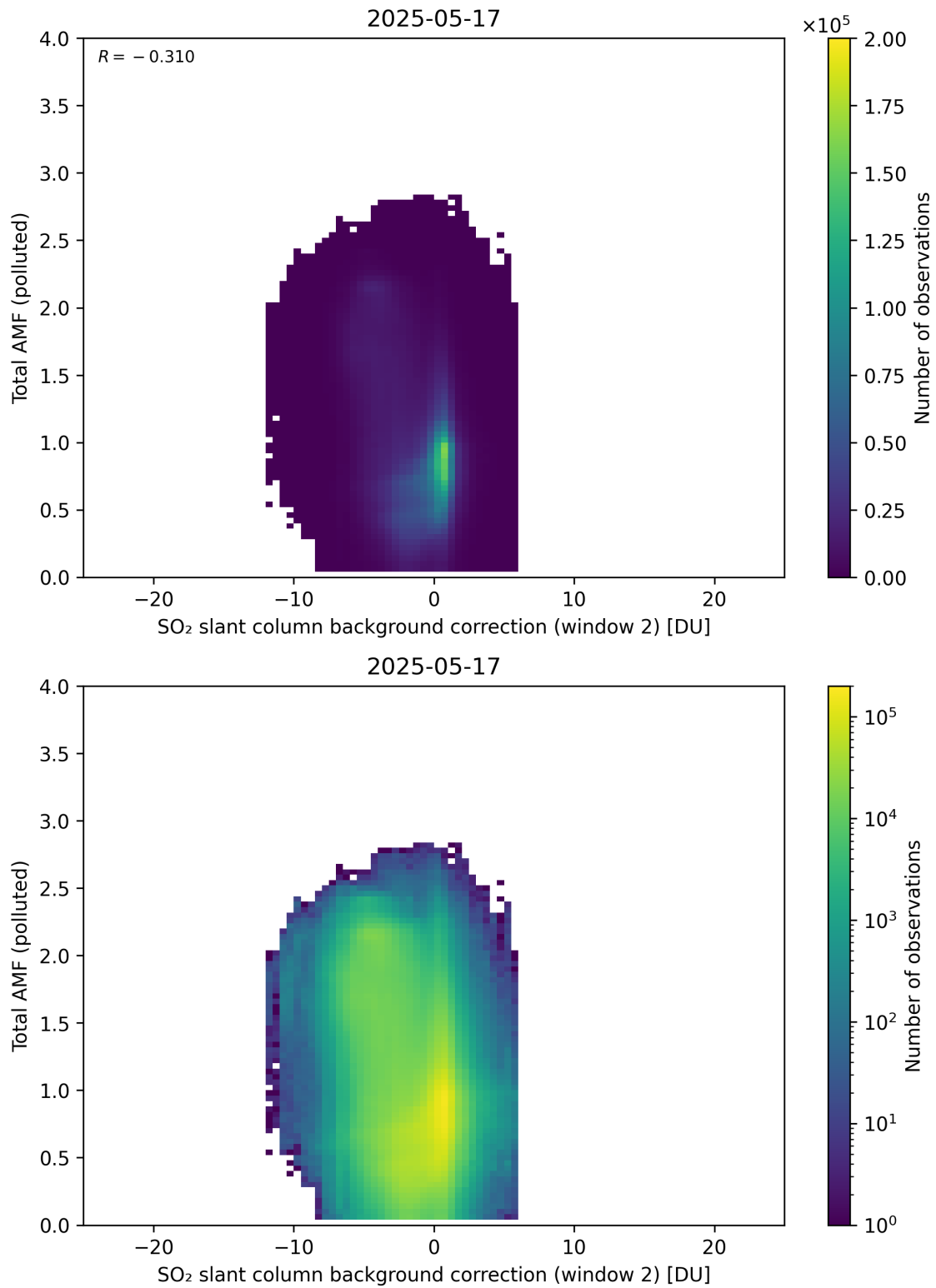
Figure 130: Scatter density plot of “SO 2 slant column background correction (window 2)” against “Total AMF (polluted)” for 2025-05-16 to 2025-05-18.
