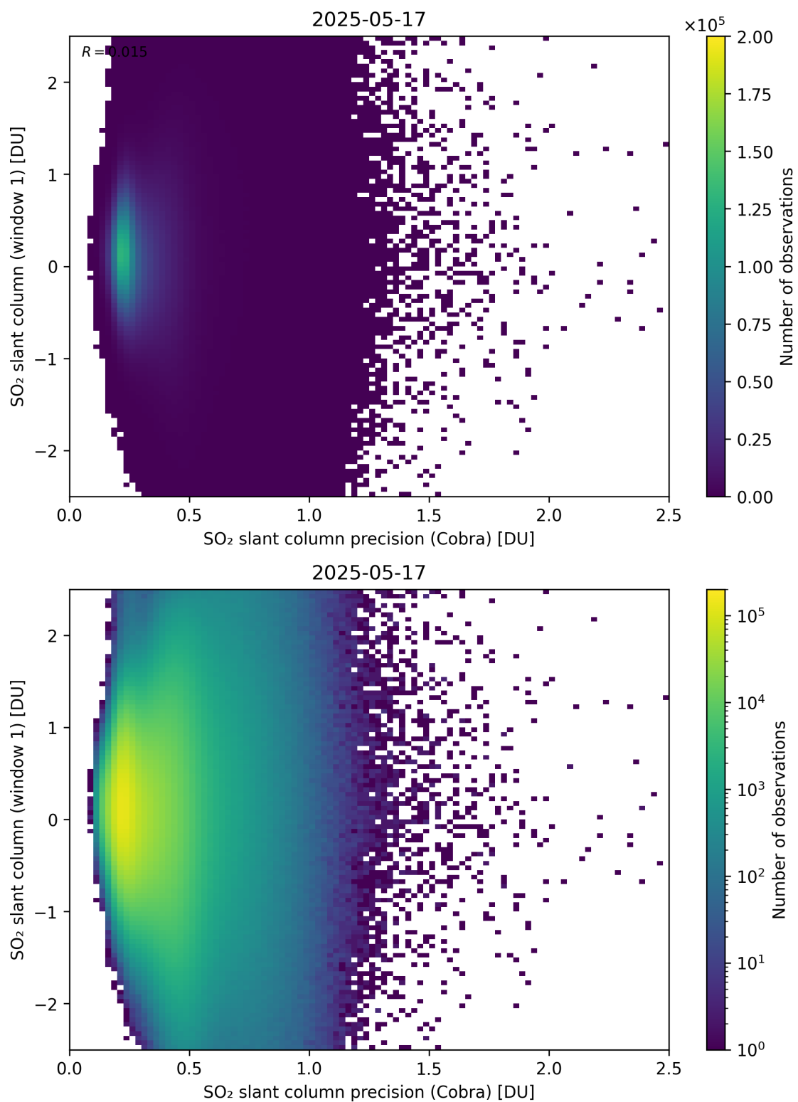
Figure 208: Scatter density plot of “SO 2 slant column precision (Cobra)” against “SO 2 slant column (window 1)” for 2025-05-16 to 2025-05-18.
