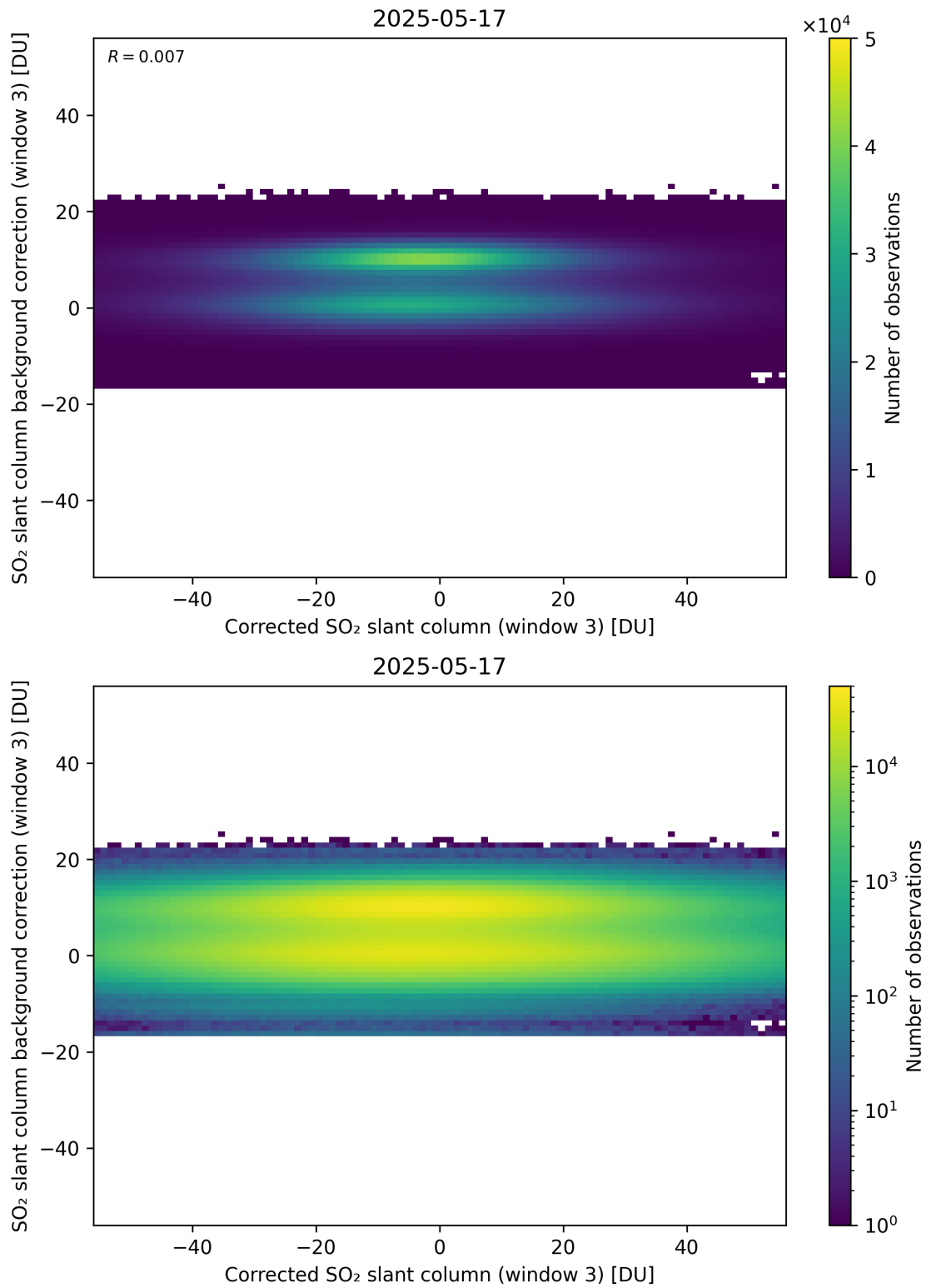
Figure 255: Scatter density plot of “Corrected SO 2 slant column (window 3)” against “SO 2 slant column background correction (window 3)” for 2025-05-16 to 2025-05-18.
