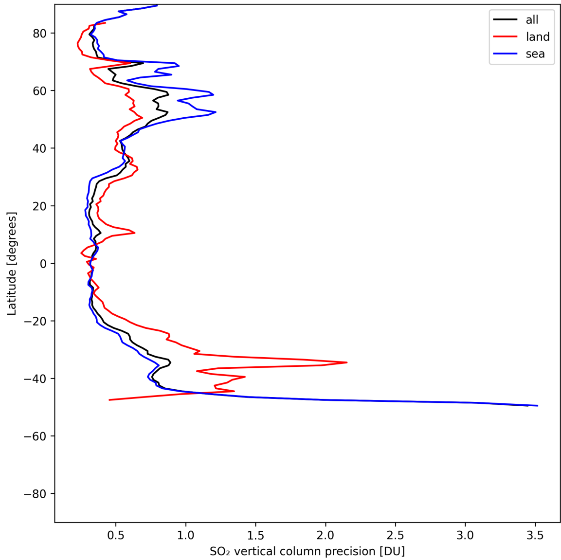
Figure 33: Zonal average of “SO 2 vertical column precision” for 2025-05-16 to 2025-05-18.
