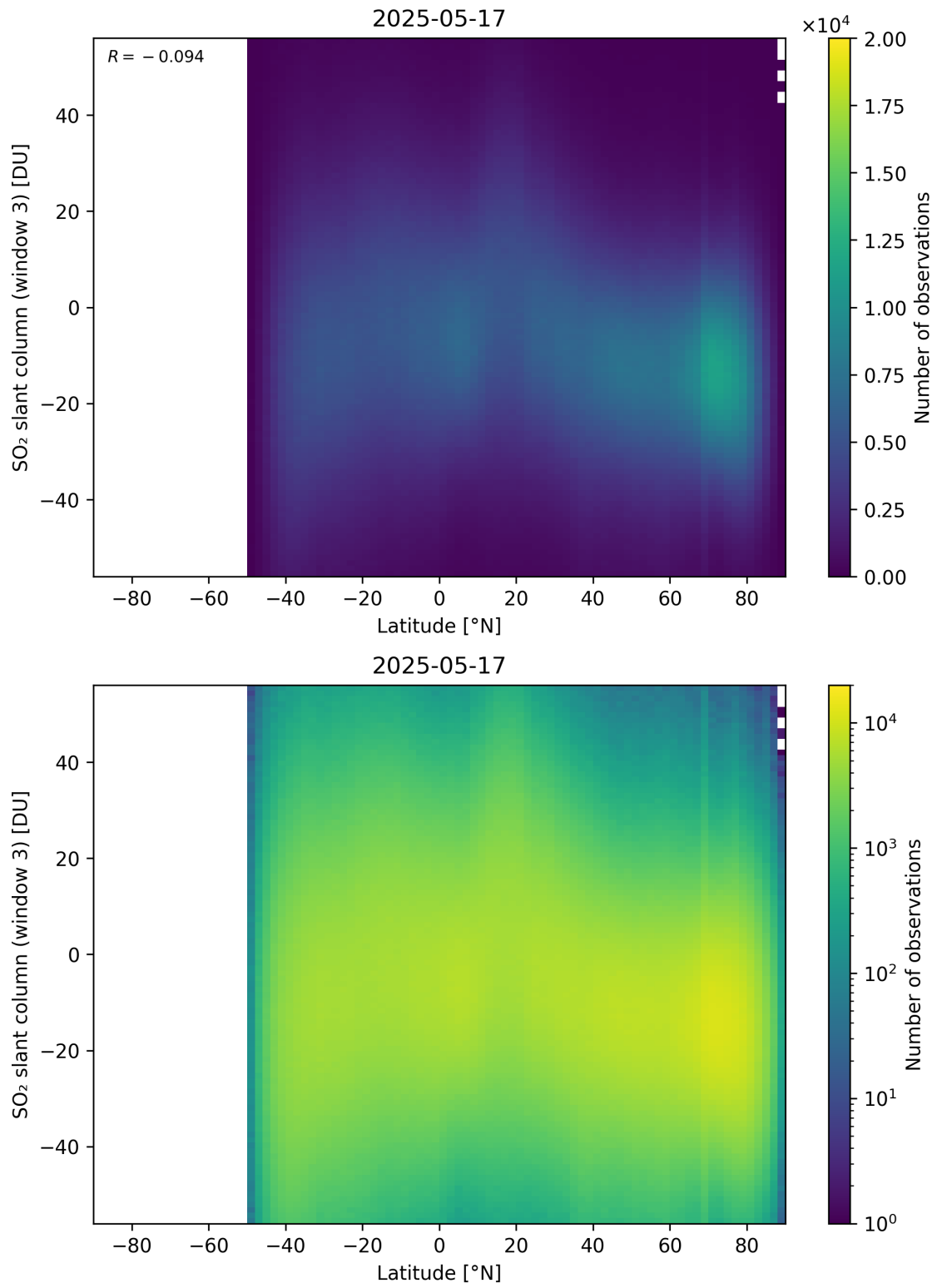
Figure 165: Scatter density plot of “Latitude” against “SO 2 slant column (window 3)” for 2025-05-16 to 2025-05-18.
