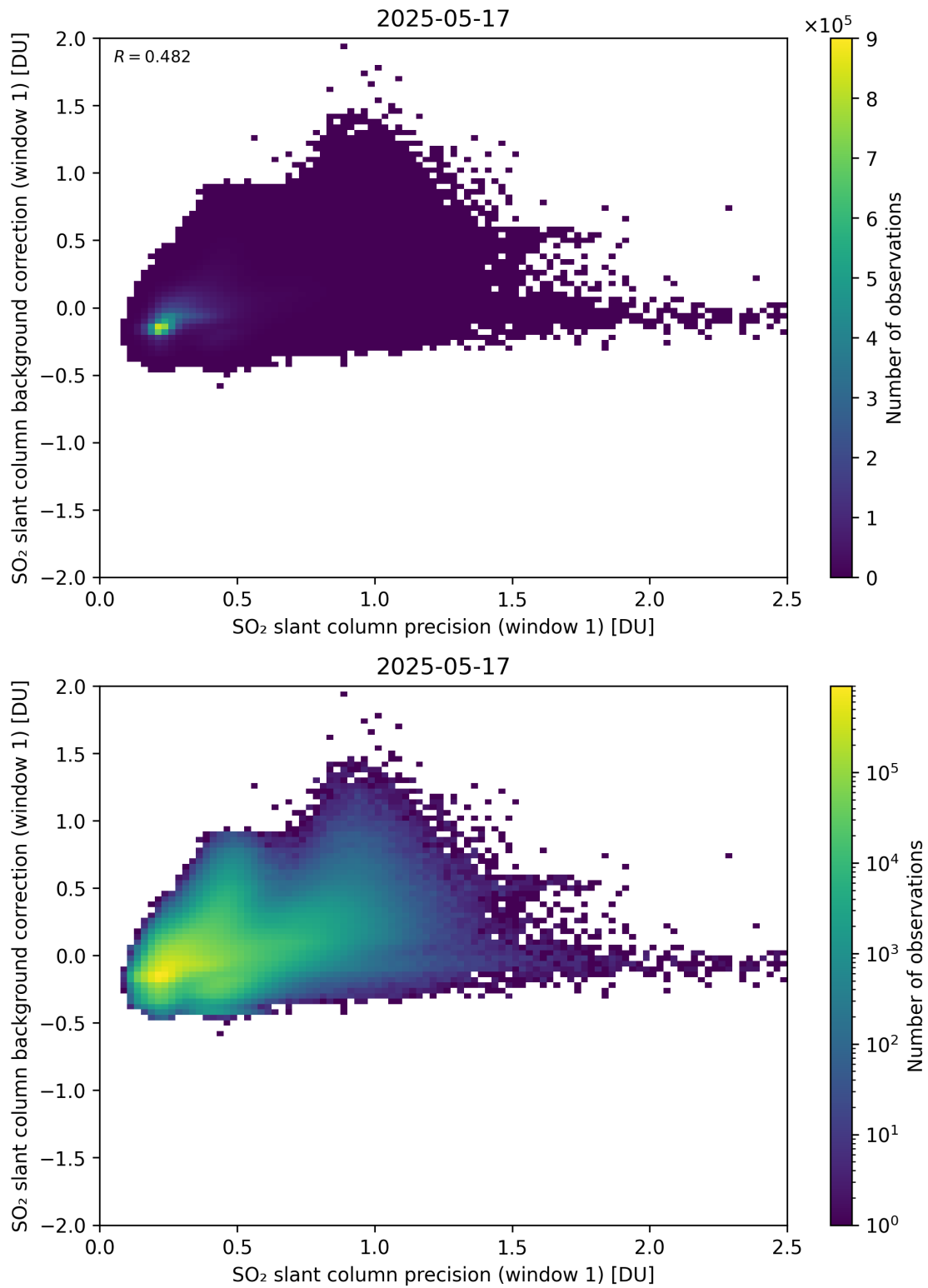
Figure 268: Scatter density plot of “SO 2 slant column precision (window 1)” against “SO 2 slant column background correction (window 1)” for 2025-05-16 to 2025-05-18.
