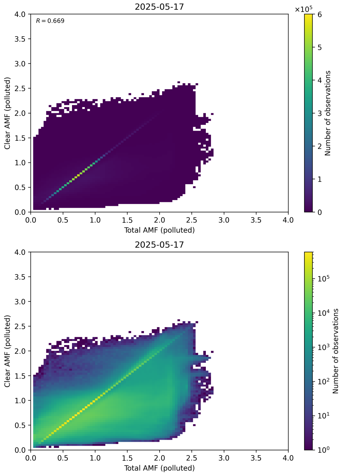
Figure 321: Scatter density plot of “Total AMF (polluted)” against “Clear AMF (polluted)” for 2025-05-16 to 2025-05-18.
