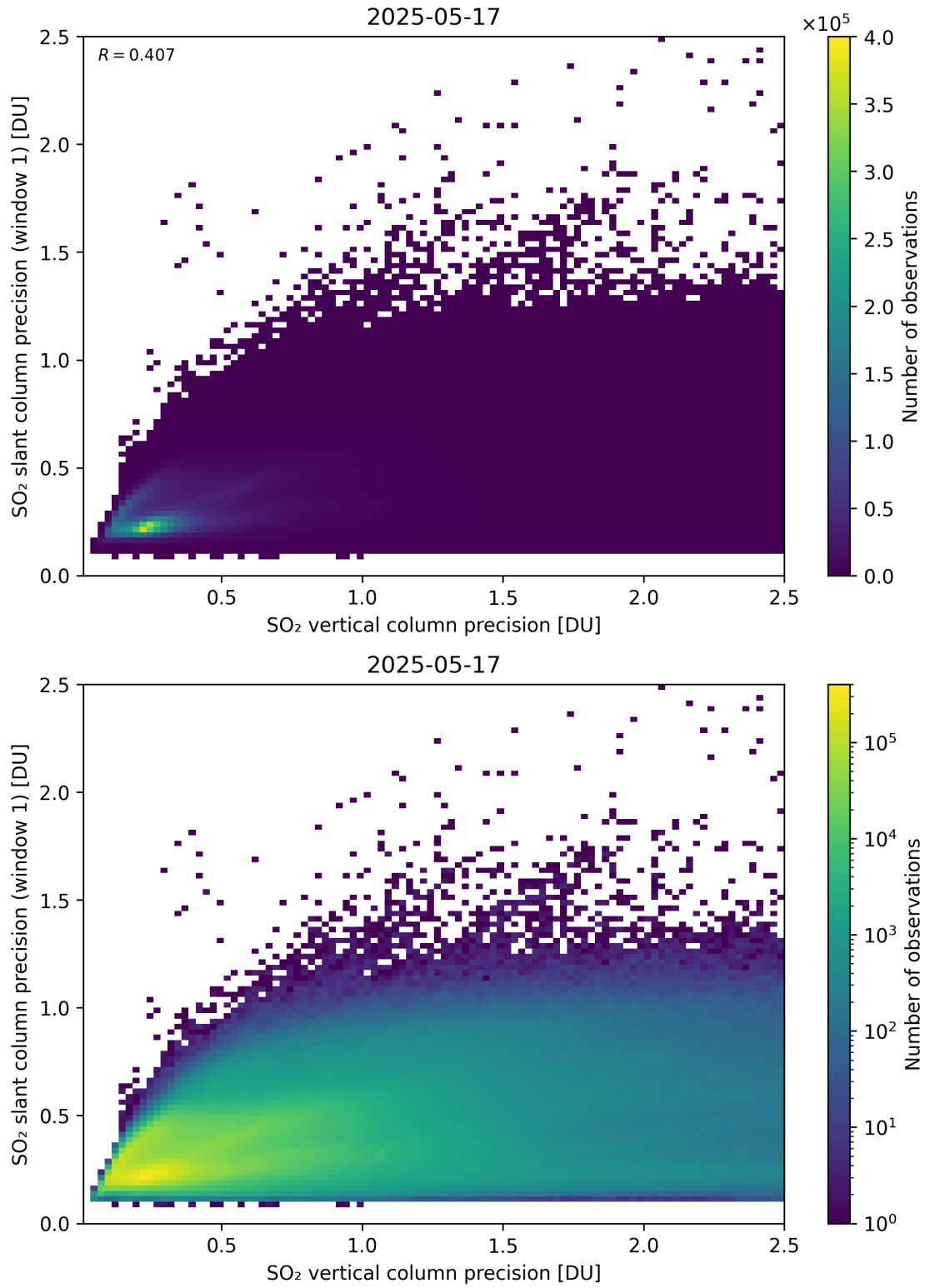
Figure 342: Scatter density plot of “SO 2 vertical column precision” against “SO 2 slant column precision (window 1)” for 2025-05-16 to 2025-05-18.
