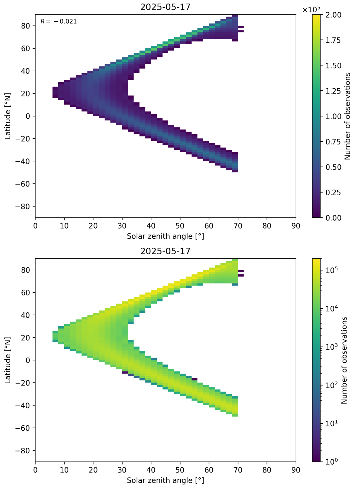
Figure 177: Scatter density plot of “Solar zenith angle” against “Latitude” for 2025-05-16 to 2025-05-18.
