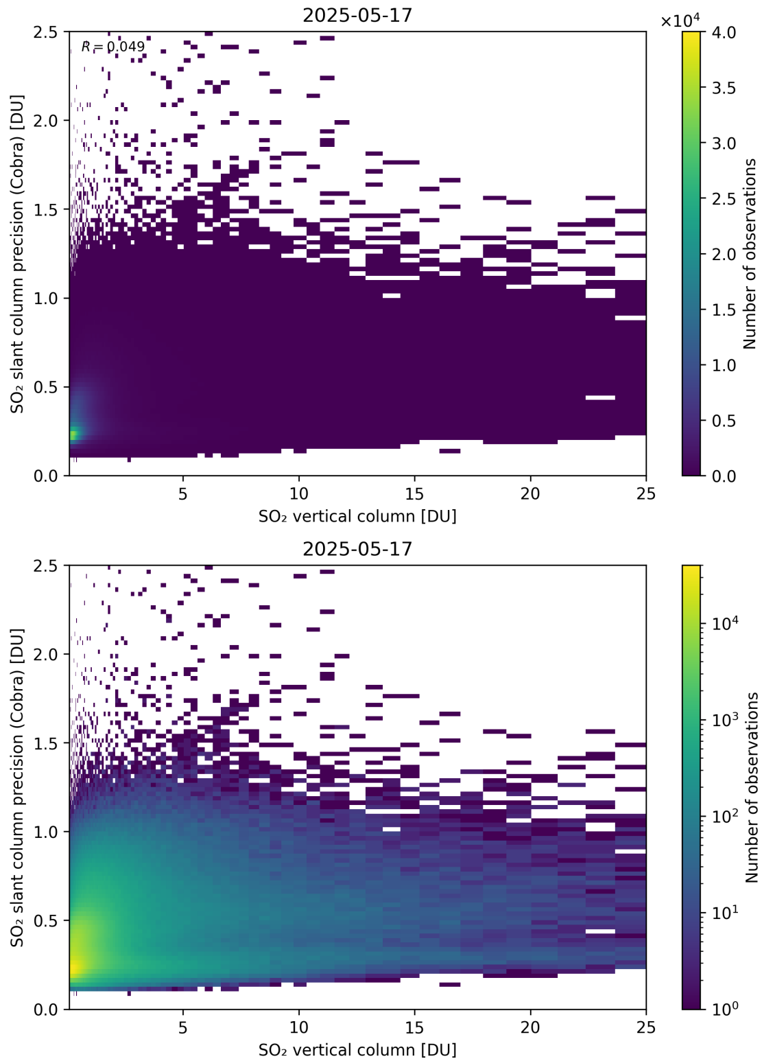
Figure 350: Scatter density plot of “SO 2 vertical column” against “SO 2 slant column precision (Cobra)” for 2025-05-16 to 2025-05-18.
