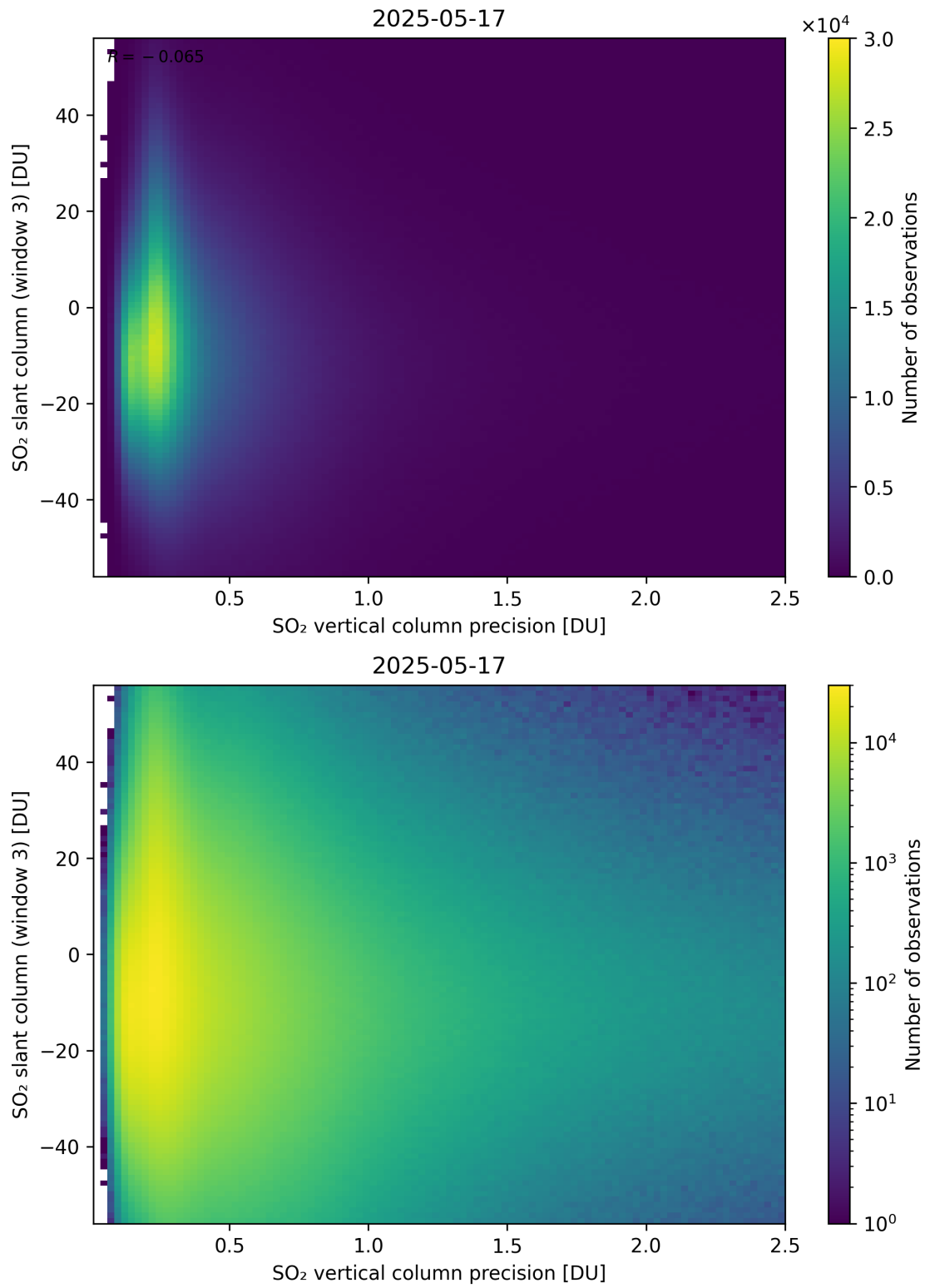
Figure 344: Scatter density plot of “SO 2 vertical column precision” against “SO 2 slant column (window 3)” for 2025-05-16 to 2025-05-18.
