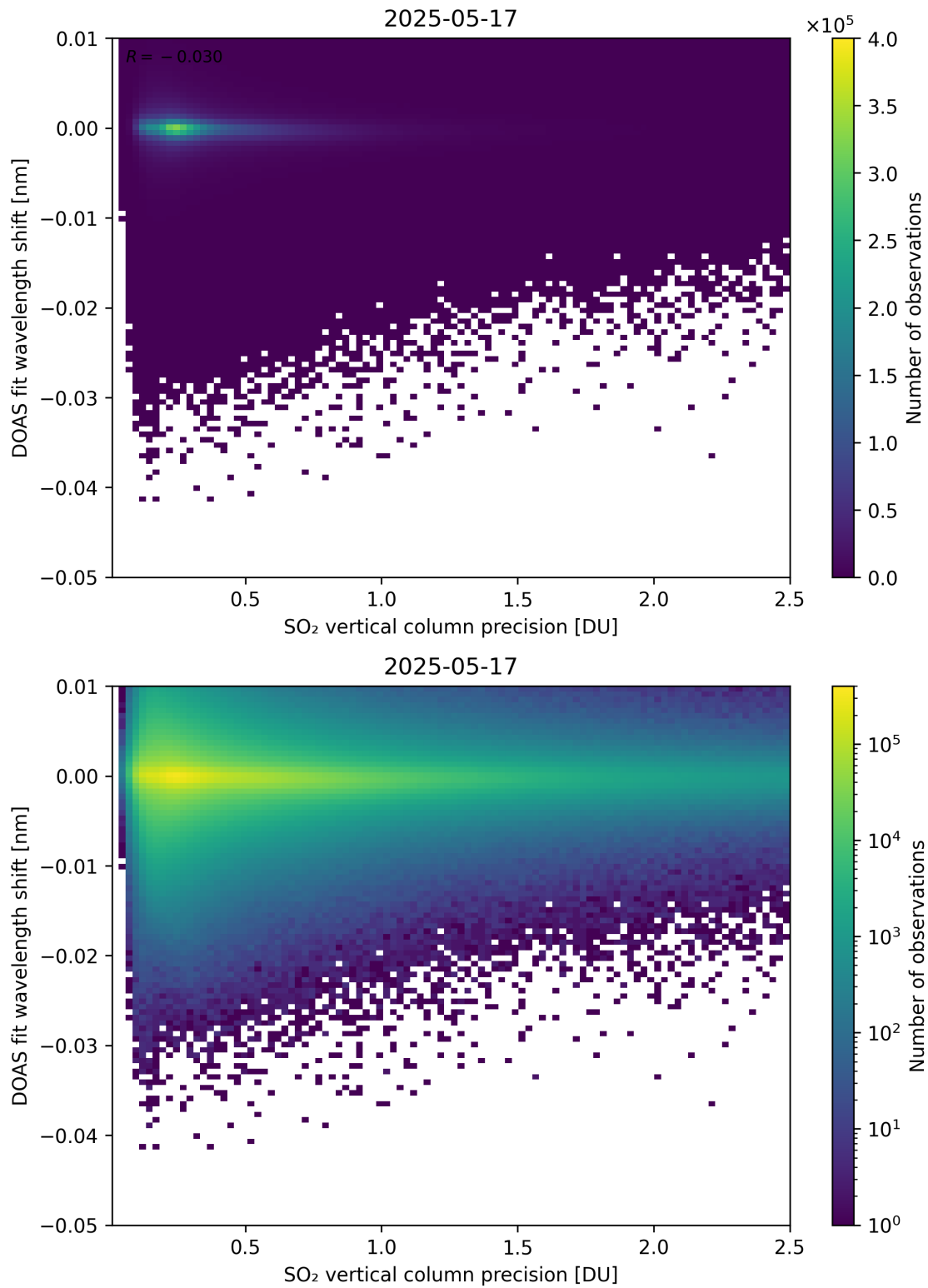
Figure 332: Scatter density plot of “SO 2 vertical column precision” against “DOAS fit wavelength shift” for 2025-05-16 to 2025-05-18.
