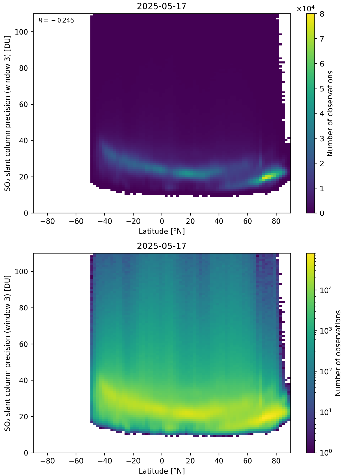
Figure 166: Scatter density plot of “Latitude” against “SO 2 slant column precision (window 3)” for 2025-05-16 to 2025-05-18.
