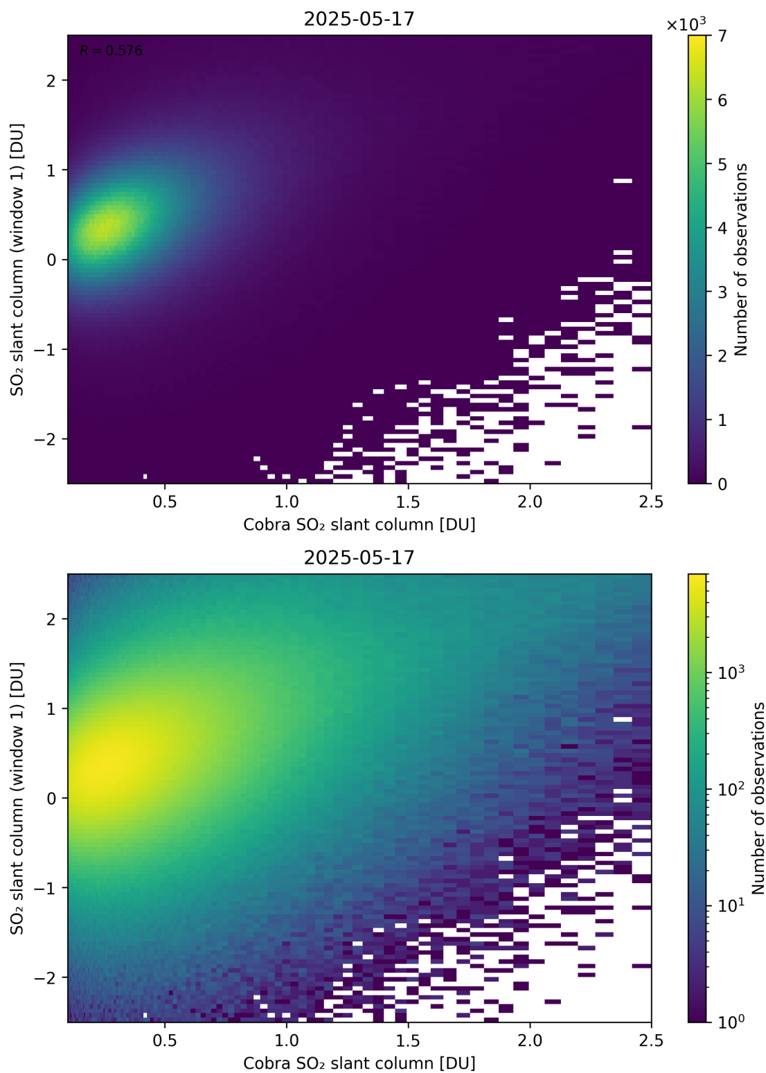
Figure 219: Scatter density plot of “Cobra SO 2 slant column” against “SO 2 slant column (window 1)” for 2025-05-16 to 2025-05-18.
