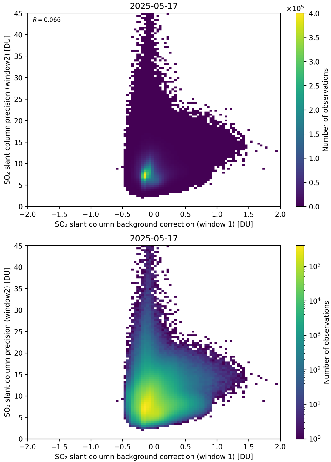
Figure 117: Scatter density plot of “SO 2 slant column background correction (window 1)” against “SO 2 slant column precision (window2)” for 2025-05-16 to 2025-05-18.
