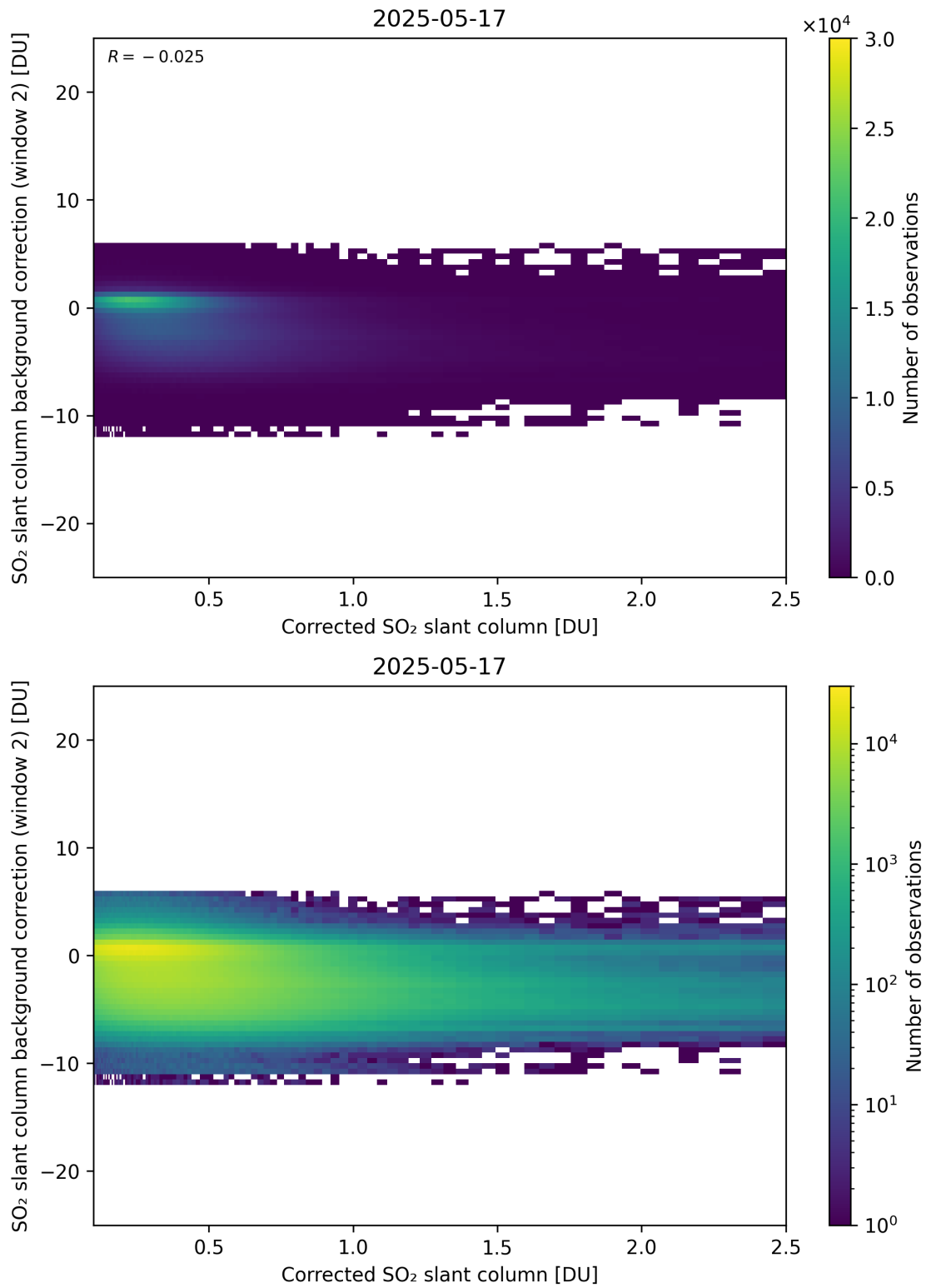
Figure 227: Scatter density plot of “Corrected SO 2 slant column” against “SO 2 slant column background correction (window 2)” for 2025-05-16 to 2025-05-18.
