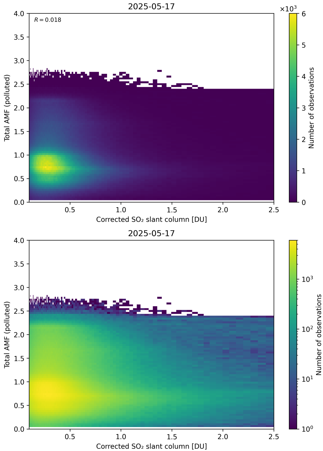
Figure 242: Scatter density plot of “Corrected SO 2 slant column” against “Total AMF (polluted)” for 2025-05-16 to 2025-05-18.
