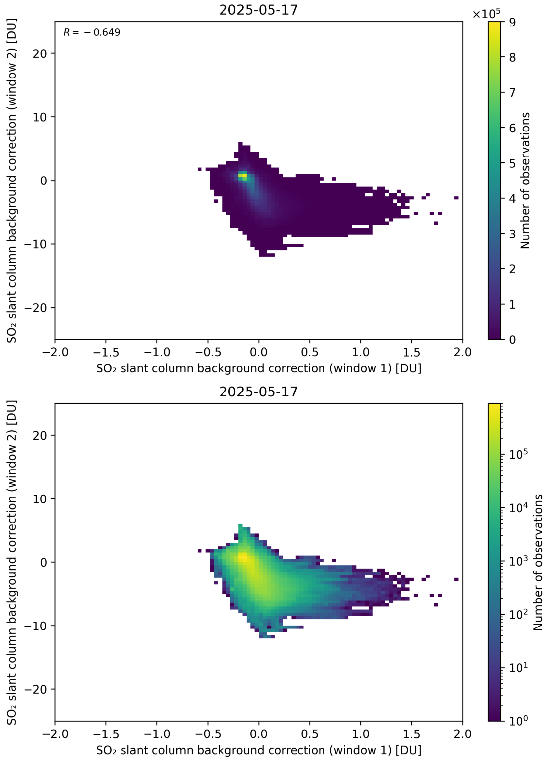
Figure 109: Scatter density plot of “SO 2 slant column background correction (window 1)” against “SO 2 slant column background correction (window 2)” for 2025-05-16 to 2025-05-18.
