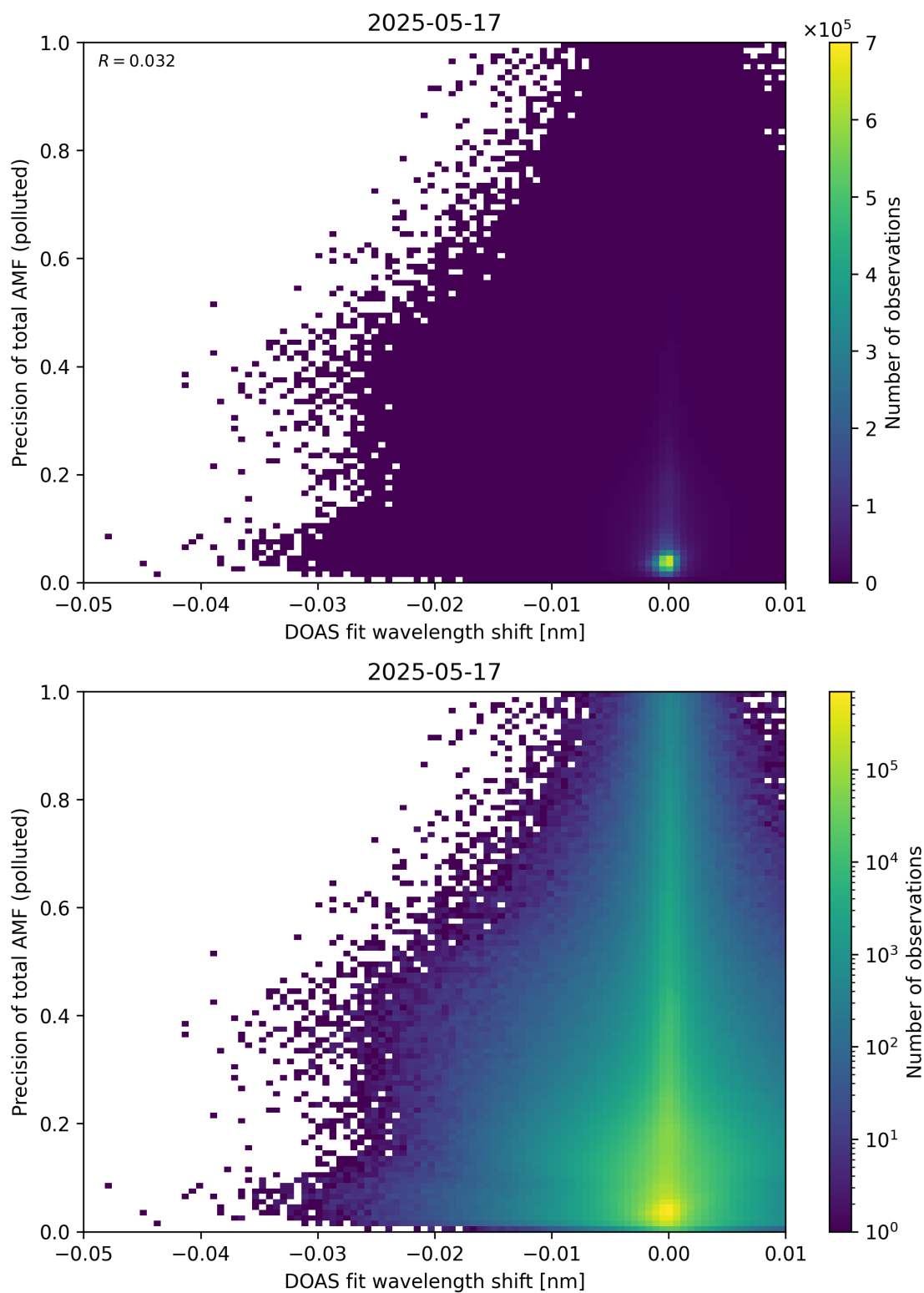
Figure 142: Scatter density plot of “DOAS fit wavelength shift” against “Precision of total AMF (polluted)” for 2025-05-16 to 2025-05-18.
