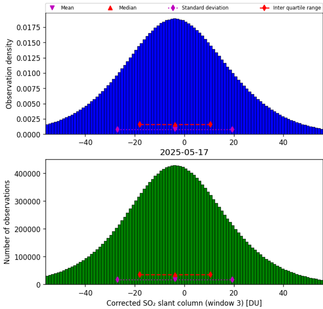
Figure 73: Histogram of “Corrected SO 2 slant column (window 3)” for 2025-05-16 to 2025-05-18
