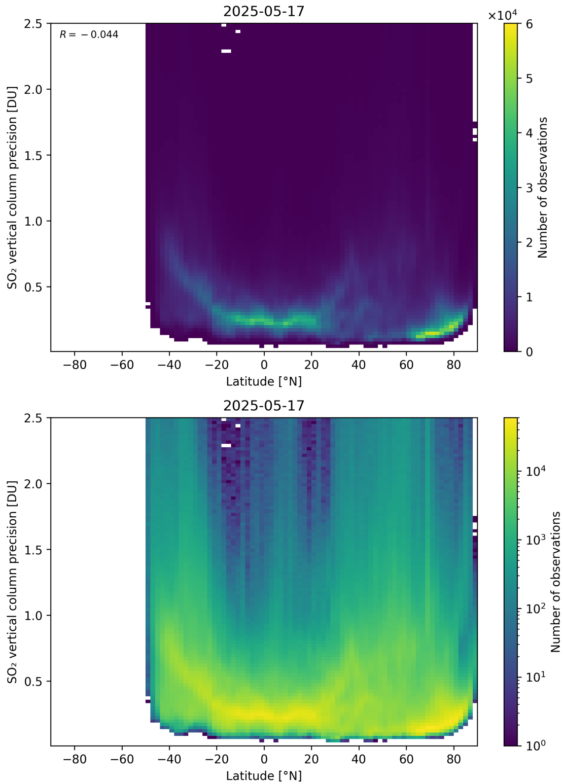
Figure 170: Scatter density plot of “Latitude” against “SO 2 vertical column precision” for 2025-05-16 to 2025-05-18.
