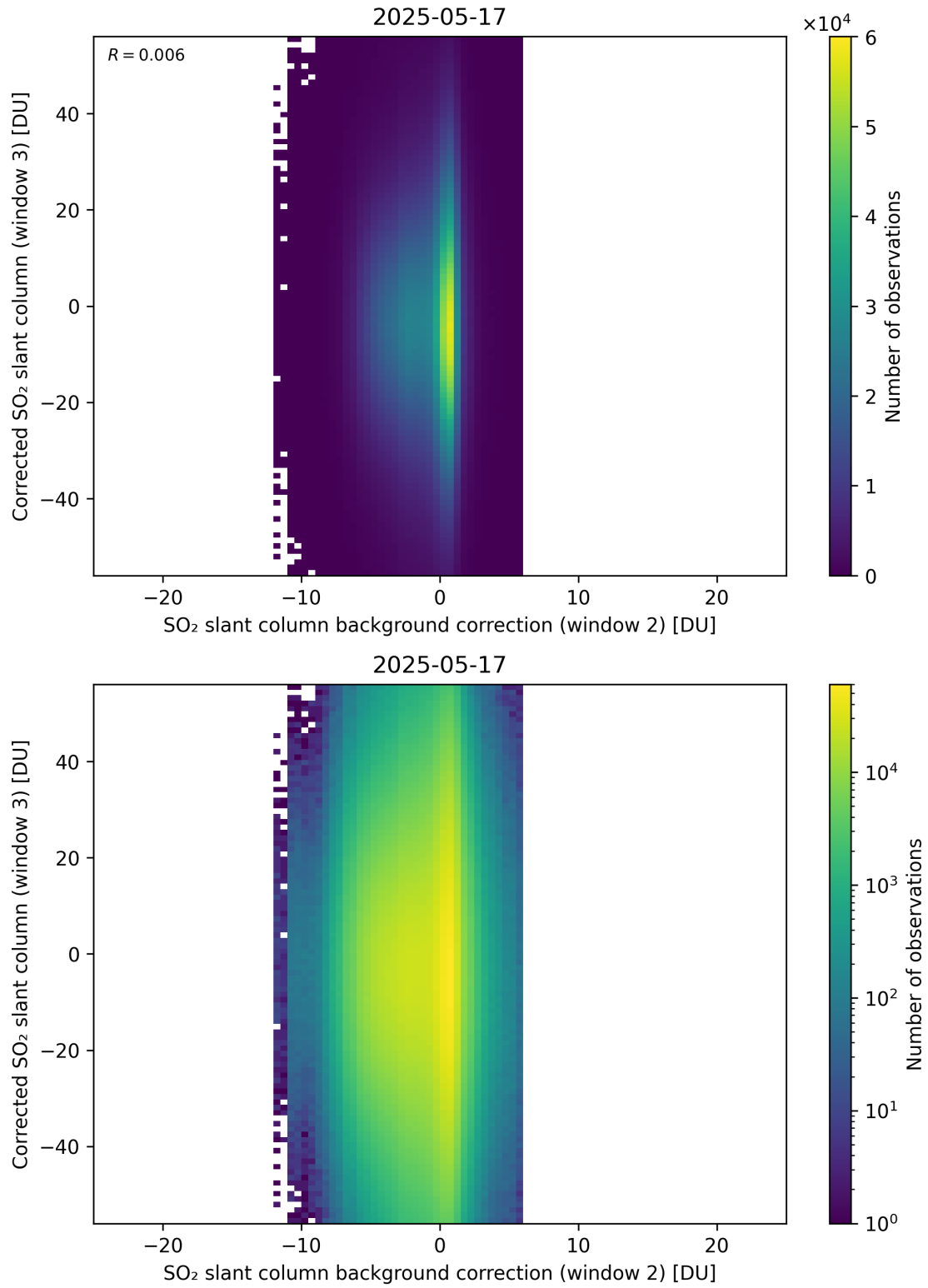
Figure 127: Scatter density plot of “SO 2 slant column background correction (window 2)” against “Corrected SO 2 slant column (window 3)” for 2025-05-16 to 2025-05-18.
