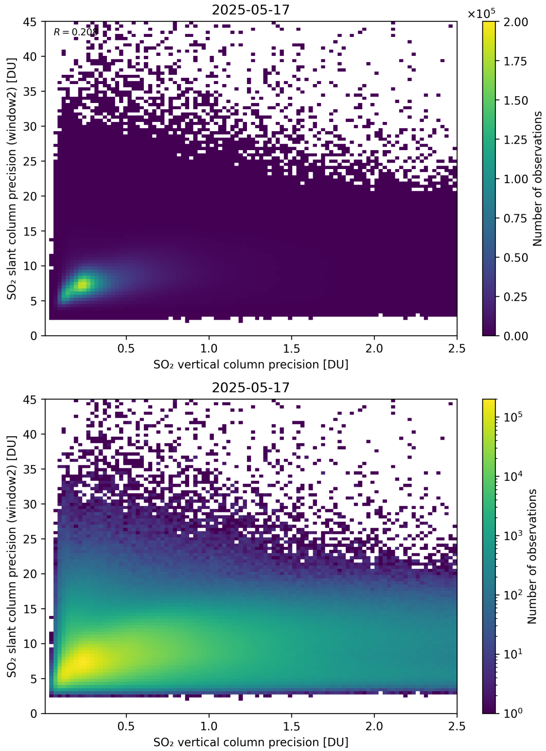
Figure 343: Scatter density plot of “SO 2 vertical column precision” against “SO 2 slant column precision (window2)” for 2025-05-16 to 2025-05-18.
