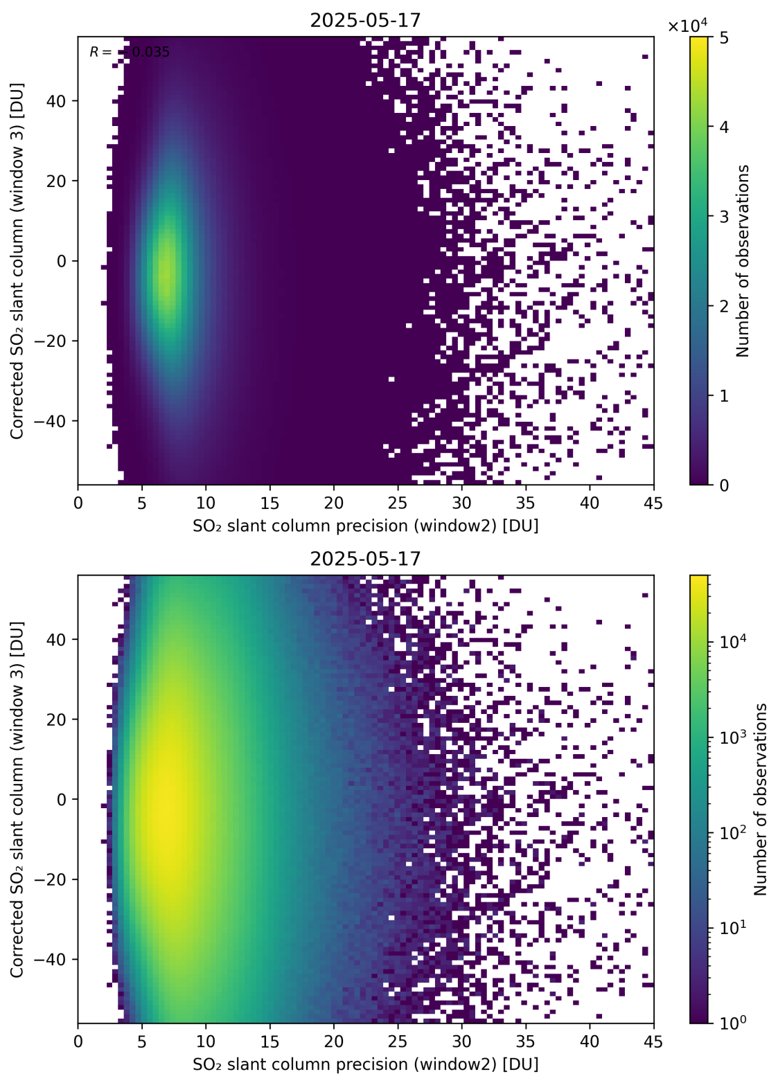
Figure 298: Scatter density plot of “SO 2 slant column precision (window2)” against “Corrected SO 2 slant column (window 3)” for 2025-05-16 to 2025-05-18.
