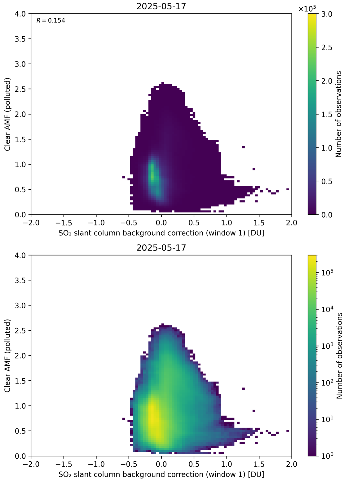
Figure 114: Scatter density plot of “SO 2 slant column background correction (window 1)” against “Clear AMF (polluted)” for 2025-05-16 to 2025-05-18.
