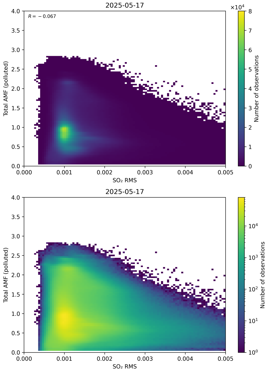
Figure 148: Scatter density plot of “SO 2 RMS” against “Total AMF (polluted)” for 2025-05-16 to 2025-05-18.
