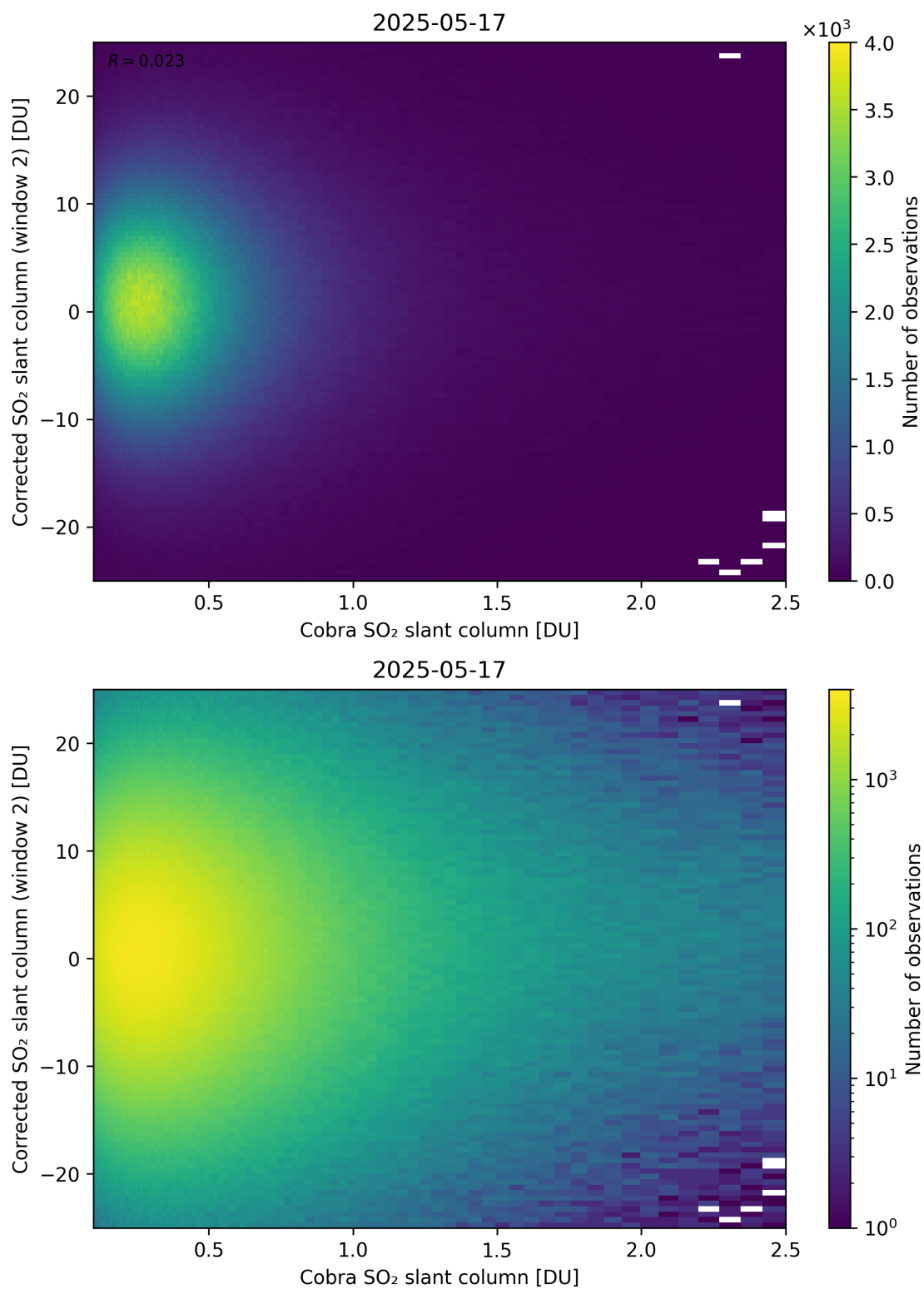
Figure 217: Scatter density plot of “Cobra SO 2 slant column” against “Corrected SO 2 slant column (window 2)” for 2025-05-16 to 2025-05-18.
