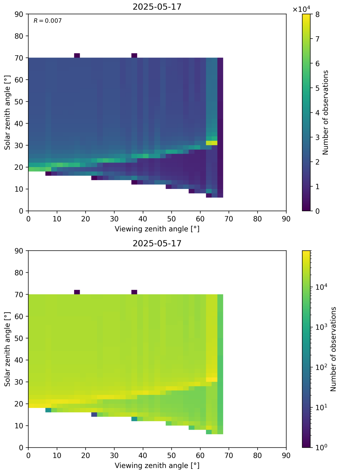
Figure 369: Scatter density plot of “Viewing zenith angle” against “Solar zenith angle” for 2025-05-16 to 2025-05-18.
