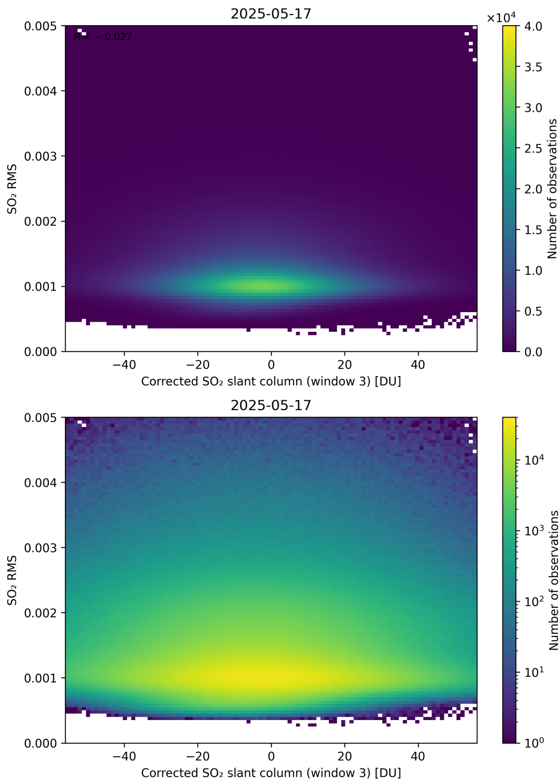
Figure 258: Scatter density plot of “Corrected SO 2 slant column (window 3)” against “SO 2 RMS” for 2025-05-16 to 2025-05-18.
