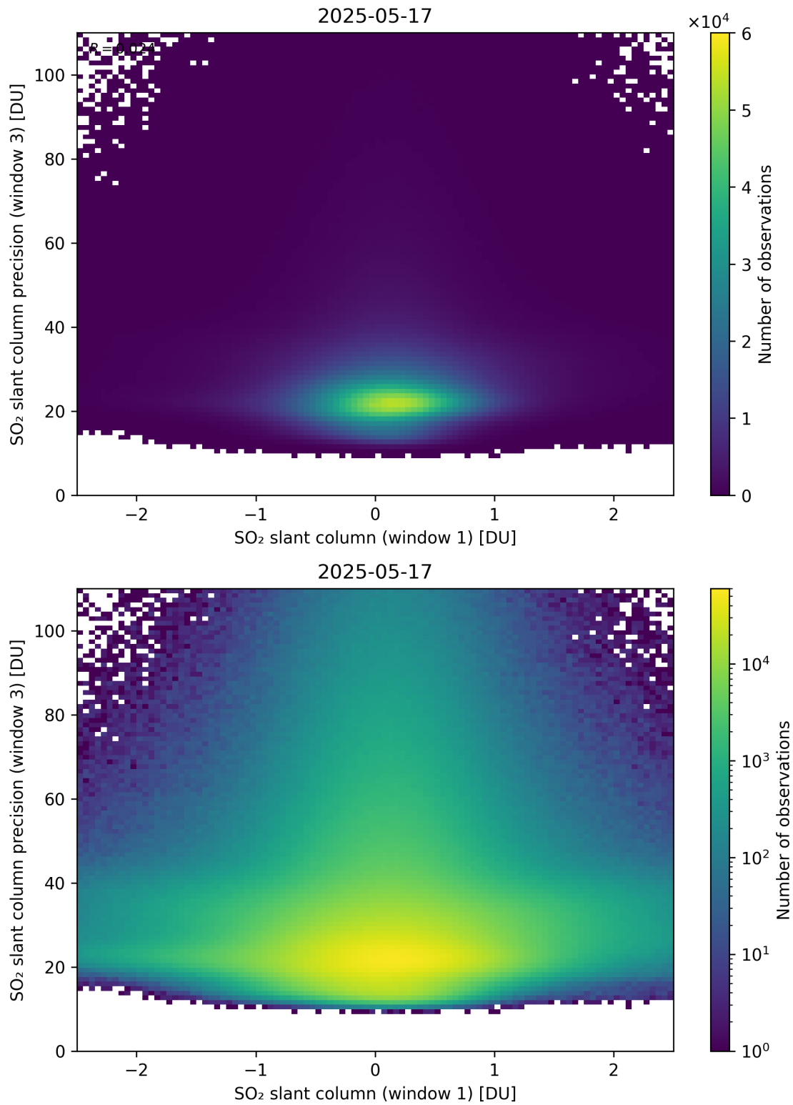
Figure 288: Scatter density plot of “SO 2 slant column (window 1)” against “SO 2 slant column precision (window 3)” for 2025-05-16 to 2025-05-18.
