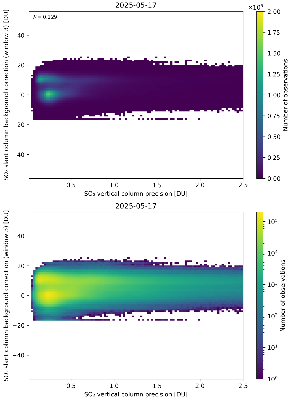
Figure 331: Scatter density plot of “SO 2 vertical column precision” against “SO 2 slant column background correction (window 3)” for 2025-05-16 to 2025-05-18.
