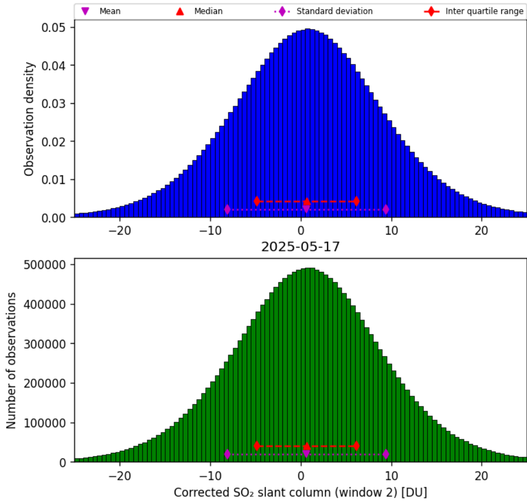
Figure 69: Histogram of “Corrected SO 2 slant column (window 2)” for 2025-05-16 to 2025-05-18
