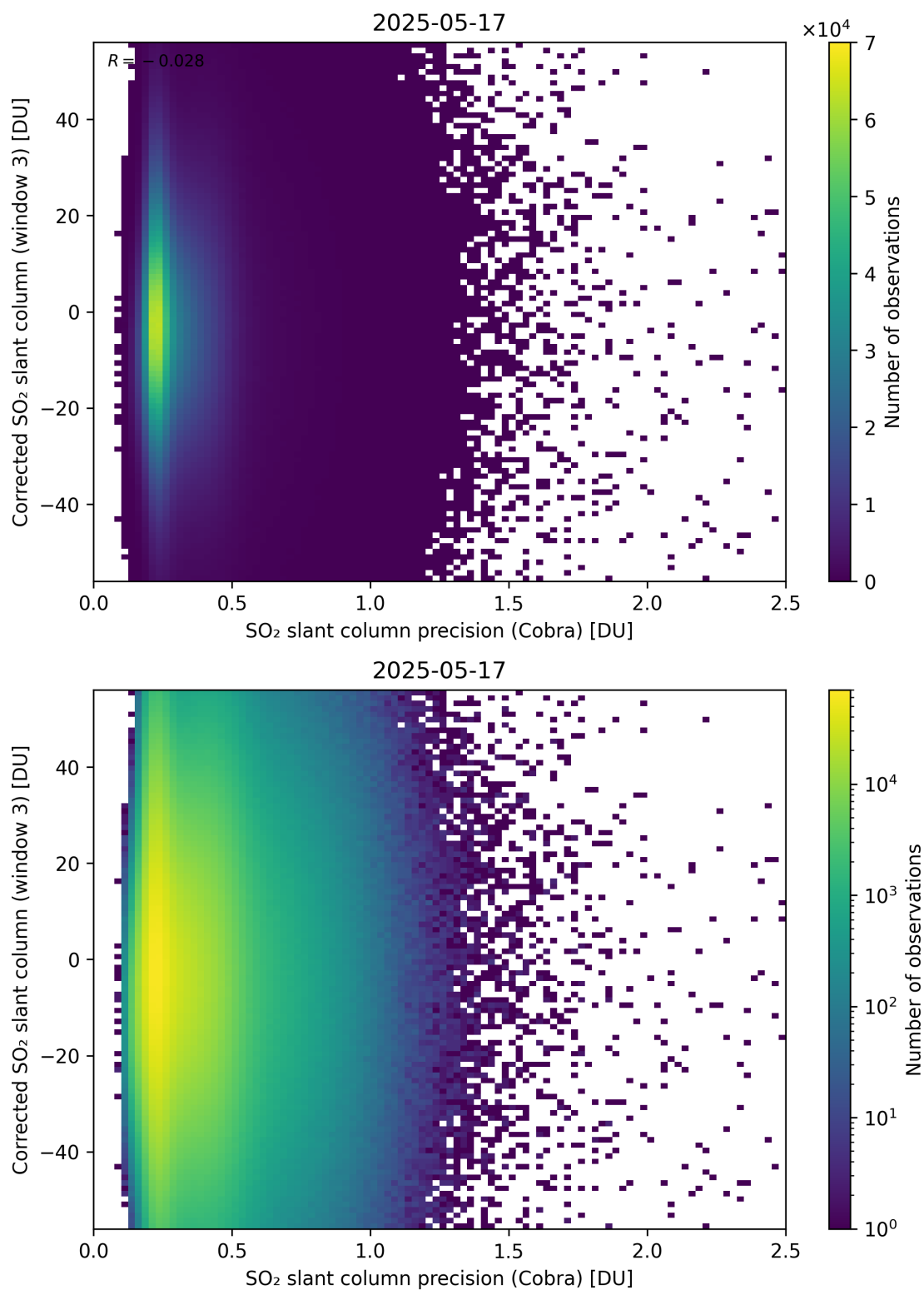
Figure 207: Scatter density plot of “SO 2 slant column precision (Cobra)” against “Corrected SO 2 slant column (window 3)” for 2025-05-16 to 2025-05-18.
