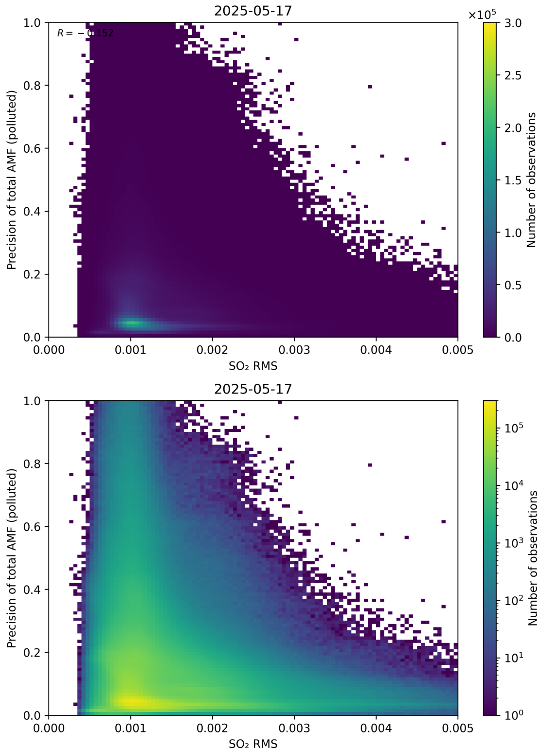
Figure 149: Scatter density plot of “SO 2 RMS” against “Precision of total AMF (polluted)” for 2025-05-16 to 2025-05-18.
