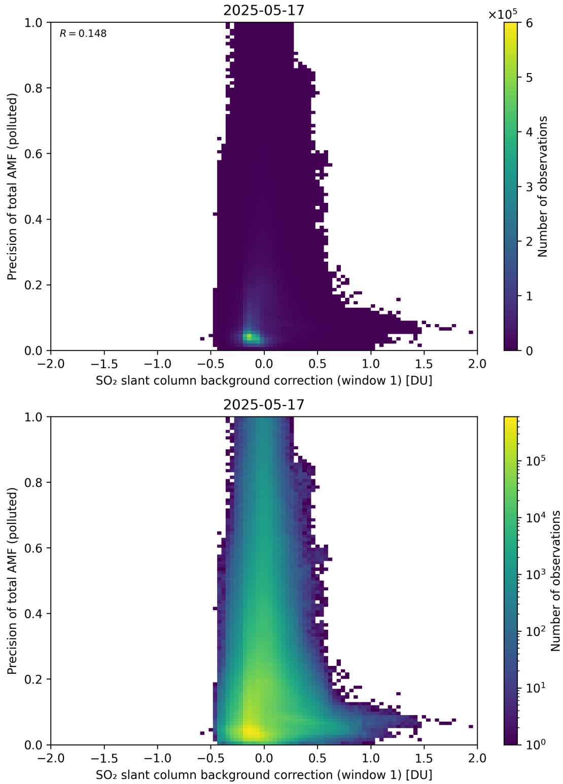
Figure 121: Scatter density plot of “SO 2 slant column background correction (window 1)” against “Precision of total AMF (polluted)” for 2025-05-16 to 2025-05-18.
