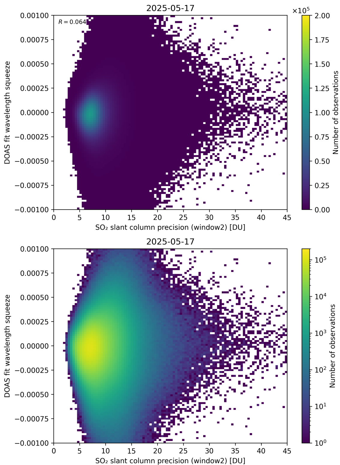
Figure 294: Scatter density plot of “SO 2 slant column precision (window2)” against “DOAS fit wavelength squeeze” for 2025-05-16 to 2025-05-18.
