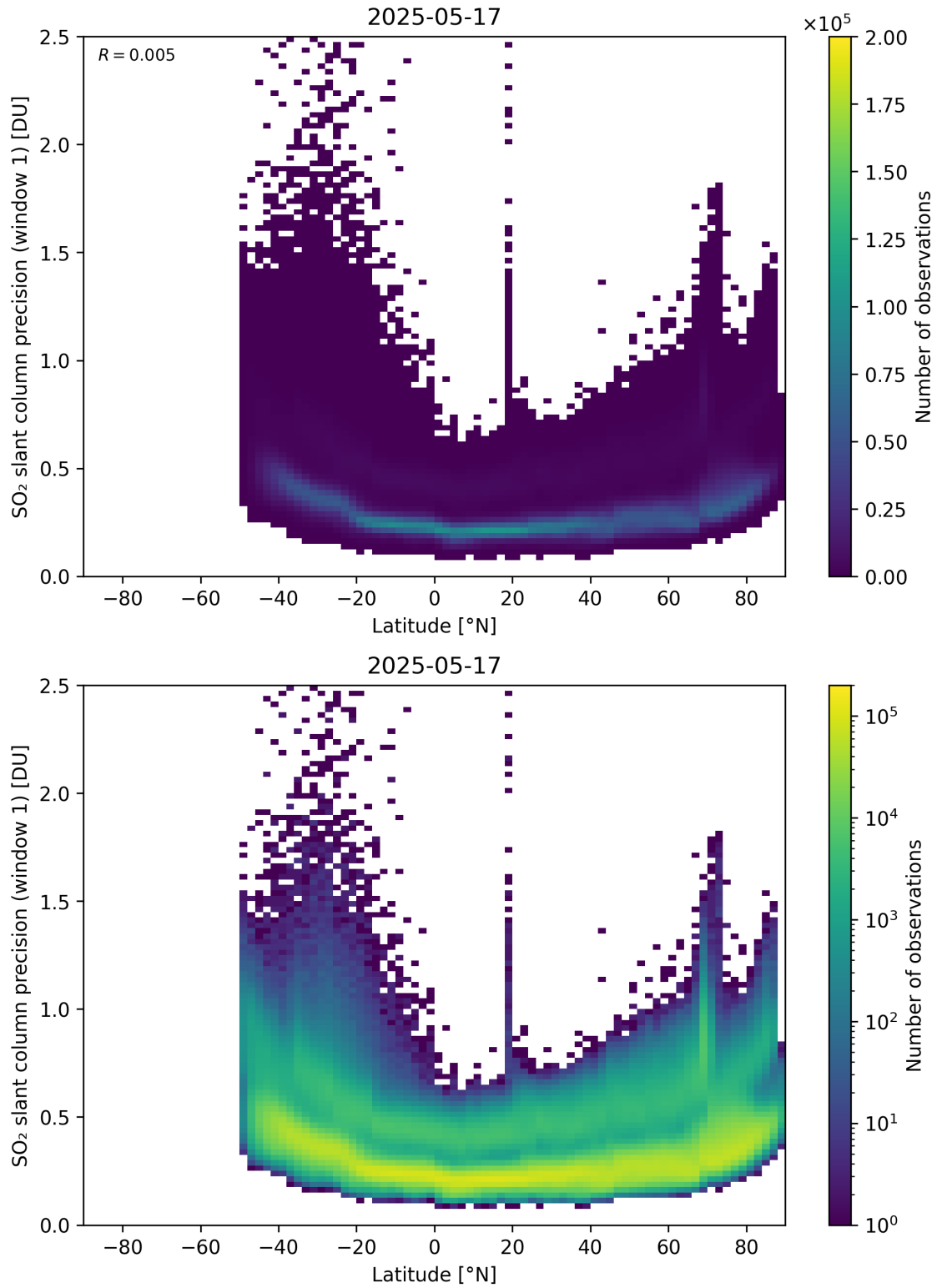
Figure 163: Scatter density plot of “Latitude” against “SO 2 slant column precision (window 1)” for 2025-05-16 to 2025-05-18.
