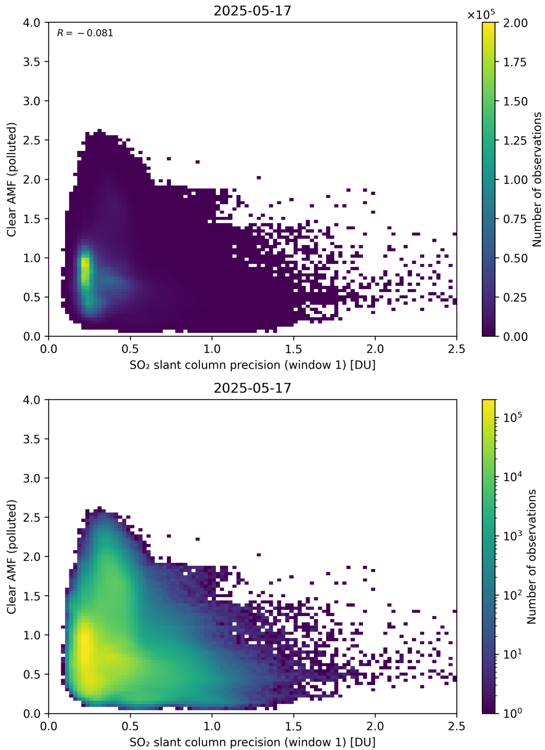
Figure 274: Scatter density plot of “SO 2 slant column precision (window 1)” against “Clear AMF (polluted)” for 2025-05-16 to 2025-05-18.
