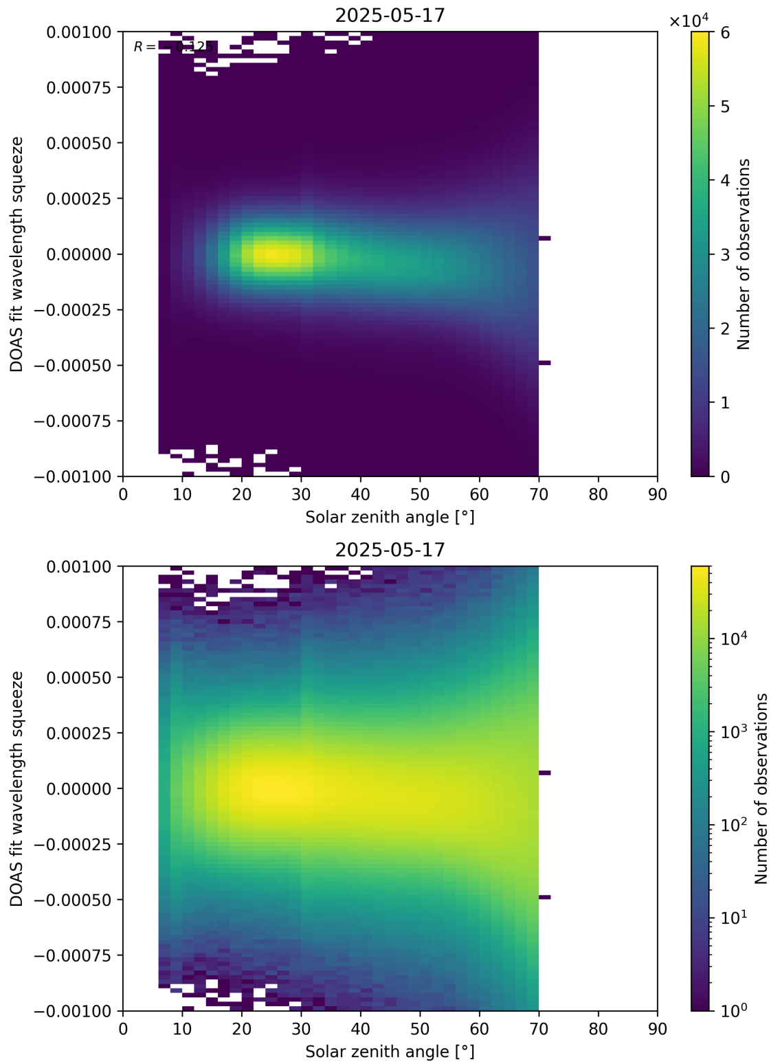
Figure 175: Scatter density plot of “Solar zenith angle” against “DOAS fit wavelength squeeze” for 2025-05-16 to 2025-05-18.
