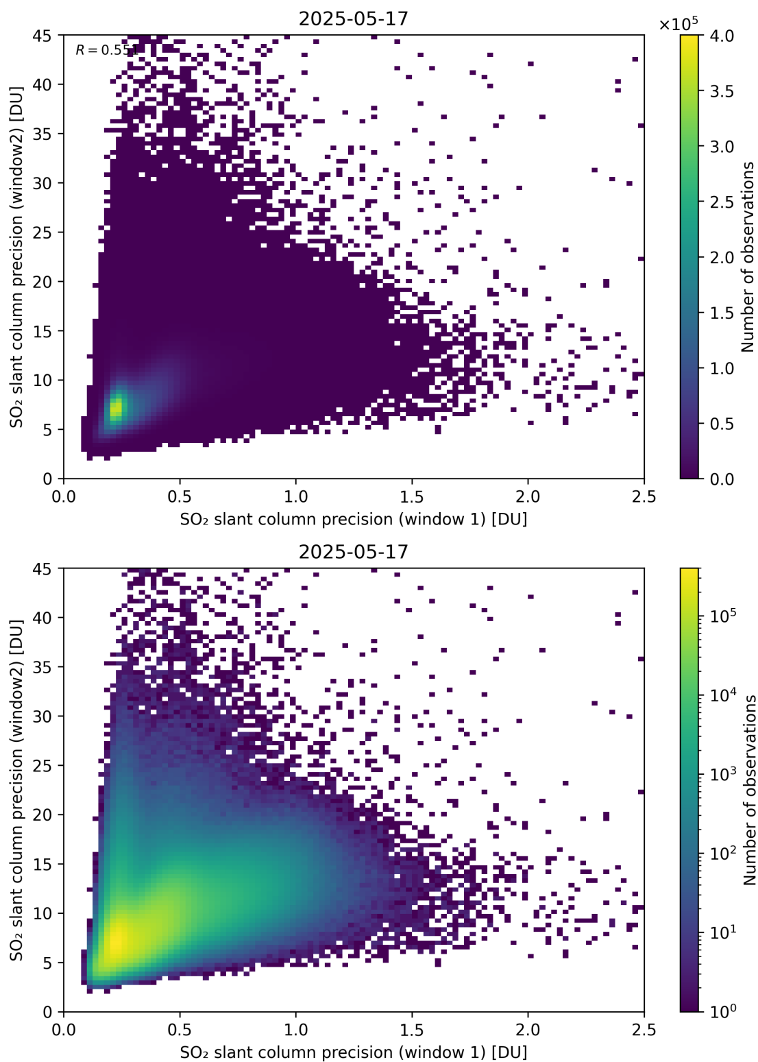
Figure 277: Scatter density plot of “SO 2 slant column precision (window 1)” against “SO 2 slant column precision (window2)” for 2025-05-16 to 2025-05-18.
