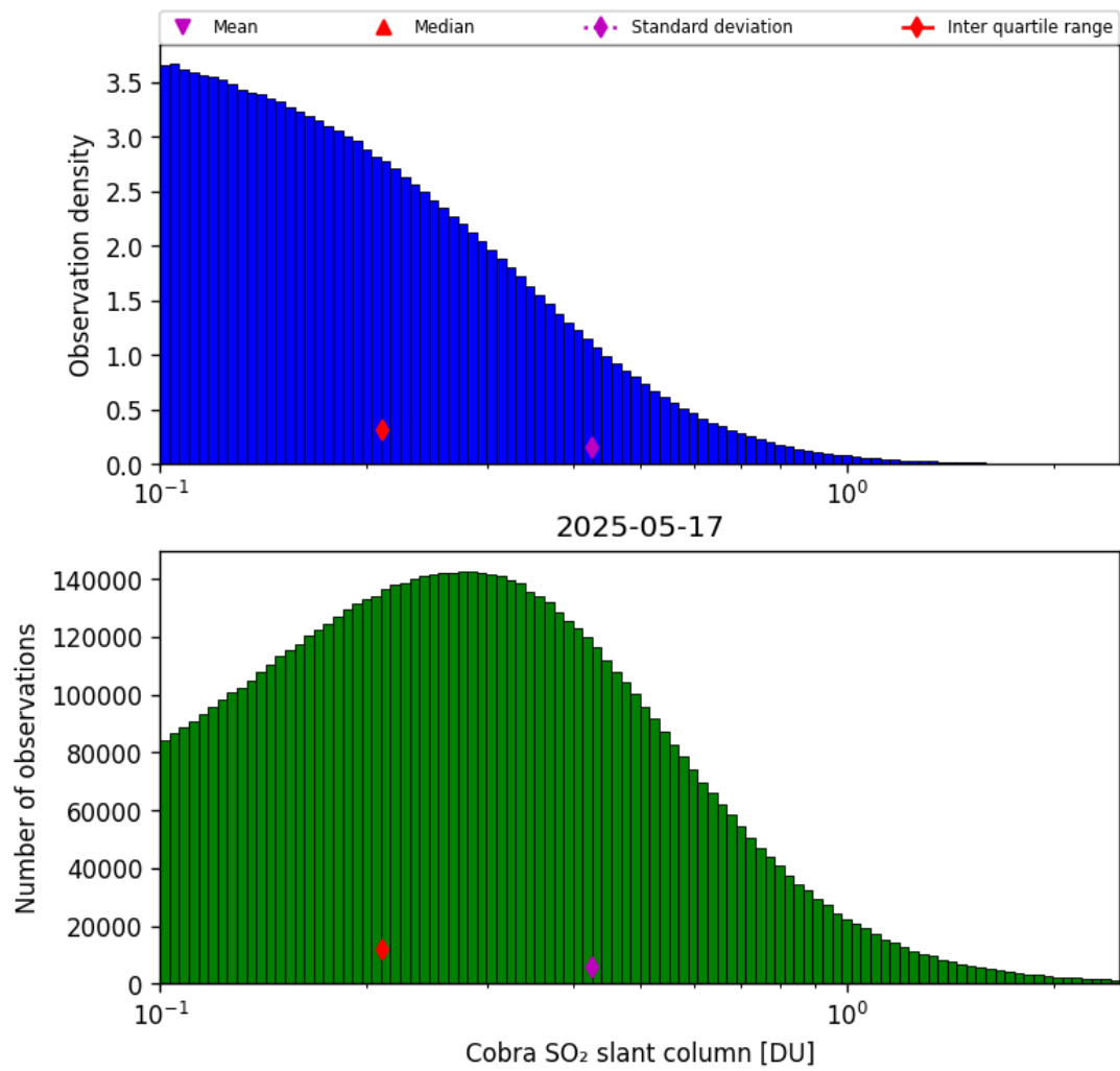
Figure 61: Histogram of “Cobra SO 2 slant column” for 2025-05-16 to 2025-05-18
