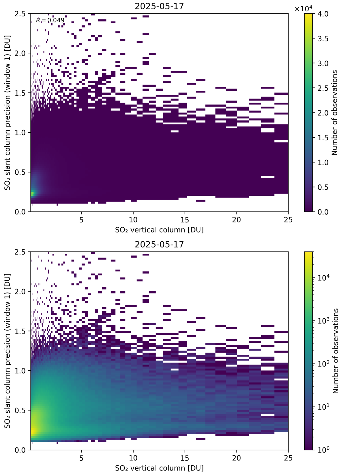
Figure 355: Scatter density plot of “SO 2 vertical column” against “SO 2 slant column precision (window 1)” for 2025-05-16 to 2025-05-18.
