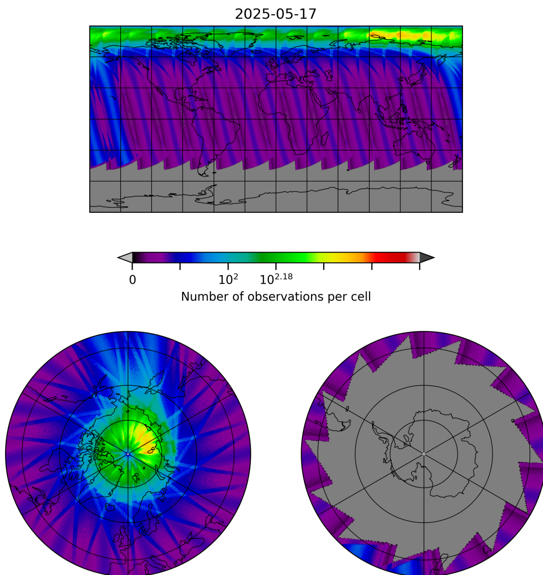
Figure 30: Map of the number of observations for 2025-05-16 to 2025-05-18
