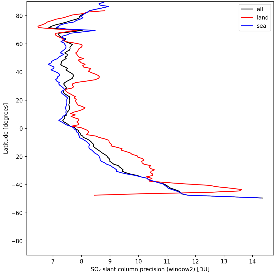
Figure 42: Zonal average of “SO 2 slant column precision (window2)” for 2025-05-16 to 2025-05-18.
