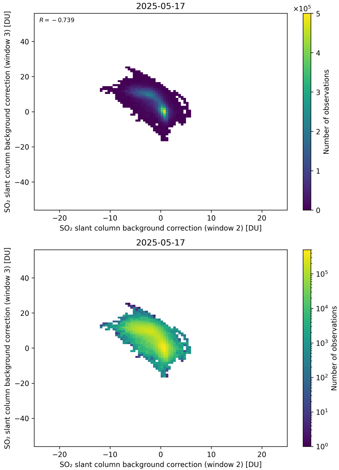
Figure 122: Scatter density plot of “SO 2 slant column background correction (window 2)” against “SO 2 slant column background correction (window 3)” for 2025-05-16 to 2025-05-18.
