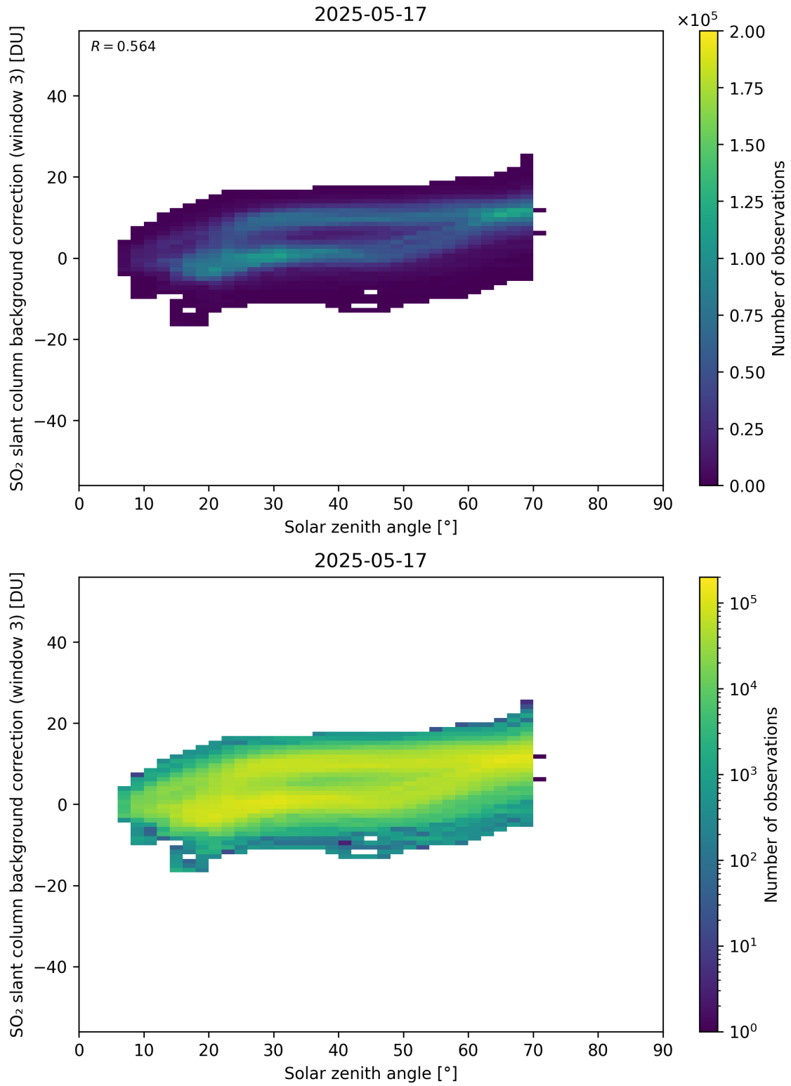
Figure 173: Scatter density plot of “Solar zenith angle” against “SO 2 slant column background correction (window 3)” for 2025-05-16 to 2025-05-18.
