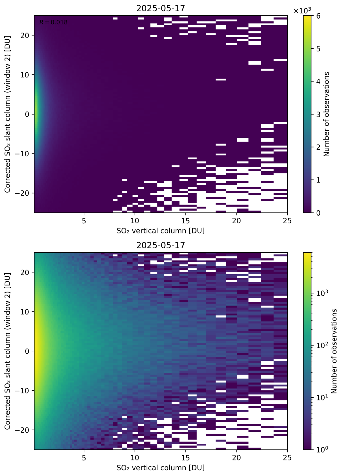
Figure 352: Scatter density plot of “SO 2 vertical column” against “Corrected SO 2 slant column (window 2)” for 2025-05-16 to 2025-05-18.
