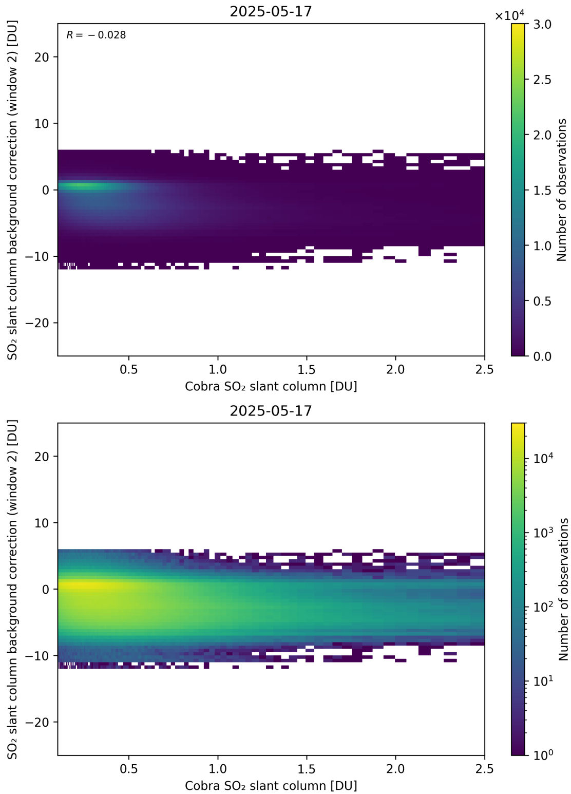
Figure 194: Scatter density plot of “Cobra SO 2 slant column” against “SO 2 slant column background correction (window 2)” for 2025-05-16 to 2025-05-18.
