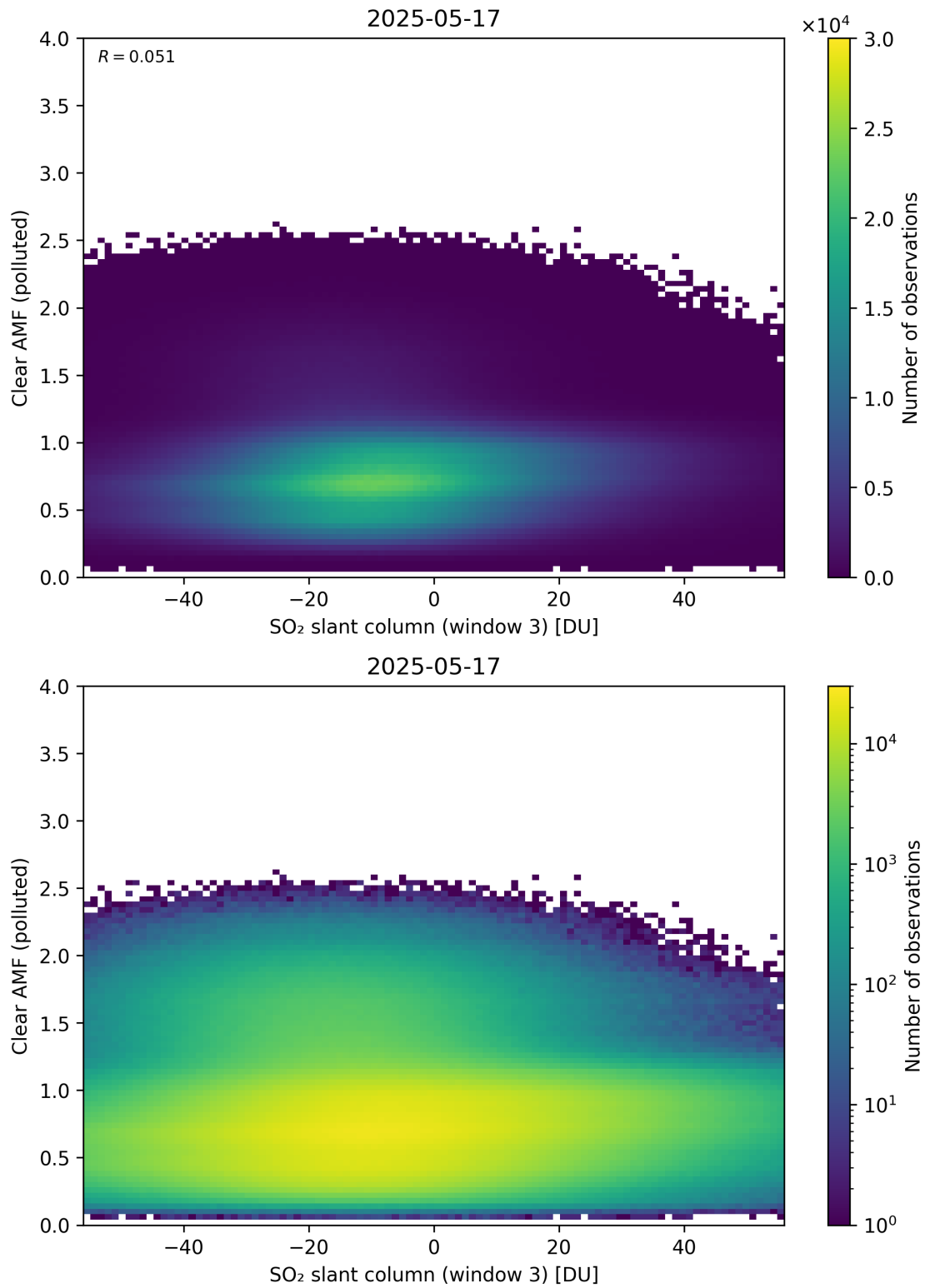
Figure 315: Scatter density plot of “SO 2 slant column (window 3)” against “Clear AMF (polluted)” for 2025-05-16 to 2025-05-18.
