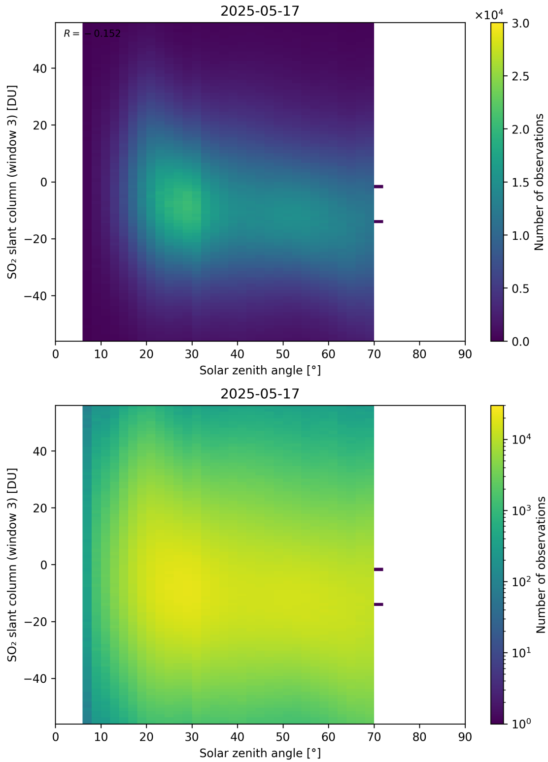
Figure 187: Scatter density plot of “Solar zenith angle” against “SO 2 slant column (window 3)” for 2025-05-16 to 2025-05-18.
