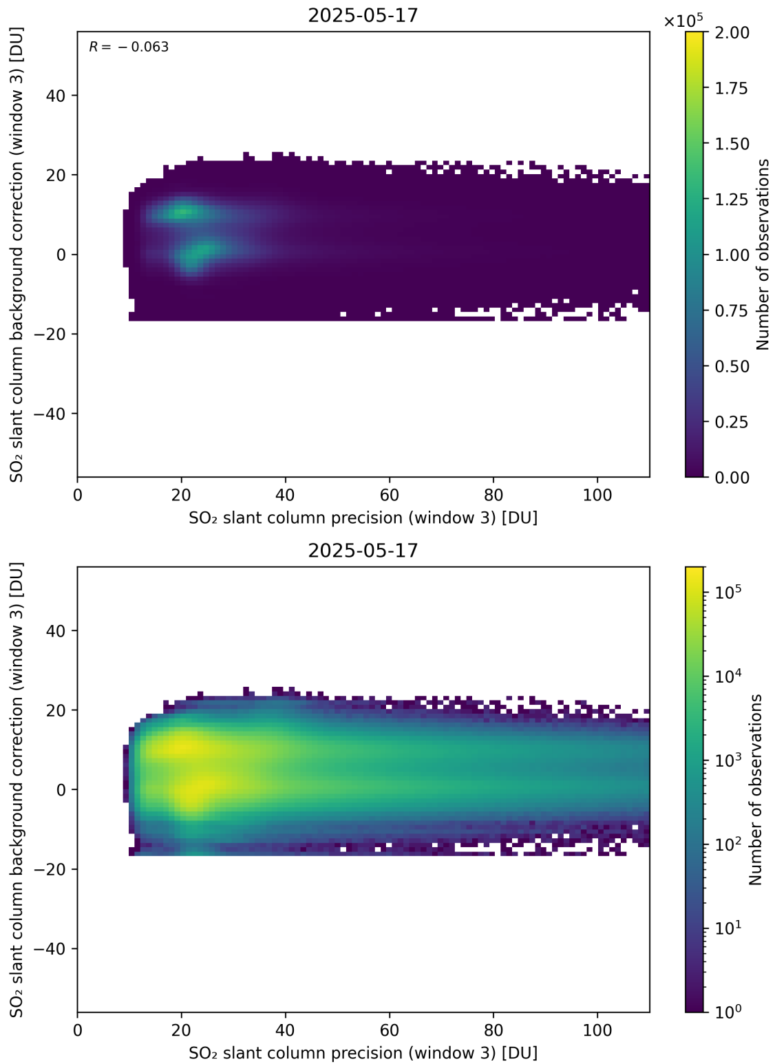
Figure 307: Scatter density plot of “SO 2 slant column precision (window 3)” against “SO 2 slant column background correction (window 3)” for 2025-05-16 to 2025-05-18.
