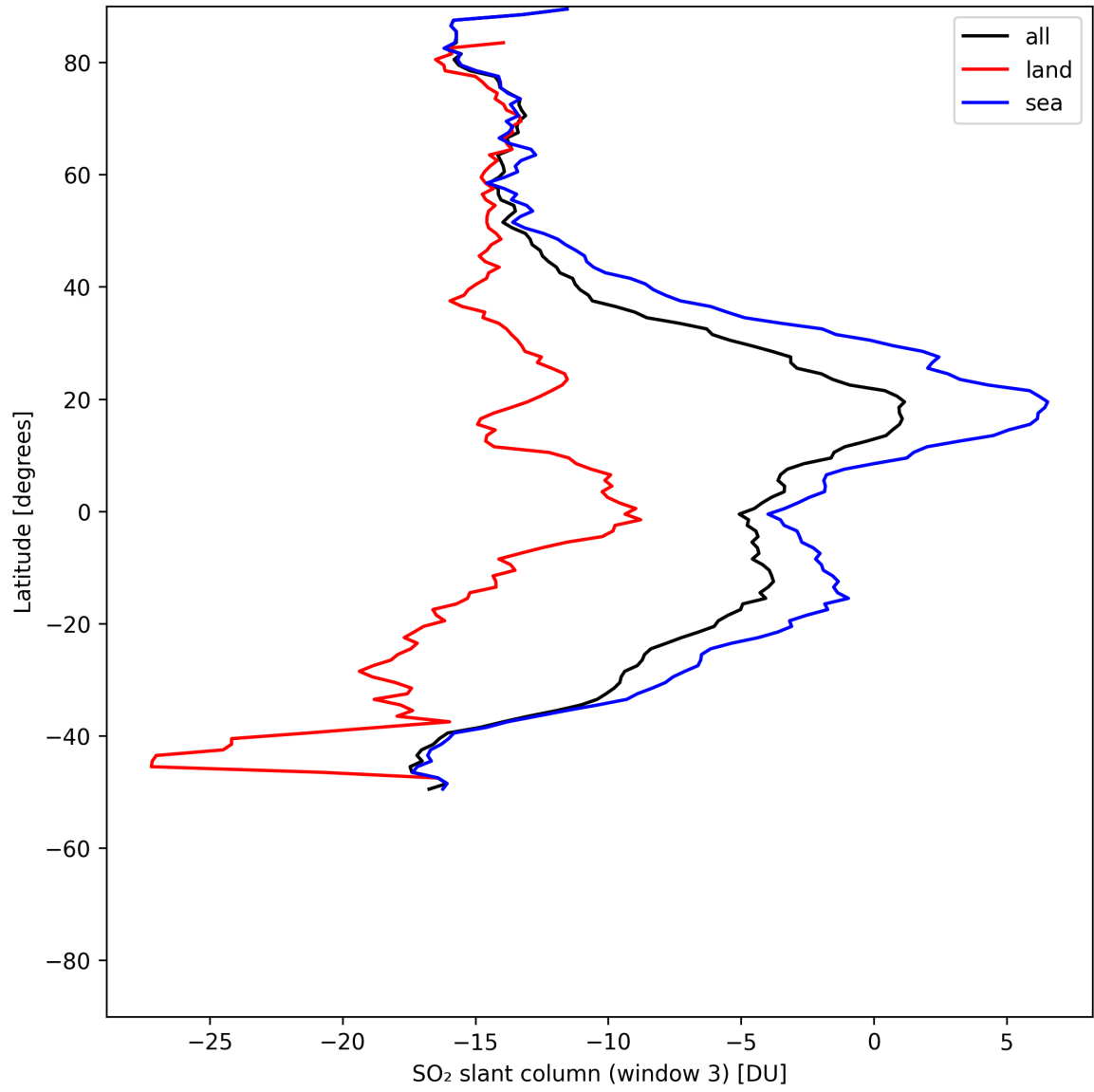
Figure 45: Zonal average of “SO 2 slant column (window 3)” for 2025-05-16 to 2025-05-18.
