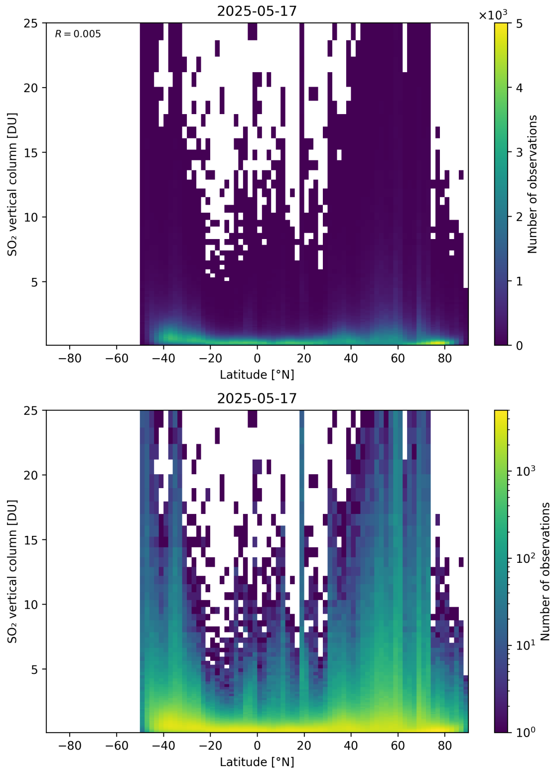
Figure 169: Scatter density plot of “Latitude” against “SO 2 vertical column” for 2025-05-16 to 2025-05-18.
