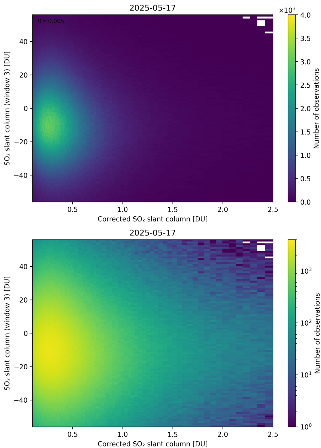
Figure 240: Scatter density plot of “Corrected SO 2 slant column” against “SO 2 slant column (window 3)” for 2025-05-16 to 2025-05-18.
