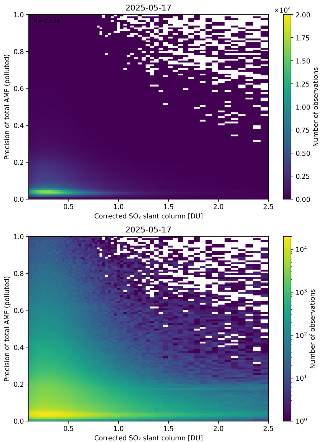
Figure 243: Scatter density plot of “Corrected SO 2 slant column” against “Precision of total AMF (polluted)” for 2025-05-16 to 2025-05-18.
