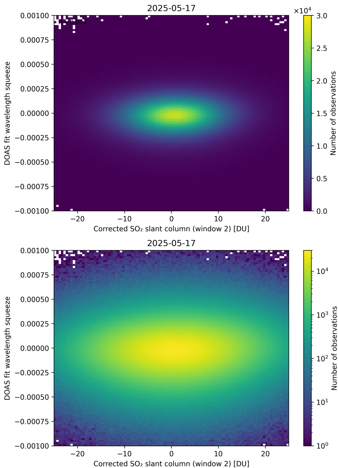
Figure 247: Scatter density plot of “Corrected SO 2 slant column (window 2)” against “DOAS fit wavelength squeeze” for 2025-05-16 to 2025-05-18.
