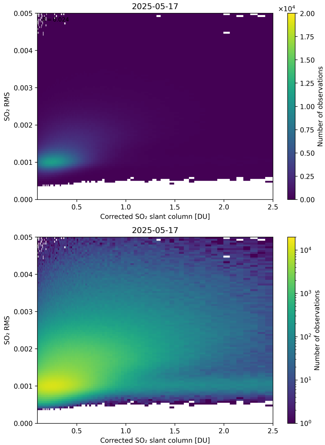
Figure 231: Scatter density plot of “Corrected SO 2 slant column” against “SO 2 RMS” for 2025-05-16 to 2025-05-18.
