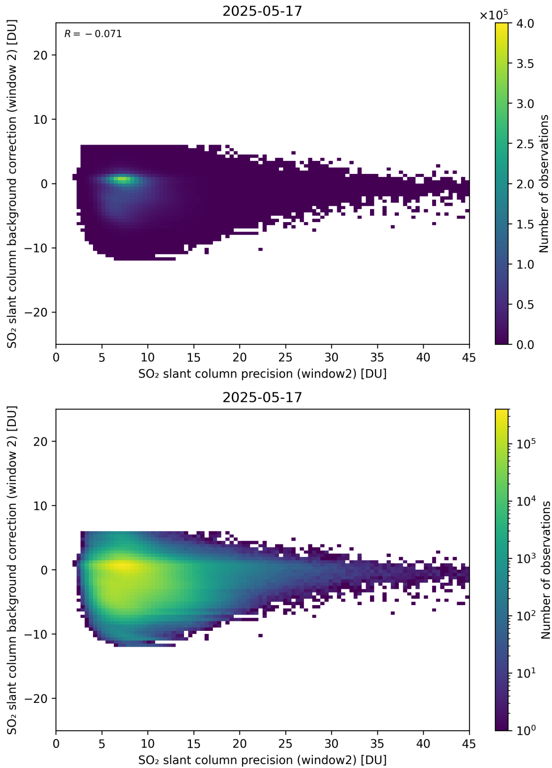
Figure 291: Scatter density plot of “SO 2 slant column precision (window2)” against “SO 2 slant column background correction (window 2)” for 2025-05-16 to 2025-05-18.
