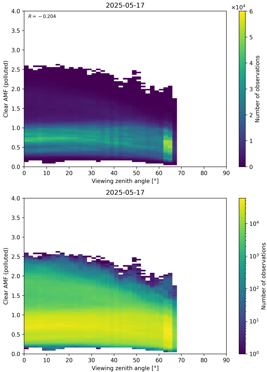
Figure 370: Scatter density plot of “Viewing zenith angle” against “Clear AMF (polluted)” for 2025-05-16 to 2025-05-18.
