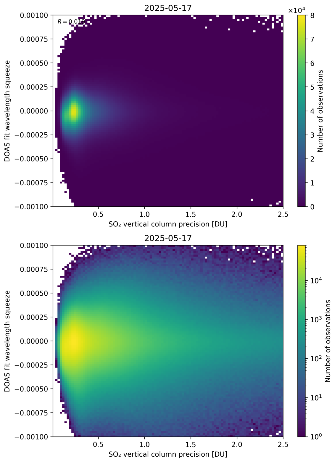
Figure 333: Scatter density plot of “SO 2 vertical column precision” against “DOAS fit wavelength squeeze” for 2025-05-16 to 2025-05-18.
