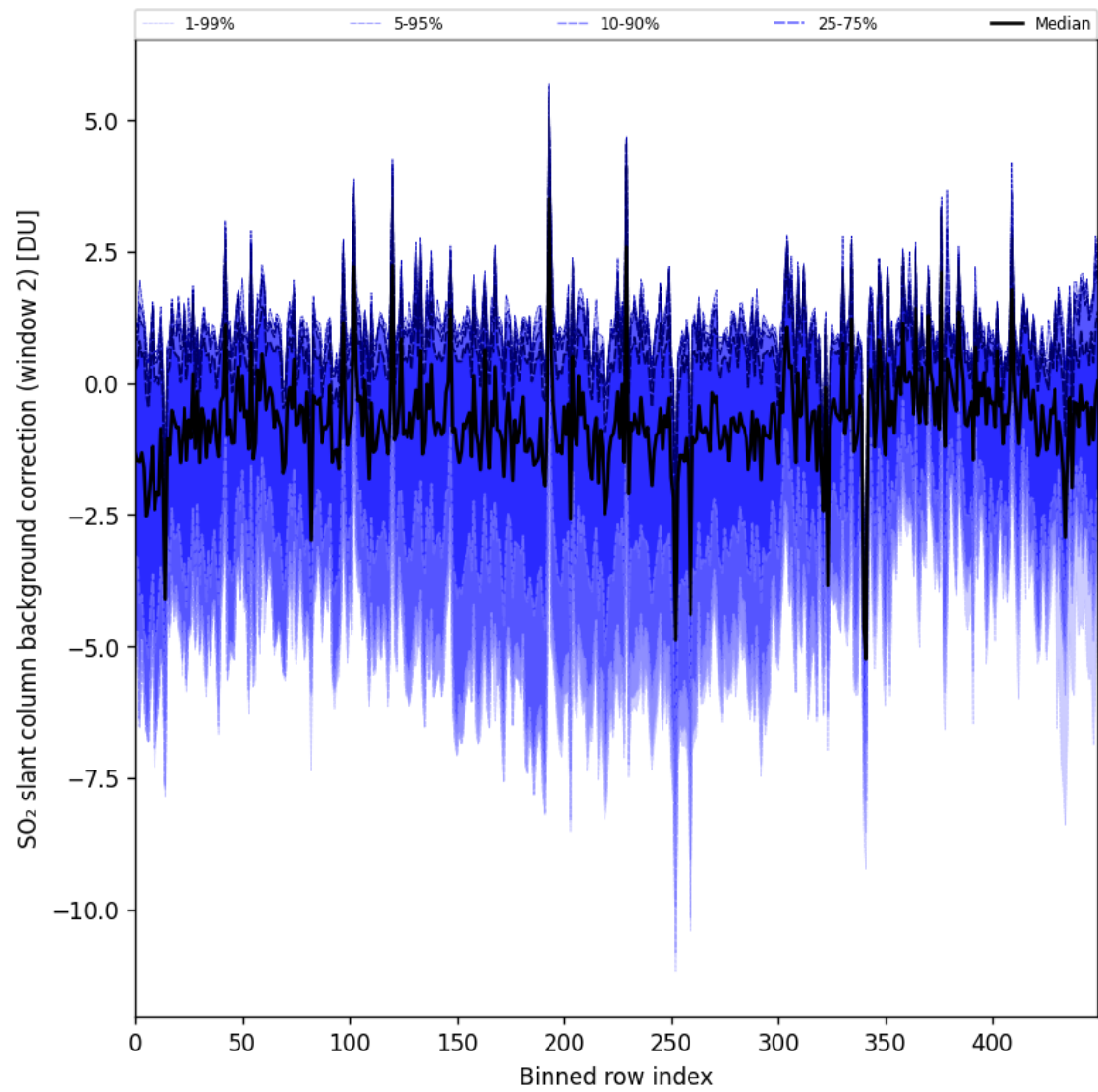
Figure 96: Along track statistics of “SO 2 slant column background correction (window 2)” for 2025-05-16 to 2025-05-18
