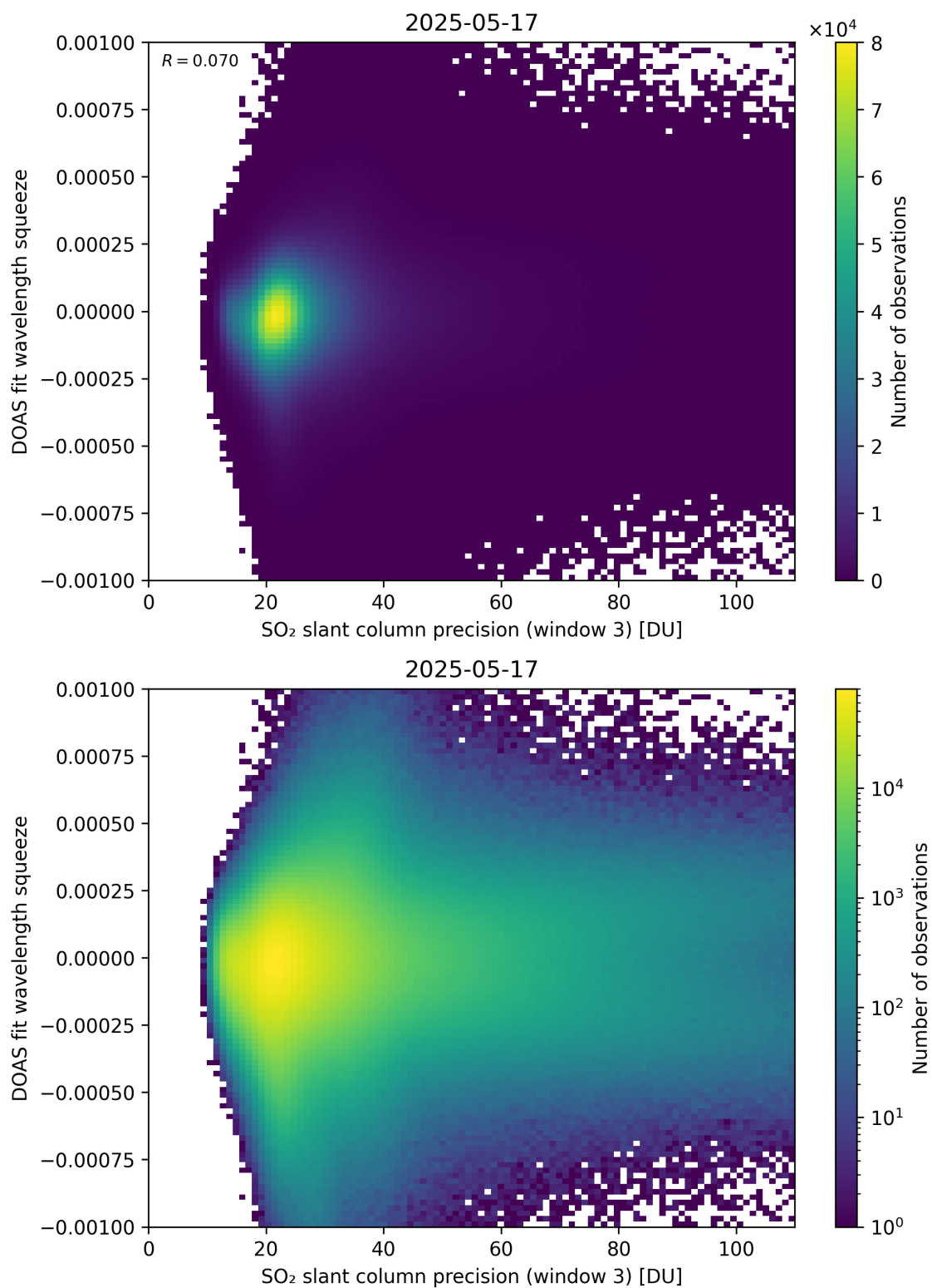
Figure 309: Scatter density plot of “SO 2 slant column precision (window 3)” against “DOAS fit wavelength squeeze” for 2025-05-16 to 2025-05-18.
