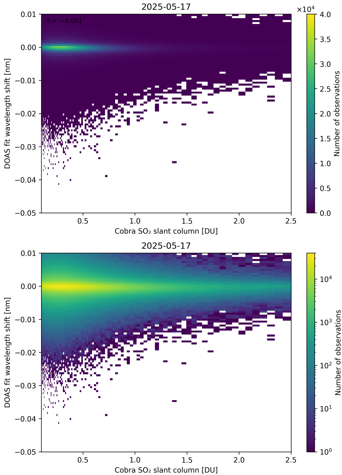
Figure 196: Scatter density plot of “Cobra SO 2 slant column” against “DOAS fit wavelength shift” for 2025-05-16 to 2025-05-18.
