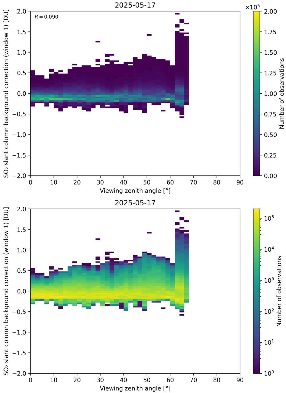
Figure 362: Scatter density plot of “Viewing zenith angle” against “SO 2 slant column background correction (window 1)” for 2025-05-16 to 2025-05-18.
