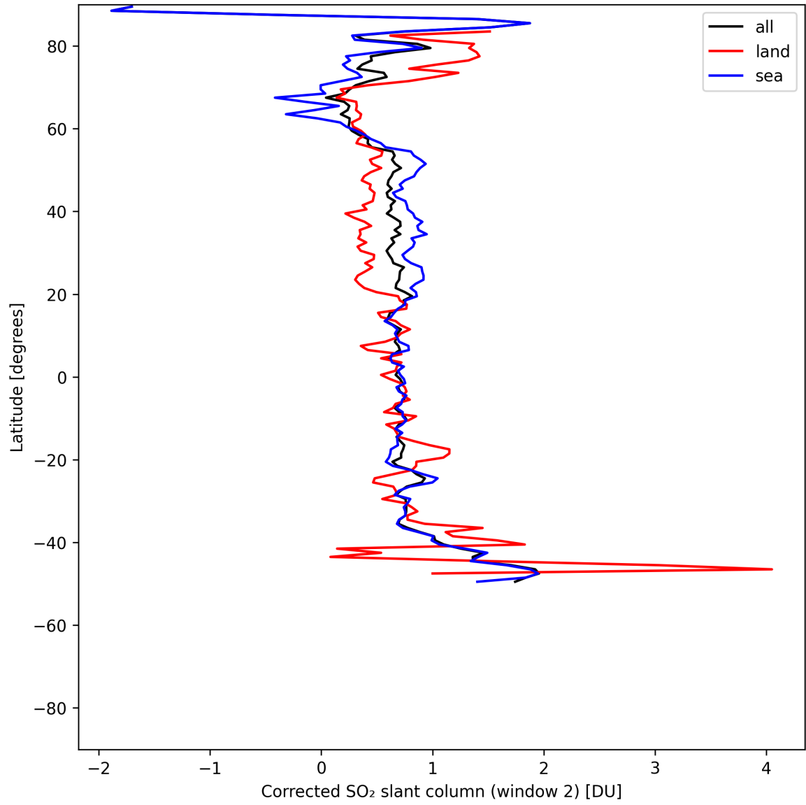
Figure 43: Zonal average of “Corrected SO 2 slant column (window 2)” for 2025-05-16 to 2025-05-18.
