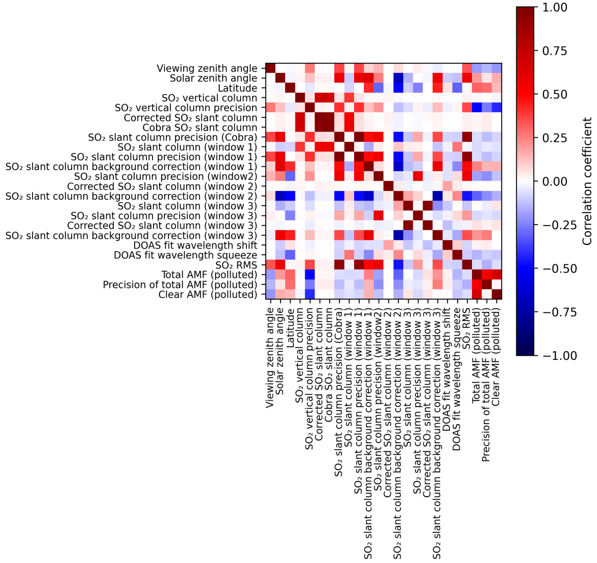
Figure 2: Map of correlation matrix for 2025-05-16 to 2025-05-18.
