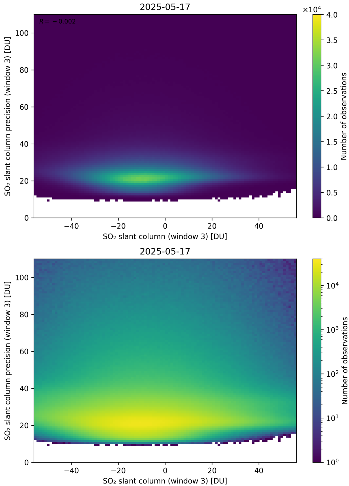
Figure 317: Scatter density plot of “SO 2 slant column (window 3)” against “SO 2 slant column precision (window 3)” for 2025-05-16 to 2025-05-18.
