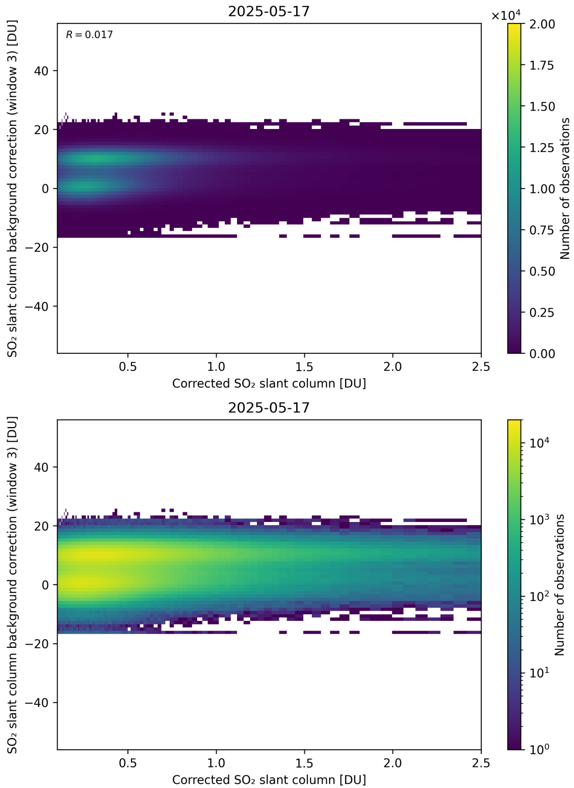
Figure 228: Scatter density plot of “Corrected SO 2 slant column” against “SO 2 slant column background correction (window 3)” for 2025-05-16 to 2025-05-18.
