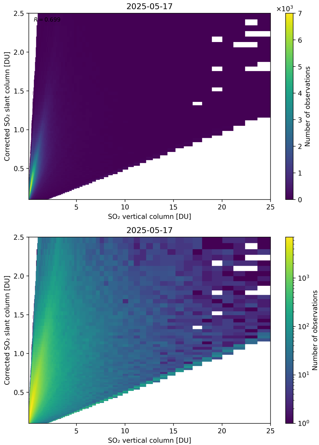
Figure 351: Scatter density plot of “SO 2 vertical column” against “Corrected SO 2 slant column” for 2025-05-16 to 2025-05-18.
