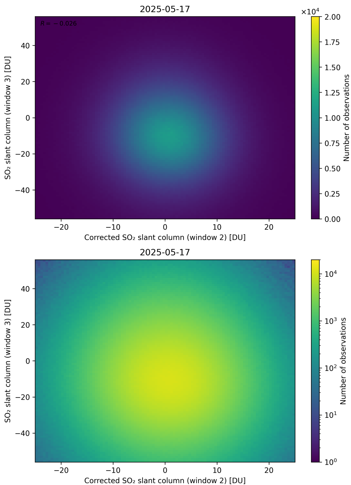
Figure 251: Scatter density plot of “Corrected SO 2 slant column (window 2)” against “SO 2 slant column (window 3)” for 2025-05-16 to 2025-05-18.
