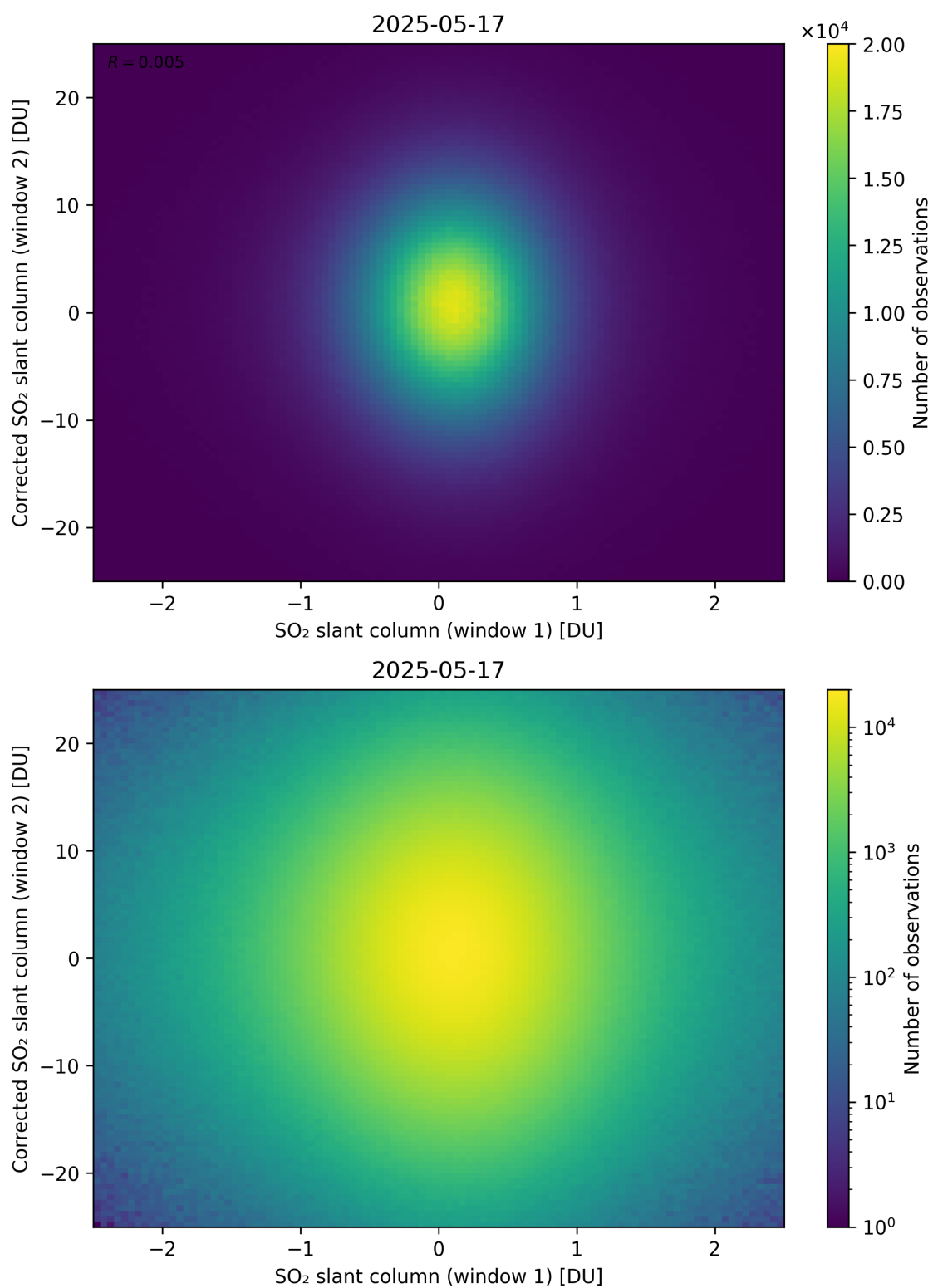
Figure 283: Scatter density plot of “SO 2 slant column (window 1)” against “Corrected SO 2 slant column (window 2)” for 2025-05-16 to 2025-05-18.
