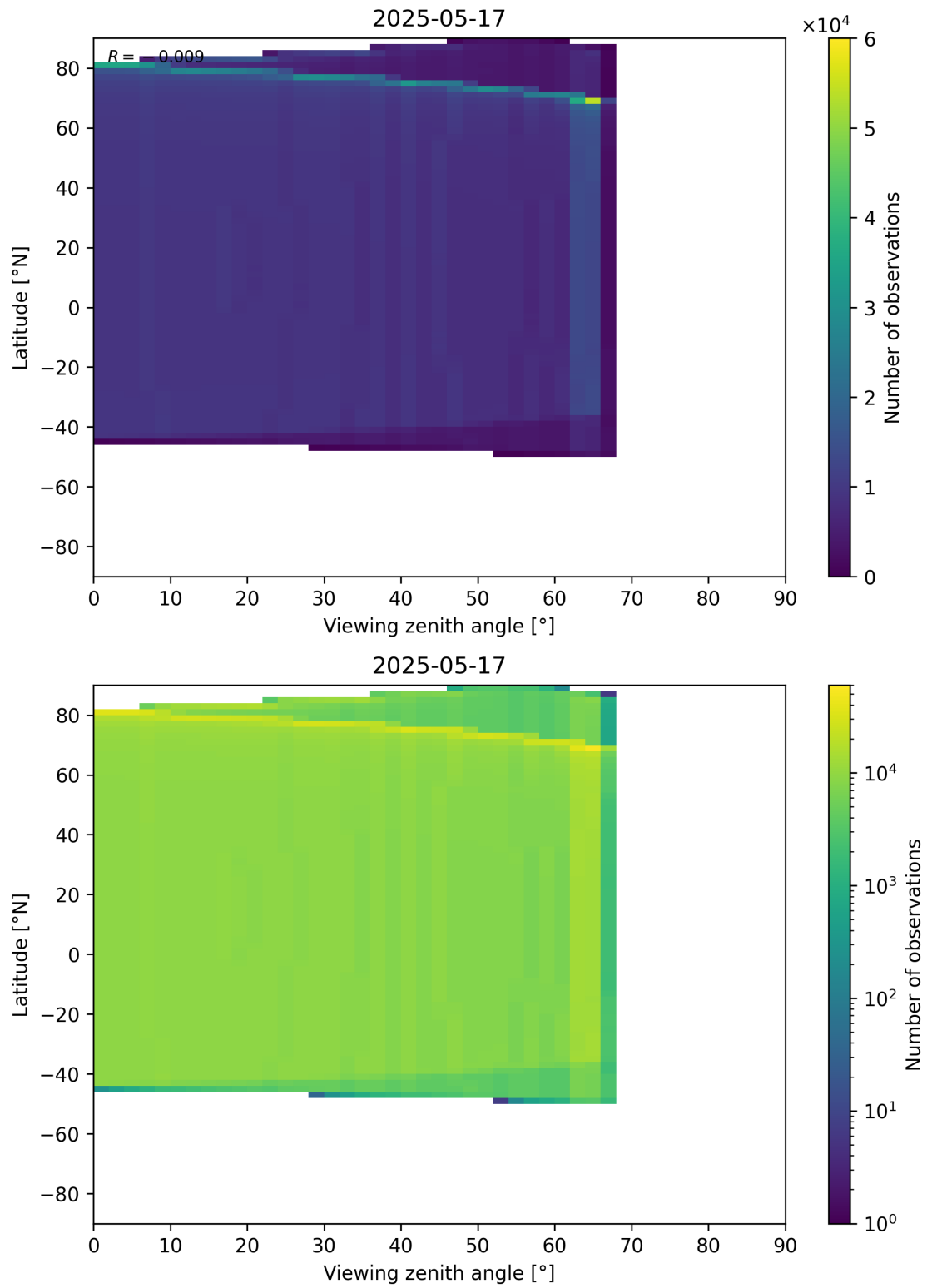
Figure 368: Scatter density plot of “Viewing zenith angle” against “Latitude” for 2025-05-16 to 2025-05-18.
