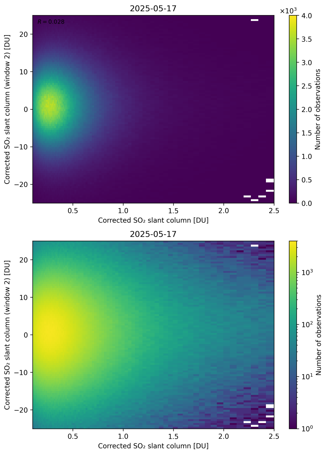
Figure 235: Scatter density plot of “Corrected SO 2 slant column” against “Corrected SO 2 slant column (window 2)” for 2025-05-16 to 2025-05-18.
