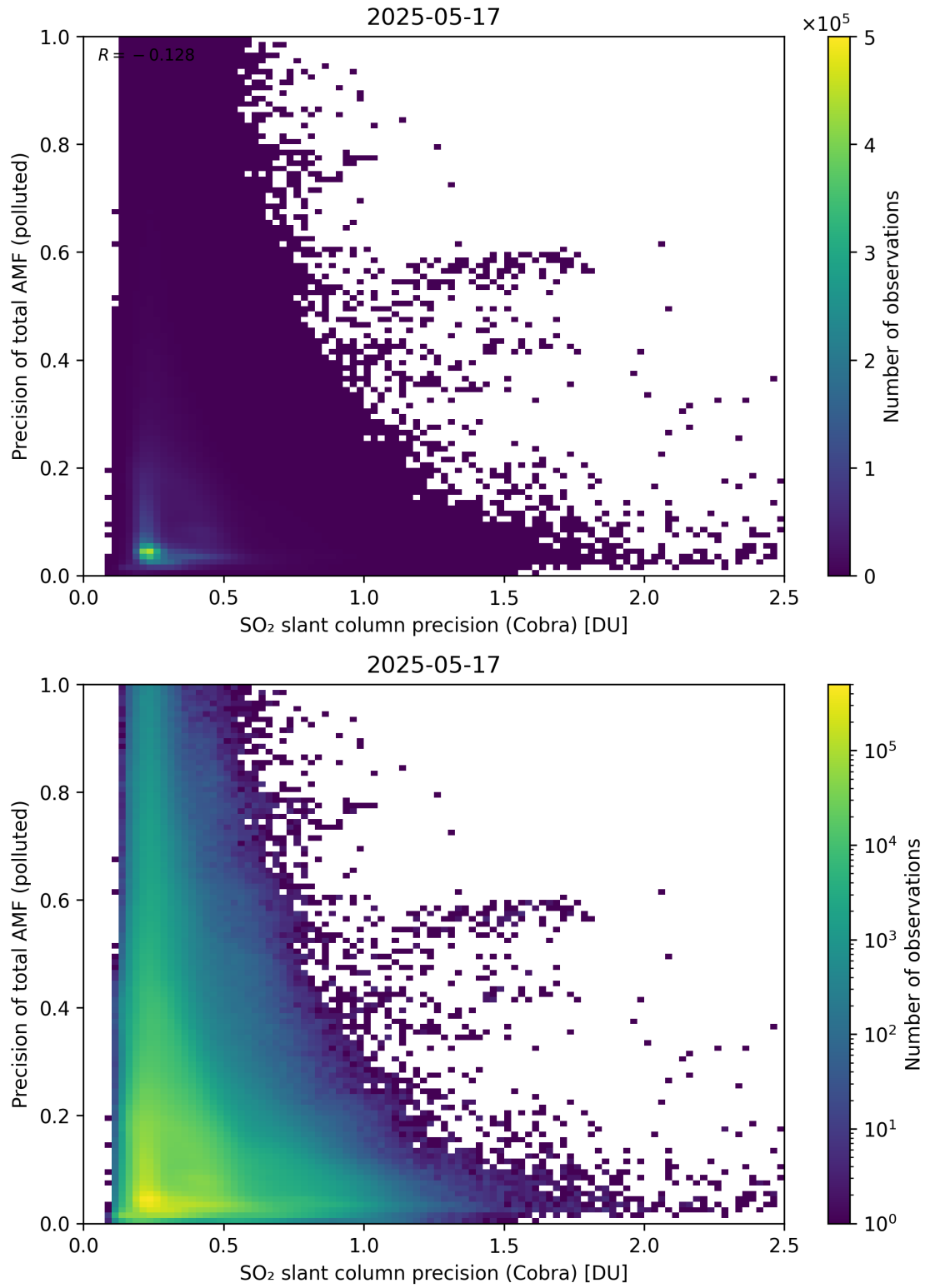
Figure 214: Scatter density plot of “SO 2 slant column precision (Cobra)” against “Precision of total AMF (polluted)” for 2025-05-16 to 2025-05-18.
