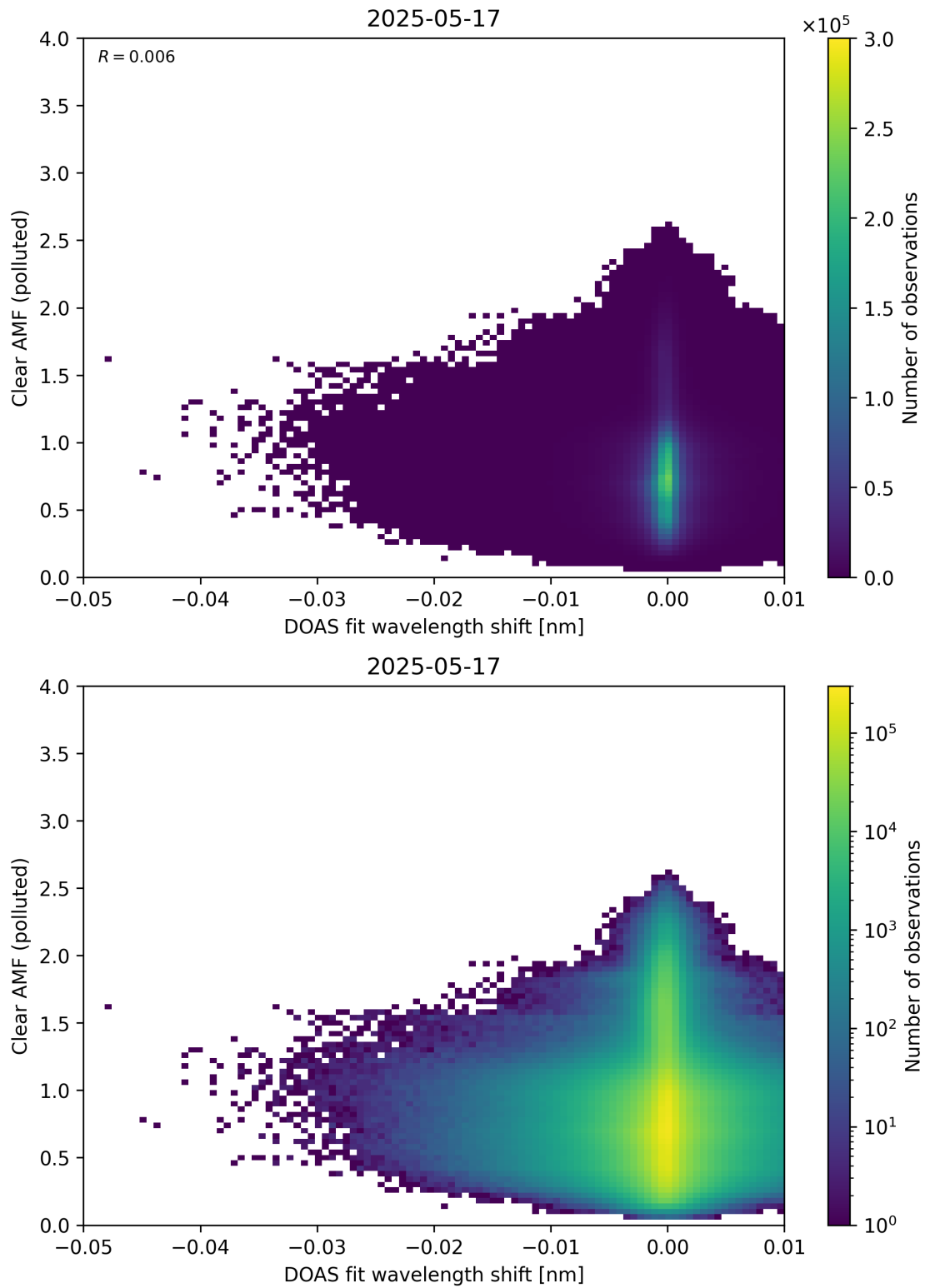
Figure 140: Scatter density plot of “DOAS fit wavelength shift” against “Clear AMF (polluted)” for 2025-05-16 to 2025-05-18.
