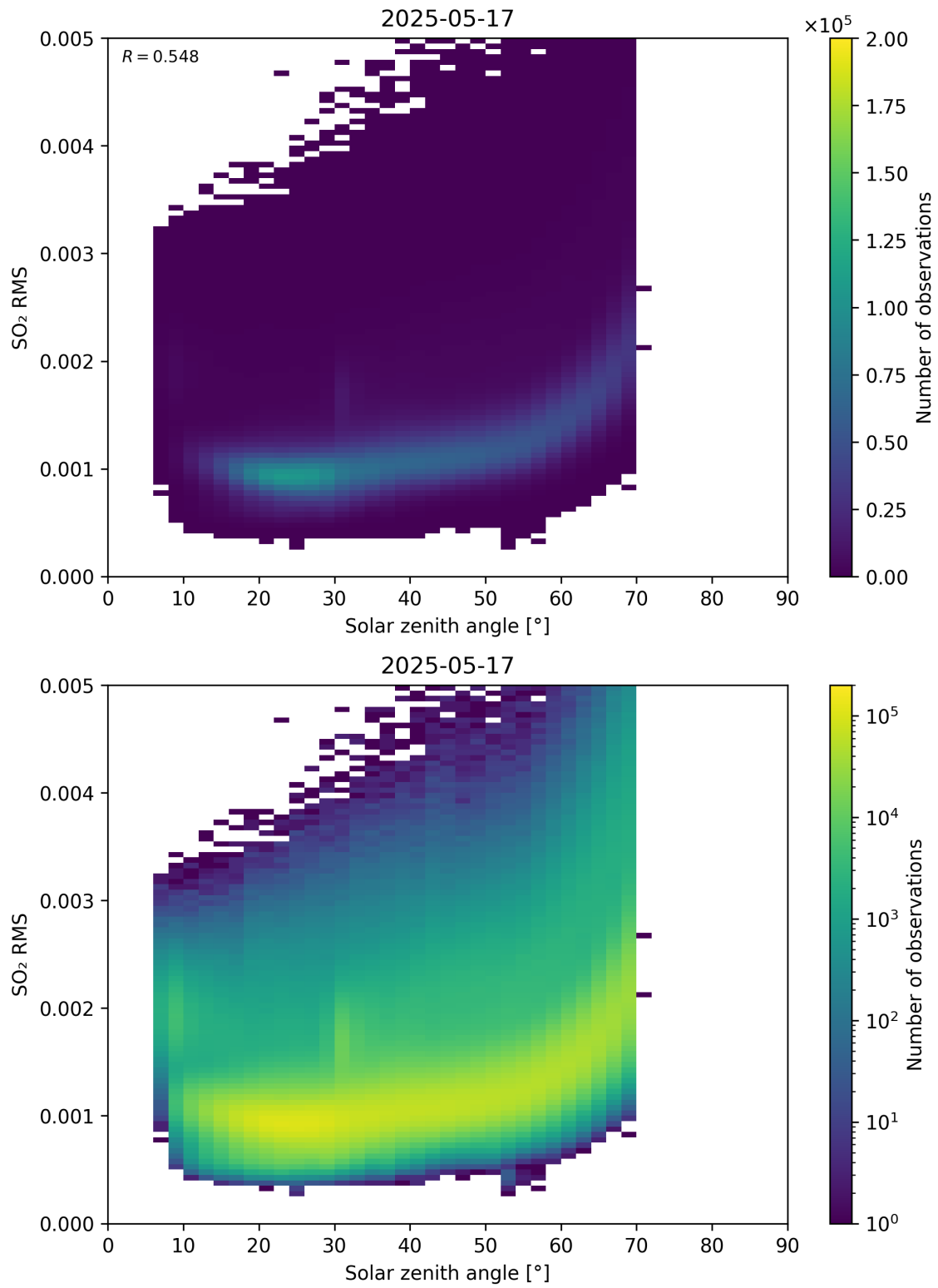
Figure 176: Scatter density plot of “Solar zenith angle” against “SO 2 RMS” for 2025-05-16 to 2025-05-18.
