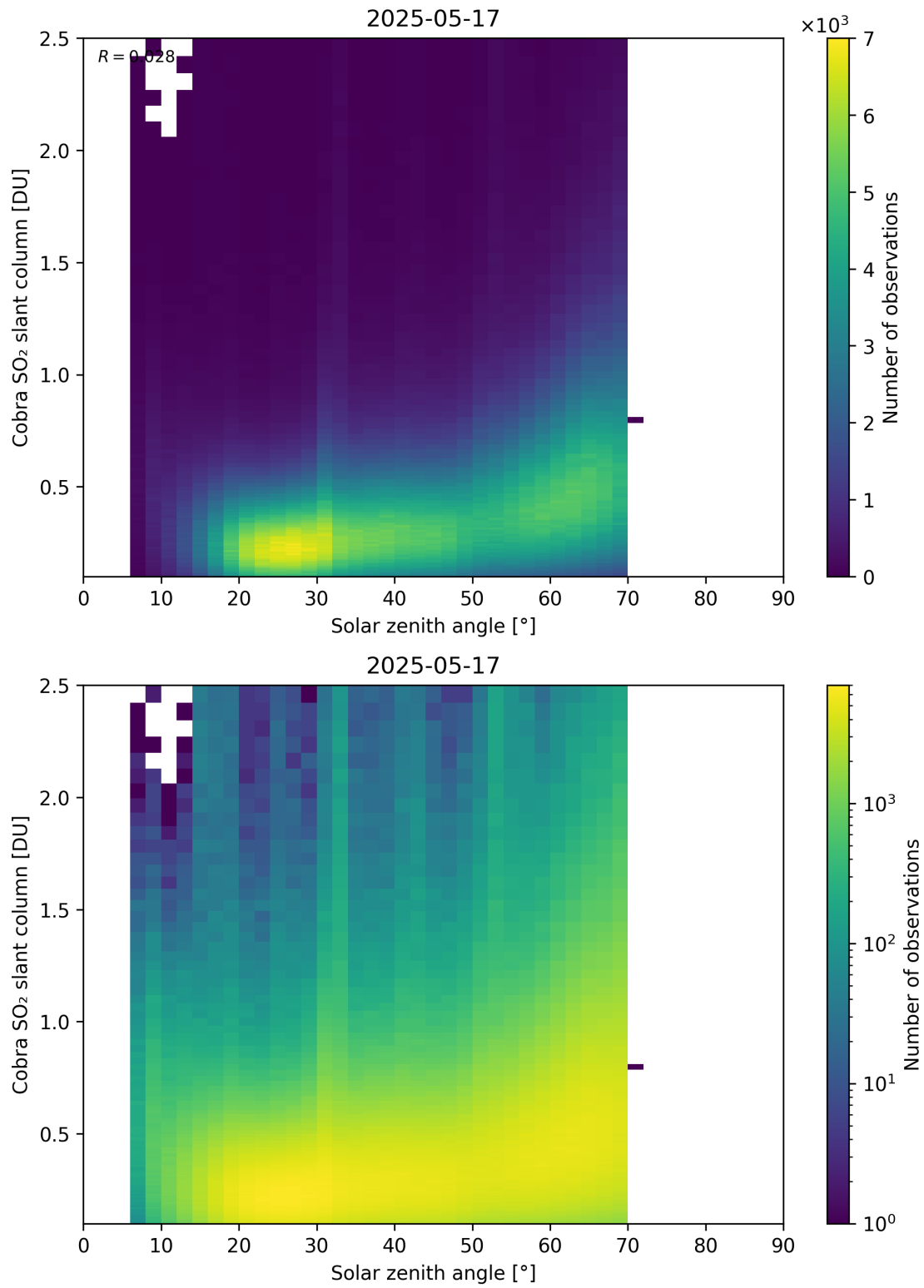
Figure 179: Scatter density plot of “Solar zenith angle” against “Cobra SO 2 slant column” for 2025-05-16 to 2025-05-18.
