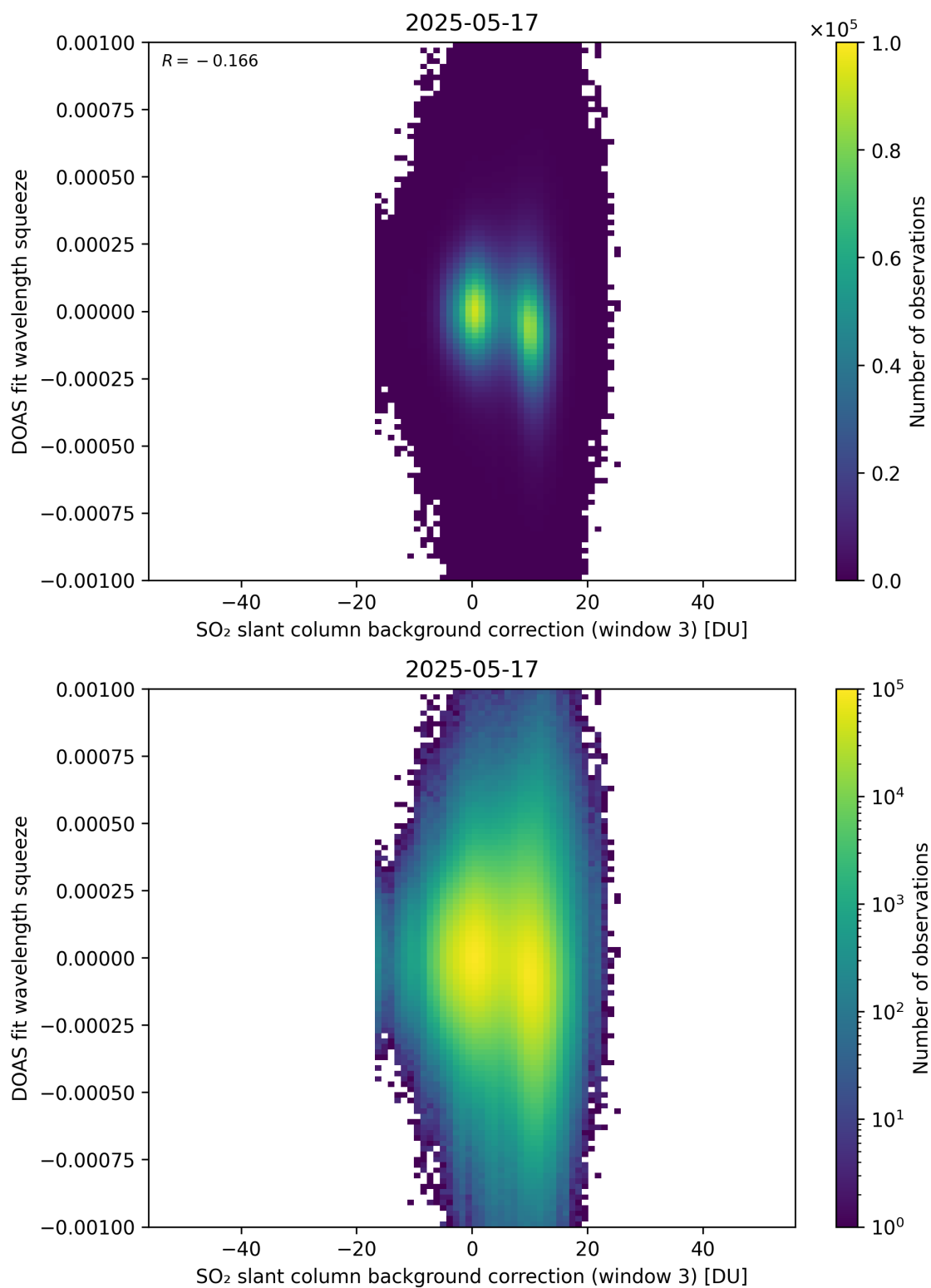
Figure 133: Scatter density plot of “SO 2 slant column background correction (window 3)” against “DOAS fit wavelength squeeze” for 2025-05-16 to 2025-05-18.
