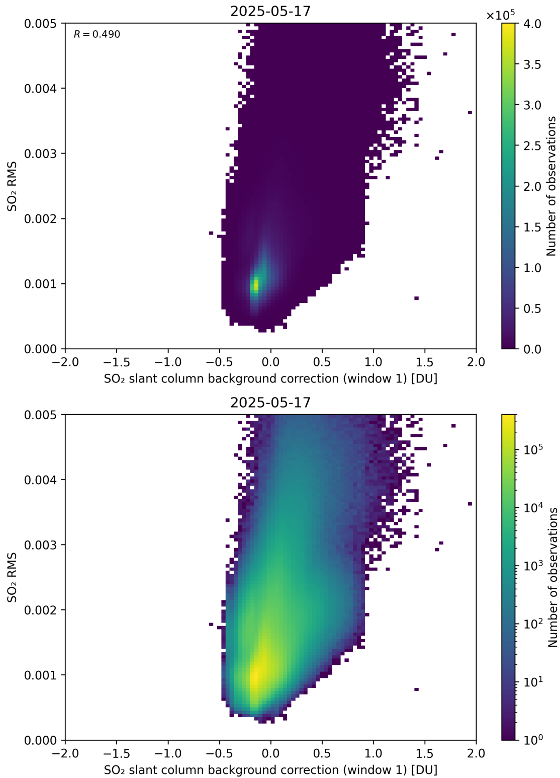
Figure 113: Scatter density plot of “SO 2 slant column background correction (window 1)” against “SO 2 RMS” for 2025-05-16 to 2025-05-18.
