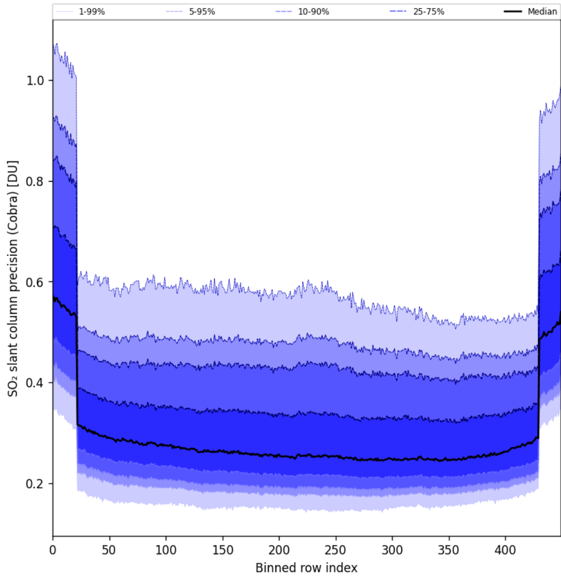
Figure 88: Along track statistics of “SO 2 slant column precision (Cobra)” for 2025-05-16 to 2025-05-18
