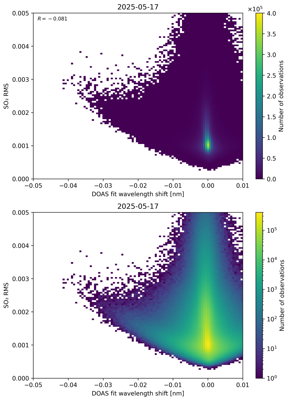
Figure 139: Scatter density plot of “DOAS fit wavelength shift” against “SO 2 RMS” for 2025-05-16 to 2025-05-18.
