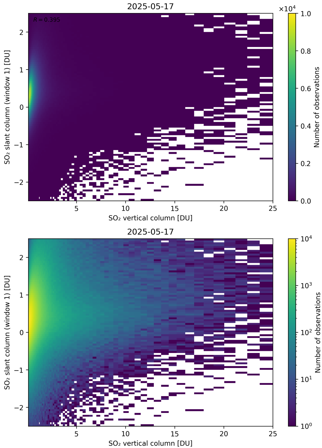
Figure 354: Scatter density plot of “SO 2 vertical column” against “SO 2 slant column (window 1)” for 2025-05-16 to 2025-05-18.
