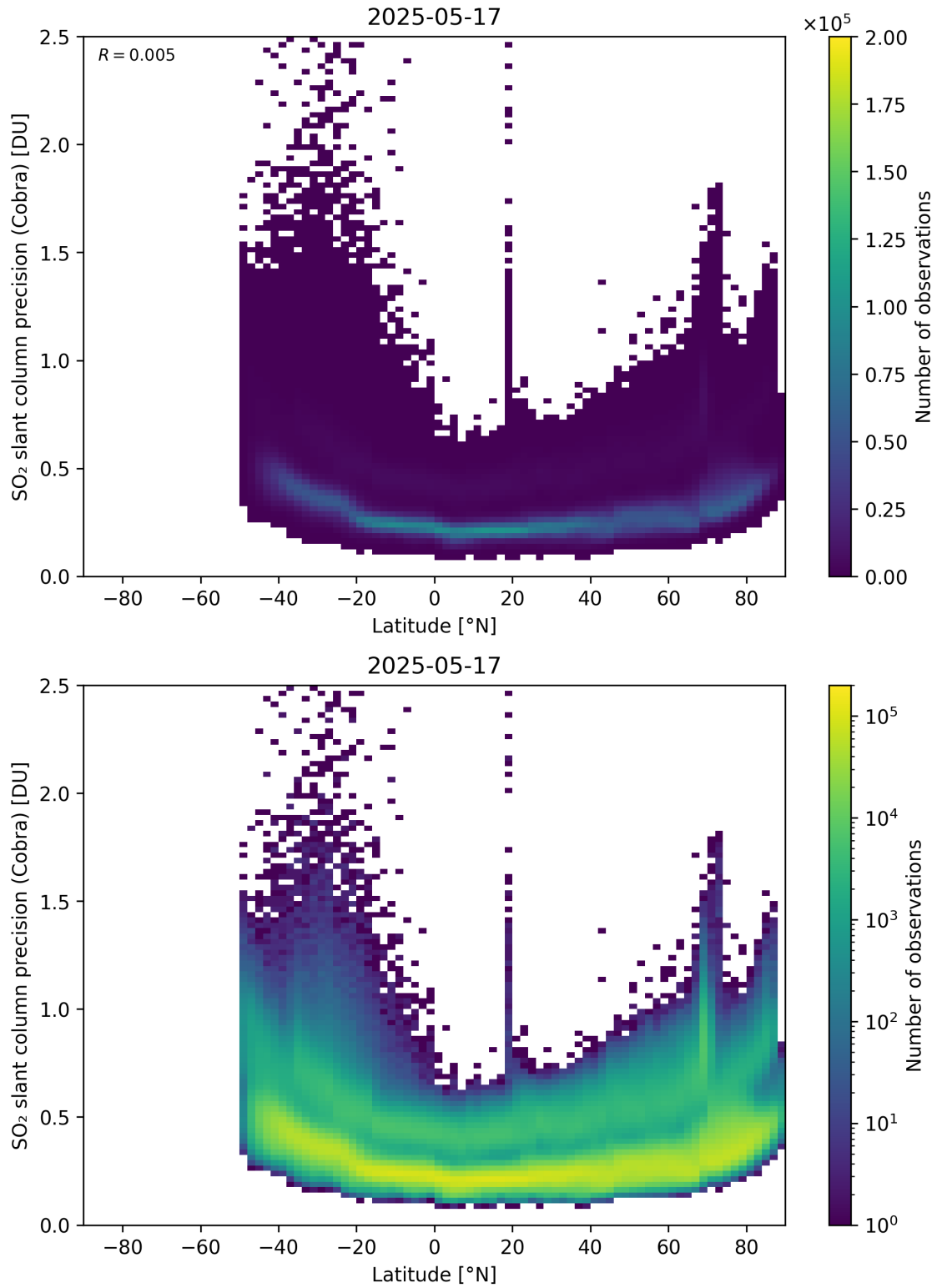
Figure 158: Scatter density plot of “Latitude” against “SO 2 slant column precision (Cobra)” for 2025-05-16 to 2025-05-18.
