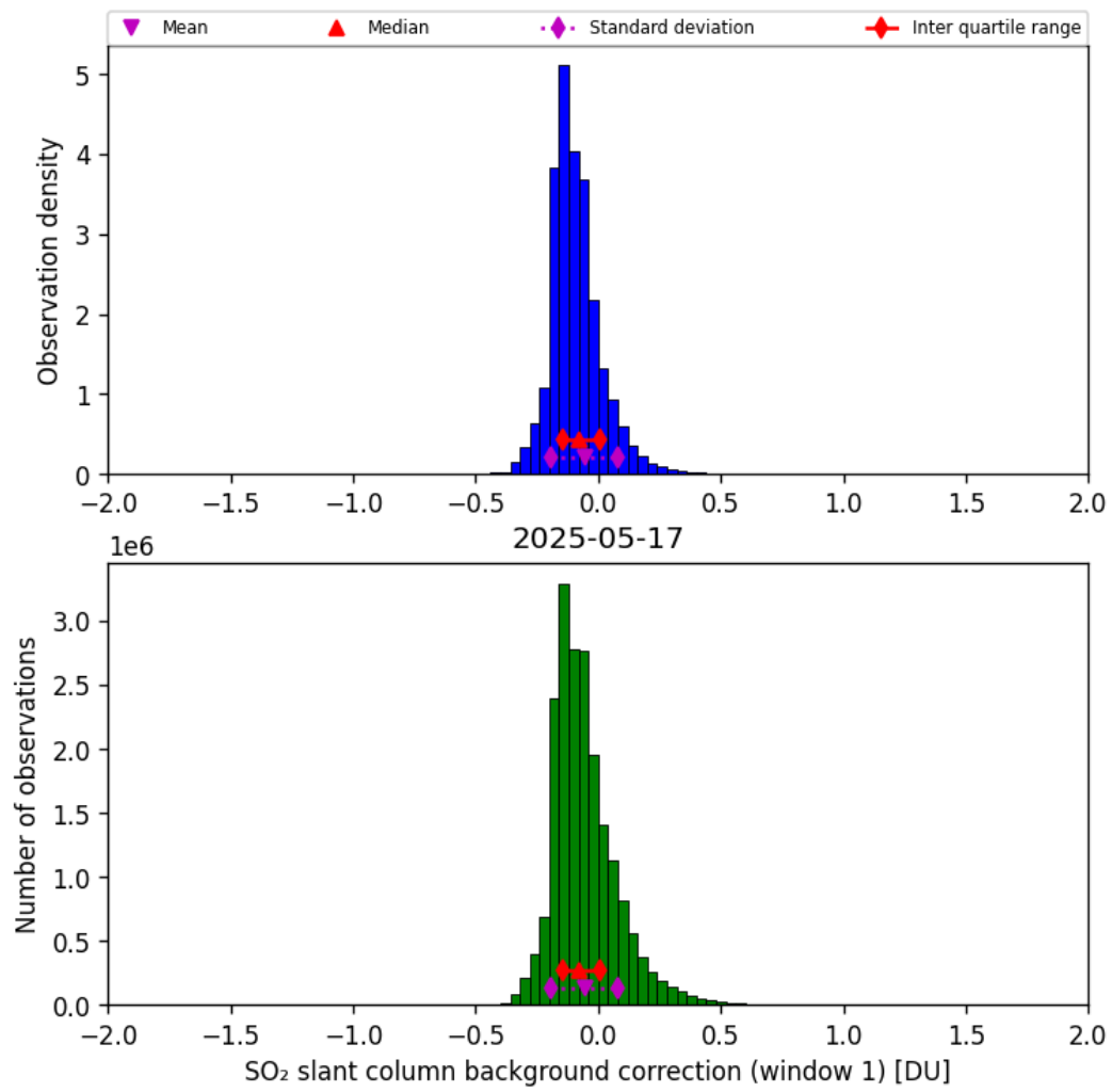
Figure 66: Histogram of “SO 2 slant column background correction (window 1)” for 2025-05-16 to 2025-05-18
