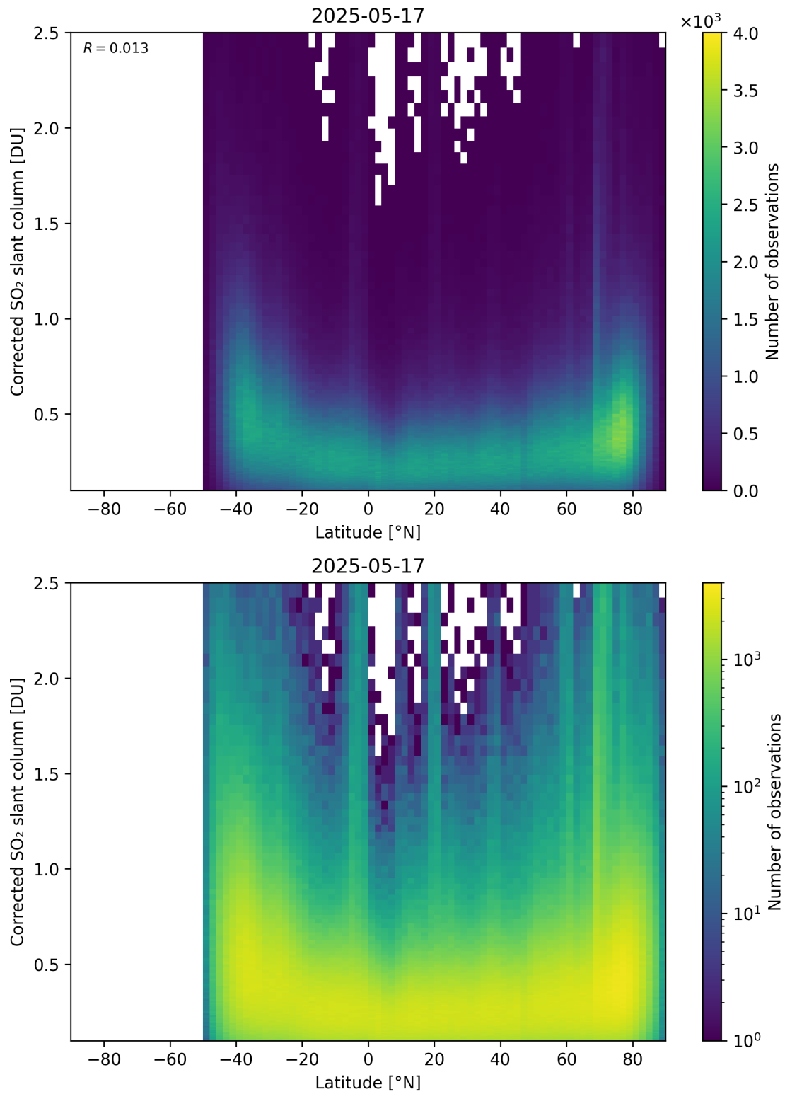
Figure 159: Scatter density plot of “Latitude” against “Corrected SO 2 slant column” for 2025-05-16 to 2025-05-18.
