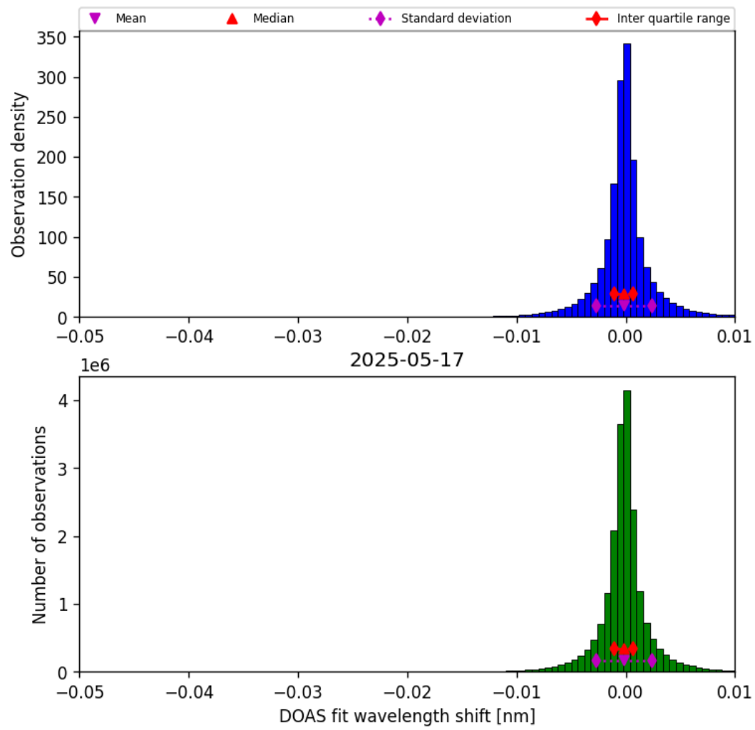
Figure 76: Histogram of “DOAS fit wavelength shift” for 2025-05-16 to 2025-05-18
