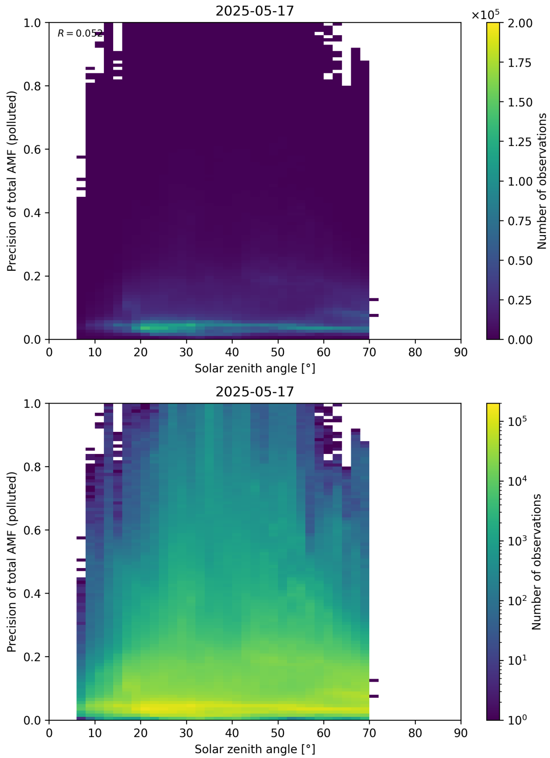
Figure 190: Scatter density plot of “Solar zenith angle” against “Precision of total AMF (polluted)” for 2025-05-16 to 2025-05-18.
