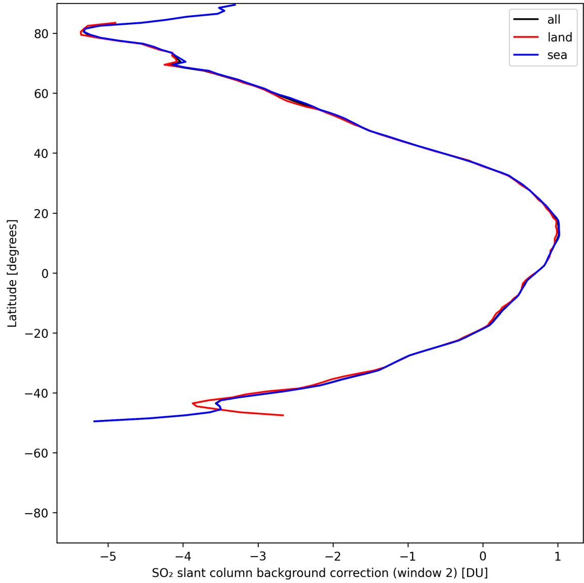
Figure 44: Zonal average of “SO 2 slant column background correction (window 2)” for 2025-05-16 to 2025-05-18.
