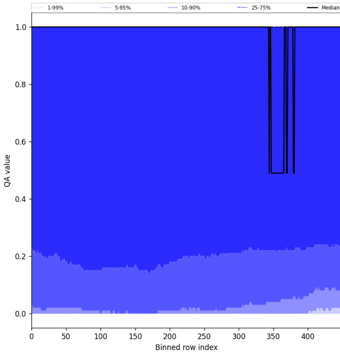
Figure 83: Along track statistics of “QA value” for 2025-05-16 to 2025-05-18
