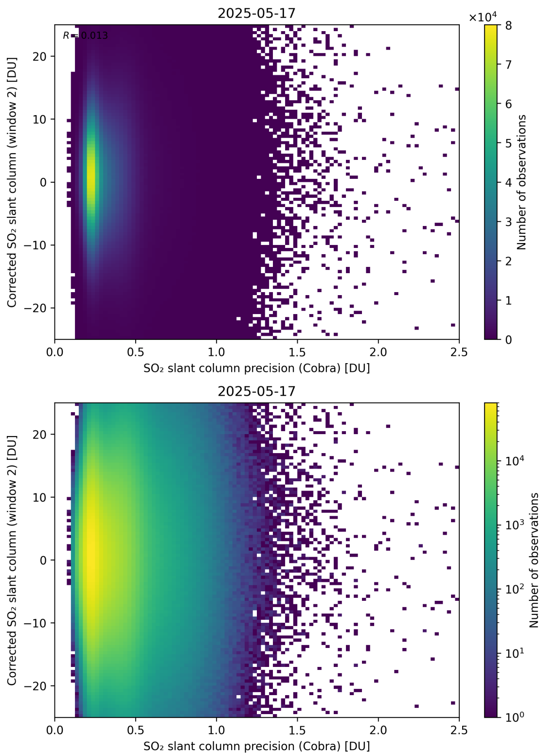
Figure 206: Scatter density plot of “SO 2 slant column precision (Cobra)” against “Corrected SO 2 slant column (window 2)” for 2025-05-16 to 2025-05-18.
