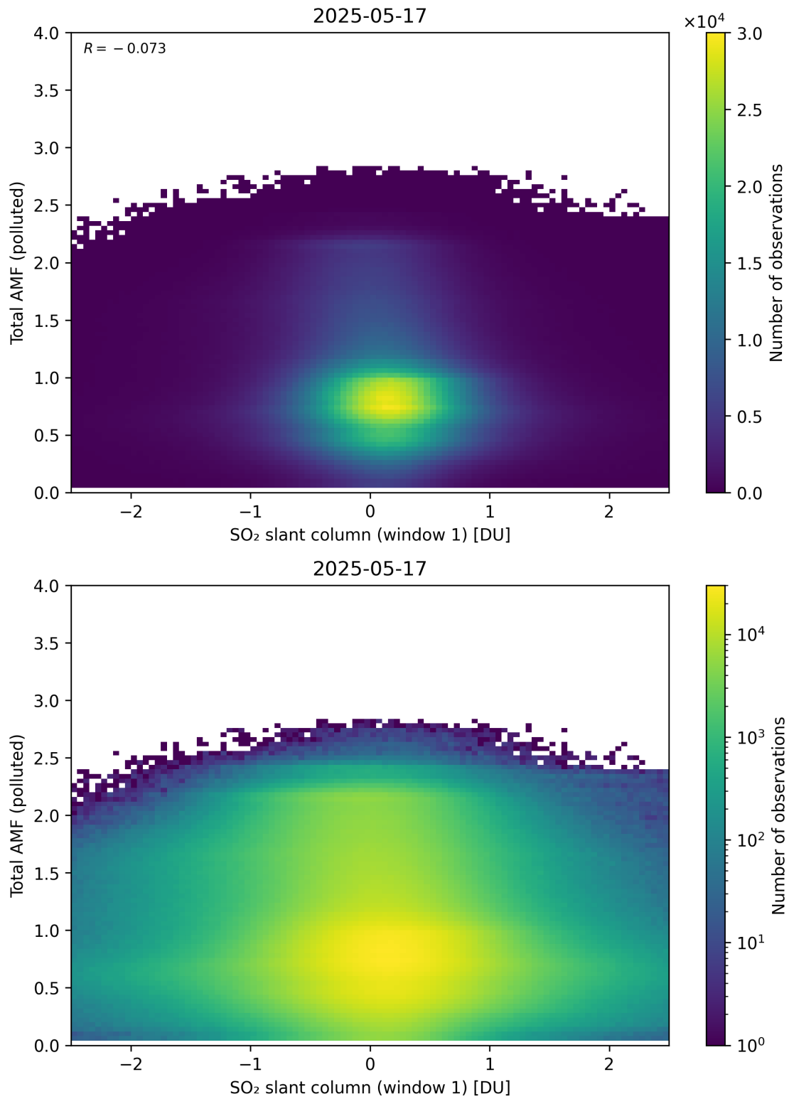
Figure 289: Scatter density plot of “SO 2 slant column (window 1)” against “Total AMF (polluted)” for 2025-05-16 to 2025-05-18.
