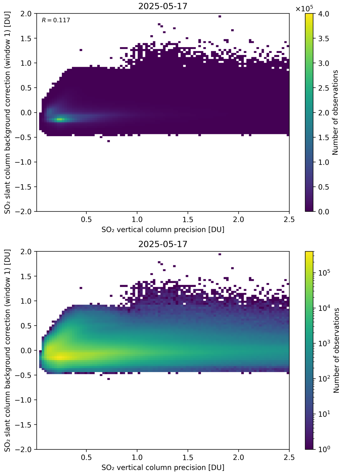
Figure 329: Scatter density plot of “SO 2 vertical column precision” against “SO 2 slant column background correction (window 1)” for 2025-05-16 to 2025-05-18.
