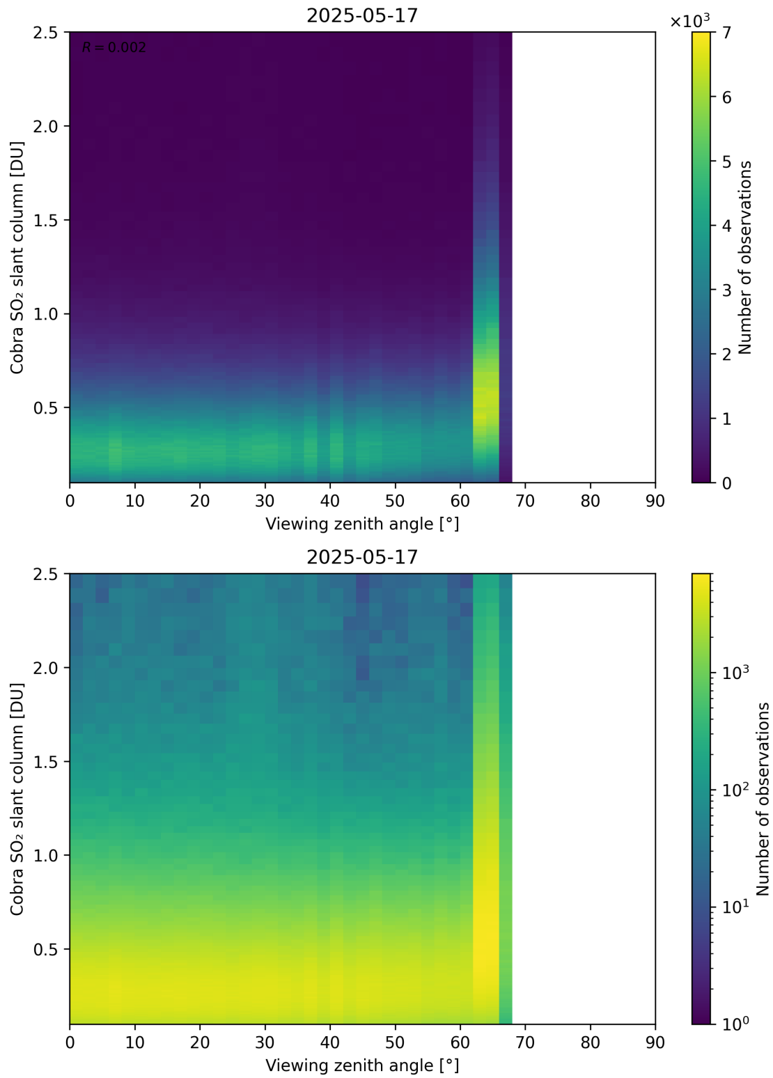
Figure 371: Scatter density plot of “Viewing zenith angle” against “Cobra SO 2 slant column” for 2025-05-16 to 2025-05-18.
