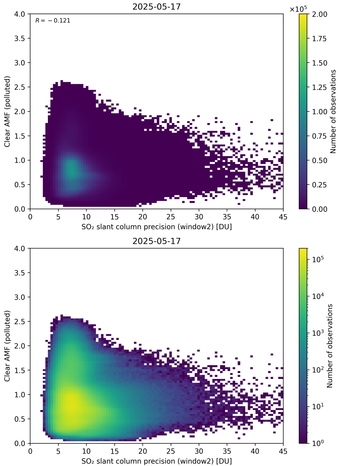
Figure 296: Scatter density plot of “SO 2 slant column precision (window2)” against “Clear AMF (polluted)” for 2025-05-16 to 2025-05-18.
