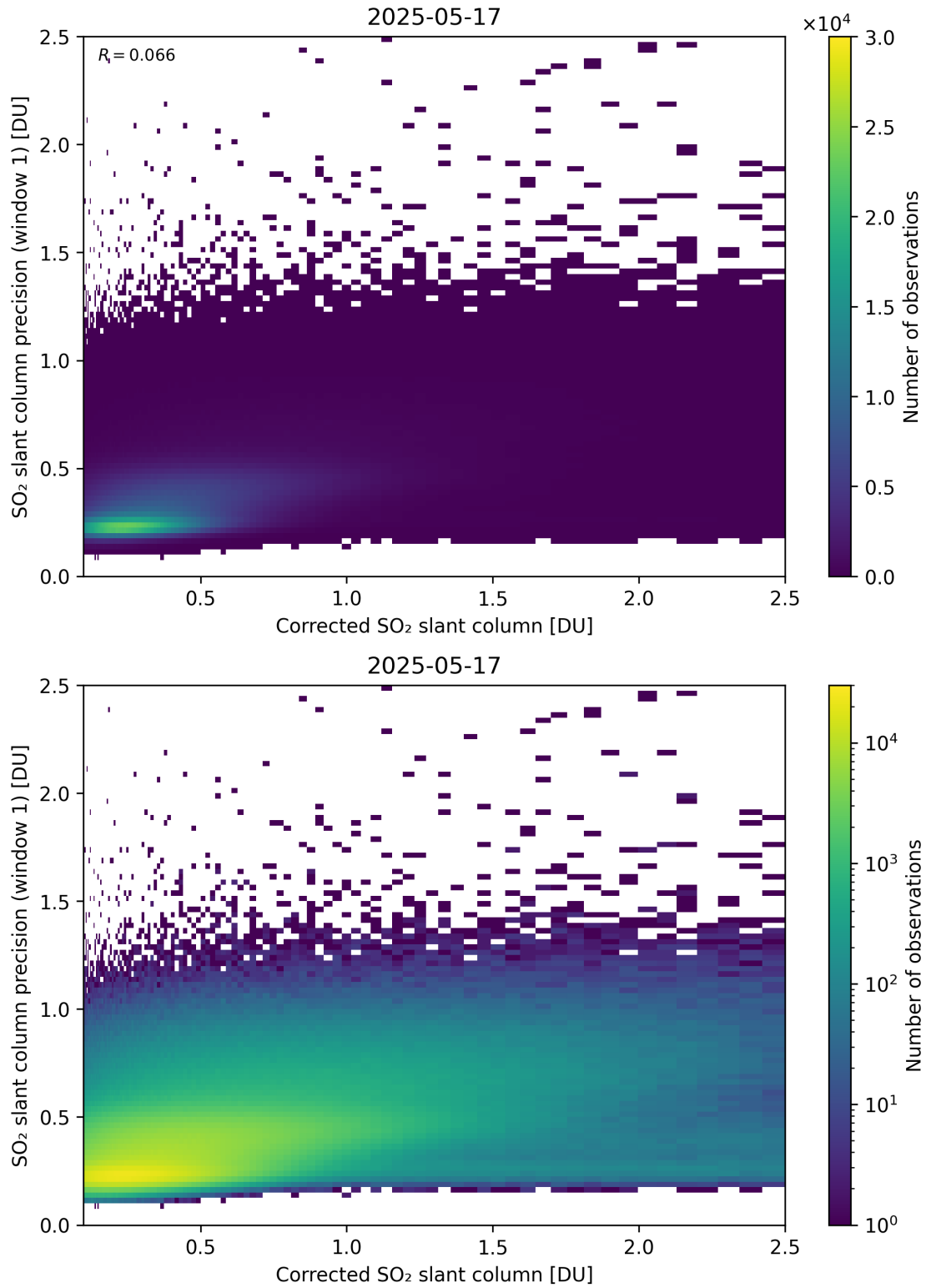
Figure 238: Scatter density plot of “Corrected SO 2 slant column” against “SO 2 slant column precision (window 1)” for 2025-05-16 to 2025-05-18.
