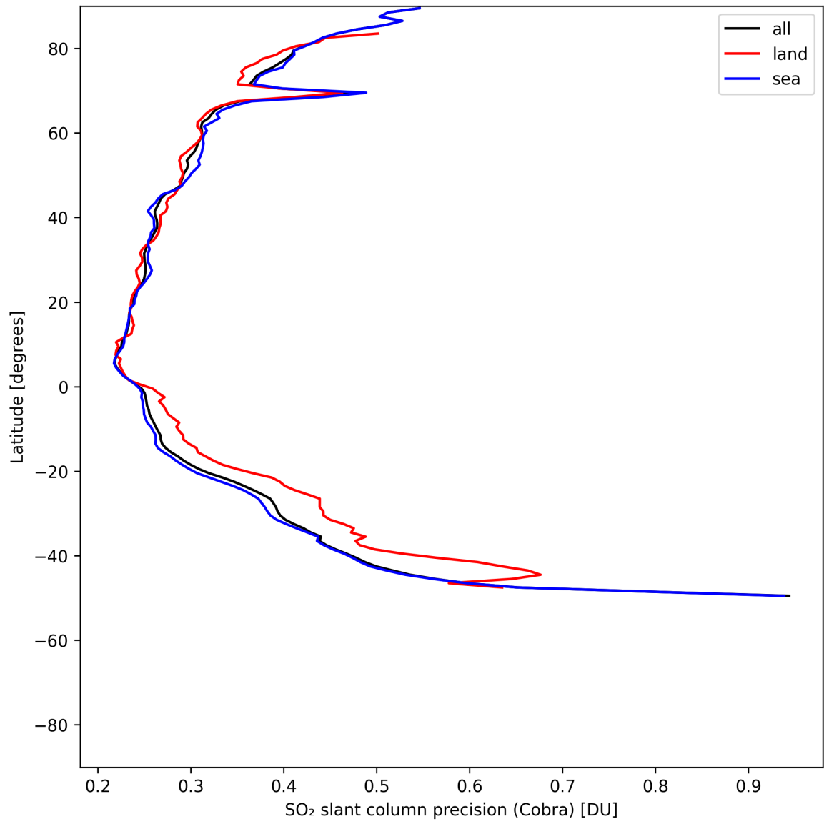
Figure 36: Zonal average of “SO 2 slant column precision (Cobra)” for 2025-05-16 to 2025-05-18.
