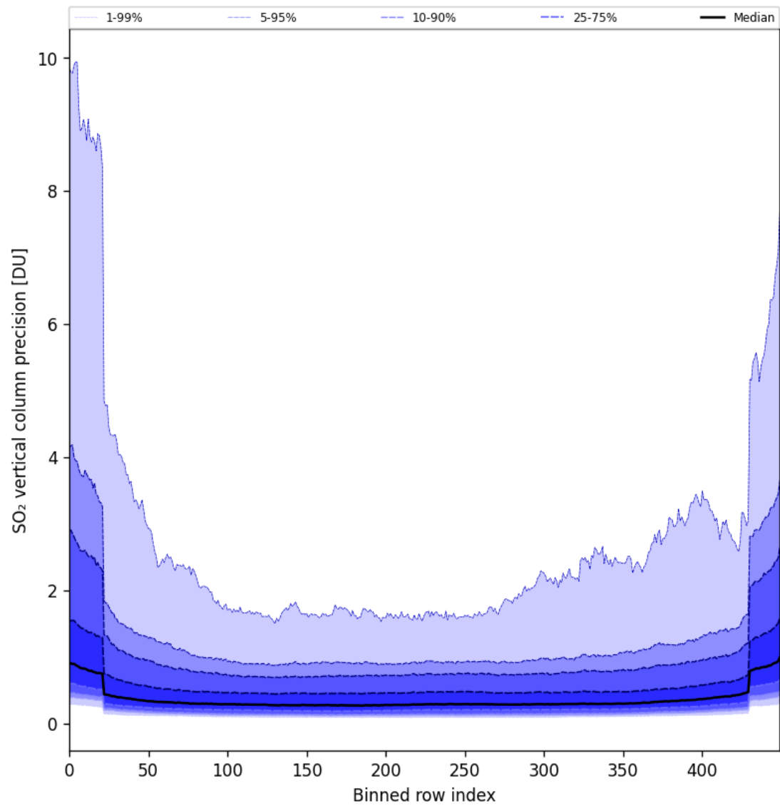
Figure 85: Along track statistics of “SO 2 vertical column precision” for 2025-05-16 to 2025-05-18
