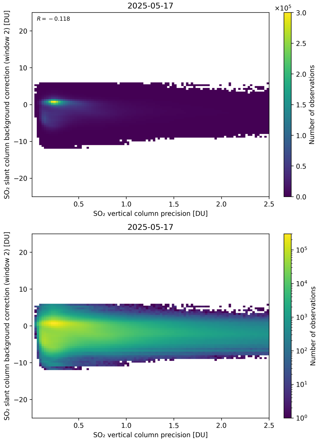
Figure 330: Scatter density plot of “SO 2 vertical column precision” against “SO 2 slant column background correction (window 2)” for 2025-05-16 to 2025-05-18.
