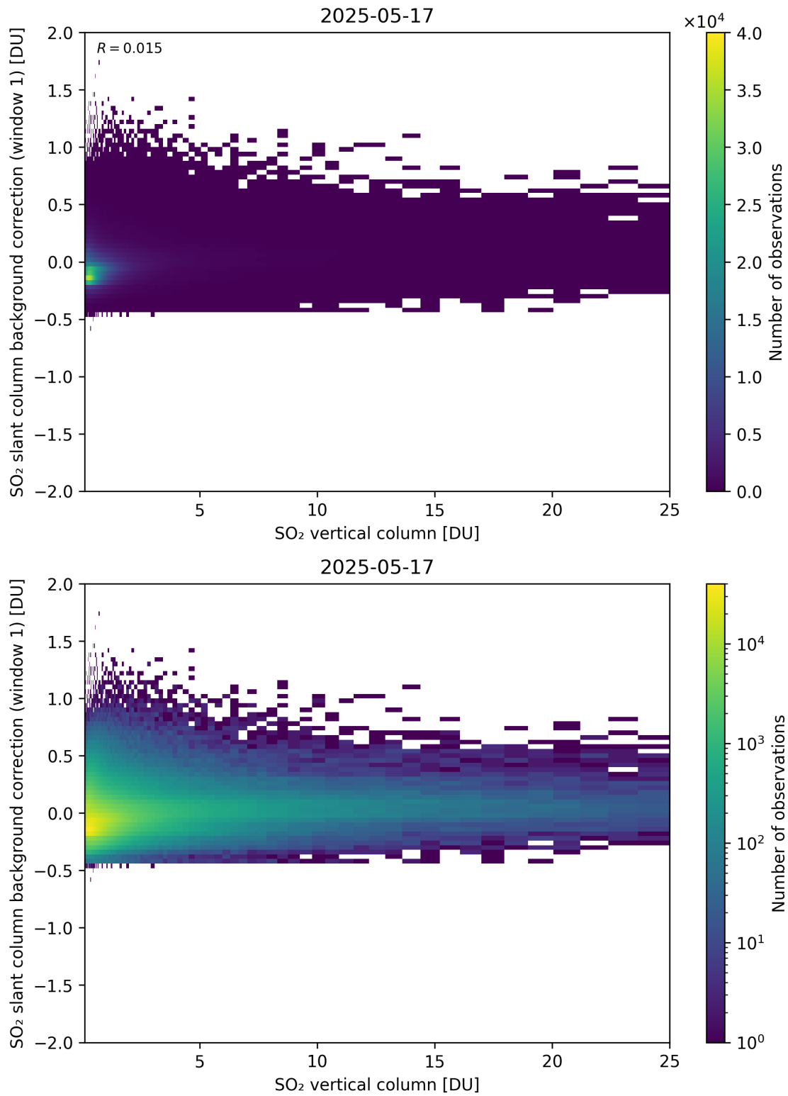
Figure 323: Scatter density plot of “SO 2 vertical column” against “SO 2 slant column background correction (window 1)” for 2025-05-16 to 2025-05-18.
