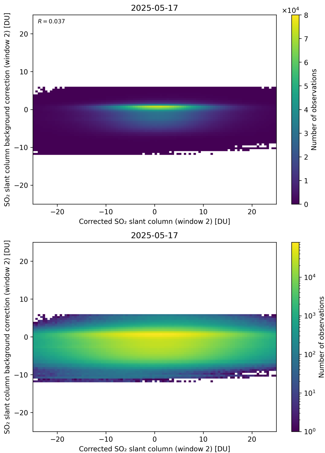
Figure 244: Scatter density plot of “Corrected SO 2 slant column (window 2)” against “SO 2 slant column background correction (window 2)” for 2025-05-16 to 2025-05-18.
