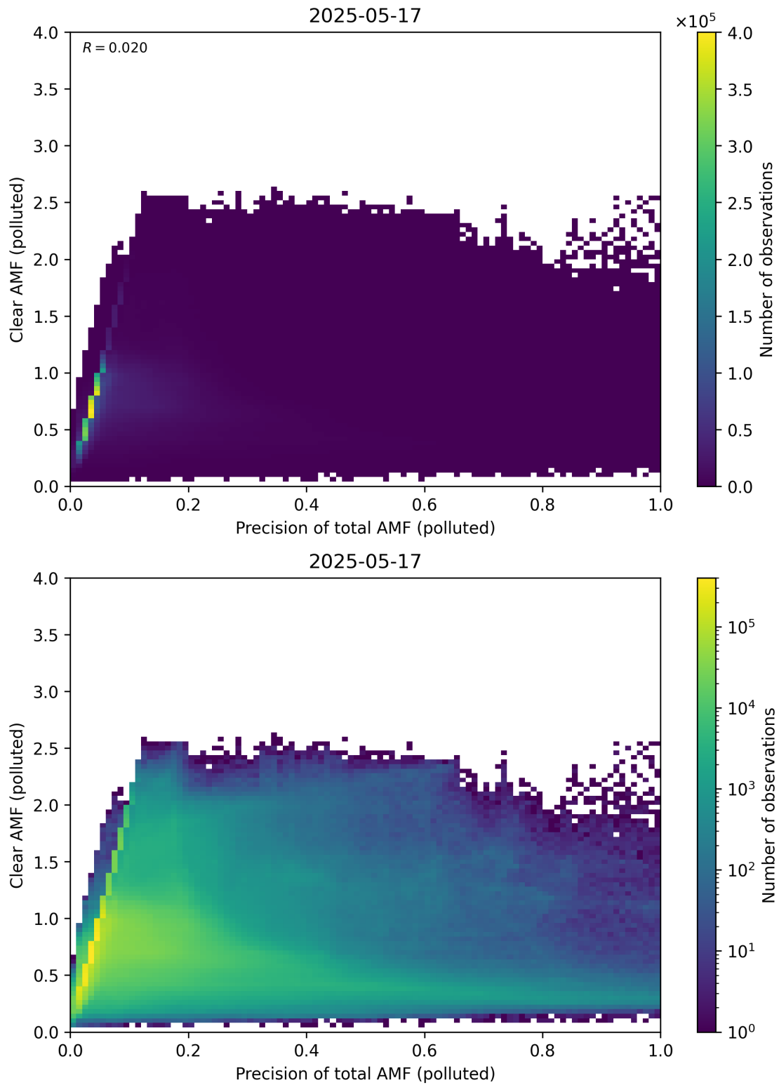
Figure 320: Scatter density plot of “Precision of total AMF (polluted)” against “Clear AMF (polluted)” for 2025-05-16 to 2025-05-18.
