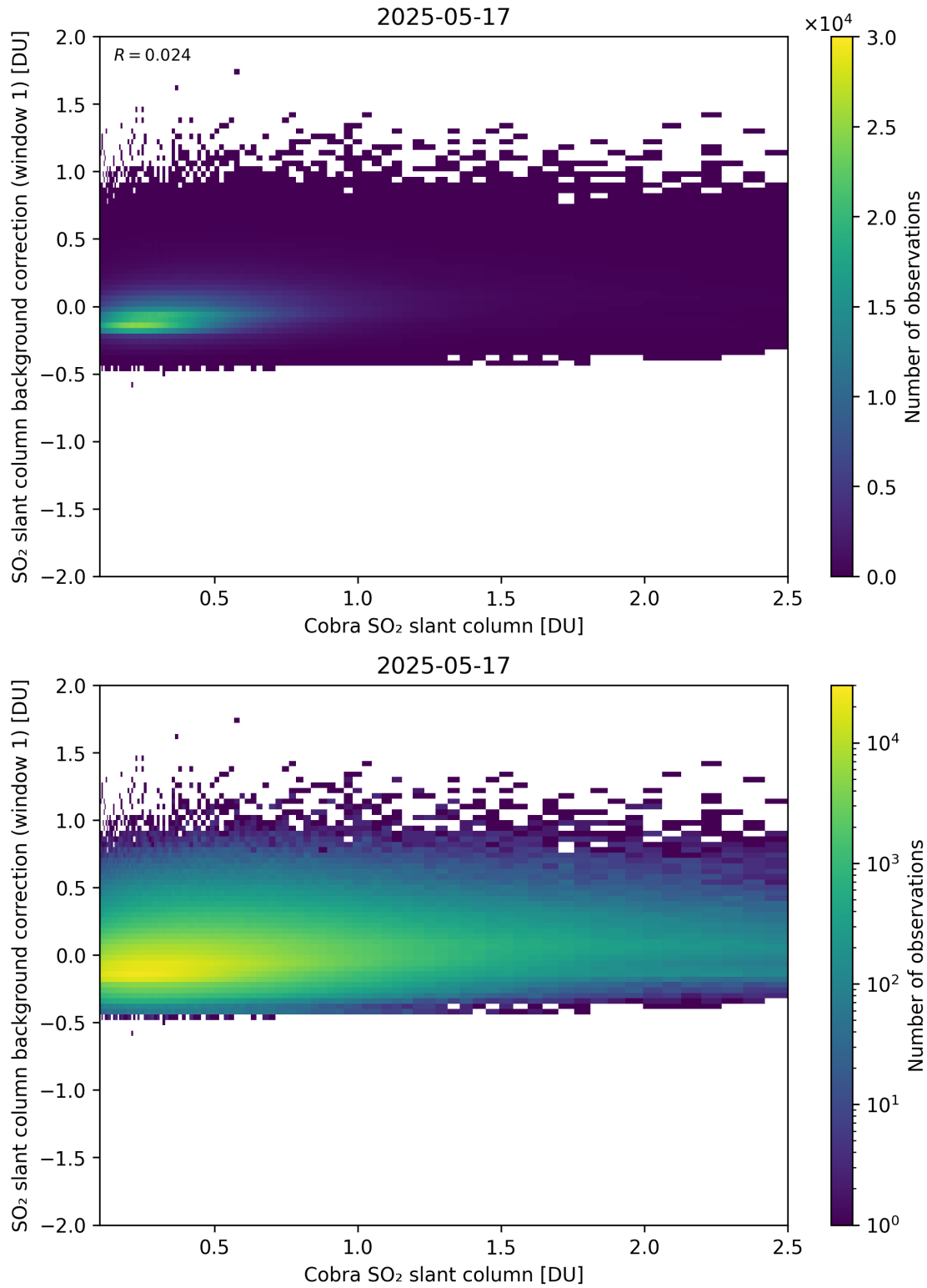
Figure 193: Scatter density plot of “Cobra SO 2 slant column” against “SO 2 slant column background correction (window 1)” for 2025-05-16 to 2025-05-18.
