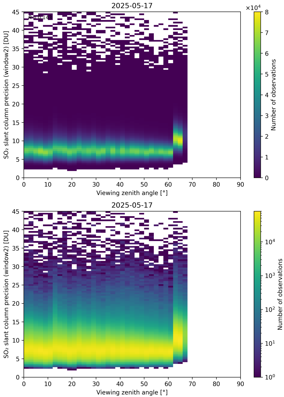
Figure 378: Scatter density plot of “Viewing zenith angle” against “SO 2 slant column precision (window2)” for 2025-05-16 to 2025-05-18.
