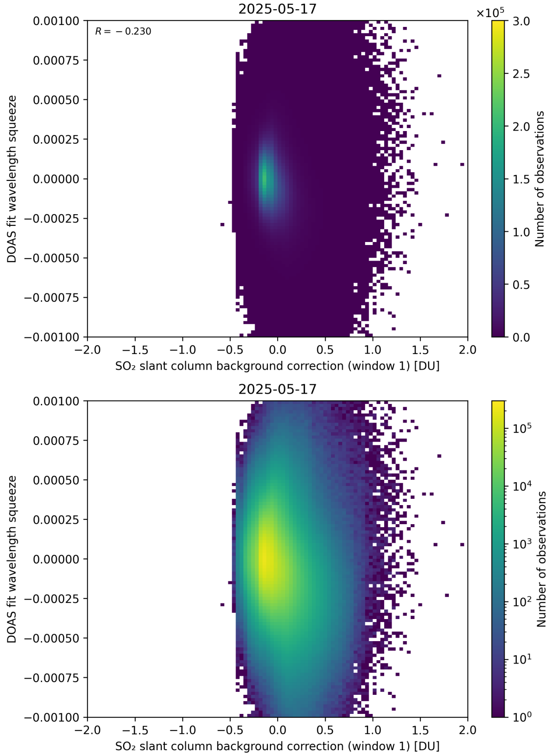
Figure 112: Scatter density plot of “SO 2 slant column background correction (window 1)” against “DOAS fit wavelength squeeze” for 2025-05-16 to 2025-05-18.
