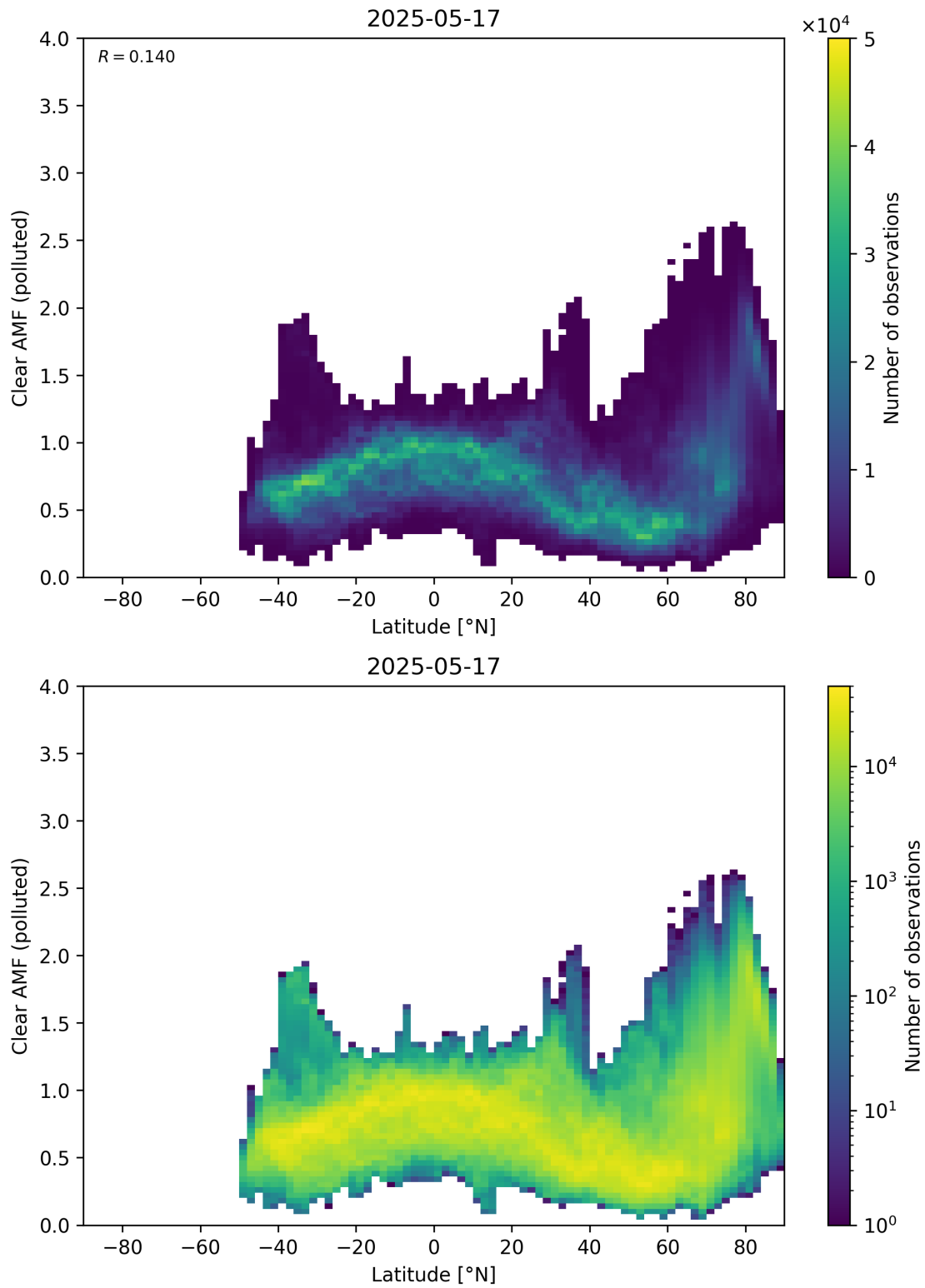
Figure 156: Scatter density plot of “Latitude” against “Clear AMF (polluted)” for 2025-05-16 to 2025-05-18.
