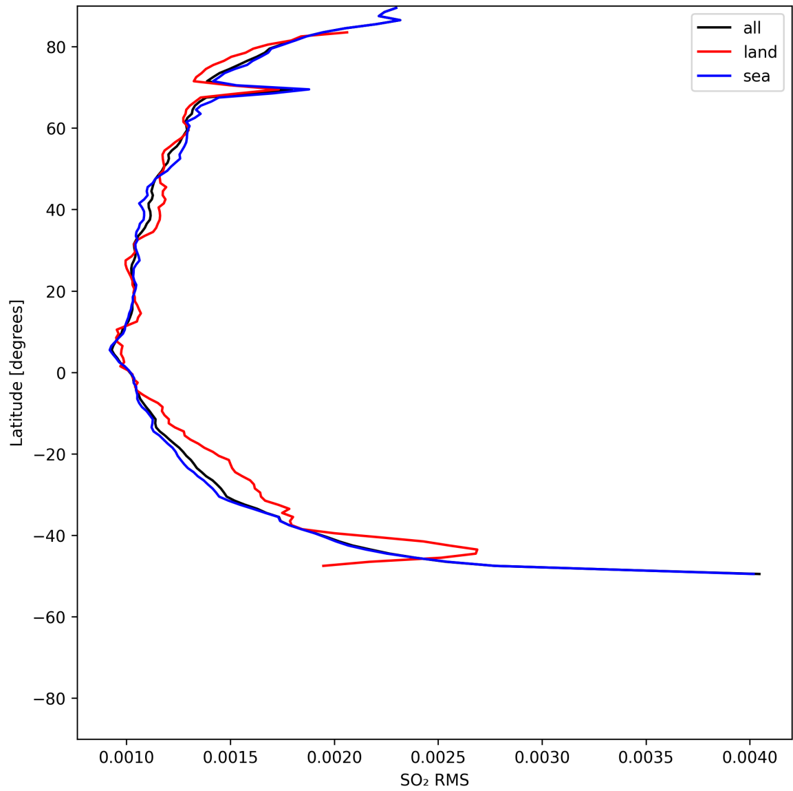
Figure 52: Zonal average of “SO 2 RMS” for 2025-05-16 to 2025-05-18.
