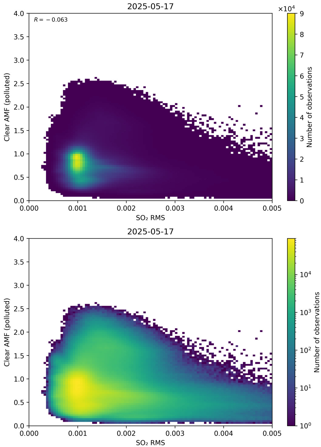
Figure 147: Scatter density plot of “SO 2 RMS” against “Clear AMF (polluted)” for 2025-05-16 to 2025-05-18.
