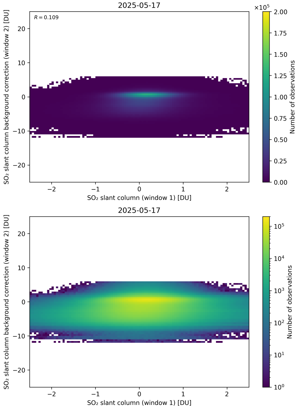
Figure 263: Scatter density plot of “SO 2 slant column (window 1)” against “SO 2 slant column background correction (window 2)” for 2025-05-16 to 2025-05-18.
