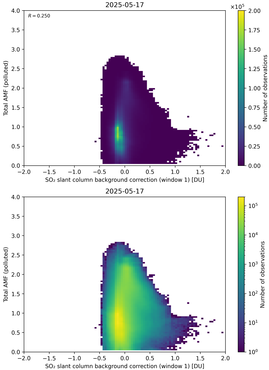
Figure 120: Scatter density plot of “SO 2 slant column background correction (window 1)” against “Total AMF (polluted)” for 2025-05-16 to 2025-05-18.
