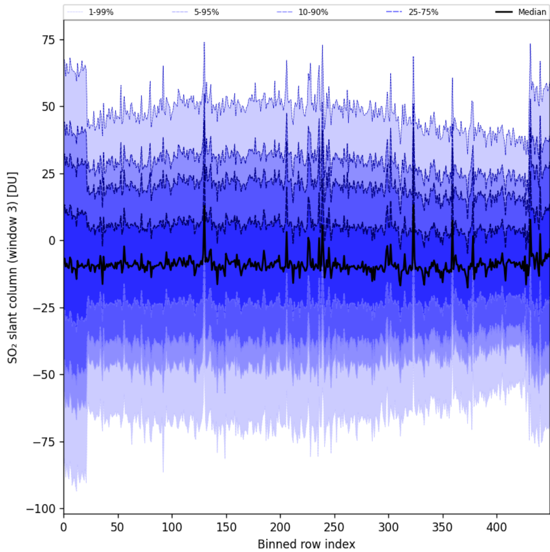
Figure 97: Along track statistics of “SO 2 slant column (window 3)” for 2025-05-16 to 2025-05-18
