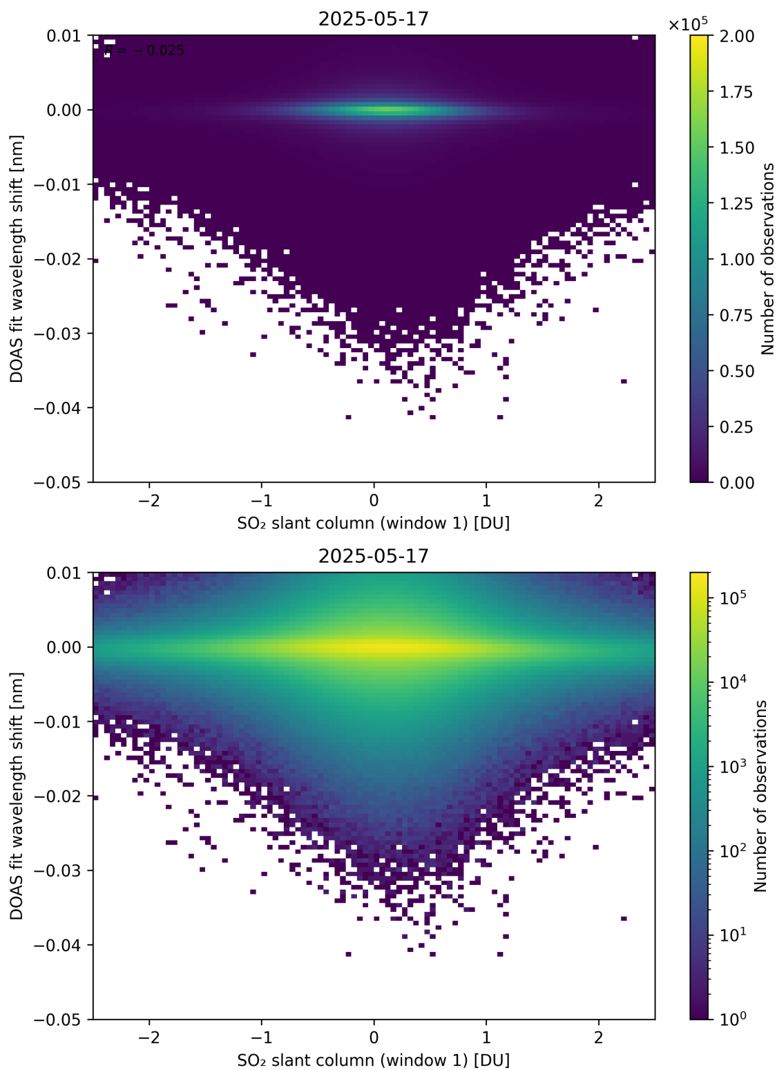
Figure 265: Scatter density plot of “SO 2 slant column (window 1)” against “DOAS fit wavelength shift” for 2025-05-16 to 2025-05-18.
