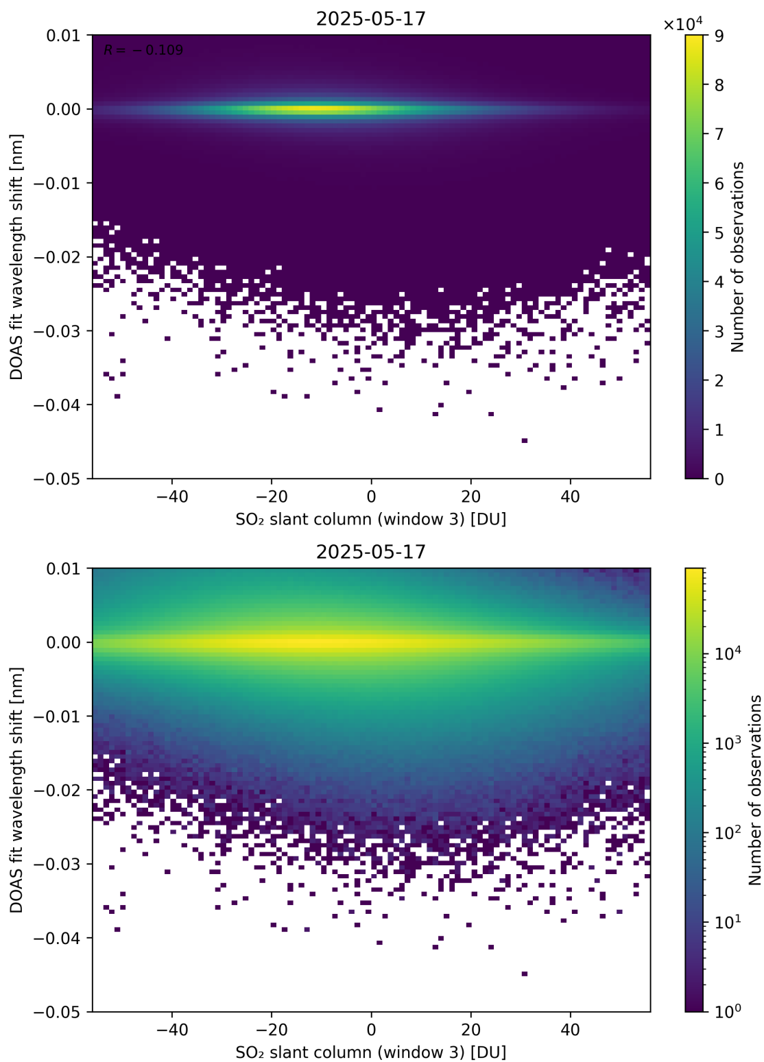
Figure 304: Scatter density plot of “SO 2 slant column (window 3)” against “DOAS fit wavelength shift” for 2025-05-16 to 2025-05-18.
