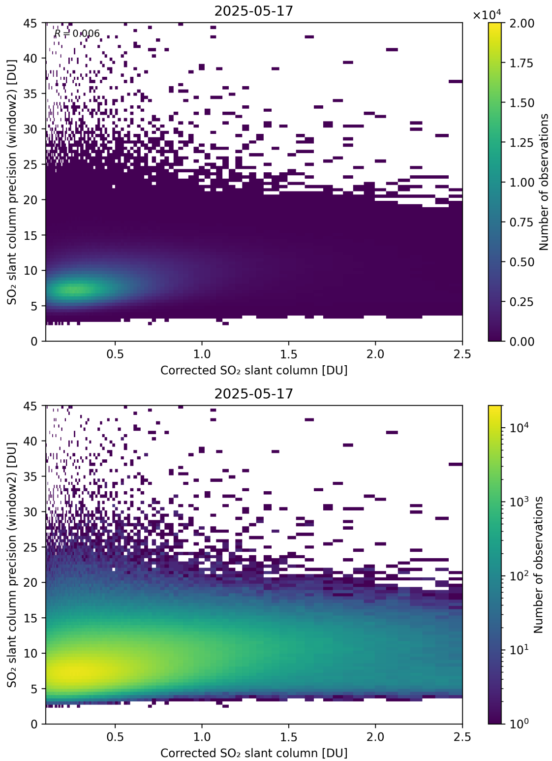
Figure 239: Scatter density plot of “Corrected SO 2 slant column” against “SO 2 slant column precision (window2)” for 2025-05-16 to 2025-05-18.
