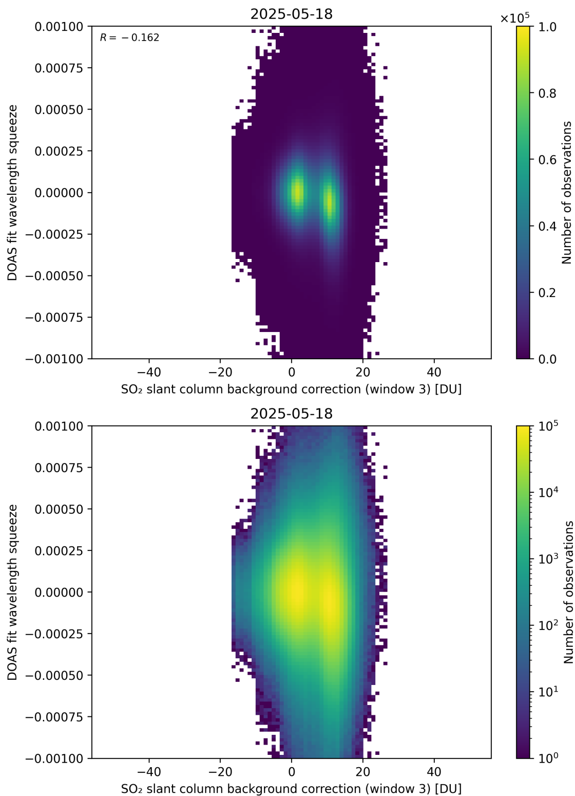
Figure 133: Scatter density plot of “SO 2 slant column background correction (window 3)” against “DOAS fit wavelength squeeze” for 2025-05-17 to 2025-05-19.
