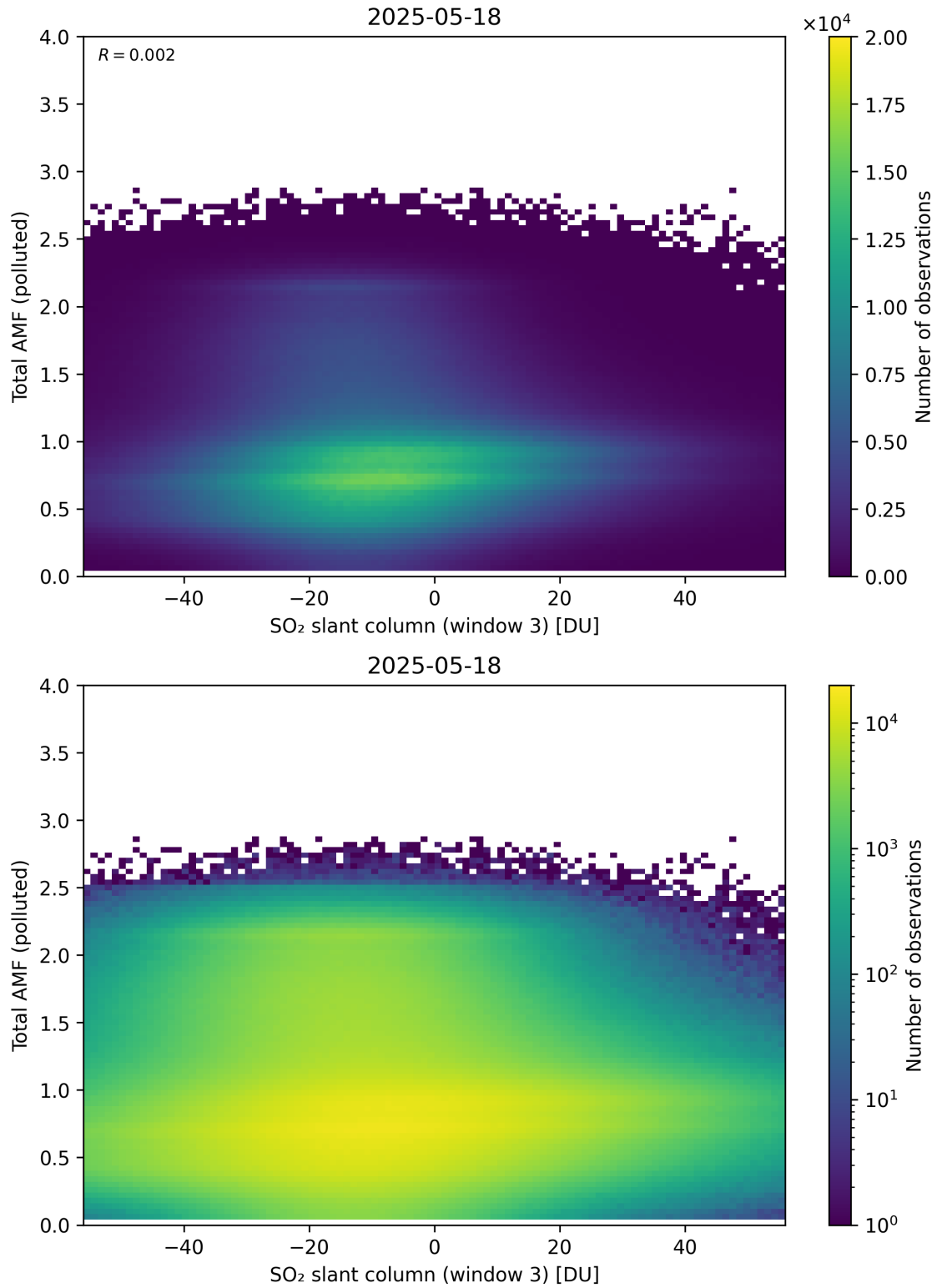
Figure 318: Scatter density plot of “SO 2 slant column (window 3)” against “Total AMF (polluted)” for 2025-05-17 to 2025-05-19.
