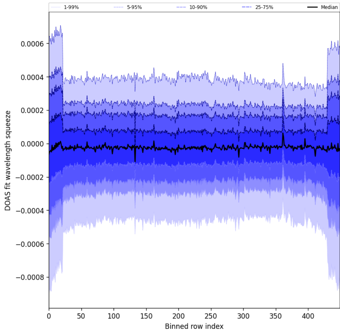
Figure 103: Along track statistics of “DOAS fit wavelength squeeze” for 2025-05-17 to 2025-05-19
