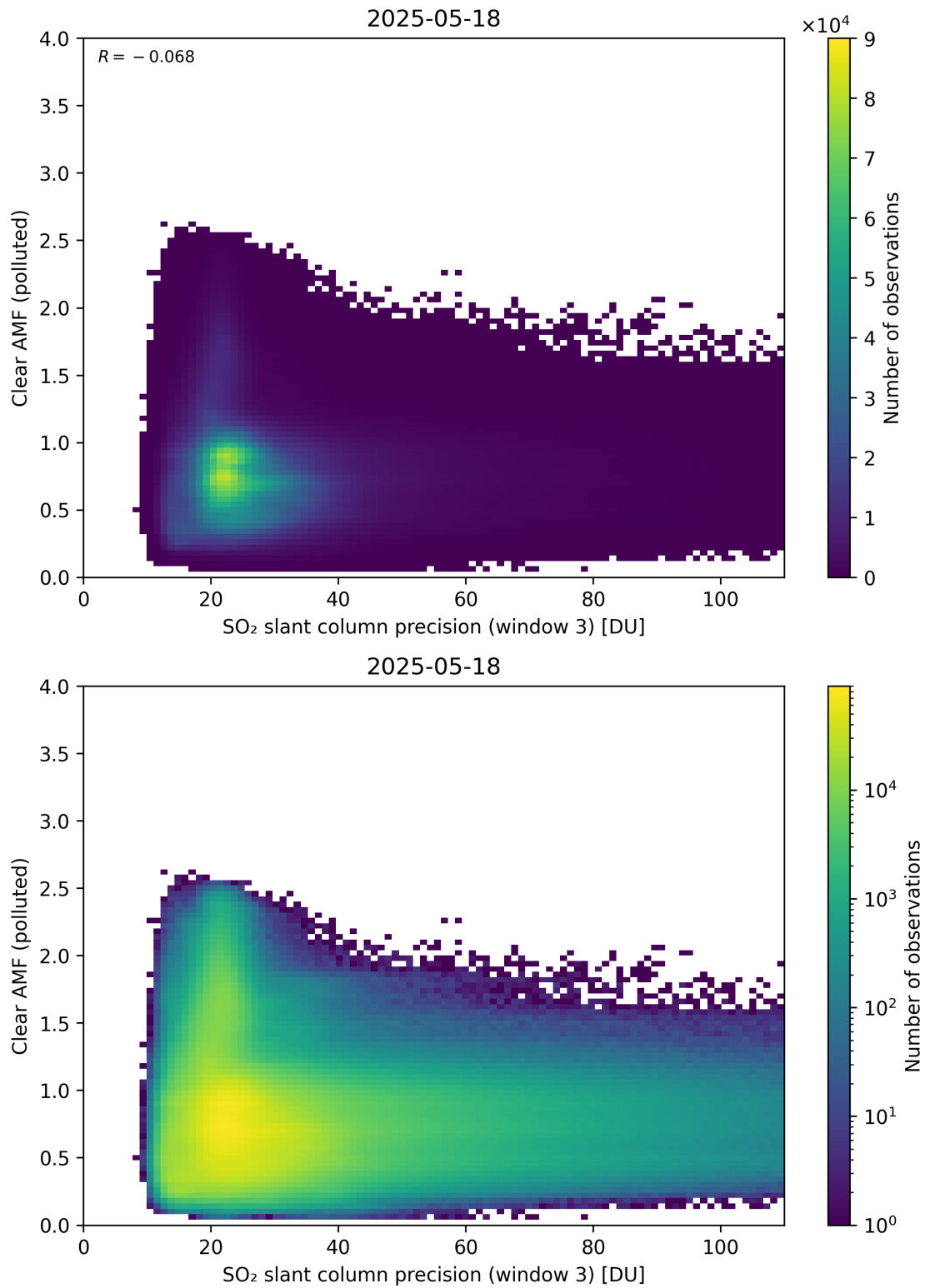
Figure 311: Scatter density plot of “SO 2 slant column precision (window 3)” against “Clear AMF (polluted)” for 2025-05-17 to 2025-05-19.
