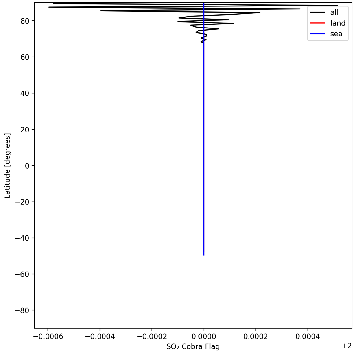
Figure 49: Zonal average of "SO 2 Cobra Flag" for 2025-05-17 to 2025-05-19.
