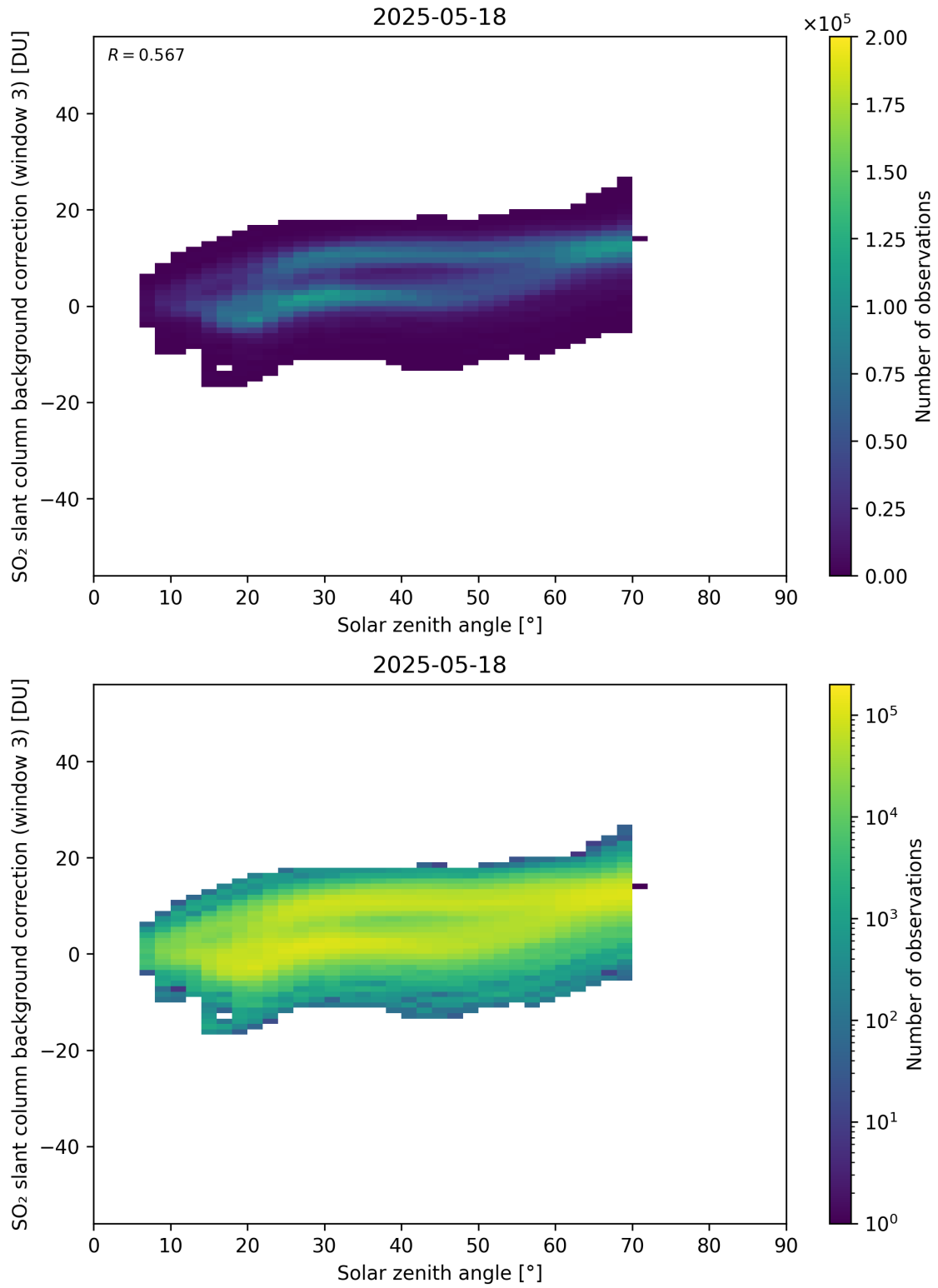
Figure 173: Scatter density plot of “Solar zenith angle” against “SO 2 slant column background correction (window 3)” for 2025-05-17 to 2025-05-19.
