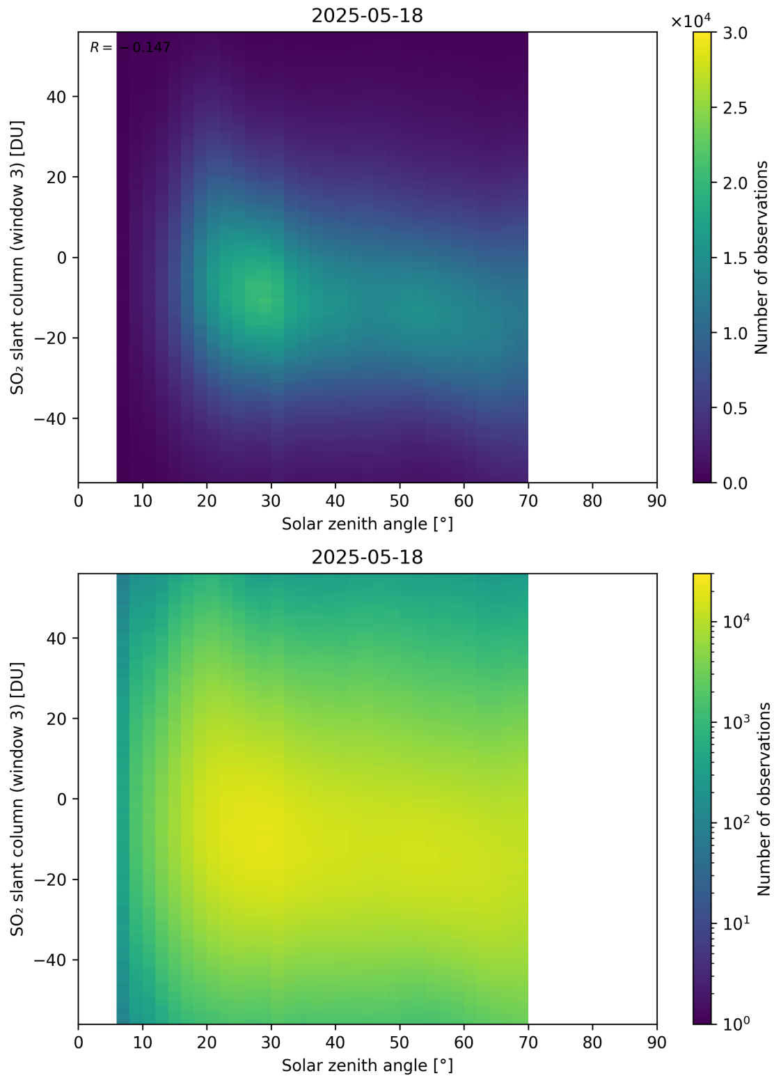
Figure 187: Scatter density plot of “Solar zenith angle” against “SO 2 slant column (window 3)” for 2025-05-17 to 2025-05-19.
