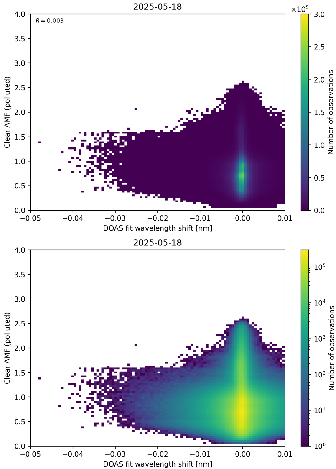
Figure 140: Scatter density plot of “DOAS fit wavelength shift” against “Clear AMF (polluted)” for 2025-05-17 to 2025-05-19.
