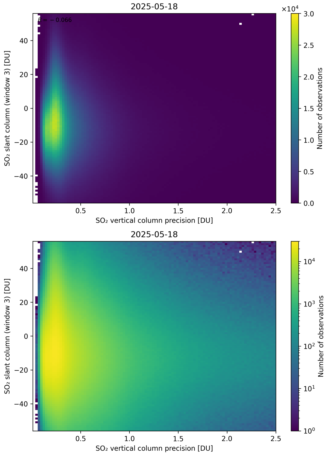
Figure 344: Scatter density plot of “SO 2 vertical column precision” against “SO 2 slant column (window 3)” for 2025-05-17 to 2025-05-19.
