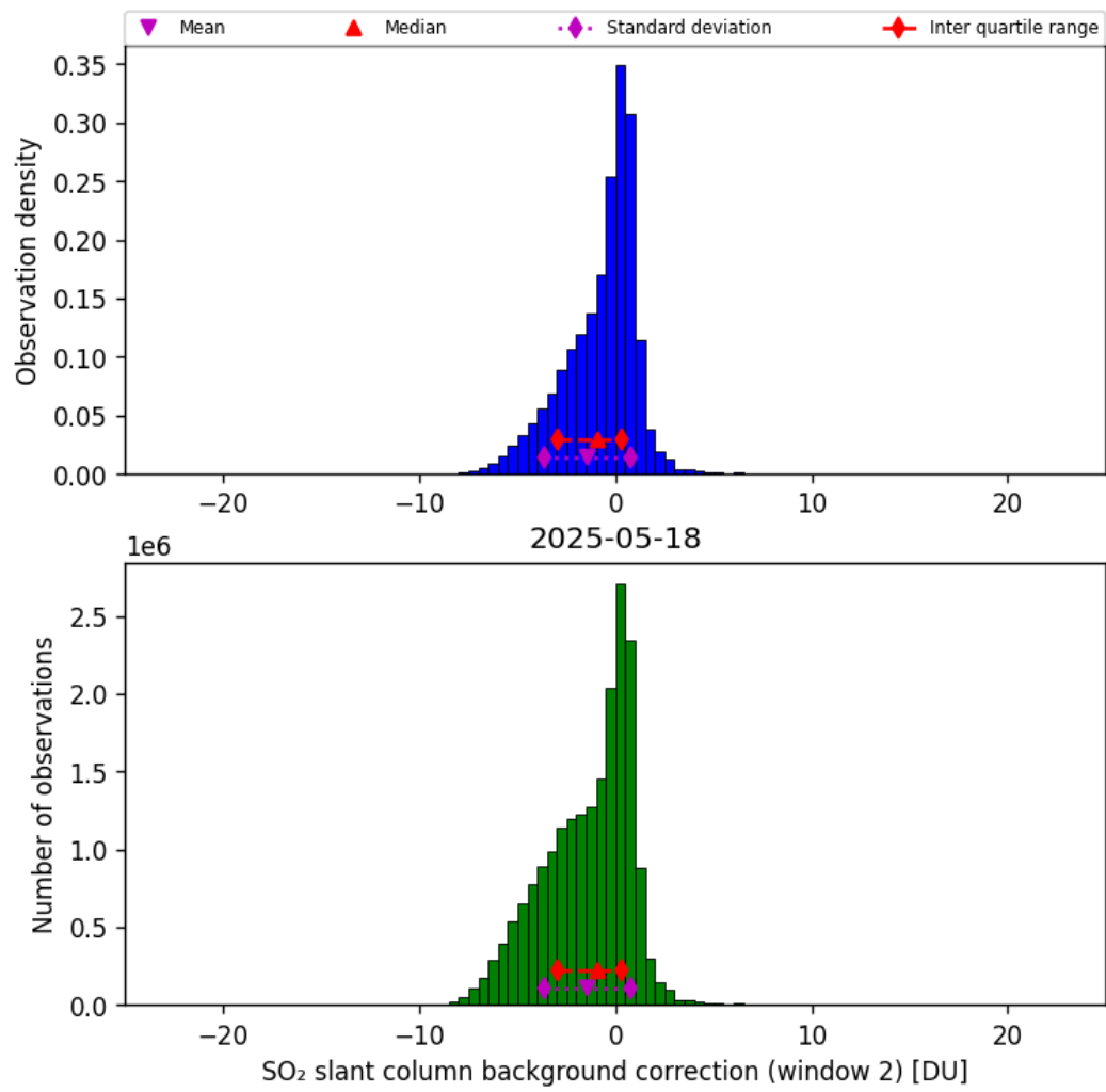
Figure 70: Histogram of “SO 2 slant column background correction (window 2)” for 2025-05-17 to 2025-05-19
