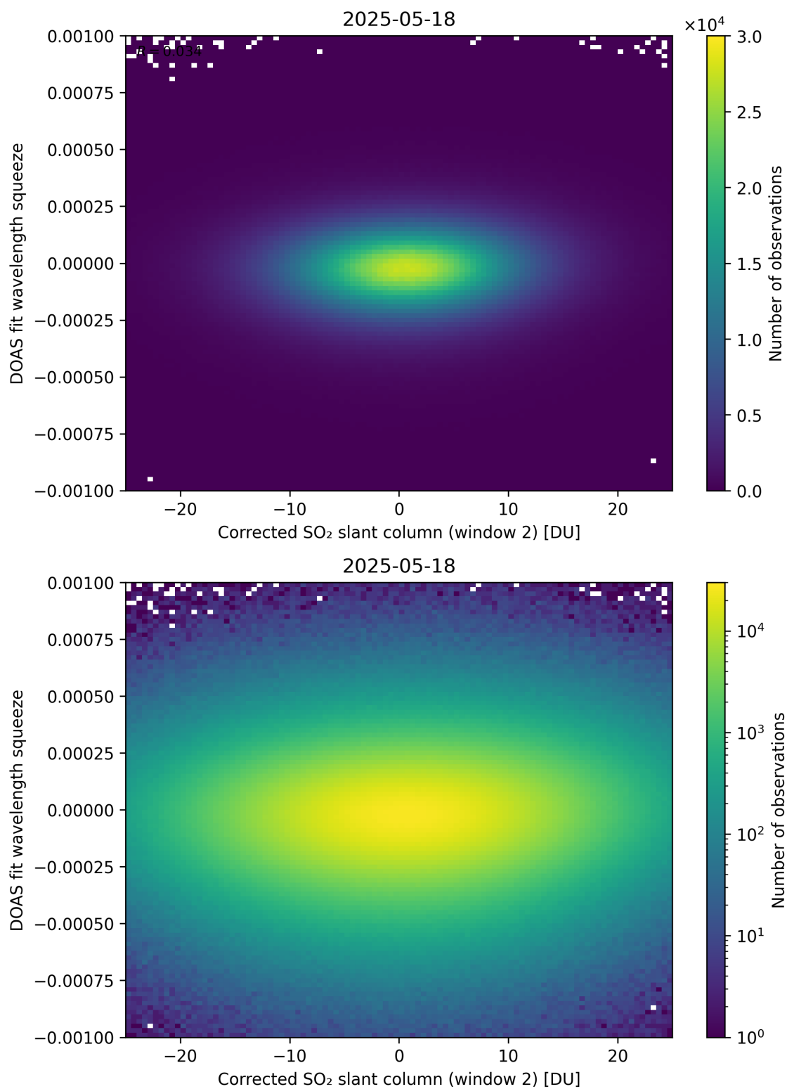
Figure 247: Scatter density plot of “Corrected SO 2 slant column (window 2)” against “DOAS fit wavelength squeeze” for 2025-05-17 to 2025-05-19.
