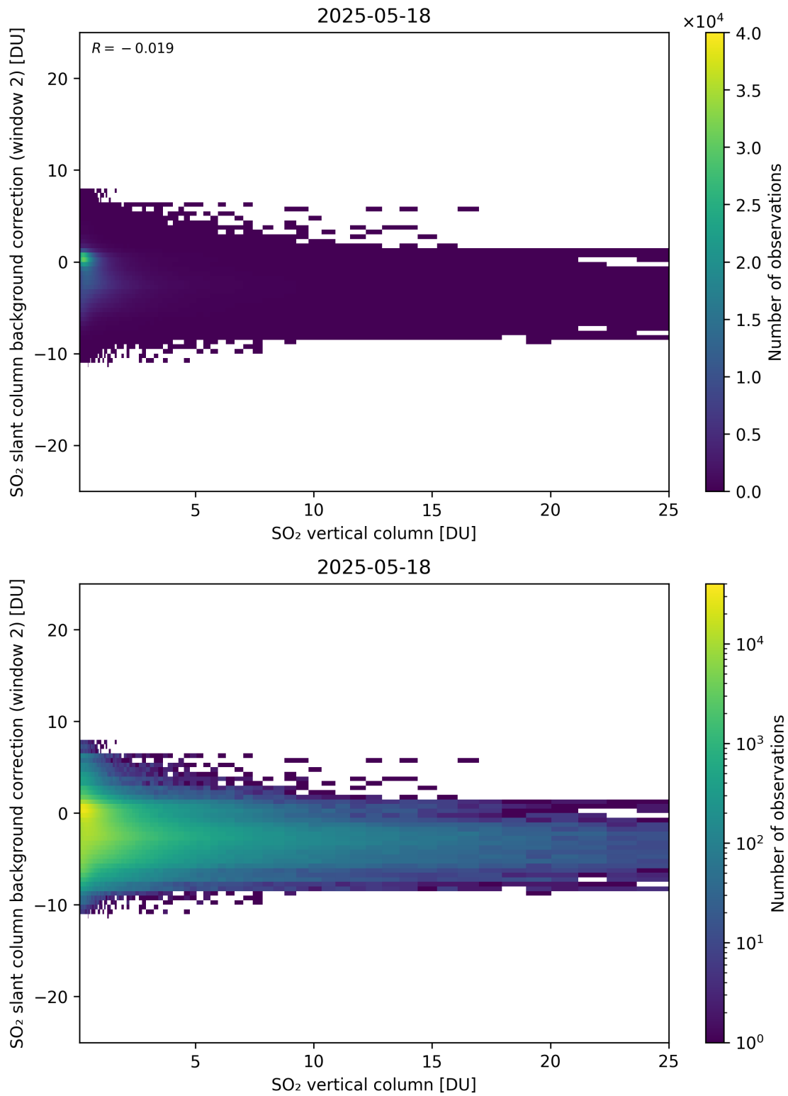
Figure 324: Scatter density plot of “SO 2 vertical column” against “SO 2 slant column background correction (window 2)” for 2025-05-17 to 2025-05-19.
