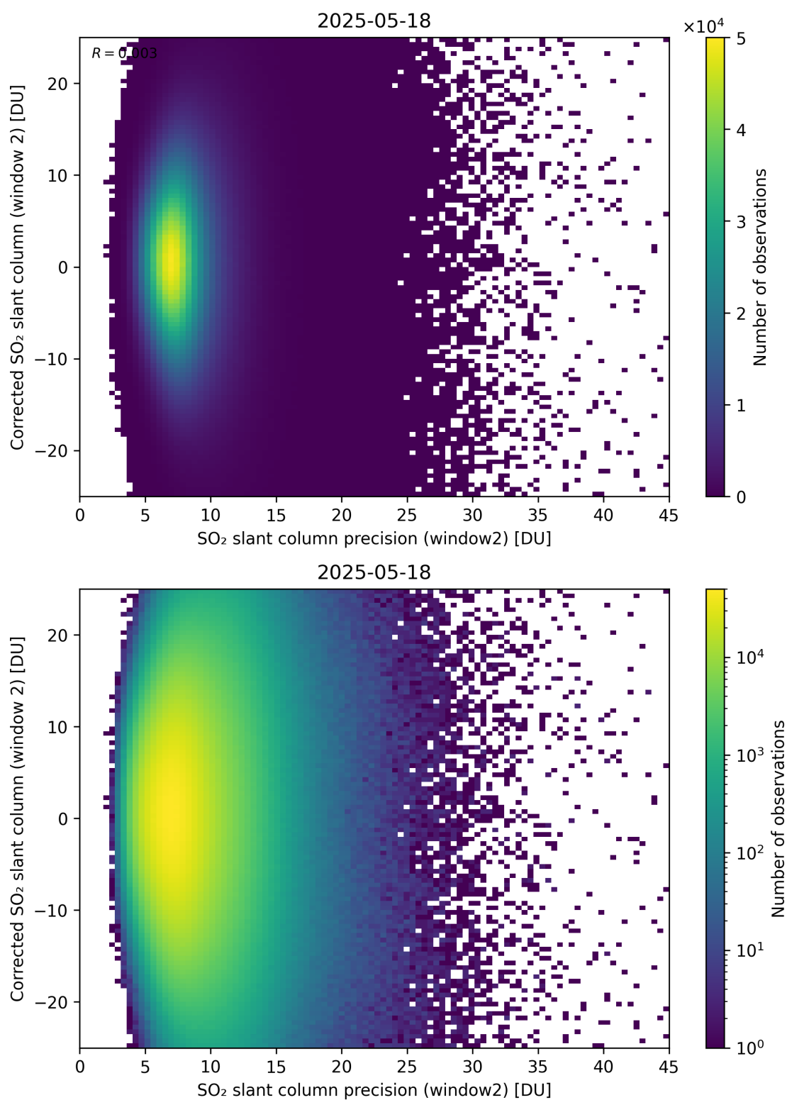
Figure 297: Scatter density plot of “SO 2 slant column precision (window2)” against “Corrected SO 2 slant column (window 2)” for 2025-05-17 to 2025-05-19.
