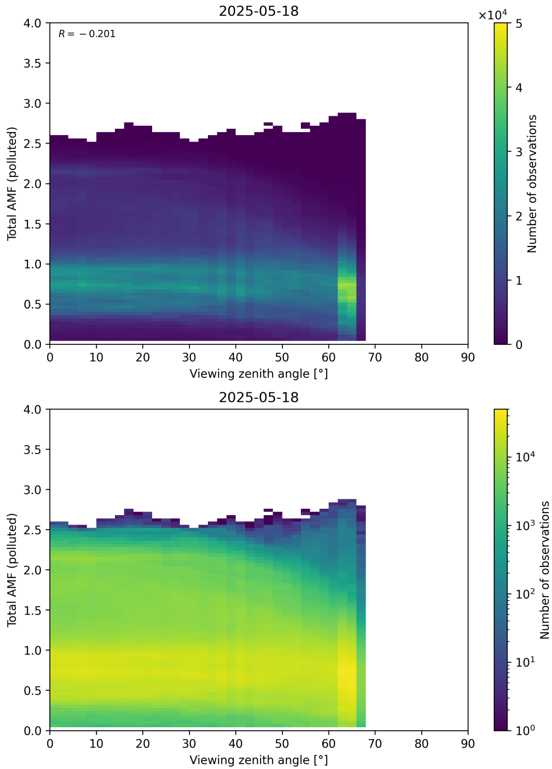
Figure 381: Scatter density plot of “Viewing zenith angle” against “Total AMF (polluted)” for 2025-05-17 to 2025-05-19.
