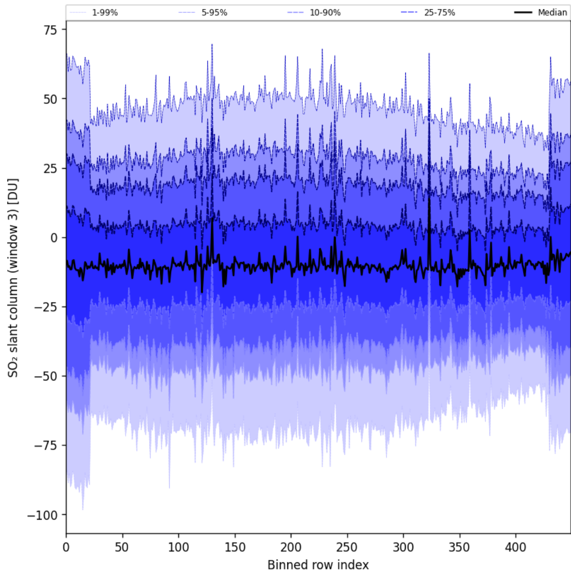
Figure 97: Along track statistics of “SO 2 slant column (window 3)” for 2025-05-17 to 2025-05-19
