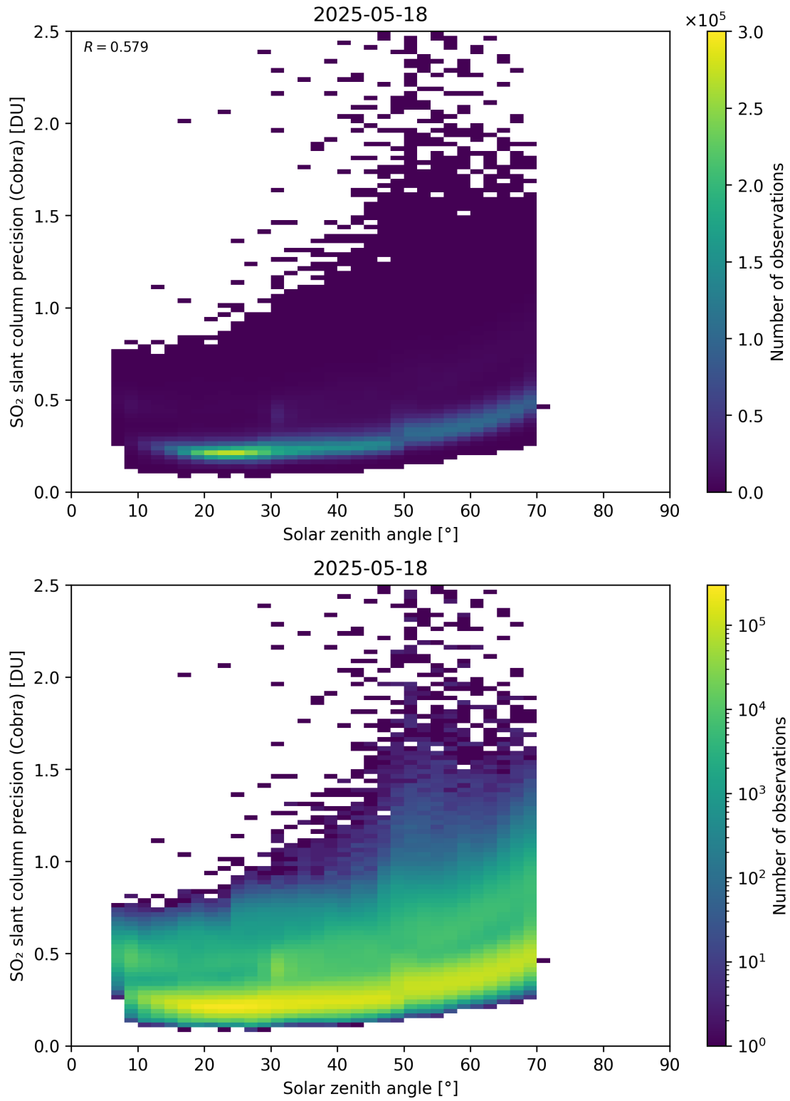
Figure 180: Scatter density plot of “Solar zenith angle” against “SO 2 slant column precision (Cobra)” for 2025-05-17 to 2025-05-19.
