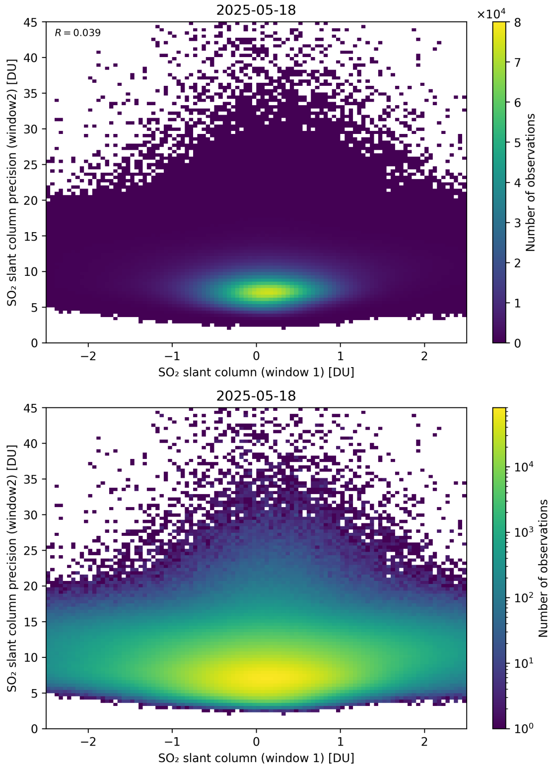
Figure 286: Scatter density plot of “SO 2 slant column (window 1)” against “SO 2 slant column precision (window2)” for 2025-05-17 to 2025-05-19.
