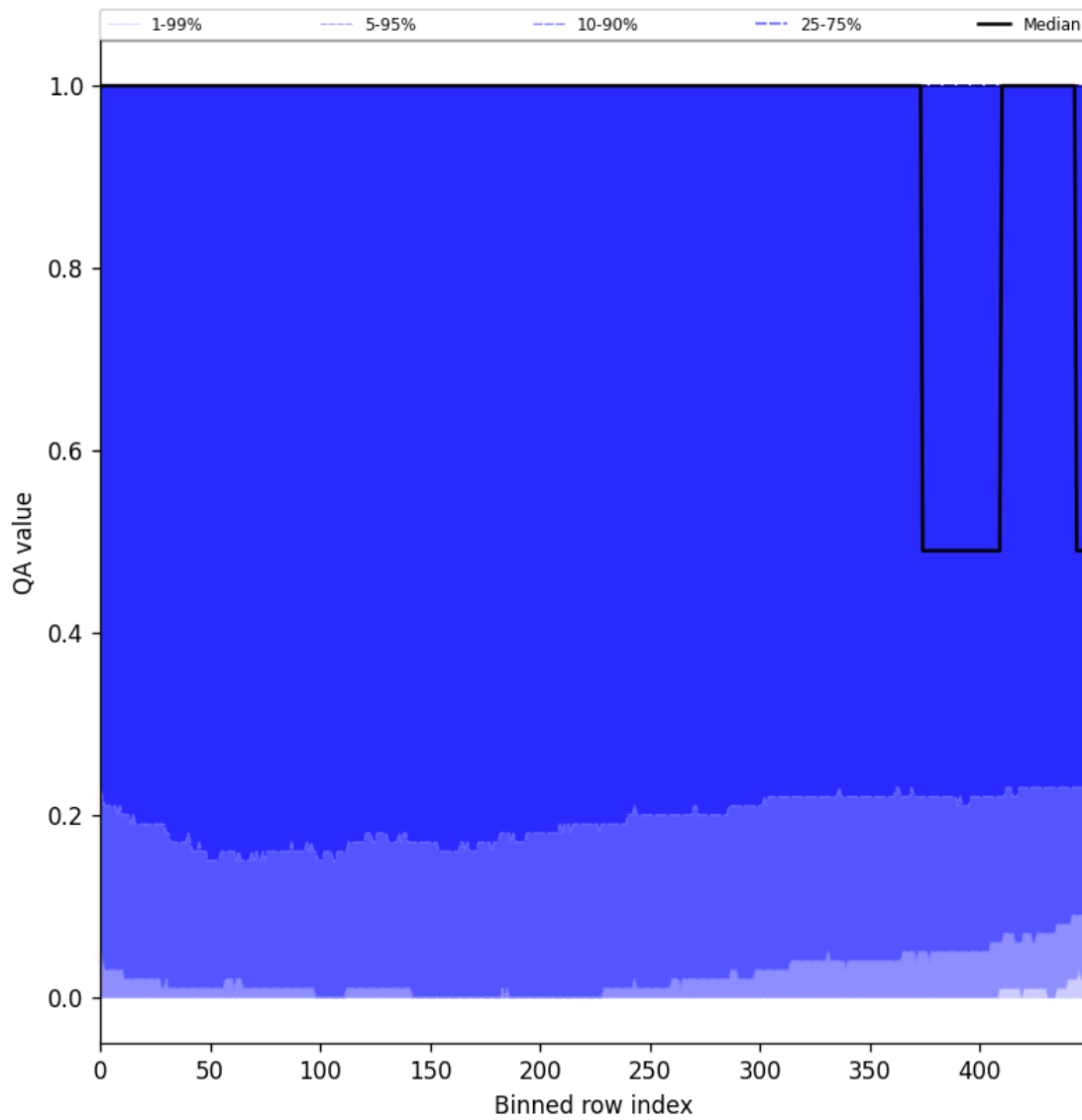
Figure 83: Along track statistics of “QA value” for 2025-05-17 to 2025-05-19
