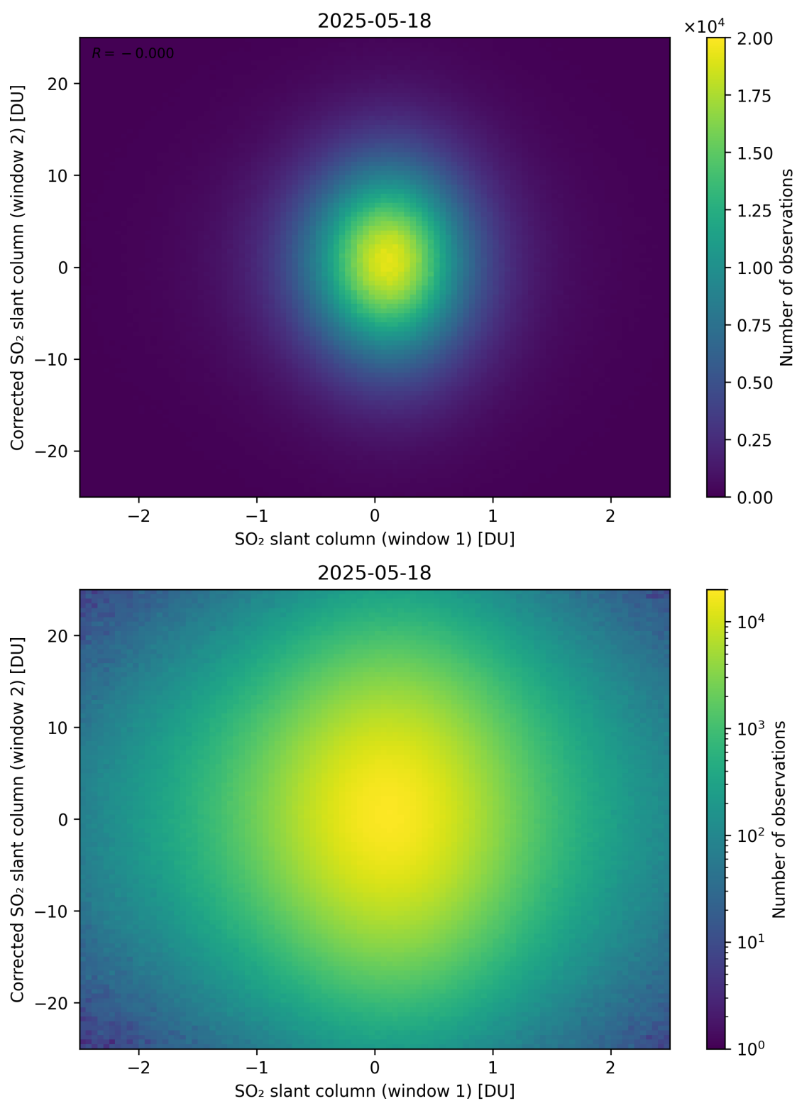
Figure 283: Scatter density plot of “SO 2 slant column (window 1)” against “Corrected SO 2 slant column (window 2)” for 2025-05-17 to 2025-05-19.
