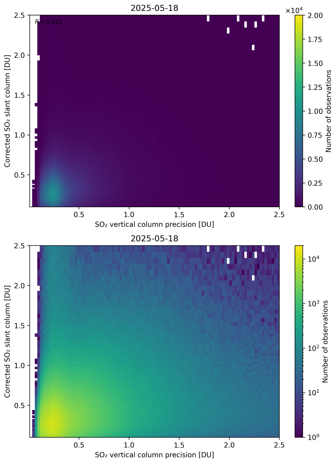
Figure 338: Scatter density plot of “SO 2 vertical column precision” against “Corrected SO 2 slant column” for 2025-05-17 to 2025-05-19.
