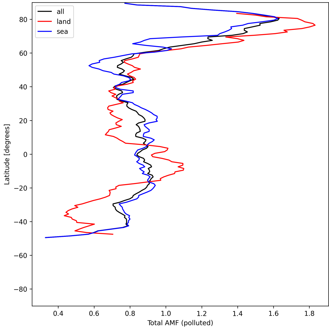
Figure 53: Zonal average of “Total AMF (polluted)” for 2025-05-17 to 2025-05-19.
