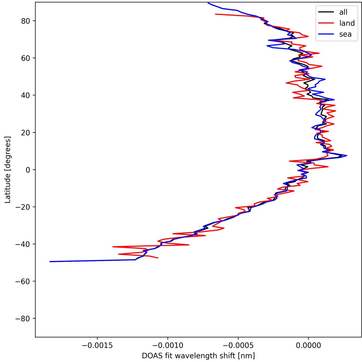
Figure 50: Zonal average of “DOAS fit wavelength shift” for 2025-05-17 to 2025-05-19.
