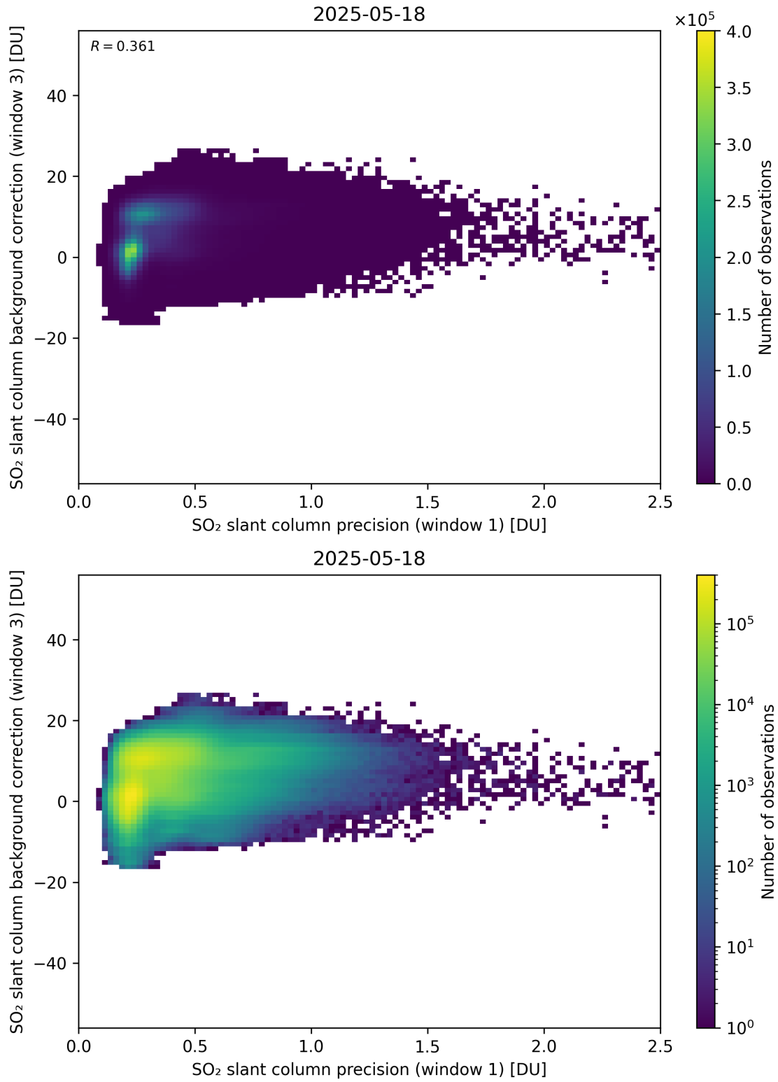
Figure 270: Scatter density plot of “SO 2 slant column precision (window 1)” against “SO 2 slant column background correction (window 3)” for 2025-05-17 to 2025-05-19.
