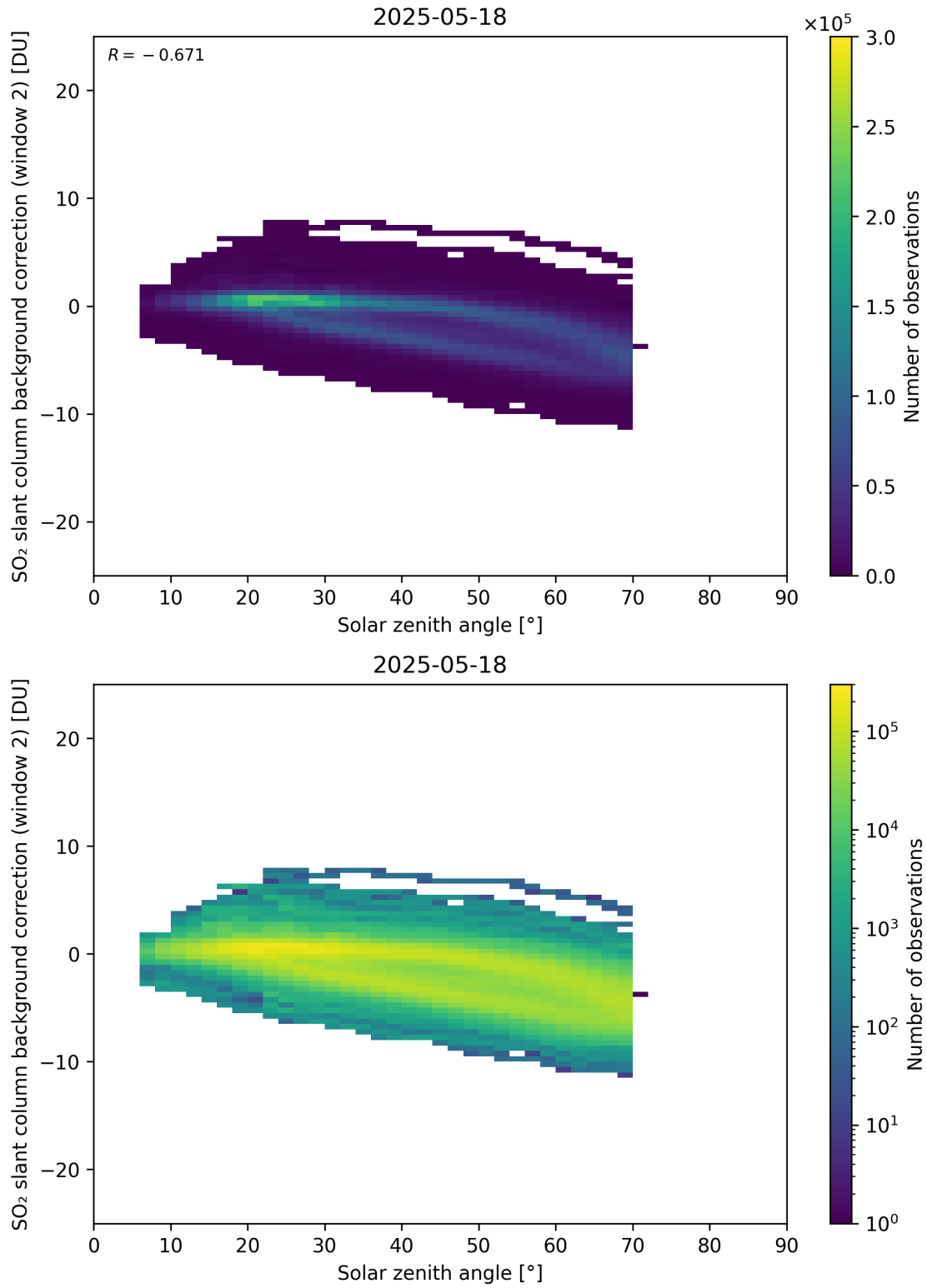
Figure 172: Scatter density plot of “Solar zenith angle” against “SO 2 slant column background correction (window 2)” for 2025-05-17 to 2025-05-19.
