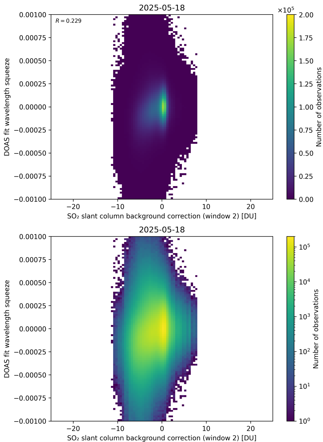
Figure 124: Scatter density plot of “SO 2 slant column background correction (window 2)” against “DOAS fit wavelength squeeze” for 2025-05-17 to 2025-05-19.
