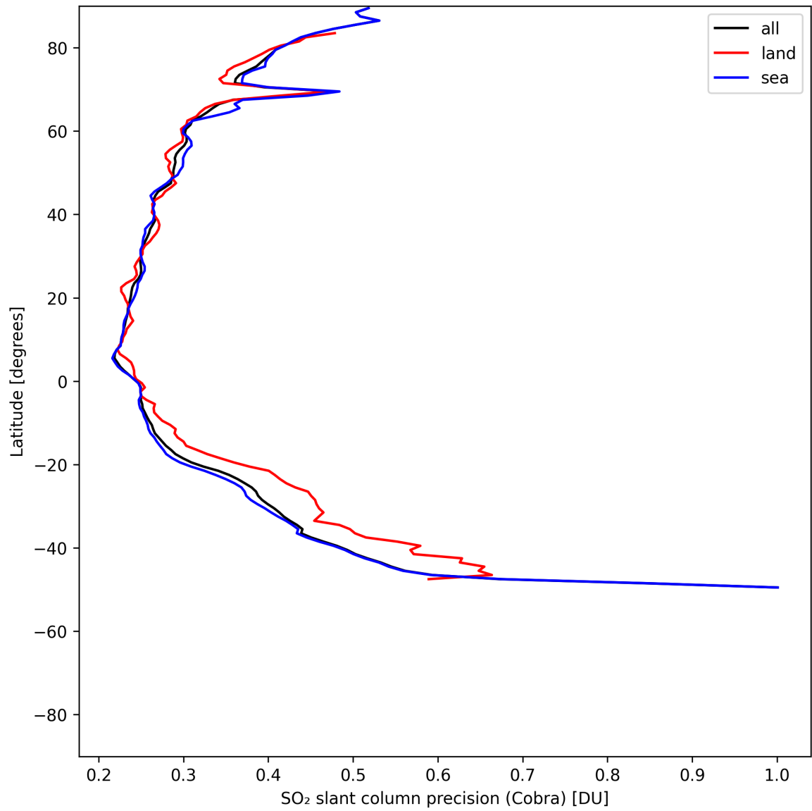
Figure 36: Zonal average of “SO 2 slant column precision (Cobra)” for 2025-05-17 to 2025-05-19.
