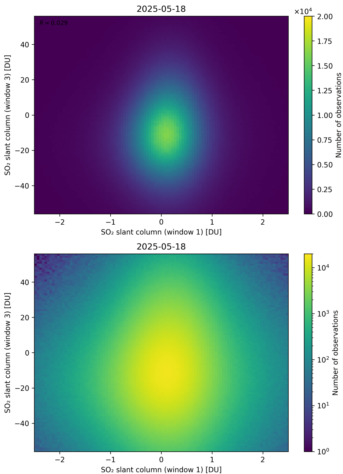
Figure 287: Scatter density plot of “SO 2 slant column (window 1)” against “SO 2 slant column (window 3)” for 2025-05-17 to 2025-05-19.
