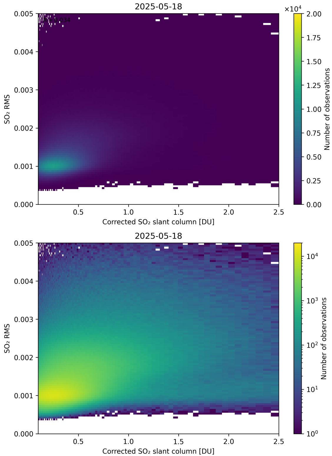
Figure 231: Scatter density plot of “Corrected SO 2 slant column” against “SO 2 RMS” for 2025-05-17 to 2025-05-19.
