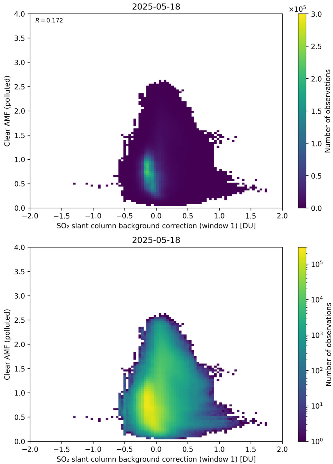
Figure 114: Scatter density plot of “SO 2 slant column background correction (window 1)” against “Clear AMF (polluted)” for 2025-05-17 to 2025-05-19.
