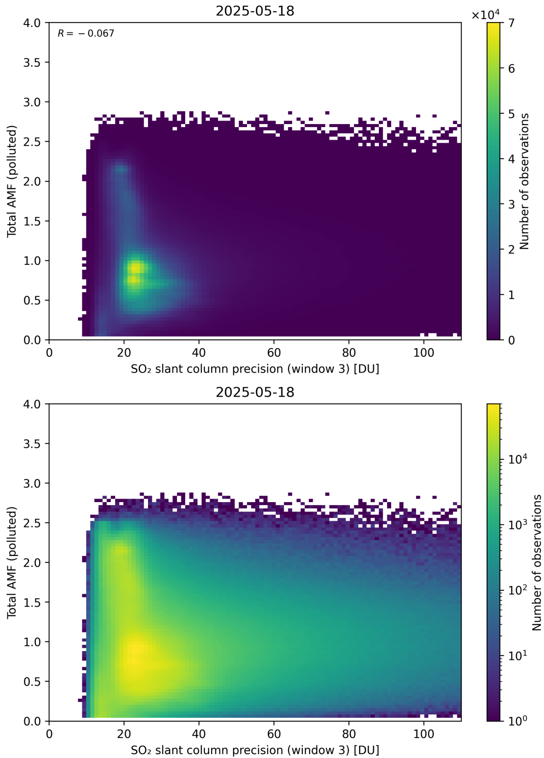
Figure 313: Scatter density plot of “SO 2 slant column precision (window 3)” against “Total AMF (polluted)” for 2025-05-17 to 2025-05-19.
