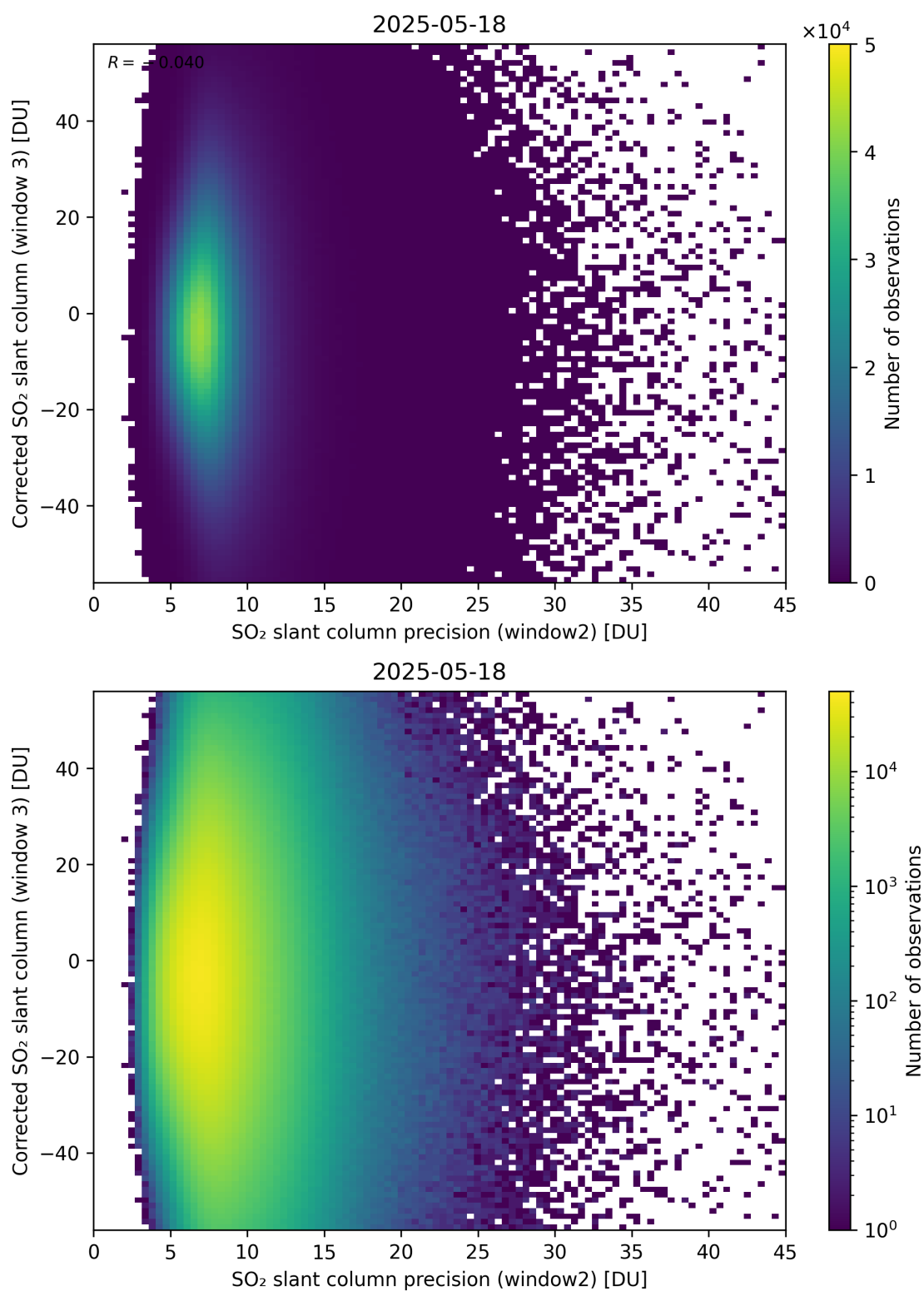
Figure 298: Scatter density plot of “SO 2 slant column precision (window2)” against “Corrected SO 2 slant column (window 3)” for 2025-05-17 to 2025-05-19.
