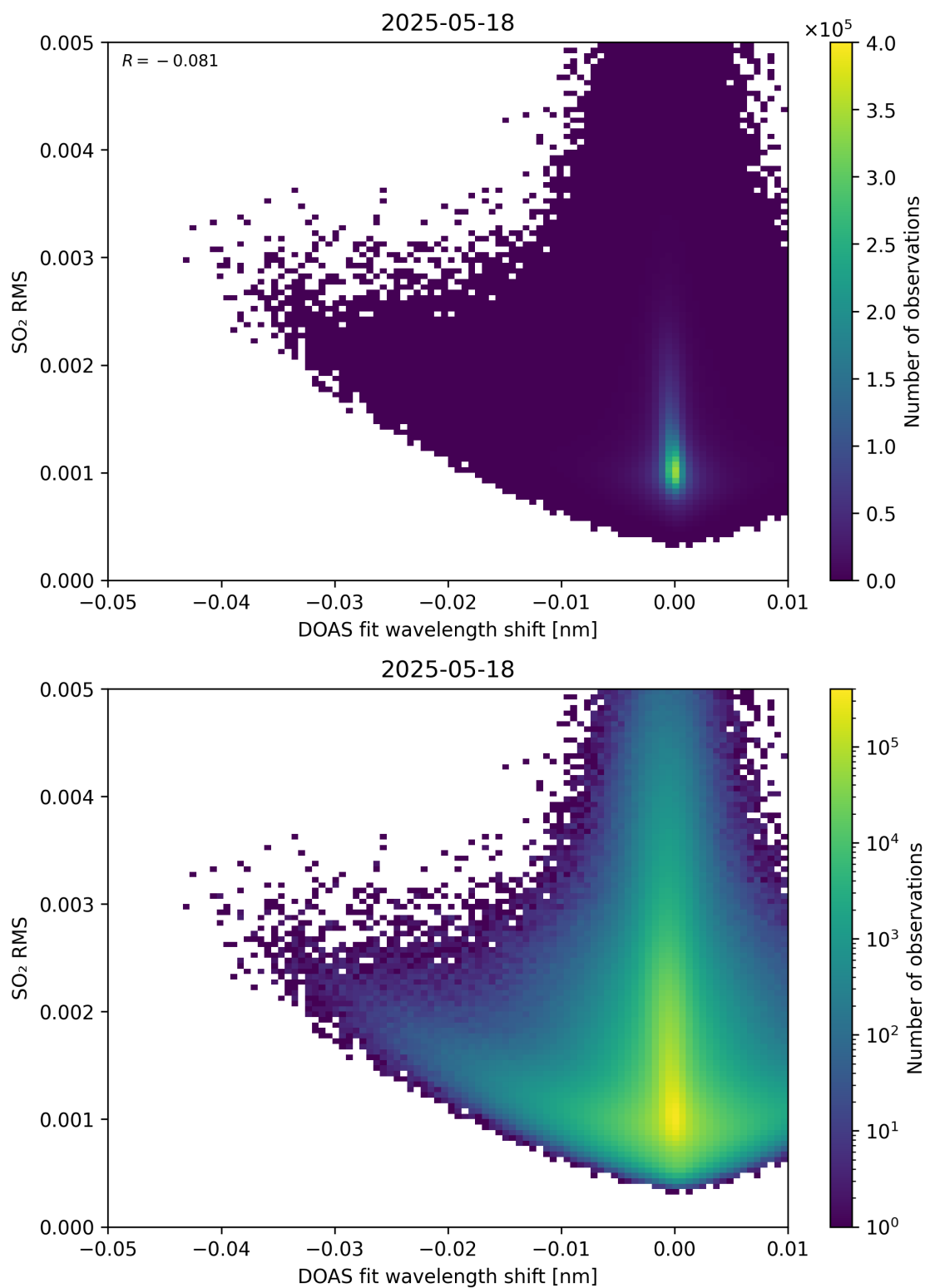
Figure 139: Scatter density plot of “DOAS fit wavelength shift” against “SO 2 RMS” for 2025-05-17 to 2025-05-19.
