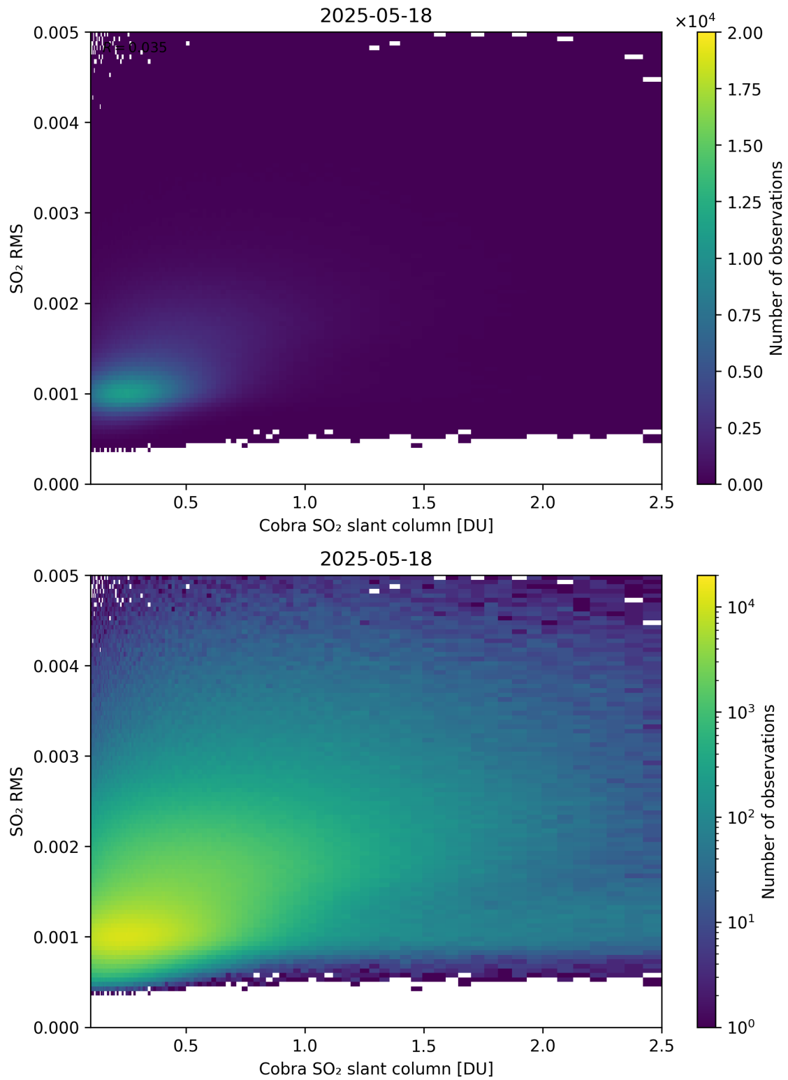
Figure 198: Scatter density plot of “Cobra SO 2 slant column” against “SO 2 RMS” for 2025-05-17 to 2025-05-19.
