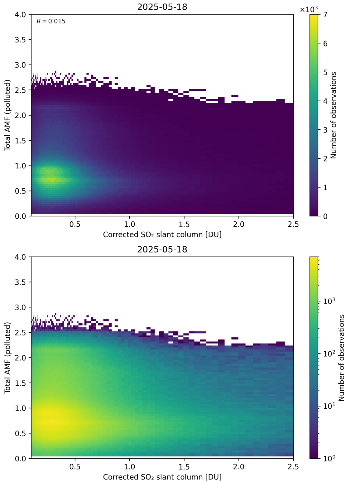
Figure 242: Scatter density plot of “Corrected SO 2 slant column” against “Total AMF (polluted)” for 2025-05-17 to 2025-05-19.
