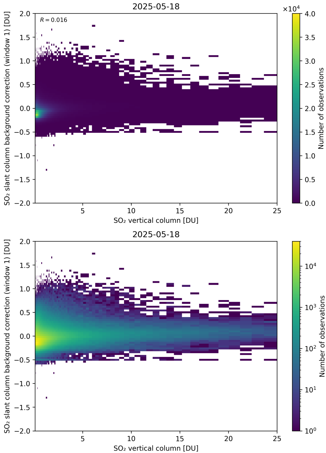
Figure 323: Scatter density plot of “SO 2 vertical column” against “SO 2 slant column background correction (window 1)” for 2025-05-17 to 2025-05-19.
