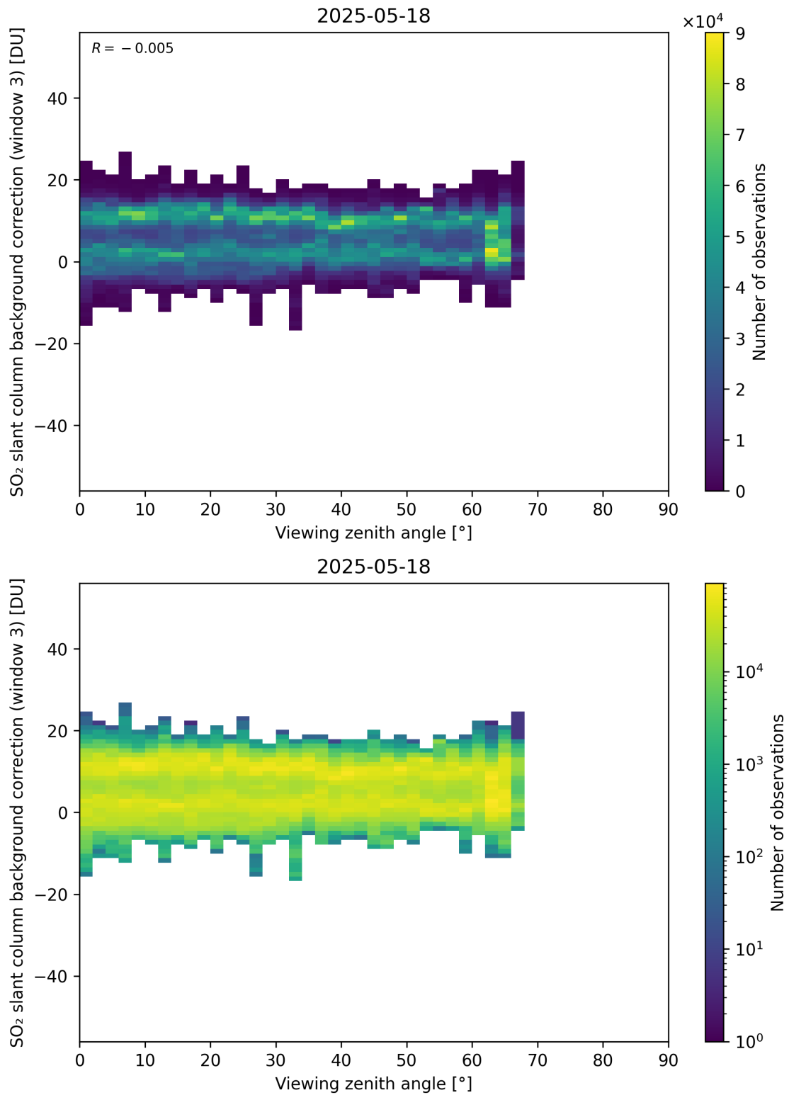
Figure 364: Scatter density plot of “Viewing zenith angle” against “SO 2 slant column background correction (window 3)” for 2025-05-17 to 2025-05-19.
