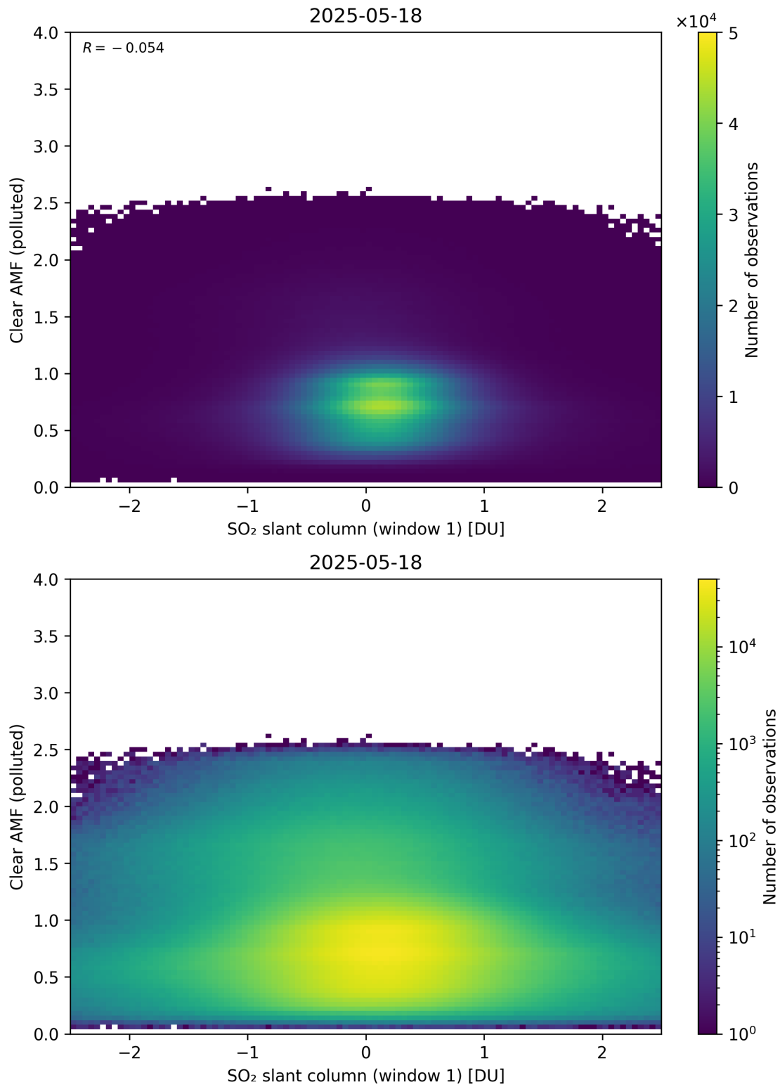
Figure 282: Scatter density plot of “SO 2 slant column (window 1)” against “Clear AMF (polluted)” for 2025-05-17 to 2025-05-19.
