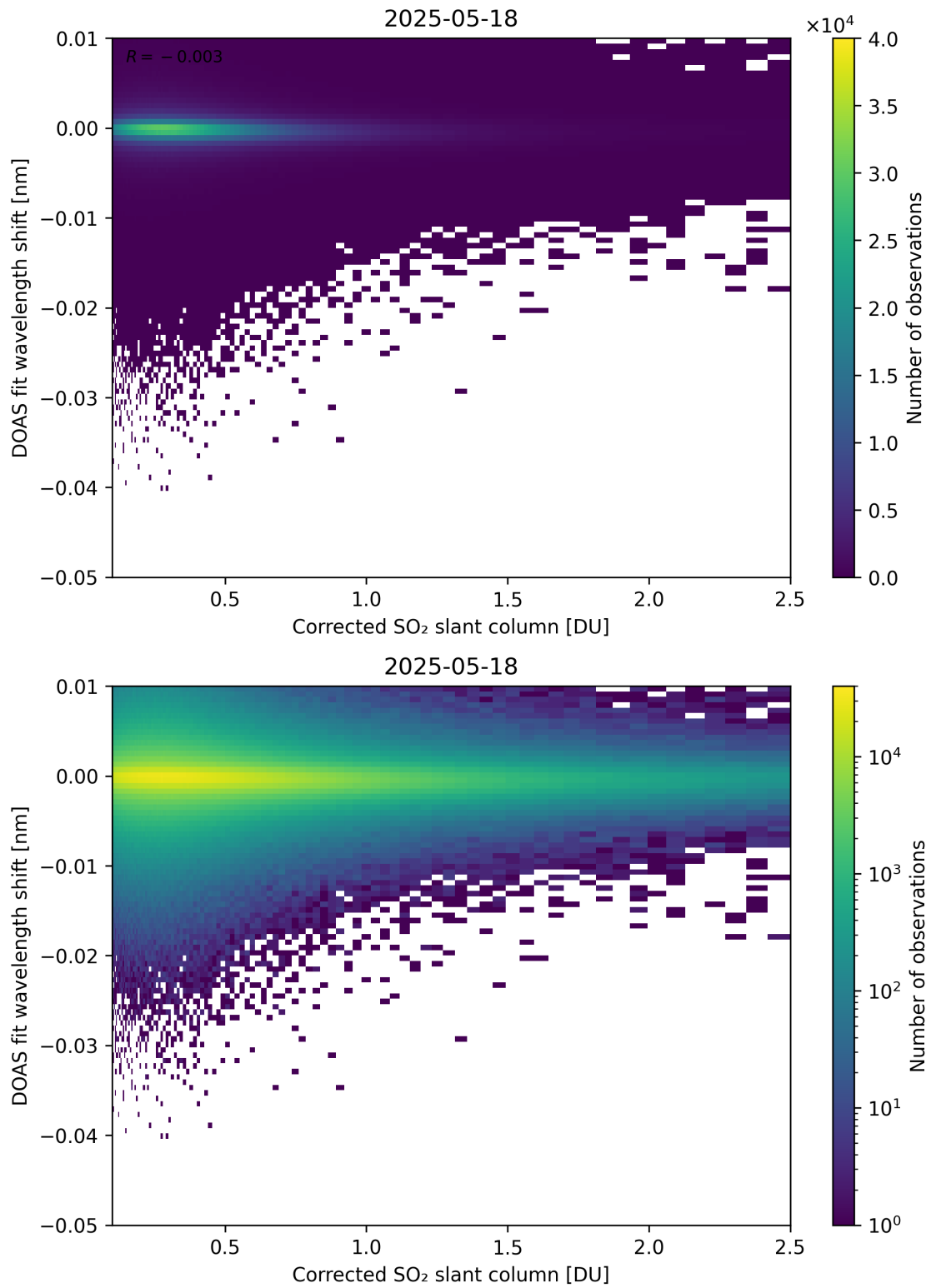
Figure 229: Scatter density plot of “Corrected SO 2 slant column” against “DOAS fit wavelength shift” for 2025-05-17 to 2025-05-19.
