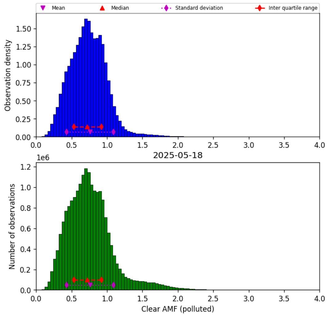
Figure 81: Histogram of “Clear AMF (polluted)” for 2025-05-17 to 2025-05-19
