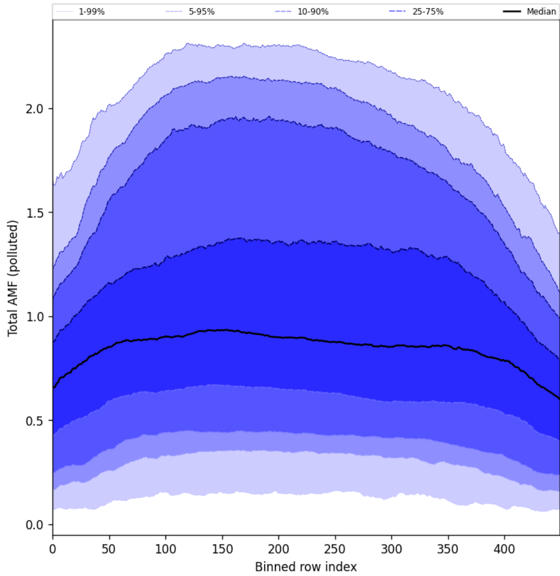
Figure 105: Along track statistics of “Total AMF (polluted)” for 2025-05-17 to 2025-05-19
