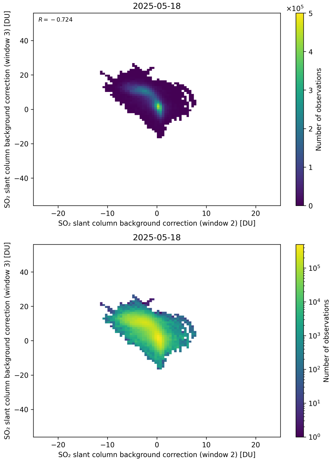
Figure 122: Scatter density plot of “SO 2 slant column background correction (window 2)” against “SO 2 slant column background correction (window 3)” for 2025-05-17 to 2025-05-19.
