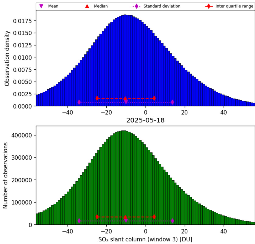
Figure 71: Histogram of “SO 2 slant column (window 3)” for 2025-05-17 to 2025-05-19
