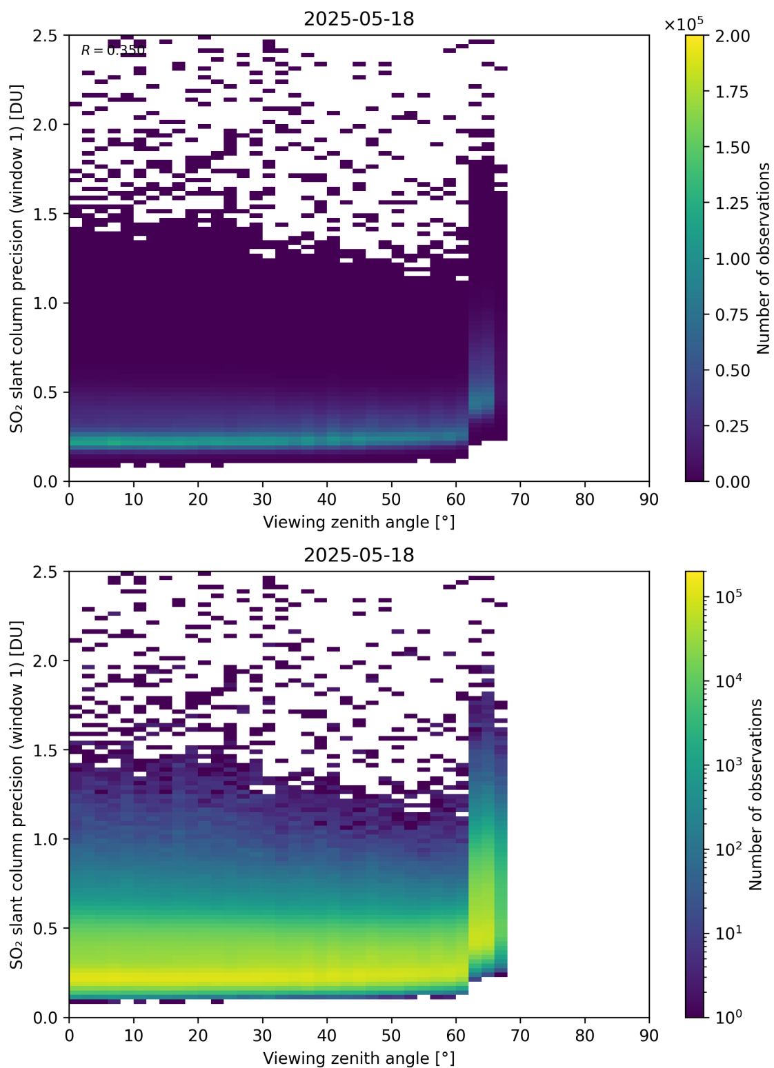
Figure 377: Scatter density plot of “Viewing zenith angle” against “SO 2 slant column precision (window 1)” for 2025-05-17 to 2025-05-19.
