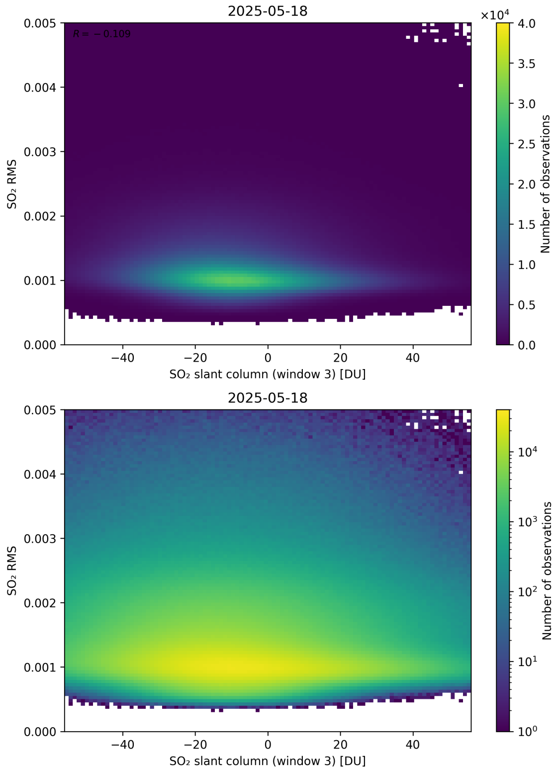
Figure 306: Scatter density plot of “SO 2 slant column (window 3)” against “SO 2 RMS” for 2025-05-17 to 2025-05-19.
