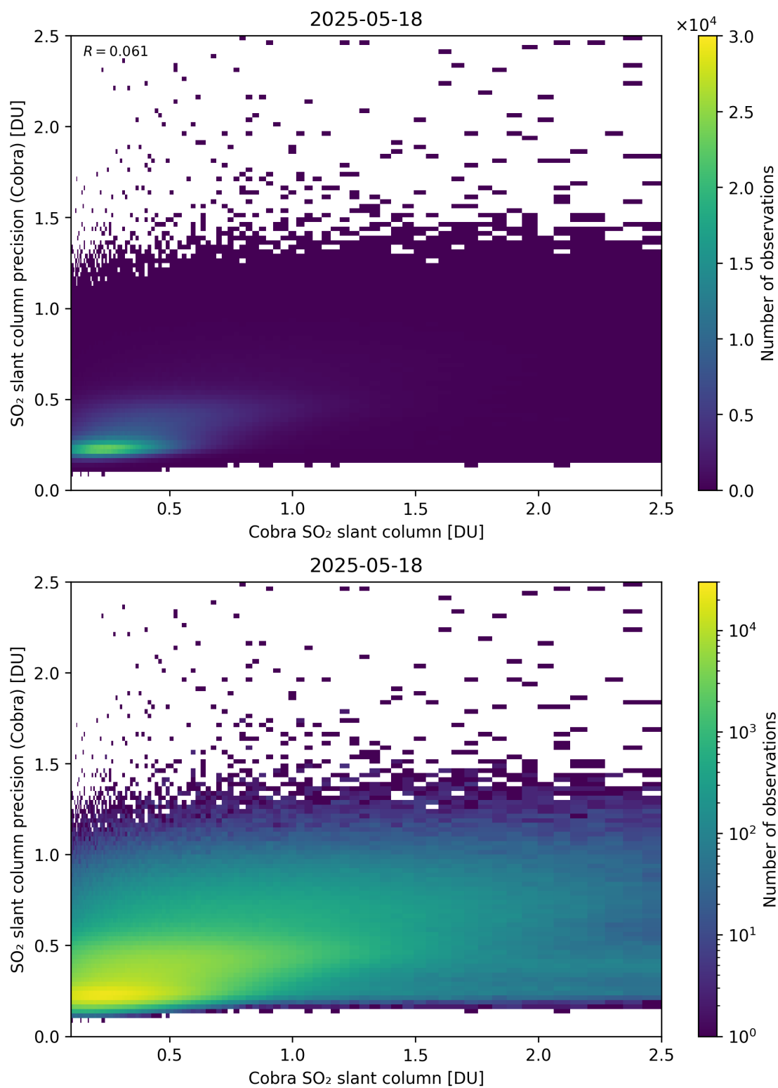
Figure 216: Scatter density plot of “Cobra SO 2 slant column” against “SO 2 slant column precision (Cobra)” for 2025-05-17 to 2025-05-19.
