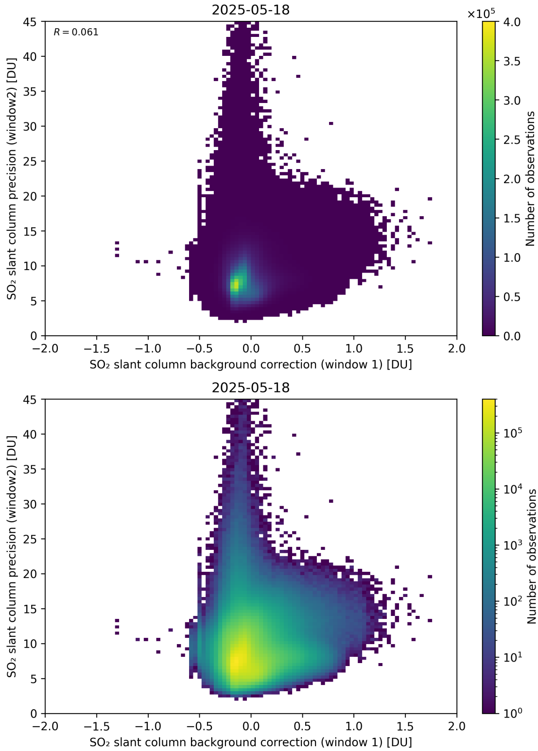
Figure 117: Scatter density plot of “SO 2 slant column background correction (window 1)” against “SO 2 slant column precision (window2)” for 2025-05-17 to 2025-05-19.
