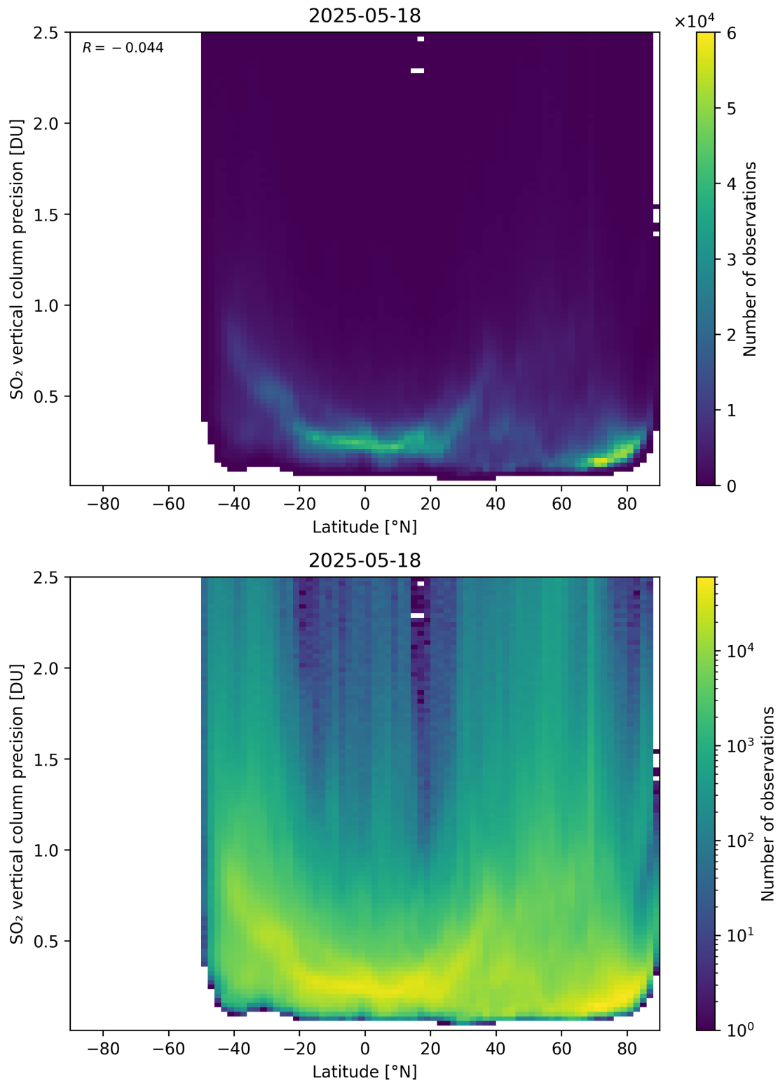
Figure 170: Scatter density plot of “Latitude” against “SO 2 vertical column precision” for 2025-05-17 to 2025-05-19.
