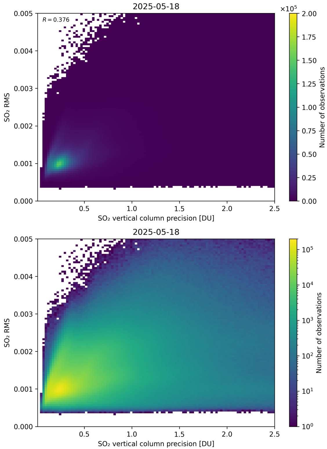
Figure 334: Scatter density plot of “SO 2 vertical column precision” against “SO 2 RMS” for 2025-05-17 to 2025-05-19.
