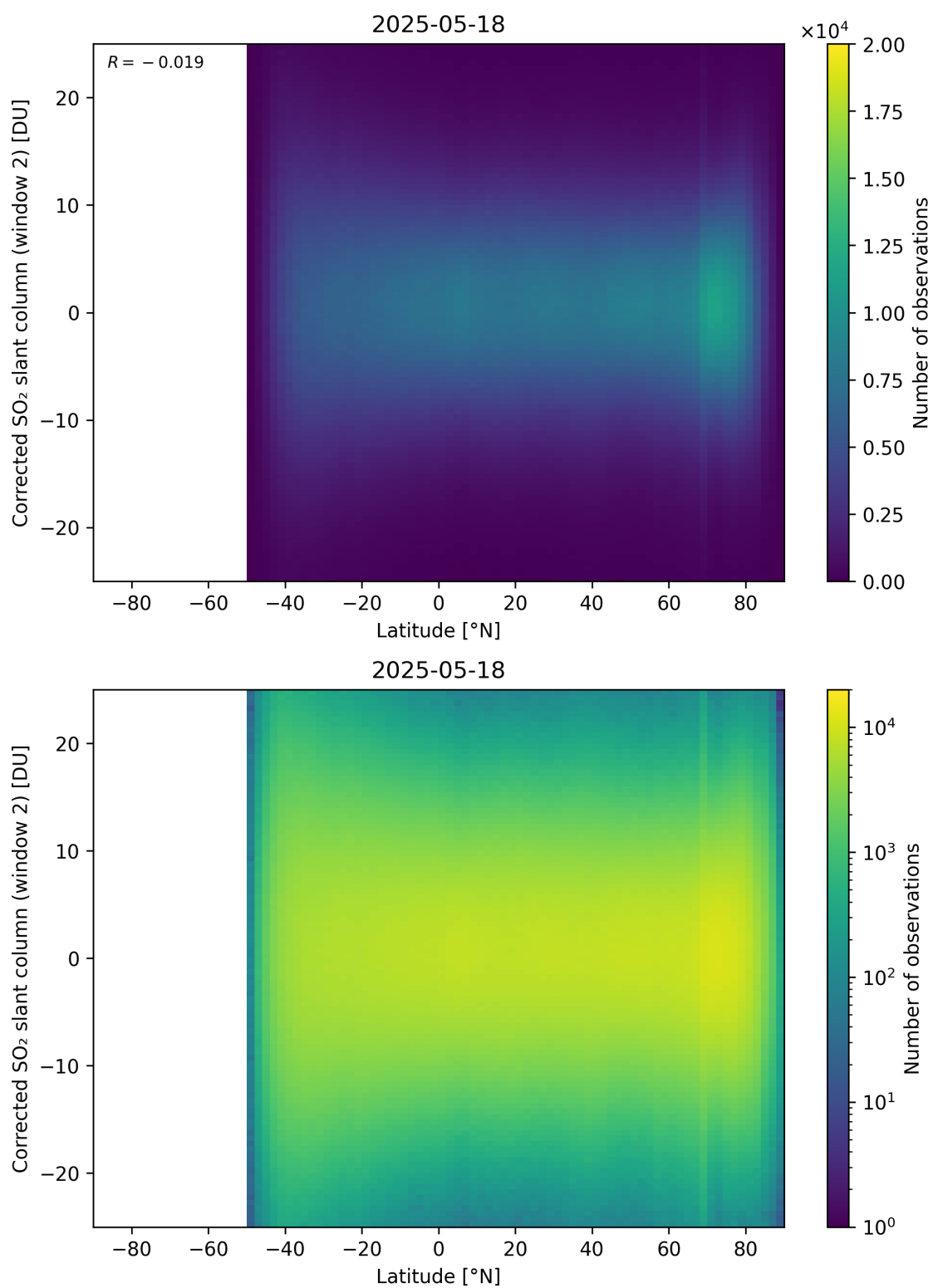
Figure 160: Scatter density plot of “Latitude” against “Corrected SO 2 slant column (window 2)” for 2025-05-17 to 2025-05-19.
