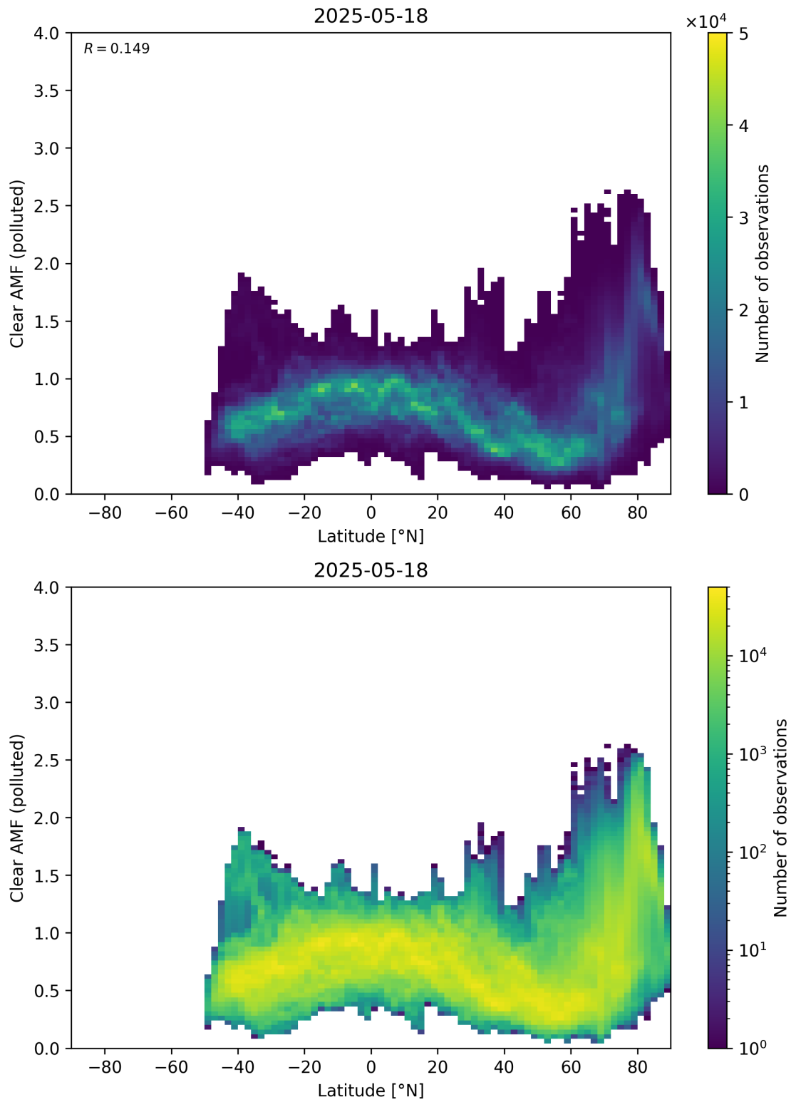
Figure 156: Scatter density plot of “Latitude” against “Clear AMF (polluted)” for 2025-05-17 to 2025-05-19.
