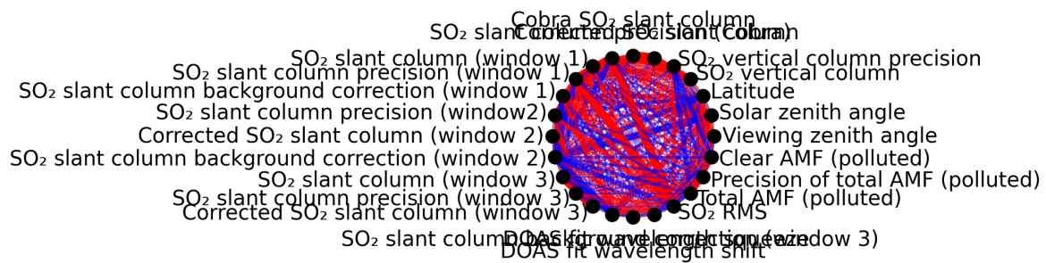
Figure 1: Map of correlation graph for 2025-05-17 to 2025-05-19.
