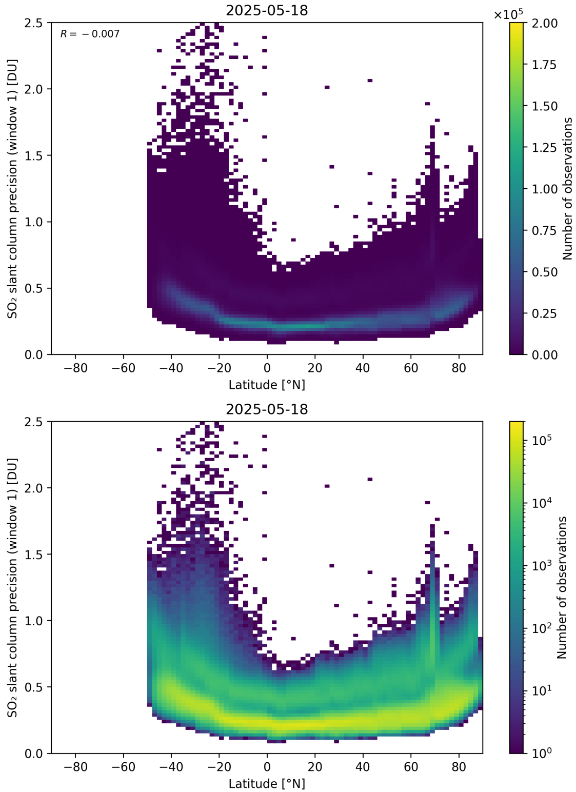
Figure 163: Scatter density plot of “Latitude” against “SO 2 slant column precision (window 1)” for 2025-05-17 to 2025-05-19.
