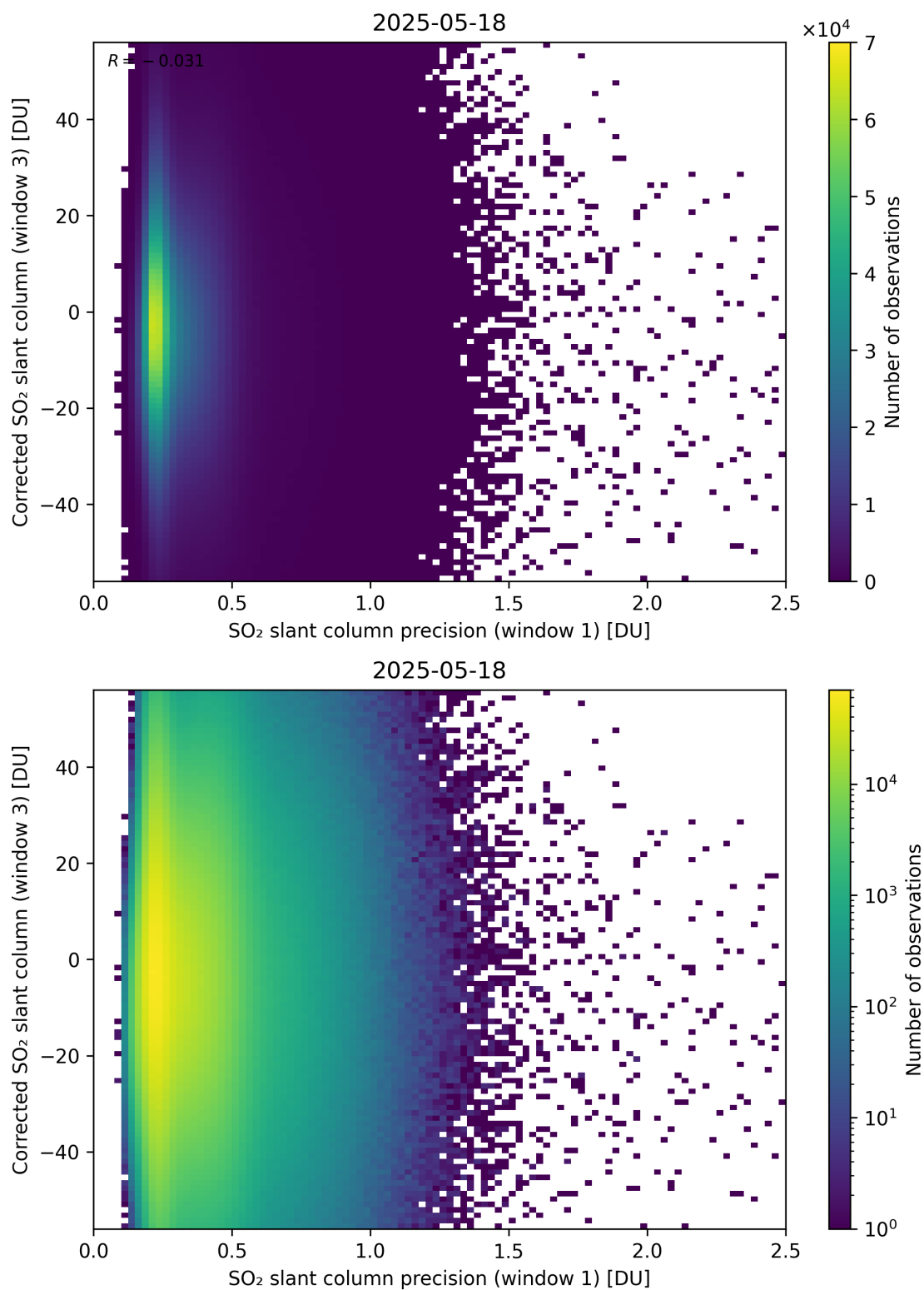
Figure 276: Scatter density plot of “SO 2 slant column precision (window 1)” against “Corrected SO 2 slant column (window 3)” for 2025-05-17 to 2025-05-19.
