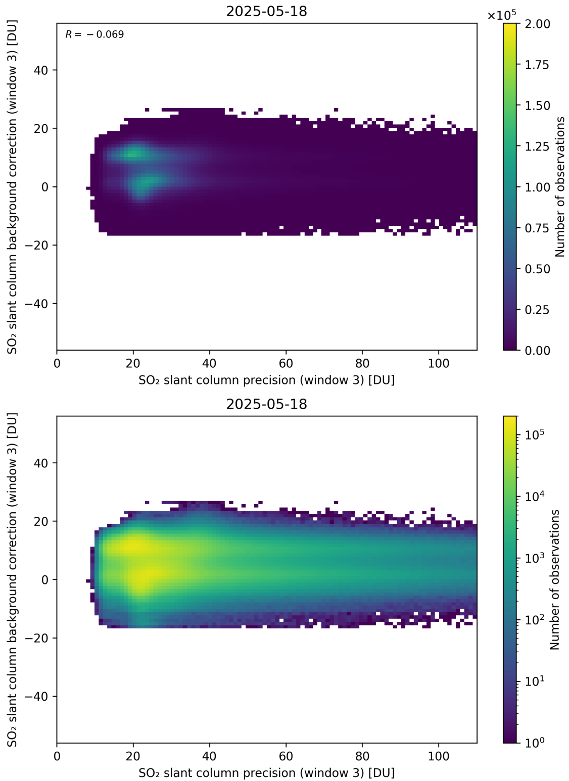
Figure 307: Scatter density plot of “SO 2 slant column precision (window 3)” against “SO 2 slant column background correction (window 3)” for 2025-05-17 to 2025-05-19.
