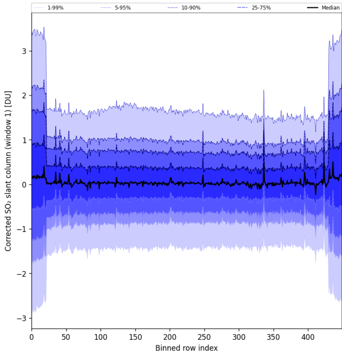
Figure 91: Along track statistics of “Corrected SO 2 slant column (window 1)” for 2025-05-17 to 2025-05-19
