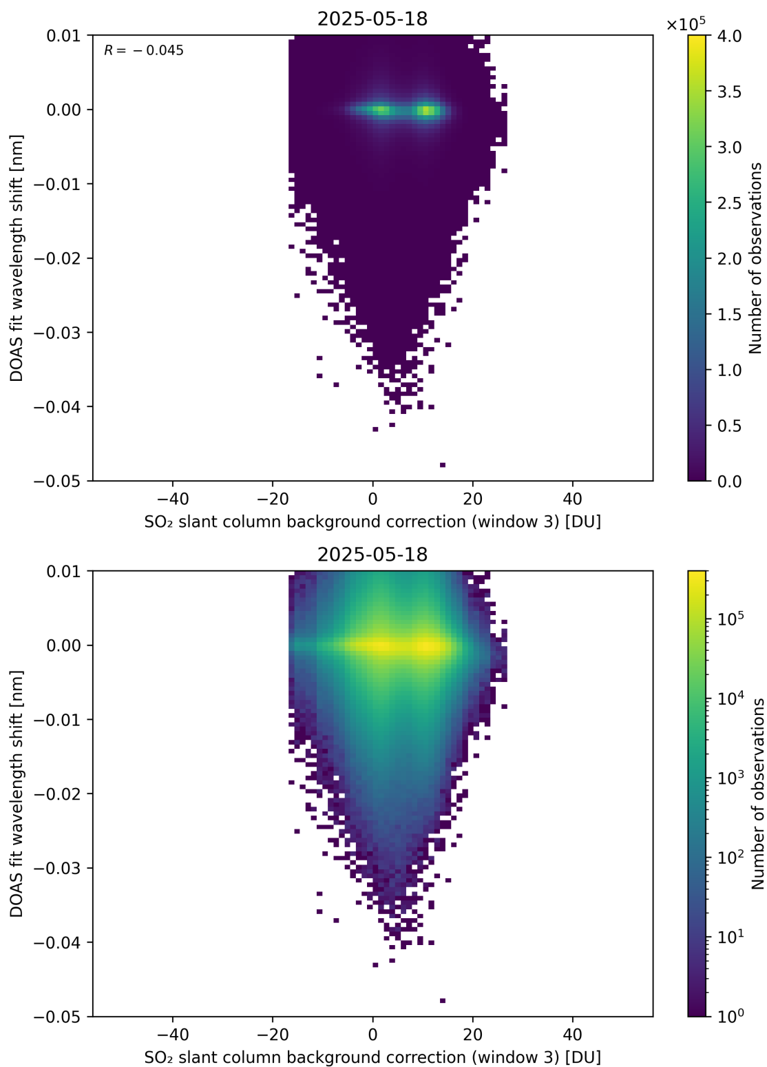
Figure 132: Scatter density plot of “SO 2 slant column background correction (window 3)” against “DOAS fit wavelength shift” for 2025-05-17 to 2025-05-19.
