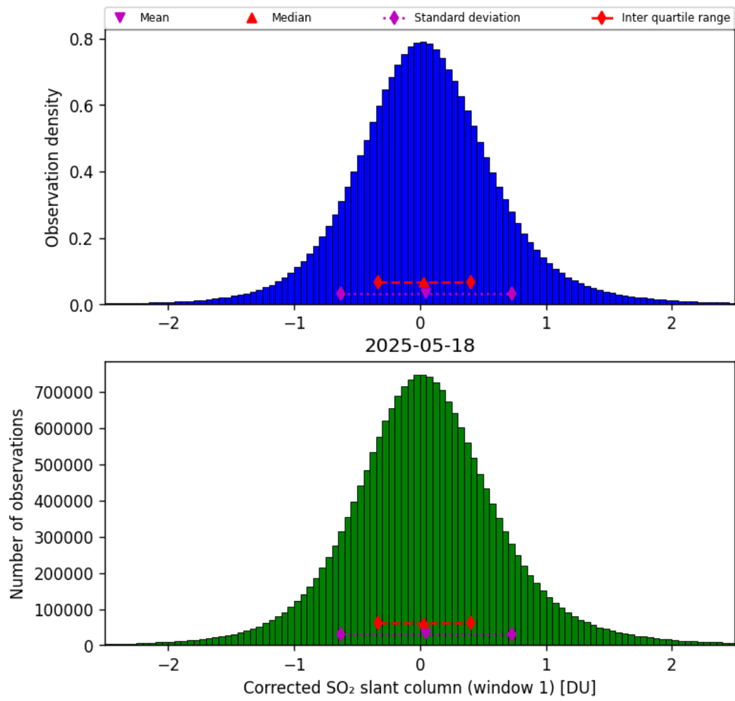
Figure 65: Histogram of “Corrected SO 2 slant column (window 1)” for 2025-05-17 to 2025-05-19
