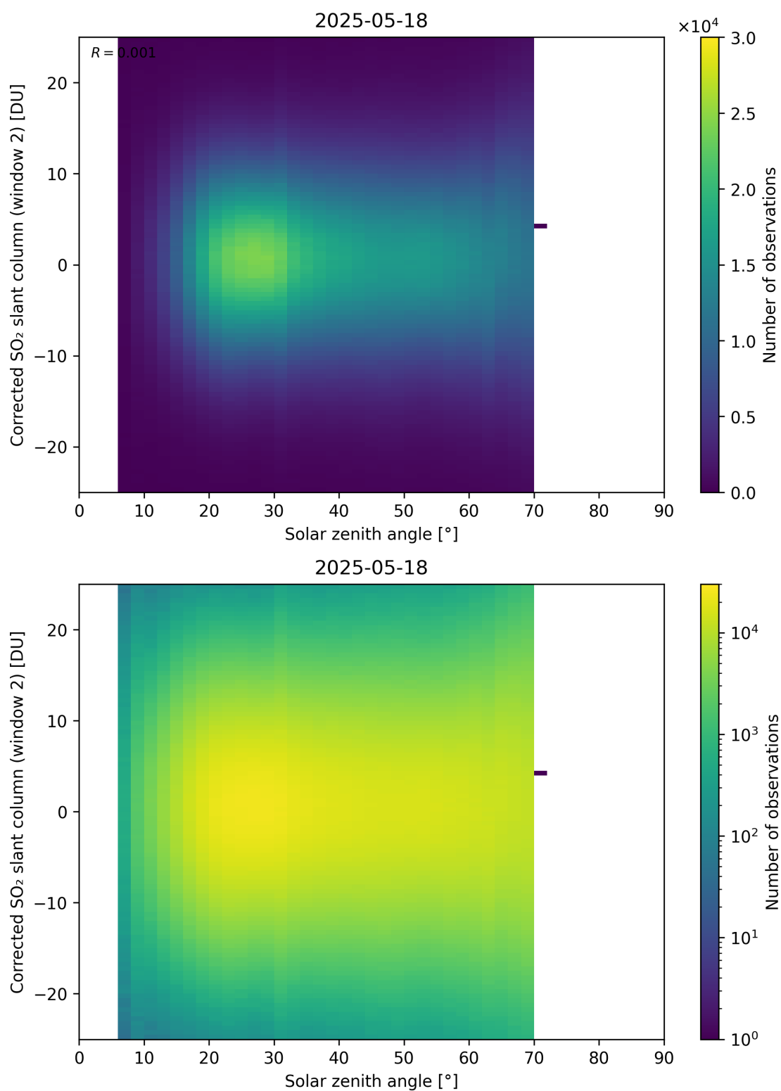
Figure 182: Scatter density plot of “Solar zenith angle” against “Corrected SO 2 slant column (window 2)” for 2025-05-17 to 2025-05-19.
