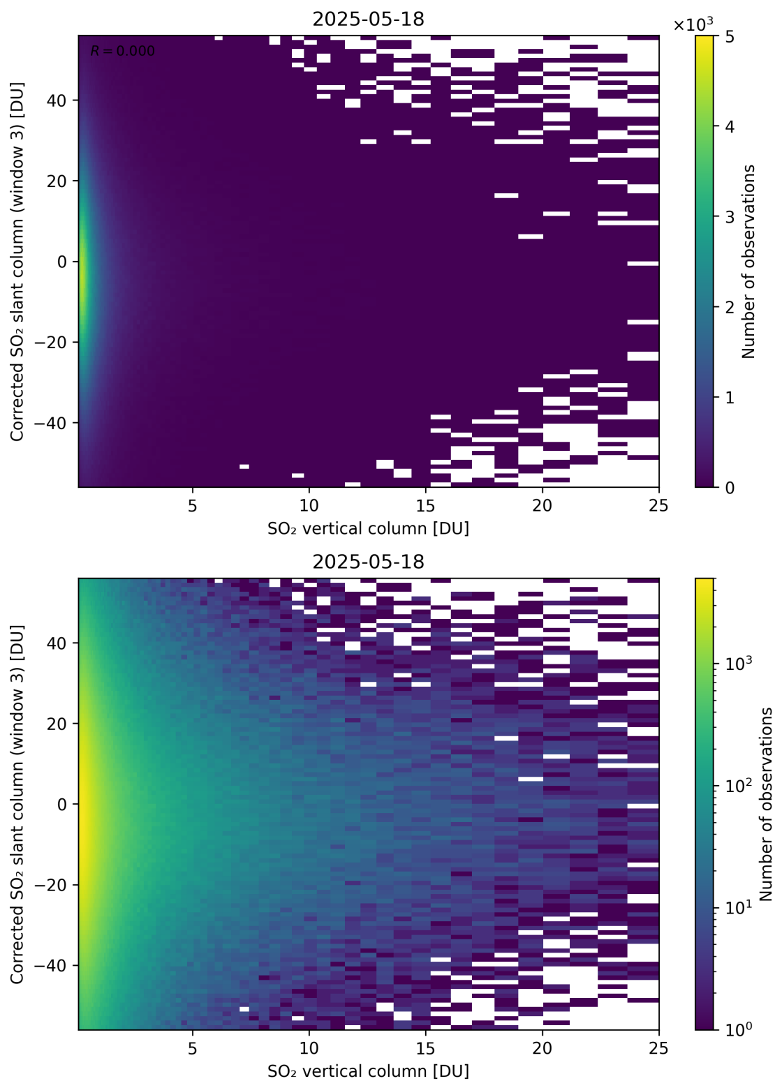
Figure 353: Scatter density plot of “SO 2 vertical column” against “Corrected SO 2 slant column (window 3)” for 2025-05-17 to 2025-05-19.
