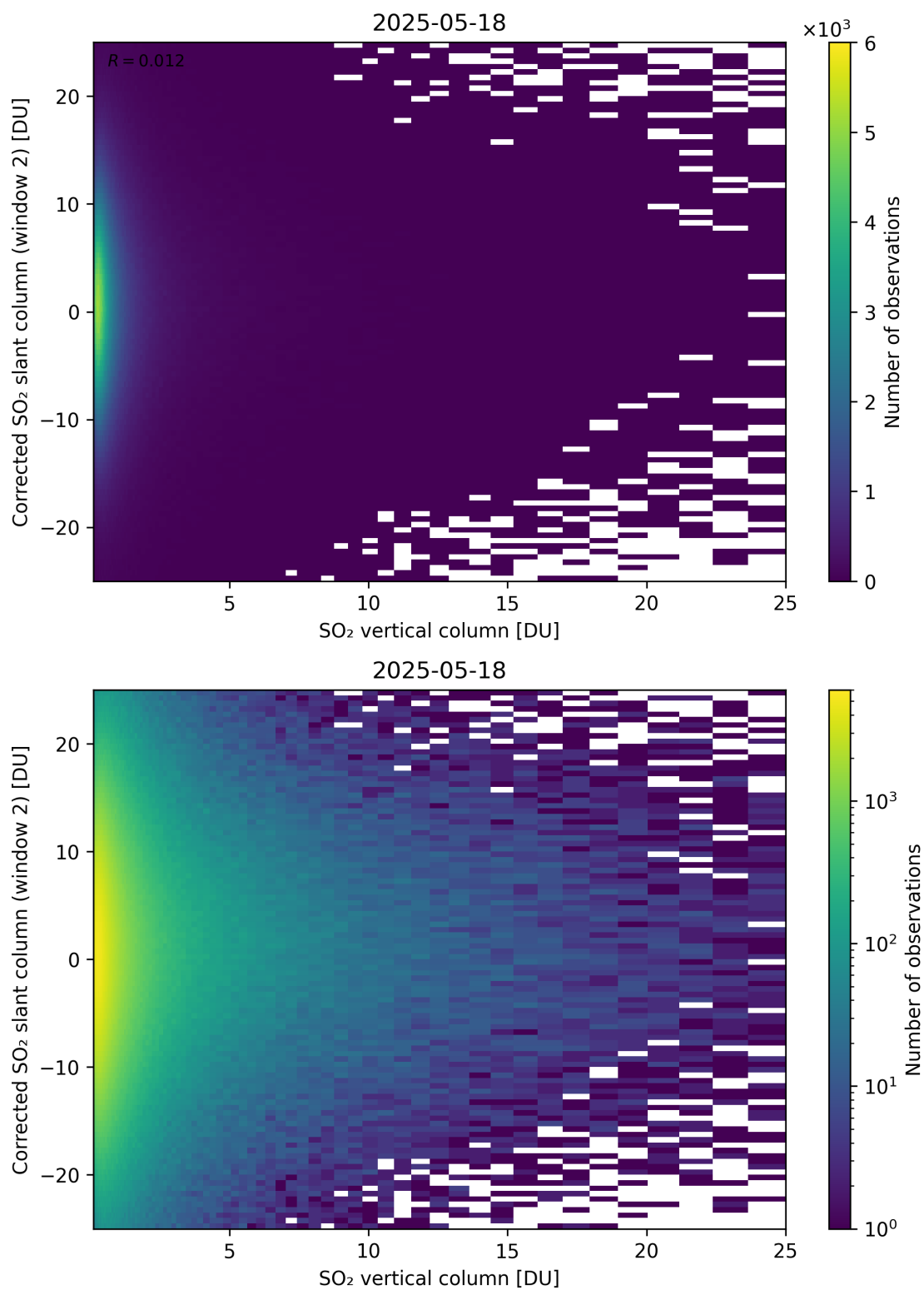
Figure 352: Scatter density plot of “SO 2 vertical column” against “Corrected SO 2 slant column (window 2)” for 2025-05-17 to 2025-05-19.
