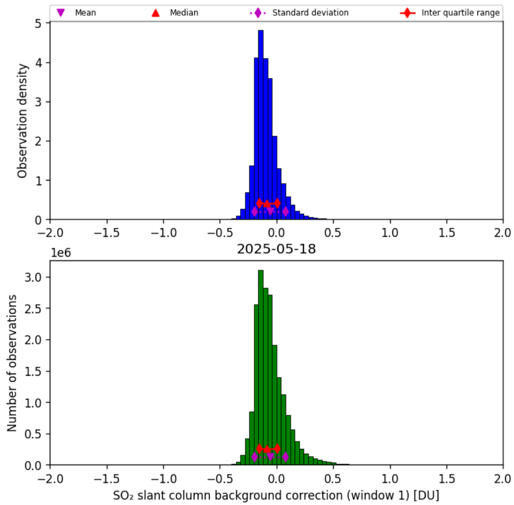
Figure 66: Histogram of “SO 2 slant column background correction (window 1)” for 2025-05-17 to 2025-05-19
