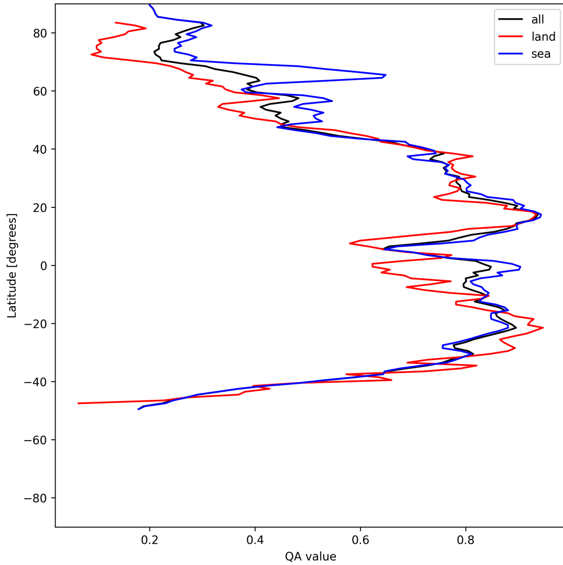
Figure 31: Zonal average of “QA value” for 2025-05-17 to 2025-05-19.
