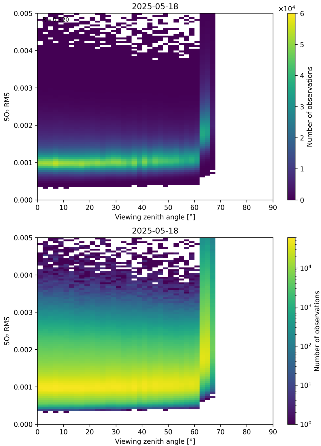
Figure 367: Scatter density plot of “Viewing zenith angle” against “SO 2 RMS” for 2025-05-17 to 2025-05-19.
