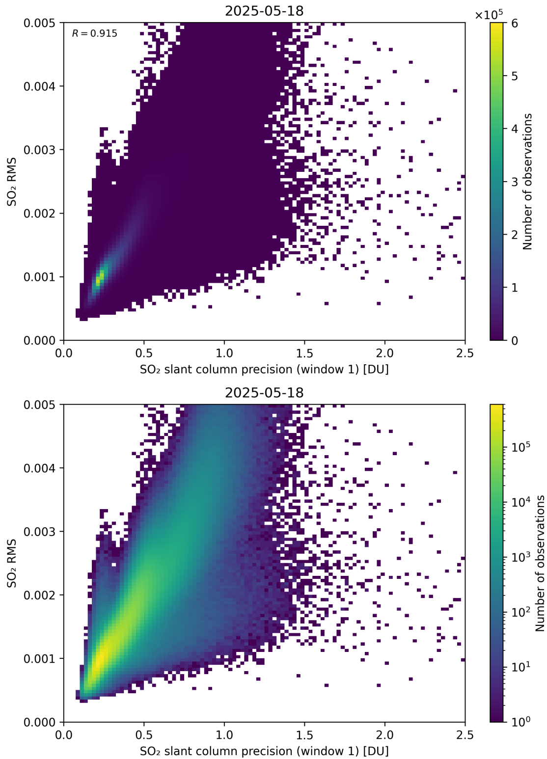
Figure 273: Scatter density plot of “SO 2 slant column precision (window 1)” against “SO 2 RMS” for 2025-05-17 to 2025-05-19.
