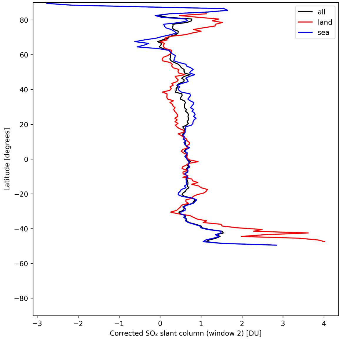
Figure 43: Zonal average of “Corrected SO 2 slant column (window 2)” for 2025-05-17 to 2025-05-19.
