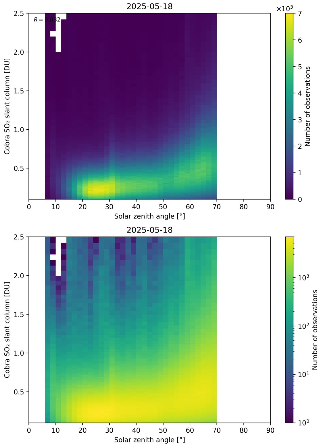
Figure 179: Scatter density plot of “Solar zenith angle” against “Cobra SO 2 slant column” for 2025-05-17 to 2025-05-19.
