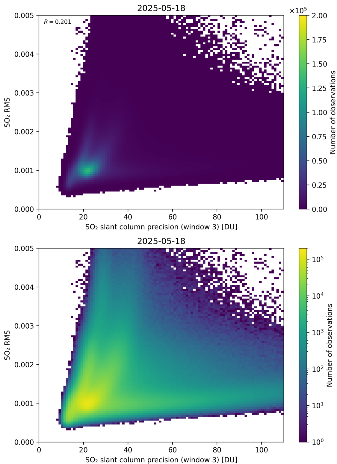
Figure 310: Scatter density plot of “SO 2 slant column precision (window 3)” against “SO 2 RMS” for 2025-05-17 to 2025-05-19.
