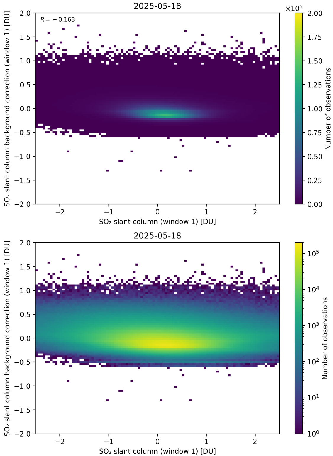
Figure 262: Scatter density plot of “SO 2 slant column (window 1)” against “SO 2 slant column background correction (window 1)” for 2025-05-17 to 2025-05-19.
