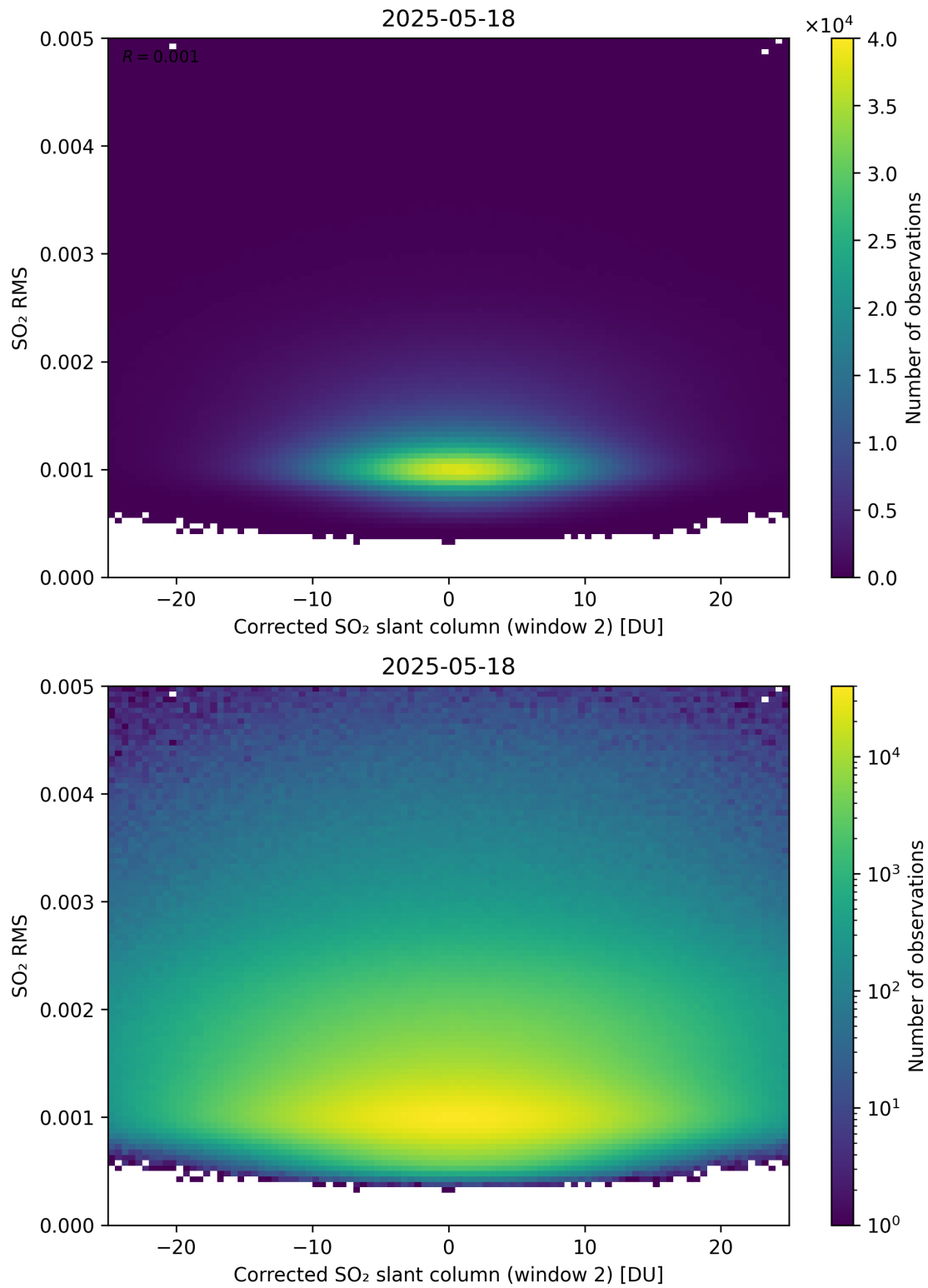
Figure 248: Scatter density plot of “Corrected SO 2 slant column (window 2)” against “SO 2 RMS” for 2025-05-17 to 2025-05-19.
