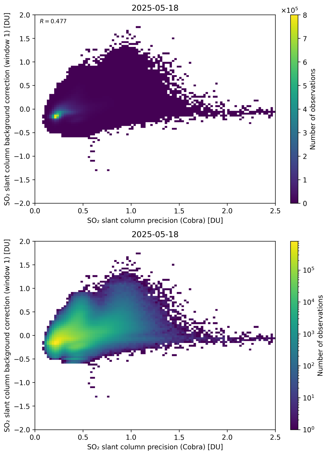
Figure 199: Scatter density plot of “SO 2 slant column precision (Cobra)” against “SO 2 slant column background correction (window 1)” for 2025-05-17 to 2025-05-19.
