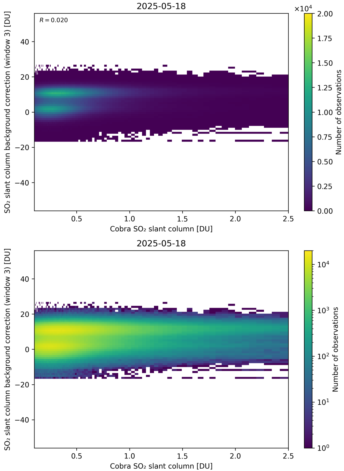
Figure 195: Scatter density plot of “Cobra SO 2 slant column” against “SO 2 slant column background correction (window 3)” for 2025-05-17 to 2025-05-19.
