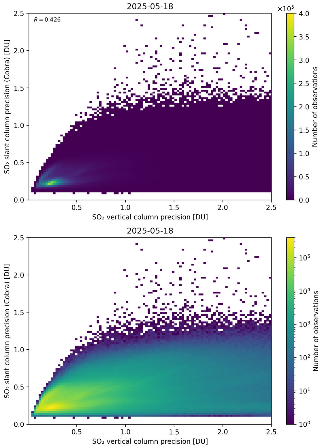
Figure 337: Scatter density plot of “SO 2 vertical column precision” against “SO 2 slant column precision (Cobra)” for 2025-05-17 to 2025-05-19.
