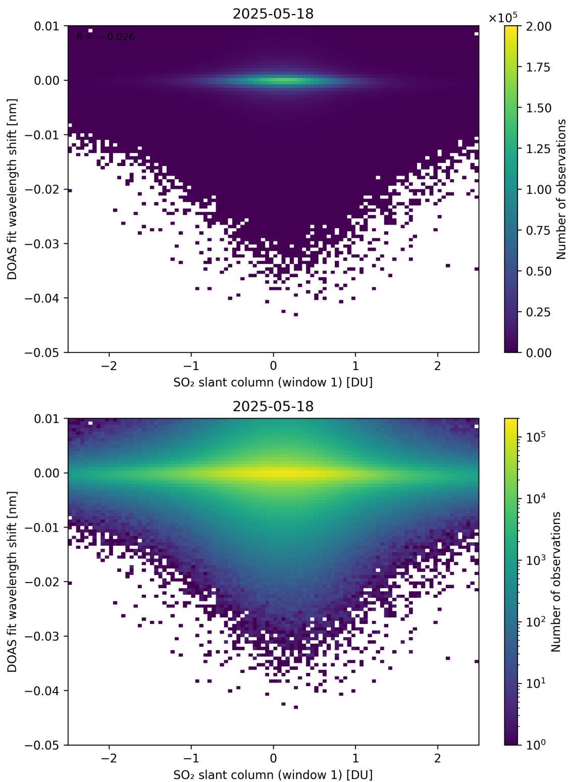
Figure 265: Scatter density plot of “SO 2 slant column (window 1)” against “DOAS fit wavelength shift” for 2025-05-17 to 2025-05-19.
