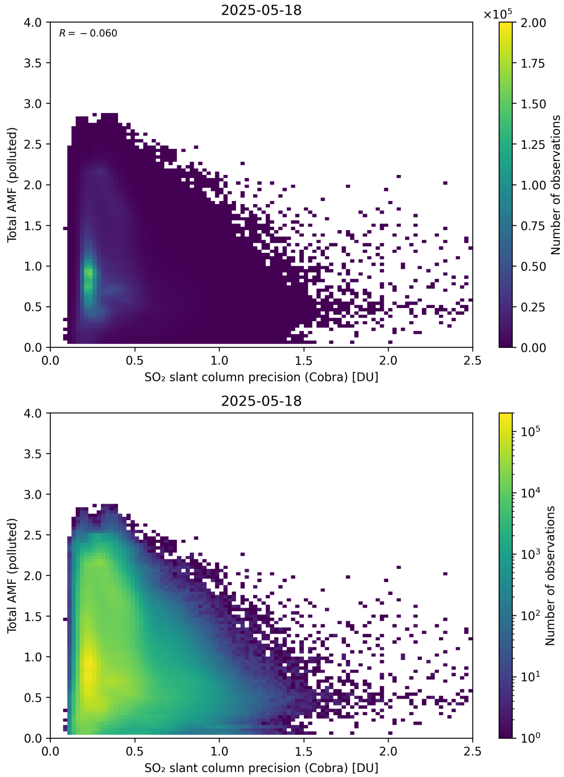
Figure 213: Scatter density plot of “SO 2 slant column precision (Cobra)” against “Total AMF (polluted)” for 2025-05-17 to 2025-05-19.
