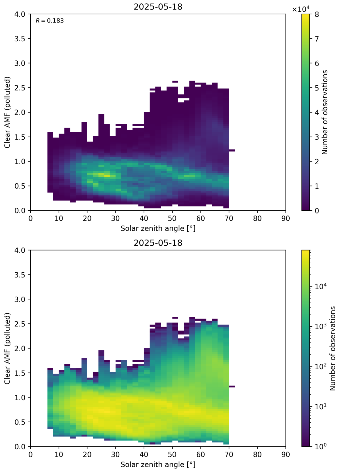
Figure 178: Scatter density plot of “Solar zenith angle” against “Clear AMF (polluted)” for 2025-05-17 to 2025-05-19.
