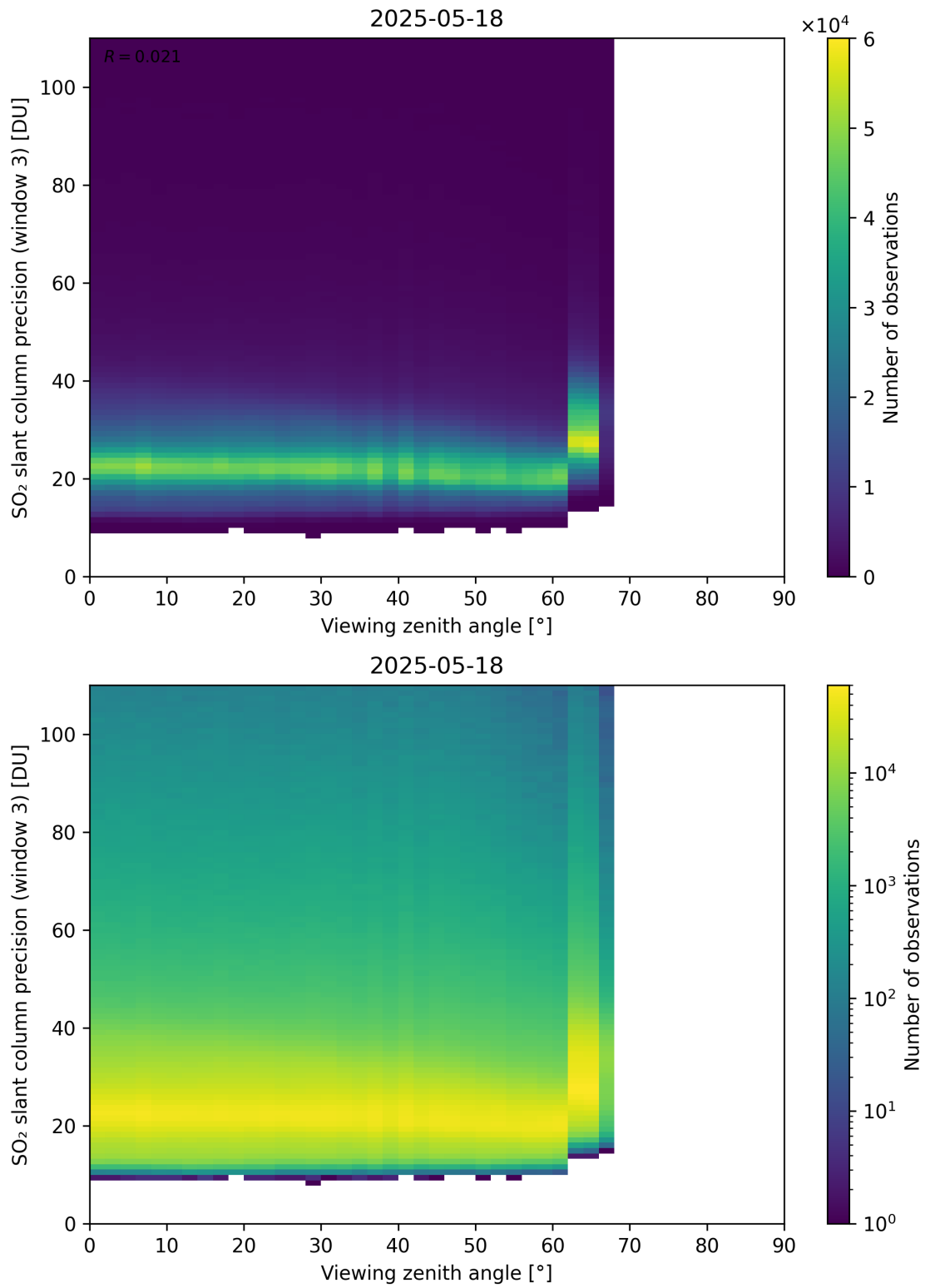
Figure 380: Scatter density plot of “Viewing zenith angle” against “SO 2 slant column precision (window 3)” for 2025-05-17 to 2025-05-19.
