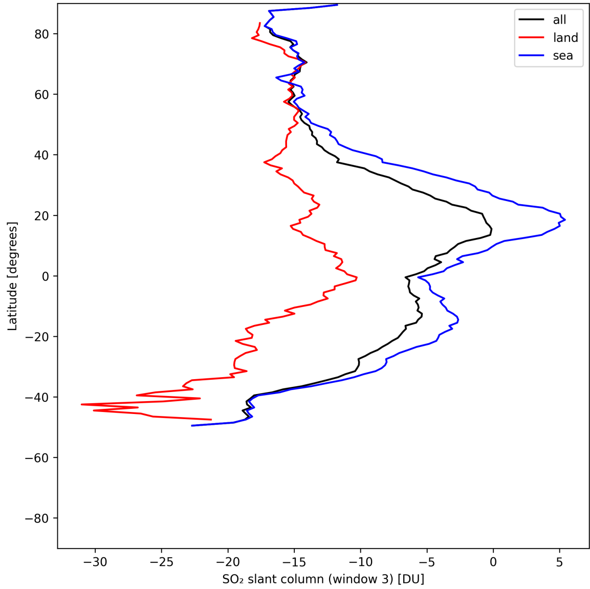
Figure 45: Zonal average of “SO 2 slant column (window 3)” for 2025-05-17 to 2025-05-19.
