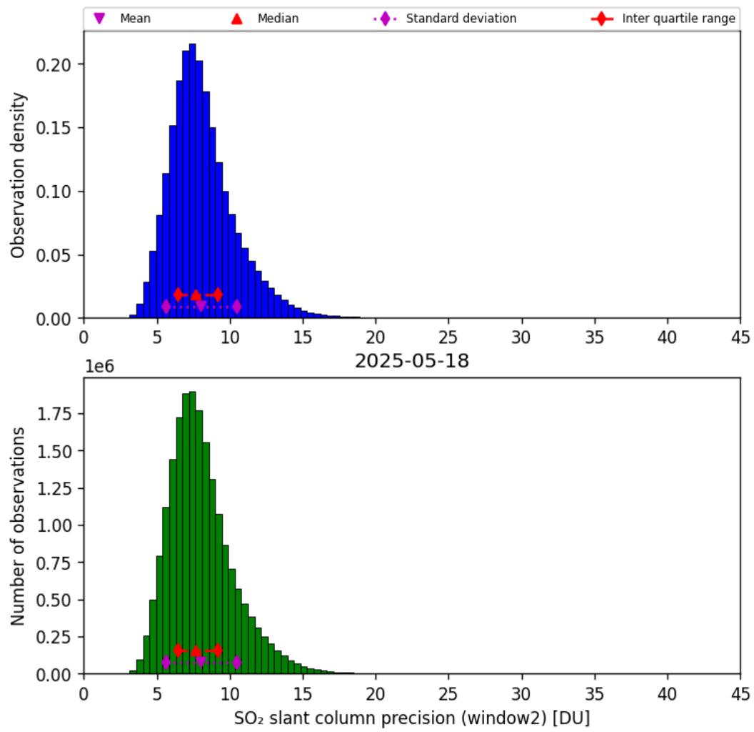
Figure 68: Histogram of “SO 2 slant column precision (window2)” for 2025-05-17 to 2025-05-19
