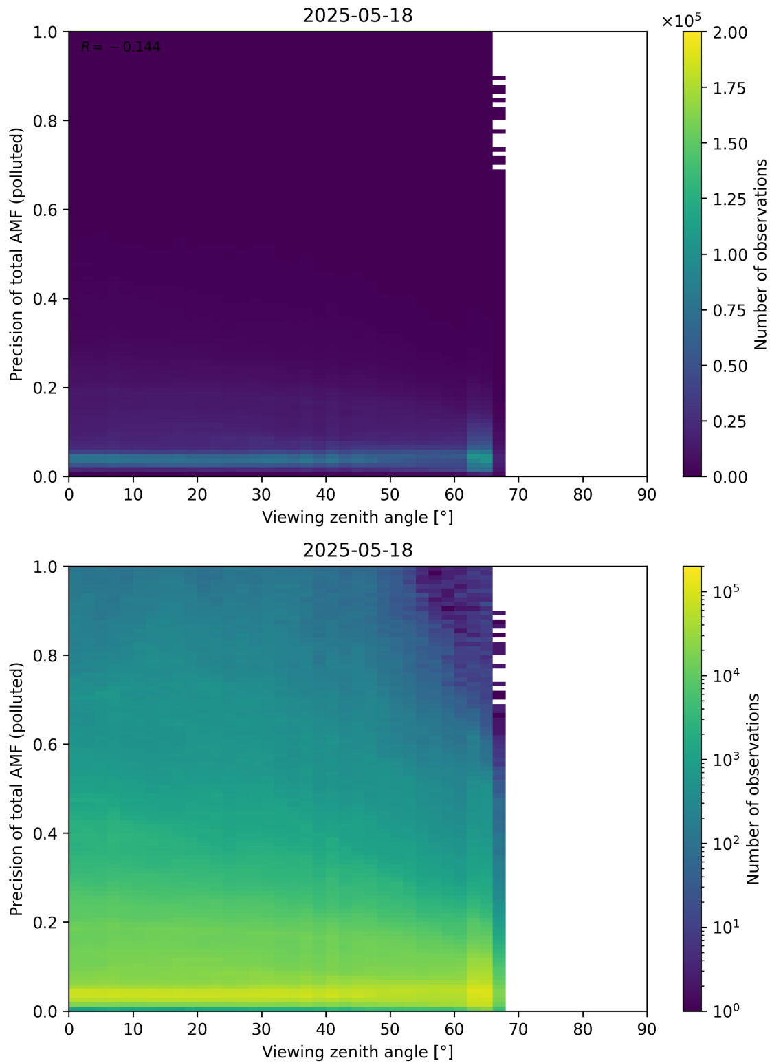
Figure 382: Scatter density plot of “Viewing zenith angle” against “Precision of total AMF (polluted)” for 2025-05-17 to 2025-05-19.
