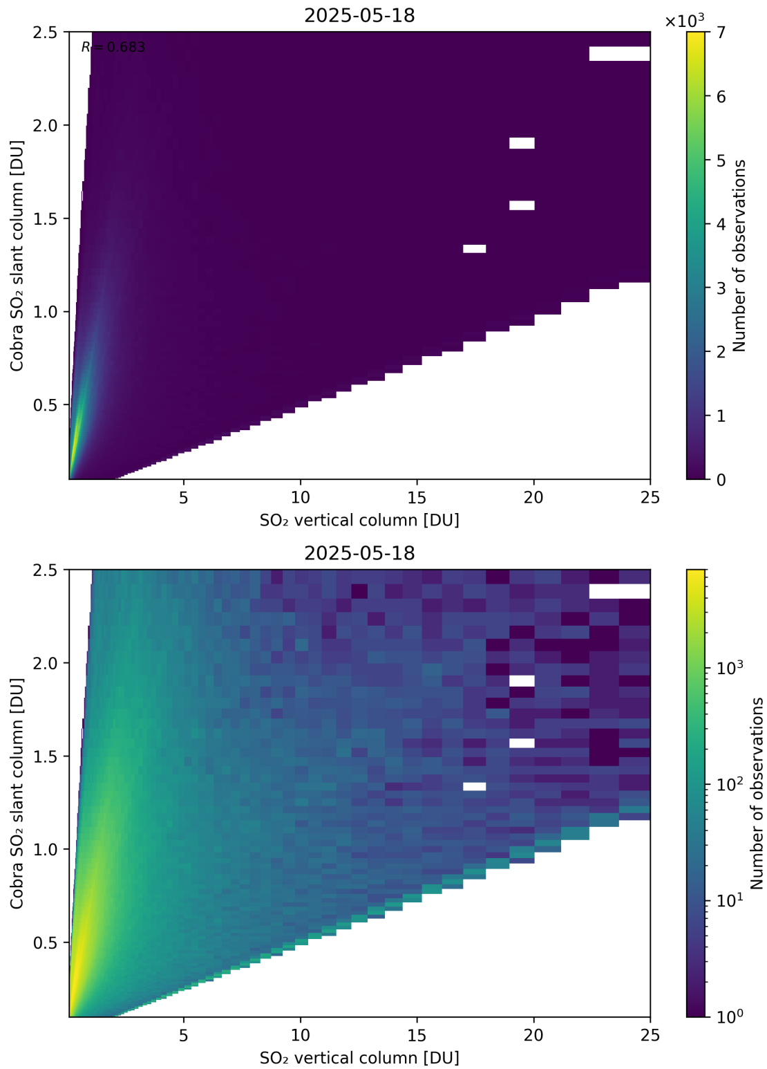
Figure 349: Scatter density plot of “SO 2 vertical column” against “Cobra SO 2 slant column” for 2025-05-17 to 2025-05-19.
