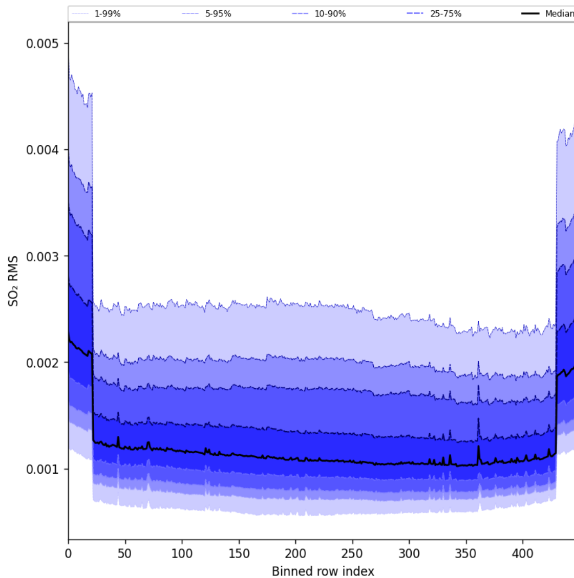
Figure 104: Along track statistics of “SO 2 RMS” for 2025-05-17 to 2025-05-19
