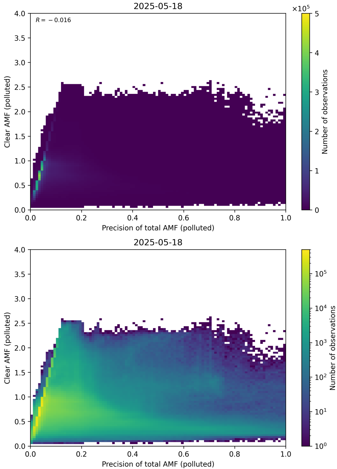
Figure 320: Scatter density plot of “Precision of total AMF (polluted)” against “Clear AMF (polluted)” for 2025-05-17 to 2025-05-19.
