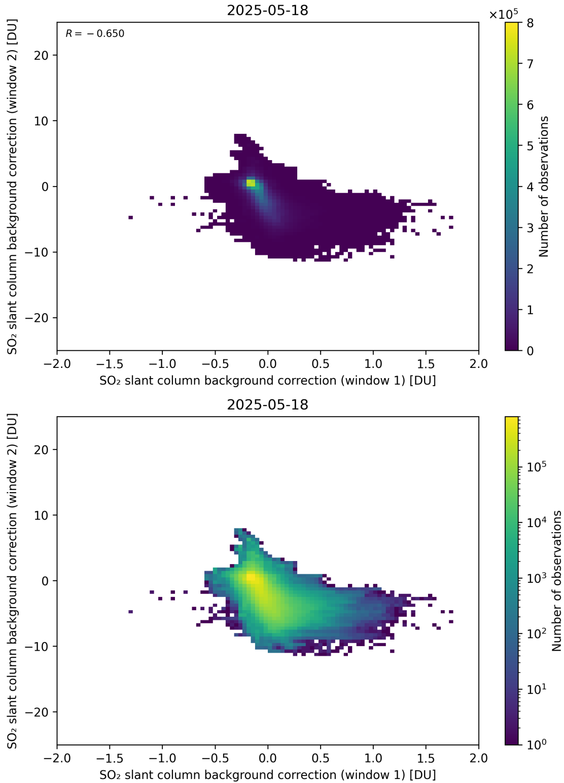
Figure 109: Scatter density plot of “SO 2 slant column background correction (window 1)” against “SO 2 slant column background correction (window 2)” for 2025-05-17 to 2025-05-19.
