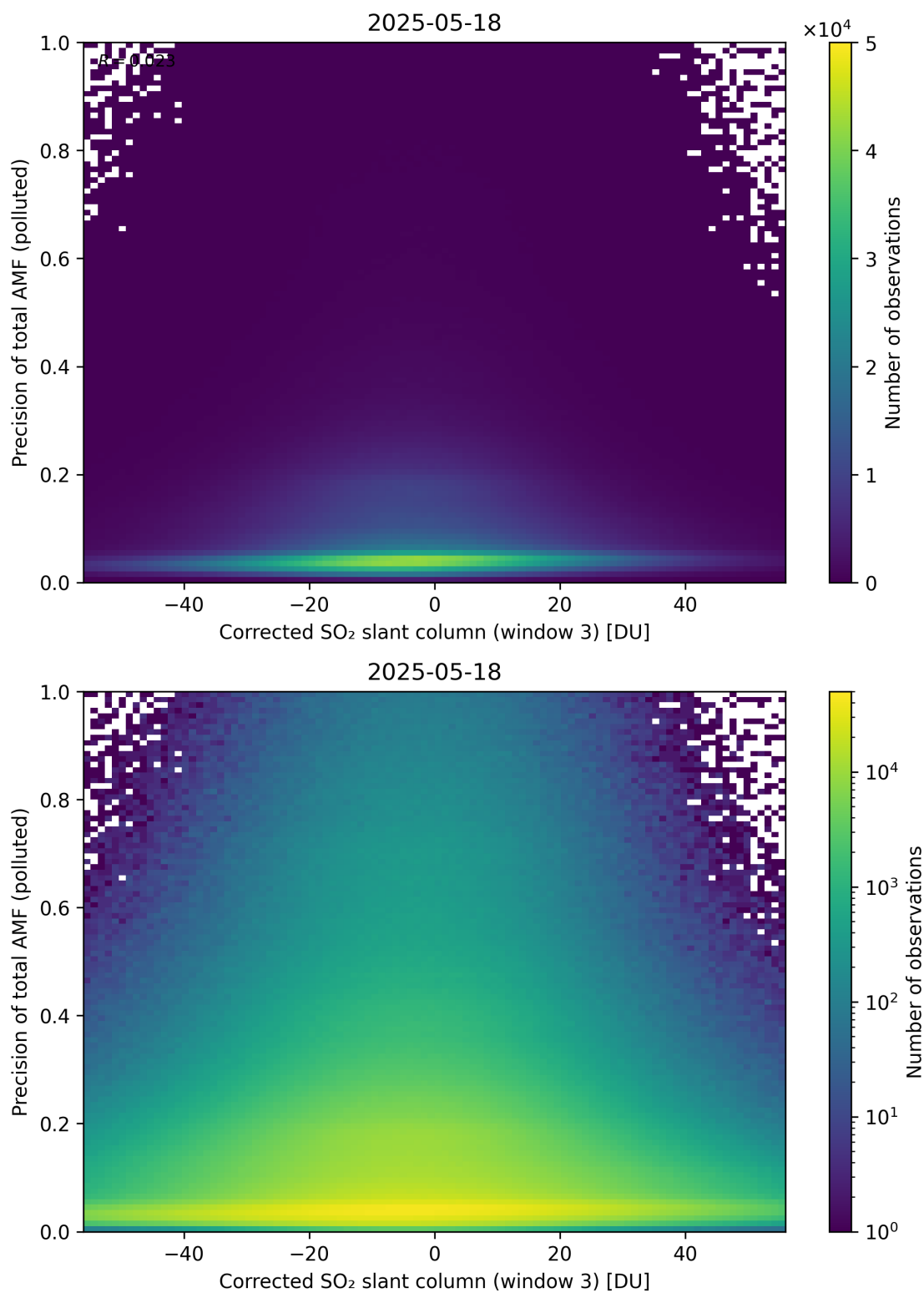
Figure 261: Scatter density plot of “Corrected SO 2 slant column (window 3)” against “Precision of total AMF (polluted)” for 2025-05-17 to 2025-05-19.
