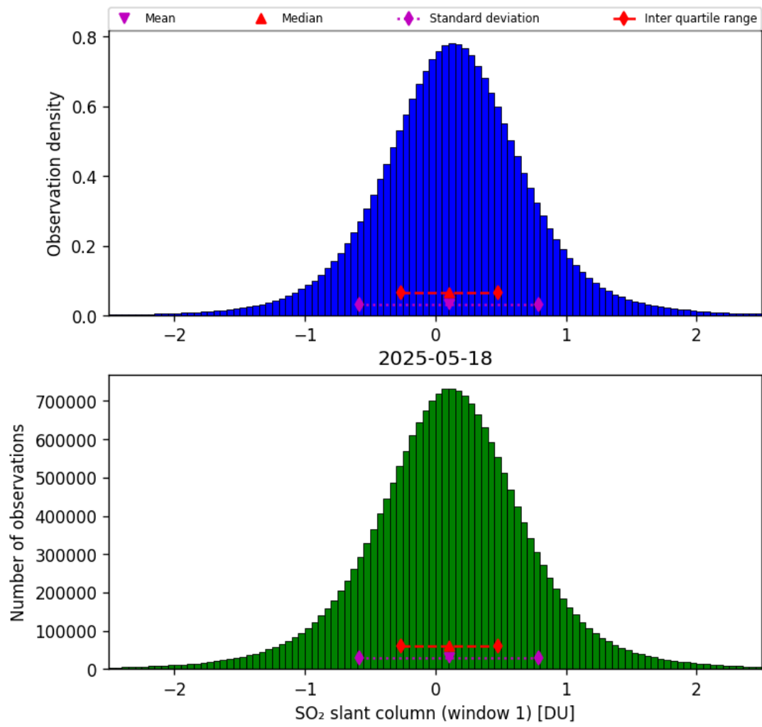
Figure 63: Histogram of “SO 2 slant column (window 1)” for 2025-05-17 to 2025-05-19
