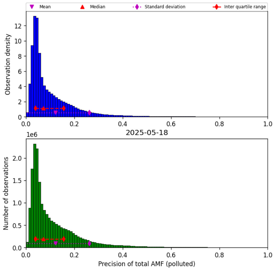
Figure 80: Histogram of “Precision of total AMF (polluted)” for 2025-05-17 to 2025-05-19
