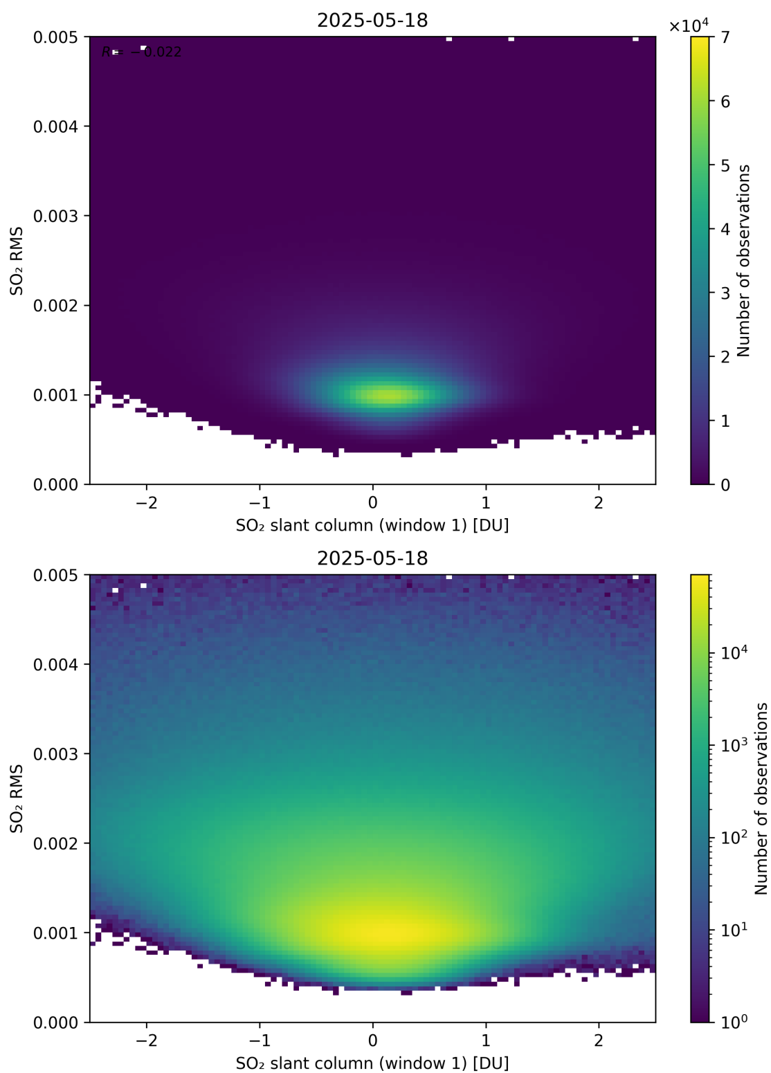
Figure 267: Scatter density plot of “SO 2 slant column (window 1)” against “SO 2 RMS” for 2025-05-17 to 2025-05-19.
