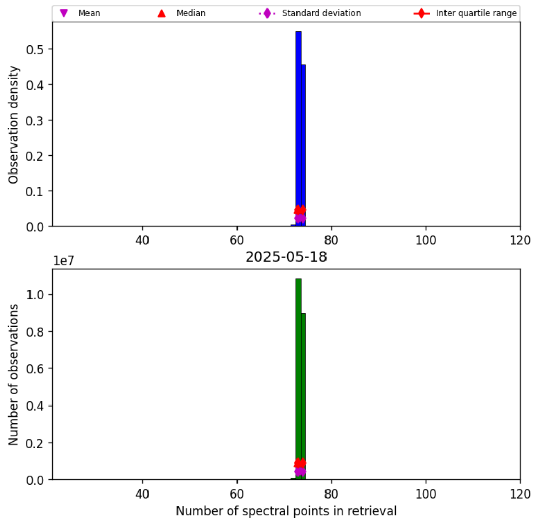
Figure 82: Histogram of “Number of spectral points in retrieval” for 2025-05-17 to 2025-05-19
