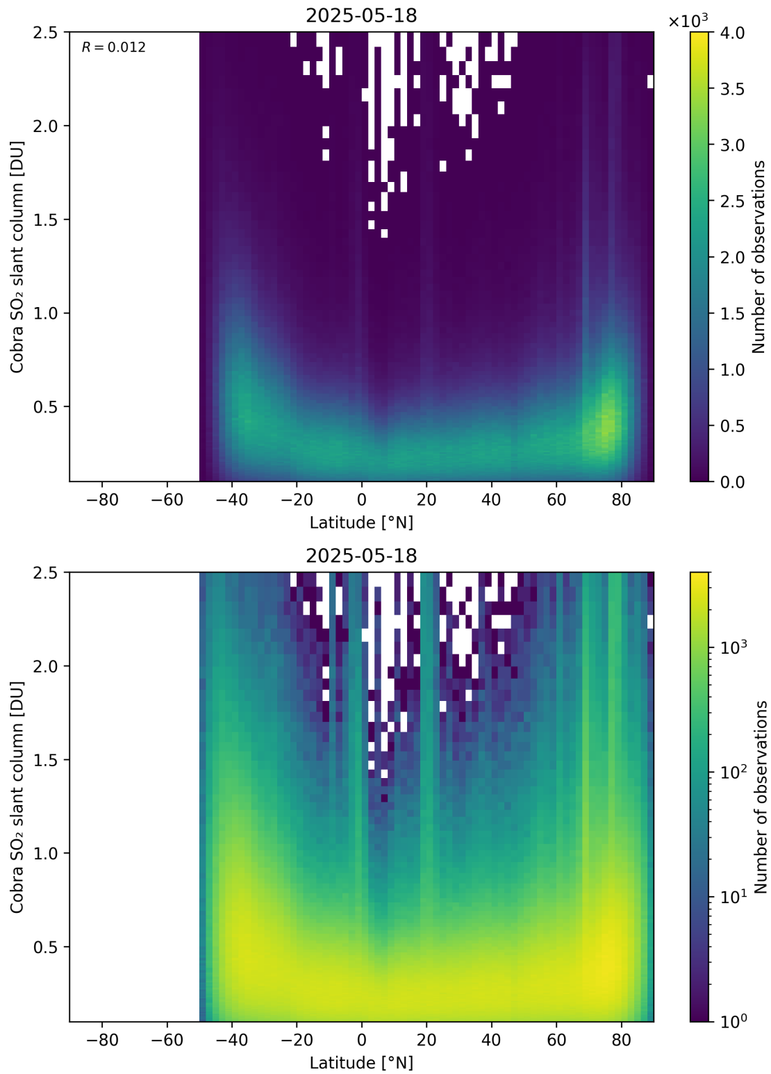
Figure 157: Scatter density plot of “Latitude” against “Cobra SO 2 slant column” for 2025-05-17 to 2025-05-19.
