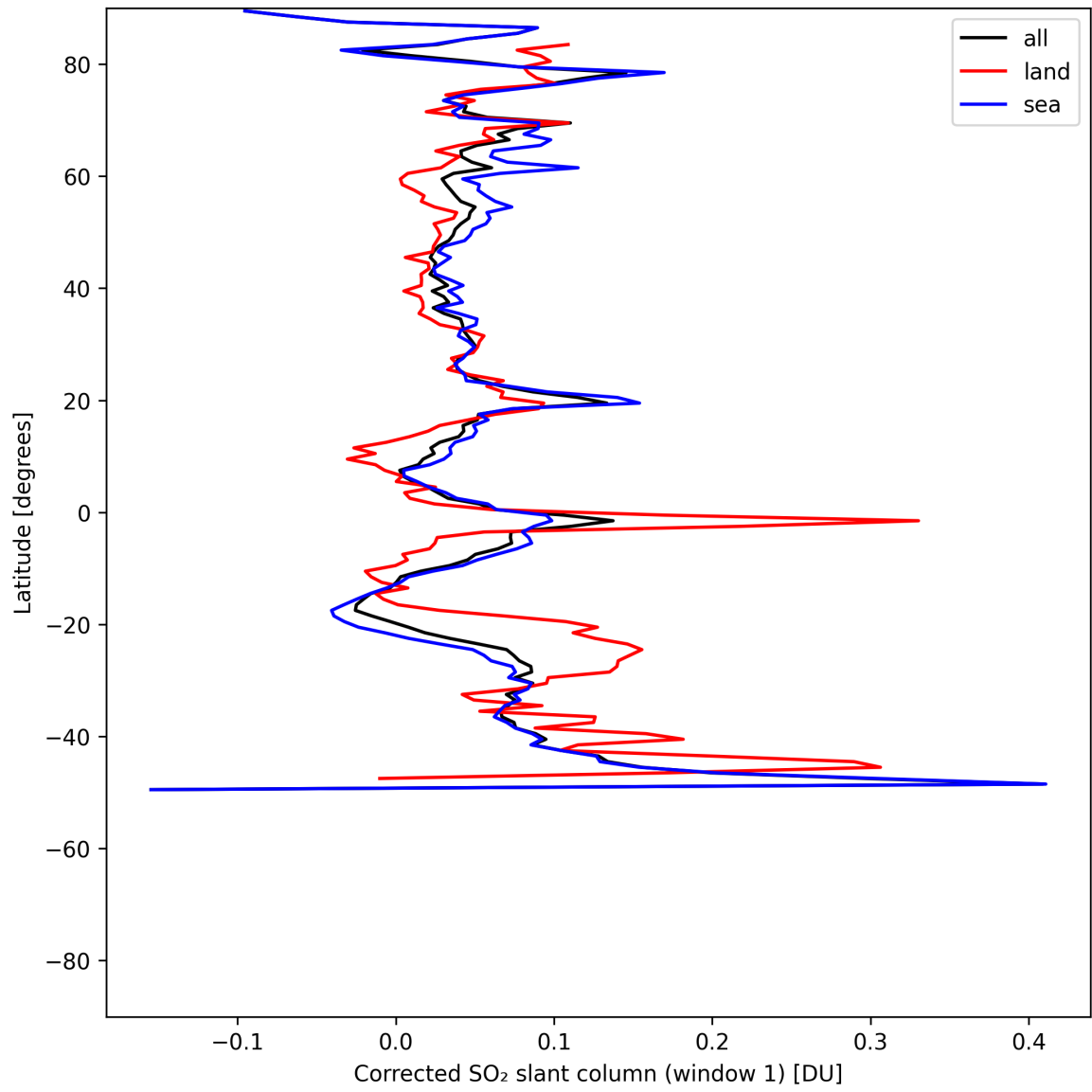
Figure 39: Zonal average of “Corrected SO 2 slant column (window 1)” for 2025-05-17 to 2025-05-19.
