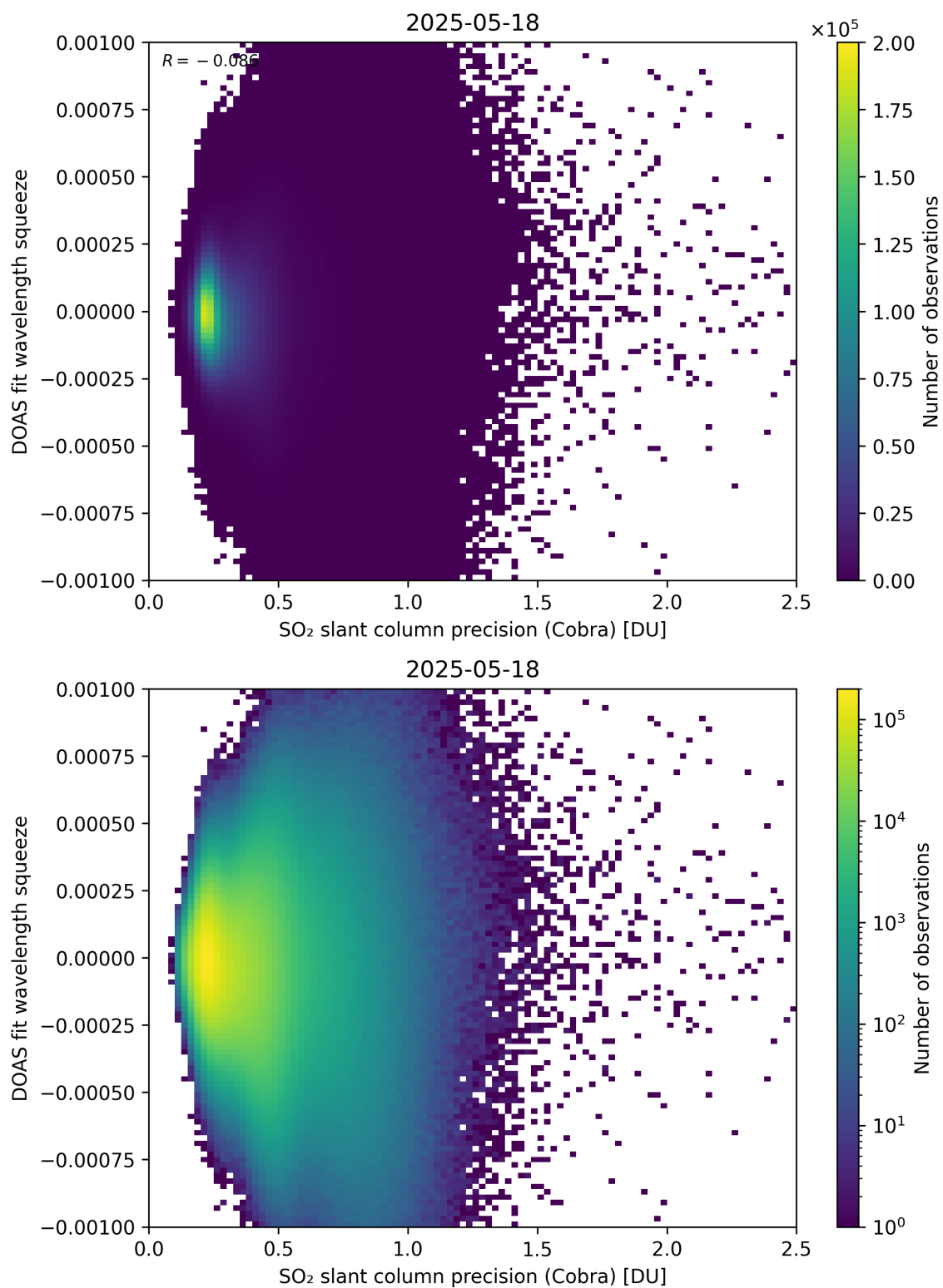
Figure 203: Scatter density plot of “SO 2 slant column precision (Cobra)” against “DOAS fit wavelength squeeze” for 2025-05-17 to 2025-05-19.
