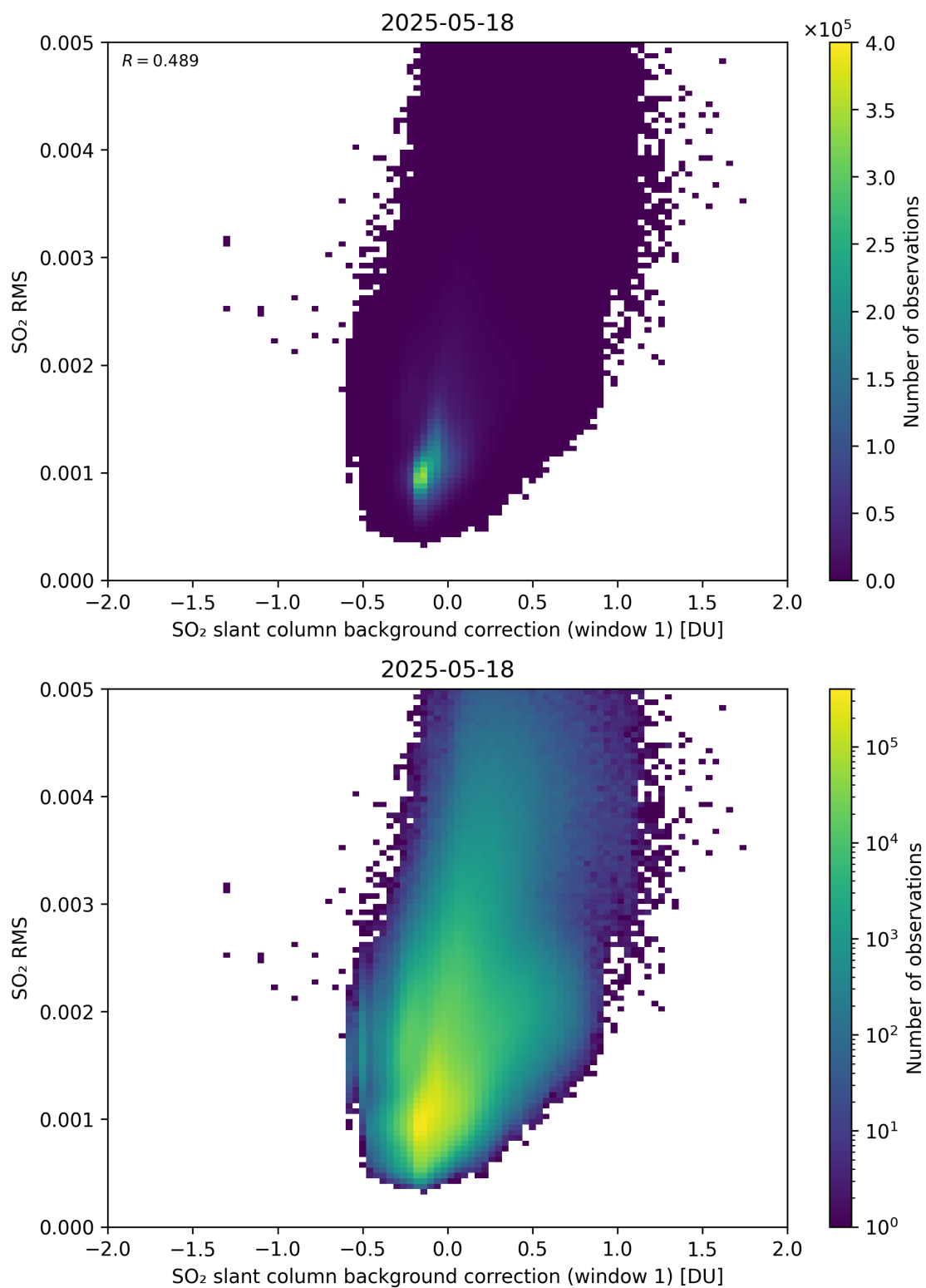
Figure 113: Scatter density plot of “SO 2 slant column background correction (window 1)” against “SO 2 RMS” for 2025-05-17 to 2025-05-19.
