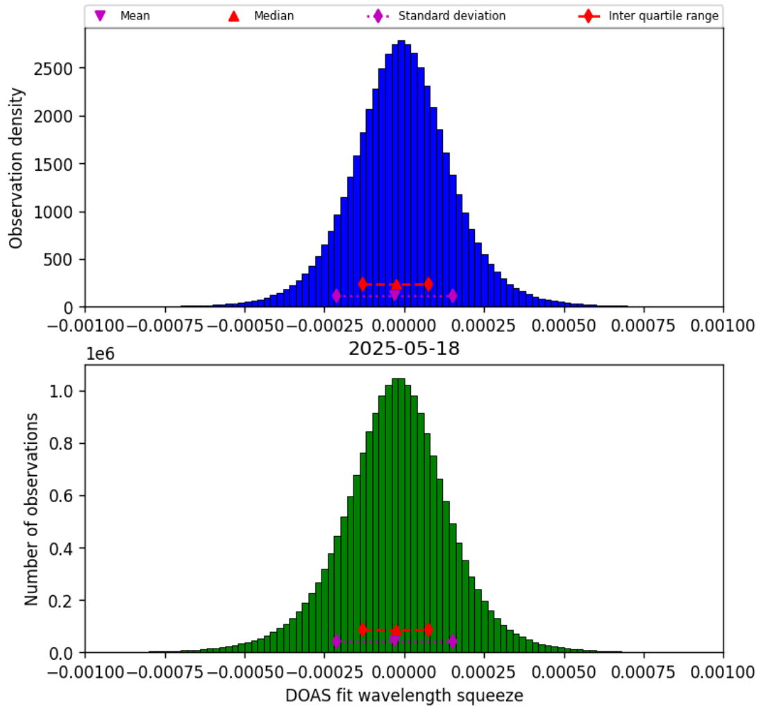
Figure 77: Histogram of “DOAS fit wavelength squeeze” for 2025-05-17 to 2025-05-19
