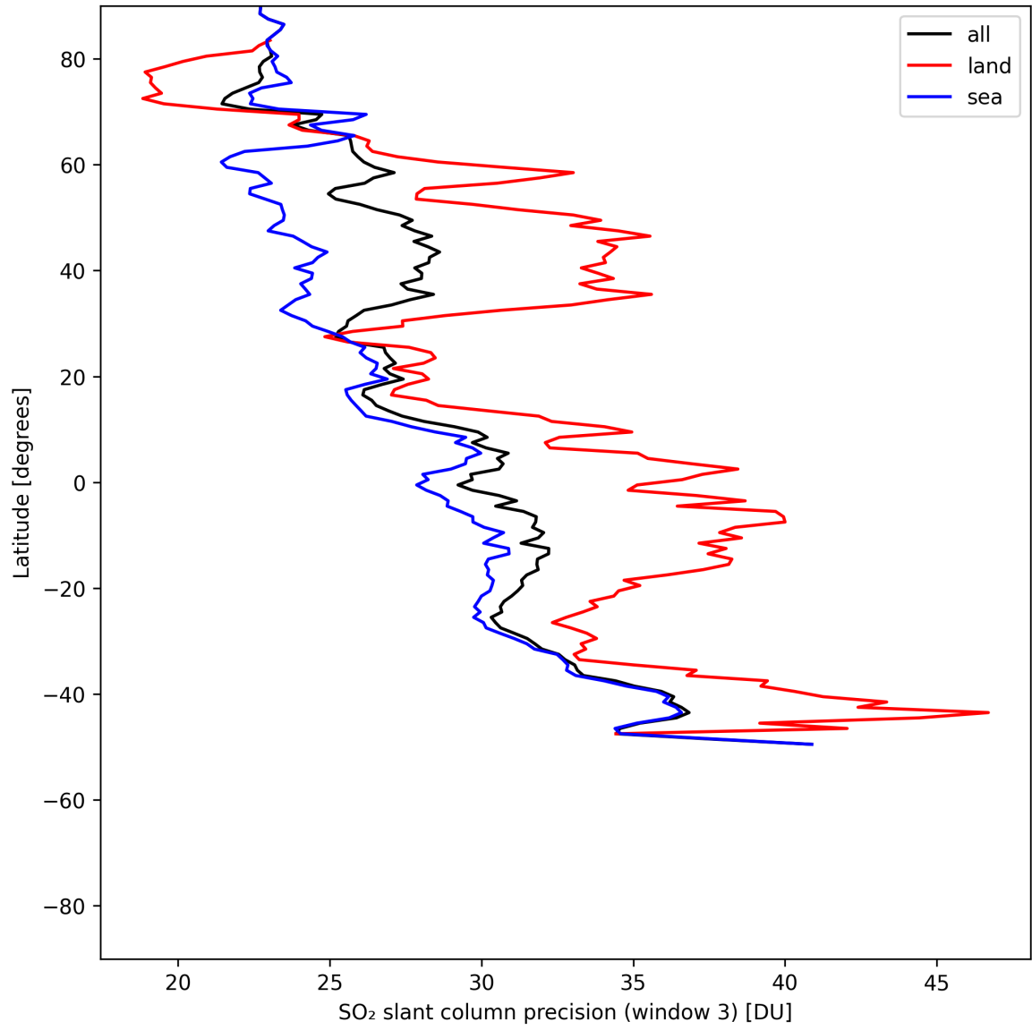
Figure 46: Zonal average of “SO 2 slant column precision (window 3)” for 2025-05-17 to 2025-05-19.
