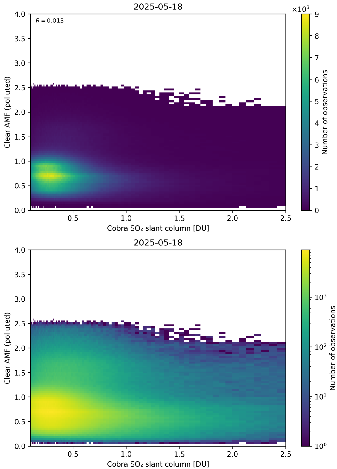
Figure 215: Scatter density plot of “Cobra SO 2 slant column” against “Clear AMF (polluted)” for 2025-05-17 to 2025-05-19.
