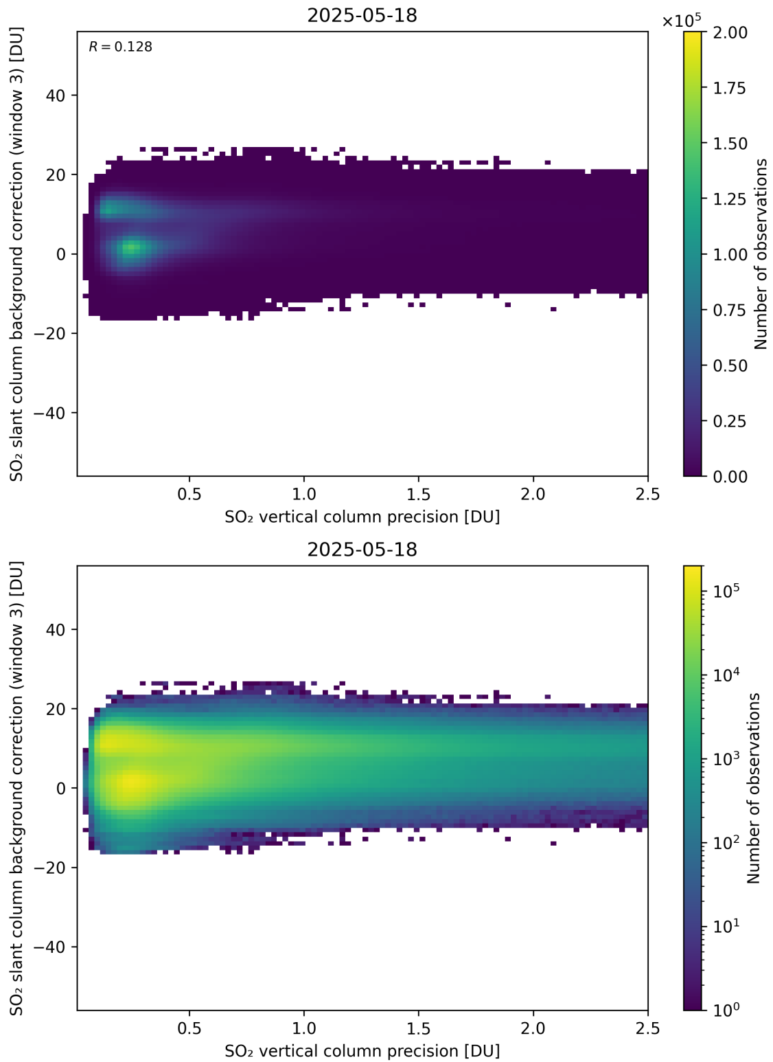
Figure 331: Scatter density plot of “SO 2 vertical column precision” against “SO 2 slant column background correction (window 3)” for 2025-05-17 to 2025-05-19.
