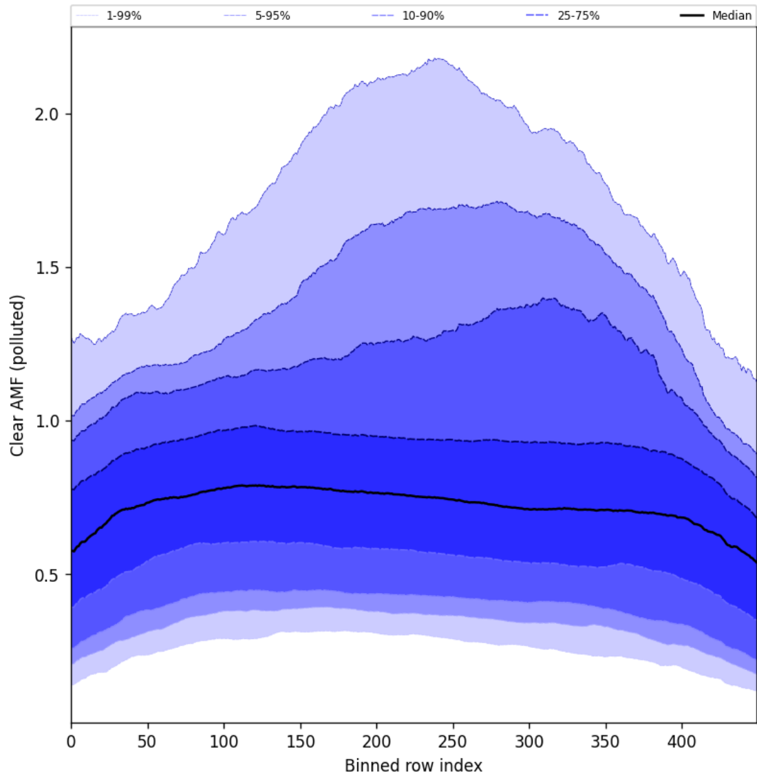
Figure 107: Along track statistics of “Clear AMF (polluted)” for 2025-05-17 to 2025-05-19
