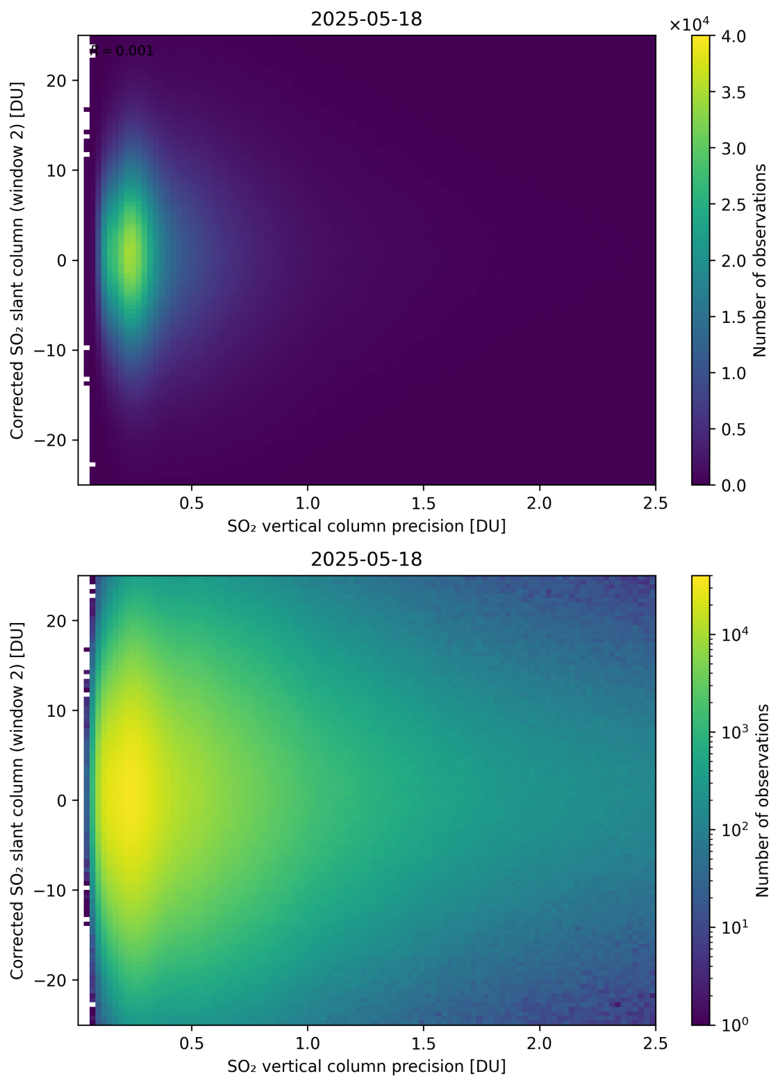
Figure 339: Scatter density plot of “SO 2 vertical column precision” against “Corrected SO 2 slant column (window 2)” for 2025-05-17 to 2025-05-19.
