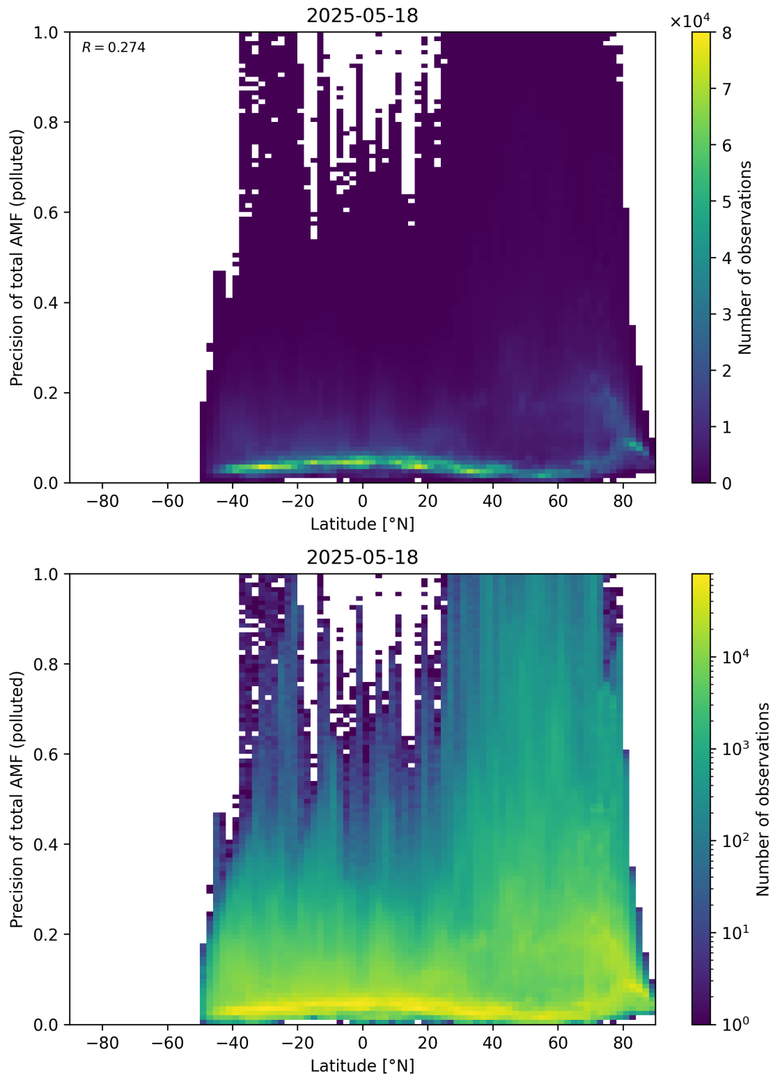
Figure 168: Scatter density plot of “Latitude” against “Precision of total AMF (polluted)” for 2025-05-17 to 2025-05-19.
