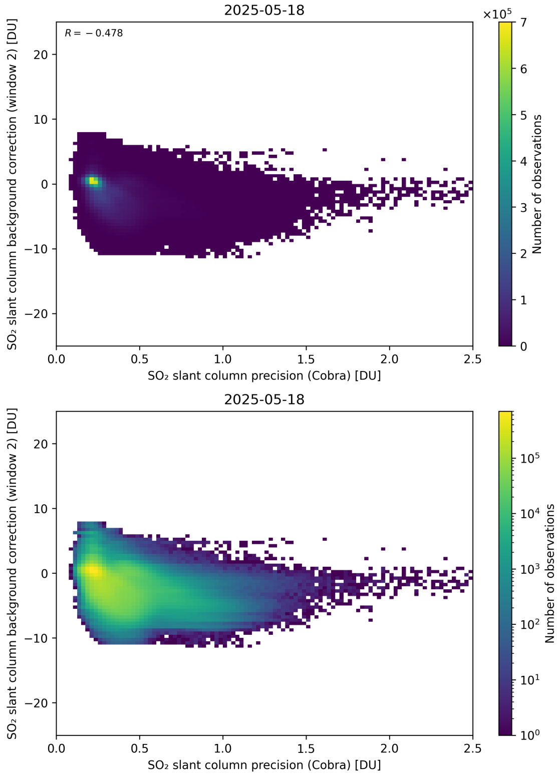
Figure 200: Scatter density plot of “SO 2 slant column precision (Cobra)” against “SO 2 slant column background correction (window 2)” for 2025-05-17 to 2025-05-19.
