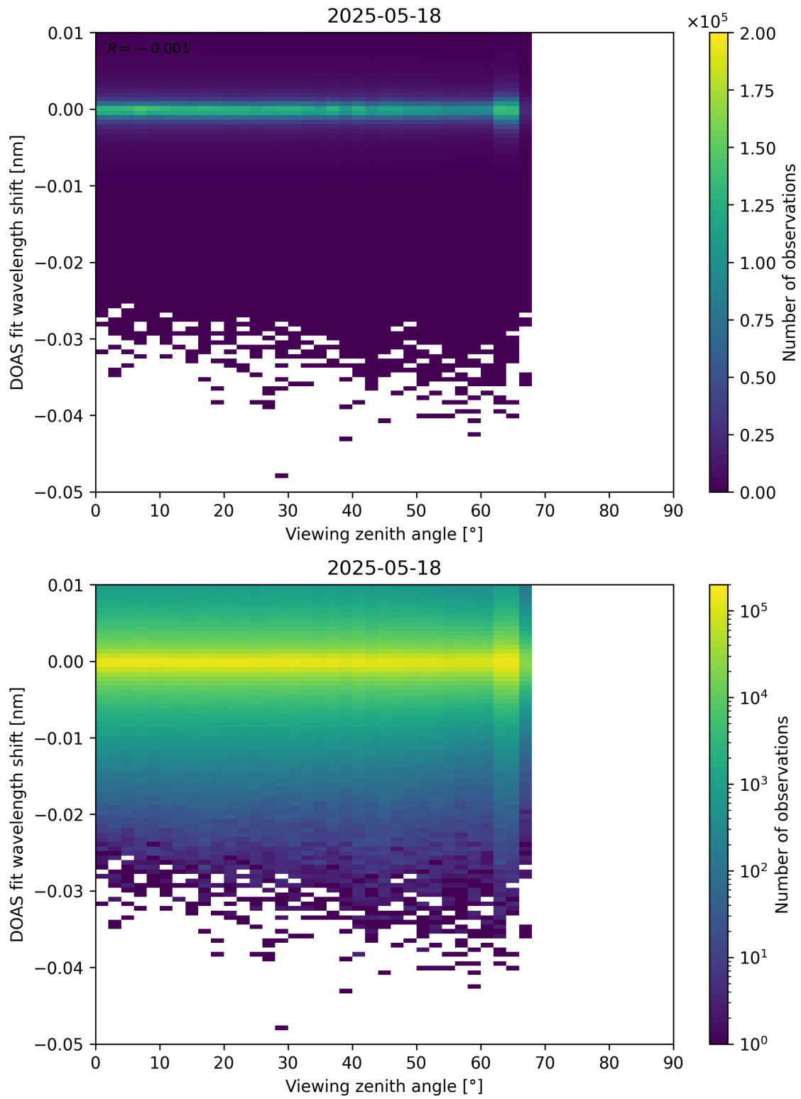
Figure 365: Scatter density plot of “Viewing zenith angle” against “DOAS fit wavelength shift” for 2025-05-17 to 2025-05-19.
