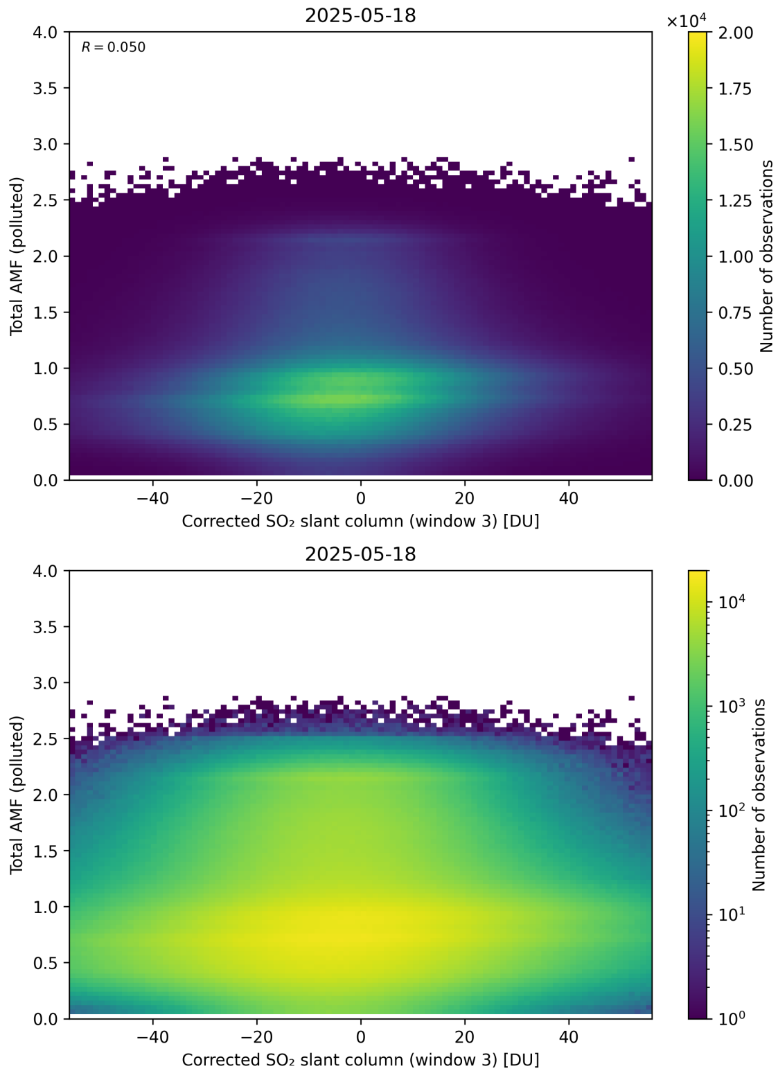
Figure 260: Scatter density plot of “Corrected SO 2 slant column (window 3)” against “Total AMF (polluted)” for 2025-05-17 to 2025-05-19.
