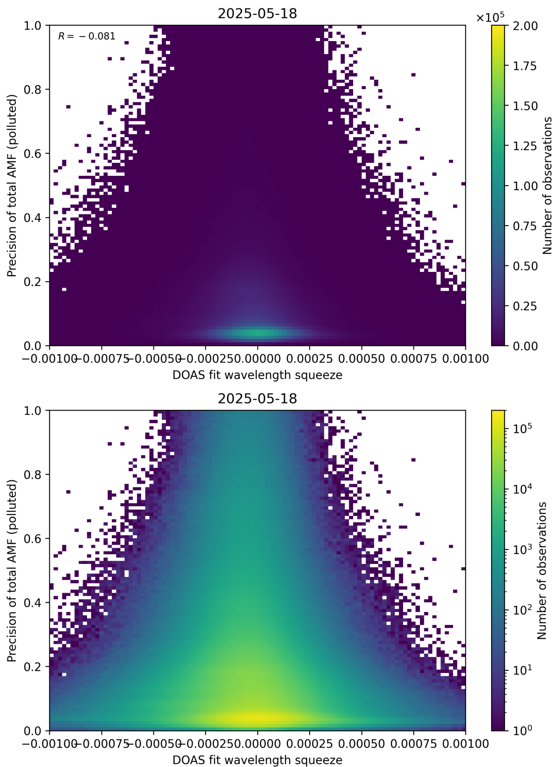
Figure 146: Scatter density plot of “DOAS fit wavelength squeeze” against “Precision of total AMF (polluted)” for 2025-05-17 to 2025-05-19.
