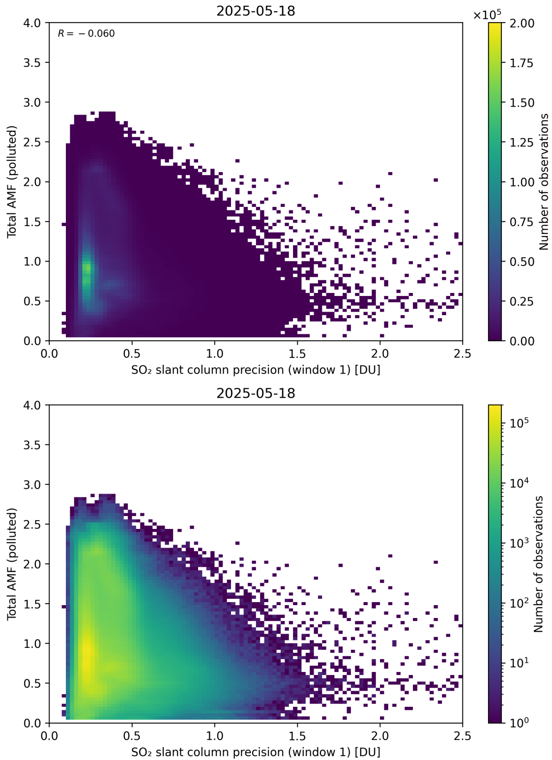
Figure 280: Scatter density plot of “SO 2 slant column precision (window 1)” against “Total AMF (polluted)” for 2025-05-17 to 2025-05-19.
