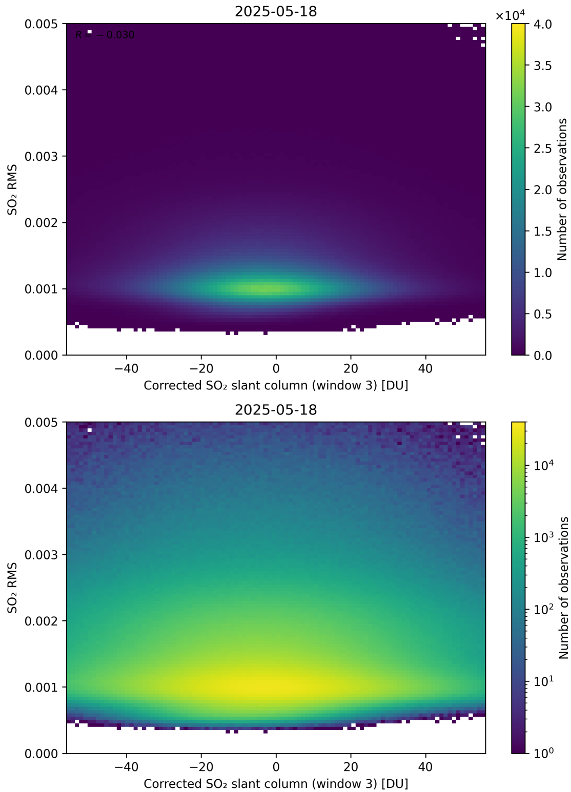
Figure 258: Scatter density plot of “Corrected SO 2 slant column (window 3)” against “SO 2 RMS” for 2025-05-17 to 2025-05-19.
