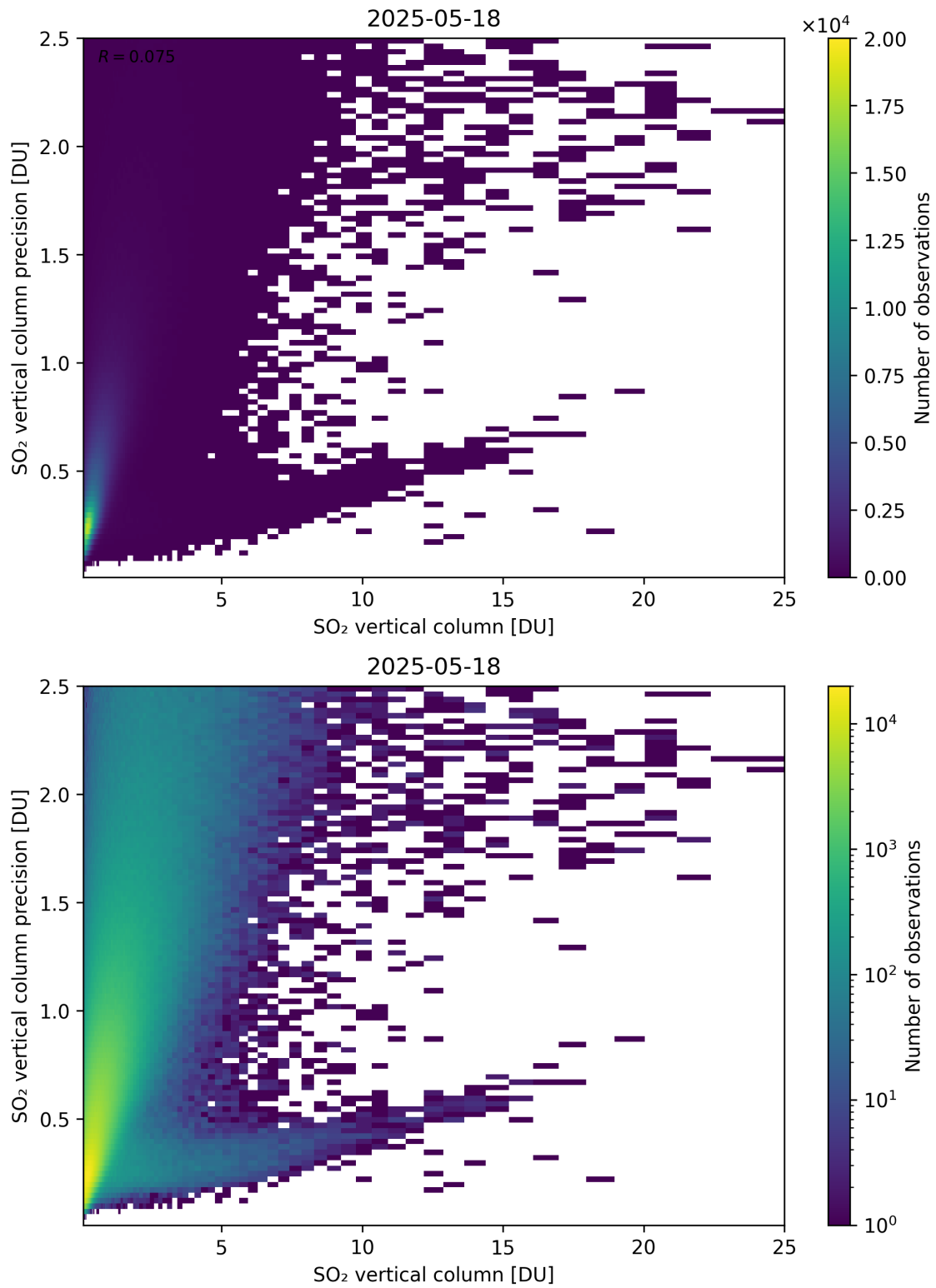
Figure 361: Scatter density plot of “SO 2 vertical column” against “SO 2 vertical column precision” for 2025-05-17 to 2025-05-19.
