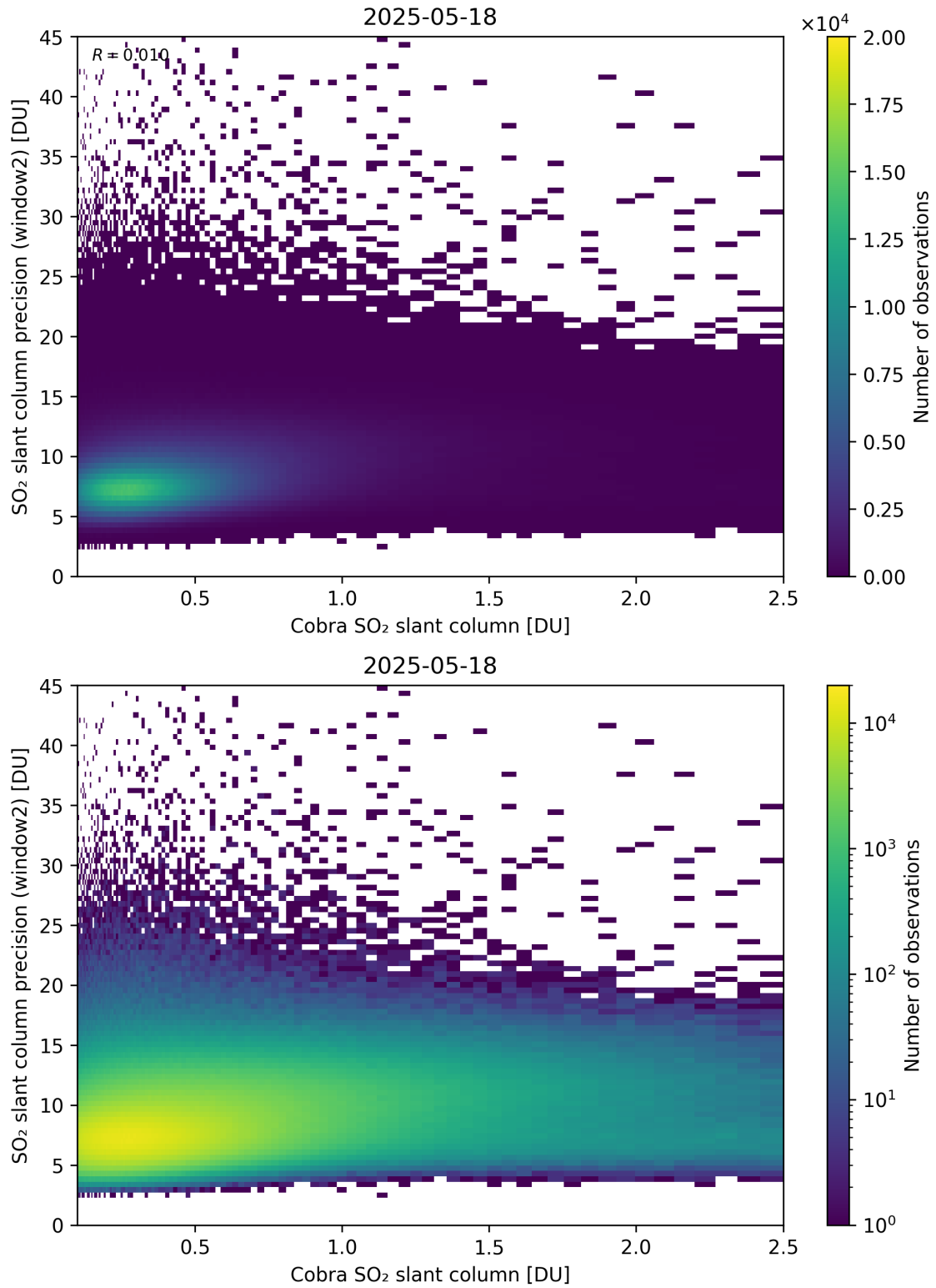
Figure 221: Scatter density plot of “Cobra SO 2 slant column” against “SO 2 slant column precision (window2)” for 2025-05-17 to 2025-05-19.
