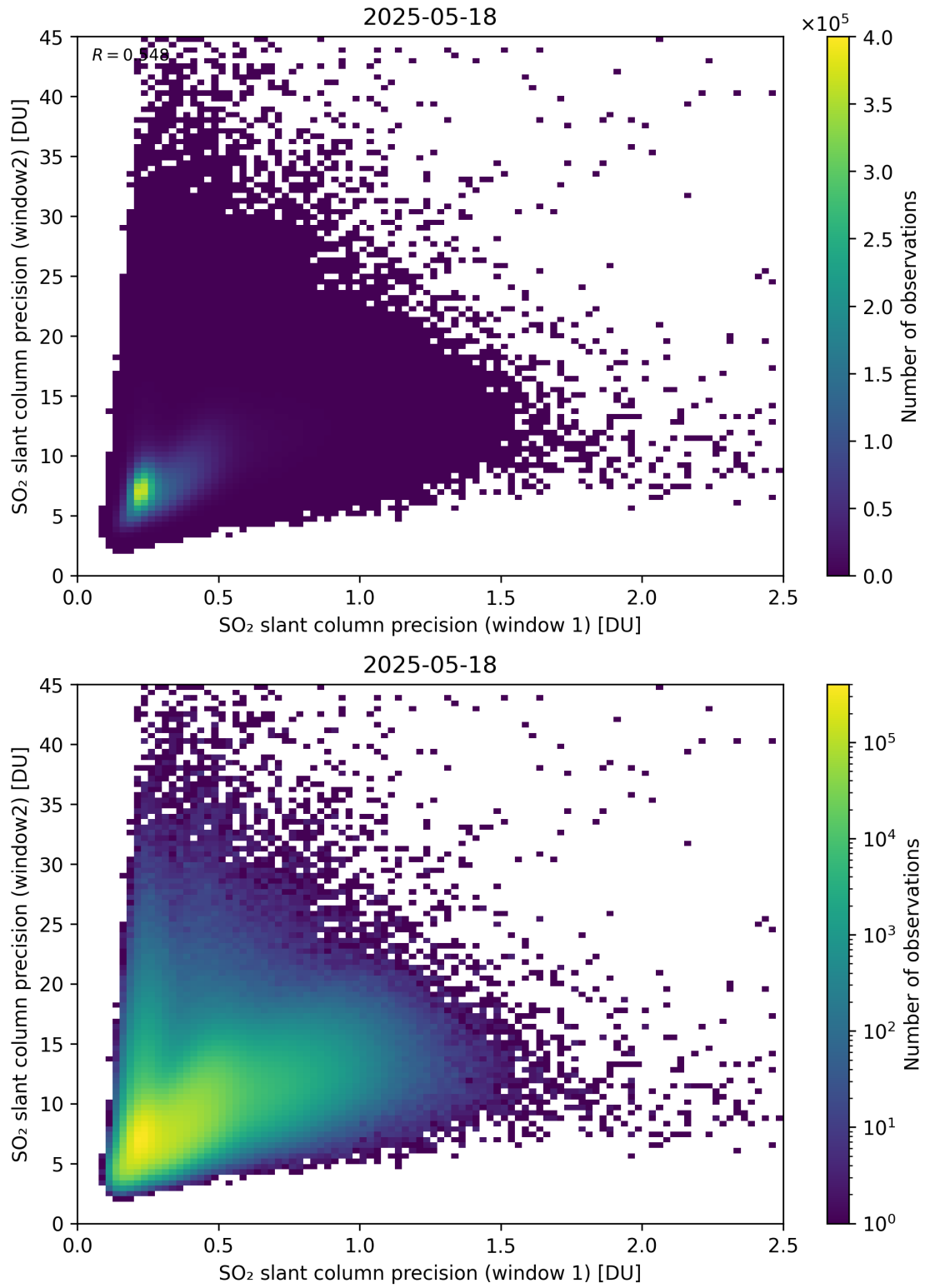
Figure 277: Scatter density plot of “SO 2 slant column precision (window 1)” against “SO 2 slant column precision (window2)” for 2025-05-17 to 2025-05-19.
