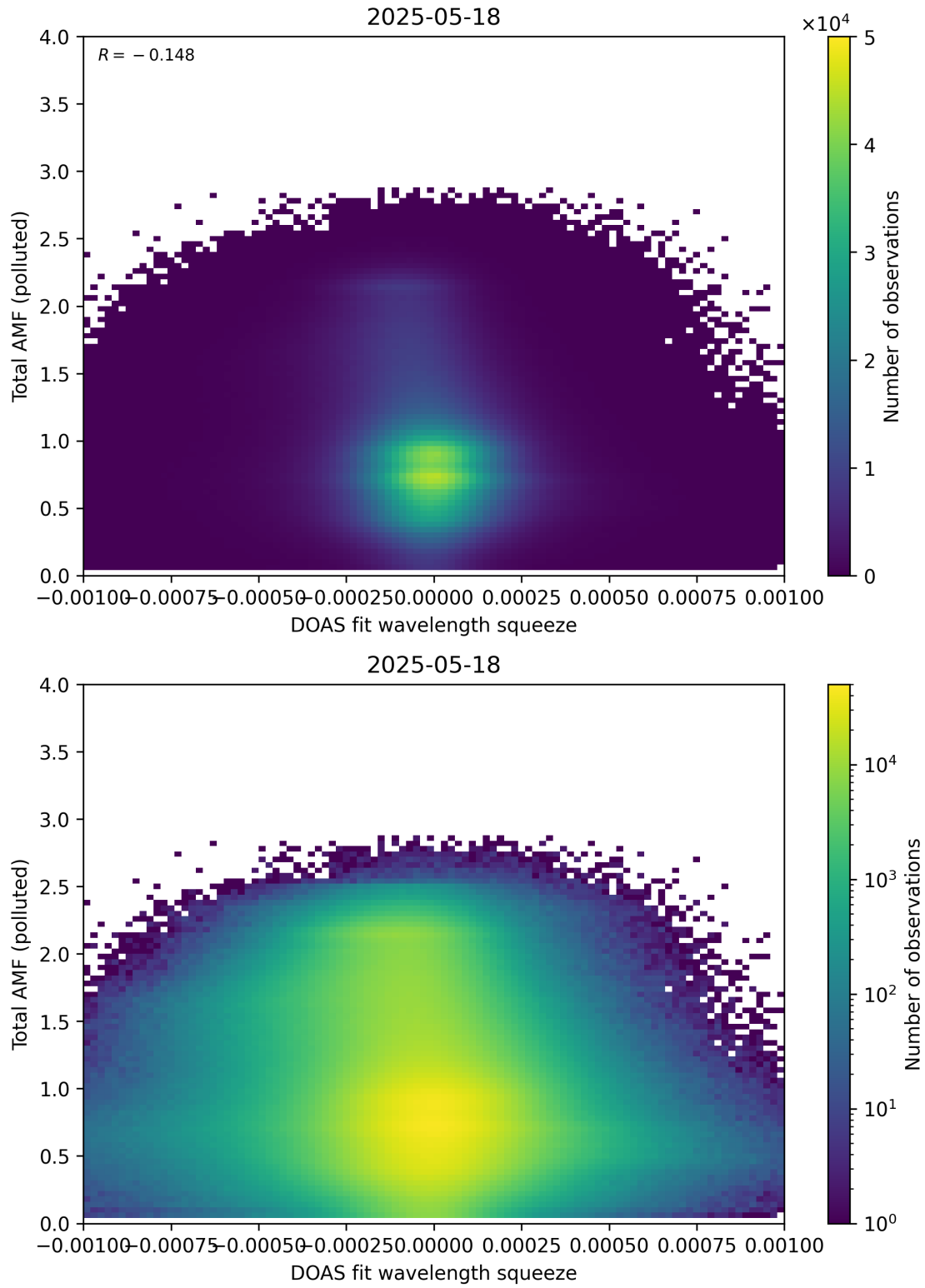
Figure 145: Scatter density plot of “DOAS fit wavelength squeeze” against “Total AMF (polluted)” for 2025-05-17 to 2025-05-19.
