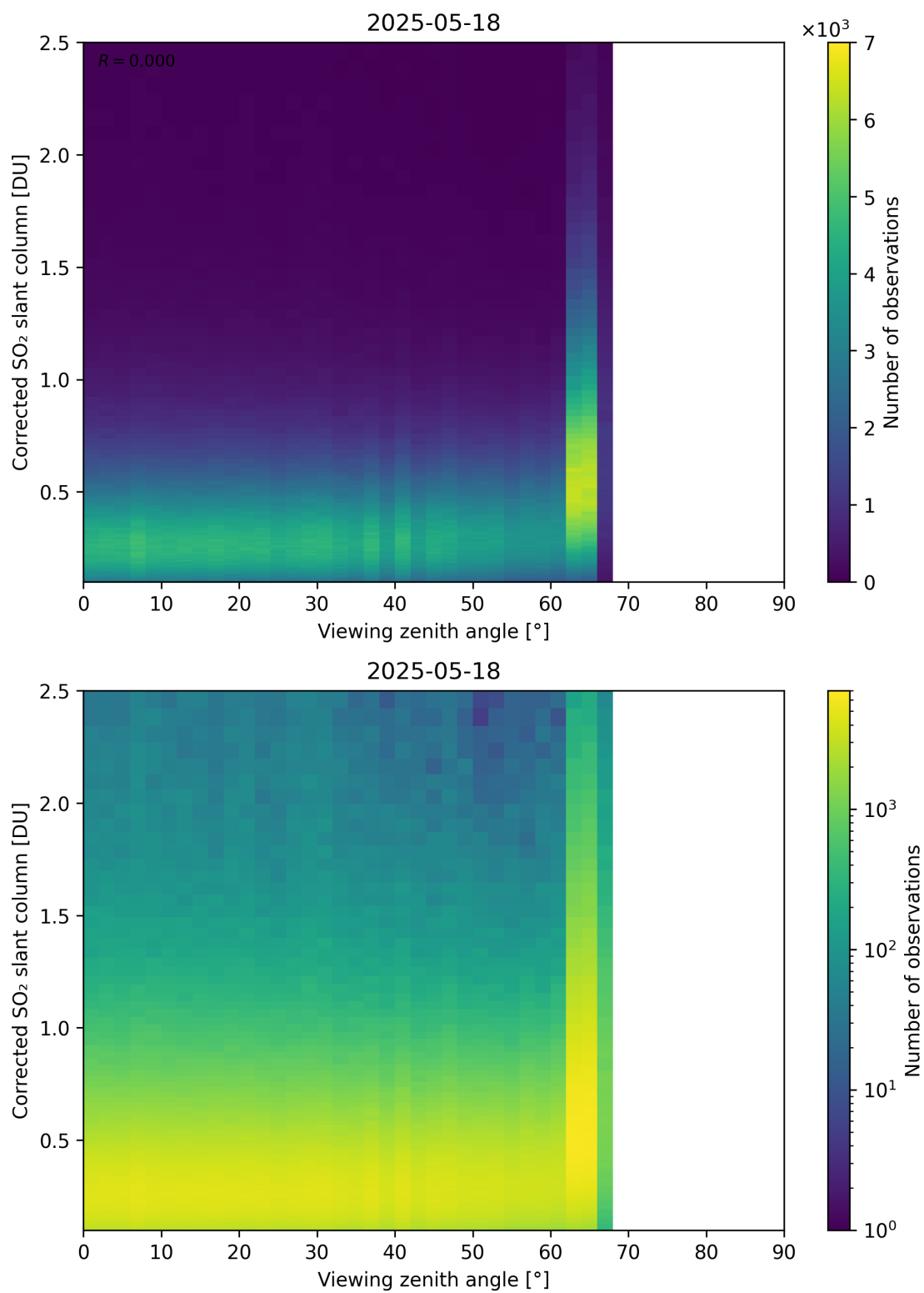
Figure 373: Scatter density plot of “Viewing zenith angle” against “Corrected SO 2 slant column” for 2025-05-17 to 2025-05-19.
