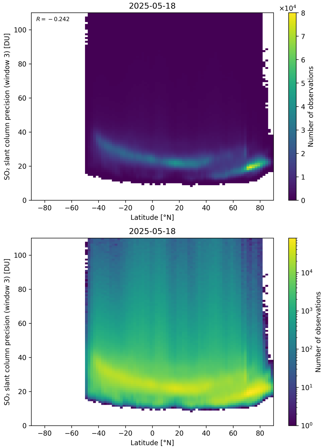
Figure 166: Scatter density plot of “Latitude” against “SO 2 slant column precision (window 3)” for 2025-05-17 to 2025-05-19.
