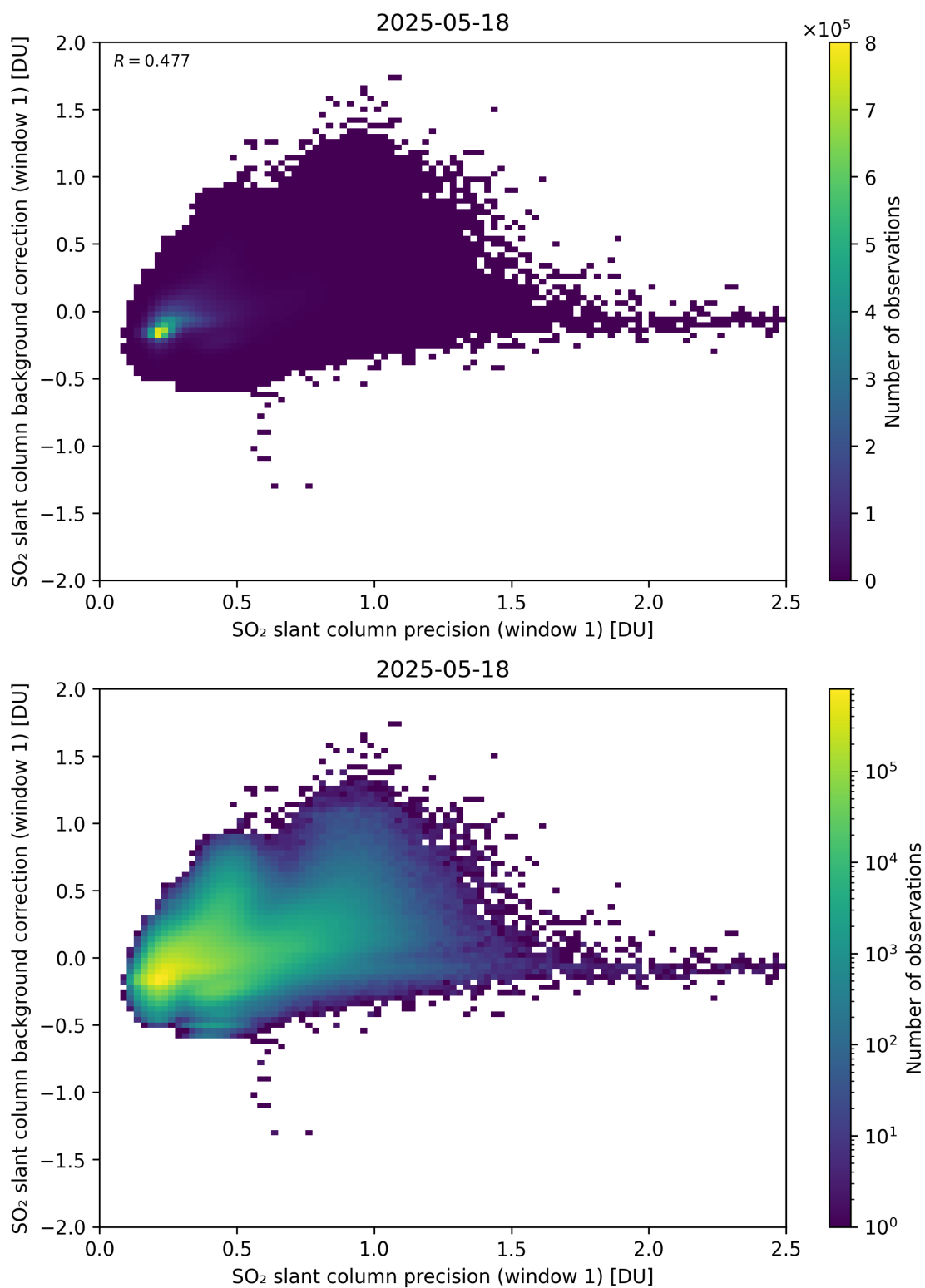
Figure 268: Scatter density plot of “SO 2 slant column precision (window 1)” against “SO 2 slant column background correction (window 1)” for 2025-05-17 to 2025-05-19.
