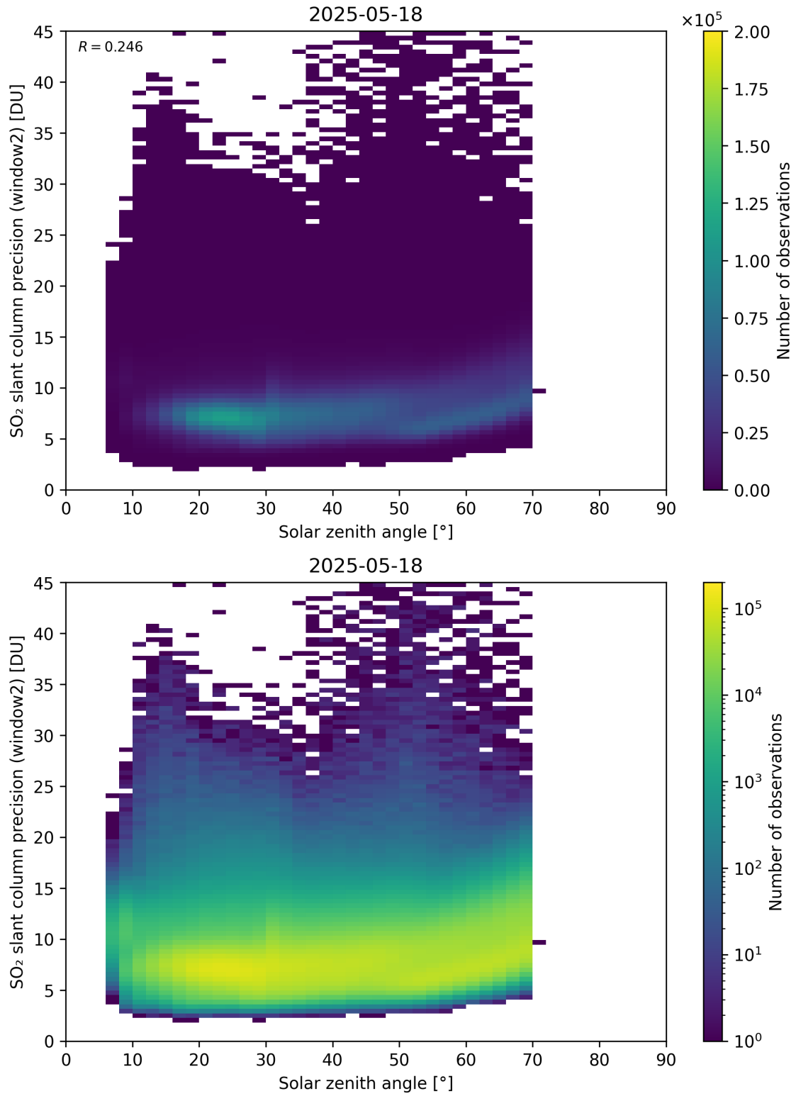
Figure 186: Scatter density plot of “Solar zenith angle” against “SO 2 slant column precision (window2)” for 2025-05-17 to 2025-05-19.
