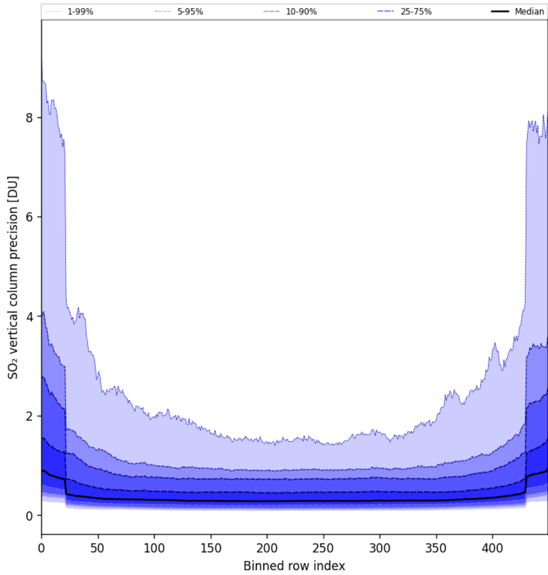
Figure 85: Along track statistics of “SO 2 vertical column precision” for 2025-05-17 to 2025-05-19
