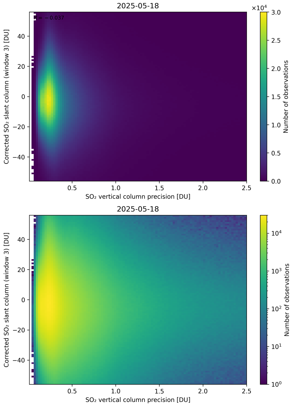
Figure 340: Scatter density plot of “SO 2 vertical column precision” against “Corrected SO 2 slant column (window 3)” for 2025-05-17 to 2025-05-19.
