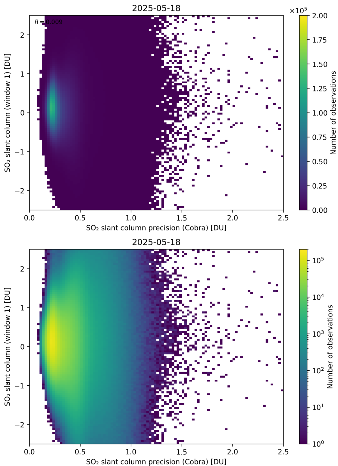
Figure 208: Scatter density plot of “SO 2 slant column precision (Cobra)” against “SO 2 slant column (window 1)” for 2025-05-17 to 2025-05-19.
