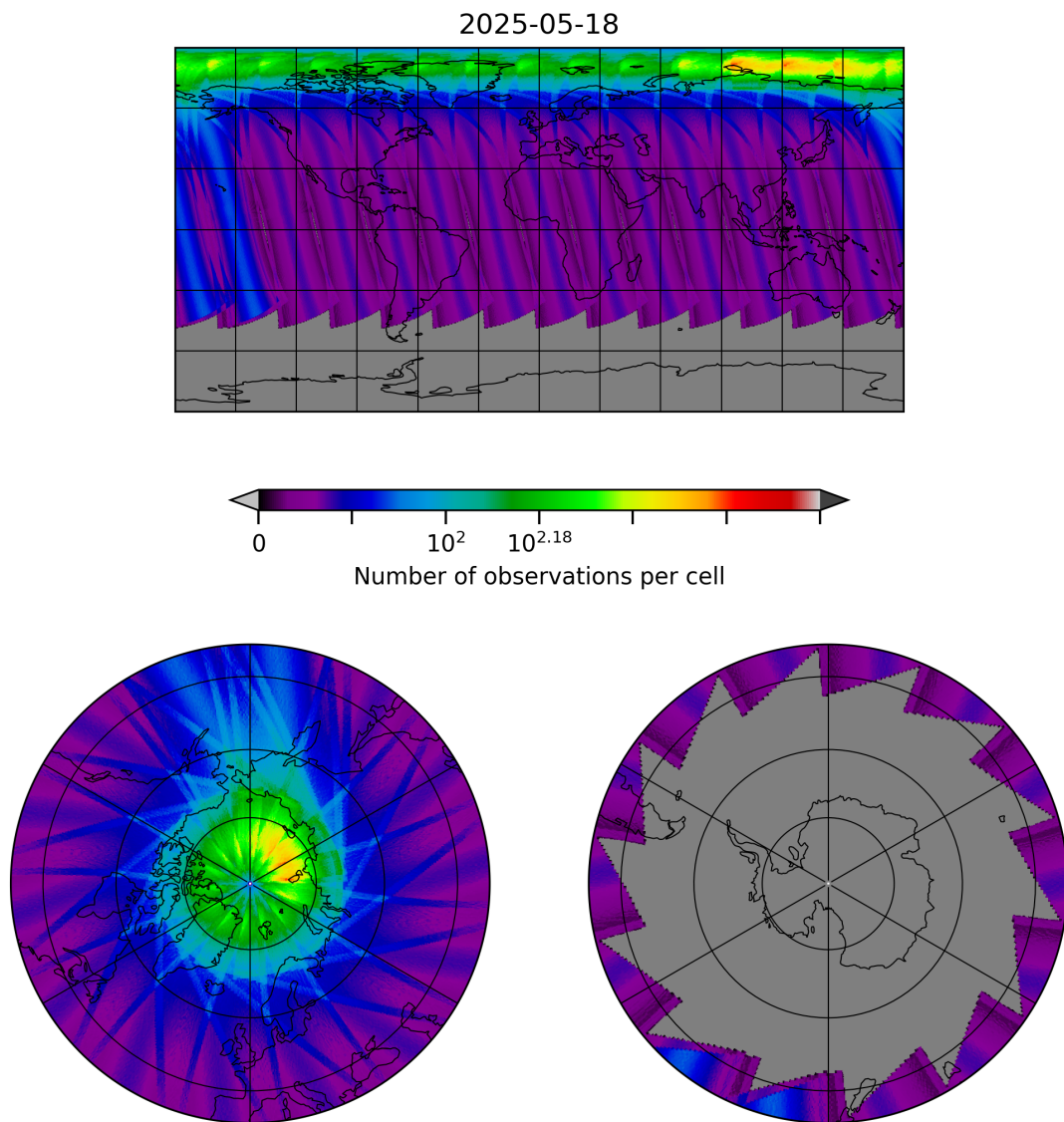
Figure 30: Map of the number of observations for 2025-05-17 to 2025-05-19
