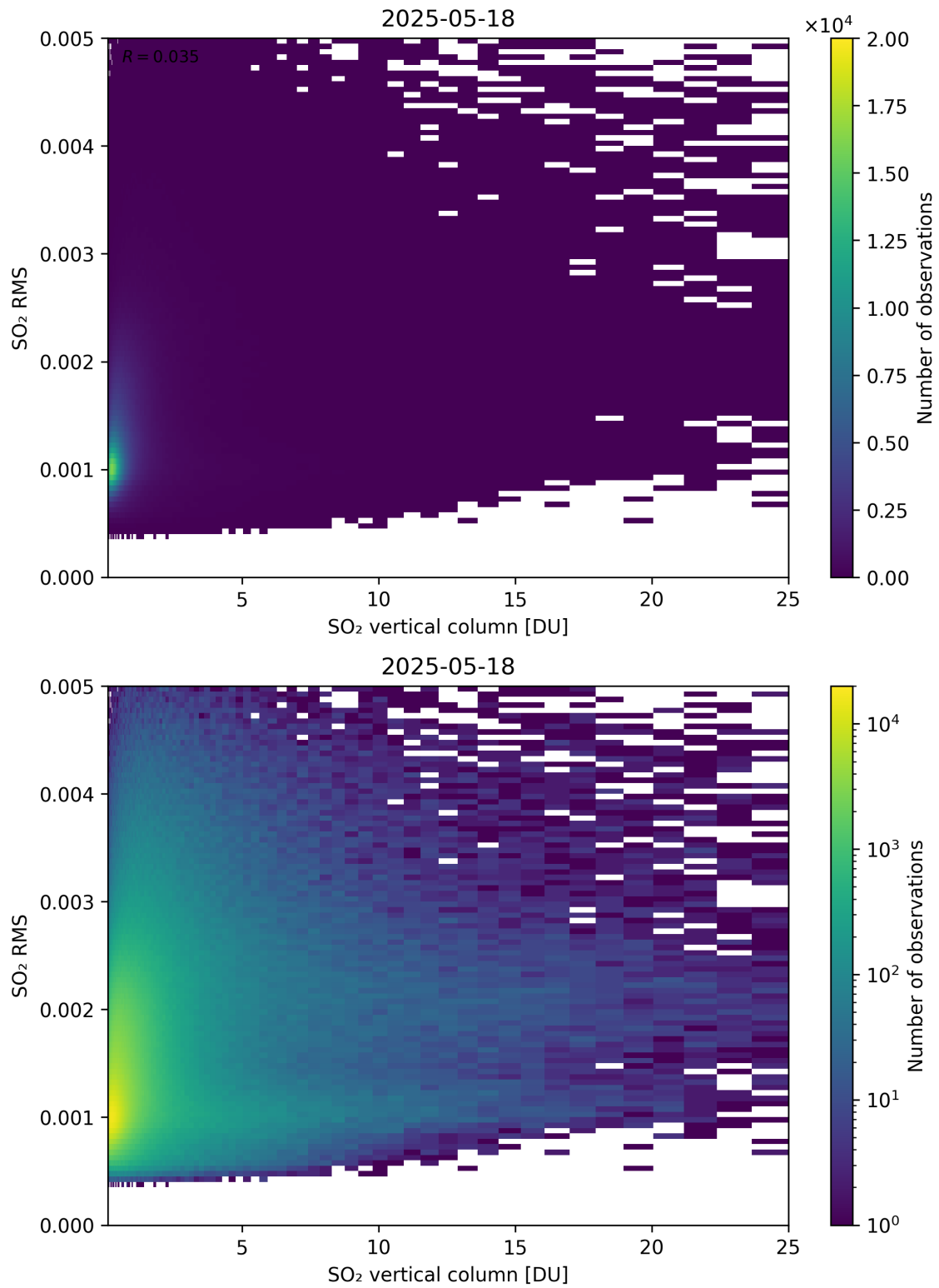
Figure 328: Scatter density plot of “SO 2 vertical column” against “SO 2 RMS” for 2025-05-17 to 2025-05-19.
