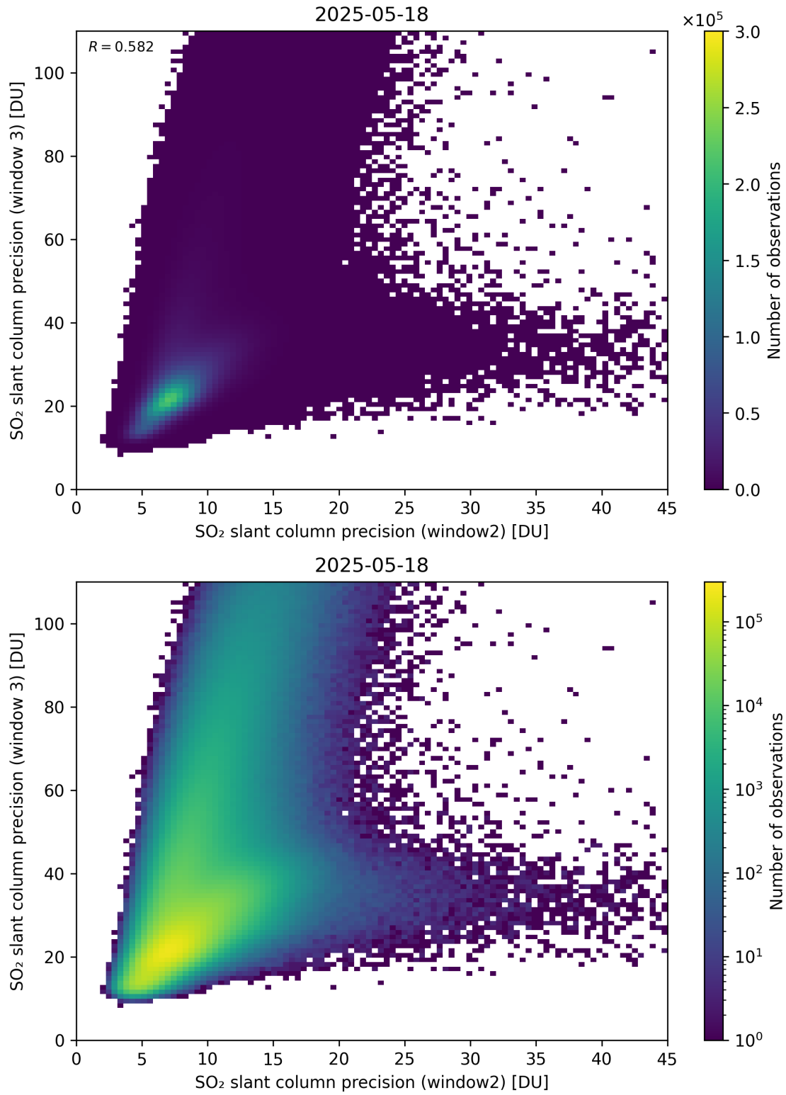
Figure 300: Scatter density plot of “SO 2 slant column precision (window2)” against “SO 2 slant column precision (window 3)” for 2025-05-17 to 2025-05-19.
