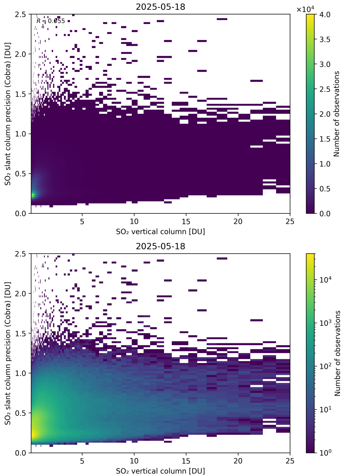
Figure 350: Scatter density plot of “SO 2 vertical column” against “SO 2 slant column precision (Cobra)” for 2025-05-17 to 2025-05-19.
