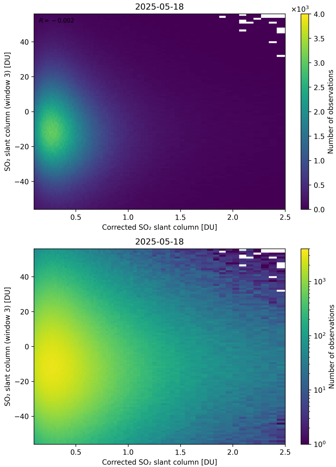
Figure 240: Scatter density plot of “Corrected SO 2 slant column” against “SO 2 slant column (window 3)” for 2025-05-17 to 2025-05-19.
