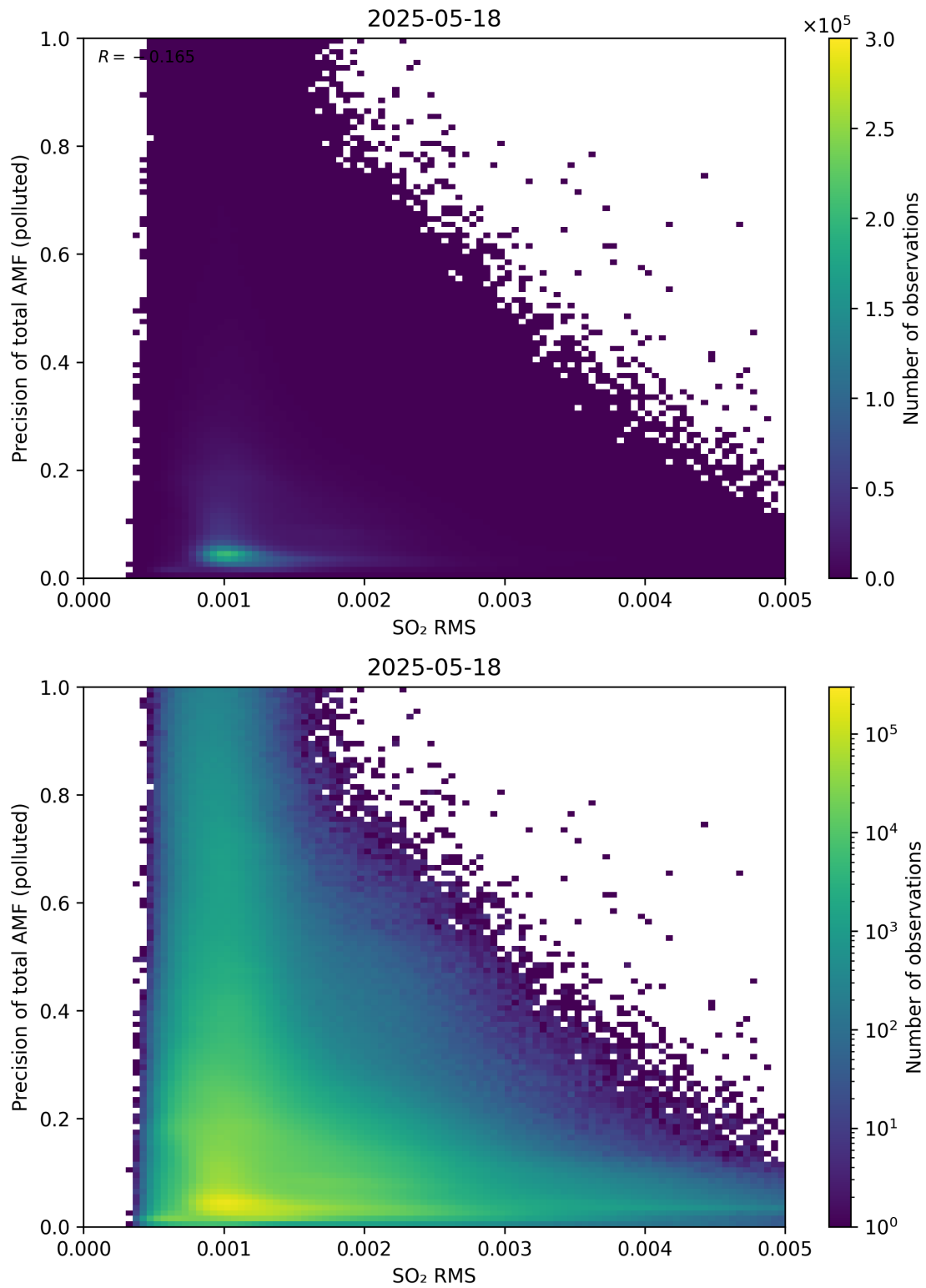
Figure 149: Scatter density plot of “SO 2 RMS” against “Precision of total AMF (polluted)” for 2025-05-17 to 2025-05-19.
