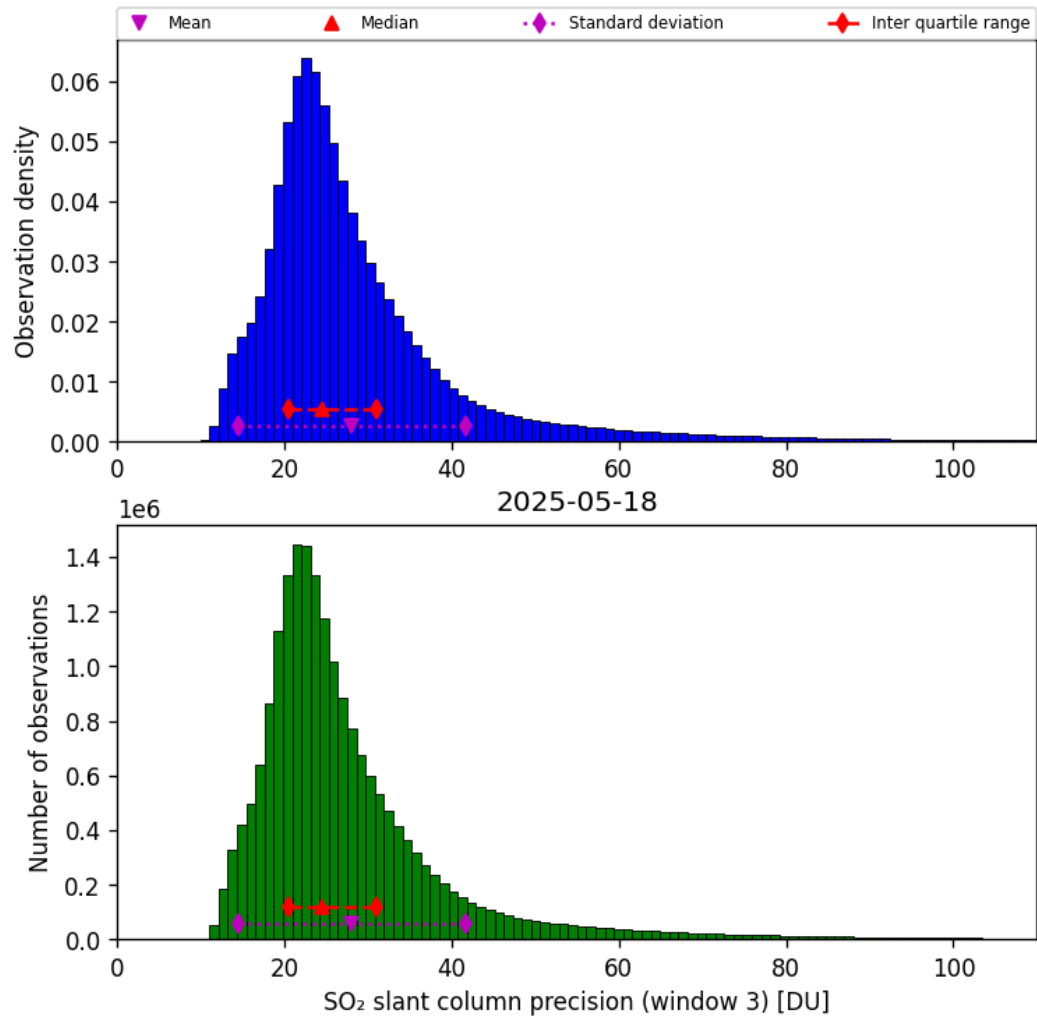
Figure 72: Histogram of “SO 2 slant column precision (window 3)” for 2025-05-17 to 2025-05-19
