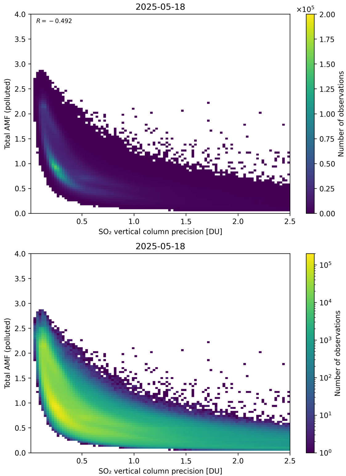
Figure 346: Scatter density plot of “SO 2 vertical column precision” against “Total AMF (polluted)” for 2025-05-17 to 2025-05-19.
