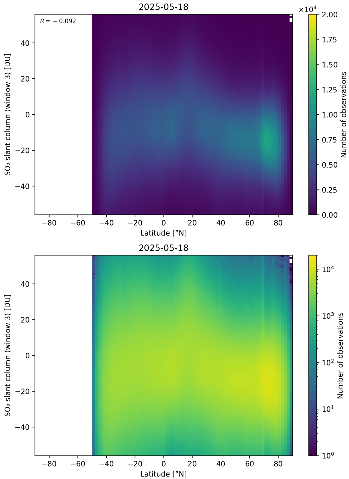
Figure 165: Scatter density plot of “Latitude” against “SO 2 slant column (window 3)” for 2025-05-17 to 2025-05-19.
