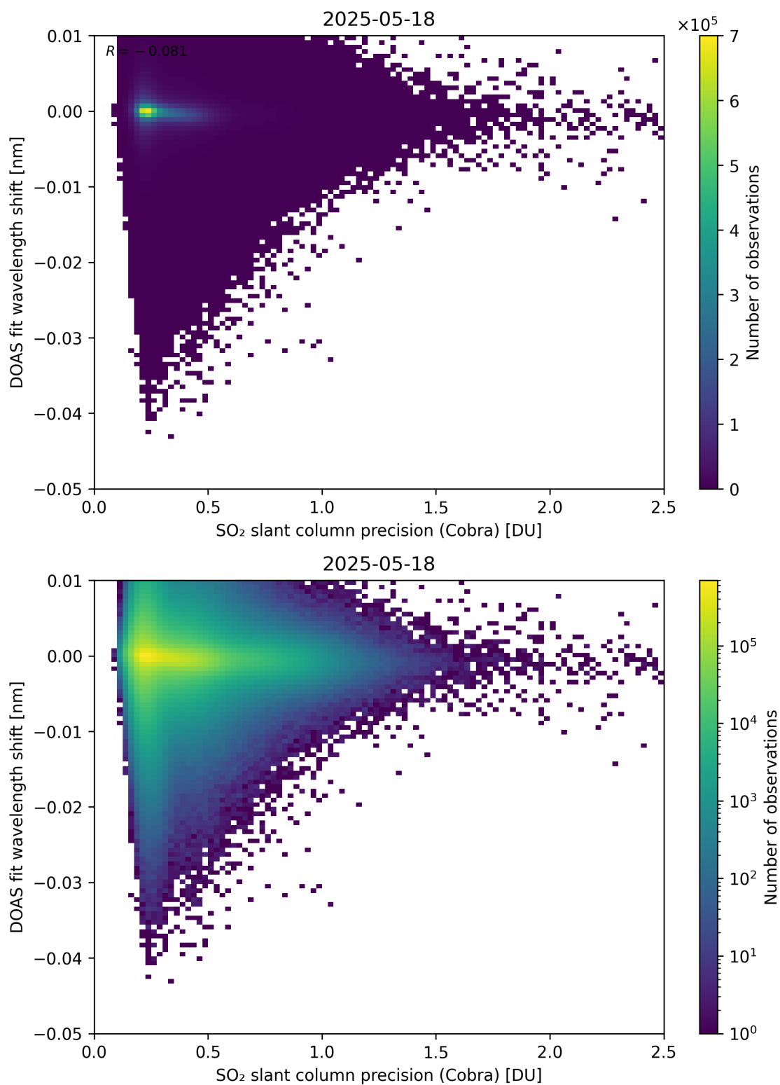
Figure 202: Scatter density plot of “SO 2 slant column precision (Cobra)” against “DOAS fit wavelength shift” for 2025-05-17 to 2025-05-19.
