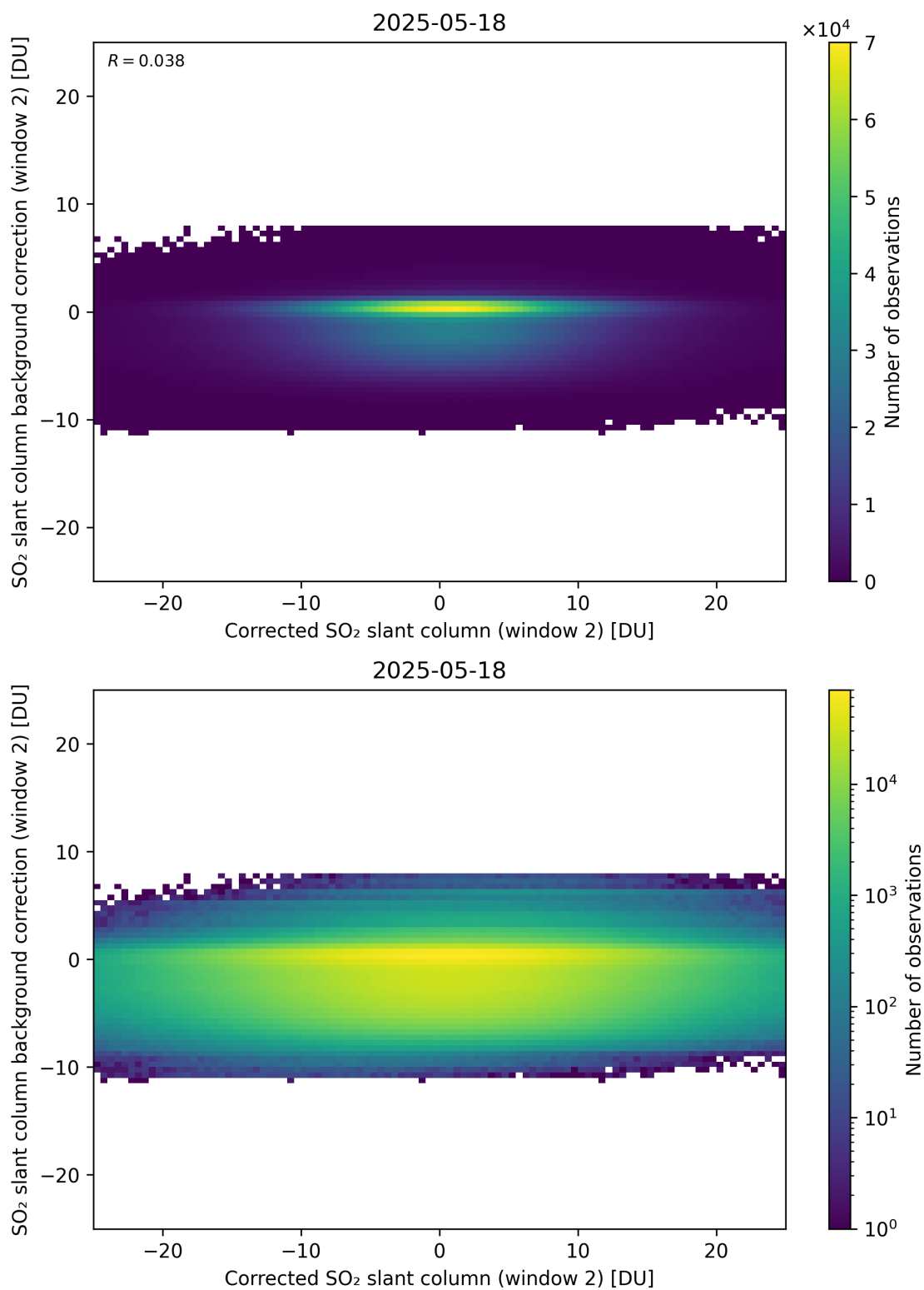
Figure 244: Scatter density plot of “Corrected SO 2 slant column (window 2)” against “SO 2 slant column background correction (window 2)” for 2025-05-17 to 2025-05-19.
