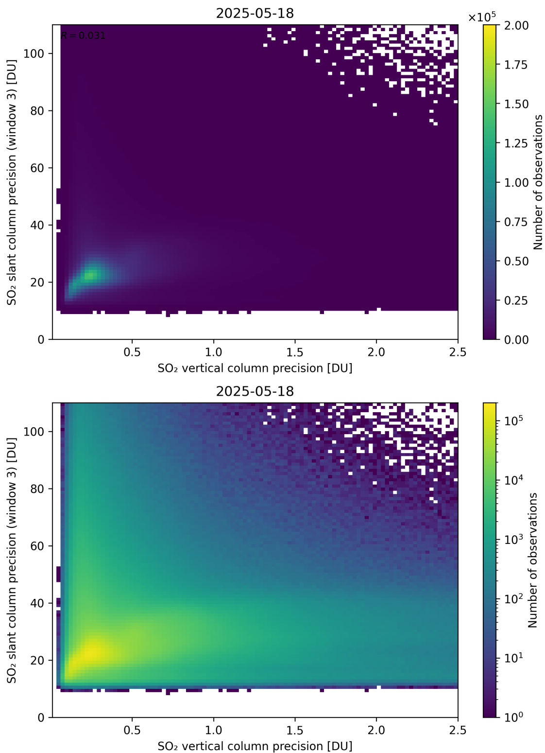
Figure 345: Scatter density plot of “SO 2 vertical column precision” against “SO 2 slant column precision (window 3)” for 2025-05-17 to 2025-05-19.
