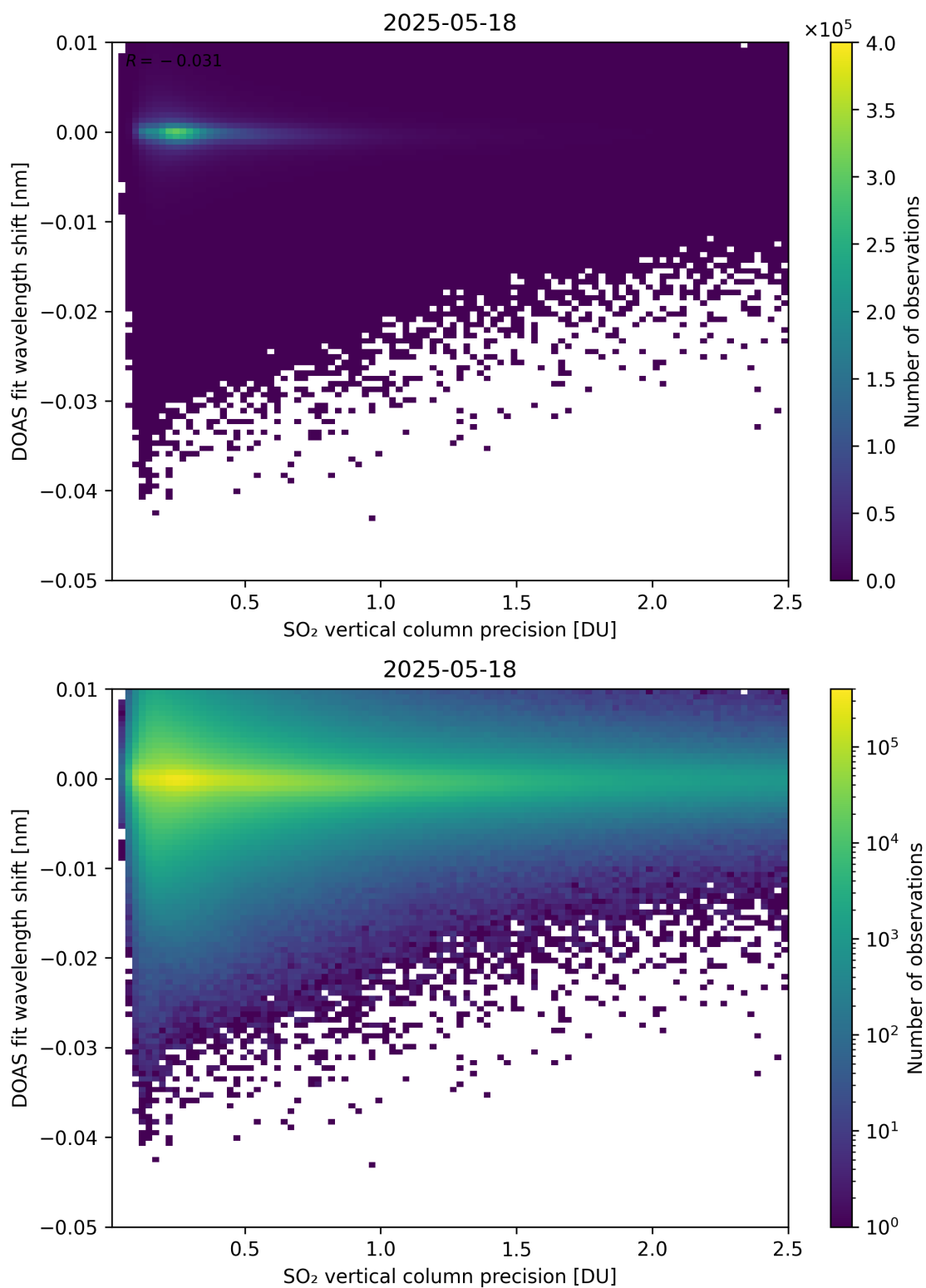
Figure 332: Scatter density plot of “SO 2 vertical column precision” against “DOAS fit wavelength shift” for 2025-05-17 to 2025-05-19.
