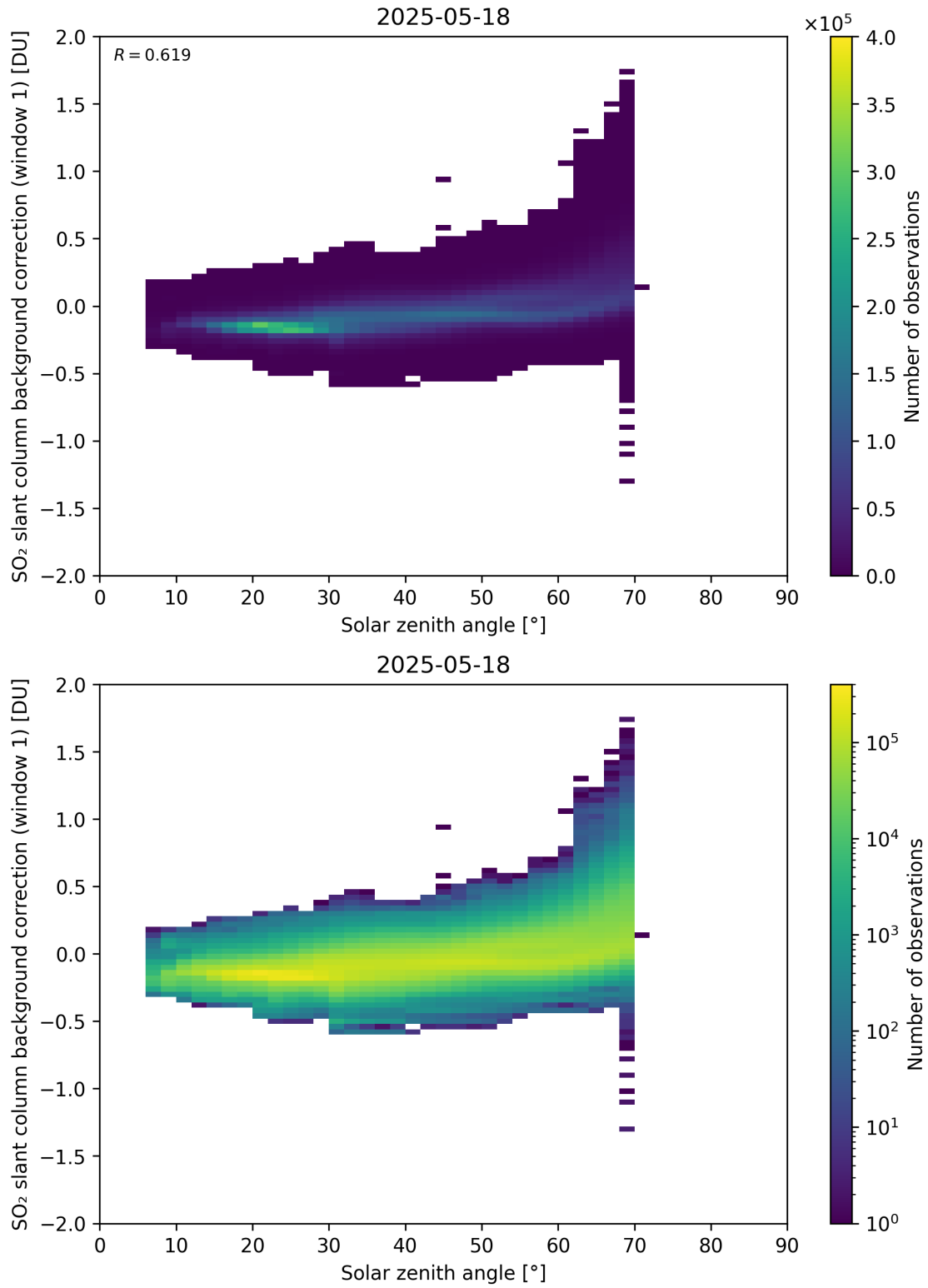
Figure 171: Scatter density plot of “Solar zenith angle” against “SO 2 slant column background correction (window 1)” for 2025-05-17 to 2025-05-19.
