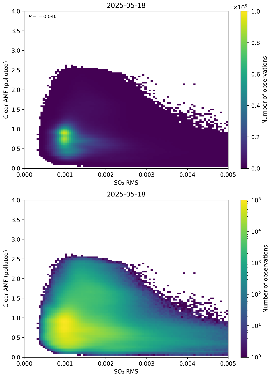
Figure 147: Scatter density plot of “SO 2 RMS” against “Clear AMF (polluted)” for 2025-05-17 to 2025-05-19.
