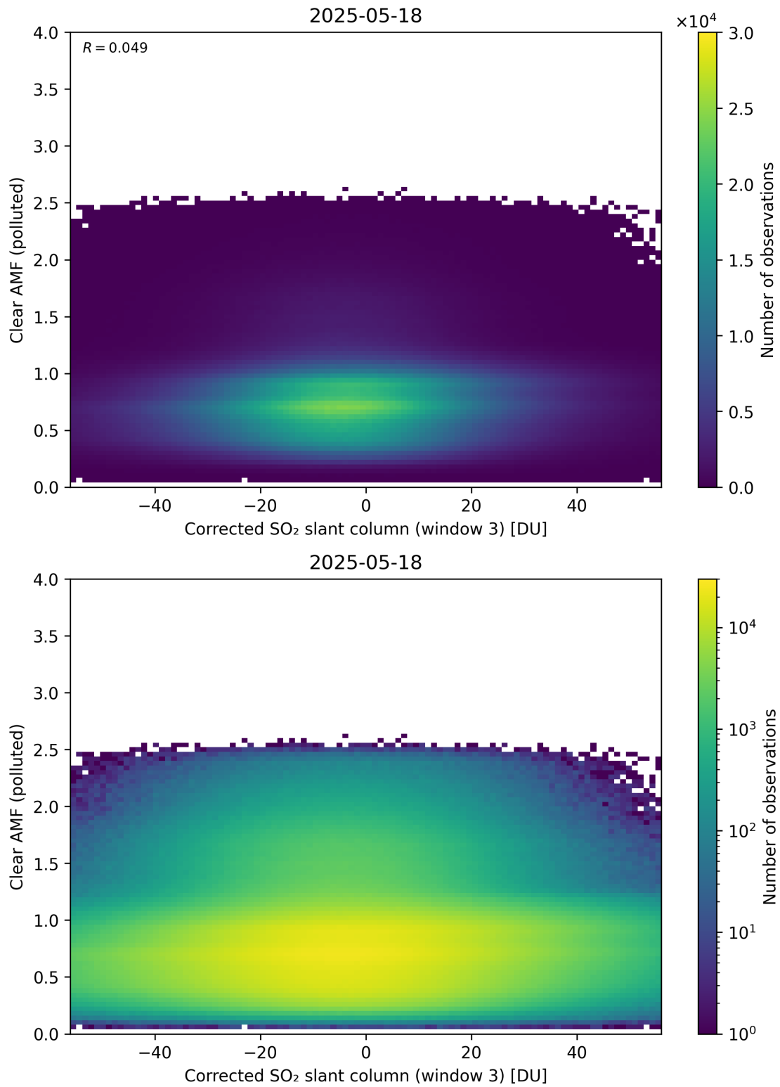
Figure 259: Scatter density plot of “Corrected SO 2 slant column (window 3)” against “Clear AMF (polluted)” for 2025-05-17 to 2025-05-19.
