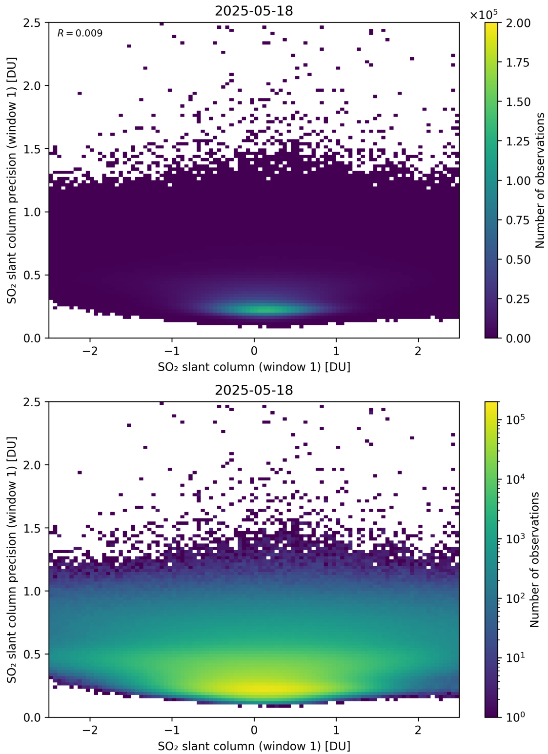
Figure 285: Scatter density plot of “SO 2 slant column (window 1)” against “SO 2 slant column precision (window 1)” for 2025-05-17 to 2025-05-19.
