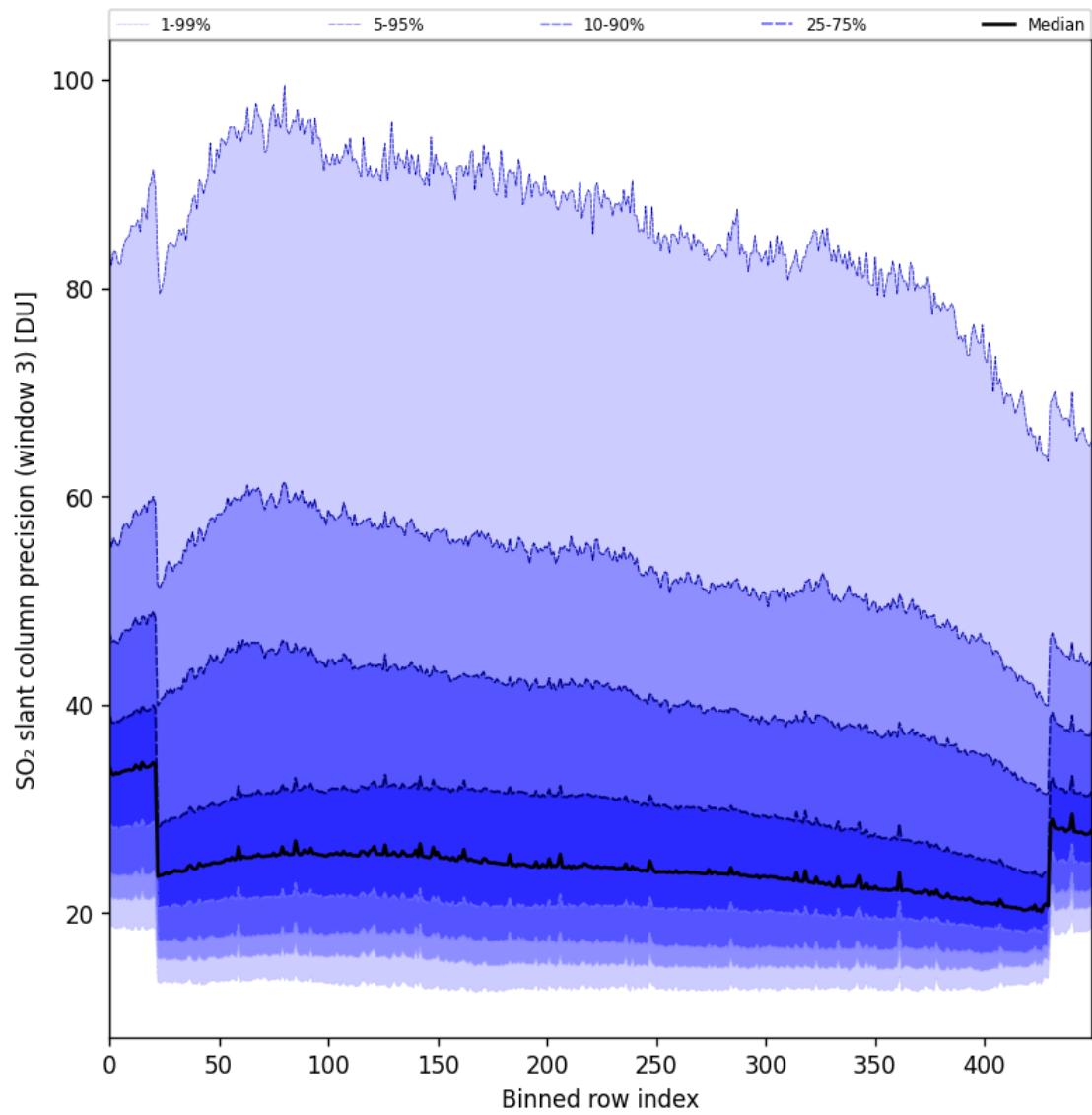
Figure 98: Along track statistics of “SO 2 slant column precision (window 3)” for 2025-05-17 to 2025-05-19
