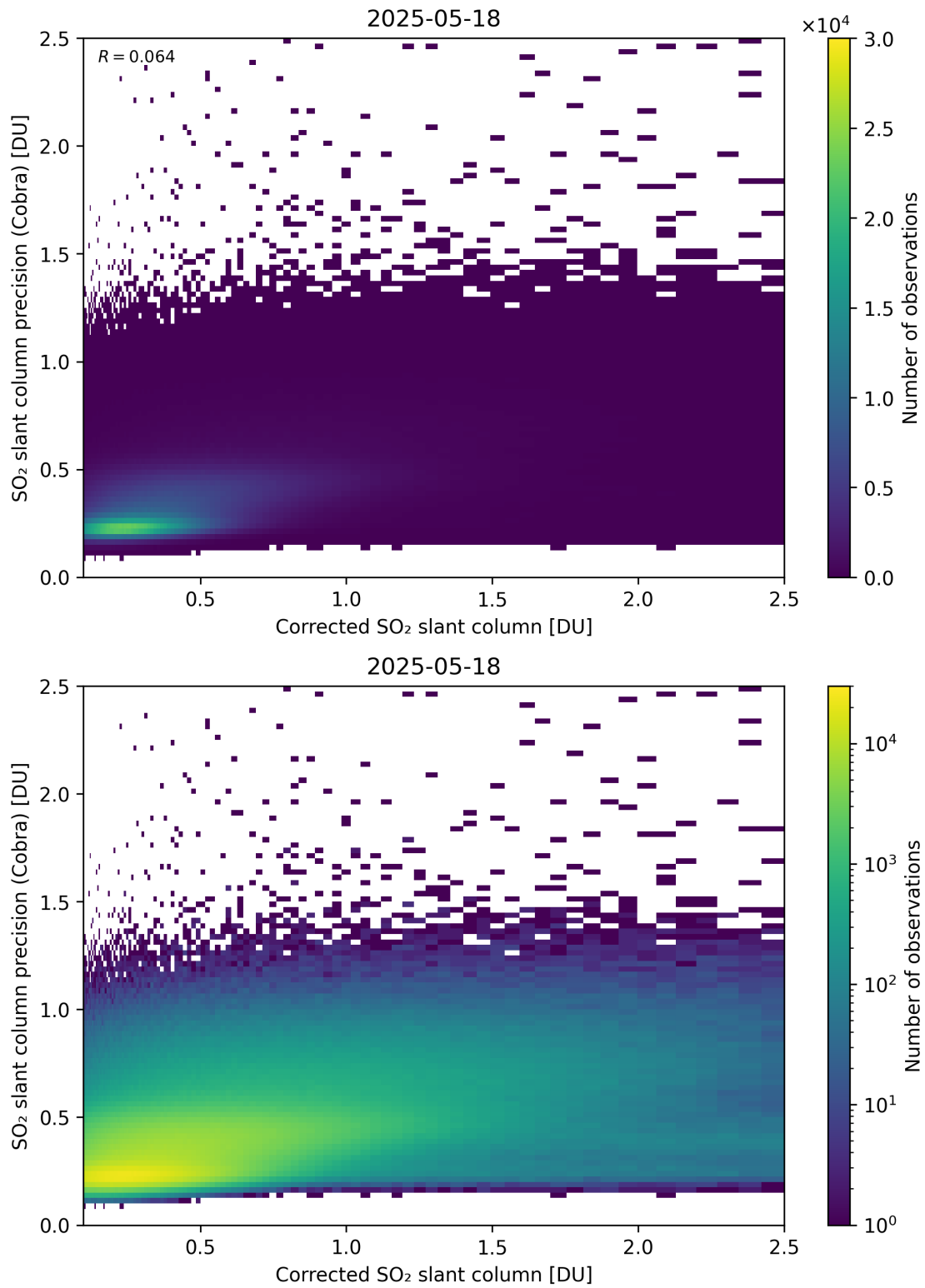
Figure 234: Scatter density plot of “Corrected SO 2 slant column” against “SO 2 slant column precision (Cobra)” for 2025-05-17 to 2025-05-19.
