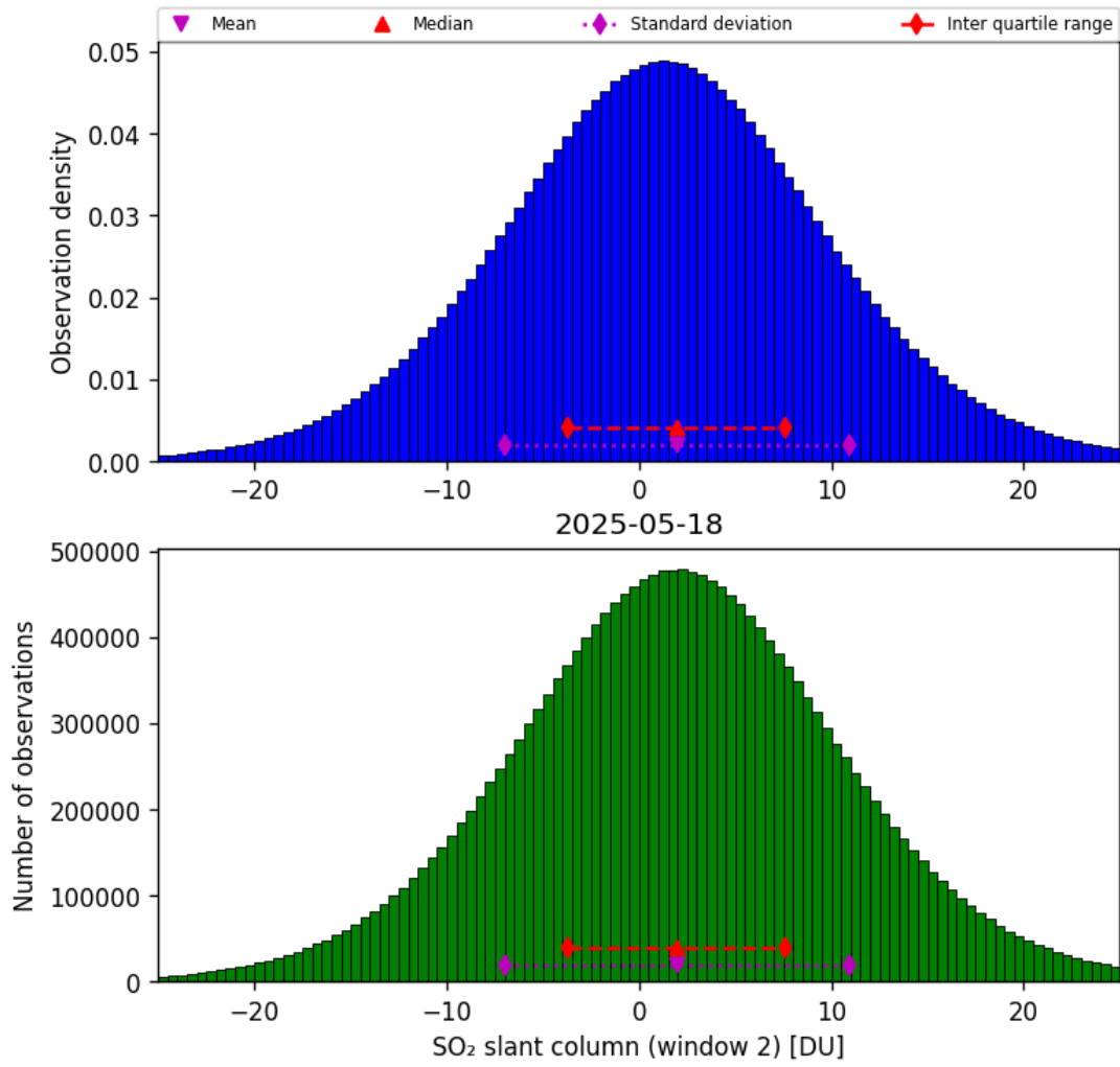
Figure 67: Histogram of “SO 2 slant column (window 2)” for 2025-05-17 to 2025-05-19
