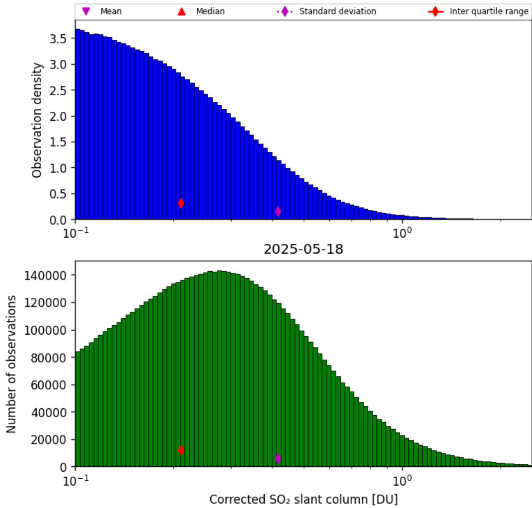
Figure 60: Histogram of “Corrected SO 2 slant column” for 2025-05-17 to 2025-05-19
