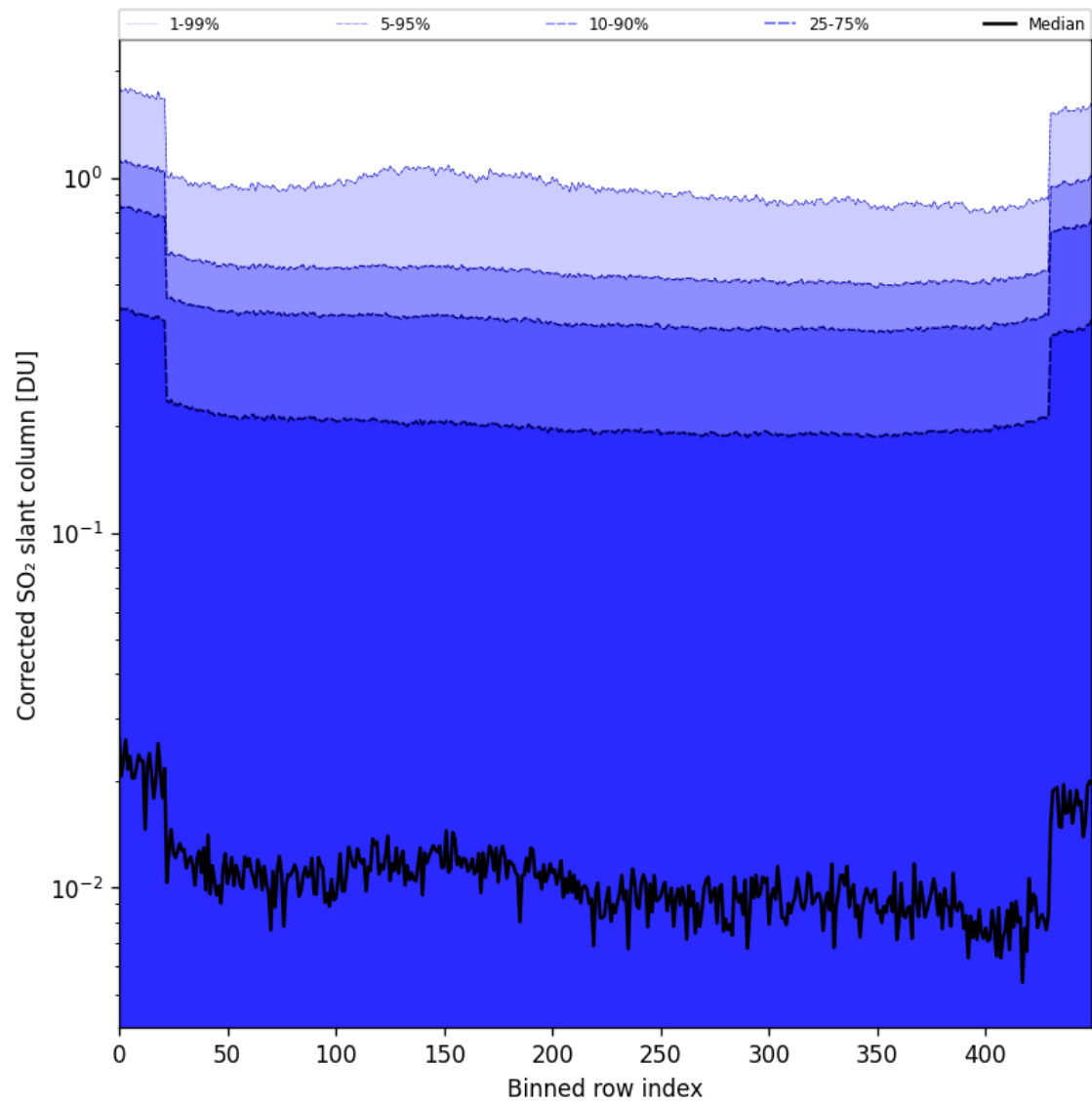
Figure 86: Along track statistics of “Corrected SO 2 slant column” for 2025-05-17 to 2025-05-19
