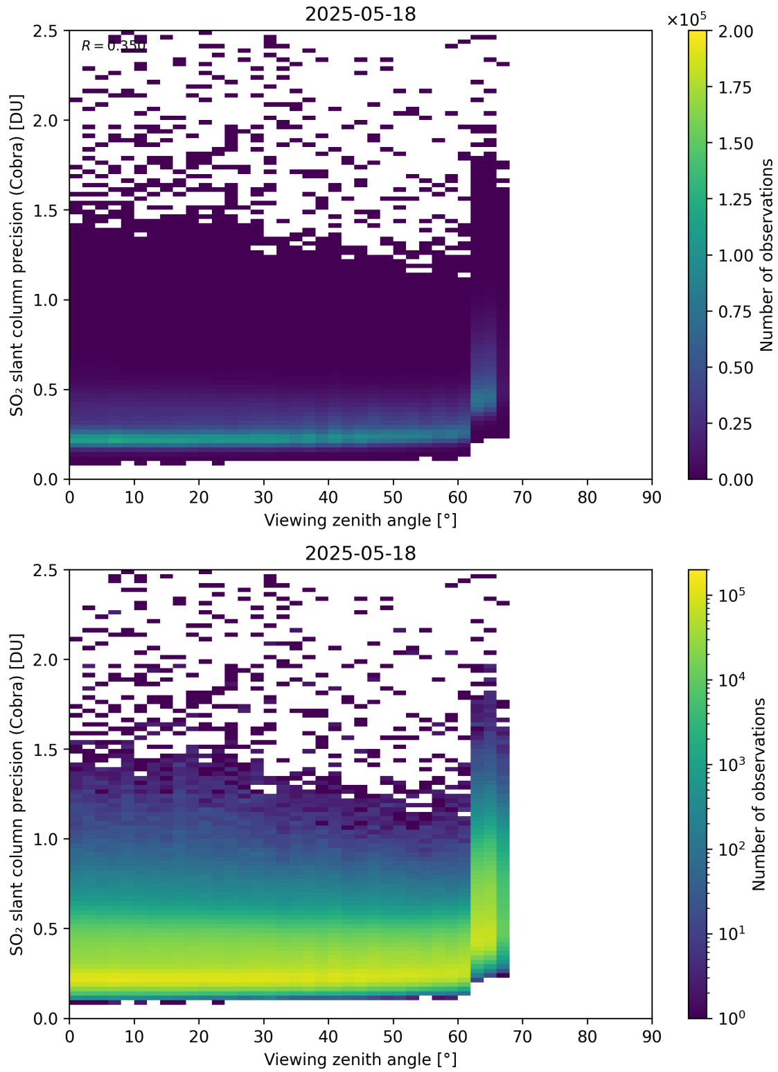
Figure 372: Scatter density plot of “Viewing zenith angle” against “SO 2 slant column precision (Cobra)” for 2025-05-17 to 2025-05-19.
