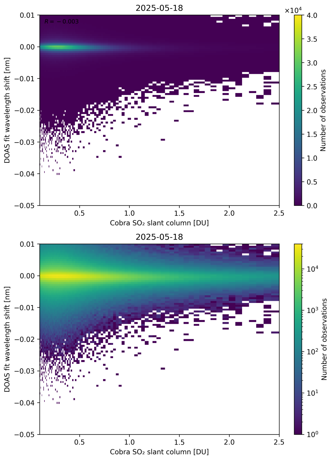
Figure 196: Scatter density plot of “Cobra SO 2 slant column” against “DOAS fit wavelength shift” for 2025-05-17 to 2025-05-19.
