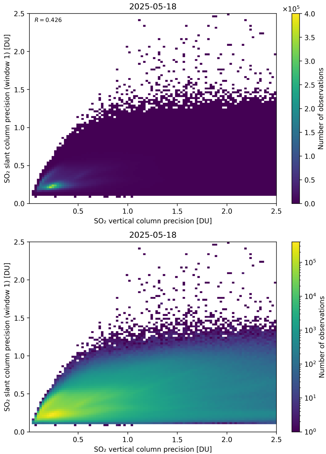
Figure 342: Scatter density plot of “SO 2 vertical column precision” against “SO 2 slant column precision (window 1)” for 2025-05-17 to 2025-05-19.
