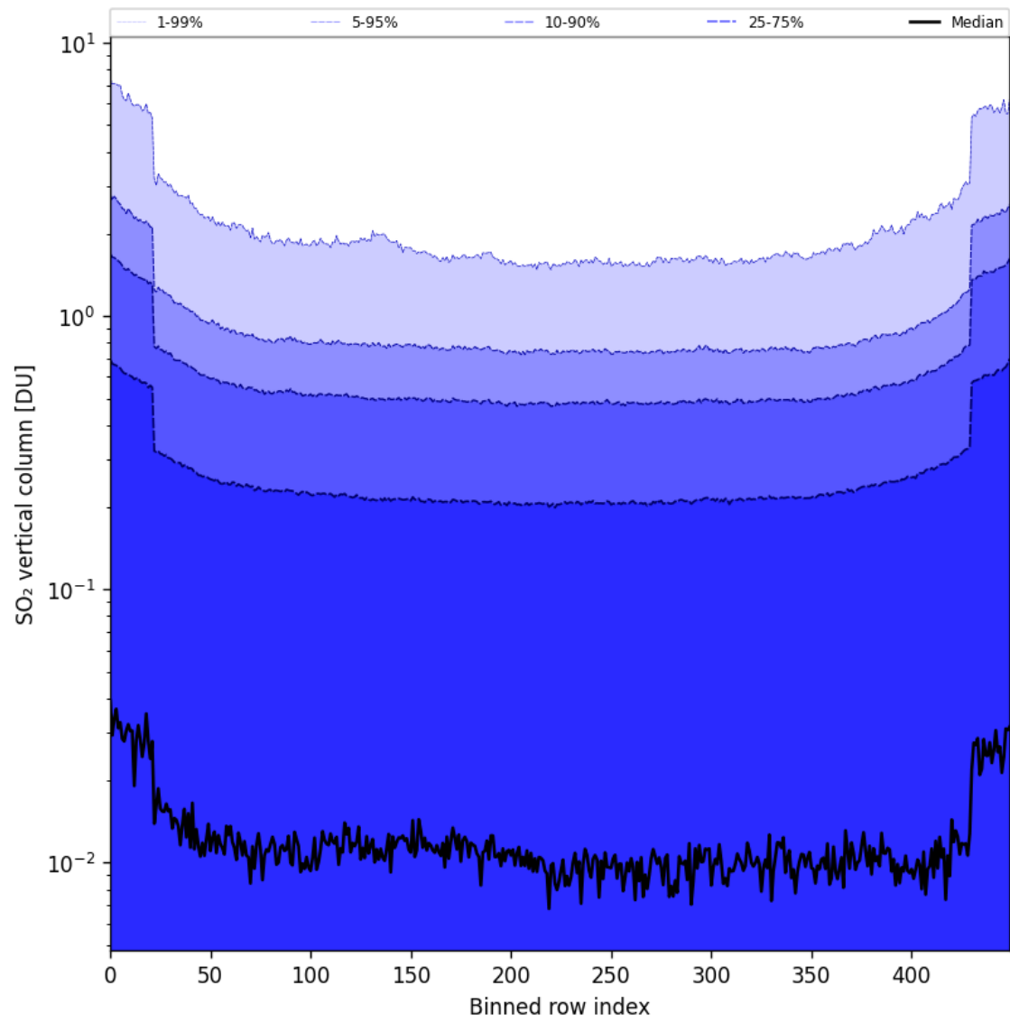
Figure 84: Along track statistics of “SO 2 vertical column” for 2025-05-17 to 2025-05-19
