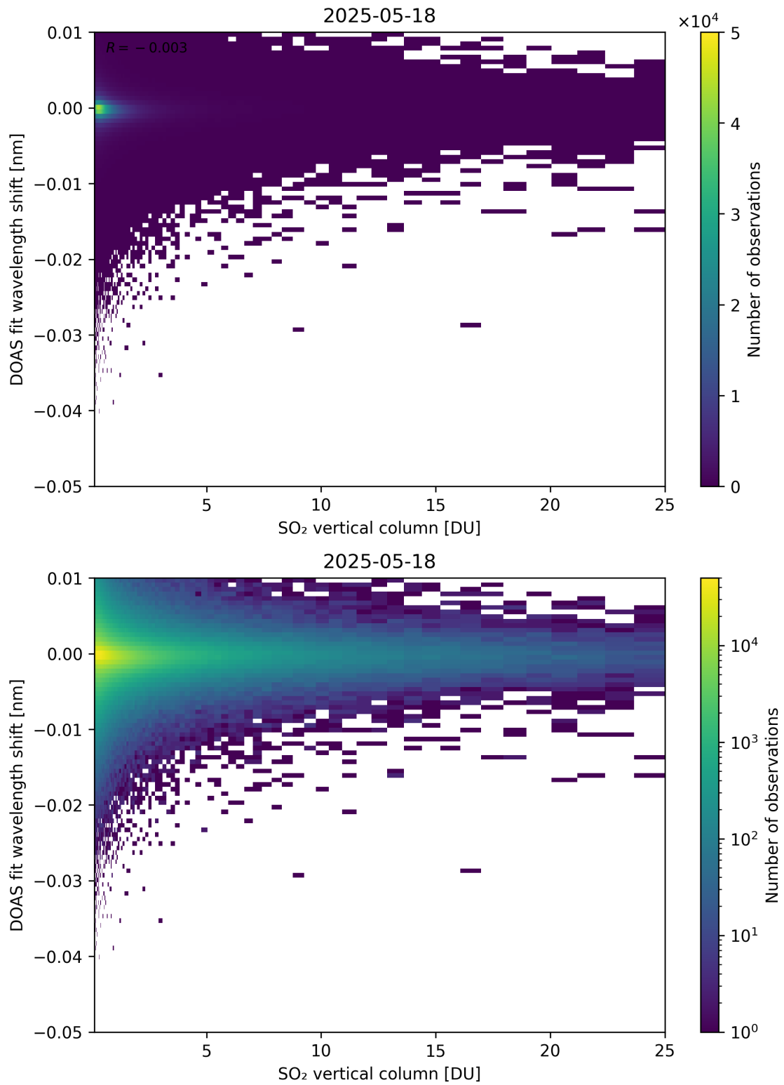
Figure 326: Scatter density plot of “SO 2 vertical column” against “DOAS fit wavelength shift” for 2025-05-17 to 2025-05-19.
