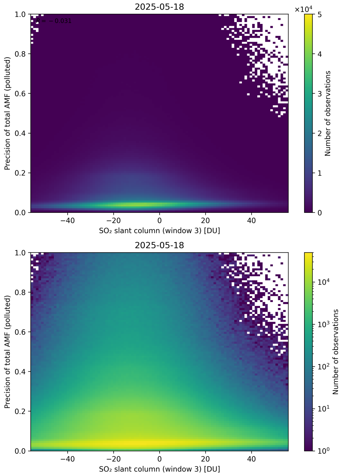
Figure 319: Scatter density plot of “SO 2 slant column (window 3)” against “Precision of total AMF (polluted)” for 2025-05-17 to 2025-05-19.
