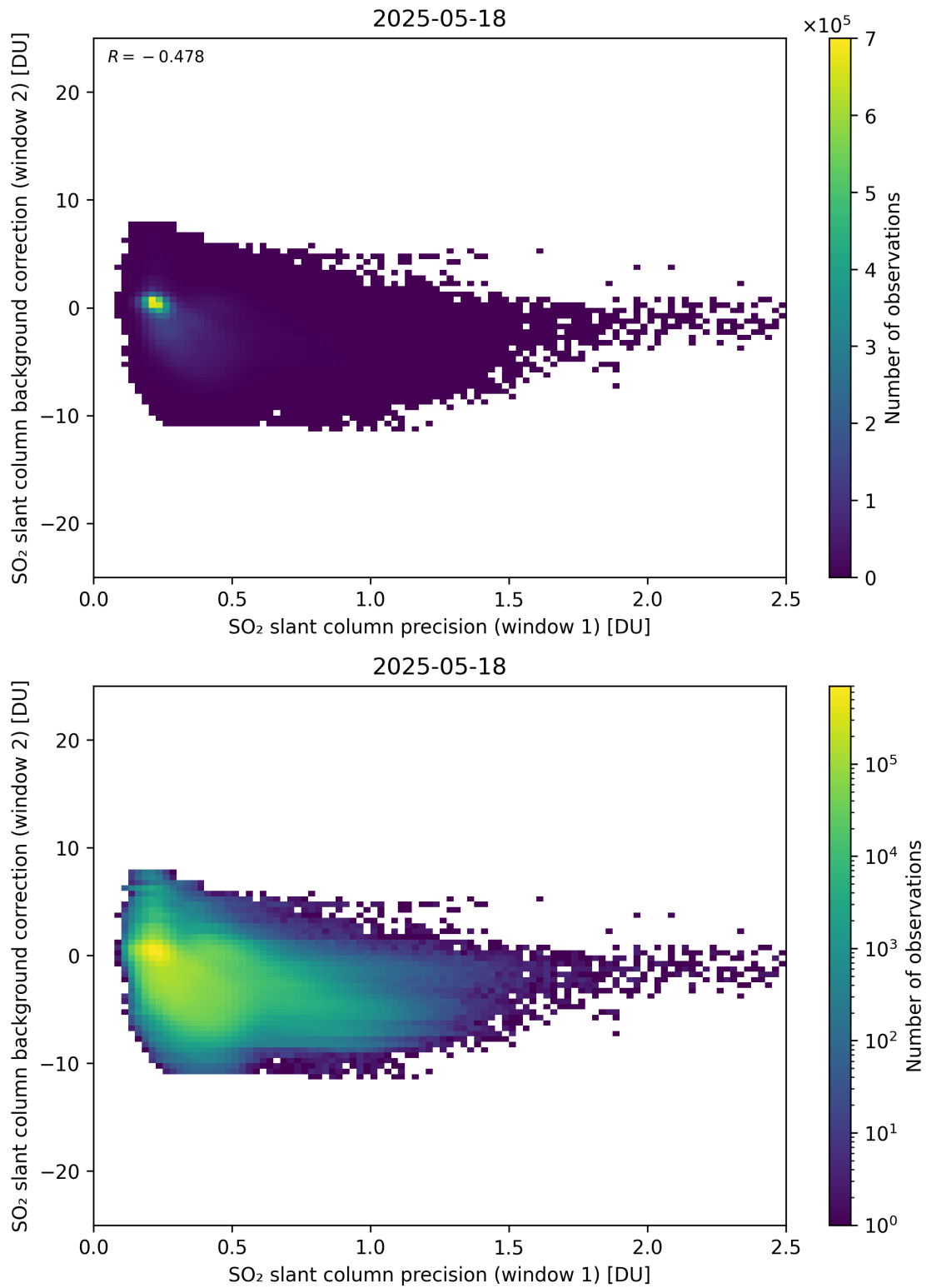
Figure 269: Scatter density plot of “SO 2 slant column precision (window 1)” against “SO 2 slant column background correction (window 2)” for 2025-05-17 to 2025-05-19.
