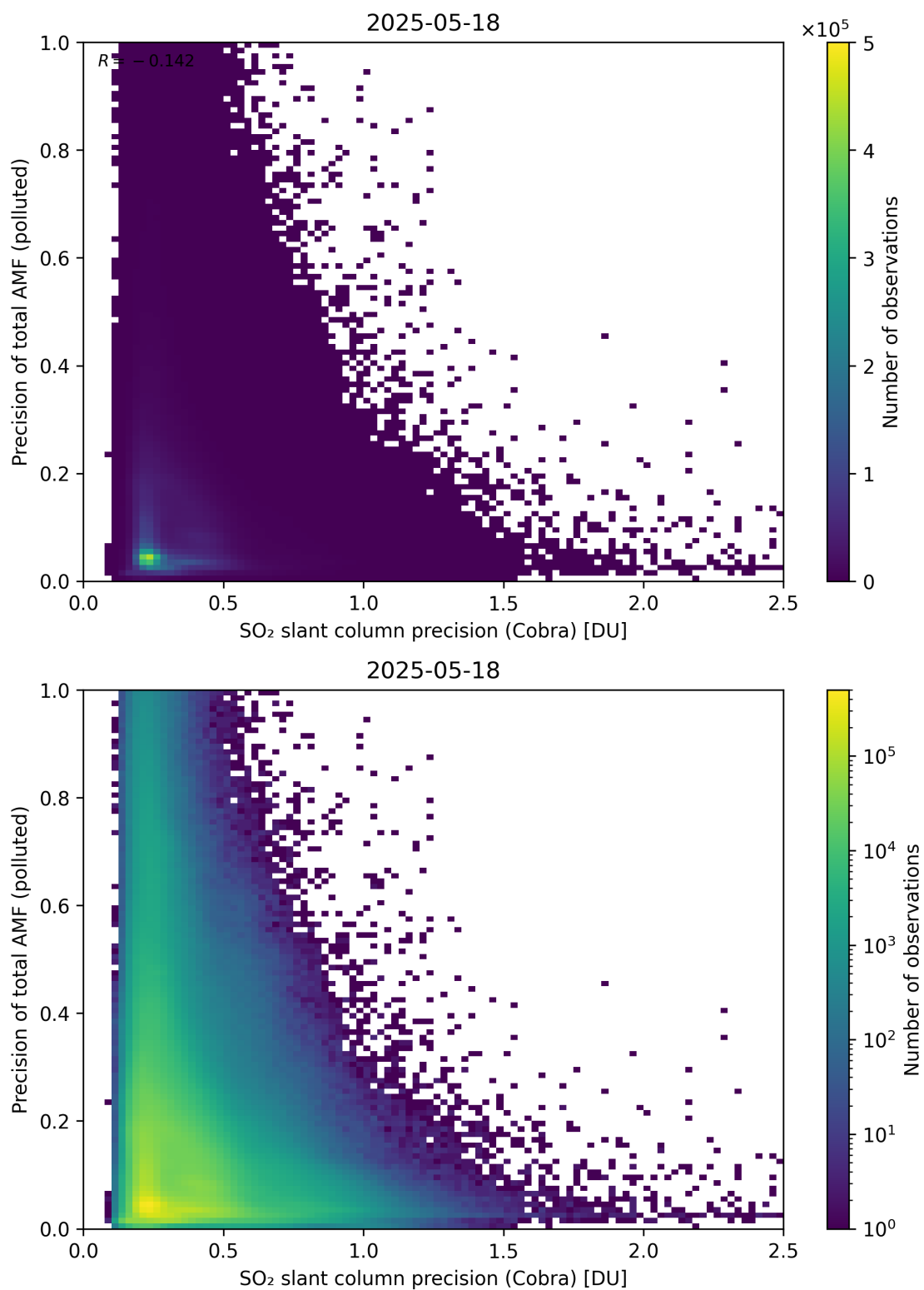
Figure 214: Scatter density plot of “SO 2 slant column precision (Cobra)” against “Precision of total AMF (polluted)” for 2025-05-17 to 2025-05-19.
