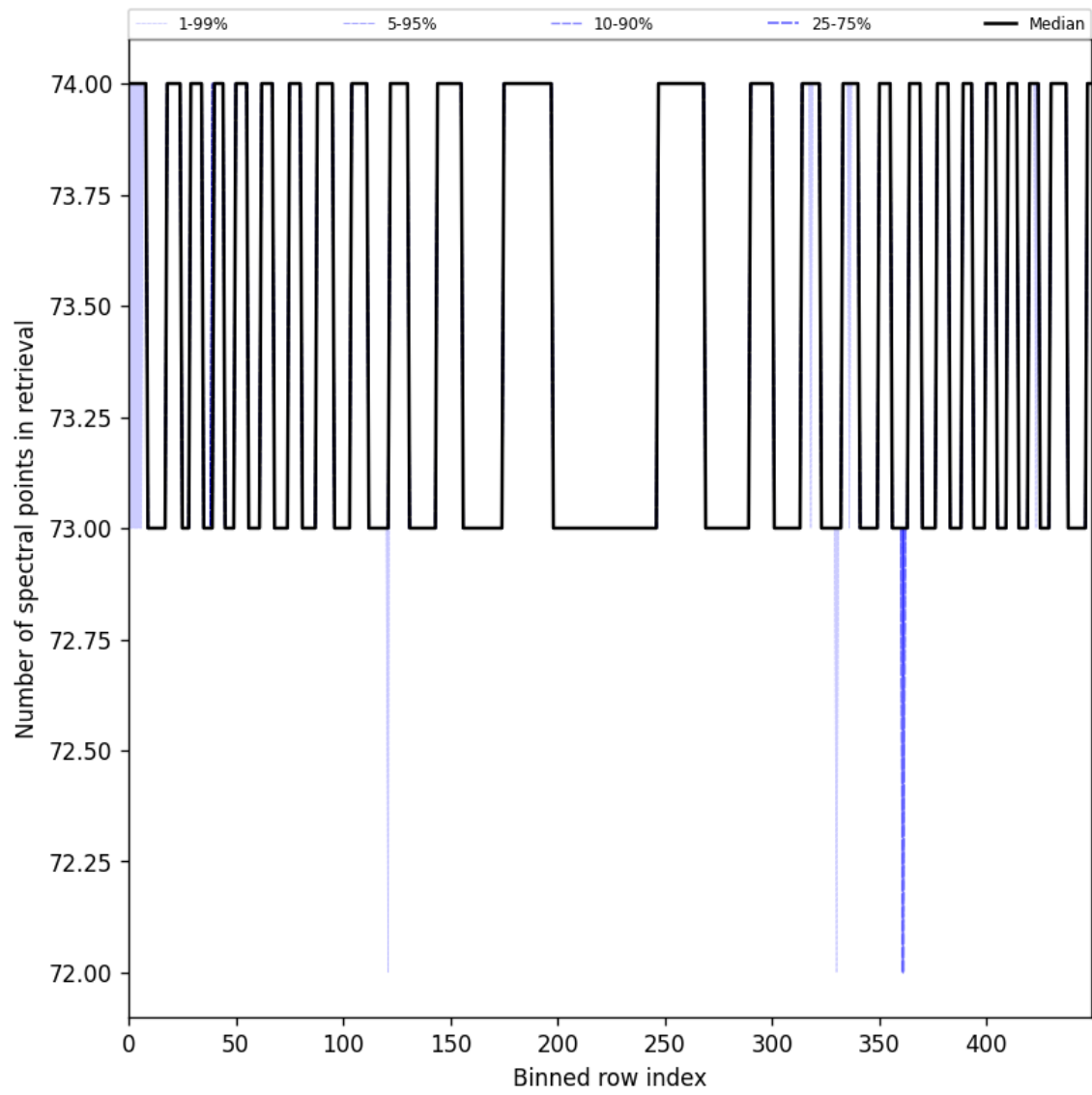
Figure 108: Along track statistics of “Number of spectral points in retrieval” for 2025-05-17 to 2025-05-19
