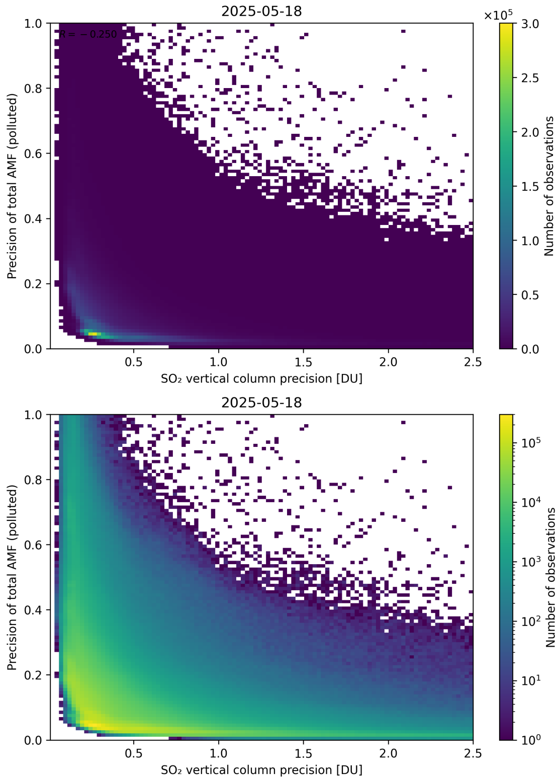
Figure 347: Scatter density plot of “SO 2 vertical column precision” against “Precision of total AMF (polluted)” for 2025-05-17 to 2025-05-19.
