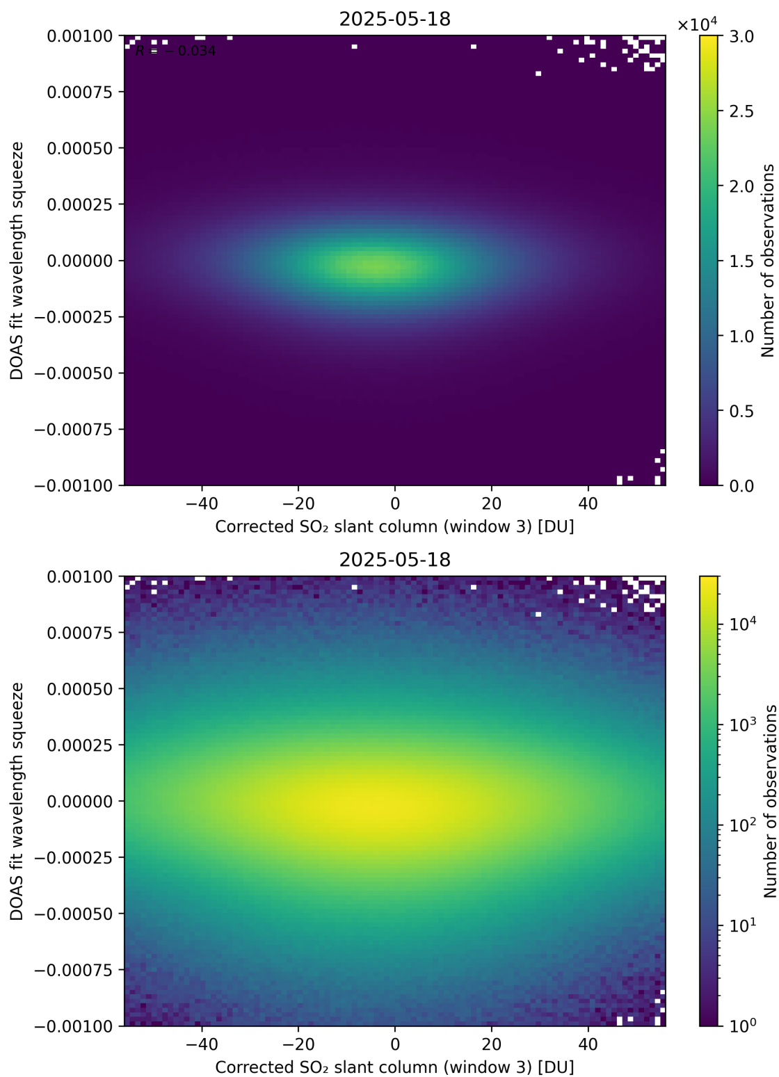
Figure 257: Scatter density plot of “Corrected SO 2 slant column (window 3)” against “DOAS fit wavelength squeeze” for 2025-05-17 to 2025-05-19.
