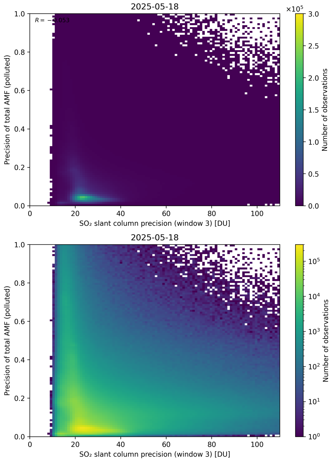
Figure 314: Scatter density plot of “SO 2 slant column precision (window 3)” against “Precision of total AMF (polluted)” for 2025-05-17 to 2025-05-19.
