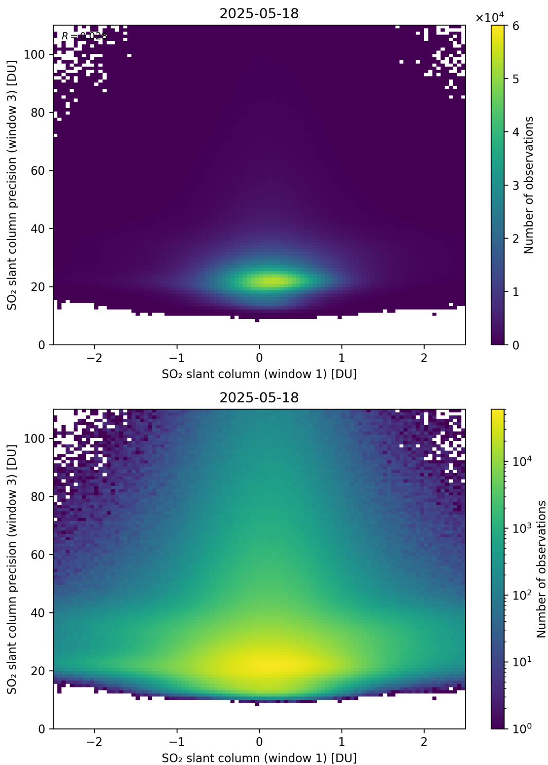
Figure 288: Scatter density plot of “SO 2 slant column (window 1)” against “SO 2 slant column precision (window 3)” for 2025-05-17 to 2025-05-19.
