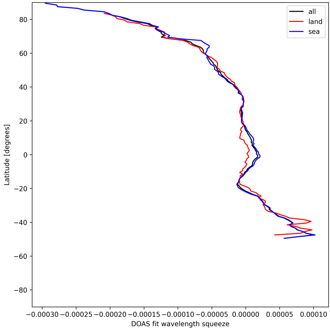
Figure 51: Zonal average of “DOAS fit wavelength squeeze” for 2025-05-17 to 2025-05-19.
