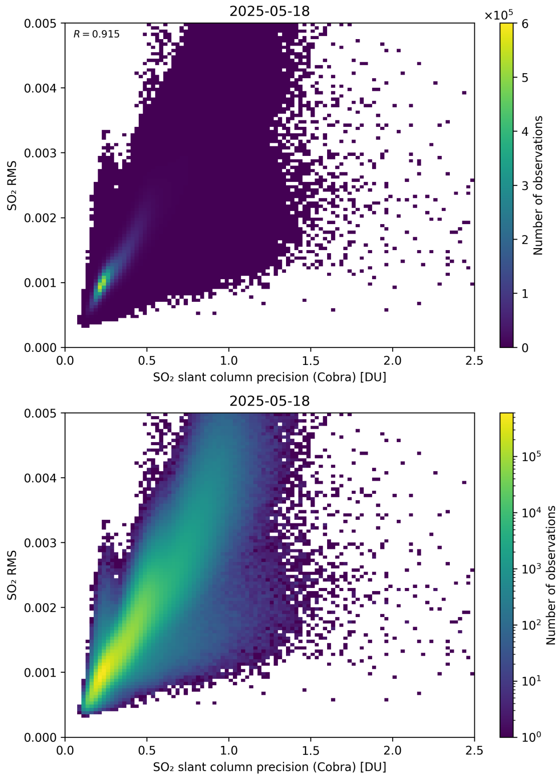
Figure 204: Scatter density plot of “SO 2 slant column precision (Cobra)” against “SO 2 RMS” for 2025-05-17 to 2025-05-19.
