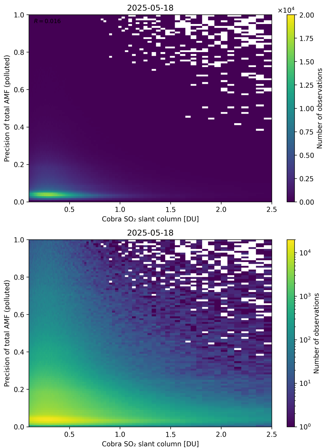
Figure 225: Scatter density plot of “Cobra SO 2 slant column” against “Precision of total AMF (polluted)” for 2025-05-17 to 2025-05-19.
