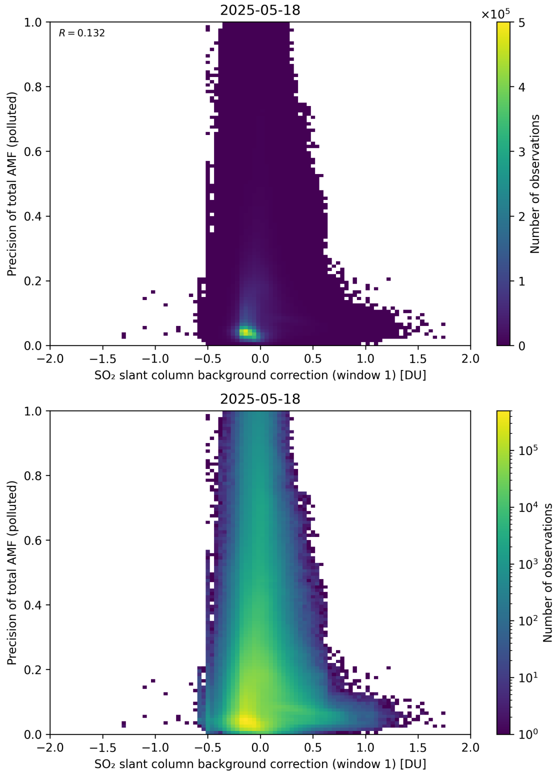
Figure 121: Scatter density plot of “SO 2 slant column background correction (window 1)” against “Precision of total AMF (polluted)” for 2025-05-17 to 2025-05-19.
