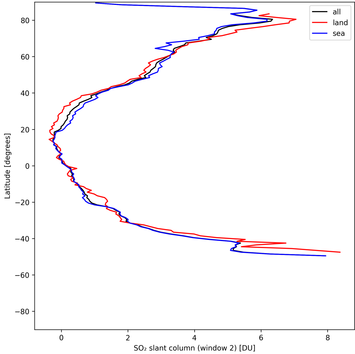
Figure 41: Zonal average of “SO 2 slant column (window 2)” for 2025-05-17 to 2025-05-19.
