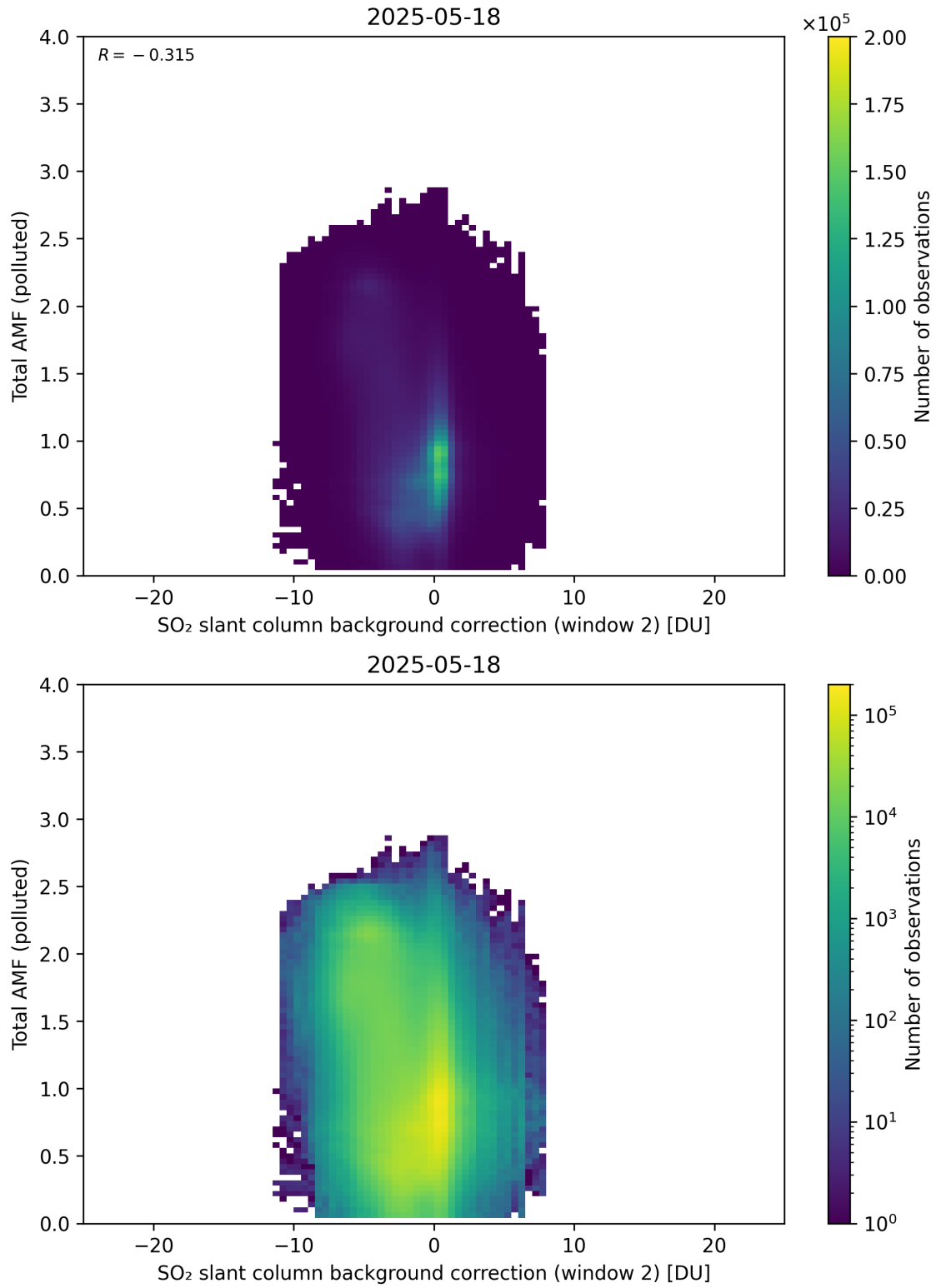
Figure 130: Scatter density plot of “SO 2 slant column background correction (window 2)” against “Total AMF (polluted)” for 2025-05-17 to 2025-05-19.
