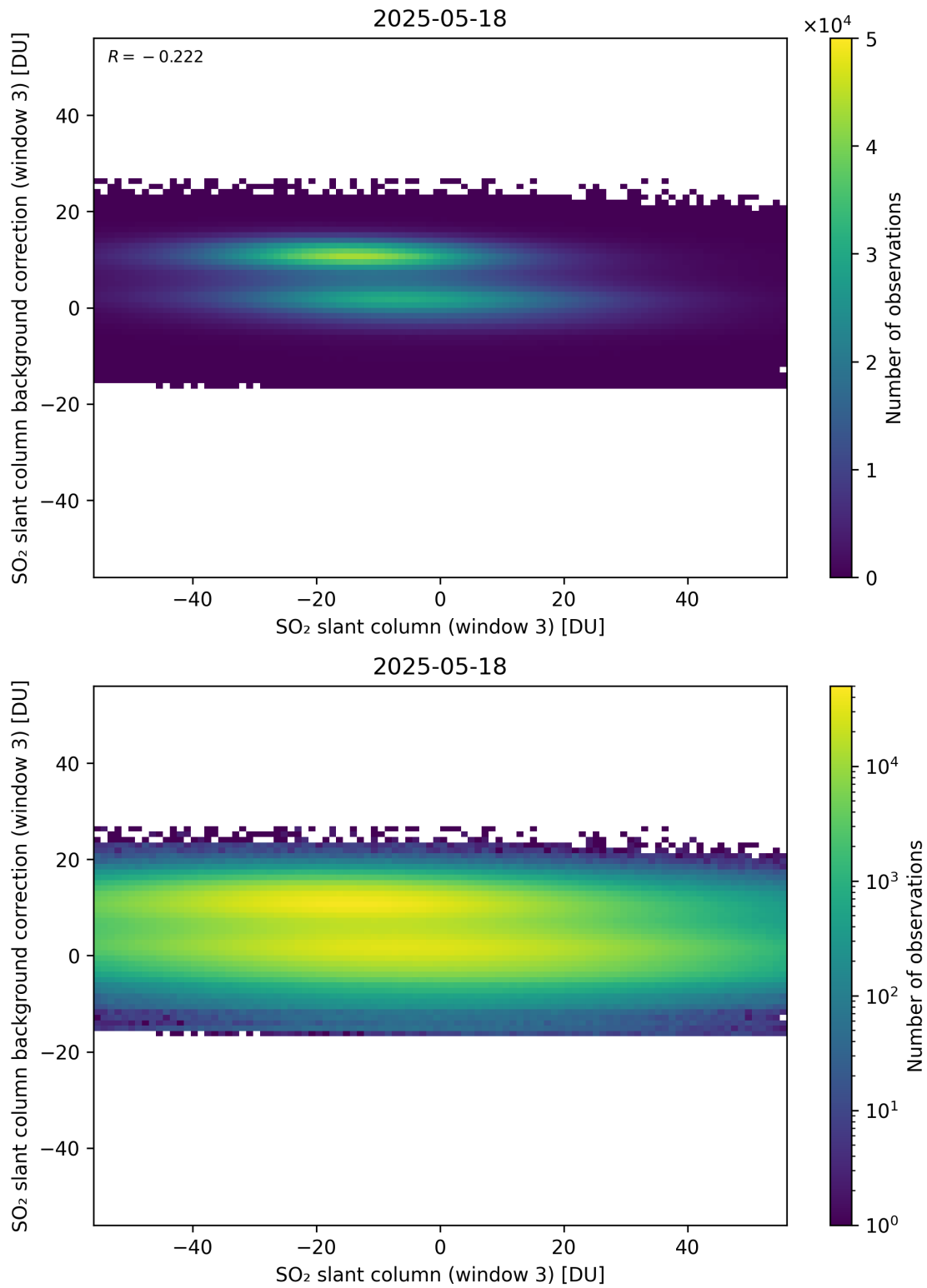
Figure 303: Scatter density plot of “SO 2 slant column (window 3)” against “SO 2 slant column background correction (window 3)” for 2025-05-17 to 2025-05-19.
