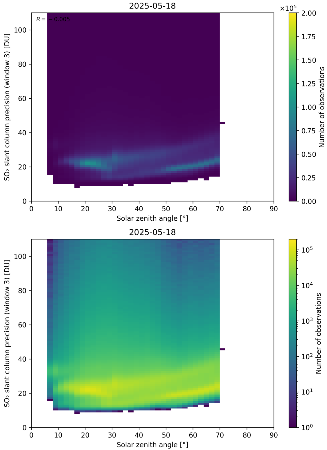
Figure 188: Scatter density plot of “Solar zenith angle” against “SO 2 slant column precision (window 3)” for 2025-05-17 to 2025-05-19.
