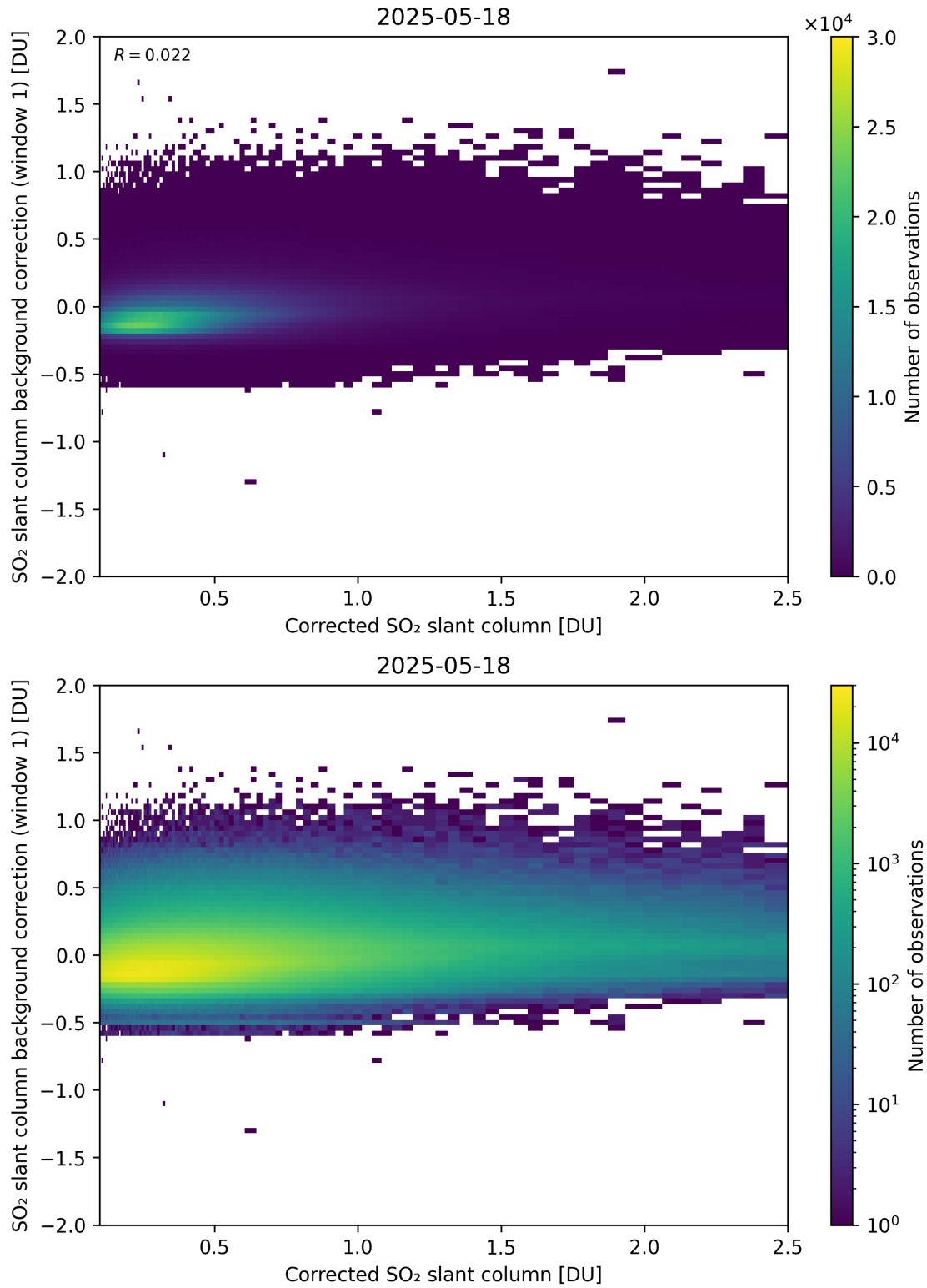
Figure 226: Scatter density plot of “Corrected SO 2 slant column” against “SO 2 slant column background correction (window 1)” for 2025-05-17 to 2025-05-19.
