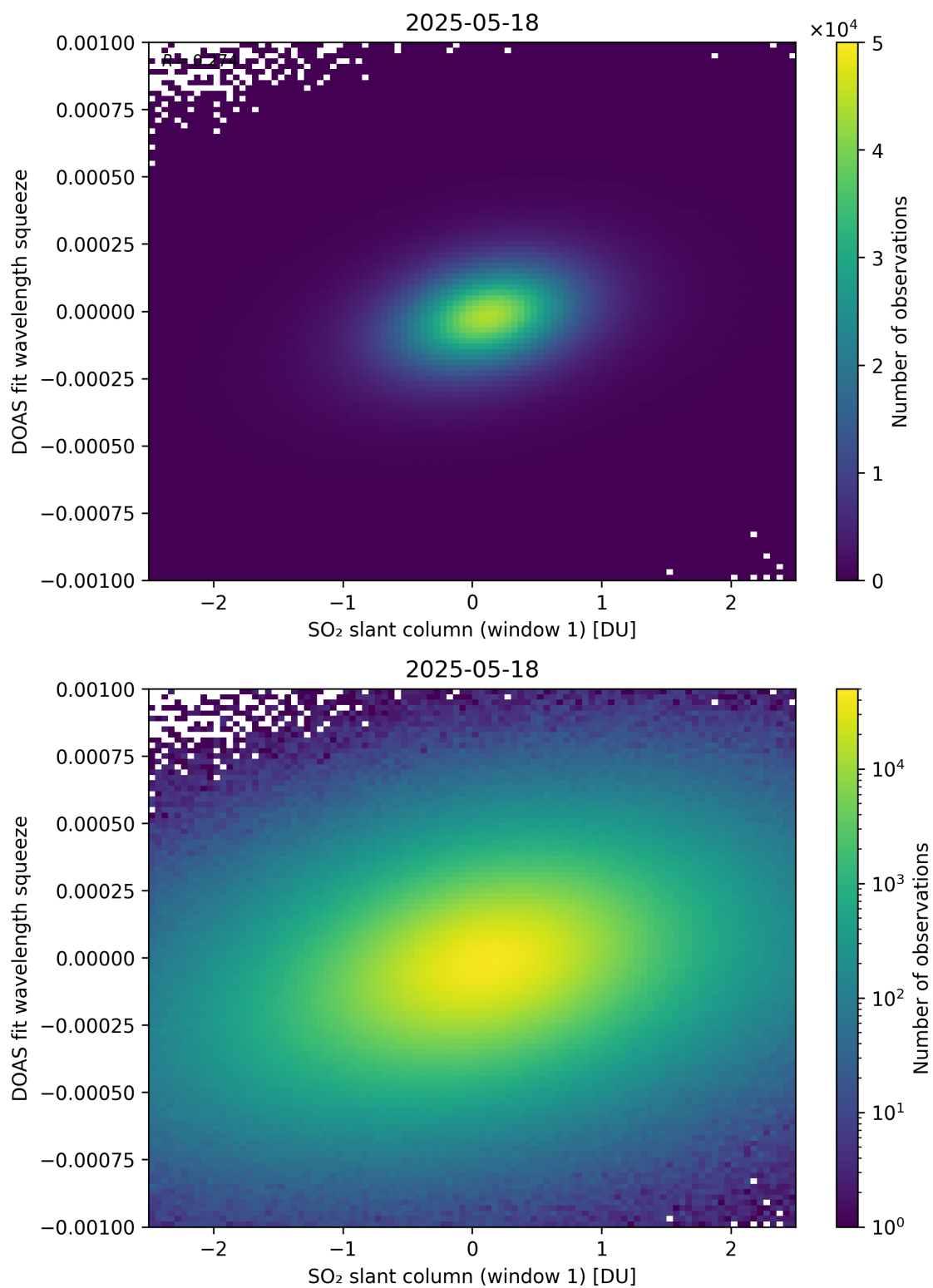
Figure 266: Scatter density plot of “SO 2 slant column (window 1)” against “DOAS fit wavelength squeeze” for 2025-05-17 to 2025-05-19.
