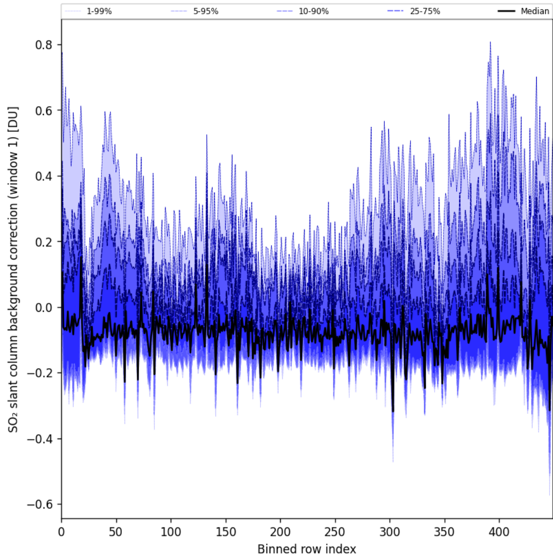
Figure 92: Along track statistics of “SO 2 slant column background correction (window 1)” for 2025-05-17 to 2025-05-19
