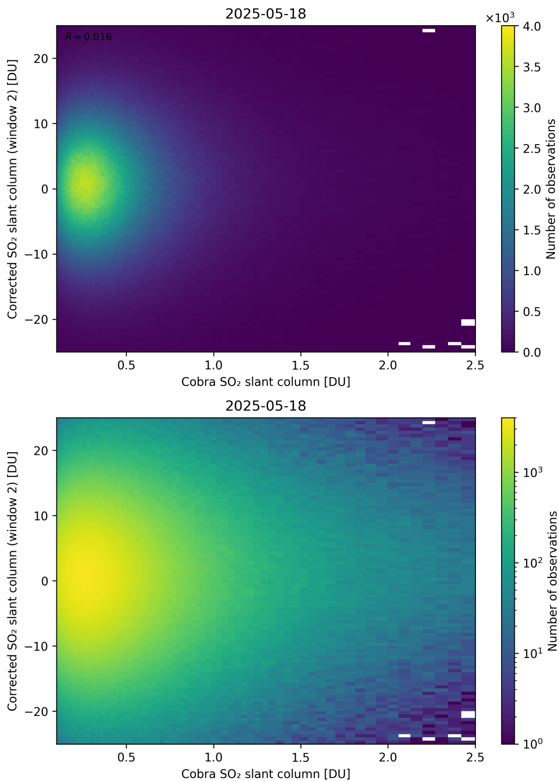
Figure 217: Scatter density plot of “Cobra SO 2 slant column” against “Corrected SO 2 slant column (window 2)” for 2025-05-17 to 2025-05-19.
