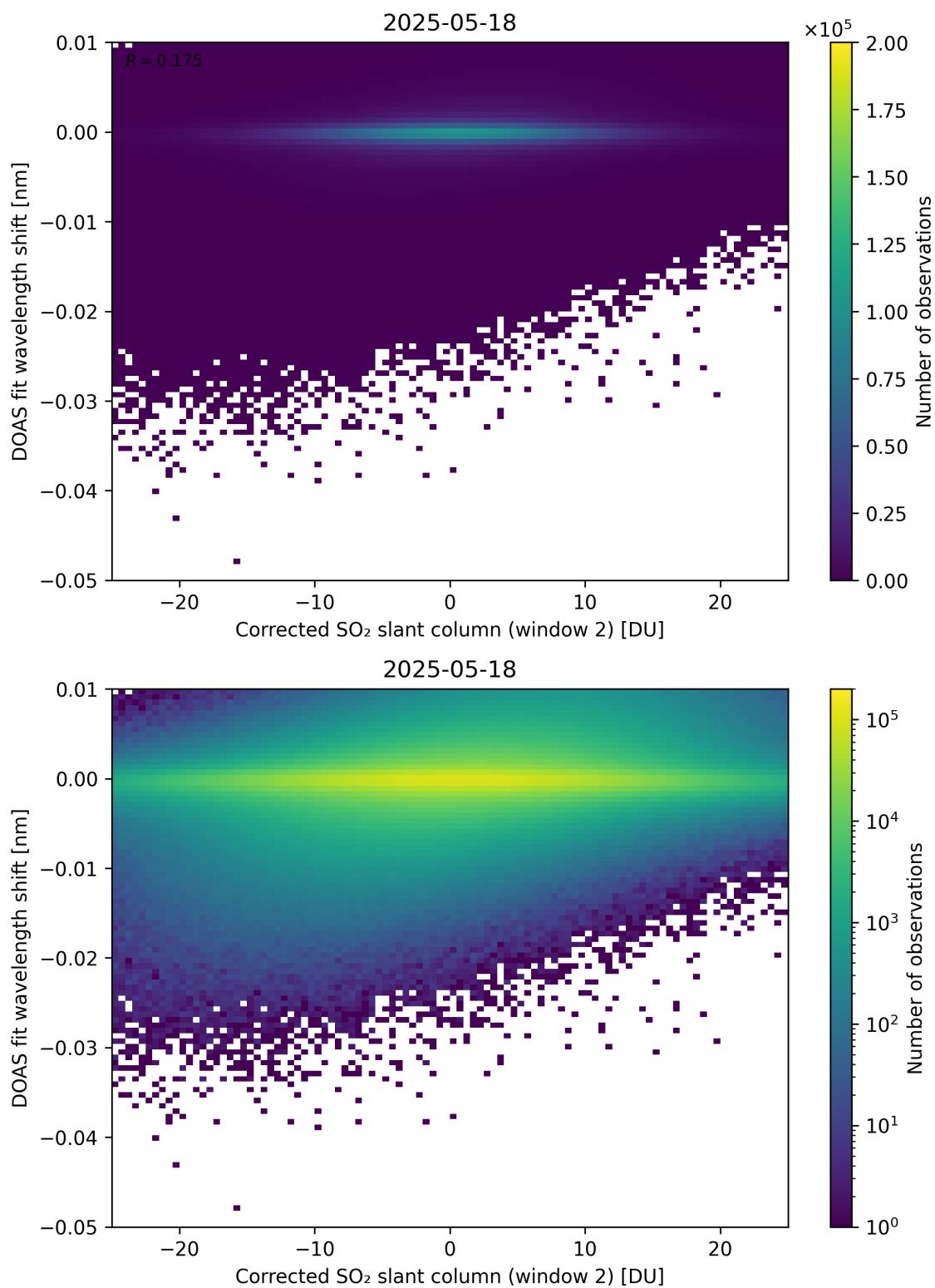
Figure 246: Scatter density plot of “Corrected SO 2 slant column (window 2)” against “DOAS fit wavelength shift” for 2025-05-17 to 2025-05-19.
