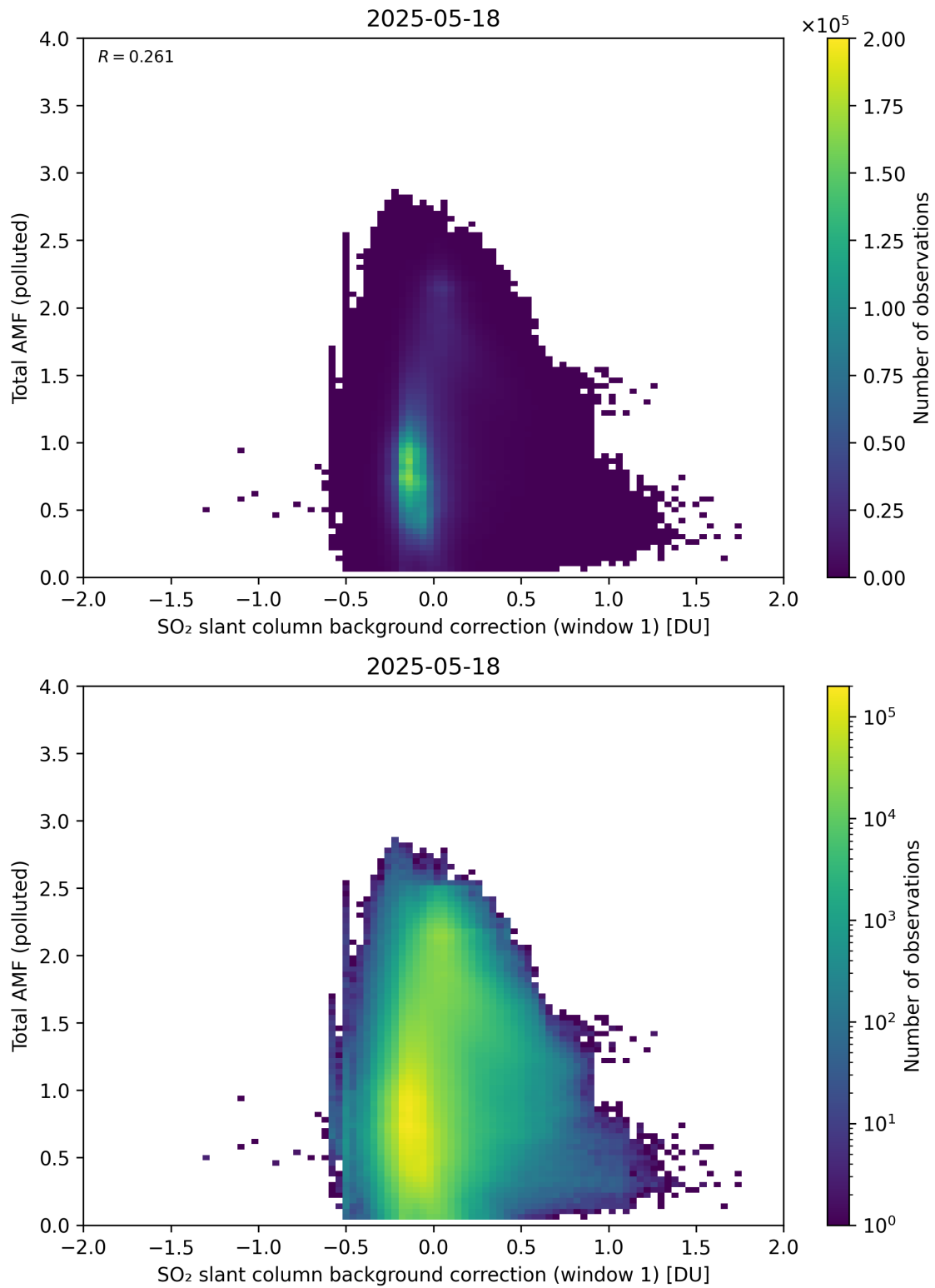
Figure 120: Scatter density plot of “SO 2 slant column background correction (window 1)” against “Total AMF (polluted)” for 2025-05-17 to 2025-05-19.
