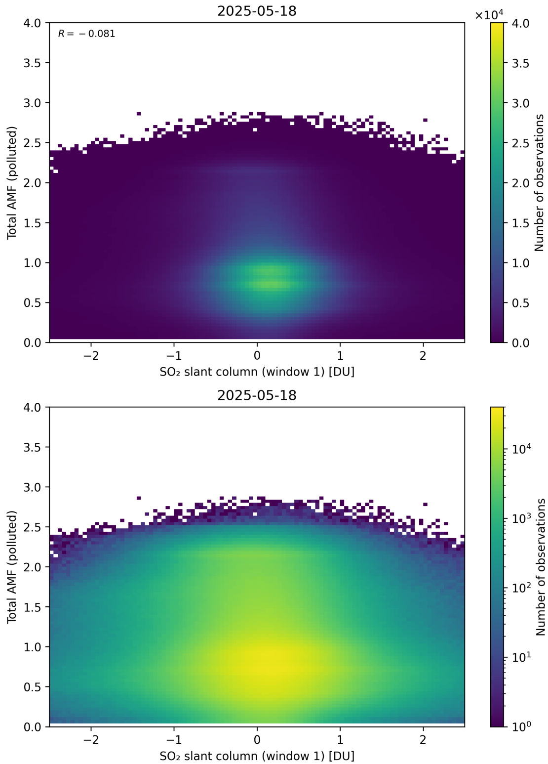
Figure 289: Scatter density plot of “SO 2 slant column (window 1)” against “Total AMF (polluted)” for 2025-05-17 to 2025-05-19.
