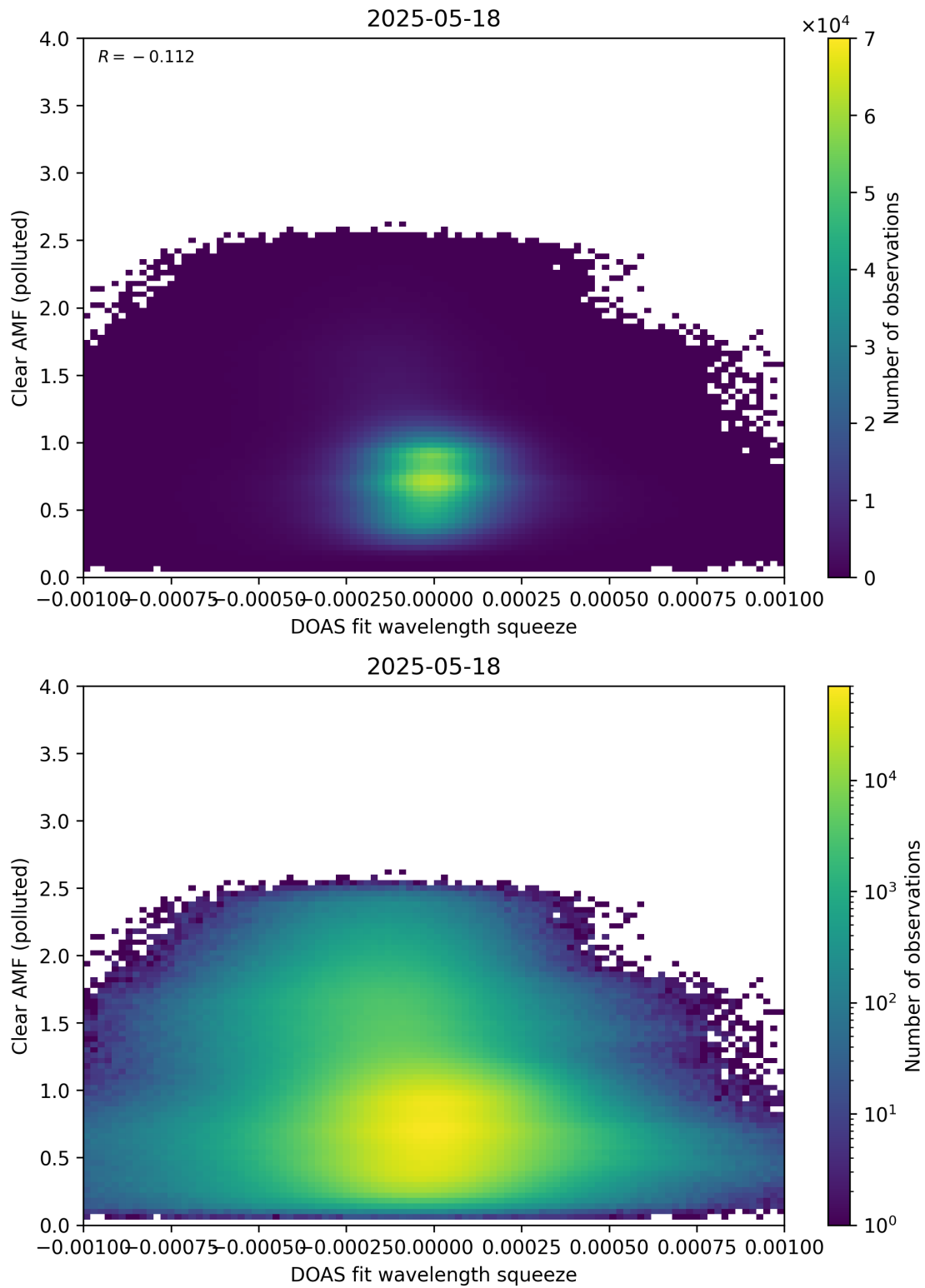
Figure 144: Scatter density plot of “DOAS fit wavelength squeeze” against “Clear AMF (polluted)” for 2025-05-17 to 2025-05-19.
