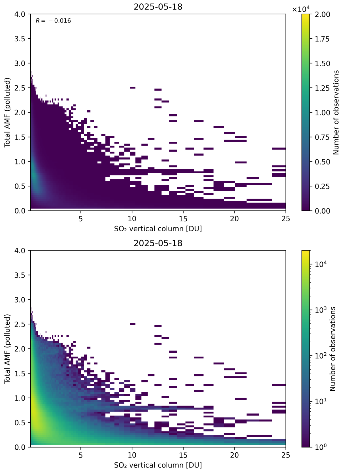
Figure 359: Scatter density plot of “SO 2 vertical column” against “Total AMF (polluted)” for 2025-05-17 to 2025-05-19.
