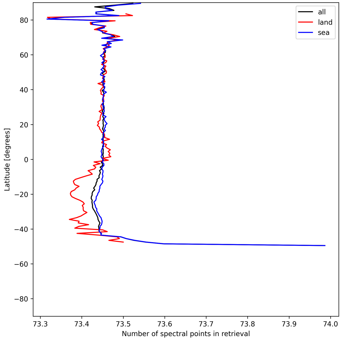
Figure 56: Zonal average of “Number of spectral points in retrieval” for 2025-05-17 to 2025-05-19.
