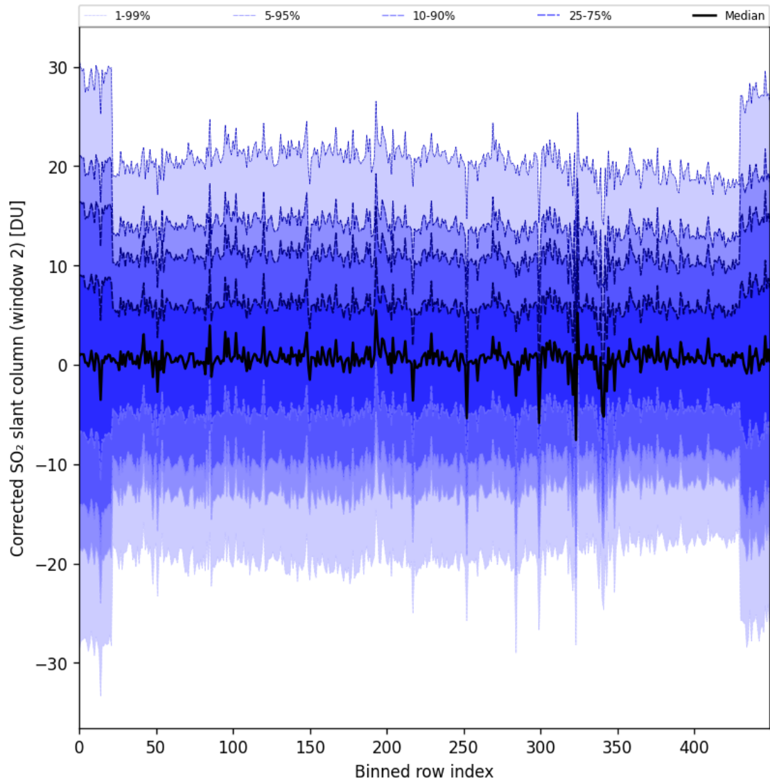
Figure 95: Along track statistics of “Corrected SO 2 slant column (window 2)” for 2025-05-17 to 2025-05-19
