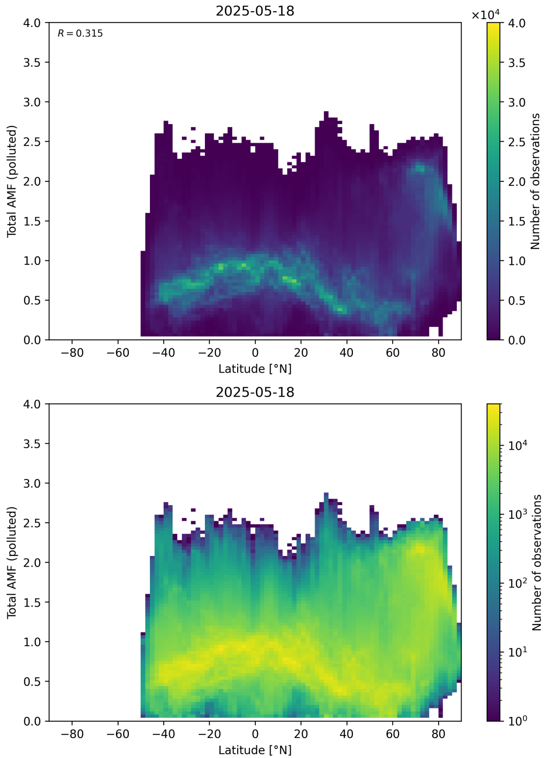
Figure 167: Scatter density plot of “Latitude” against “Total AMF (polluted)” for 2025-05-17 to 2025-05-19.
