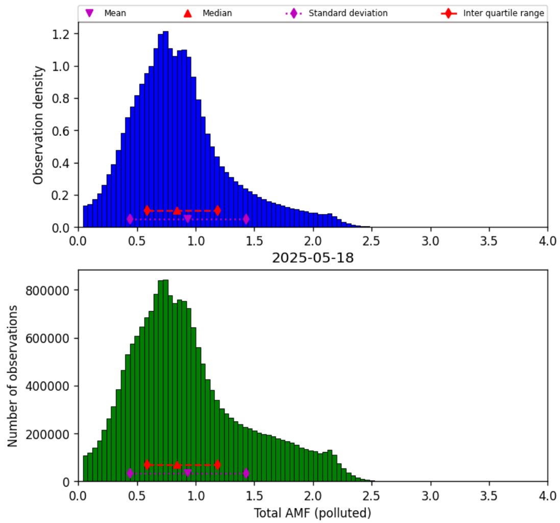
Figure 79: Histogram of “Total AMF (polluted)” for 2025-05-17 to 2025-05-19
