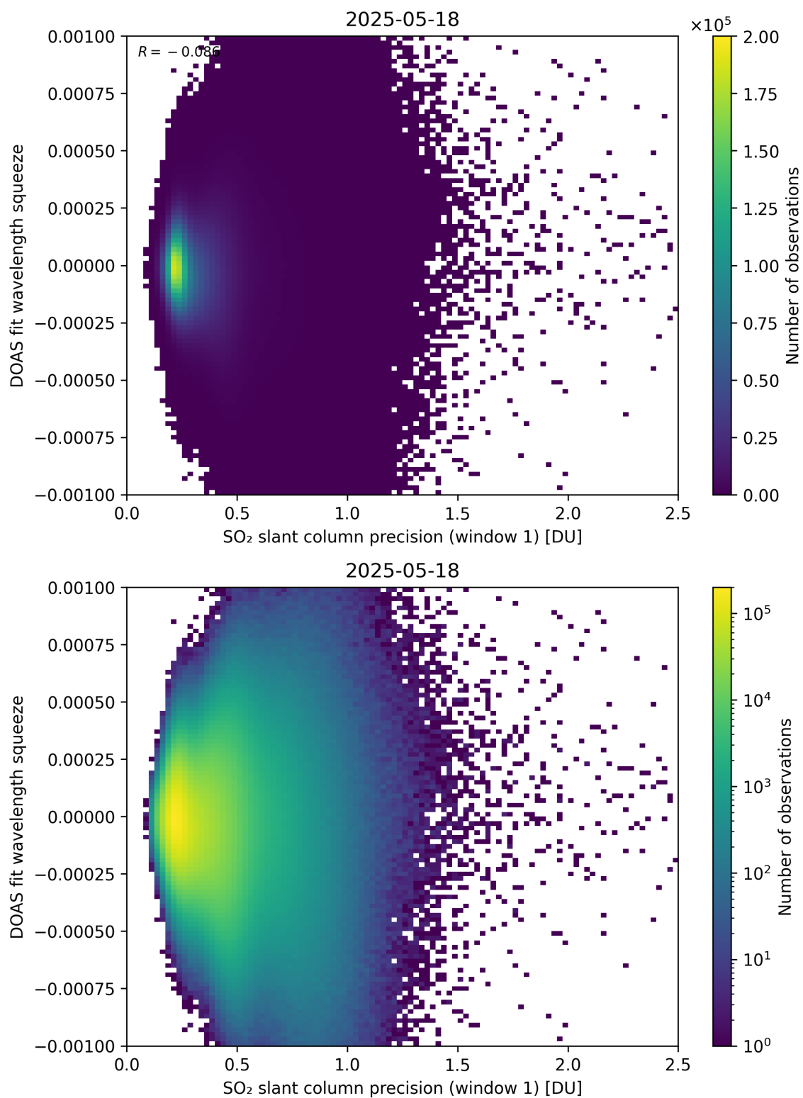
Figure 272: Scatter density plot of “SO 2 slant column precision (window 1)” against “DOAS fit wavelength squeeze” for 2025-05-17 to 2025-05-19.
