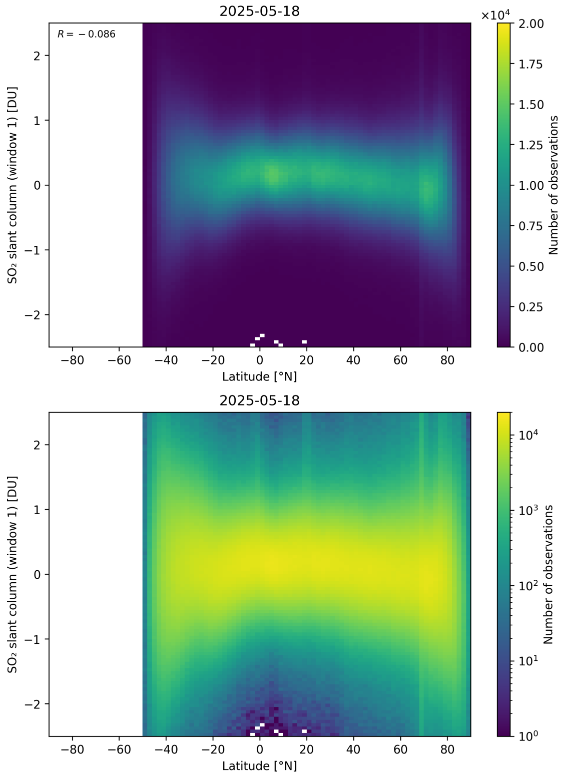
Figure 162: Scatter density plot of “Latitude” against “SO 2 slant column (window 1)” for 2025-05-17 to 2025-05-19.
