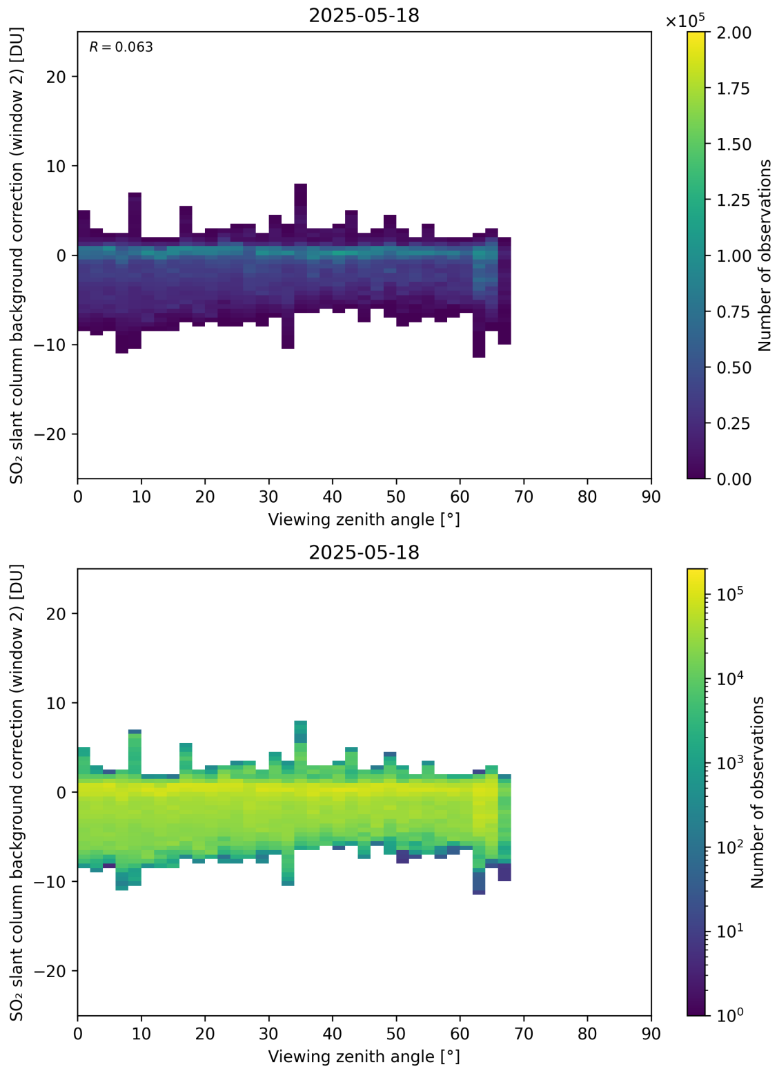
Figure 363: Scatter density plot of “Viewing zenith angle” against “SO 2 slant column background correction (window 2)” for 2025-05-17 to 2025-05-19.
