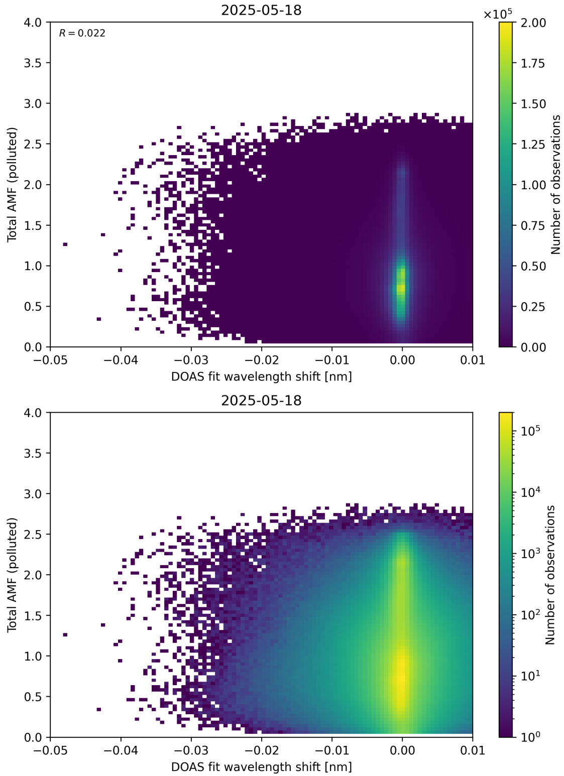
Figure 141: Scatter density plot of “DOAS fit wavelength shift” against “Total AMF (polluted)” for 2025-05-17 to 2025-05-19.
