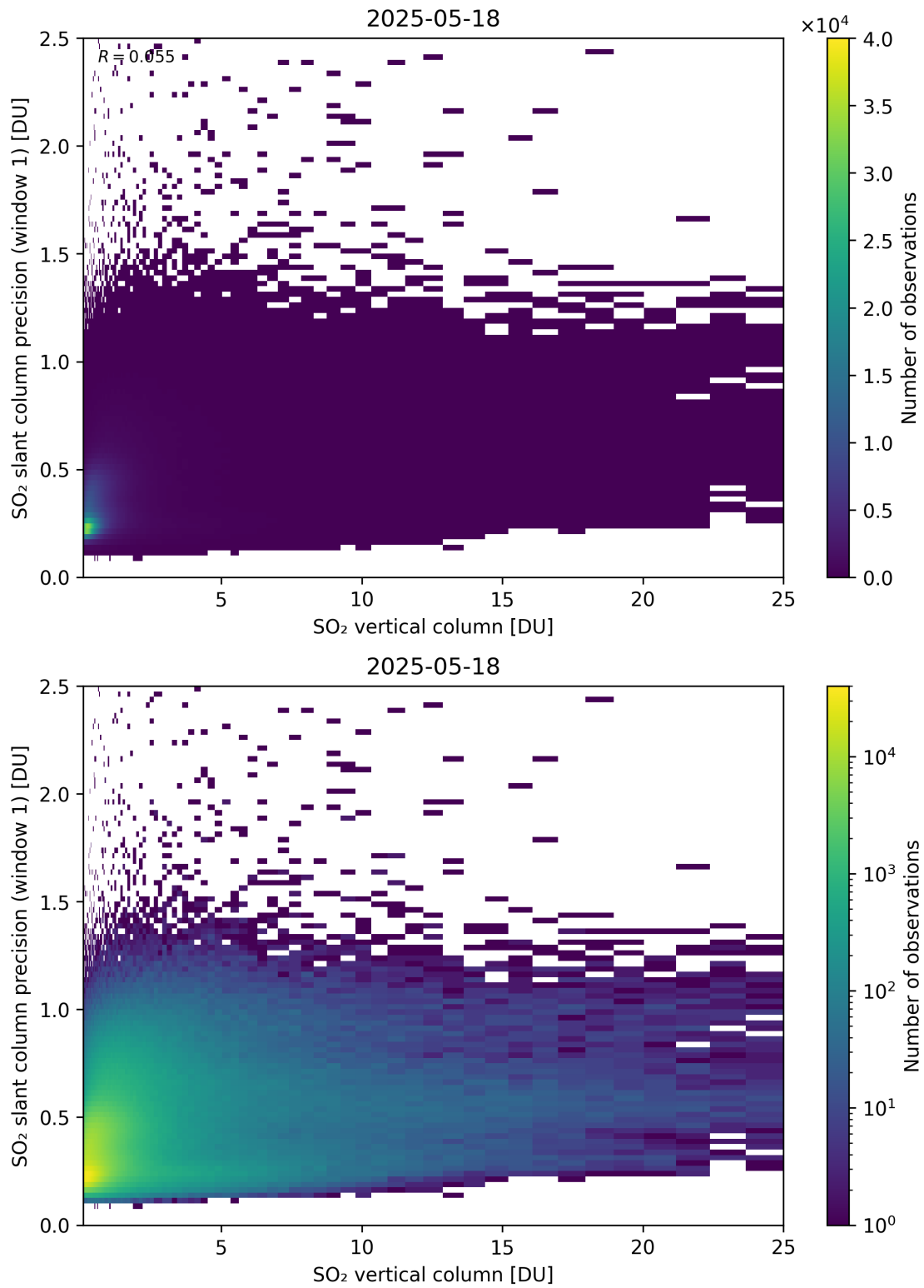
Figure 355: Scatter density plot of “SO 2 vertical column” against “SO 2 slant column precision (window 1)” for 2025-05-17 to 2025-05-19.
