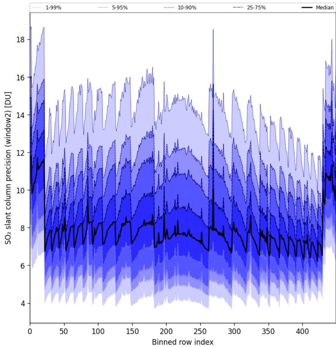
Figure 94: Along track statistics of “SO 2 slant column precision (window2)” for 2025-05-17 to 2025-05-19
