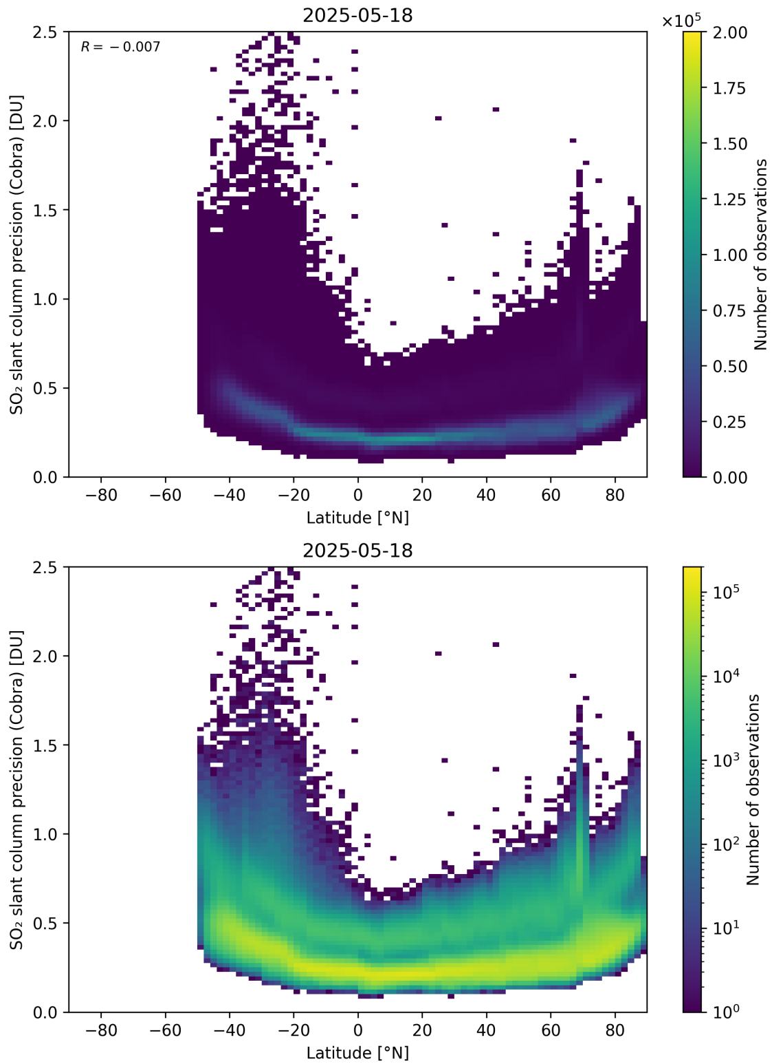
Figure 158: Scatter density plot of “Latitude” against “SO 2 slant column precision (Cobra)” for 2025-05-17 to 2025-05-19.
