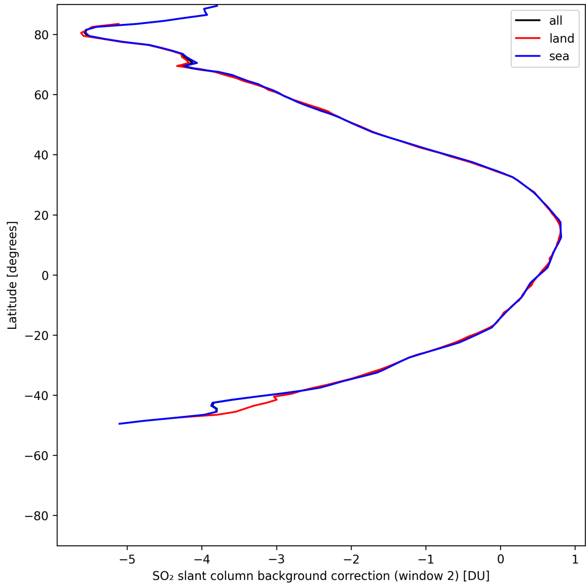
Figure 44: Zonal average of “SO 2 slant column background correction (window 2)” for 2025-05-17 to 2025-05-19.
