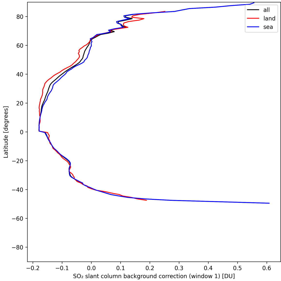
Figure 40: Zonal average of "SO 2 slant column background correction (window 1)" for 2025-05-17 to 2025-05-19.
