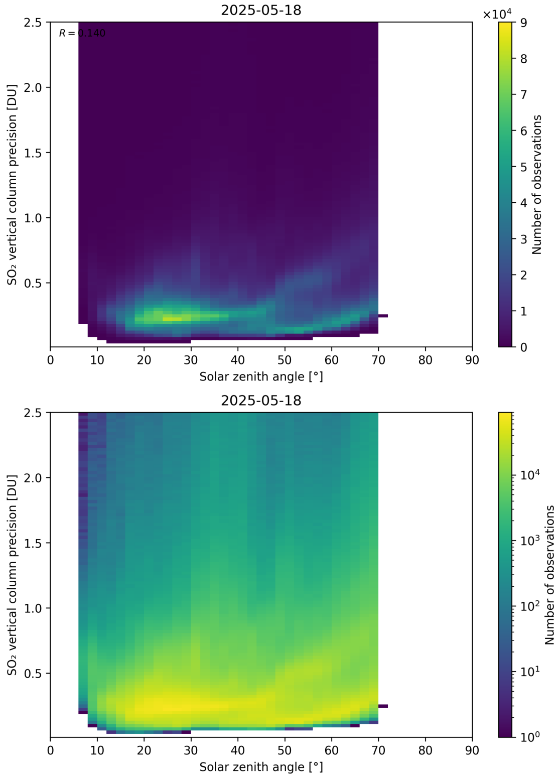
Figure 192: Scatter density plot of “Solar zenith angle” against “SO 2 vertical column precision” for 2025-05-17 to 2025-05-19.
