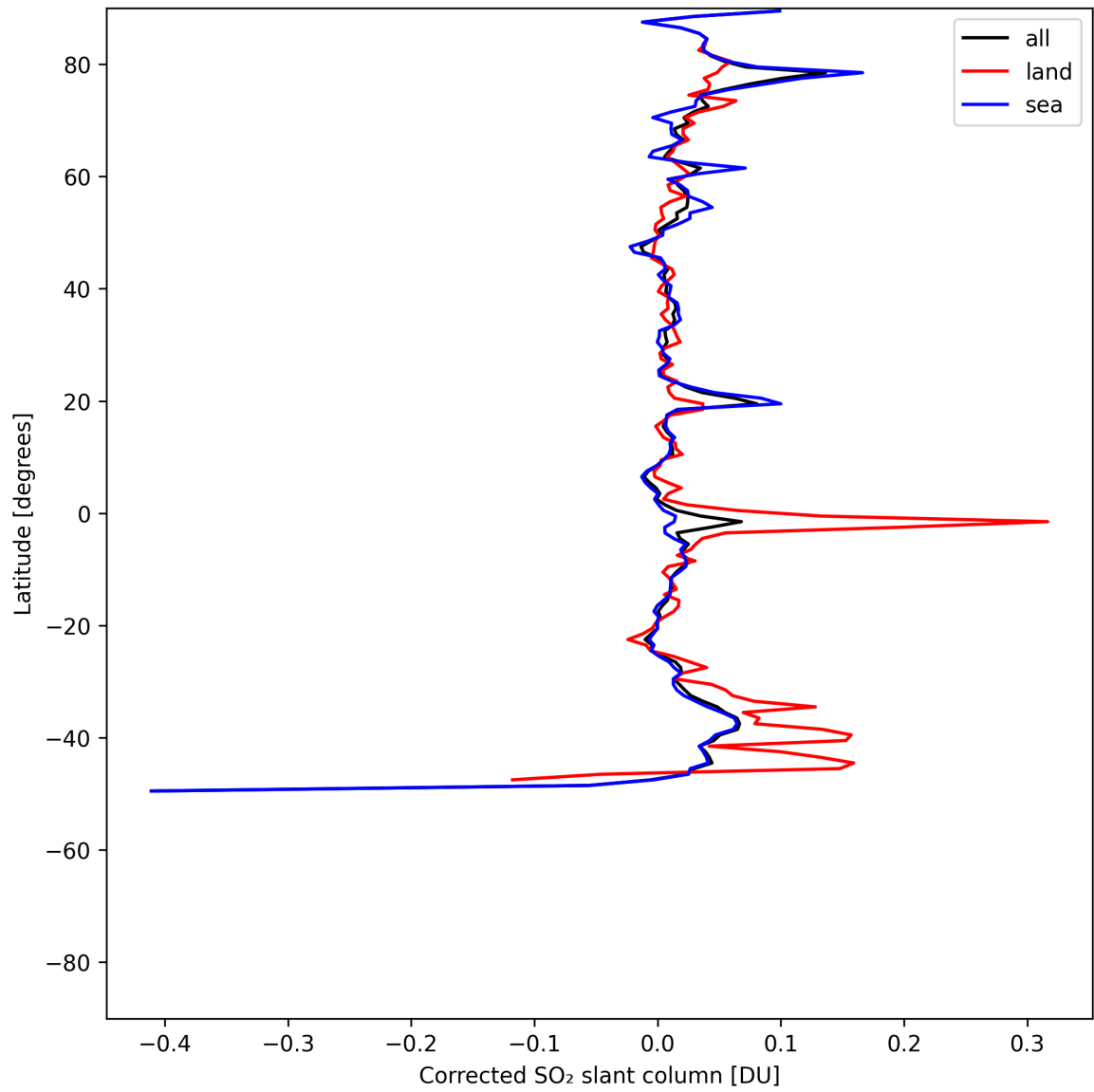
Figure 34: Zonal average of “Corrected SO 2 slant column” for 2025-05-17 to 2025-05-19.
