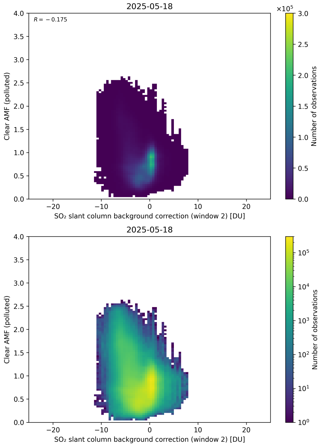
Figure 126: Scatter density plot of “SO 2 slant column background correction (window 2)” against “Clear AMF (polluted)” for 2025-05-17 to 2025-05-19.
