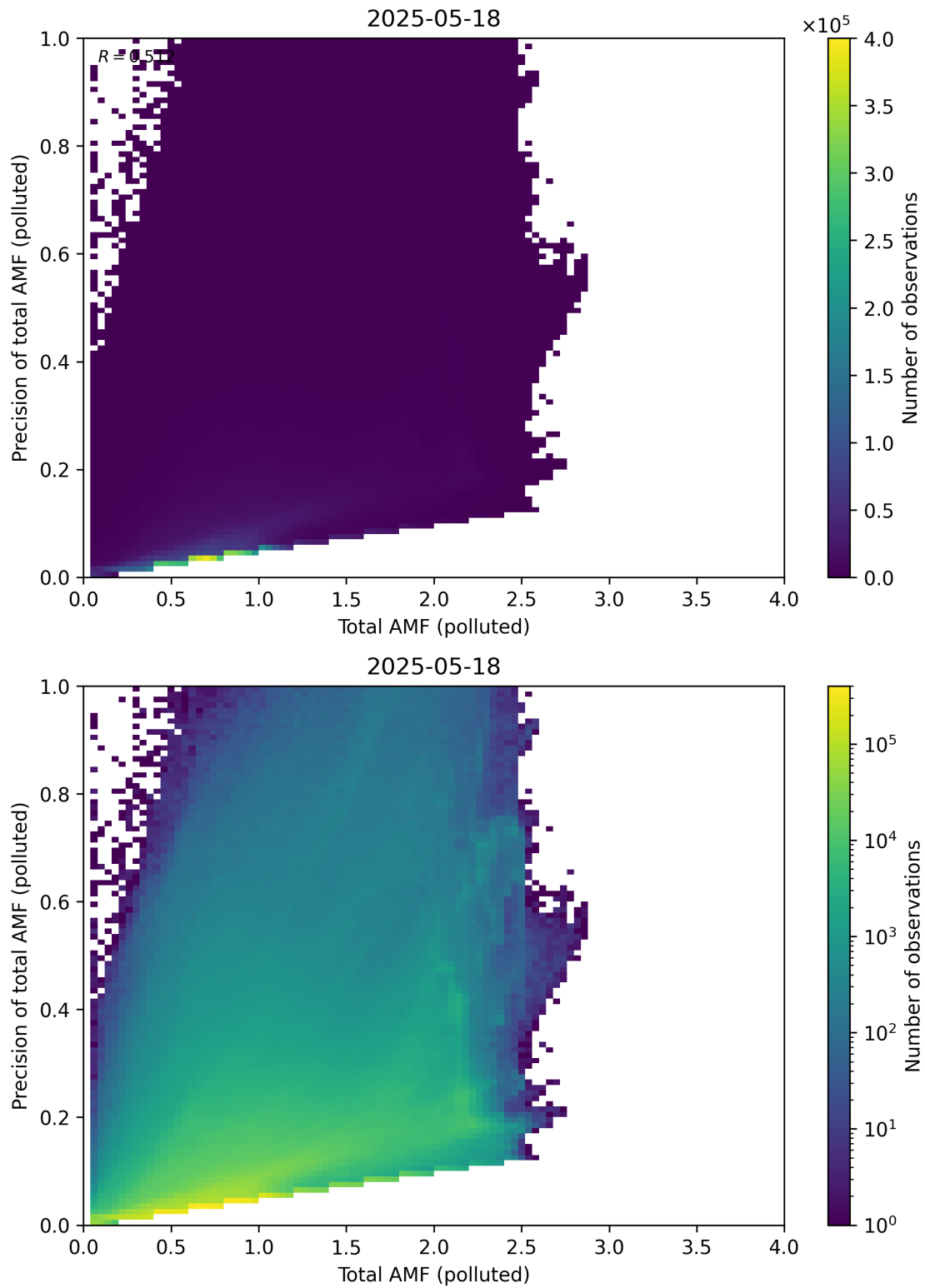
Figure 322: Scatter density plot of “Total AMF (polluted)” against “Precision of total AMF (polluted)” for 2025-05-17 to 2025-05-19.
