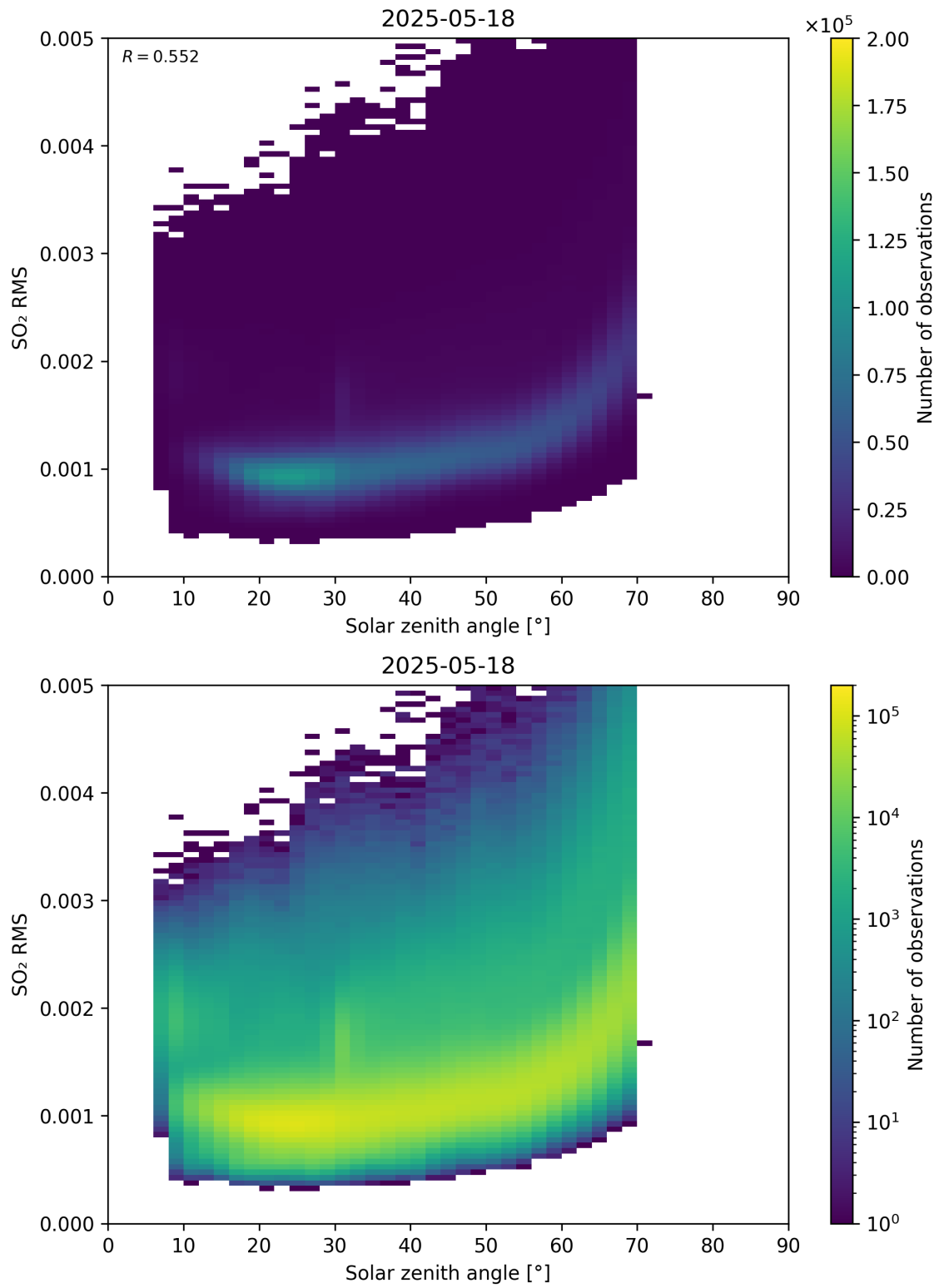
Figure 176: Scatter density plot of “Solar zenith angle” against “SO 2 RMS” for 2025-05-17 to 2025-05-19.
