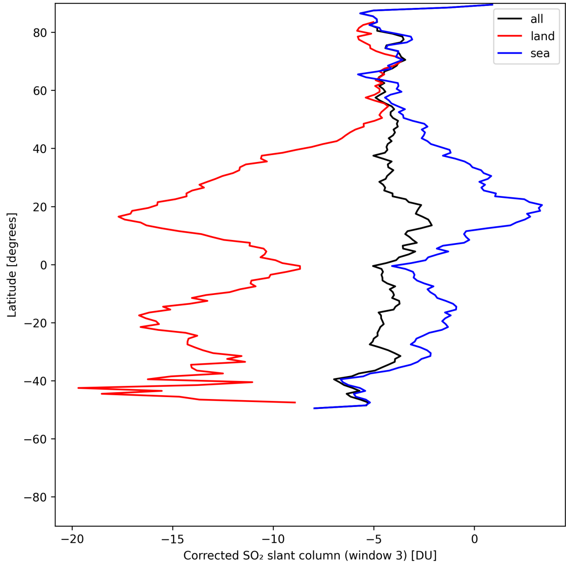
Figure 47: Zonal average of “Corrected SO 2 slant column (window 3)” for 2025-05-17 to 2025-05-19.
