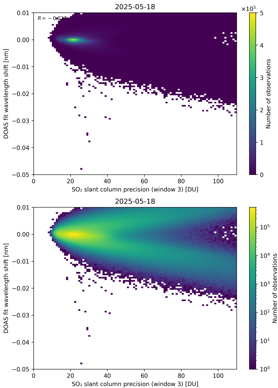
Figure 308: Scatter density plot of “SO 2 slant column precision (window 3)” against “DOAS fit wavelength shift” for 2025-05-17 to 2025-05-19.
