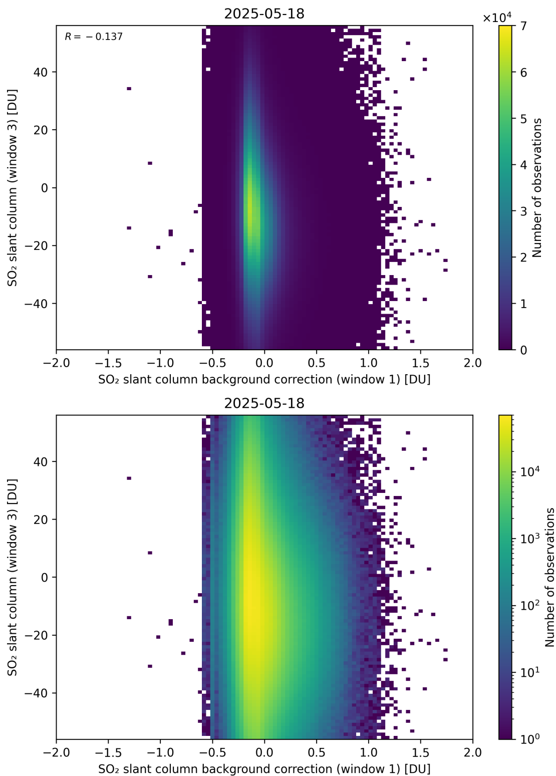
Figure 118: Scatter density plot of “SO 2 slant column background correction (window 1)” against “SO 2 slant column (window 3)” for 2025-05-17 to 2025-05-19.
