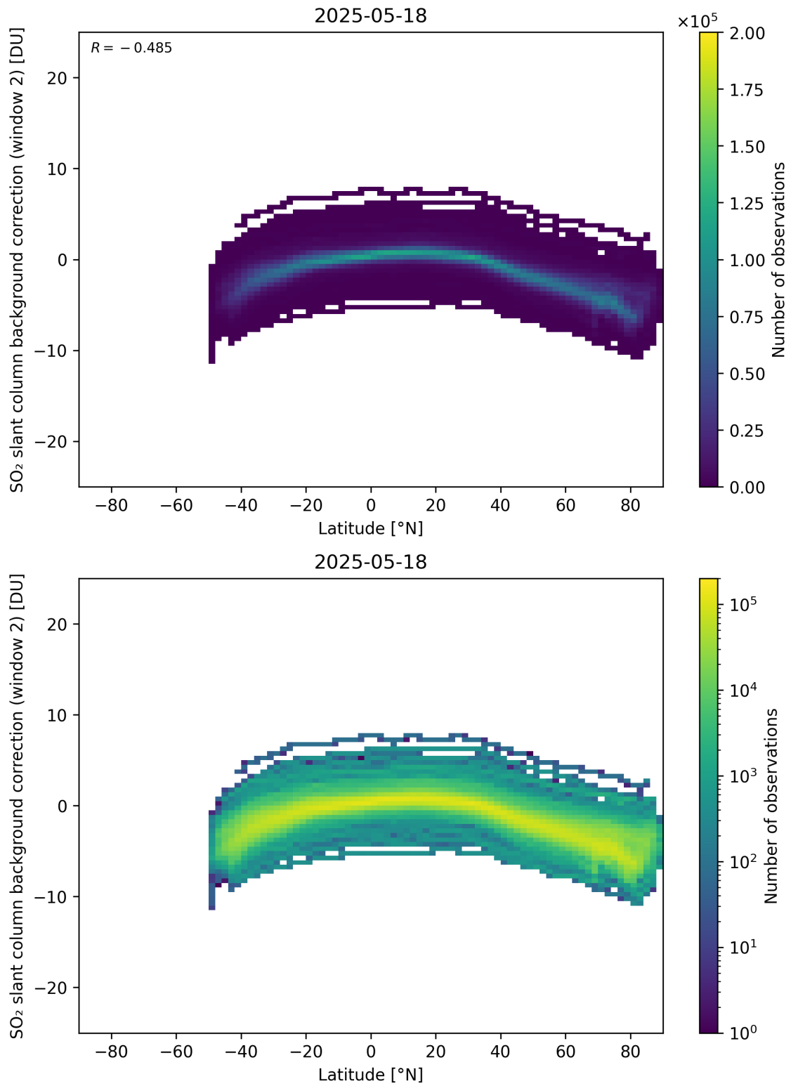
Figure 151: Scatter density plot of “Latitude” against “SO 2 slant column background correction (window 2)” for 2025-05-17 to 2025-05-19.
