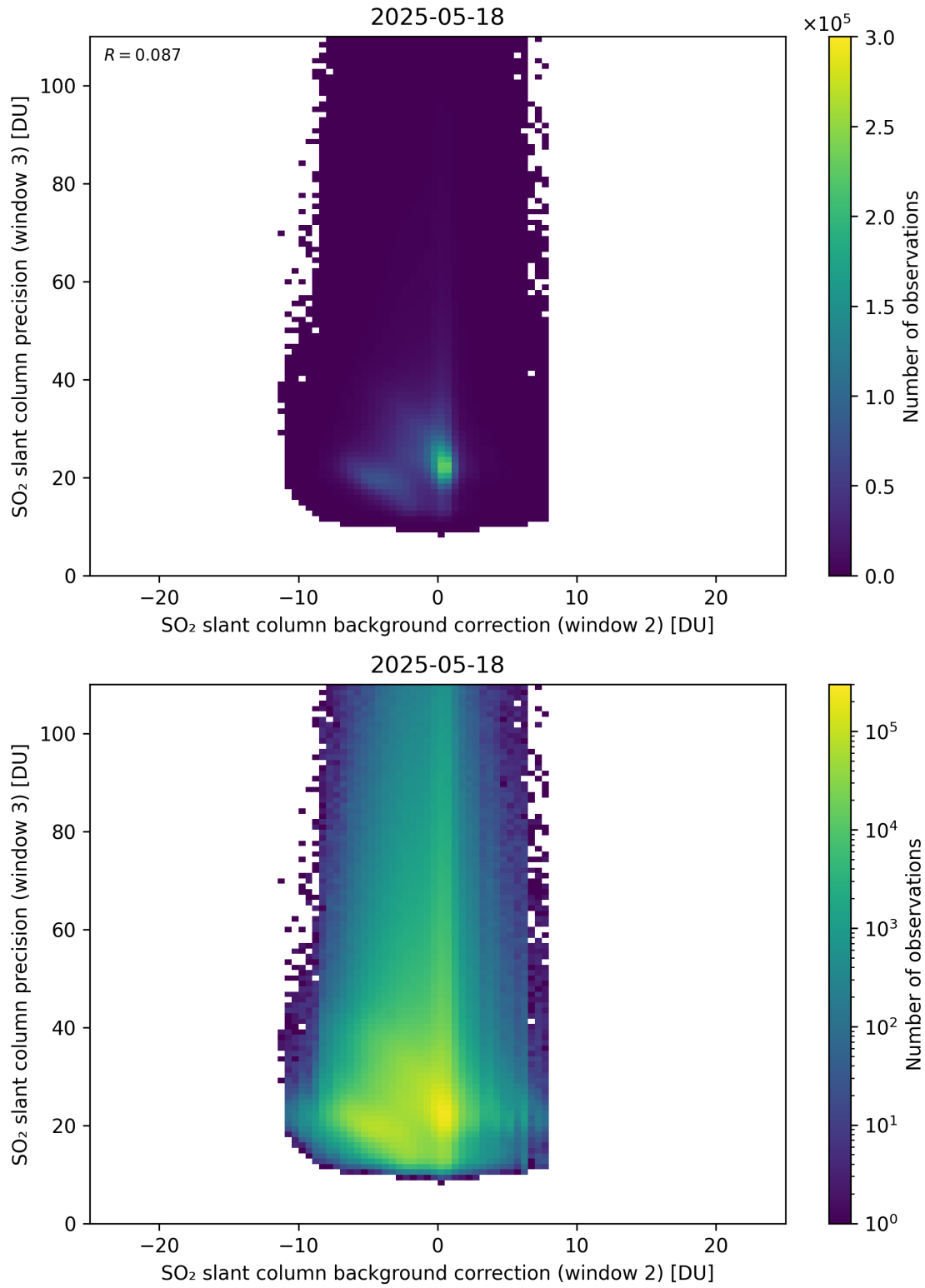
Figure 129: Scatter density plot of “SO 2 slant column background correction (window 2)” against “SO 2 slant column precision (window 3)” for 2025-05-17 to 2025-05-19.
