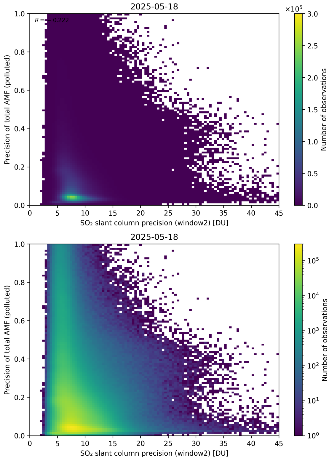
Figure 302: Scatter density plot of “SO 2 slant column precision (window2)” against “Precision of total AMF (polluted)” for 2025-05-17 to 2025-05-19.
