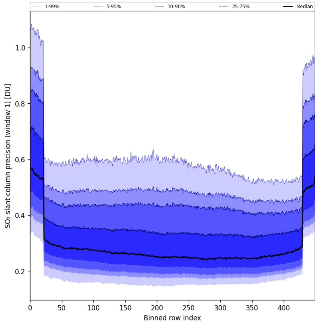
Figure 90: Along track statistics of “SO 2 slant column precision (window 1)” for 2025-05-17 to 2025-05-19
