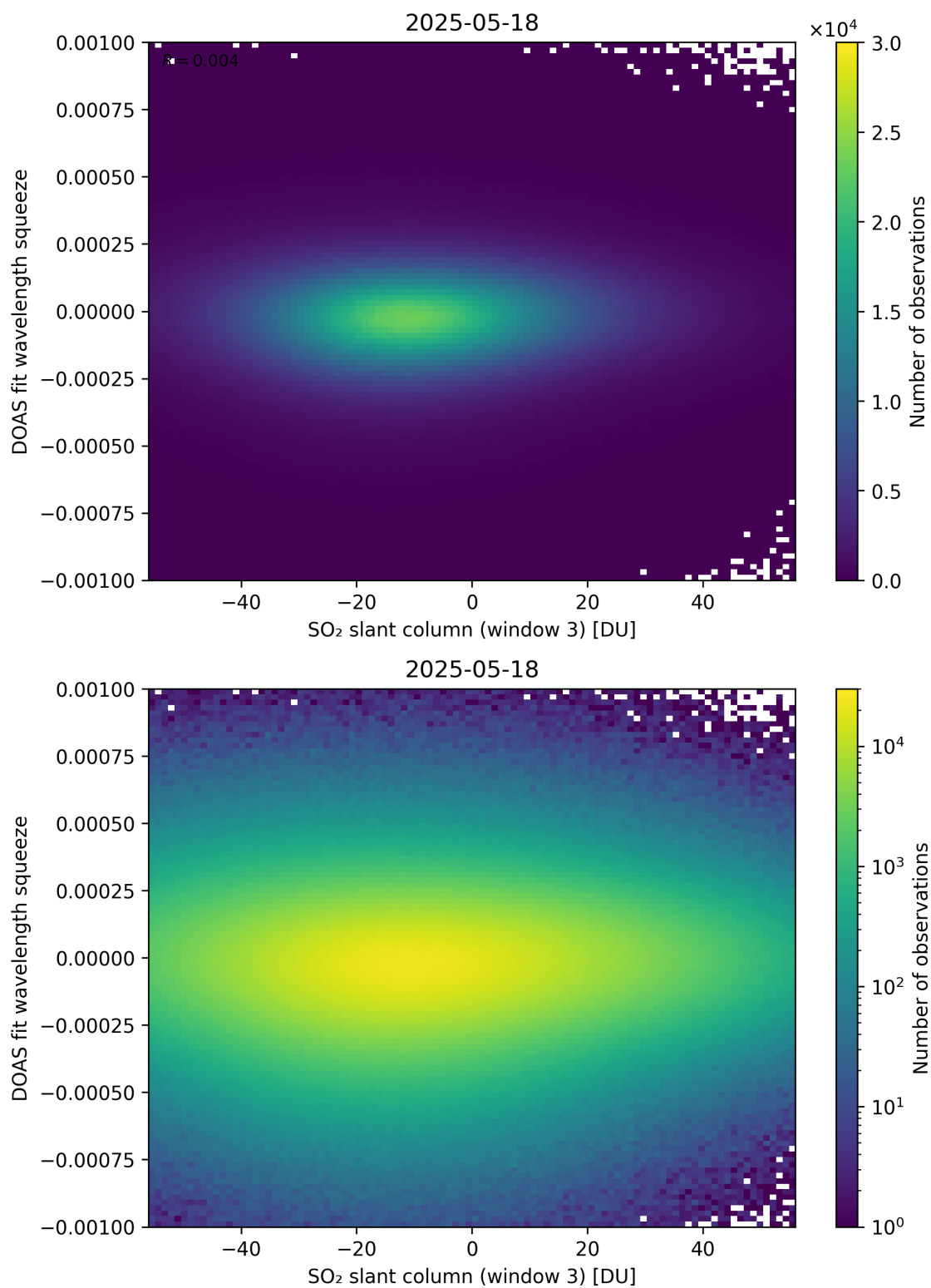
Figure 305: Scatter density plot of “SO 2 slant column (window 3)” against “DOAS fit wavelength squeeze” for 2025-05-17 to 2025-05-19.
