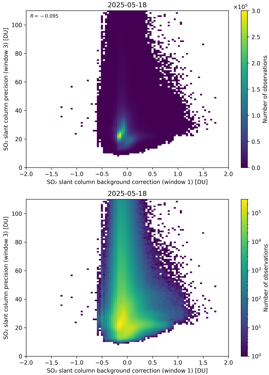
Figure 119: Scatter density plot of “SO 2 slant column background correction (window 1)” against “SO 2 slant column precision (window 3)” for 2025-05-17 to 2025-05-19.
