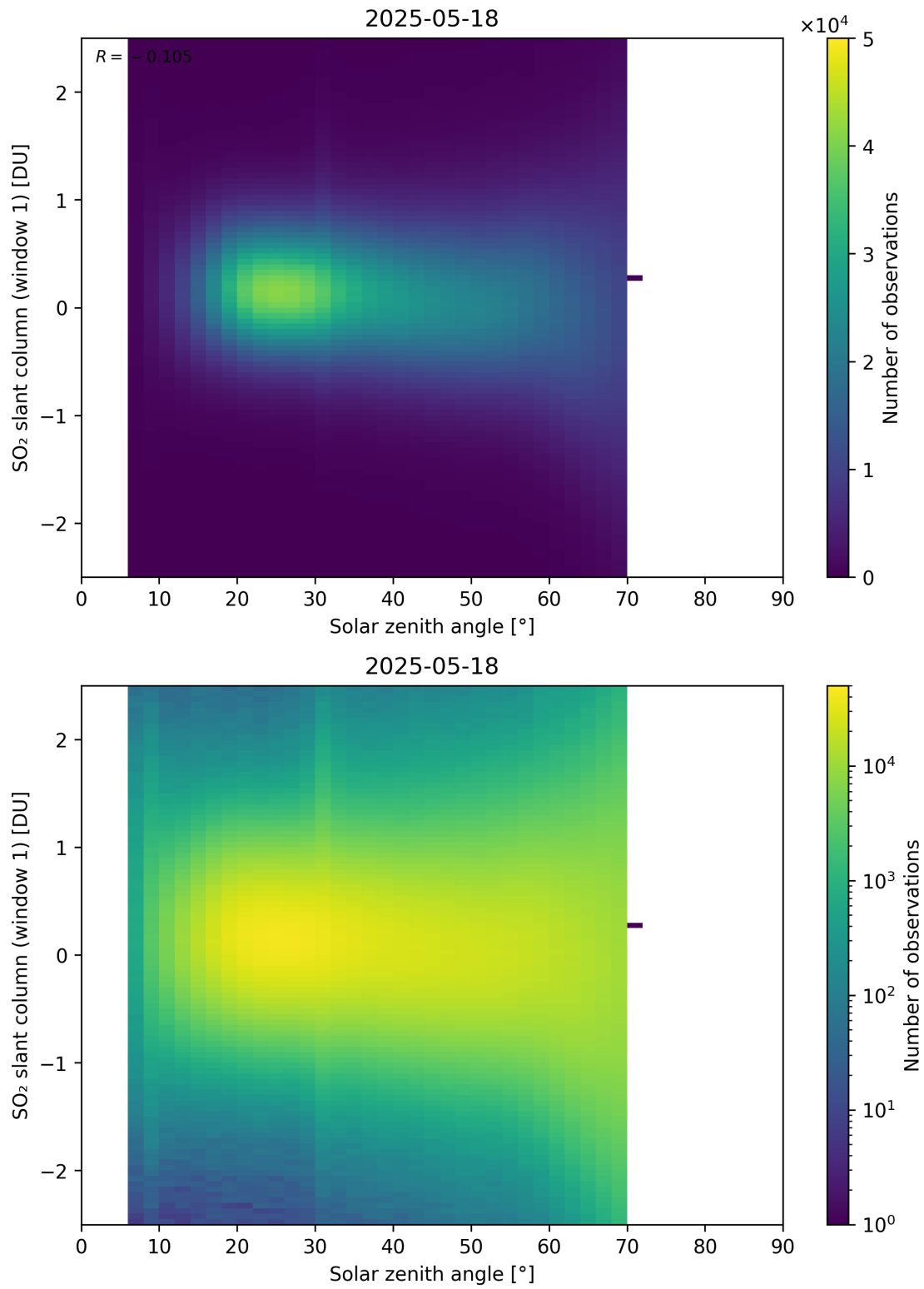
Figure 184: Scatter density plot of “Solar zenith angle” against “SO 2 slant column (window 1)” for 2025-05-17 to 2025-05-19.
