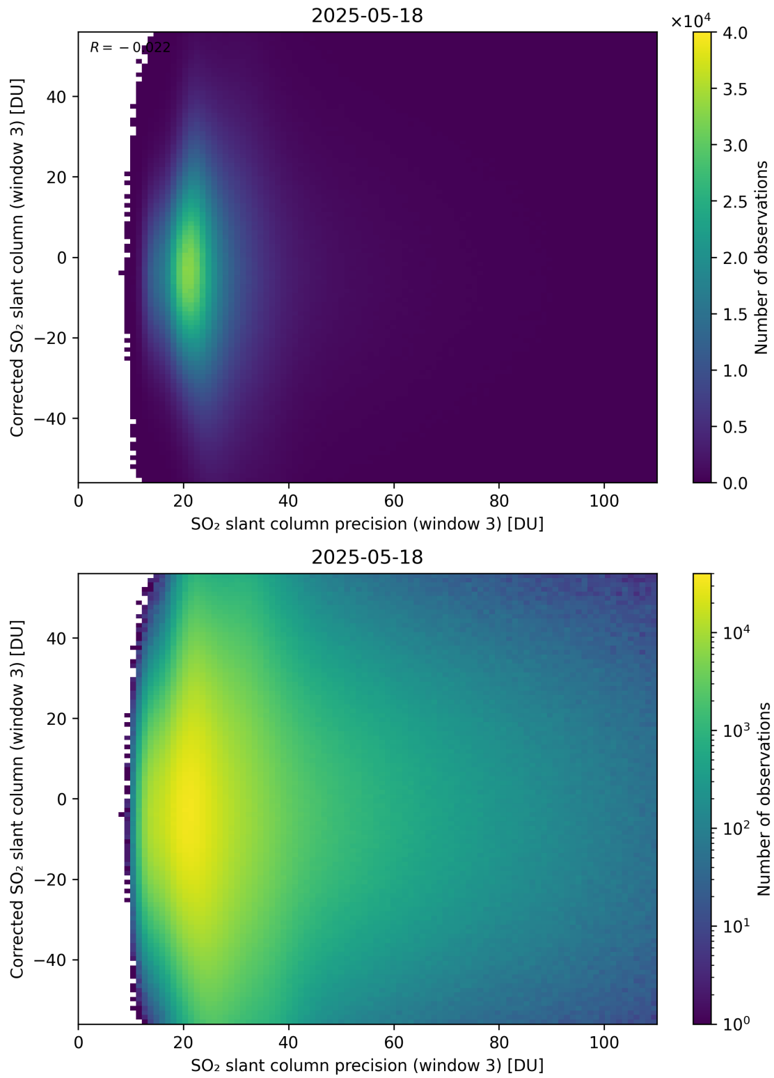
Figure 312: Scatter density plot of “SO 2 slant column precision (window 3)” against “Corrected SO 2 slant column (window 3)” for 2025-05-17 to 2025-05-19.
