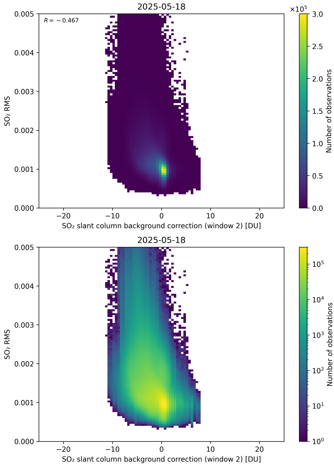
Figure 125: Scatter density plot of “SO 2 slant column background correction (window 2)” against “SO 2 RMS” for 2025-05-17 to 2025-05-19.
