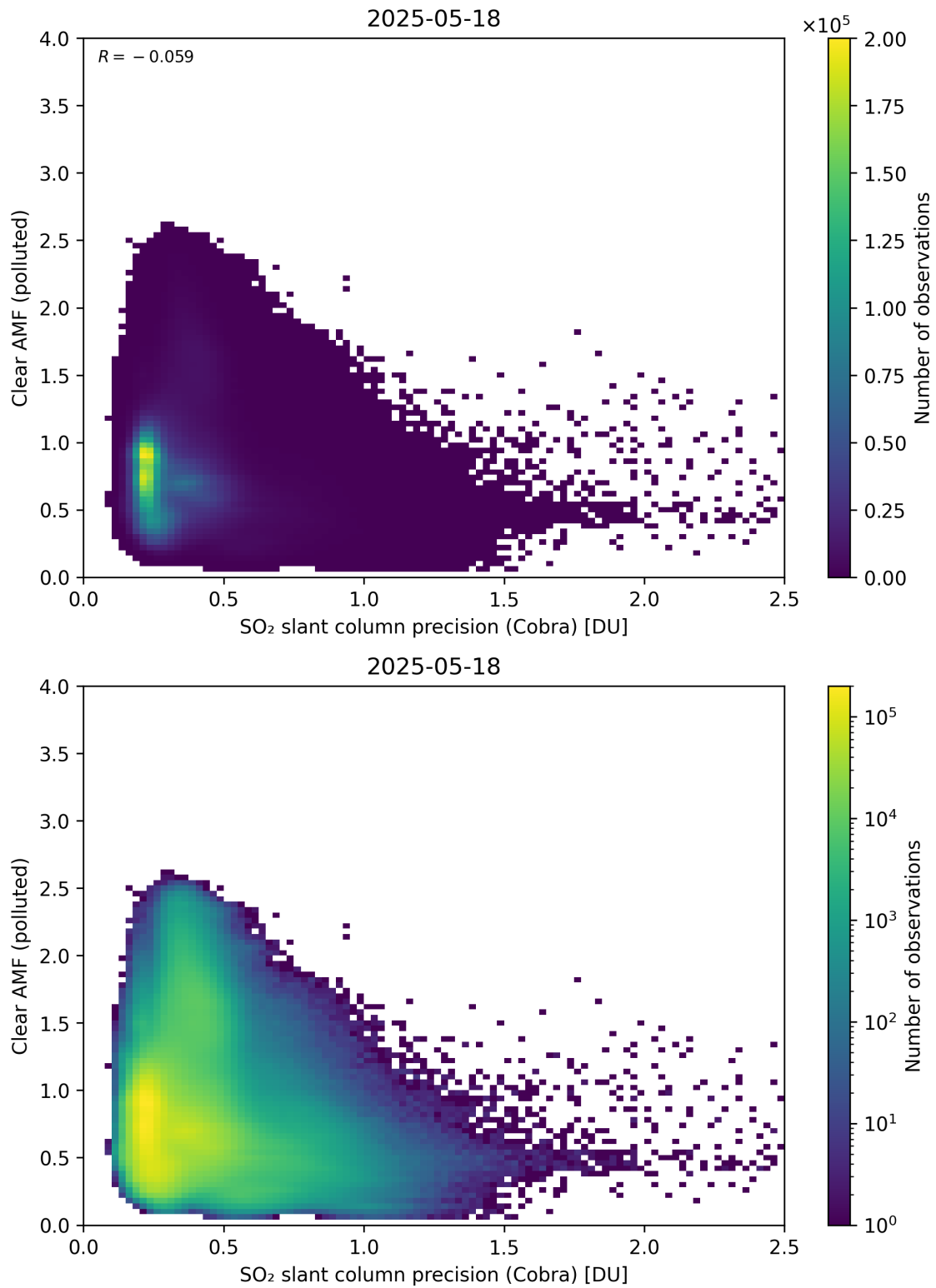
Figure 205: Scatter density plot of “SO 2 slant column precision (Cobra)” against “Clear AMF (polluted)” for 2025-05-17 to 2025-05-19.
