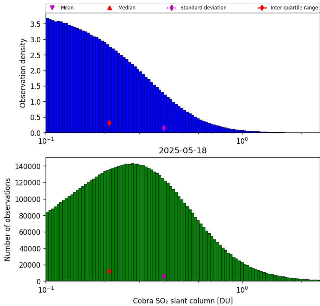
Figure 61: Histogram of “Cobra SO 2 slant column” for 2025-05-17 to 2025-05-19
