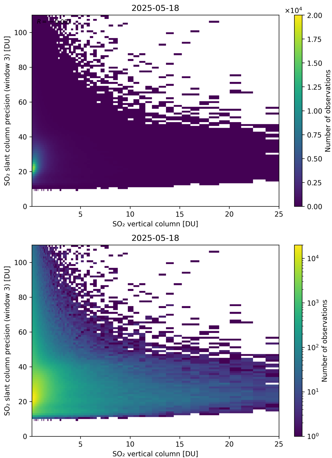
Figure 358: Scatter density plot of “SO 2 vertical column” against “SO 2 slant column precision (window 3)” for 2025-05-17 to 2025-05-19.
