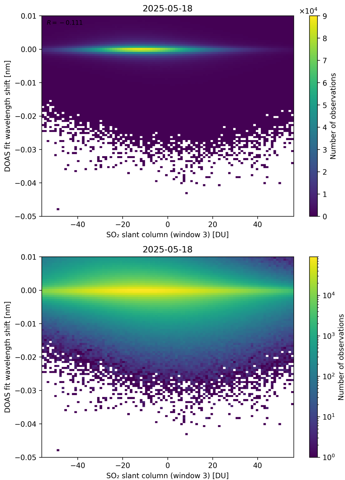
Figure 304: Scatter density plot of “SO 2 slant column (window 3)” against “DOAS fit wavelength shift” for 2025-05-17 to 2025-05-19.
