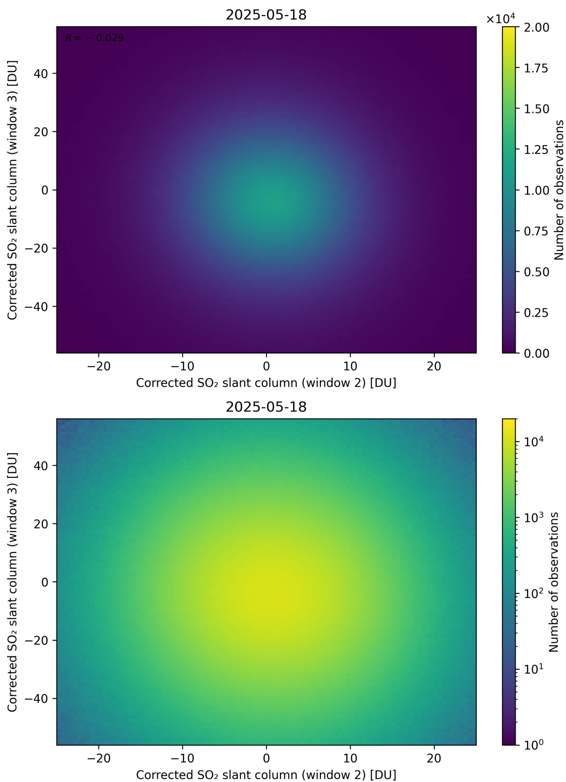
Figure 250: Scatter density plot of “Corrected SO 2 slant column (window 2)” against “Corrected SO 2 slant column (window 3)” for 2025-05-17 to 2025-05-19.
