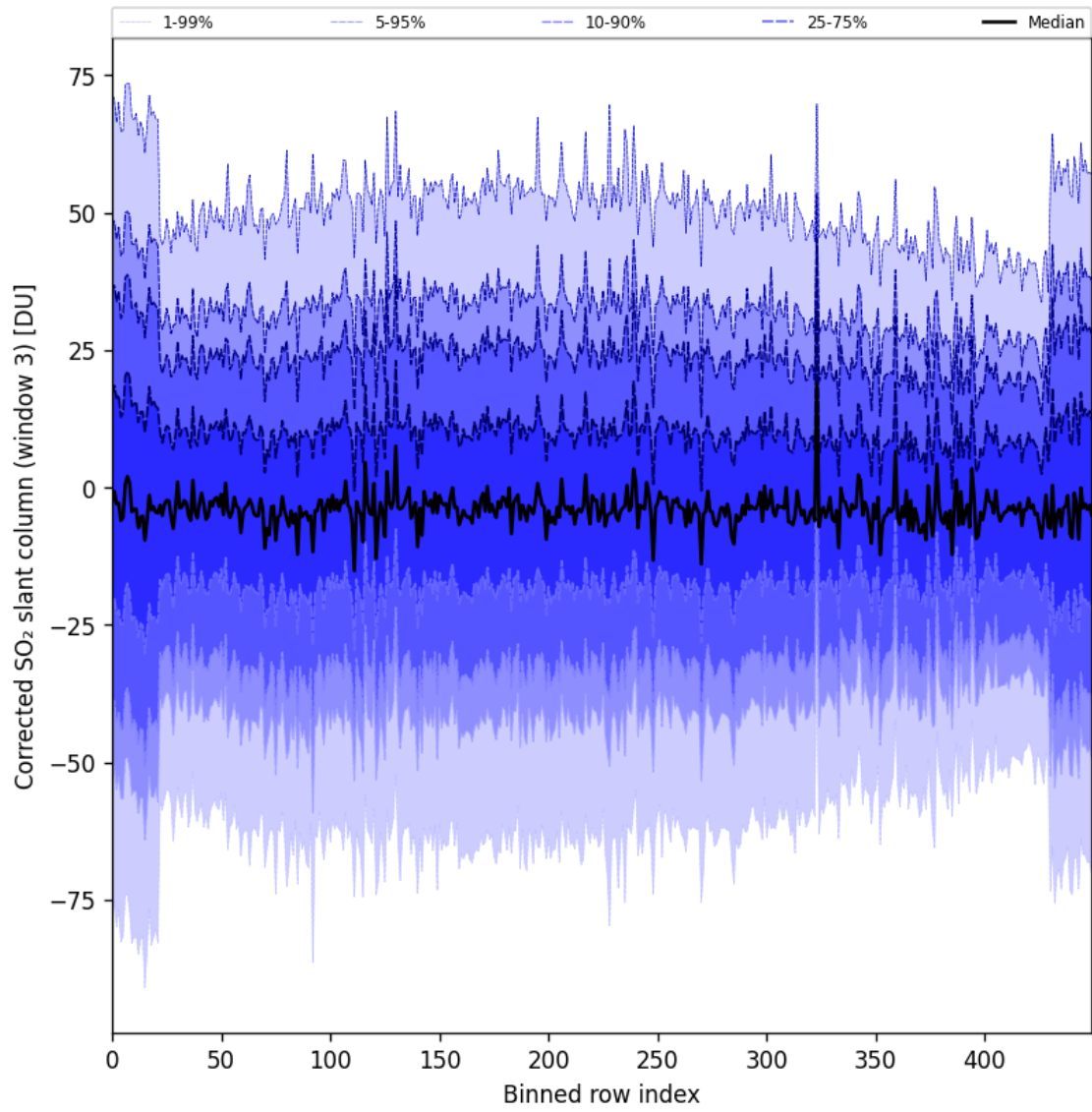
Figure 99: Along track statistics of “Corrected SO 2 slant column (window 3)” for 2025-05-17 to 2025-05-19
