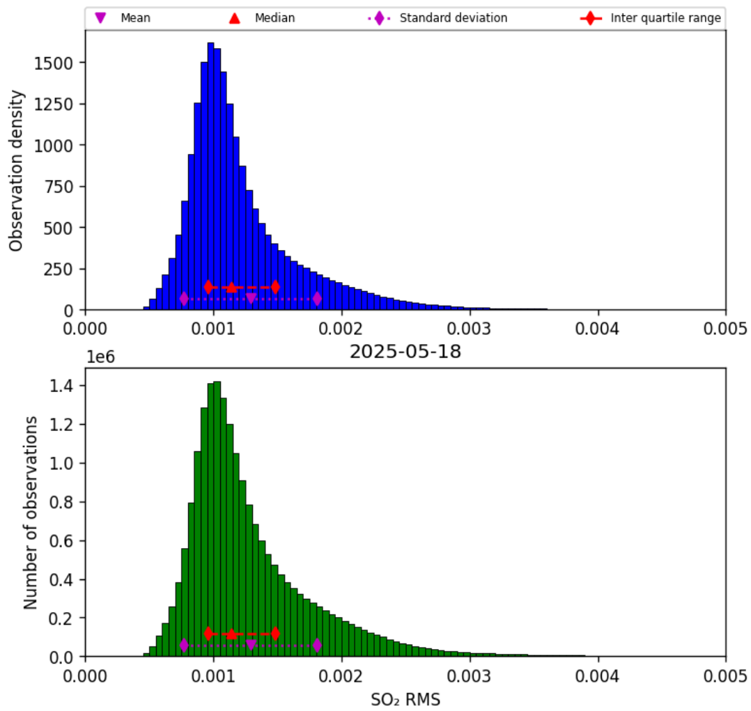
Figure 78: Histogram of “SO 2 RMS” for 2025-05-17 to 2025-05-19
