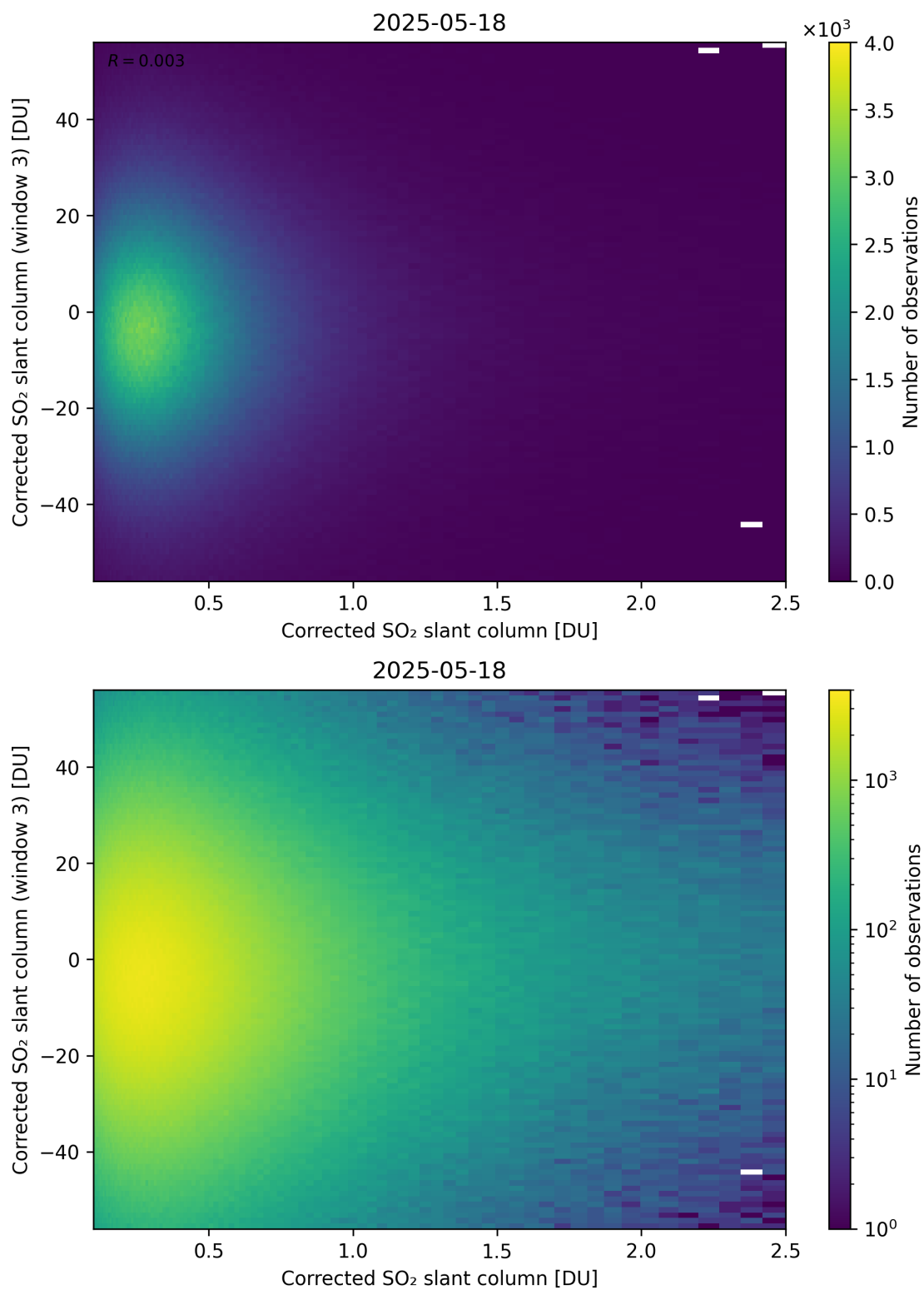
Figure 236: Scatter density plot of “Corrected SO 2 slant column” against “Corrected SO 2 slant column (window 3)” for 2025-05-17 to 2025-05-19.
