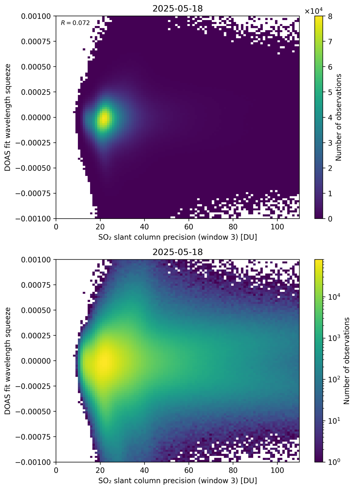
Figure 309: Scatter density plot of “SO 2 slant column precision (window 3)” against “DOAS fit wavelength squeeze” for 2025-05-17 to 2025-05-19.
