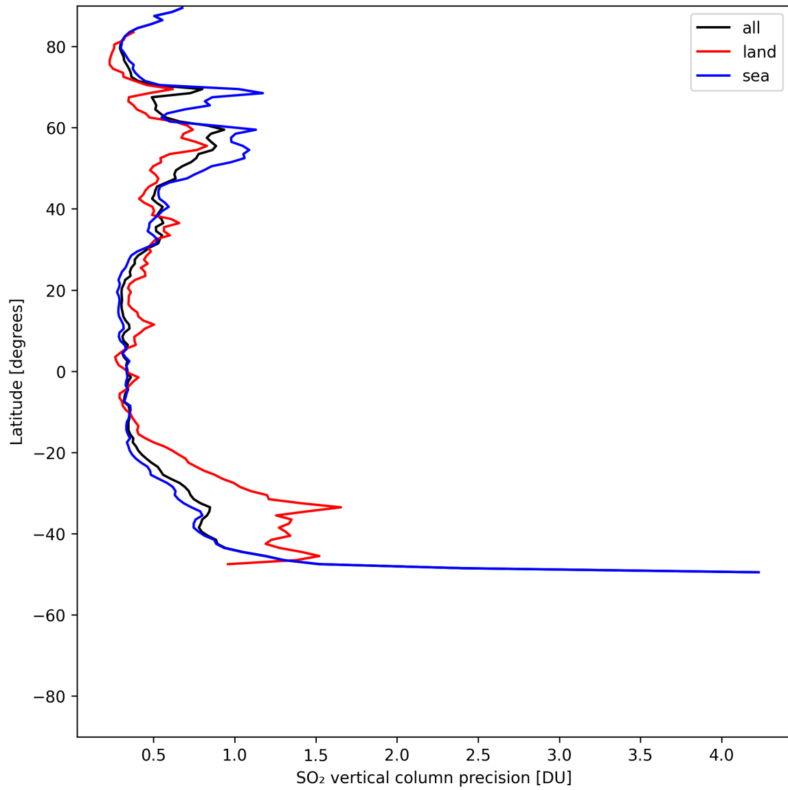
Figure 33: Zonal average of “SO 2 vertical column precision” for 2025-05-17 to 2025-05-19.
