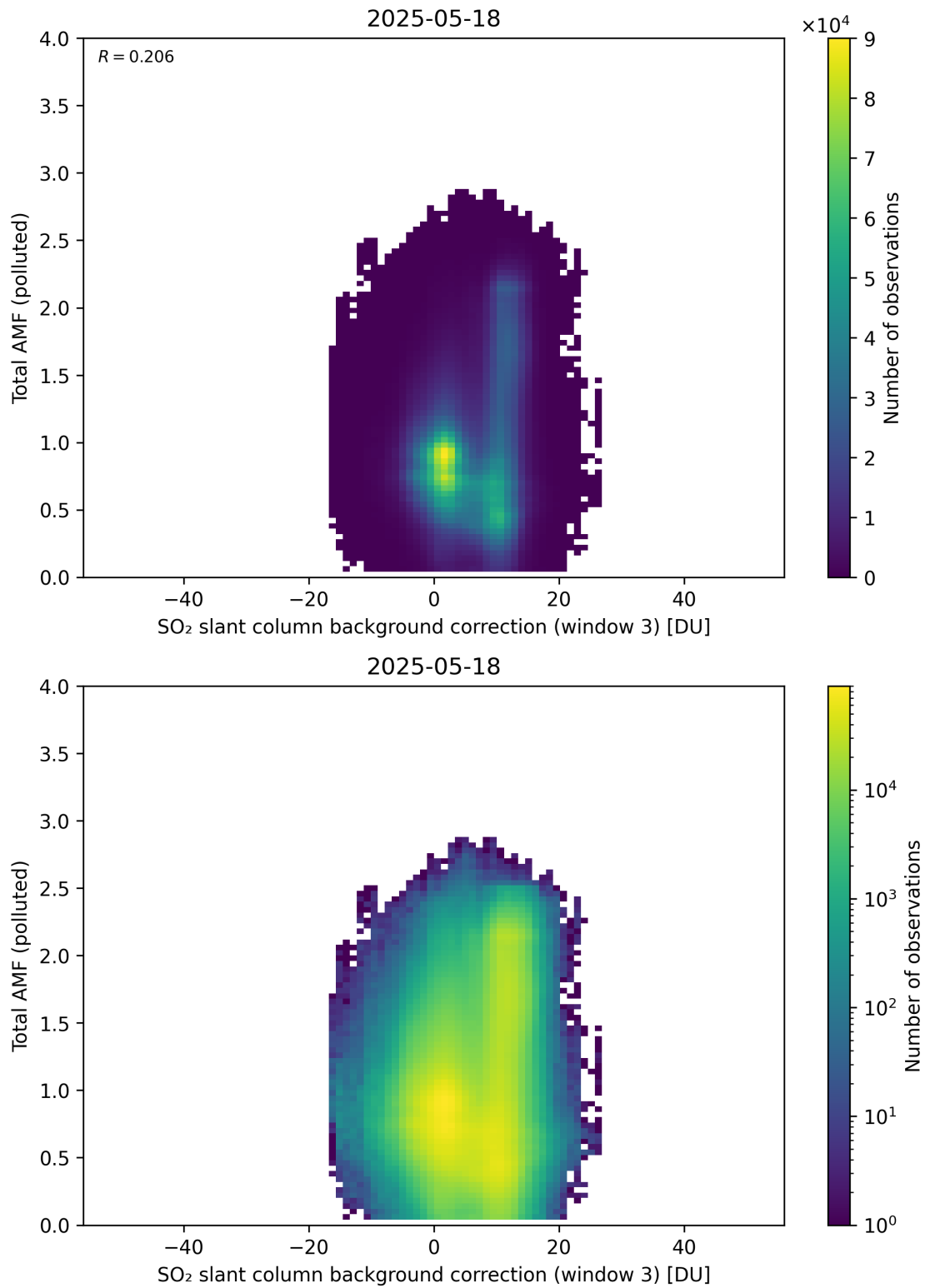
Figure 136: Scatter density plot of “SO 2 slant column background correction (window 3)” against “Total AMF (polluted)” for 2025-05-17 to 2025-05-19.
