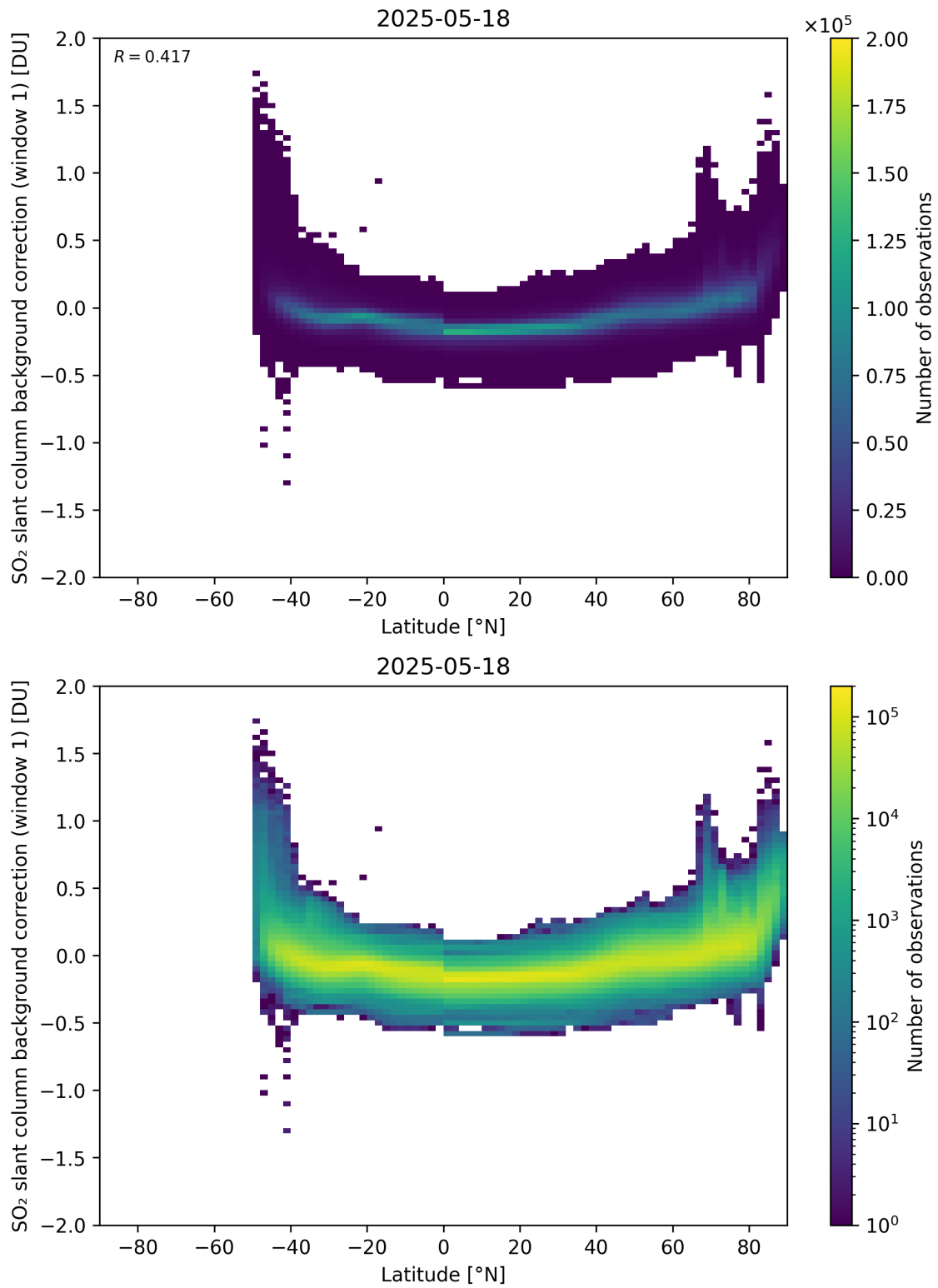
Figure 150: Scatter density plot of “Latitude” against “SO 2 slant column background correction (window 1)” for 2025-05-17 to 2025-05-19.
