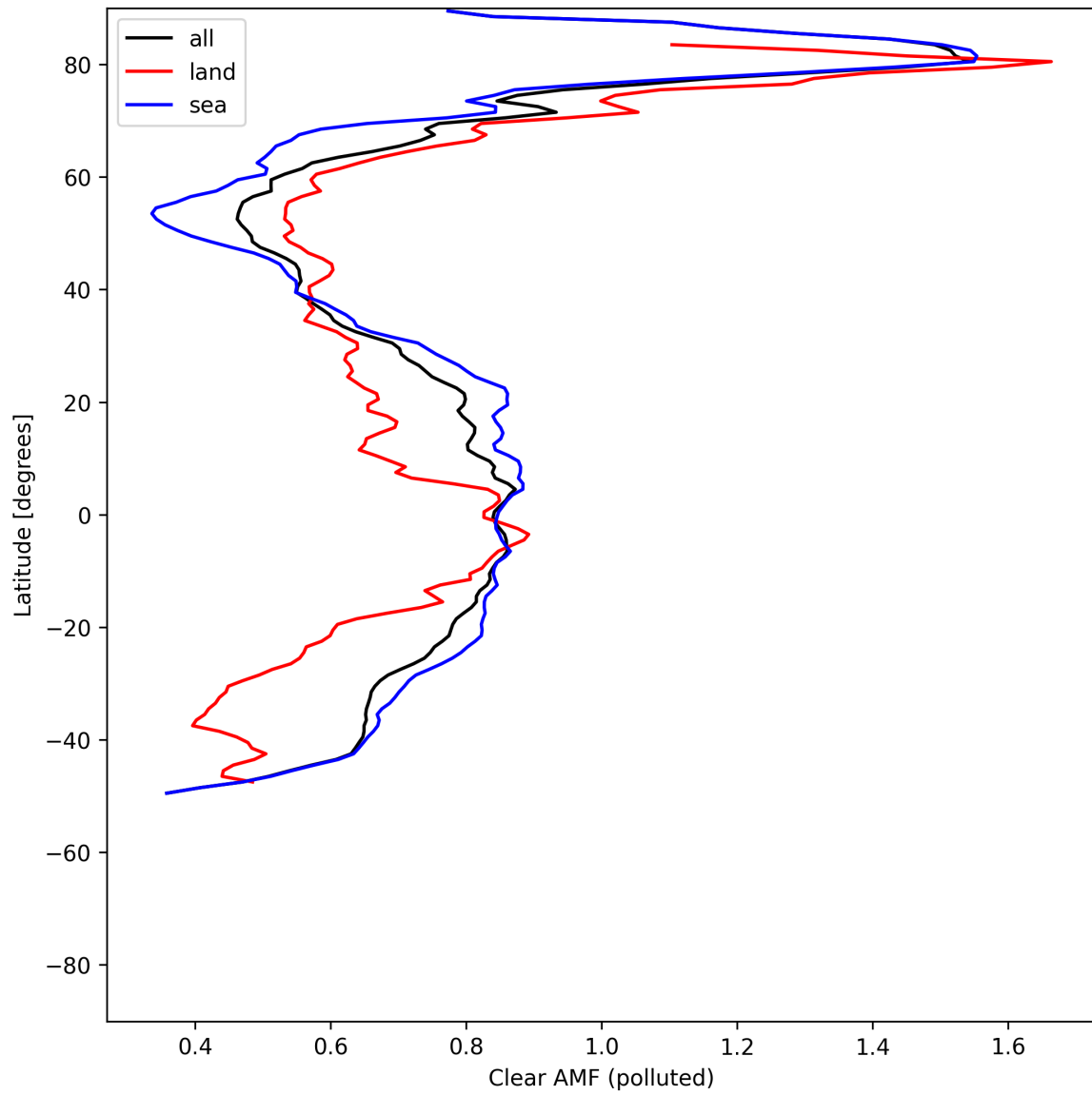
Figure 55: Zonal average of “Clear AMF (polluted)” for 2025-05-17 to 2025-05-19.
