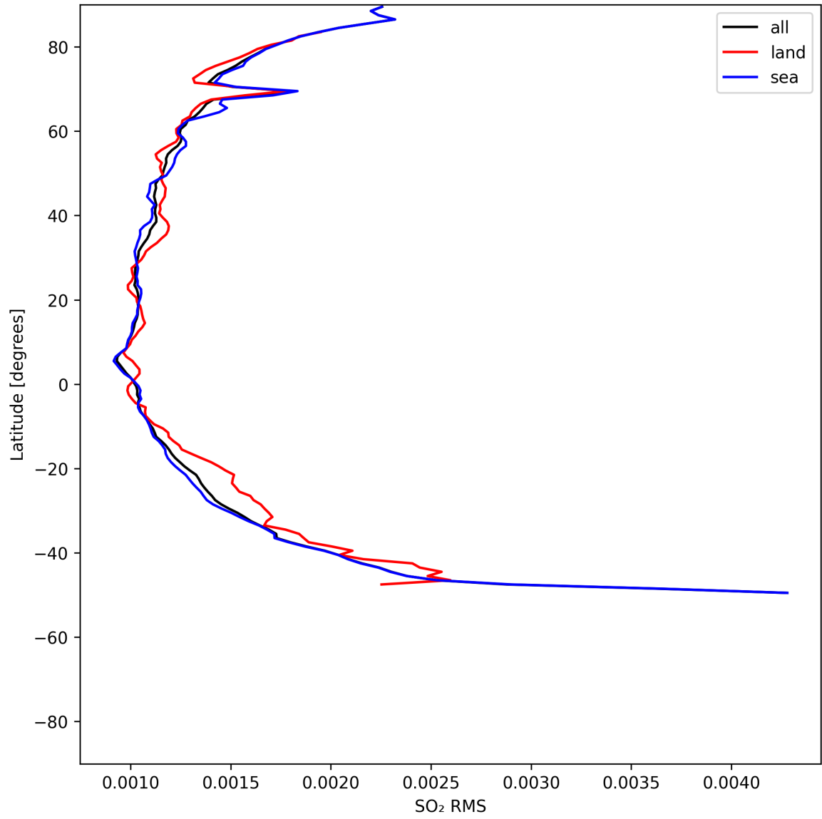
Figure 52: Zonal average of “SO 2 RMS” for 2025-05-17 to 2025-05-19.
