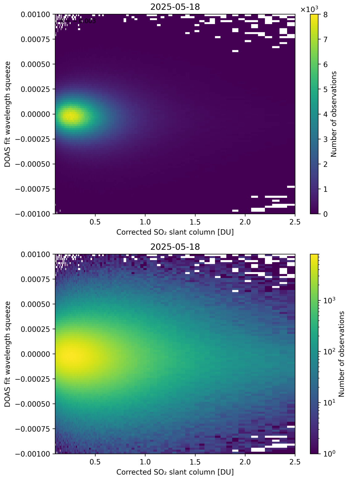
Figure 230: Scatter density plot of “Corrected SO 2 slant column” against “DOAS fit wavelength squeeze” for 2025-05-17 to 2025-05-19.
