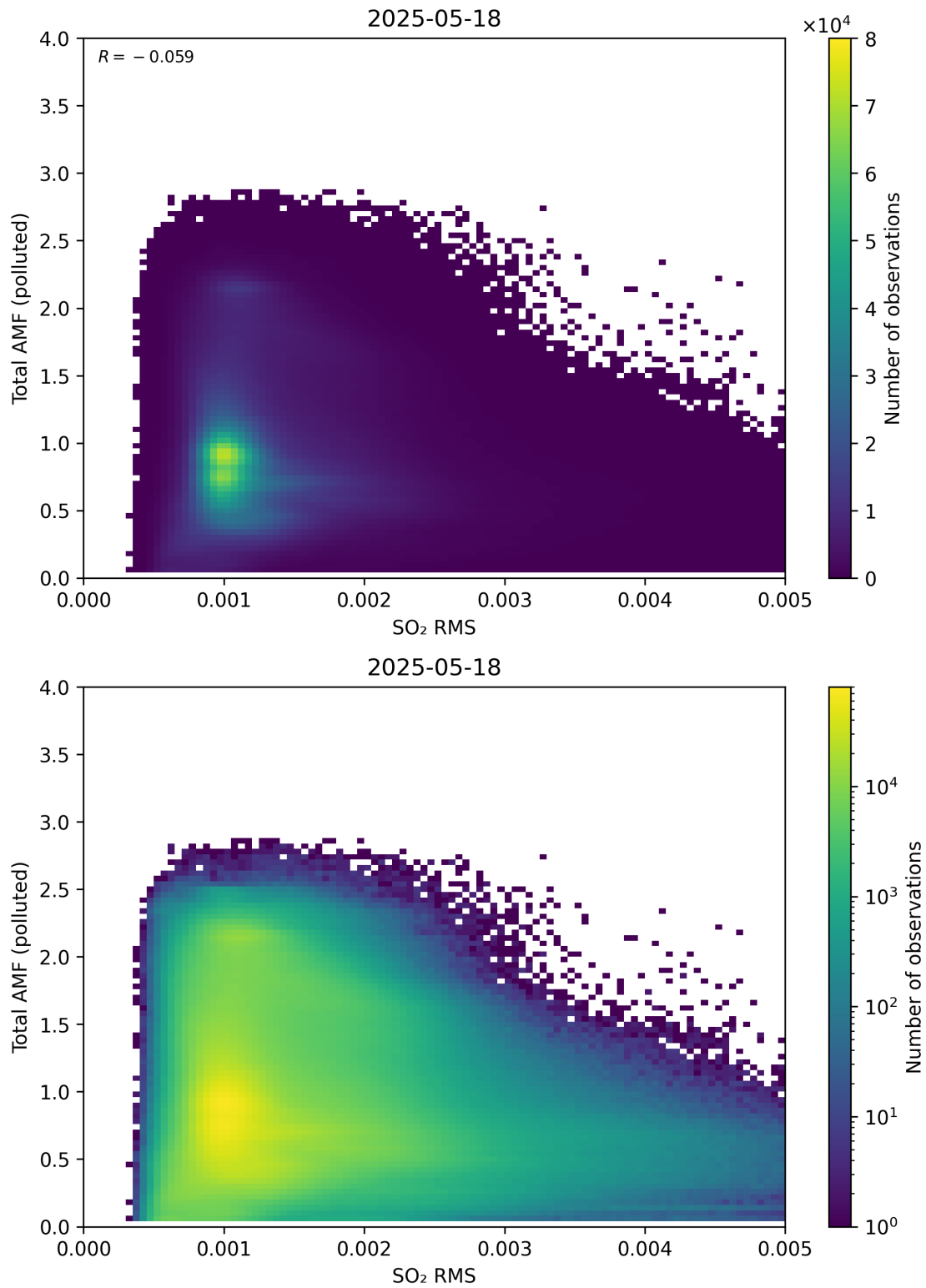
Figure 148: Scatter density plot of “SO 2 RMS” against “Total AMF (polluted)” for 2025-05-17 to 2025-05-19.
