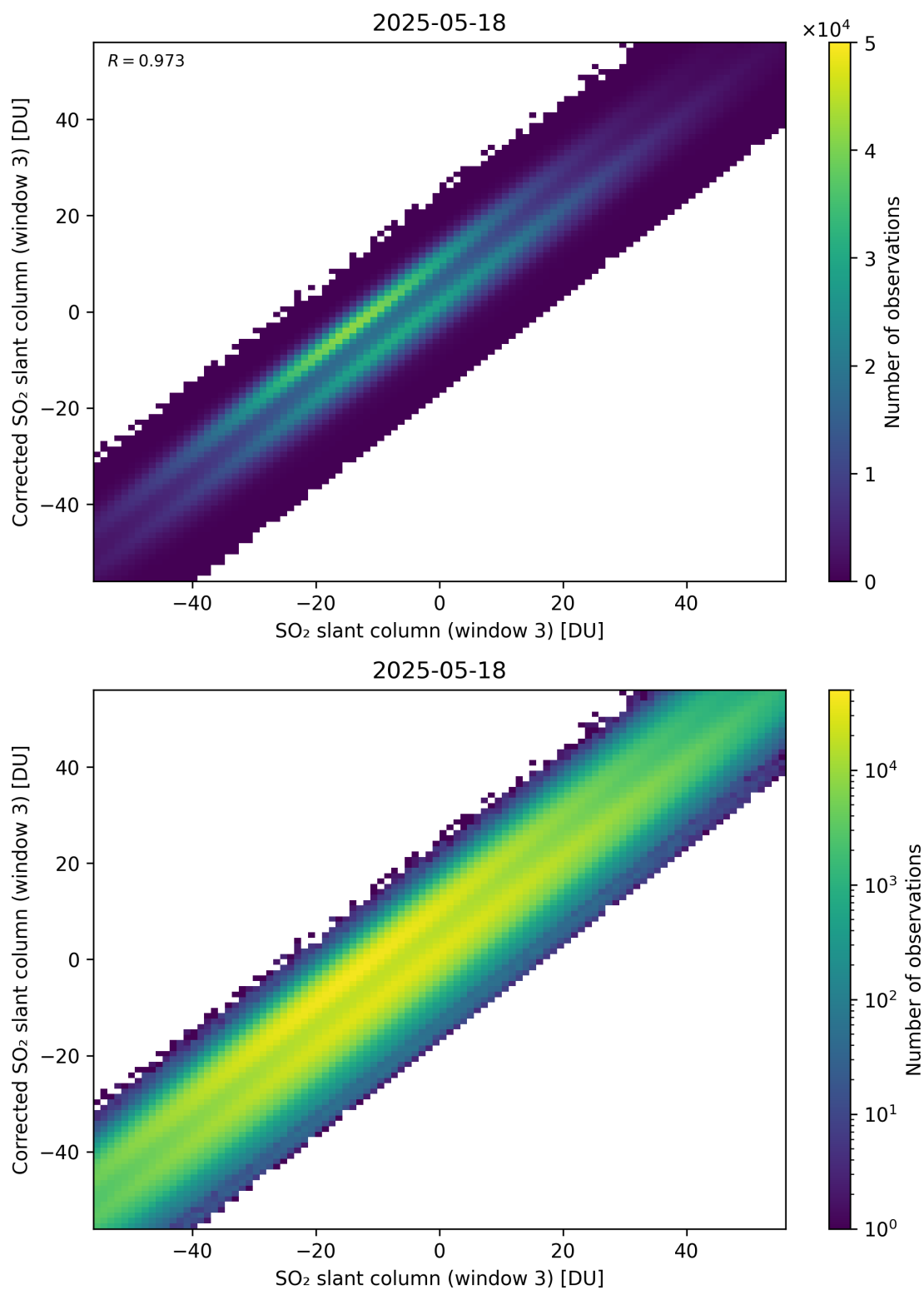
Figure 316: Scatter density plot of “SO 2 slant column (window 3)” against “Corrected SO 2 slant column (window 3)” for 2025-05-17 to 2025-05-19.
