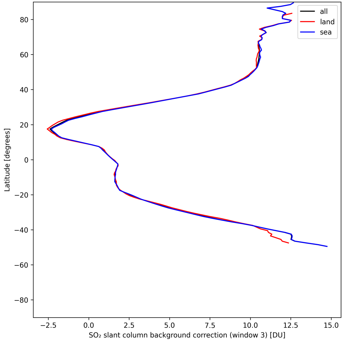
Figure 48: Zonal average of “SO 2 slant column background correction (window 3)” for 2025-05-17 to 2025-05-19.
