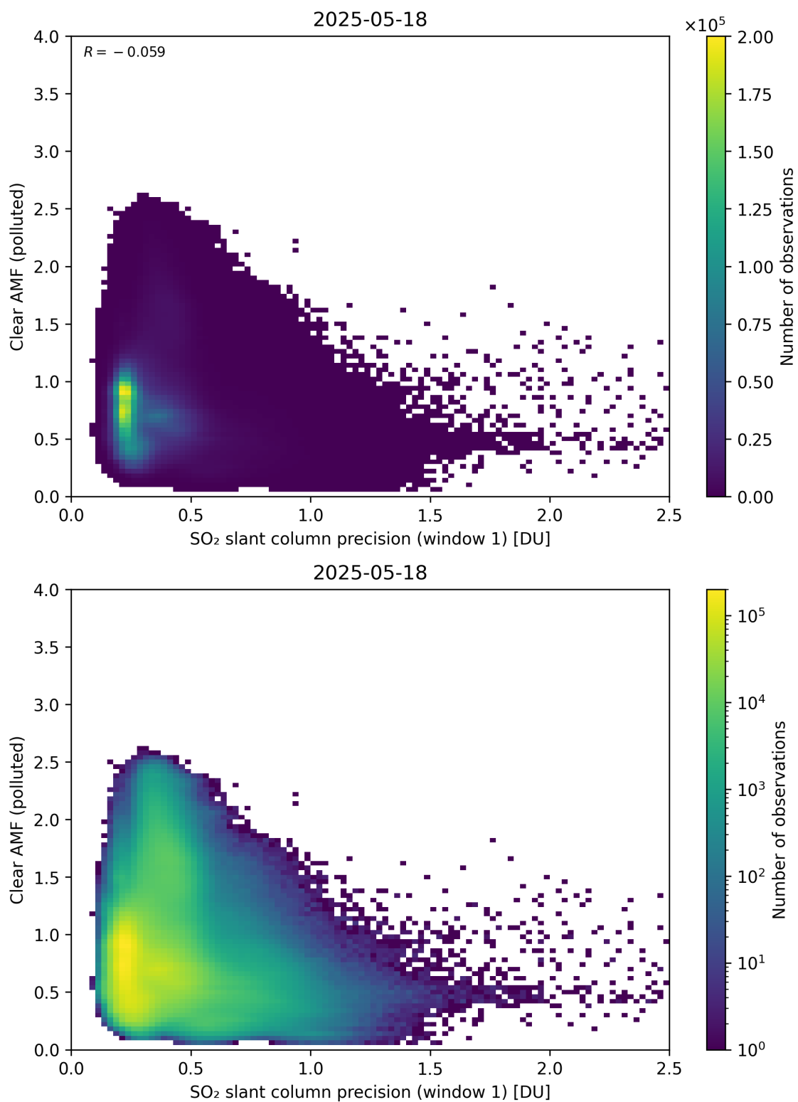
Figure 274: Scatter density plot of “SO 2 slant column precision (window 1)” against “Clear AMF (polluted)” for 2025-05-17 to 2025-05-19.
