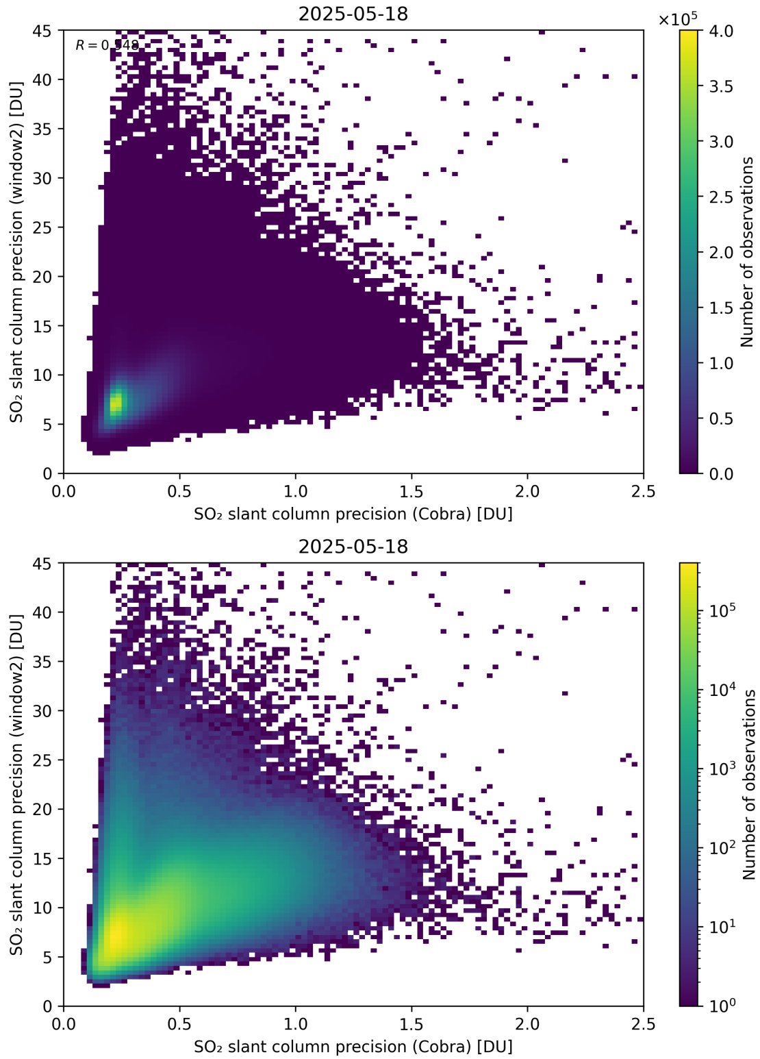
Figure 210: Scatter density plot of “SO 2 slant column precision (Cobra)” against “SO 2 slant column precision (window2)” for 2025-05-17 to 2025-05-19.
