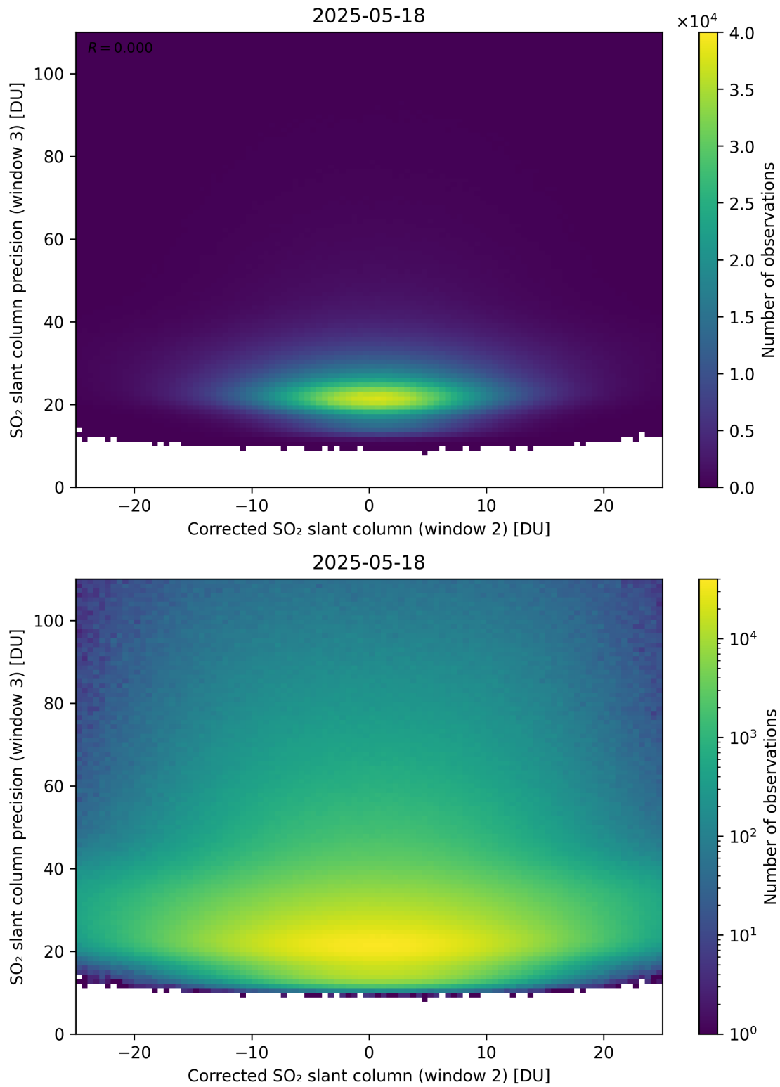
Figure 252: Scatter density plot of “Corrected SO 2 slant column (window 2)” against “SO 2 slant column precision (window 3)” for 2025-05-17 to 2025-05-19.
