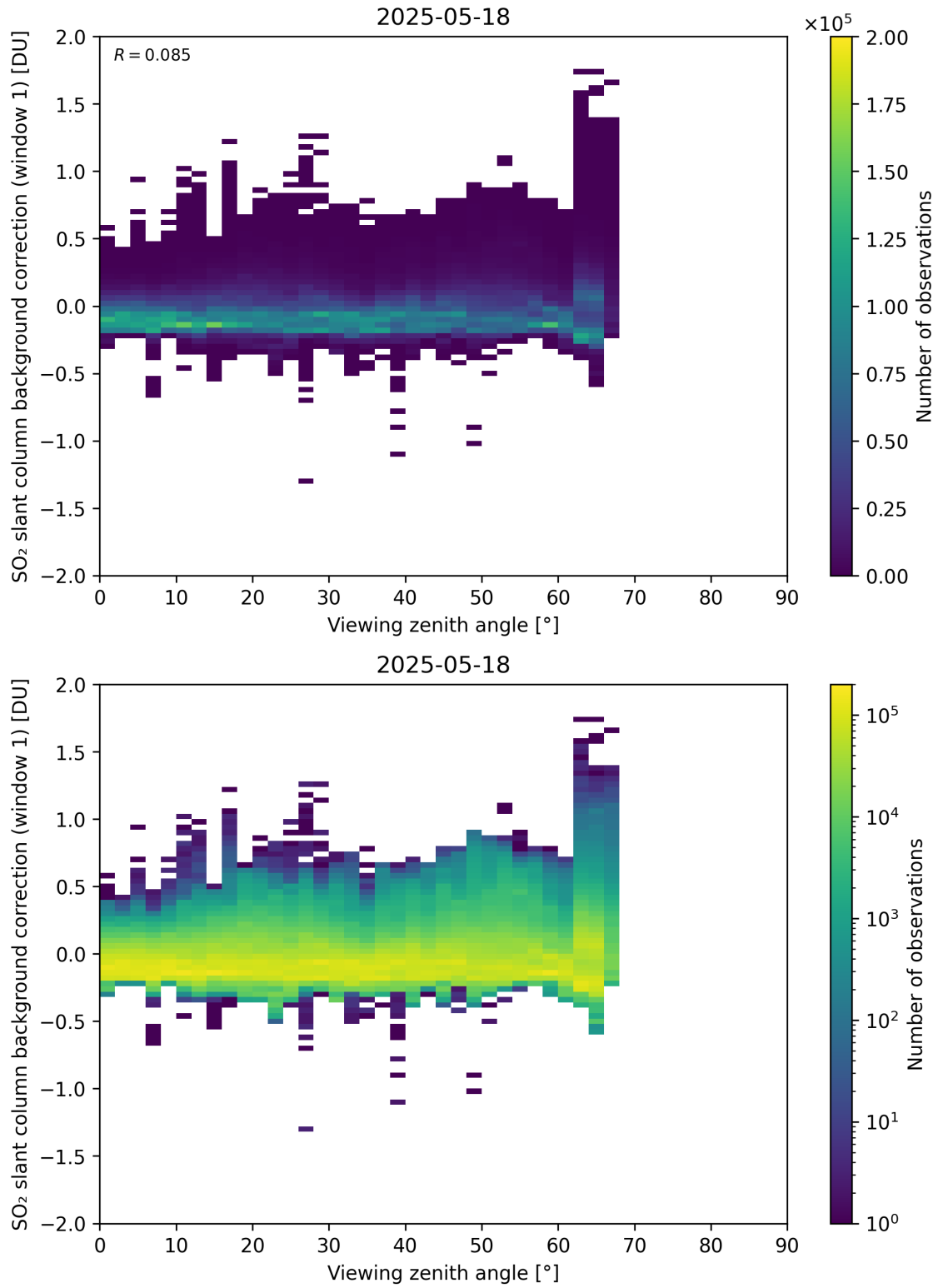
Figure 362: Scatter density plot of “Viewing zenith angle” against “SO 2 slant column background correction (window 1)” for 2025-05-17 to 2025-05-19.
