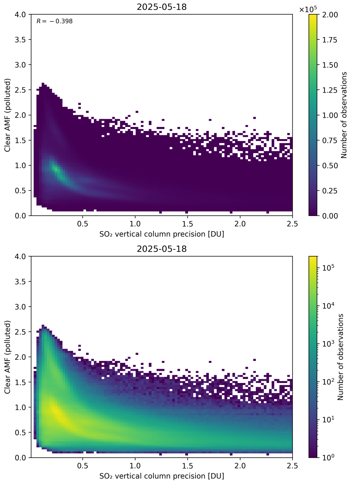
Figure 335: Scatter density plot of “SO 2 vertical column precision” against “Clear AMF (polluted)” for 2025-05-17 to 2025-05-19.
