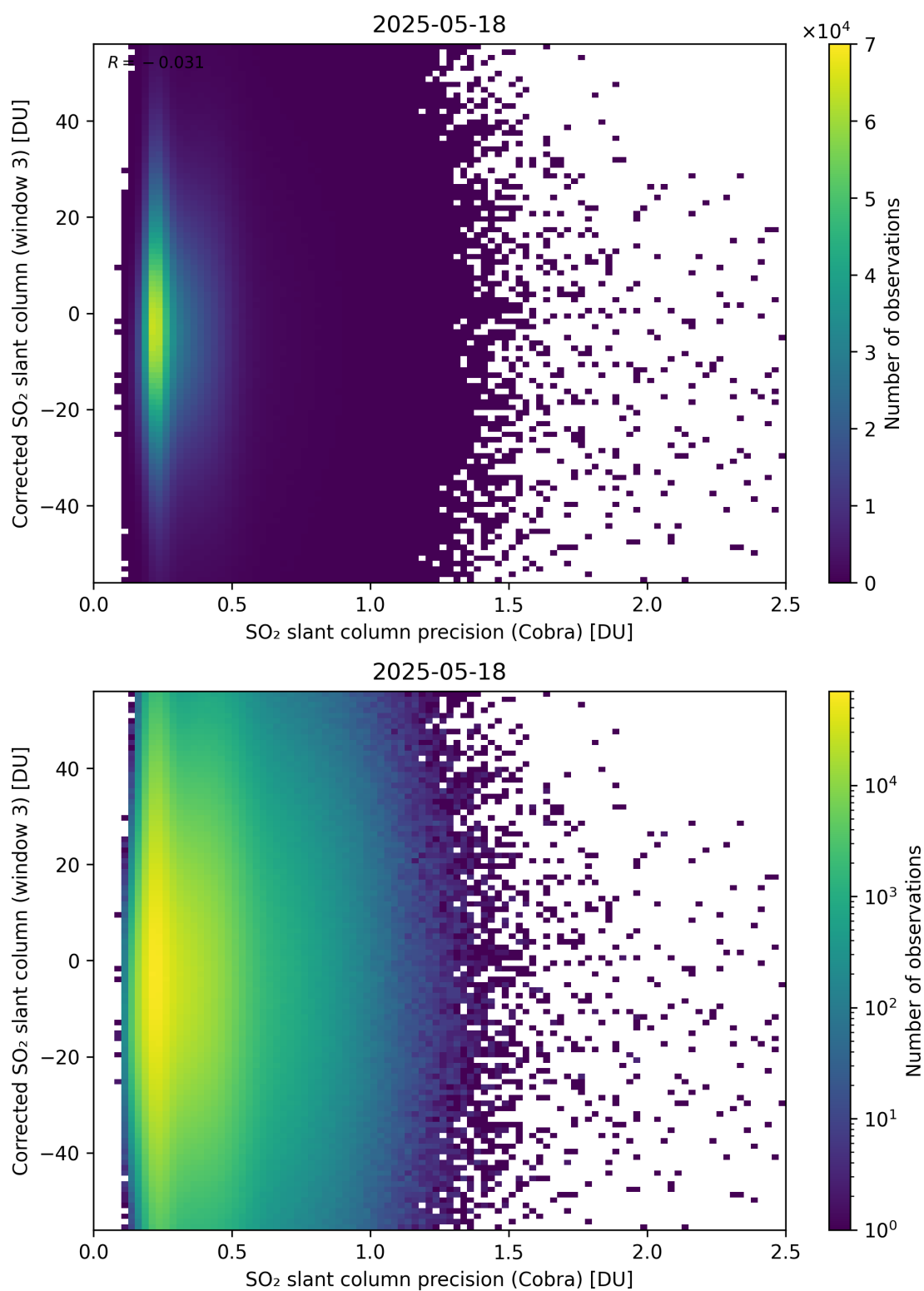
Figure 207: Scatter density plot of “SO 2 slant column precision (Cobra)” against “Corrected SO 2 slant column (window 3)” for 2025-05-17 to 2025-05-19.
