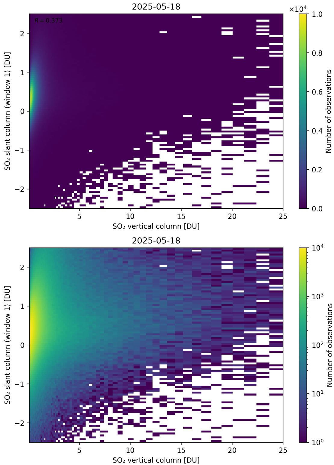
Figure 354: Scatter density plot of “SO 2 vertical column” against “SO 2 slant column (window 1)” for 2025-05-17 to 2025-05-19.
