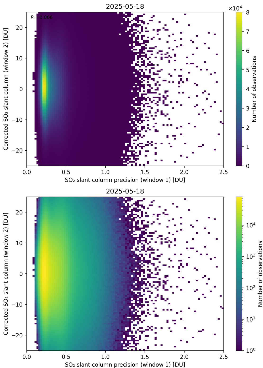
Figure 275: Scatter density plot of “SO 2 slant column precision (window 1)” against “Corrected SO 2 slant column (window 2)” for 2025-05-17 to 2025-05-19.
