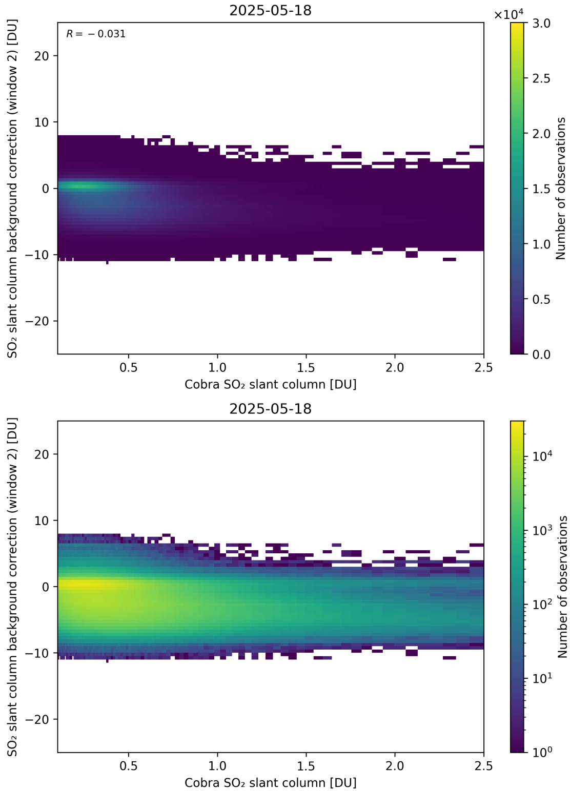
Figure 194: Scatter density plot of “Cobra SO 2 slant column” against “SO 2 slant column background correction (window 2)” for 2025-05-17 to 2025-05-19.
