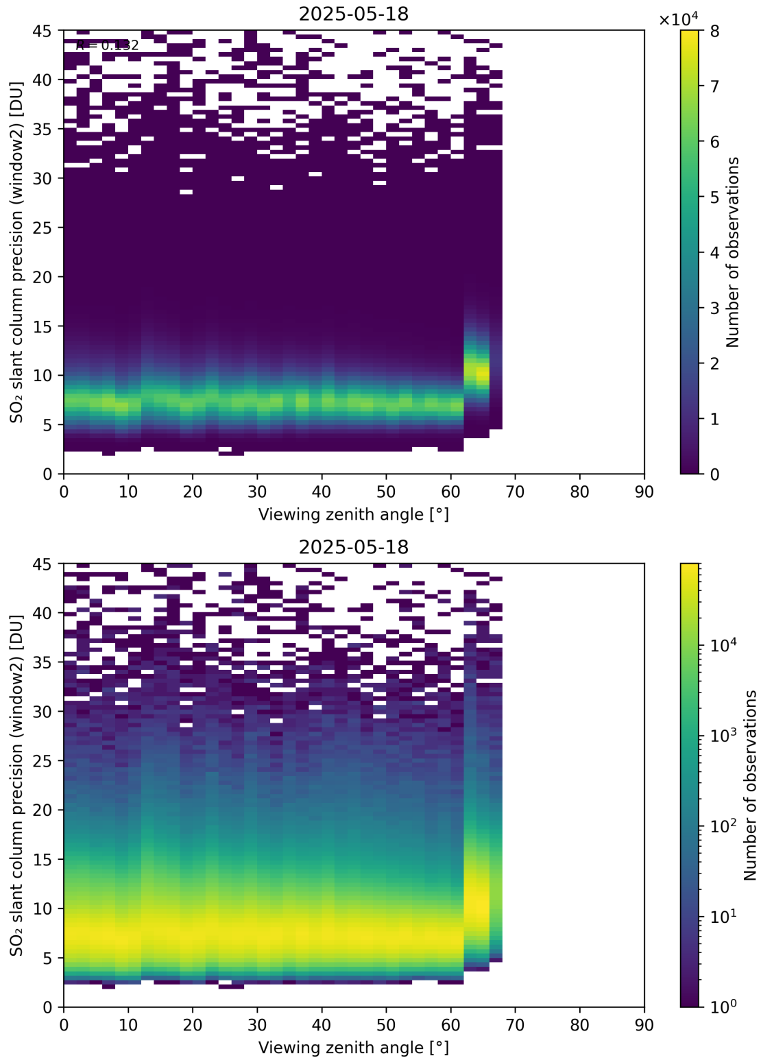
Figure 378: Scatter density plot of “Viewing zenith angle” against “SO 2 slant column precision (window2)” for 2025-05-17 to 2025-05-19.
