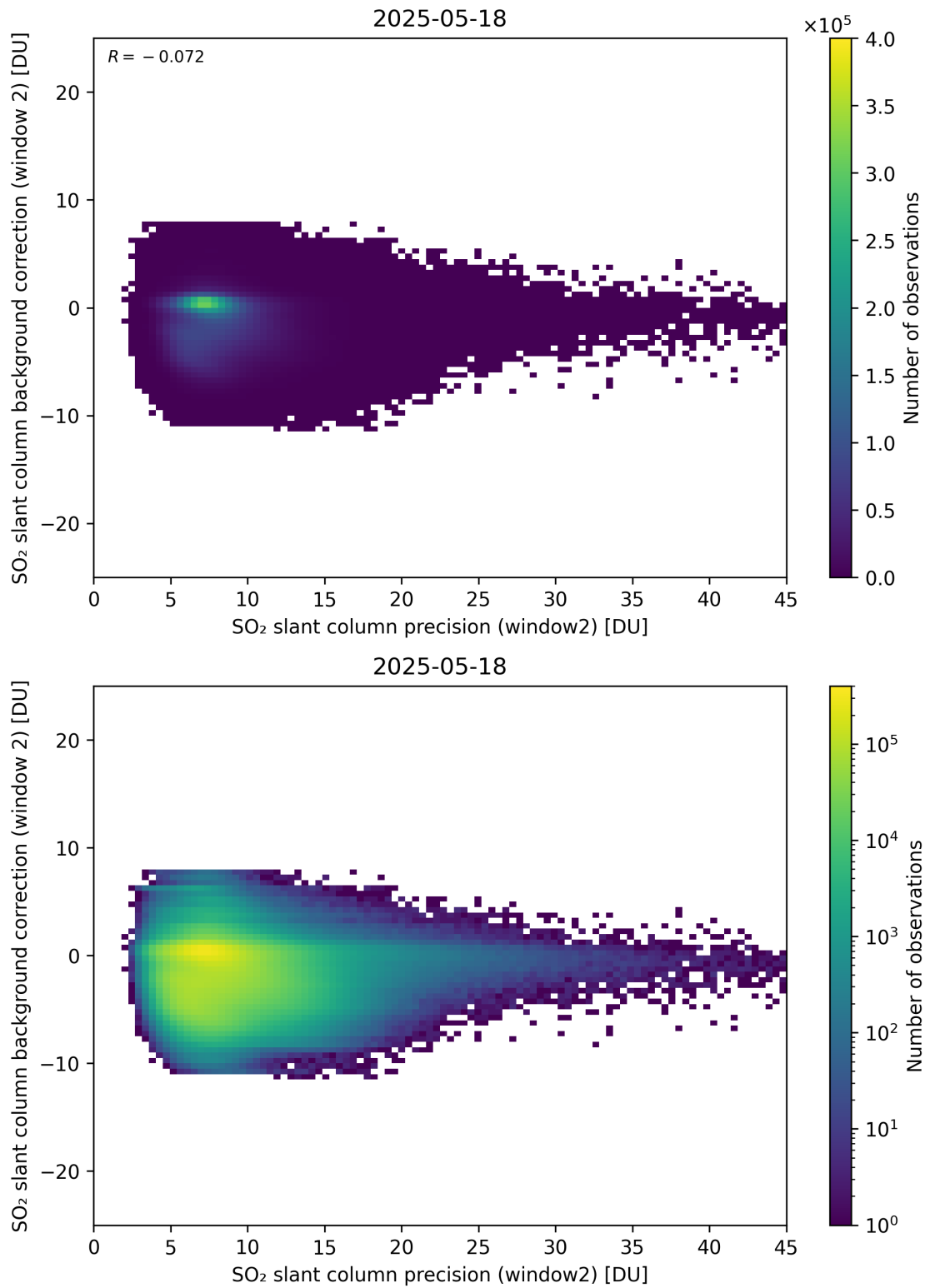
Figure 291: Scatter density plot of “SO 2 slant column precision (window2)” against “SO 2 slant column background correction (window 2)” for 2025-05-17 to 2025-05-19.
