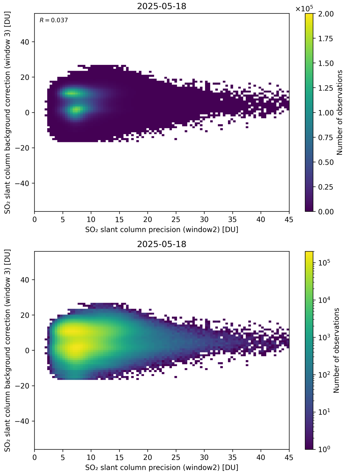
Figure 292: Scatter density plot of “SO 2 slant column precision (window2)” against “SO 2 slant column background correction (window 3)” for 2025-05-17 to 2025-05-19.
