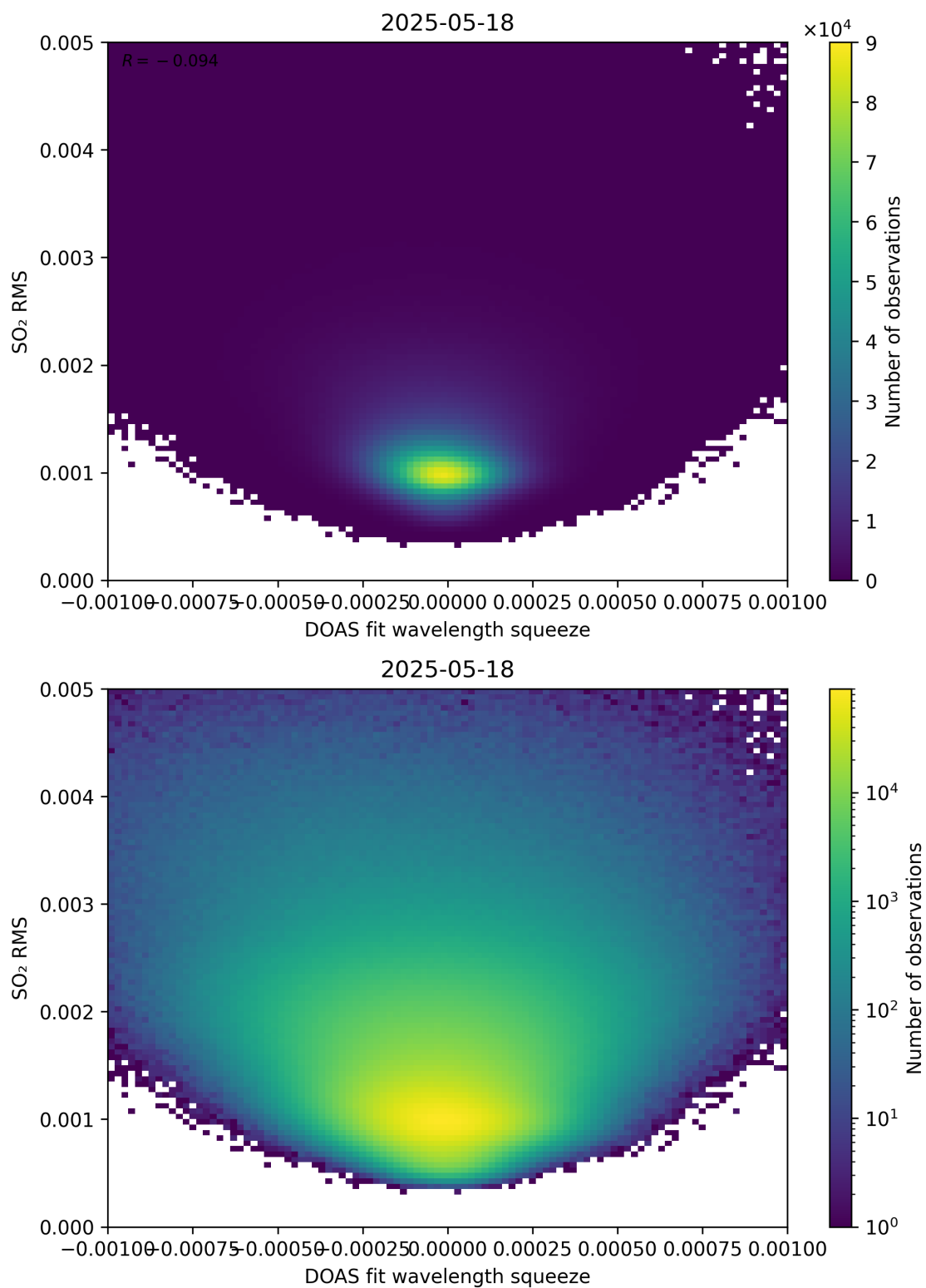
Figure 143: Scatter density plot of “DOAS fit wavelength squeeze” against “SO 2 RMS” for 2025-05-17 to 2025-05-19.
