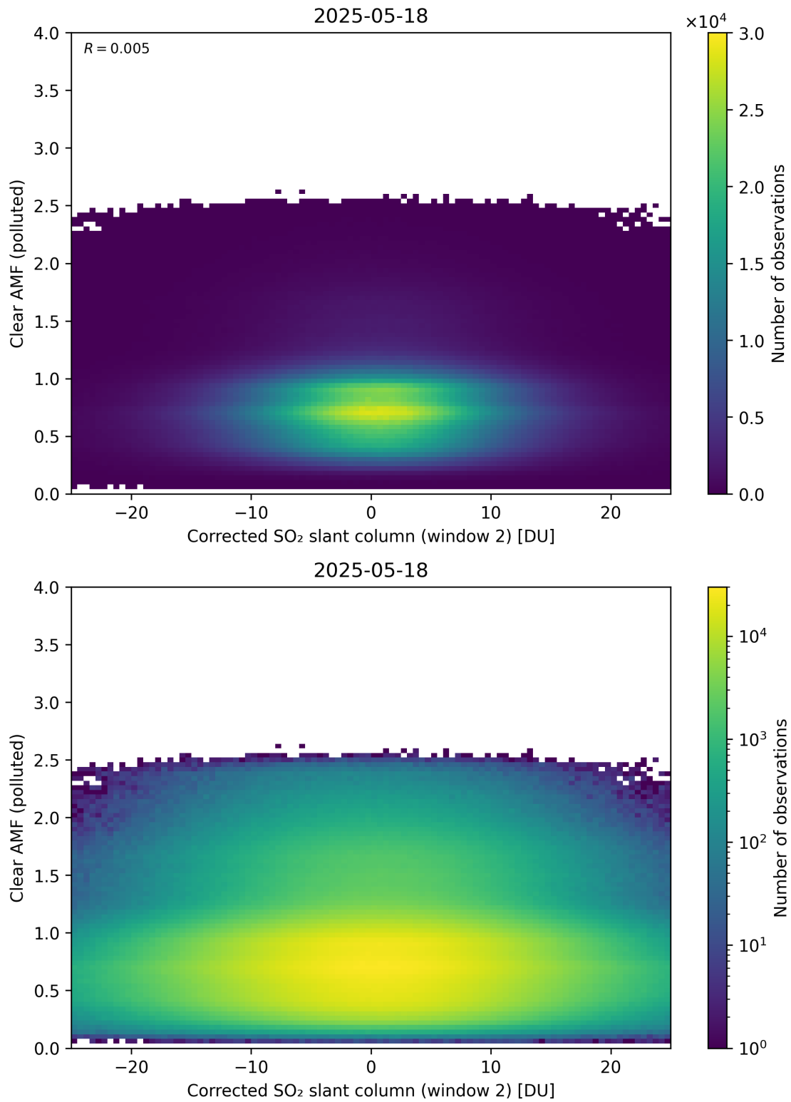
Figure 249: Scatter density plot of “Corrected SO 2 slant column (window 2)” against “Clear AMF (polluted)” for 2025-05-17 to 2025-05-19.
