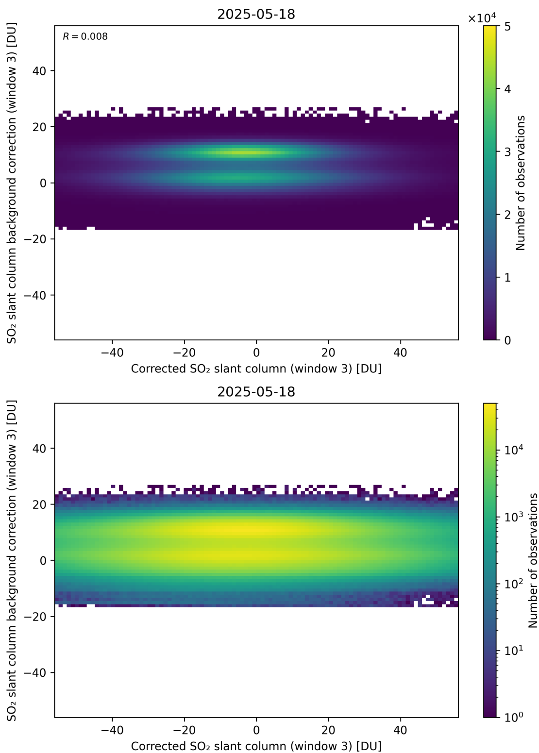
Figure 255: Scatter density plot of “Corrected SO 2 slant column (window 3)” against “SO 2 slant column background correction (window 3)” for 2025-05-17 to 2025-05-19.
