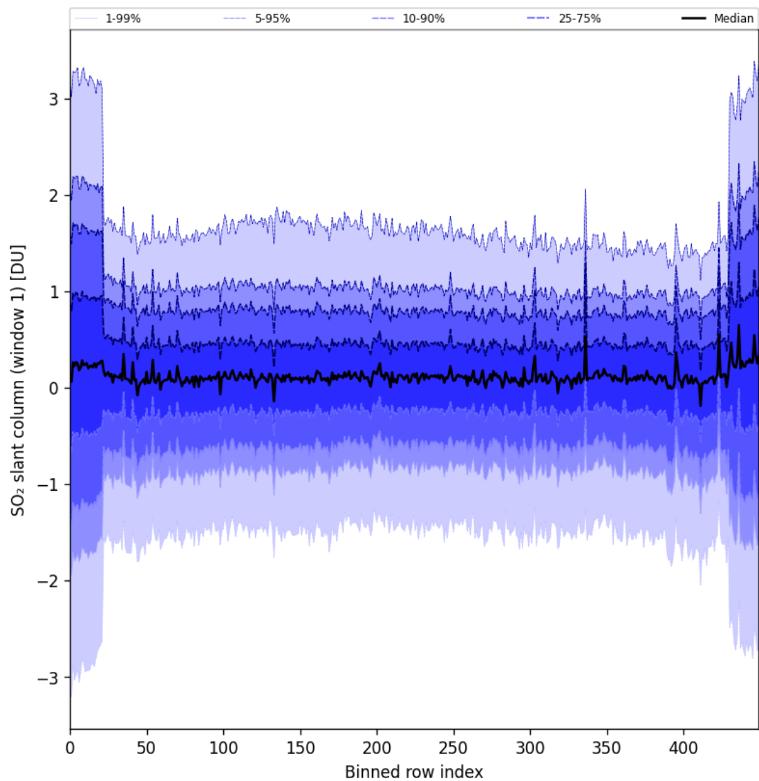
Figure 89: Along track statistics of “SO 2 slant column (window 1)” for 2025-05-17 to 2025-05-19
