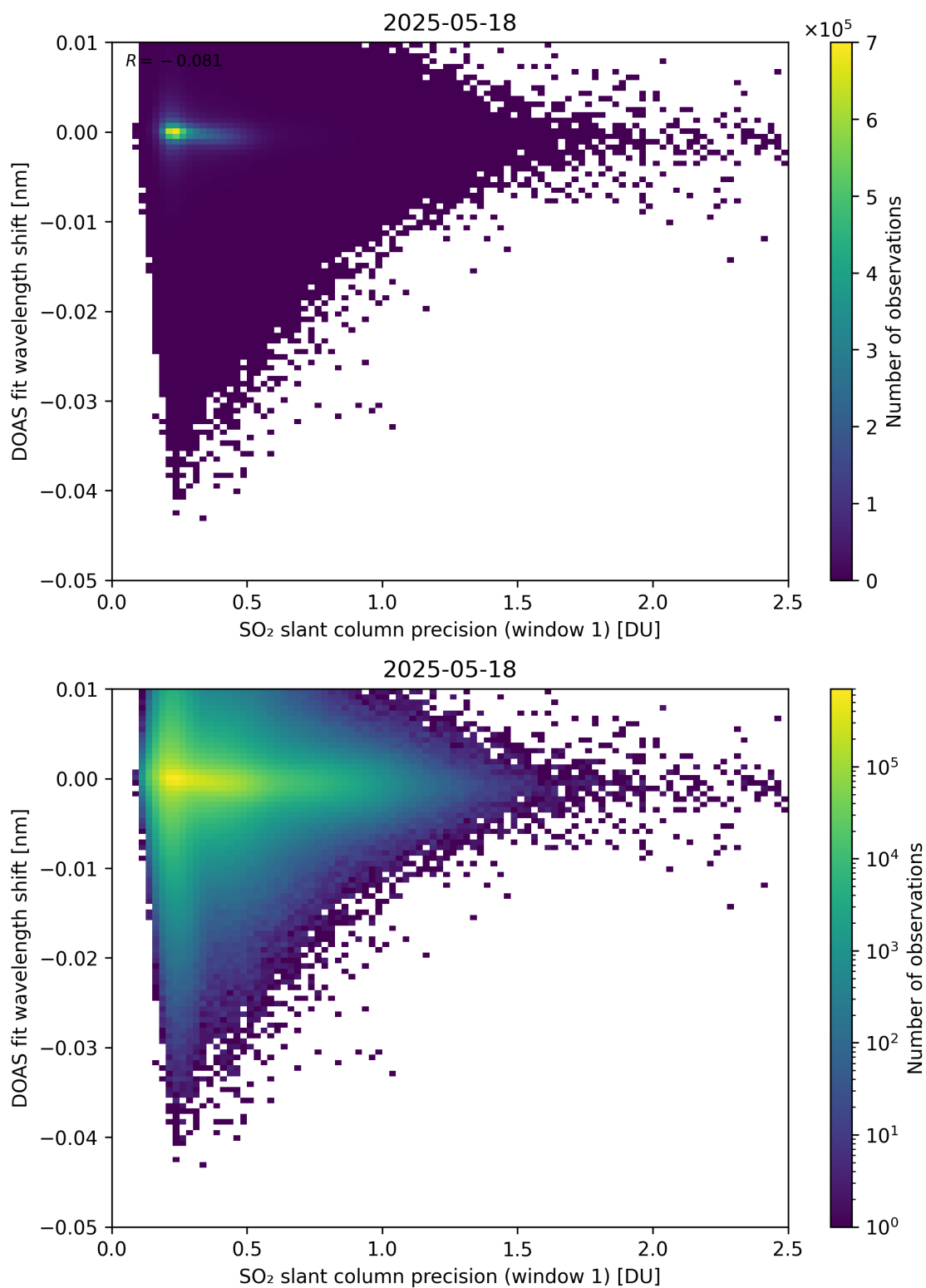
Figure 271: Scatter density plot of “SO 2 slant column precision (window 1)” against “DOAS fit wavelength shift” for 2025-05-17 to 2025-05-19.
