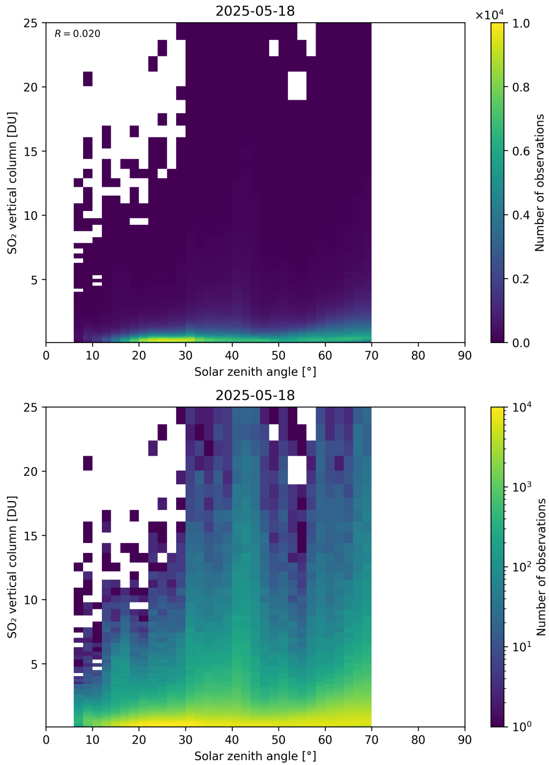
Figure 191: Scatter density plot of “Solar zenith angle” against “SO 2 vertical column” for 2025-05-17 to 2025-05-19.
