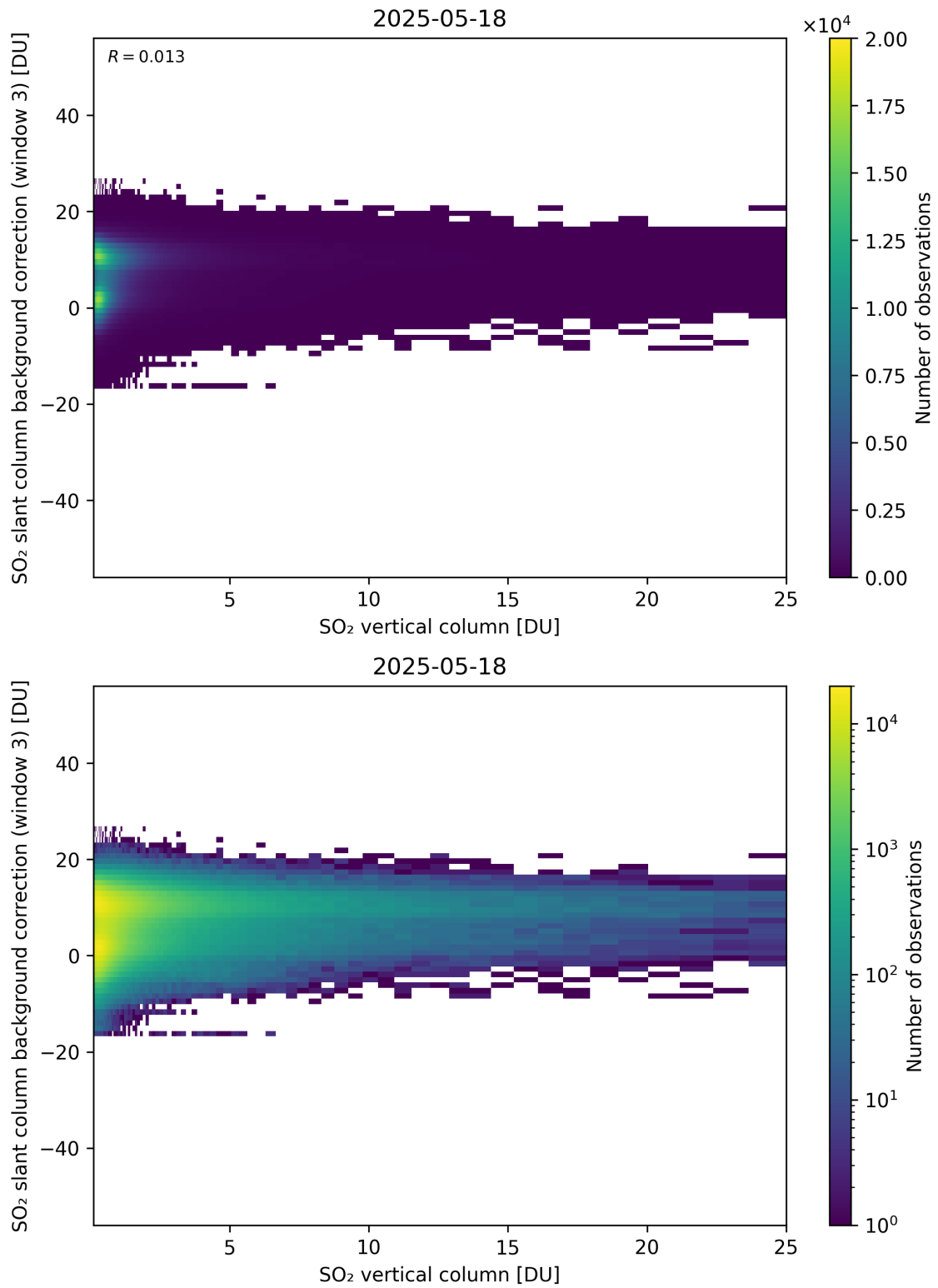
Figure 325: Scatter density plot of “SO 2 vertical column” against “SO 2 slant column background correction (window 3)” for 2025-05-17 to 2025-05-19.
