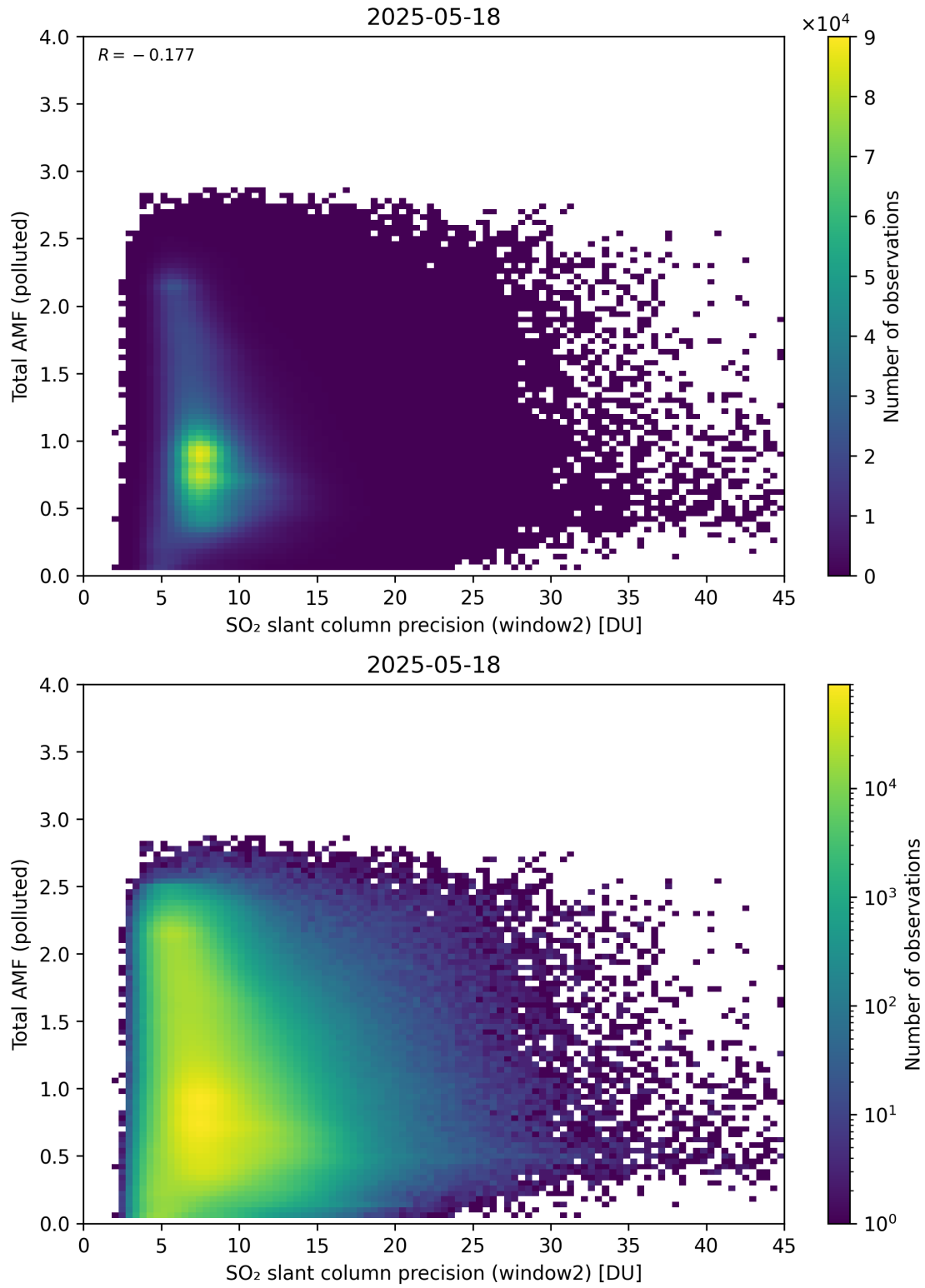
Figure 301: Scatter density plot of “SO 2 slant column precision (window2)” against “Total AMF (polluted)” for 2025-05-17 to 2025-05-19.
