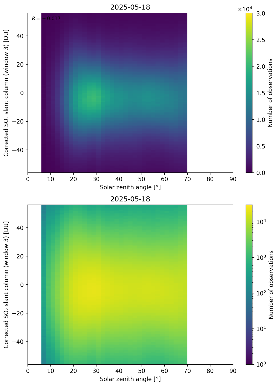
Figure 183: Scatter density plot of “Solar zenith angle” against “Corrected SO 2 slant column (window 3)” for 2025-05-17 to 2025-05-19.
