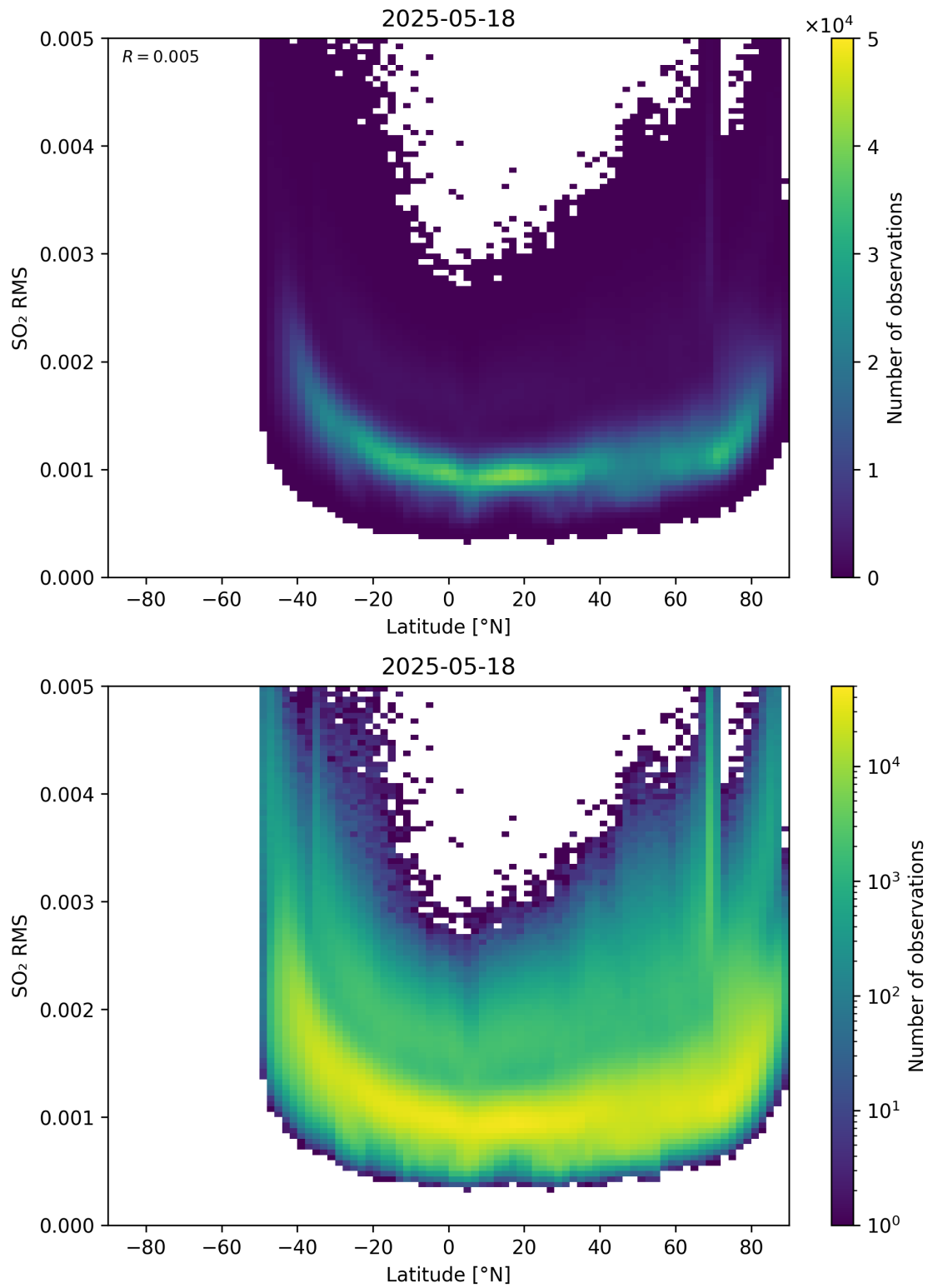
Figure 155: Scatter density plot of “Latitude” against “SO 2 RMS” for 2025-05-17 to 2025-05-19.
