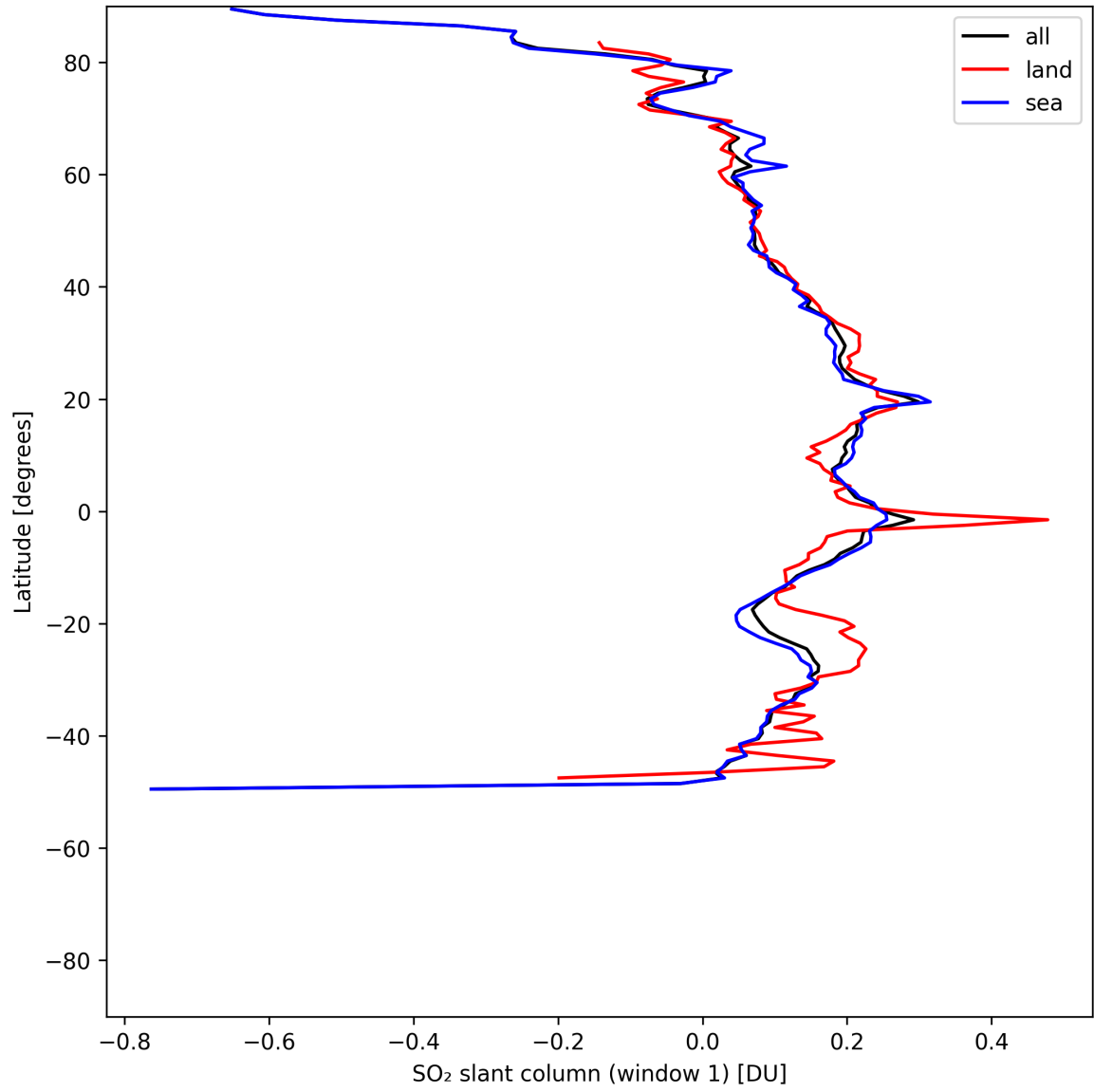
Figure 37: Zonal average of “SO 2 slant column (window 1)” for 2025-05-17 to 2025-05-19.
