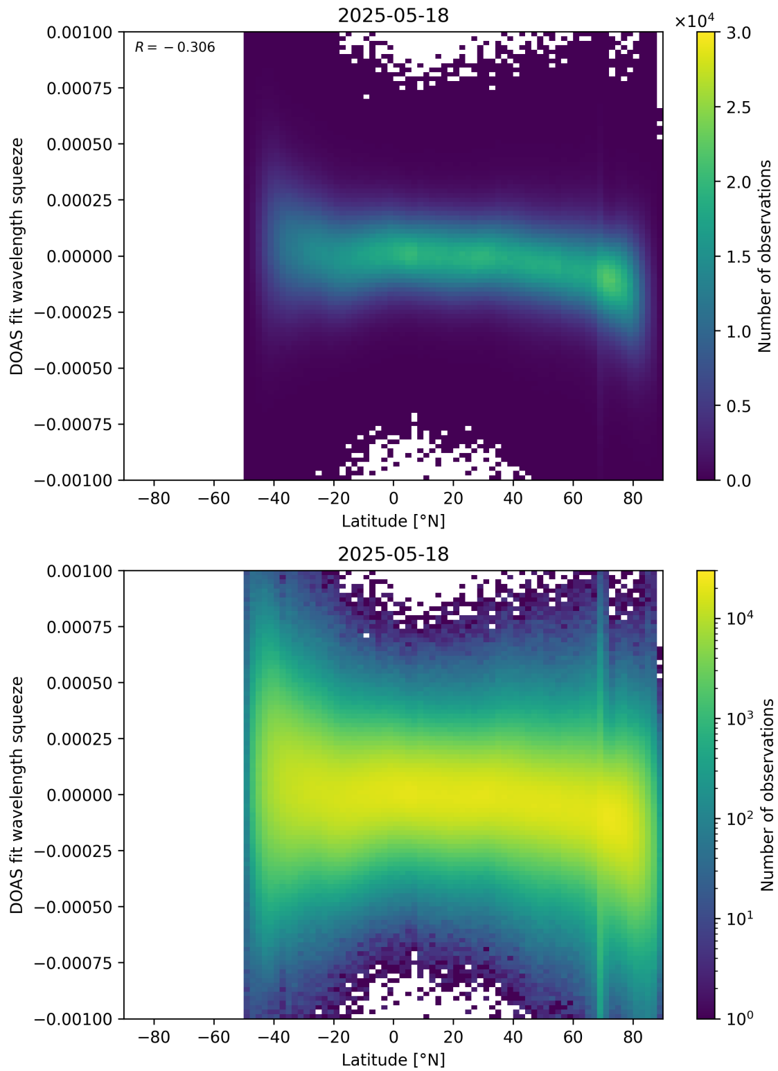
Figure 154: Scatter density plot of “Latitude” against “DOAS fit wavelength squeeze” for 2025-05-17 to 2025-05-19.
