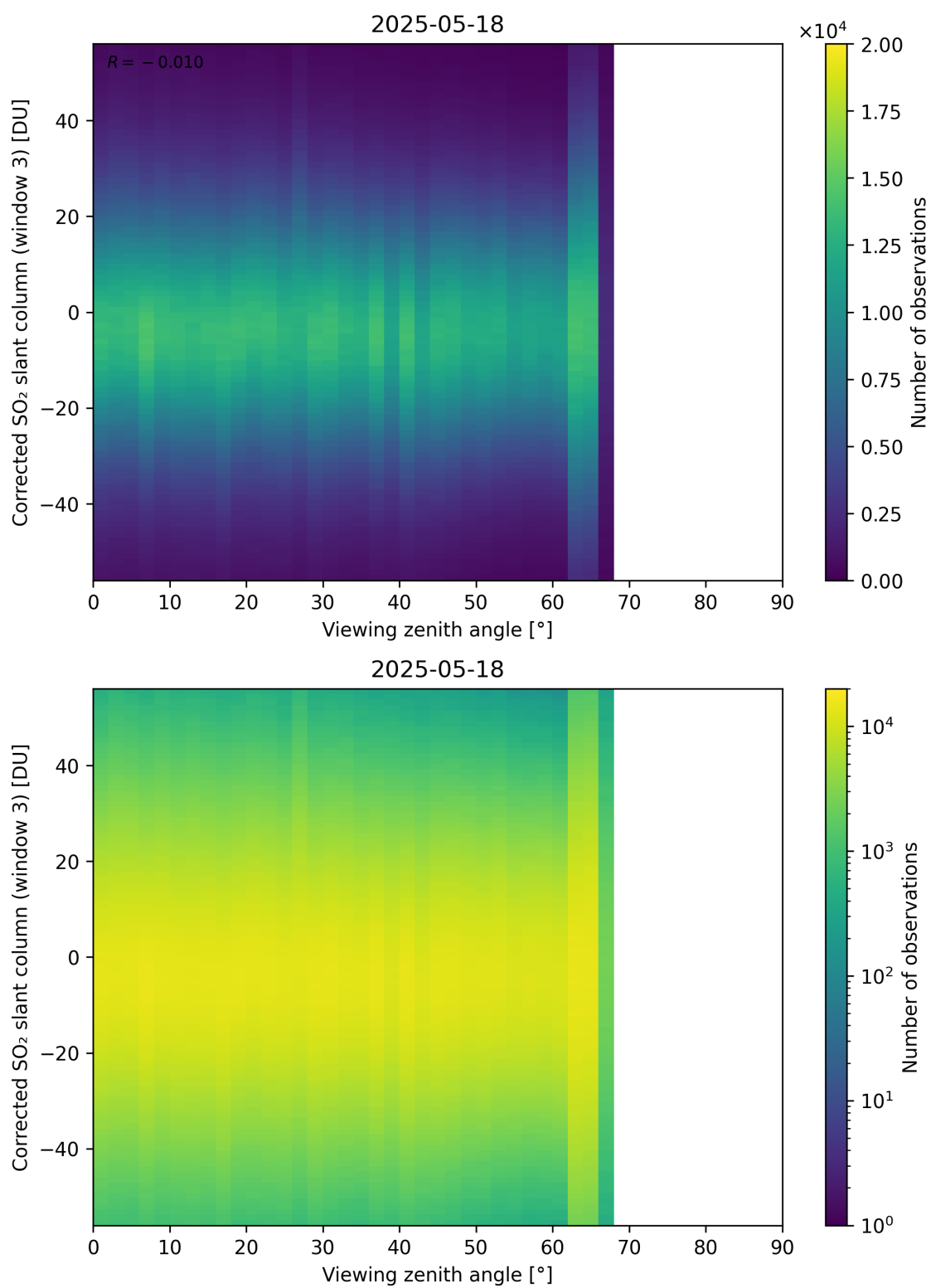
Figure 375: Scatter density plot of “Viewing zenith angle” against “Corrected SO 2 slant column (window 3)” for 2025-05-17 to 2025-05-19.
