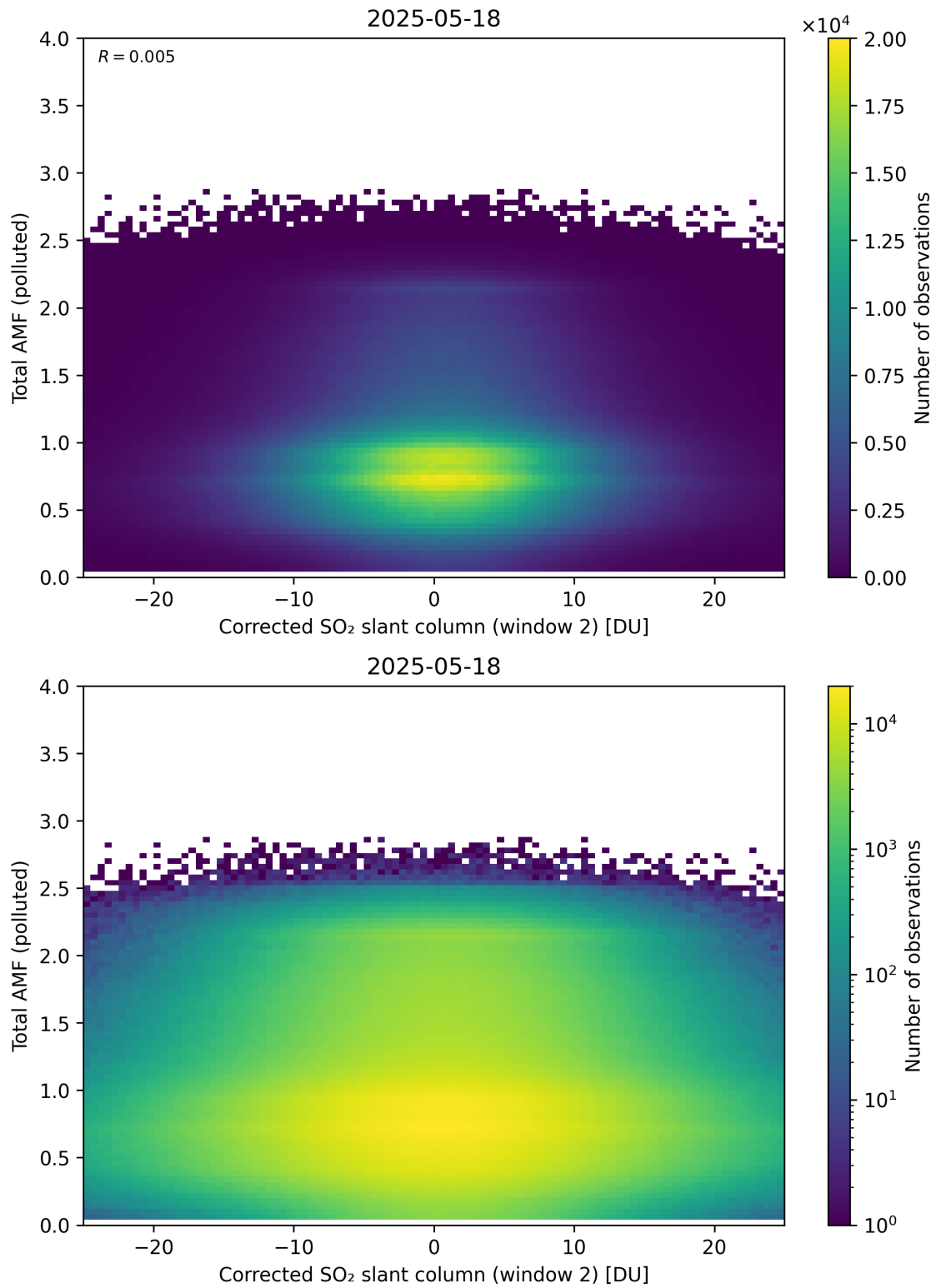
Figure 253: Scatter density plot of “Corrected SO 2 slant column (window 2)” against “Total AMF (polluted)” for 2025-05-17 to 2025-05-19.
