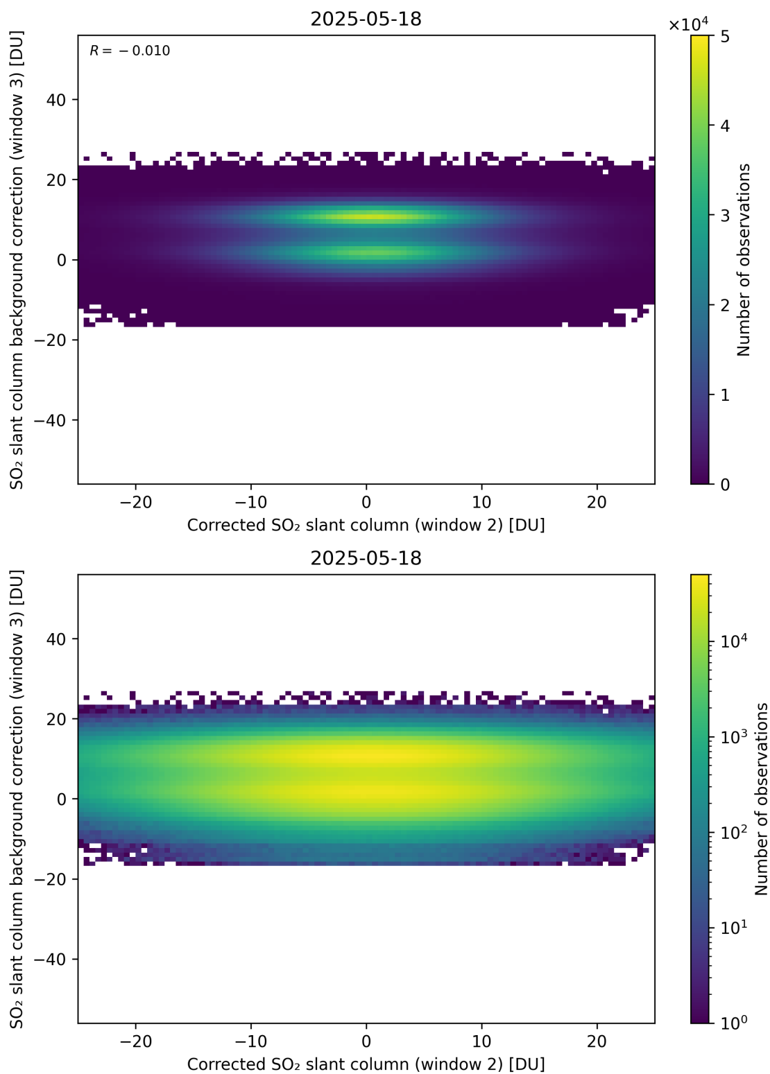
Figure 245: Scatter density plot of “Corrected SO 2 slant column (window 2)” against “SO 2 slant column background correction (window 3)” for 2025-05-17 to 2025-05-19.
