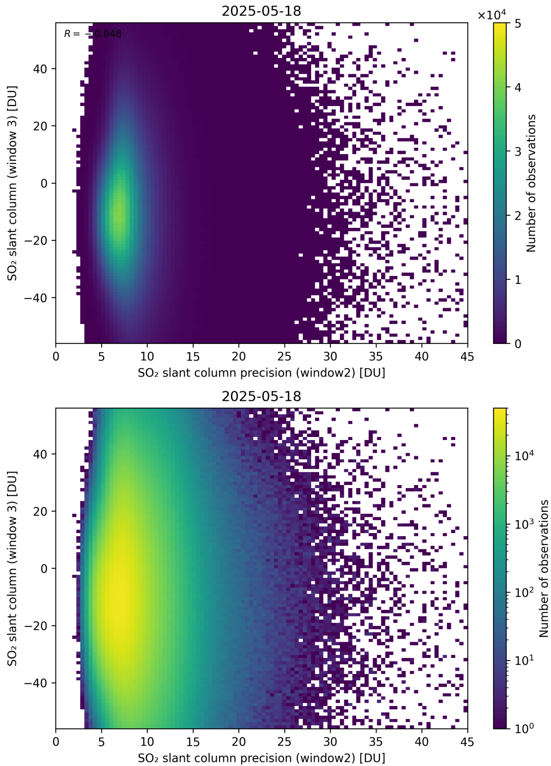
Figure 299: Scatter density plot of “SO 2 slant column precision (window2)” against “SO 2 slant column (window 3)” for 2025-05-17 to 2025-05-19.
