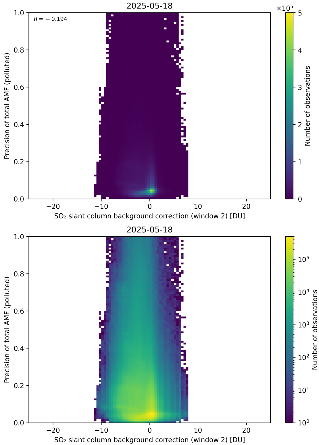
Figure 131: Scatter density plot of “SO 2 slant column background correction (window 2)” against “Precision of total AMF (polluted)” for 2025-05-17 to 2025-05-19.
