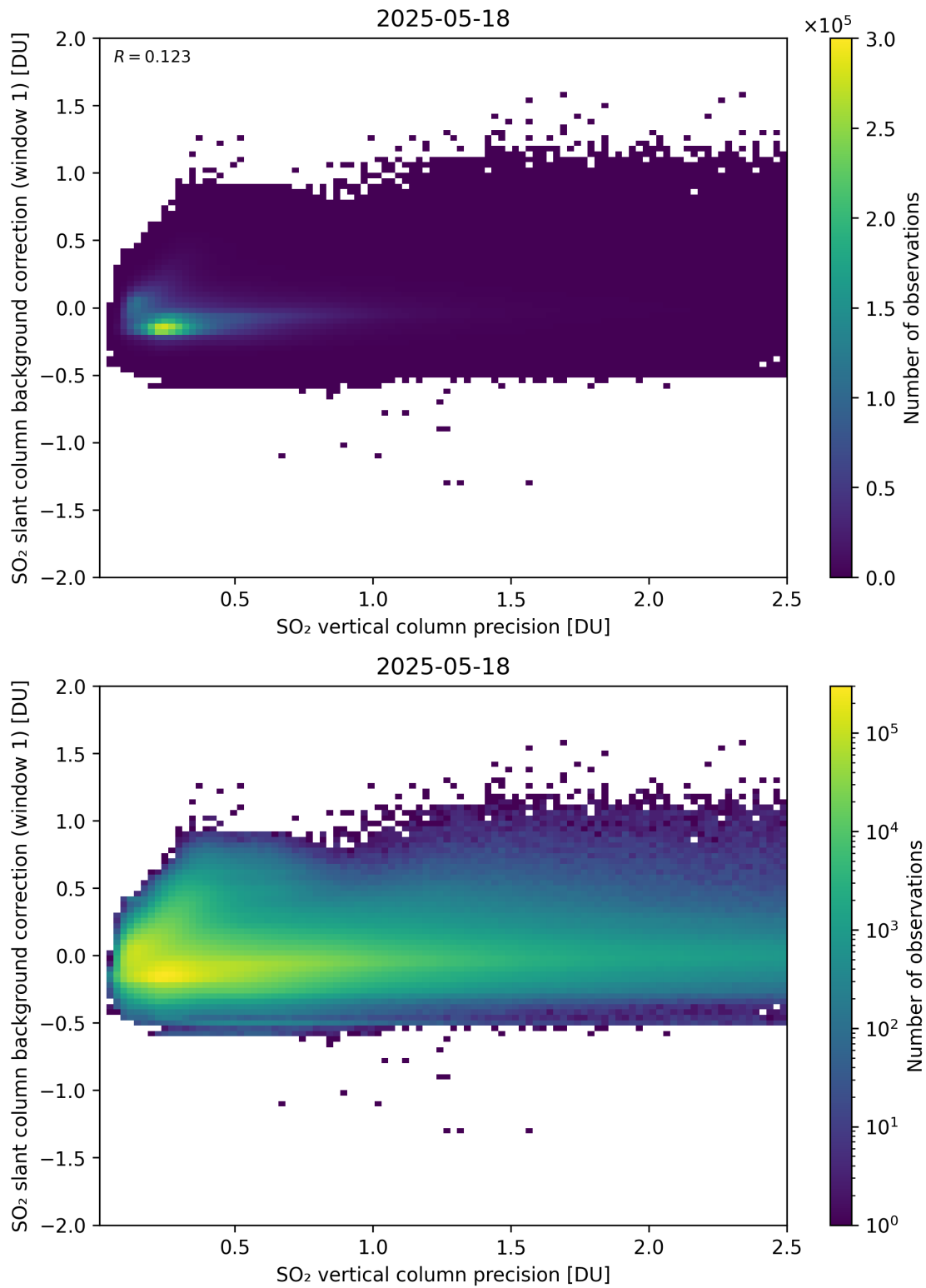
Figure 329: Scatter density plot of “SO 2 vertical column precision” against “SO 2 slant column background correction (window 1)” for 2025-05-17 to 2025-05-19.
