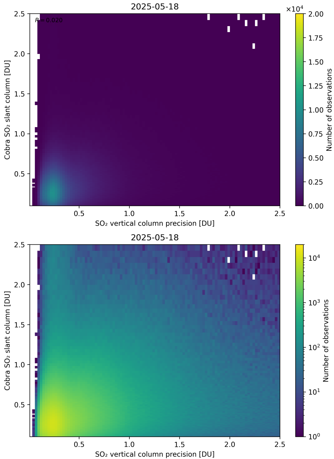
Figure 336: Scatter density plot of “SO 2 vertical column precision” against “Cobra SO 2 slant column” for 2025-05-17 to 2025-05-19.
