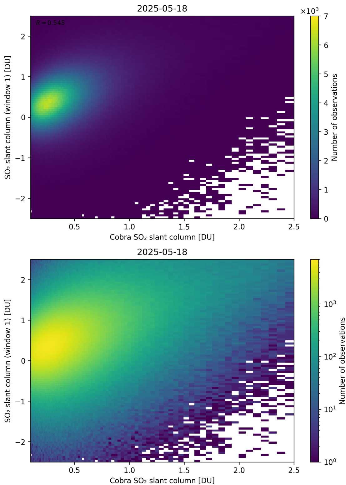
Figure 219: Scatter density plot of “Cobra SO 2 slant column” against “SO 2 slant column (window 1)” for 2025-05-17 to 2025-05-19.
