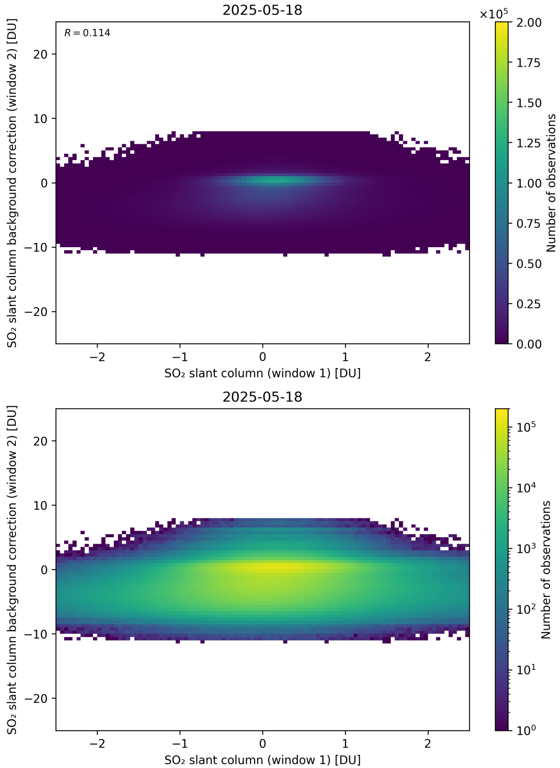
Figure 263: Scatter density plot of “SO 2 slant column (window 1)” against “SO 2 slant column background correction (window 2)” for 2025-05-17 to 2025-05-19.
