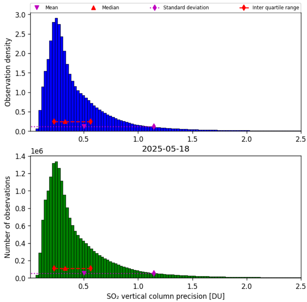
Figure 59: Histogram of “SO 2 vertical column precision” for 2025-05-17 to 2025-05-19
