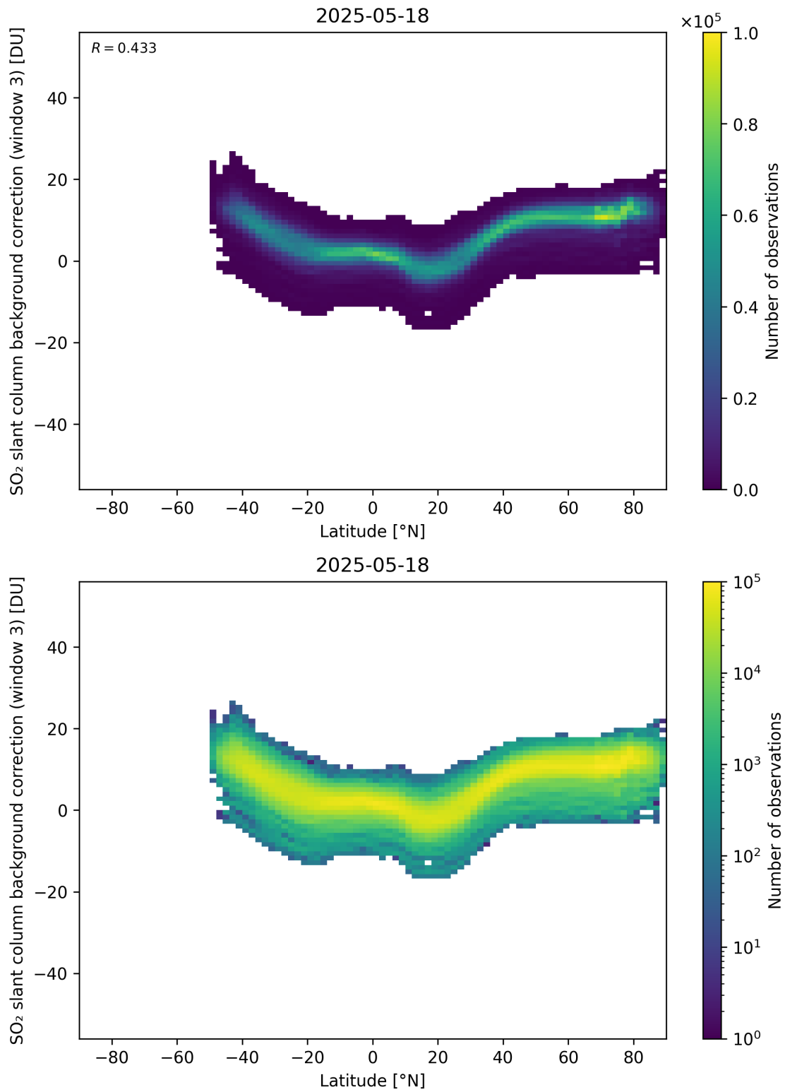
Figure 152: Scatter density plot of “Latitude” against “SO 2 slant column background correction (window 3)” for 2025-05-17 to 2025-05-19.
