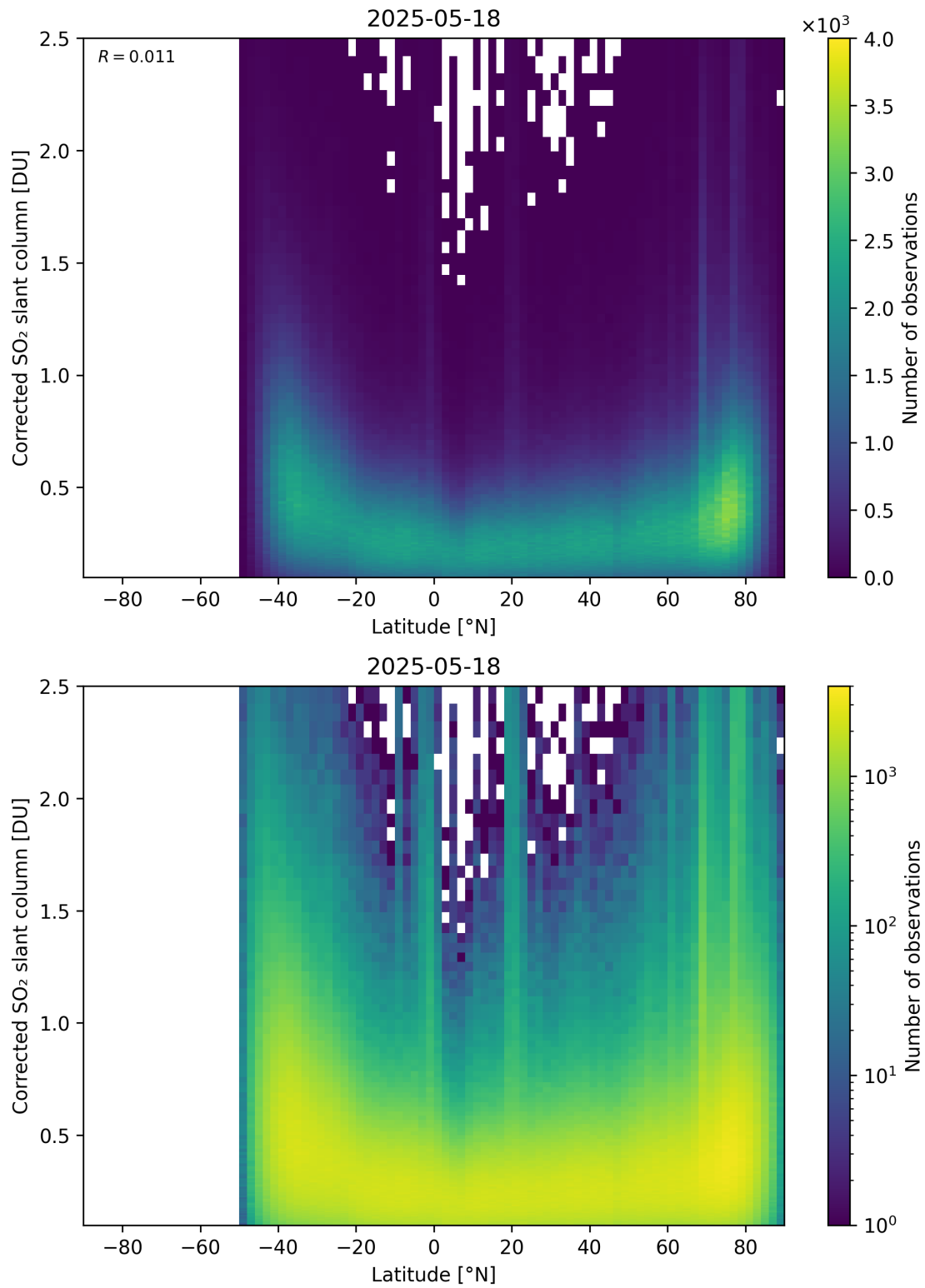
Figure 159: Scatter density plot of “Latitude” against “Corrected SO 2 slant column” for 2025-05-17 to 2025-05-19.
