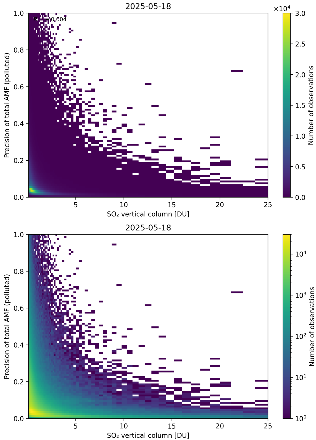
Figure 360: Scatter density plot of “SO 2 vertical column” against “Precision of total AMF (polluted)” for 2025-05-17 to 2025-05-19.
