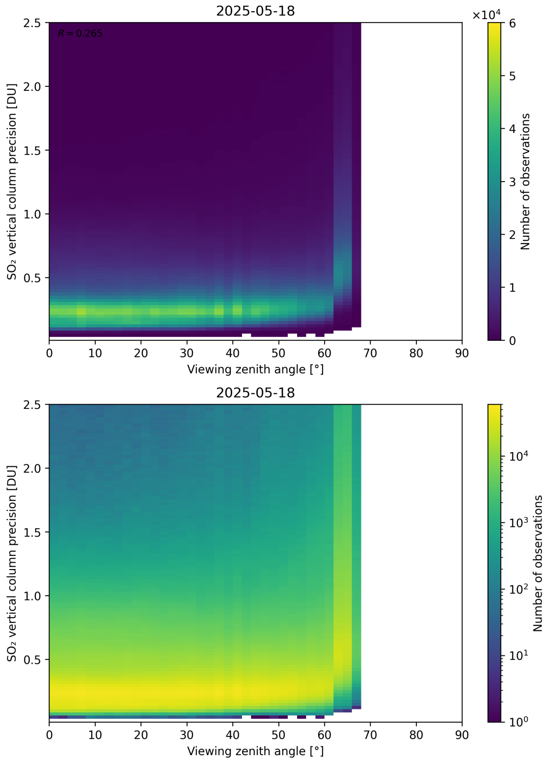
Figure 384: Scatter density plot of “Viewing zenith angle” against “SO 2 vertical column precision” for 2025-05-17 to 2025-05-19.
