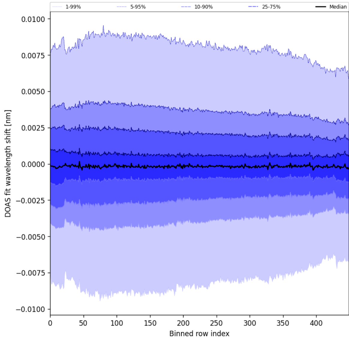
Figure 102: Along track statistics of “DOAS fit wavelength shift” for 2025-05-17 to 2025-05-19
