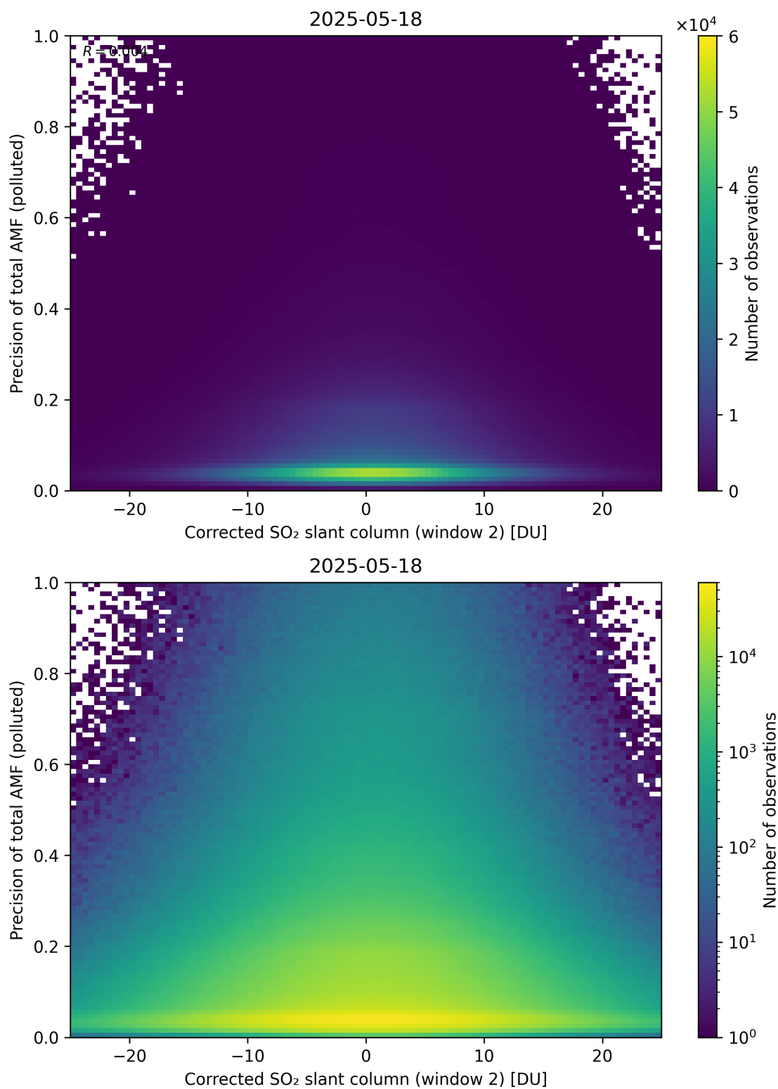
Figure 254: Scatter density plot of “Corrected SO 2 slant column (window 2)” against “Precision of total AMF (polluted)” for 2025-05-17 to 2025-05-19.
