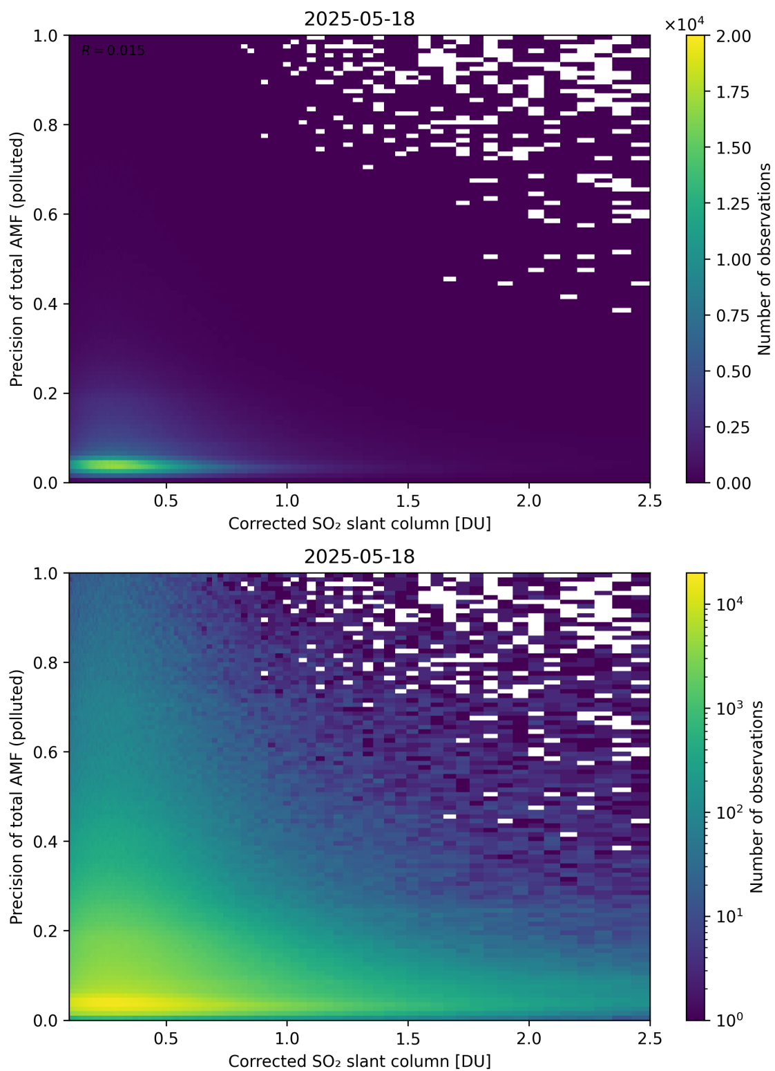
Figure 243: Scatter density plot of “Corrected SO 2 slant column” against “Precision of total AMF (polluted)” for 2025-05-17 to 2025-05-19.
