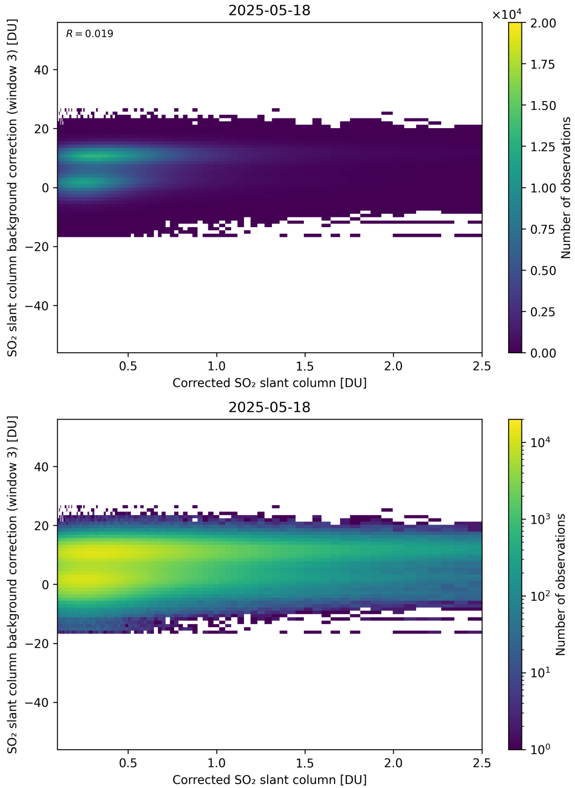
Figure 228: Scatter density plot of “Corrected SO 2 slant column” against “SO 2 slant column background correction (window 3)” for 2025-05-17 to 2025-05-19.
