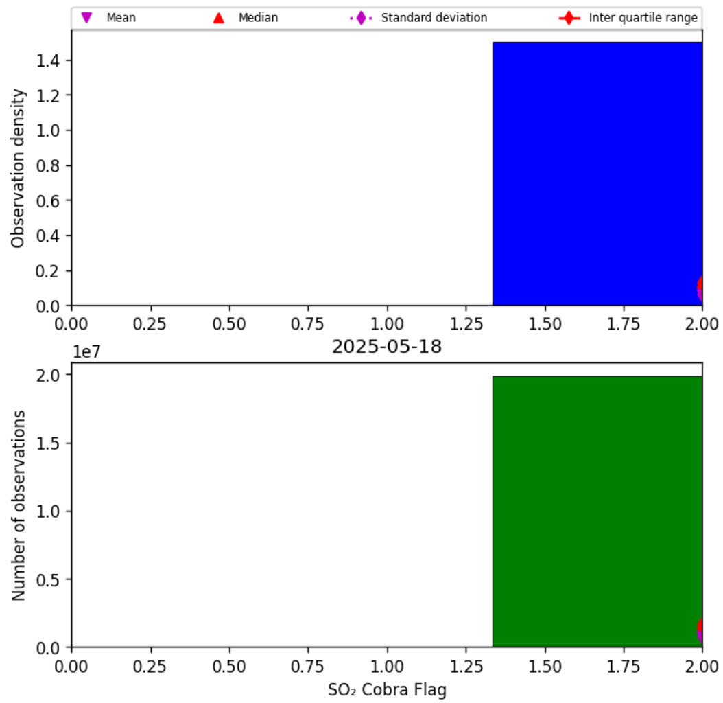
Figure 75: Histogram of “SO 2 Cobra Flag” for 2025-05-17 to 2025-05-19
