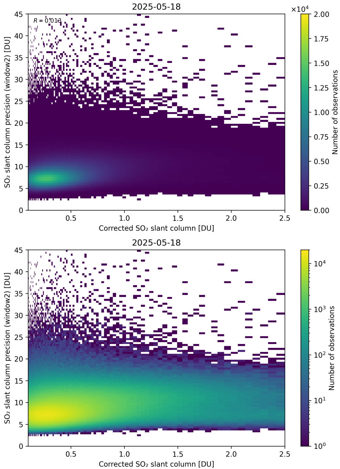
Figure 239: Scatter density plot of “Corrected SO 2 slant column” against “SO 2 slant column precision (window2)” for 2025-05-17 to 2025-05-19.
