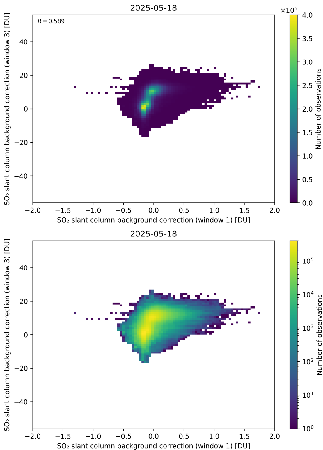
Figure 110: Scatter density plot of “SO 2 slant column background correction (window 1)” against “SO 2 slant column background correction (window 3)” for 2025-05-17 to 2025-05-19.
