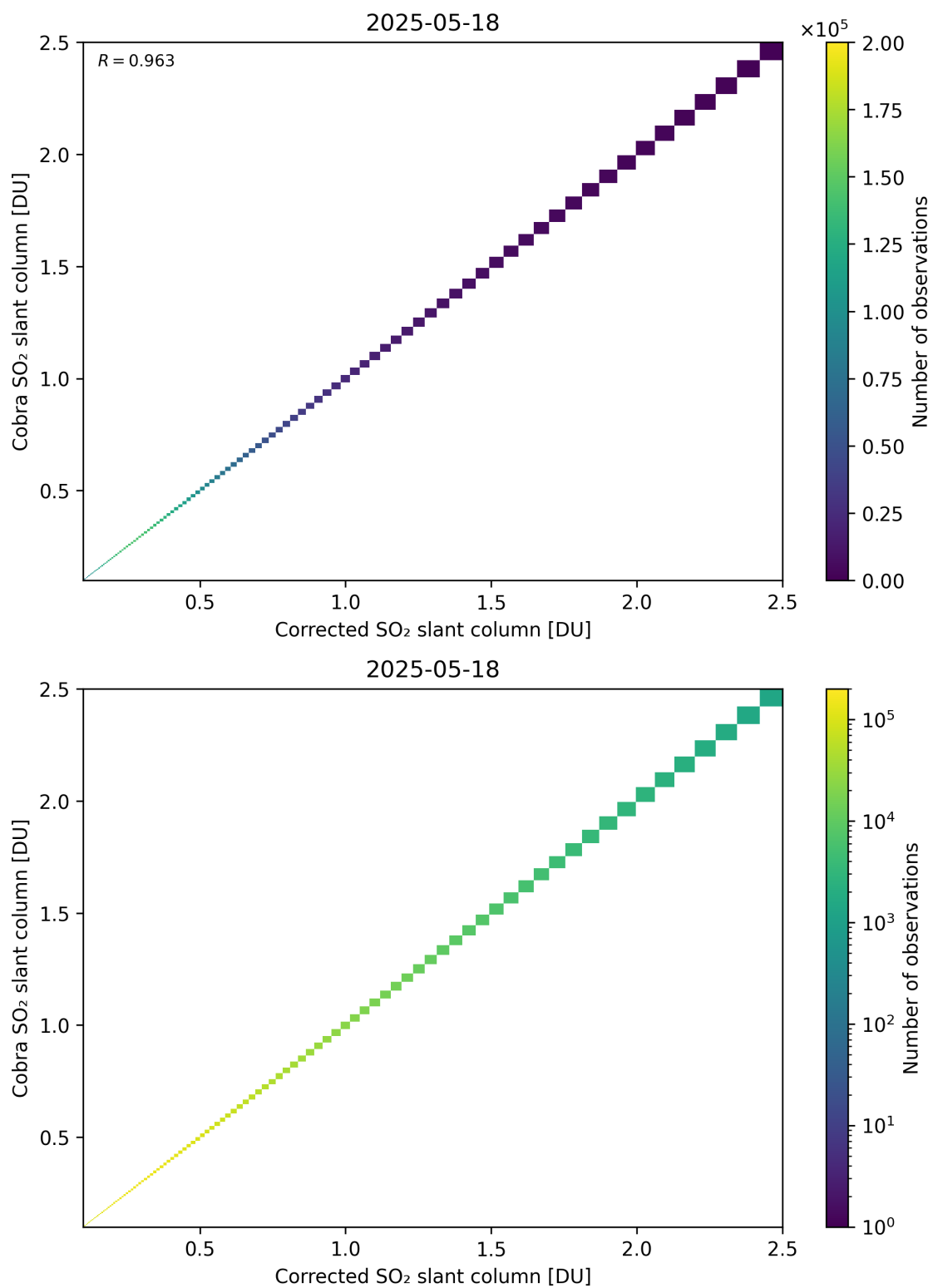
Figure 233: Scatter density plot of “Corrected SO 2 slant column” against “Cobra SO 2 slant column” for 2025-05-17 to 2025-05-19.
