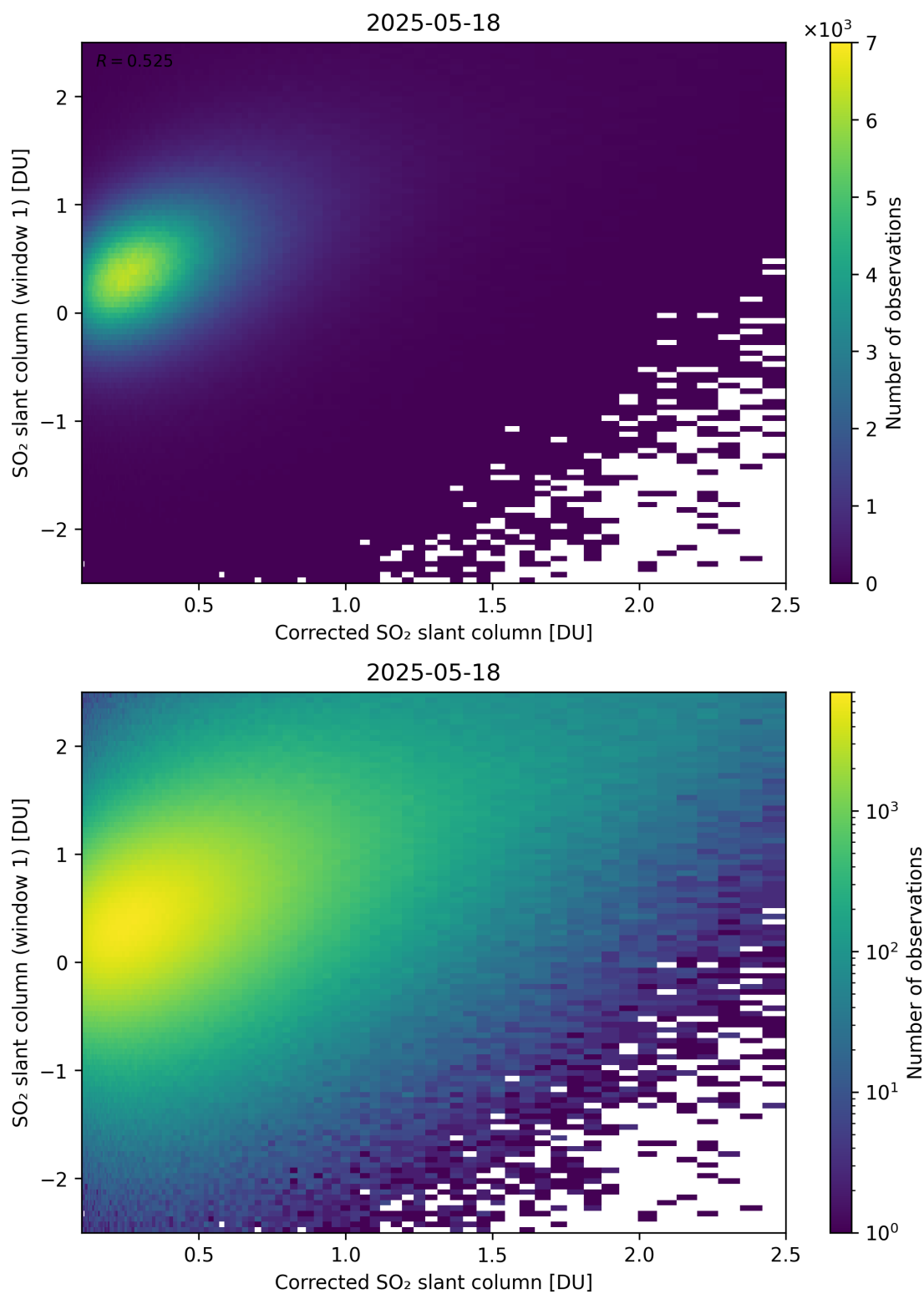
Figure 237: Scatter density plot of “Corrected SO 2 slant column” against “SO 2 slant column (window 1)” for 2025-05-17 to 2025-05-19.
