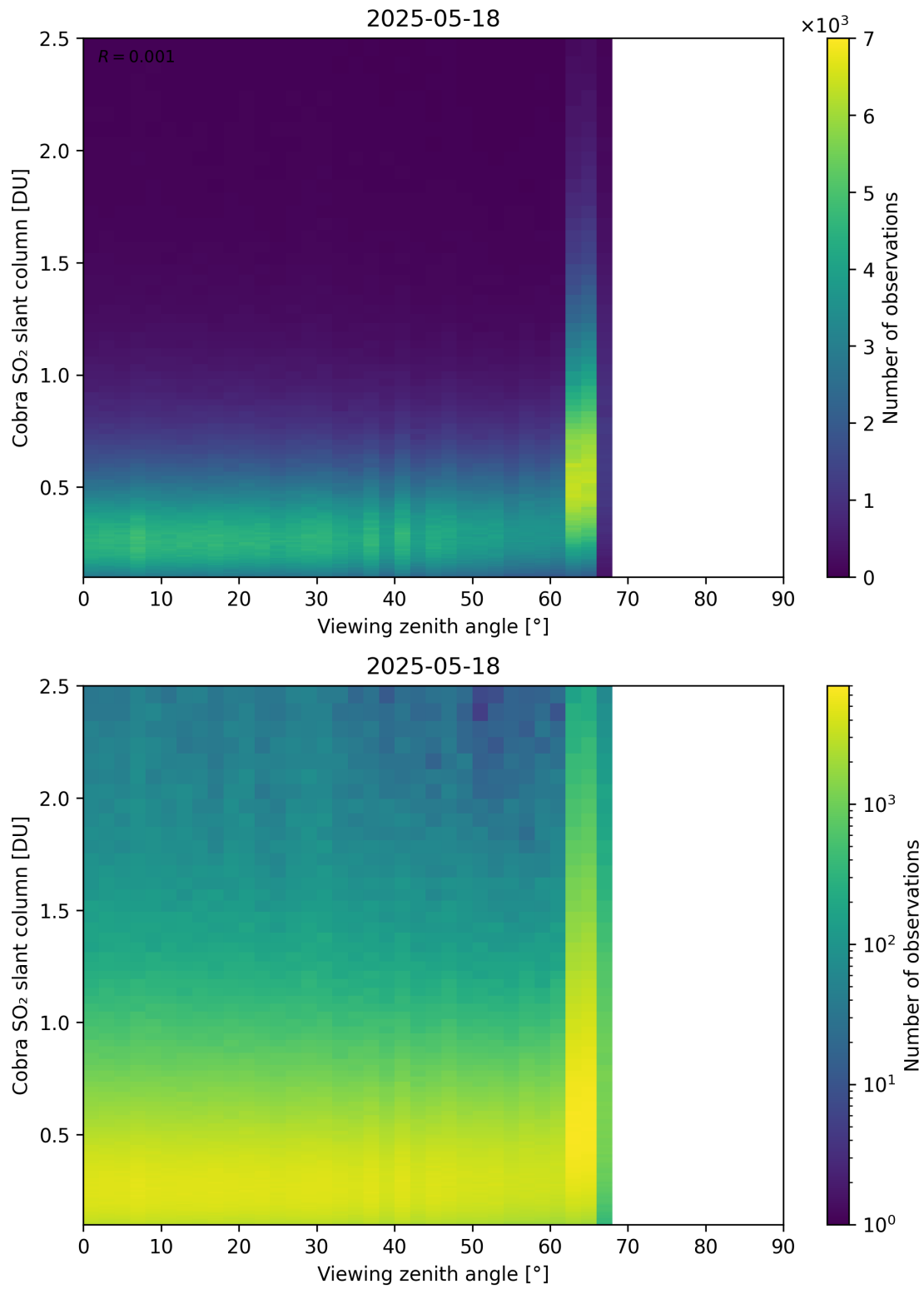
Figure 371: Scatter density plot of “Viewing zenith angle” against “Cobra SO 2 slant column” for 2025-05-17 to 2025-05-19.
