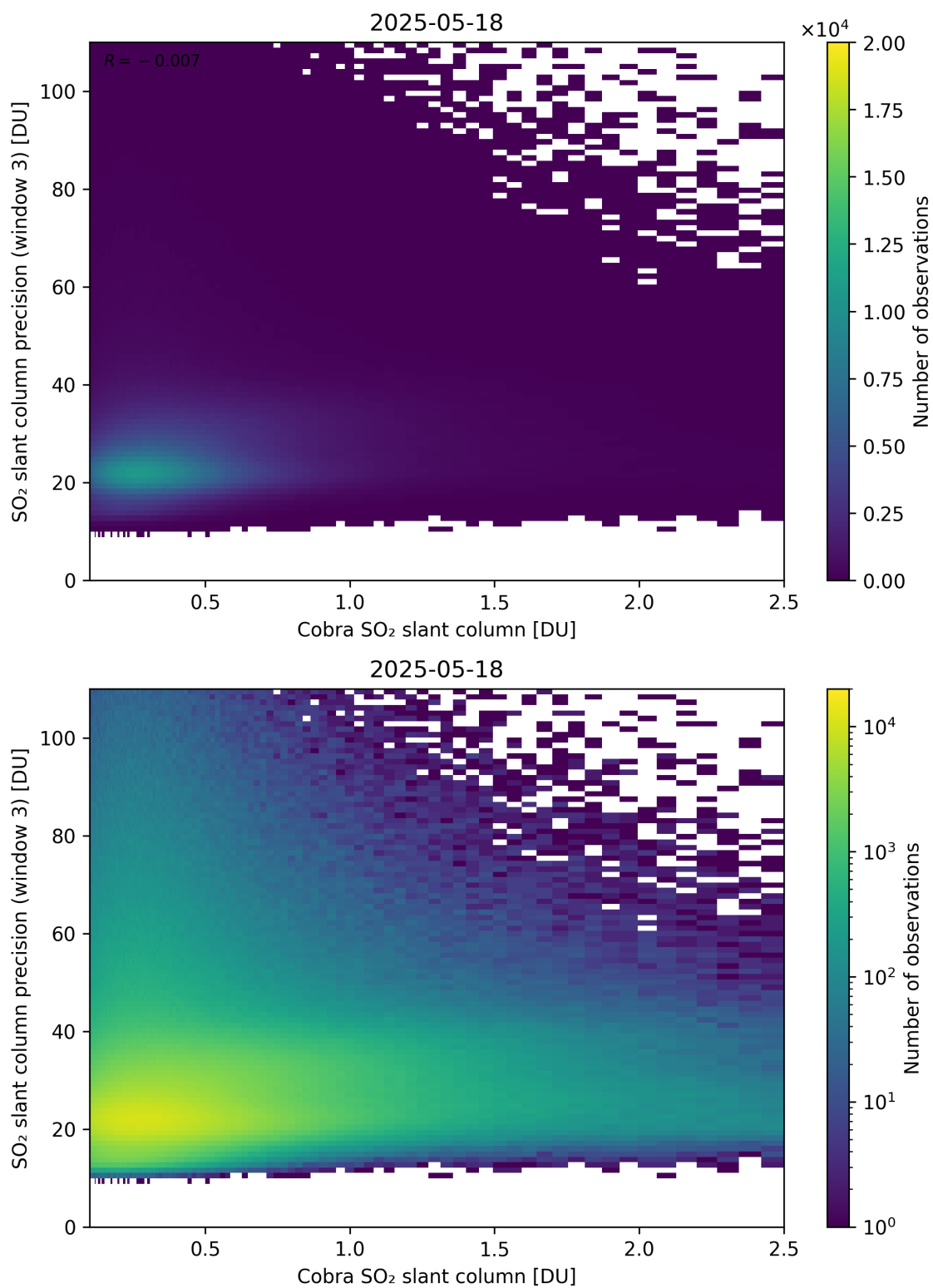
Figure 223: Scatter density plot of “Cobra SO 2 slant column” against “SO 2 slant column precision (window 3)” for 2025-05-17 to 2025-05-19.
