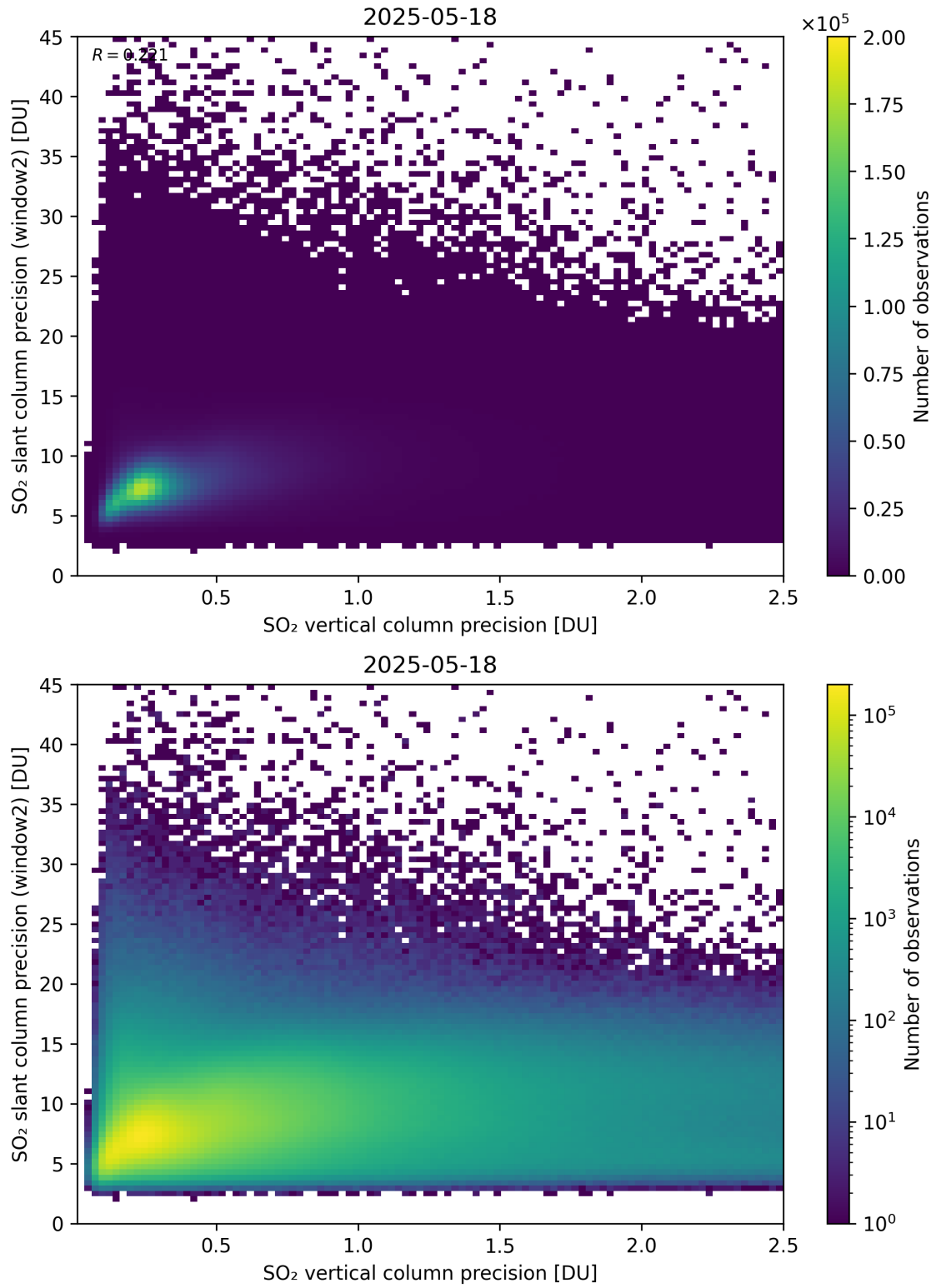
Figure 343: Scatter density plot of “SO 2 vertical column precision” against “SO 2 slant column precision (window2)” for 2025-05-17 to 2025-05-19.
