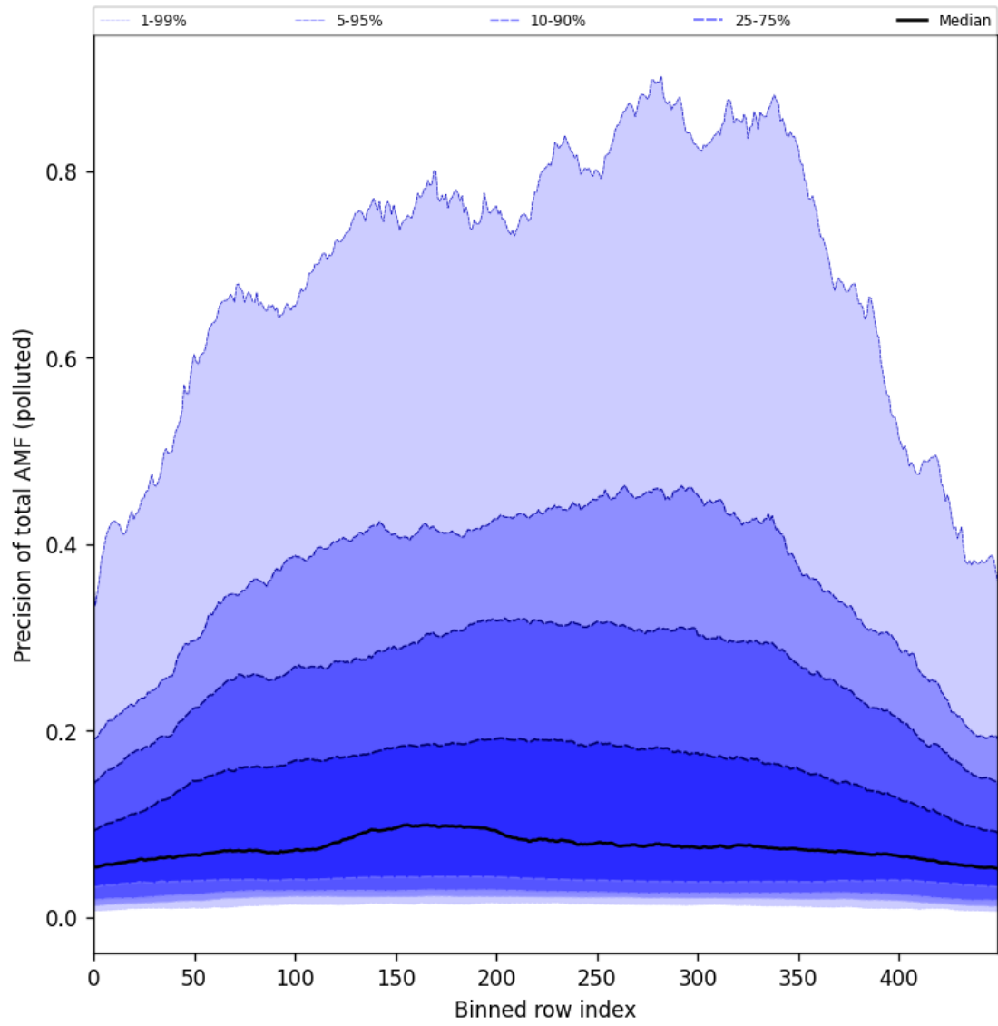
Figure 106: Along track statistics of “Precision of total AMF (polluted)” for 2025-05-17 to 2025-05-19
