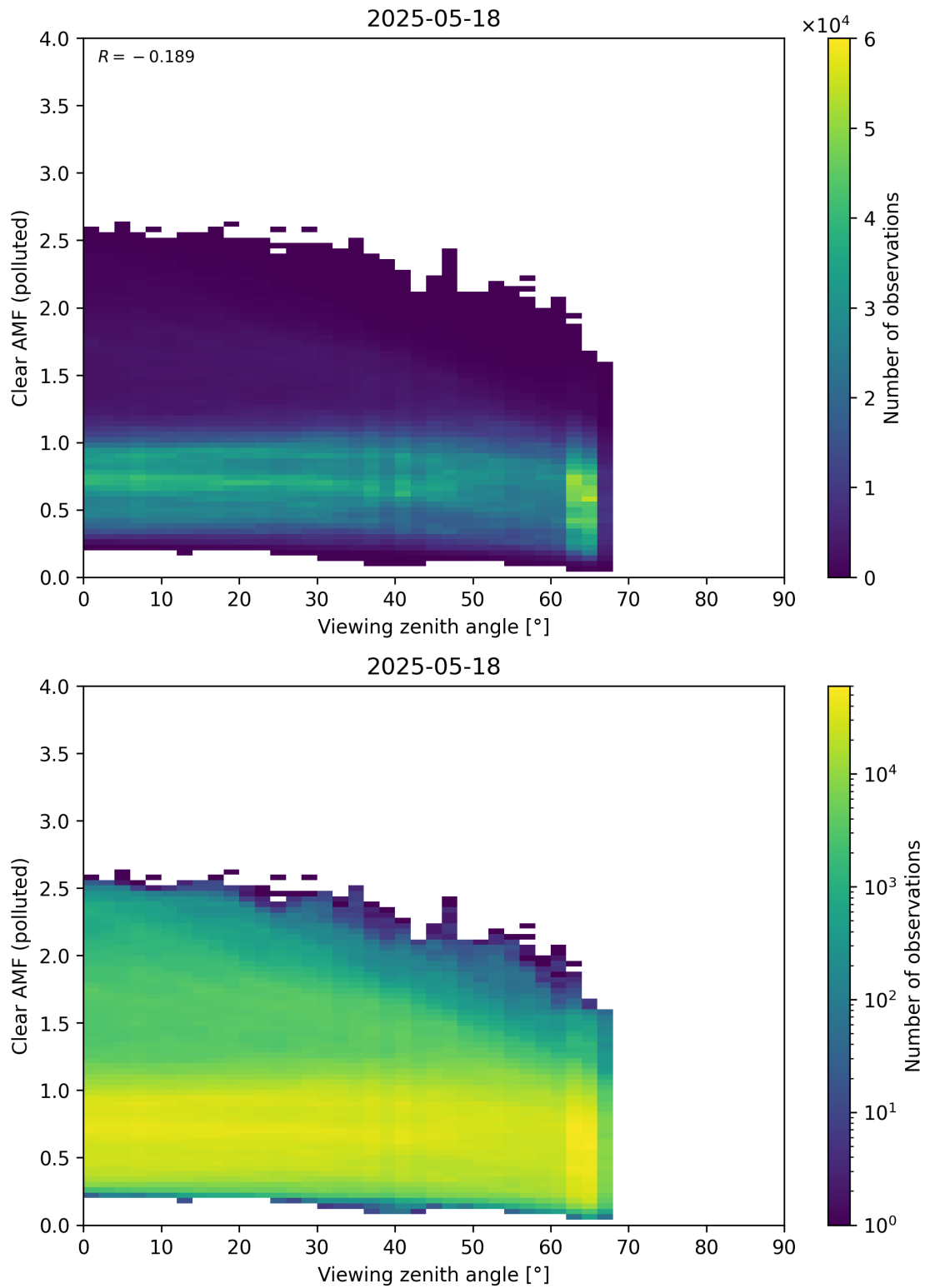
Figure 370: Scatter density plot of “Viewing zenith angle” against “Clear AMF (polluted)” for 2025-05-17 to 2025-05-19.
