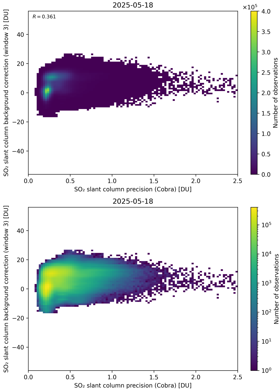
Figure 201: Scatter density plot of “SO 2 slant column precision (Cobra)” against “SO 2 slant column background correction (window 3)” for 2025-05-17 to 2025-05-19.
