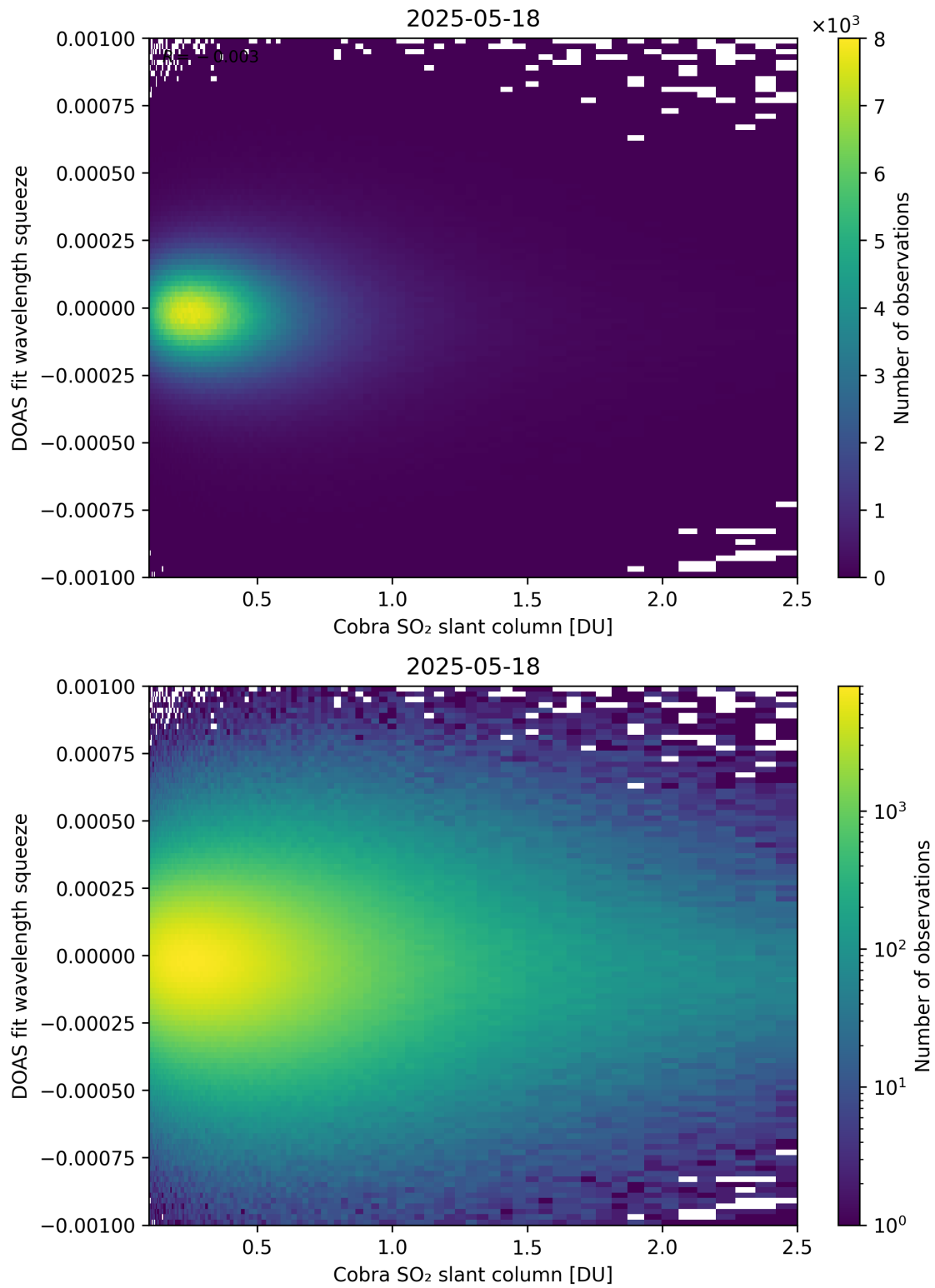
Figure 197: Scatter density plot of “Cobra SO 2 slant column” against “DOAS fit wavelength squeeze” for 2025-05-17 to 2025-05-19.
