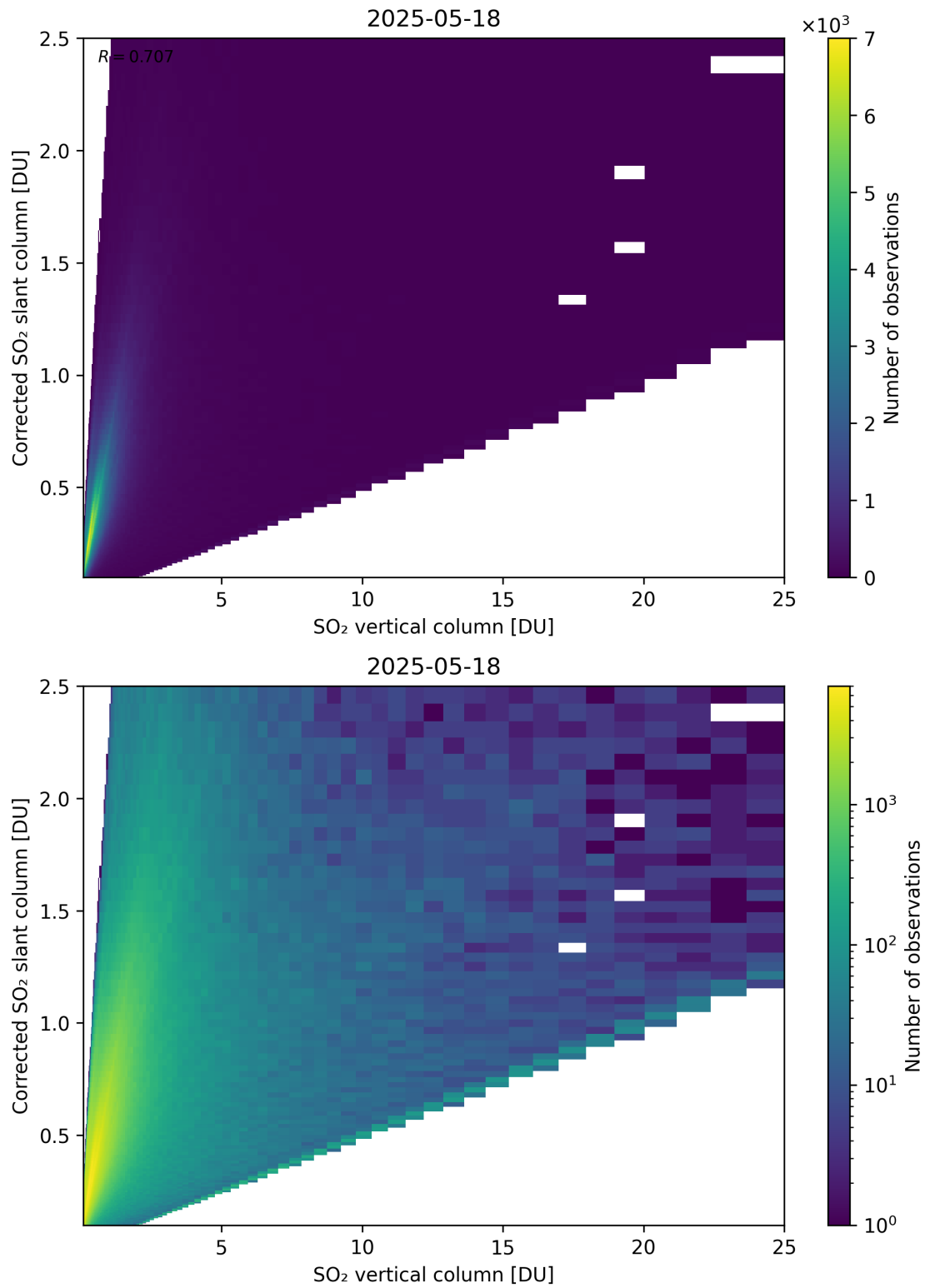
Figure 351: Scatter density plot of “SO 2 vertical column” against “Corrected SO 2 slant column” for 2025-05-17 to 2025-05-19.
