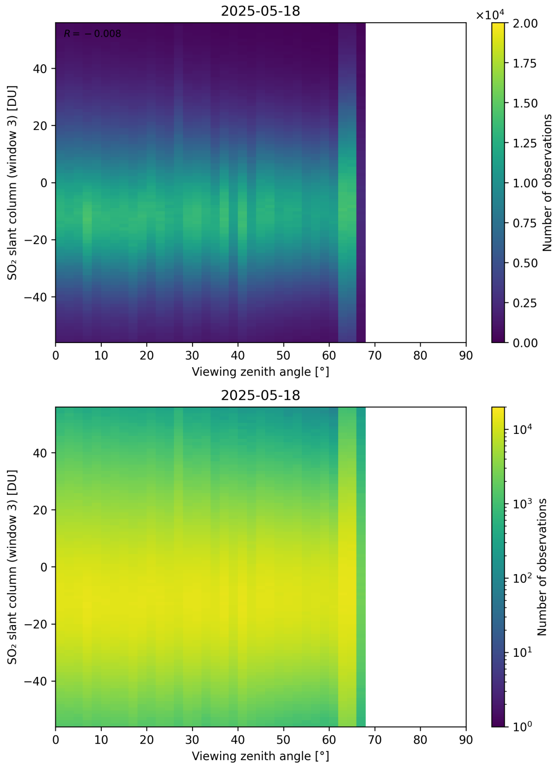
Figure 379: Scatter density plot of “Viewing zenith angle” against “SO 2 slant column (window 3)” for 2025-05-17 to 2025-05-19.
