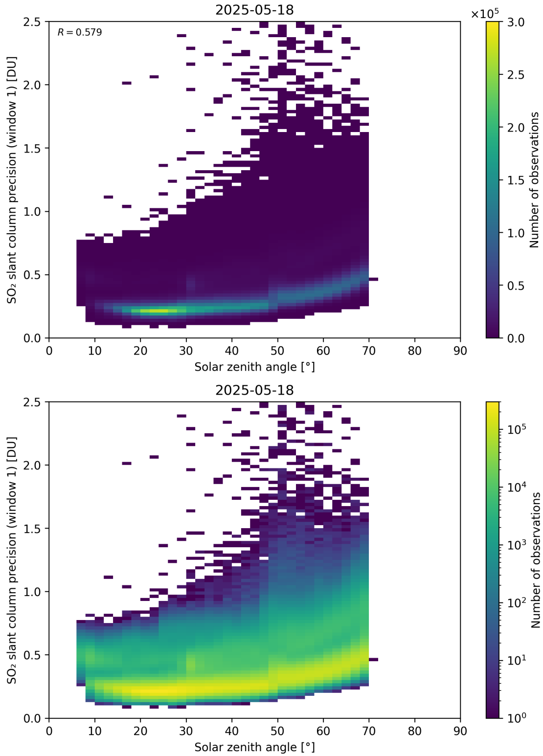
Figure 185: Scatter density plot of “Solar zenith angle” against “SO 2 slant column precision (window 1)” for 2025-05-17 to 2025-05-19.
