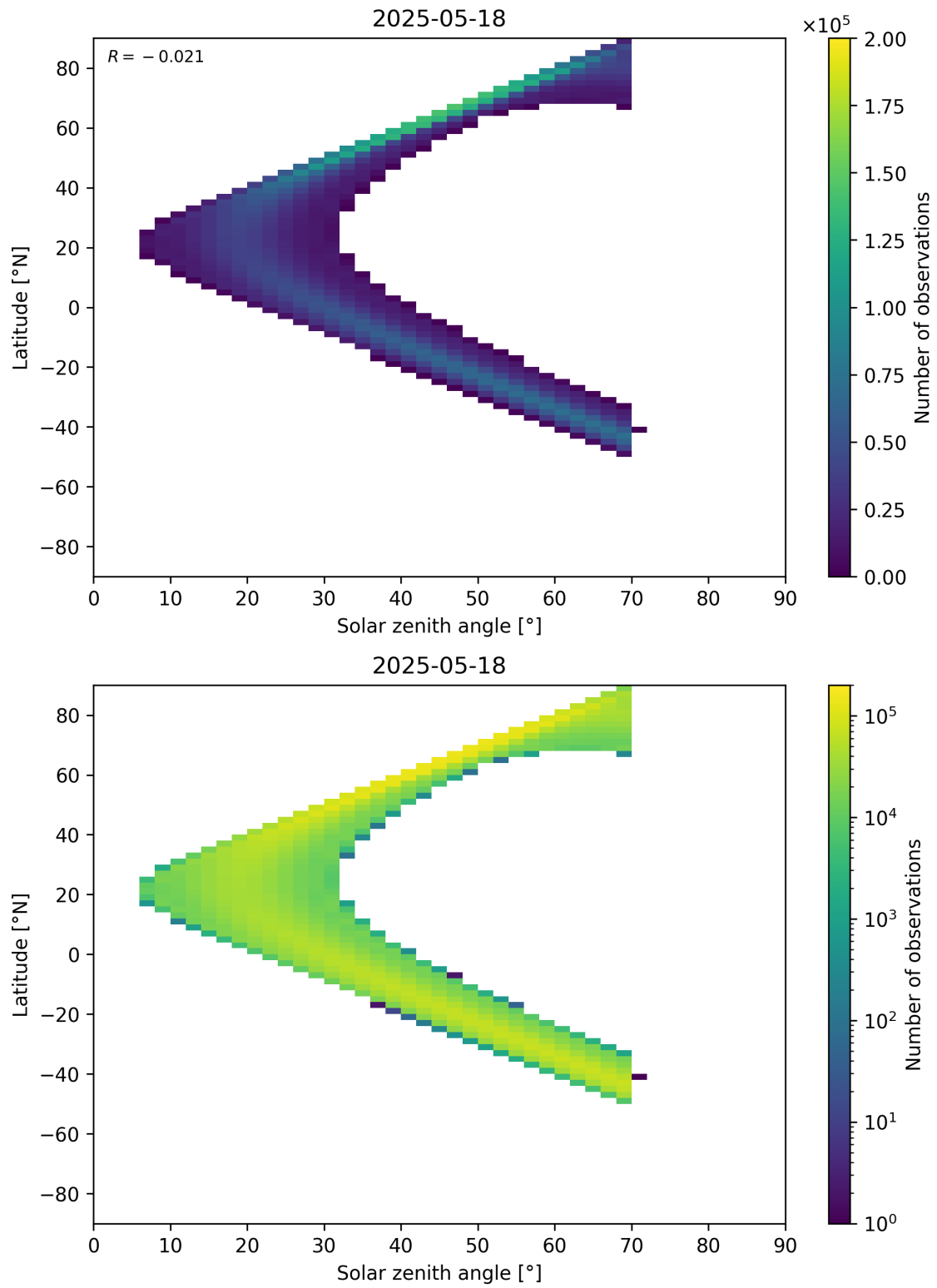
Figure 177: Scatter density plot of “Solar zenith angle” against “Latitude” for 2025-05-17 to 2025-05-19.
