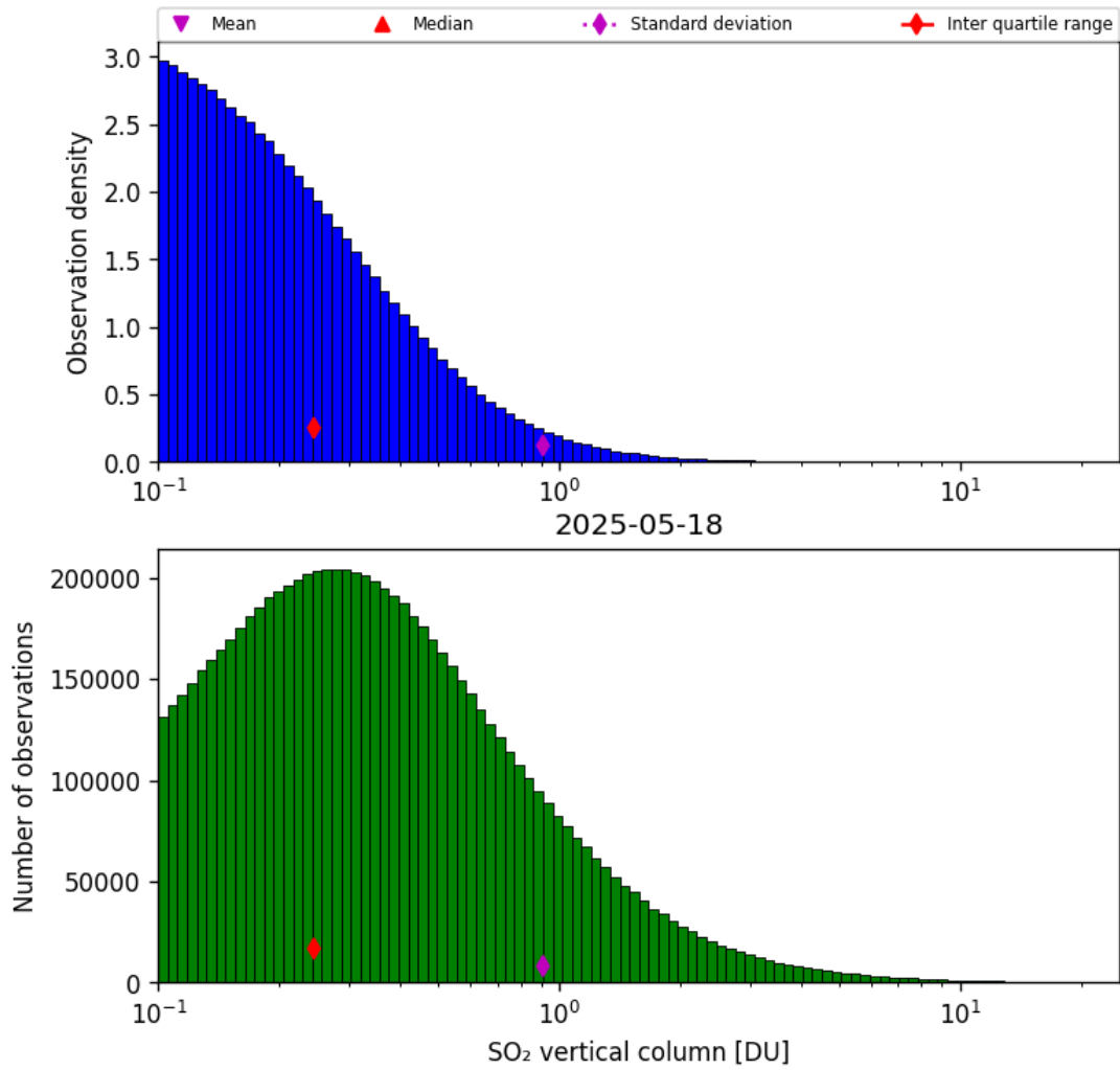
Figure 58: Histogram of “SO 2 vertical column” for 2025-05-17 to 2025-05-19
