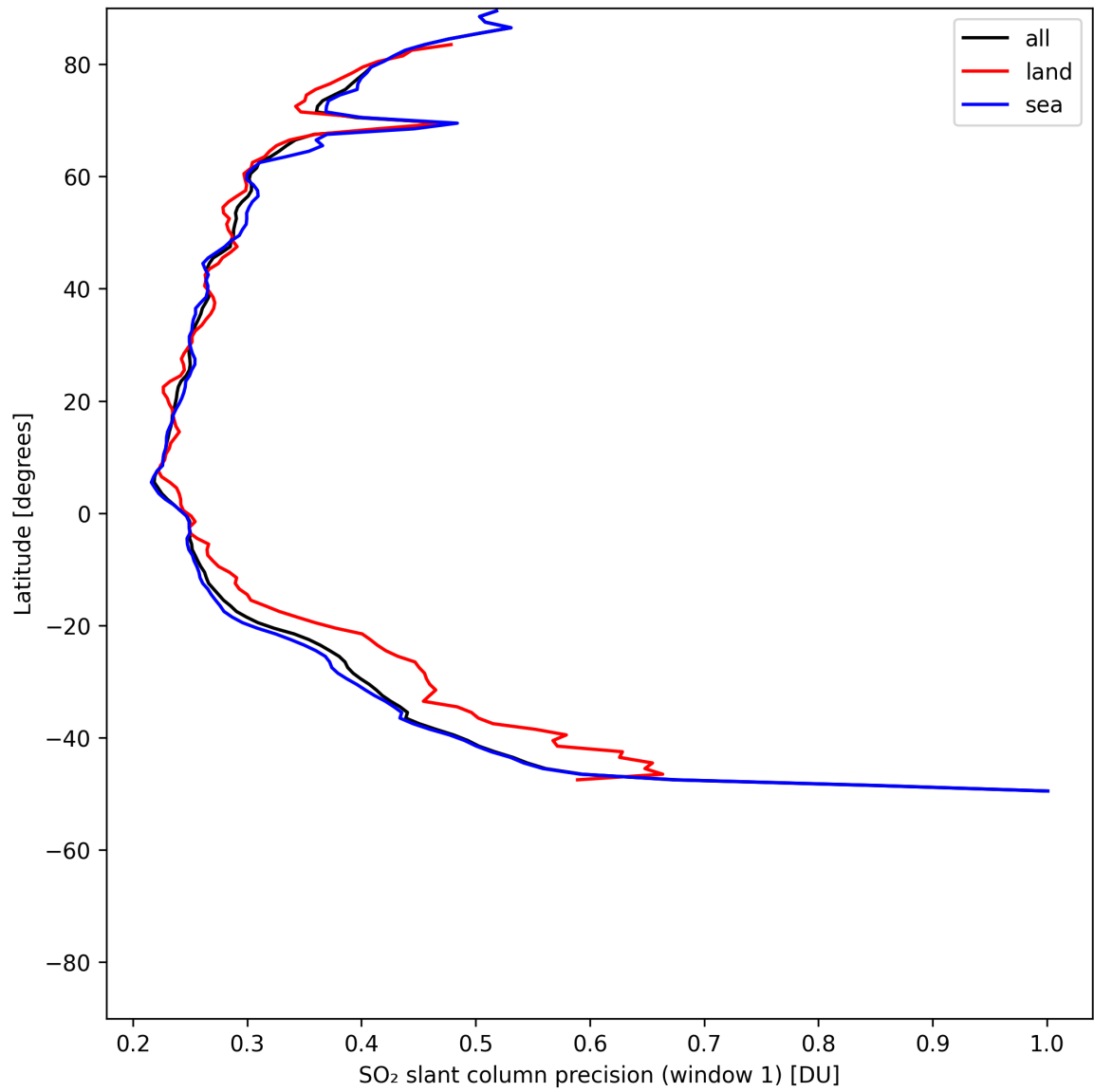
Figure 38: Zonal average of “SO 2 slant column precision (window 1)” for 2025-05-17 to 2025-05-19.
