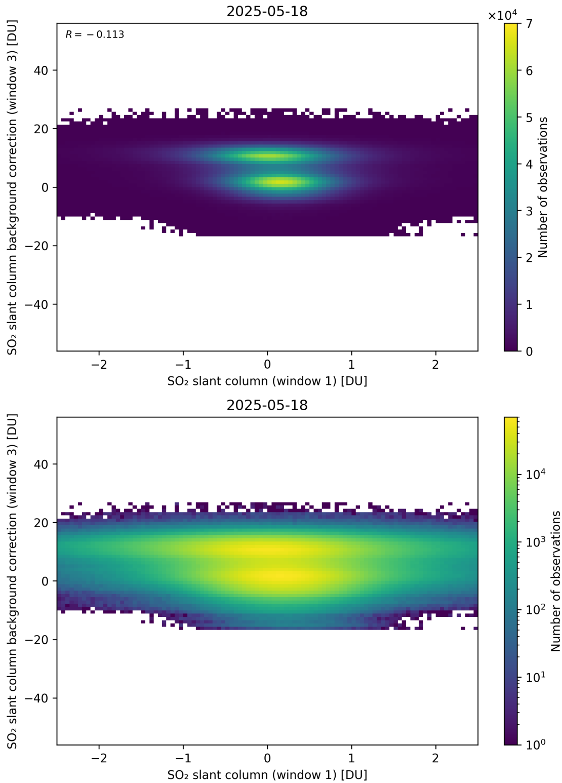
Figure 264: Scatter density plot of “SO 2 slant column (window 1)” against “SO 2 slant column background correction (window 3)” for 2025-05-17 to 2025-05-19.
