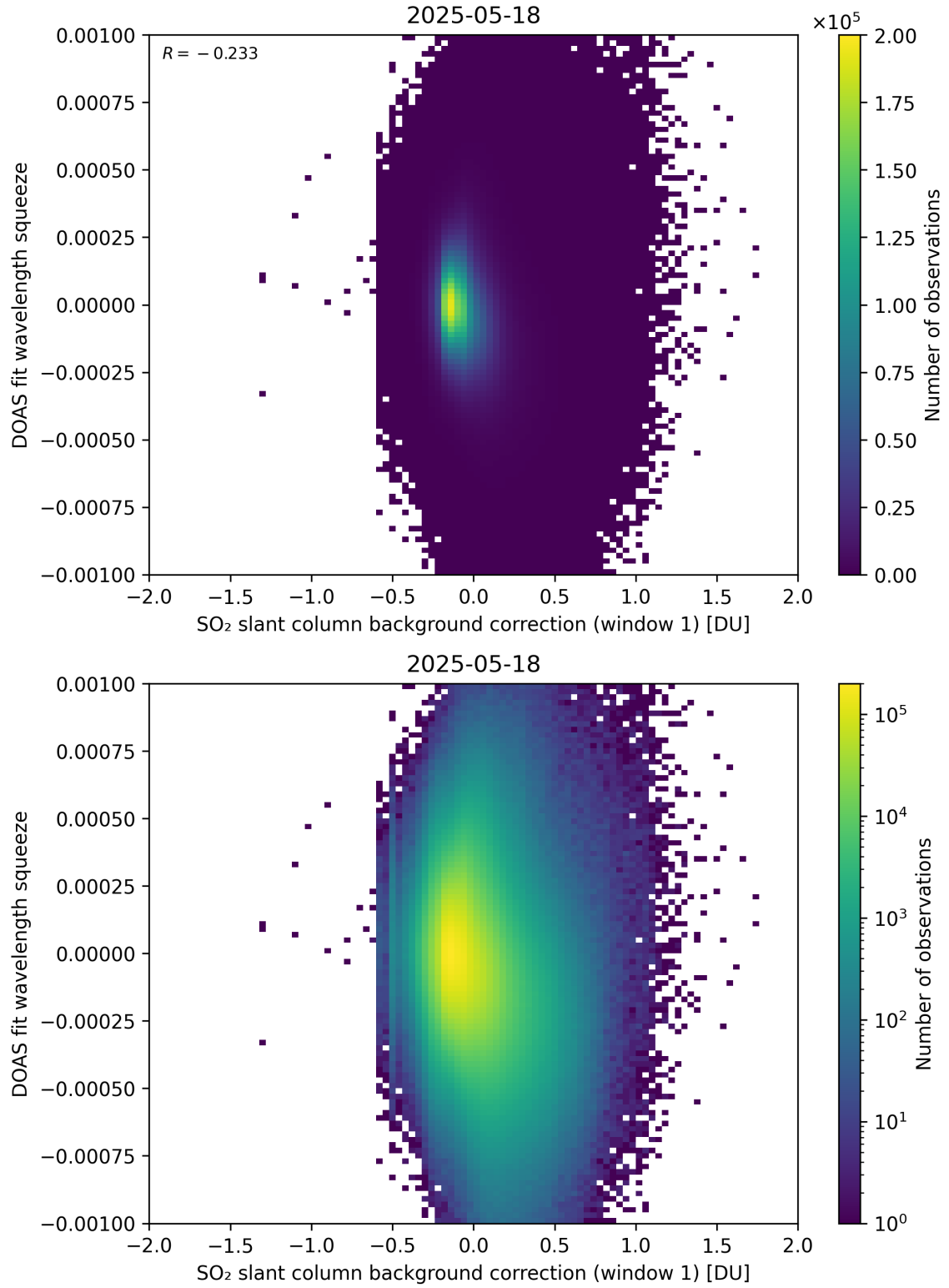
Figure 112: Scatter density plot of “SO 2 slant column background correction (window 1)” against “DOAS fit wavelength squeeze” for 2025-05-17 to 2025-05-19.
