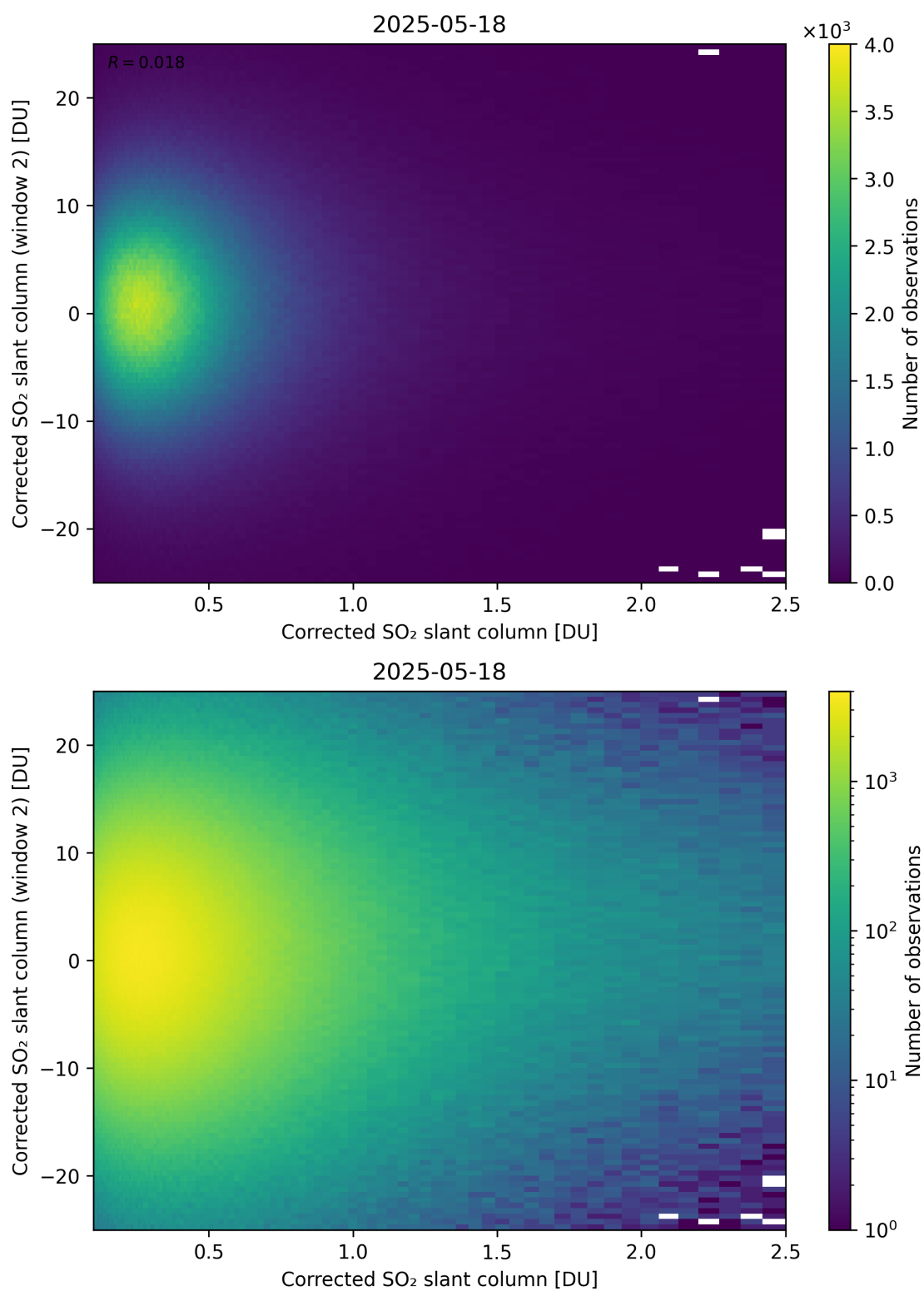
Figure 235: Scatter density plot of “Corrected SO 2 slant column” against “Corrected SO 2 slant column (window 2)” for 2025-05-17 to 2025-05-19.
