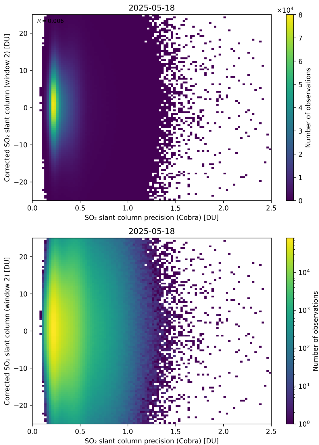
Figure 206: Scatter density plot of “SO 2 slant column precision (Cobra)” against “Corrected SO 2 slant column (window 2)” for 2025-05-17 to 2025-05-19.
