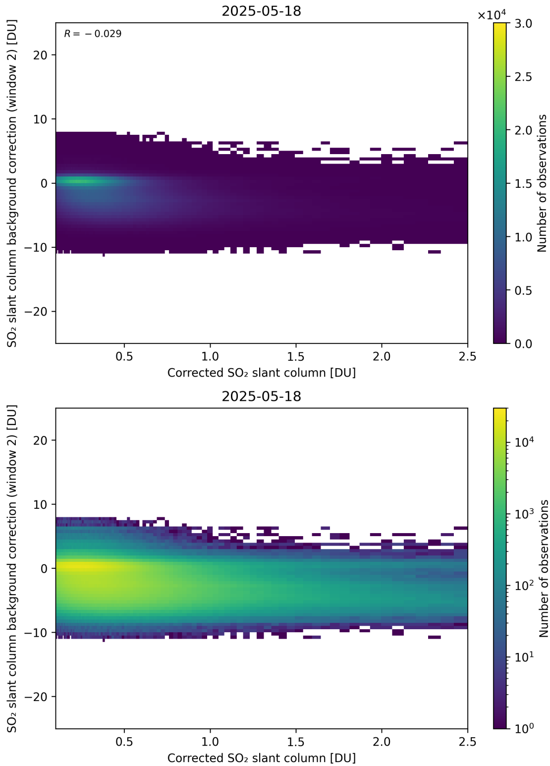
Figure 227: Scatter density plot of “Corrected SO 2 slant column” against “SO 2 slant column background correction (window 2)” for 2025-05-17 to 2025-05-19.
