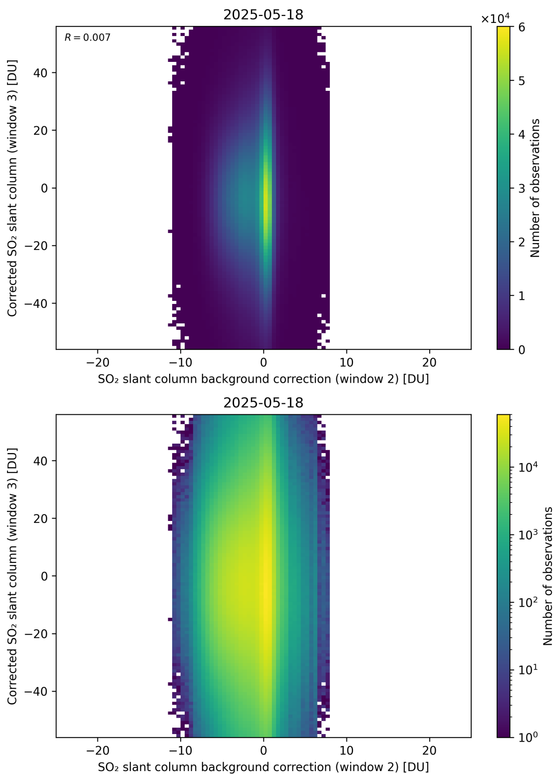
Figure 127: Scatter density plot of “SO 2 slant column background correction (window 2)” against “Corrected SO 2 slant column (window 3)” for 2025-05-17 to 2025-05-19.
