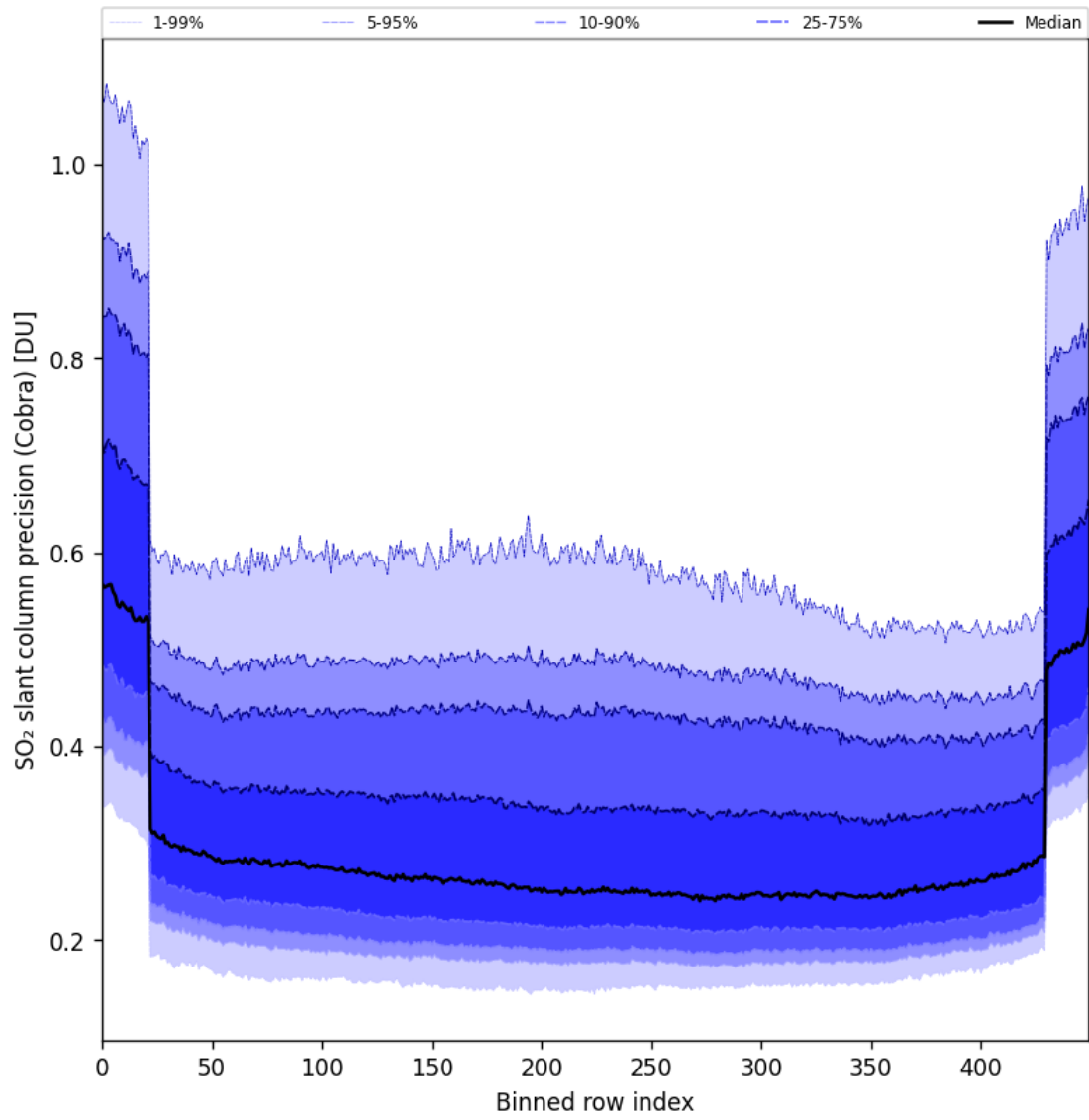
Figure 88: Along track statistics of “SO 2 slant column precision (Cobra)” for 2025-05-17 to 2025-05-19
