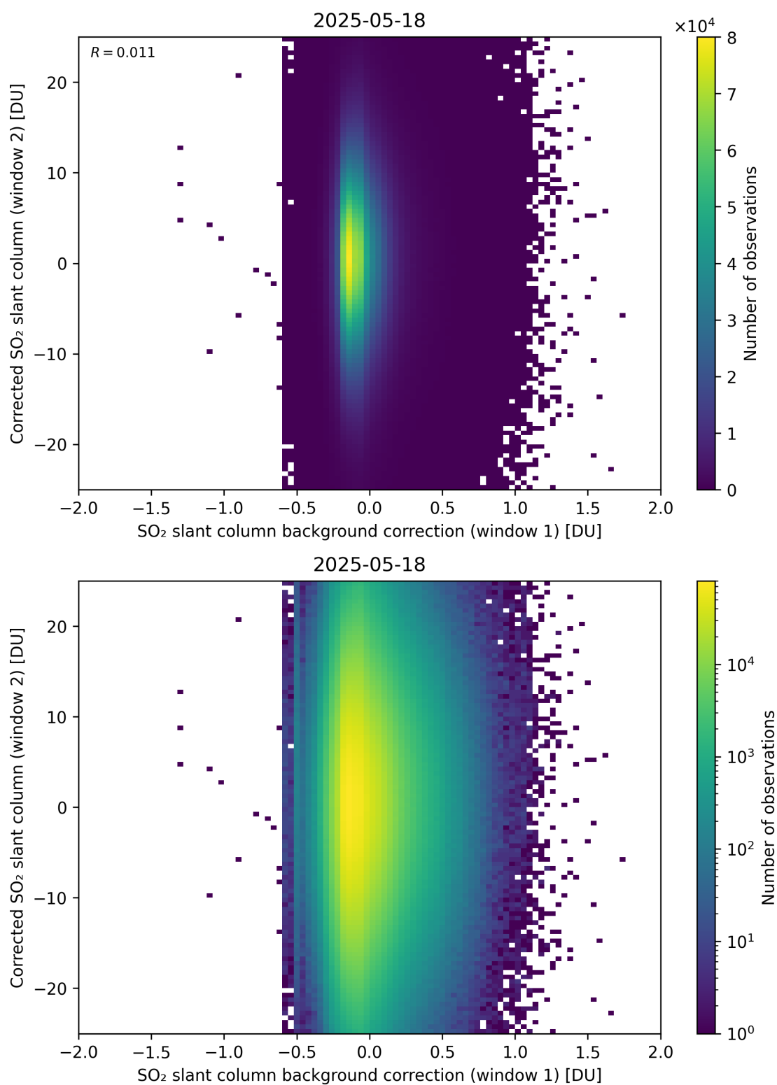
Figure 115: Scatter density plot of “SO 2 slant column background correction (window 1)” against “Corrected SO 2 slant column (window 2)” for 2025-05-17 to 2025-05-19.
