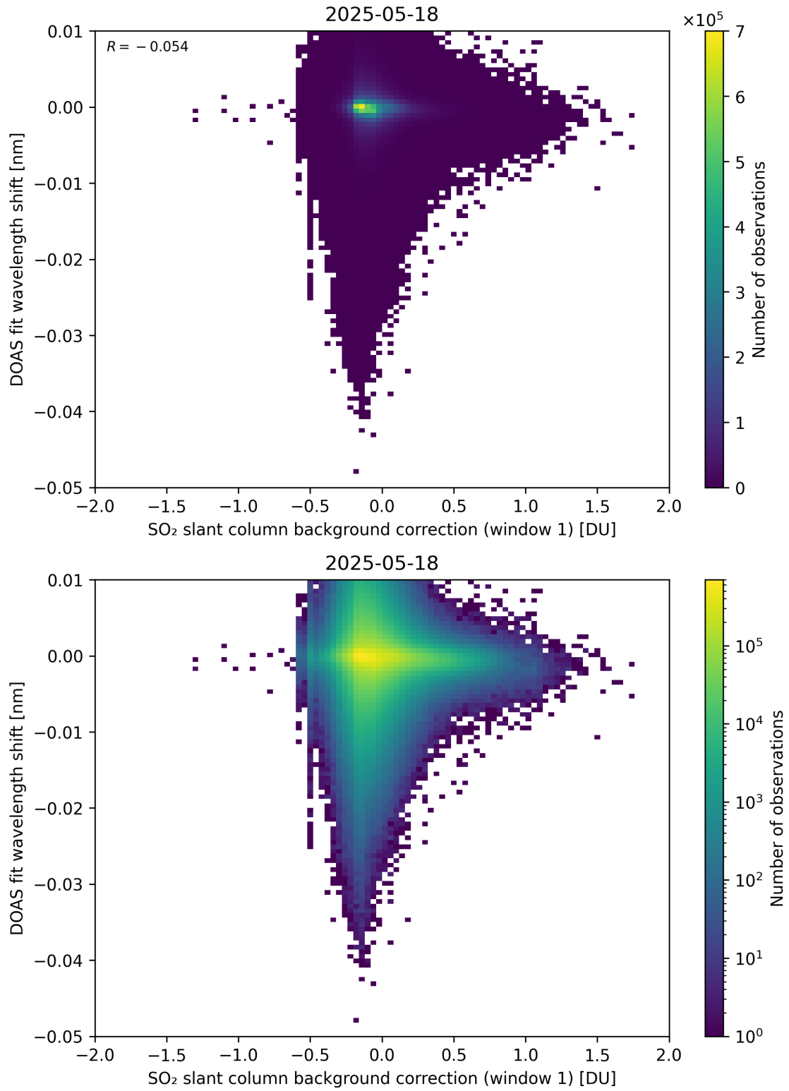
Figure 111: Scatter density plot of “SO 2 slant column background correction (window 1)” against “DOAS fit wavelength shift” for 2025-05-17 to 2025-05-19.
