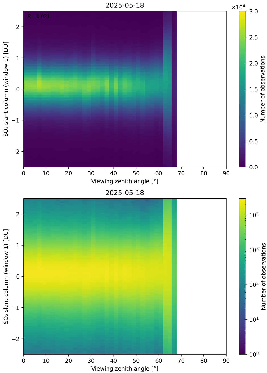
Figure 376: Scatter density plot of “Viewing zenith angle” against “SO 2 slant column (window 1)” for 2025-05-17 to 2025-05-19.
