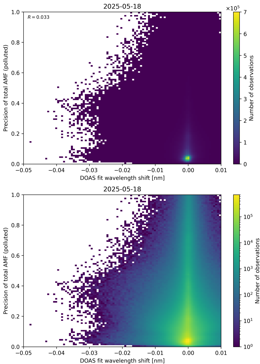
Figure 142: Scatter density plot of “DOAS fit wavelength shift” against “Precision of total AMF (polluted)” for 2025-05-17 to 2025-05-19.
