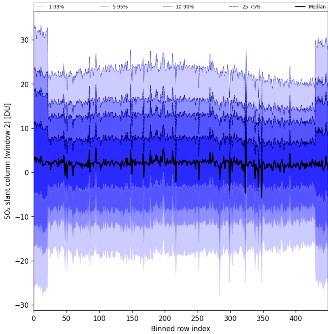
Figure 93: Along track statistics of “SO 2 slant column (window 2)” for 2025-05-17 to 2025-05-19
