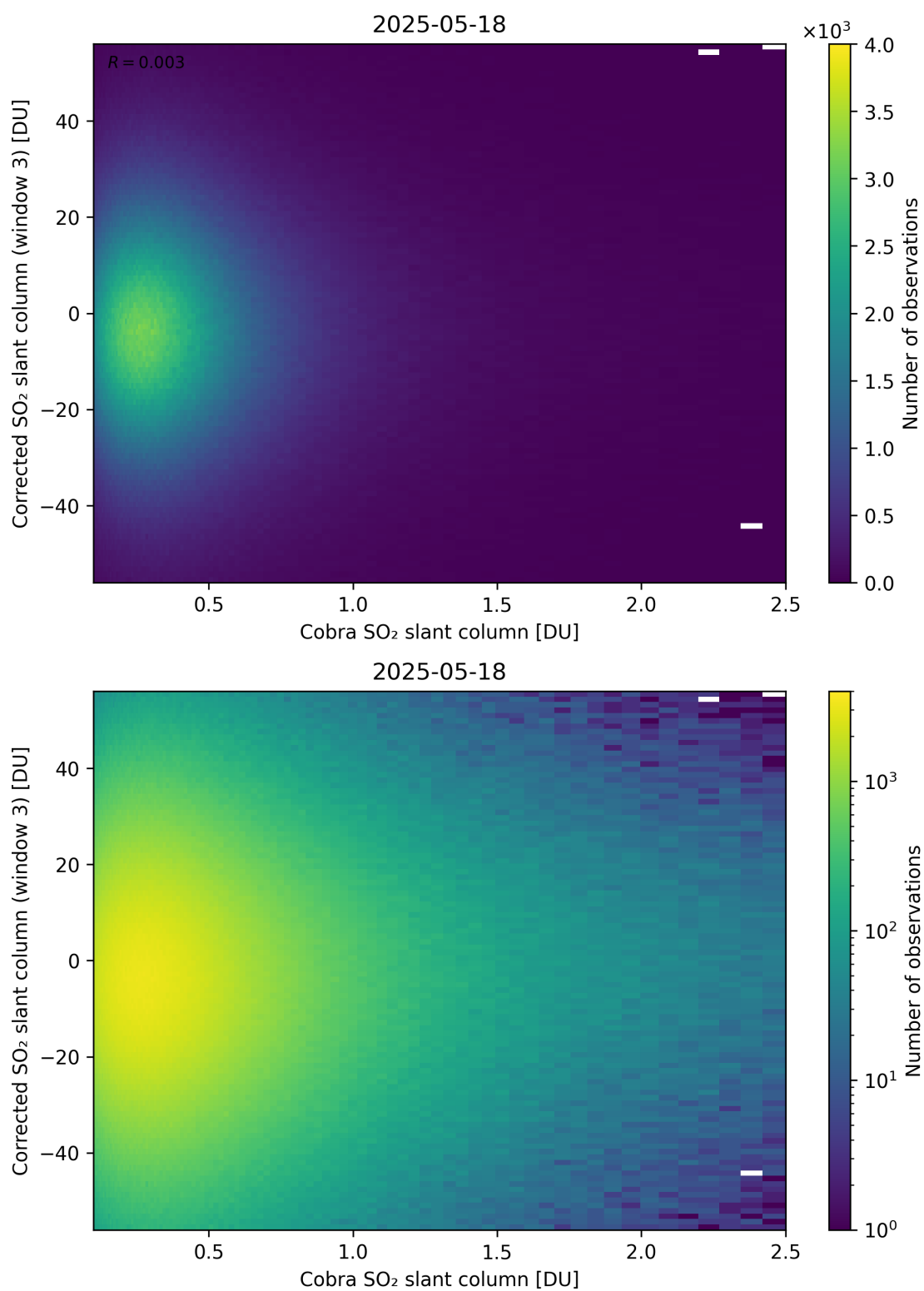
Figure 218: Scatter density plot of “Cobra SO 2 slant column” against “Corrected SO 2 slant column (window 3)” for 2025-05-17 to 2025-05-19.
