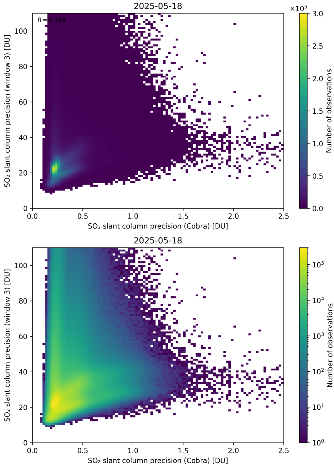
Figure 212: Scatter density plot of “SO 2 slant column precision (Cobra)” against “SO 2 slant column precision (window 3)” for 2025-05-17 to 2025-05-19.
