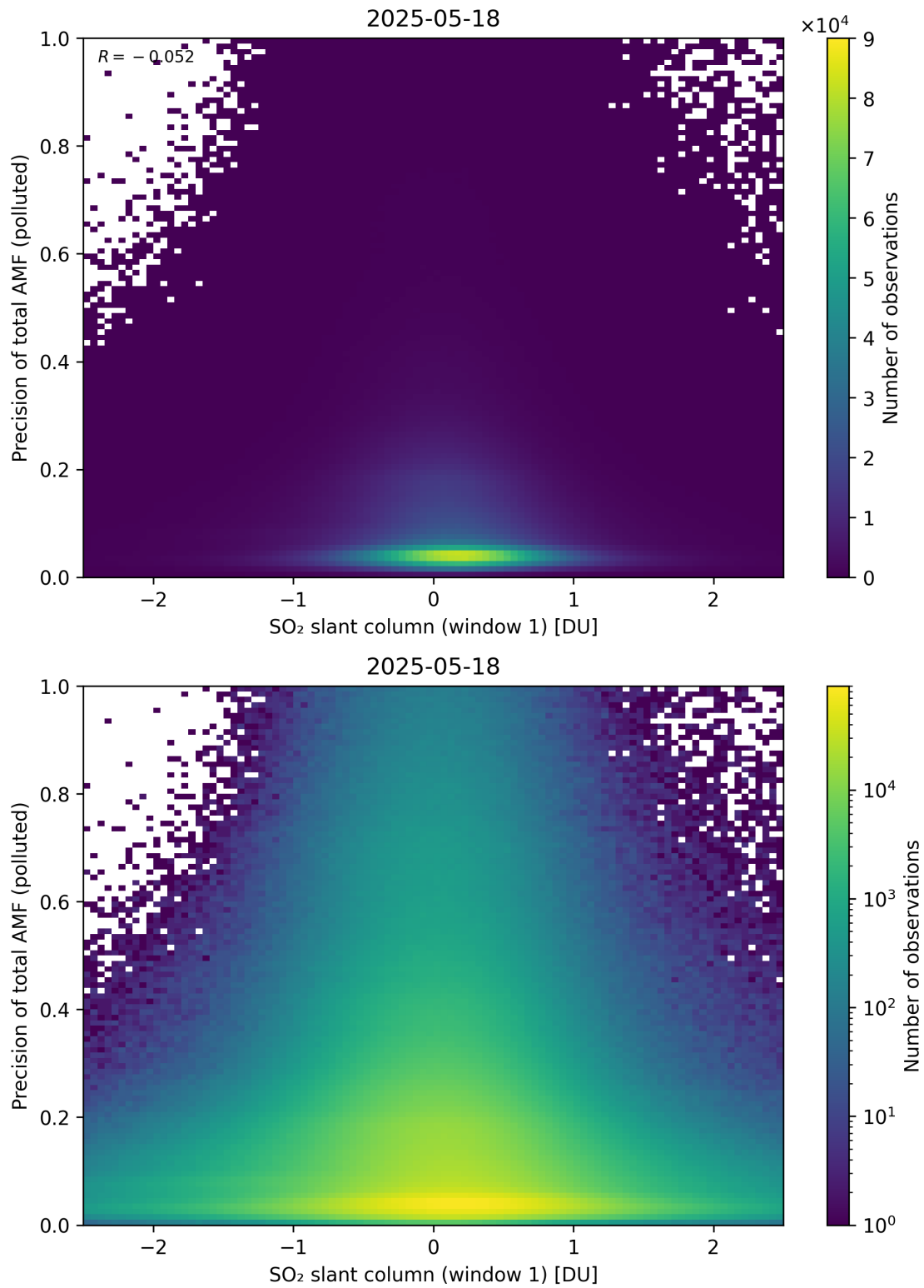
Figure 290: Scatter density plot of “SO 2 slant column (window 1)” against “Precision of total AMF (polluted)” for 2025-05-17 to 2025-05-19.
