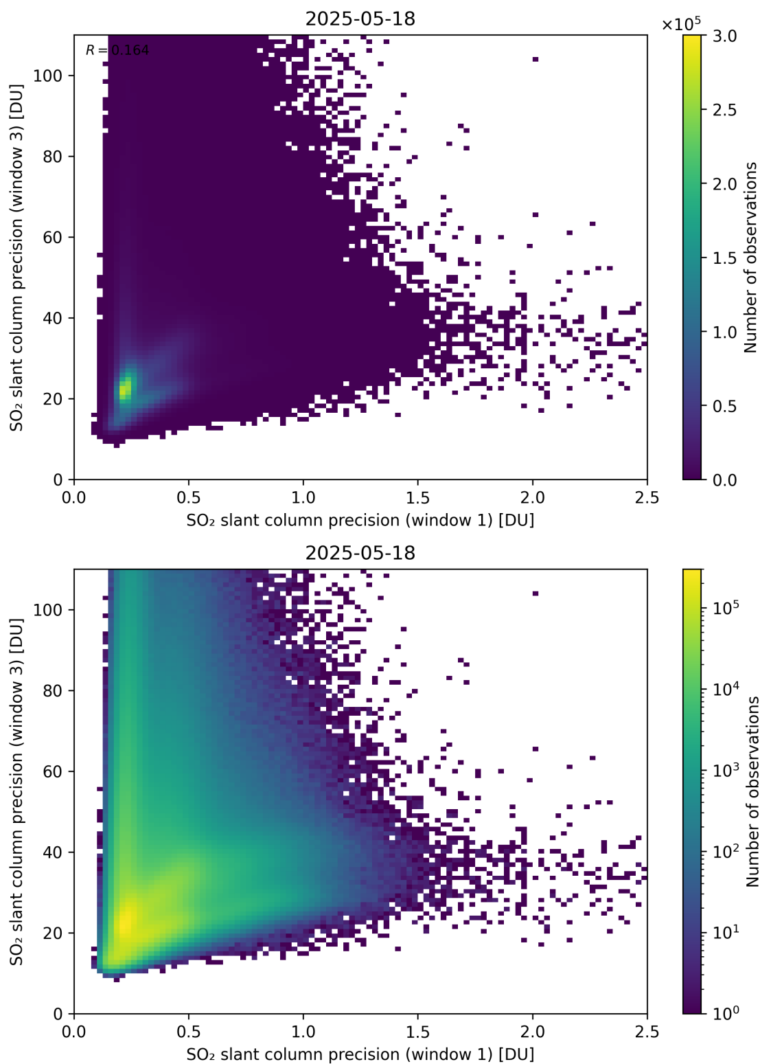
Figure 279: Scatter density plot of “SO 2 slant column precision (window 1)” against “SO 2 slant column precision (window 3)” for 2025-05-17 to 2025-05-19.
