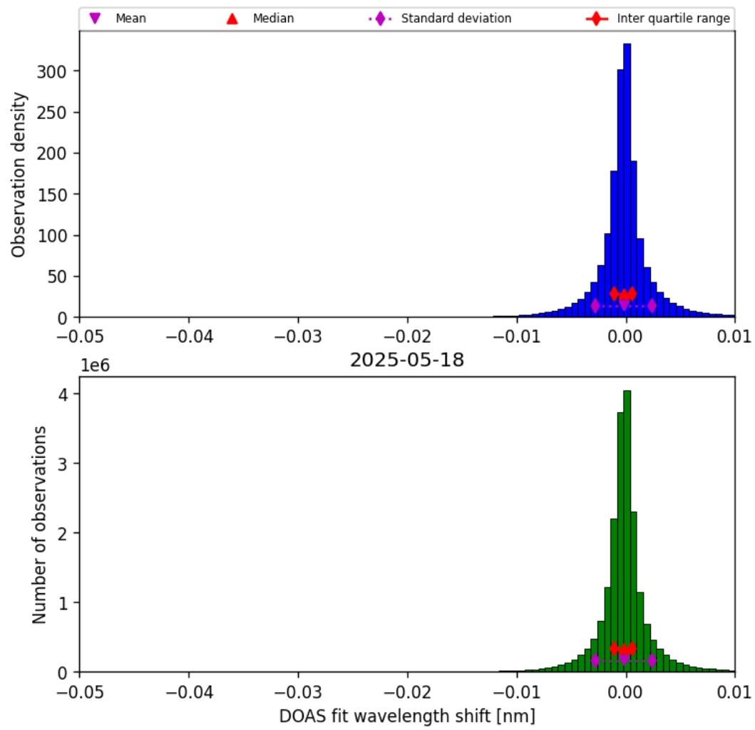
Figure 76: Histogram of “DOAS fit wavelength shift” for 2025-05-17 to 2025-05-19
