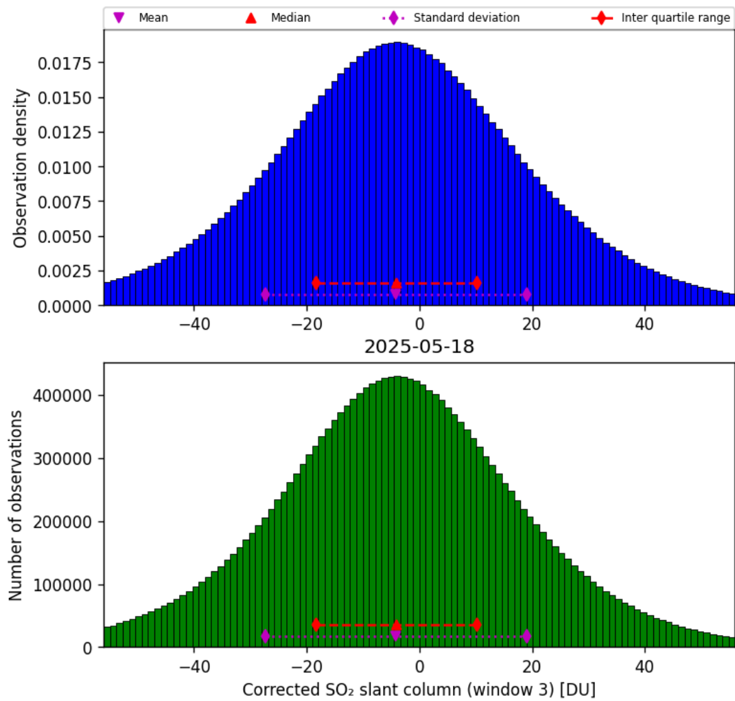
Figure 73: Histogram of “Corrected SO 2 slant column (window 3)” for 2025-05-17 to 2025-05-19
