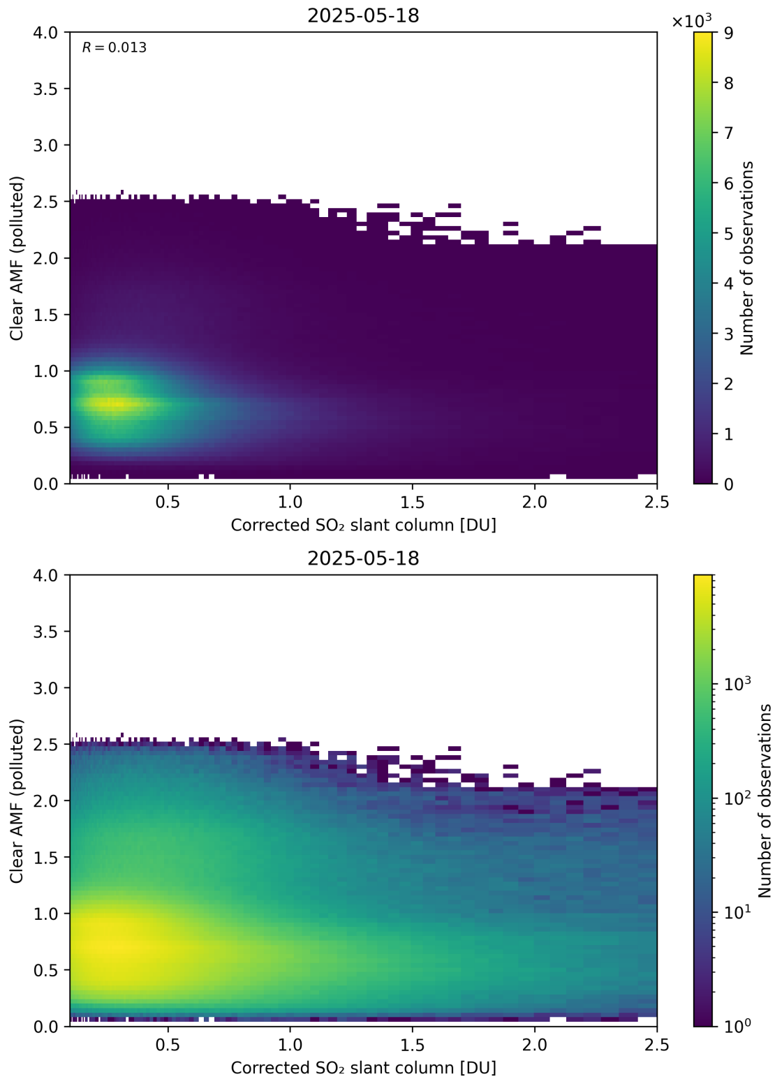
Figure 232: Scatter density plot of “Corrected SO 2 slant column” against “Clear AMF (polluted)” for 2025-05-17 to 2025-05-19.
