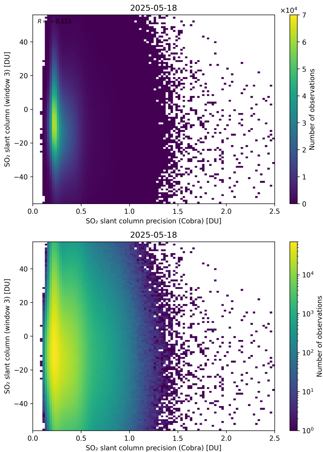
Figure 211: Scatter density plot of “SO 2 slant column precision (Cobra)” against “SO 2 slant column (window 3)” for 2025-05-17 to 2025-05-19.
