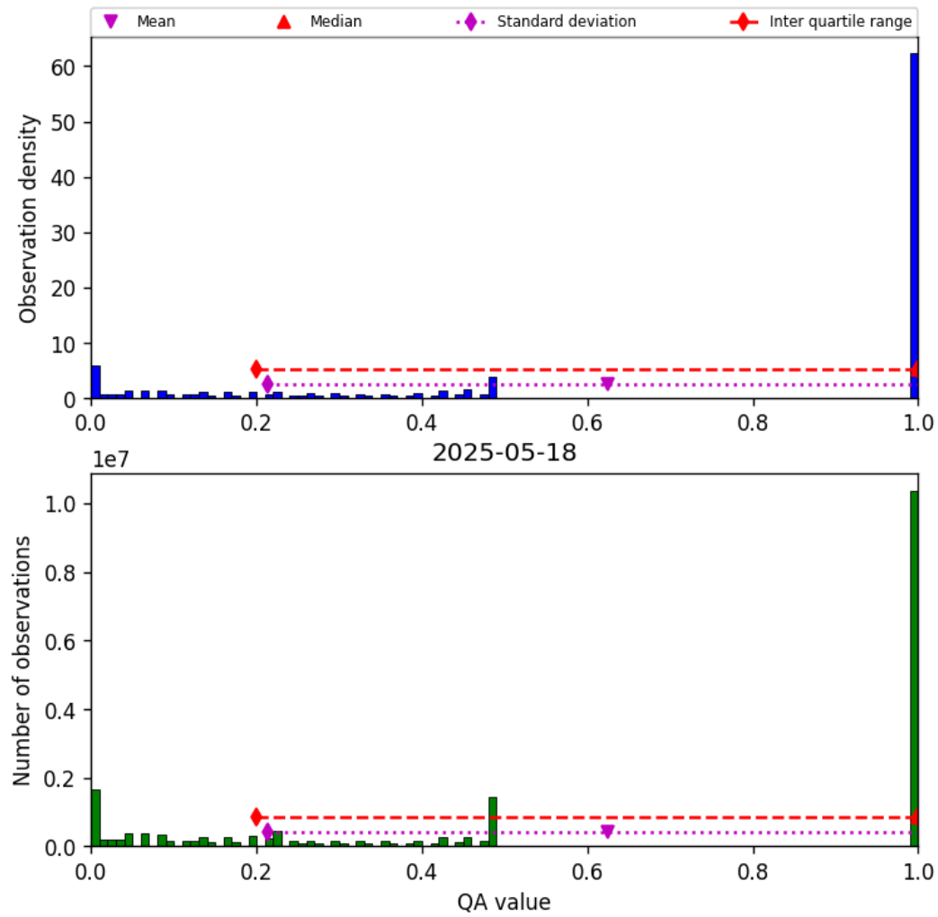
Figure 57: Histogram of “QA value” for 2025-05-17 to 2025-05-19
