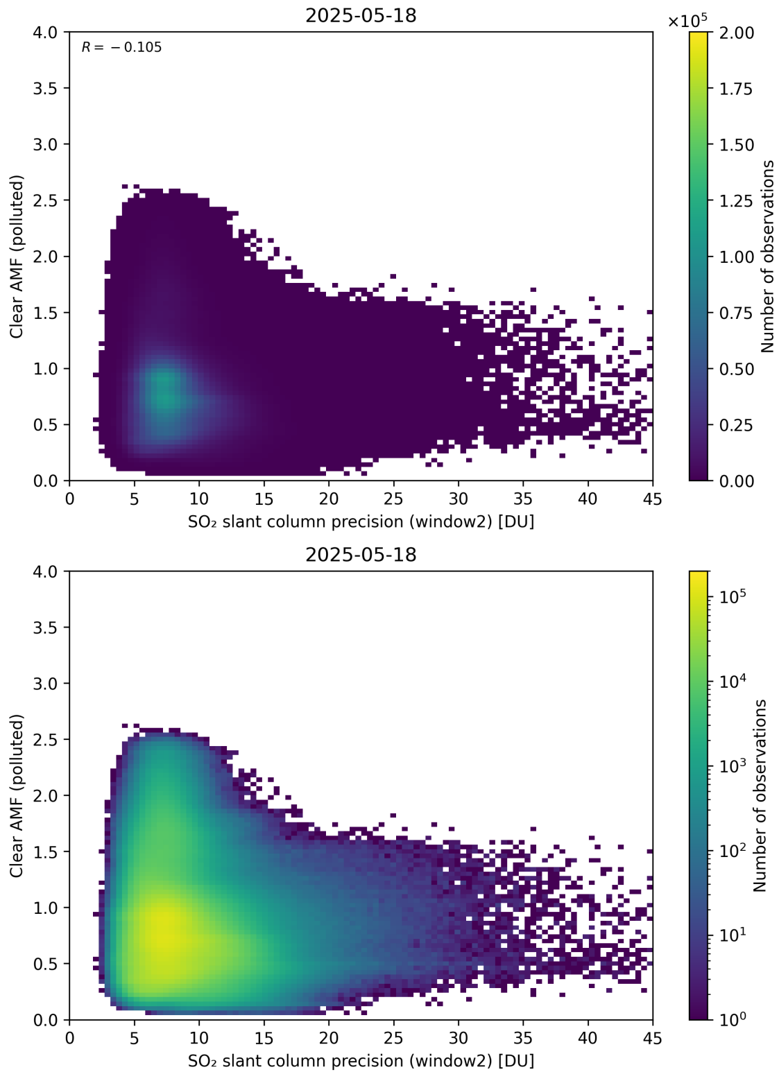
Figure 296: Scatter density plot of “SO 2 slant column precision (window2)” against “Clear AMF (polluted)” for 2025-05-17 to 2025-05-19.
