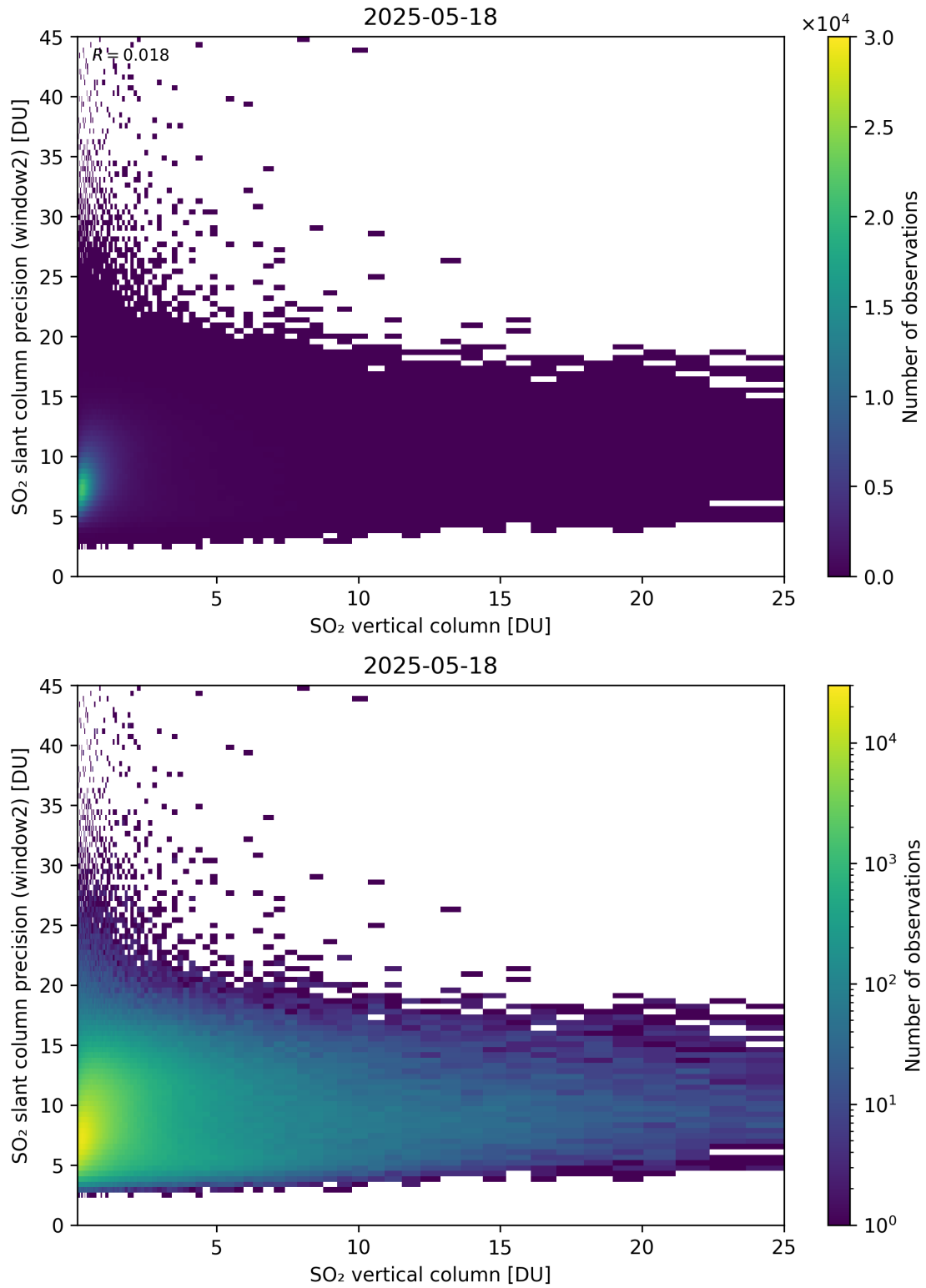
Figure 356: Scatter density plot of “SO 2 vertical column” against “SO 2 slant column precision (window2)” for 2025-05-17 to 2025-05-19.
