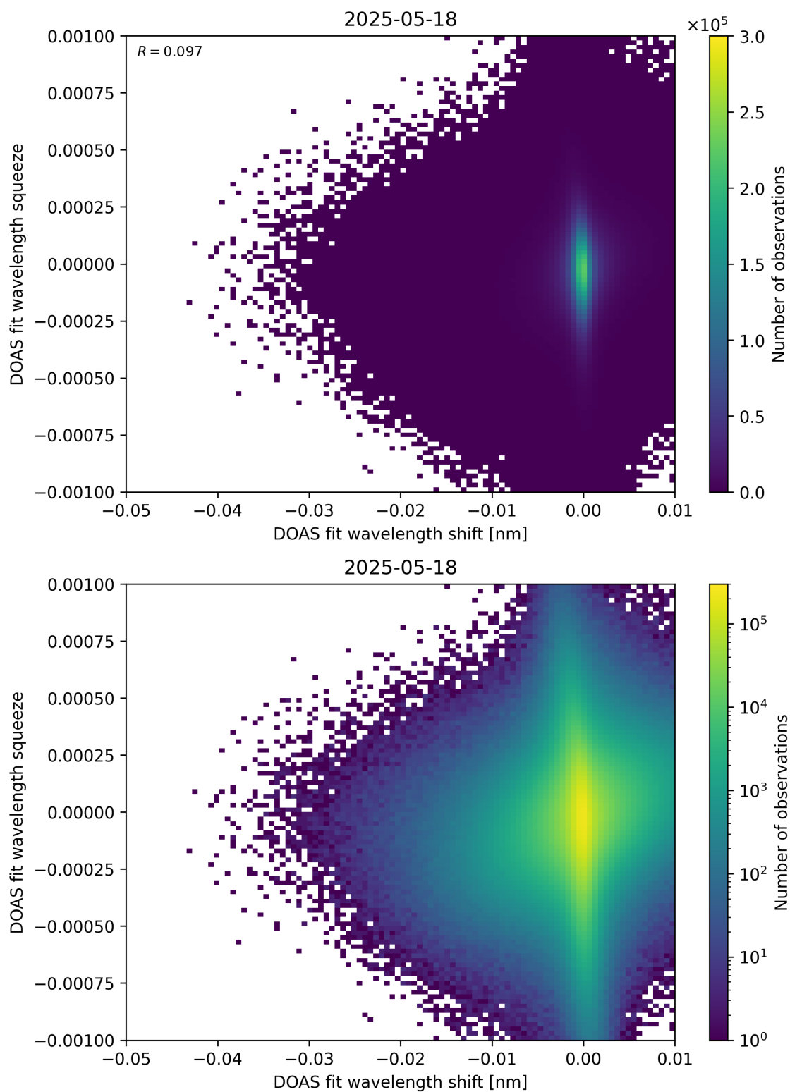
Figure 138: Scatter density plot of “DOAS fit wavelength shift” against “DOAS fit wavelength squeeze” for 2025-05-17 to 2025-05-19.
