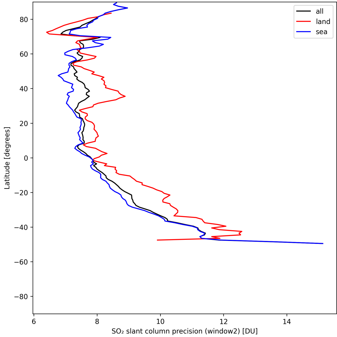
Figure 42: Zonal average of “SO 2 slant column precision (window2)” for 2025-05-17 to 2025-05-19.
