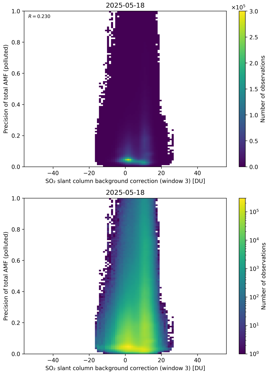
Figure 137: Scatter density plot of “SO 2 slant column background correction (window 3)” against “Precision of total AMF (polluted)” for 2025-05-17 to 2025-05-19.
