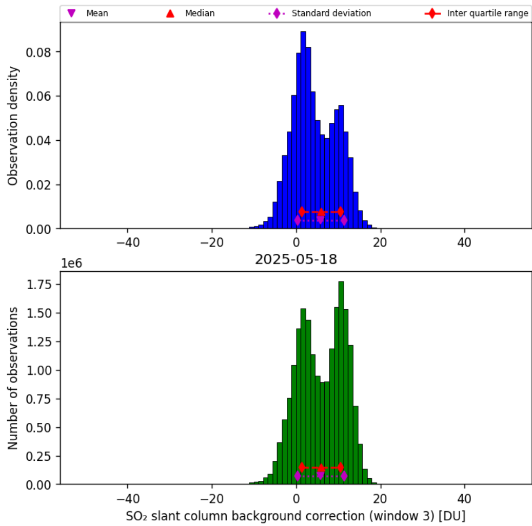
Figure 74: Histogram of “SO 2 slant column background correction (window 3)” for 2025-05-17 to 2025-05-19
