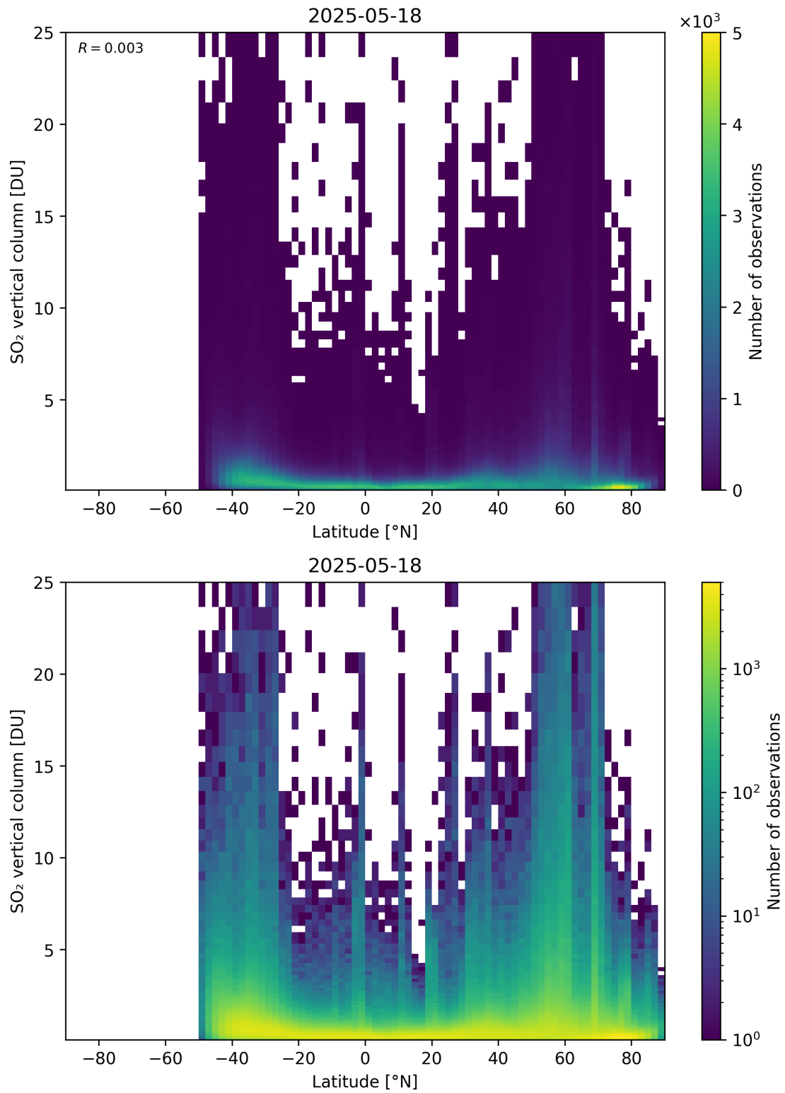
Figure 169: Scatter density plot of “Latitude” against “SO 2 vertical column” for 2025-05-17 to 2025-05-19.
