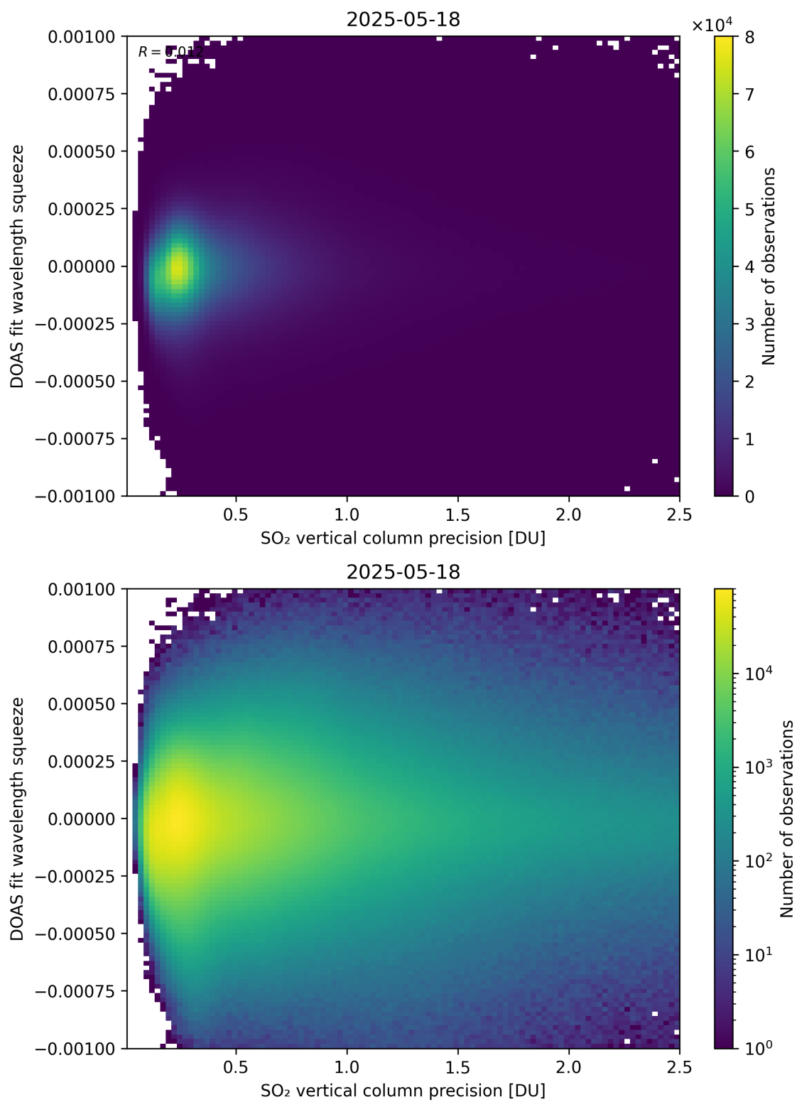
Figure 333: Scatter density plot of “SO 2 vertical column precision” against “DOAS fit wavelength squeeze” for 2025-05-17 to 2025-05-19.
