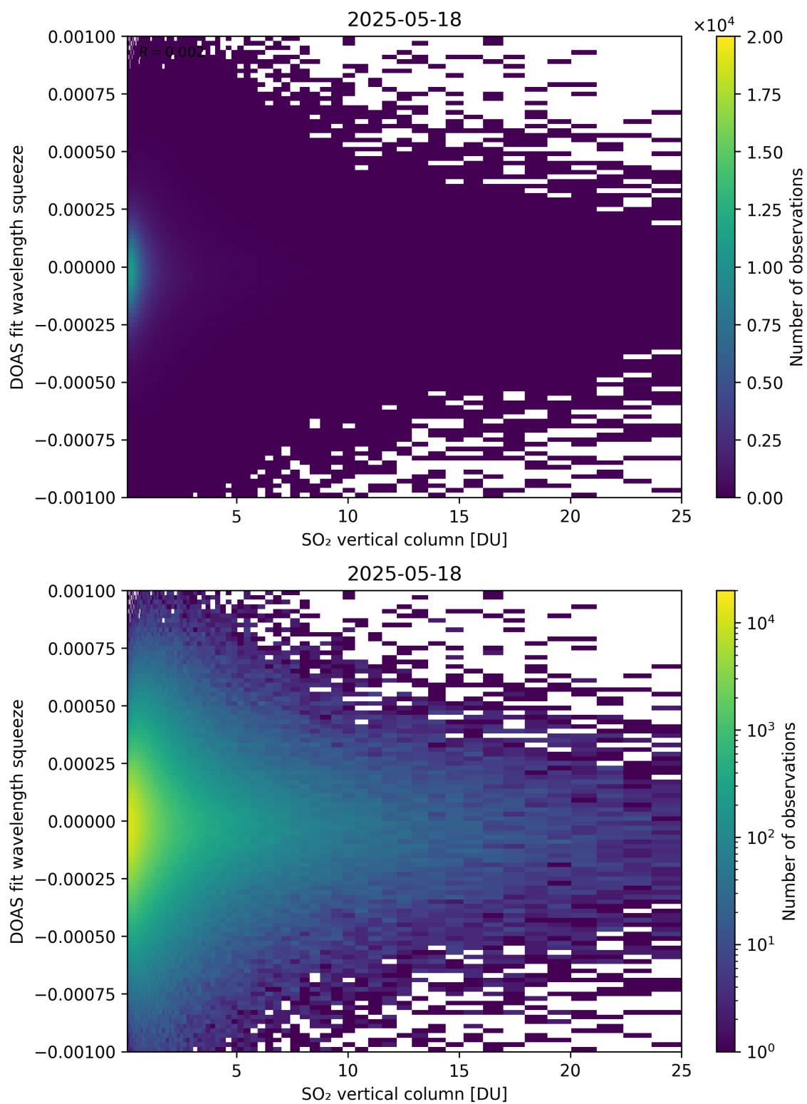
Figure 327: Scatter density plot of “SO 2 vertical column” against “DOAS fit wavelength squeeze” for 2025-05-17 to 2025-05-19.
