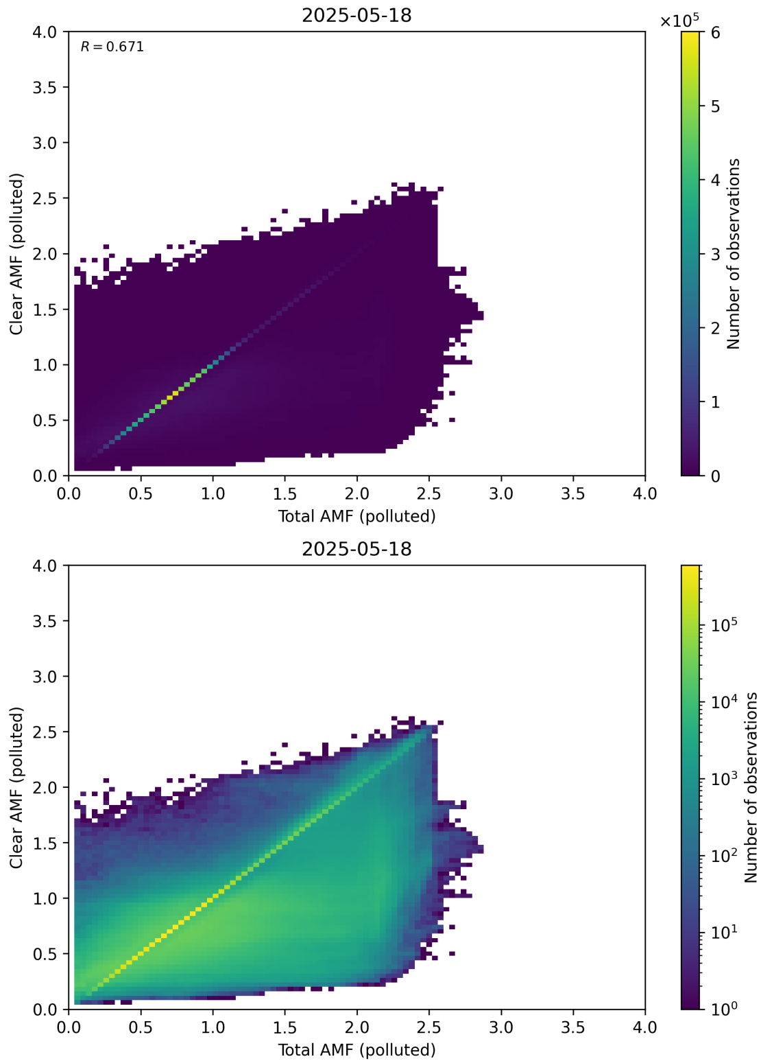
Figure 321: Scatter density plot of “Total AMF (polluted)” against “Clear AMF (polluted)” for 2025-05-17 to 2025-05-19.
