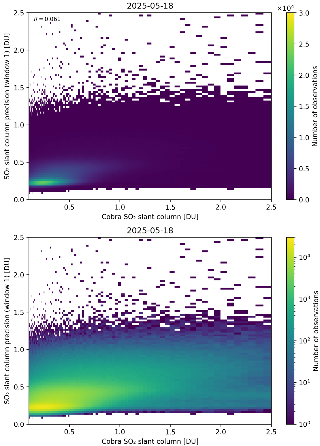
Figure 220: Scatter density plot of “Cobra SO 2 slant column” against “SO 2 slant column precision (window 1)” for 2025-05-17 to 2025-05-19.
