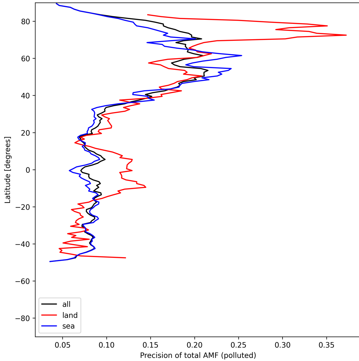
Figure 54: Zonal average of “Precision of total AMF (polluted)” for 2025-05-17 to 2025-05-19.
