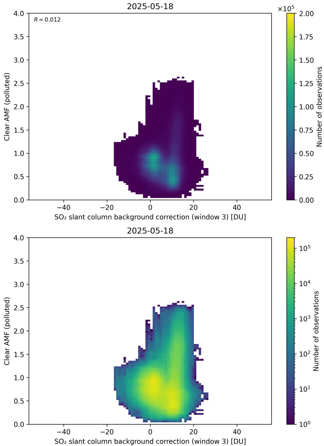
Figure 135: Scatter density plot of “SO 2 slant column background correction (window 3)” against “Clear AMF (polluted)” for 2025-05-17 to 2025-05-19.
