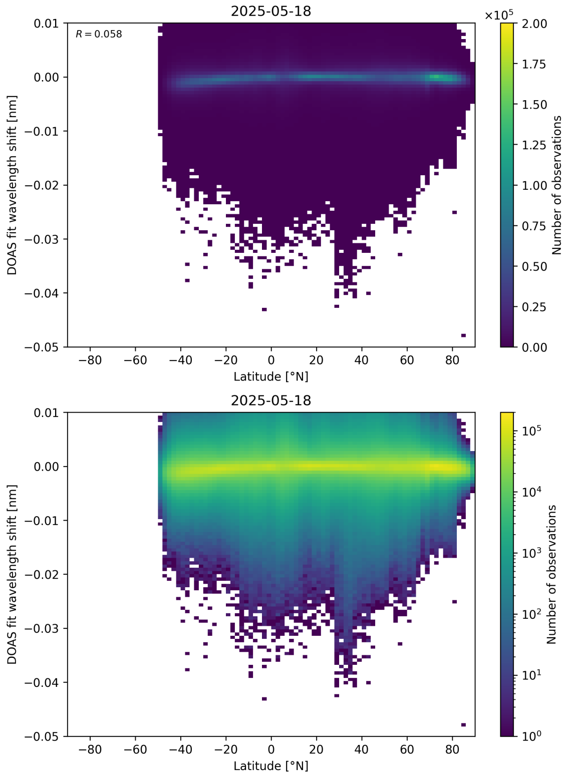
Figure 153: Scatter density plot of “Latitude” against “DOAS fit wavelength shift” for 2025-05-17 to 2025-05-19.
