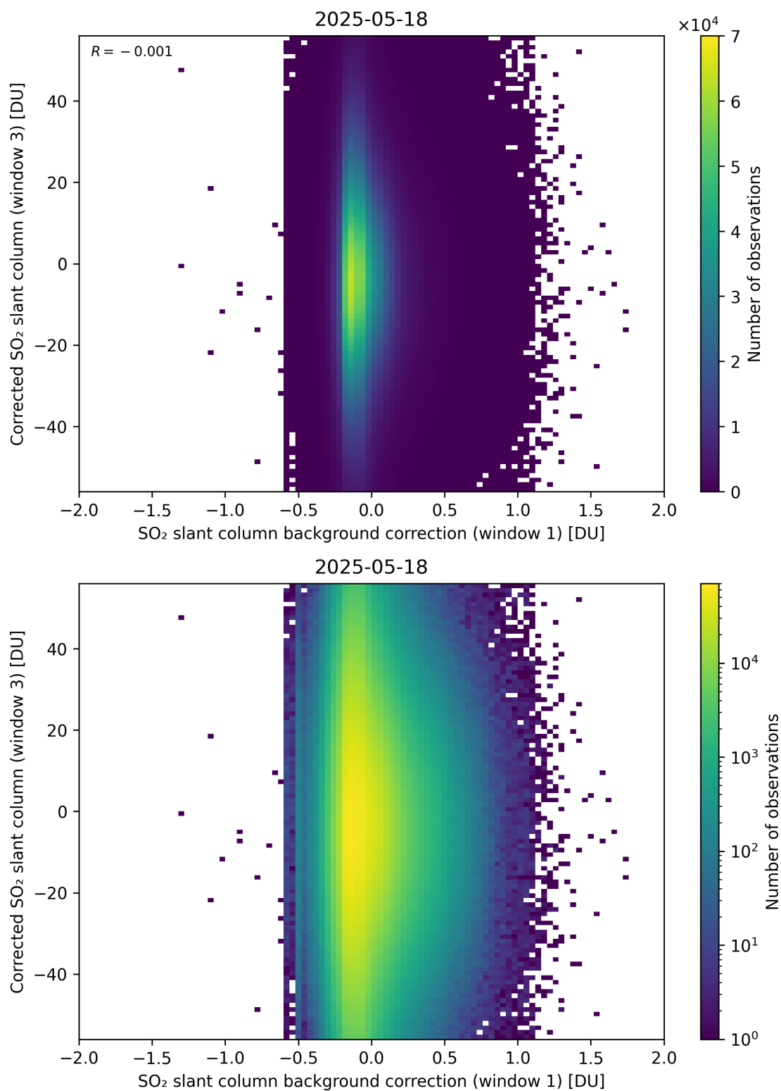
Figure 116: Scatter density plot of “SO 2 slant column background correction (window 1)” against “Corrected SO 2 slant column (window 3)” for 2025-05-17 to 2025-05-19.
