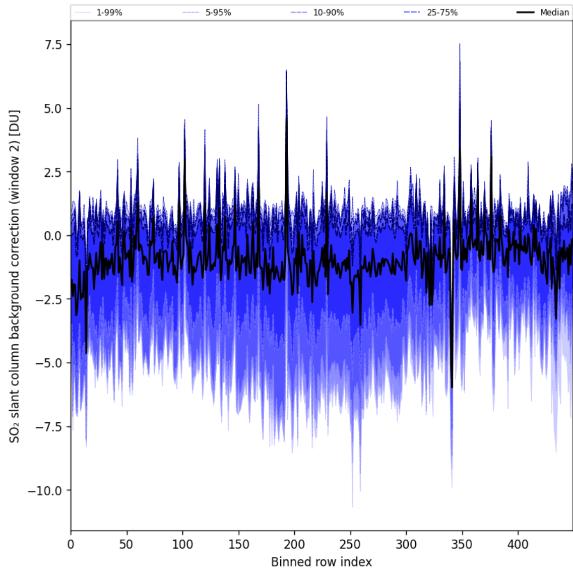
Figure 96: Along track statistics of “SO 2 slant column background correction (window 2)” for 2025-05-17 to 2025-05-19
