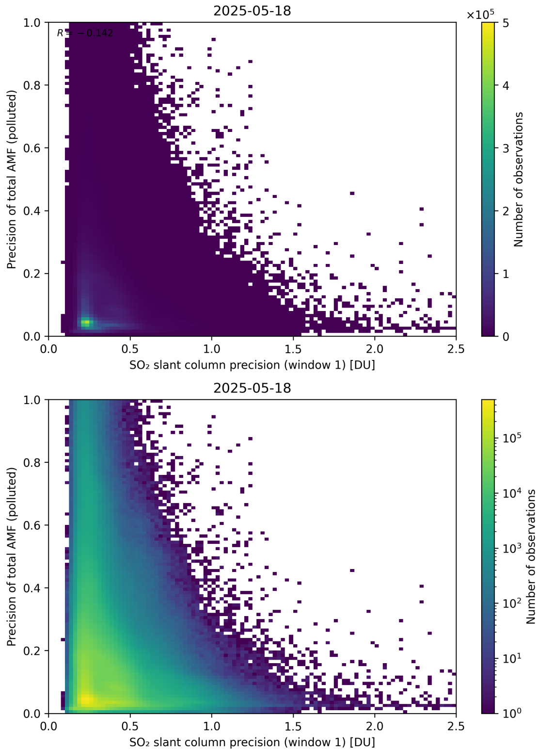
Figure 281: Scatter density plot of “SO 2 slant column precision (window 1)” against “Precision of total AMF (polluted)” for 2025-05-17 to 2025-05-19.
