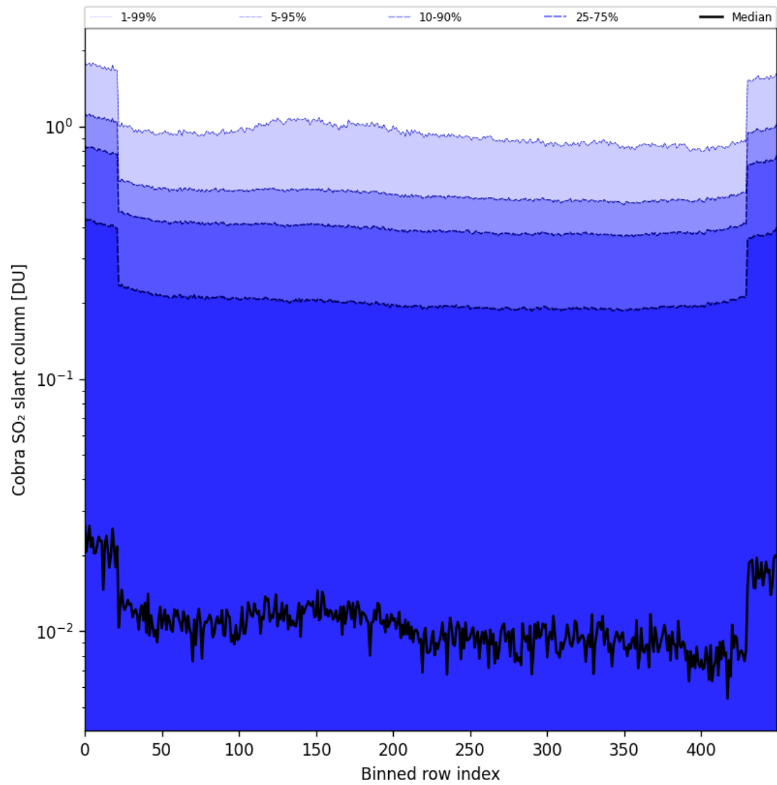
Figure 87: Along track statistics of “Cobra SO 2 slant column” for 2025-05-17 to 2025-05-19
