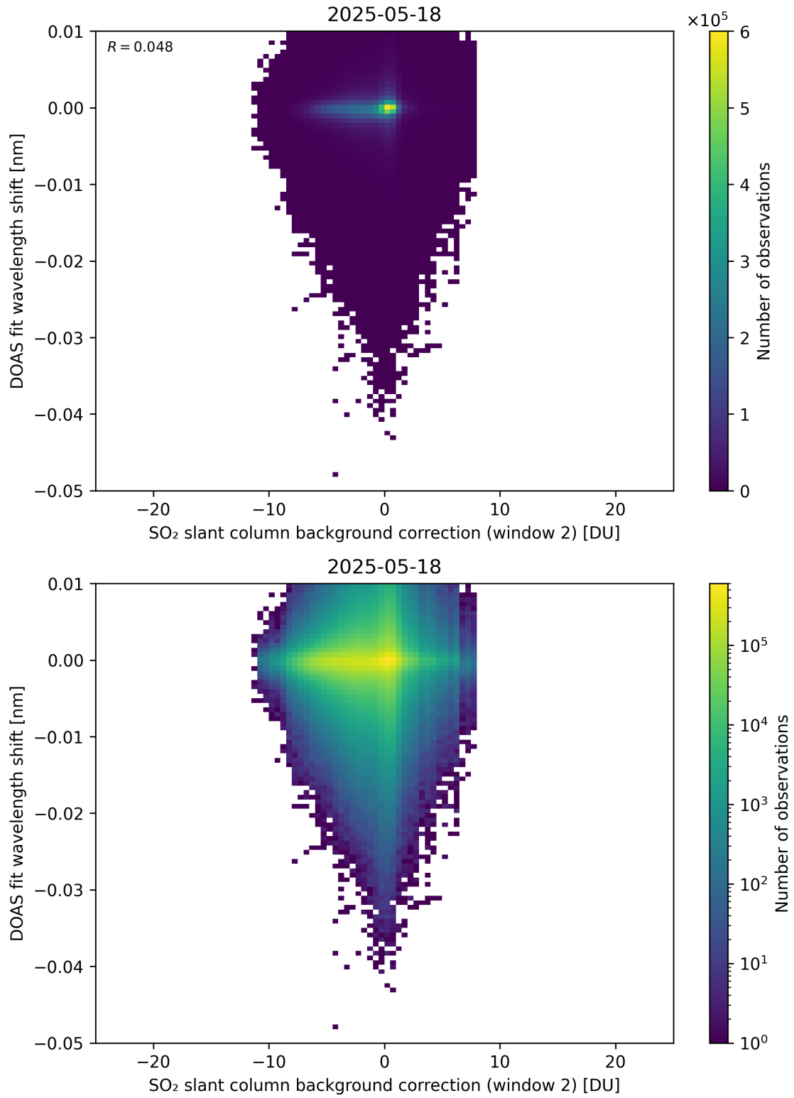
Figure 123: Scatter density plot of “SO 2 slant column background correction (window 2)” against “DOAS fit wavelength shift” for 2025-05-17 to 2025-05-19.
