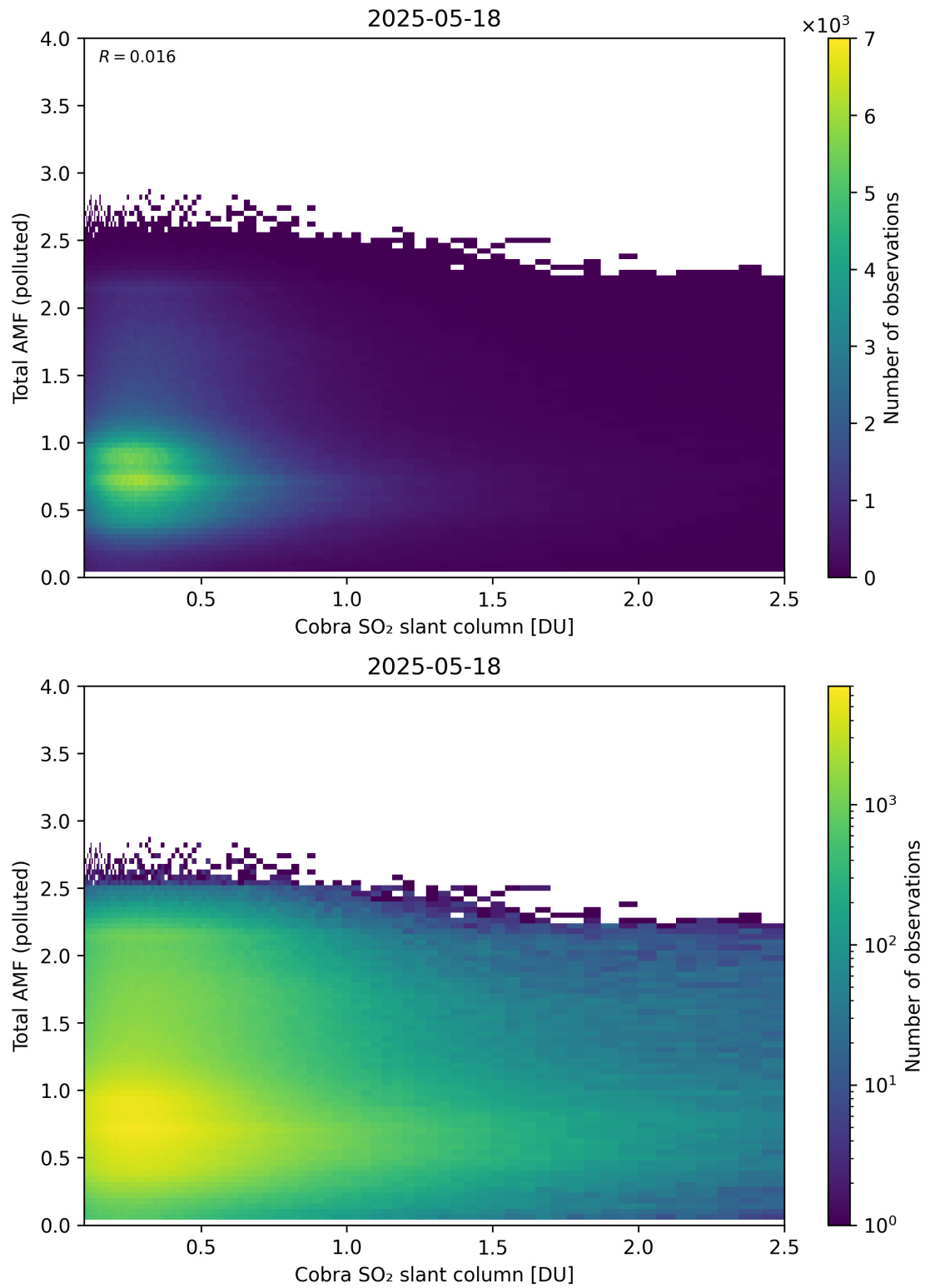
Figure 224: Scatter density plot of “Cobra SO 2 slant column” against “Total AMF (polluted)” for 2025-05-17 to 2025-05-19.
