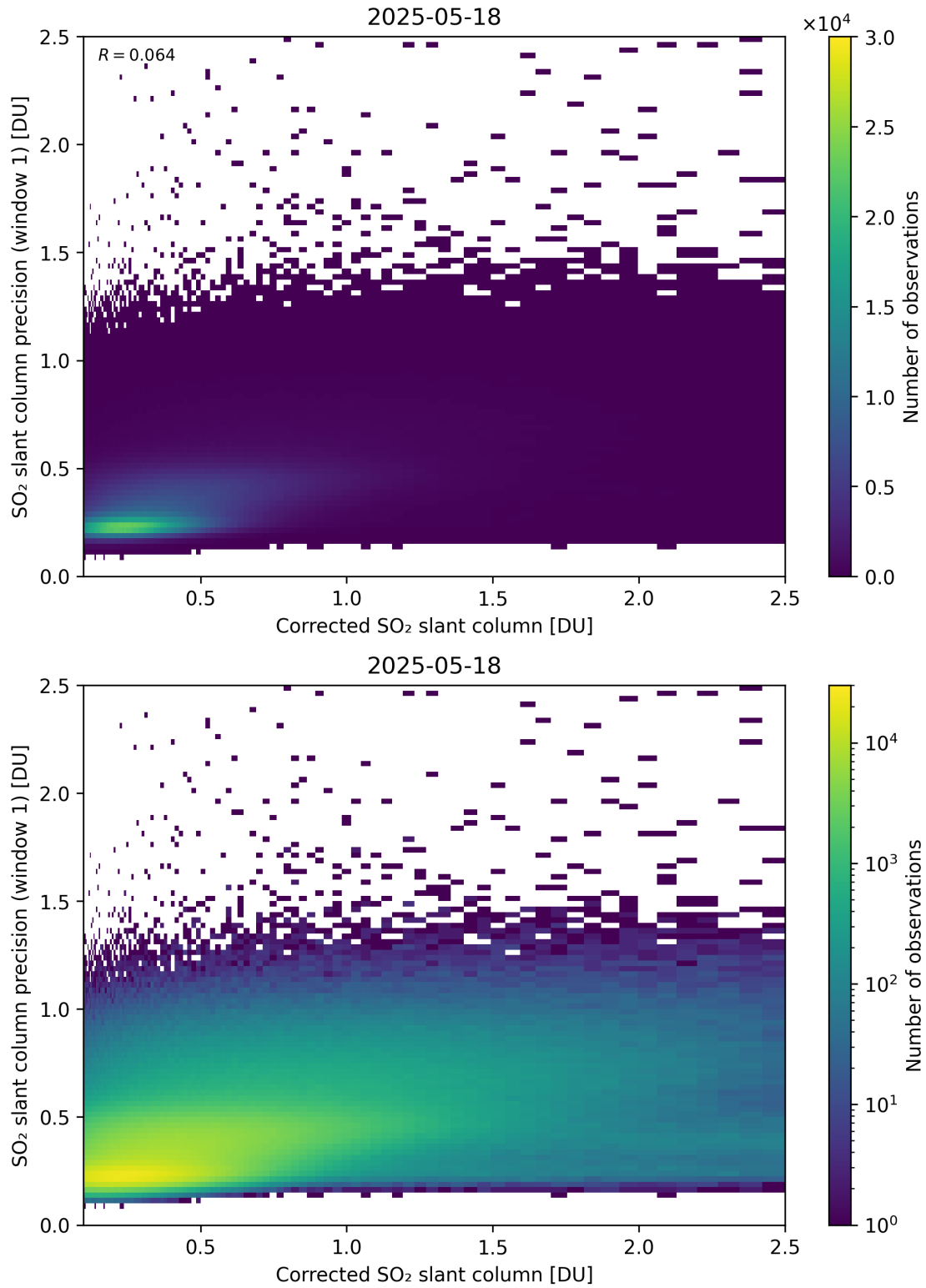
Figure 238: Scatter density plot of “Corrected SO 2 slant column” against “SO 2 slant column precision (window 1)” for 2025-05-17 to 2025-05-19.
