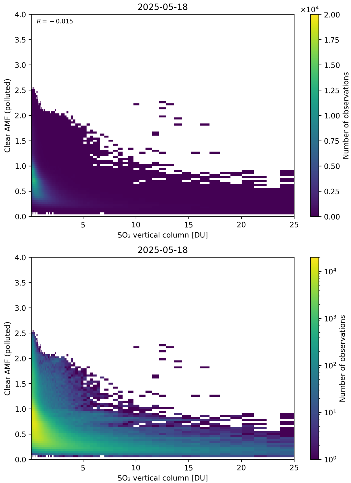
Figure 348: Scatter density plot of “SO 2 vertical column” against “Clear AMF (polluted)” for 2025-05-17 to 2025-05-19.
