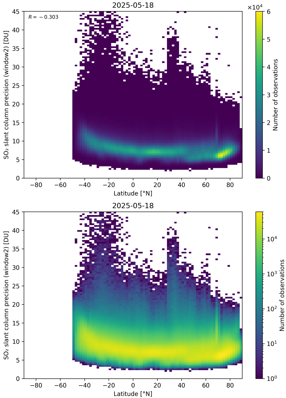
Figure 164: Scatter density plot of “Latitude” against “SO 2 slant column precision (window2)” for 2025-05-17 to 2025-05-19.
