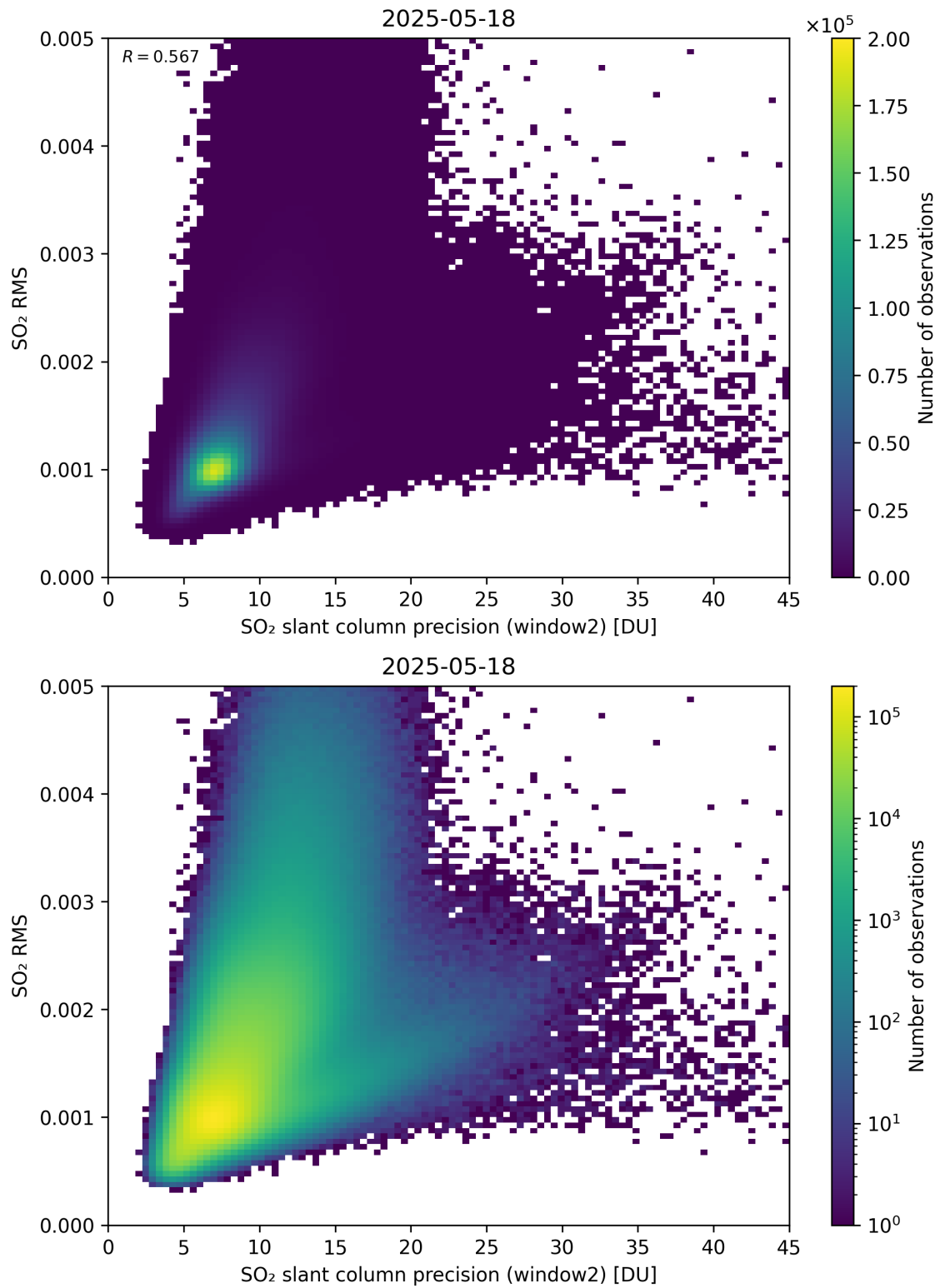
Figure 295: Scatter density plot of “SO 2 slant column precision (window2)” against “SO 2 RMS” for 2025-05-17 to 2025-05-19.
