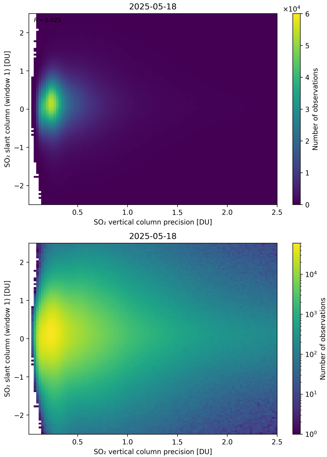
Figure 341: Scatter density plot of “SO 2 vertical column precision” against “SO 2 slant column (window 1)” for 2025-05-17 to 2025-05-19.
