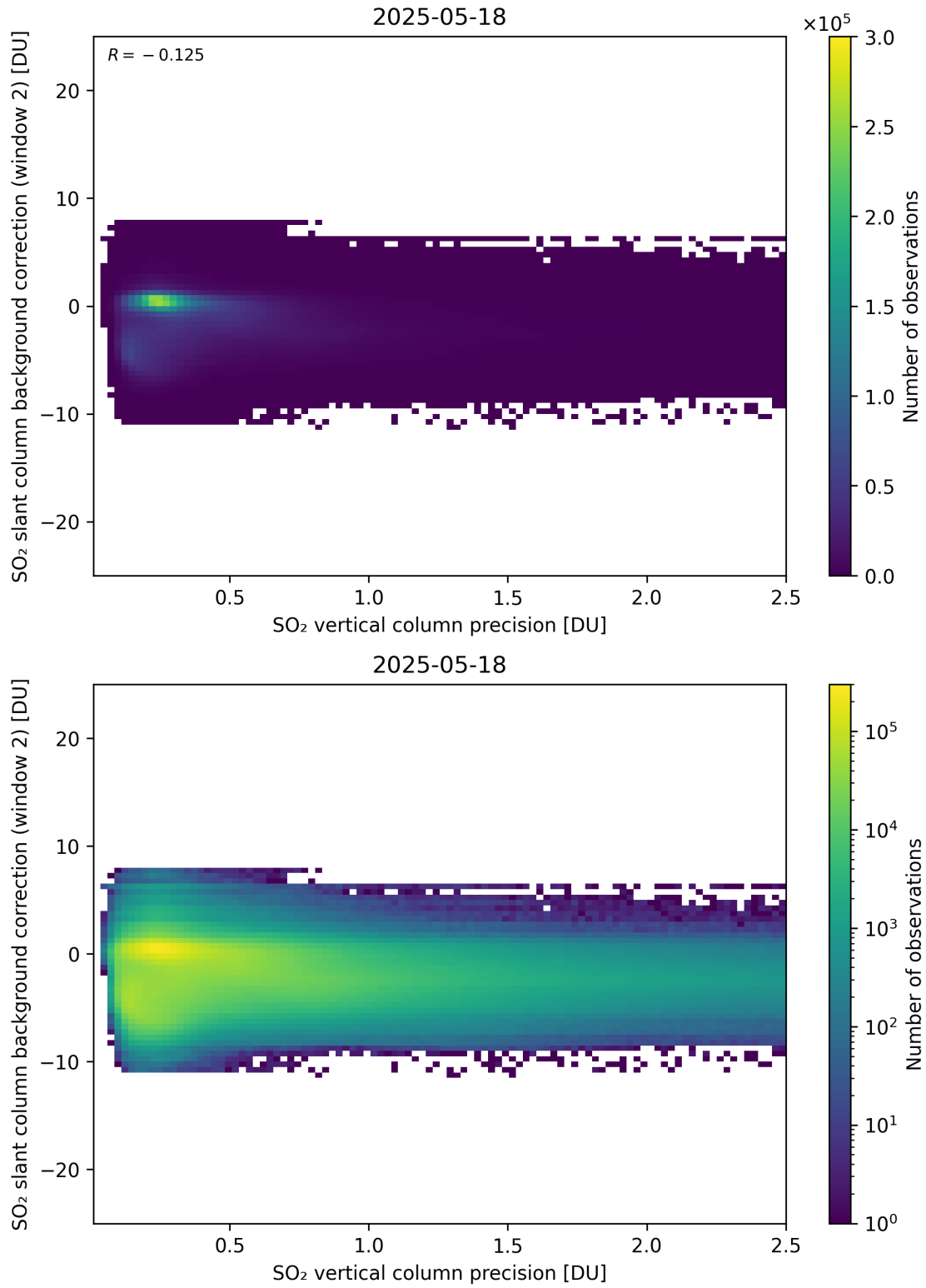
Figure 330: Scatter density plot of “SO 2 vertical column precision” against “SO 2 slant column background correction (window 2)” for 2025-05-17 to 2025-05-19.
