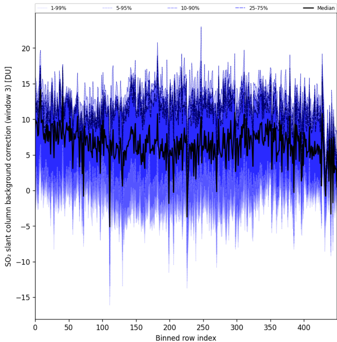
Figure 100: Along track statistics of “SO 2 slant column background correction (window 3)” for 2025-05-17 to 2025-05-19
