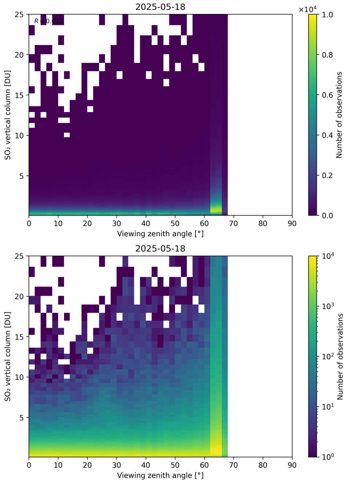
Figure 383: Scatter density plot of “Viewing zenith angle” against “SO 2 vertical column” for 2025-05-17 to 2025-05-19.
