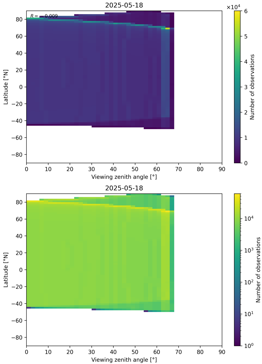
Figure 368: Scatter density plot of “Viewing zenith angle” against “Latitude” for 2025-05-17 to 2025-05-19.
