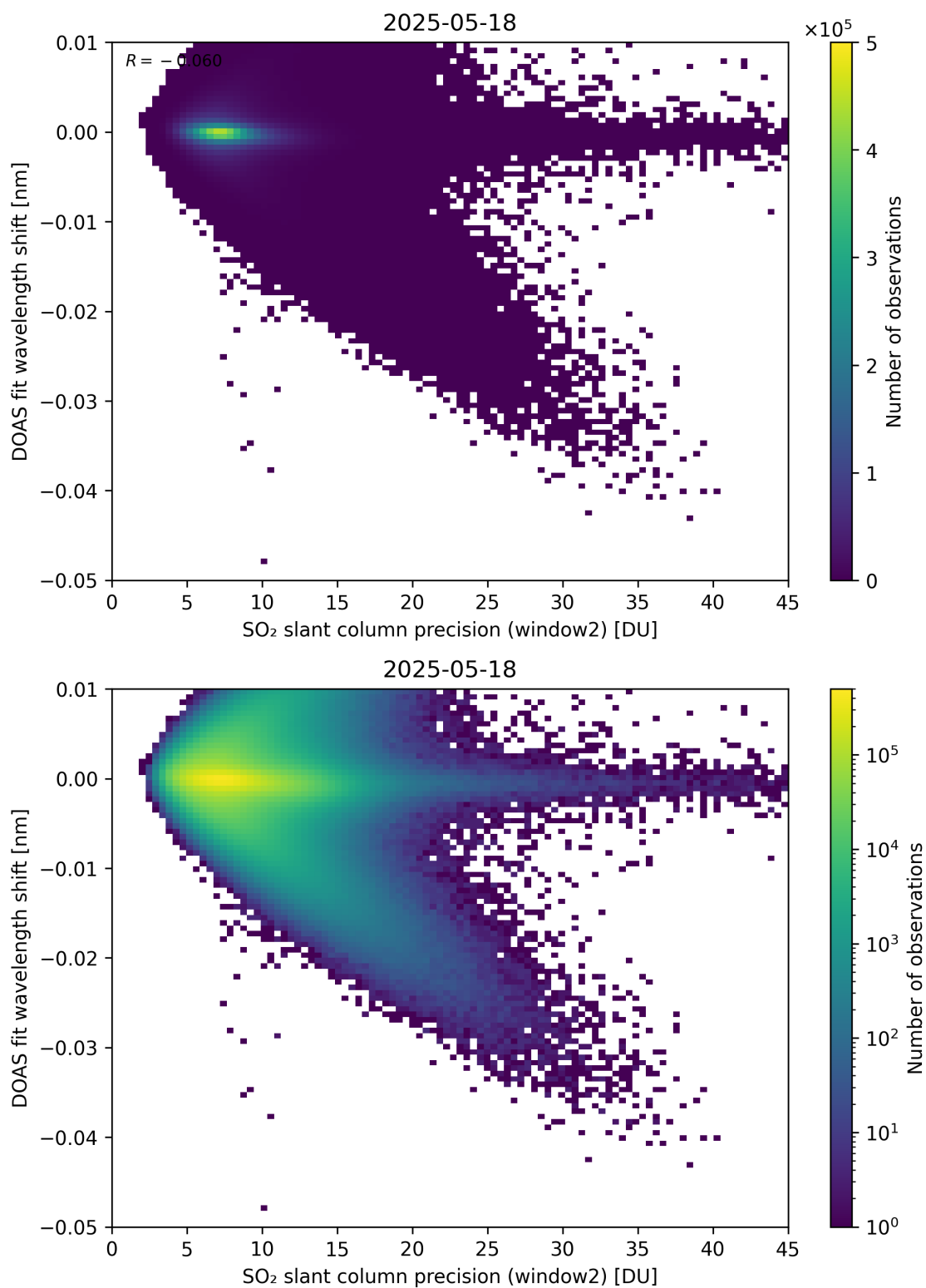
Figure 293: Scatter density plot of “SO 2 slant column precision (window2)” against “DOAS fit wavelength shift” for 2025-05-17 to 2025-05-19.
