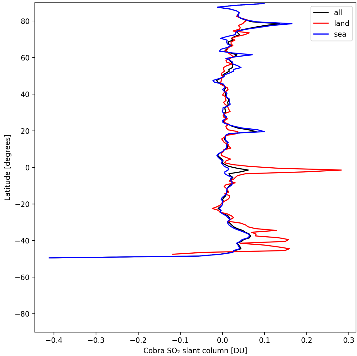
Figure 35: Zonal average of “Cobra SO 2 slant column” for 2025-05-17 to 2025-05-19.
