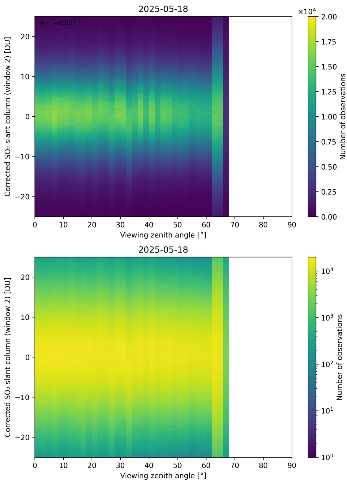
Figure 374: Scatter density plot of “Viewing zenith angle” against “Corrected SO 2 slant column (window 2)” for 2025-05-17 to 2025-05-19.
