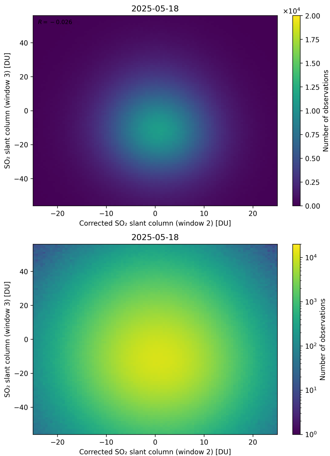
Figure 251: Scatter density plot of “Corrected SO 2 slant column (window 2)” against “SO 2 slant column (window 3)” for 2025-05-17 to 2025-05-19.
