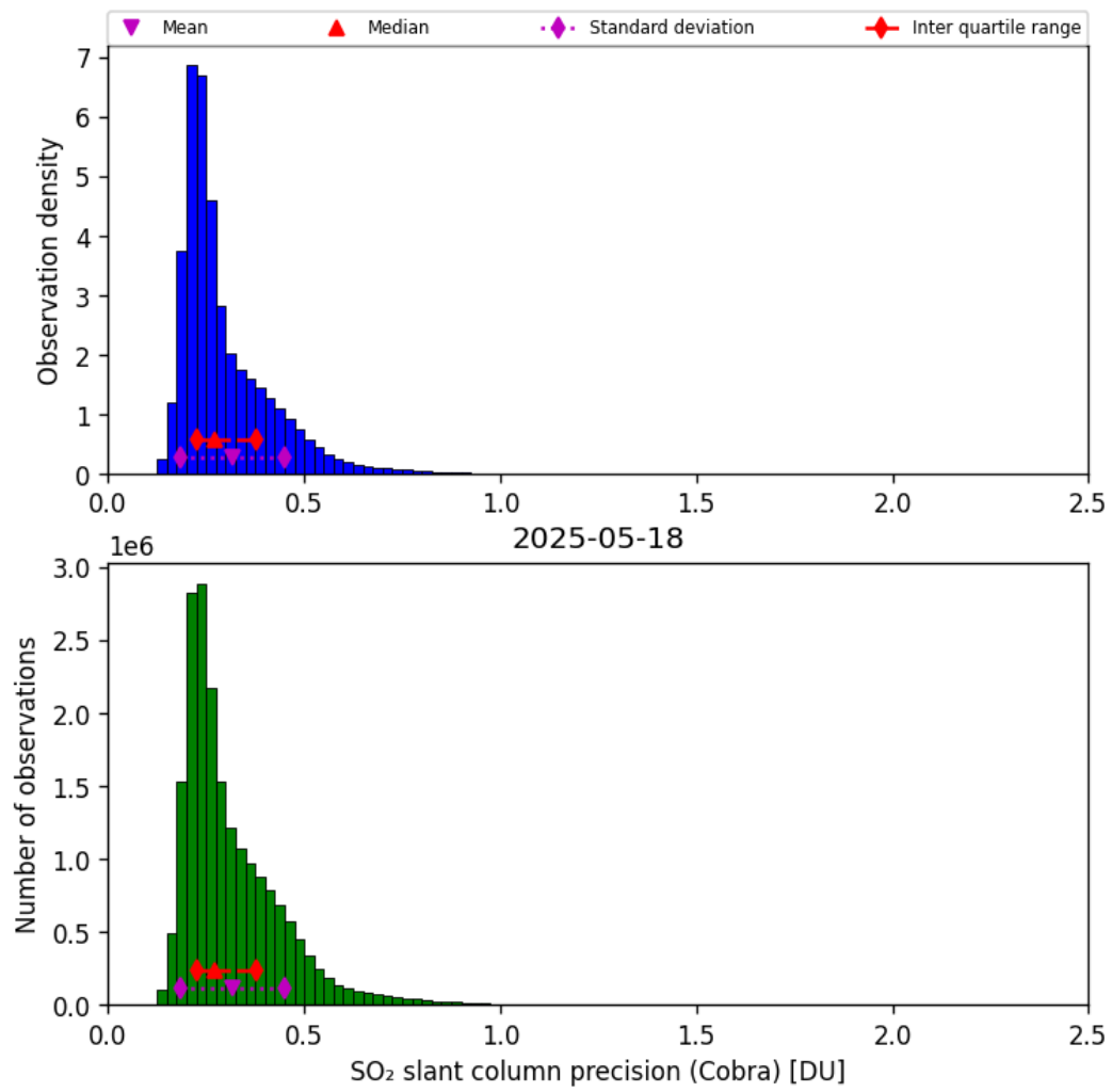
Figure 62: Histogram of “SO 2 slant column precision (Cobra)” for 2025-05-17 to 2025-05-19
