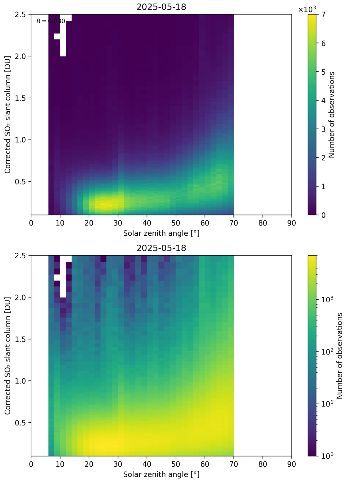
Figure 181: Scatter density plot of “Solar zenith angle” against “Corrected SO 2 slant column” for 2025-05-17 to 2025-05-19.
