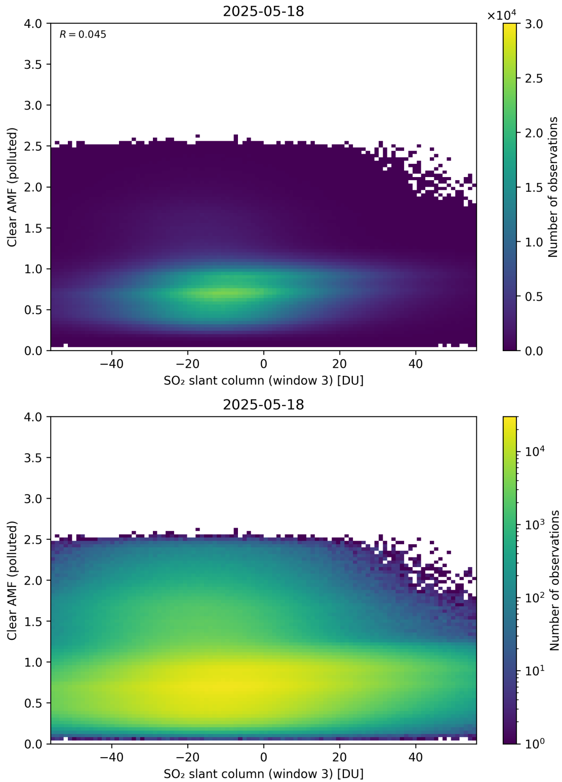
Figure 315: Scatter density plot of “SO 2 slant column (window 3)” against “Clear AMF (polluted)” for 2025-05-17 to 2025-05-19.
