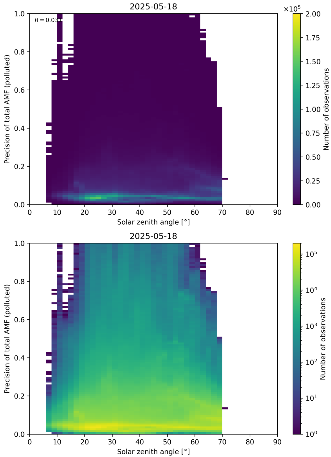
Figure 190: Scatter density plot of “Solar zenith angle” against “Precision of total AMF (polluted)” for 2025-05-17 to 2025-05-19.
