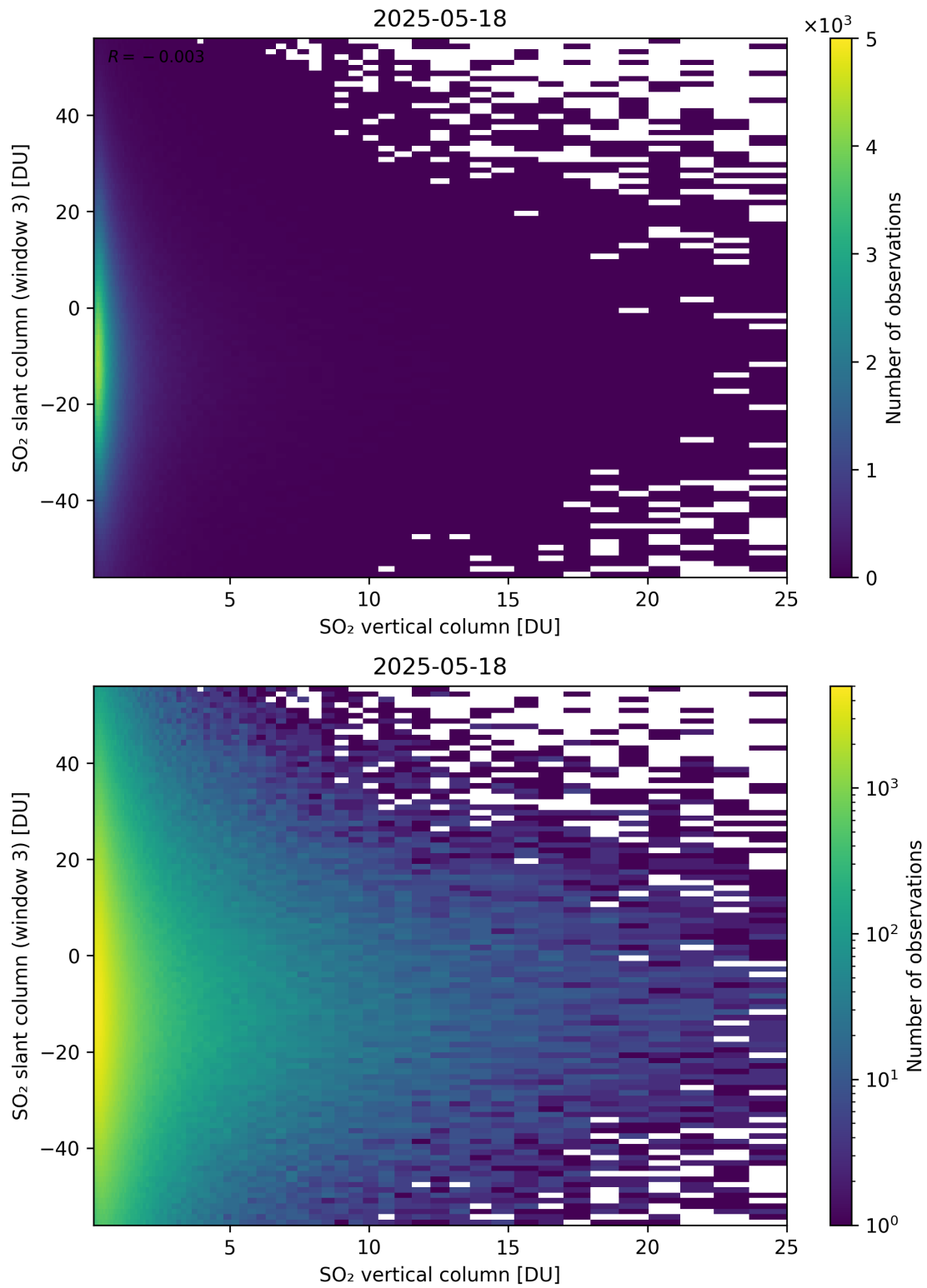
Figure 357: Scatter density plot of “SO 2 vertical column” against “SO 2 slant column (window 3)” for 2025-05-17 to 2025-05-19.
