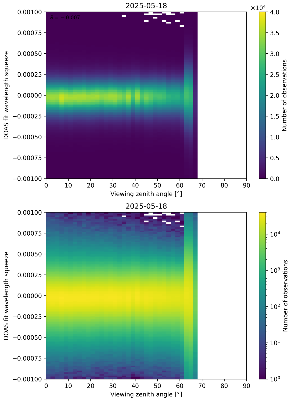
Figure 366: Scatter density plot of “Viewing zenith angle” against “DOAS fit wavelength squeeze” for 2025-05-17 to 2025-05-19.
