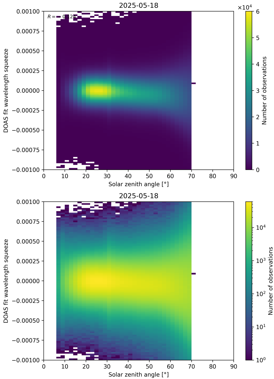
Figure 175: Scatter density plot of “Solar zenith angle” against “DOAS fit wavelength squeeze” for 2025-05-17 to 2025-05-19.
