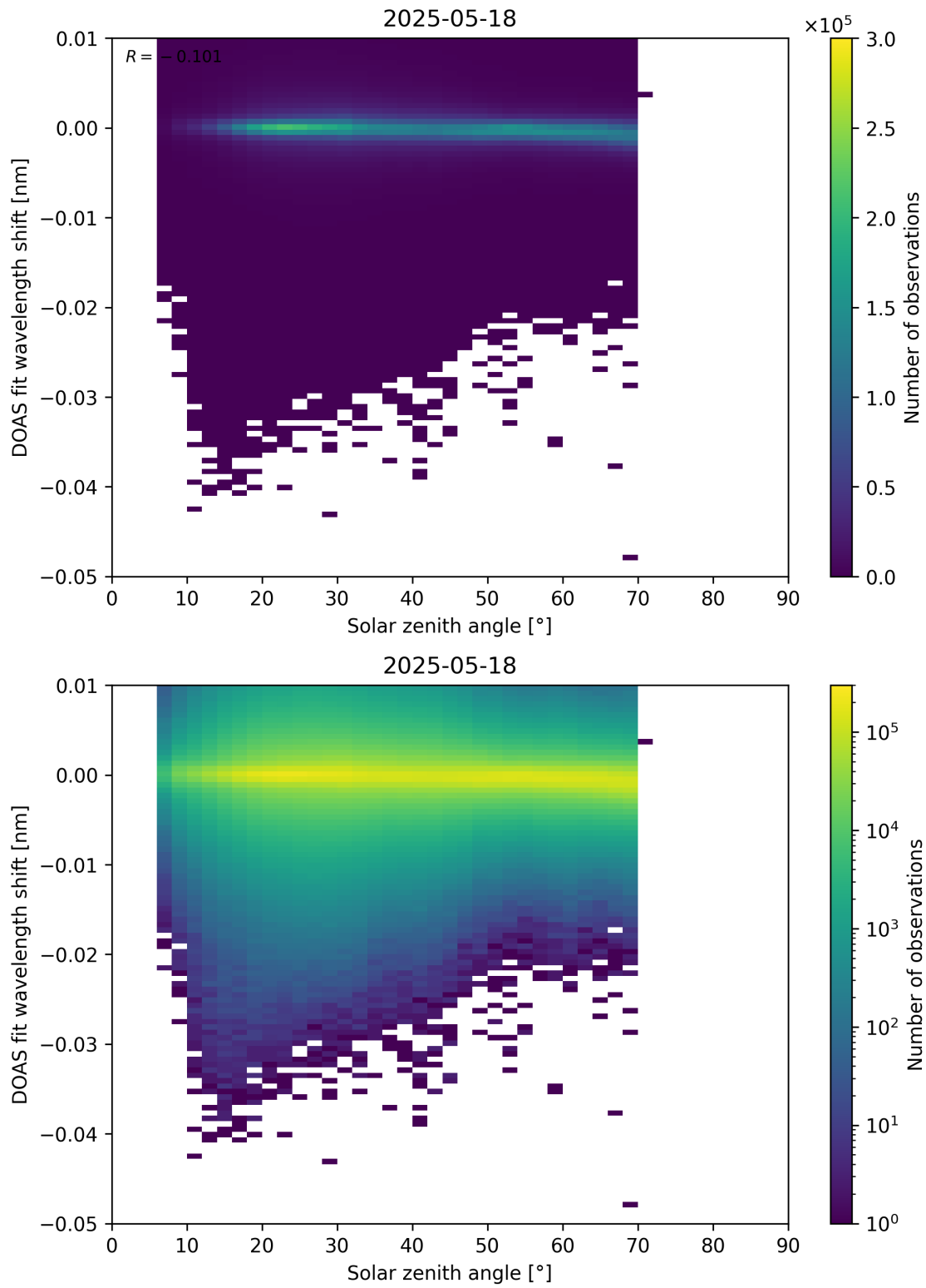
Figure 174: Scatter density plot of “Solar zenith angle” against “DOAS fit wavelength shift” for 2025-05-17 to 2025-05-19.
