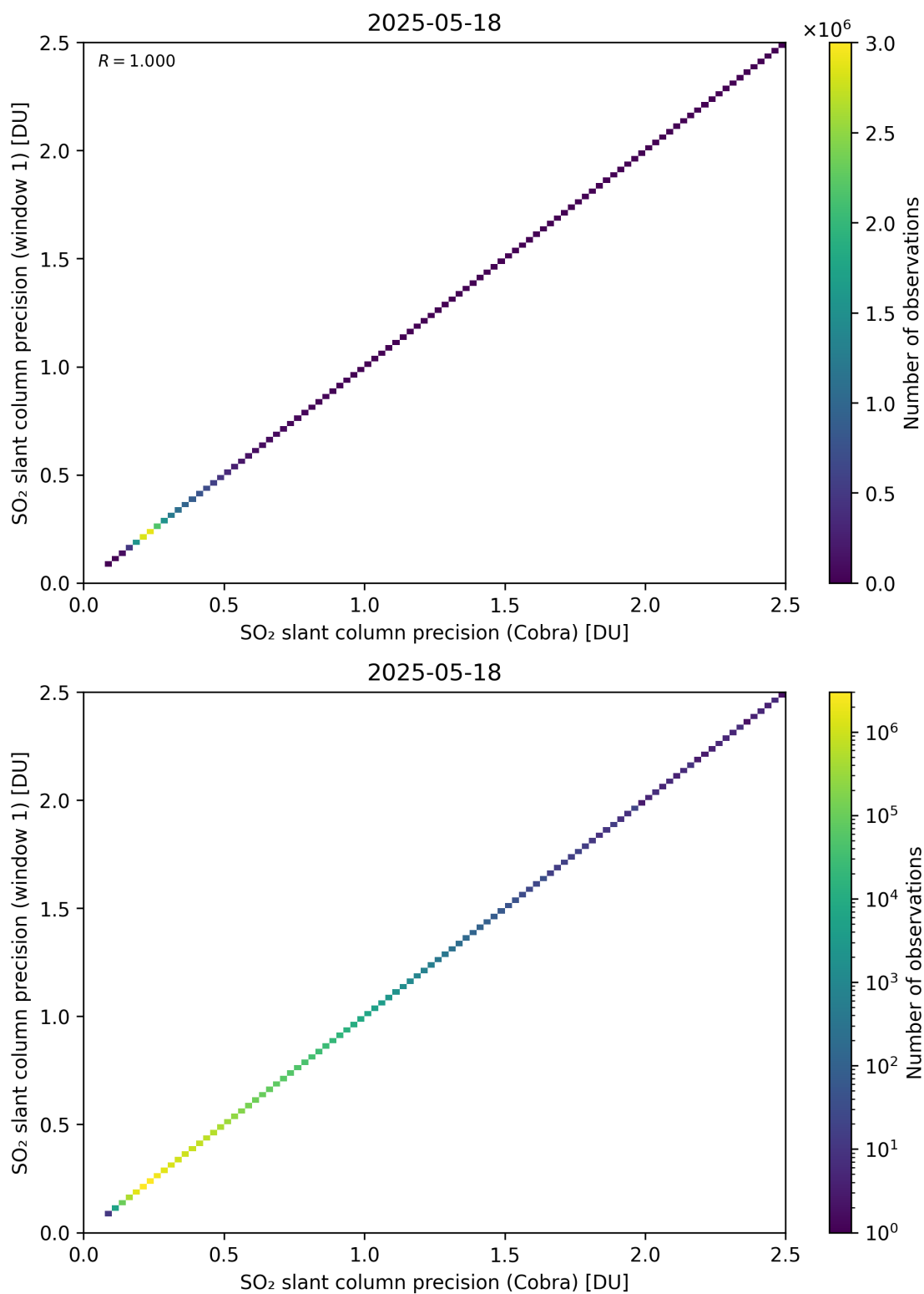
Figure 209: Scatter density plot of “SO 2 slant column precision (Cobra)” against “SO 2 slant column precision (window 1)” for 2025-05-17 to 2025-05-19.
