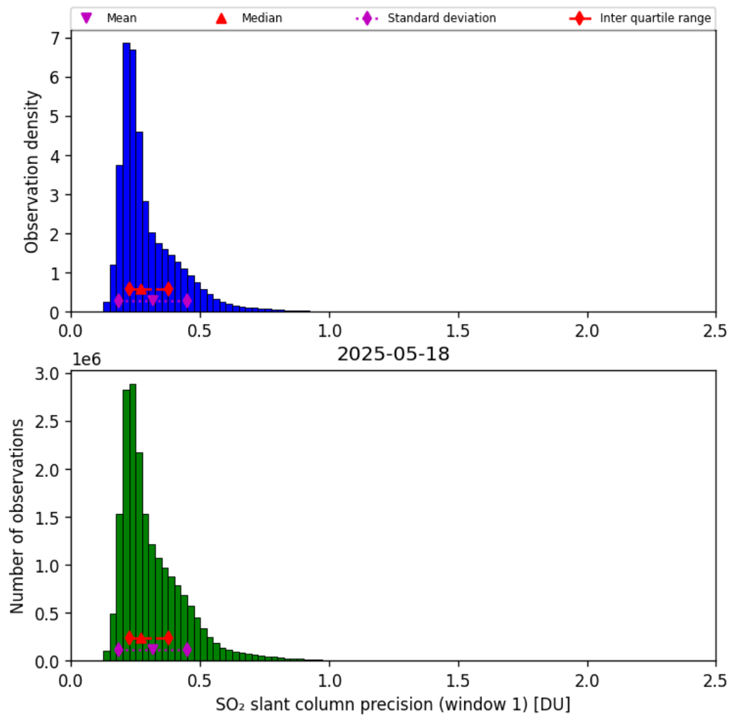
Figure 64: Histogram of “SO 2 slant column precision (window 1)” for 2025-05-17 to 2025-05-19
