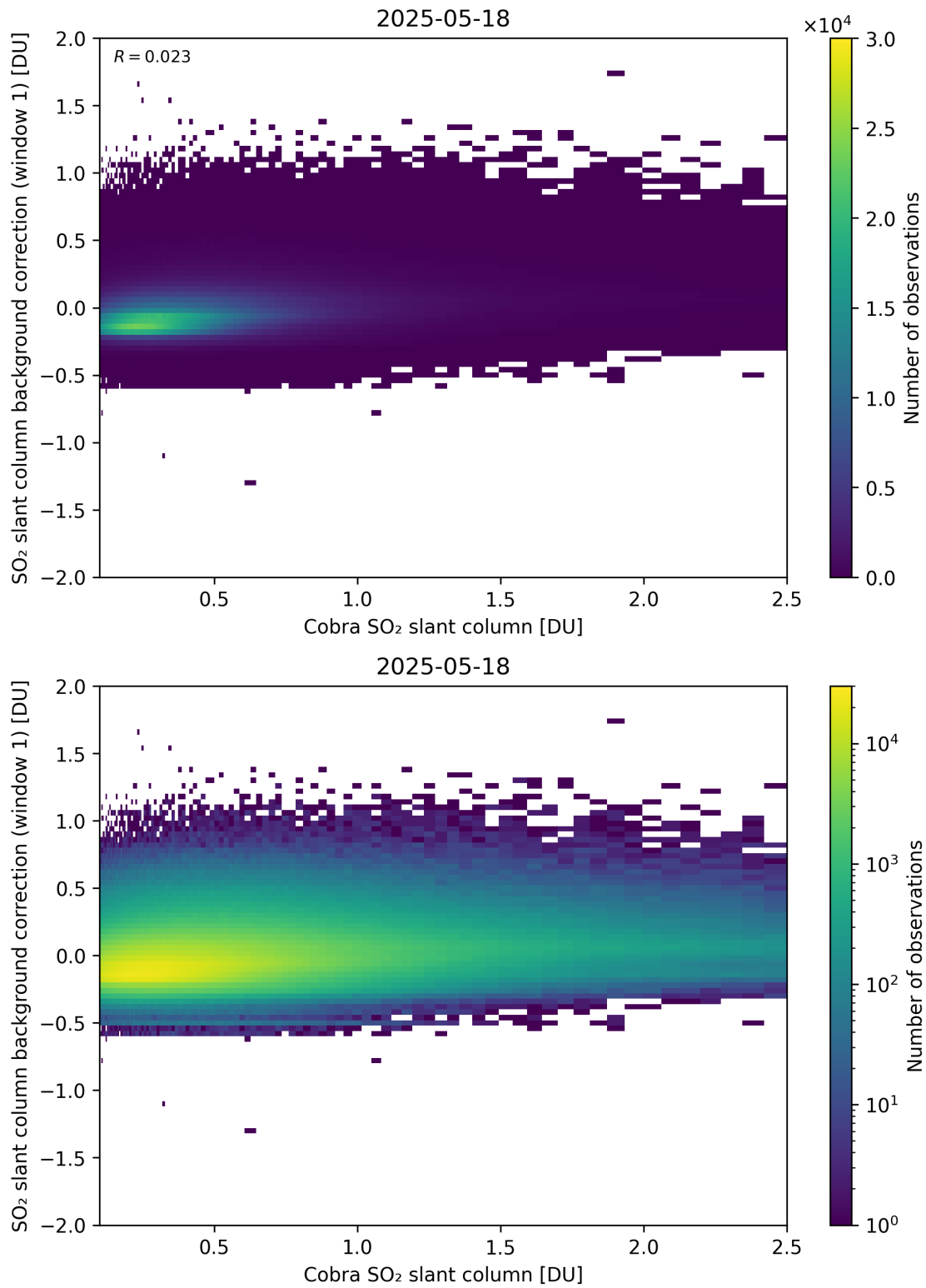
Figure 193: Scatter density plot of “Cobra SO 2 slant column” against “SO 2 slant column background correction (window 1)” for 2025-05-17 to 2025-05-19.
