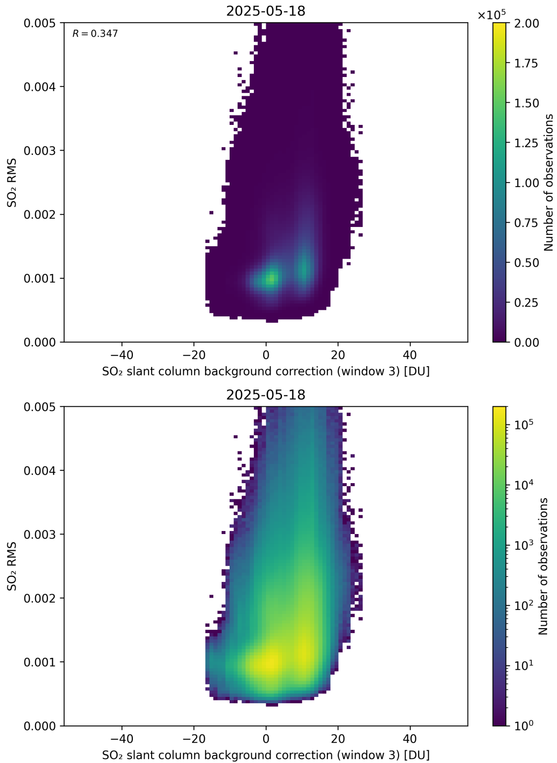
Figure 134: Scatter density plot of “SO 2 slant column background correction (window 3)” against “SO 2 RMS” for 2025-05-17 to 2025-05-19.
