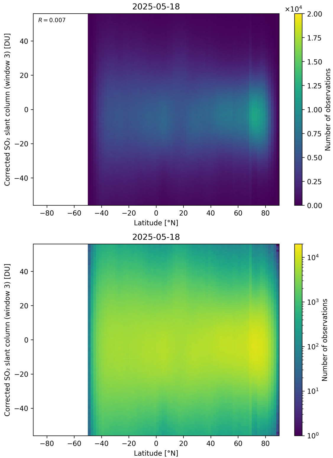
Figure 161: Scatter density plot of “Latitude” against “Corrected SO 2 slant column (window 3)” for 2025-05-17 to 2025-05-19.
