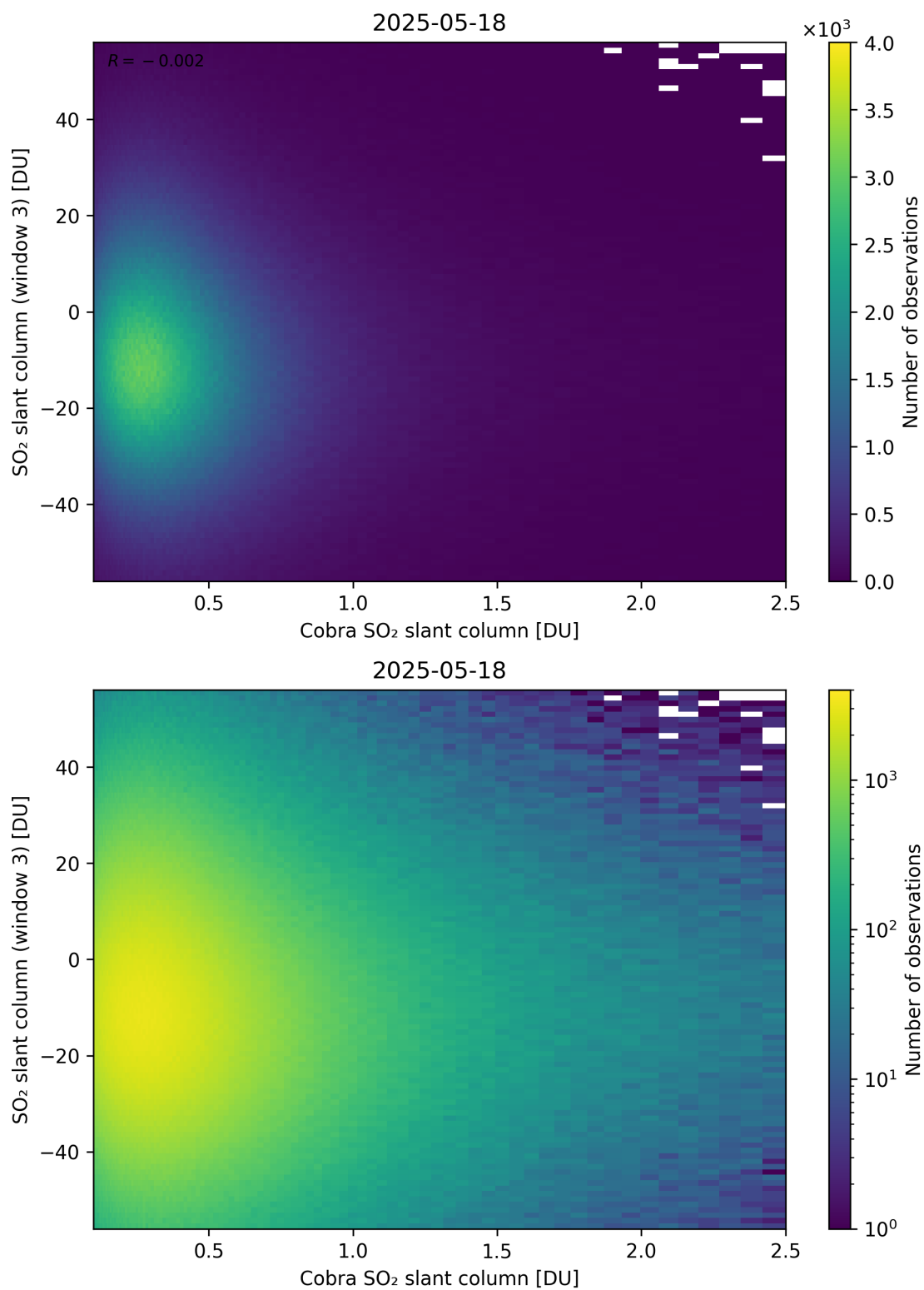
Figure 222: Scatter density plot of “Cobra SO 2 slant column” against “SO 2 slant column (window 3)” for 2025-05-17 to 2025-05-19.
