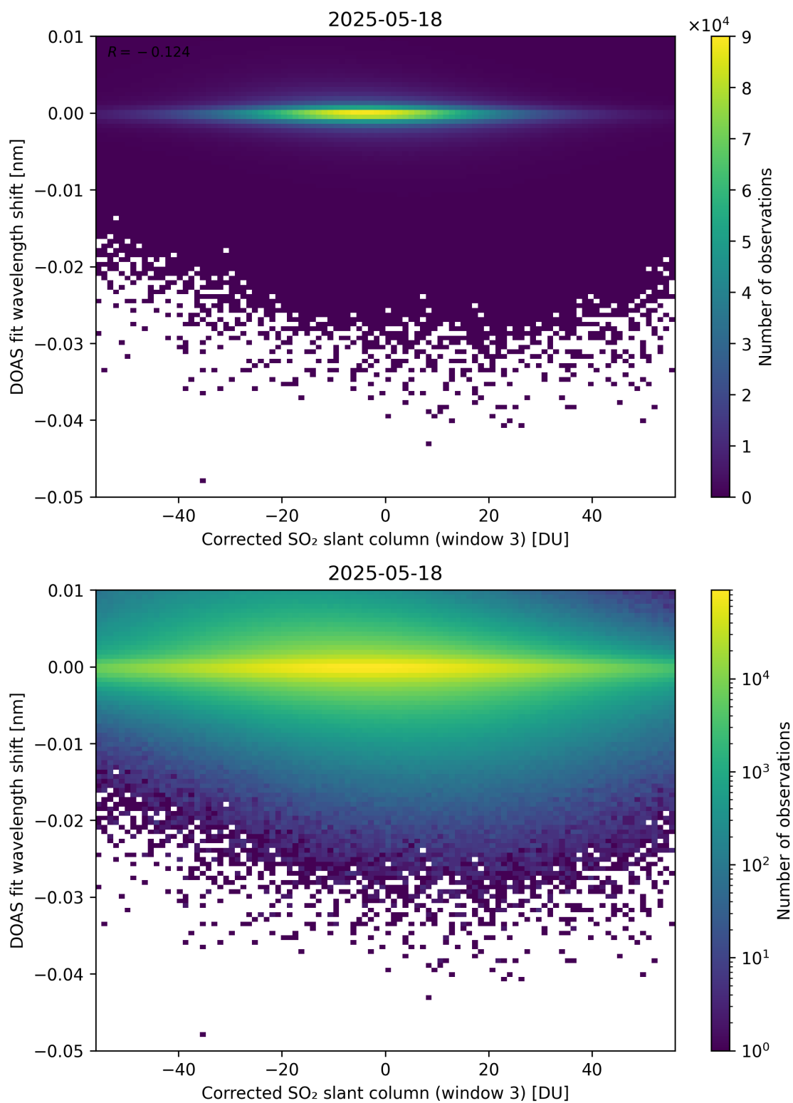
Figure 256: Scatter density plot of “Corrected SO 2 slant column (window 3)” against “DOAS fit wavelength shift” for 2025-05-17 to 2025-05-19.
