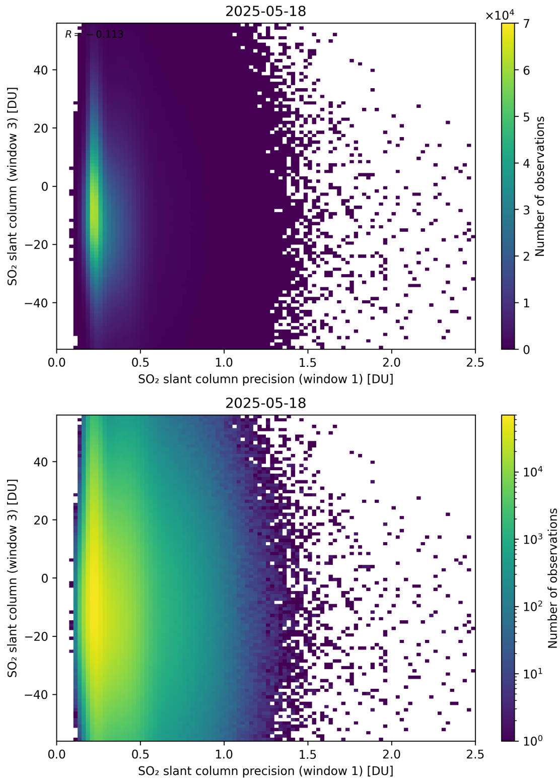
Figure 278: Scatter density plot of “SO 2 slant column precision (window 1)” against “SO 2 slant column (window 3)” for 2025-05-17 to 2025-05-19.
