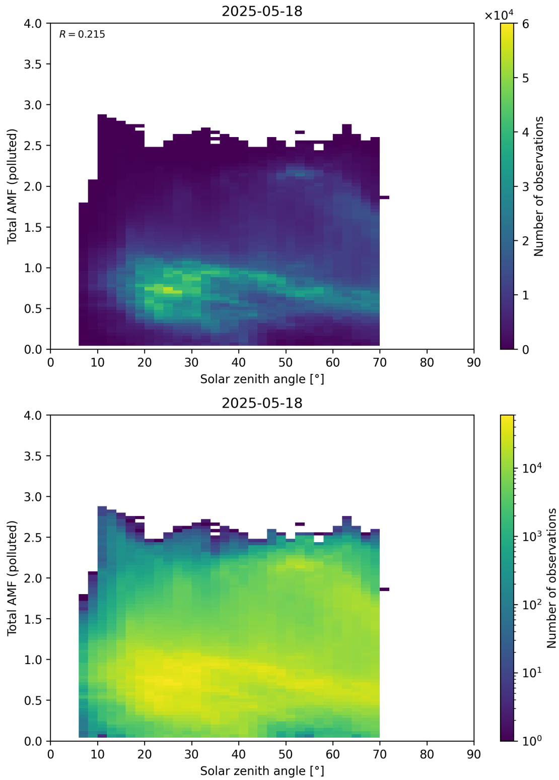
Figure 189: Scatter density plot of “Solar zenith angle” against “Total AMF (polluted)” for 2025-05-17 to 2025-05-19.
