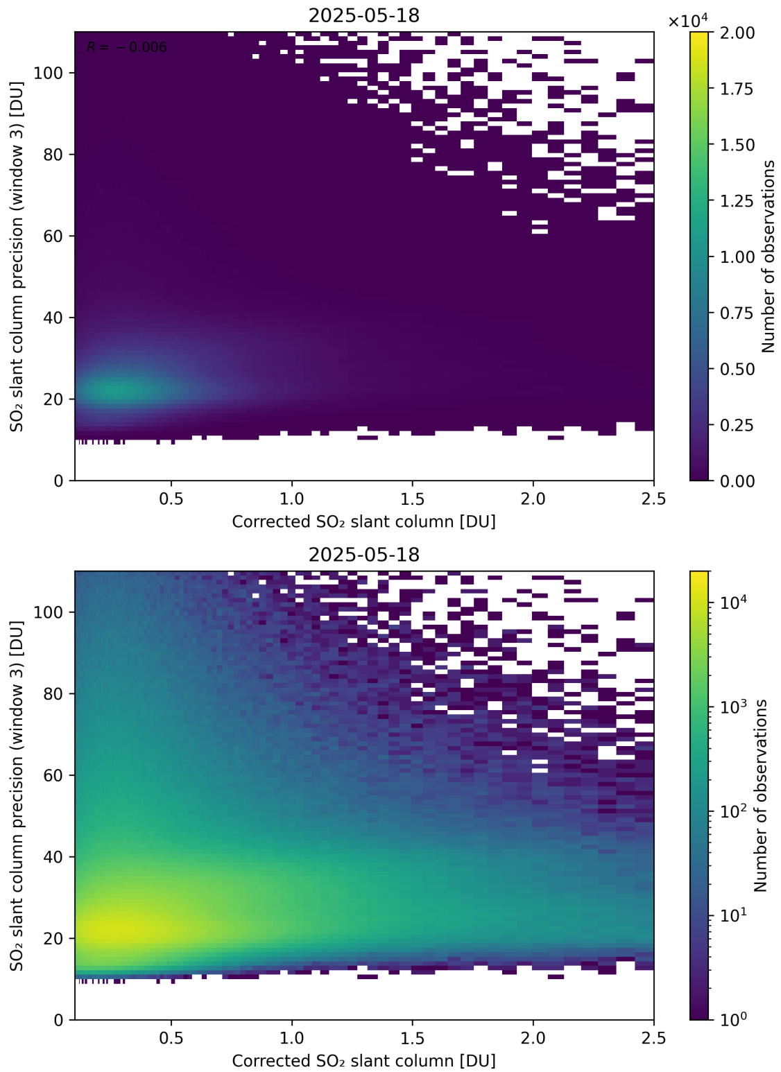
Figure 241: Scatter density plot of “Corrected SO 2 slant column” against “SO 2 slant column precision (window 3)” for 2025-05-17 to 2025-05-19.
