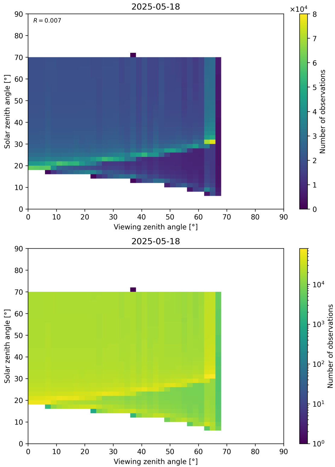
Figure 369: Scatter density plot of “Viewing zenith angle” against “Solar zenith angle” for 2025-05-17 to 2025-05-19.
