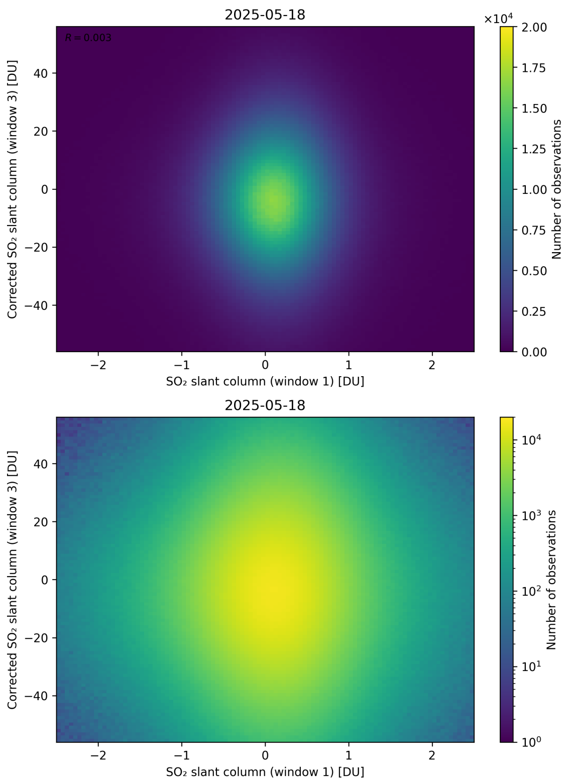
Figure 284: Scatter density plot of “SO 2 slant column (window 1)” against “Corrected SO 2 slant column (window 3)” for 2025-05-17 to 2025-05-19.
