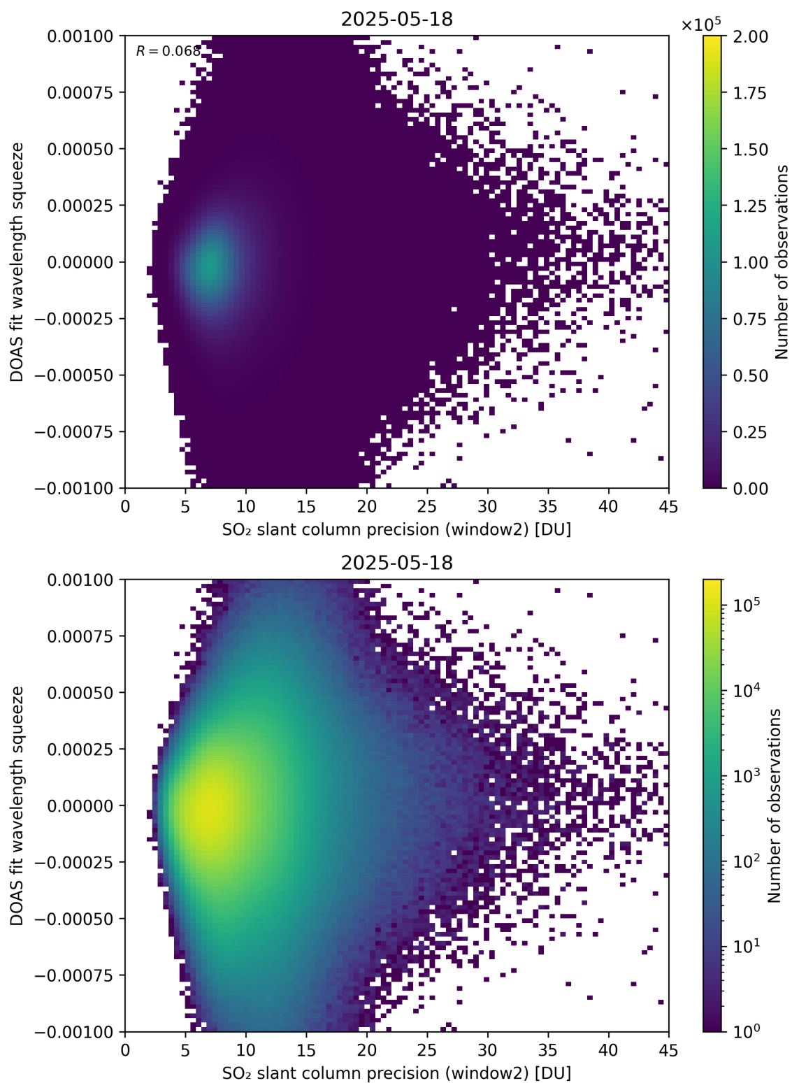
Figure 294: Scatter density plot of “SO 2 slant column precision (window2)” against “DOAS fit wavelength squeeze” for 2025-05-17 to 2025-05-19.
