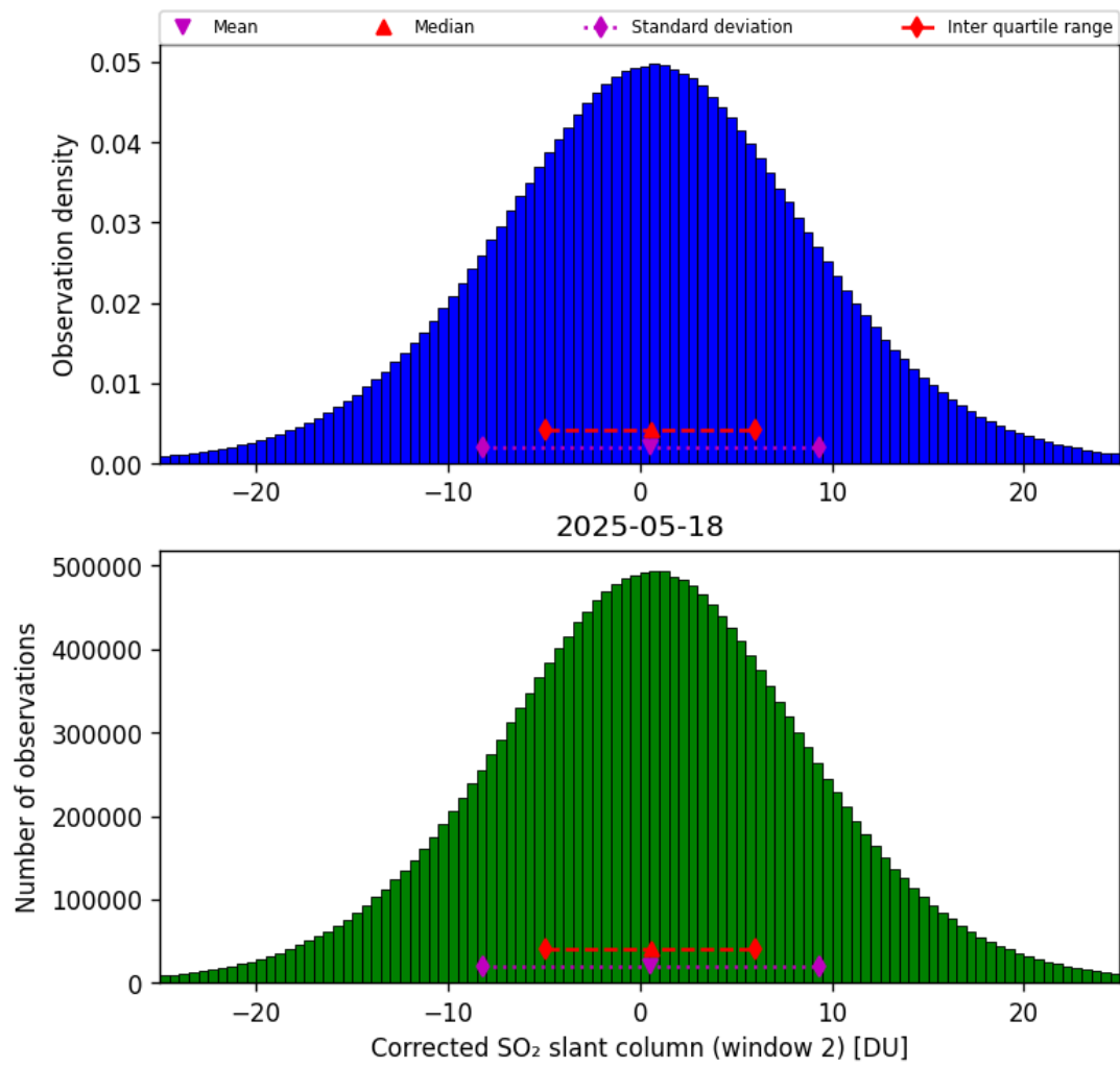
Figure 69: Histogram of “Corrected SO 2 slant column (window 2)” for 2025-05-17 to 2025-05-19
