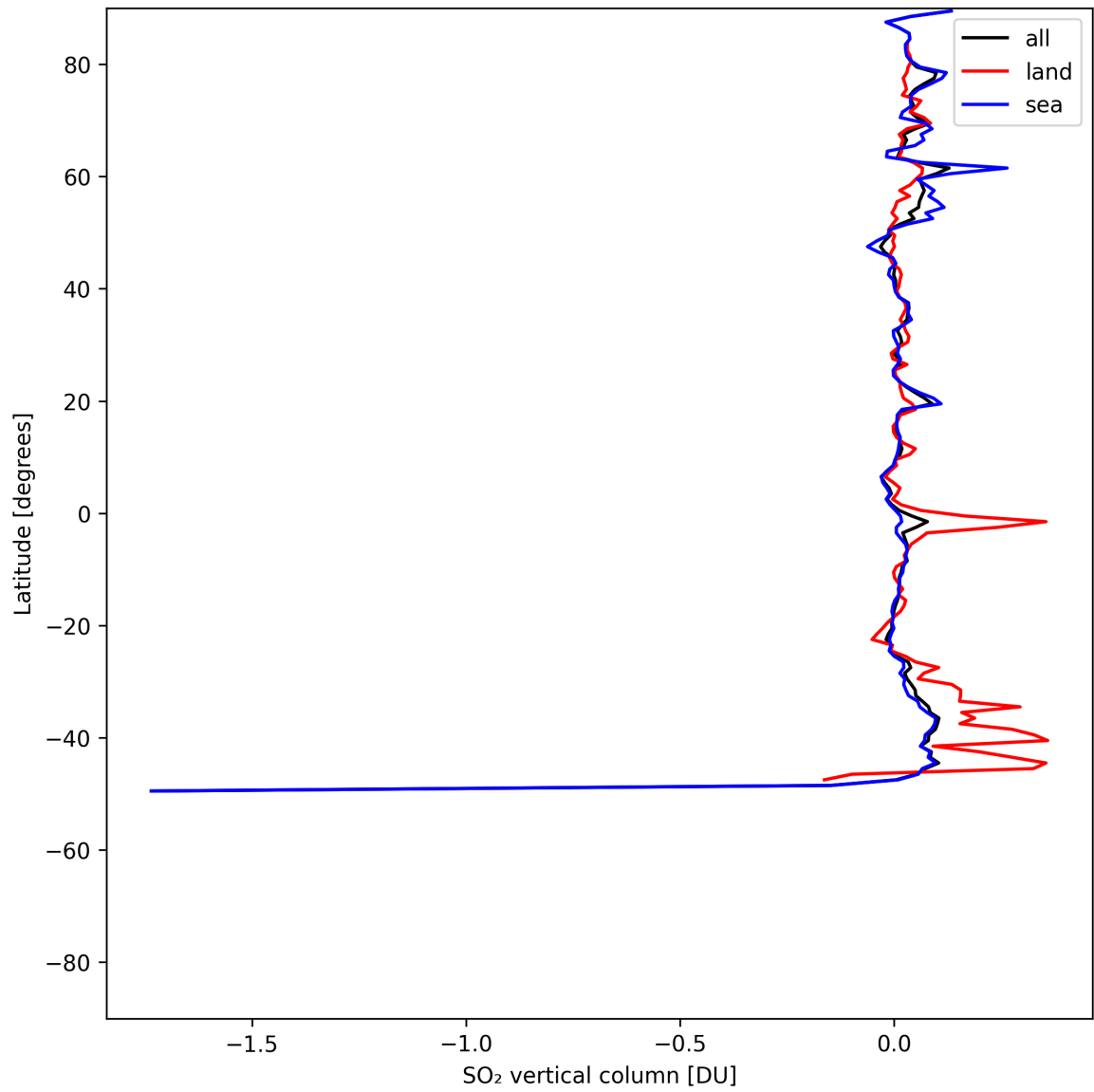
Figure 32: Zonal average of “SO 2 vertical column” for 2025-05-17 to 2025-05-19.
