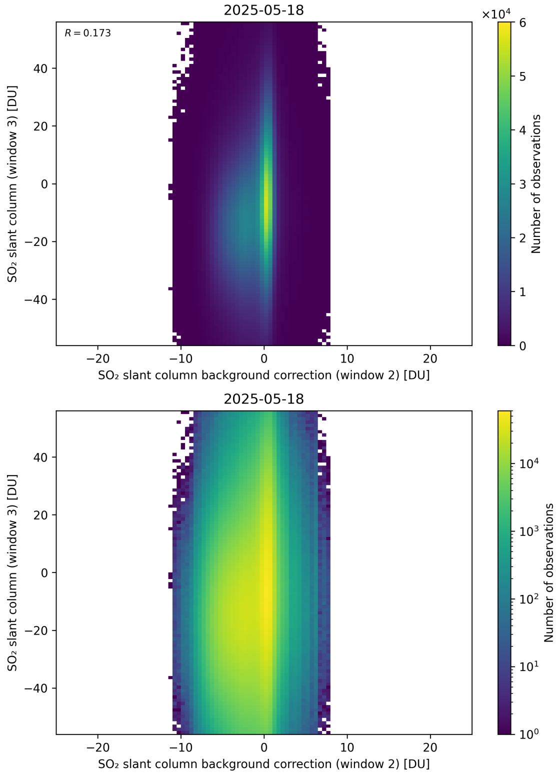
Figure 128: Scatter density plot of “SO 2 slant column background correction (window 2)” against “SO 2 slant column (window 3)” for 2025-05-17 to 2025-05-19.
