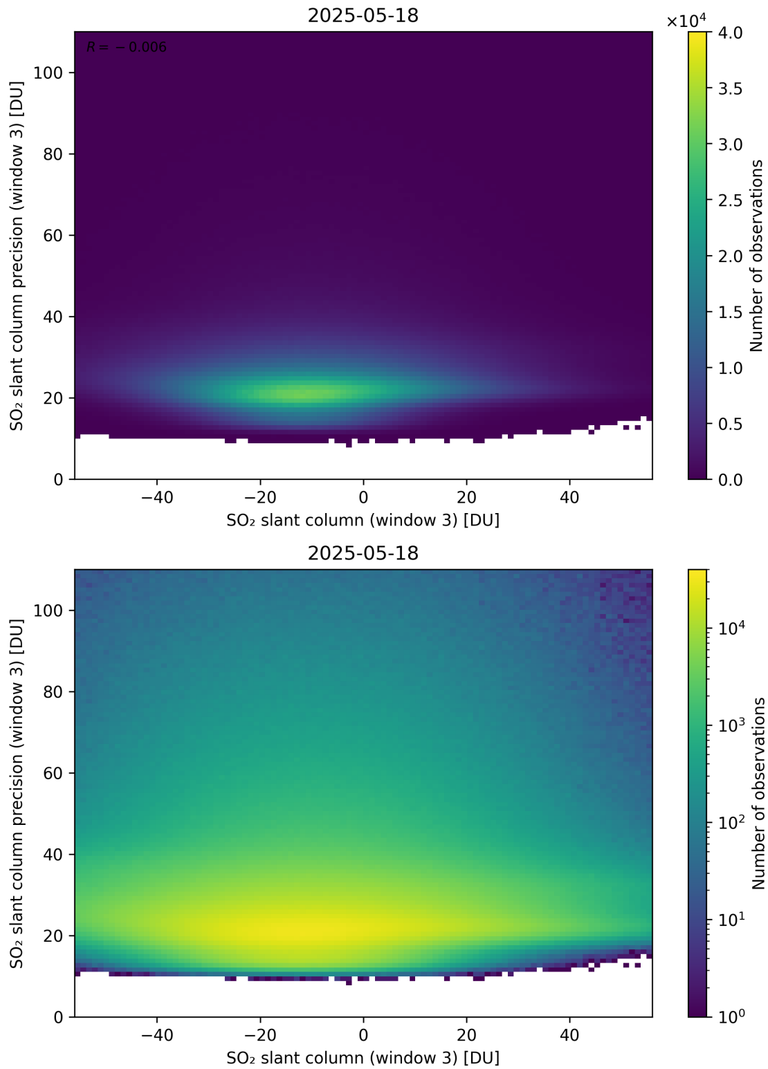
Figure 317: Scatter density plot of “SO 2 slant column (window 3)” against “SO 2 slant column precision (window 3)” for 2025-05-17 to 2025-05-19.
