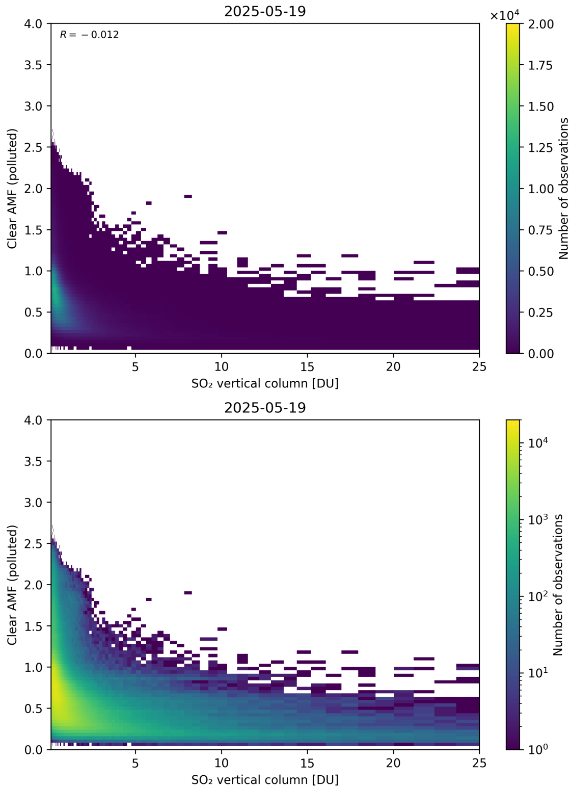
Figure 348: Scatter density plot of “SO 2 vertical column” against “Clear AMF (polluted)” for 2025-05-18 to 2025-05-20.
