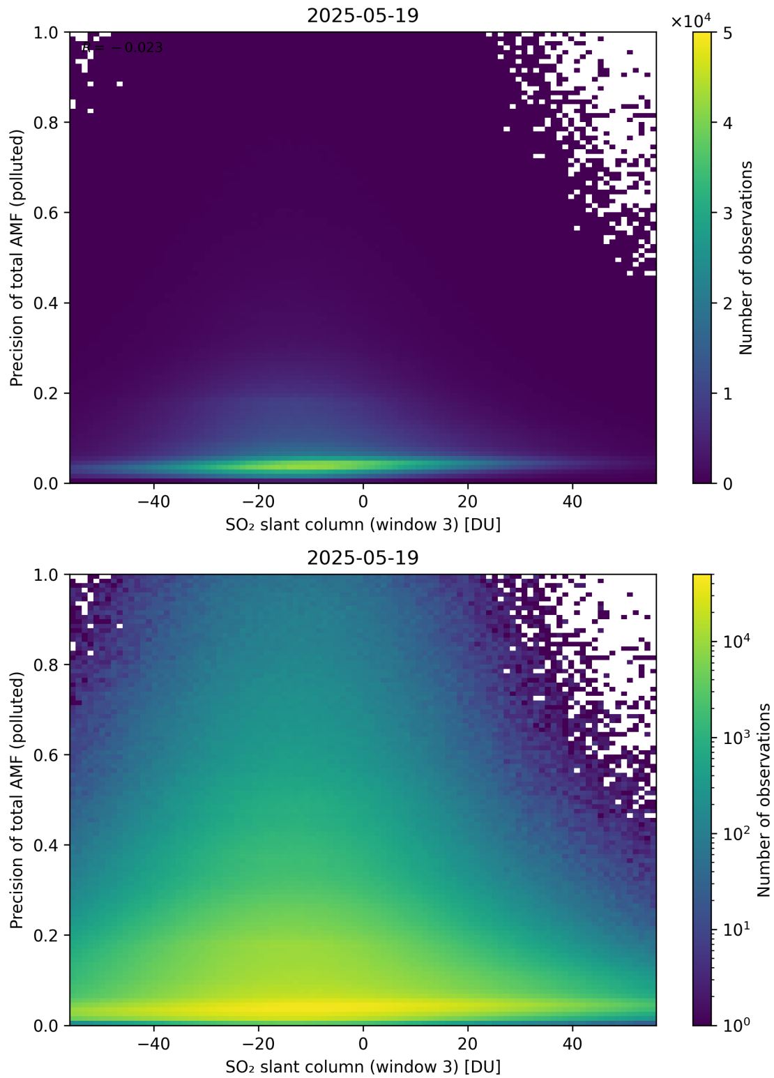
Figure 319: Scatter density plot of “SO 2 slant column (window 3)” against “Precision of total AMF (polluted)” for 2025-05-18 to 2025-05-20.
