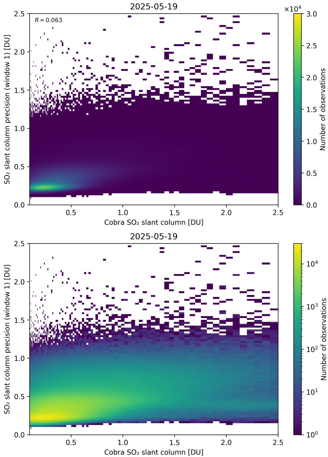
Figure 220: Scatter density plot of “Cobra SO 2 slant column” against “SO 2 slant column precision (window 1)” for 2025-05-18 to 2025-05-20.
