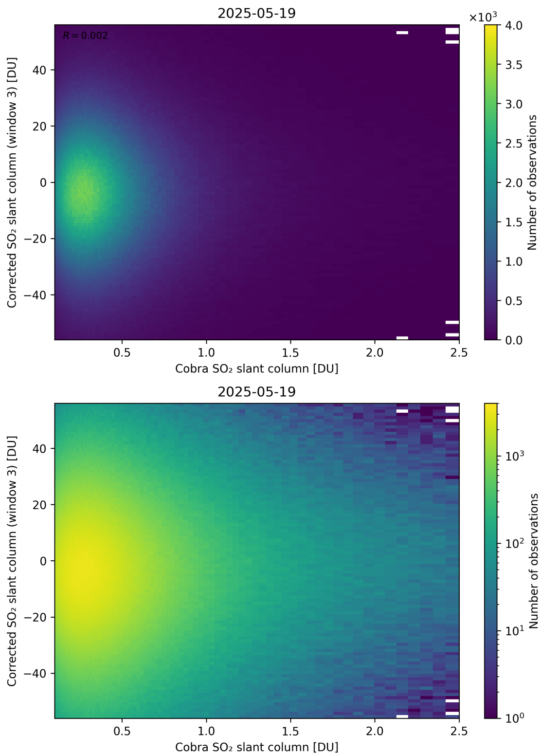
Figure 218: Scatter density plot of “Cobra SO 2 slant column” against “Corrected SO 2 slant column (window 3)” for 2025-05-18 to 2025-05-20.
