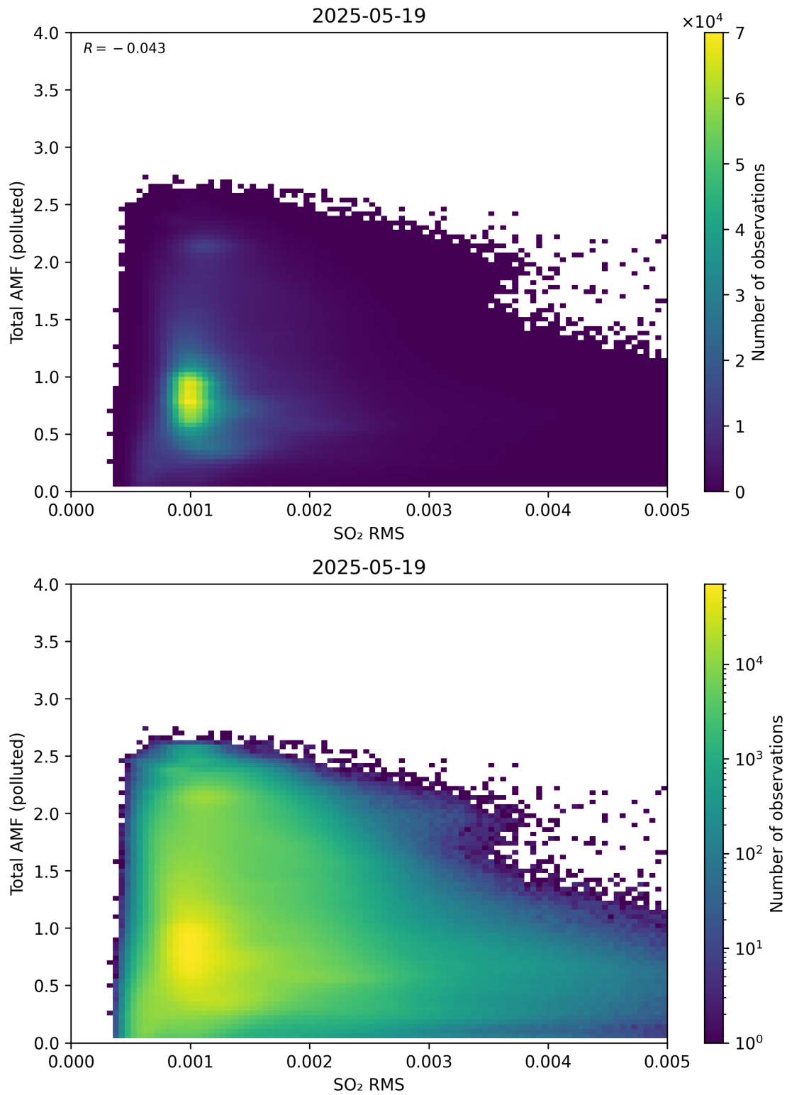
Figure 148: Scatter density plot of “SO 2 RMS” against “Total AMF (polluted)” for 2025-05-18 to 2025-05-20.
