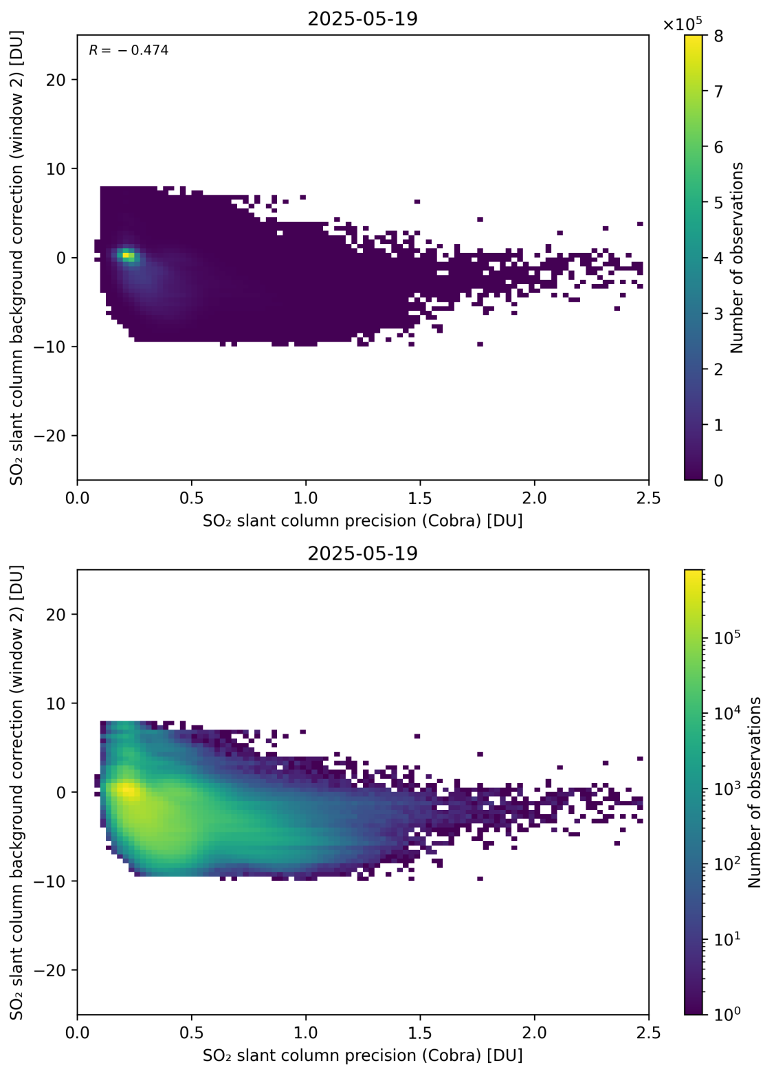
Figure 200: Scatter density plot of “SO 2 slant column precision (Cobra)” against “SO 2 slant column background correction (window 2)” for 2025-05-18 to 2025-05-20.
