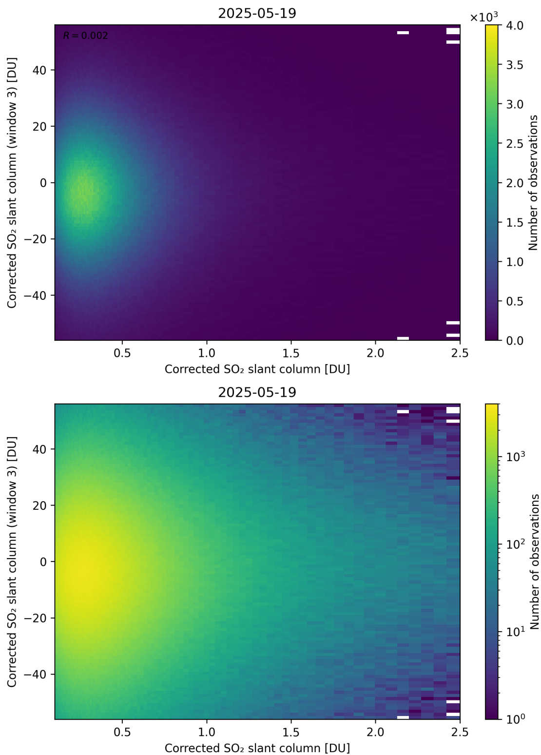
Figure 236: Scatter density plot of “Corrected SO 2 slant column” against “Corrected SO 2 slant column (window 3)” for 2025-05-18 to 2025-05-20.
