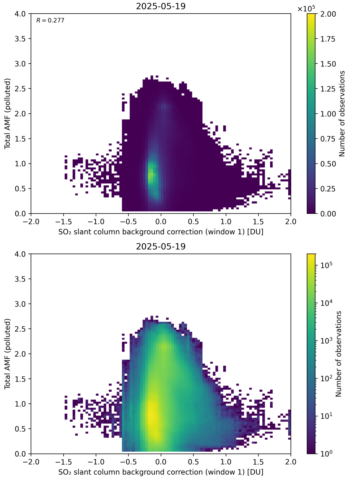
Figure 120: Scatter density plot of “SO 2 slant column background correction (window 1)” against “Total AMF (polluted)” for 2025-05-18 to 2025-05-20.
