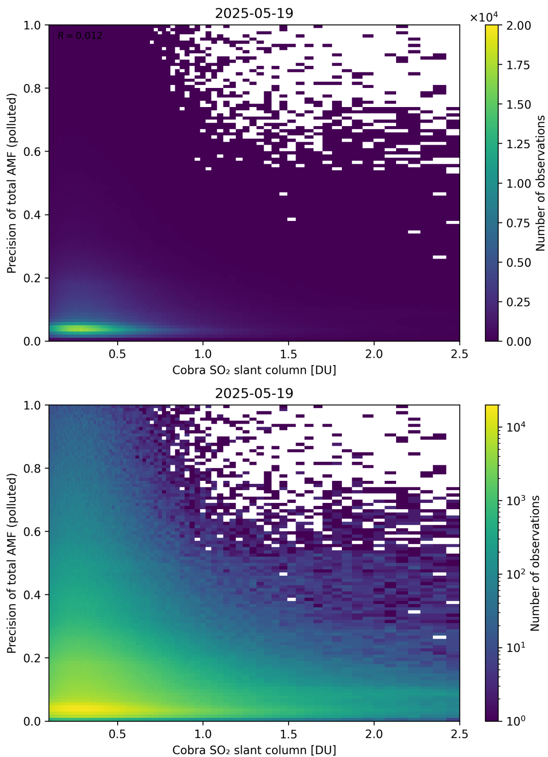
Figure 225: Scatter density plot of “Cobra SO 2 slant column” against “Precision of total AMF (polluted)” for 2025-05-18 to 2025-05-20.
