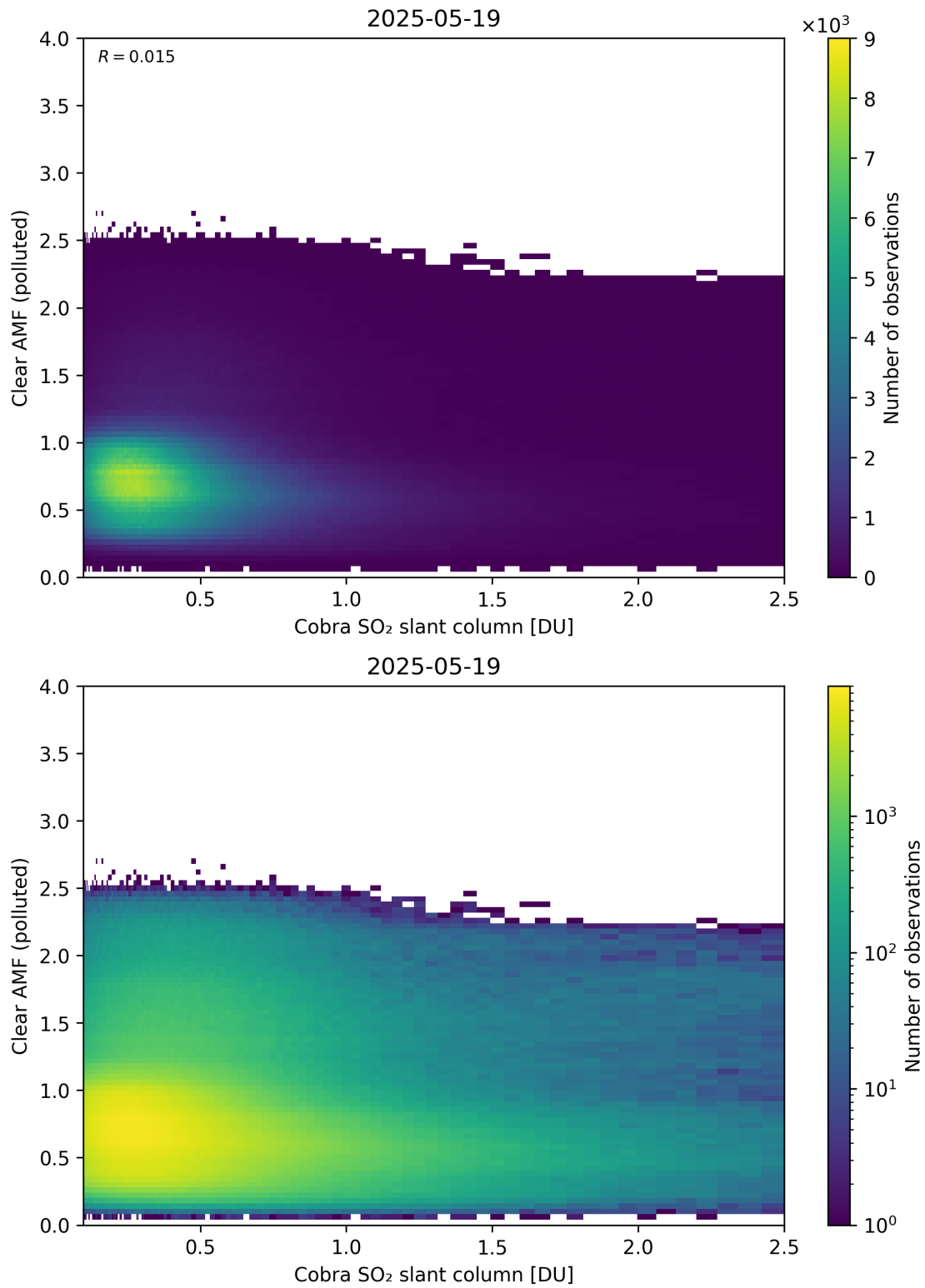
Figure 215: Scatter density plot of “Cobra SO 2 slant column” against “Clear AMF (polluted)” for 2025-05-18 to 2025-05-20.
