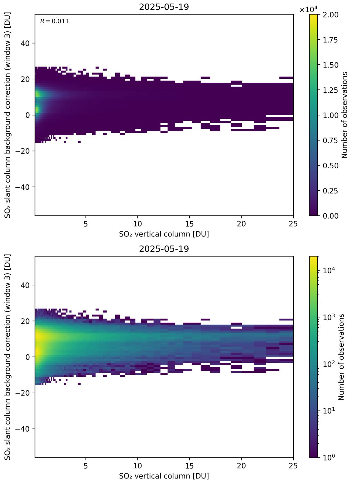
Figure 325: Scatter density plot of “SO 2 vertical column” against “SO 2 slant column background correction (window 3)” for 2025-05-18 to 2025-05-20.
