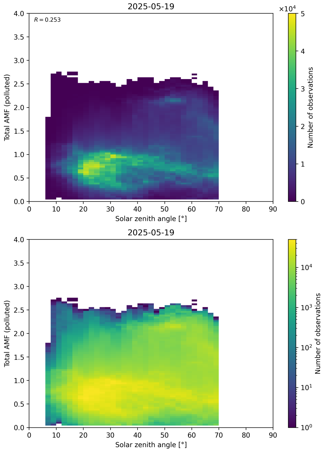
Figure 189: Scatter density plot of “Solar zenith angle” against “Total AMF (polluted)” for 2025-05-18 to 2025-05-20.
