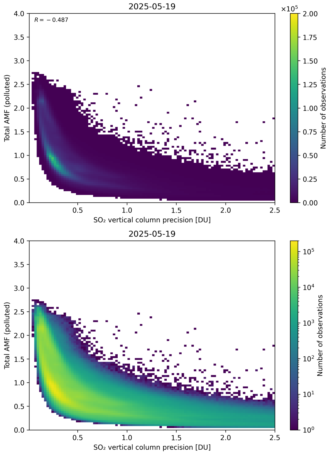
Figure 346: Scatter density plot of “SO 2 vertical column precision” against “Total AMF (polluted)” for 2025-05-18 to 2025-05-20.
