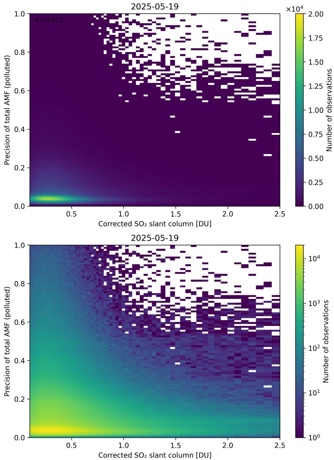
Figure 243: Scatter density plot of “Corrected SO 2 slant column” against “Precision of total AMF (polluted)” for 2025-05-18 to 2025-05-20.
