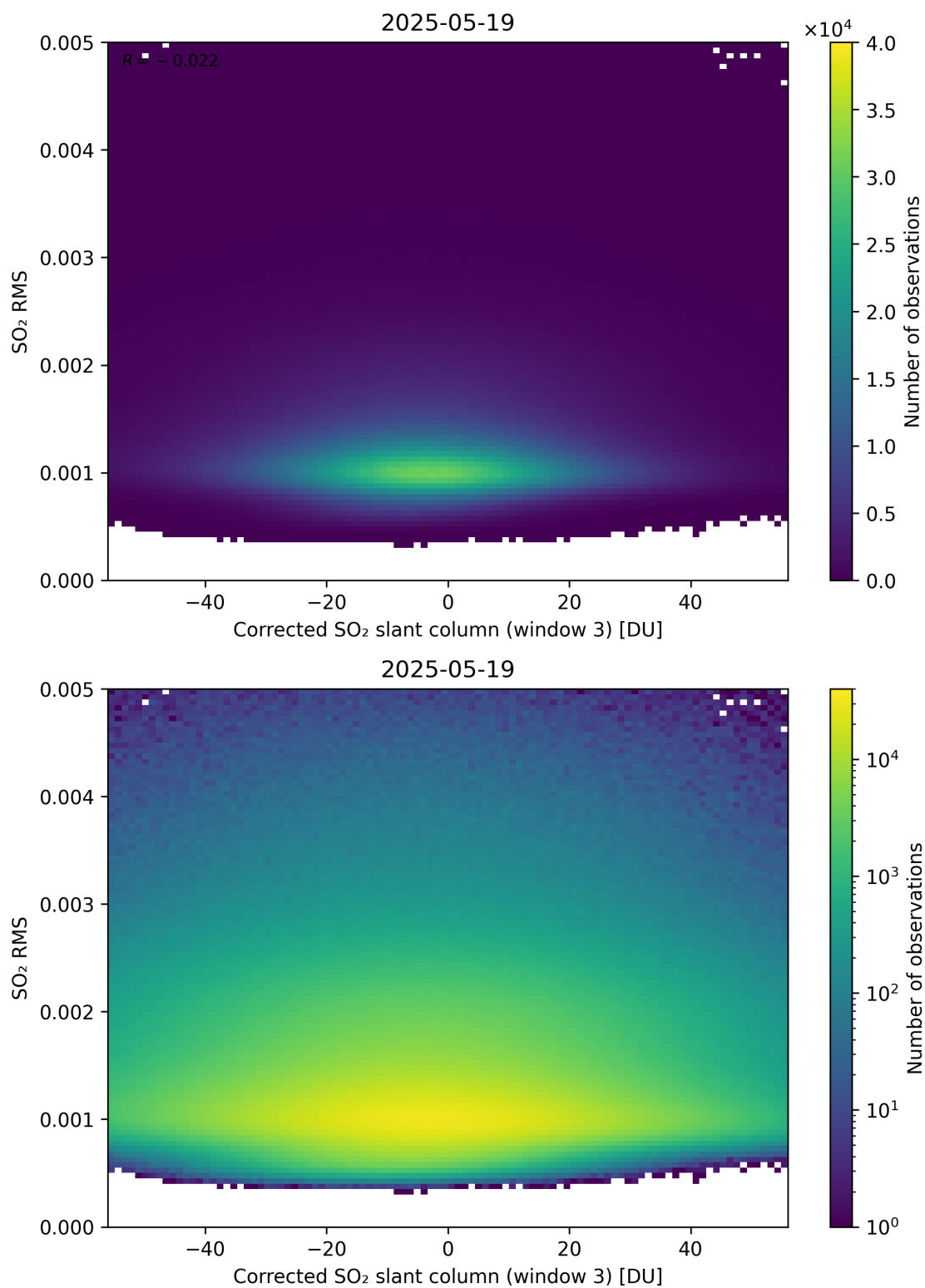
Figure 258: Scatter density plot of “Corrected SO 2 slant column (window 3)” against “SO 2 RMS” for 2025-05-18 to 2025-05-20.
