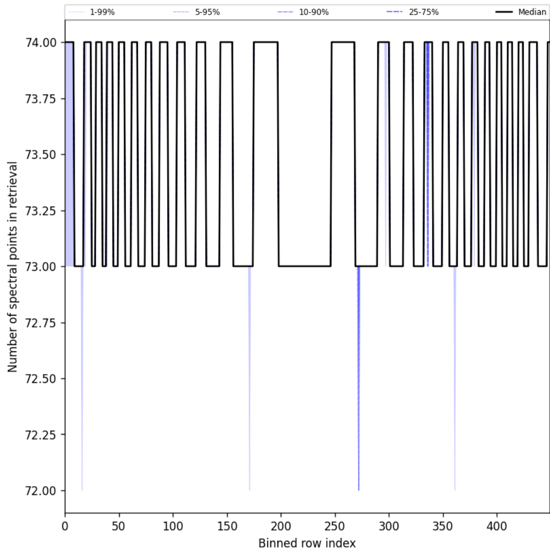
Figure 108: Along track statistics of “Number of spectral points in retrieval” for 2025-05-18 to 2025-05-20
