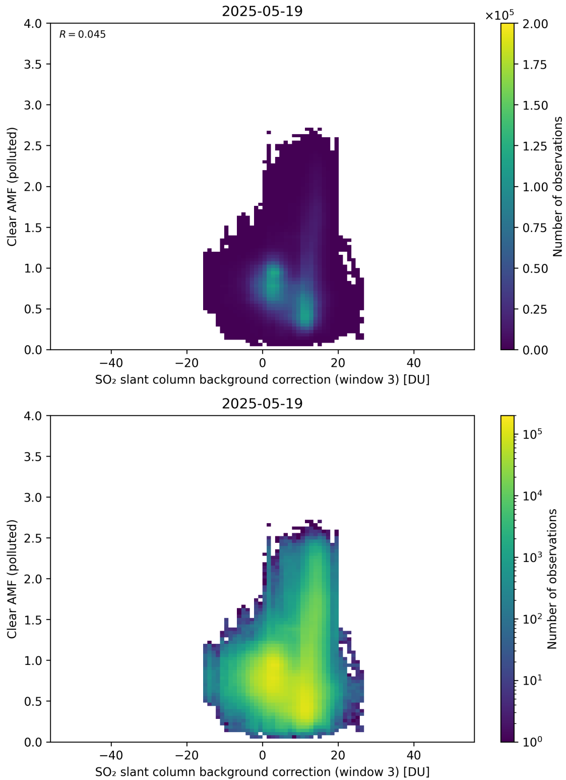
Figure 135: Scatter density plot of “SO 2 slant column background correction (window 3)” against “Clear AMF (polluted)” for 2025-05-18 to 2025-05-20.
