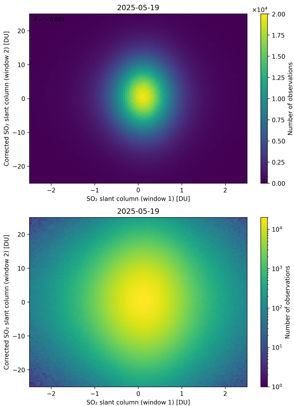
Figure 283: Scatter density plot of “SO 2 slant column (window 1)” against “Corrected SO 2 slant column (window 2)” for 2025-05-18 to 2025-05-20.
