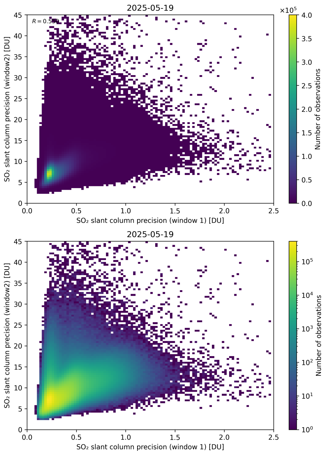
Figure 277: Scatter density plot of “SO 2 slant column precision (window 1)” against “SO 2 slant column precision (window2)” for 2025-05-18 to 2025-05-20.
