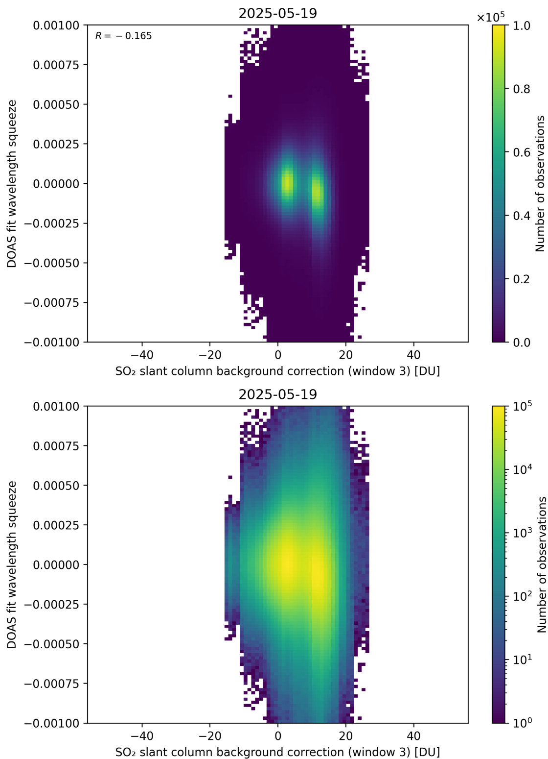
Figure 133: Scatter density plot of “SO 2 slant column background correction (window 3)” against “DOAS fit wavelength squeeze” for 2025-05-18 to 2025-05-20.
