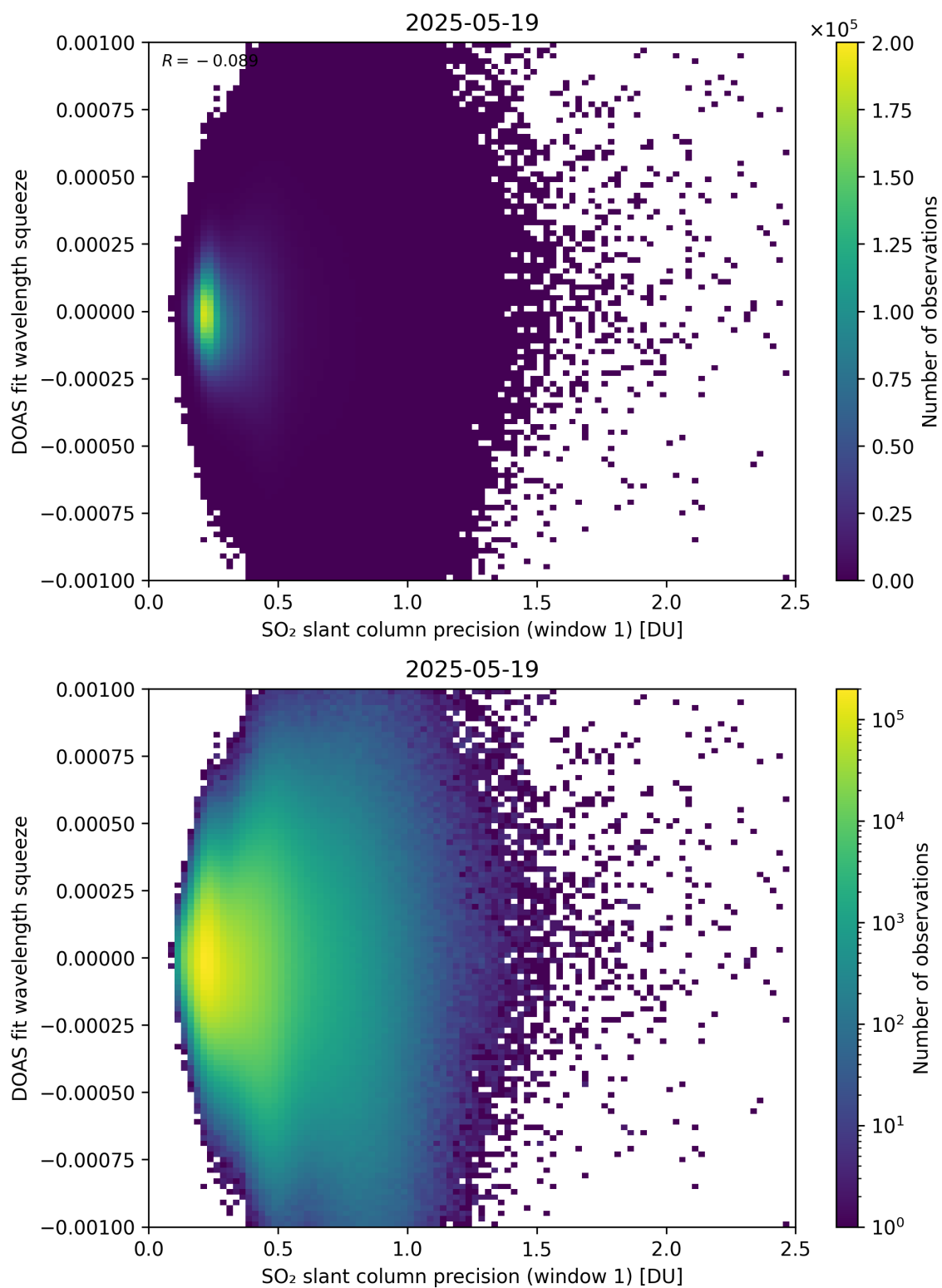
Figure 272: Scatter density plot of “SO 2 slant column precision (window 1)” against “DOAS fit wavelength squeeze” for 2025-05-18 to 2025-05-20.
