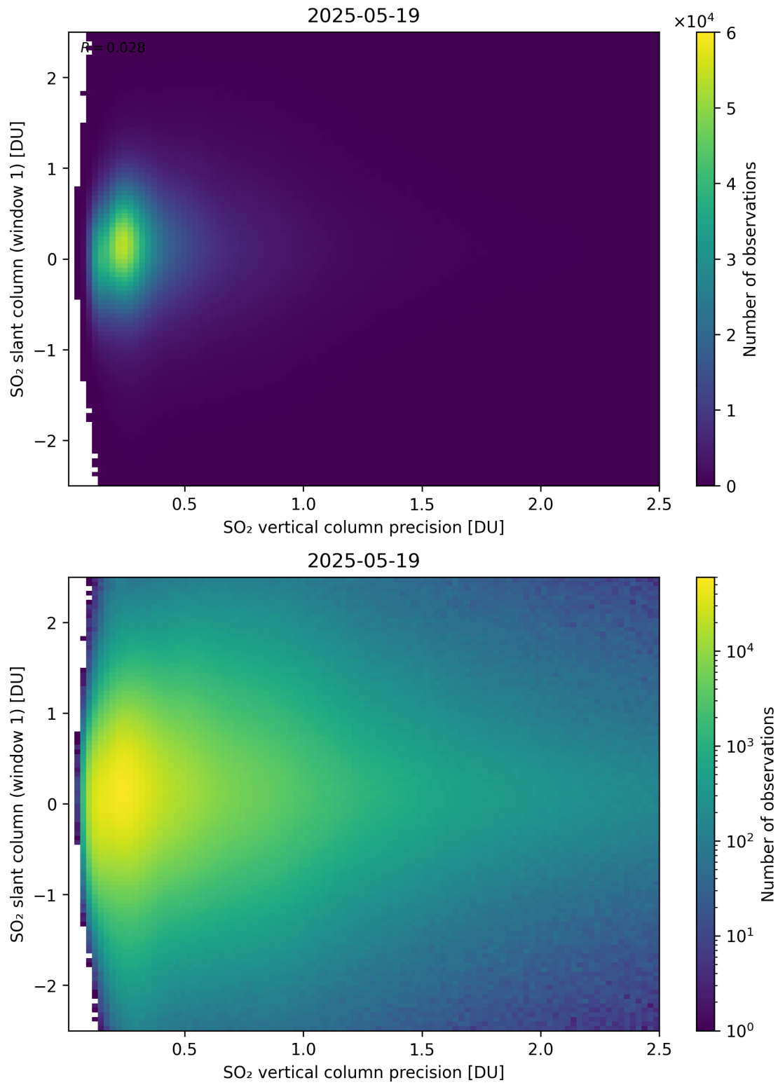
Figure 341: Scatter density plot of “SO 2 vertical column precision” against “SO 2 slant column (window 1)” for 2025-05-18 to 2025-05-20.
