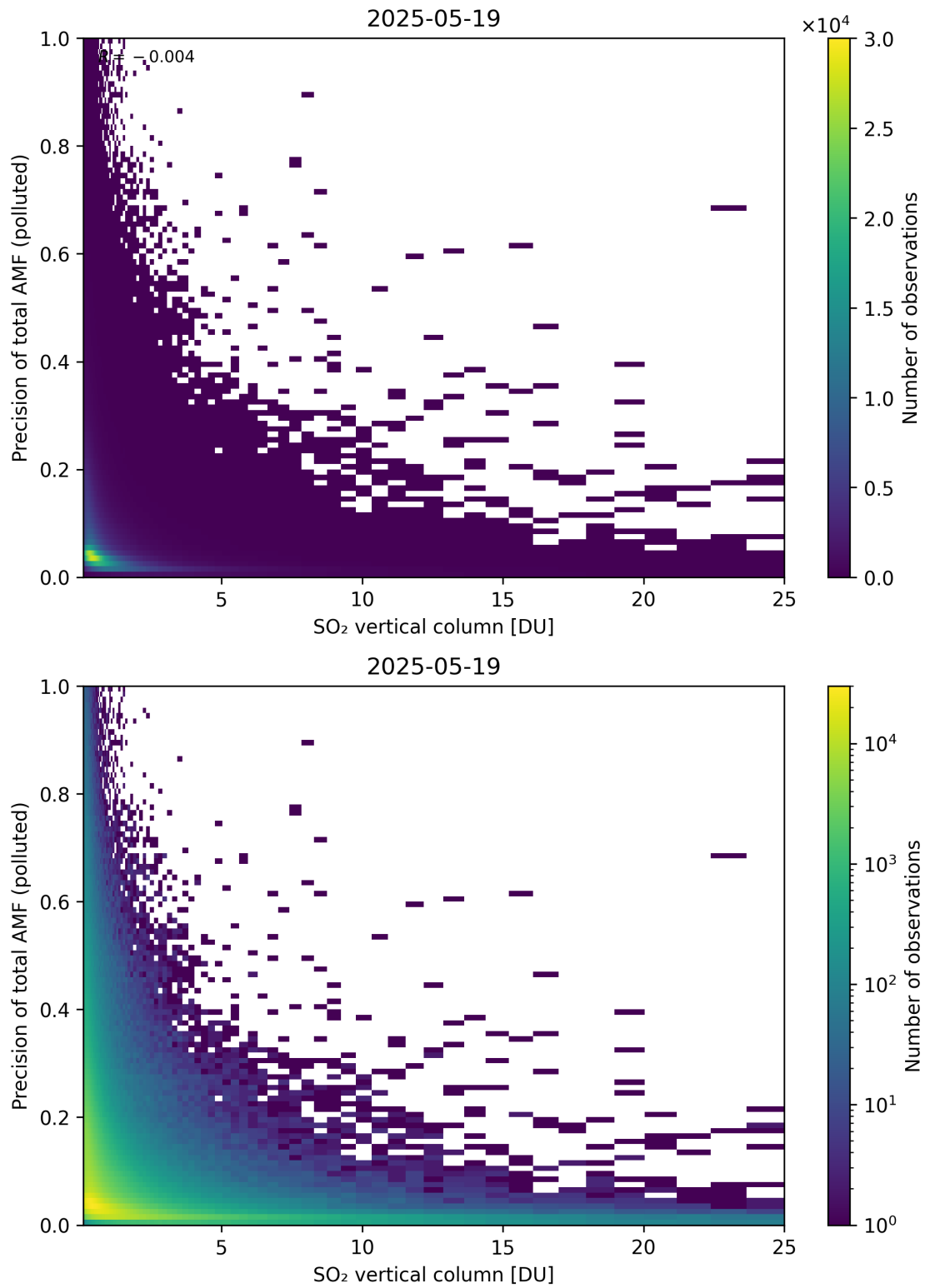
Figure 360: Scatter density plot of “SO 2 vertical column” against “Precision of total AMF (polluted)” for 2025-05-18 to 2025-05-20.
