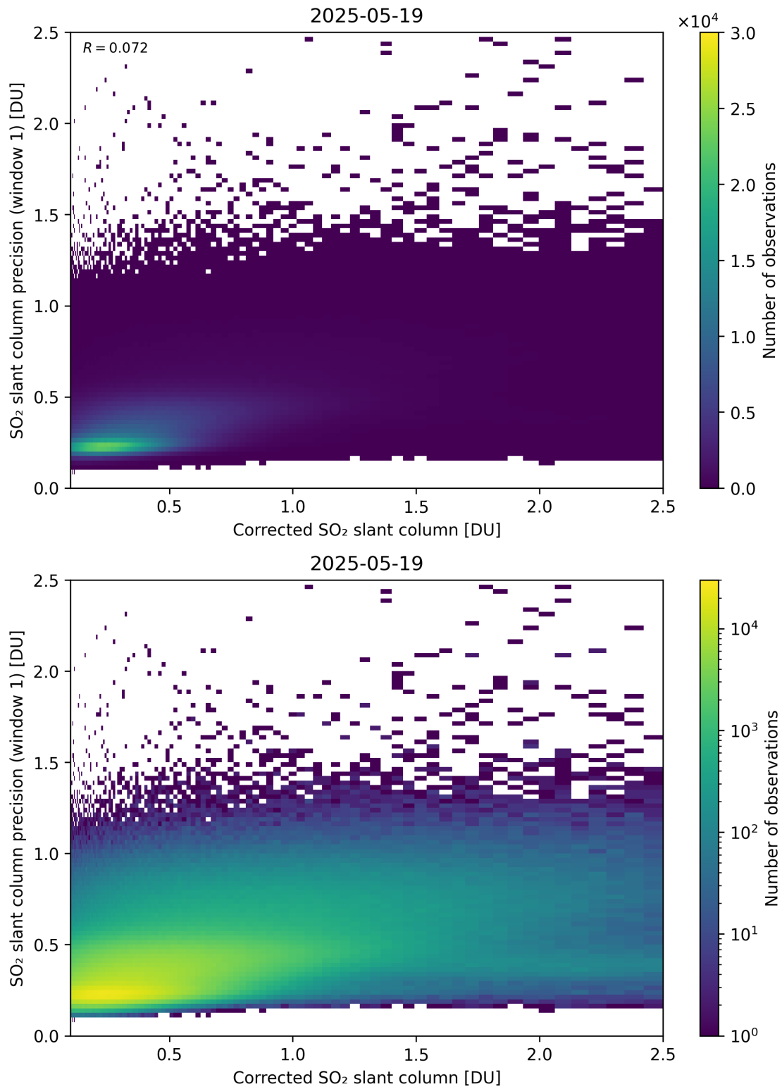
Figure 238: Scatter density plot of “Corrected SO 2 slant column” against “SO 2 slant column precision (window 1)” for 2025-05-18 to 2025-05-20.
