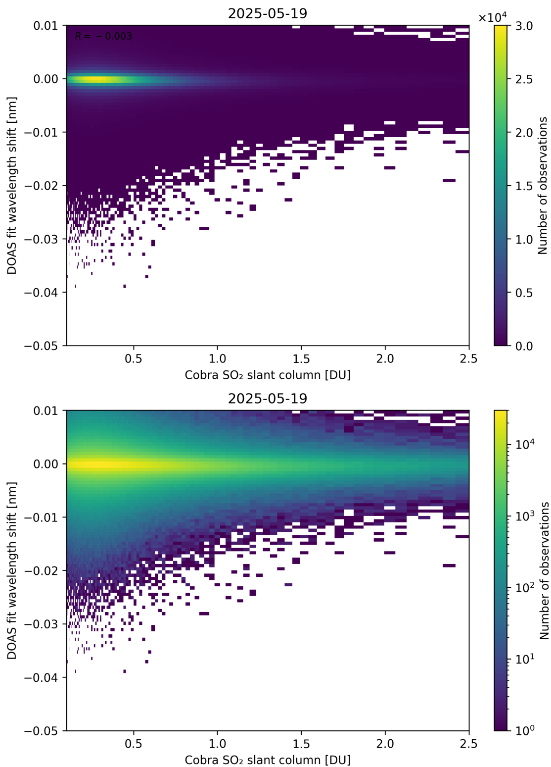
Figure 196: Scatter density plot of “Cobra SO 2 slant column” against “DOAS fit wavelength shift” for 2025-05-18 to 2025-05-20.
