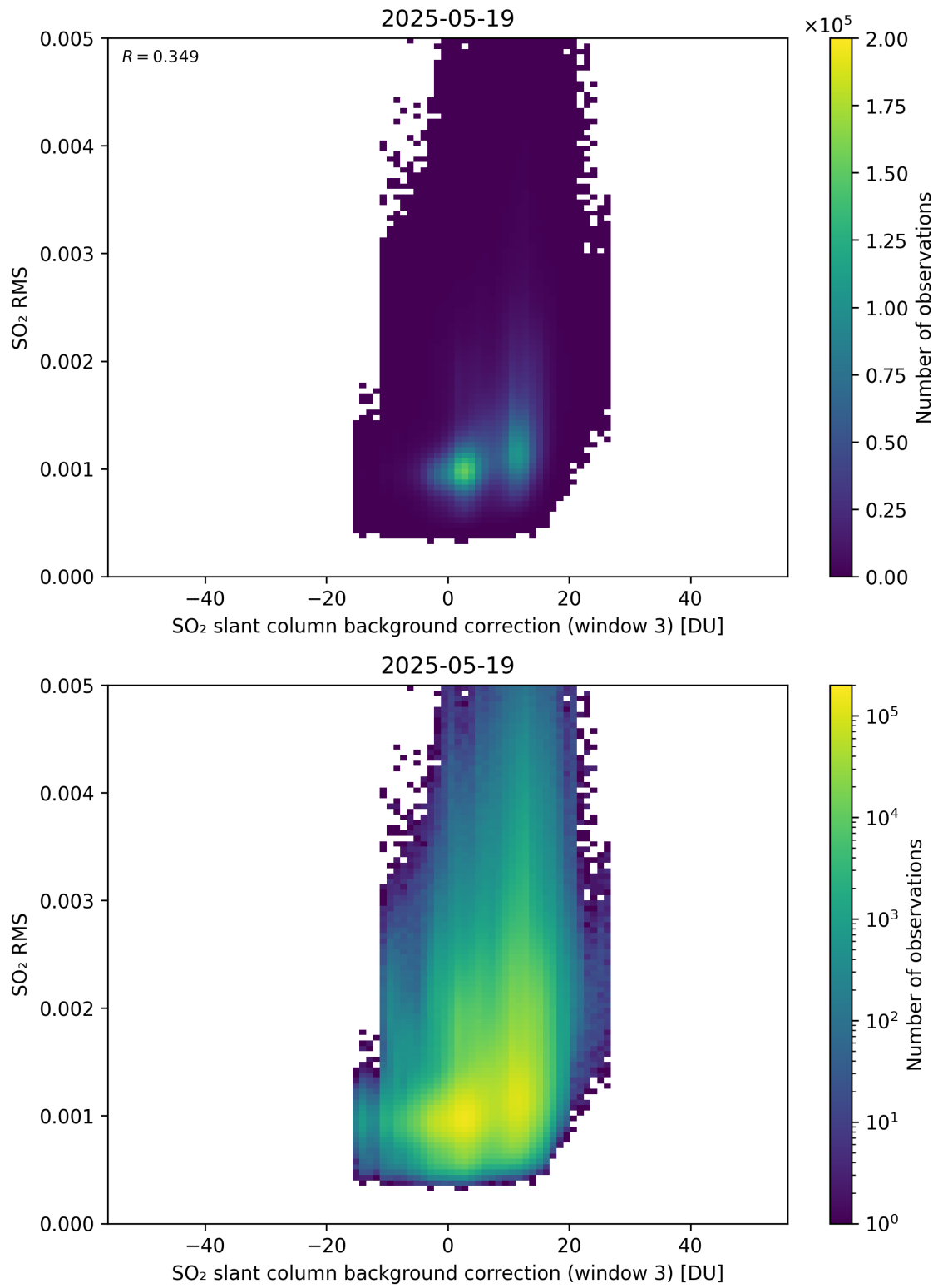
Figure 134: Scatter density plot of “SO 2 slant column background correction (window 3)” against “SO 2 RMS” for 2025-05-18 to 2025-05-20.
