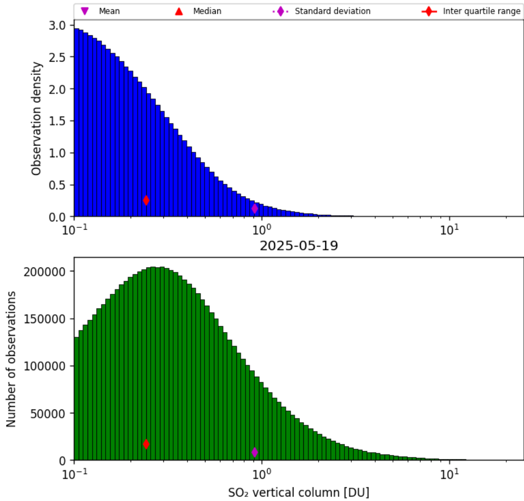
Figure 58: Histogram of “SO 2 vertical column” for 2025-05-18 to 2025-05-20
