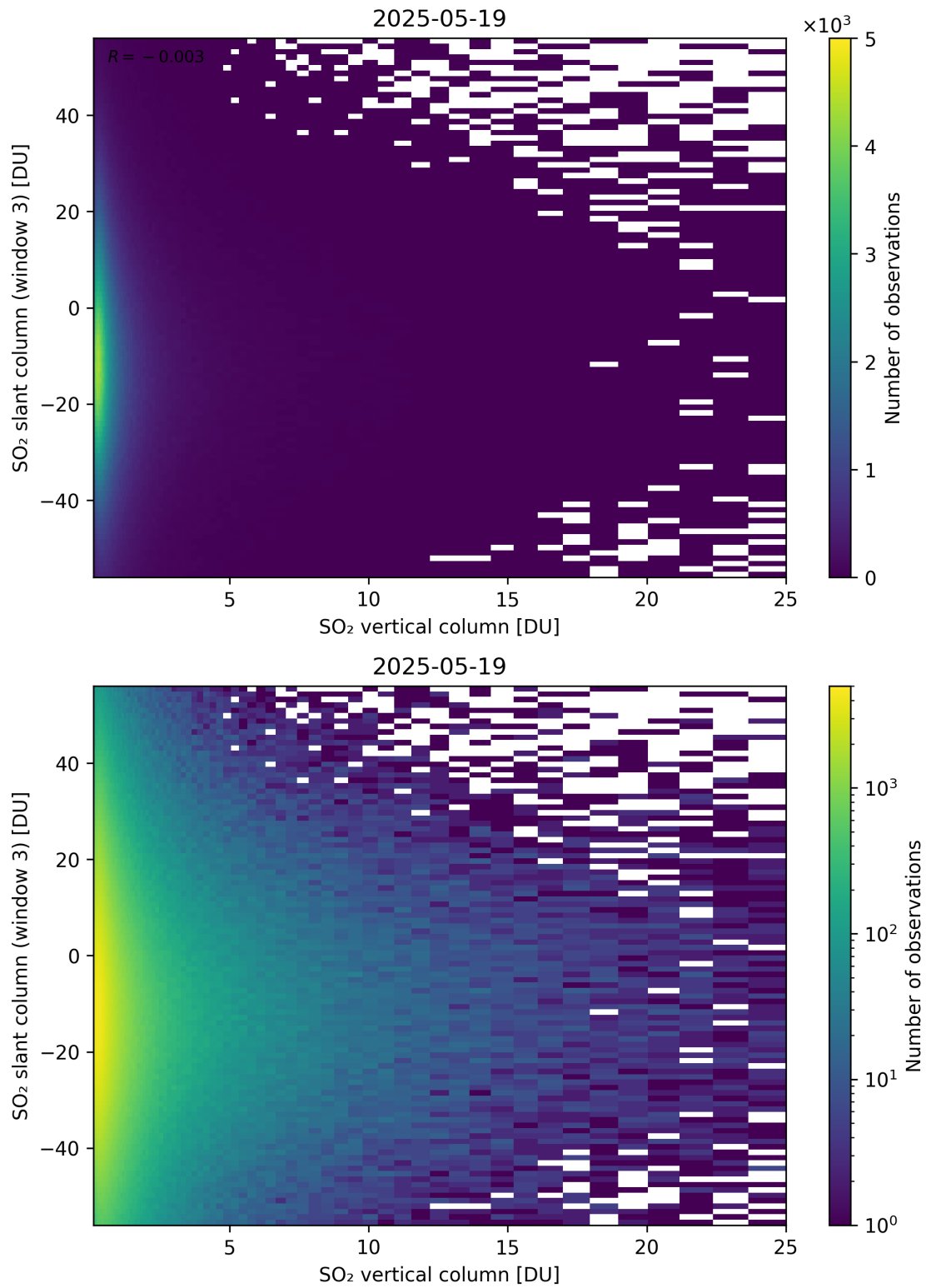
Figure 357: Scatter density plot of “SO 2 vertical column” against “SO 2 slant column (window 3)” for 2025-05-18 to 2025-05-20.
