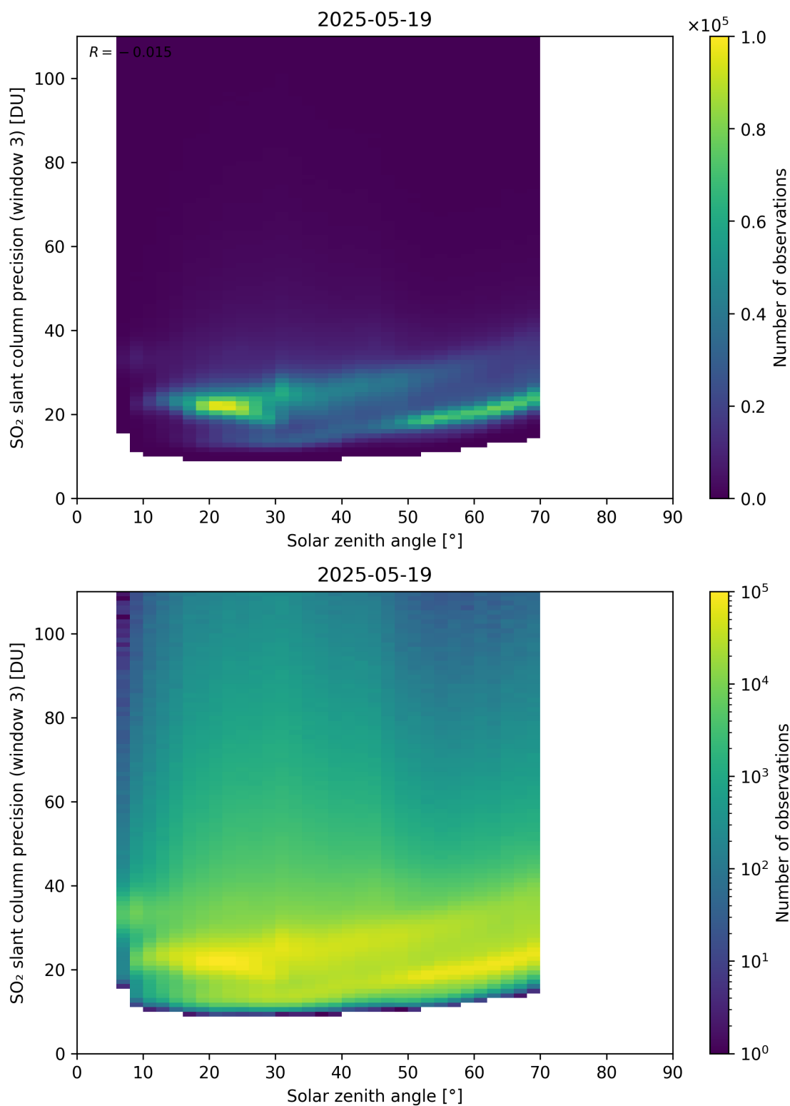
Figure 188: Scatter density plot of “Solar zenith angle” against “SO 2 slant column precision (window 3)” for 2025-05-18 to 2025-05-20.
