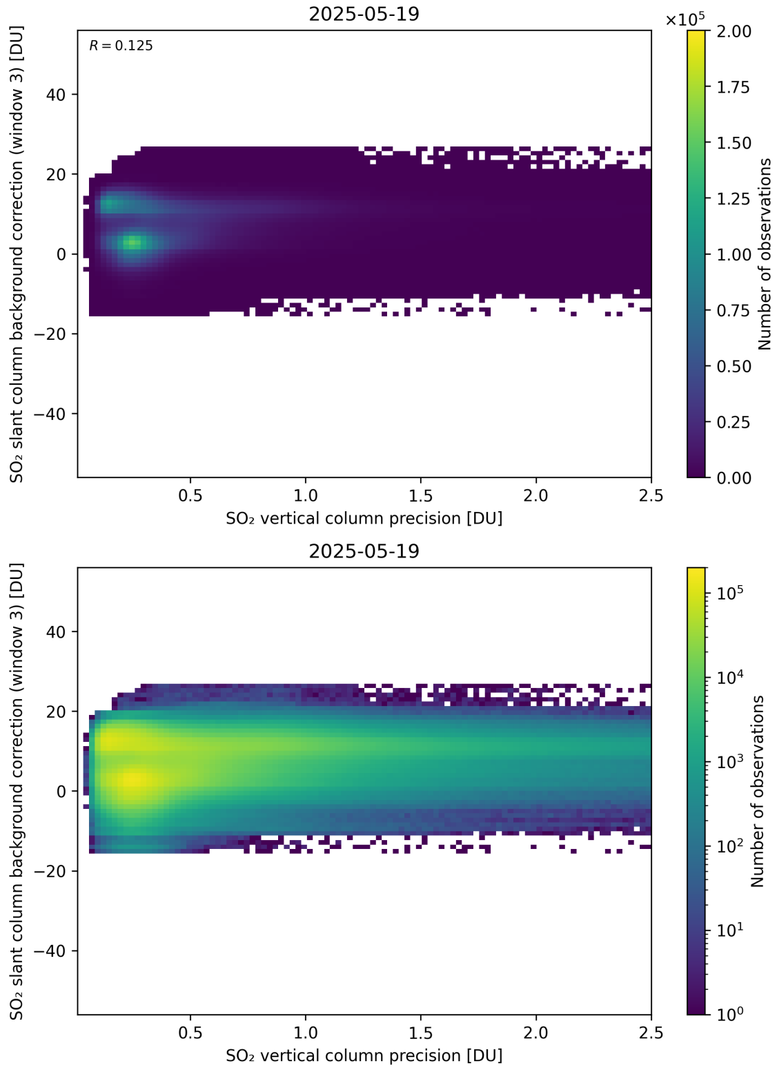
Figure 331: Scatter density plot of “SO 2 vertical column precision” against “SO 2 slant column background correction (window 3)” for 2025-05-18 to 2025-05-20.
