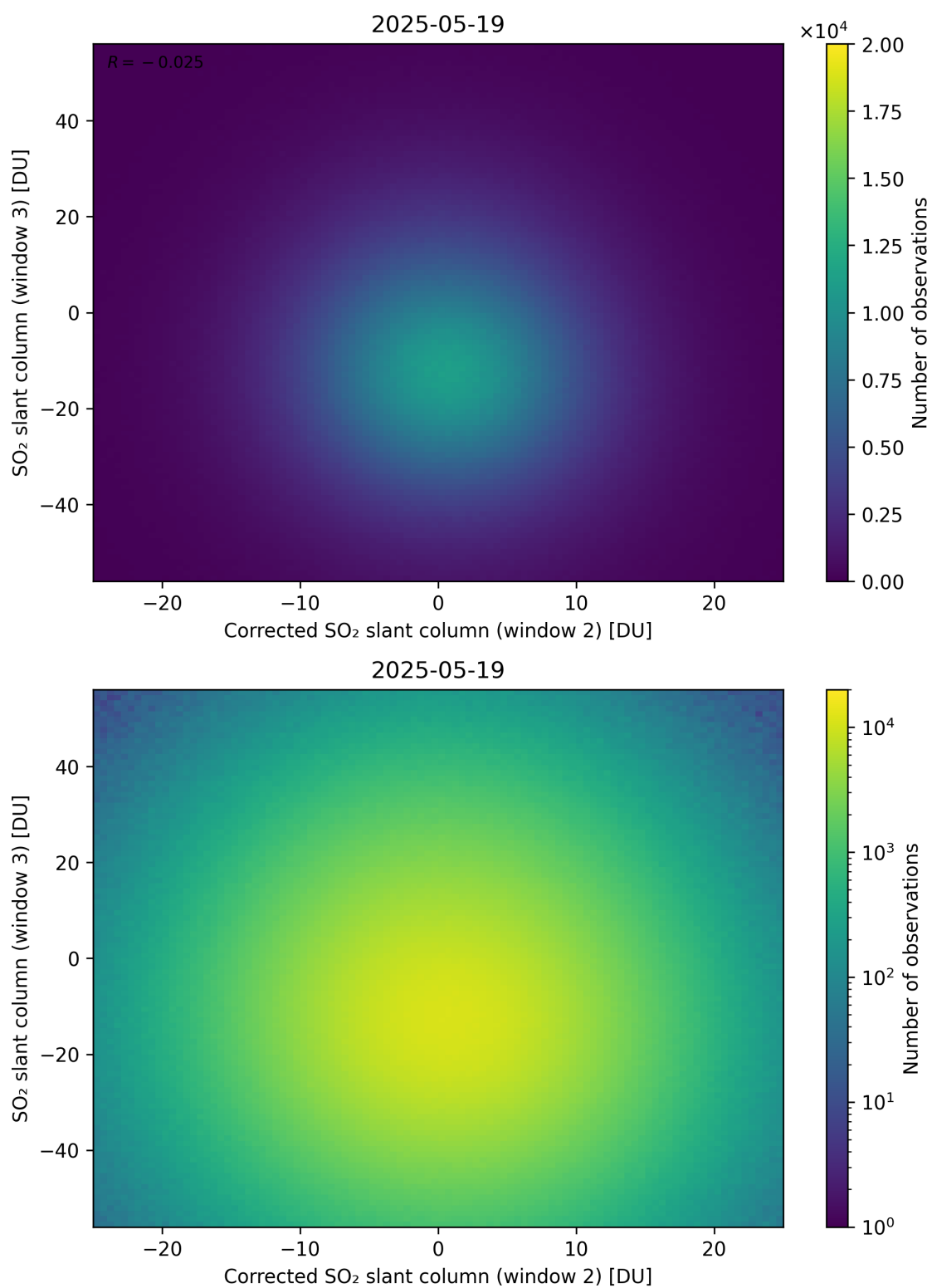
Figure 251: Scatter density plot of “Corrected SO 2 slant column (window 2)” against “SO 2 slant column (window 3)” for 2025-05-18 to 2025-05-20.
