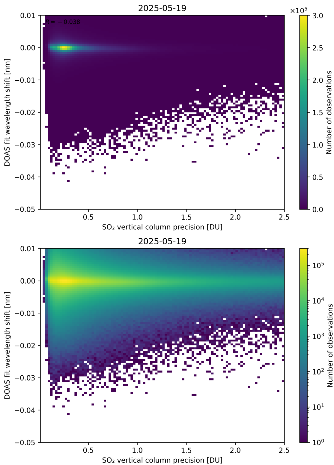
Figure 332: Scatter density plot of “SO 2 vertical column precision” against “DOAS fit wavelength shift” for 2025-05-18 to 2025-05-20.
