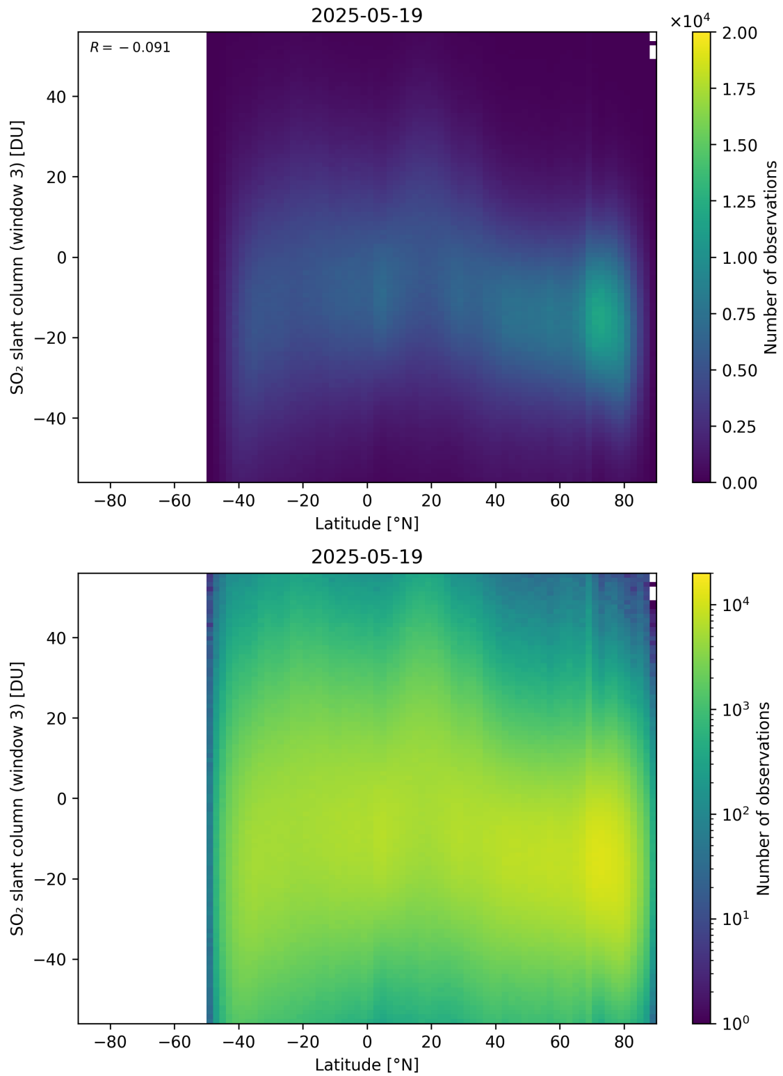
Figure 165: Scatter density plot of “Latitude” against “SO 2 slant column (window 3)” for 2025-05-18 to 2025-05-20.
