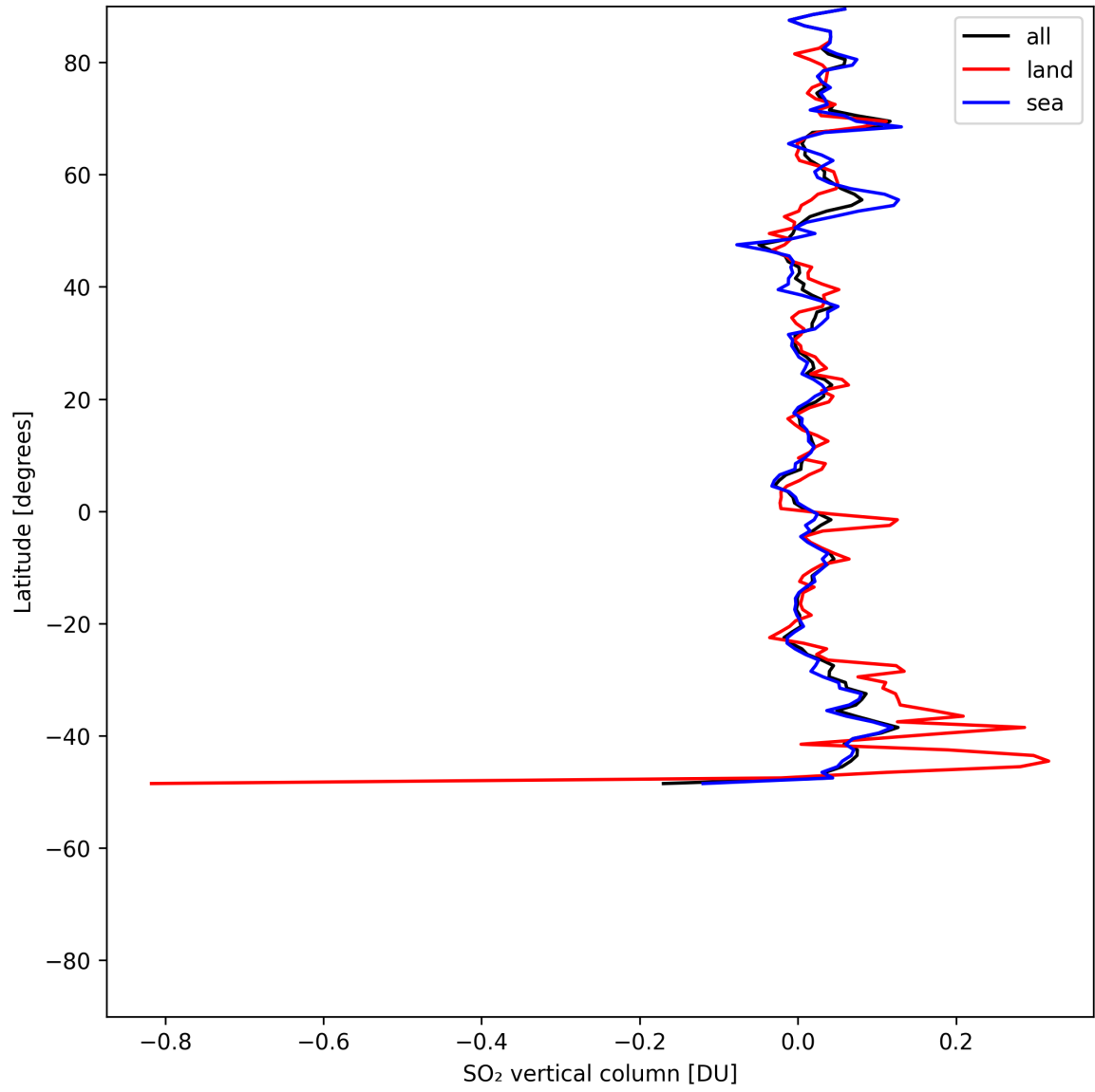
Figure 32: Zonal average of “SO 2 vertical column” for 2025-05-18 to 2025-05-20.
