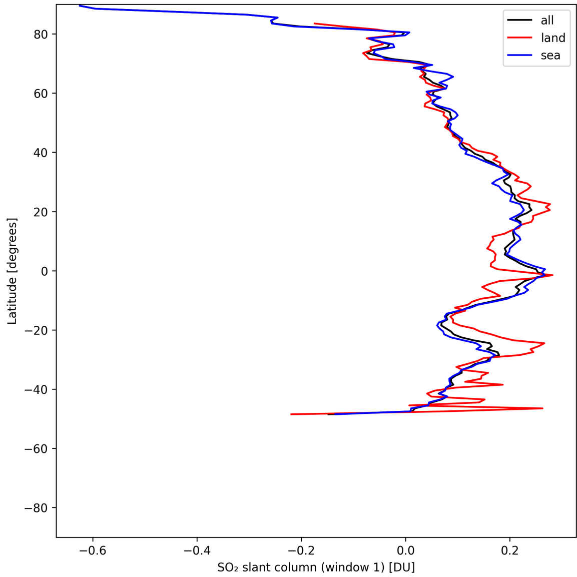
Figure 37: Zonal average of “SO 2 slant column (window 1)” for 2025-05-18 to 2025-05-20.
