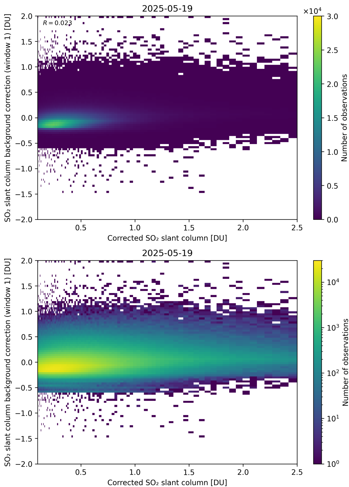
Figure 226: Scatter density plot of “Corrected SO 2 slant column” against “SO 2 slant column background correction (window 1)” for 2025-05-18 to 2025-05-20.
