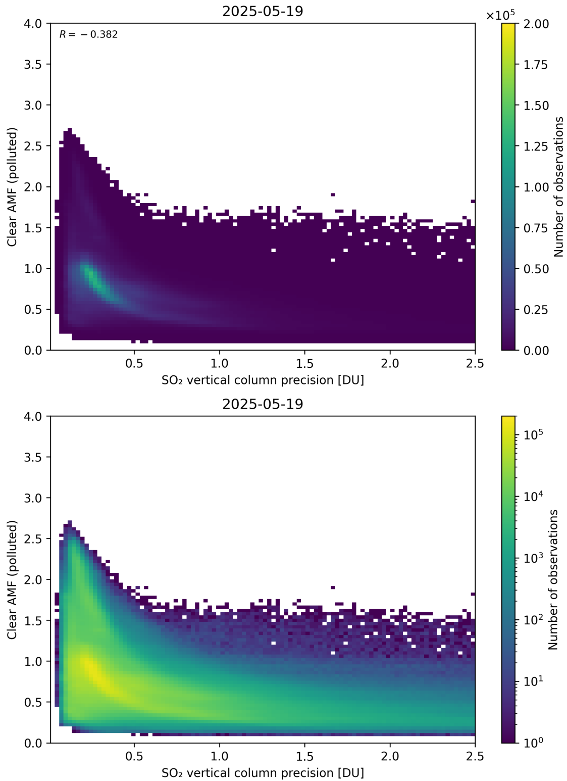
Figure 335: Scatter density plot of “SO 2 vertical column precision” against “Clear AMF (polluted)” for 2025-05-18 to 2025-05-20.
