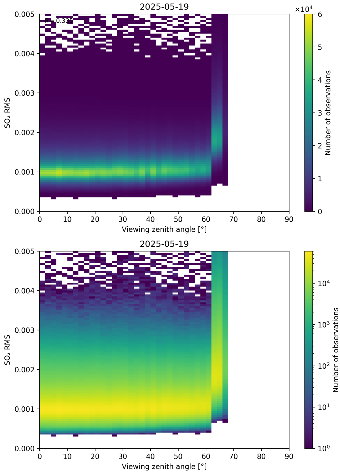
Figure 367: Scatter density plot of “Viewing zenith angle” against “SO 2 RMS” for 2025-05-18 to 2025-05-20.
