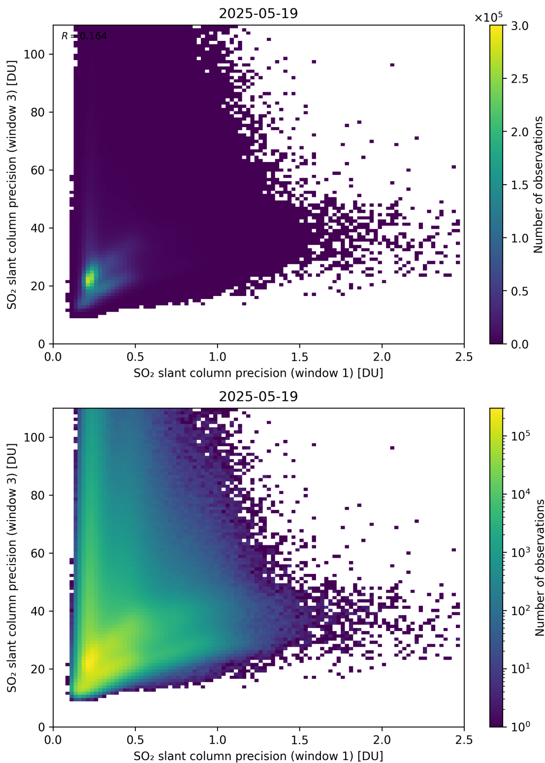
Figure 279: Scatter density plot of “SO 2 slant column precision (window 1)” against “SO 2 slant column precision (window 3)” for 2025-05-18 to 2025-05-20.
