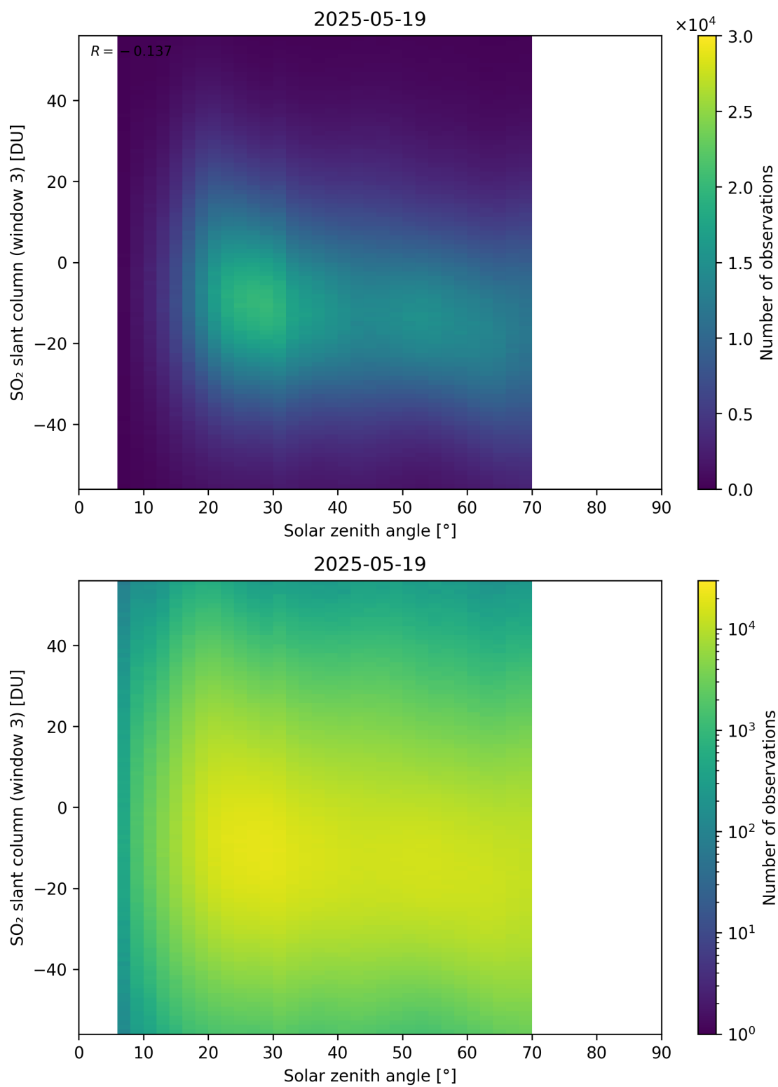
Figure 187: Scatter density plot of “Solar zenith angle” against “SO 2 slant column (window 3)” for 2025-05-18 to 2025-05-20.
