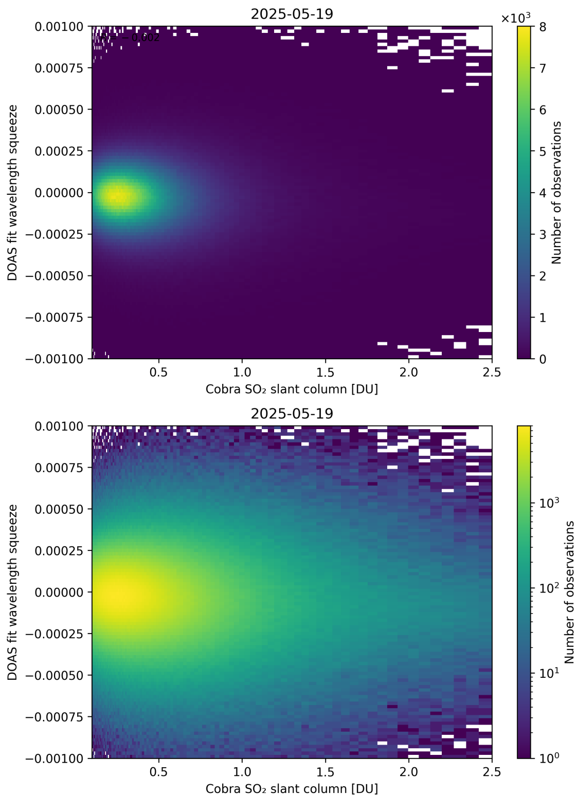
Figure 197: Scatter density plot of “Cobra SO 2 slant column” against “DOAS fit wavelength squeeze” for 2025-05-18 to 2025-05-20.
