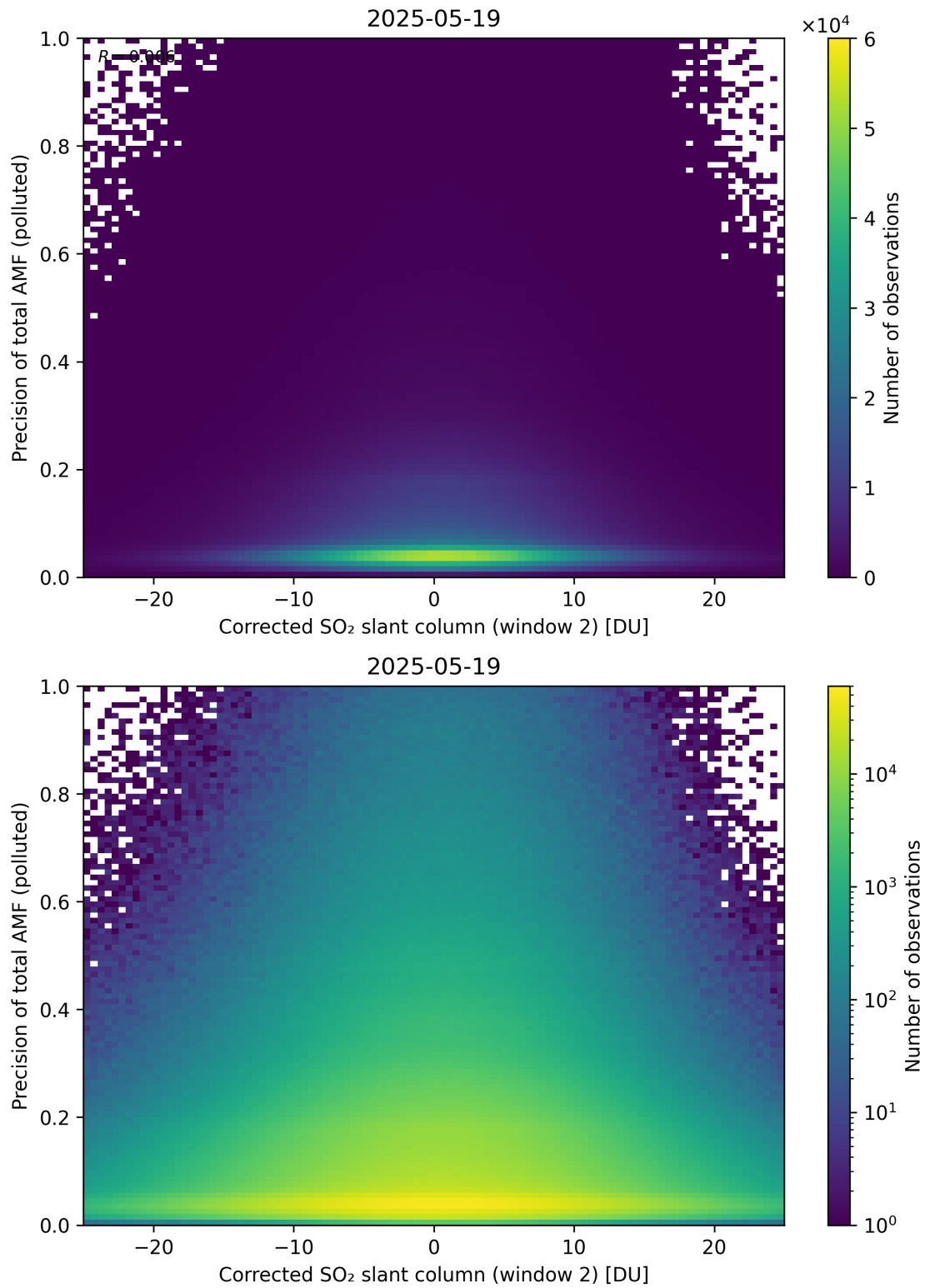
Figure 254: Scatter density plot of “Corrected SO 2 slant column (window 2)” against “Precision of total AMF (polluted)” for 2025-05-18 to 2025-05-20.
