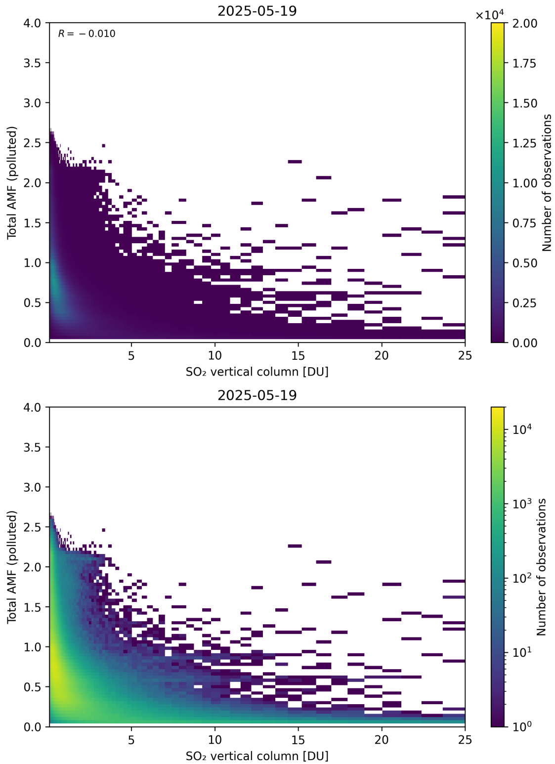
Figure 359: Scatter density plot of “SO 2 vertical column” against “Total AMF (polluted)” for 2025-05-18 to 2025-05-20.
