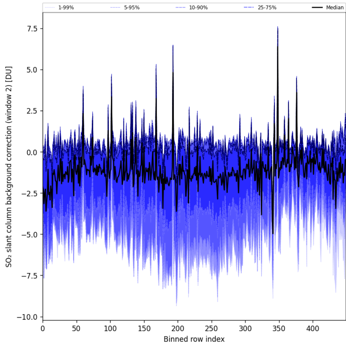
Figure 96: Along track statistics of “SO 2 slant column background correction (window 2)” for 2025-05-18 to 2025-05-20
