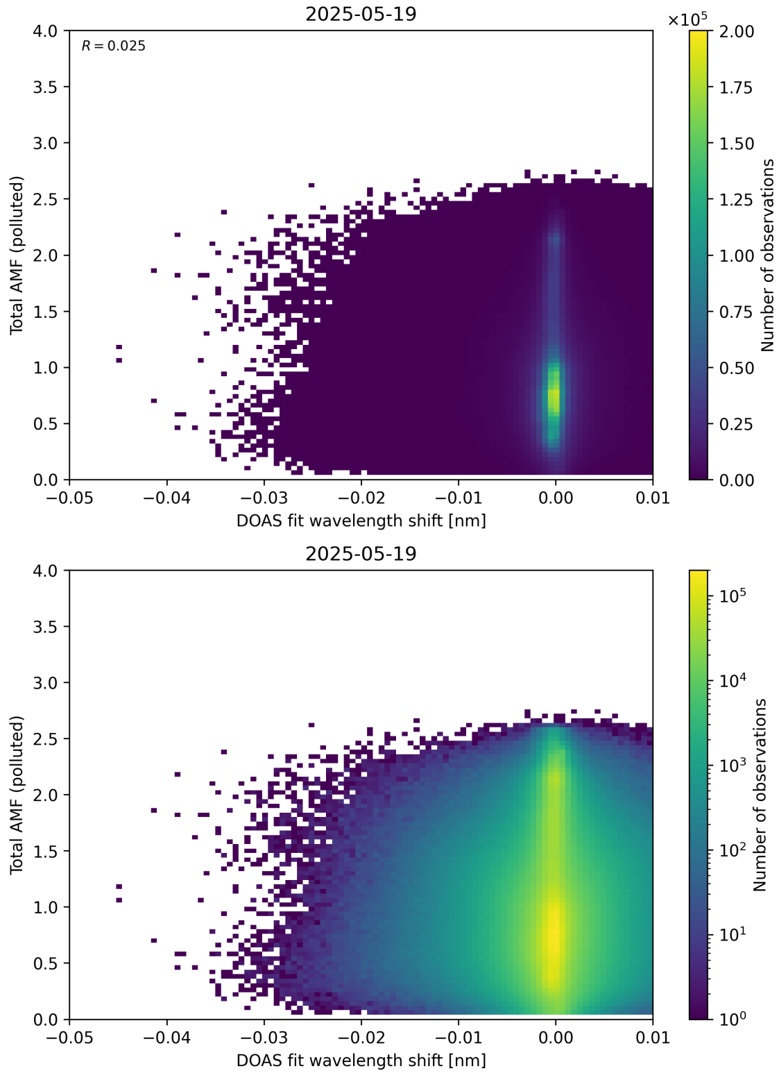
Figure 141: Scatter density plot of “DOAS fit wavelength shift” against “Total AMF (polluted)” for 2025-05-18 to 2025-05-20.
