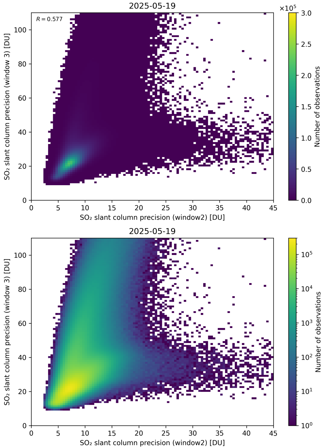
Figure 300: Scatter density plot of “SO 2 slant column precision (window2)” against “SO 2 slant column precision (window 3)” for 2025-05-18 to 2025-05-20.
