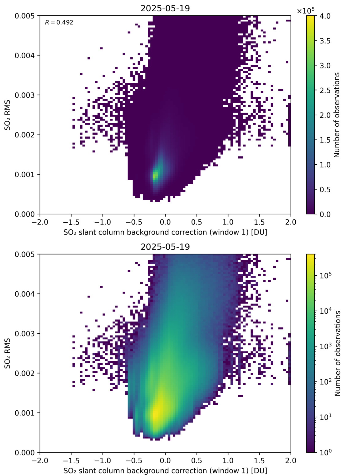
Figure 113: Scatter density plot of “SO 2 slant column background correction (window 1)” against “SO 2 RMS” for 2025-05-18 to 2025-05-20.
