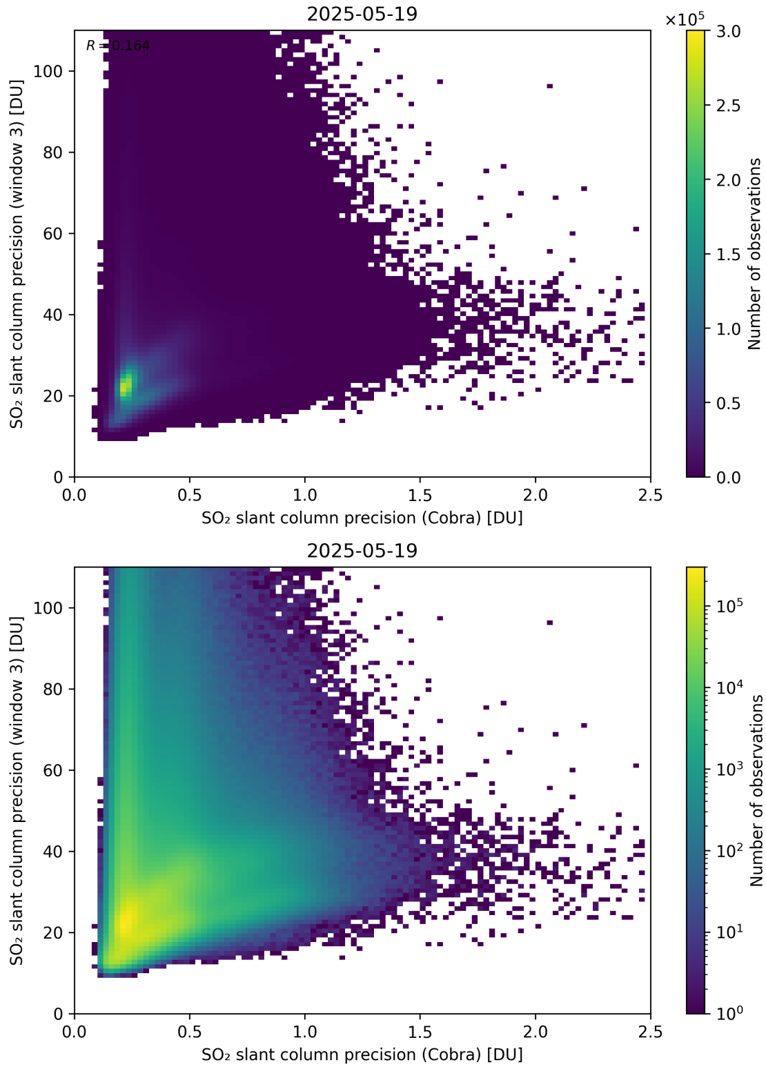
Figure 212: Scatter density plot of “SO 2 slant column precision (Cobra)” against “SO 2 slant column precision (window 3)” for 2025-05-18 to 2025-05-20.
