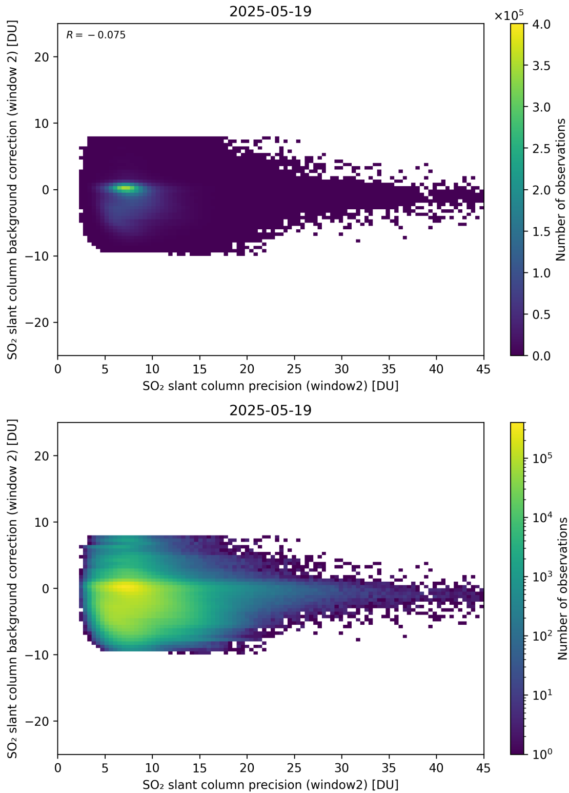
Figure 291: Scatter density plot of “SO 2 slant column precision (window2)” against “SO 2 slant column background correction (window 2)” for 2025-05-18 to 2025-05-20.
