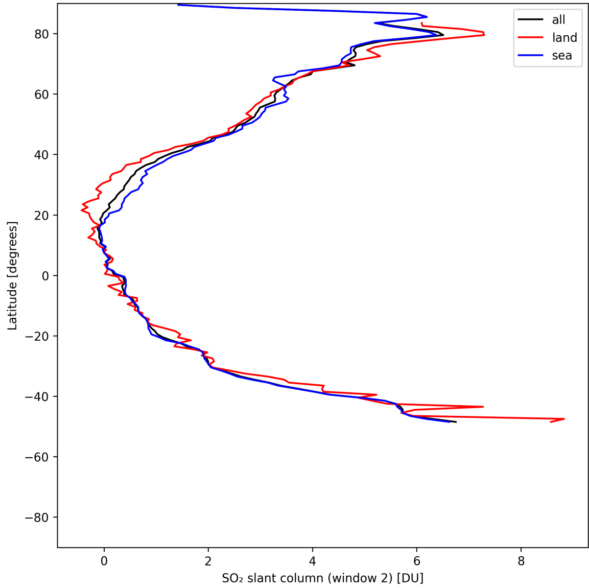
Figure 41: Zonal average of “SO 2 slant column (window 2)” for 2025-05-18 to 2025-05-20.
