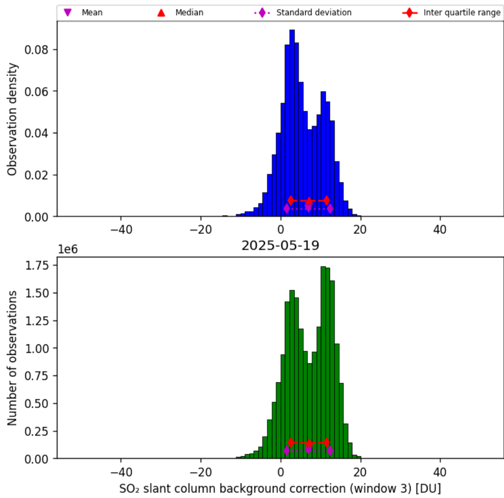
Figure 74: Histogram of “SO 2 slant column background correction (window 3)” for 2025-05-18 to 2025-05-20
