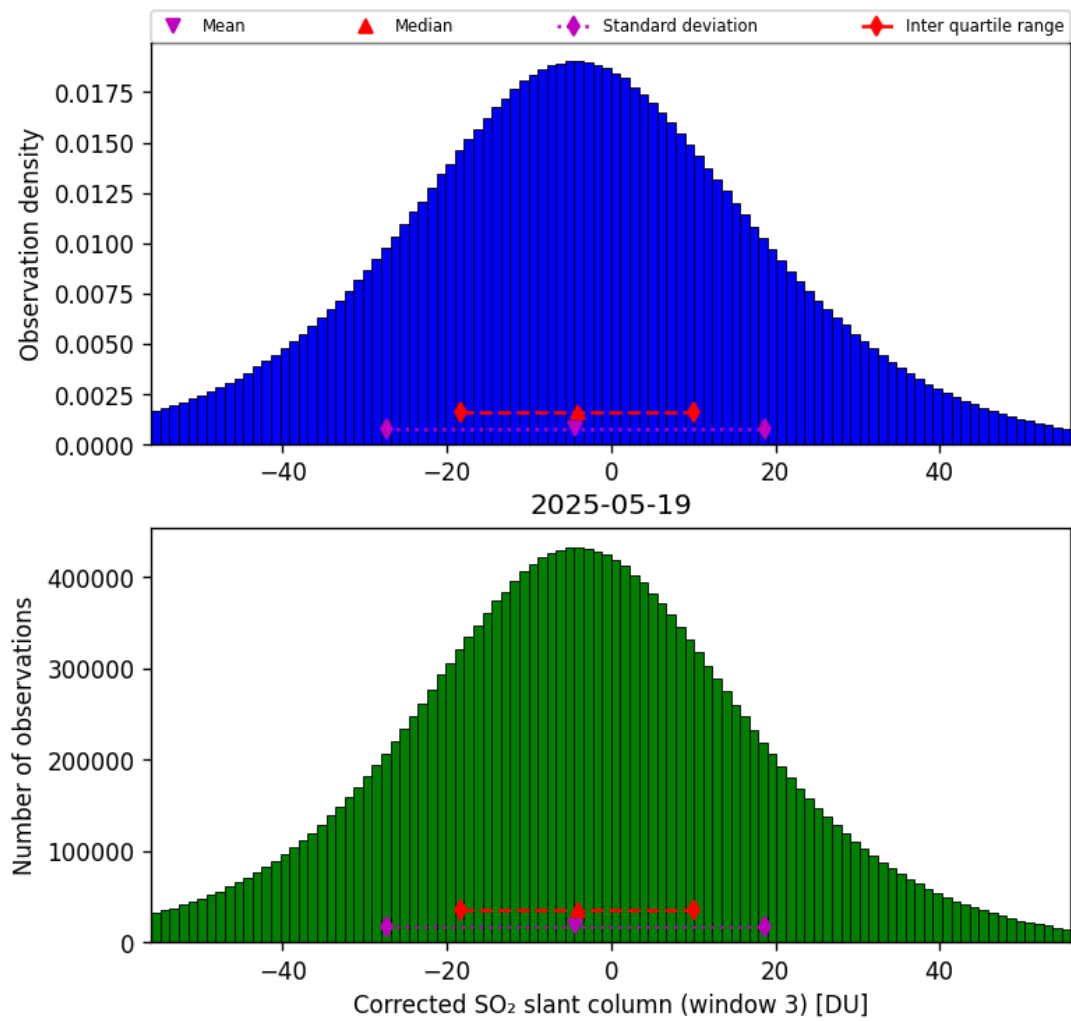
Figure 73: Histogram of “Corrected SO 2 slant column (window 3)” for 2025-05-18 to 2025-05-20
