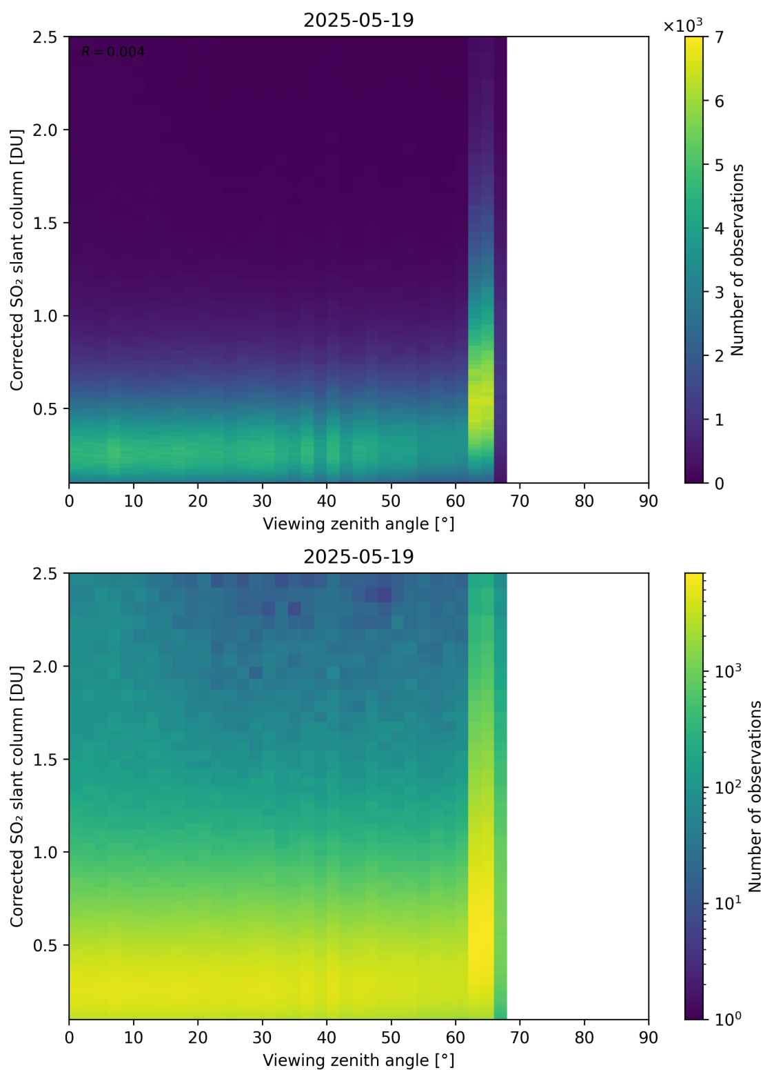
Figure 373: Scatter density plot of “Viewing zenith angle” against “Corrected SO 2 slant column” for 2025-05-18 to 2025-05-20.
