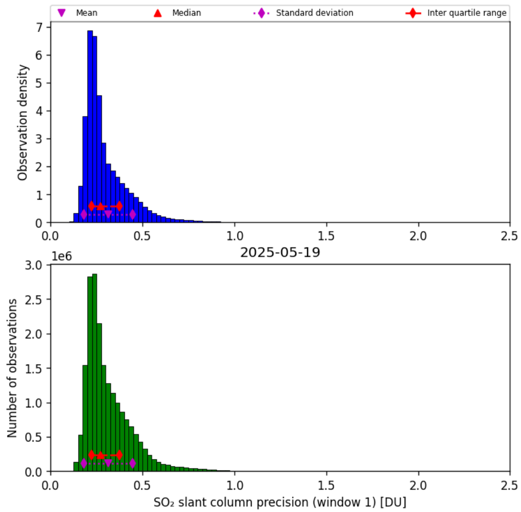
Figure 64: Histogram of “SO 2 slant column precision (window 1)” for 2025-05-18 to 2025-05-20
