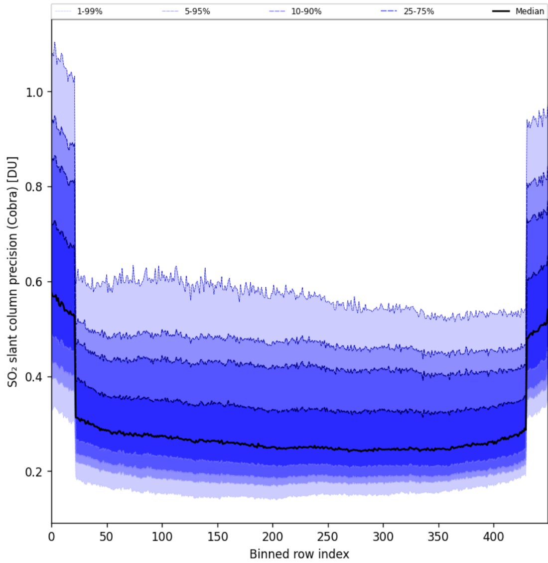
Figure 88: Along track statistics of “SO 2 slant column precision (Cobra)” for 2025-05-18 to 2025-05-20
