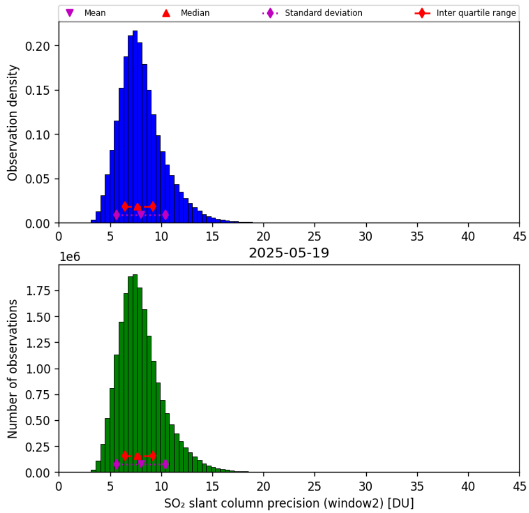
Figure 68: Histogram of “SO 2 slant column precision (window2)” for 2025-05-18 to 2025-05-20
