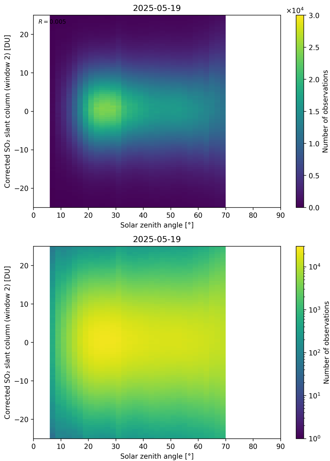
Figure 182: Scatter density plot of “Solar zenith angle” against “Corrected SO 2 slant column (window 2)” for 2025-05-18 to 2025-05-20.
