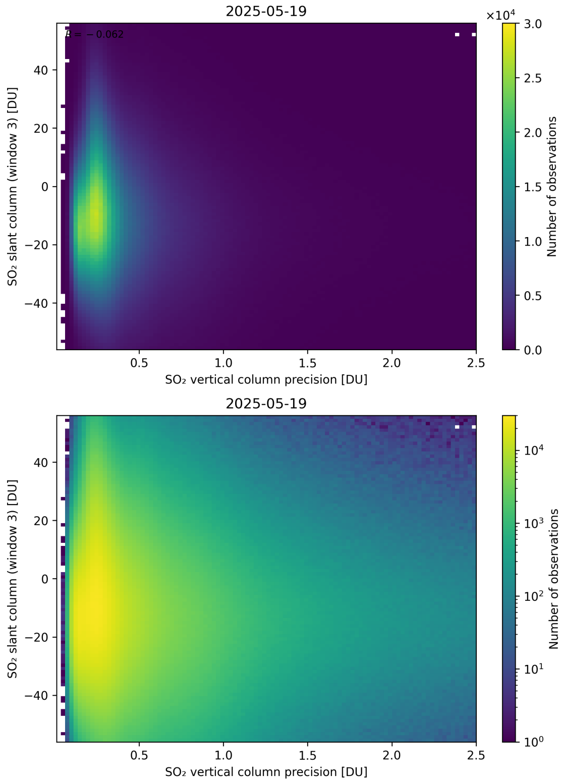
Figure 344: Scatter density plot of “SO 2 vertical column precision” against “SO 2 slant column (window 3)” for 2025-05-18 to 2025-05-20.
