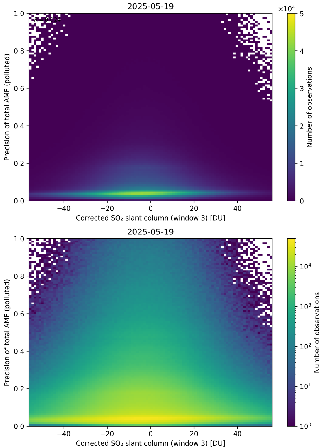
Figure 261: Scatter density plot of “Corrected SO 2 slant column (window 3)” against “Precision of total AMF (polluted)” for 2025-05-18 to 2025-05-20.
