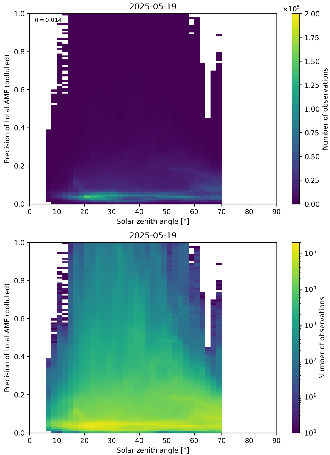
Figure 190: Scatter density plot of “Solar zenith angle” against “Precision of total AMF (polluted)” for 2025-05-18 to 2025-05-20.
