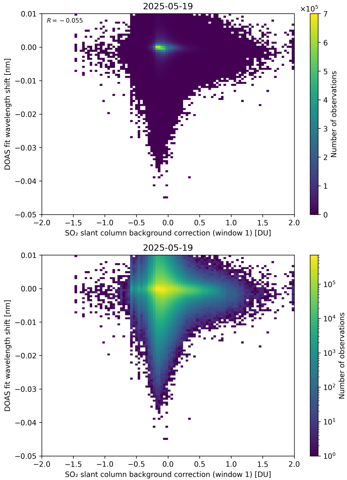
Figure 111: Scatter density plot of “SO 2 slant column background correction (window 1)” against “DOAS fit wavelength shift” for 2025-05-18 to 2025-05-20.
