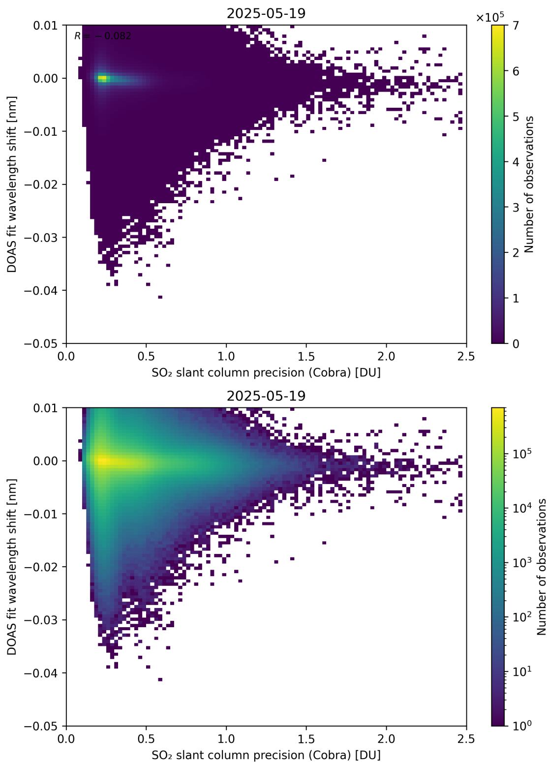
Figure 202: Scatter density plot of “SO 2 slant column precision (Cobra)” against “DOAS fit wavelength shift” for 2025-05-18 to 2025-05-20.
