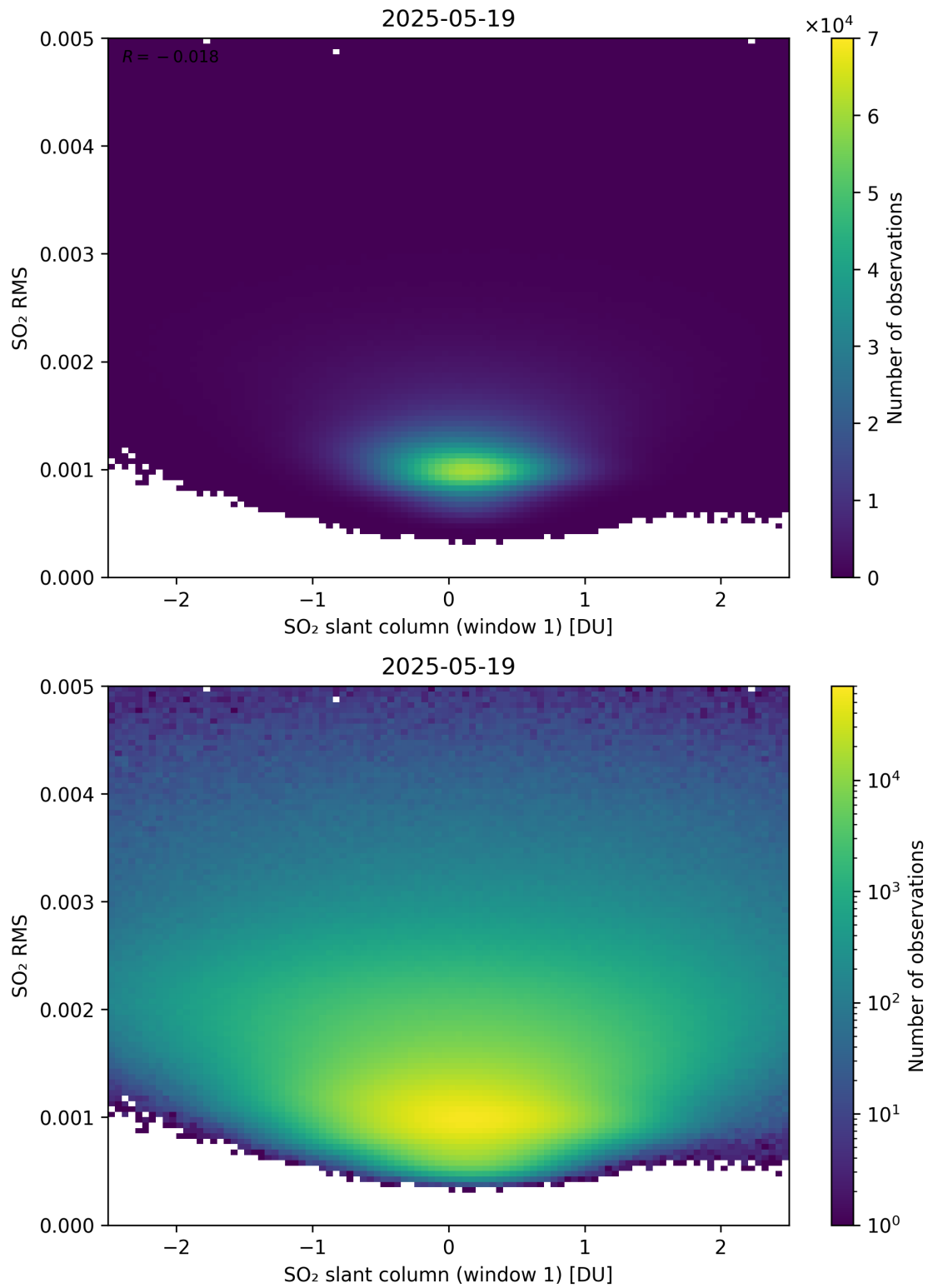
Figure 267: Scatter density plot of “SO 2 slant column (window 1)” against “SO 2 RMS” for 2025-05-18 to 2025-05-20.
