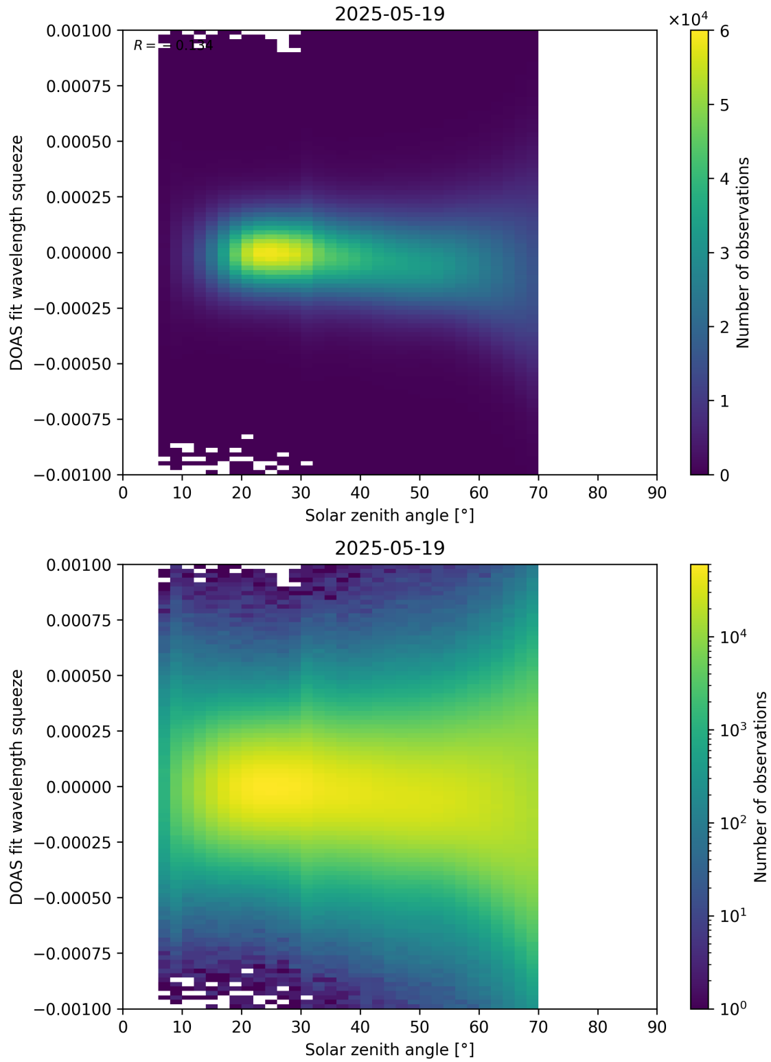
Figure 175: Scatter density plot of “Solar zenith angle” against “DOAS fit wavelength squeeze” for 2025-05-18 to 2025-05-20.
