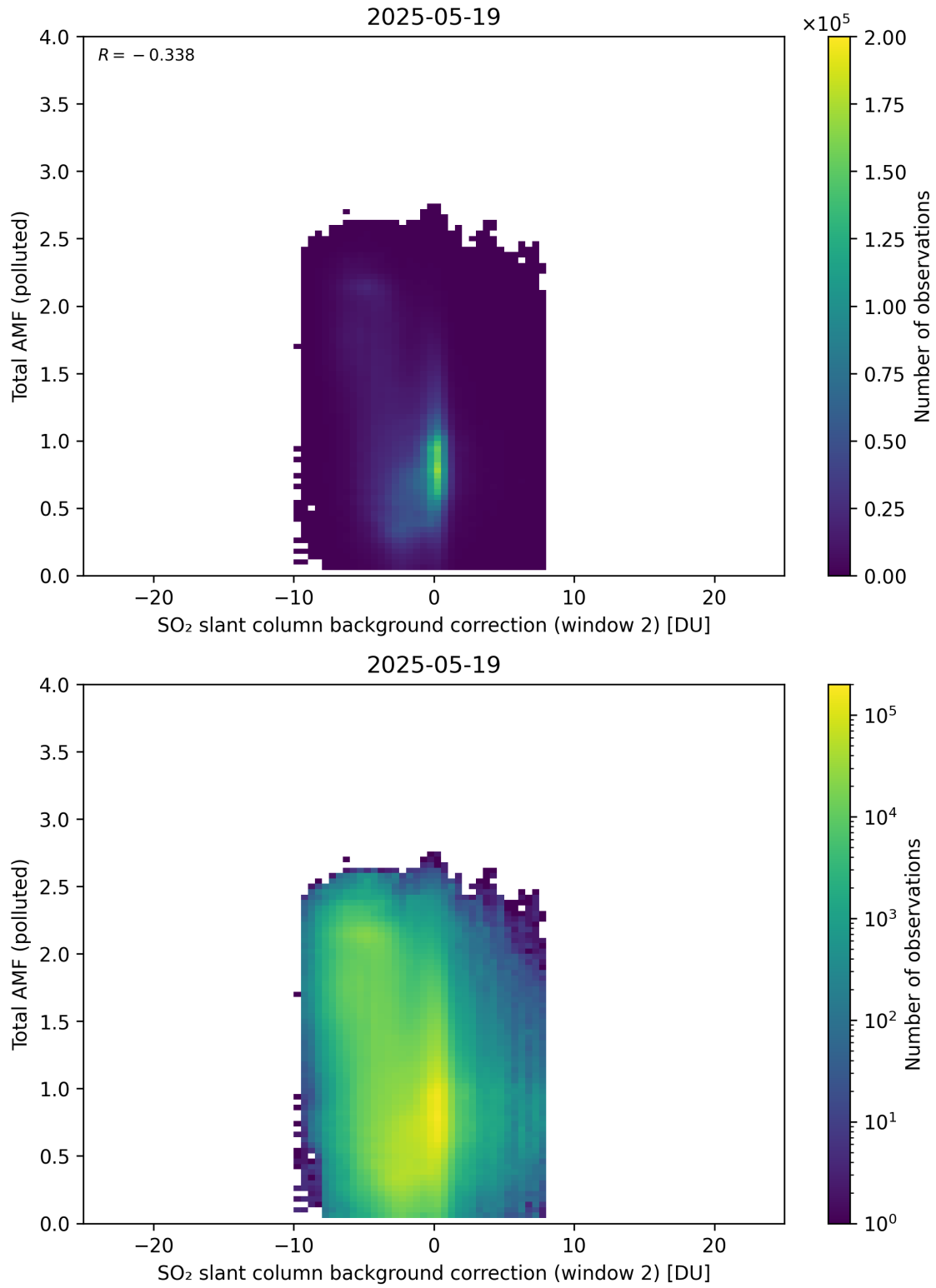
Figure 130: Scatter density plot of “SO 2 slant column background correction (window 2)” against “Total AMF (polluted)” for 2025-05-18 to 2025-05-20.
