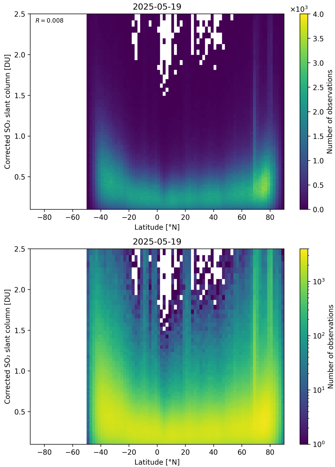
Figure 159: Scatter density plot of “Latitude” against “Corrected SO 2 slant column” for 2025-05-18 to 2025-05-20.
