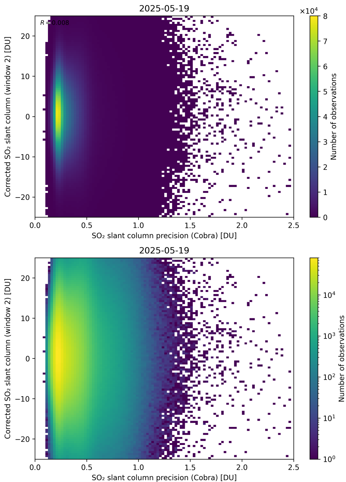
Figure 206: Scatter density plot of “SO 2 slant column precision (Cobra)” against “Corrected SO 2 slant column (window 2)” for 2025-05-18 to 2025-05-20.
