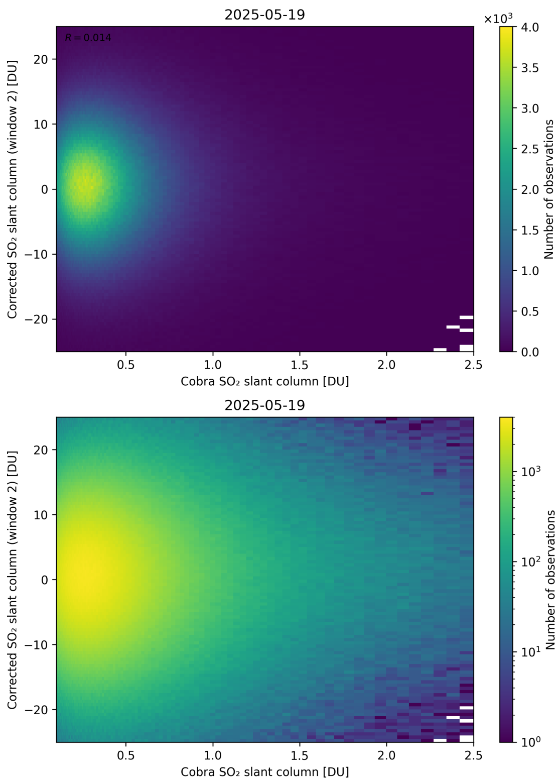
Figure 217: Scatter density plot of “Cobra SO 2 slant column” against “Corrected SO 2 slant column (window 2)” for 2025-05-18 to 2025-05-20.
