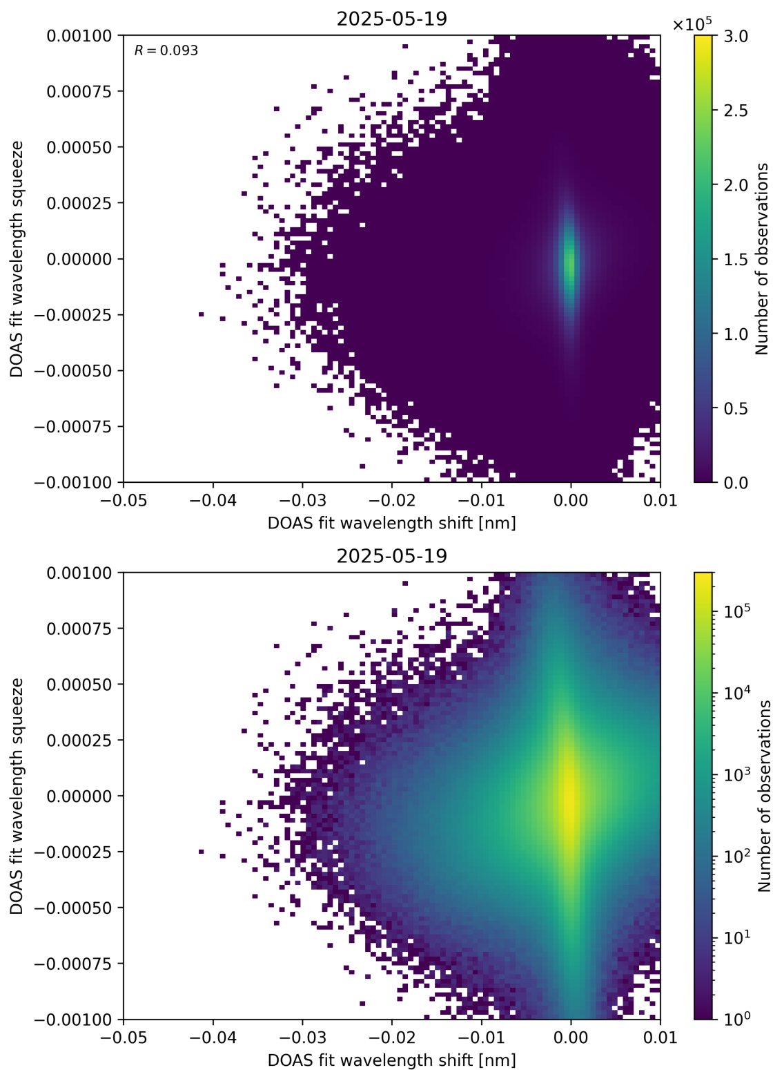
Figure 138: Scatter density plot of “DOAS fit wavelength shift” against “DOAS fit wavelength squeeze” for 2025-05-18 to 2025-05-20.
