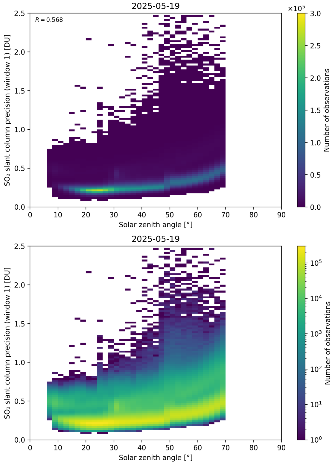
Figure 185: Scatter density plot of “Solar zenith angle” against “SO 2 slant column precision (window 1)” for 2025-05-18 to 2025-05-20.
