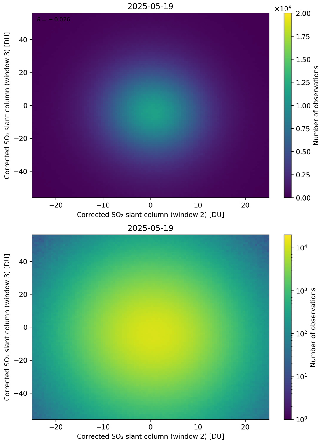
Figure 250: Scatter density plot of “Corrected SO 2 slant column (window 2)” against “Corrected SO 2 slant column (window 3)” for 2025-05-18 to 2025-05-20.
