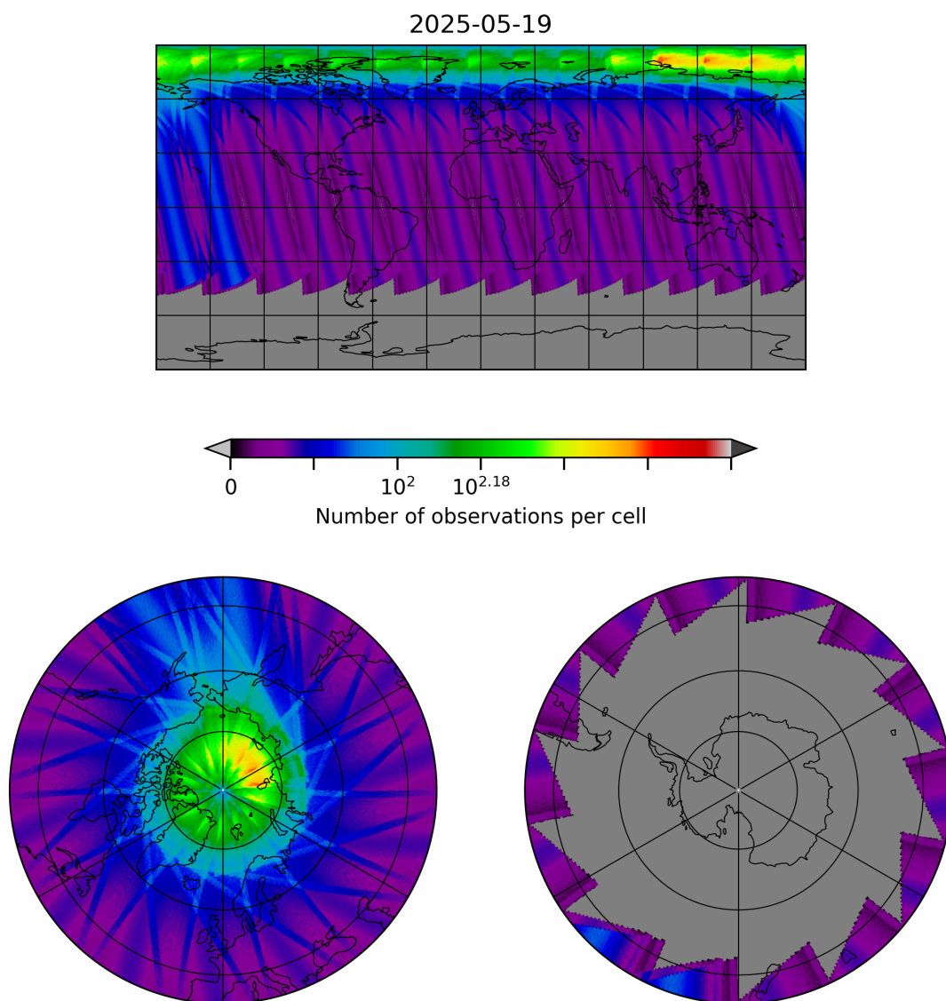
Figure 30: Map of the number of observations for 2025-05-18 to 2025-05-20
