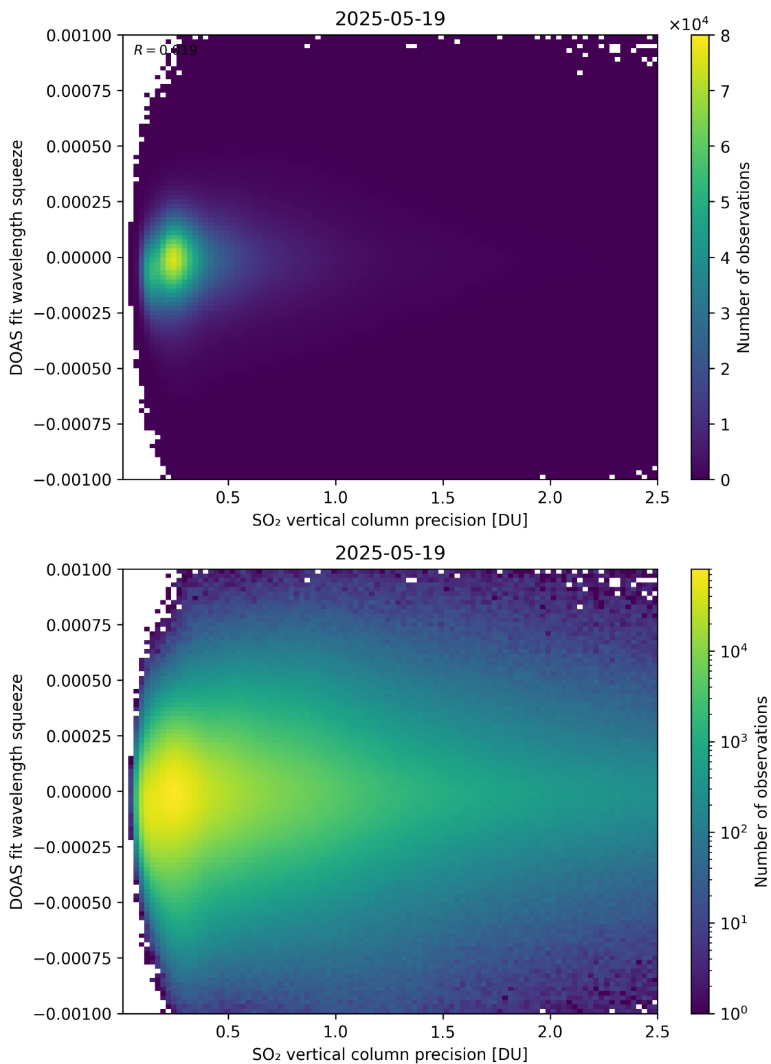
Figure 333: Scatter density plot of “SO 2 vertical column precision” against “DOAS fit wavelength squeeze” for 2025-05-18 to 2025-05-20.
