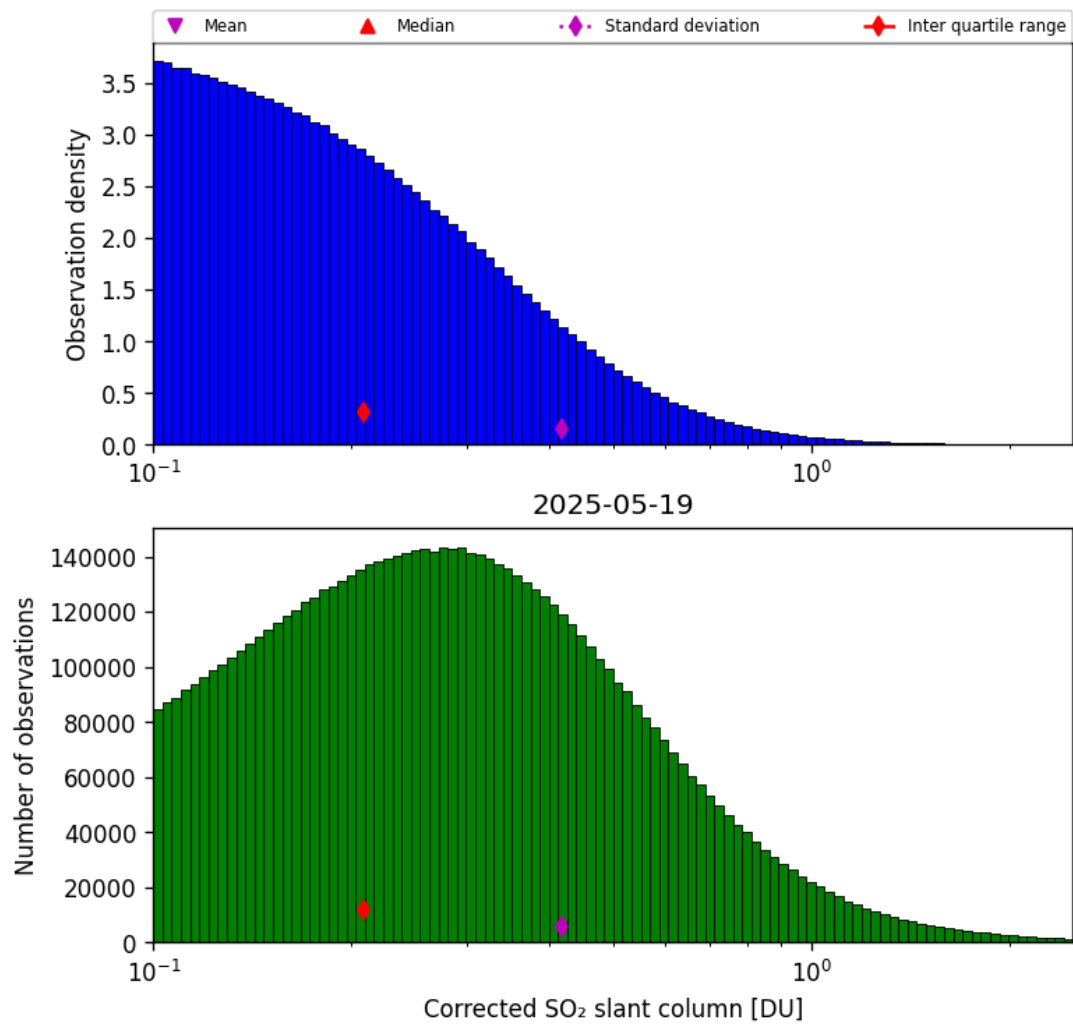
Figure 60: Histogram of “Corrected SO 2 slant column” for 2025-05-18 to 2025-05-20
