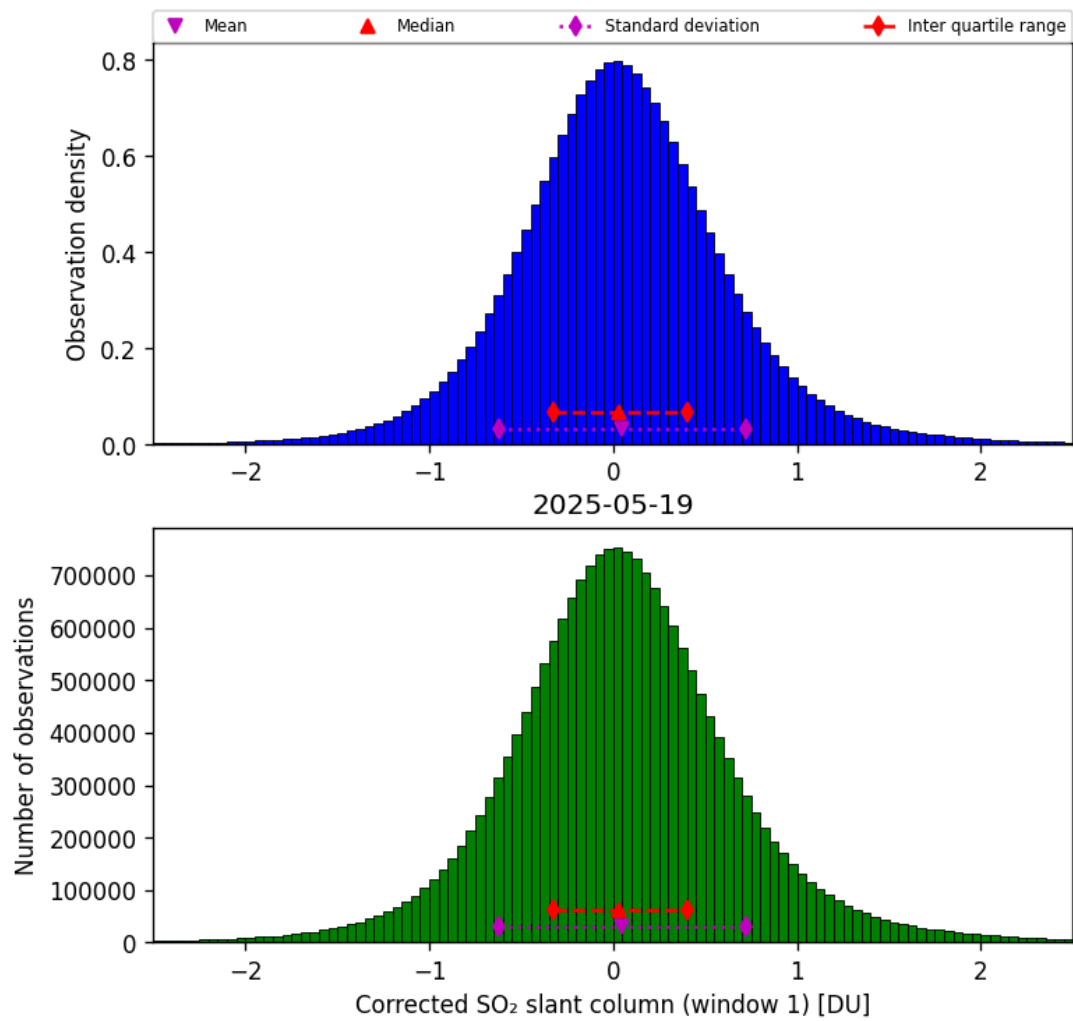
Figure 65: Histogram of “Corrected SO 2 slant column (window 1)” for 2025-05-18 to 2025-05-20
