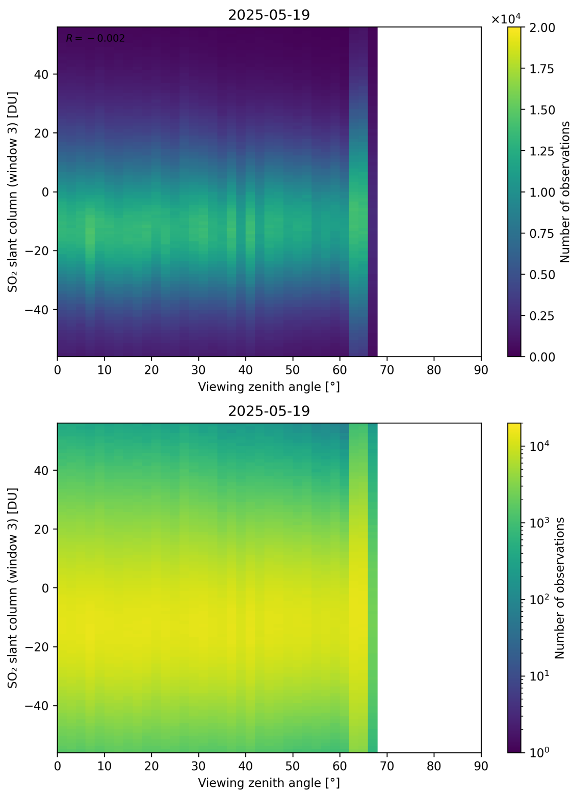
Figure 379: Scatter density plot of “Viewing zenith angle” against “SO 2 slant column (window 3)” for 2025-05-18 to 2025-05-20.
