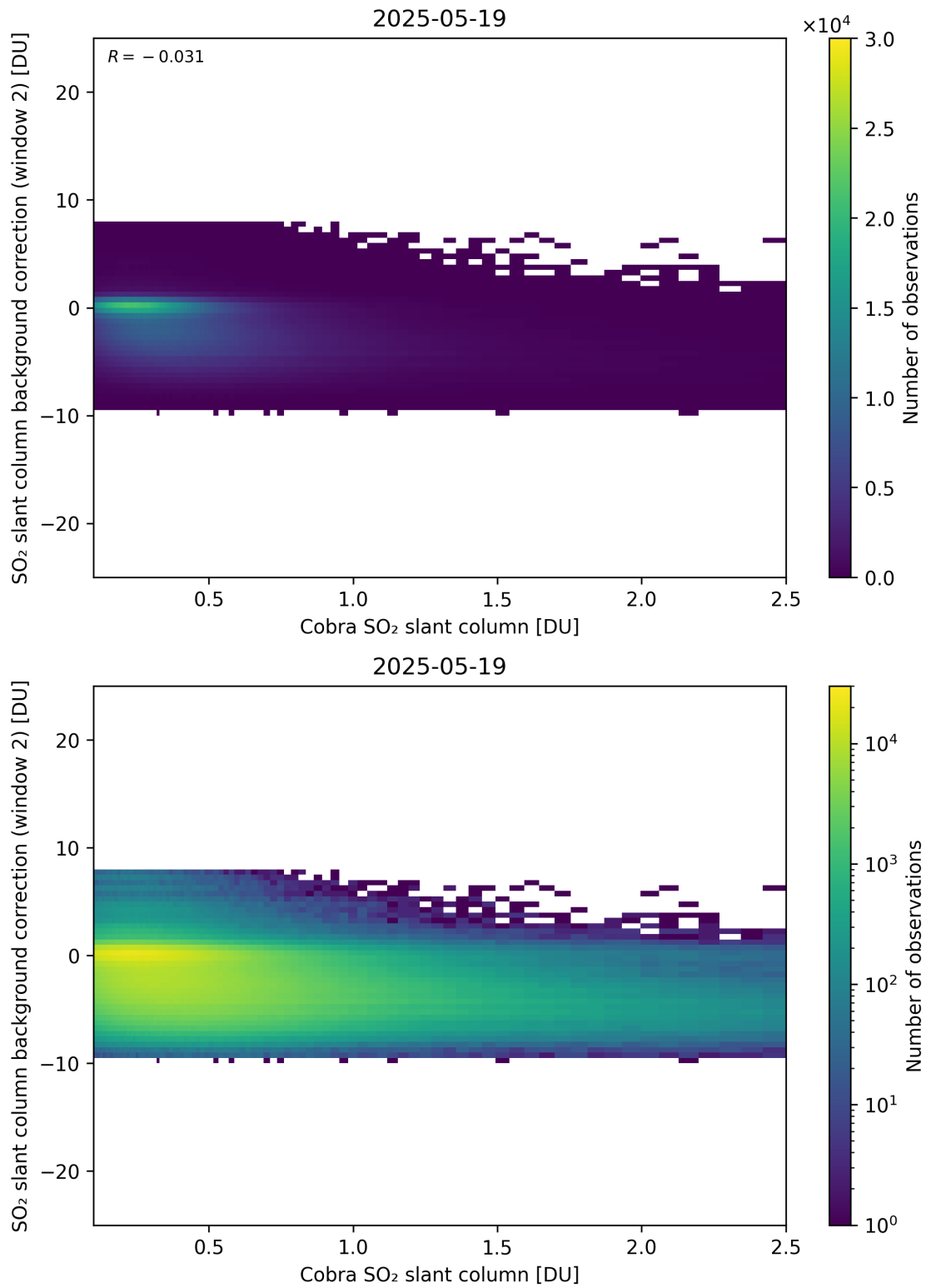
Figure 194: Scatter density plot of “Cobra SO 2 slant column” against “SO 2 slant column background correction (window 2)” for 2025-05-18 to 2025-05-20.
