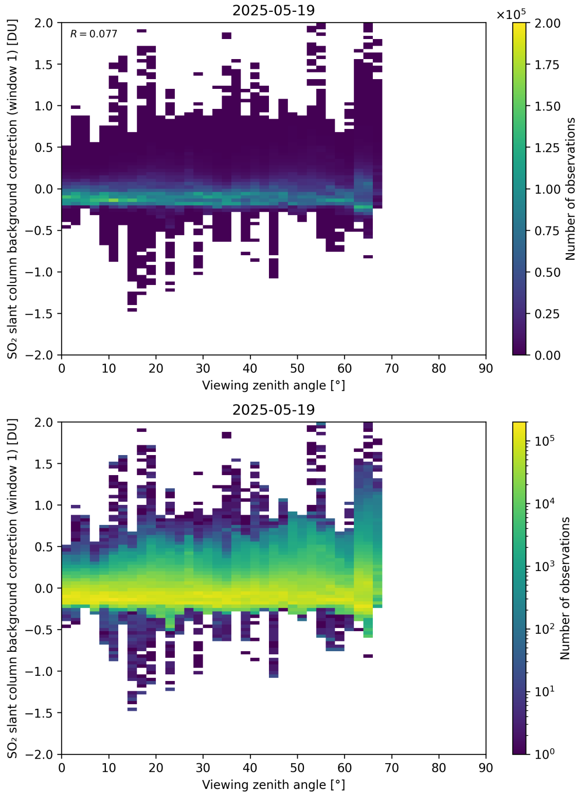
Figure 362: Scatter density plot of “Viewing zenith angle” against “SO 2 slant column background correction (window 1)” for 2025-05-18 to 2025-05-20.
