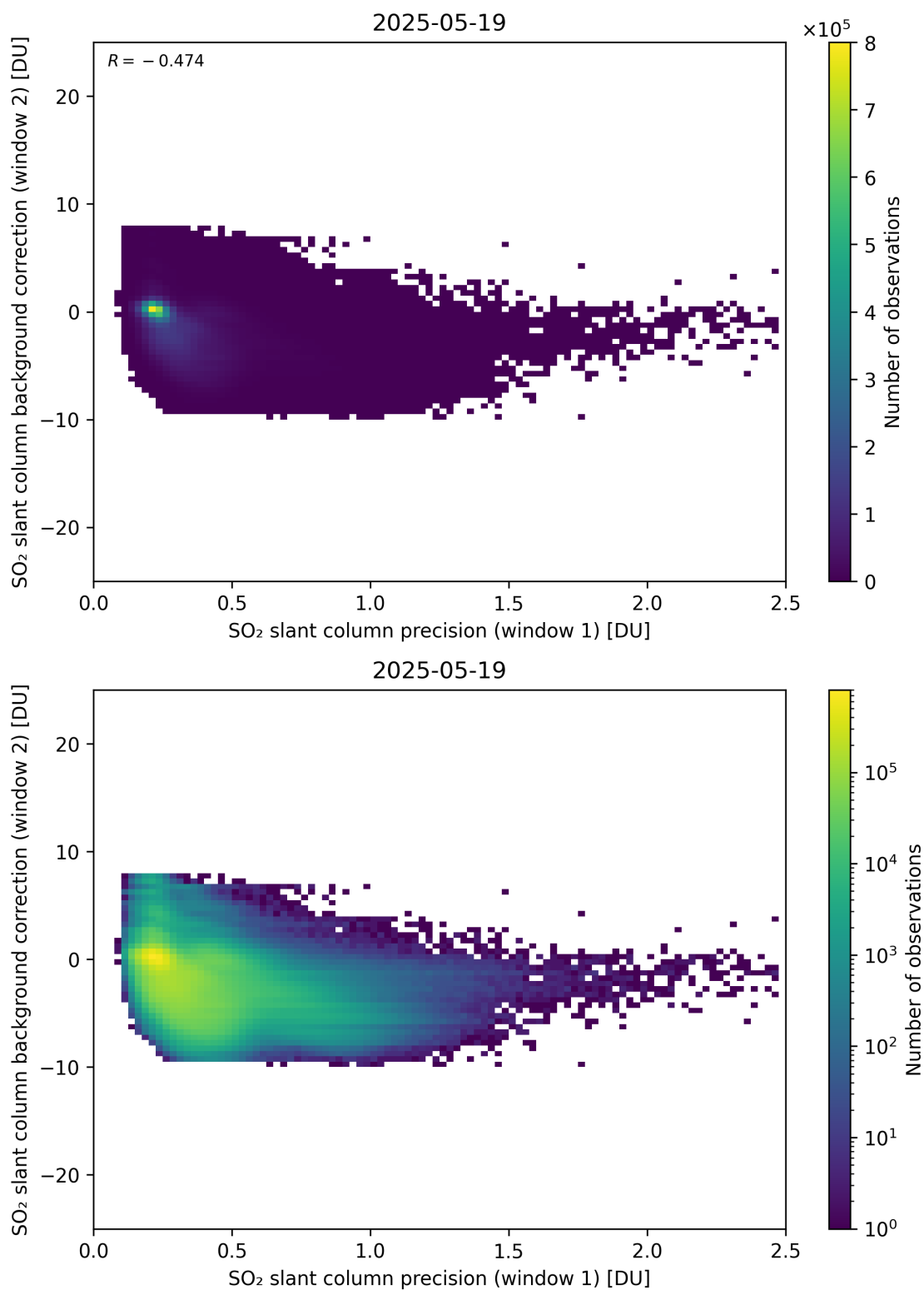
Figure 269: Scatter density plot of “SO 2 slant column precision (window 1)” against “SO 2 slant column background correction (window 2)” for 2025-05-18 to 2025-05-20.
