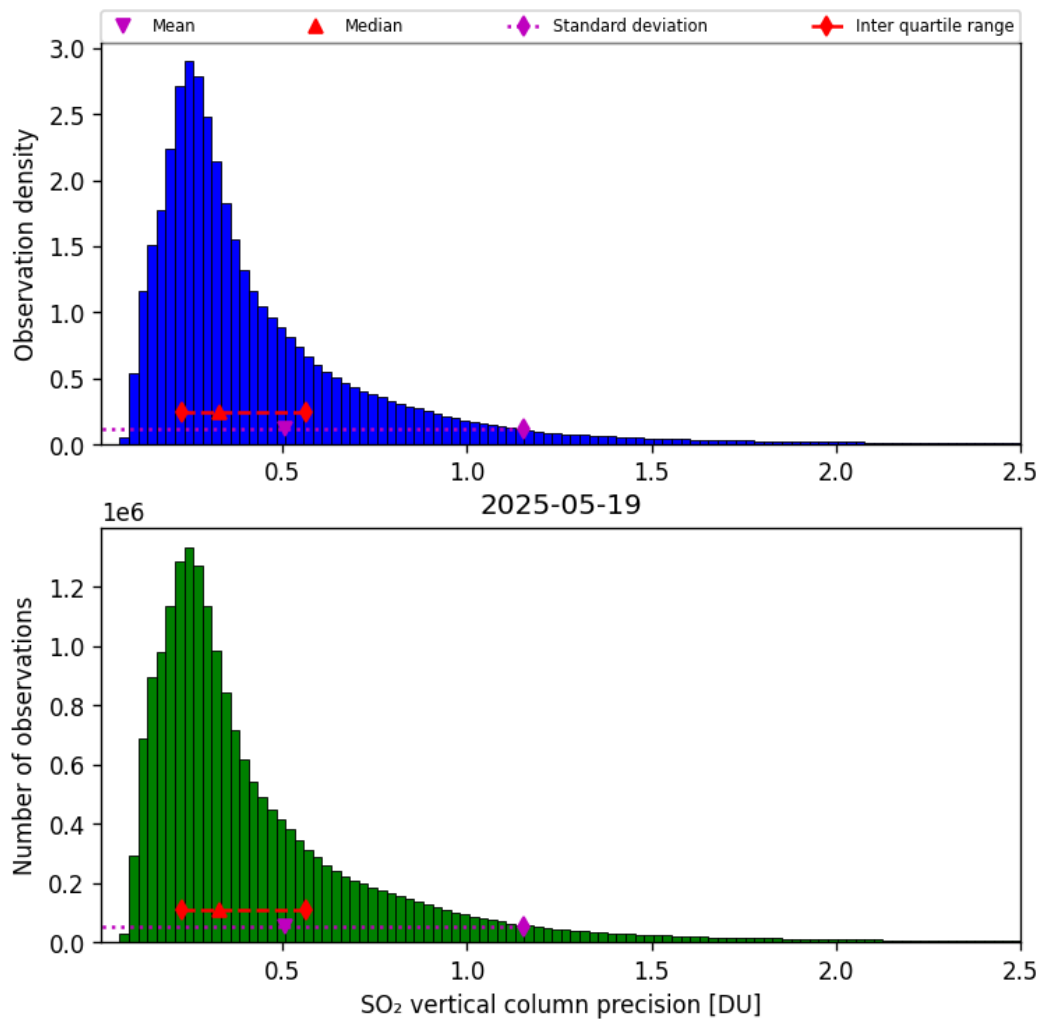
Figure 59: Histogram of “SO 2 vertical column precision” for 2025-05-18 to 2025-05-20
