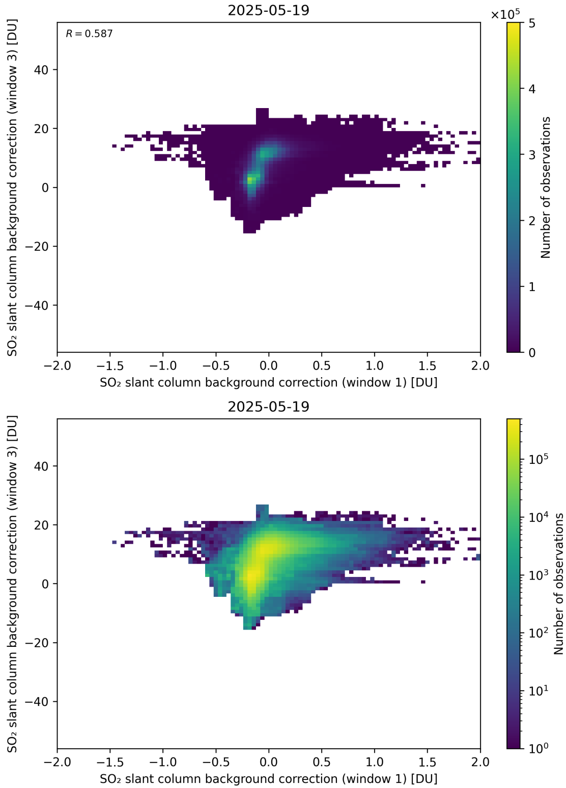
Figure 110: Scatter density plot of “SO 2 slant column background correction (window 1)” against “SO 2 slant column background correction (window 3)” for 2025-05-18 to 2025-05-20.
