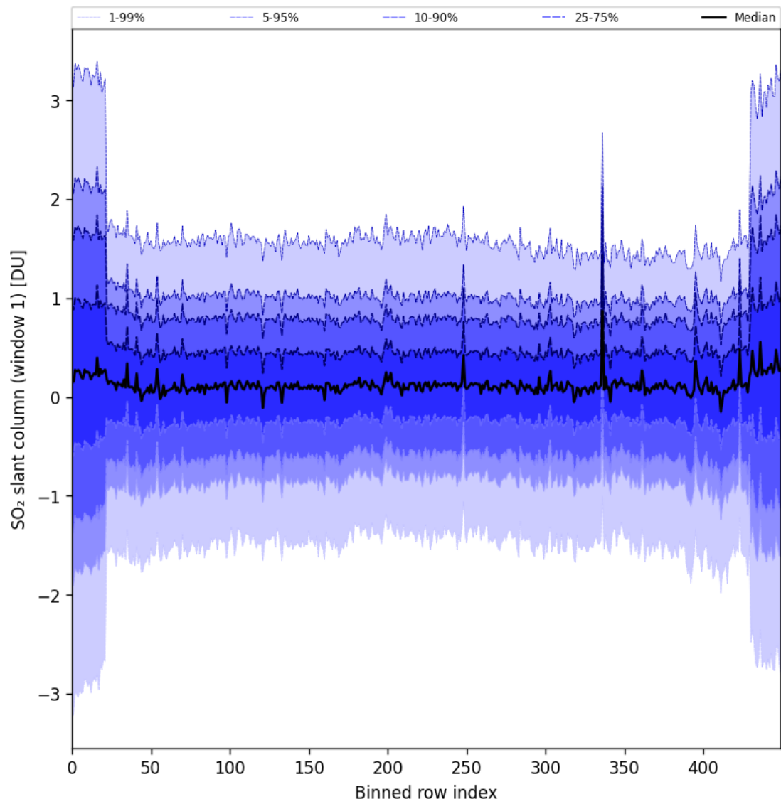
Figure 89: Along track statistics of “SO 2 slant column (window 1)” for 2025-05-18 to 2025-05-20
