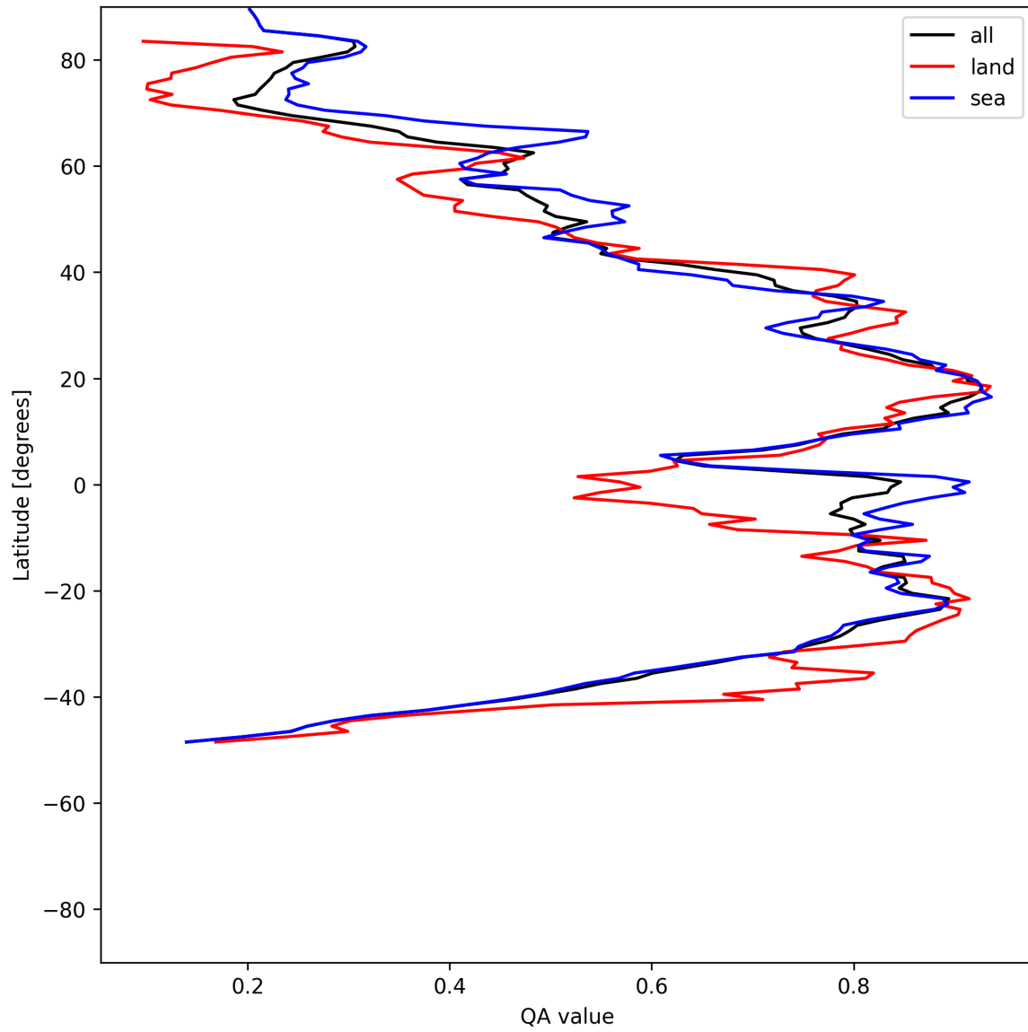
Figure 31: Zonal average of “QA value” for 2025-05-18 to 2025-05-20.
