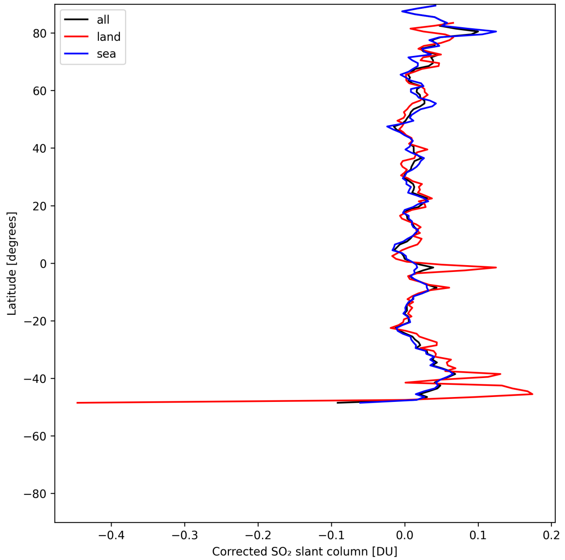
Figure 34: Zonal average of “Corrected SO 2 slant column” for 2025-05-18 to 2025-05-20.
