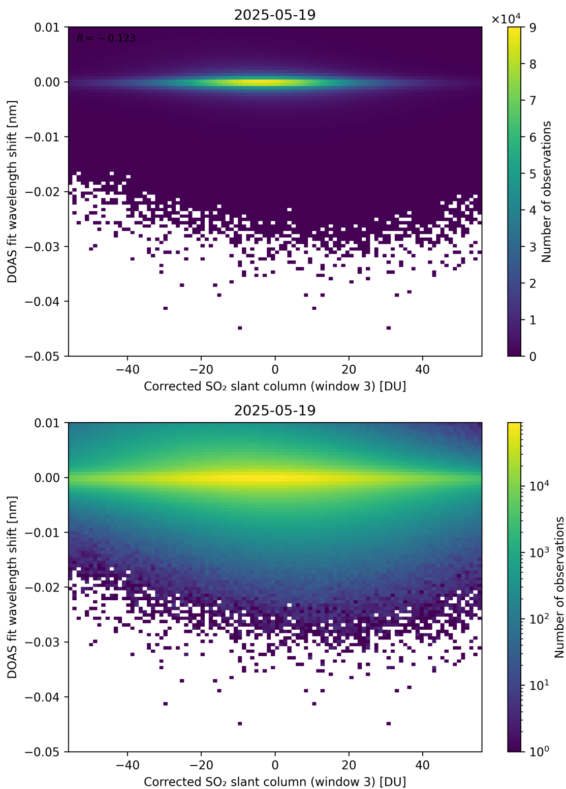
Figure 256: Scatter density plot of “Corrected SO 2 slant column (window 3)” against “DOAS fit wavelength shift” for 2025-05-18 to 2025-05-20.
