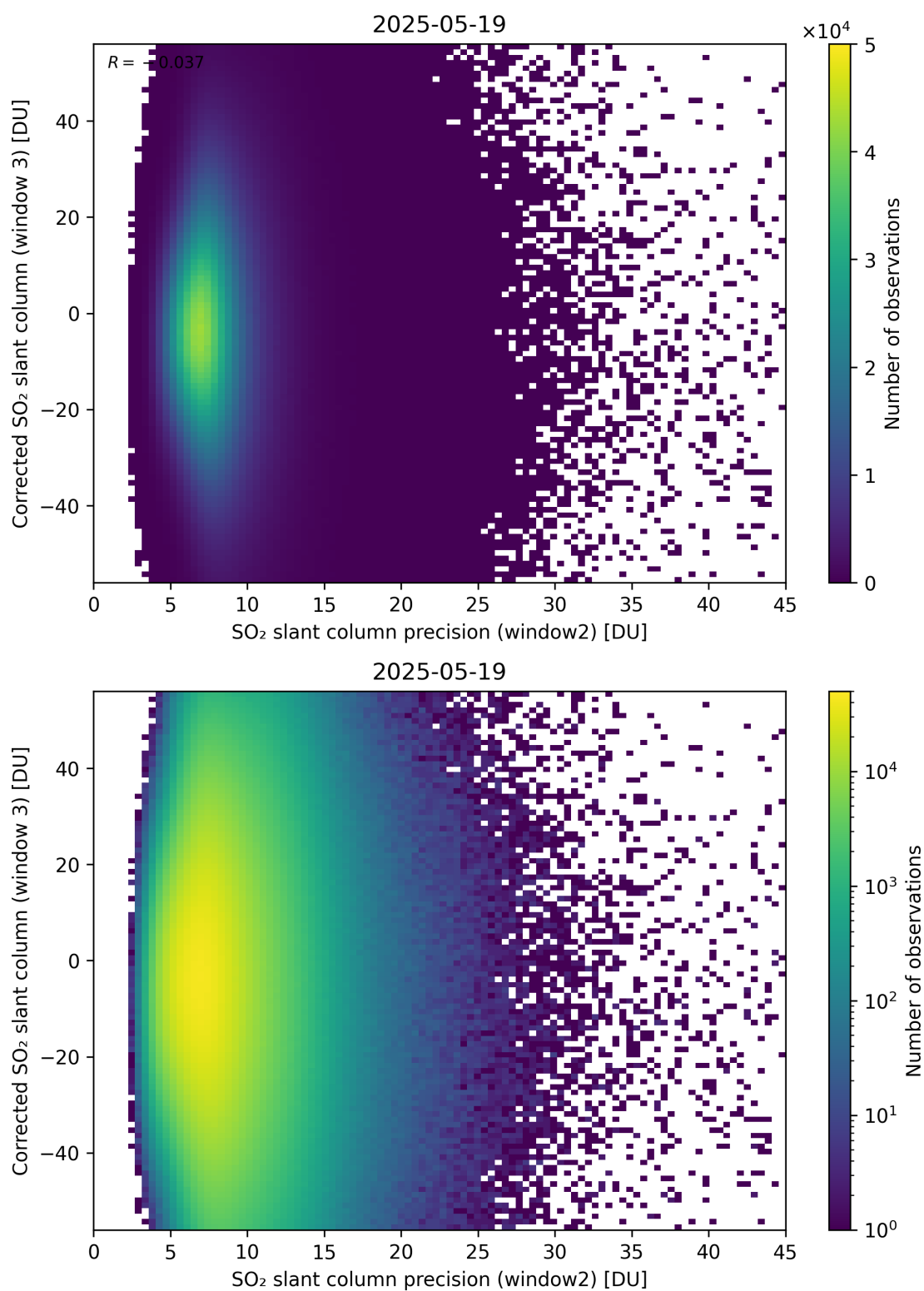
Figure 298: Scatter density plot of “SO 2 slant column precision (window2)” against “Corrected SO 2 slant column (window 3)” for 2025-05-18 to 2025-05-20.
