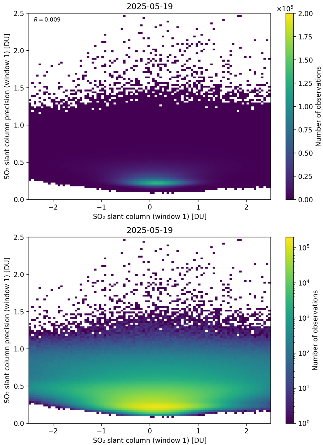
Figure 285: Scatter density plot of “SO 2 slant column (window 1)” against “SO 2 slant column precision (window 1)” for 2025-05-18 to 2025-05-20.
