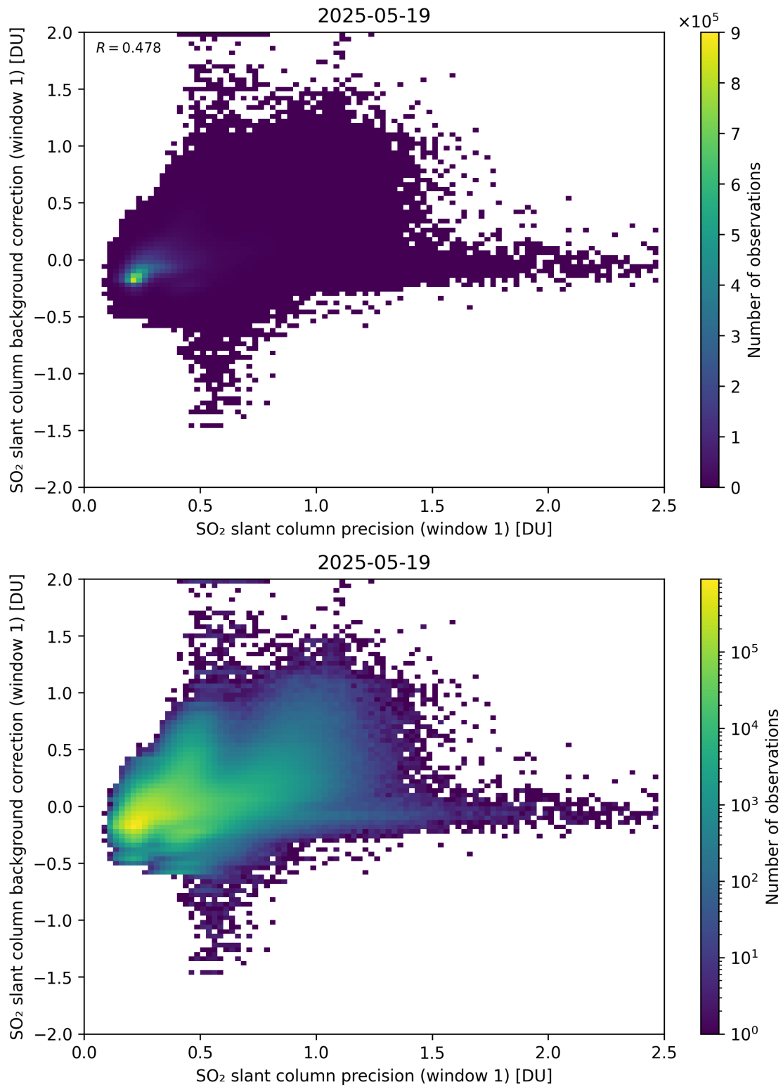
Figure 268: Scatter density plot of “SO 2 slant column precision (window 1)” against “SO 2 slant column background correction (window 1)” for 2025-05-18 to 2025-05-20.
