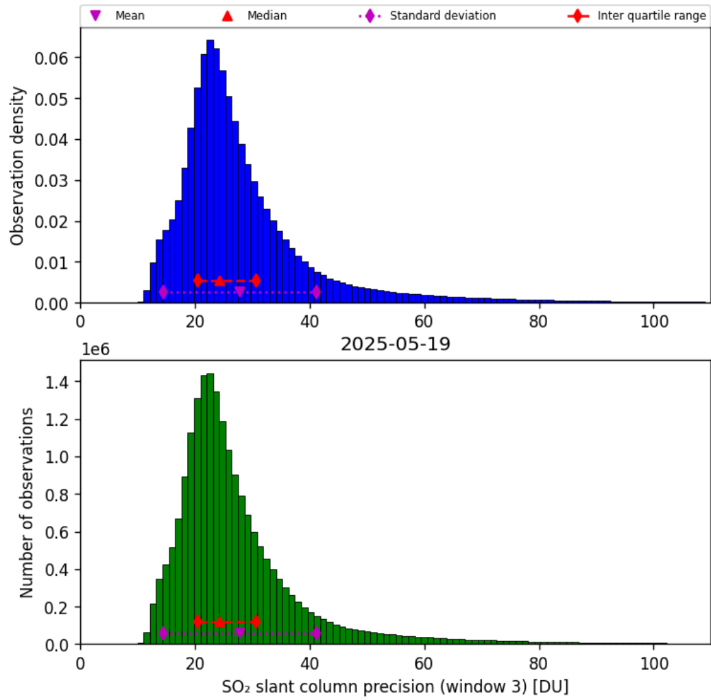
Figure 72: Histogram of “SO 2 slant column precision (window 3)” for 2025-05-18 to 2025-05-20
