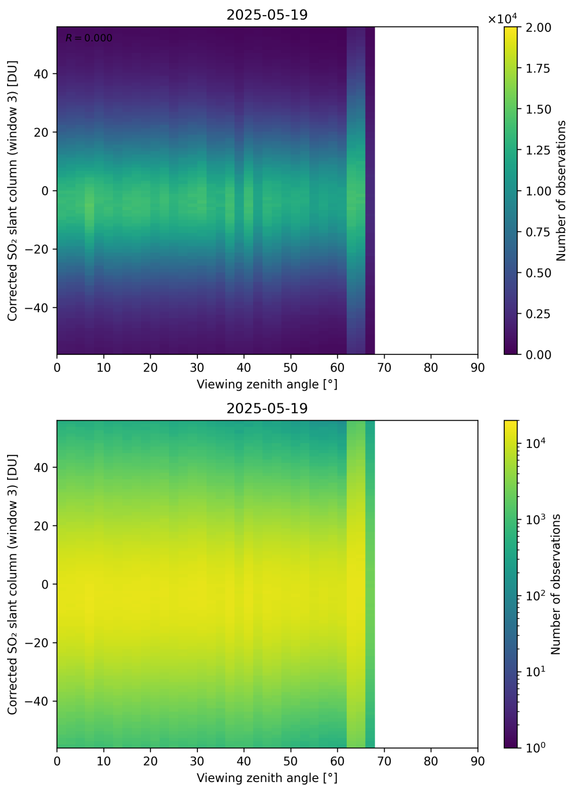
Figure 375: Scatter density plot of “Viewing zenith angle” against “Corrected SO 2 slant column (window 3)” for 2025-05-18 to 2025-05-20.
