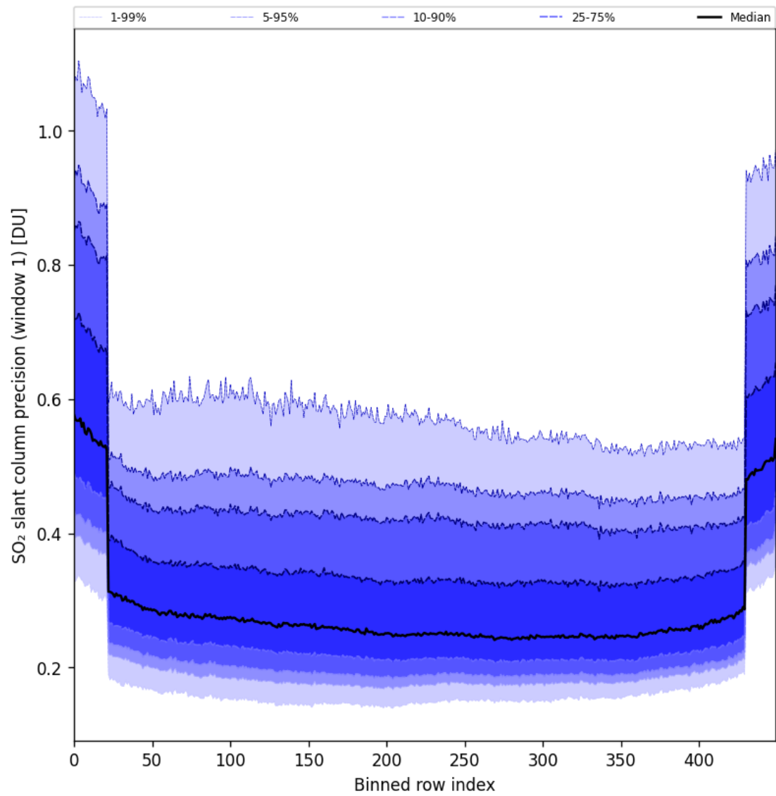
Figure 90: Along track statistics of "SO 2 slant column precision (window 1)" for 2025-05-18 to 2025-05-20
