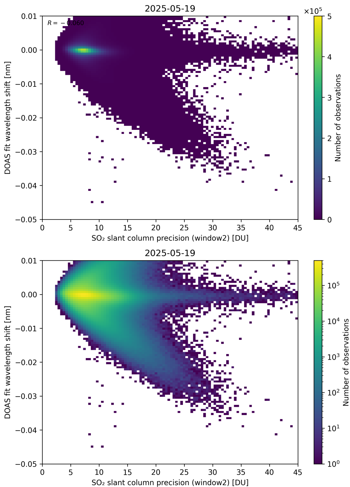
Figure 293: Scatter density plot of “SO 2 slant column precision (window2)” against “DOAS fit wavelength shift” for 2025-05-18 to 2025-05-20.
