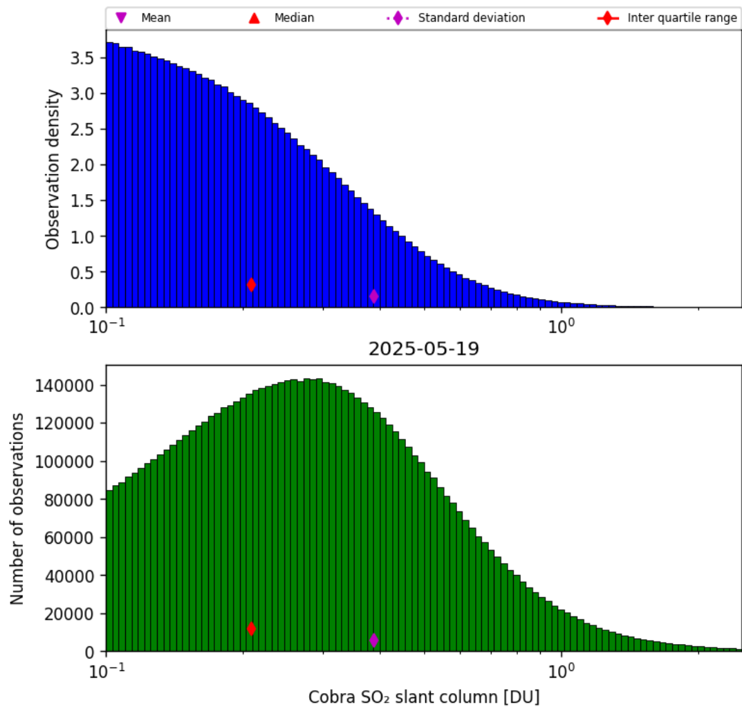
Figure 61: Histogram of “Cobra SO 2 slant column” for 2025-05-18 to 2025-05-20
