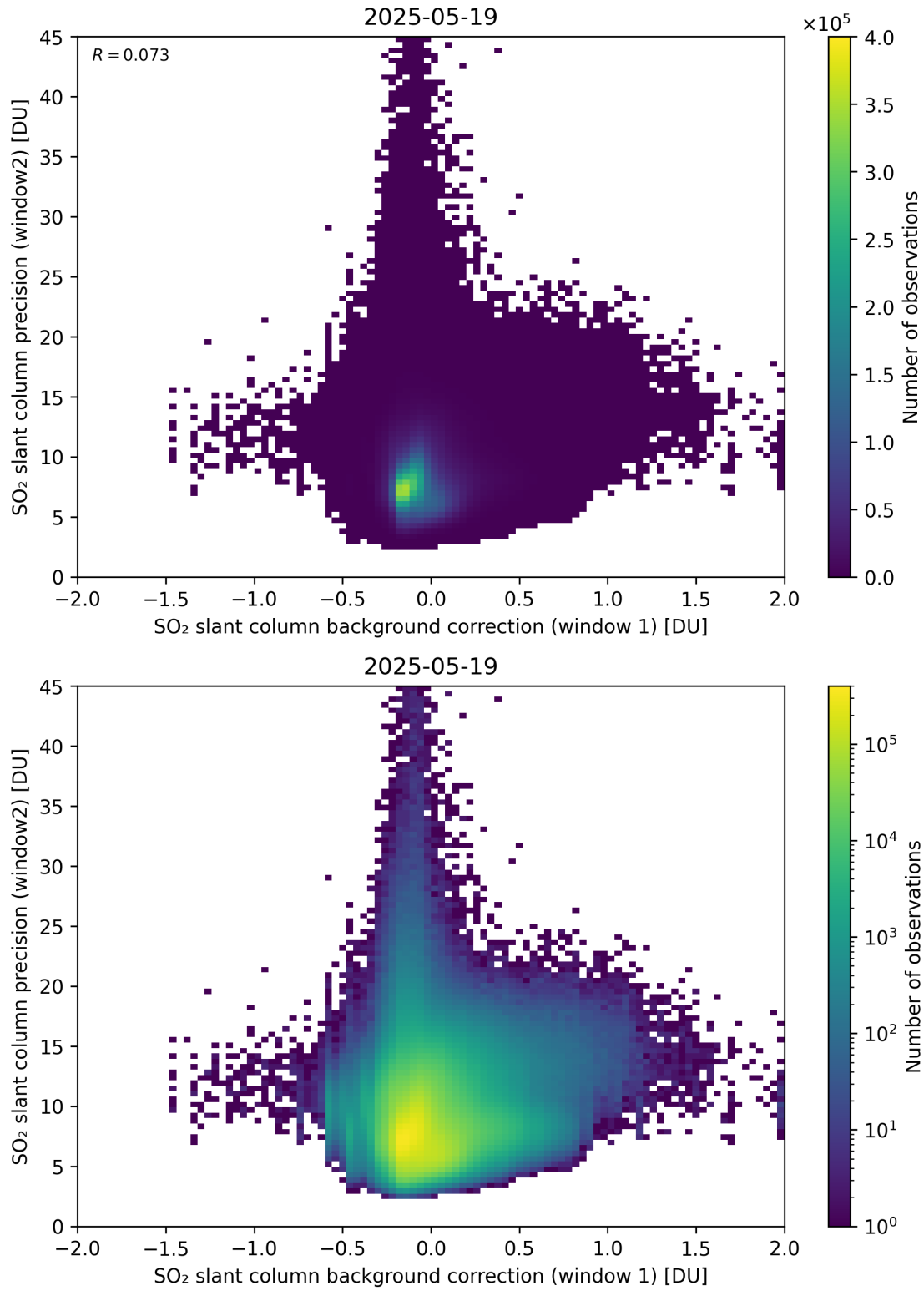
Figure 117: Scatter density plot of “SO 2 slant column background correction (window 1)” against “SO 2 slant column precision (window2)” for 2025-05-18 to 2025-05-20.
