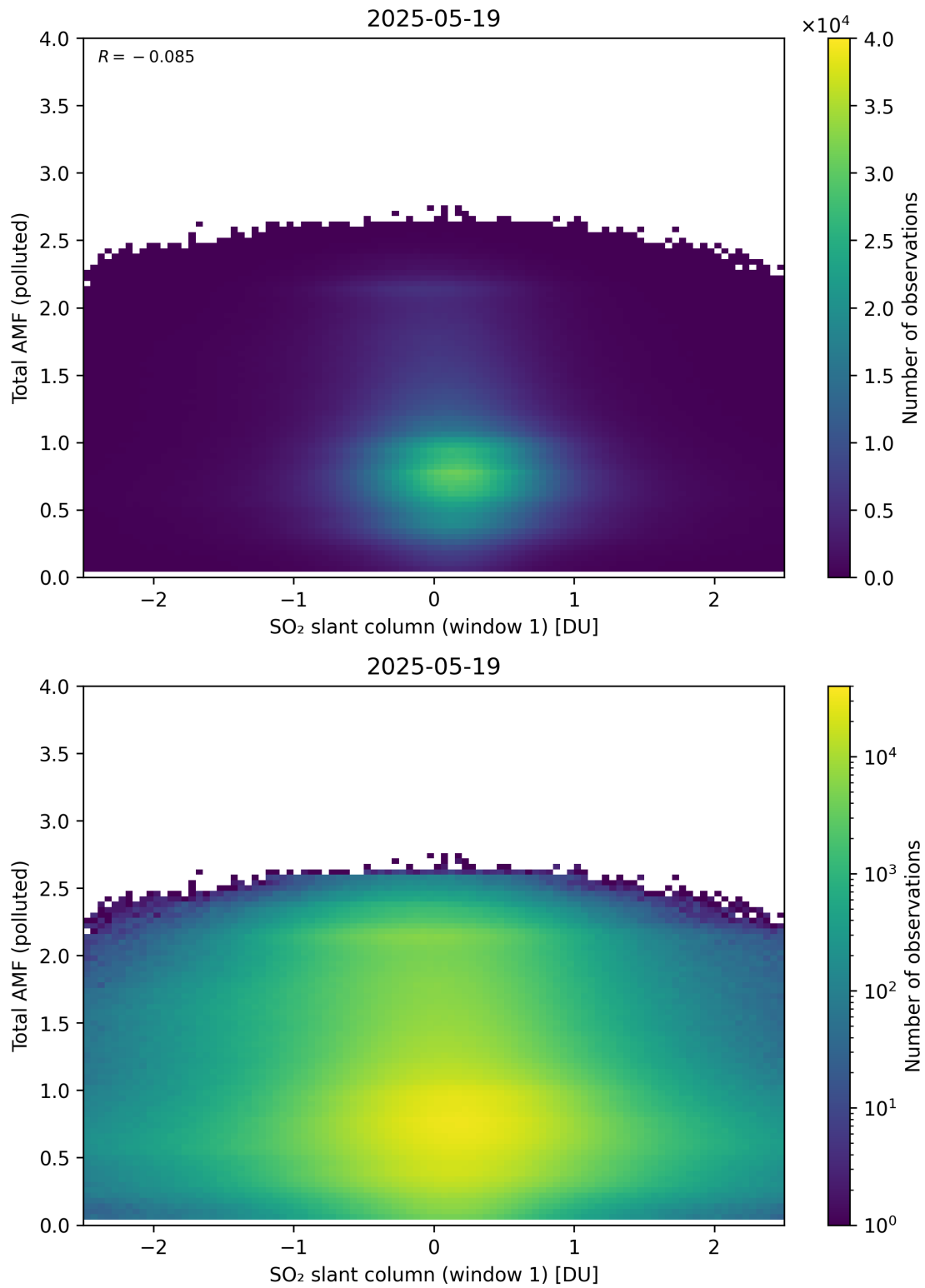
Figure 289: Scatter density plot of “SO 2 slant column (window 1)” against “Total AMF (polluted)” for 2025-05-18 to 2025-05-20.
