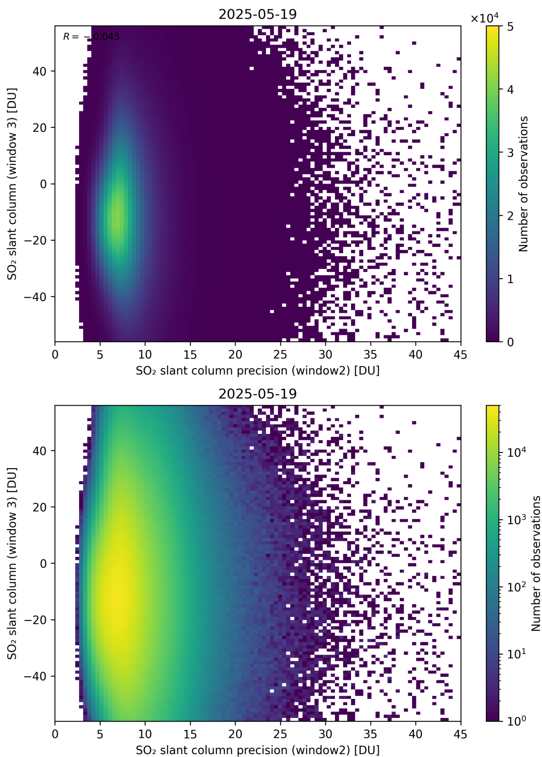
Figure 299: Scatter density plot of “SO 2 slant column precision (window2)” against “SO 2 slant column (window 3)” for 2025-05-18 to 2025-05-20.
