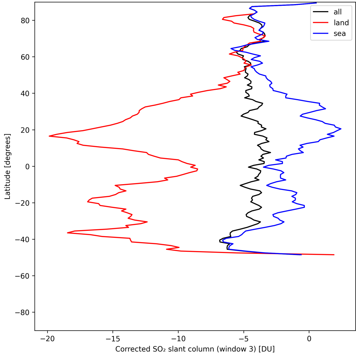
Figure 47: Zonal average of “Corrected SO 2 slant column (window 3)” for 2025-05-18 to 2025-05-20.
