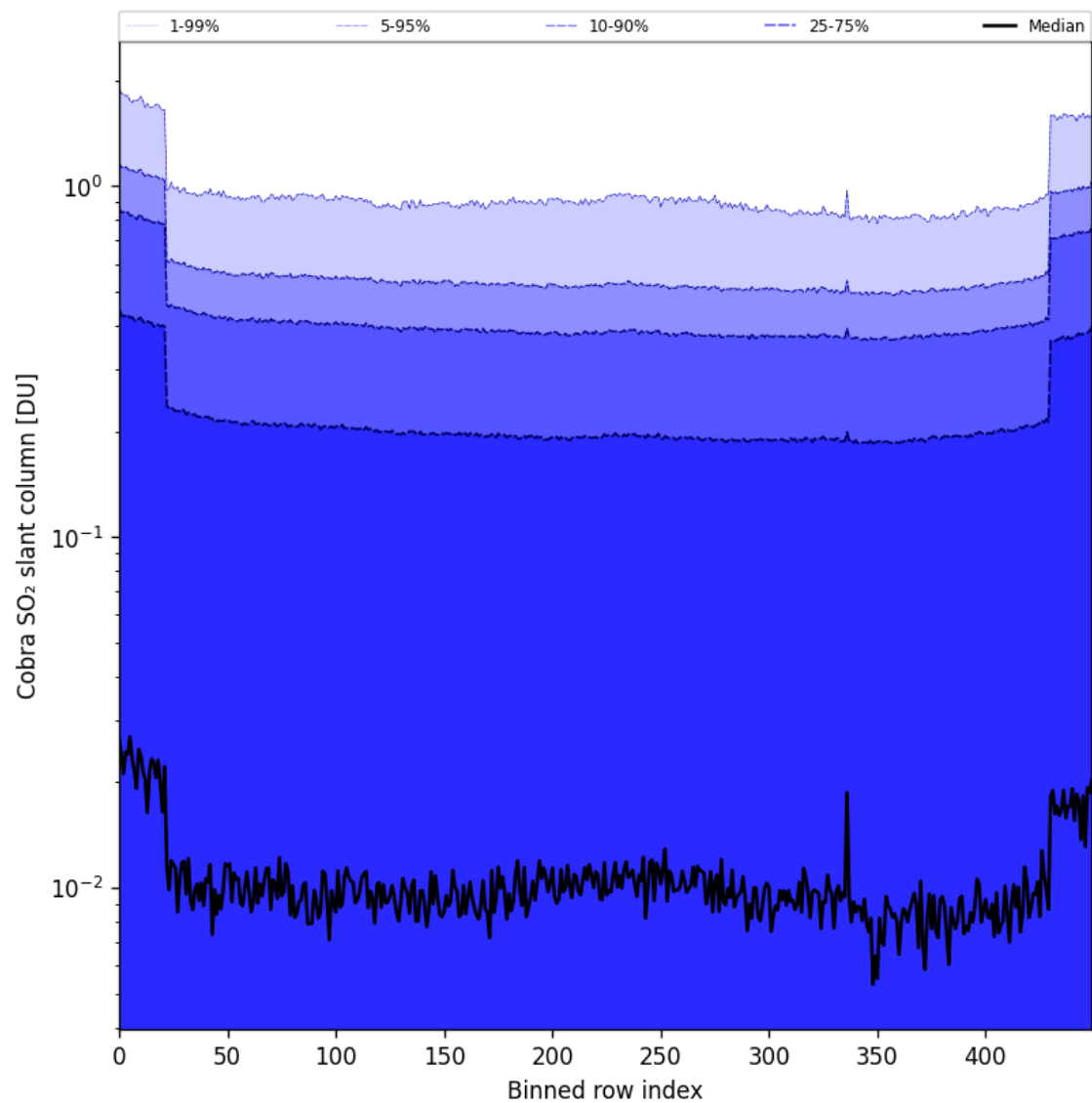
Figure 87: Along track statistics of “Cobra SO 2 slant column” for 2025-05-18 to 2025-05-20
