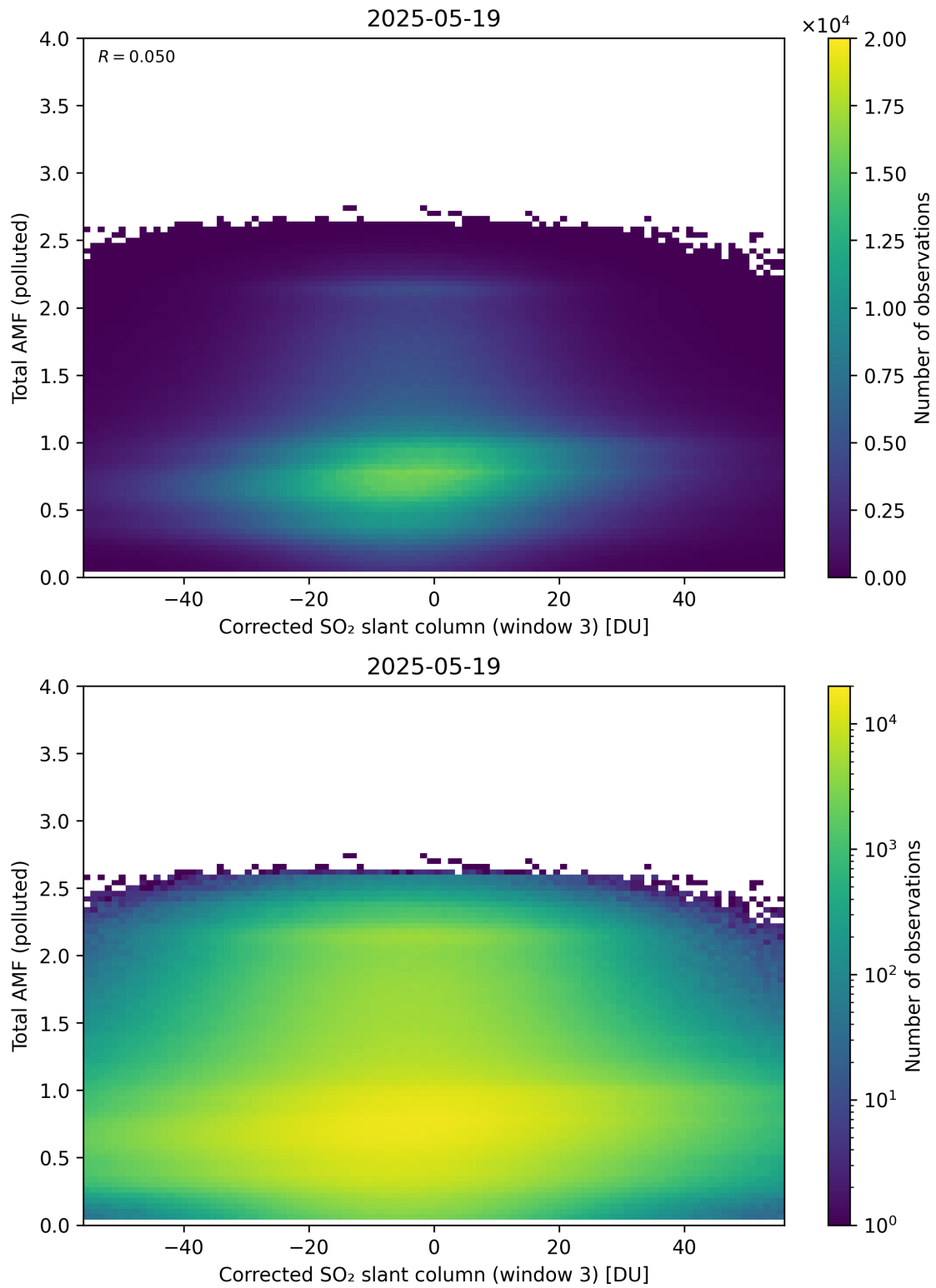
Figure 260: Scatter density plot of “Corrected SO 2 slant column (window 3)” against “Total AMF (polluted)” for 2025-05-18 to 2025-05-20.
