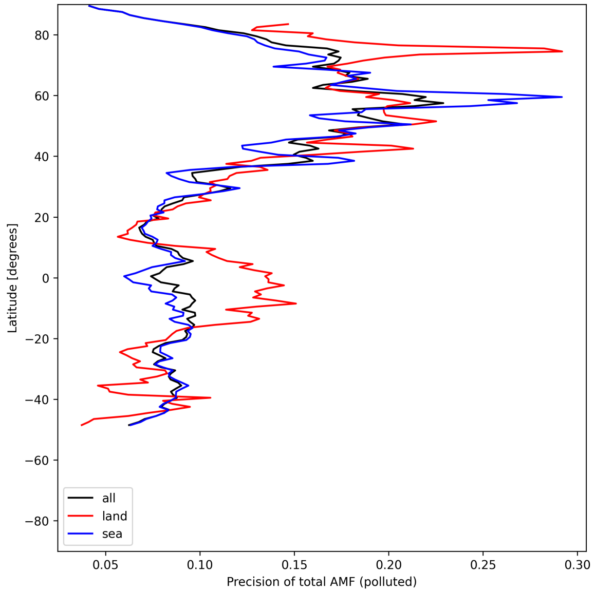
Figure 54: Zonal average of “Precision of total AMF (polluted)” for 2025-05-18 to 2025-05-20.
