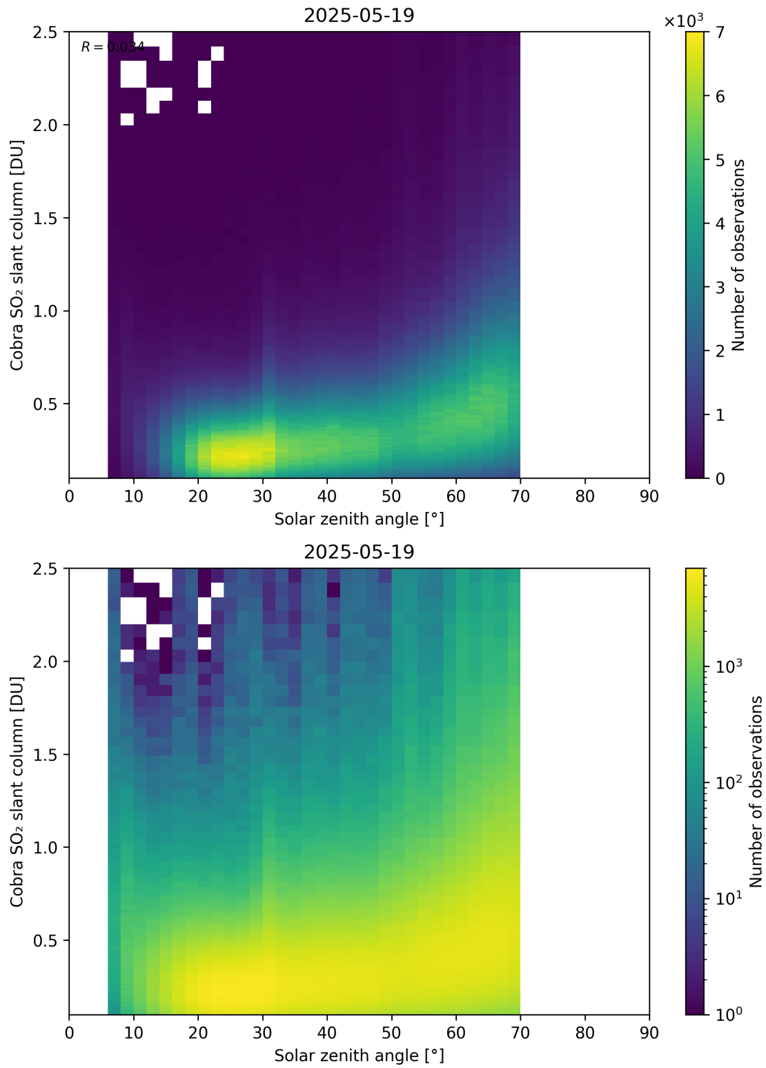
Figure 179: Scatter density plot of “Solar zenith angle” against “Cobra SO 2 slant column” for 2025-05-18 to 2025-05-20.
