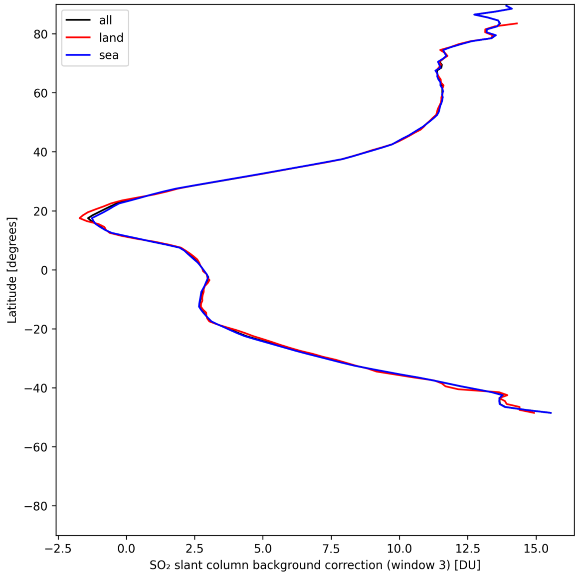
Figure 48: Zonal average of “SO 2 slant column background correction (window 3)” for 2025-05-18 to 2025-05-20.
