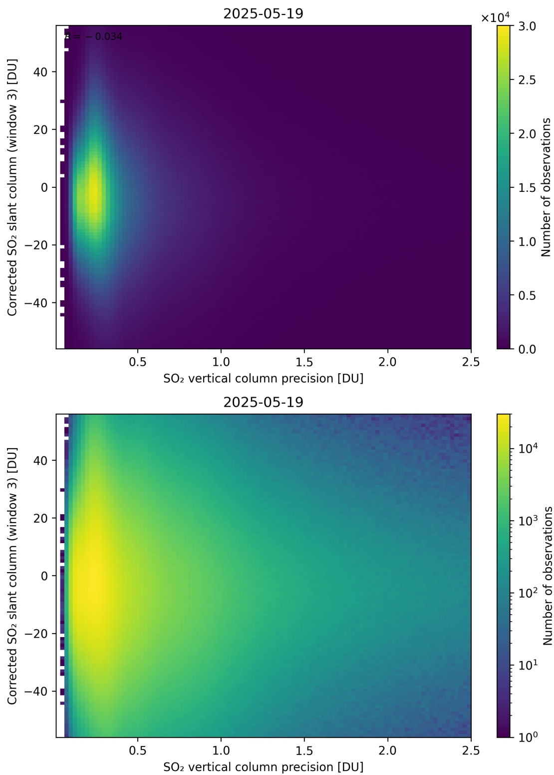
Figure 340: Scatter density plot of “SO 2 vertical column precision” against “Corrected SO 2 slant column (window 3)” for 2025-05-18 to 2025-05-20.
