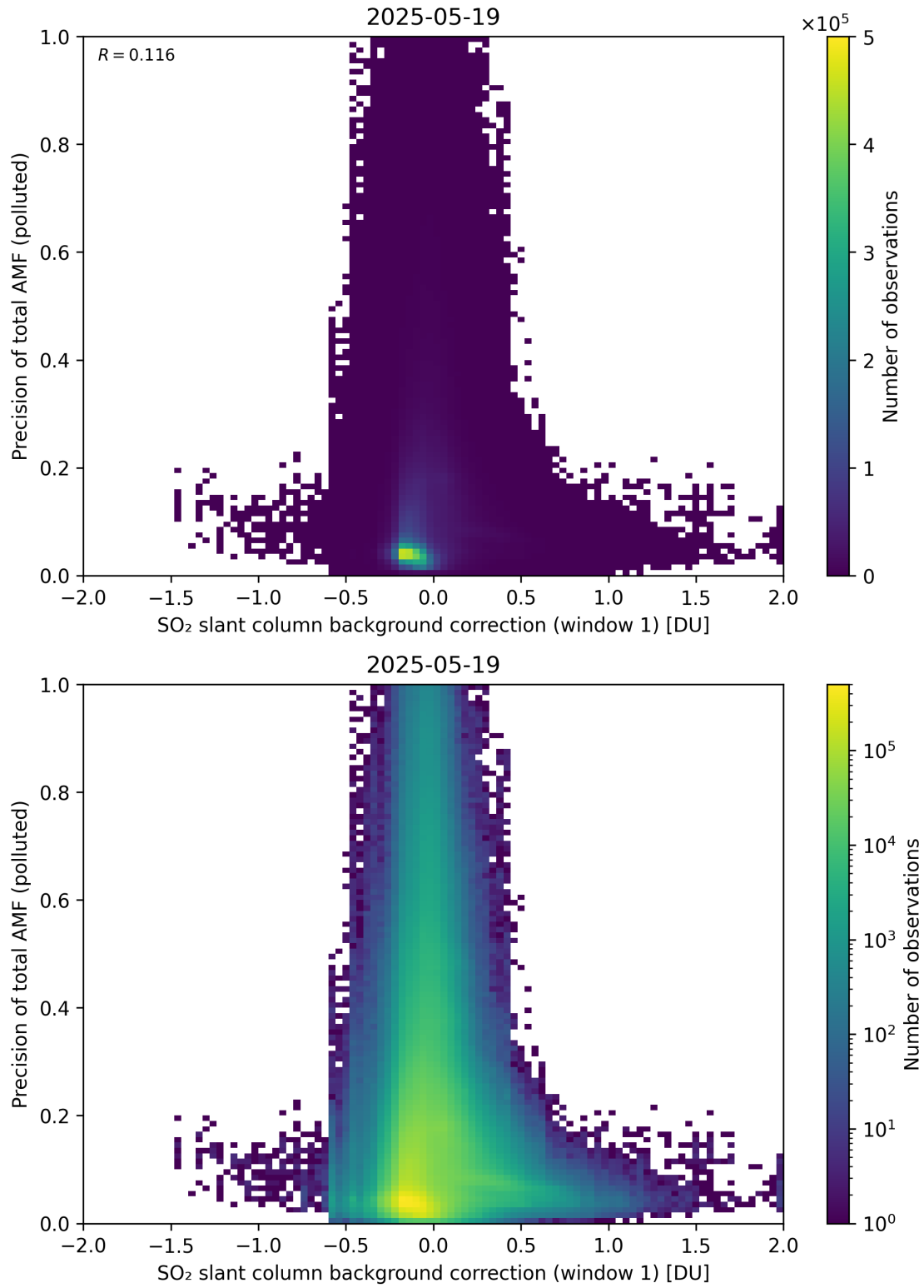
Figure 121: Scatter density plot of “SO 2 slant column background correction (window 1)” against “Precision of total AMF (polluted)” for 2025-05-18 to 2025-05-20.
