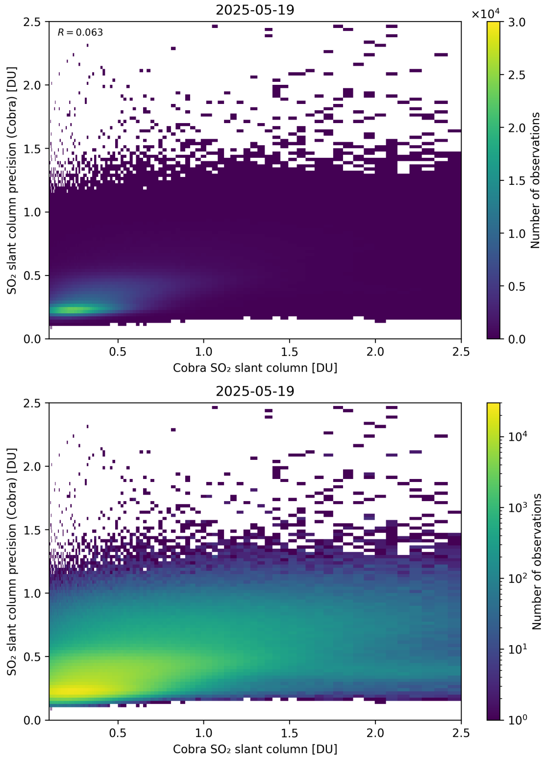
Figure 216: Scatter density plot of “Cobra SO 2 slant column” against “SO 2 slant column precision (Cobra)” for 2025-05-18 to 2025-05-20.
