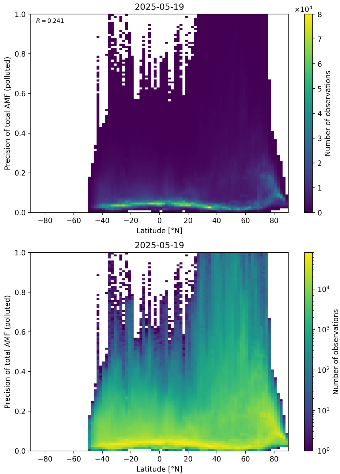
Figure 168: Scatter density plot of “Latitude” against “Precision of total AMF (polluted)” for 2025-05-18 to 2025-05-20.
