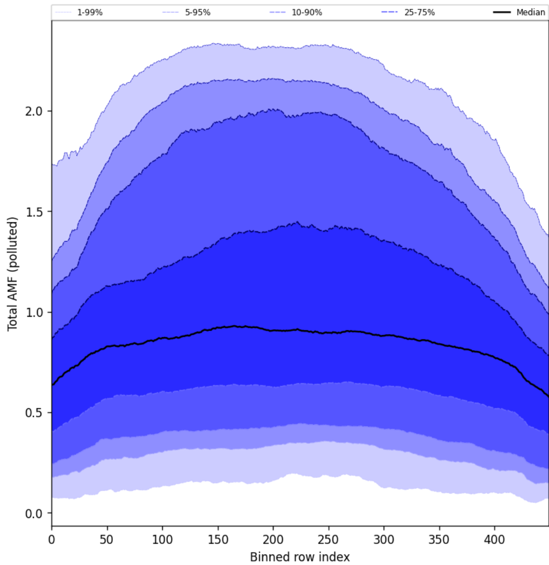
Figure 105: Along track statistics of “Total AMF (polluted)” for 2025-05-18 to 2025-05-20
