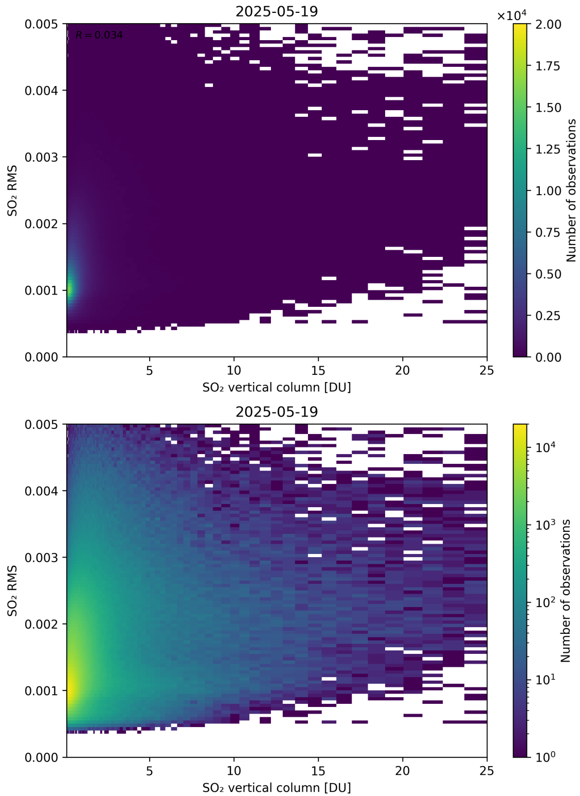
Figure 328: Scatter density plot of “SO 2 vertical column” against “SO 2 RMS” for 2025-05-18 to 2025-05-20.
