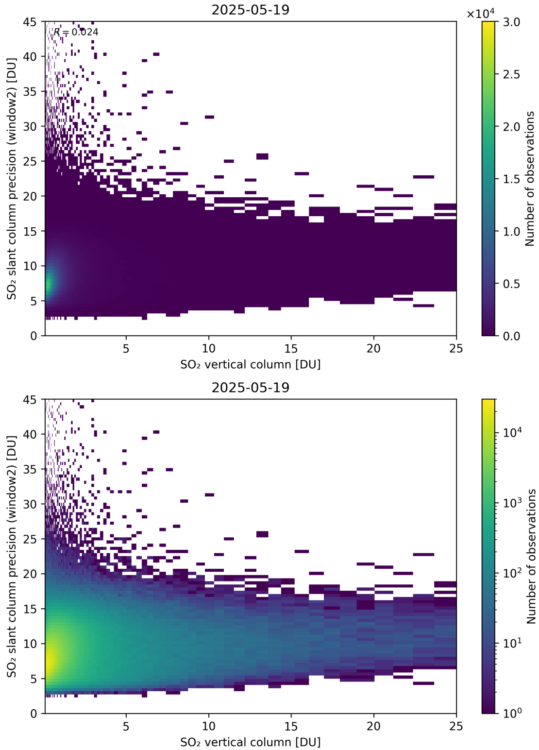
Figure 356: Scatter density plot of “SO 2 vertical column” against “SO 2 slant column precision (window2)” for 2025-05-18 to 2025-05-20.
