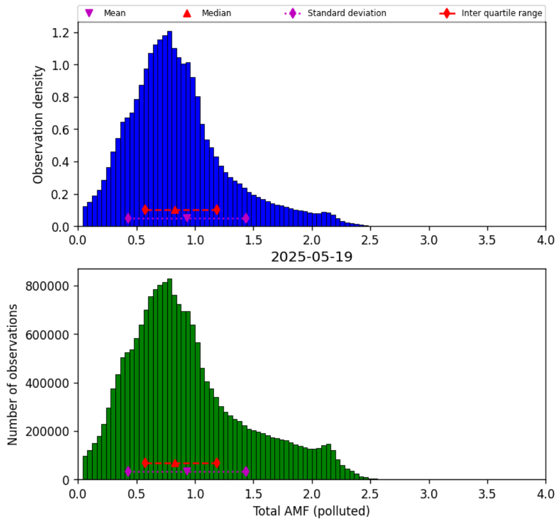
Figure 79: Histogram of “Total AMF (polluted)” for 2025-05-18 to 2025-05-20
