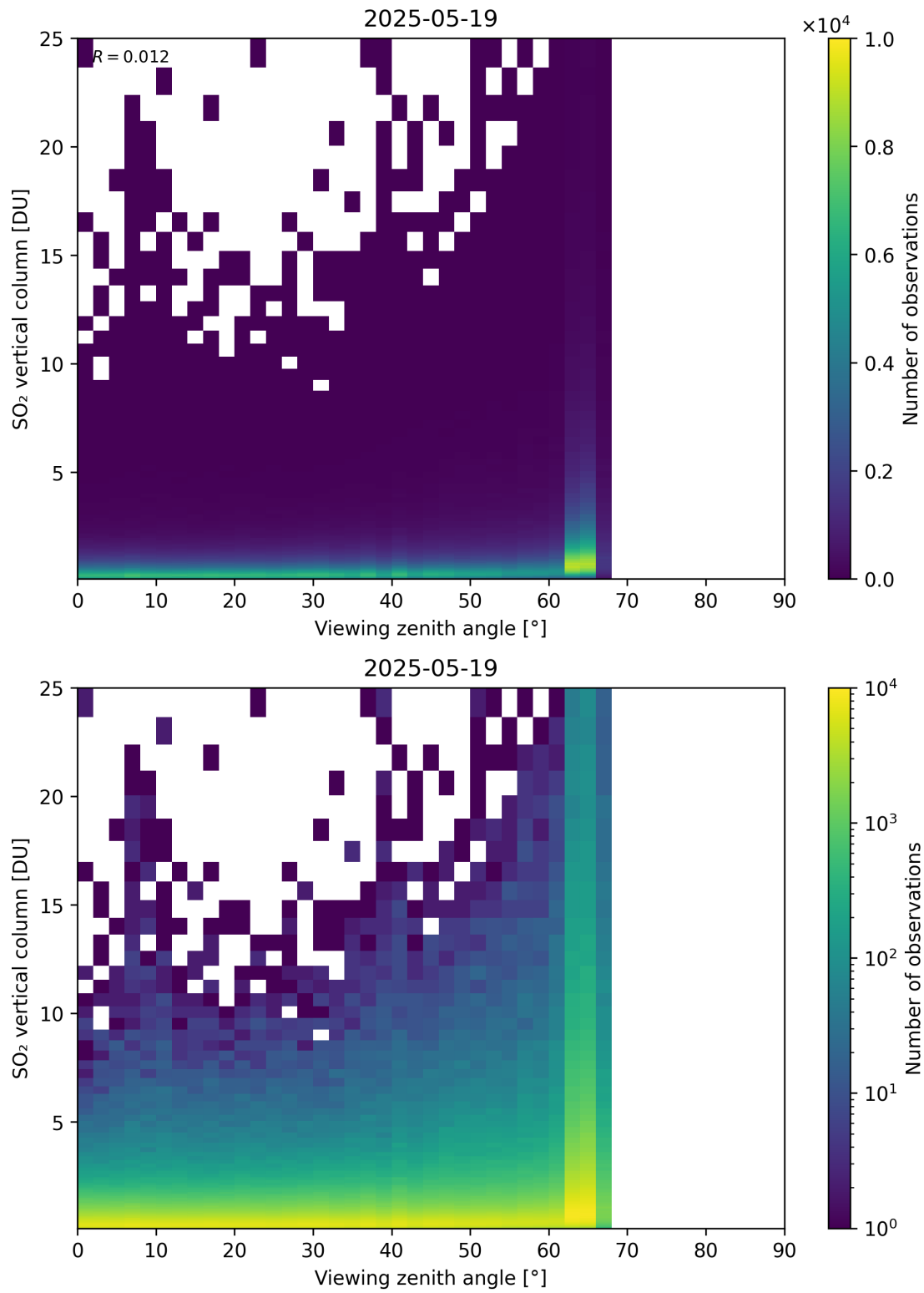
Figure 383: Scatter density plot of “Viewing zenith angle” against “SO 2 vertical column” for 2025-05-18 to 2025-05-20.
