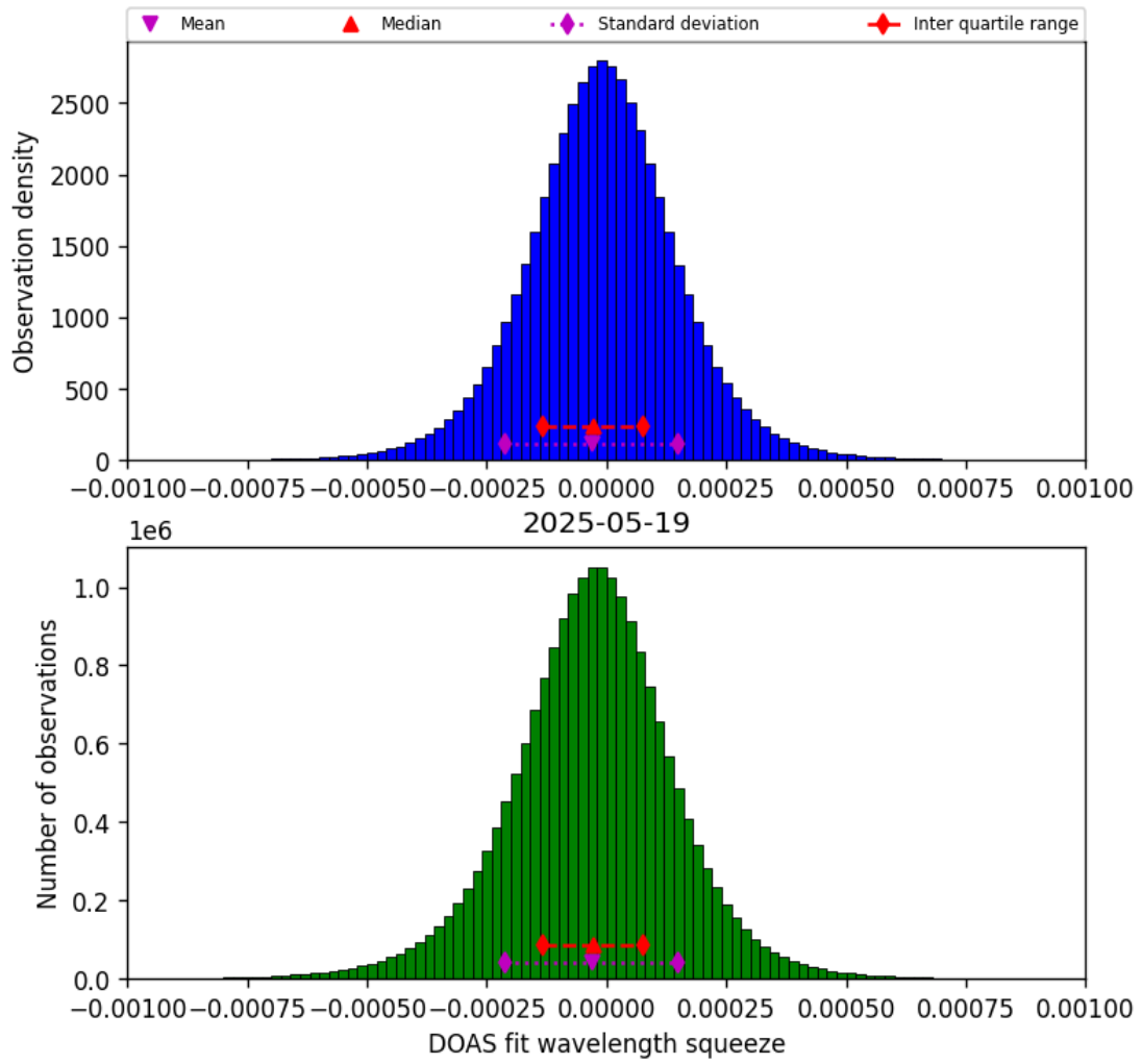
Figure 77: Histogram of “DOAS fit wavelength squeeze” for 2025-05-18 to 2025-05-20
