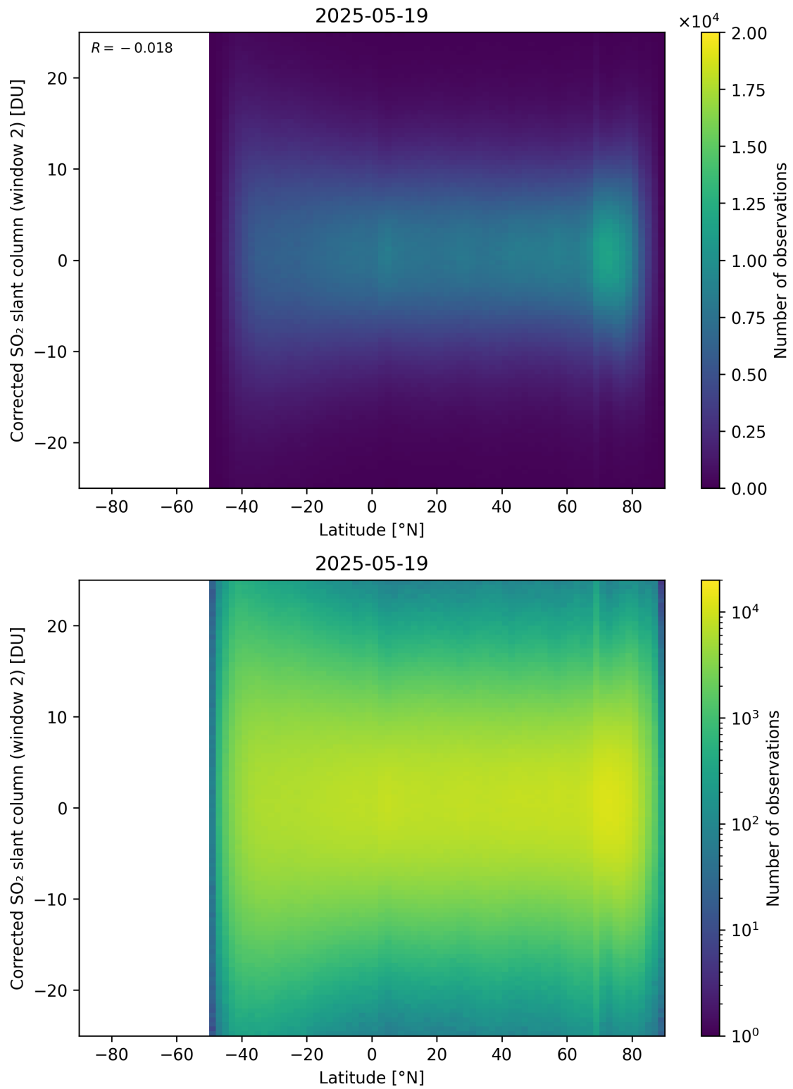
Figure 160: Scatter density plot of “Latitude” against “Corrected SO 2 slant column (window 2)” for 2025-05-18 to 2025-05-20.
