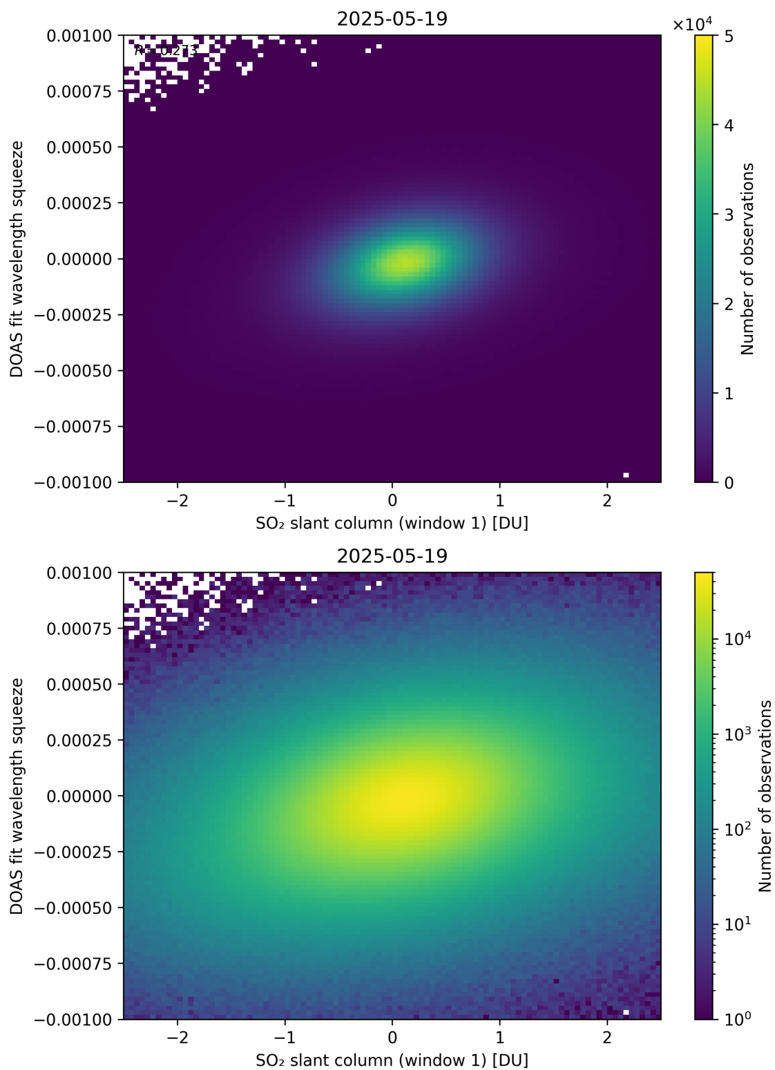
Figure 266: Scatter density plot of “SO 2 slant column (window 1)” against “DOAS fit wavelength squeeze” for 2025-05-18 to 2025-05-20.
