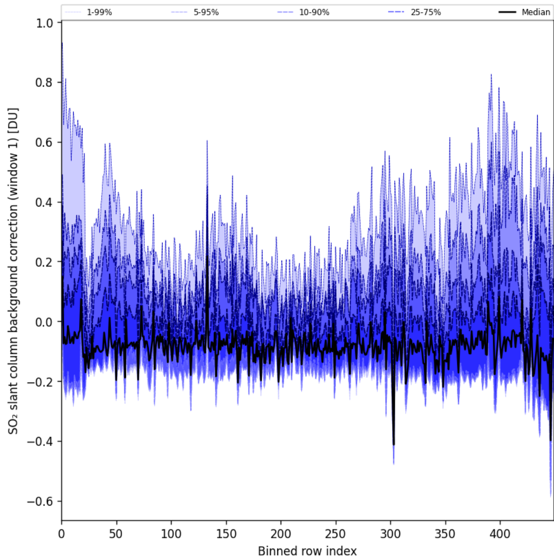
Figure 92: Along track statistics of “SO 2 slant column background correction (window 1)” for 2025-05-18 to 2025-05-20
