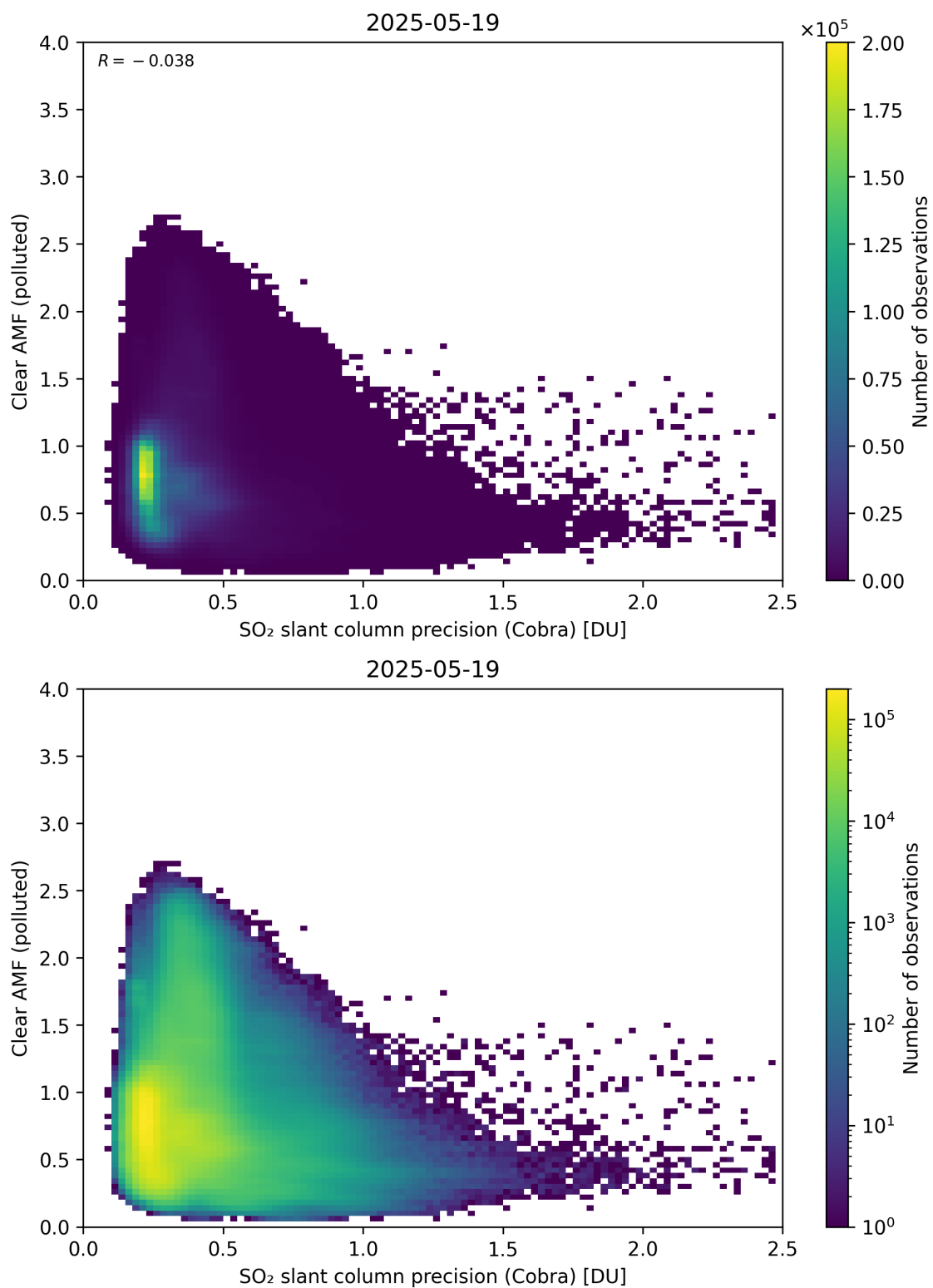
Figure 205: Scatter density plot of “SO 2 slant column precision (Cobra)” against “Clear AMF (polluted)” for 2025-05-18 to 2025-05-20.
