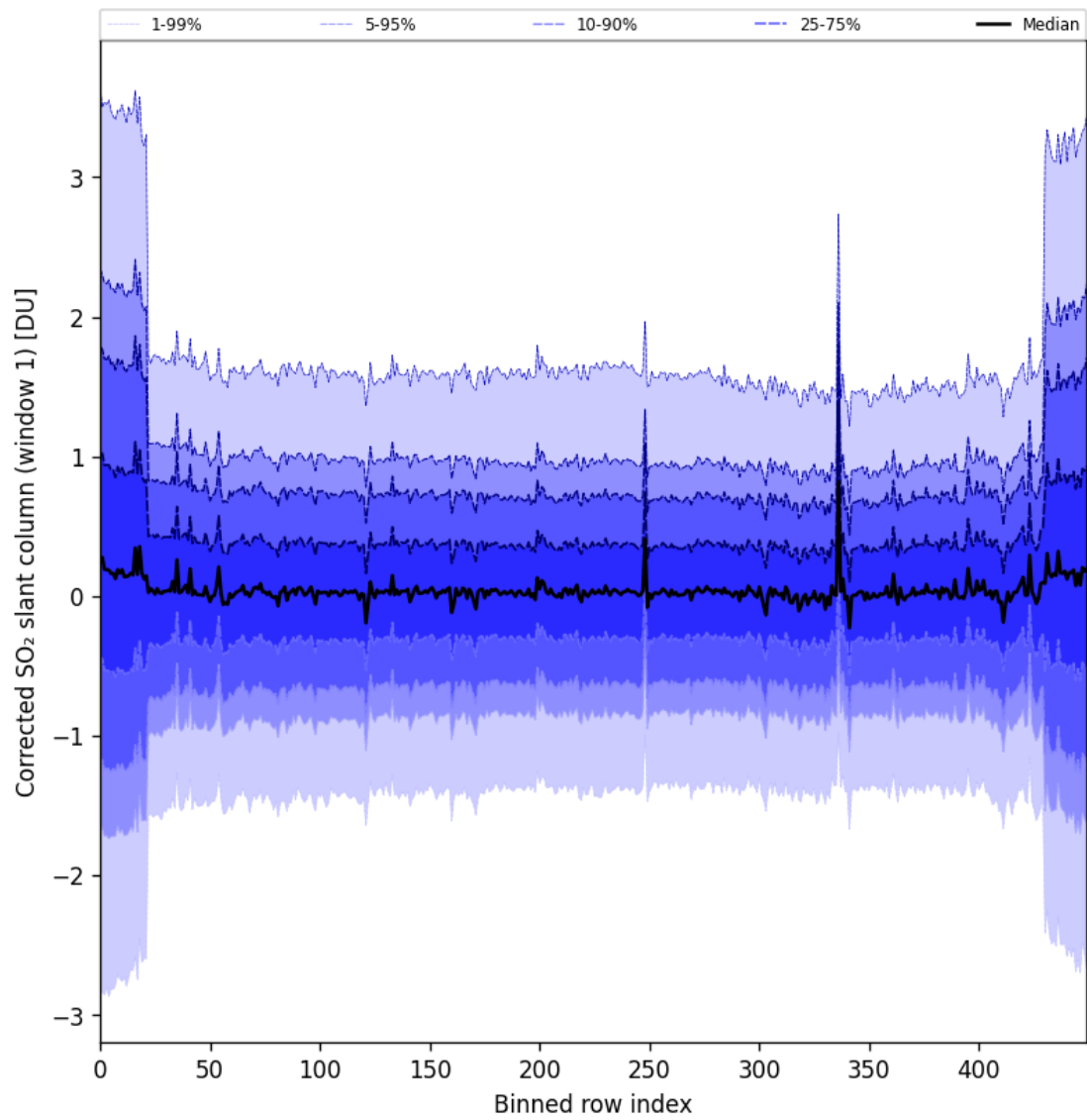
Figure 91: Along track statistics of “Corrected SO 2 slant column (window 1)” for 2025-05-18 to 2025-05-20
