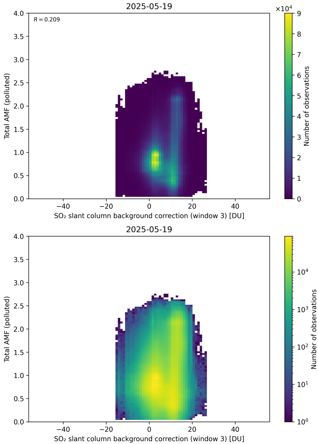
Figure 136: Scatter density plot of “SO 2 slant column background correction (window 3)” against “Total AMF (polluted)” for 2025-05-18 to 2025-05-20.
