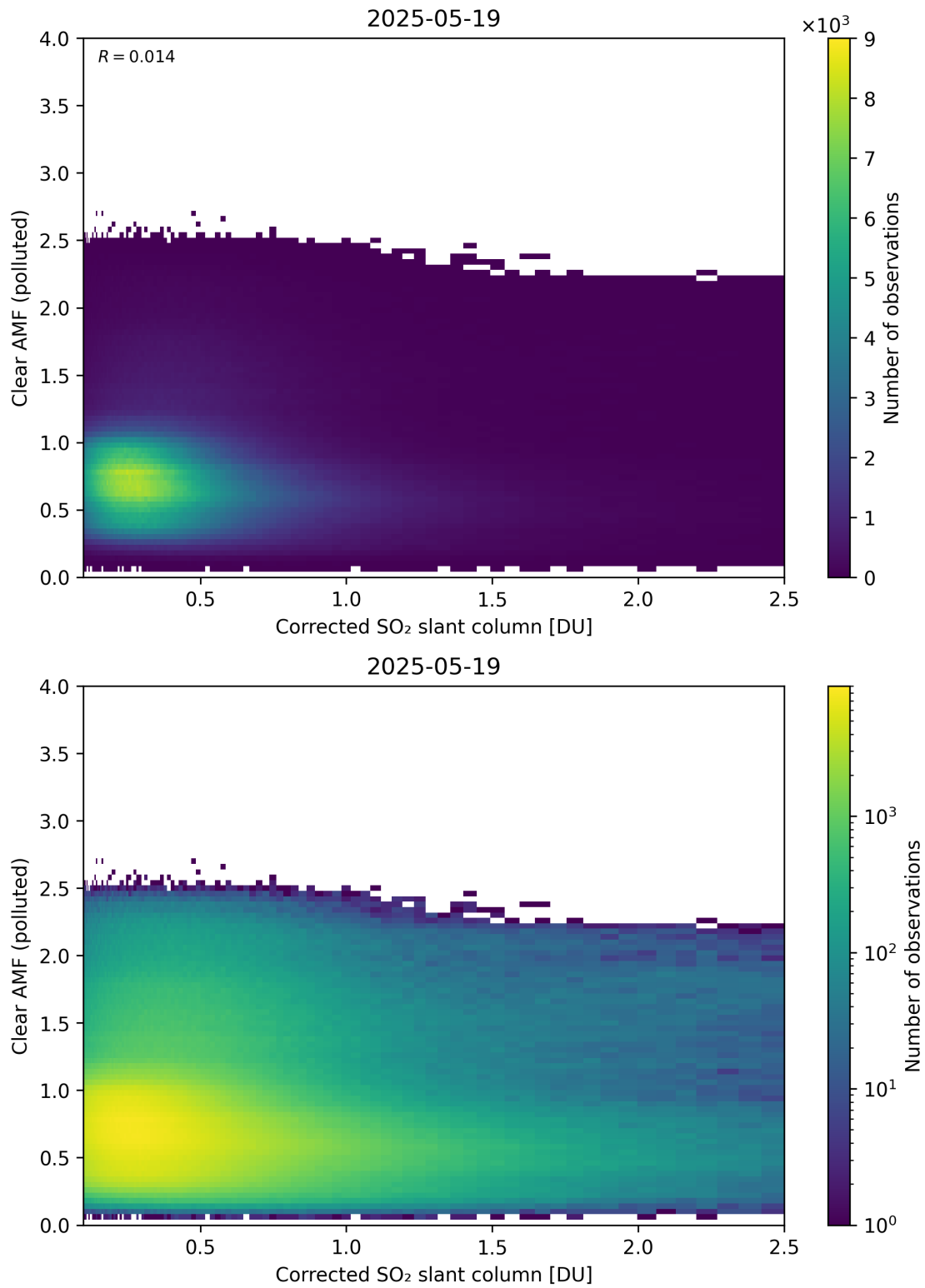
Figure 232: Scatter density plot of “Corrected SO 2 slant column” against “Clear AMF (polluted)” for 2025-05-18 to 2025-05-20.
