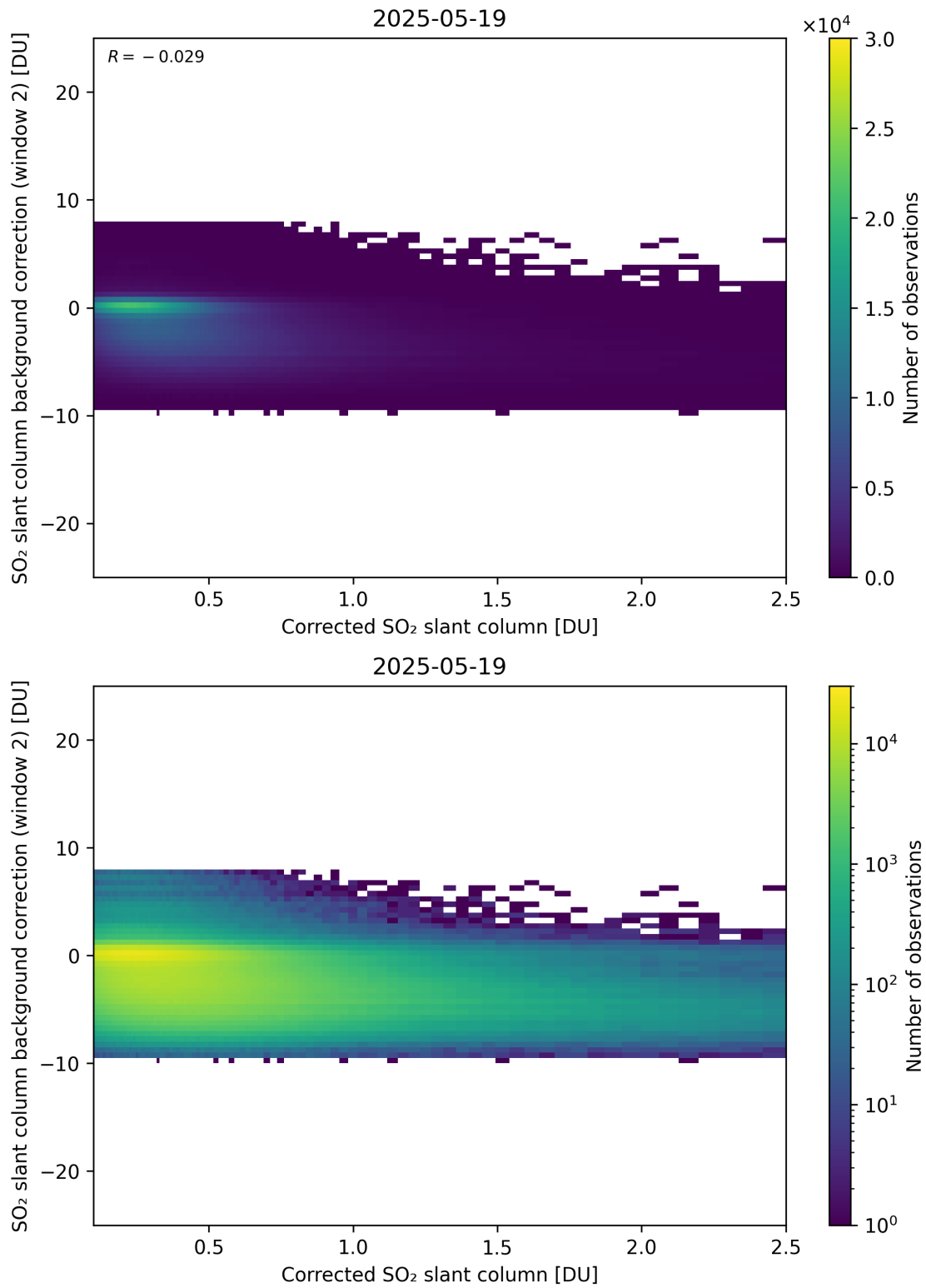
Figure 227: Scatter density plot of “Corrected SO 2 slant column” against “SO 2 slant column background correction (window 2)” for 2025-05-18 to 2025-05-20.
