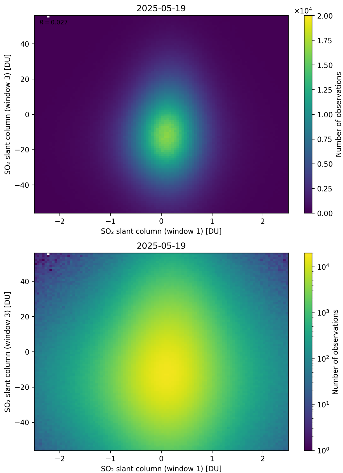
Figure 287: Scatter density plot of “SO 2 slant column (window 1)” against “SO 2 slant column (window 3)” for 2025-05-18 to 2025-05-20.
