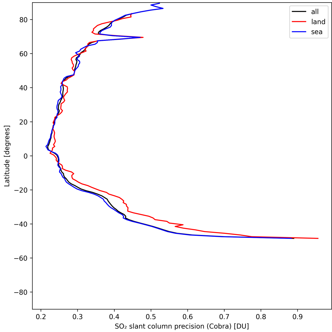
Figure 36: Zonal average of “SO 2 slant column precision (Cobra)” for 2025-05-18 to 2025-05-20.
