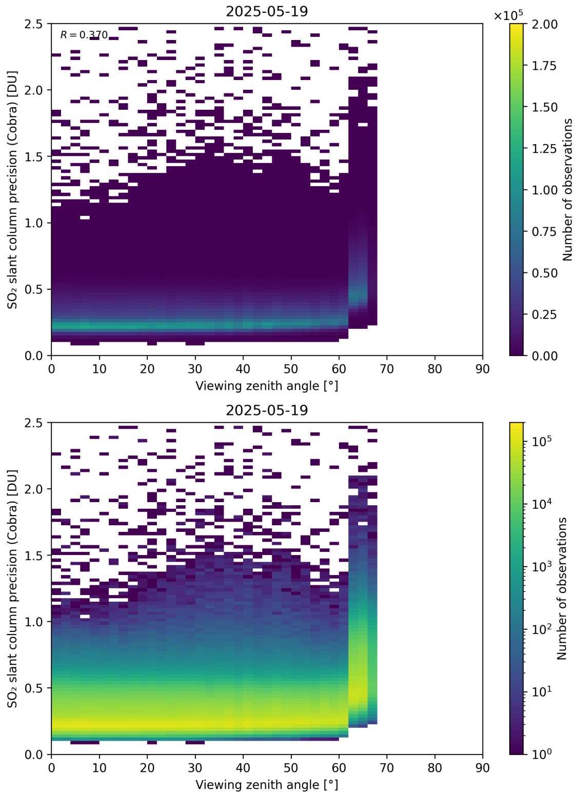
Figure 372: Scatter density plot of “Viewing zenith angle” against “SO 2 slant column precision (Cobra)” for 2025-05-18 to 2025-05-20.
