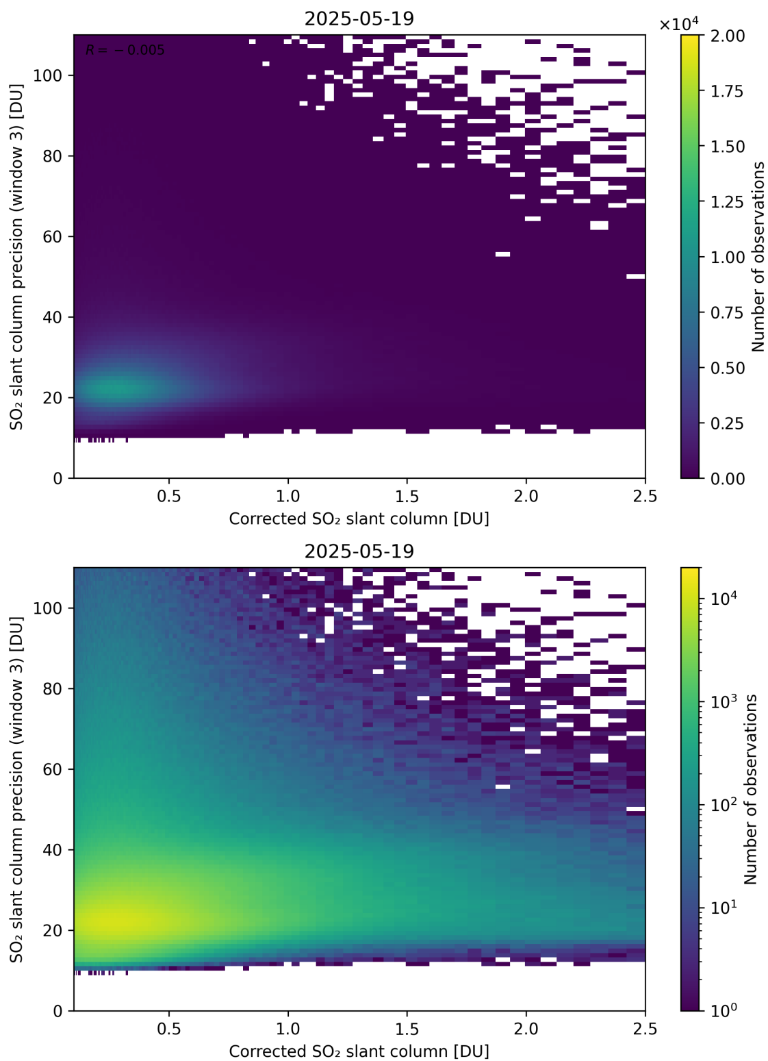
Figure 241: Scatter density plot of “Corrected SO 2 slant column” against “SO 2 slant column precision (window 3)” for 2025-05-18 to 2025-05-20.
