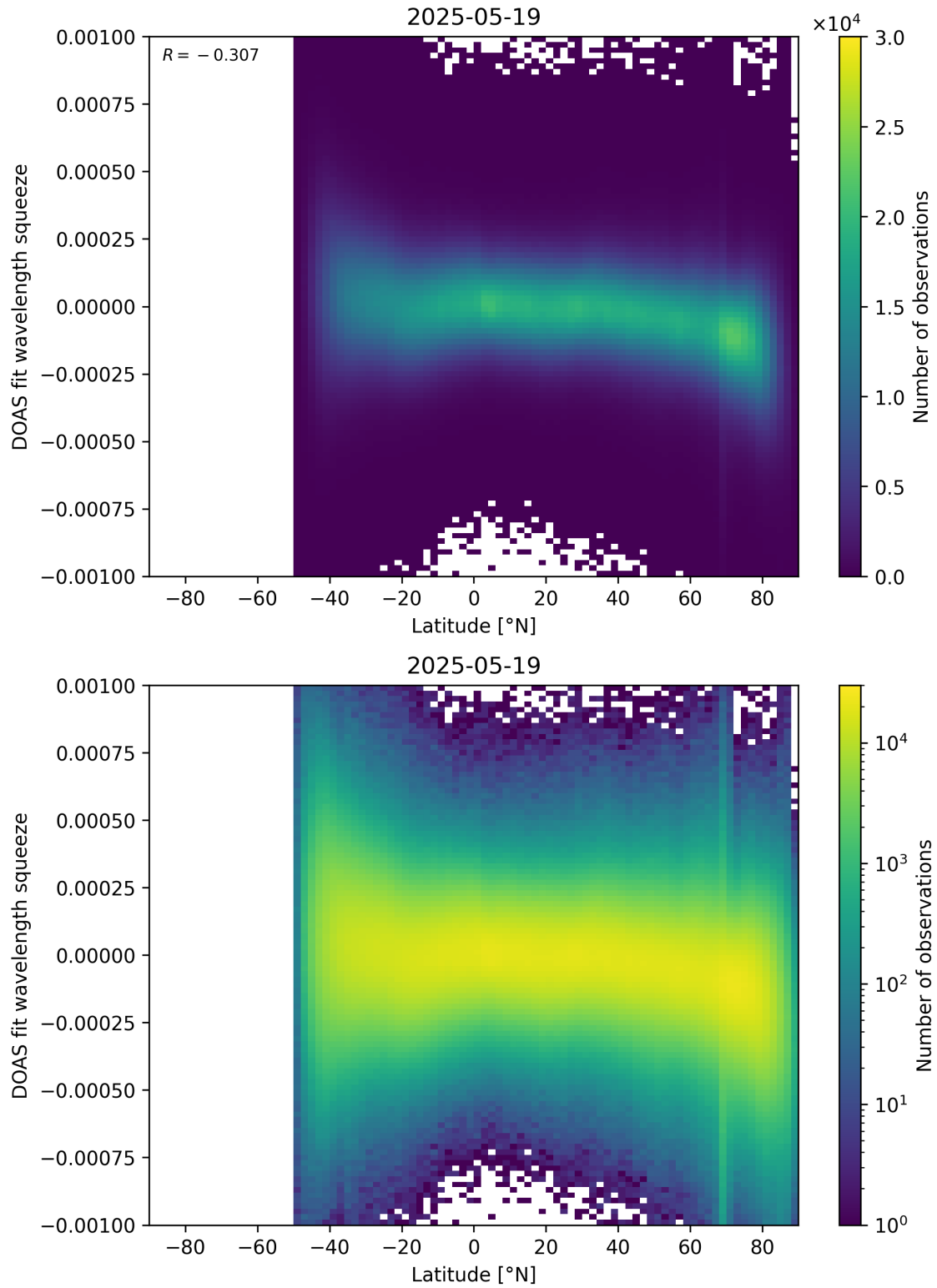
Figure 154: Scatter density plot of “Latitude” against “DOAS fit wavelength squeeze” for 2025-05-18 to 2025-05-20.
