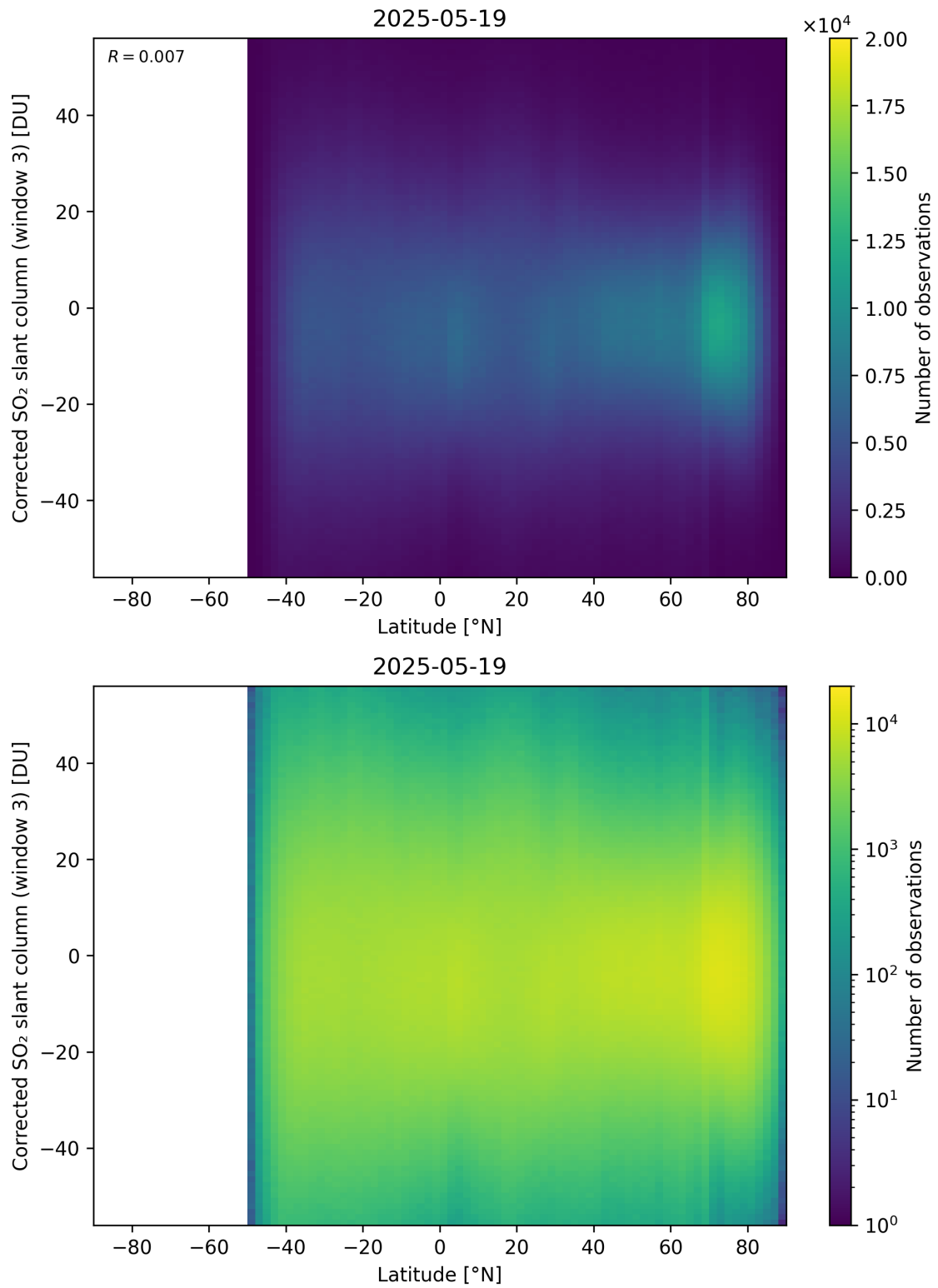
Figure 161: Scatter density plot of “Latitude” against “Corrected SO 2 slant column (window 3)” for 2025-05-18 to 2025-05-20.
