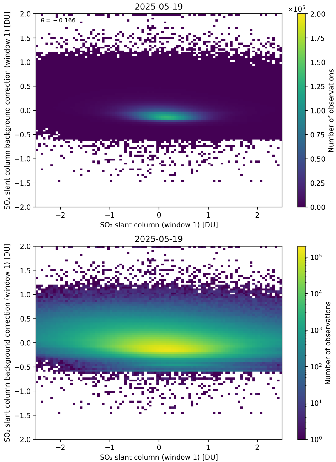
Figure 262: Scatter density plot of “SO 2 slant column (window 1)” against “SO 2 slant column background correction (window 1)” for 2025-05-18 to 2025-05-20.
