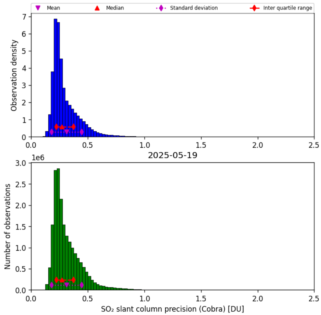
Figure 62: Histogram of “SO 2 slant column precision (Cobra)” for 2025-05-18 to 2025-05-20
