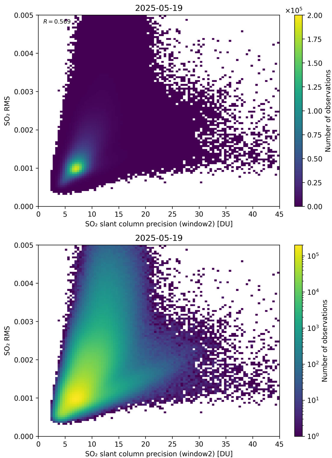
Figure 295: Scatter density plot of “SO 2 slant column precision (window2)” against “SO 2 RMS” for 2025-05-18 to 2025-05-20.
