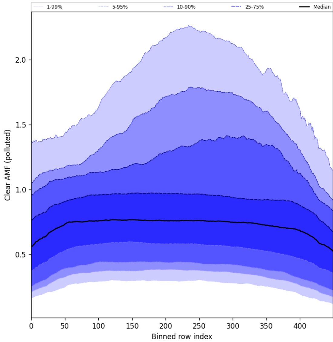
Figure 107: Along track statistics of “Clear AMF (polluted)” for 2025-05-18 to 2025-05-20
