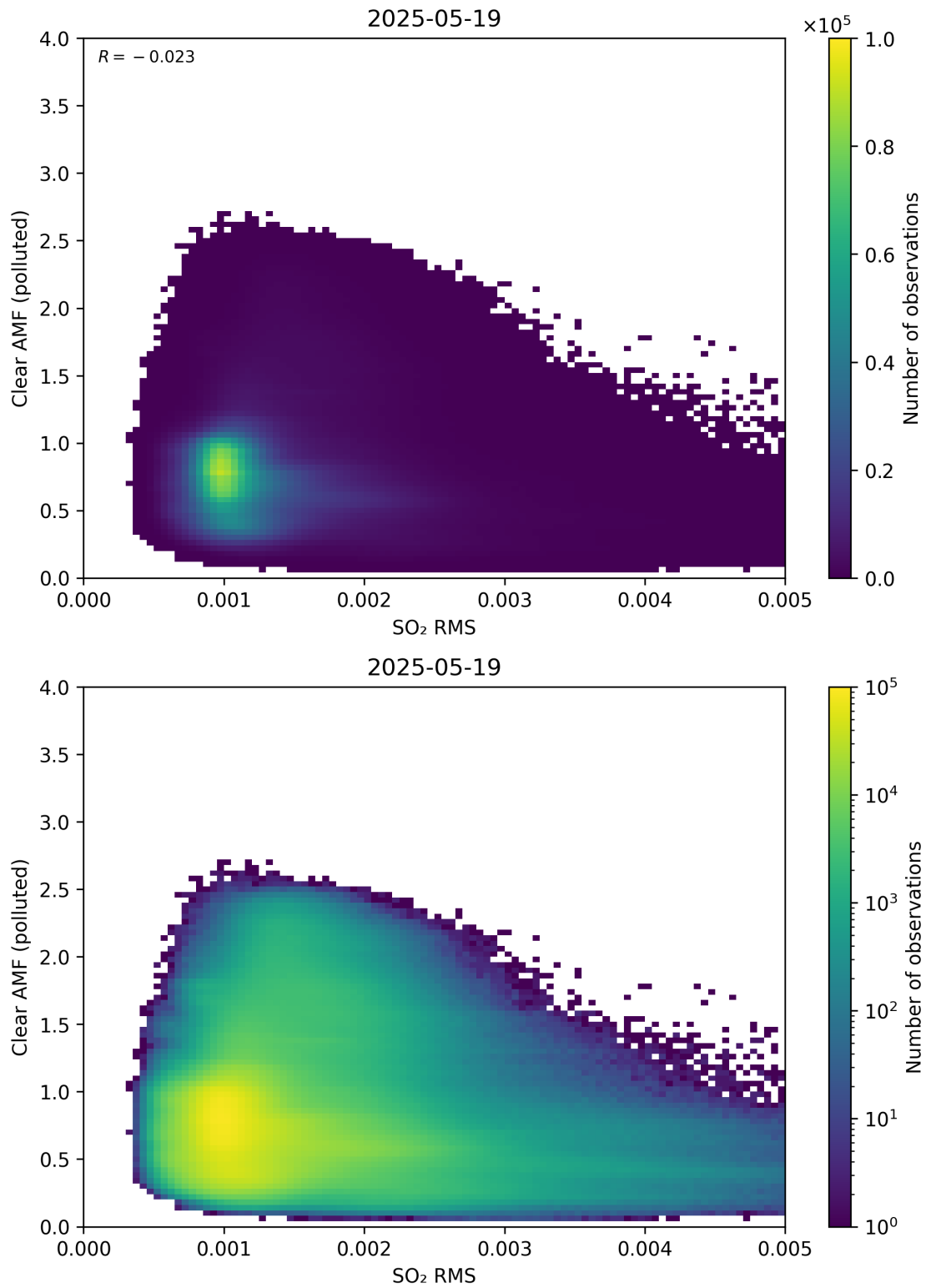
Figure 147: Scatter density plot of “SO 2 RMS” against “Clear AMF (polluted)” for 2025-05-18 to 2025-05-20.
