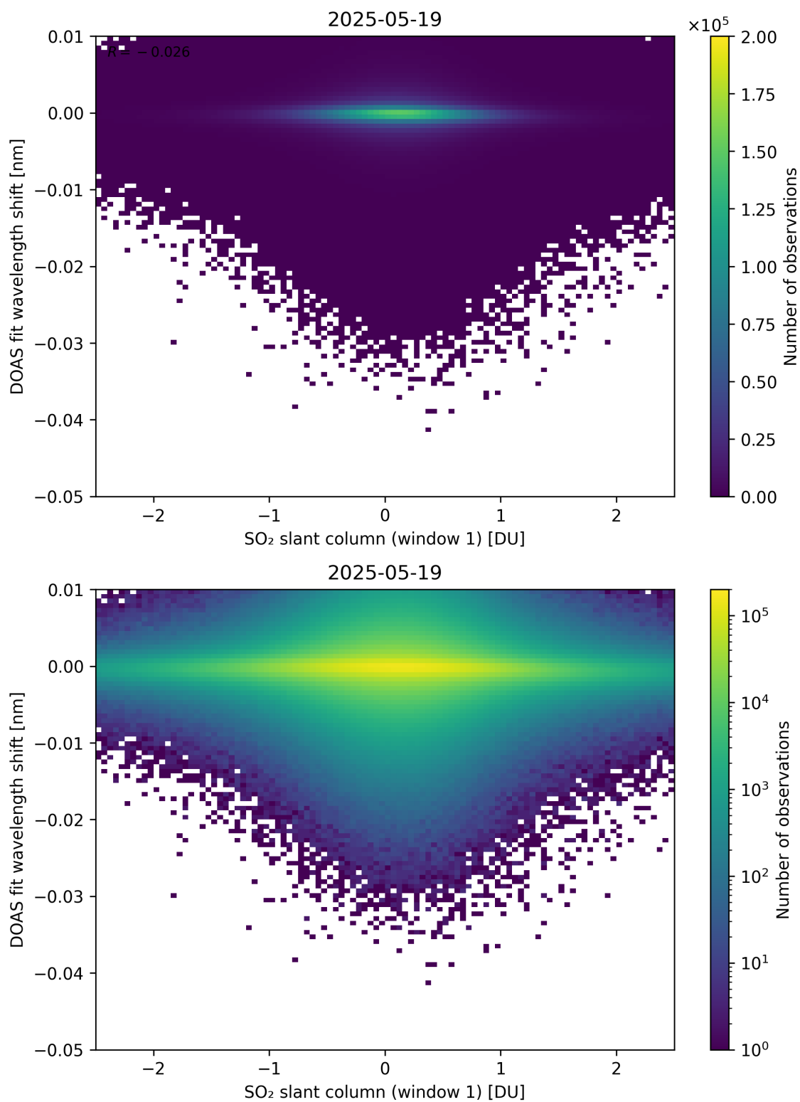
Figure 265: Scatter density plot of “SO 2 slant column (window 1)” against “DOAS fit wavelength shift” for 2025-05-18 to 2025-05-20.
