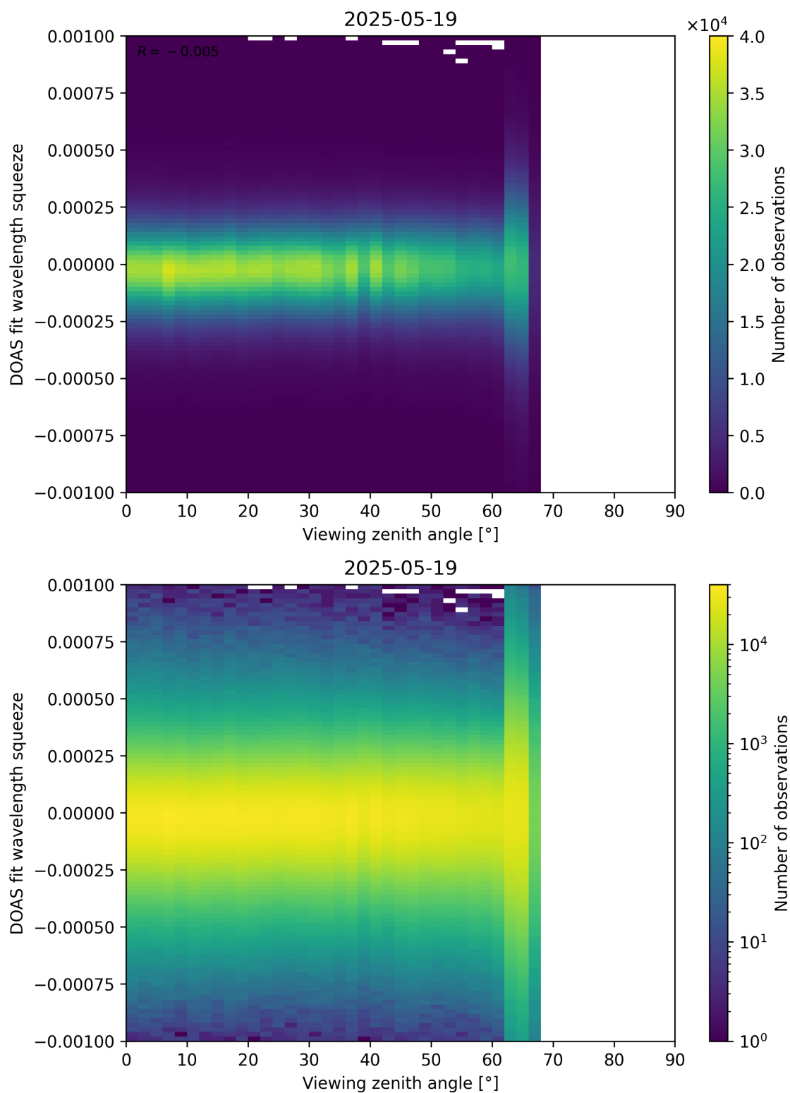
Figure 366: Scatter density plot of “Viewing zenith angle” against “DOAS fit wavelength squeeze” for 2025-05-18 to 2025-05-20.
