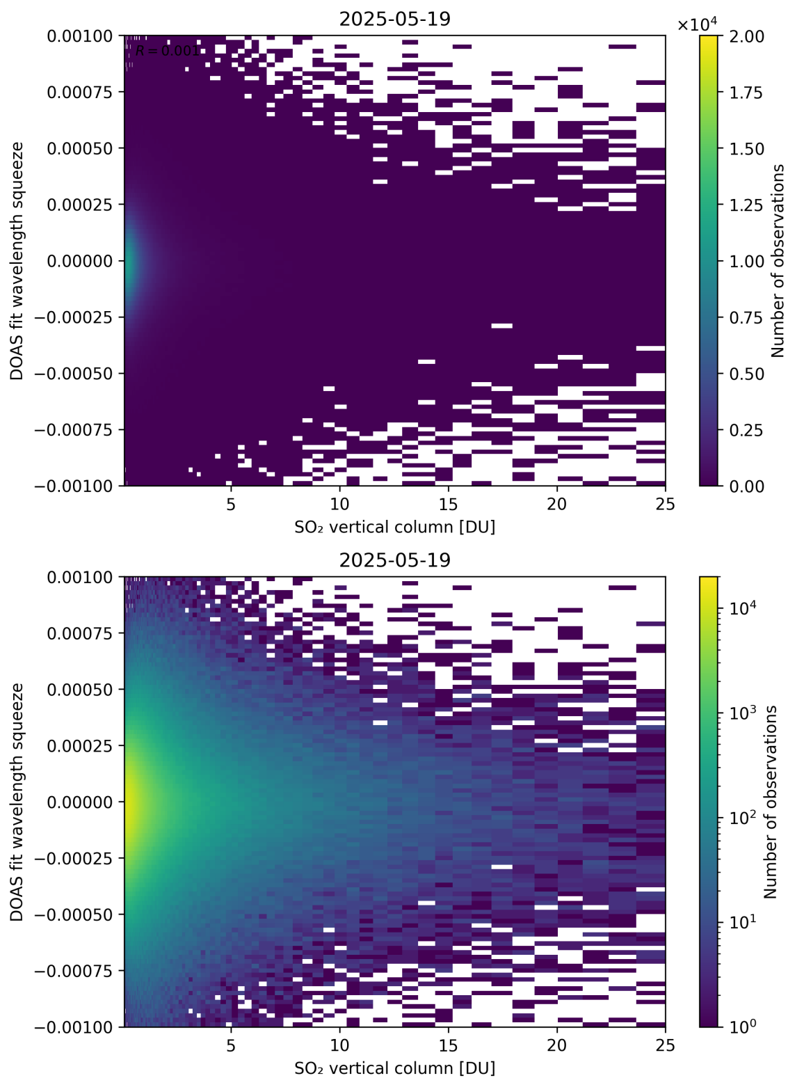
Figure 327: Scatter density plot of “SO 2 vertical column” against “DOAS fit wavelength squeeze” for 2025-05-18 to 2025-05-20.
