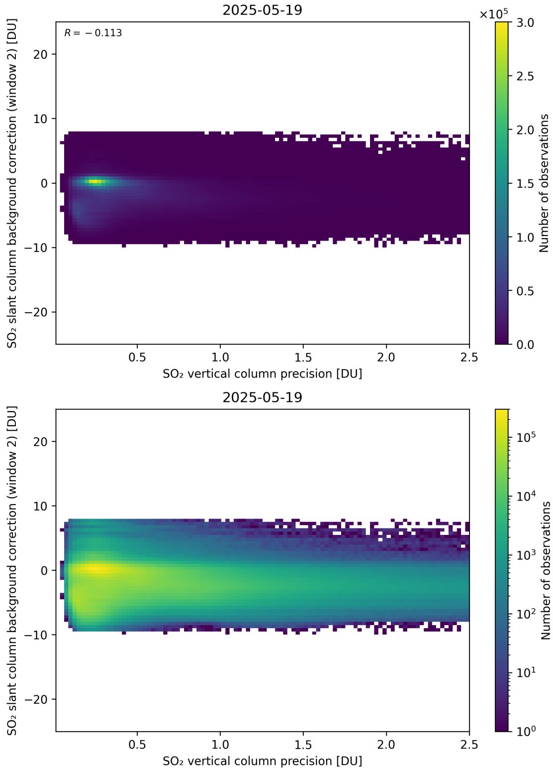
Figure 330: Scatter density plot of “SO 2 vertical column precision” against “SO 2 slant column background correction (window 2)” for 2025-05-18 to 2025-05-20.
