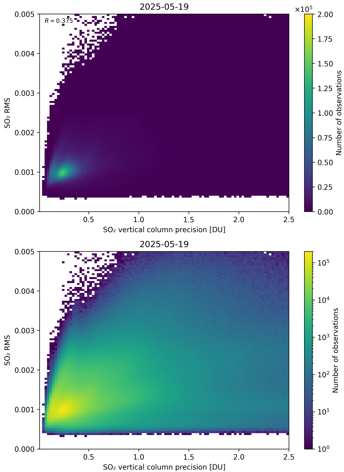
Figure 334: Scatter density plot of “SO 2 vertical column precision” against “SO 2 RMS” for 2025-05-18 to 2025-05-20.
