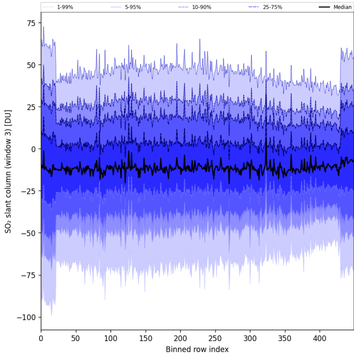
Figure 97: Along track statistics of “SO 2 slant column (window 3)” for 2025-05-18 to 2025-05-20
