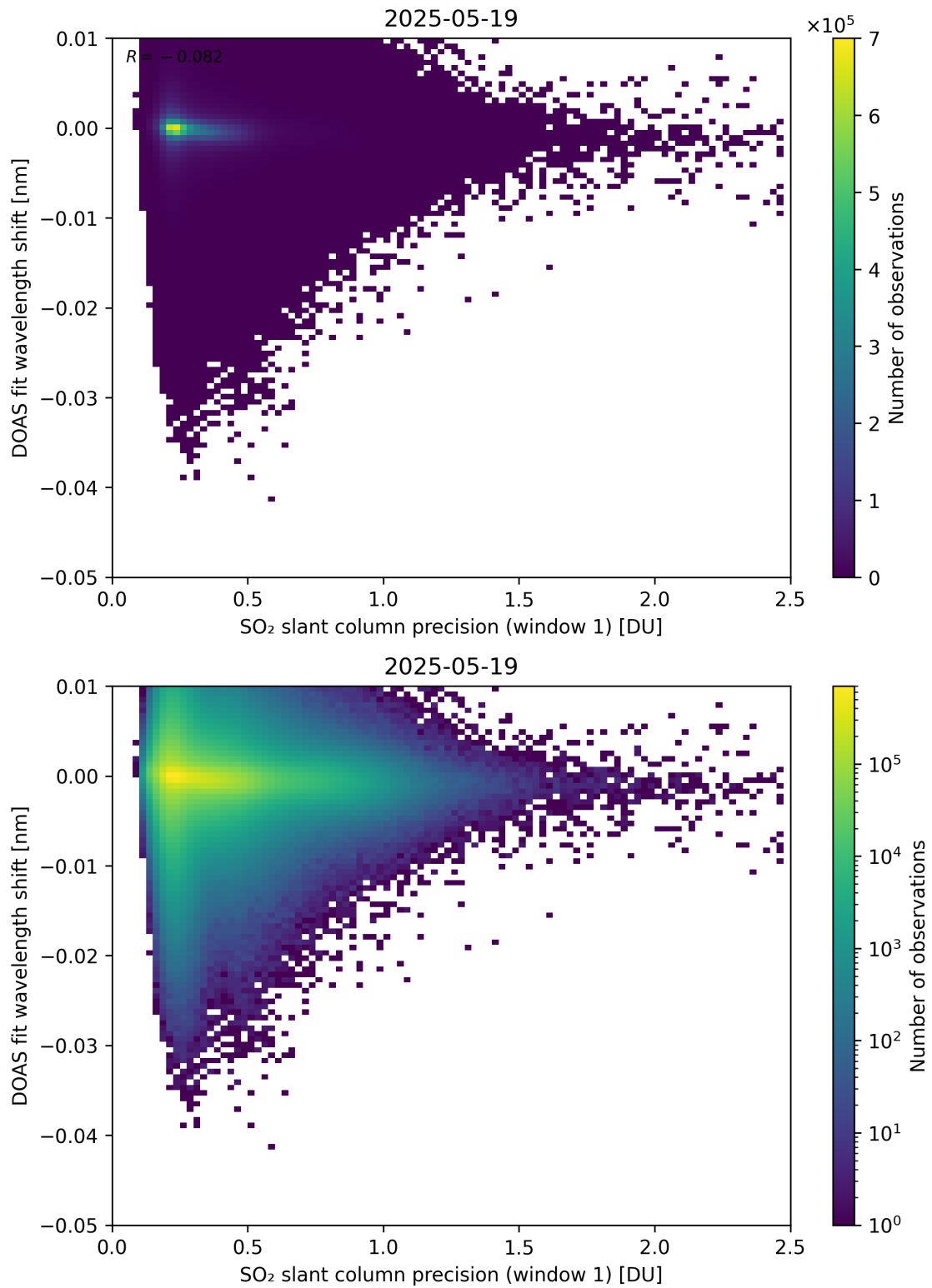
Figure 271: Scatter density plot of “SO 2 slant column precision (window 1)” against “DOAS fit wavelength shift” for 2025-05-18 to 2025-05-20.
