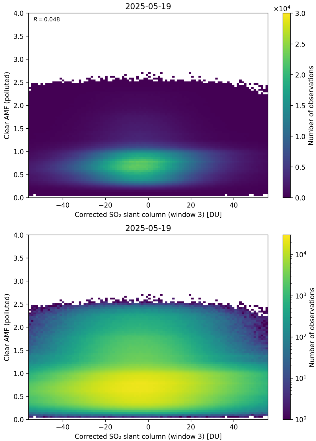
Figure 259: Scatter density plot of “Corrected SO 2 slant column (window 3)” against “Clear AMF (polluted)” for 2025-05-18 to 2025-05-20.
