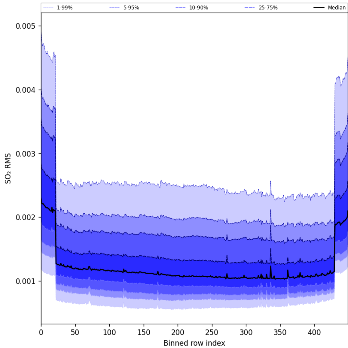
Figure 104: Along track statistics of “SO 2 RMS” for 2025-05-18 to 2025-05-20
