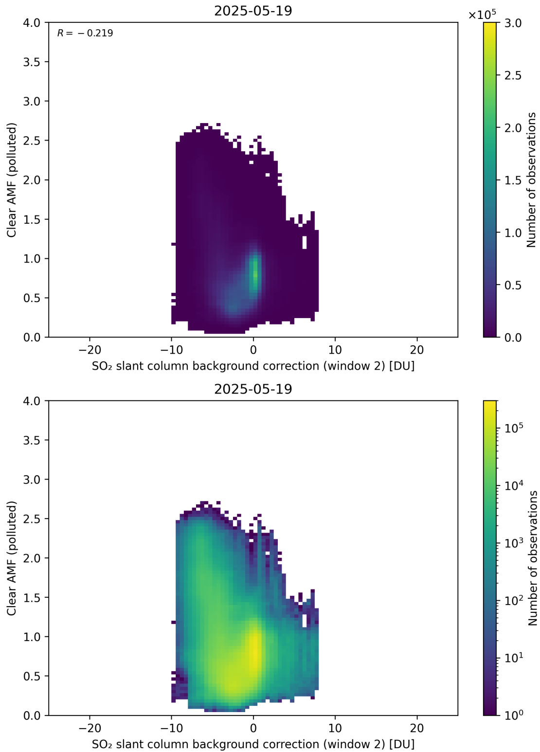
Figure 126: Scatter density plot of “SO 2 slant column background correction (window 2)” against “Clear AMF (polluted)” for 2025-05-18 to 2025-05-20.
