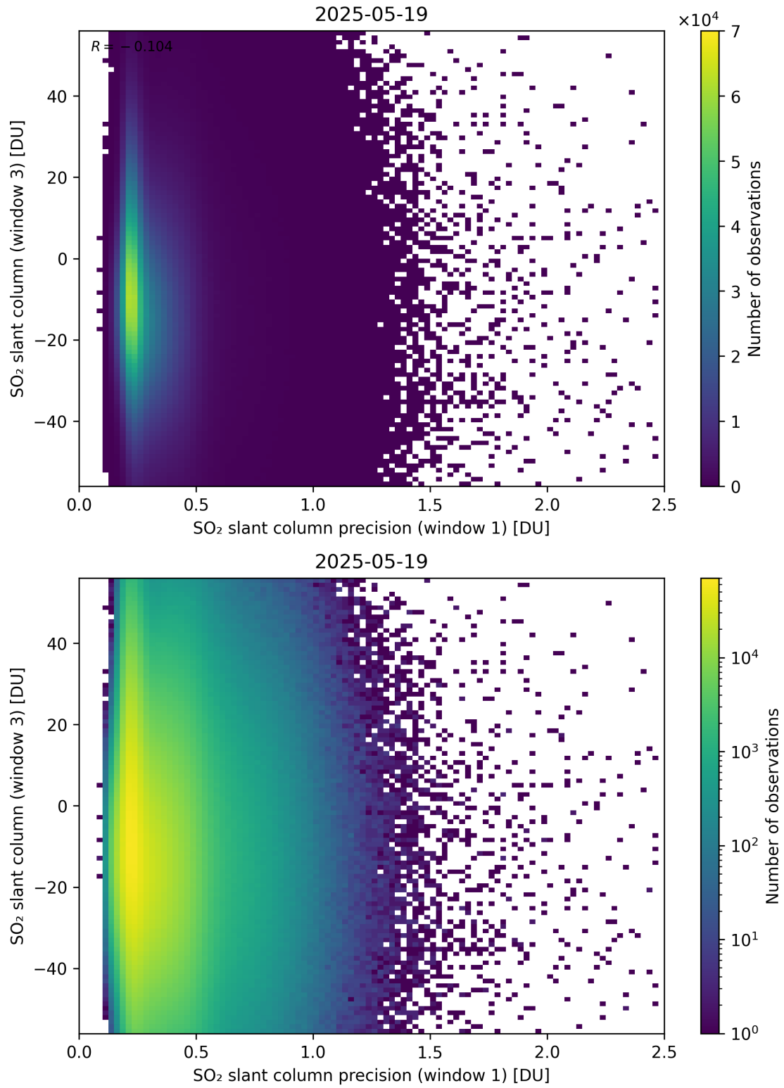
Figure 278: Scatter density plot of “SO 2 slant column precision (window 1)” against “SO 2 slant column (window 3)” for 2025-05-18 to 2025-05-20.
