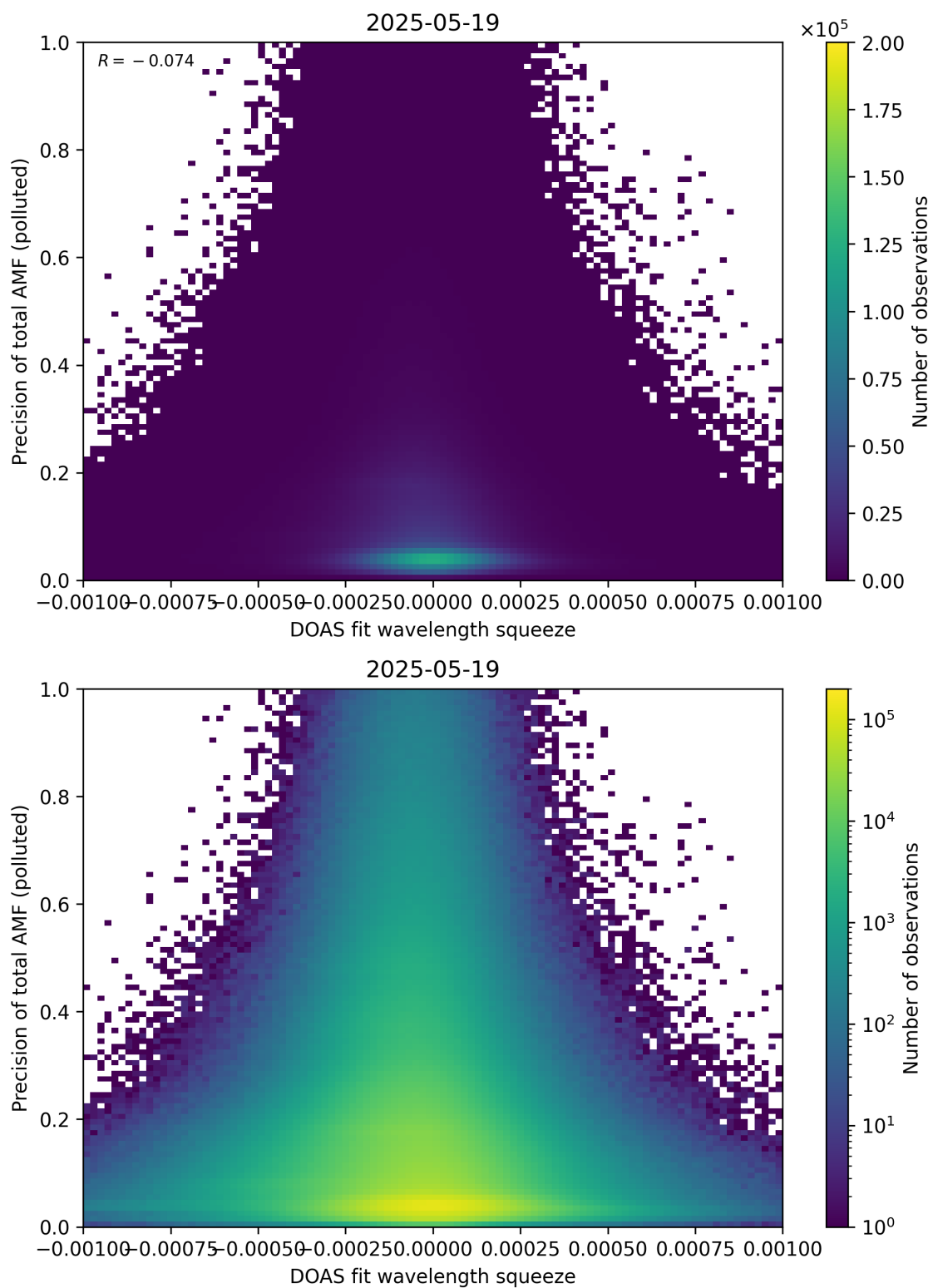
Figure 146: Scatter density plot of “DOAS fit wavelength squeeze” against “Precision of total AMF (polluted)” for 2025-05-18 to 2025-05-20.
