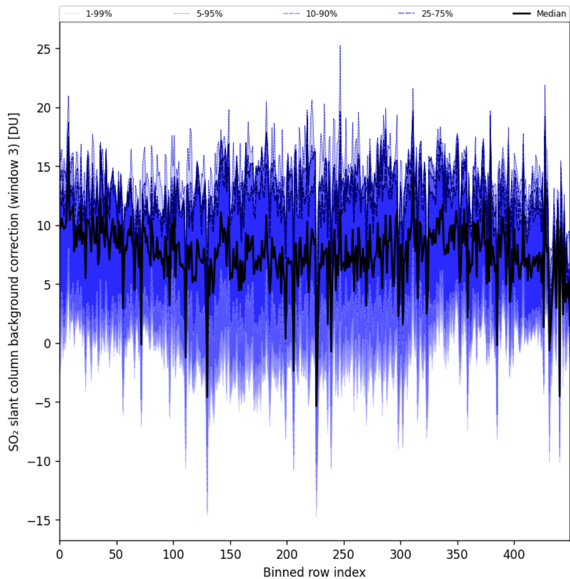
Figure 100: Along track statistics of “SO 2 slant column background correction (window 3)” for 2025-05-18 to 2025-05-20
