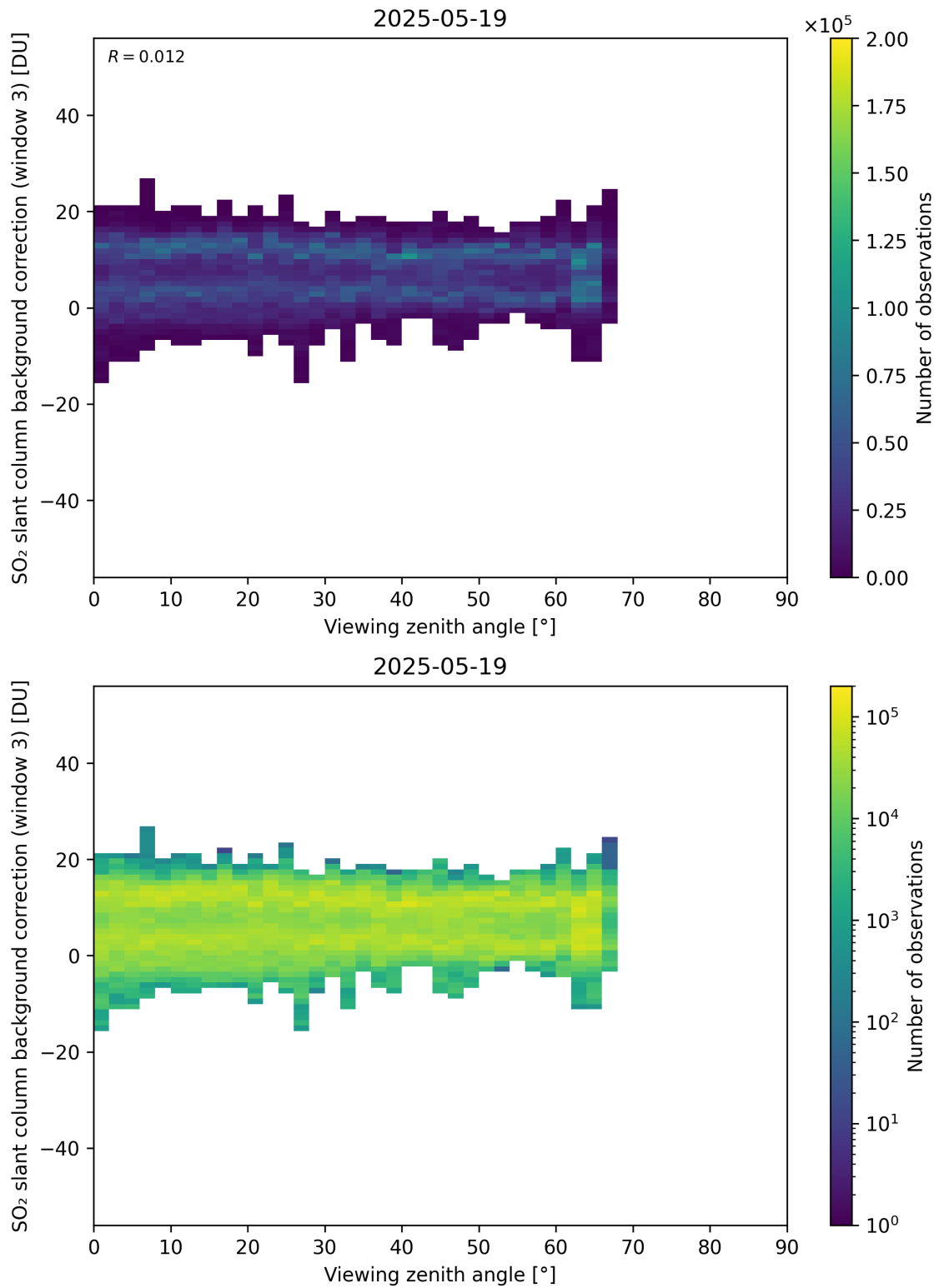
Figure 364: Scatter density plot of “Viewing zenith angle” against “SO 2 slant column background correction (window 3)” for 2025-05-18 to 2025-05-20.
