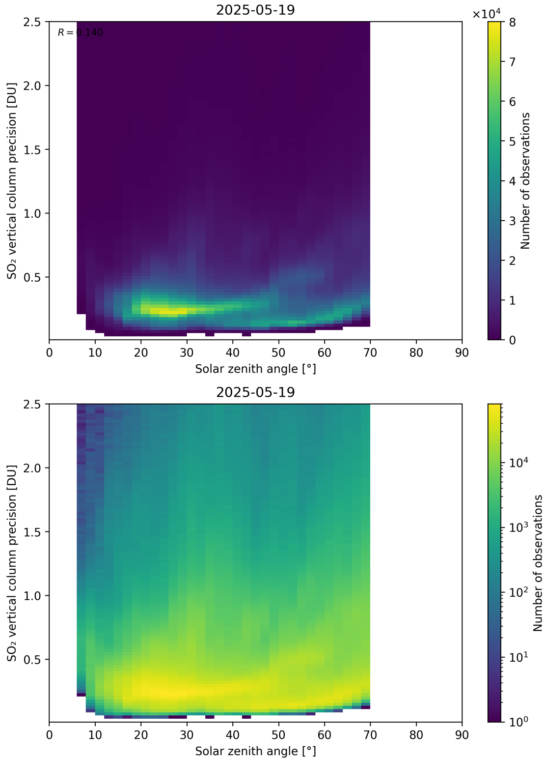
Figure 192: Scatter density plot of “Solar zenith angle” against “SO 2 vertical column precision” for 2025-05-18 to 2025-05-20.
