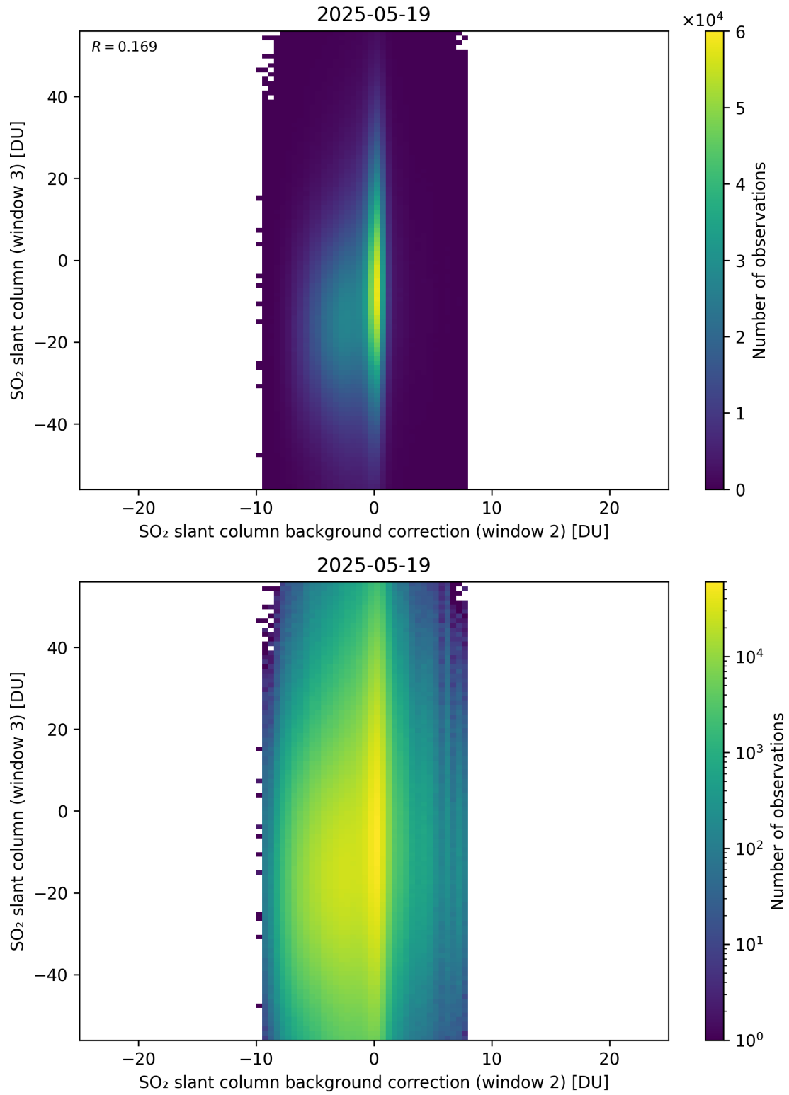
Figure 128: Scatter density plot of “SO 2 slant column background correction (window 2)” against “SO 2 slant column (window 3)” for 2025-05-18 to 2025-05-20.
