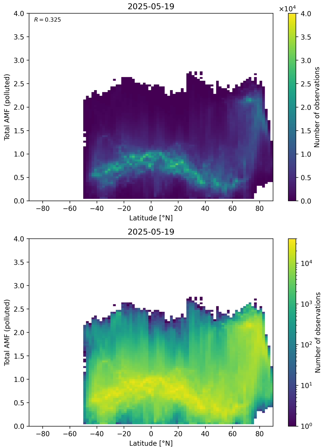
Figure 167: Scatter density plot of “Latitude” against “Total AMF (polluted)” for 2025-05-18 to 2025-05-20.
