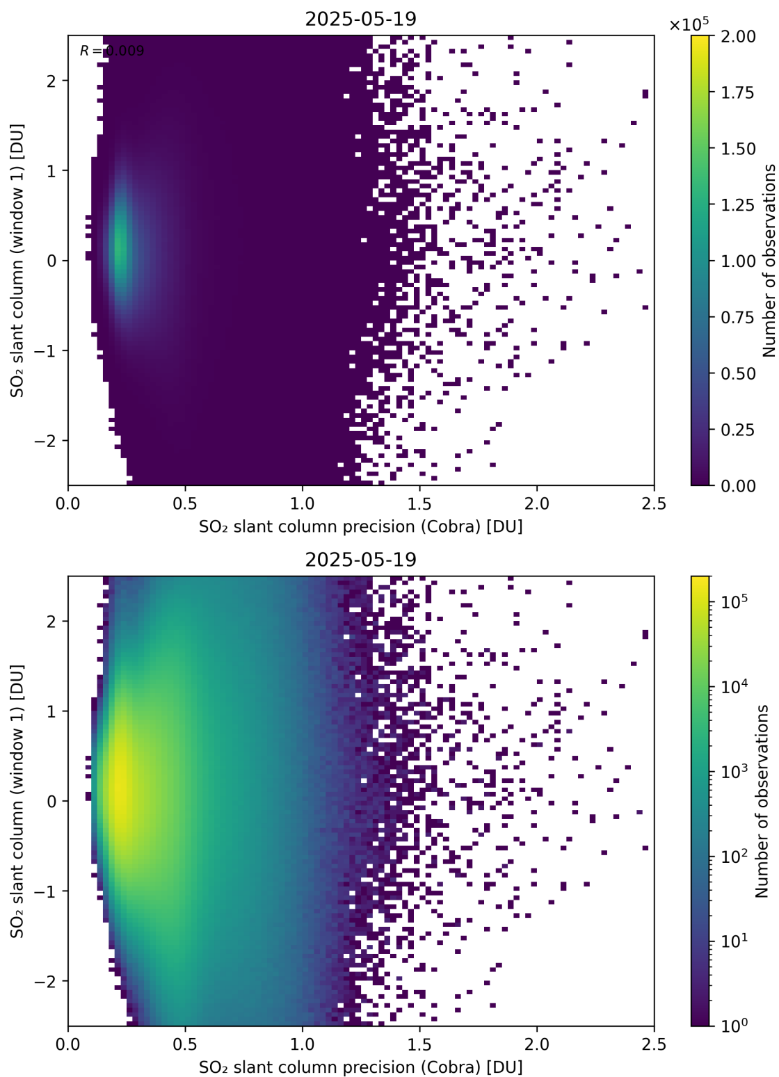
Figure 208: Scatter density plot of “SO 2 slant column precision (Cobra)” against “SO 2 slant column (window 1)” for 2025-05-18 to 2025-05-20.
