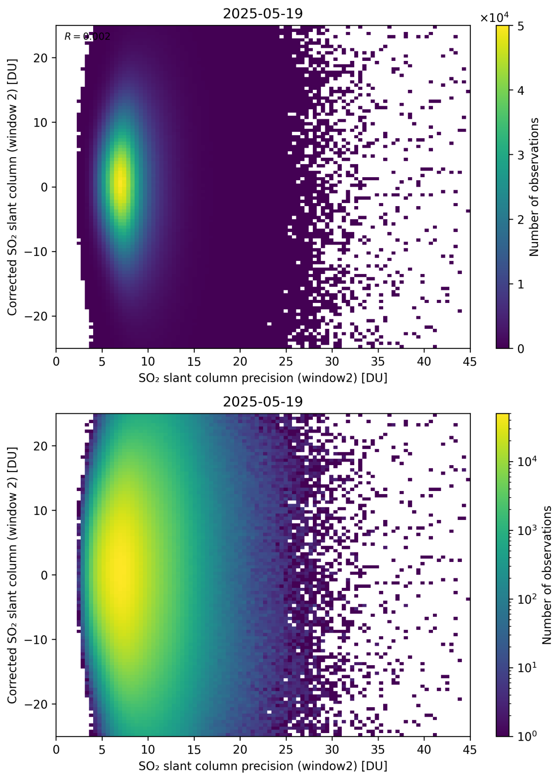
Figure 297: Scatter density plot of “SO 2 slant column precision (window2)” against “Corrected SO 2 slant column (window 2)” for 2025-05-18 to 2025-05-20.
