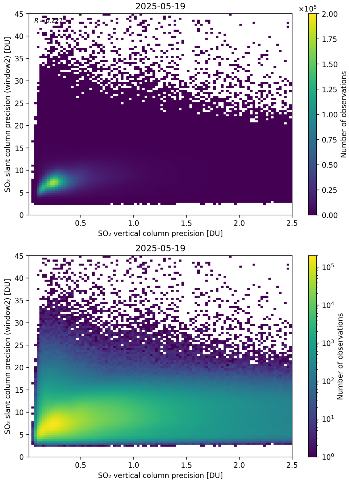
Figure 343: Scatter density plot of “SO 2 vertical column precision” against “SO 2 slant column precision (window2)” for 2025-05-18 to 2025-05-20.
