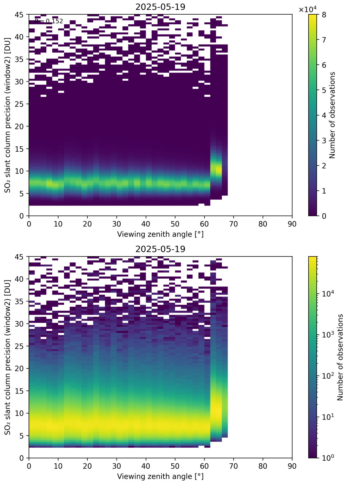
Figure 378: Scatter density plot of “Viewing zenith angle” against “SO 2 slant column precision (window2)” for 2025-05-18 to 2025-05-20.
