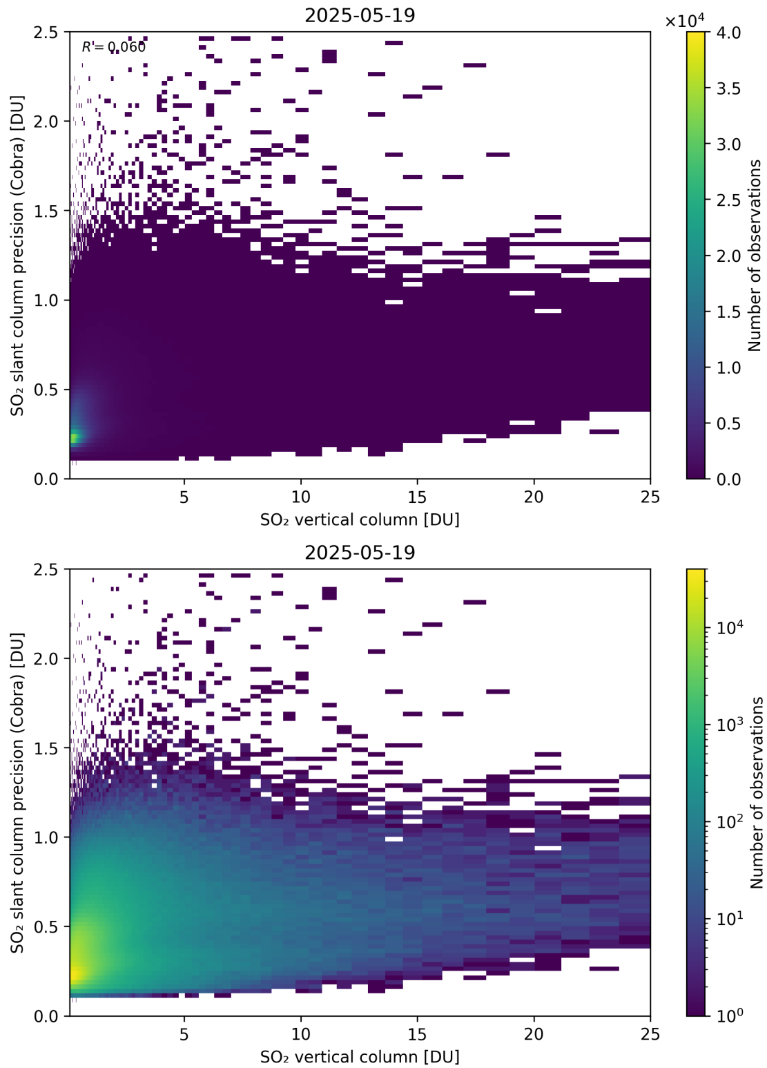
Figure 350: Scatter density plot of “SO 2 vertical column” against “SO 2 slant column precision (Cobra)” for 2025-05-18 to 2025-05-20.
