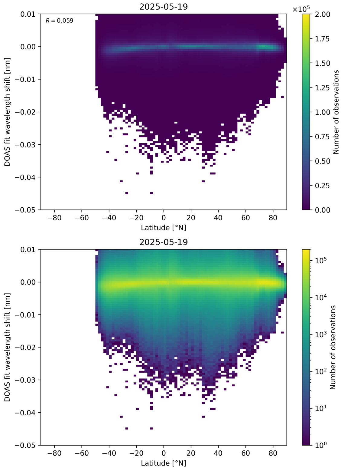
Figure 153: Scatter density plot of “Latitude” against “DOAS fit wavelength shift” for 2025-05-18 to 2025-05-20.
