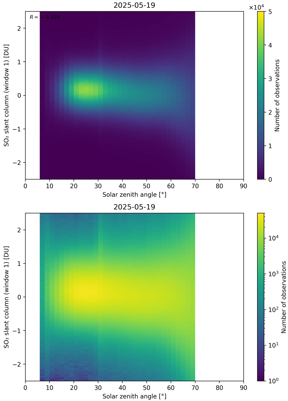
Figure 184: Scatter density plot of “Solar zenith angle” against “SO 2 slant column (window 1)” for 2025-05-18 to 2025-05-20.
