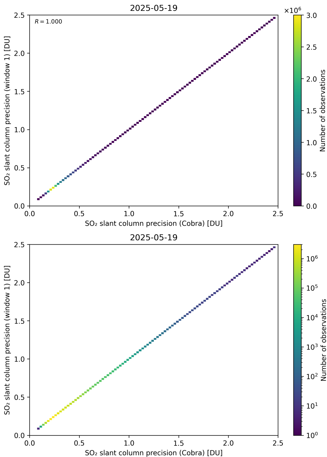
Figure 209: Scatter density plot of “SO 2 slant column precision (Cobra)” against “SO 2 slant column precision (window 1)” for 2025-05-18 to 2025-05-20.
