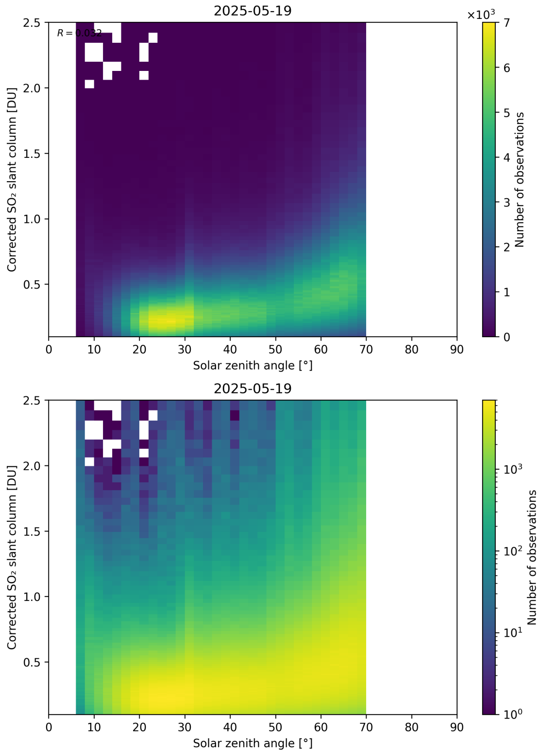
Figure 181: Scatter density plot of “Solar zenith angle” against “Corrected SO 2 slant column” for 2025-05-18 to 2025-05-20.
