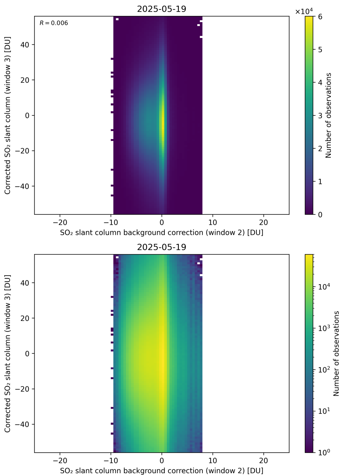
Figure 127: Scatter density plot of “SO 2 slant column background correction (window 2)” against “Corrected SO 2 slant column (window 3)” for 2025-05-18 to 2025-05-20.
