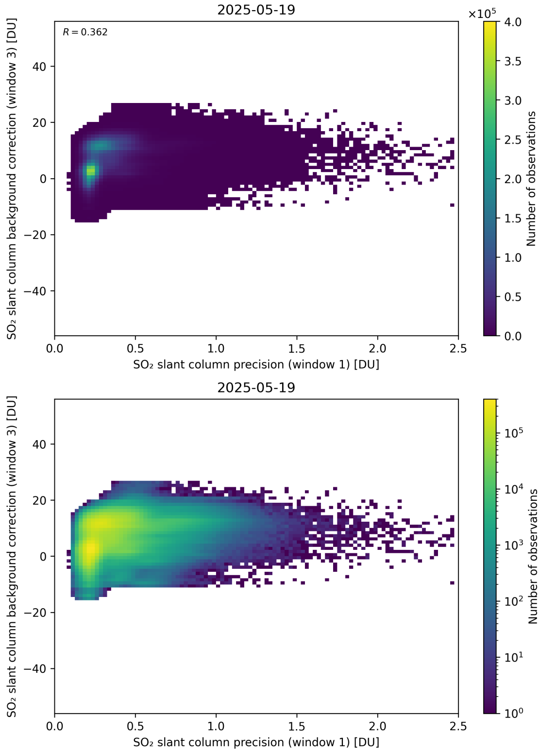
Figure 270: Scatter density plot of “SO 2 slant column precision (window 1)” against “SO 2 slant column background correction (window 3)” for 2025-05-18 to 2025-05-20.
