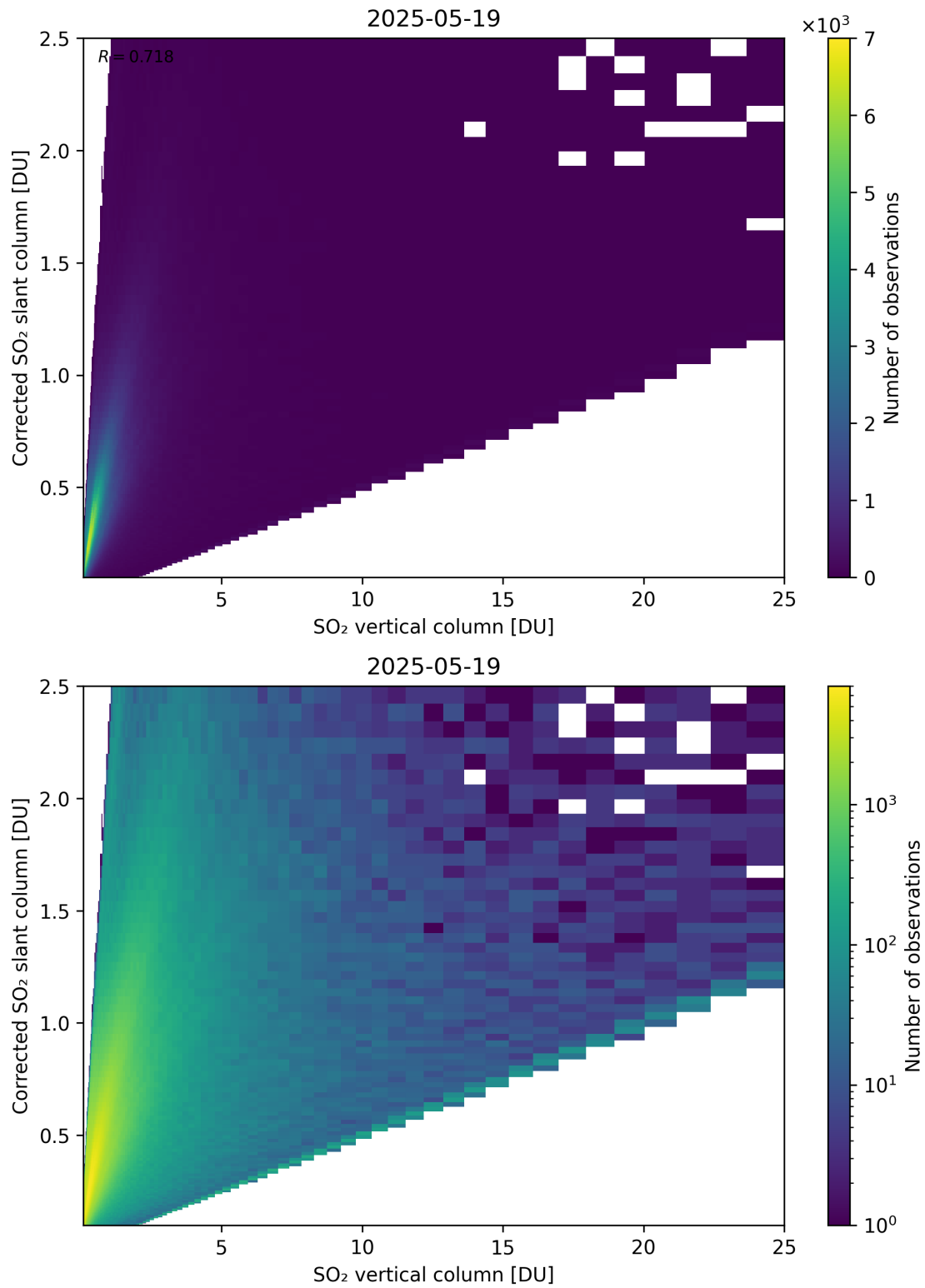
Figure 351: Scatter density plot of “SO 2 vertical column” against “Corrected SO 2 slant column” for 2025-05-18 to 2025-05-20.
