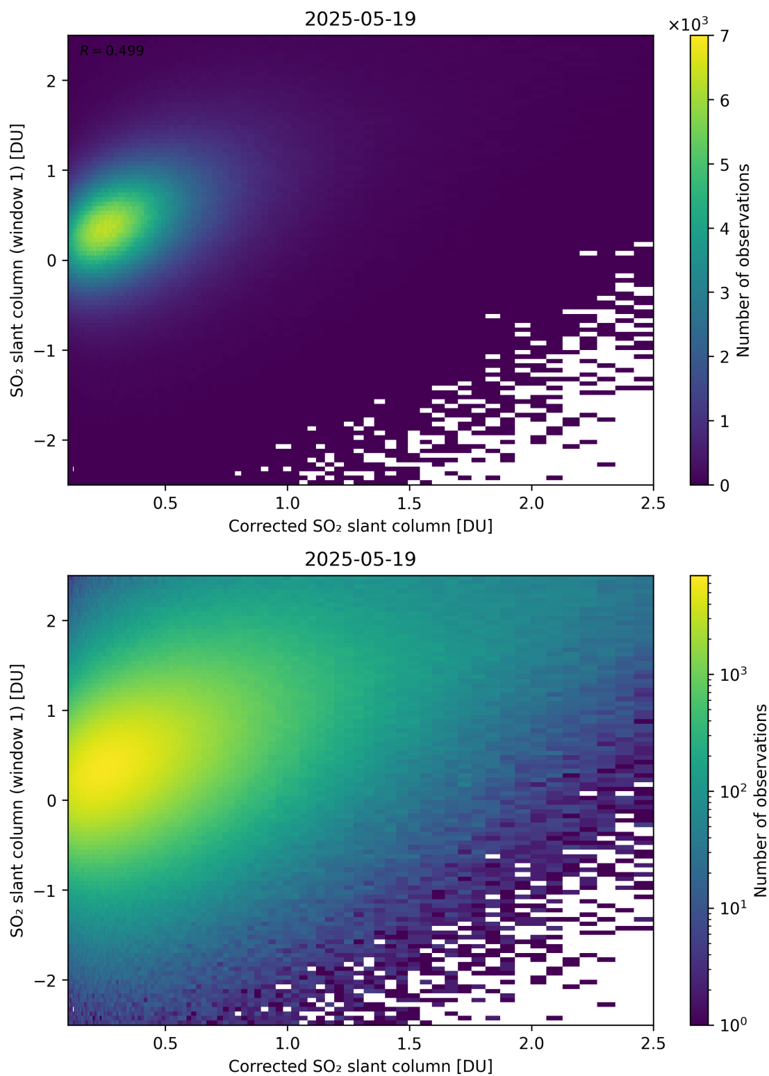
Figure 237: Scatter density plot of “Corrected SO 2 slant column” against “SO 2 slant column (window 1)” for 2025-05-18 to 2025-05-20.
