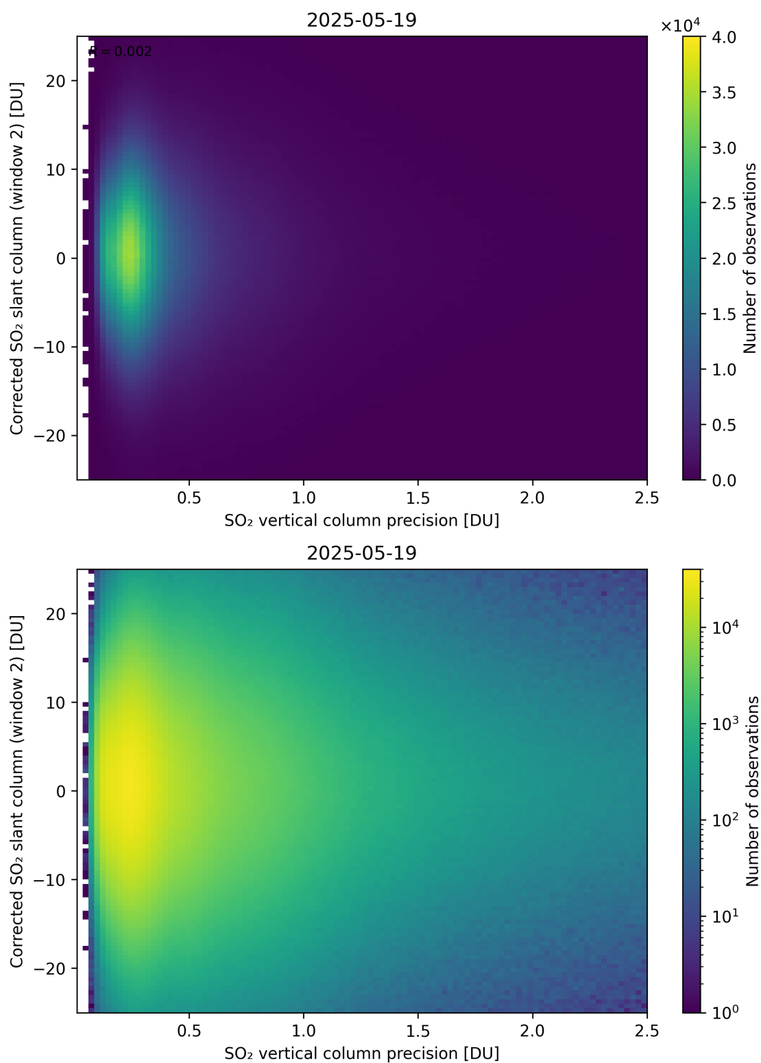
Figure 339: Scatter density plot of “SO 2 vertical column precision” against “Corrected SO 2 slant column (window 2)” for 2025-05-18 to 2025-05-20.
