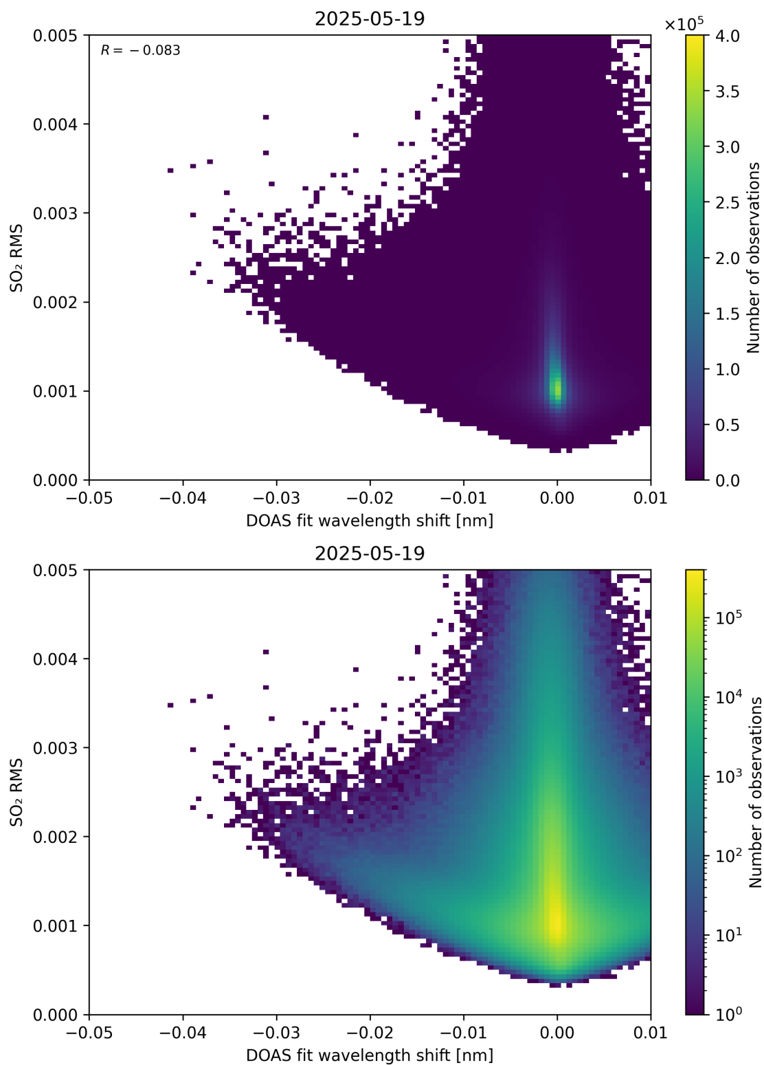
Figure 139: Scatter density plot of “DOAS fit wavelength shift” against “SO 2 RMS” for 2025-05-18 to 2025-05-20.
