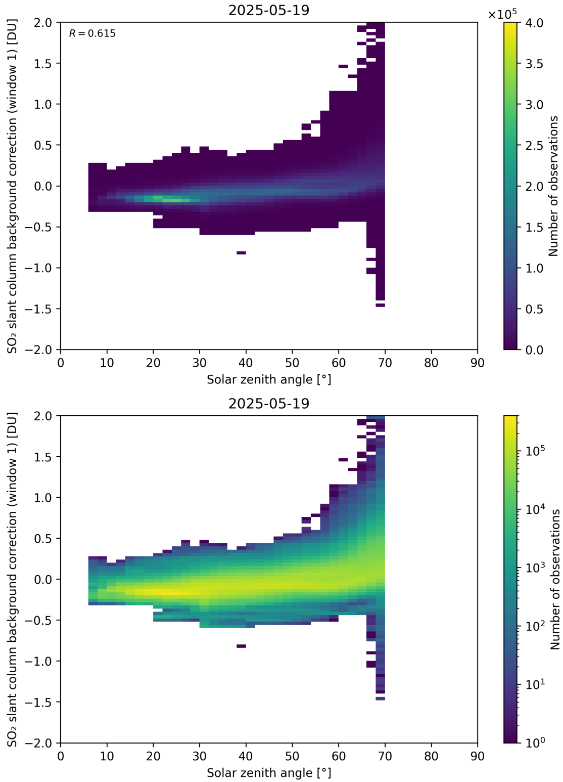
Figure 171: Scatter density plot of “Solar zenith angle” against “SO 2 slant column background correction (window 1)” for 2025-05-18 to 2025-05-20.
