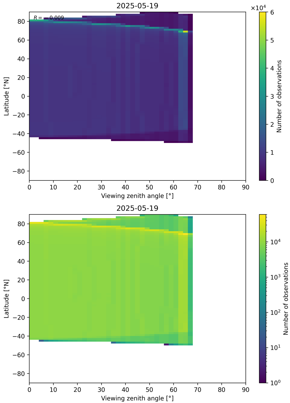
Figure 368: Scatter density plot of “Viewing zenith angle” against “Latitude” for 2025-05-18 to 2025-05-20.
