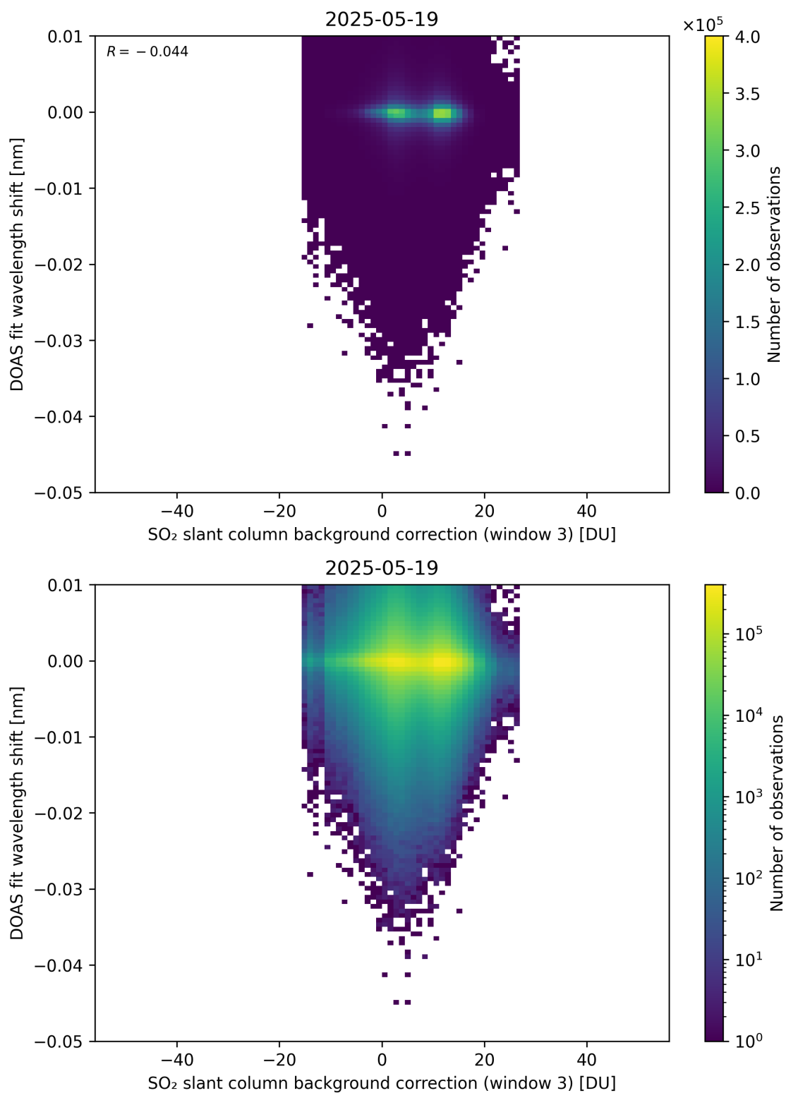
Figure 132: Scatter density plot of “SO 2 slant column background correction (window 3)” against “DOAS fit wavelength shift” for 2025-05-18 to 2025-05-20.
