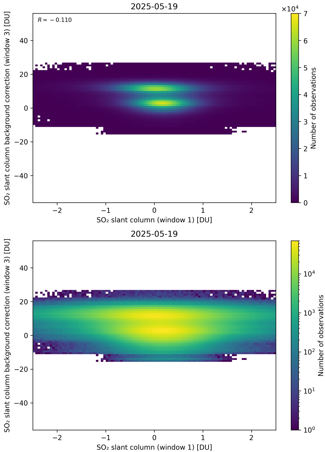
Figure 264: Scatter density plot of “SO 2 slant column (window 1)” against “SO 2 slant column background correction (window 3)” for 2025-05-18 to 2025-05-20.
