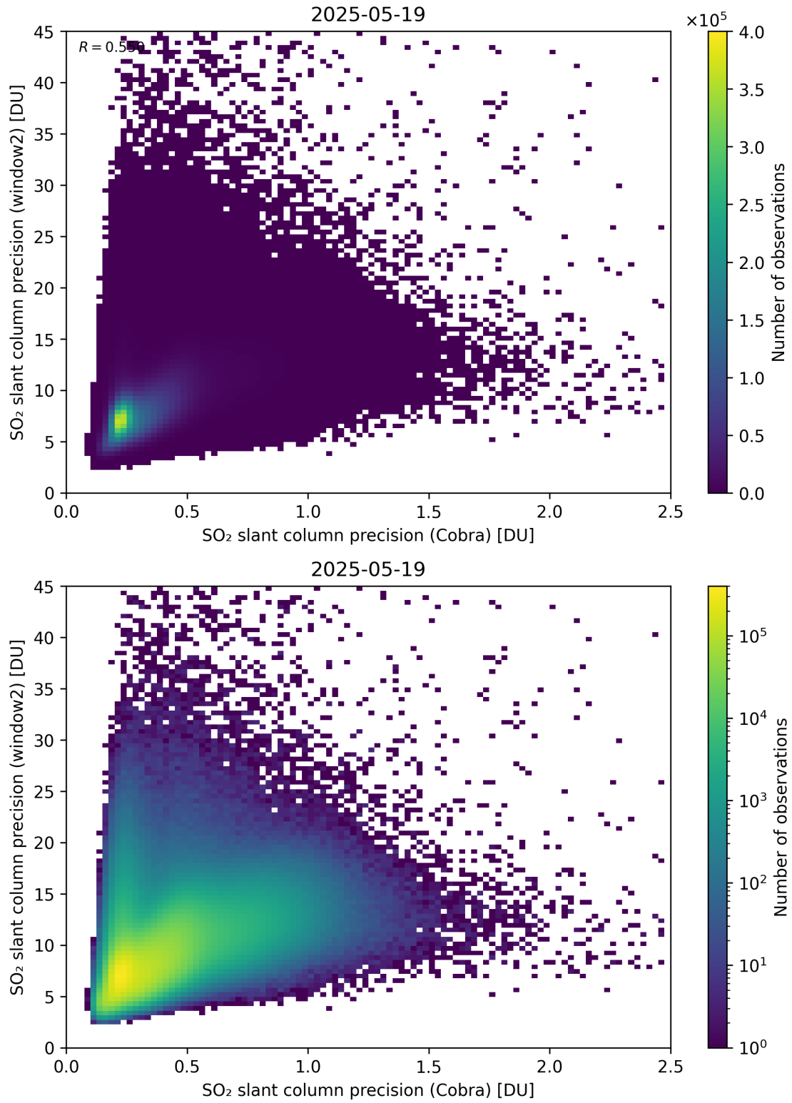
Figure 210: Scatter density plot of “SO 2 slant column precision (Cobra)” against “SO 2 slant column precision (window2)” for 2025-05-18 to 2025-05-20.
