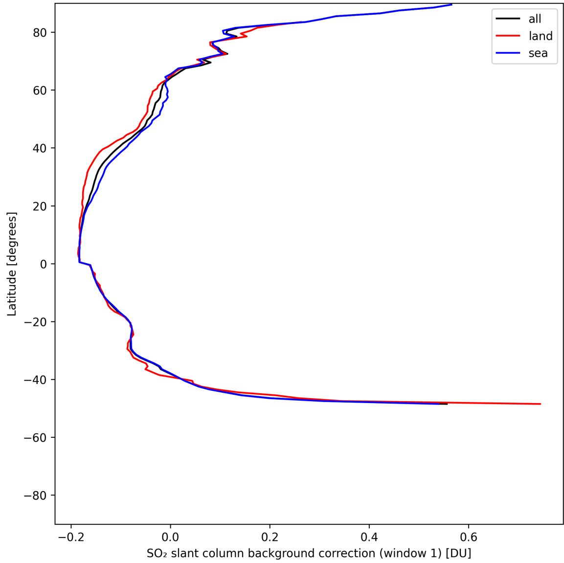
Figure 40: Zonal average of "SO 2 slant column background correction (window 1)" for 2025-05-18 to 2025-05-20.
