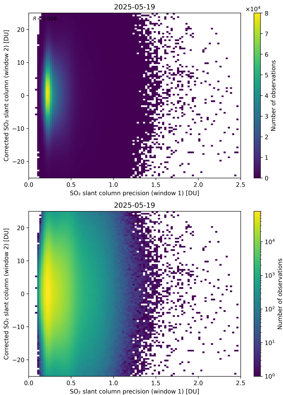
Figure 275: Scatter density plot of “SO 2 slant column precision (window 1)” against “Corrected SO 2 slant column (window 2)” for 2025-05-18 to 2025-05-20.
