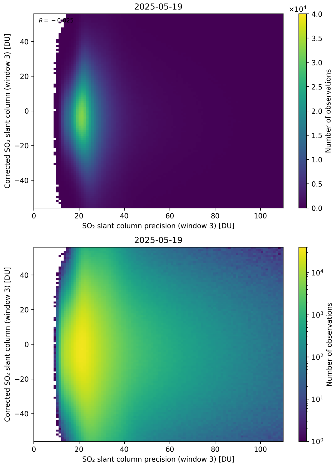
Figure 312: Scatter density plot of “SO 2 slant column precision (window 3)” against “Corrected SO 2 slant column (window 3)” for 2025-05-18 to 2025-05-20.
