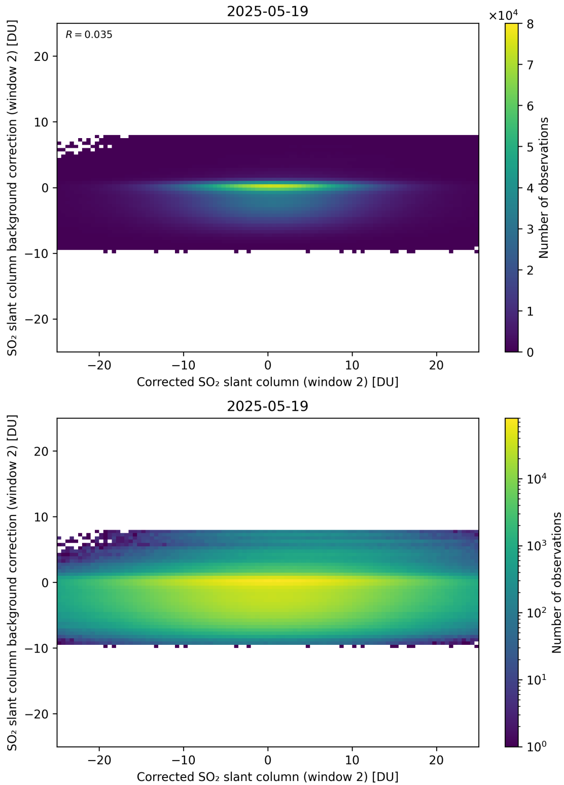
Figure 244: Scatter density plot of “Corrected SO 2 slant column (window 2)” against “SO 2 slant column background correction (window 2)” for 2025-05-18 to 2025-05-20.
