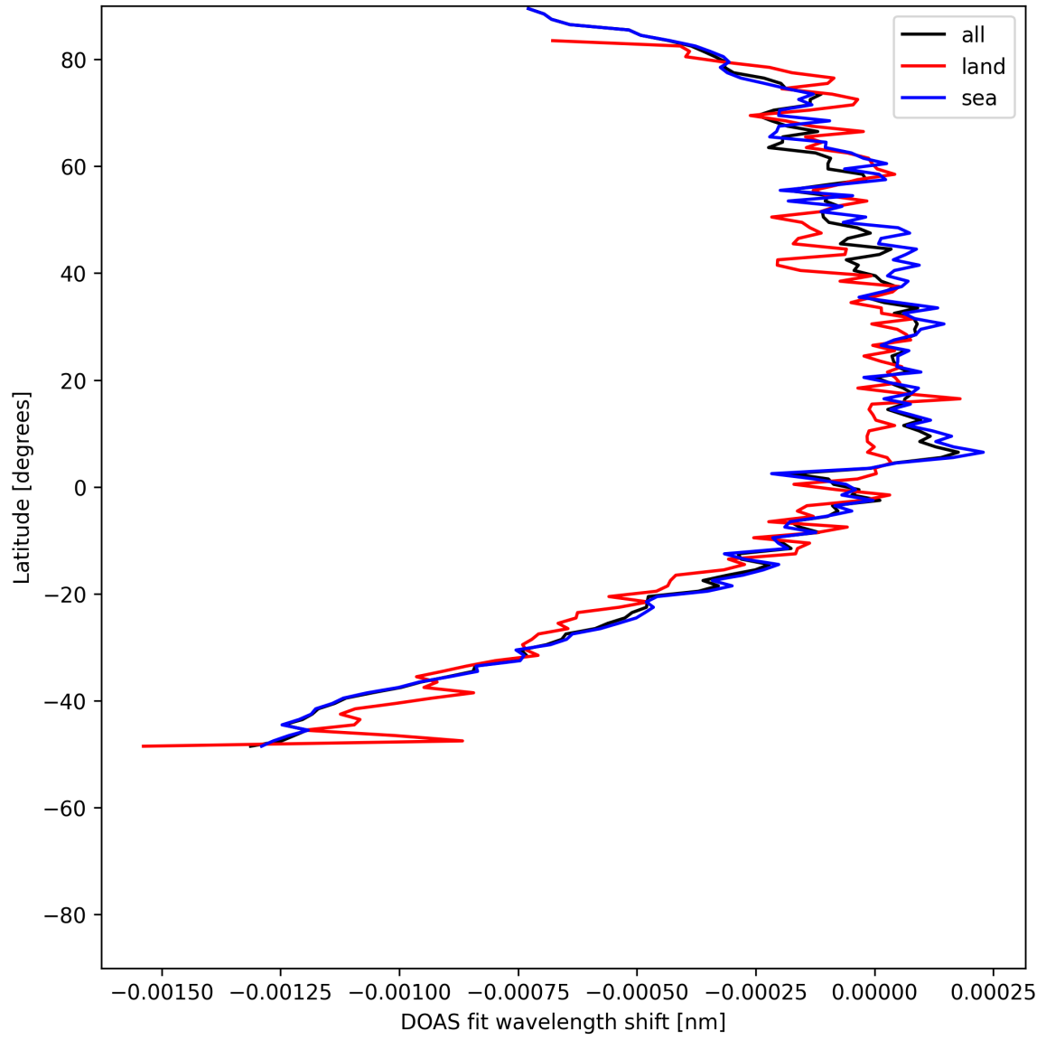
Figure 50: Zonal average of “DOAS fit wavelength shift” for 2025-05-18 to 2025-05-20.
