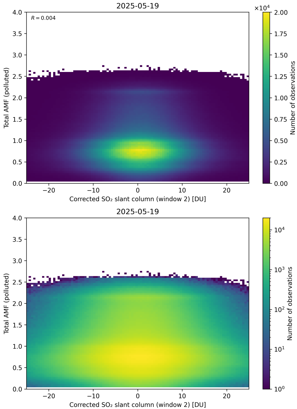
Figure 253: Scatter density plot of “Corrected SO 2 slant column (window 2)” against “Total AMF (polluted)” for 2025-05-18 to 2025-05-20.
