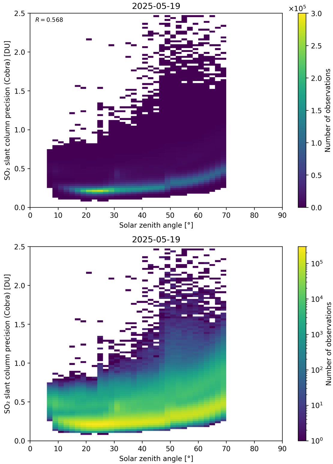
Figure 180: Scatter density plot of “Solar zenith angle” against “SO 2 slant column precision (Cobra)” for 2025-05-18 to 2025-05-20.
