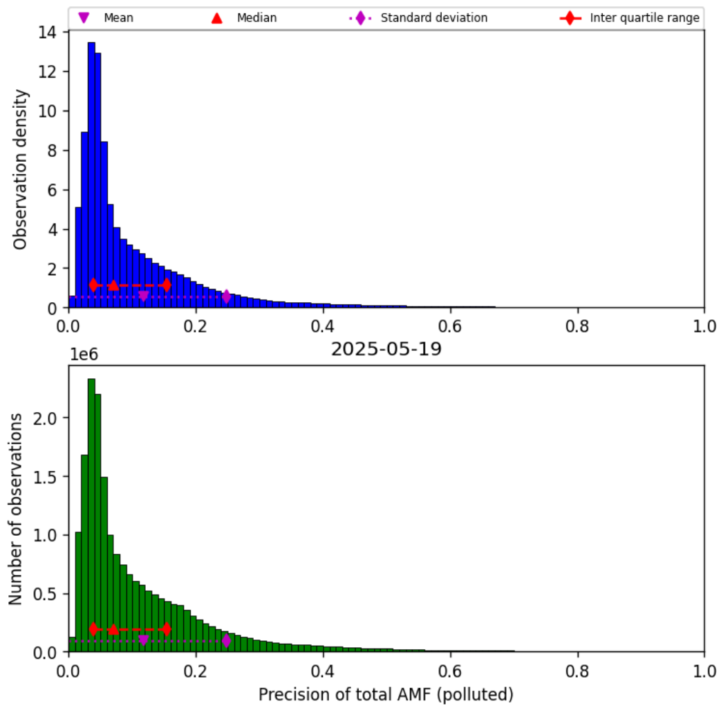
Figure 80: Histogram of “Precision of total AMF (polluted)” for 2025-05-18 to 2025-05-20
