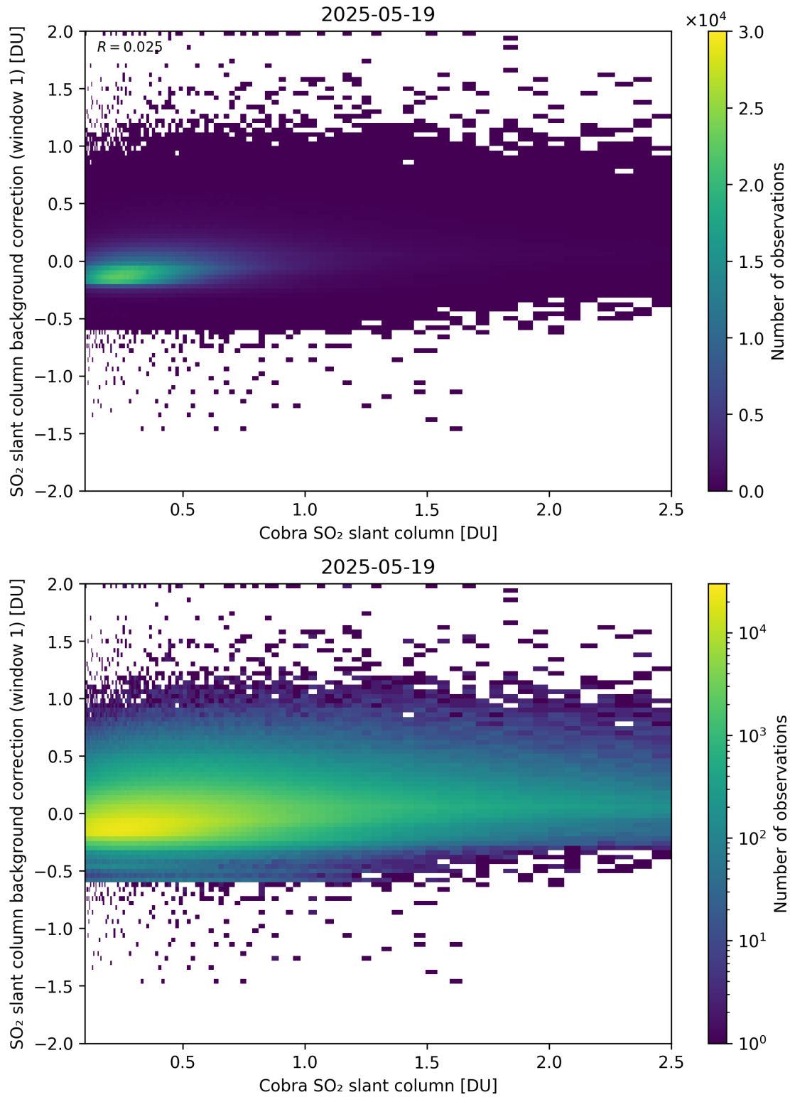
Figure 193: Scatter density plot of “Cobra SO 2 slant column” against “SO 2 slant column background correction (window 1)” for 2025-05-18 to 2025-05-20.
