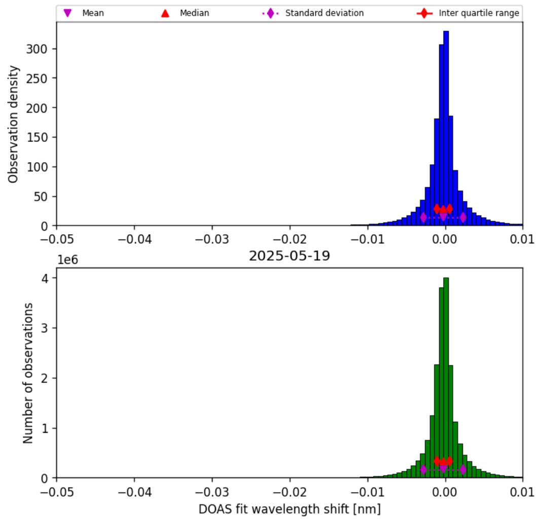
Figure 76: Histogram of “DOAS fit wavelength shift” for 2025-05-18 to 2025-05-20
