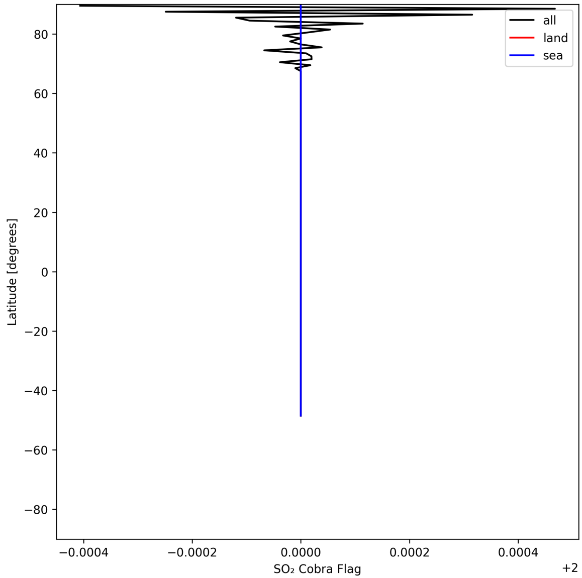
Figure 49: Zonal average of “SO 2 Cobra Flag” for 2025-05-18 to 2025-05-20.
