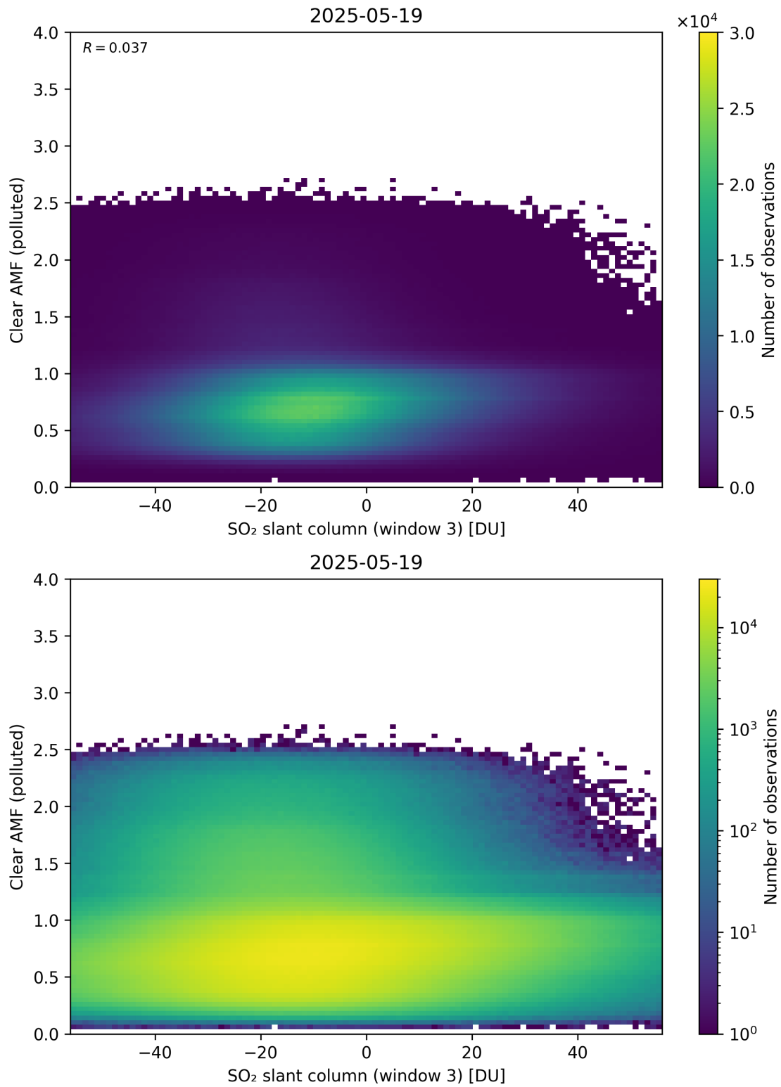
Figure 315: Scatter density plot of “SO 2 slant column (window 3)” against “Clear AMF (polluted)” for 2025-05-18 to 2025-05-20.
