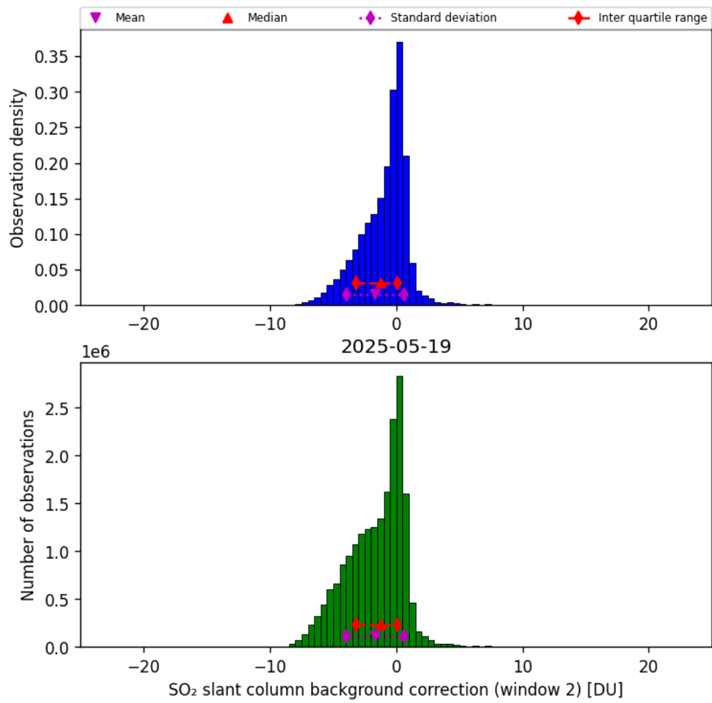
Figure 70: Histogram of “SO 2 slant column background correction (window 2)” for 2025-05-18 to 2025-05-20
