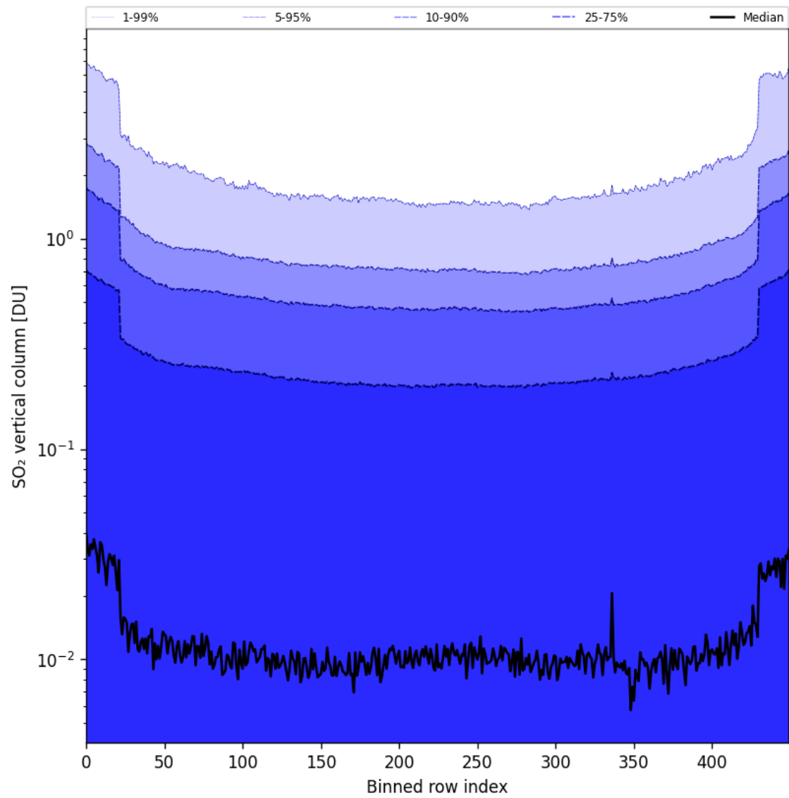
Figure 84: Along track statistics of “SO 2 vertical column” for 2025-05-18 to 2025-05-20
