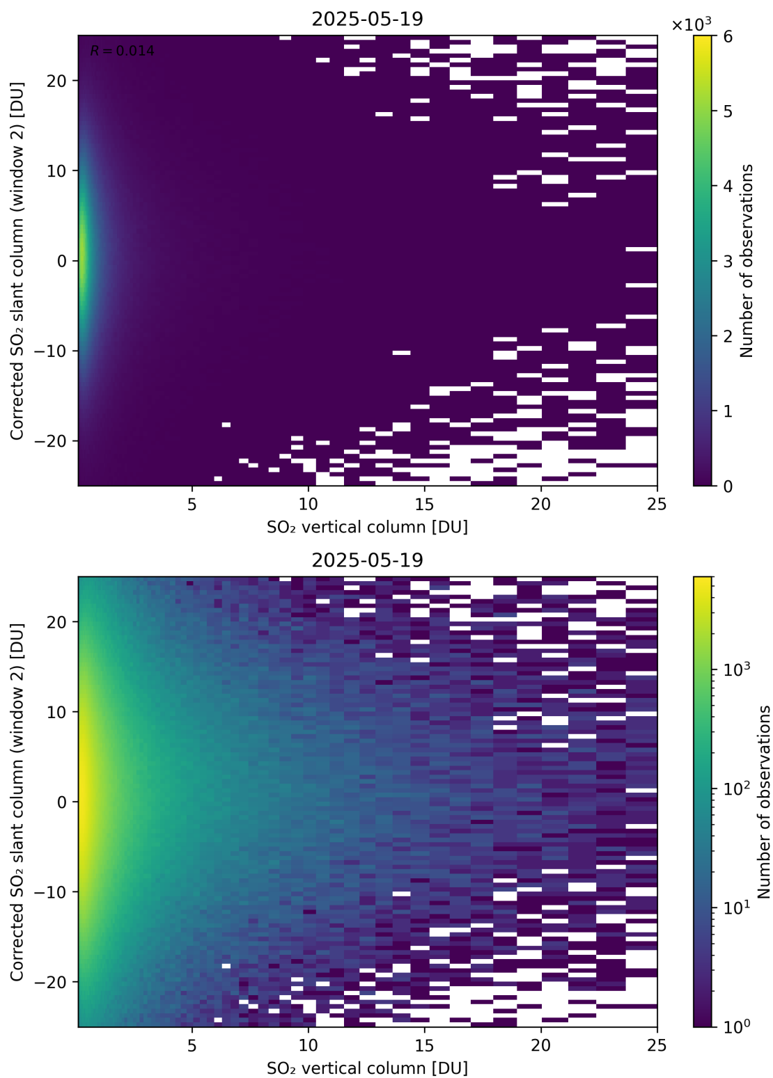
Figure 352: Scatter density plot of “SO 2 vertical column” against “Corrected SO 2 slant column (window 2)” for 2025-05-18 to 2025-05-20.
