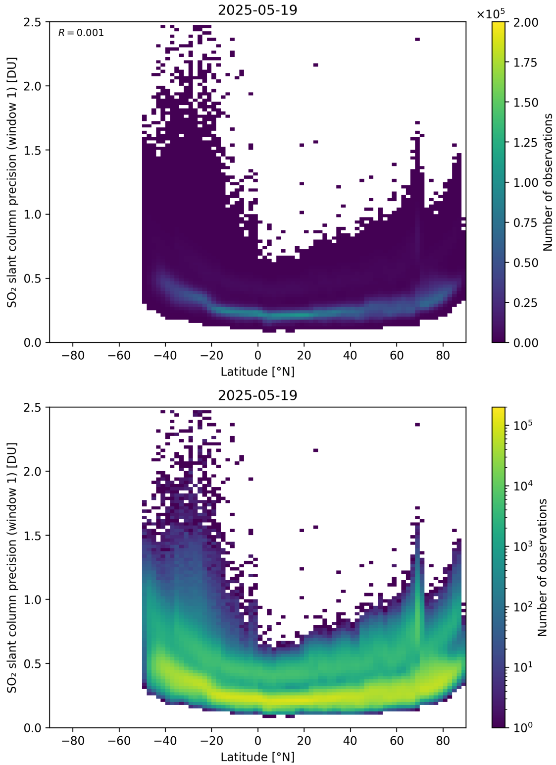
Figure 163: Scatter density plot of “Latitude” against “SO 2 slant column precision (window 1)” for 2025-05-18 to 2025-05-20.
