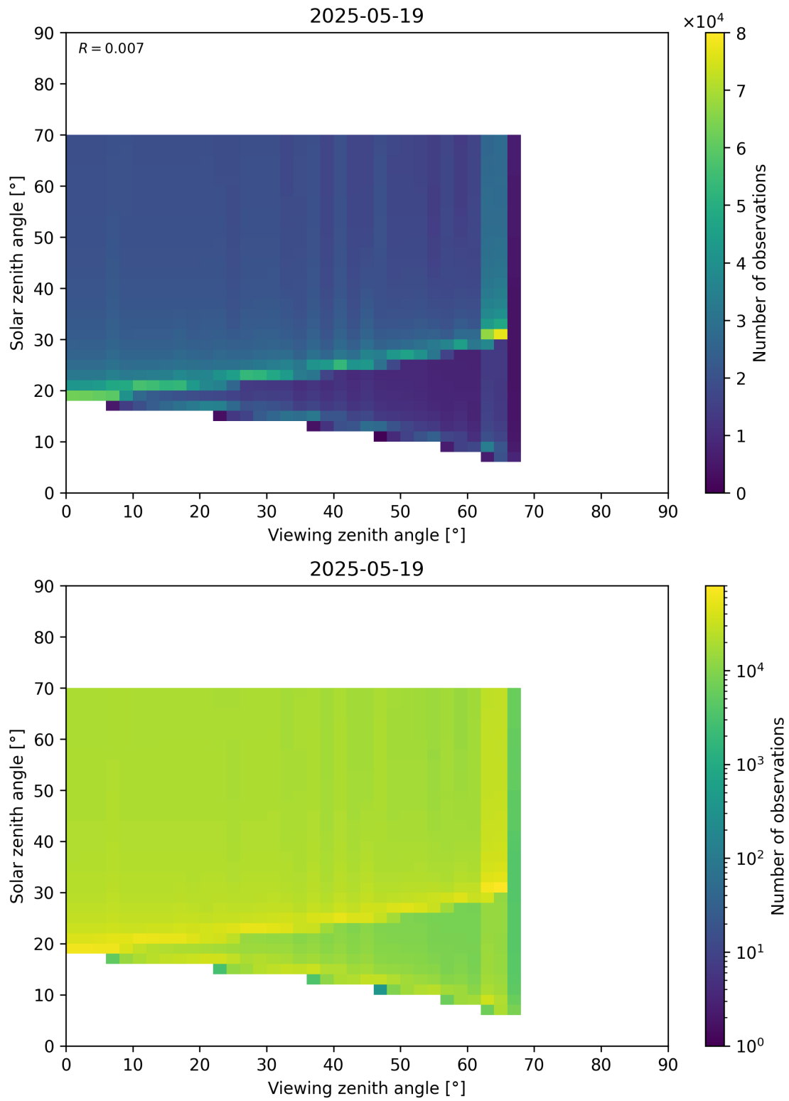
Figure 369: Scatter density plot of “Viewing zenith angle” against “Solar zenith angle” for 2025-05-18 to 2025-05-20.
