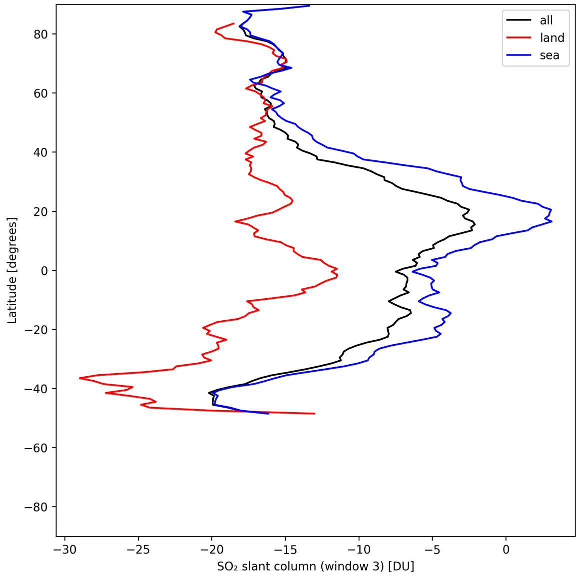
Figure 45: Zonal average of “SO 2 slant column (window 3)” for 2025-05-18 to 2025-05-20.
