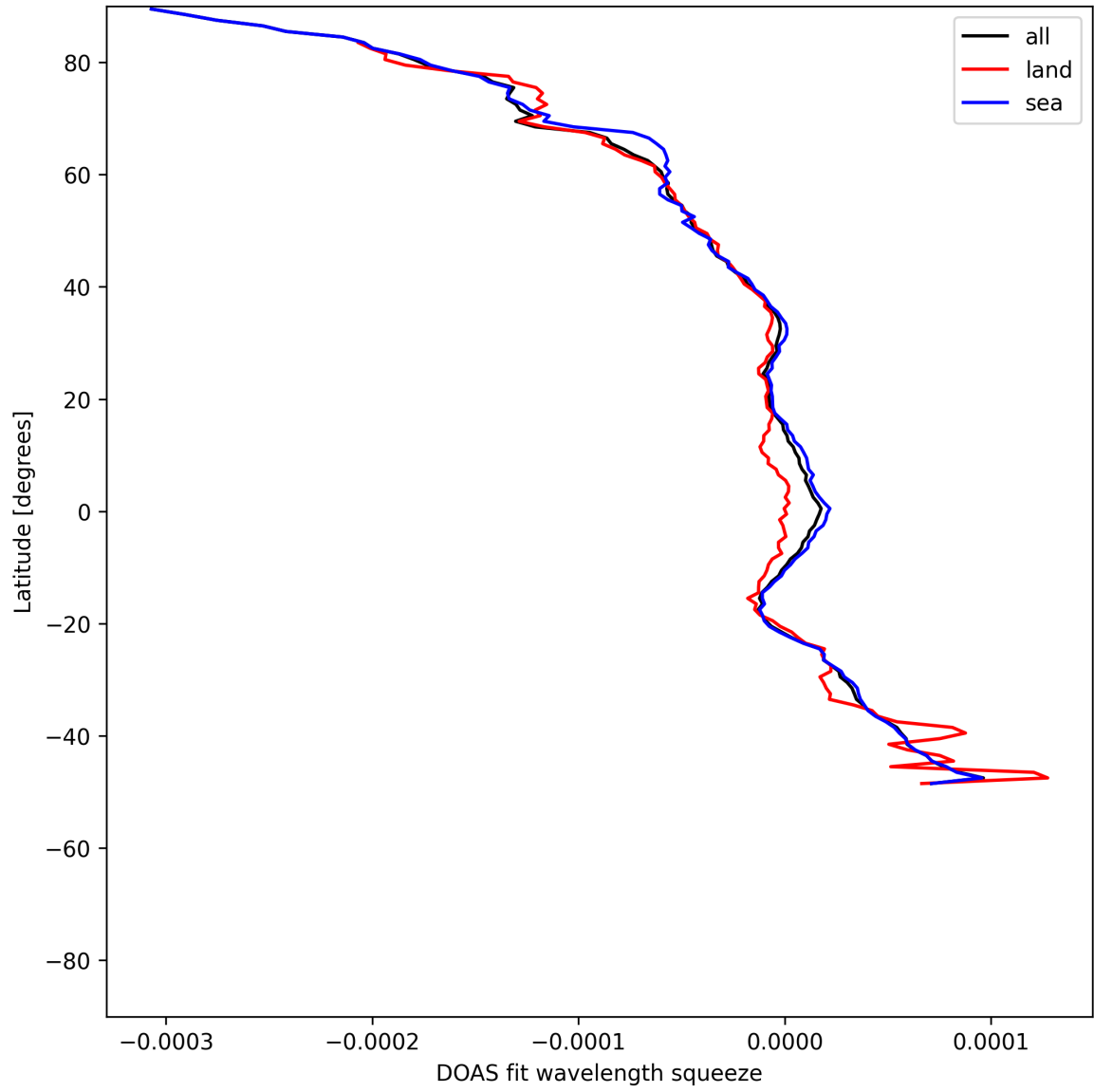
Figure 51: Zonal average of “DOAS fit wavelength squeeze” for 2025-05-18 to 2025-05-20.
