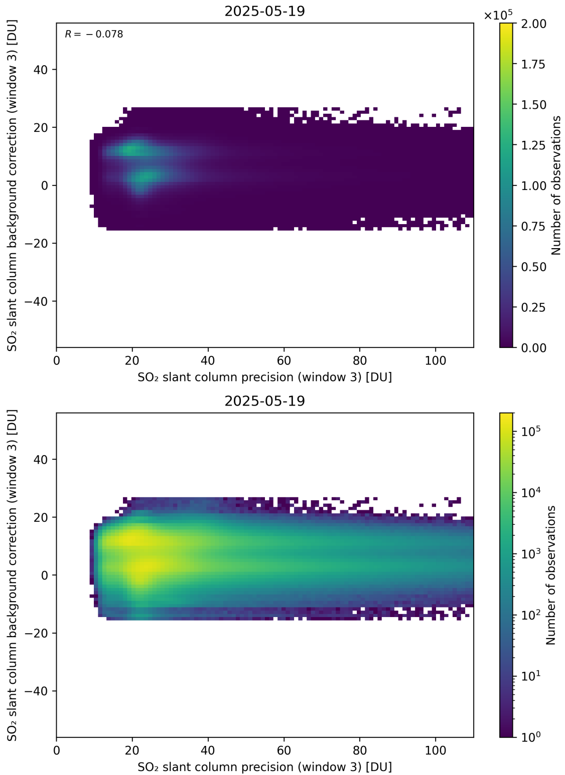
Figure 307: Scatter density plot of “SO 2 slant column precision (window 3)” against “SO 2 slant column background correction (window 3)” for 2025-05-18 to 2025-05-20.
