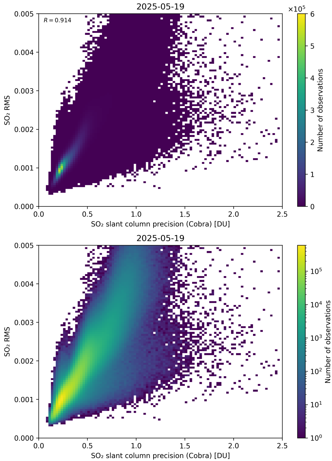
Figure 204: Scatter density plot of “SO 2 slant column precision (Cobra)” against “SO 2 RMS” for 2025-05-18 to 2025-05-20.
