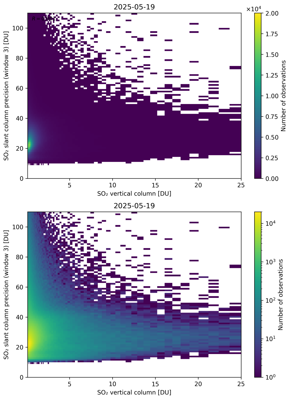
Figure 358: Scatter density plot of “SO 2 vertical column” against “SO 2 slant column precision (window 3)” for 2025-05-18 to 2025-05-20.
