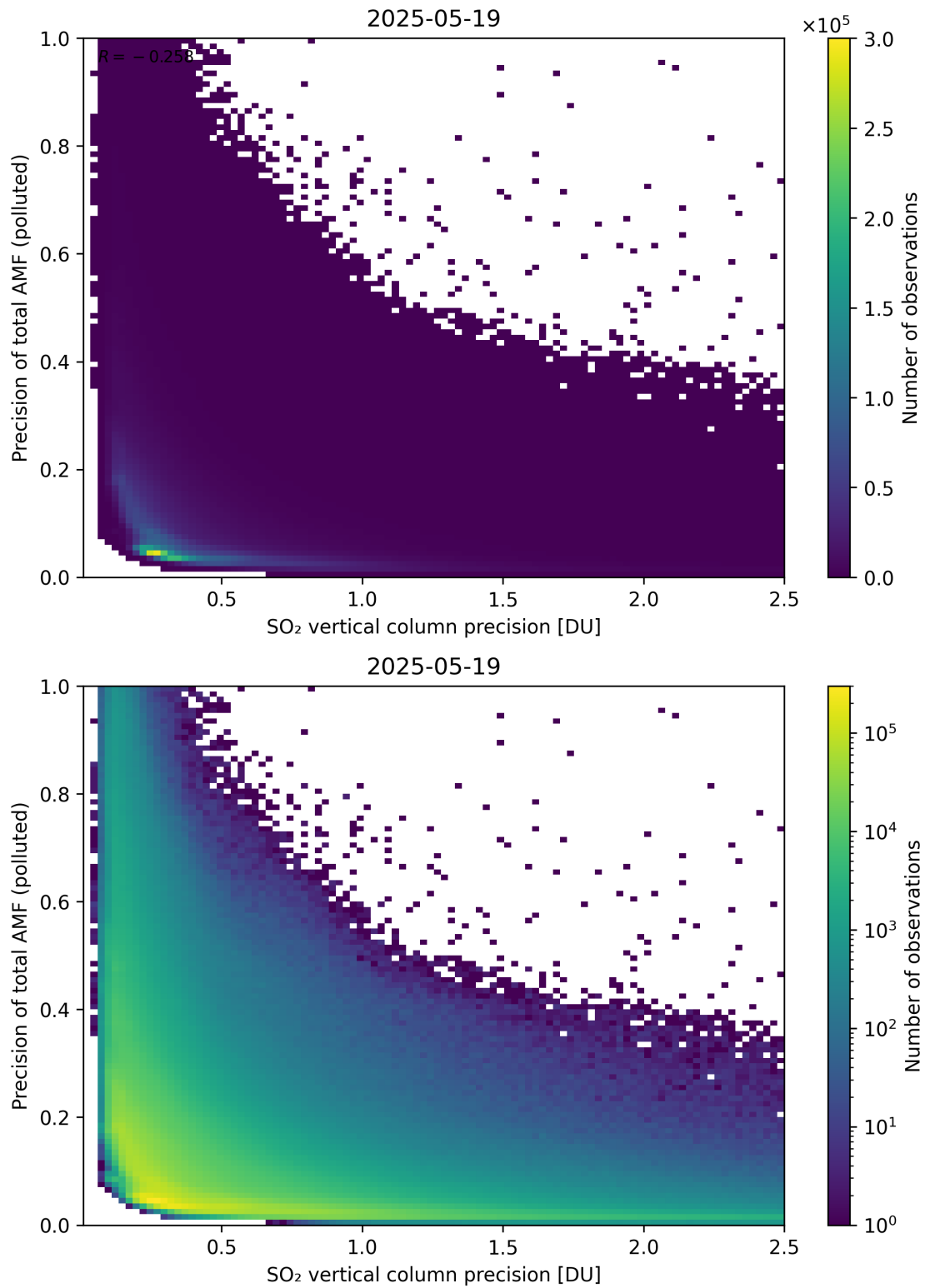
Figure 347: Scatter density plot of “SO 2 vertical column precision” against “Precision of total AMF (polluted)” for 2025-05-18 to 2025-05-20.
