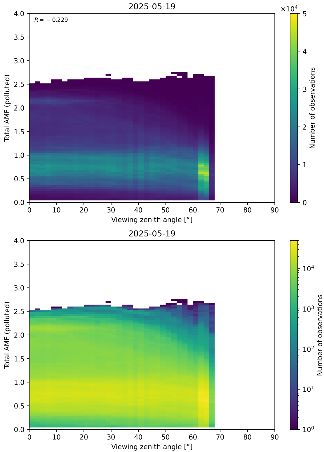
Figure 381: Scatter density plot of “Viewing zenith angle” against “Total AMF (polluted)” for 2025-05-18 to 2025-05-20.
