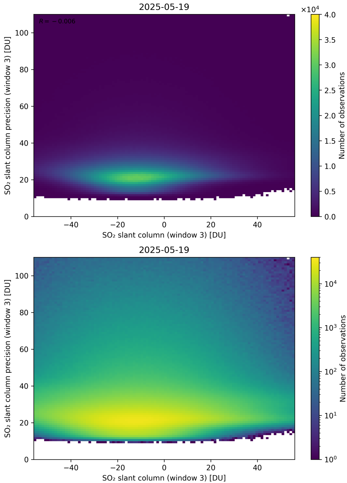
Figure 317: Scatter density plot of “SO 2 slant column (window 3)” against “SO 2 slant column precision (window 3)” for 2025-05-18 to 2025-05-20.
