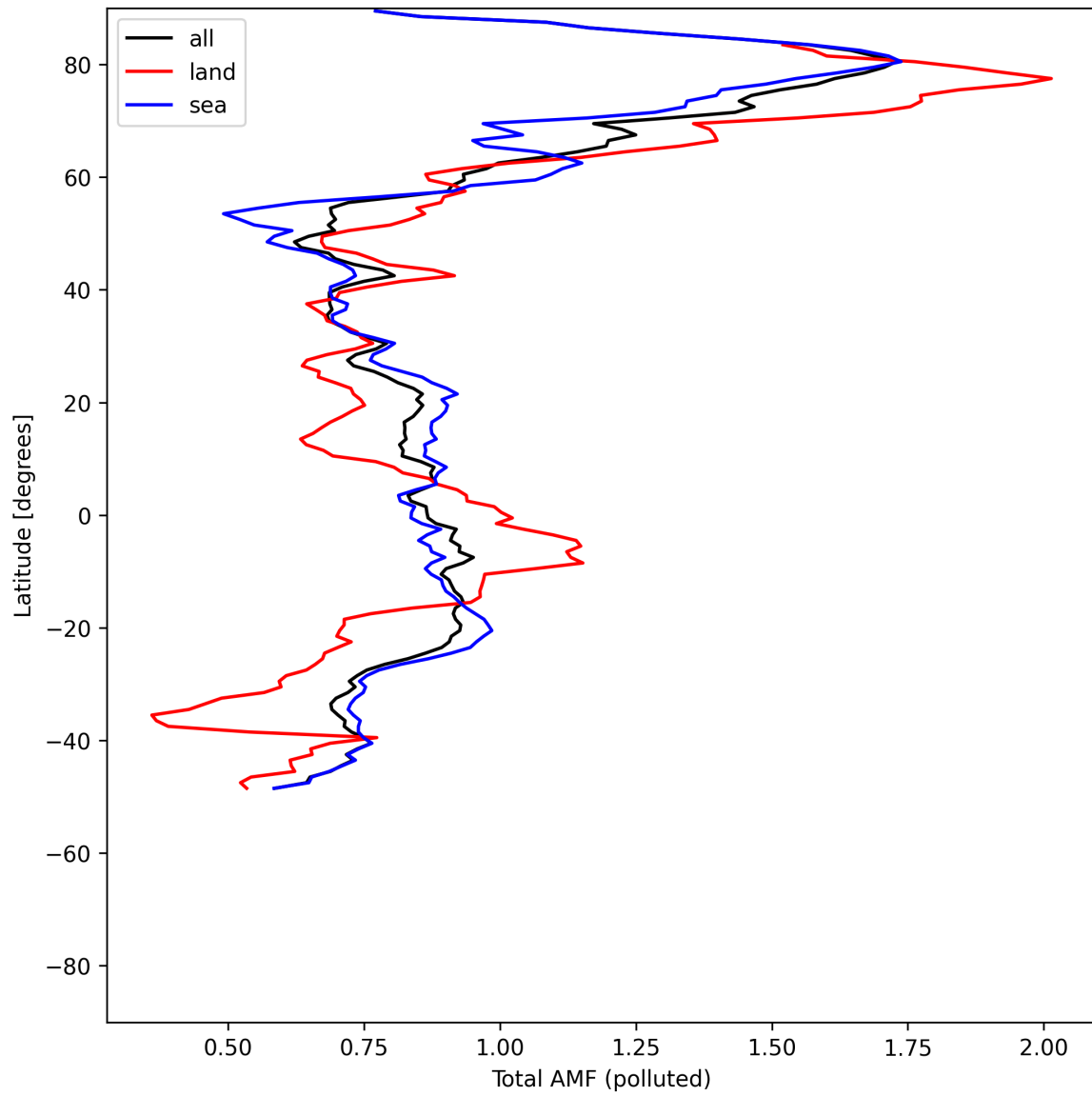
Figure 53: Zonal average of “Total AMF (polluted)” for 2025-05-18 to 2025-05-20.
