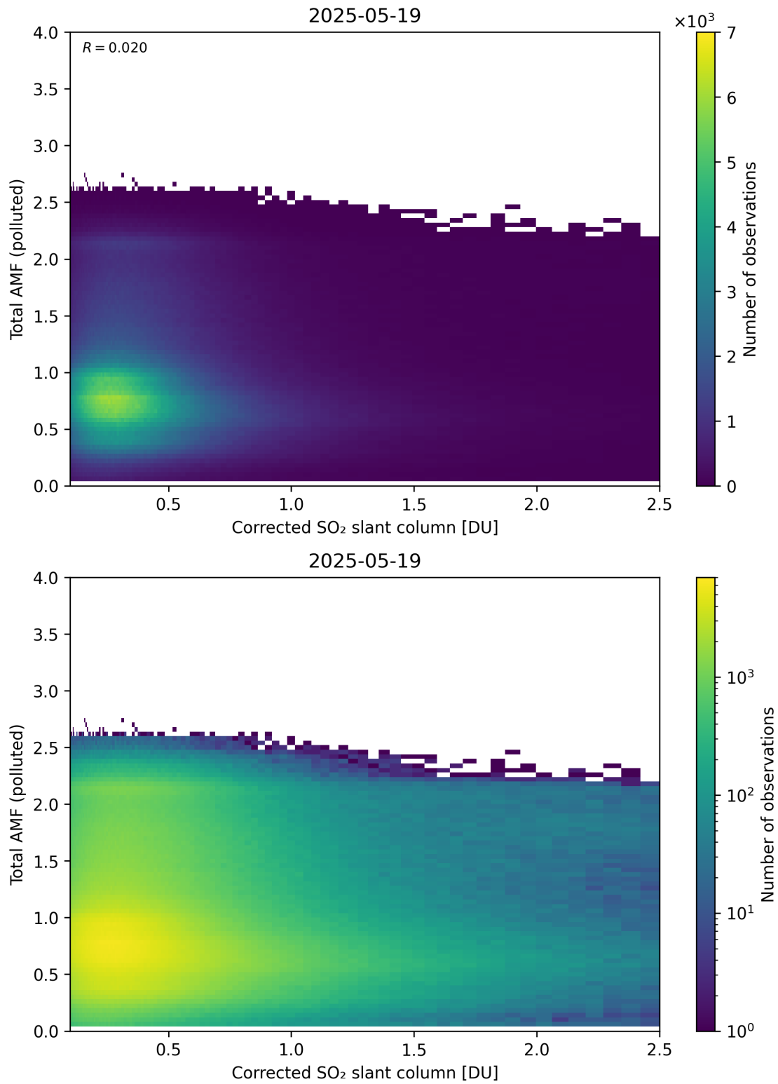
Figure 242: Scatter density plot of “Corrected SO 2 slant column” against “Total AMF (polluted)” for 2025-05-18 to 2025-05-20.
