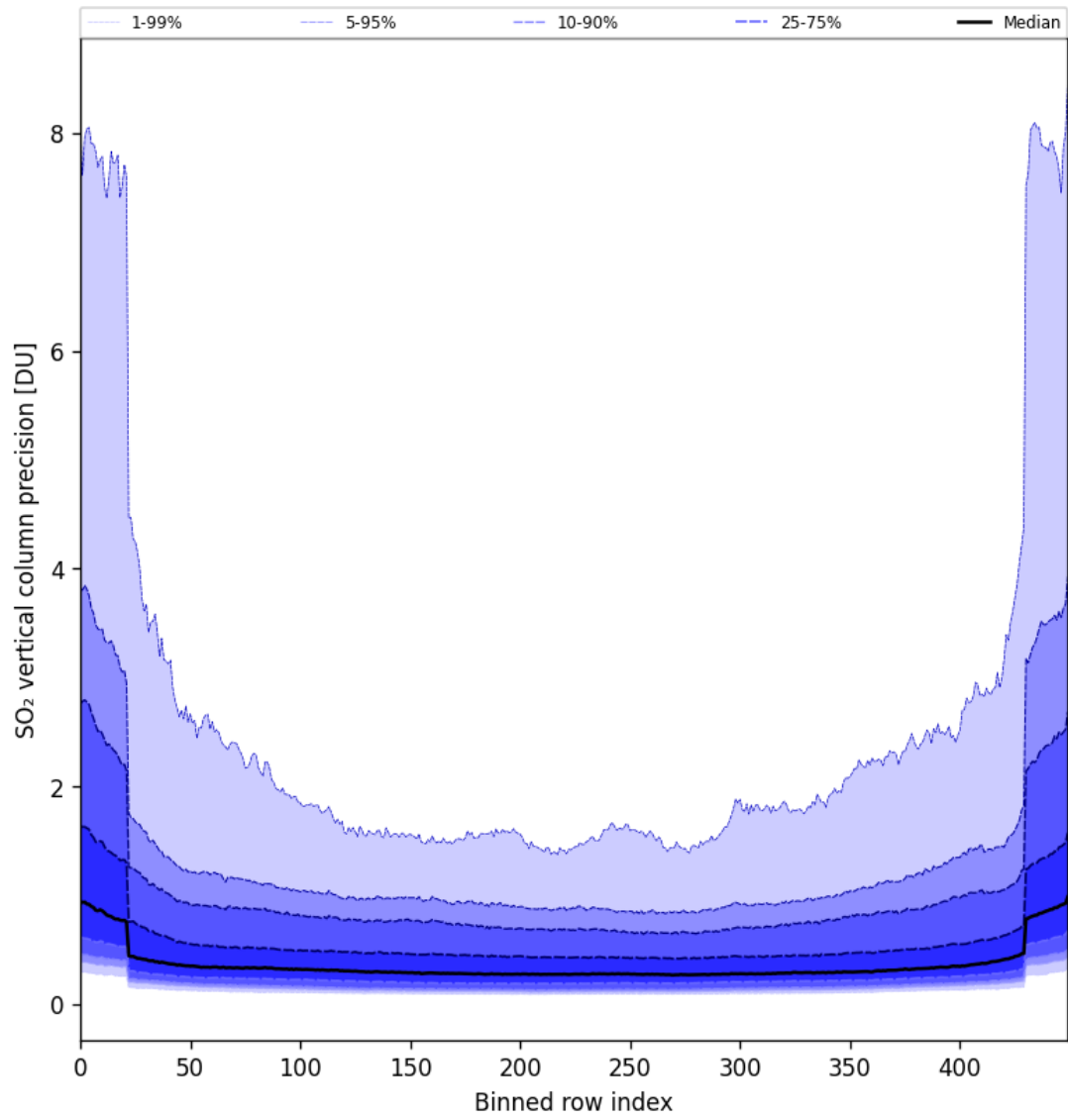
Figure 85: Along track statistics of “SO 2 vertical column precision” for 2025-05-18 to 2025-05-20
