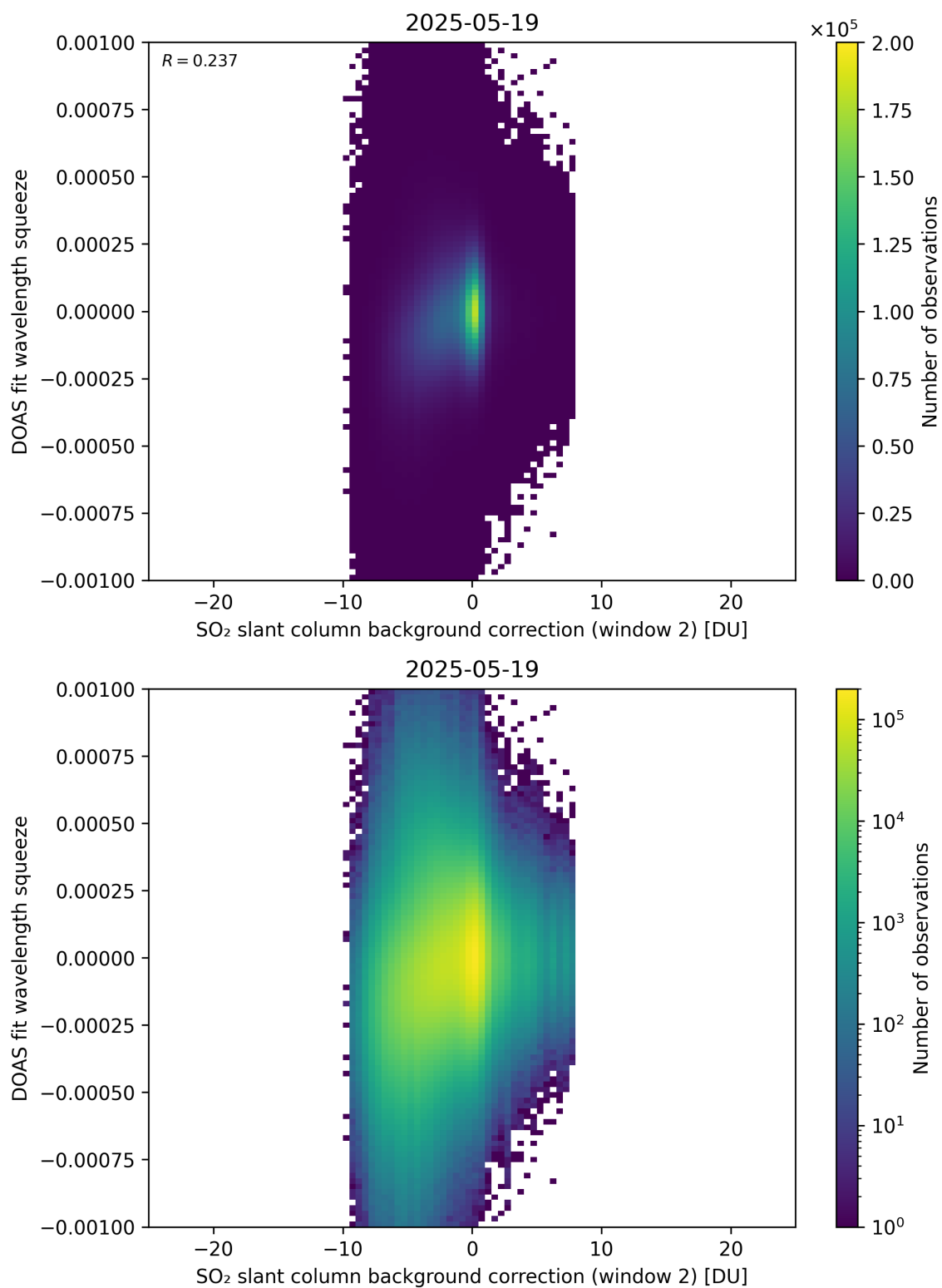
Figure 124: Scatter density plot of “SO 2 slant column background correction (window 2)” against “DOAS fit wavelength squeeze” for 2025-05-18 to 2025-05-20.
