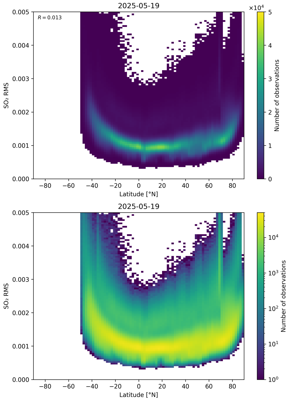
Figure 155: Scatter density plot of “Latitude” against “SO 2 RMS” for 2025-05-18 to 2025-05-20.
