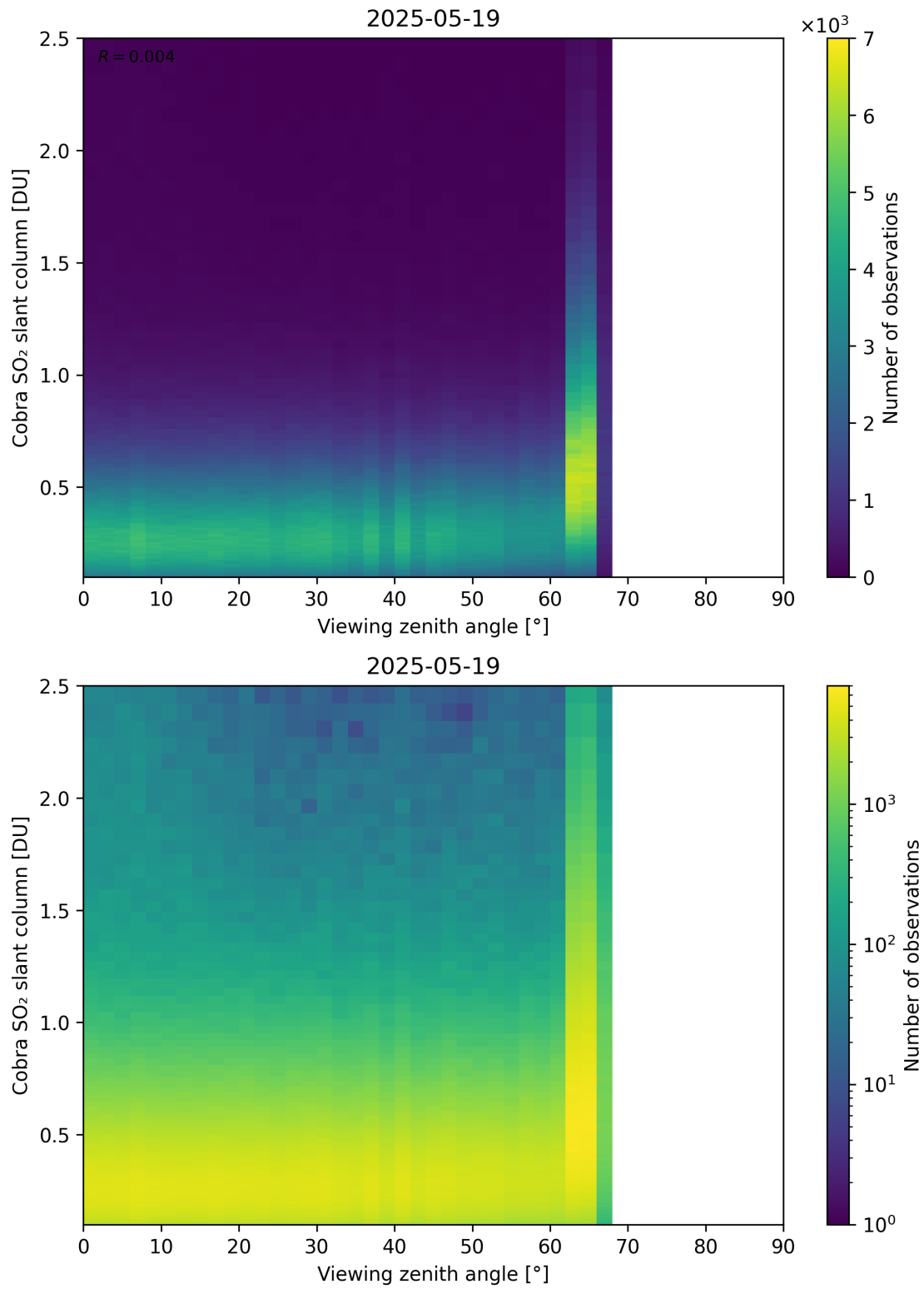
Figure 371: Scatter density plot of “Viewing zenith angle” against “Cobra SO 2 slant column” for 2025-05-18 to 2025-05-20.
