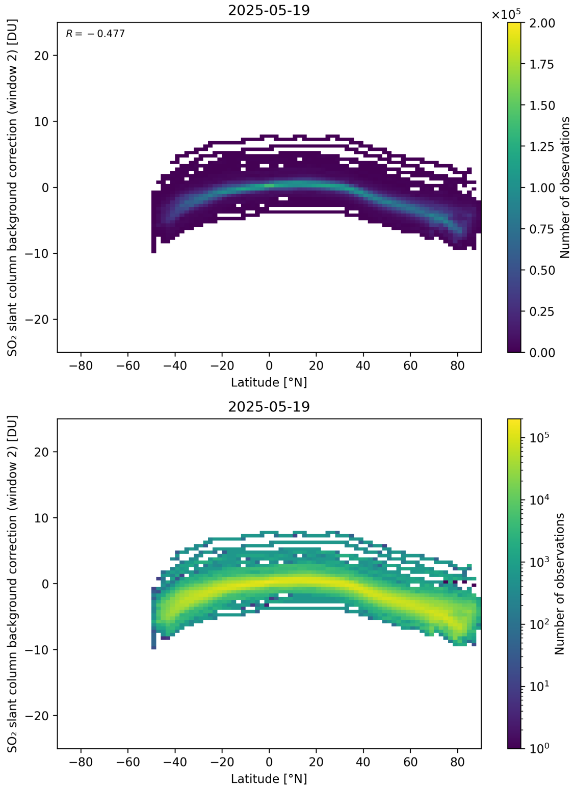
Figure 151: Scatter density plot of “Latitude” against “SO 2 slant column background correction (window 2)” for 2025-05-18 to 2025-05-20.
