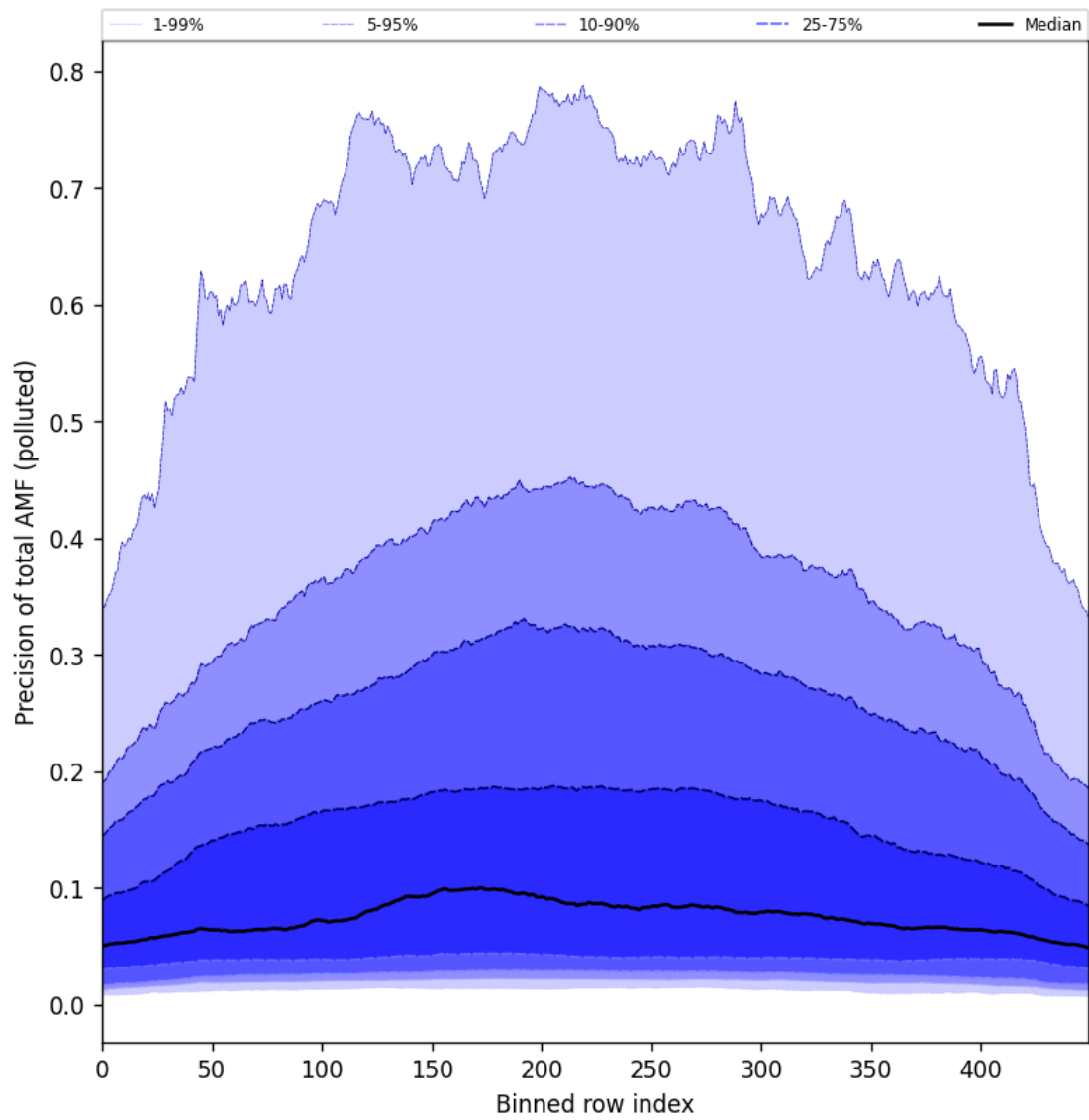
Figure 106: Along track statistics of “Precision of total AMF (polluted)” for 2025-05-18 to 2025-05-20
