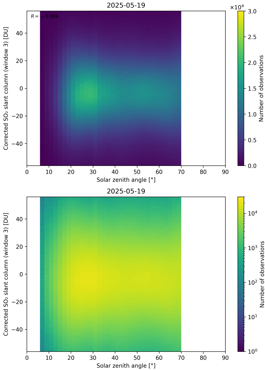
Figure 183: Scatter density plot of “Solar zenith angle” against “Corrected SO 2 slant column (window 3)” for 2025-05-18 to 2025-05-20.
