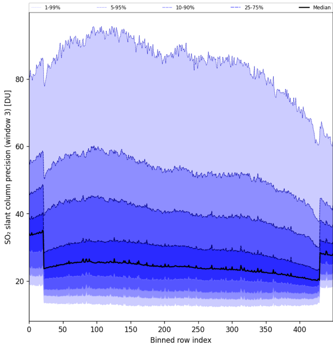
Figure 98: Along track statistics of “SO 2 slant column precision (window 3)” for 2025-05-18 to 2025-05-20
