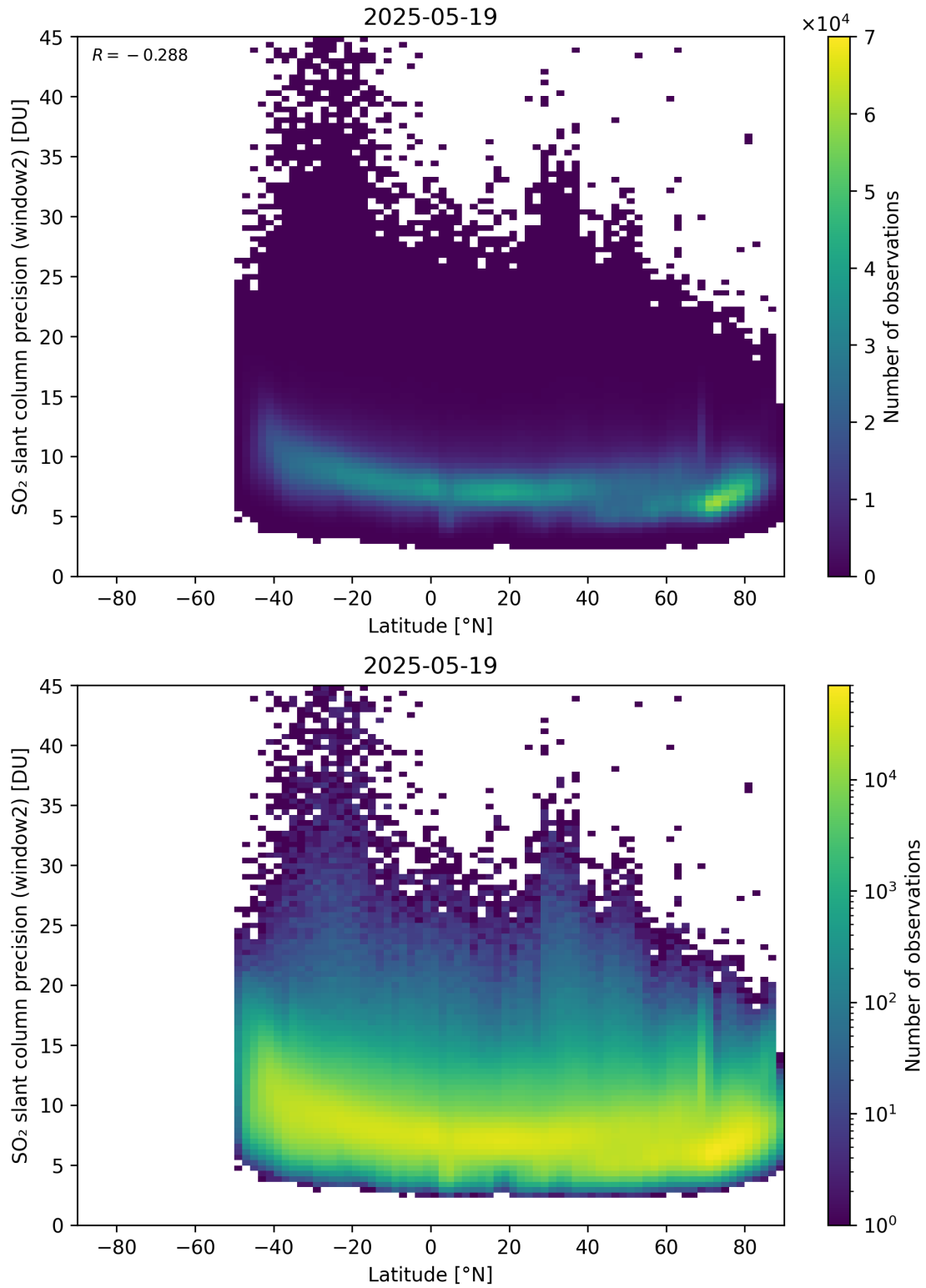
Figure 164: Scatter density plot of “Latitude” against “SO 2 slant column precision (window2)” for 2025-05-18 to 2025-05-20.
