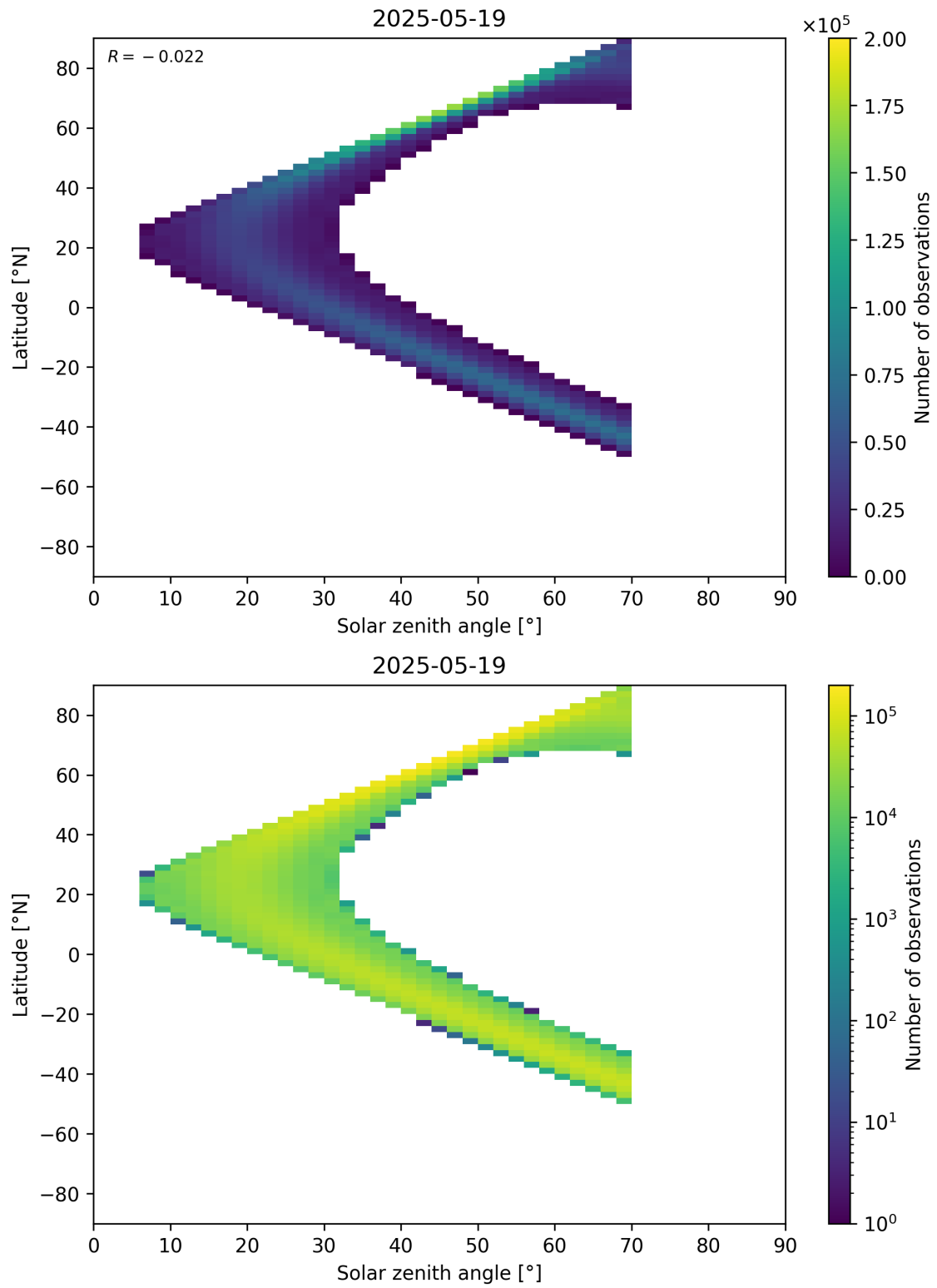
Figure 177: Scatter density plot of “Solar zenith angle” against “Latitude” for 2025-05-18 to 2025-05-20.
