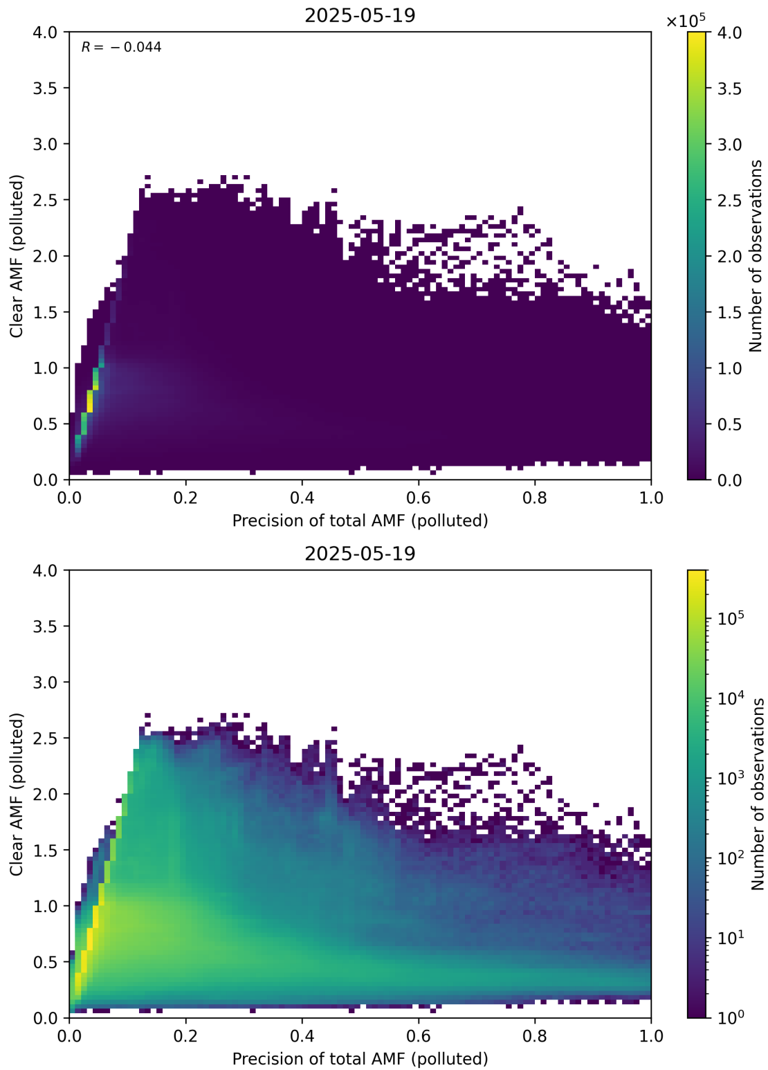
Figure 320: Scatter density plot of “Precision of total AMF (polluted)” against “Clear AMF (polluted)” for 2025-05-18 to 2025-05-20.
