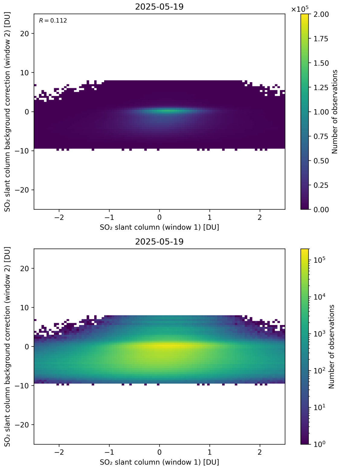
Figure 263: Scatter density plot of “SO 2 slant column (window 1)” against “SO 2 slant column background correction (window 2)” for 2025-05-18 to 2025-05-20.
