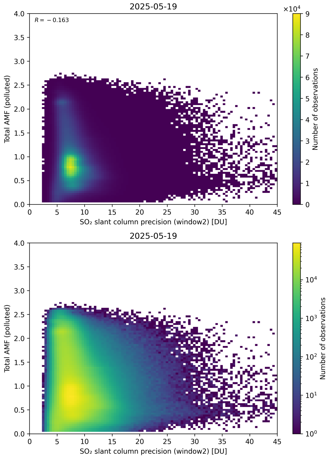
Figure 301: Scatter density plot of “SO 2 slant column precision (window2)” against “Total AMF (polluted)” for 2025-05-18 to 2025-05-20.
