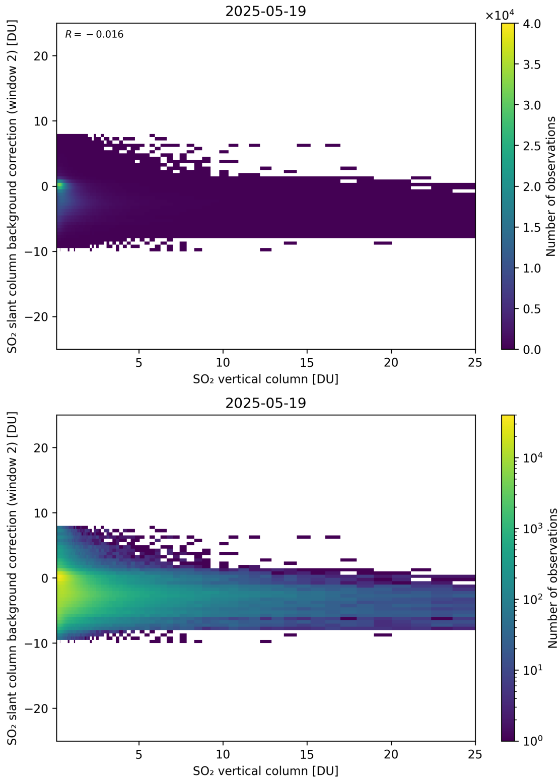
Figure 324: Scatter density plot of “SO 2 vertical column” against “SO 2 slant column background correction (window 2)” for 2025-05-18 to 2025-05-20.
