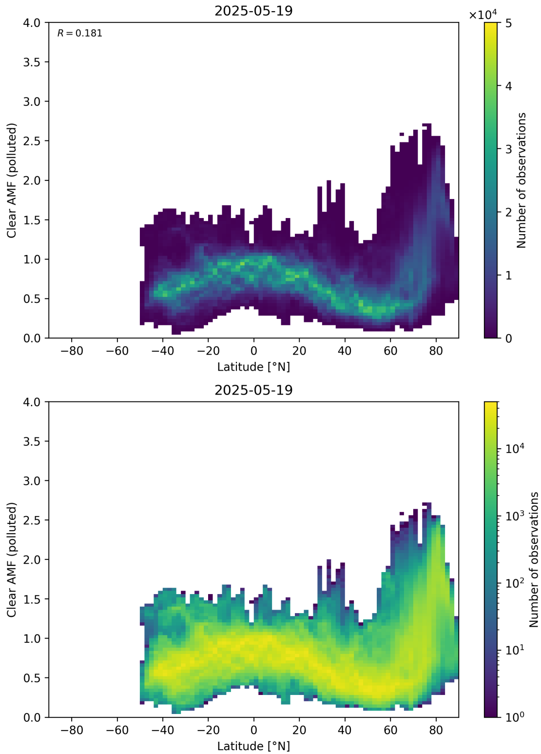
Figure 156: Scatter density plot of “Latitude” against “Clear AMF (polluted)” for 2025-05-18 to 2025-05-20.
