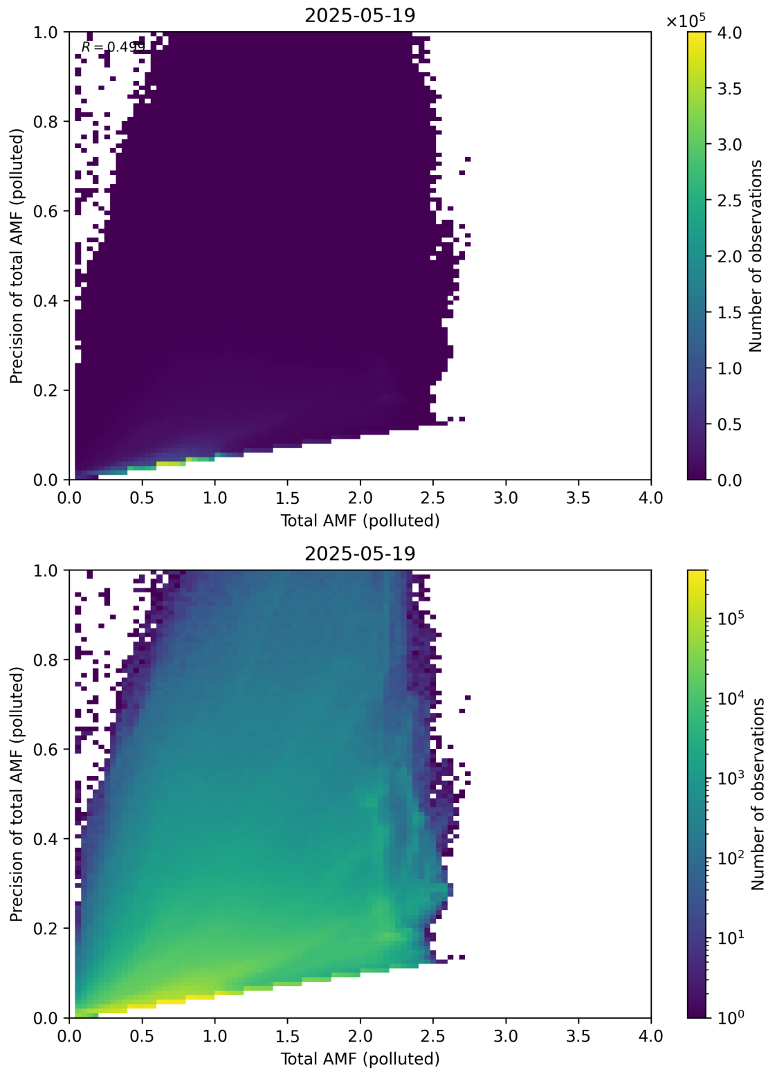
Figure 322: Scatter density plot of “Total AMF (polluted)” against “Precision of total AMF (polluted)” for 2025-05-18 to 2025-05-20.
