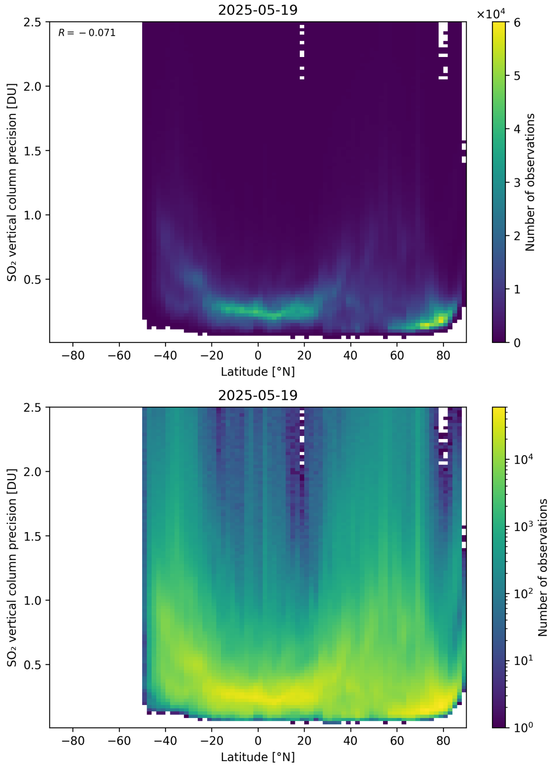
Figure 170: Scatter density plot of “Latitude” against “SO 2 vertical column precision” for 2025-05-18 to 2025-05-20.
