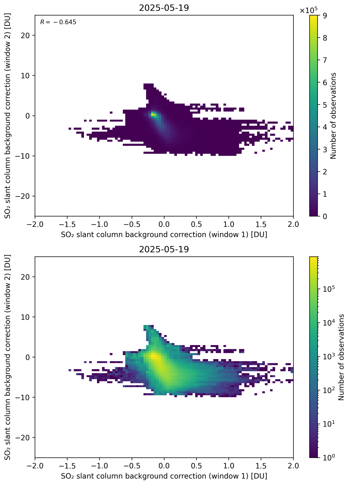
Figure 109: Scatter density plot of “SO 2 slant column background correction (window 1)” against “SO 2 slant column background correction (window 2)” for 2025-05-18 to 2025-05-20.
