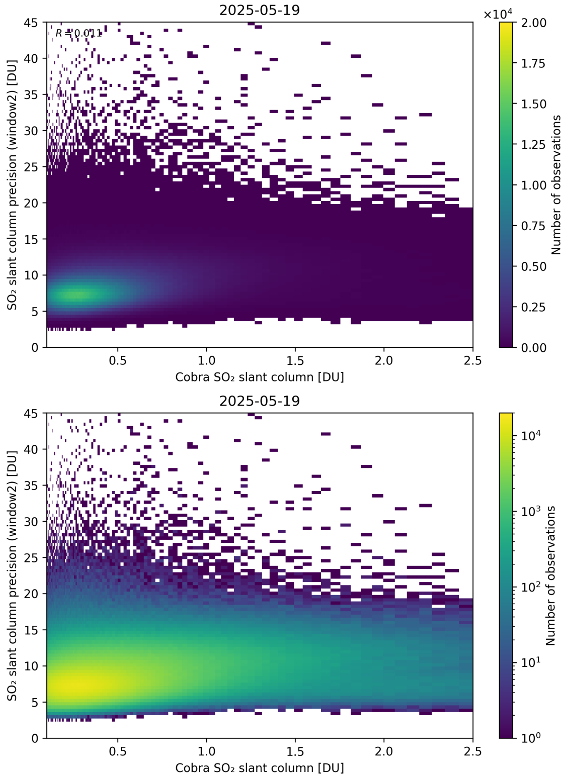
Figure 221: Scatter density plot of “Cobra SO 2 slant column” against “SO 2 slant column precision (window2)” for 2025-05-18 to 2025-05-20.
