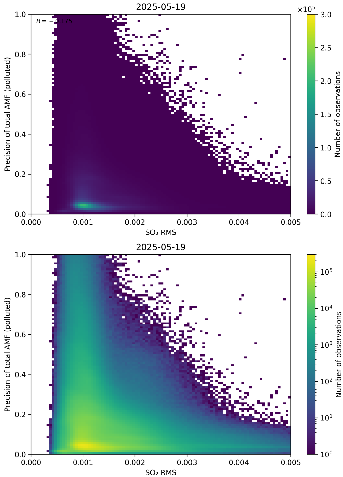
Figure 149: Scatter density plot of “SO 2 RMS” against “Precision of total AMF (polluted)” for 2025-05-18 to 2025-05-20.
