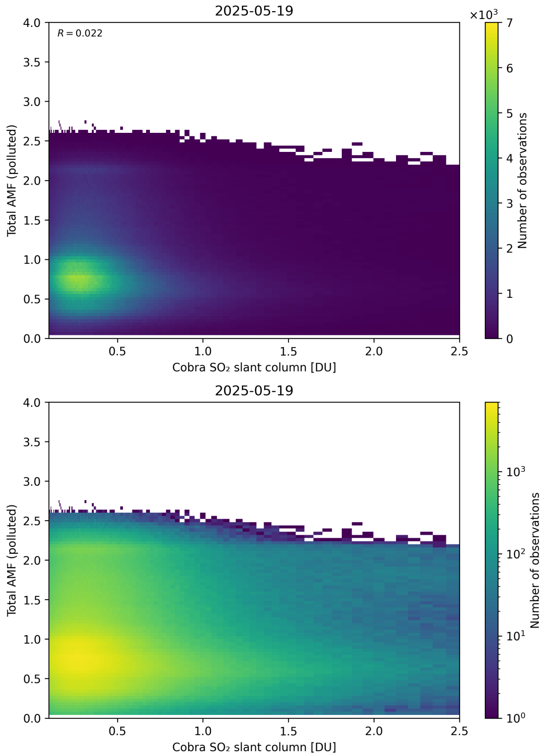
Figure 224: Scatter density plot of “Cobra SO 2 slant column” against “Total AMF (polluted)” for 2025-05-18 to 2025-05-20.
