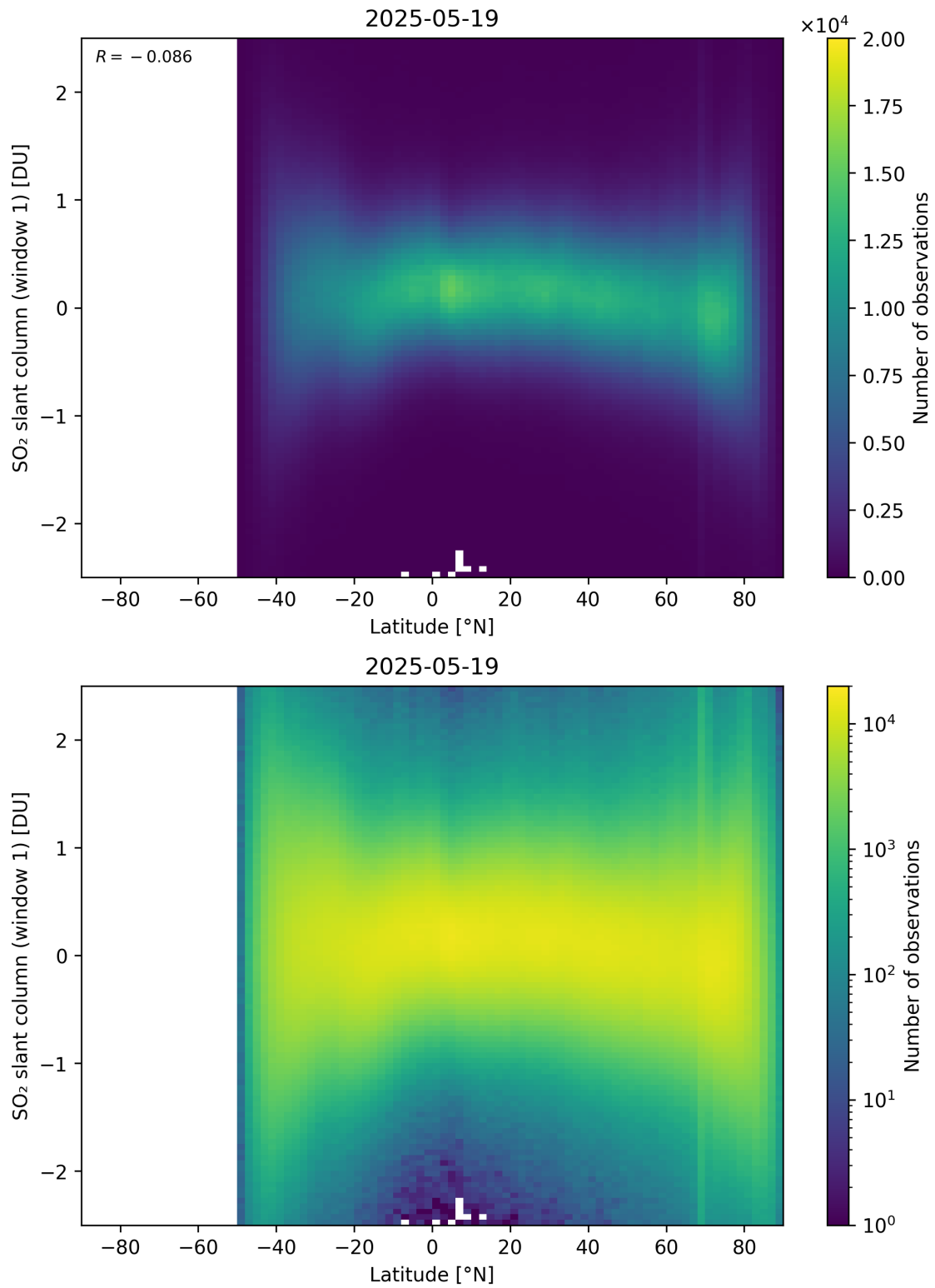
Figure 162: Scatter density plot of “Latitude” against “SO 2 slant column (window 1)” for 2025-05-18 to 2025-05-20.
