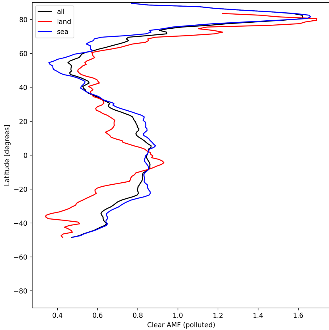
Figure 55: Zonal average of “Clear AMF (polluted)” for 2025-05-18 to 2025-05-20.
