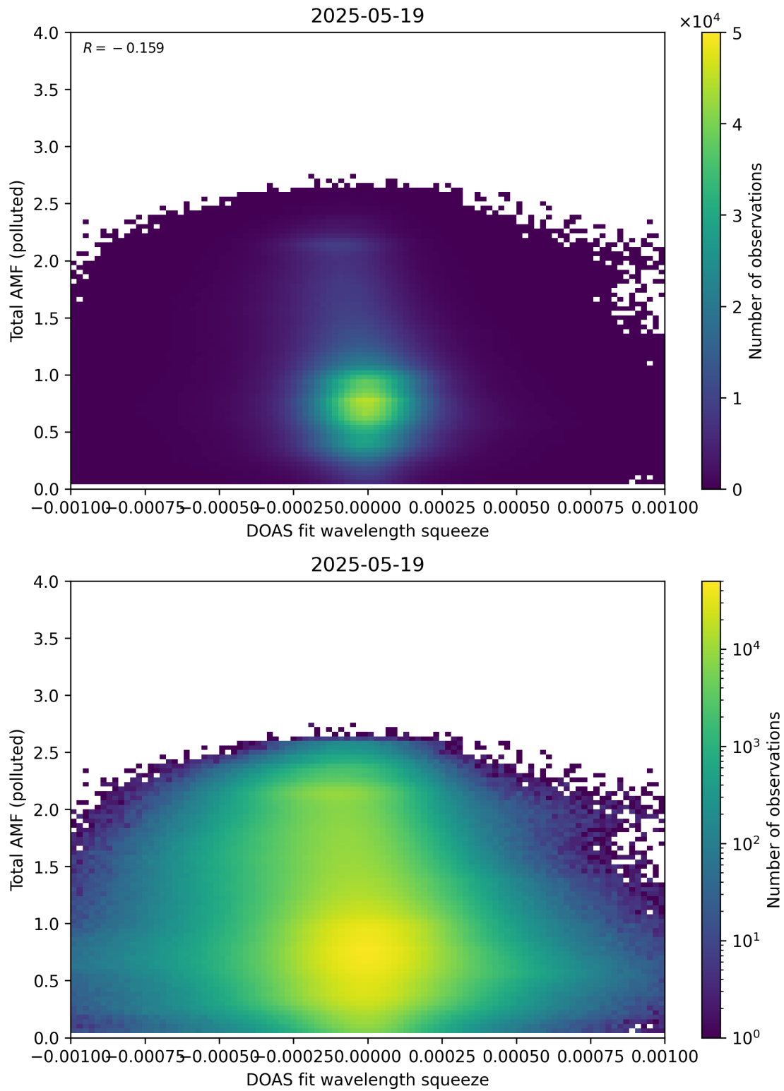
Figure 145: Scatter density plot of “DOAS fit wavelength squeeze” against “Total AMF (polluted)” for 2025-05-18 to 2025-05-20.
