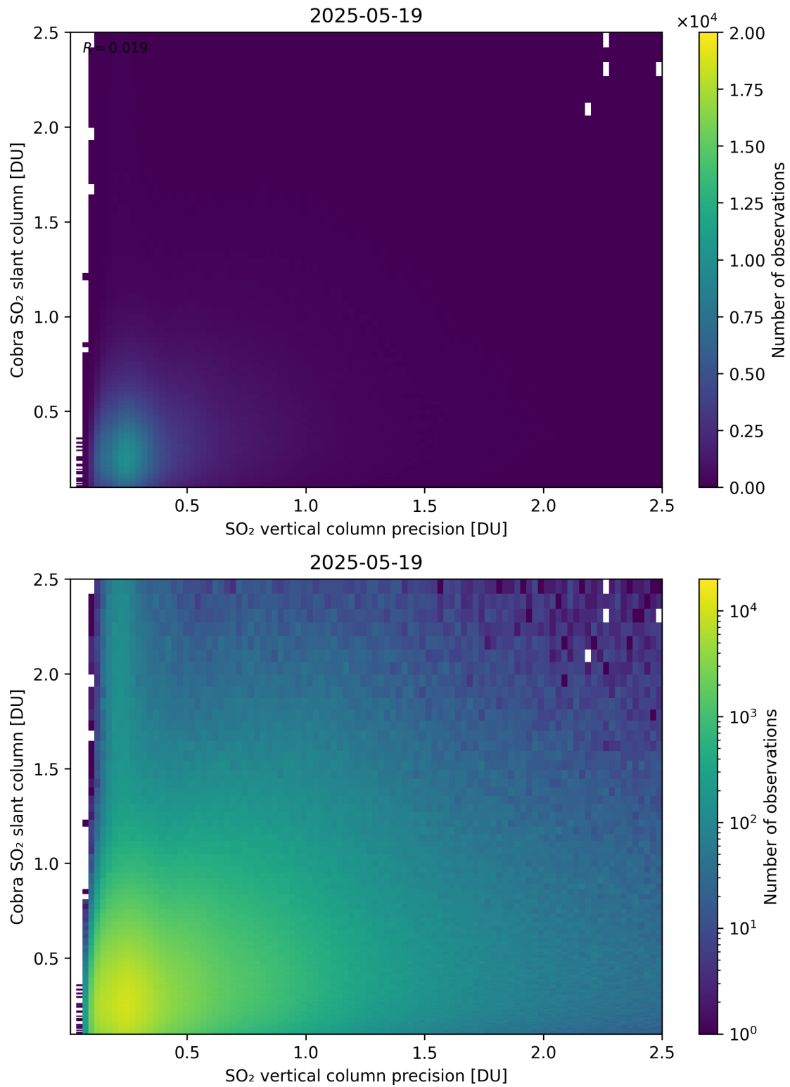
Figure 336: Scatter density plot of “SO 2 vertical column precision” against “Cobra SO 2 slant column” for 2025-05-18 to 2025-05-20.
