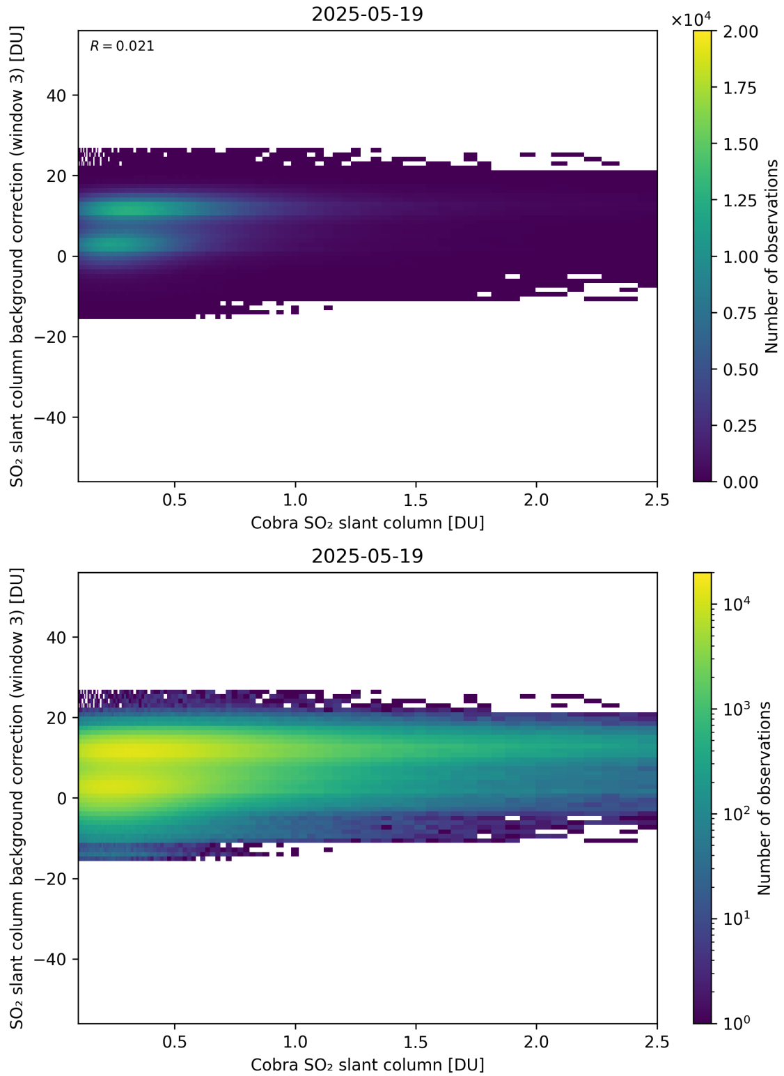
Figure 195: Scatter density plot of “Cobra SO 2 slant column” against “SO 2 slant column background correction (window 3)” for 2025-05-18 to 2025-05-20.
