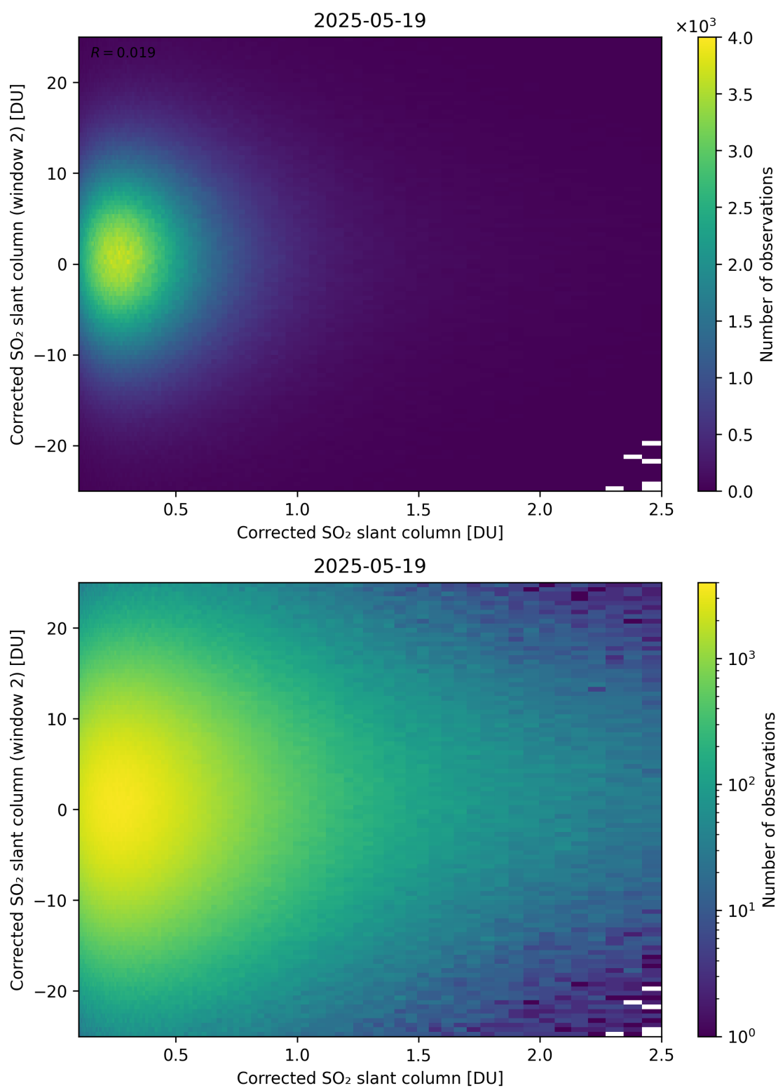
Figure 235: Scatter density plot of “Corrected SO 2 slant column” against “Corrected SO 2 slant column (window 2)” for 2025-05-18 to 2025-05-20.
