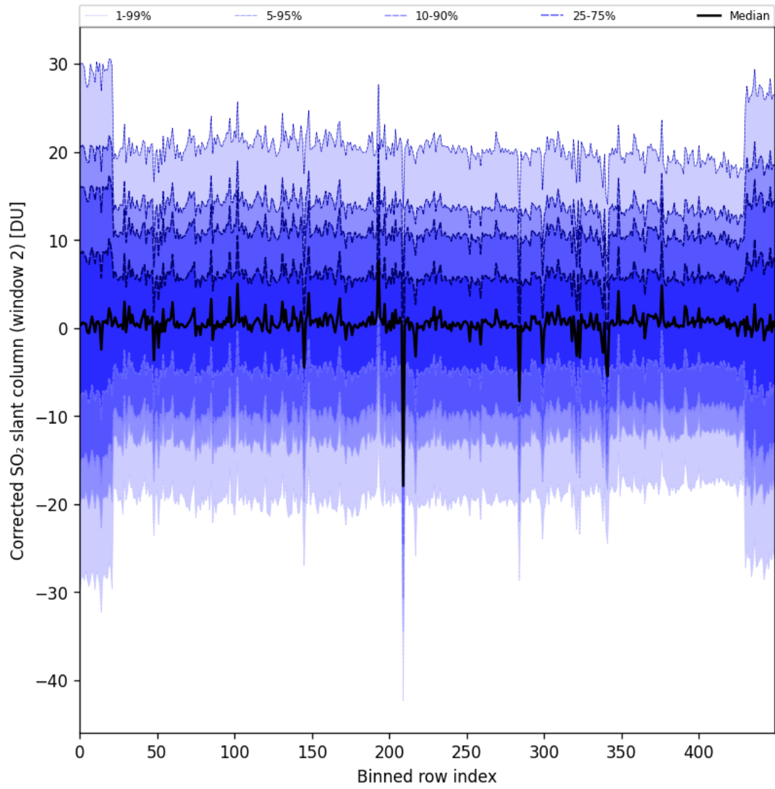
Figure 95: Along track statistics of “Corrected SO 2 slant column (window 2)” for 2025-05-18 to 2025-05-20
