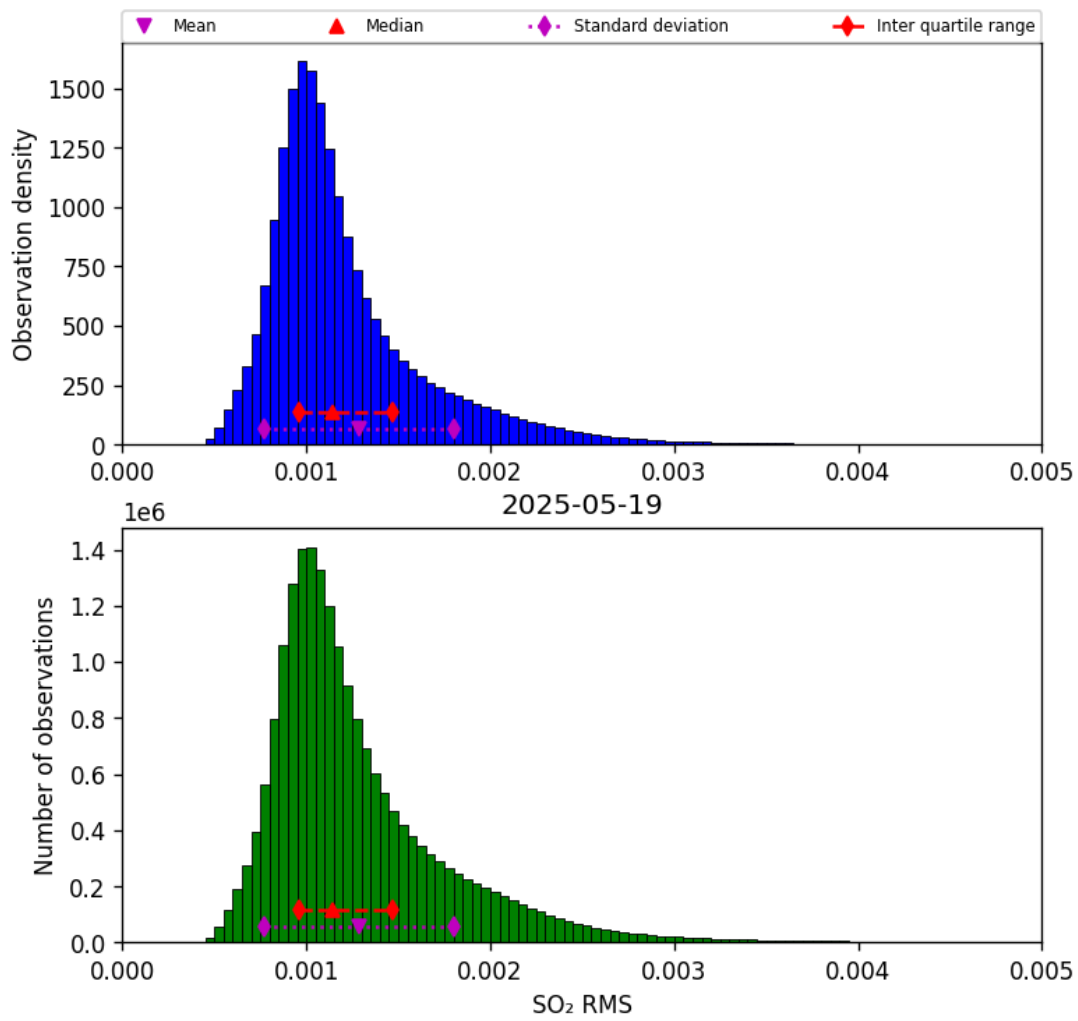
Figure 78: Histogram of “SO 2 RMS” for 2025-05-18 to 2025-05-20
