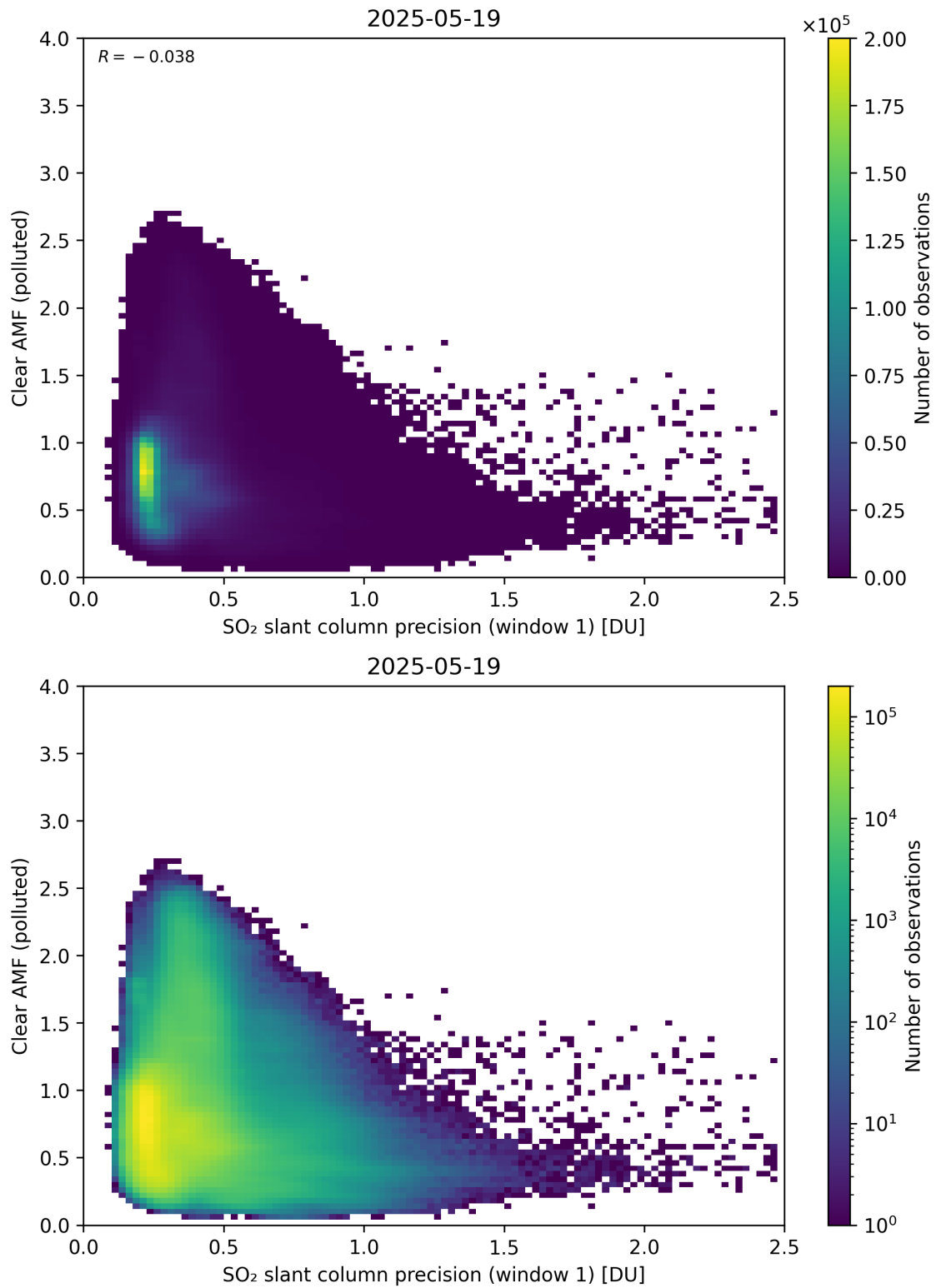
Figure 274: Scatter density plot of “SO 2 slant column precision (window 1)” against “Clear AMF (polluted)” for 2025-05-18 to 2025-05-20.
