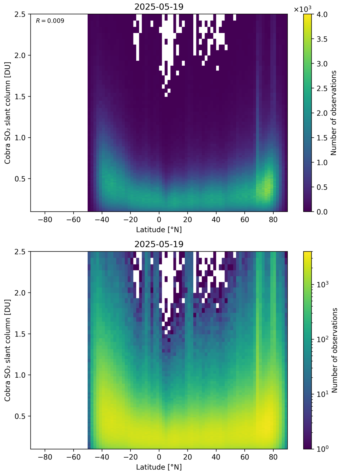
Figure 157: Scatter density plot of “Latitude” against “Cobra SO 2 slant column” for 2025-05-18 to 2025-05-20.
