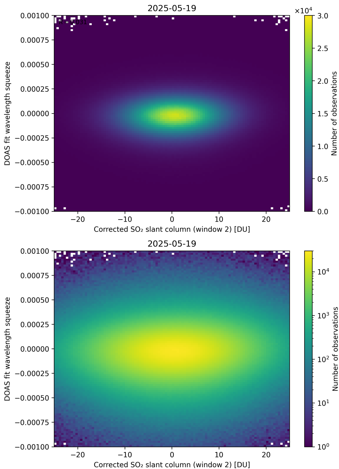
Figure 247: Scatter density plot of “Corrected SO 2 slant column (window 2)” against “DOAS fit wavelength squeeze” for 2025-05-18 to 2025-05-20.
