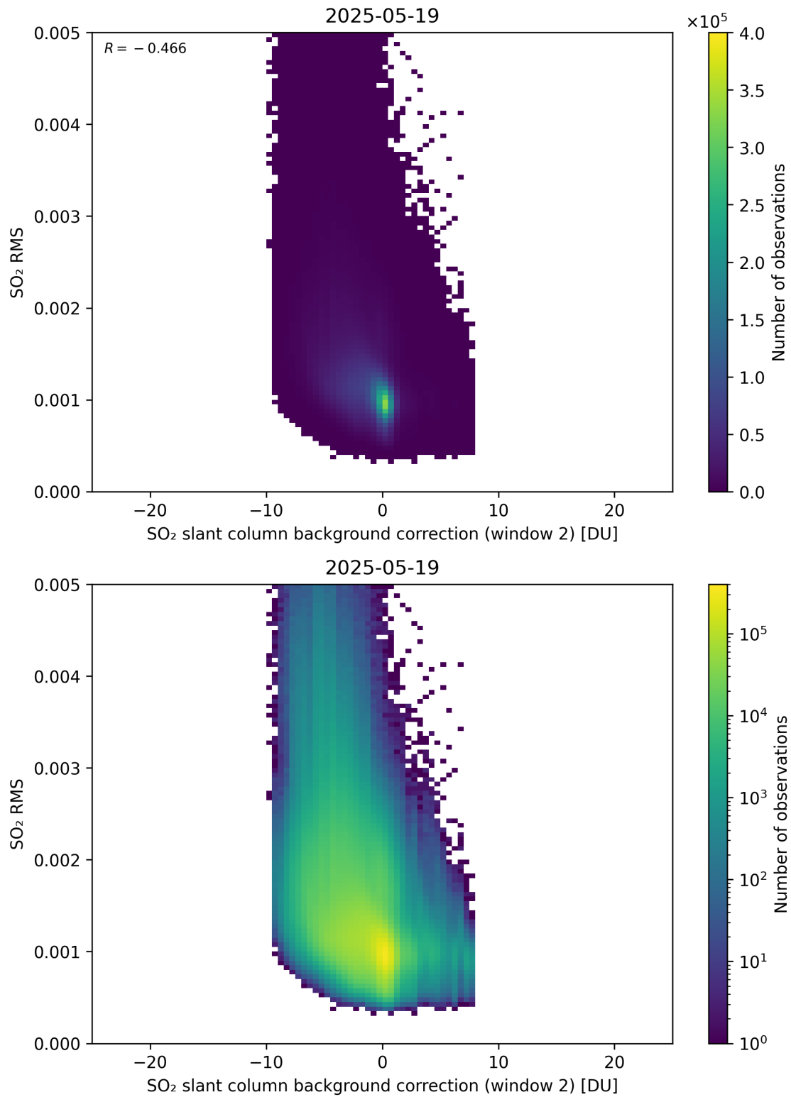
Figure 125: Scatter density plot of “SO 2 slant column background correction (window 2)” against “SO 2 RMS” for 2025-05-18 to 2025-05-20.
