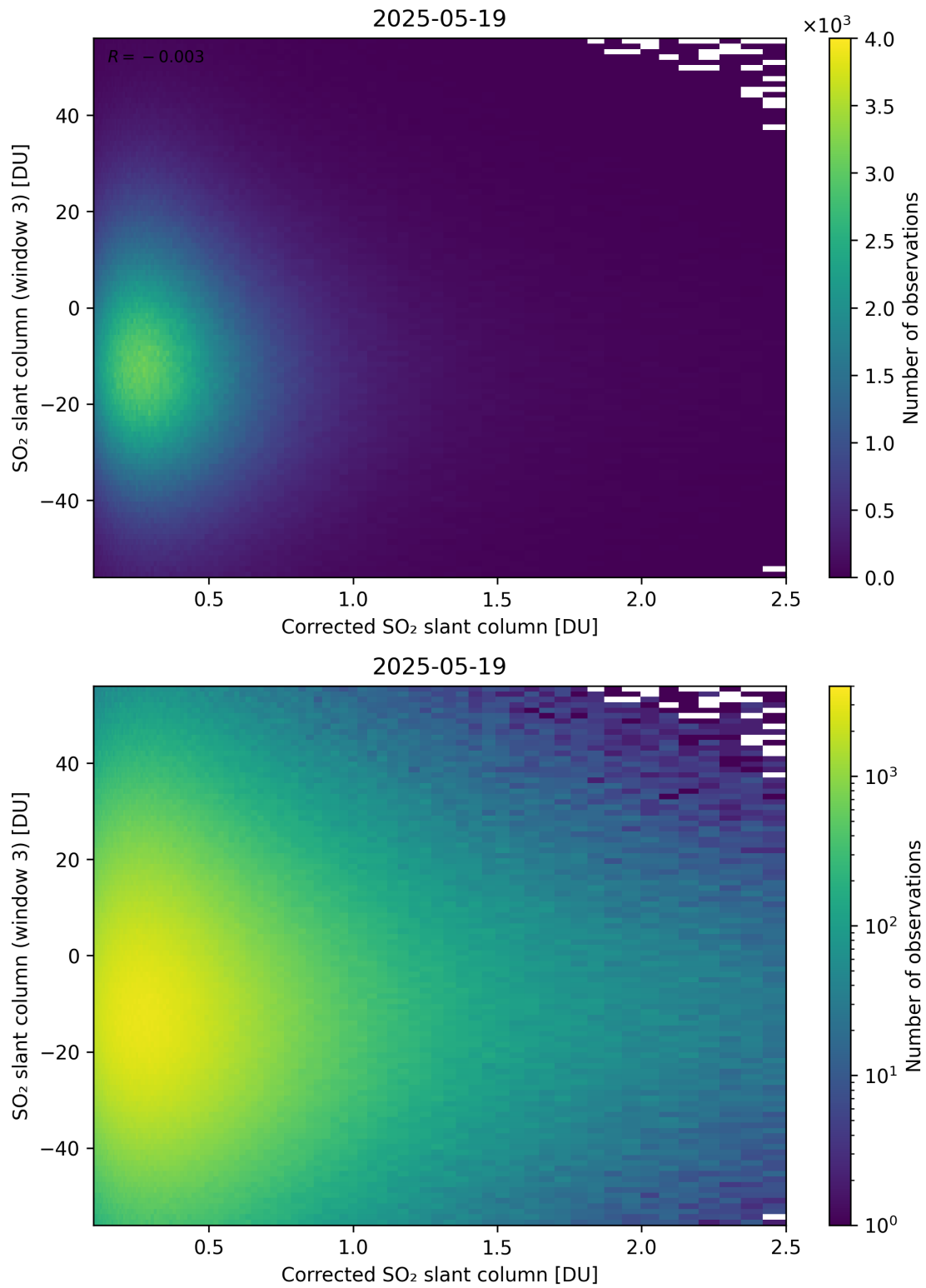
Figure 240: Scatter density plot of “Corrected SO 2 slant column” against “SO 2 slant column (window 3)” for 2025-05-18 to 2025-05-20.
