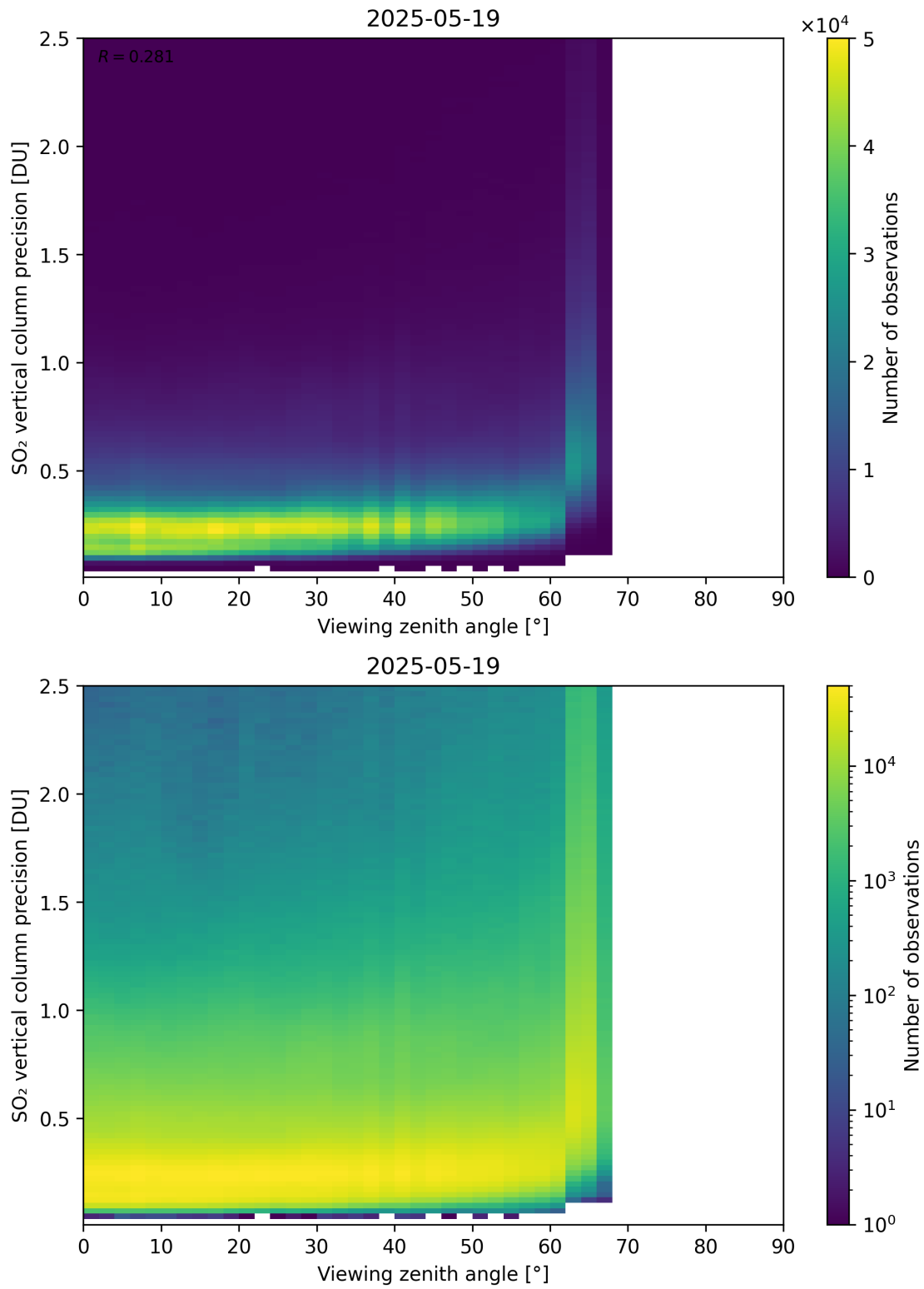
Figure 384: Scatter density plot of “Viewing zenith angle” against “SO 2 vertical column precision” for 2025-05-18 to 2025-05-20.
