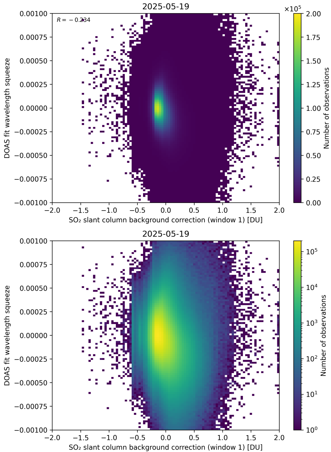
Figure 112: Scatter density plot of “SO 2 slant column background correction (window 1)” against “DOAS fit wavelength squeeze” for 2025-05-18 to 2025-05-20.
