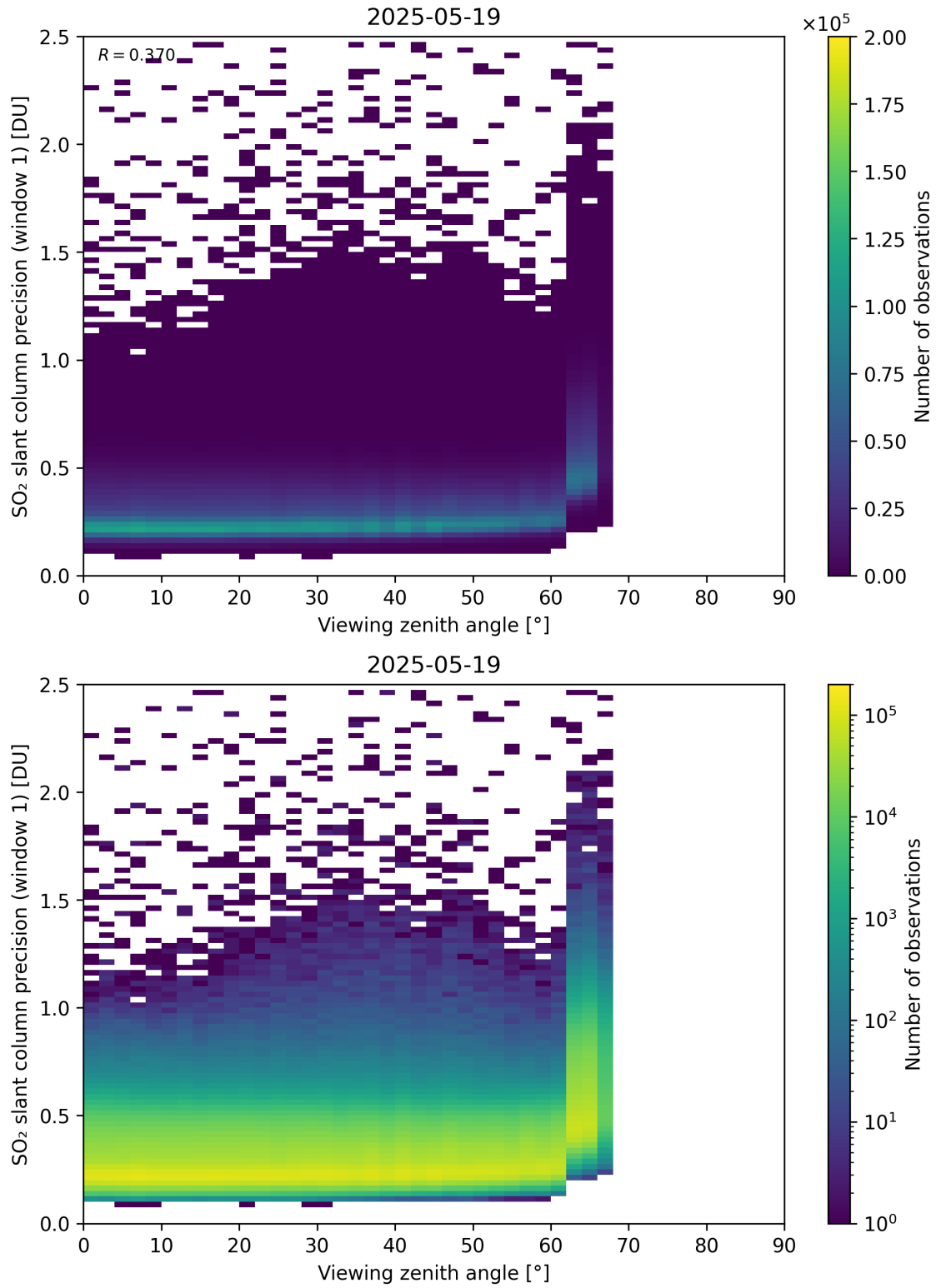
Figure 377: Scatter density plot of “Viewing zenith angle” against “SO 2 slant column precision (window 1)” for 2025-05-18 to 2025-05-20.
