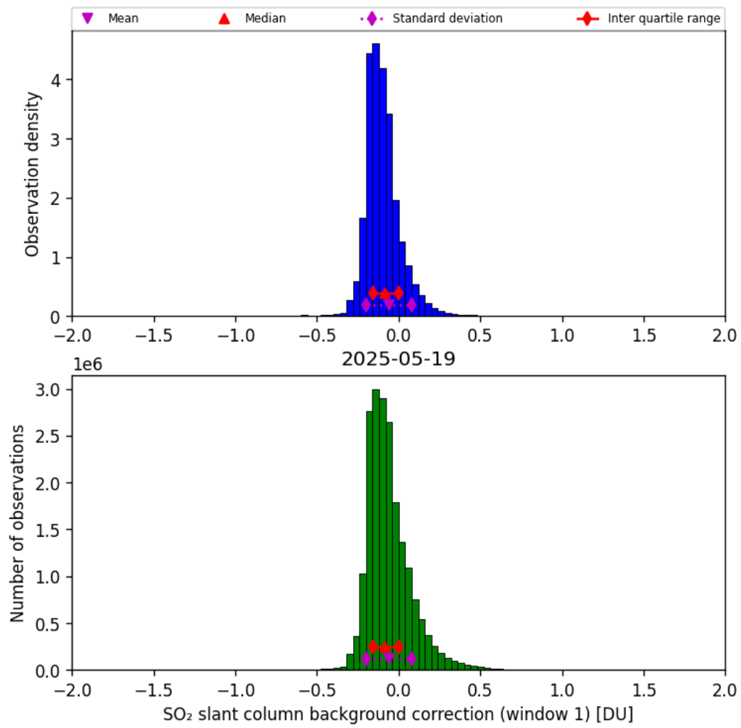
Figure 66: Histogram of “SO 2 slant column background correction (window 1)” for 2025-05-18 to 2025-05-20
