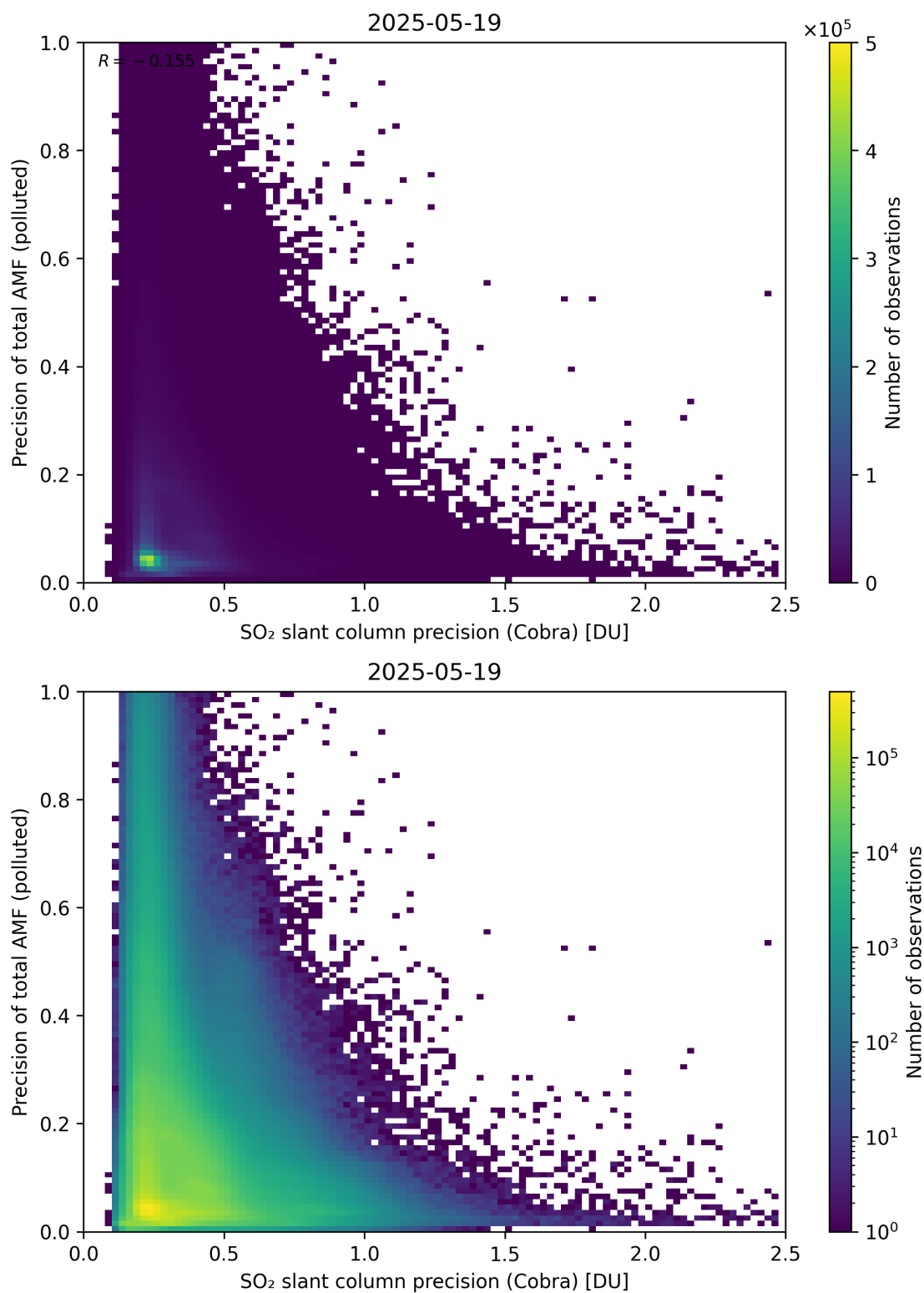
Figure 214: Scatter density plot of “SO 2 slant column precision (Cobra)” against “Precision of total AMF (polluted)” for 2025-05-18 to 2025-05-20.
