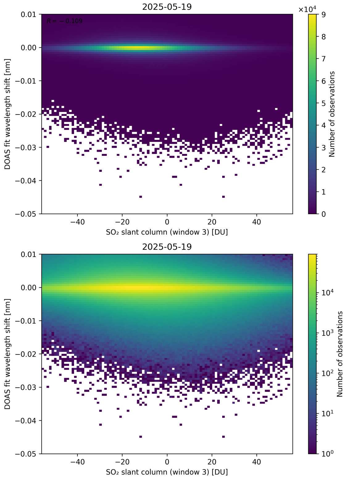
Figure 304: Scatter density plot of “SO 2 slant column (window 3)” against “DOAS fit wavelength shift” for 2025-05-18 to 2025-05-20.
