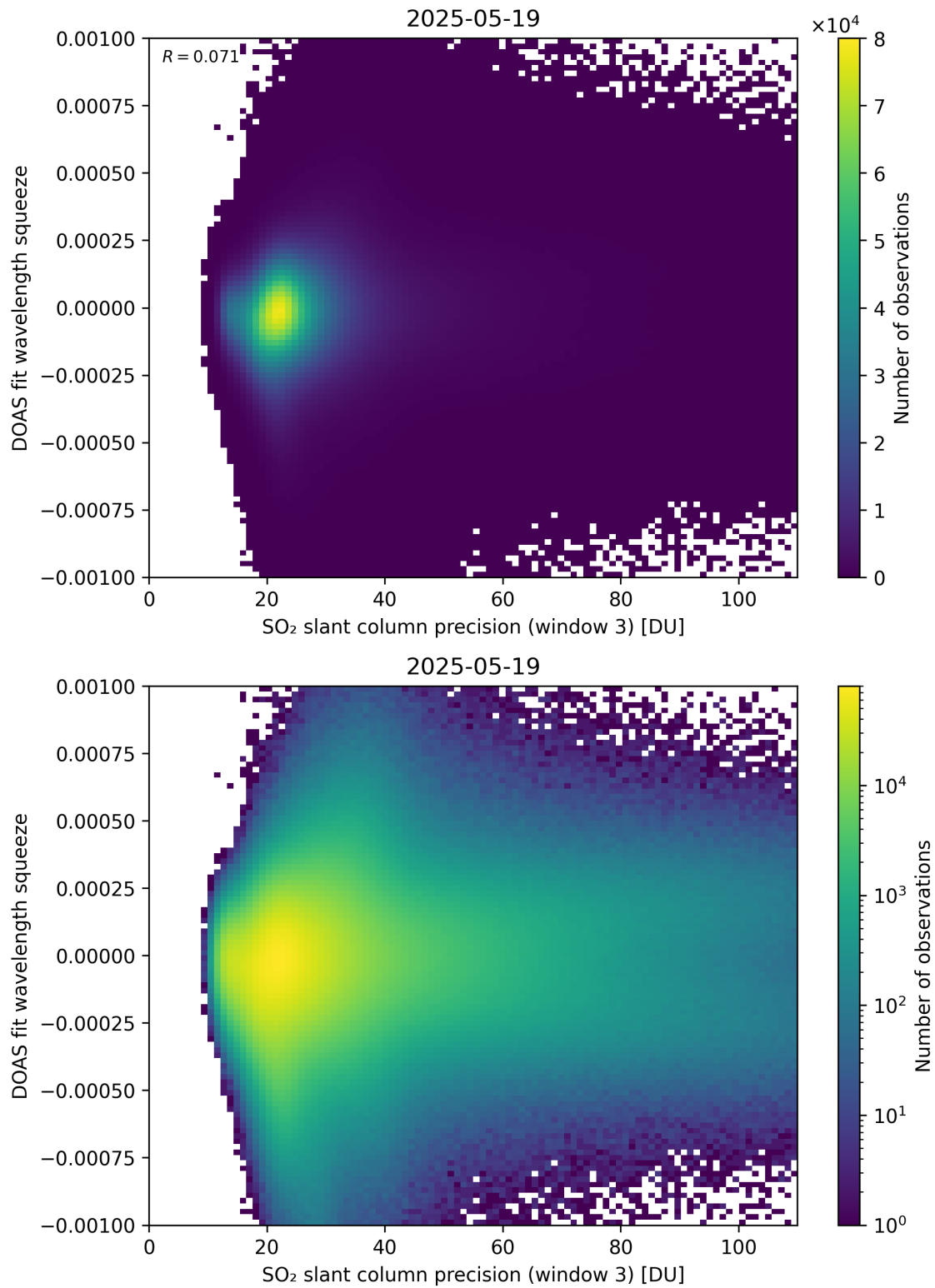
Figure 309: Scatter density plot of “SO 2 slant column precision (window 3)” against “DOAS fit wavelength squeeze” for 2025-05-18 to 2025-05-20.
