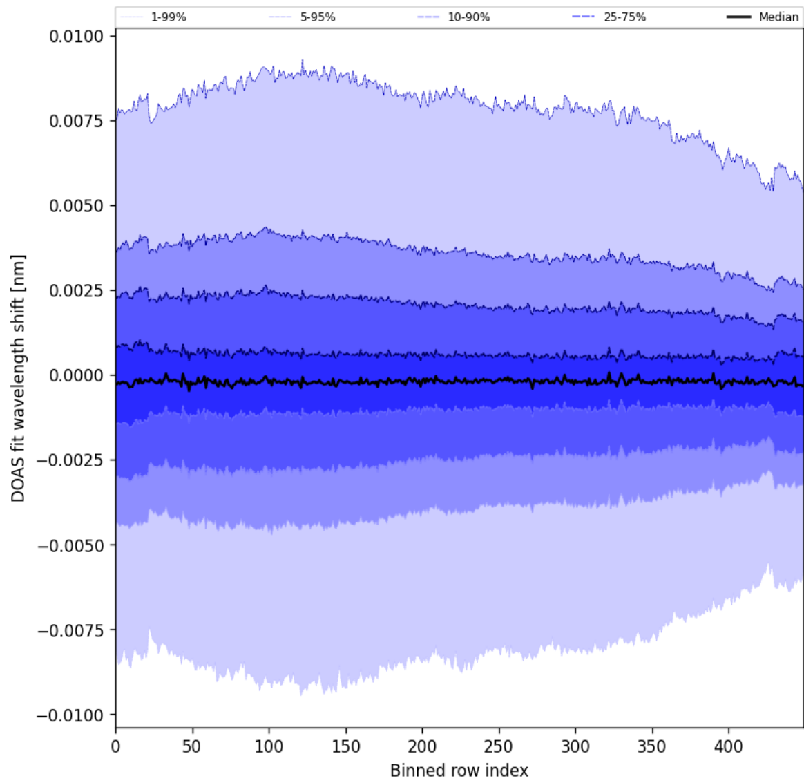
Figure 102: Along track statistics of “DOAS fit wavelength shift” for 2025-05-18 to 2025-05-20
