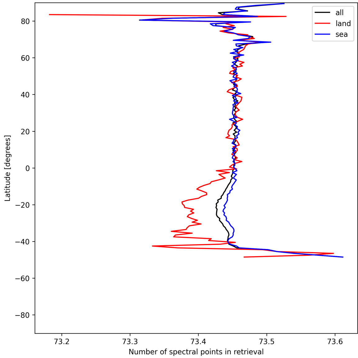
Figure 56: Zonal average of “Number of spectral points in retrieval” for 2025-05-18 to 2025-05-20.
