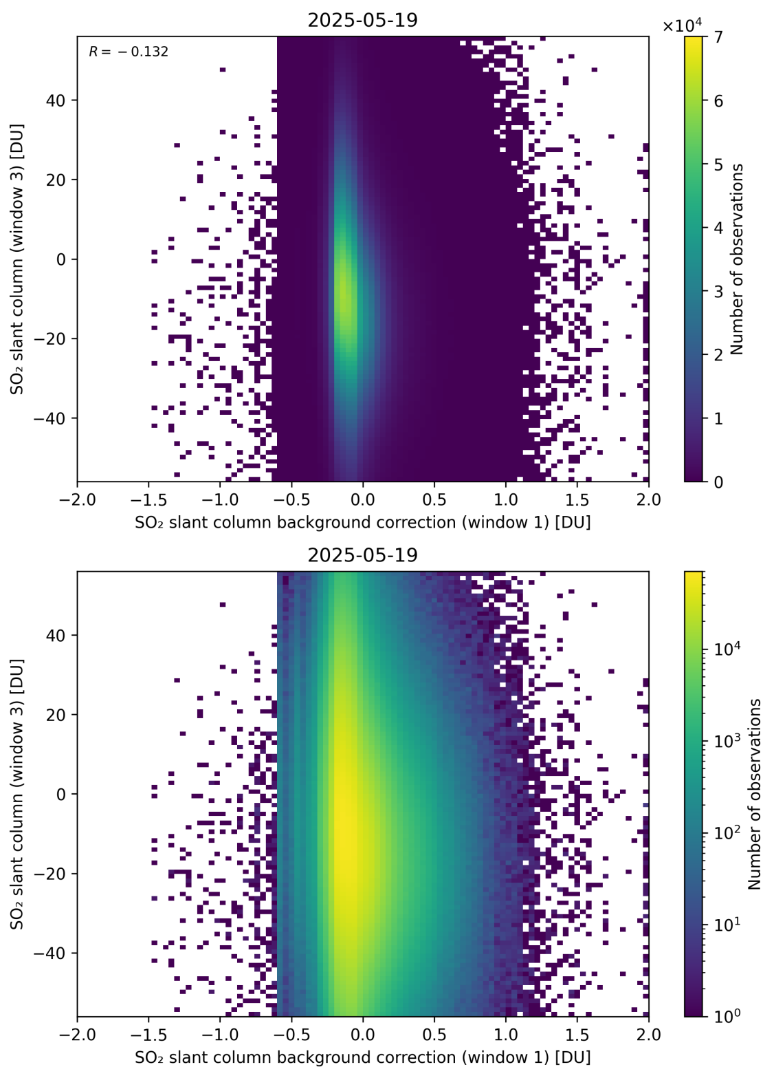
Figure 118: Scatter density plot of “SO 2 slant column background correction (window 1)” against “SO 2 slant column (window 3)” for 2025-05-18 to 2025-05-20.
