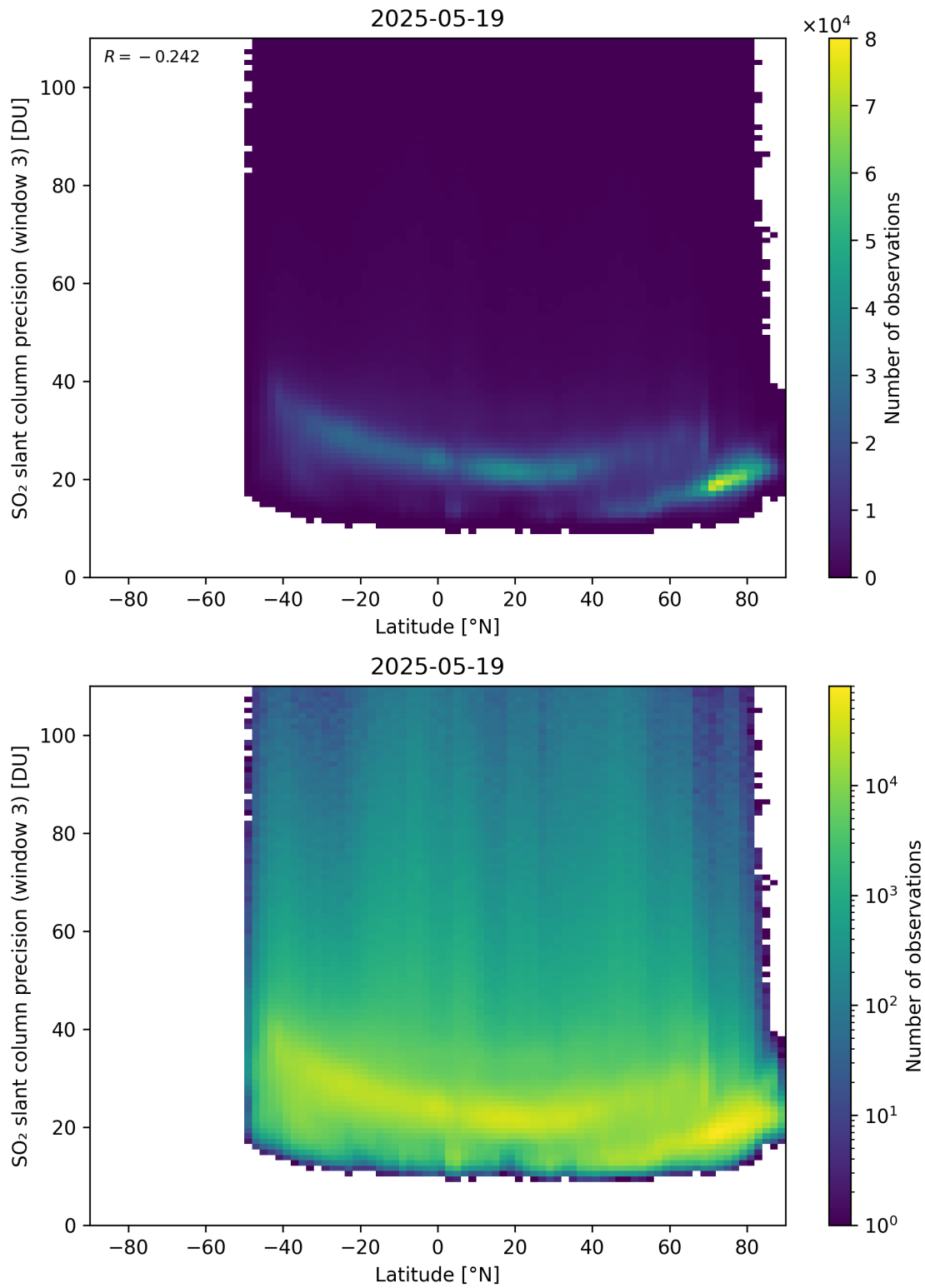
Figure 166: Scatter density plot of “Latitude” against “SO 2 slant column precision (window 3)” for 2025-05-18 to 2025-05-20.
