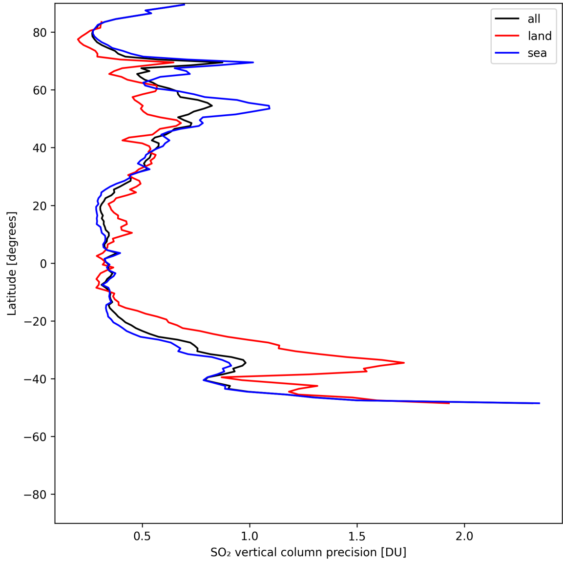
Figure 33: Zonal average of “SO 2 vertical column precision” for 2025-05-18 to 2025-05-20.
