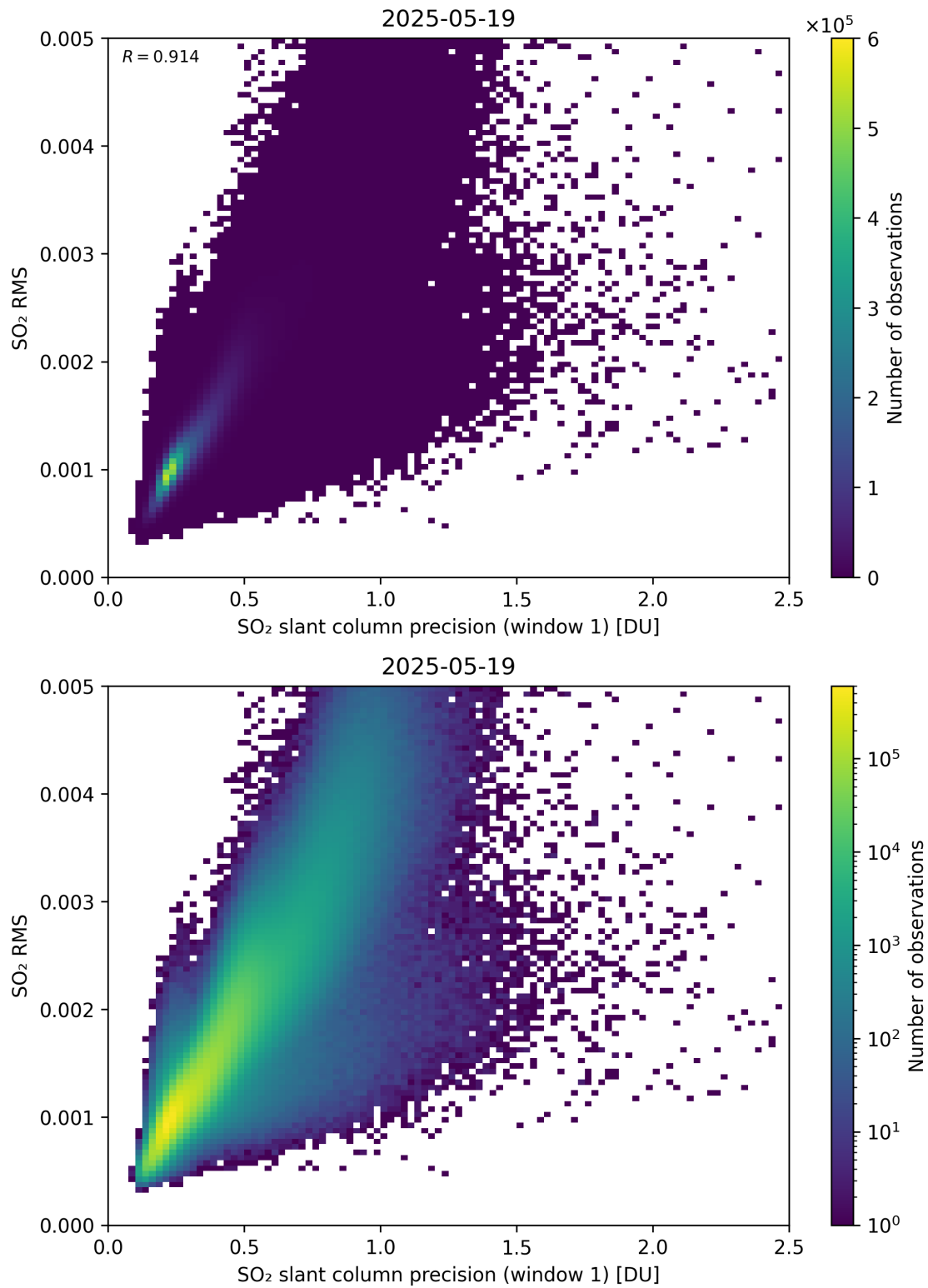
Figure 273: Scatter density plot of “SO 2 slant column precision (window 1)” against “SO 2 RMS” for 2025-05-18 to 2025-05-20.
