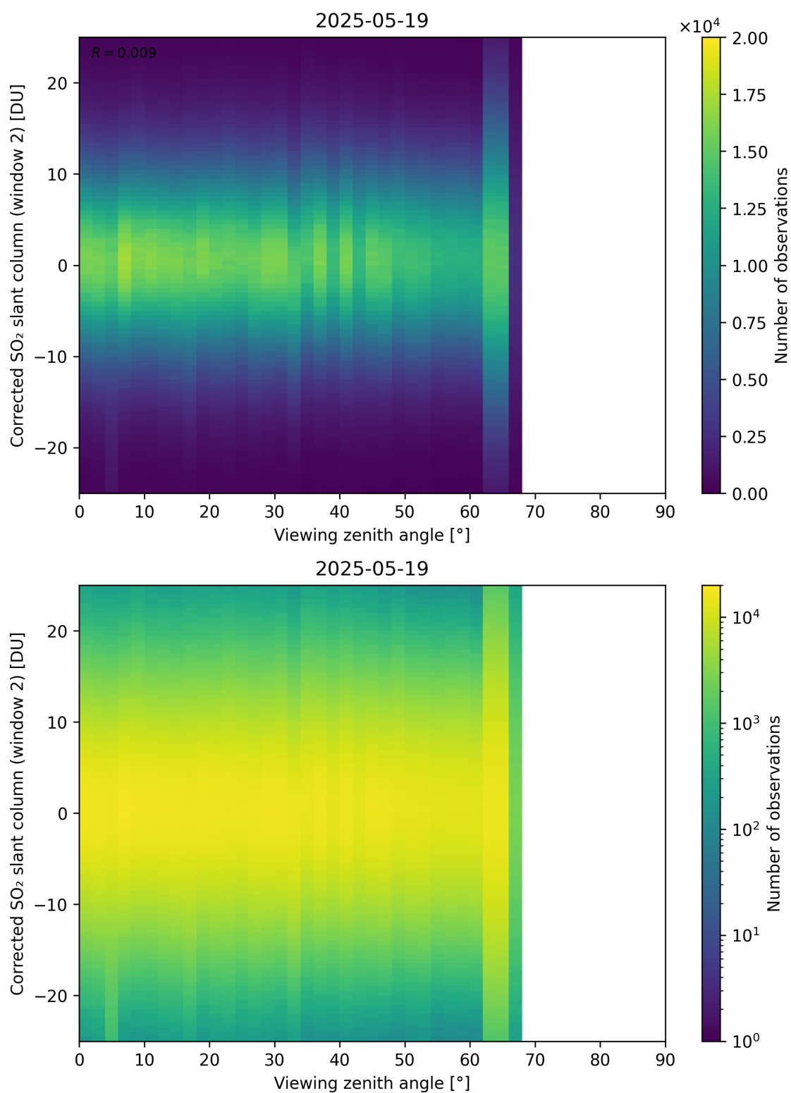
Figure 374: Scatter density plot of “Viewing zenith angle” against “Corrected SO 2 slant column (window 2)” for 2025-05-18 to 2025-05-20.
