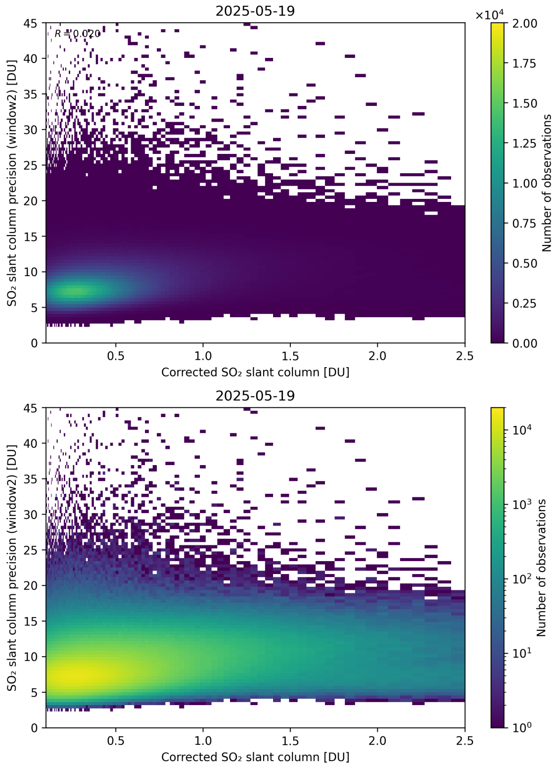
Figure 239: Scatter density plot of “Corrected SO 2 slant column” against “SO 2 slant column precision (window2)” for 2025-05-18 to 2025-05-20.
