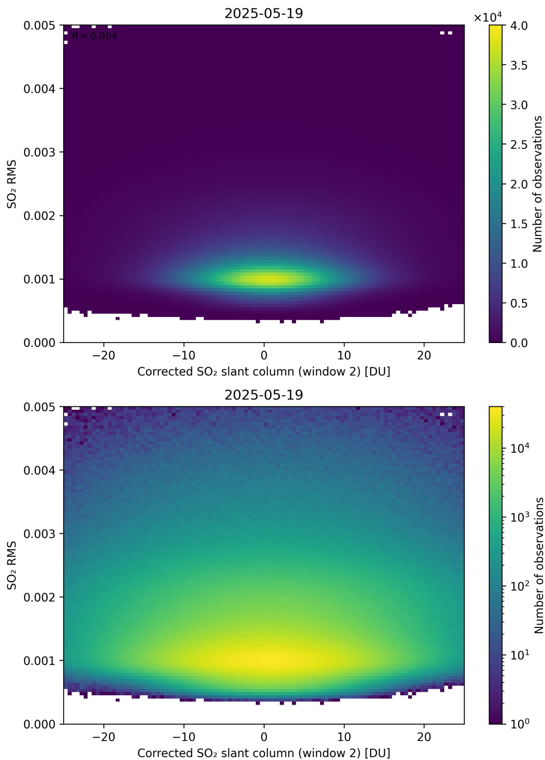
Figure 248: Scatter density plot of “Corrected SO 2 slant column (window 2)” against “SO 2 RMS” for 2025-05-18 to 2025-05-20.
