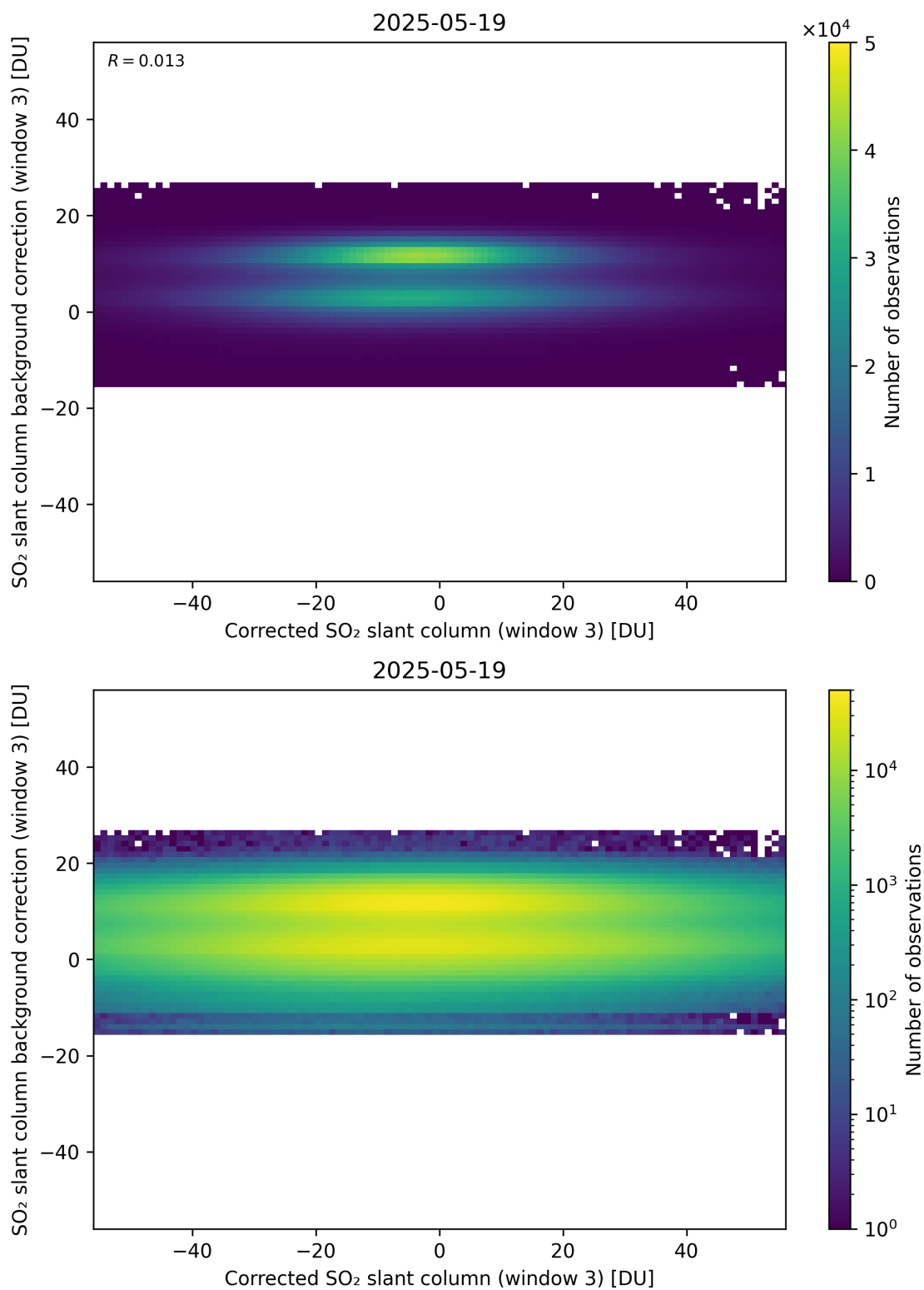
Figure 255: Scatter density plot of “Corrected SO 2 slant column (window 3)” against “SO 2 slant column background correction (window 3)” for 2025-05-18 to 2025-05-20.
