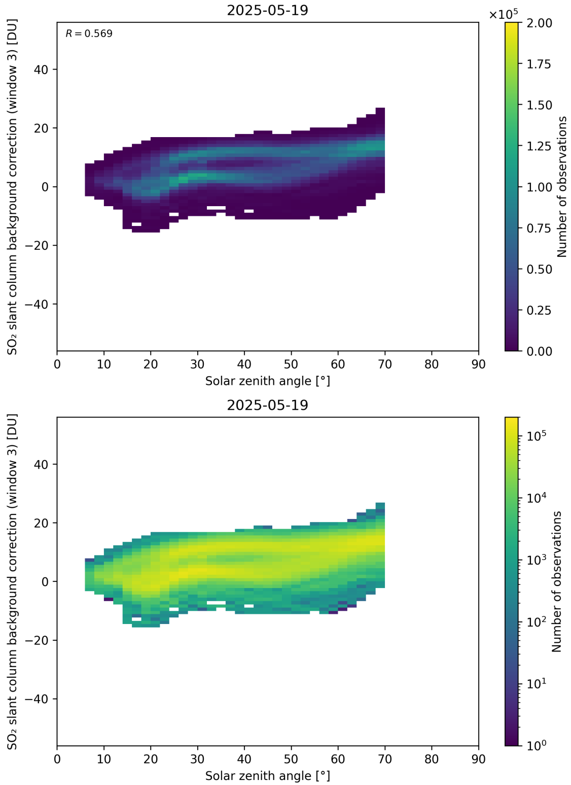
Figure 173: Scatter density plot of “Solar zenith angle” against “SO 2 slant column background correction (window 3)” for 2025-05-18 to 2025-05-20.
