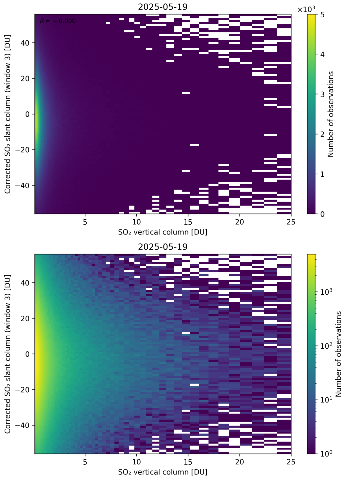
Figure 353: Scatter density plot of “SO 2 vertical column” against “Corrected SO 2 slant column (window 3)” for 2025-05-18 to 2025-05-20.
