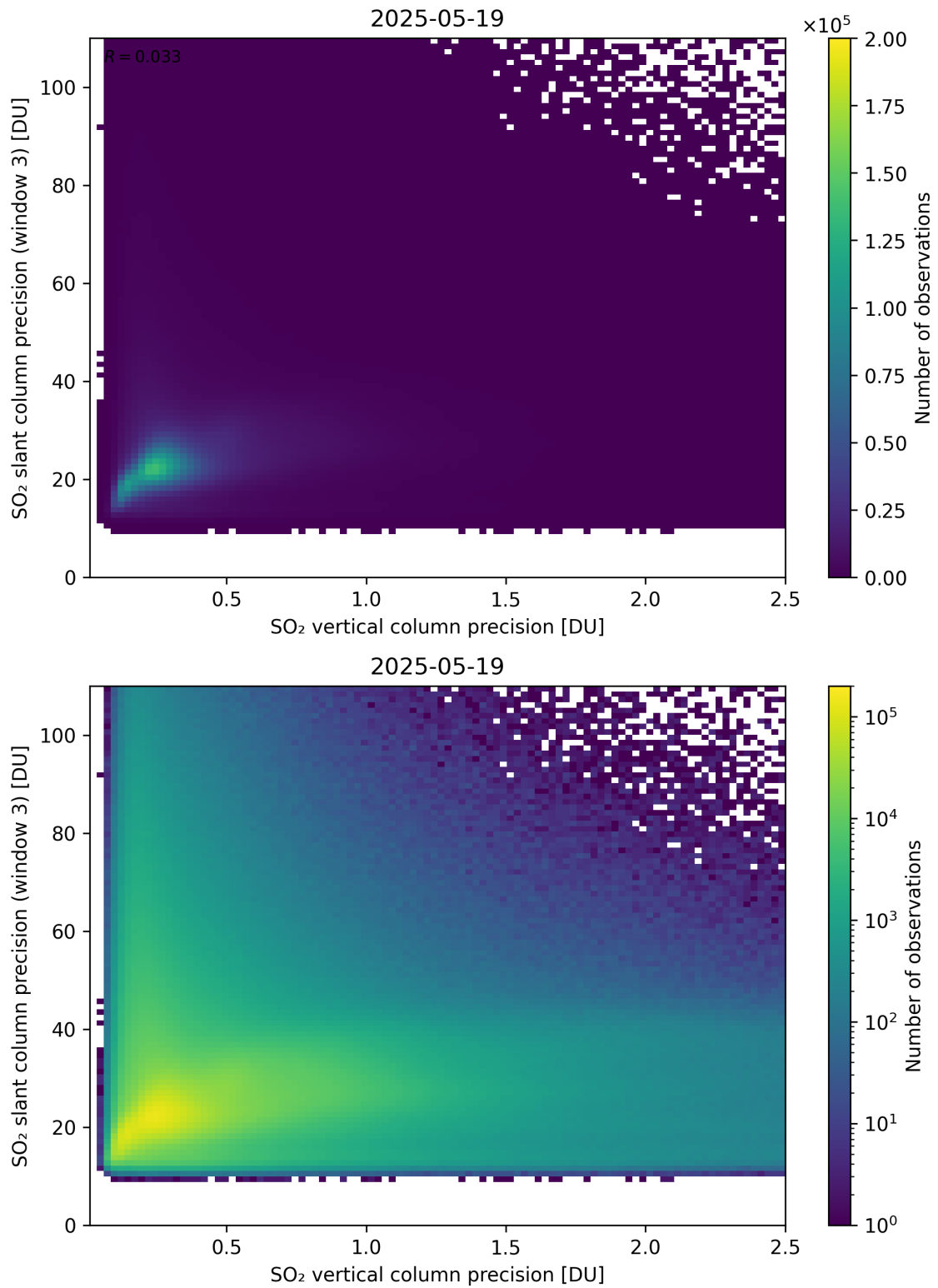
Figure 345: Scatter density plot of “SO 2 vertical column precision” against “SO 2 slant column precision (window 3)” for 2025-05-18 to 2025-05-20.
