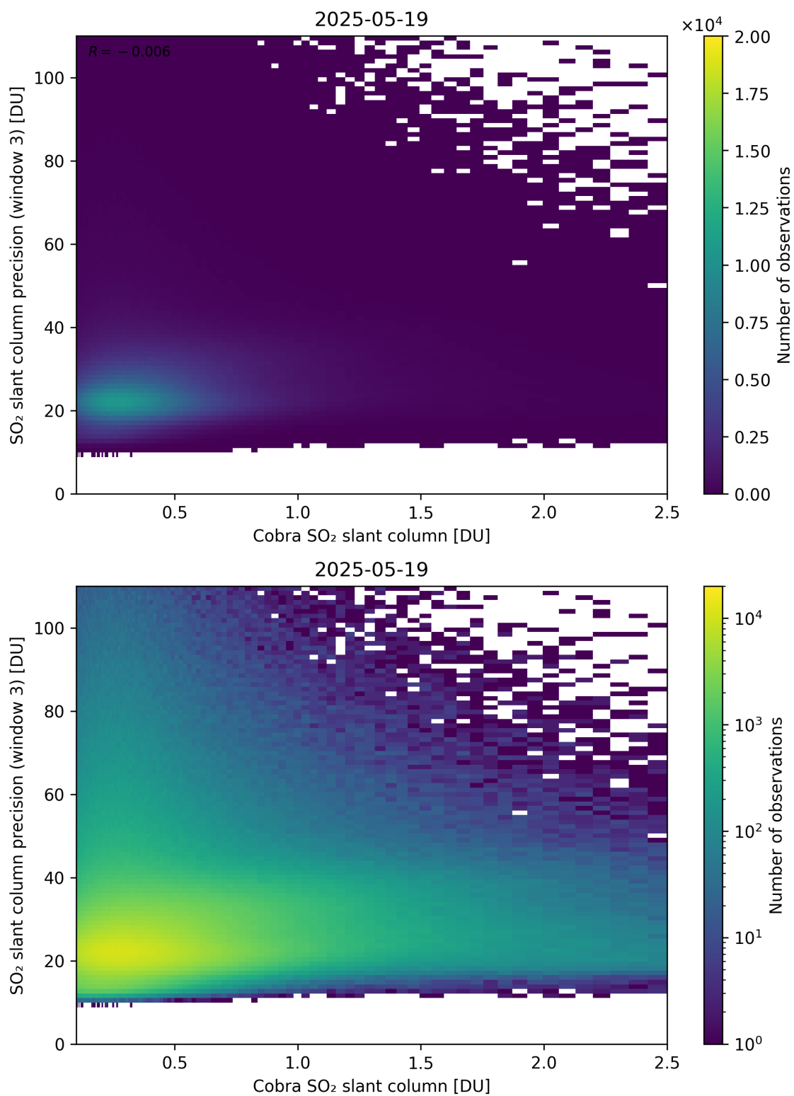
Figure 223: Scatter density plot of “Cobra SO 2 slant column” against “SO 2 slant column precision (window 3)” for 2025-05-18 to 2025-05-20.
