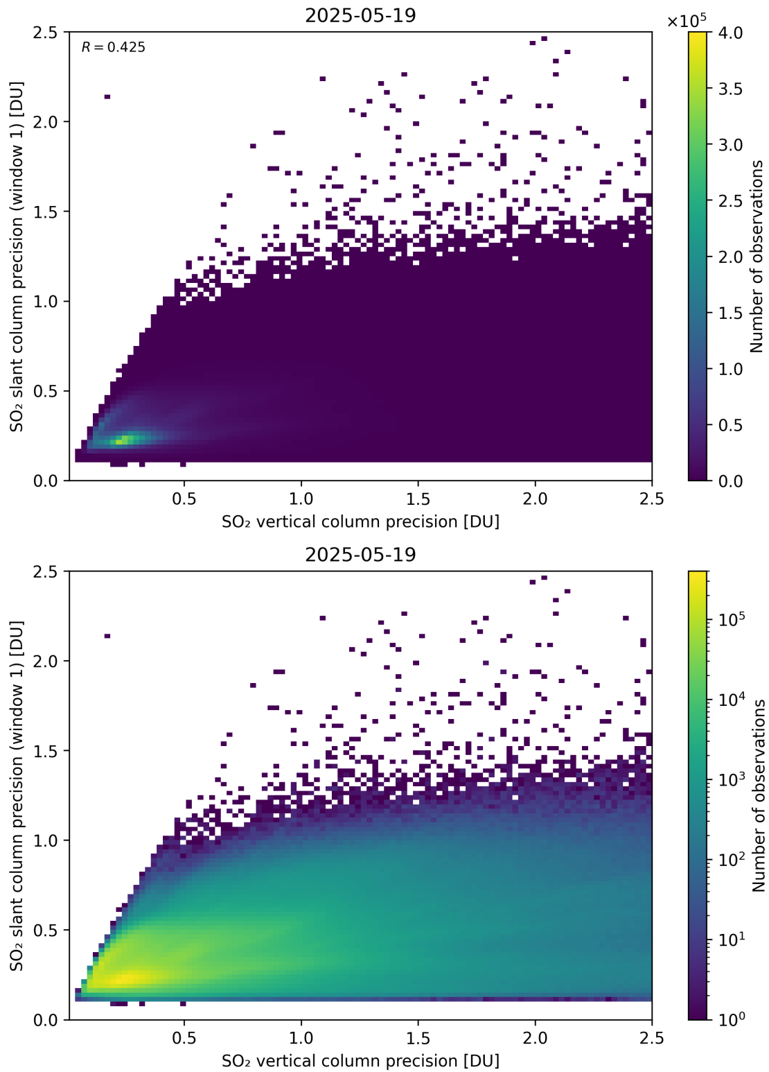
Figure 342: Scatter density plot of “SO 2 vertical column precision” against “SO 2 slant column precision (window 1)” for 2025-05-18 to 2025-05-20.
