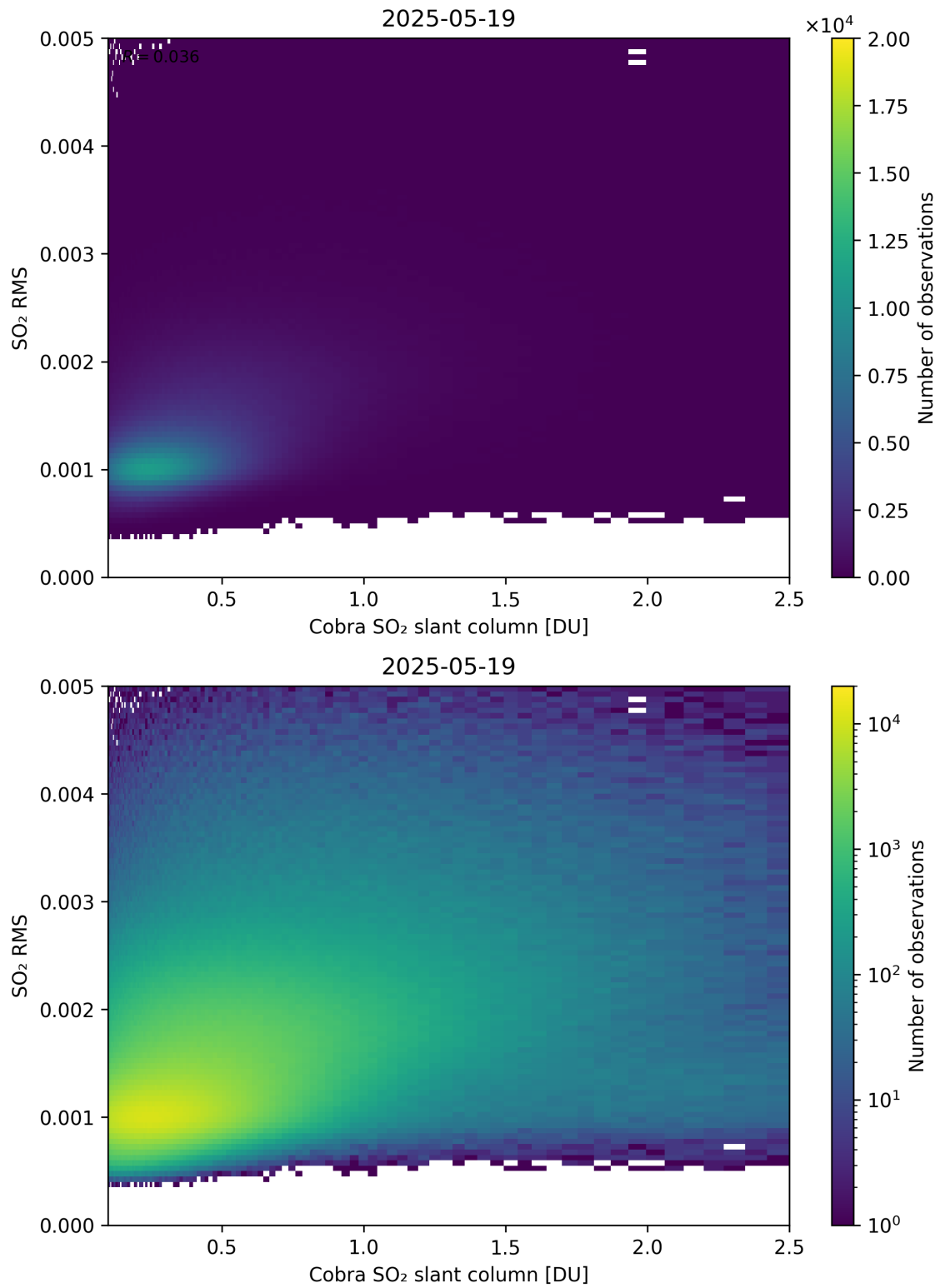
Figure 198: Scatter density plot of “Cobra SO 2 slant column” against “SO 2 RMS” for 2025-05-18 to 2025-05-20.
