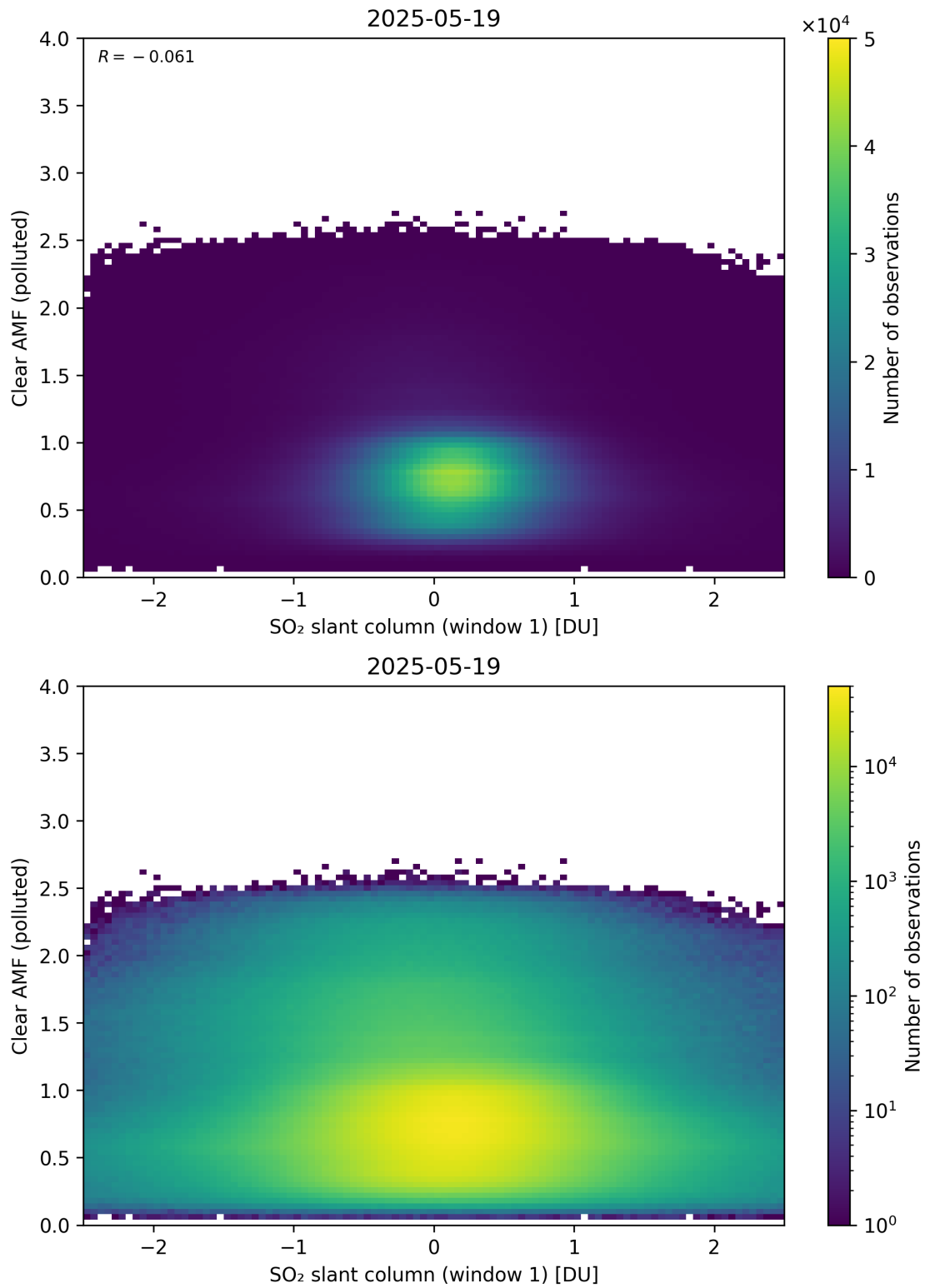
Figure 282: Scatter density plot of “SO 2 slant column (window 1)” against “Clear AMF (polluted)” for 2025-05-18 to 2025-05-20.
