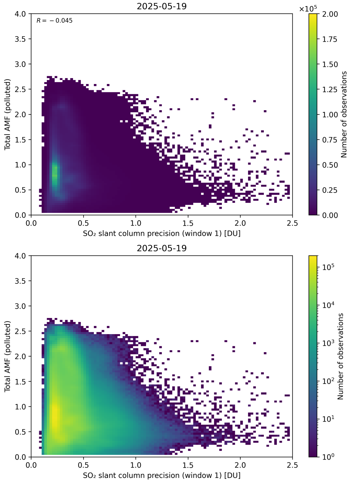
Figure 280: Scatter density plot of “SO 2 slant column precision (window 1)” against “Total AMF (polluted)” for 2025-05-18 to 2025-05-20.
