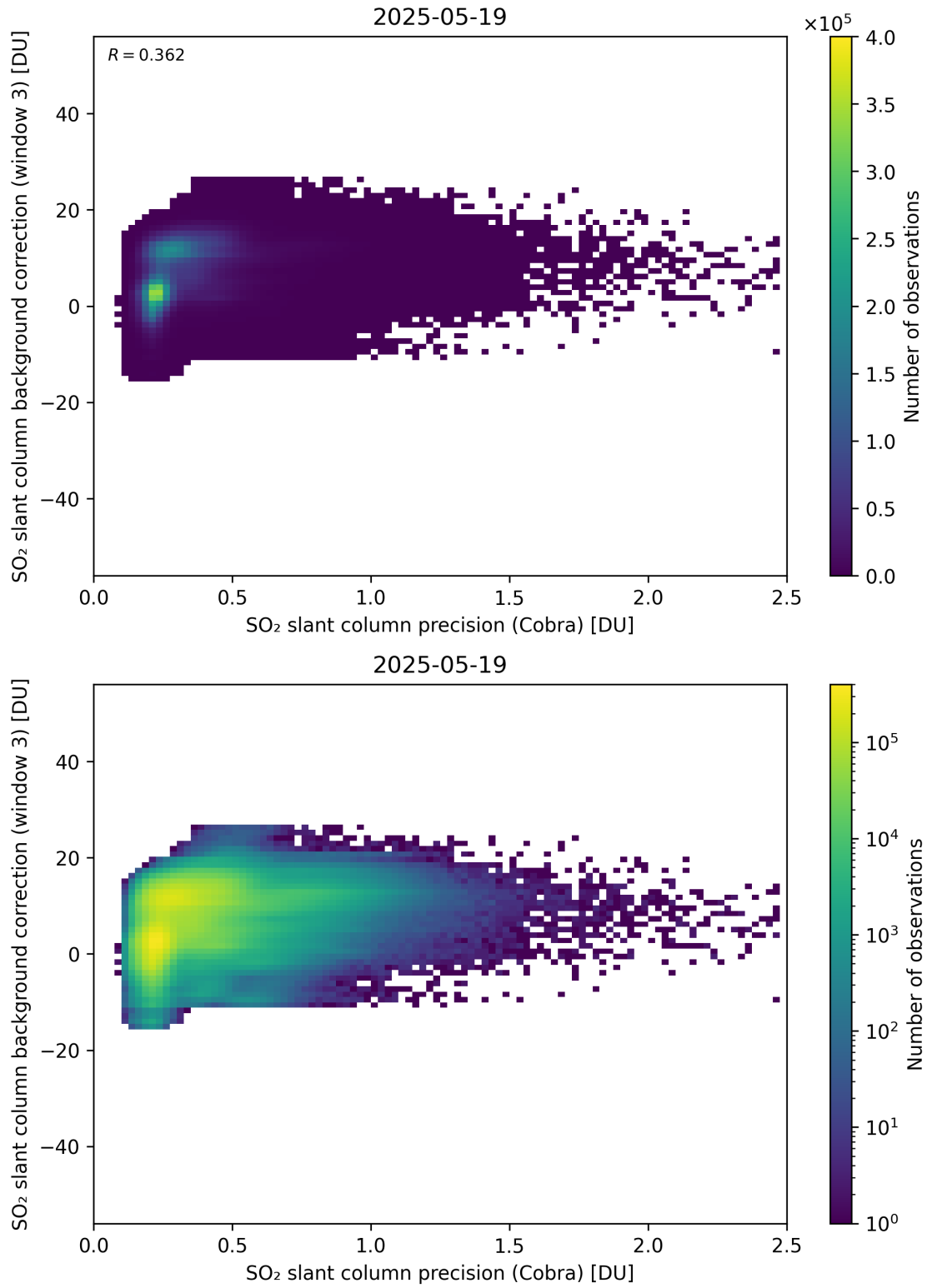
Figure 201: Scatter density plot of “SO 2 slant column precision (Cobra)” against “SO 2 slant column background correction (window 3)” for 2025-05-18 to 2025-05-20.
