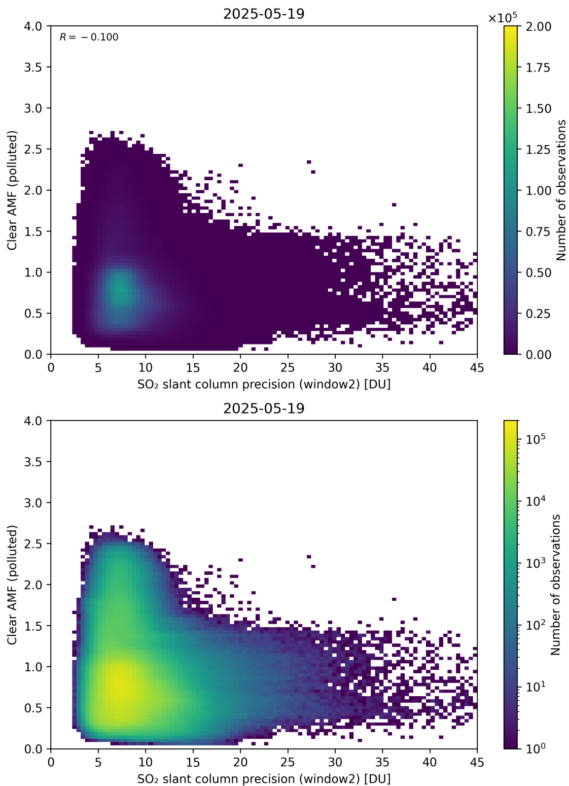
Figure 296: Scatter density plot of “SO 2 slant column precision (window2)” against “Clear AMF (polluted)” for 2025-05-18 to 2025-05-20.
