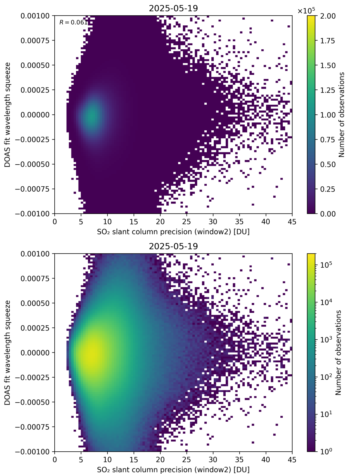
Figure 294: Scatter density plot of “SO 2 slant column precision (window2)” against “DOAS fit wavelength squeeze” for 2025-05-18 to 2025-05-20.
