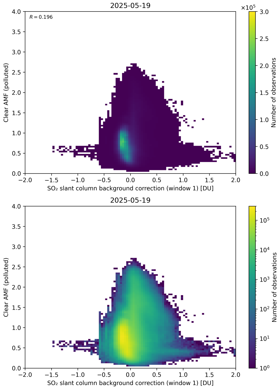
Figure 114: Scatter density plot of “SO 2 slant column background correction (window 1)” against “Clear AMF (polluted)” for 2025-05-18 to 2025-05-20.
