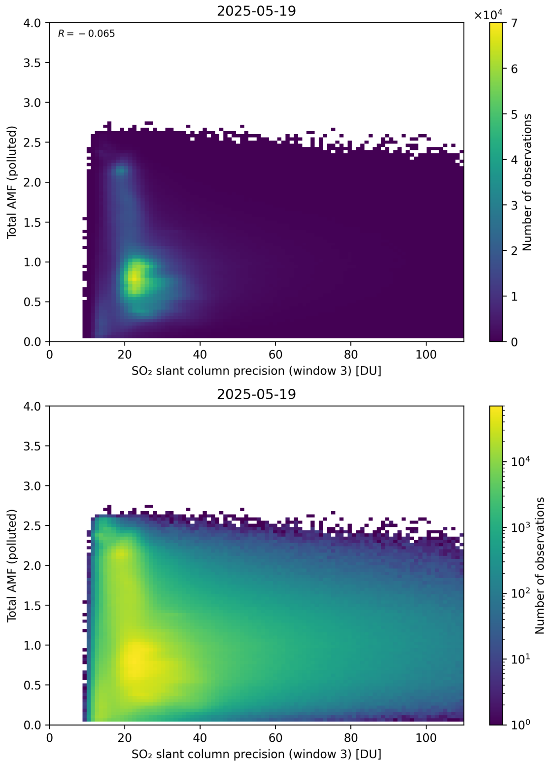
Figure 313: Scatter density plot of “SO 2 slant column precision (window 3)” against “Total AMF (polluted)” for 2025-05-18 to 2025-05-20.
