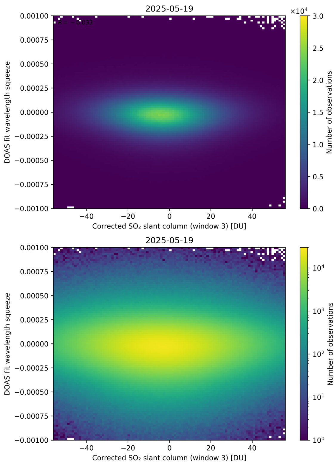
Figure 257: Scatter density plot of “Corrected SO 2 slant column (window 3)” against “DOAS fit wavelength squeeze” for 2025-05-18 to 2025-05-20.
