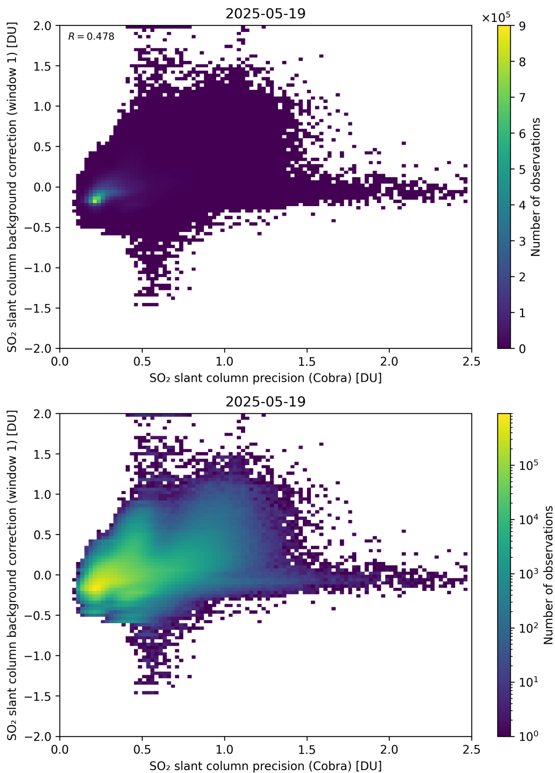
Figure 199: Scatter density plot of “SO 2 slant column precision (Cobra)” against “SO 2 slant column background correction (window 1)” for 2025-05-18 to 2025-05-20.
