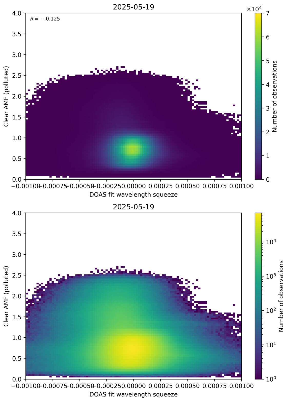
Figure 144: Scatter density plot of “DOAS fit wavelength squeeze” against “Clear AMF (polluted)” for 2025-05-18 to 2025-05-20.
