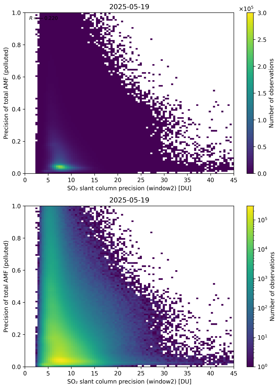
Figure 302: Scatter density plot of “SO 2 slant column precision (window2)” against “Precision of total AMF (polluted)” for 2025-05-18 to 2025-05-20.
