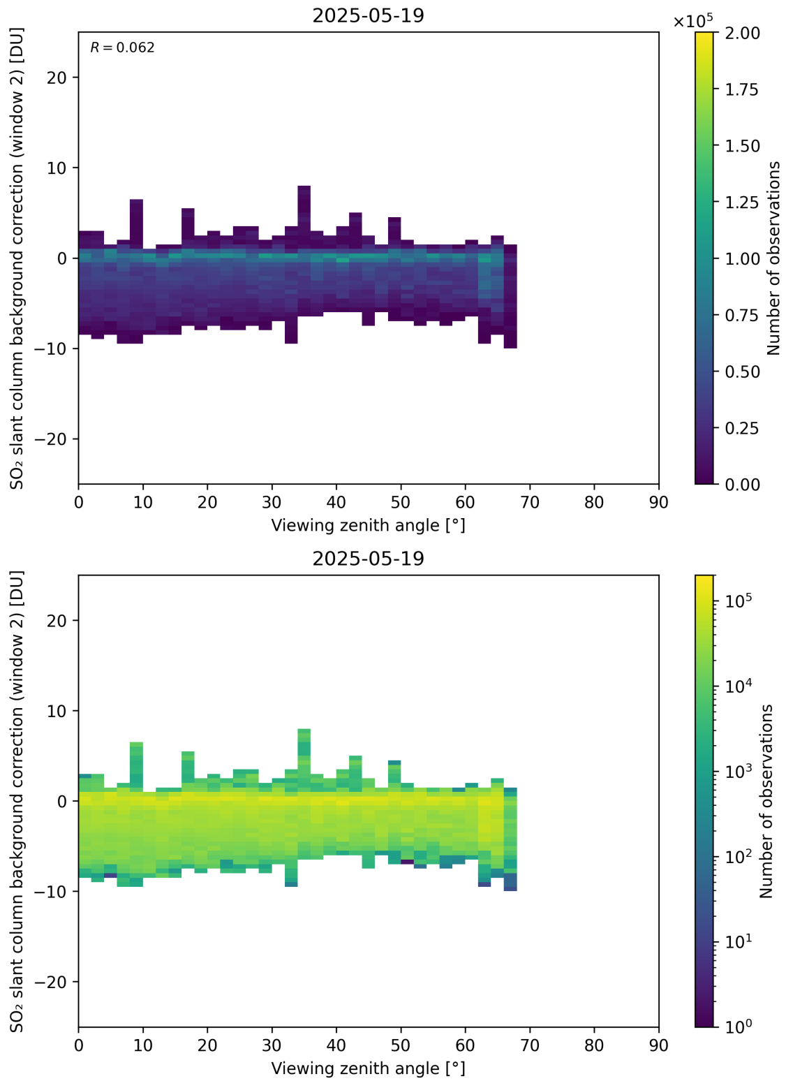
Figure 363: Scatter density plot of “Viewing zenith angle” against “SO 2 slant column background correction (window 2)” for 2025-05-18 to 2025-05-20.
