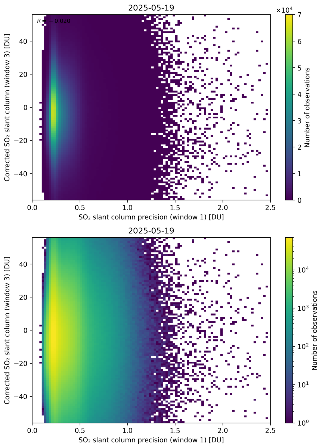
Figure 276: Scatter density plot of “SO 2 slant column precision (window 1)” against “Corrected SO 2 slant column (window 3)” for 2025-05-18 to 2025-05-20.
