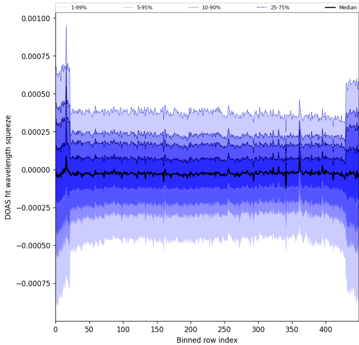
Figure 103: Along track statistics of “DOAS fit wavelength squeeze” for 2025-05-18 to 2025-05-20
