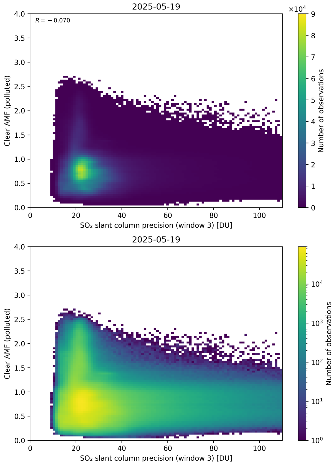
Figure 311: Scatter density plot of “SO 2 slant column precision (window 3)” against “Clear AMF (polluted)” for 2025-05-18 to 2025-05-20.
