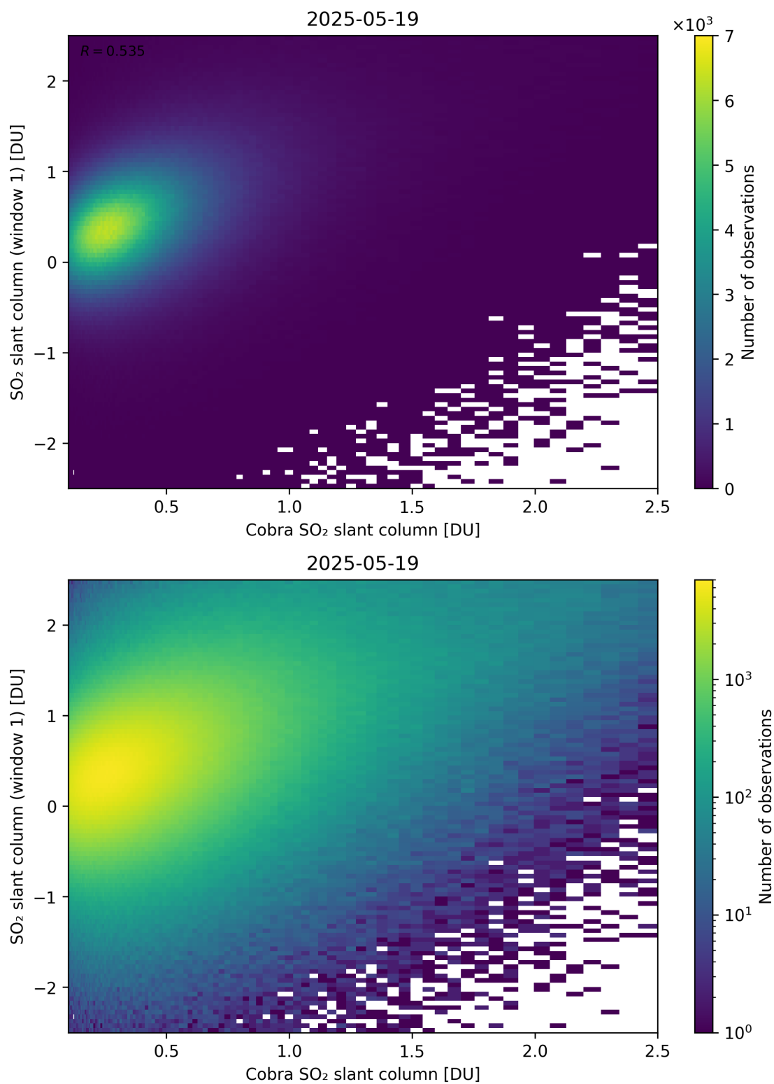
Figure 219: Scatter density plot of “Cobra SO 2 slant column” against “SO 2 slant column (window 1)” for 2025-05-18 to 2025-05-20.
