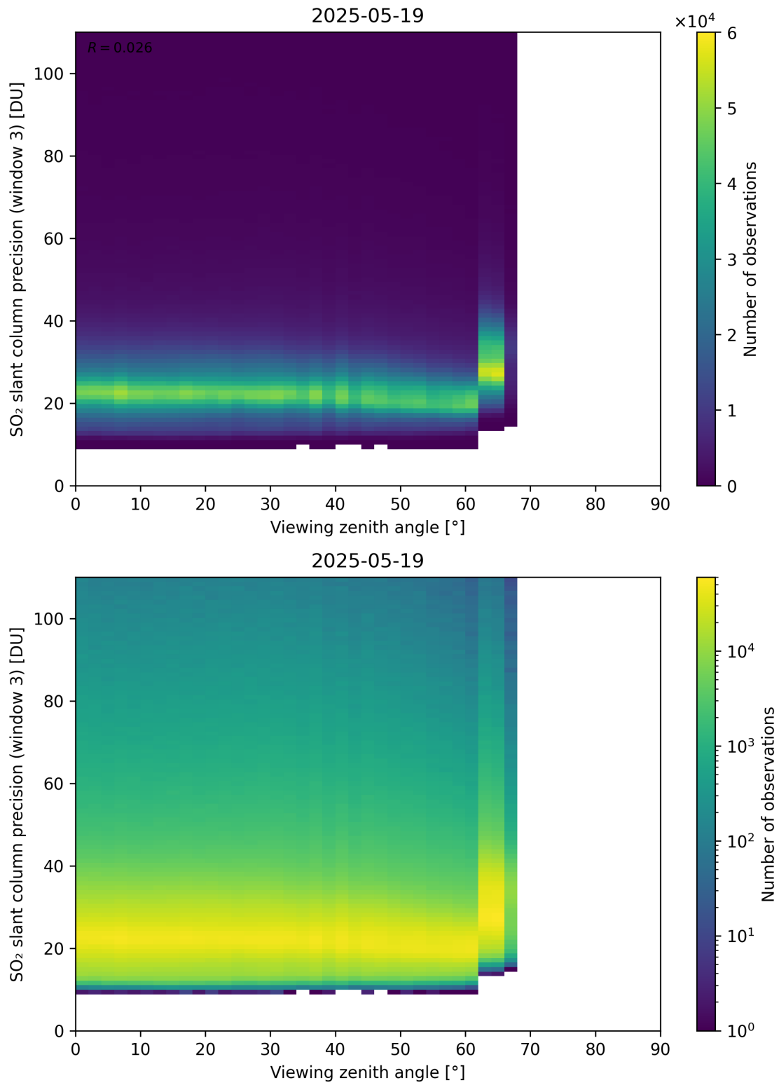
Figure 380: Scatter density plot of “Viewing zenith angle” against “SO 2 slant column precision (window 3)” for 2025-05-18 to 2025-05-20.
