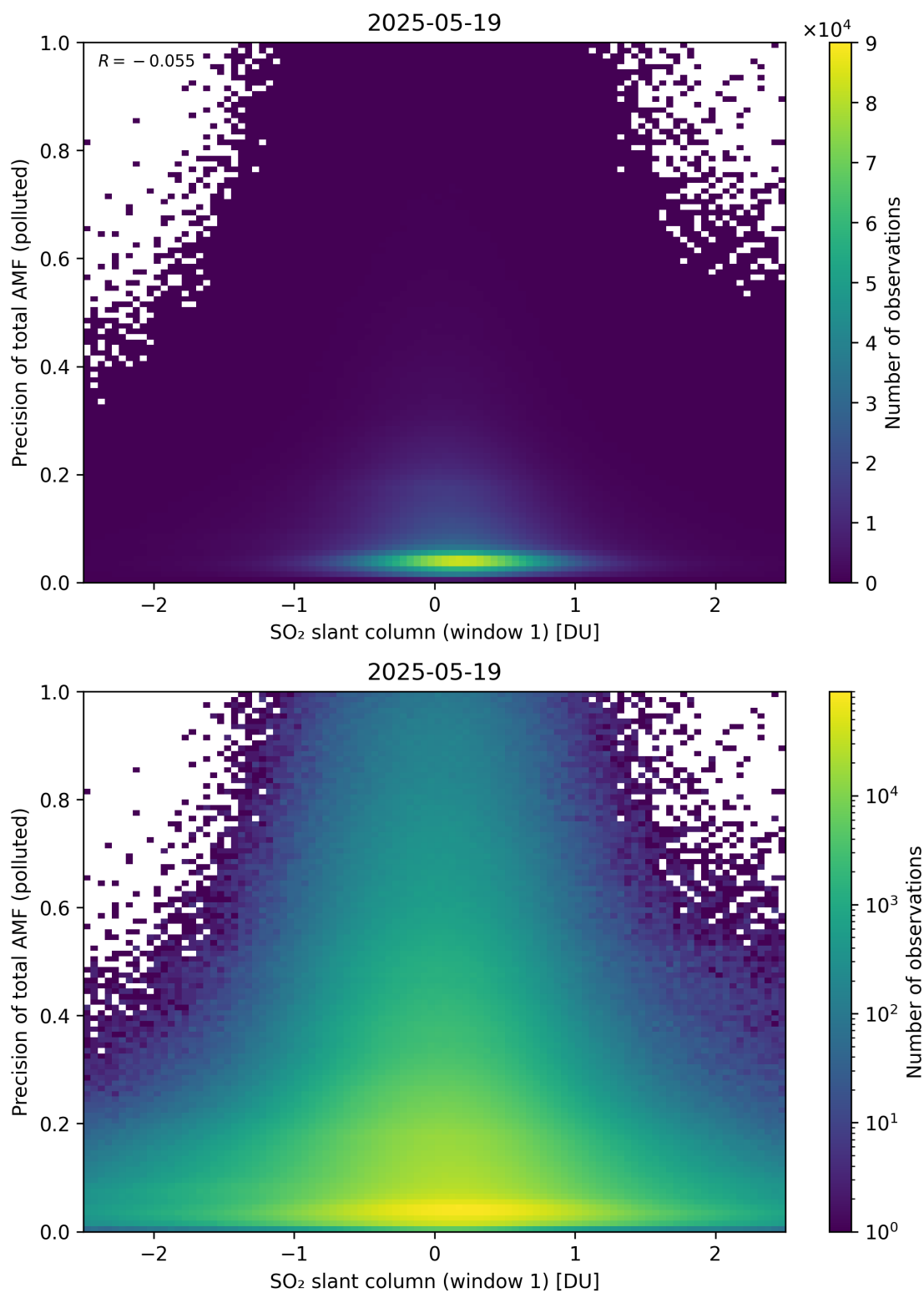
Figure 290: Scatter density plot of “SO 2 slant column (window 1)” against “Precision of total AMF (polluted)” for 2025-05-18 to 2025-05-20.
