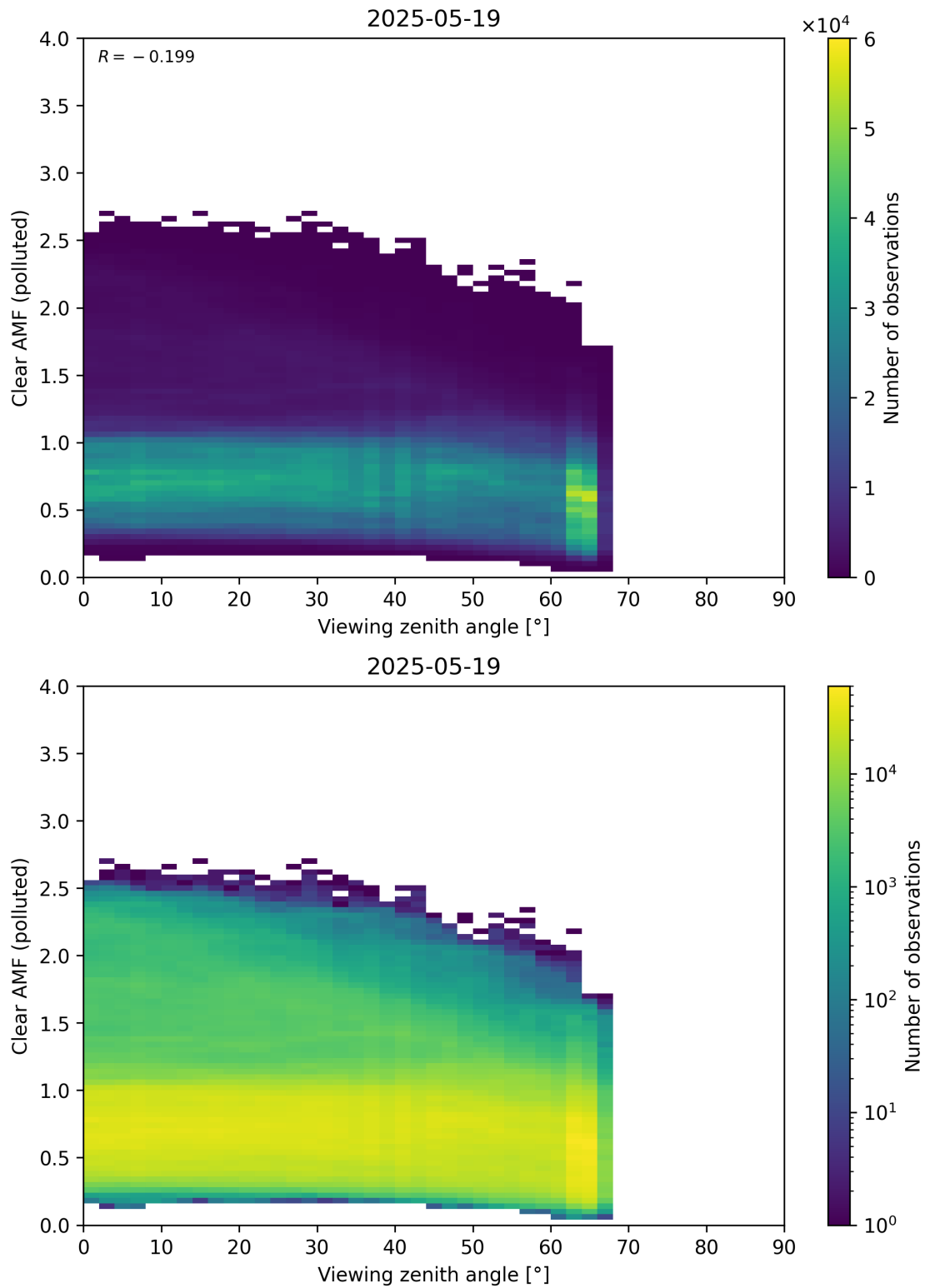
Figure 370: Scatter density plot of “Viewing zenith angle” against “Clear AMF (polluted)” for 2025-05-18 to 2025-05-20.
