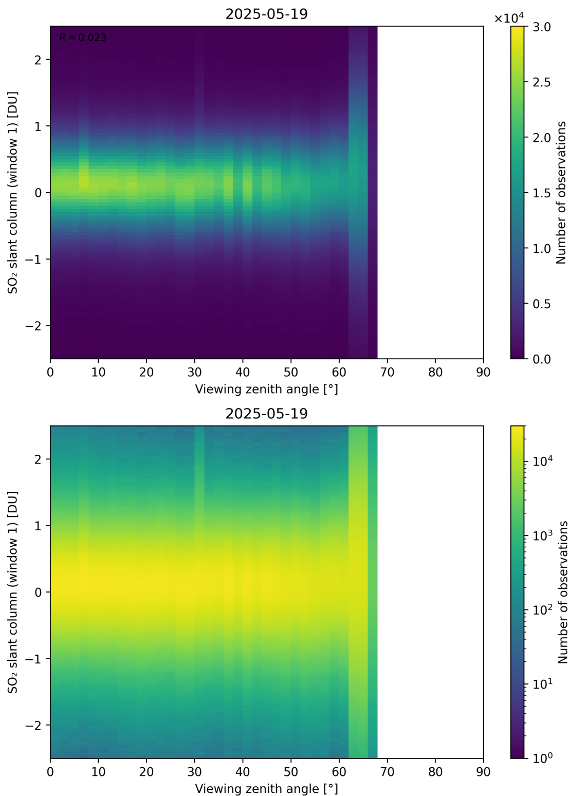
Figure 376: Scatter density plot of “Viewing zenith angle” against “SO 2 slant column (window 1)” for 2025-05-18 to 2025-05-20.
