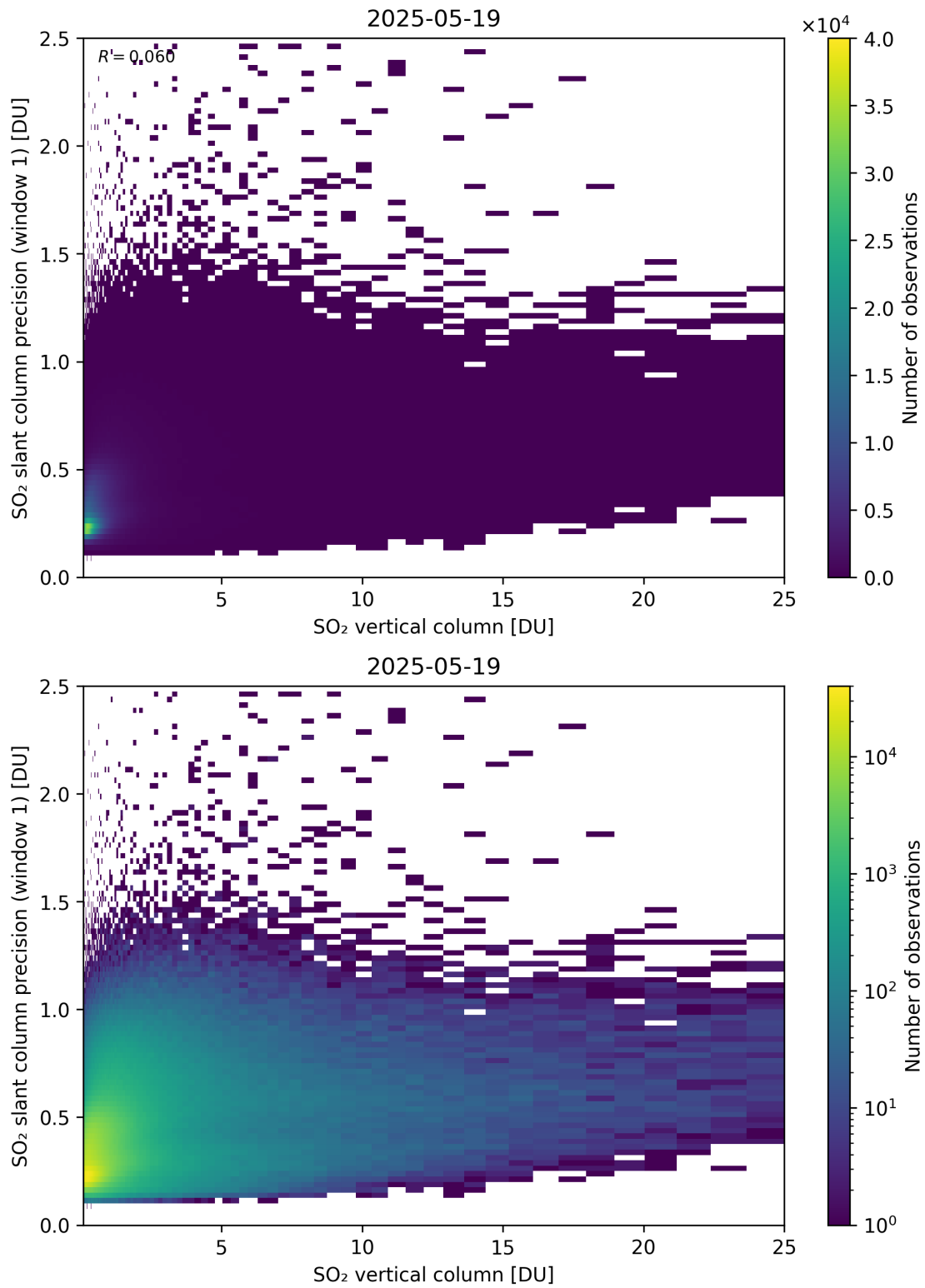
Figure 355: Scatter density plot of “SO 2 vertical column” against “SO 2 slant column precision (window 1)” for 2025-05-18 to 2025-05-20.
