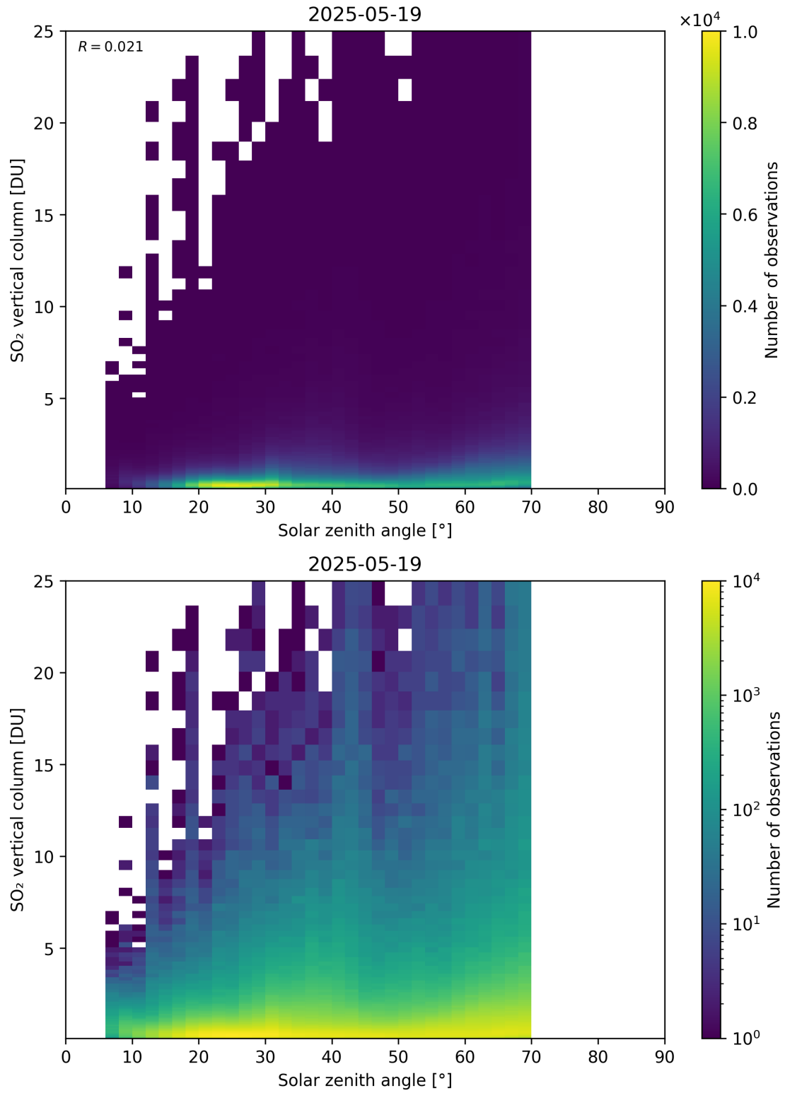
Figure 191: Scatter density plot of “Solar zenith angle” against “SO 2 vertical column” for 2025-05-18 to 2025-05-20.
