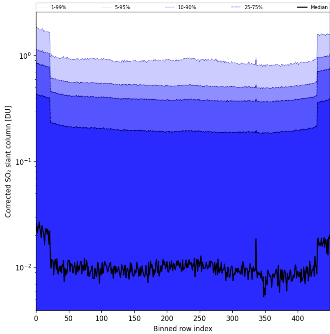
Figure 86: Along track statistics of “Corrected SO 2 slant column” for 2025-05-18 to 2025-05-20
