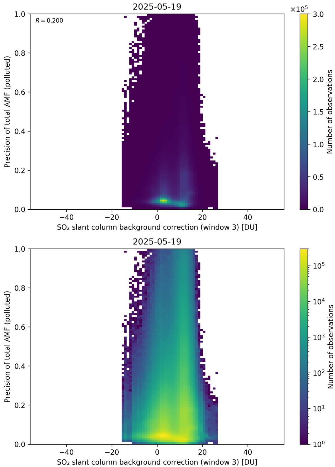
Figure 137: Scatter density plot of “SO 2 slant column background correction (window 3)” against “Precision of total AMF (polluted)” for 2025-05-18 to 2025-05-20.
