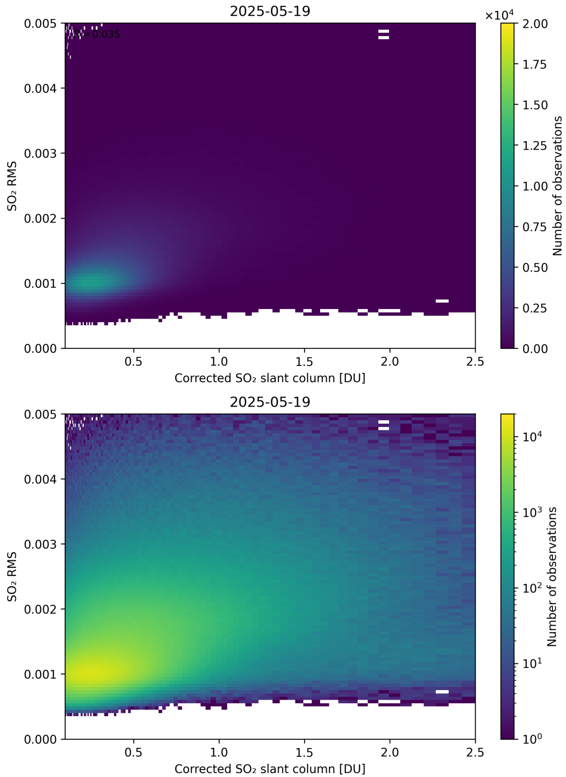
Figure 231: Scatter density plot of “Corrected SO 2 slant column” against “SO 2 RMS” for 2025-05-18 to 2025-05-20.
