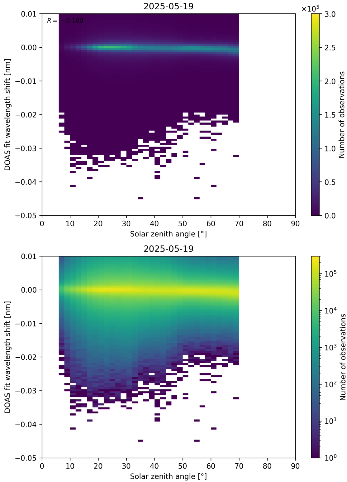
Figure 174: Scatter density plot of “Solar zenith angle” against “DOAS fit wavelength shift” for 2025-05-18 to 2025-05-20.
