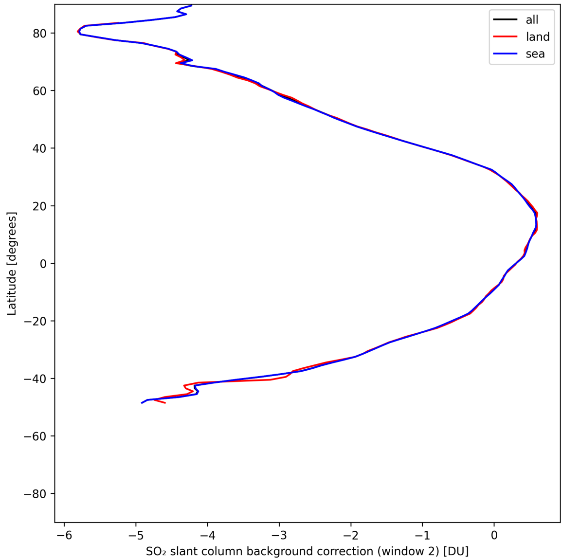
Figure 44: Zonal average of “SO 2 slant column background correction (window 2)” for 2025-05-18 to 2025-05-20.
