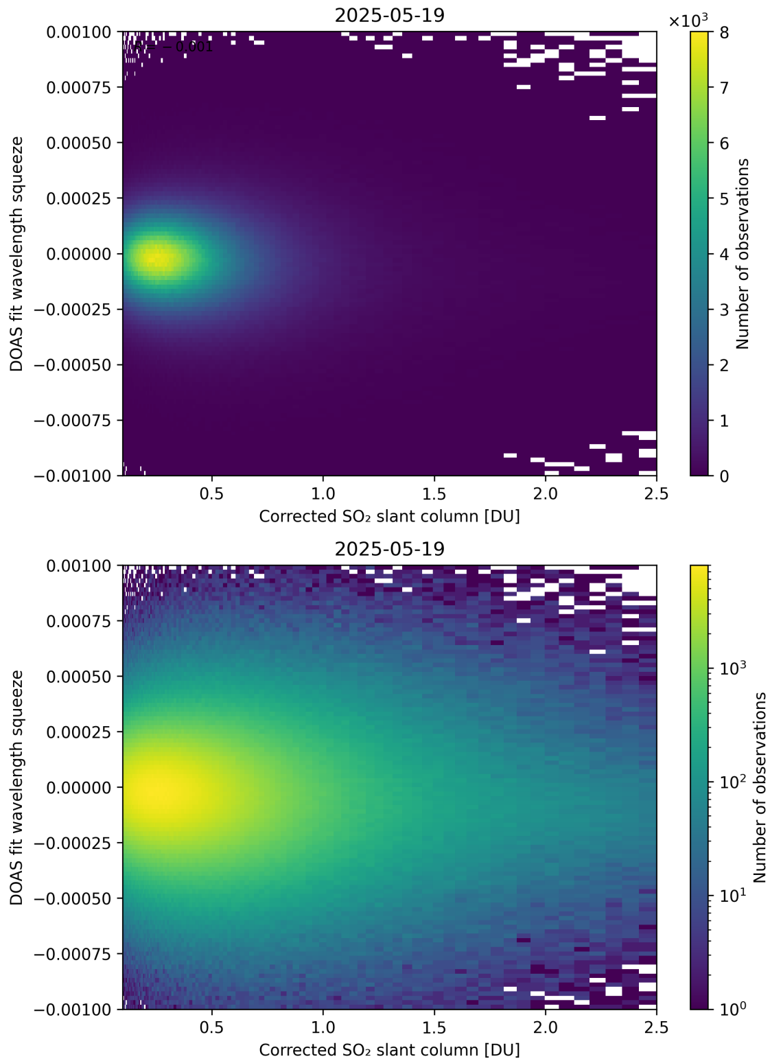
Figure 230: Scatter density plot of “Corrected SO 2 slant column” against “DOAS fit wavelength squeeze” for 2025-05-18 to 2025-05-20.
