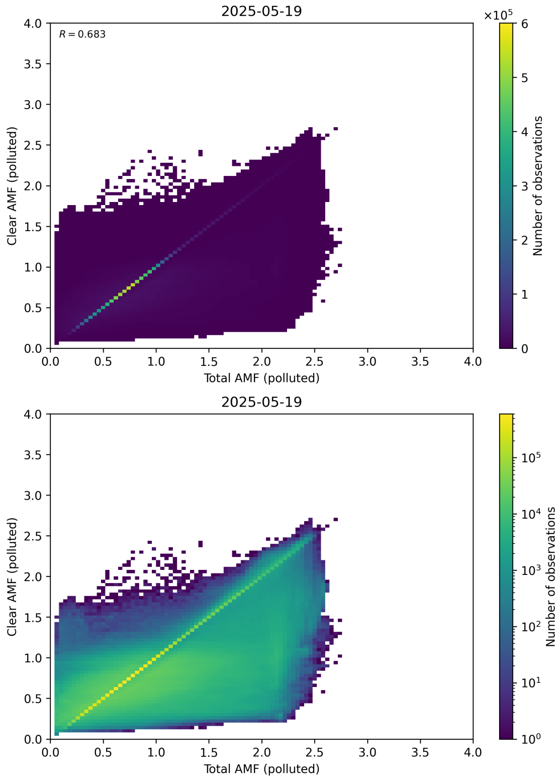
Figure 321: Scatter density plot of “Total AMF (polluted)” against “Clear AMF (polluted)” for 2025-05-18 to 2025-05-20.
