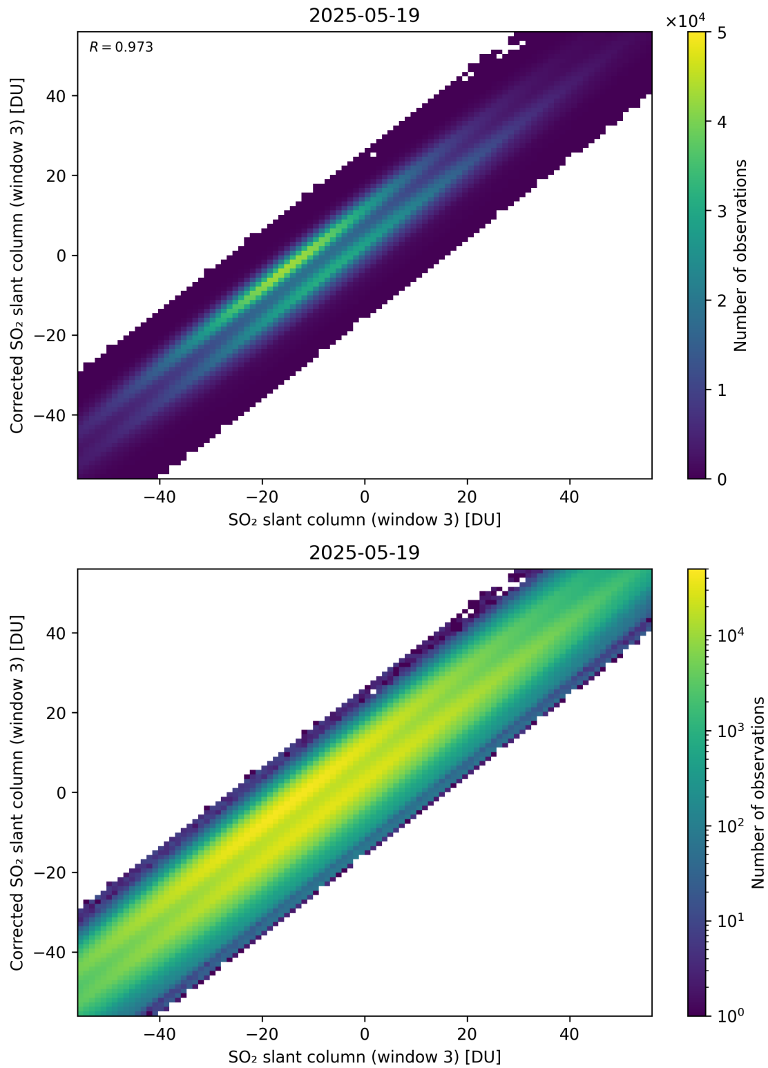
Figure 316: Scatter density plot of “SO 2 slant column (window 3)” against “Corrected SO 2 slant column (window 3)” for 2025-05-18 to 2025-05-20.
