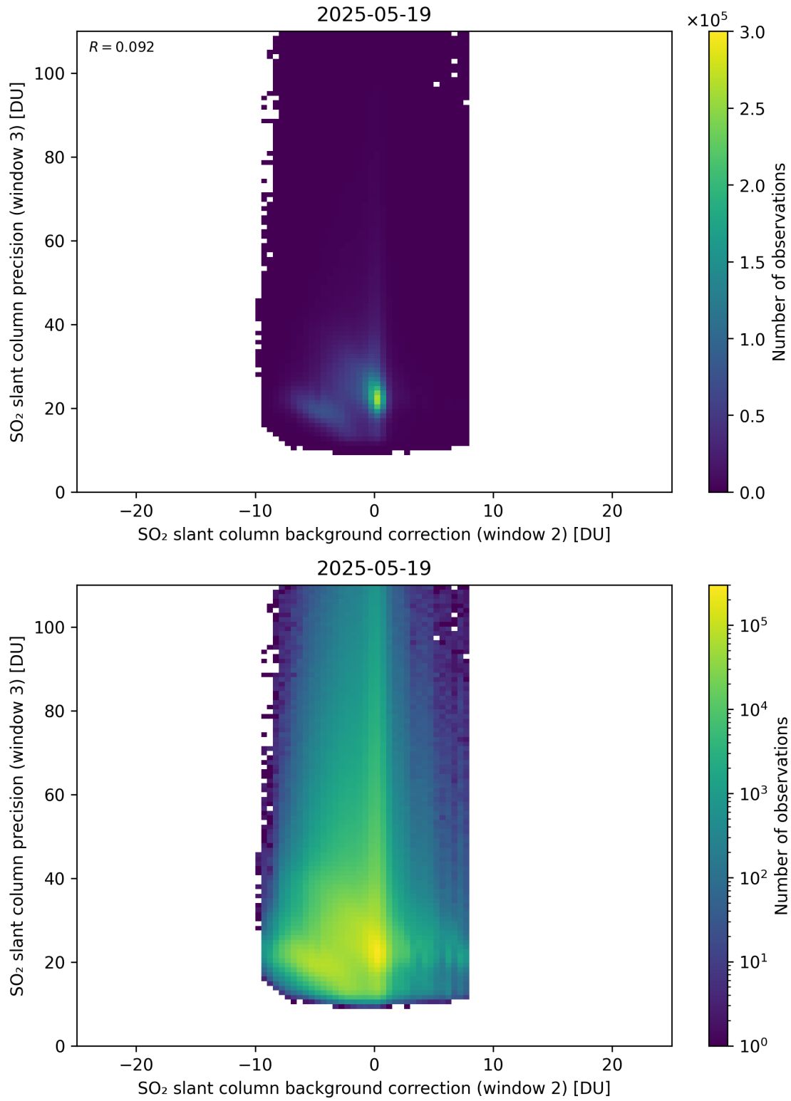
Figure 129: Scatter density plot of “SO 2 slant column background correction (window 2)” against “SO 2 slant column precision (window 3)” for 2025-05-18 to 2025-05-20.
