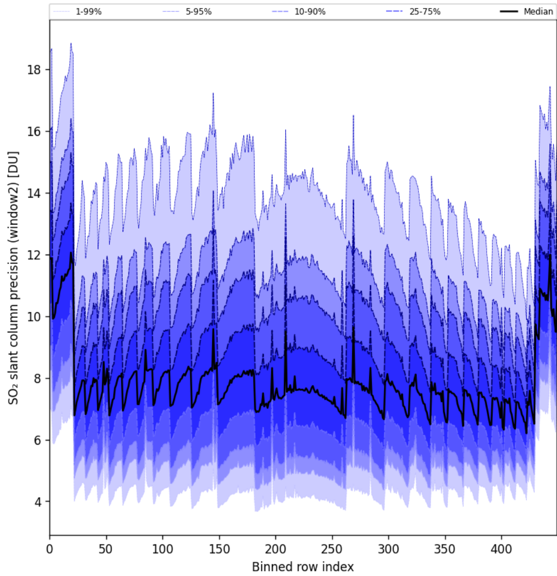
Figure 94: Along track statistics of “SO 2 slant column precision (window2)” for 2025-05-18 to 2025-05-20
