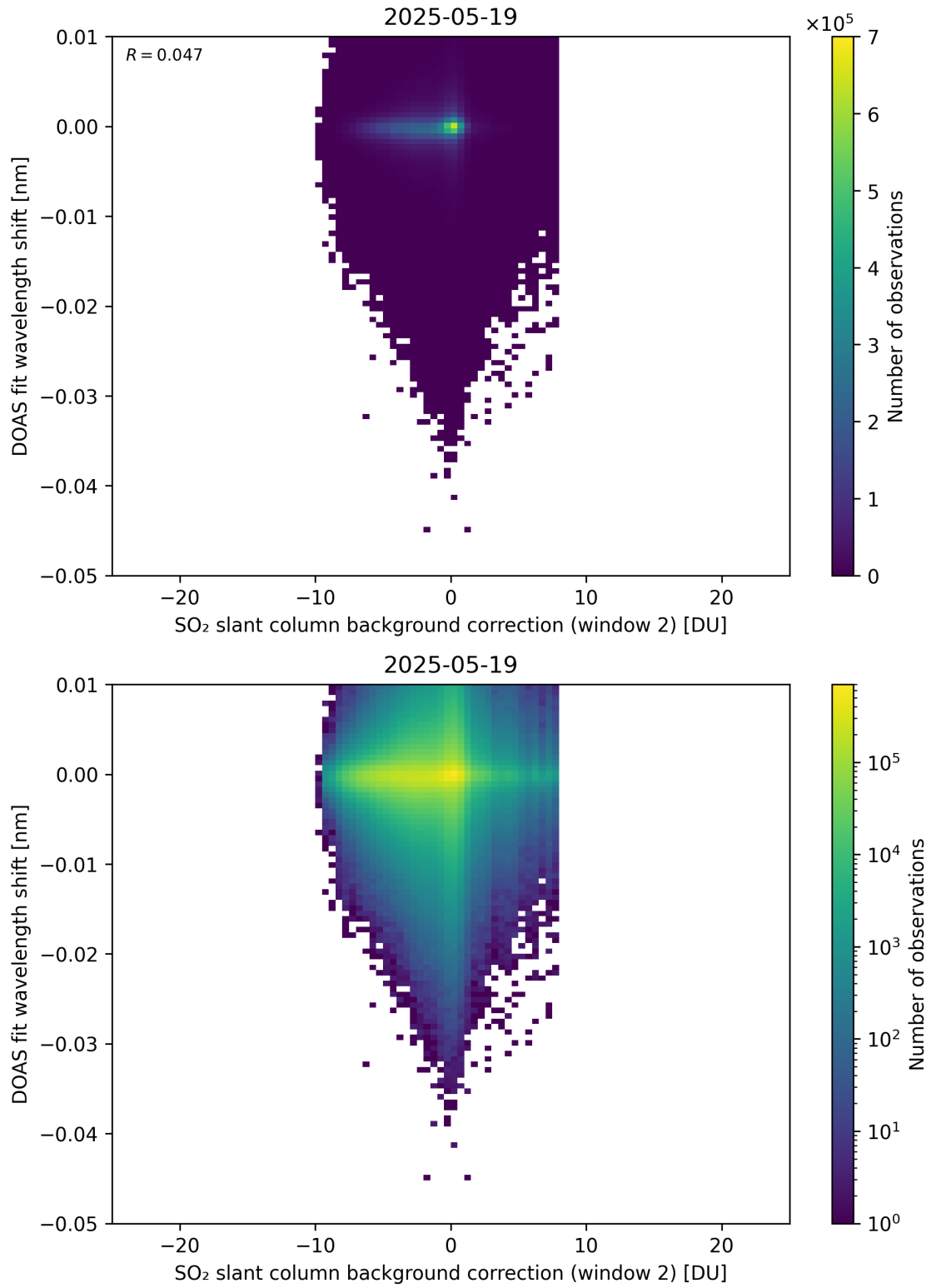
Figure 123: Scatter density plot of “SO 2 slant column background correction (window 2)” against “DOAS fit wavelength shift” for 2025-05-18 to 2025-05-20.
