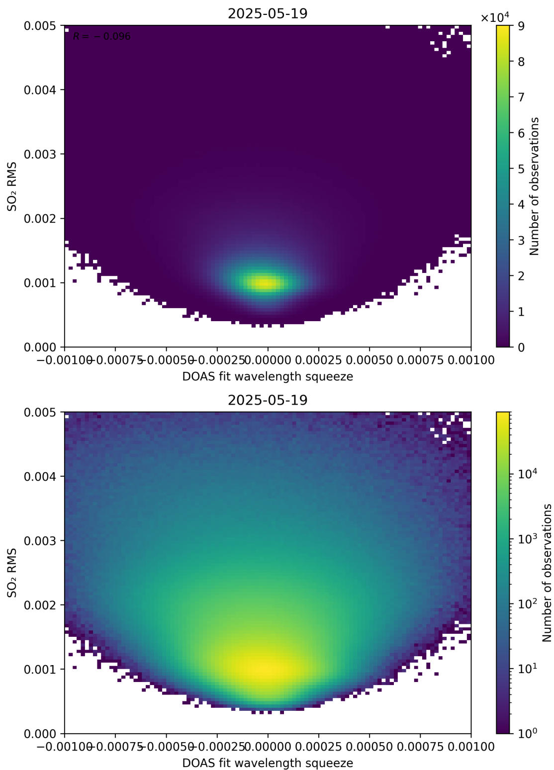
Figure 143: Scatter density plot of “DOAS fit wavelength squeeze” against “SO 2 RMS” for 2025-05-18 to 2025-05-20.
