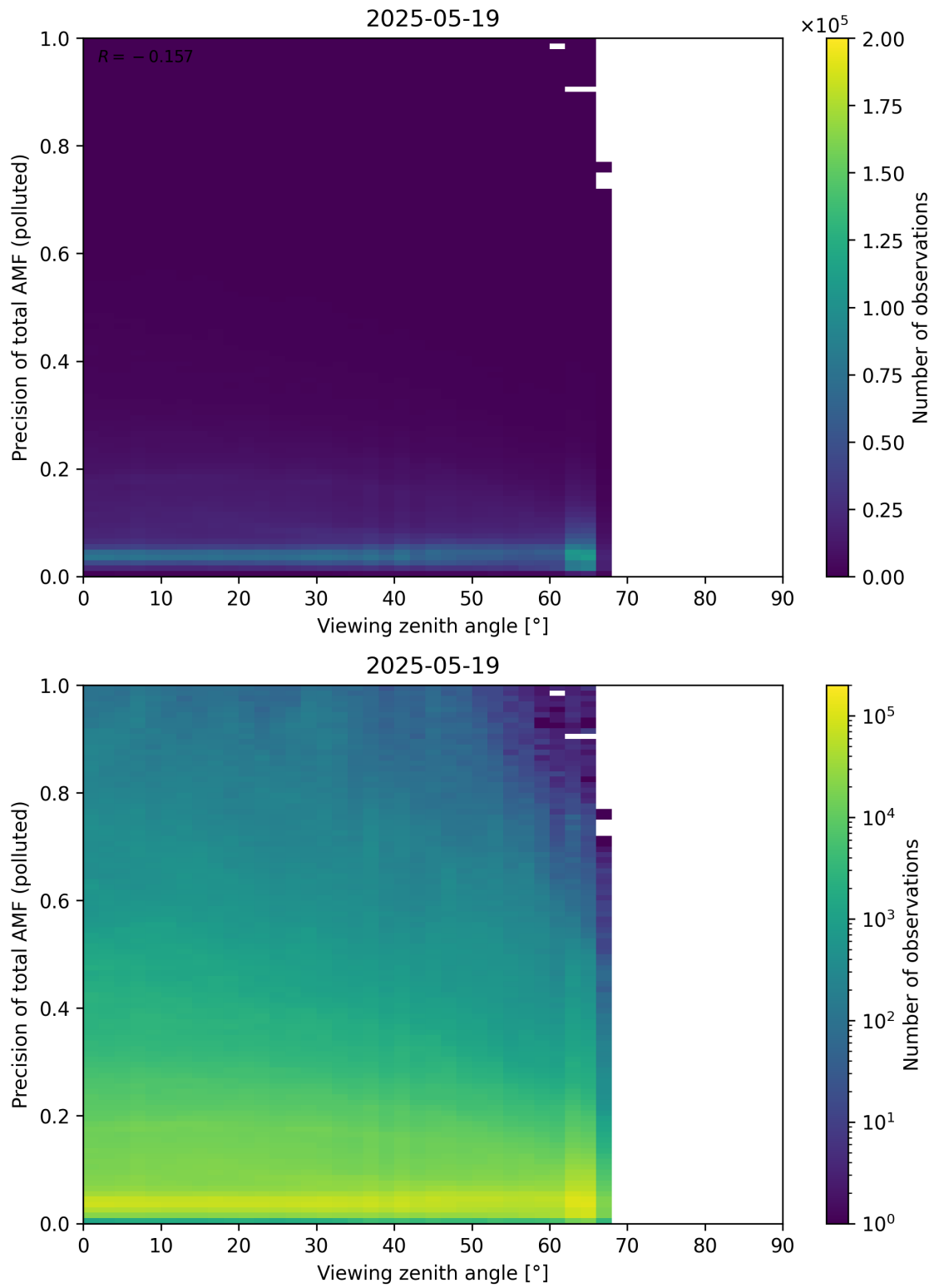
Figure 382: Scatter density plot of “Viewing zenith angle” against “Precision of total AMF (polluted)” for 2025-05-18 to 2025-05-20.
