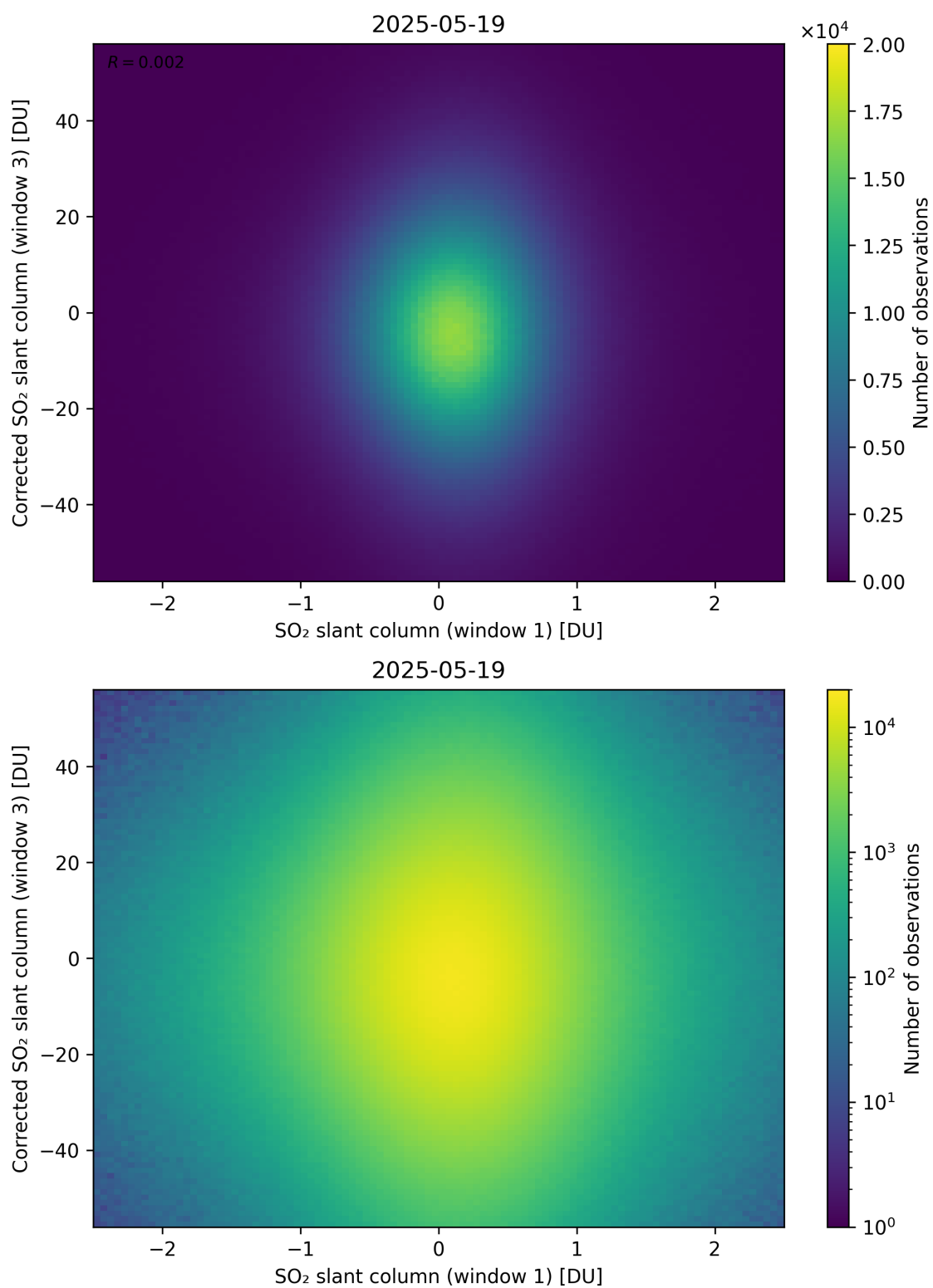
Figure 284: Scatter density plot of “SO 2 slant column (window 1)” against “Corrected SO 2 slant column (window 3)” for 2025-05-18 to 2025-05-20.
