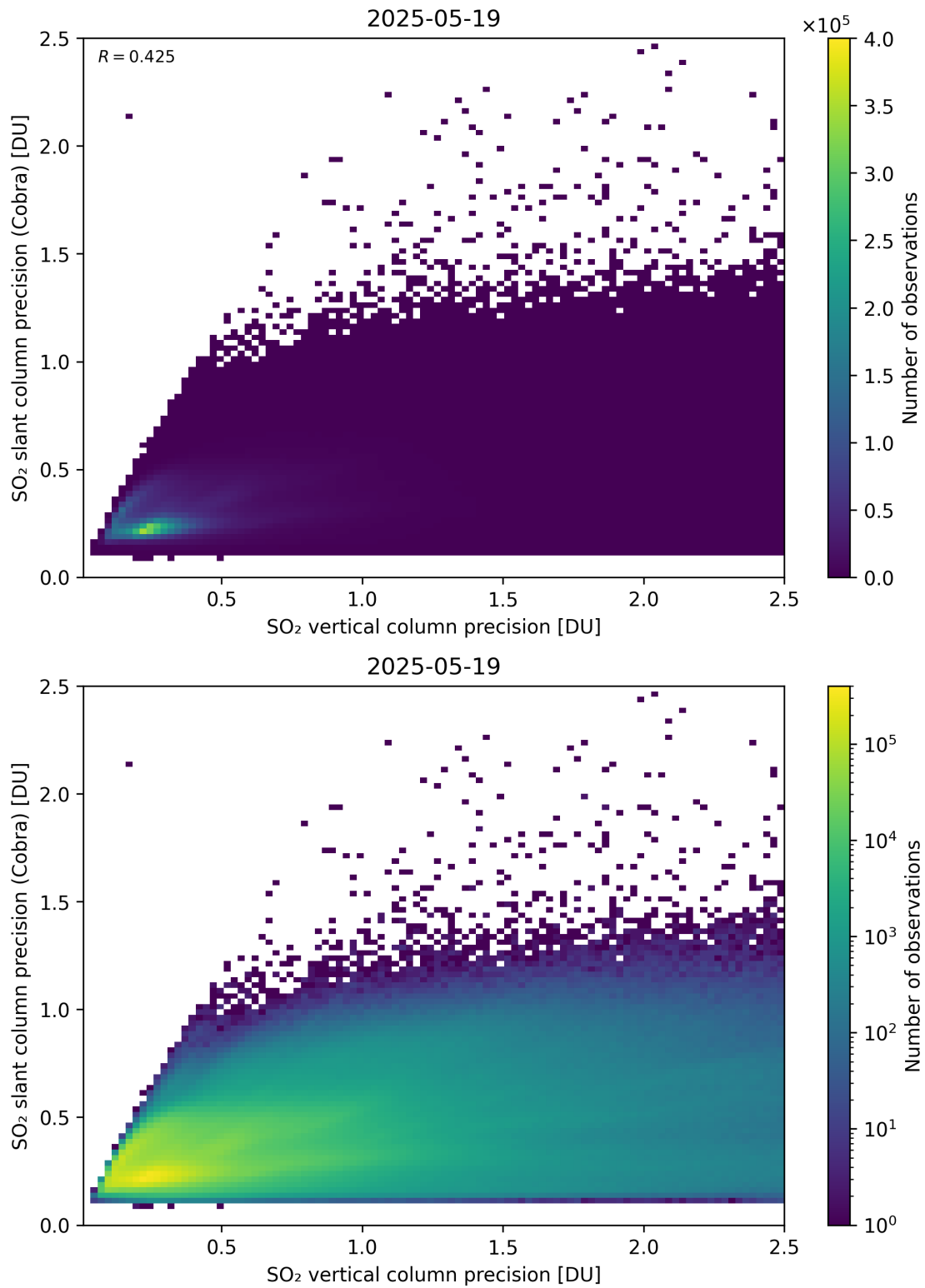
Figure 337: Scatter density plot of “SO 2 vertical column precision” against “SO 2 slant column precision (Cobra)” for 2025-05-18 to 2025-05-20.
