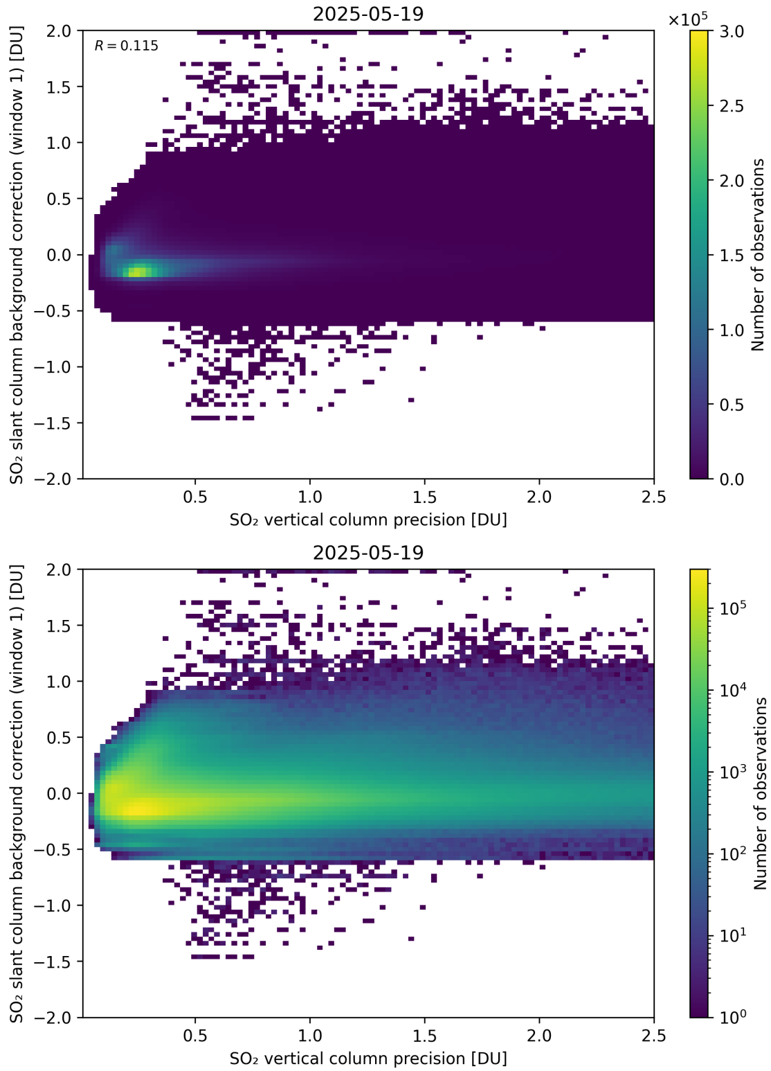
Figure 329: Scatter density plot of “SO 2 vertical column precision” against “SO 2 slant column background correction (window 1)” for 2025-05-18 to 2025-05-20.
