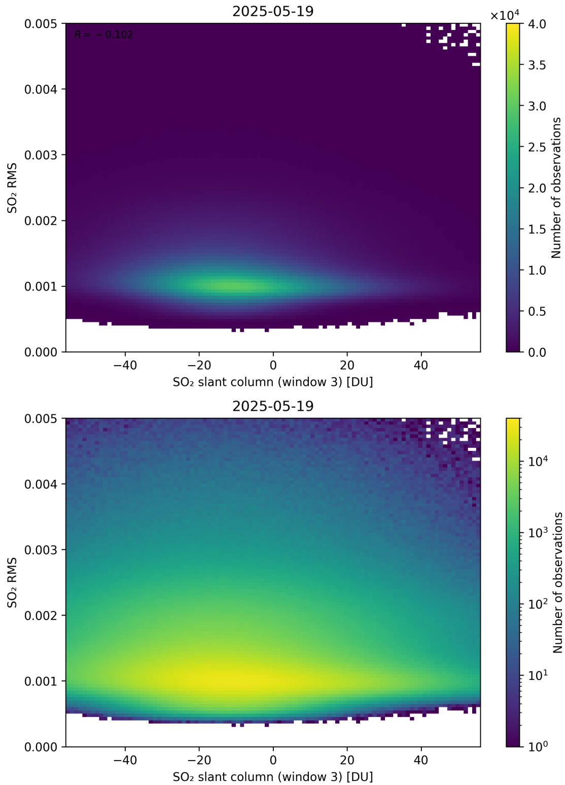
Figure 306: Scatter density plot of “SO 2 slant column (window 3)” against “SO 2 RMS” for 2025-05-18 to 2025-05-20.
