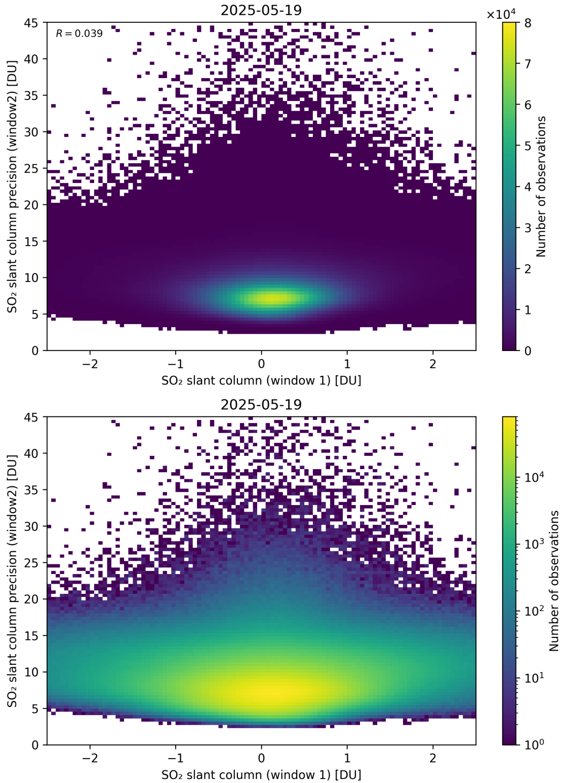
Figure 286: Scatter density plot of “SO 2 slant column (window 1)” against “SO 2 slant column precision (window2)” for 2025-05-18 to 2025-05-20.
