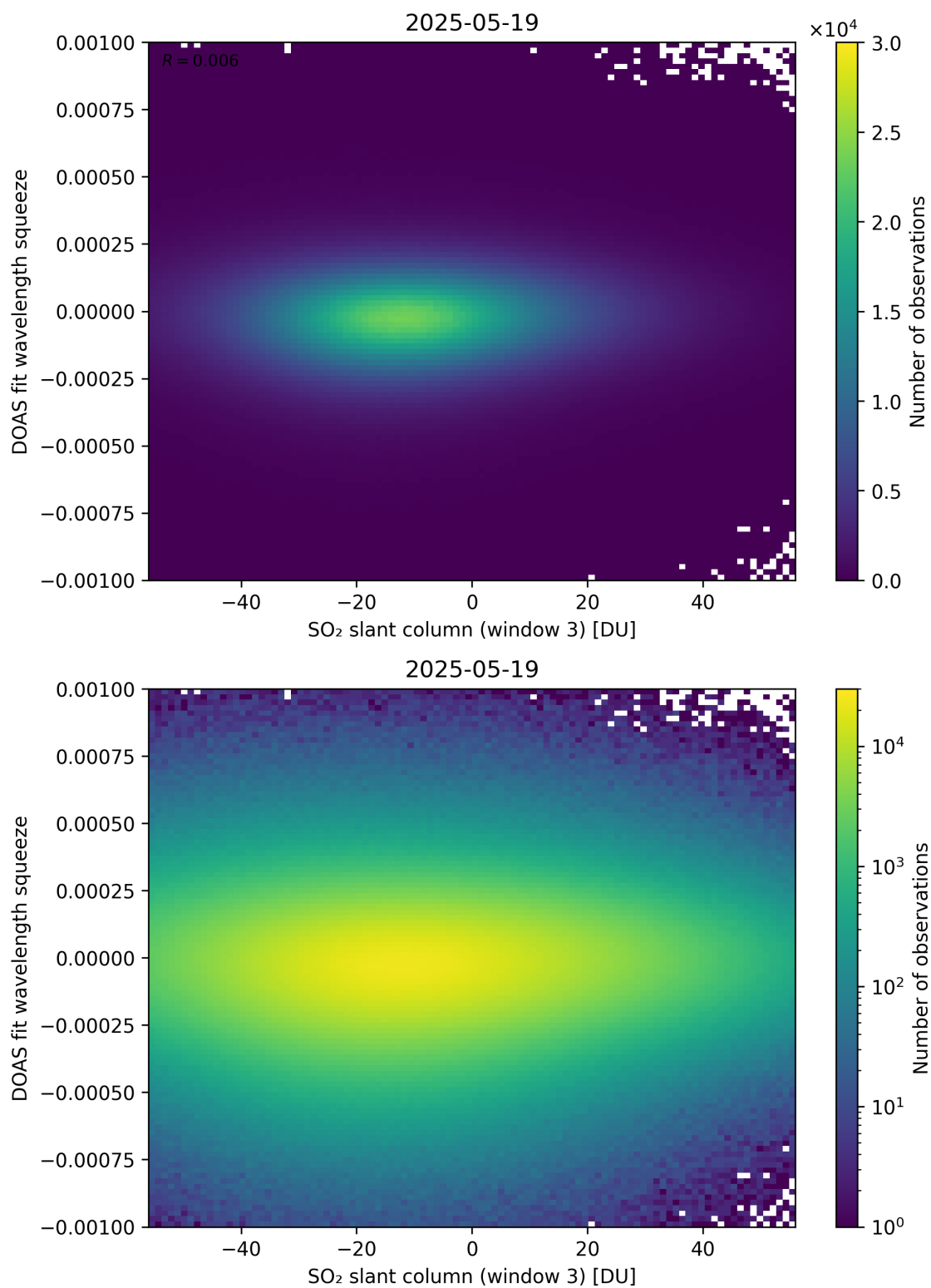
Figure 305: Scatter density plot of “SO 2 slant column (window 3)” against “DOAS fit wavelength squeeze” for 2025-05-18 to 2025-05-20.
