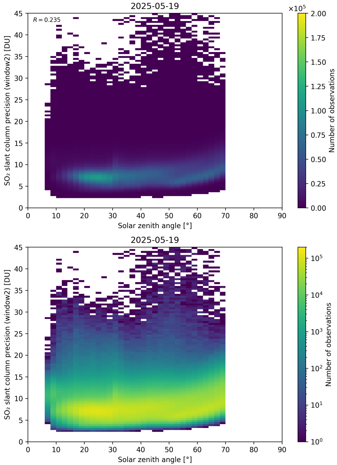
Figure 186: Scatter density plot of “Solar zenith angle” against “SO 2 slant column precision (window2)” for 2025-05-18 to 2025-05-20.
