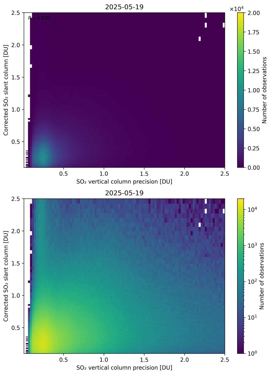
Figure 338: Scatter density plot of “SO 2 vertical column precision” against “Corrected SO 2 slant column” for 2025-05-18 to 2025-05-20.
