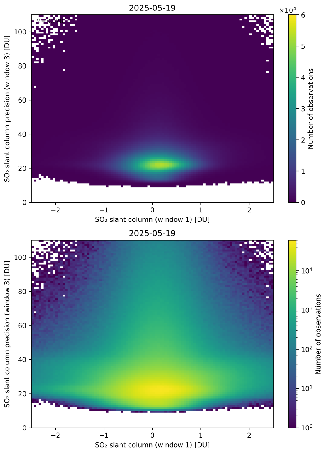
Figure 288: Scatter density plot of “SO 2 slant column (window 1)” against “SO 2 slant column precision (window 3)” for 2025-05-18 to 2025-05-20.
