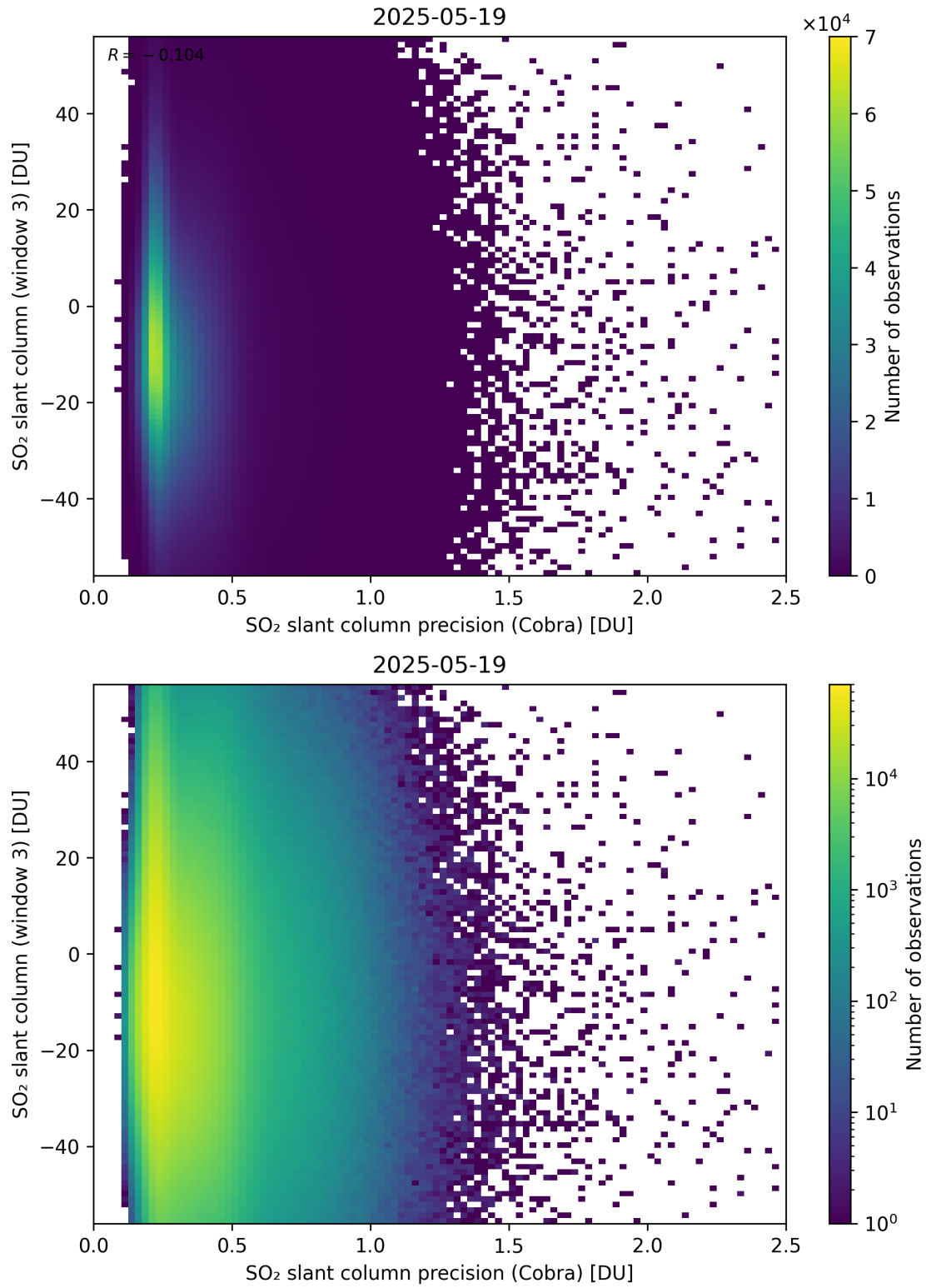
Figure 211: Scatter density plot of “SO 2 slant column precision (Cobra)” against “SO 2 slant column (window 3)” for 2025-05-18 to 2025-05-20.
