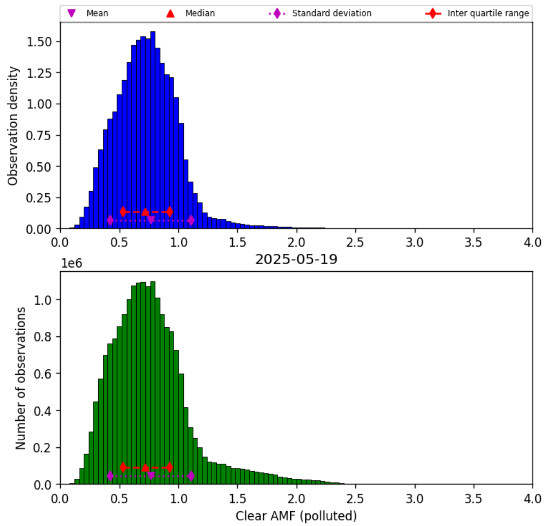
Figure 81: Histogram of “Clear AMF (polluted)” for 2025-05-18 to 2025-05-20
