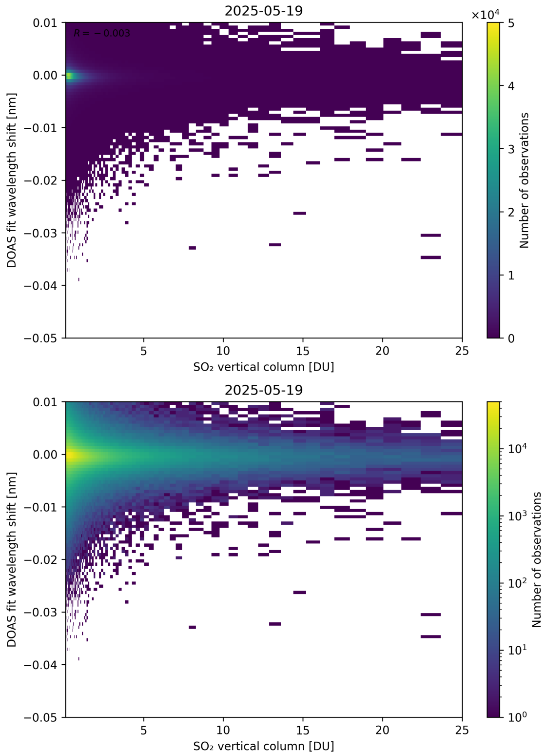
Figure 326: Scatter density plot of “SO 2 vertical column” against “DOAS fit wavelength shift” for 2025-05-18 to 2025-05-20.
