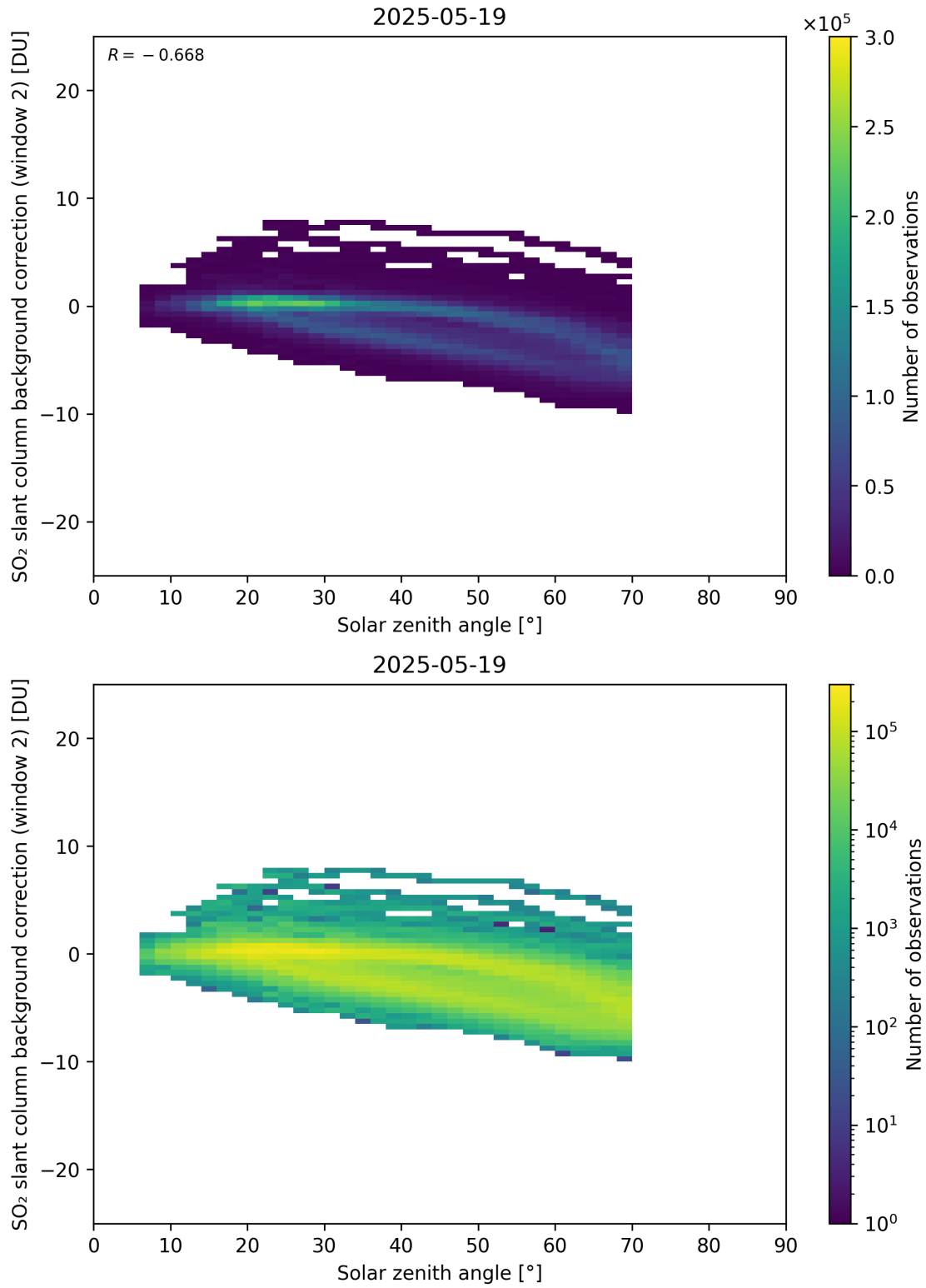
Figure 172: Scatter density plot of “Solar zenith angle” against “SO 2 slant column background correction (window 2)” for 2025-05-18 to 2025-05-20.
