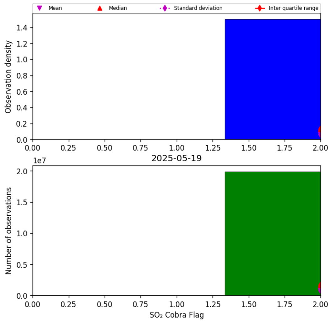
Figure 75: Histogram of “SO 2 Cobra Flag” for 2025-05-18 to 2025-05-20
