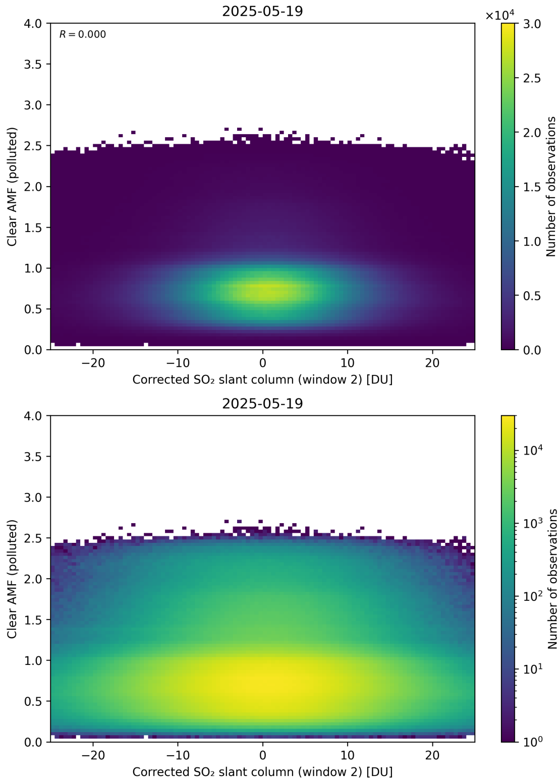
Figure 249: Scatter density plot of “Corrected SO 2 slant column (window 2)” against “Clear AMF (polluted)” for 2025-05-18 to 2025-05-20.
