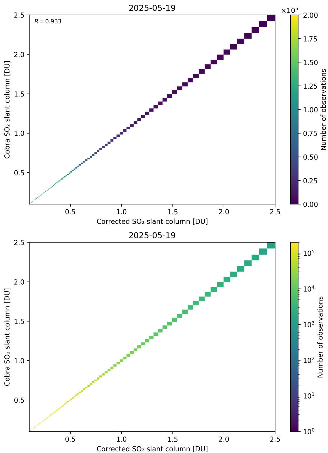
Figure 233: Scatter density plot of “Corrected SO 2 slant column” against “Cobra SO 2 slant column” for 2025-05-18 to 2025-05-20.
