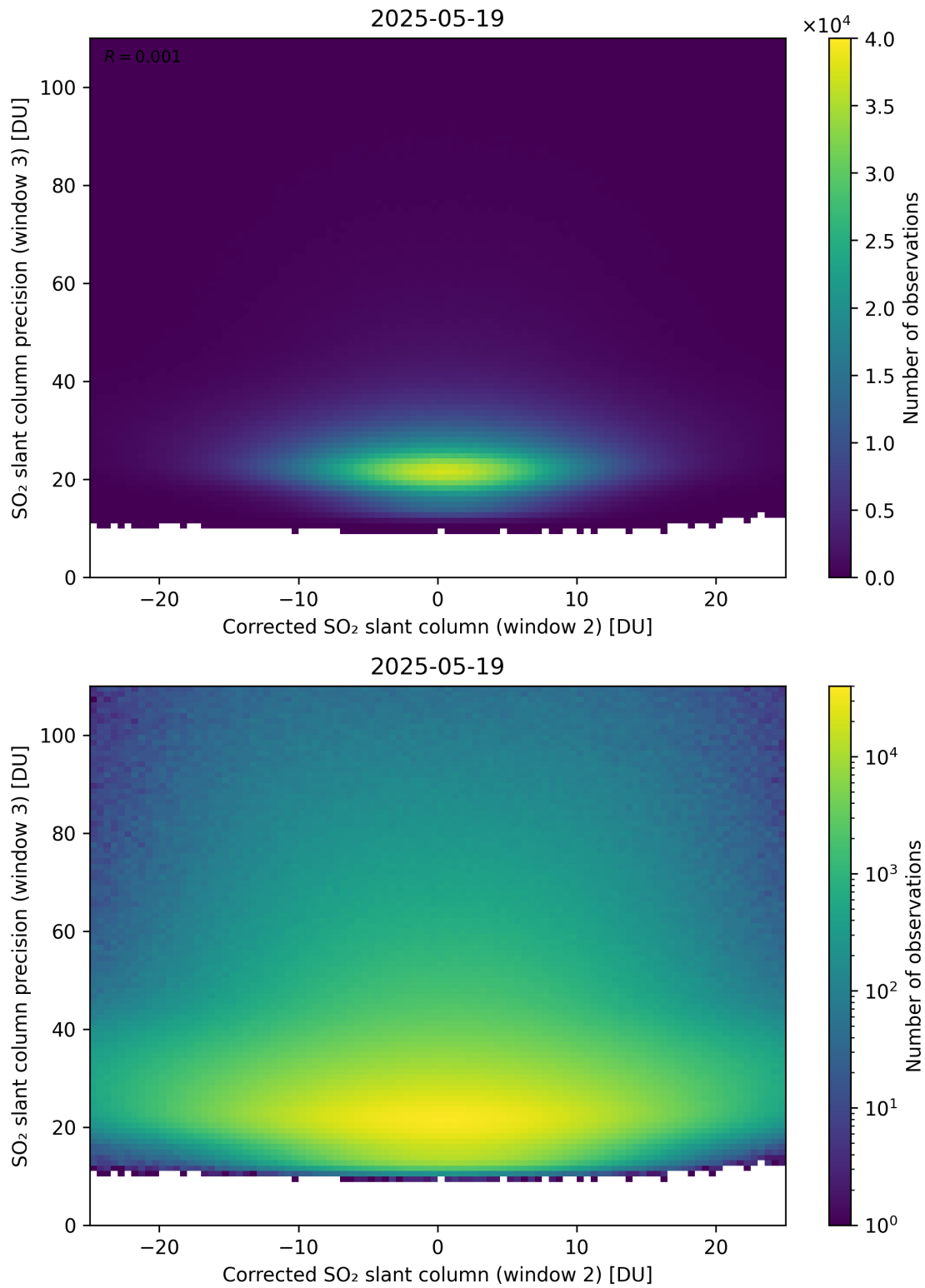
Figure 252: Scatter density plot of “Corrected SO 2 slant column (window 2)” against “SO 2 slant column precision (window 3)” for 2025-05-18 to 2025-05-20.
