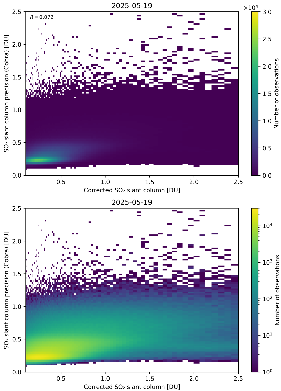
Figure 234: Scatter density plot of “Corrected SO 2 slant column” against “SO 2 slant column precision (Cobra)” for 2025-05-18 to 2025-05-20.
