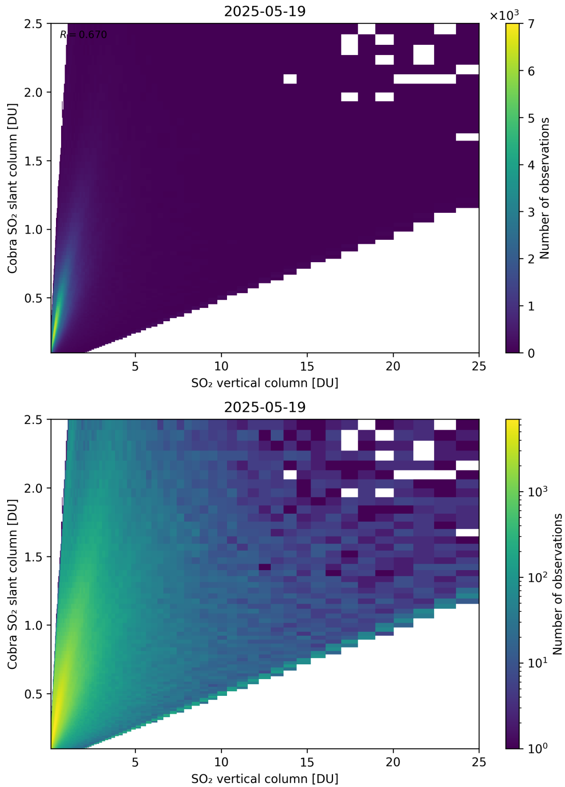
Figure 349: Scatter density plot of “SO 2 vertical column” against “Cobra SO 2 slant column” for 2025-05-18 to 2025-05-20.
