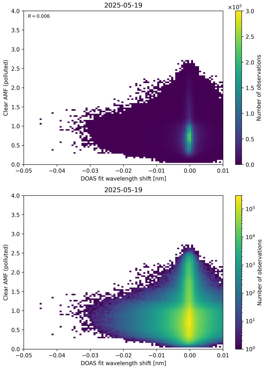
Figure 140: Scatter density plot of “DOAS fit wavelength shift” against “Clear AMF (polluted)” for 2025-05-18 to 2025-05-20.
