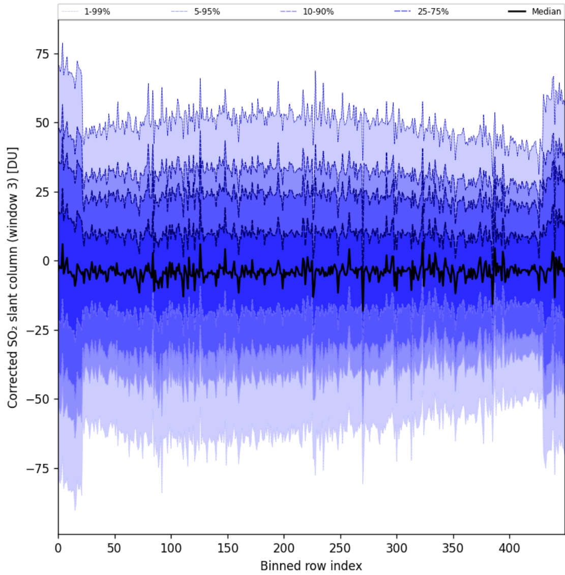
Figure 99: Along track statistics of “Corrected SO 2 slant column (window 3)” for 2025-05-18 to 2025-05-20
