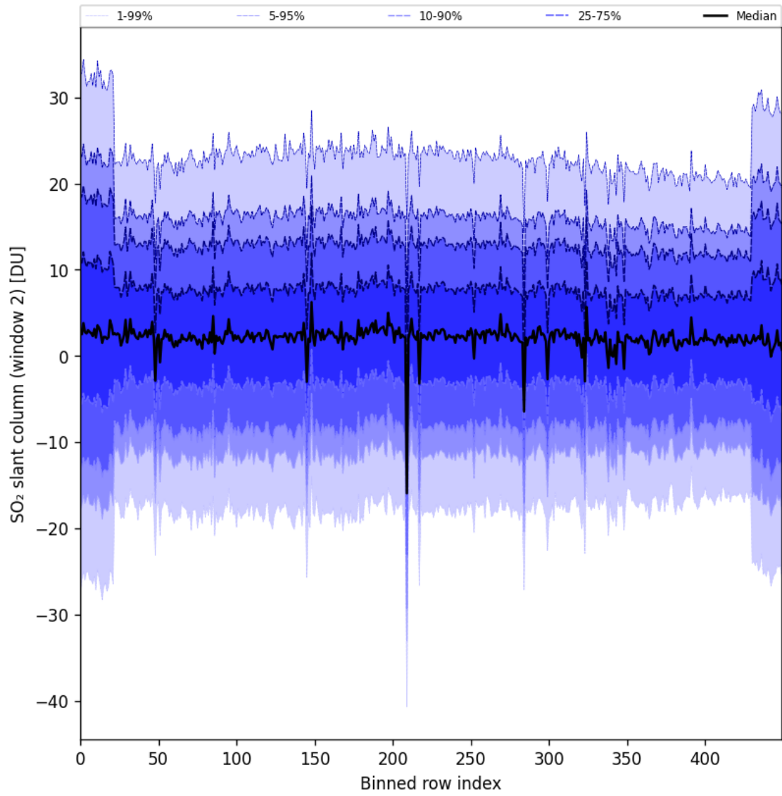
Figure 93: Along track statistics of “SO 2 slant column (window 2)” for 2025-05-18 to 2025-05-20
