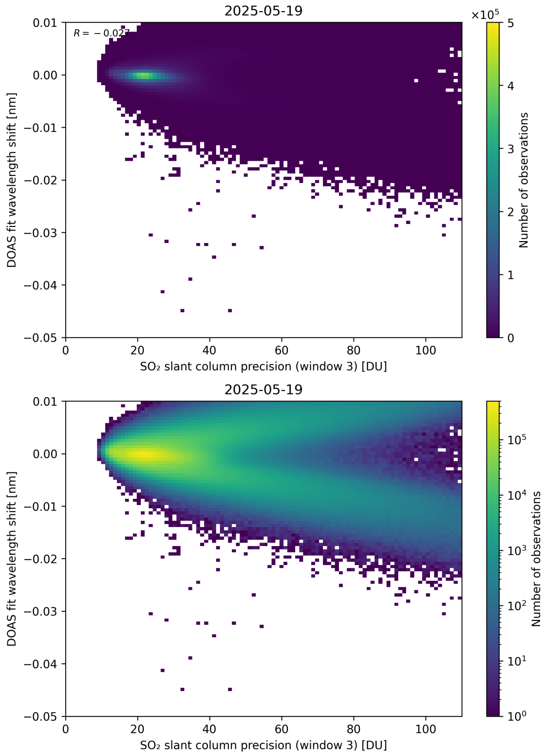
Figure 308: Scatter density plot of “SO 2 slant column precision (window 3)” against “DOAS fit wavelength shift” for 2025-05-18 to 2025-05-20.
