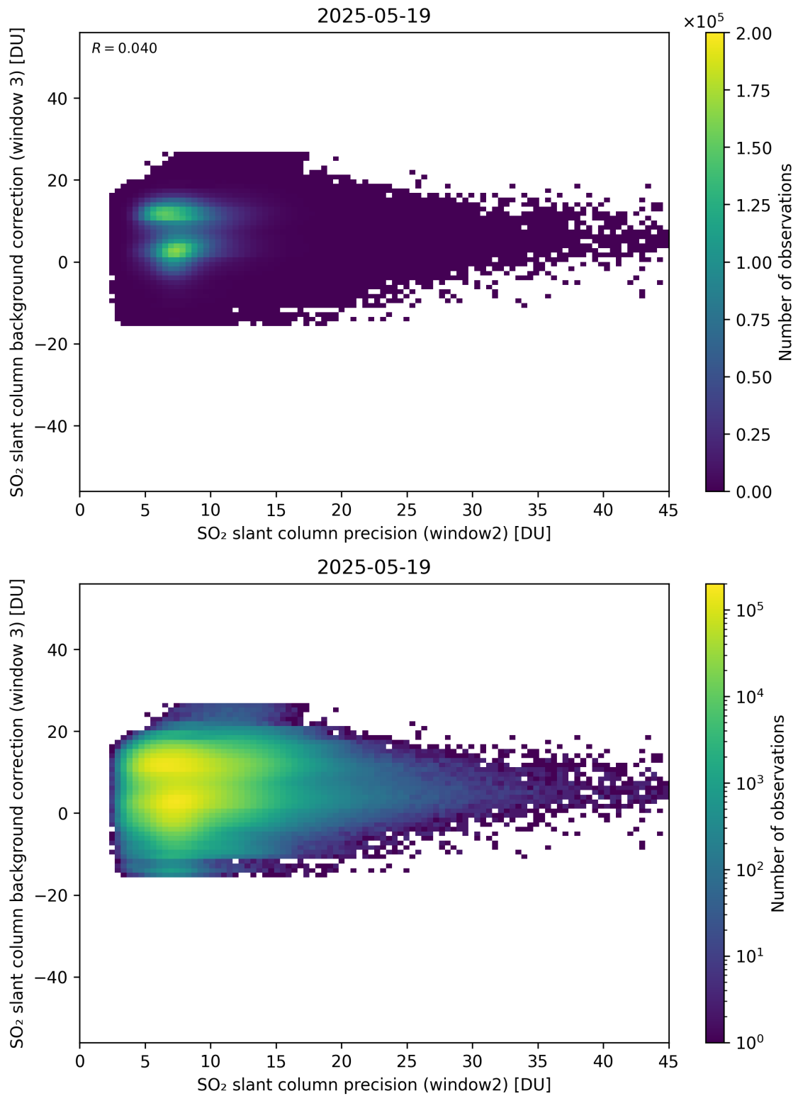
Figure 292: Scatter density plot of “SO 2 slant column precision (window2)” against “SO 2 slant column background correction (window 3)” for 2025-05-18 to 2025-05-20.
