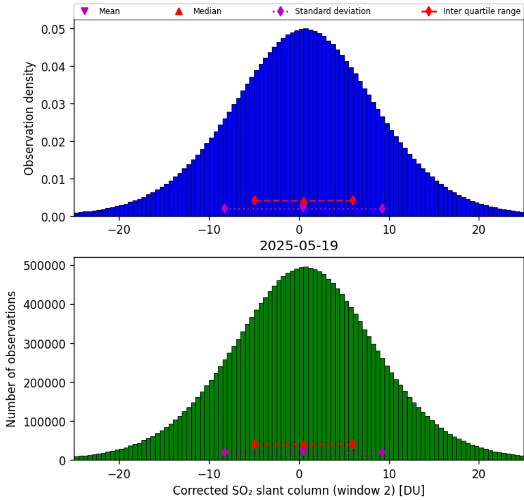
Figure 69: Histogram of “Corrected SO 2 slant column (window 2)” for 2025-05-18 to 2025-05-20
