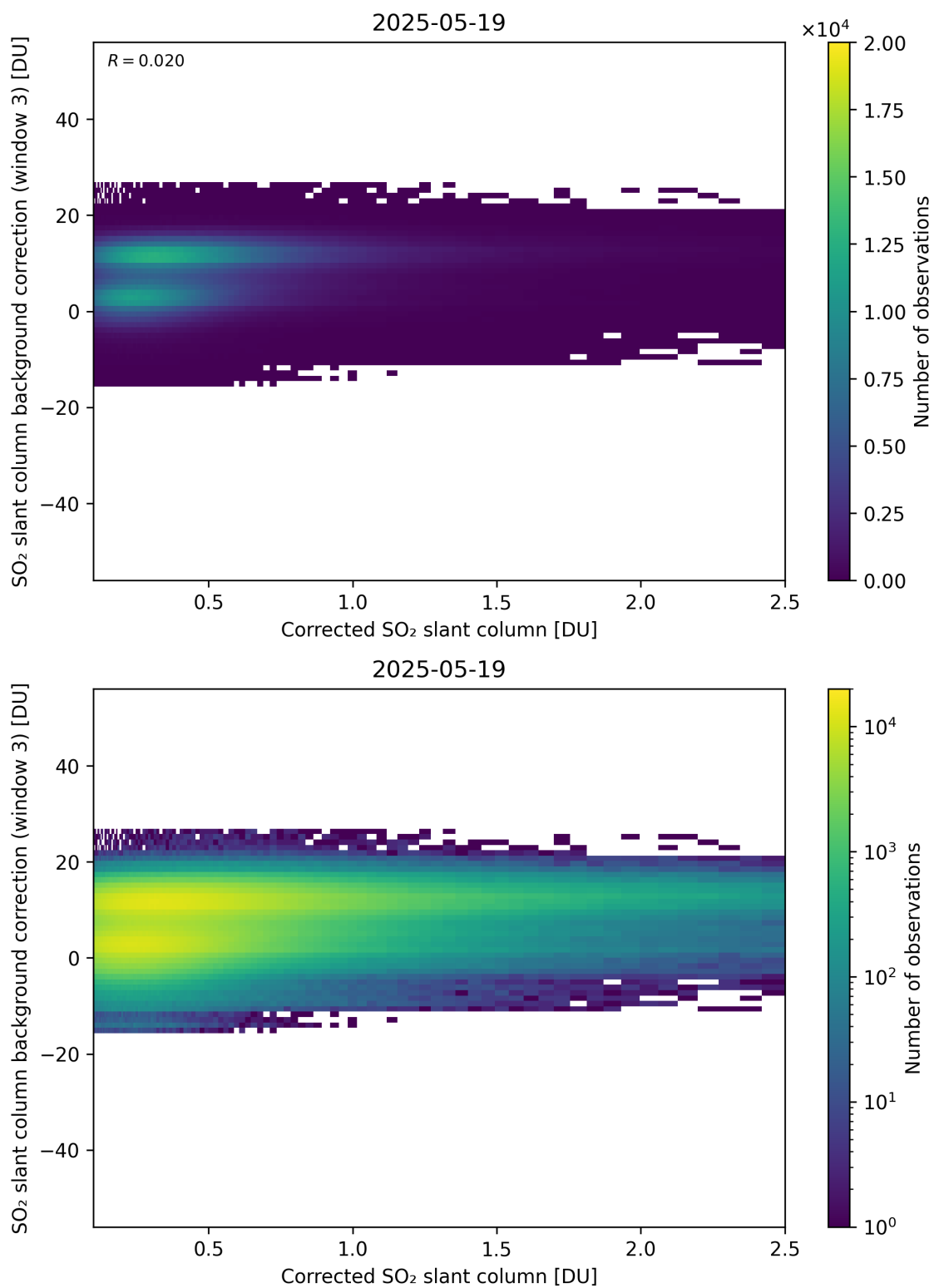
Figure 228: Scatter density plot of “Corrected SO 2 slant column” against “SO 2 slant column background correction (window 3)” for 2025-05-18 to 2025-05-20.
