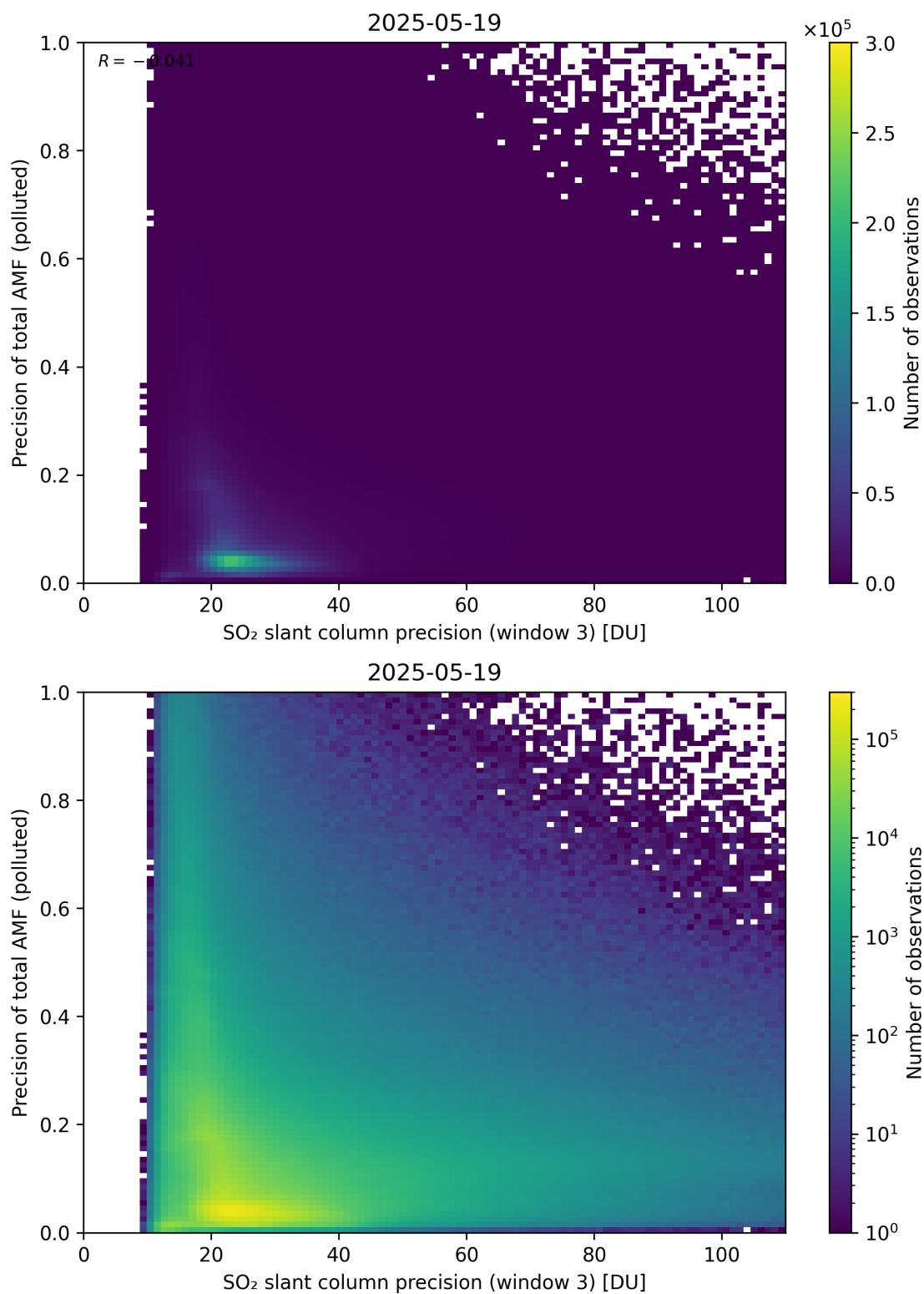
Figure 314: Scatter density plot of “SO 2 slant column precision (window 3)” against “Precision of total AMF (polluted)” for 2025-05-18 to 2025-05-20.
