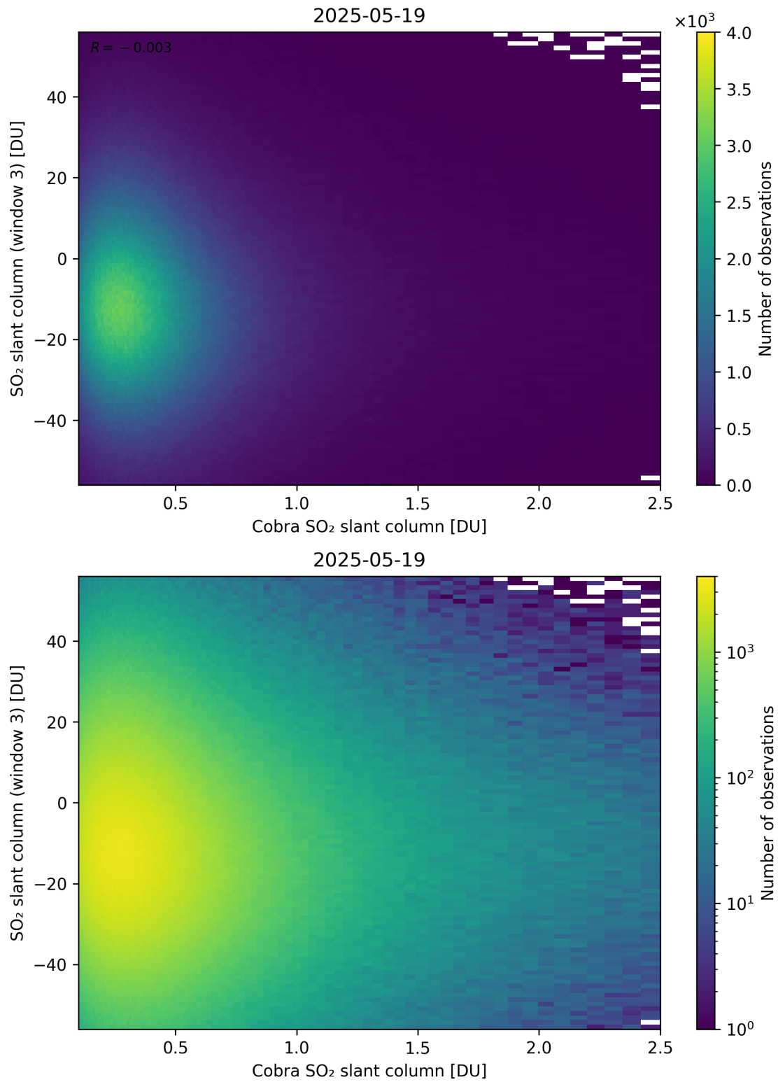
Figure 222: Scatter density plot of “Cobra SO 2 slant column” against “SO 2 slant column (window 3)” for 2025-05-18 to 2025-05-20.
