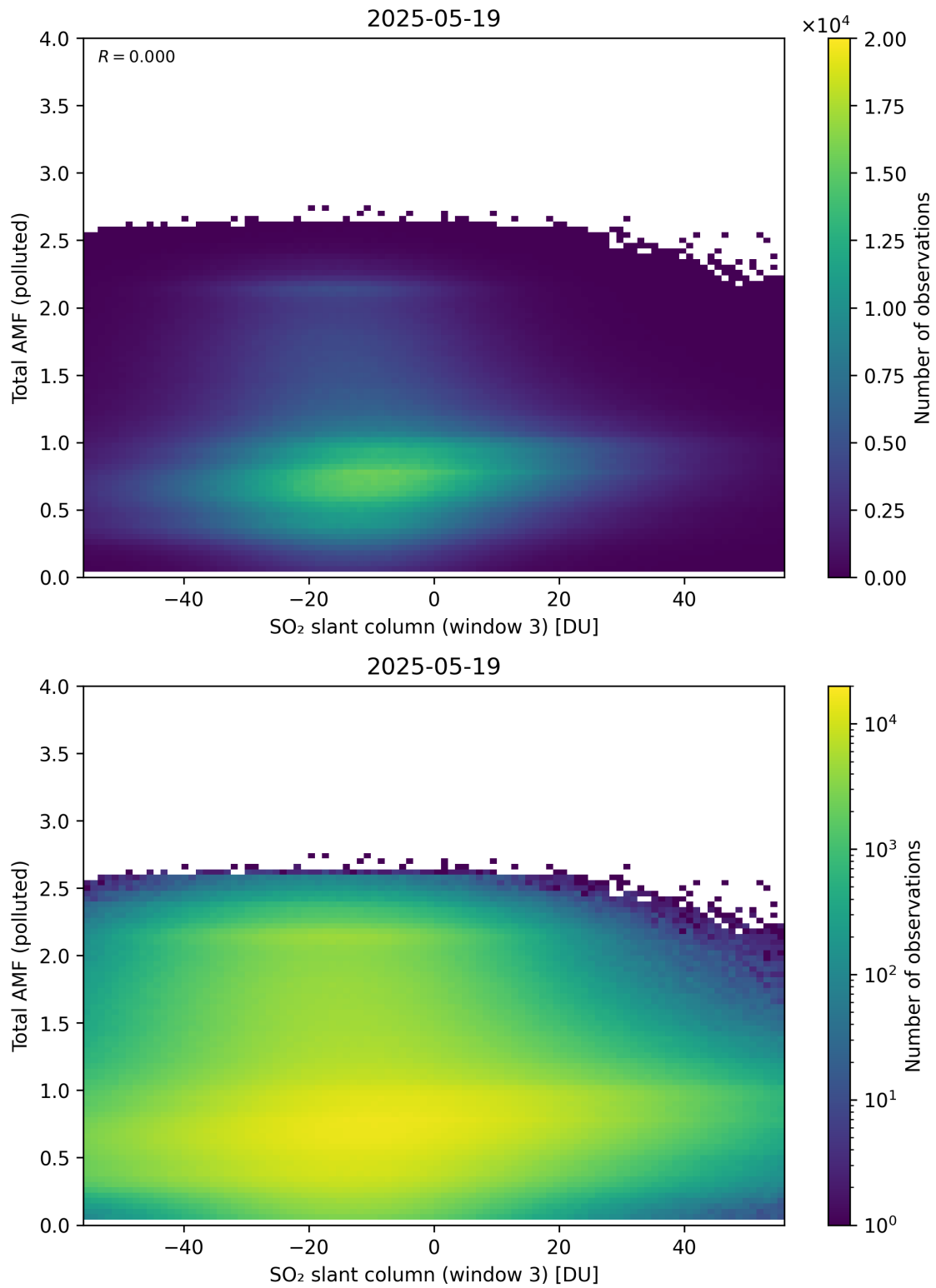
Figure 318: Scatter density plot of “SO 2 slant column (window 3)” against “Total AMF (polluted)” for 2025-05-18 to 2025-05-20.
