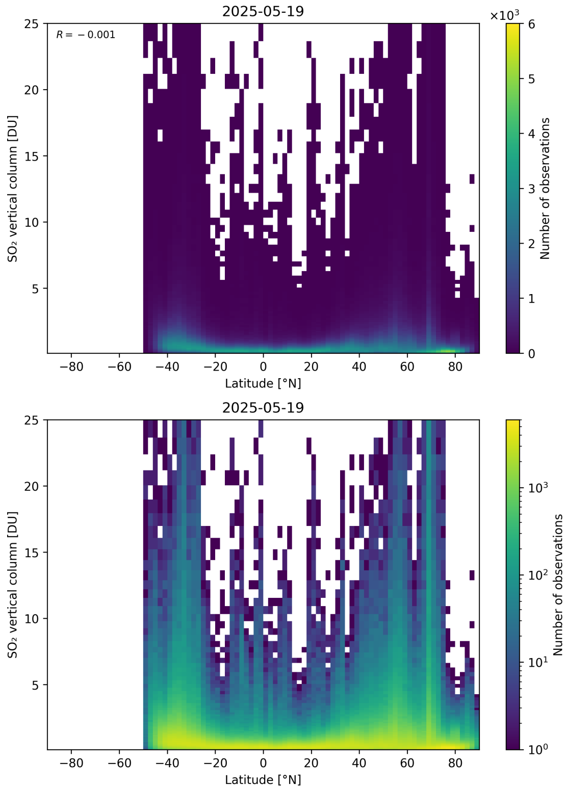
Figure 169: Scatter density plot of “Latitude” against “SO 2 vertical column” for 2025-05-18 to 2025-05-20.
