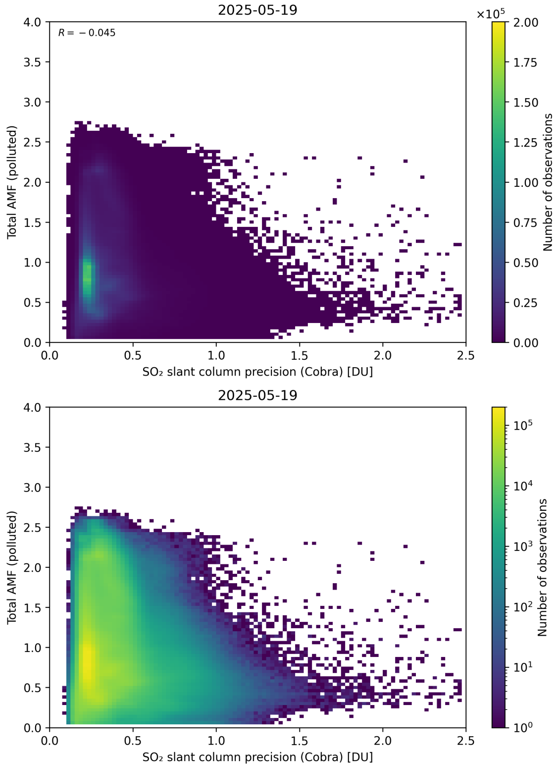
Figure 213: Scatter density plot of “SO 2 slant column precision (Cobra)” against “Total AMF (polluted)” for 2025-05-18 to 2025-05-20.
