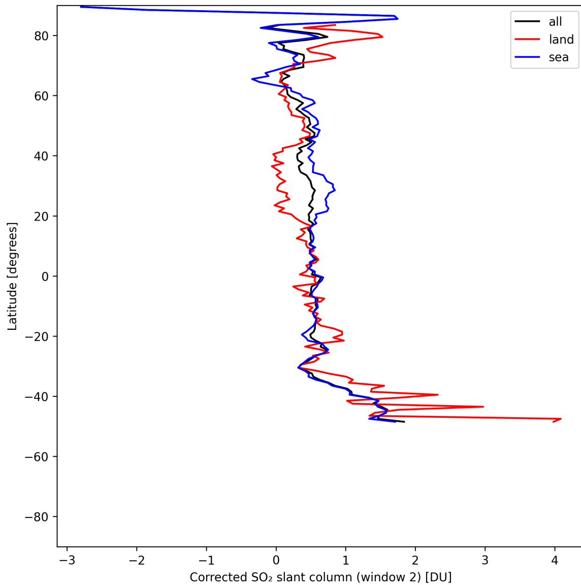
Figure 43: Zonal average of “Corrected SO 2 slant column (window 2)” for 2025-05-18 to 2025-05-20.
