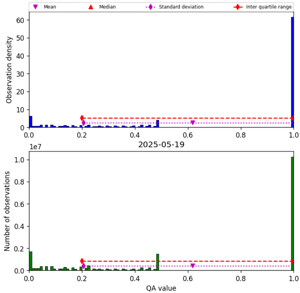
Figure 57: Histogram of “QA value” for 2025-05-18 to 2025-05-20
