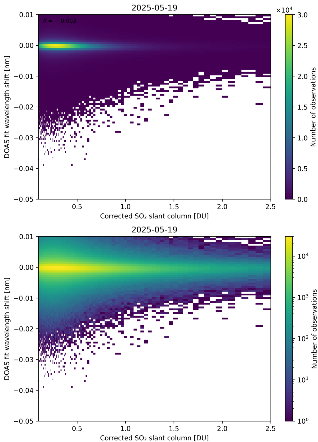
Figure 229: Scatter density plot of “Corrected SO 2 slant column” against “DOAS fit wavelength shift” for 2025-05-18 to 2025-05-20.
