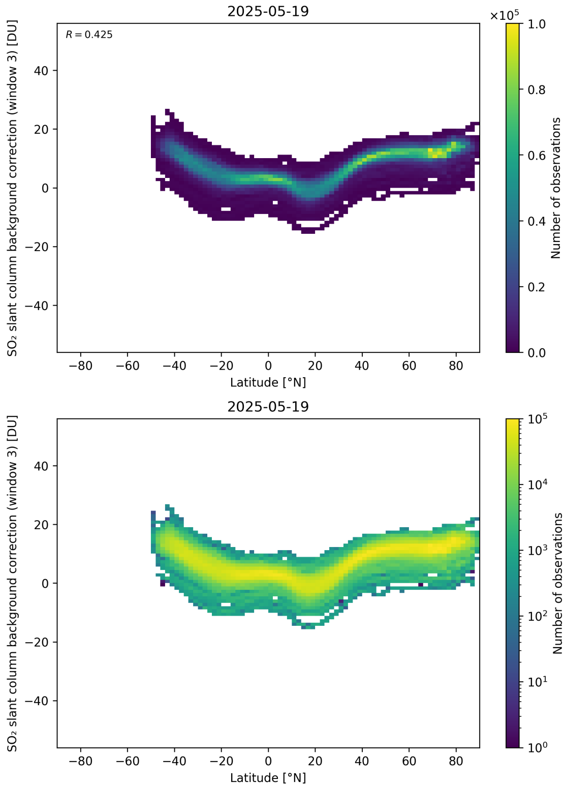
Figure 152: Scatter density plot of “Latitude” against “SO 2 slant column background correction (window 3)” for 2025-05-18 to 2025-05-20.
