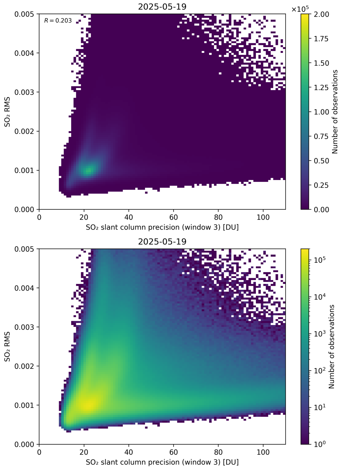
Figure 310: Scatter density plot of “SO 2 slant column precision (window 3)” against “SO 2 RMS” for 2025-05-18 to 2025-05-20.
