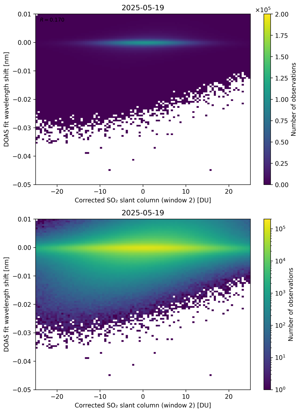
Figure 246: Scatter density plot of “Corrected SO 2 slant column (window 2)” against “DOAS fit wavelength shift” for 2025-05-18 to 2025-05-20.
