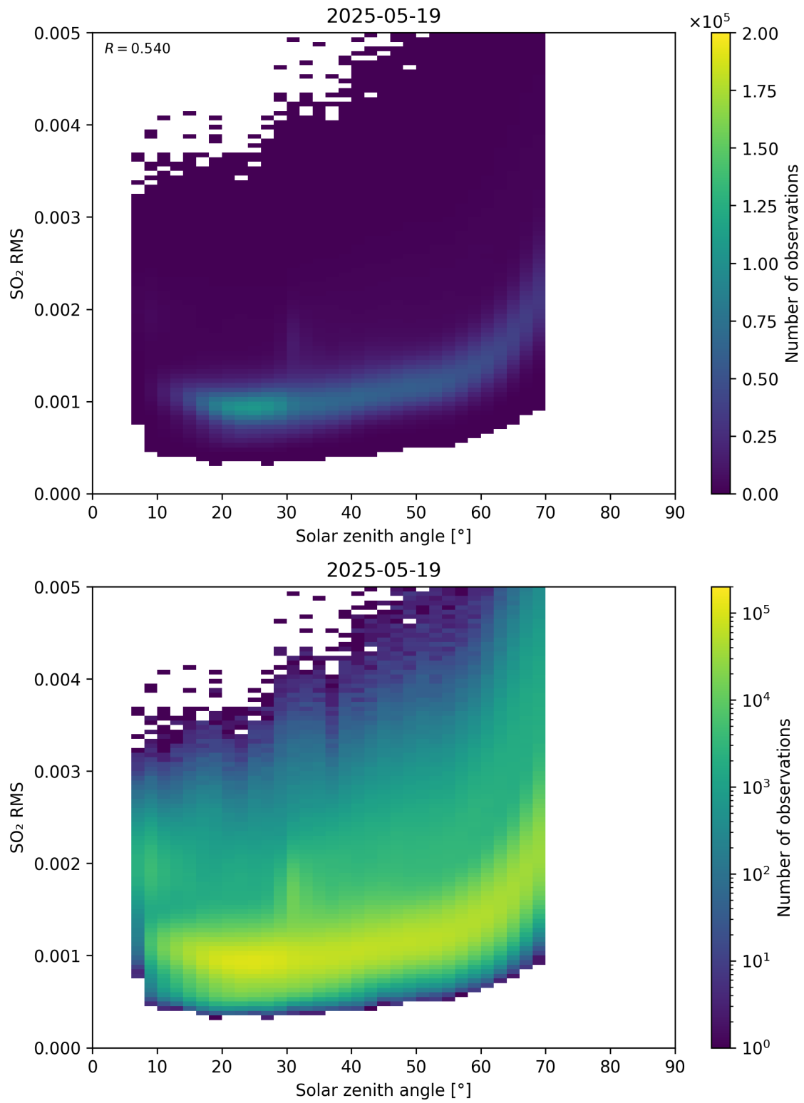
Figure 176: Scatter density plot of “Solar zenith angle” against “SO 2 RMS” for 2025-05-18 to 2025-05-20.
