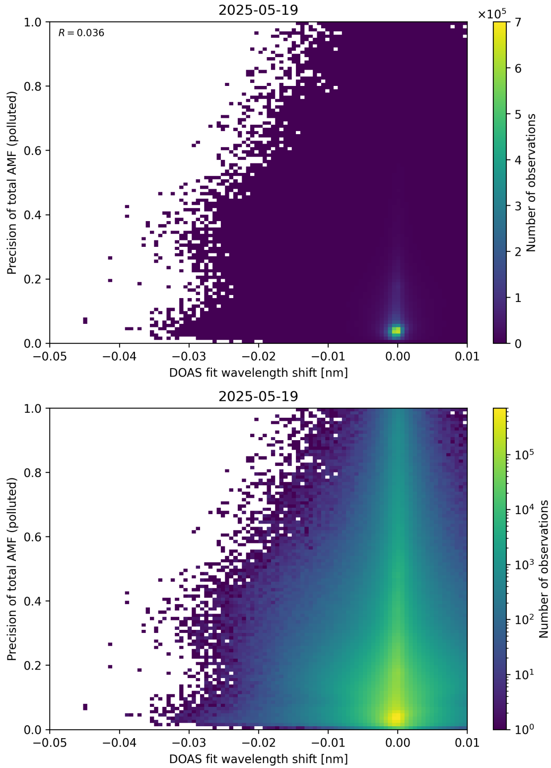
Figure 142: Scatter density plot of “DOAS fit wavelength shift” against “Precision of total AMF (polluted)” for 2025-05-18 to 2025-05-20.
