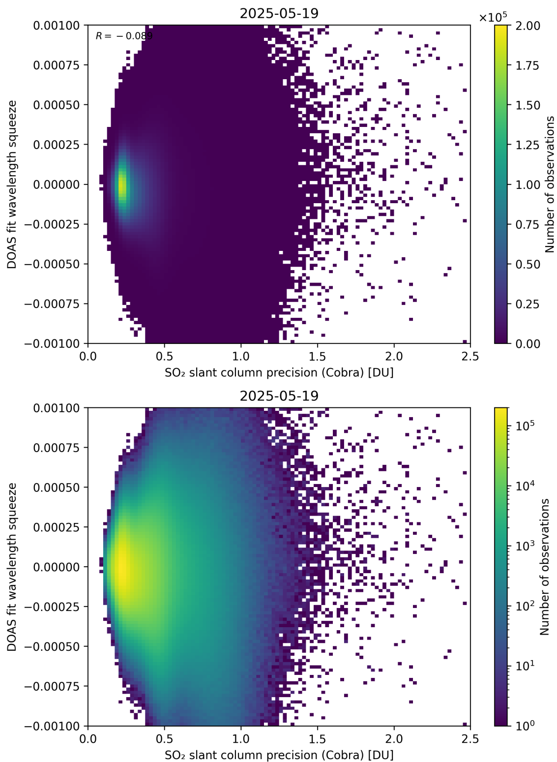
Figure 203: Scatter density plot of “SO 2 slant column precision (Cobra)” against “DOAS fit wavelength squeeze” for 2025-05-18 to 2025-05-20.
