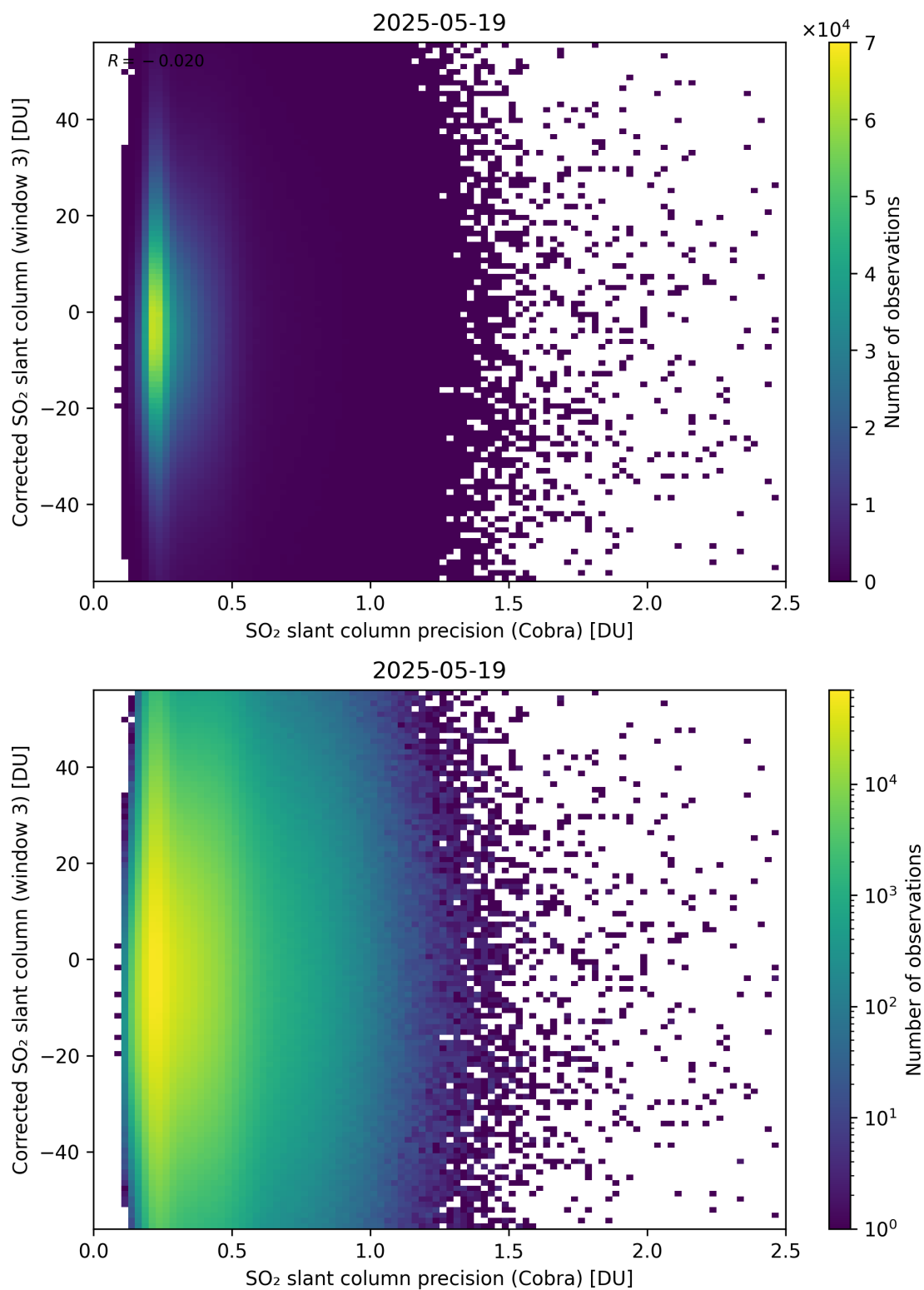
Figure 207: Scatter density plot of “SO 2 slant column precision (Cobra)” against “Corrected SO 2 slant column (window 3)” for 2025-05-18 to 2025-05-20.
