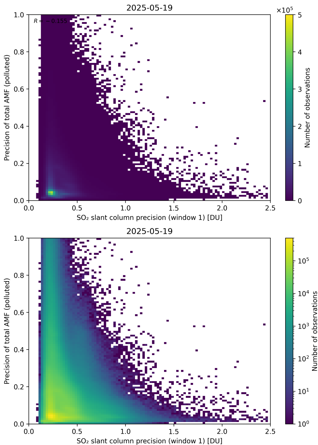
Figure 281: Scatter density plot of “SO 2 slant column precision (window 1)” against “Precision of total AMF (polluted)” for 2025-05-18 to 2025-05-20.
