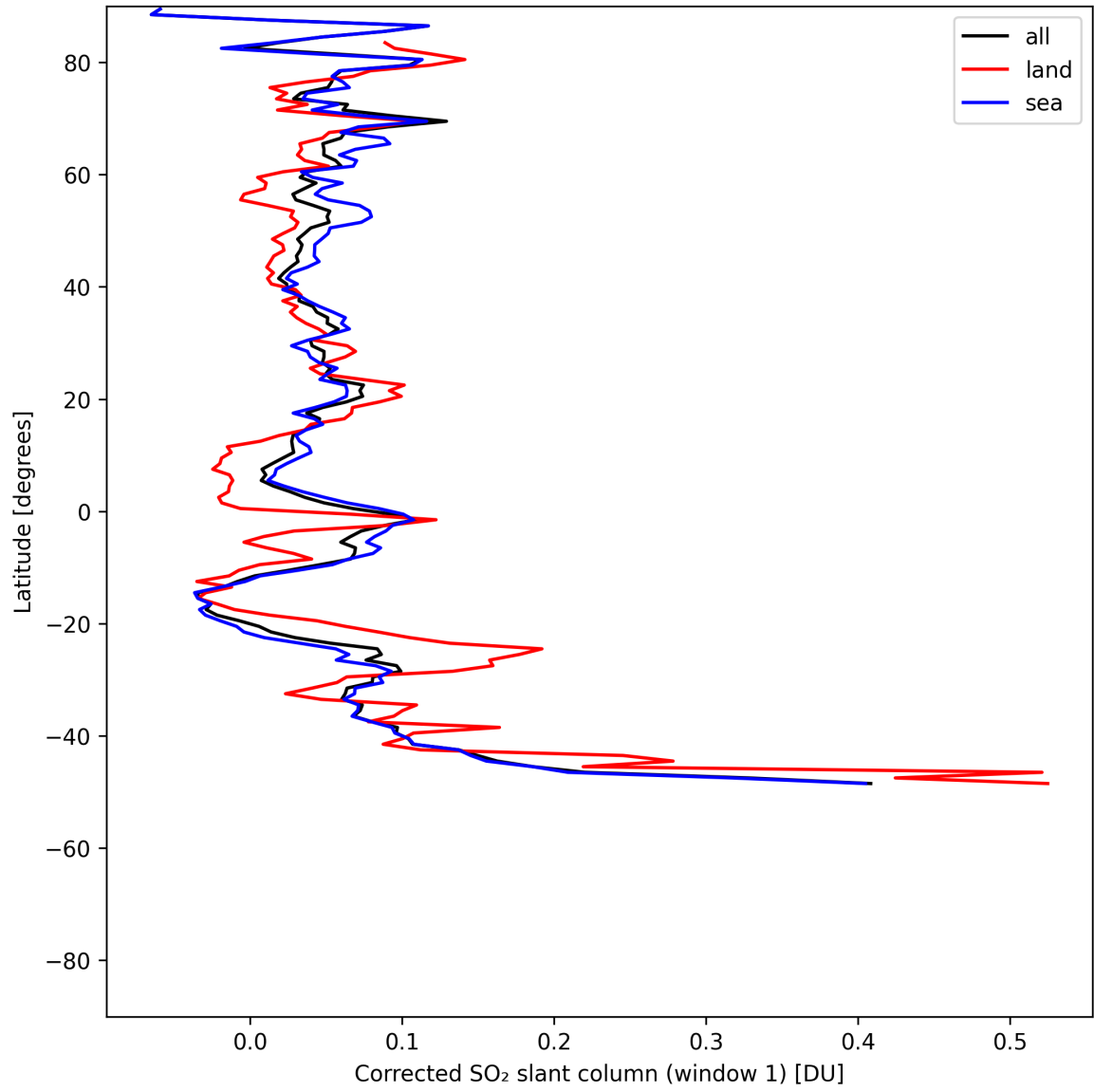
Figure 39: Zonal average of “Corrected SO 2 slant column (window 1)” for 2025-05-18 to 2025-05-20.
