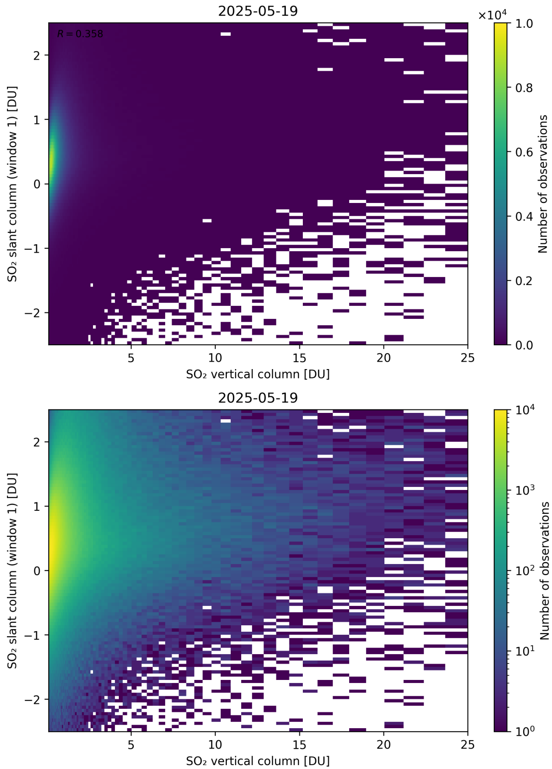
Figure 354: Scatter density plot of “SO 2 vertical column” against “SO 2 slant column (window 1)” for 2025-05-18 to 2025-05-20.
