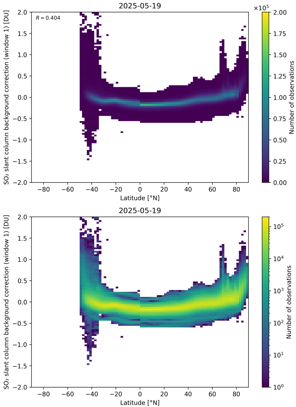
Figure 150: Scatter density plot of “Latitude” against “SO 2 slant column background correction (window 1)” for 2025-05-18 to 2025-05-20.
