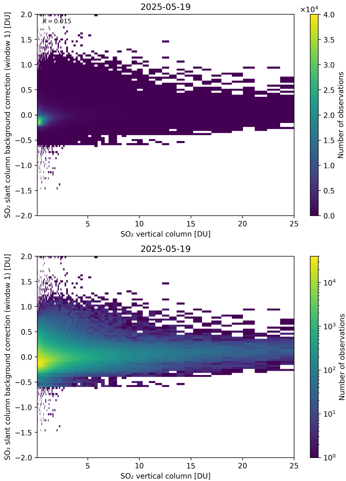
Figure 323: Scatter density plot of “SO 2 vertical column” against “SO 2 slant column background correction (window 1)” for 2025-05-18 to 2025-05-20.
