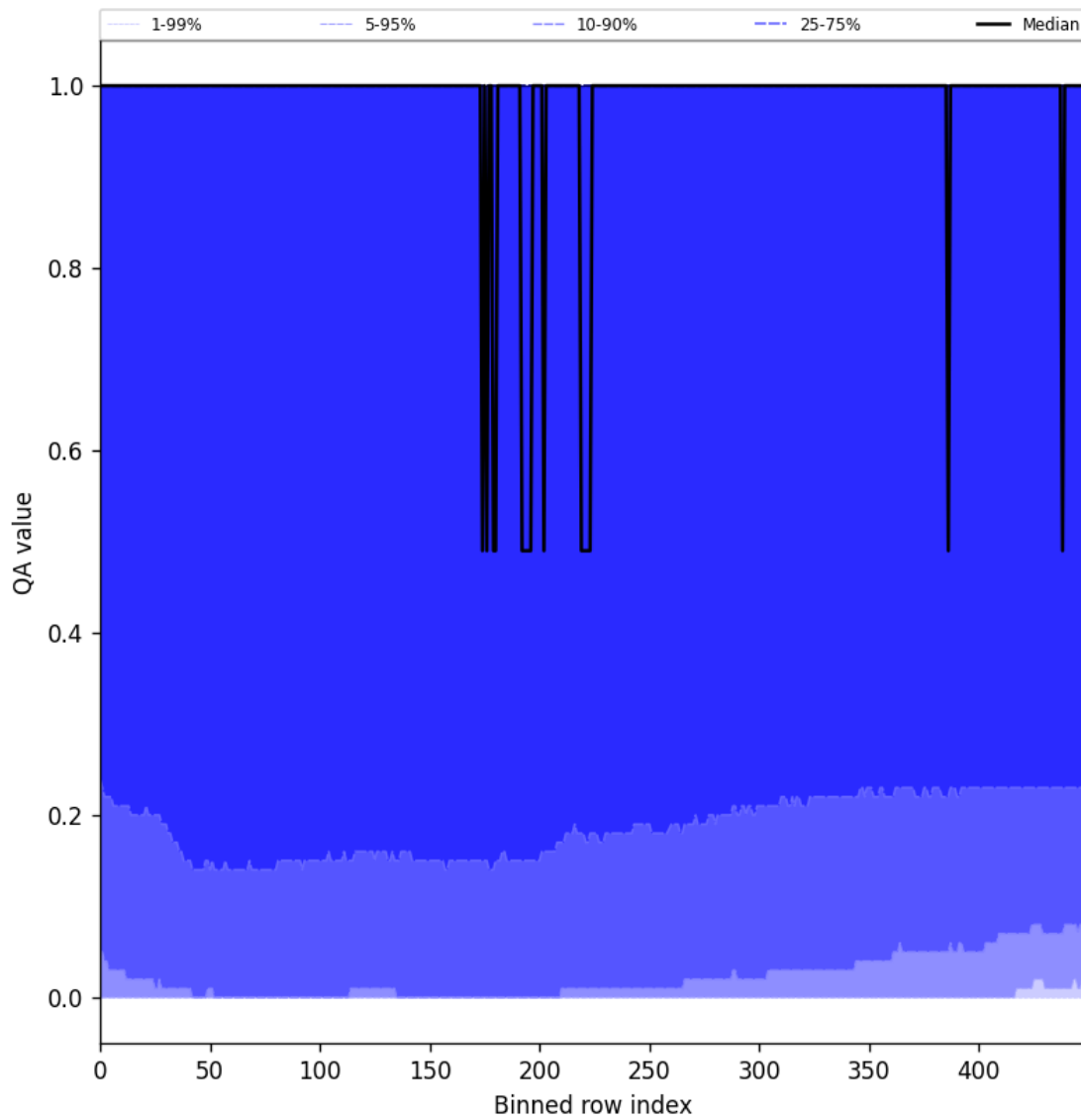
Figure 83: Along track statistics of “QA value” for 2025-05-18 to 2025-05-20
