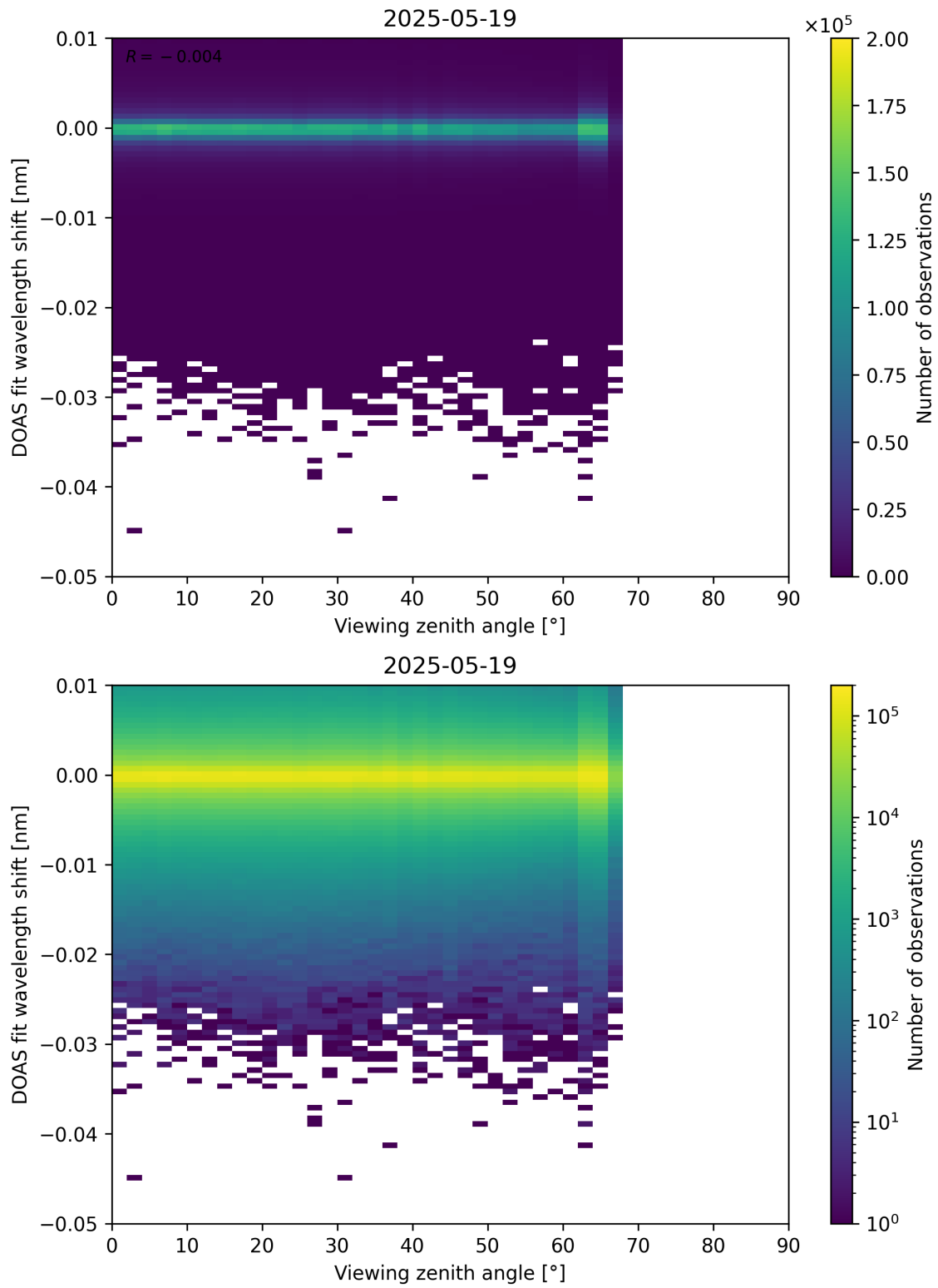
Figure 365: Scatter density plot of “Viewing zenith angle” against “DOAS fit wavelength shift” for 2025-05-18 to 2025-05-20.
