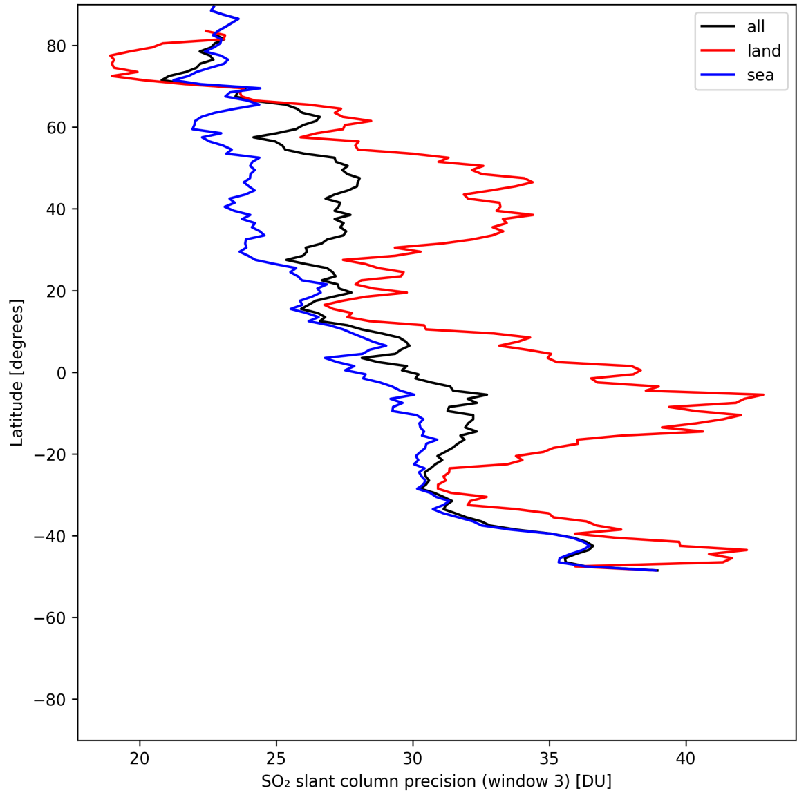
Figure 46: Zonal average of “SO 2 slant column precision (window 3)” for 2025-05-18 to 2025-05-20.
