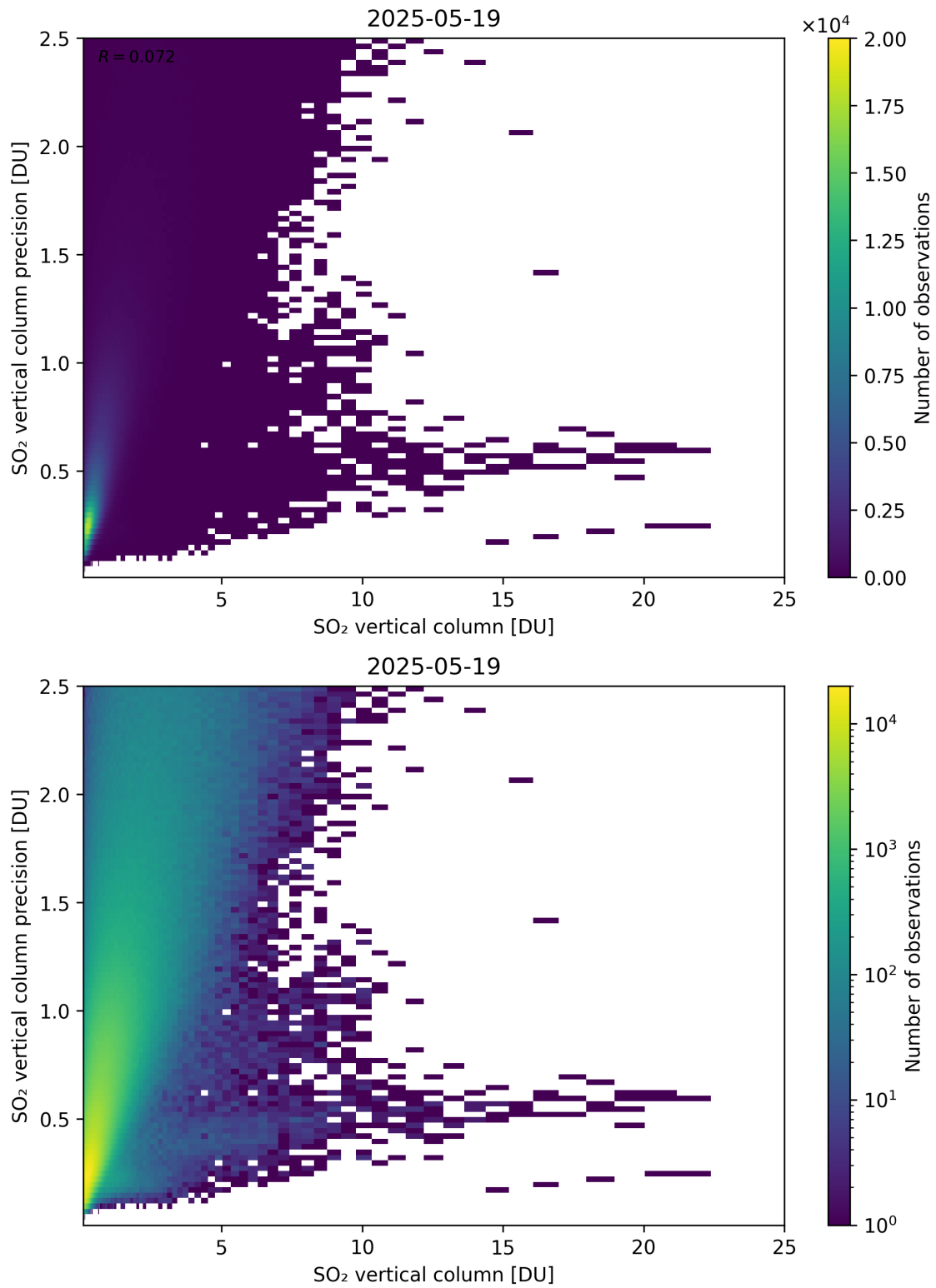
Figure 361: Scatter density plot of “SO 2 vertical column” against “SO 2 vertical column precision” for 2025-05-18 to 2025-05-20.
