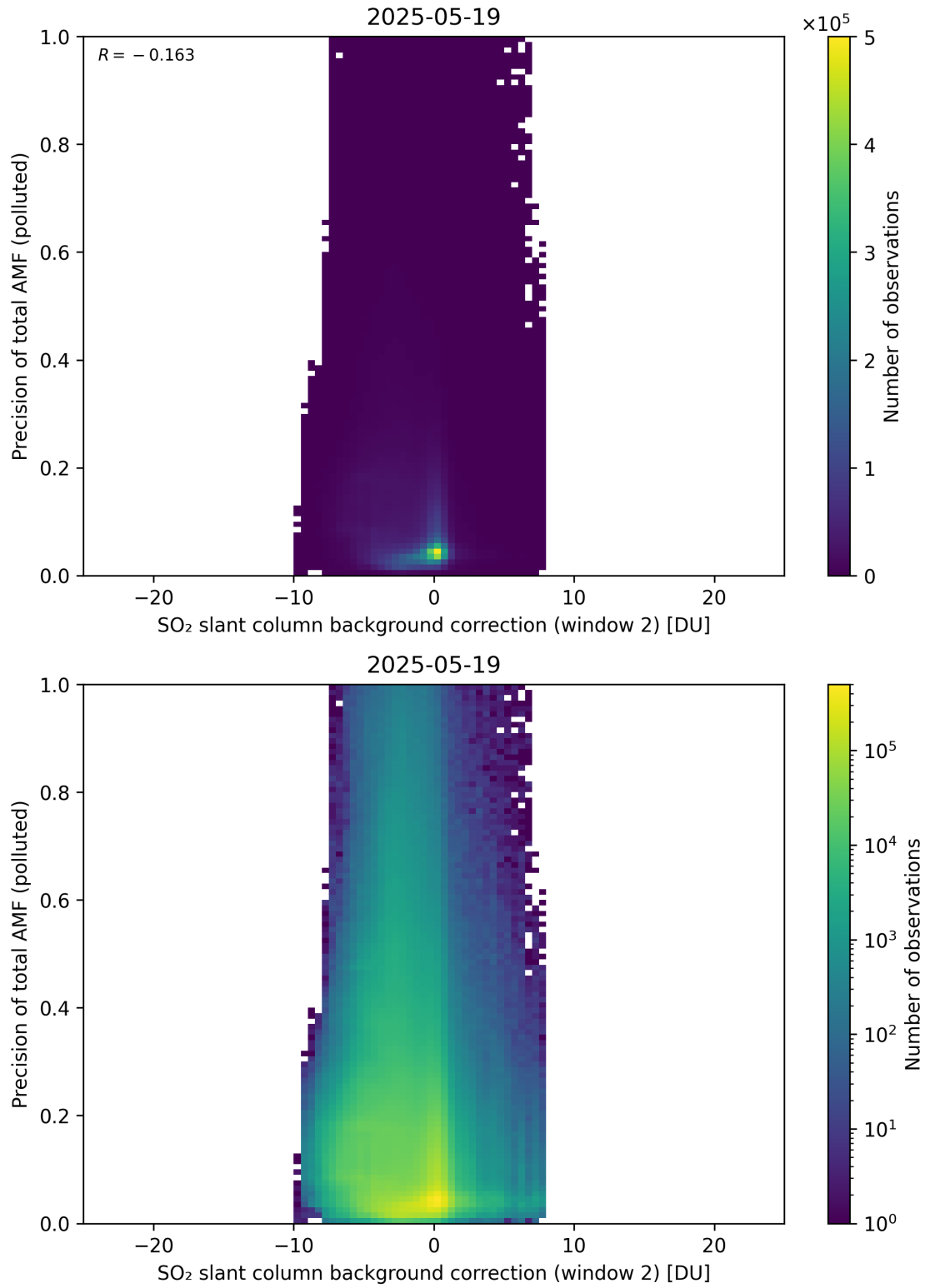
Figure 131: Scatter density plot of “SO 2 slant column background correction (window 2)” against “Precision of total AMF (polluted)” for 2025-05-18 to 2025-05-20.
