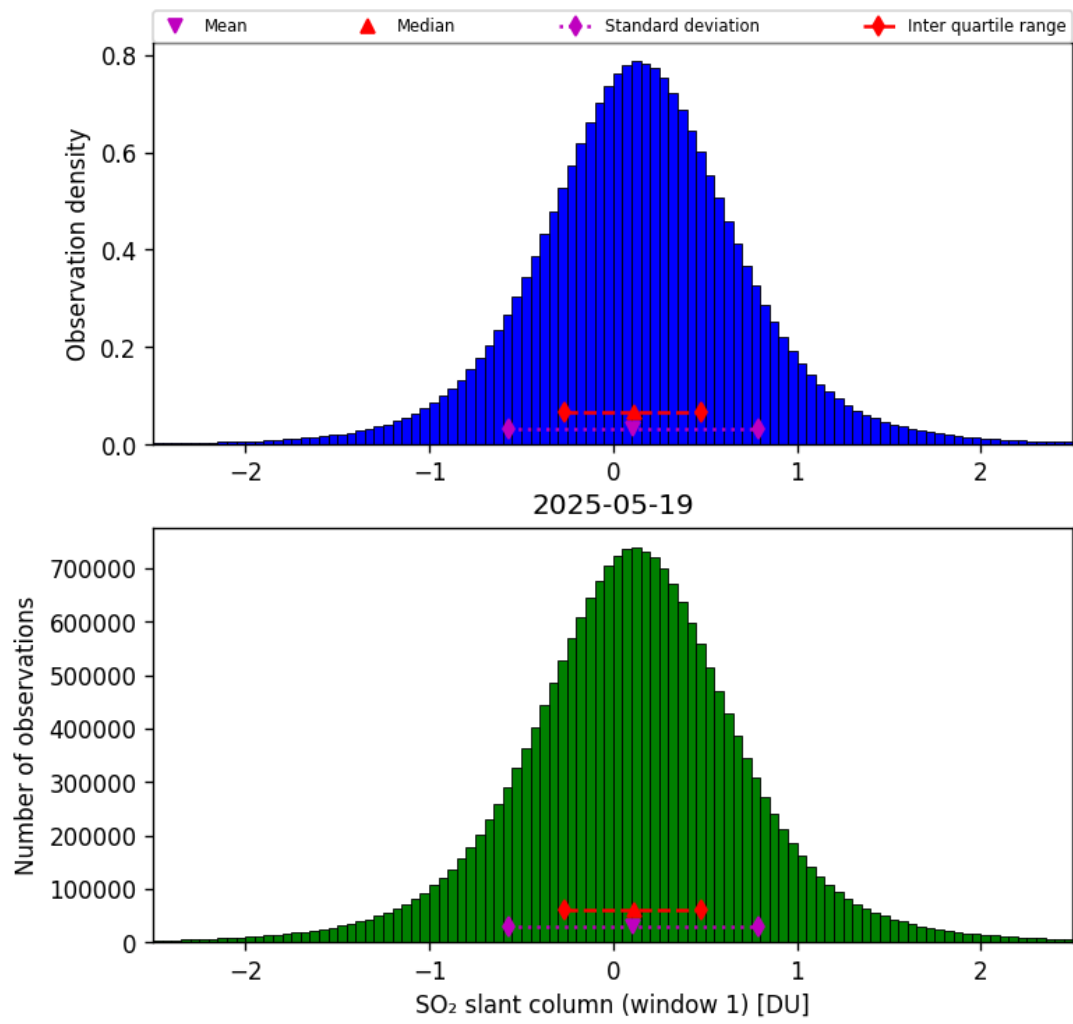
Figure 63: Histogram of “SO 2 slant column (window 1)” for 2025-05-18 to 2025-05-20
