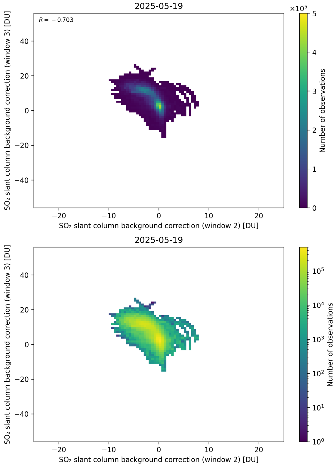
Figure 122: Scatter density plot of “SO 2 slant column background correction (window 2)” against “SO 2 slant column background correction (window 3)” for 2025-05-18 to 2025-05-20.
