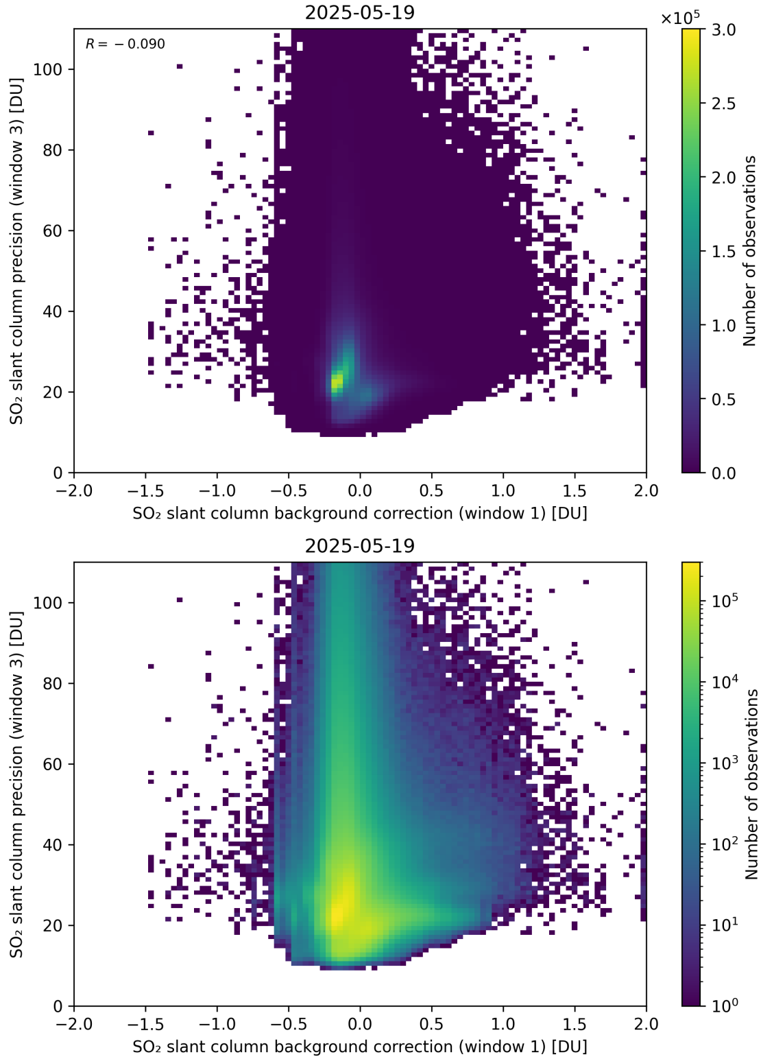
Figure 119: Scatter density plot of “SO 2 slant column background correction (window 1)” against “SO 2 slant column precision (window 3)” for 2025-05-18 to 2025-05-20.
