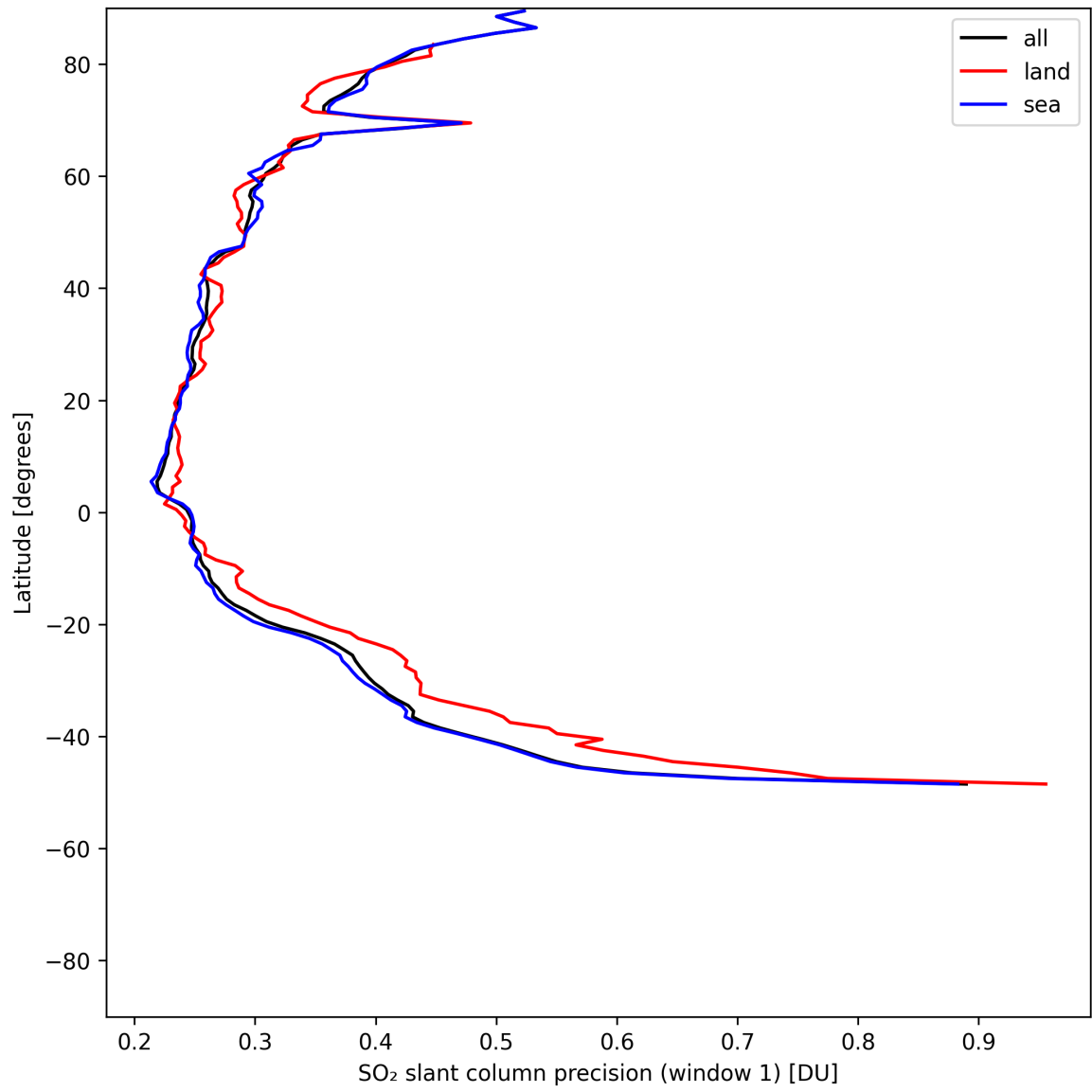
Figure 38: Zonal average of “SO 2 slant column precision (window 1)” for 2025-05-18 to 2025-05-20.
