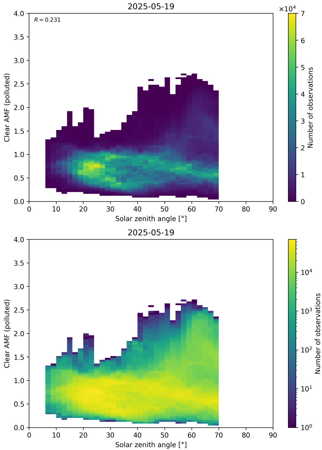
Figure 178: Scatter density plot of “Solar zenith angle” against “Clear AMF (polluted)” for 2025-05-18 to 2025-05-20.
