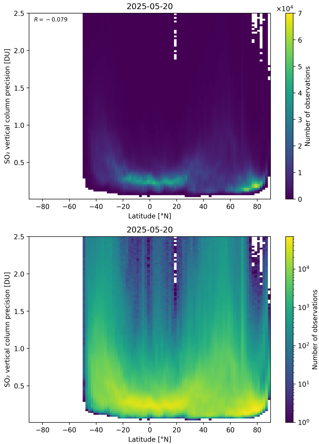
Figure 170: Scatter density plot of “Latitude” against “SO 2 vertical column precision” for 2025-05-19 to 2025-05-21.
