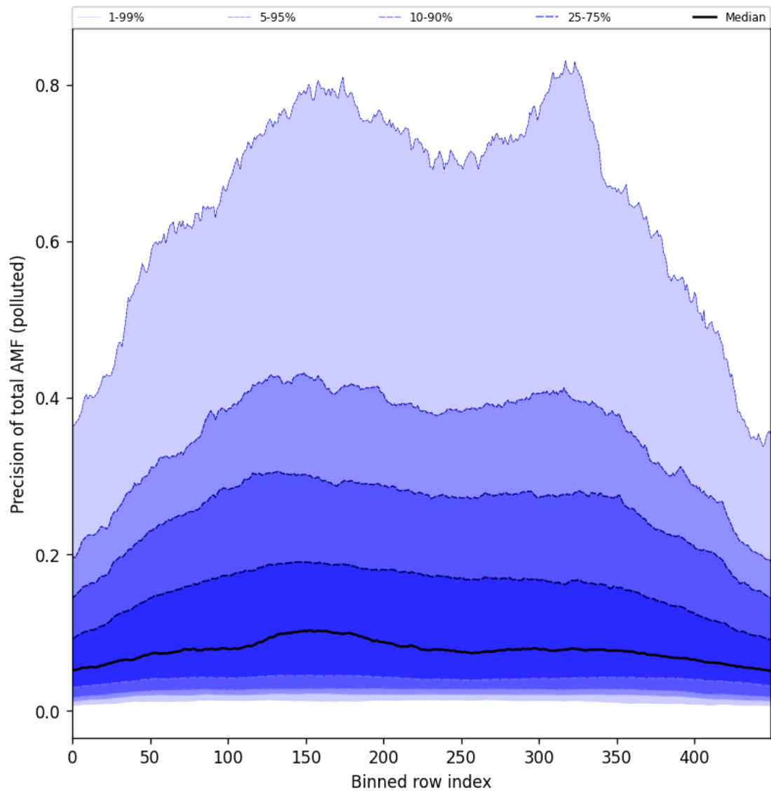
Figure 106: Along track statistics of “Precision of total AMF (polluted)” for 2025-05-19 to 2025-05-21
