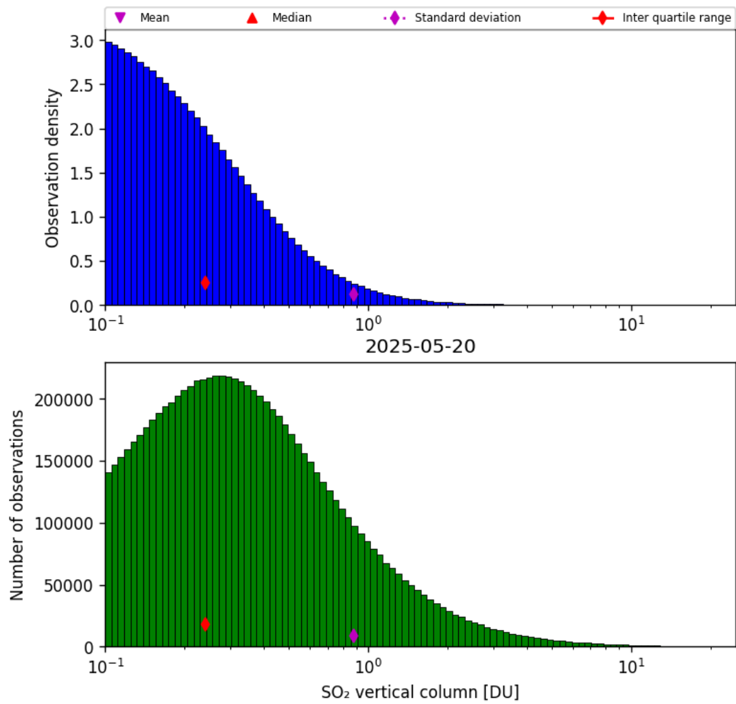
Figure 58: Histogram of “SO 2 vertical column” for 2025-05-19 to 2025-05-21
