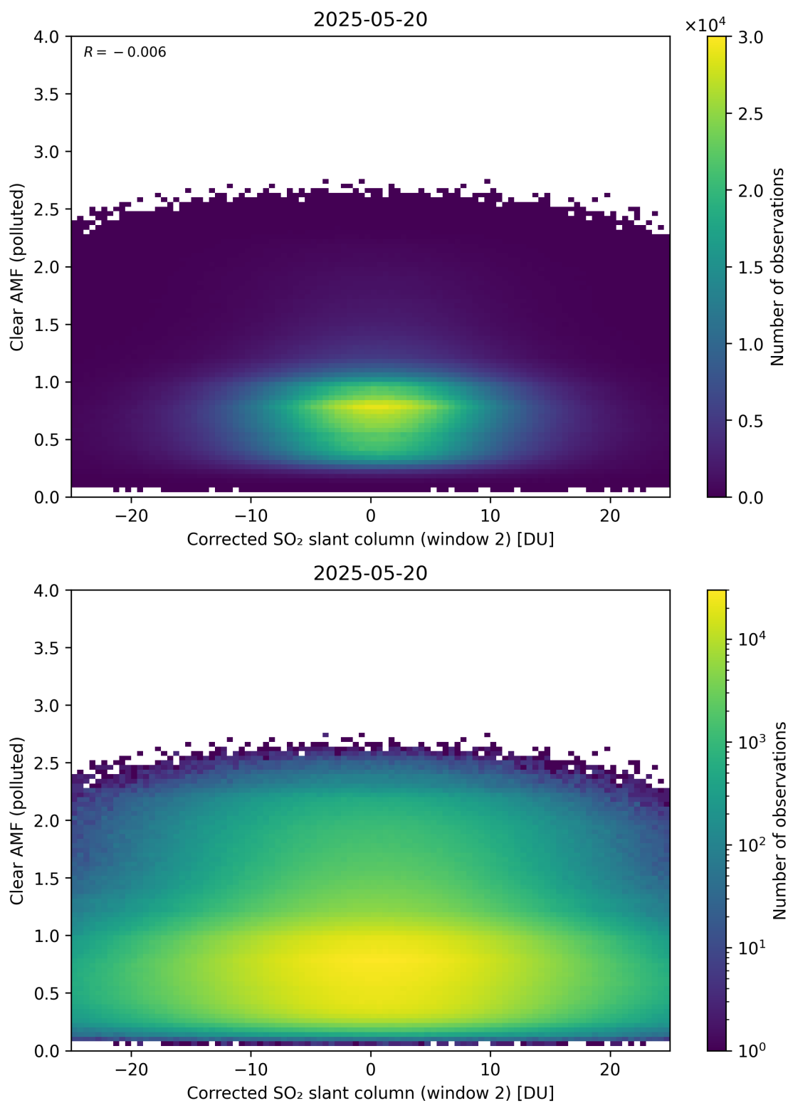
Figure 249: Scatter density plot of “Corrected SO 2 slant column (window 2)” against “Clear AMF (polluted)” for 2025-05-19 to 2025-05-21.
