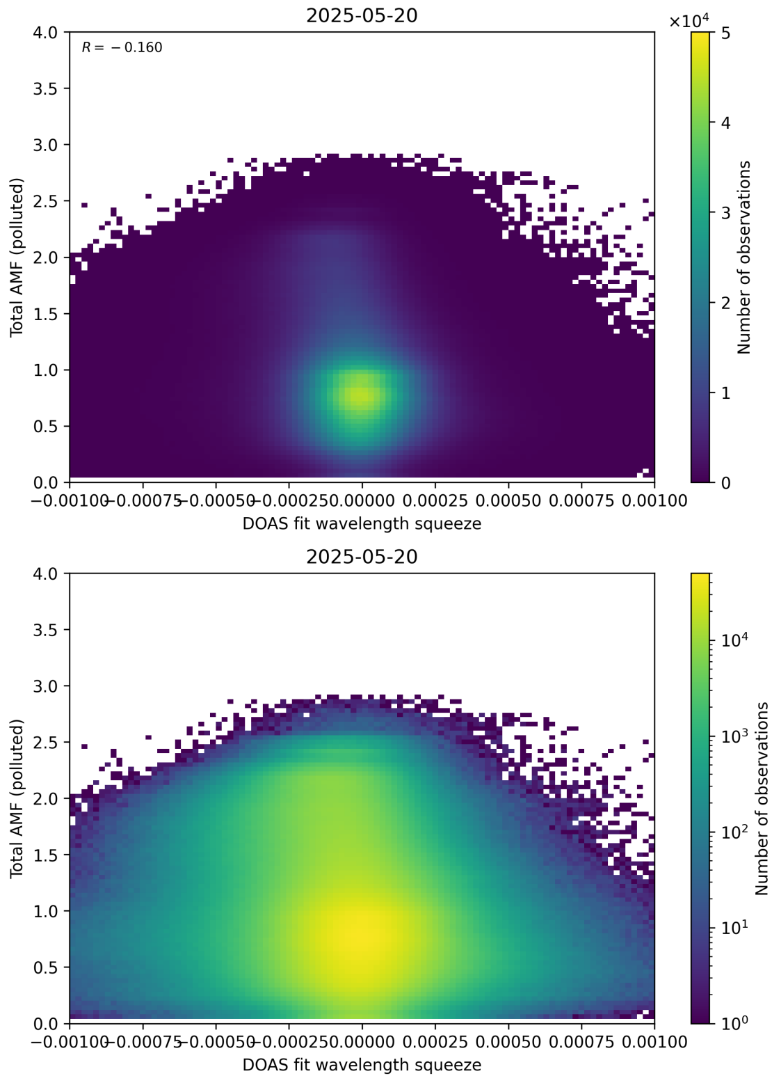
Figure 145: Scatter density plot of “DOAS fit wavelength squeeze” against “Total AMF (polluted)” for 2025-05-19 to 2025-05-21.
