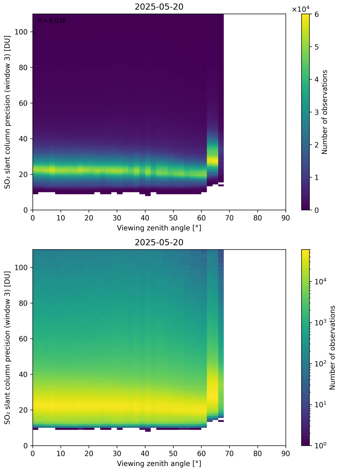
Figure 380: Scatter density plot of “Viewing zenith angle” against “SO 2 slant column precision (window 3)” for 2025-05-19 to 2025-05-21.
