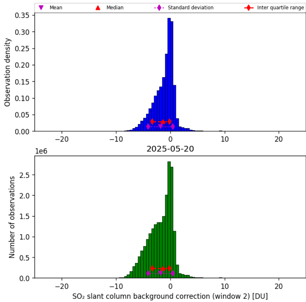
Figure 70: Histogram of “SO 2 slant column background correction (window 2)” for 2025-05-19 to 2025-05-21
