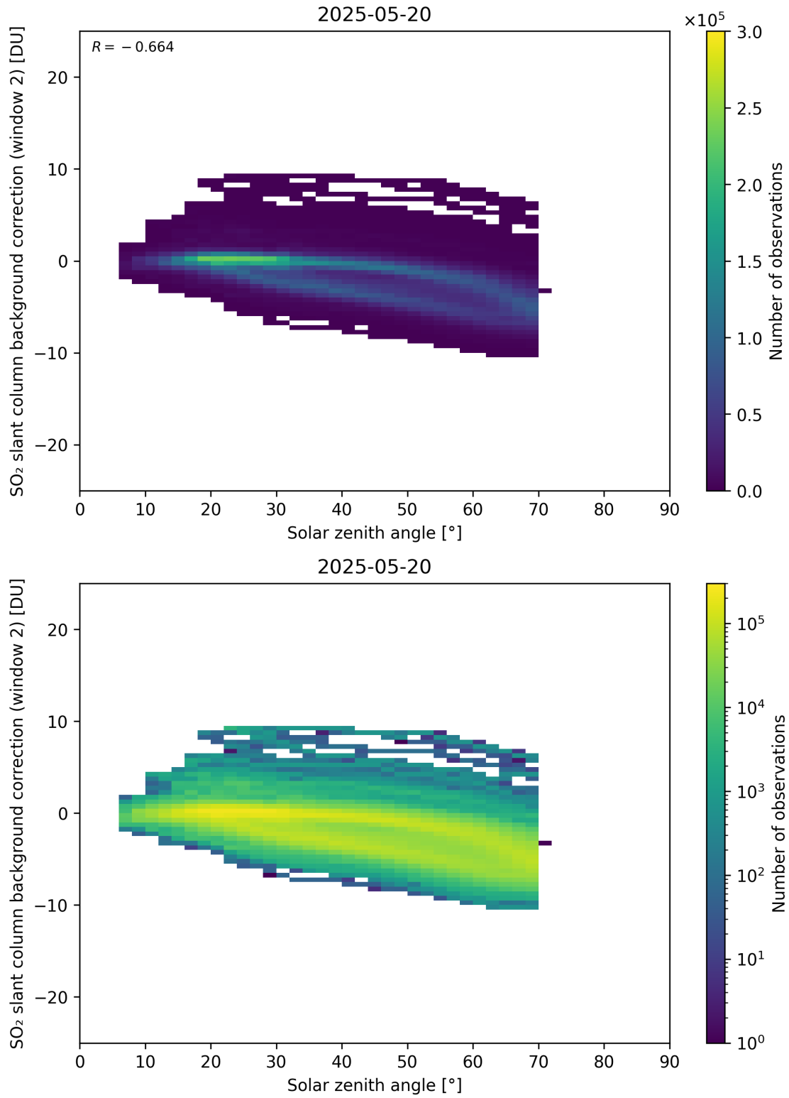
Figure 172: Scatter density plot of “Solar zenith angle” against “SO 2 slant column background correction (window 2)” for 2025-05-19 to 2025-05-21.
