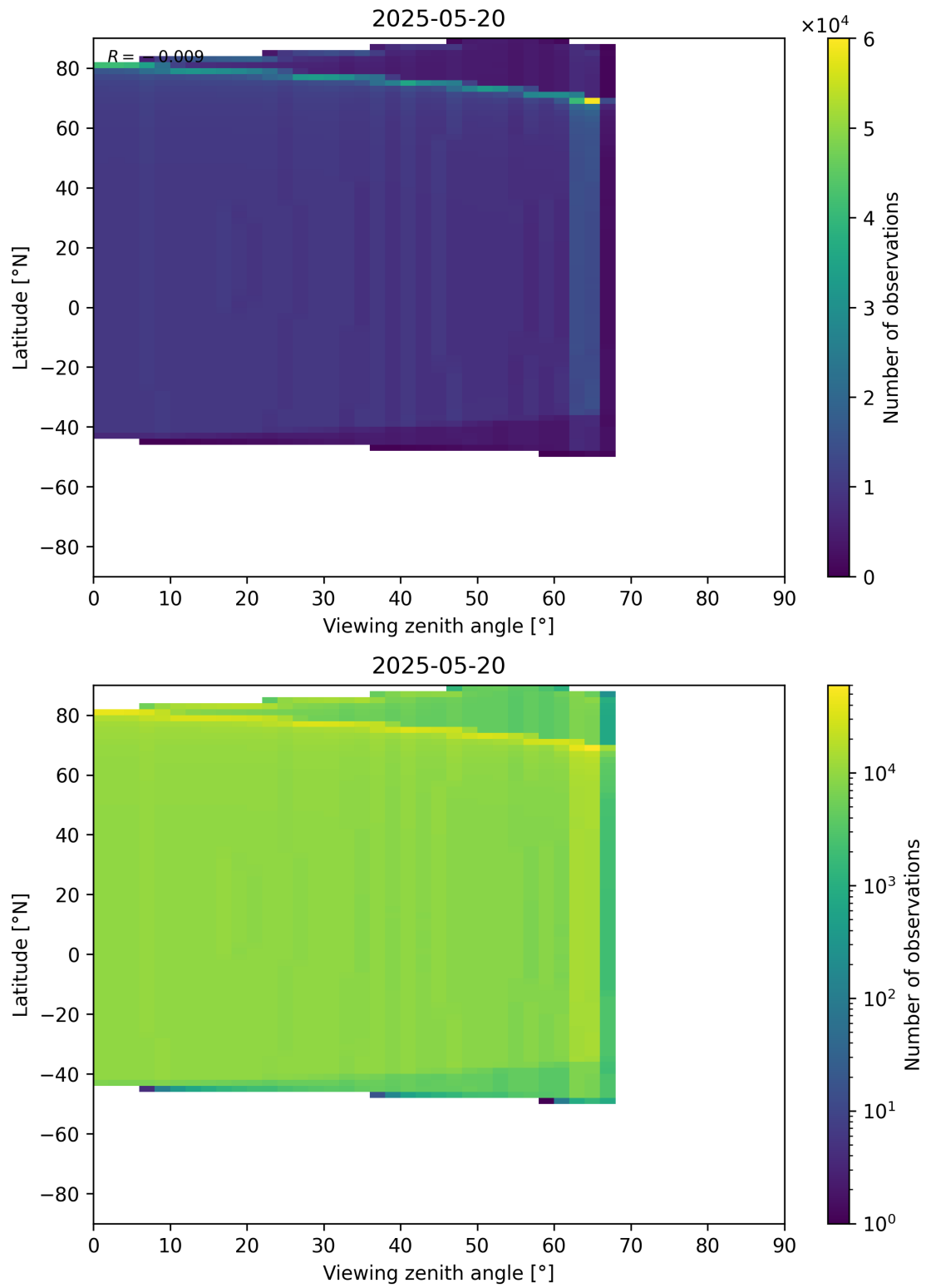
Figure 368: Scatter density plot of “Viewing zenith angle” against “Latitude” for 2025-05-19 to 2025-05-21.
