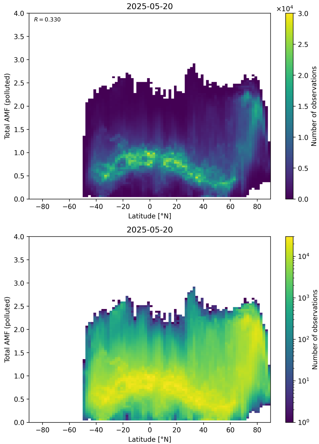
Figure 167: Scatter density plot of “Latitude” against “Total AMF (polluted)” for 2025-05-19 to 2025-05-21.
