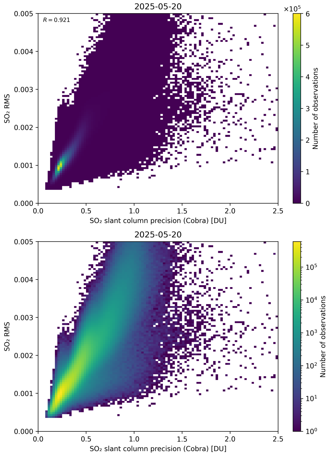
Figure 204: Scatter density plot of “SO 2 slant column precision (Cobra)” against “SO 2 RMS” for 2025-05-19 to 2025-05-21.
