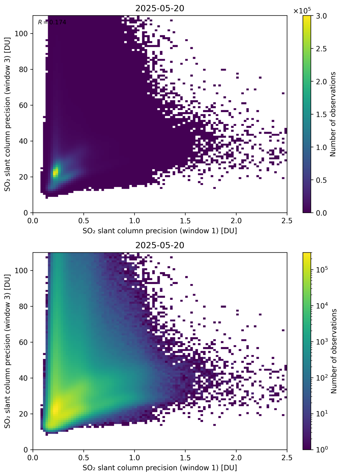
Figure 279: Scatter density plot of “SO 2 slant column precision (window 1)” against “SO 2 slant column precision (window 3)” for 2025-05-19 to 2025-05-21.
