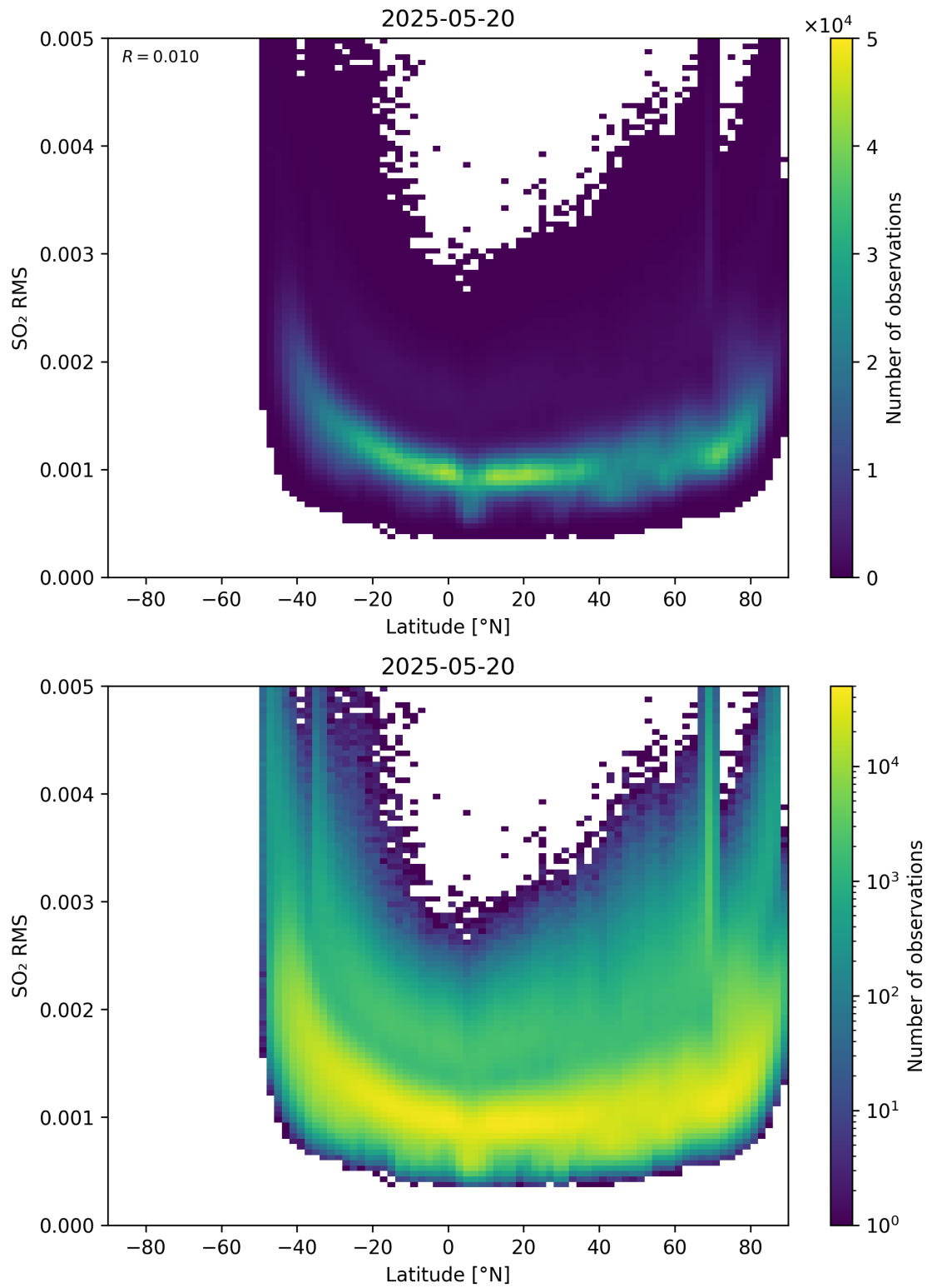
Figure 155: Scatter density plot of “Latitude” against “SO 2 RMS” for 2025-05-19 to 2025-05-21.
