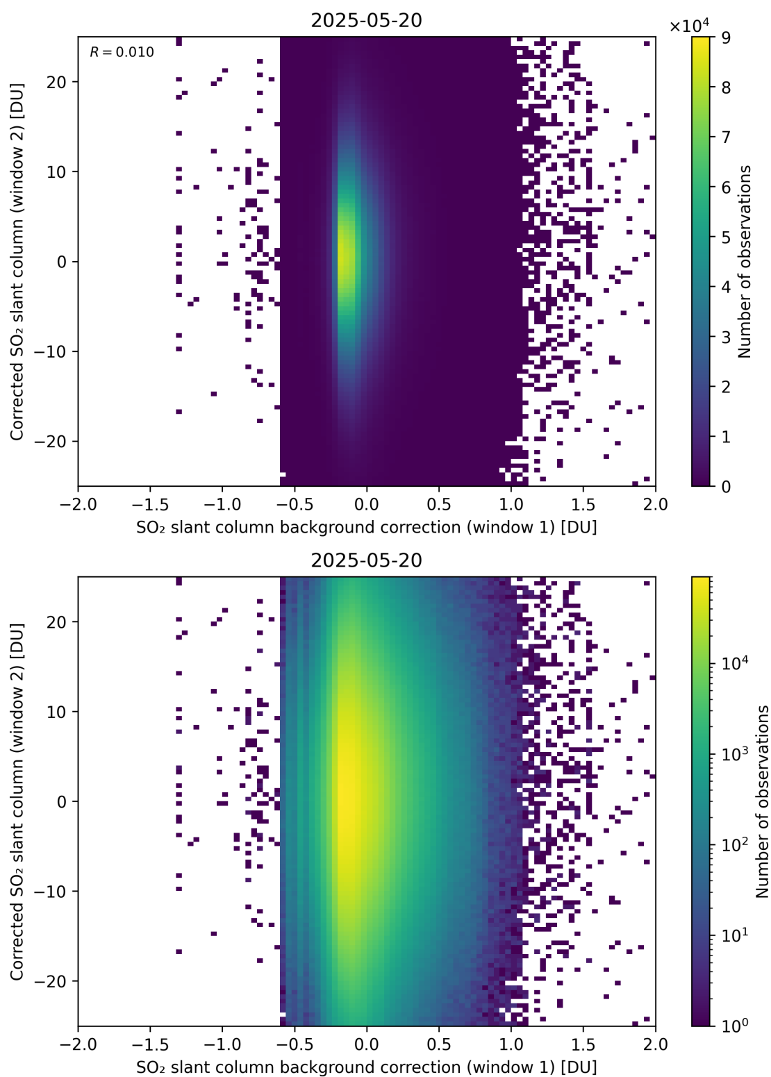
Figure 115: Scatter density plot of “SO 2 slant column background correction (window 1)” against “Corrected SO 2 slant column (window 2)” for 2025-05-19 to 2025-05-21.
