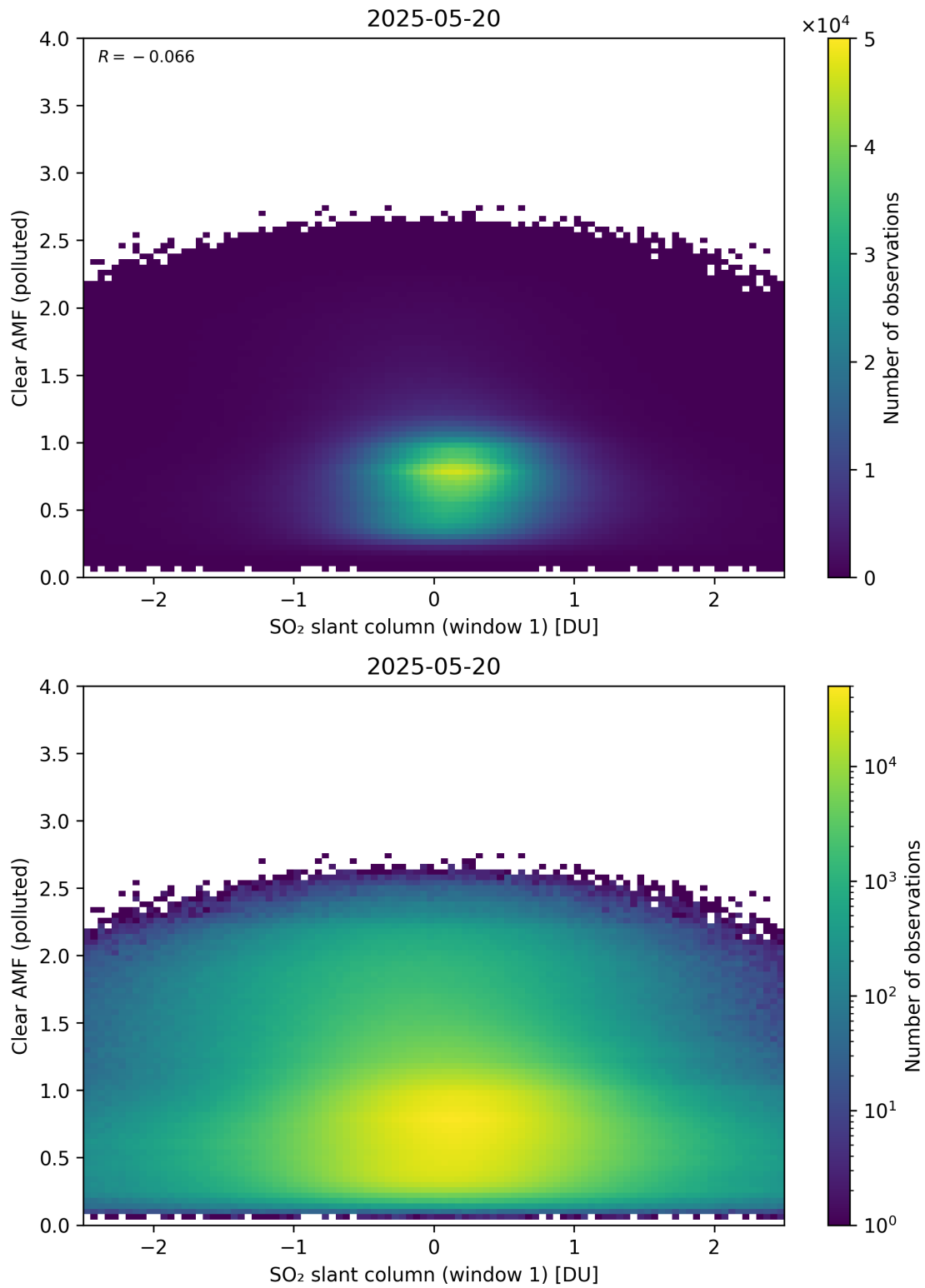
Figure 282: Scatter density plot of “SO 2 slant column (window 1)” against “Clear AMF (polluted)” for 2025-05-19 to 2025-05-21.
