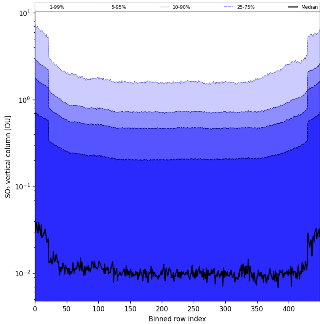
Figure 84: Along track statistics of “SO 2 vertical column” for 2025-05-19 to 2025-05-21
