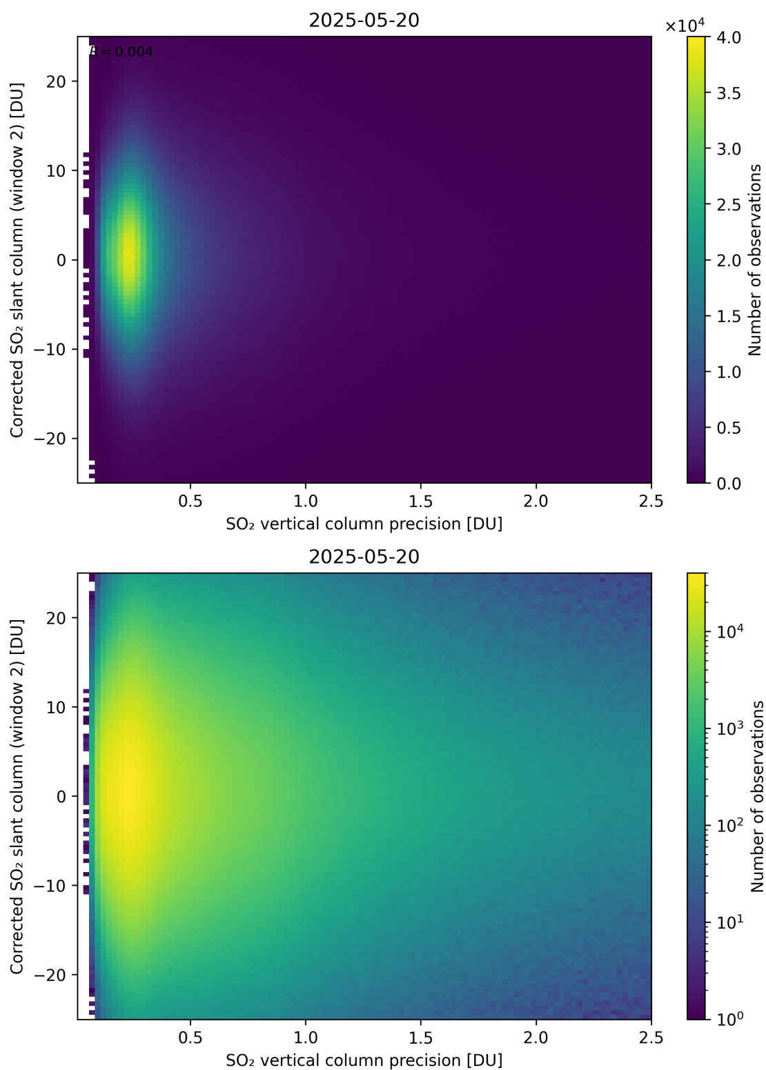
Figure 339: Scatter density plot of “SO 2 vertical column precision” against “Corrected SO 2 slant column (window 2)” for 2025-05-19 to 2025-05-21.
