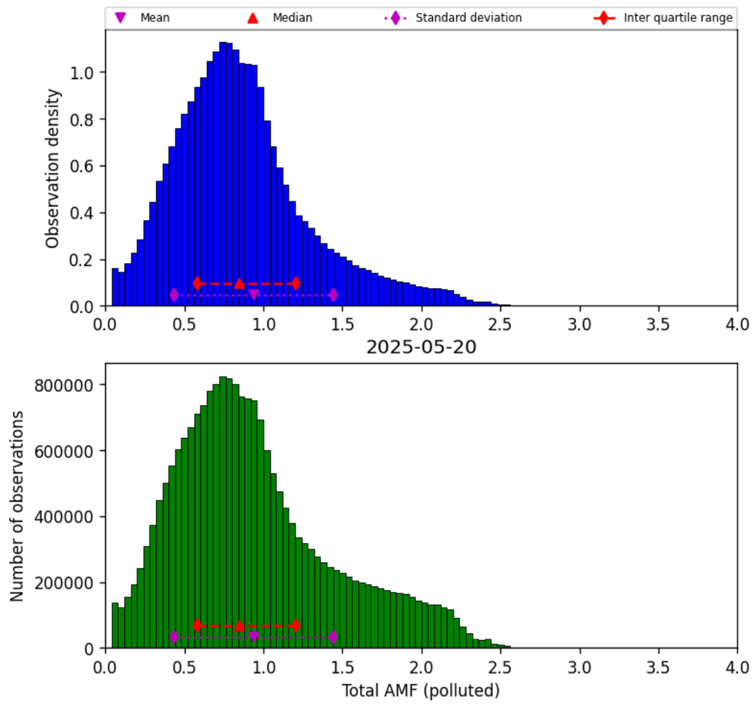
Figure 79: Histogram of “Total AMF (polluted)” for 2025-05-19 to 2025-05-21
