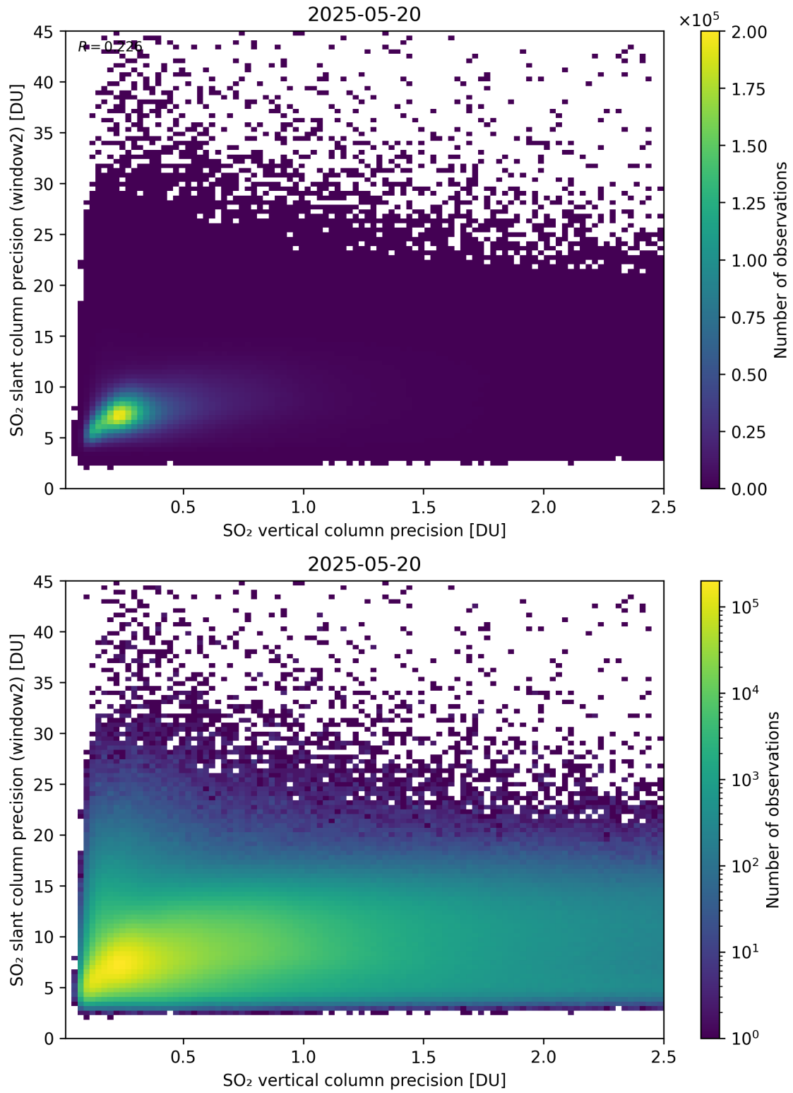
Figure 343: Scatter density plot of “SO 2 vertical column precision” against “SO 2 slant column precision (window2)” for 2025-05-19 to 2025-05-21.
