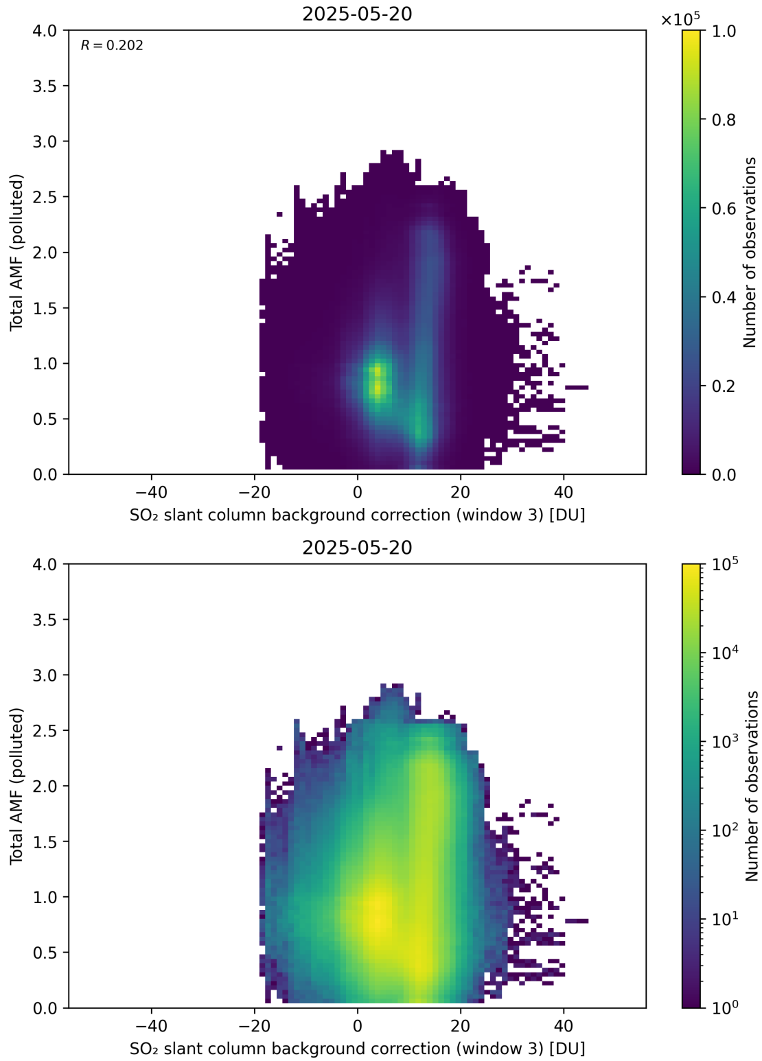
Figure 136: Scatter density plot of “SO 2 slant column background correction (window 3)” against “Total AMF (polluted)” for 2025-05-19 to 2025-05-21.
