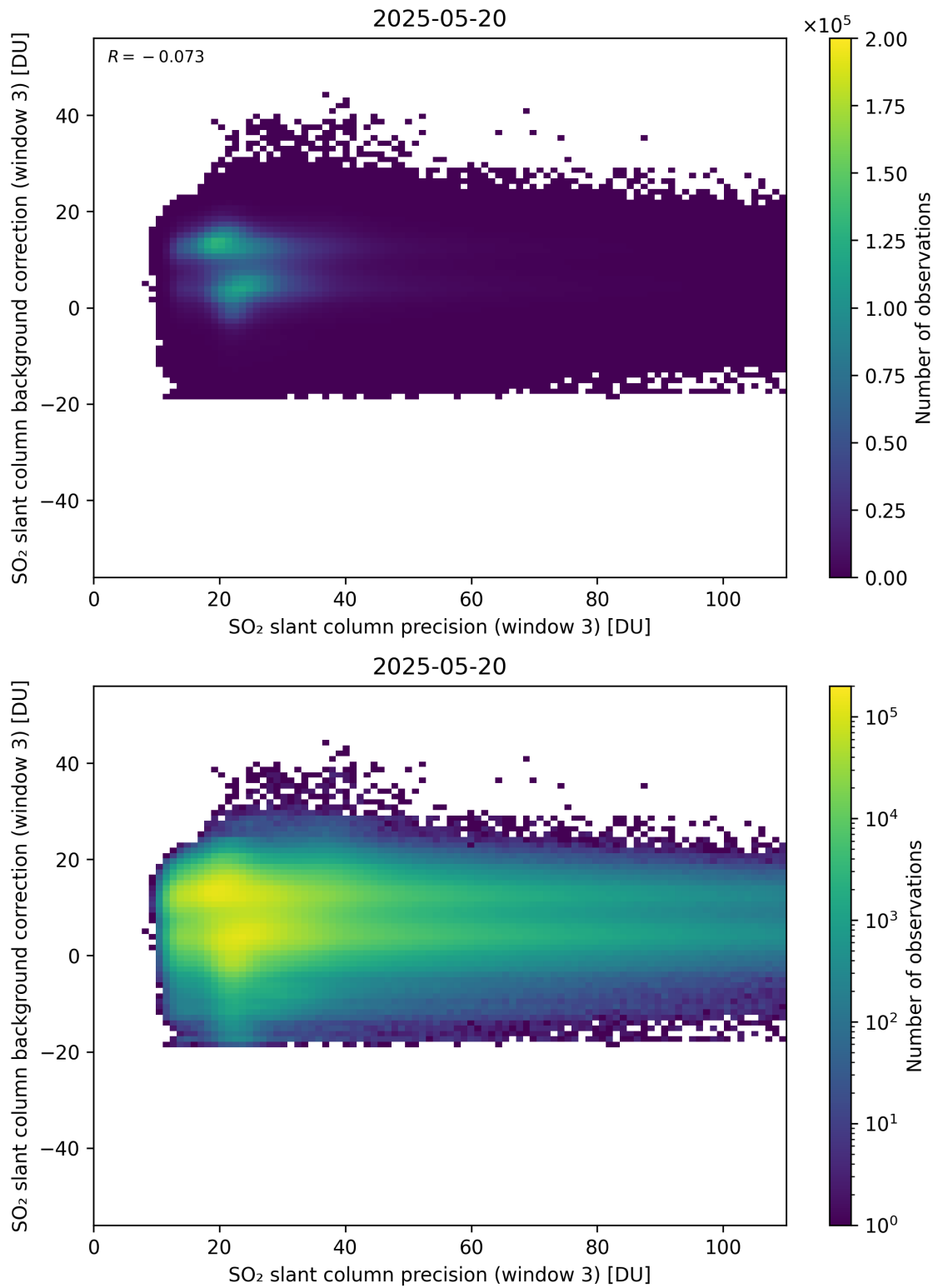
Figure 307: Scatter density plot of “SO 2 slant column precision (window 3)” against “SO 2 slant column background correction (window 3)” for 2025-05-19 to 2025-05-21.
