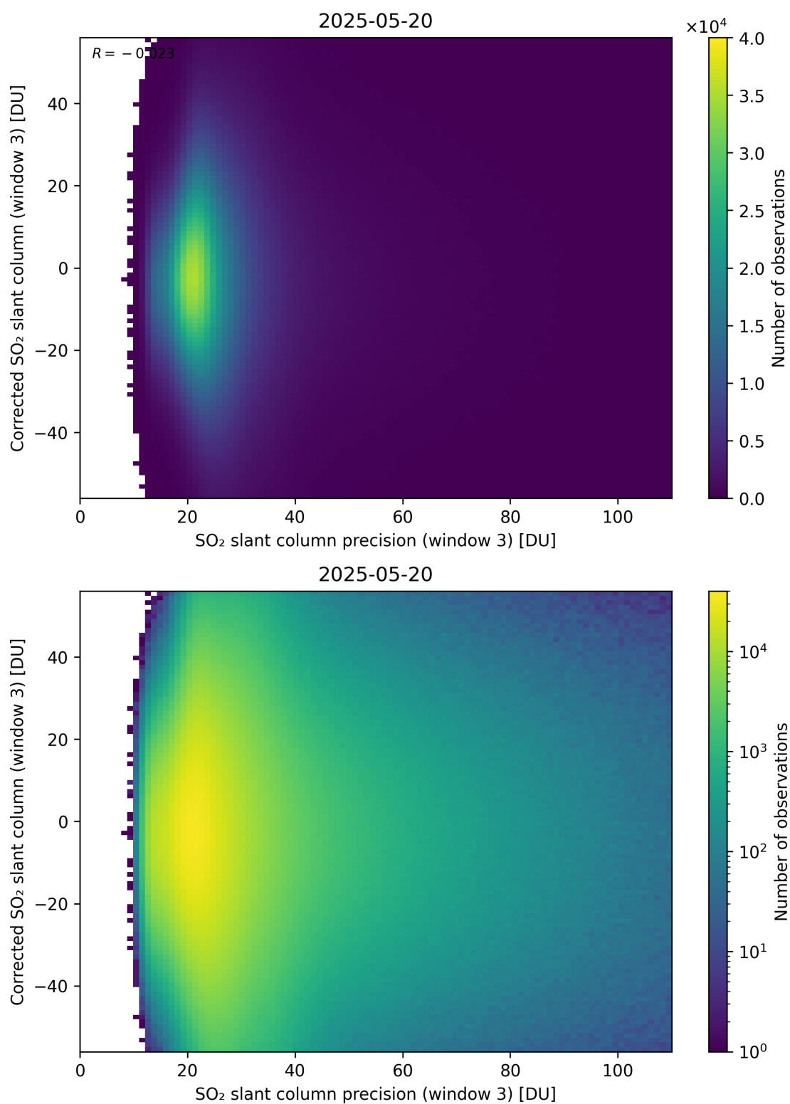
Figure 312: Scatter density plot of “SO 2 slant column precision (window 3)” against “Corrected SO 2 slant column (window 3)” for 2025-05-19 to 2025-05-21.
