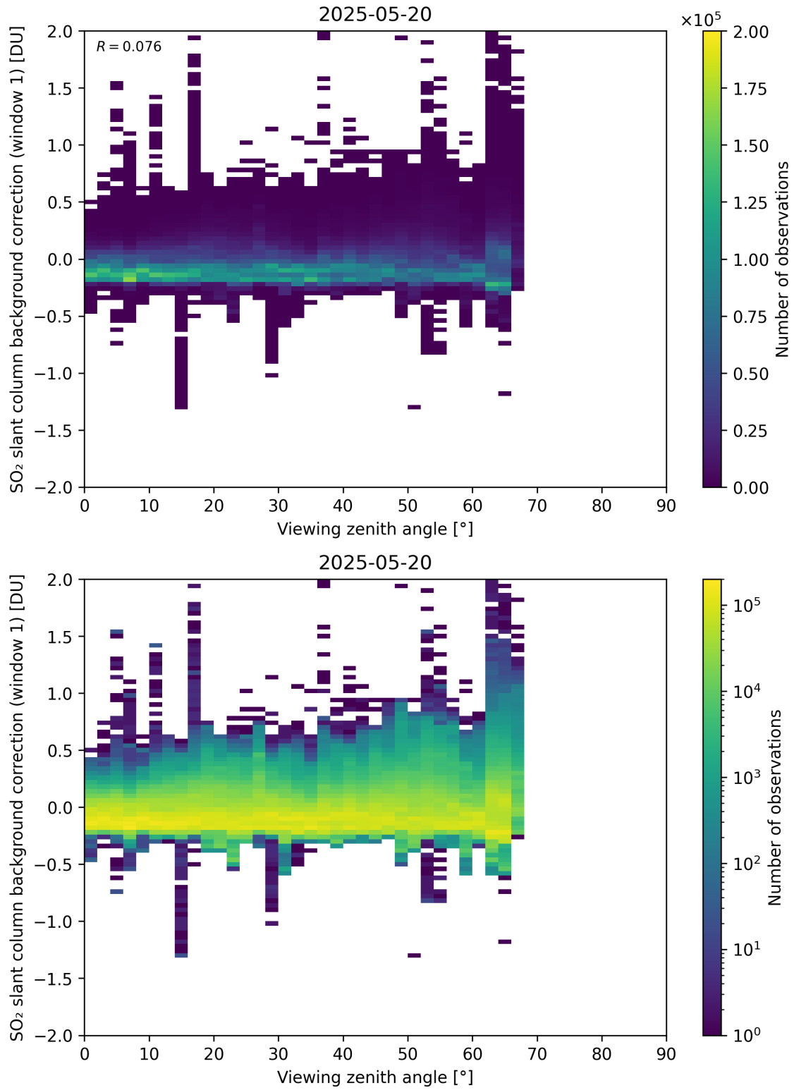
Figure 362: Scatter density plot of “Viewing zenith angle” against “SO 2 slant column background correction (window 1)” for 2025-05-19 to 2025-05-21.
