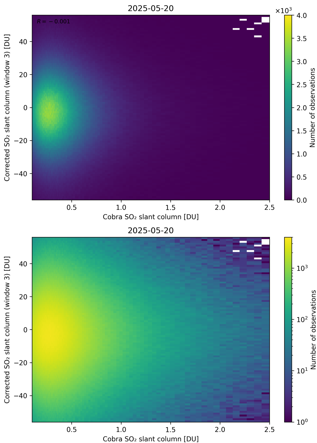
Figure 218: Scatter density plot of “Cobra SO 2 slant column” against “Corrected SO 2 slant column (window 3)” for 2025-05-19 to 2025-05-21.
