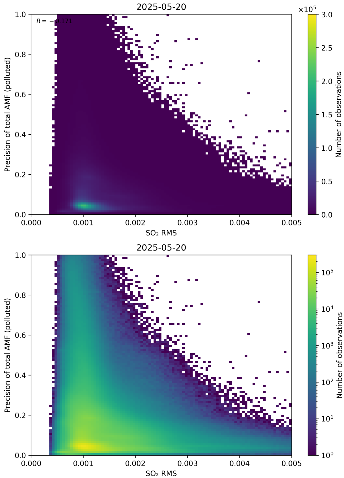
Figure 149: Scatter density plot of “SO 2 RMS” against “Precision of total AMF (polluted)” for 2025-05-19 to 2025-05-21.
