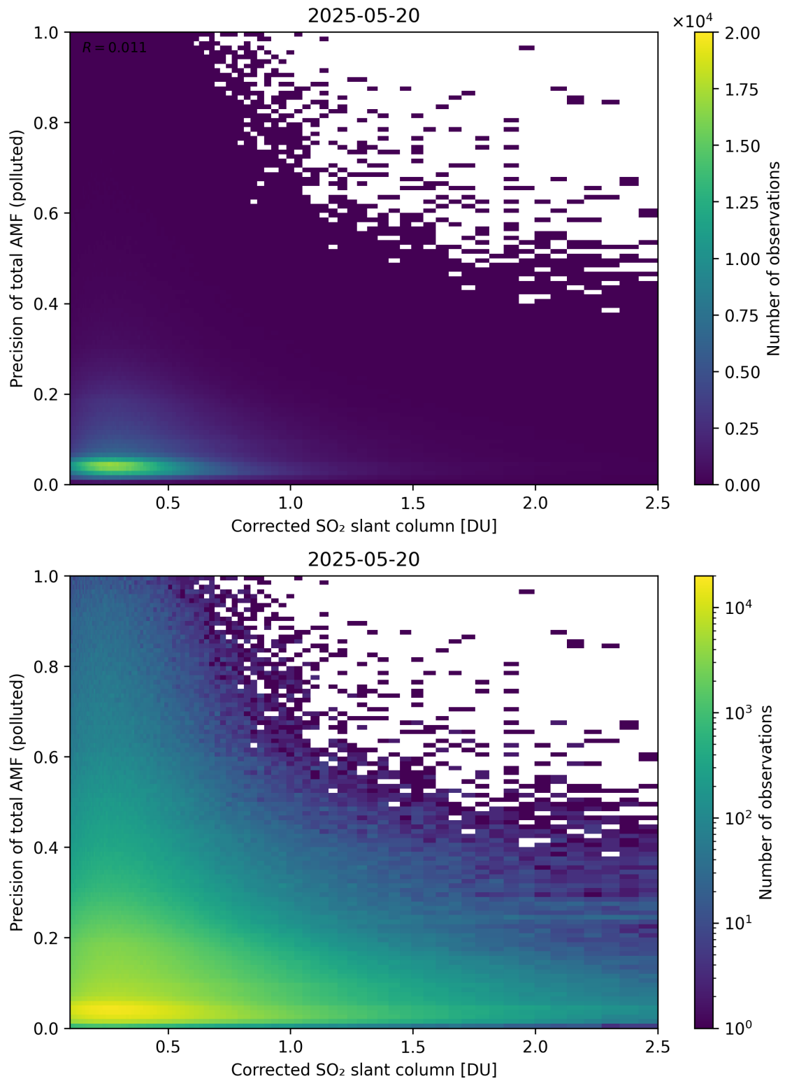
Figure 243: Scatter density plot of “Corrected SO 2 slant column” against “Precision of total AMF (polluted)” for 2025-05-19 to 2025-05-21.
