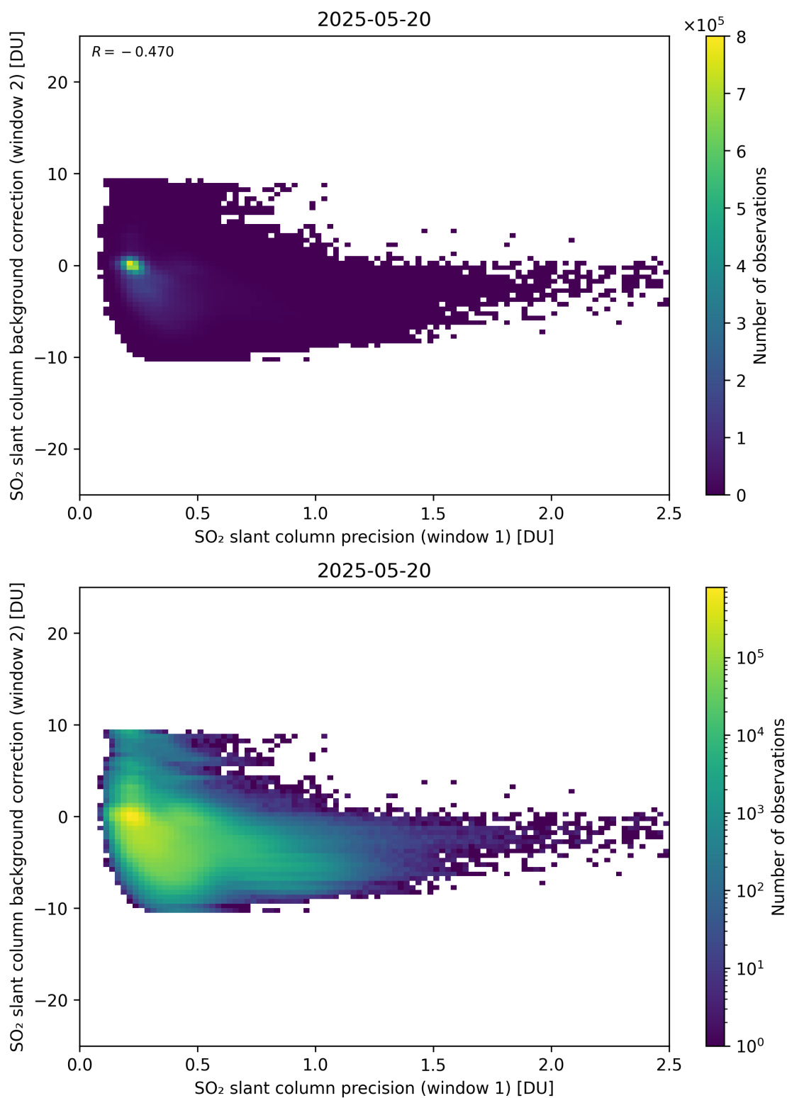
Figure 269: Scatter density plot of “SO 2 slant column precision (window 1)” against “SO 2 slant column background correction (window 2)” for 2025-05-19 to 2025-05-21.
