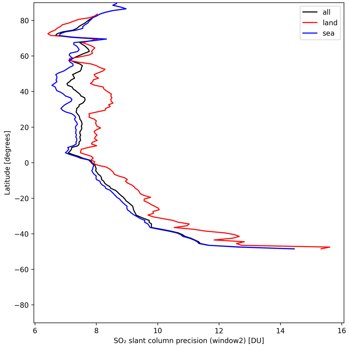
Figure 42: Zonal average of “SO 2 slant column precision (window2)” for 2025-05-19 to 2025-05-21.
