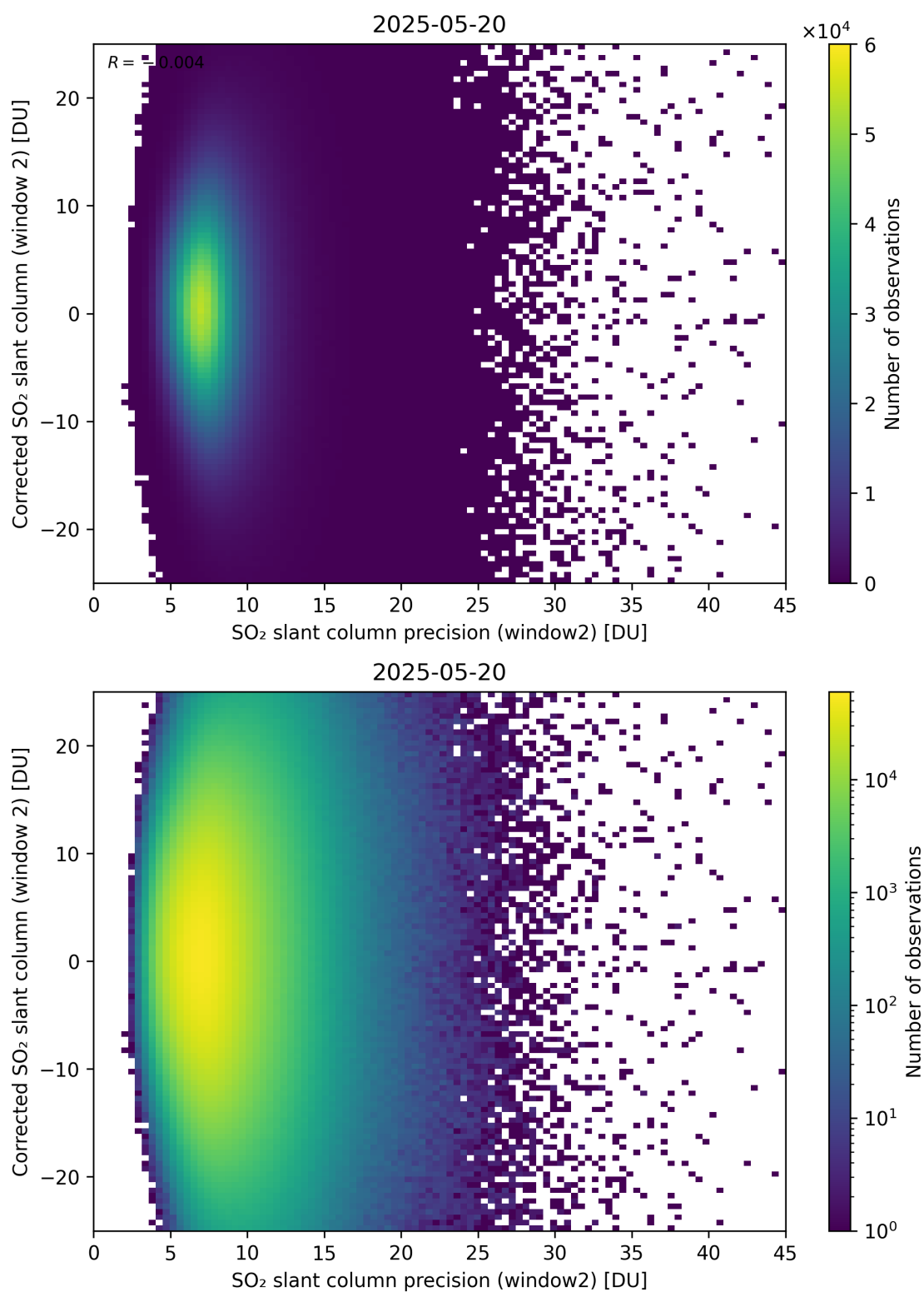
Figure 297: Scatter density plot of “SO 2 slant column precision (window2)” against “Corrected SO 2 slant column (window 2)” for 2025-05-19 to 2025-05-21.
