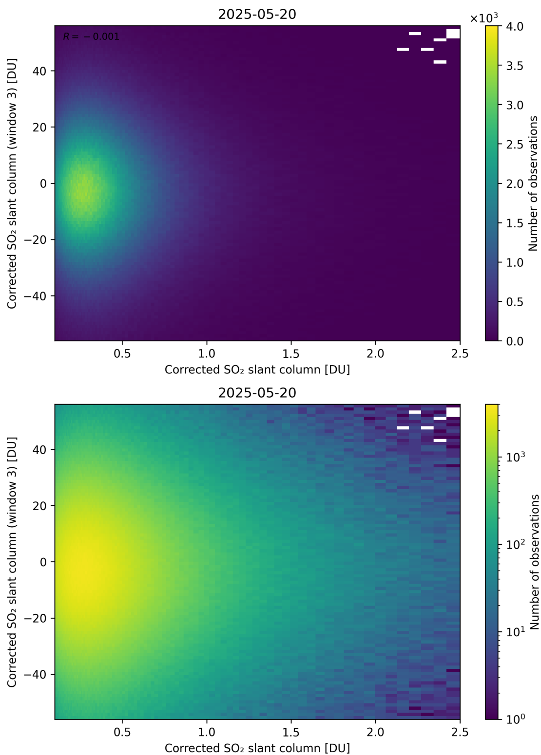
Figure 236: Scatter density plot of “Corrected SO 2 slant column” against “Corrected SO 2 slant column (window 3)” for 2025-05-19 to 2025-05-21.
