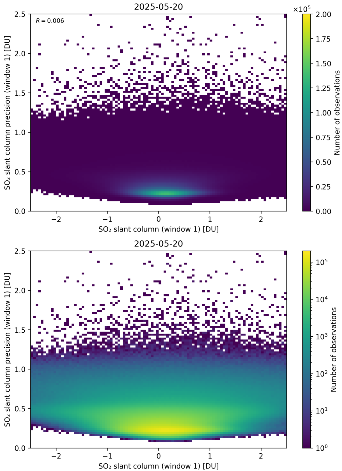
Figure 285: Scatter density plot of “SO 2 slant column (window 1)” against “SO 2 slant column precision (window 1)” for 2025-05-19 to 2025-05-21.
