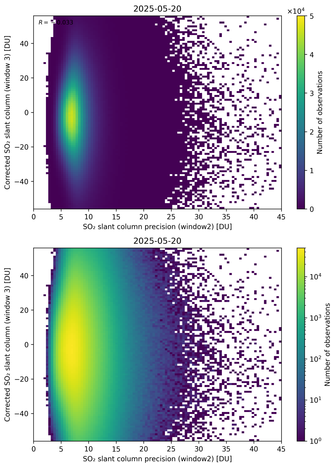
Figure 298: Scatter density plot of “SO 2 slant column precision (window2)” against “Corrected SO 2 slant column (window 3)” for 2025-05-19 to 2025-05-21.
