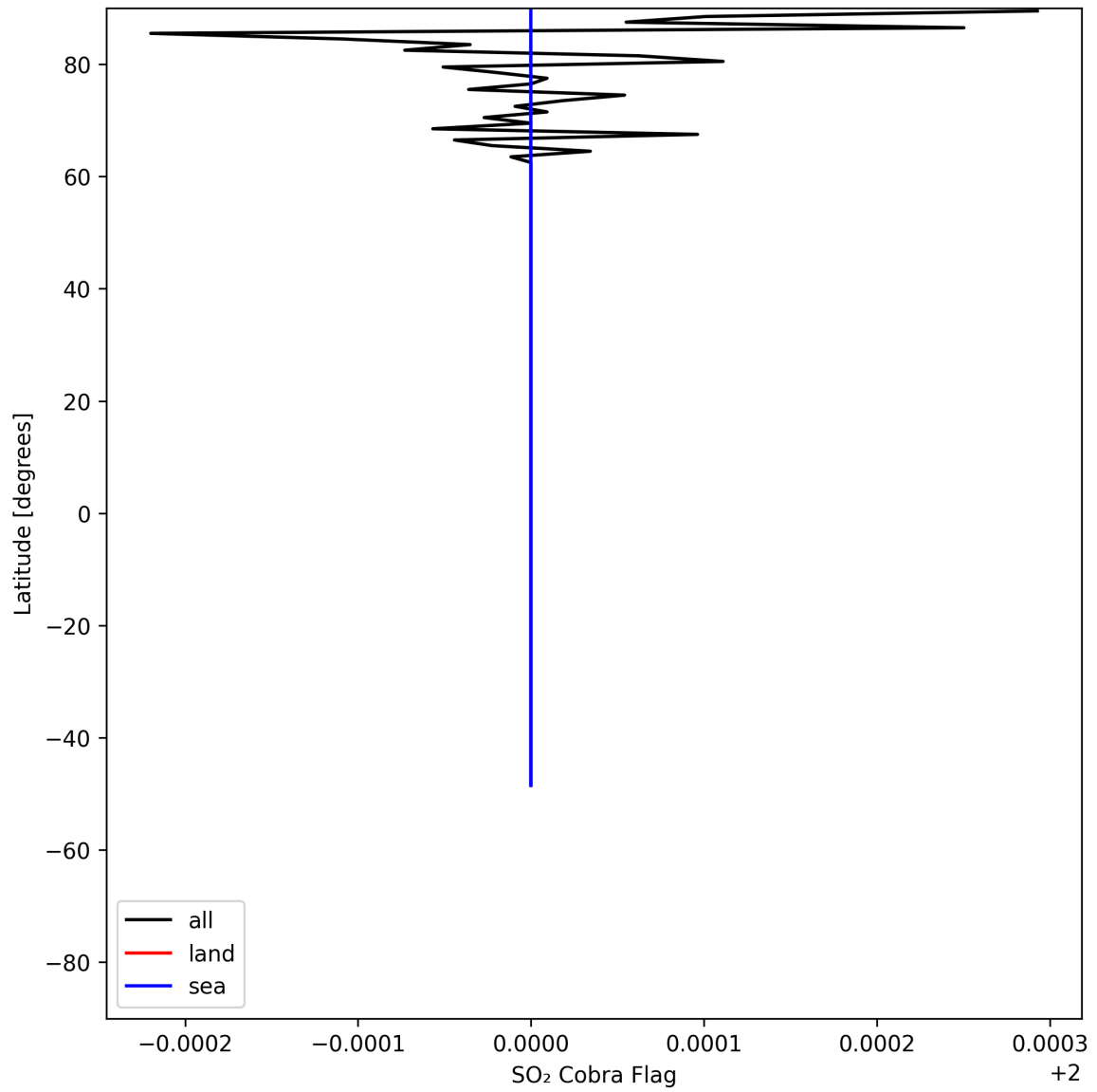
Figure 49: Zonal average of "SO 2 Cobra Flag" for 2025-05-19 to 2025-05-21.
