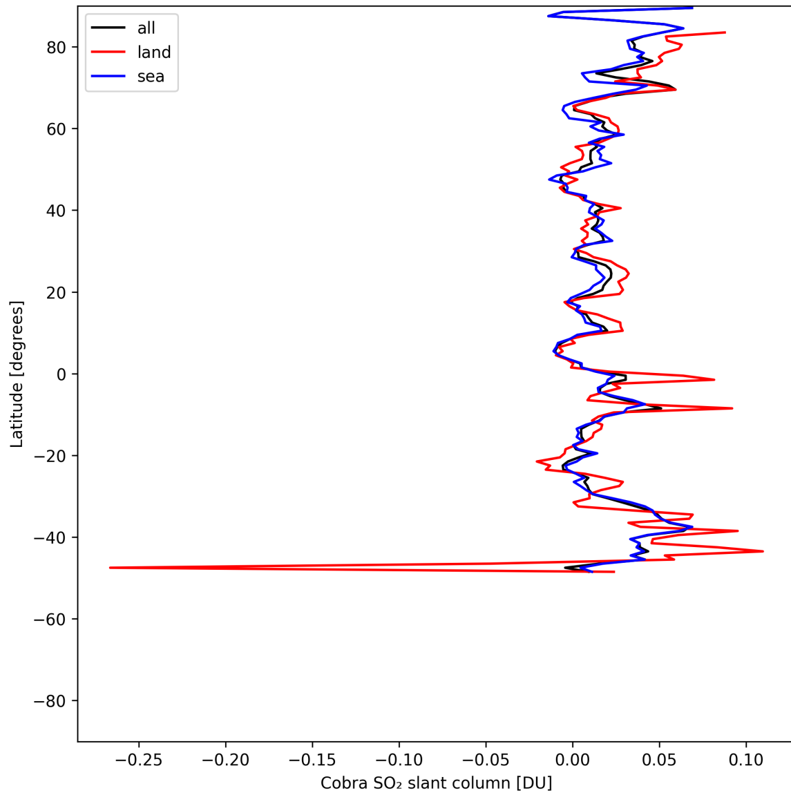
Figure 35: Zonal average of “Cobra SO 2 slant column” for 2025-05-19 to 2025-05-21.
