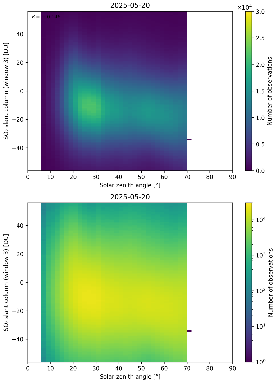
Figure 187: Scatter density plot of “Solar zenith angle” against “SO 2 slant column (window 3)” for 2025-05-19 to 2025-05-21.
