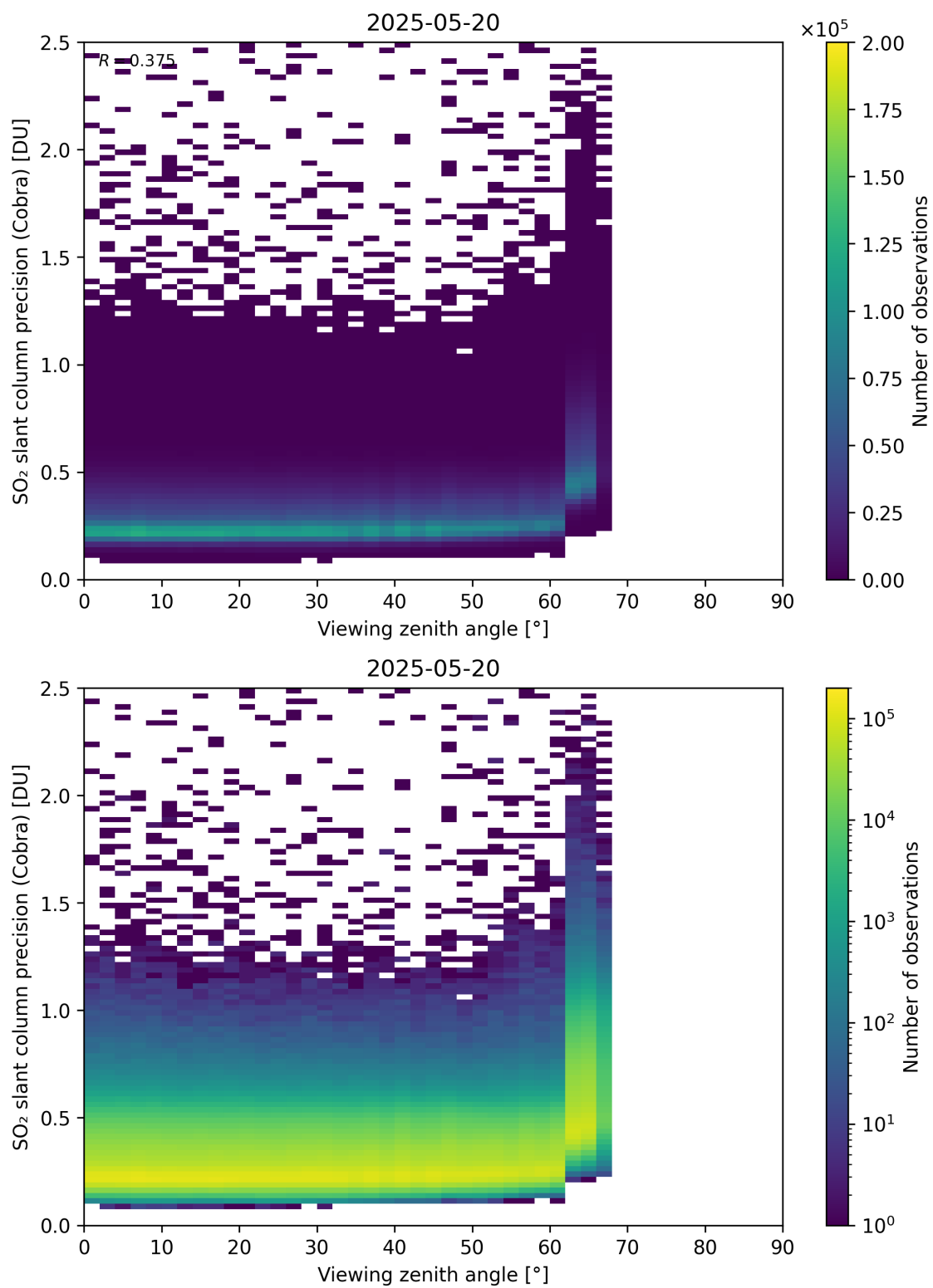
Figure 372: Scatter density plot of “Viewing zenith angle” against “SO 2 slant column precision (Cobra)” for 2025-05-19 to 2025-05-21.
