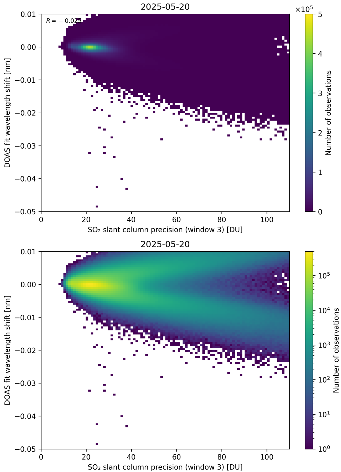
Figure 308: Scatter density plot of “SO 2 slant column precision (window 3)” against “DOAS fit wavelength shift” for 2025-05-19 to 2025-05-21.
