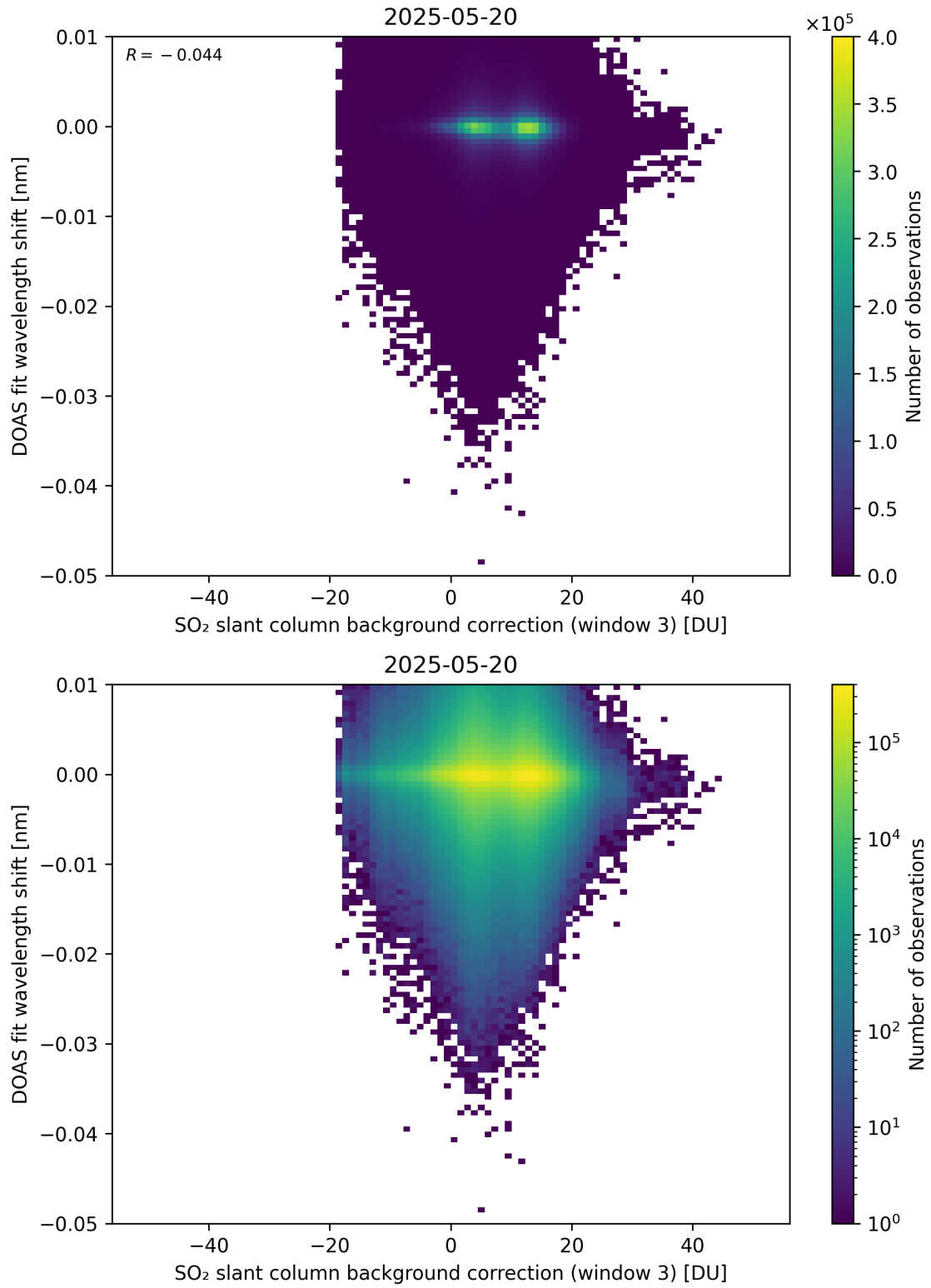
Figure 132: Scatter density plot of “SO 2 slant column background correction (window 3)” against “DOAS fit wavelength shift” for 2025-05-19 to 2025-05-21.
