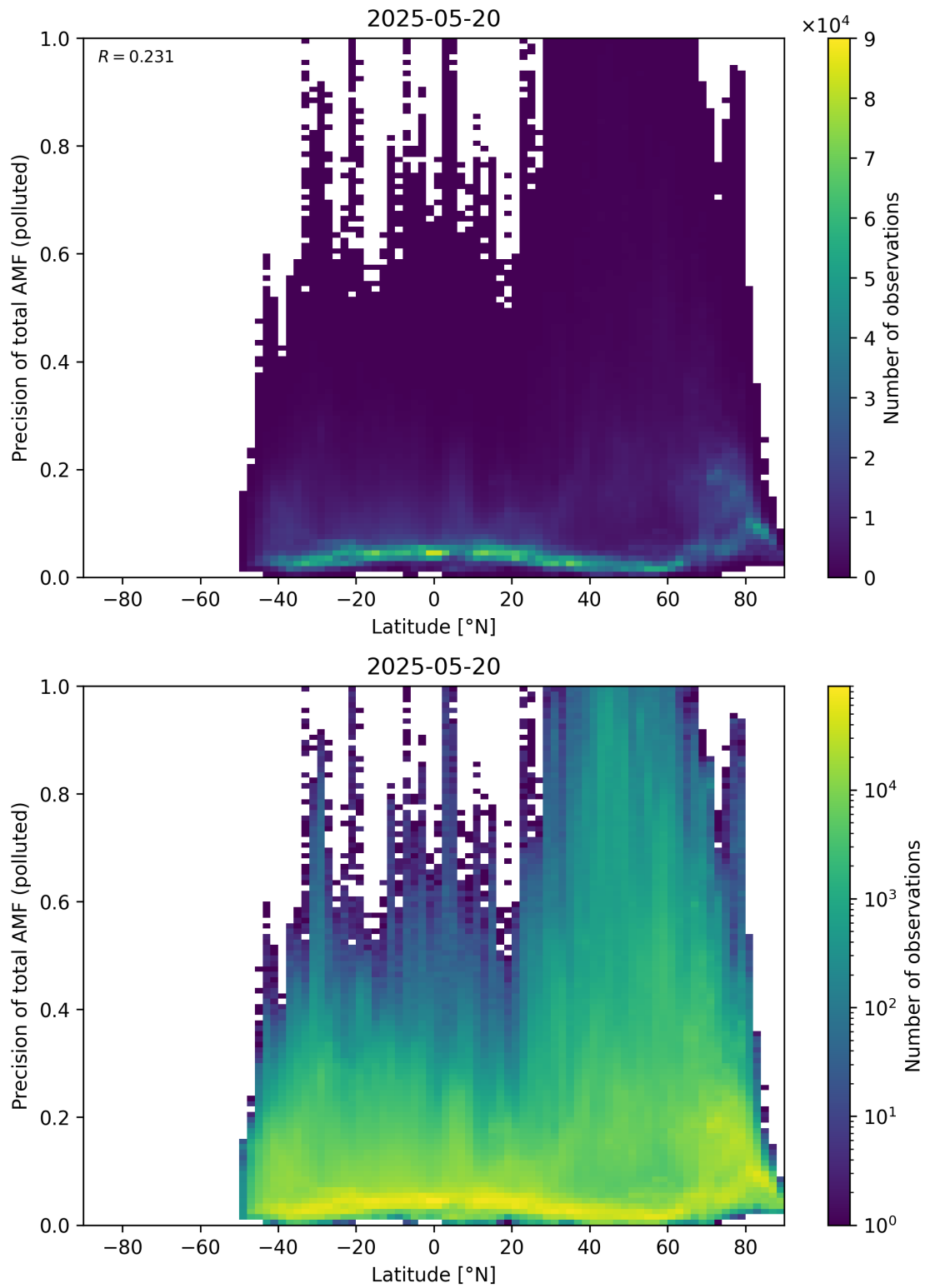
Figure 168: Scatter density plot of “Latitude” against “Precision of total AMF (polluted)” for 2025-05-19 to 2025-05-21.
