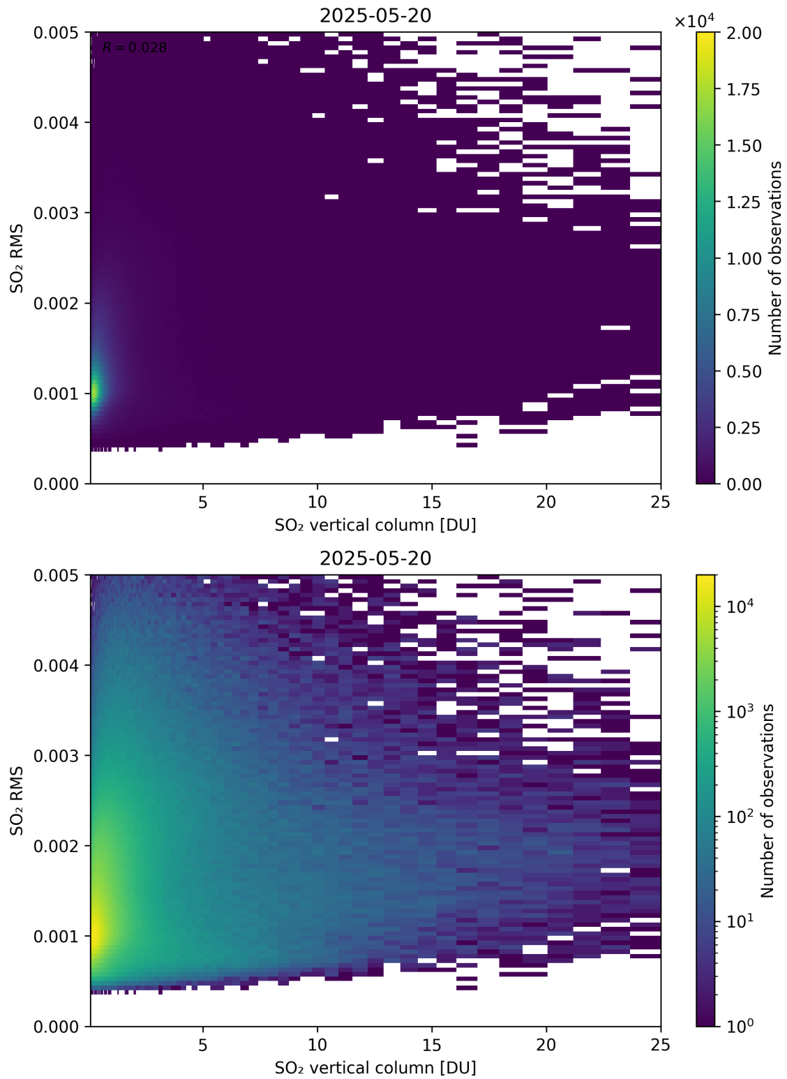
Figure 328: Scatter density plot of “SO 2 vertical column” against “SO 2 RMS” for 2025-05-19 to 2025-05-21.
