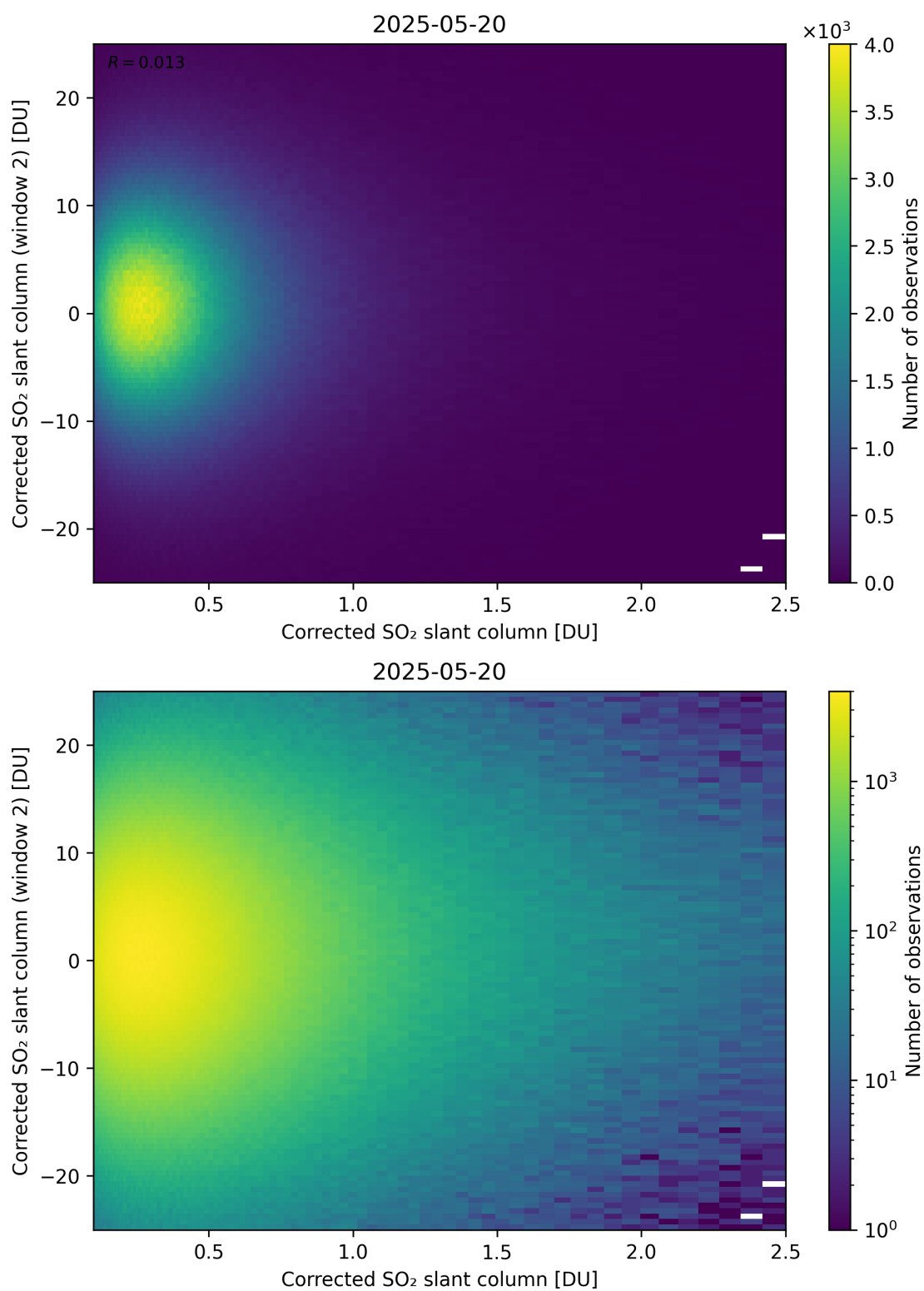
Figure 235: Scatter density plot of “Corrected SO 2 slant column” against “Corrected SO 2 slant column (window 2)” for 2025-05-19 to 2025-05-21.
