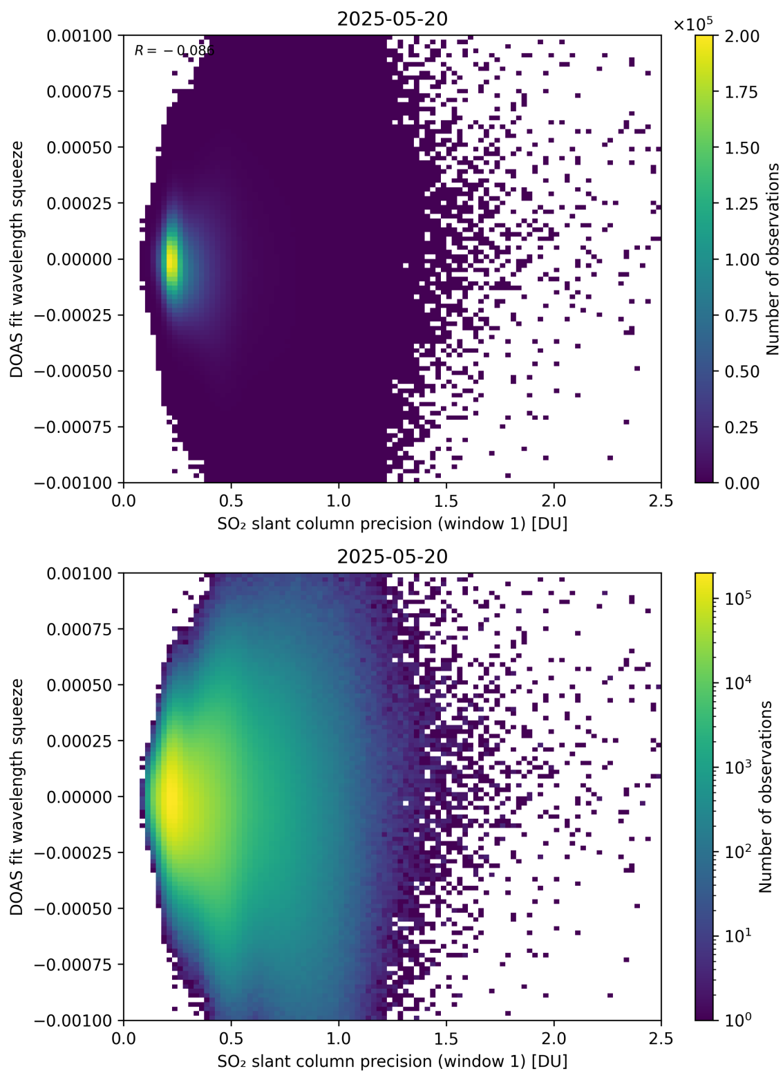
Figure 272: Scatter density plot of “SO 2 slant column precision (window 1)” against “DOAS fit wavelength squeeze” for 2025-05-19 to 2025-05-21.
