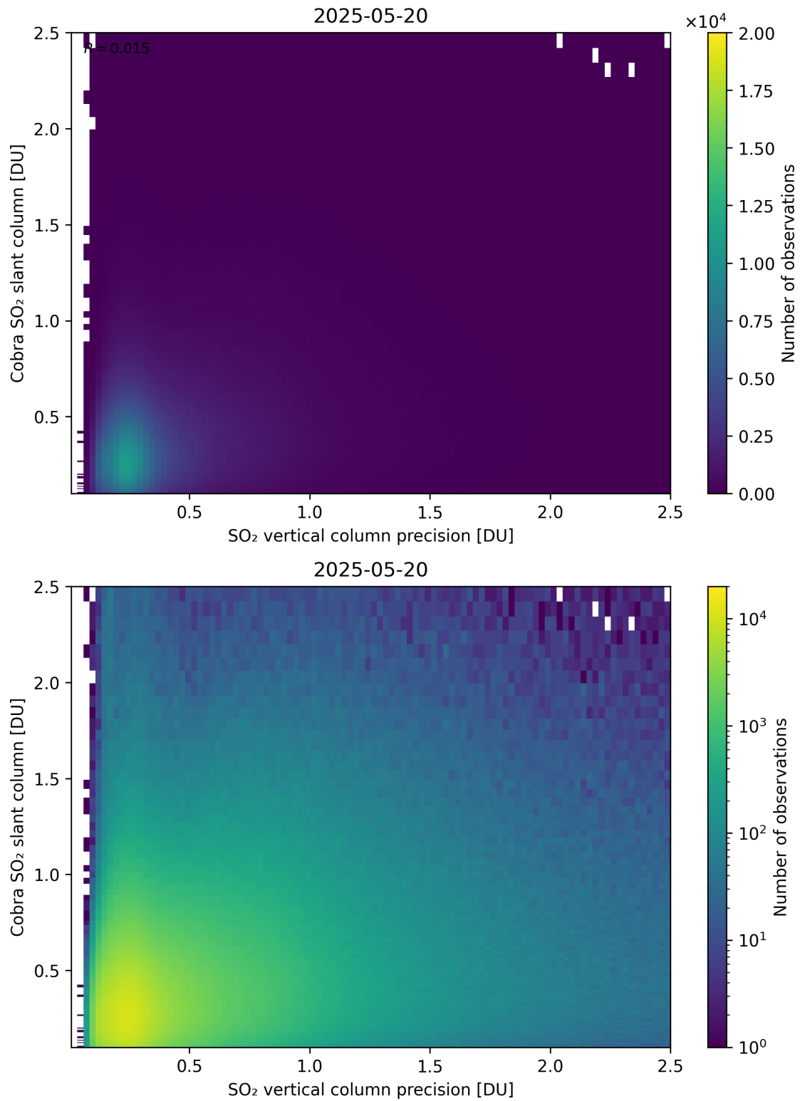
Figure 336: Scatter density plot of “SO 2 vertical column precision” against “Cobra SO 2 slant column” for 2025-05-19 to 2025-05-21.
