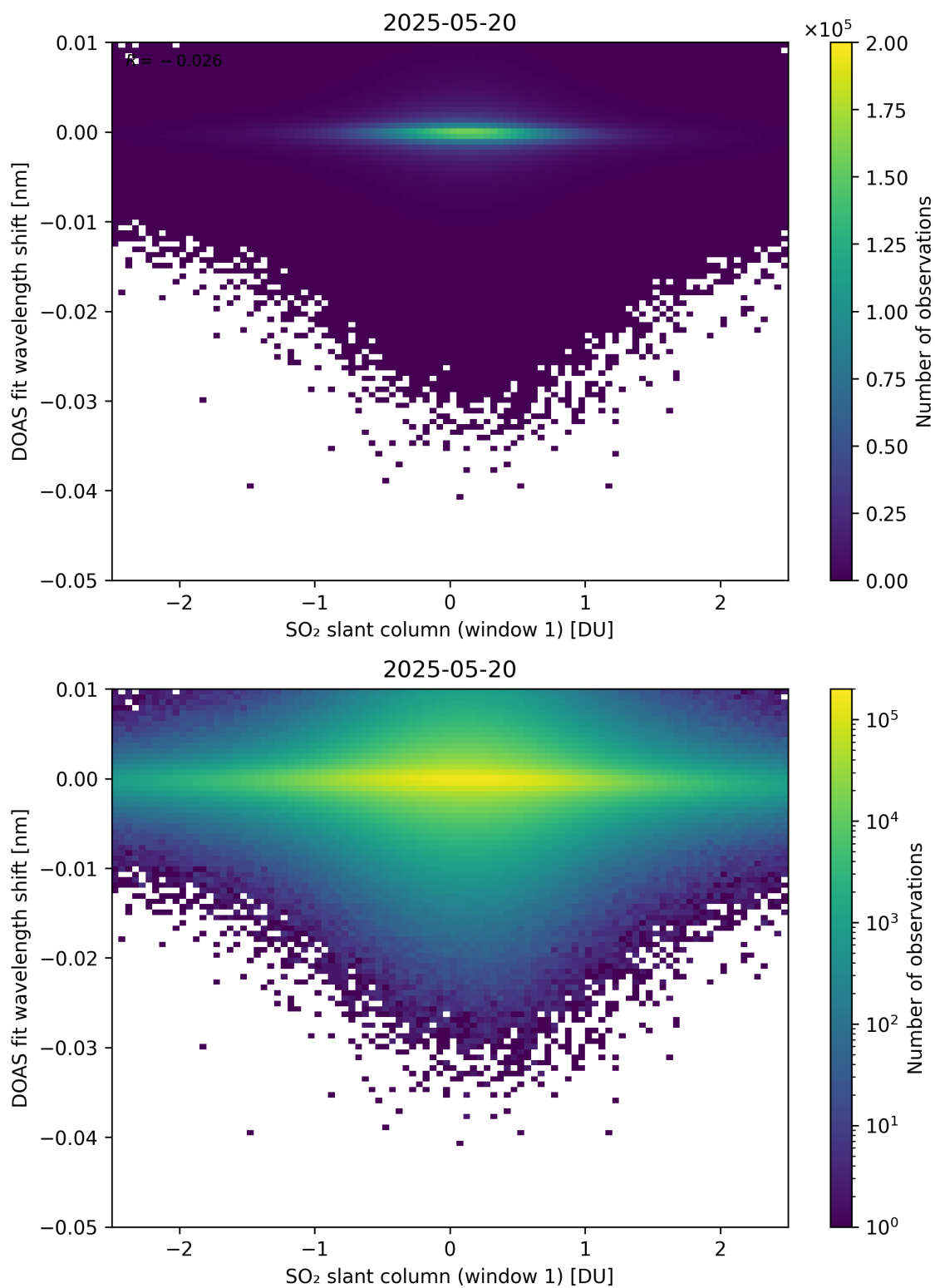
Figure 265: Scatter density plot of “SO 2 slant column (window 1)” against “DOAS fit wavelength shift” for 2025-05-19 to 2025-05-21.
