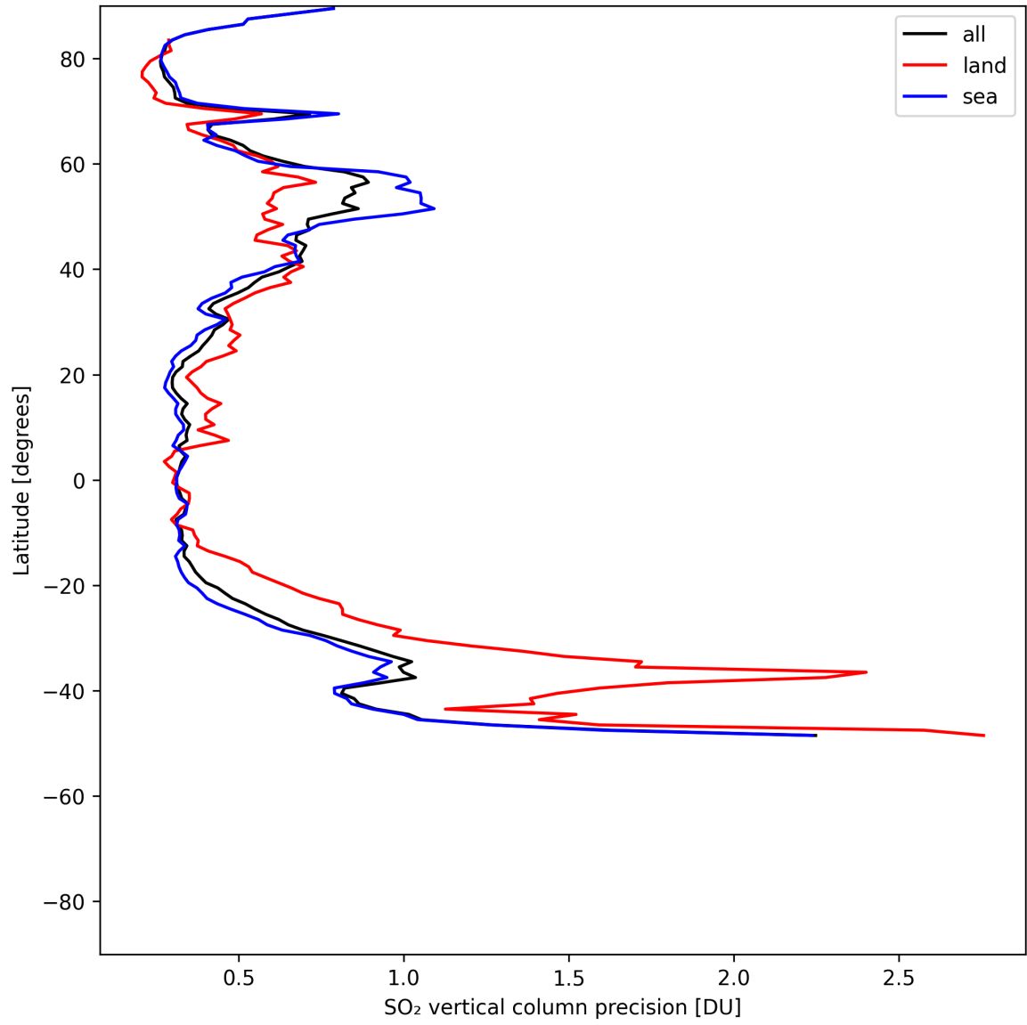
Figure 33: Zonal average of “SO 2 vertical column precision” for 2025-05-19 to 2025-05-21.
