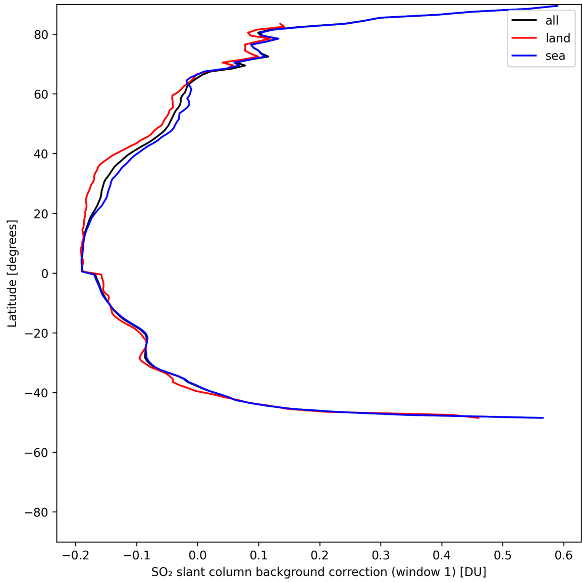
Figure 40: Zonal average of "SO 2 slant column background correction (window 1)" for 2025-05-19 to 2025-05-21.
