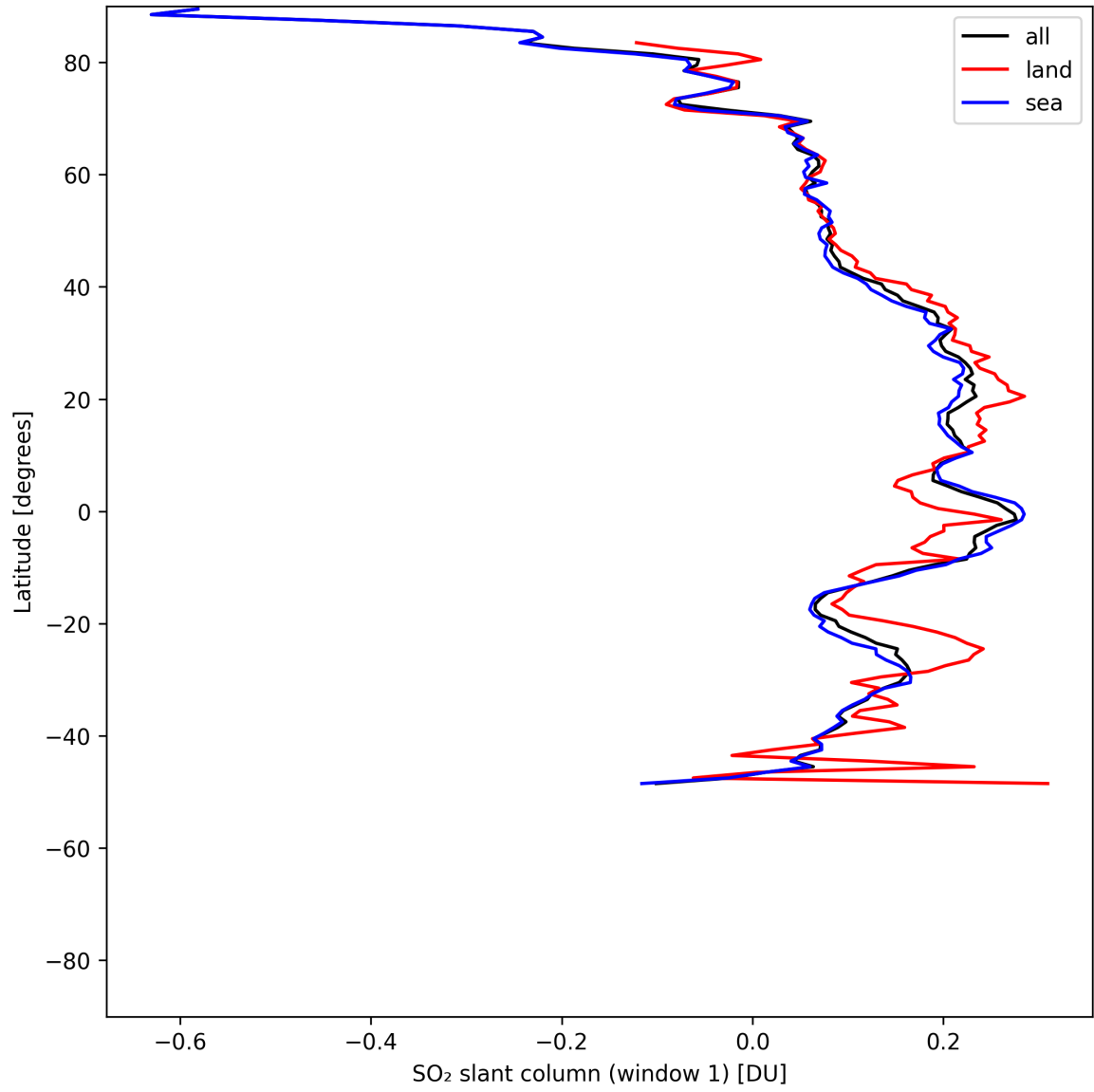
Figure 37: Zonal average of “SO 2 slant column (window 1)” for 2025-05-19 to 2025-05-21.
