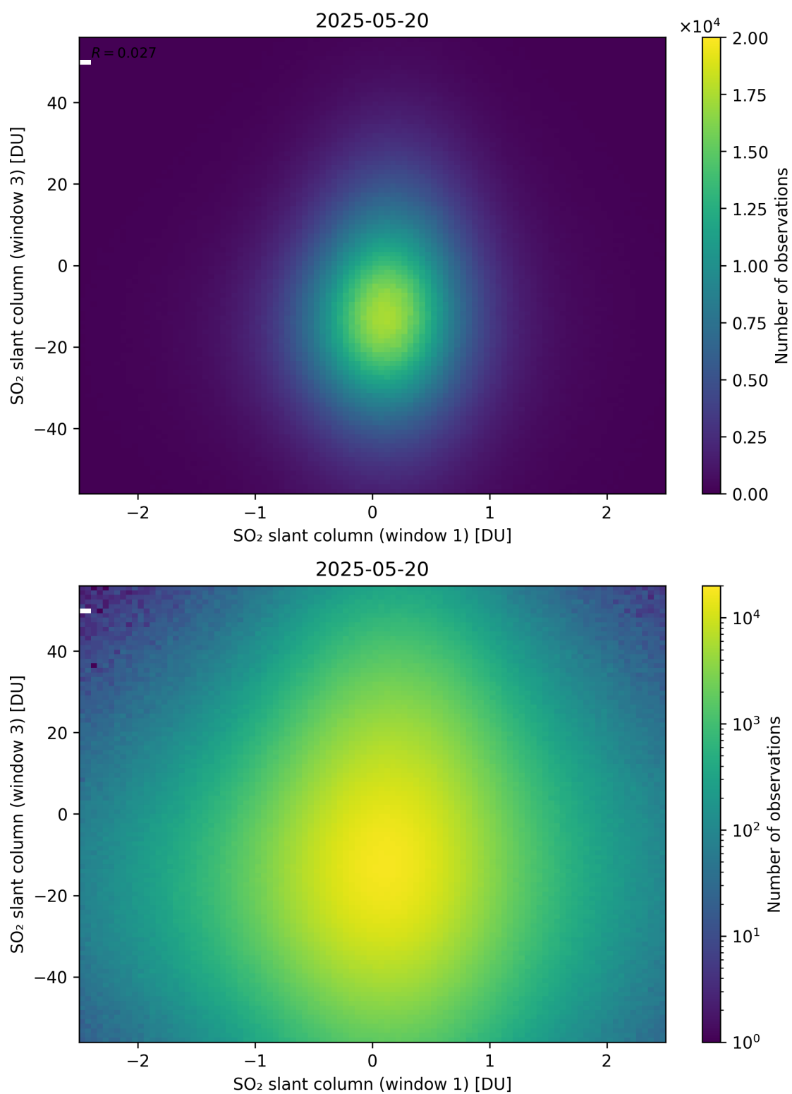
Figure 287: Scatter density plot of “SO 2 slant column (window 1)” against “SO 2 slant column (window 3)” for 2025-05-19 to 2025-05-21.
