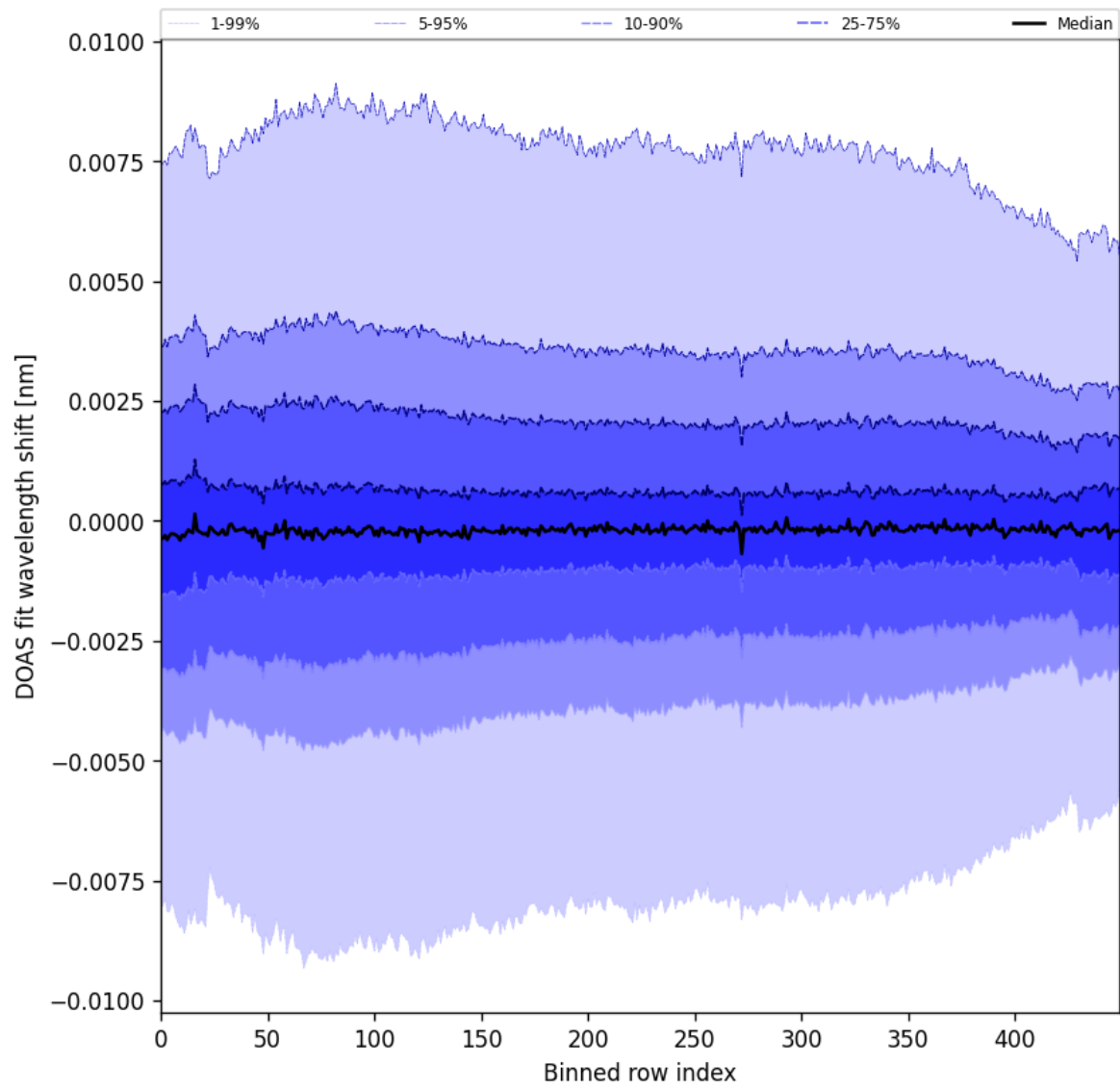
Figure 102: Along track statistics of “DOAS fit wavelength shift” for 2025-05-19 to 2025-05-21
