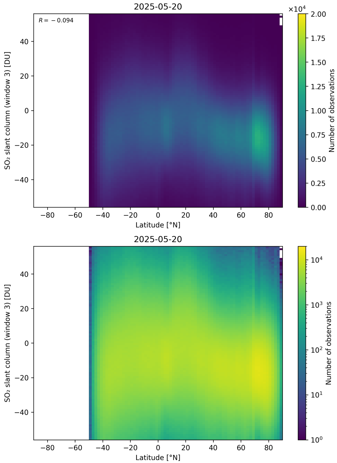
Figure 165: Scatter density plot of “Latitude” against “SO 2 slant column (window 3)” for 2025-05-19 to 2025-05-21.
