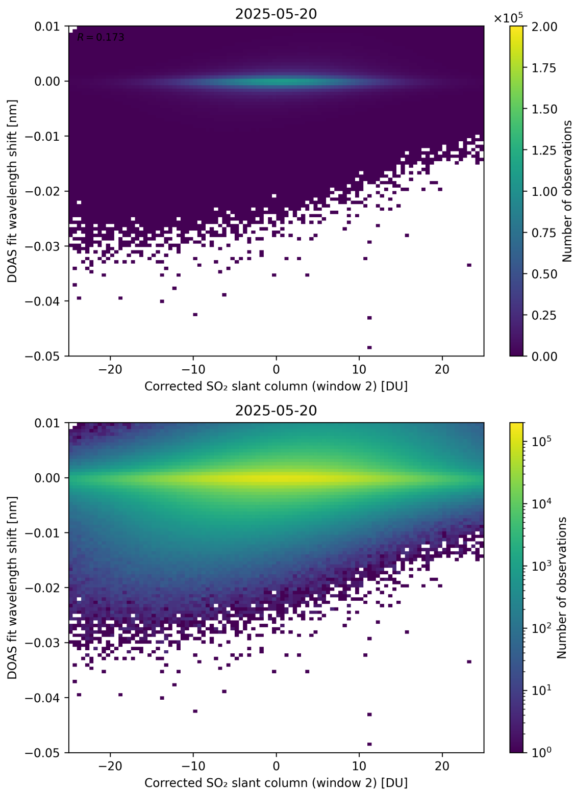
Figure 246: Scatter density plot of “Corrected SO 2 slant column (window 2)” against “DOAS fit wavelength shift” for 2025-05-19 to 2025-05-21.
