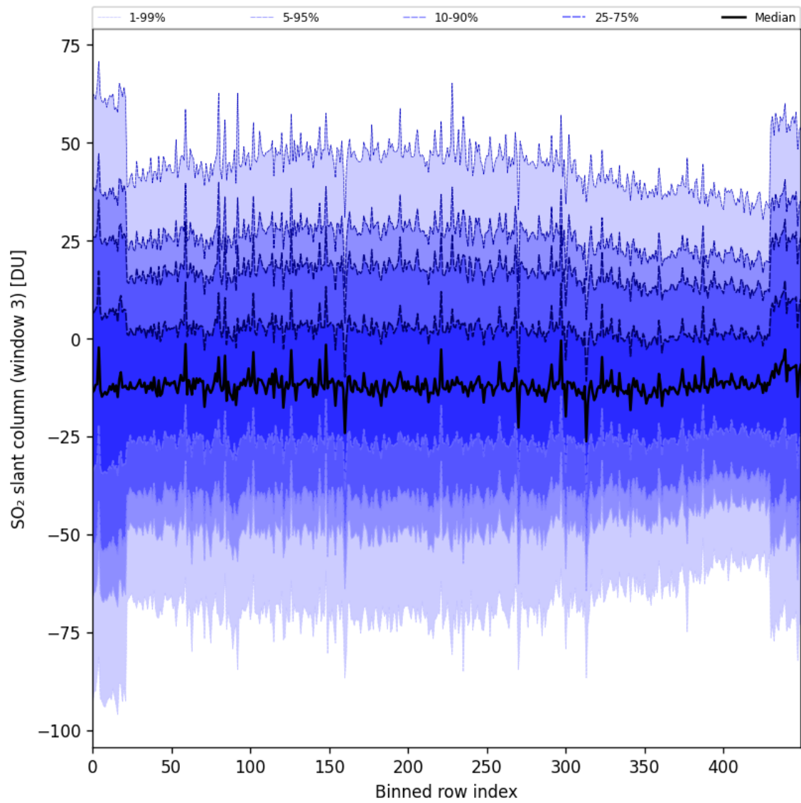
Figure 97: Along track statistics of “SO 2 slant column (window 3)” for 2025-05-19 to 2025-05-21
