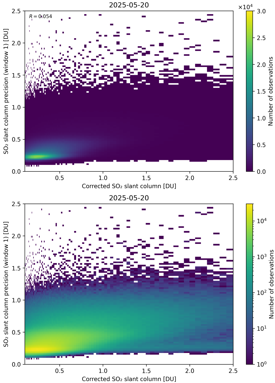
Figure 238: Scatter density plot of “Corrected SO 2 slant column” against “SO 2 slant column precision (window 1)” for 2025-05-19 to 2025-05-21.
