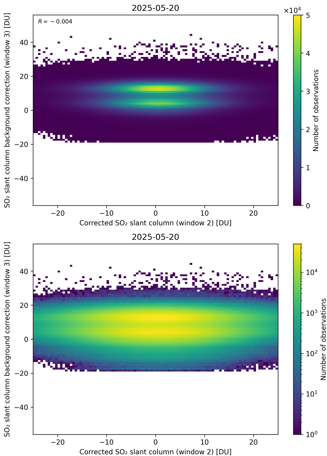
Figure 245: Scatter density plot of “Corrected SO 2 slant column (window 2)” against “SO 2 slant column background correction (window 3)” for 2025-05-19 to 2025-05-21.
