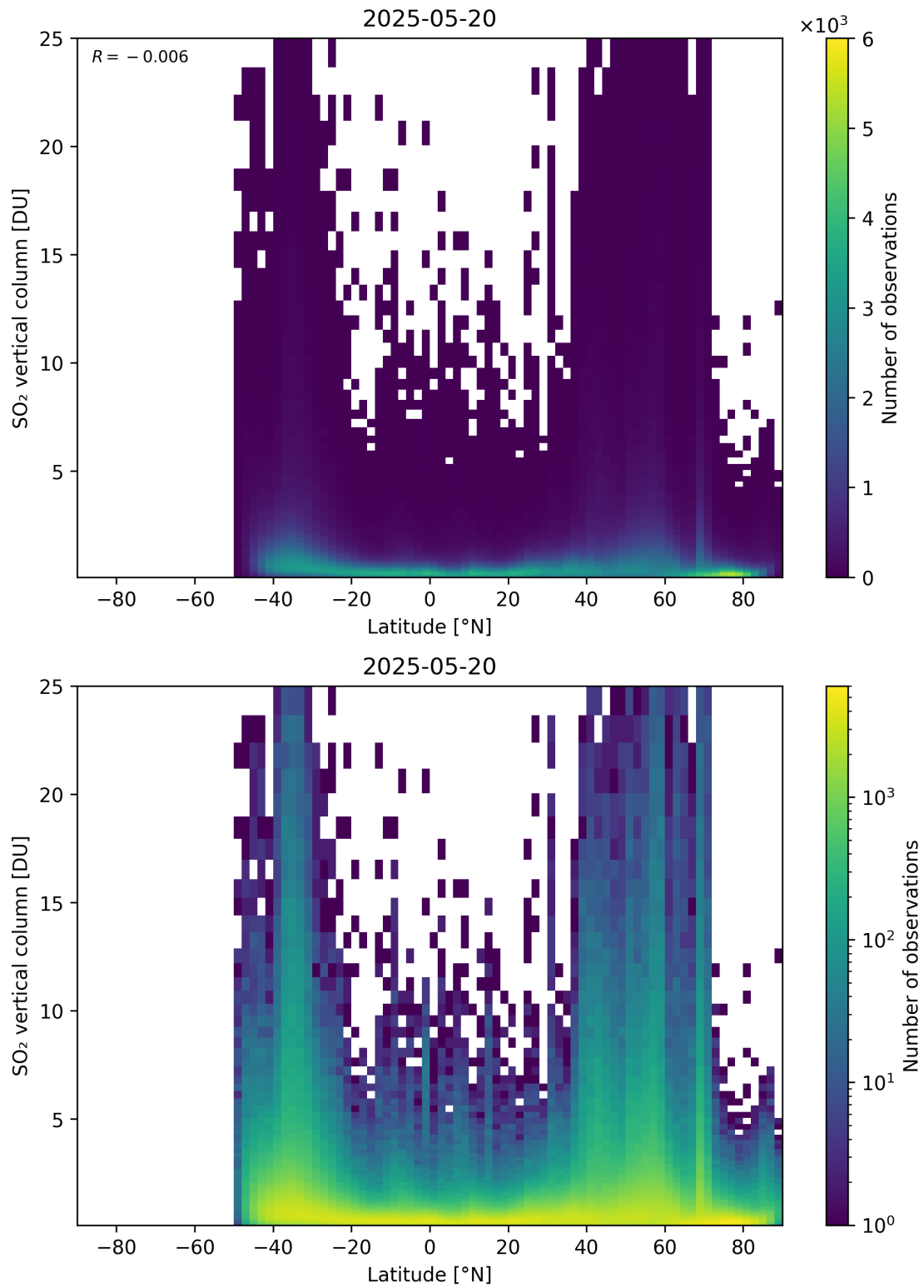
Figure 169: Scatter density plot of “Latitude” against “SO 2 vertical column” for 2025-05-19 to 2025-05-21.
