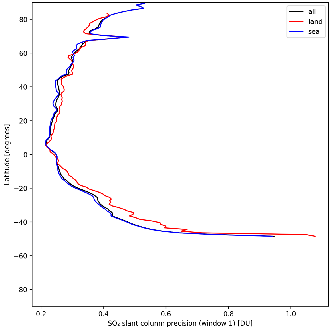
Figure 38: Zonal average of “SO 2 slant column precision (window 1)” for 2025-05-19 to 2025-05-21.
