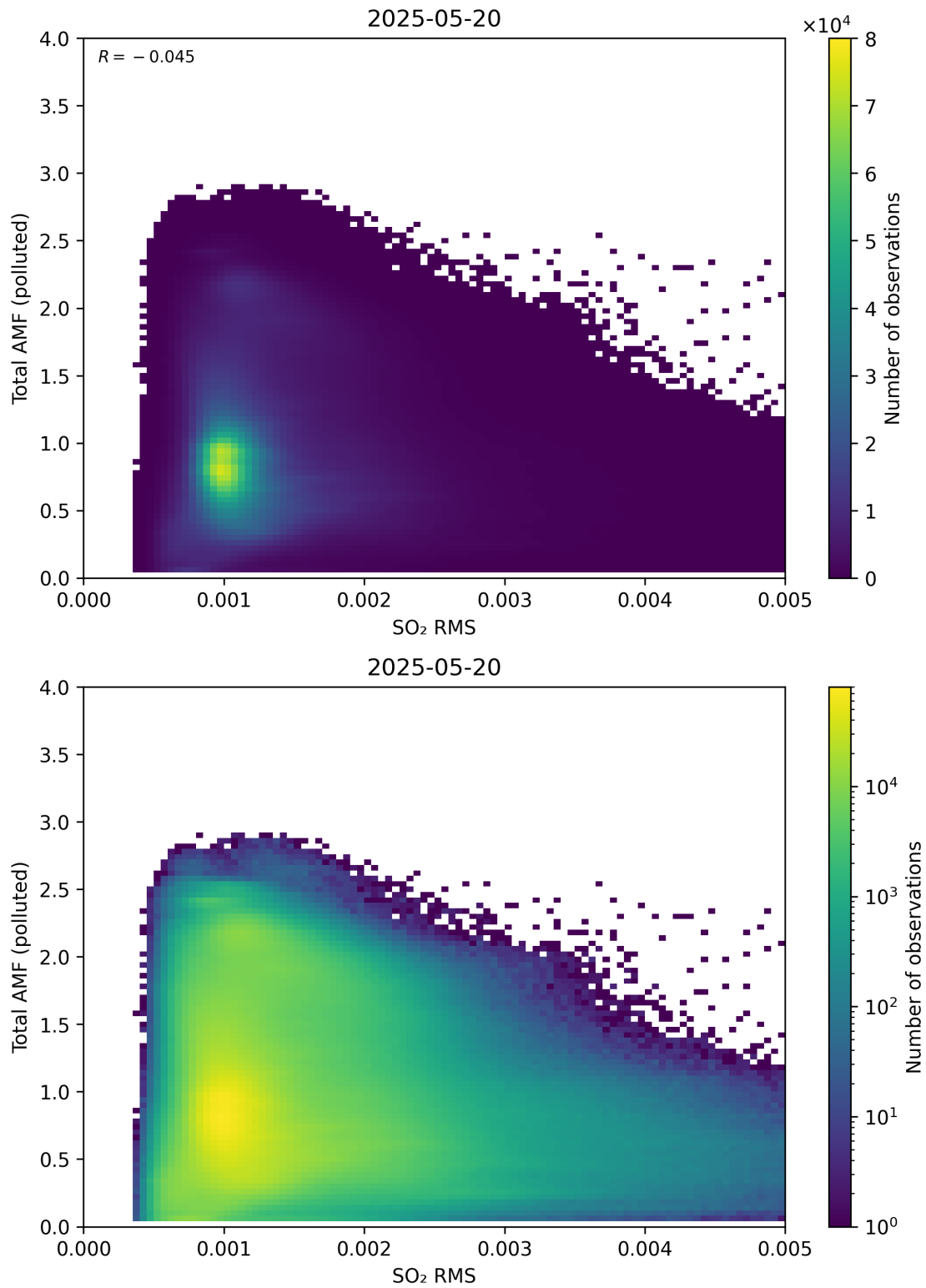
Figure 148: Scatter density plot of “SO 2 RMS” against “Total AMF (polluted)” for 2025-05-19 to 2025-05-21.
