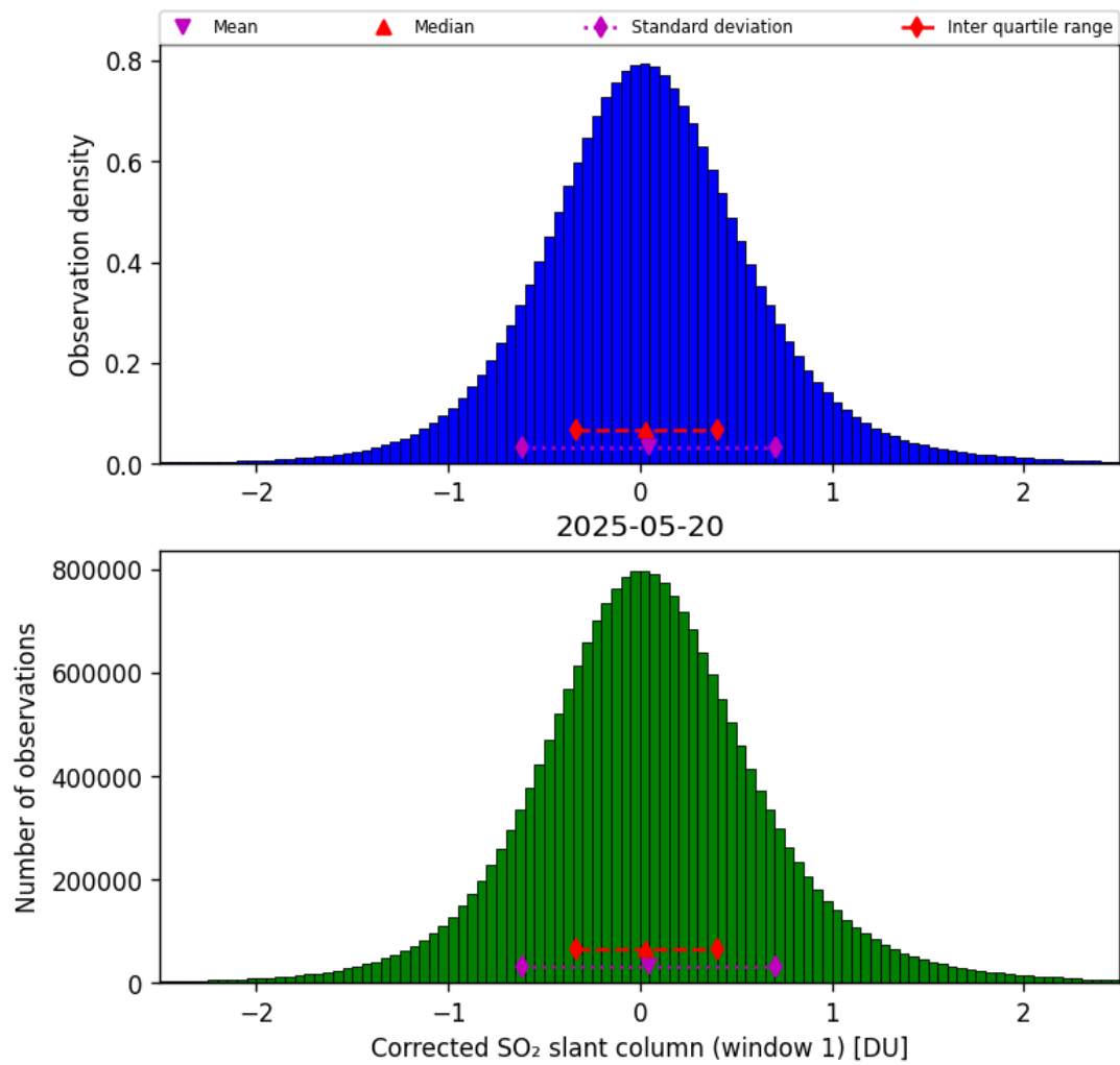
Figure 65: Histogram of “Corrected SO 2 slant column (window 1)” for 2025-05-19 to 2025-05-21
