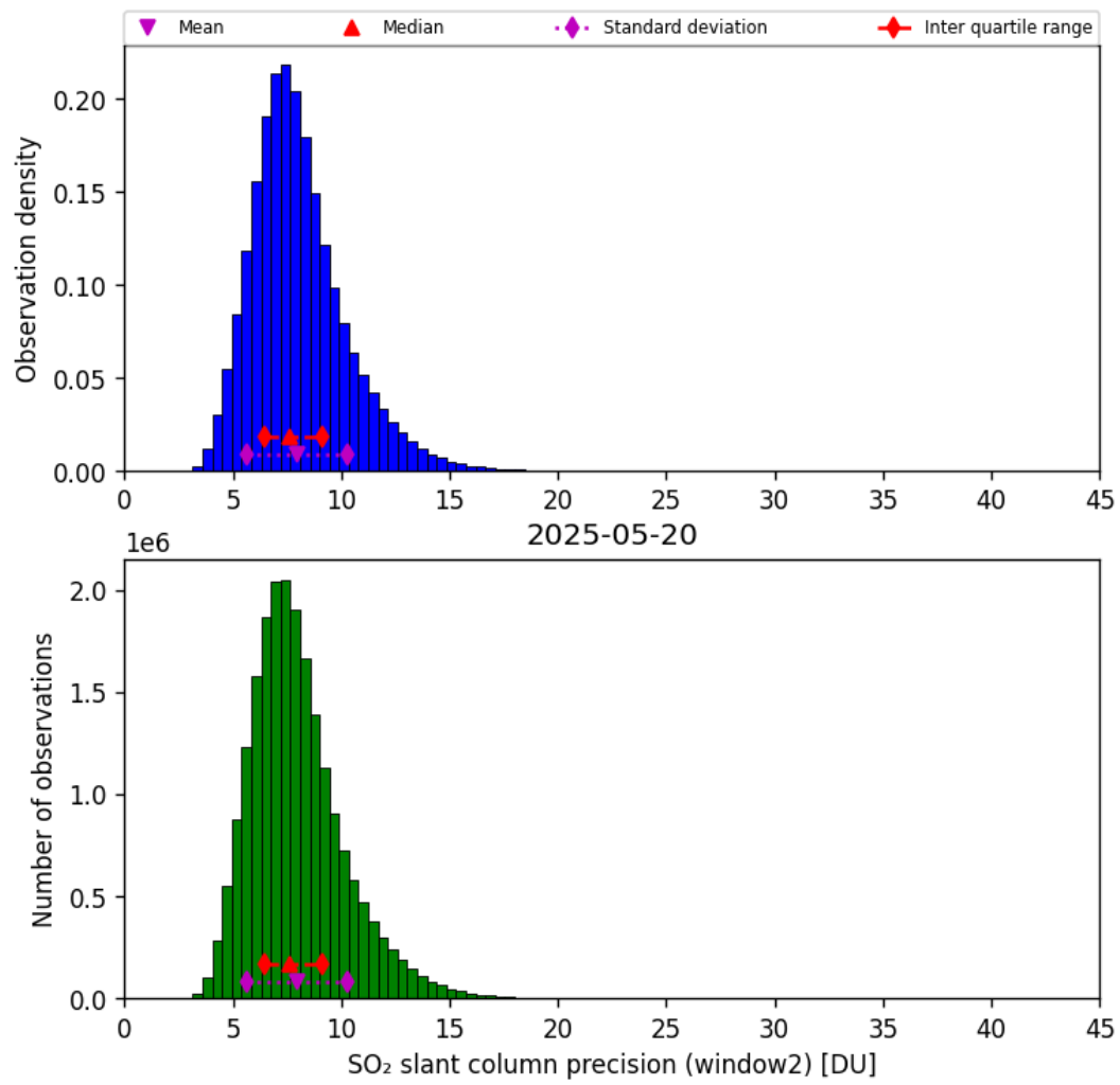
Figure 68: Histogram of “SO 2 slant column precision (window2)” for 2025-05-19 to 2025-05-21
