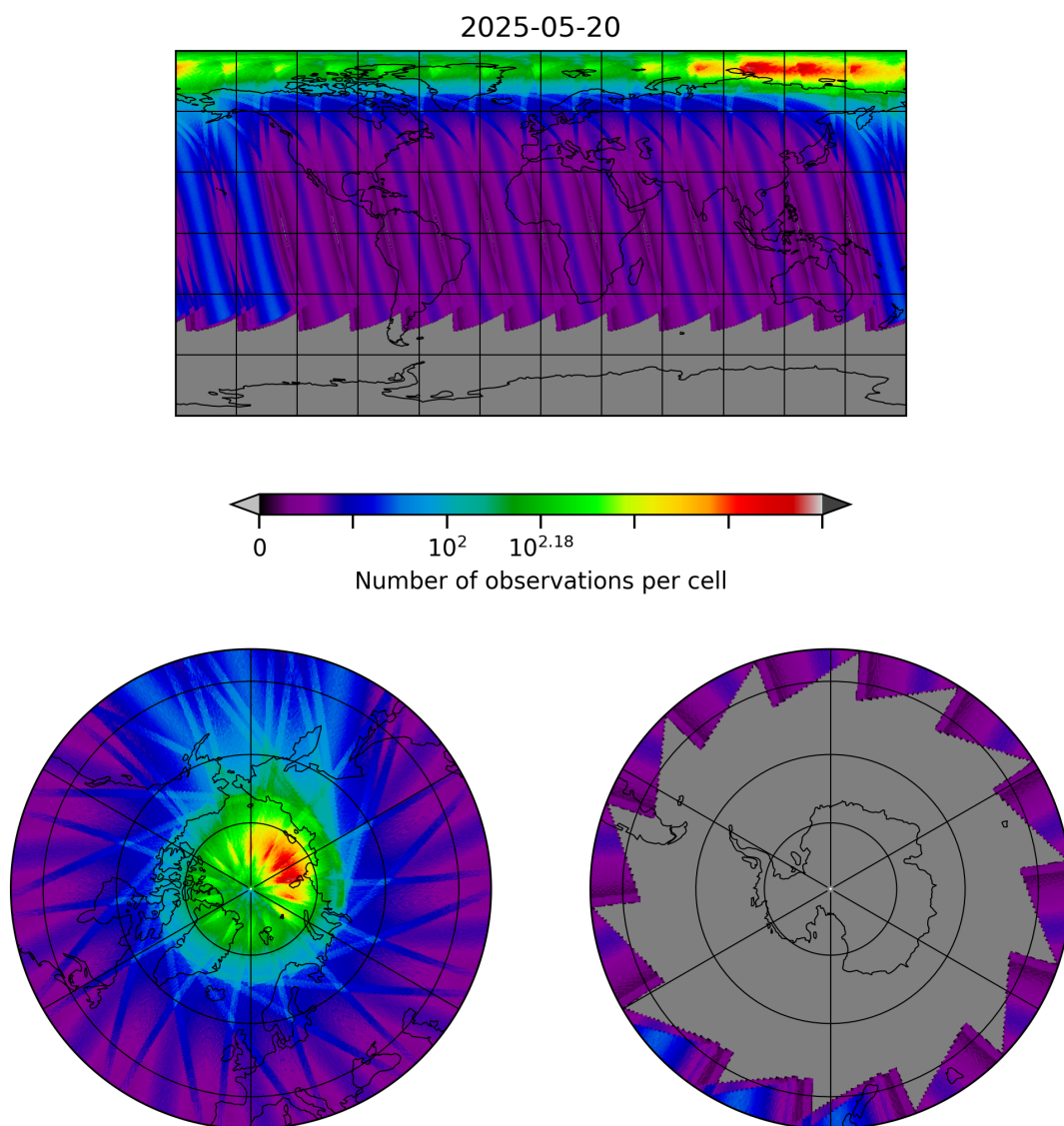
Figure 30: Map of the number of observations for 2025-05-19 to 2025-05-21
