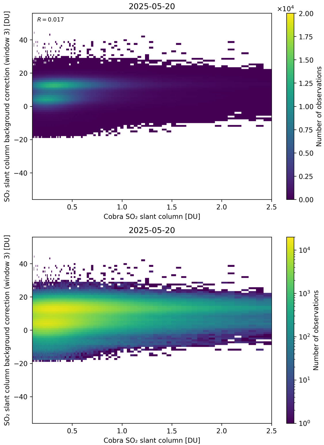
Figure 195: Scatter density plot of “Cobra SO 2 slant column” against “SO 2 slant column background correction (window 3)” for 2025-05-19 to 2025-05-21.
