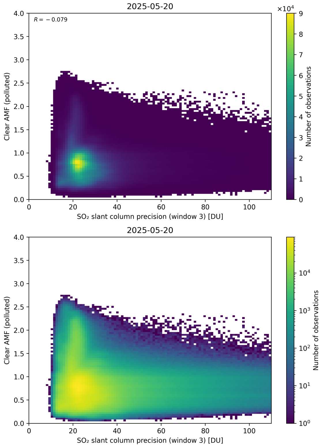
Figure 311: Scatter density plot of “SO 2 slant column precision (window 3)” against “Clear AMF (polluted)” for 2025-05-19 to 2025-05-21.
