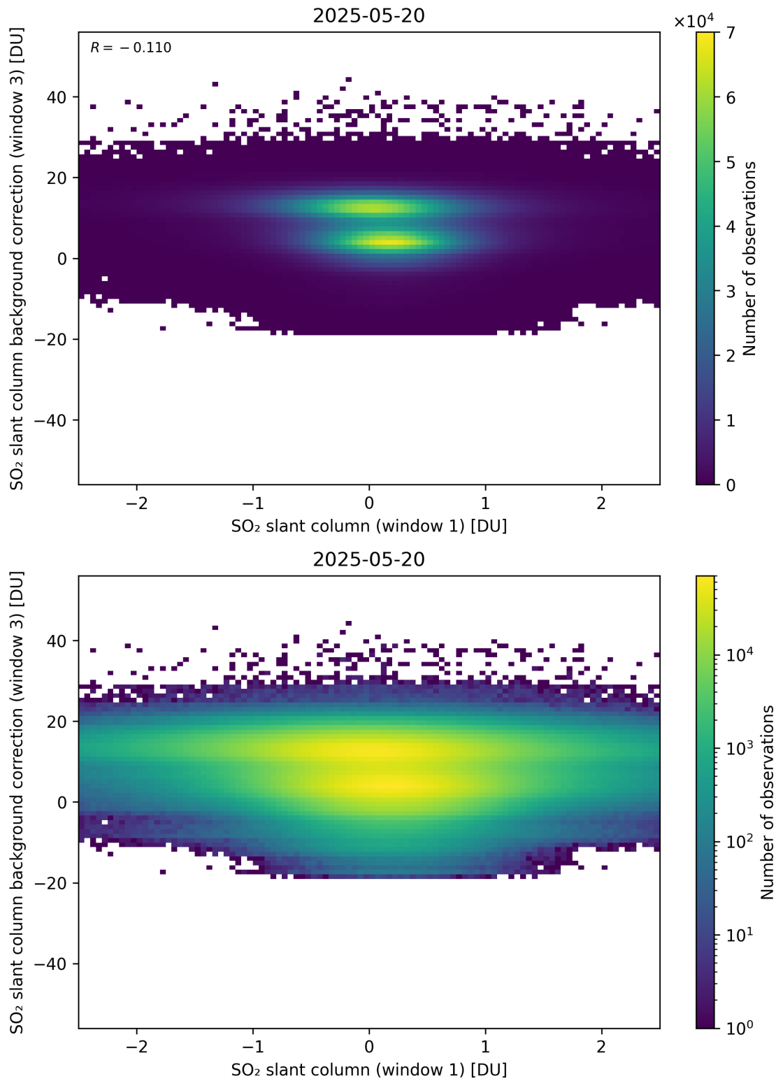
Figure 264: Scatter density plot of “SO 2 slant column (window 1)” against “SO 2 slant column background correction (window 3)” for 2025-05-19 to 2025-05-21.
