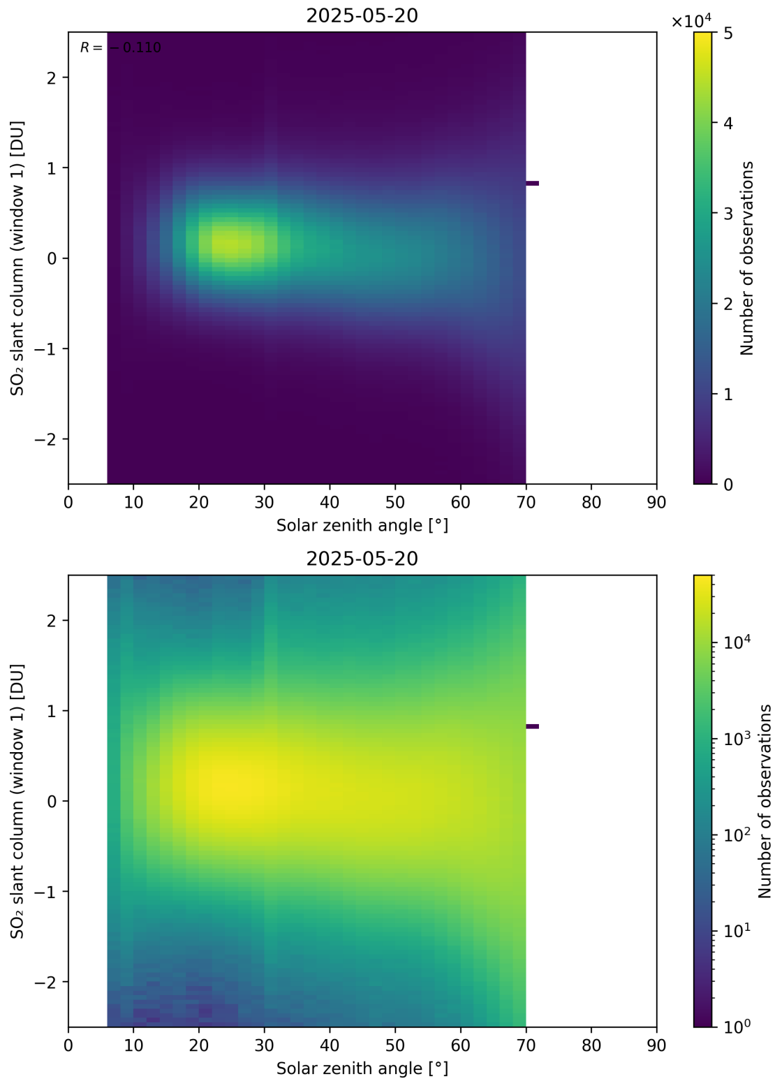
Figure 184: Scatter density plot of “Solar zenith angle” against “SO 2 slant column (window 1)” for 2025-05-19 to 2025-05-21.
