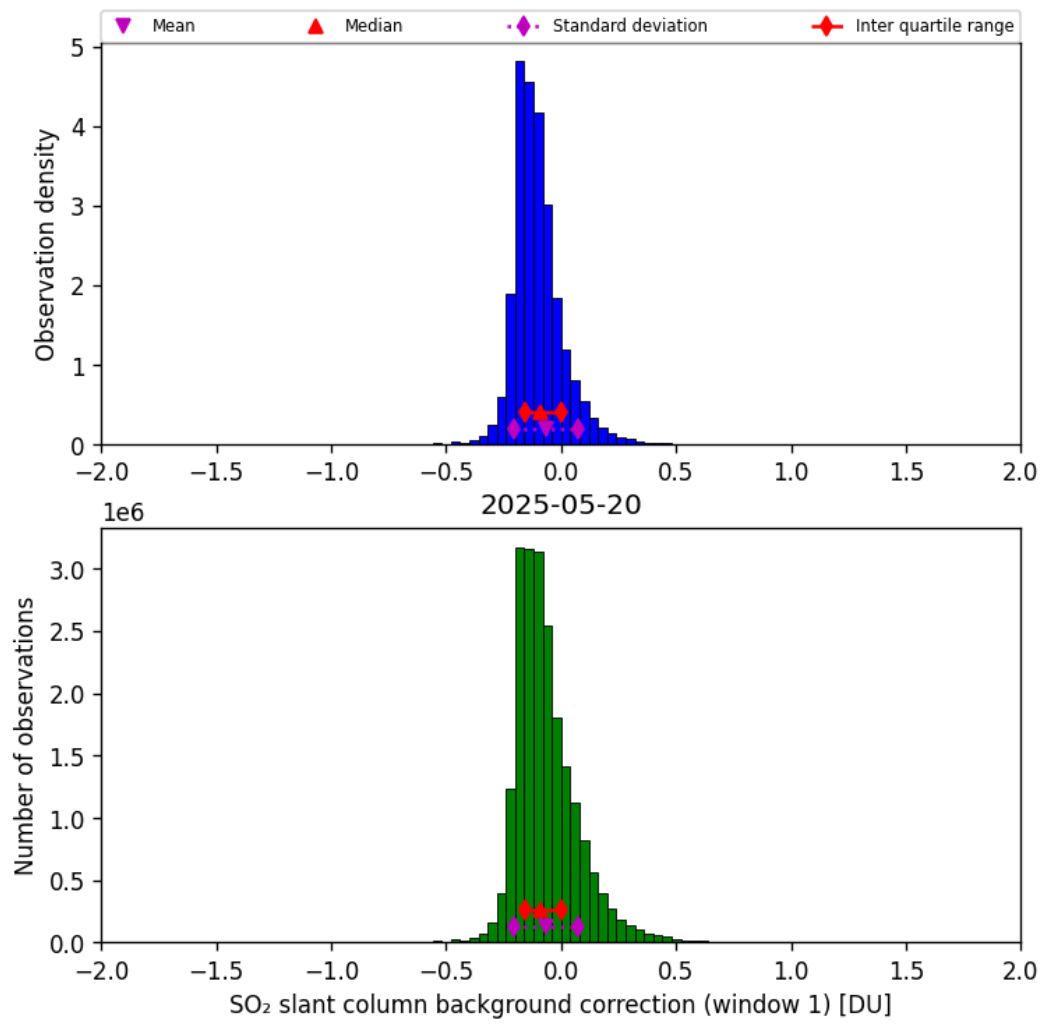
Figure 66: Histogram of “SO 2 slant column background correction (window 1)” for 2025-05-19 to 2025-05-21
