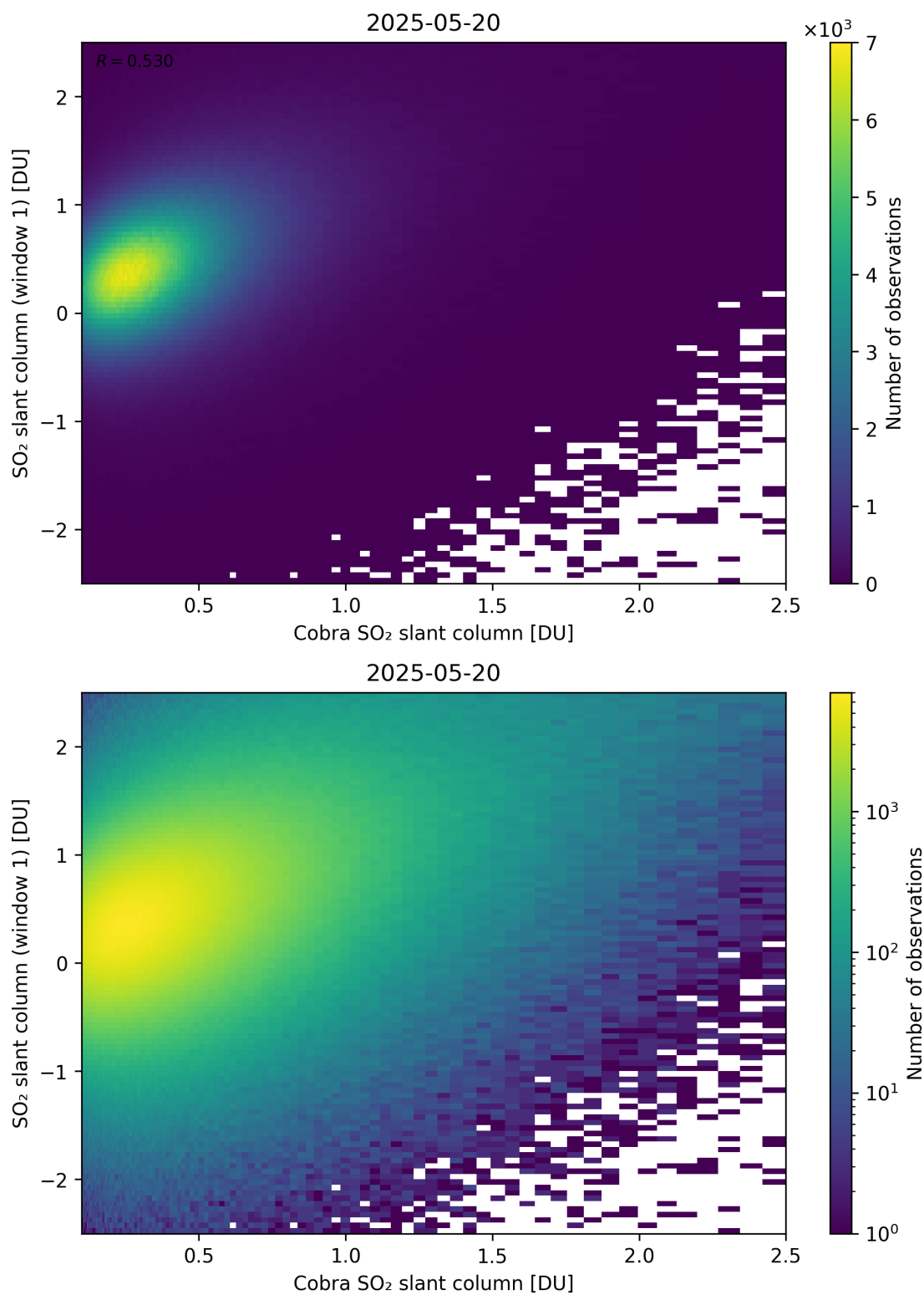
Figure 219: Scatter density plot of “Cobra SO 2 slant column” against “SO 2 slant column (window 1)” for 2025-05-19 to 2025-05-21.
