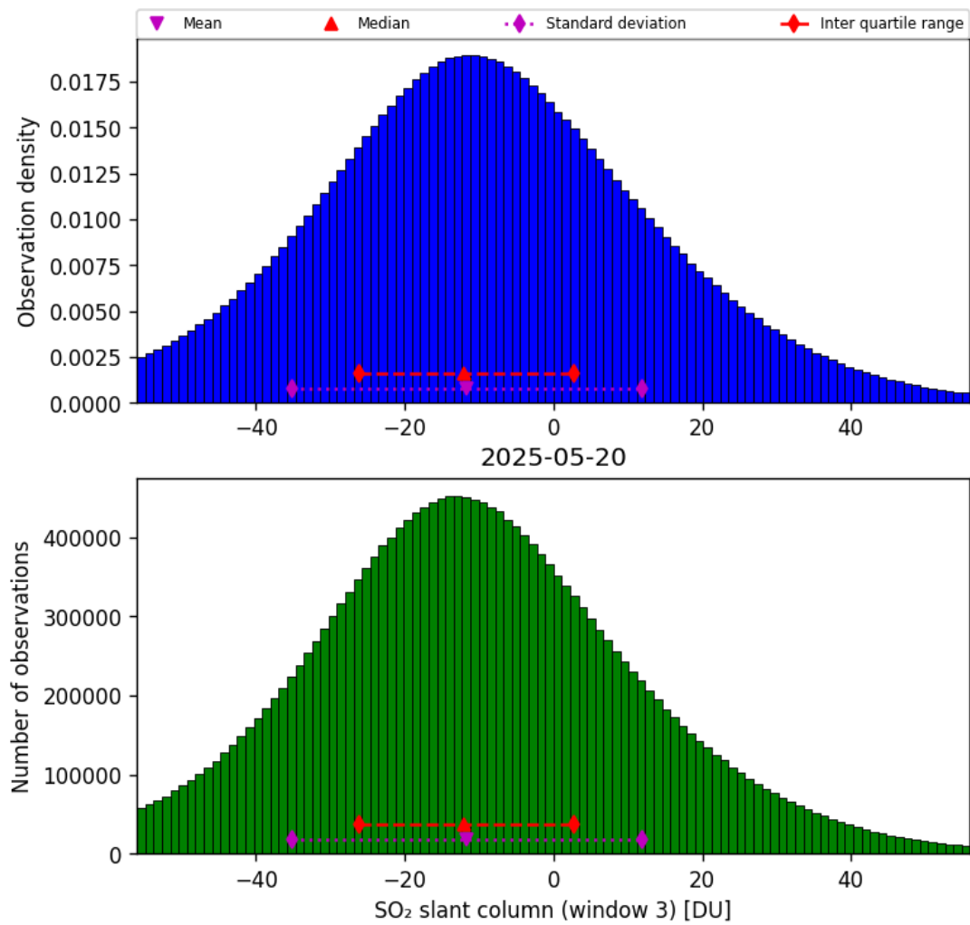
Figure 71: Histogram of “SO 2 slant column (window 3)” for 2025-05-19 to 2025-05-21
