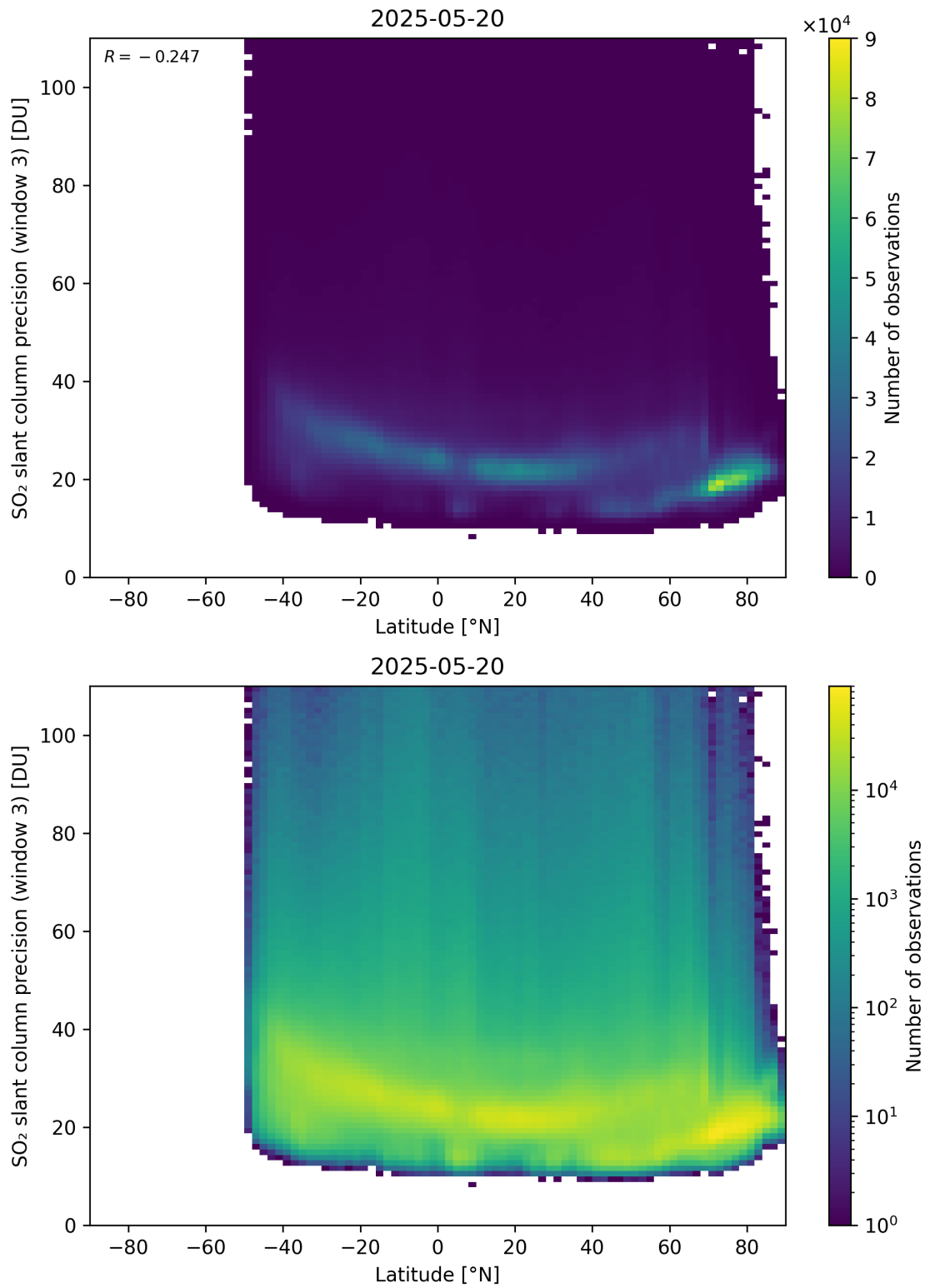
Figure 166: Scatter density plot of “Latitude” against “SO 2 slant column precision (window 3)” for 2025-05-19 to 2025-05-21.
