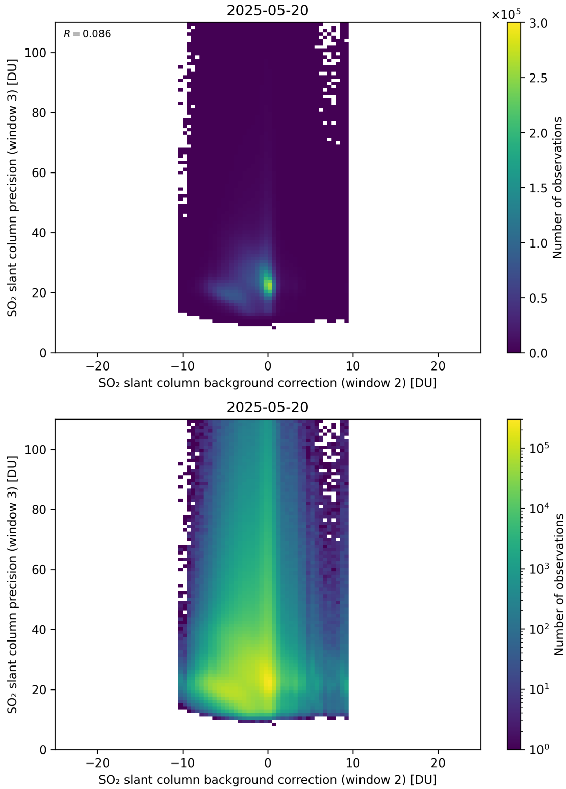
Figure 129: Scatter density plot of “SO 2 slant column background correction (window 2)” against “SO 2 slant column precision (window 3)” for 2025-05-19 to 2025-05-21.
