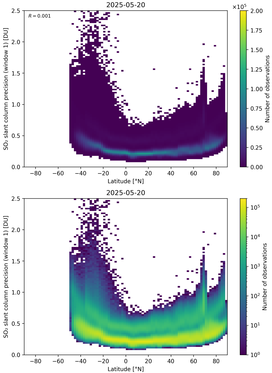
Figure 163: Scatter density plot of “Latitude” against “SO 2 slant column precision (window 1)” for 2025-05-19 to 2025-05-21.
