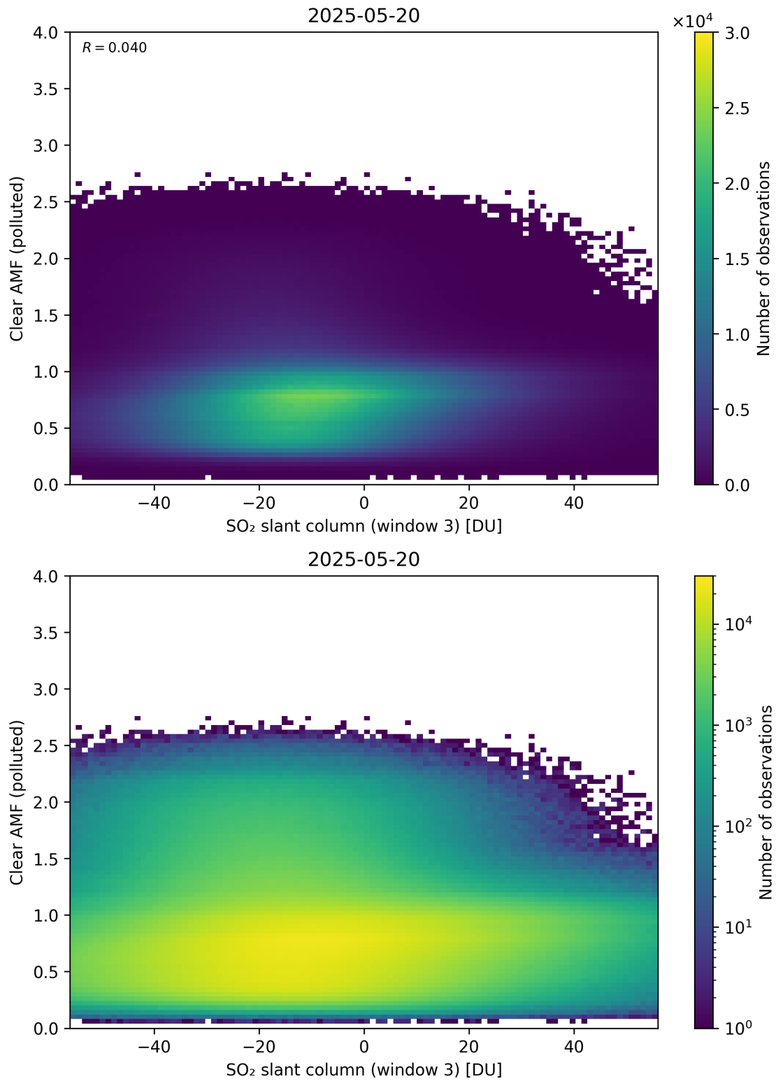
Figure 315: Scatter density plot of “SO 2 slant column (window 3)” against “Clear AMF (polluted)” for 2025-05-19 to 2025-05-21.
