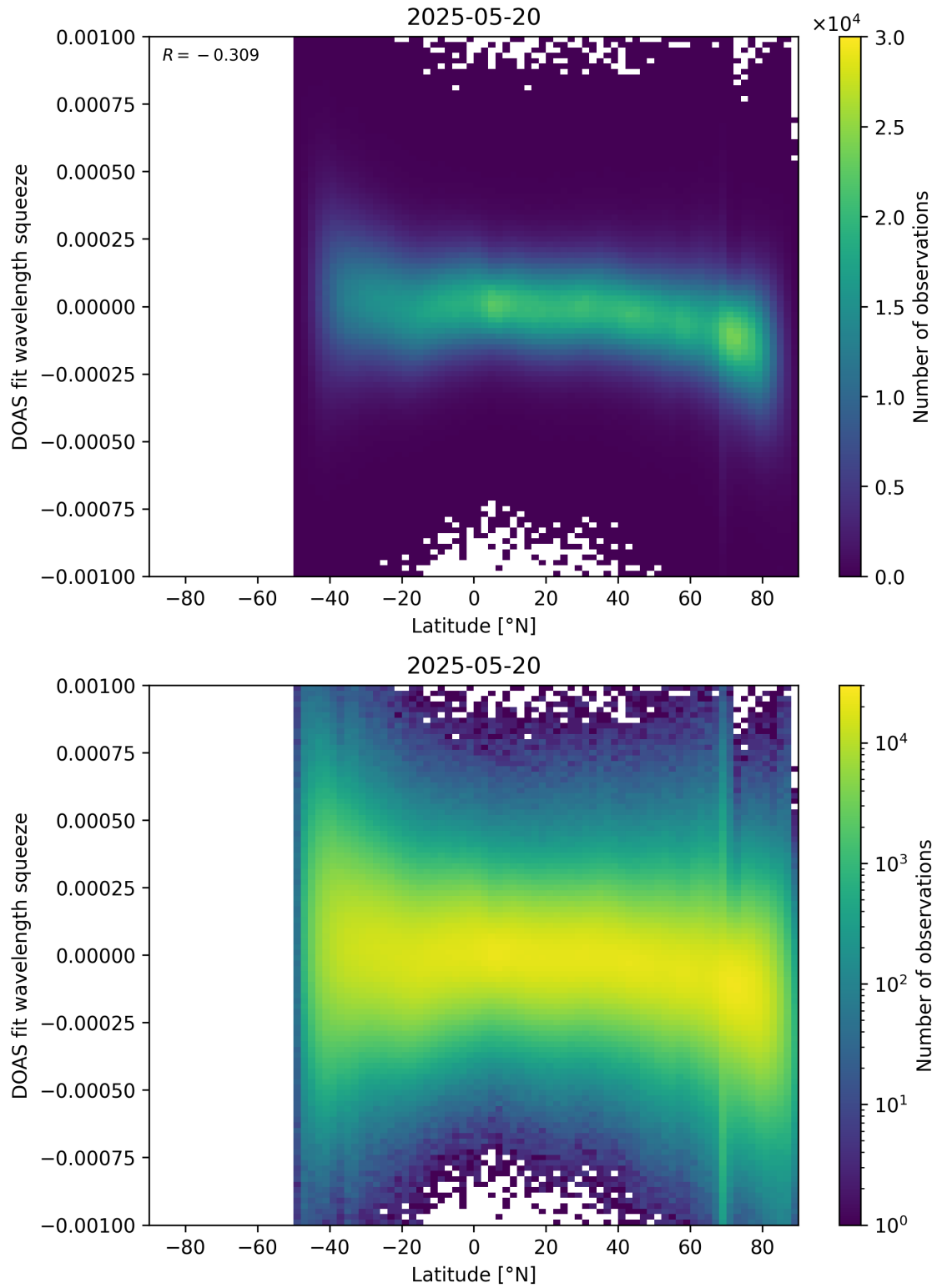
Figure 154: Scatter density plot of “Latitude” against “DOAS fit wavelength squeeze” for 2025-05-19 to 2025-05-21.
