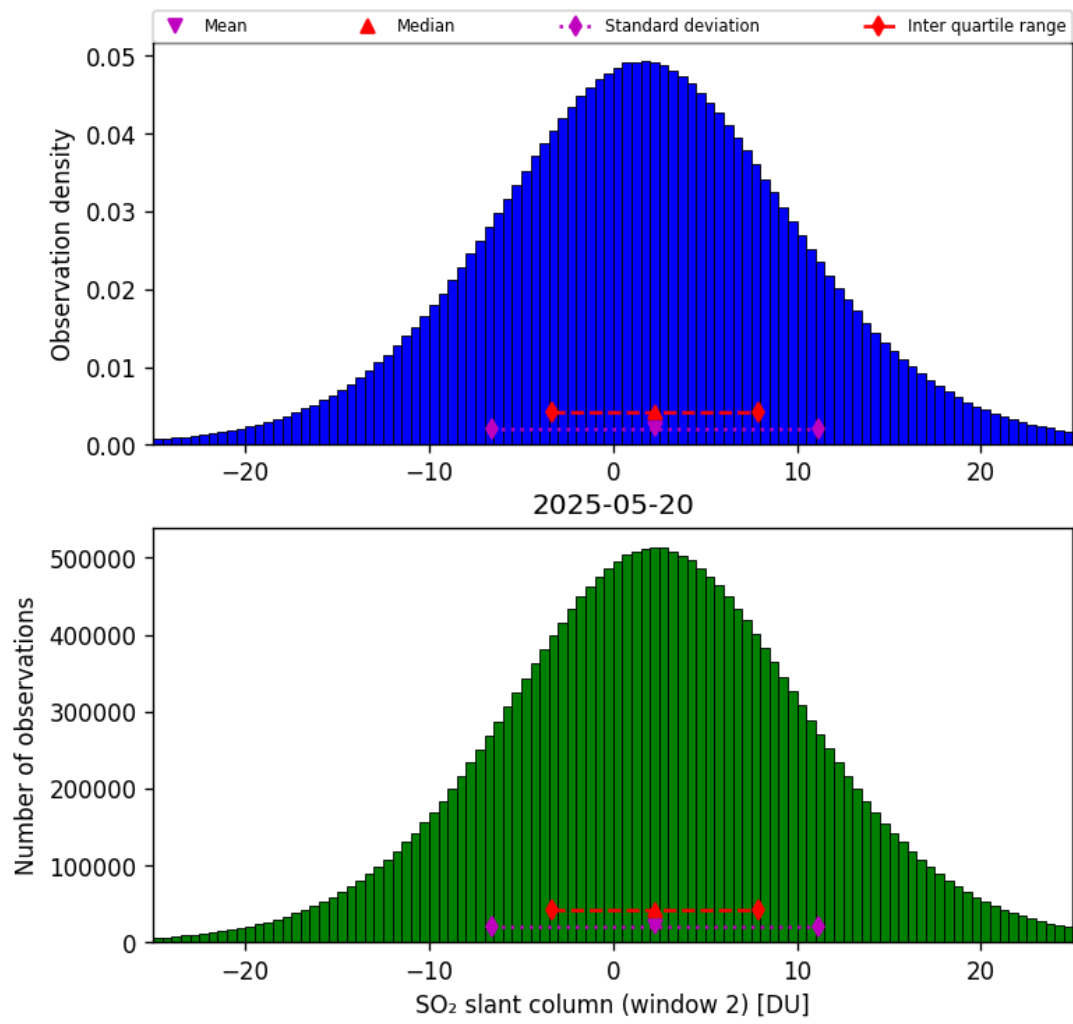
Figure 67: Histogram of “SO 2 slant column (window 2)” for 2025-05-19 to 2025-05-21
