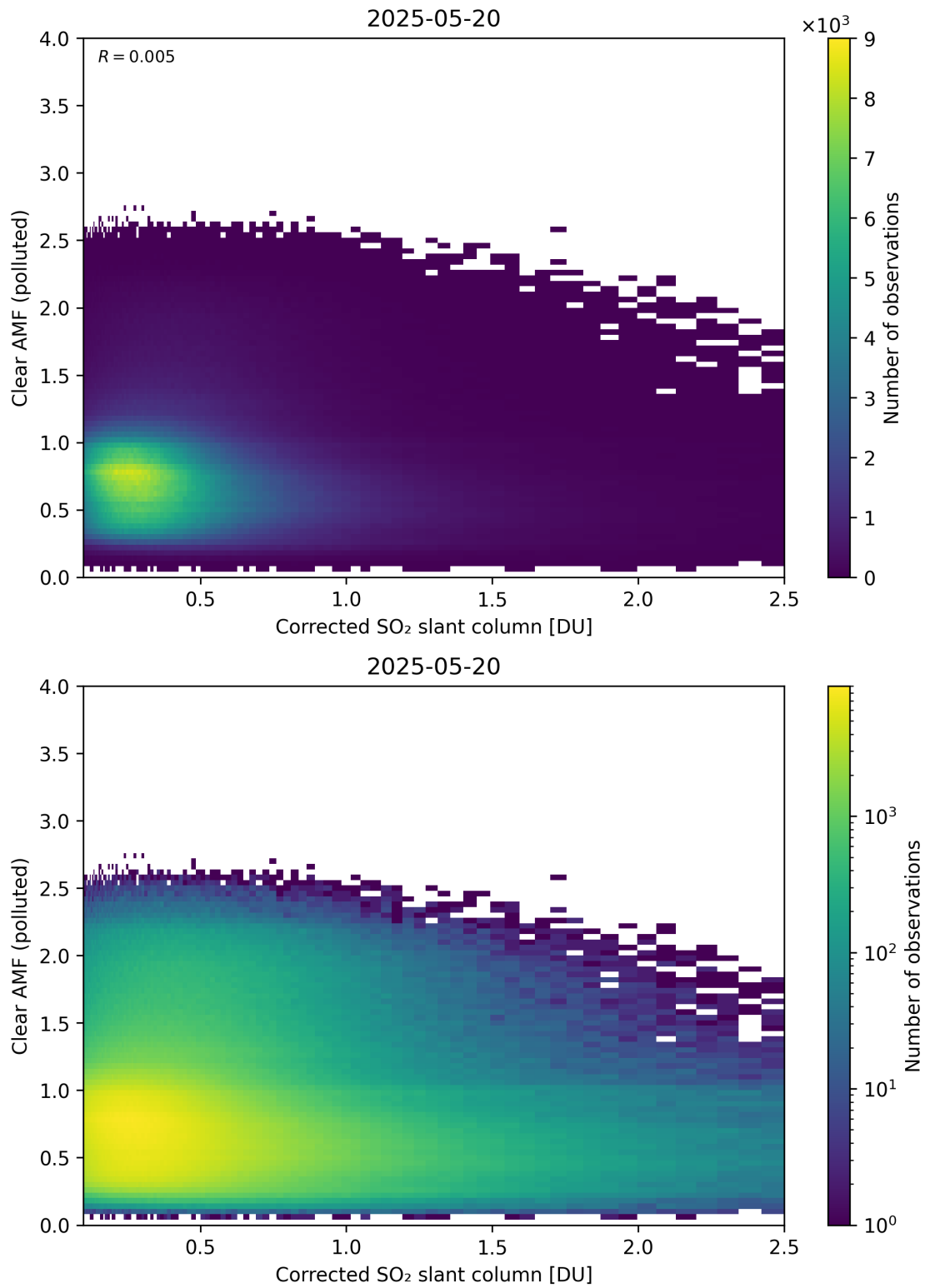
Figure 232: Scatter density plot of “Corrected SO 2 slant column” against “Clear AMF (polluted)” for 2025-05-19 to 2025-05-21.
