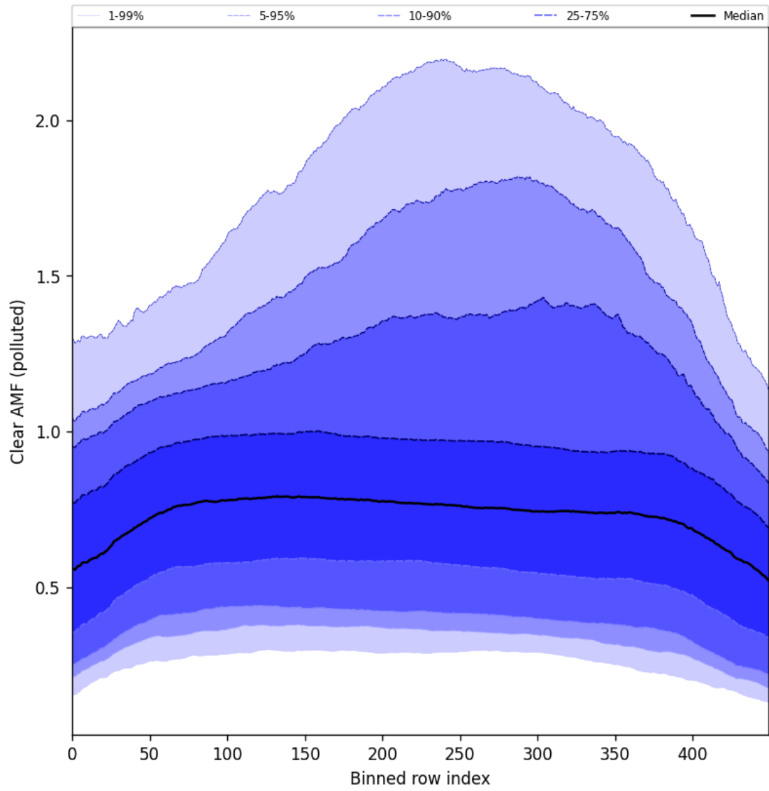
Figure 107: Along track statistics of “Clear AMF (polluted)” for 2025-05-19 to 2025-05-21
