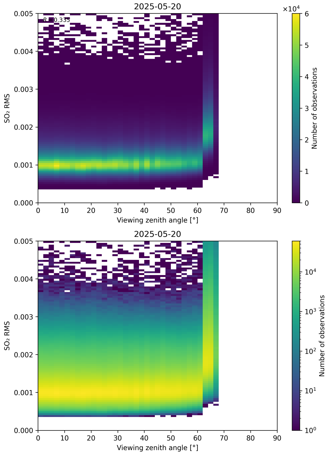
Figure 367: Scatter density plot of “Viewing zenith angle” against “SO 2 RMS” for 2025-05-19 to 2025-05-21.
