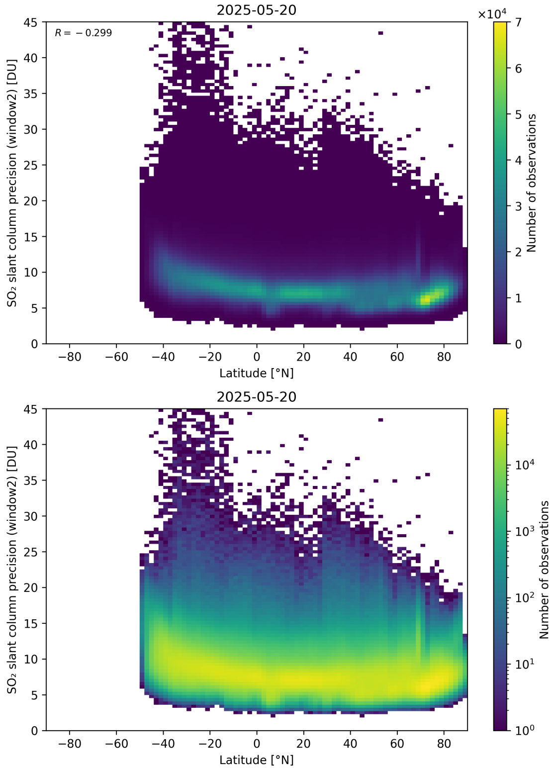
Figure 164: Scatter density plot of “Latitude” against “SO 2 slant column precision (window2)” for 2025-05-19 to 2025-05-21.
