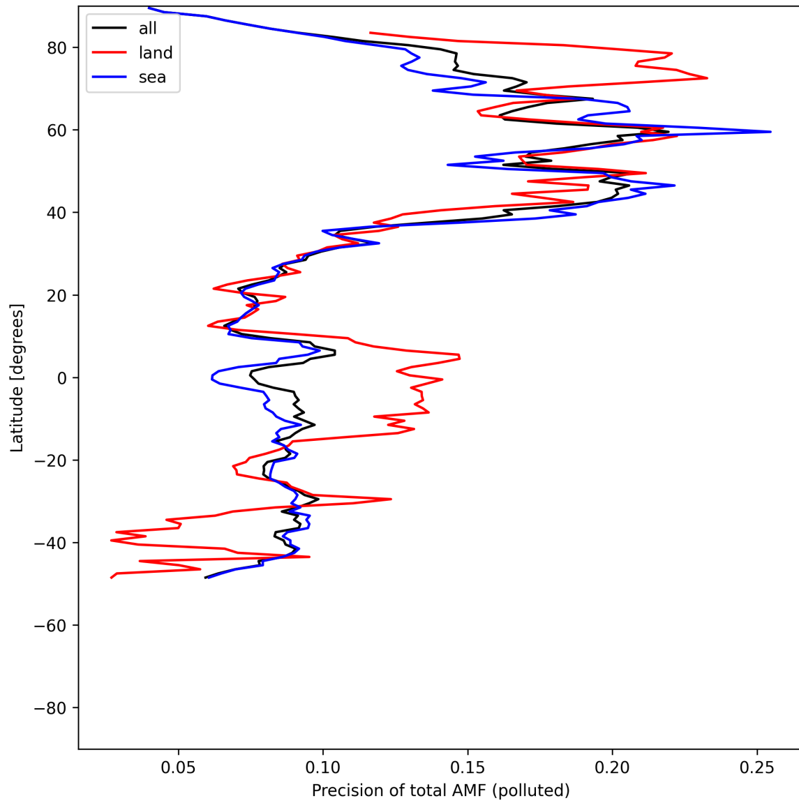
Figure 54: Zonal average of “Precision of total AMF (polluted)” for 2025-05-19 to 2025-05-21.
