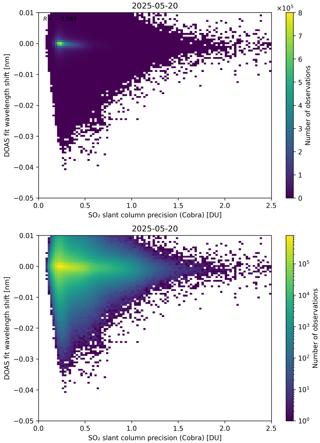
Figure 202: Scatter density plot of “SO 2 slant column precision (Cobra)” against “DOAS fit wavelength shift” for 2025-05-19 to 2025-05-21.
