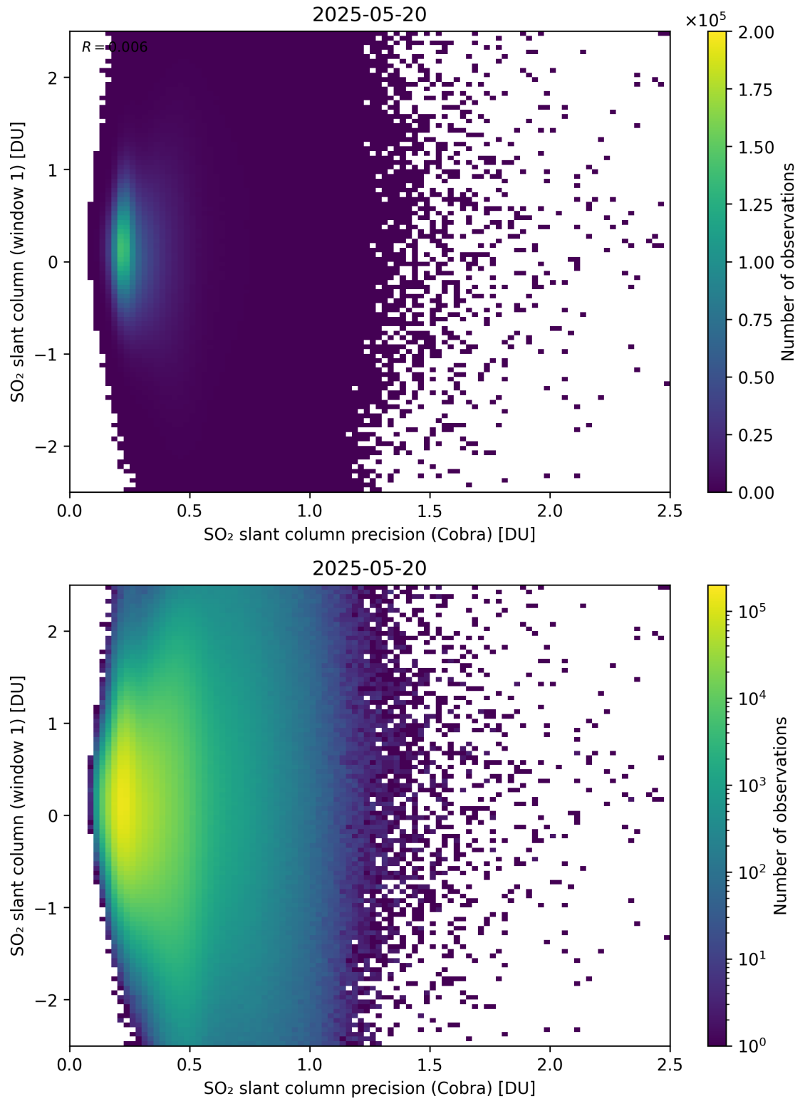
Figure 208: Scatter density plot of “SO 2 slant column precision (Cobra)” against “SO 2 slant column (window 1)” for 2025-05-19 to 2025-05-21.
