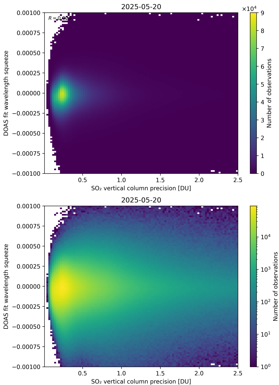
Figure 333: Scatter density plot of “SO 2 vertical column precision” against “DOAS fit wavelength squeeze” for 2025-05-19 to 2025-05-21.
