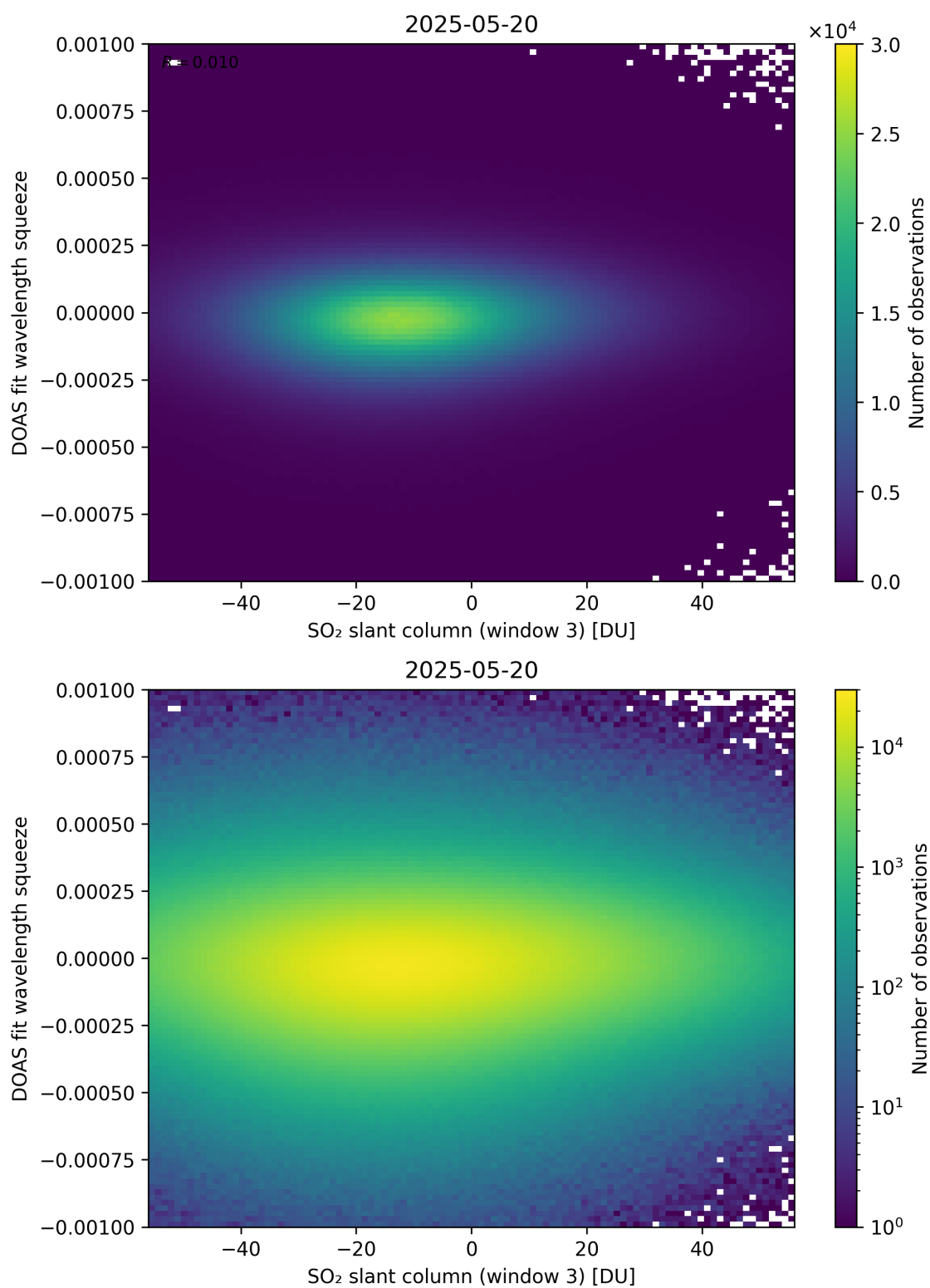
Figure 305: Scatter density plot of “SO 2 slant column (window 3)” against “DOAS fit wavelength squeeze” for 2025-05-19 to 2025-05-21.
