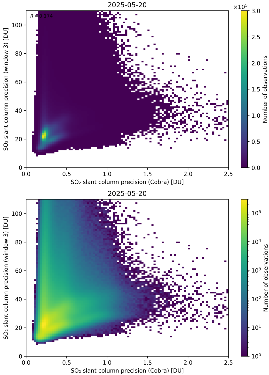
Figure 212: Scatter density plot of “SO 2 slant column precision (Cobra)” against “SO 2 slant column precision (window 3)” for 2025-05-19 to 2025-05-21.
