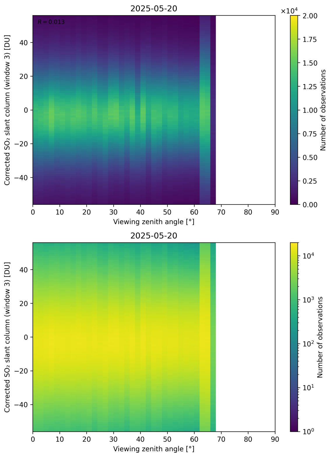
Figure 375: Scatter density plot of “Viewing zenith angle” against “Corrected SO 2 slant column (window 3)” for 2025-05-19 to 2025-05-21.
