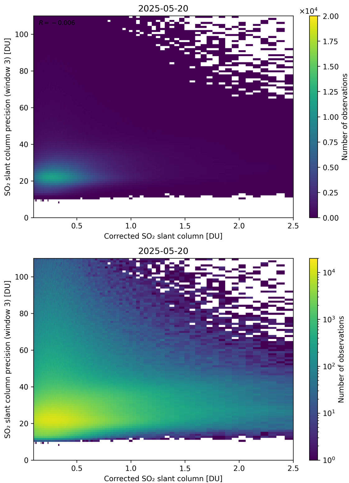
Figure 241: Scatter density plot of “Corrected SO 2 slant column” against “SO 2 slant column precision (window 3)” for 2025-05-19 to 2025-05-21.
