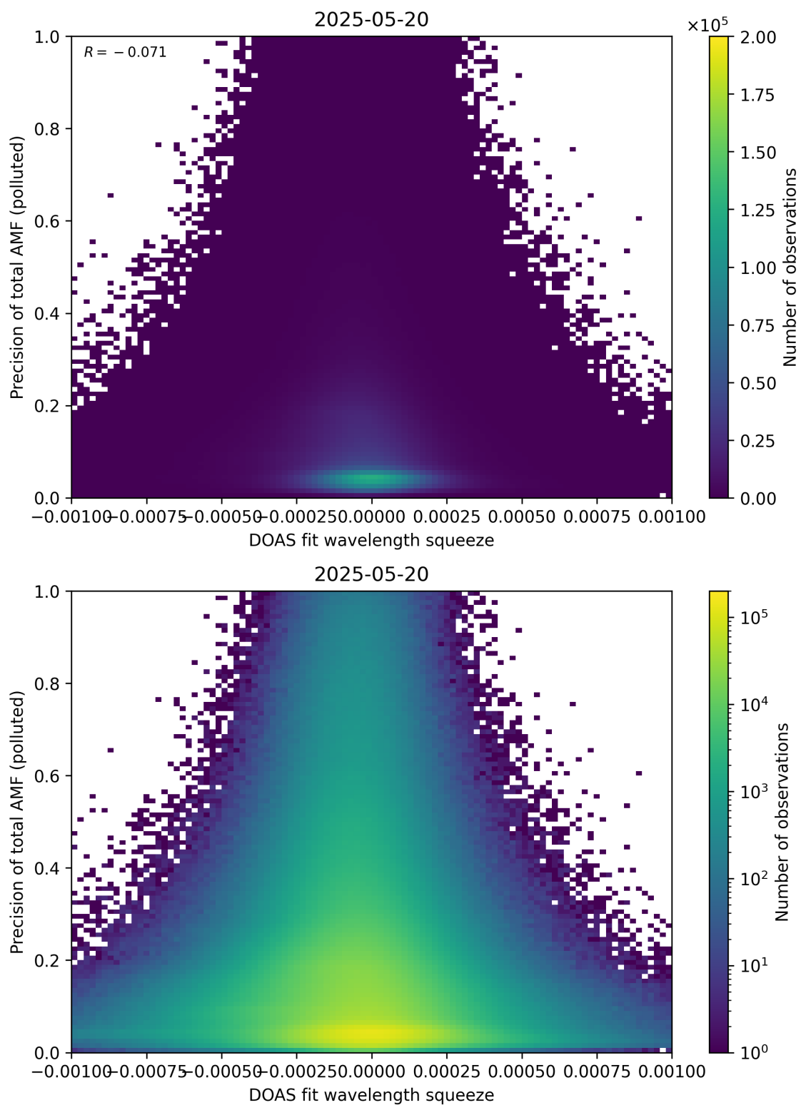
Figure 146: Scatter density plot of “DOAS fit wavelength squeeze” against “Precision of total AMF (polluted)” for 2025-05-19 to 2025-05-21.
