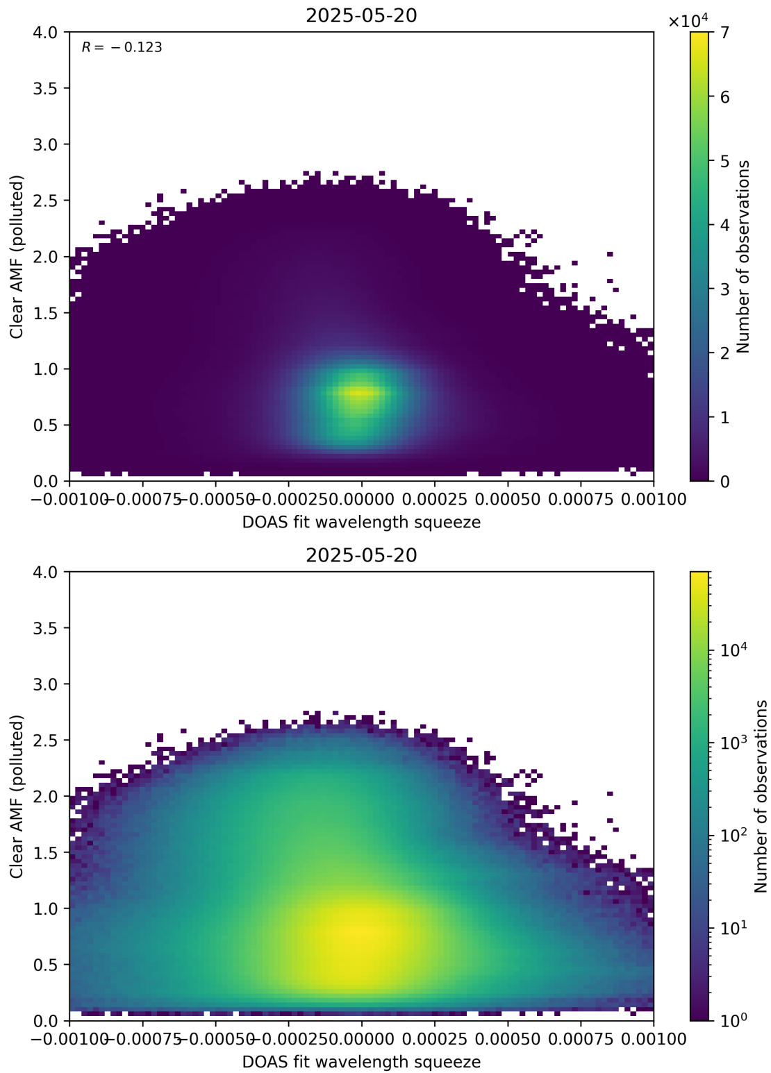
Figure 144: Scatter density plot of “DOAS fit wavelength squeeze” against “Clear AMF (polluted)” for 2025-05-19 to 2025-05-21.
