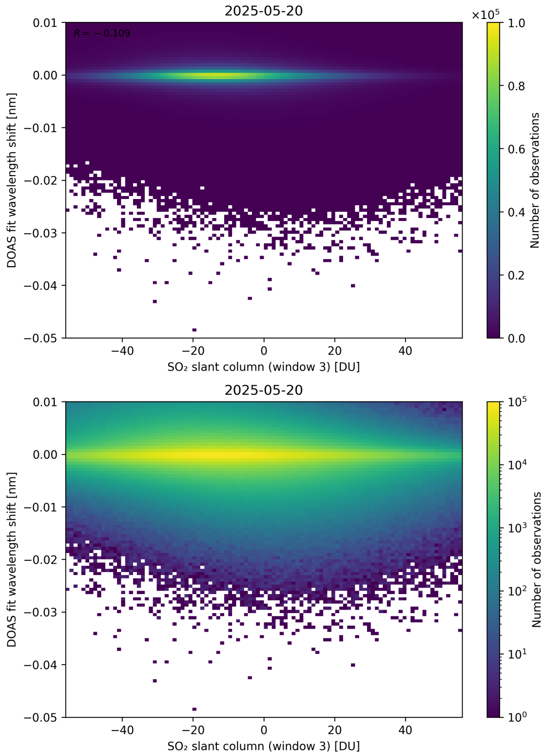
Figure 304: Scatter density plot of “SO 2 slant column (window 3)” against “DOAS fit wavelength shift” for 2025-05-19 to 2025-05-21.
