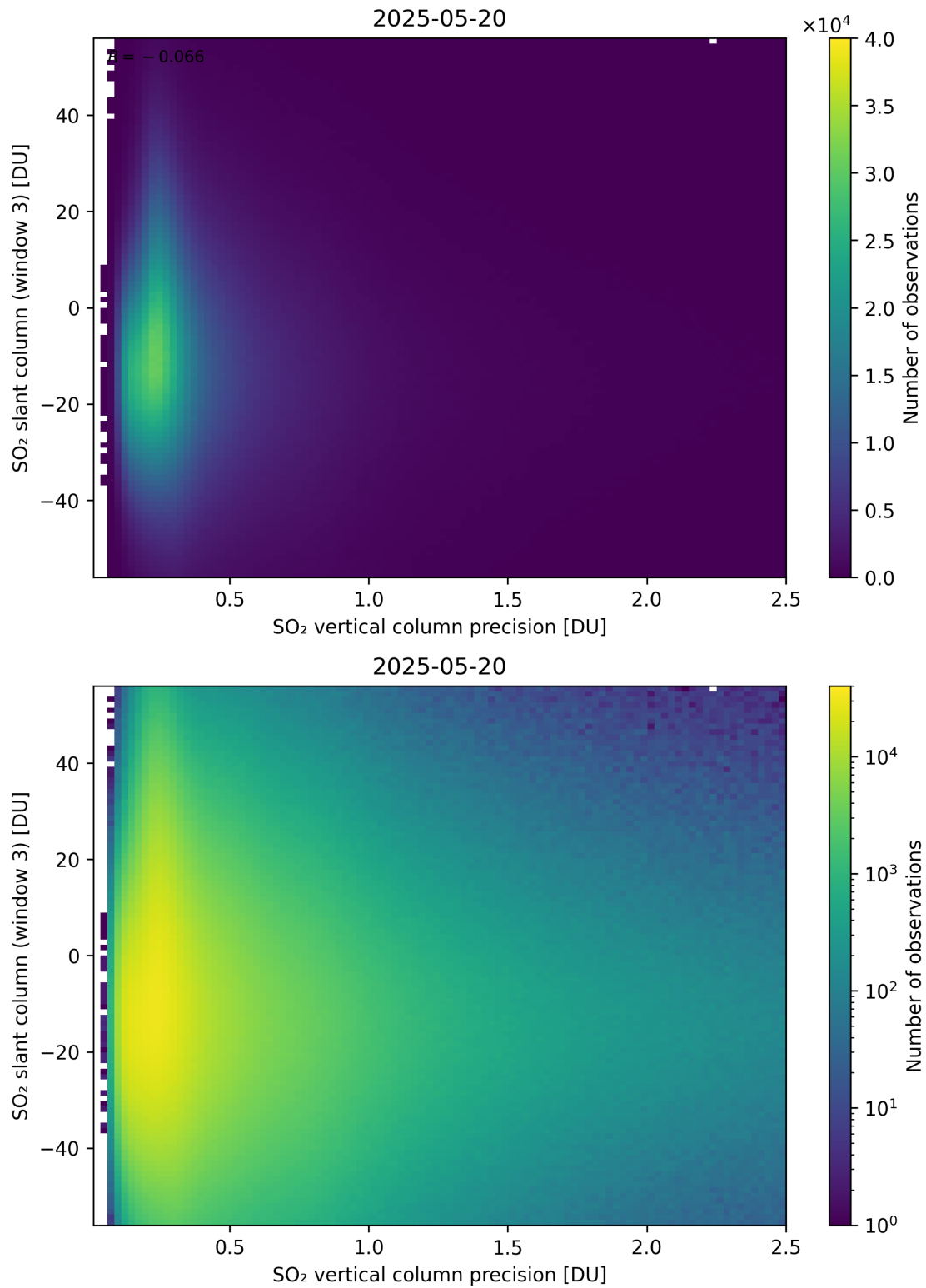
Figure 344: Scatter density plot of “SO 2 vertical column precision” against “SO 2 slant column (window 3)” for 2025-05-19 to 2025-05-21.
