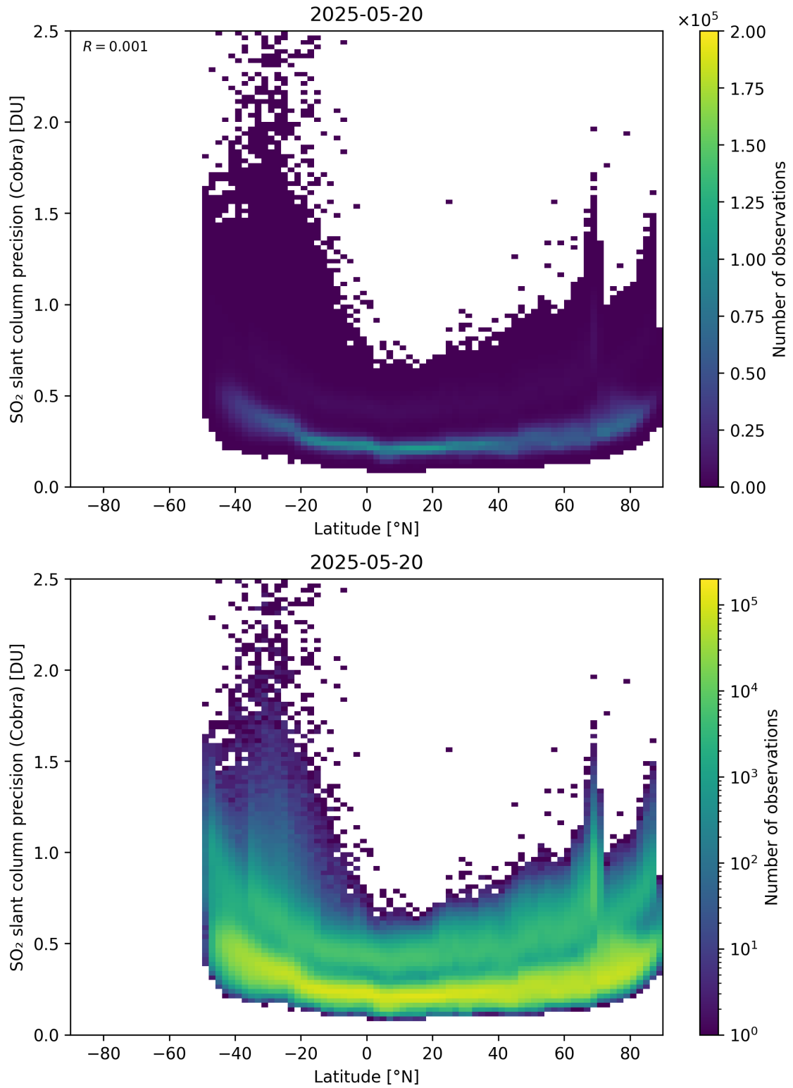
Figure 158: Scatter density plot of “Latitude” against “SO 2 slant column precision (Cobra)” for 2025-05-19 to 2025-05-21.
