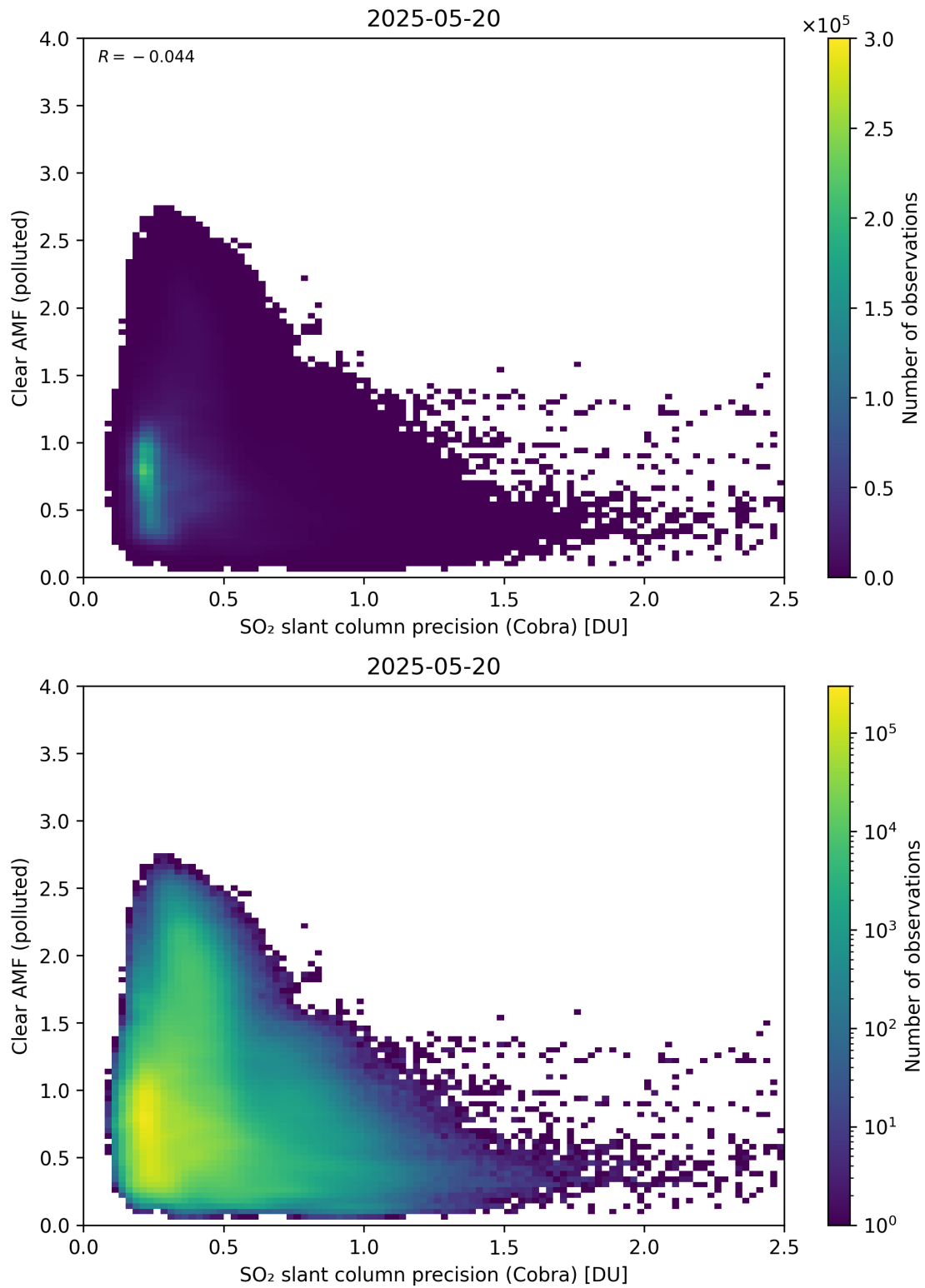
Figure 205: Scatter density plot of “SO 2 slant column precision (Cobra)” against “Clear AMF (polluted)” for 2025-05-19 to 2025-05-21.
