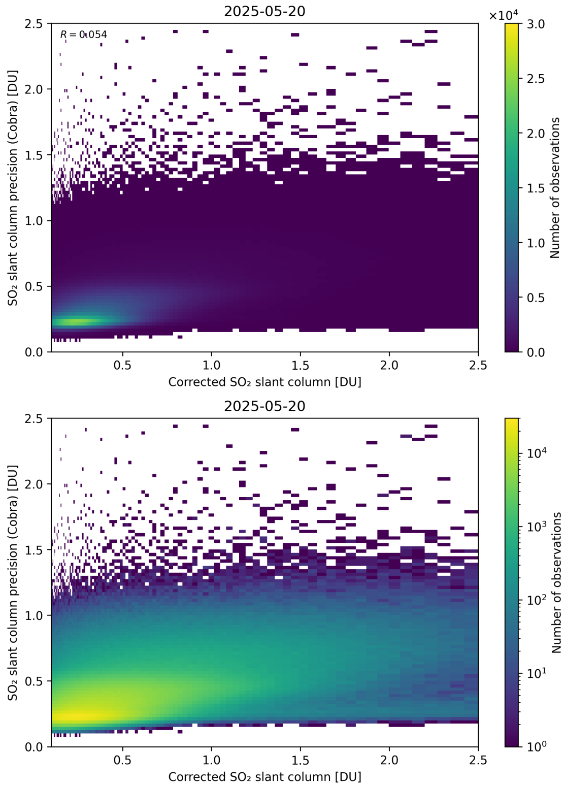
Figure 234: Scatter density plot of “Corrected SO 2 slant column” against “SO 2 slant column precision (Cobra)” for 2025-05-19 to 2025-05-21.
