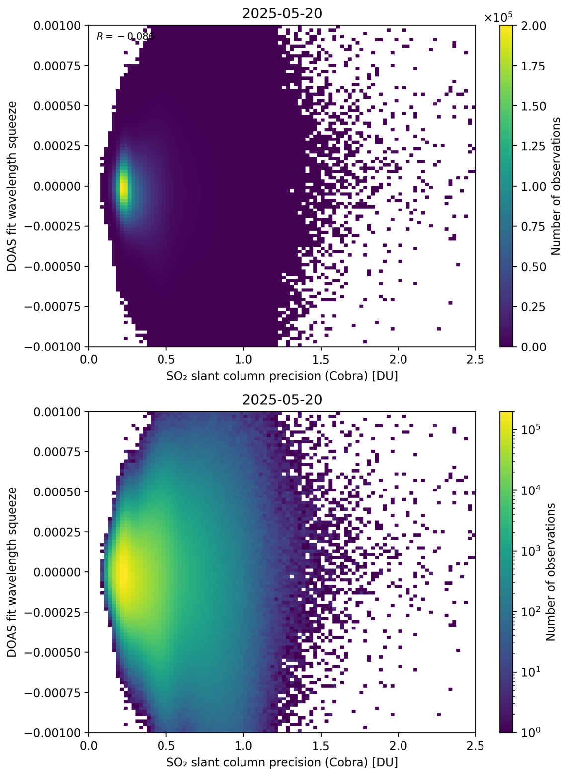
Figure 203: Scatter density plot of “SO 2 slant column precision (Cobra)” against “DOAS fit wavelength squeeze” for 2025-05-19 to 2025-05-21.
