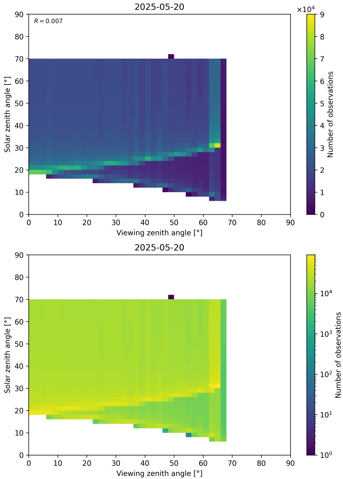
Figure 369: Scatter density plot of “Viewing zenith angle” against “Solar zenith angle” for 2025-05-19 to 2025-05-21.
