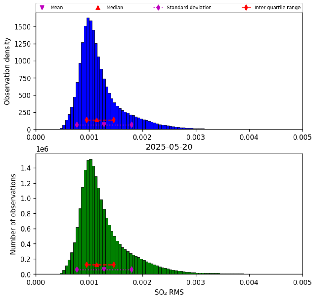
Figure 78: Histogram of “SO 2 RMS” for 2025-05-19 to 2025-05-21
