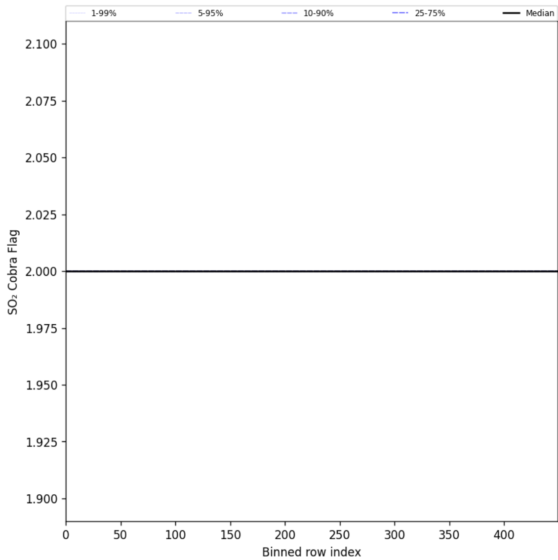
Figure 101: Along track statistics of “SO 2 Cobra Flag” for 2025-05-19 to 2025-05-21
