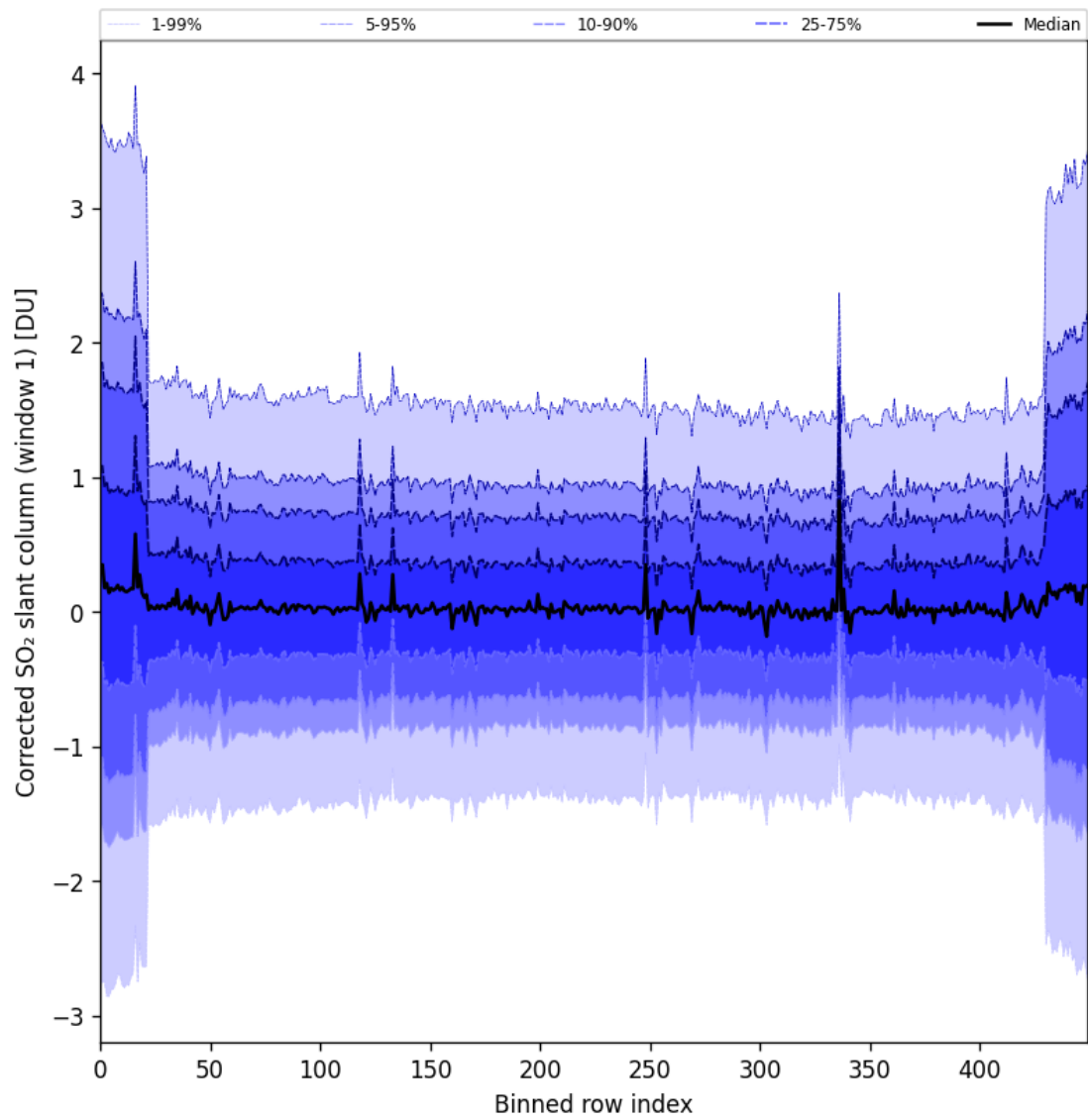
Figure 91: Along track statistics of “Corrected SO 2 slant column (window 1)” for 2025-05-19 to 2025-05-21
