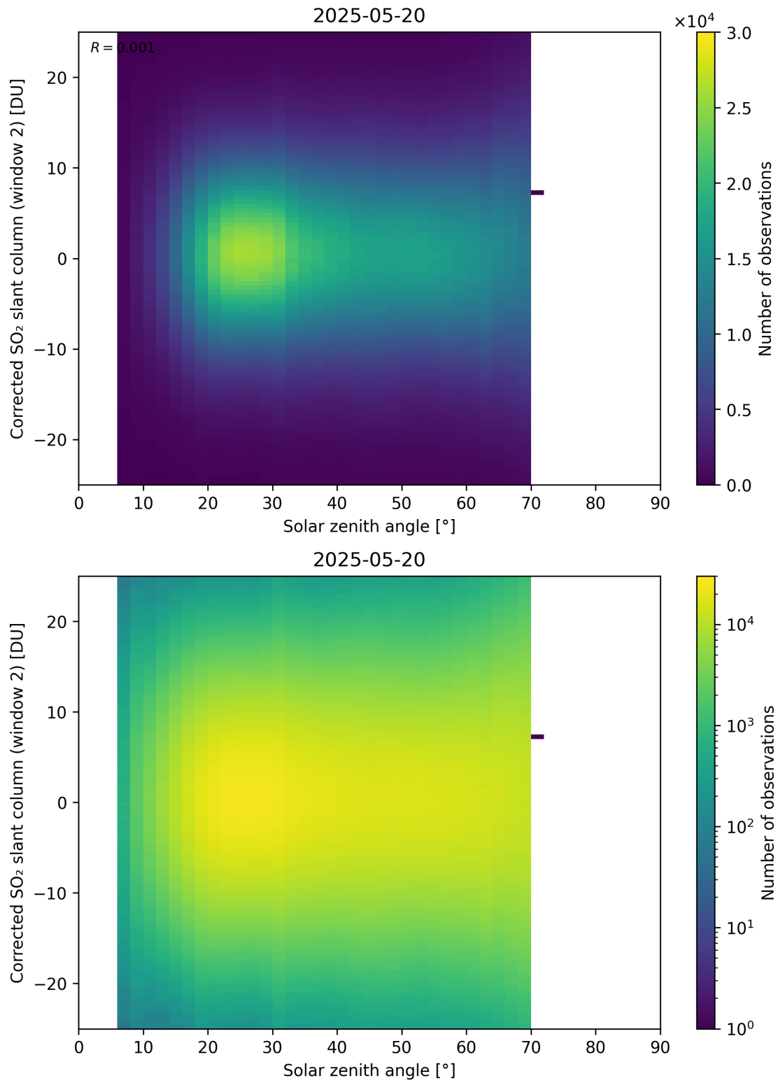
Figure 182: Scatter density plot of “Solar zenith angle” against “Corrected SO 2 slant column (window 2)” for 2025-05-19 to 2025-05-21.
