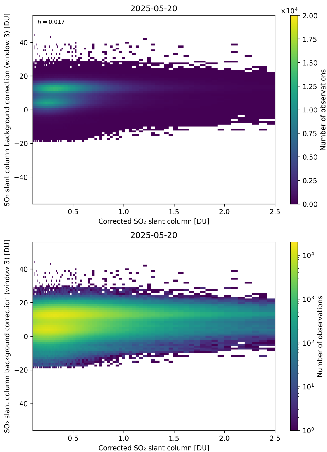
Figure 228: Scatter density plot of “Corrected SO 2 slant column” against “SO 2 slant column background correction (window 3)” for 2025-05-19 to 2025-05-21.
