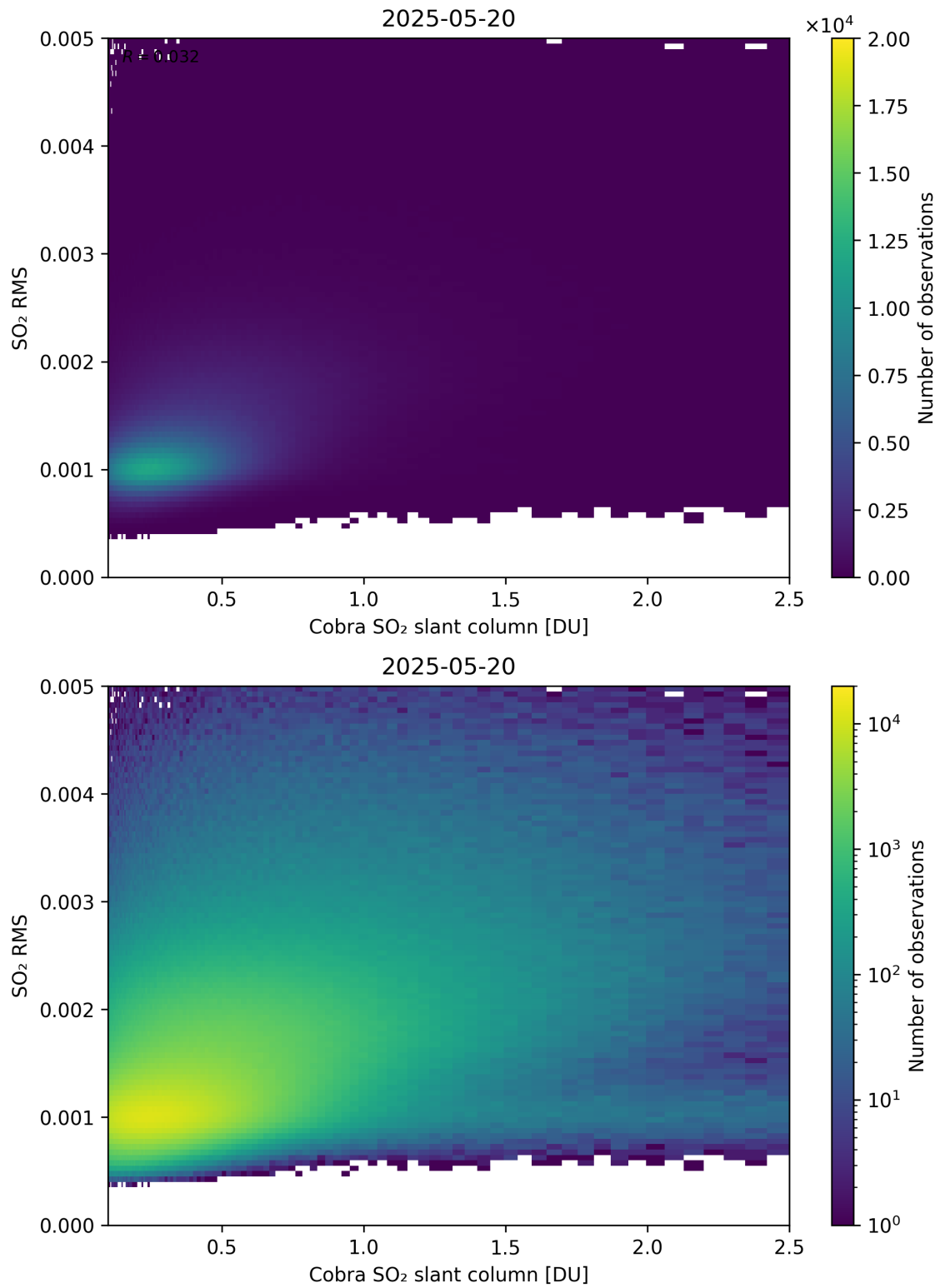
Figure 198: Scatter density plot of “Cobra SO 2 slant column” against “SO 2 RMS” for 2025-05-19 to 2025-05-21.
