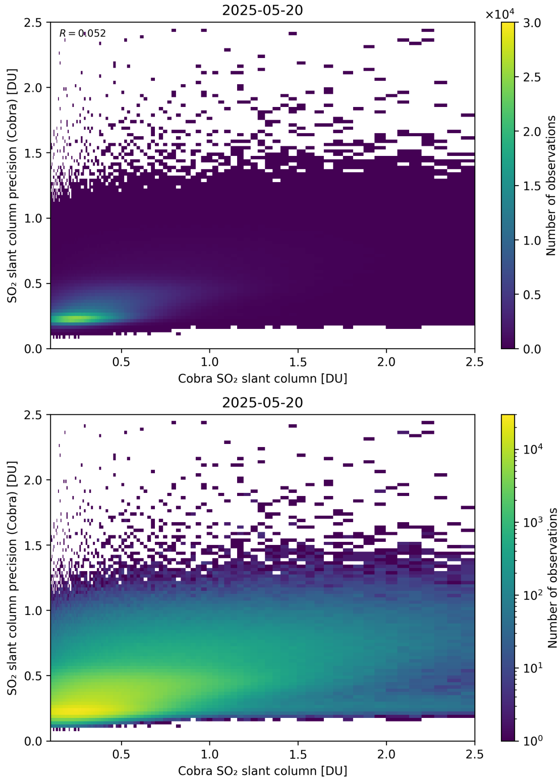
Figure 216: Scatter density plot of “Cobra SO 2 slant column” against “SO 2 slant column precision (Cobra)” for 2025-05-19 to 2025-05-21.
