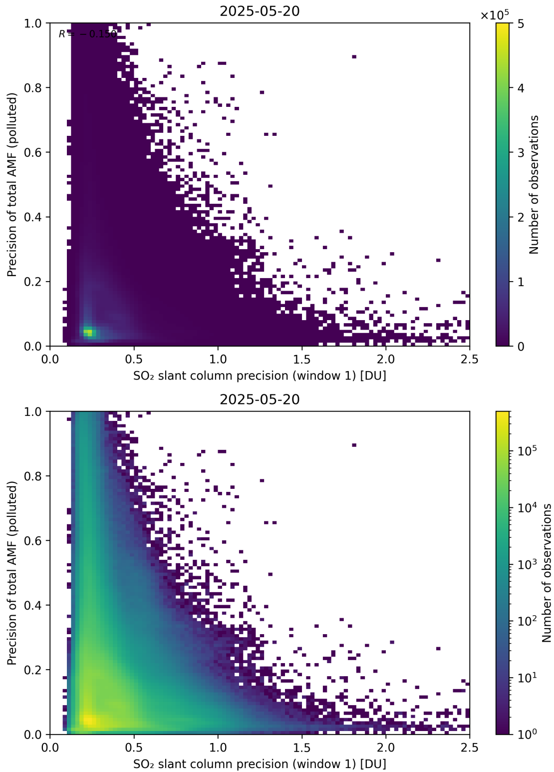
Figure 281: Scatter density plot of “SO 2 slant column precision (window 1)” against “Precision of total AMF (polluted)” for 2025-05-19 to 2025-05-21.
