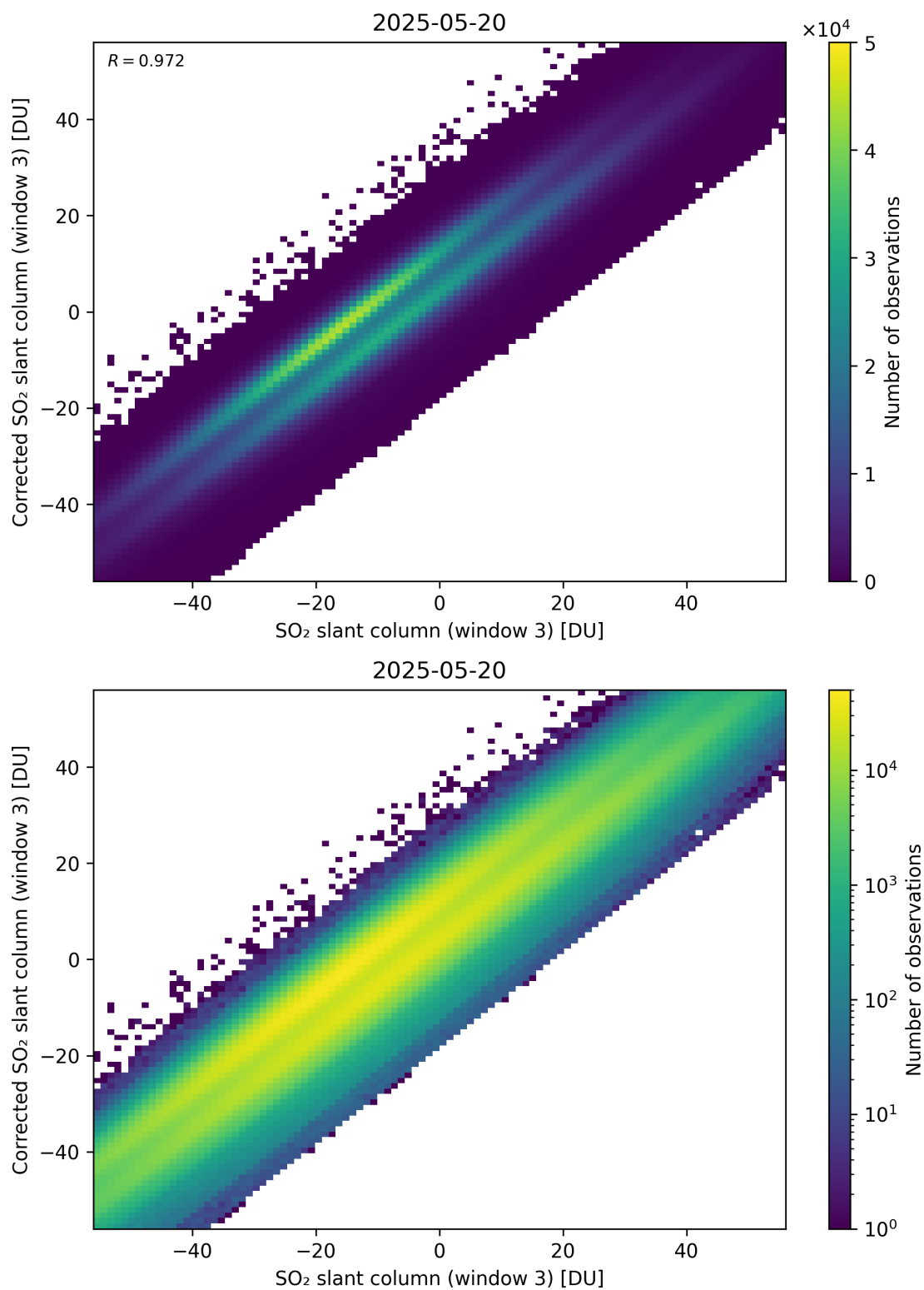
Figure 316: Scatter density plot of “SO 2 slant column (window 3)” against “Corrected SO 2 slant column (window 3)” for 2025-05-19 to 2025-05-21.
