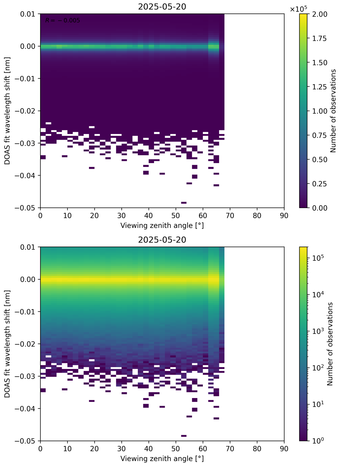
Figure 365: Scatter density plot of “Viewing zenith angle” against “DOAS fit wavelength shift” for 2025-05-19 to 2025-05-21.
