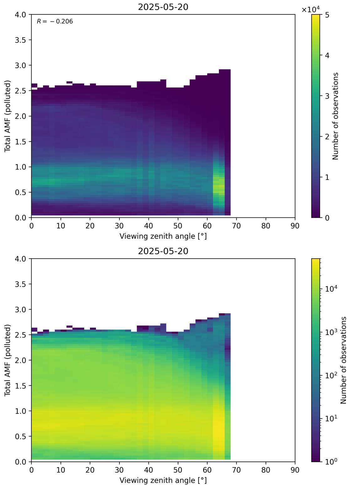
Figure 381: Scatter density plot of “Viewing zenith angle” against “Total AMF (polluted)” for 2025-05-19 to 2025-05-21.
