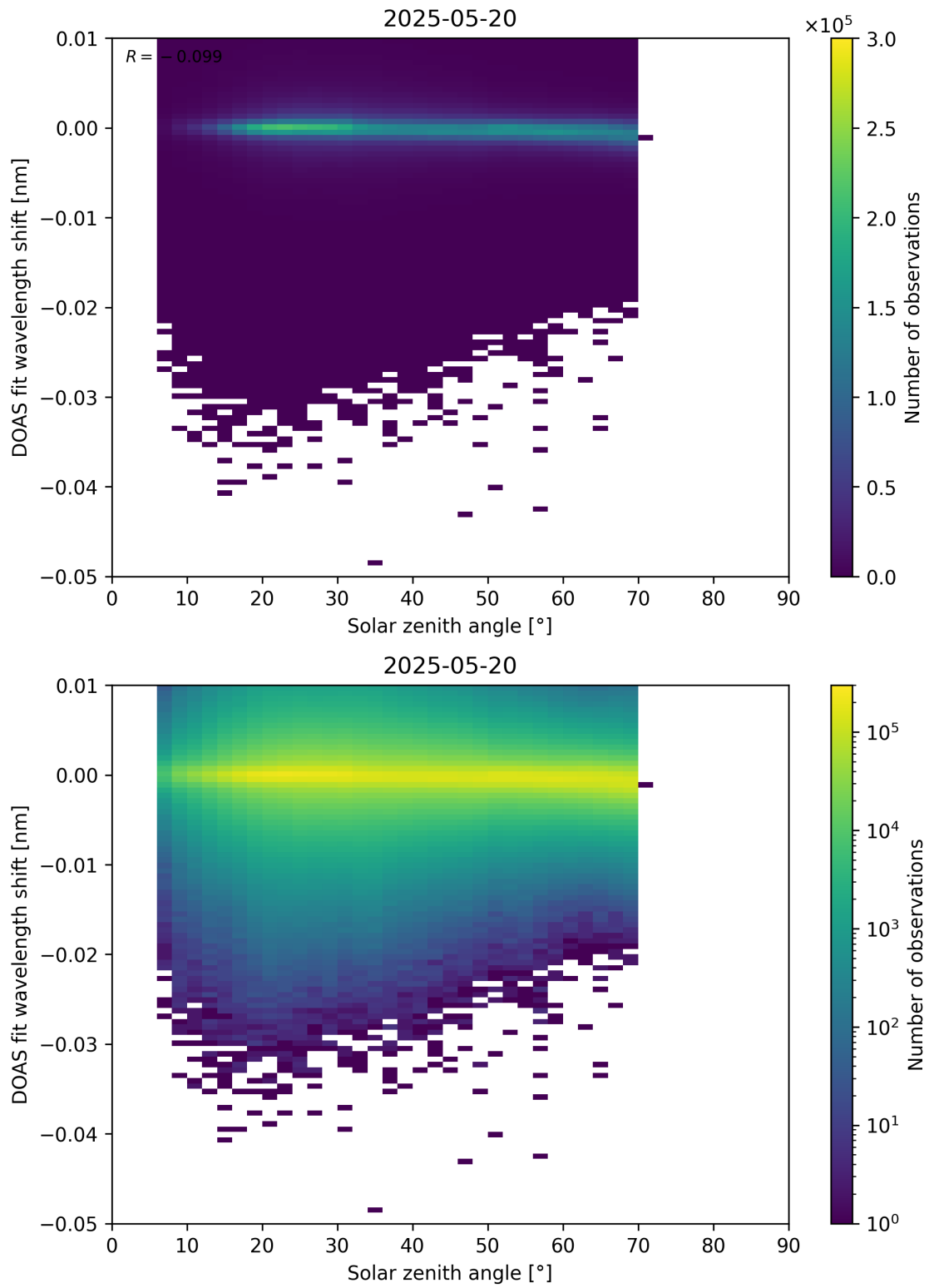
Figure 174: Scatter density plot of “Solar zenith angle” against “DOAS fit wavelength shift” for 2025-05-19 to 2025-05-21.
