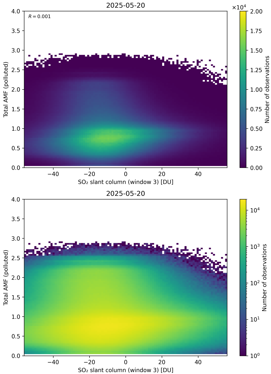
Figure 318: Scatter density plot of “SO 2 slant column (window 3)” against “Total AMF (polluted)” for 2025-05-19 to 2025-05-21.
