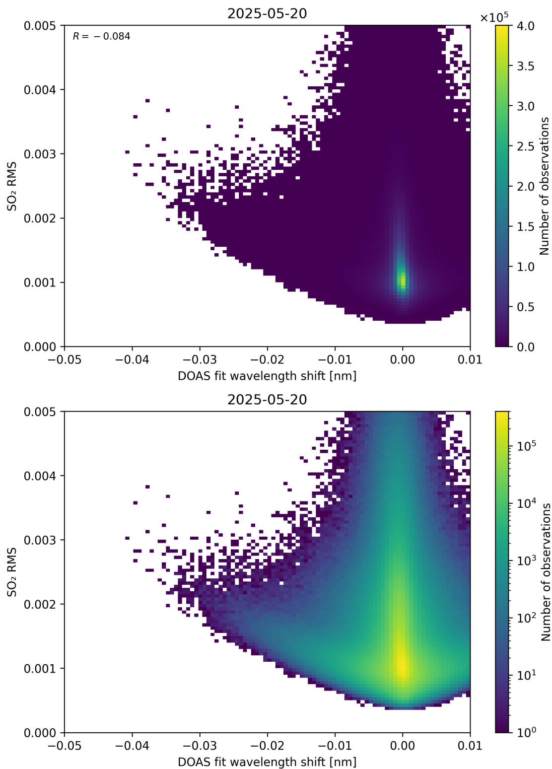
Figure 139: Scatter density plot of “DOAS fit wavelength shift” against “SO 2 RMS” for 2025-05-19 to 2025-05-21.
