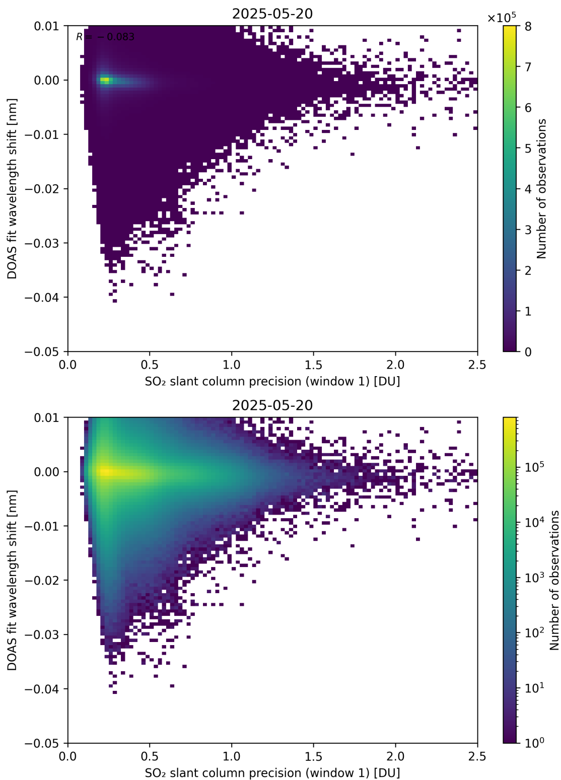
Figure 271: Scatter density plot of “SO 2 slant column precision (window 1)” against “DOAS fit wavelength shift” for 2025-05-19 to 2025-05-21.
