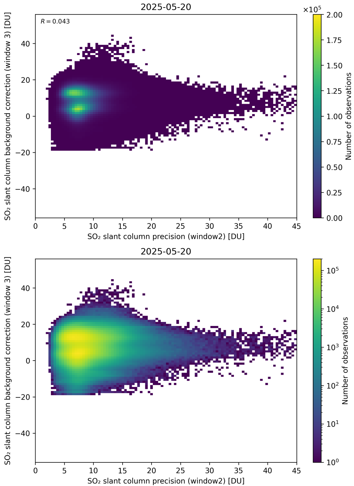
Figure 292: Scatter density plot of “SO 2 slant column precision (window2)” against “SO 2 slant column background correction (window 3)” for 2025-05-19 to 2025-05-21.
