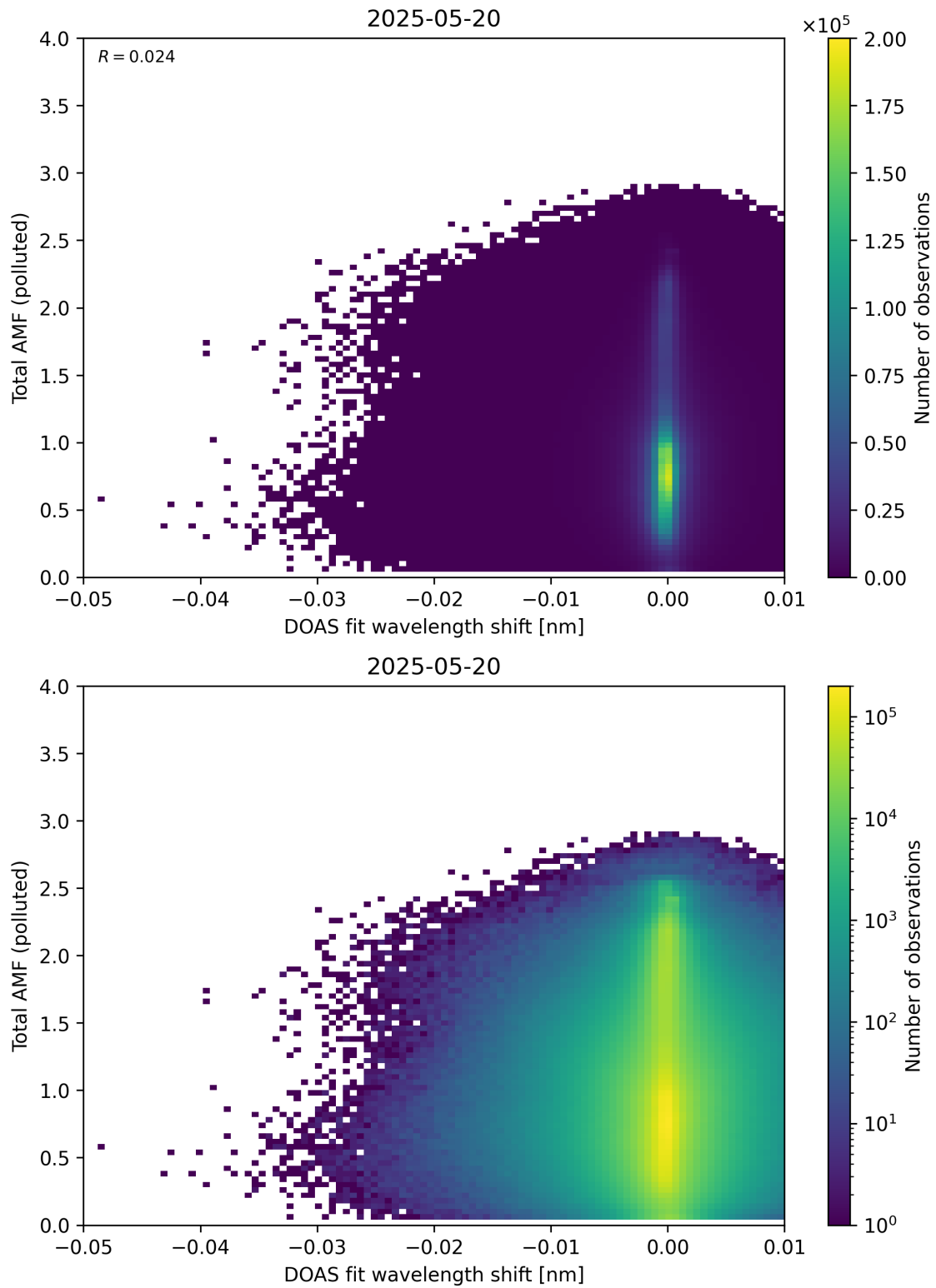
Figure 141: Scatter density plot of “DOAS fit wavelength shift” against “Total AMF (polluted)” for 2025-05-19 to 2025-05-21.
