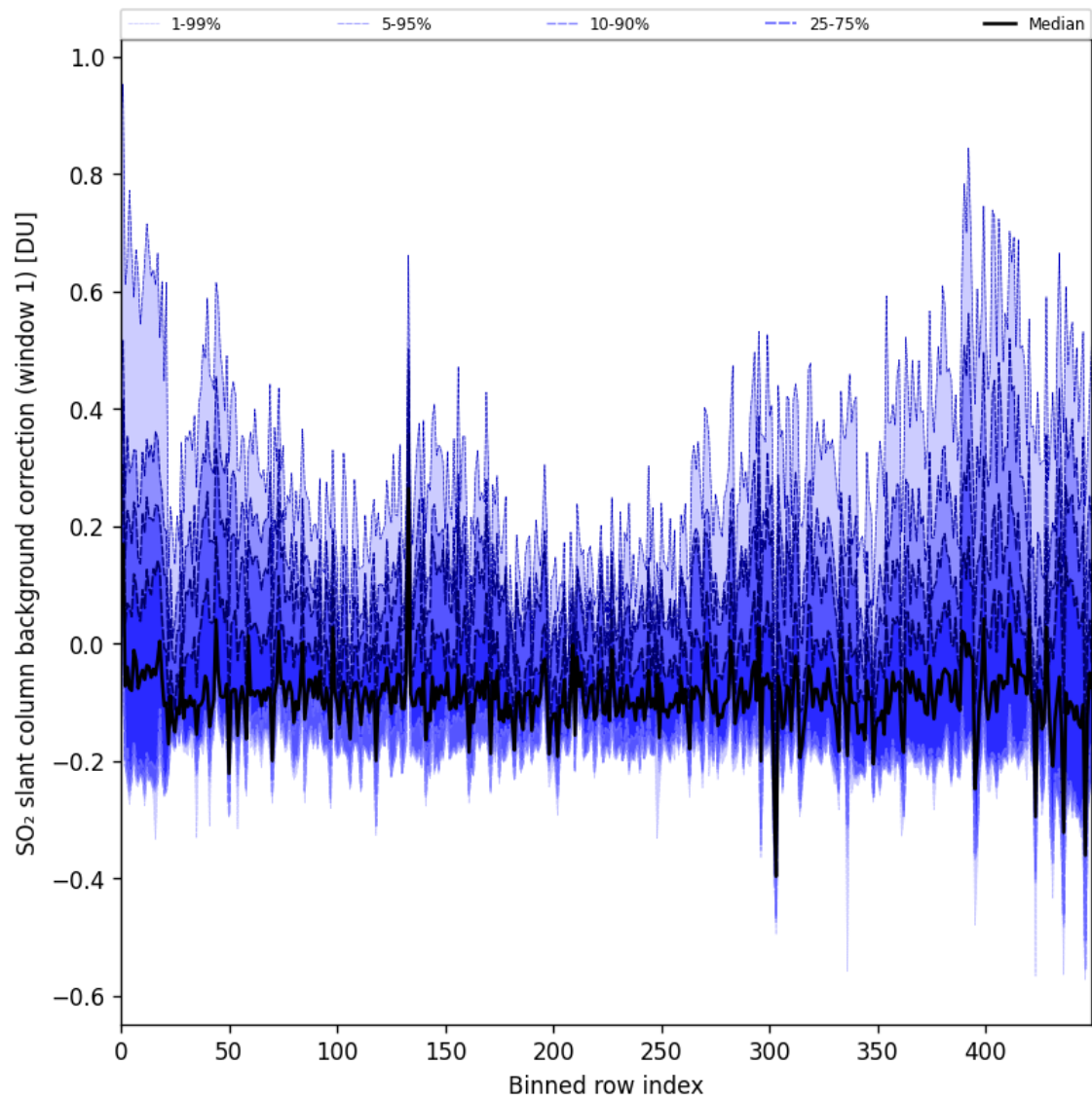
Figure 92: Along track statistics of “SO 2 slant column background correction (window 1)” for 2025-05-19 to 2025-05-21
