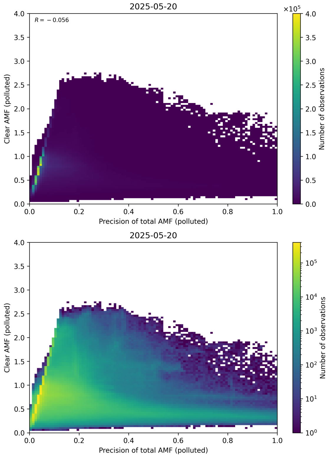
Figure 320: Scatter density plot of “Precision of total AMF (polluted)” against “Clear AMF (polluted)” for 2025-05-19 to 2025-05-21.
