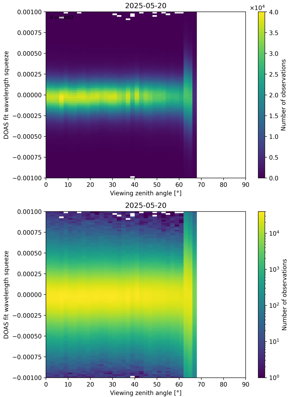
Figure 366: Scatter density plot of “Viewing zenith angle” against “DOAS fit wavelength squeeze” for 2025-05-19 to 2025-05-21.
