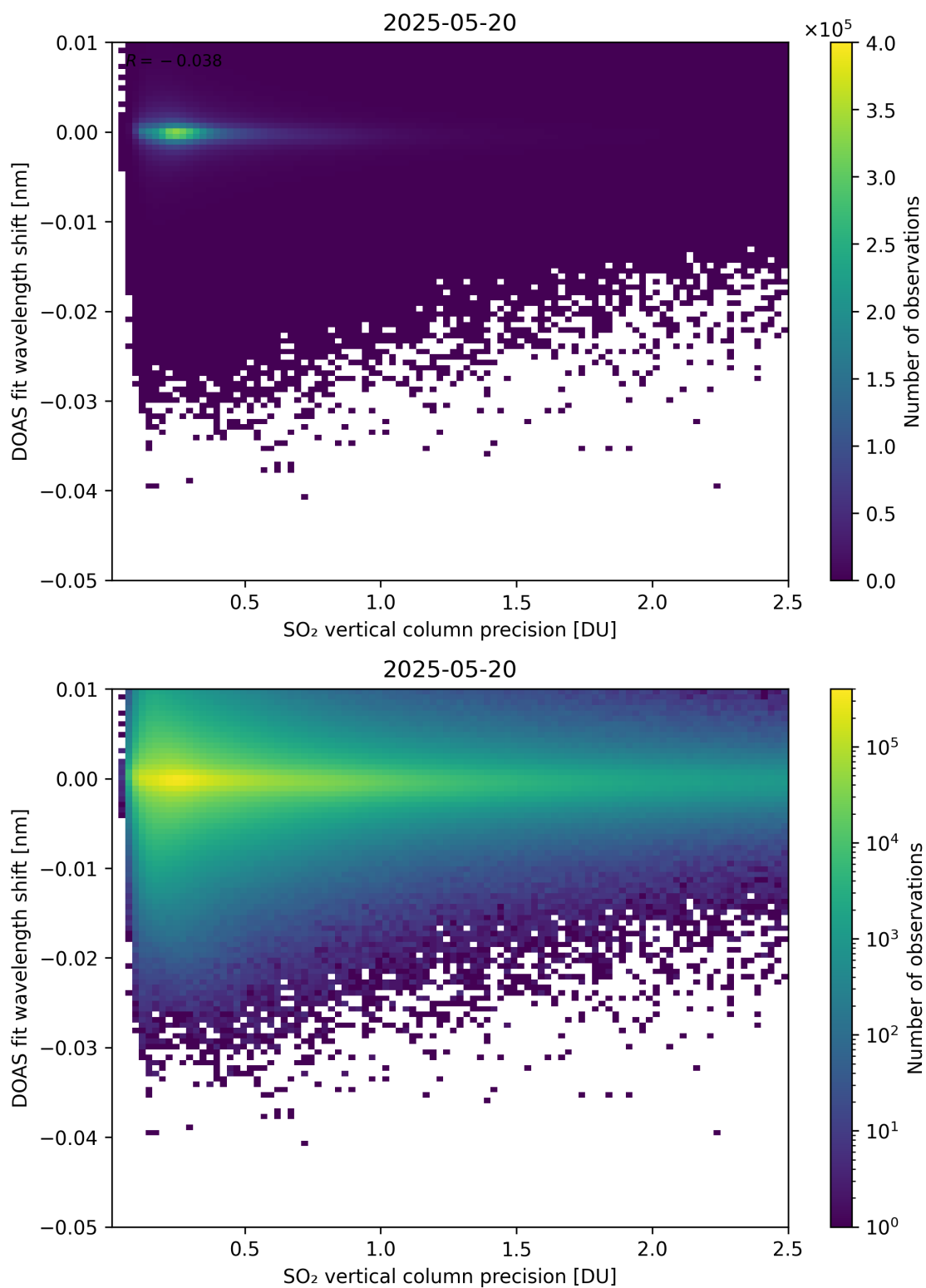
Figure 332: Scatter density plot of “SO 2 vertical column precision” against “DOAS fit wavelength shift” for 2025-05-19 to 2025-05-21.
