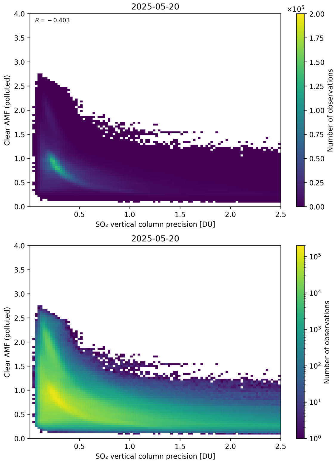
Figure 335: Scatter density plot of “SO 2 vertical column precision” against “Clear AMF (polluted)” for 2025-05-19 to 2025-05-21.
