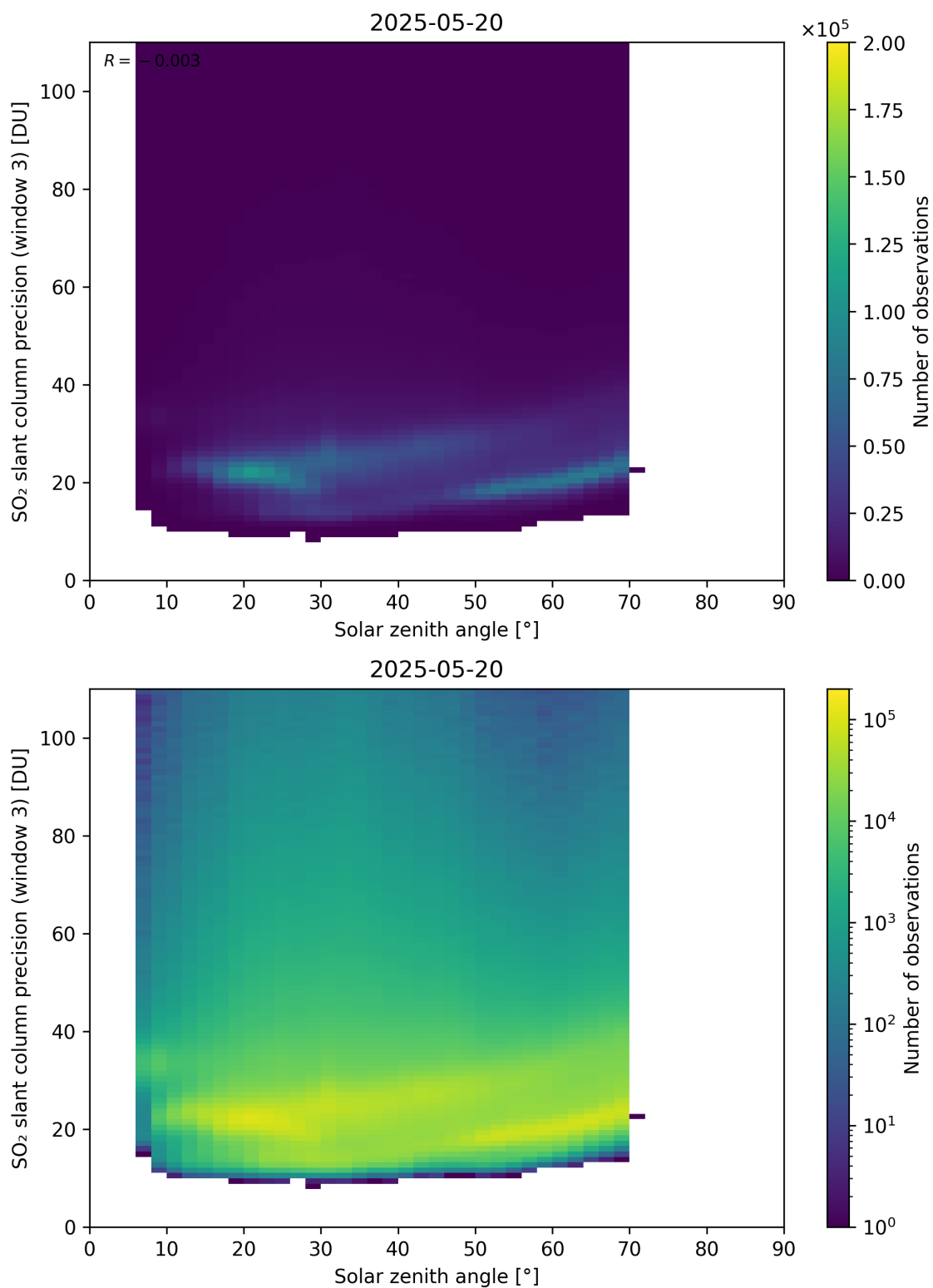
Figure 188: Scatter density plot of “Solar zenith angle” against “SO 2 slant column precision (window 3)” for 2025-05-19 to 2025-05-21.
