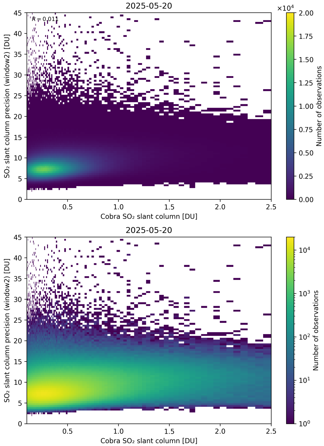
Figure 221: Scatter density plot of “Cobra SO 2 slant column” against “SO 2 slant column precision (window2)” for 2025-05-19 to 2025-05-21.
