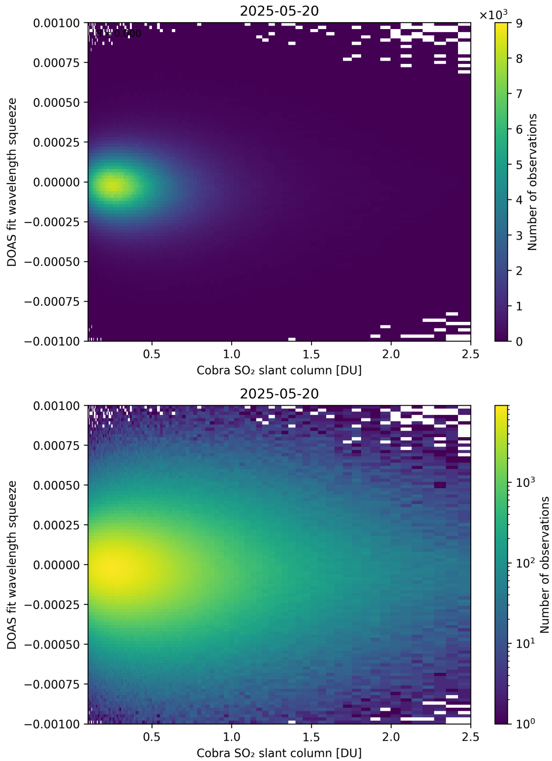
Figure 197: Scatter density plot of “Cobra SO 2 slant column” against “DOAS fit wavelength squeeze” for 2025-05-19 to 2025-05-21.
