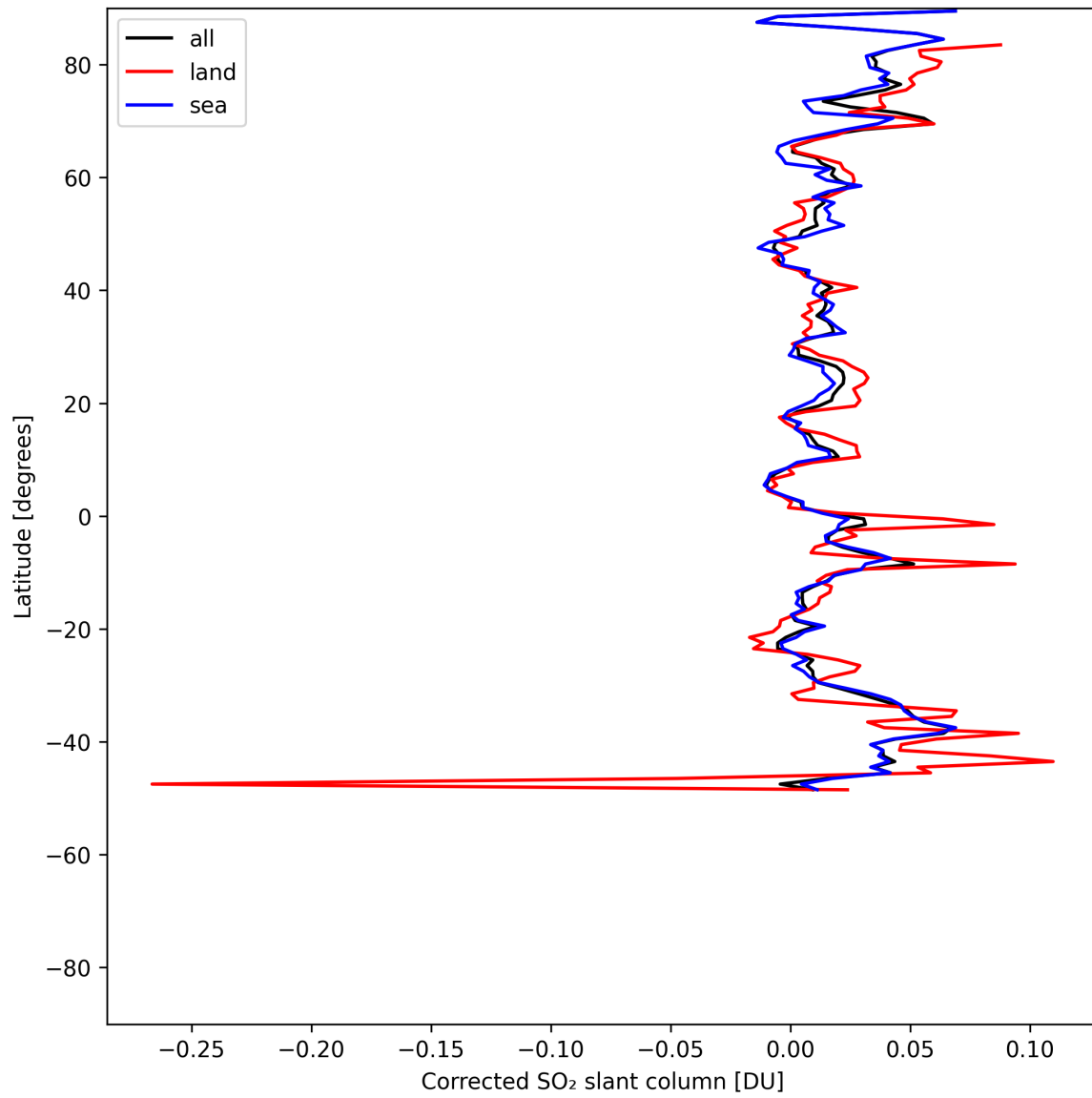
Figure 34: Zonal average of “Corrected SO 2 slant column” for 2025-05-19 to 2025-05-21.
