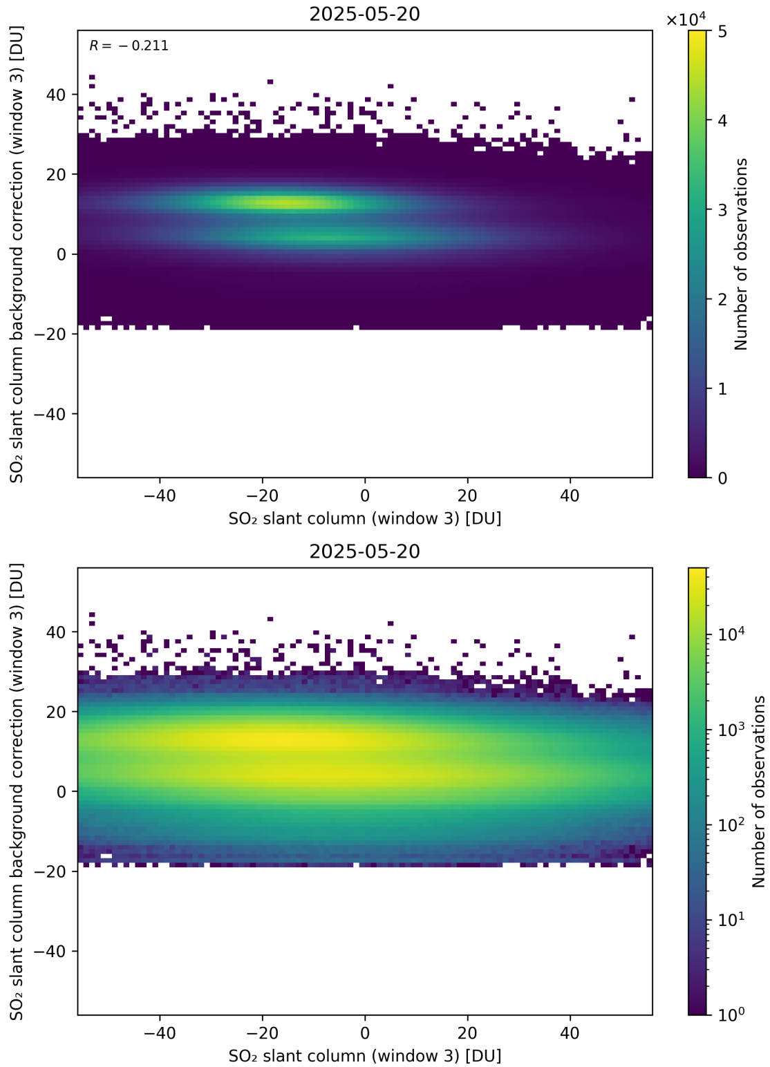
Figure 303: Scatter density plot of “SO 2 slant column (window 3)” against “SO 2 slant column background correction (window 3)” for 2025-05-19 to 2025-05-21.
