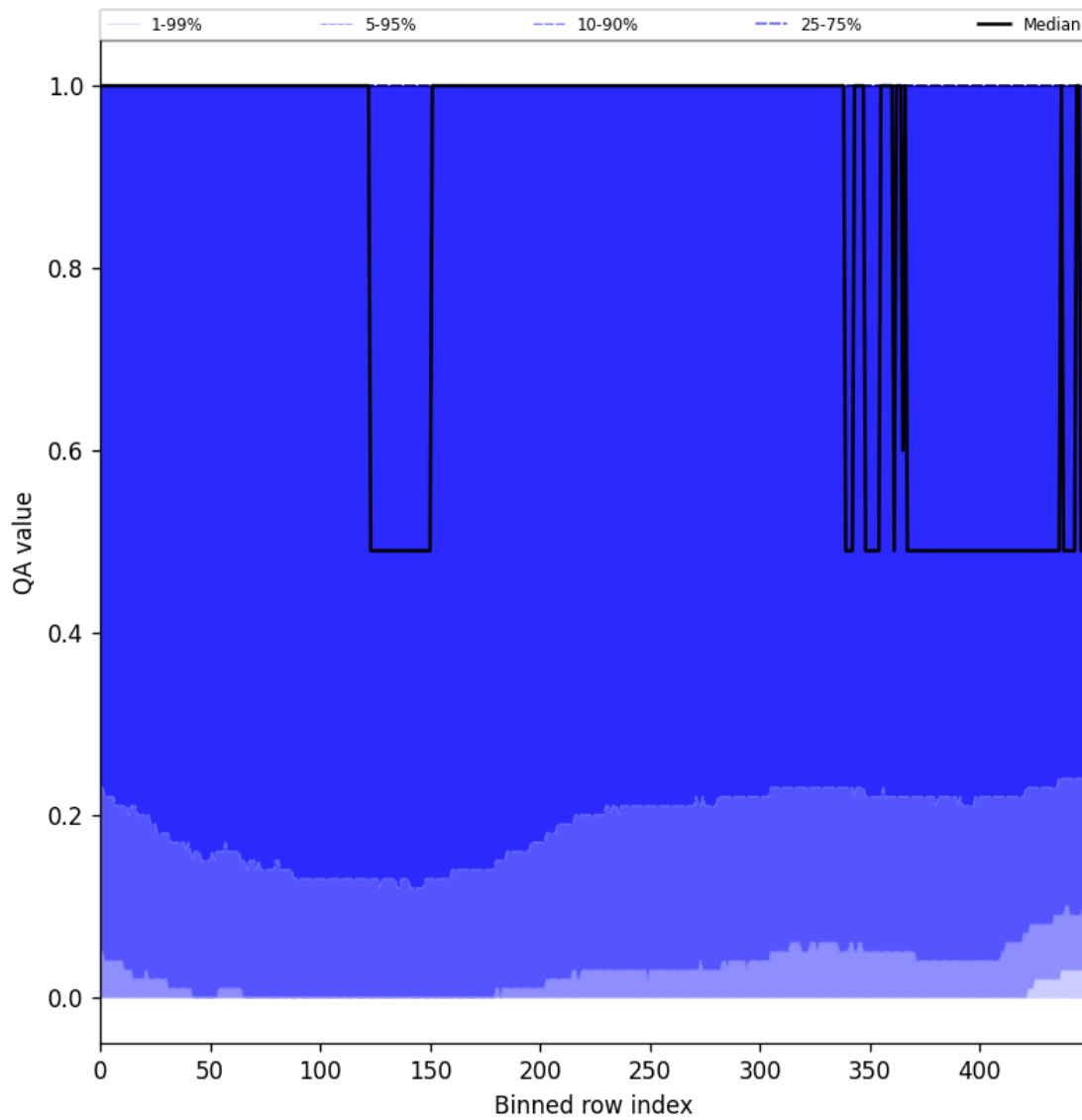
Figure 83: Along track statistics of “QA value” for 2025-05-19 to 2025-05-21
