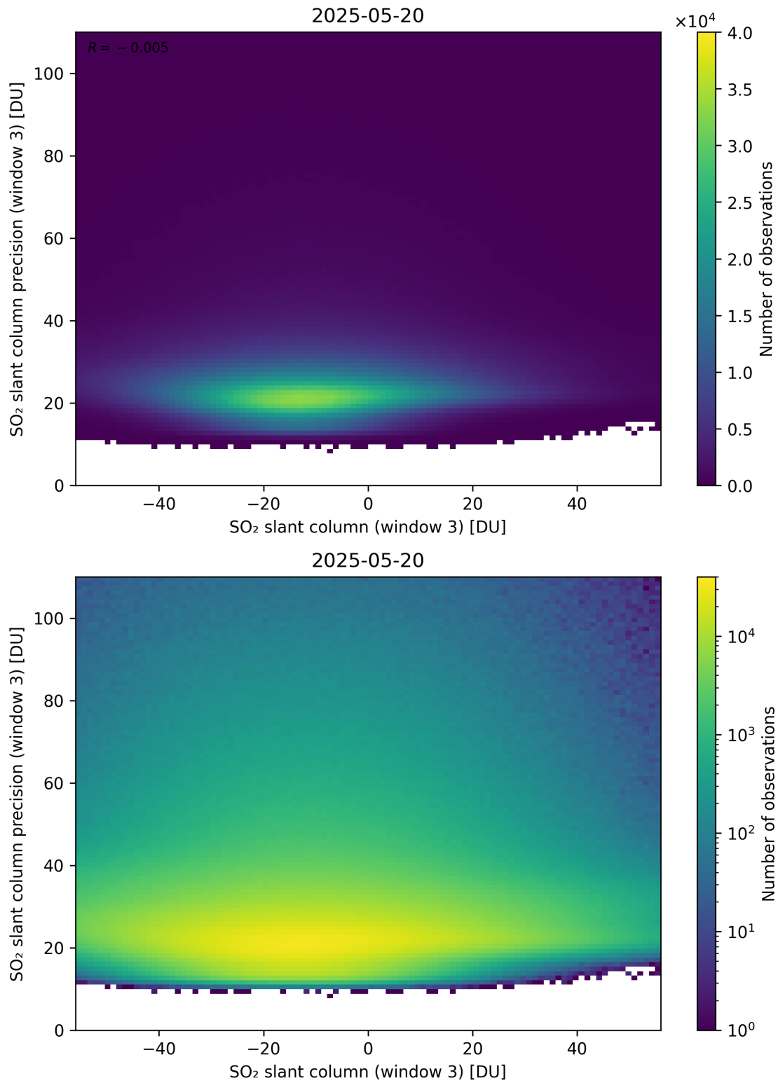
Figure 317: Scatter density plot of “SO 2 slant column (window 3)” against “SO 2 slant column precision (window 3)” for 2025-05-19 to 2025-05-21.
