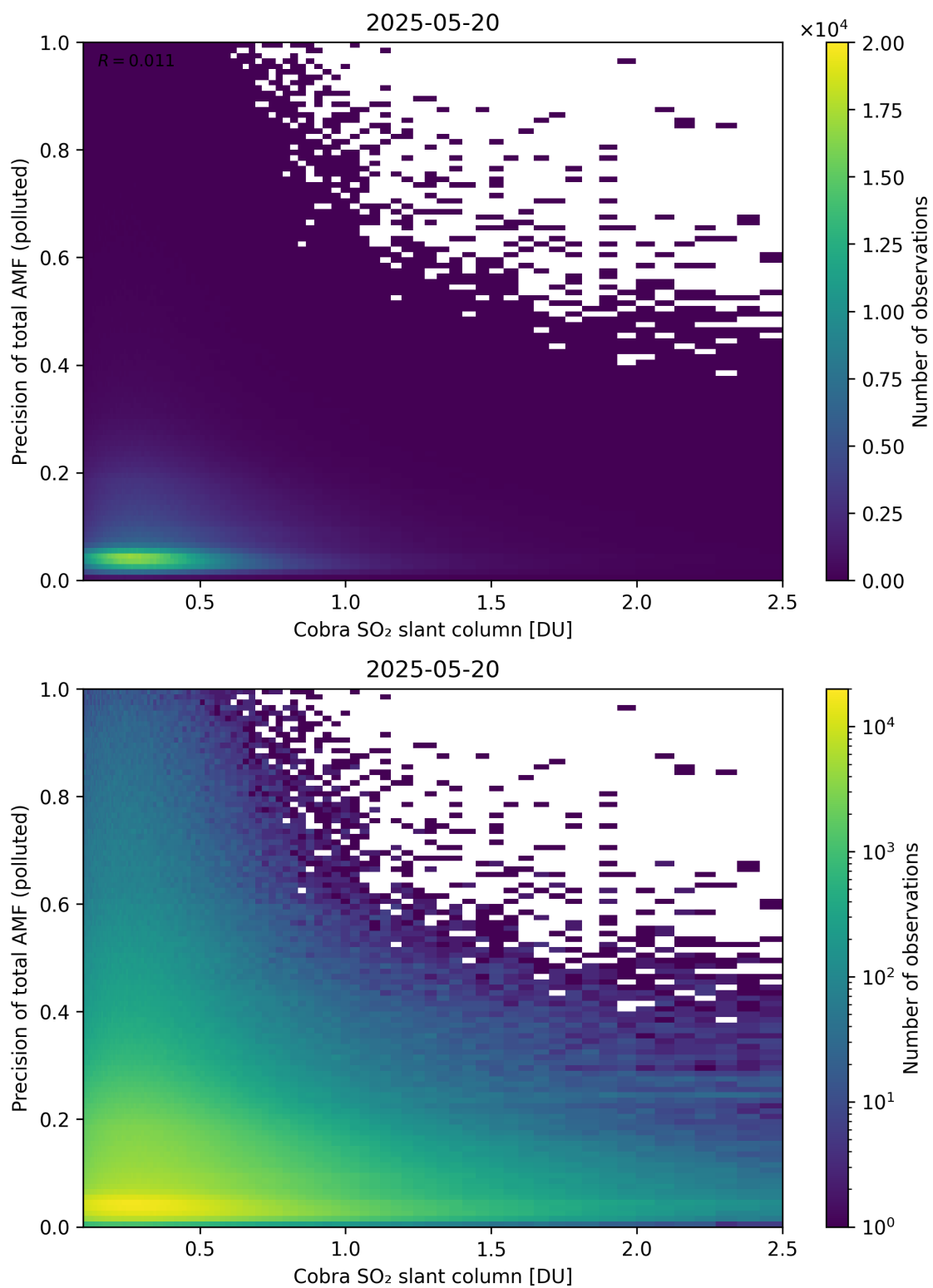
Figure 225: Scatter density plot of “Cobra SO 2 slant column” against “Precision of total AMF (polluted)” for 2025-05-19 to 2025-05-21.
