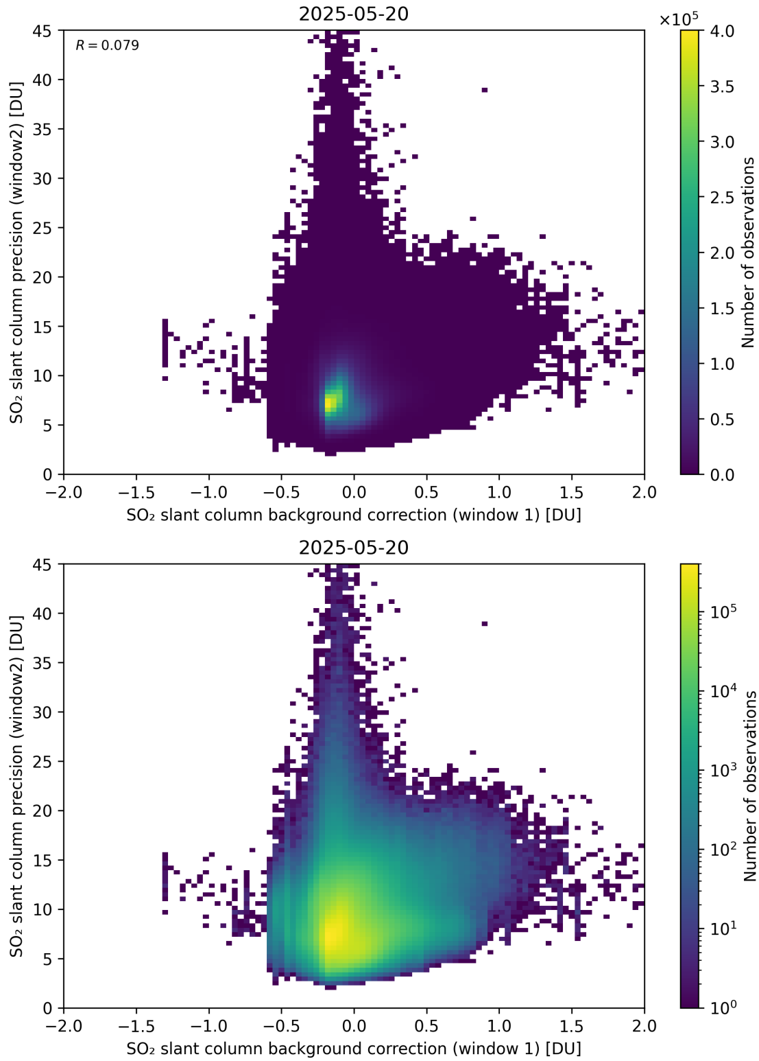
Figure 117: Scatter density plot of “SO 2 slant column background correction (window 1)” against “SO 2 slant column precision (window2)” for 2025-05-19 to 2025-05-21.
