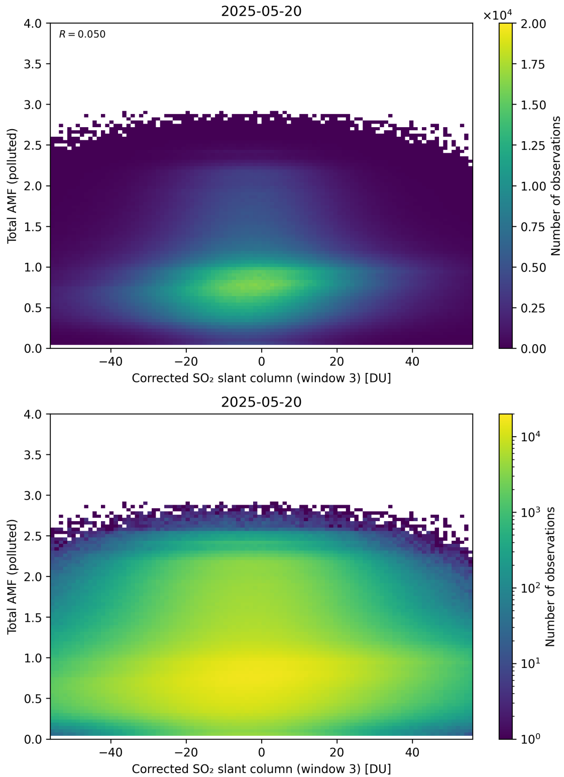
Figure 260: Scatter density plot of “Corrected SO 2 slant column (window 3)” against “Total AMF (polluted)” for 2025-05-19 to 2025-05-21.
