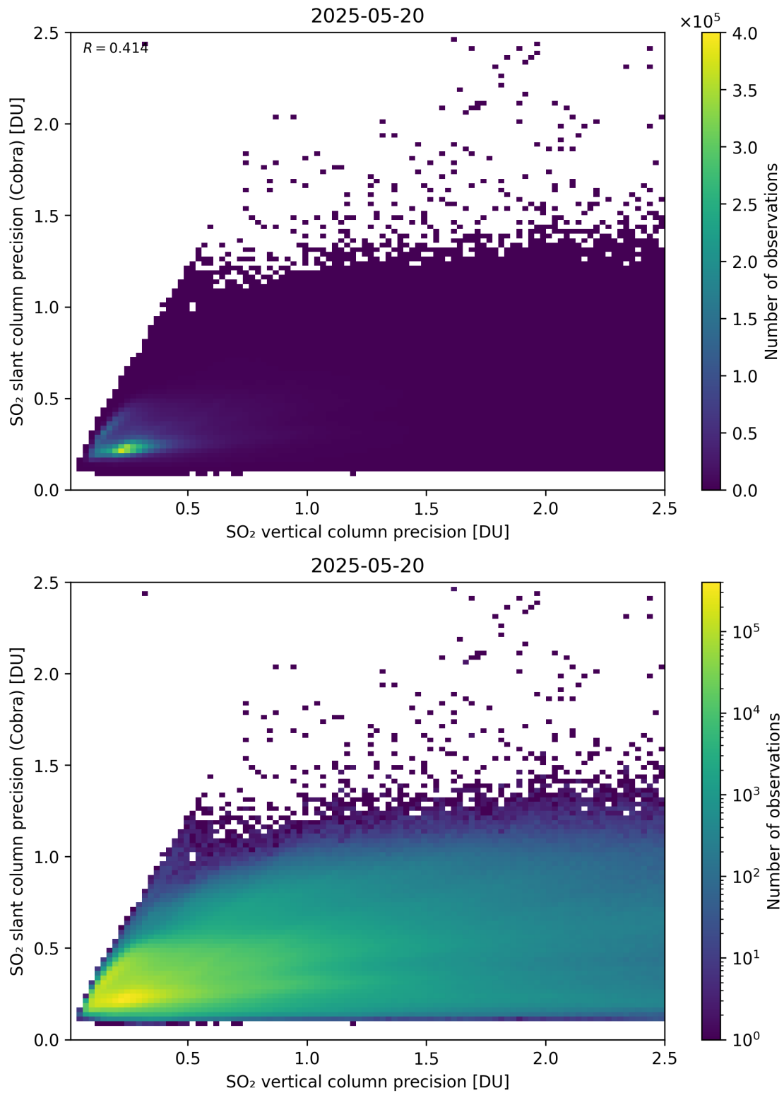
Figure 337: Scatter density plot of “SO 2 vertical column precision” against “SO 2 slant column precision (Cobra)” for 2025-05-19 to 2025-05-21.
