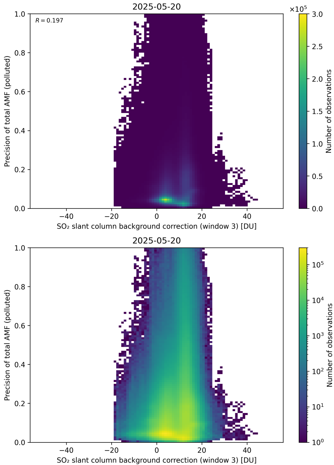
Figure 137: Scatter density plot of “SO 2 slant column background correction (window 3)” against “Precision of total AMF (polluted)” for 2025-05-19 to 2025-05-21.
