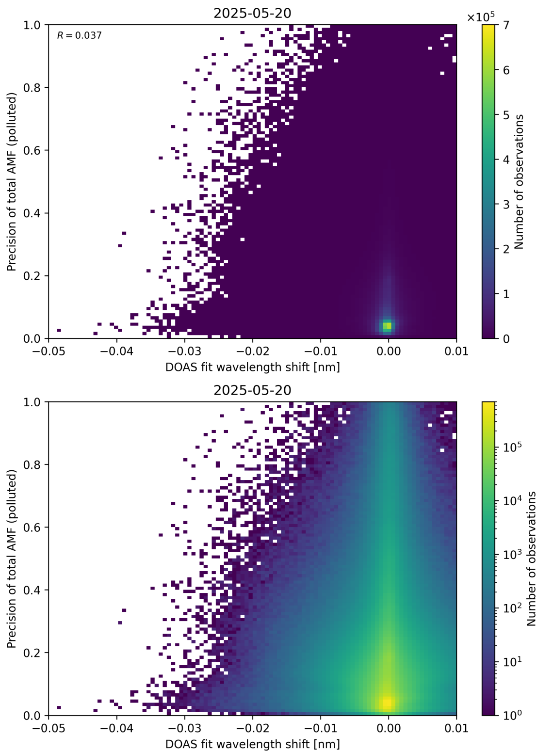
Figure 142: Scatter density plot of “DOAS fit wavelength shift” against “Precision of total AMF (polluted)” for 2025-05-19 to 2025-05-21.
