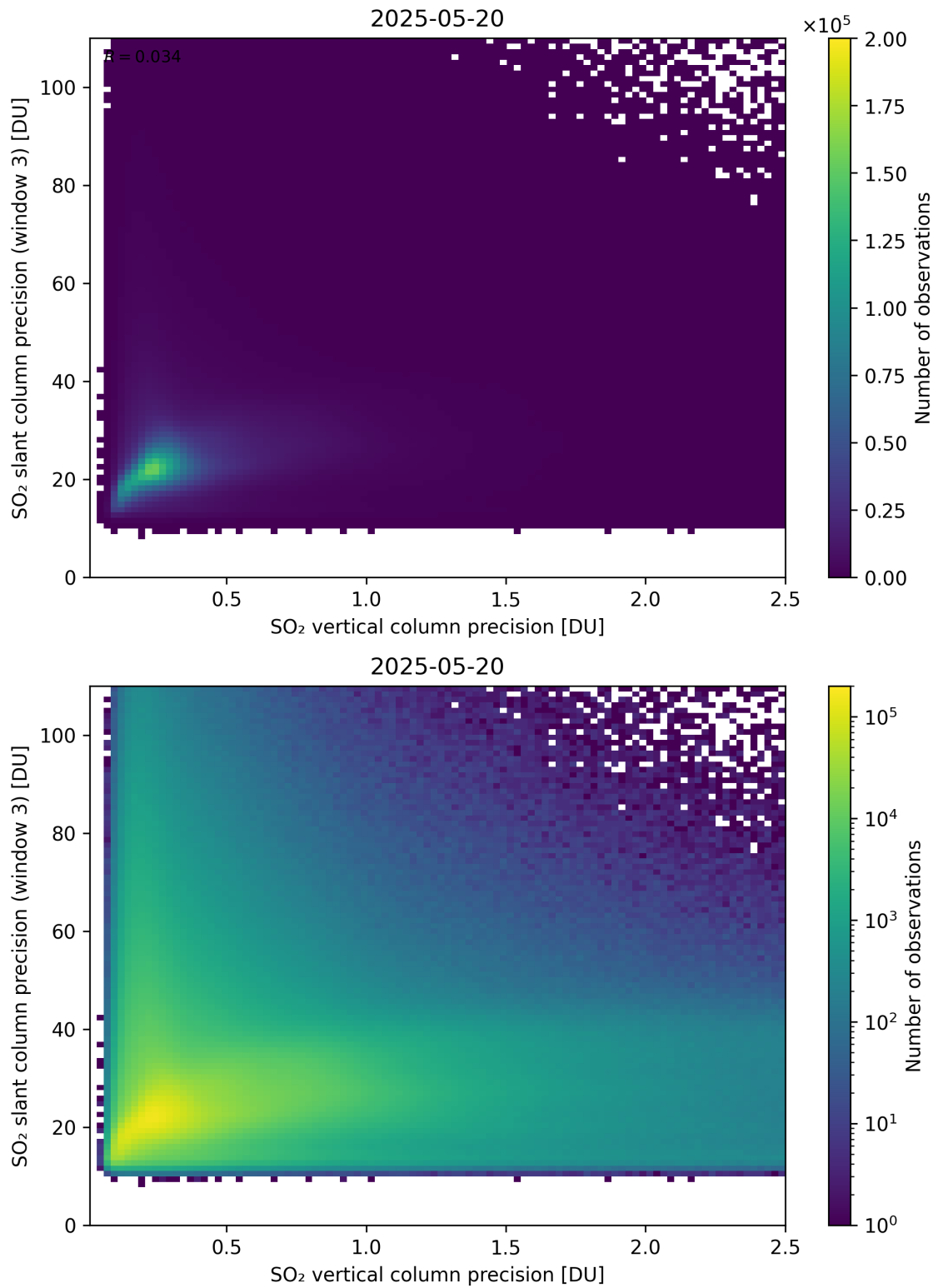
Figure 345: Scatter density plot of “SO 2 vertical column precision” against “SO 2 slant column precision (window 3)” for 2025-05-19 to 2025-05-21.
