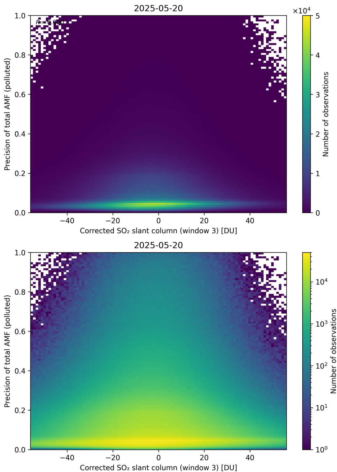
Figure 261: Scatter density plot of “Corrected SO 2 slant column (window 3)” against “Precision of total AMF (polluted)” for 2025-05-19 to 2025-05-21.
