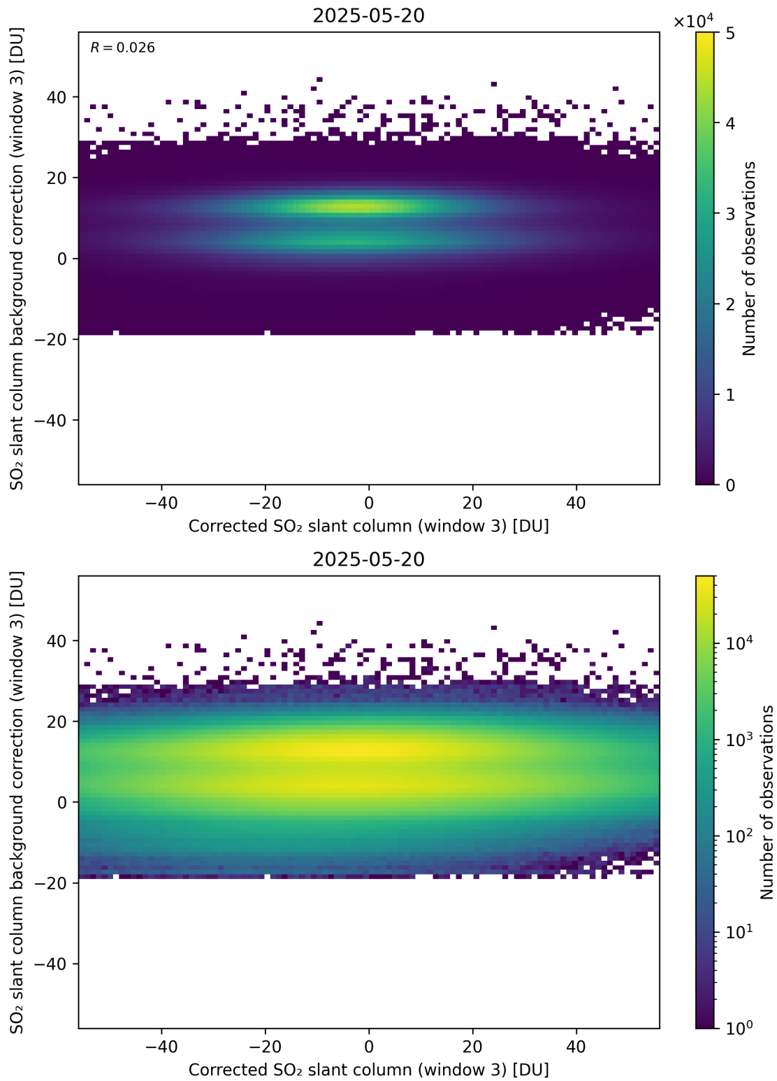
Figure 255: Scatter density plot of “Corrected SO 2 slant column (window 3)” against “SO 2 slant column background correction (window 3)” for 2025-05-19 to 2025-05-21.
