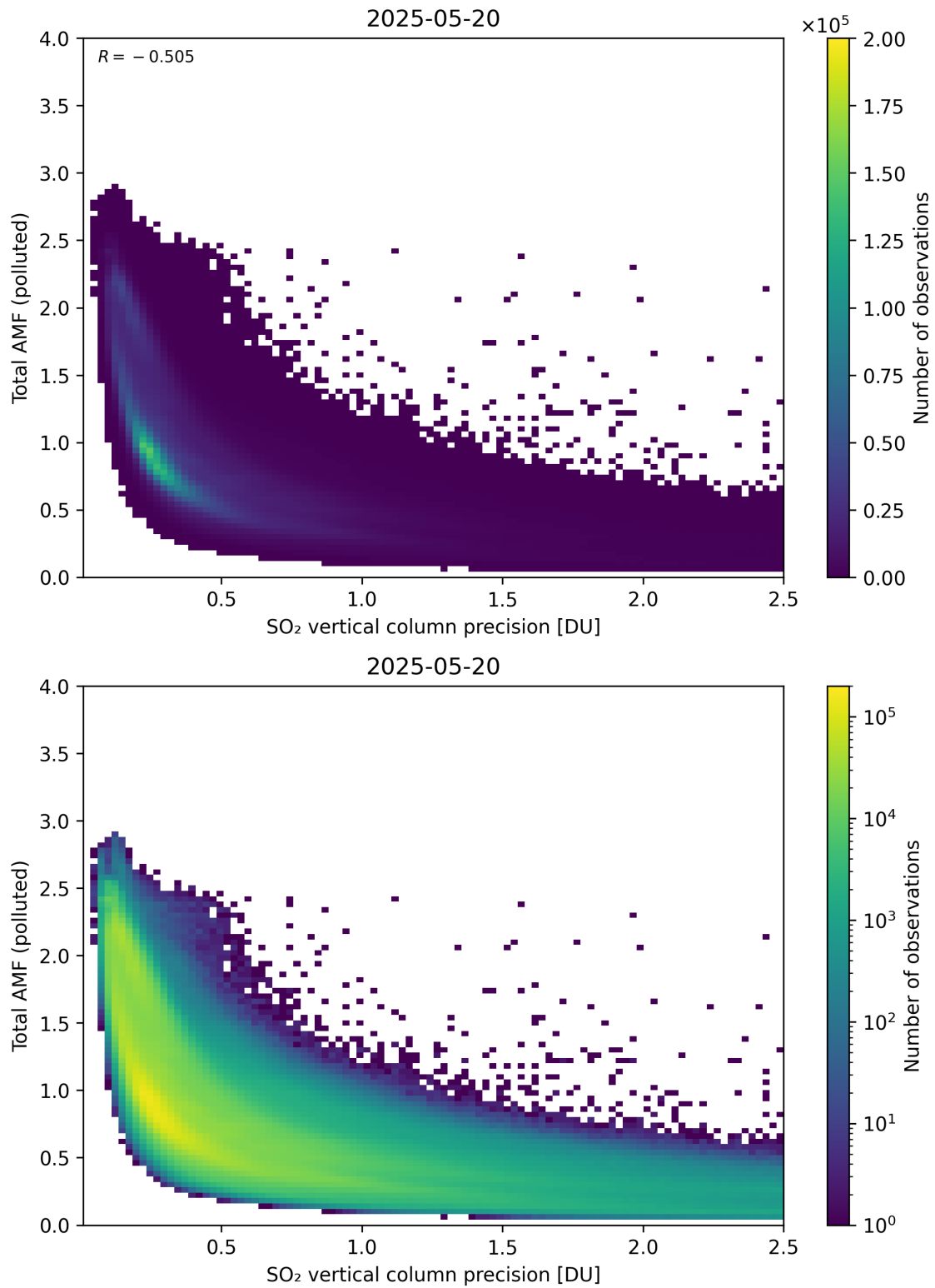
Figure 346: Scatter density plot of “SO 2 vertical column precision” against “Total AMF (polluted)” for 2025-05-19 to 2025-05-21.
