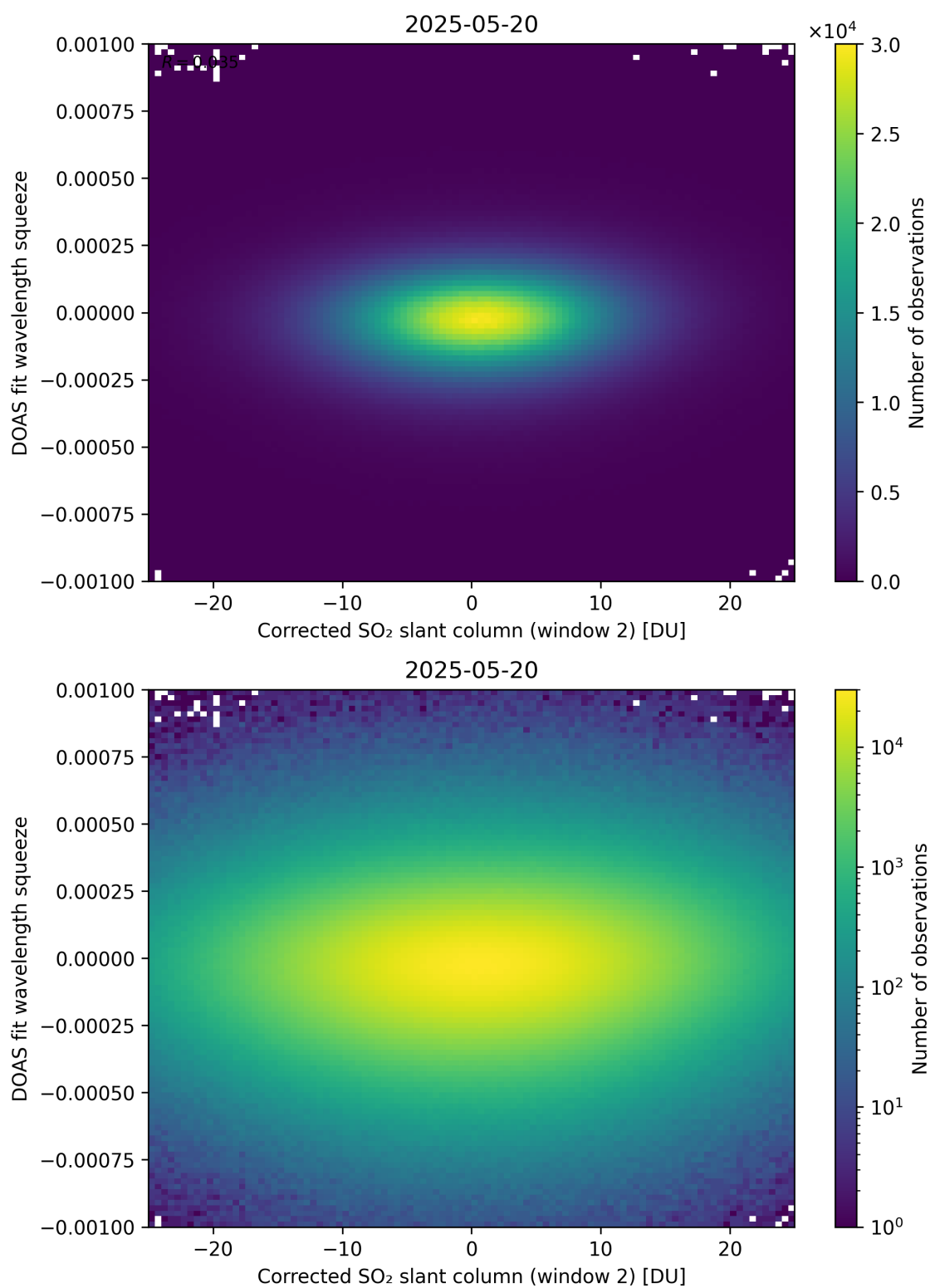
Figure 247: Scatter density plot of “Corrected SO 2 slant column (window 2)” against “DOAS fit wavelength squeeze” for 2025-05-19 to 2025-05-21.
