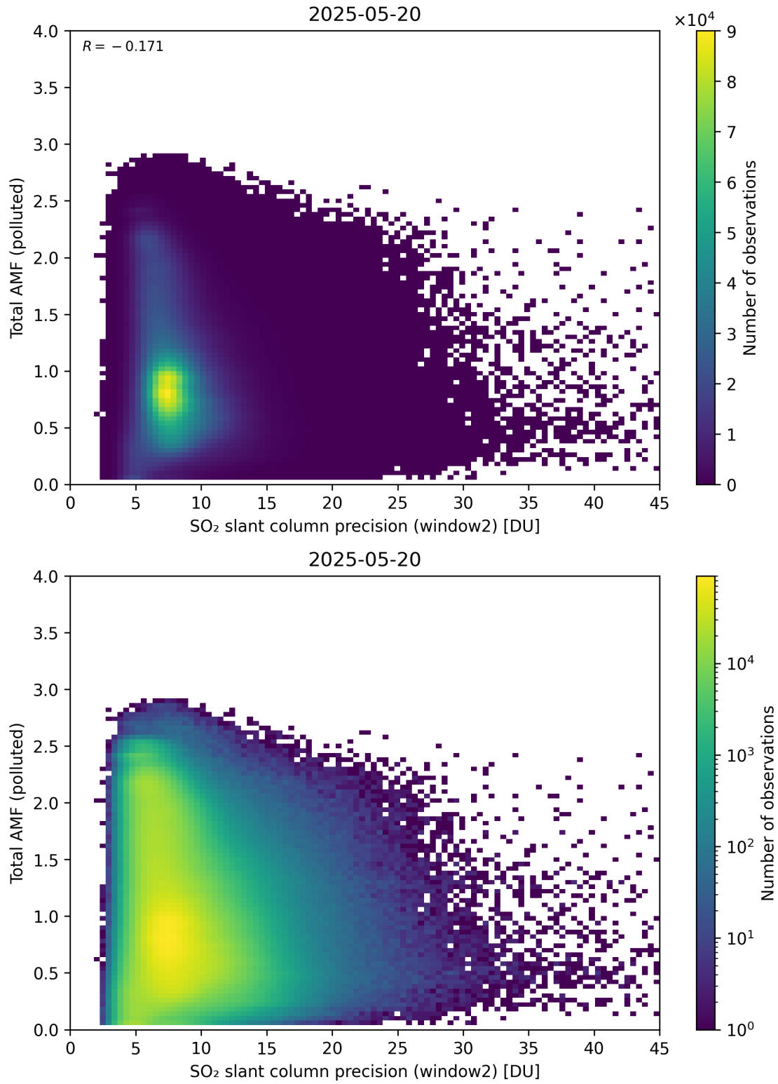
Figure 301: Scatter density plot of “SO 2 slant column precision (window2)” against “Total AMF (polluted)” for 2025-05-19 to 2025-05-21.
