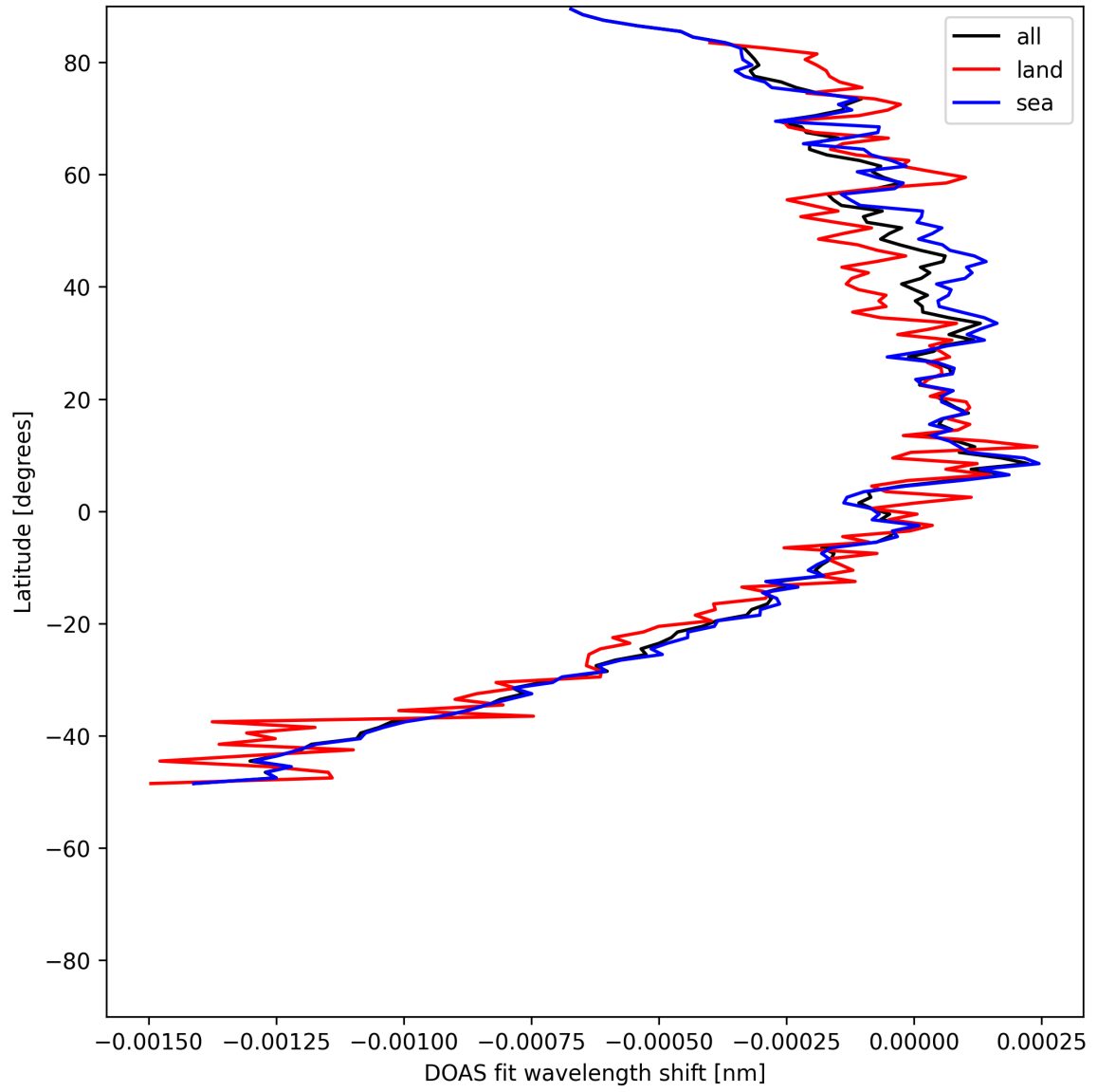
Figure 50: Zonal average of “DOAS fit wavelength shift” for 2025-05-19 to 2025-05-21.
