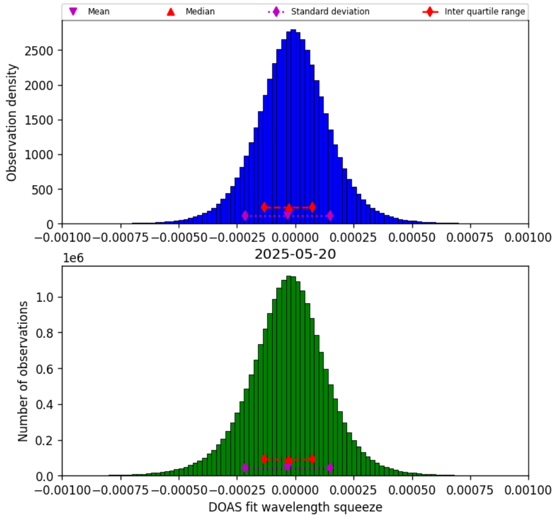
Figure 77: Histogram of “DOAS fit wavelength squeeze” for 2025-05-19 to 2025-05-21
