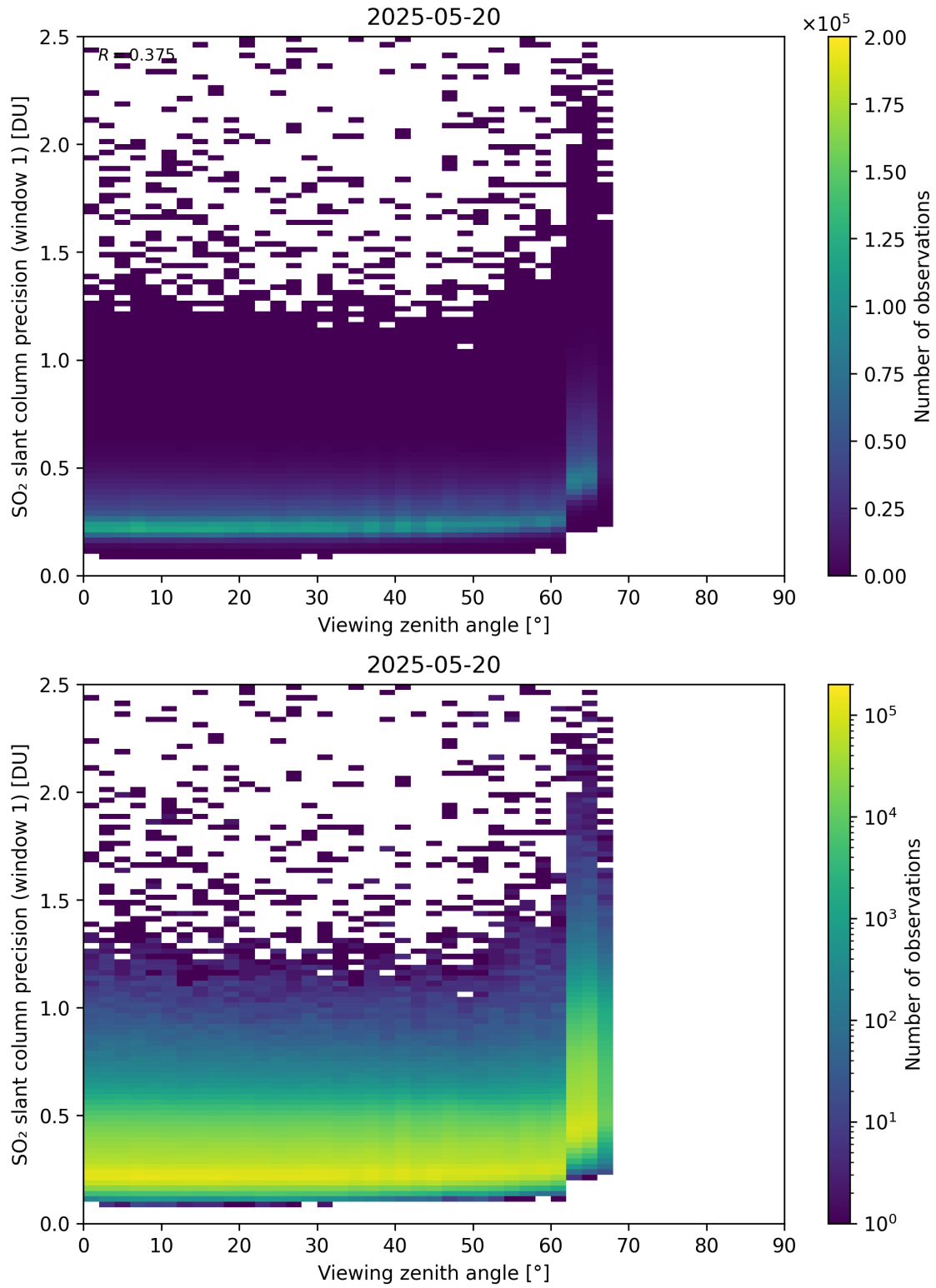
Figure 377: Scatter density plot of “Viewing zenith angle” against “SO 2 slant column precision (window 1)” for 2025-05-19 to 2025-05-21.
