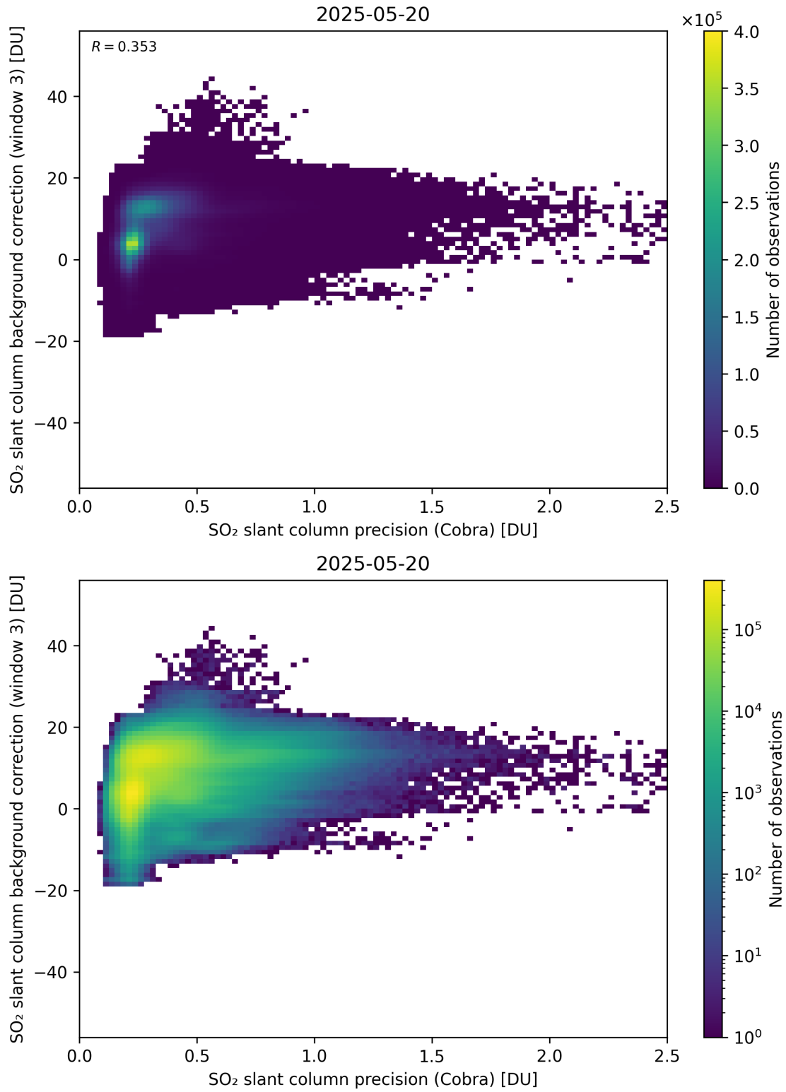
Figure 201: Scatter density plot of “SO 2 slant column precision (Cobra)” against “SO 2 slant column background correction (window 3)” for 2025-05-19 to 2025-05-21.
