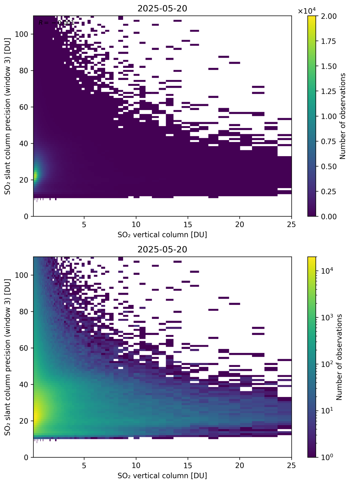
Figure 358: Scatter density plot of “SO 2 vertical column” against “SO 2 slant column precision (window 3)” for 2025-05-19 to 2025-05-21.
