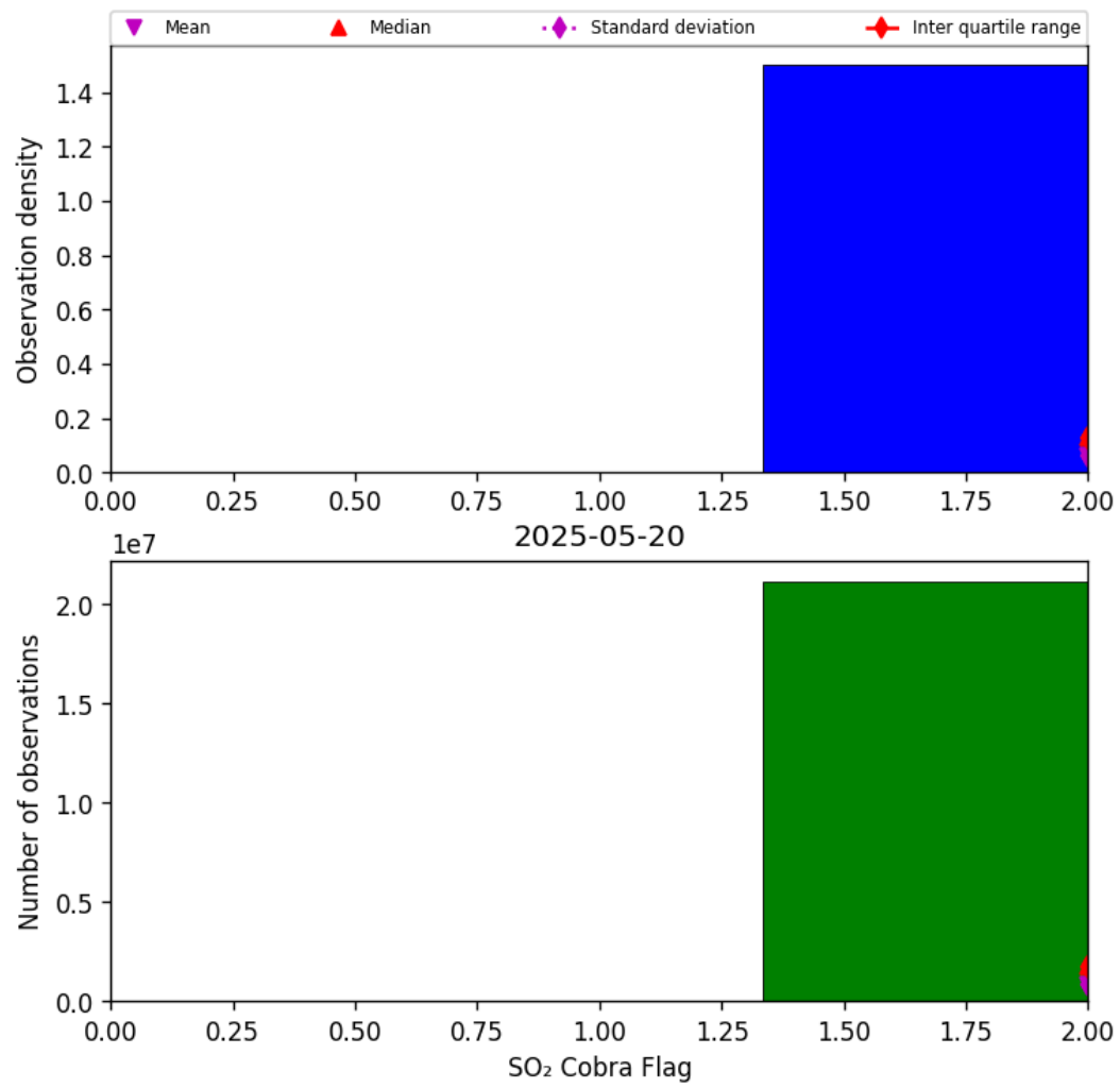
Figure 75: Histogram of “SO 2 Cobra Flag” for 2025-05-19 to 2025-05-21
