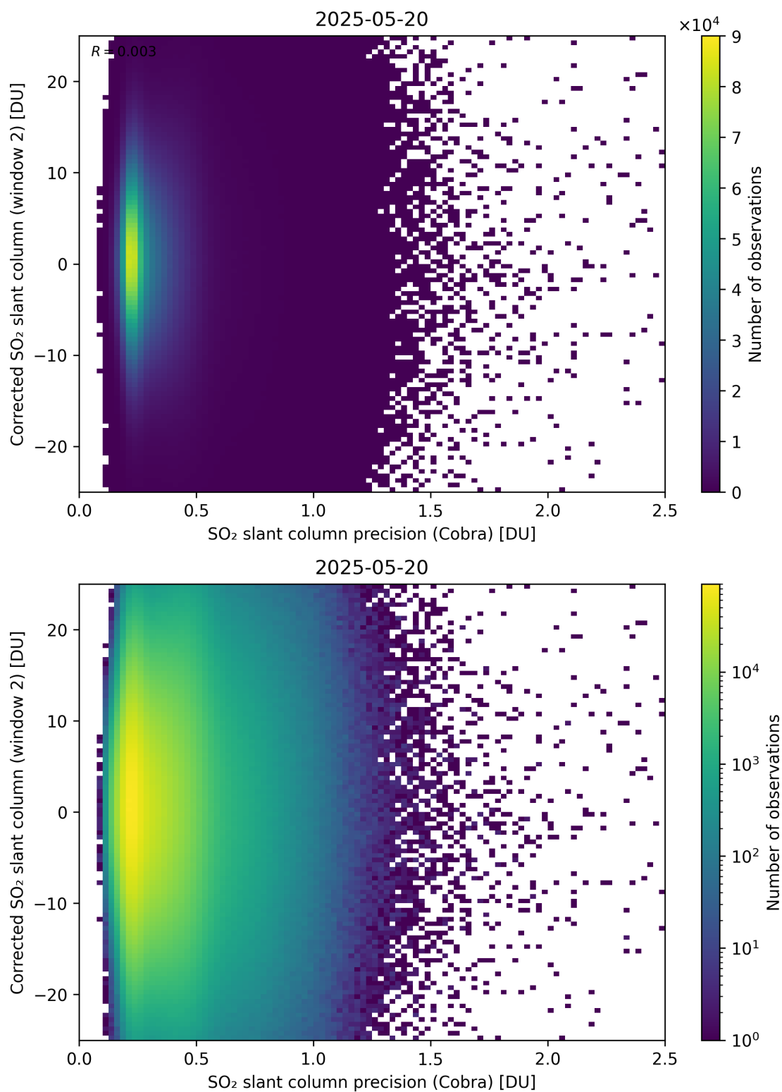
Figure 206: Scatter density plot of “SO 2 slant column precision (Cobra)” against “Corrected SO 2 slant column (window 2)” for 2025-05-19 to 2025-05-21.
