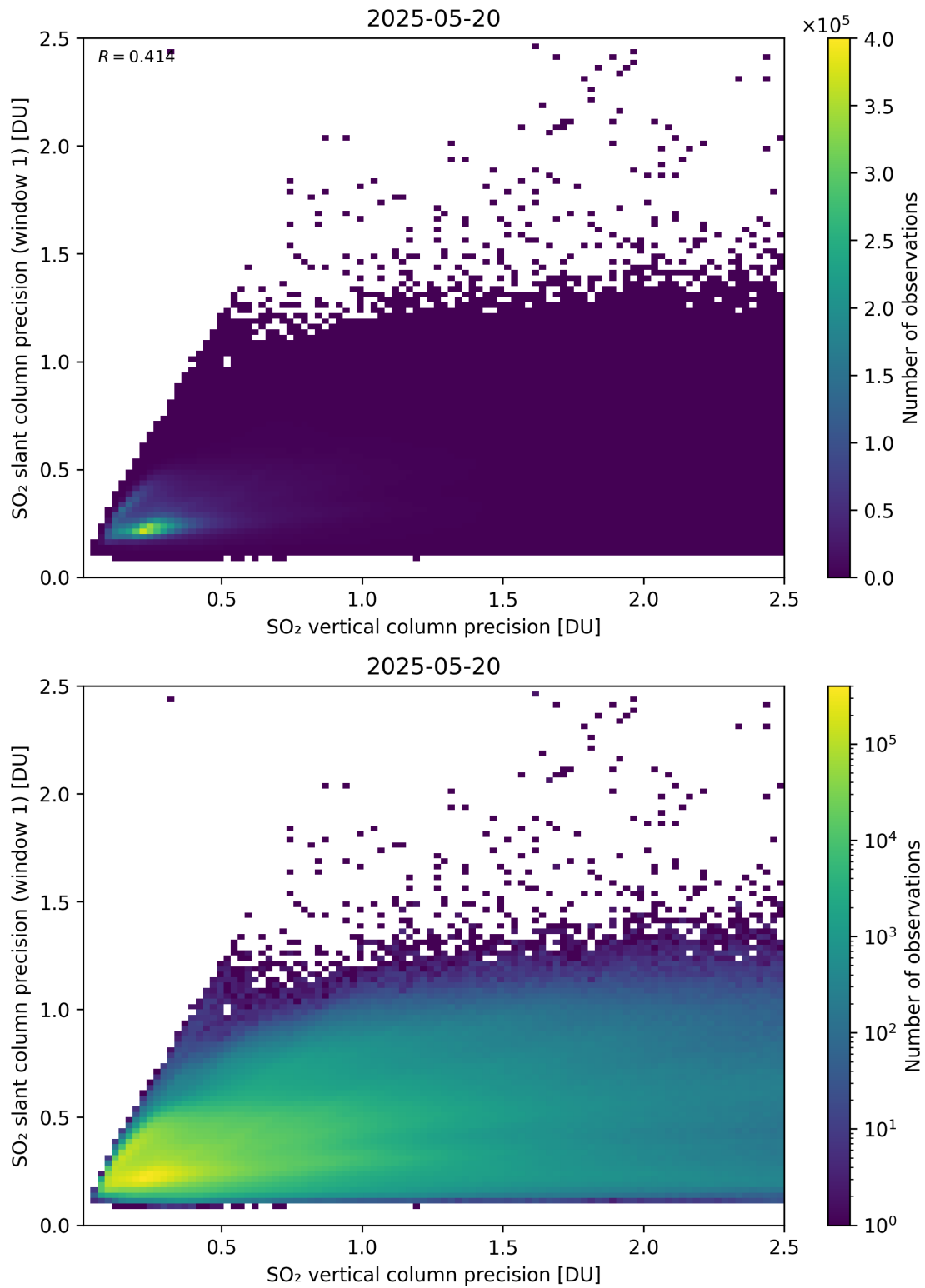
Figure 342: Scatter density plot of “SO 2 vertical column precision” against “SO 2 slant column precision (window 1)” for 2025-05-19 to 2025-05-21.
