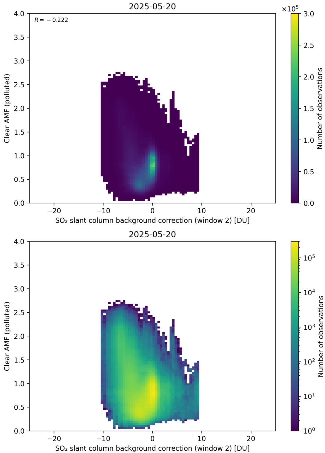
Figure 126: Scatter density plot of “SO 2 slant column background correction (window 2)” against “Clear AMF (polluted)” for 2025-05-19 to 2025-05-21.
