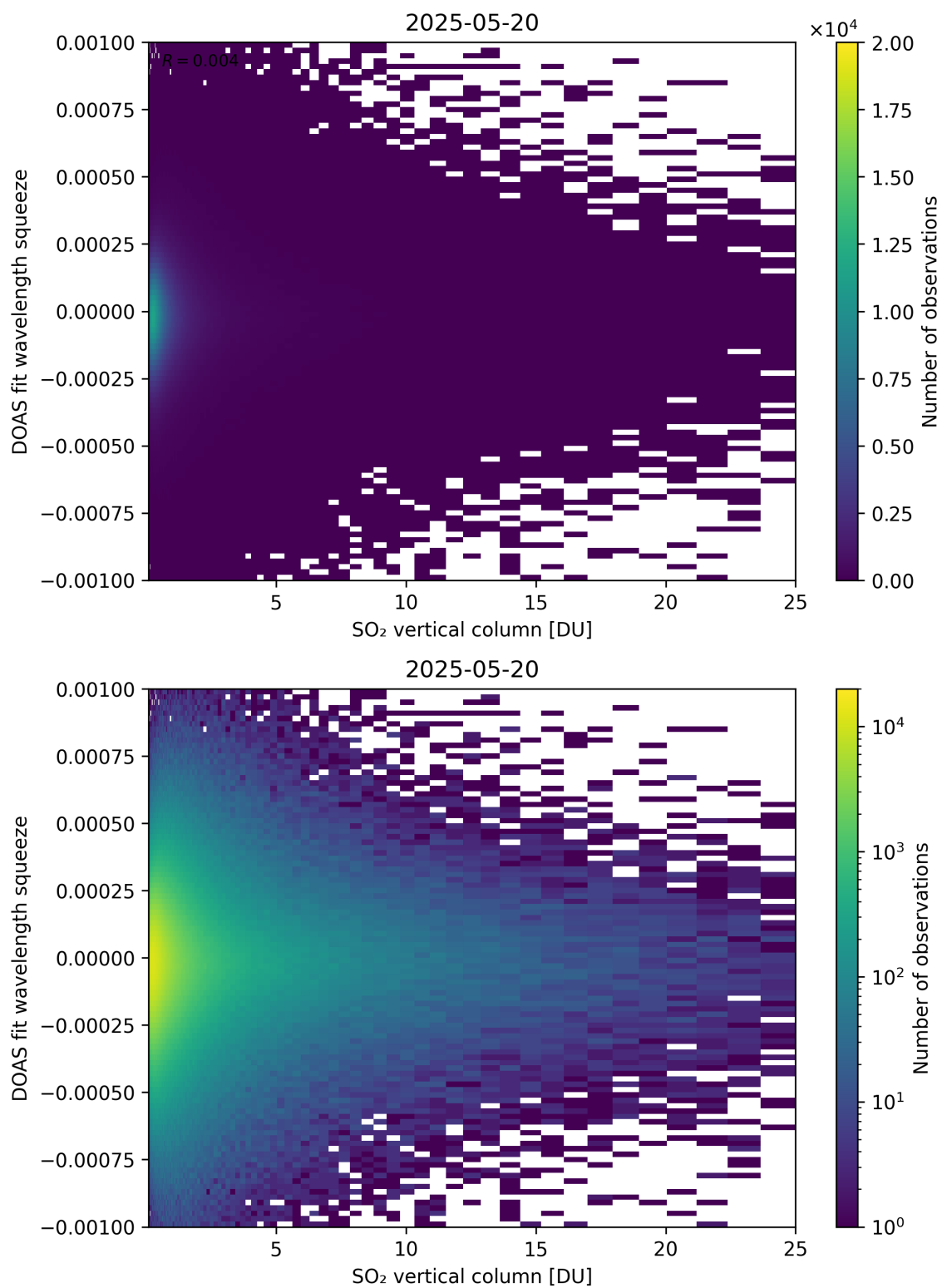
Figure 327: Scatter density plot of “SO 2 vertical column” against “DOAS fit wavelength squeeze” for 2025-05-19 to 2025-05-21.
