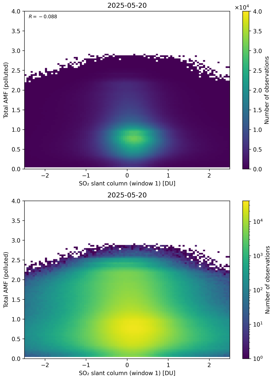
Figure 289: Scatter density plot of “SO 2 slant column (window 1)” against “Total AMF (polluted)” for 2025-05-19 to 2025-05-21.
