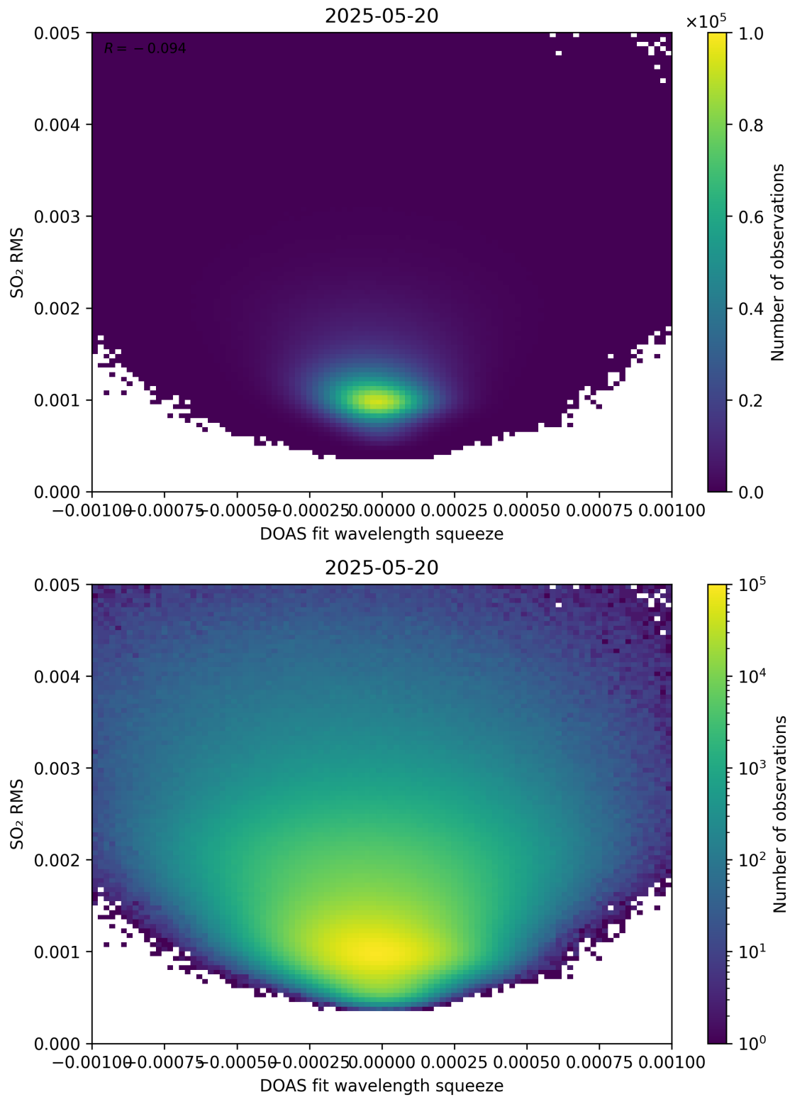
Figure 143: Scatter density plot of “DOAS fit wavelength squeeze” against “SO 2 RMS” for 2025-05-19 to 2025-05-21.
