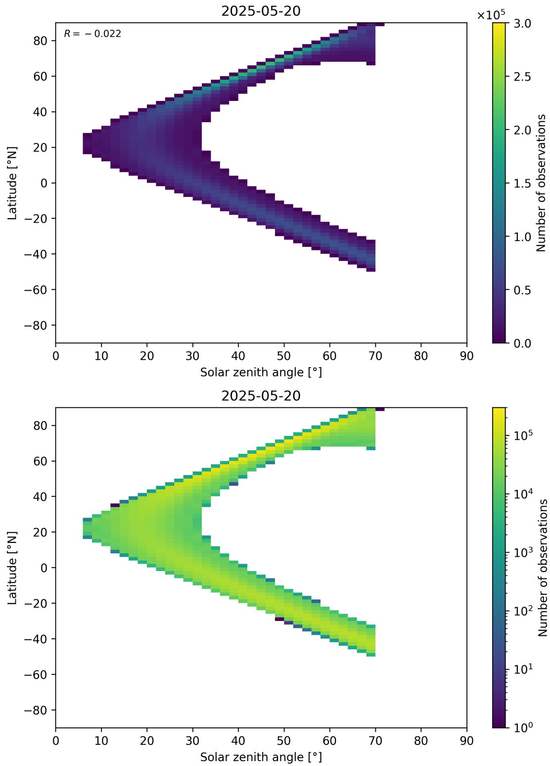
Figure 177: Scatter density plot of “Solar zenith angle” against “Latitude” for 2025-05-19 to 2025-05-21.
