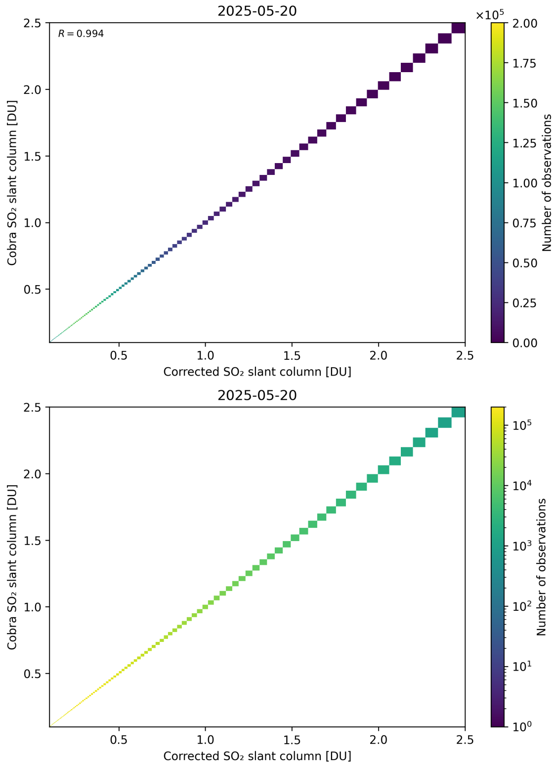
Figure 233: Scatter density plot of “Corrected SO 2 slant column” against “Cobra SO 2 slant column” for 2025-05-19 to 2025-05-21.
