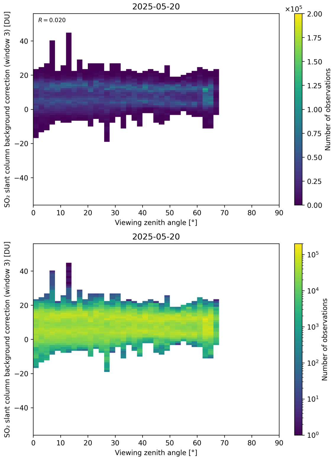
Figure 364: Scatter density plot of “Viewing zenith angle” against “SO 2 slant column background correction (window 3)” for 2025-05-19 to 2025-05-21.
