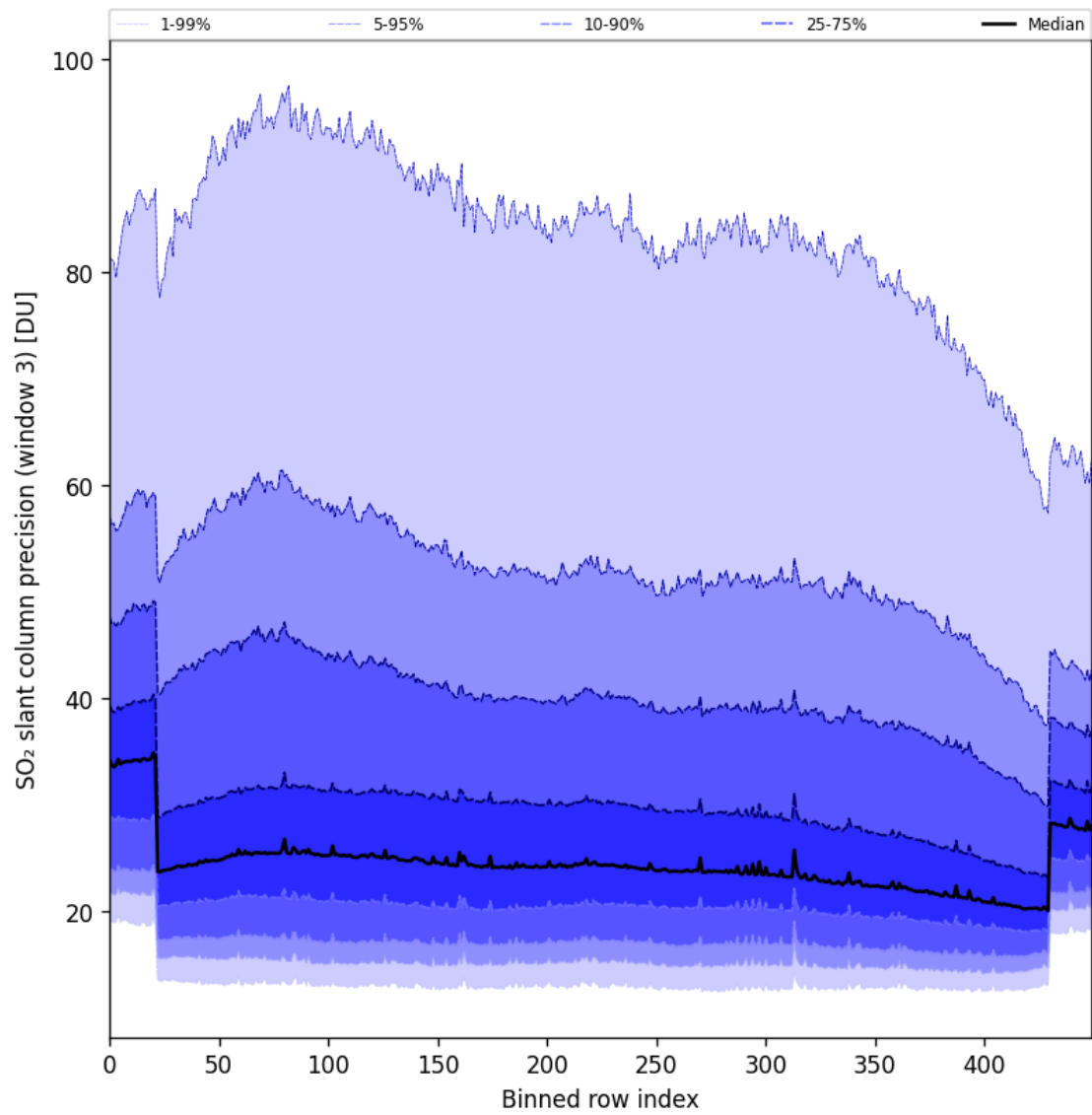
Figure 98: Along track statistics of “SO 2 slant column precision (window 3)” for 2025-05-19 to 2025-05-21
