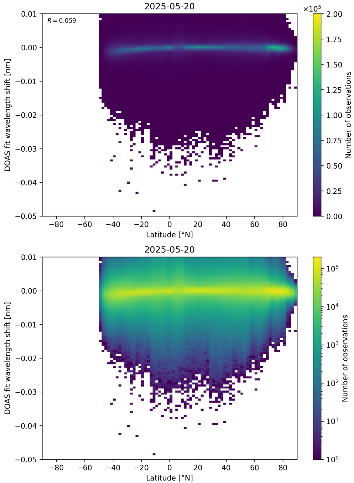
Figure 153: Scatter density plot of “Latitude” against “DOAS fit wavelength shift” for 2025-05-19 to 2025-05-21.
