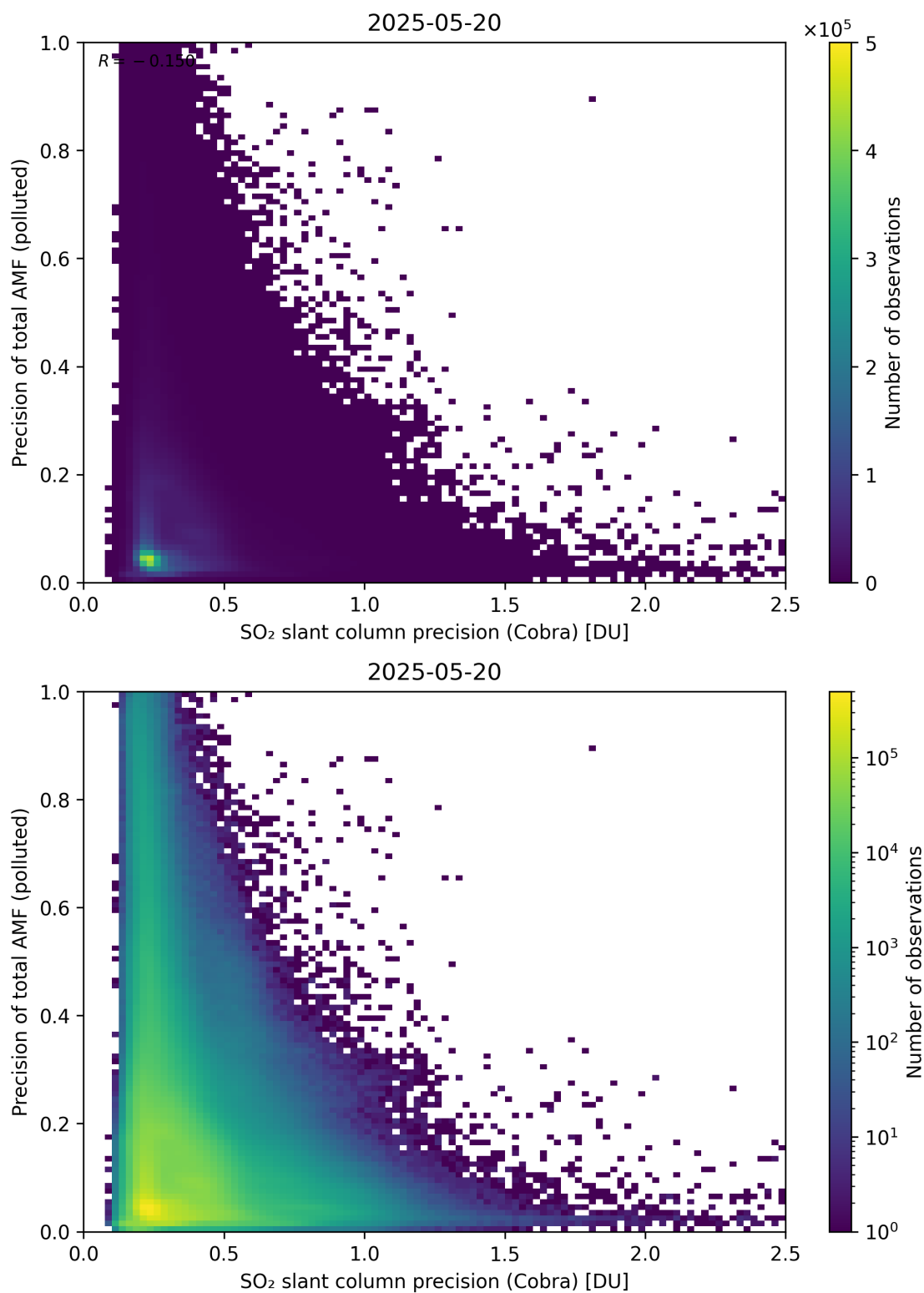
Figure 214: Scatter density plot of “SO 2 slant column precision (Cobra)” against “Precision of total AMF (polluted)” for 2025-05-19 to 2025-05-21.
