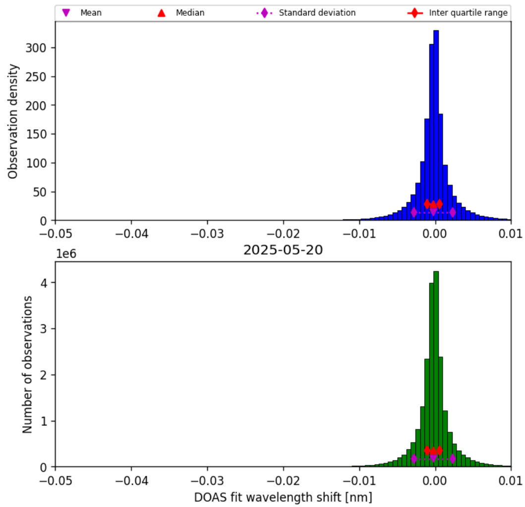
Figure 76: Histogram of “DOAS fit wavelength shift” for 2025-05-19 to 2025-05-21
