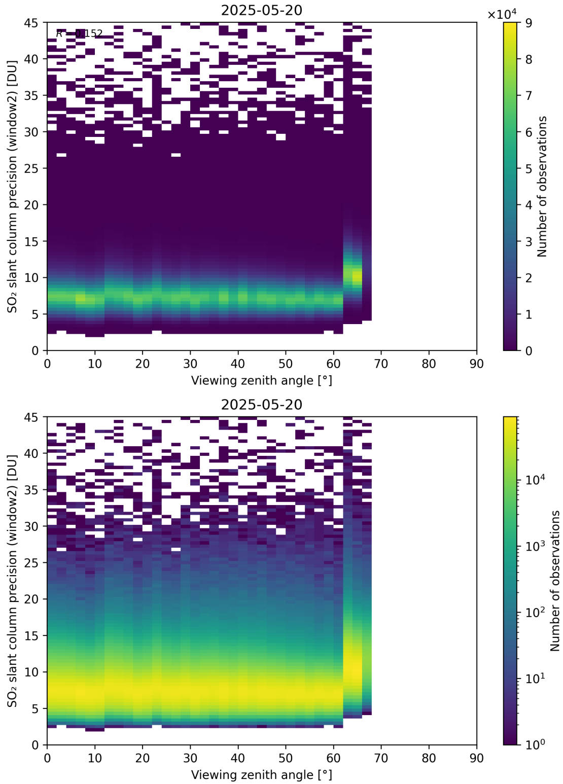
Figure 378: Scatter density plot of “Viewing zenith angle” against “SO 2 slant column precision (window2)” for 2025-05-19 to 2025-05-21.
