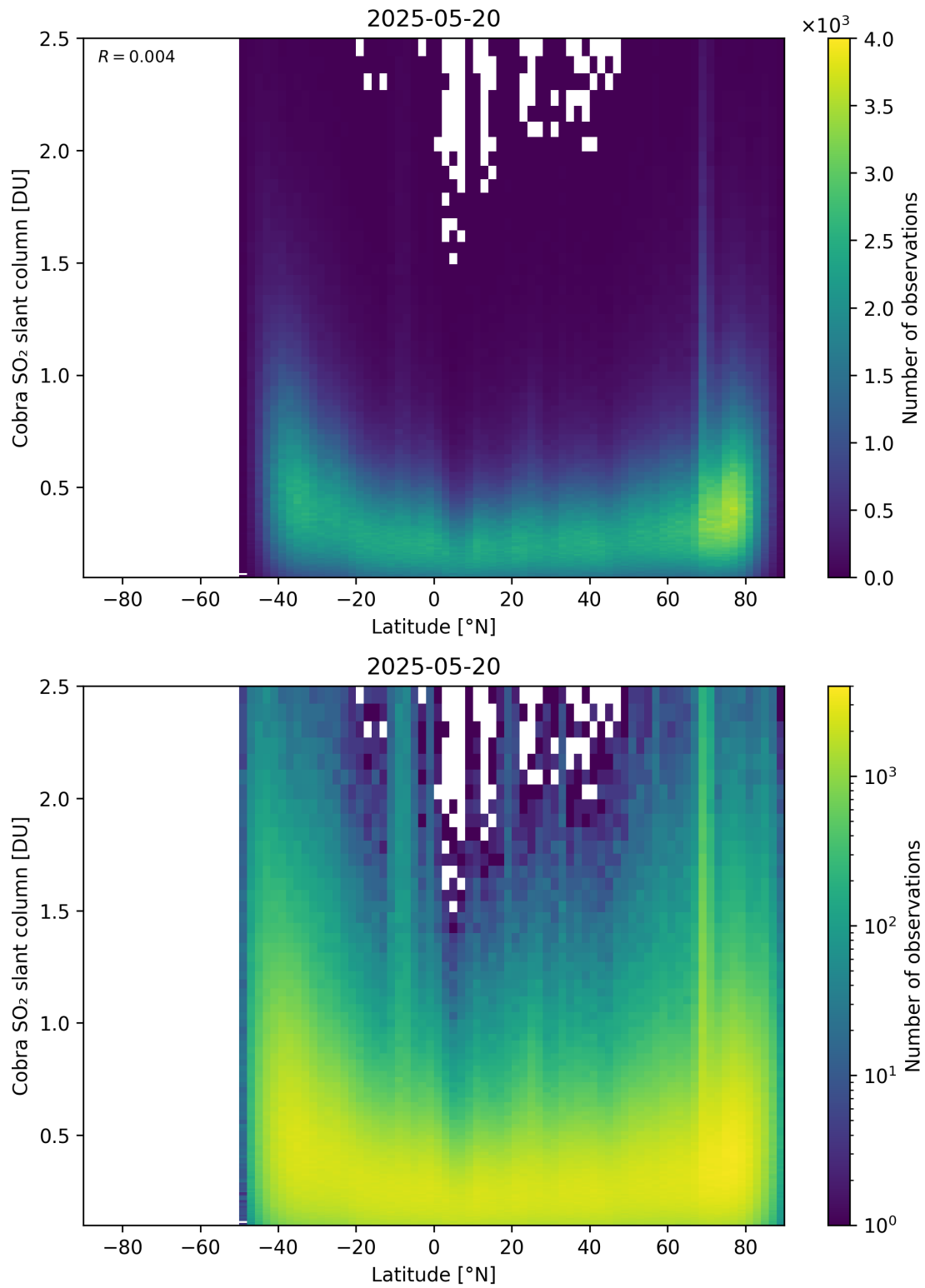
Figure 157: Scatter density plot of “Latitude” against “Cobra SO 2 slant column” for 2025-05-19 to 2025-05-21.
