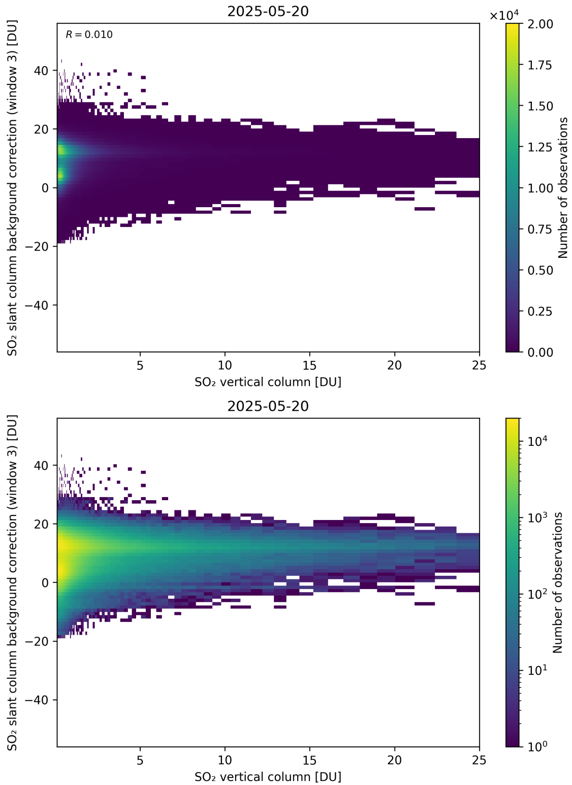
Figure 325: Scatter density plot of “SO 2 vertical column” against “SO 2 slant column background correction (window 3)” for 2025-05-19 to 2025-05-21.
