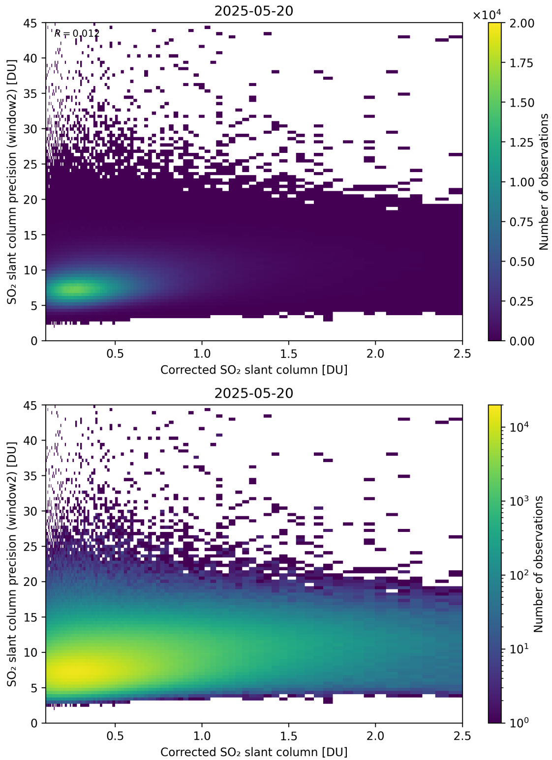
Figure 239: Scatter density plot of “Corrected SO 2 slant column” against “SO 2 slant column precision (window2)” for 2025-05-19 to 2025-05-21.
