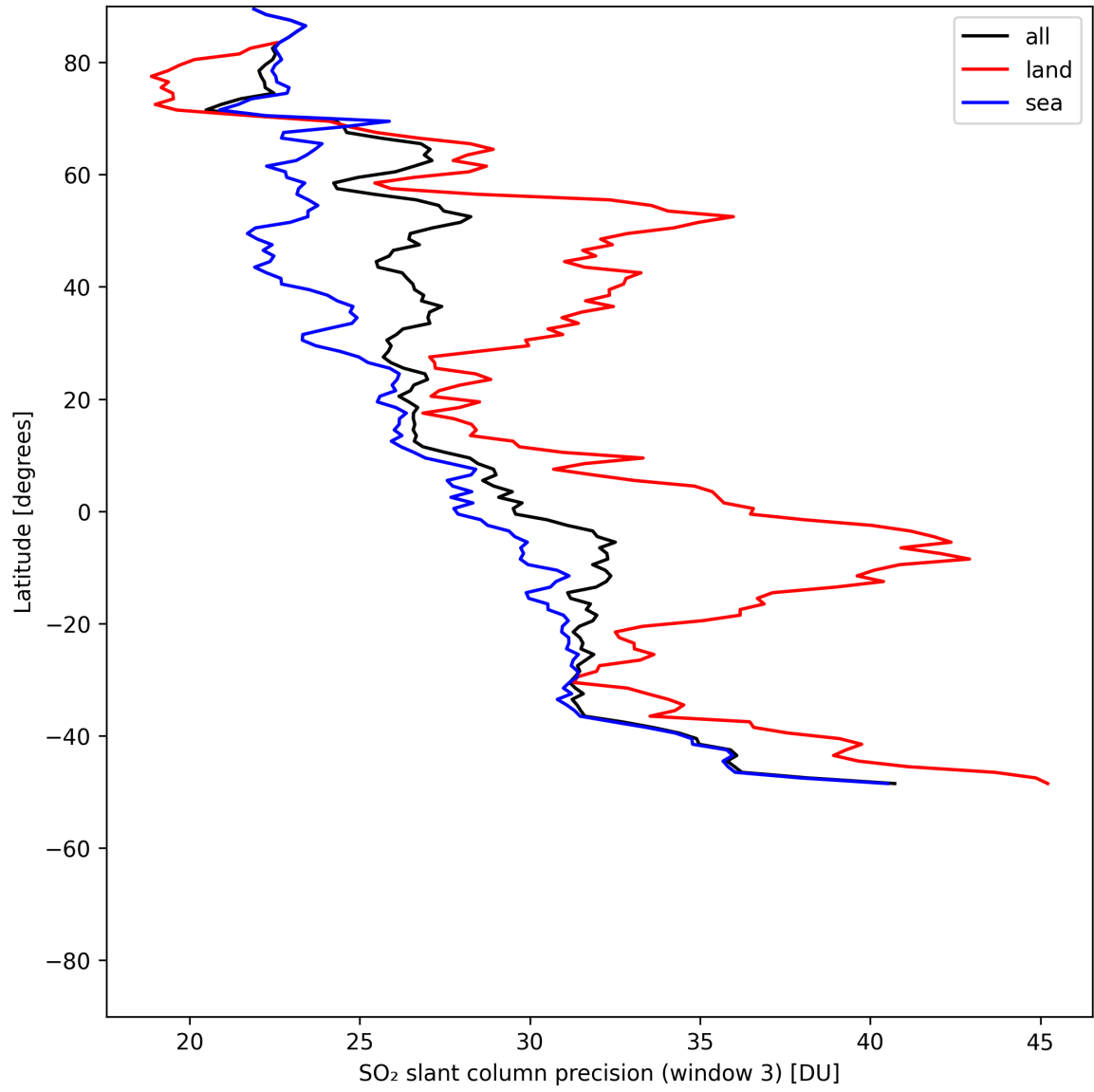
Figure 46: Zonal average of “SO 2 slant column precision (window 3)” for 2025-05-19 to 2025-05-21.
