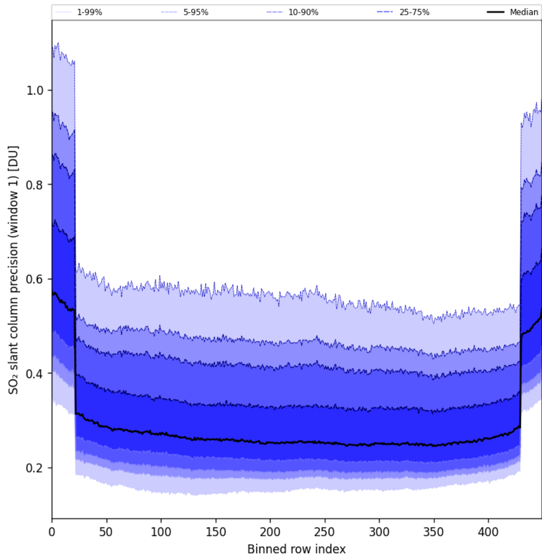
Figure 90: Along track statistics of “SO 2 slant column precision (window 1)” for 2025-05-19 to 2025-05-21
