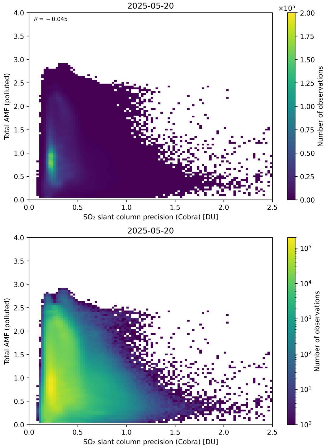
Figure 213: Scatter density plot of “SO 2 slant column precision (Cobra)” against “Total AMF (polluted)” for 2025-05-19 to 2025-05-21.
