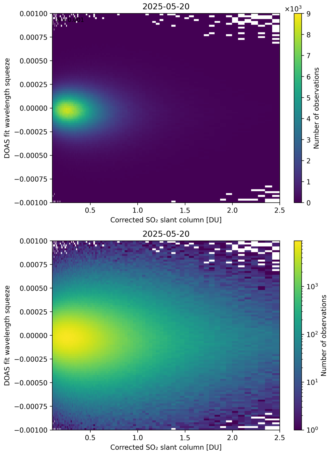
Figure 230: Scatter density plot of “Corrected SO 2 slant column” against “DOAS fit wavelength squeeze” for 2025-05-19 to 2025-05-21.
