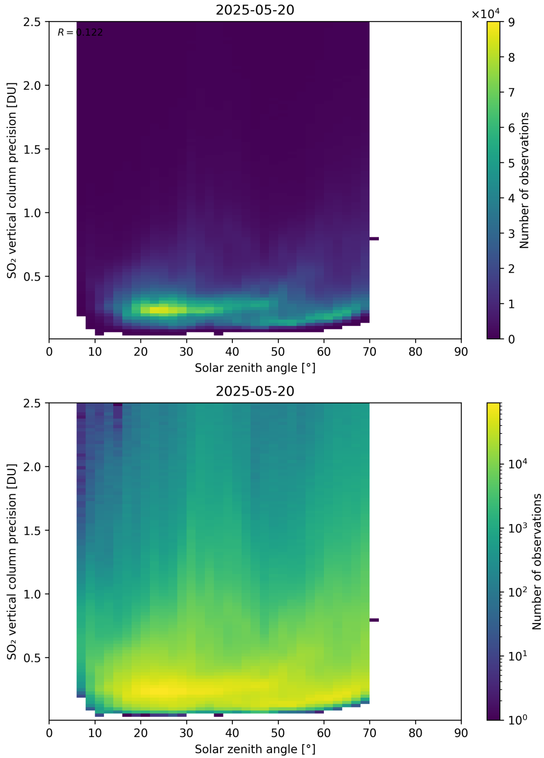
Figure 192: Scatter density plot of “Solar zenith angle” against “SO 2 vertical column precision” for 2025-05-19 to 2025-05-21.
