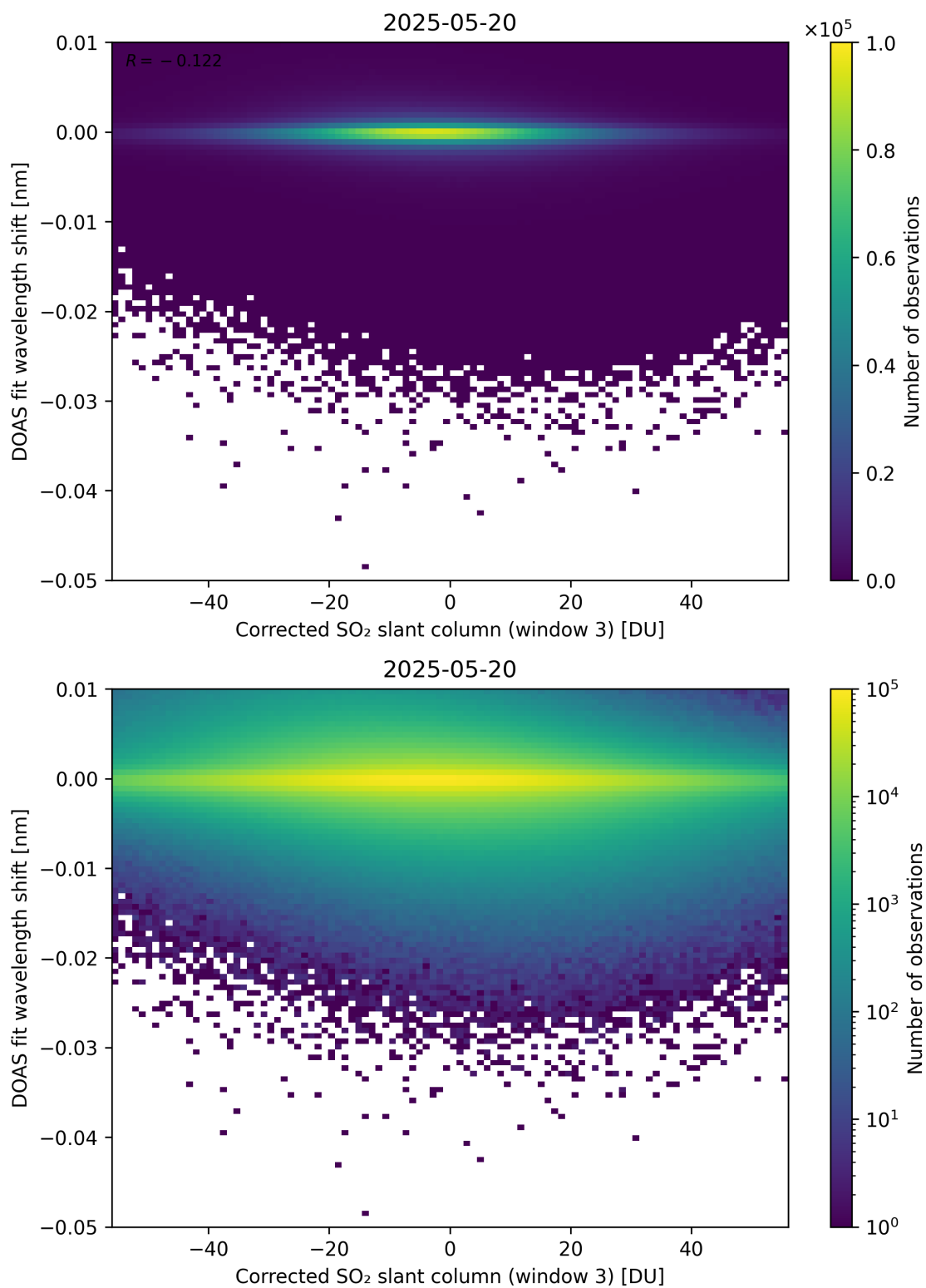
Figure 256: Scatter density plot of “Corrected SO 2 slant column (window 3)” against “DOAS fit wavelength shift” for 2025-05-19 to 2025-05-21.
