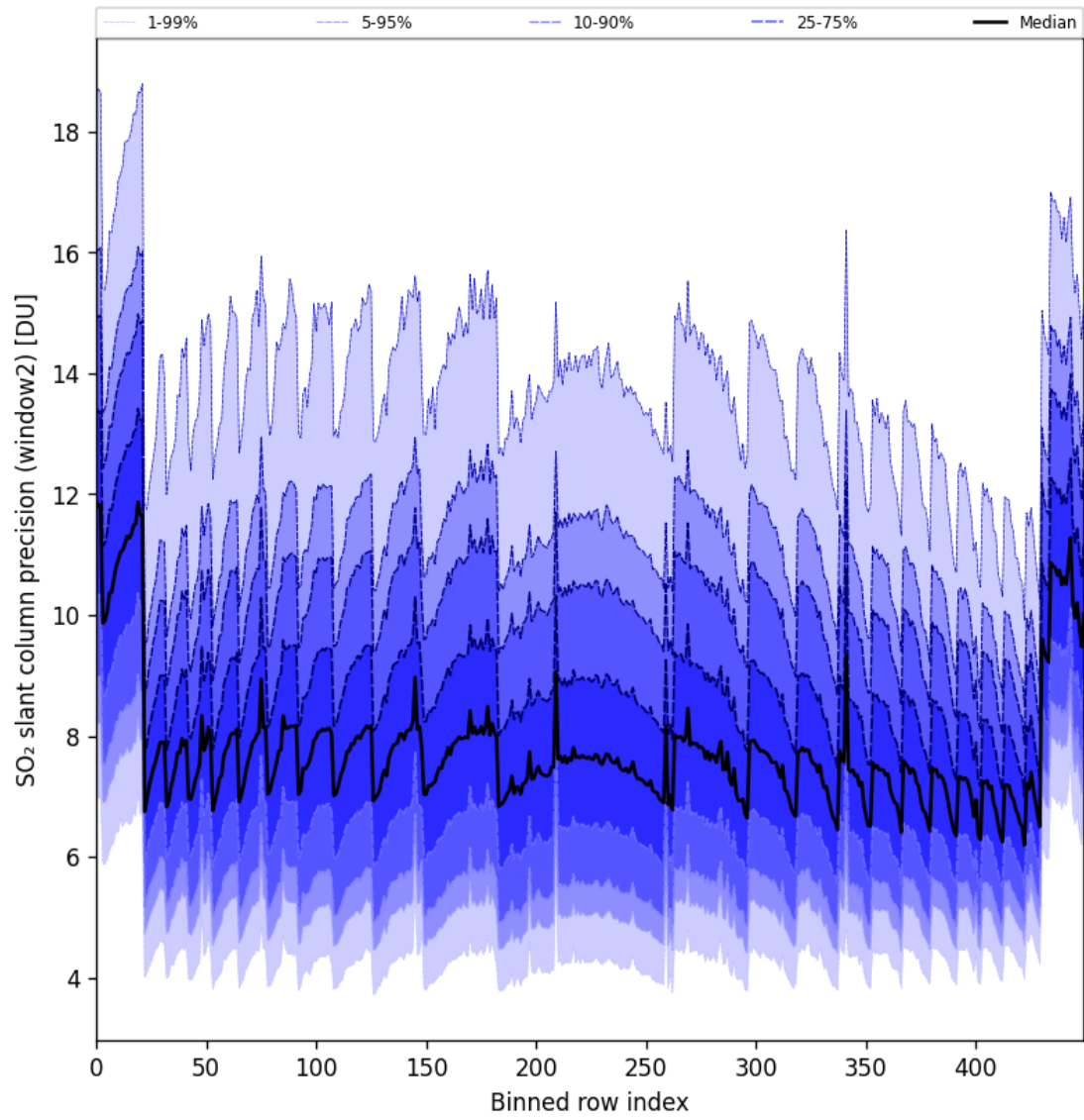
Figure 94: Along track statistics of “SO 2 slant column precision (window2)” for 2025-05-19 to 2025-05-21
