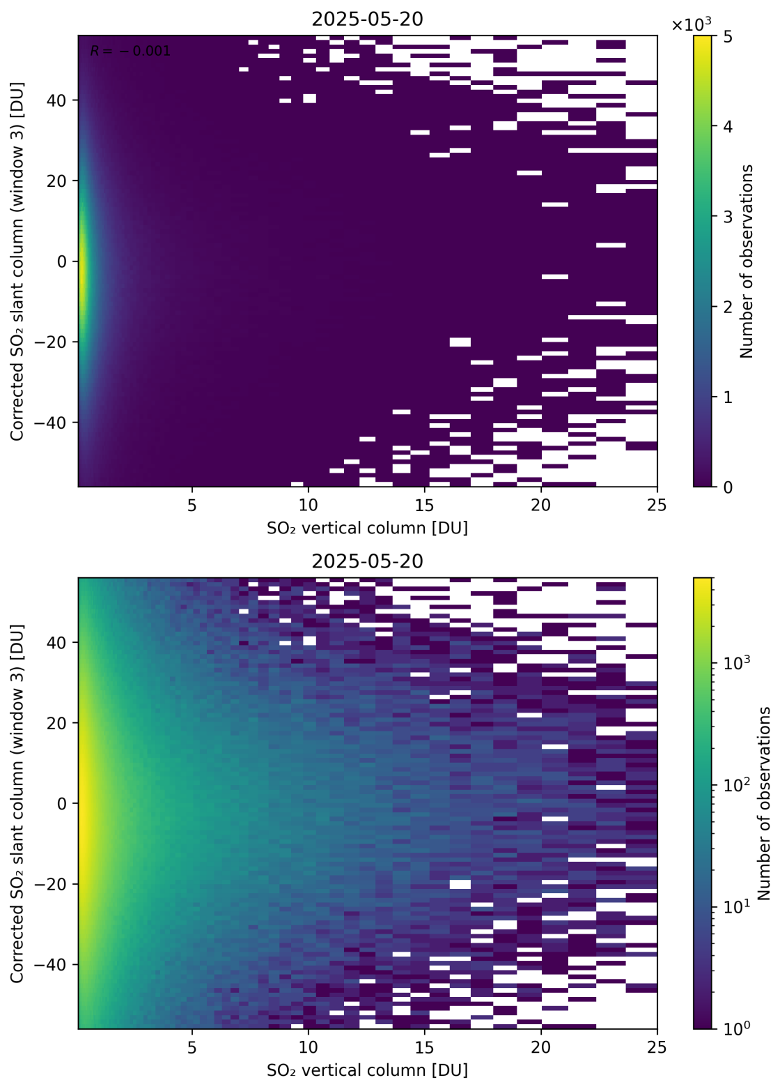
Figure 353: Scatter density plot of “SO 2 vertical column” against “Corrected SO 2 slant column (window 3)” for 2025-05-19 to 2025-05-21.
