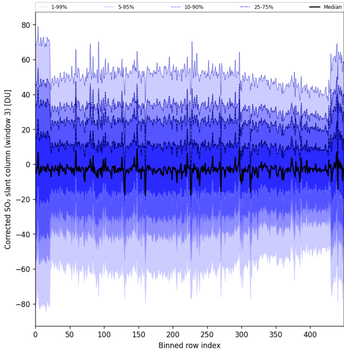
Figure 99: Along track statistics of “Corrected SO 2 slant column (window 3)” for 2025-05-19 to 2025-05-21
