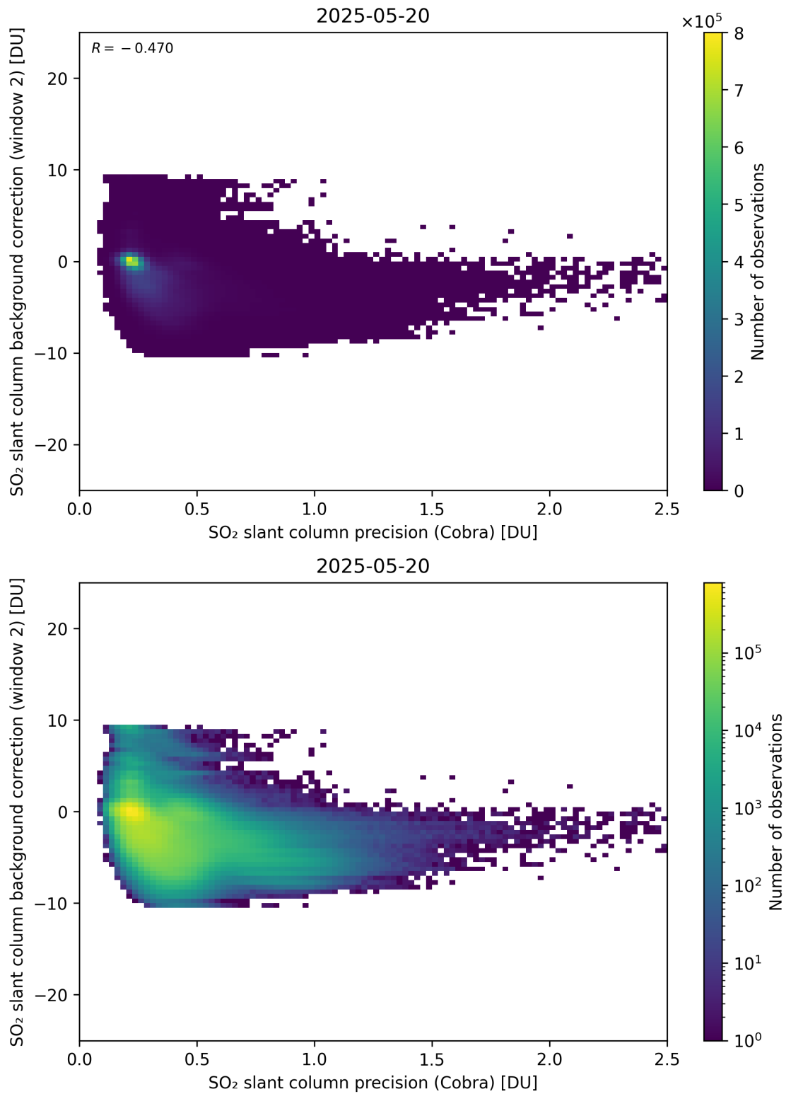
Figure 200: Scatter density plot of “SO 2 slant column precision (Cobra)” against “SO 2 slant column background correction (window 2)” for 2025-05-19 to 2025-05-21.
