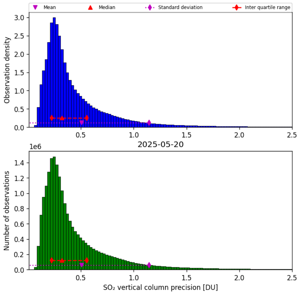
Figure 59: Histogram of “SO 2 vertical column precision” for 2025-05-19 to 2025-05-21
