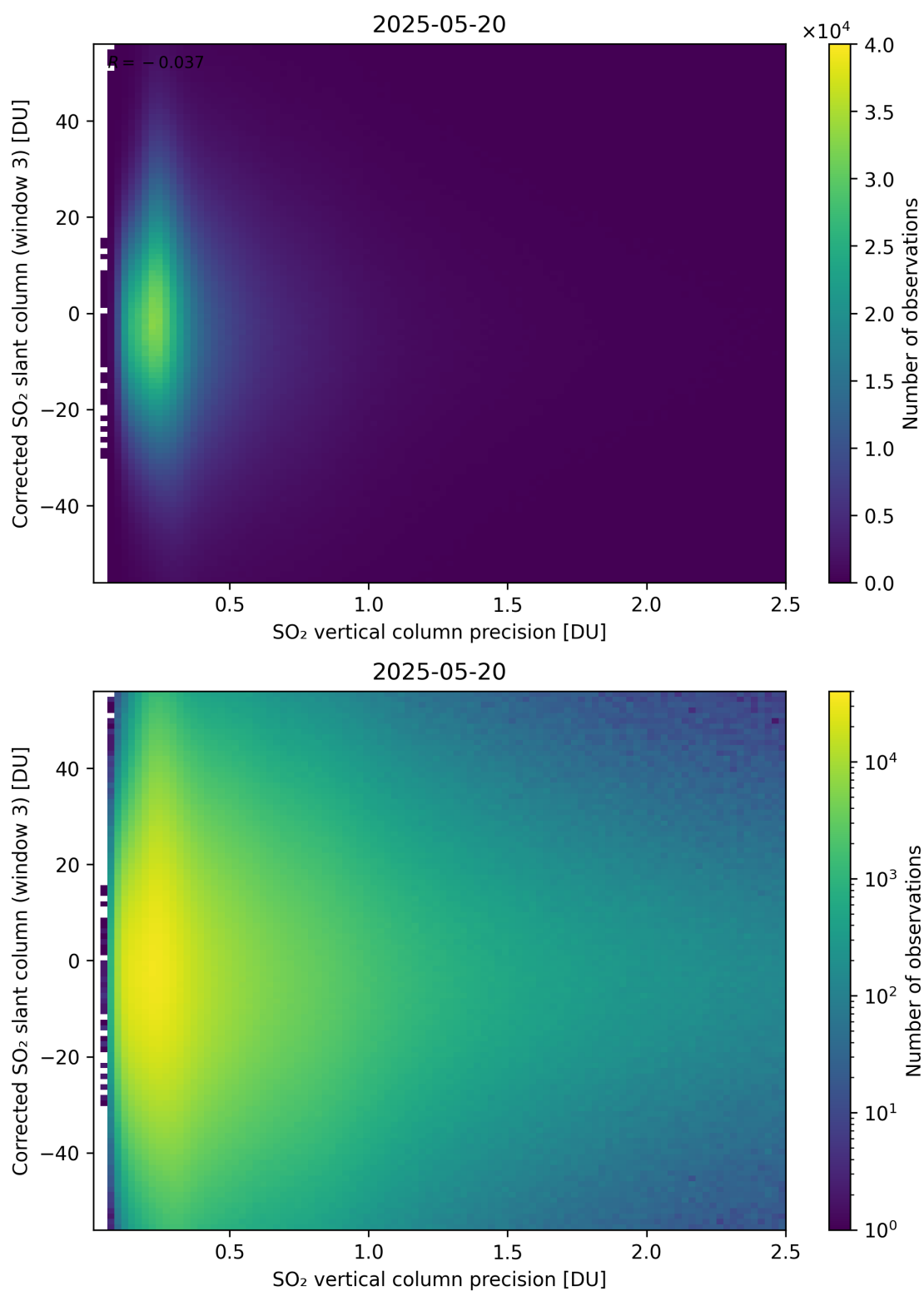
Figure 340: Scatter density plot of “SO 2 vertical column precision” against “Corrected SO 2 slant column (window 3)” for 2025-05-19 to 2025-05-21.
