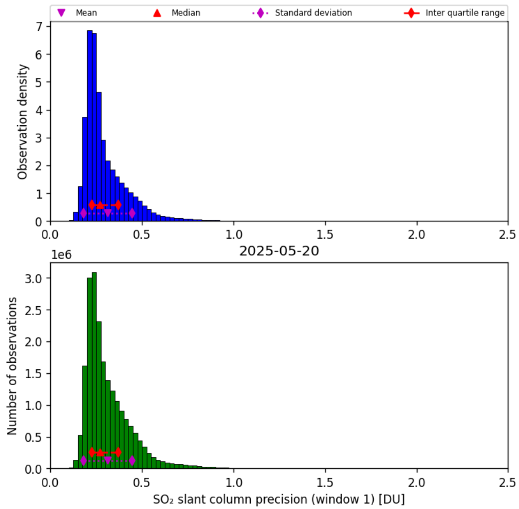
Figure 64: Histogram of “SO 2 slant column precision (window 1)” for 2025-05-19 to 2025-05-21
