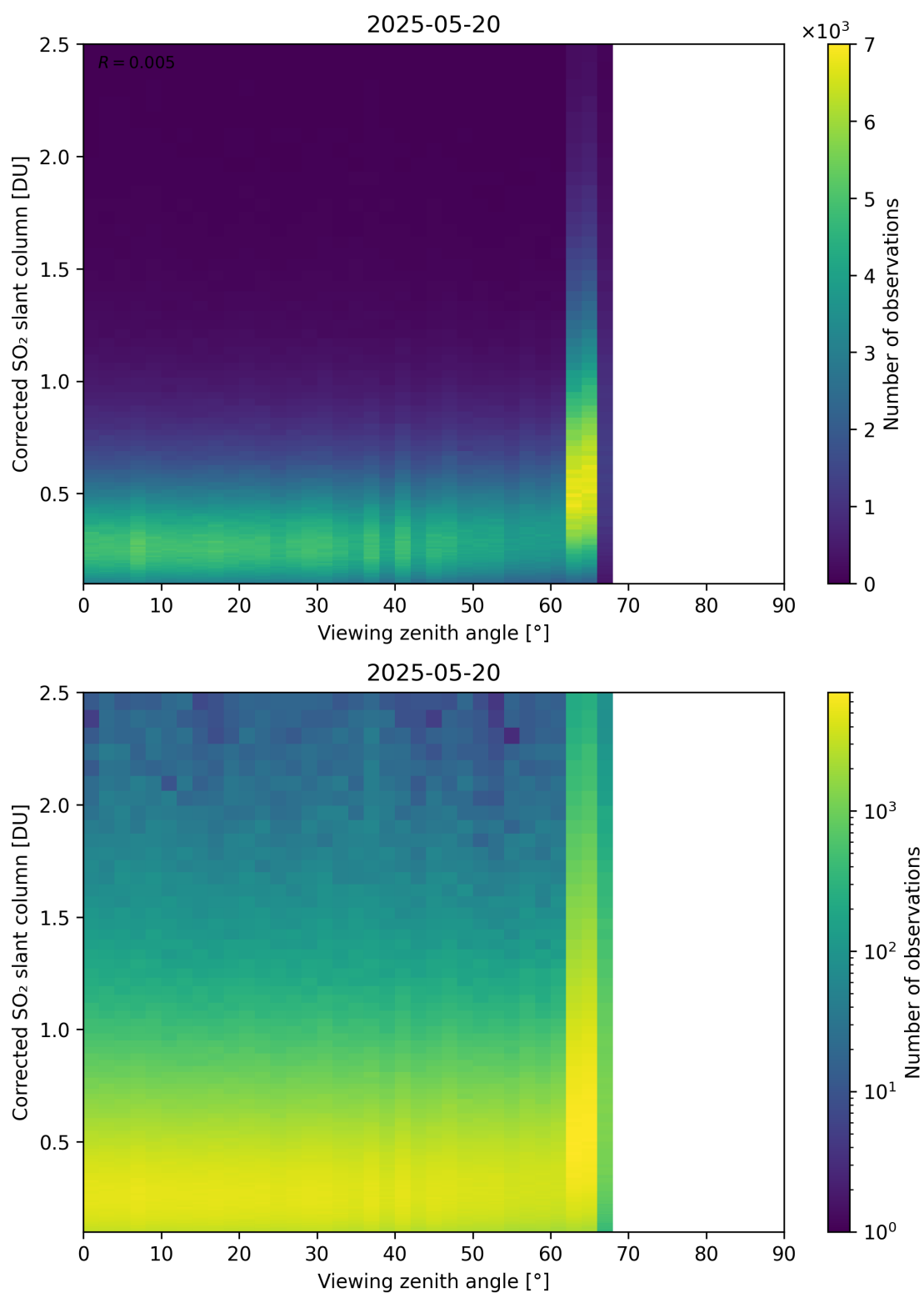
Figure 373: Scatter density plot of “Viewing zenith angle” against “Corrected SO 2 slant column” for 2025-05-19 to 2025-05-21.
