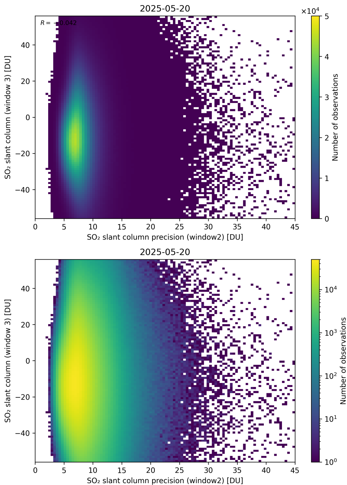
Figure 299: Scatter density plot of “SO 2 slant column precision (window2)” against “SO 2 slant column (window 3)” for 2025-05-19 to 2025-05-21.
