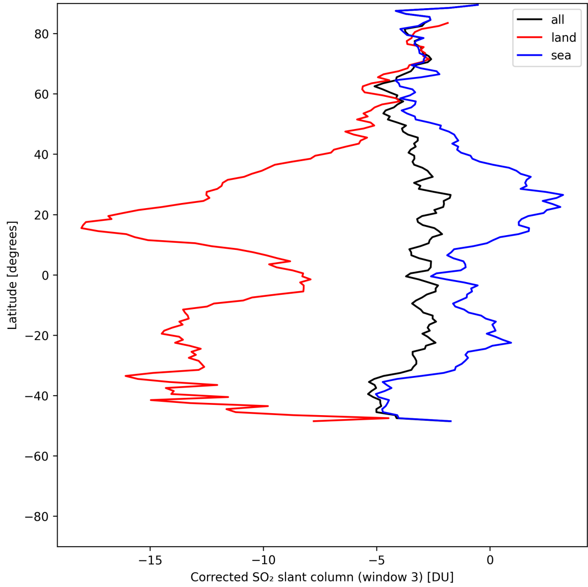
Figure 47: Zonal average of “Corrected SO 2 slant column (window 3)” for 2025-05-19 to 2025-05-21.
