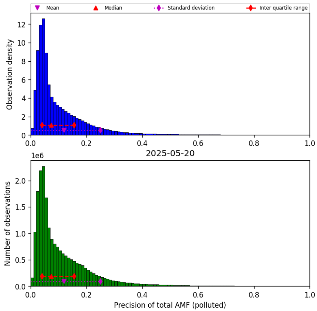
Figure 80: Histogram of “Precision of total AMF (polluted)” for 2025-05-19 to 2025-05-21
