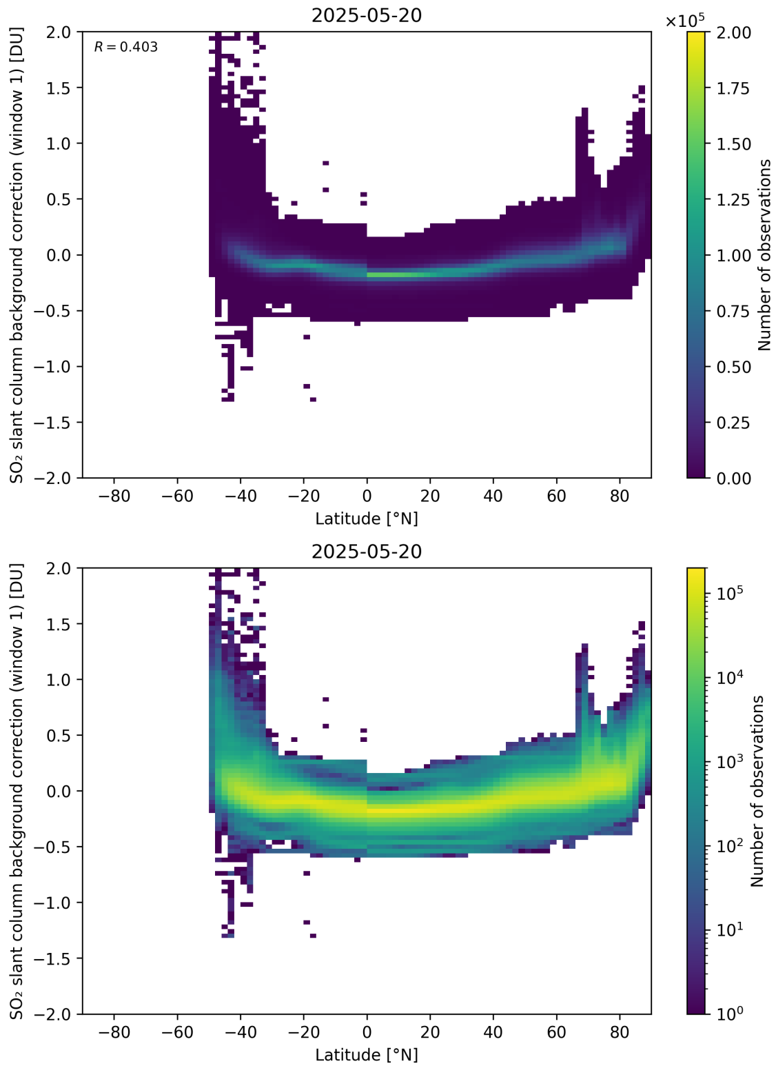
Figure 150: Scatter density plot of “Latitude” against “SO 2 slant column background correction (window 1)” for 2025-05-19 to 2025-05-21.
