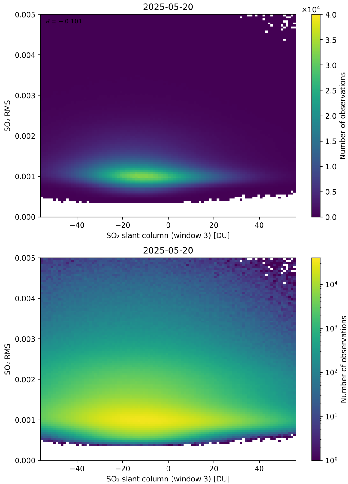
Figure 306: Scatter density plot of “SO 2 slant column (window 3)” against “SO 2 RMS” for 2025-05-19 to 2025-05-21.
