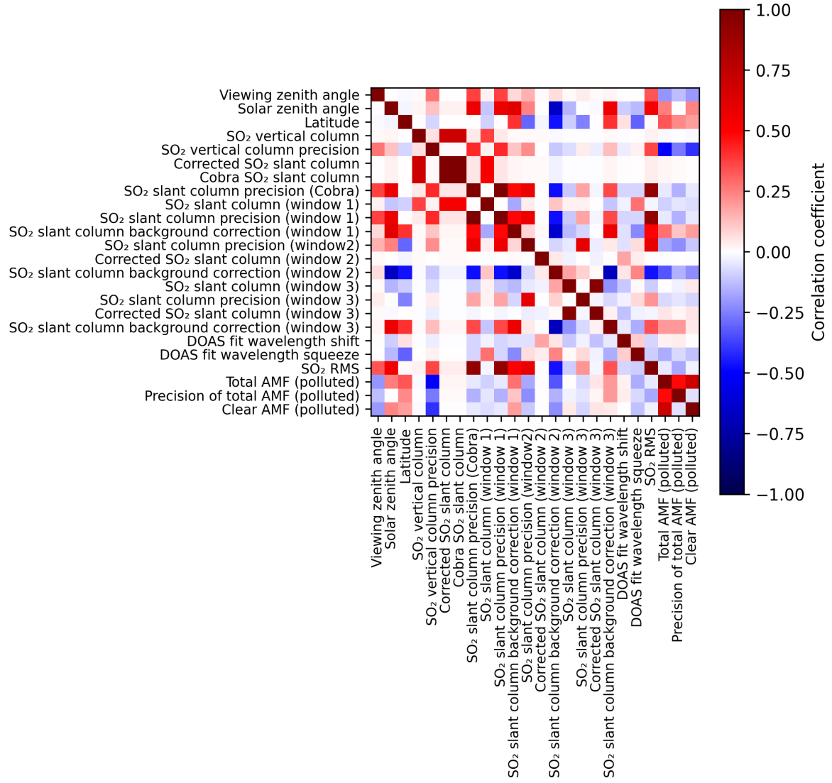
Figure 2: Map of correlation matrix for 2025-05-19 to 2025-05-21.
