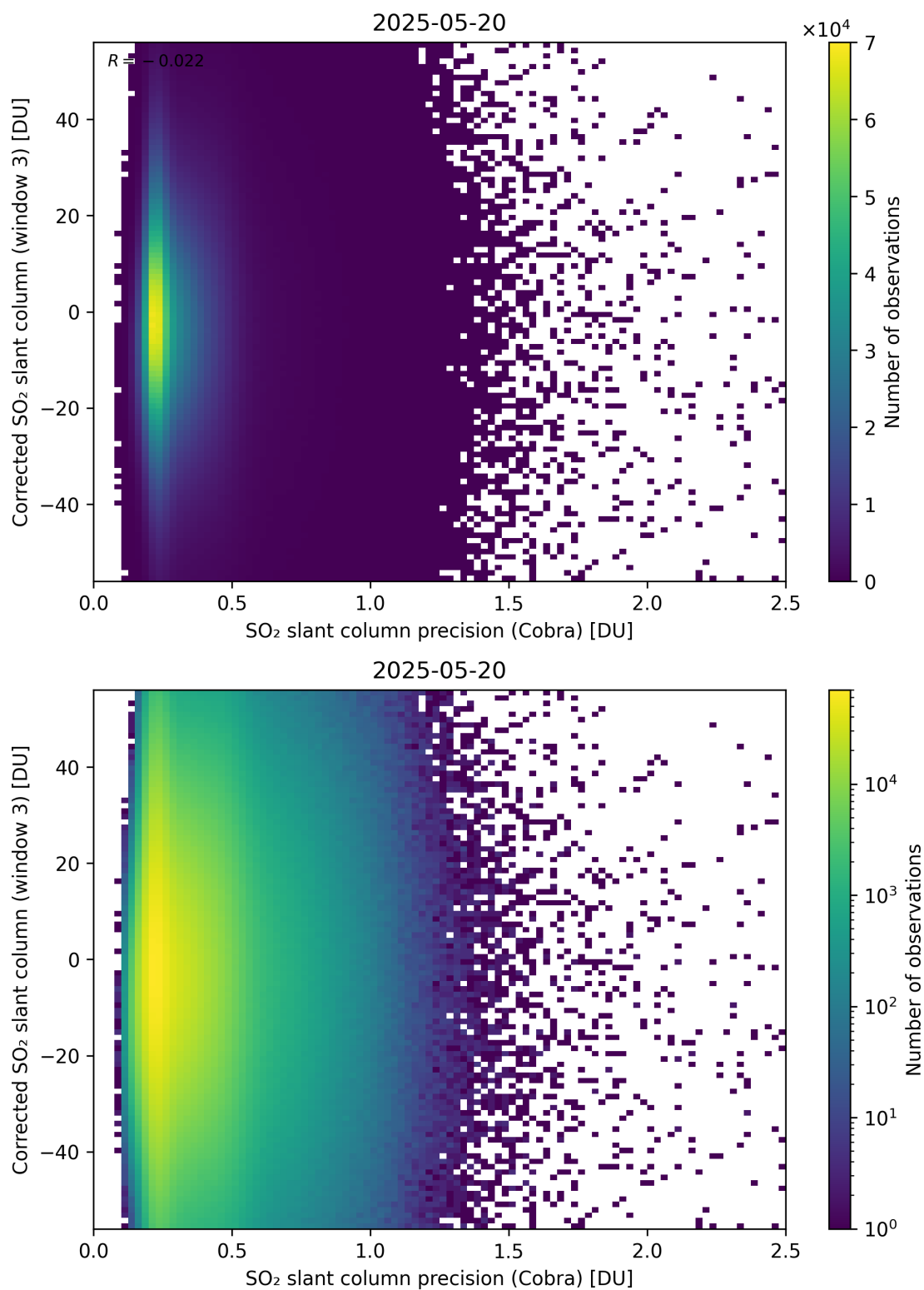
Figure 207: Scatter density plot of “SO 2 slant column precision (Cobra)” against “Corrected SO 2 slant column (window 3)” for 2025-05-19 to 2025-05-21.
