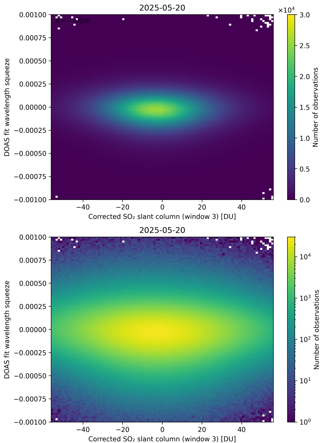
Figure 257: Scatter density plot of “Corrected SO 2 slant column (window 3)” against “DOAS fit wavelength squeeze” for 2025-05-19 to 2025-05-21.
