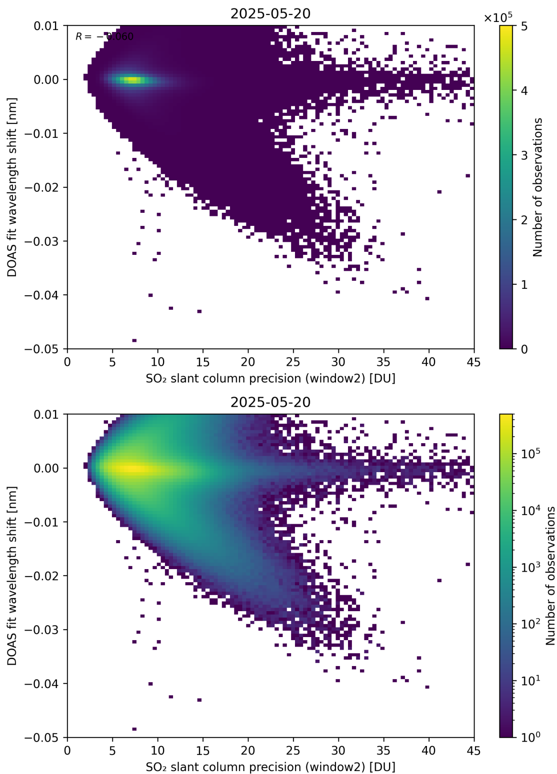
Figure 293: Scatter density plot of “SO 2 slant column precision (window2)” against “DOAS fit wavelength shift” for 2025-05-19 to 2025-05-21.
