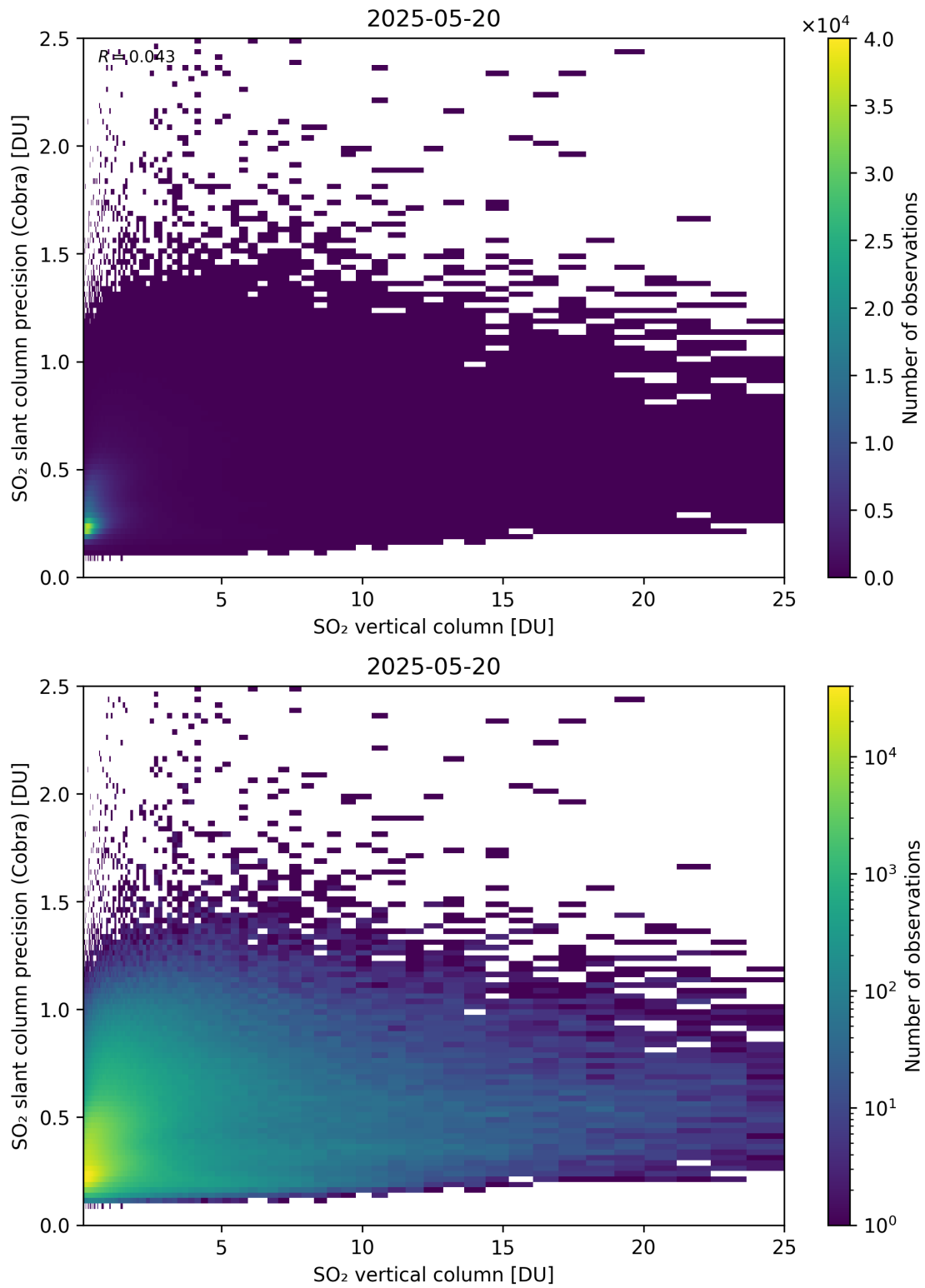
Figure 350: Scatter density plot of “SO 2 vertical column” against “SO 2 slant column precision (Cobra)” for 2025-05-19 to 2025-05-21.
