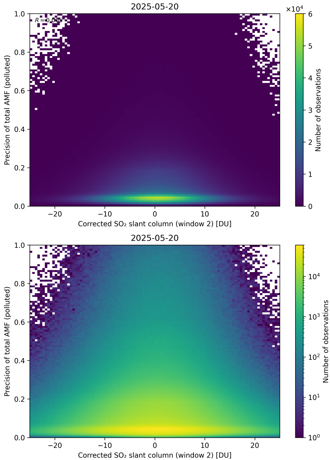
Figure 254: Scatter density plot of “Corrected SO 2 slant column (window 2)” against “Precision of total AMF (polluted)” for 2025-05-19 to 2025-05-21.
