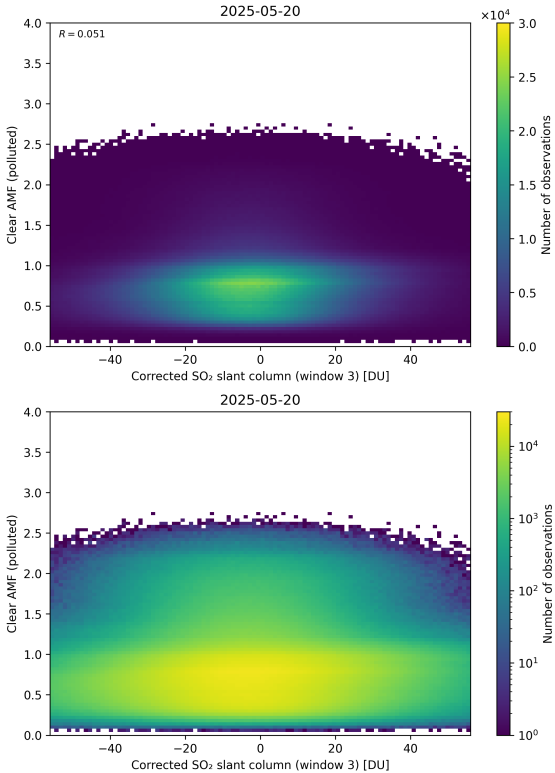
Figure 259: Scatter density plot of “Corrected SO 2 slant column (window 3)” against “Clear AMF (polluted)” for 2025-05-19 to 2025-05-21.
