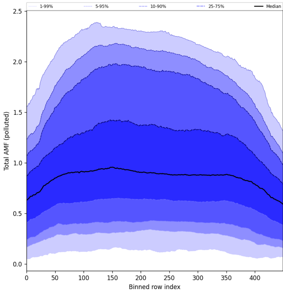
Figure 105: Along track statistics of “Total AMF (polluted)” for 2025-05-19 to 2025-05-21
