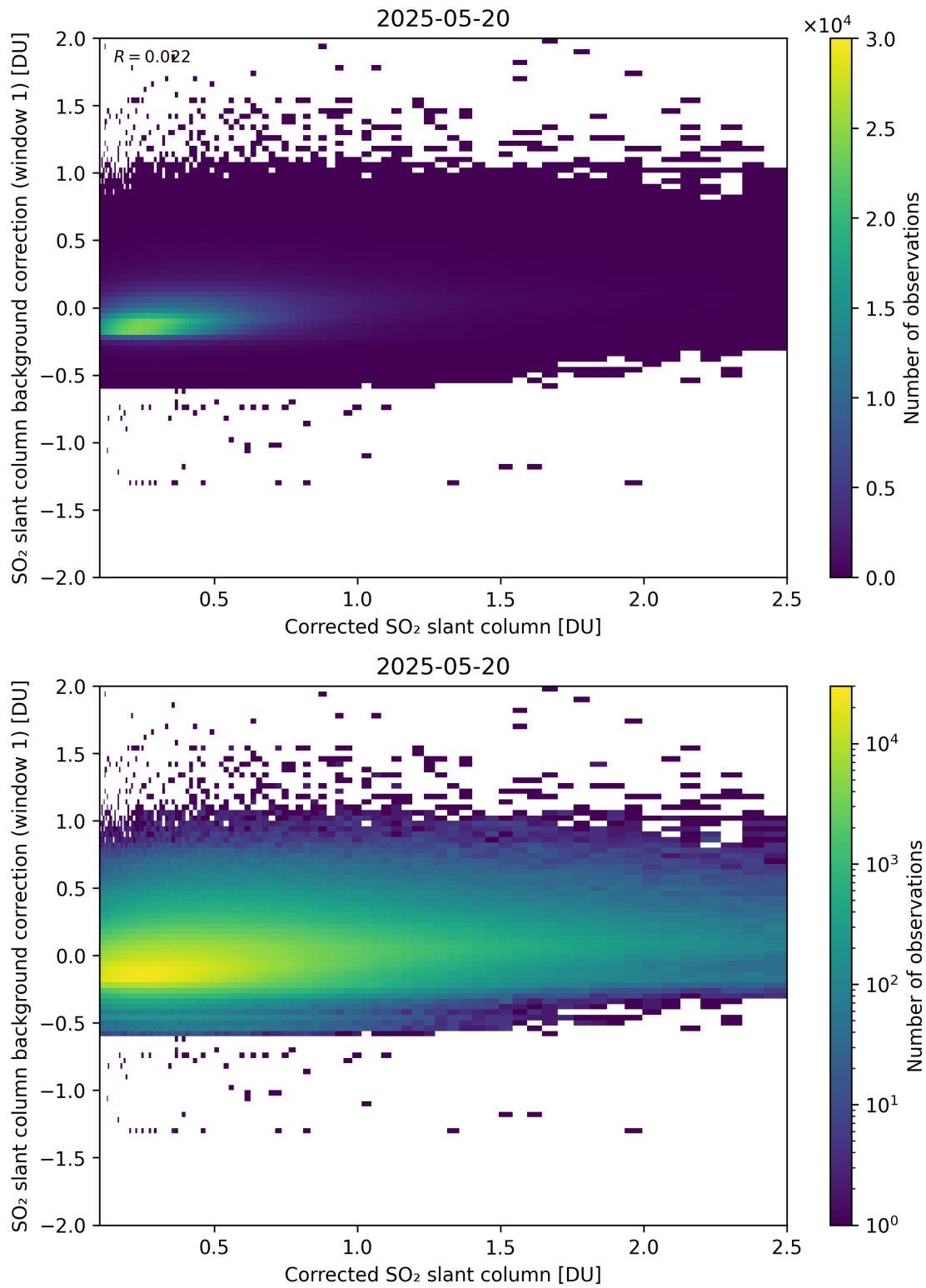
Figure 226: Scatter density plot of “Corrected SO 2 slant column” against “SO 2 slant column background correction (window 1)” for 2025-05-19 to 2025-05-21.
