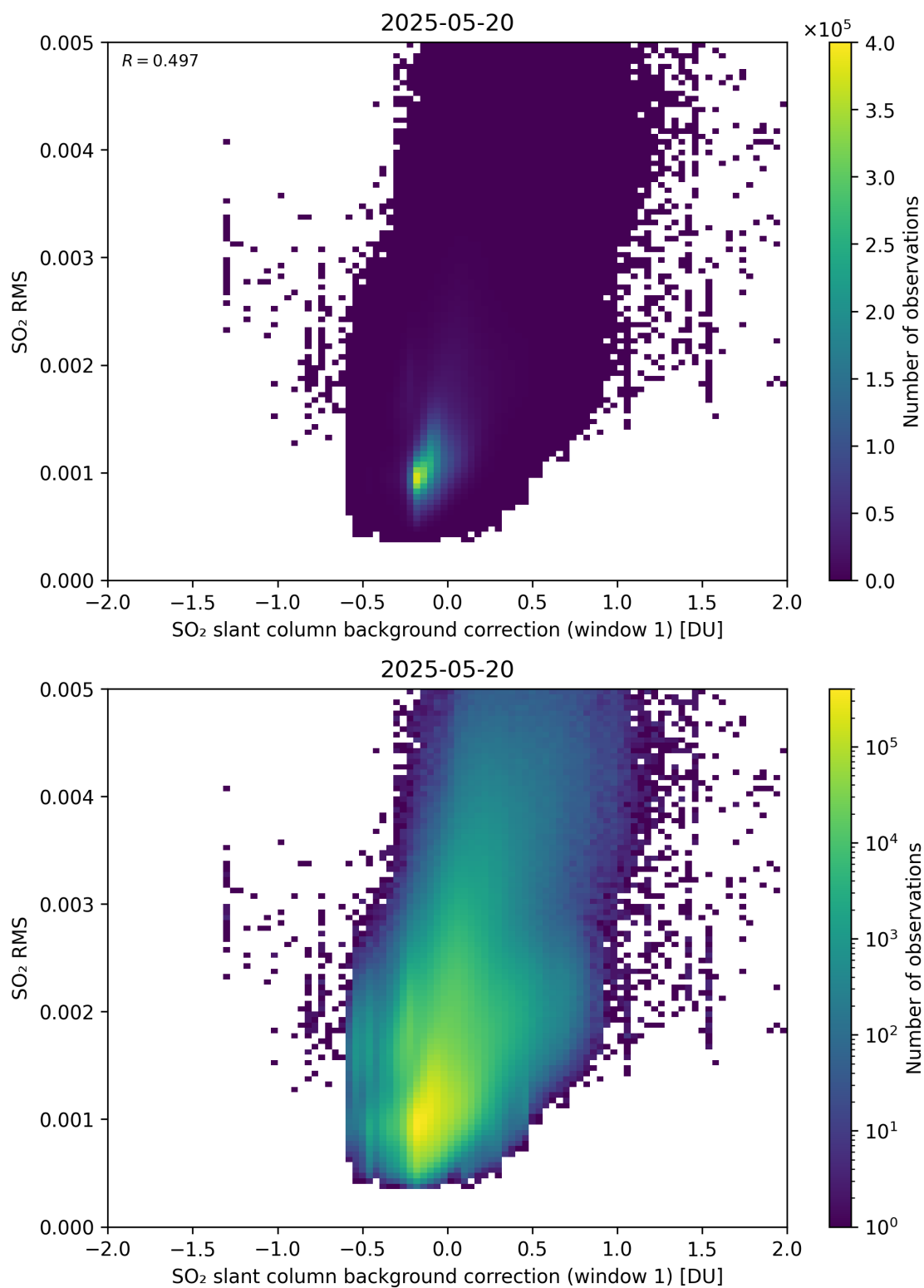
Figure 113: Scatter density plot of “SO 2 slant column background correction (window 1)” against “SO 2 RMS” for 2025-05-19 to 2025-05-21.
