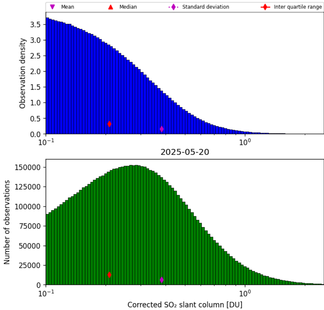
Figure 60: Histogram of "Corrected SO 2 slant column" for 2025-05-19 to 2025-05-21
