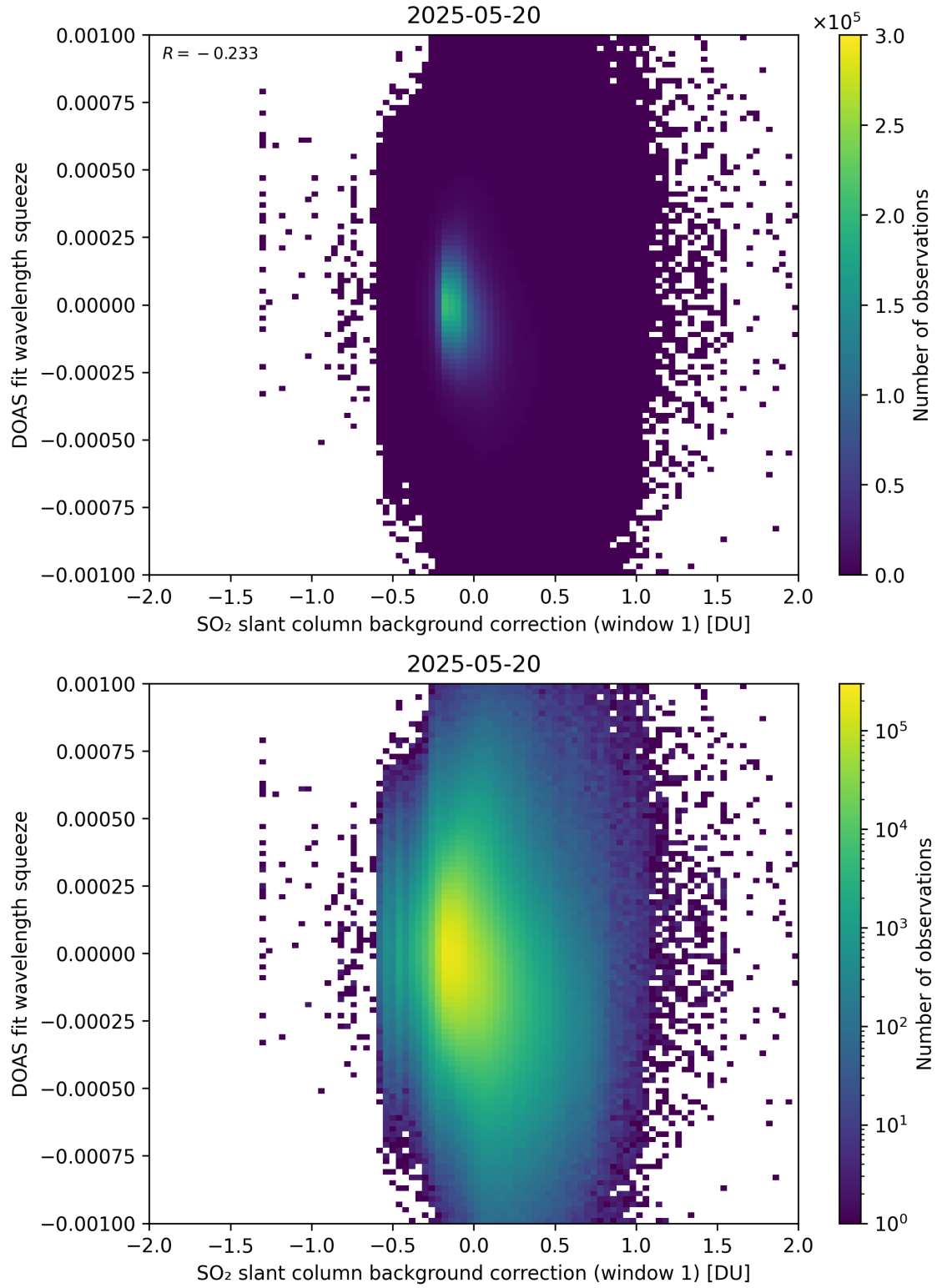
Figure 112: Scatter density plot of “SO 2 slant column background correction (window 1)” against “DOAS fit wavelength squeeze” for 2025-05-19 to 2025-05-21.
