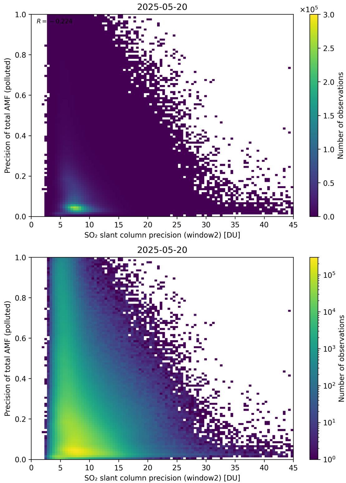
Figure 302: Scatter density plot of “SO 2 slant column precision (window2)” against “Precision of total AMF (polluted)” for 2025-05-19 to 2025-05-21.
