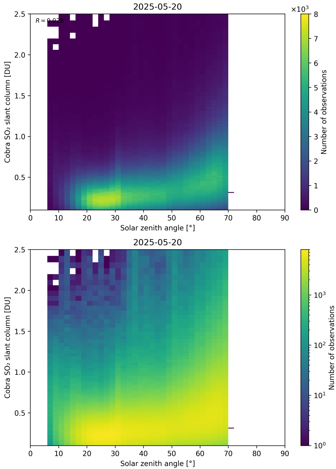
Figure 179: Scatter density plot of “Solar zenith angle” against “Cobra SO 2 slant column” for 2025-05-19 to 2025-05-21.
