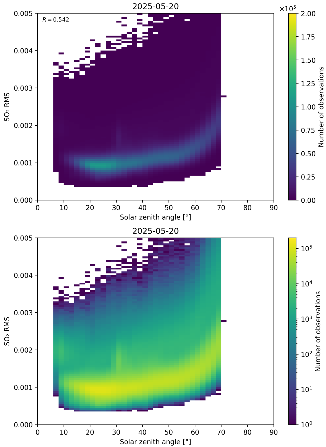
Figure 176: Scatter density plot of “Solar zenith angle” against “SO 2 RMS” for 2025-05-19 to 2025-05-21.
