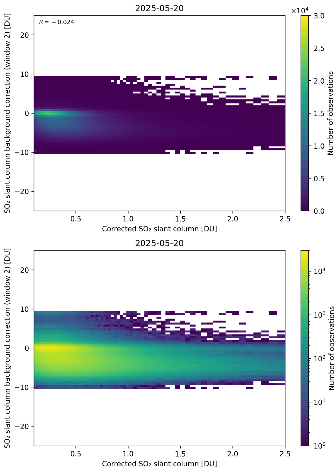
Figure 227: Scatter density plot of “Corrected SO 2 slant column” against “SO 2 slant column background correction (window 2)” for 2025-05-19 to 2025-05-21.
