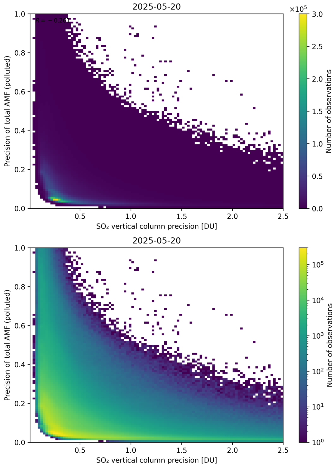
Figure 347: Scatter density plot of “SO 2 vertical column precision” against “Precision of total AMF (polluted)” for 2025-05-19 to 2025-05-21.
