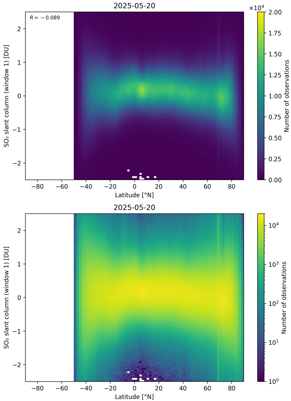
Figure 162: Scatter density plot of “Latitude” against “SO 2 slant column (window 1)” for 2025-05-19 to 2025-05-21.
