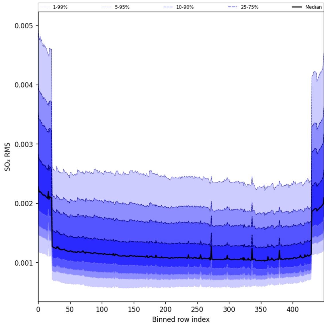
Figure 104: Along track statistics of “SO 2 RMS” for 2025-05-19 to 2025-05-21
