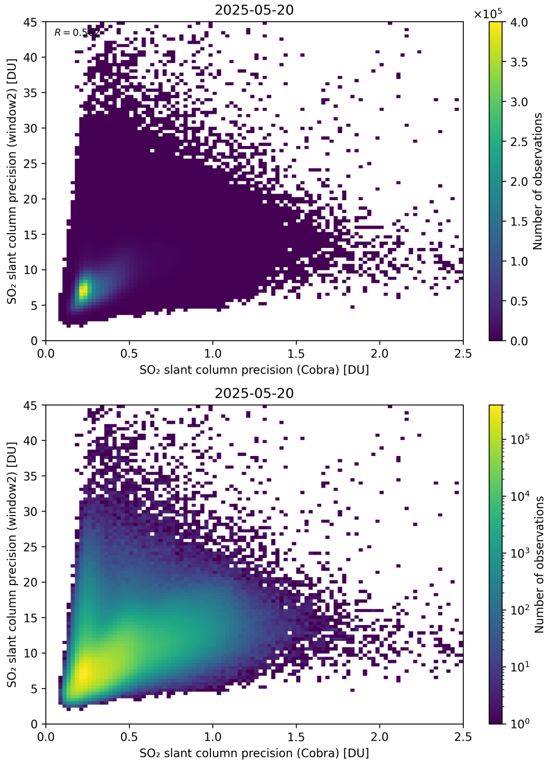
Figure 210: Scatter density plot of “SO 2 slant column precision (Cobra)” against “SO 2 slant column precision (window2)” for 2025-05-19 to 2025-05-21.
