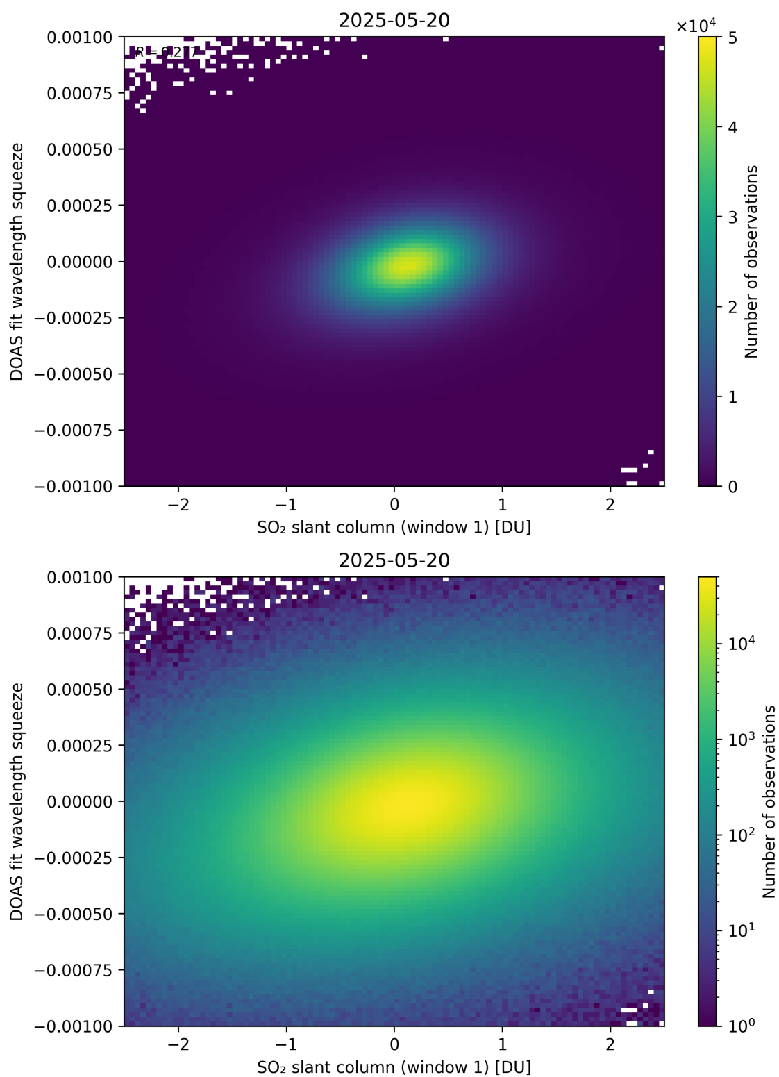
Figure 266: Scatter density plot of “SO 2 slant column (window 1)” against “DOAS fit wavelength squeeze” for 2025-05-19 to 2025-05-21.
