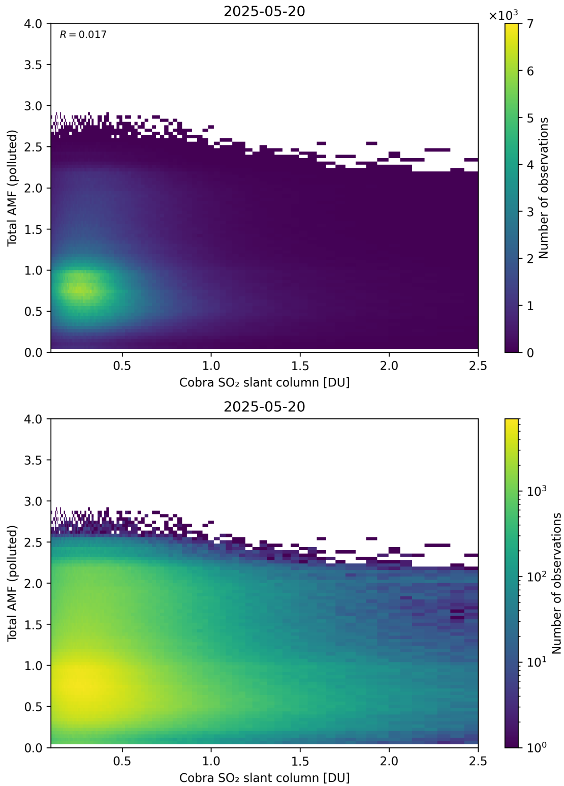
Figure 224: Scatter density plot of “Cobra SO 2 slant column” against “Total AMF (polluted)” for 2025-05-19 to 2025-05-21.
