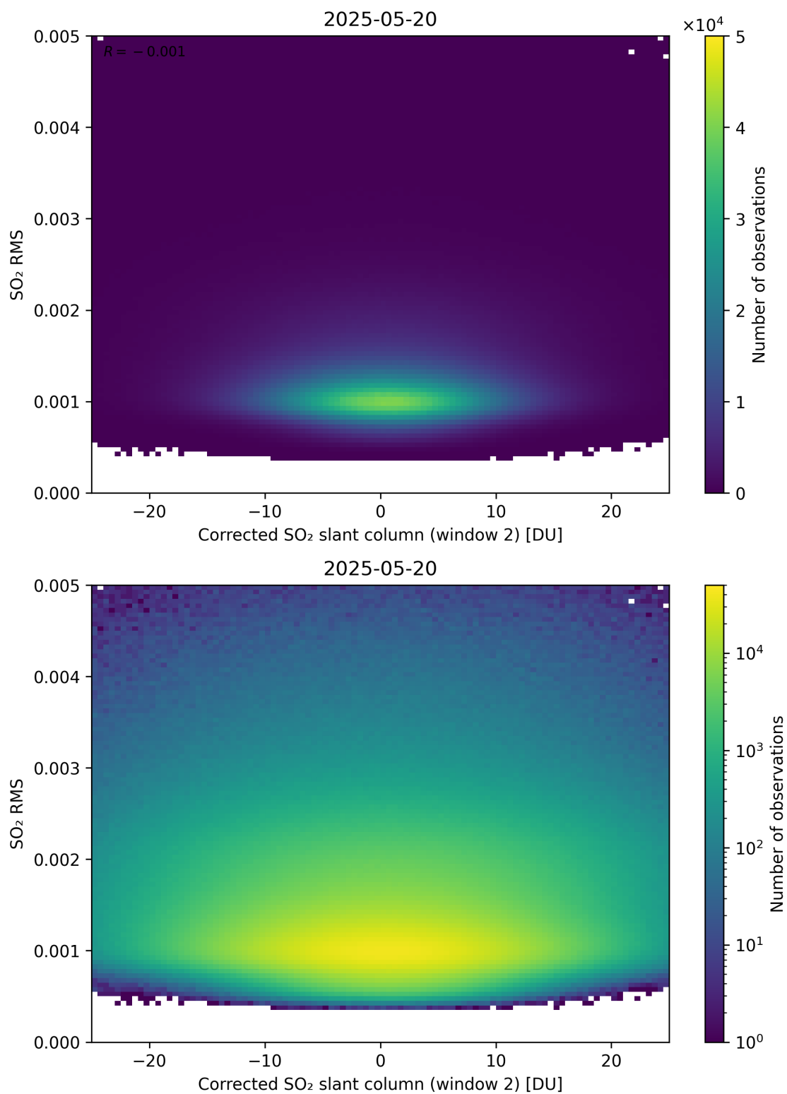
Figure 248: Scatter density plot of “Corrected SO 2 slant column (window 2)” against “SO 2 RMS” for 2025-05-19 to 2025-05-21.
