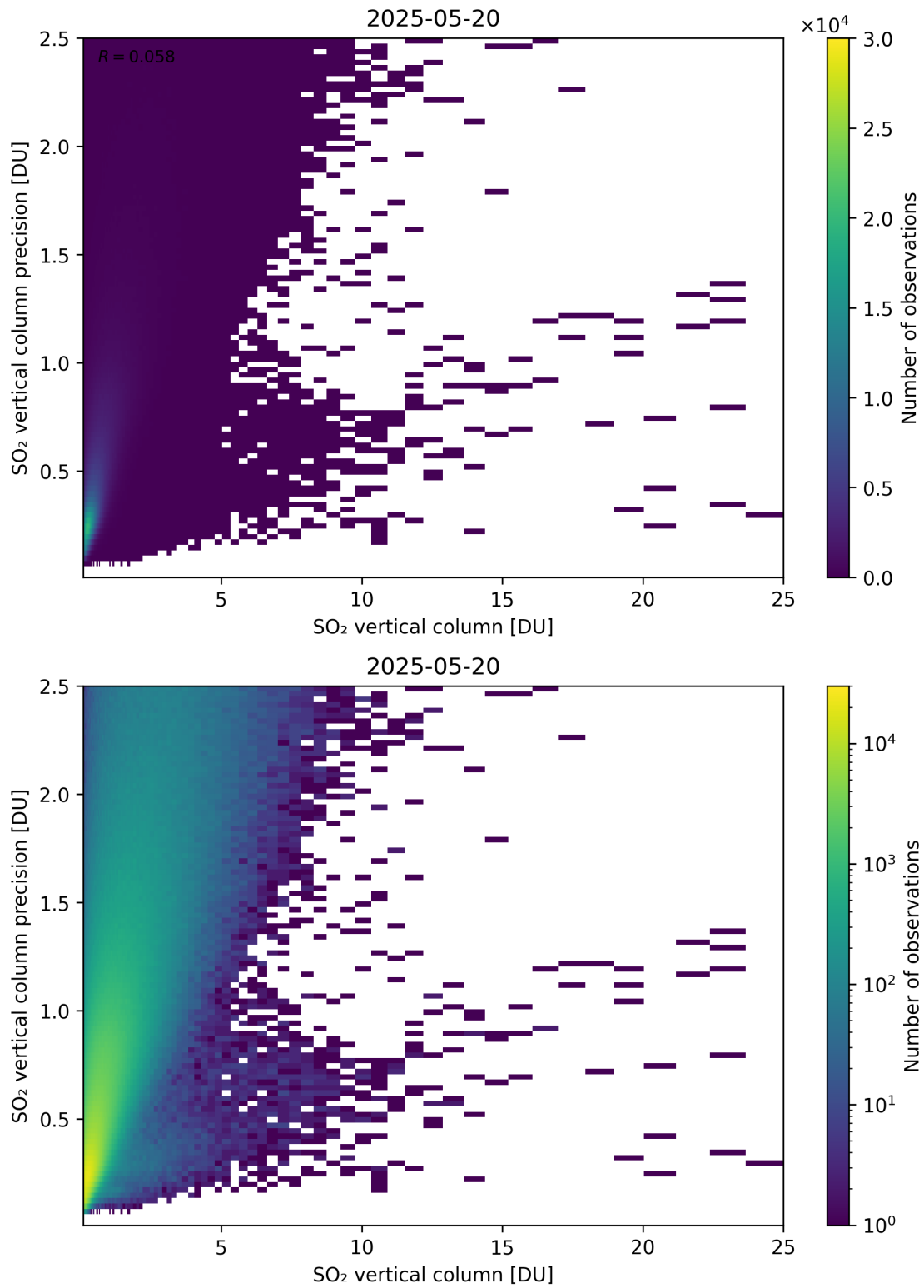
Figure 361: Scatter density plot of “SO 2 vertical column” against “SO 2 vertical column precision” for 2025-05-19 to 2025-05-21.
