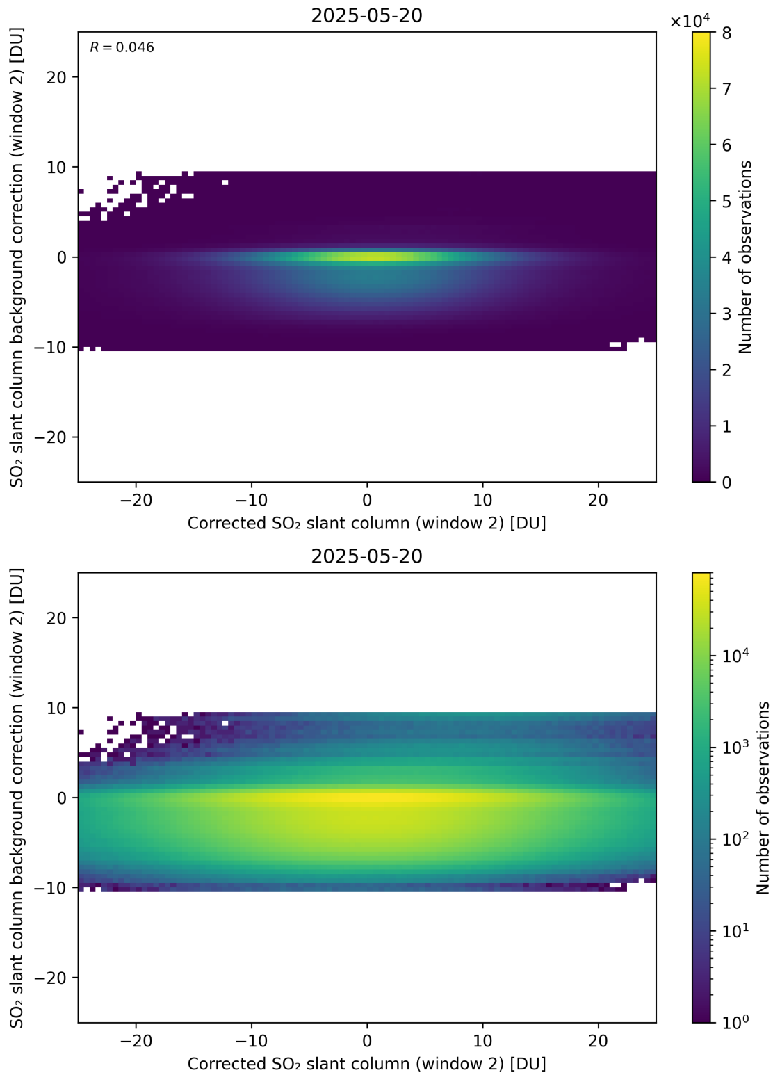
Figure 244: Scatter density plot of “Corrected SO 2 slant column (window 2)” against “SO 2 slant column background correction (window 2)” for 2025-05-19 to 2025-05-21.
