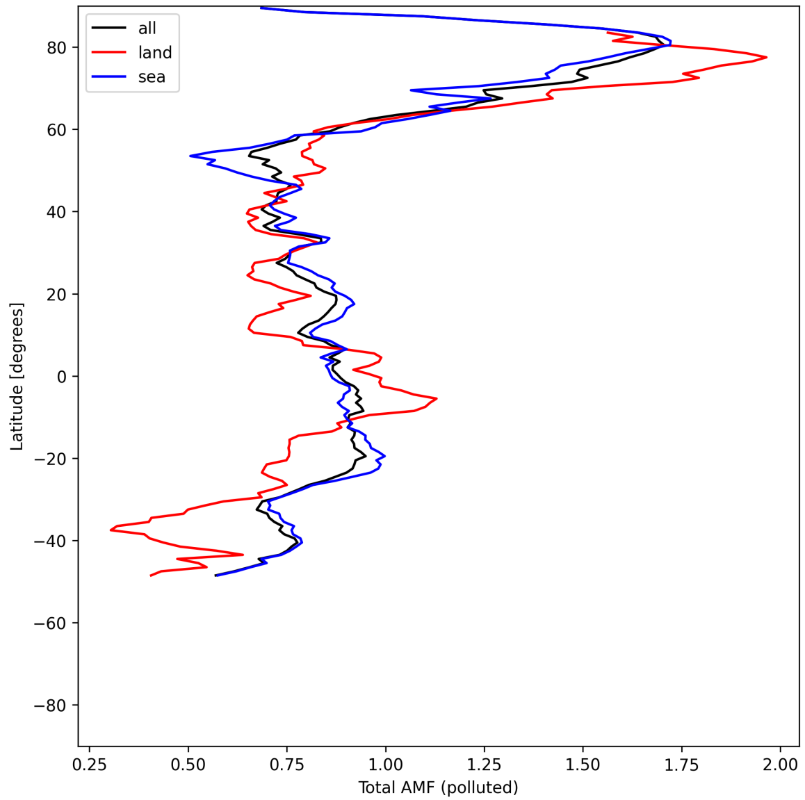
Figure 53: Zonal average of “Total AMF (polluted)” for 2025-05-19 to 2025-05-21.
