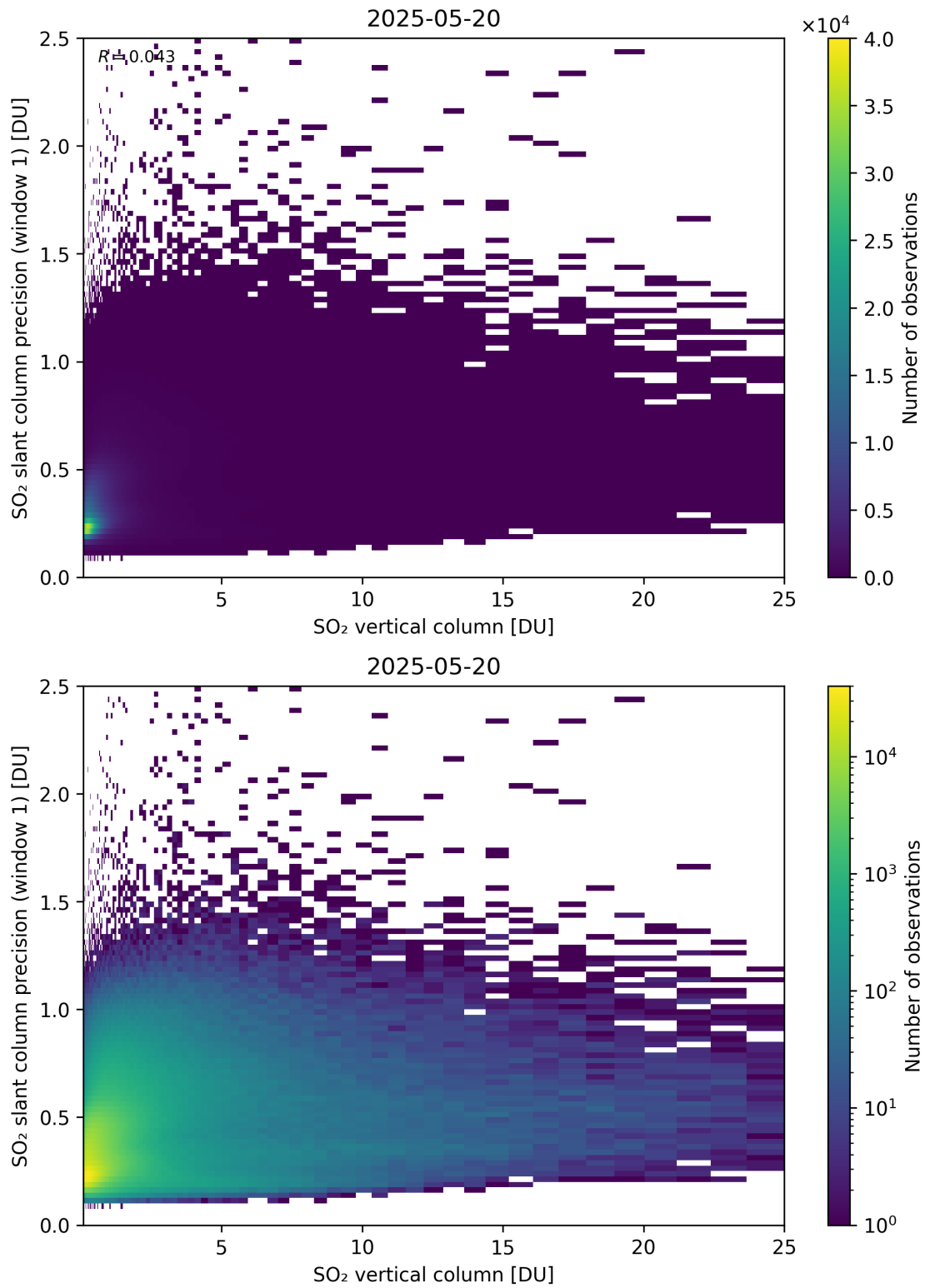
Figure 355: Scatter density plot of “SO 2 vertical column” against “SO 2 slant column precision (window 1)” for 2025-05-19 to 2025-05-21.
