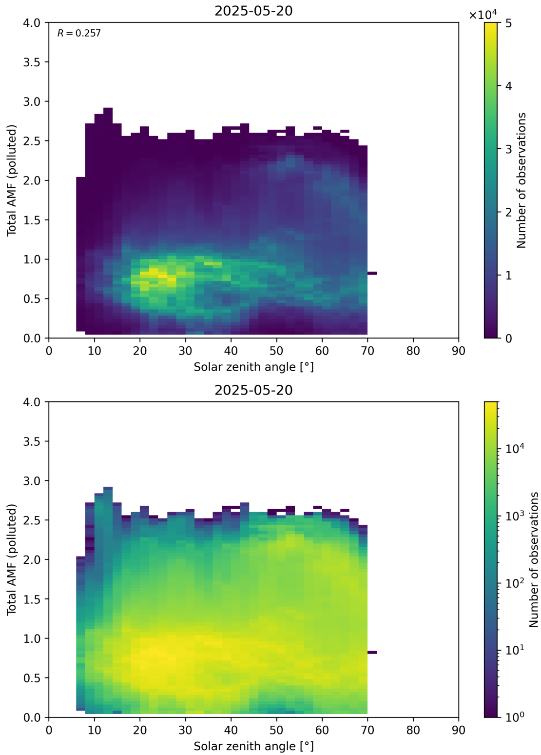
Figure 189: Scatter density plot of “Solar zenith angle” against “Total AMF (polluted)” for 2025-05-19 to 2025-05-21.
