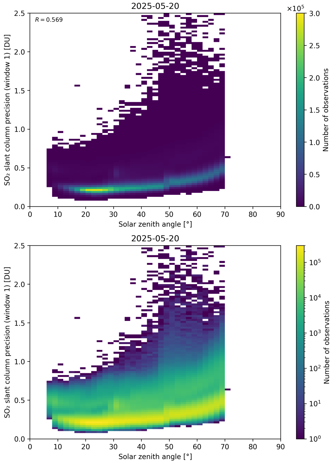
Figure 185: Scatter density plot of “Solar zenith angle” against “SO 2 slant column precision (window 1)” for 2025-05-19 to 2025-05-21.
