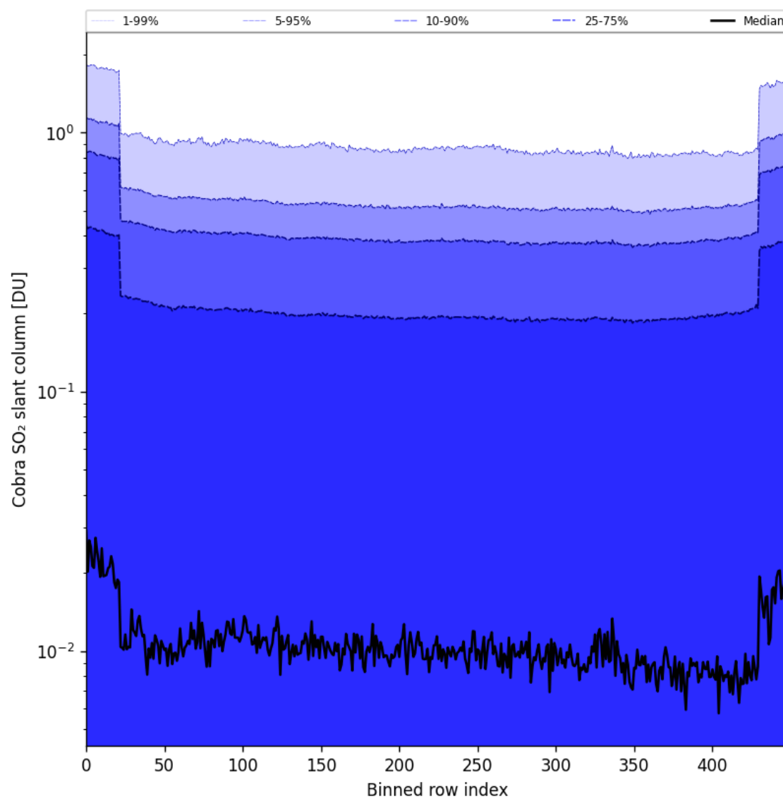
Figure 87: Along track statistics of “Cobra SO 2 slant column” for 2025-05-19 to 2025-05-21
