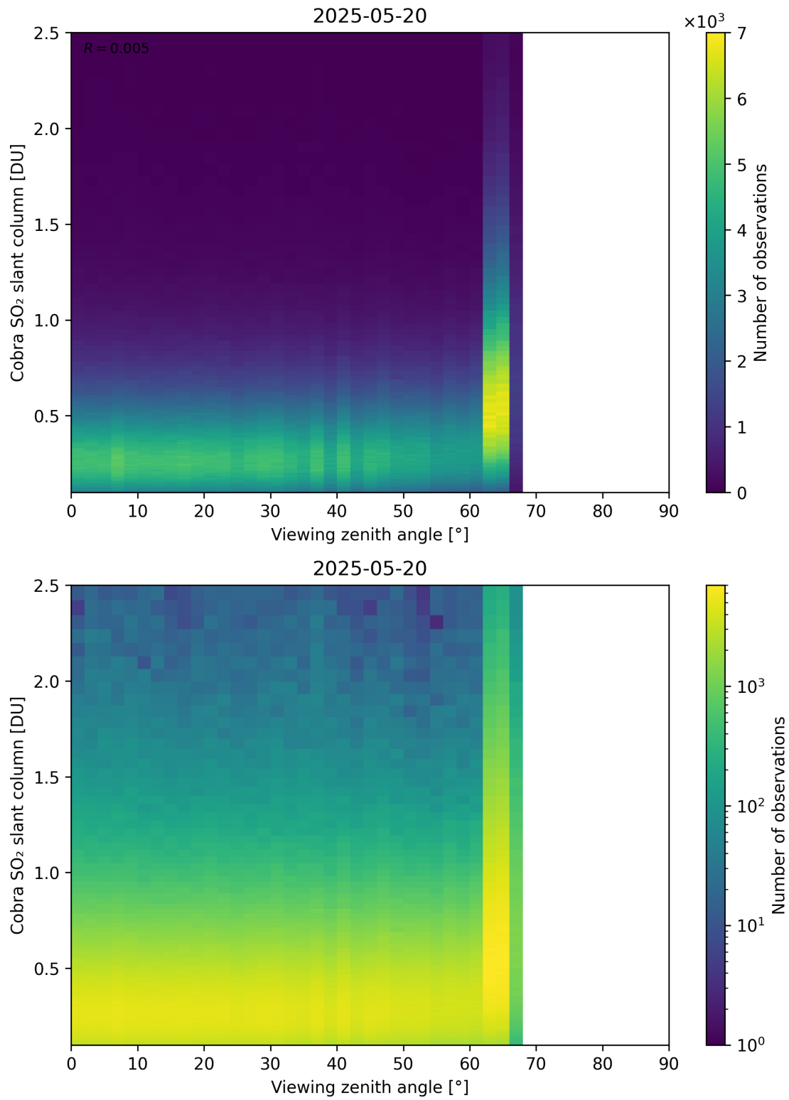
Figure 371: Scatter density plot of “Viewing zenith angle” against “Cobra SO 2 slant column” for 2025-05-19 to 2025-05-21.
