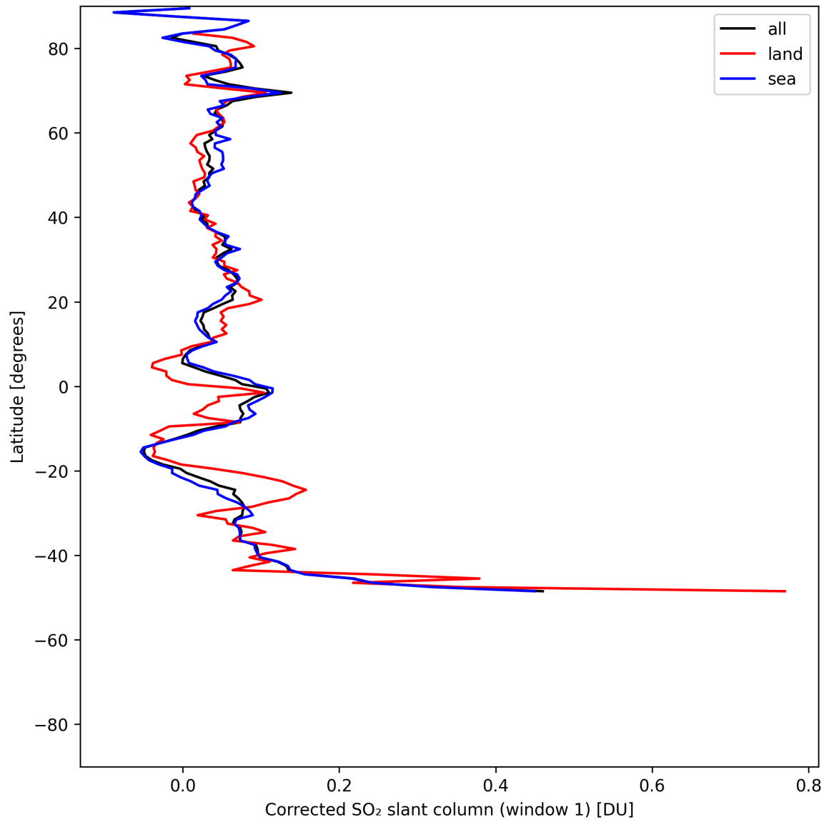
Figure 39: Zonal average of “Corrected SO 2 slant column (window 1)” for 2025-05-19 to 2025-05-21.
