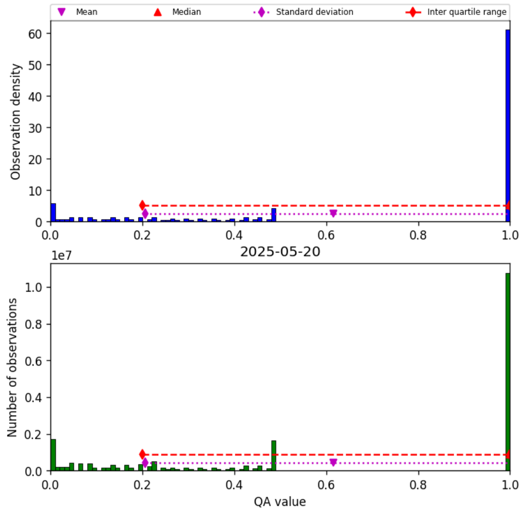
Figure 57: Histogram of “QA value” for 2025-05-19 to 2025-05-21
