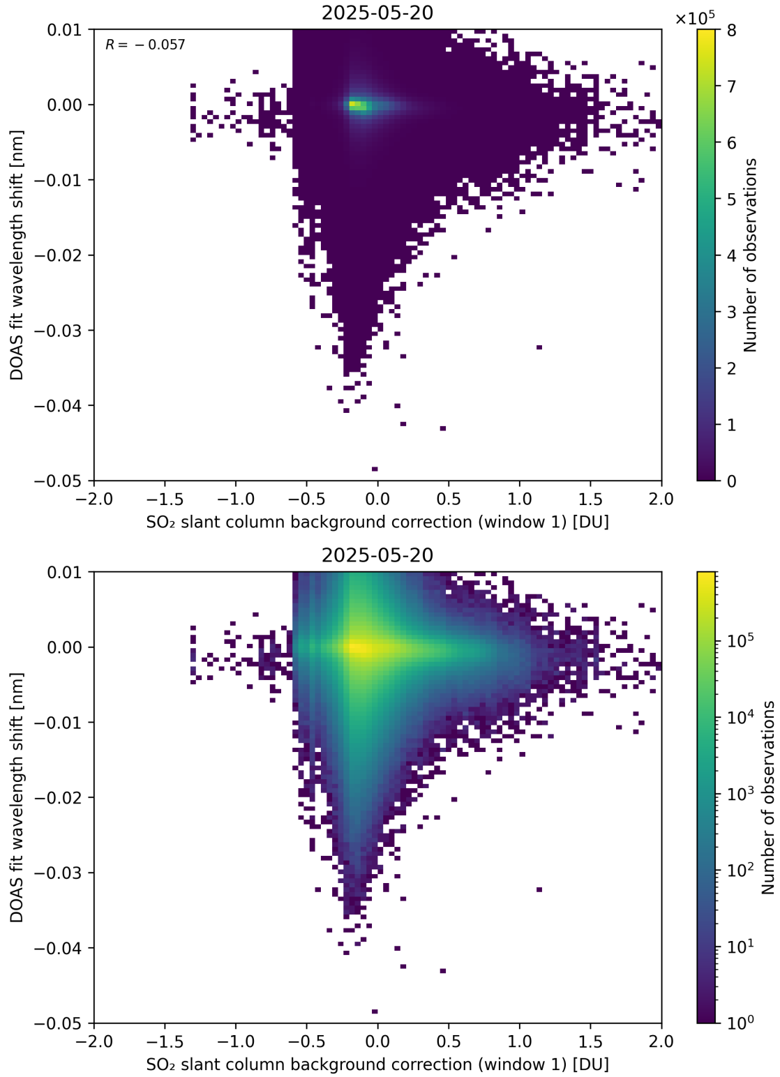
Figure 111: Scatter density plot of “SO 2 slant column background correction (window 1)” against “DOAS fit wavelength shift” for 2025-05-19 to 2025-05-21.
