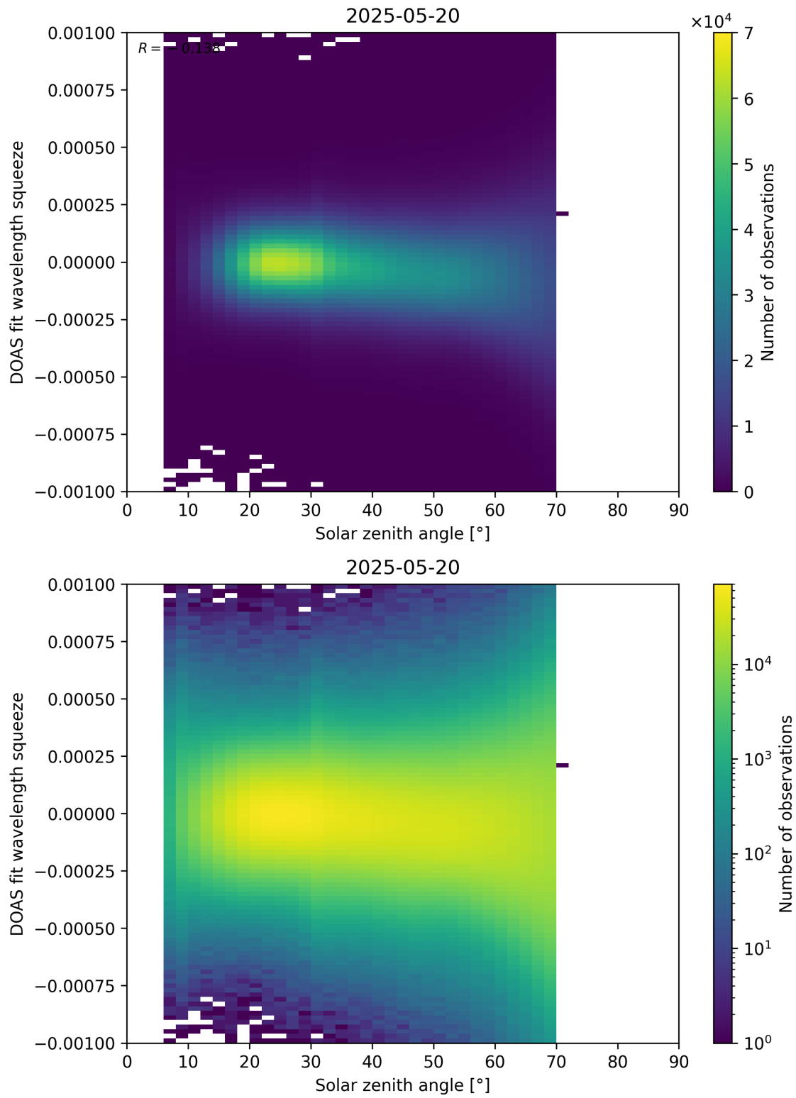
Figure 175: Scatter density plot of “Solar zenith angle” against “DOAS fit wavelength squeeze” for 2025-05-19 to 2025-05-21.
