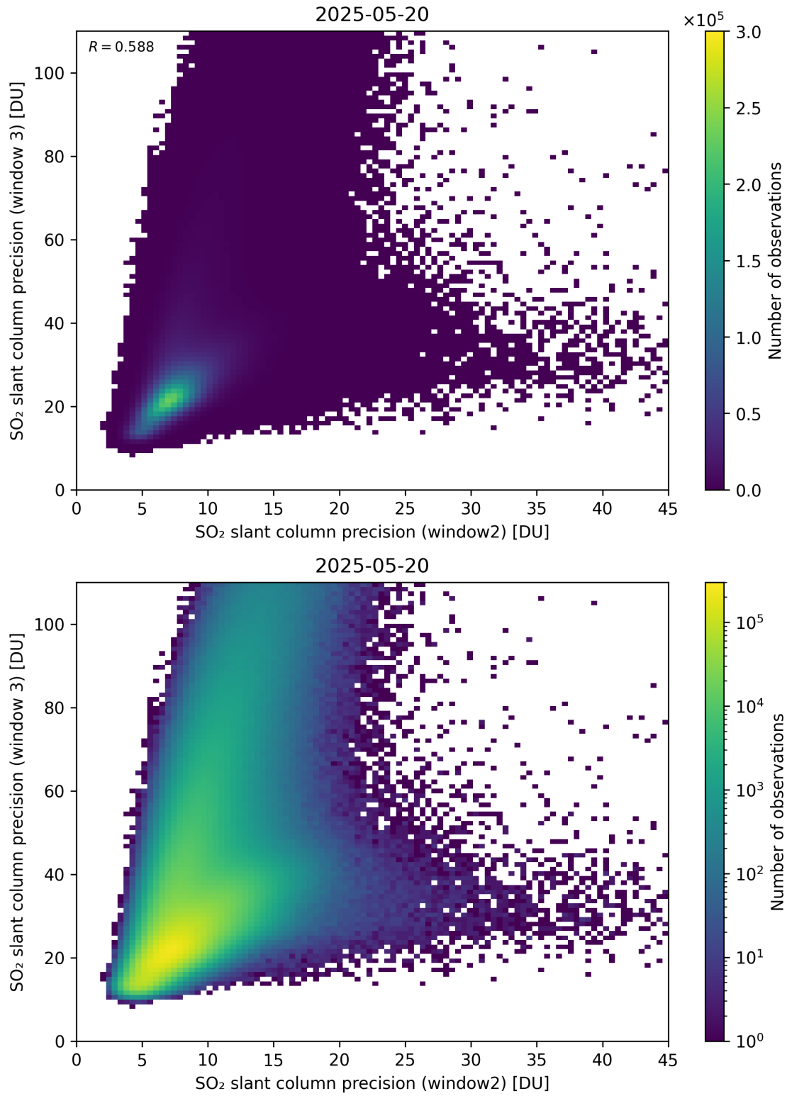
Figure 300: Scatter density plot of “SO 2 slant column precision (window2)” against “SO 2 slant column precision (window 3)” for 2025-05-19 to 2025-05-21.
