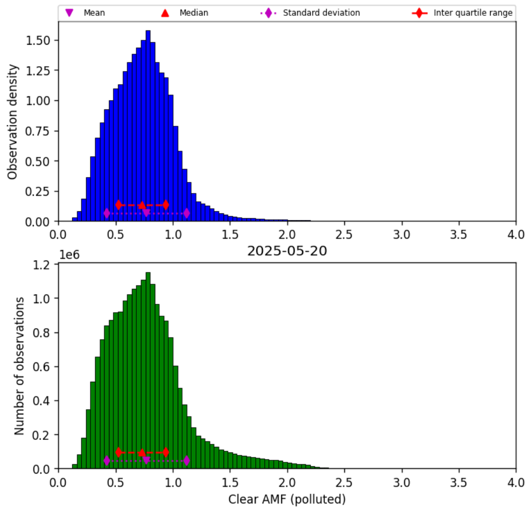
Figure 81: Histogram of “Clear AMF (polluted)” for 2025-05-19 to 2025-05-21
