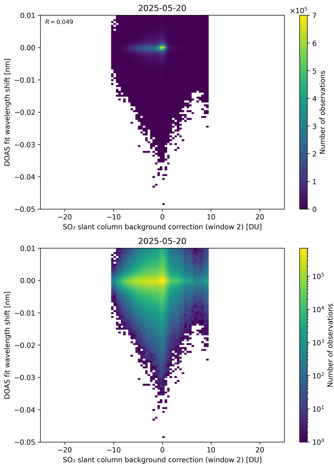
Figure 123: Scatter density plot of “SO 2 slant column background correction (window 2)” against “DOAS fit wavelength shift” for 2025-05-19 to 2025-05-21.
