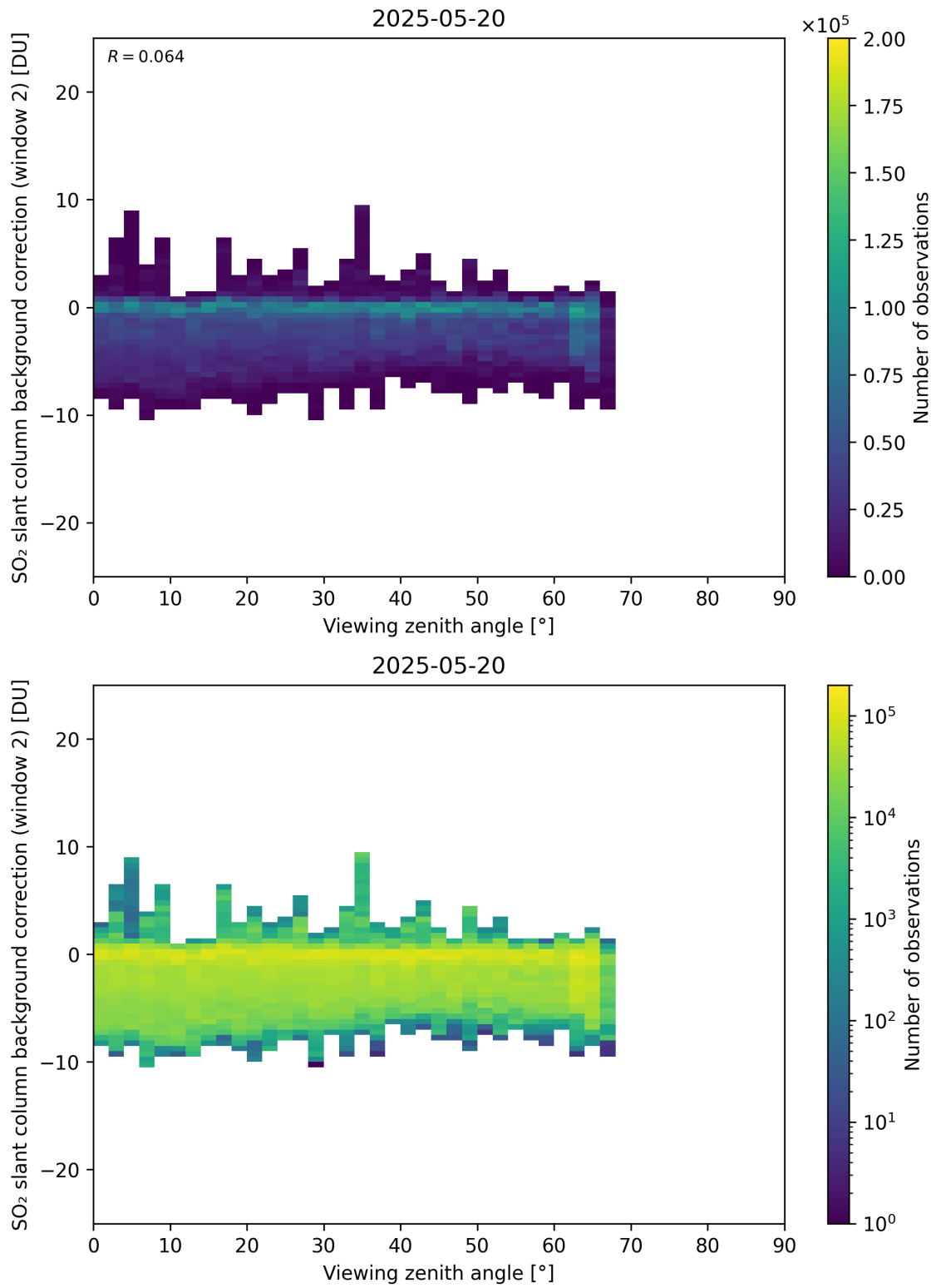
Figure 363: Scatter density plot of “Viewing zenith angle” against “SO 2 slant column background correction (window 2)” for 2025-05-19 to 2025-05-21.
