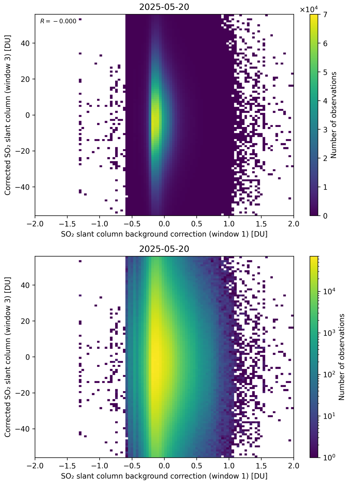
Figure 116: Scatter density plot of “SO 2 slant column background correction (window 1)” against “Corrected SO 2 slant column (window 3)” for 2025-05-19 to 2025-05-21.
