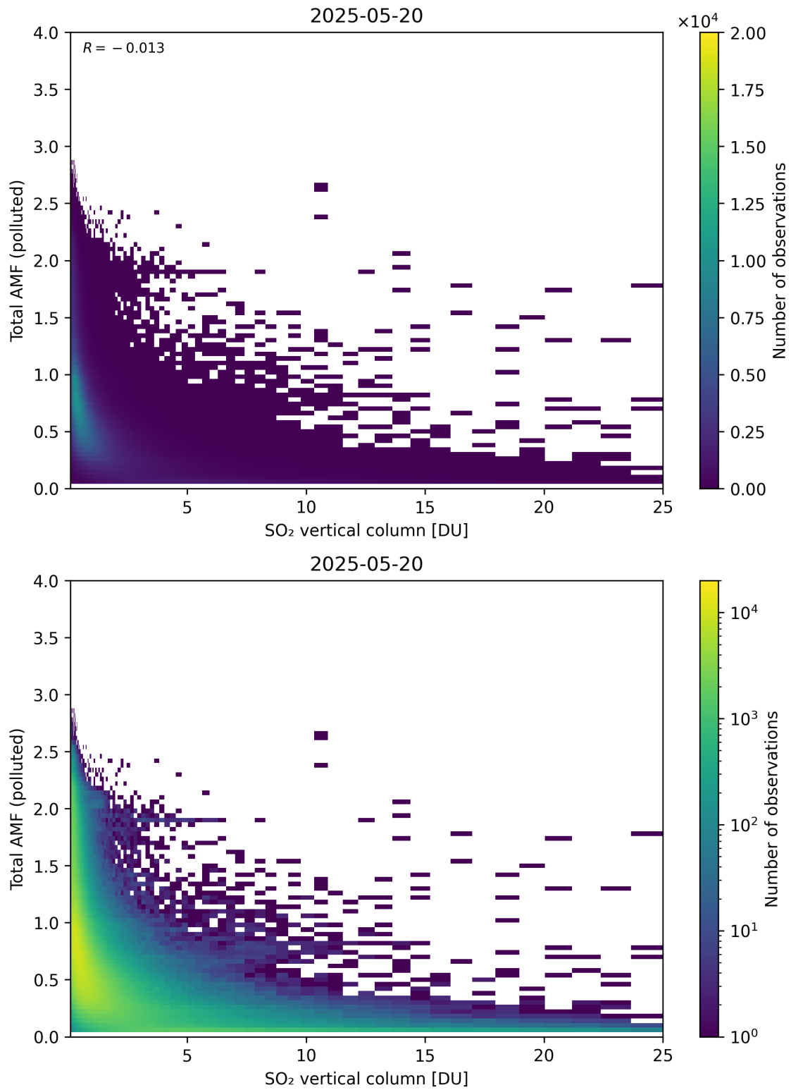
Figure 359: Scatter density plot of “SO 2 vertical column” against “Total AMF (polluted)” for 2025-05-19 to 2025-05-21.
