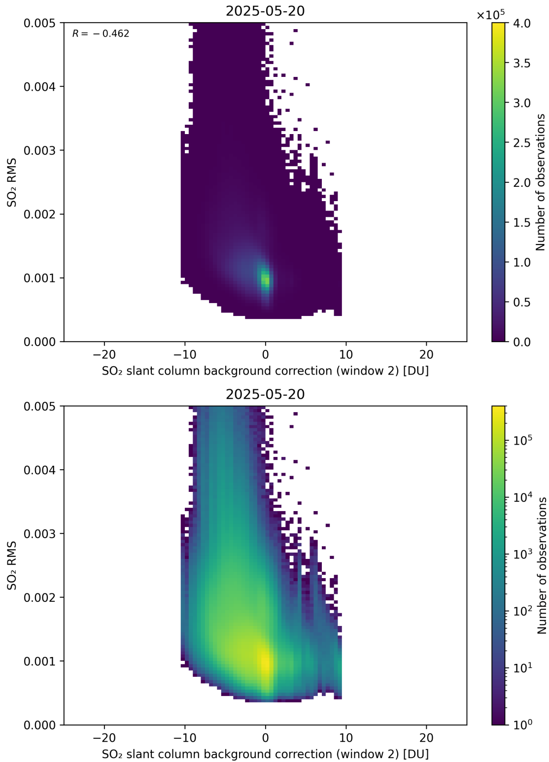
Figure 125: Scatter density plot of “SO 2 slant column background correction (window 2)” against “SO 2 RMS” for 2025-05-19 to 2025-05-21.
