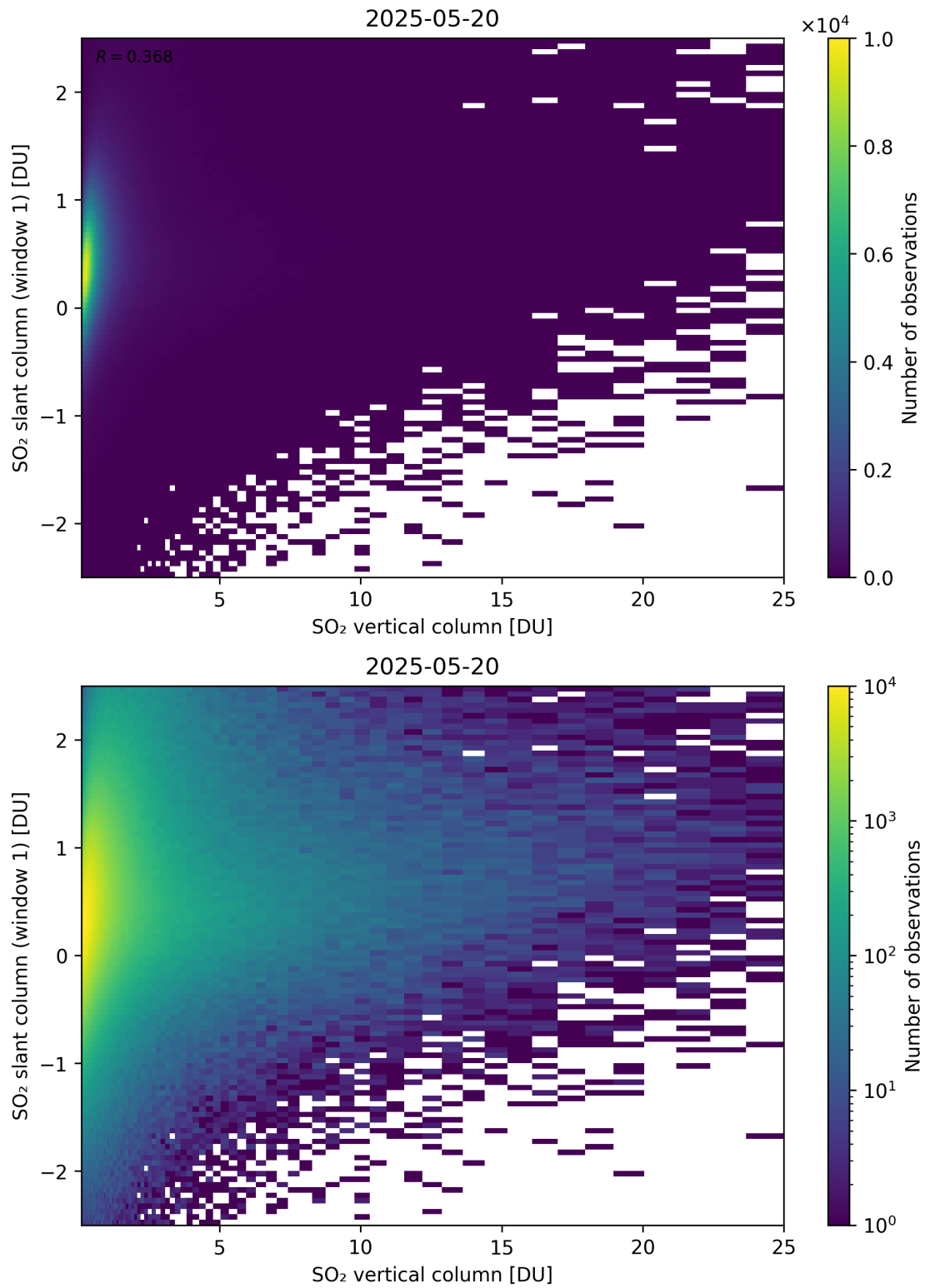
Figure 354: Scatter density plot of “SO 2 vertical column” against “SO 2 slant column (window 1)” for 2025-05-19 to 2025-05-21.
