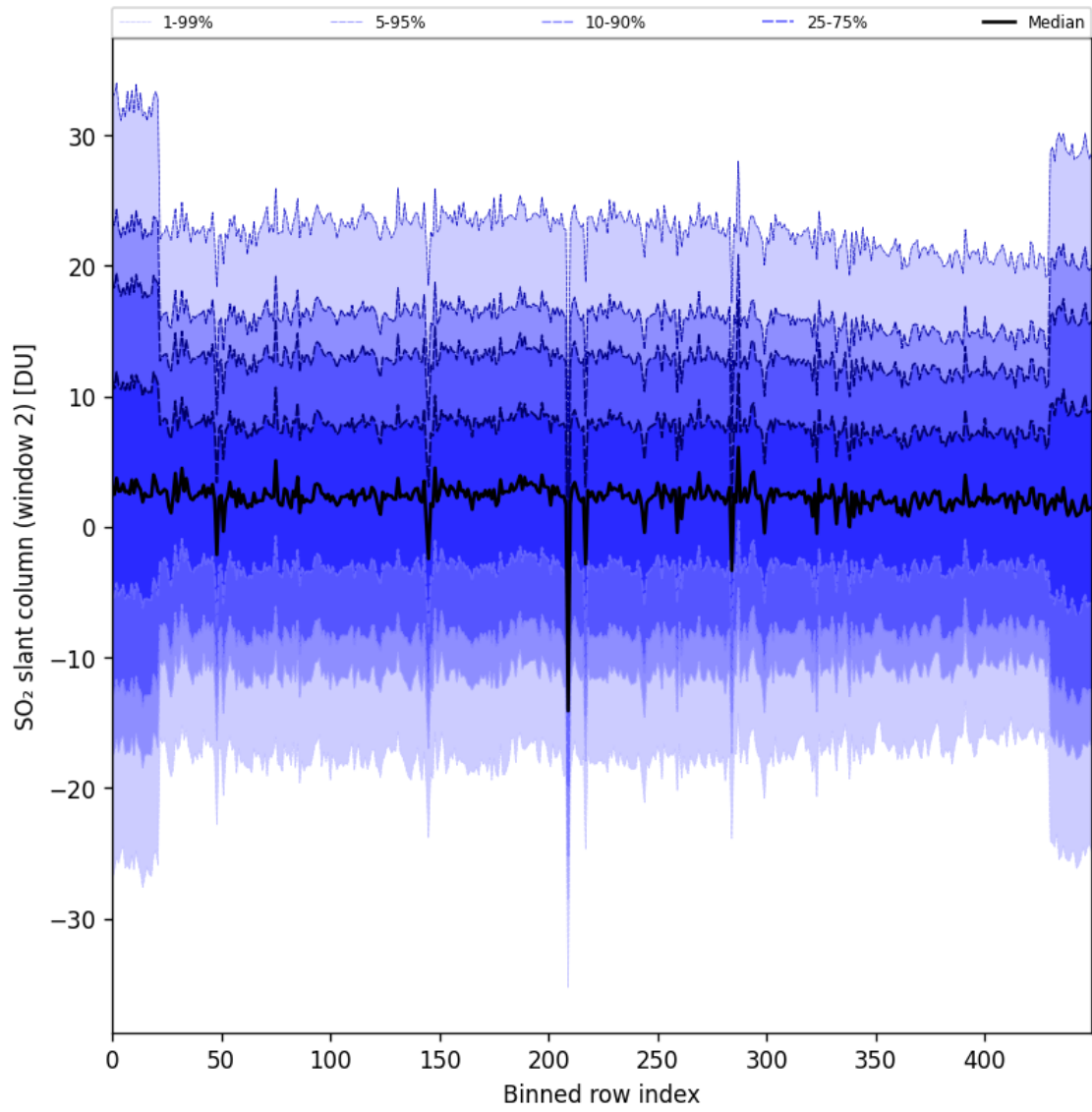
Figure 93: Along track statistics of “SO 2 slant column (window 2)” for 2025-05-19 to 2025-05-21
