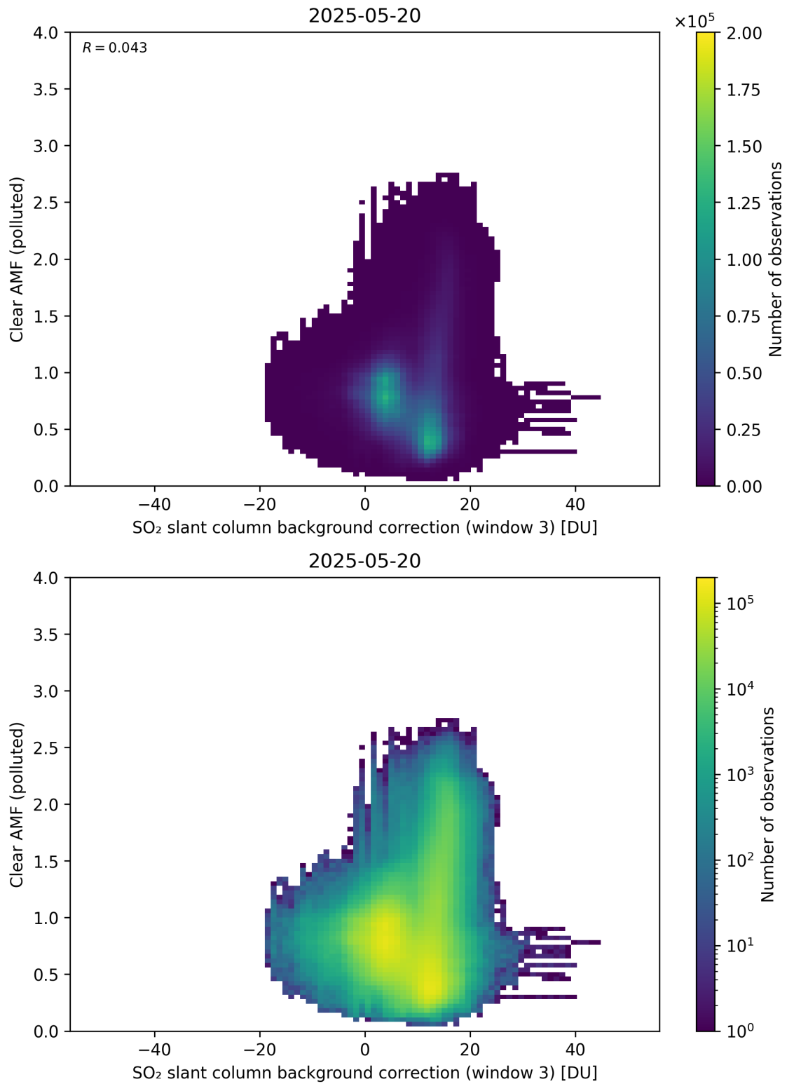
Figure 135: Scatter density plot of “SO 2 slant column background correction (window 3)” against “Clear AMF (polluted)” for 2025-05-19 to 2025-05-21.
