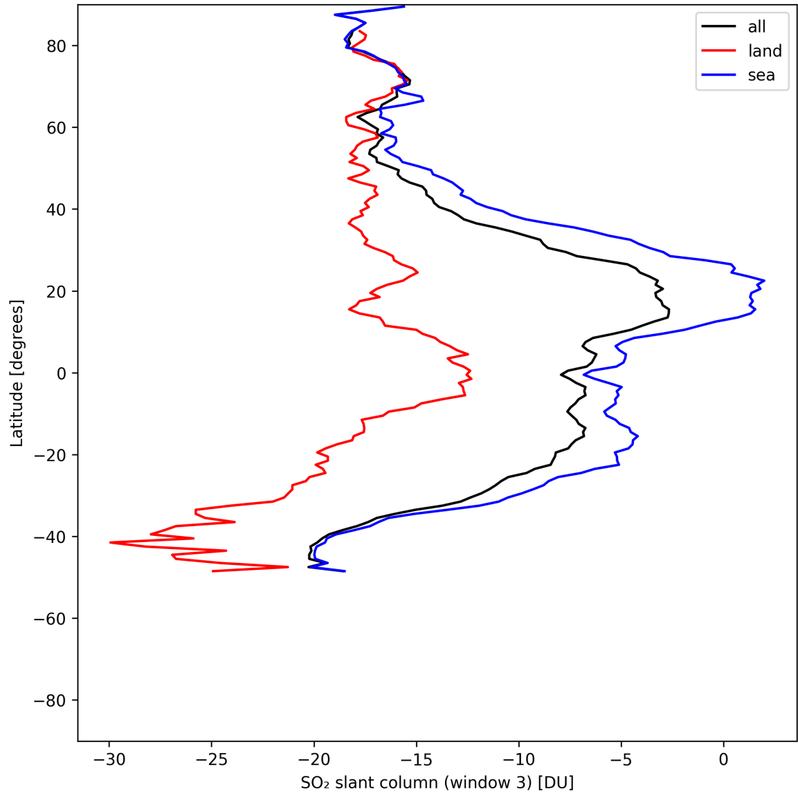
Figure 45: Zonal average of “SO 2 slant column (window 3)” for 2025-05-19 to 2025-05-21.
