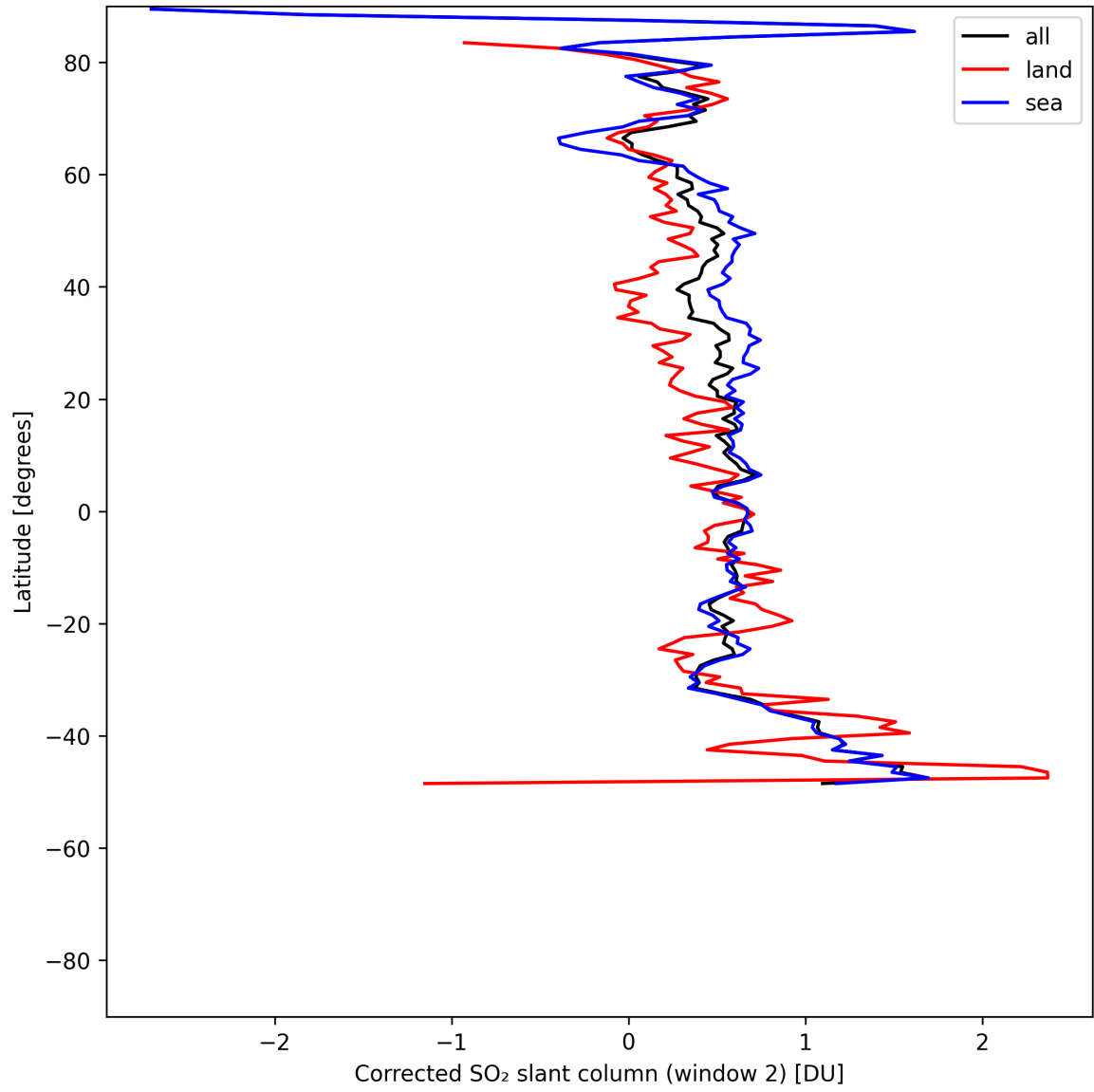
Figure 43: Zonal average of “Corrected SO 2 slant column (window 2)” for 2025-05-19 to 2025-05-21.
