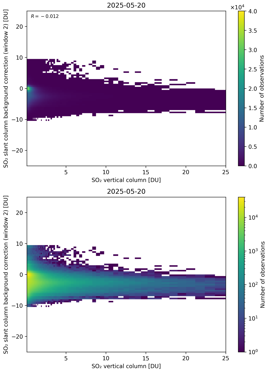
Figure 324: Scatter density plot of “SO 2 vertical column” against “SO 2 slant column background correction (window 2)” for 2025-05-19 to 2025-05-21.
