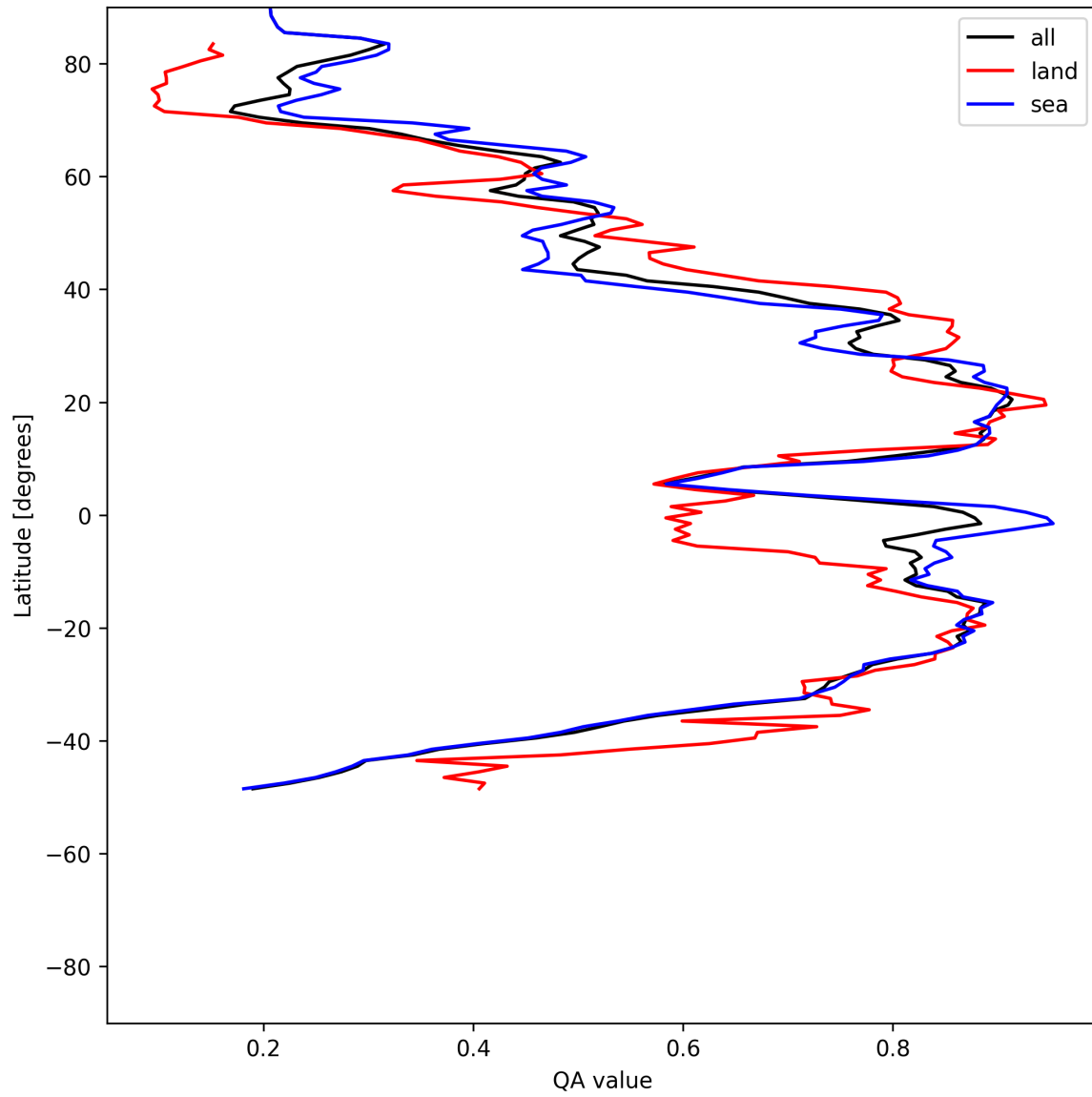
Figure 31: Zonal average of “QA value” for 2025-05-19 to 2025-05-21.
