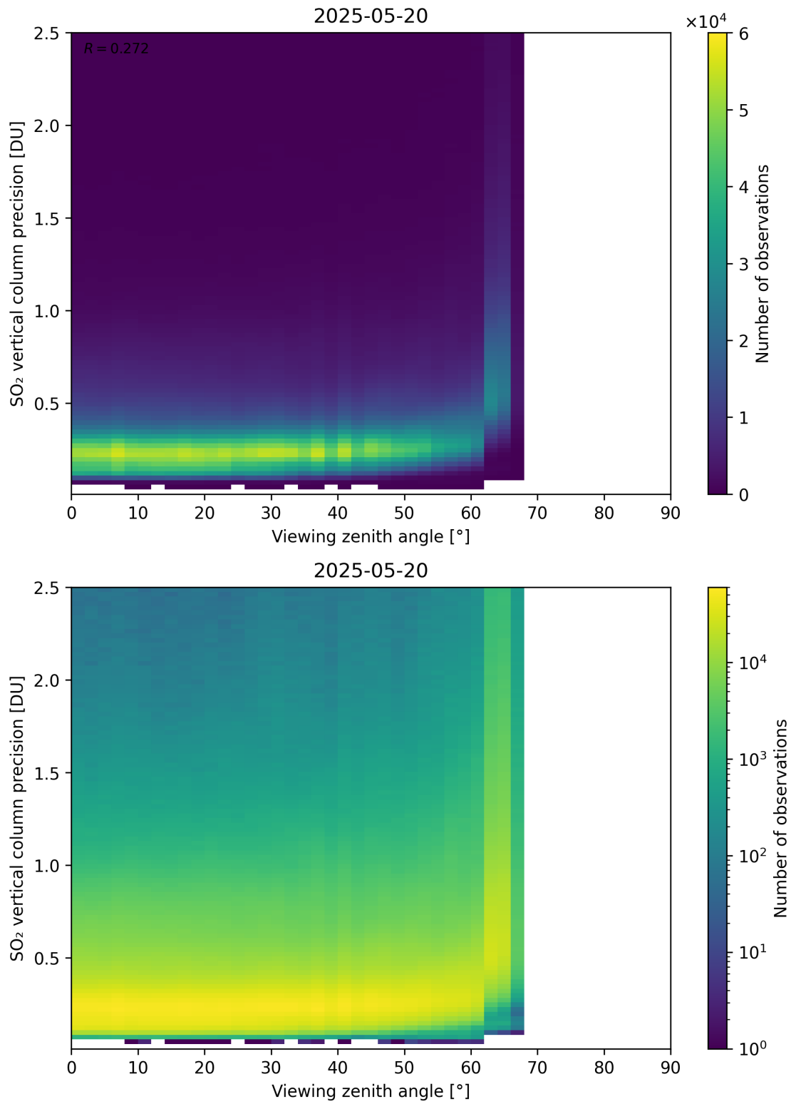
Figure 384: Scatter density plot of “Viewing zenith angle” against “SO 2 vertical column precision” for 2025-05-19 to 2025-05-21.
