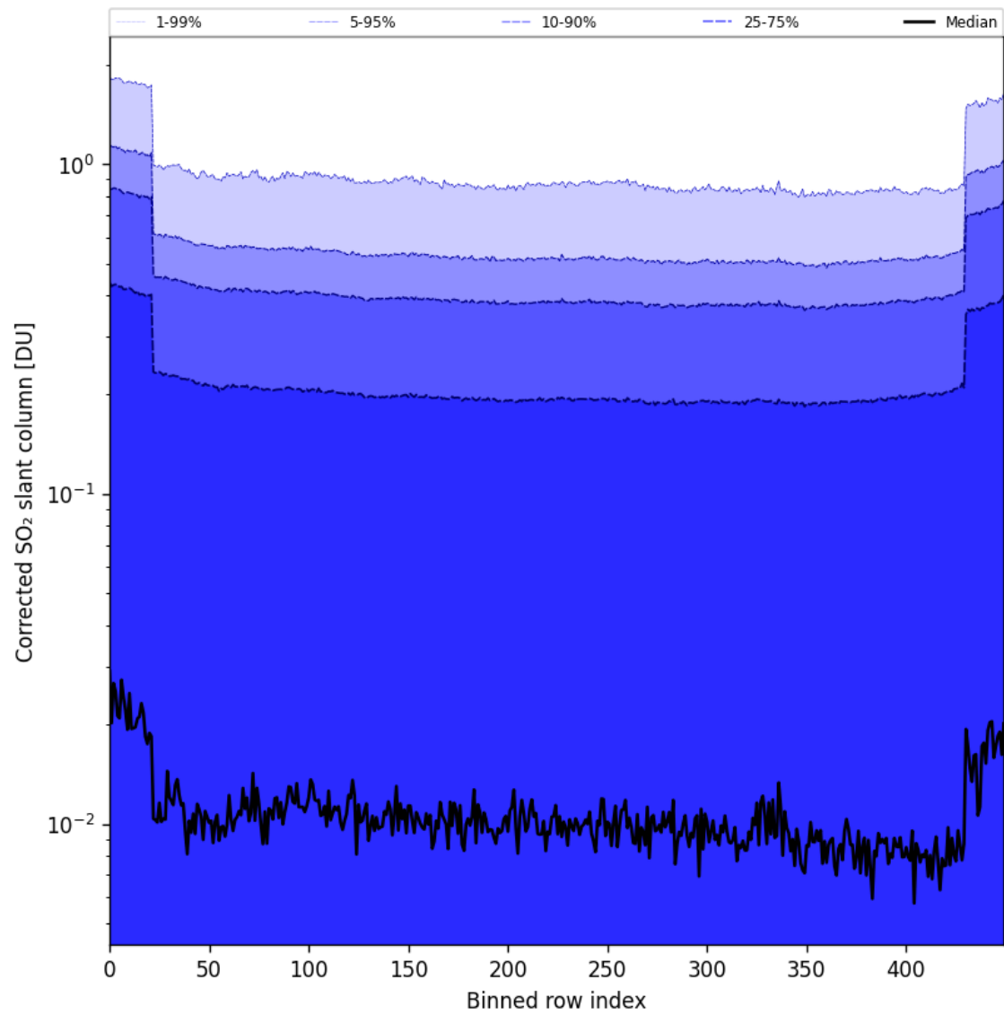
Figure 86: Along track statistics of “Corrected SO 2 slant column” for 2025-05-19 to 2025-05-21
