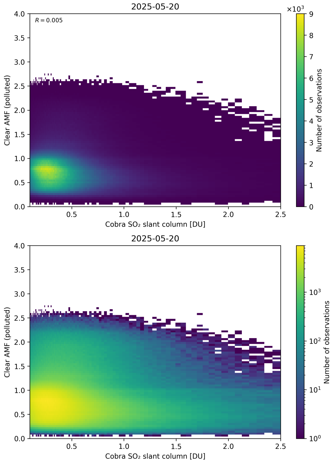
Figure 215: Scatter density plot of “Cobra SO 2 slant column” against “Clear AMF (polluted)” for 2025-05-19 to 2025-05-21.
