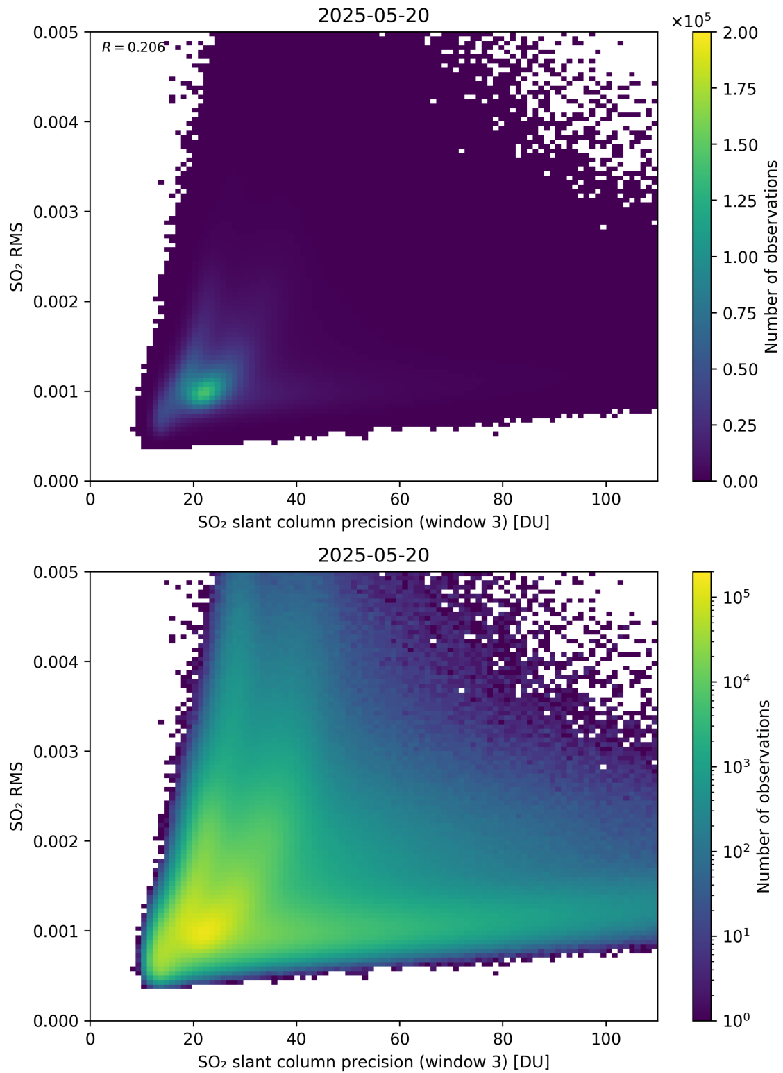
Figure 310: Scatter density plot of “SO 2 slant column precision (window 3)” against “SO 2 RMS” for 2025-05-19 to 2025-05-21.
