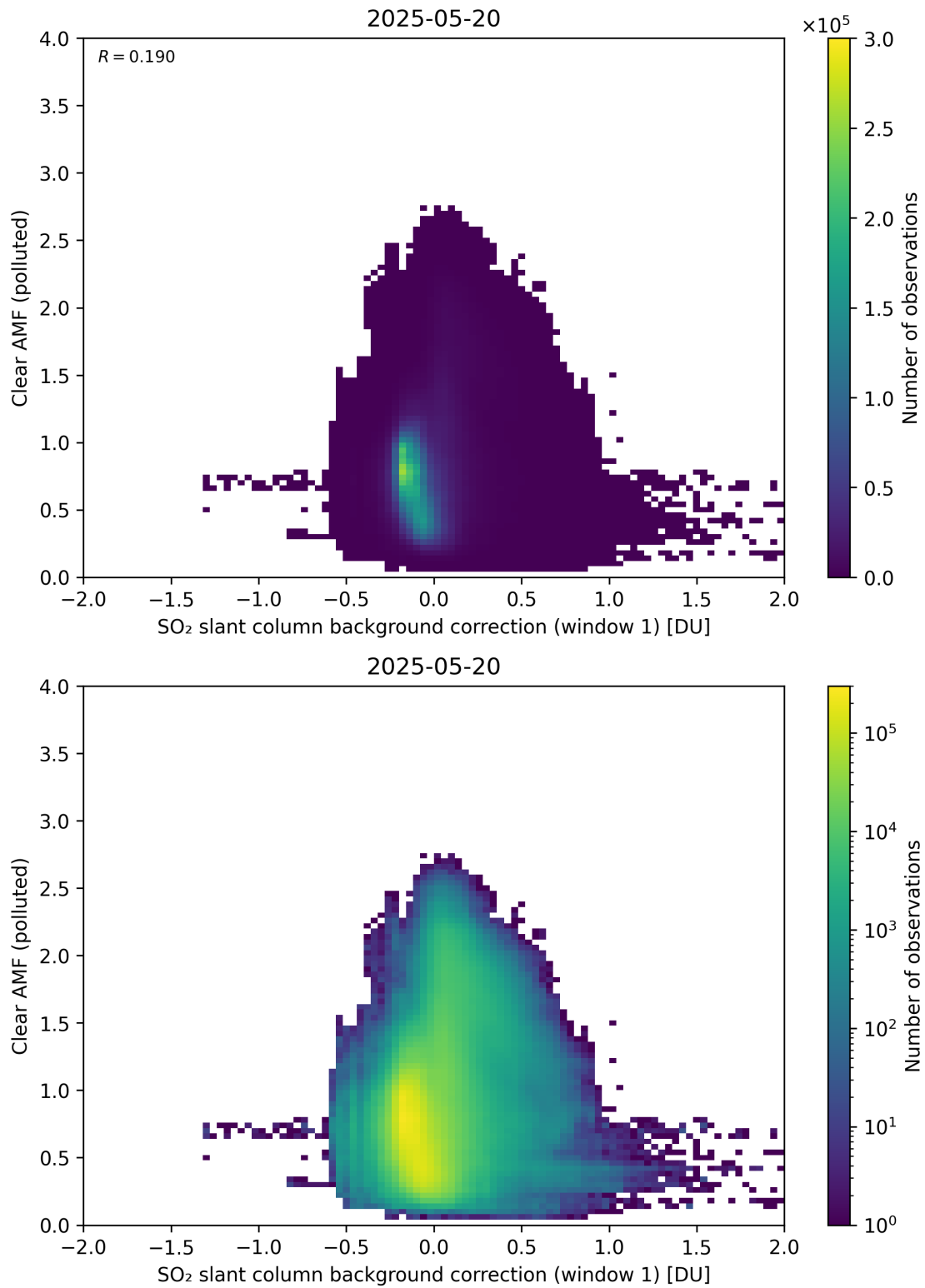
Figure 114: Scatter density plot of “SO 2 slant column background correction (window 1)” against “Clear AMF (polluted)” for 2025-05-19 to 2025-05-21.
