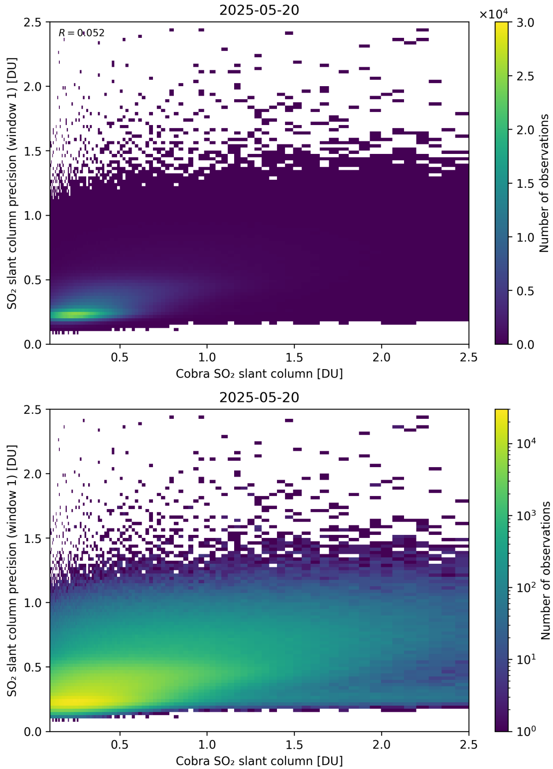
Figure 220: Scatter density plot of “Cobra SO 2 slant column” against “SO 2 slant column precision (window 1)” for 2025-05-19 to 2025-05-21.
