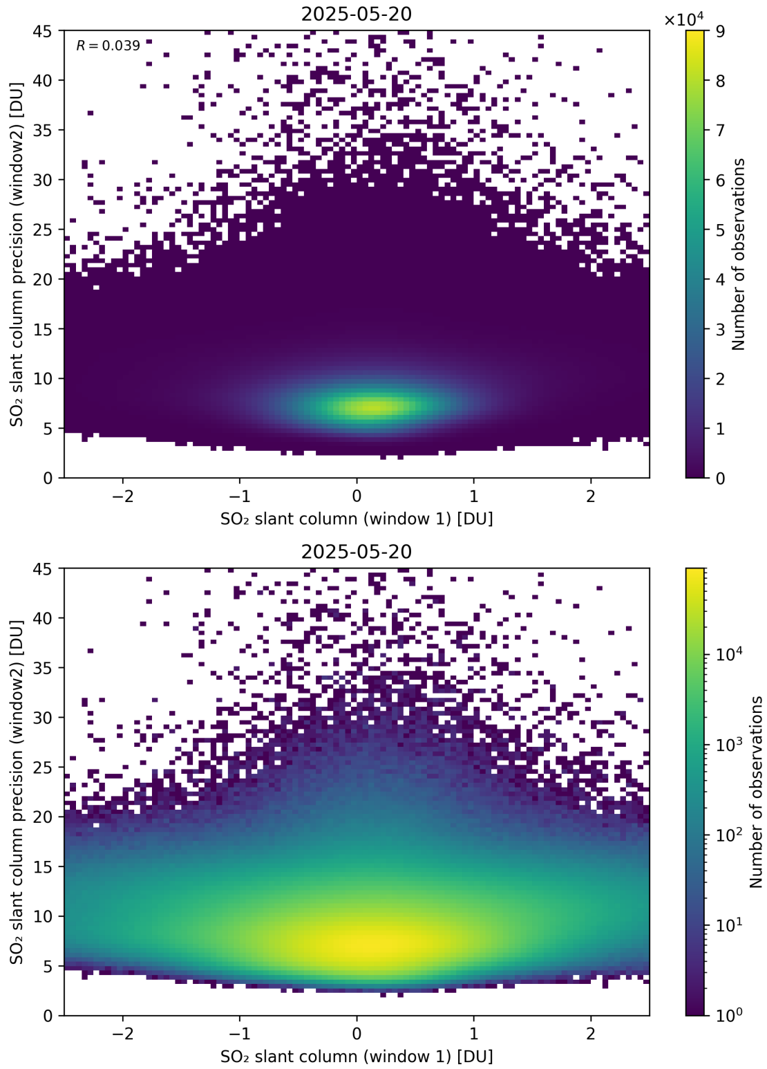
Figure 286: Scatter density plot of “SO 2 slant column (window 1)” against “SO 2 slant column precision (window2)” for 2025-05-19 to 2025-05-21.
