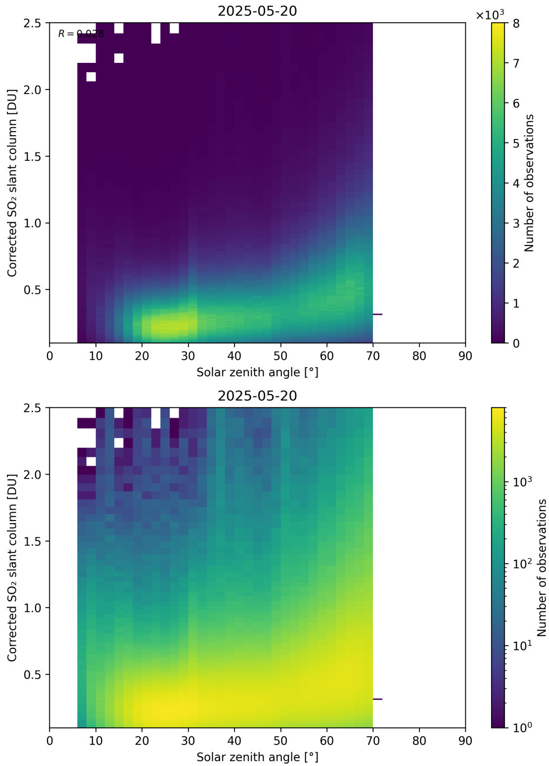
Figure 181: Scatter density plot of “Solar zenith angle” against “Corrected SO 2 slant column” for 2025-05-19 to 2025-05-21.
