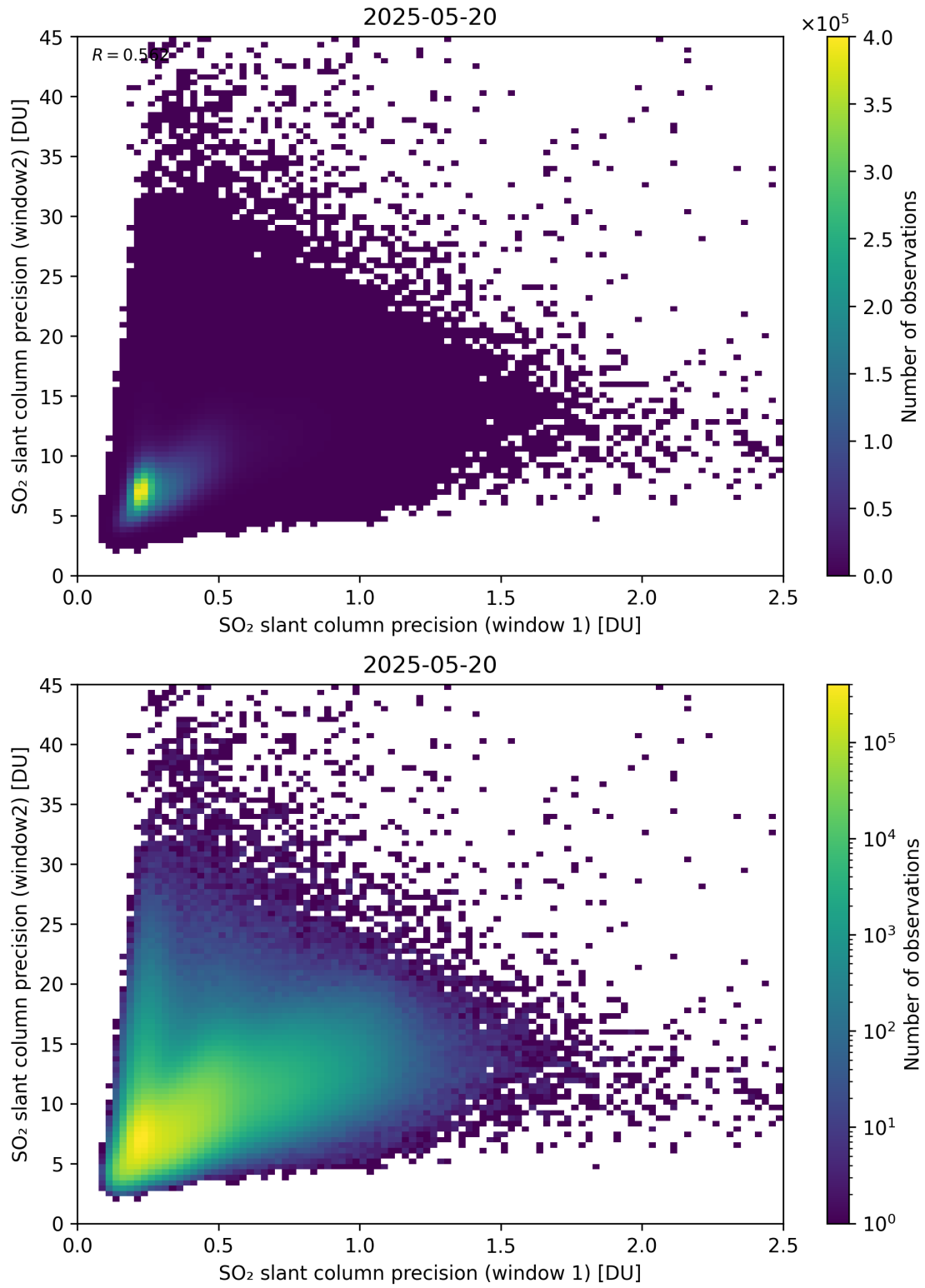
Figure 277: Scatter density plot of “SO 2 slant column precision (window 1)” against “SO 2 slant column precision (window2)” for 2025-05-19 to 2025-05-21.
