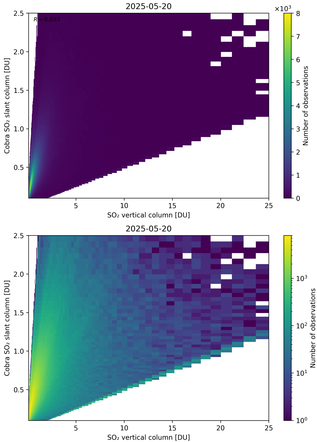
Figure 349: Scatter density plot of “SO 2 vertical column” against “Cobra SO 2 slant column” for 2025-05-19 to 2025-05-21.
