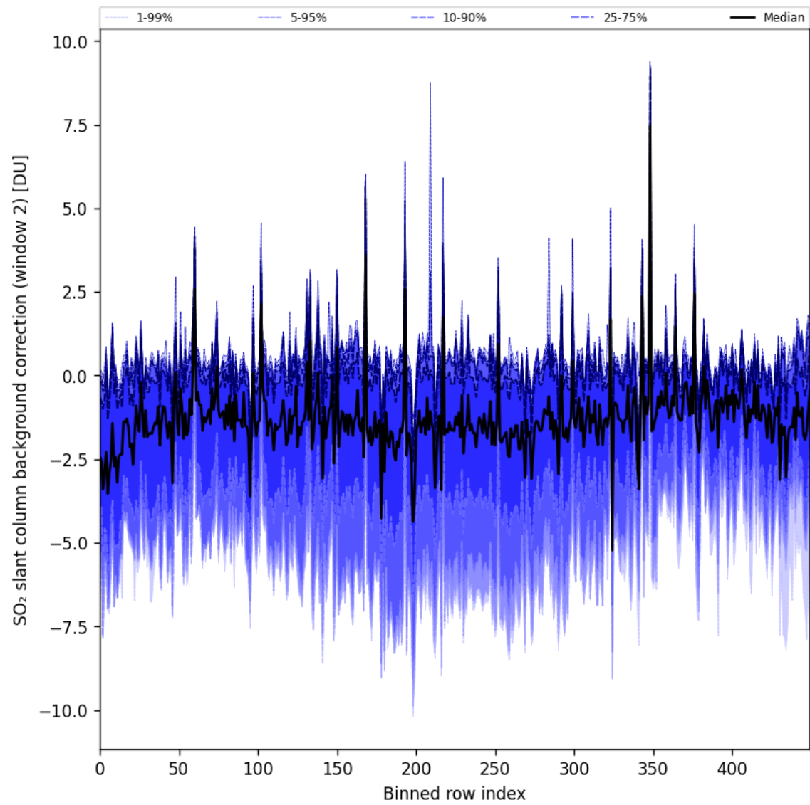
Figure 96: Along track statistics of “SO 2 slant column background correction (window 2)” for 2025-05-19 to 2025-05-21
