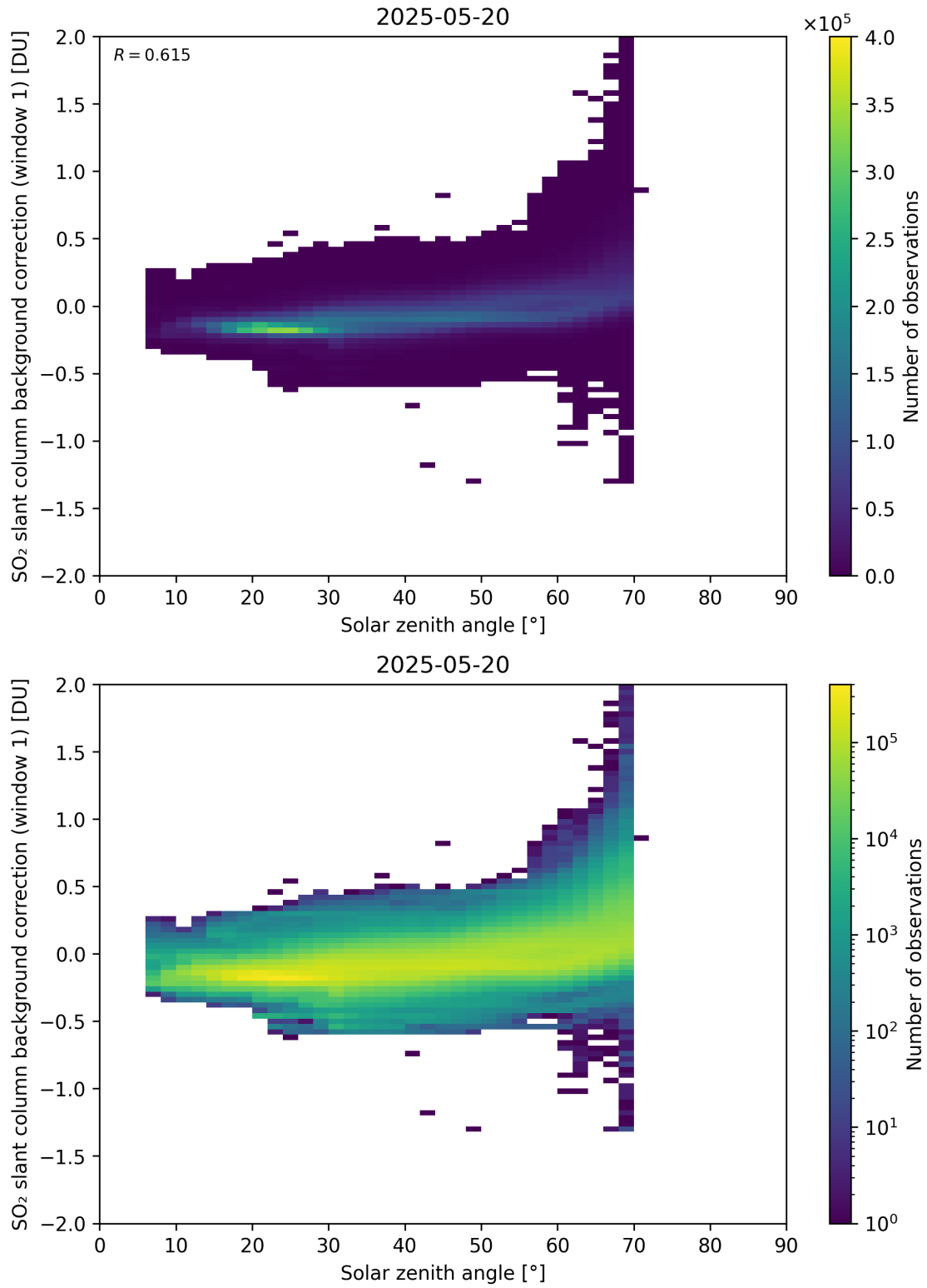
Figure 171: Scatter density plot of “Solar zenith angle” against “SO 2 slant column background correction (window 1)” for 2025-05-19 to 2025-05-21.
