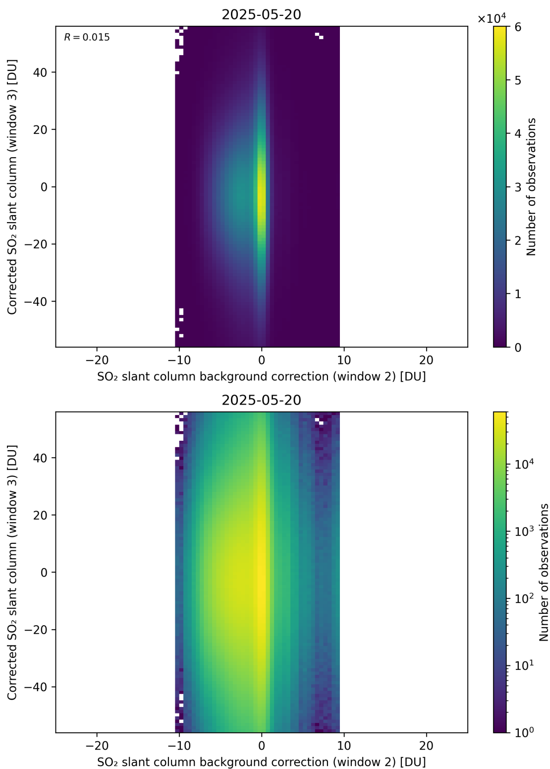
Figure 127: Scatter density plot of “SO 2 slant column background correction (window 2)” against “Corrected SO 2 slant column (window 3)” for 2025-05-19 to 2025-05-21.
