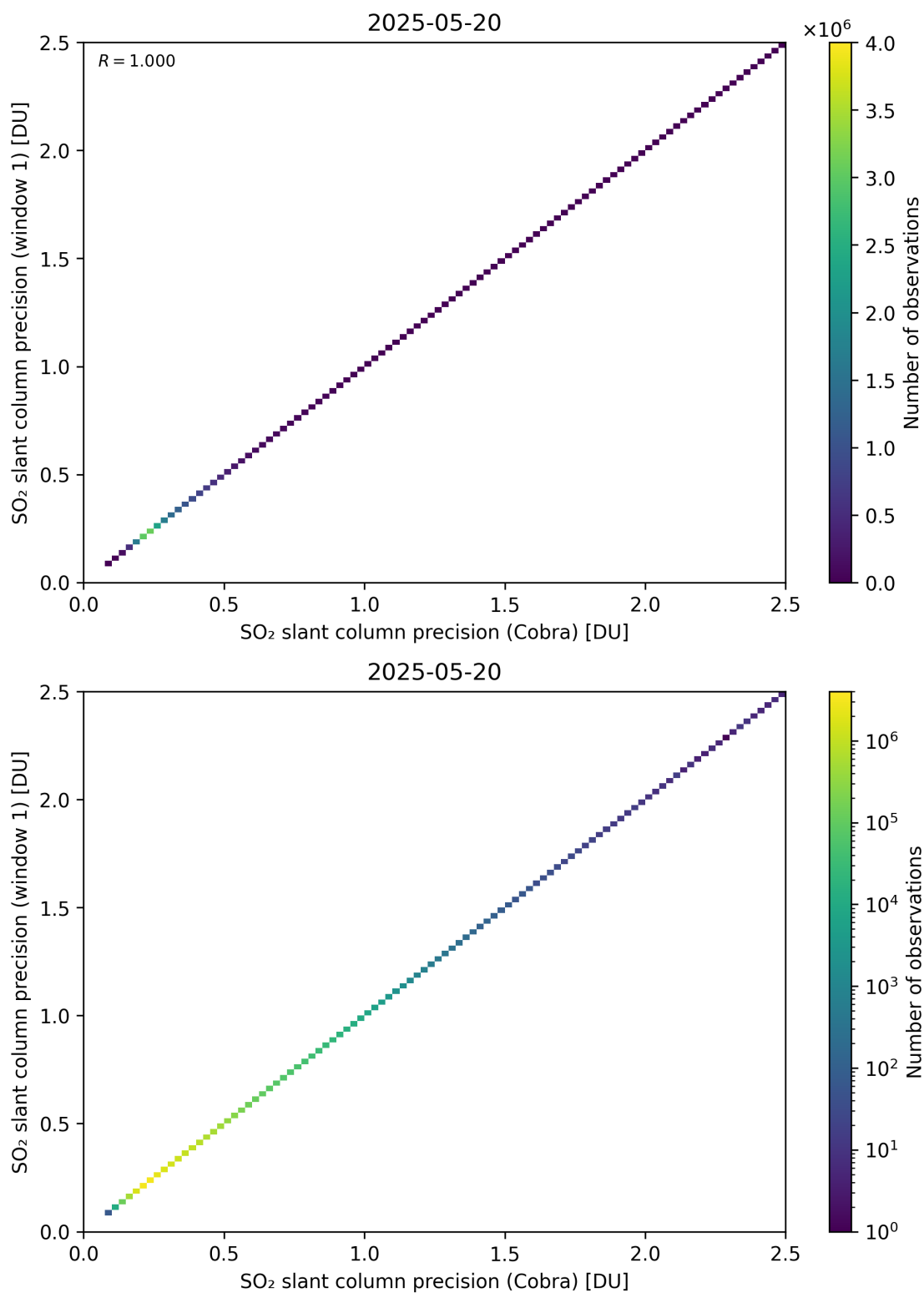
Figure 209: Scatter density plot of “SO 2 slant column precision (Cobra)” against “SO 2 slant column precision (window 1)” for 2025-05-19 to 2025-05-21.
