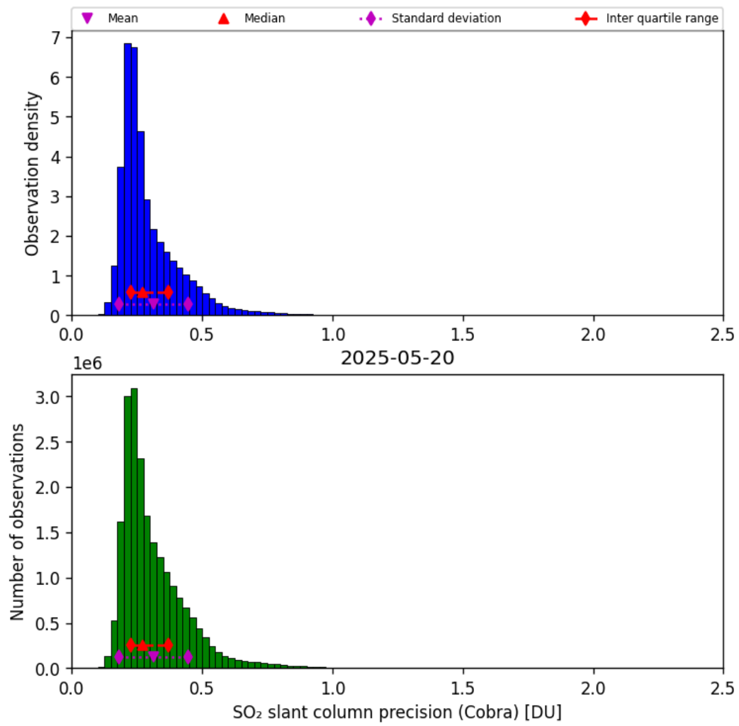
Figure 62: Histogram of “SO 2 slant column precision (Cobra)” for 2025-05-19 to 2025-05-21
