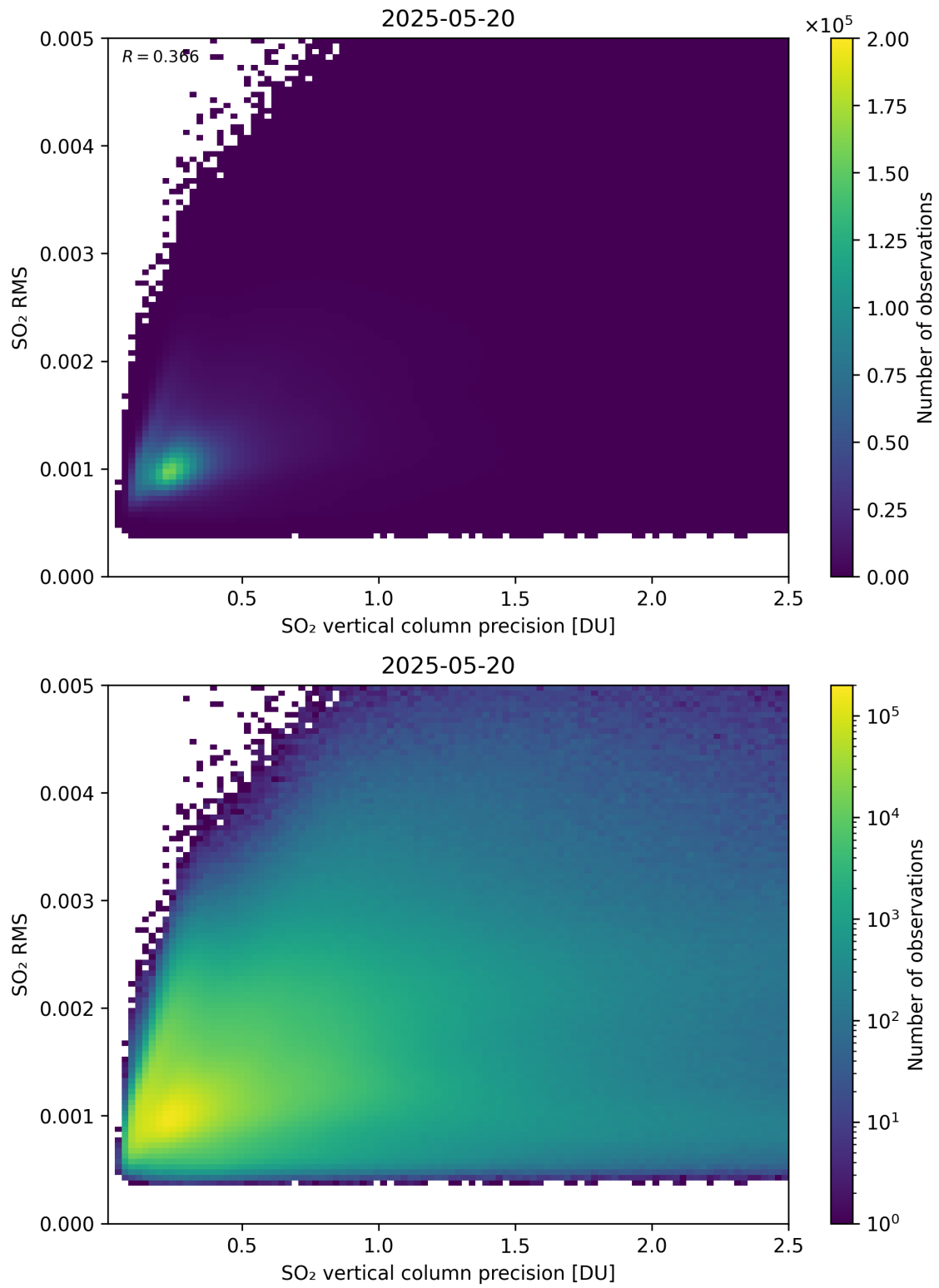
Figure 334: Scatter density plot of “SO 2 vertical column precision” against “SO 2 RMS” for 2025-05-19 to 2025-05-21.
