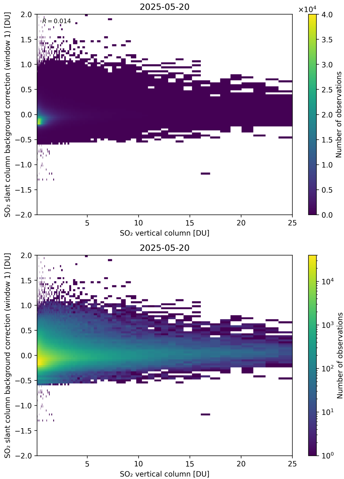
Figure 323: Scatter density plot of “SO 2 vertical column” against “SO 2 slant column background correction (window 1)” for 2025-05-19 to 2025-05-21.
