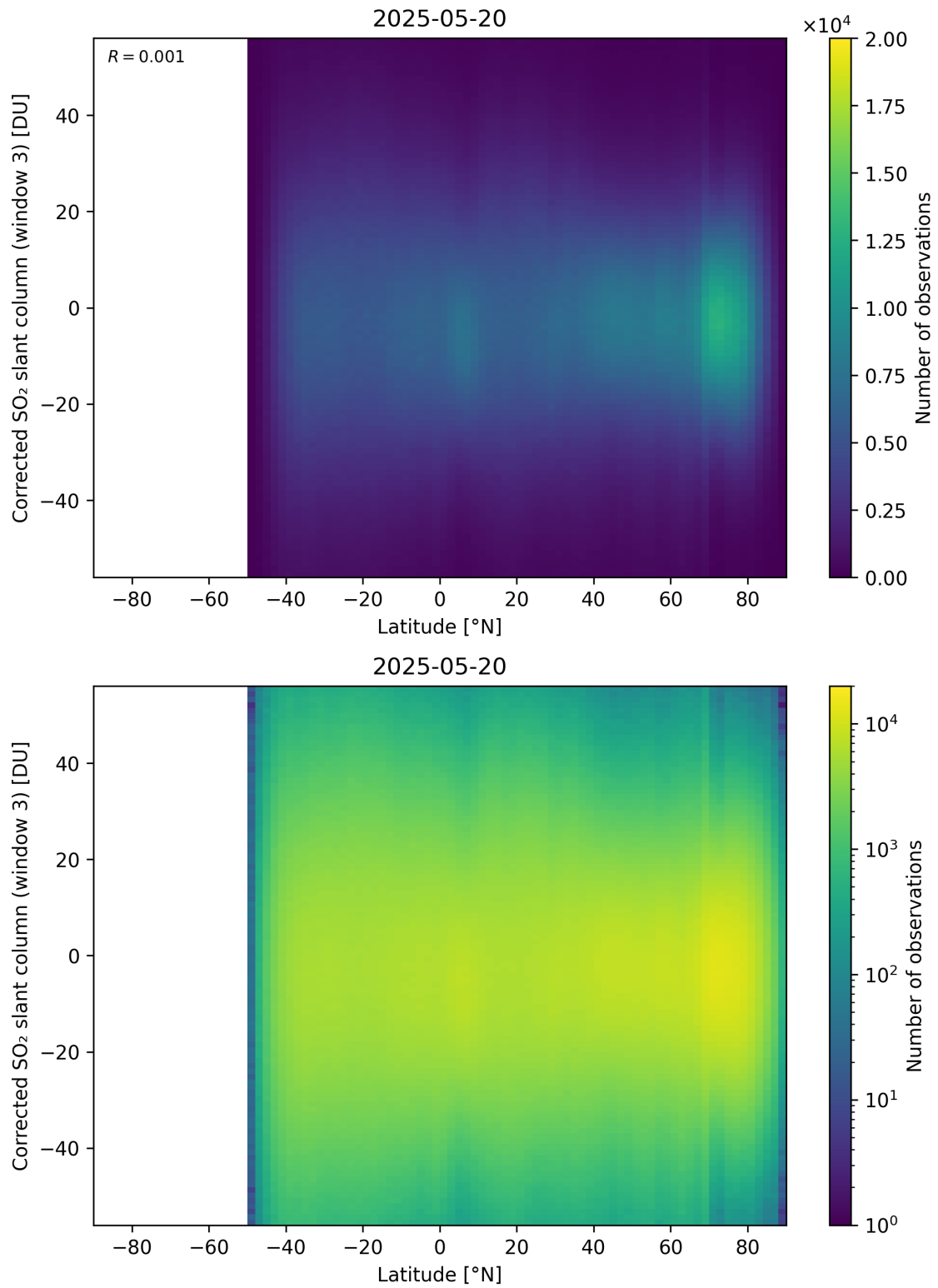
Figure 161: Scatter density plot of “Latitude” against “Corrected SO 2 slant column (window 3)” for 2025-05-19 to 2025-05-21.
