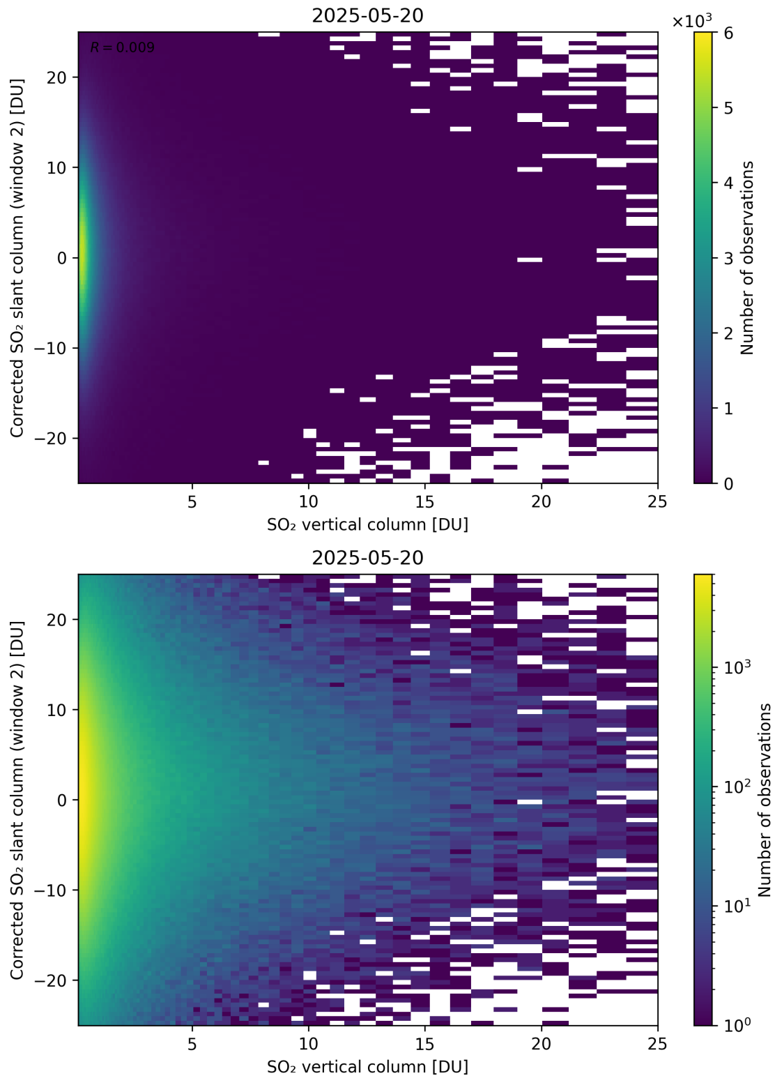
Figure 352: Scatter density plot of “SO 2 vertical column” against “Corrected SO 2 slant column (window 2)” for 2025-05-19 to 2025-05-21.
