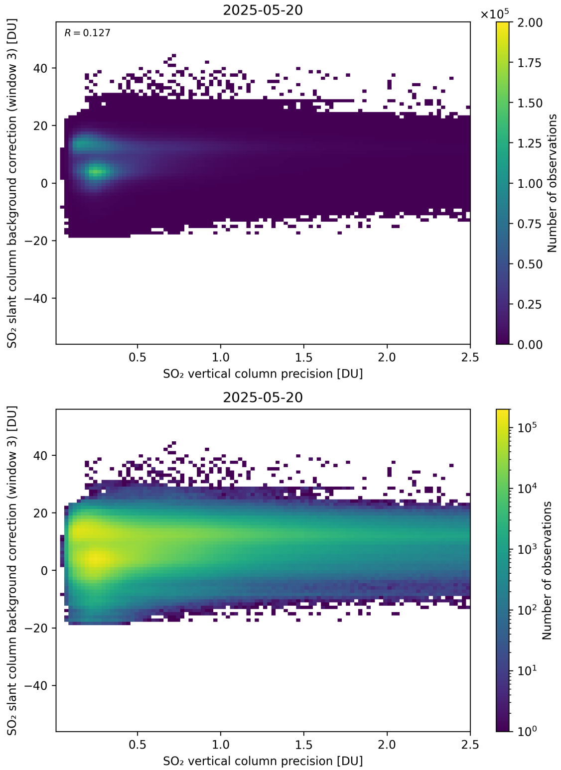
Figure 331: Scatter density plot of “SO 2 vertical column precision” against “SO 2 slant column background correction (window 3)” for 2025-05-19 to 2025-05-21.
