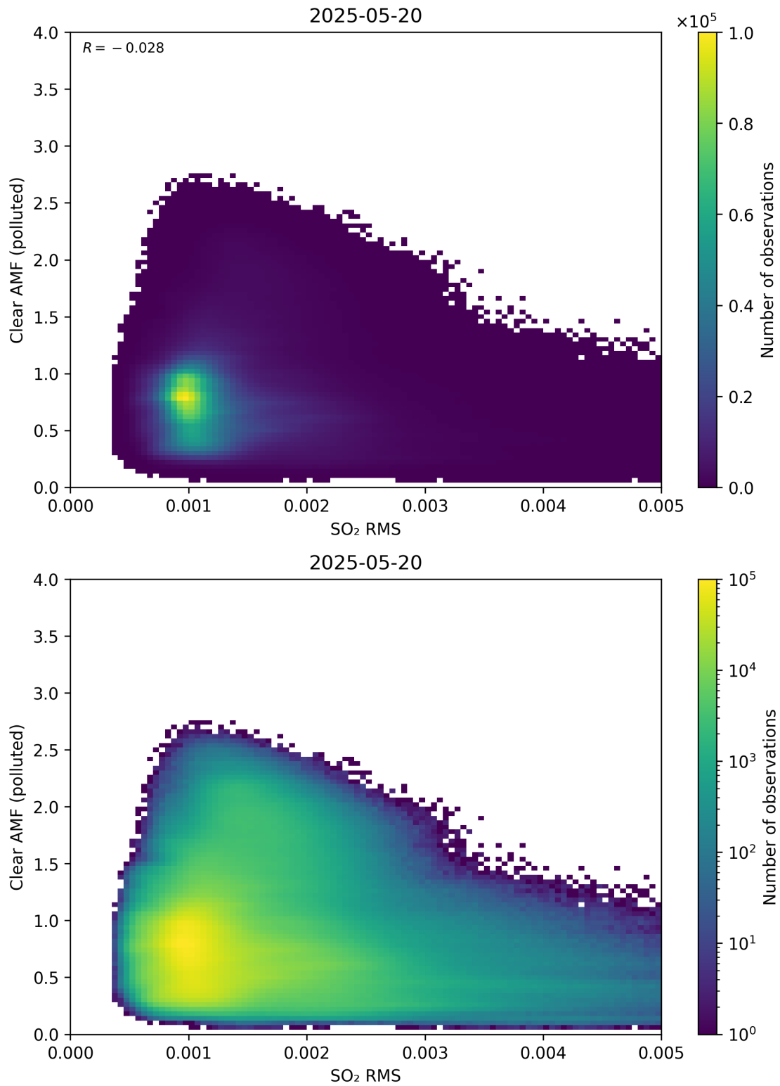
Figure 147: Scatter density plot of “SO 2 RMS” against “Clear AMF (polluted)” for 2025-05-19 to 2025-05-21.
