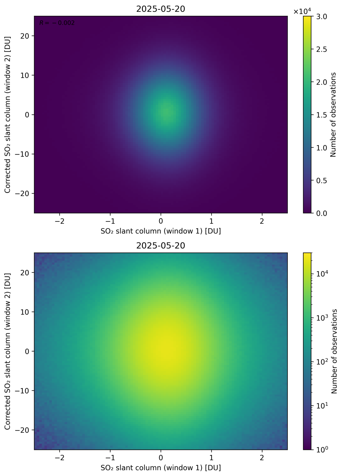
Figure 283: Scatter density plot of “SO 2 slant column (window 1)” against “Corrected SO 2 slant column (window 2)” for 2025-05-19 to 2025-05-21.
