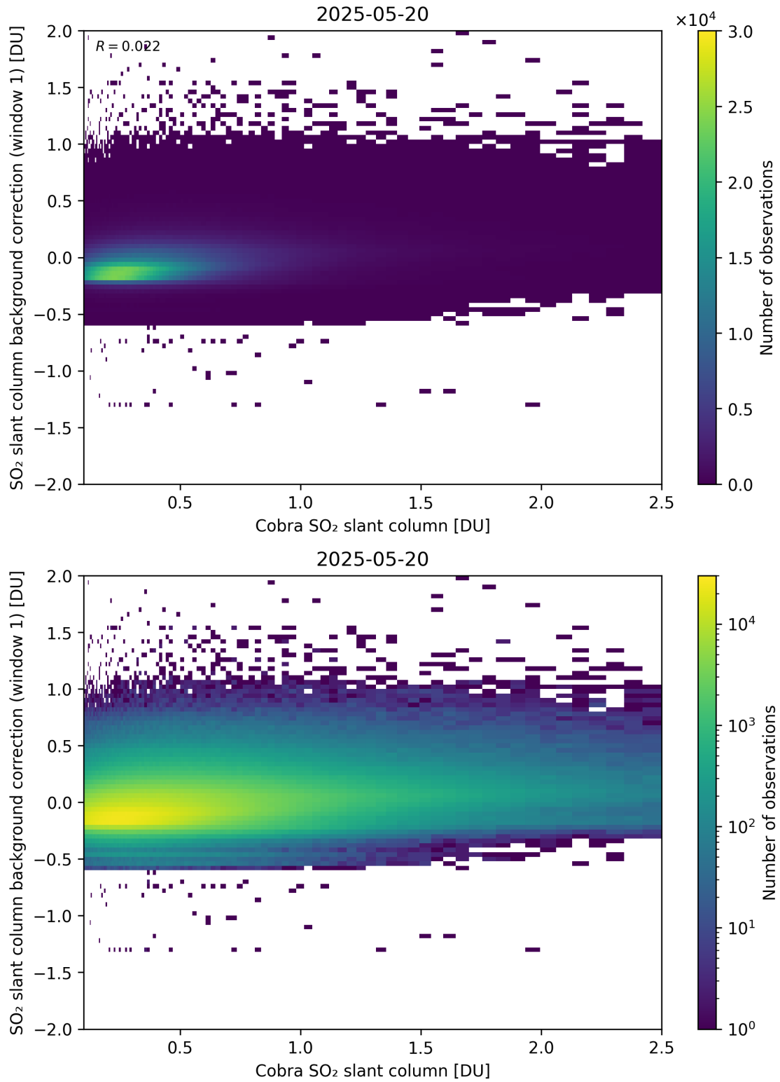
Figure 193: Scatter density plot of “Cobra SO 2 slant column” against “SO 2 slant column background correction (window 1)” for 2025-05-19 to 2025-05-21.
