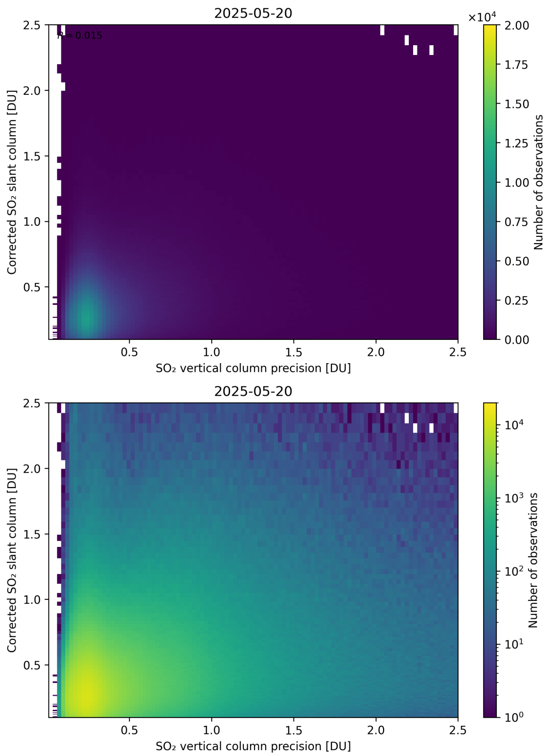
Figure 338: Scatter density plot of “SO 2 vertical column precision” against “Corrected SO 2 slant column” for 2025-05-19 to 2025-05-21.
