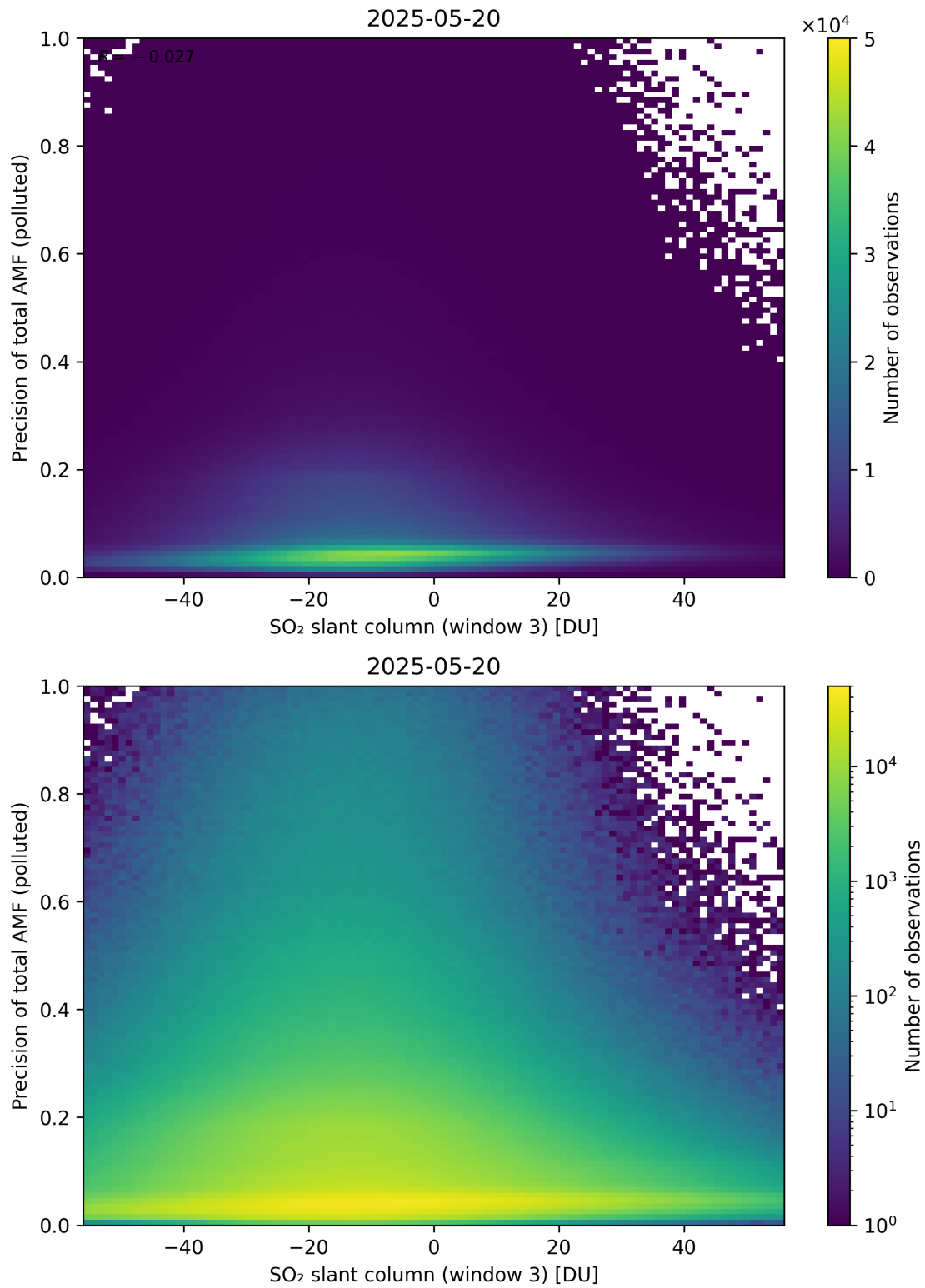
Figure 319: Scatter density plot of “SO 2 slant column (window 3)” against “Precision of total AMF (polluted)” for 2025-05-19 to 2025-05-21.
