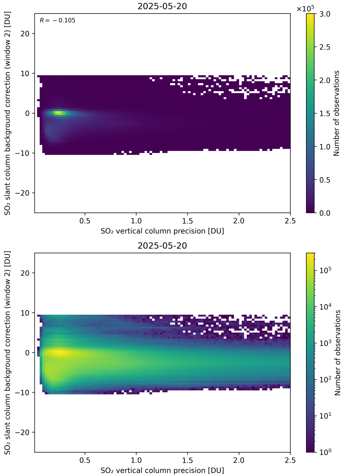
Figure 330: Scatter density plot of “SO 2 vertical column precision” against “SO 2 slant column background correction (window 2)” for 2025-05-19 to 2025-05-21.
