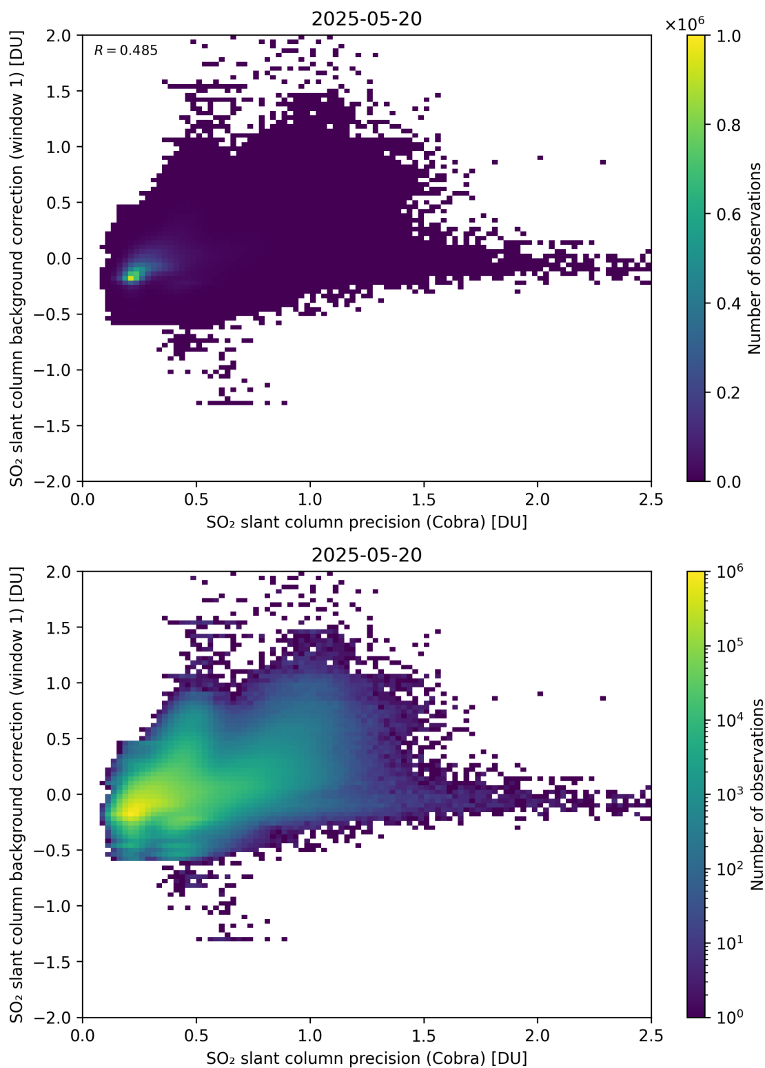
Figure 199: Scatter density plot of “SO 2 slant column precision (Cobra)” against “SO 2 slant column background correction (window 1)” for 2025-05-19 to 2025-05-21.
