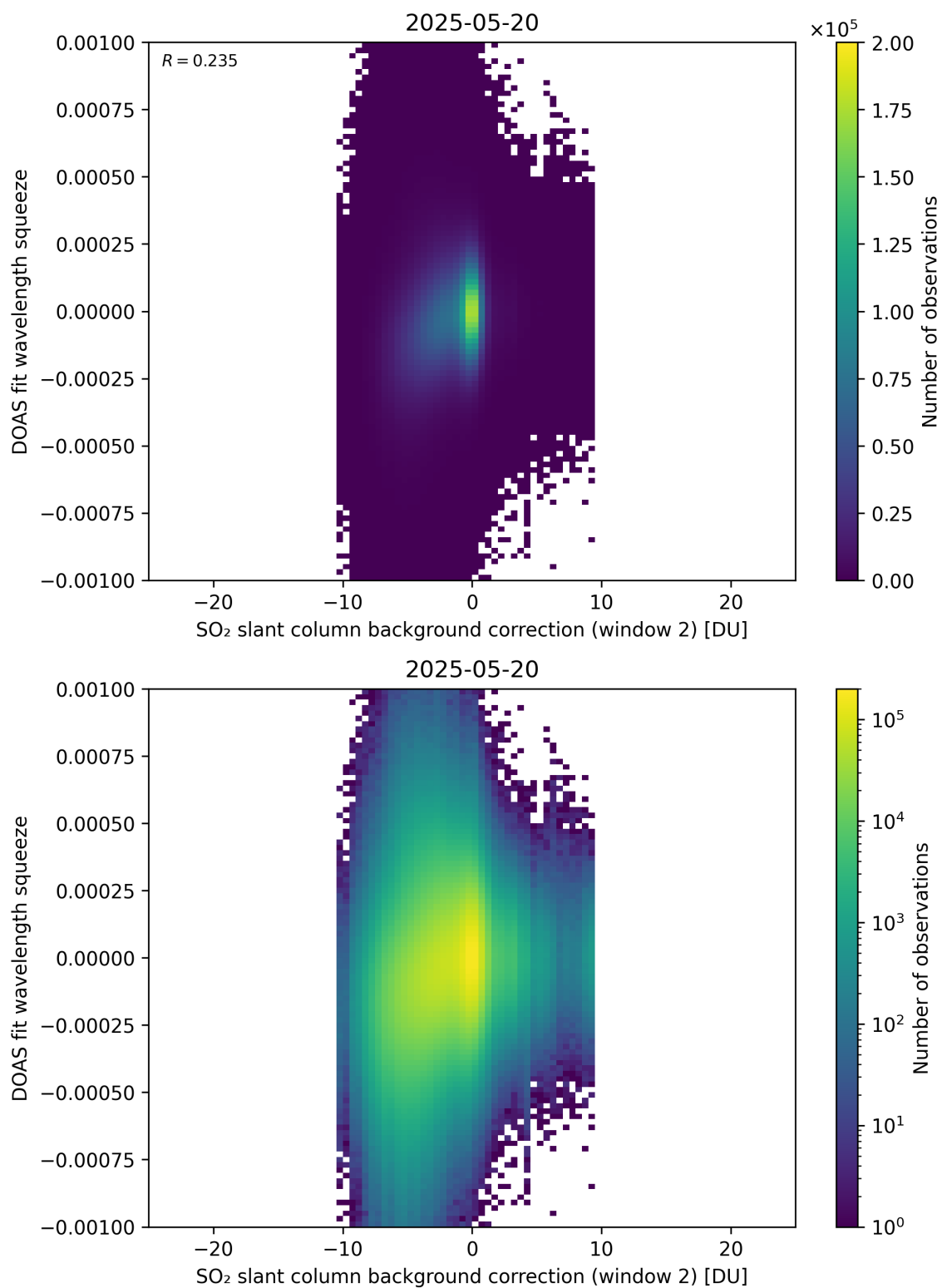
Figure 124: Scatter density plot of “SO 2 slant column background correction (window 2)” against “DOAS fit wavelength squeeze” for 2025-05-19 to 2025-05-21.
