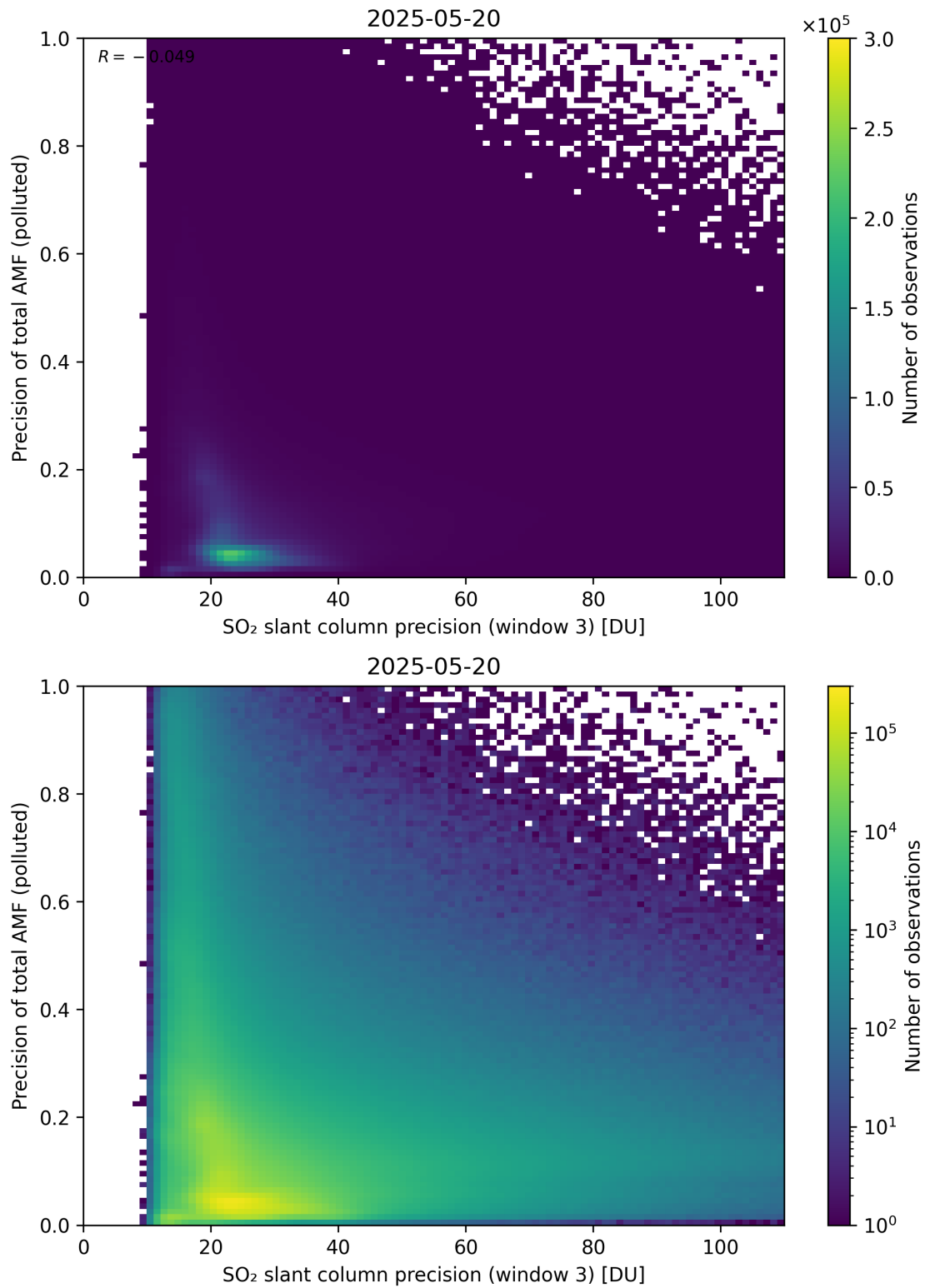
Figure 314: Scatter density plot of “SO 2 slant column precision (window 3)” against “Precision of total AMF (polluted)” for 2025-05-19 to 2025-05-21.
