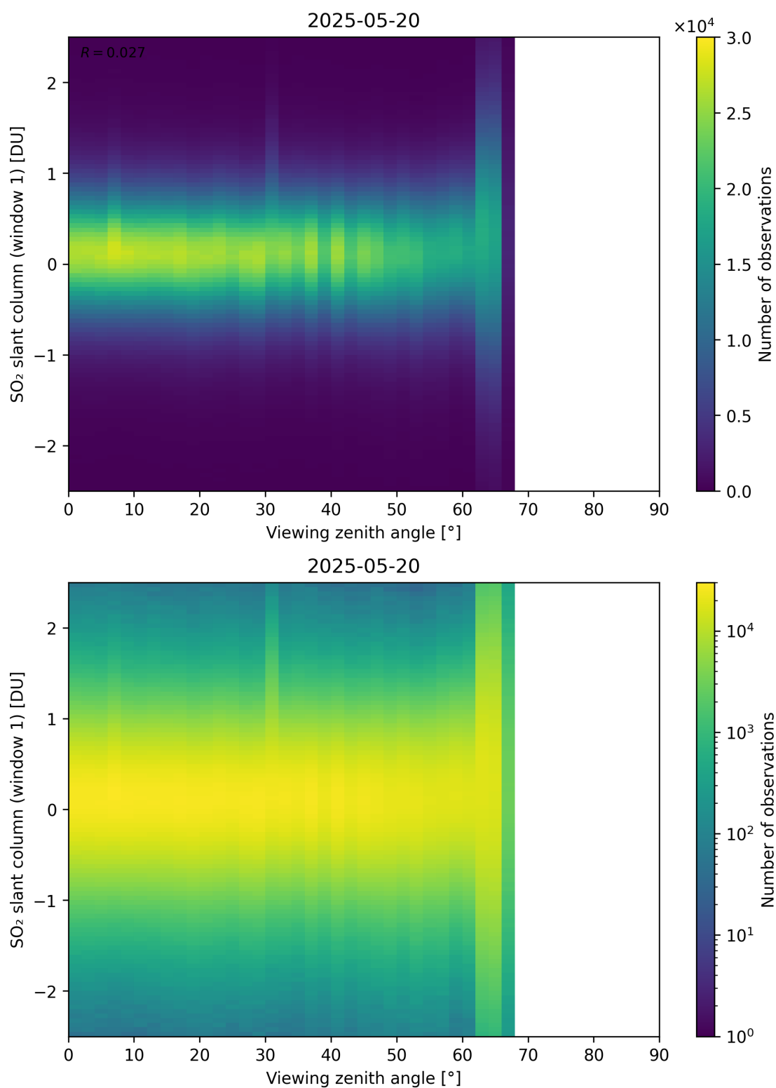
Figure 376: Scatter density plot of “Viewing zenith angle” against “SO 2 slant column (window 1)” for 2025-05-19 to 2025-05-21.
