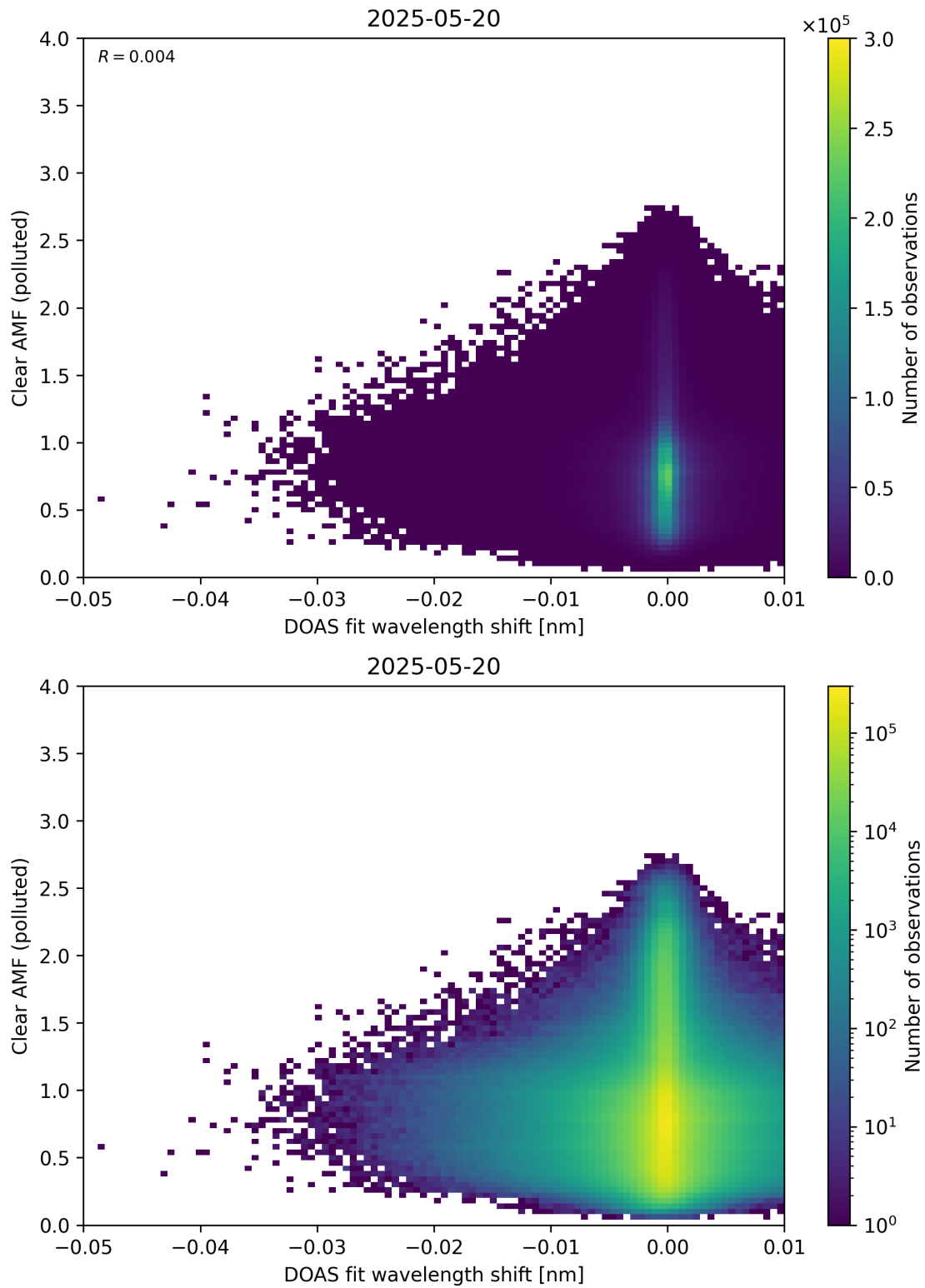
Figure 140: Scatter density plot of “DOAS fit wavelength shift” against “Clear AMF (polluted)” for 2025-05-19 to 2025-05-21.
