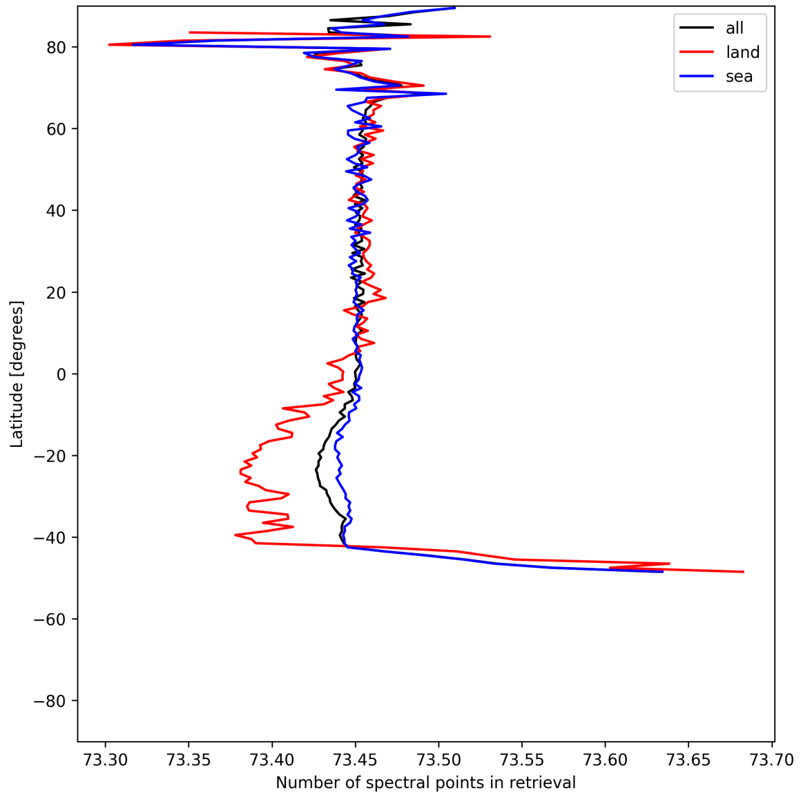
Figure 56: Zonal average of “Number of spectral points in retrieval” for 2025-05-19 to 2025-05-21.
