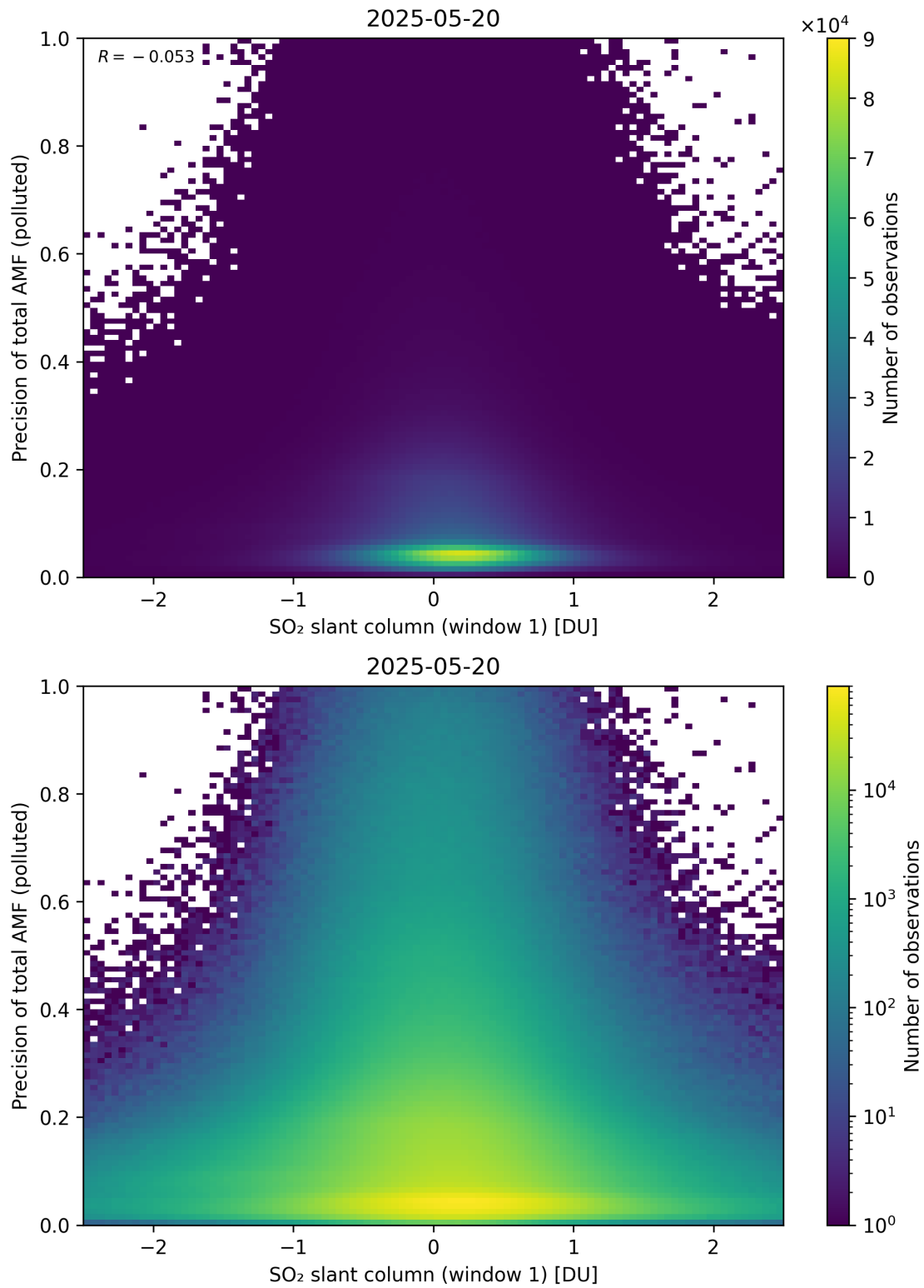
Figure 290: Scatter density plot of “SO 2 slant column (window 1)” against “Precision of total AMF (polluted)” for 2025-05-19 to 2025-05-21.
