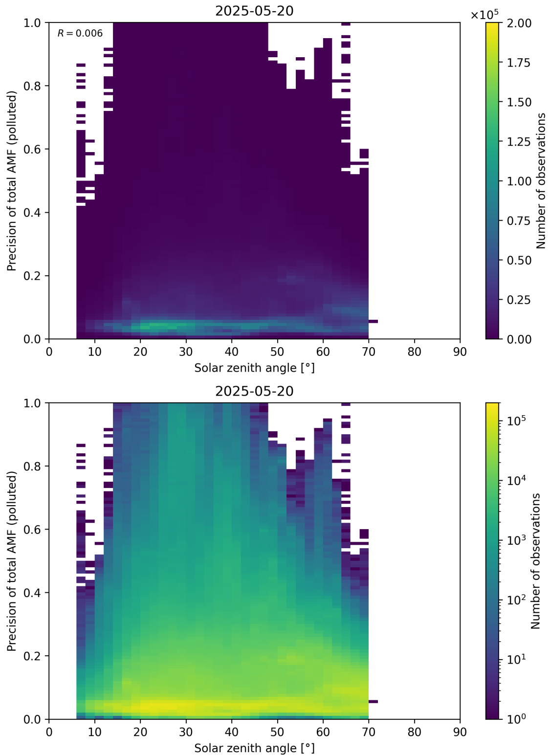
Figure 190: Scatter density plot of “Solar zenith angle” against “Precision of total AMF (polluted)” for 2025-05-19 to 2025-05-21.
