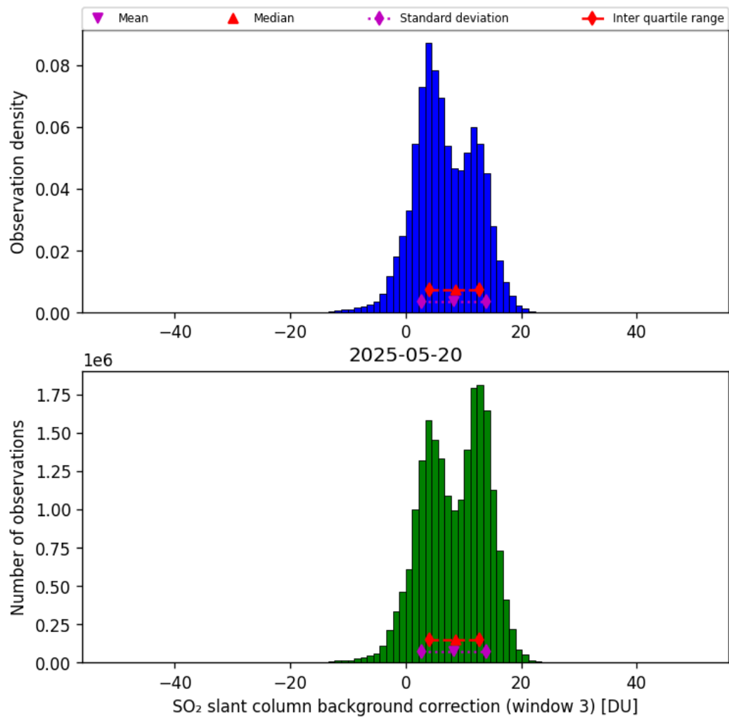
Figure 74: Histogram of “SO 2 slant column background correction (window 3)” for 2025-05-19 to 2025-05-21
