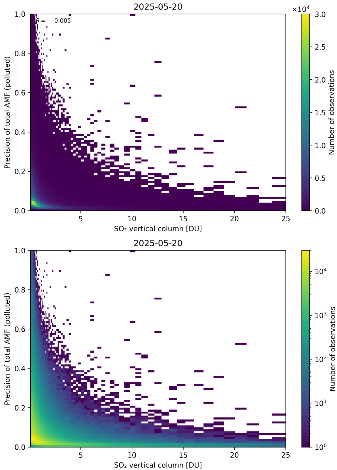
Figure 360: Scatter density plot of “SO 2 vertical column” against “Precision of total AMF (polluted)” for 2025-05-19 to 2025-05-21.
