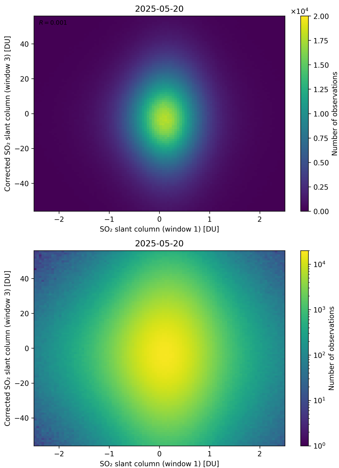
Figure 284: Scatter density plot of “SO 2 slant column (window 1)” against “Corrected SO 2 slant column (window 3)” for 2025-05-19 to 2025-05-21.
