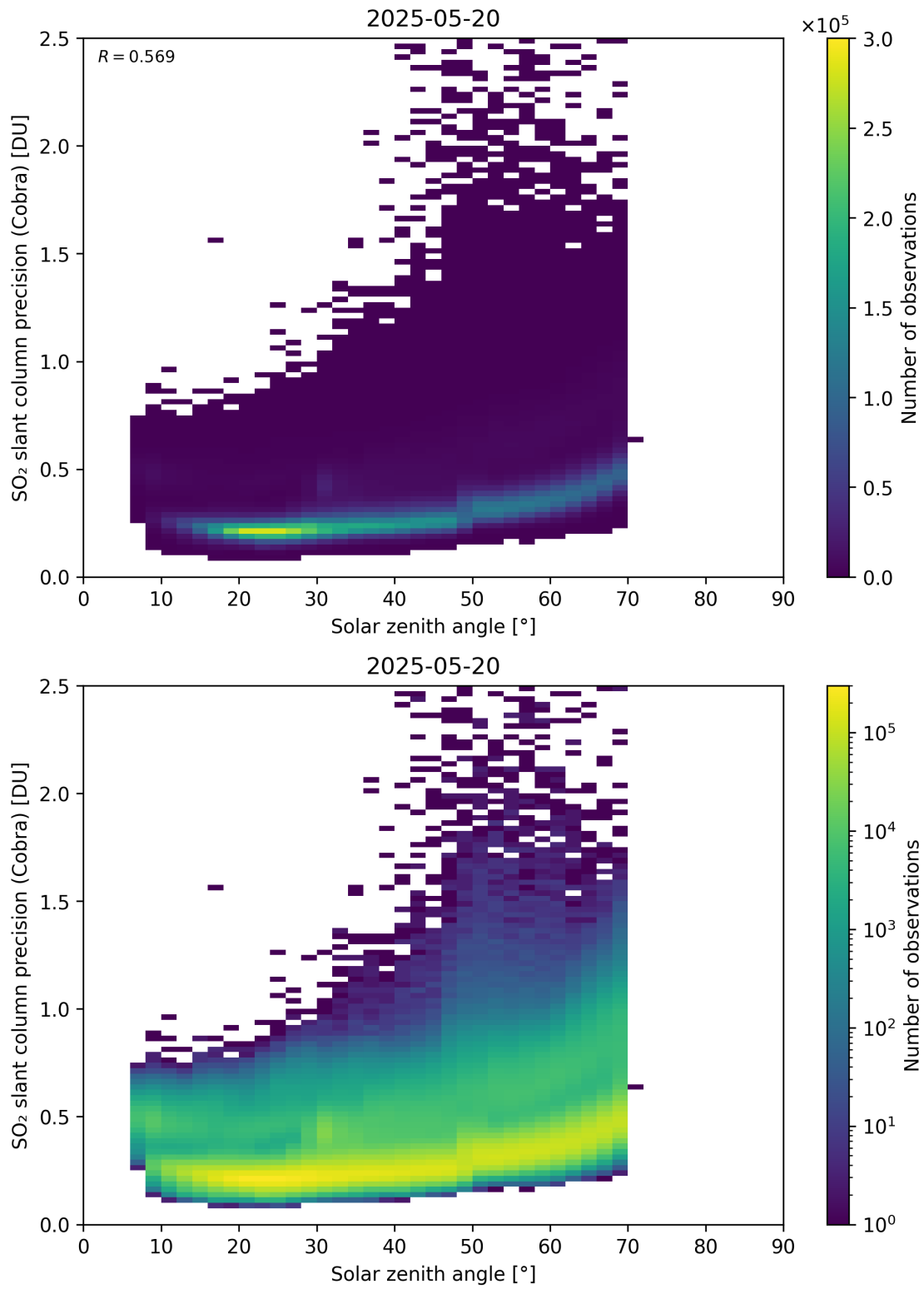
Figure 180: Scatter density plot of “Solar zenith angle” against “SO 2 slant column precision (Cobra)” for 2025-05-19 to 2025-05-21.
