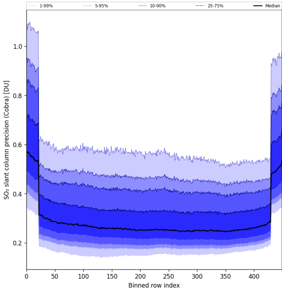
Figure 88: Along track statistics of “SO 2 slant column precision (Cobra)” for 2025-05-19 to 2025-05-21
