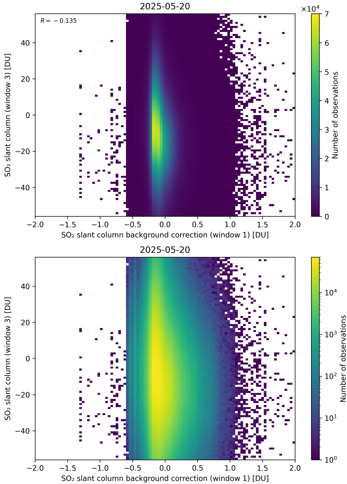
Figure 118: Scatter density plot of “SO 2 slant column background correction (window 1)” against “SO 2 slant column (window 3)” for 2025-05-19 to 2025-05-21.
