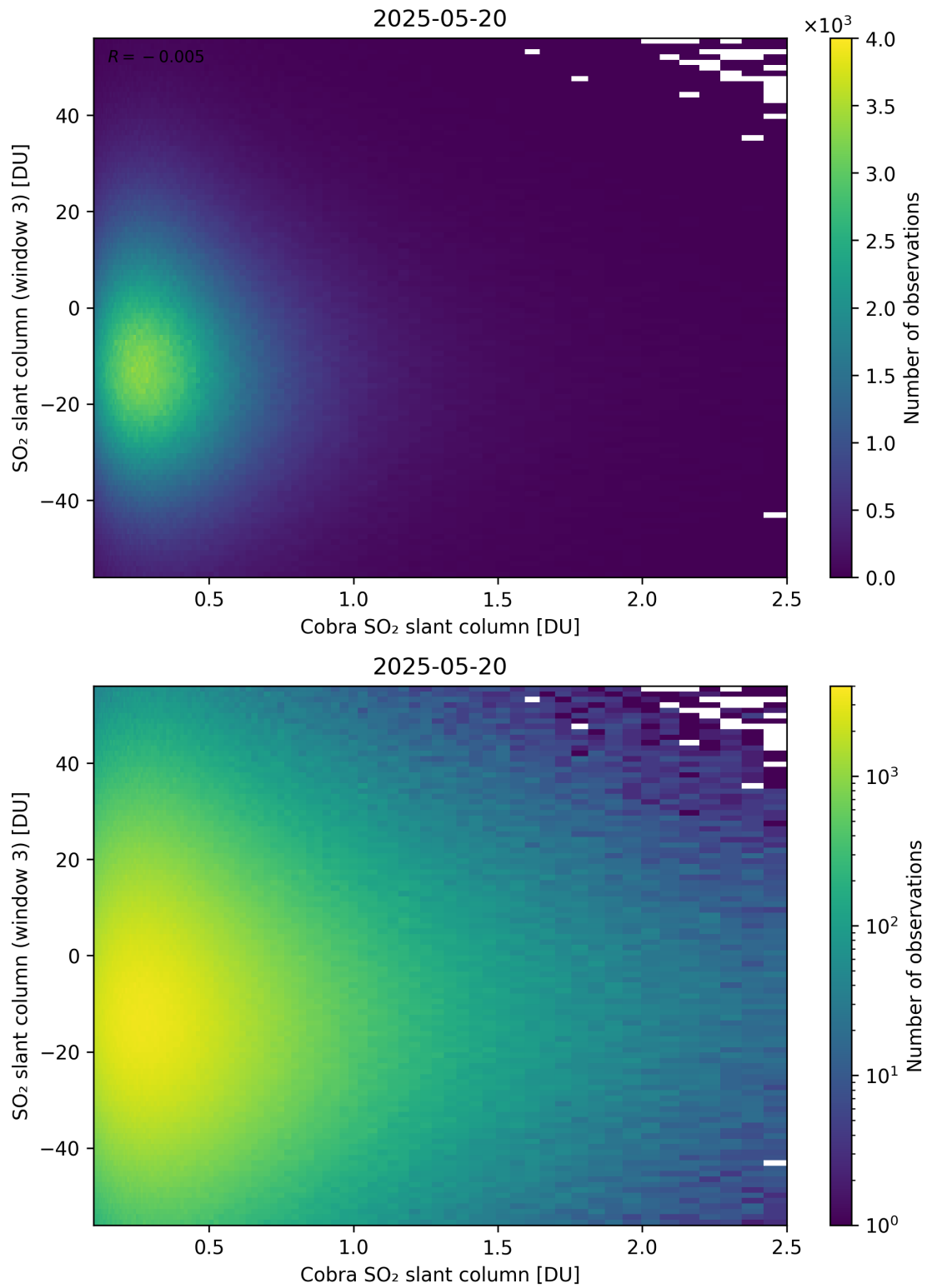
Figure 222: Scatter density plot of “Cobra SO 2 slant column” against “SO 2 slant column (window 3)” for 2025-05-19 to 2025-05-21.
