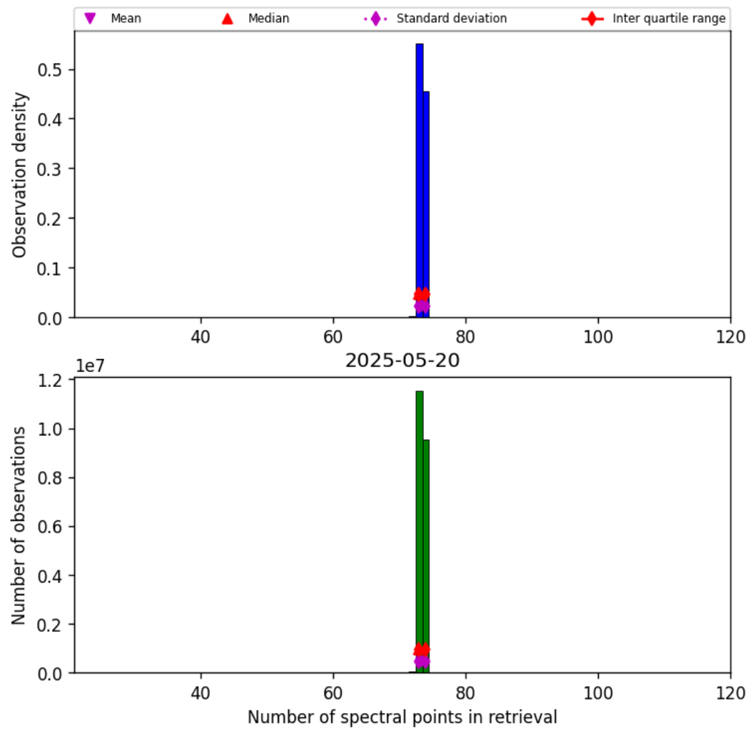
Figure 82: Histogram of “Number of spectral points in retrieval” for 2025-05-19 to 2025-05-21
