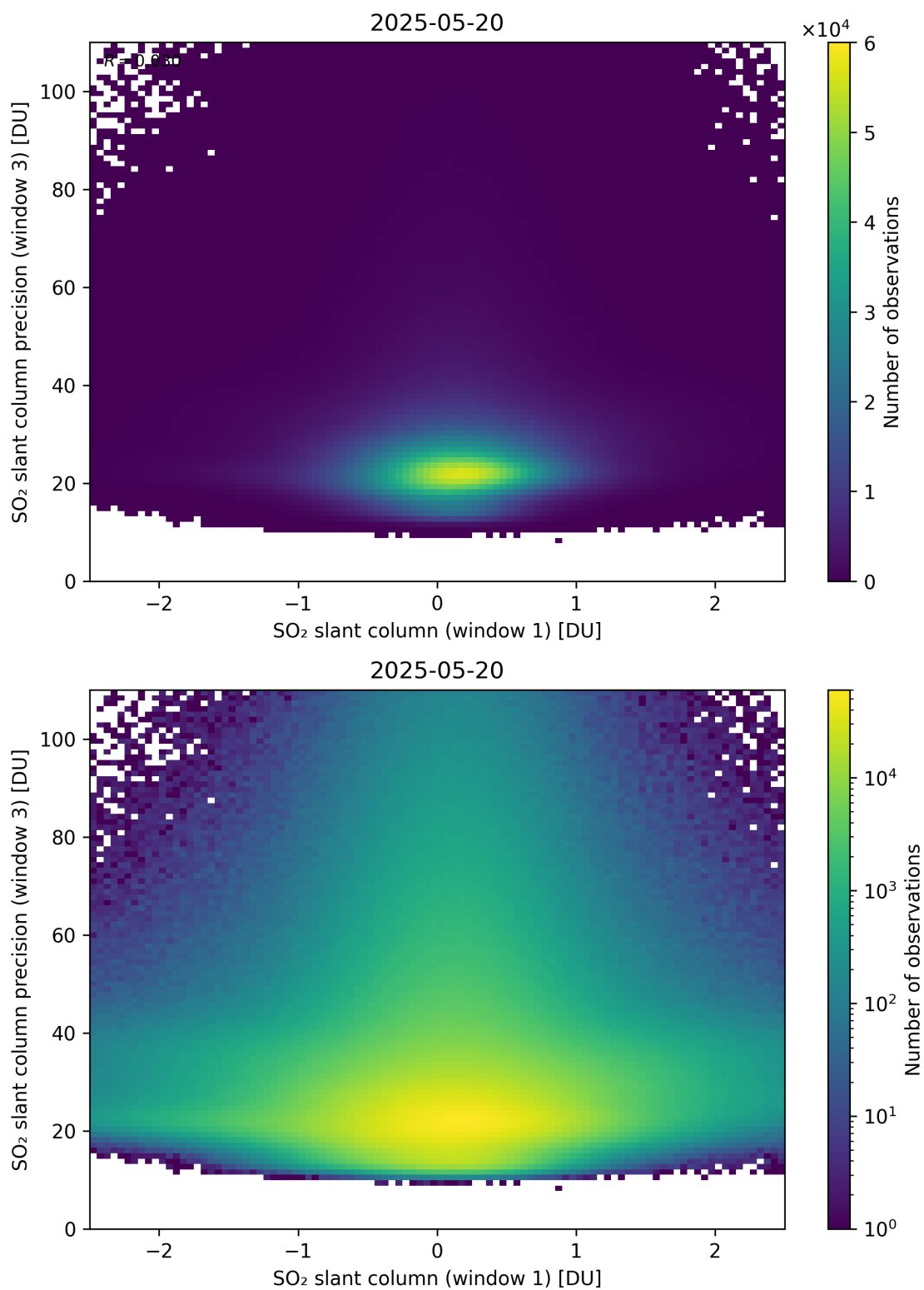
Figure 288: Scatter density plot of “SO 2 slant column (window 1)” against “SO 2 slant column precision (window 3)” for 2025-05-19 to 2025-05-21.
