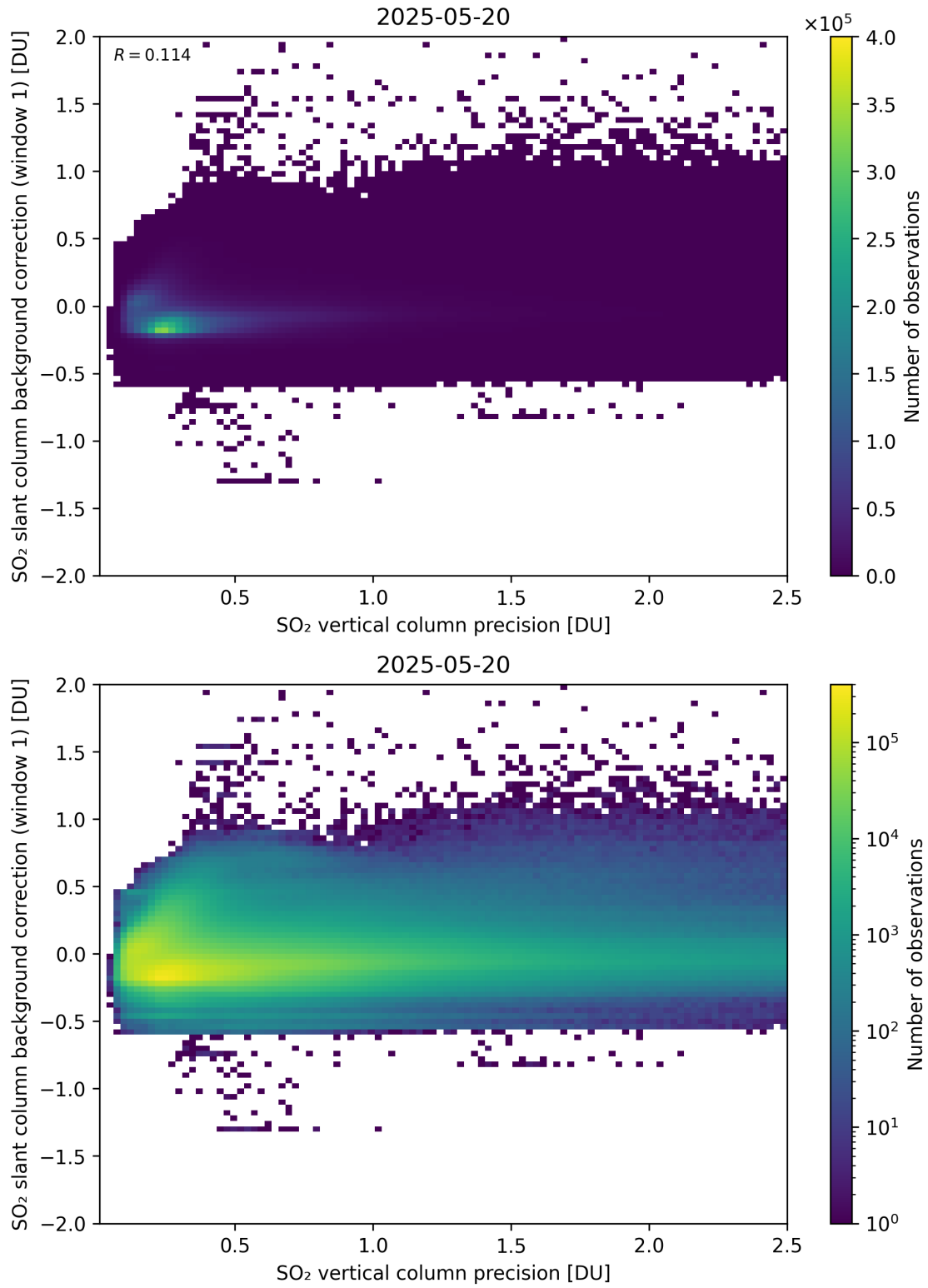
Figure 329: Scatter density plot of “SO 2 vertical column precision” against “SO 2 slant column background correction (window 1)” for 2025-05-19 to 2025-05-21.
