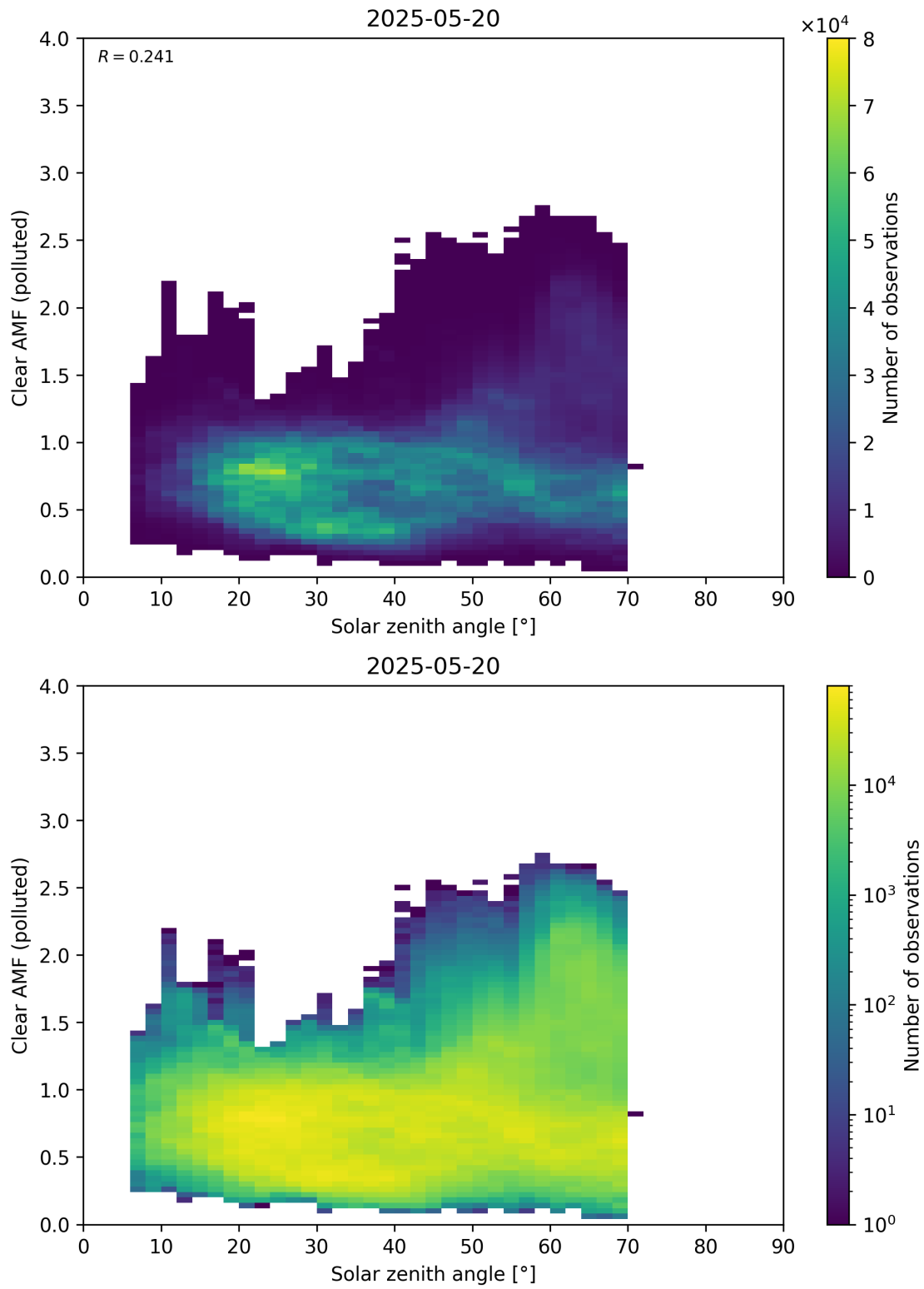
Figure 178: Scatter density plot of “Solar zenith angle” against “Clear AMF (polluted)” for 2025-05-19 to 2025-05-21.
