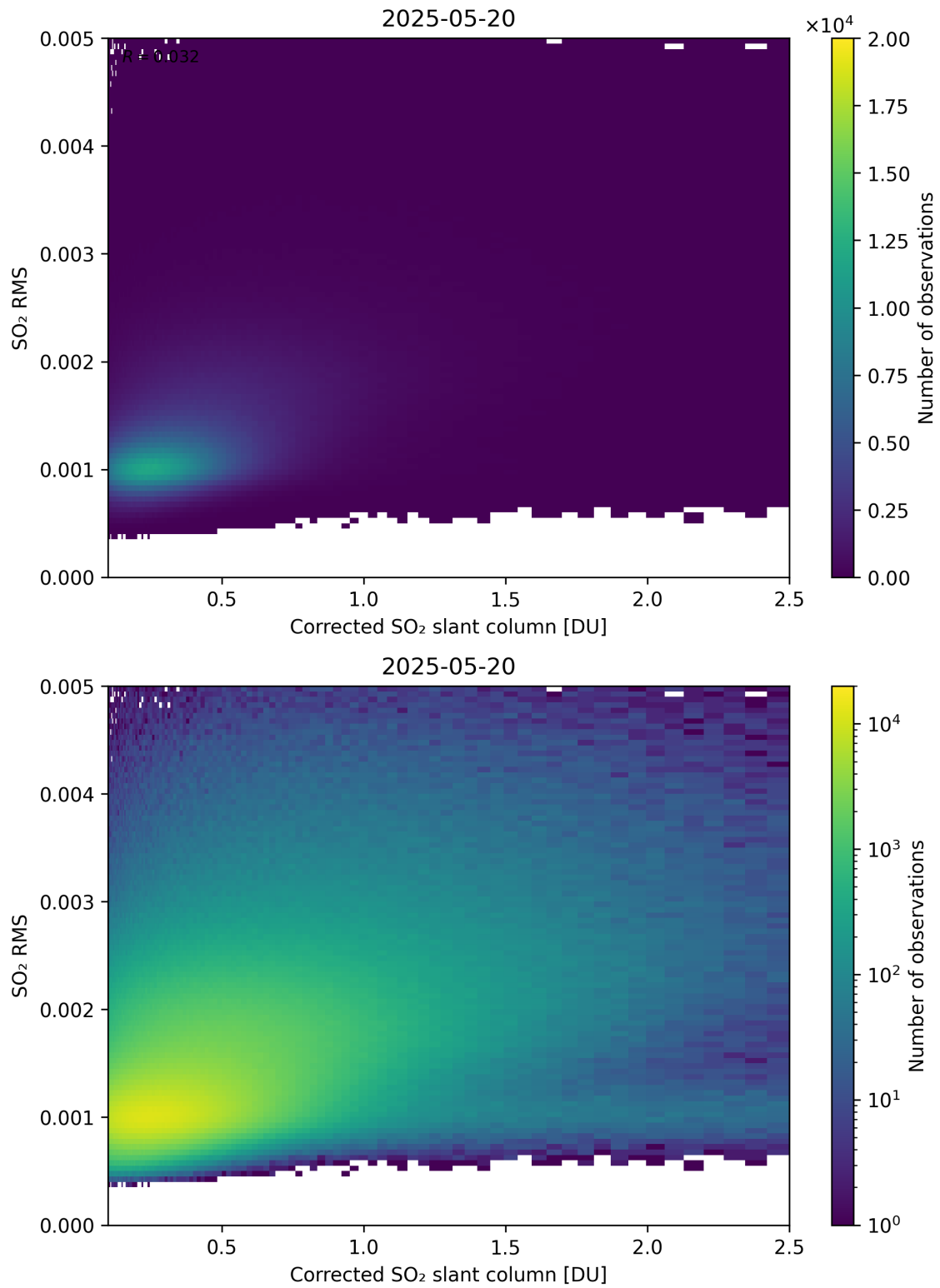
Figure 231: Scatter density plot of “Corrected SO 2 slant column” against “SO 2 RMS” for 2025-05-19 to 2025-05-21.
