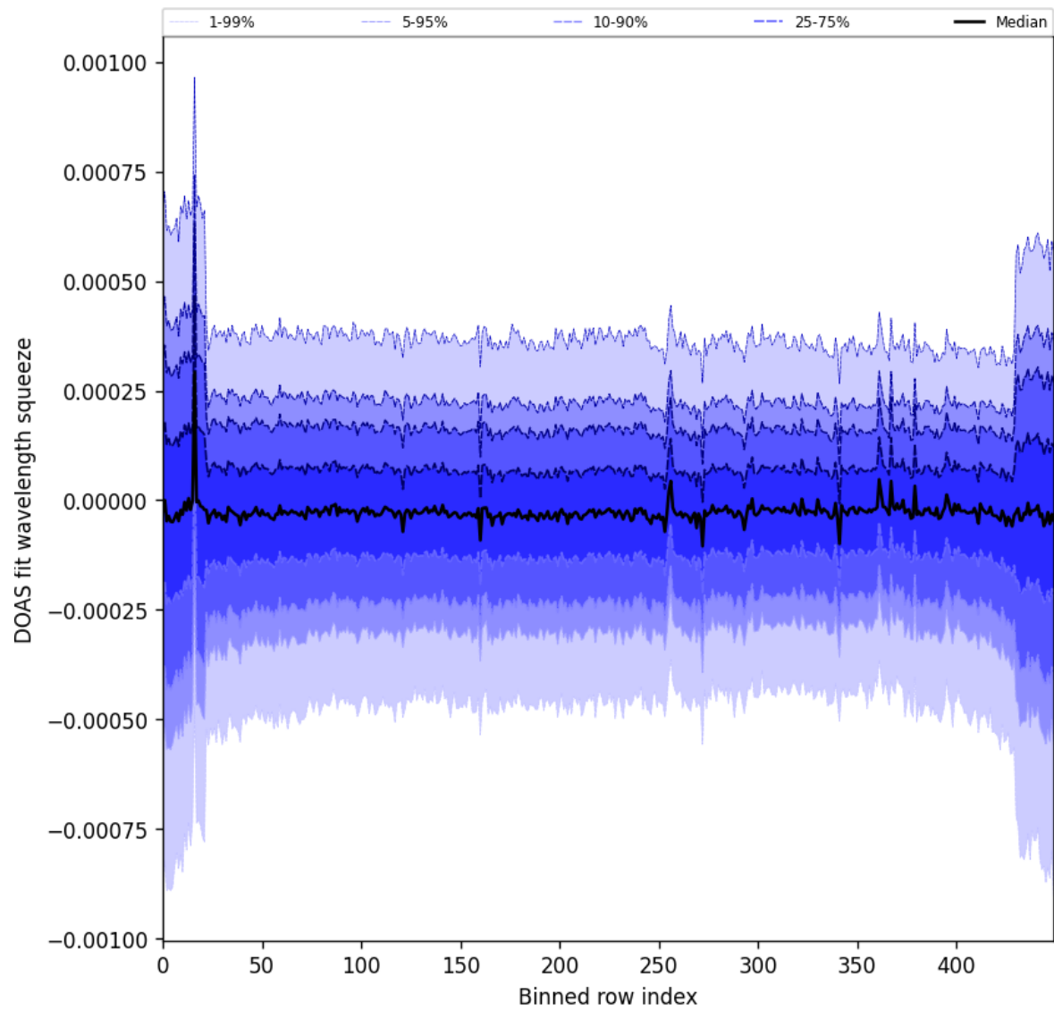
Figure 103: Along track statistics of “DOAS fit wavelength squeeze” for 2025-05-19 to 2025-05-21
