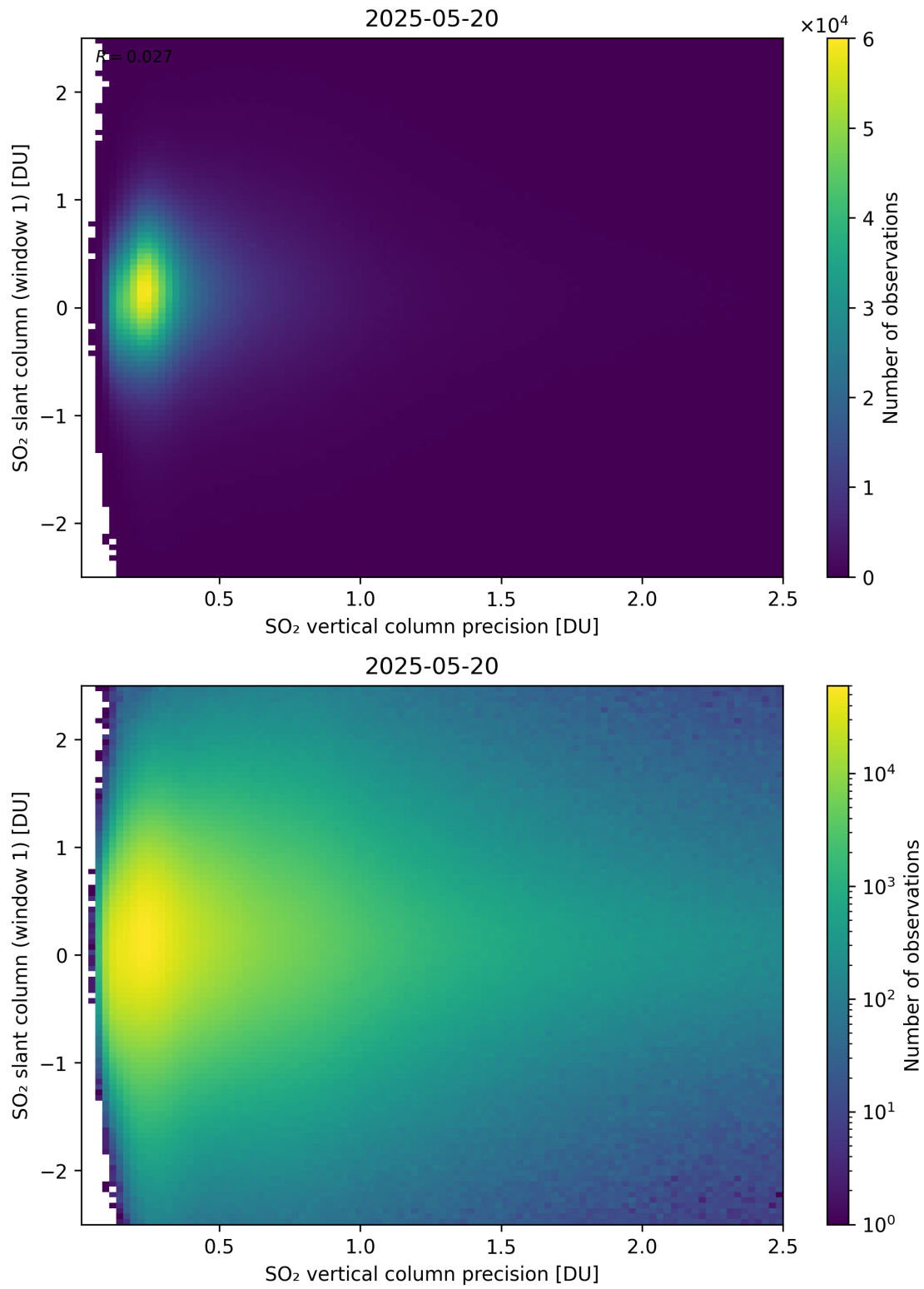
Figure 341: Scatter density plot of “SO 2 vertical column precision” against “SO 2 slant column (window 1)” for 2025-05-19 to 2025-05-21.
