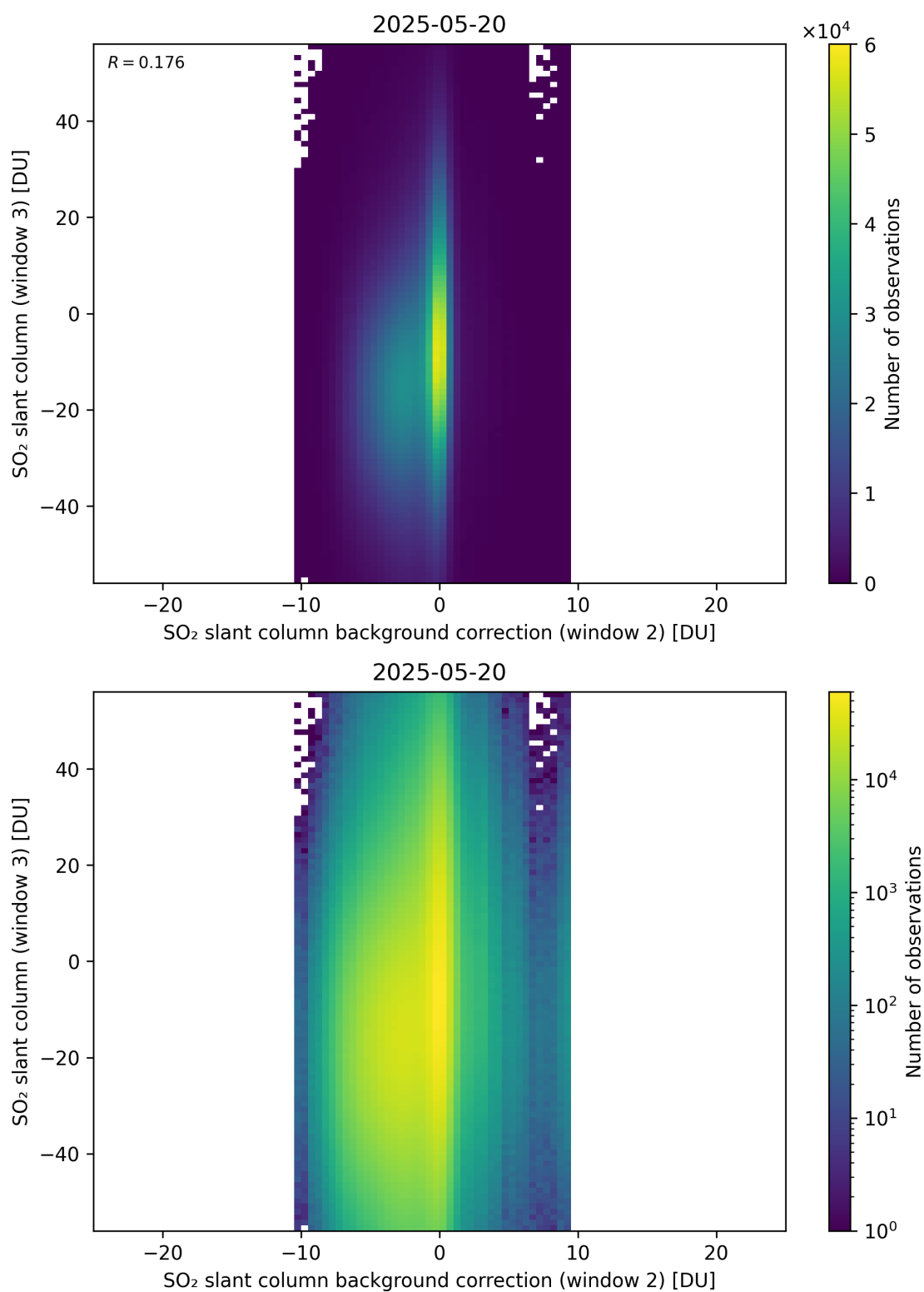
Figure 128: Scatter density plot of “SO 2 slant column background correction (window 2)” against “SO 2 slant column (window 3)” for 2025-05-19 to 2025-05-21.
