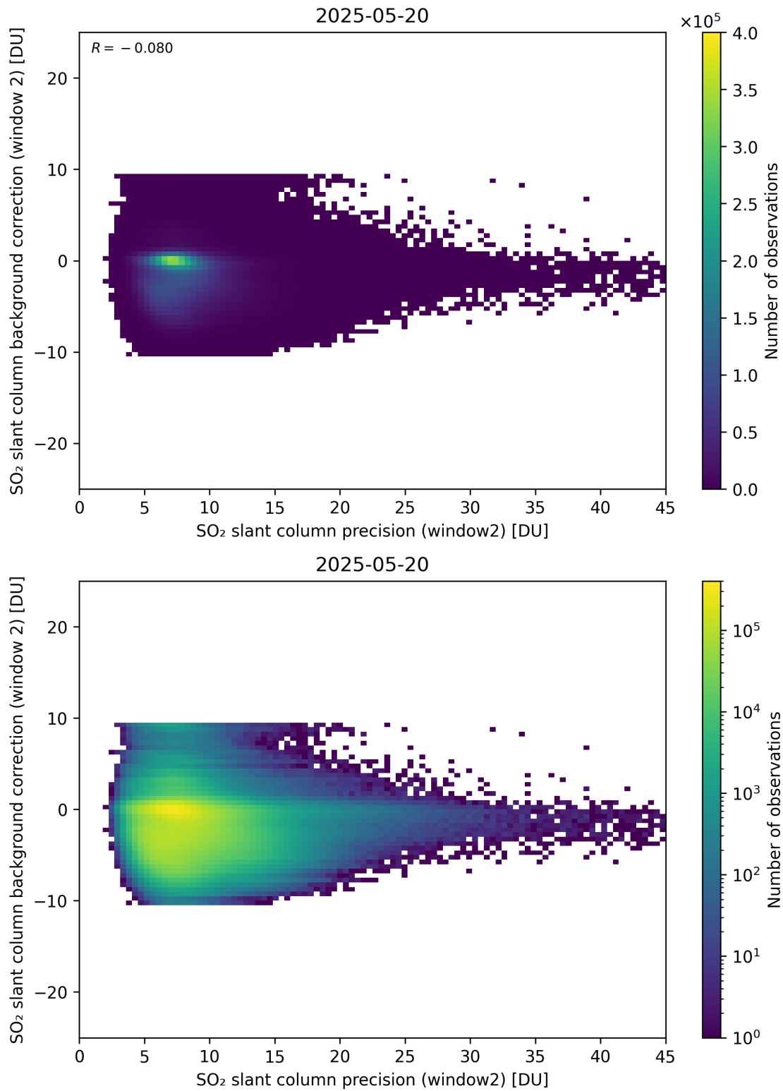
Figure 291: Scatter density plot of “SO 2 slant column precision (window2)” against “SO 2 slant column background correction (window 2)” for 2025-05-19 to 2025-05-21.
