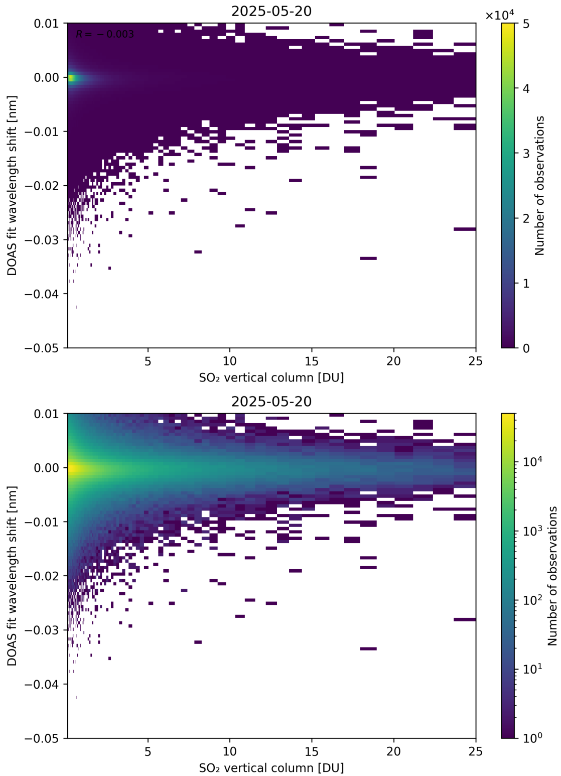
Figure 326: Scatter density plot of “SO 2 vertical column” against “DOAS fit wavelength shift” for 2025-05-19 to 2025-05-21.
