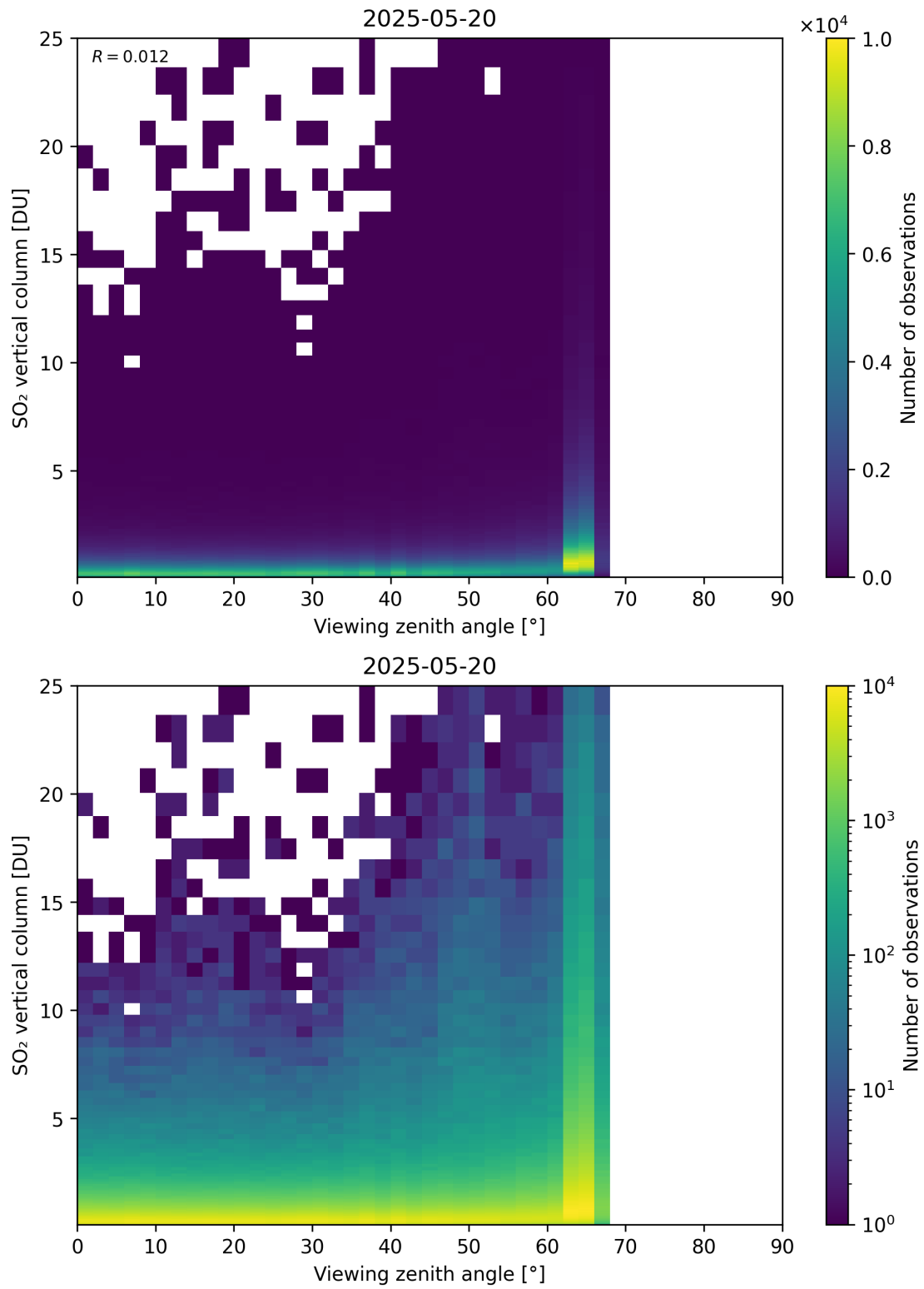
Figure 383: Scatter density plot of “Viewing zenith angle” against “SO 2 vertical column” for 2025-05-19 to 2025-05-21.
