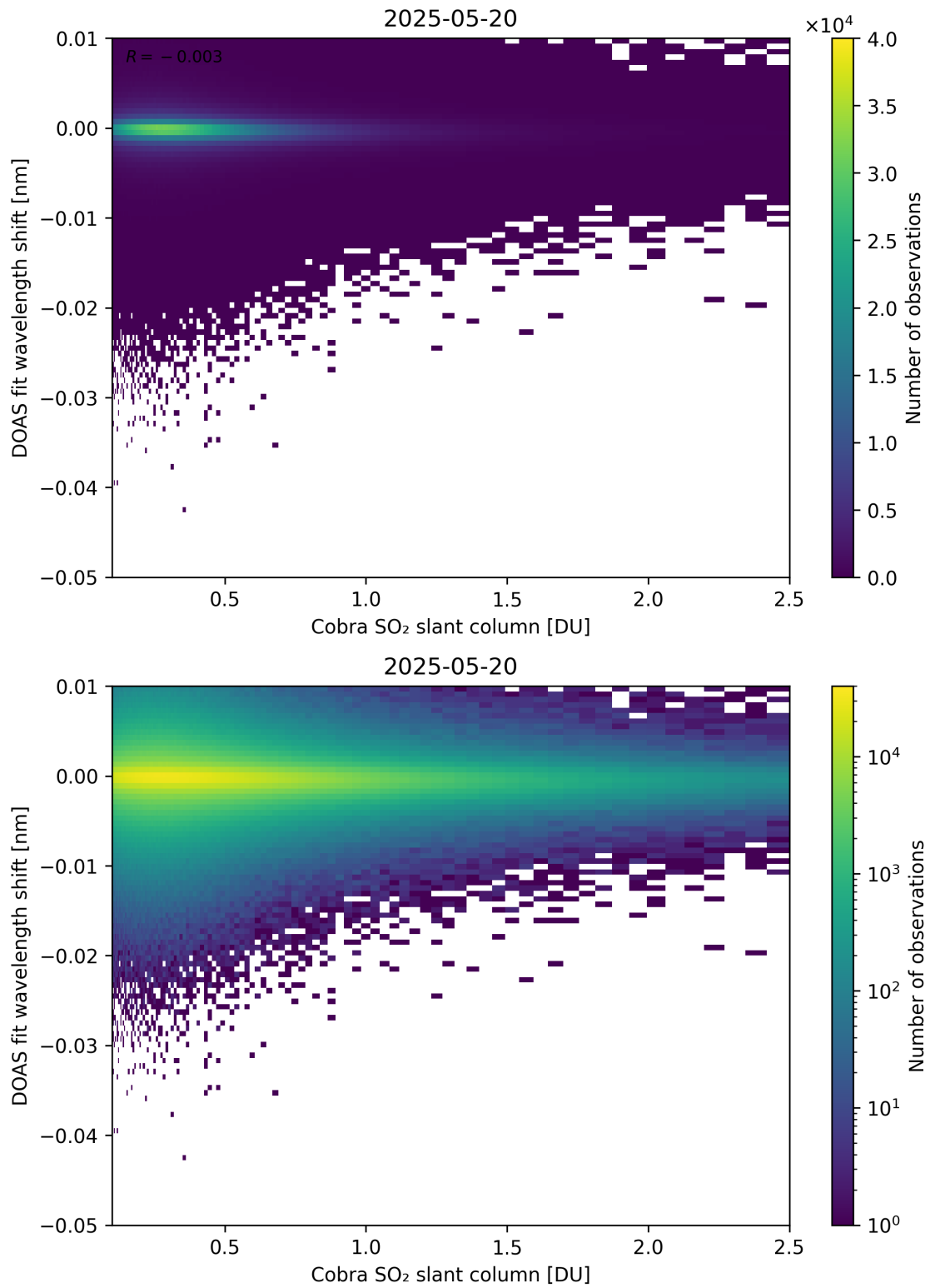
Figure 196: Scatter density plot of “Cobra SO 2 slant column” against “DOAS fit wavelength shift” for 2025-05-19 to 2025-05-21.
