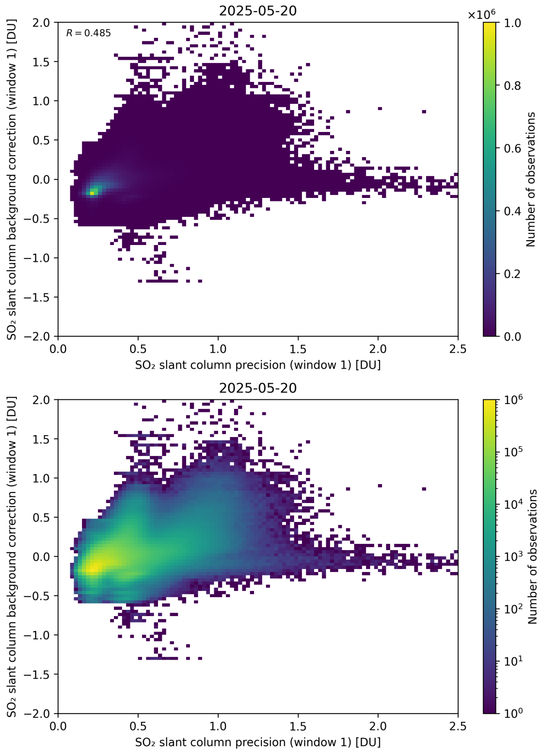
Figure 268: Scatter density plot of “SO 2 slant column precision (window 1)” against “SO 2 slant column background correction (window 1)” for 2025-05-19 to 2025-05-21.
