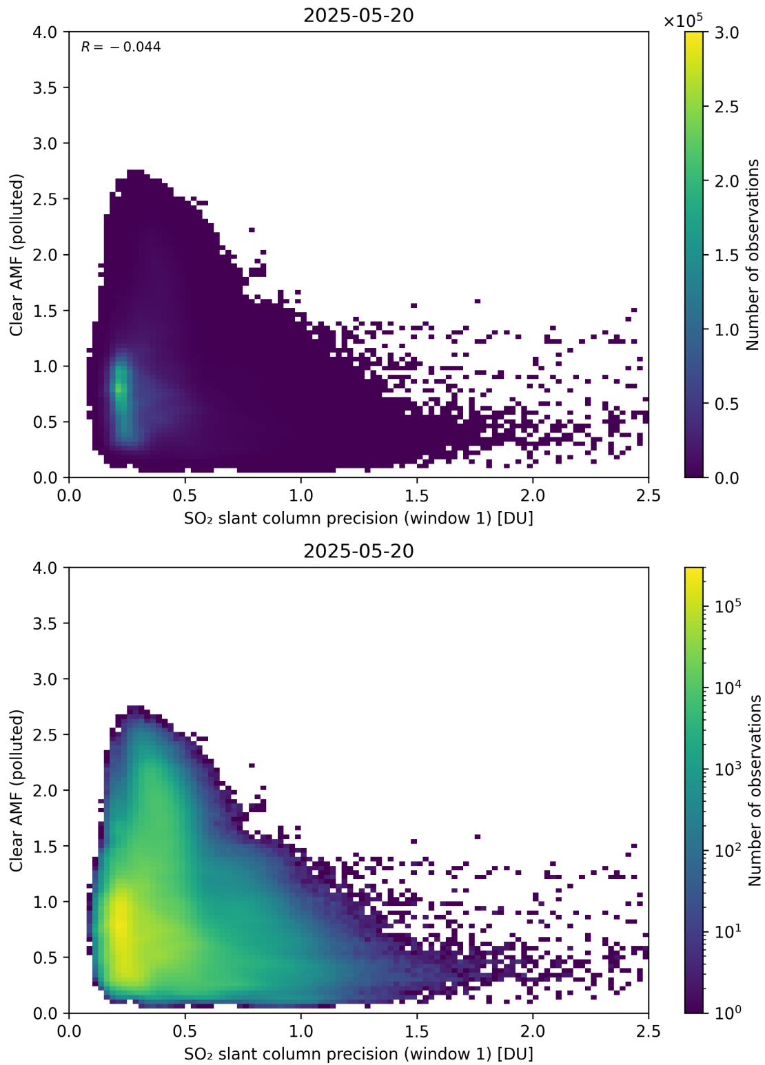
Figure 274: Scatter density plot of “SO 2 slant column precision (window 1)” against “Clear AMF (polluted)” for 2025-05-19 to 2025-05-21.
