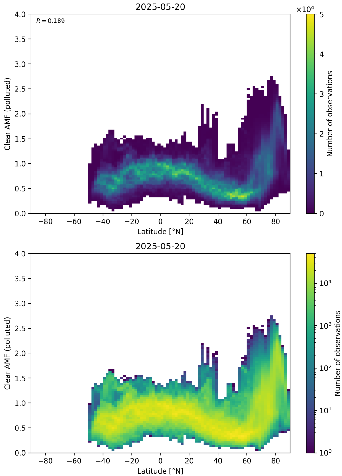
Figure 156: Scatter density plot of “Latitude” against “Clear AMF (polluted)” for 2025-05-19 to 2025-05-21.
