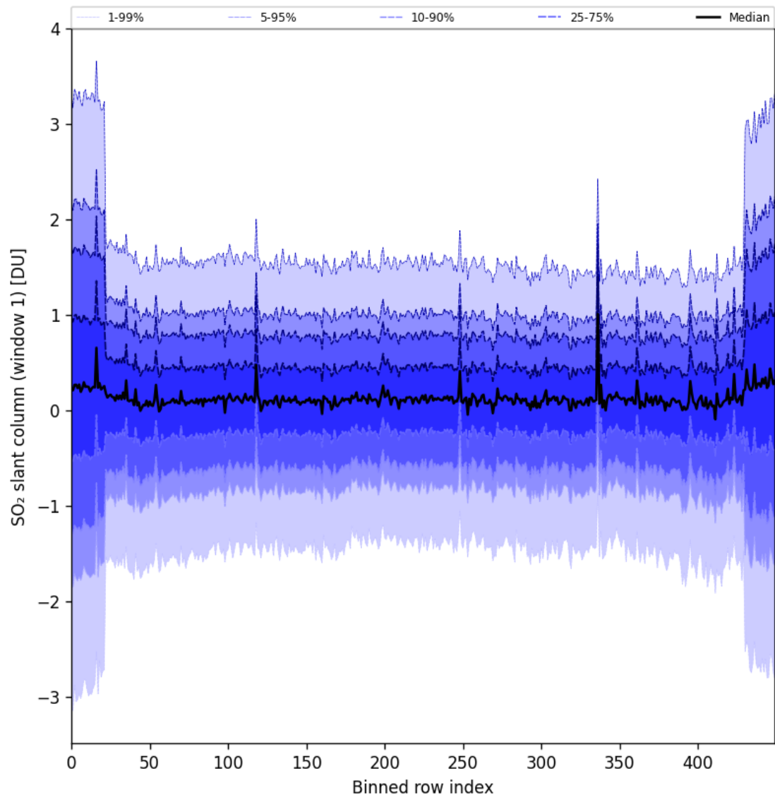
Figure 89: Along track statistics of “SO 2 slant column (window 1)” for 2025-05-19 to 2025-05-21
