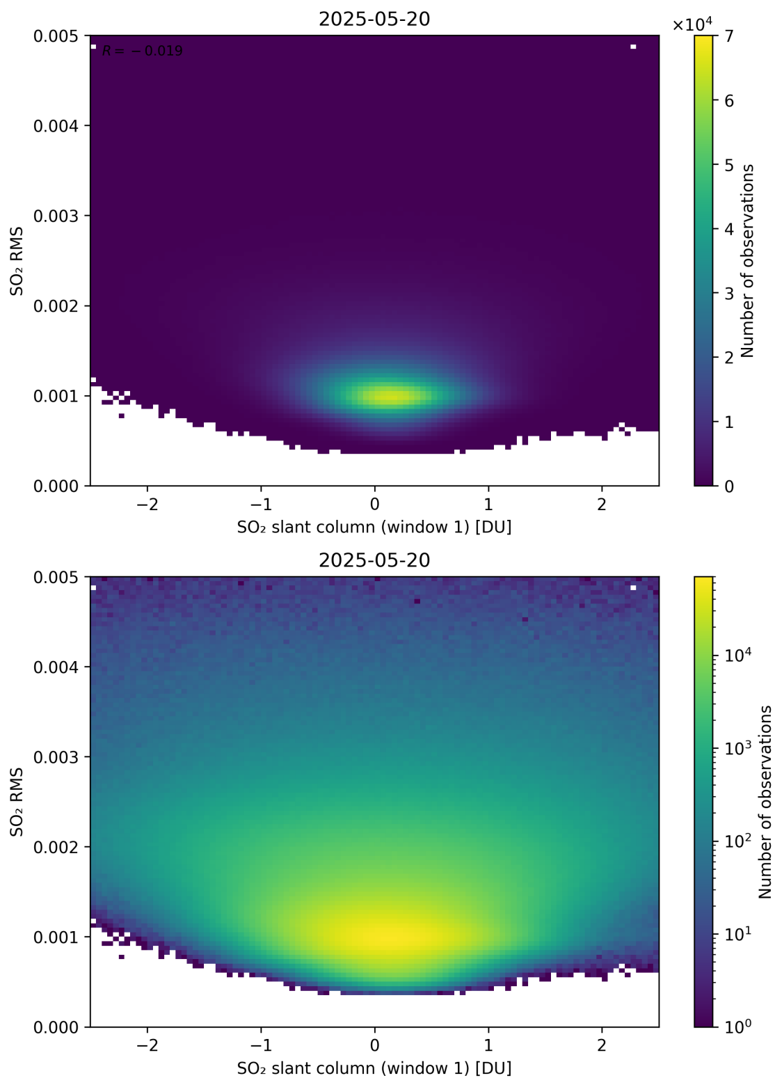
Figure 267: Scatter density plot of “SO 2 slant column (window 1)” against “SO 2 RMS” for 2025-05-19 to 2025-05-21.
