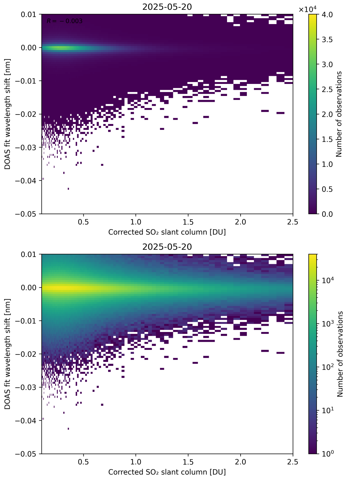
Figure 229: Scatter density plot of “Corrected SO 2 slant column” against “DOAS fit wavelength shift” for 2025-05-19 to 2025-05-21.
