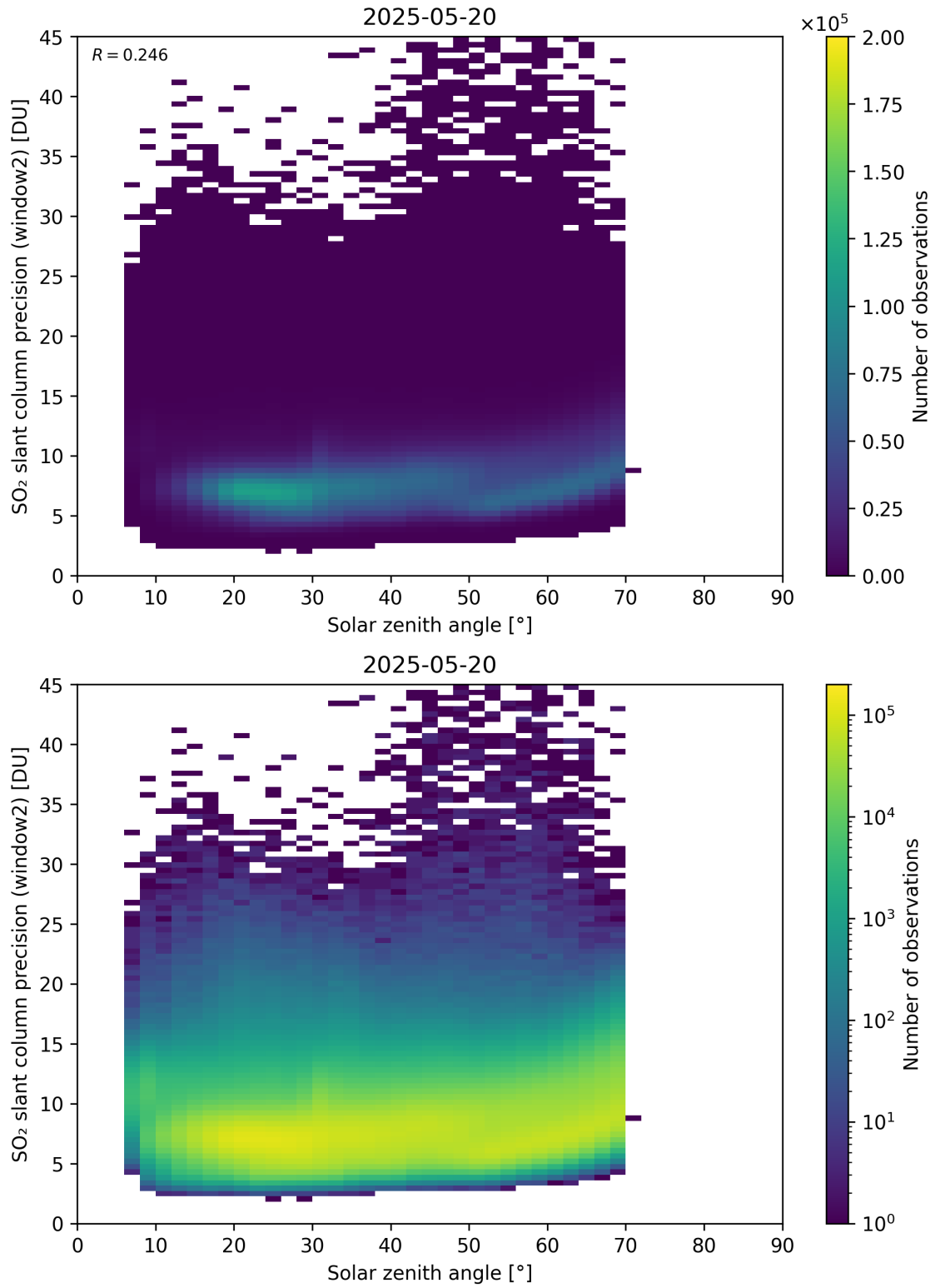
Figure 186: Scatter density plot of “Solar zenith angle” against “SO 2 slant column precision (window2)” for 2025-05-19 to 2025-05-21.
