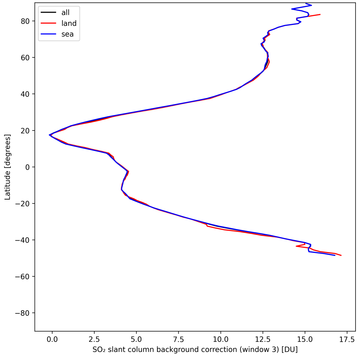
Figure 48: Zonal average of “SO 2 slant column background correction (window 3)” for 2025-05-19 to 2025-05-21.
