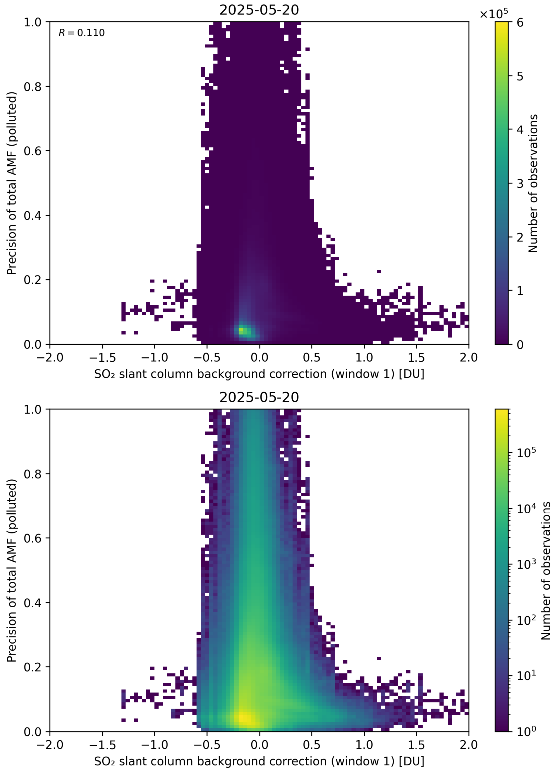
Figure 121: Scatter density plot of “SO 2 slant column background correction (window 1)” against “Precision of total AMF (polluted)” for 2025-05-19 to 2025-05-21.
