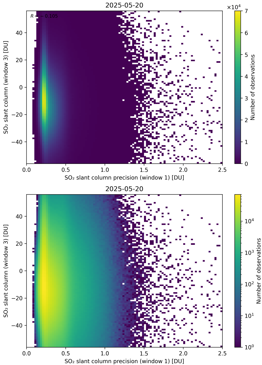
Figure 278: Scatter density plot of “SO 2 slant column precision (window 1)” against “SO 2 slant column (window 3)” for 2025-05-19 to 2025-05-21.
