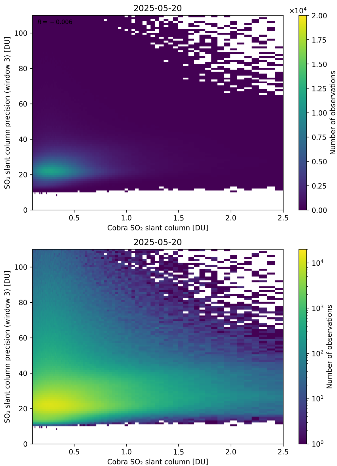
Figure 223: Scatter density plot of “Cobra SO 2 slant column” against “SO 2 slant column precision (window 3)” for 2025-05-19 to 2025-05-21.
