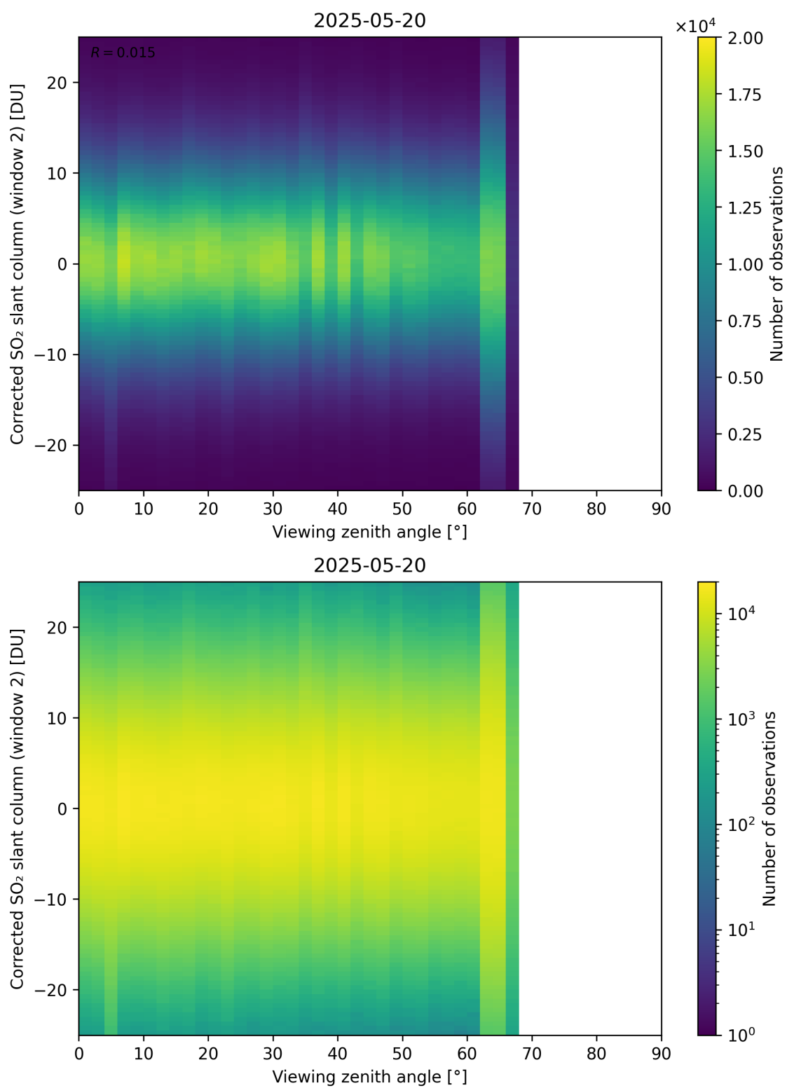
Figure 374: Scatter density plot of “Viewing zenith angle” against “Corrected SO 2 slant column (window 2)” for 2025-05-19 to 2025-05-21.
