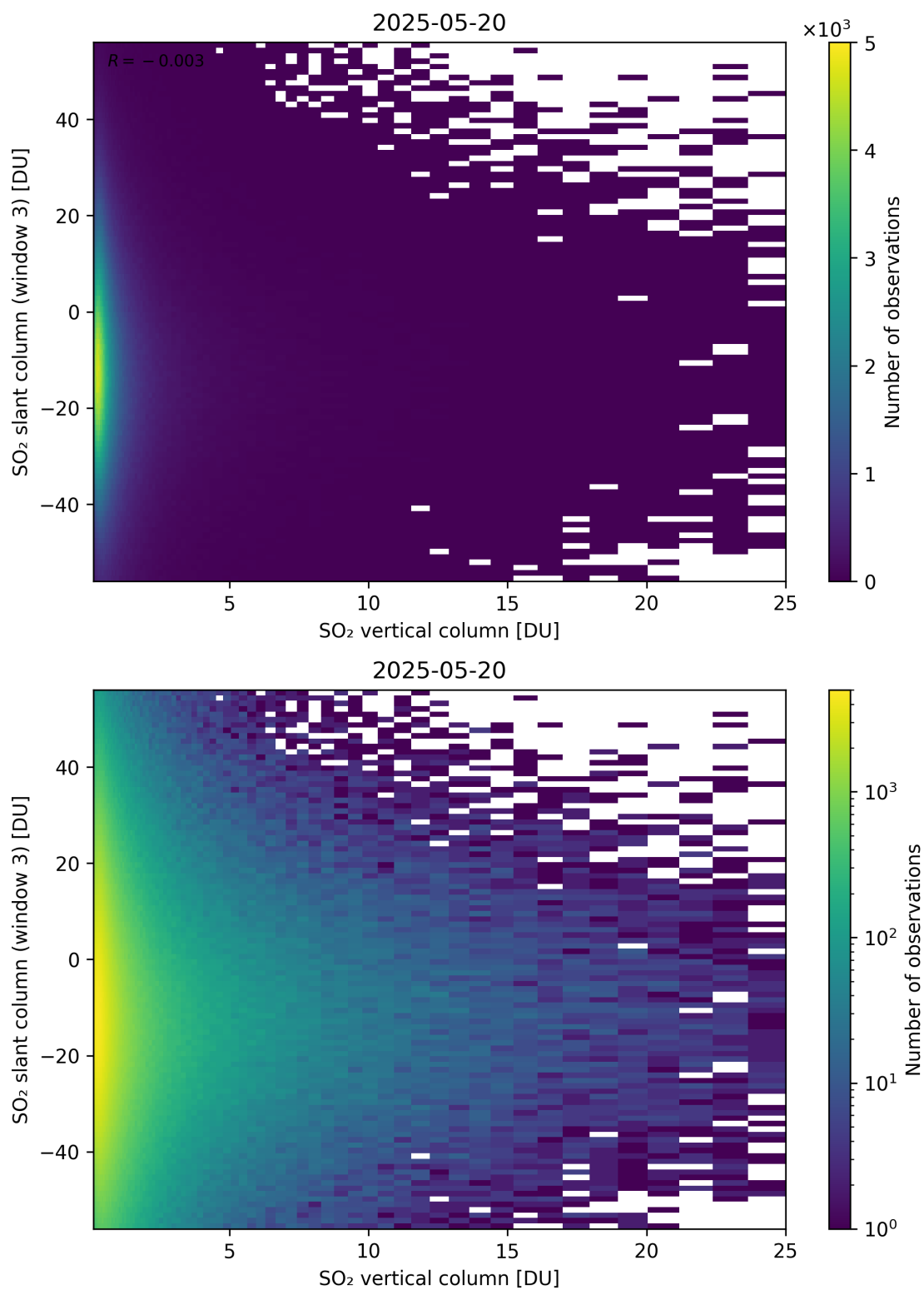
Figure 357: Scatter density plot of “SO 2 vertical column” against “SO 2 slant column (window 3)” for 2025-05-19 to 2025-05-21.
