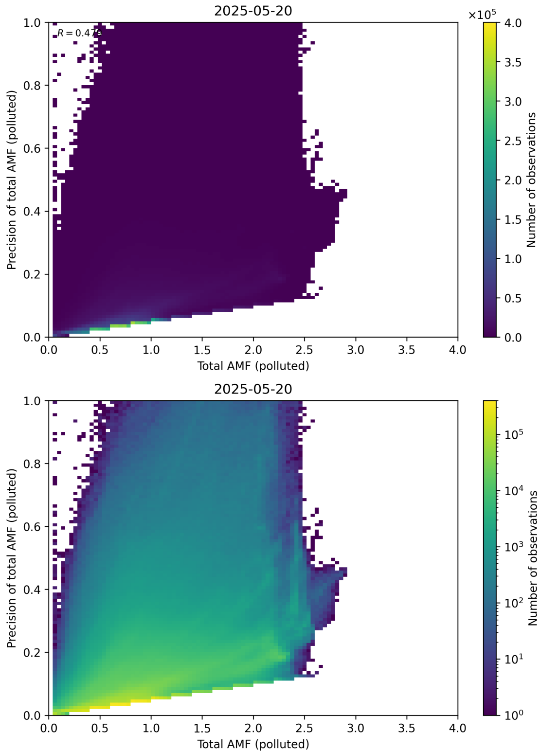
Figure 322: Scatter density plot of “Total AMF (polluted)” against “Precision of total AMF (polluted)” for 2025-05-19 to 2025-05-21.
