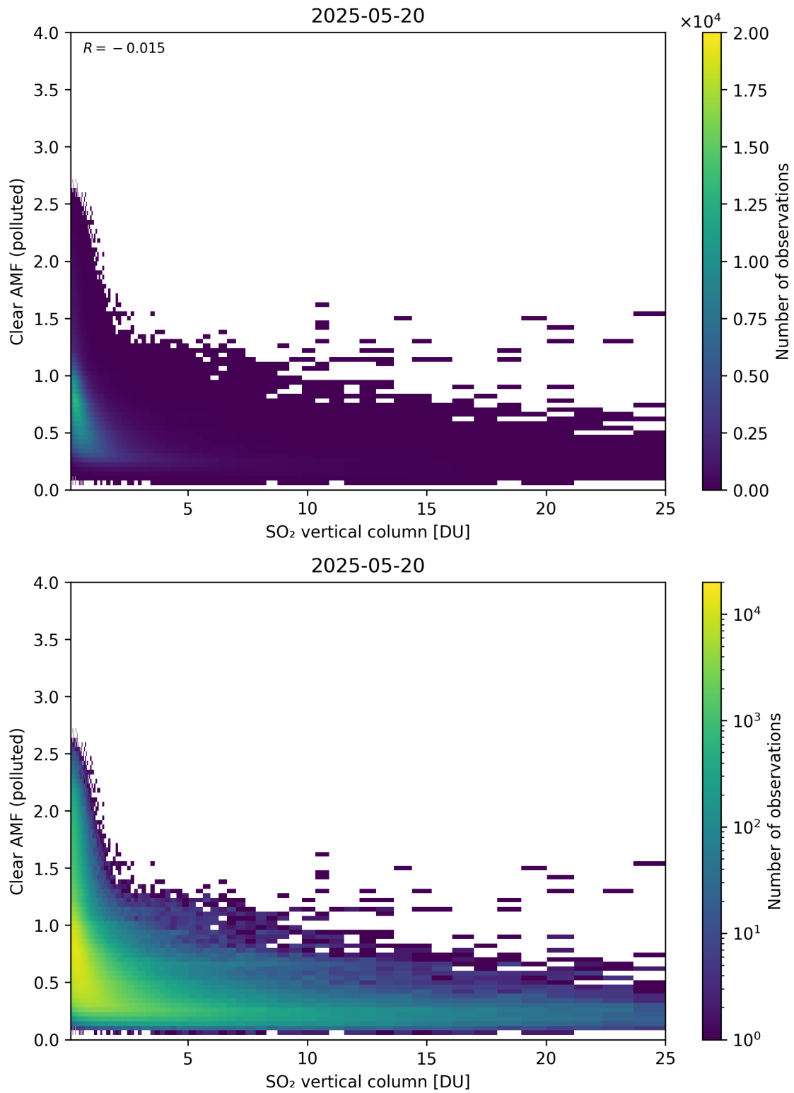
Figure 348: Scatter density plot of “SO 2 vertical column” against “Clear AMF (polluted)” for 2025-05-19 to 2025-05-21.
