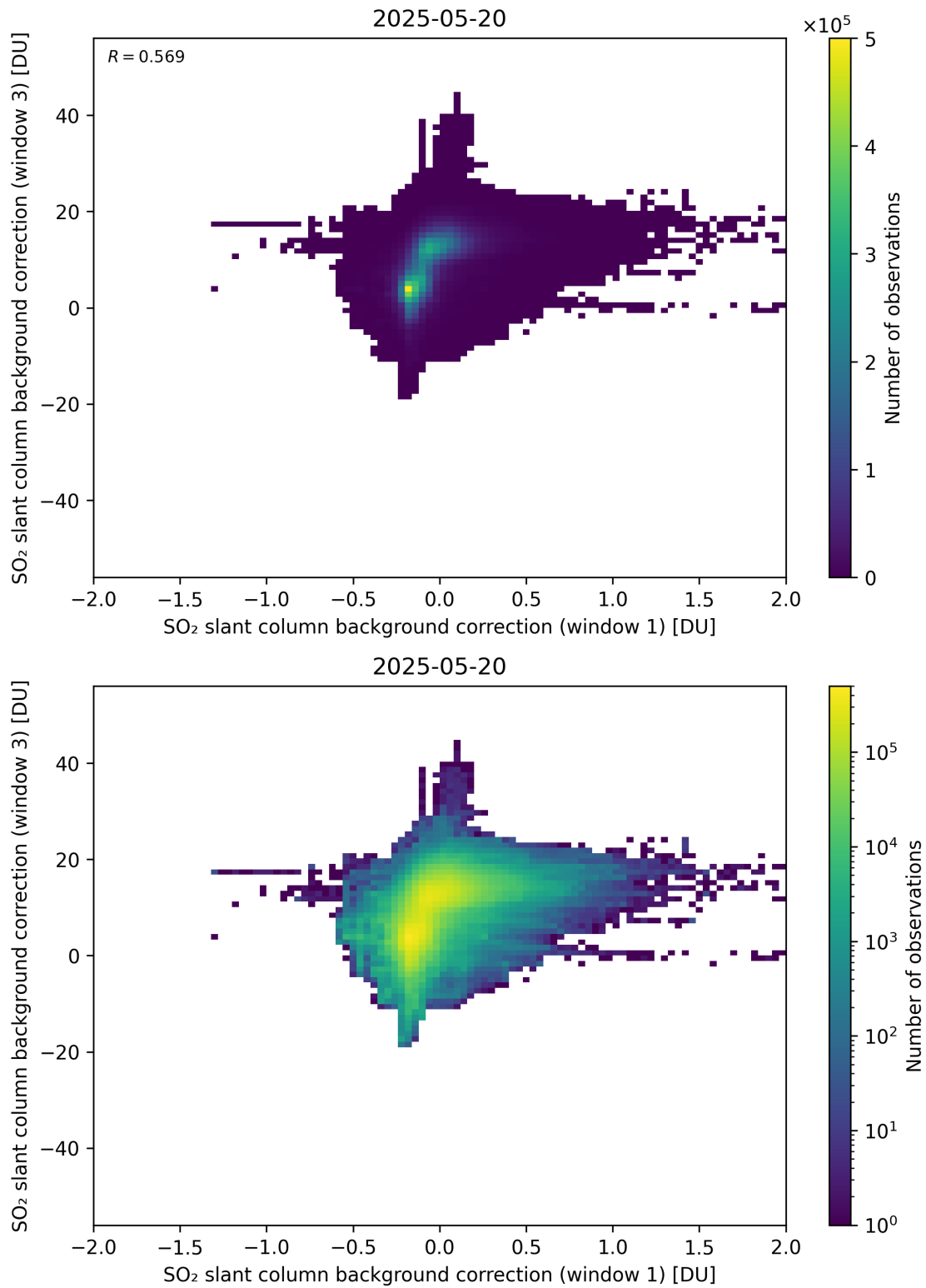
Figure 110: Scatter density plot of “SO 2 slant column background correction (window 1)” against “SO 2 slant column background correction (window 3)” for 2025-05-19 to 2025-05-21.
