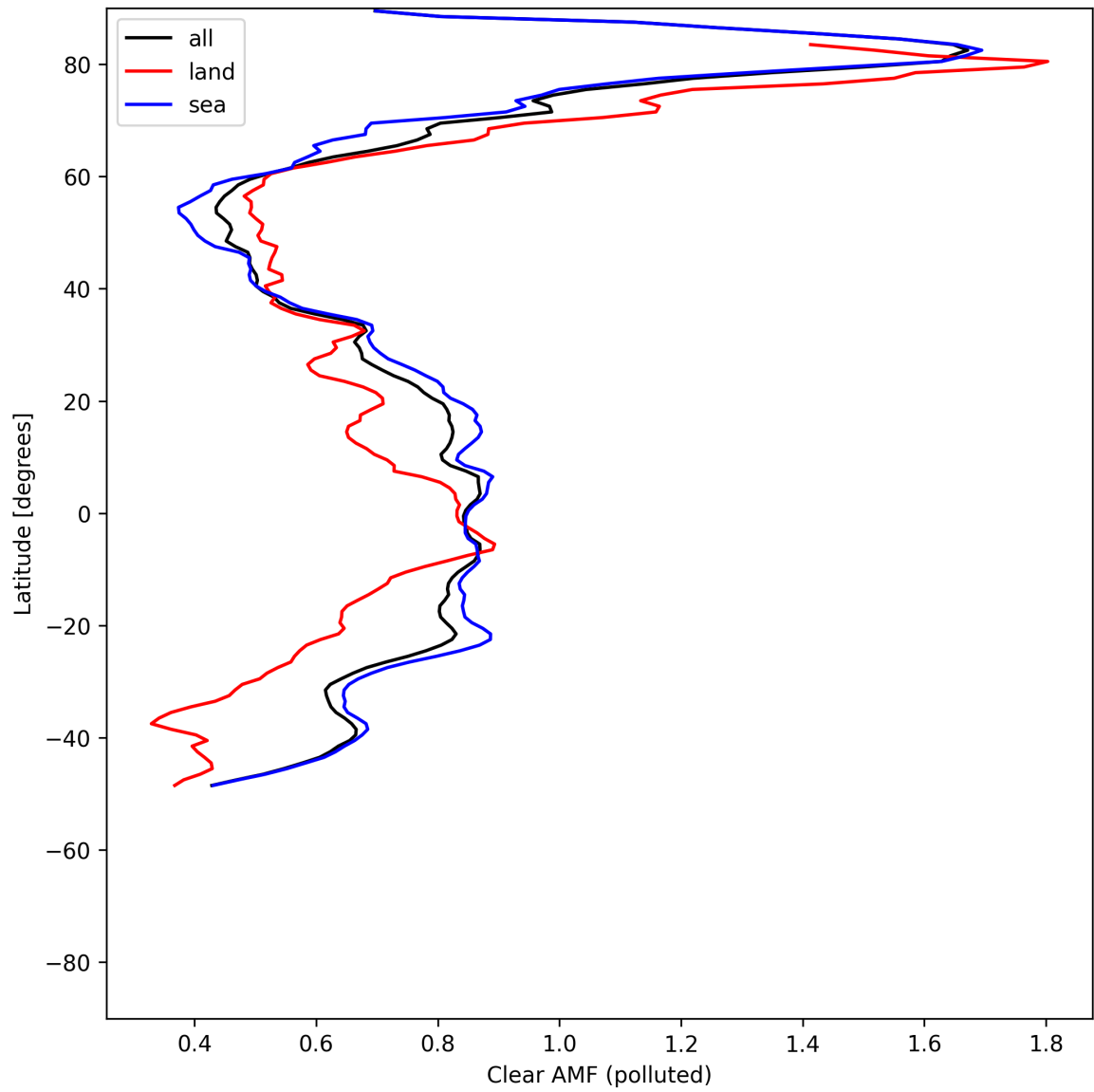
Figure 55: Zonal average of “Clear AMF (polluted)” for 2025-05-19 to 2025-05-21.
