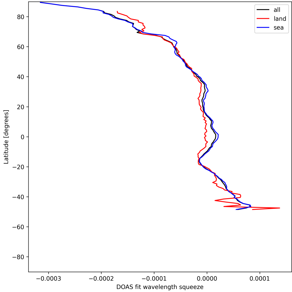
Figure 51: Zonal average of “DOAS fit wavelength squeeze” for 2025-05-19 to 2025-05-21.
