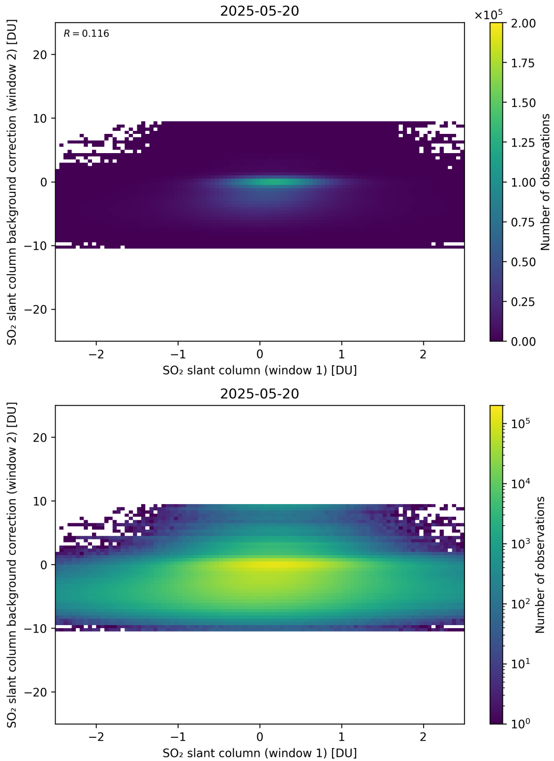
Figure 263: Scatter density plot of “SO 2 slant column (window 1)” against “SO 2 slant column background correction (window 2)” for 2025-05-19 to 2025-05-21.
