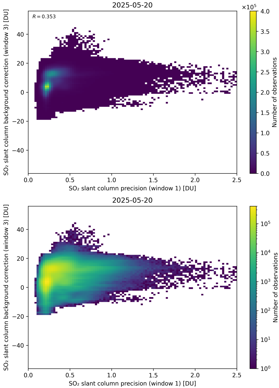
Figure 270: Scatter density plot of “SO 2 slant column precision (window 1)” against “SO 2 slant column background correction (window 3)” for 2025-05-19 to 2025-05-21.
