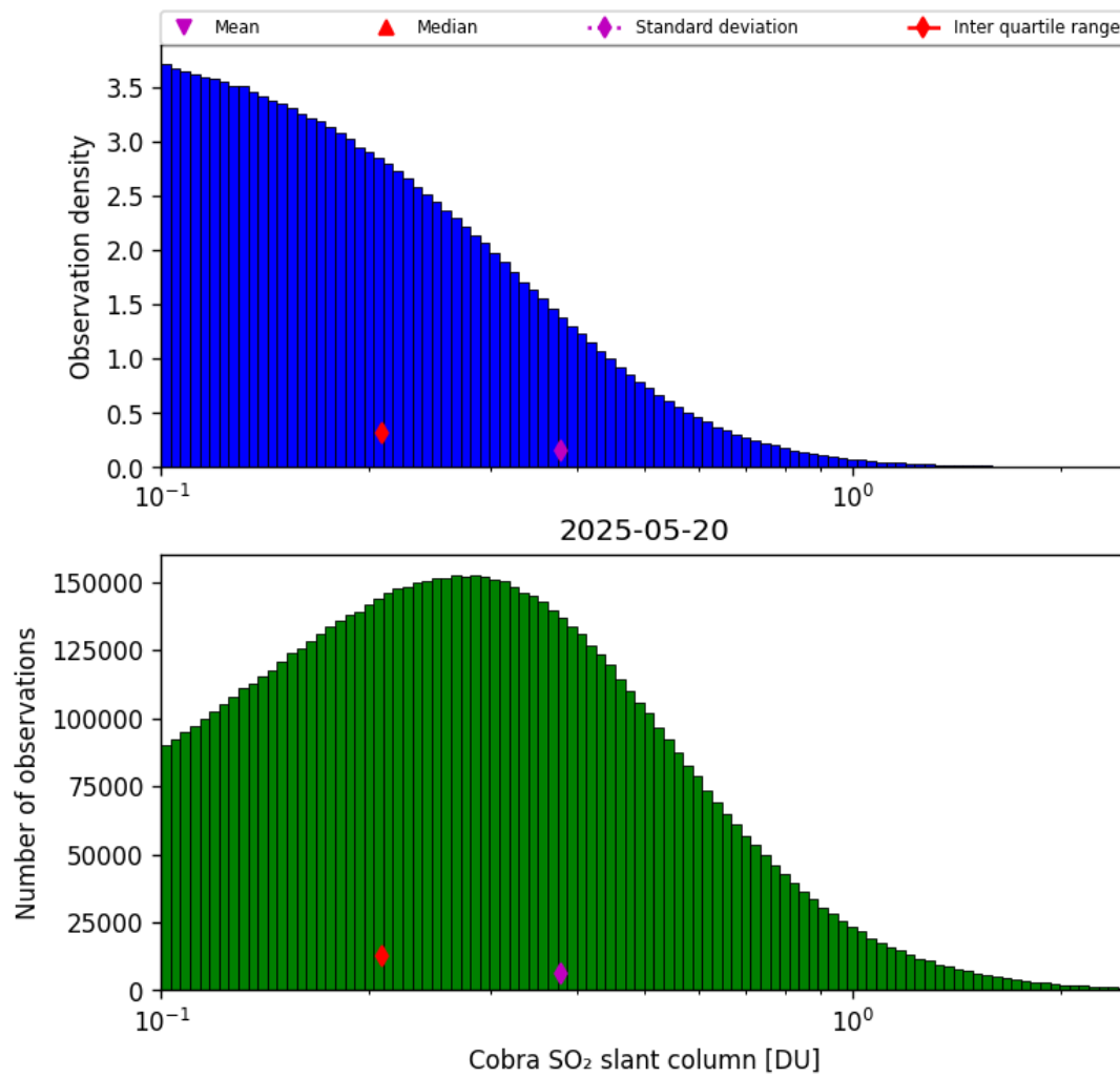
Figure 61: Histogram of “Cobra SO 2 slant column” for 2025-05-19 to 2025-05-21
