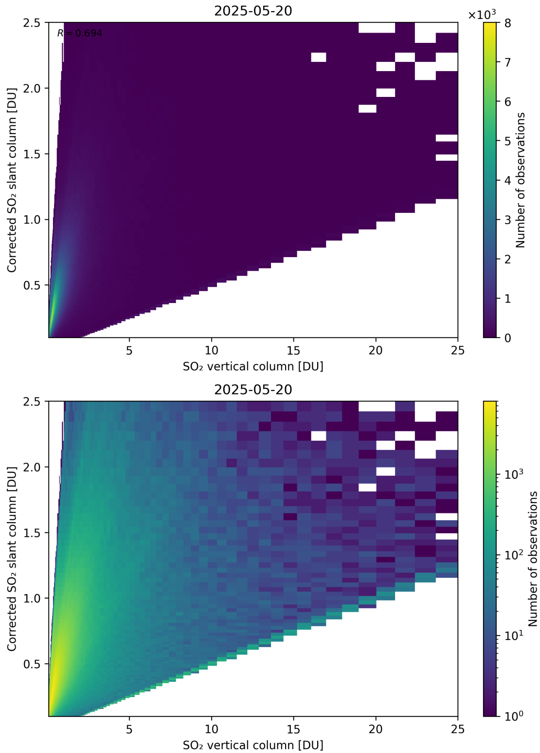
Figure 351: Scatter density plot of “SO 2 vertical column” against “Corrected SO 2 slant column” for 2025-05-19 to 2025-05-21.
