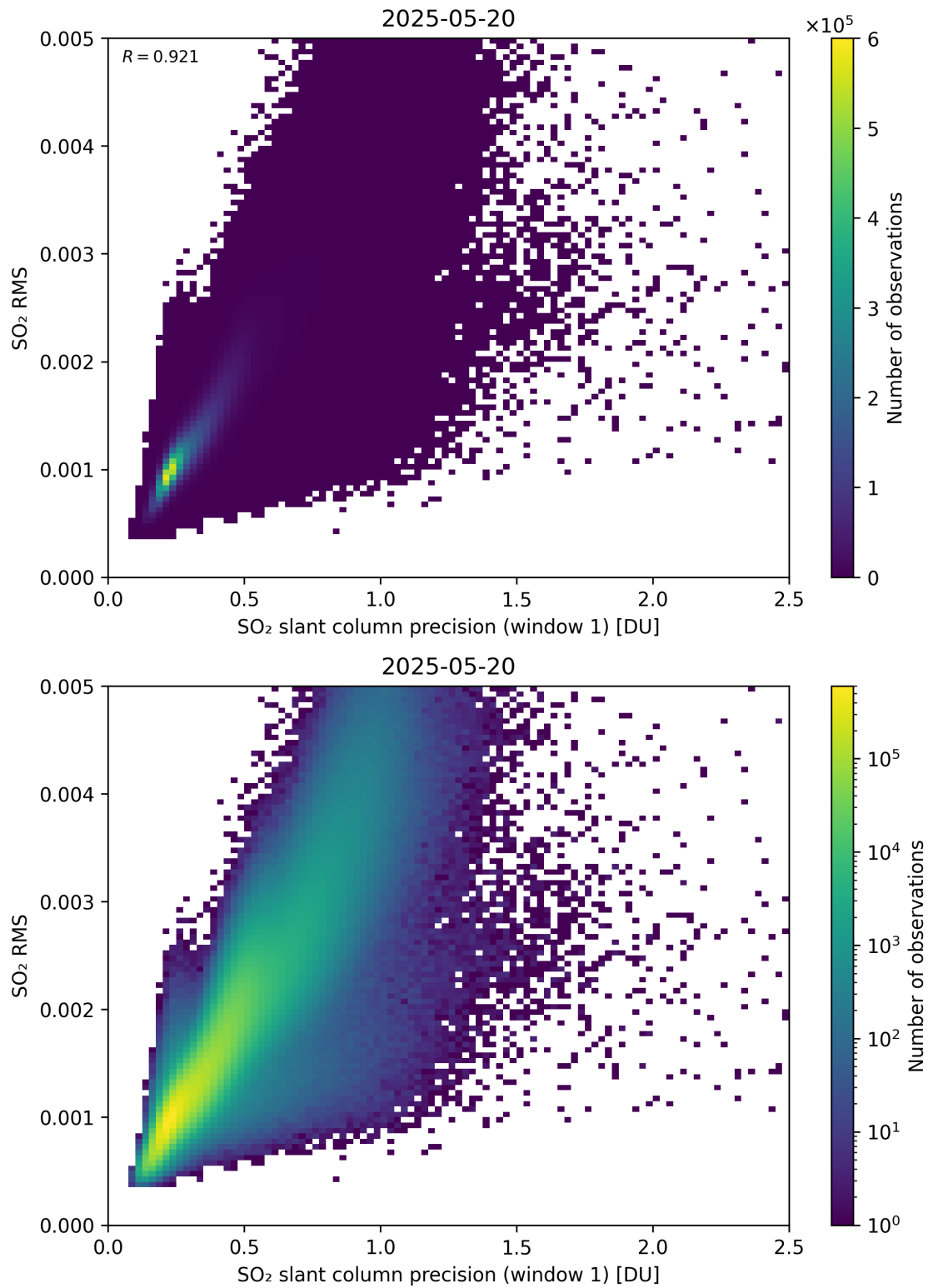
Figure 273: Scatter density plot of “SO 2 slant column precision (window 1)” against “SO 2 RMS” for 2025-05-19 to 2025-05-21.
