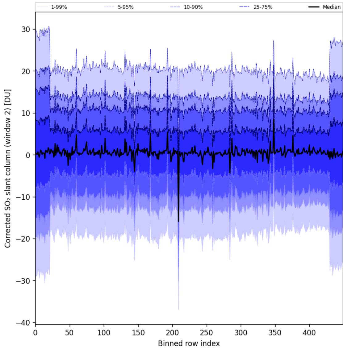
Figure 95: Along track statistics of “Corrected SO 2 slant column (window 2)” for 2025-05-19 to 2025-05-21
