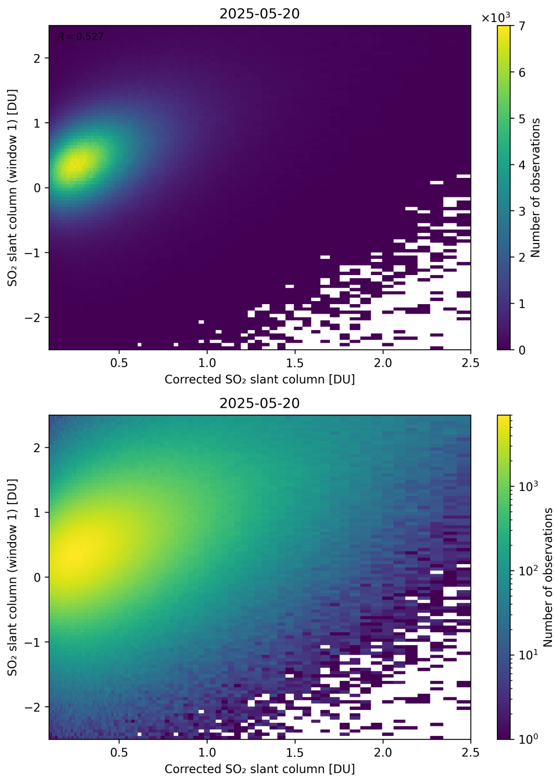
Figure 237: Scatter density plot of “Corrected SO 2 slant column” against “SO 2 slant column (window 1)” for 2025-05-19 to 2025-05-21.
