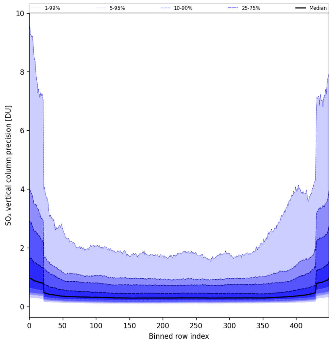
Figure 85: Along track statistics of “SO 2 vertical column precision” for 2025-05-19 to 2025-05-21
