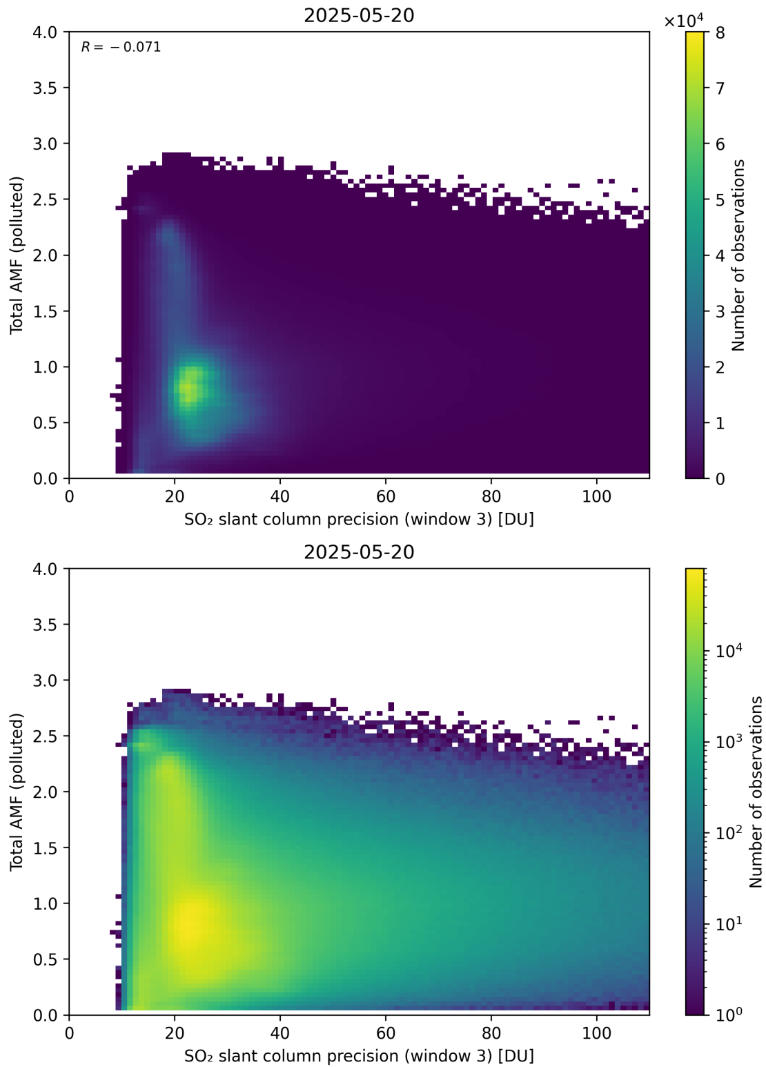
Figure 313: Scatter density plot of “SO 2 slant column precision (window 3)” against “Total AMF (polluted)” for 2025-05-19 to 2025-05-21.
