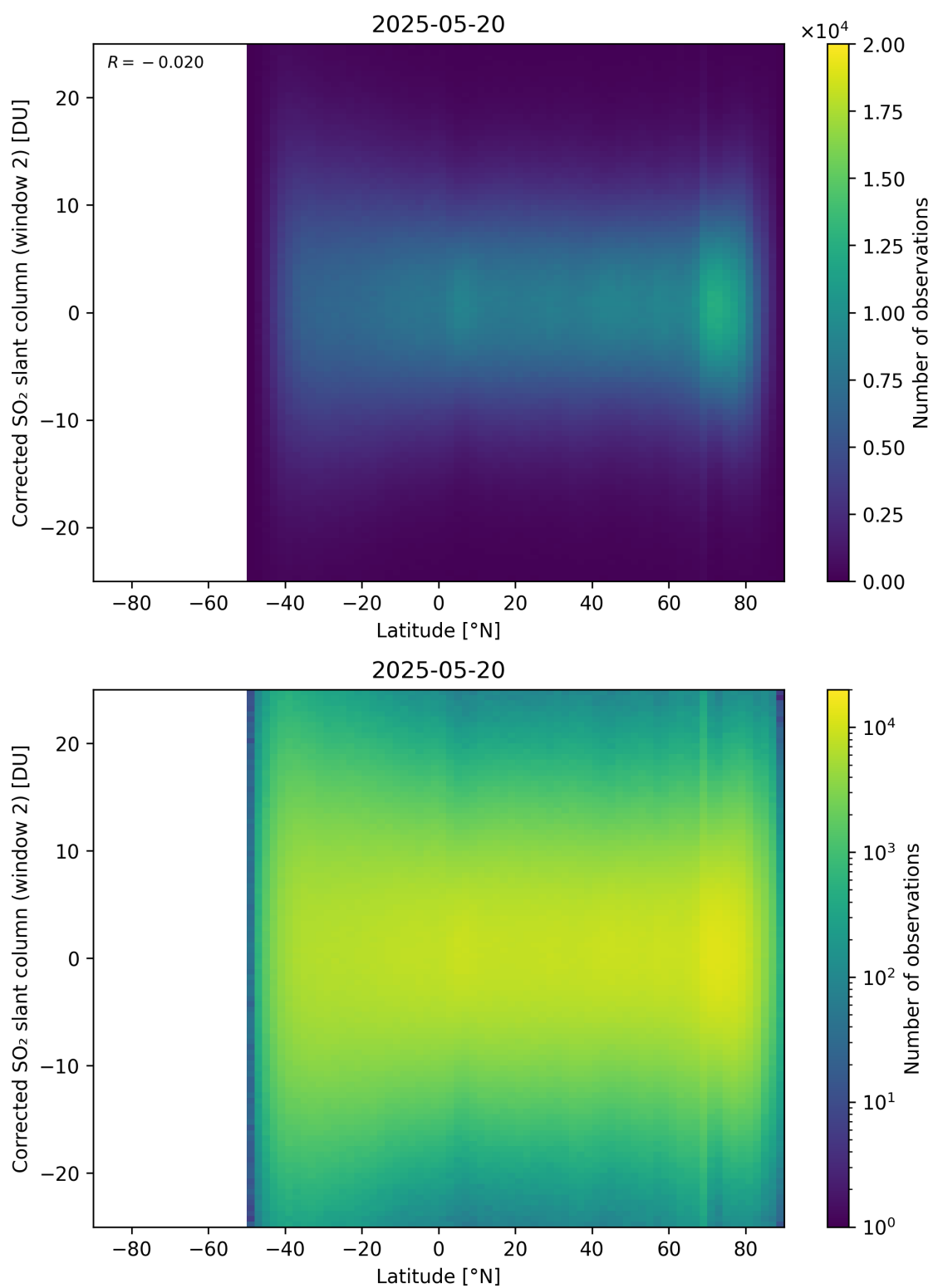
Figure 160: Scatter density plot of “Latitude” against “Corrected SO 2 slant column (window 2)” for 2025-05-19 to 2025-05-21.
