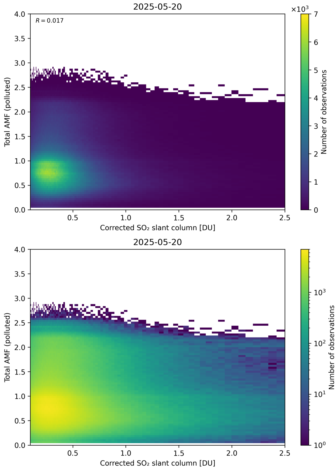
Figure 242: Scatter density plot of “Corrected SO 2 slant column” against “Total AMF (polluted)” for 2025-05-19 to 2025-05-21.
