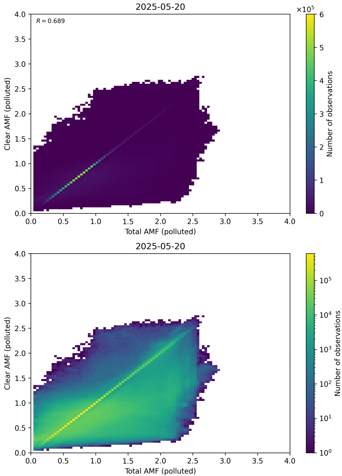
Figure 321: Scatter density plot of “Total AMF (polluted)” against “Clear AMF (polluted)” for 2025-05-19 to 2025-05-21.
