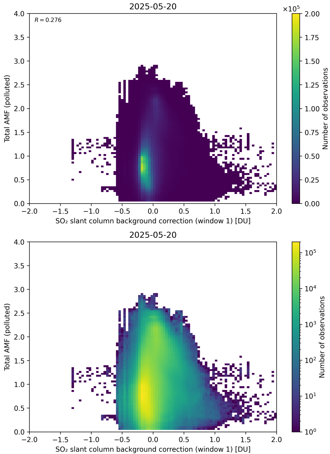
Figure 120: Scatter density plot of “SO 2 slant column background correction (window 1)” against “Total AMF (polluted)” for 2025-05-19 to 2025-05-21.
