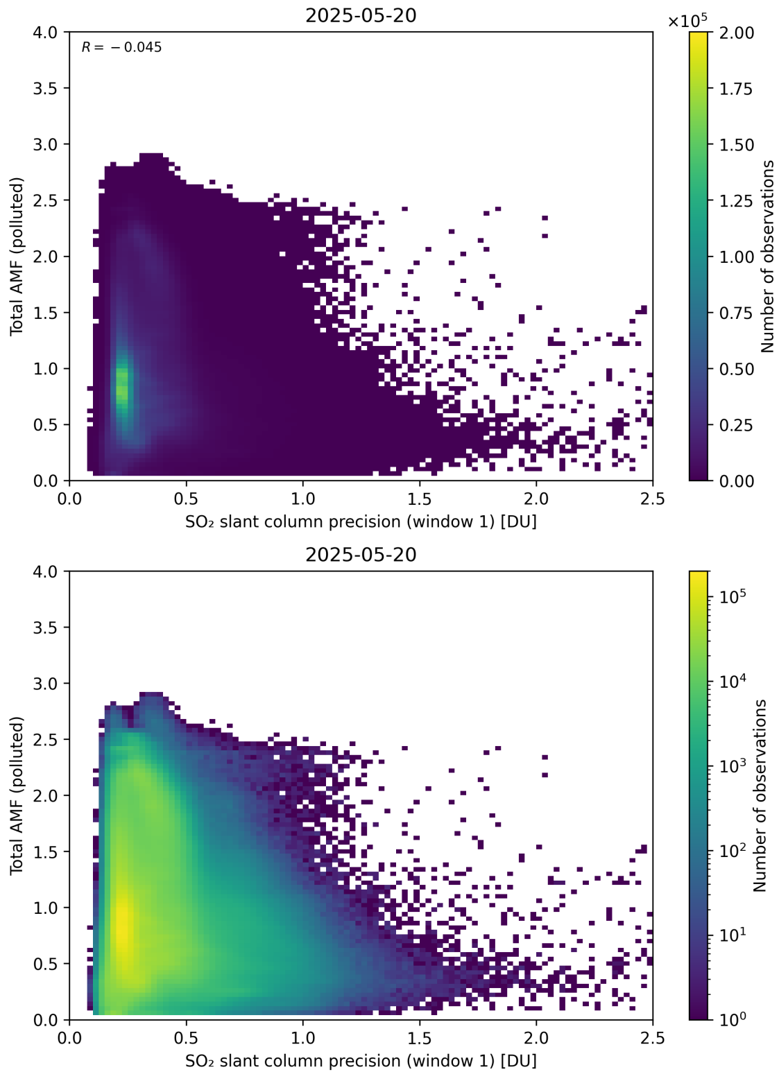
Figure 280: Scatter density plot of “SO 2 slant column precision (window 1)” against “Total AMF (polluted)” for 2025-05-19 to 2025-05-21.
