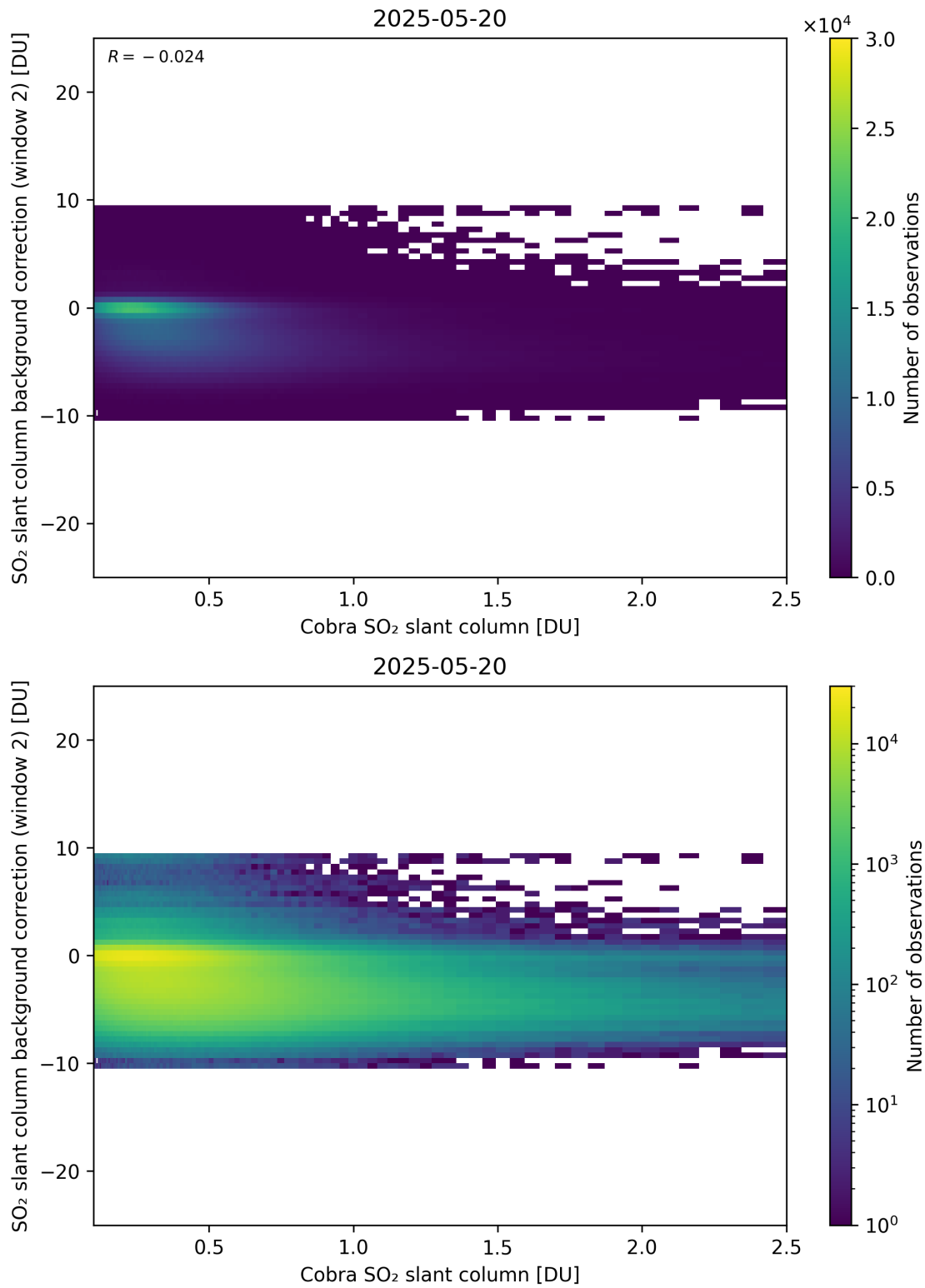
Figure 194: Scatter density plot of “Cobra SO 2 slant column” against “SO 2 slant column background correction (window 2)” for 2025-05-19 to 2025-05-21.
