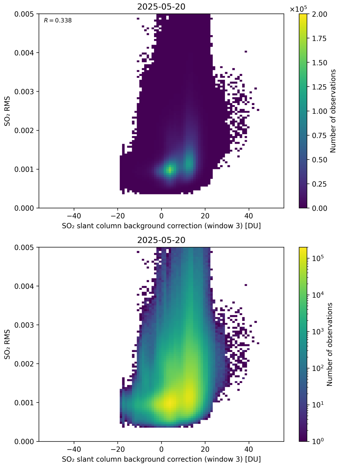
Figure 134: Scatter density plot of “SO 2 slant column background correction (window 3)” against “SO 2 RMS” for 2025-05-19 to 2025-05-21.
