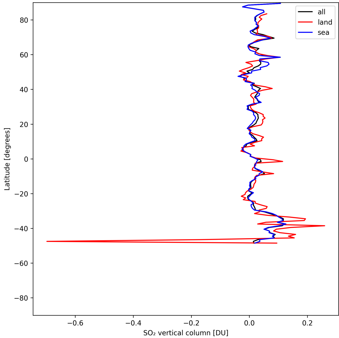
Figure 32: Zonal average of “SO 2 vertical column” for 2025-05-19 to 2025-05-21.
