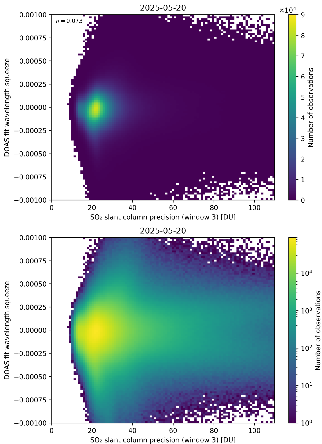
Figure 309: Scatter density plot of “SO 2 slant column precision (window 3)” against “DOAS fit wavelength squeeze” for 2025-05-19 to 2025-05-21.
