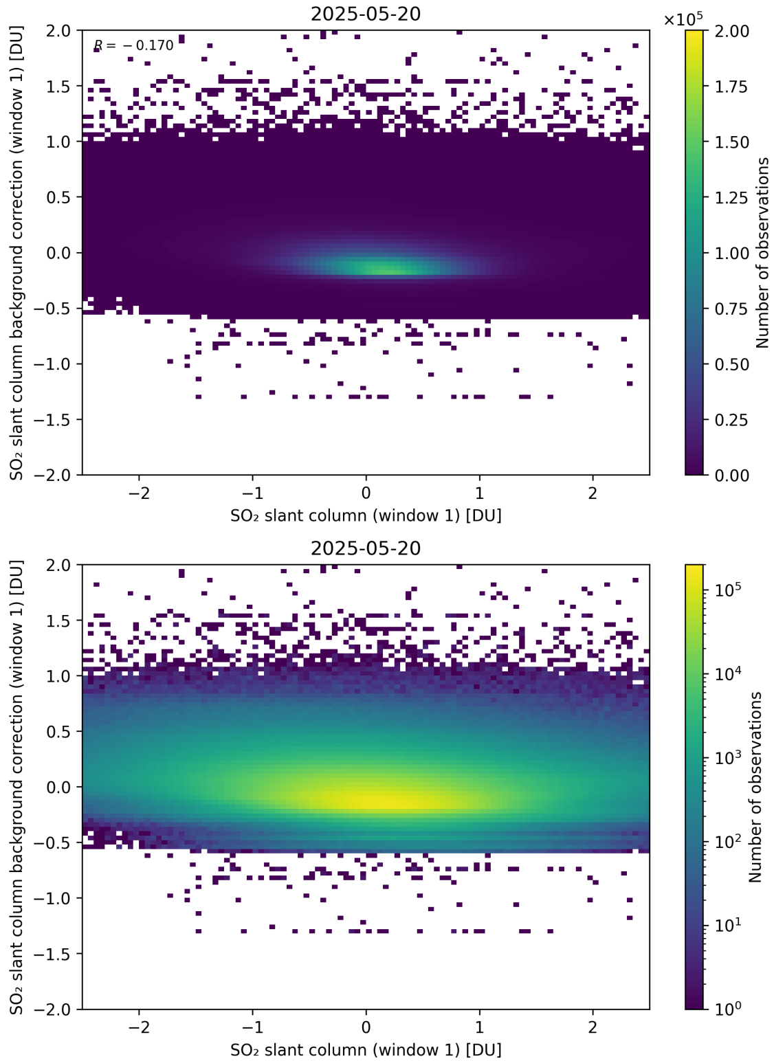
Figure 262: Scatter density plot of “SO 2 slant column (window 1)” against “SO 2 slant column background correction (window 1)” for 2025-05-19 to 2025-05-21.
