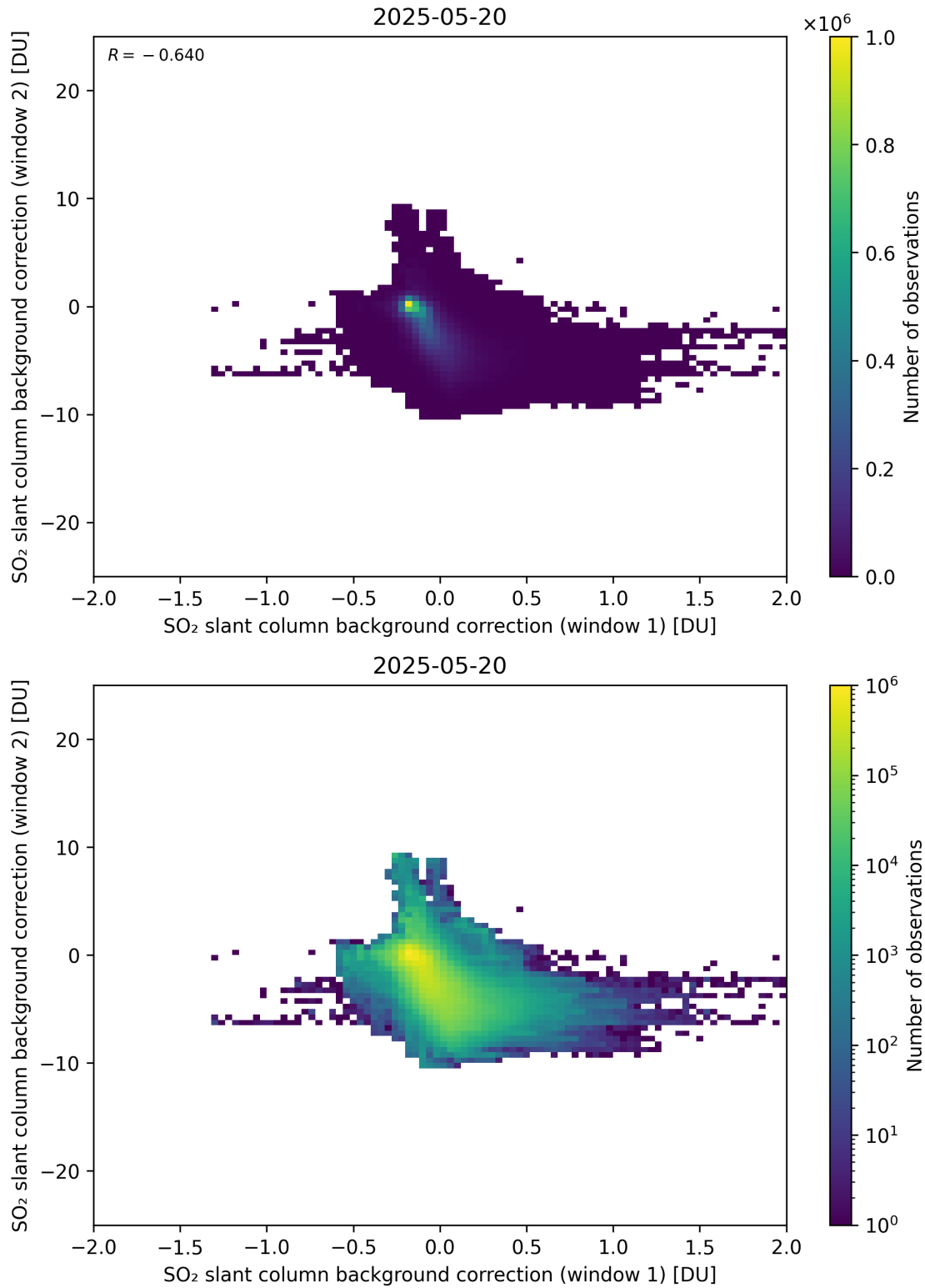
Figure 109: Scatter density plot of “SO 2 slant column background correction (window 1)” against “SO 2 slant column background correction (window 2)” for 2025-05-19 to 2025-05-21.
