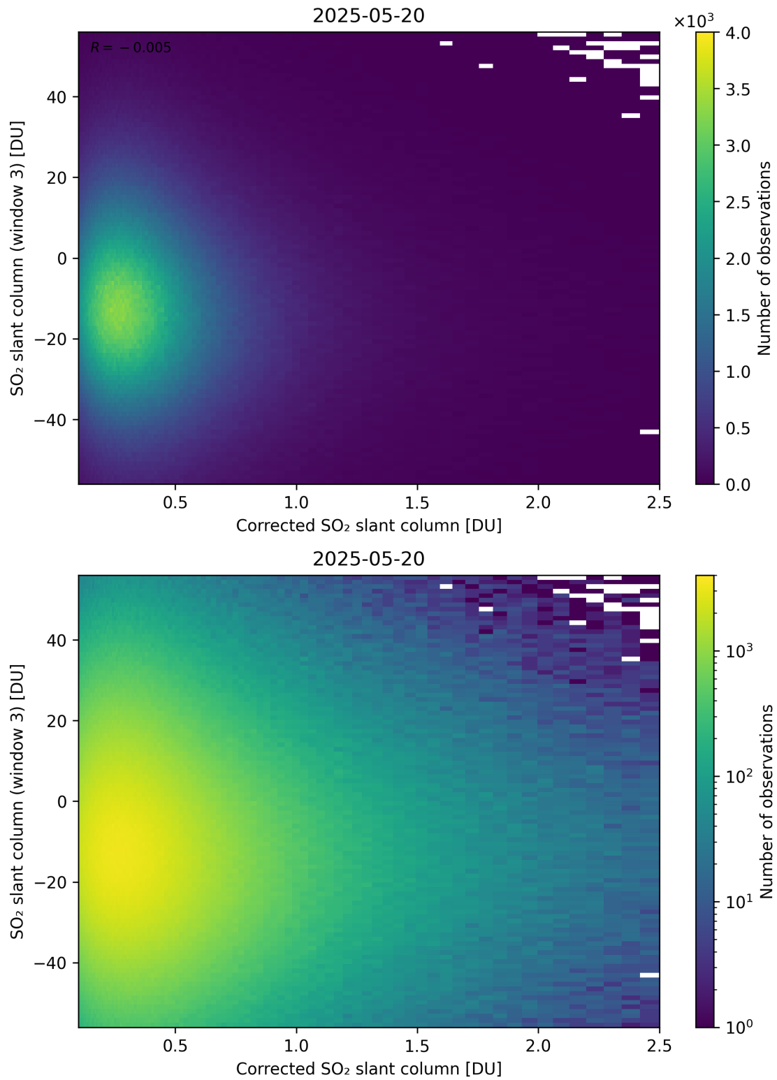
Figure 240: Scatter density plot of “Corrected SO 2 slant column” against “SO 2 slant column (window 3)” for 2025-05-19 to 2025-05-21.
