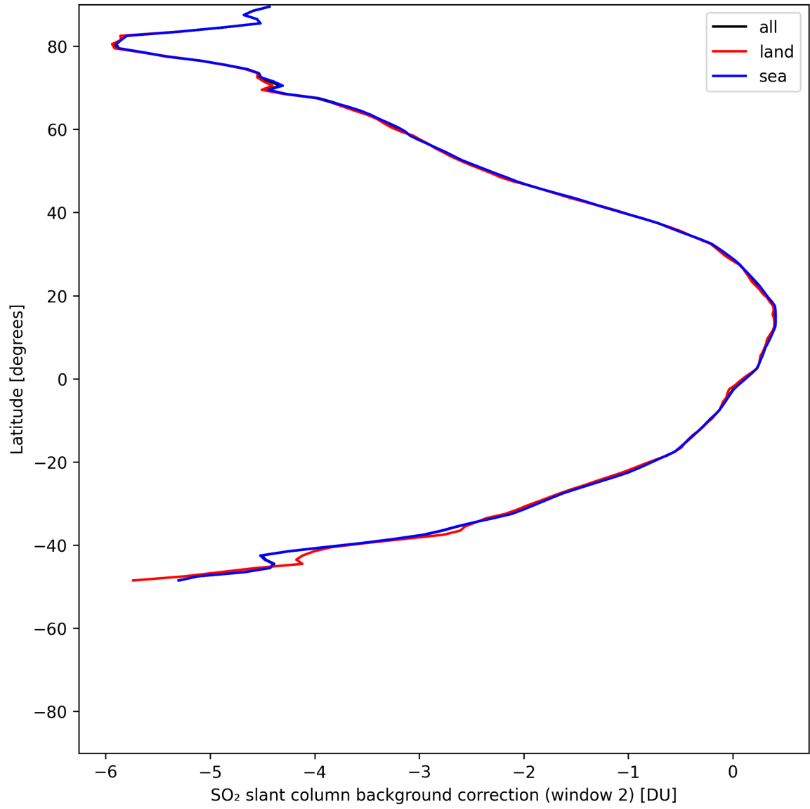
Figure 44: Zonal average of “SO 2 slant column background correction (window 2)” for 2025-05-19 to 2025-05-21.
