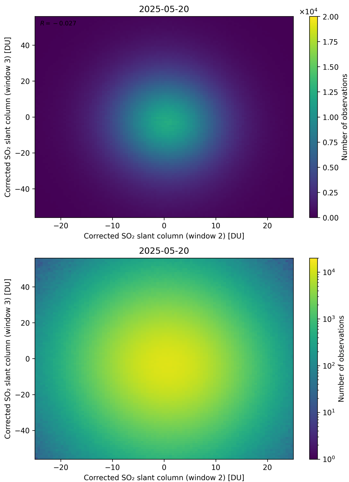
Figure 250: Scatter density plot of “Corrected SO 2 slant column (window 2)” against “Corrected SO 2 slant column (window 3)” for 2025-05-19 to 2025-05-21.
