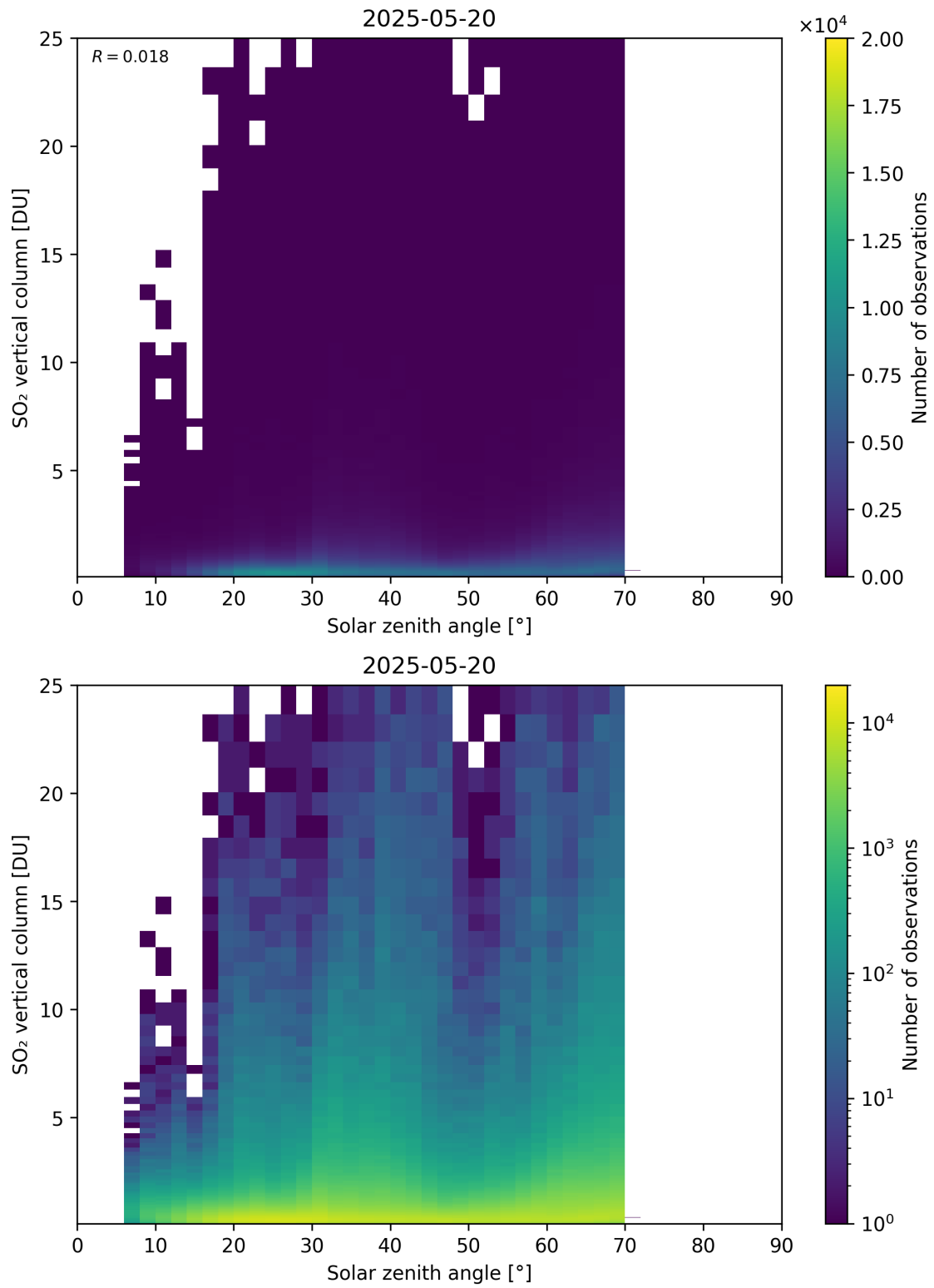
Figure 191: Scatter density plot of “Solar zenith angle” against “SO 2 vertical column” for 2025-05-19 to 2025-05-21.
