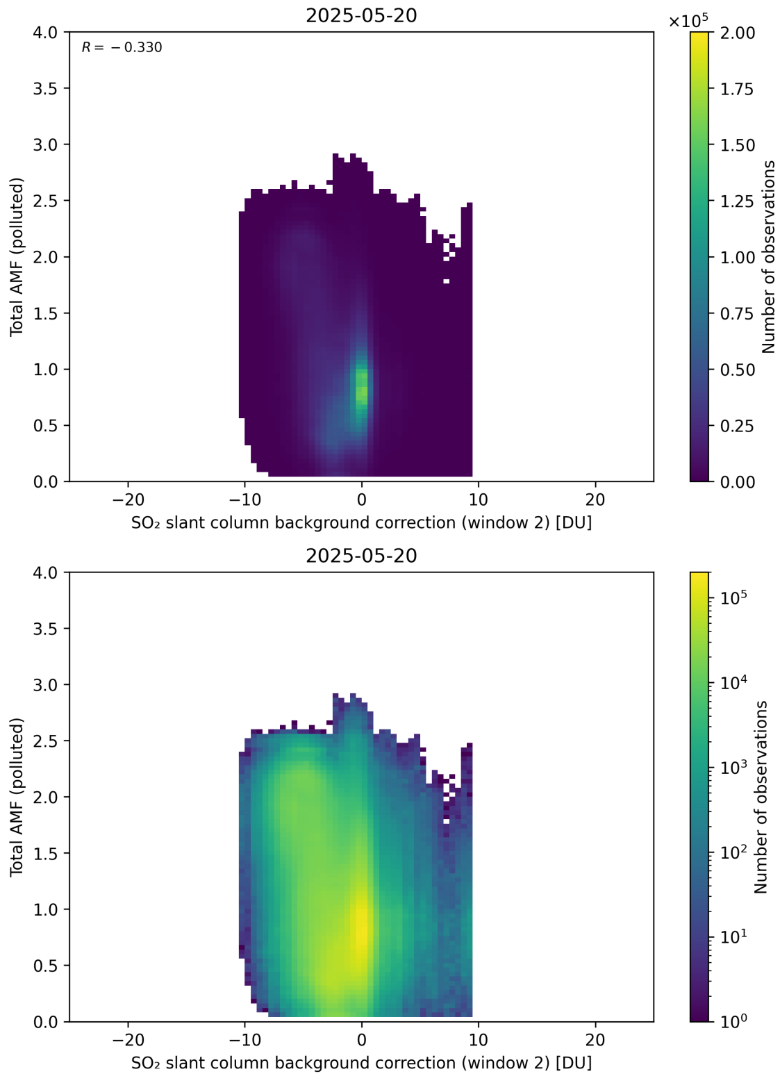
Figure 130: Scatter density plot of “SO 2 slant column background correction (window 2)” against “Total AMF (polluted)” for 2025-05-19 to 2025-05-21.
