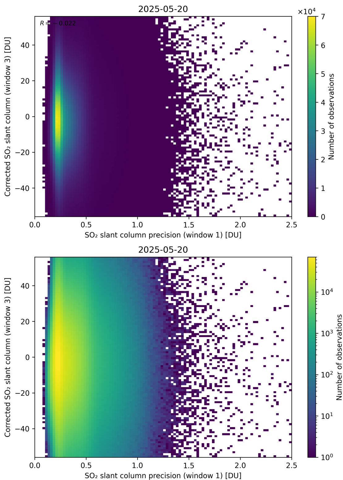
Figure 276: Scatter density plot of “SO 2 slant column precision (window 1)” against “Corrected SO 2 slant column (window 3)” for 2025-05-19 to 2025-05-21.
