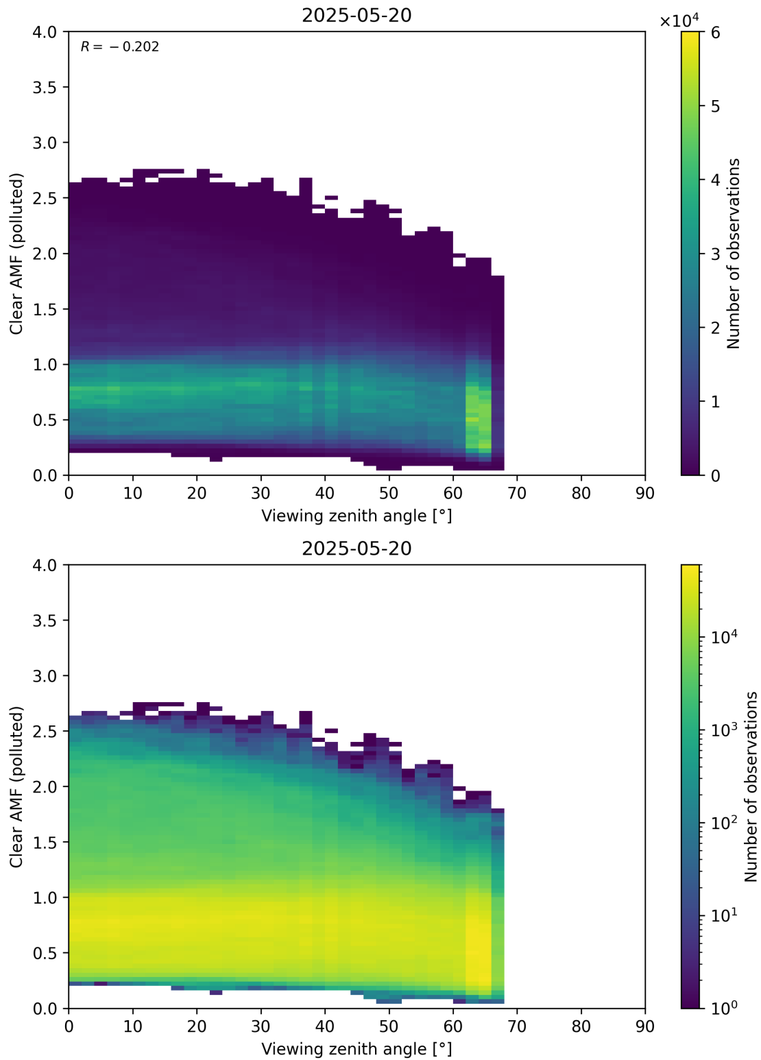
Figure 370: Scatter density plot of “Viewing zenith angle” against “Clear AMF (polluted)” for 2025-05-19 to 2025-05-21.
