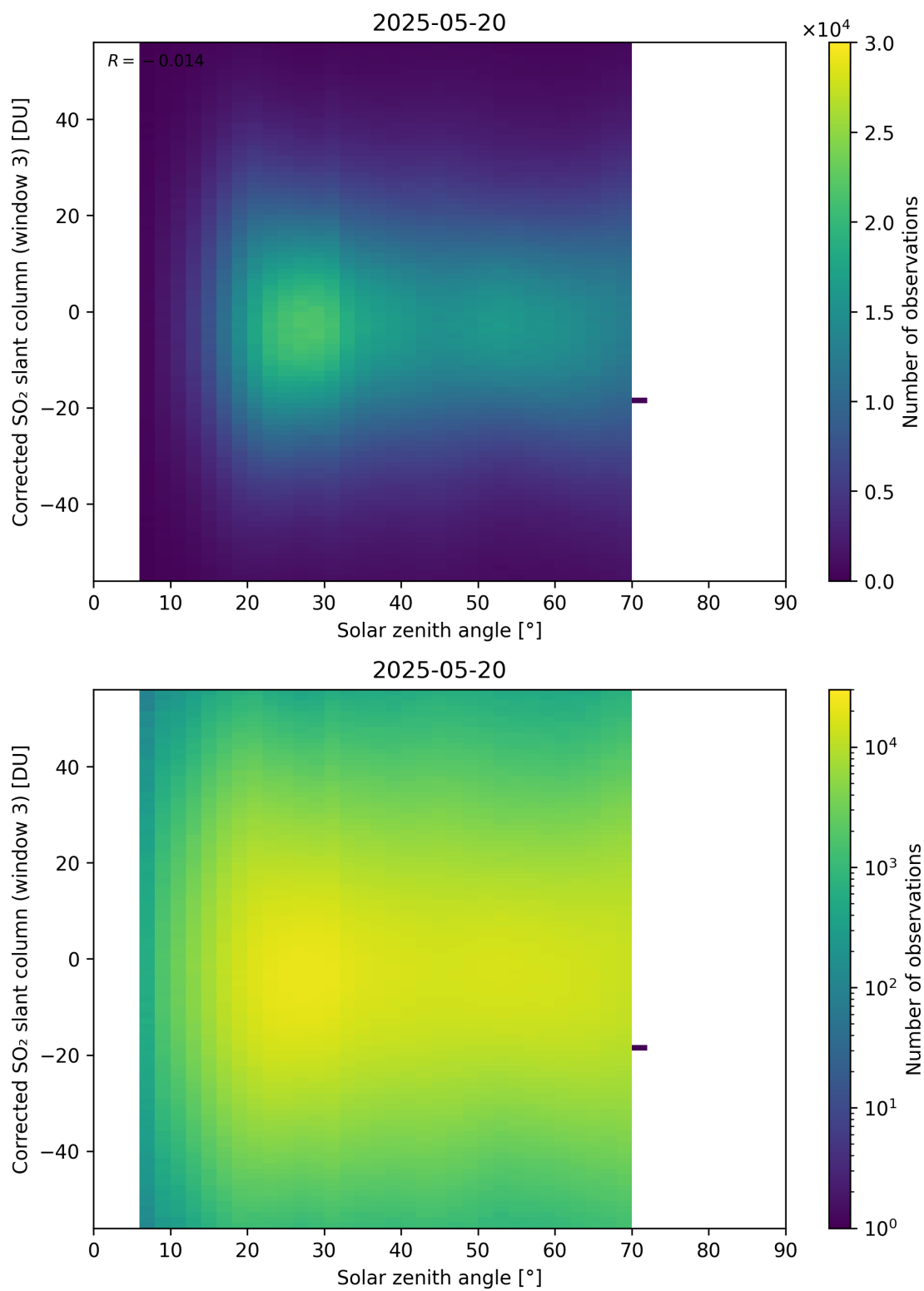
Figure 183: Scatter density plot of “Solar zenith angle” against “Corrected SO 2 slant column (window 3)” for 2025-05-19 to 2025-05-21.
