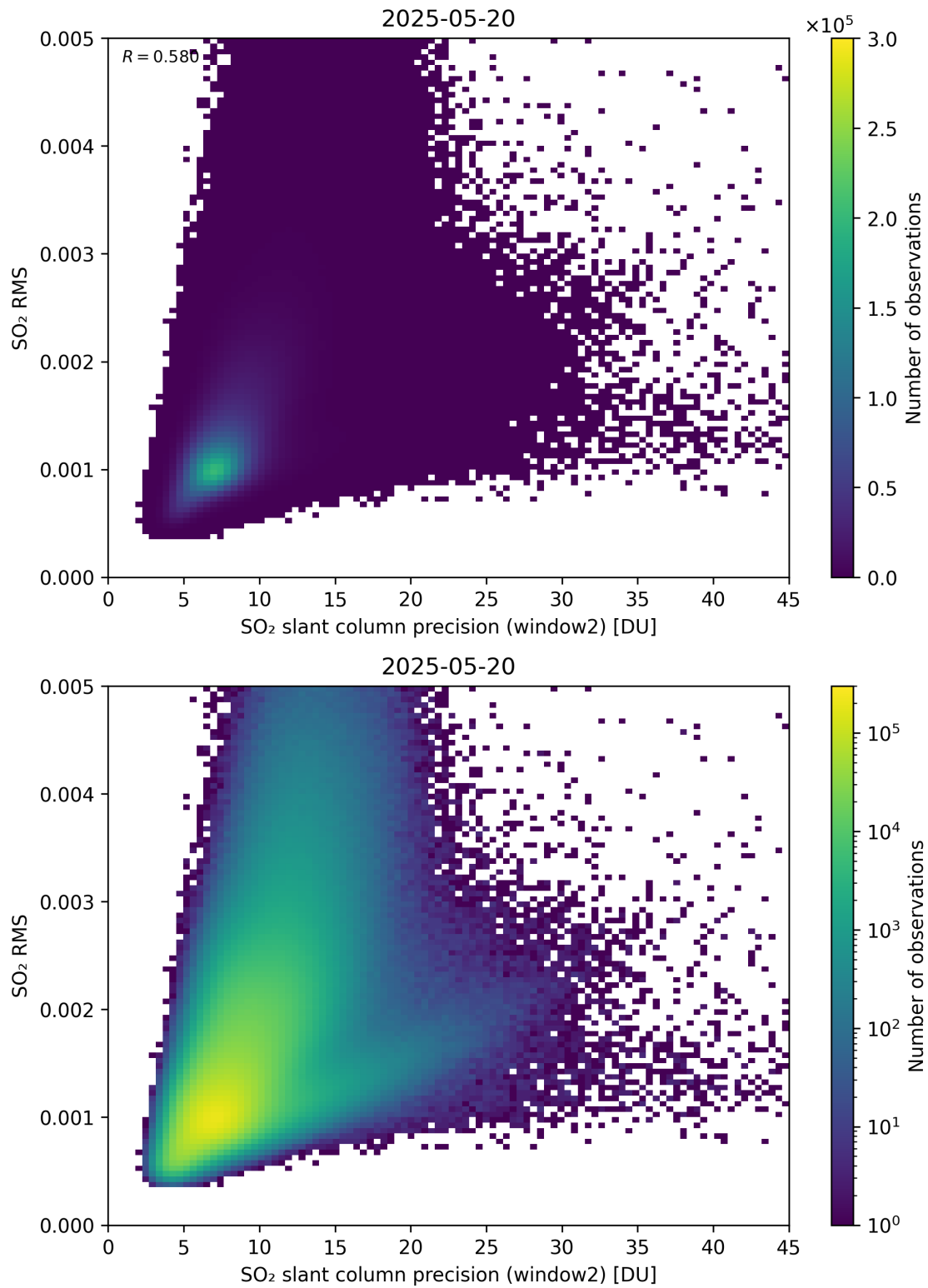
Figure 295: Scatter density plot of “SO 2 slant column precision (window2)” against “SO 2 RMS” for 2025-05-19 to 2025-05-21.
