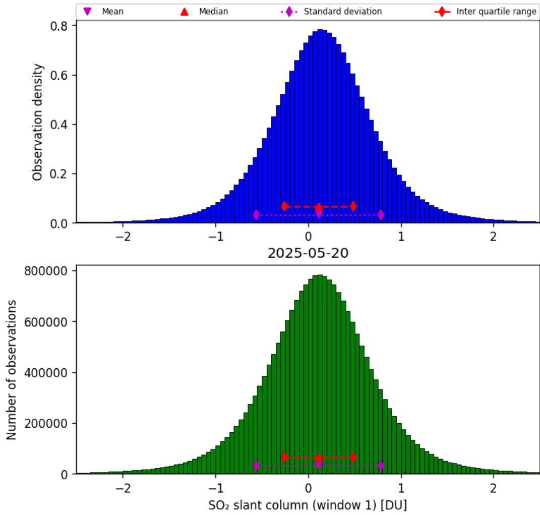
Figure 63: Histogram of “SO 2 slant column (window 1)” for 2025-05-19 to 2025-05-21
