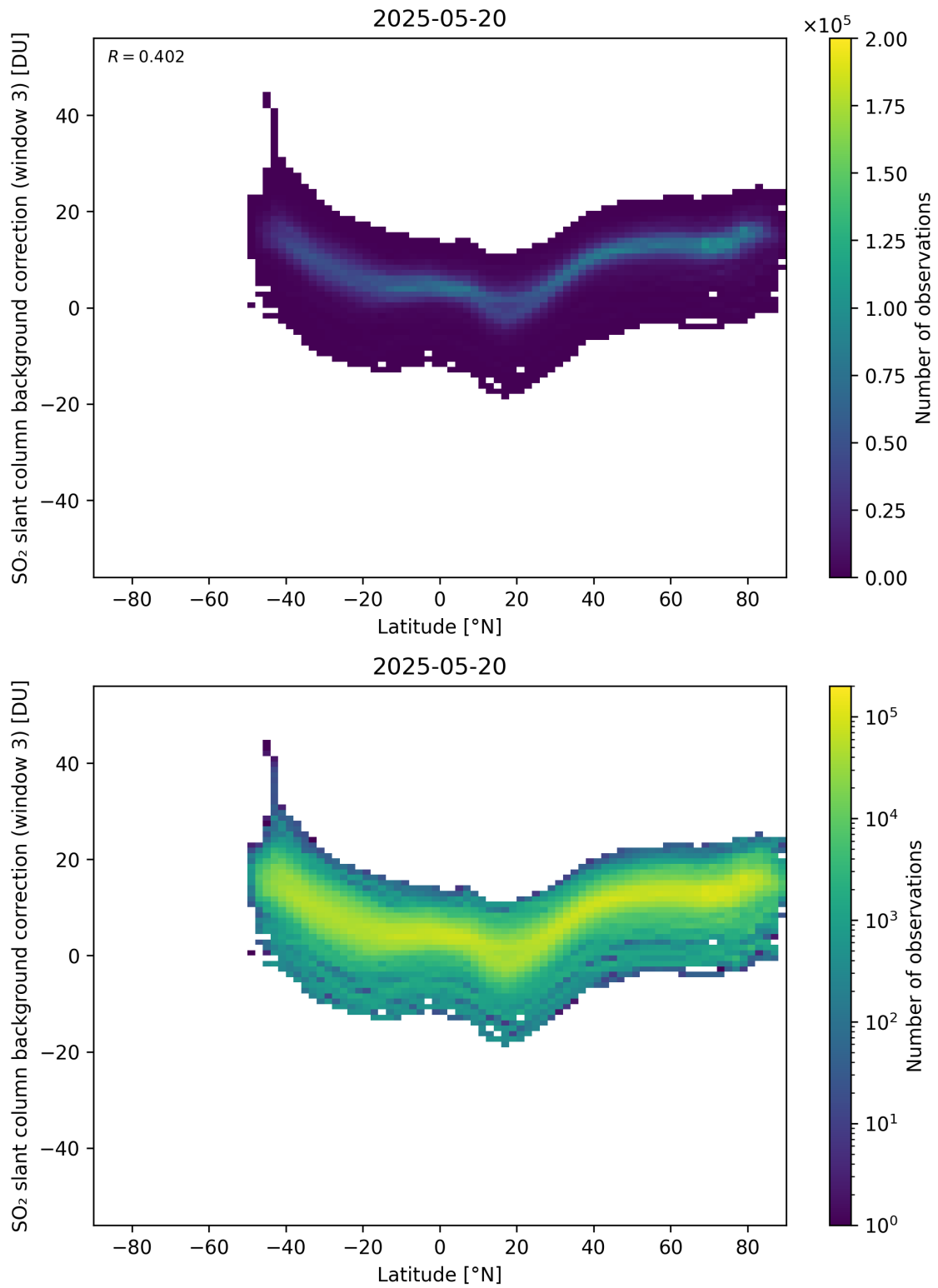
Figure 152: Scatter density plot of “Latitude” against “SO 2 slant column background correction (window 3)” for 2025-05-19 to 2025-05-21.
