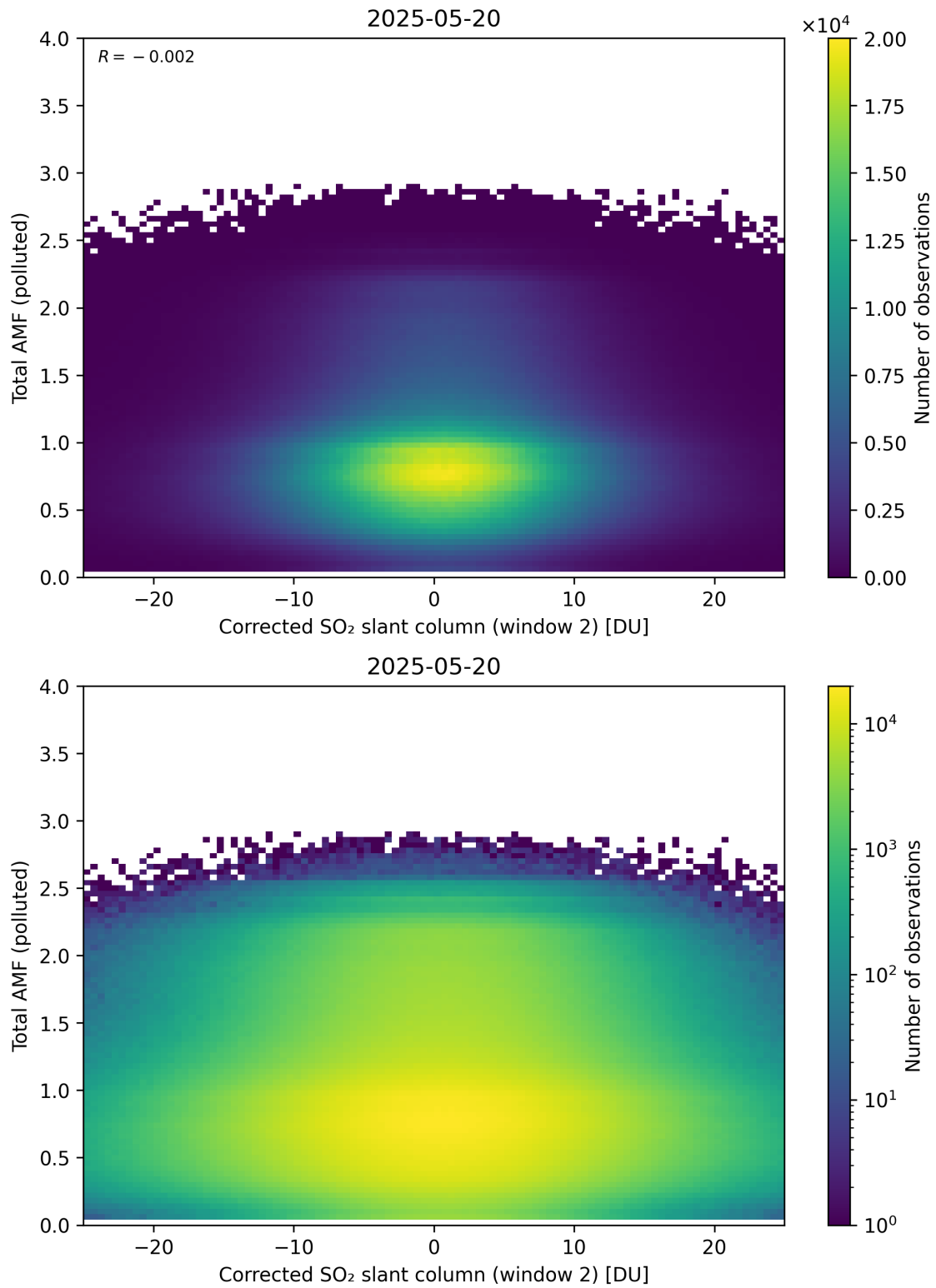
Figure 253: Scatter density plot of “Corrected SO 2 slant column (window 2)” against “Total AMF (polluted)” for 2025-05-19 to 2025-05-21.
