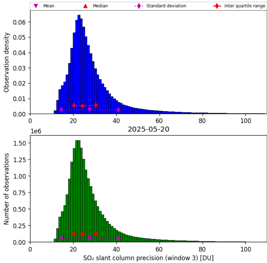
Figure 72: Histogram of “SO 2 slant column precision (window 3)” for 2025-05-19 to 2025-05-21
