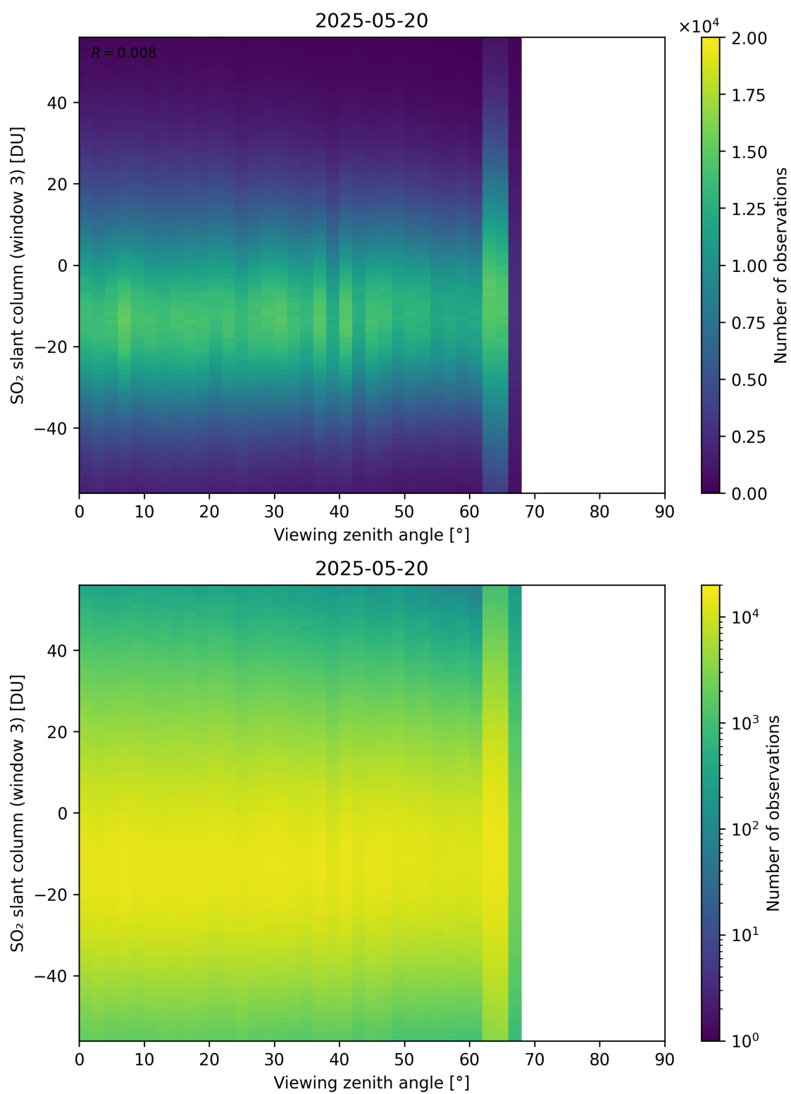
Figure 379: Scatter density plot of “Viewing zenith angle” against “SO 2 slant column (window 3)” for 2025-05-19 to 2025-05-21.
