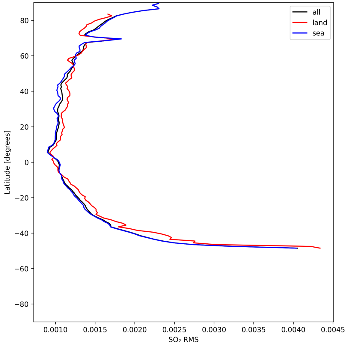
Figure 52: Zonal average of “SO 2 RMS” for 2025-05-19 to 2025-05-21.
