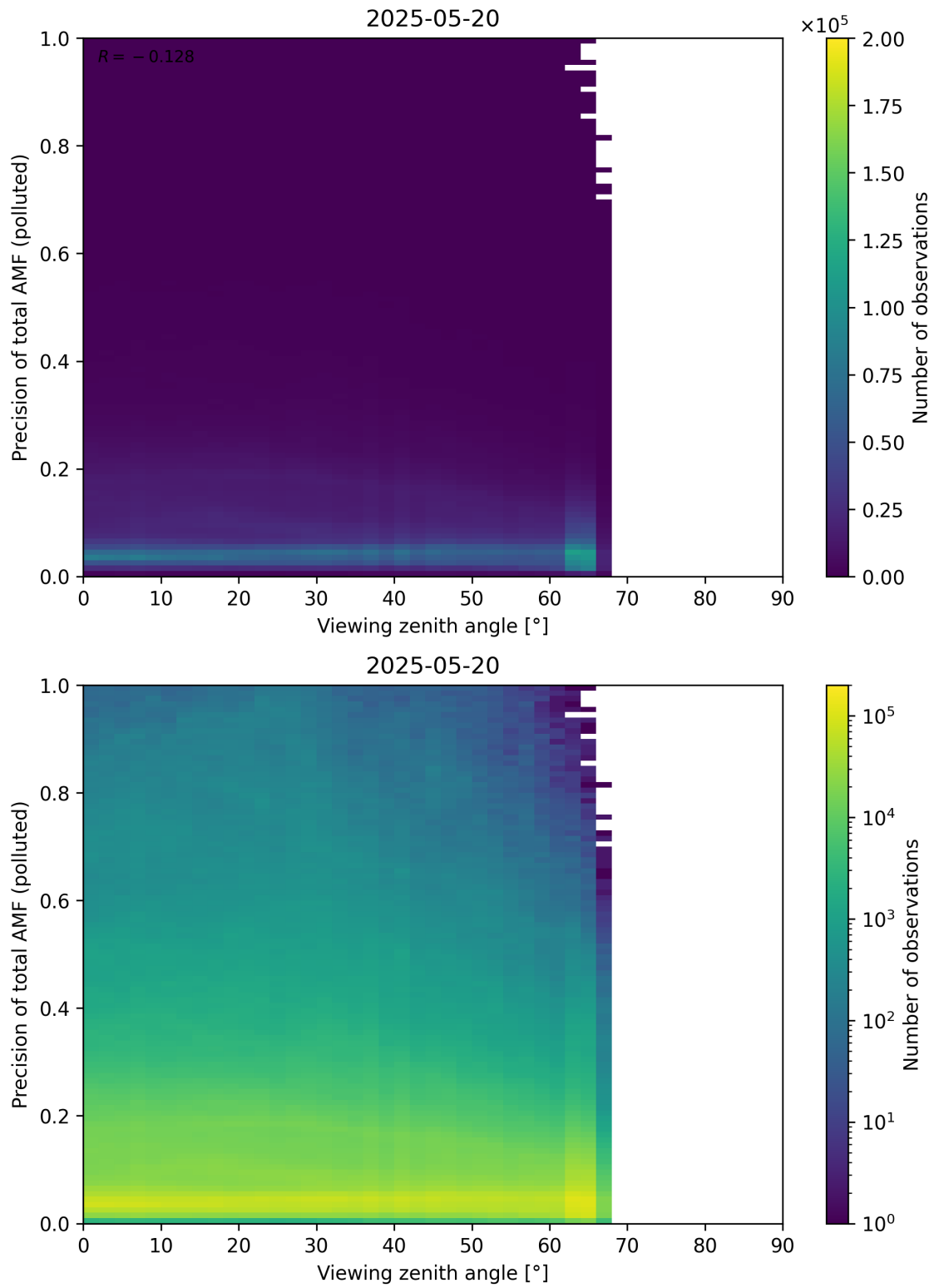
Figure 382: Scatter density plot of “Viewing zenith angle” against “Precision of total AMF (polluted)” for 2025-05-19 to 2025-05-21.
