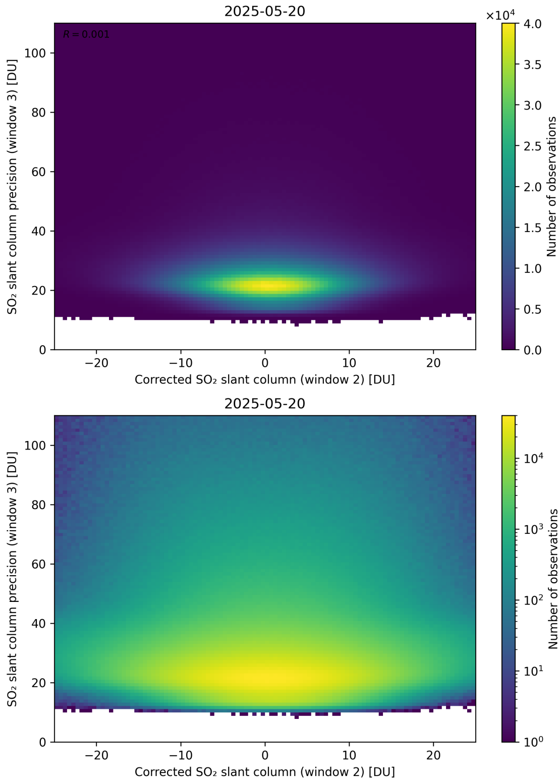
Figure 252: Scatter density plot of “Corrected SO 2 slant column (window 2)” against “SO 2 slant column precision (window 3)” for 2025-05-19 to 2025-05-21.
