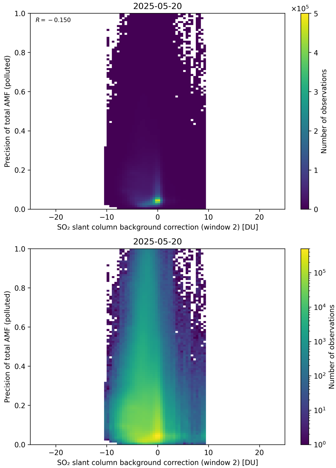
Figure 131: Scatter density plot of “SO 2 slant column background correction (window 2)” against “Precision of total AMF (polluted)” for 2025-05-19 to 2025-05-21.
