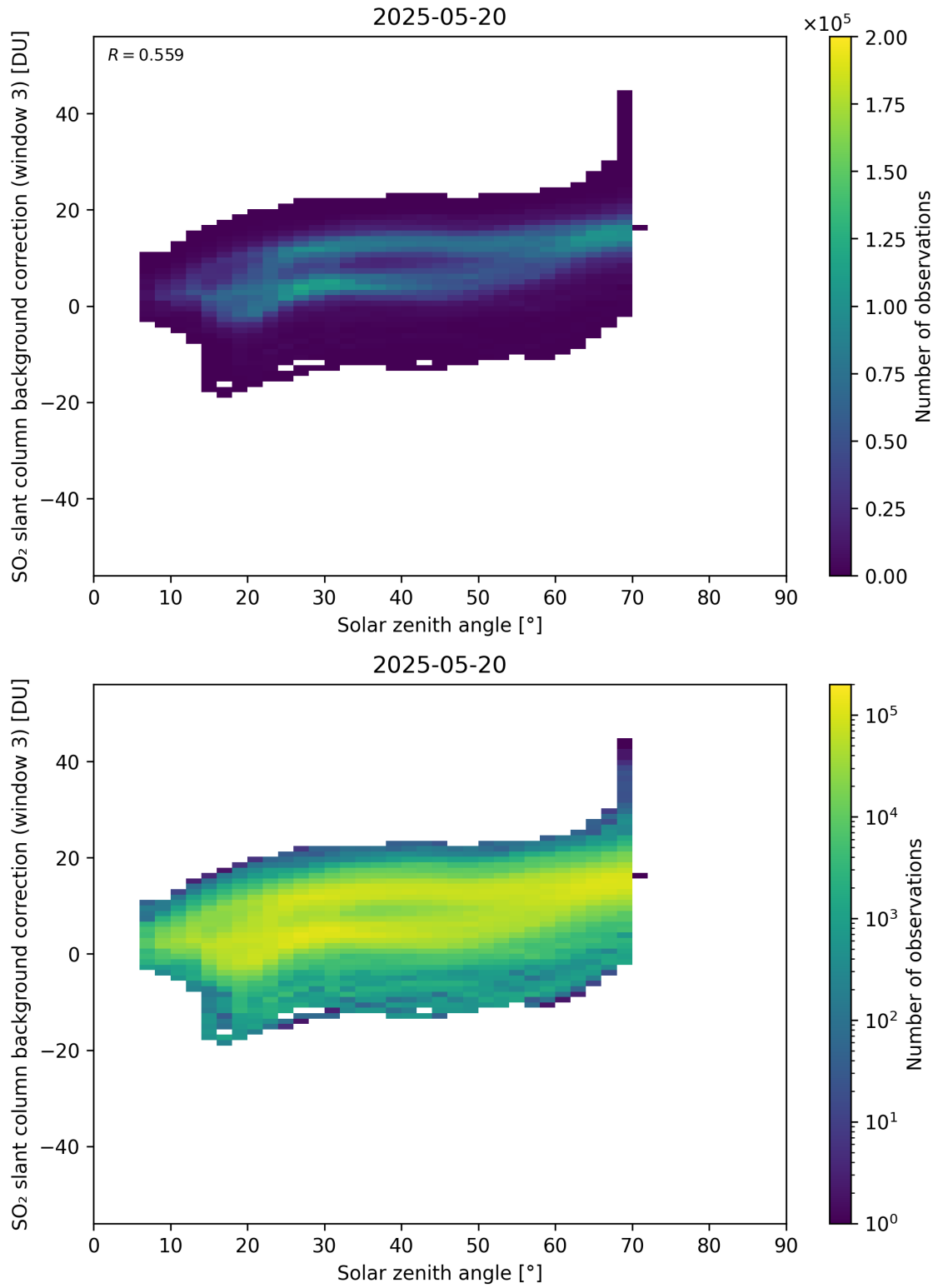
Figure 173: Scatter density plot of “Solar zenith angle” against “SO 2 slant column background correction (window 3)” for 2025-05-19 to 2025-05-21.
