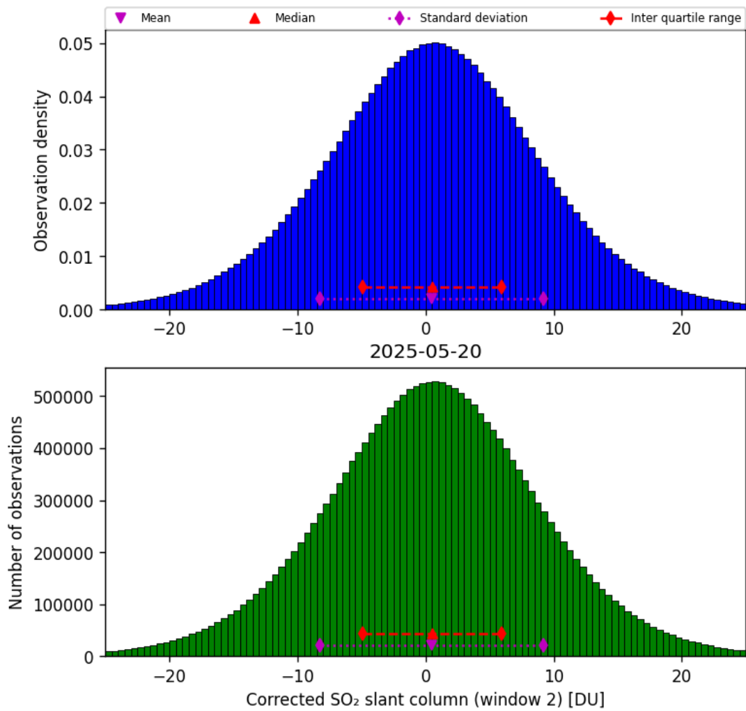
Figure 69: Histogram of “Corrected SO 2 slant column (window 2)” for 2025-05-19 to 2025-05-21
