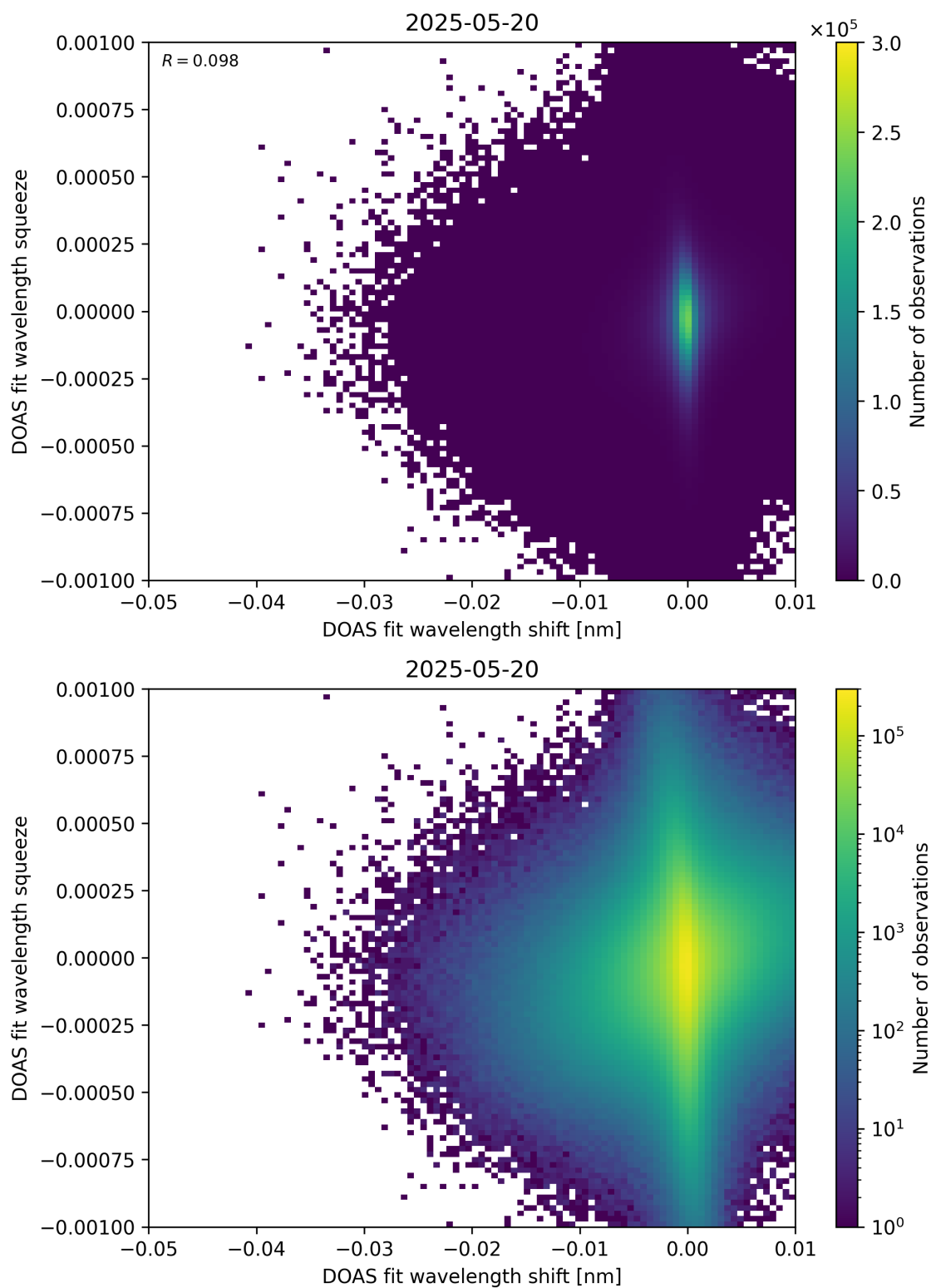
Figure 138: Scatter density plot of “DOAS fit wavelength shift” against “DOAS fit wavelength squeeze” for 2025-05-19 to 2025-05-21.
