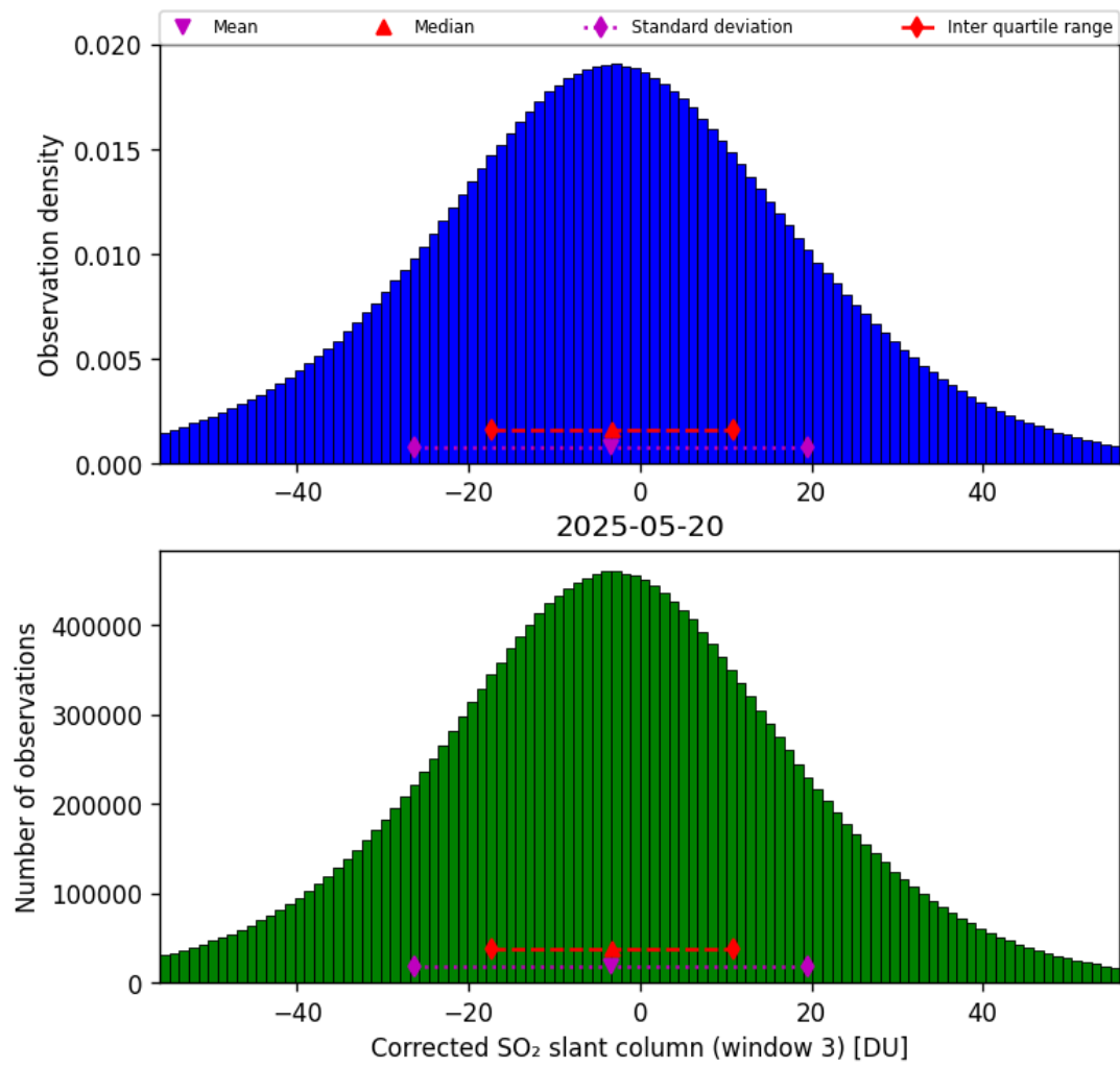
Figure 73: Histogram of “Corrected SO 2 slant column (window 3)” for 2025-05-19 to 2025-05-21
