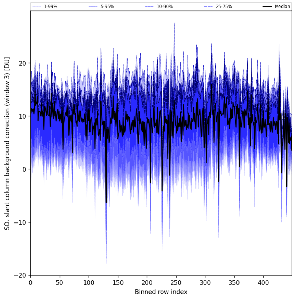
Figure 100: Along track statistics of “SO 2 slant column background correction (window 3)” for 2025-05-19 to 2025-05-21
