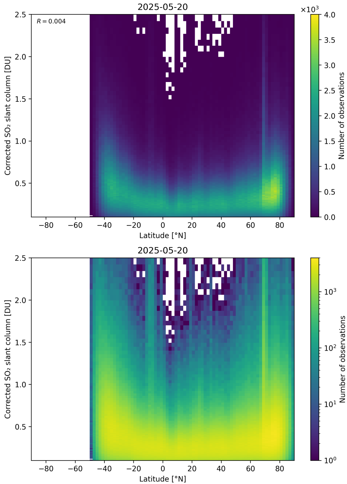
Figure 159: Scatter density plot of “Latitude” against “Corrected SO 2 slant column” for 2025-05-19 to 2025-05-21.
