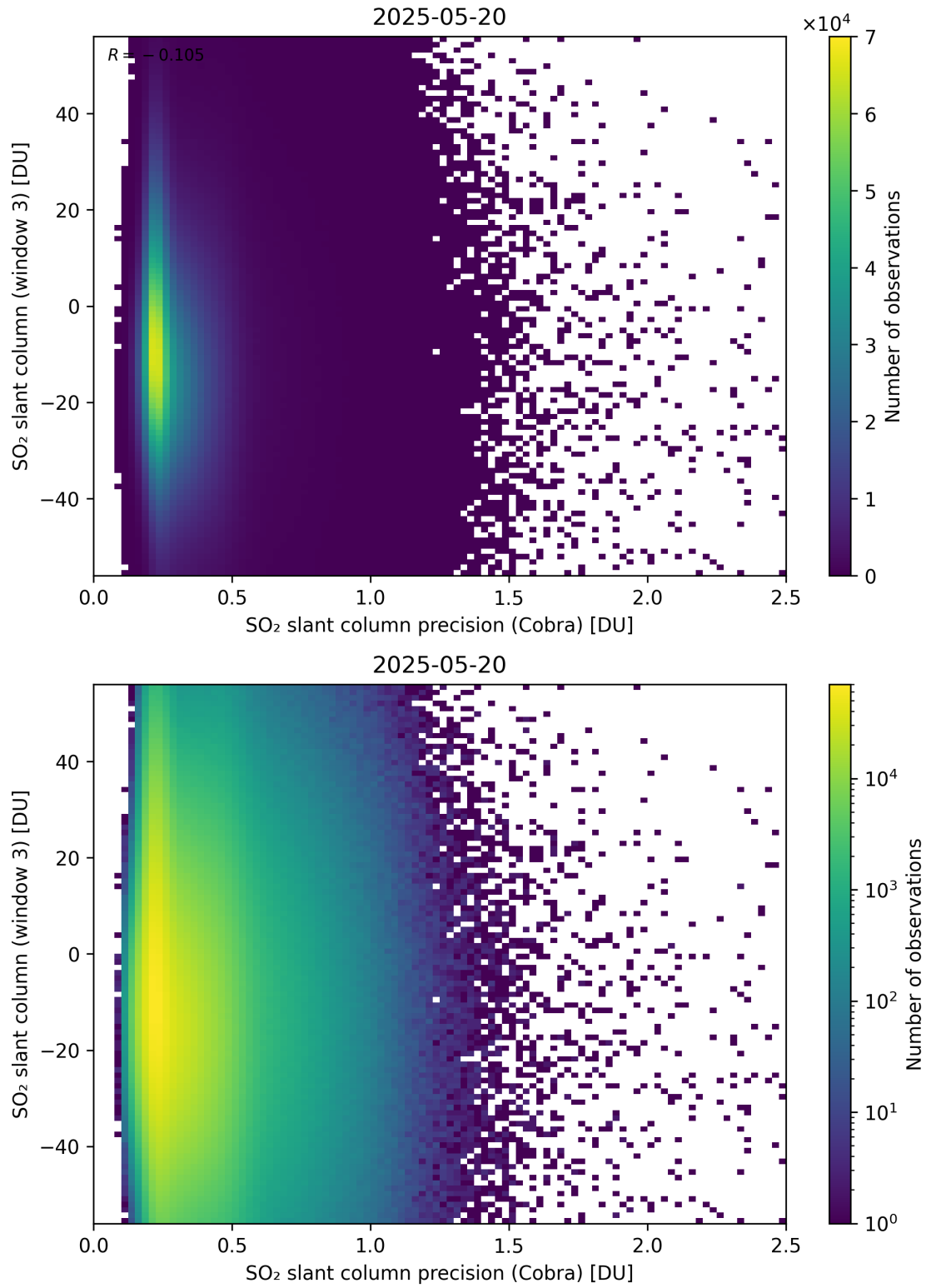
Figure 211: Scatter density plot of “SO 2 slant column precision (Cobra)” against “SO 2 slant column (window 3)” for 2025-05-19 to 2025-05-21.
