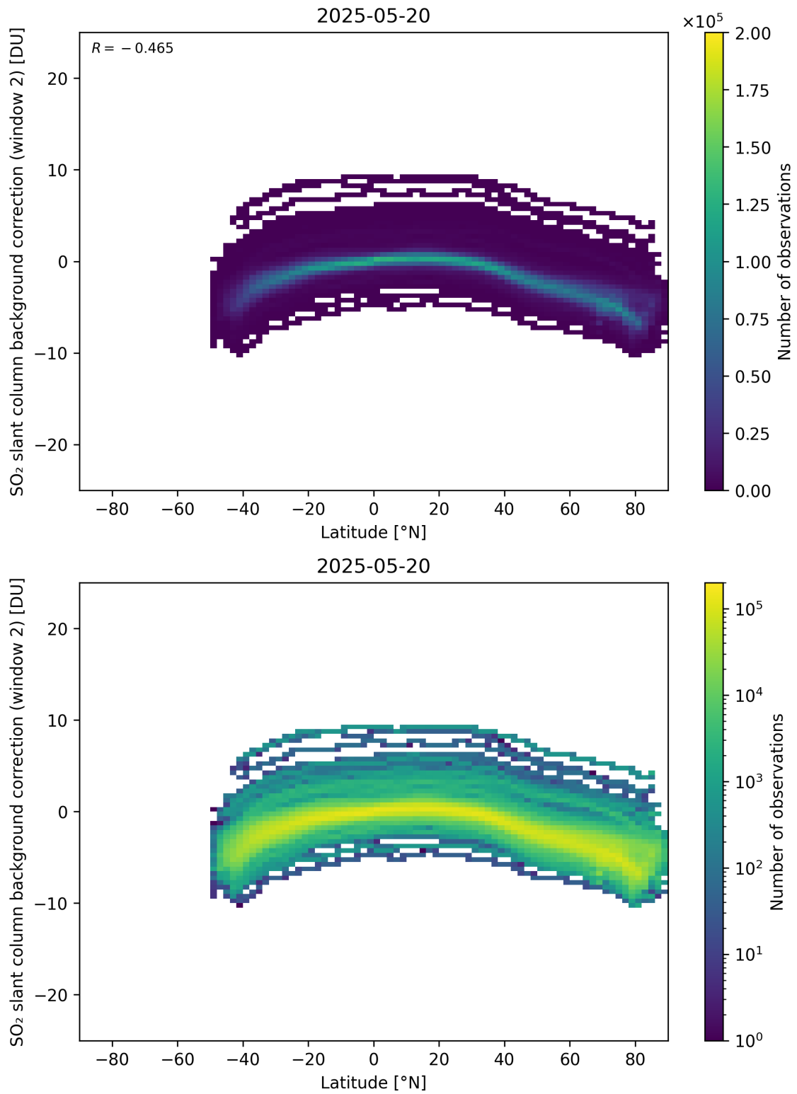
Figure 151: Scatter density plot of “Latitude” against “SO 2 slant column background correction (window 2)” for 2025-05-19 to 2025-05-21.
