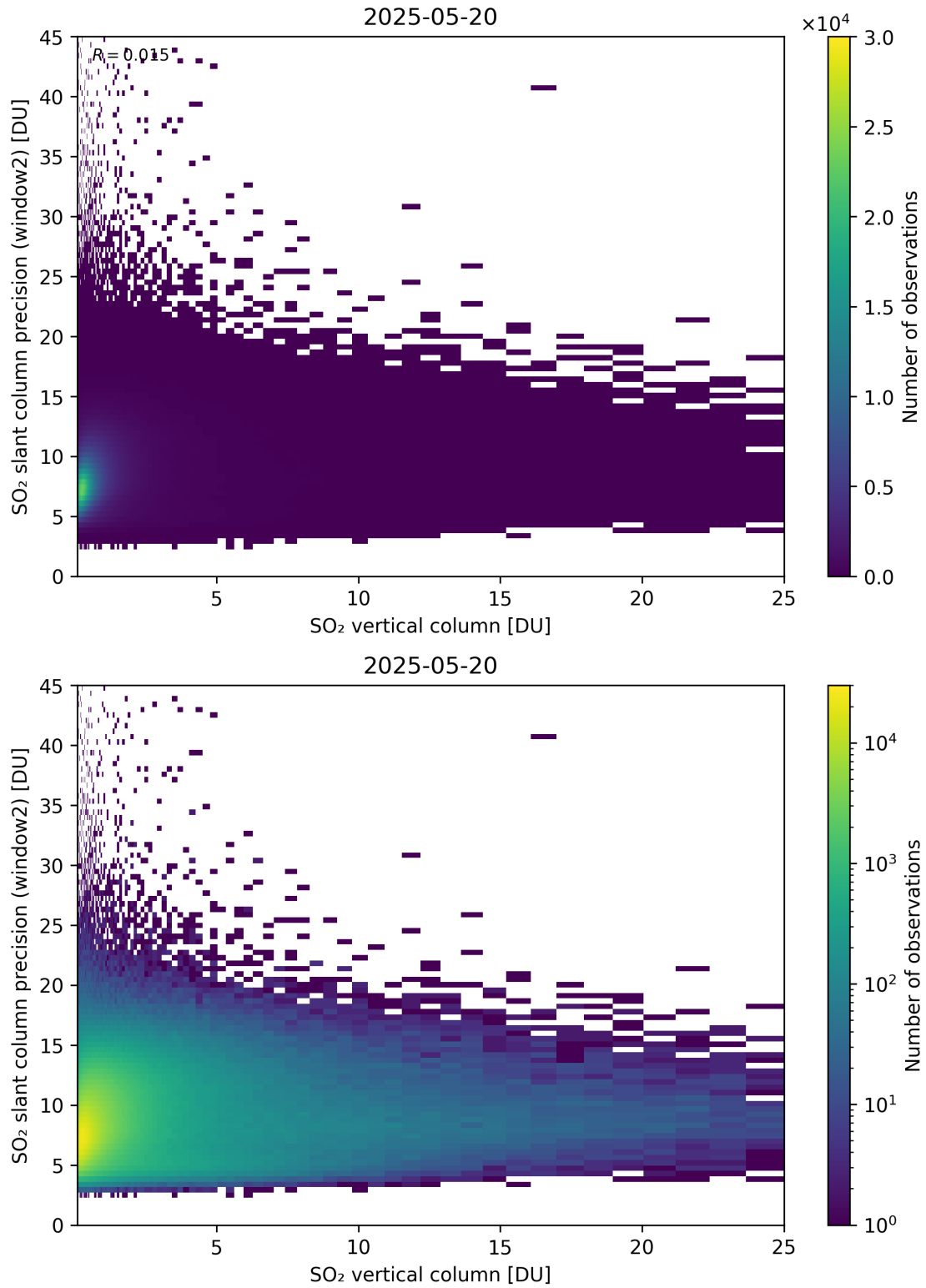
Figure 356: Scatter density plot of “SO 2 vertical column” against “SO 2 slant column precision (window2)” for 2025-05-19 to 2025-05-21.
