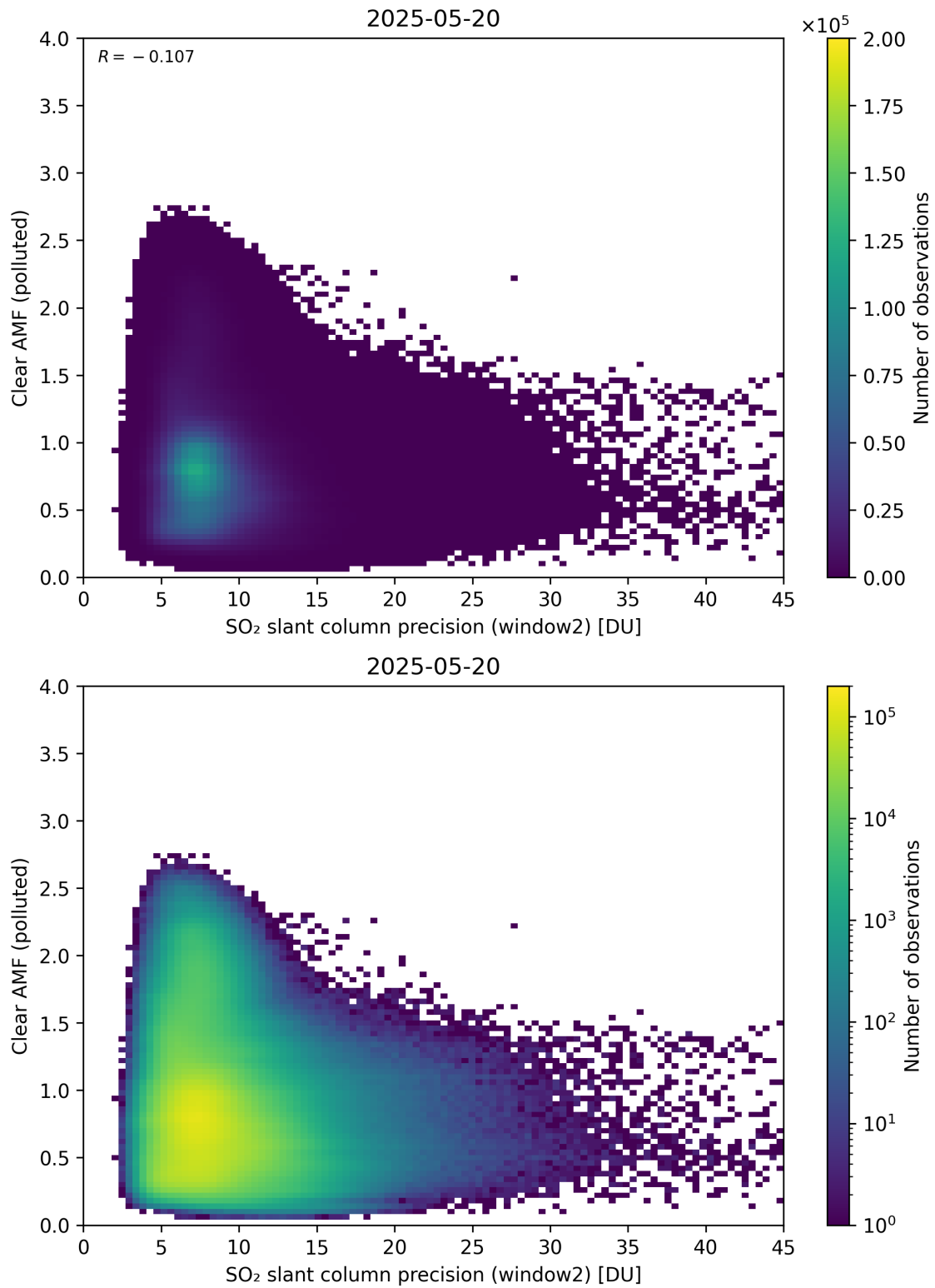
Figure 296: Scatter density plot of “SO 2 slant column precision (window2)” against “Clear AMF (polluted)” for 2025-05-19 to 2025-05-21.
