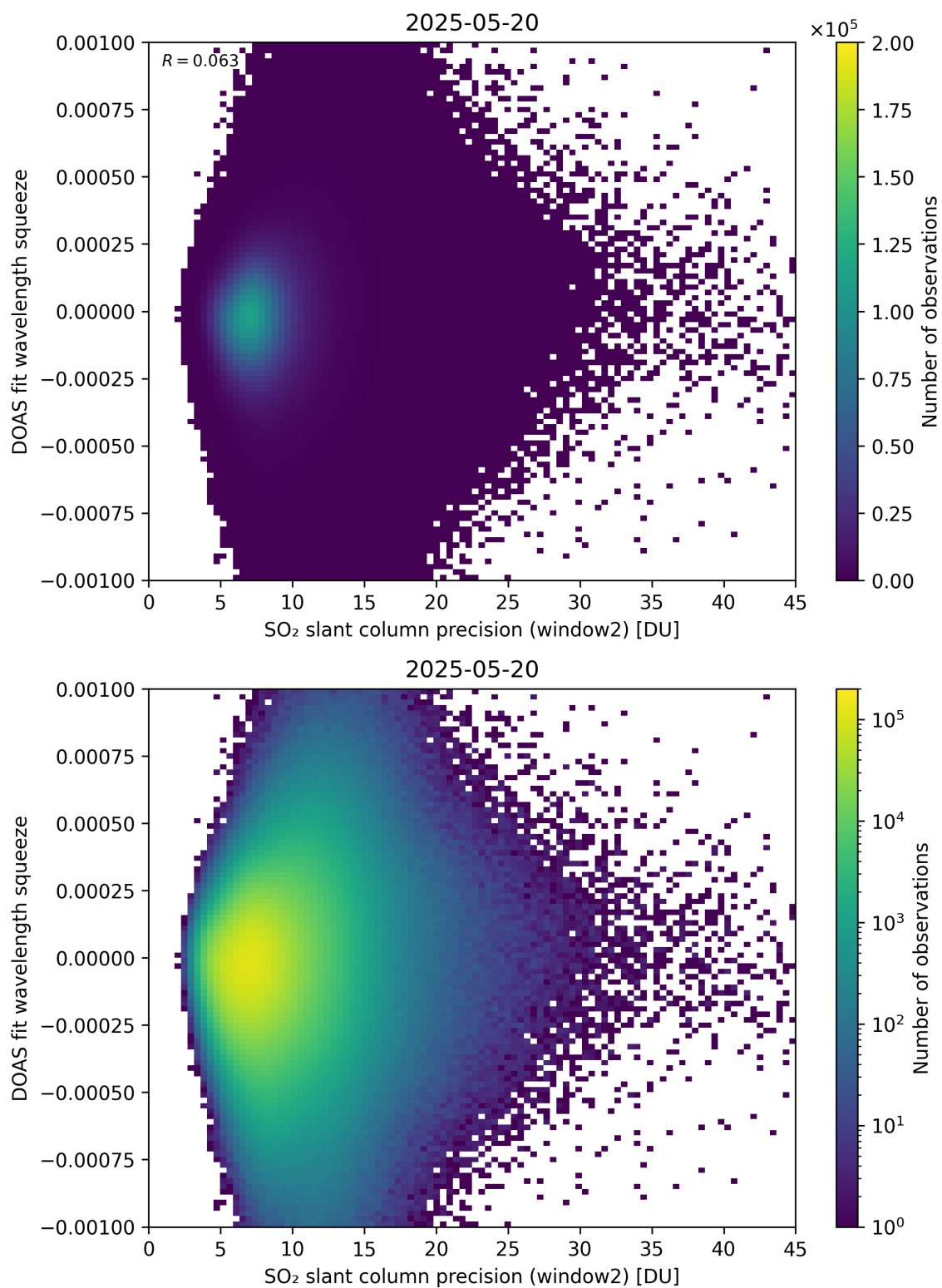
Figure 294: Scatter density plot of “SO 2 slant column precision (window2)” against “DOAS fit wavelength squeeze” for 2025-05-19 to 2025-05-21.
