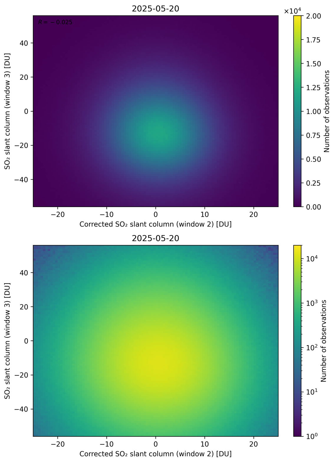
Figure 251: Scatter density plot of “Corrected SO 2 slant column (window 2)” against “SO 2 slant column (window 3)” for 2025-05-19 to 2025-05-21.
