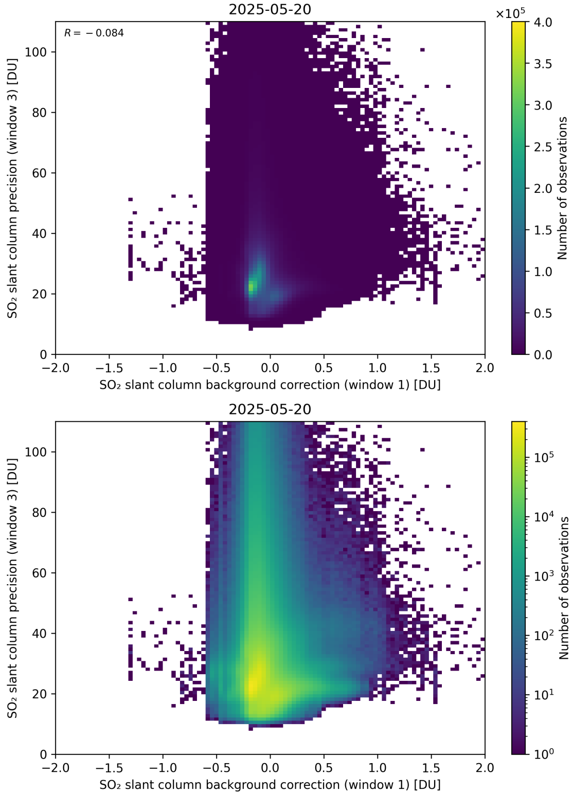
Figure 119: Scatter density plot of “SO 2 slant column background correction (window 1)” against “SO 2 slant column precision (window 3)” for 2025-05-19 to 2025-05-21.
