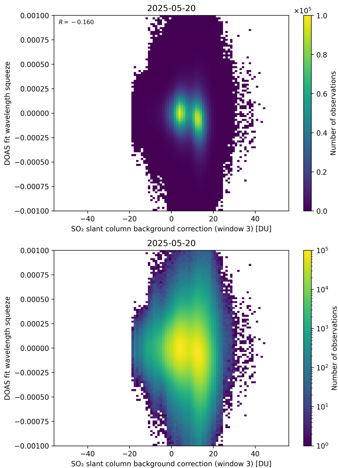
Figure 133: Scatter density plot of “SO 2 slant column background correction (window 3)” against “DOAS fit wavelength squeeze” for 2025-05-19 to 2025-05-21.
