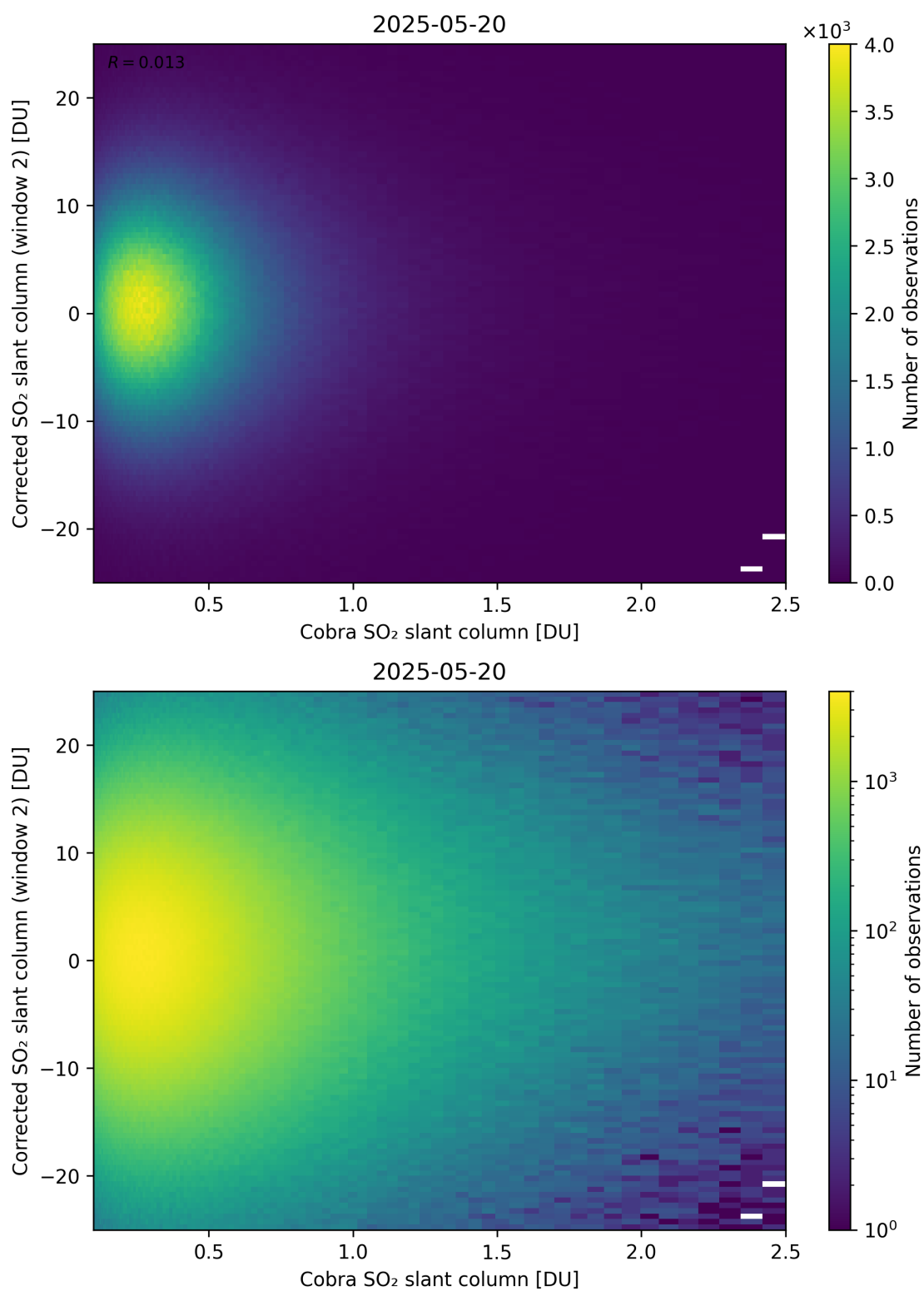
Figure 217: Scatter density plot of “Cobra SO 2 slant column” against “Corrected SO 2 slant column (window 2)” for 2025-05-19 to 2025-05-21.
