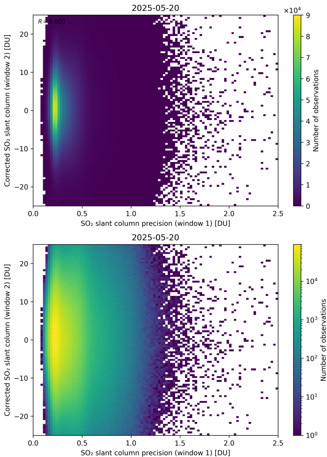
Figure 275: Scatter density plot of “SO 2 slant column precision (window 1)” against “Corrected SO 2 slant column (window 2)” for 2025-05-19 to 2025-05-21.
