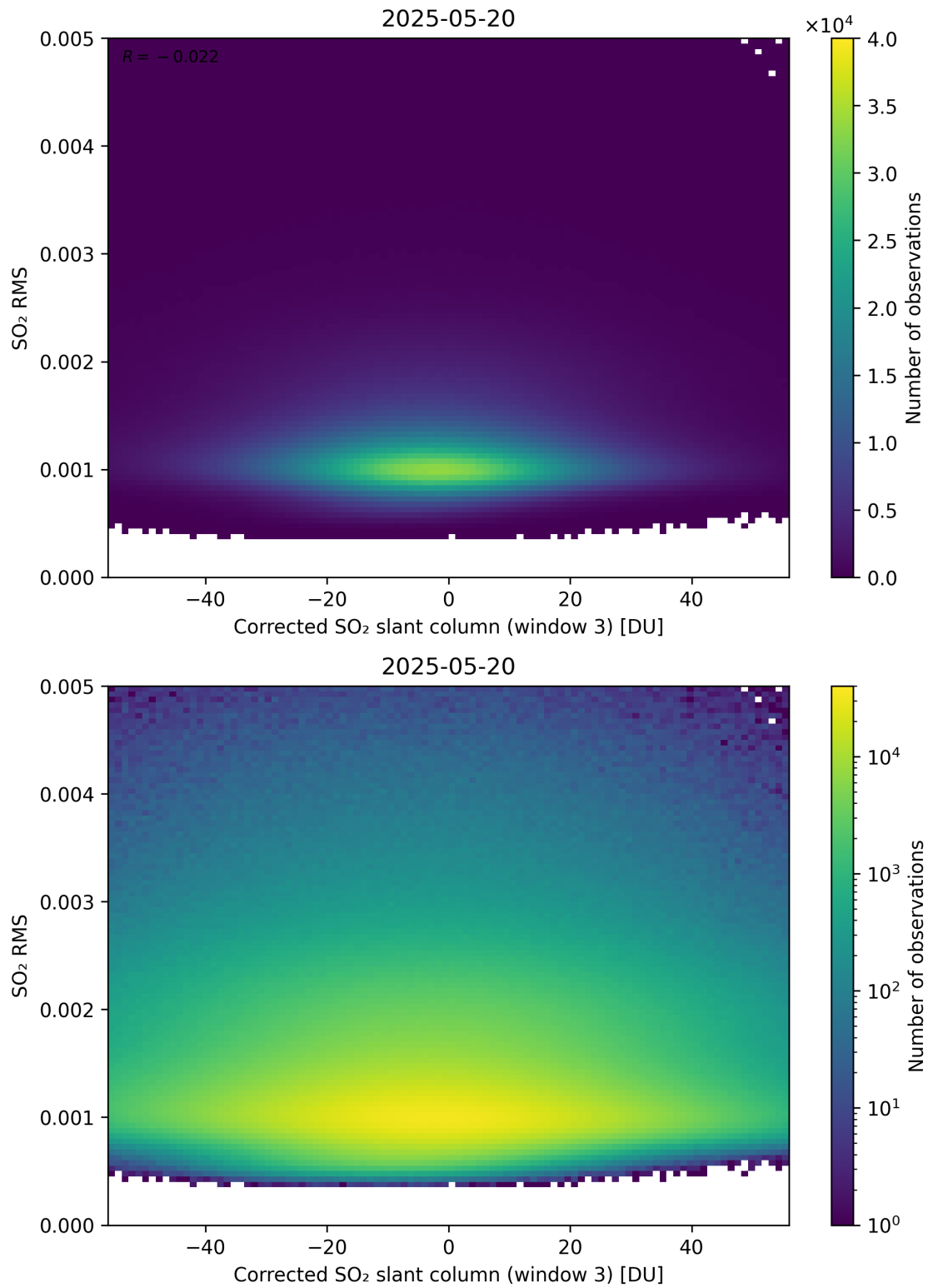
Figure 258: Scatter density plot of “Corrected SO 2 slant column (window 3)” against “SO 2 RMS” for 2025-05-19 to 2025-05-21.
