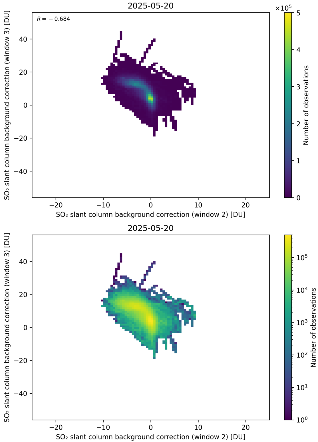
Figure 122: Scatter density plot of “SO 2 slant column background correction (window 2)” against “SO 2 slant column background correction (window 3)” for 2025-05-19 to 2025-05-21.
