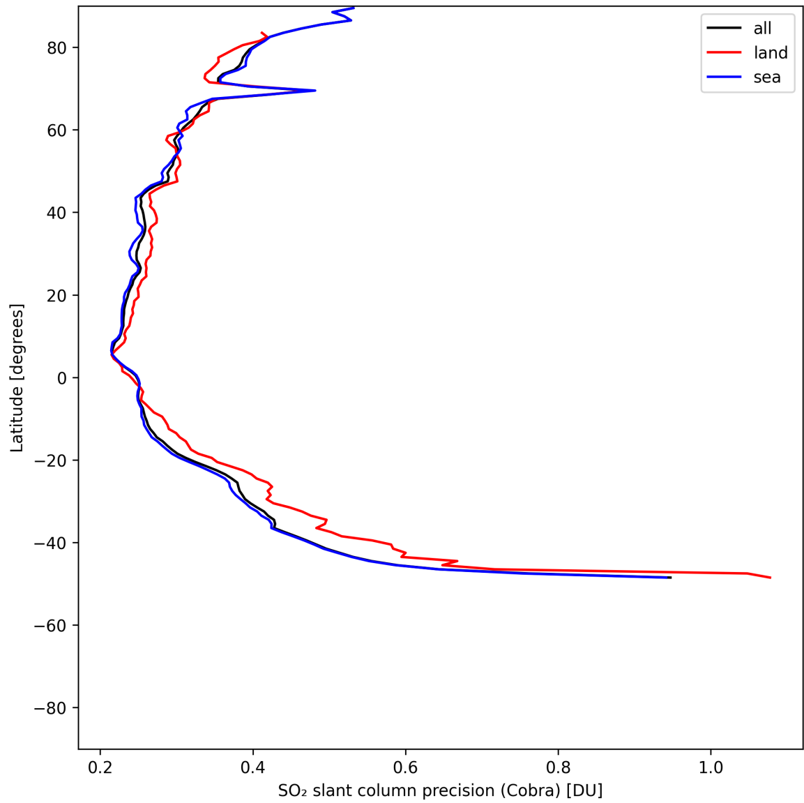
Figure 36: Zonal average of “SO 2 slant column precision (Cobra)” for 2025-05-19 to 2025-05-21.
