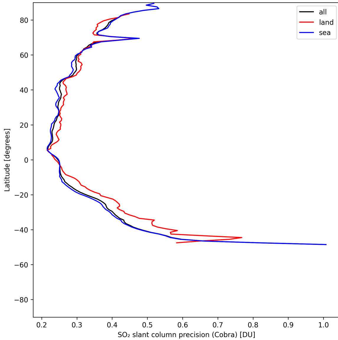
Figure 36: Zonal average of “SO 2 slant column precision (Cobra)” for 2025-05-21 to 2025-05-22.
