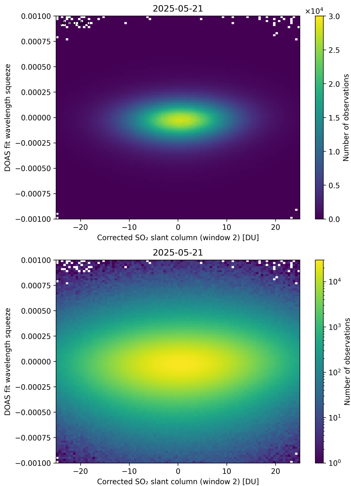
Figure 247: Scatter density plot of “Corrected SO 2 slant column (window 2)” against “DOAS fit wavelength squeeze” for 2025-05-21 to 2025-05-22.
