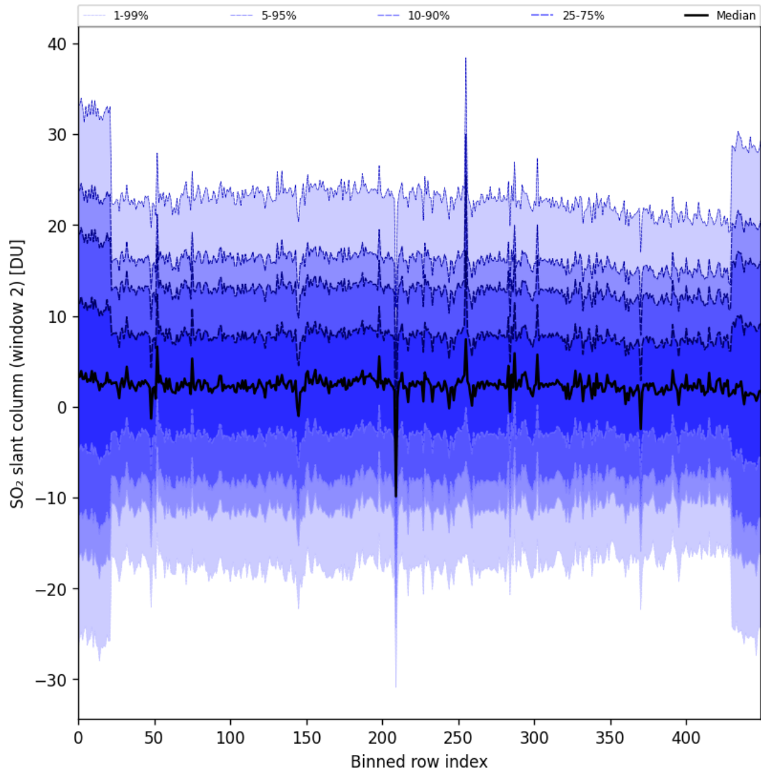
Figure 93: Along track statistics of “SO 2 slant column (window 2)” for 2025-05-21 to 2025-05-22
