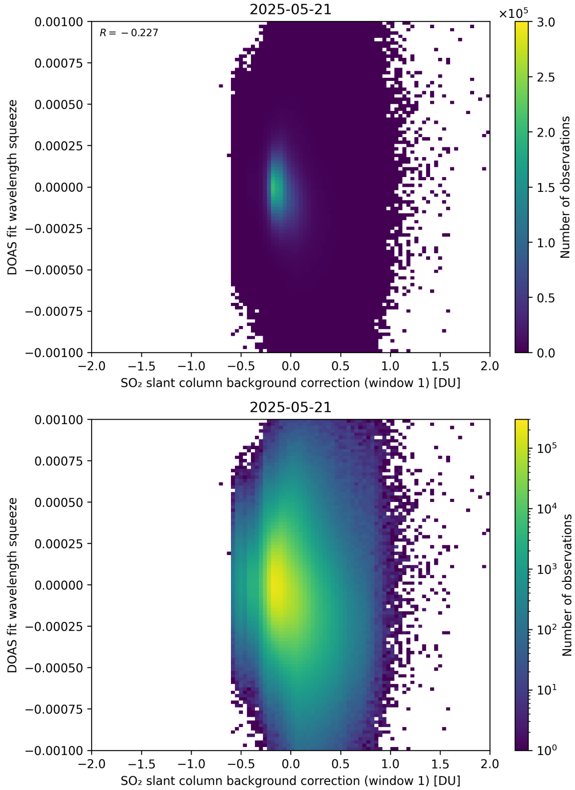
Figure 112: Scatter density plot of “SO 2 slant column background correction (window 1)” against “DOAS fit wavelength squeeze” for 2025-05-21 to 2025-05-22.
