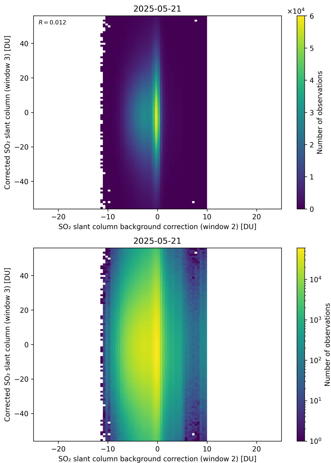
Figure 127: Scatter density plot of “SO 2 slant column background correction (window 2)” against “Corrected SO 2 slant column (window 3)” for 2025-05-21 to 2025-05-22.
