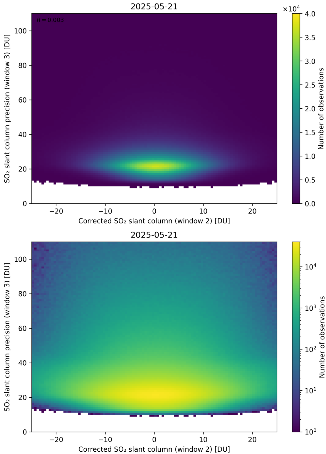
Figure 252: Scatter density plot of “Corrected SO 2 slant column (window 2)” against “SO 2 slant column precision (window 3)” for 2025-05-21 to 2025-05-22.
