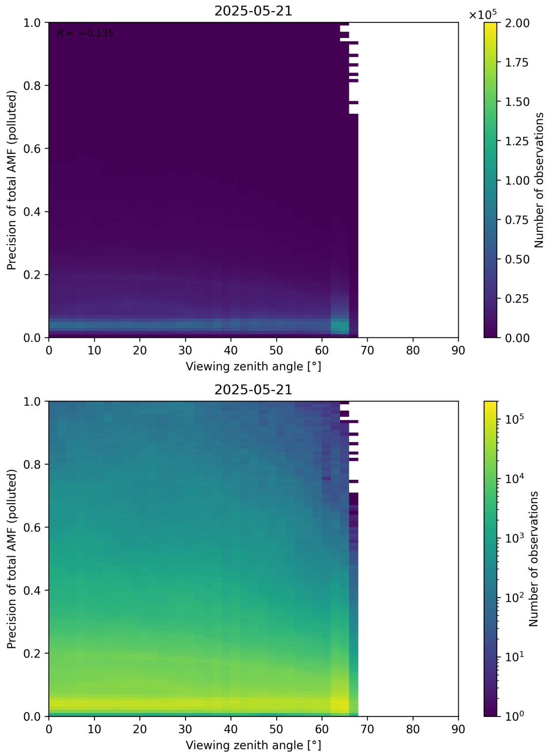
Figure 382: Scatter density plot of “Viewing zenith angle” against “Precision of total AMF (polluted)” for 2025-05-21 to 2025-05-22.
