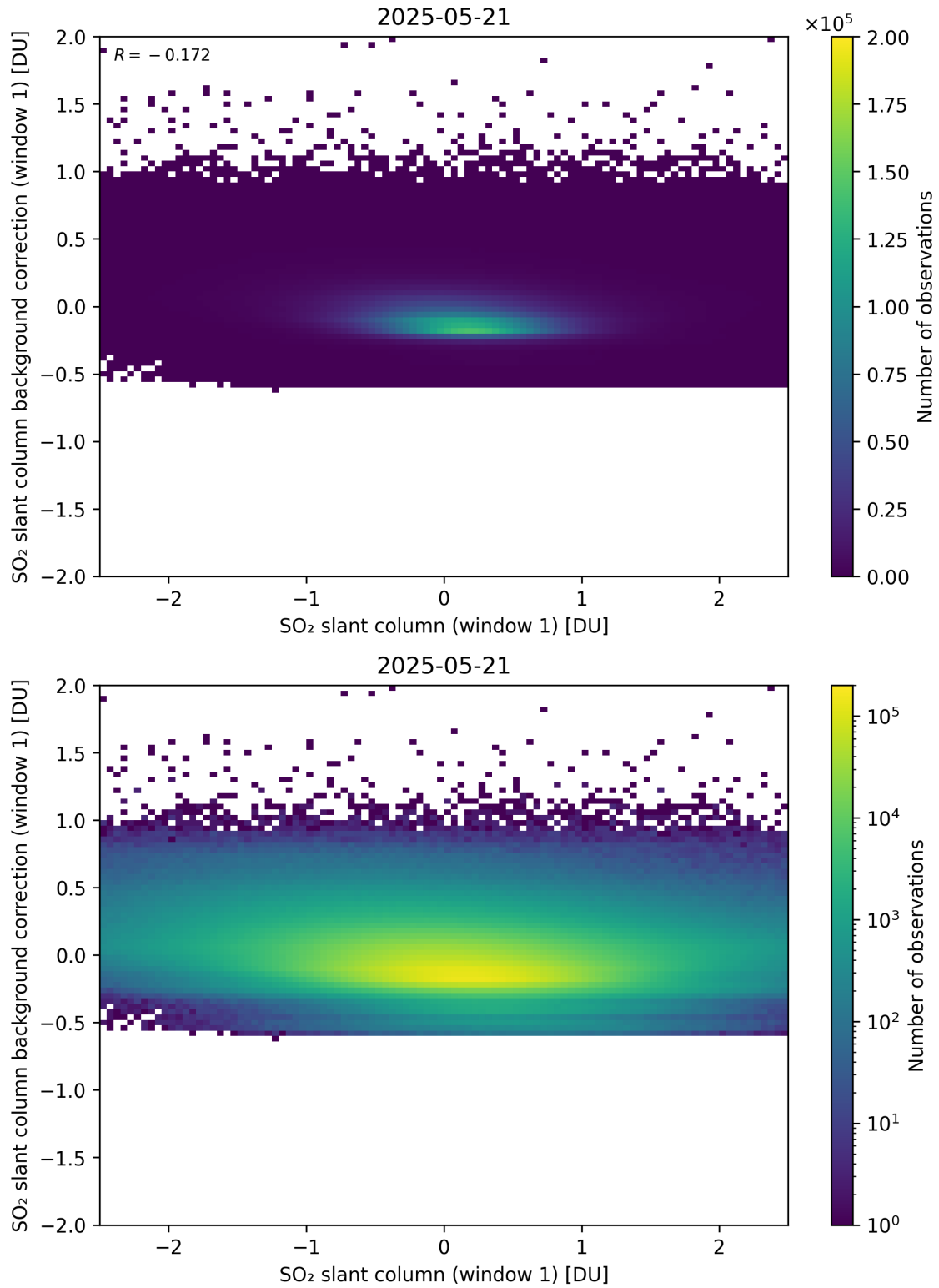
Figure 262: Scatter density plot of “SO 2 slant column (window 1)” against “SO 2 slant column background correction (window 1)” for 2025-05-21 to 2025-05-22.
