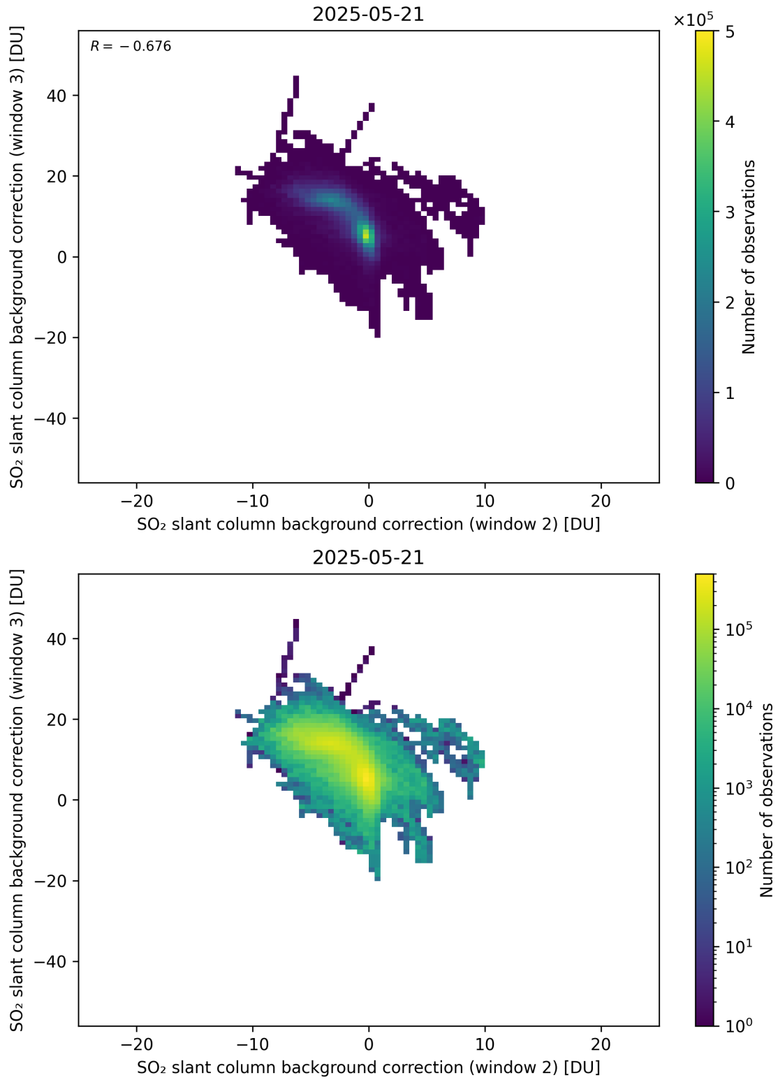
Figure 122: Scatter density plot of “SO 2 slant column background correction (window 2)” against “SO 2 slant column background correction (window 3)” for 2025-05-21 to 2025-05-22.
