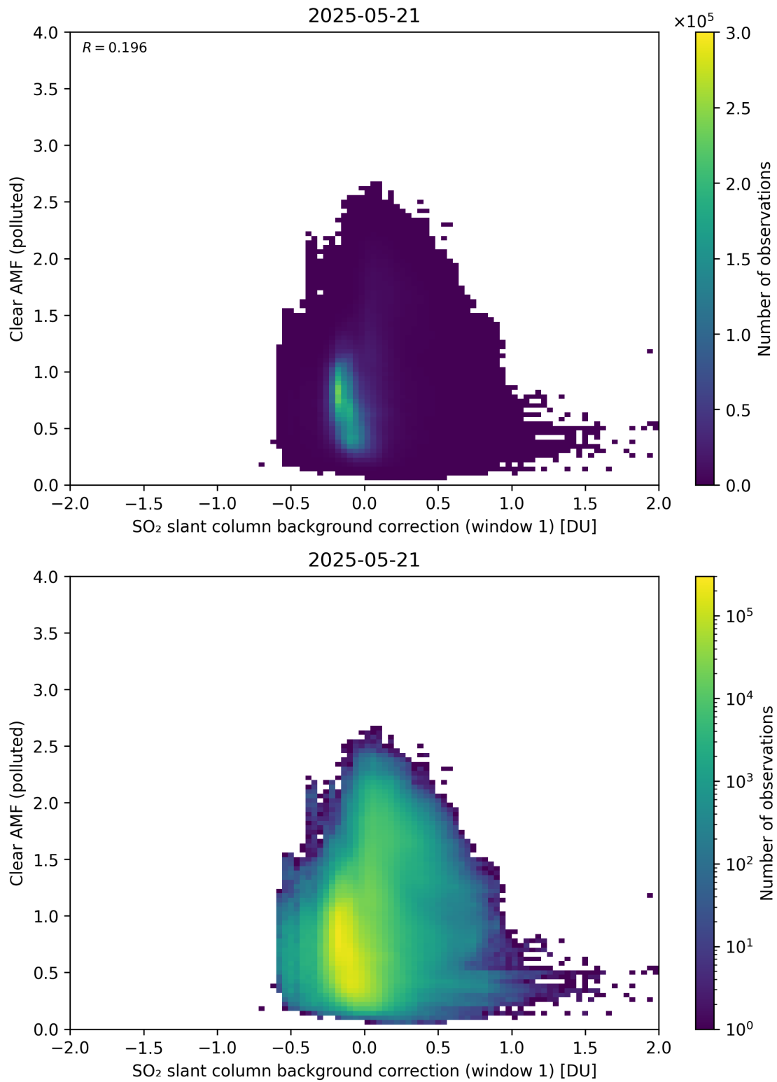
Figure 114: Scatter density plot of “SO 2 slant column background correction (window 1)” against “Clear AMF (polluted)” for 2025-05-21 to 2025-05-22.
