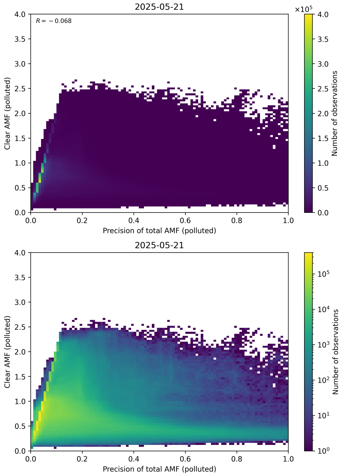
Figure 320: Scatter density plot of “Precision of total AMF (polluted)” against “Clear AMF (polluted)” for 2025-05-21 to 2025-05-22.
