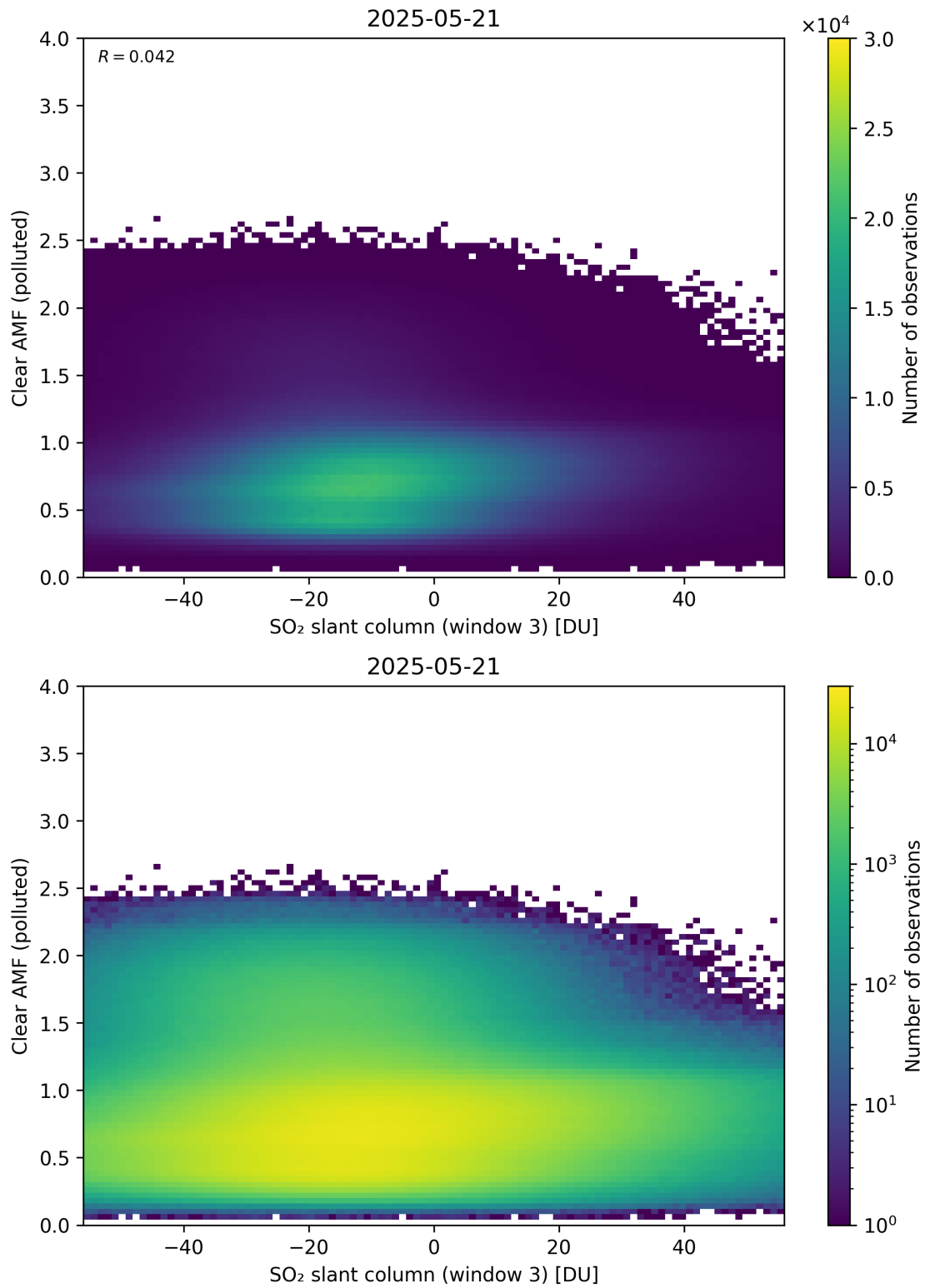
Figure 315: Scatter density plot of “SO 2 slant column (window 3)” against “Clear AMF (polluted)” for 2025-05-21 to 2025-05-22.
