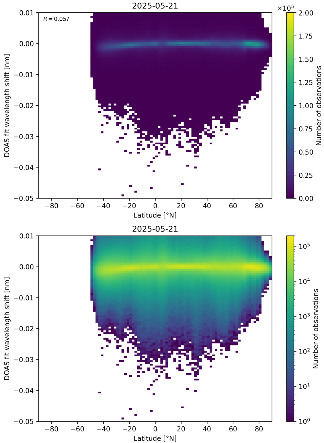
Figure 153: Scatter density plot of “Latitude” against “DOAS fit wavelength shift” for 2025-05-21 to 2025-05-22.
