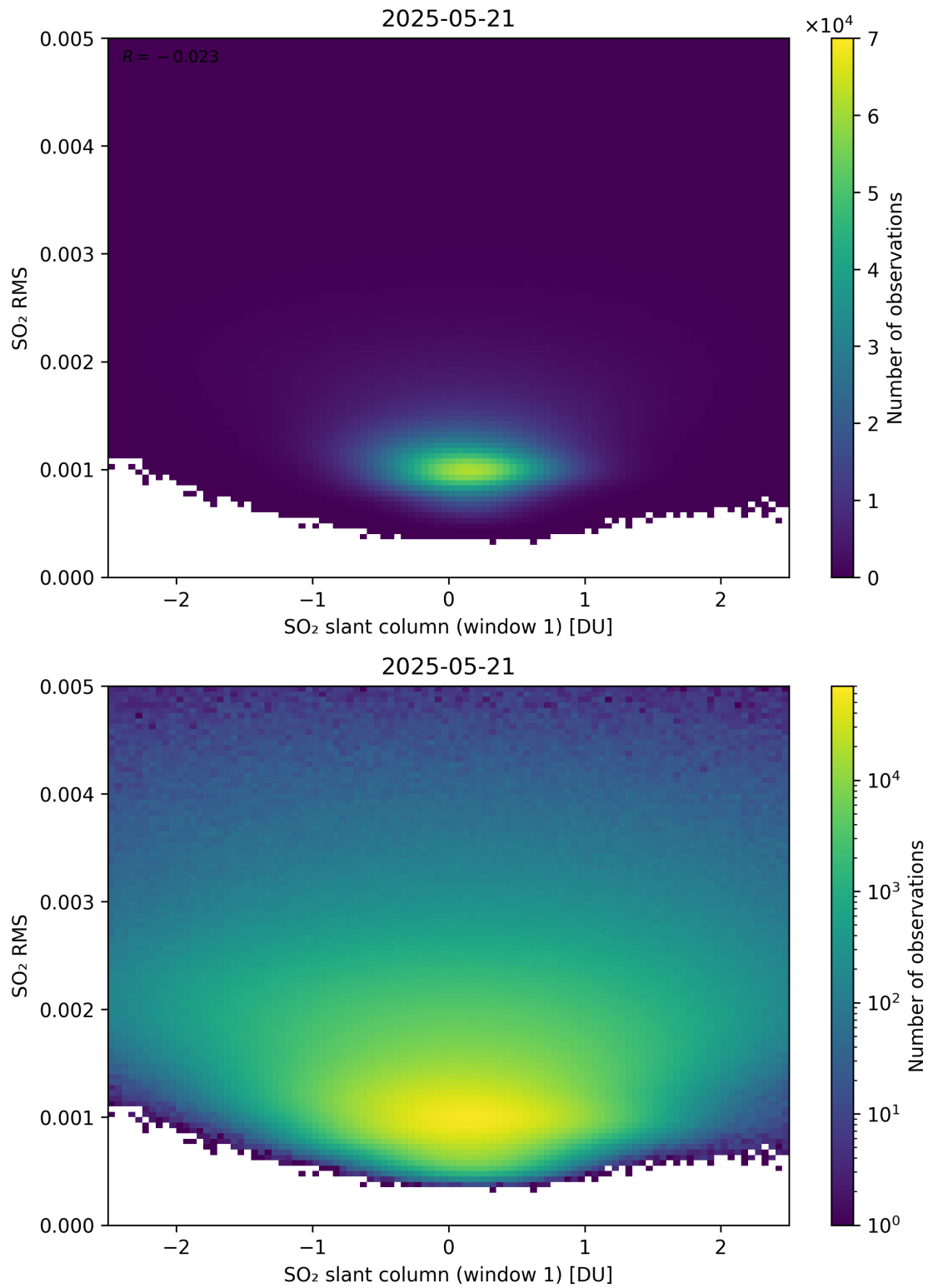
Figure 267: Scatter density plot of “SO 2 slant column (window 1)” against “SO 2 RMS” for 2025-05-21 to 2025-05-22.
