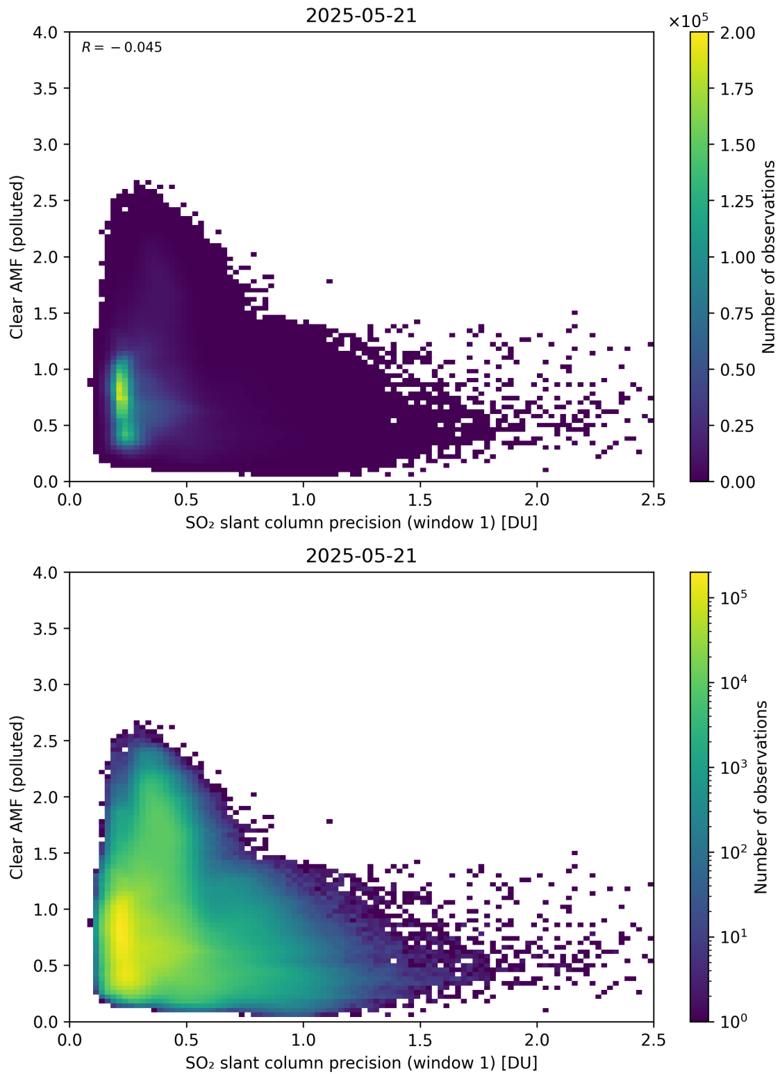
Figure 274: Scatter density plot of “SO 2 slant column precision (window 1)” against “Clear AMF (polluted)” for 2025-05-21 to 2025-05-22.
