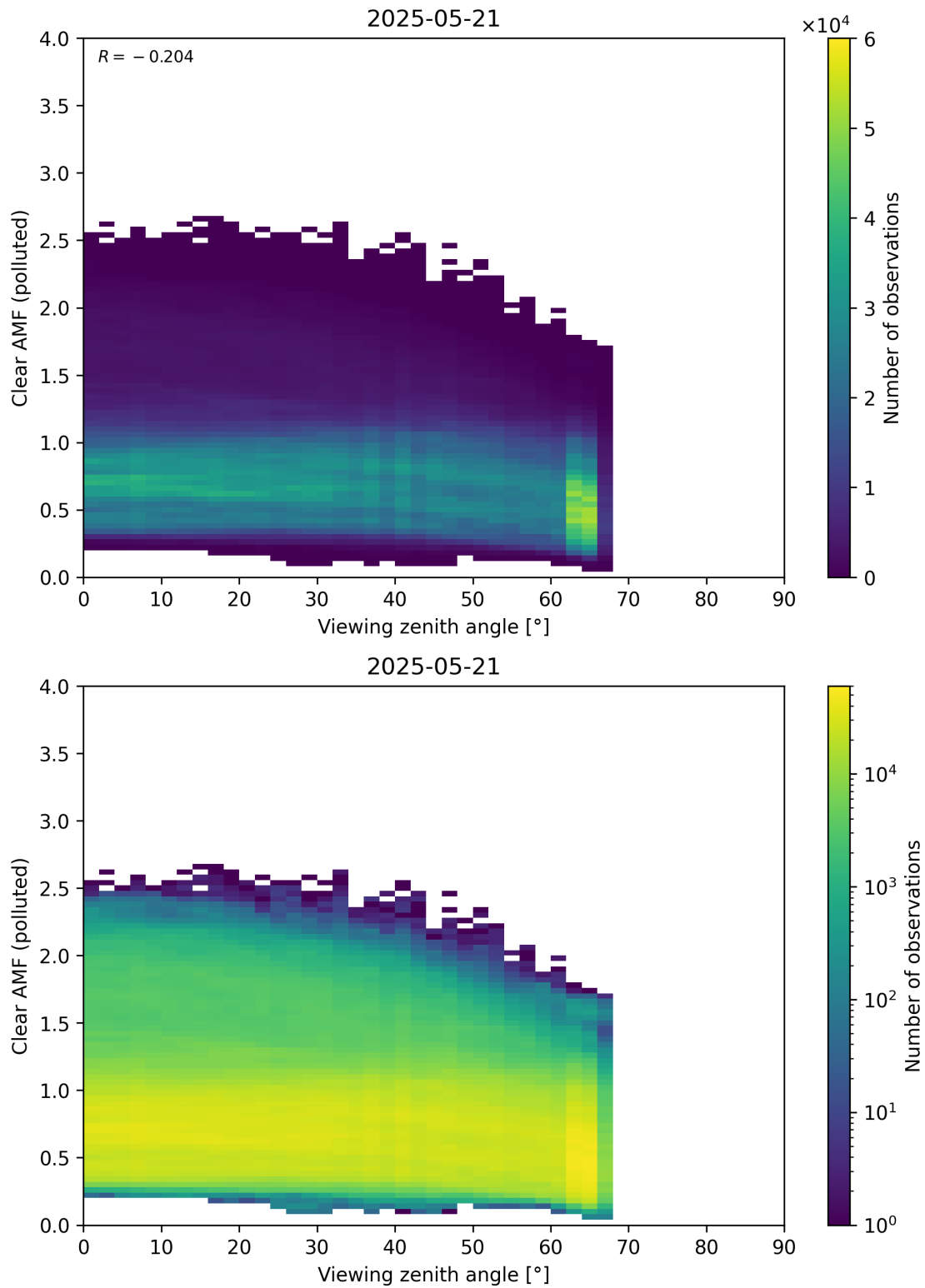
Figure 370: Scatter density plot of “Viewing zenith angle” against “Clear AMF (polluted)” for 2025-05-21 to 2025-05-22.
