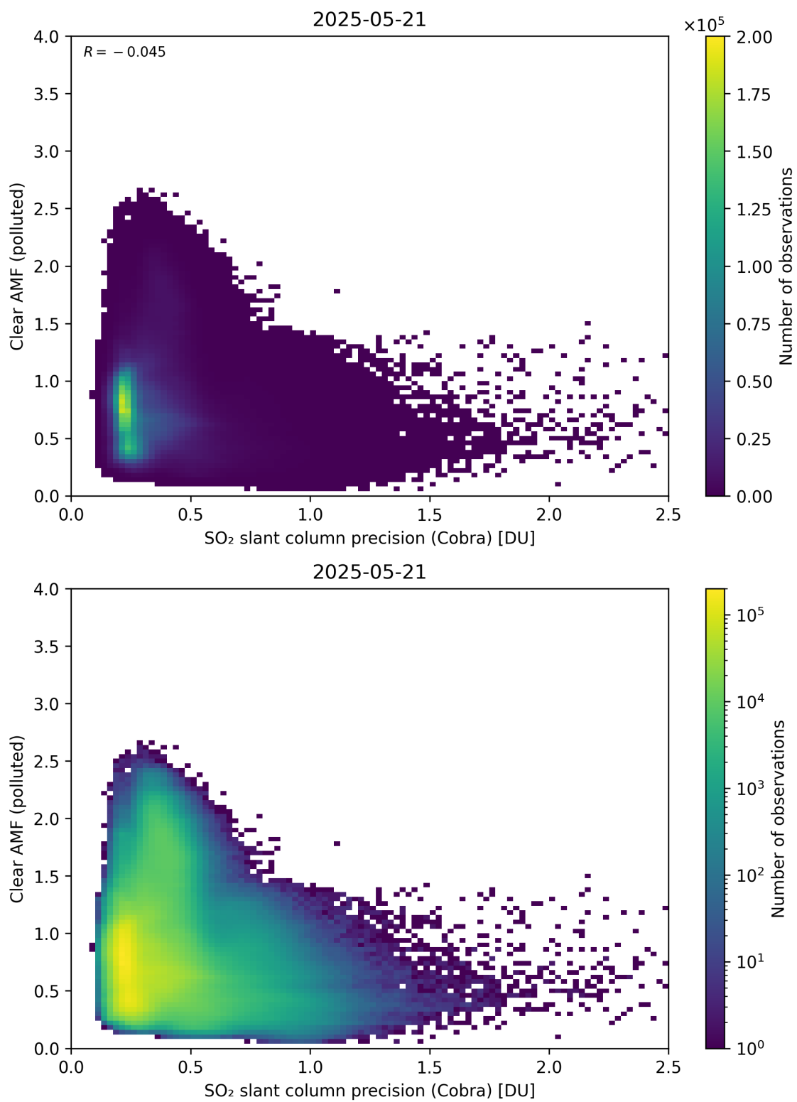
Figure 205: Scatter density plot of “SO 2 slant column precision (Cobra)” against “Clear AMF (polluted)” for 2025-05-21 to 2025-05-22.
