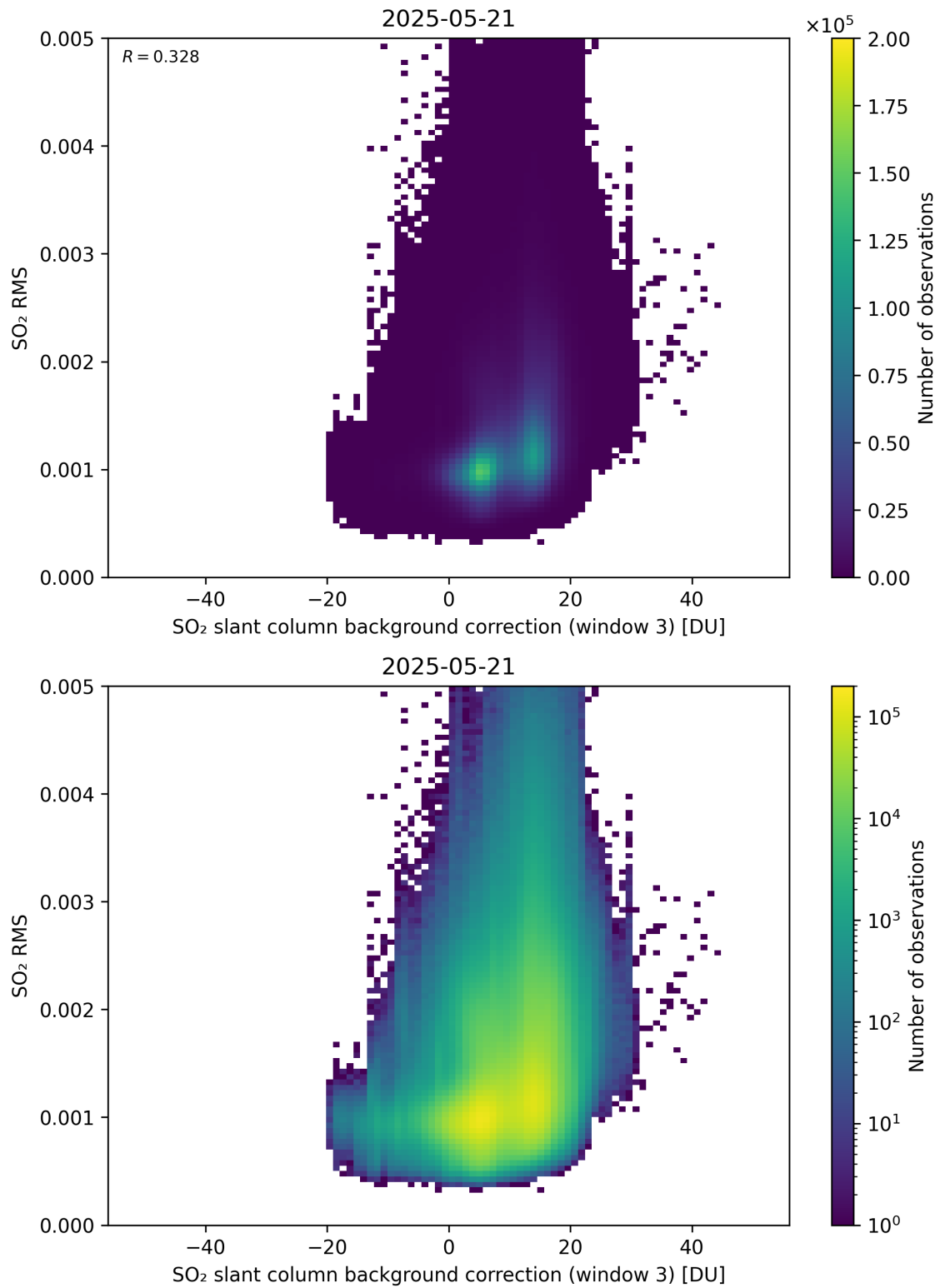
Figure 134: Scatter density plot of “SO 2 slant column background correction (window 3)” against “SO 2 RMS” for 2025-05-21 to 2025-05-22.
