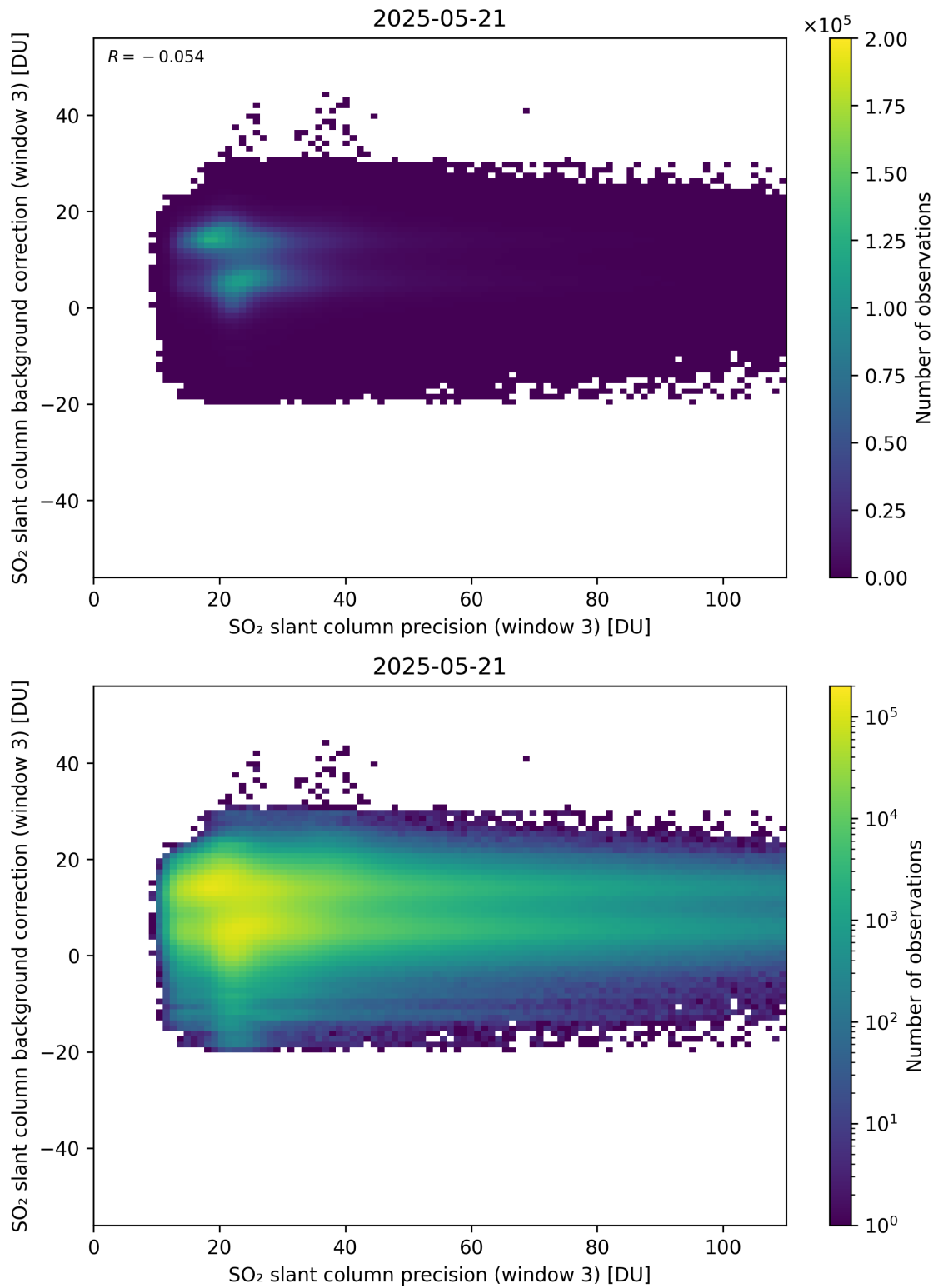
Figure 307: Scatter density plot of “SO 2 slant column precision (window 3)” against “SO 2 slant column background correction (window 3)” for 2025-05-21 to 2025-05-22.
