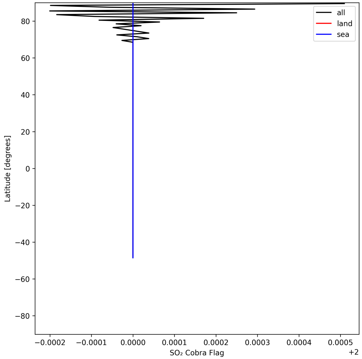
Figure 49: Zonal average of "SO 2 Cobra Flag" for 2025-05-21 to 2025-05-22.
