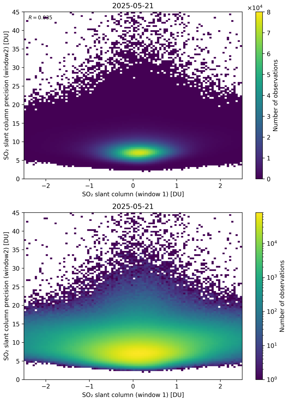
Figure 286: Scatter density plot of “SO 2 slant column (window 1)” against “SO 2 slant column precision (window2)” for 2025-05-21 to 2025-05-22.
