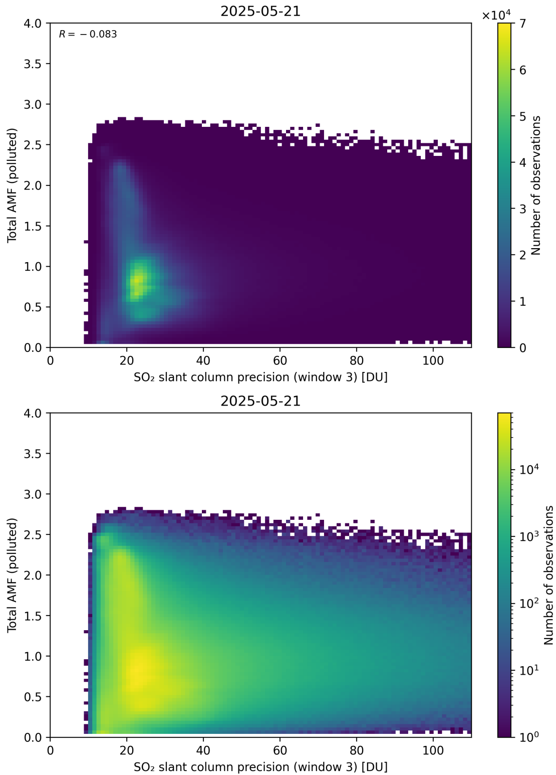
Figure 313: Scatter density plot of “SO 2 slant column precision (window 3)” against “Total AMF (polluted)” for 2025-05-21 to 2025-05-22.
