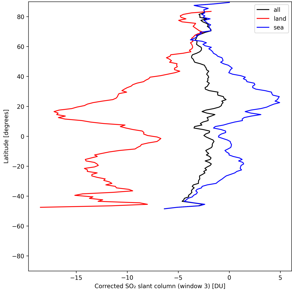
Figure 47: Zonal average of “Corrected SO 2 slant column (window 3)” for 2025-05-21 to 2025-05-22.
