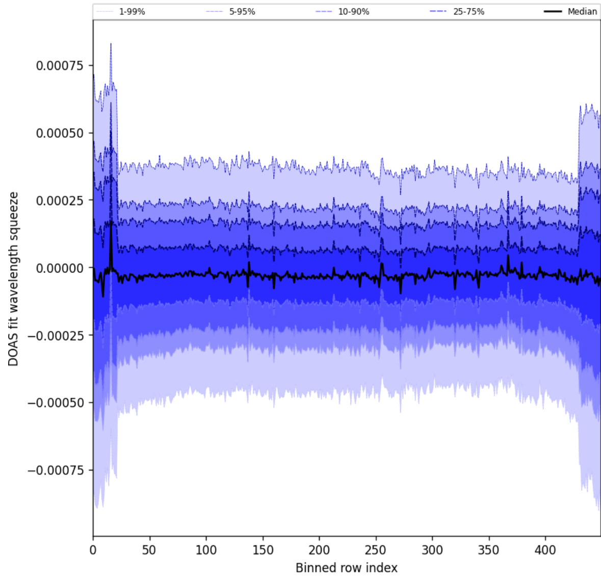
Figure 103: Along track statistics of “DOAS fit wavelength squeeze” for 2025-05-21 to 2025-05-22
