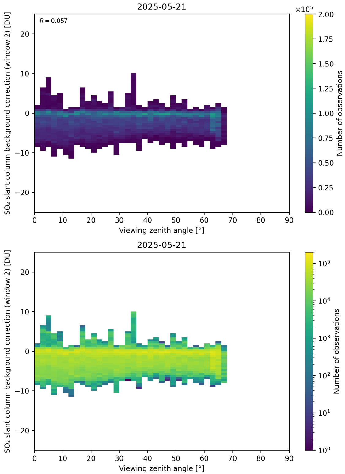
Figure 363: Scatter density plot of “Viewing zenith angle” against “SO 2 slant column background correction (window 2)” for 2025-05-21 to 2025-05-22.
