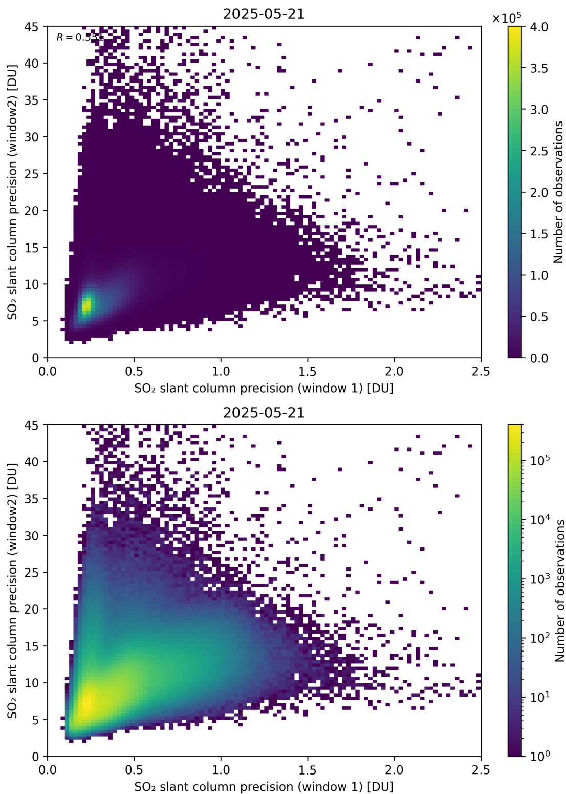
Figure 277: Scatter density plot of “SO 2 slant column precision (window 1)” against “SO 2 slant column precision (window2)” for 2025-05-21 to 2025-05-22.
