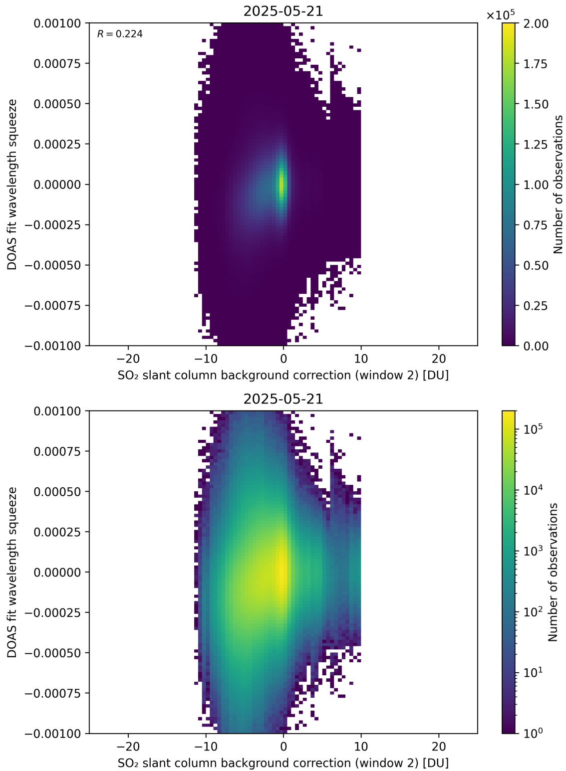
Figure 124: Scatter density plot of “SO 2 slant column background correction (window 2)” against “DOAS fit wavelength squeeze” for 2025-05-21 to 2025-05-22.
