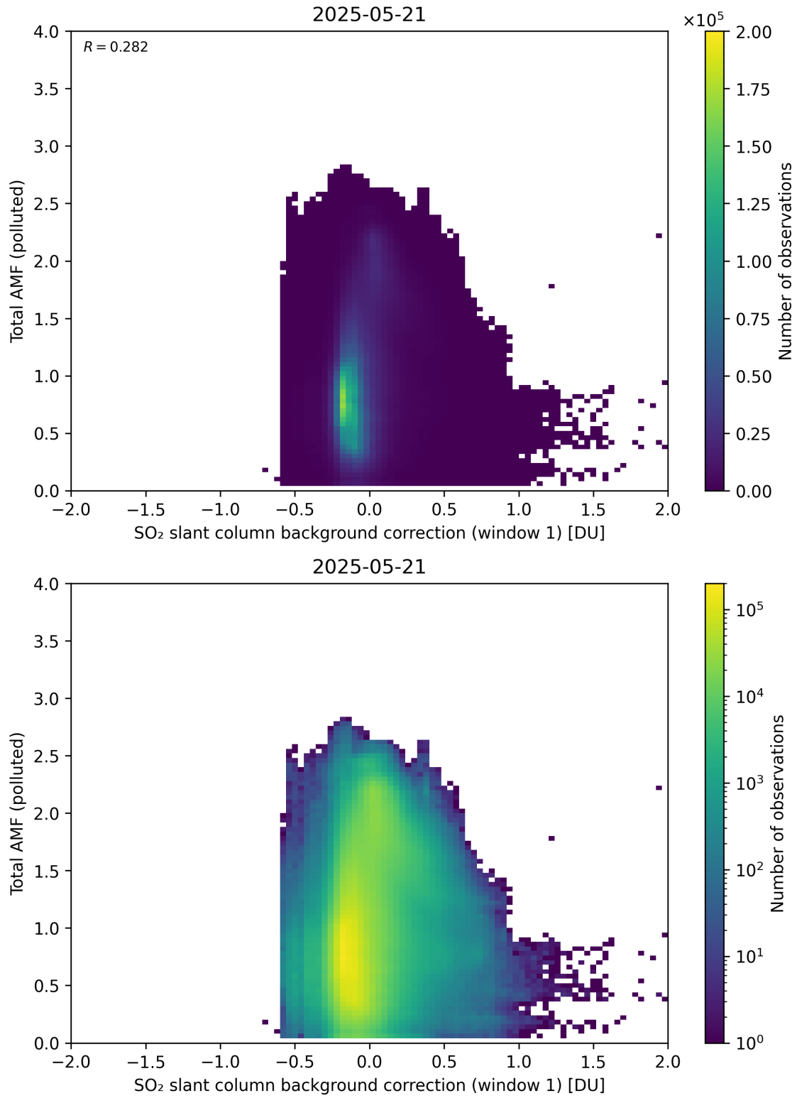
Figure 120: Scatter density plot of “SO 2 slant column background correction (window 1)” against “Total AMF (polluted)” for 2025-05-21 to 2025-05-22.
