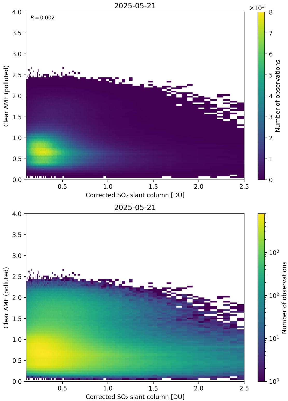
Figure 232: Scatter density plot of “Corrected SO 2 slant column” against “Clear AMF (polluted)” for 2025-05-21 to 2025-05-22.
