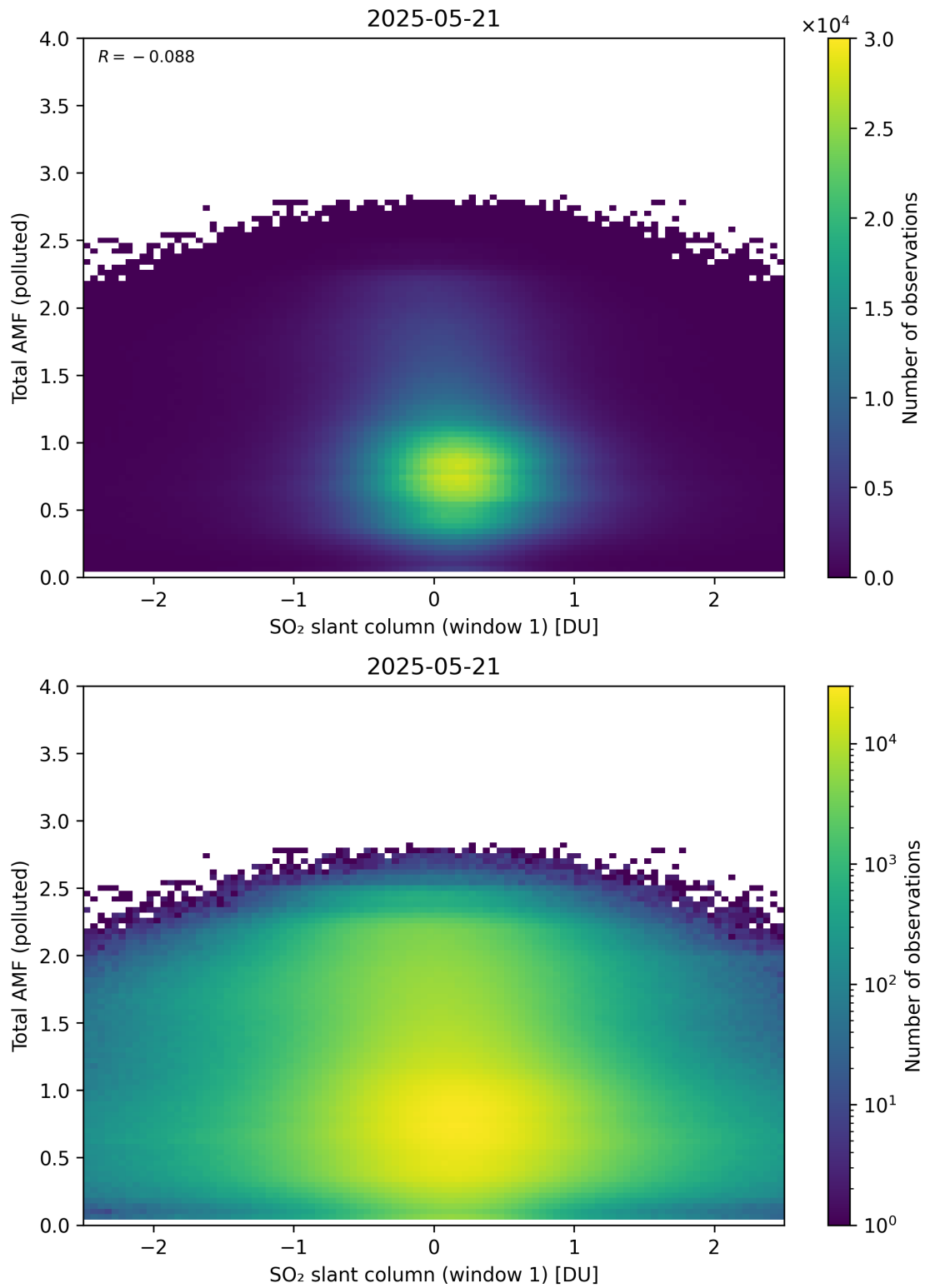
Figure 289: Scatter density plot of “SO 2 slant column (window 1)” against “Total AMF (polluted)” for 2025-05-21 to 2025-05-22.
