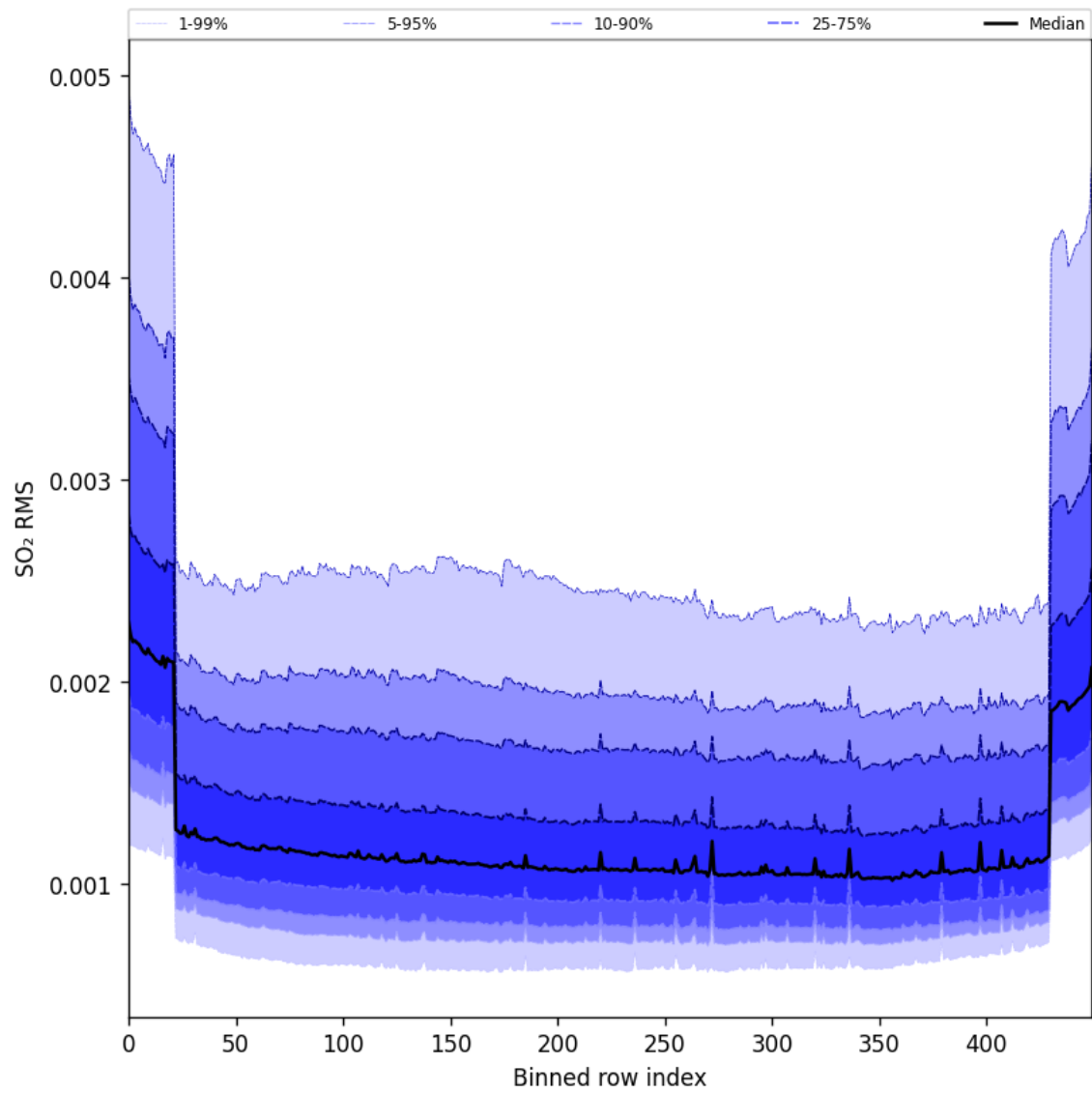
Figure 104: Along track statistics of “SO 2 RMS” for 2025-05-21 to 2025-05-22
