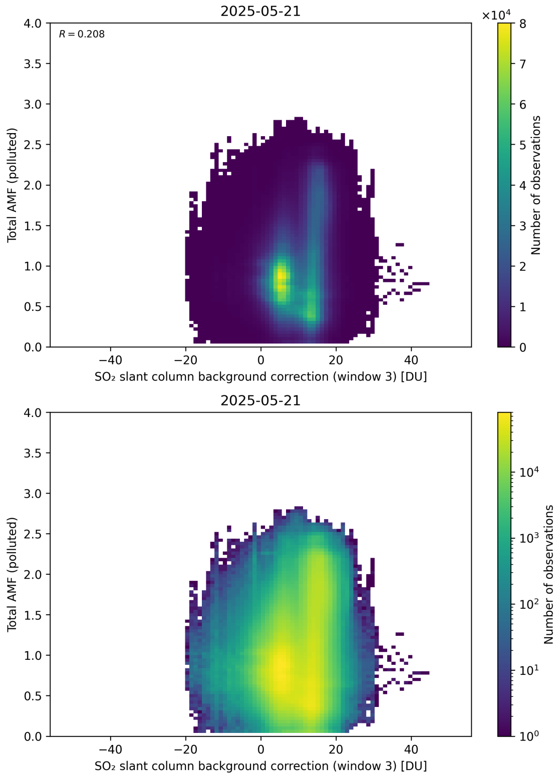
Figure 136: Scatter density plot of “SO 2 slant column background correction (window 3)” against “Total AMF (polluted)” for 2025-05-21 to 2025-05-22.
