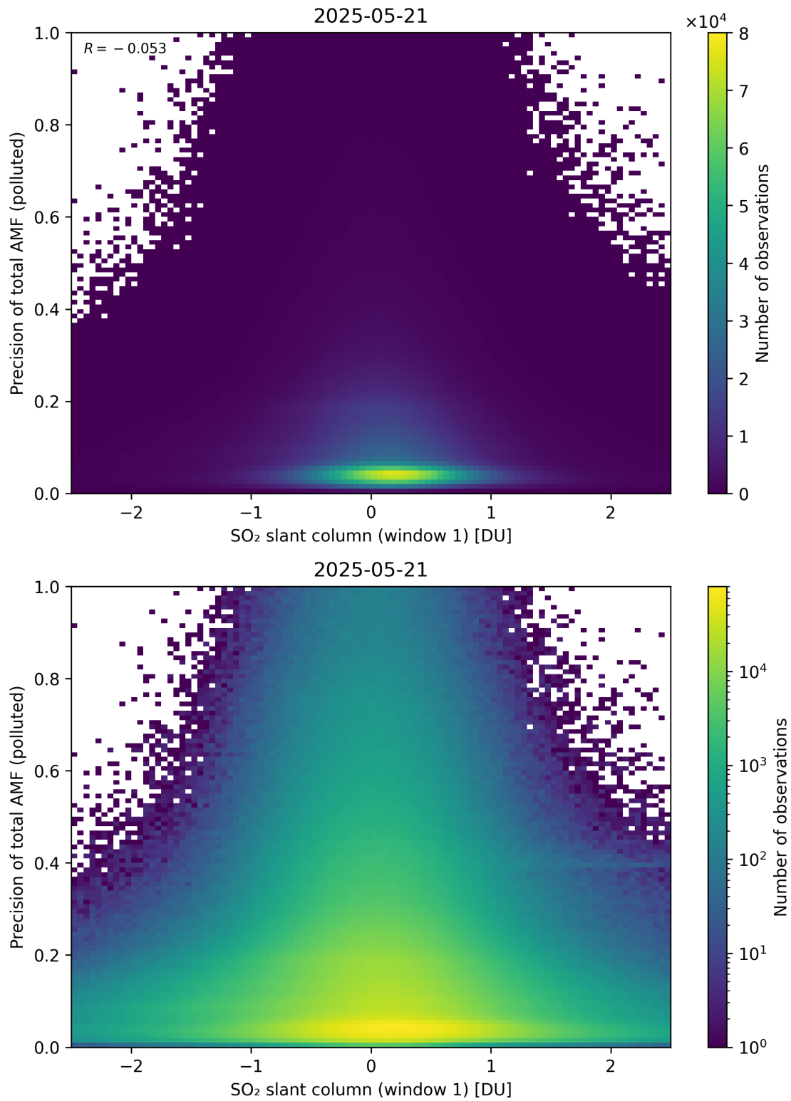
Figure 290: Scatter density plot of “SO 2 slant column (window 1)” against “Precision of total AMF (polluted)” for 2025-05-21 to 2025-05-22.
