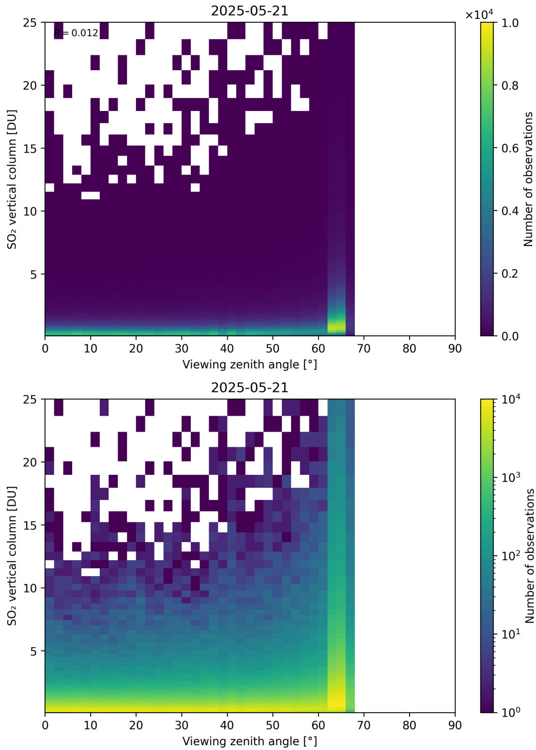
Figure 383: Scatter density plot of “Viewing zenith angle” against “SO 2 vertical column” for 2025-05-21 to 2025-05-22.
