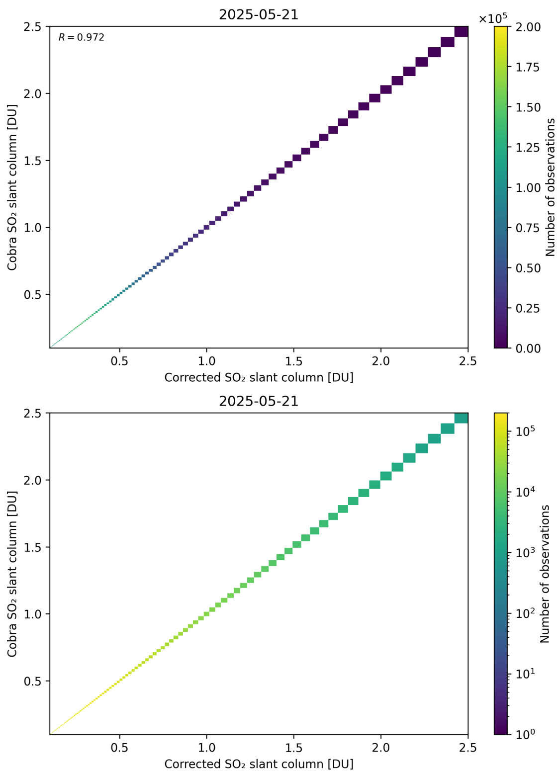
Figure 233: Scatter density plot of “Corrected SO 2 slant column” against “Cobra SO 2 slant column” for 2025-05-21 to 2025-05-22.
