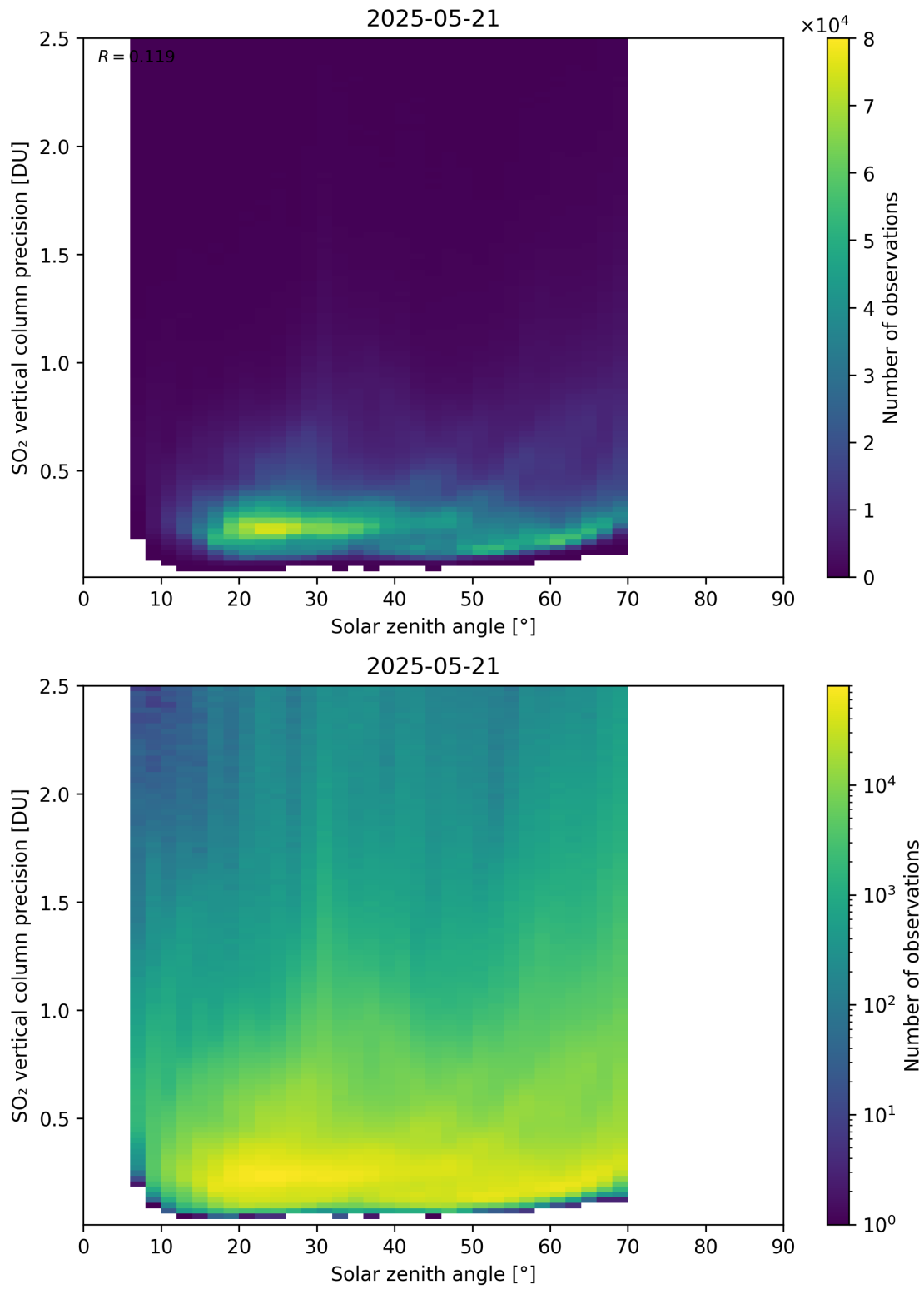
Figure 192: Scatter density plot of “Solar zenith angle” against “SO 2 vertical column precision” for 2025-05-21 to 2025-05-22.
