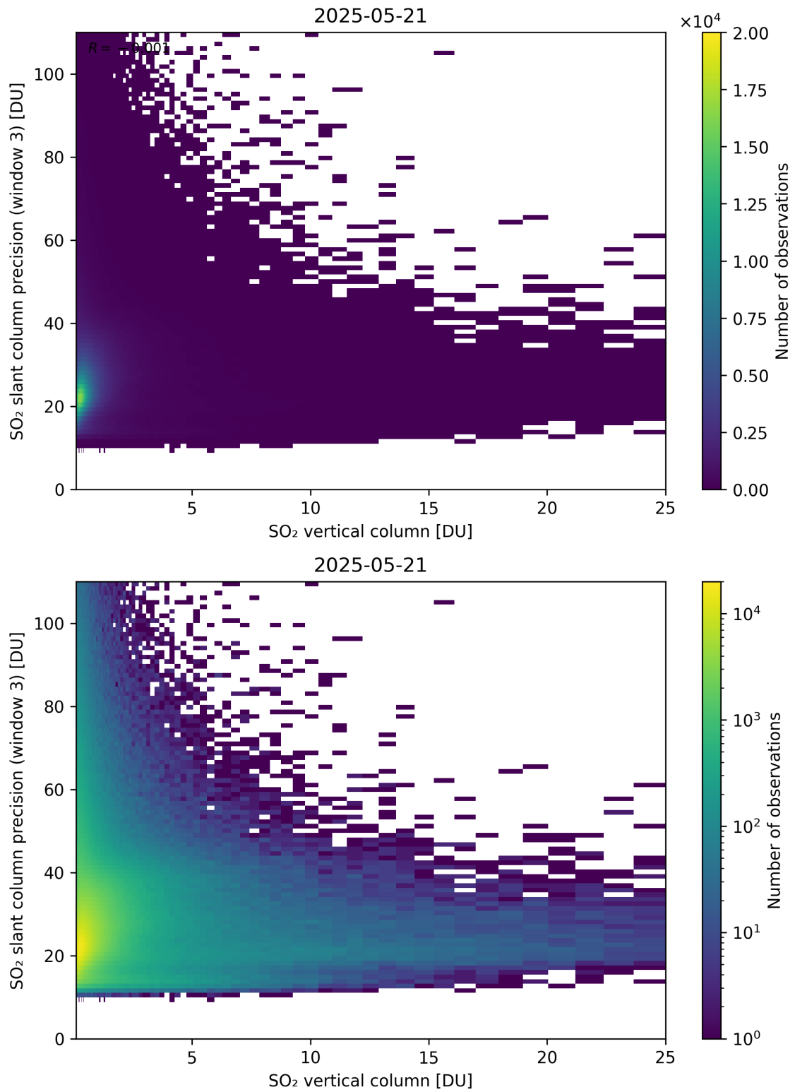
Figure 358: Scatter density plot of “SO 2 vertical column” against “SO 2 slant column precision (window 3)” for 2025-05-21 to 2025-05-22.
