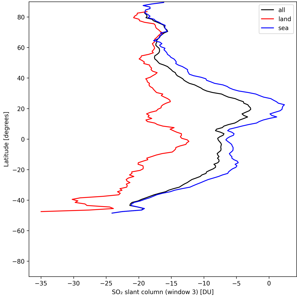
Figure 45: Zonal average of “SO 2 slant column (window 3)” for 2025-05-21 to 2025-05-22.
