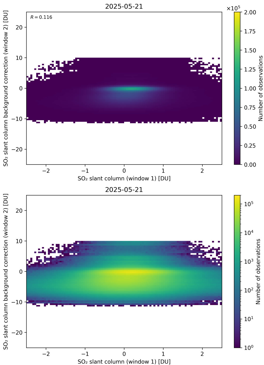
Figure 263: Scatter density plot of “SO 2 slant column (window 1)” against “SO 2 slant column background correction (window 2)” for 2025-05-21 to 2025-05-22.
