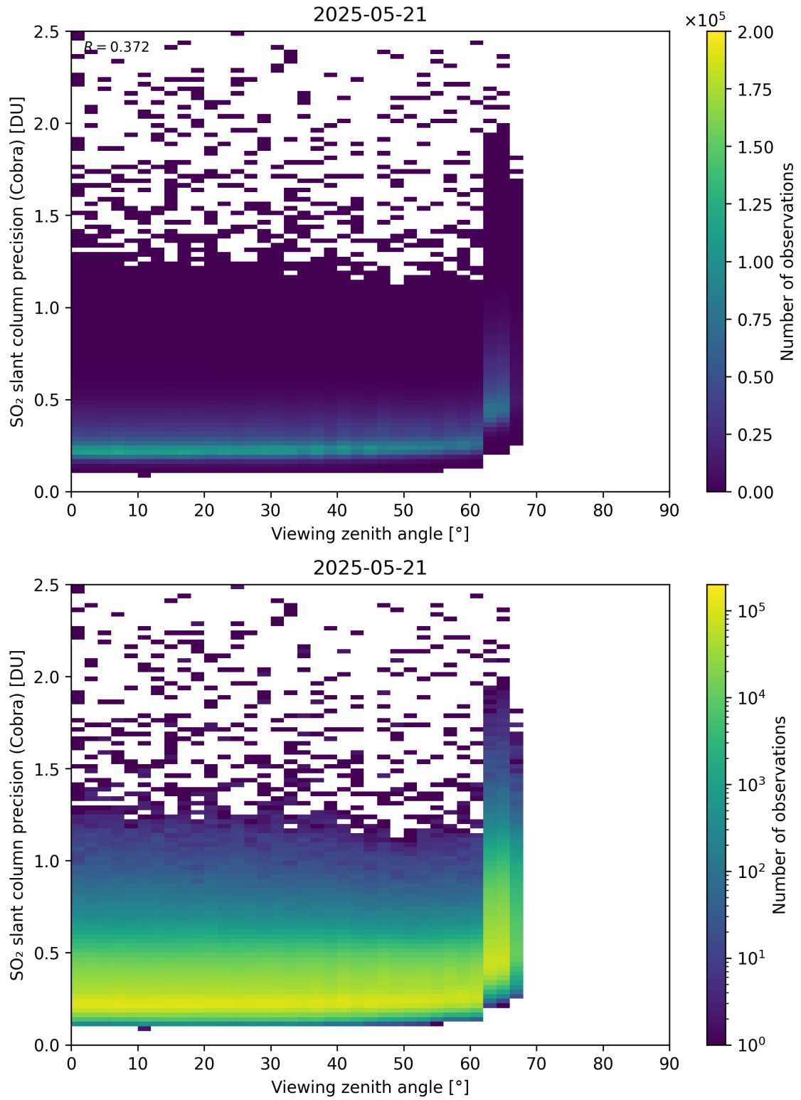
Figure 372: Scatter density plot of “Viewing zenith angle” against “SO 2 slant column precision (Cobra)” for 2025-05-21 to 2025-05-22.
