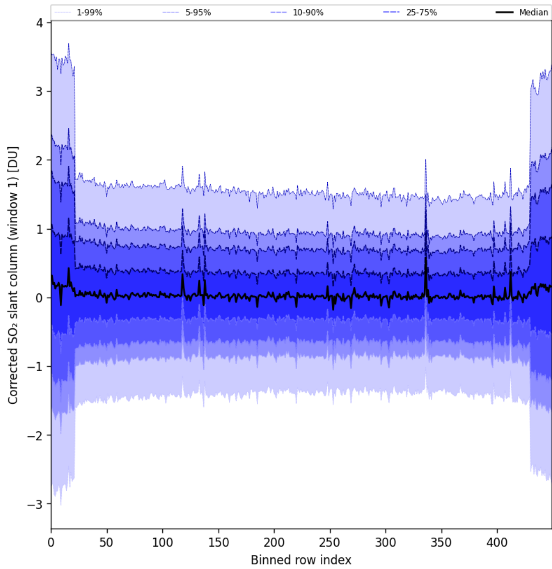
Figure 91: Along track statistics of “Corrected SO 2 slant column (window 1)” for 2025-05-21 to 2025-05-22
