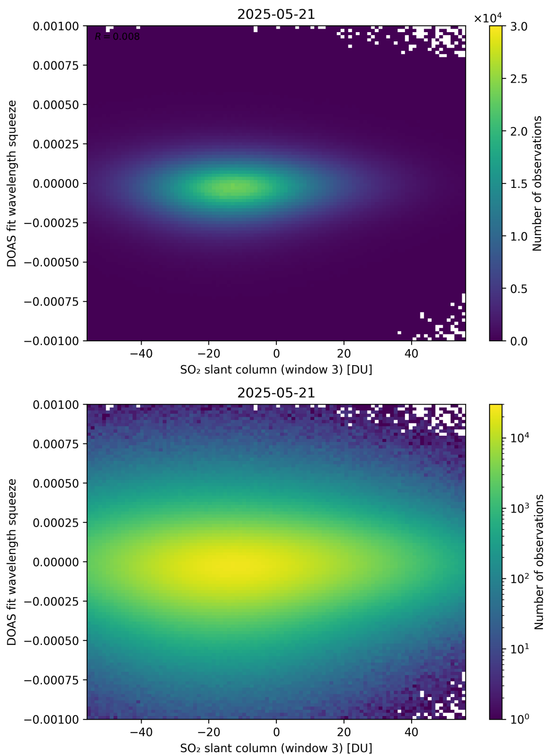
Figure 305: Scatter density plot of “SO 2 slant column (window 3)” against “DOAS fit wavelength squeeze” for 2025-05-21 to 2025-05-22.
