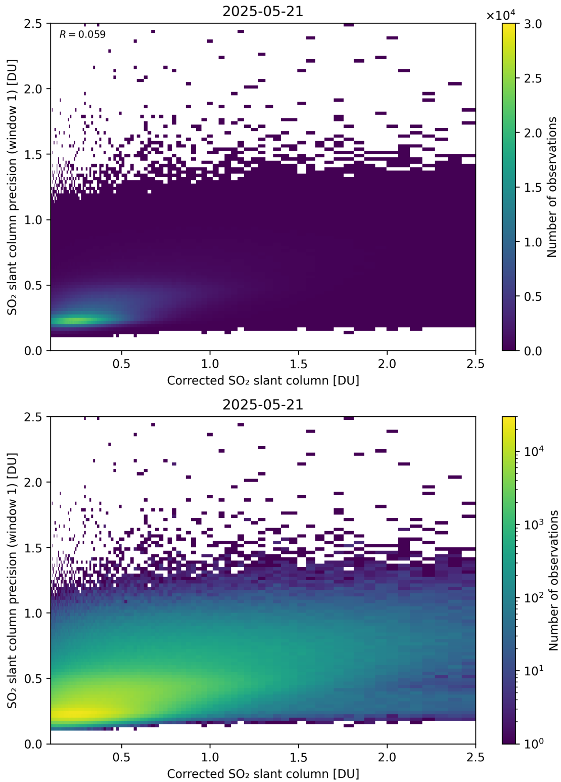
Figure 238: Scatter density plot of “Corrected SO 2 slant column” against “SO 2 slant column precision (window 1)” for 2025-05-21 to 2025-05-22.
