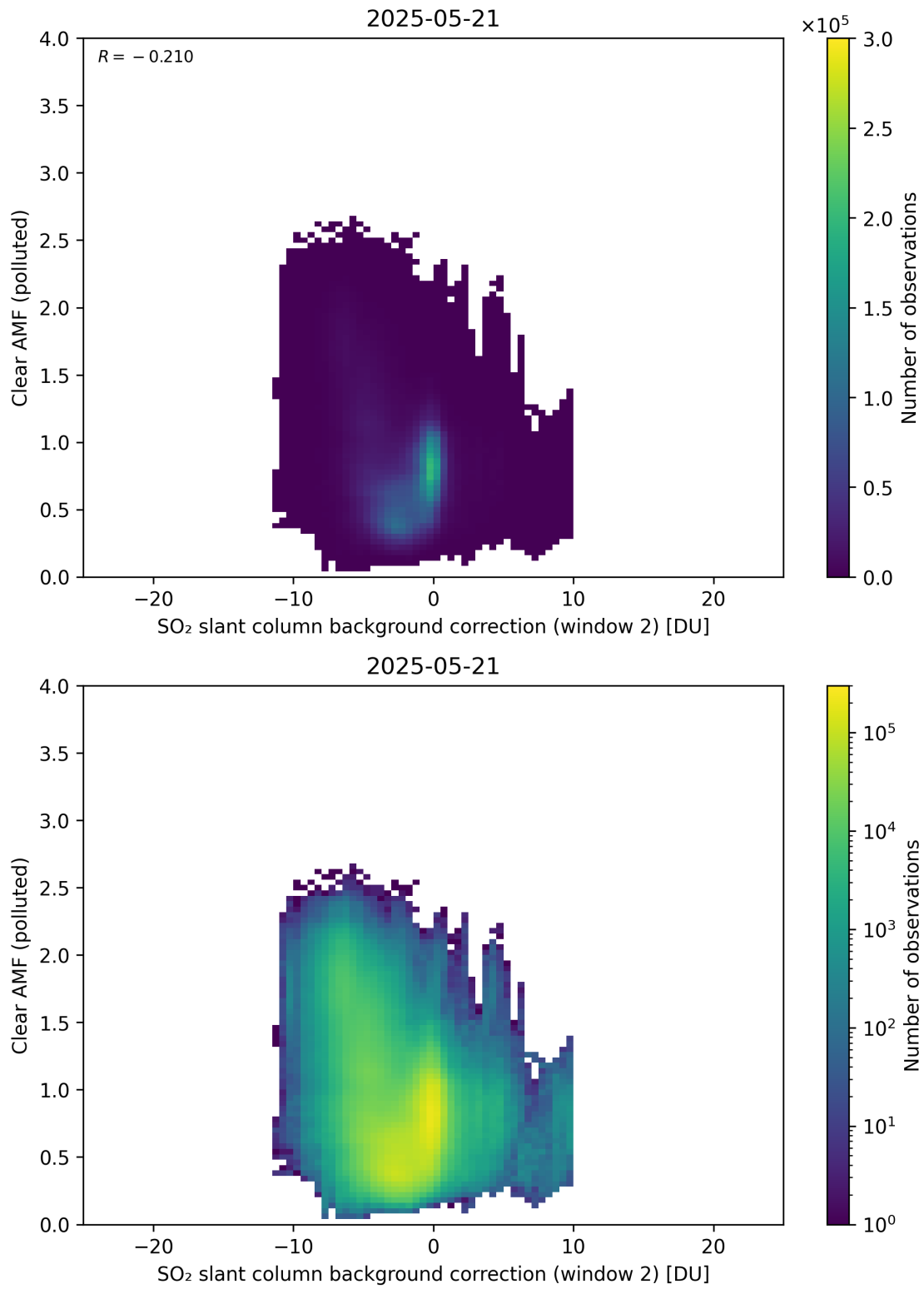
Figure 126: Scatter density plot of “SO 2 slant column background correction (window 2)” against “Clear AMF (polluted)” for 2025-05-21 to 2025-05-22.
