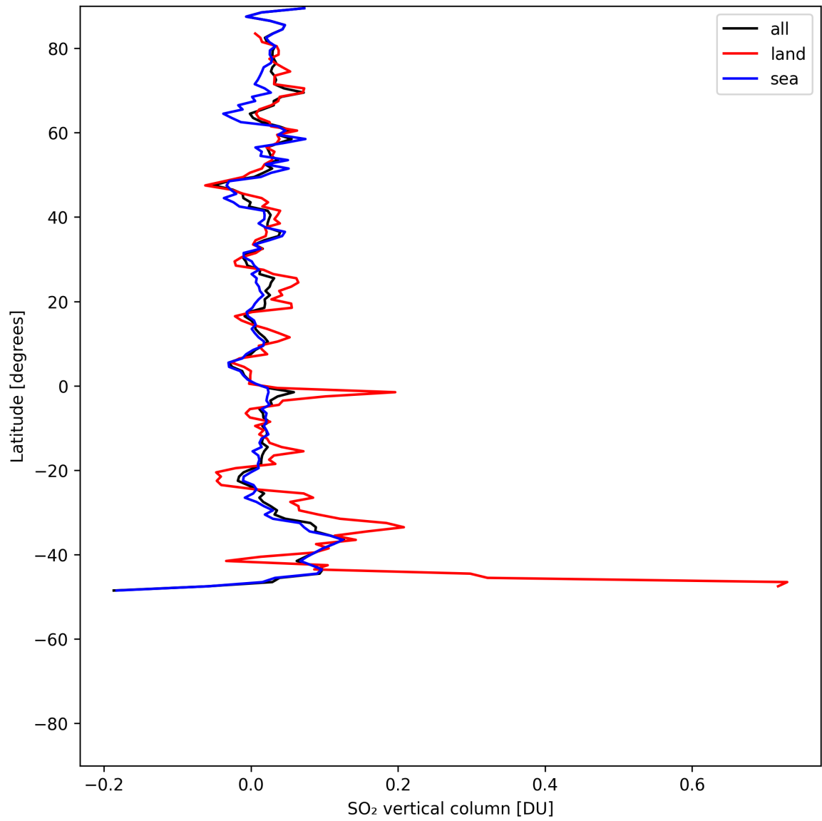
Figure 32: Zonal average of “SO 2 vertical column” for 2025-05-21 to 2025-05-22.
