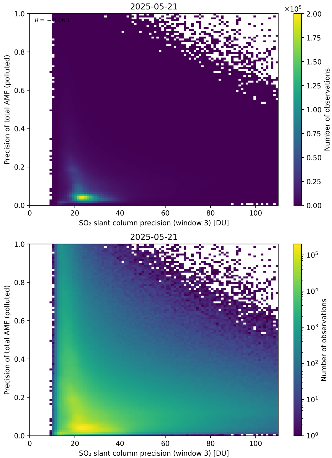
Figure 314: Scatter density plot of “SO 2 slant column precision (window 3)” against “Precision of total AMF (polluted)” for 2025-05-21 to 2025-05-22.
