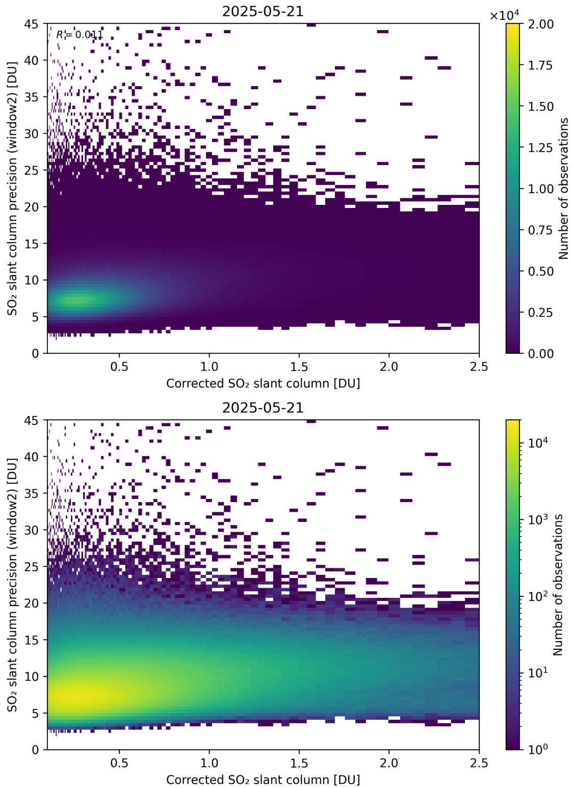
Figure 239: Scatter density plot of “Corrected SO 2 slant column” against “SO 2 slant column precision (window2)” for 2025-05-21 to 2025-05-22.
