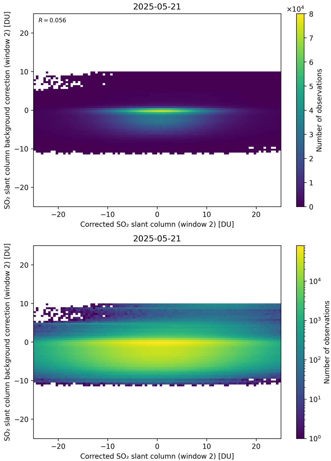
Figure 244: Scatter density plot of “Corrected SO 2 slant column (window 2)” against “SO 2 slant column background correction (window 2)” for 2025-05-21 to 2025-05-22.
