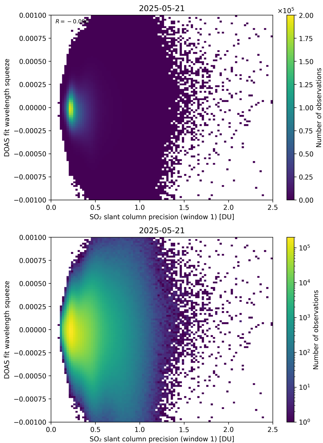
Figure 272: Scatter density plot of “SO 2 slant column precision (window 1)” against “DOAS fit wavelength squeeze” for 2025-05-21 to 2025-05-22.
