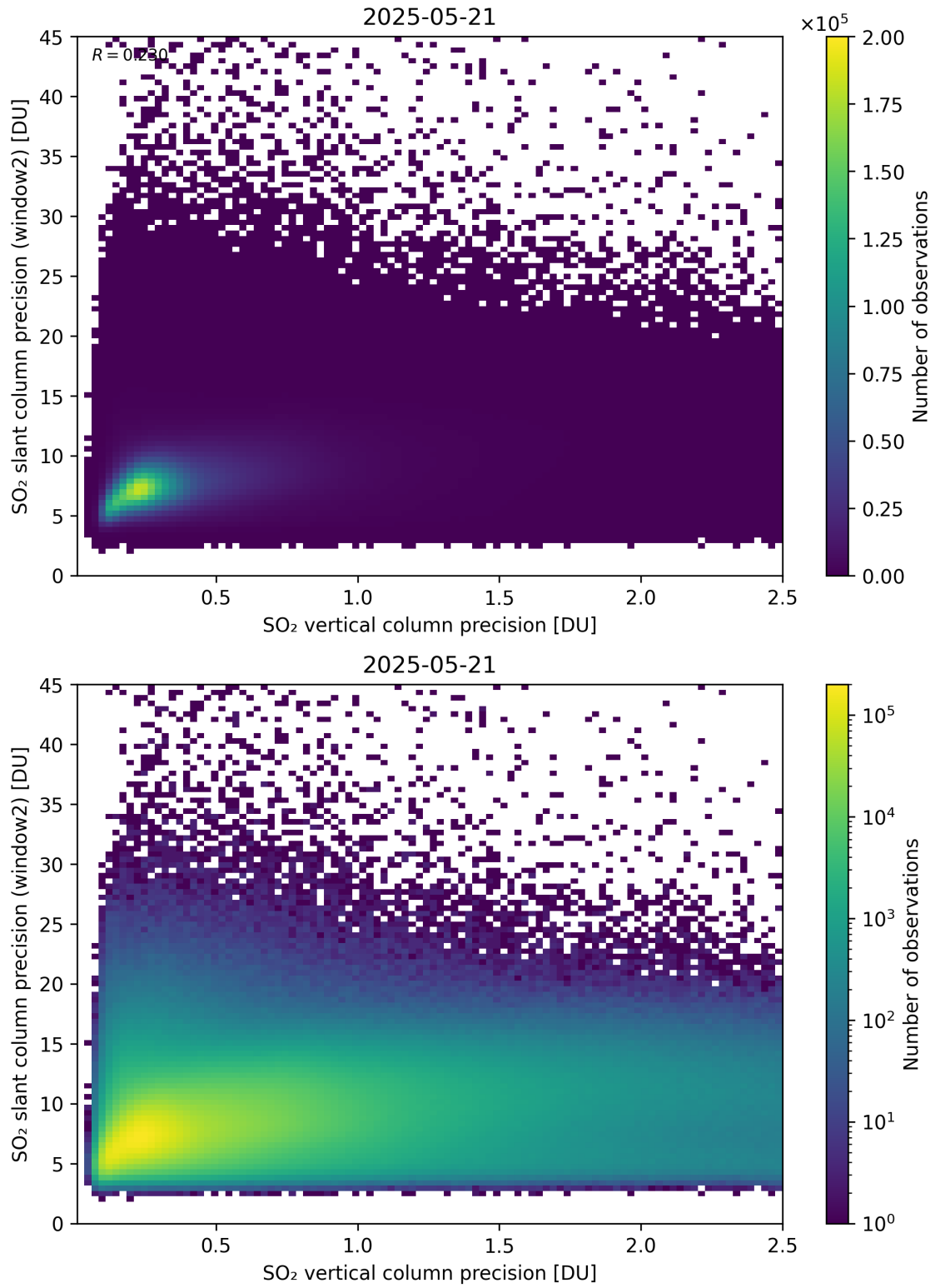
Figure 343: Scatter density plot of “SO 2 vertical column precision” against “SO 2 slant column precision (window2)” for 2025-05-21 to 2025-05-22.
