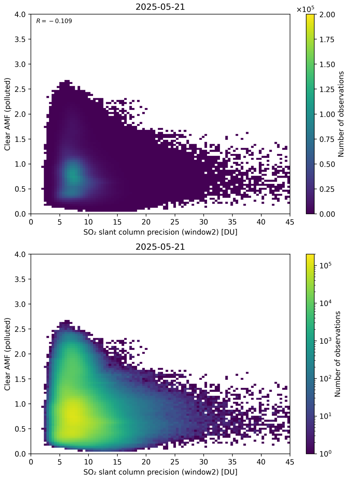
Figure 296: Scatter density plot of “SO 2 slant column precision (window2)” against “Clear AMF (polluted)” for 2025-05-21 to 2025-05-22.
