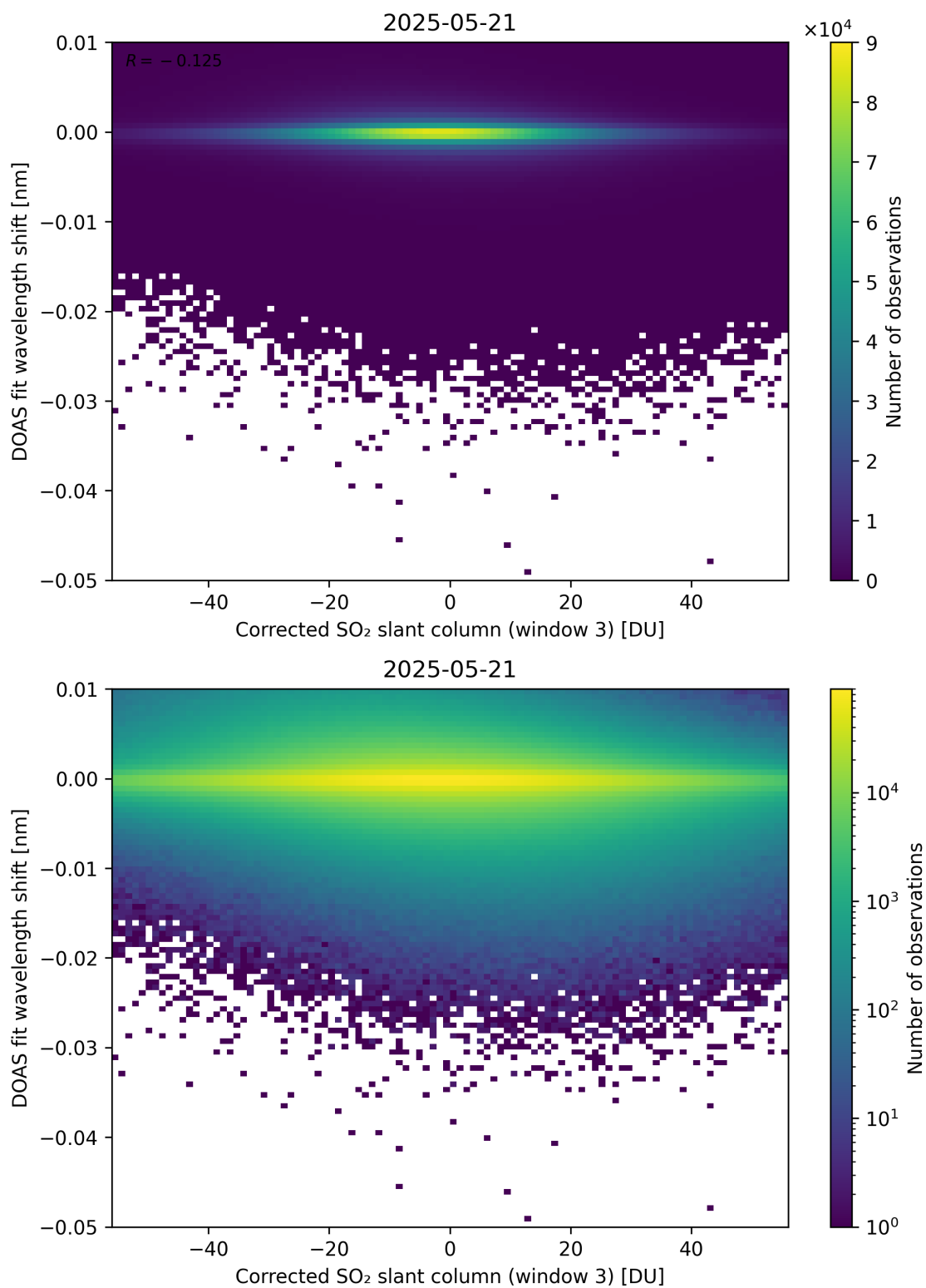
Figure 256: Scatter density plot of “Corrected SO 2 slant column (window 3)” against “DOAS fit wavelength shift” for 2025-05-21 to 2025-05-22.
