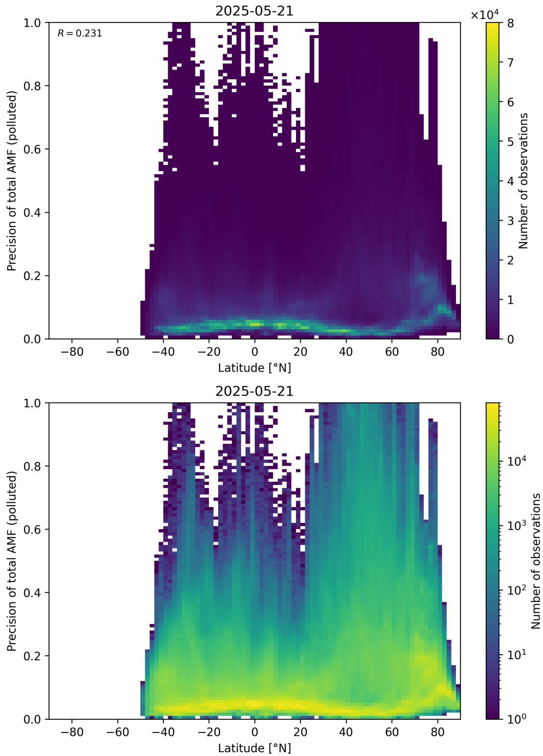
Figure 168: Scatter density plot of “Latitude” against “Precision of total AMF (polluted)” for 2025-05-21 to 2025-05-22.
