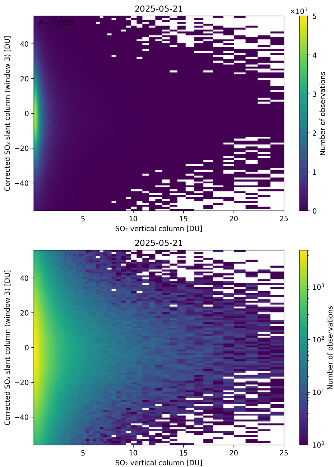
Figure 353: Scatter density plot of “SO 2 vertical column” against “Corrected SO 2 slant column (window 3)” for 2025-05-21 to 2025-05-22.
