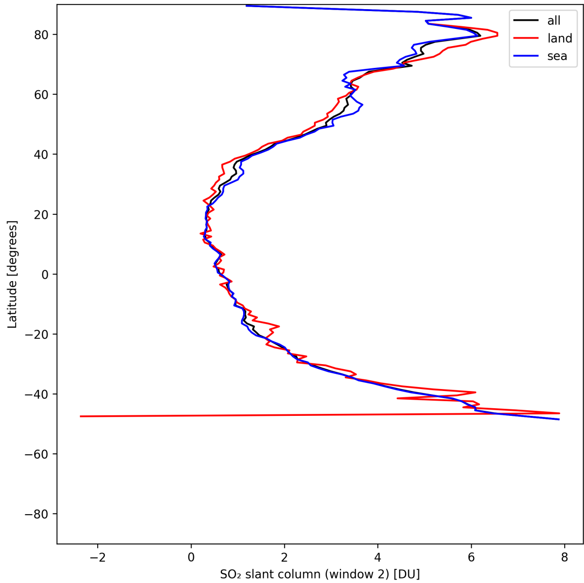
Figure 41: Zonal average of “SO 2 slant column (window 2)” for 2025-05-21 to 2025-05-22.
