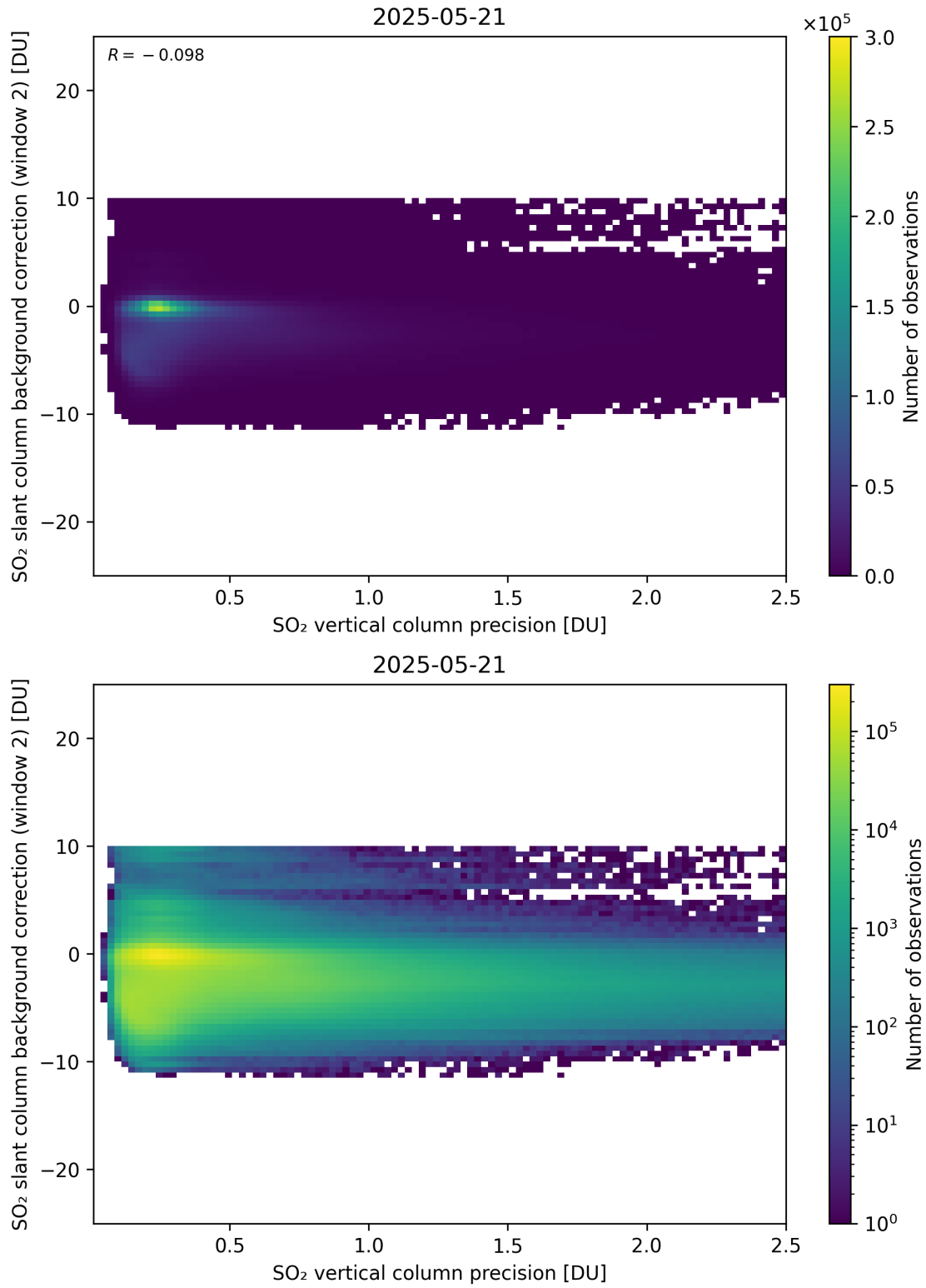
Figure 330: Scatter density plot of “SO 2 vertical column precision” against “SO 2 slant column background correction (window 2)” for 2025-05-21 to 2025-05-22.
