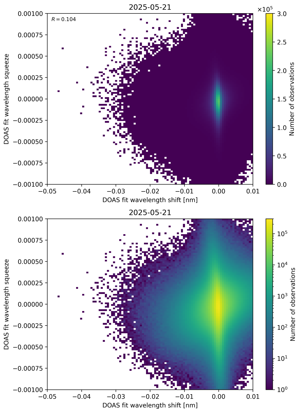
Figure 138: Scatter density plot of “DOAS fit wavelength shift” against “DOAS fit wavelength squeeze” for 2025-05-21 to 2025-05-22.
