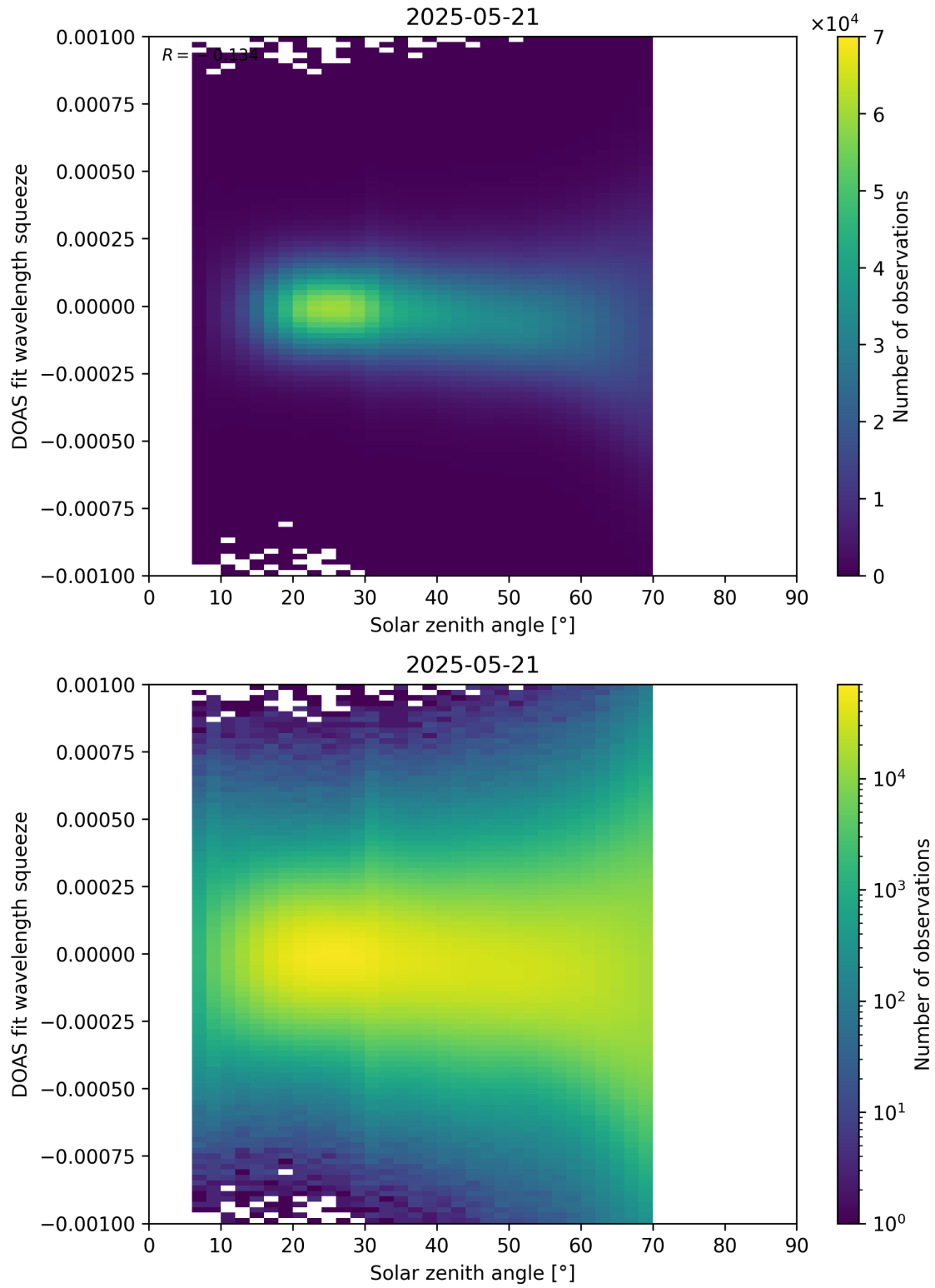
Figure 175: Scatter density plot of “Solar zenith angle” against “DOAS fit wavelength squeeze” for 2025-05-21 to 2025-05-22.
