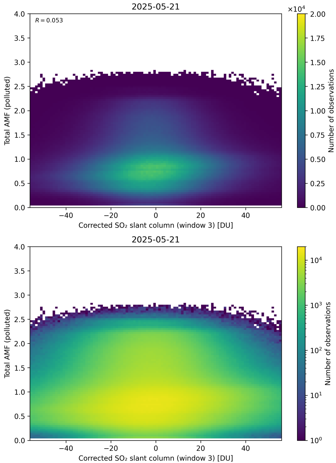
Figure 260: Scatter density plot of “Corrected SO 2 slant column (window 3)” against “Total AMF (polluted)” for 2025-05-21 to 2025-05-22.
