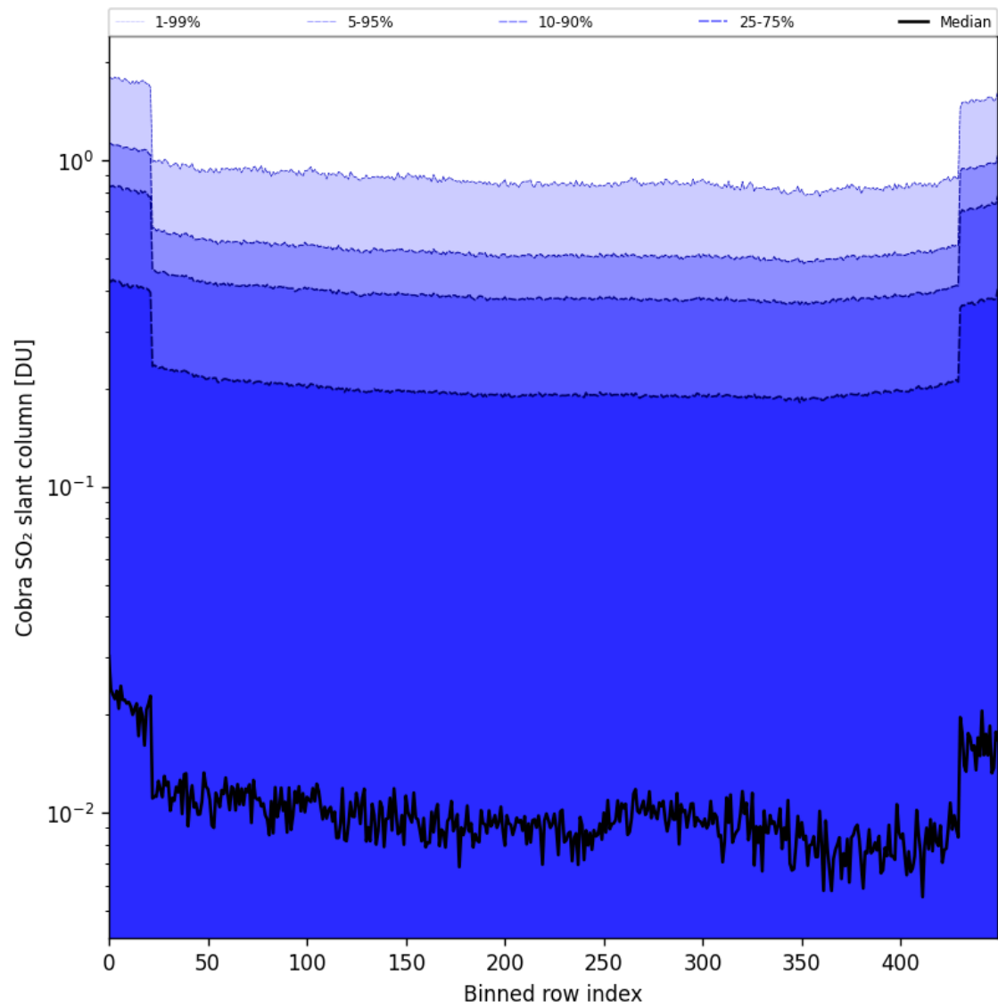
Figure 87: Along track statistics of “Cobra SO 2 slant column” for 2025-05-21 to 2025-05-22
