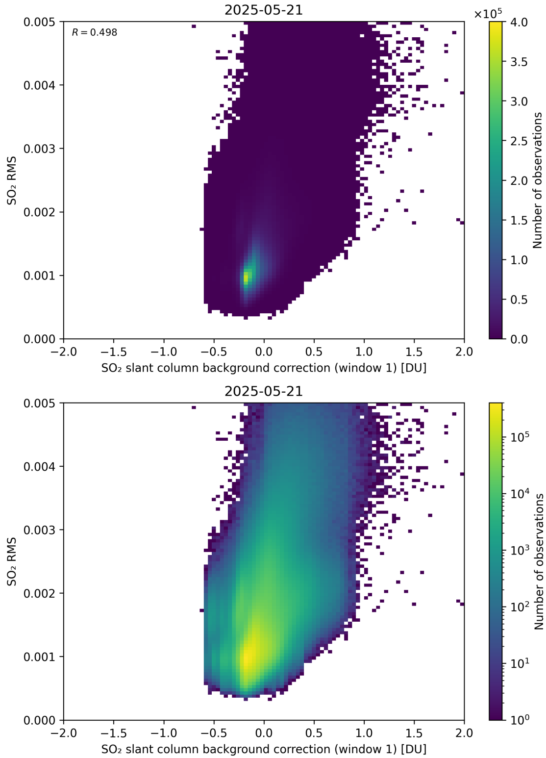
Figure 113: Scatter density plot of “SO 2 slant column background correction (window 1)” against “SO 2 RMS” for 2025-05-21 to 2025-05-22.
