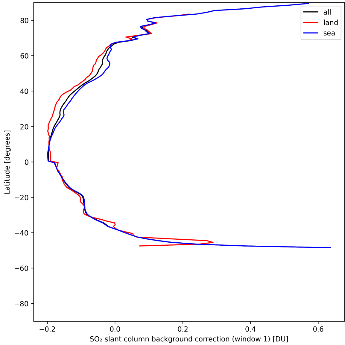
Figure 40: Zonal average of “SO 2 slant column background correction (window 1)” for 2025-05-21 to 2025-05-22.
