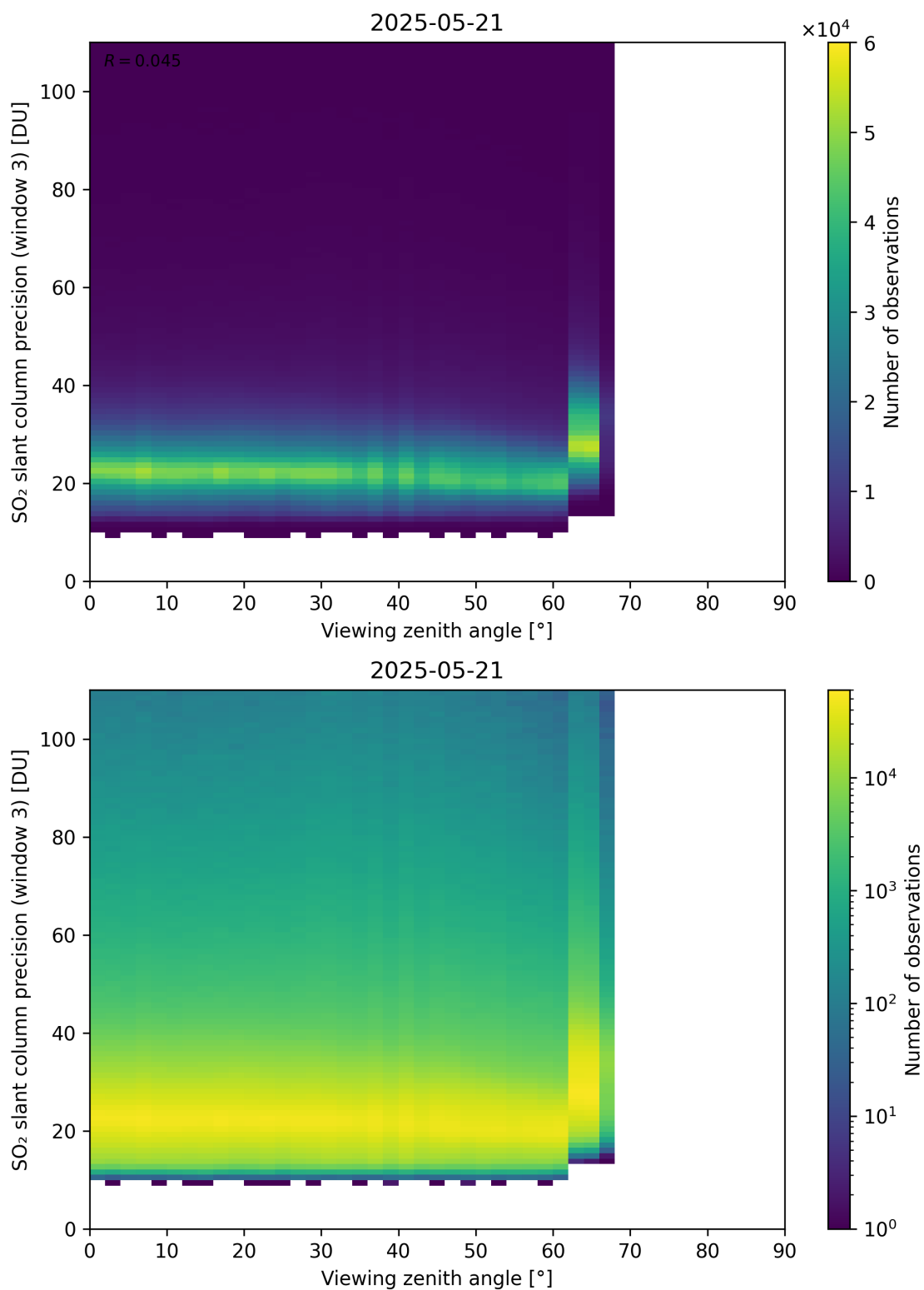
Figure 380: Scatter density plot of “Viewing zenith angle” against “SO 2 slant column precision (window 3)” for 2025-05-21 to 2025-05-22.
