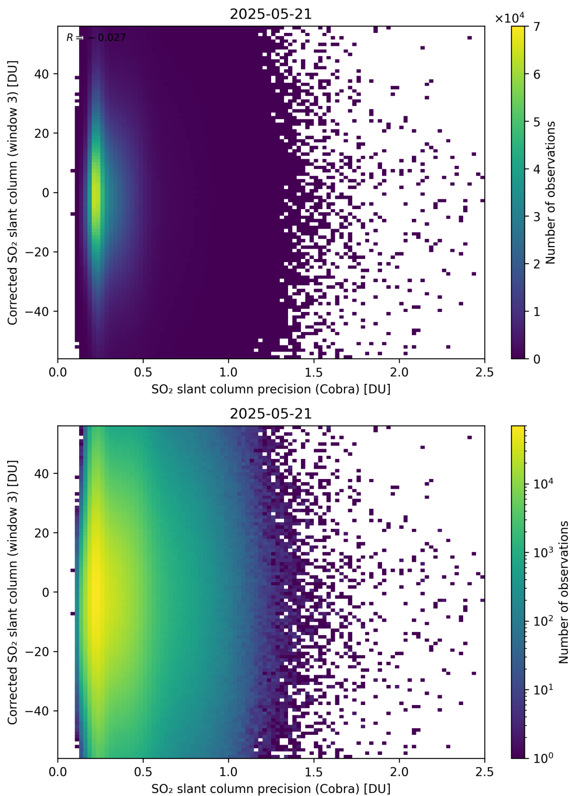
Figure 207: Scatter density plot of “SO 2 slant column precision (Cobra)” against “Corrected SO 2 slant column (window 3)” for 2025-05-21 to 2025-05-22.
