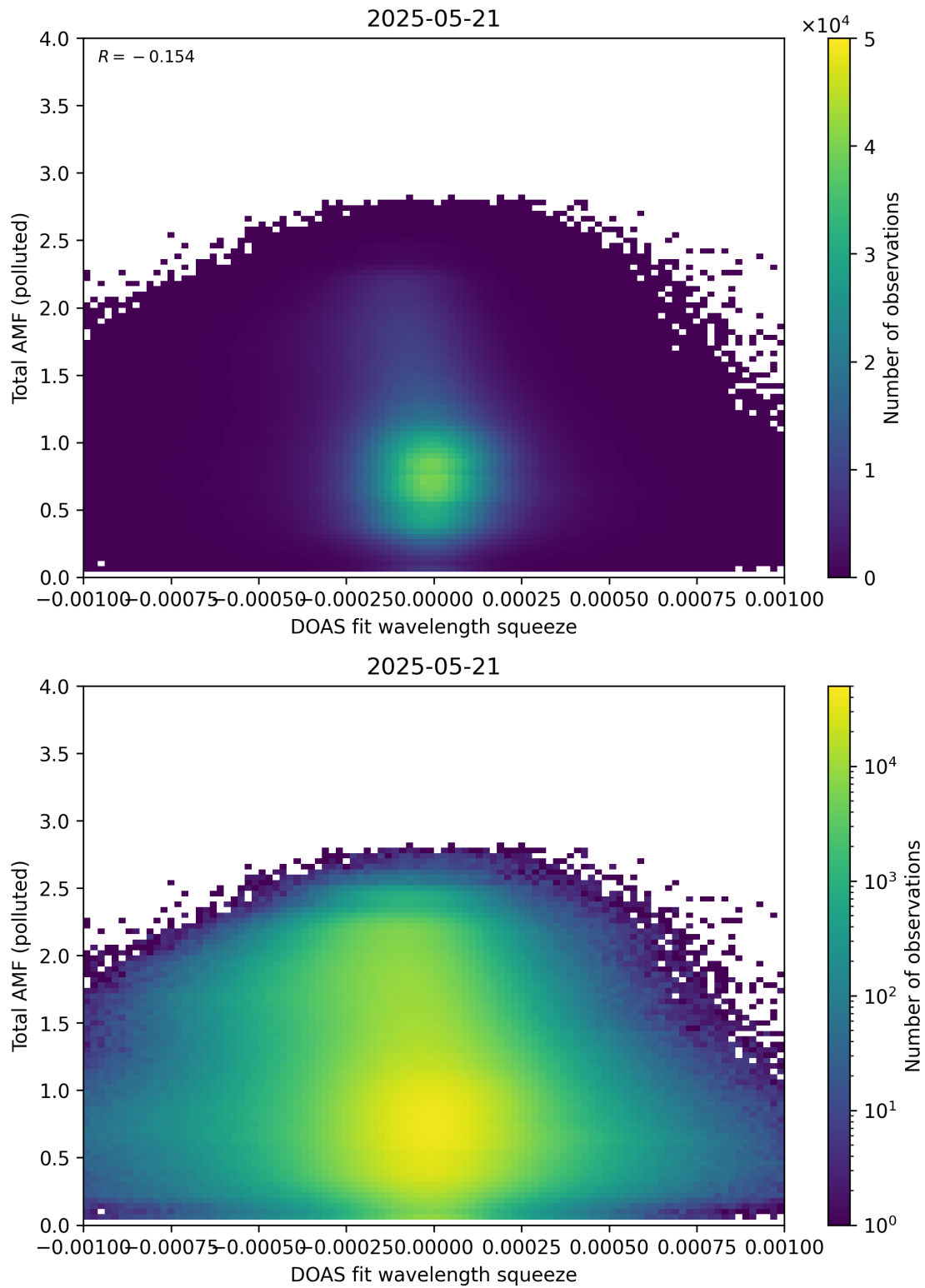
Figure 145: Scatter density plot of “DOAS fit wavelength squeeze” against “Total AMF (polluted)” for 2025-05-21 to 2025-05-22.
