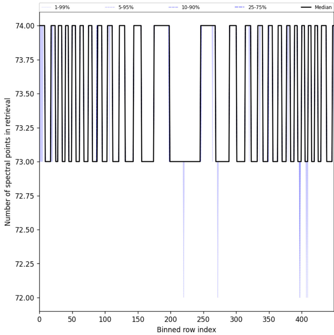
Figure 108: Along track statistics of “Number of spectral points in retrieval” for 2025-05-21 to 2025-05-22
