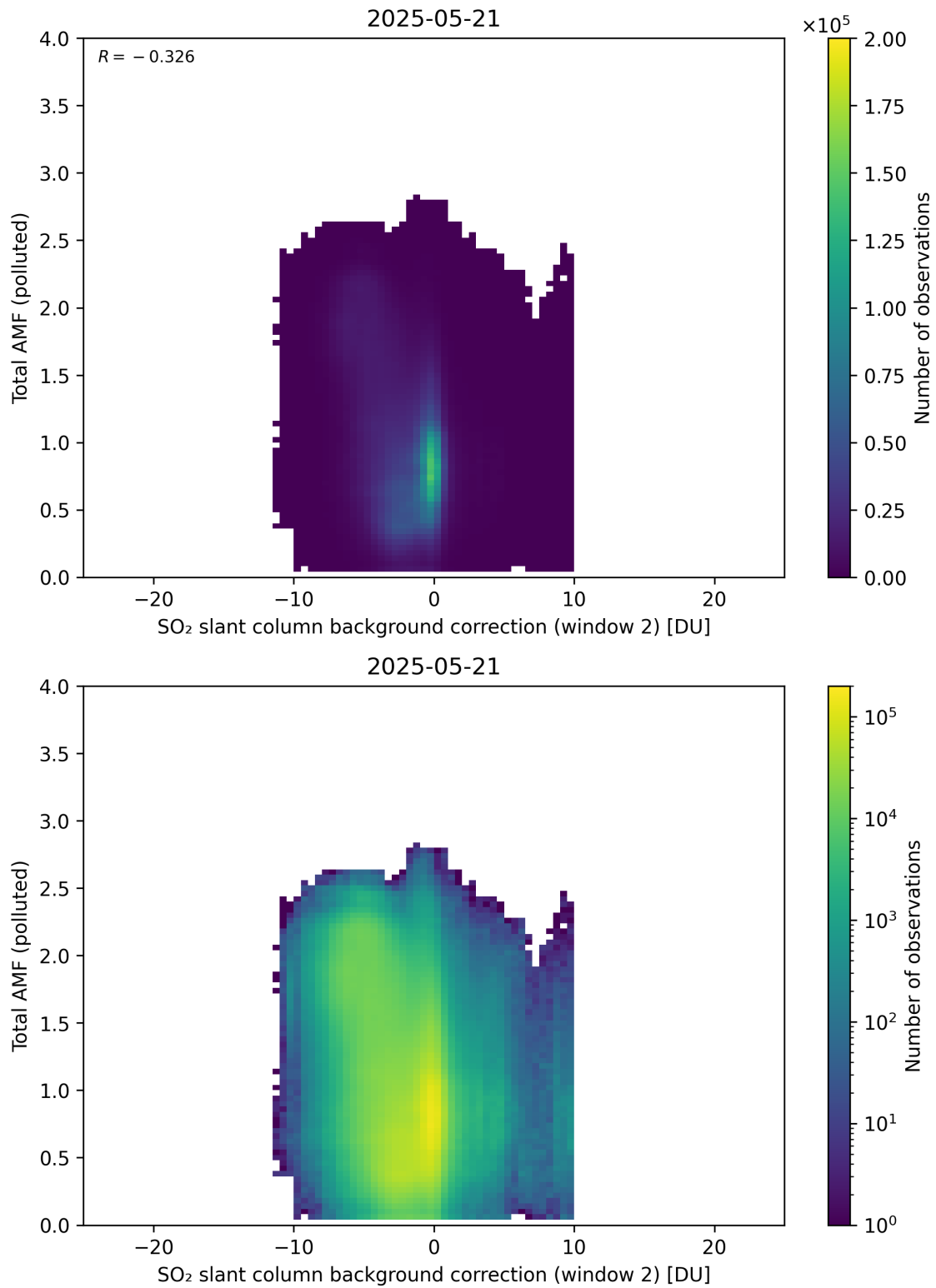
Figure 130: Scatter density plot of “SO 2 slant column background correction (window 2)” against “Total AMF (polluted)” for 2025-05-21 to 2025-05-22.
