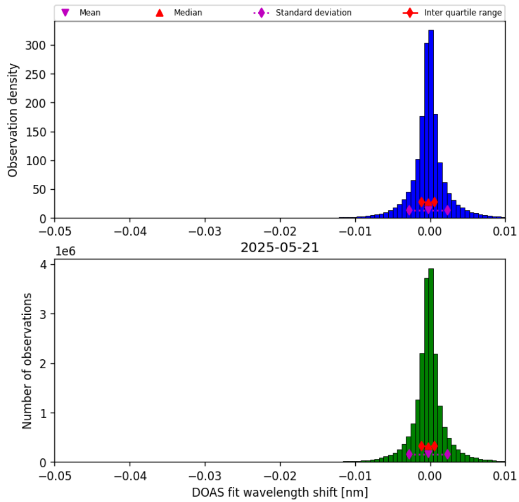
Figure 76: Histogram of “DOAS fit wavelength shift” for 2025-05-21 to 2025-05-22
