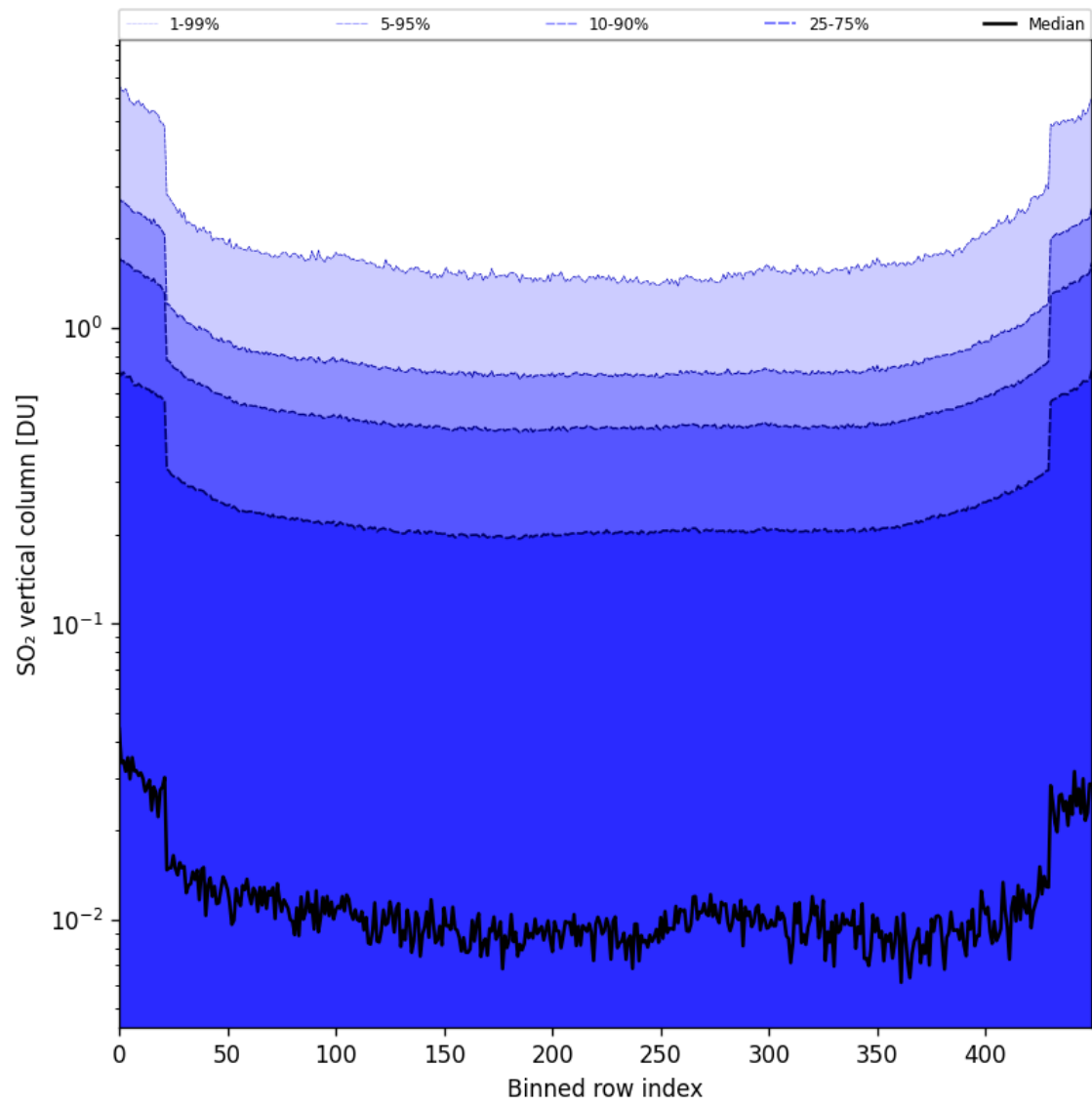
Figure 84: Along track statistics of “SO 2 vertical column” for 2025-05-21 to 2025-05-22
