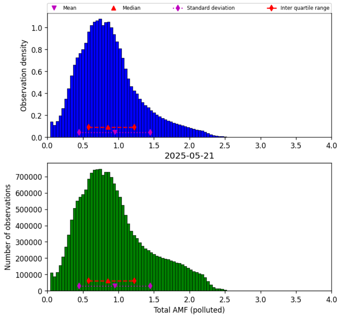
Figure 79: Histogram of “Total AMF (polluted)” for 2025-05-21 to 2025-05-22
