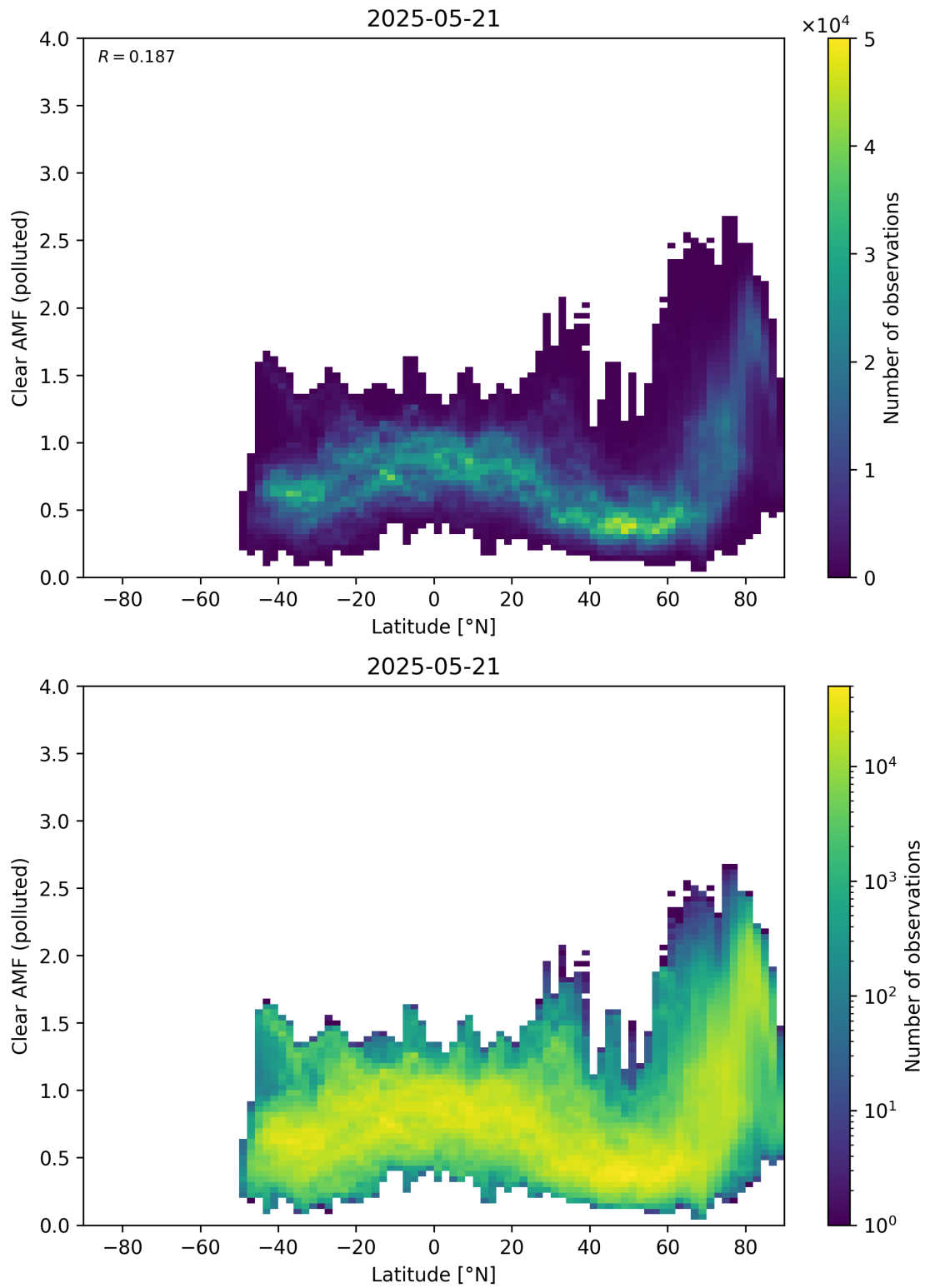
Figure 156: Scatter density plot of “Latitude” against “Clear AMF (polluted)” for 2025-05-21 to 2025-05-22.
