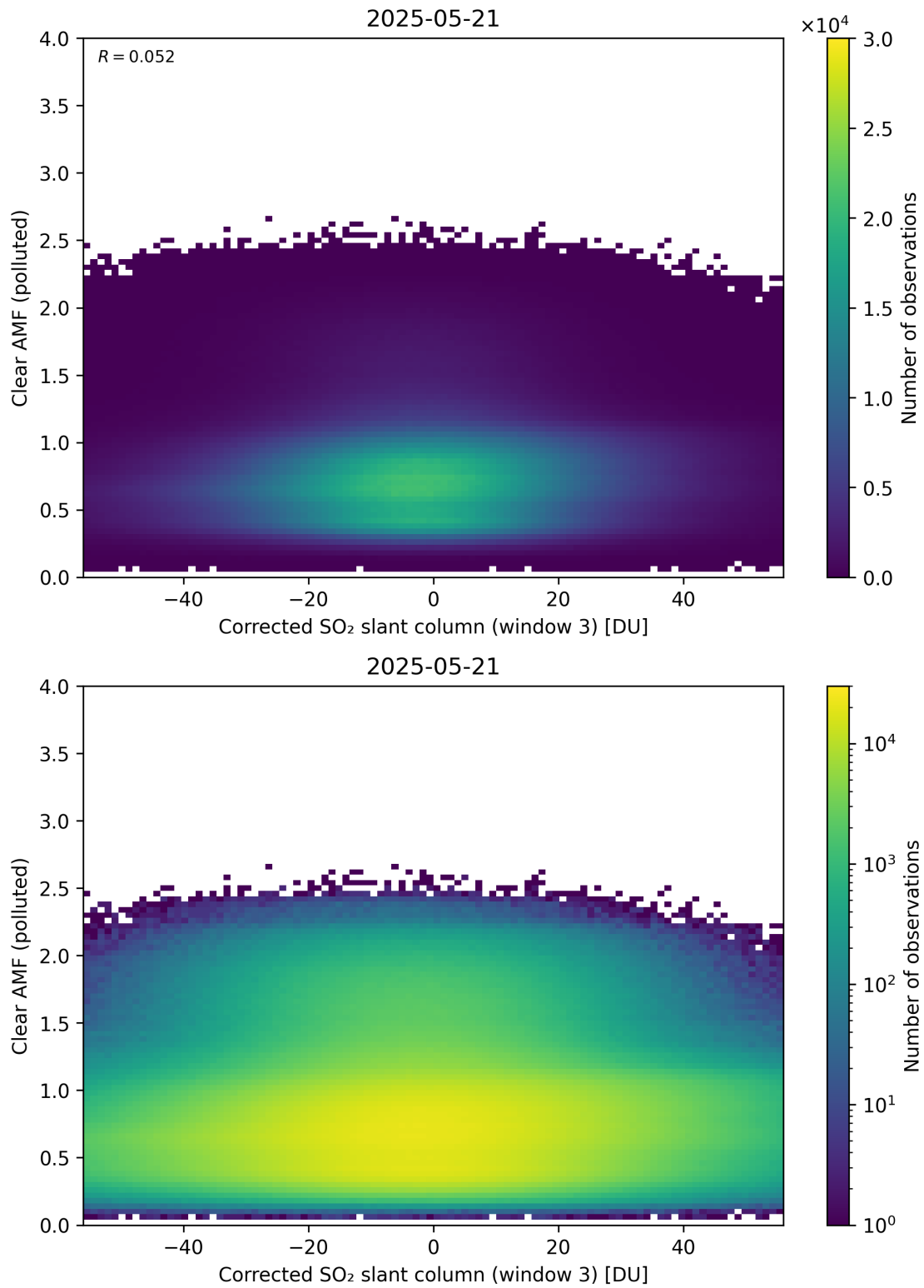
Figure 259: Scatter density plot of “Corrected SO 2 slant column (window 3)” against “Clear AMF (polluted)” for 2025-05-21 to 2025-05-22.
