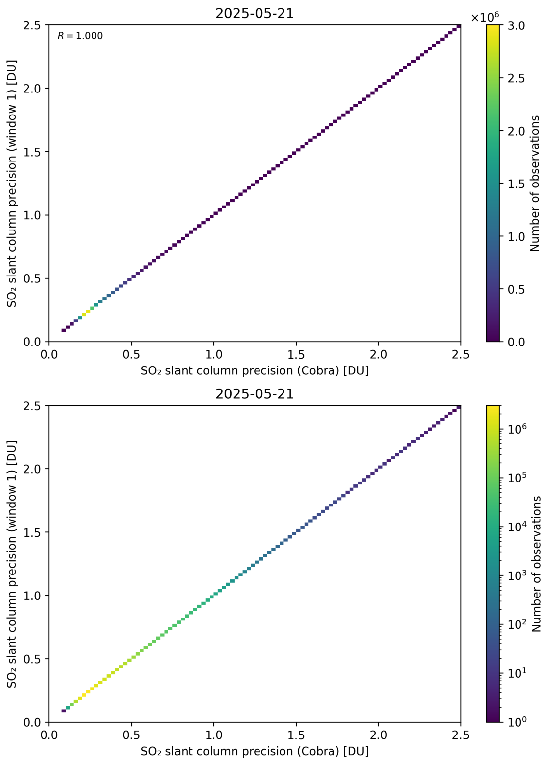
Figure 209: Scatter density plot of “SO 2 slant column precision (Cobra)” against “SO 2 slant column precision (window 1)” for 2025-05-21 to 2025-05-22.
