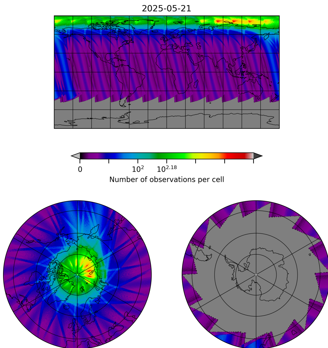
Figure 30: Map of the number of observations for 2025-05-21 to 2025-05-22
