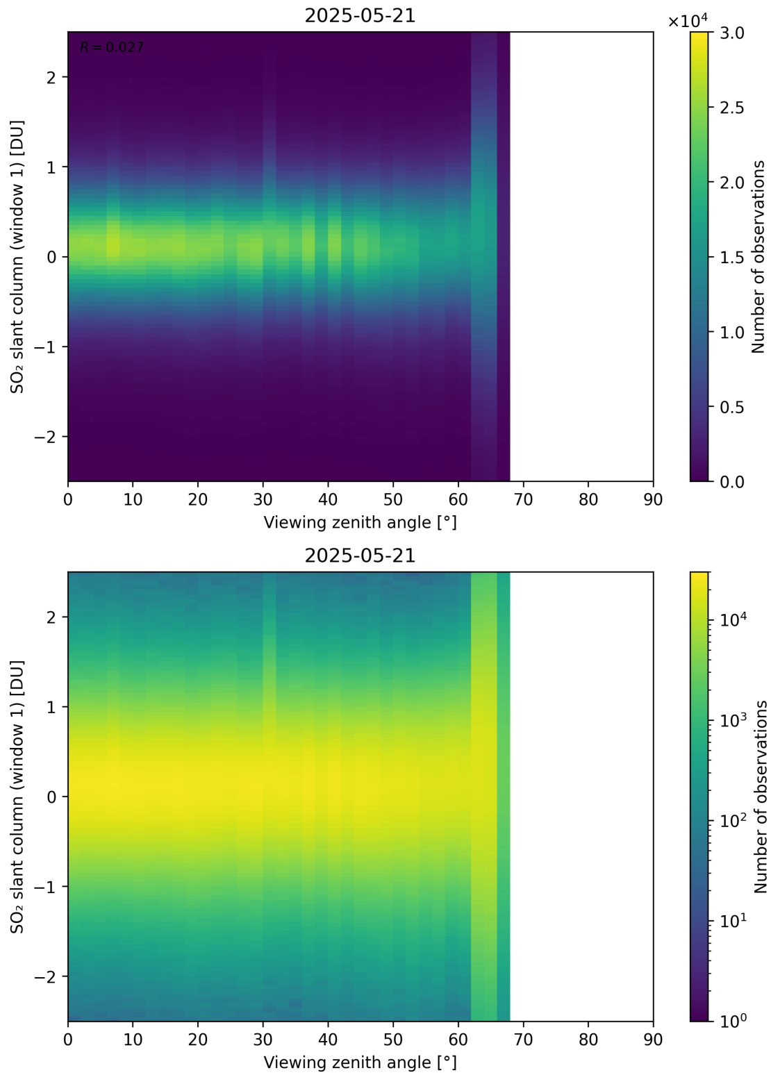
Figure 376: Scatter density plot of “Viewing zenith angle” against “SO 2 slant column (window 1)” for 2025-05-21 to 2025-05-22.
