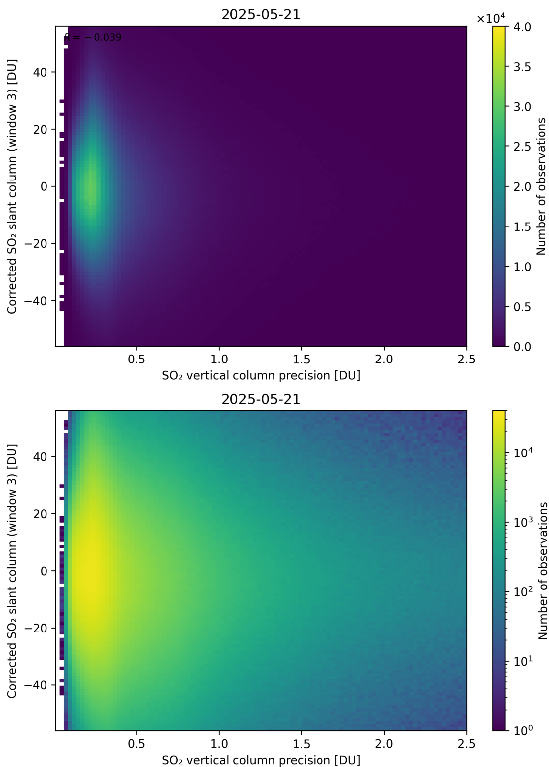
Figure 340: Scatter density plot of “SO 2 vertical column precision” against “Corrected SO 2 slant column (window 3)” for 2025-05-21 to 2025-05-22.
