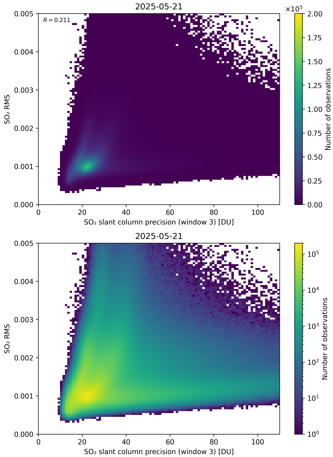
Figure 310: Scatter density plot of “SO 2 slant column precision (window 3)” against “SO 2 RMS” for 2025-05-21 to 2025-05-22.
