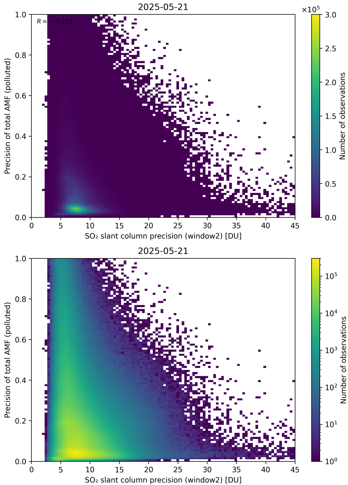
Figure 302: Scatter density plot of “SO 2 slant column precision (window2)” against “Precision of total AMF (polluted)” for 2025-05-21 to 2025-05-22.
