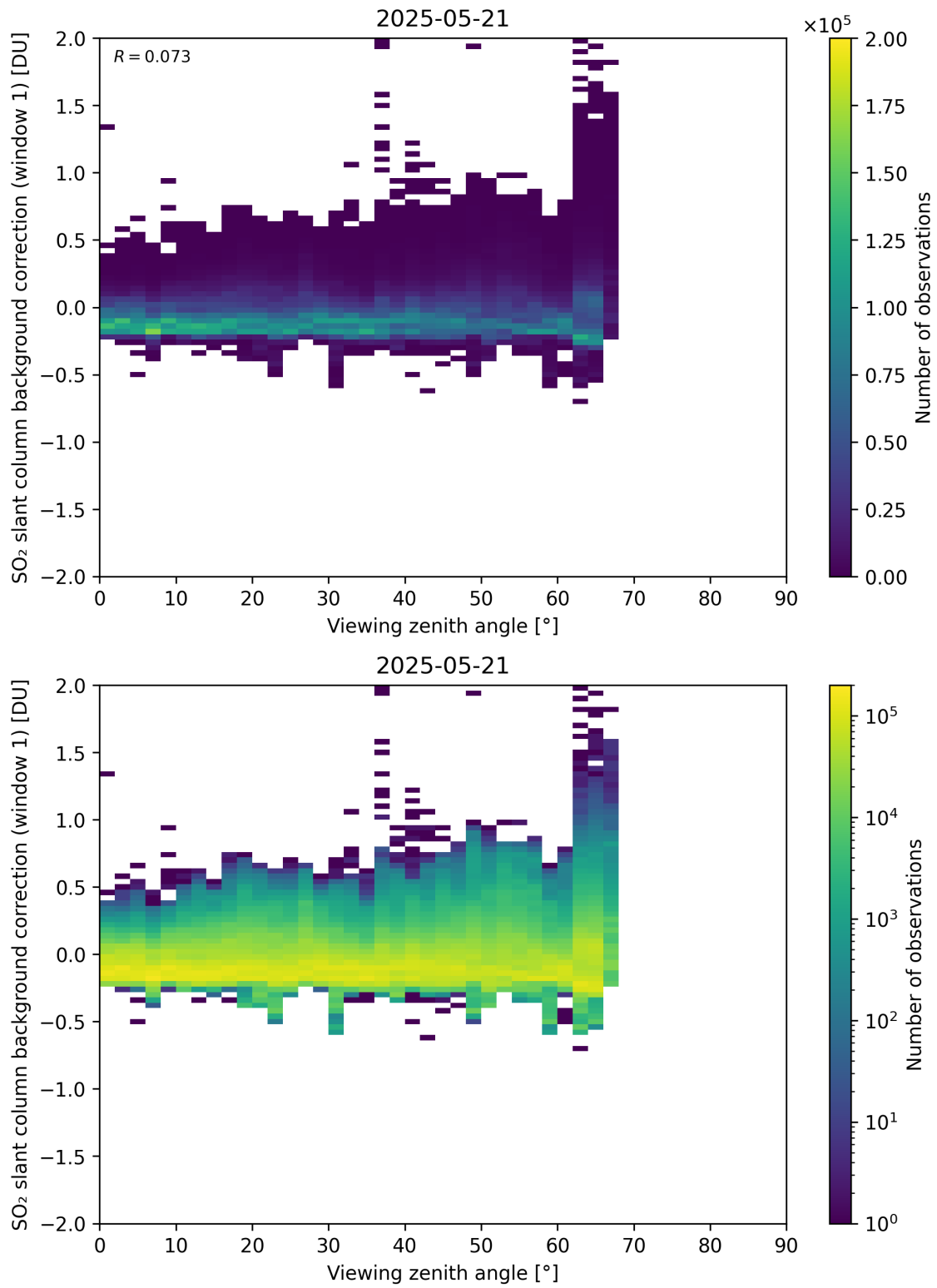
Figure 362: Scatter density plot of “Viewing zenith angle” against “SO 2 slant column background correction (window 1)” for 2025-05-21 to 2025-05-22.
