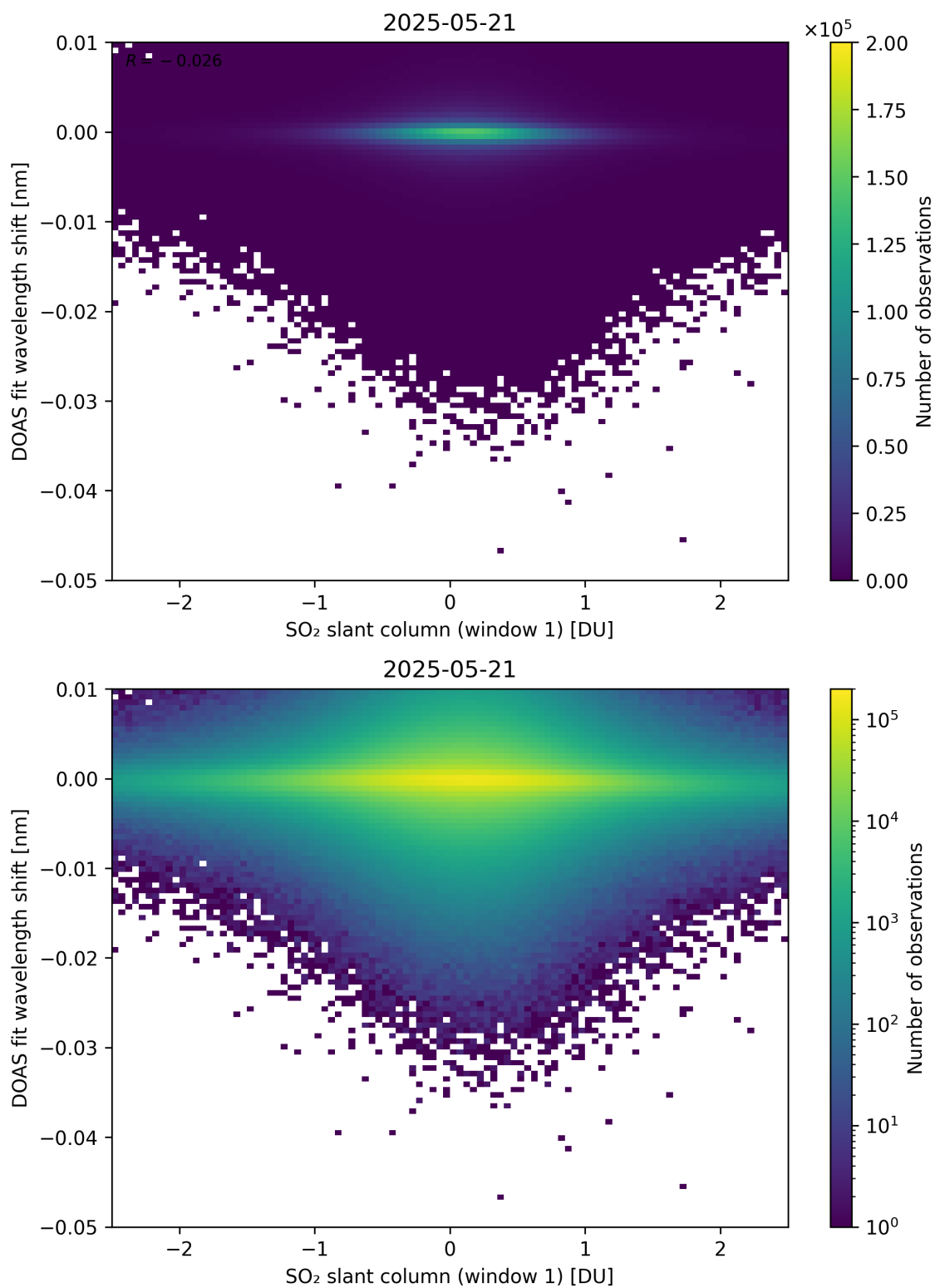
Figure 265: Scatter density plot of “SO 2 slant column (window 1)” against “DOAS fit wavelength shift” for 2025-05-21 to 2025-05-22.
