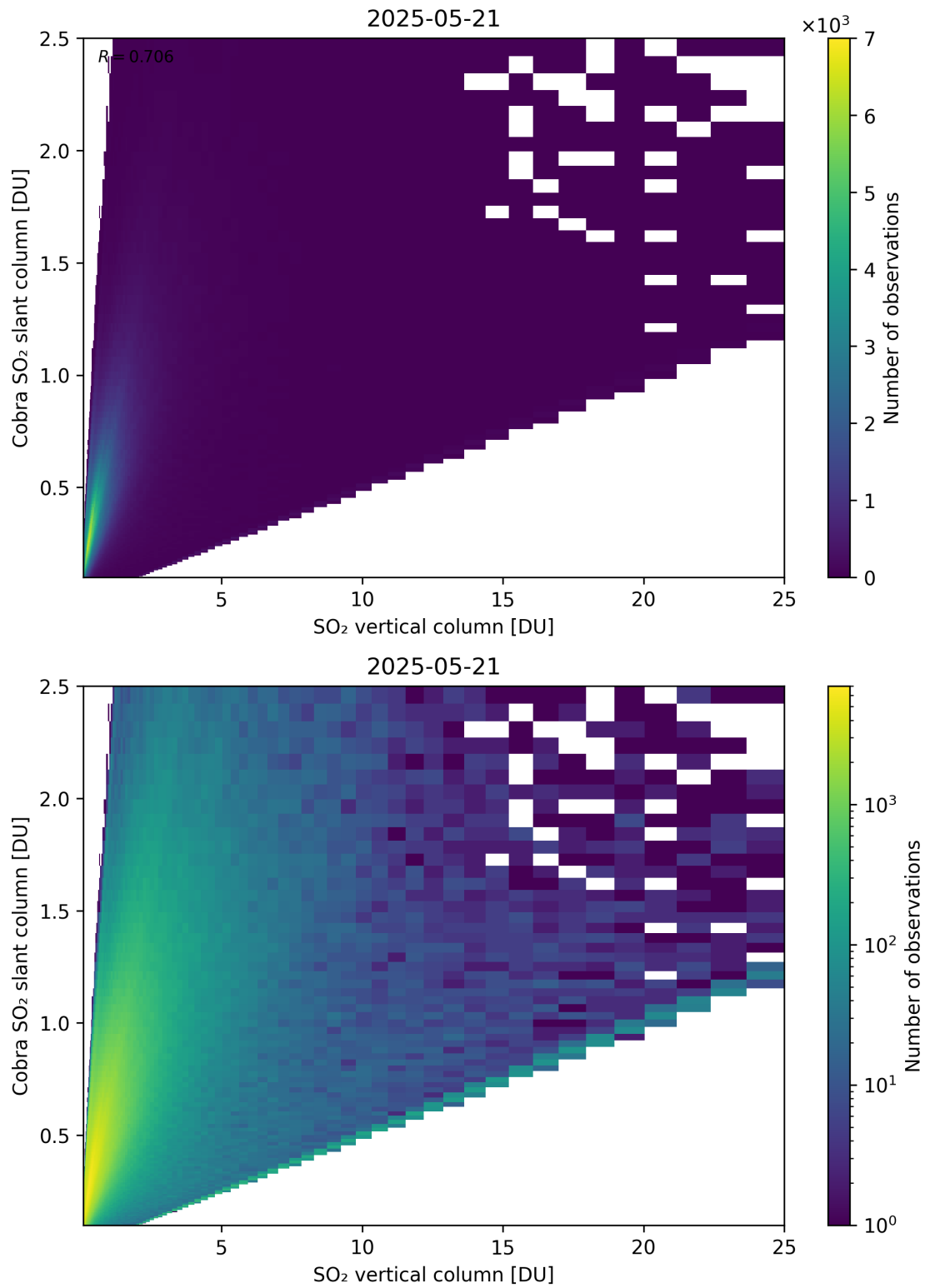
Figure 349: Scatter density plot of “SO 2 vertical column” against “Cobra SO 2 slant column” for 2025-05-21 to 2025-05-22.
