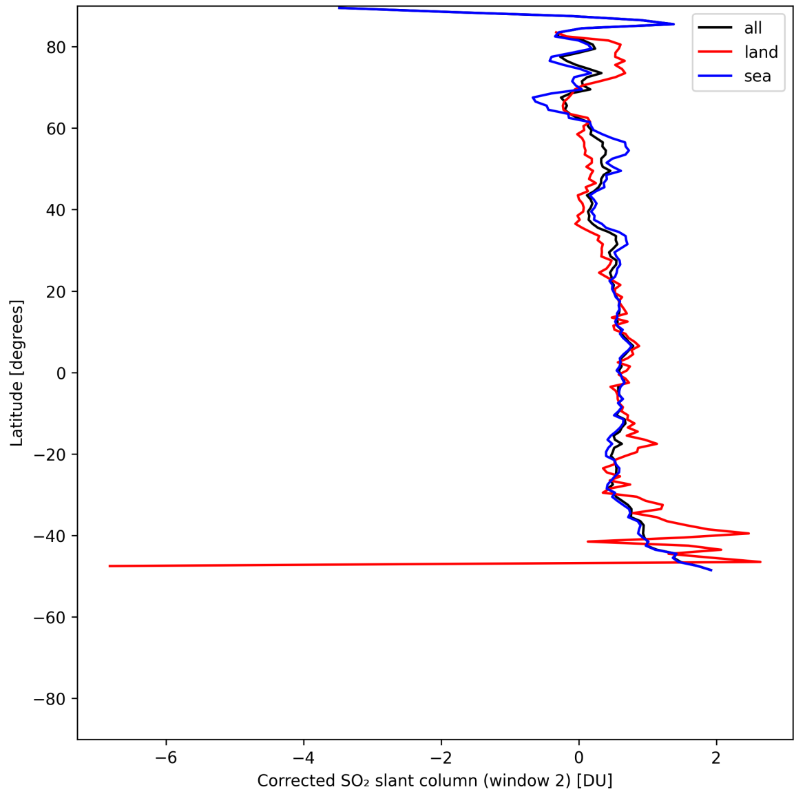
Figure 43: Zonal average of “Corrected SO 2 slant column (window 2)” for 2025-05-21 to 2025-05-22.
