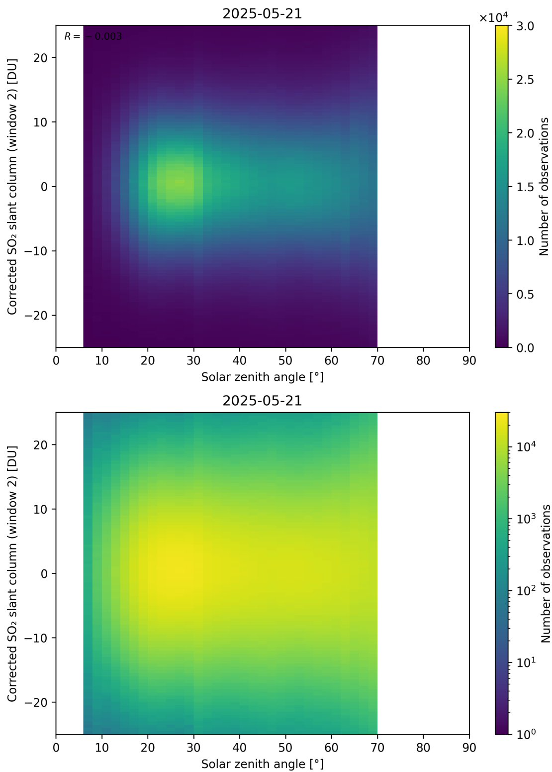
Figure 182: Scatter density plot of “Solar zenith angle” against “Corrected SO 2 slant column (window 2)” for 2025-05-21 to 2025-05-22.
