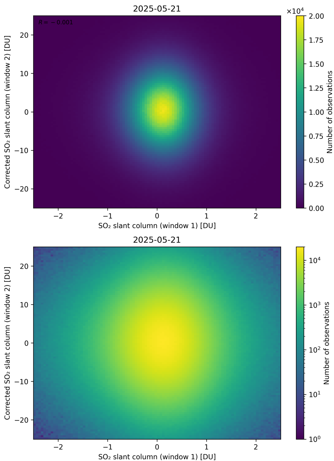
Figure 283: Scatter density plot of “SO 2 slant column (window 1)” against “Corrected SO 2 slant column (window 2)” for 2025-05-21 to 2025-05-22.
