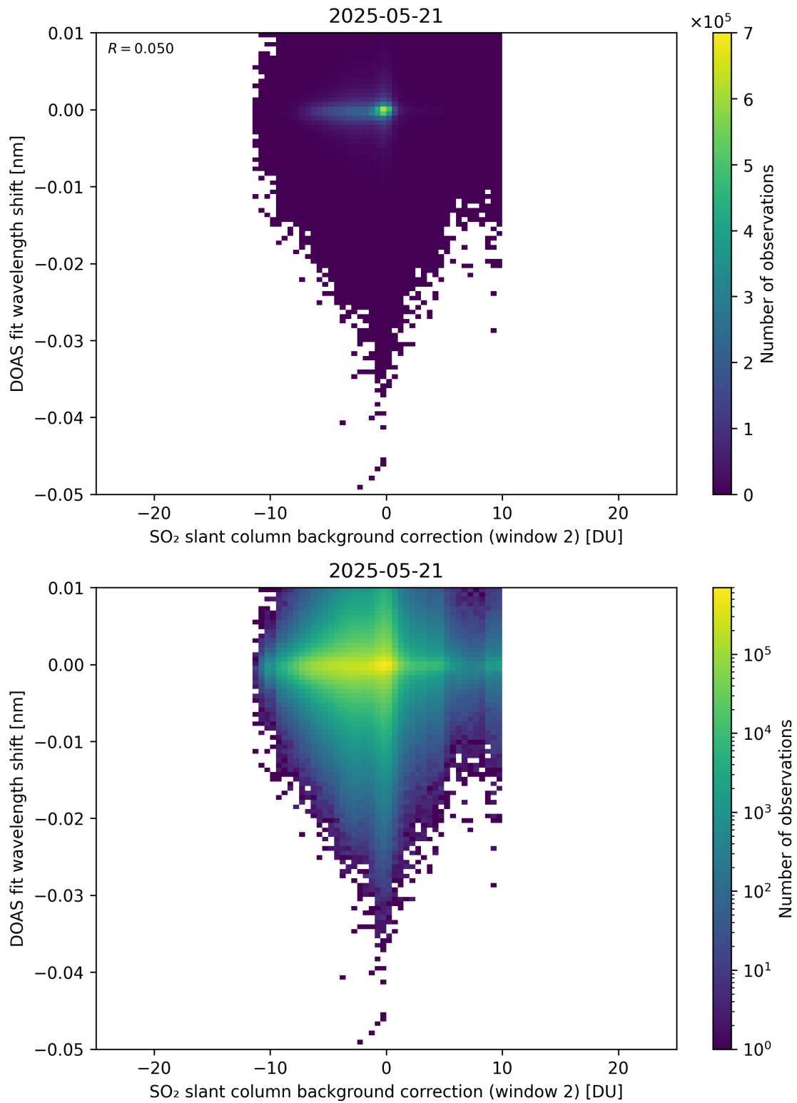
Figure 123: Scatter density plot of “SO 2 slant column background correction (window 2)” against “DOAS fit wavelength shift” for 2025-05-21 to 2025-05-22.
