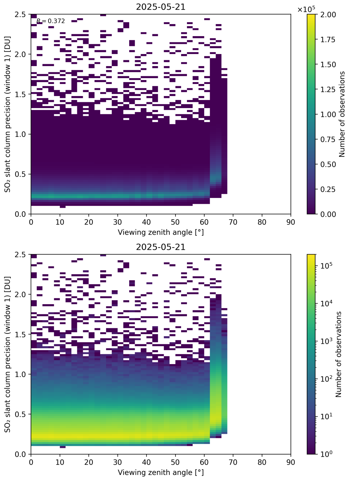
Figure 377: Scatter density plot of “Viewing zenith angle” against “SO 2 slant column precision (window 1)” for 2025-05-21 to 2025-05-22.
