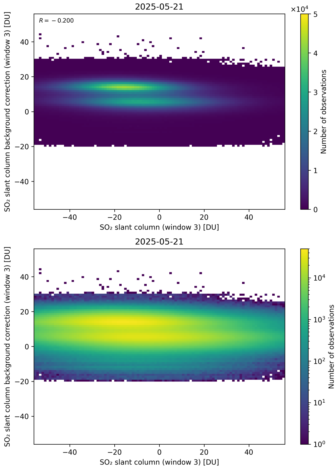
Figure 303: Scatter density plot of “SO 2 slant column (window 3)” against “SO 2 slant column background correction (window 3)” for 2025-05-21 to 2025-05-22.
