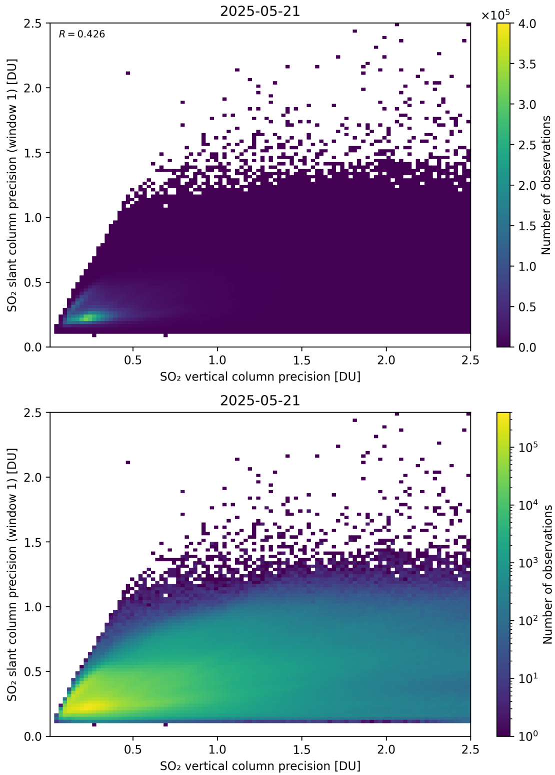
Figure 342: Scatter density plot of “SO 2 vertical column precision” against “SO 2 slant column precision (window 1)” for 2025-05-21 to 2025-05-22.
