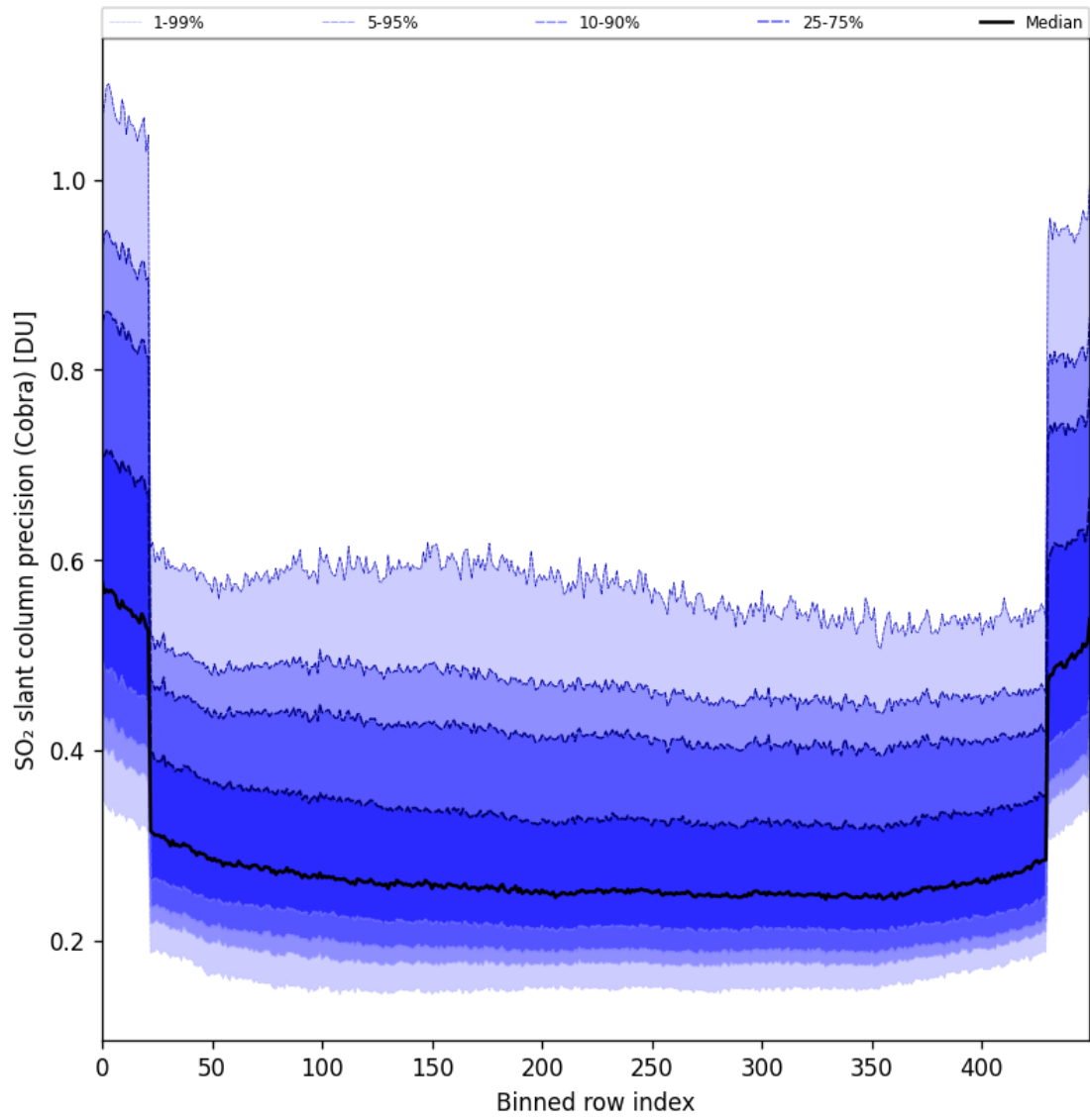
Figure 88: Along track statistics of “SO 2 slant column precision (Cobra)” for 2025-05-21 to 2025-05-22
