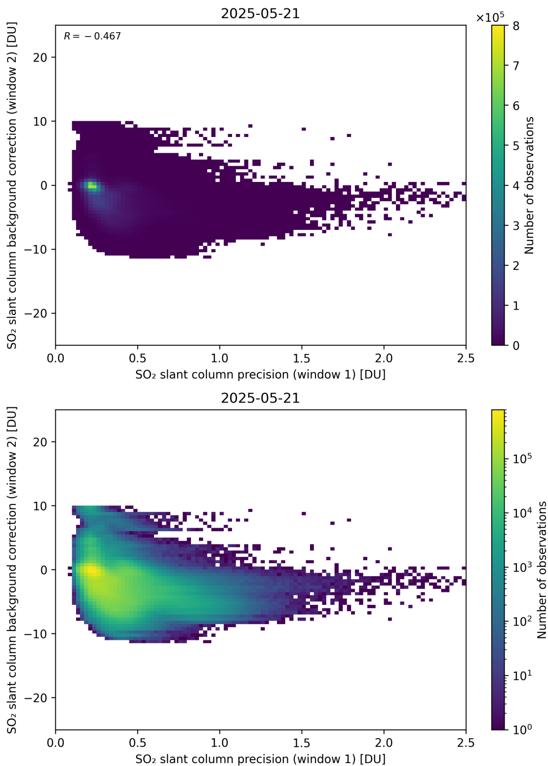
Figure 269: Scatter density plot of “SO 2 slant column precision (window 1)” against “SO 2 slant column background correction (window 2)” for 2025-05-21 to 2025-05-22.
