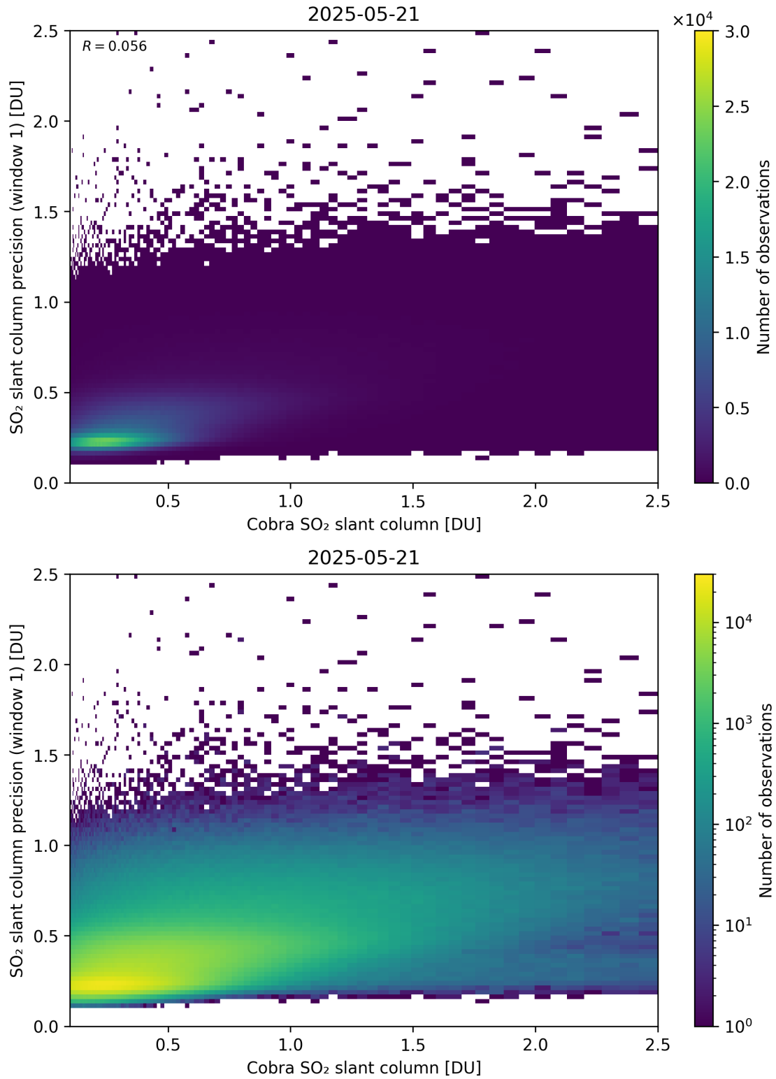
Figure 220: Scatter density plot of “Cobra SO 2 slant column” against “SO 2 slant column precision (window 1)” for 2025-05-21 to 2025-05-22.
