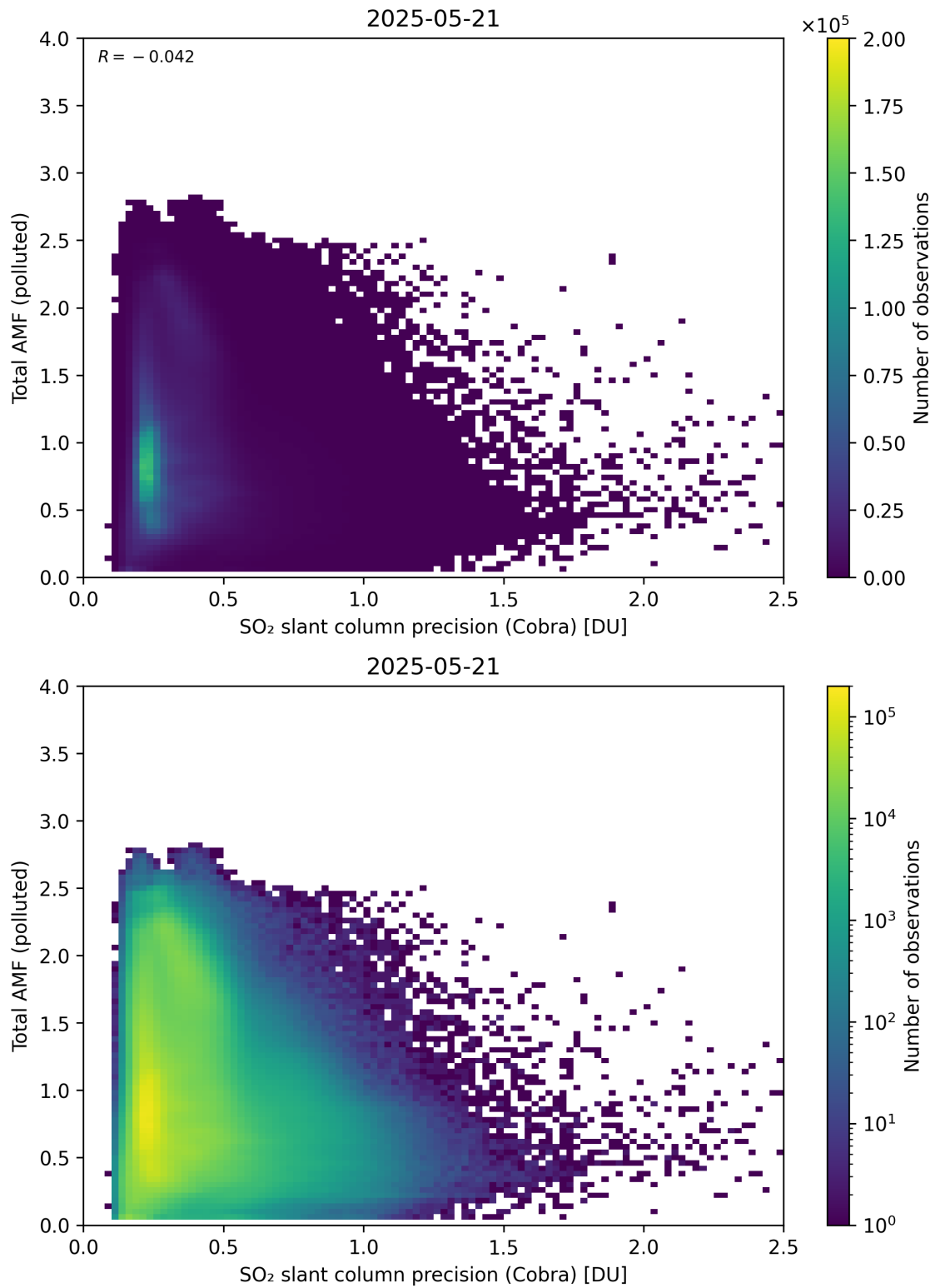
Figure 213: Scatter density plot of “SO 2 slant column precision (Cobra)” against “Total AMF (polluted)” for 2025-05-21 to 2025-05-22.
