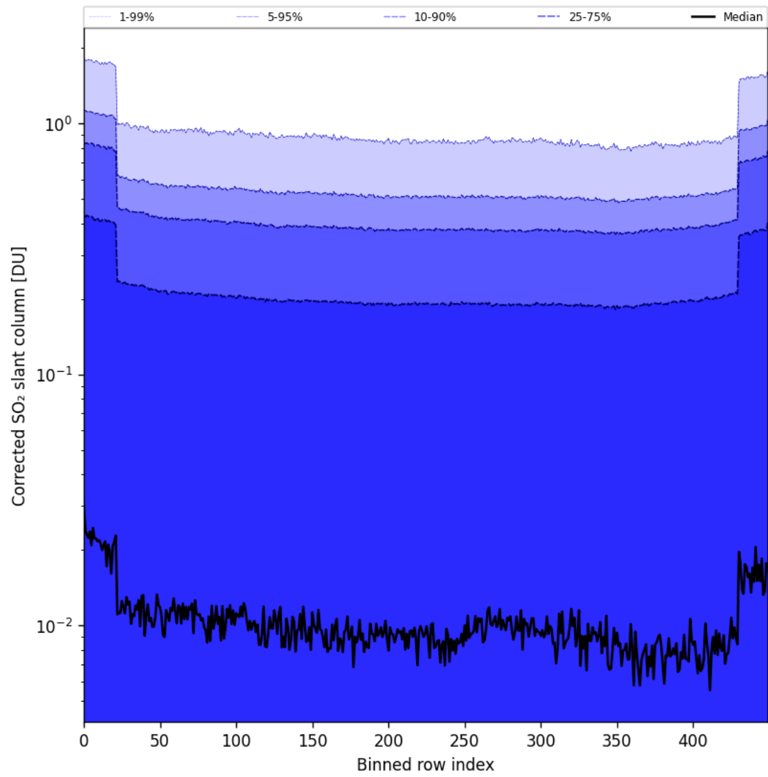
Figure 86: Along track statistics of “Corrected SO 2 slant column” for 2025-05-21 to 2025-05-22
