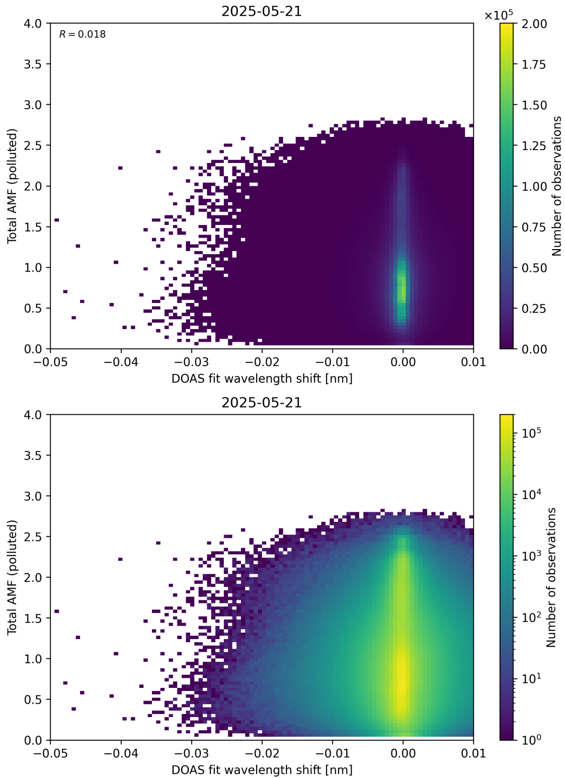
Figure 141: Scatter density plot of “DOAS fit wavelength shift” against “Total AMF (polluted)” for 2025-05-21 to 2025-05-22.
