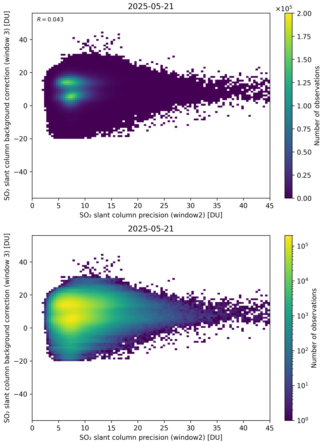
Figure 292: Scatter density plot of “SO 2 slant column precision (window2)” against “SO 2 slant column background correction (window 3)” for 2025-05-21 to 2025-05-22.
