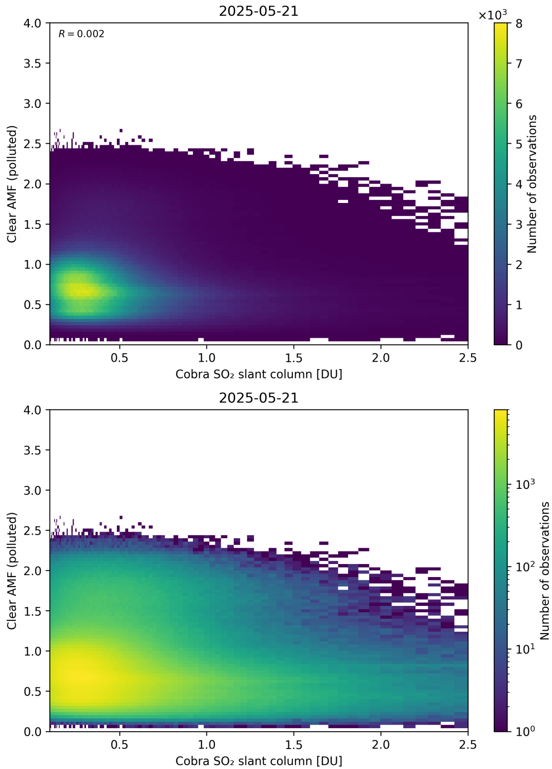
Figure 215: Scatter density plot of “Cobra SO 2 slant column” against “Clear AMF (polluted)” for 2025-05-21 to 2025-05-22.
