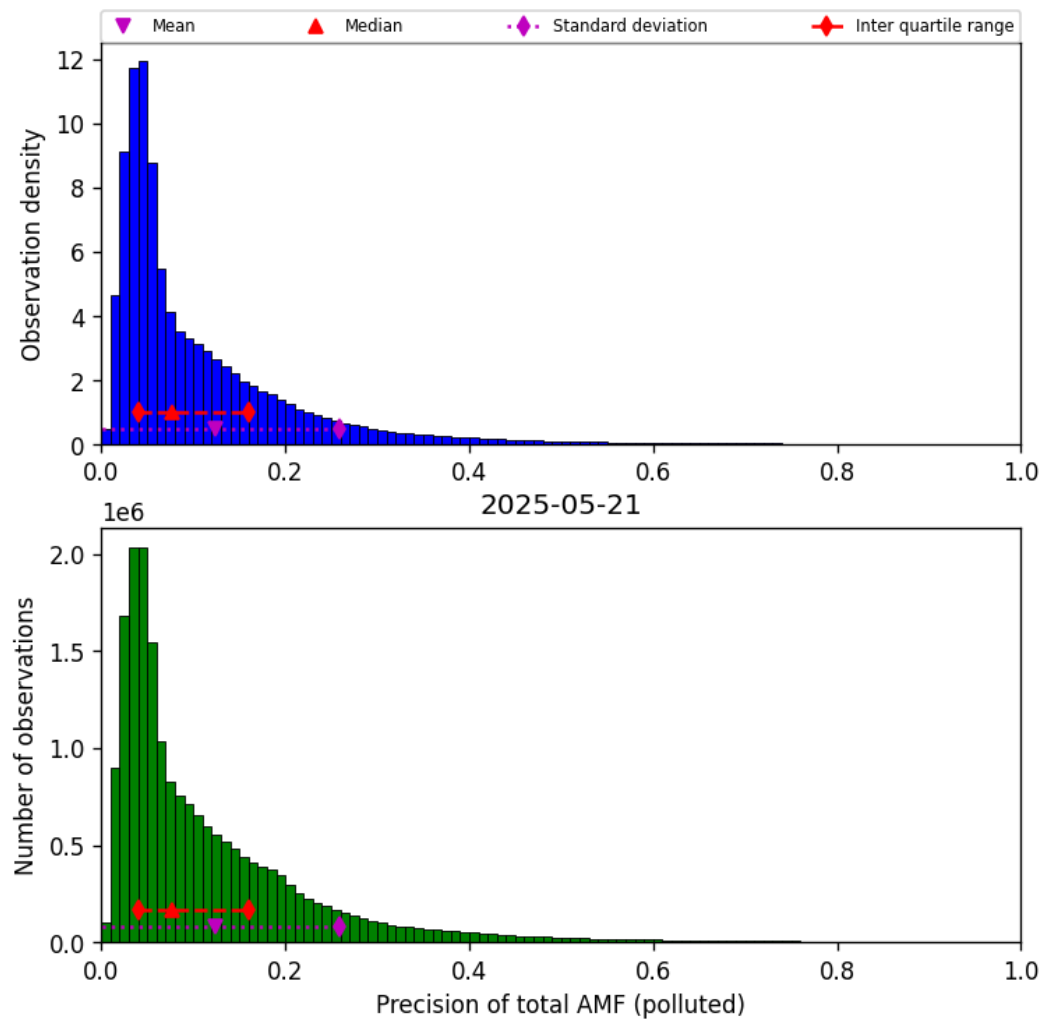
Figure 80: Histogram of “Precision of total AMF (polluted)” for 2025-05-21 to 2025-05-22
