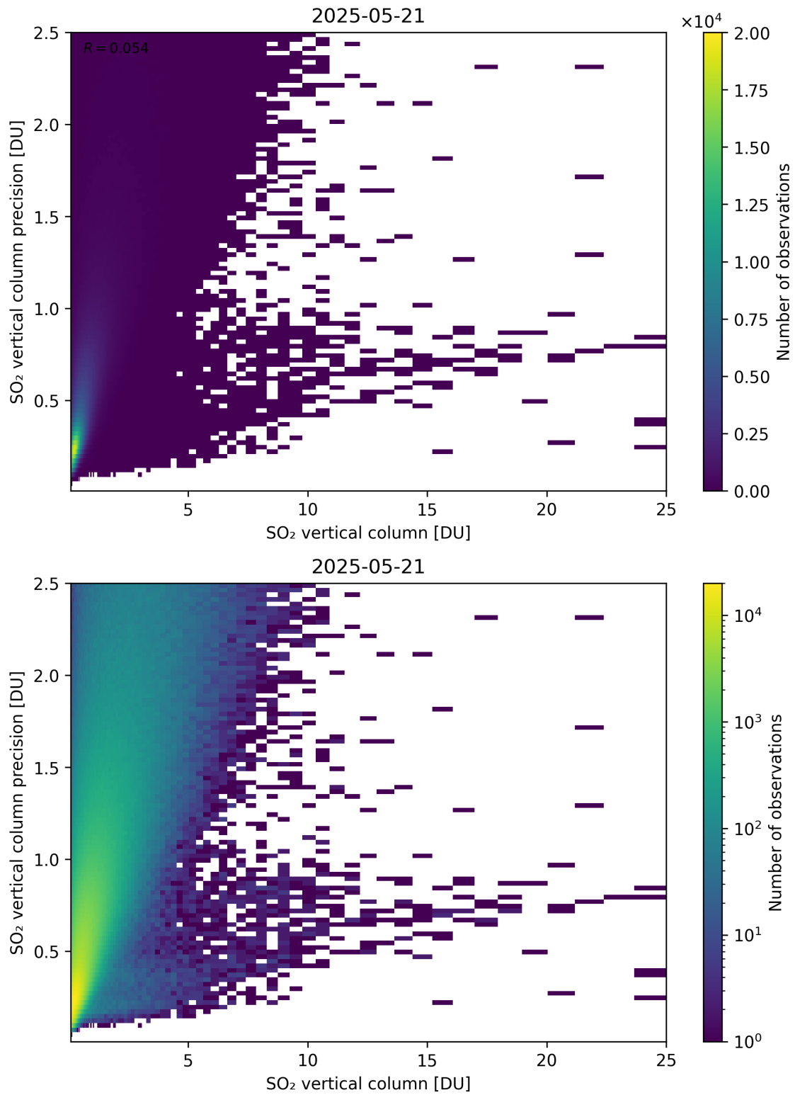
Figure 361: Scatter density plot of “SO 2 vertical column” against “SO 2 vertical column precision” for 2025-05-21 to 2025-05-22.
