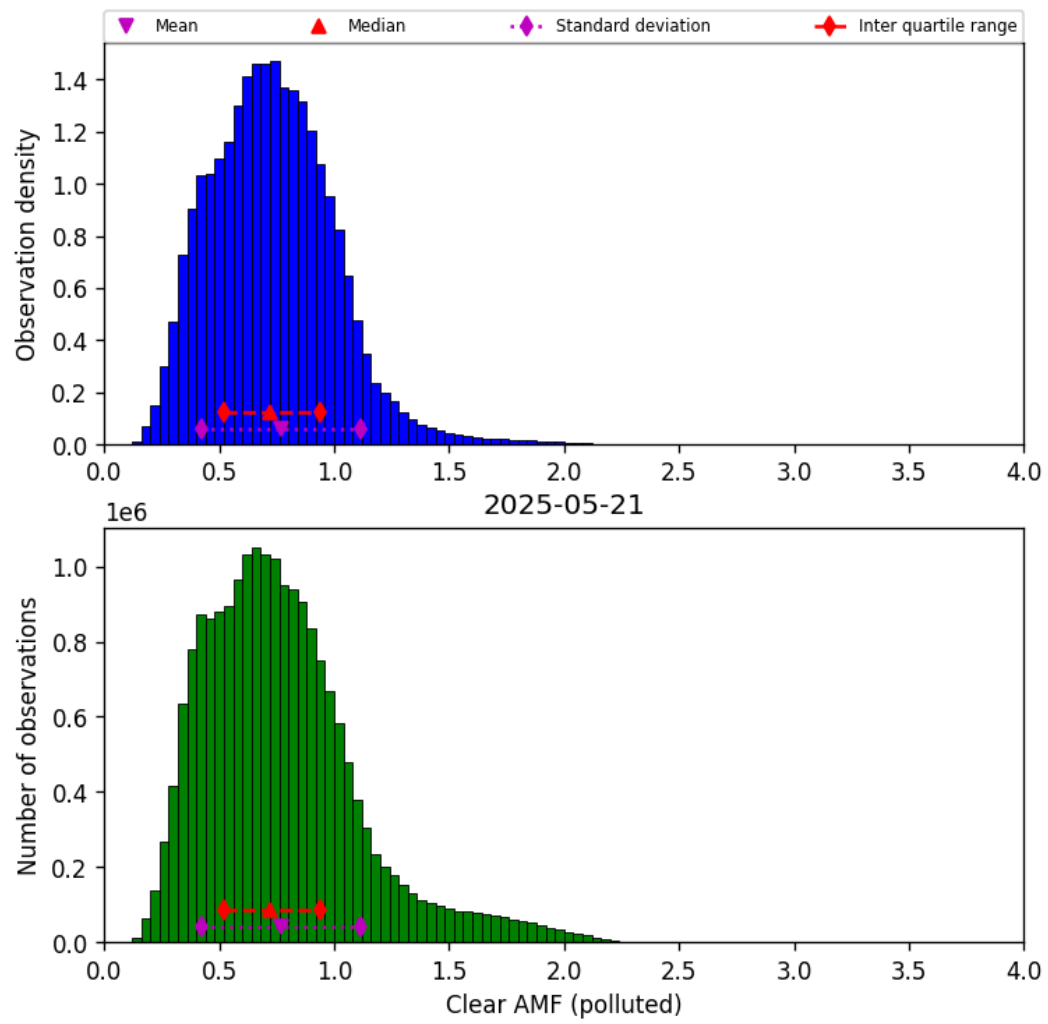
Figure 81: Histogram of “Clear AMF (polluted)” for 2025-05-21 to 2025-05-22
