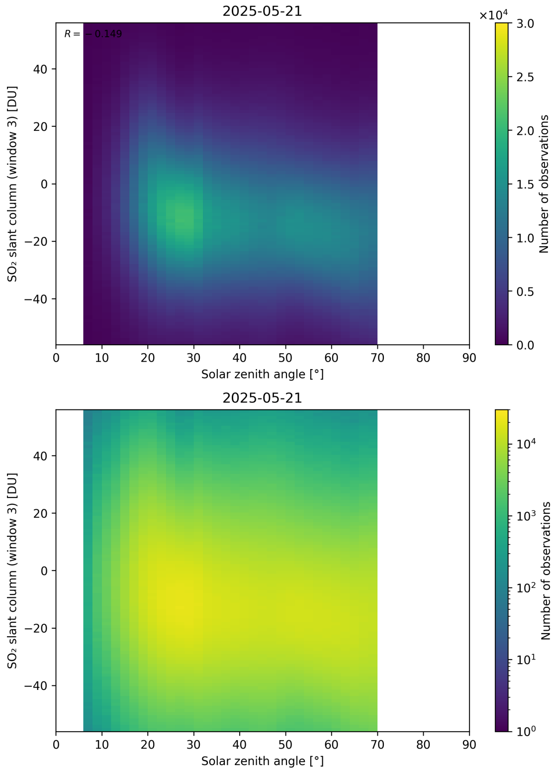
Figure 187: Scatter density plot of “Solar zenith angle” against “SO 2 slant column (window 3)” for 2025-05-21 to 2025-05-22.
