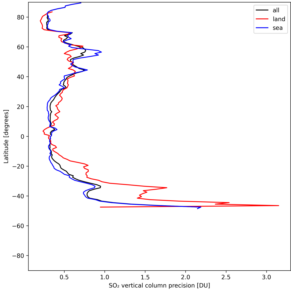
Figure 33: Zonal average of “SO 2 vertical column precision” for 2025-05-21 to 2025-05-22.
