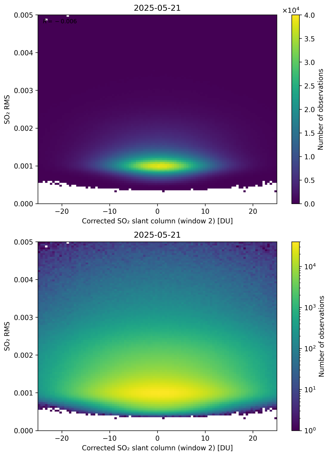
Figure 248: Scatter density plot of “Corrected SO 2 slant column (window 2)” against “SO 2 RMS” for 2025-05-21 to 2025-05-22.
