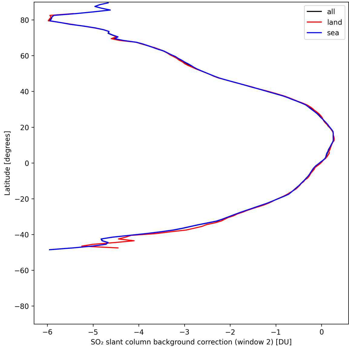
Figure 44: Zonal average of “SO 2 slant column background correction (window 2)” for 2025-05-21 to 2025-05-22.
