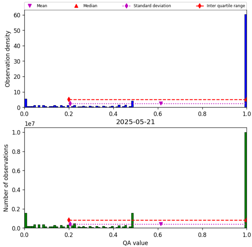
Figure 57: Histogram of “QA value” for 2025-05-21 to 2025-05-22
