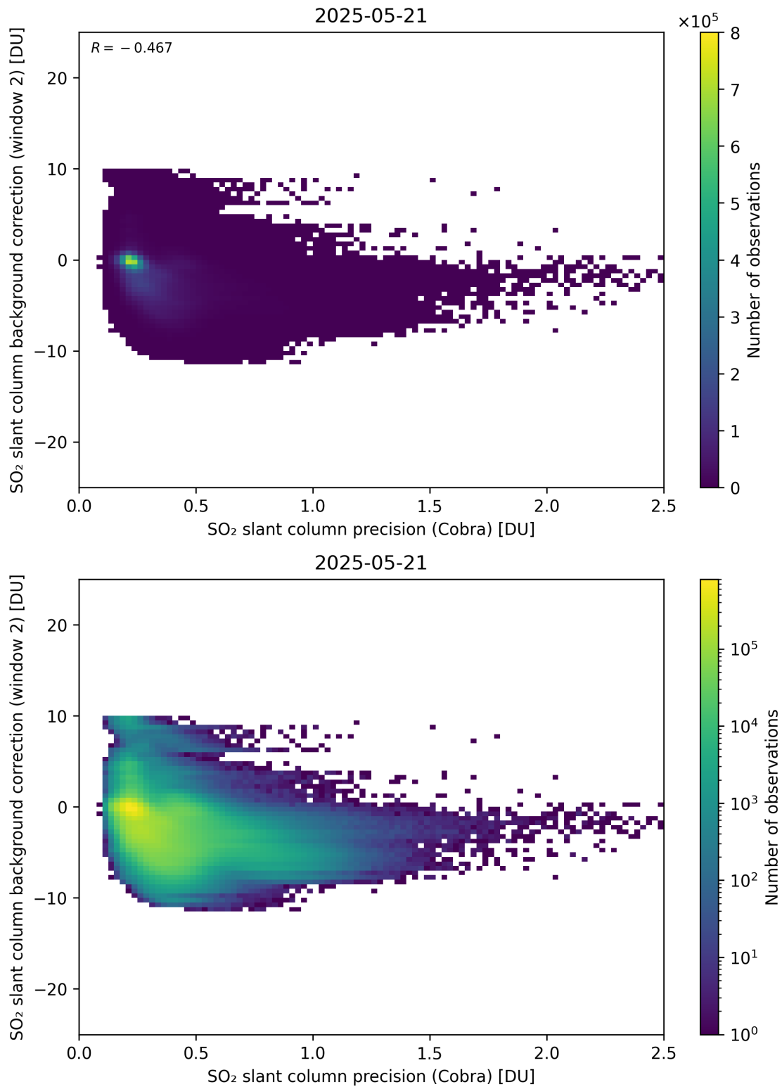
Figure 200: Scatter density plot of “SO 2 slant column precision (Cobra)” against “SO 2 slant column background correction (window 2)” for 2025-05-21 to 2025-05-22.
