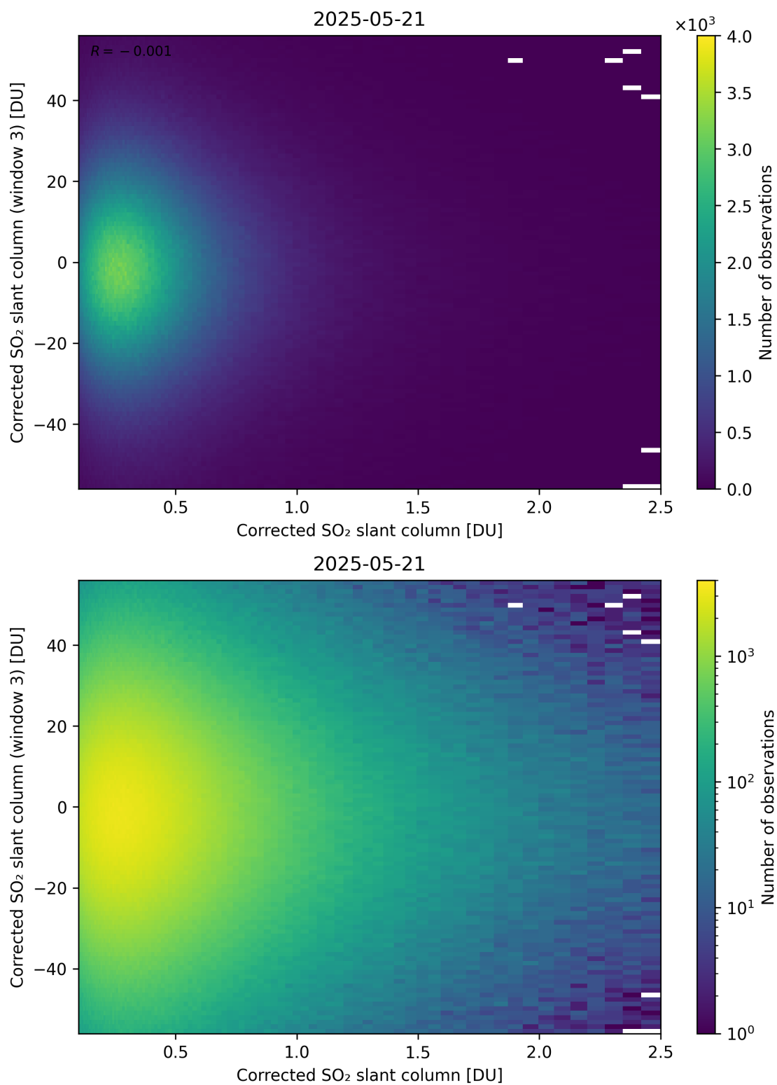
Figure 236: Scatter density plot of “Corrected SO 2 slant column” against “Corrected SO 2 slant column (window 3)” for 2025-05-21 to 2025-05-22.
