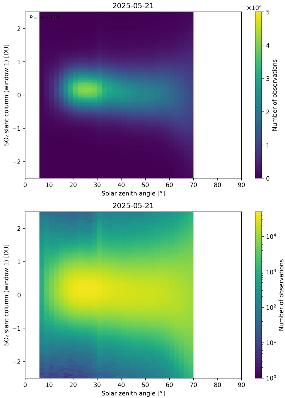
Figure 184: Scatter density plot of “Solar zenith angle” against “SO 2 slant column (window 1)” for 2025-05-21 to 2025-05-22.
