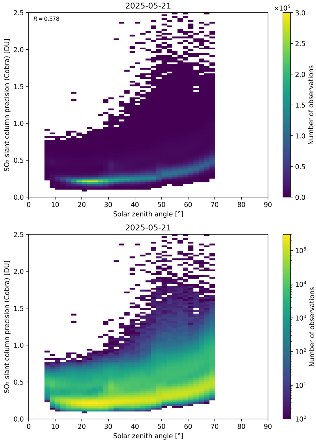
Figure 180: Scatter density plot of “Solar zenith angle” against “SO 2 slant column precision (Cobra)” for 2025-05-21 to 2025-05-22.
