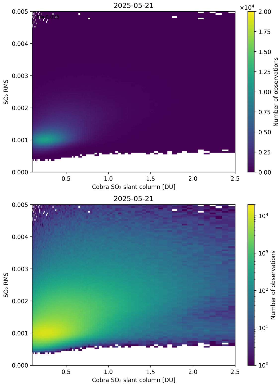
Figure 198: Scatter density plot of “Cobra SO 2 slant column” against “SO 2 RMS” for 2025-05-21 to 2025-05-22.
