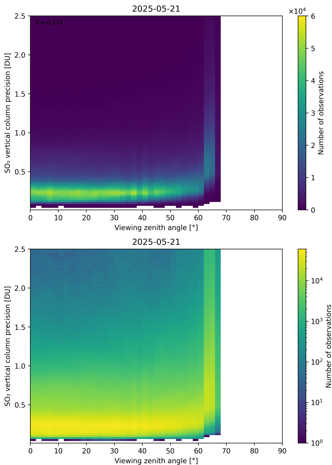
Figure 384: Scatter density plot of “Viewing zenith angle” against “SO 2 vertical column precision” for 2025-05-21 to 2025-05-22.
