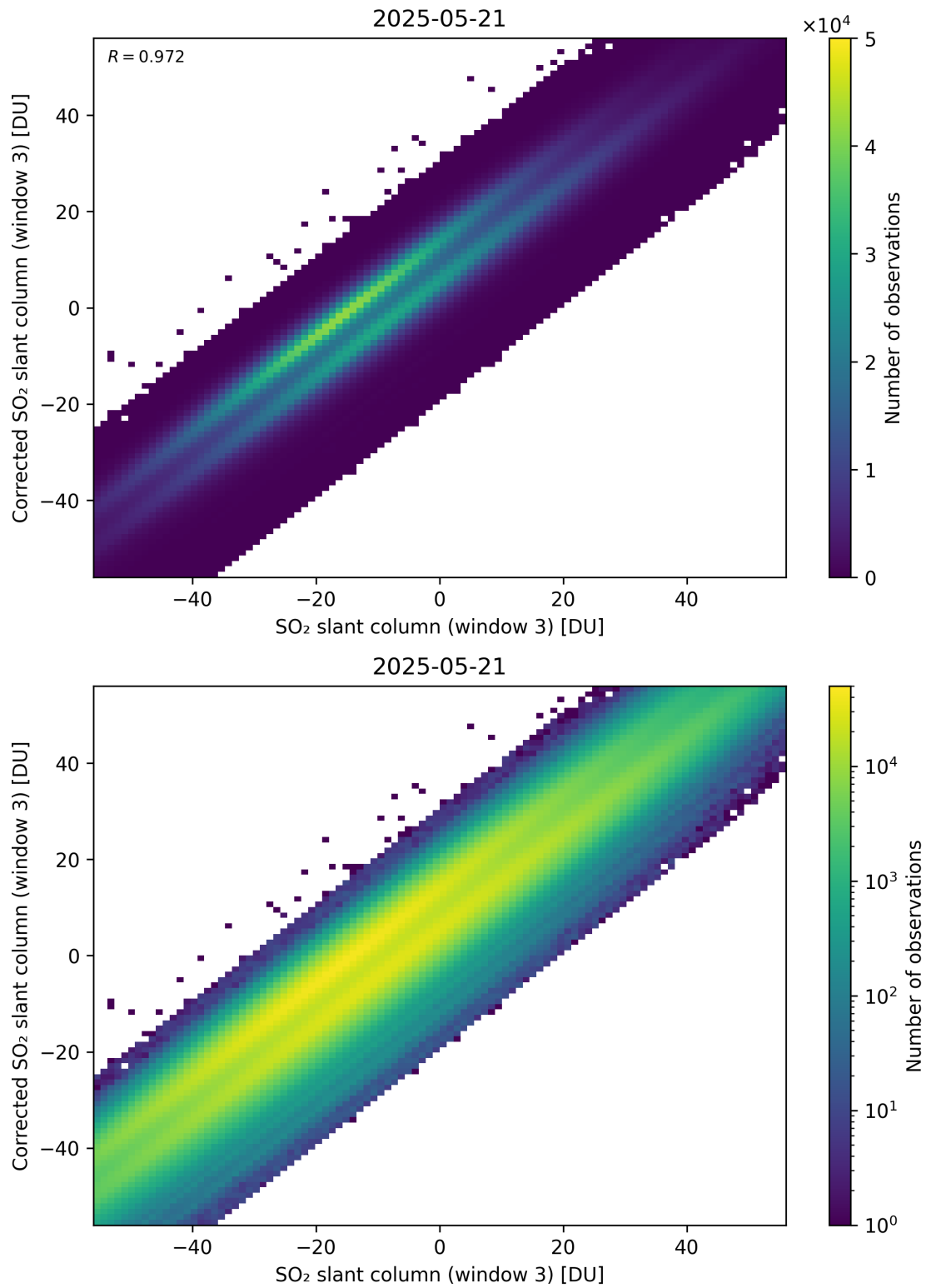
Figure 316: Scatter density plot of “SO 2 slant column (window 3)” against “Corrected SO 2 slant column (window 3)” for 2025-05-21 to 2025-05-22.
