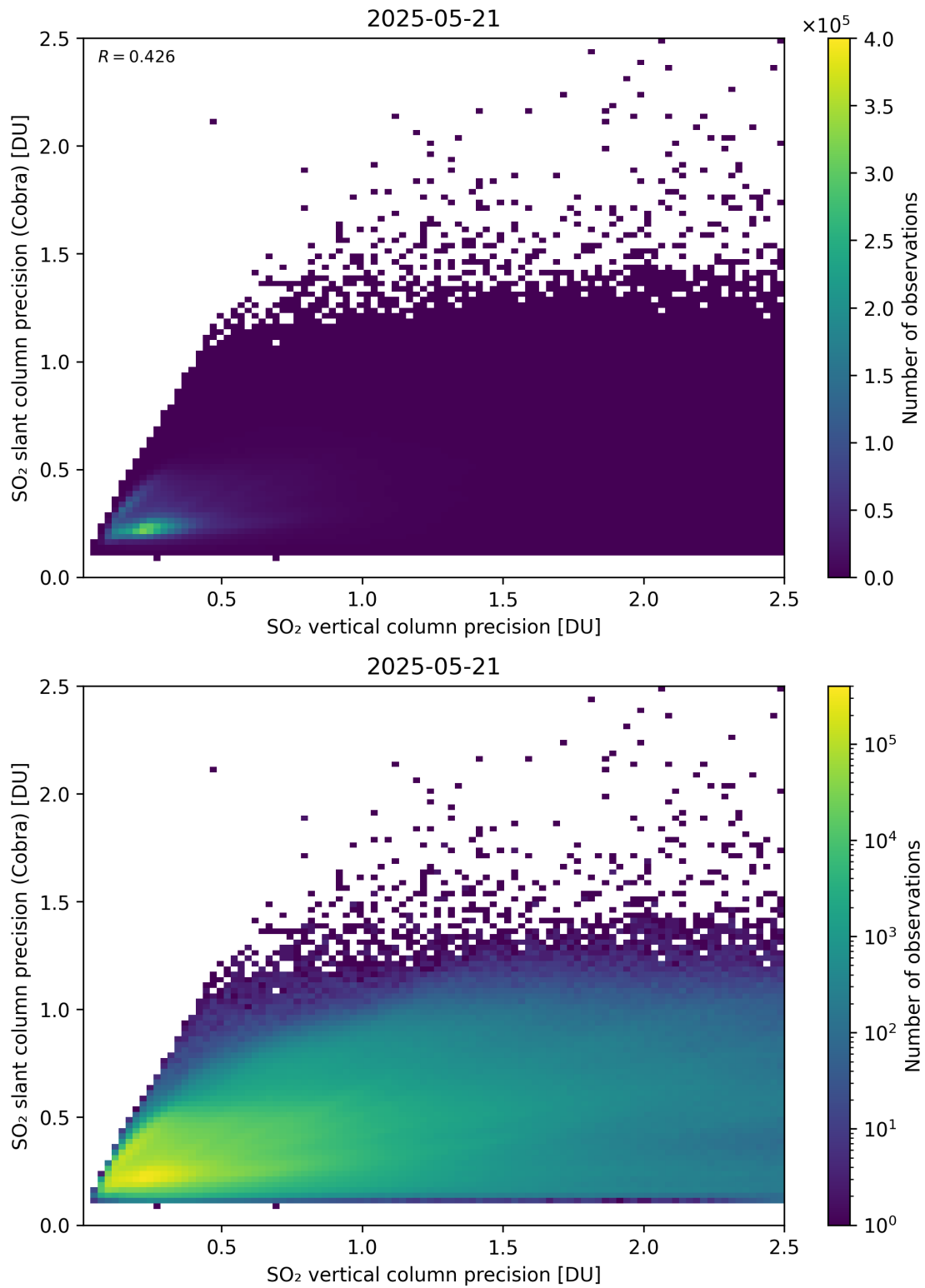
Figure 337: Scatter density plot of “SO 2 vertical column precision” against “SO 2 slant column precision (Cobra)” for 2025-05-21 to 2025-05-22.
