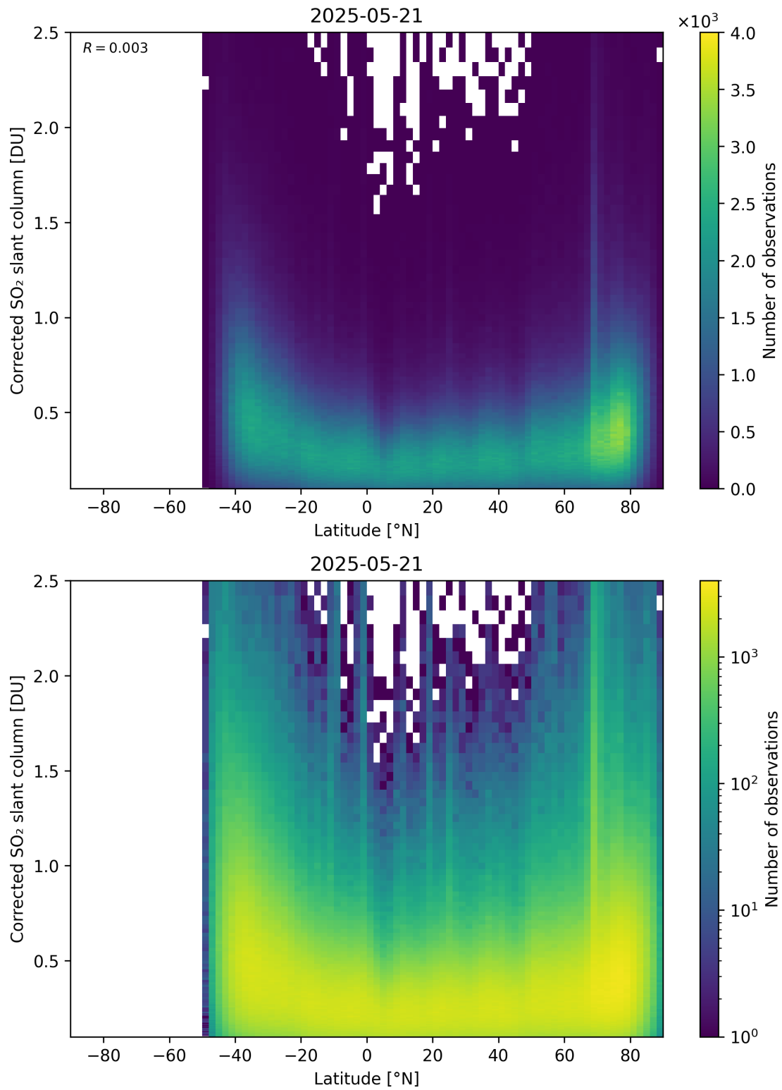
Figure 159: Scatter density plot of “Latitude” against “Corrected SO 2 slant column” for 2025-05-21 to 2025-05-22.
