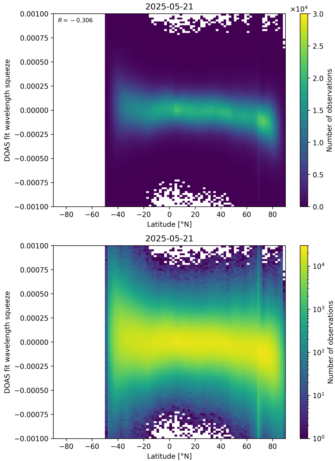
Figure 154: Scatter density plot of “Latitude” against “DOAS fit wavelength squeeze” for 2025-05-21 to 2025-05-22.
