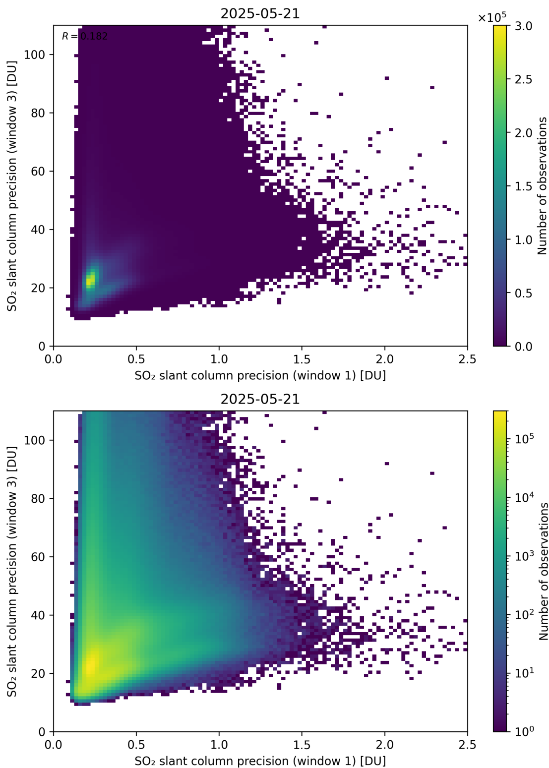
Figure 279: Scatter density plot of “SO 2 slant column precision (window 1)” against “SO 2 slant column precision (window 3)” for 2025-05-21 to 2025-05-22.
