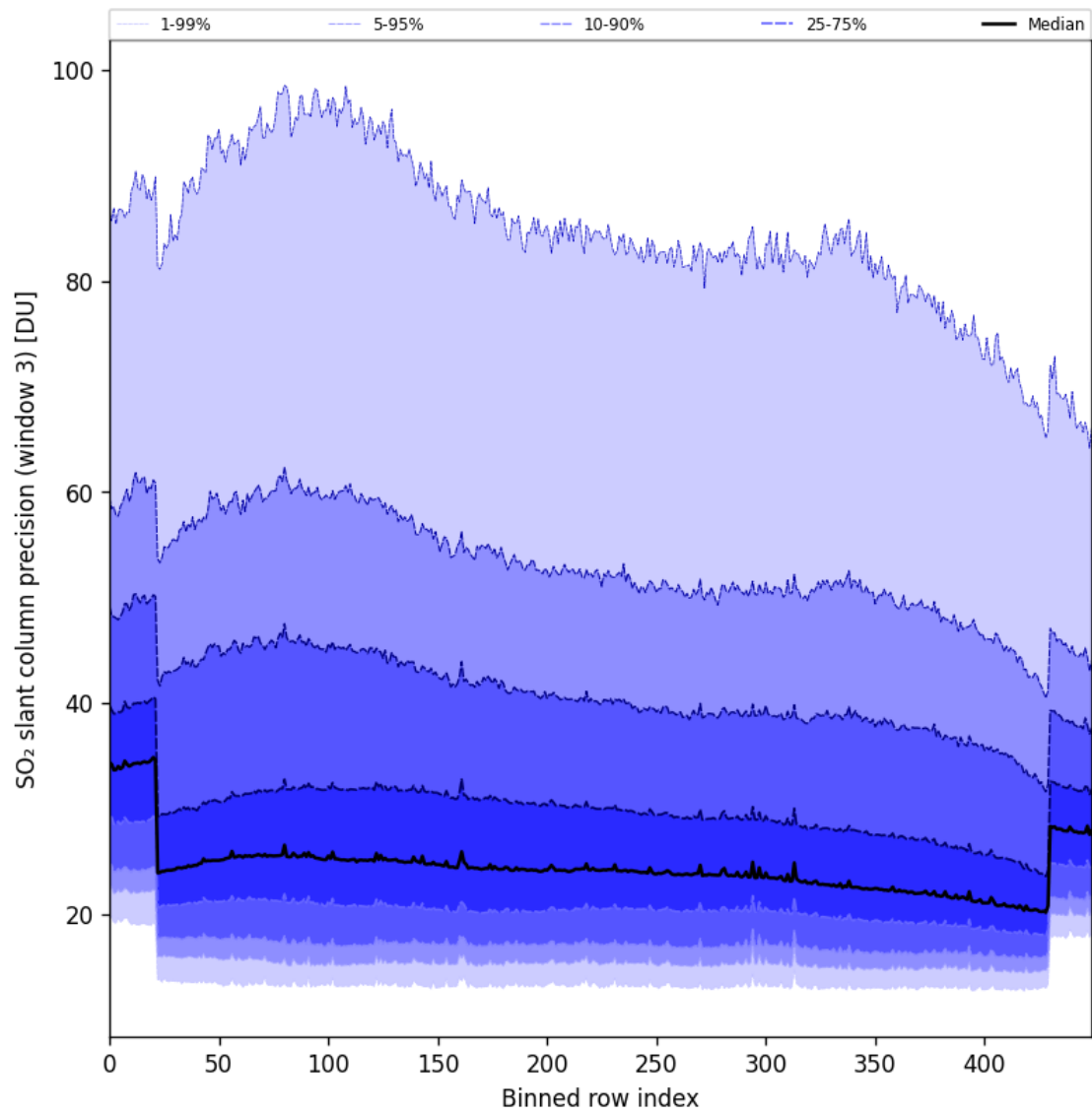
Figure 98: Along track statistics of “SO 2 slant column precision (window 3)” for 2025-05-21 to 2025-05-22
