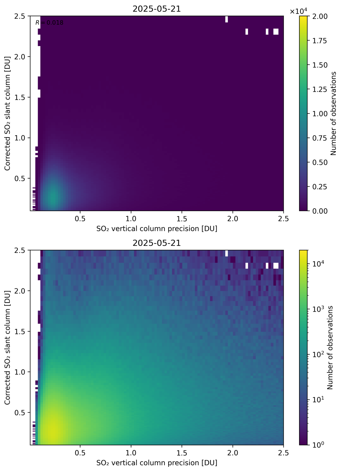
Figure 338: Scatter density plot of “SO 2 vertical column precision” against “Corrected SO 2 slant column” for 2025-05-21 to 2025-05-22.
