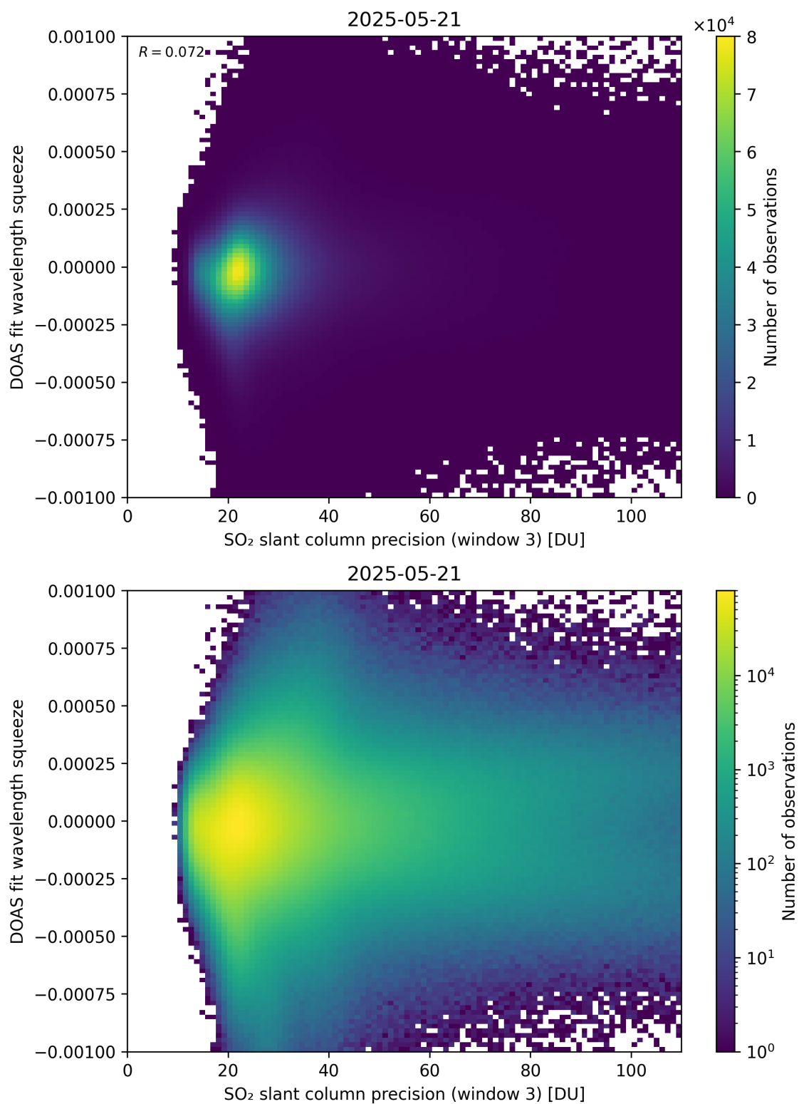
Figure 309: Scatter density plot of “SO 2 slant column precision (window 3)” against “DOAS fit wavelength squeeze” for 2025-05-21 to 2025-05-22.
