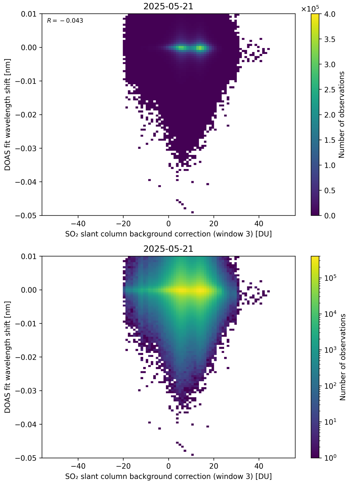
Figure 132: Scatter density plot of “SO 2 slant column background correction (window 3)” against “DOAS fit wavelength shift” for 2025-05-21 to 2025-05-22.
