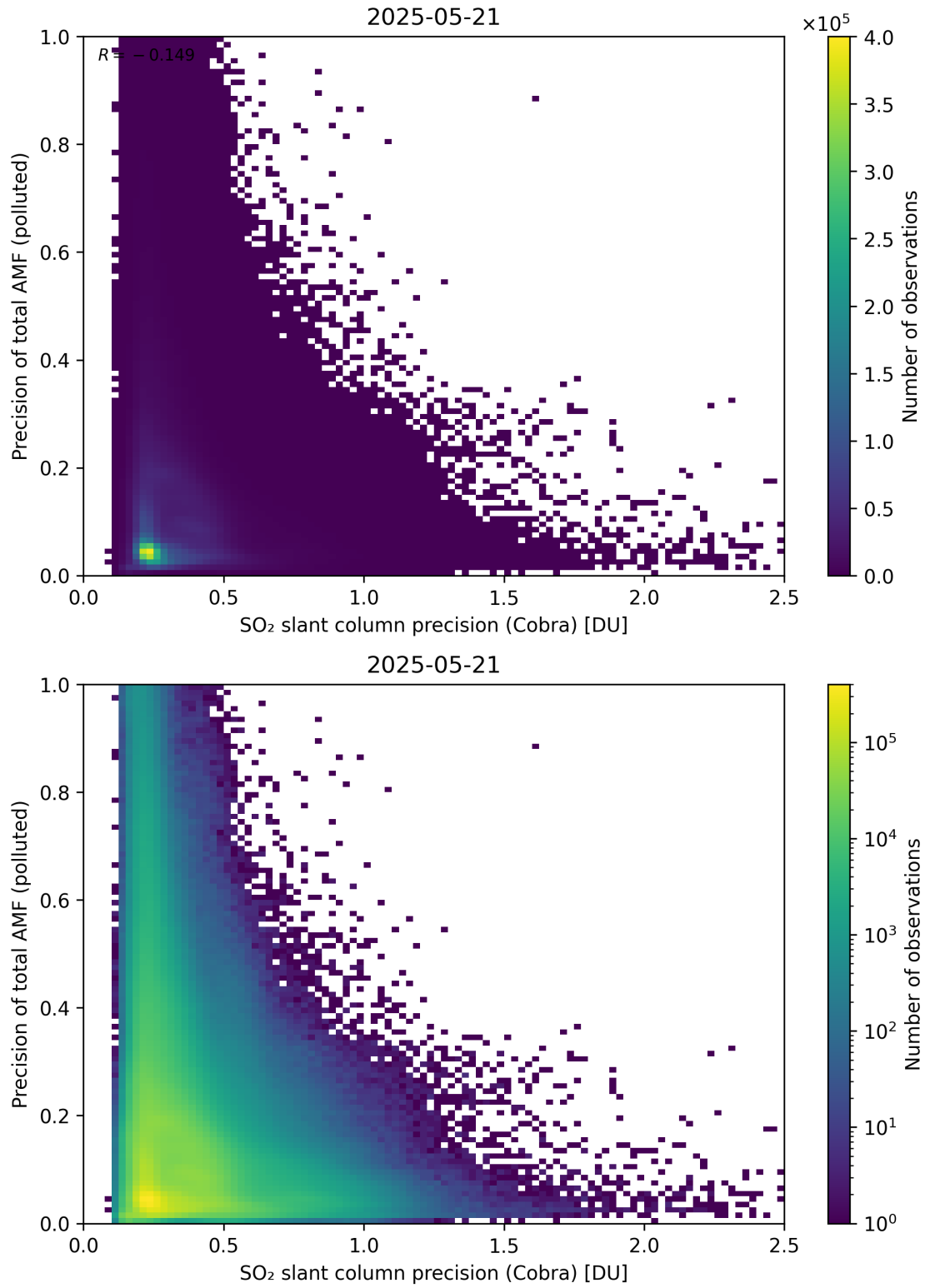
Figure 214: Scatter density plot of “SO 2 slant column precision (Cobra)” against “Precision of total AMF (polluted)” for 2025-05-21 to 2025-05-22.
