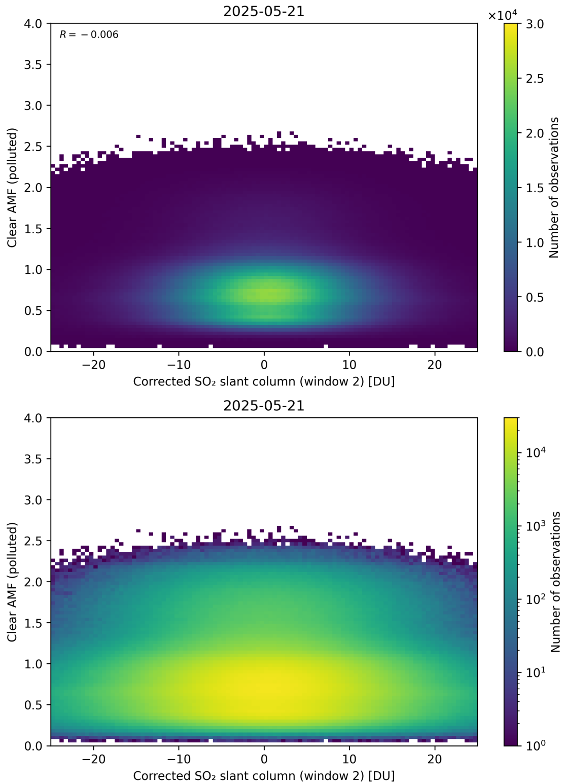
Figure 249: Scatter density plot of “Corrected SO 2 slant column (window 2)” against “Clear AMF (polluted)” for 2025-05-21 to 2025-05-22.
