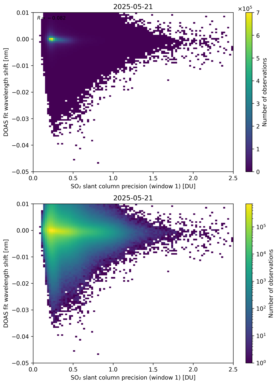
Figure 271: Scatter density plot of “SO 2 slant column precision (window 1)” against “DOAS fit wavelength shift” for 2025-05-21 to 2025-05-22.
