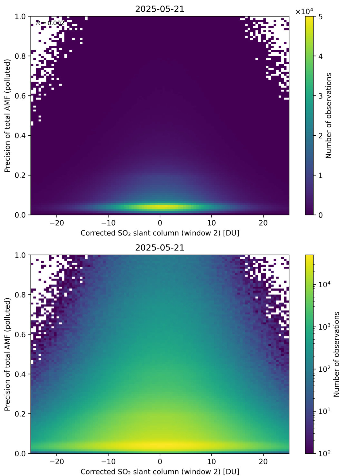
Figure 254: Scatter density plot of “Corrected SO 2 slant column (window 2)” against “Precision of total AMF (polluted)” for 2025-05-21 to 2025-05-22.
