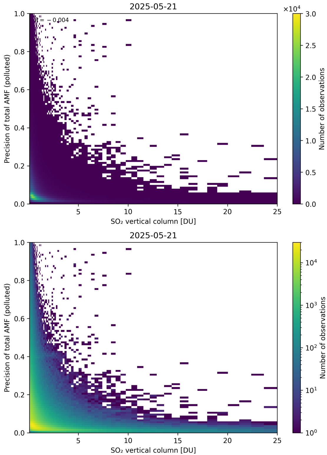
Figure 360: Scatter density plot of “SO 2 vertical column” against “Precision of total AMF (polluted)” for 2025-05-21 to 2025-05-22.
