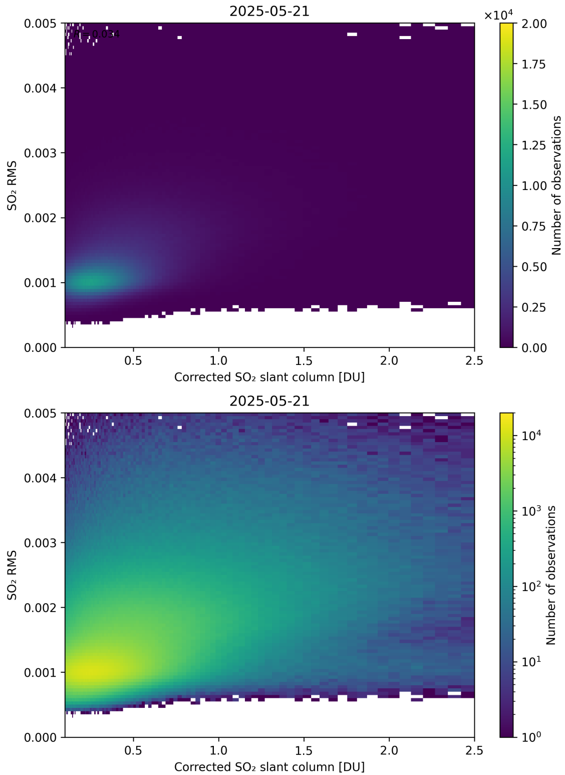
Figure 231: Scatter density plot of “Corrected SO 2 slant column” against “SO 2 RMS” for 2025-05-21 to 2025-05-22.
