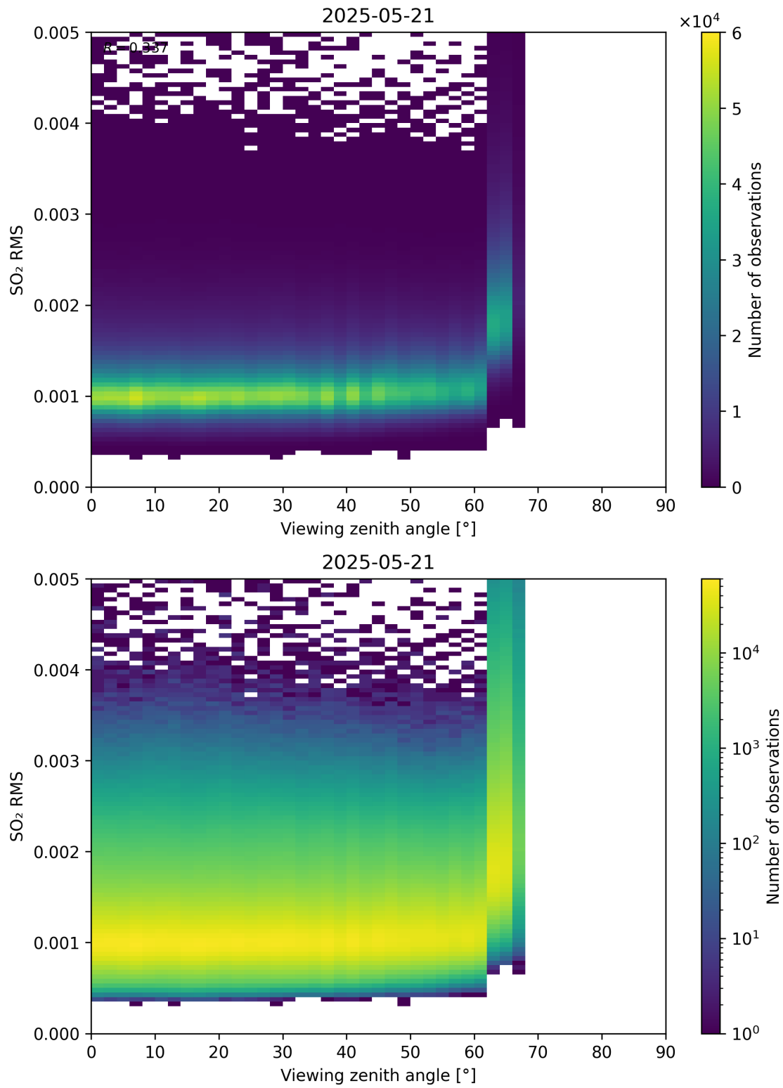
Figure 367: Scatter density plot of “Viewing zenith angle” against “SO 2 RMS” for 2025-05-21 to 2025-05-22.
