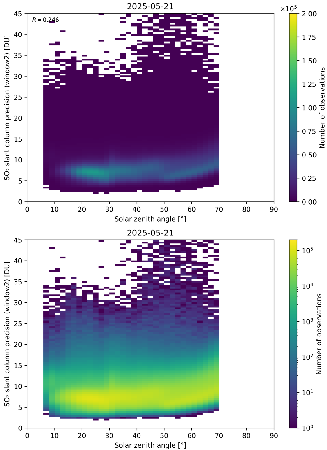
Figure 186: Scatter density plot of “Solar zenith angle” against “SO 2 slant column precision (window2)” for 2025-05-21 to 2025-05-22.
