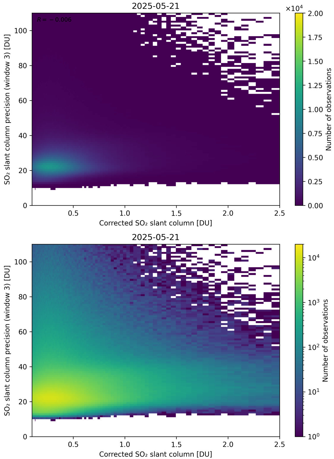
Figure 241: Scatter density plot of “Corrected SO 2 slant column” against “SO 2 slant column precision (window 3)” for 2025-05-21 to 2025-05-22.
