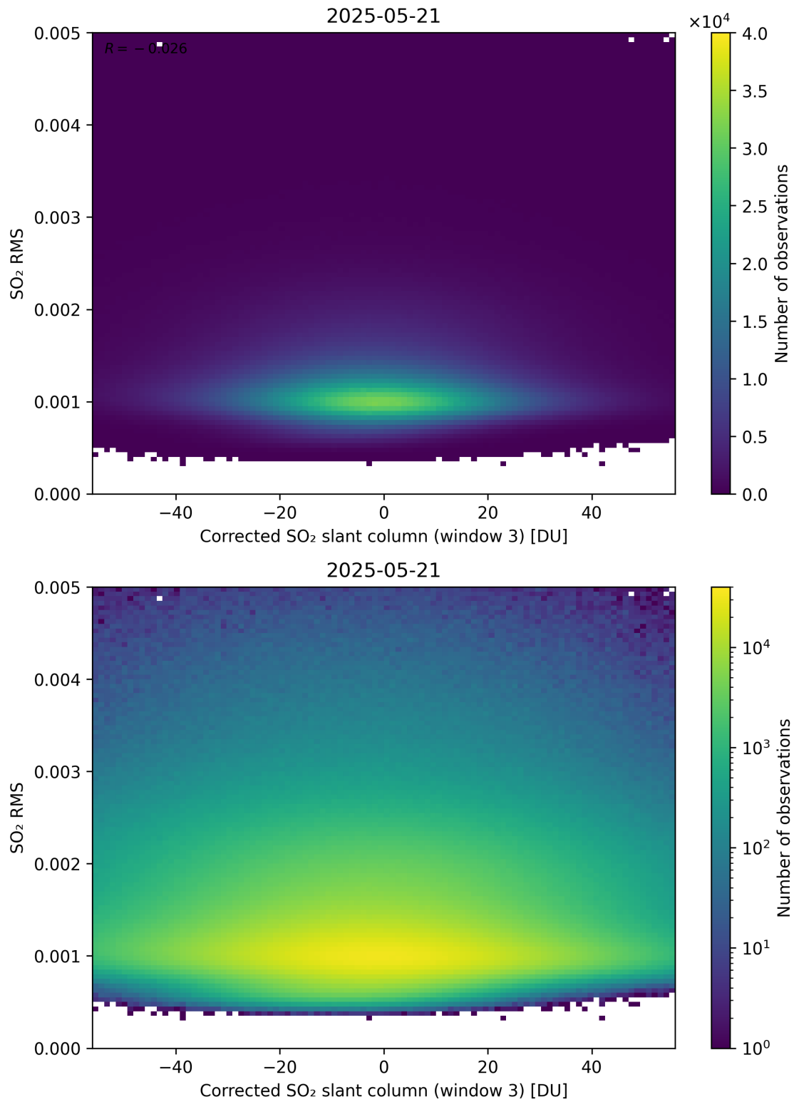
Figure 258: Scatter density plot of “Corrected SO 2 slant column (window 3)” against “SO 2 RMS” for 2025-05-21 to 2025-05-22.
