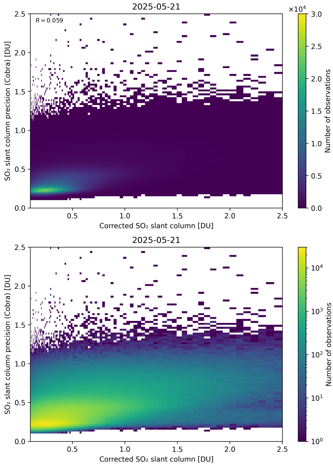
Figure 234: Scatter density plot of “Corrected SO 2 slant column” against “SO 2 slant column precision (Cobra)” for 2025-05-21 to 2025-05-22.
