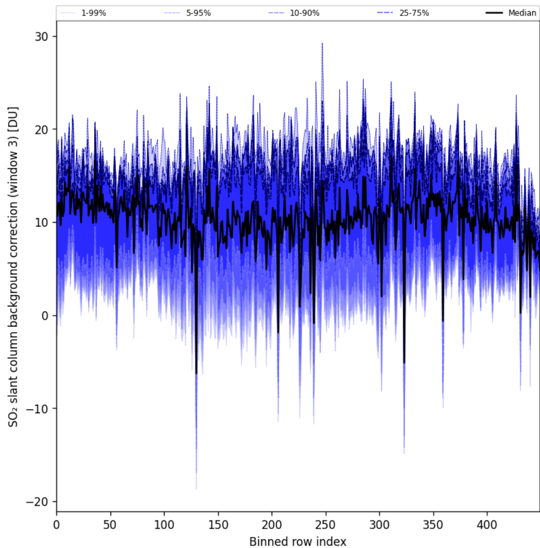
Figure 100: Along track statistics of “SO 2 slant column background correction (window 3)” for 2025-05-21 to 2025-05-22
