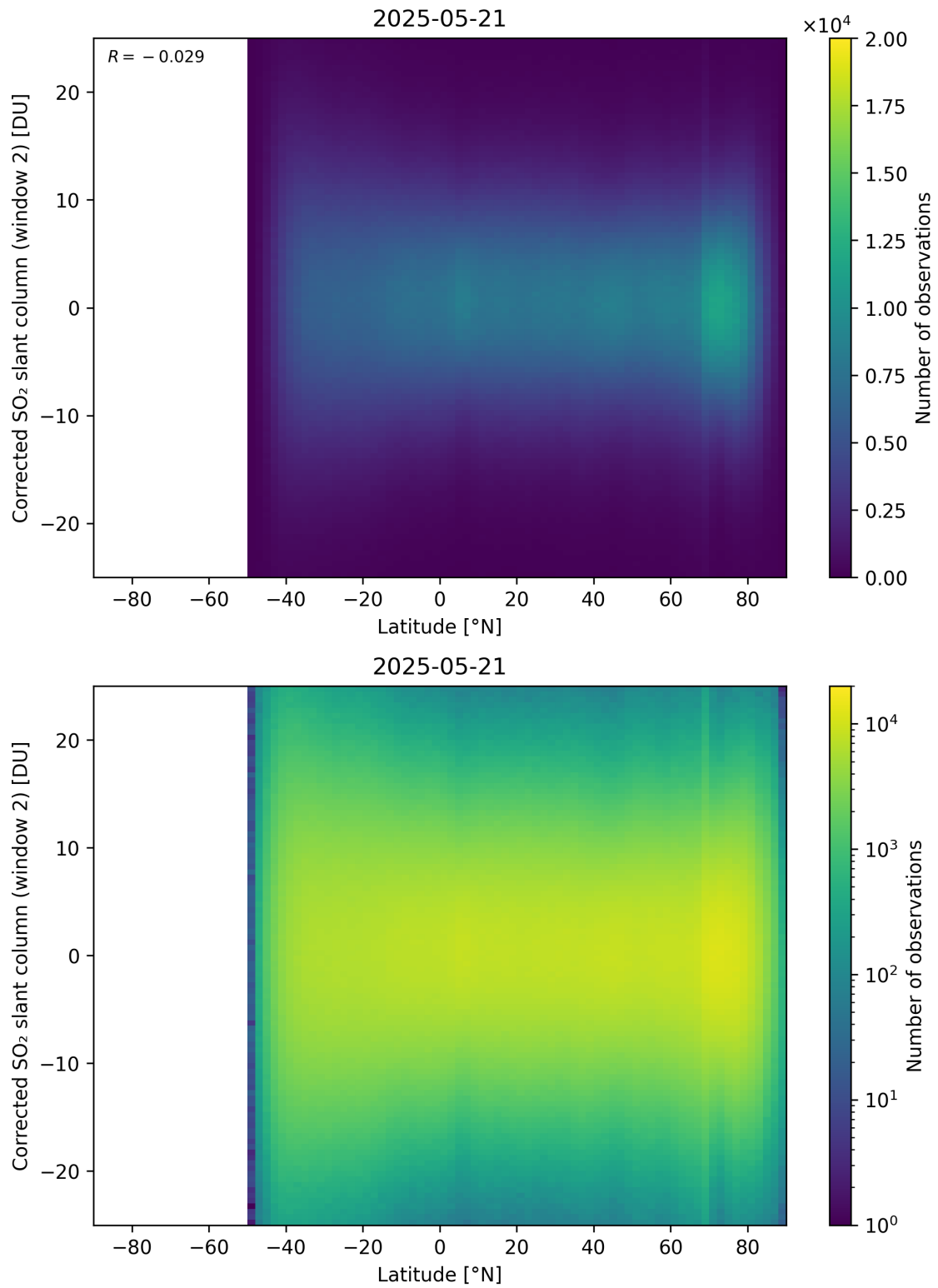
Figure 160: Scatter density plot of “Latitude” against “Corrected SO 2 slant column (window 2)” for 2025-05-21 to 2025-05-22.
