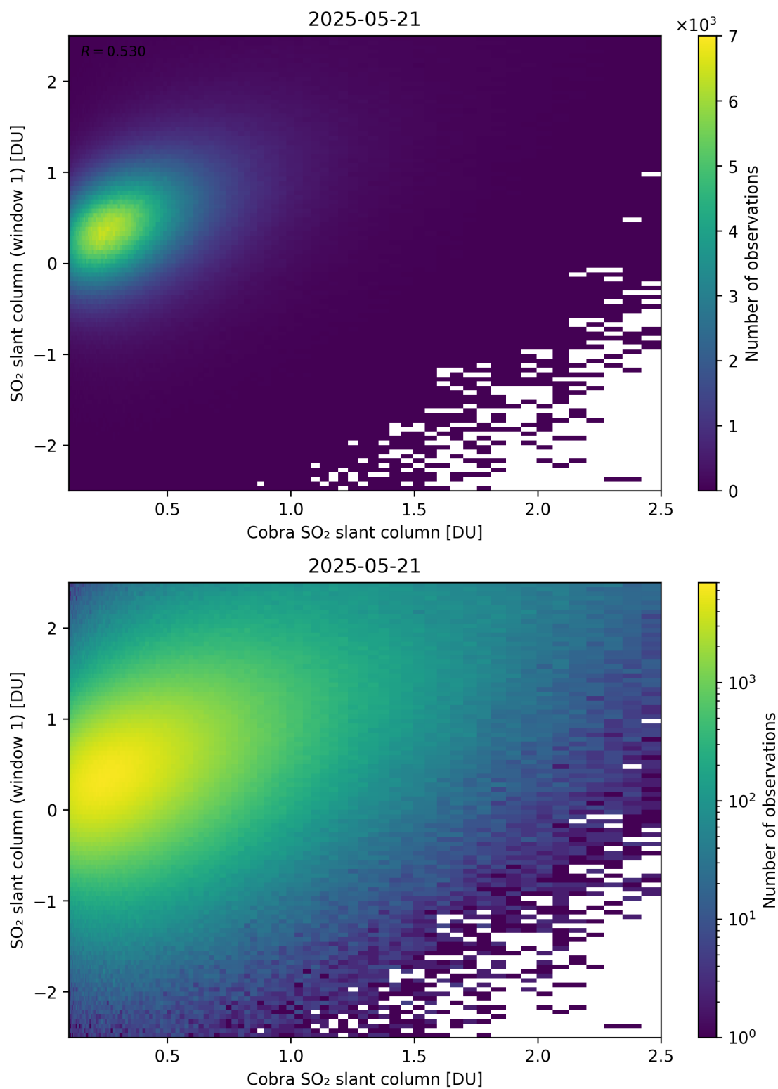
Figure 219: Scatter density plot of “Cobra SO 2 slant column” against “SO 2 slant column (window 1)” for 2025-05-21 to 2025-05-22.
