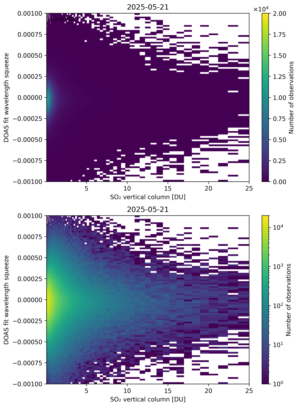
Figure 327: Scatter density plot of “SO 2 vertical column” against “DOAS fit wavelength squeeze” for 2025-05-21 to 2025-05-22.
