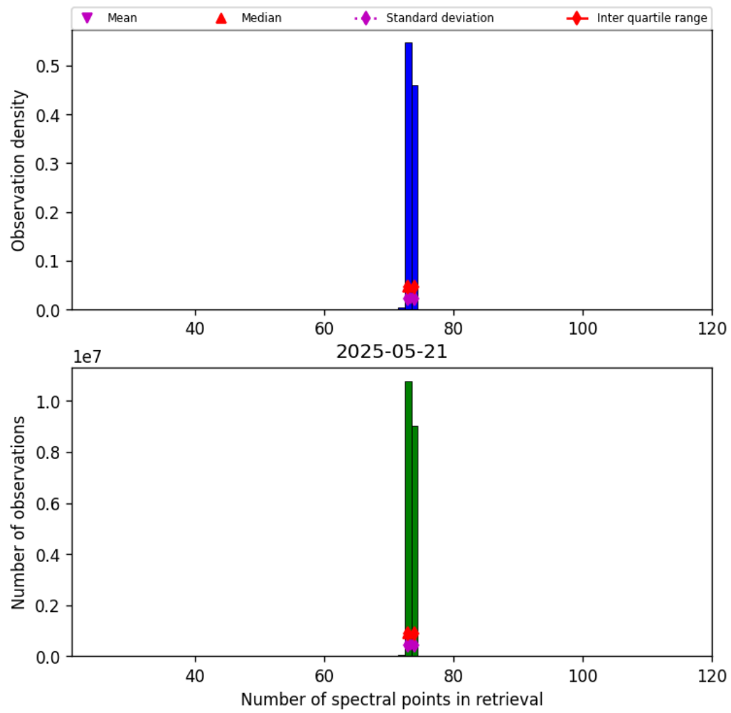
Figure 82: Histogram of “Number of spectral points in retrieval” for 2025-05-21 to 2025-05-22
