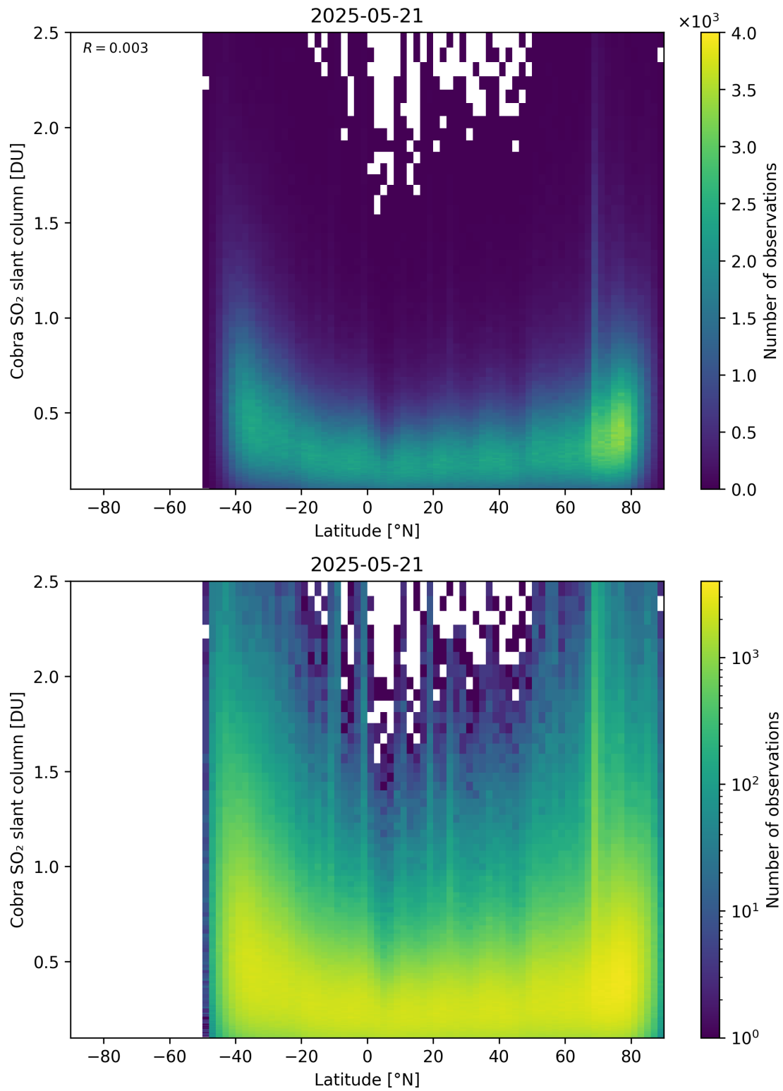
Figure 157: Scatter density plot of “Latitude” against “Cobra SO 2 slant column” for 2025-05-21 to 2025-05-22.
