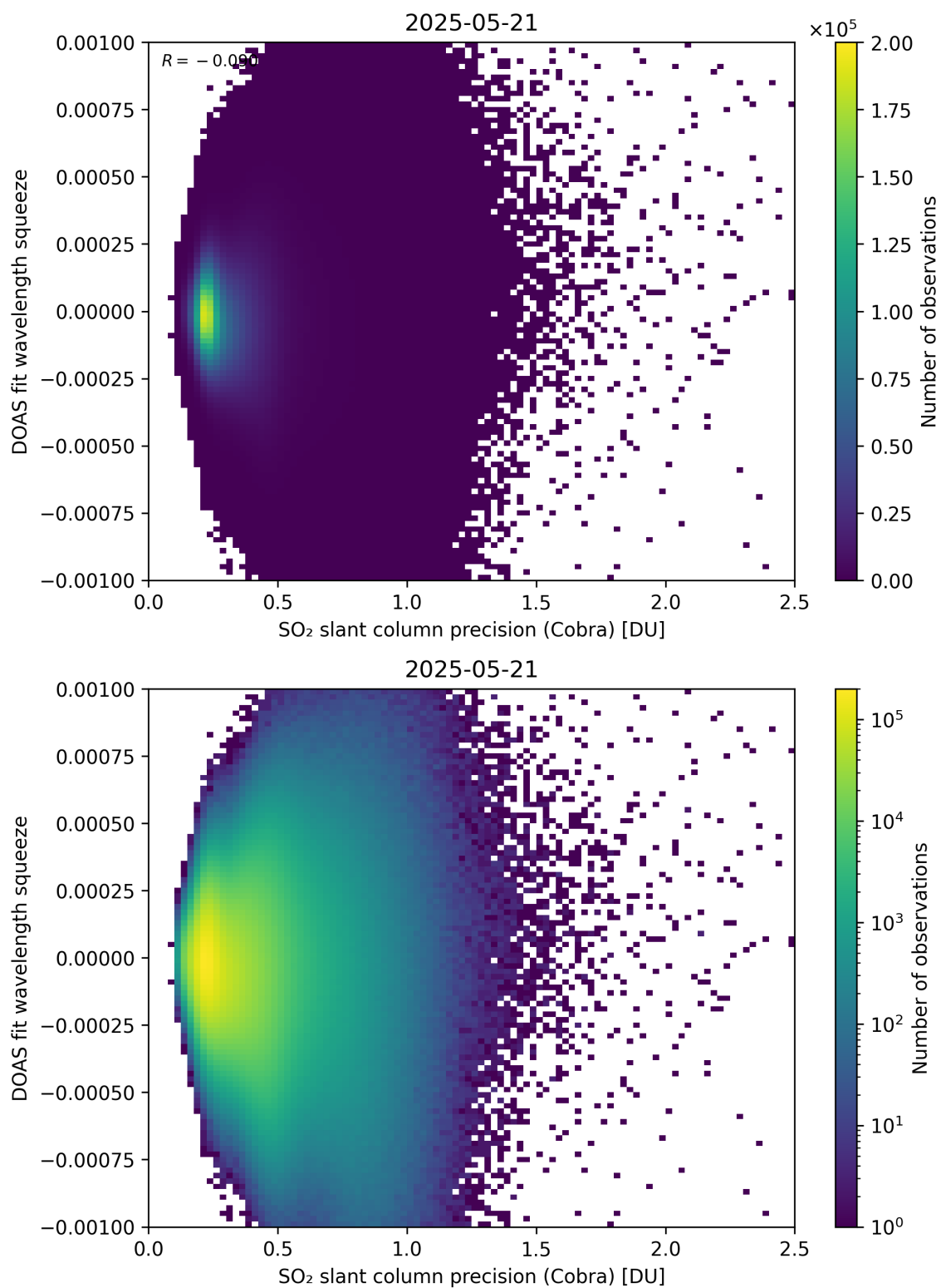
Figure 203: Scatter density plot of “SO 2 slant column precision (Cobra)” against “DOAS fit wavelength squeeze” for 2025-05-21 to 2025-05-22.
