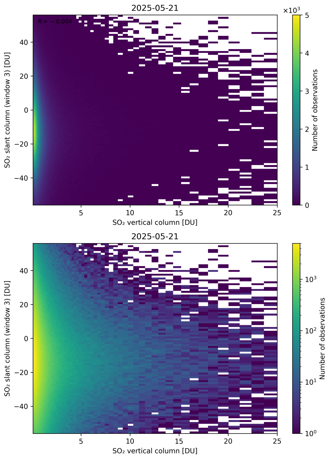
Figure 357: Scatter density plot of “SO 2 vertical column” against “SO 2 slant column (window 3)” for 2025-05-21 to 2025-05-22.
