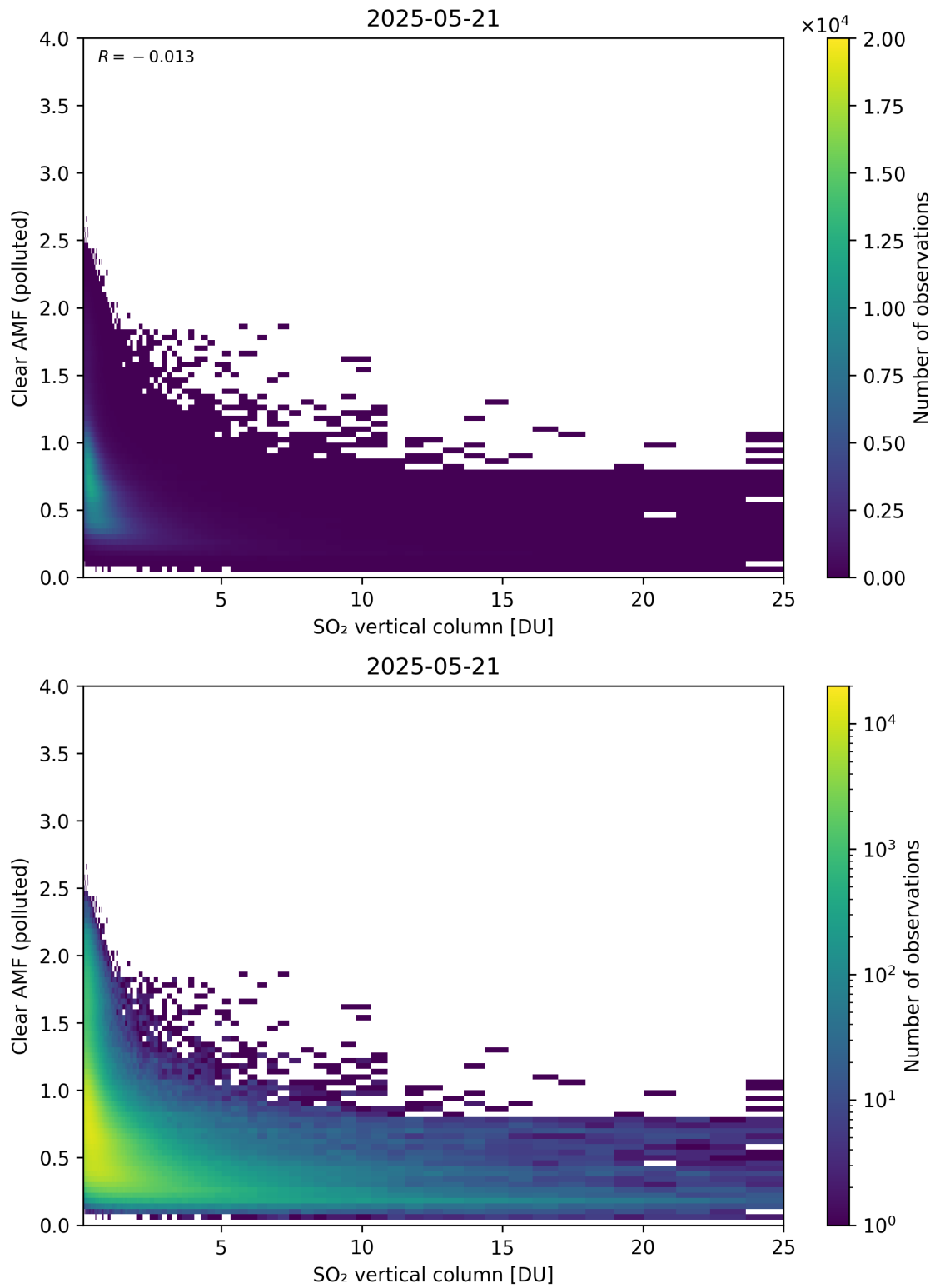
Figure 348: Scatter density plot of “SO 2 vertical column” against “Clear AMF (polluted)” for 2025-05-21 to 2025-05-22.
