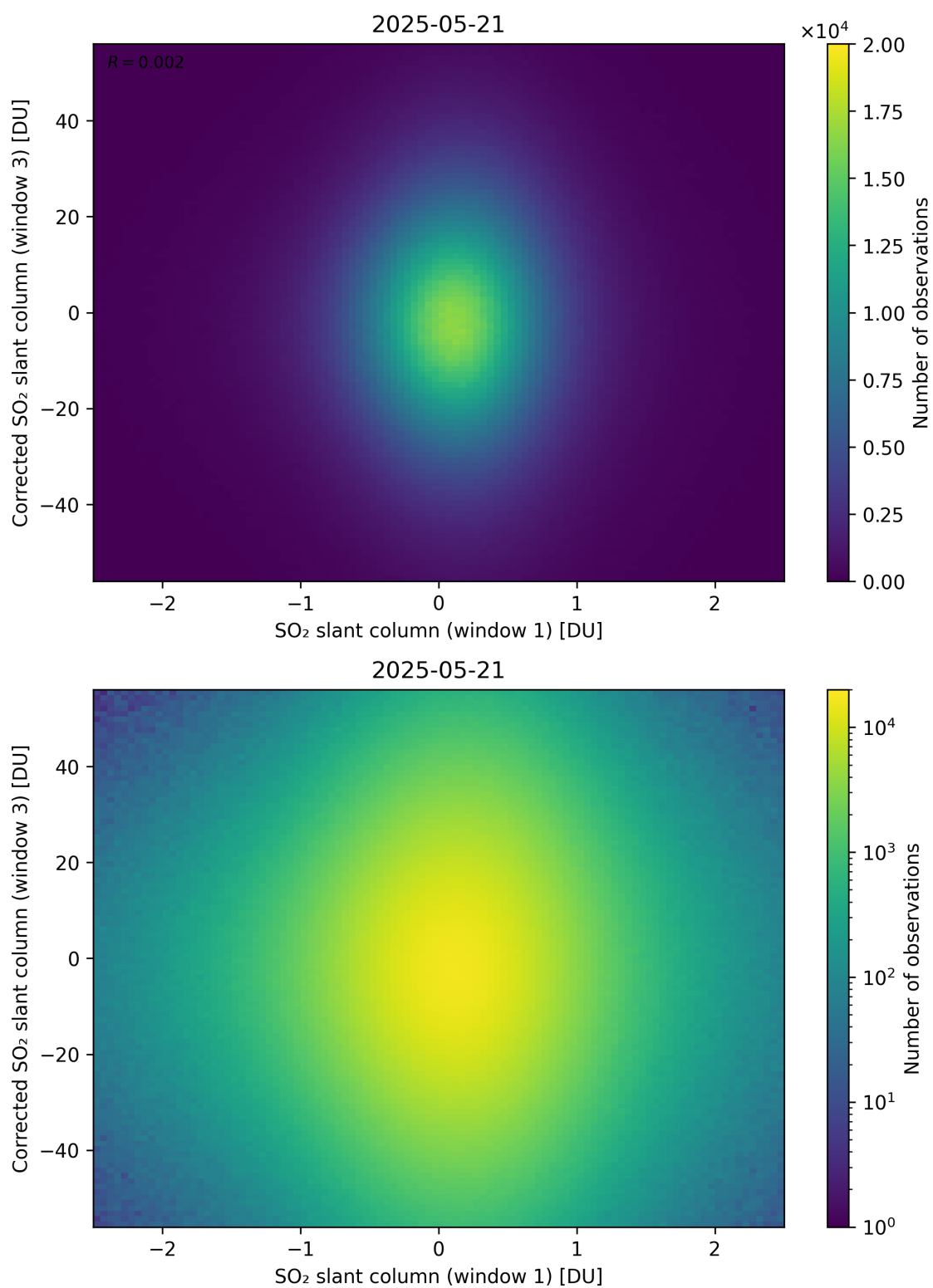
Figure 284: Scatter density plot of “SO 2 slant column (window 1)” against “Corrected SO 2 slant column (window 3)” for 2025-05-21 to 2025-05-22.
