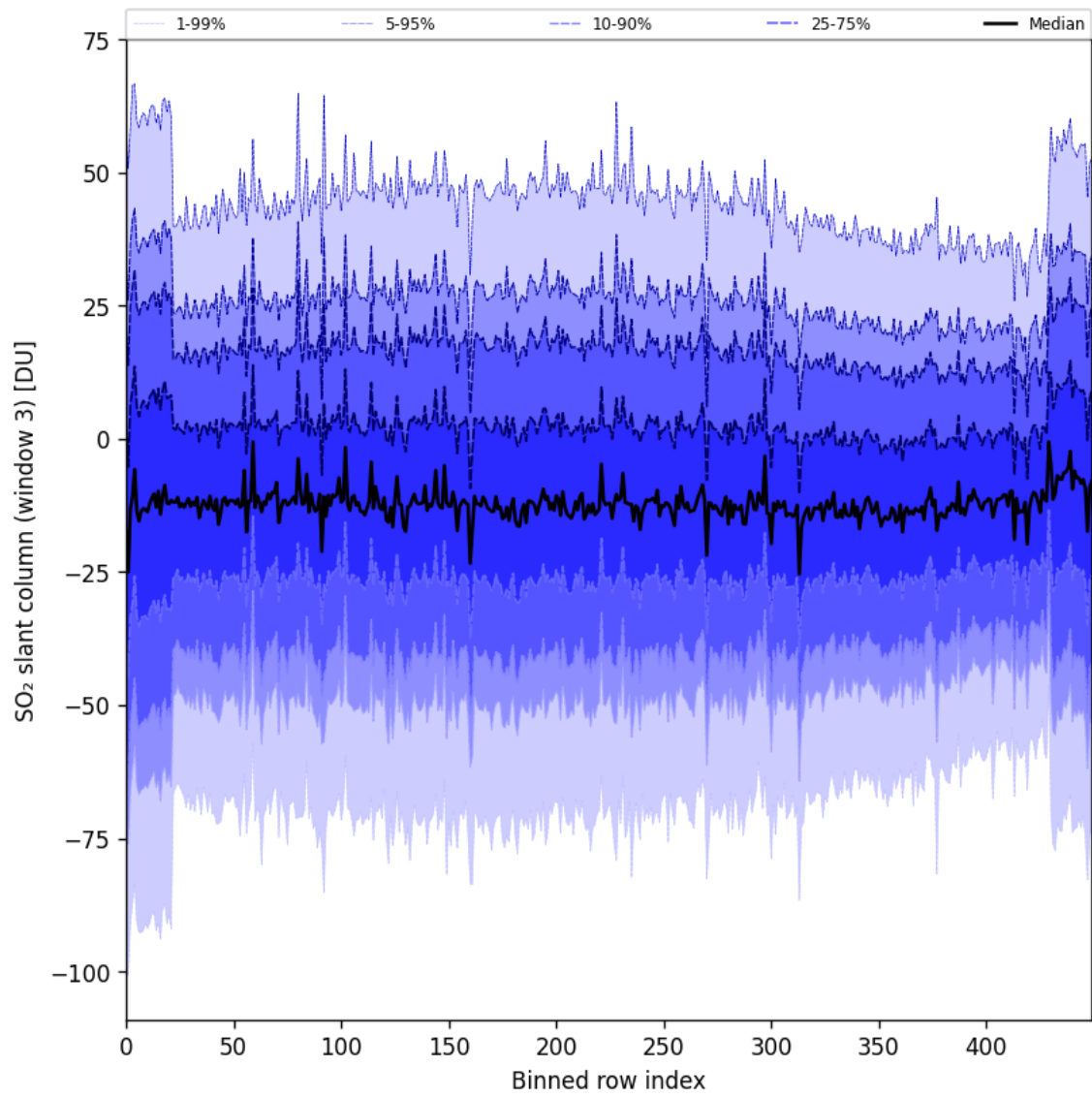
Figure 97: Along track statistics of “SO 2 slant column (window 3)” for 2025-05-21 to 2025-05-22
