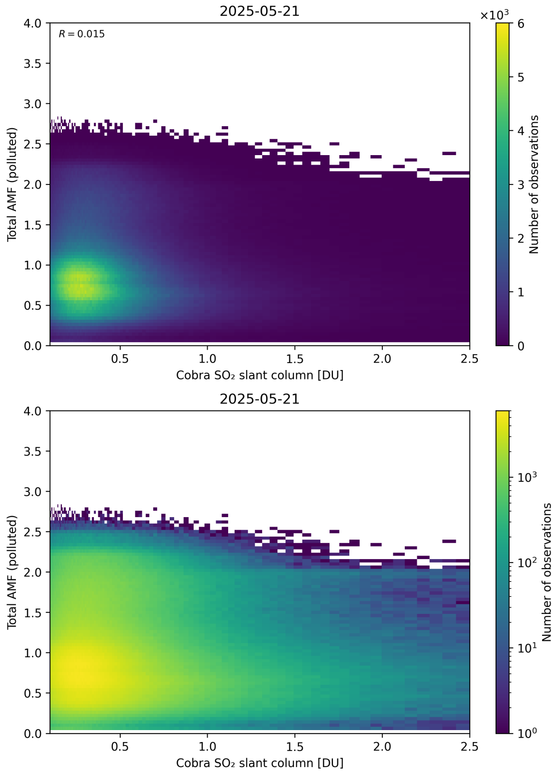
Figure 224: Scatter density plot of “Cobra SO 2 slant column” against “Total AMF (polluted)” for 2025-05-21 to 2025-05-22.
