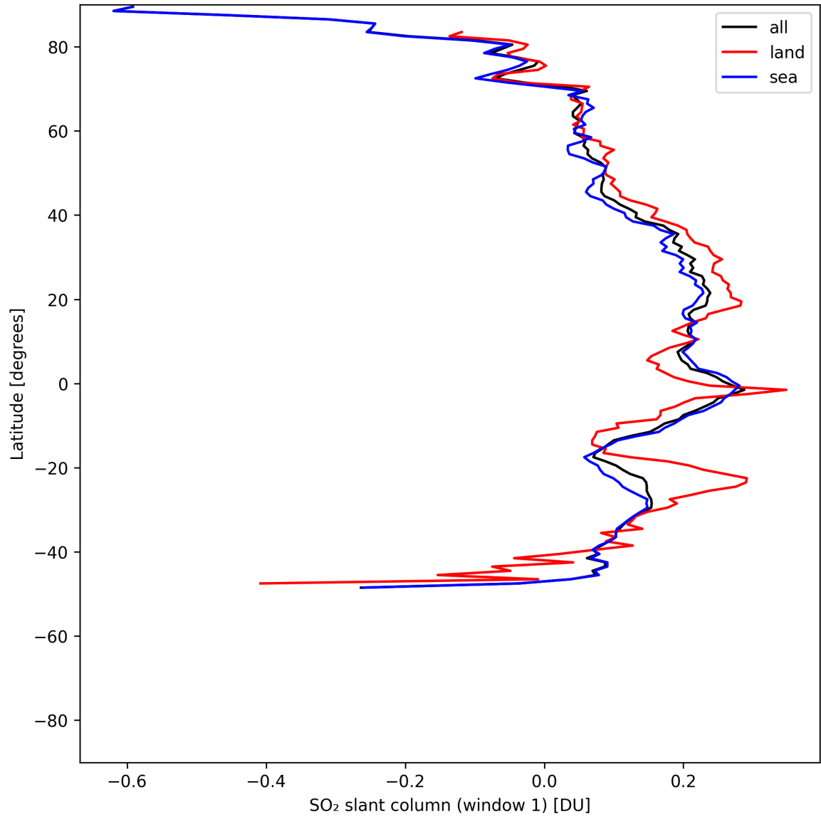
Figure 37: Zonal average of “SO 2 slant column (window 1)” for 2025-05-21 to 2025-05-22.
