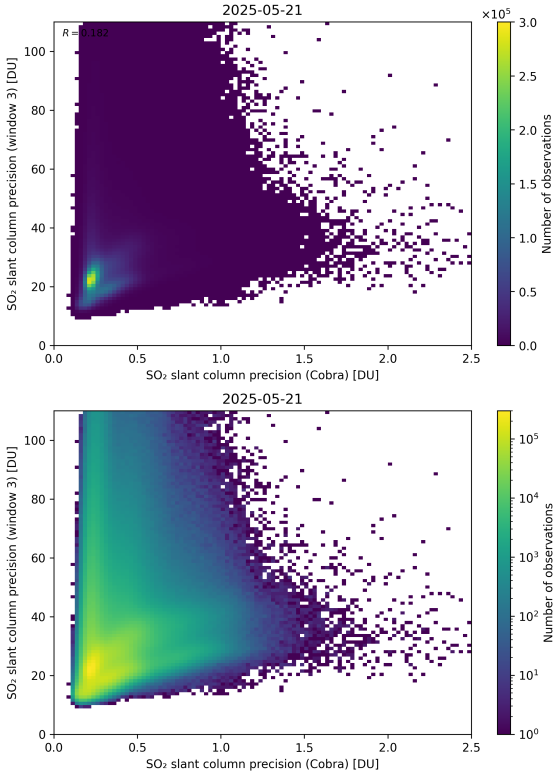
Figure 212: Scatter density plot of “SO 2 slant column precision (Cobra)” against “SO 2 slant column precision (window 3)” for 2025-05-21 to 2025-05-22.
