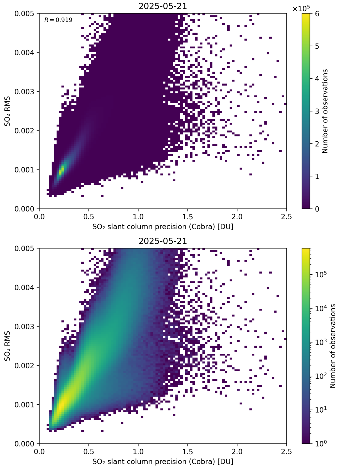
Figure 204: Scatter density plot of “SO 2 slant column precision (Cobra)” against “SO 2 RMS” for 2025-05-21 to 2025-05-22.
