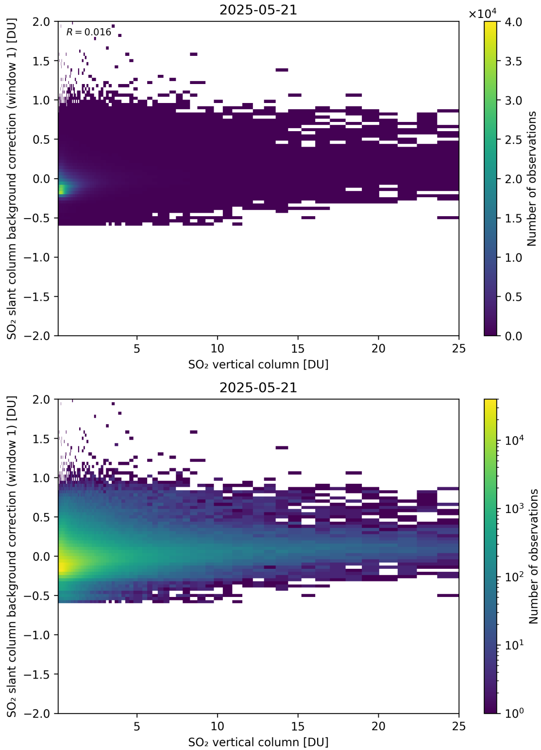
Figure 323: Scatter density plot of “SO 2 vertical column” against “SO 2 slant column background correction (window 1)” for 2025-05-21 to 2025-05-22.
