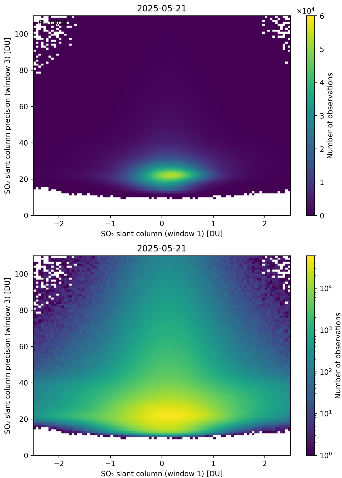
Figure 288: Scatter density plot of “SO 2 slant column (window 1)” against “SO 2 slant column precision (window 3)” for 2025-05-21 to 2025-05-22.
