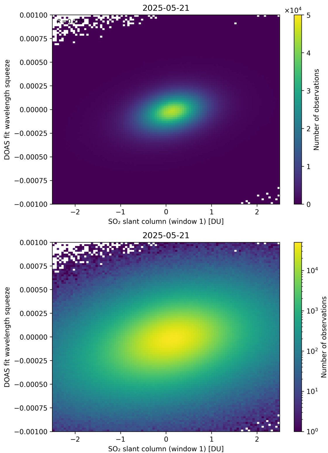
Figure 266: Scatter density plot of “SO 2 slant column (window 1)” against “DOAS fit wavelength squeeze” for 2025-05-21 to 2025-05-22.
