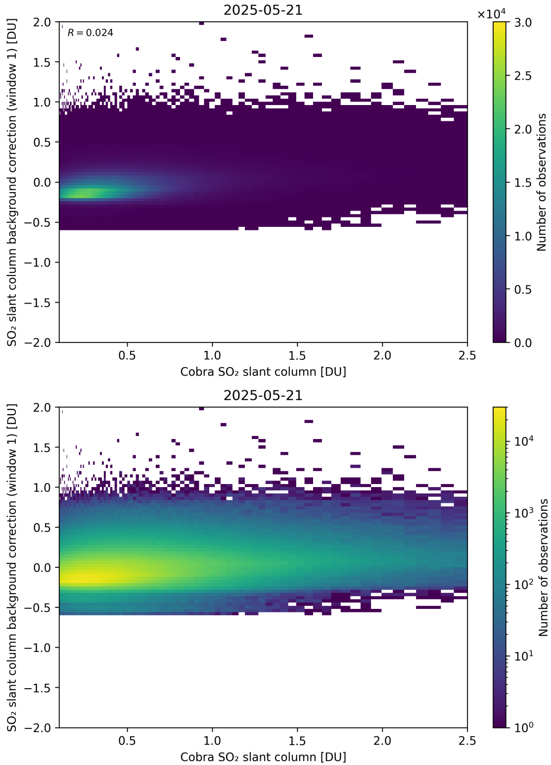
Figure 193: Scatter density plot of “Cobra SO 2 slant column” against “SO 2 slant column background correction (window 1)” for 2025-05-21 to 2025-05-22.
