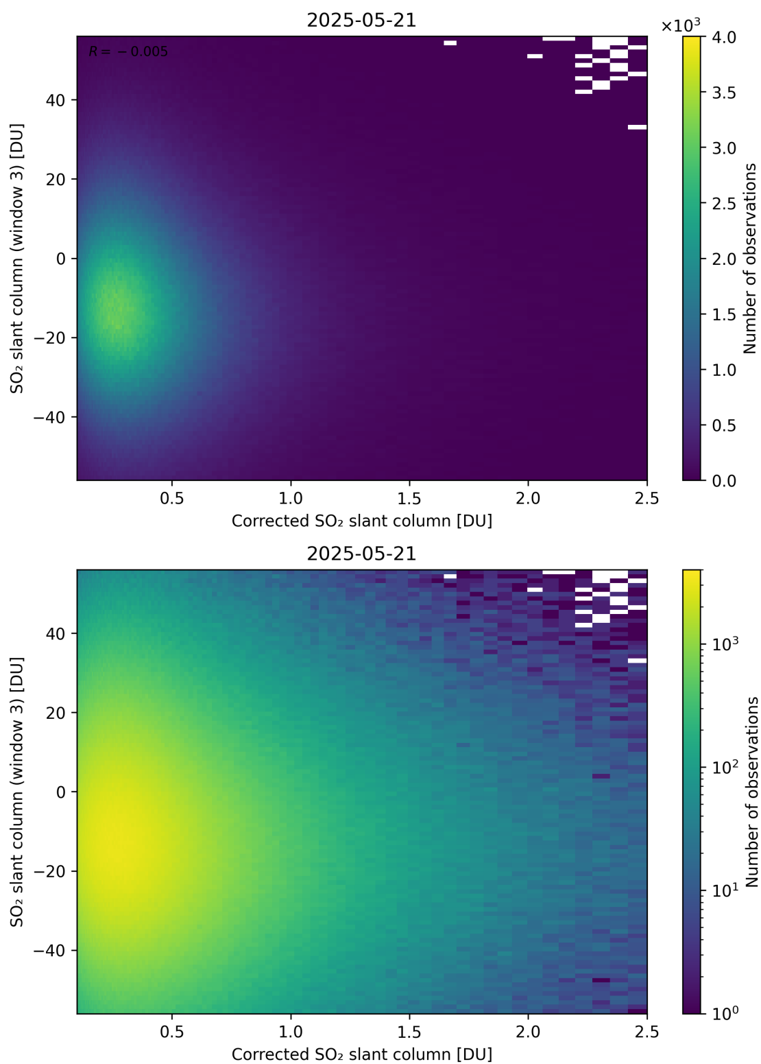
Figure 240: Scatter density plot of “Corrected SO 2 slant column” against “SO 2 slant column (window 3)” for 2025-05-21 to 2025-05-22.
