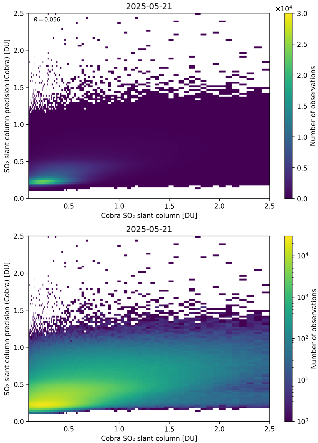
Figure 216: Scatter density plot of “Cobra SO 2 slant column” against “SO 2 slant column precision (Cobra)” for 2025-05-21 to 2025-05-22.
