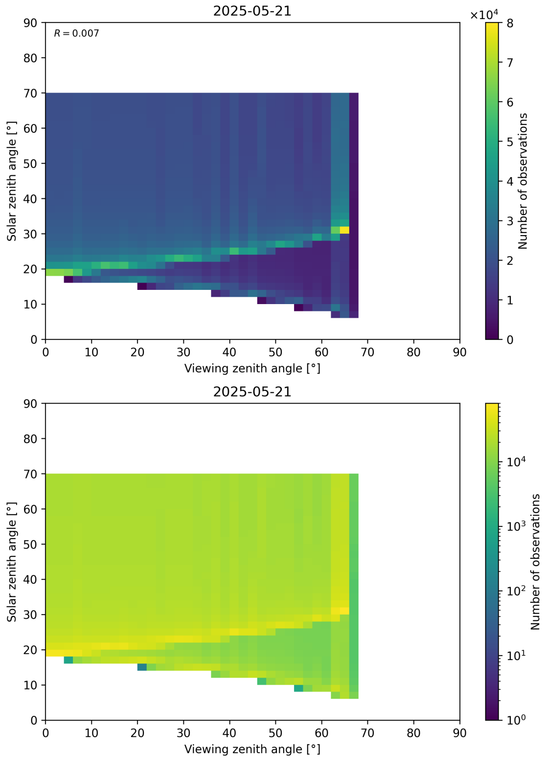
Figure 369: Scatter density plot of “Viewing zenith angle” against “Solar zenith angle” for 2025-05-21 to 2025-05-22.
