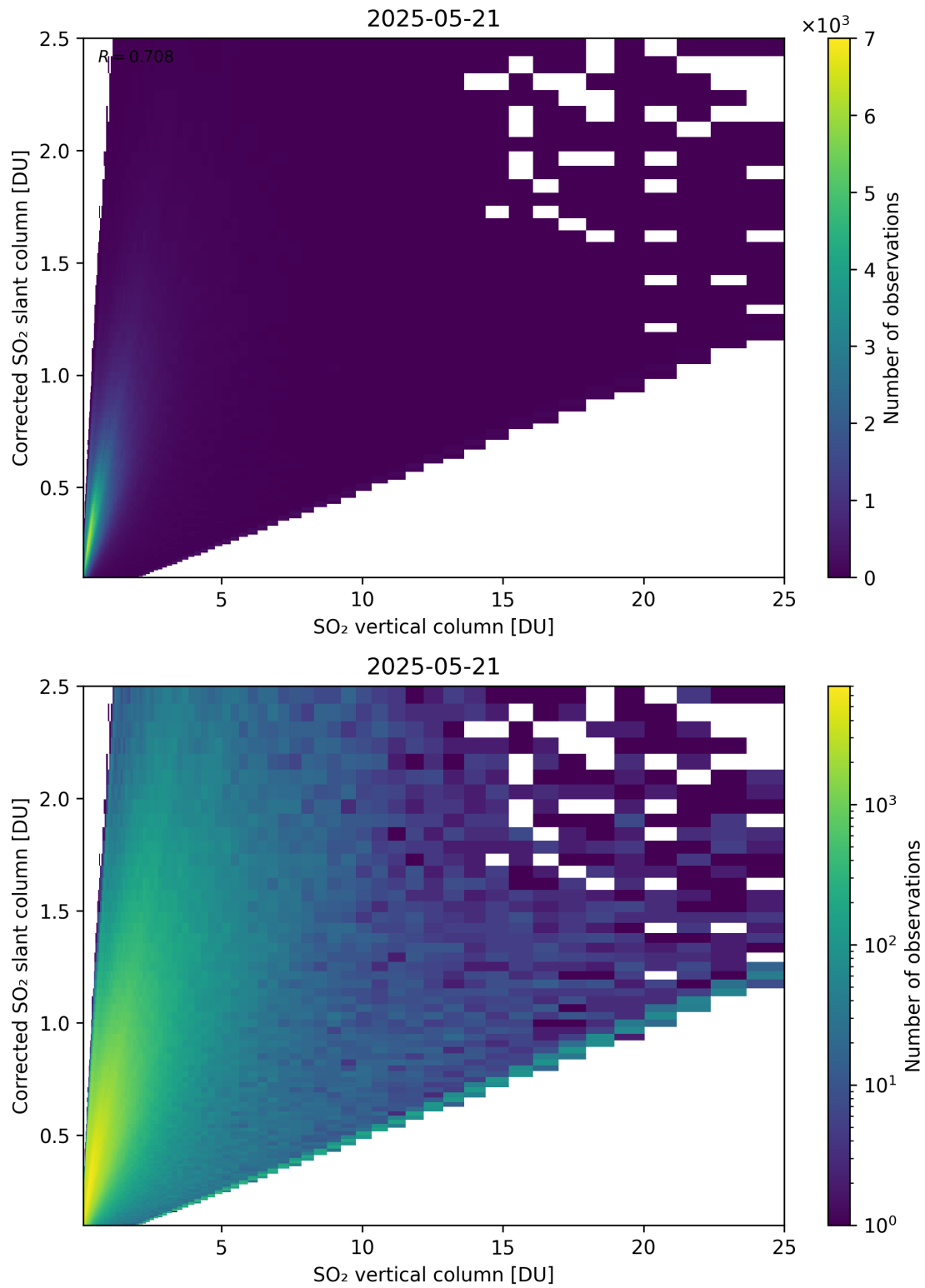
Figure 351: Scatter density plot of “SO 2 vertical column” against “Corrected SO 2 slant column” for 2025-05-21 to 2025-05-22.
