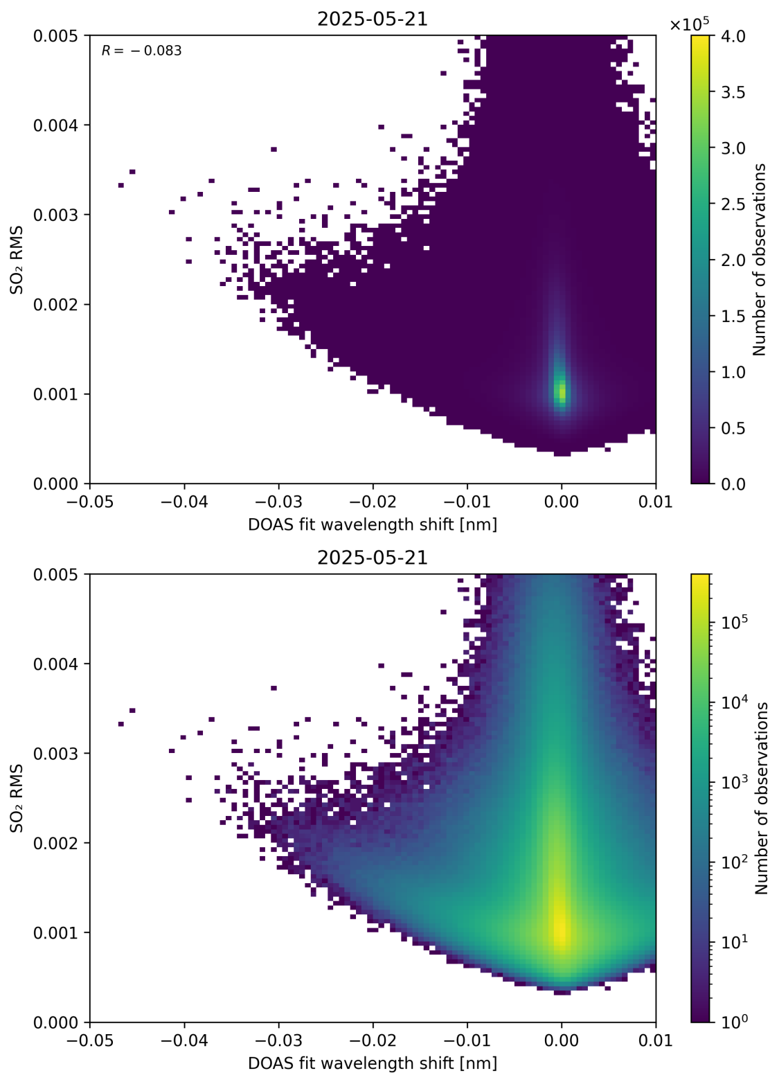
Figure 139: Scatter density plot of “DOAS fit wavelength shift” against “SO 2 RMS” for 2025-05-21 to 2025-05-22.
