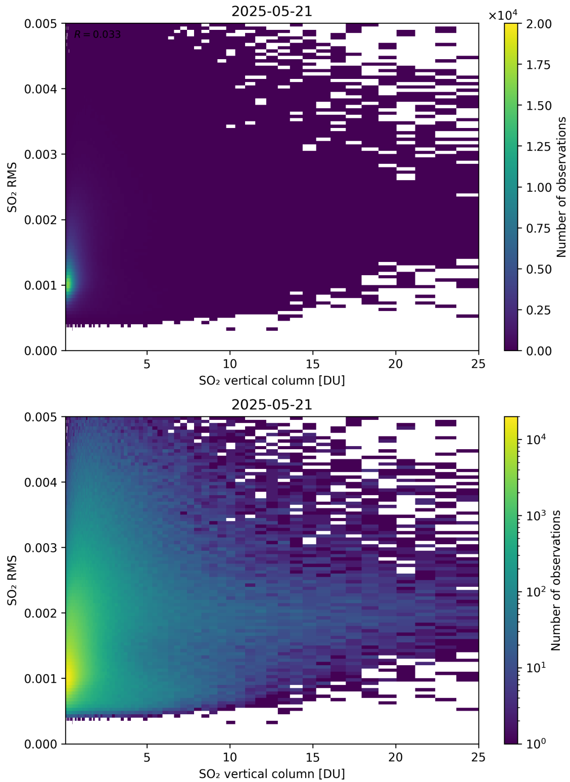
Figure 328: Scatter density plot of “SO 2 vertical column” against “SO 2 RMS” for 2025-05-21 to 2025-05-22.
