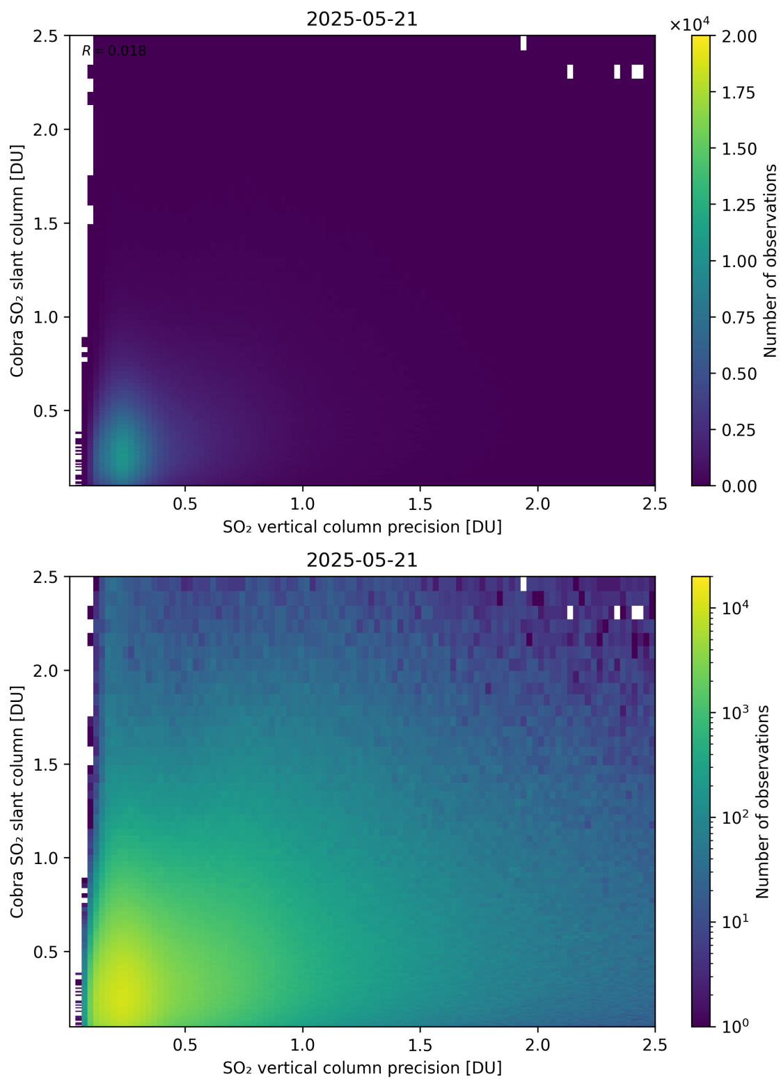
Figure 336: Scatter density plot of “SO 2 vertical column precision” against “Cobra SO 2 slant column” for 2025-05-21 to 2025-05-22.
