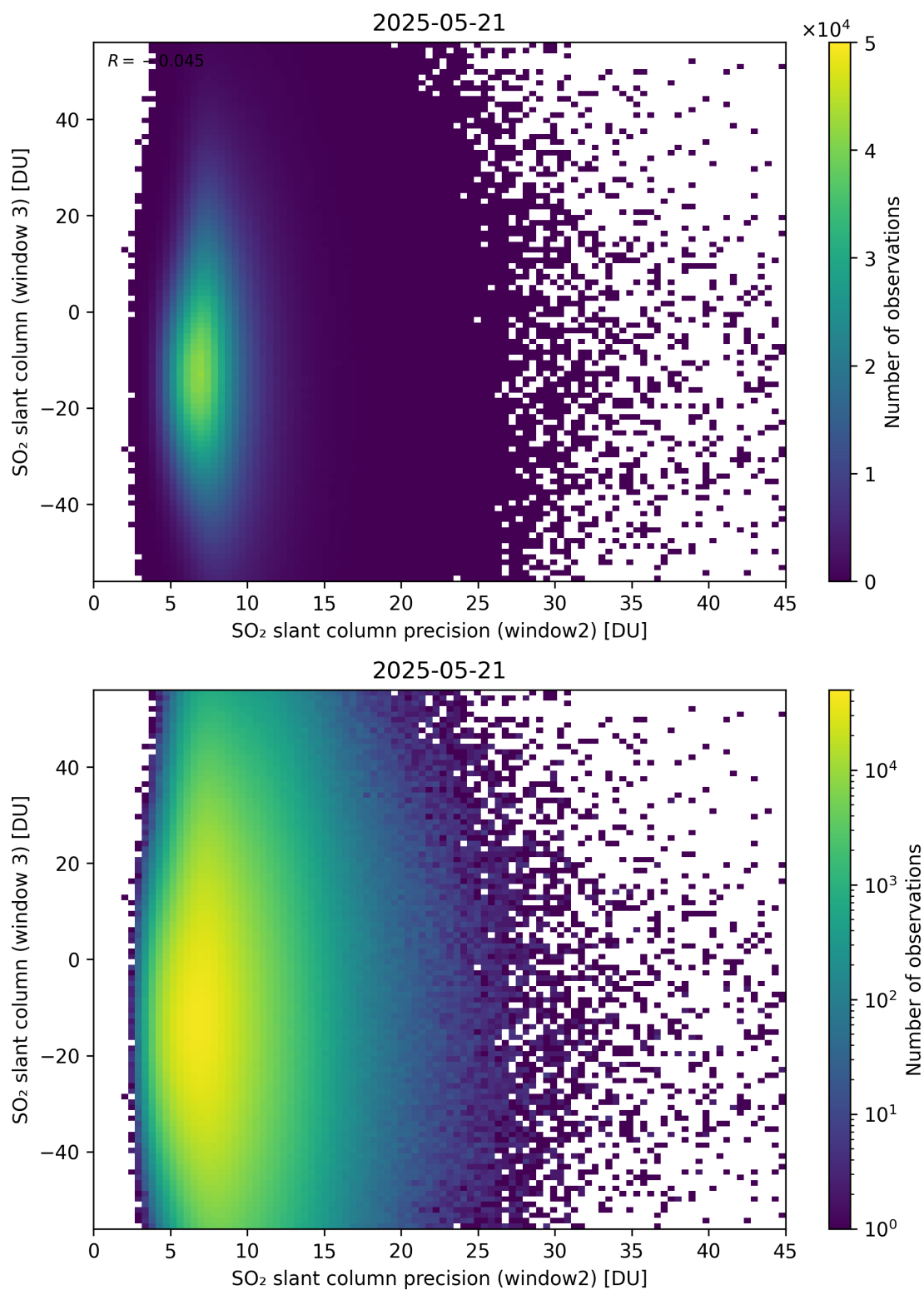
Figure 299: Scatter density plot of “SO 2 slant column precision (window2)” against “SO 2 slant column (window 3)” for 2025-05-21 to 2025-05-22.
