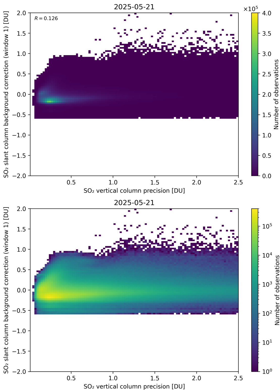
Figure 329: Scatter density plot of “SO 2 vertical column precision” against “SO 2 slant column background correction (window 1)” for 2025-05-21 to 2025-05-22.
