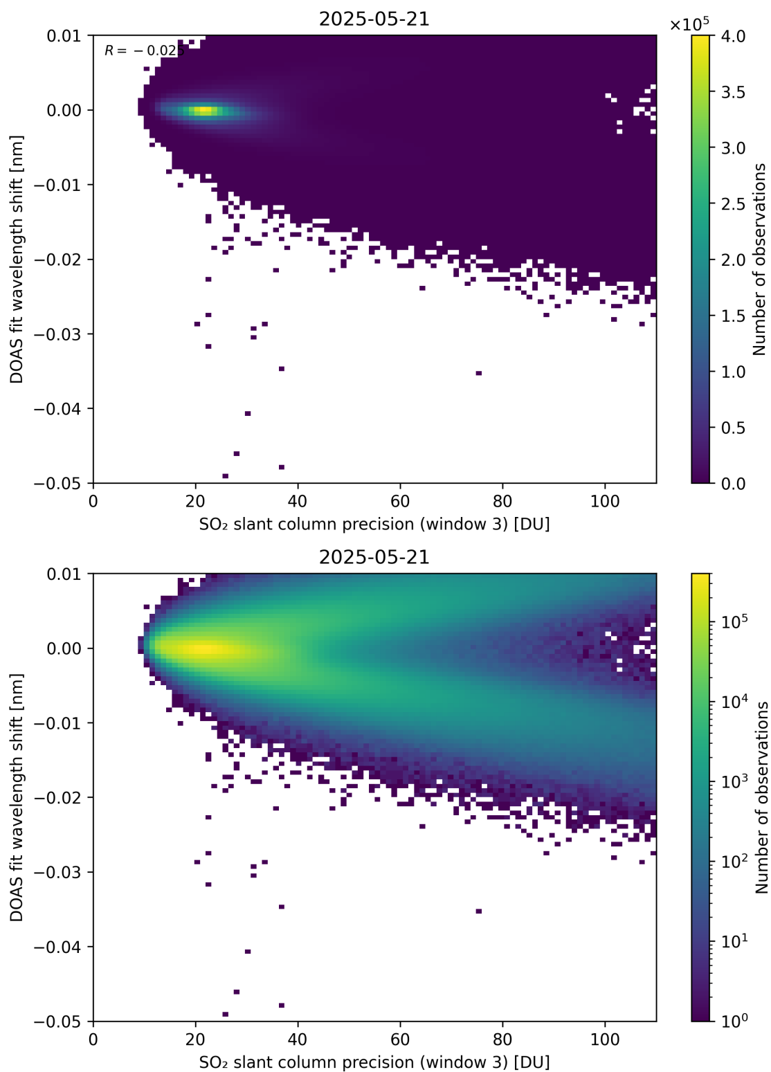
Figure 308: Scatter density plot of “SO 2 slant column precision (window 3)” against “DOAS fit wavelength shift” for 2025-05-21 to 2025-05-22.
