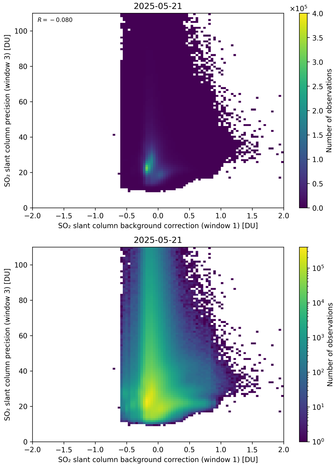
Figure 119: Scatter density plot of “SO 2 slant column background correction (window 1)” against “SO 2 slant column precision (window 3)” for 2025-05-21 to 2025-05-22.
