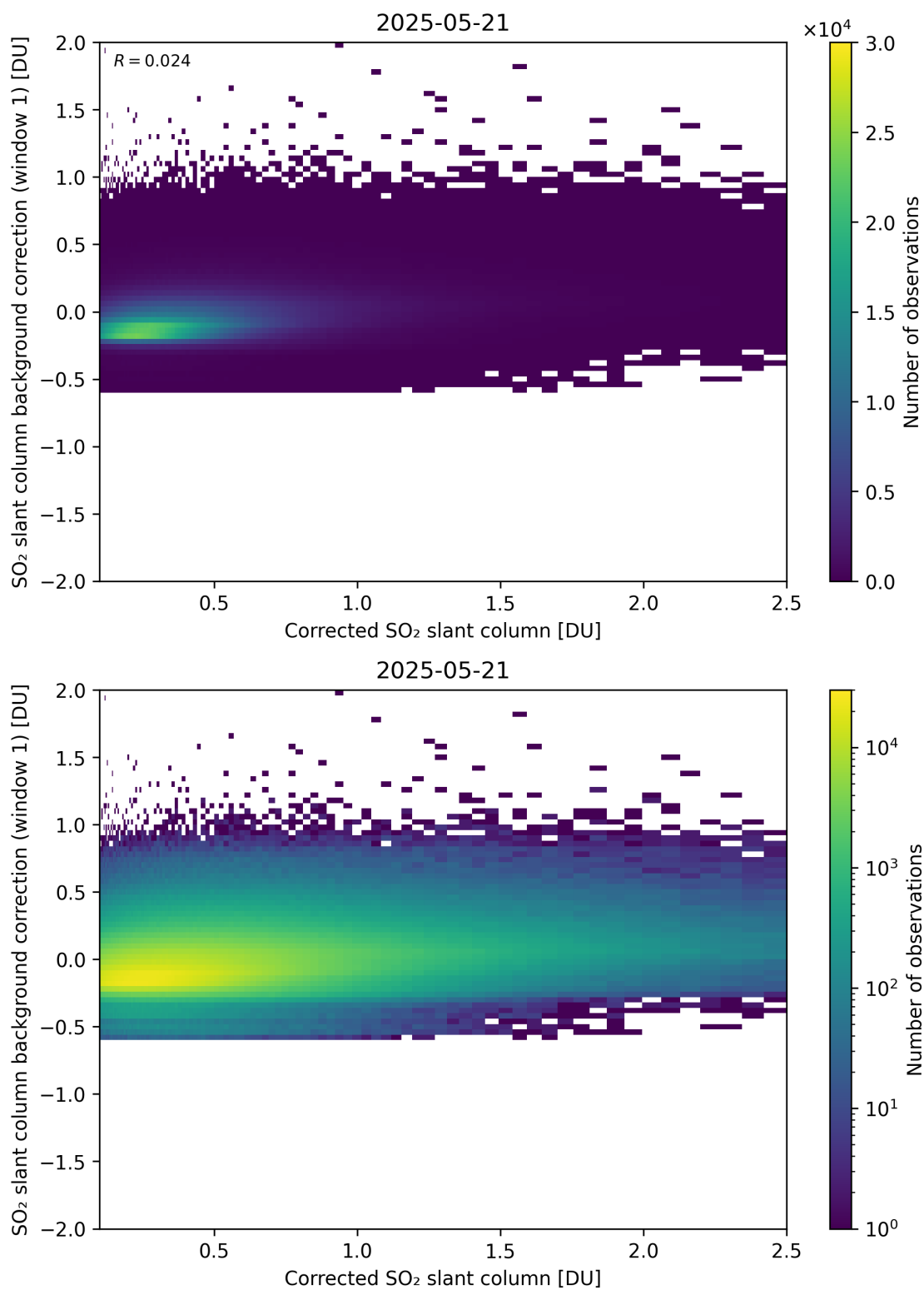
Figure 226: Scatter density plot of “Corrected SO 2 slant column” against “SO 2 slant column background correction (window 1)” for 2025-05-21 to 2025-05-22.
