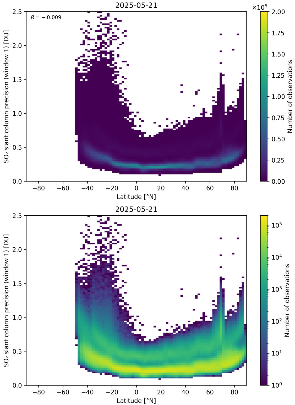
Figure 163: Scatter density plot of “Latitude” against “SO 2 slant column precision (window 1)” for 2025-05-21 to 2025-05-22.
