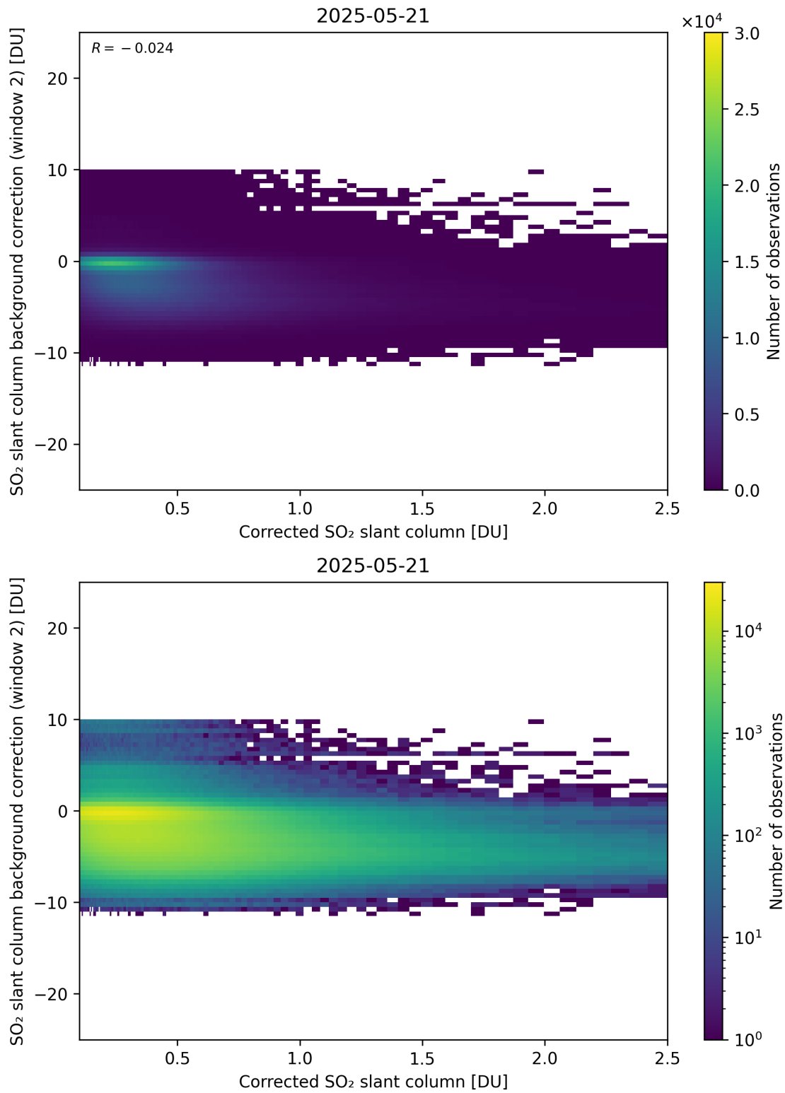
Figure 227: Scatter density plot of “Corrected SO 2 slant column” against “SO 2 slant column background correction (window 2)” for 2025-05-21 to 2025-05-22.
