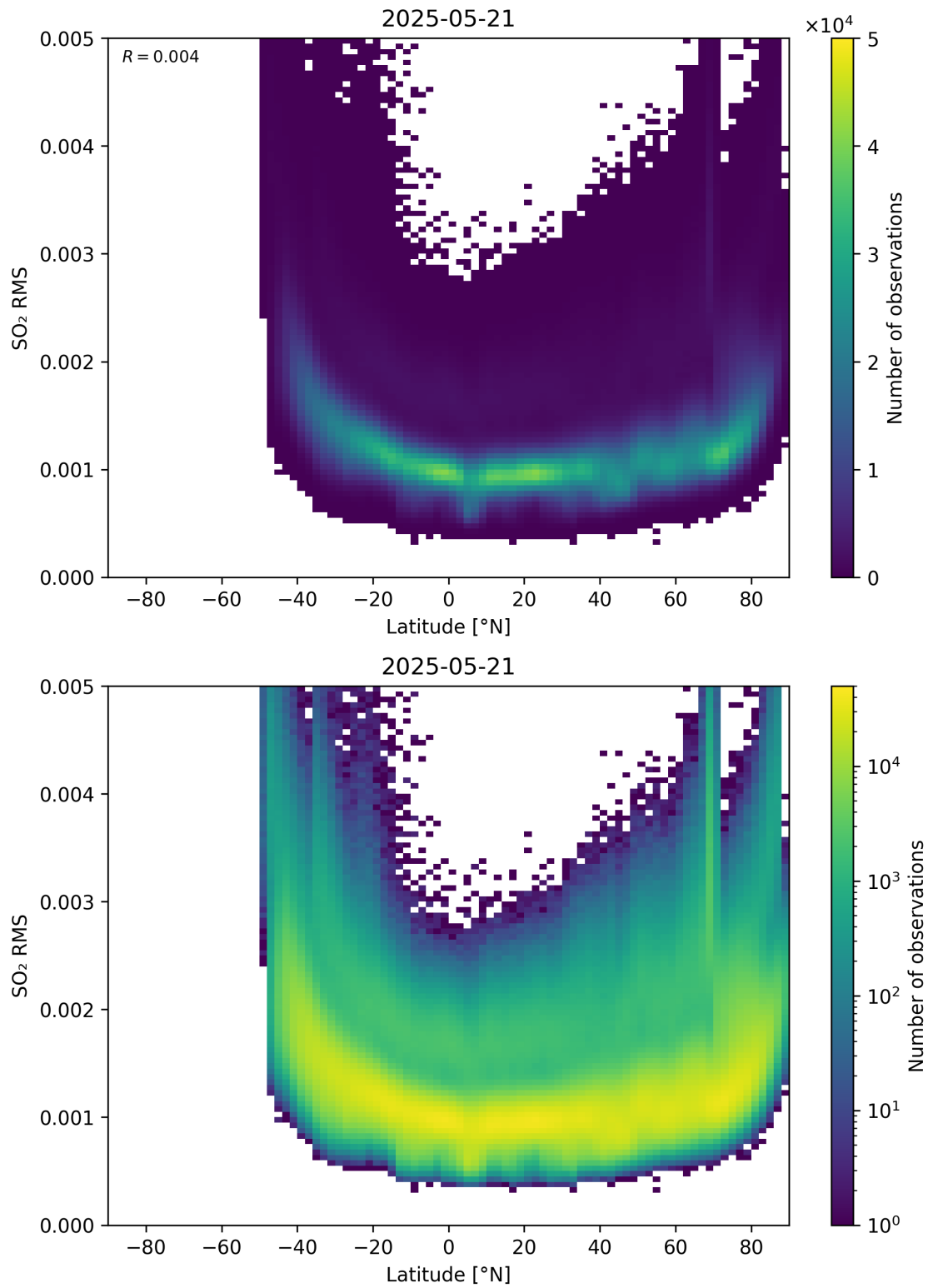
Figure 155: Scatter density plot of “Latitude” against “SO 2 RMS” for 2025-05-21 to 2025-05-22.
