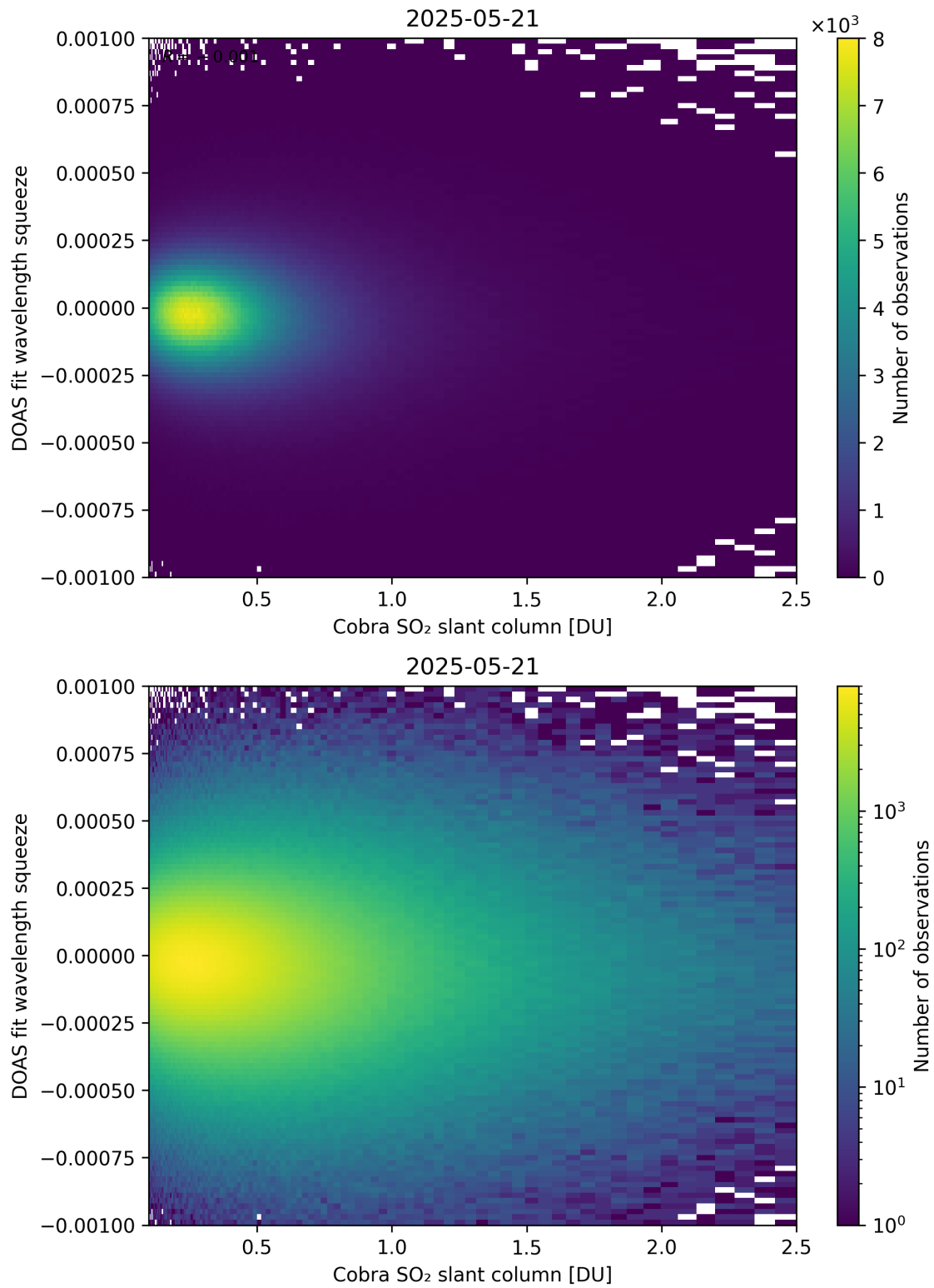
Figure 197: Scatter density plot of “Cobra SO 2 slant column” against “DOAS fit wavelength squeeze” for 2025-05-21 to 2025-05-22.
