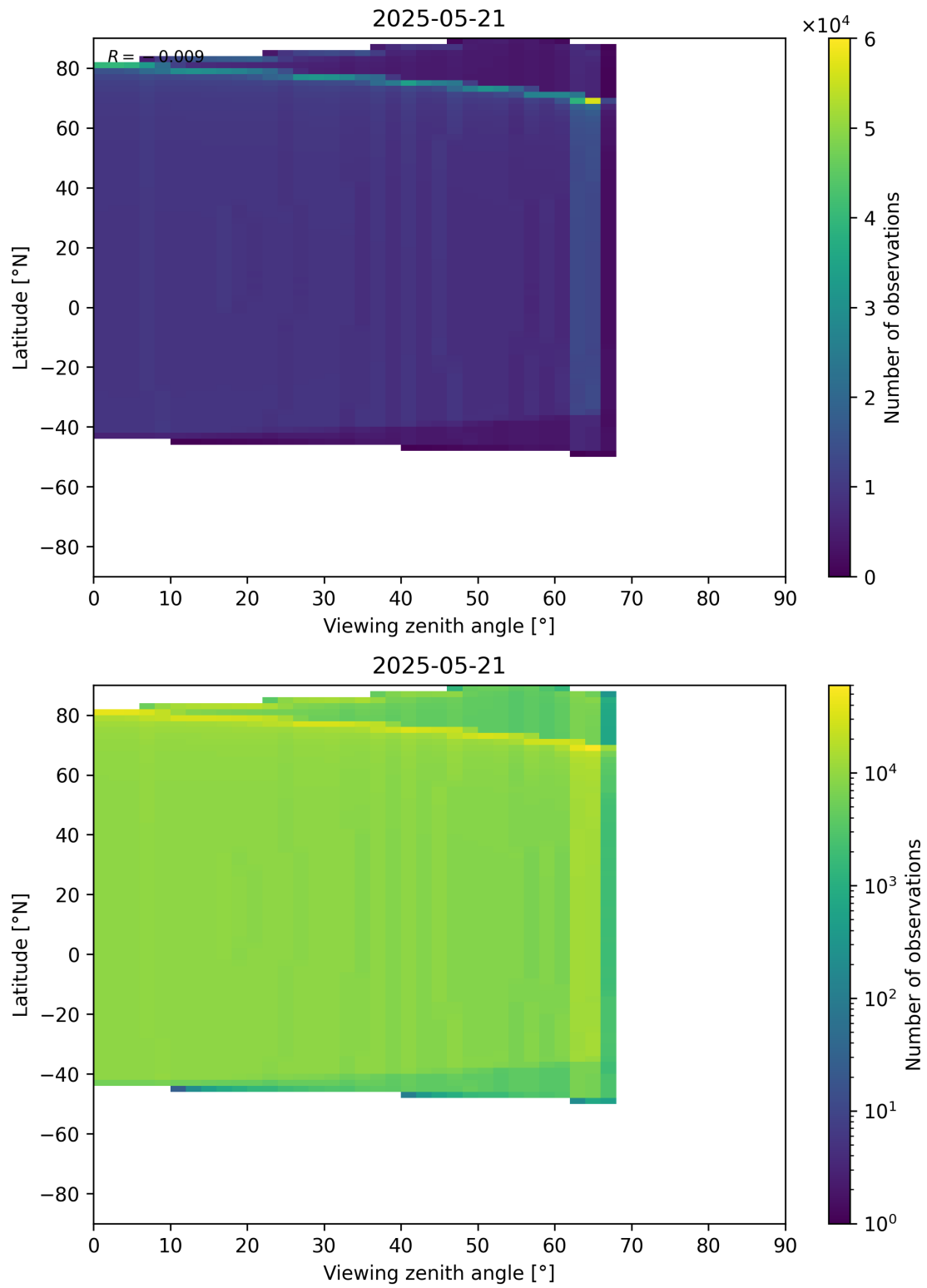
Figure 368: Scatter density plot of “Viewing zenith angle” against “Latitude” for 2025-05-21 to 2025-05-22.
