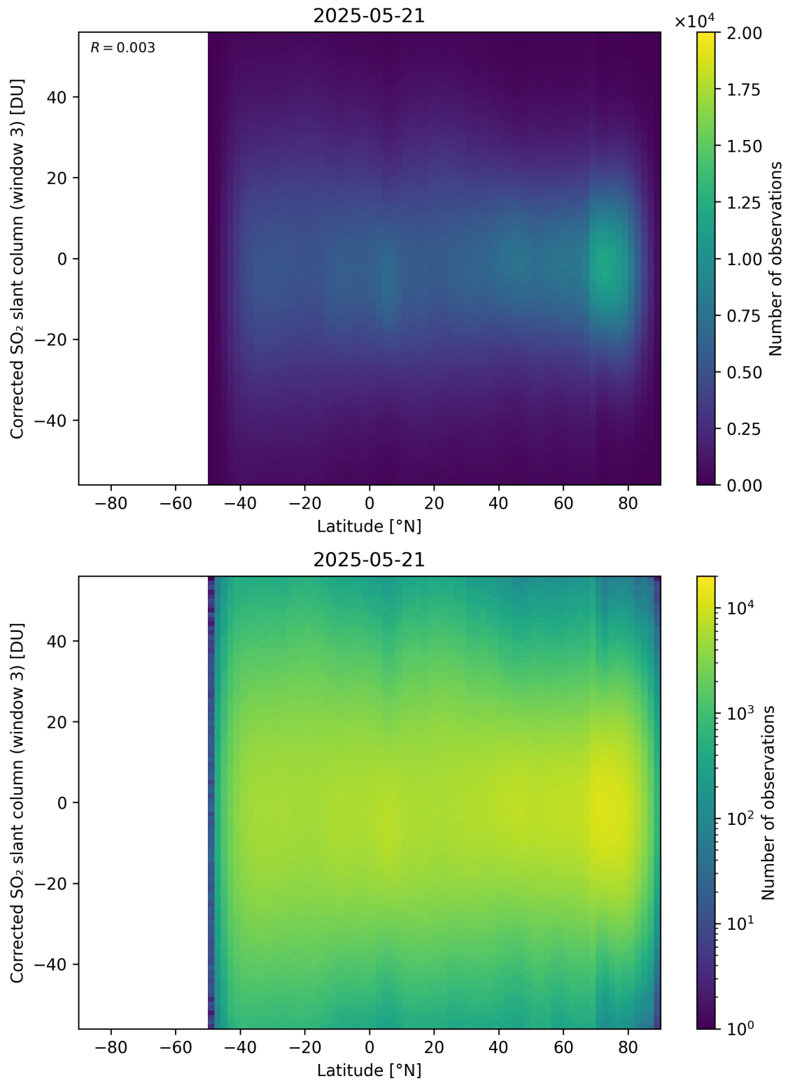
Figure 161: Scatter density plot of “Latitude” against “Corrected SO 2 slant column (window 3)” for 2025-05-21 to 2025-05-22.
