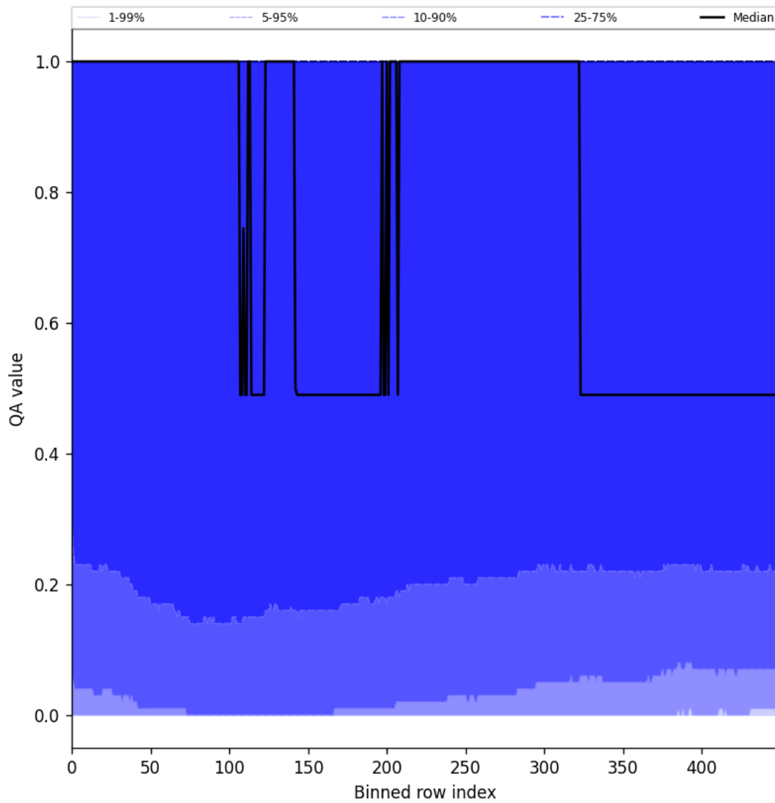
Figure 83: Along track statistics of “QA value” for 2025-05-21 to 2025-05-22
