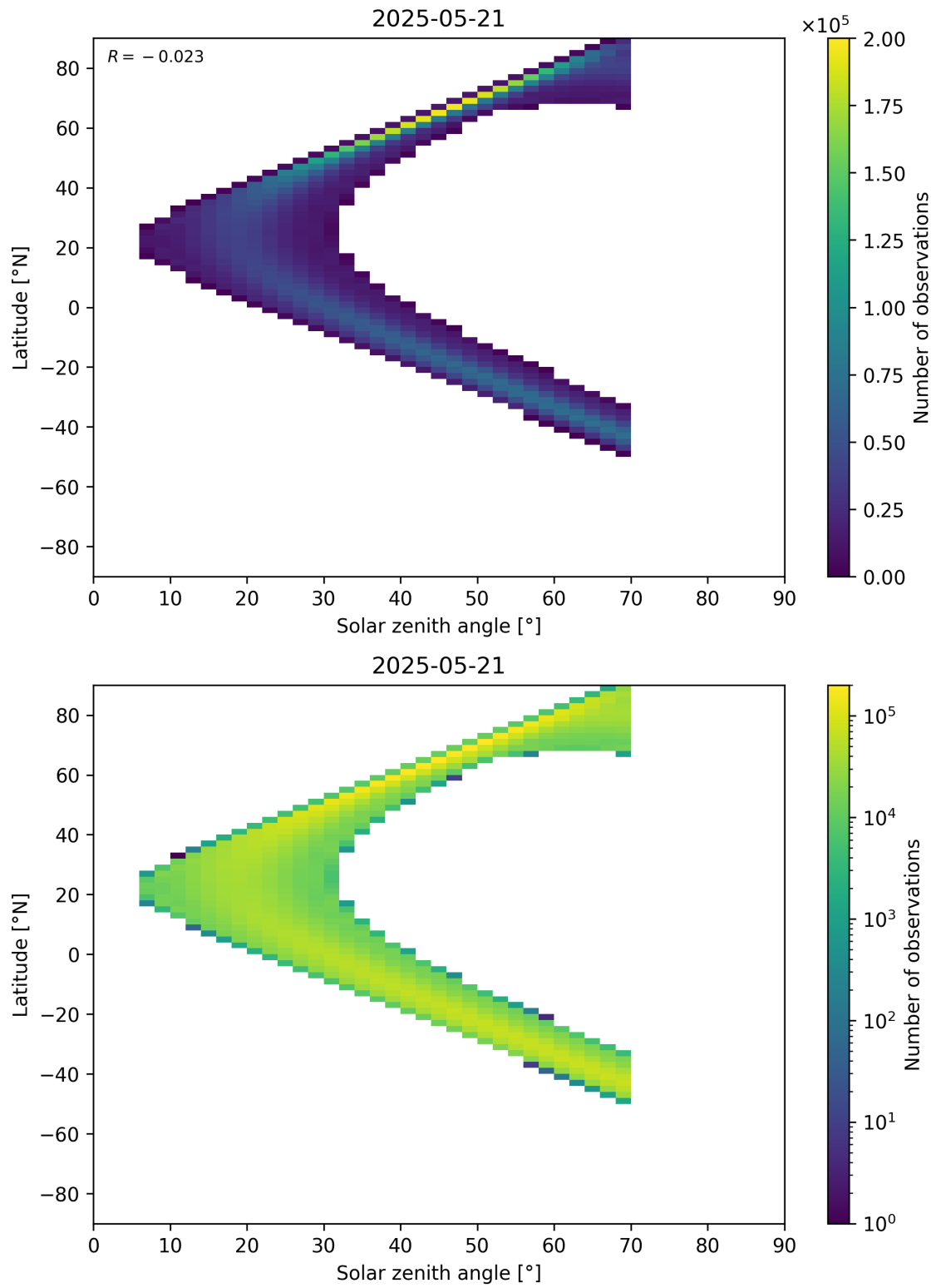
Figure 177: Scatter density plot of “Solar zenith angle” against “Latitude” for 2025-05-21 to 2025-05-22.
