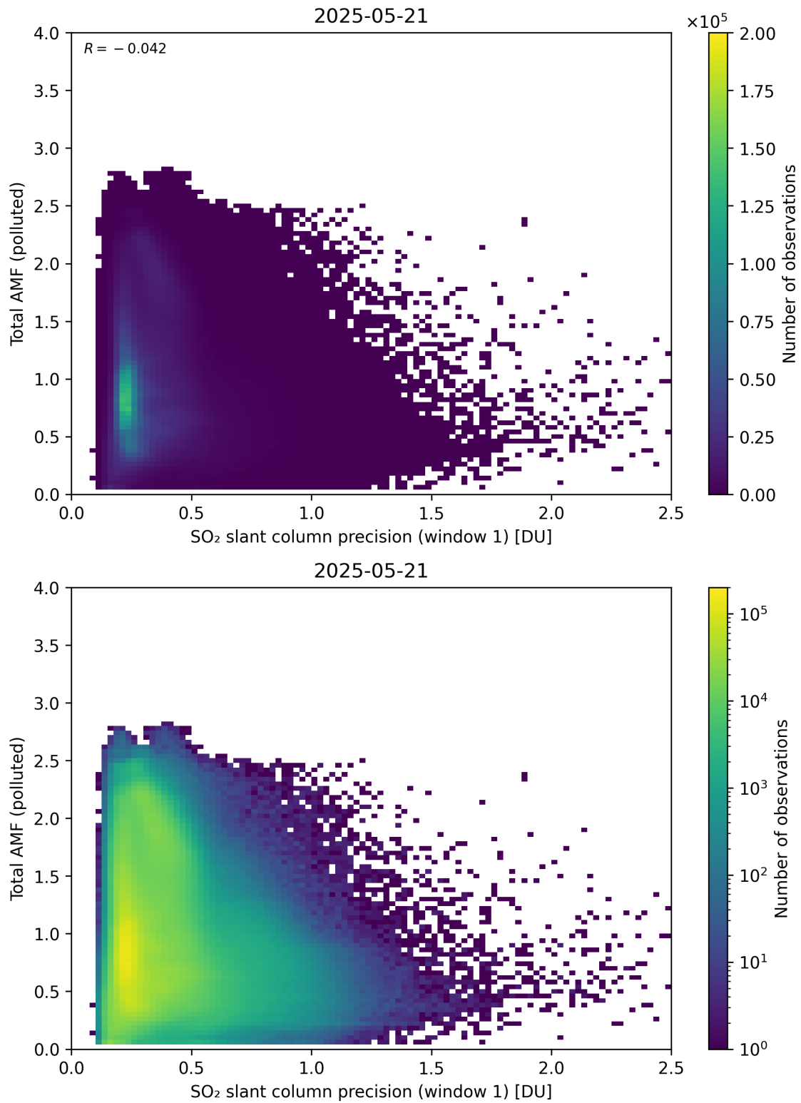
Figure 280: Scatter density plot of “SO 2 slant column precision (window 1)” against “Total AMF (polluted)” for 2025-05-21 to 2025-05-22.
