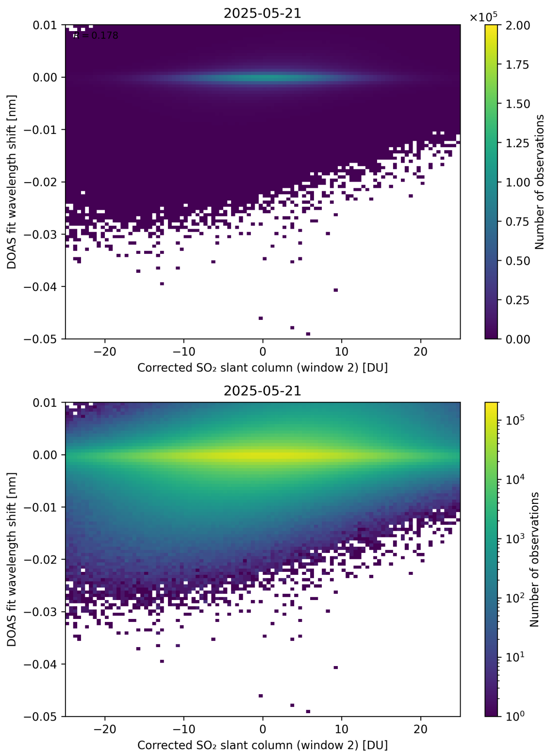
Figure 246: Scatter density plot of “Corrected SO 2 slant column (window 2)” against “DOAS fit wavelength shift” for 2025-05-21 to 2025-05-22.
