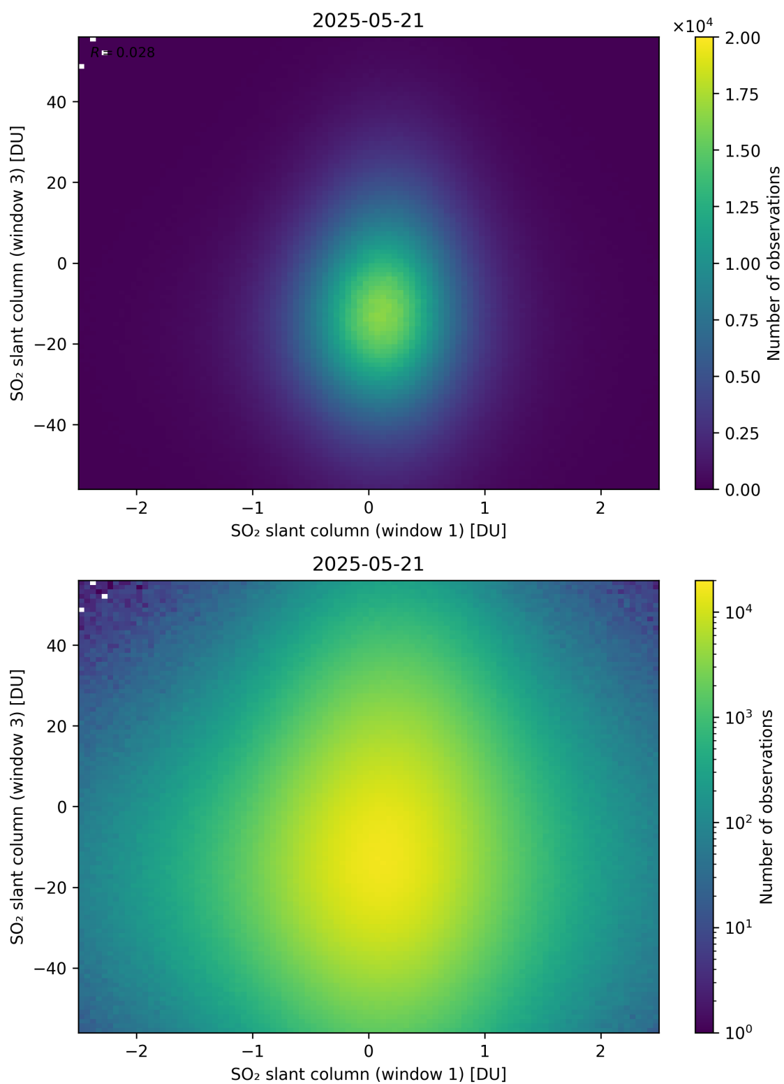
Figure 287: Scatter density plot of “SO 2 slant column (window 1)” against “SO 2 slant column (window 3)” for 2025-05-21 to 2025-05-22.
