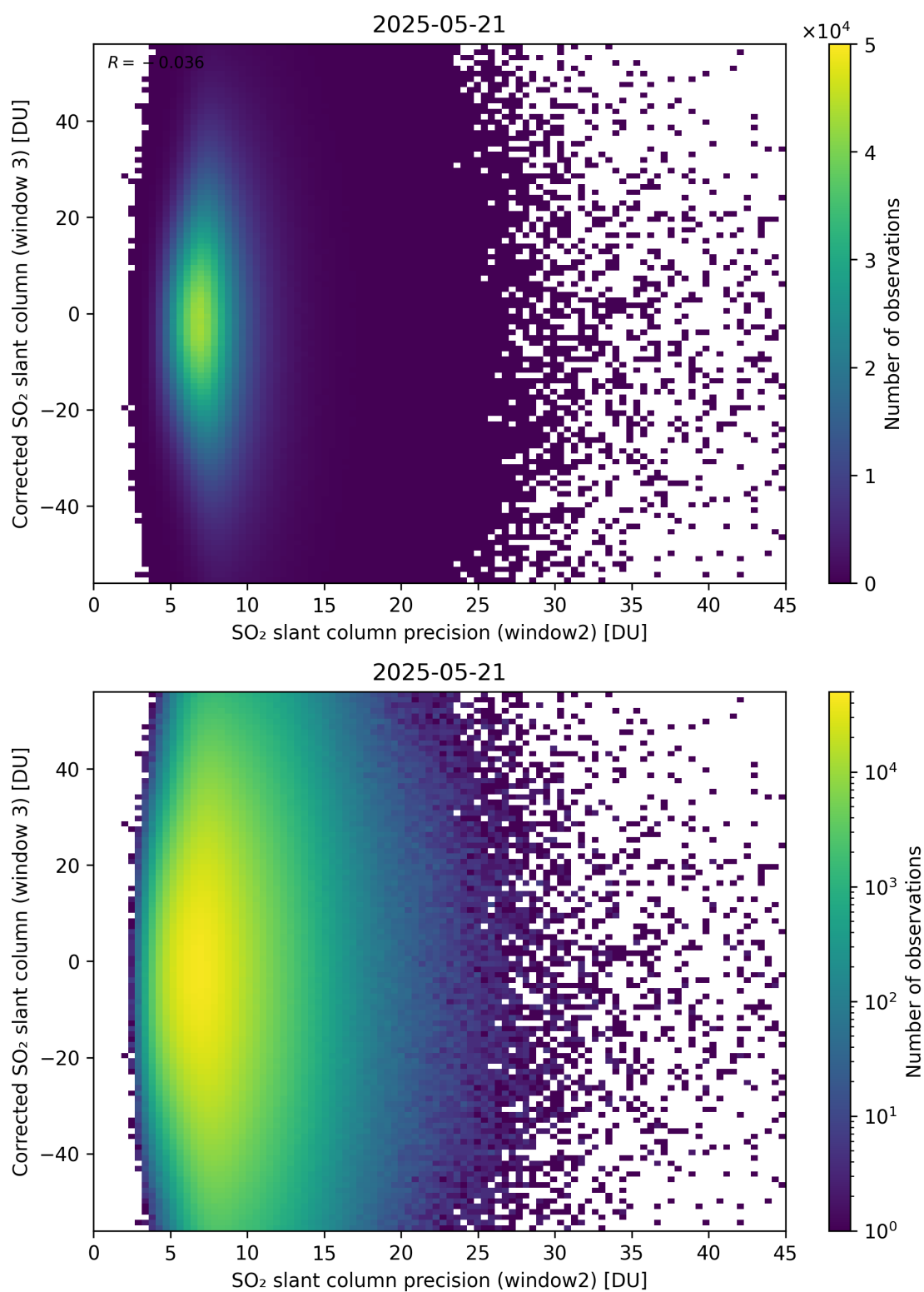
Figure 298: Scatter density plot of “SO 2 slant column precision (window2)” against “Corrected SO 2 slant column (window 3)” for 2025-05-21 to 2025-05-22.
