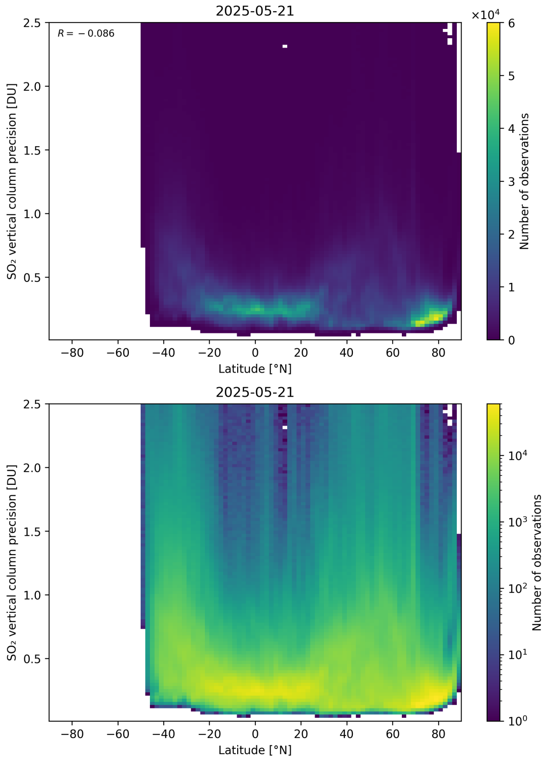
Figure 170: Scatter density plot of “Latitude” against “SO 2 vertical column precision” for 2025-05-21 to 2025-05-22.
