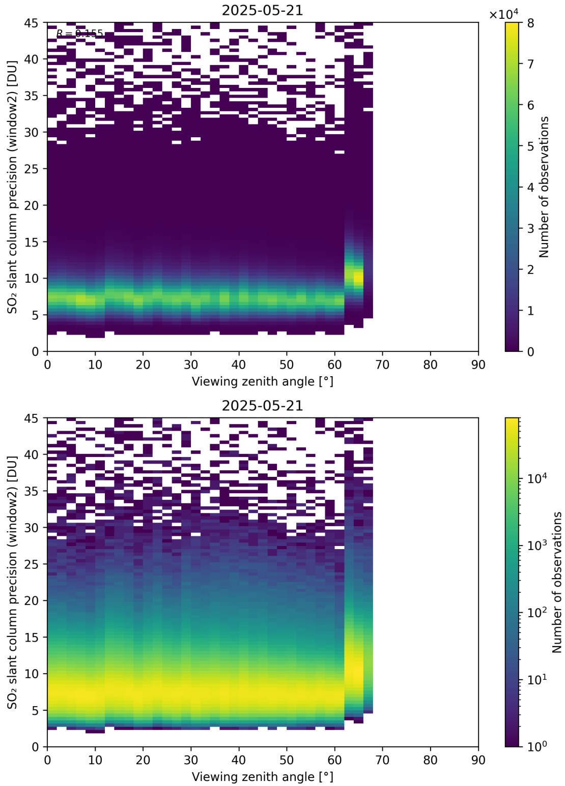
Figure 378: Scatter density plot of “Viewing zenith angle” against “SO 2 slant column precision (window2)” for 2025-05-21 to 2025-05-22.
