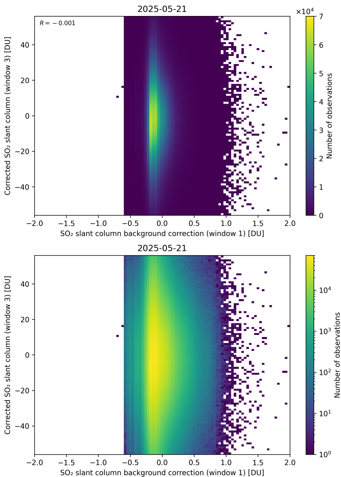
Figure 116: Scatter density plot of “SO 2 slant column background correction (window 1)” against “Corrected SO 2 slant column (window 3)” for 2025-05-21 to 2025-05-22.
