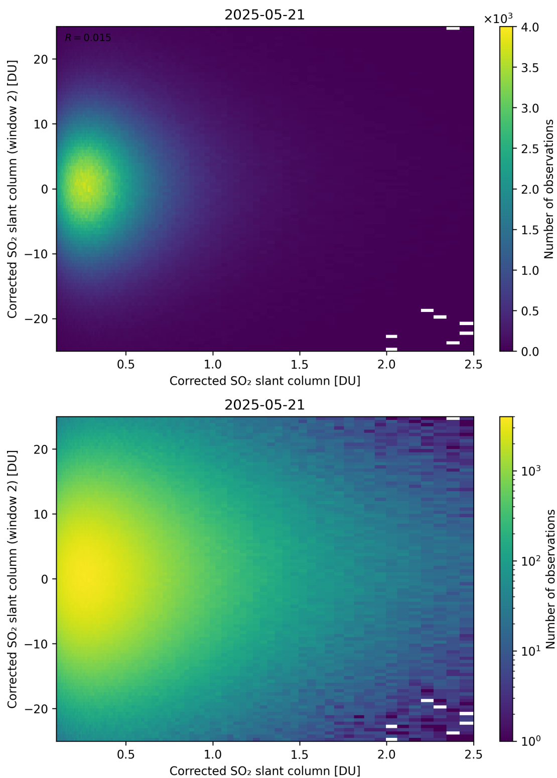
Figure 235: Scatter density plot of “Corrected SO 2 slant column” against “Corrected SO 2 slant column (window 2)” for 2025-05-21 to 2025-05-22.
