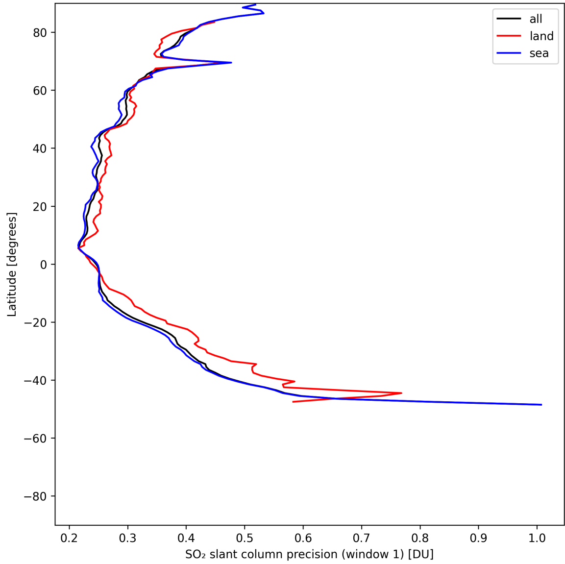
Figure 38: Zonal average of “SO 2 slant column precision (window 1)” for 2025-05-21 to 2025-05-22.
