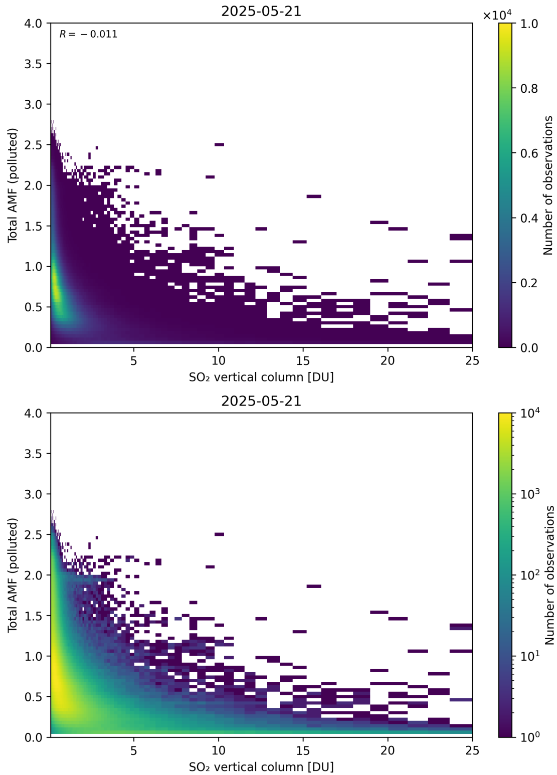
Figure 359: Scatter density plot of “SO 2 vertical column” against “Total AMF (polluted)” for 2025-05-21 to 2025-05-22.
