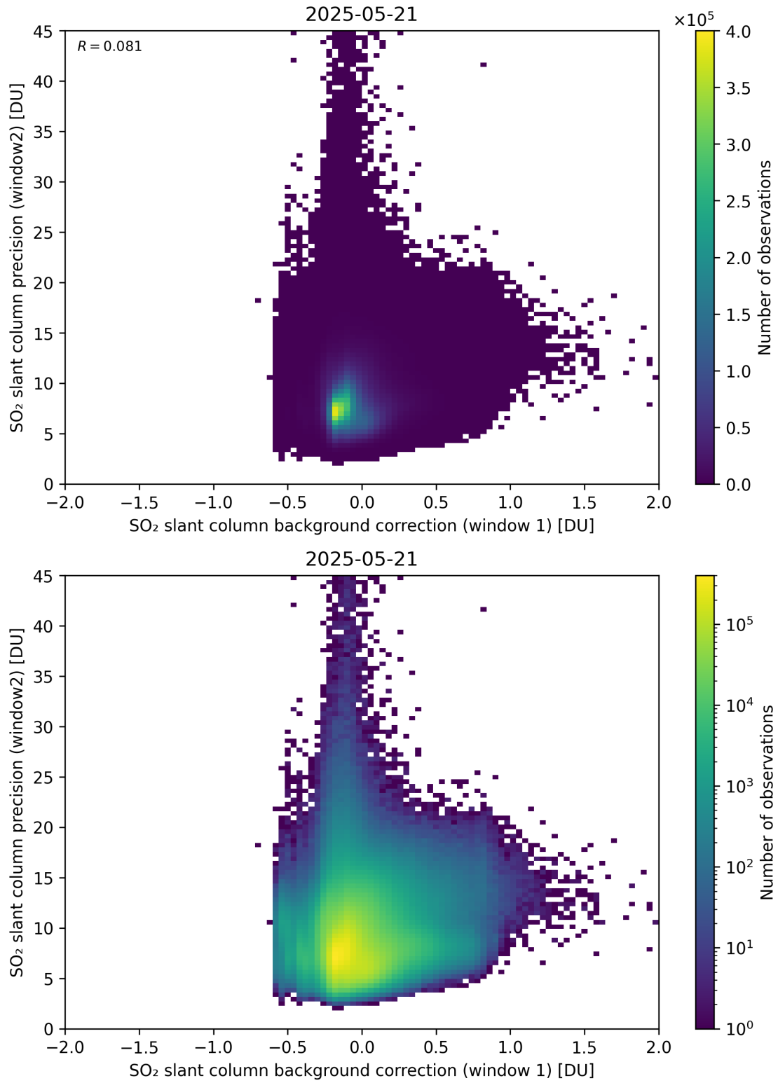
Figure 117: Scatter density plot of “SO 2 slant column background correction (window 1)” against “SO 2 slant column precision (window2)” for 2025-05-21 to 2025-05-22.
