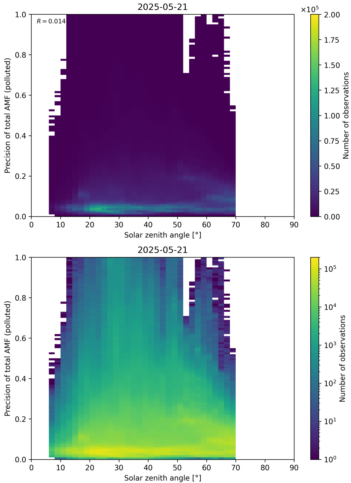
Figure 190: Scatter density plot of “Solar zenith angle” against “Precision of total AMF (polluted)” for 2025-05-21 to 2025-05-22.
