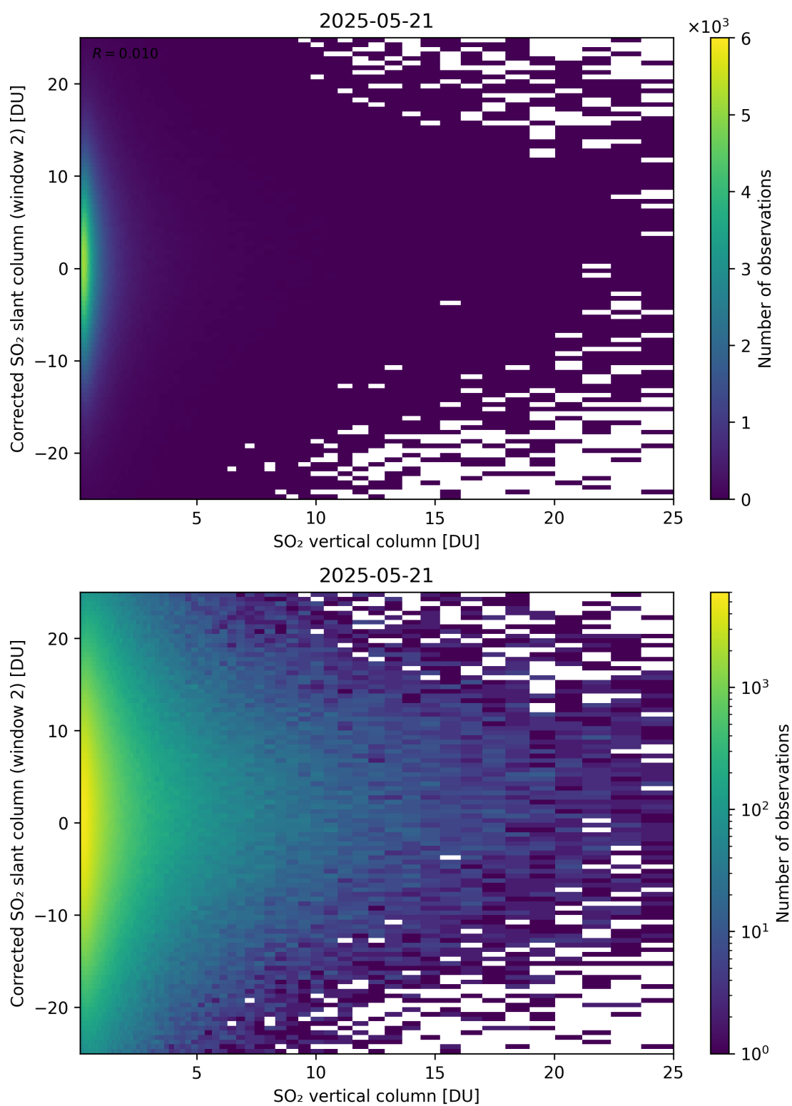
Figure 352: Scatter density plot of “SO 2 vertical column” against “Corrected SO 2 slant column (window 2)” for 2025-05-21 to 2025-05-22.
