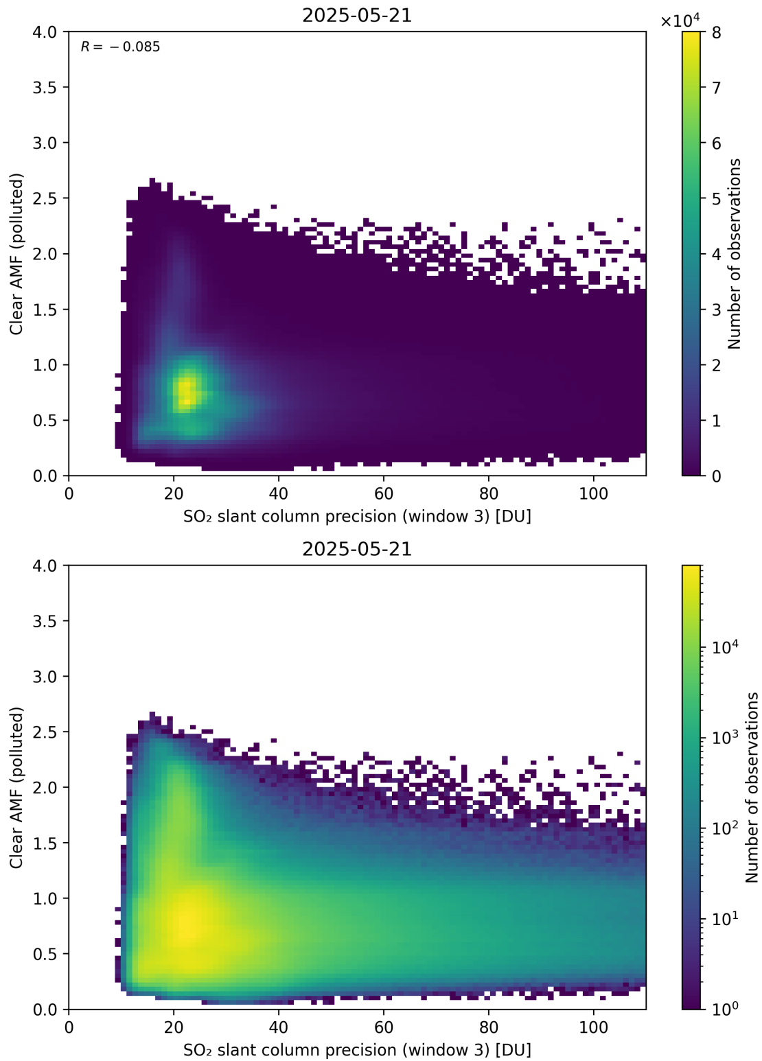
Figure 311: Scatter density plot of “SO 2 slant column precision (window 3)” against “Clear AMF (polluted)” for 2025-05-21 to 2025-05-22.
