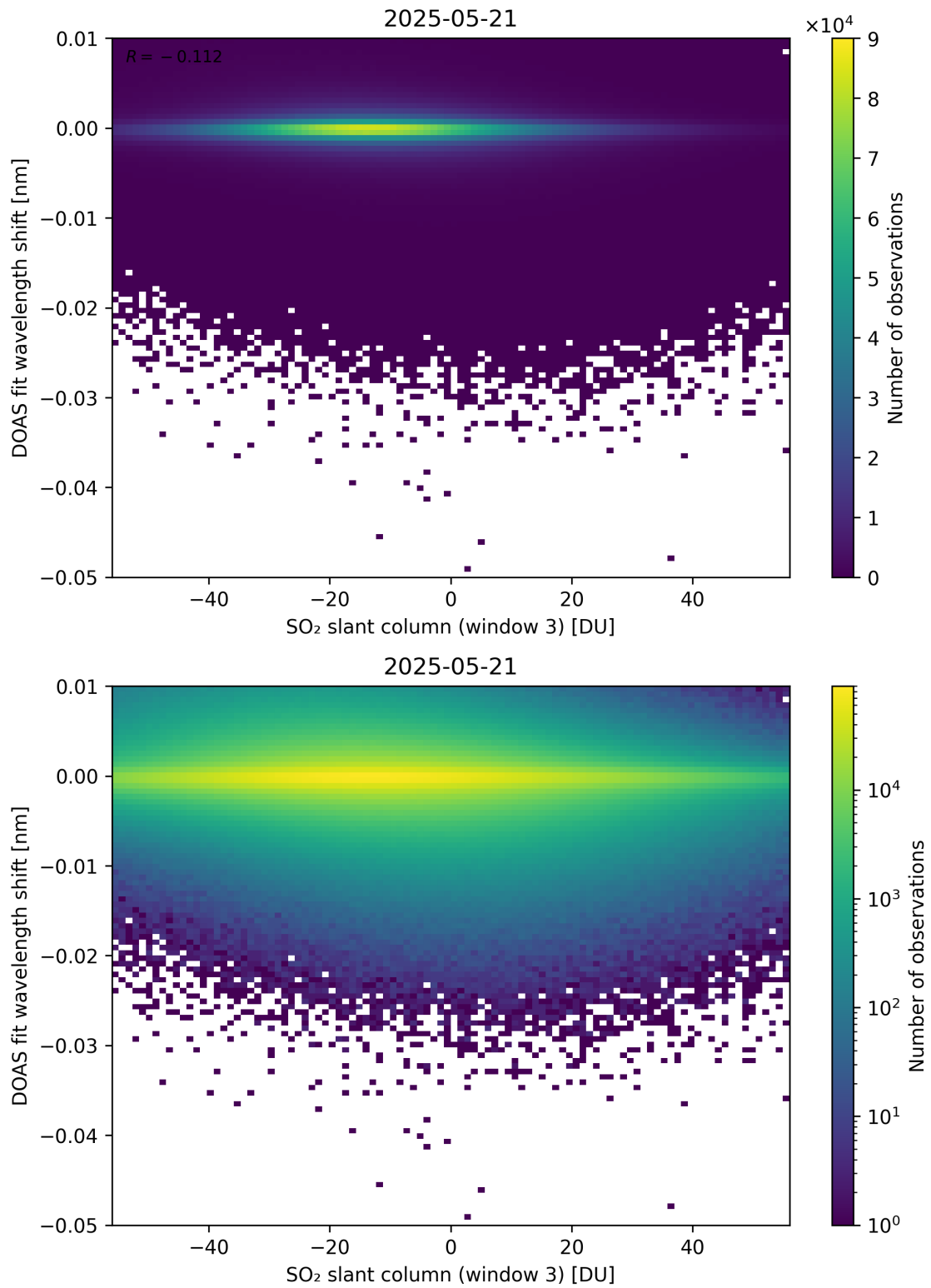
Figure 304: Scatter density plot of “SO 2 slant column (window 3)” against “DOAS fit wavelength shift” for 2025-05-21 to 2025-05-22.
