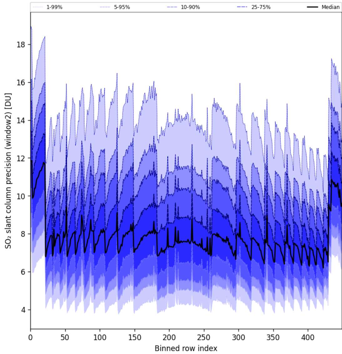
Figure 94: Along track statistics of “SO 2 slant column precision (window2)” for 2025-05-21 to 2025-05-22
