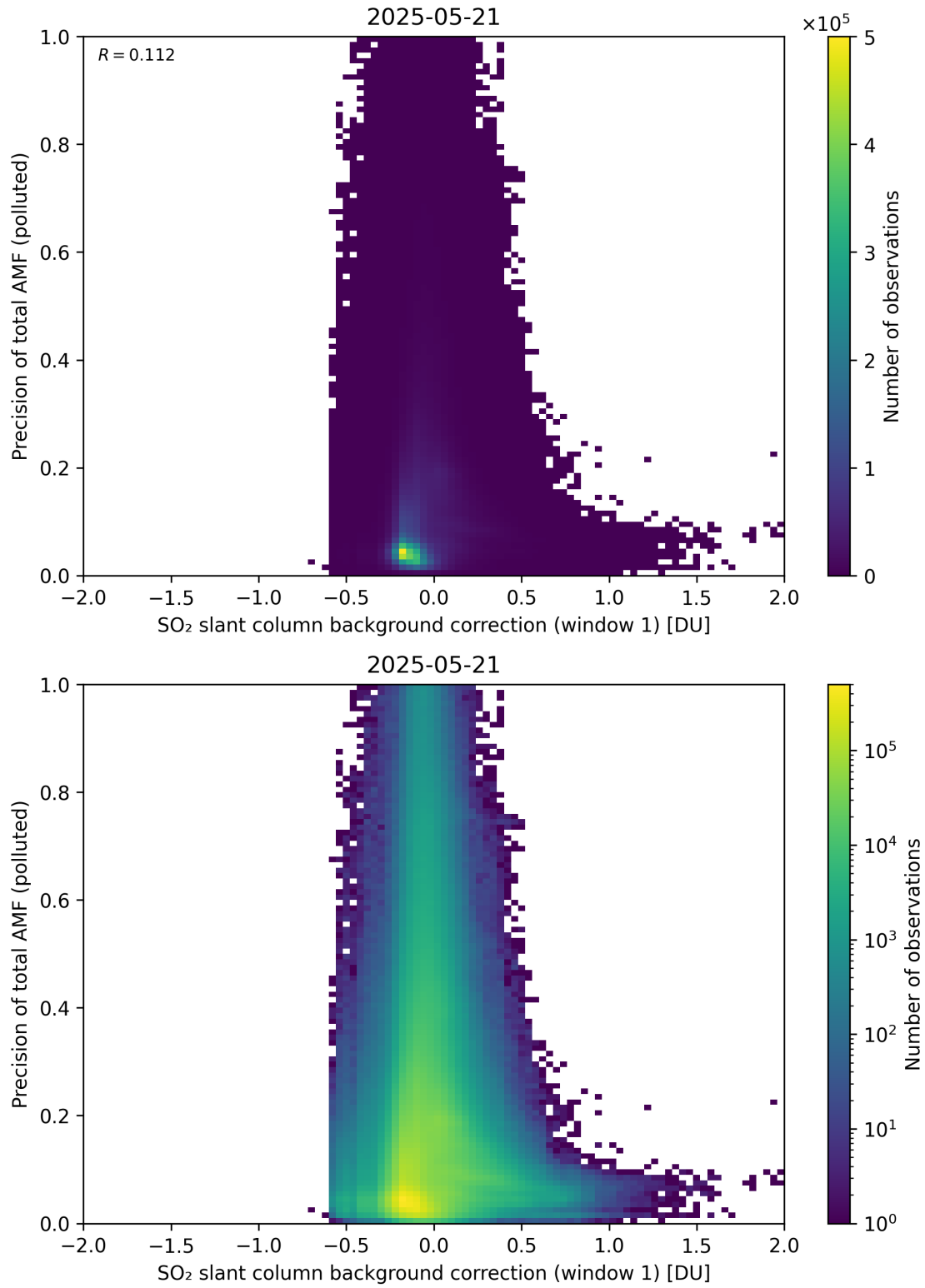
Figure 121: Scatter density plot of “SO 2 slant column background correction (window 1)” against “Precision of total AMF (polluted)” for 2025-05-21 to 2025-05-22.
