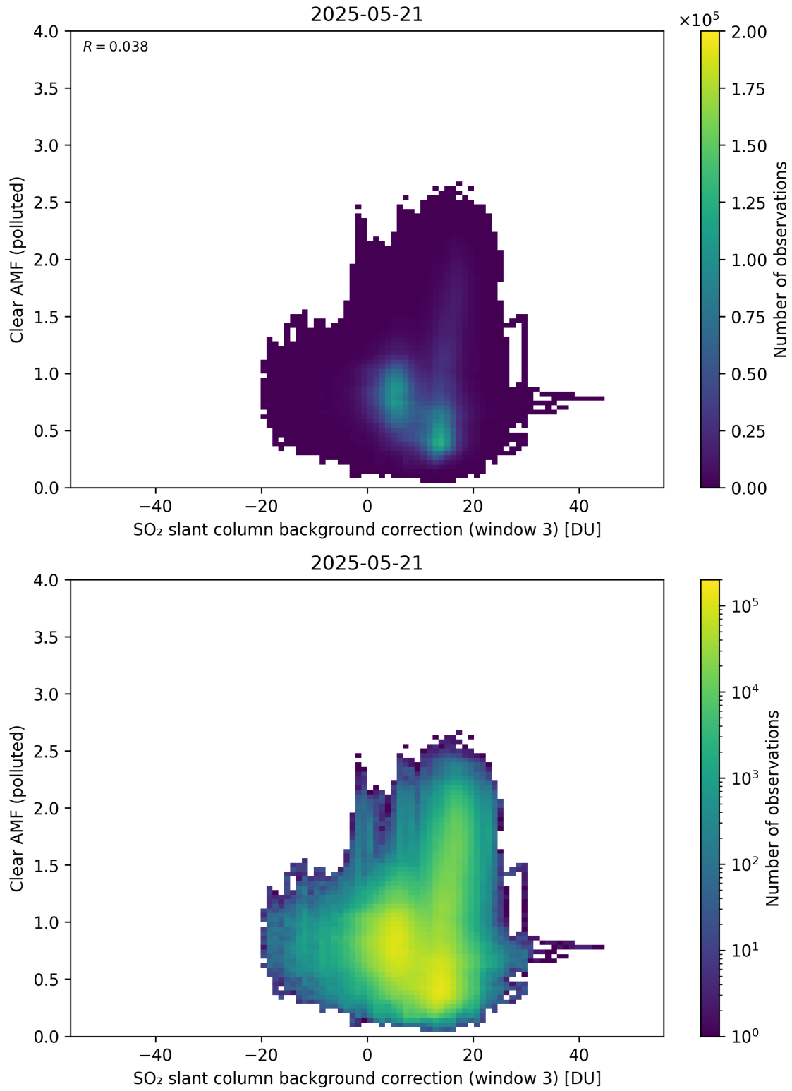
Figure 135: Scatter density plot of “SO 2 slant column background correction (window 3)” against “Clear AMF (polluted)” for 2025-05-21 to 2025-05-22.
