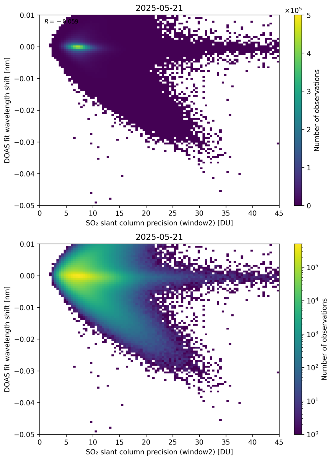
Figure 293: Scatter density plot of “SO 2 slant column precision (window2)” against “DOAS fit wavelength shift” for 2025-05-21 to 2025-05-22.
