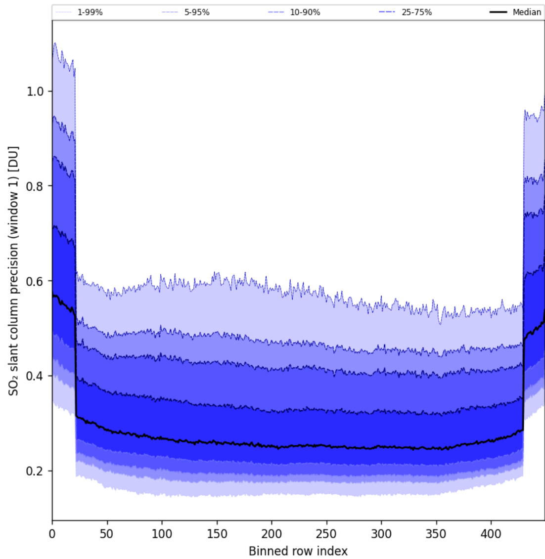
Figure 90: Along track statistics of “SO 2 slant column precision (window 1)” for 2025-05-21 to 2025-05-22
