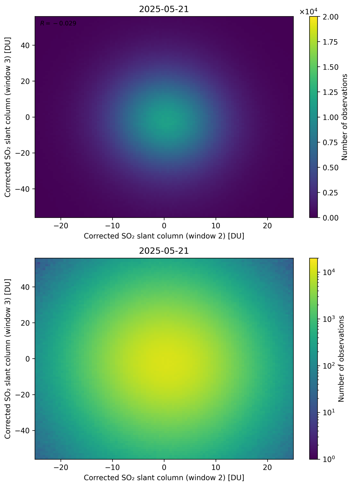
Figure 250: Scatter density plot of “Corrected SO 2 slant column (window 2)” against “Corrected SO 2 slant column (window 3)” for 2025-05-21 to 2025-05-22.
