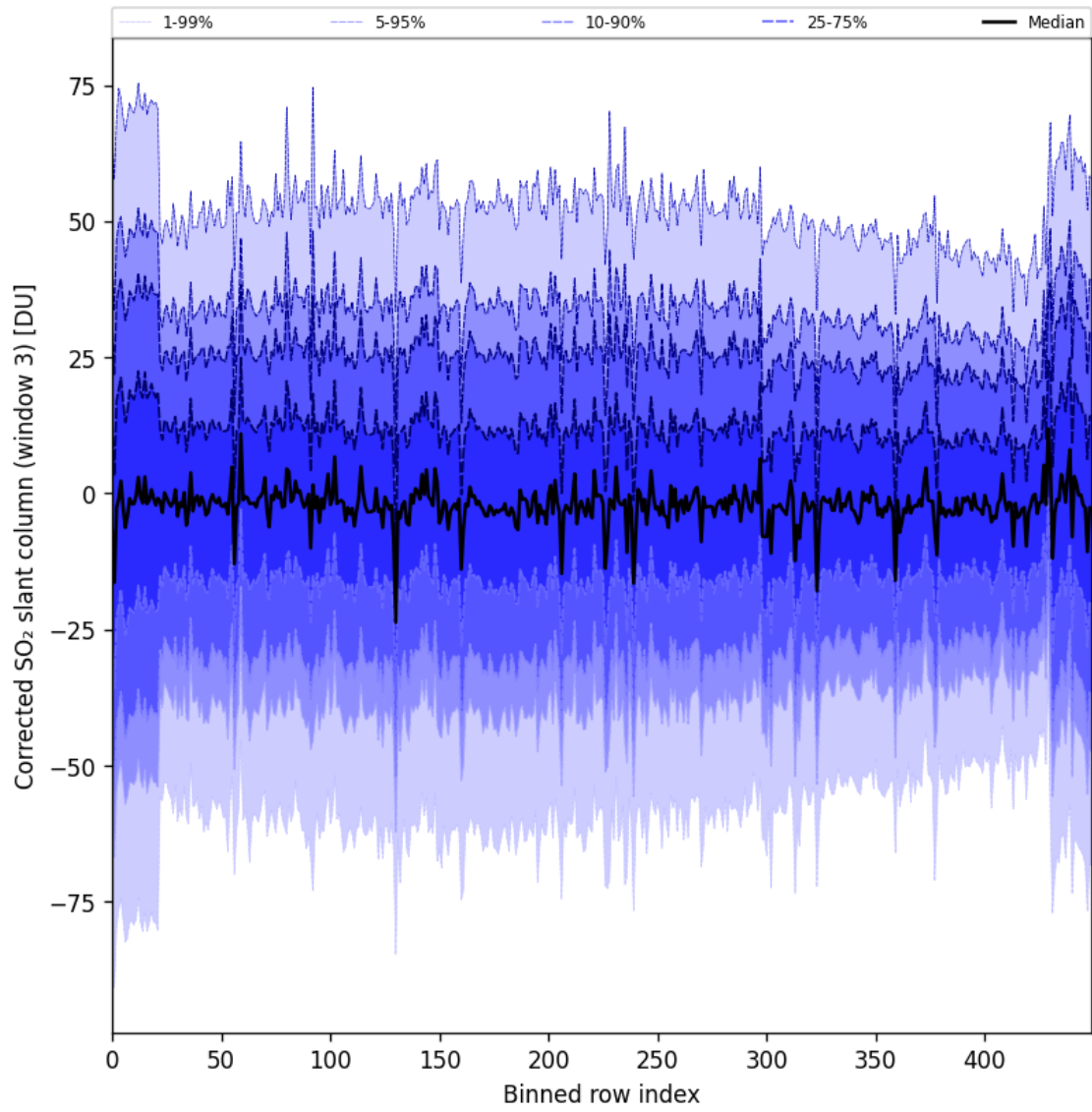
Figure 99: Along track statistics of “Corrected SO 2 slant column (window 3)” for 2025-05-21 to 2025-05-22
