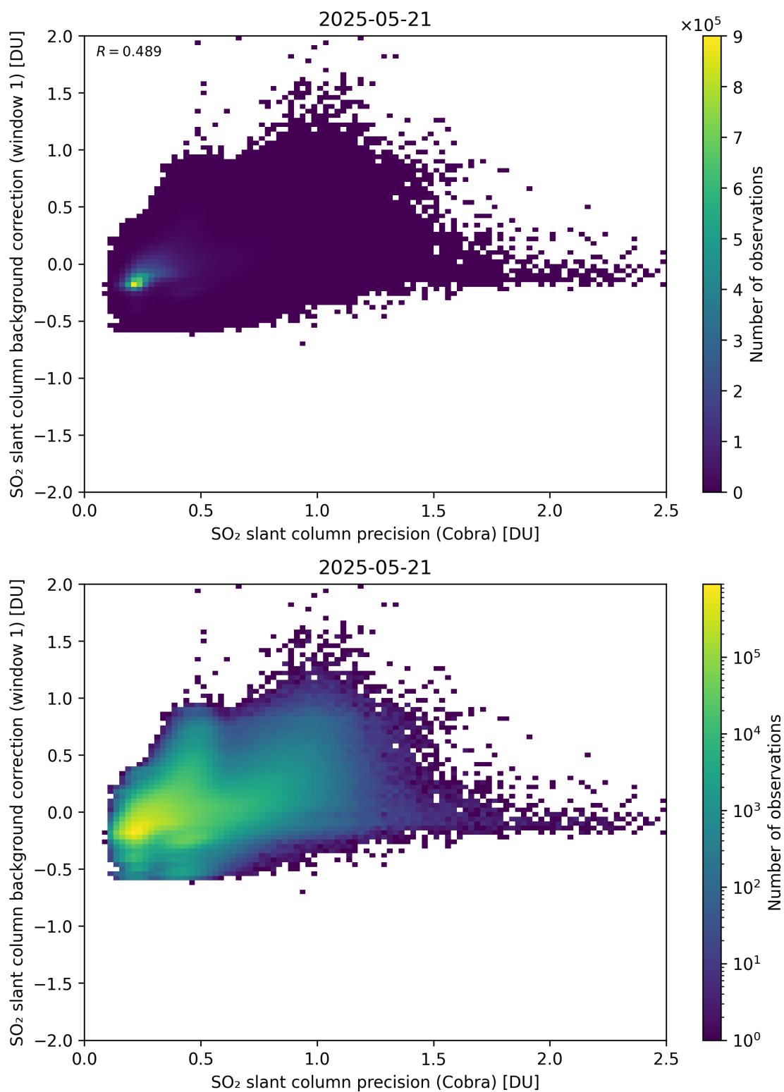
Figure 199: Scatter density plot of “SO 2 slant column precision (Cobra)” against “SO 2 slant column background correction (window 1)” for 2025-05-21 to 2025-05-22.
