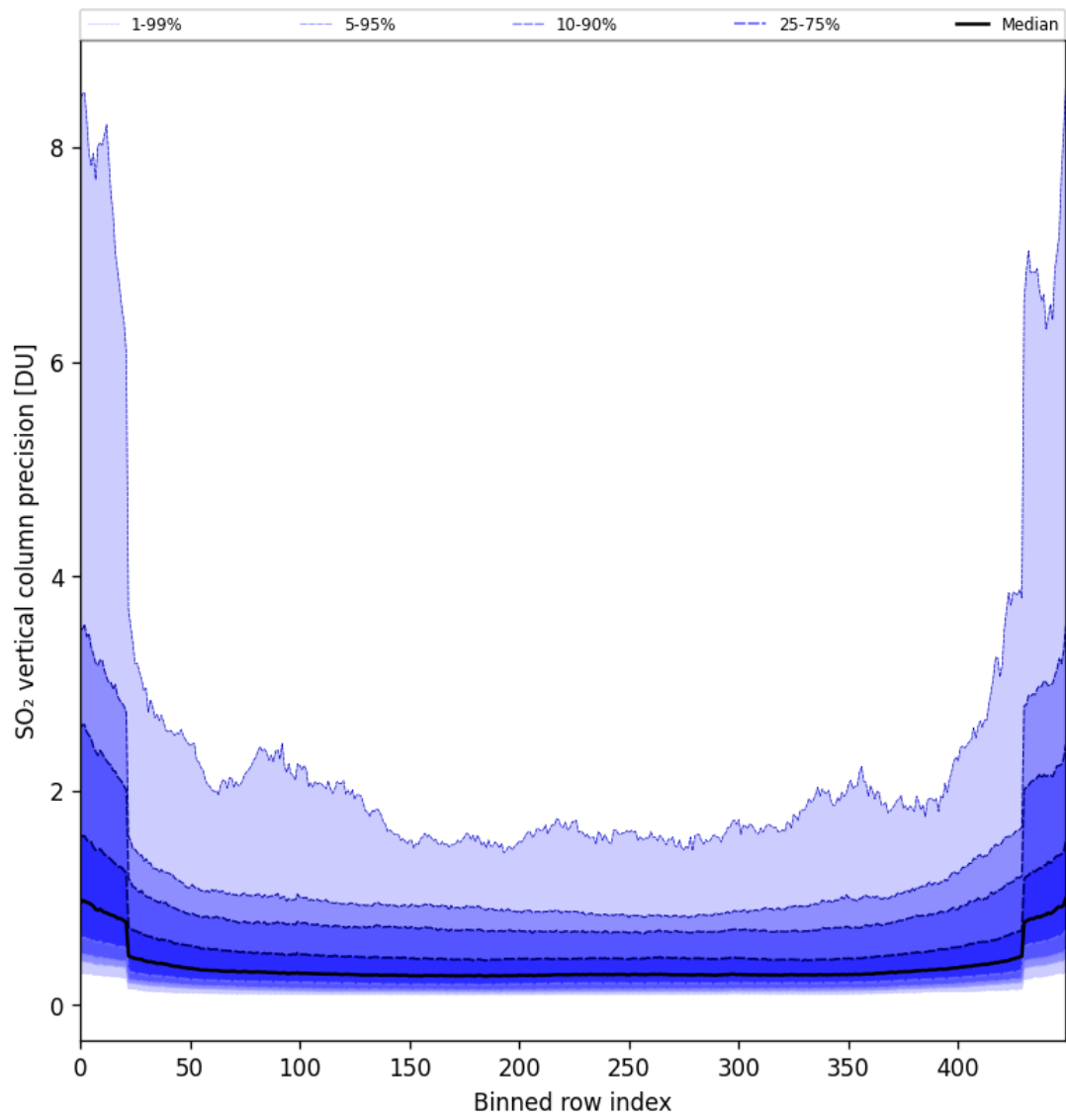
Figure 85: Along track statistics of “SO 2 vertical column precision” for 2025-05-21 to 2025-05-22
