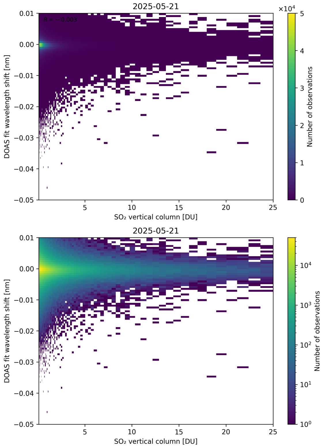
Figure 326: Scatter density plot of “SO 2 vertical column” against “DOAS fit wavelength shift” for 2025-05-21 to 2025-05-22.
