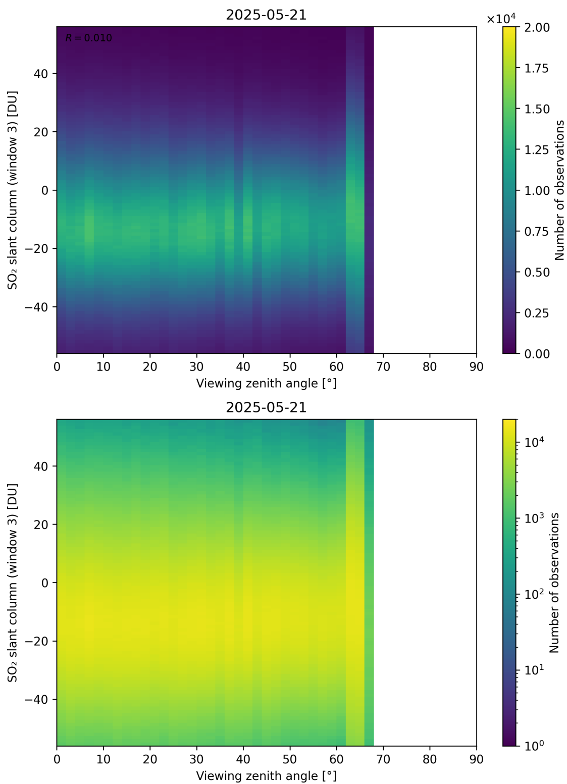
Figure 379: Scatter density plot of “Viewing zenith angle” against “SO 2 slant column (window 3)” for 2025-05-21 to 2025-05-22.
