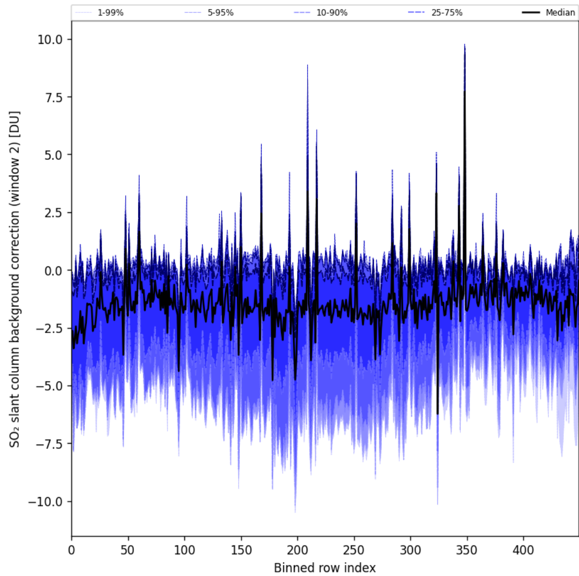
Figure 96: Along track statistics of “SO 2 slant column background correction (window 2)” for 2025-05-21 to 2025-05-22
