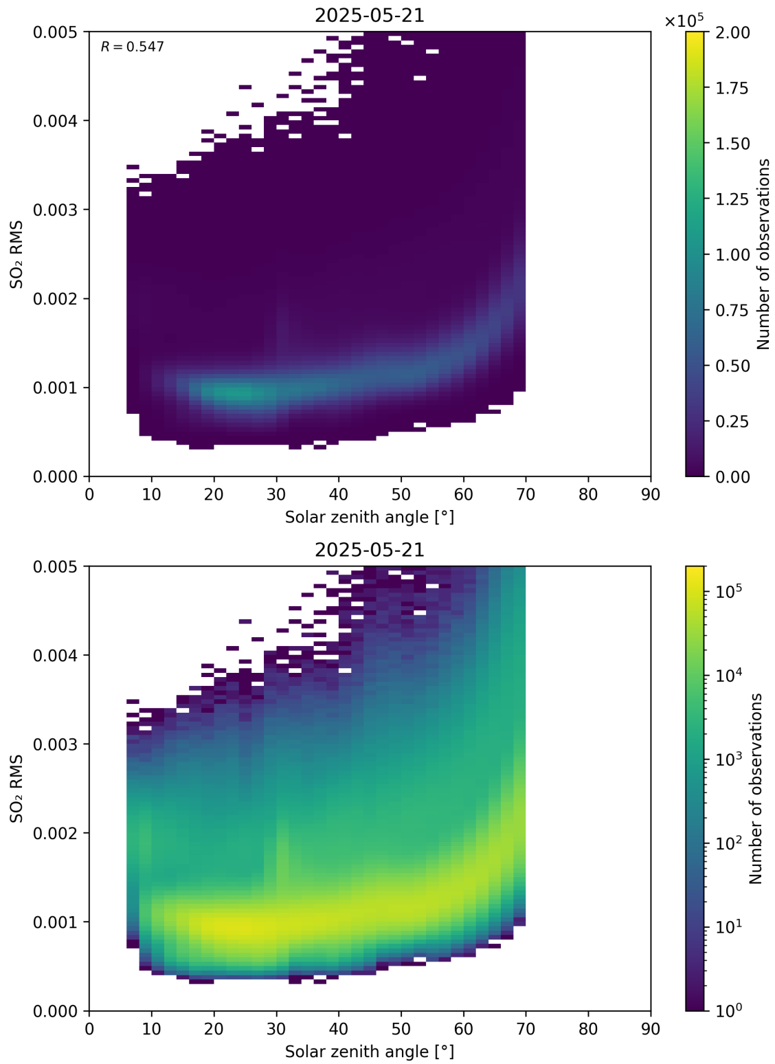
Figure 176: Scatter density plot of “Solar zenith angle” against “SO 2 RMS” for 2025-05-21 to 2025-05-22.
