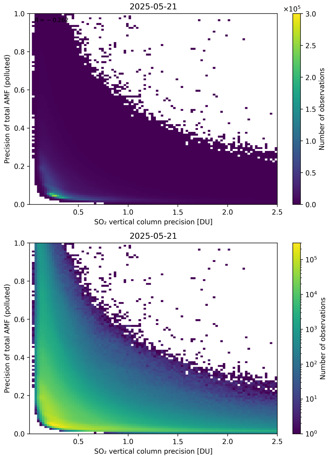
Figure 347: Scatter density plot of “SO 2 vertical column precision” against “Precision of total AMF (polluted)” for 2025-05-21 to 2025-05-22.
