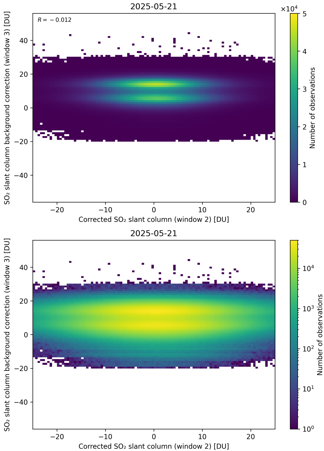
Figure 245: Scatter density plot of “Corrected SO 2 slant column (window 2)” against “SO 2 slant column background correction (window 3)” for 2025-05-21 to 2025-05-22.
