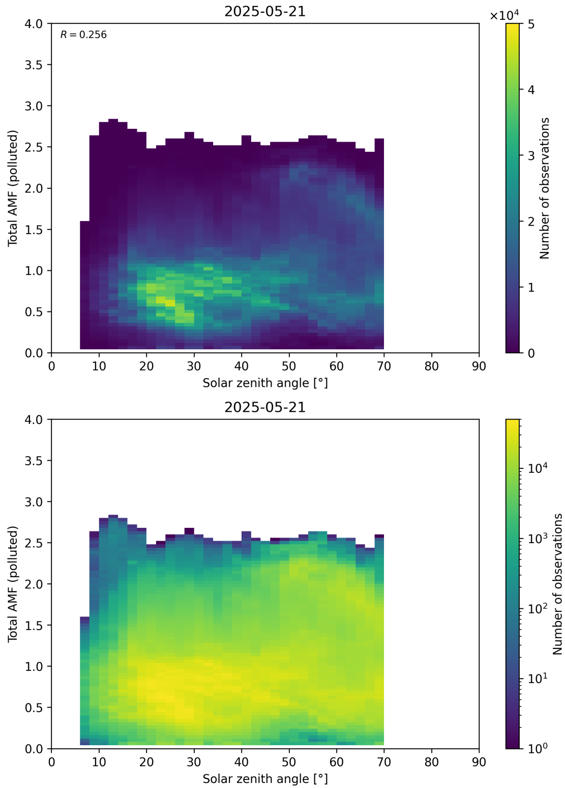
Figure 189: Scatter density plot of “Solar zenith angle” against “Total AMF (polluted)” for 2025-05-21 to 2025-05-22.
