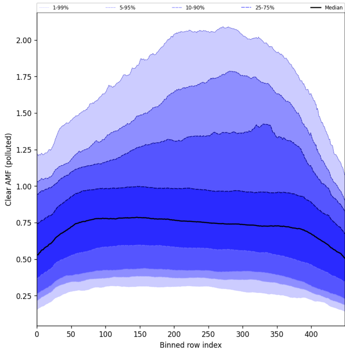
Figure 107: Along track statistics of “Clear AMF (polluted)” for 2025-05-21 to 2025-05-22
