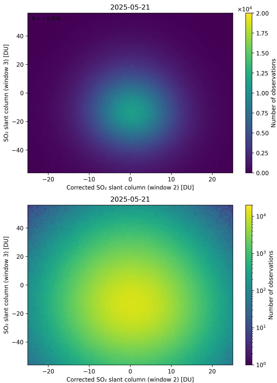
Figure 251: Scatter density plot of “Corrected SO 2 slant column (window 2)” against “SO 2 slant column (window 3)” for 2025-05-21 to 2025-05-22.
