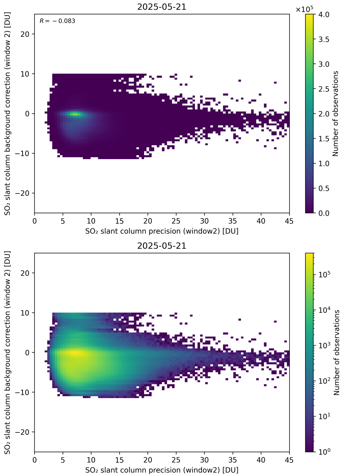
Figure 291: Scatter density plot of “SO 2 slant column precision (window2)” against “SO 2 slant column background correction (window 2)” for 2025-05-21 to 2025-05-22.
