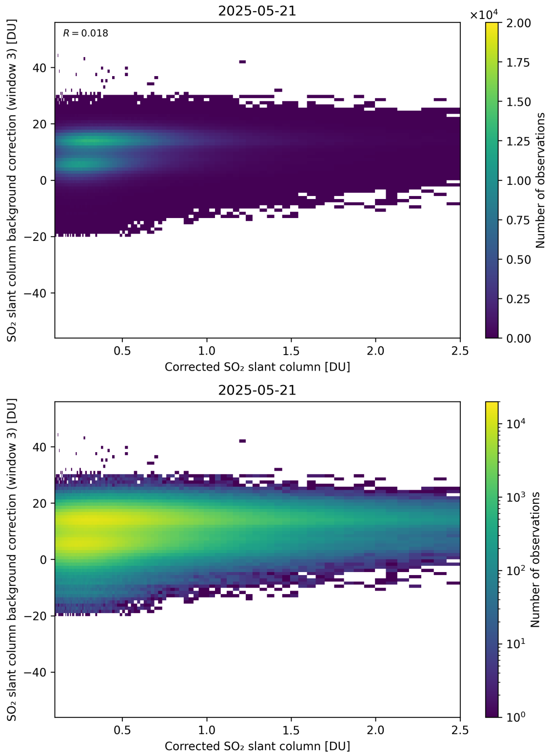
Figure 228: Scatter density plot of “Corrected SO 2 slant column” against “SO 2 slant column background correction (window 3)” for 2025-05-21 to 2025-05-22.
