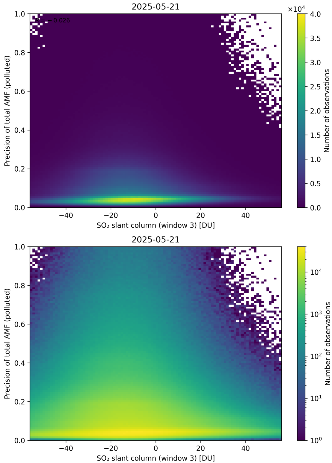
Figure 319: Scatter density plot of “SO 2 slant column (window 3)” against “Precision of total AMF (polluted)” for 2025-05-21 to 2025-05-22.
