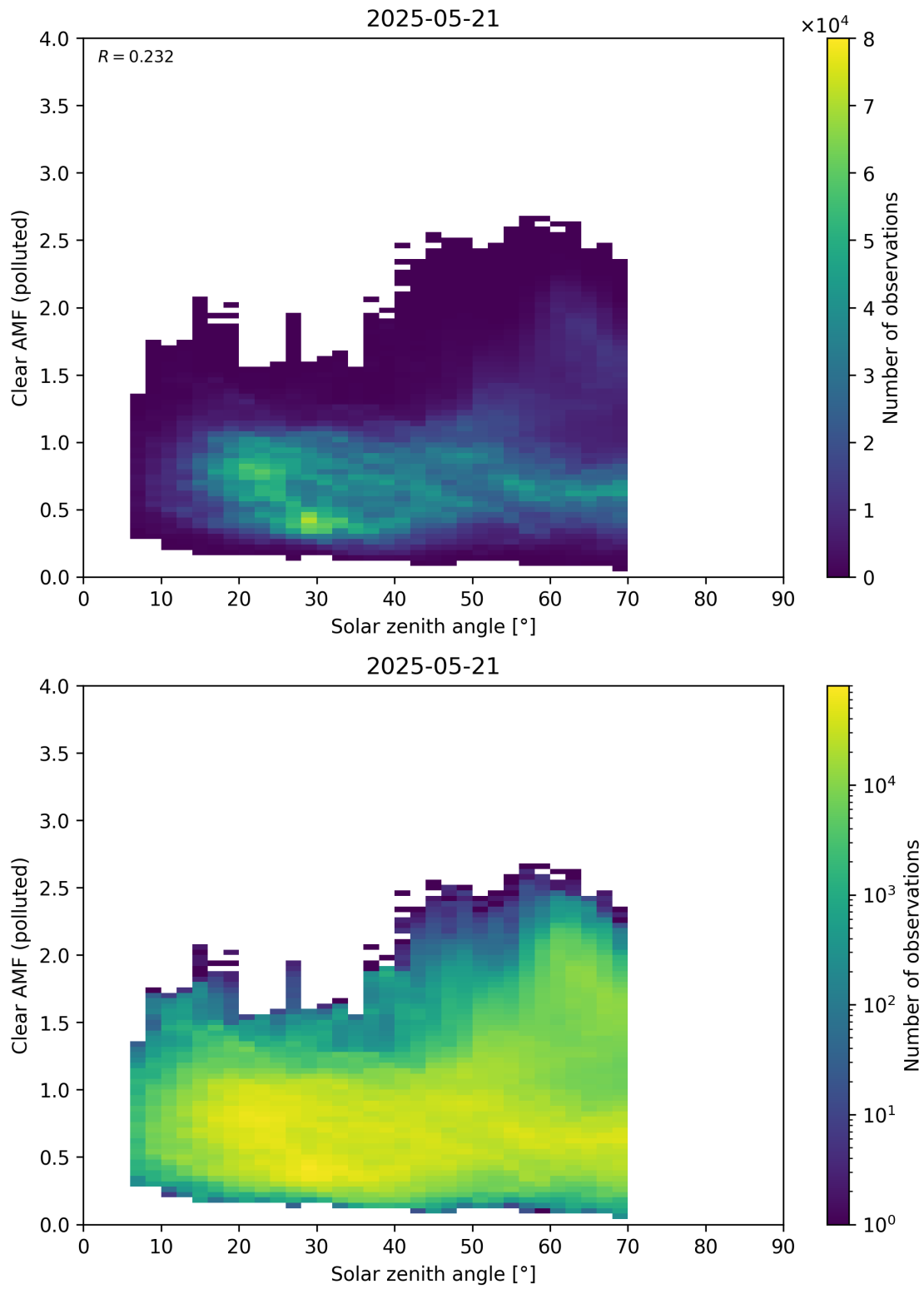
Figure 178: Scatter density plot of “Solar zenith angle” against “Clear AMF (polluted)” for 2025-05-21 to 2025-05-22.
