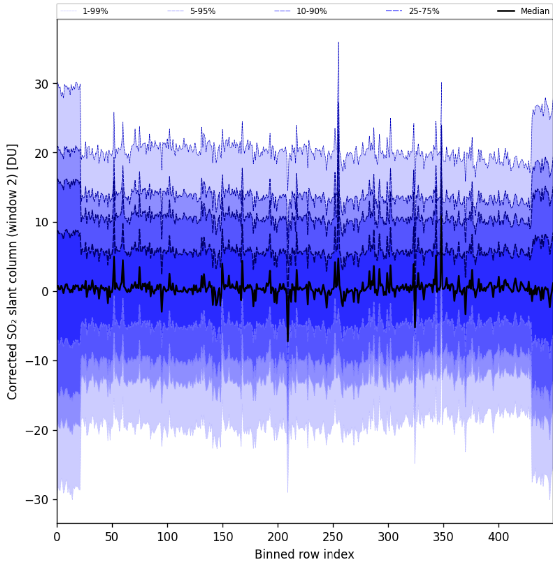
Figure 95: Along track statistics of “Corrected SO 2 slant column (window 2)” for 2025-05-21 to 2025-05-22
