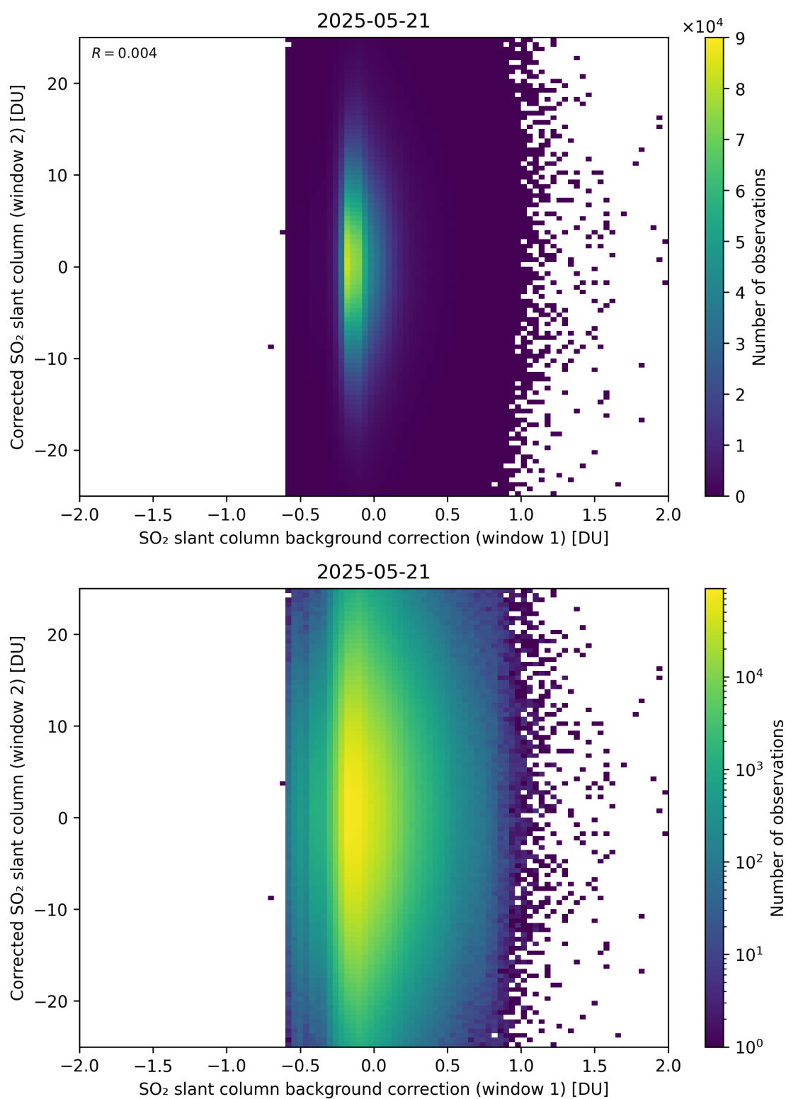
Figure 115: Scatter density plot of “SO 2 slant column background correction (window 1)” against “Corrected SO 2 slant column (window 2)” for 2025-05-21 to 2025-05-22.
