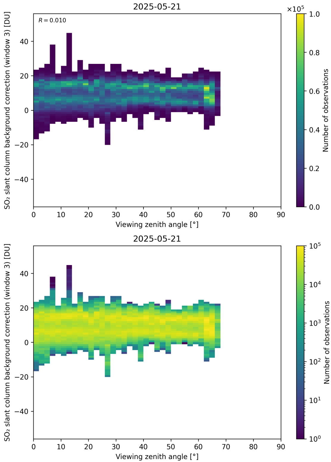
Figure 364: Scatter density plot of “Viewing zenith angle” against “SO 2 slant column background correction (window 3)” for 2025-05-21 to 2025-05-22.
