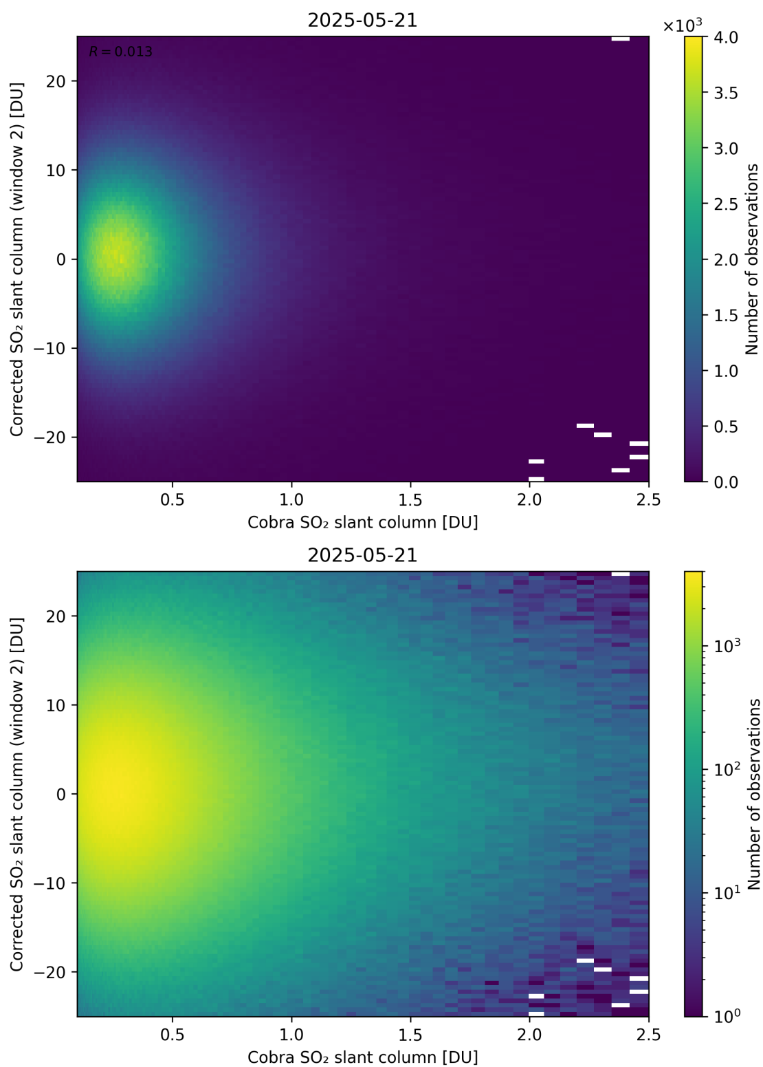
Figure 217: Scatter density plot of “Cobra SO 2 slant column” against “Corrected SO 2 slant column (window 2)” for 2025-05-21 to 2025-05-22.
