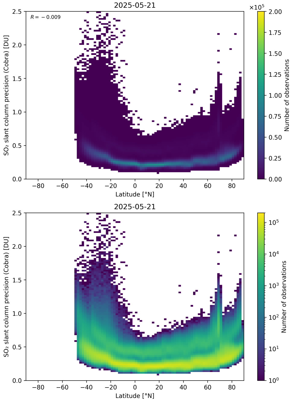
Figure 158: Scatter density plot of “Latitude” against “SO 2 slant column precision (Cobra)” for 2025-05-21 to 2025-05-22.
