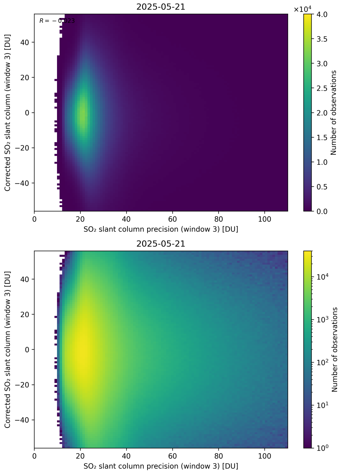
Figure 312: Scatter density plot of “SO 2 slant column precision (window 3)” against “Corrected SO 2 slant column (window 3)” for 2025-05-21 to 2025-05-22.
