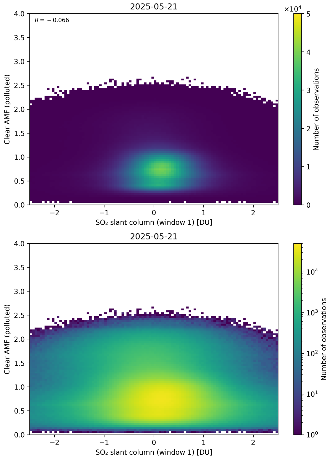
Figure 282: Scatter density plot of “SO 2 slant column (window 1)” against “Clear AMF (polluted)” for 2025-05-21 to 2025-05-22.
