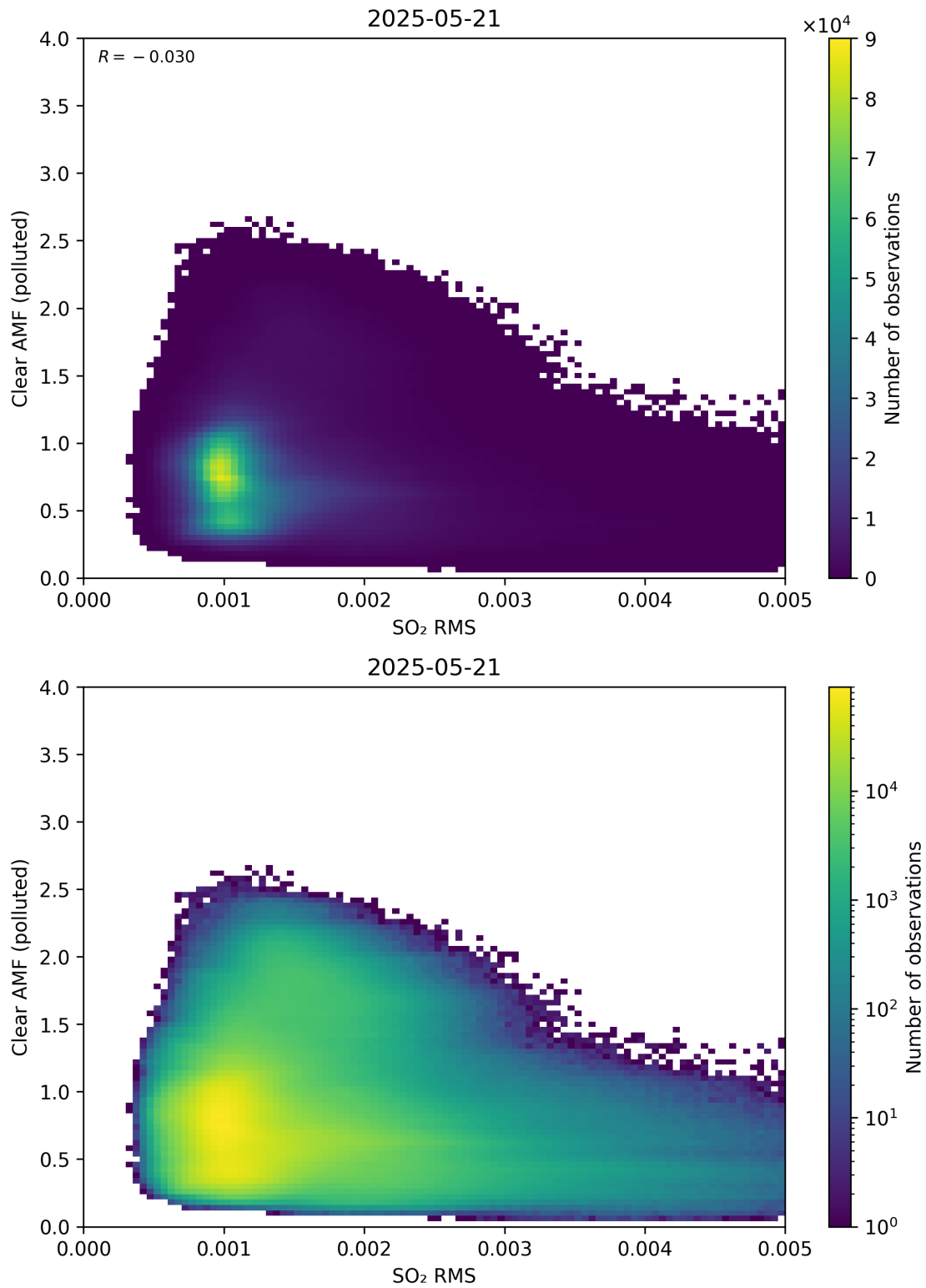
Figure 147: Scatter density plot of “SO 2 RMS” against “Clear AMF (polluted)” for 2025-05-21 to 2025-05-22.
