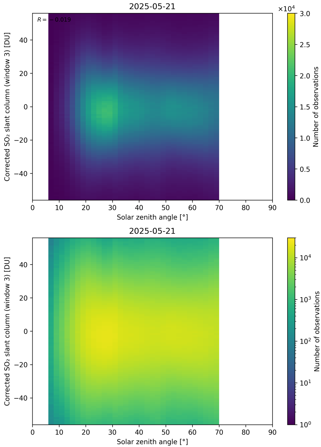
Figure 183: Scatter density plot of “Solar zenith angle” against “Corrected SO 2 slant column (window 3)” for 2025-05-21 to 2025-05-22.
