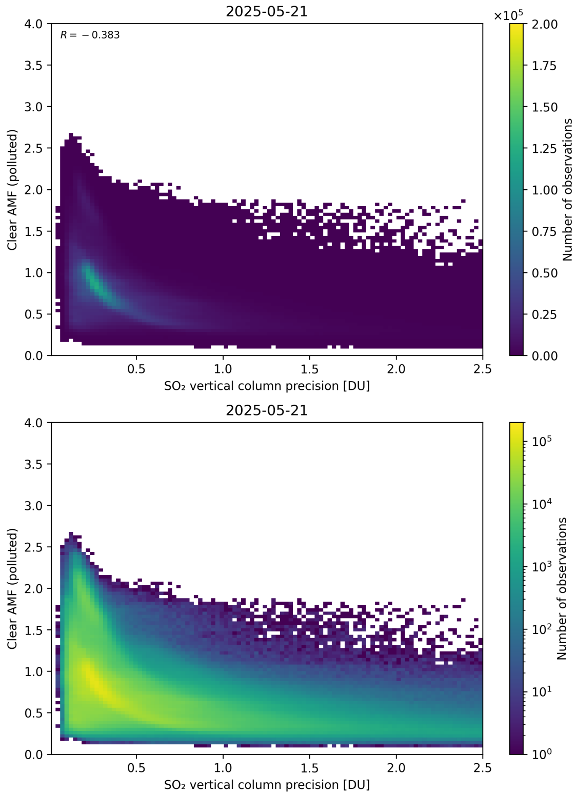
Figure 335: Scatter density plot of “SO 2 vertical column precision” against “Clear AMF (polluted)” for 2025-05-21 to 2025-05-22.
