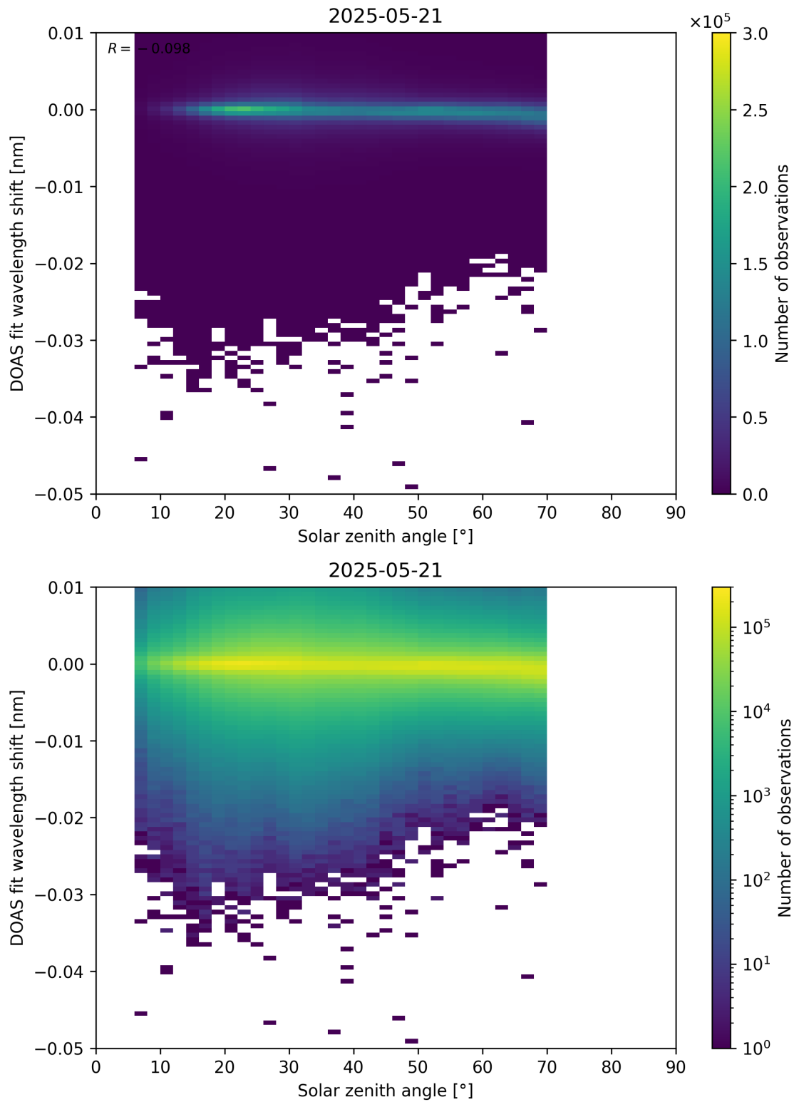
Figure 174: Scatter density plot of “Solar zenith angle” against “DOAS fit wavelength shift” for 2025-05-21 to 2025-05-22.
