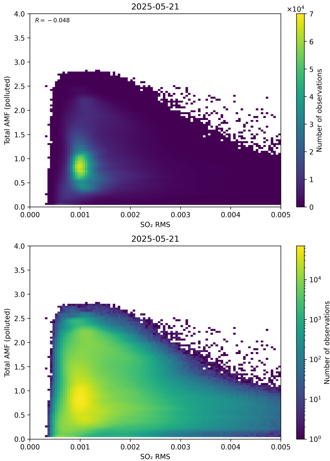
Figure 148: Scatter density plot of “SO 2 RMS” against “Total AMF (polluted)” for 2025-05-21 to 2025-05-22.
