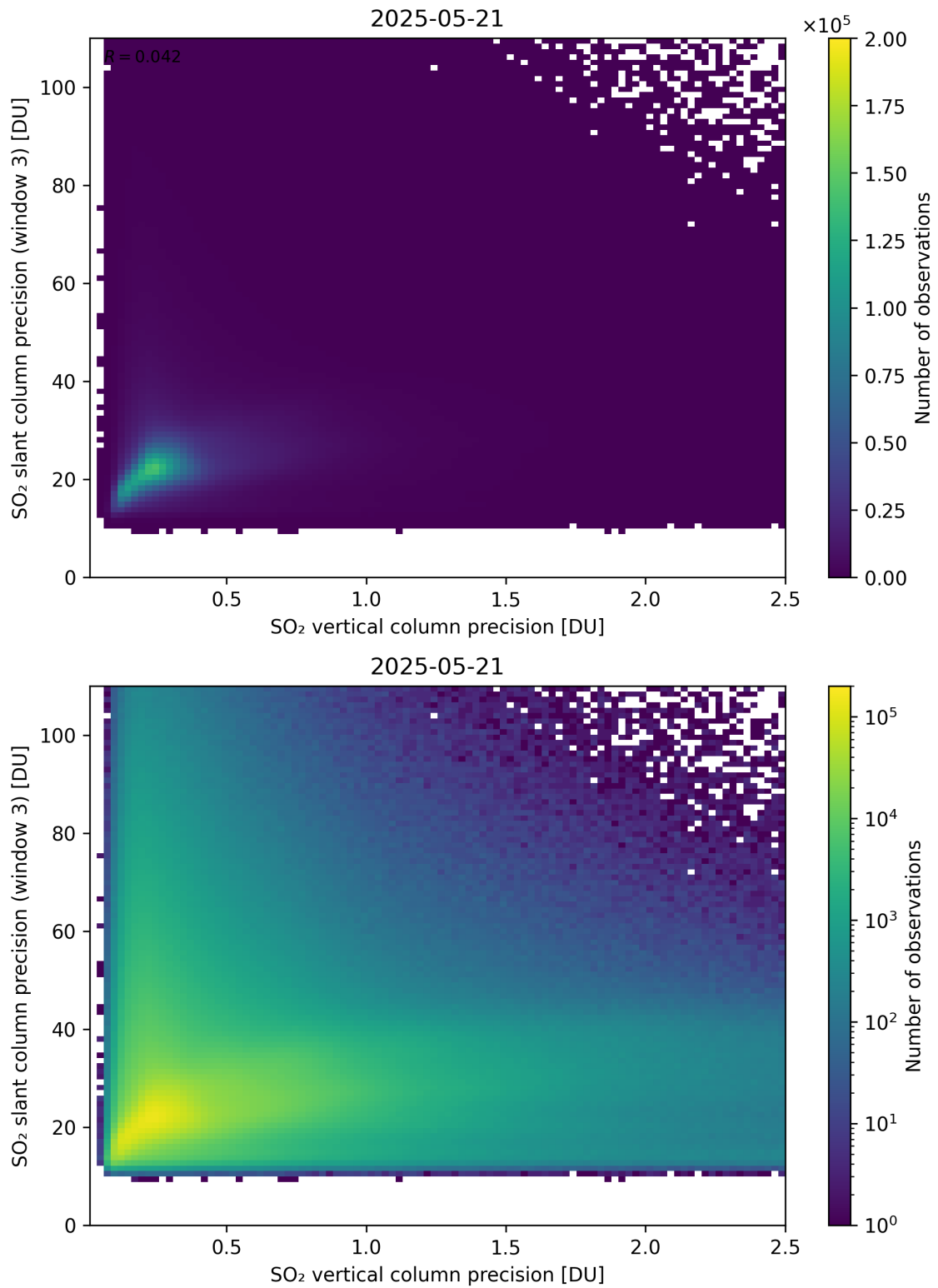
Figure 345: Scatter density plot of “SO 2 vertical column precision” against “SO 2 slant column precision (window 3)” for 2025-05-21 to 2025-05-22.
