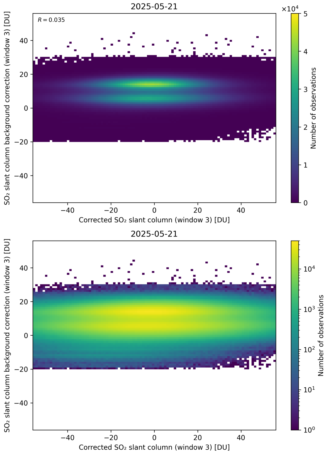
Figure 255: Scatter density plot of “Corrected SO 2 slant column (window 3)” against “SO 2 slant column background correction (window 3)” for 2025-05-21 to 2025-05-22.
