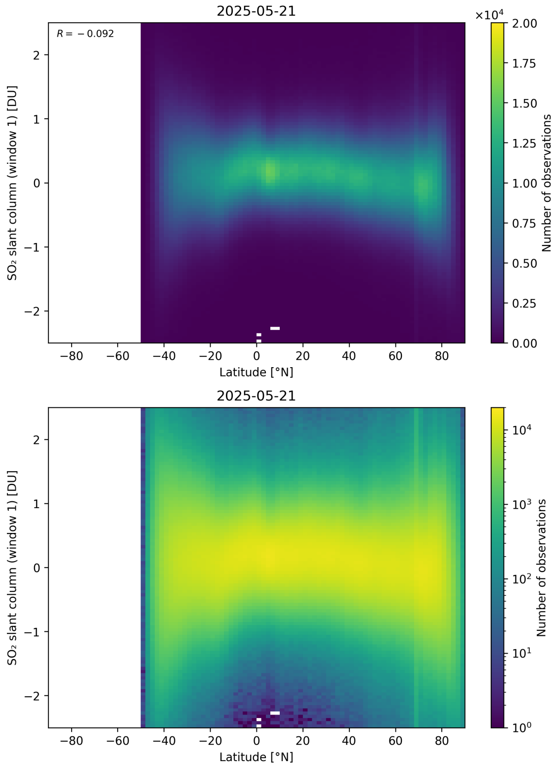
Figure 162: Scatter density plot of “Latitude” against “SO 2 slant column (window 1)” for 2025-05-21 to 2025-05-22.
