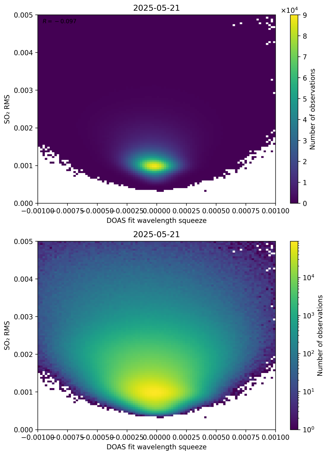
Figure 143: Scatter density plot of “DOAS fit wavelength squeeze” against “SO 2 RMS” for 2025-05-21 to 2025-05-22.
