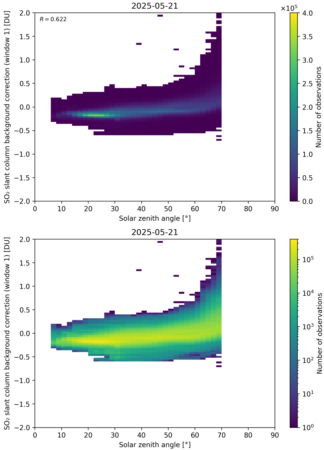
Figure 171: Scatter density plot of “Solar zenith angle” against “SO 2 slant column background correction (window 1)” for 2025-05-21 to 2025-05-22.
