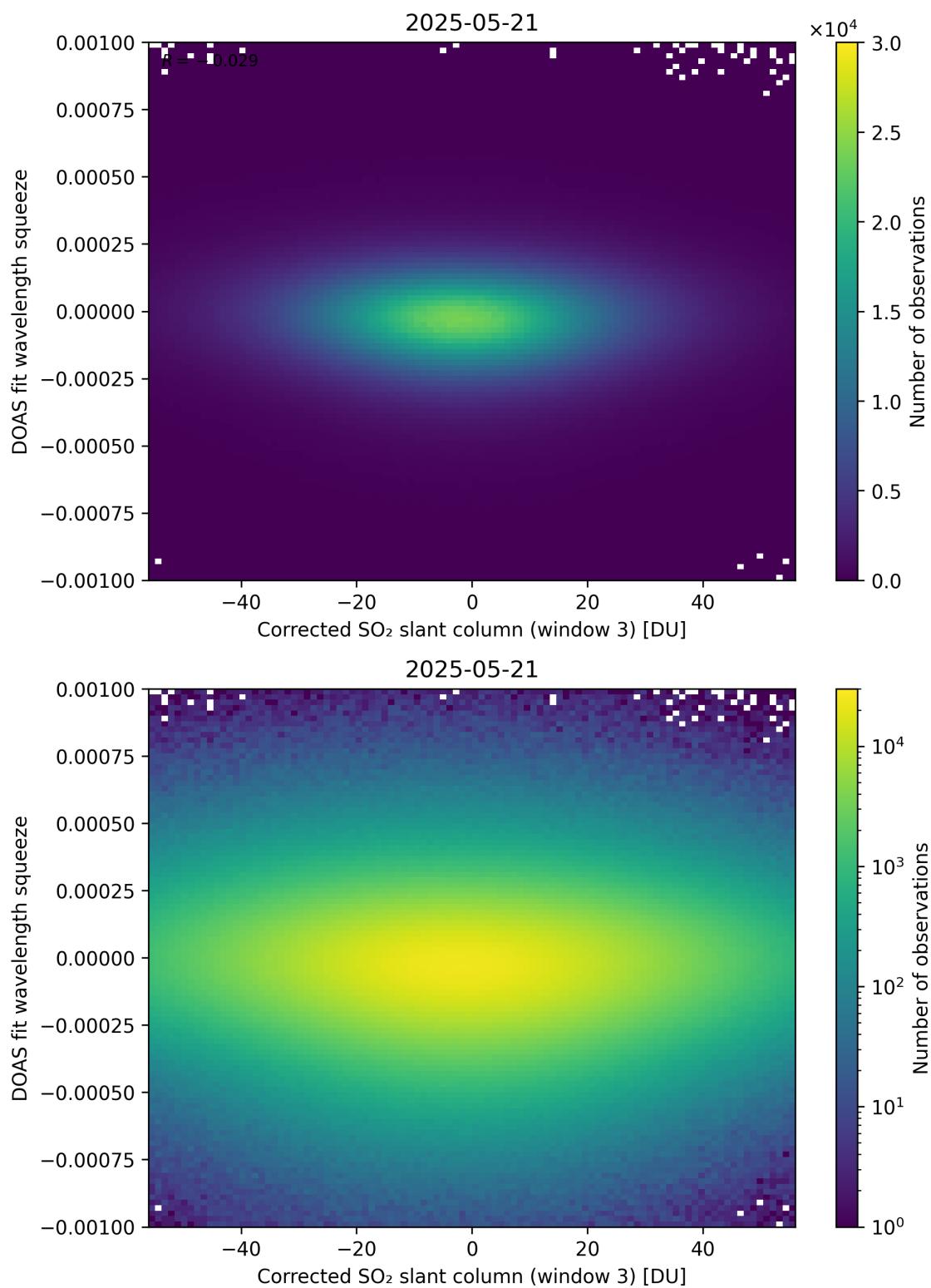
Figure 257: Scatter density plot of “Corrected SO 2 slant column (window 3)” against “DOAS fit wavelength squeeze” for 2025-05-21 to 2025-05-22.
