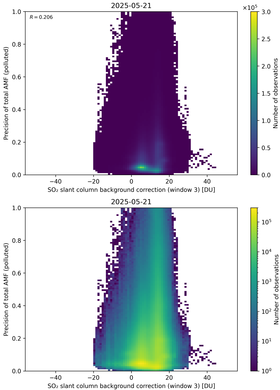
Figure 137: Scatter density plot of “SO 2 slant column background correction (window 3)” against “Precision of total AMF (polluted)” for 2025-05-21 to 2025-05-22.
