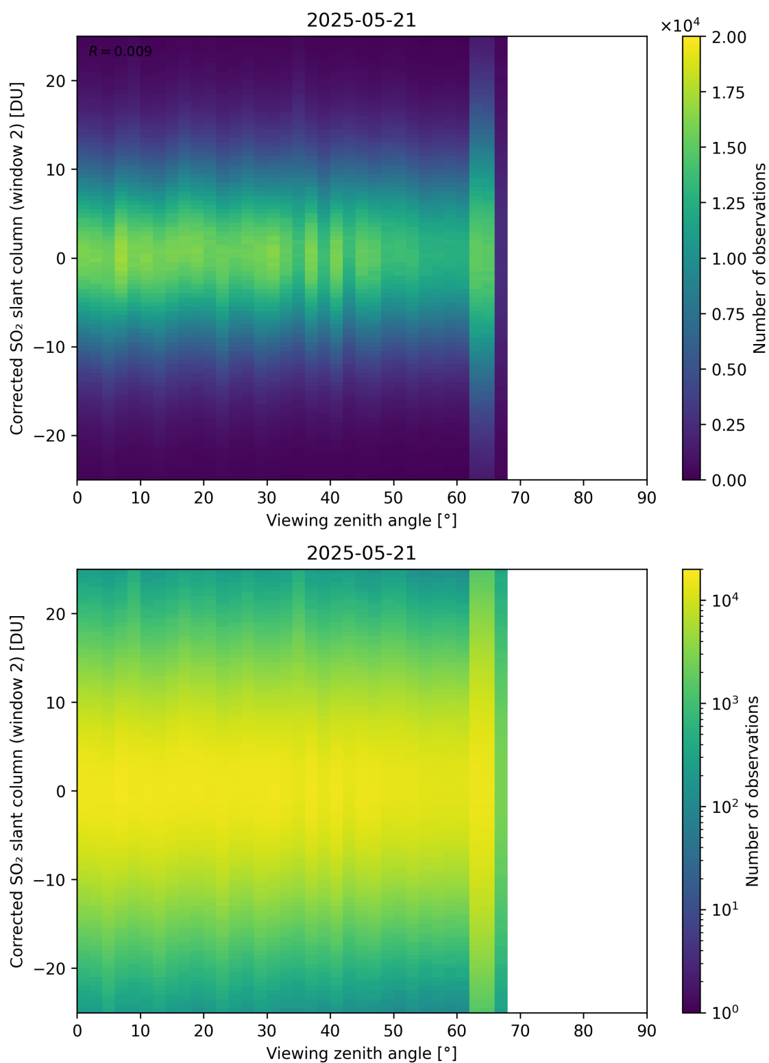
Figure 374: Scatter density plot of “Viewing zenith angle” against “Corrected SO 2 slant column (window 2)” for 2025-05-21 to 2025-05-22.
