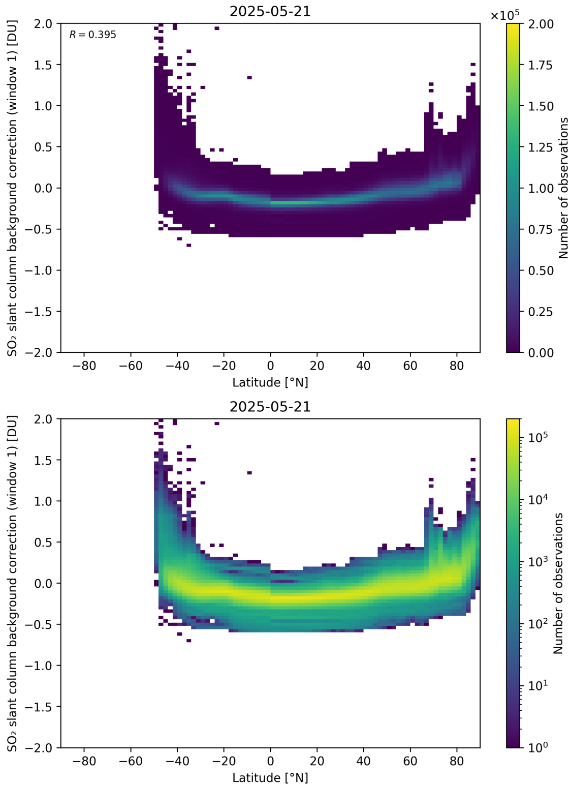
Figure 150: Scatter density plot of “Latitude” against “SO 2 slant column background correction (window 1)” for 2025-05-21 to 2025-05-22.
