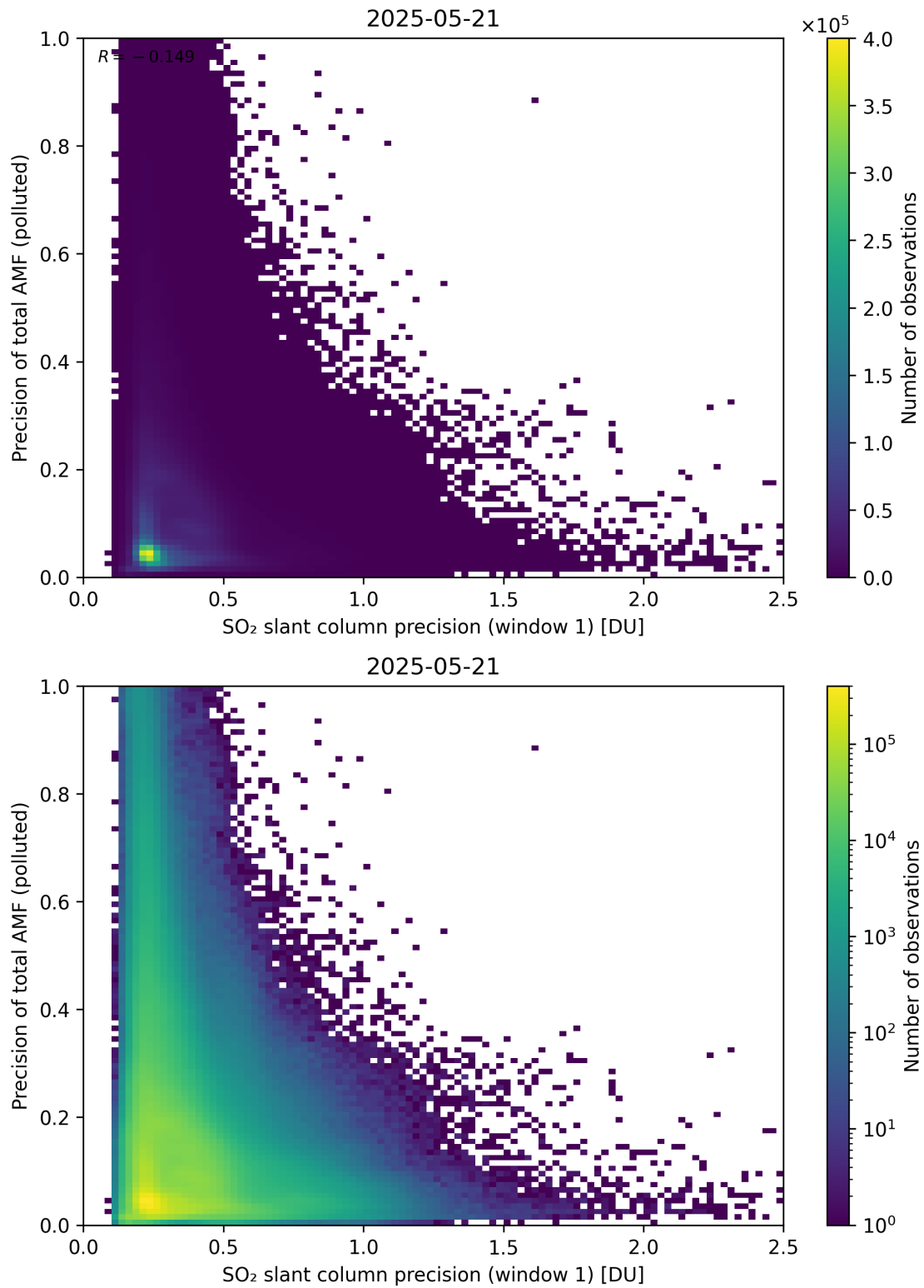
Figure 281: Scatter density plot of “SO 2 slant column precision (window 1)” against “Precision of total AMF (polluted)” for 2025-05-21 to 2025-05-22.
