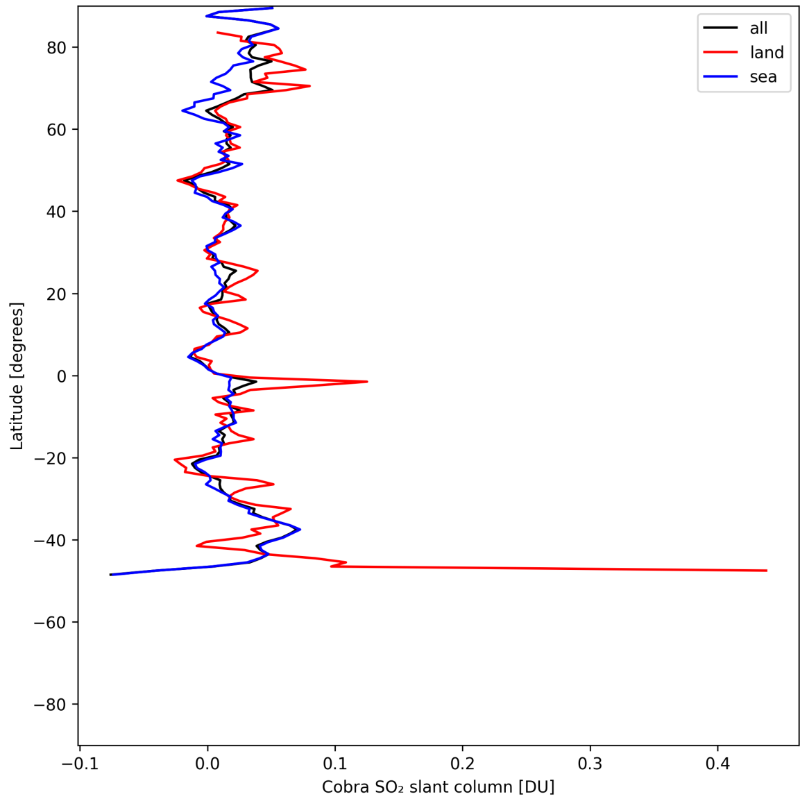
Figure 35: Zonal average of “Cobra SO 2 slant column” for 2025-05-21 to 2025-05-22.
