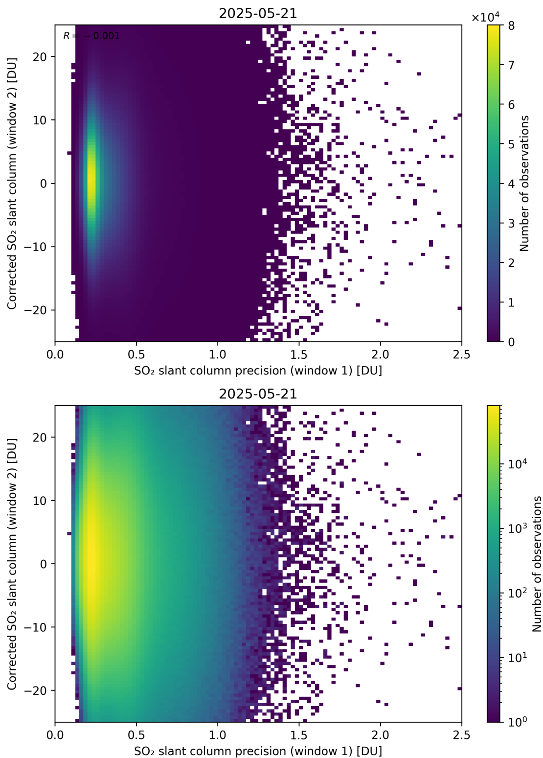
Figure 275: Scatter density plot of “SO 2 slant column precision (window 1)” against “Corrected SO 2 slant column (window 2)” for 2025-05-21 to 2025-05-22.
