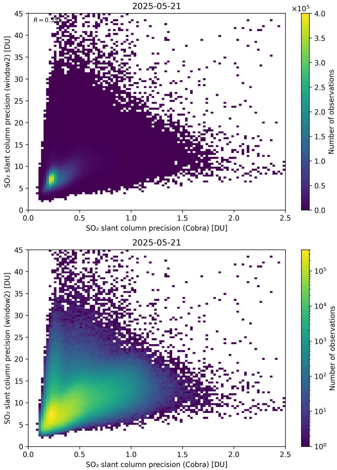
Figure 210: Scatter density plot of “SO 2 slant column precision (Cobra)” against “SO 2 slant column precision (window2)” for 2025-05-21 to 2025-05-22.
