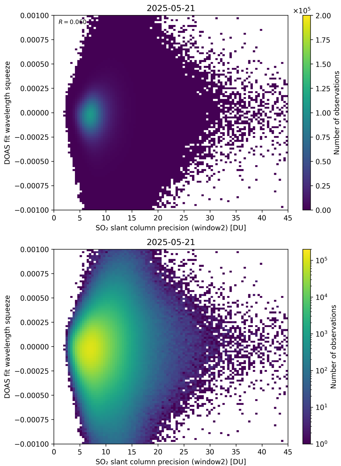
Figure 294: Scatter density plot of “SO 2 slant column precision (window2)” against “DOAS fit wavelength squeeze” for 2025-05-21 to 2025-05-22.
