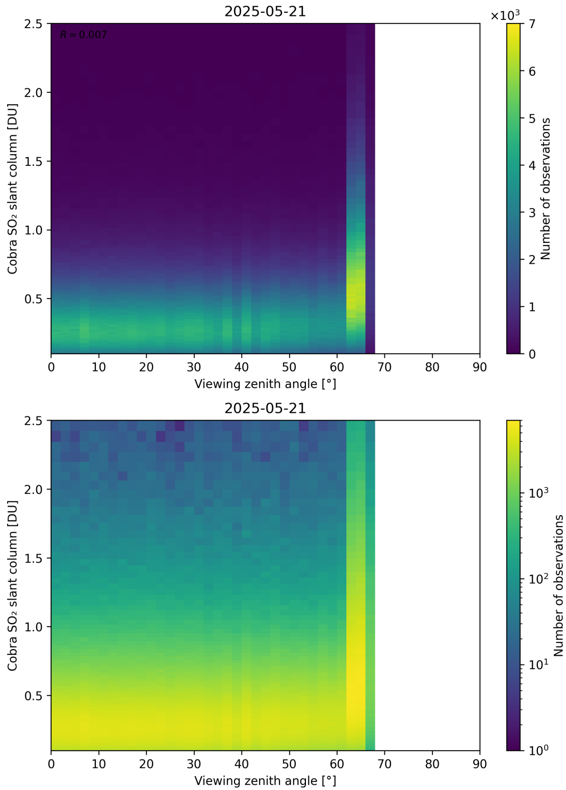
Figure 371: Scatter density plot of “Viewing zenith angle” against “Cobra SO 2 slant column” for 2025-05-21 to 2025-05-22.
