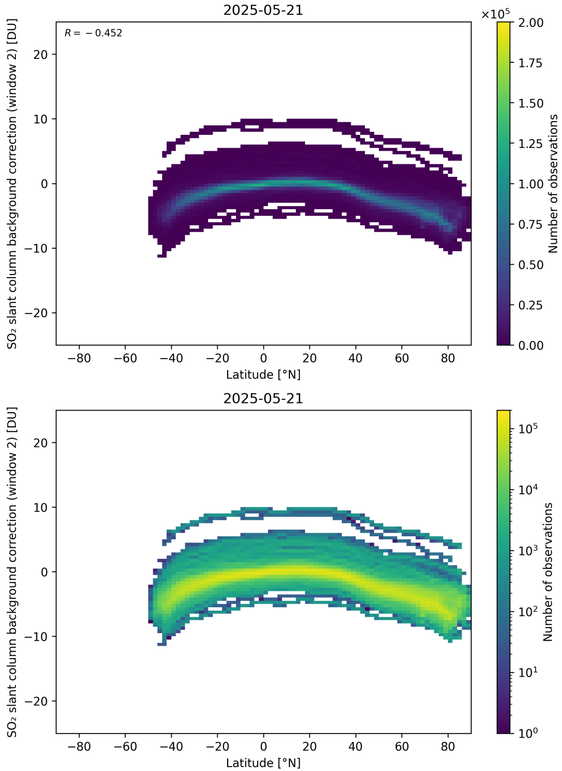
Figure 151: Scatter density plot of “Latitude” against “SO 2 slant column background correction (window 2)” for 2025-05-21 to 2025-05-22.
