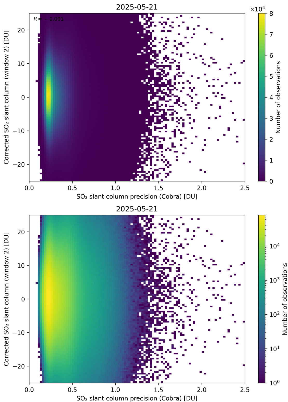
Figure 206: Scatter density plot of “SO 2 slant column precision (Cobra)” against “Corrected SO 2 slant column (window 2)” for 2025-05-21 to 2025-05-22.
