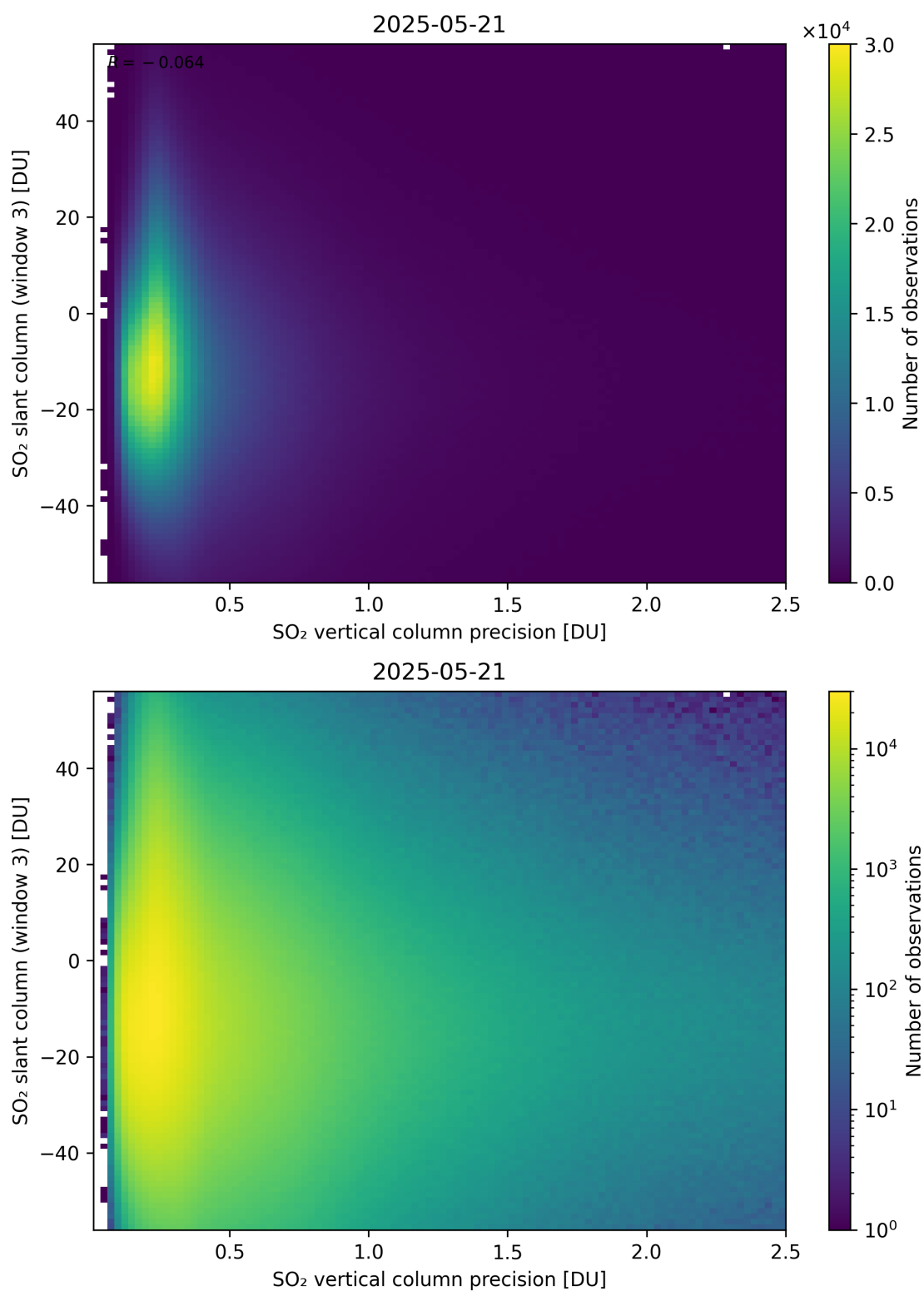
Figure 344: Scatter density plot of “SO 2 vertical column precision” against “SO 2 slant column (window 3)” for 2025-05-21 to 2025-05-22.
