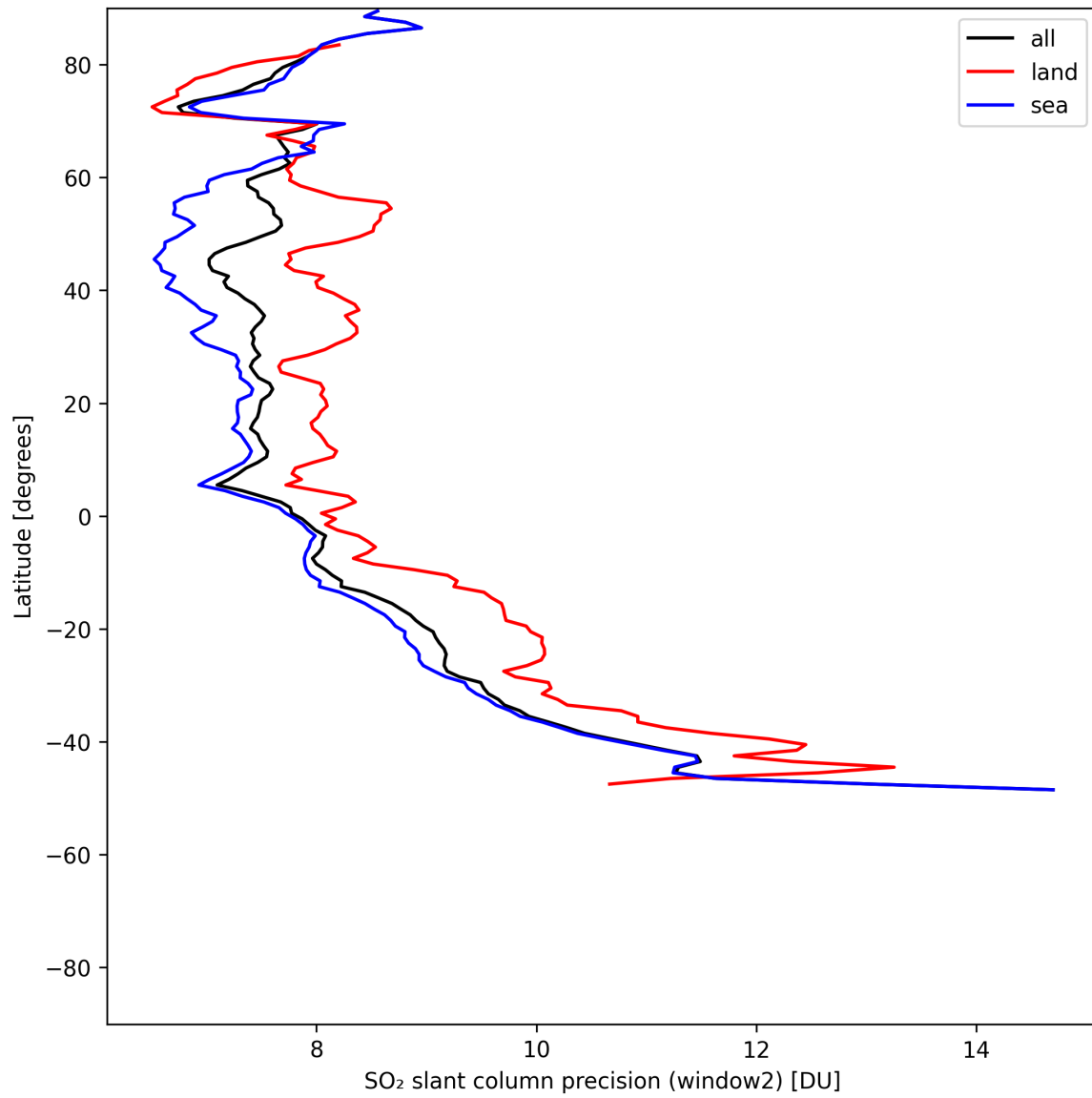
Figure 42: Zonal average of “SO 2 slant column precision (window2)” for 2025-05-21 to 2025-05-22.
