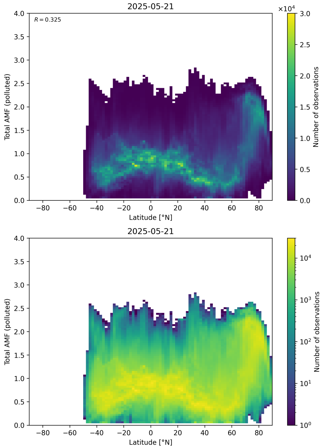
Figure 167: Scatter density plot of “Latitude” against “Total AMF (polluted)” for 2025-05-21 to 2025-05-22.
