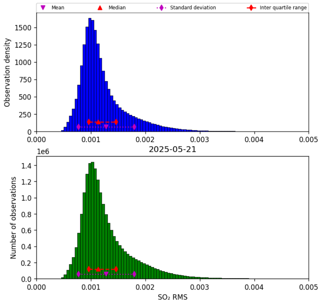
Figure 78: Histogram of "SO 2 RMS" for 2025-05-21 to 2025-05-22
