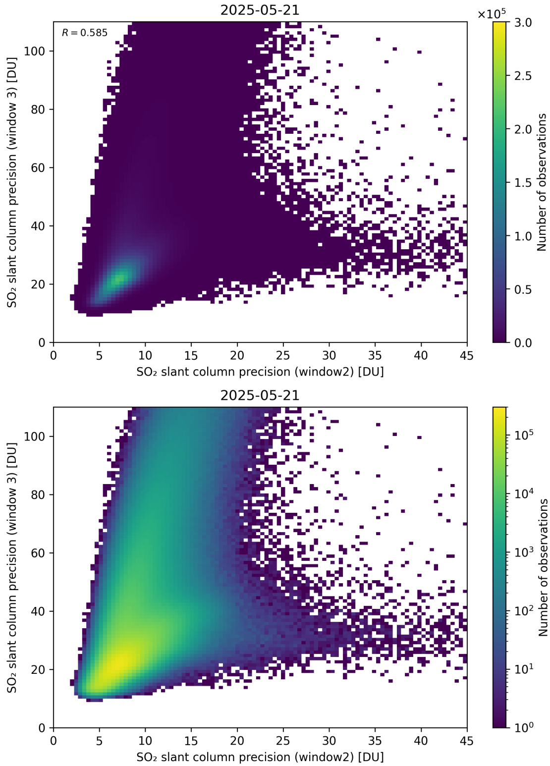
Figure 300: Scatter density plot of “SO 2 slant column precision (window2)” against “SO 2 slant column precision (window 3)” for 2025-05-21 to 2025-05-22.
