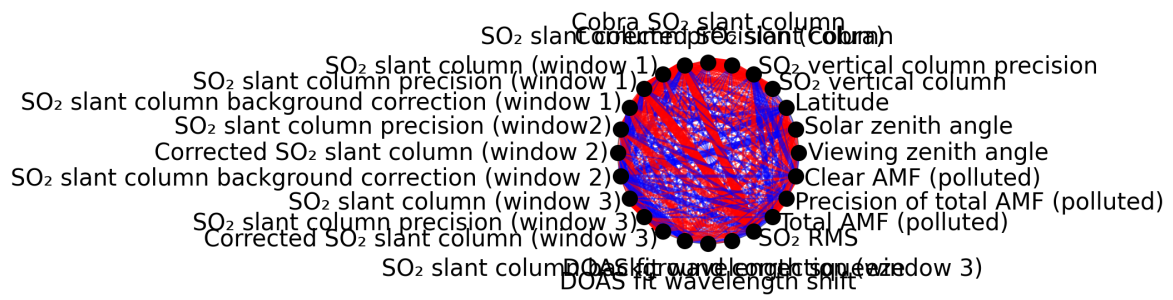
Figure 1: Map of correlation graph for 2025-05-21 to 2025-05-22.
