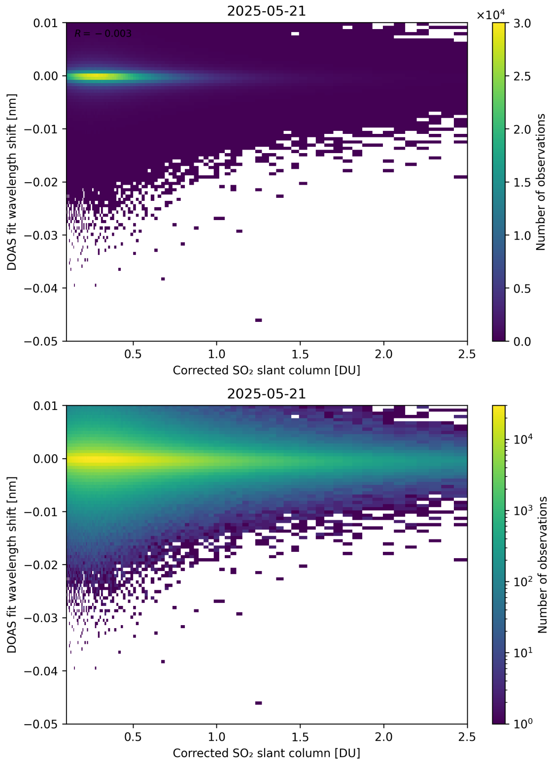
Figure 229: Scatter density plot of “Corrected SO 2 slant column” against “DOAS fit wavelength shift” for 2025-05-21 to 2025-05-22.
