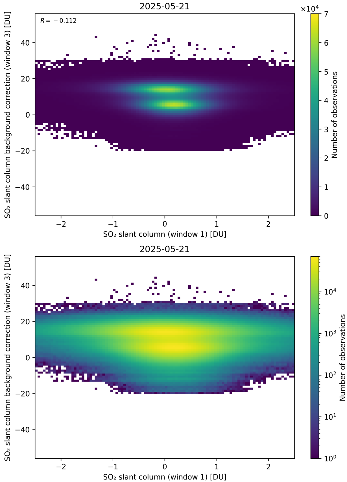
Figure 264: Scatter density plot of “SO 2 slant column (window 1)” against “SO 2 slant column background correction (window 3)” for 2025-05-21 to 2025-05-22.
