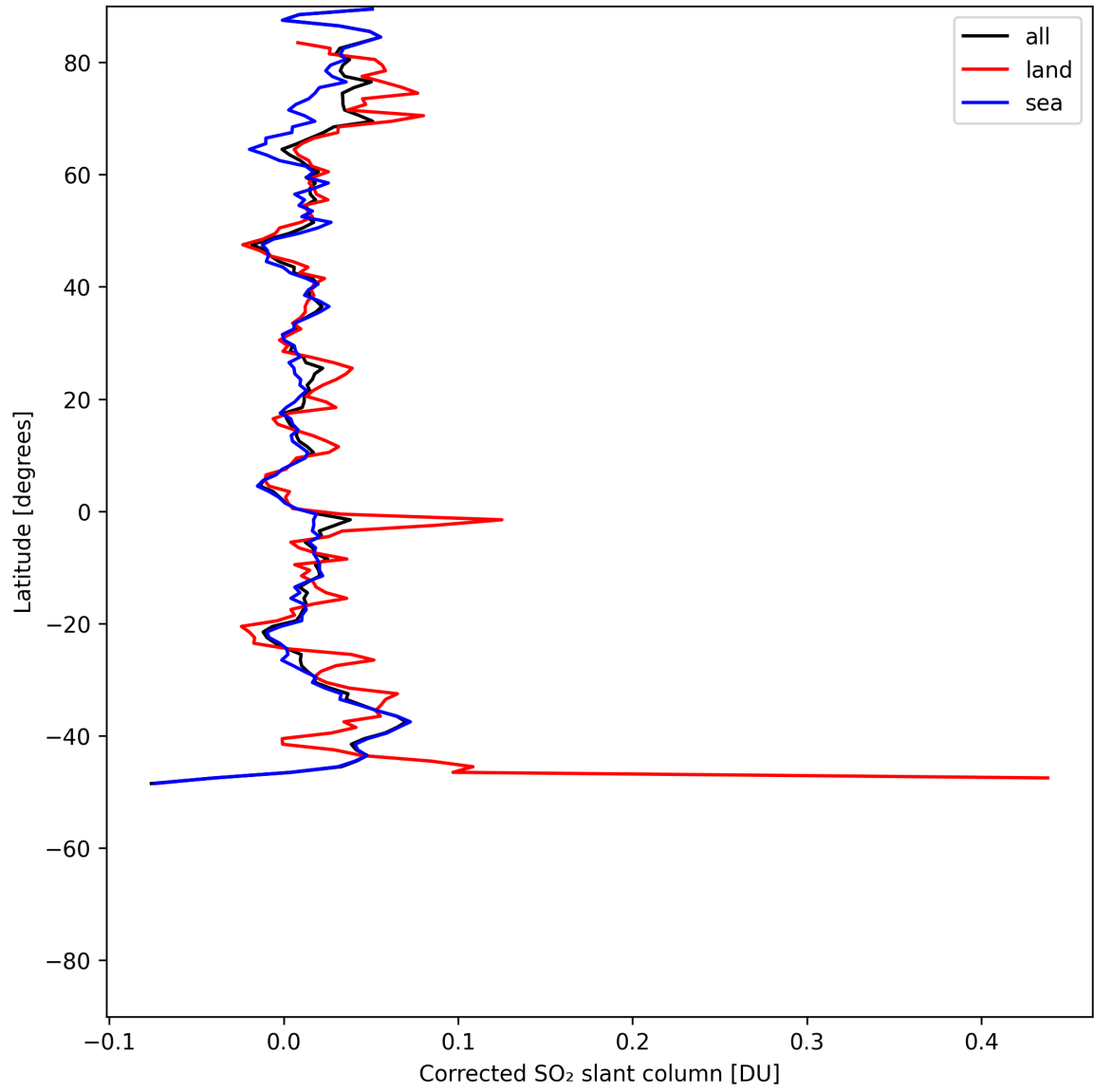
Figure 34: Zonal average of “Corrected SO 2 slant column” for 2025-05-21 to 2025-05-22.
