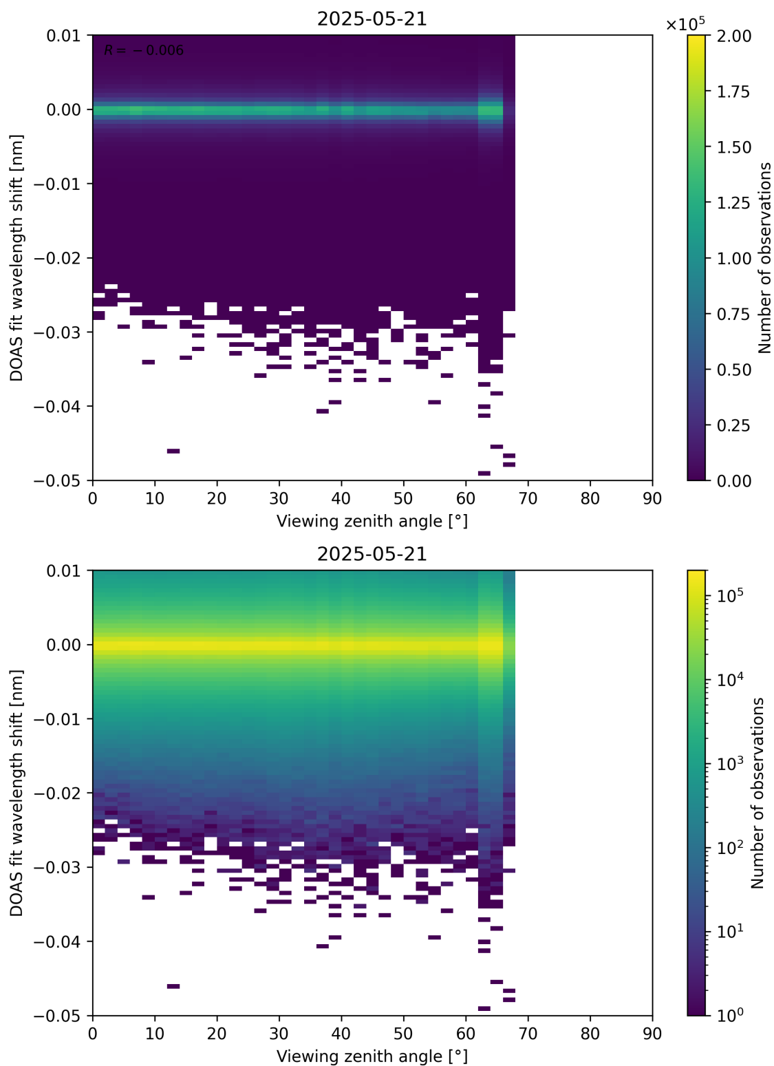
Figure 365: Scatter density plot of “Viewing zenith angle” against “DOAS fit wavelength shift” for 2025-05-21 to 2025-05-22.
