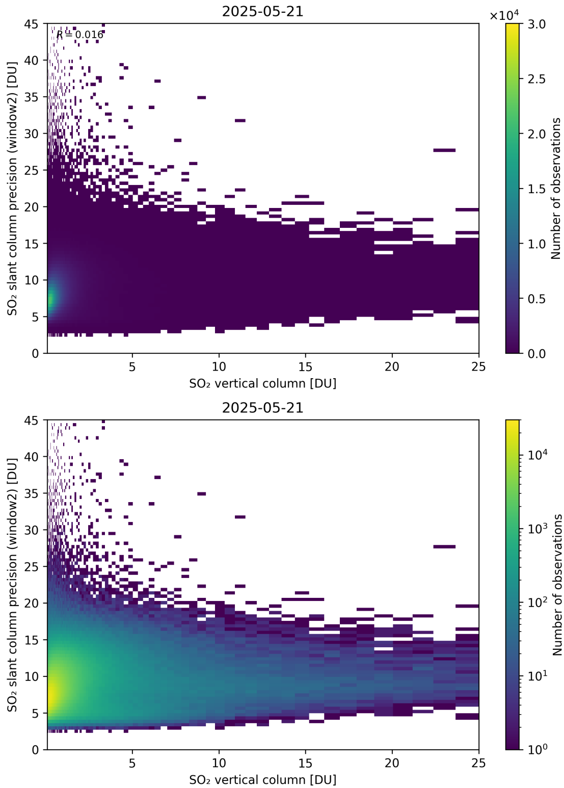
Figure 356: Scatter density plot of “SO 2 vertical column” against “SO 2 slant column precision (window2)” for 2025-05-21 to 2025-05-22.
