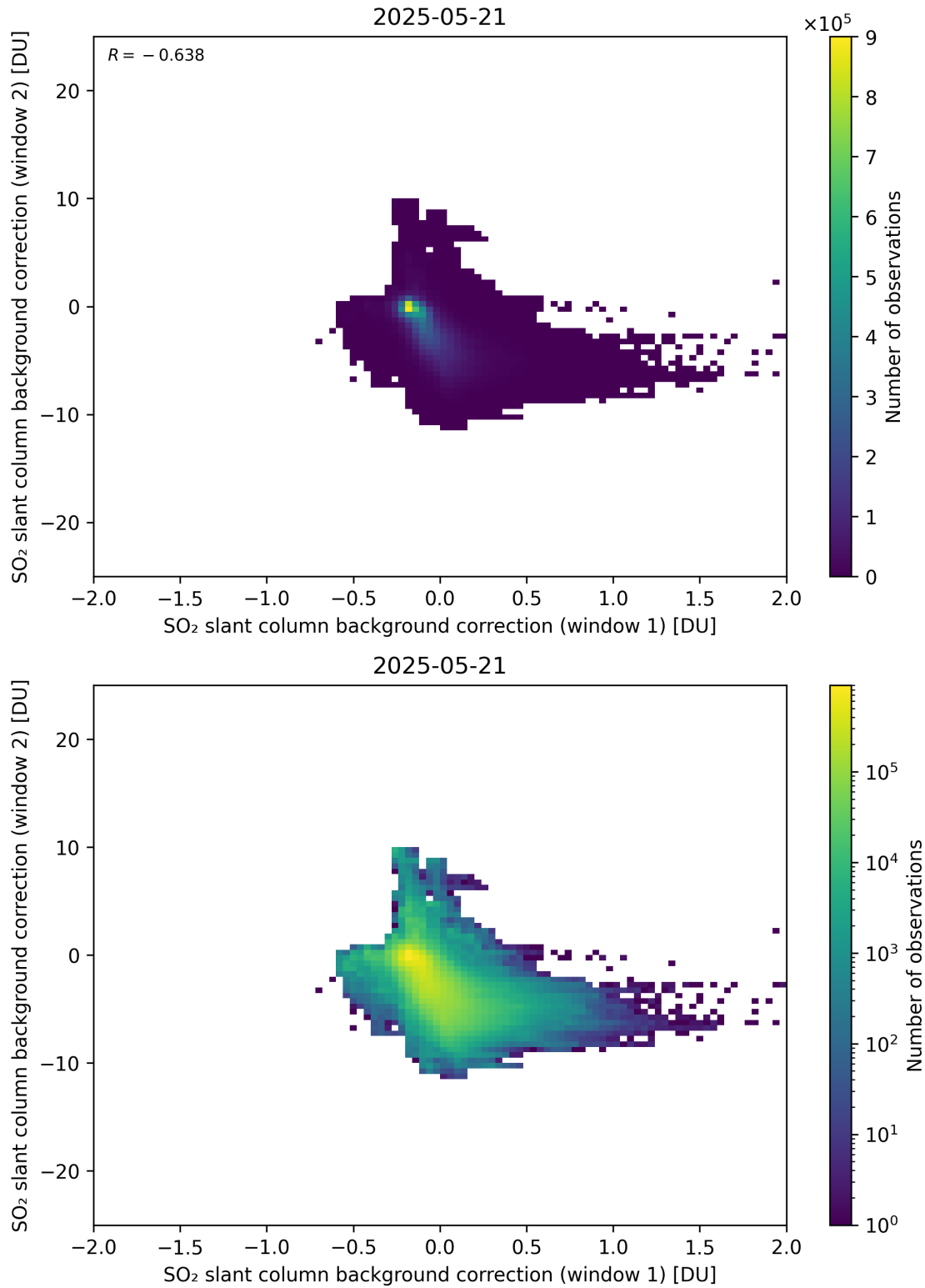
Figure 109: Scatter density plot of “SO 2 slant column background correction (window 1)” against “SO 2 slant column background correction (window 2)” for 2025-05-21 to 2025-05-22.
