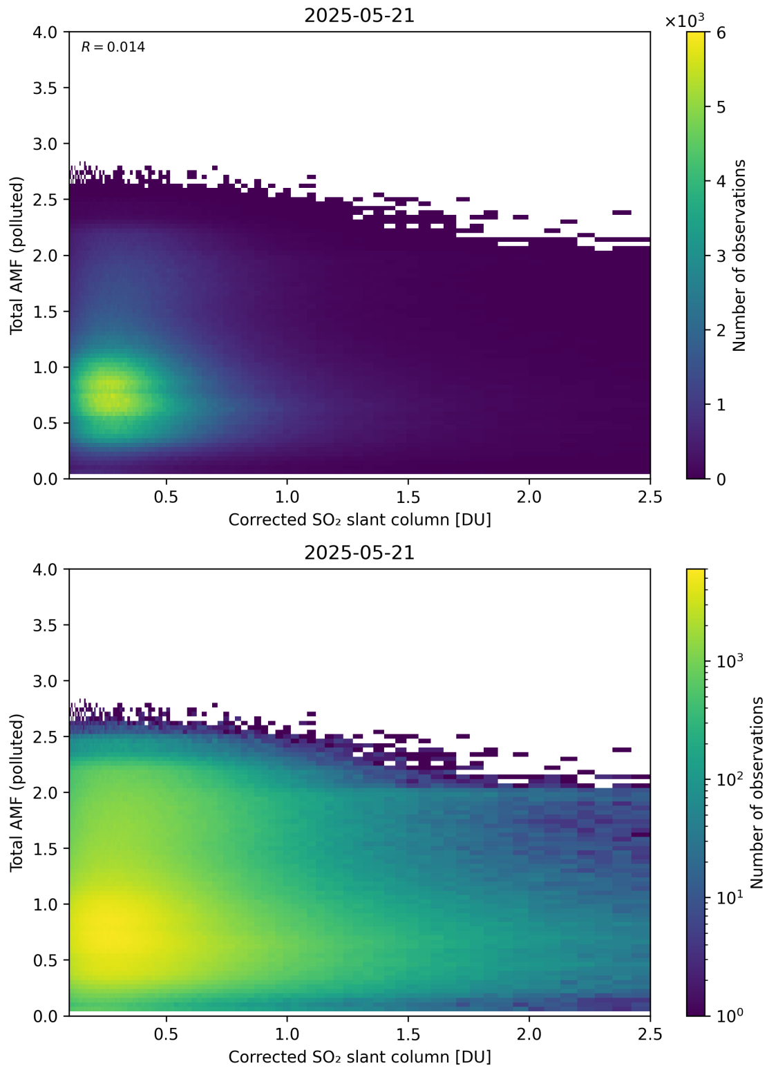
Figure 242: Scatter density plot of “Corrected SO 2 slant column” against “Total AMF (polluted)” for 2025-05-21 to 2025-05-22.
