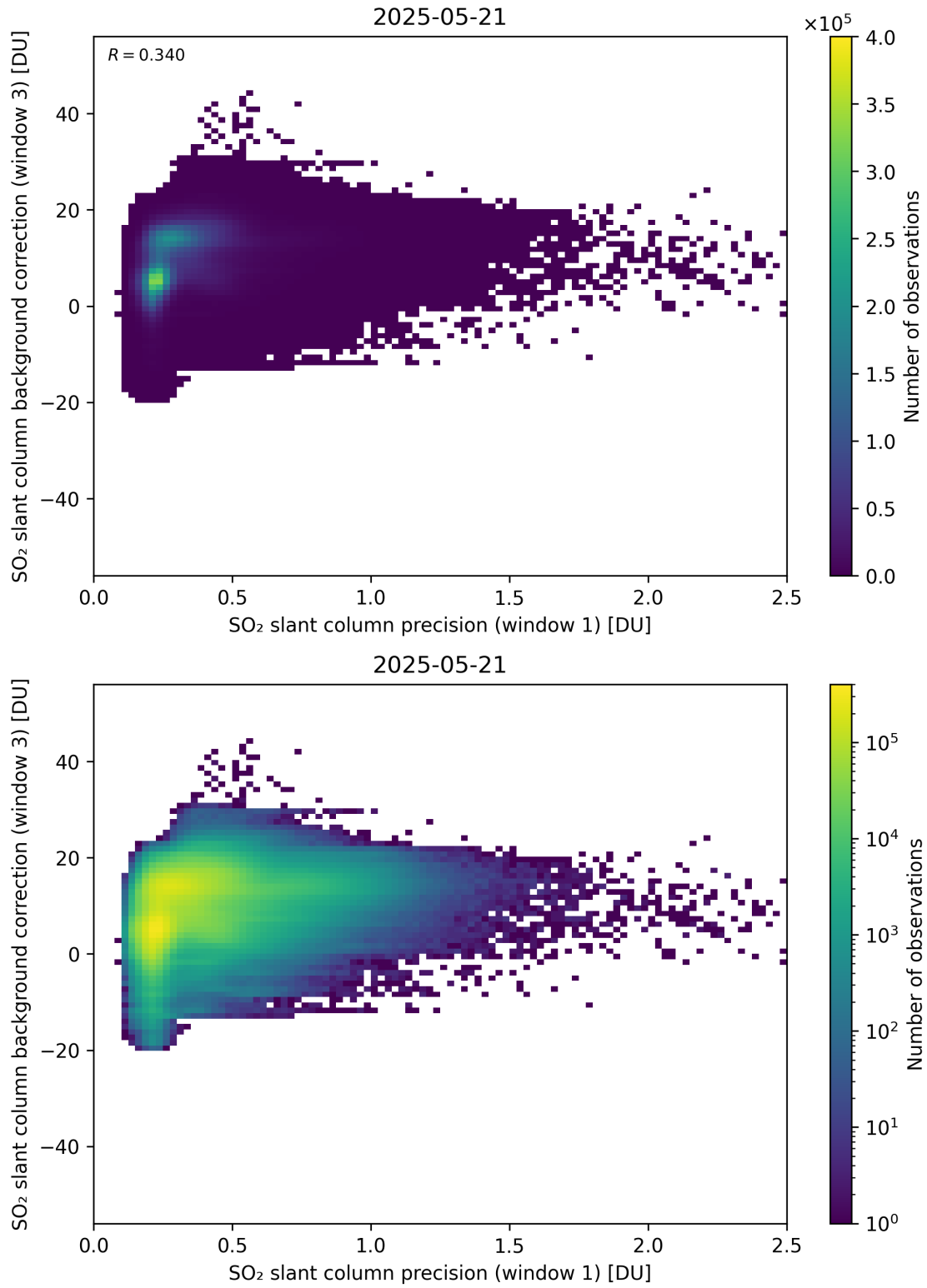
Figure 270: Scatter density plot of “SO 2 slant column precision (window 1)” against “SO 2 slant column background correction (window 3)” for 2025-05-21 to 2025-05-22.
