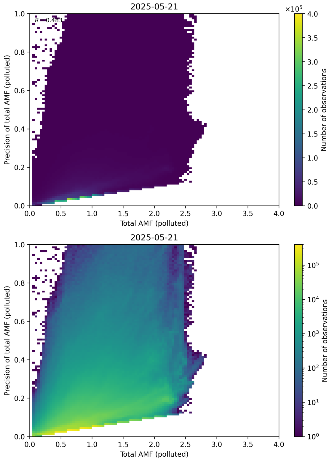
Figure 322: Scatter density plot of “Total AMF (polluted)” against “Precision of total AMF (polluted)” for 2025-05-21 to 2025-05-22.
