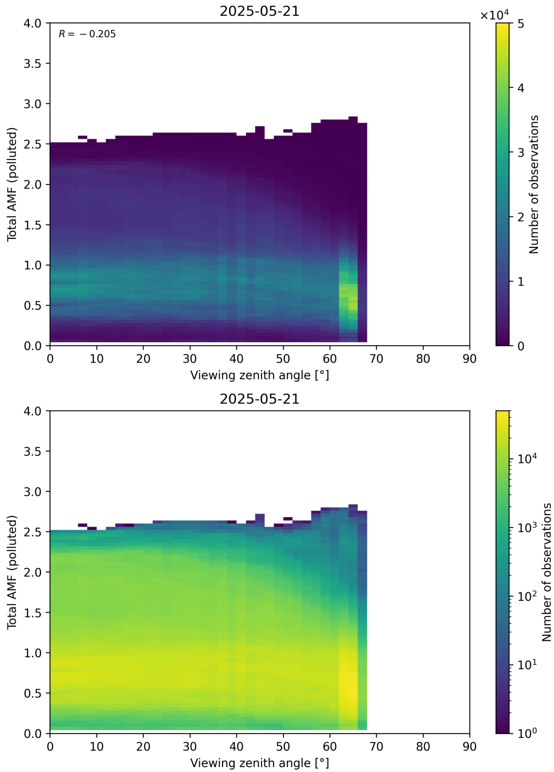
Figure 381: Scatter density plot of “Viewing zenith angle” against “Total AMF (polluted)” for 2025-05-21 to 2025-05-22.
