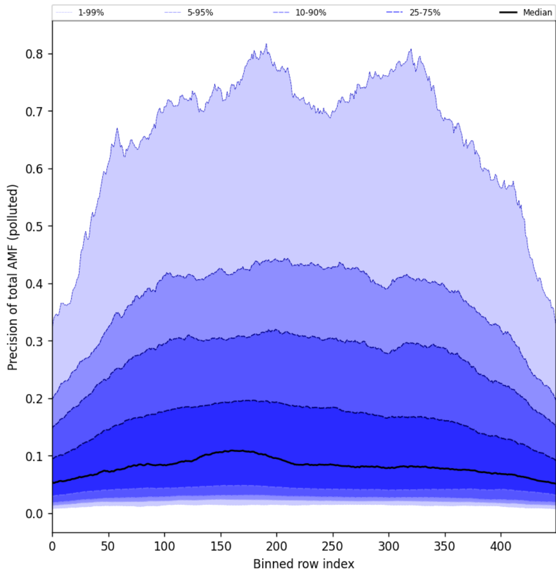
Figure 106: Along track statistics of “Precision of total AMF (polluted)” for 2025-05-21 to 2025-05-22
