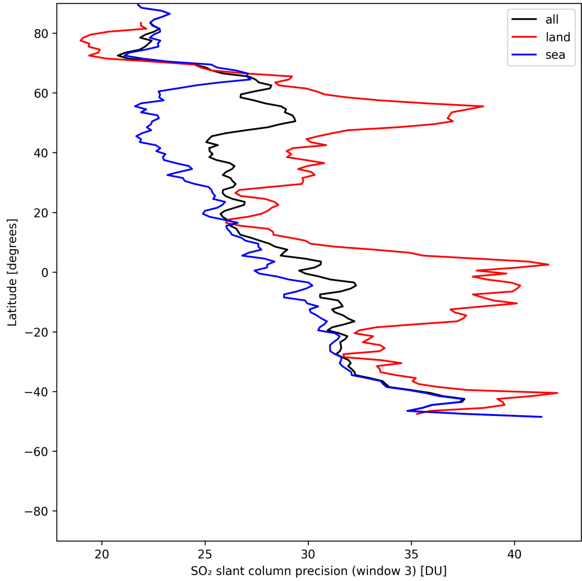
Figure 46: Zonal average of “SO 2 slant column precision (window 3)” for 2025-05-21 to 2025-05-22.
