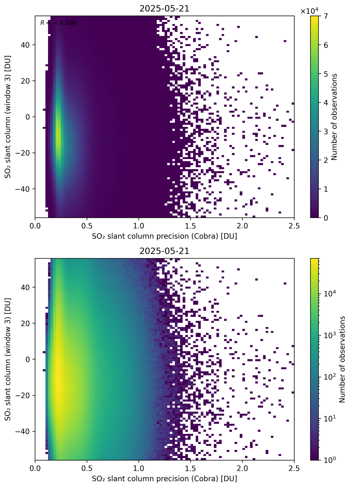
Figure 211: Scatter density plot of “SO 2 slant column precision (Cobra)” against “SO 2 slant column (window 3)” for 2025-05-21 to 2025-05-22.
