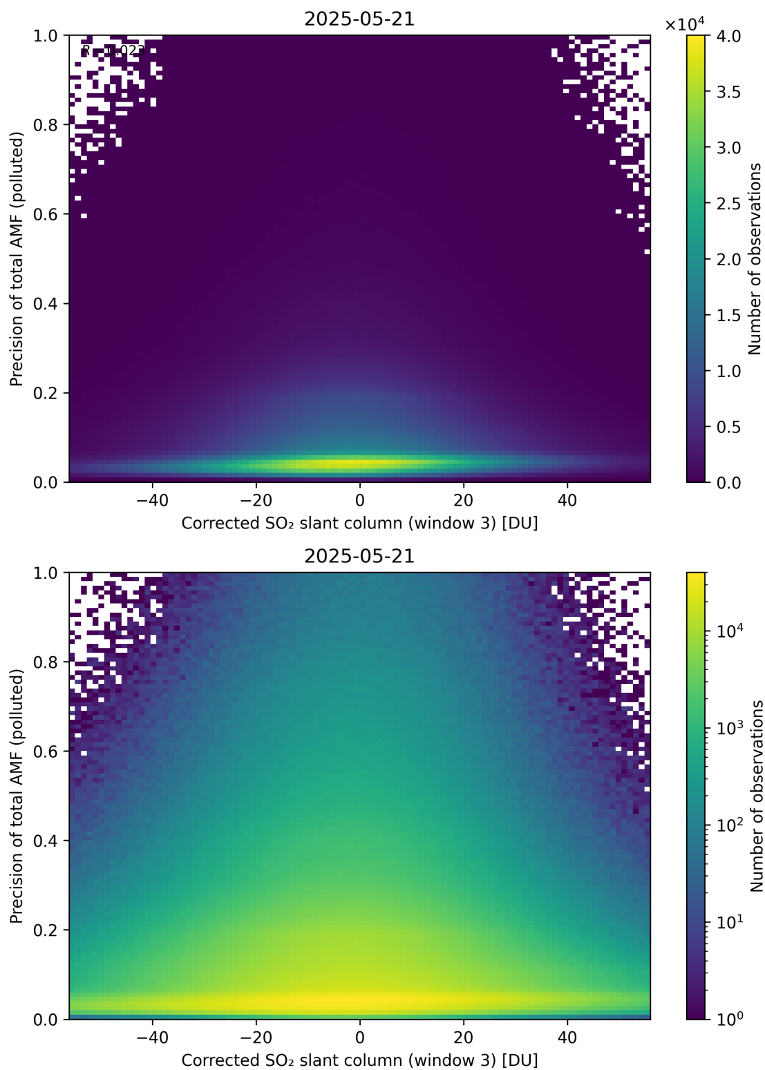
Figure 261: Scatter density plot of “Corrected SO 2 slant column (window 3)” against “Precision of total AMF (polluted)” for 2025-05-21 to 2025-05-22.
