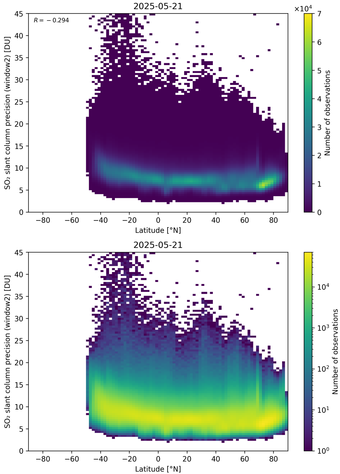
Figure 164: Scatter density plot of “Latitude” against “SO 2 slant column precision (window2)” for 2025-05-21 to 2025-05-22.
