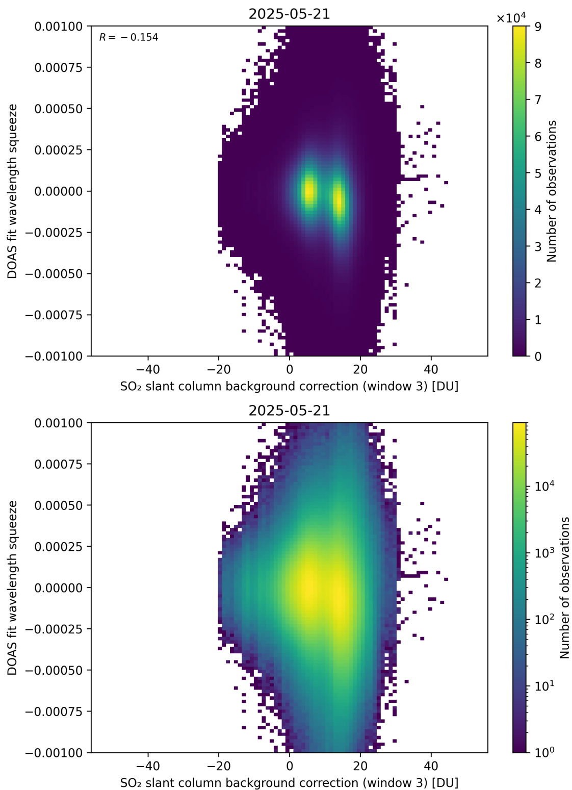
Figure 133: Scatter density plot of “SO 2 slant column background correction (window 3)” against “DOAS fit wavelength squeeze” for 2025-05-21 to 2025-05-22.
