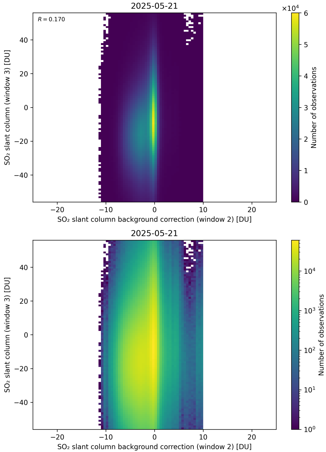
Figure 128: Scatter density plot of “SO 2 slant column background correction (window 2)” against “SO 2 slant column (window 3)” for 2025-05-21 to 2025-05-22.
