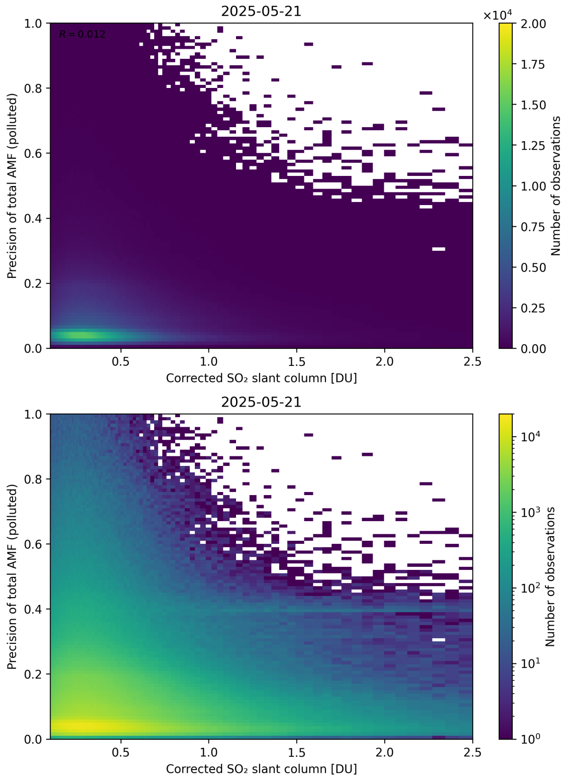
Figure 243: Scatter density plot of “Corrected SO 2 slant column” against “Precision of total AMF (polluted)” for 2025-05-21 to 2025-05-22.
