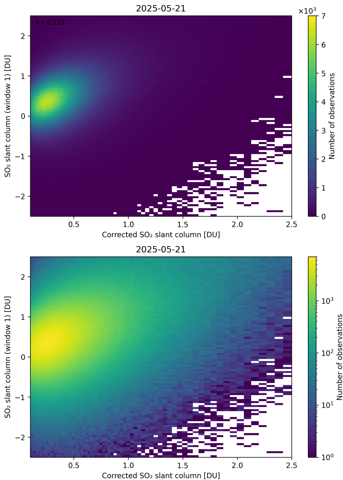
Figure 237: Scatter density plot of “Corrected SO 2 slant column” against “SO 2 slant column (window 1)” for 2025-05-21 to 2025-05-22.
