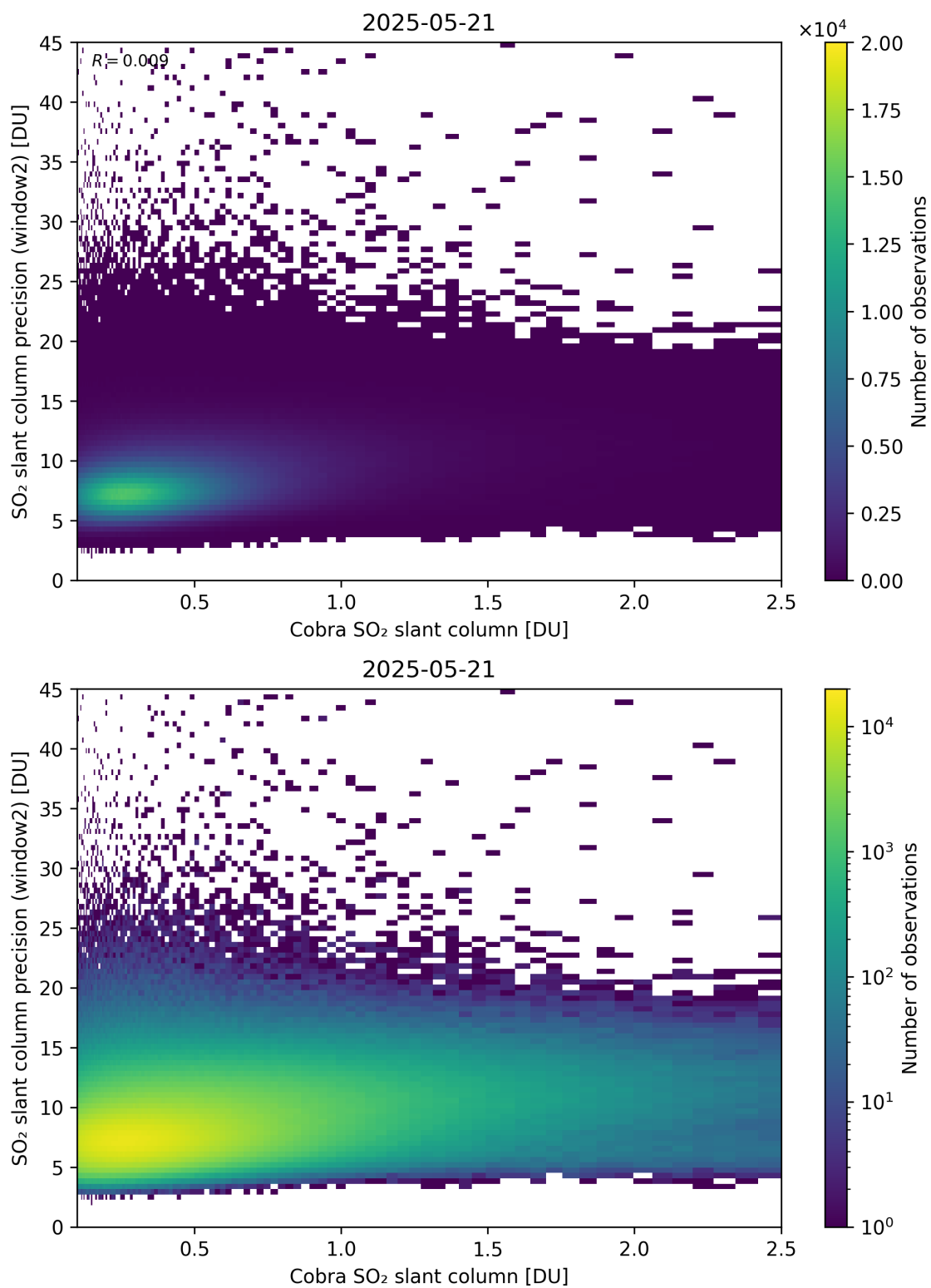
Figure 221: Scatter density plot of “Cobra SO 2 slant column” against “SO 2 slant column precision (window2)” for 2025-05-21 to 2025-05-22.
