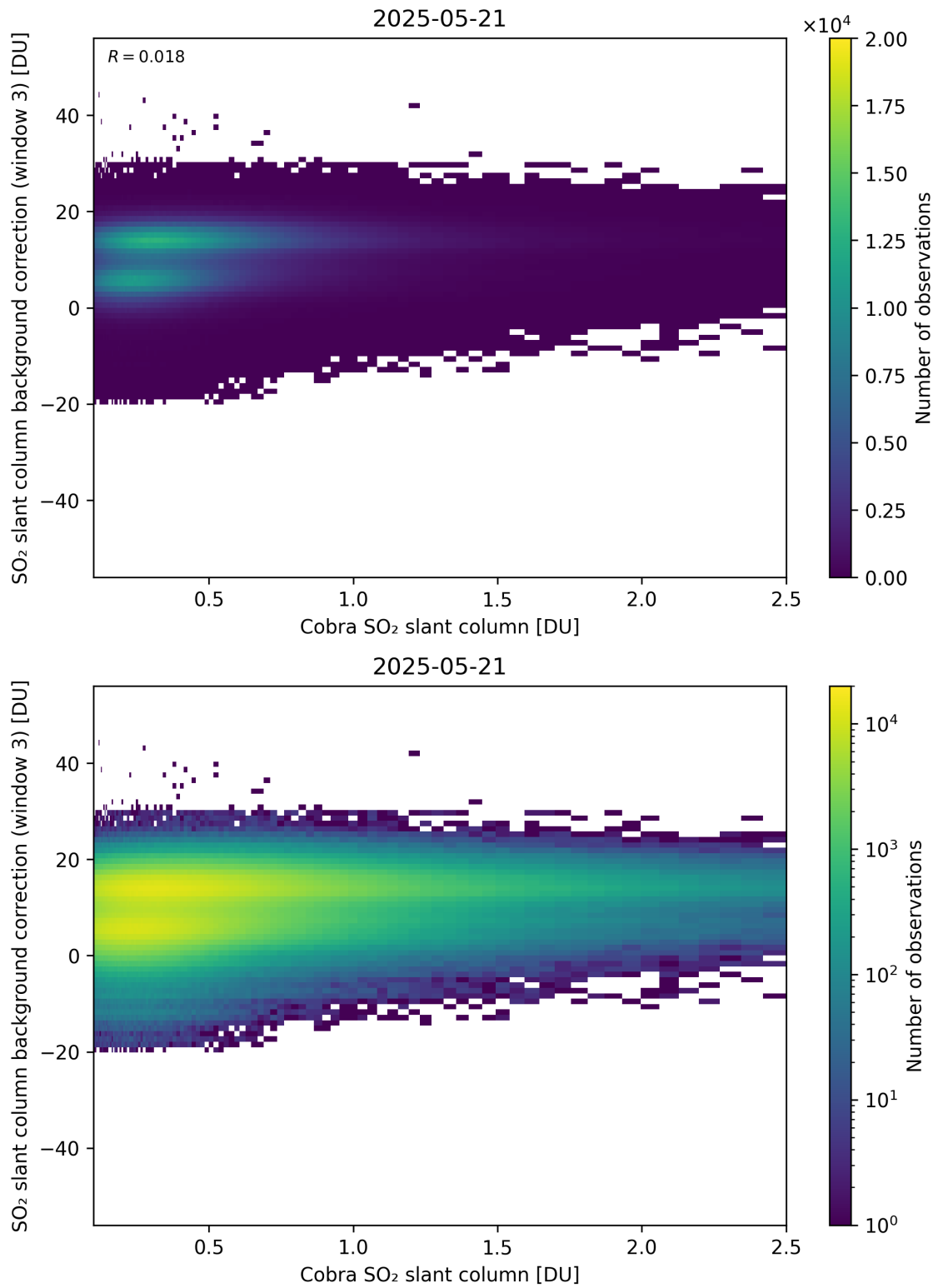
Figure 195: Scatter density plot of “Cobra SO 2 slant column” against “SO 2 slant column background correction (window 3)” for 2025-05-21 to 2025-05-22.
