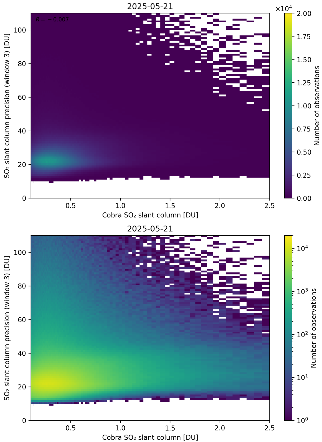
Figure 223: Scatter density plot of “Cobra SO 2 slant column” against “SO 2 slant column precision (window 3)” for 2025-05-21 to 2025-05-22.
