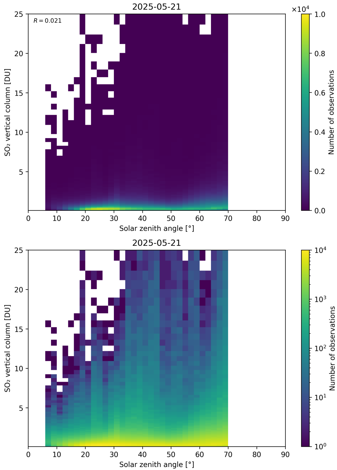
Figure 191: Scatter density plot of “Solar zenith angle” against “SO 2 vertical column” for 2025-05-21 to 2025-05-22.
