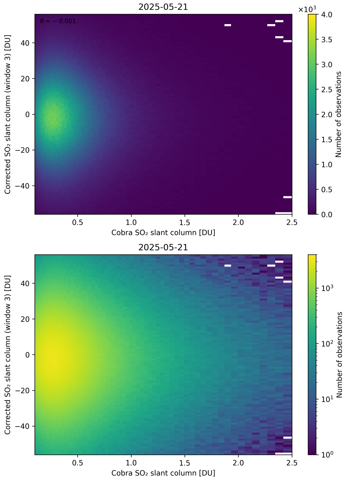
Figure 218: Scatter density plot of “Cobra SO 2 slant column” against “Corrected SO 2 slant column (window 3)” for 2025-05-21 to 2025-05-22.
