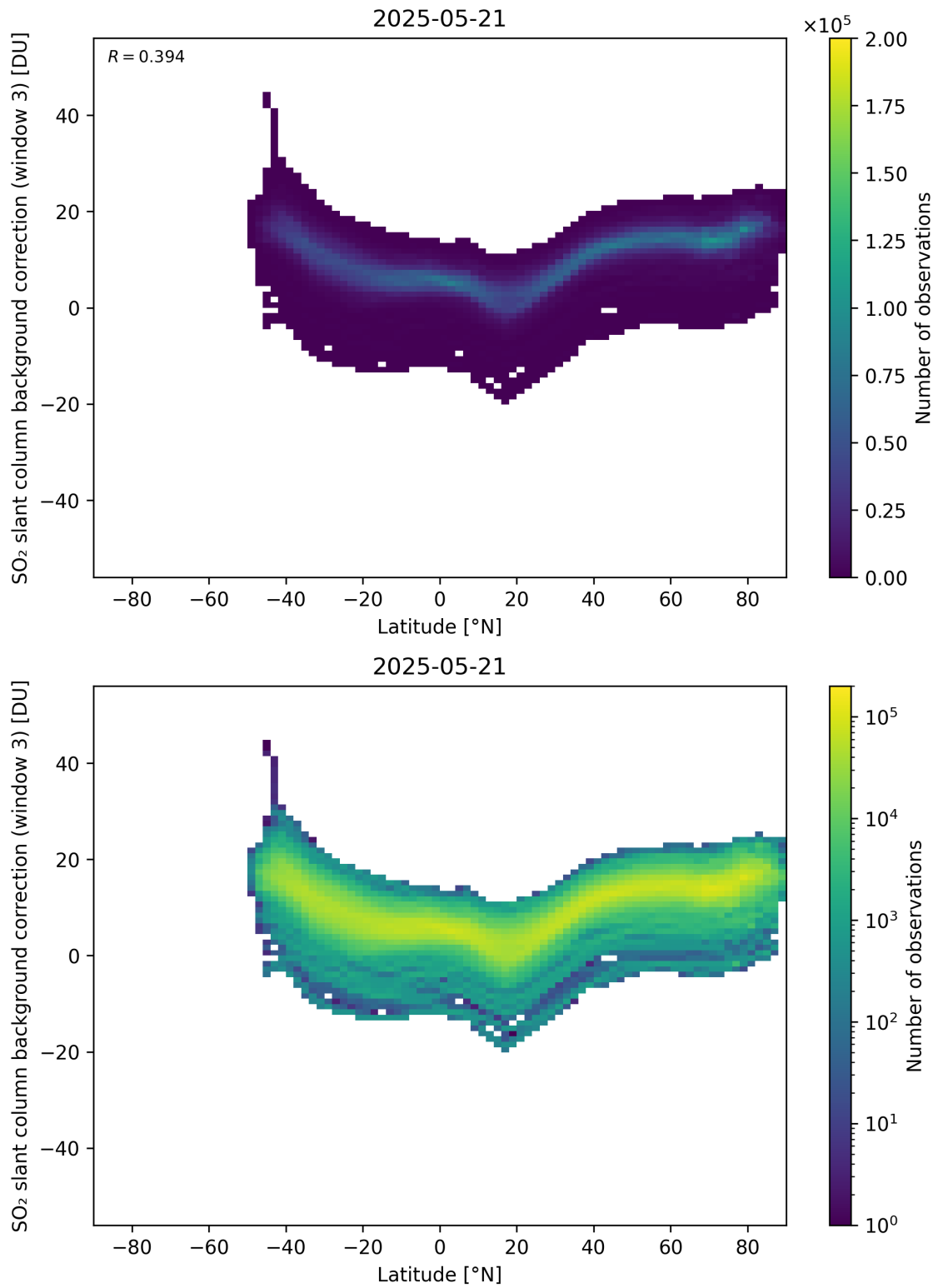
Figure 152: Scatter density plot of “Latitude” against “SO 2 slant column background correction (window 3)” for 2025-05-21 to 2025-05-22.
