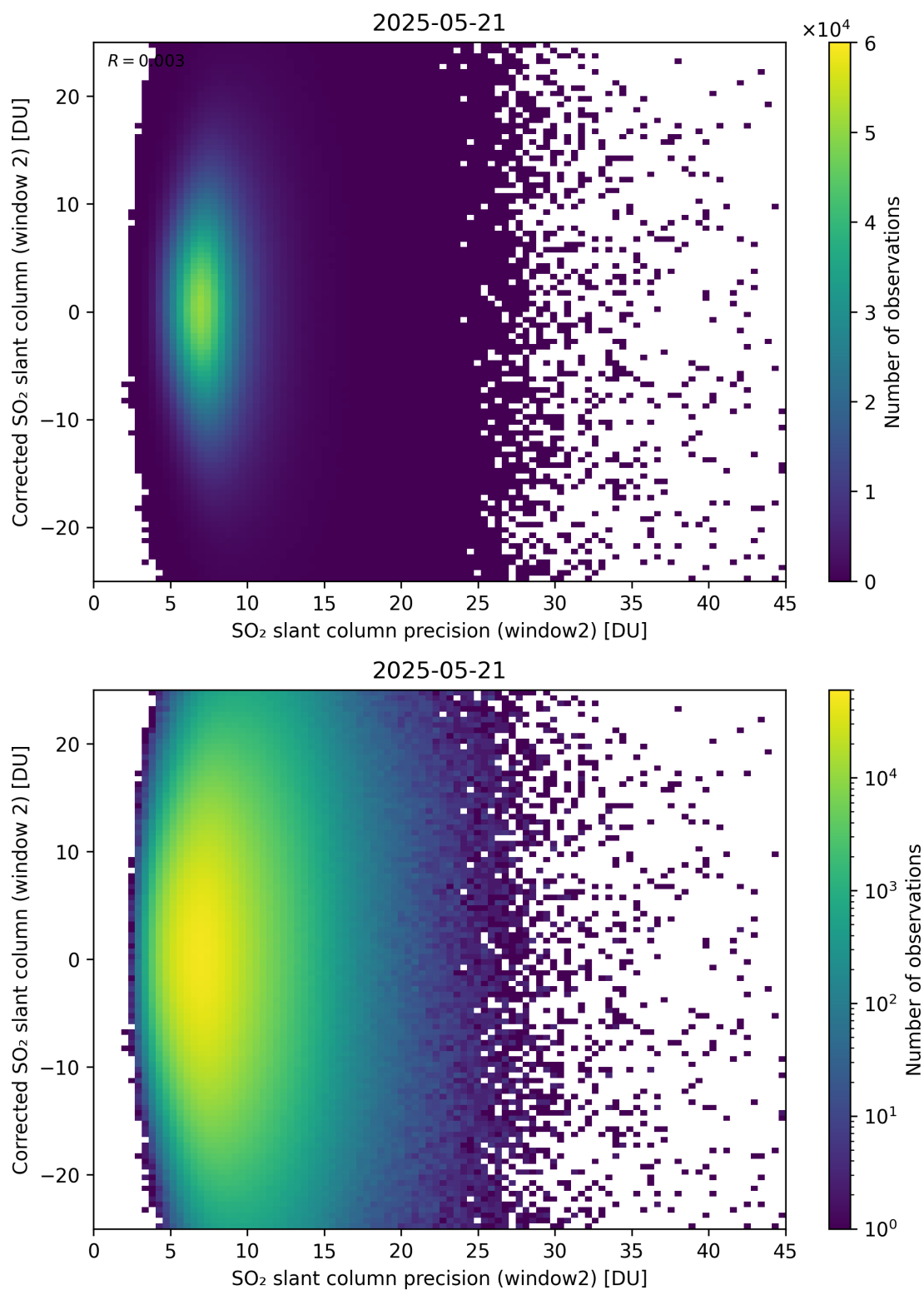
Figure 297: Scatter density plot of “SO 2 slant column precision (window2)” against “Corrected SO 2 slant column (window 2)” for 2025-05-21 to 2025-05-22.
