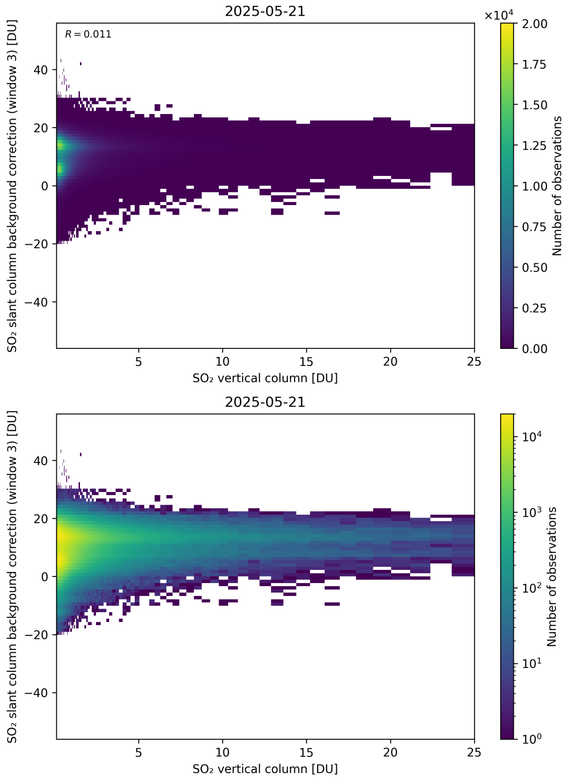
Figure 325: Scatter density plot of “SO 2 vertical column” against “SO 2 slant column background correction (window 3)” for 2025-05-21 to 2025-05-22.
