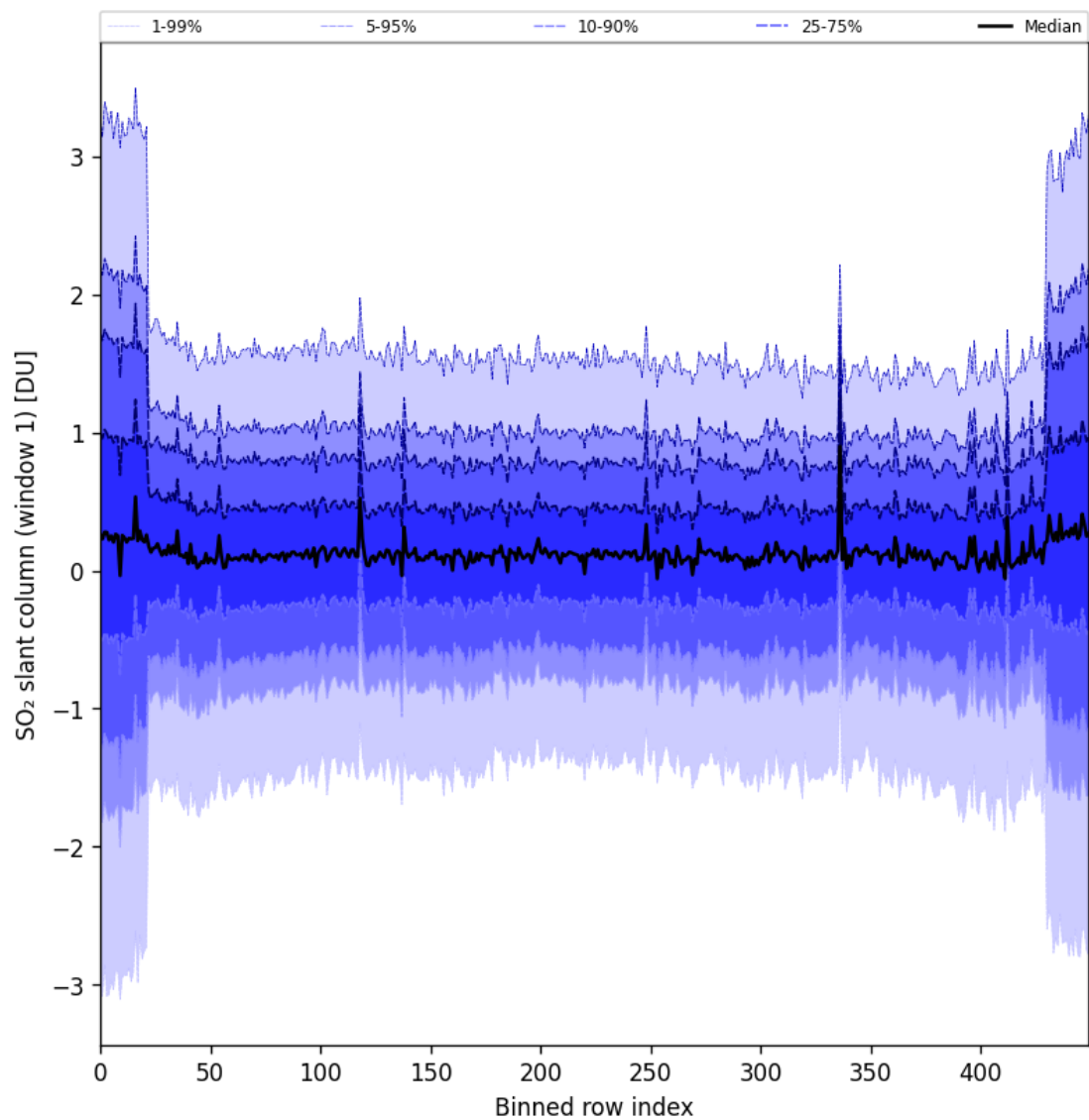
Figure 89: Along track statistics of “SO 2 slant column (window 1)” for 2025-05-21 to 2025-05-22
