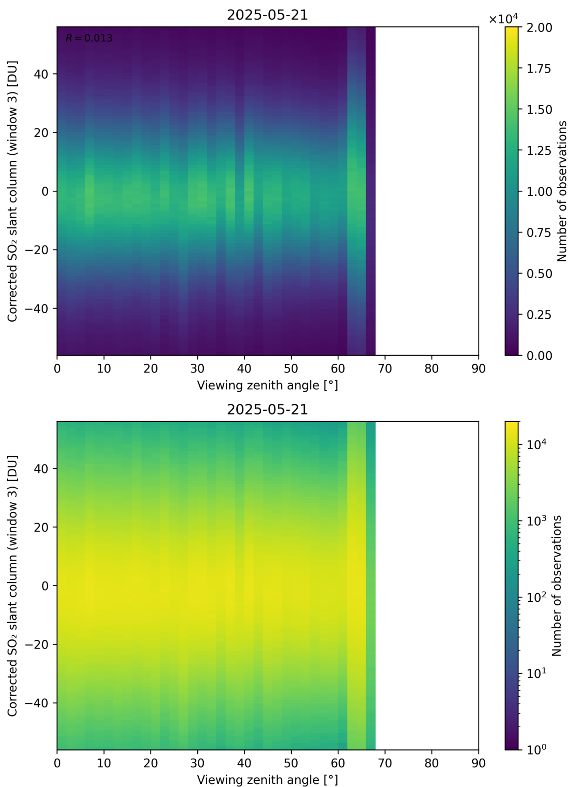
Figure 375: Scatter density plot of “Viewing zenith angle” against “Corrected SO 2 slant column (window 3)” for 2025-05-21 to 2025-05-22.
