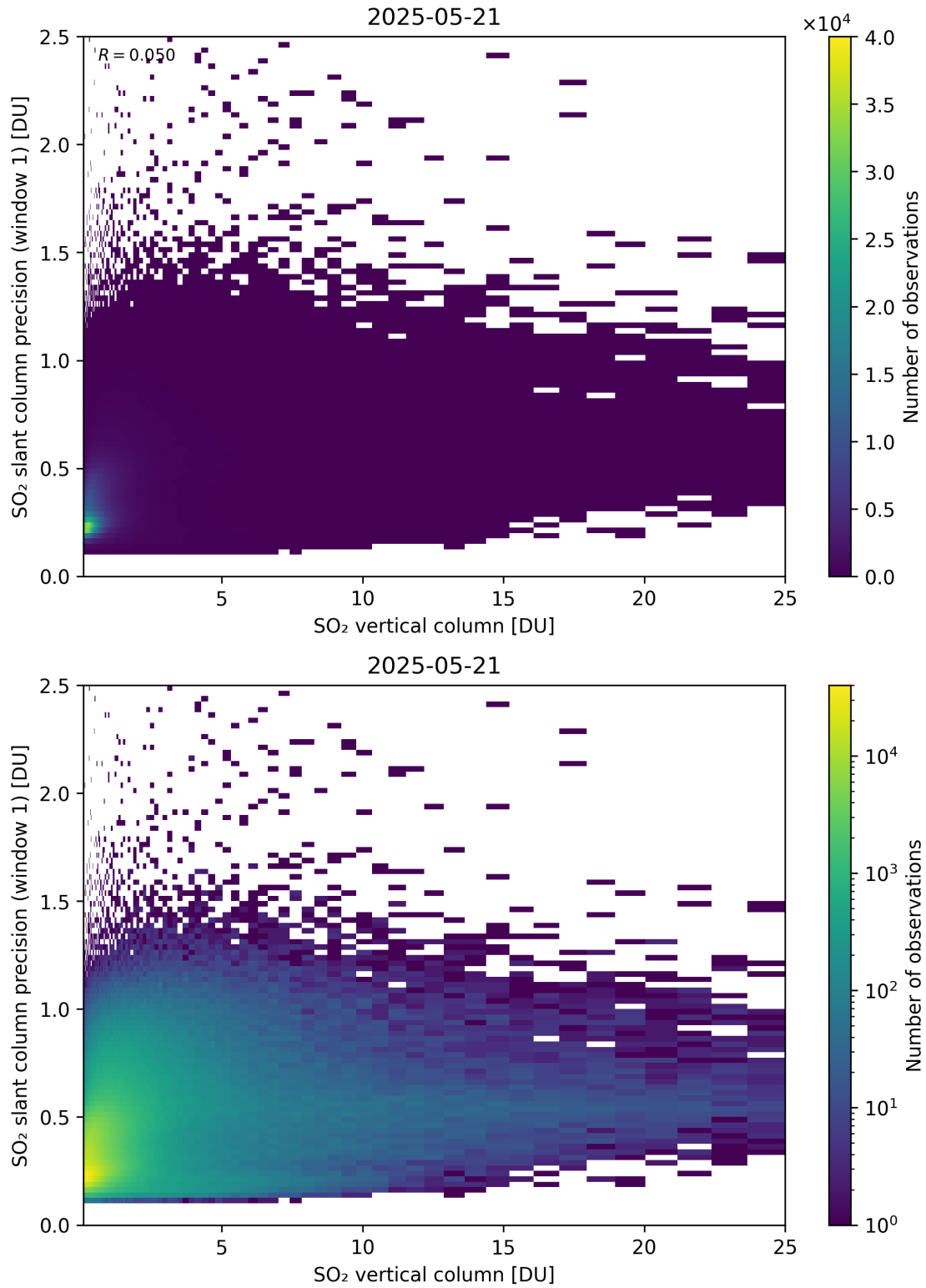
Figure 355: Scatter density plot of “SO 2 vertical column” against “SO 2 slant column precision (window 1)” for 2025-05-21 to 2025-05-22.
