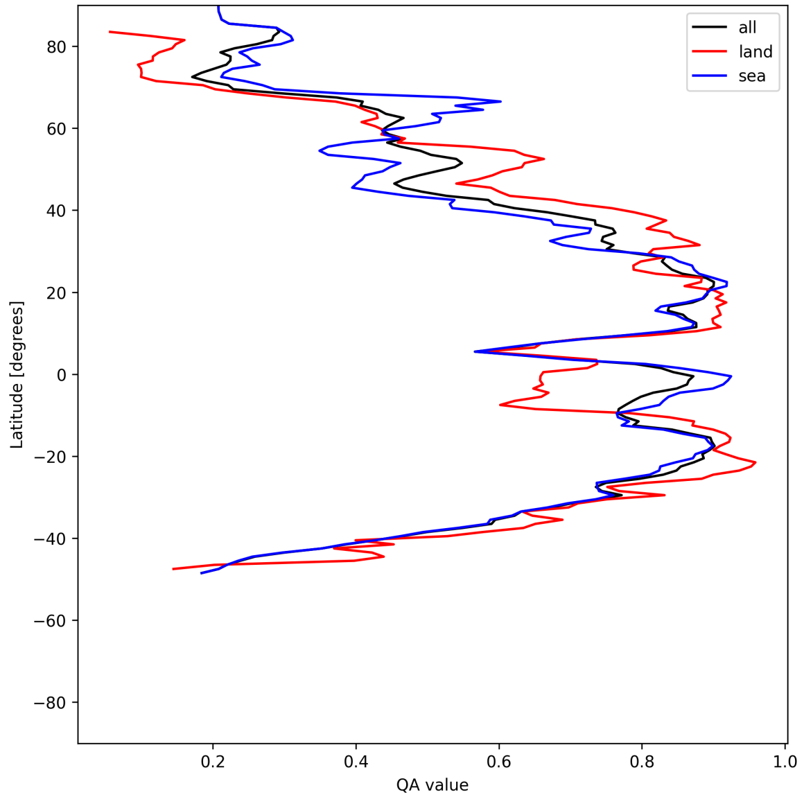
Figure 31: Zonal average of “QA value” for 2025-05-21 to 2025-05-22.
