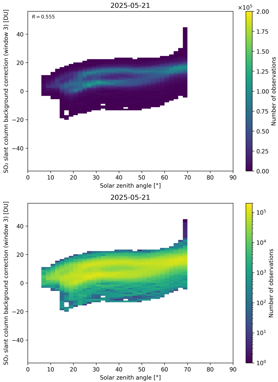
Figure 173: Scatter density plot of “Solar zenith angle” against “SO 2 slant column background correction (window 3)” for 2025-05-21 to 2025-05-22.
