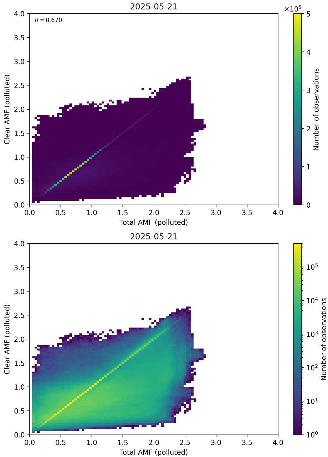
Figure 321: Scatter density plot of “Total AMF (polluted)” against “Clear AMF (polluted)” for 2025-05-21 to 2025-05-22.
