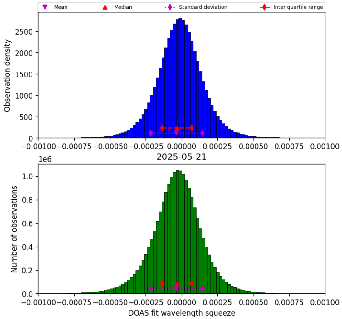
Figure 77: Histogram of “DOAS fit wavelength squeeze” for 2025-05-21 to 2025-05-22
