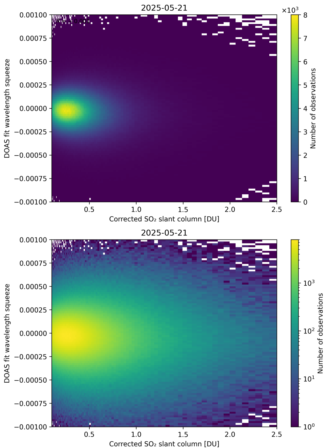
Figure 230: Scatter density plot of “Corrected SO 2 slant column” against “DOAS fit wavelength squeeze” for 2025-05-21 to 2025-05-22.
