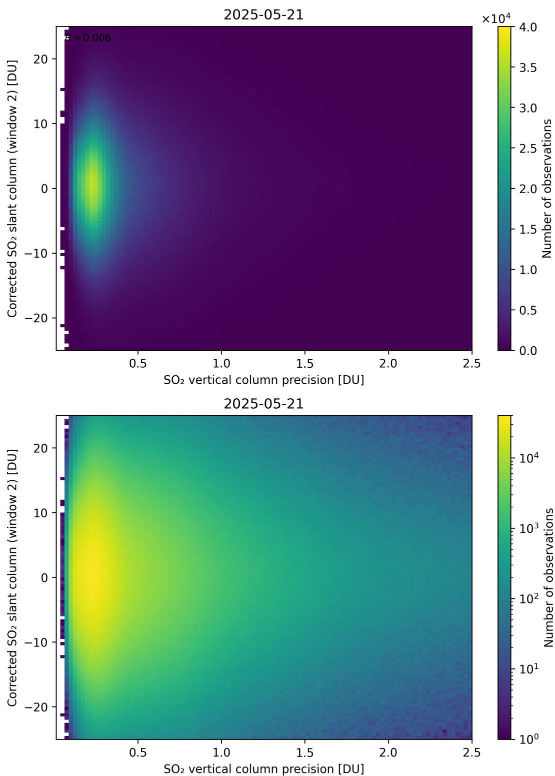
Figure 339: Scatter density plot of “SO 2 vertical column precision” against “Corrected SO 2 slant column (window 2)” for 2025-05-21 to 2025-05-22.
