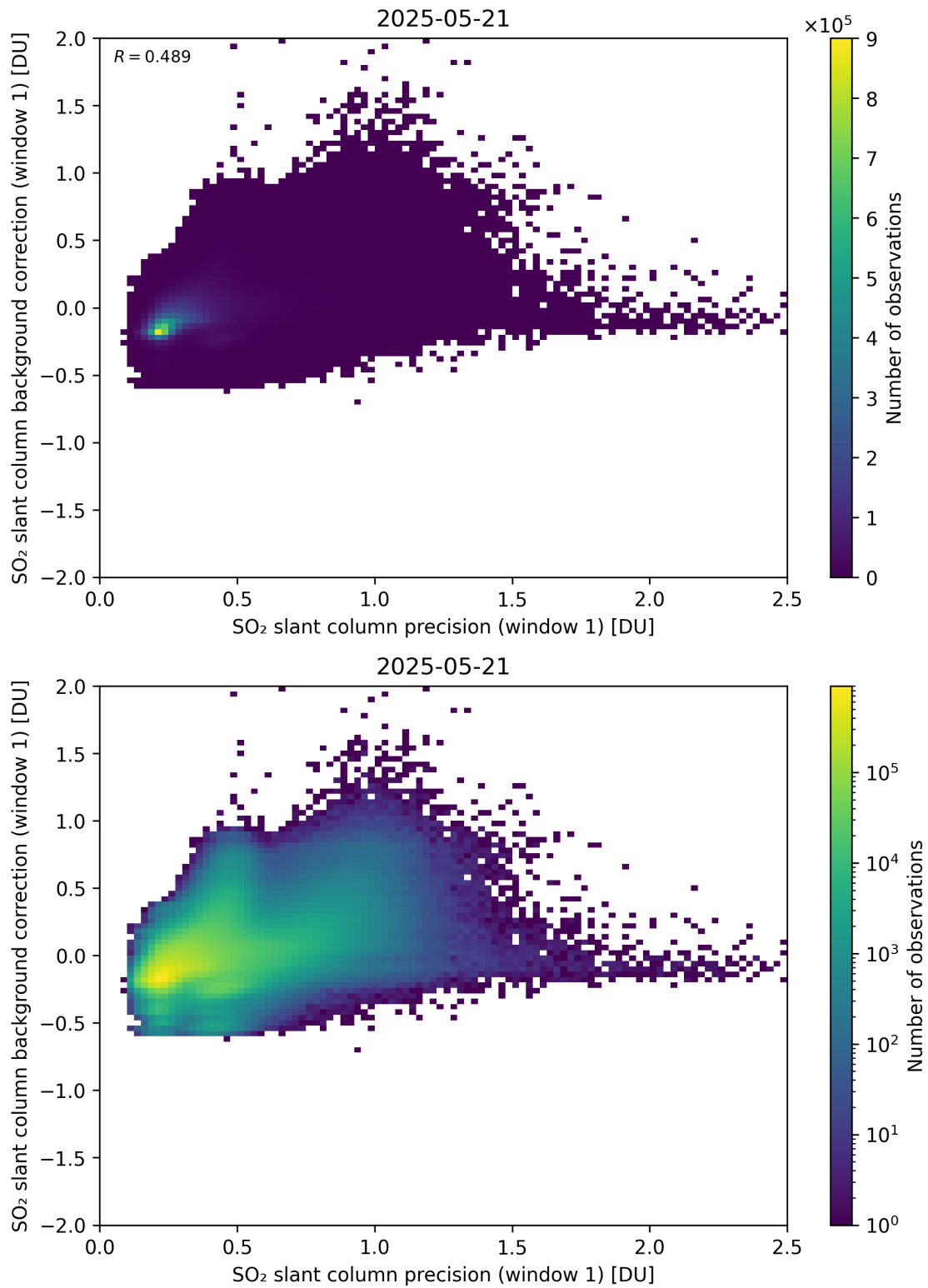
Figure 268: Scatter density plot of “SO 2 slant column precision (window 1)” against “SO 2 slant column background correction (window 1)” for 2025-05-21 to 2025-05-22.
