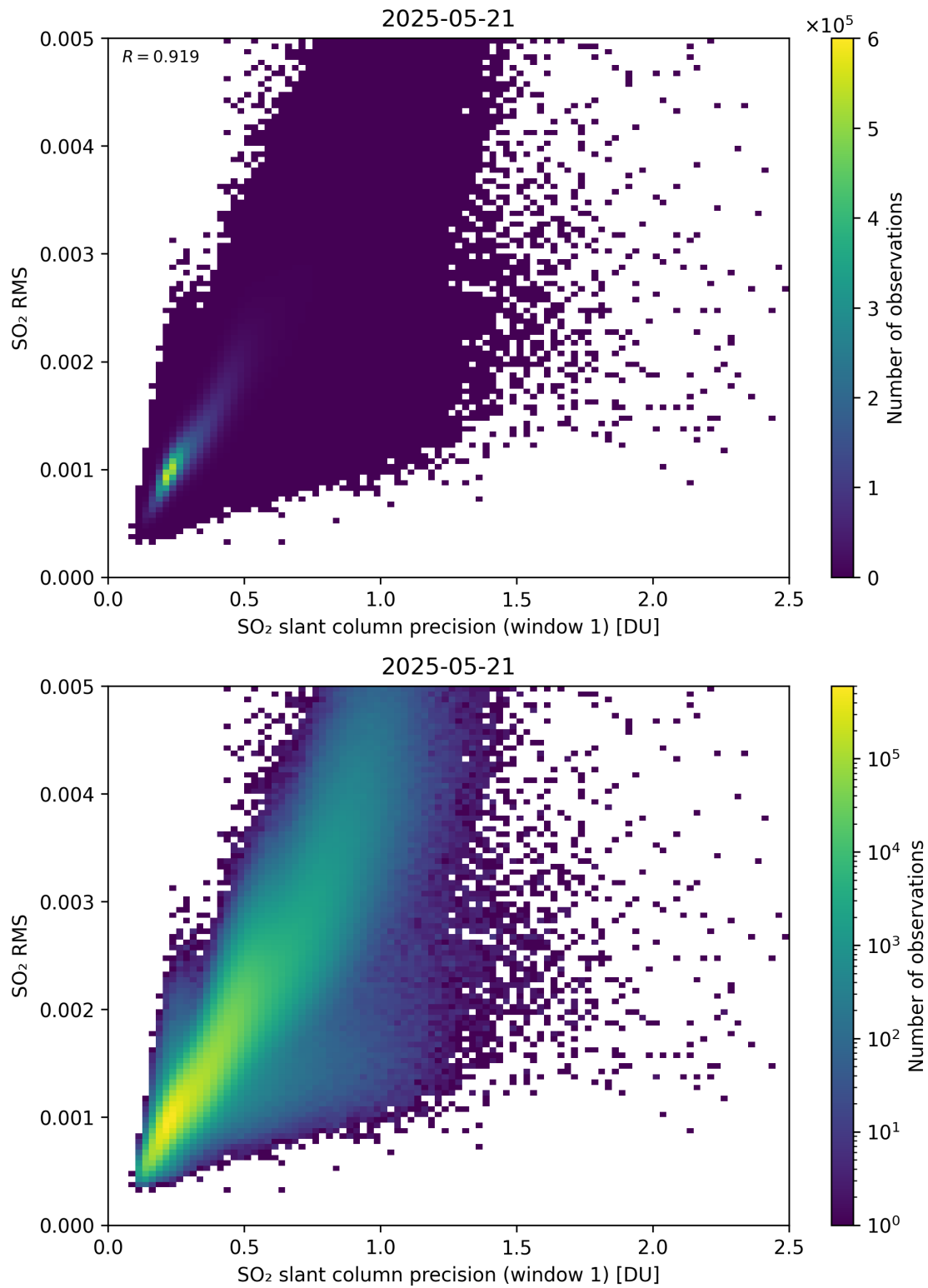
Figure 273: Scatter density plot of “SO 2 slant column precision (window 1)” against “SO 2 RMS” for 2025-05-21 to 2025-05-22.
