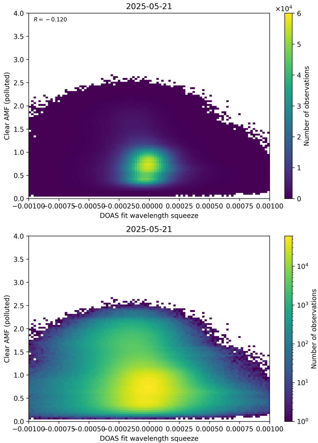
Figure 144: Scatter density plot of “DOAS fit wavelength squeeze” against “Clear AMF (polluted)” for 2025-05-21 to 2025-05-22.
