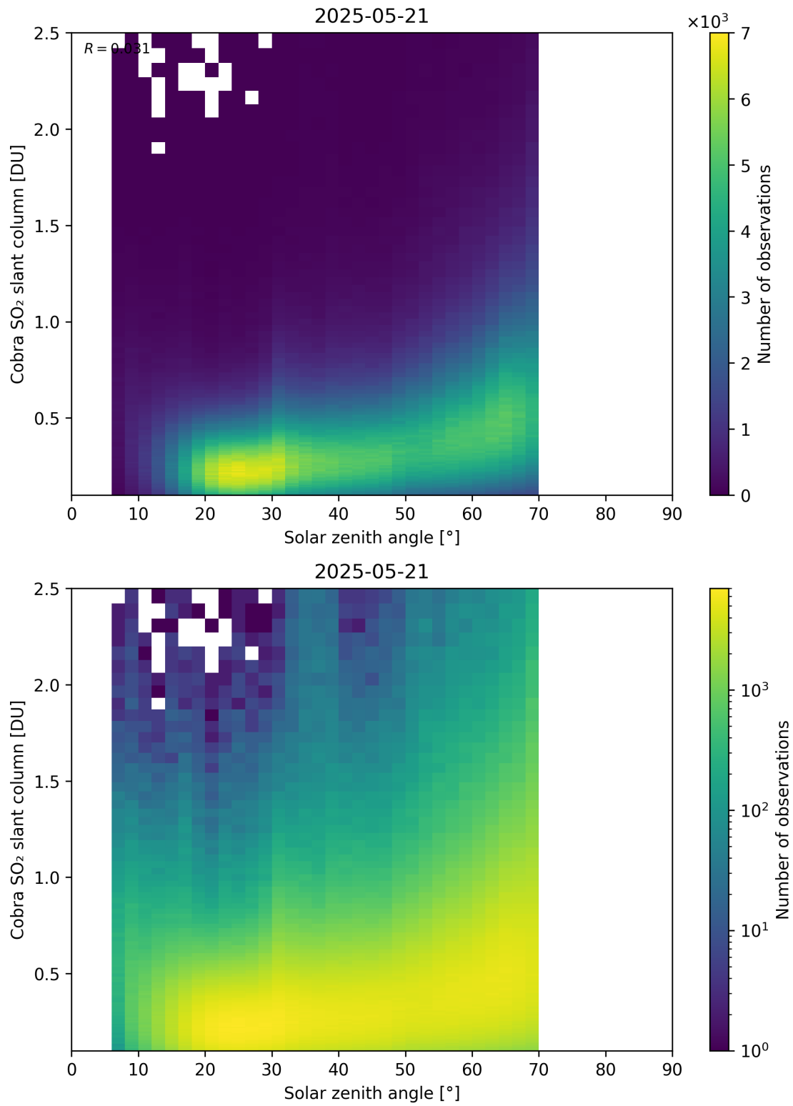
Figure 179: Scatter density plot of “Solar zenith angle” against “Cobra SO 2 slant column” for 2025-05-21 to 2025-05-22.
