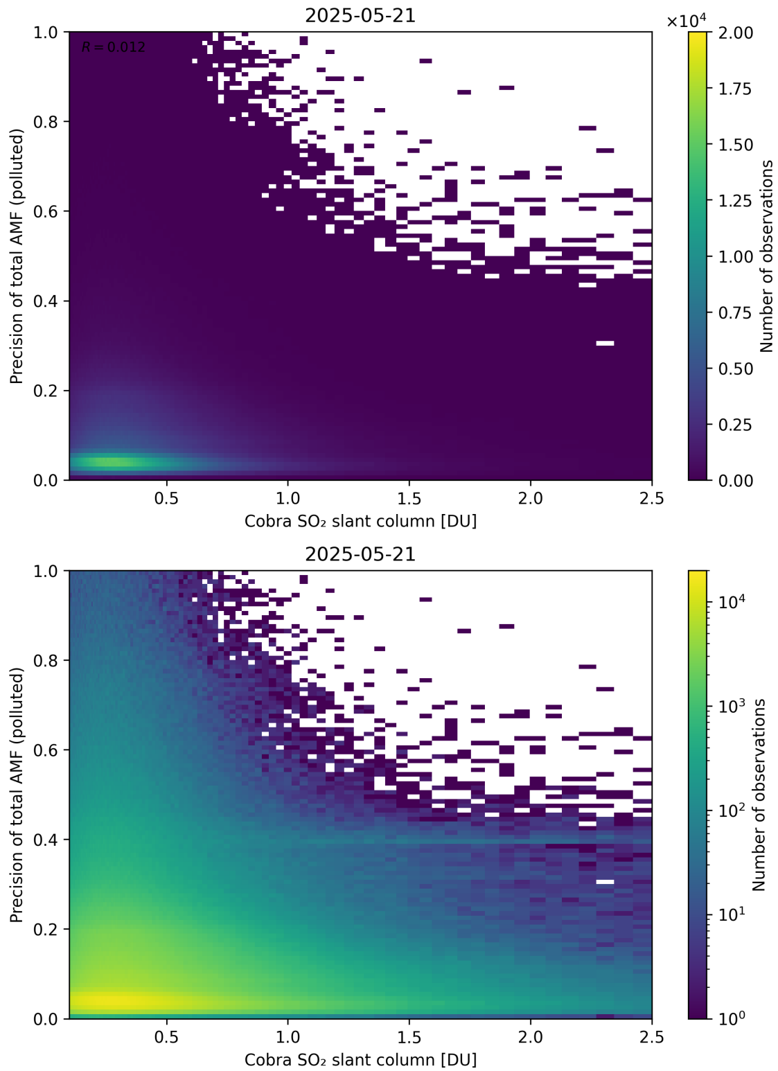
Figure 225: Scatter density plot of “Cobra SO 2 slant column” against “Precision of total AMF (polluted)” for 2025-05-21 to 2025-05-22.
