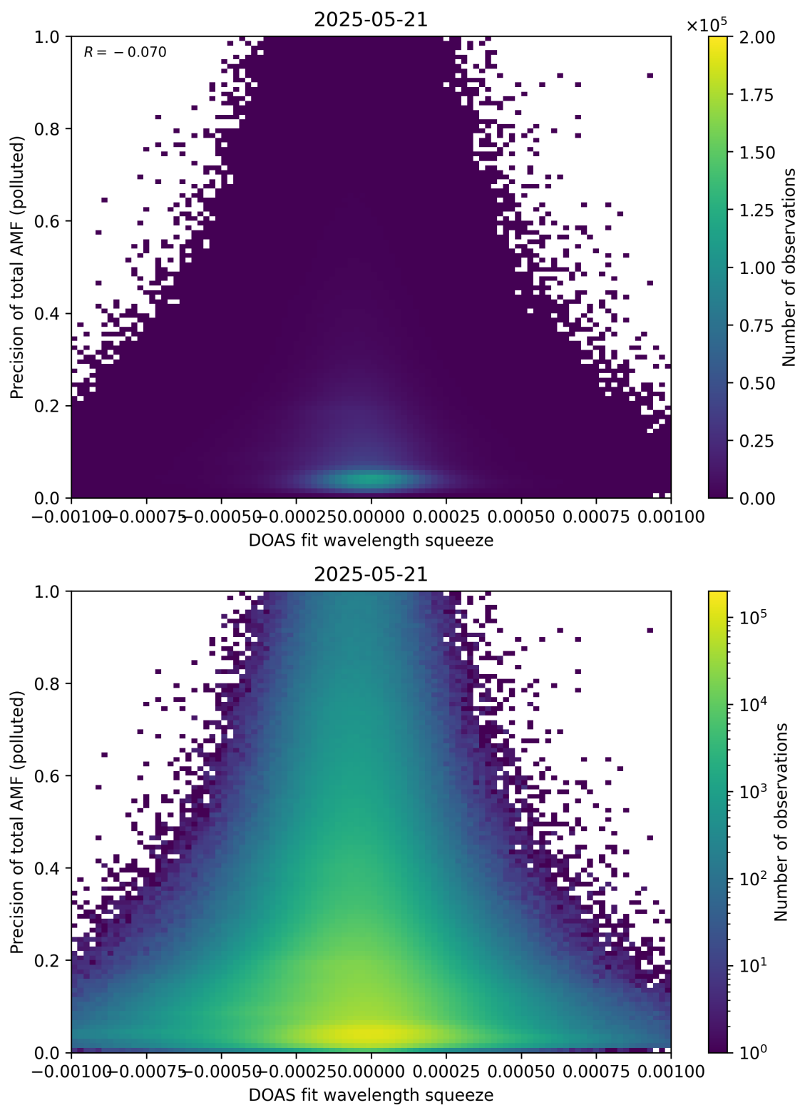
Figure 146: Scatter density plot of “DOAS fit wavelength squeeze” against “Precision of total AMF (polluted)” for 2025-05-21 to 2025-05-22.
