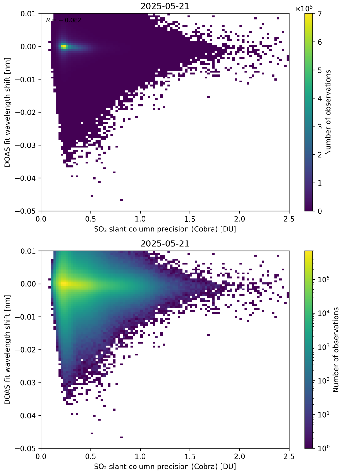
Figure 202: Scatter density plot of “SO 2 slant column precision (Cobra)” against “DOAS fit wavelength shift” for 2025-05-21 to 2025-05-22.
