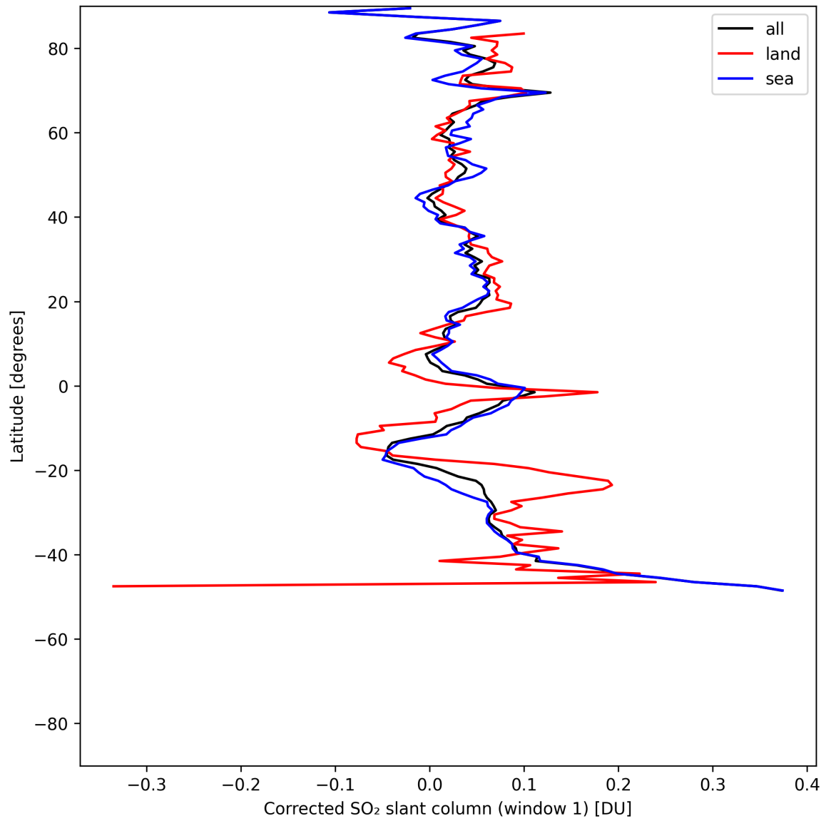
Figure 39: Zonal average of “Corrected SO 2 slant column (window 1)” for 2025-05-21 to 2025-05-22.
