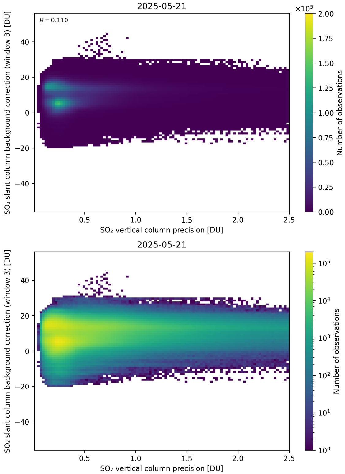
Figure 331: Scatter density plot of “SO 2 vertical column precision” against “SO 2 slant column background correction (window 3)” for 2025-05-21 to 2025-05-22.
