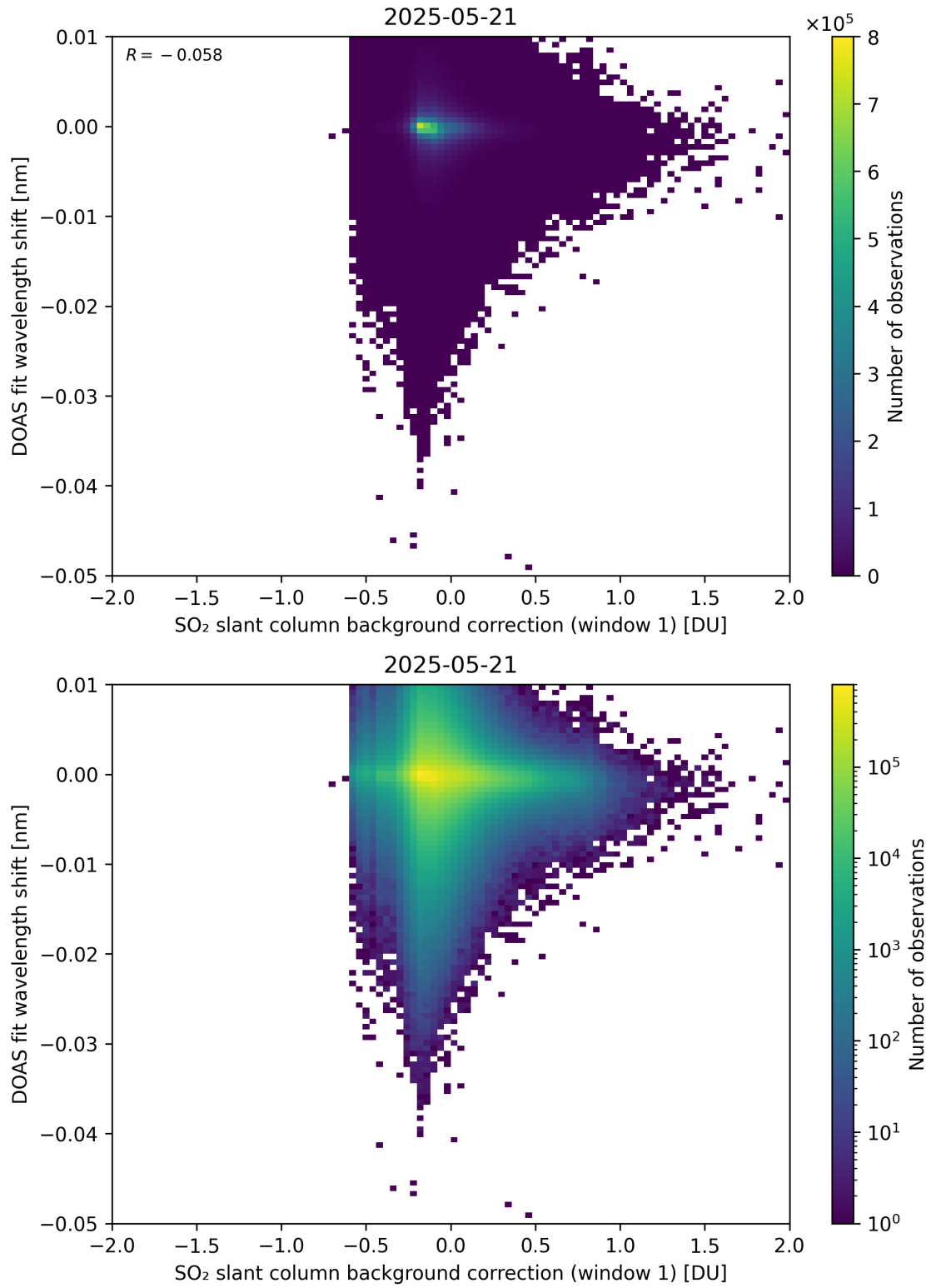
Figure 111: Scatter density plot of “SO 2 slant column background correction (window 1)” against “DOAS fit wavelength shift” for 2025-05-21 to 2025-05-22.
