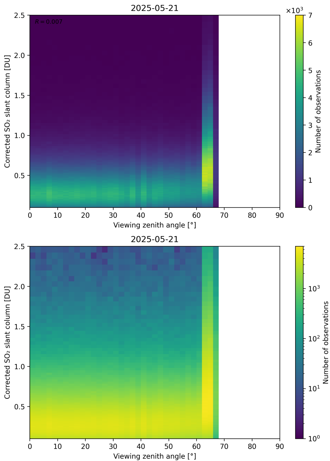
Figure 373: Scatter density plot of “Viewing zenith angle” against “Corrected SO 2 slant column” for 2025-05-21 to 2025-05-22.
