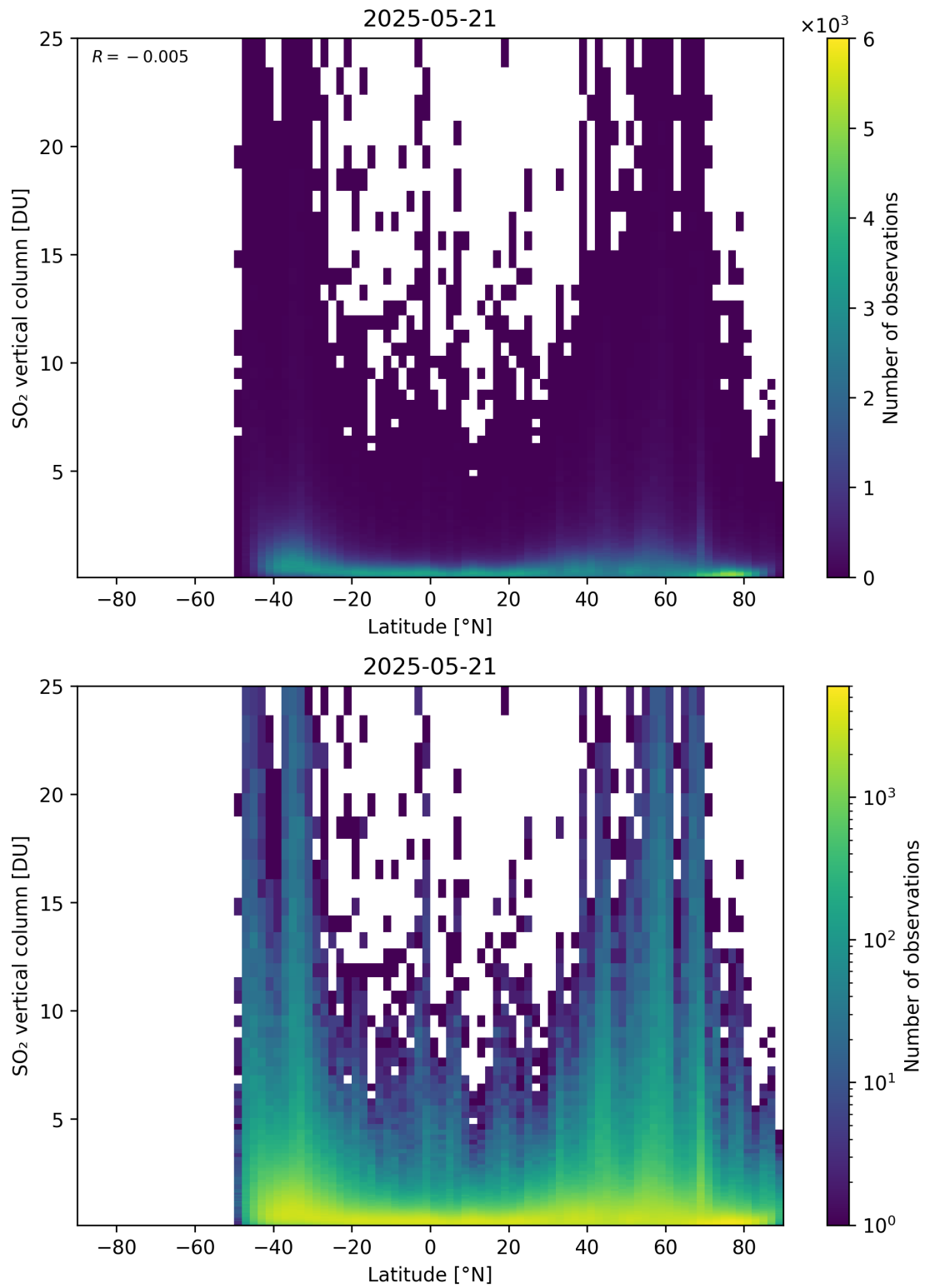
Figure 169: Scatter density plot of “Latitude” against “SO 2 vertical column” for 2025-05-21 to 2025-05-22.
