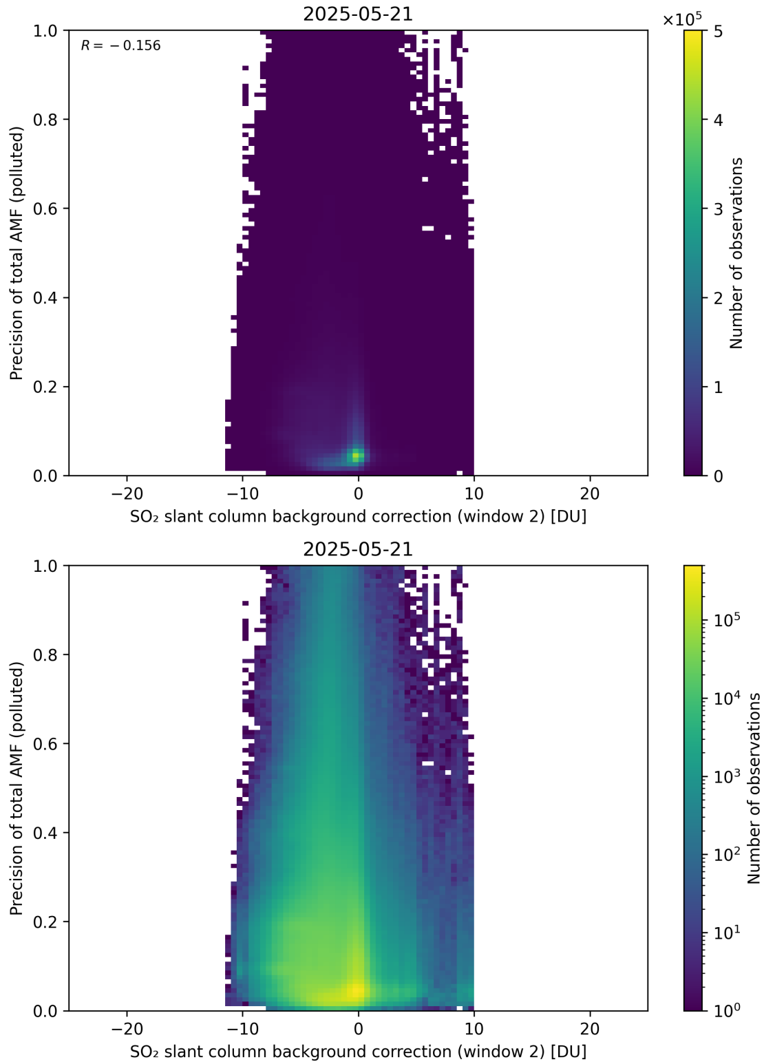
Figure 131: Scatter density plot of “SO 2 slant column background correction (window 2)” against “Precision of total AMF (polluted)” for 2025-05-21 to 2025-05-22.
