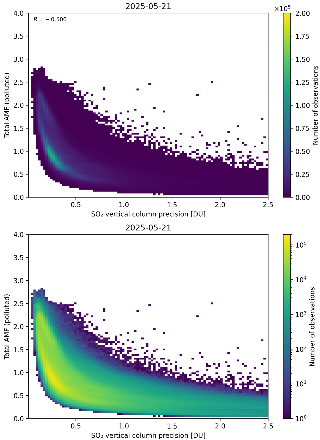
Figure 346: Scatter density plot of “SO 2 vertical column precision” against “Total AMF (polluted)” for 2025-05-21 to 2025-05-22.
