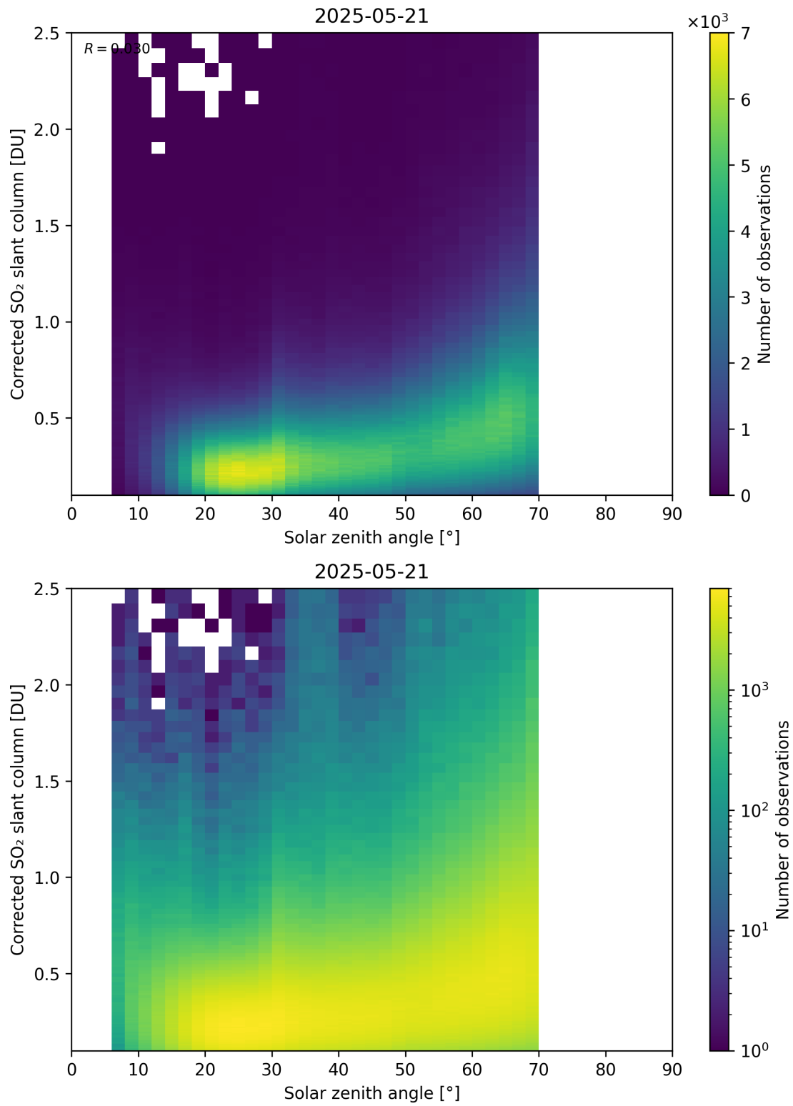
Figure 181: Scatter density plot of “Solar zenith angle” against “Corrected SO 2 slant column” for 2025-05-21 to 2025-05-22.
