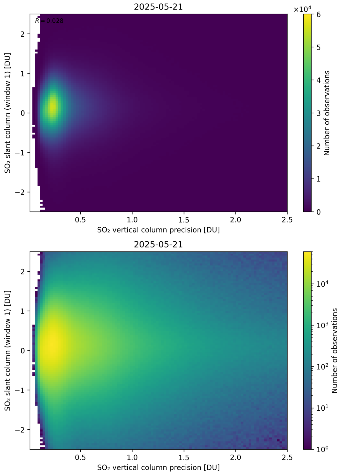
Figure 341: Scatter density plot of “SO 2 vertical column precision” against “SO 2 slant column (window 1)” for 2025-05-21 to 2025-05-22.
