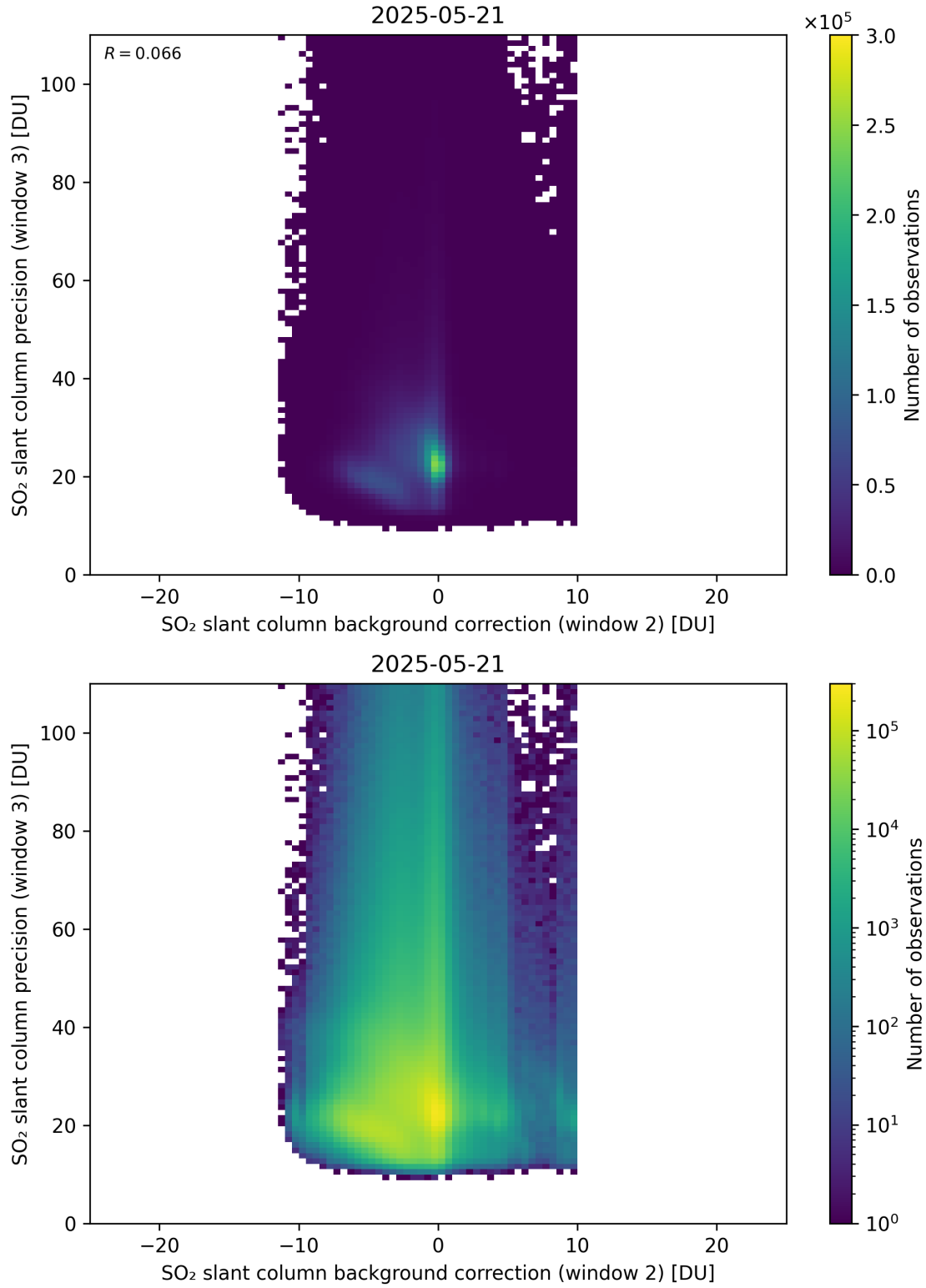
Figure 129: Scatter density plot of “SO 2 slant column background correction (window 2)” against “SO 2 slant column precision (window 3)” for 2025-05-21 to 2025-05-22.
