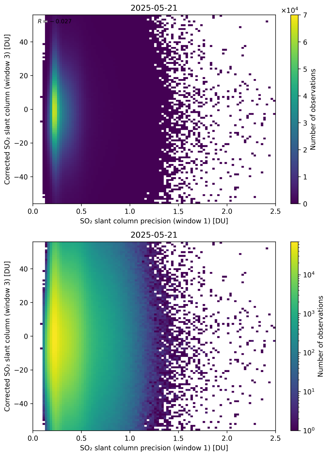
Figure 276: Scatter density plot of “SO 2 slant column precision (window 1)” against “Corrected SO 2 slant column (window 3)” for 2025-05-21 to 2025-05-22.
