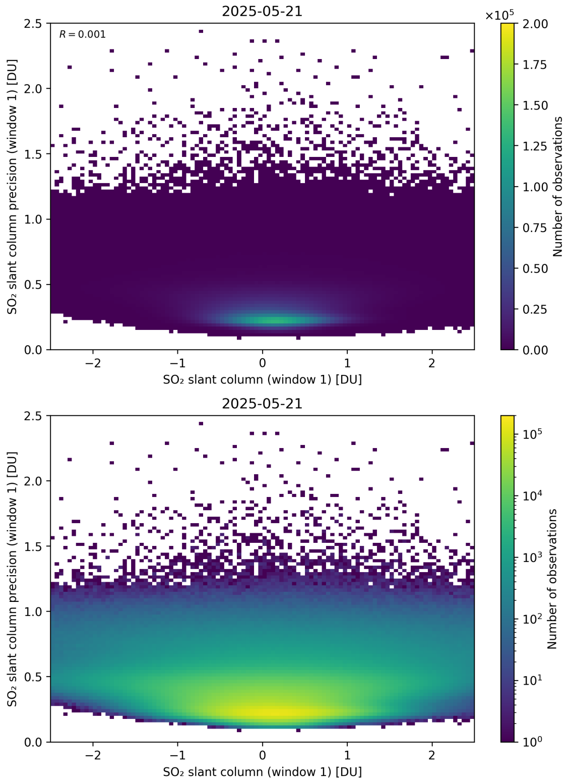
Figure 285: Scatter density plot of “SO 2 slant column (window 1)” against “SO 2 slant column precision (window 1)” for 2025-05-21 to 2025-05-22.
