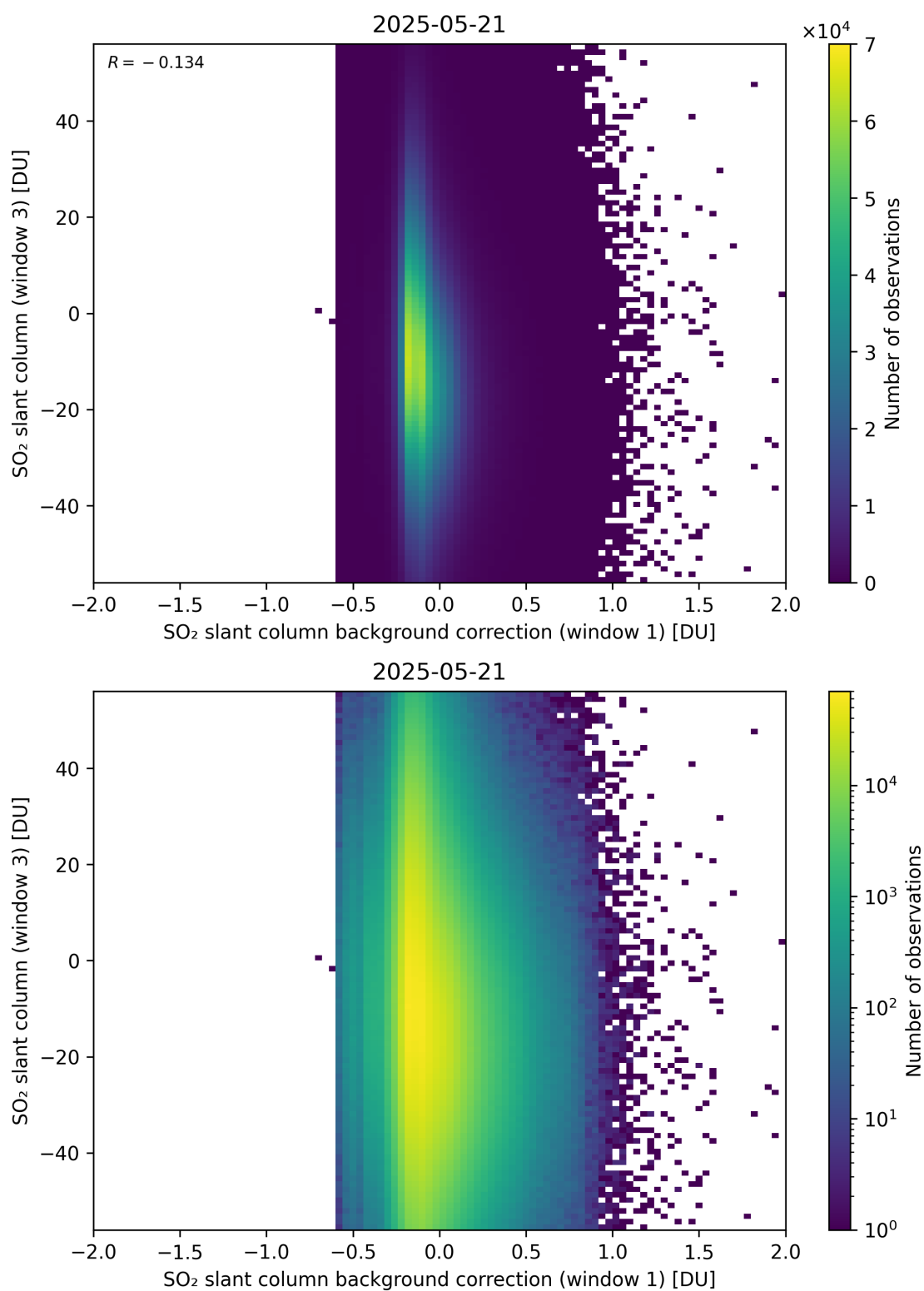
Figure 118: Scatter density plot of “SO 2 slant column background correction (window 1)” against “SO 2 slant column (window 3)” for 2025-05-21 to 2025-05-22.
