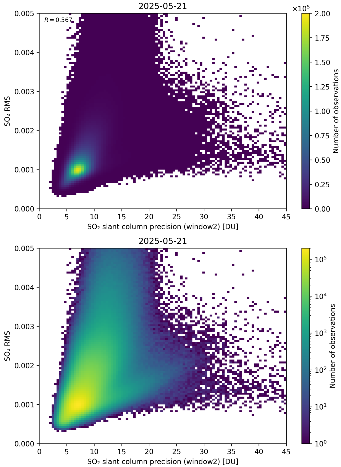
Figure 295: Scatter density plot of “SO 2 slant column precision (window2)” against “SO 2 RMS” for 2025-05-21 to 2025-05-22.
