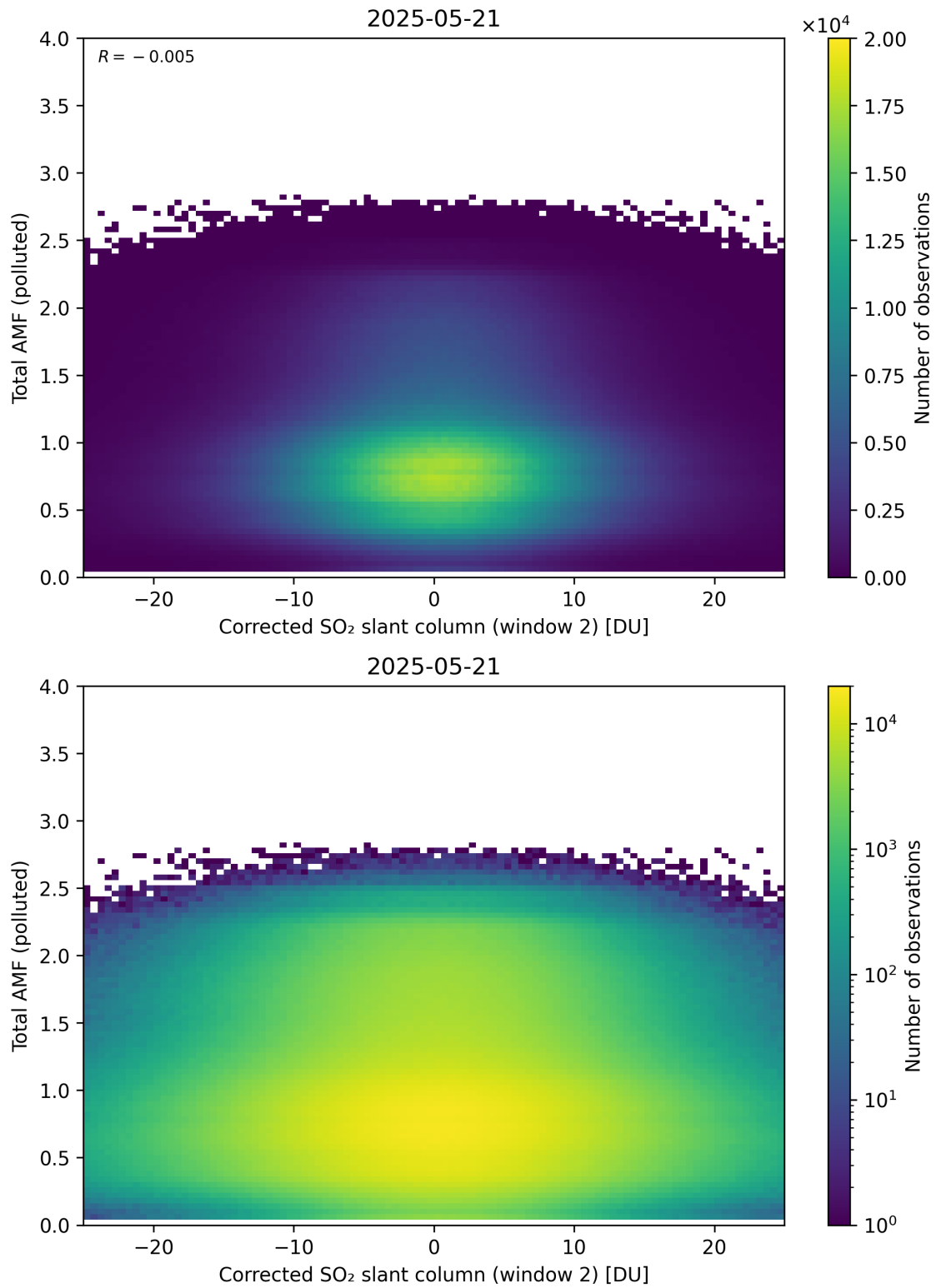
Figure 253: Scatter density plot of “Corrected SO 2 slant column (window 2)” against “Total AMF (polluted)” for 2025-05-21 to 2025-05-22.
