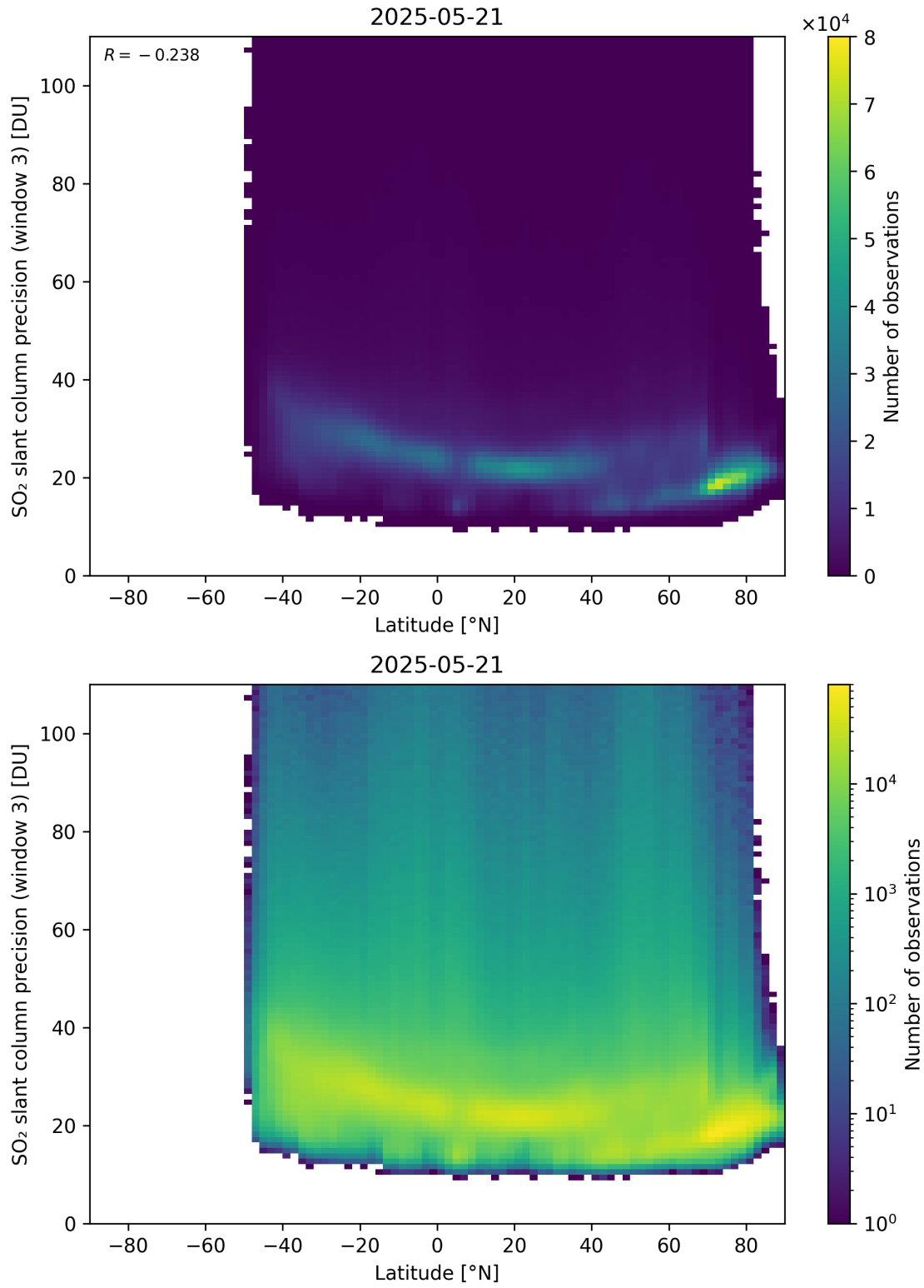
Figure 166: Scatter density plot of “Latitude” against “SO 2 slant column precision (window 3)” for 2025-05-21 to 2025-05-22.
