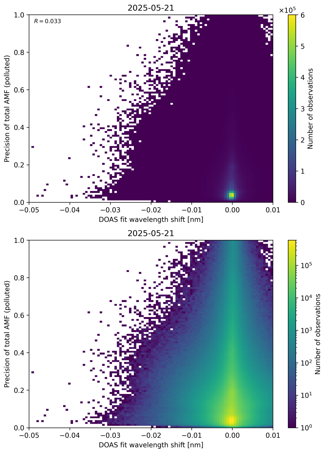
Figure 142: Scatter density plot of “DOAS fit wavelength shift” against “Precision of total AMF (polluted)” for 2025-05-21 to 2025-05-22.
