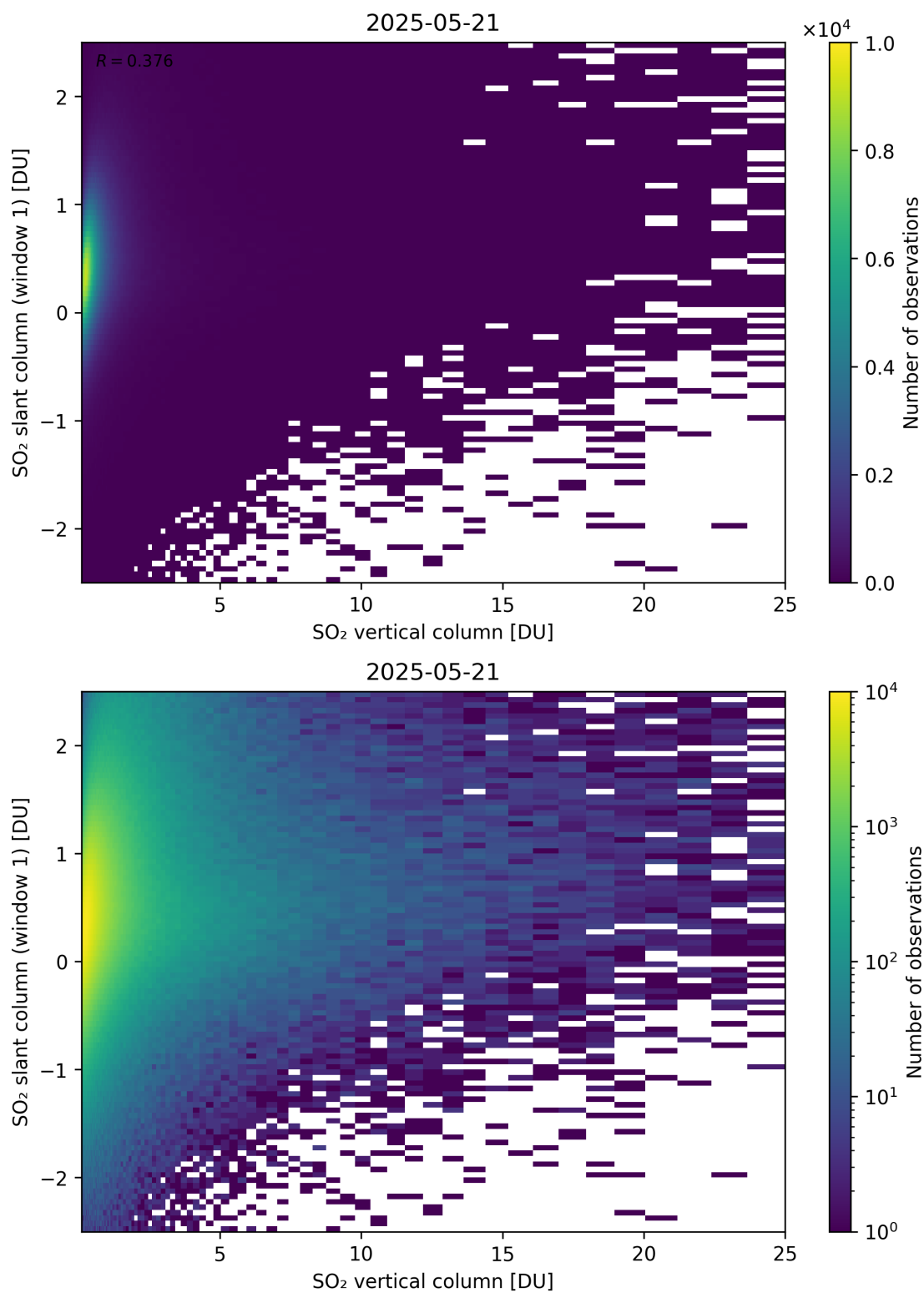
Figure 354: Scatter density plot of “SO 2 vertical column” against “SO 2 slant column (window 1)” for 2025-05-21 to 2025-05-22.
