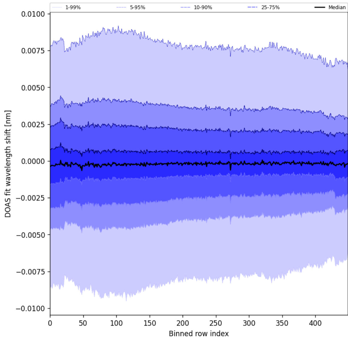
Figure 102: Along track statistics of “DOAS fit wavelength shift” for 2025-05-21 to 2025-05-22
