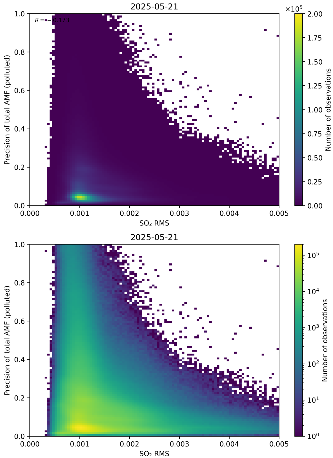
Figure 149: Scatter density plot of “SO 2 RMS” against “Precision of total AMF (polluted)” for 2025-05-21 to 2025-05-22.
