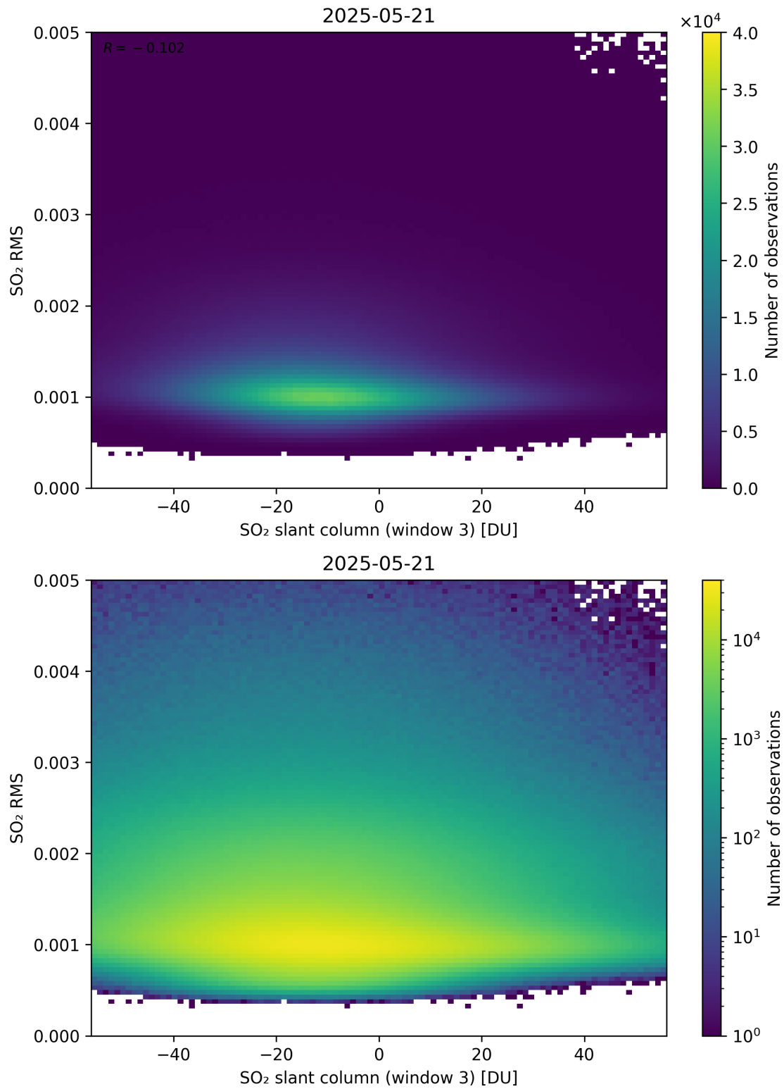
Figure 306: Scatter density plot of “SO 2 slant column (window 3)” against “SO 2 RMS” for 2025-05-21 to 2025-05-22.
