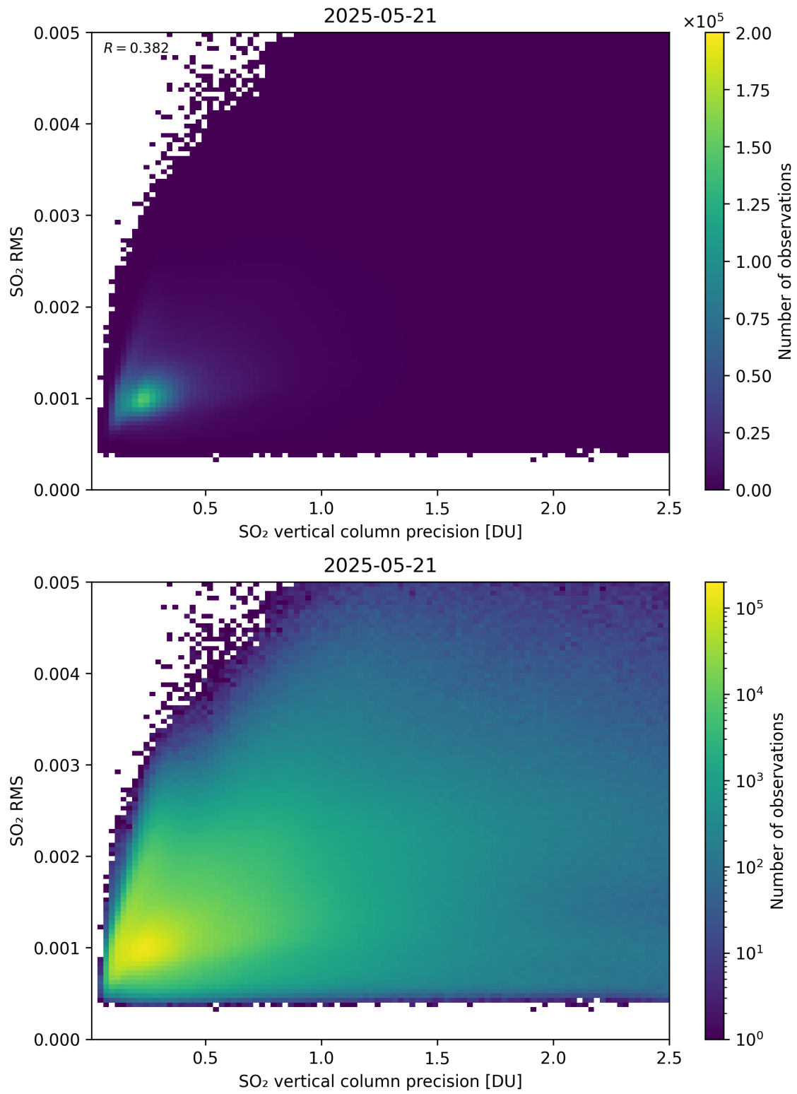
Figure 334: Scatter density plot of “SO 2 vertical column precision” against “SO 2 RMS” for 2025-05-21 to 2025-05-22.
