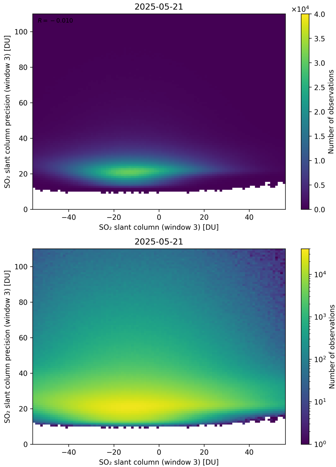
Figure 317: Scatter density plot of “SO 2 slant column (window 3)” against “SO 2 slant column precision (window 3)” for 2025-05-21 to 2025-05-22.
