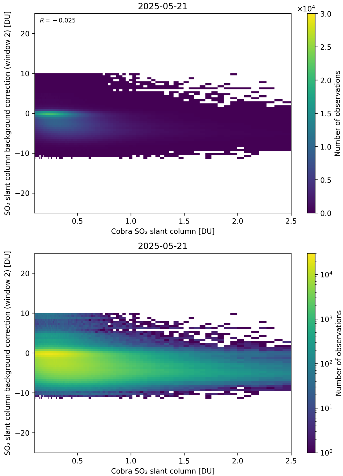
Figure 194: Scatter density plot of “Cobra SO 2 slant column” against “SO 2 slant column background correction (window 2)” for 2025-05-21 to 2025-05-22.
