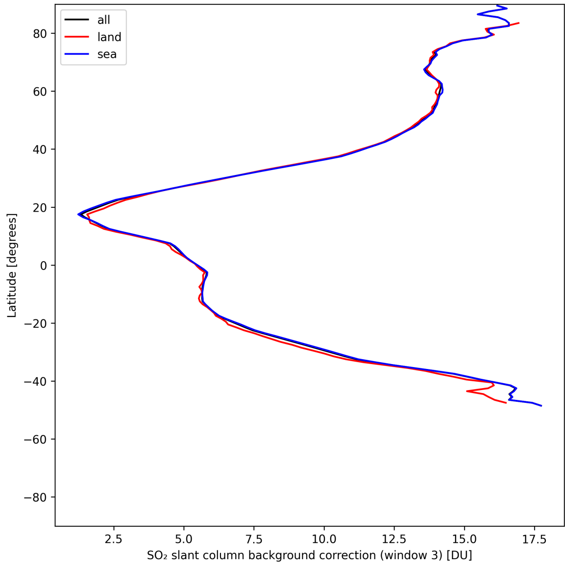
Figure 48: Zonal average of “SO 2 slant column background correction (window 3)” for 2025-05-21 to 2025-05-22.
