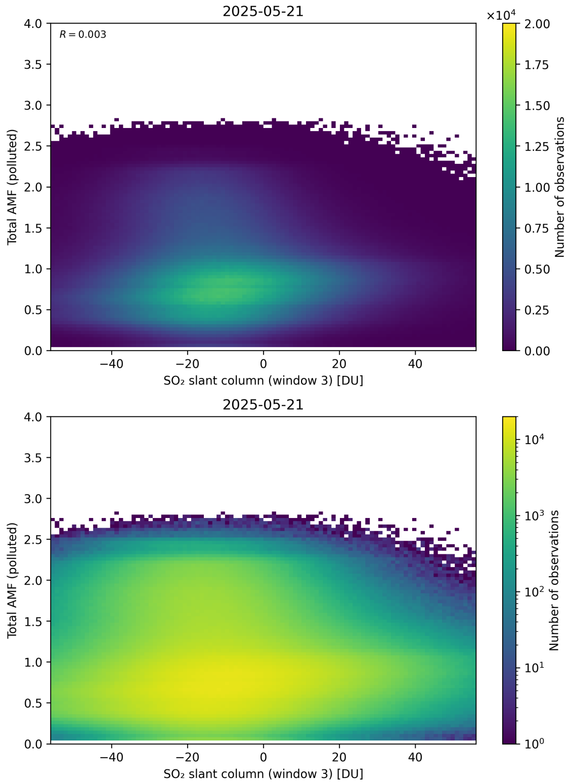
Figure 318: Scatter density plot of “SO 2 slant column (window 3)” against “Total AMF (polluted)” for 2025-05-21 to 2025-05-22.
