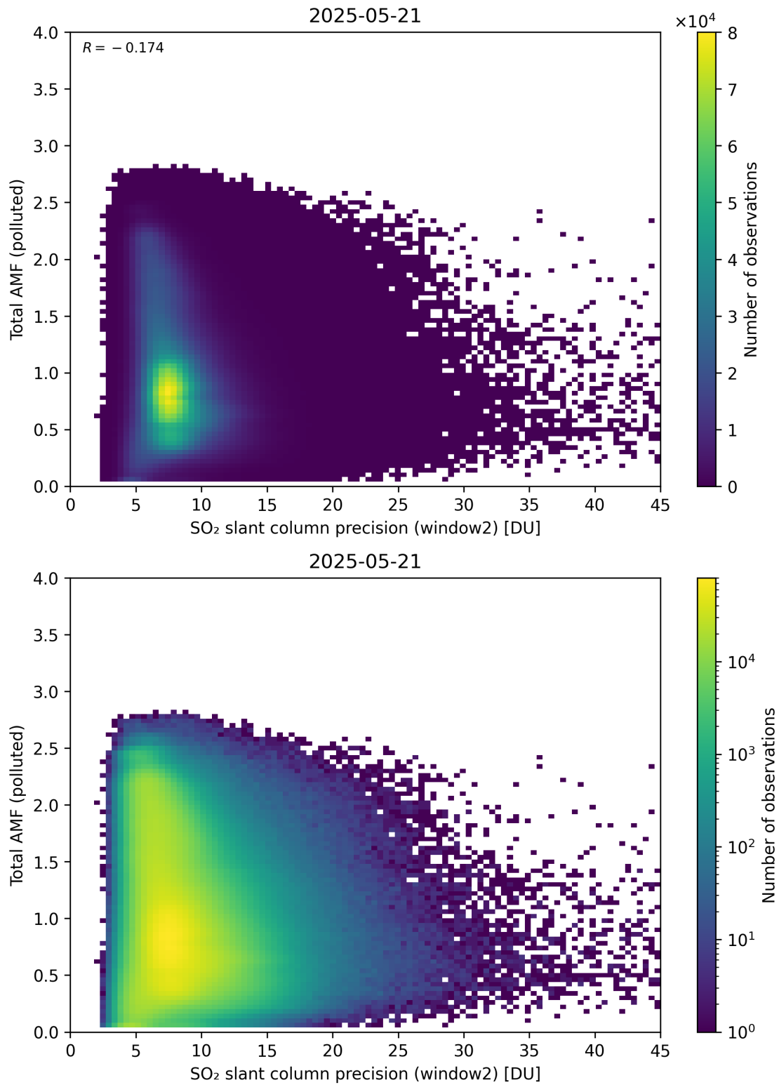
Figure 301: Scatter density plot of “SO 2 slant column precision (window2)” against “Total AMF (polluted)” for 2025-05-21 to 2025-05-22.
