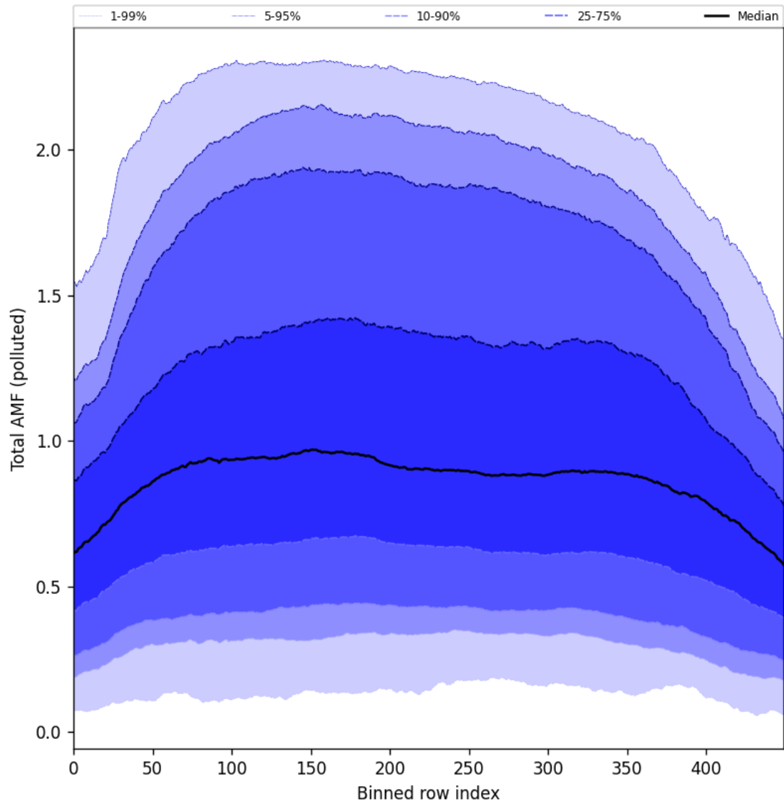
Figure 105: Along track statistics of “Total AMF (polluted)” for 2025-05-21 to 2025-05-22
