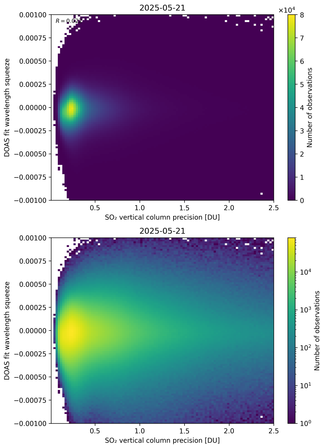
Figure 333: Scatter density plot of “SO 2 vertical column precision” against “DOAS fit wavelength squeeze” for 2025-05-21 to 2025-05-22.
