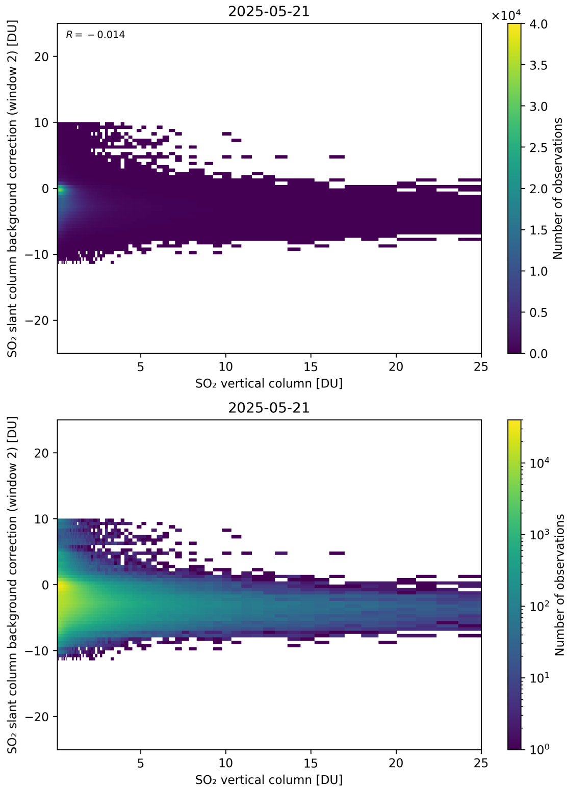
Figure 324: Scatter density plot of “SO 2 vertical column” against “SO 2 slant column background correction (window 2)” for 2025-05-21 to 2025-05-22.
