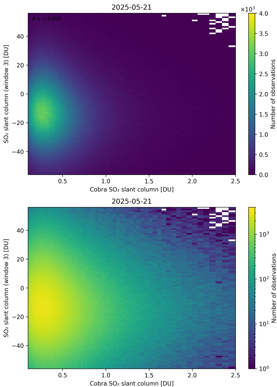
Figure 222: Scatter density plot of “Cobra SO 2 slant column” against “SO 2 slant column (window 3)” for 2025-05-21 to 2025-05-22.
