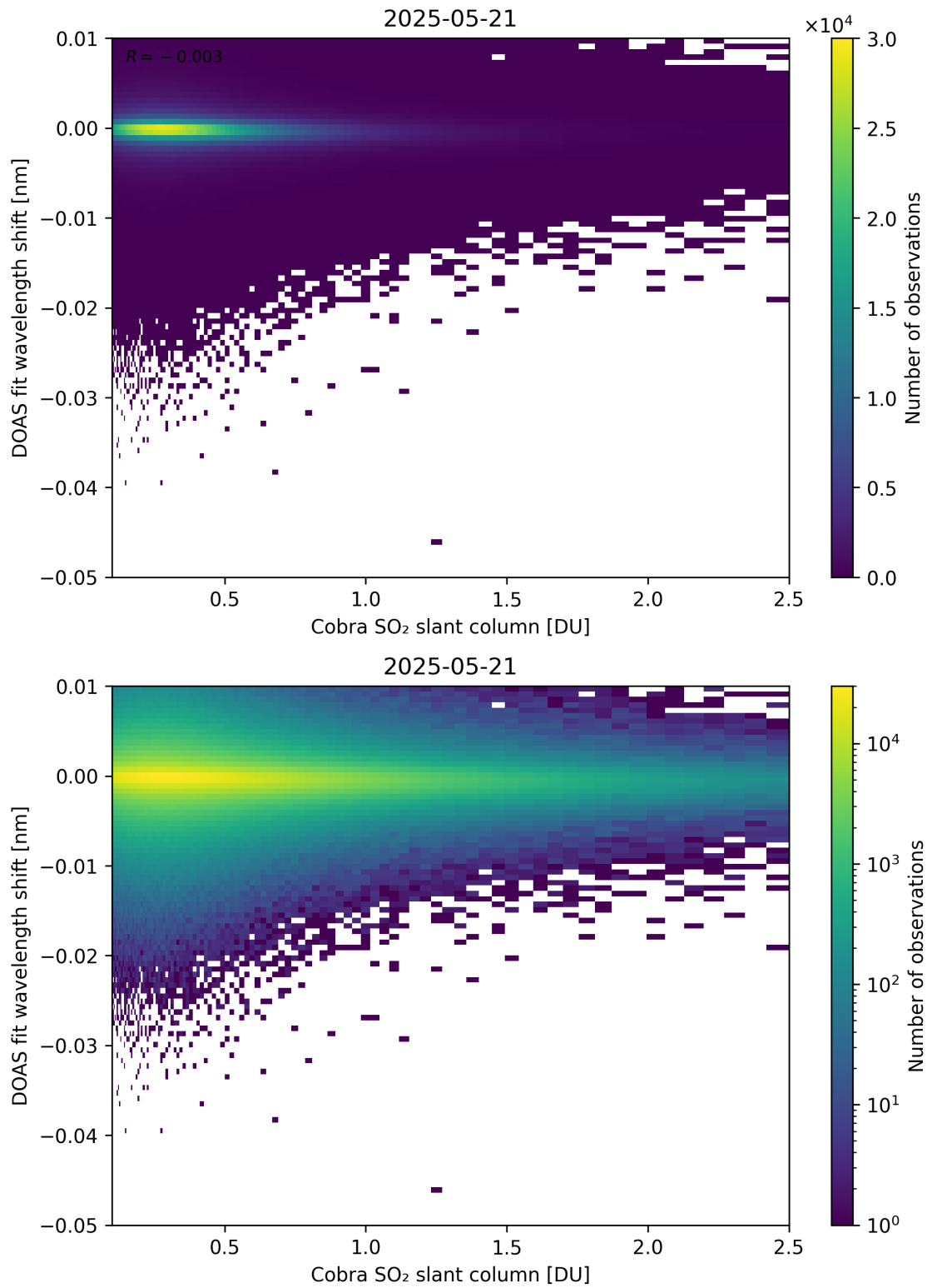
Figure 196: Scatter density plot of “Cobra SO 2 slant column” against “DOAS fit wavelength shift” for 2025-05-21 to 2025-05-22.
