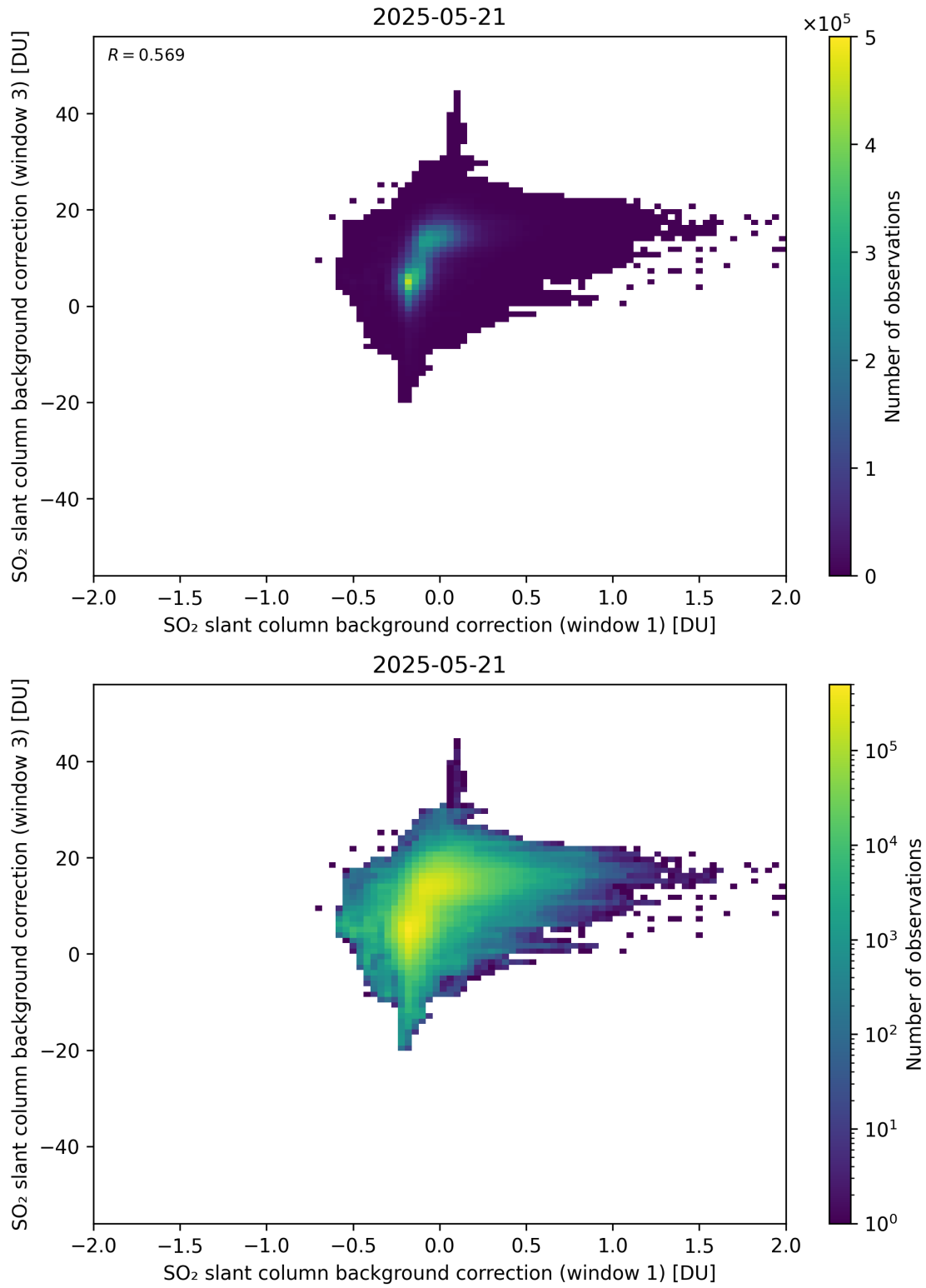
Figure 110: Scatter density plot of “SO 2 slant column background correction (window 1)” against “SO 2 slant column background correction (window 3)” for 2025-05-21 to 2025-05-22.
