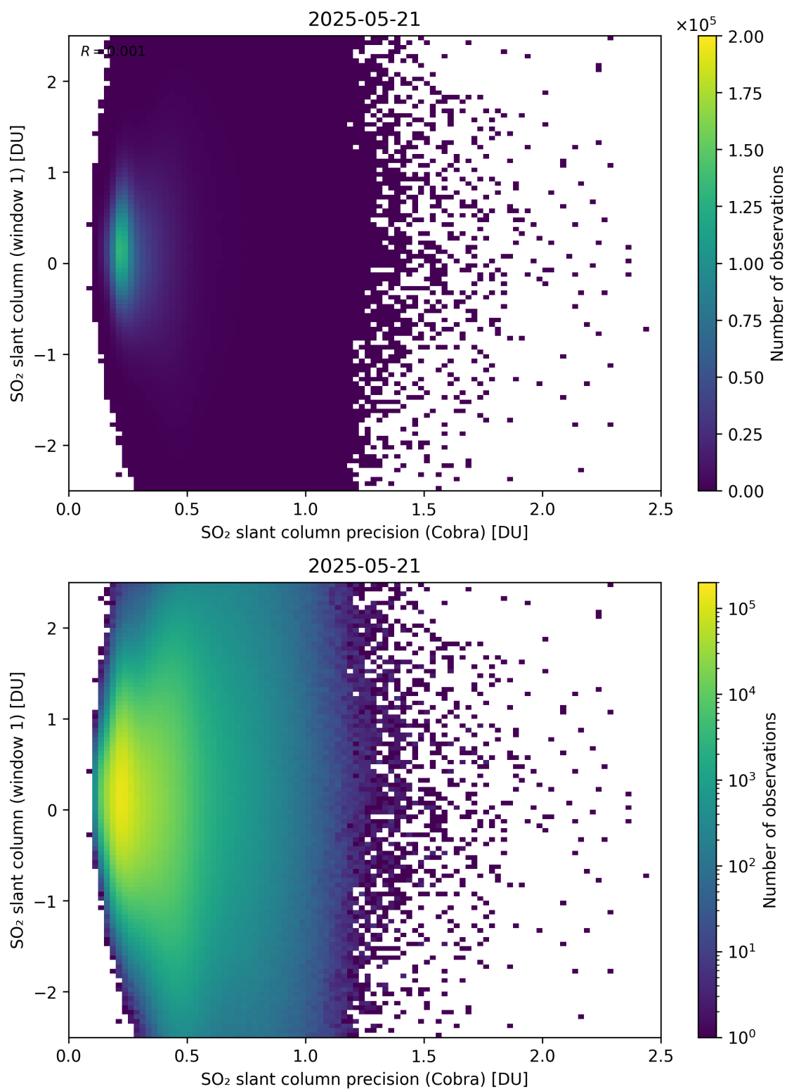
Figure 208: Scatter density plot of “SO 2 slant column precision (Cobra)” against “SO 2 slant column (window 1)” for 2025-05-21 to 2025-05-22.
