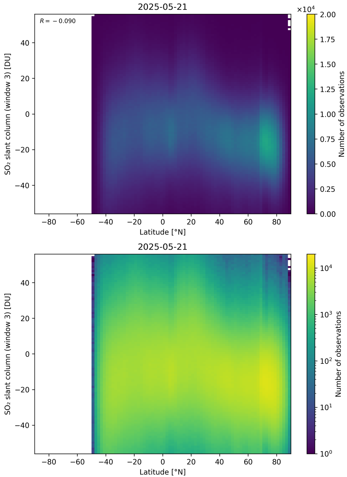
Figure 165: Scatter density plot of “Latitude” against “SO 2 slant column (window 3)” for 2025-05-21 to 2025-05-22.
