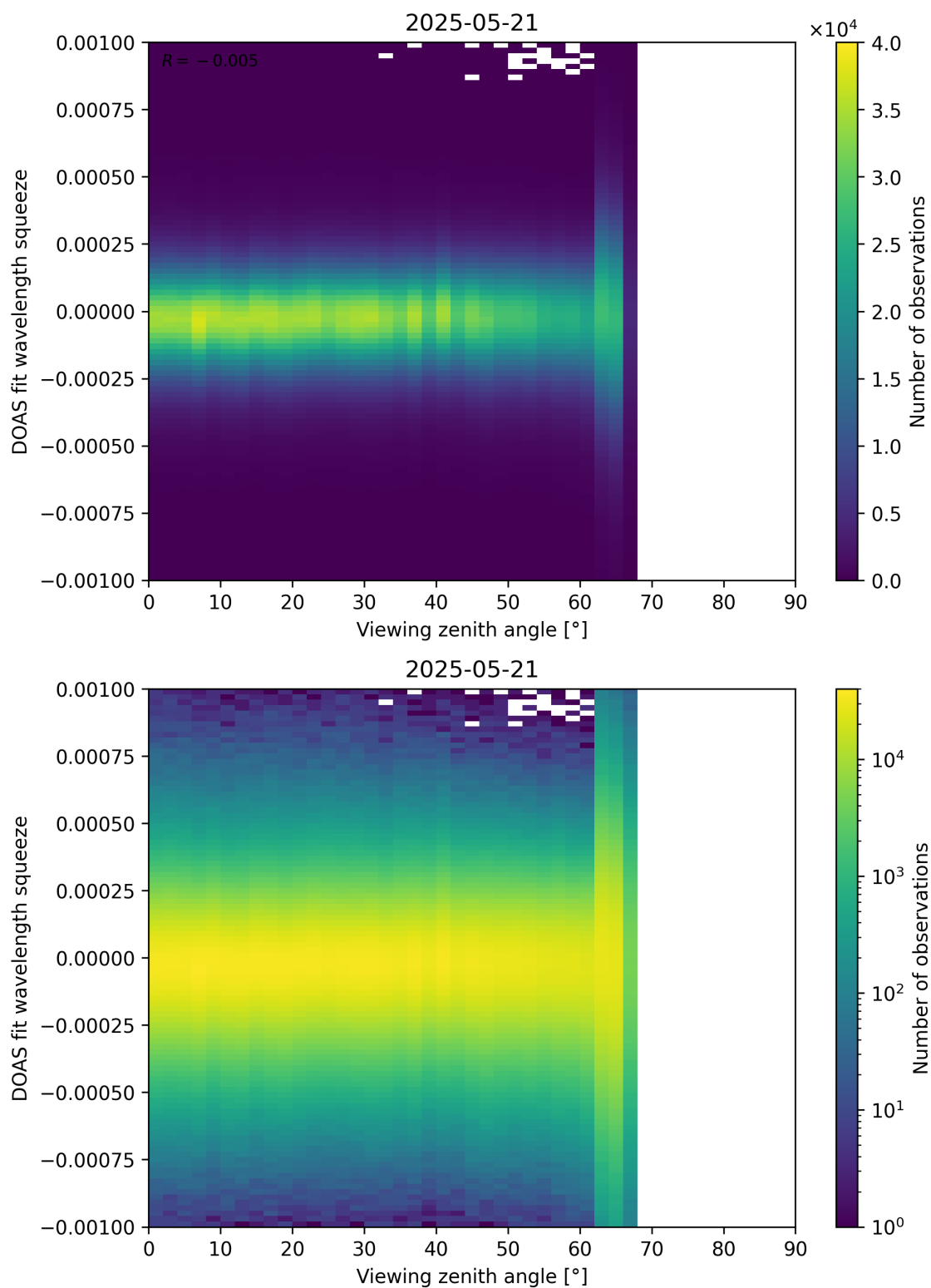
Figure 366: Scatter density plot of “Viewing zenith angle” against “DOAS fit wavelength squeeze” for 2025-05-21 to 2025-05-22.
