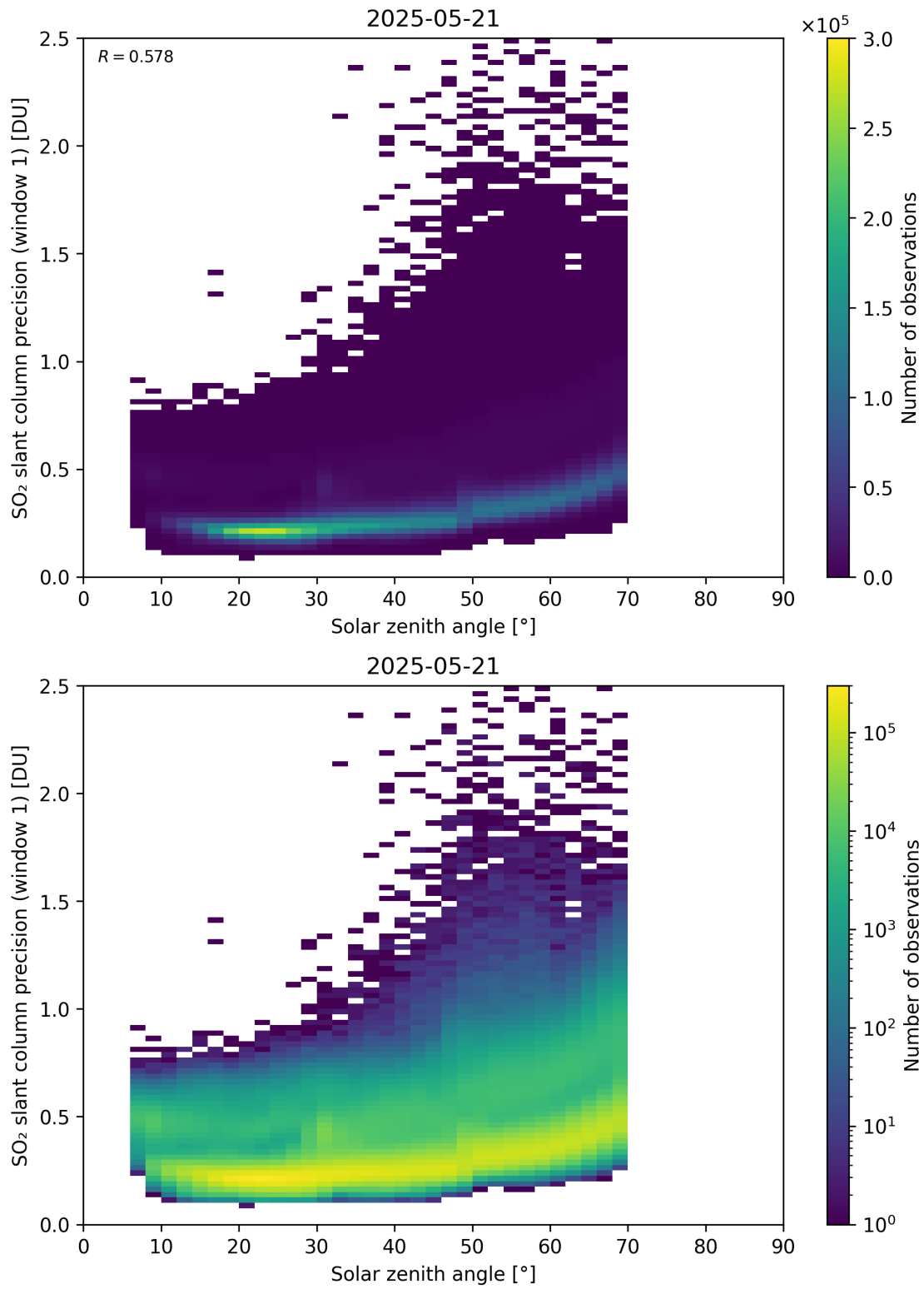
Figure 185: Scatter density plot of “Solar zenith angle” against “SO 2 slant column precision (window 1)” for 2025-05-21 to 2025-05-22.
