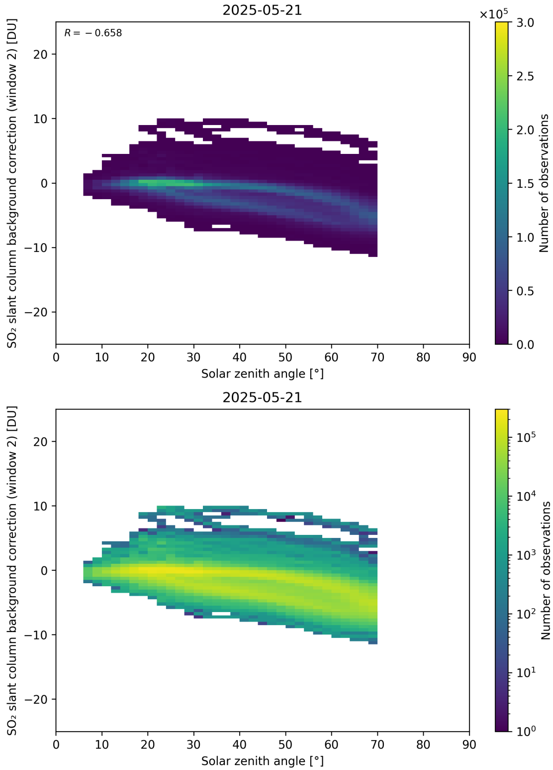
Figure 172: Scatter density plot of “Solar zenith angle” against “SO 2 slant column background correction (window 2)” for 2025-05-21 to 2025-05-22.
