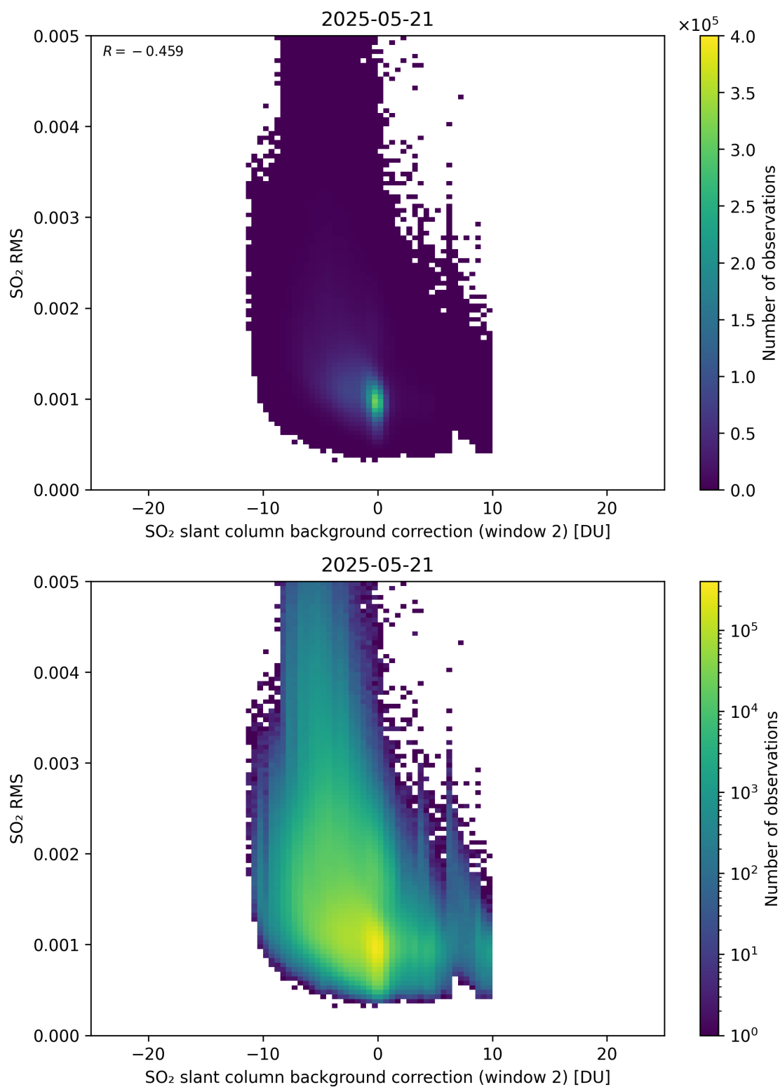
Figure 125: Scatter density plot of “SO 2 slant column background correction (window 2)” against “SO 2 RMS” for 2025-05-21 to 2025-05-22.
