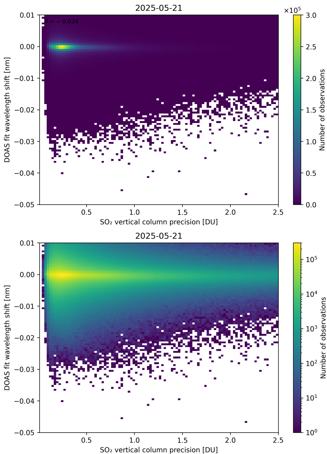
Figure 332: Scatter density plot of “SO 2 vertical column precision” against “DOAS fit wavelength shift” for 2025-05-21 to 2025-05-22.
