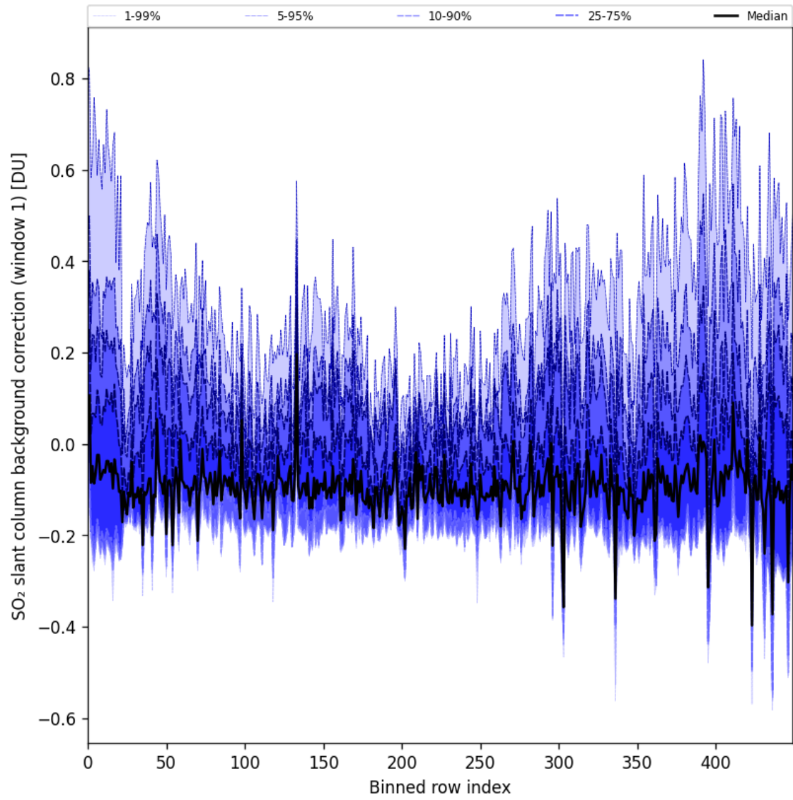
Figure 92: Along track statistics of “SO 2 slant column background correction (window 1)” for 2025-05-21 to 2025-05-22
