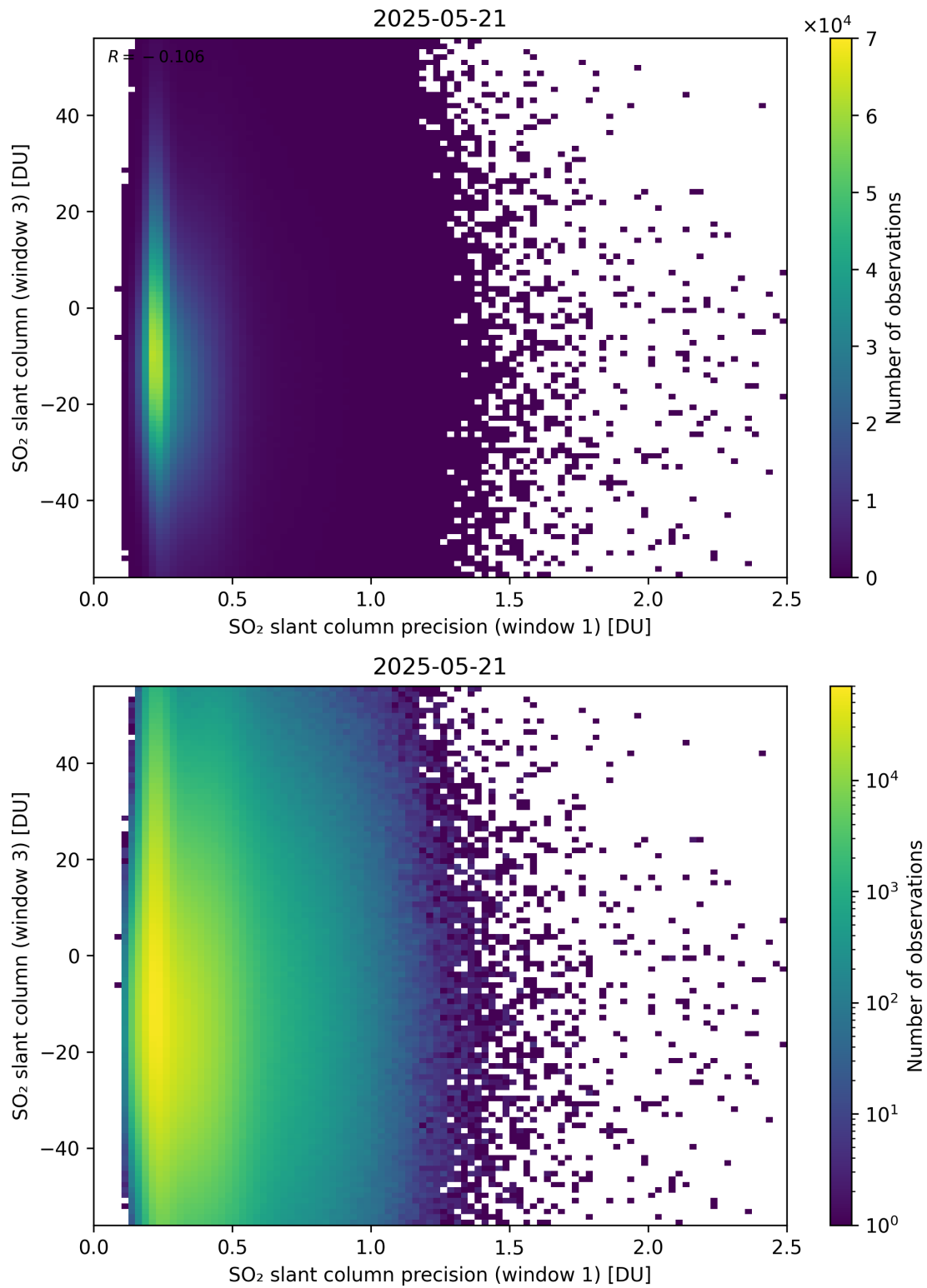
Figure 278: Scatter density plot of “SO 2 slant column precision (window 1)” against “SO 2 slant column (window 3)” for 2025-05-21 to 2025-05-22.
