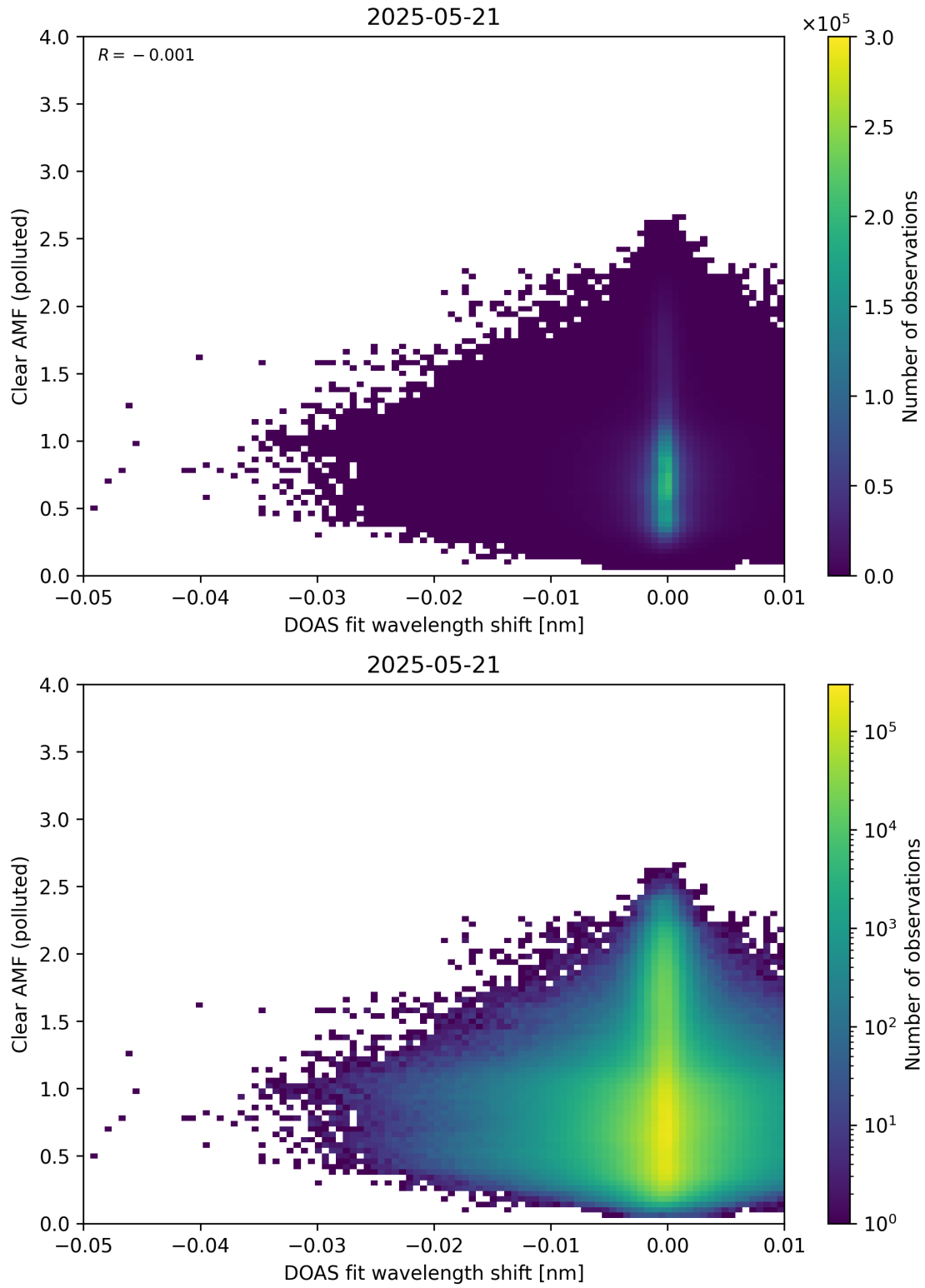
Figure 140: Scatter density plot of “DOAS fit wavelength shift” against “Clear AMF (polluted)” for 2025-05-21 to 2025-05-22.
