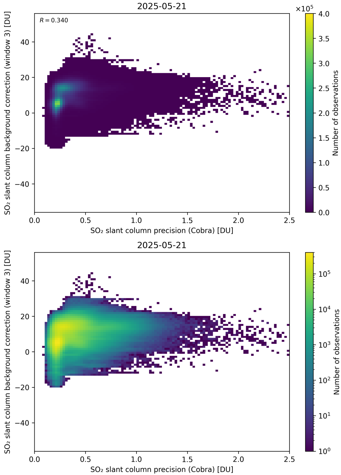
Figure 201: Scatter density plot of “SO 2 slant column precision (Cobra)” against “SO 2 slant column background correction (window 3)” for 2025-05-21 to 2025-05-22.
