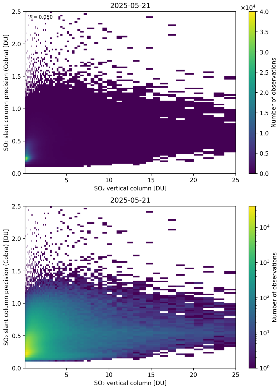
Figure 350: Scatter density plot of “SO 2 vertical column” against “SO 2 slant column precision (Cobra)” for 2025-05-21 to 2025-05-22.
