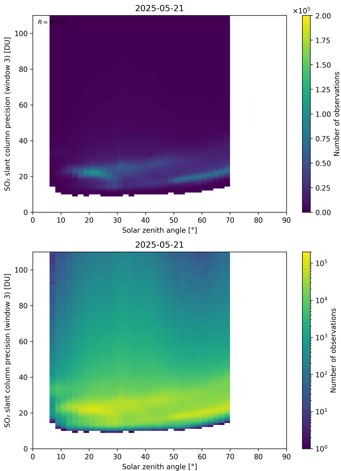
Figure 188: Scatter density plot of “Solar zenith angle” against “SO 2 slant column precision (window 3)” for 2025-05-21 to 2025-05-22.
