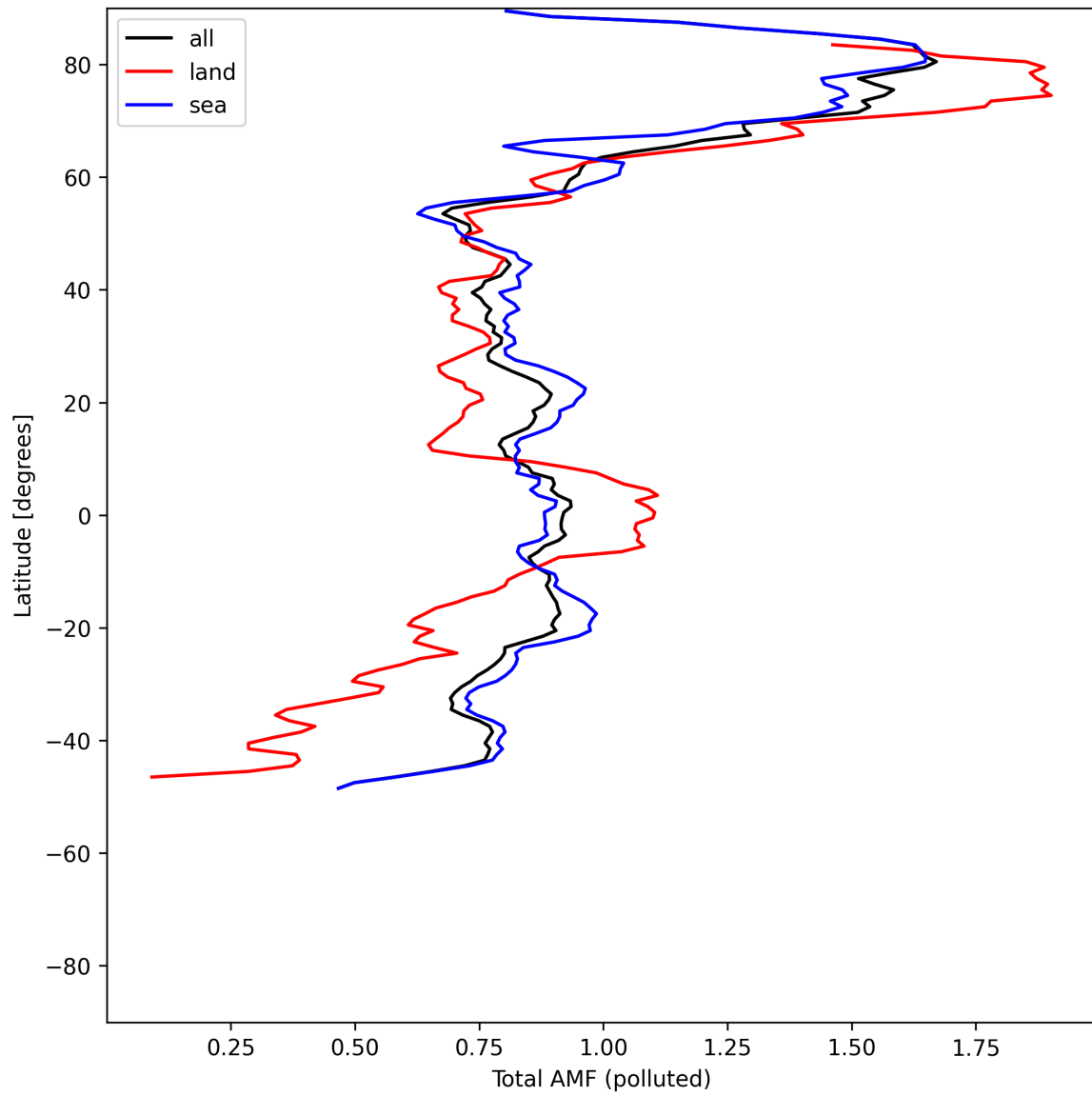
Figure 53: Zonal average of “Total AMF (polluted)” for 2025-05-21 to 2025-05-23.
