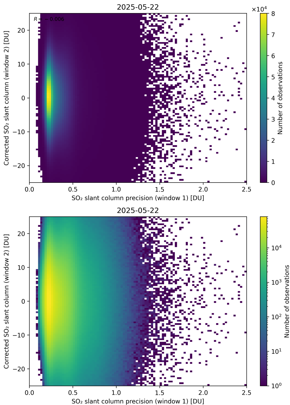
Figure 275: Scatter density plot of “SO 2 slant column precision (window 1)” against “Corrected SO 2 slant column (window 2)” for 2025-05-21 to 2025-05-23.
