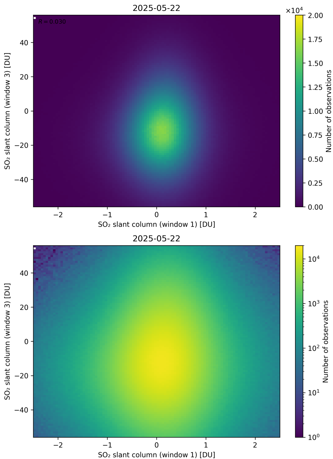
Figure 287: Scatter density plot of “SO 2 slant column (window 1)” against “SO 2 slant column (window 3)” for 2025-05-21 to 2025-05-23.
