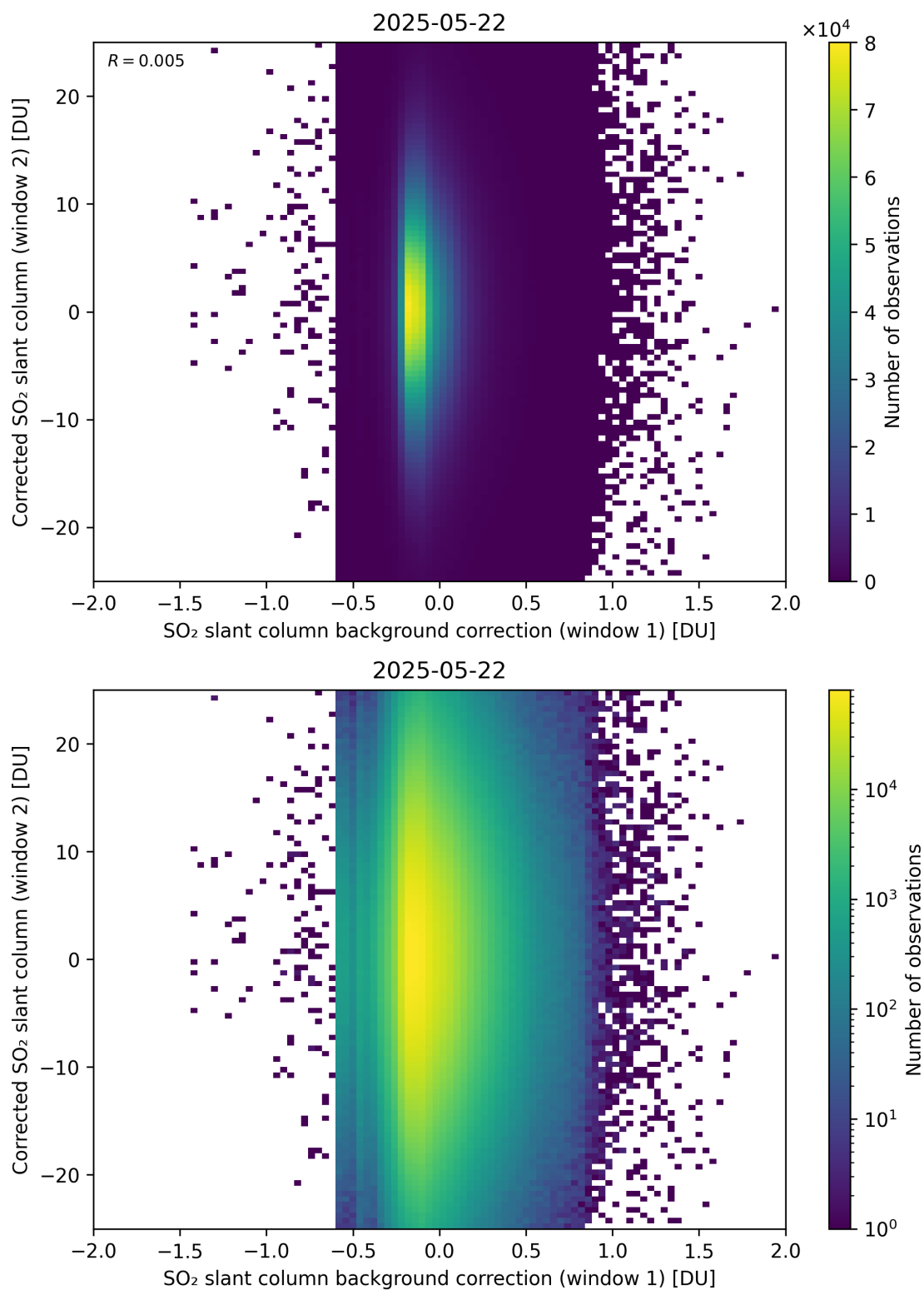
Figure 115: Scatter density plot of “SO 2 slant column background correction (window 1)” against “Corrected SO 2 slant column (window 2)” for 2025-05-21 to 2025-05-23.
