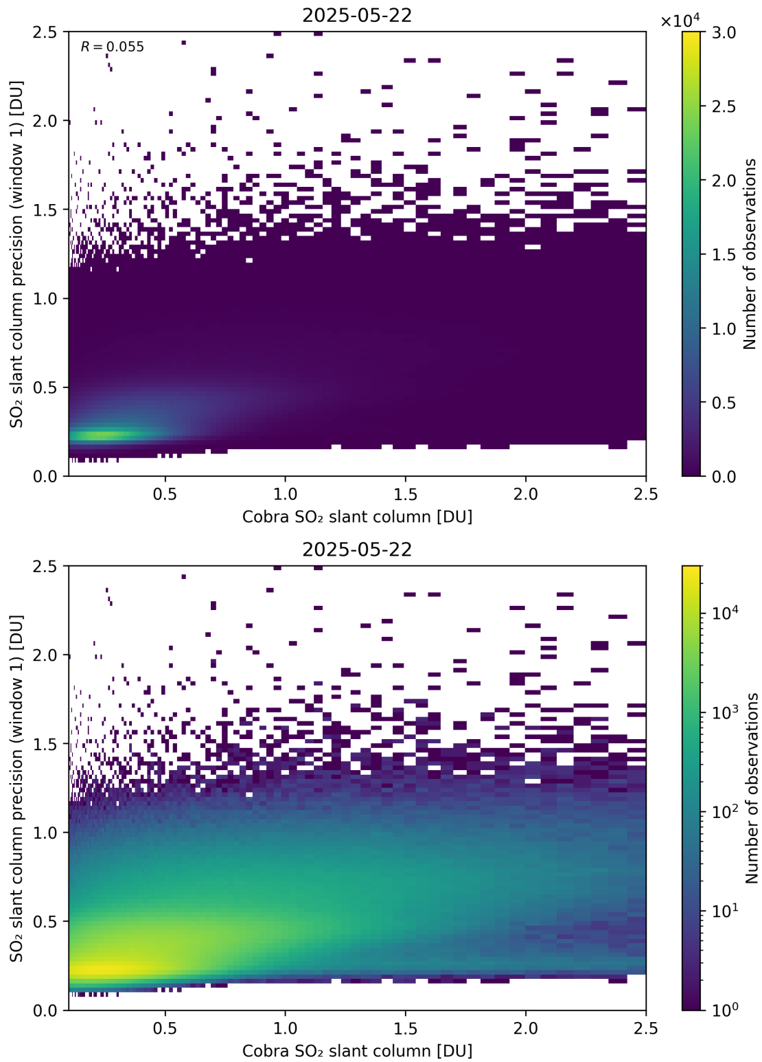
Figure 220: Scatter density plot of “Cobra SO 2 slant column” against “SO 2 slant column precision (window 1)” for 2025-05-21 to 2025-05-23.
