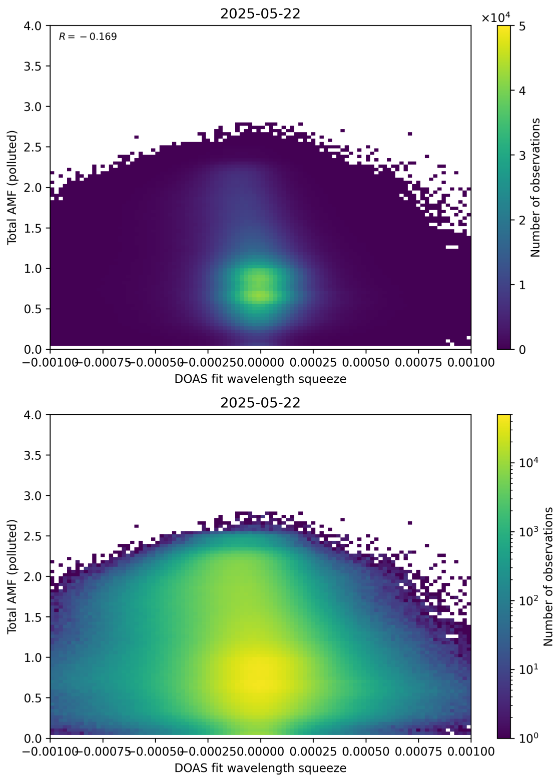
Figure 145: Scatter density plot of “DOAS fit wavelength squeeze” against “Total AMF (polluted)” for 2025-05-21 to 2025-05-23.
