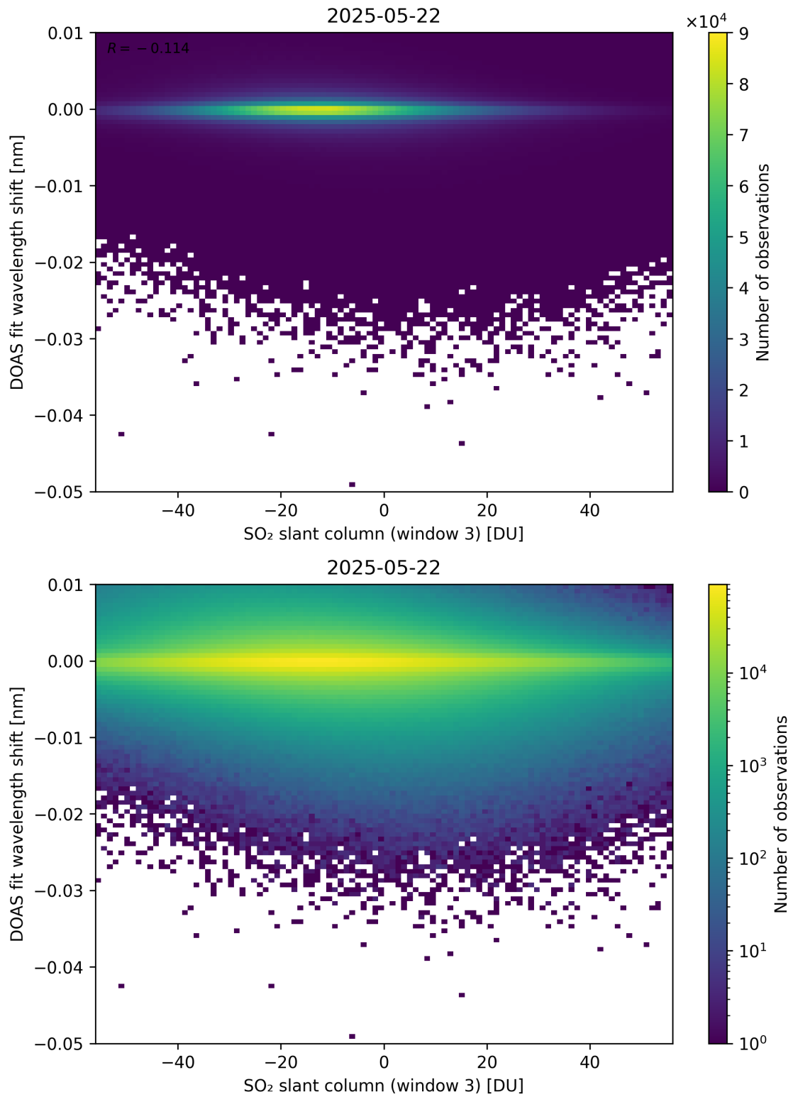
Figure 304: Scatter density plot of “SO 2 slant column (window 3)” against “DOAS fit wavelength shift” for 2025-05-21 to 2025-05-23.
