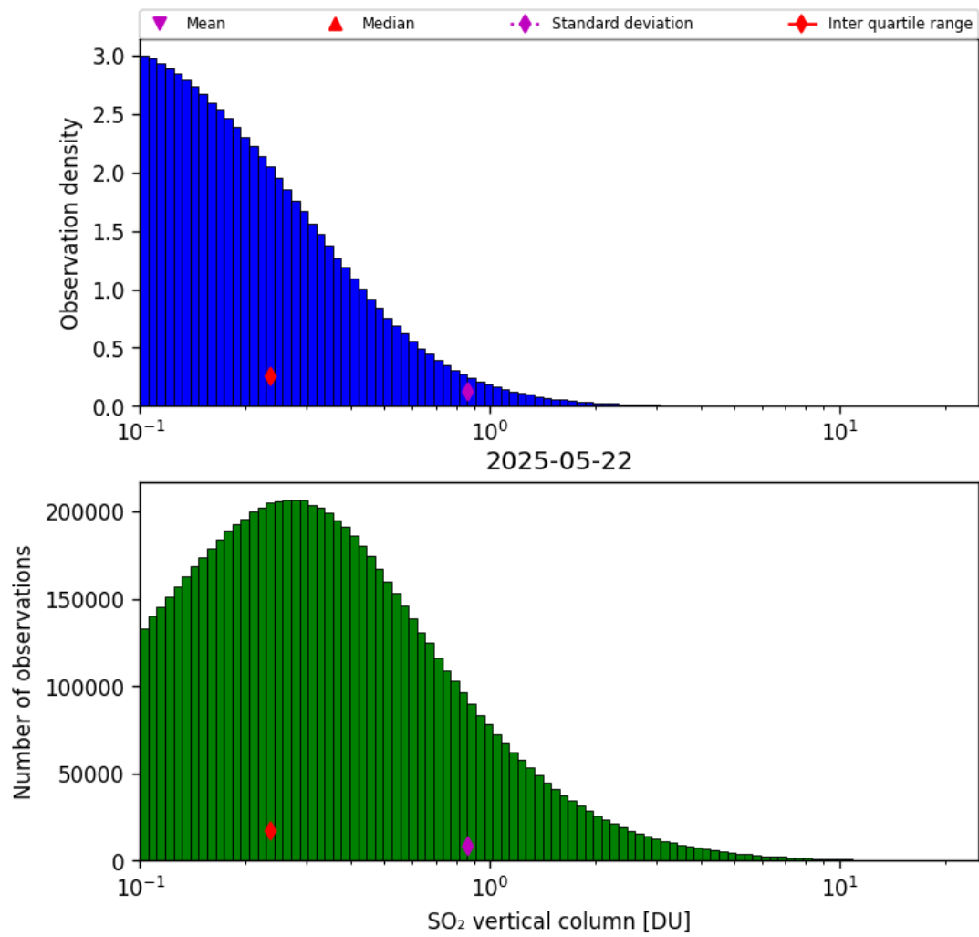
Figure 58: Histogram of “SO 2 vertical column” for 2025-05-21 to 2025-05-23
