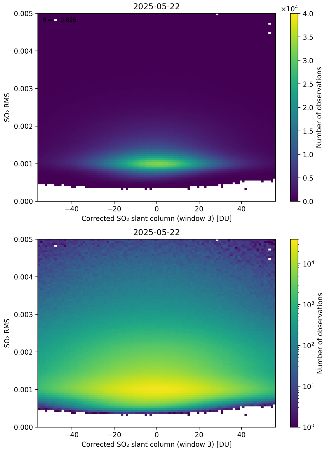
Figure 258: Scatter density plot of “Corrected SO 2 slant column (window 3)” against “SO 2 RMS” for 2025-05-21 to 2025-05-23.
