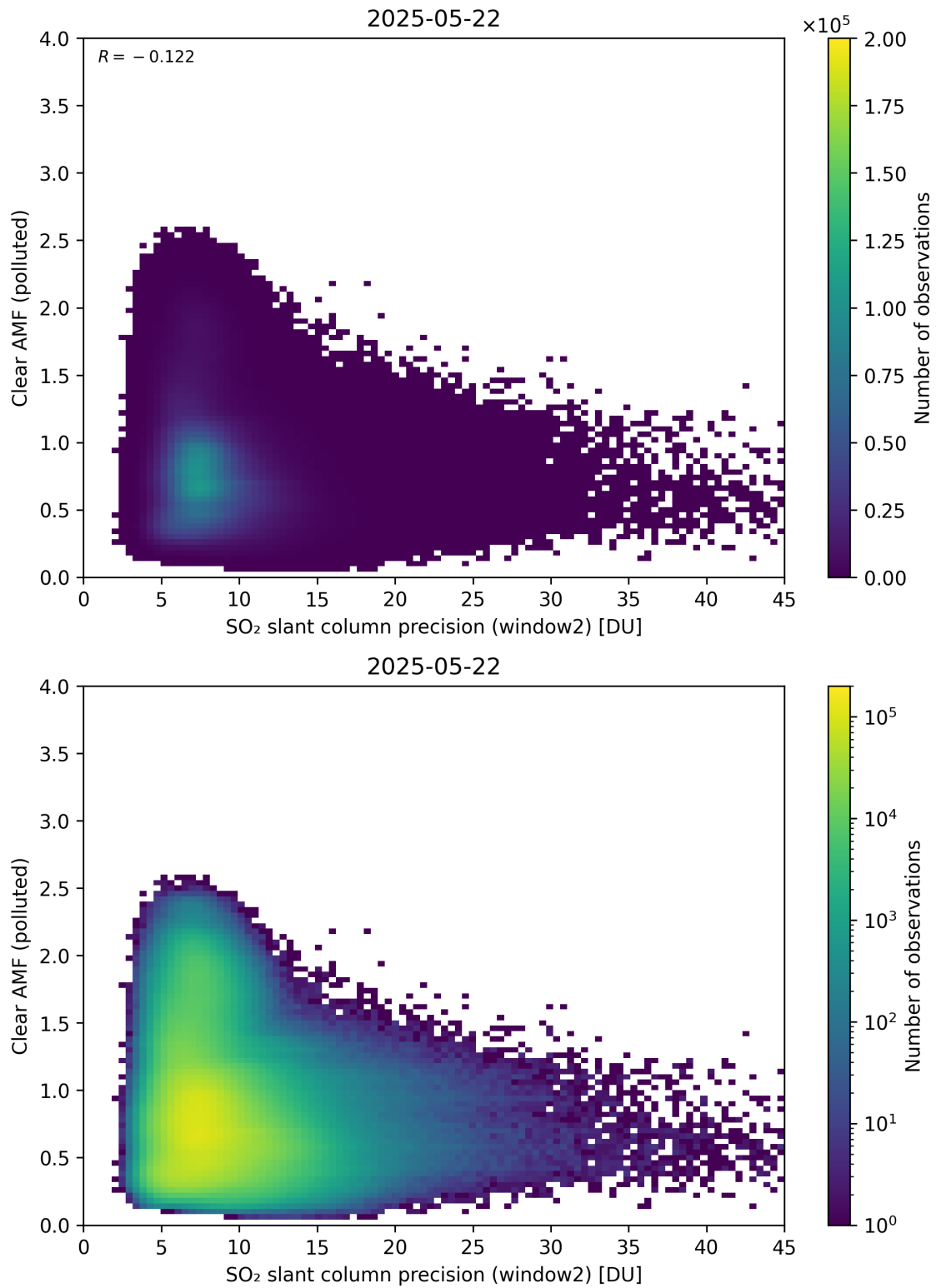
Figure 296: Scatter density plot of “SO 2 slant column precision (window2)” against “Clear AMF (polluted)” for 2025-05-21 to 2025-05-23.
