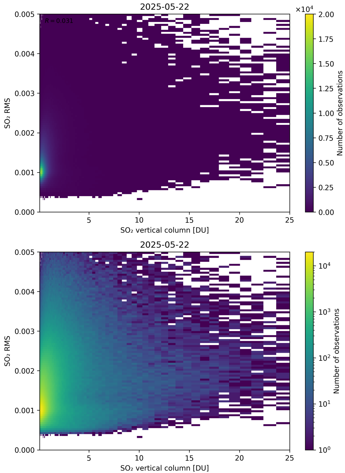
Figure 328: Scatter density plot of “SO 2 vertical column” against “SO 2 RMS” for 2025-05-21 to 2025-05-23.
