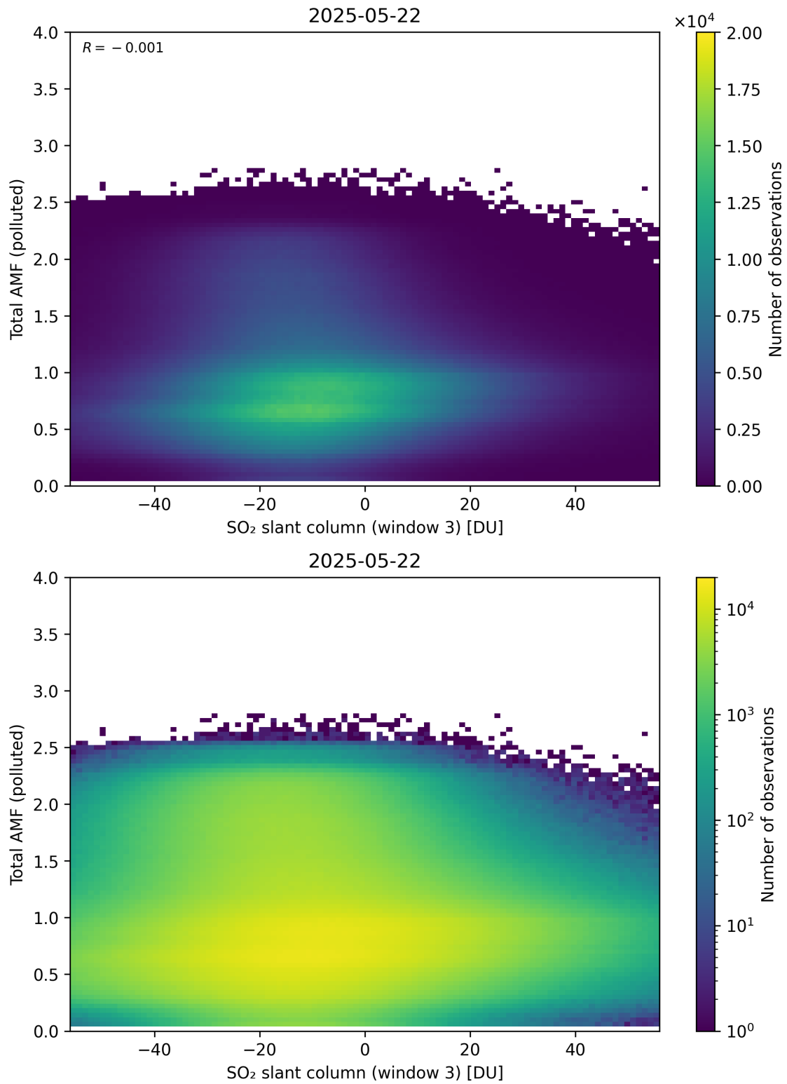
Figure 318: Scatter density plot of “SO 2 slant column (window 3)” against “Total AMF (polluted)” for 2025-05-21 to 2025-05-23.
