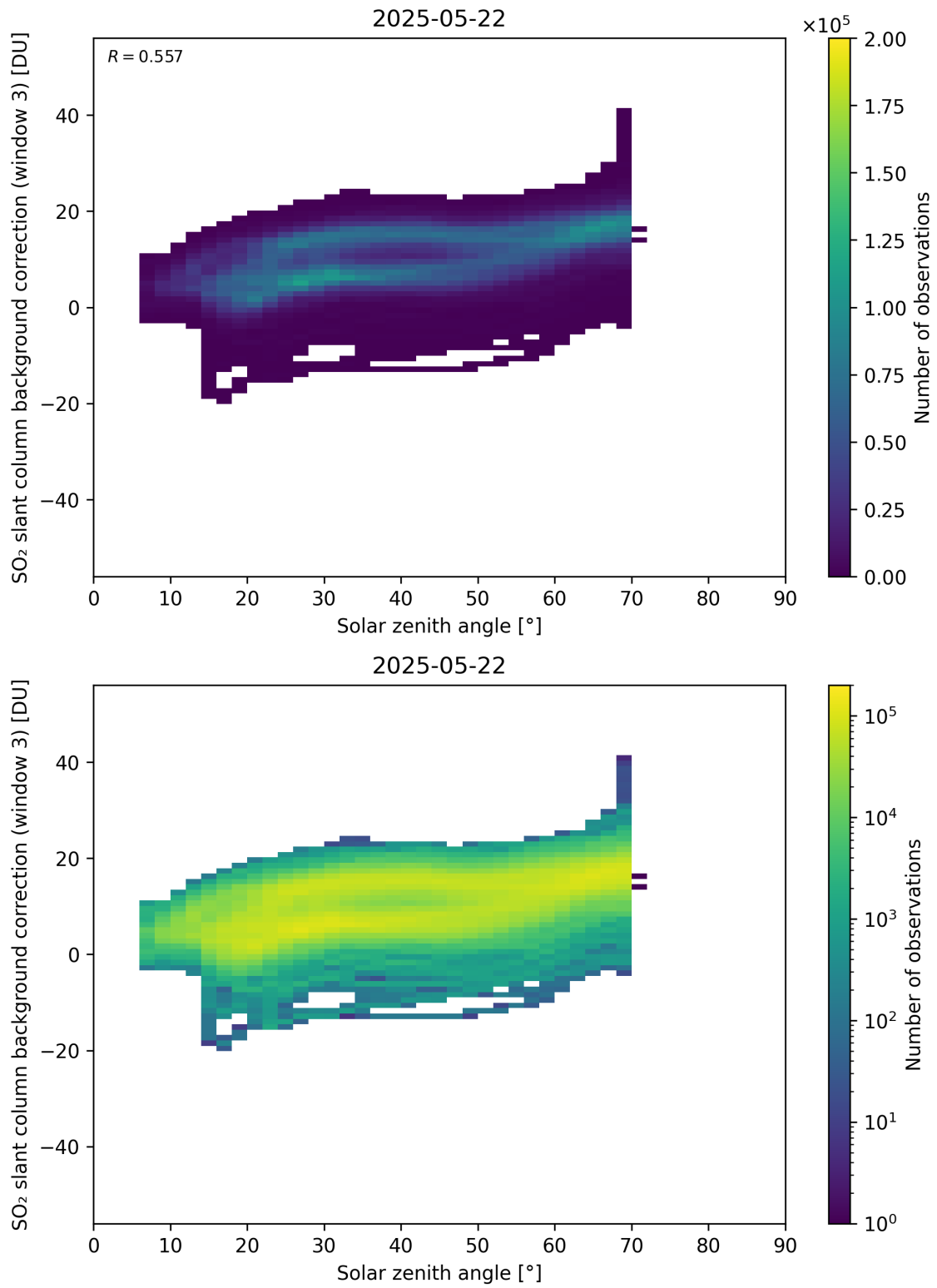
Figure 173: Scatter density plot of “Solar zenith angle” against “SO 2 slant column background correction (window 3)” for 2025-05-21 to 2025-05-23.
