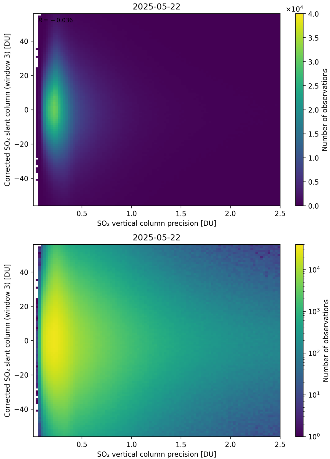
Figure 340: Scatter density plot of “SO 2 vertical column precision” against “Corrected SO 2 slant column (window 3)” for 2025-05-21 to 2025-05-23.
