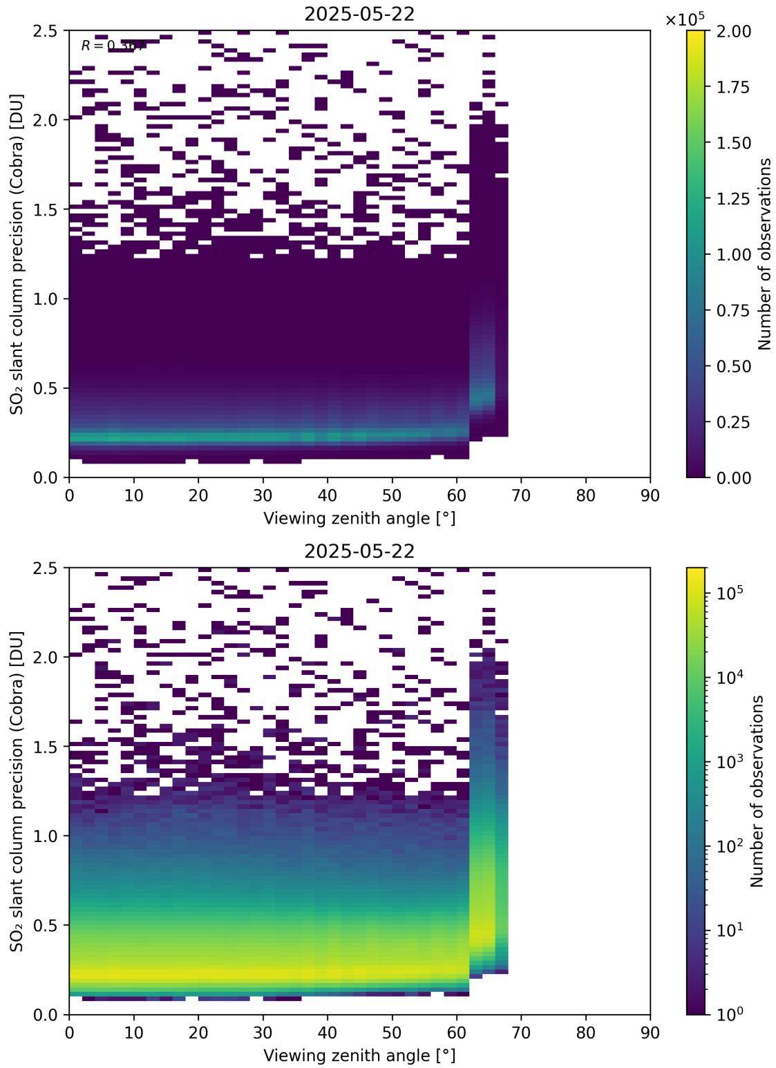
Figure 372: Scatter density plot of “Viewing zenith angle” against “SO 2 slant column precision (Cobra)” for 2025-05-21 to 2025-05-23.
