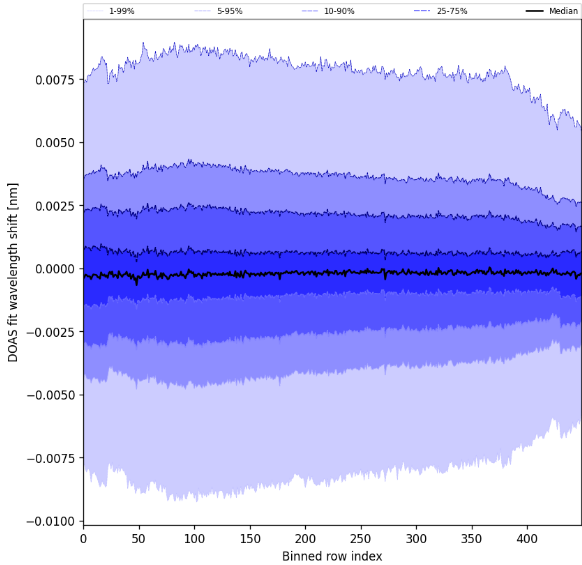
Figure 102: Along track statistics of “DOAS fit wavelength shift” for 2025-05-21 to 2025-05-23
