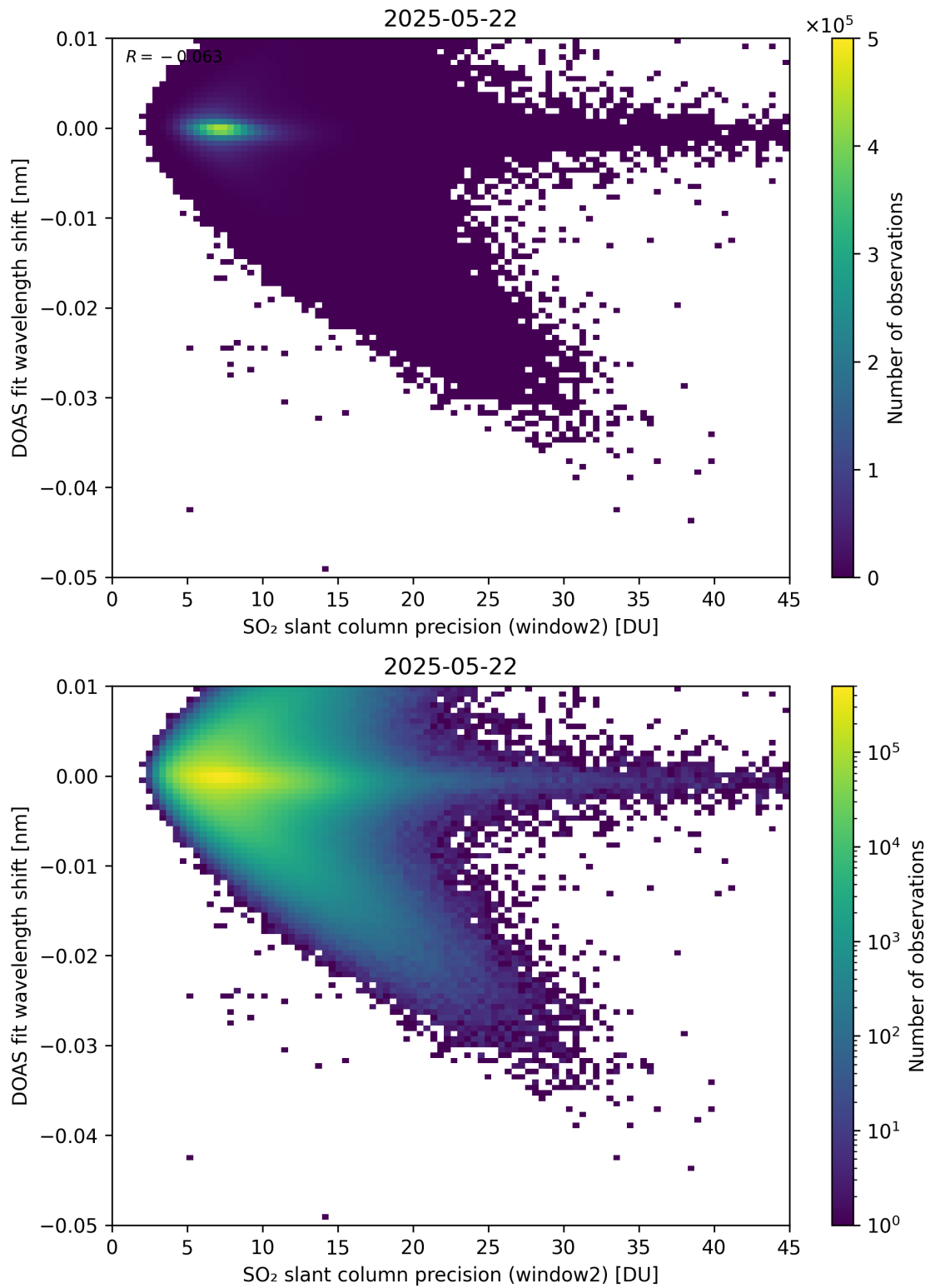
Figure 293: Scatter density plot of “SO 2 slant column precision (window2)” against “DOAS fit wavelength shift” for 2025-05-21 to 2025-05-23.
