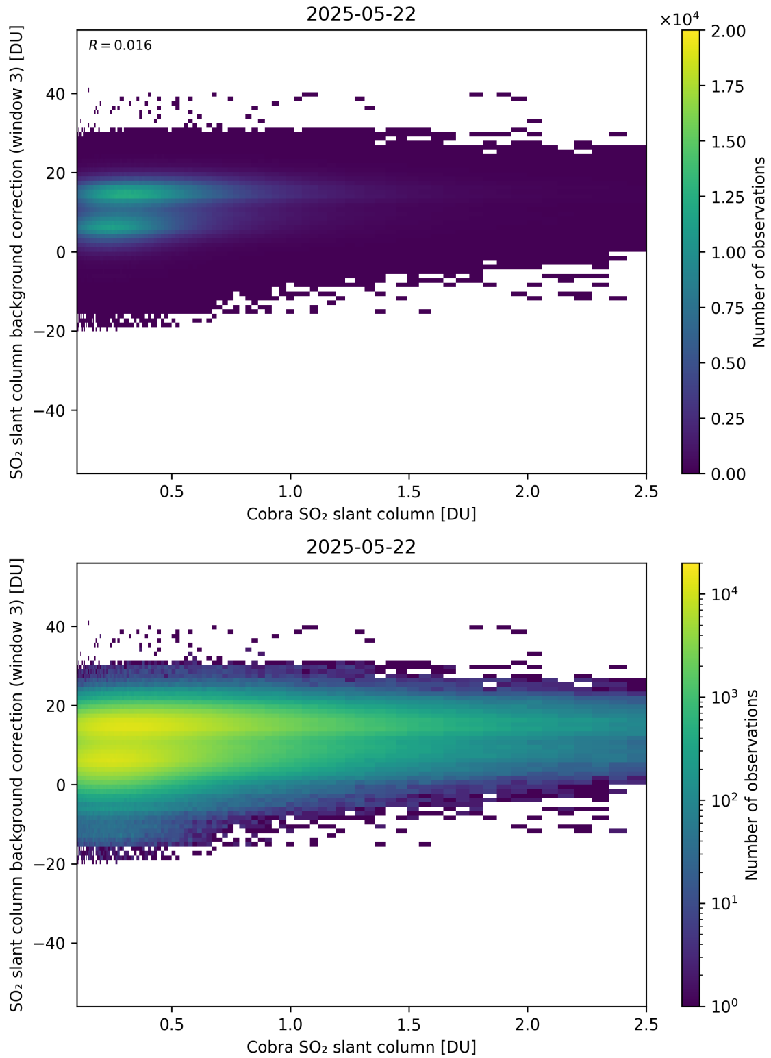
Figure 195: Scatter density plot of “Cobra SO 2 slant column” against “SO 2 slant column background correction (window 3)” for 2025-05-21 to 2025-05-23.
