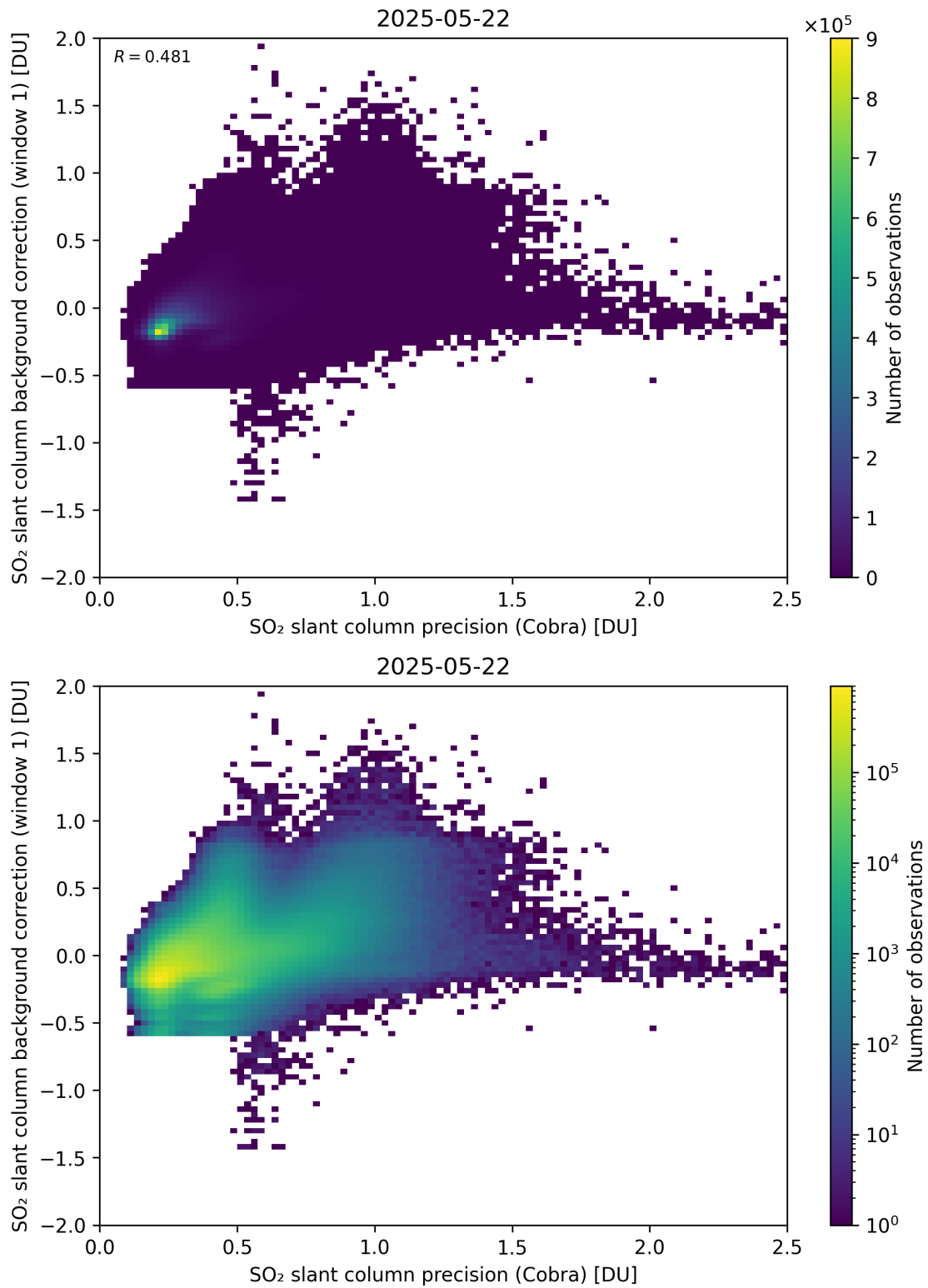
Figure 199: Scatter density plot of “SO 2 slant column precision (Cobra)” against “SO 2 slant column background correction (window 1)” for 2025-05-21 to 2025-05-23.
