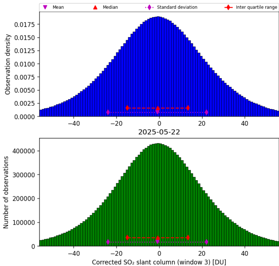
Figure 73: Histogram of “Corrected SO 2 slant column (window 3)” for 2025-05-21 to 2025-05-23
