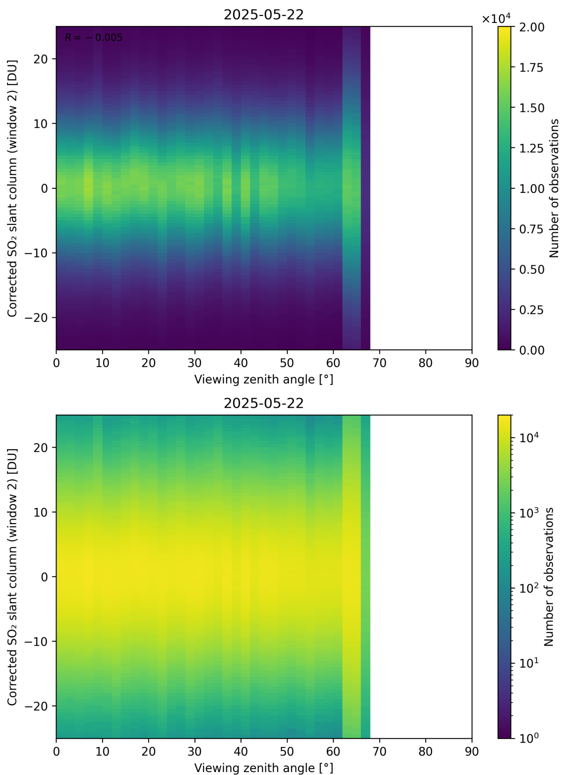
Figure 374: Scatter density plot of “Viewing zenith angle” against “Corrected SO 2 slant column (window 2)” for 2025-05-21 to 2025-05-23.
