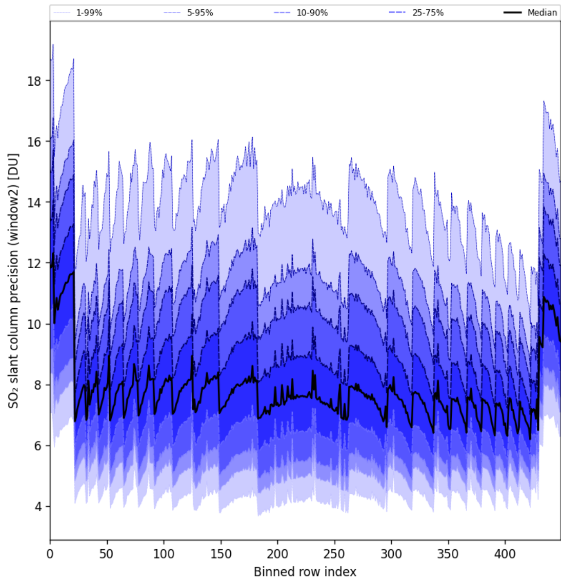
Figure 94: Along track statistics of “SO 2 slant column precision (window2)” for 2025-05-21 to 2025-05-23
