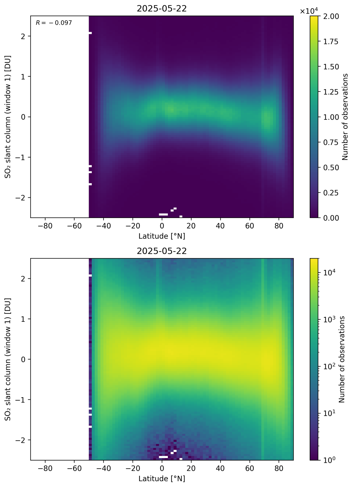
Figure 162: Scatter density plot of “Latitude” against “SO 2 slant column (window 1)” for 2025-05-21 to 2025-05-23.
