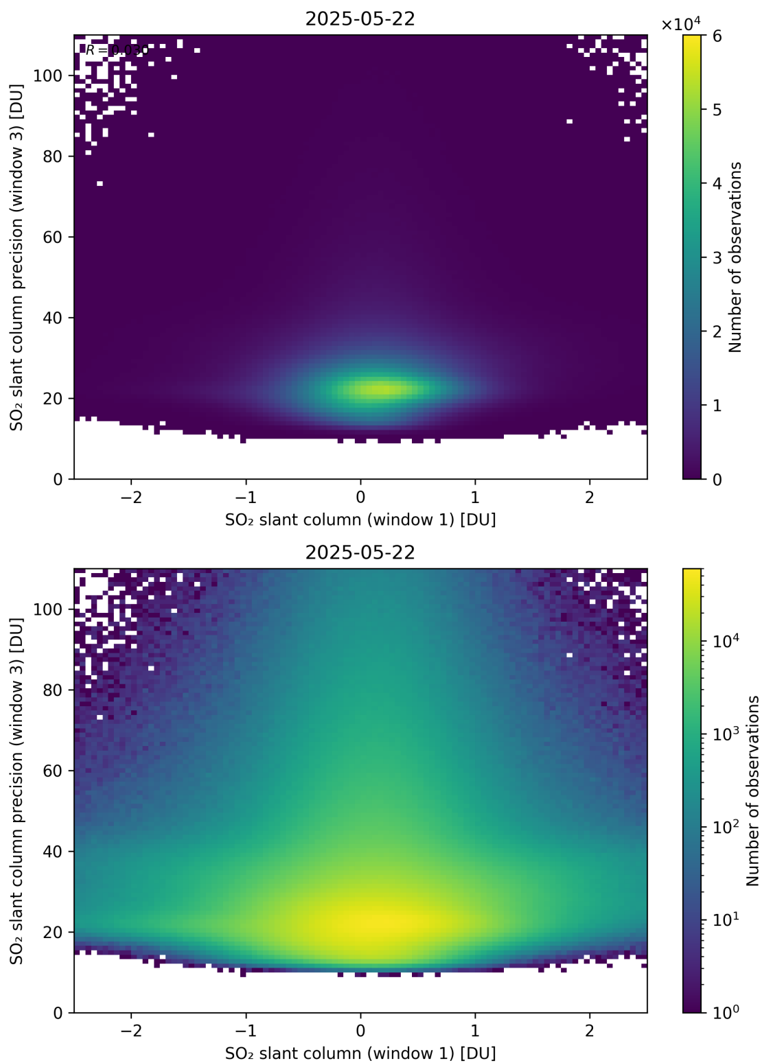
Figure 288: Scatter density plot of “SO 2 slant column (window 1)” against “SO 2 slant column precision (window 3)” for 2025-05-21 to 2025-05-23.
