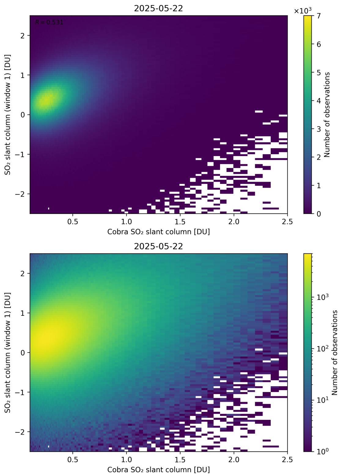
Figure 219: Scatter density plot of “Cobra SO 2 slant column” against “SO 2 slant column (window 1)” for 2025-05-21 to 2025-05-23.
