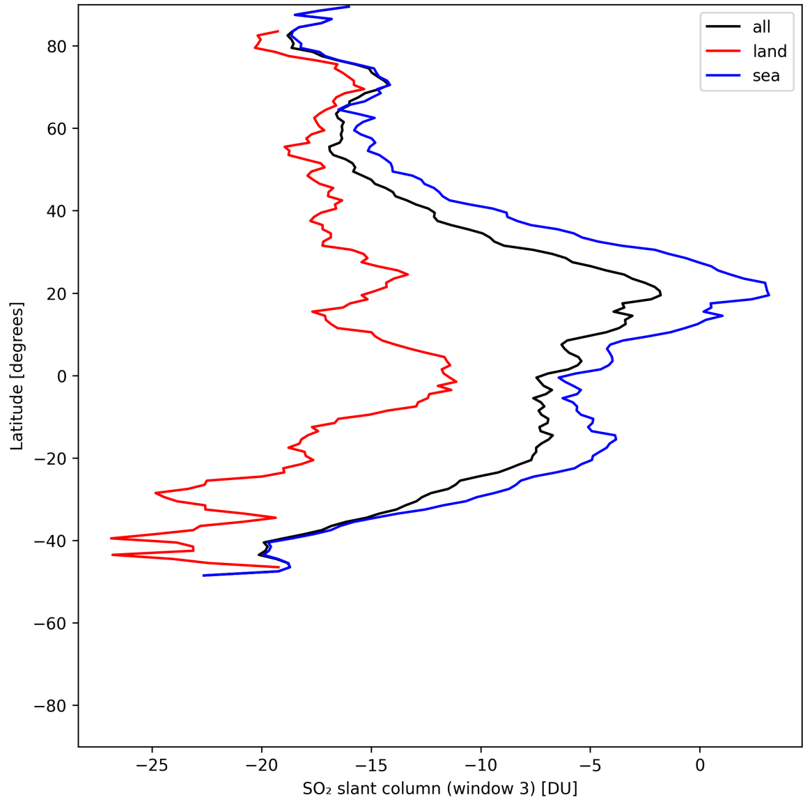
Figure 45: Zonal average of “SO 2 slant column (window 3)” for 2025-05-21 to 2025-05-23.
