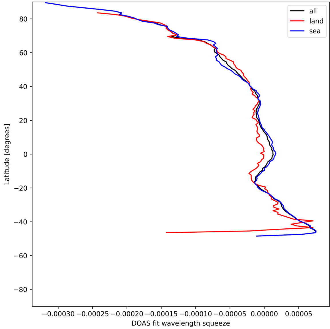
Figure 51: Zonal average of “DOAS fit wavelength squeeze” for 2025-05-21 to 2025-05-23.
