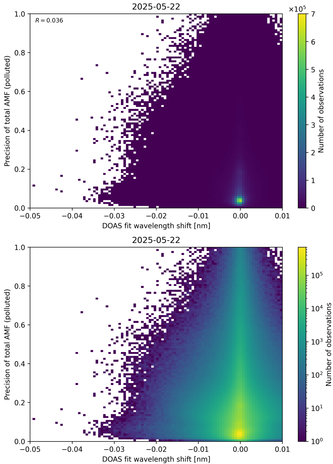
Figure 142: Scatter density plot of “DOAS fit wavelength shift” against “Precision of total AMF (polluted)” for 2025-05-21 to 2025-05-23.
