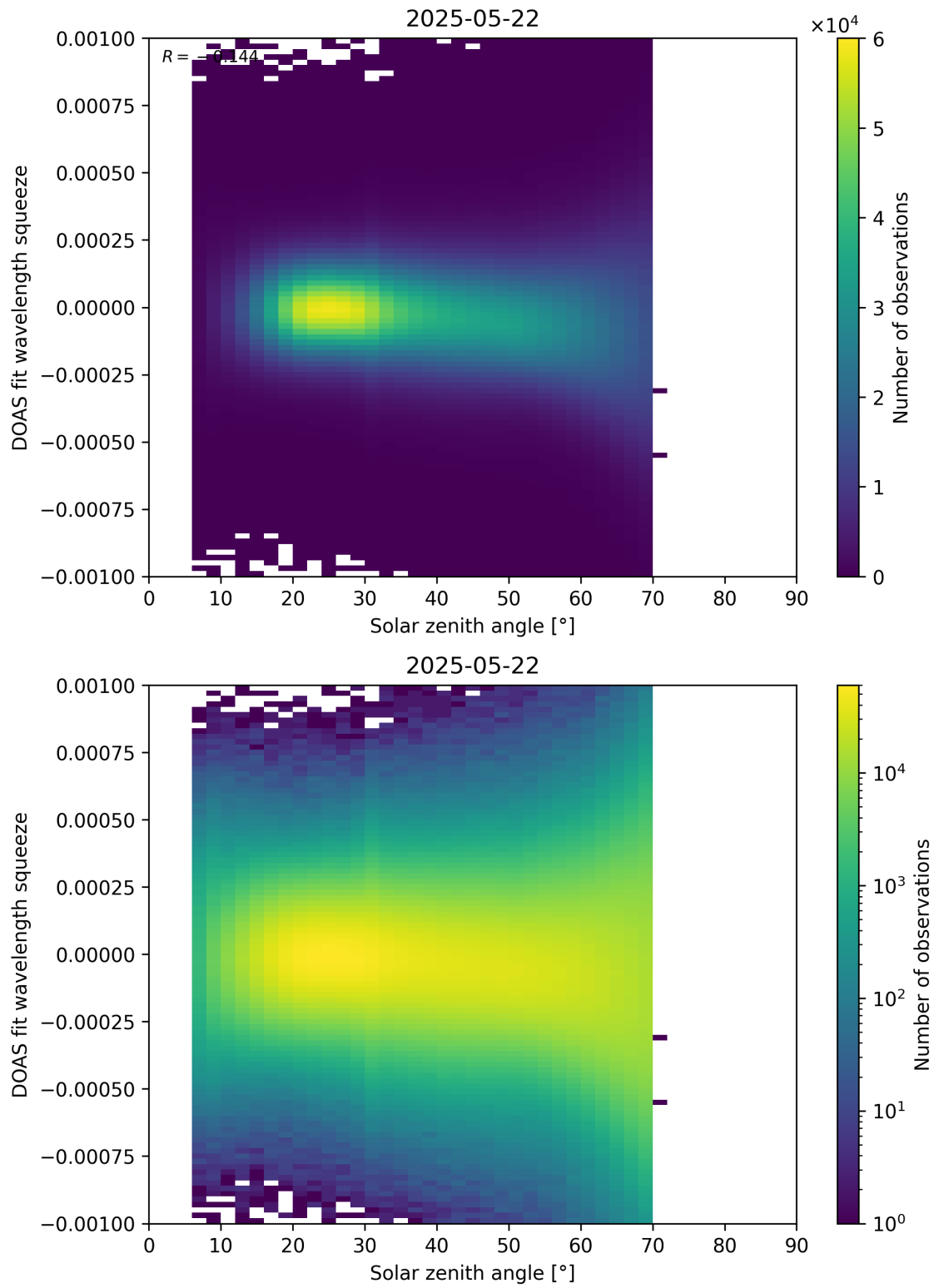
Figure 175: Scatter density plot of “Solar zenith angle” against “DOAS fit wavelength squeeze” for 2025-05-21 to 2025-05-23.
