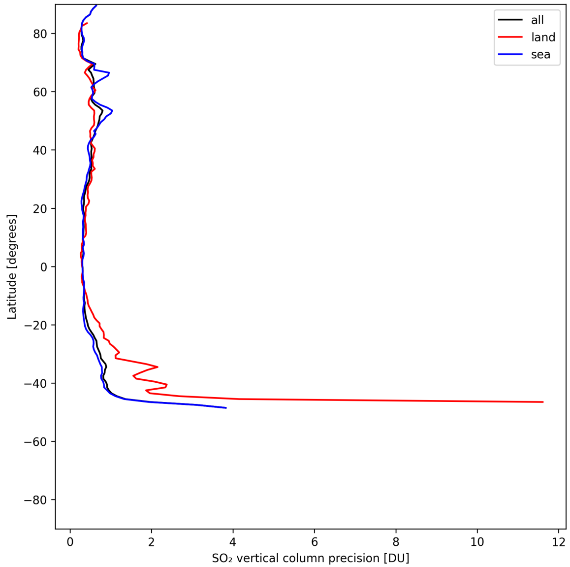
Figure 33: Zonal average of “SO 2 vertical column precision” for 2025-05-21 to 2025-05-23.
