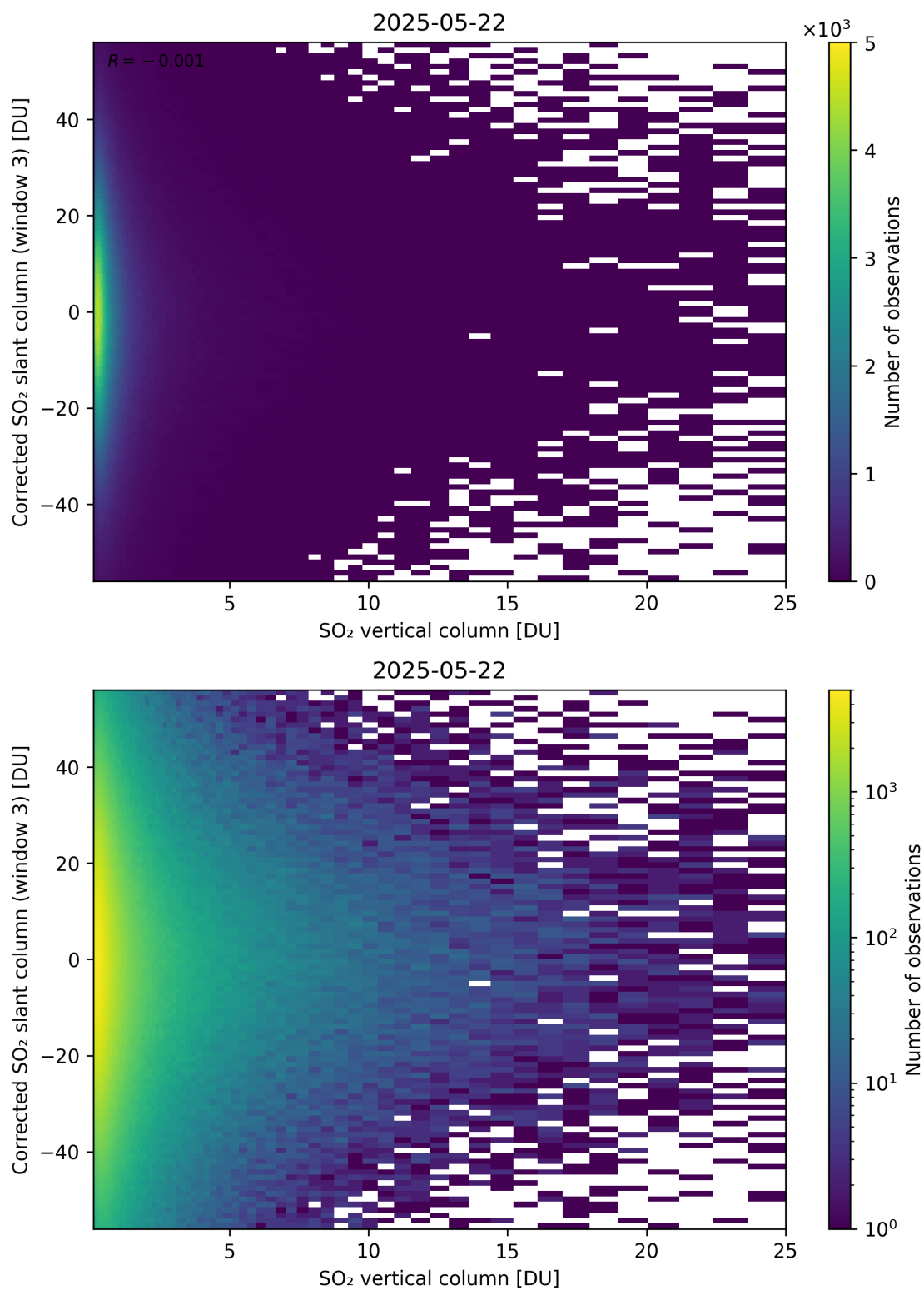
Figure 353: Scatter density plot of “SO 2 vertical column” against “Corrected SO 2 slant column (window 3)” for 2025-05-21 to 2025-05-23.
