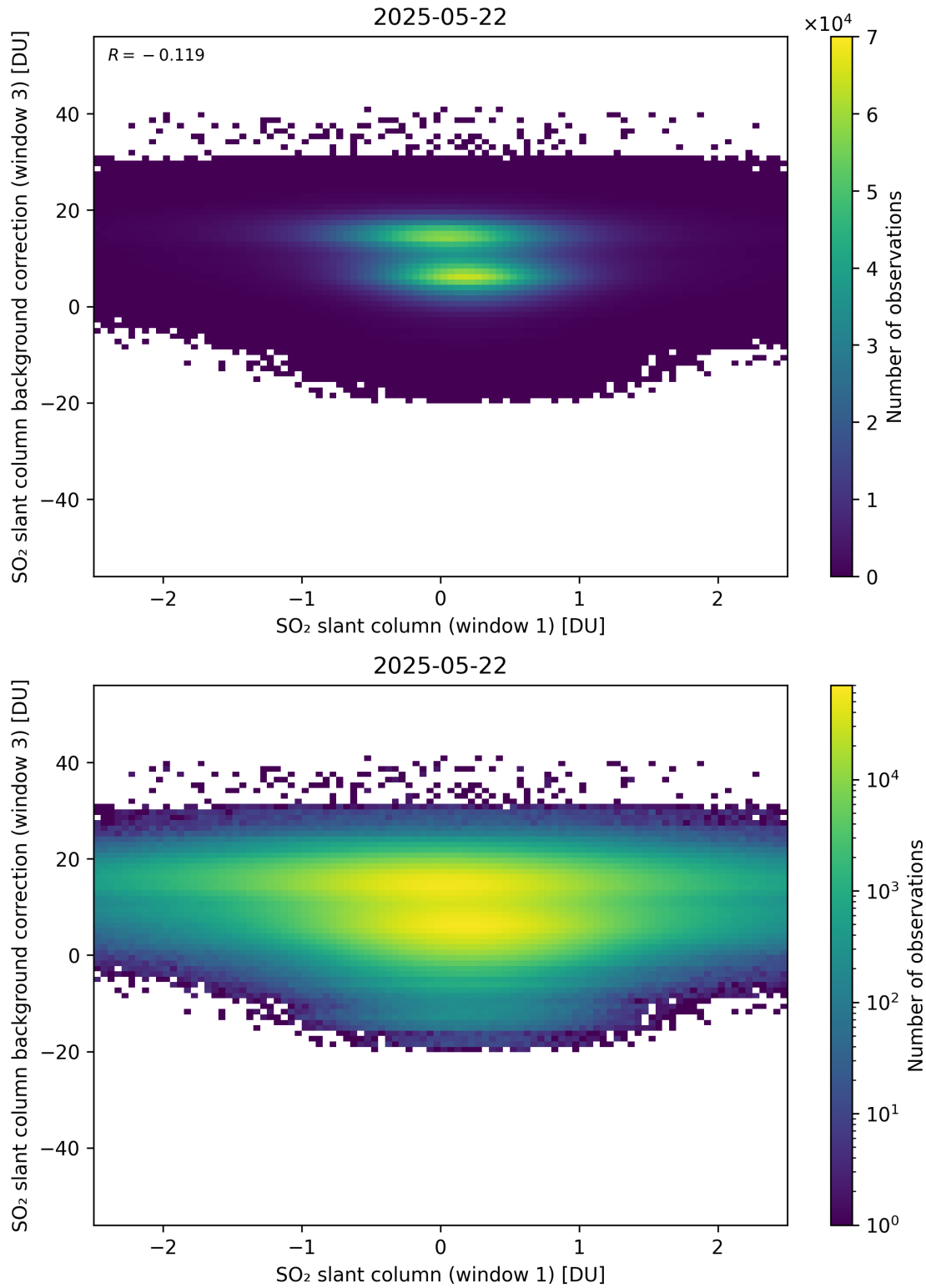
Figure 264: Scatter density plot of “SO 2 slant column (window 1)” against “SO 2 slant column background correction (window 3)” for 2025-05-21 to 2025-05-23.
