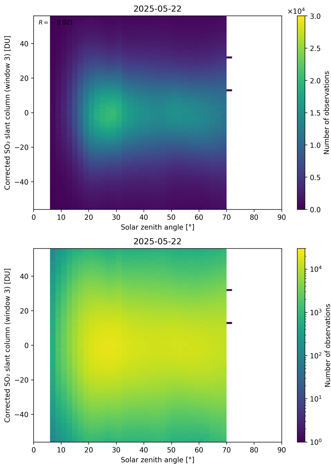
Figure 183: Scatter density plot of “Solar zenith angle” against “Corrected SO 2 slant column (window 3)” for 2025-05-21 to 2025-05-23.
