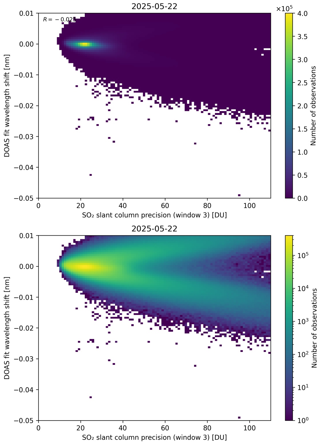
Figure 308: Scatter density plot of “SO 2 slant column precision (window 3)” against “DOAS fit wavelength shift” for 2025-05-21 to 2025-05-23.
