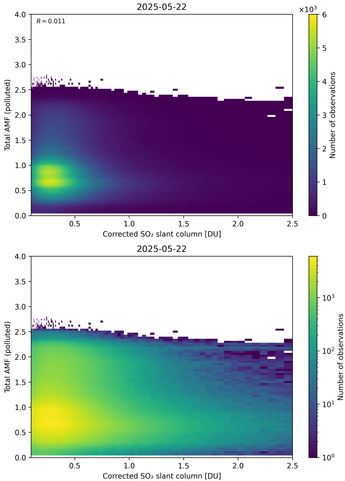
Figure 242: Scatter density plot of “Corrected SO 2 slant column” against “Total AMF (polluted)” for 2025-05-21 to 2025-05-23.
