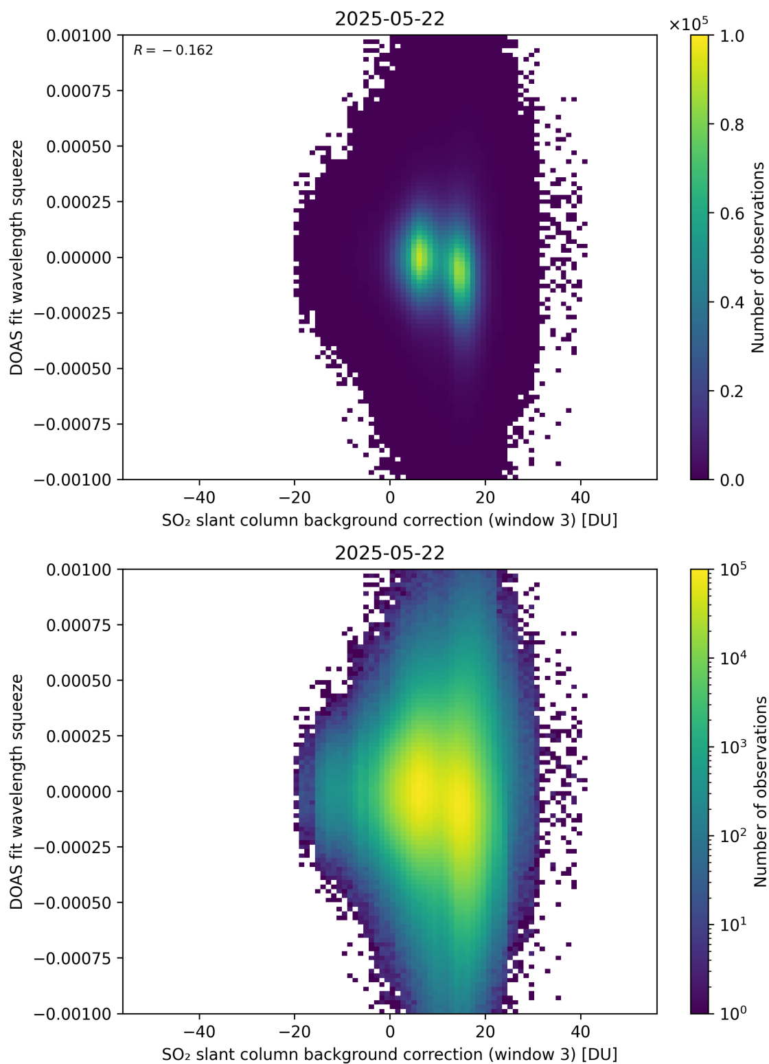
Figure 133: Scatter density plot of “SO 2 slant column background correction (window 3)” against “DOAS fit wavelength squeeze” for 2025-05-21 to 2025-05-23.
