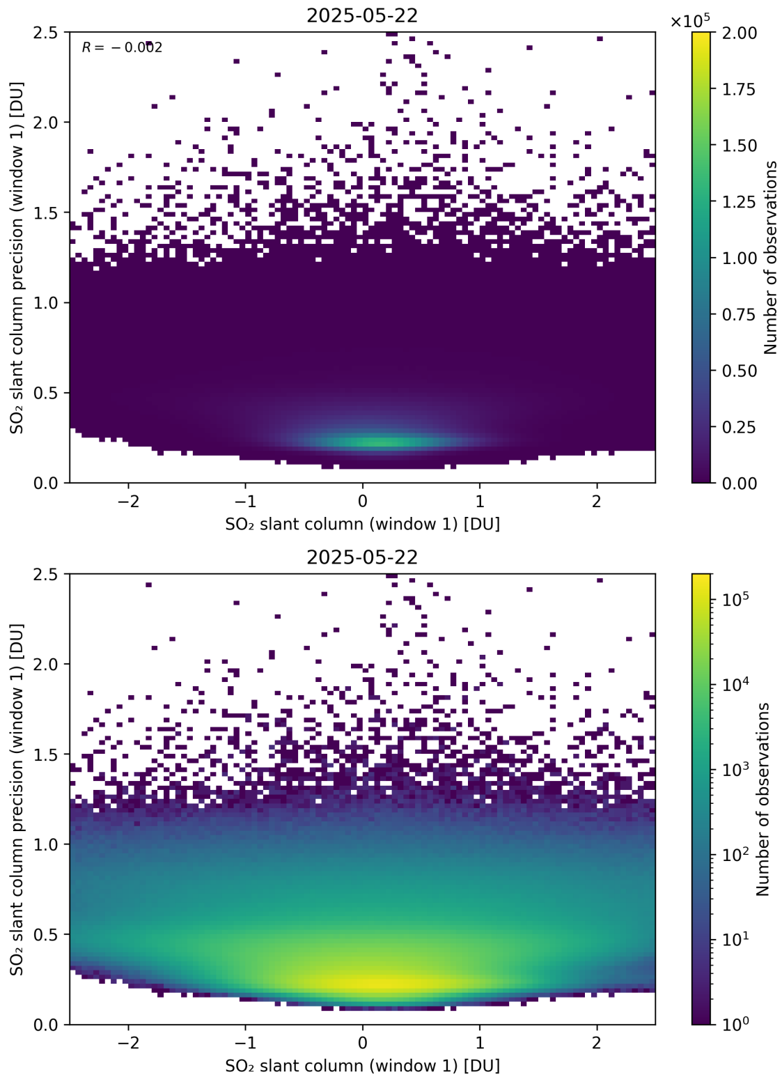
Figure 285: Scatter density plot of “SO 2 slant column (window 1)” against “SO 2 slant column precision (window 1)” for 2025-05-21 to 2025-05-23.
