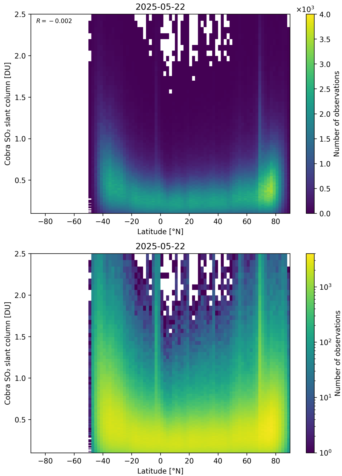
Figure 157: Scatter density plot of “Latitude” against “Cobra SO 2 slant column” for 2025-05-21 to 2025-05-23.
