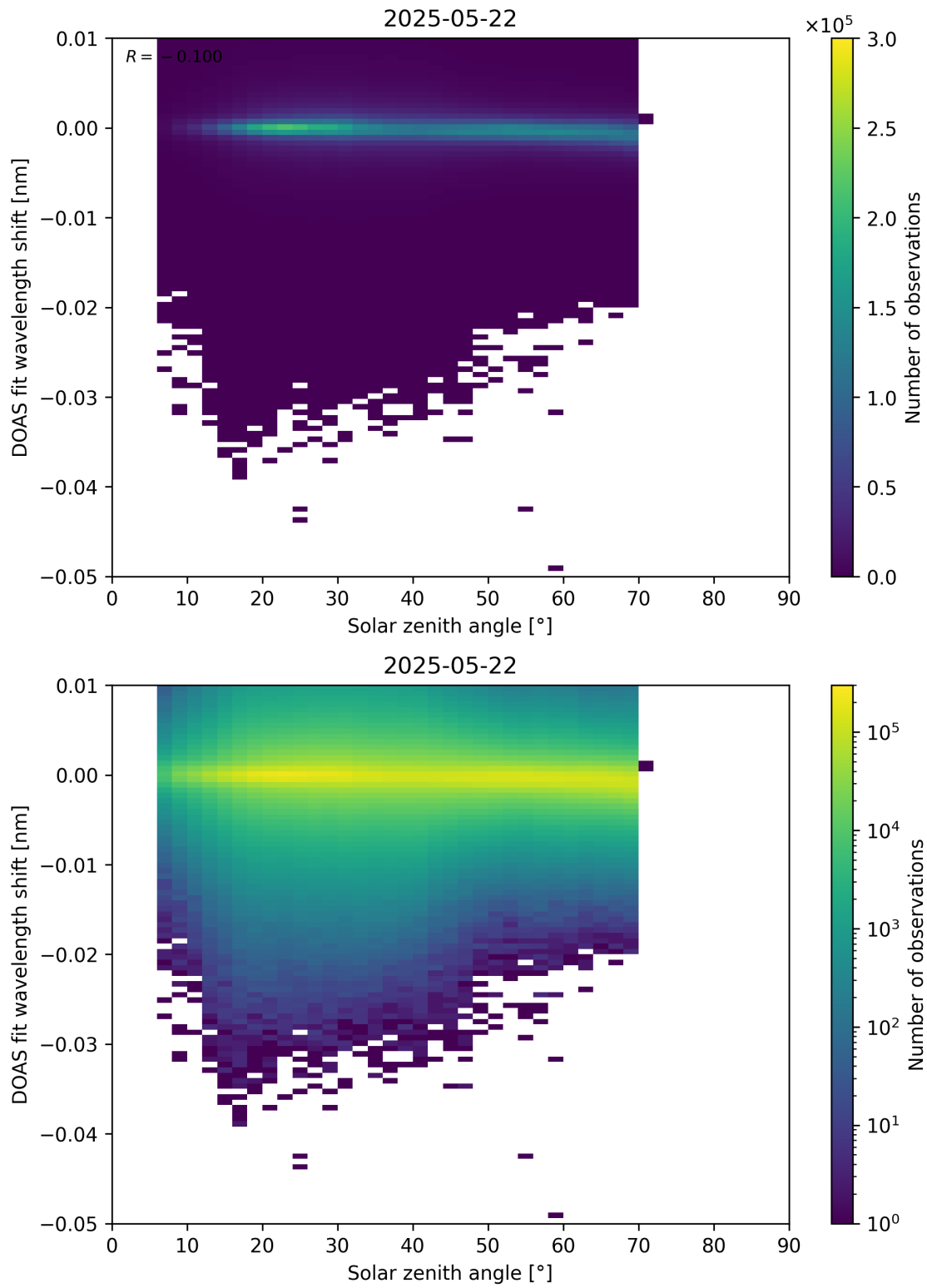
Figure 174: Scatter density plot of “Solar zenith angle” against “DOAS fit wavelength shift” for 2025-05-21 to 2025-05-23.
