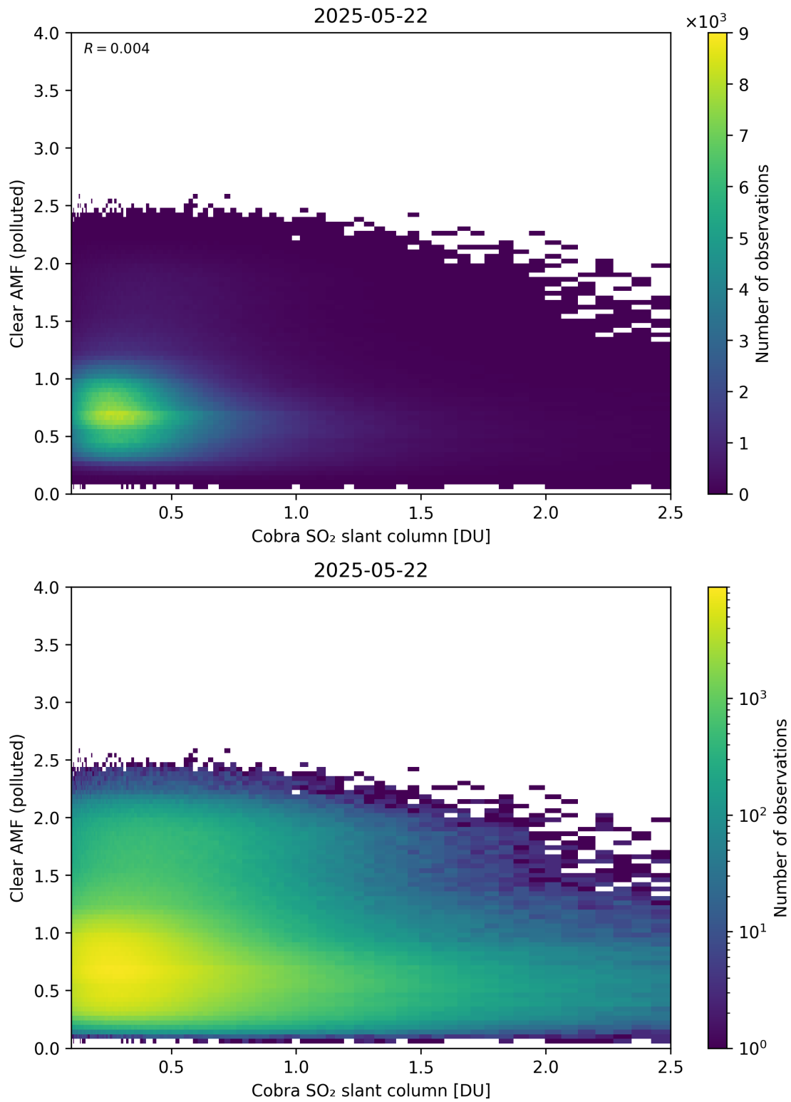
Figure 215: Scatter density plot of “Cobra SO 2 slant column” against “Clear AMF (polluted)” for 2025-05-21 to 2025-05-23.
