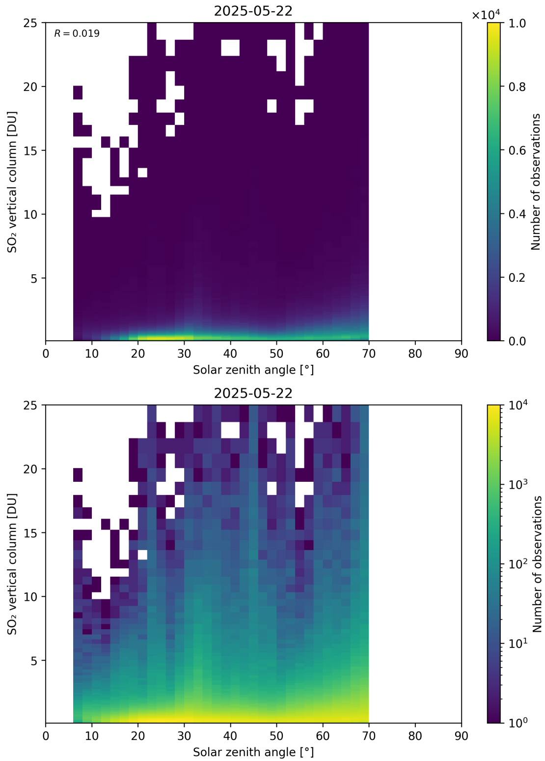
Figure 191: Scatter density plot of “Solar zenith angle” against “SO 2 vertical column” for 2025-05-21 to 2025-05-23.
