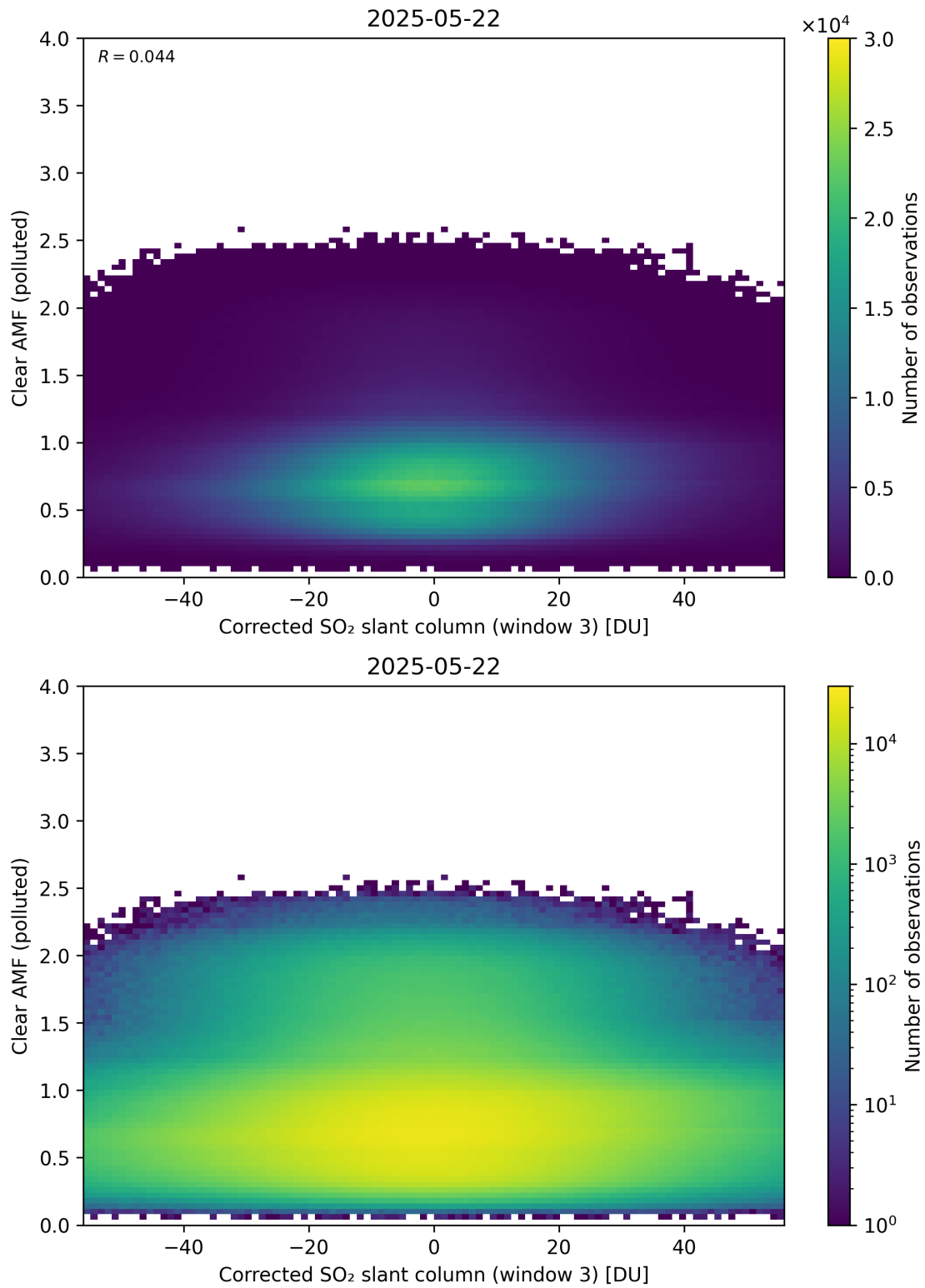
Figure 259: Scatter density plot of “Corrected SO 2 slant column (window 3)” against “Clear AMF (polluted)” for 2025-05-21 to 2025-05-23.
