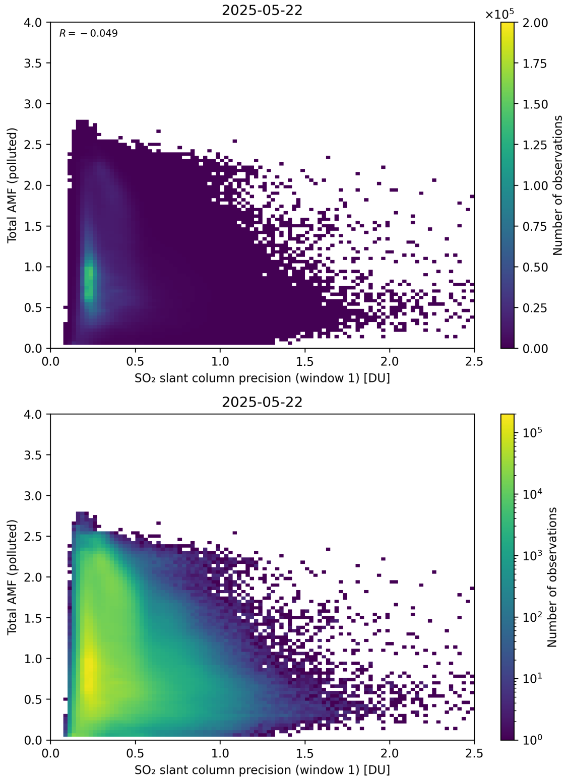
Figure 280: Scatter density plot of “SO 2 slant column precision (window 1)” against “Total AMF (polluted)” for 2025-05-21 to 2025-05-23.
