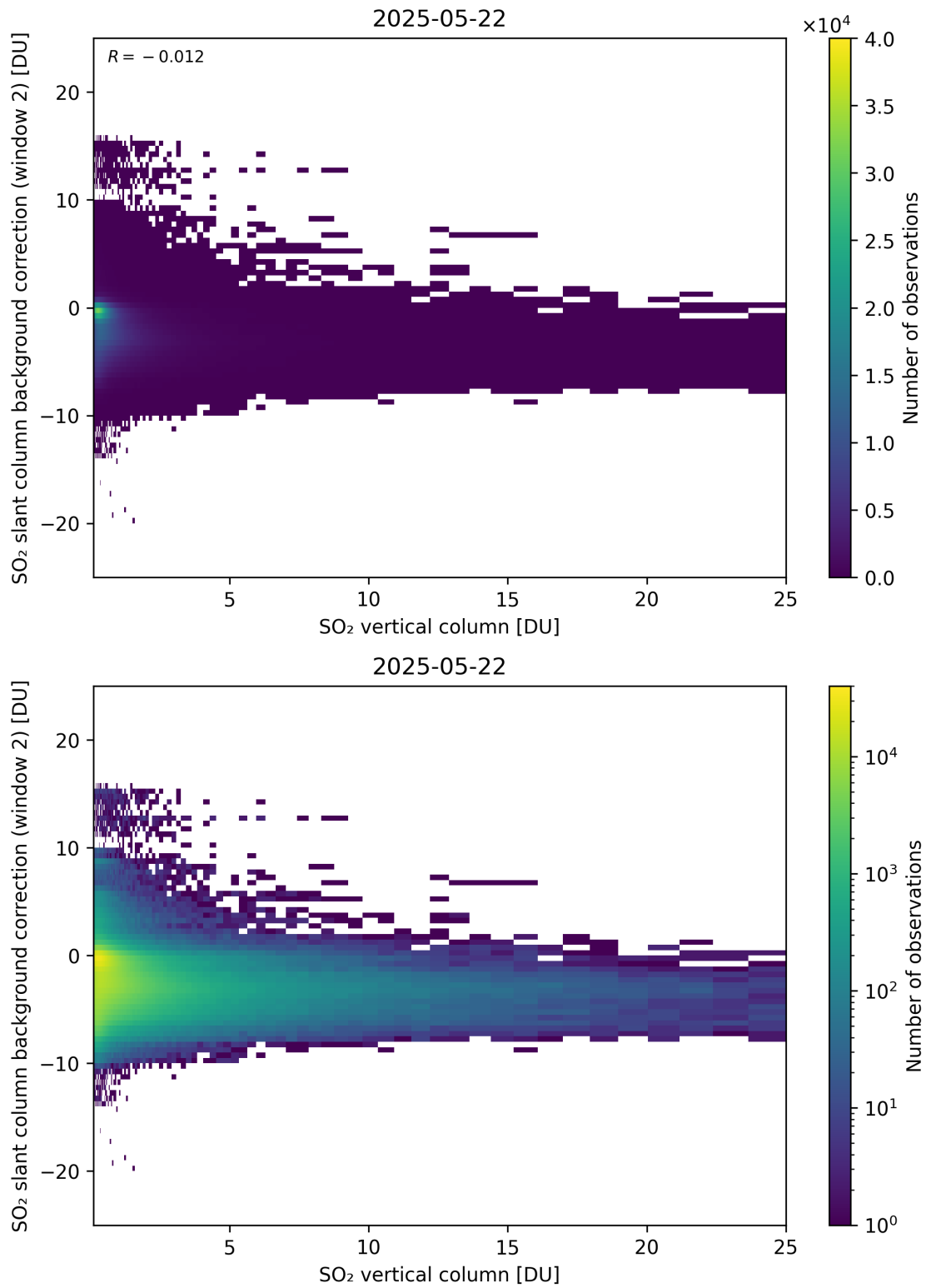
Figure 324: Scatter density plot of “SO 2 vertical column” against “SO 2 slant column background correction (window 2)” for 2025-05-21 to 2025-05-23.
