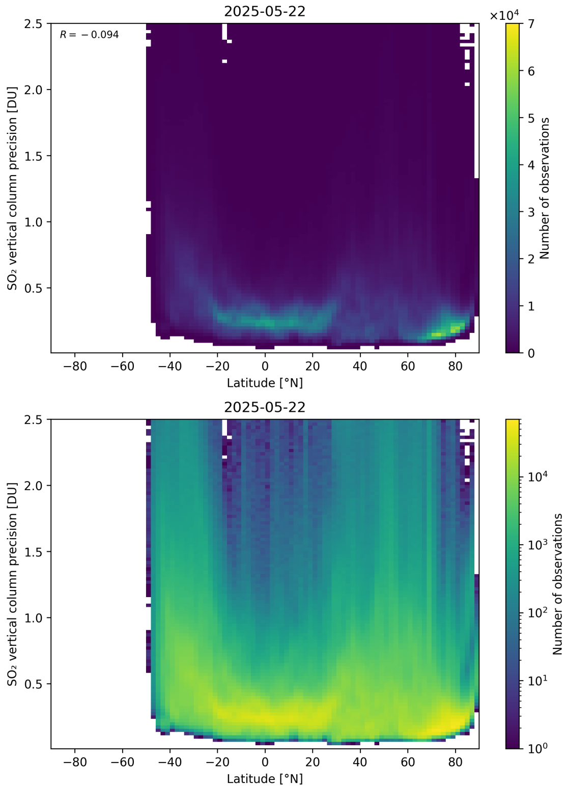
Figure 170: Scatter density plot of “Latitude” against “SO 2 vertical column precision” for 2025-05-21 to 2025-05-23.
