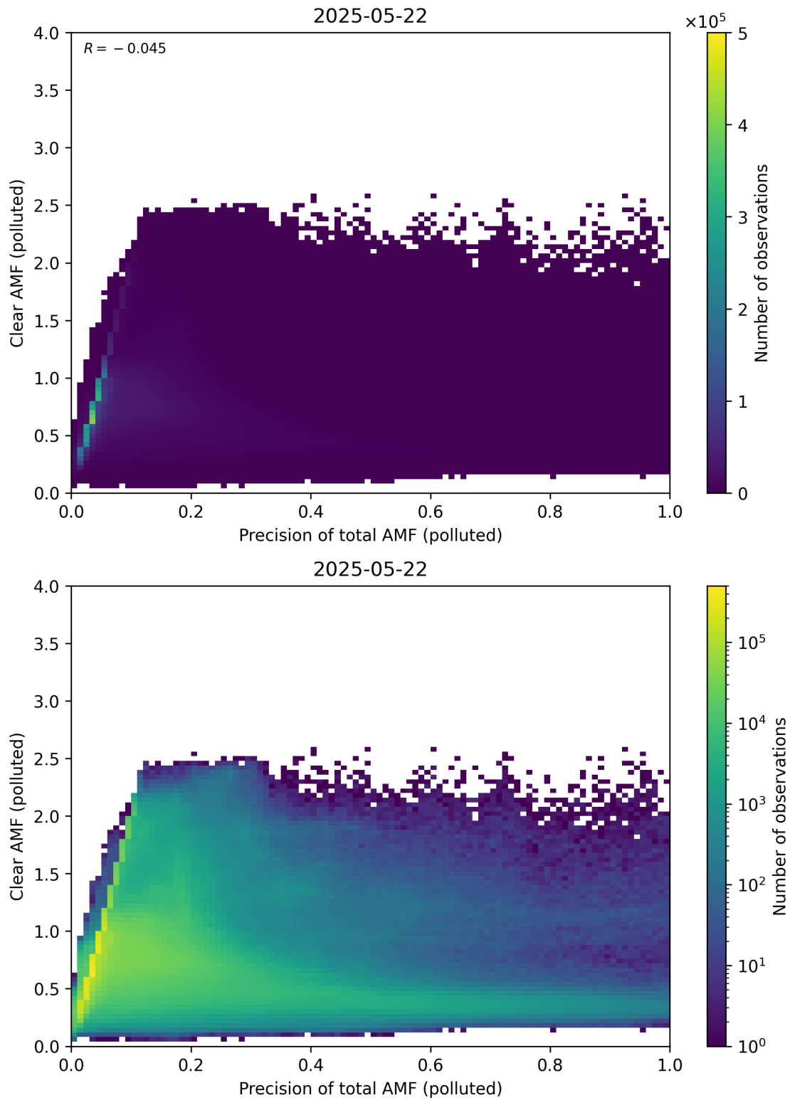
Figure 320: Scatter density plot of “Precision of total AMF (polluted)” against “Clear AMF (polluted)” for 2025-05-21 to 2025-05-23.
