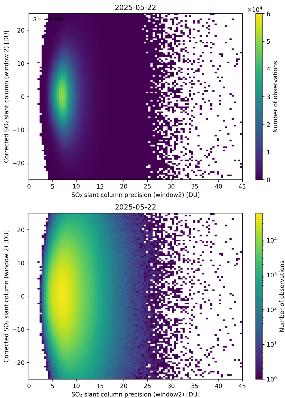
Figure 297: Scatter density plot of “SO 2 slant column precision (window2)” against “Corrected SO 2 slant column (window 2)” for 2025-05-21 to 2025-05-23.
