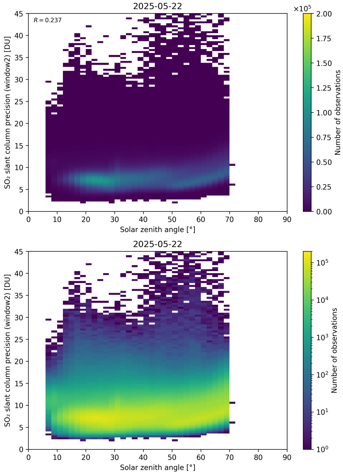
Figure 186: Scatter density plot of “Solar zenith angle” against “SO 2 slant column precision (window2)” for 2025-05-21 to 2025-05-23.
