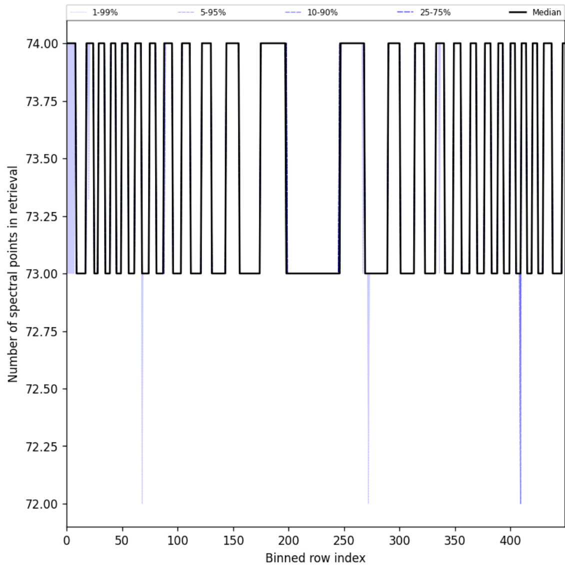
Figure 108: Along track statistics of “Number of spectral points in retrieval” for 2025-05-21 to 2025-05-23
