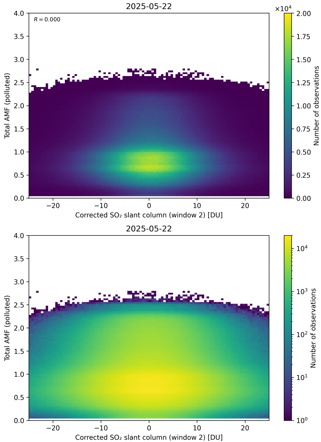
Figure 253: Scatter density plot of “Corrected SO 2 slant column (window 2)” against “Total AMF (polluted)” for 2025-05-21 to 2025-05-23.
