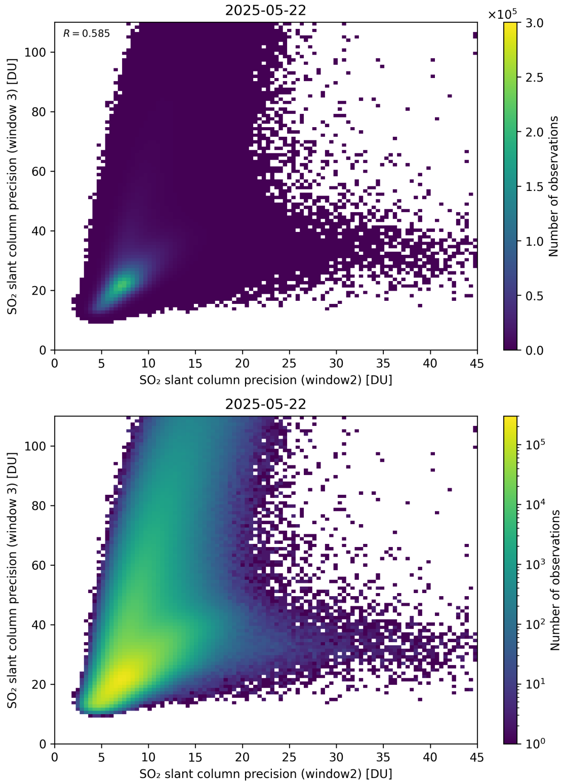
Figure 300: Scatter density plot of “SO 2 slant column precision (window2)” against “SO 2 slant column precision (window 3)” for 2025-05-21 to 2025-05-23.
