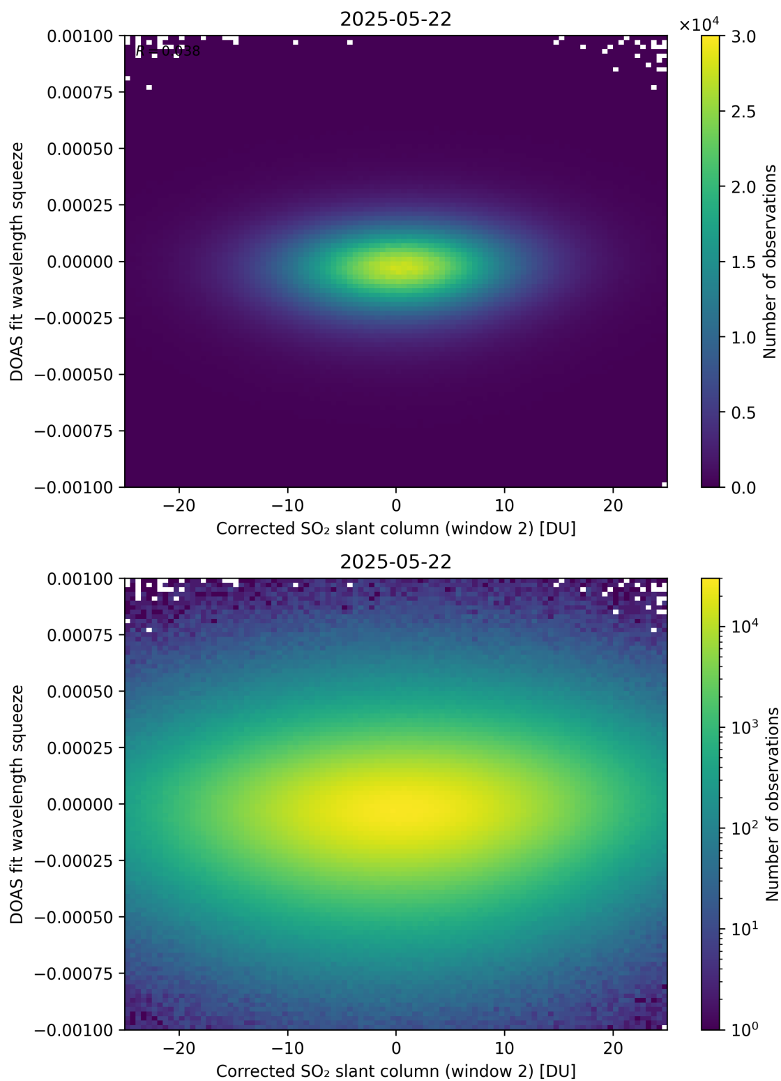
Figure 247: Scatter density plot of “Corrected SO 2 slant column (window 2)” against “DOAS fit wavelength squeeze” for 2025-05-21 to 2025-05-23.
