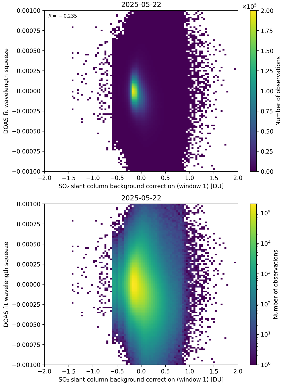
Figure 112: Scatter density plot of “SO 2 slant column background correction (window 1)” against “DOAS fit wavelength squeeze” for 2025-05-21 to 2025-05-23.
