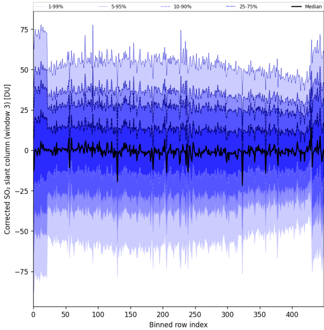
Figure 99: Along track statistics of “Corrected SO 2 slant column (window 3)” for 2025-05-21 to 2025-05-23
