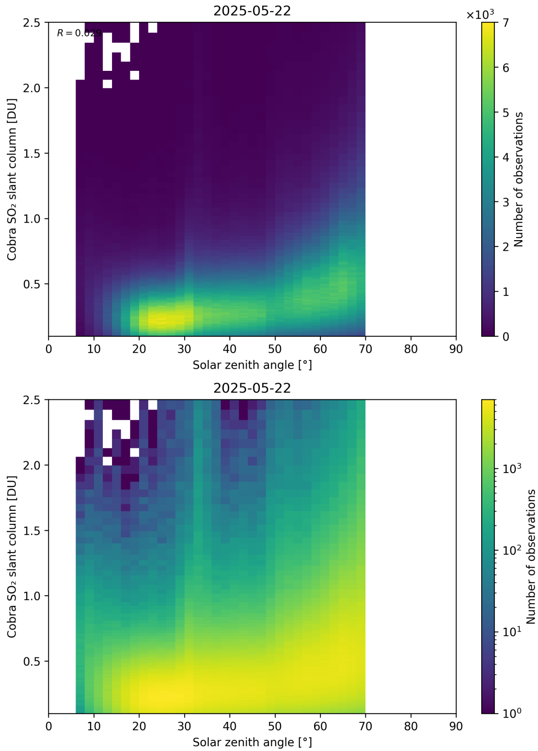
Figure 179: Scatter density plot of “Solar zenith angle” against “Cobra SO 2 slant column” for 2025-05-21 to 2025-05-23.
