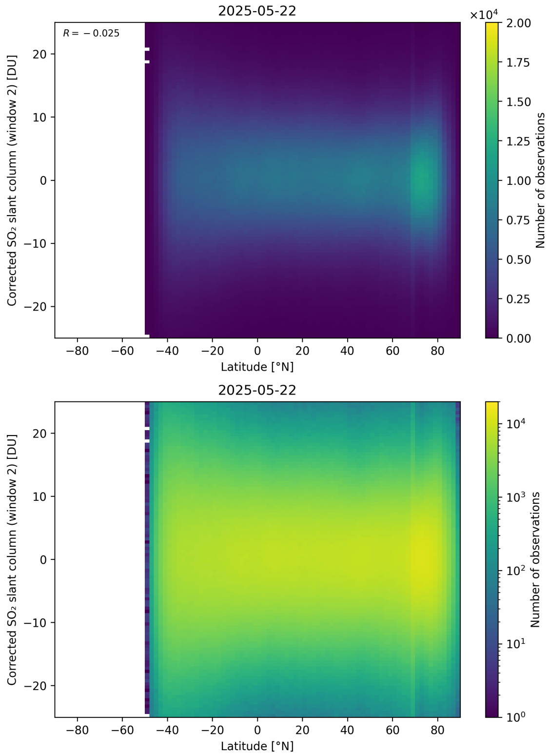
Figure 160: Scatter density plot of “Latitude” against “Corrected SO 2 slant column (window 2)” for 2025-05-21 to 2025-05-23.
