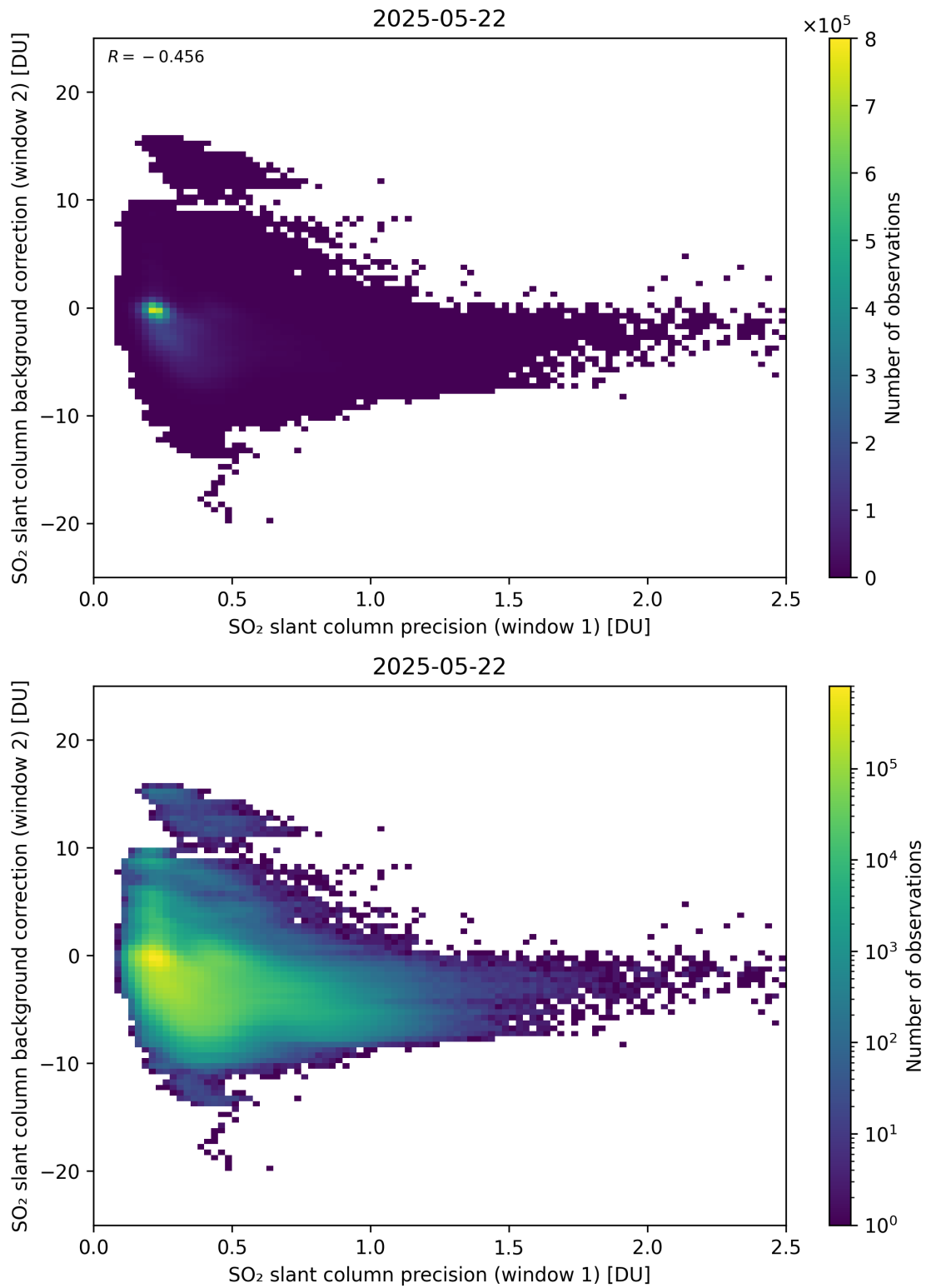
Figure 269: Scatter density plot of “SO 2 slant column precision (window 1)” against “SO 2 slant column background correction (window 2)” for 2025-05-21 to 2025-05-23.
