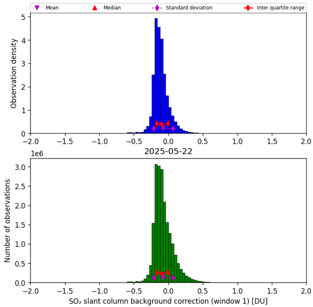
Figure 66: Histogram of “SO 2 slant column background correction (window 1)” for 2025-05-21 to 2025-05-23
