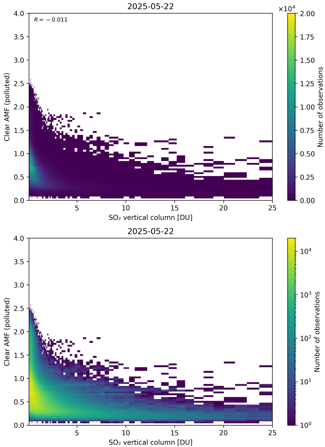
Figure 348: Scatter density plot of “SO 2 vertical column” against “Clear AMF (polluted)” for 2025-05-21 to 2025-05-23.
