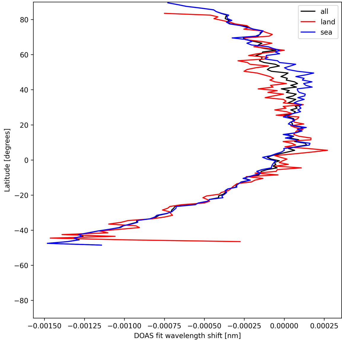
Figure 50: Zonal average of “DOAS fit wavelength shift” for 2025-05-21 to 2025-05-23.
