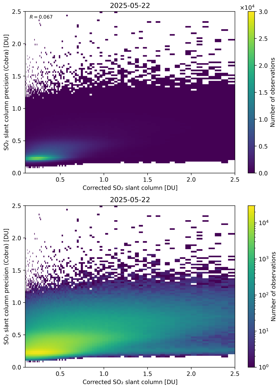
Figure 234: Scatter density plot of “Corrected SO 2 slant column” against “SO 2 slant column precision (Cobra)” for 2025-05-21 to 2025-05-23.
