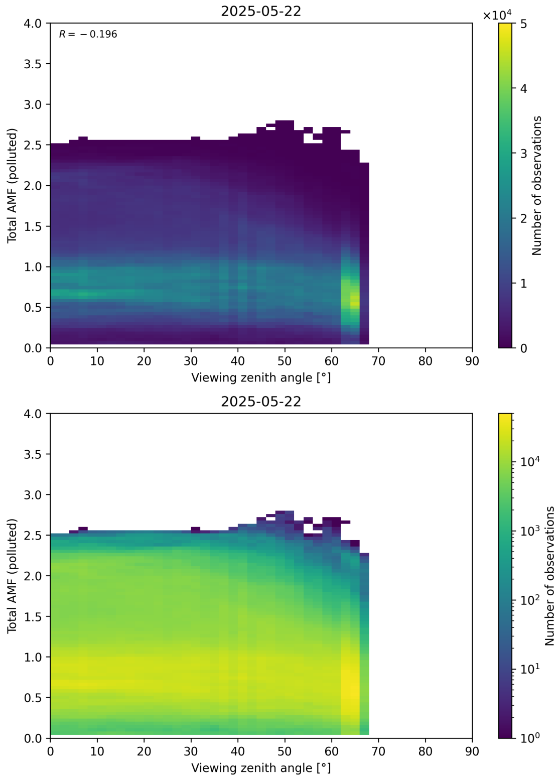
Figure 381: Scatter density plot of “Viewing zenith angle” against “Total AMF (polluted)” for 2025-05-21 to 2025-05-23.
