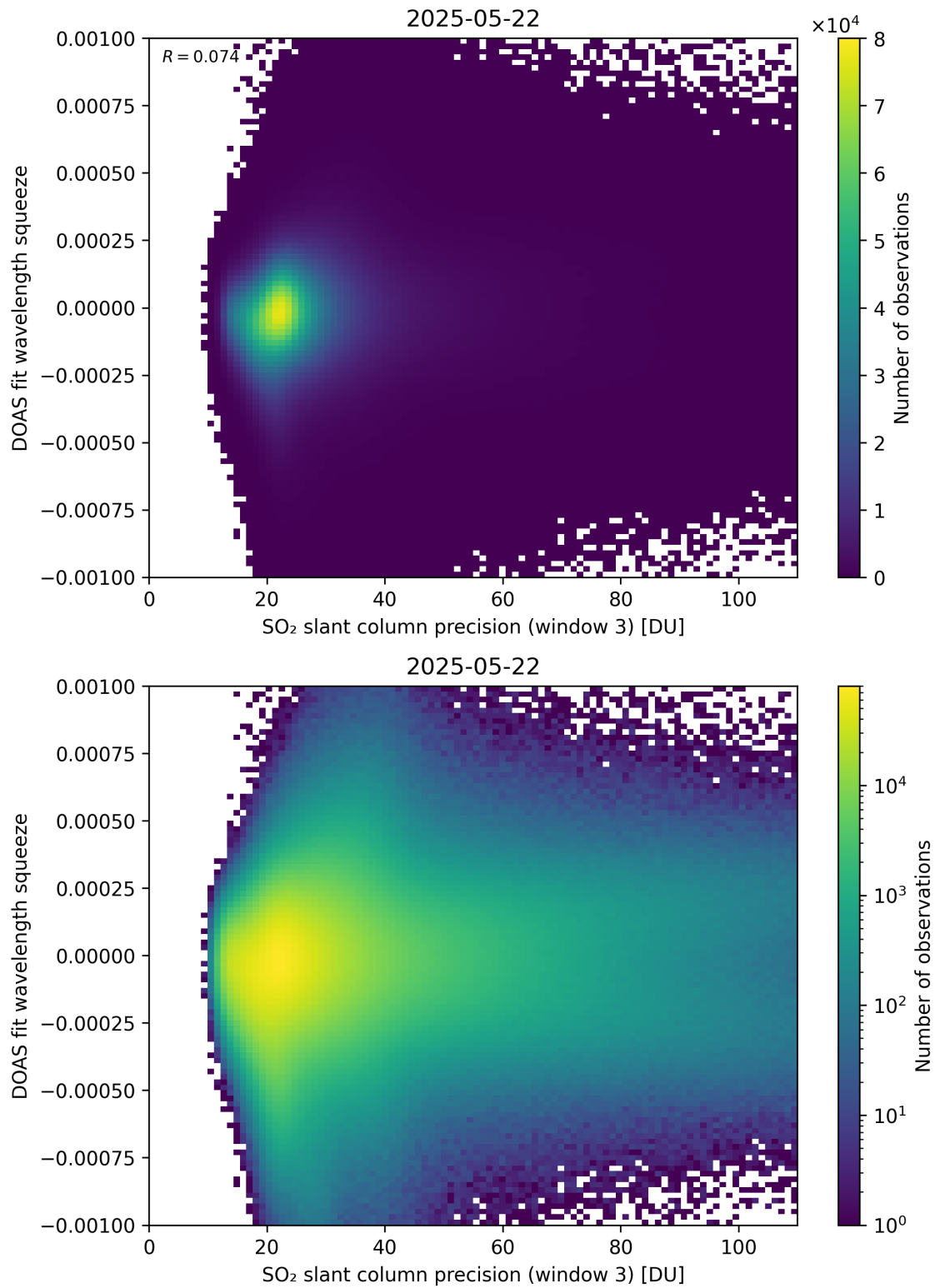
Figure 309: Scatter density plot of “SO 2 slant column precision (window 3)” against “DOAS fit wavelength squeeze” for 2025-05-21 to 2025-05-23.
