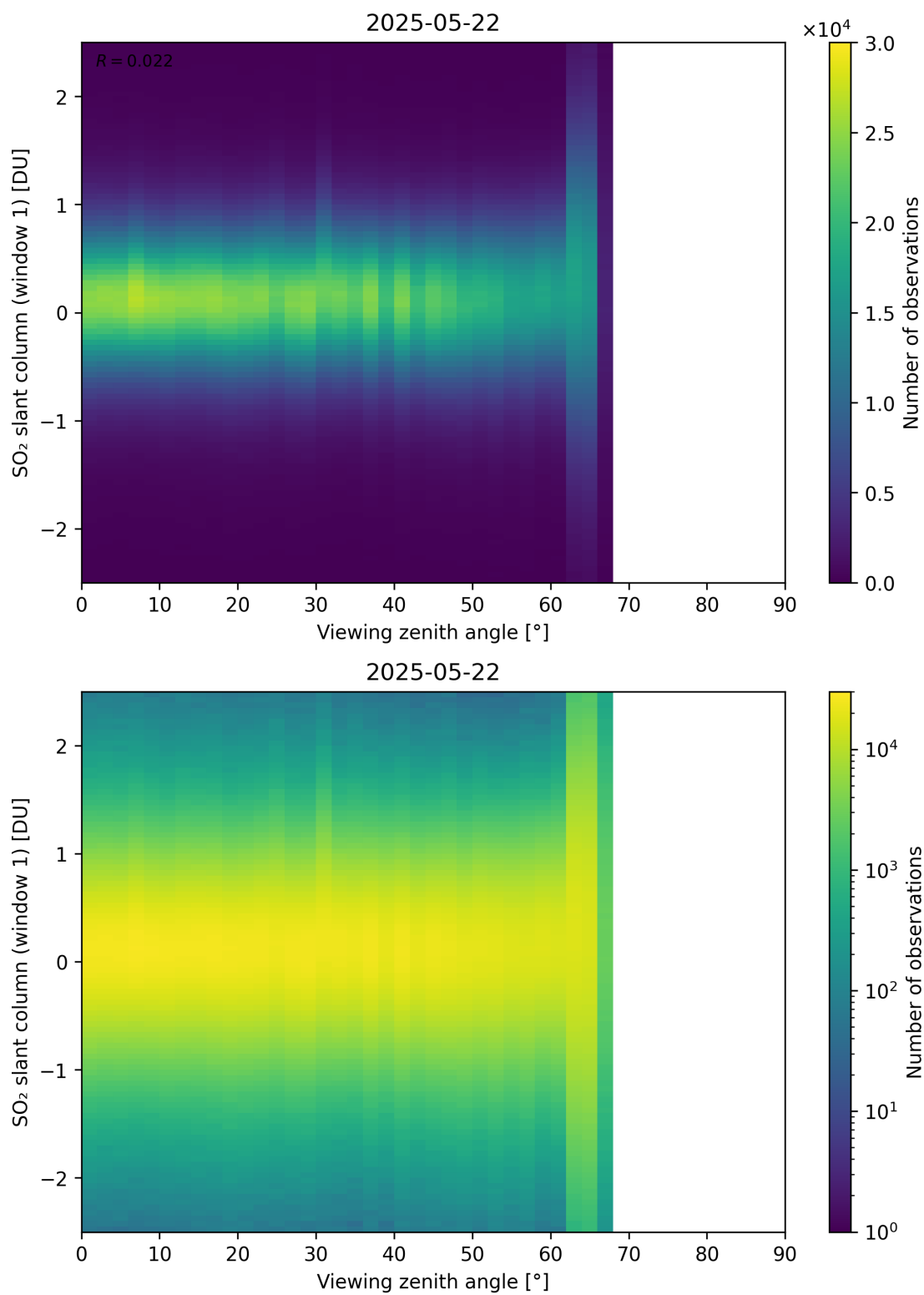
Figure 376: Scatter density plot of “Viewing zenith angle” against “SO 2 slant column (window 1)” for 2025-05-21 to 2025-05-23.
