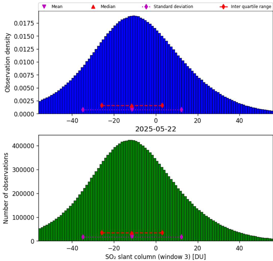
Figure 71: Histogram of “SO 2 slant column (window 3)” for 2025-05-21 to 2025-05-23
