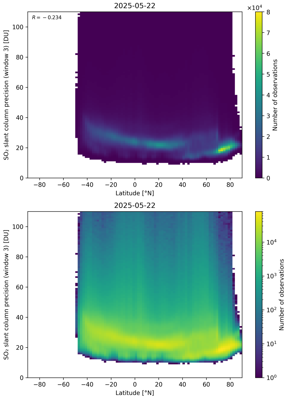
Figure 166: Scatter density plot of “Latitude” against “SO 2 slant column precision (window 3)” for 2025-05-21 to 2025-05-23.
