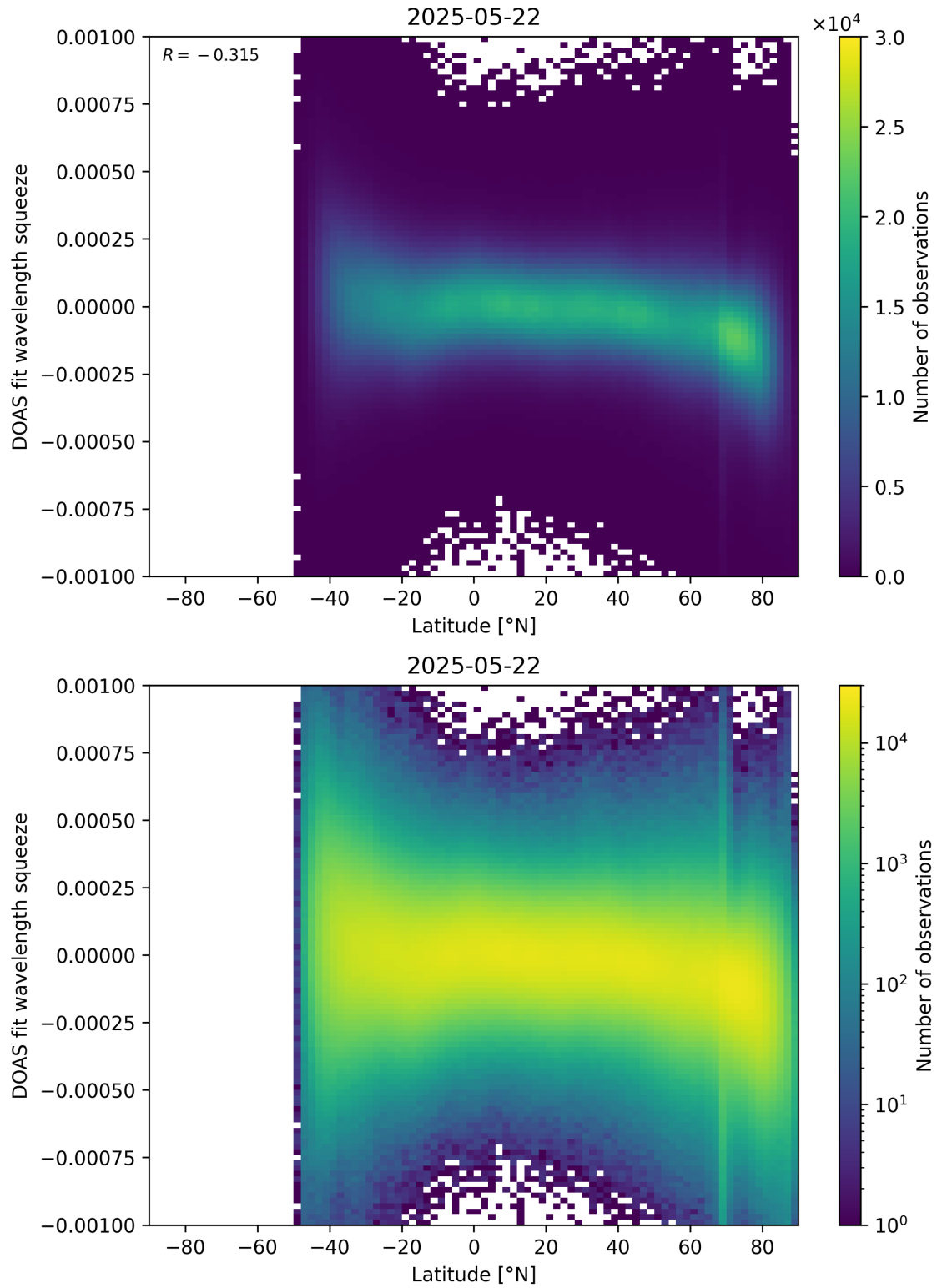
Figure 154: Scatter density plot of “Latitude” against “DOAS fit wavelength squeeze” for 2025-05-21 to 2025-05-23.
