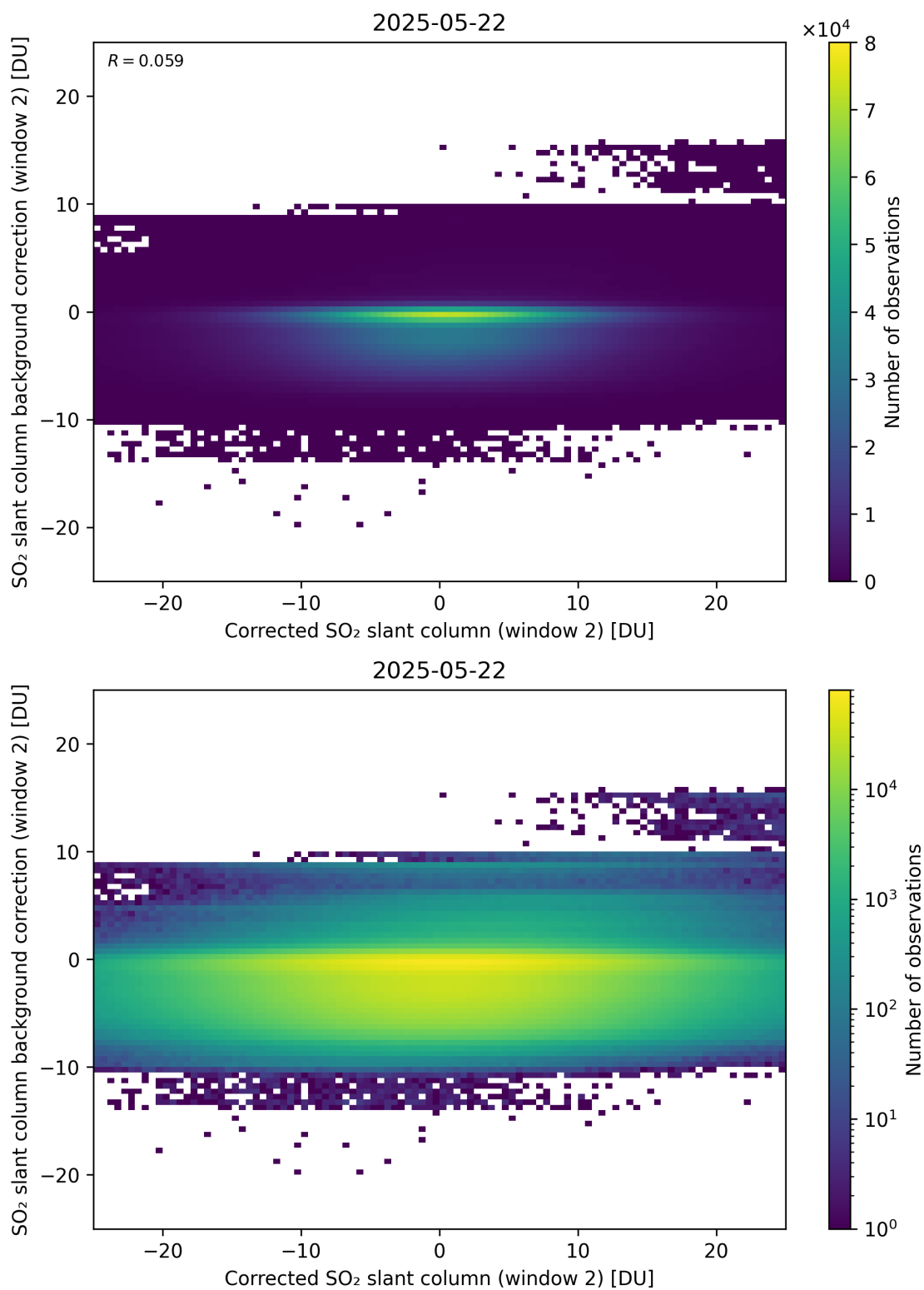
Figure 244: Scatter density plot of “Corrected SO 2 slant column (window 2)” against “SO 2 slant column background correction (window 2)” for 2025-05-21 to 2025-05-23.
