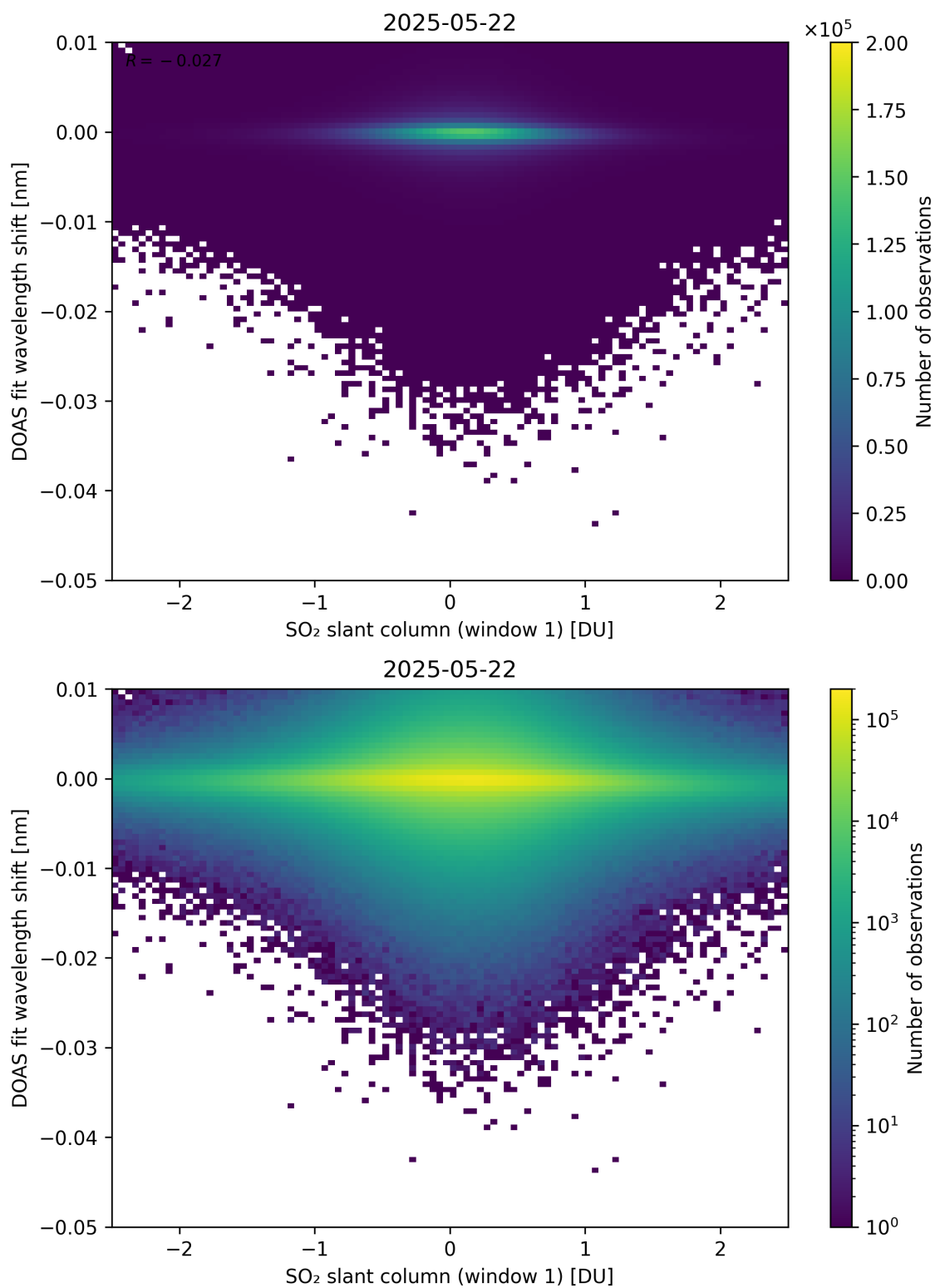
Figure 265: Scatter density plot of “SO 2 slant column (window 1)” against “DOAS fit wavelength shift” for 2025-05-21 to 2025-05-23.
