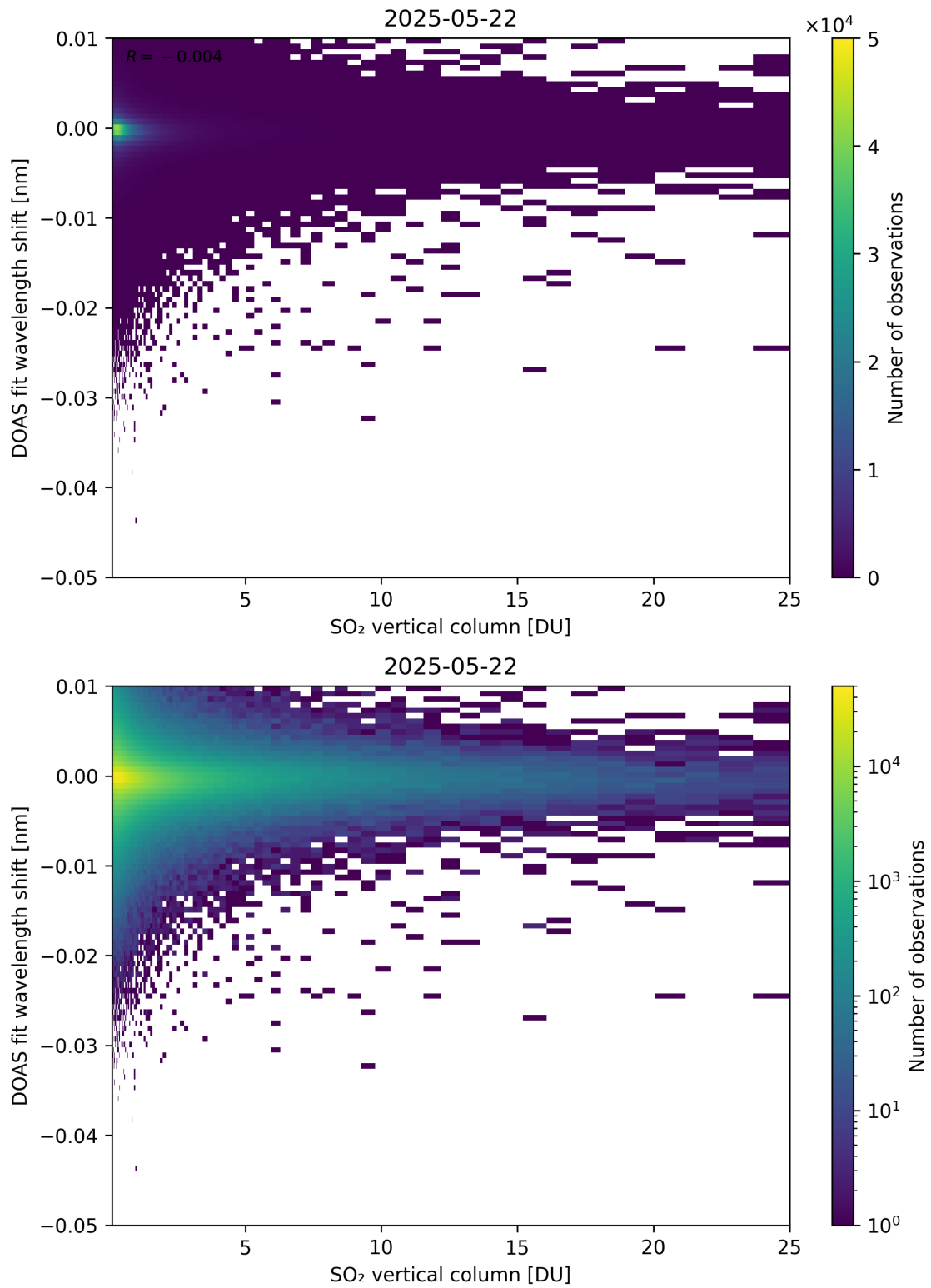
Figure 326: Scatter density plot of “SO 2 vertical column” against “DOAS fit wavelength shift” for 2025-05-21 to 2025-05-23.
