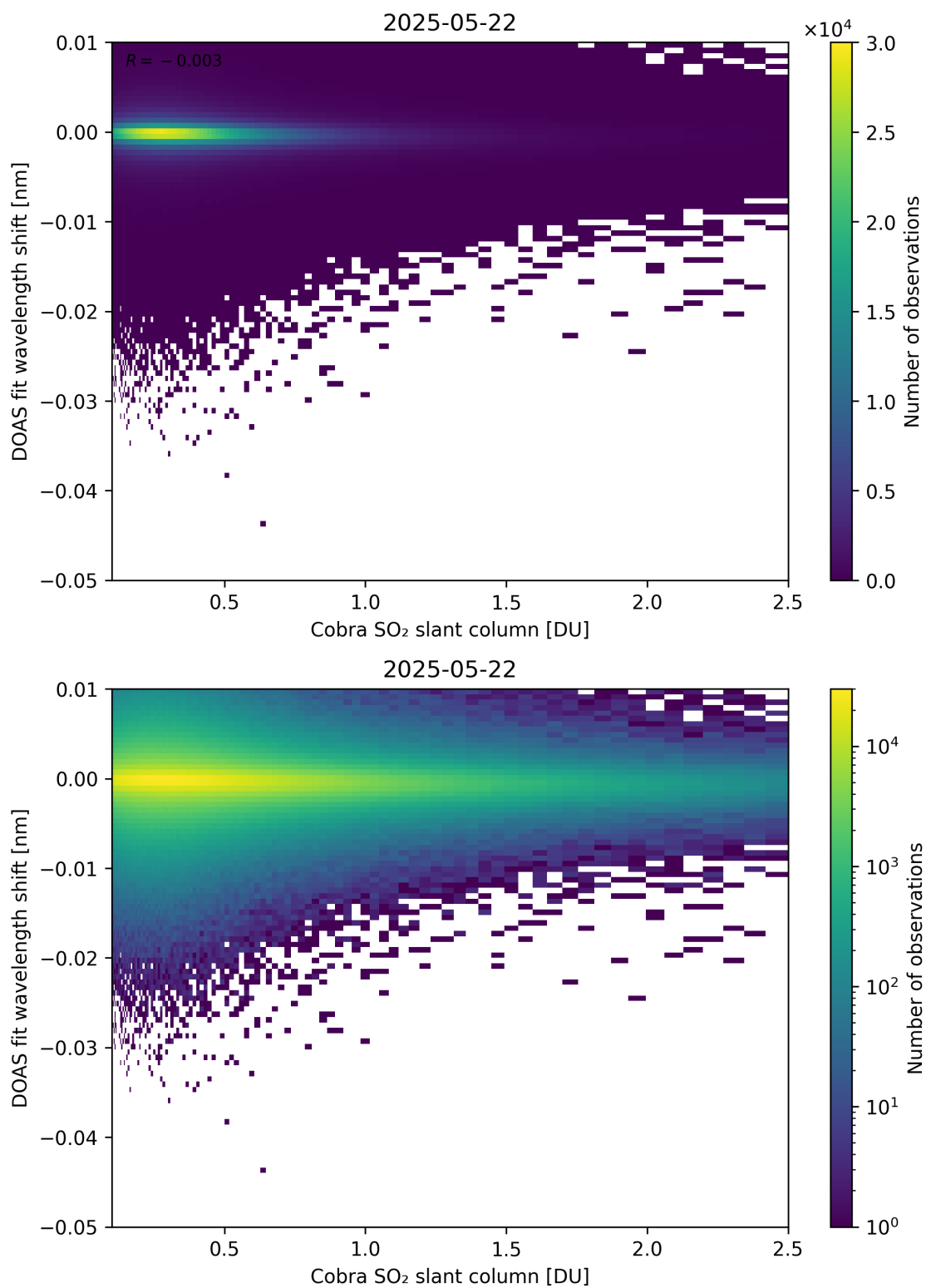
Figure 196: Scatter density plot of “Cobra SO 2 slant column” against “DOAS fit wavelength shift” for 2025-05-21 to 2025-05-23.
