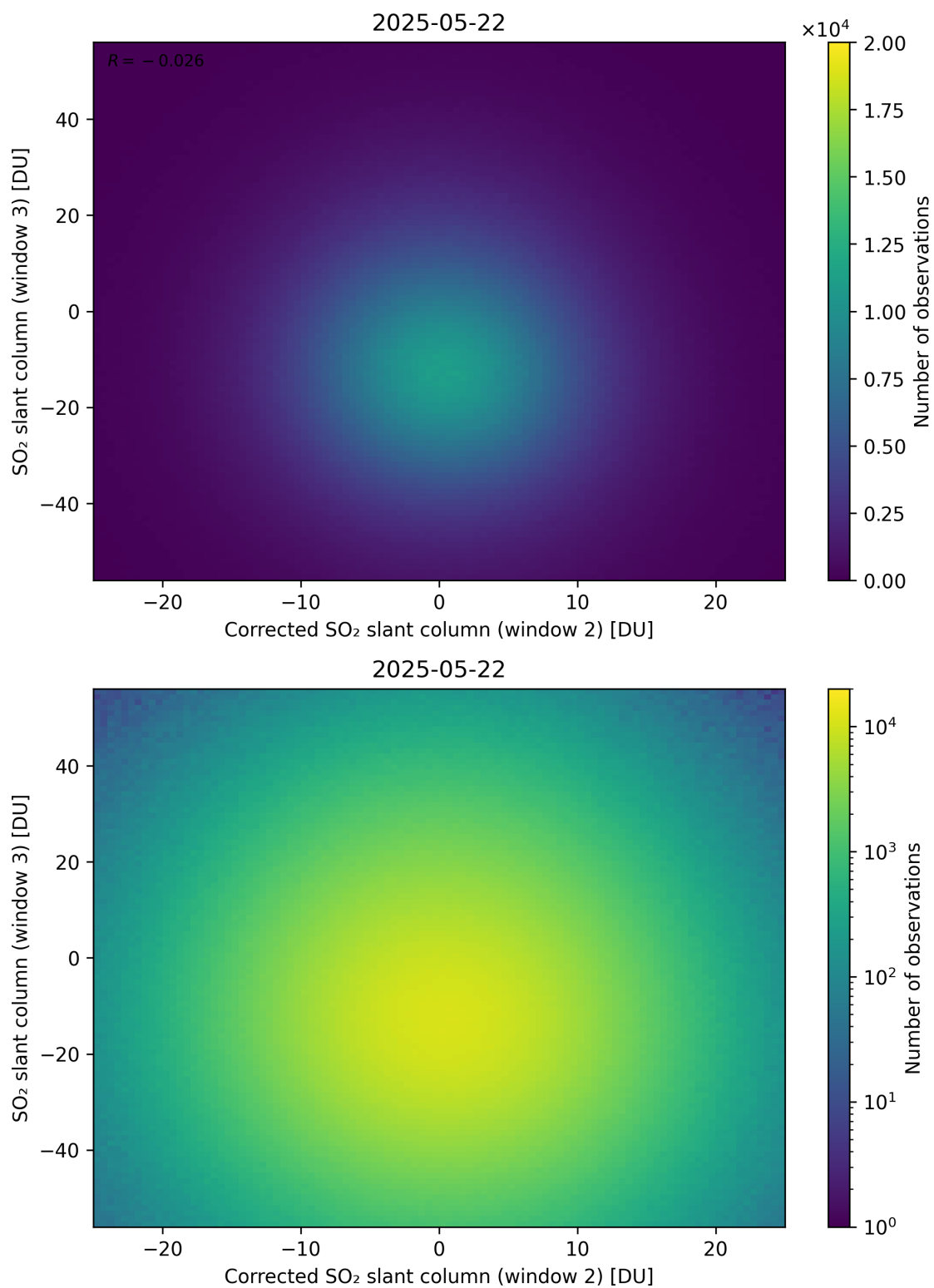
Figure 251: Scatter density plot of “Corrected SO 2 slant column (window 2)” against “SO 2 slant column (window 3)” for 2025-05-21 to 2025-05-23.
