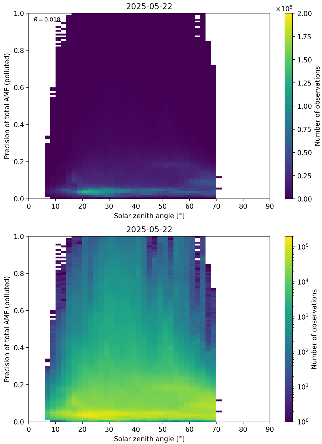
Figure 190: Scatter density plot of “Solar zenith angle” against “Precision of total AMF (polluted)” for 2025-05-21 to 2025-05-23.
