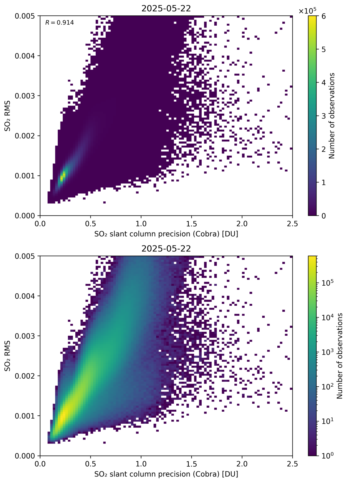
Figure 204: Scatter density plot of “SO 2 slant column precision (Cobra)” against “SO 2 RMS” for 2025-05-21 to 2025-05-23.
