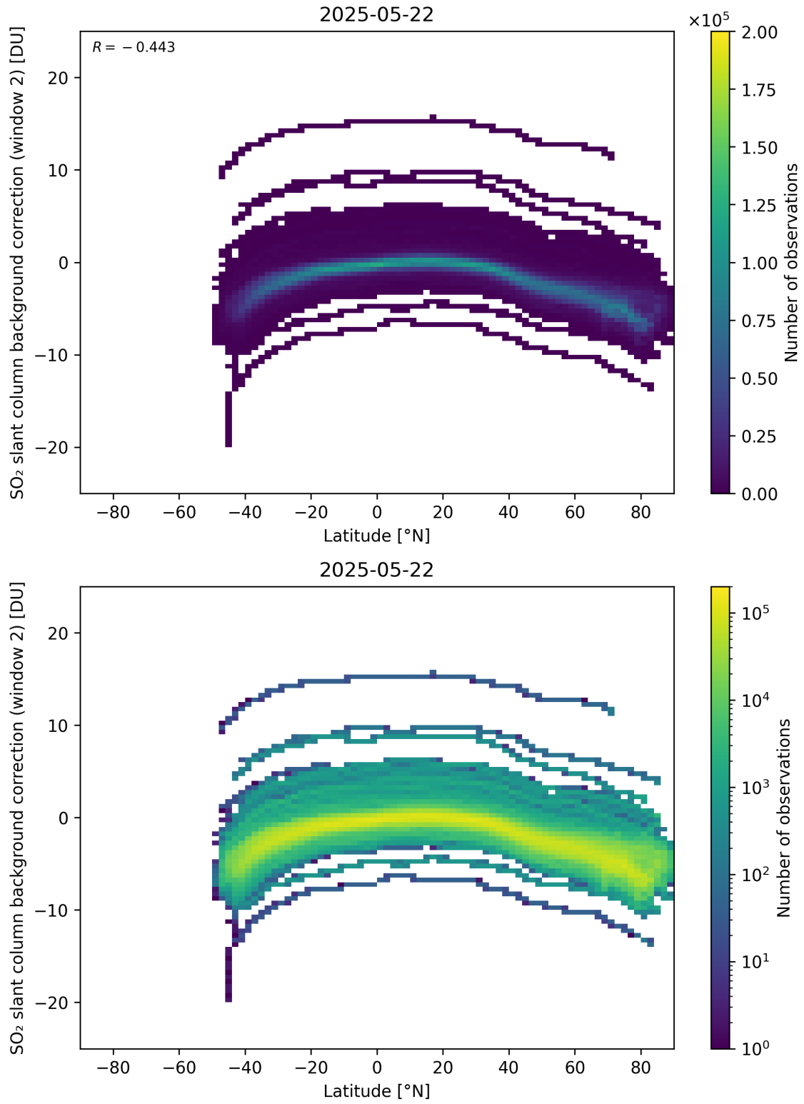
Figure 151: Scatter density plot of “Latitude” against “SO 2 slant column background correction (window 2)” for 2025-05-21 to 2025-05-23.
