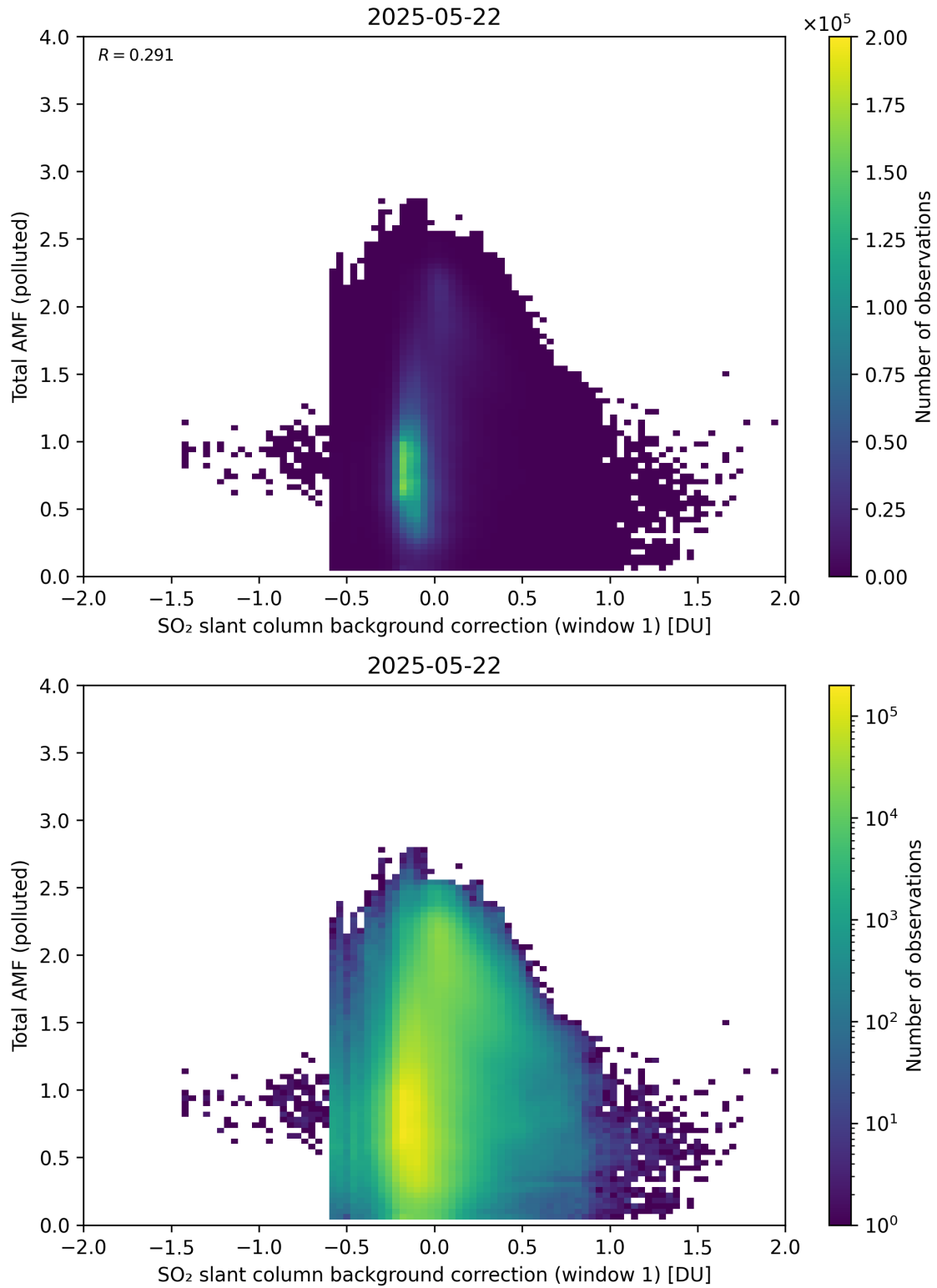
Figure 120: Scatter density plot of “SO 2 slant column background correction (window 1)” against “Total AMF (polluted)” for 2025-05-21 to 2025-05-23.
