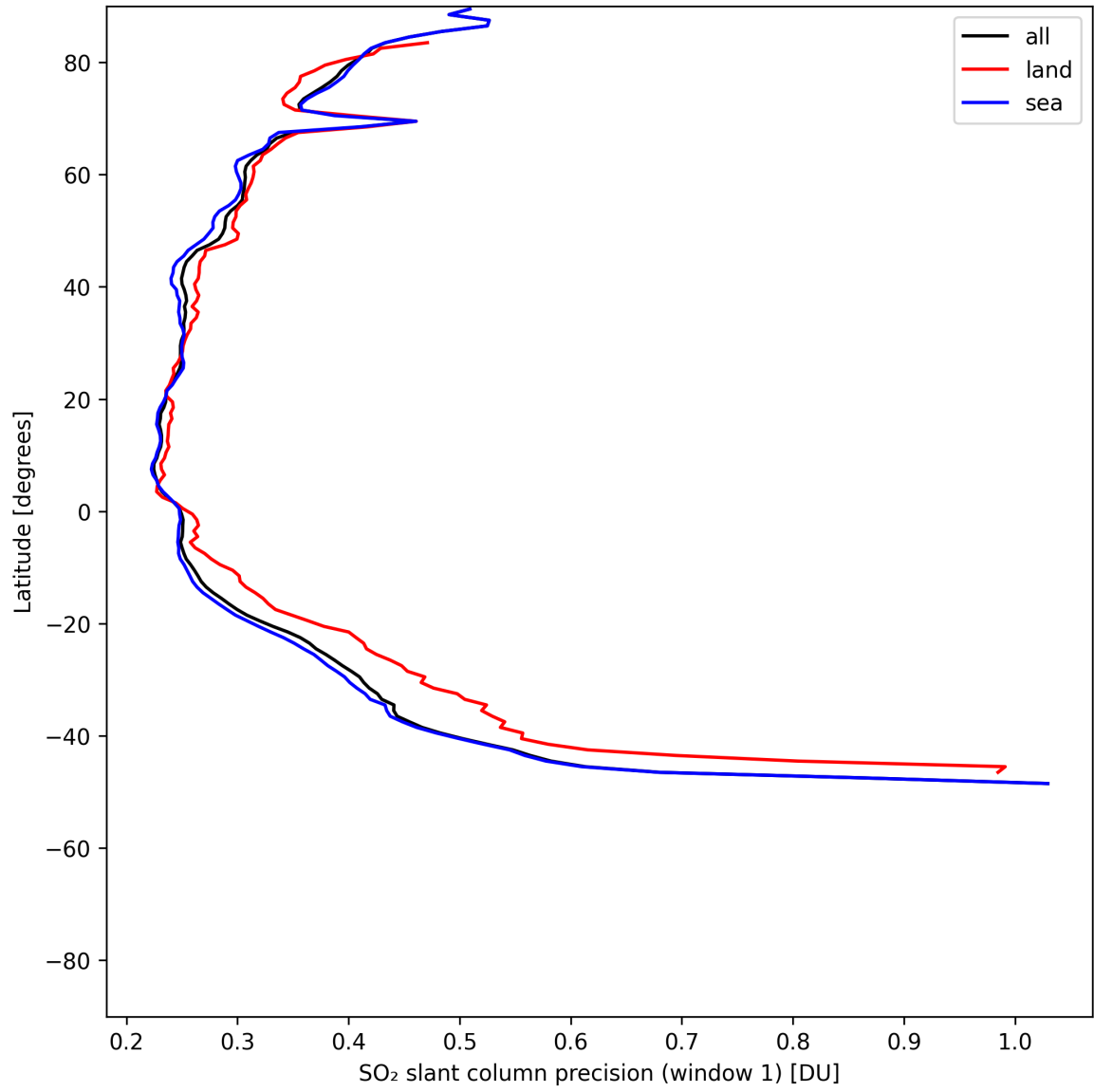
Figure 38: Zonal average of “SO 2 slant column precision (window 1)” for 2025-05-21 to 2025-05-23.
