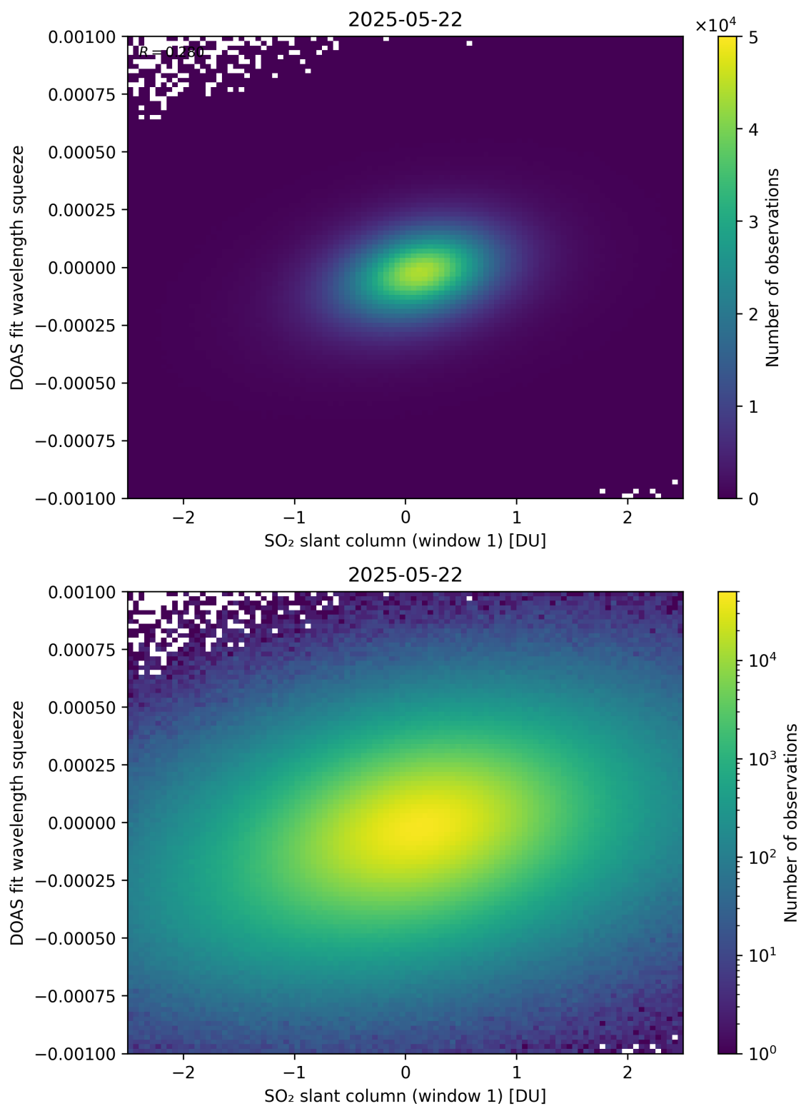
Figure 266: Scatter density plot of “SO 2 slant column (window 1)” against “DOAS fit wavelength squeeze” for 2025-05-21 to 2025-05-23.
