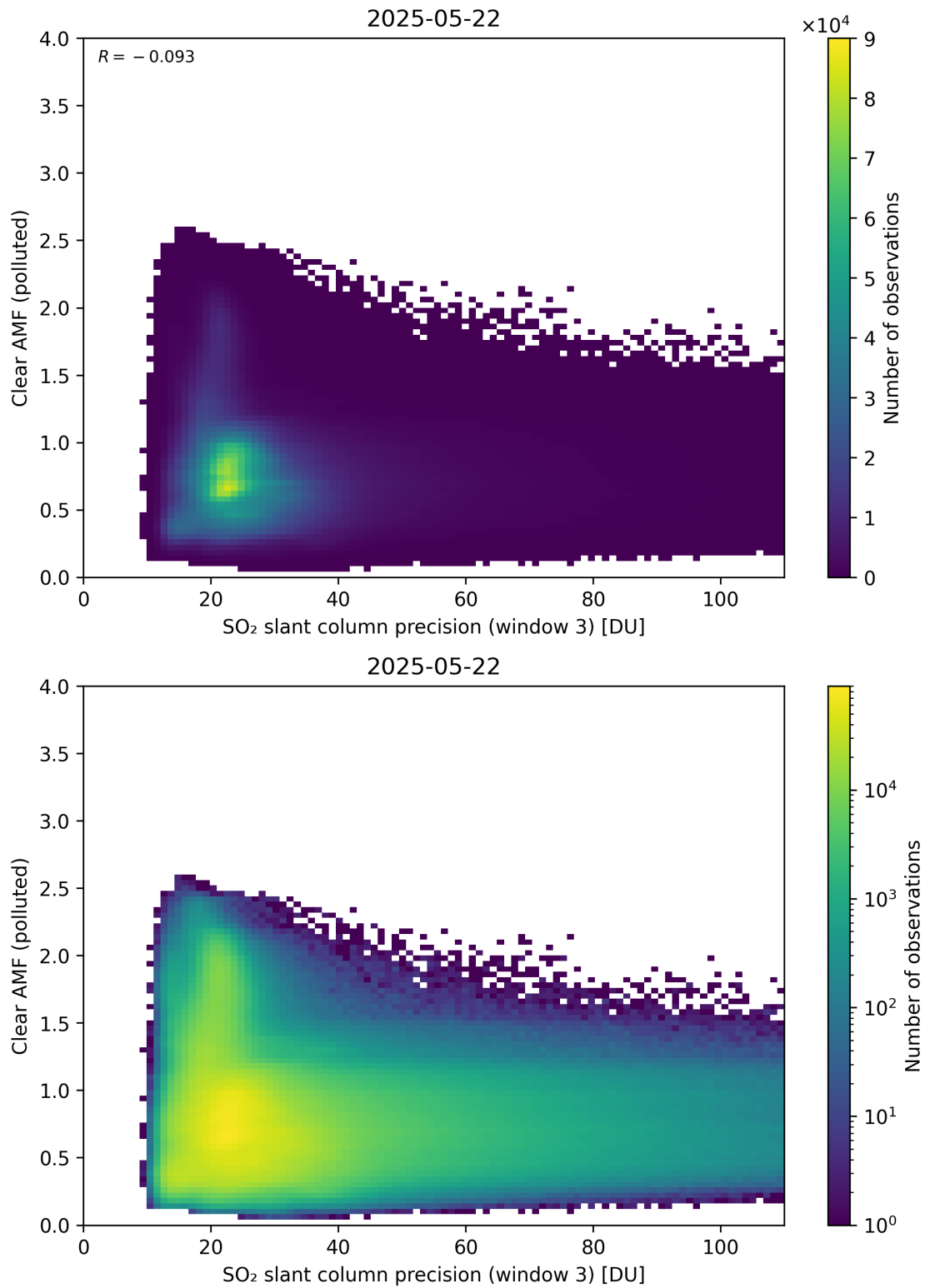
Figure 311: Scatter density plot of “SO 2 slant column precision (window 3)” against “Clear AMF (polluted)” for 2025-05-21 to 2025-05-23.
