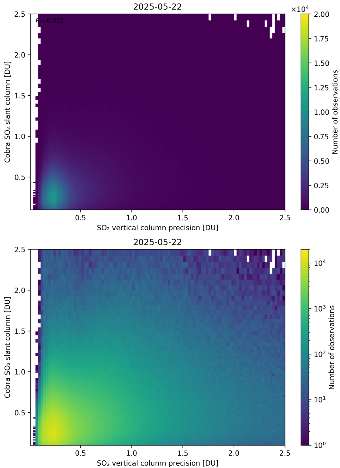
Figure 336: Scatter density plot of “SO 2 vertical column precision” against “Cobra SO 2 slant column” for 2025-05-21 to 2025-05-23.
