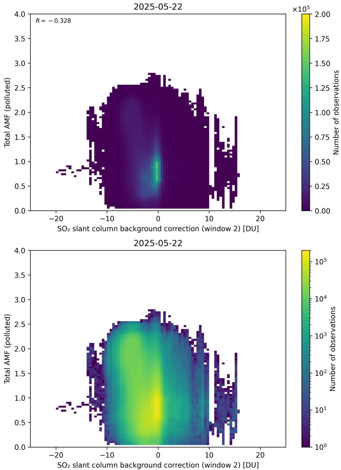
Figure 130: Scatter density plot of “SO 2 slant column background correction (window 2)” against “Total AMF (polluted)” for 2025-05-21 to 2025-05-23.
