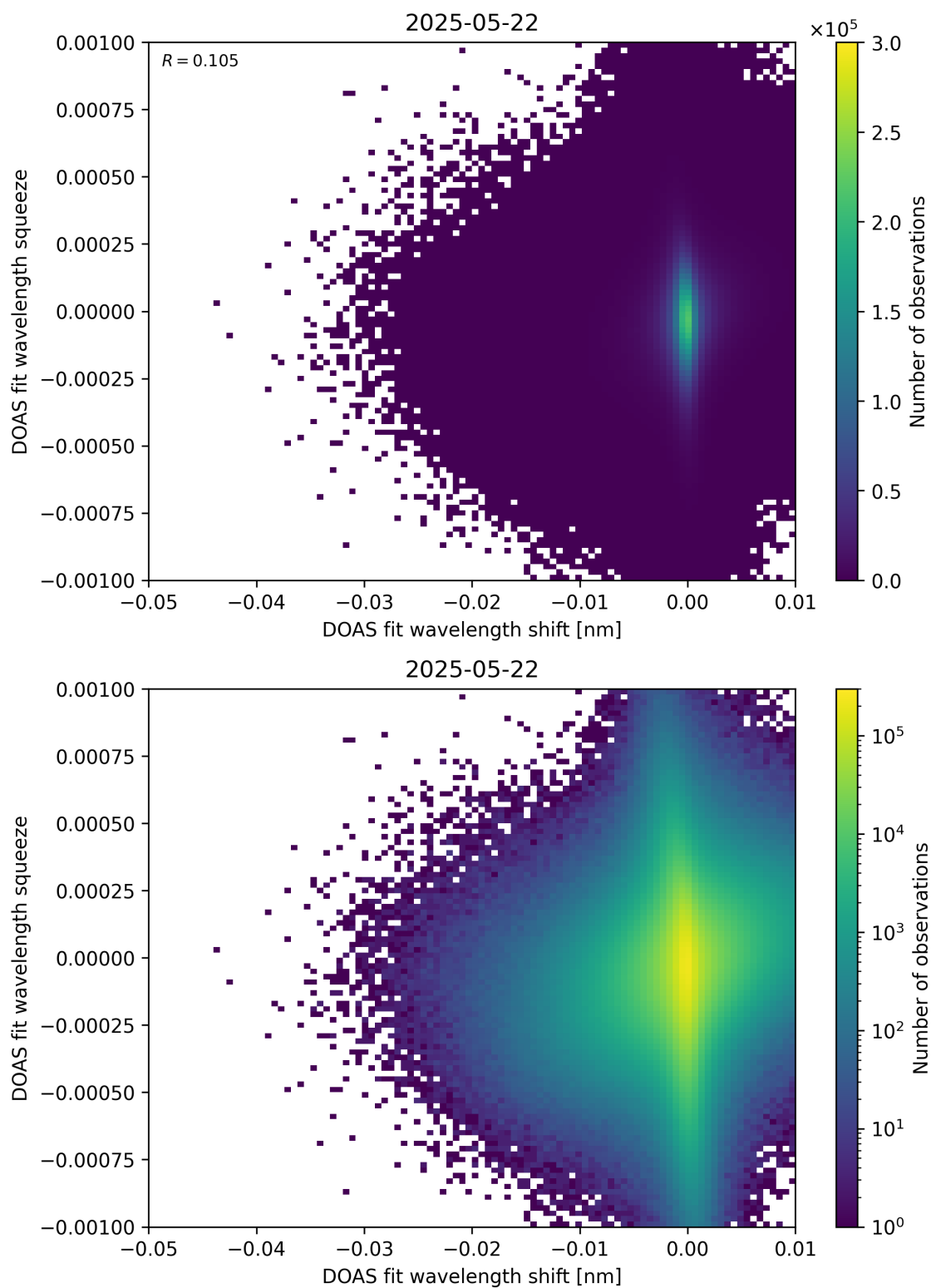
Figure 138: Scatter density plot of “DOAS fit wavelength shift” against “DOAS fit wavelength squeeze” for 2025-05-21 to 2025-05-23.
