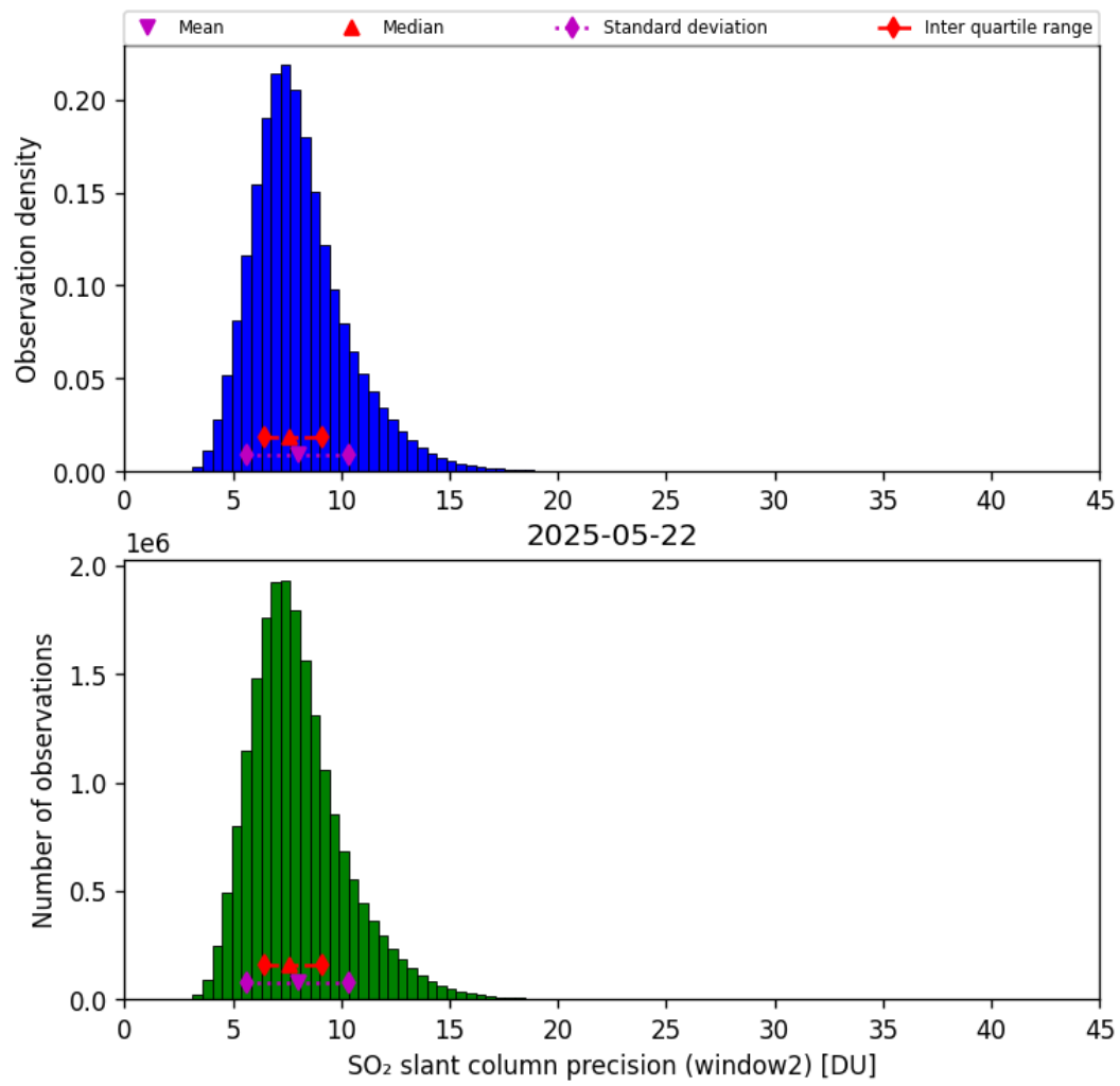
Figure 68: Histogram of “SO 2 slant column precision (window2)” for 2025-05-21 to 2025-05-23
