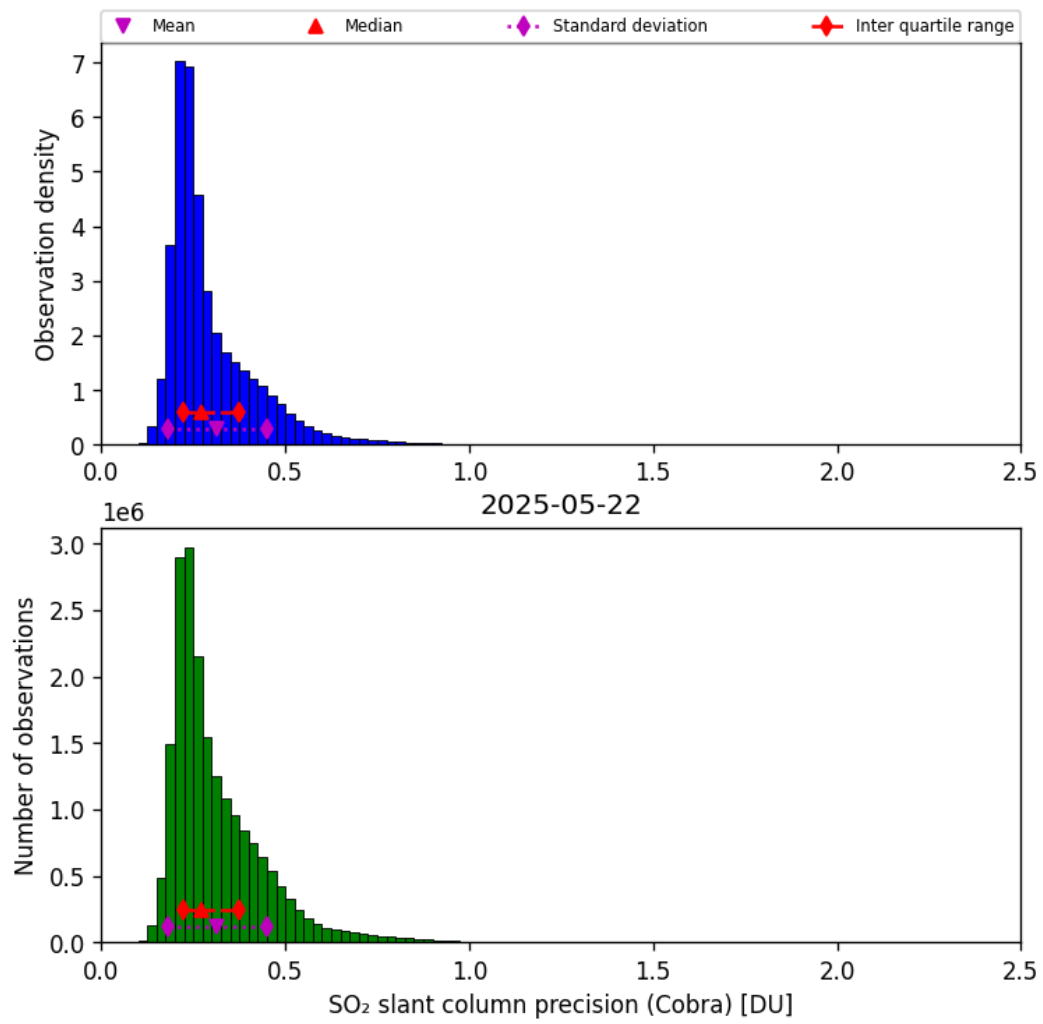
Figure 62: Histogram of “SO 2 slant column precision (Cobra)” for 2025-05-21 to 2025-05-23
