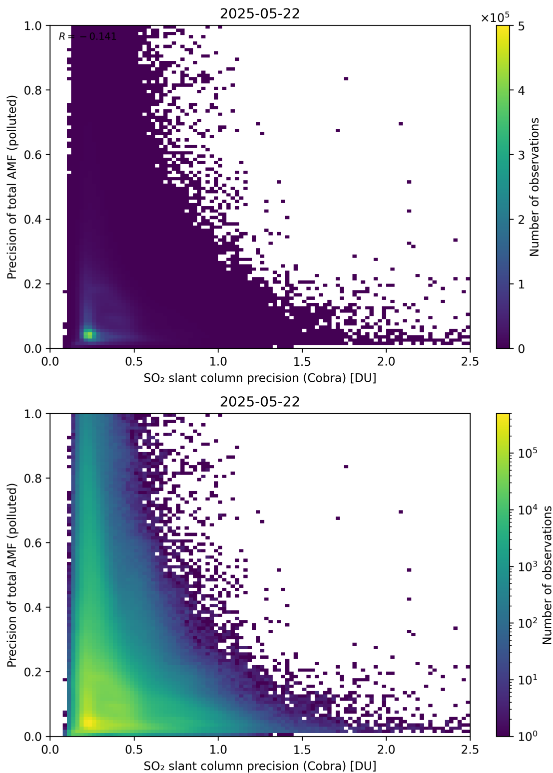
Figure 214: Scatter density plot of “SO 2 slant column precision (Cobra)” against “Precision of total AMF (polluted)” for 2025-05-21 to 2025-05-23.
