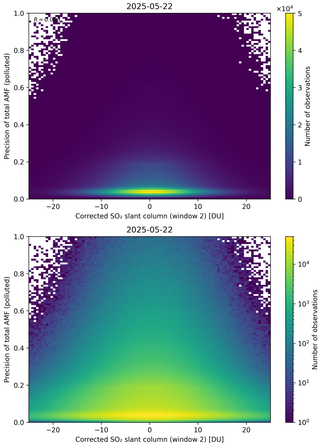
Figure 254: Scatter density plot of “Corrected SO 2 slant column (window 2)” against “Precision of total AMF (polluted)” for 2025-05-21 to 2025-05-23.
