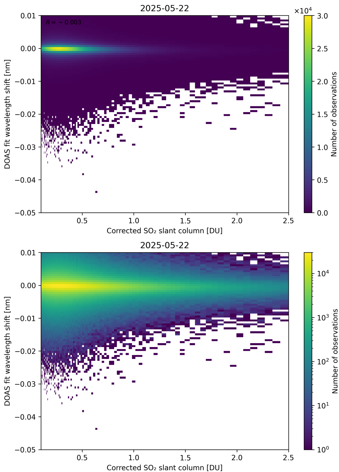
Figure 229: Scatter density plot of “Corrected SO 2 slant column” against “DOAS fit wavelength shift” for 2025-05-21 to 2025-05-23.
