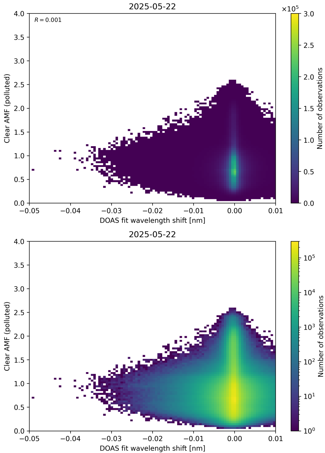
Figure 140: Scatter density plot of “DOAS fit wavelength shift” against “Clear AMF (polluted)” for 2025-05-21 to 2025-05-23.
