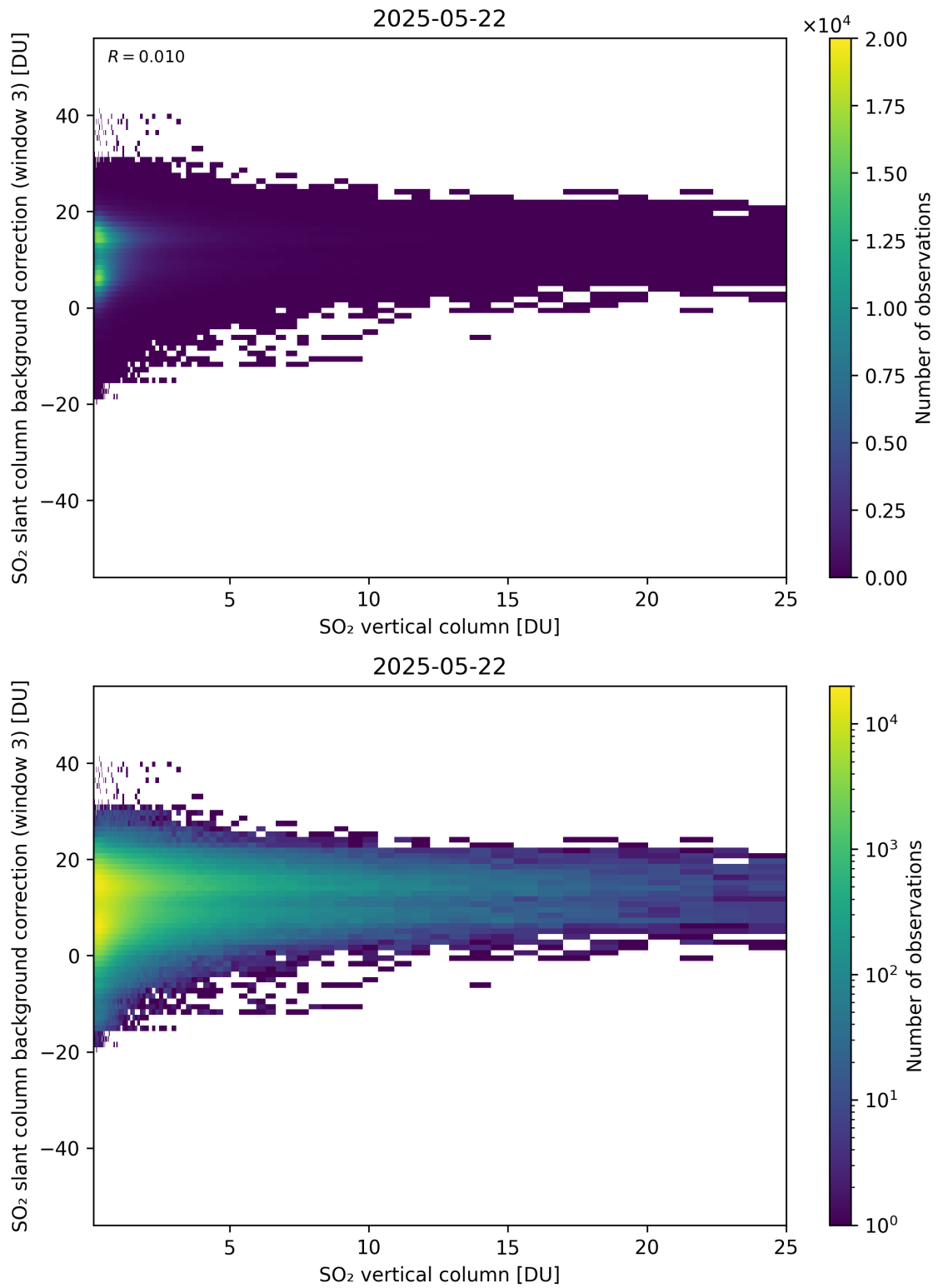
Figure 325: Scatter density plot of “SO 2 vertical column” against “SO 2 slant column background correction (window 3)” for 2025-05-21 to 2025-05-23.
