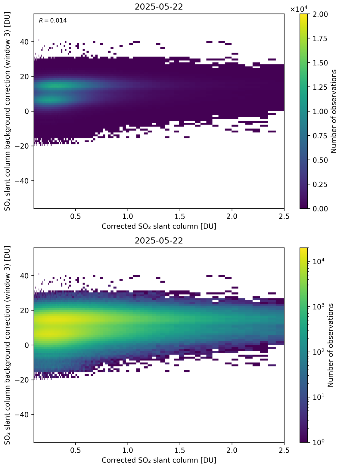
Figure 228: Scatter density plot of “Corrected SO 2 slant column” against “SO 2 slant column background correction (window 3)” for 2025-05-21 to 2025-05-23.
