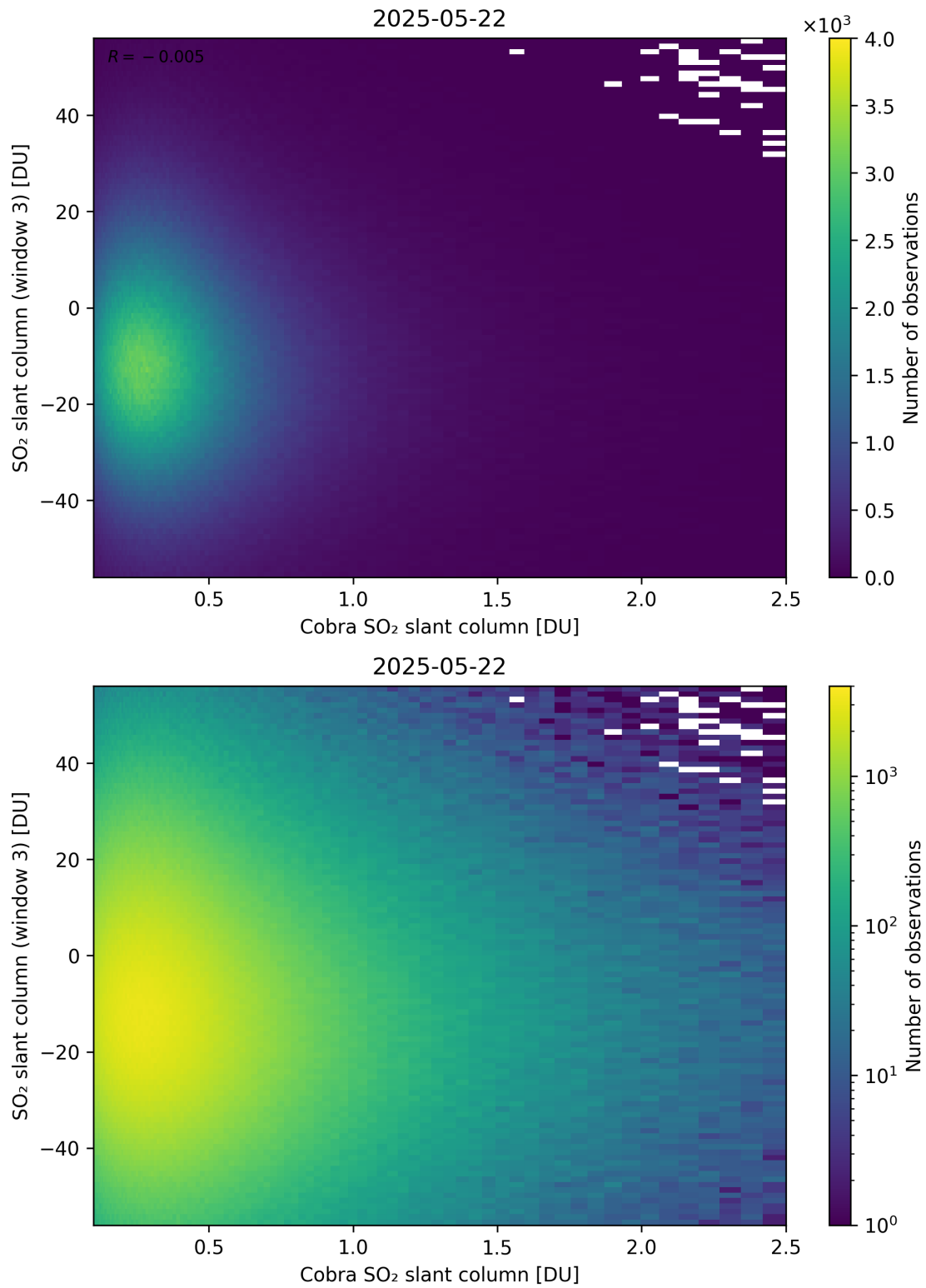
Figure 222: Scatter density plot of “Cobra SO 2 slant column” against “SO 2 slant column (window 3)” for 2025-05-21 to 2025-05-23.
