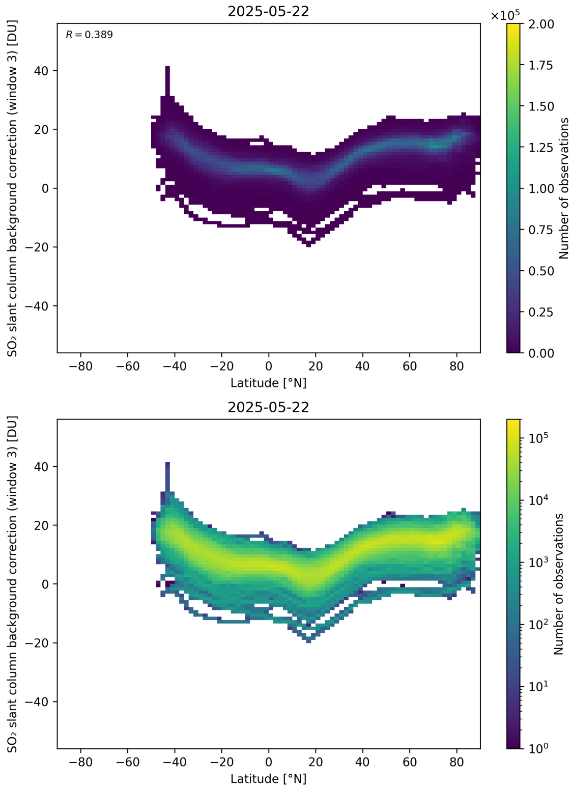
Figure 152: Scatter density plot of “Latitude” against “SO 2 slant column background correction (window 3)” for 2025-05-21 to 2025-05-23.
