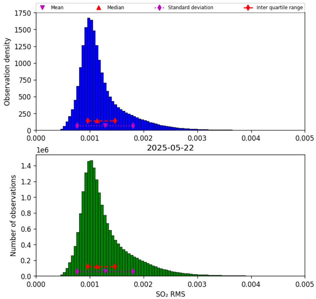
Figure 78: Histogram of “SO 2 RMS” for 2025-05-21 to 2025-05-23
