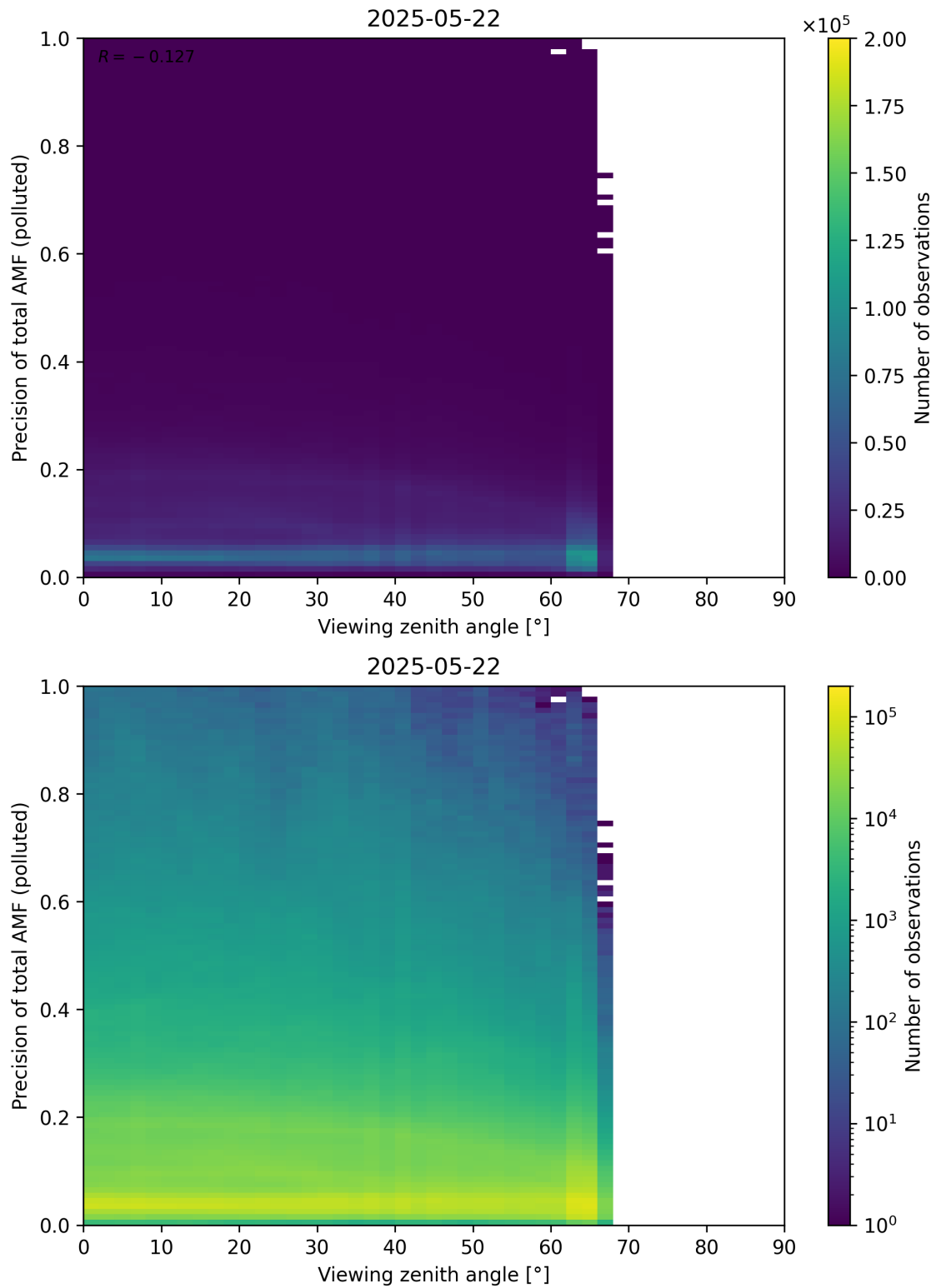
Figure 382: Scatter density plot of “Viewing zenith angle” against “Precision of total AMF (polluted)” for 2025-05-21 to 2025-05-23.
