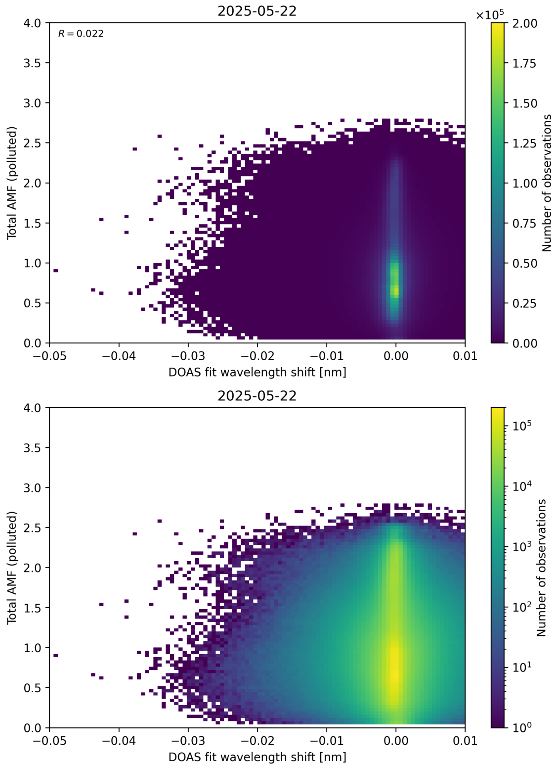
Figure 141: Scatter density plot of “DOAS fit wavelength shift” against “Total AMF (polluted)” for 2025-05-21 to 2025-05-23.
