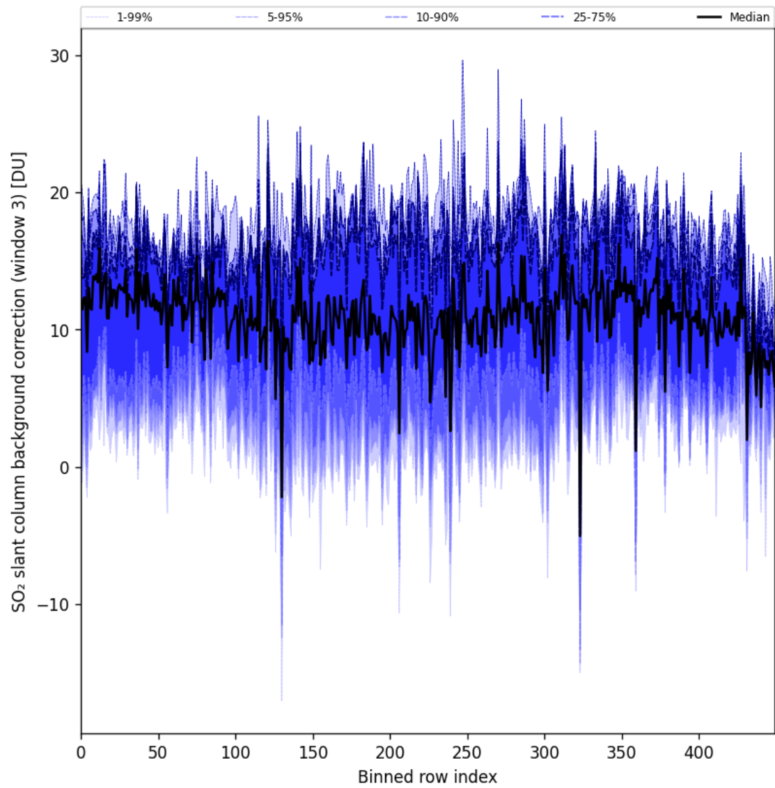
Figure 100: Along track statistics of “SO 2 slant column background correction (window 3)” for 2025-05-21 to 2025-05-23
