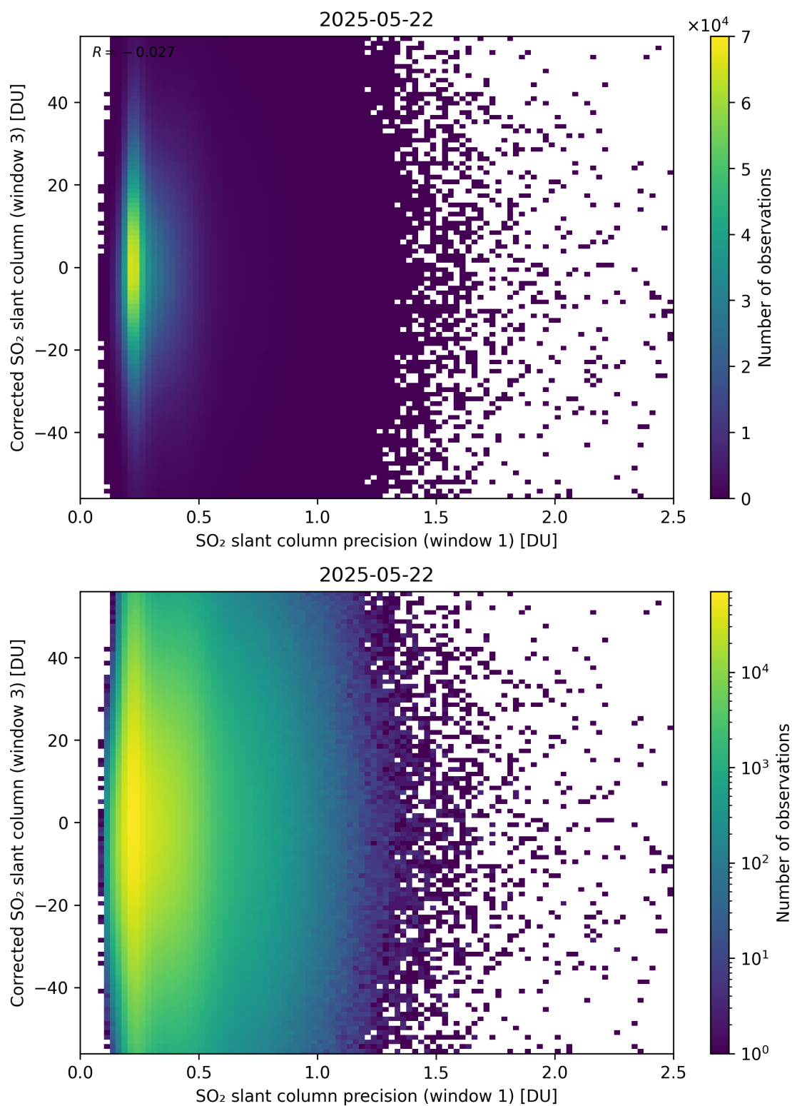
Figure 276: Scatter density plot of “SO 2 slant column precision (window 1)” against “Corrected SO 2 slant column (window 3)” for 2025-05-21 to 2025-05-23.
