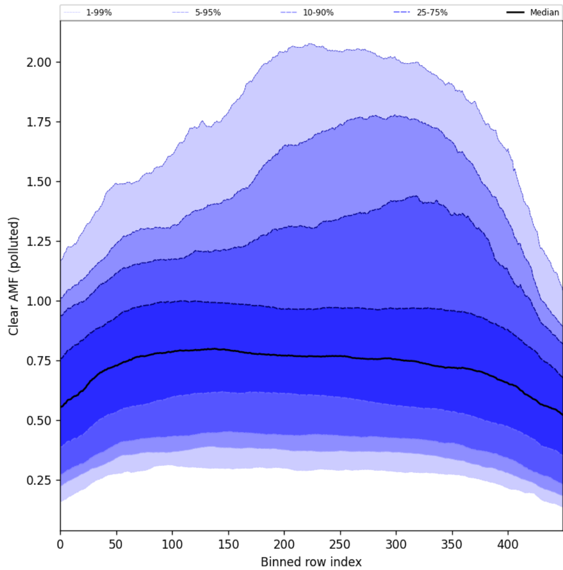
Figure 107: Along track statistics of “Clear AMF (polluted)” for 2025-05-21 to 2025-05-23
