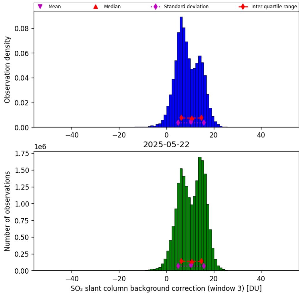
Figure 74: Histogram of “SO 2 slant column background correction (window 3)” for 2025-05-21 to 2025-05-23
