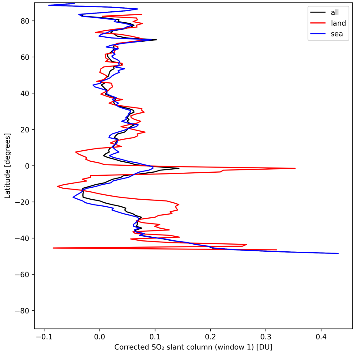
Figure 39: Zonal average of “Corrected SO 2 slant column (window 1)” for 2025-05-21 to 2025-05-23.
