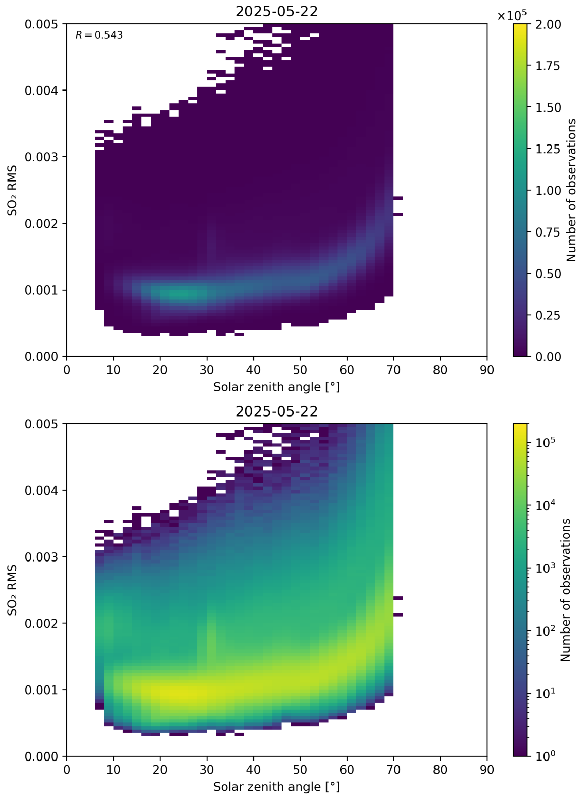
Figure 176: Scatter density plot of “Solar zenith angle” against “SO 2 RMS” for 2025-05-21 to 2025-05-23.
