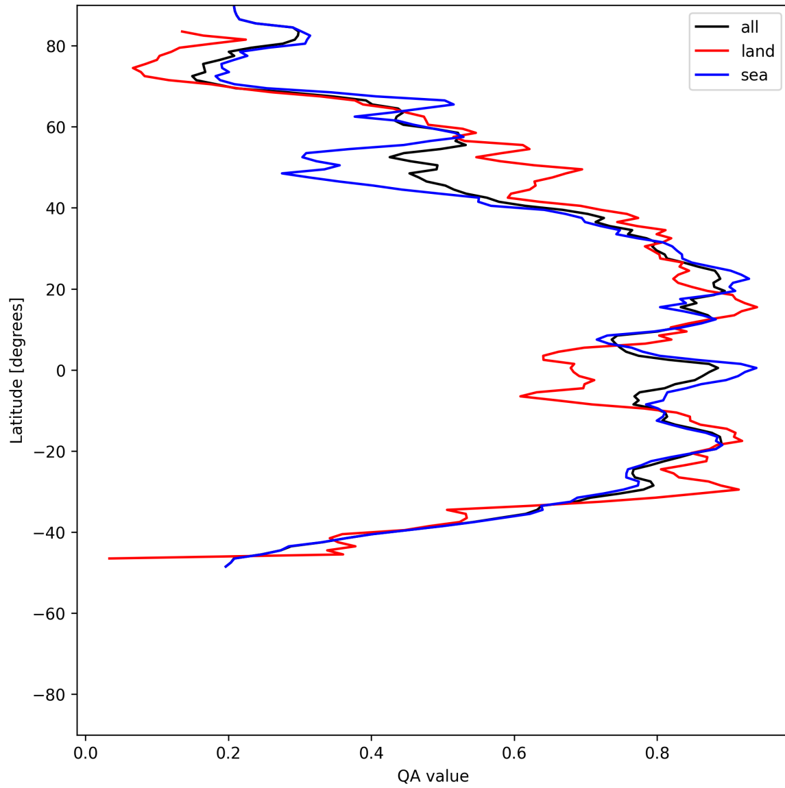
Figure 31: Zonal average of “QA value” for 2025-05-21 to 2025-05-23.
