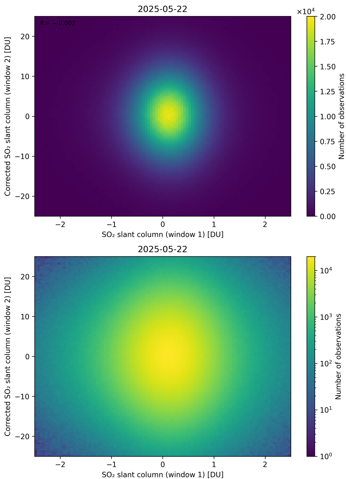
Figure 283: Scatter density plot of “SO 2 slant column (window 1)” against “Corrected SO 2 slant column (window 2)” for 2025-05-21 to 2025-05-23.
