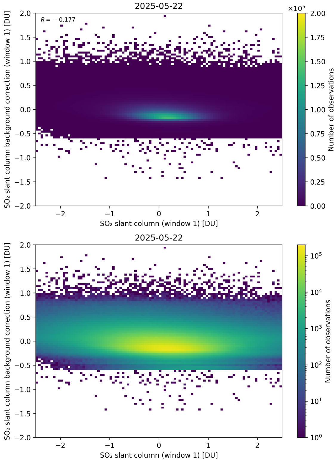
Figure 262: Scatter density plot of “SO 2 slant column (window 1)” against “SO 2 slant column background correction (window 1)” for 2025-05-21 to 2025-05-23.
