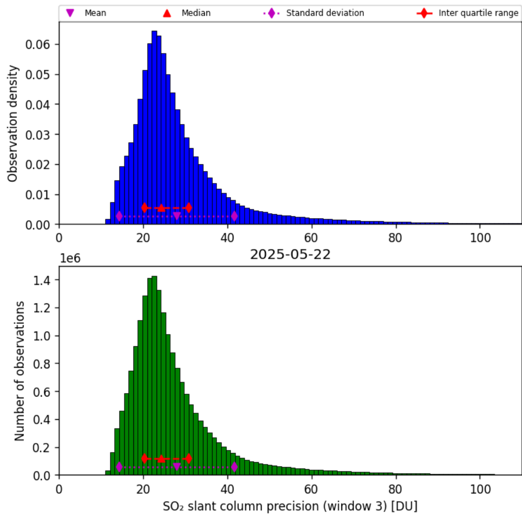
Figure 72: Histogram of “SO 2 slant column precision (window 3)” for 2025-05-21 to 2025-05-23
