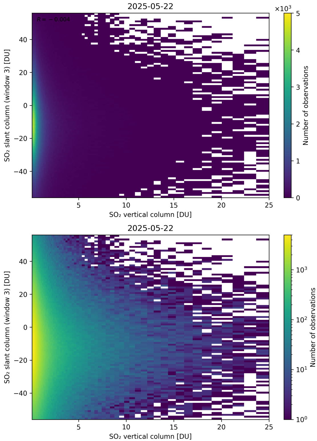
Figure 357: Scatter density plot of “SO 2 vertical column” against “SO 2 slant column (window 3)” for 2025-05-21 to 2025-05-23.
