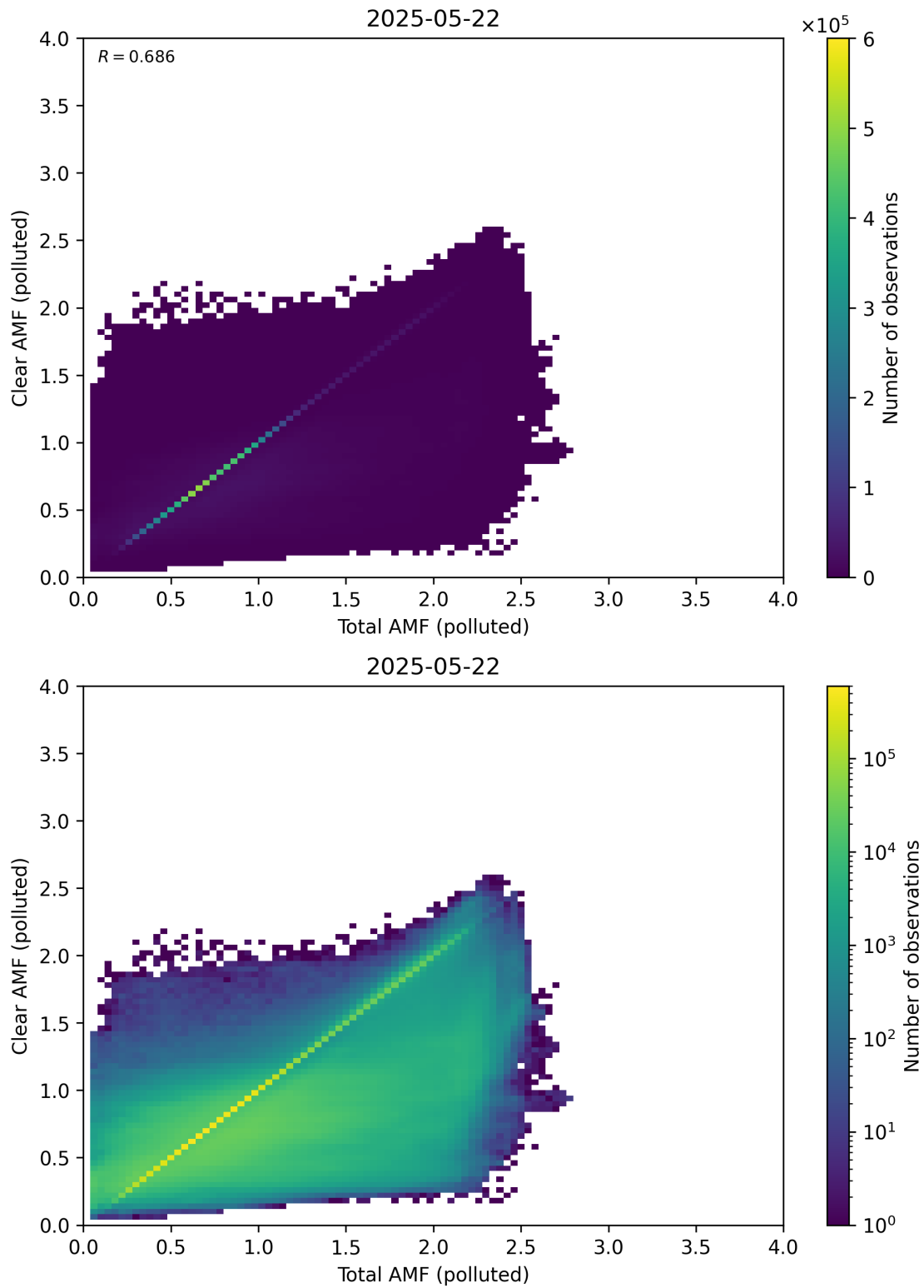
Figure 321: Scatter density plot of “Total AMF (polluted)” against “Clear AMF (polluted)” for 2025-05-21 to 2025-05-23.
