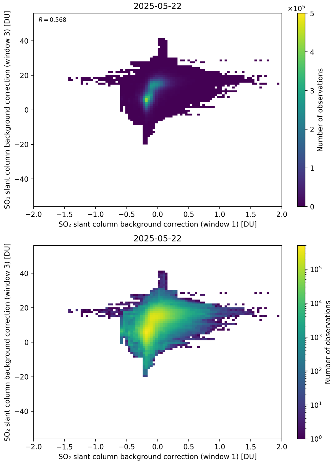
Figure 110: Scatter density plot of “SO 2 slant column background correction (window 1)” against “SO 2 slant column background correction (window 3)” for 2025-05-21 to 2025-05-23.
