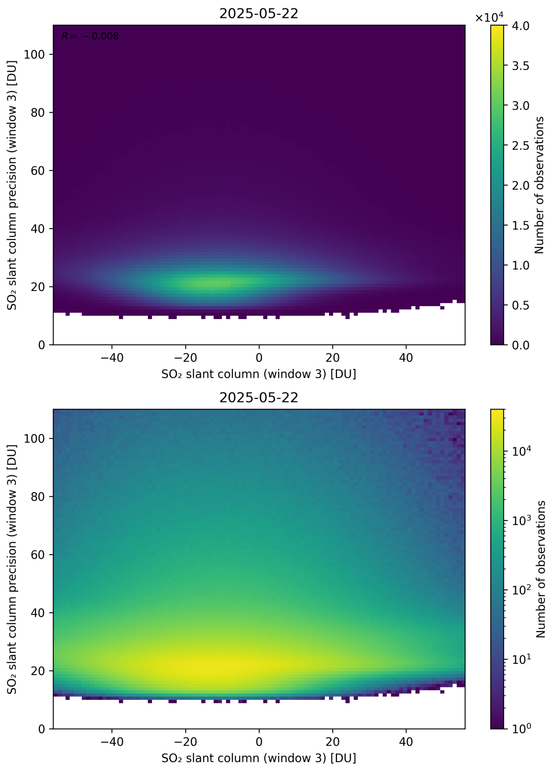
Figure 317: Scatter density plot of “SO 2 slant column (window 3)” against “SO 2 slant column precision (window 3)” for 2025-05-21 to 2025-05-23.
