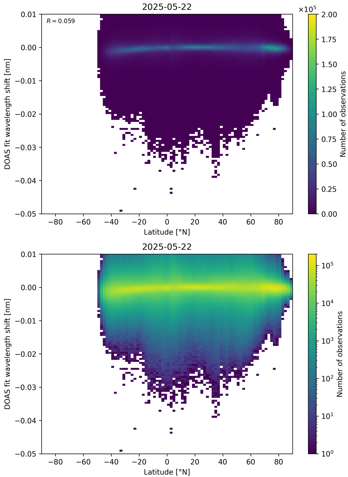
Figure 153: Scatter density plot of “Latitude” against “DOAS fit wavelength shift” for 2025-05-21 to 2025-05-23.
