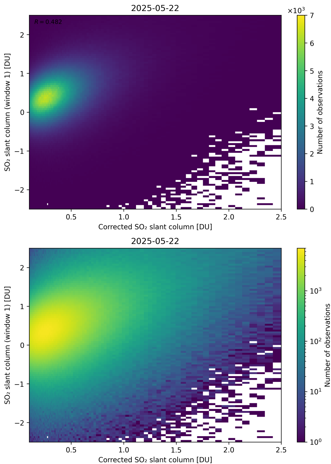
Figure 237: Scatter density plot of “Corrected SO 2 slant column” against “SO 2 slant column (window 1)” for 2025-05-21 to 2025-05-23.
