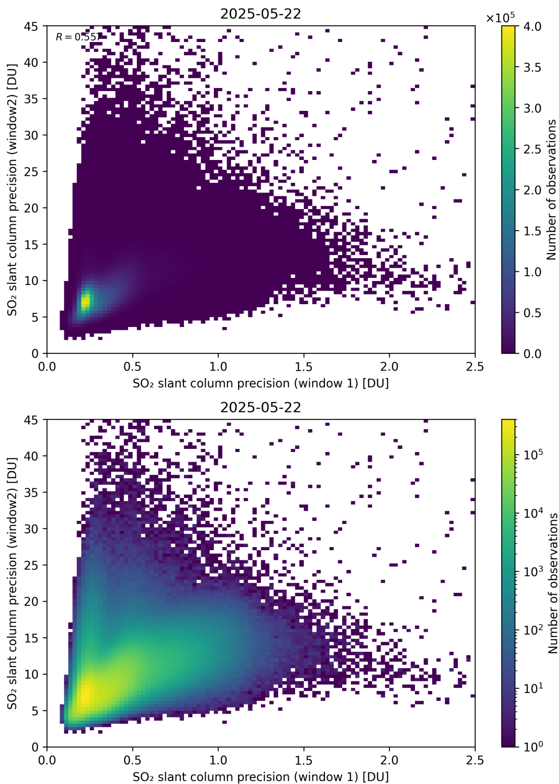
Figure 277: Scatter density plot of “SO 2 slant column precision (window 1)” against “SO 2 slant column precision (window2)” for 2025-05-21 to 2025-05-23.
