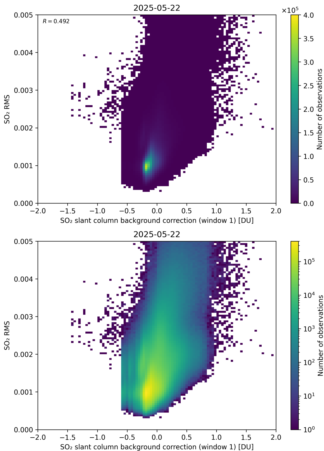
Figure 113: Scatter density plot of “SO 2 slant column background correction (window 1)” against “SO 2 RMS” for 2025-05-21 to 2025-05-23.
