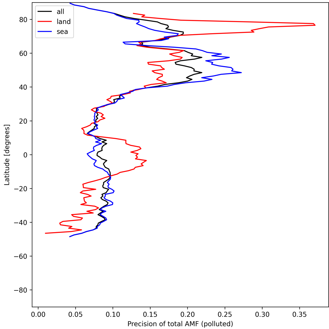
Figure 54: Zonal average of “Precision of total AMF (polluted)” for 2025-05-21 to 2025-05-23.
