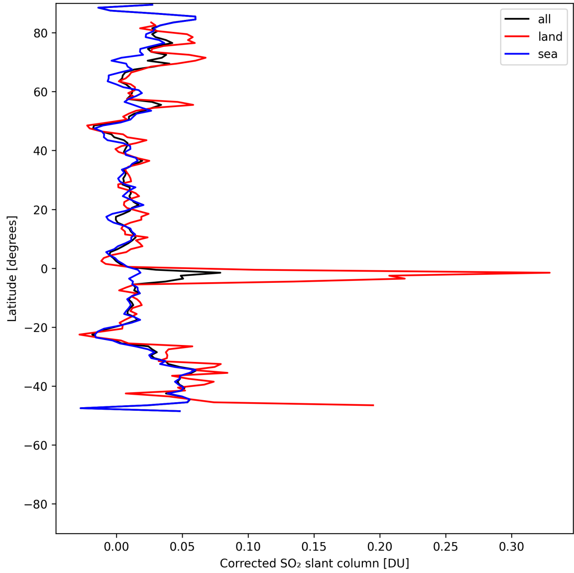
Figure 34: Zonal average of “Corrected SO 2 slant column” for 2025-05-21 to 2025-05-23.
