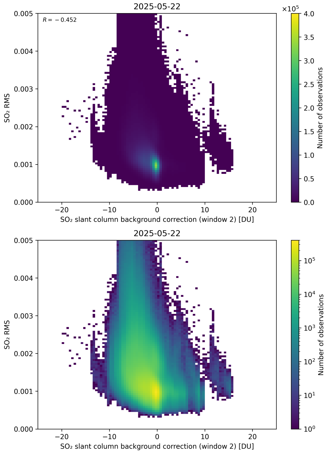
Figure 125: Scatter density plot of “SO 2 slant column background correction (window 2)” against “SO 2 RMS” for 2025-05-21 to 2025-05-23.
