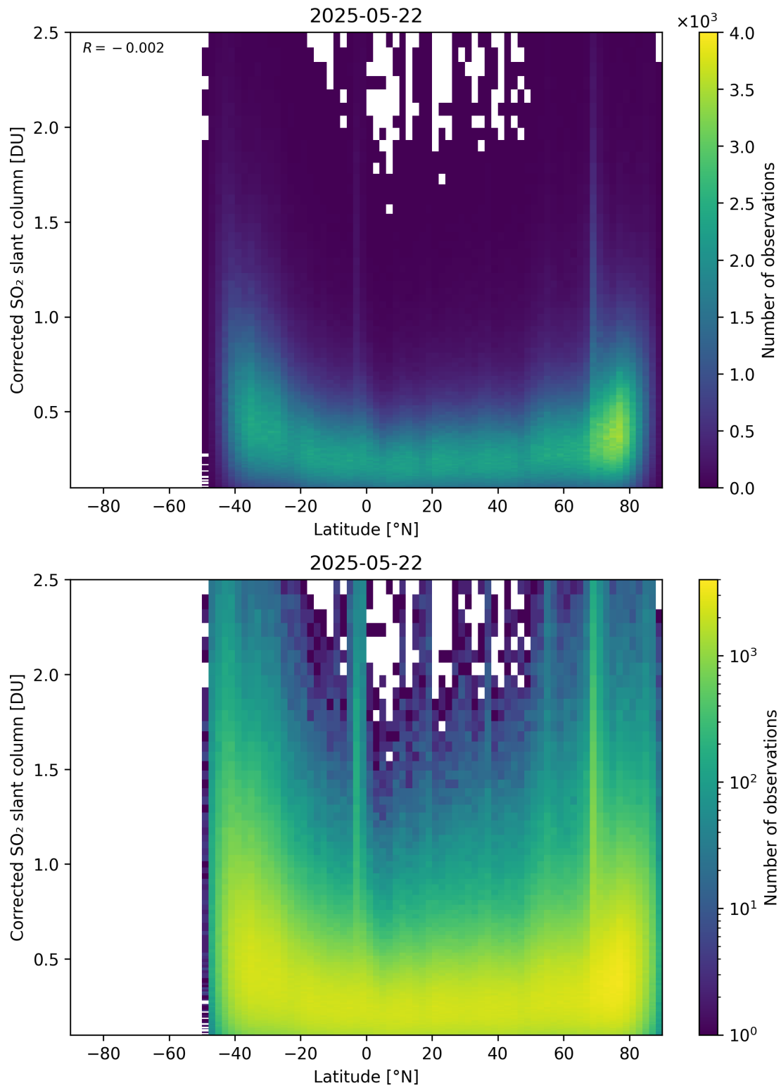
Figure 159: Scatter density plot of “Latitude” against “Corrected SO 2 slant column” for 2025-05-21 to 2025-05-23.
