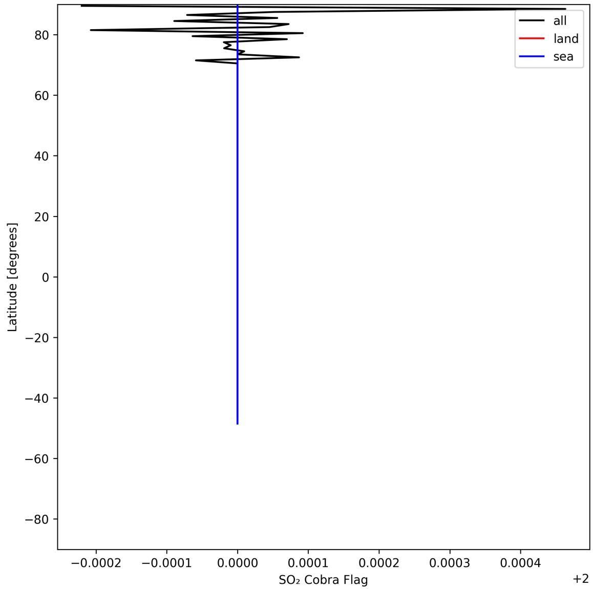
Figure 49: Zonal average of “SO 2 Cobra Flag” for 2025-05-21 to 2025-05-23.
