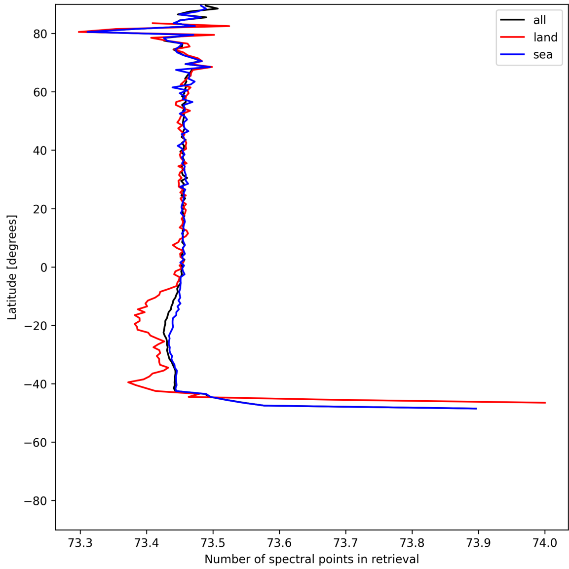
Figure 56: Zonal average of “Number of spectral points in retrieval” for 2025-05-21 to 2025-05-23.
