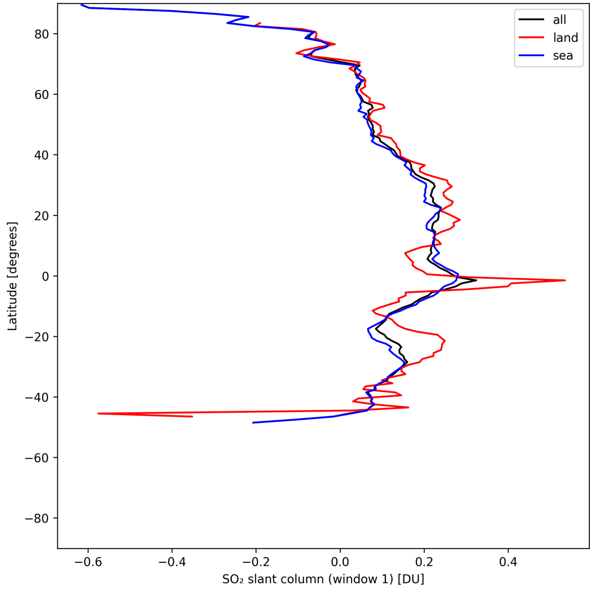
Figure 37: Zonal average of “SO 2 slant column (window 1)” for 2025-05-21 to 2025-05-23.
