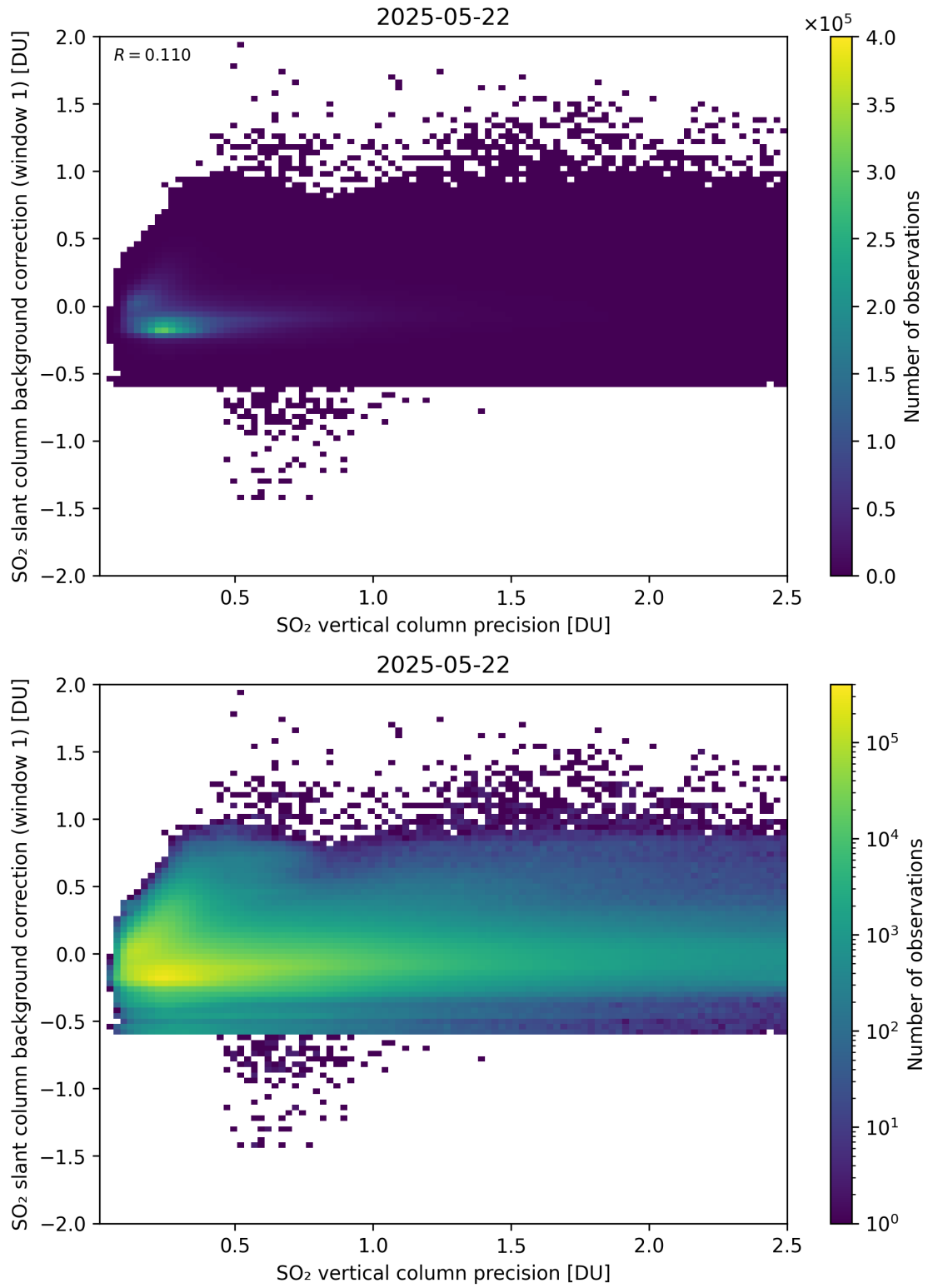
Figure 329: Scatter density plot of “SO 2 vertical column precision” against “SO 2 slant column background correction (window 1)” for 2025-05-21 to 2025-05-23.
