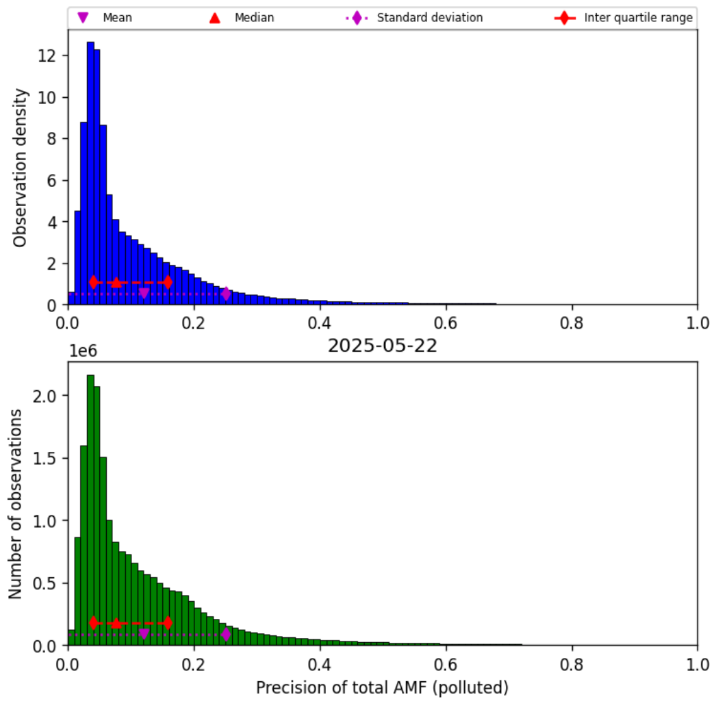
Figure 80: Histogram of “Precision of total AMF (polluted)” for 2025-05-21 to 2025-05-23
