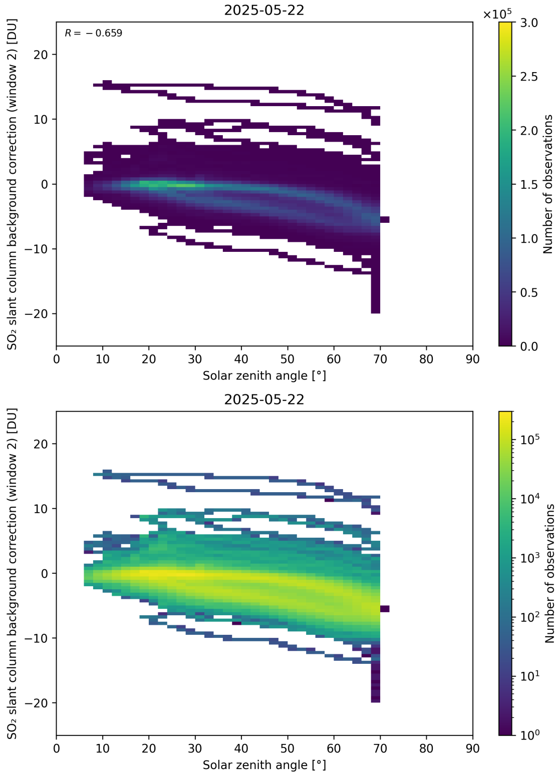
Figure 172: Scatter density plot of “Solar zenith angle” against “SO 2 slant column background correction (window 2)” for 2025-05-21 to 2025-05-23.
