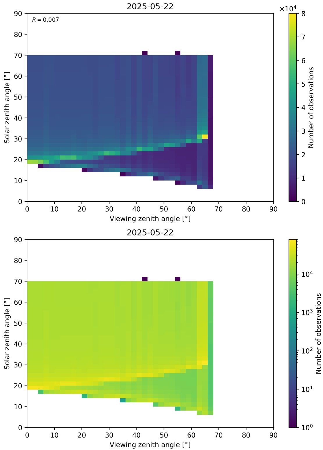
Figure 369: Scatter density plot of “Viewing zenith angle” against “Solar zenith angle” for 2025-05-21 to 2025-05-23.
