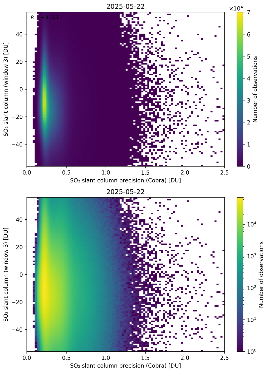
Figure 211: Scatter density plot of “SO 2 slant column precision (Cobra)” against “SO 2 slant column (window 3)” for 2025-05-21 to 2025-05-23.
