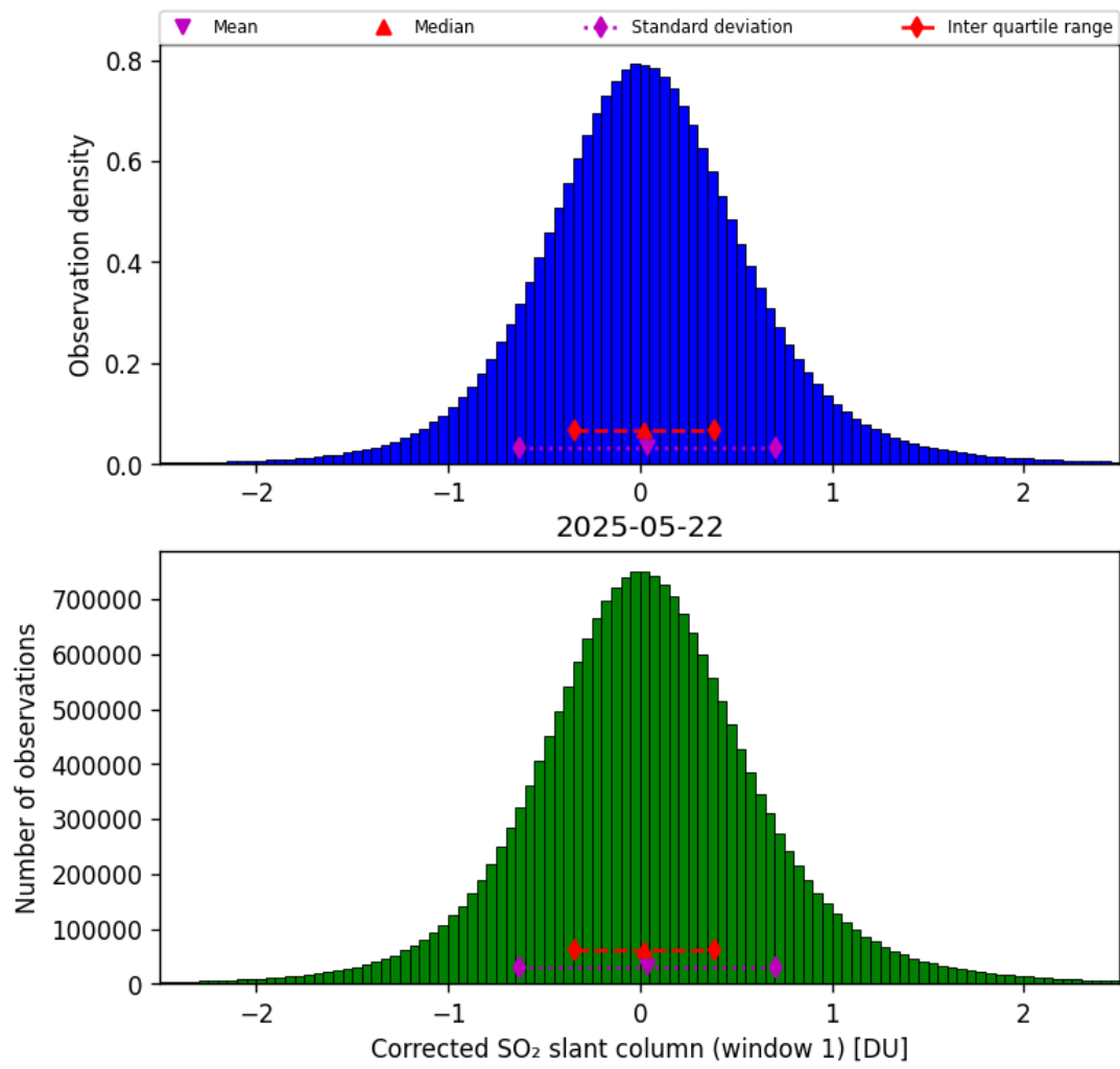
Figure 65: Histogram of “Corrected SO 2 slant column (window 1)” for 2025-05-21 to 2025-05-23
