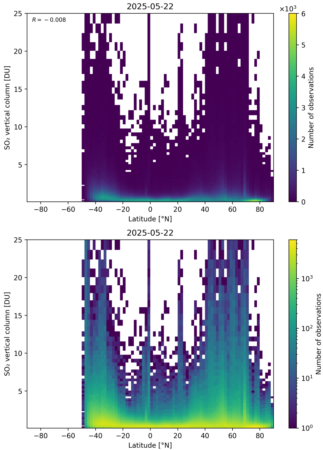
Figure 169: Scatter density plot of “Latitude” against “SO 2 vertical column” for 2025-05-21 to 2025-05-23.
