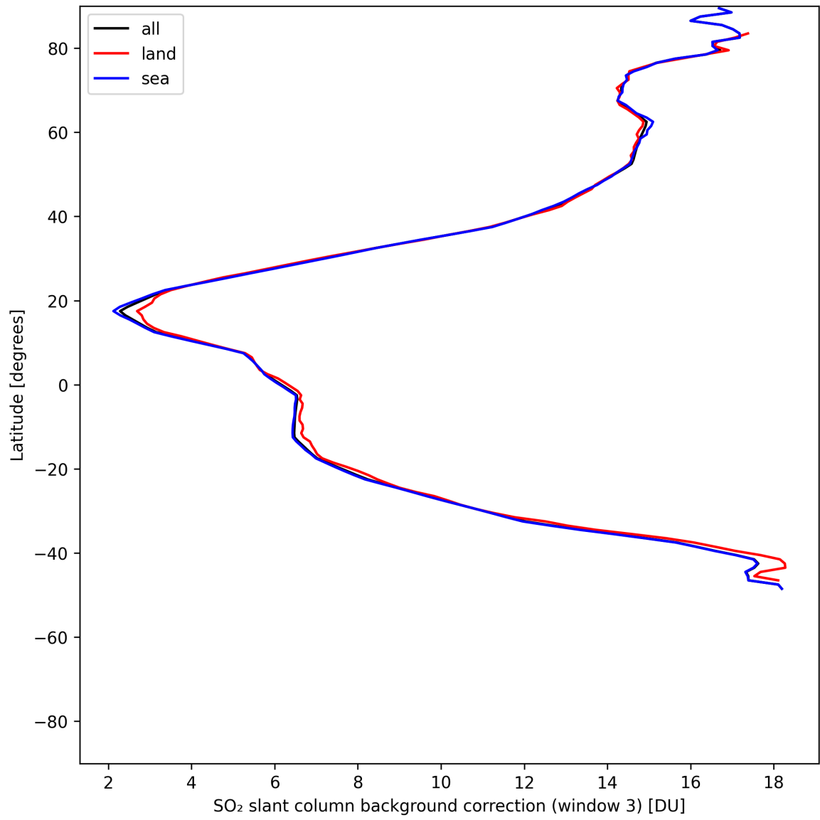
Figure 48: Zonal average of “SO 2 slant column background correction (window 3)” for 2025-05-21 to 2025-05-23.
