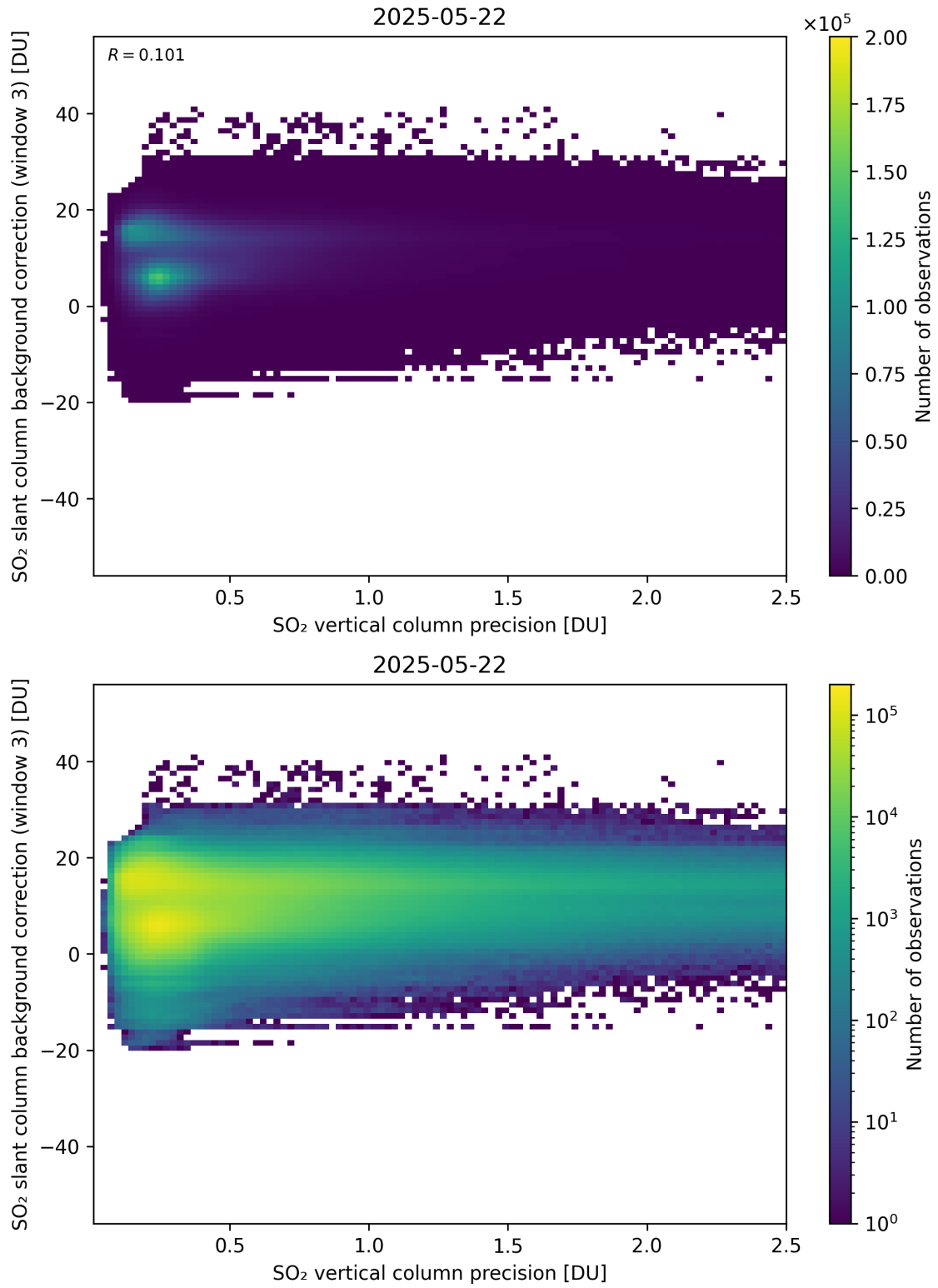
Figure 331: Scatter density plot of “SO 2 vertical column precision” against “SO 2 slant column background correction (window 3)” for 2025-05-21 to 2025-05-23.
