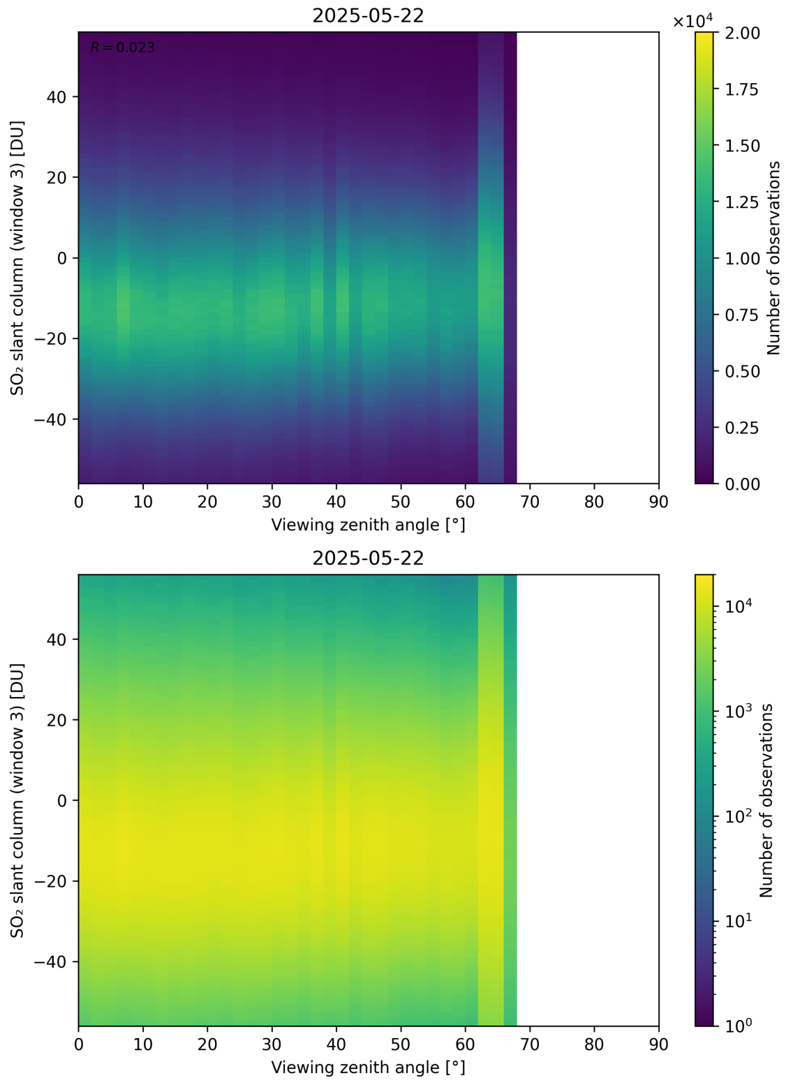
Figure 379: Scatter density plot of “Viewing zenith angle” against “SO 2 slant column (window 3)” for 2025-05-21 to 2025-05-23.
