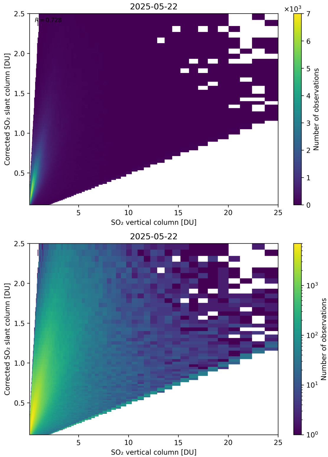
Figure 351: Scatter density plot of “SO 2 vertical column” against “Corrected SO 2 slant column” for 2025-05-21 to 2025-05-23.
