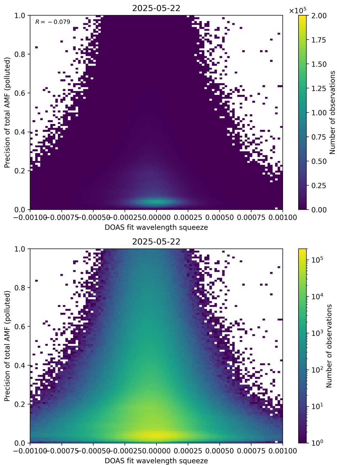
Figure 146: Scatter density plot of “DOAS fit wavelength squeeze” against “Precision of total AMF (polluted)” for 2025-05-21 to 2025-05-23.
