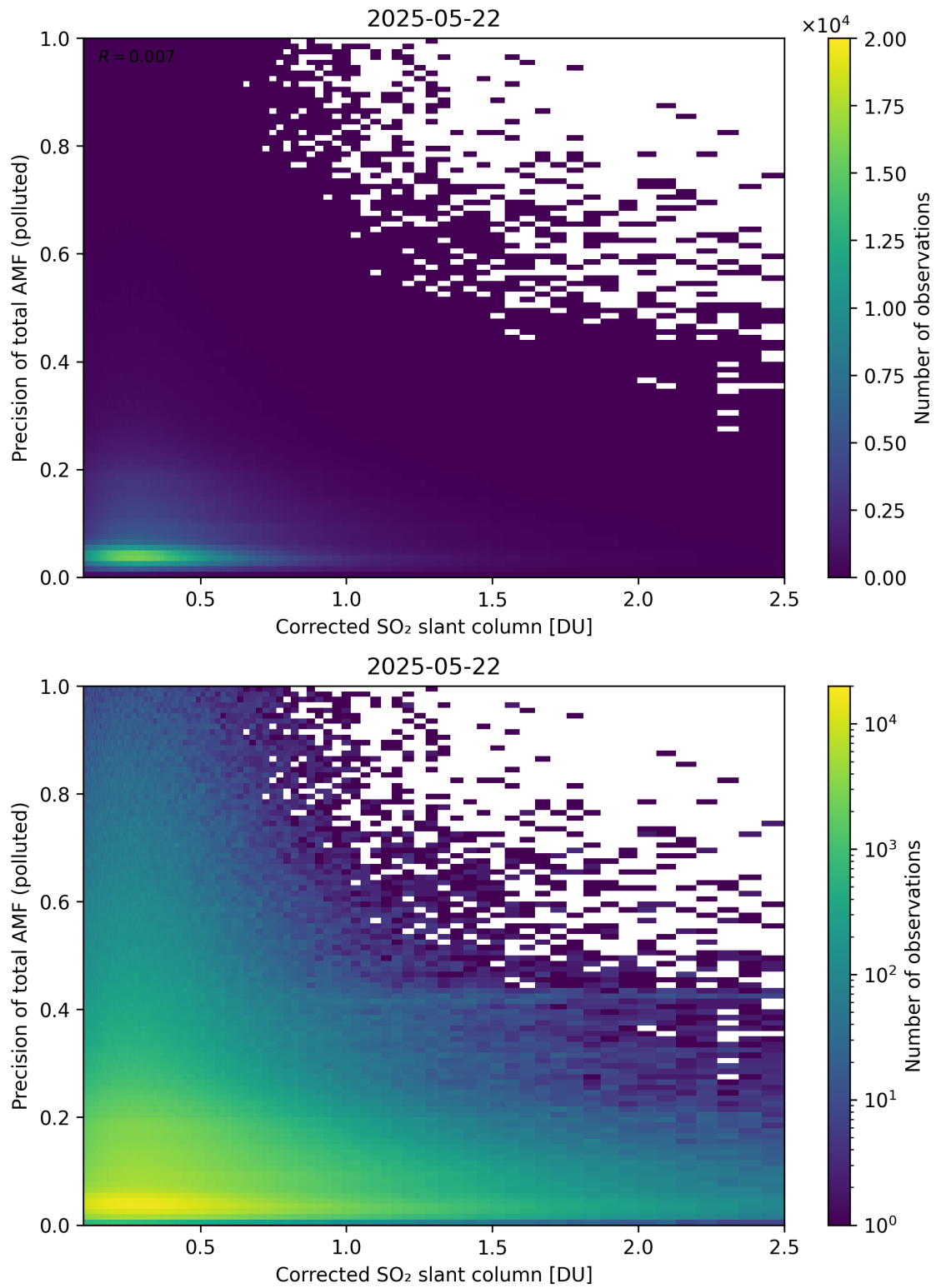
Figure 243: Scatter density plot of “Corrected SO 2 slant column” against “Precision of total AMF (polluted)” for 2025-05-21 to 2025-05-23.
