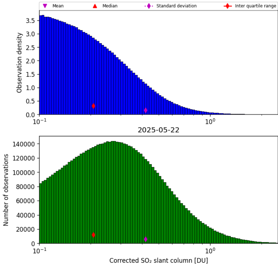
Figure 60: Histogram of "Corrected SO 2 slant column" for 2025-05-21 to 2025-05-23
