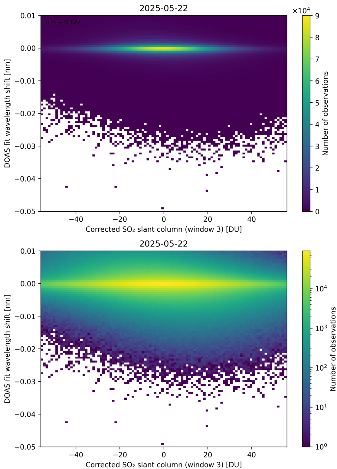
Figure 256: Scatter density plot of “Corrected SO 2 slant column (window 3)” against “DOAS fit wavelength shift” for 2025-05-21 to 2025-05-23.
