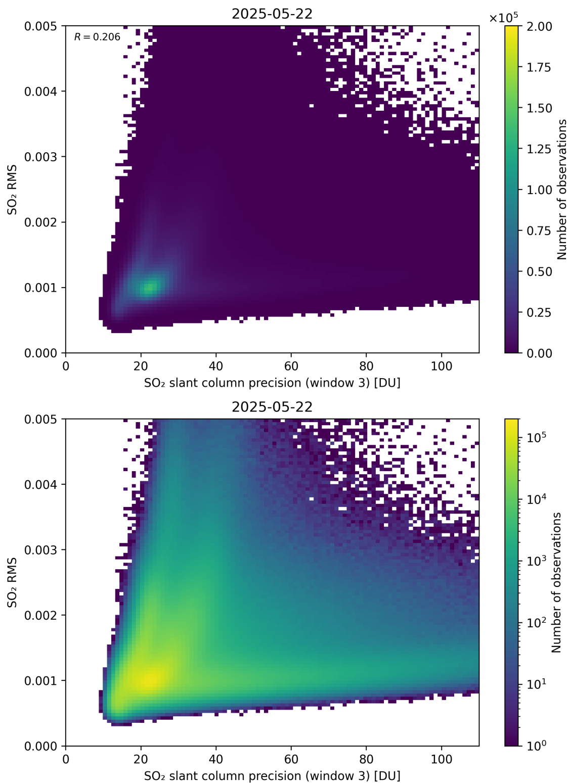
Figure 310: Scatter density plot of “SO 2 slant column precision (window 3)” against “SO 2 RMS” for 2025-05-21 to 2025-05-23.
