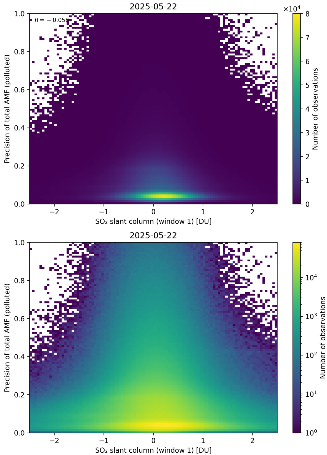
Figure 290: Scatter density plot of “SO 2 slant column (window 1)” against “Precision of total AMF (polluted)” for 2025-05-21 to 2025-05-23.
