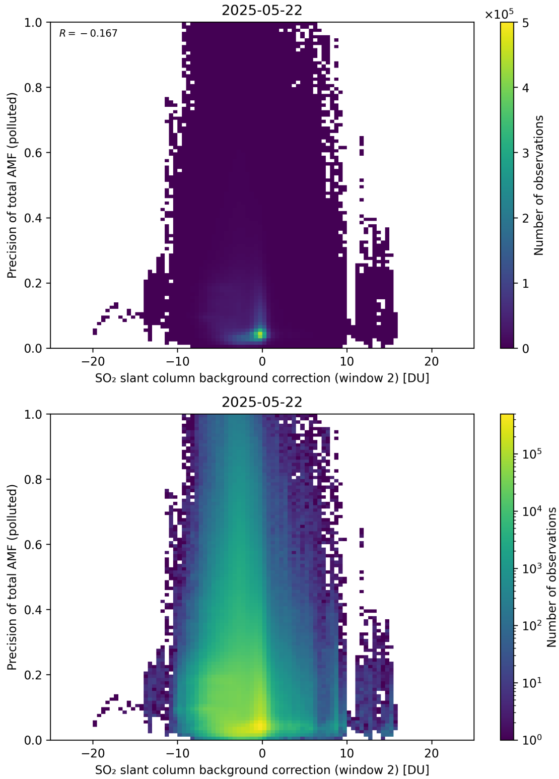
Figure 131: Scatter density plot of “SO 2 slant column background correction (window 2)” against “Precision of total AMF (polluted)” for 2025-05-21 to 2025-05-23.
