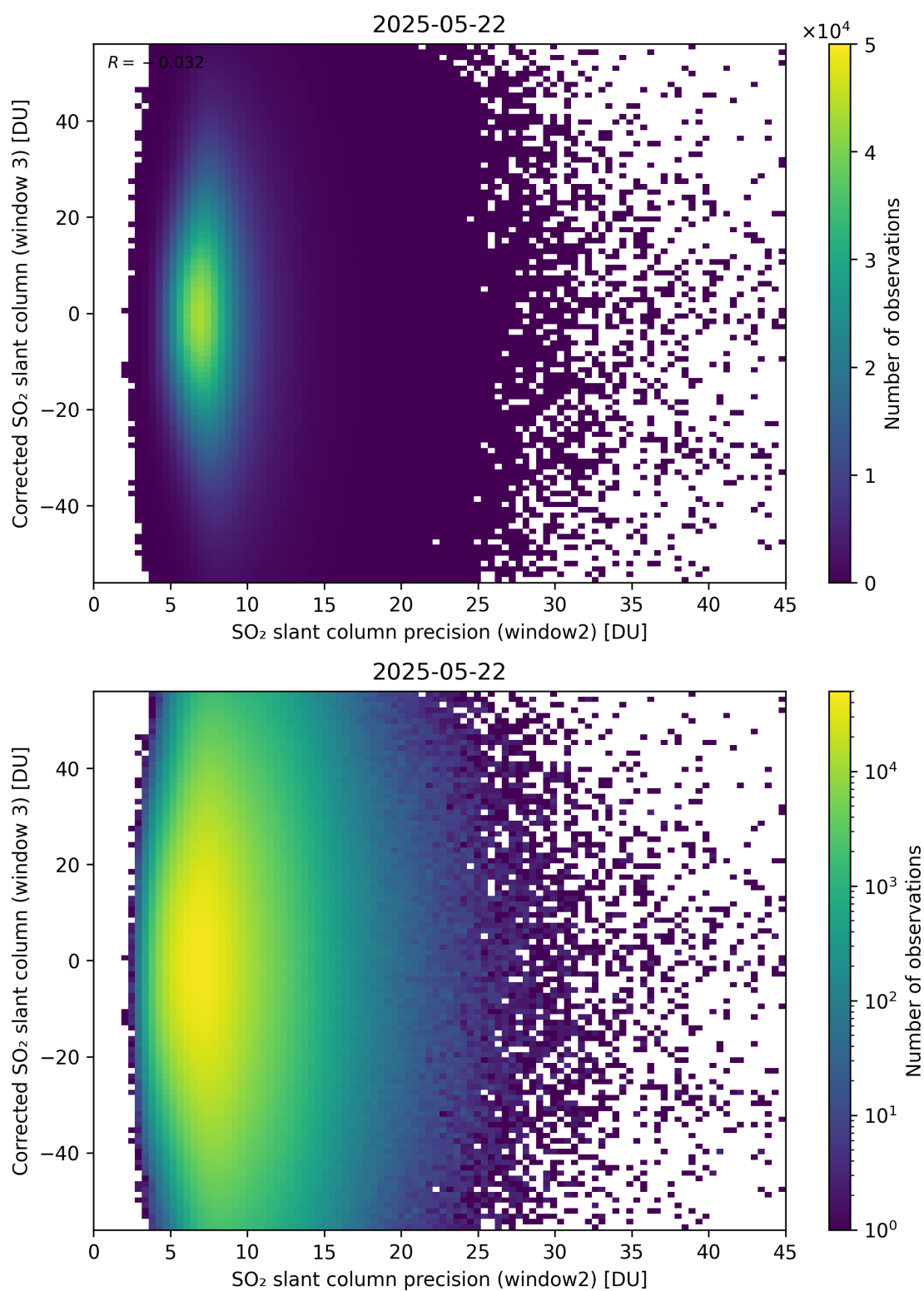
Figure 298: Scatter density plot of “SO 2 slant column precision (window2)” against “Corrected SO 2 slant column (window 3)” for 2025-05-21 to 2025-05-23.
