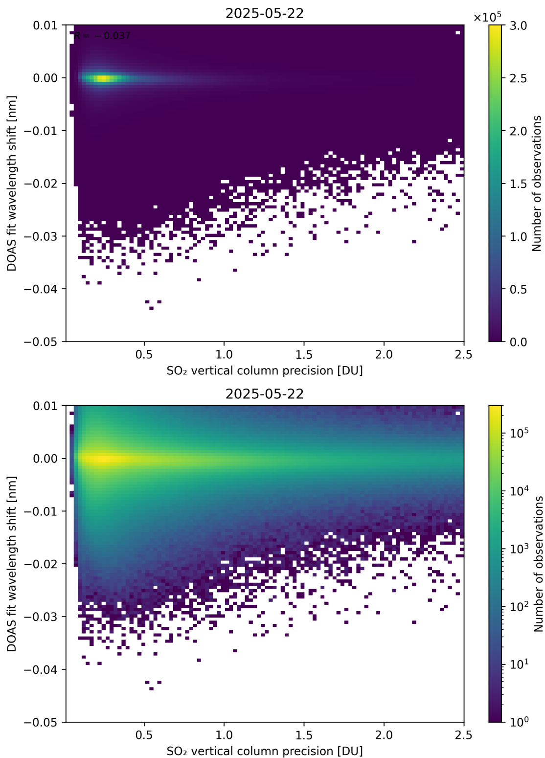
Figure 332: Scatter density plot of “SO 2 vertical column precision” against “DOAS fit wavelength shift” for 2025-05-21 to 2025-05-23.
