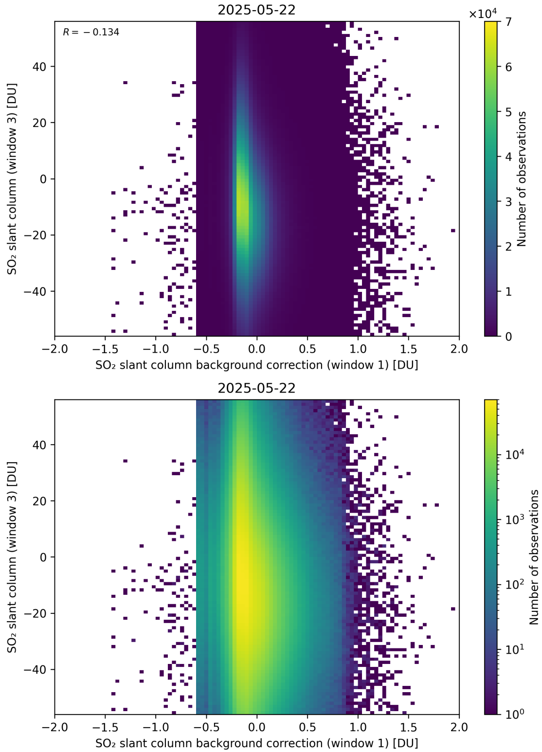
Figure 118: Scatter density plot of “SO 2 slant column background correction (window 1)” against “SO 2 slant column (window 3)” for 2025-05-21 to 2025-05-23.
