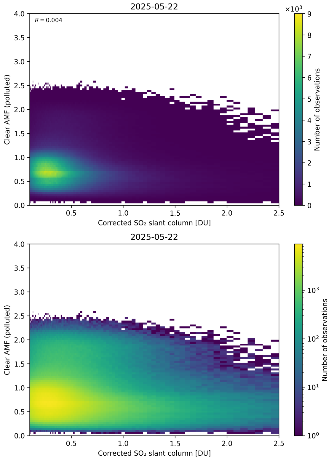
Figure 232: Scatter density plot of “Corrected SO 2 slant column” against “Clear AMF (polluted)” for 2025-05-21 to 2025-05-23.
