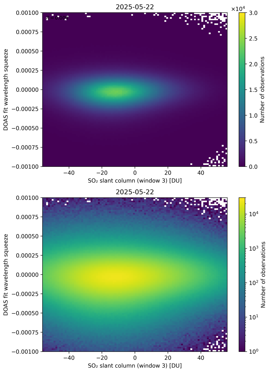
Figure 305: Scatter density plot of “SO 2 slant column (window 3)” against “DOAS fit wavelength squeeze” for 2025-05-21 to 2025-05-23.
