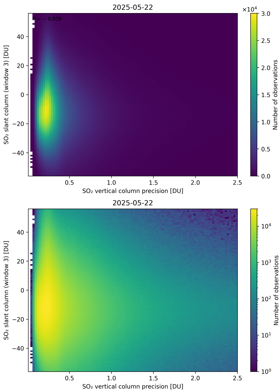
Figure 344: Scatter density plot of “SO 2 vertical column precision” against “SO 2 slant column (window 3)” for 2025-05-21 to 2025-05-23.
