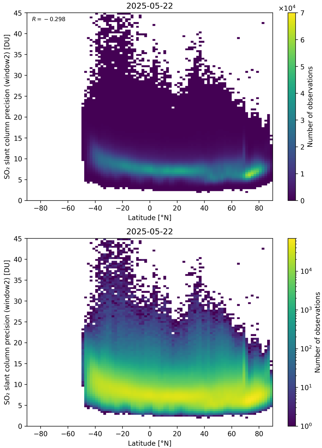
Figure 164: Scatter density plot of “Latitude” against “SO 2 slant column precision (window2)” for 2025-05-21 to 2025-05-23.
