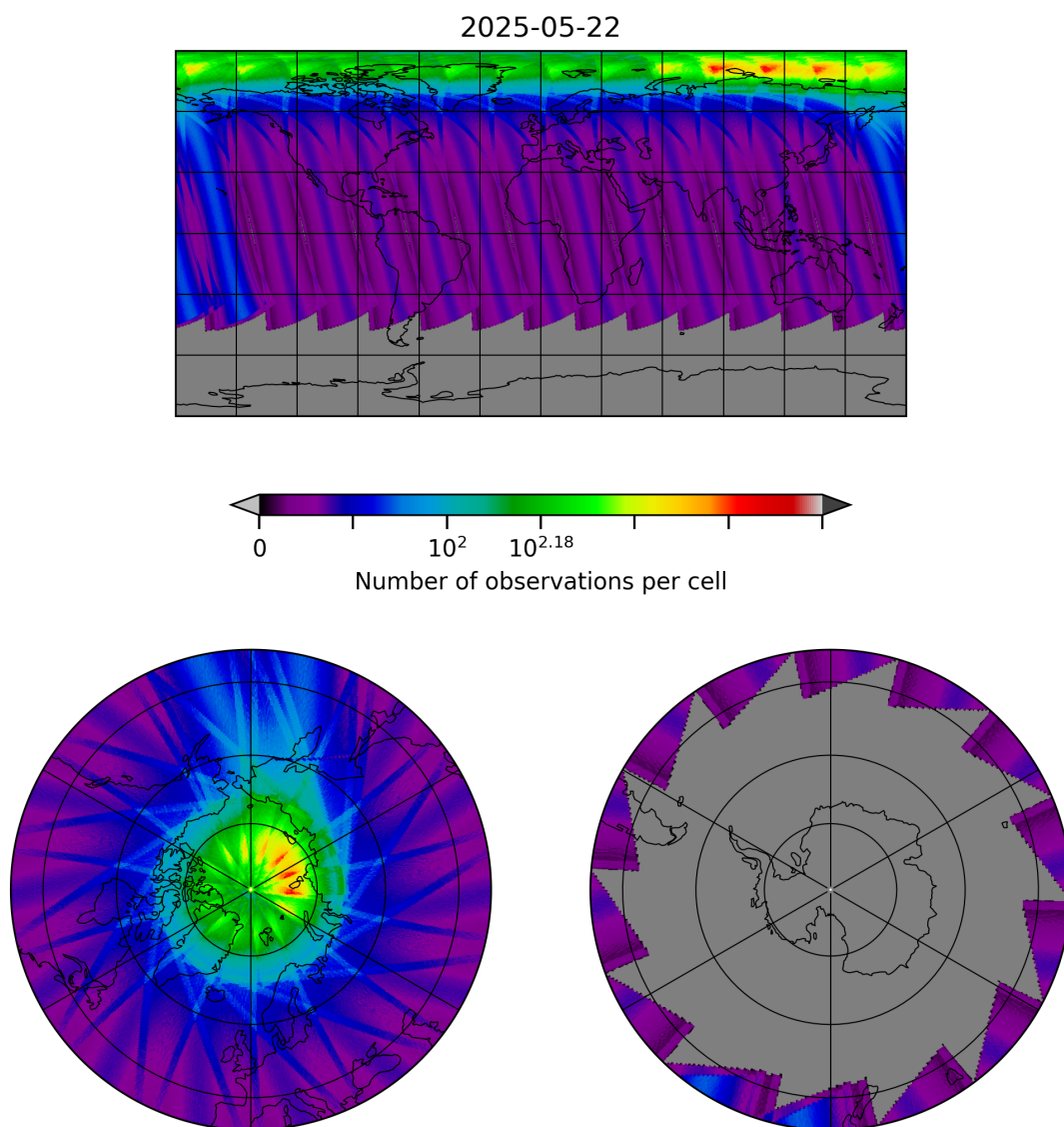
Figure 30: Map of the number of observations for 2025-05-21 to 2025-05-23
