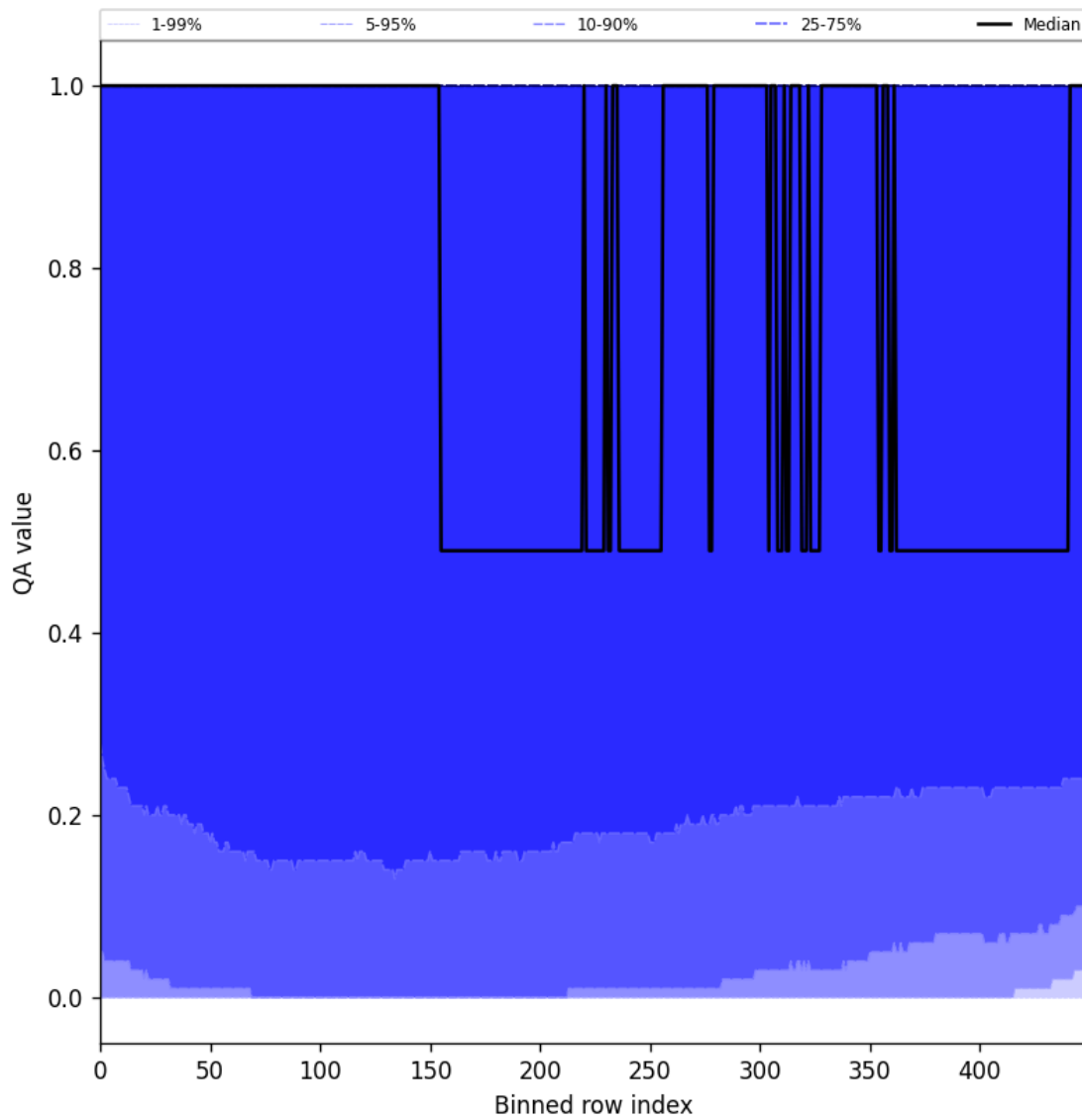
Figure 83: Along track statistics of “QA value” for 2025-05-21 to 2025-05-23
