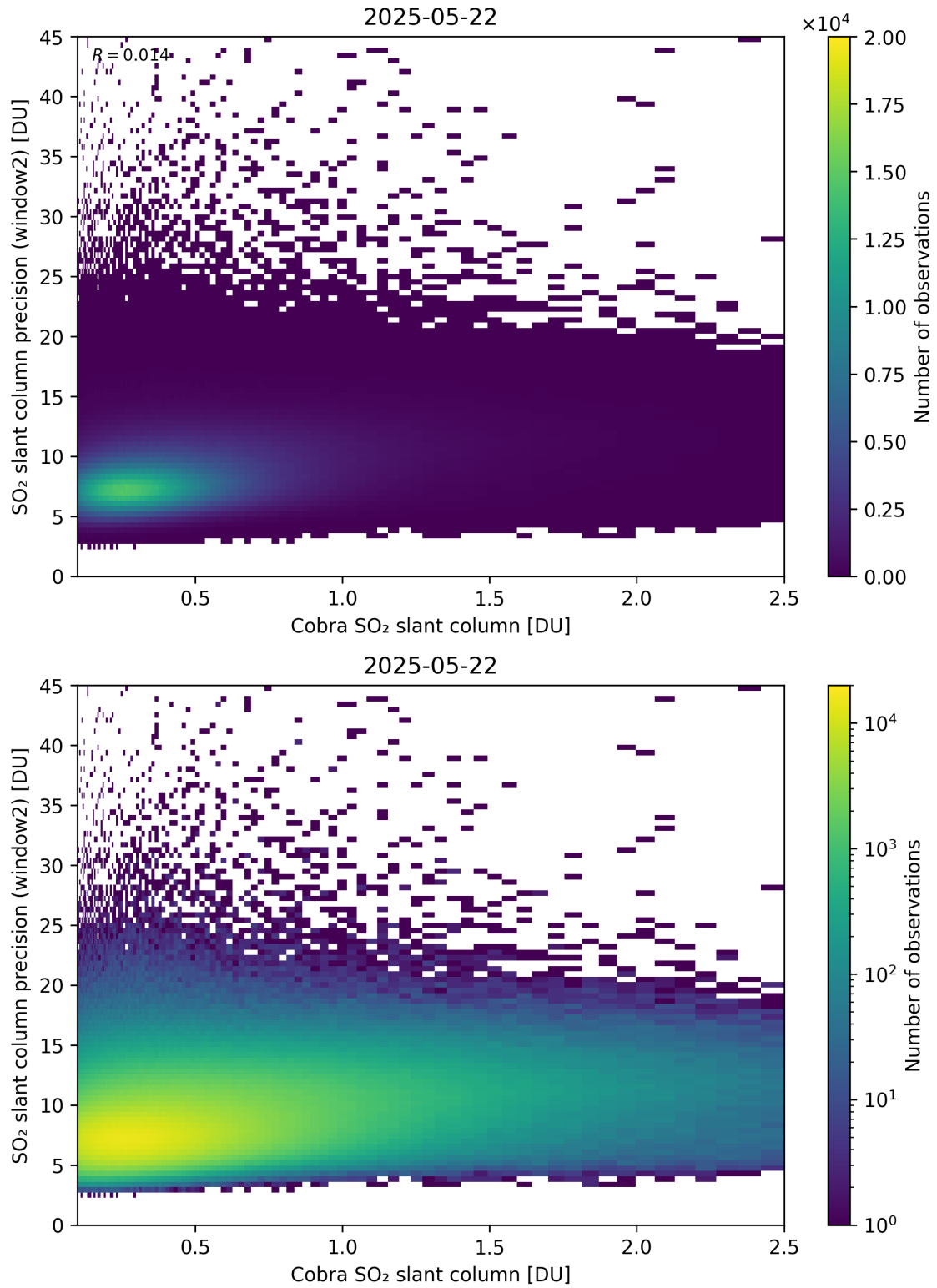
Figure 221: Scatter density plot of “Cobra SO 2 slant column” against “SO 2 slant column precision (window2)” for 2025-05-21 to 2025-05-23.
