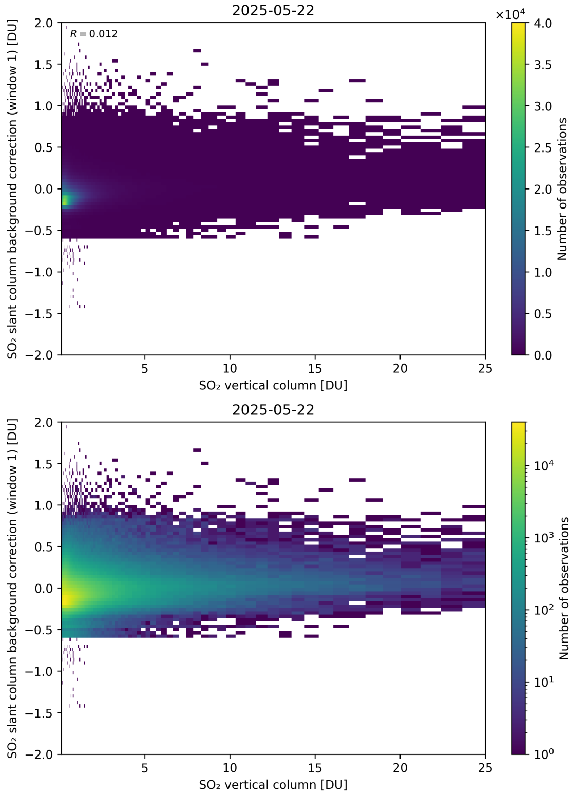
Figure 323: Scatter density plot of “SO 2 vertical column” against “SO 2 slant column background correction (window 1)” for 2025-05-21 to 2025-05-23.
