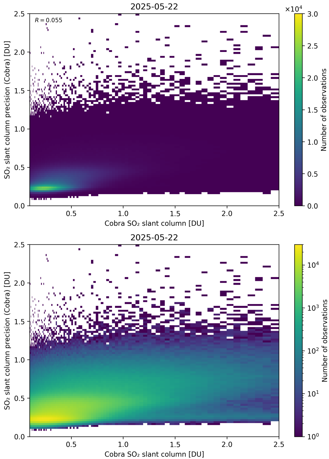
Figure 216: Scatter density plot of “Cobra SO 2 slant column” against “SO 2 slant column precision (Cobra)” for 2025-05-21 to 2025-05-23.
