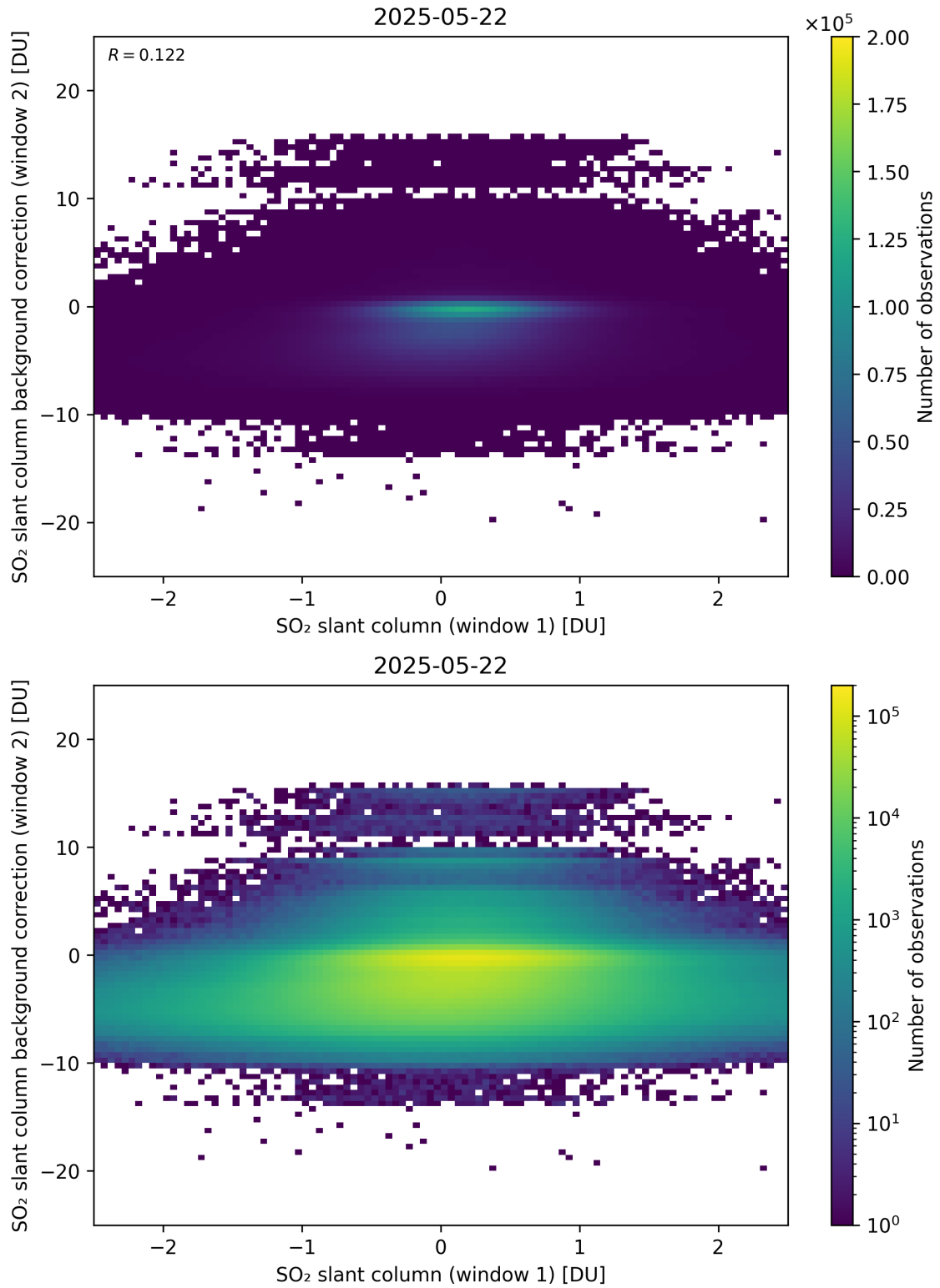
Figure 263: Scatter density plot of “SO 2 slant column (window 1)” against “SO 2 slant column background correction (window 2)” for 2025-05-21 to 2025-05-23.
