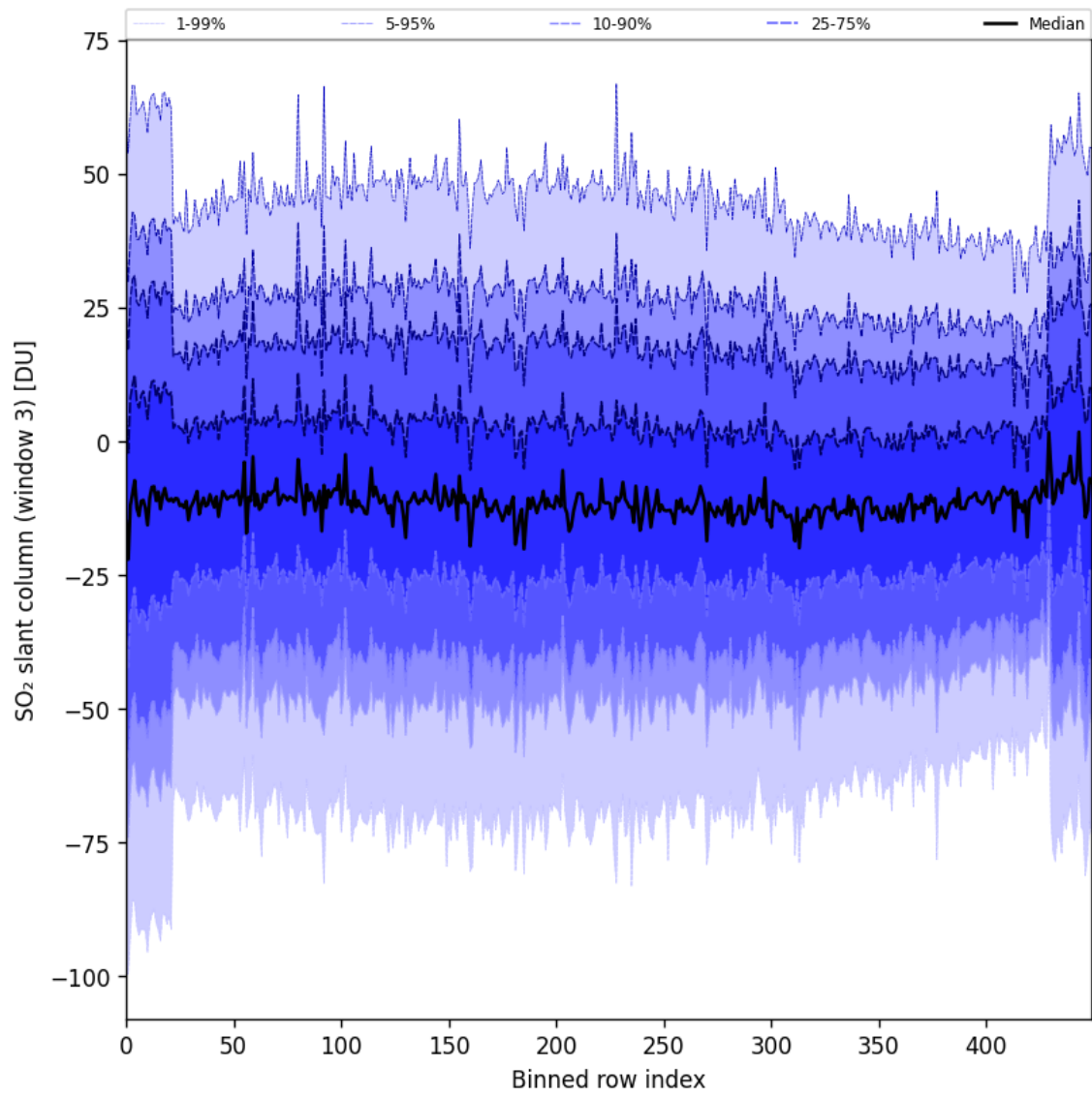
Figure 97: Along track statistics of “SO 2 slant column (window 3)” for 2025-05-21 to 2025-05-23
