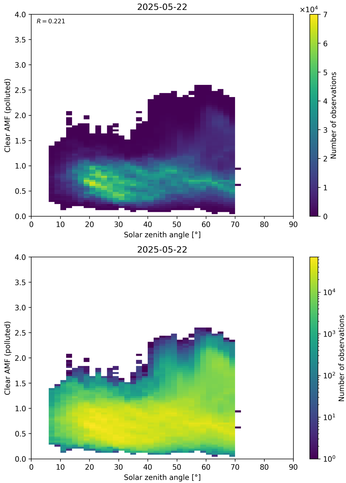
Figure 178: Scatter density plot of “Solar zenith angle” against “Clear AMF (polluted)” for 2025-05-21 to 2025-05-23.
