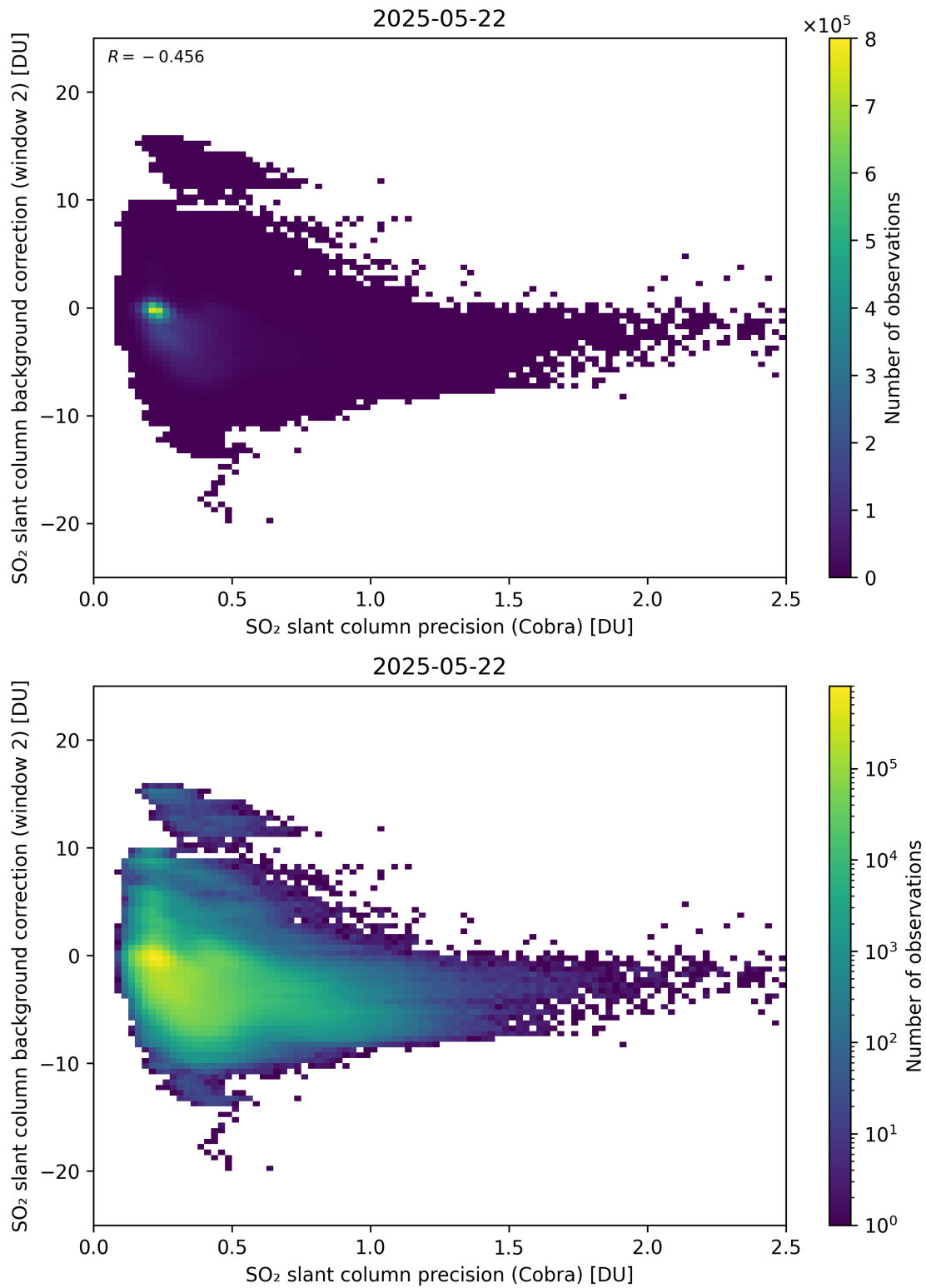
Figure 200: Scatter density plot of “SO 2 slant column precision (Cobra)” against “SO 2 slant column background correction (window 2)” for 2025-05-21 to 2025-05-23.
