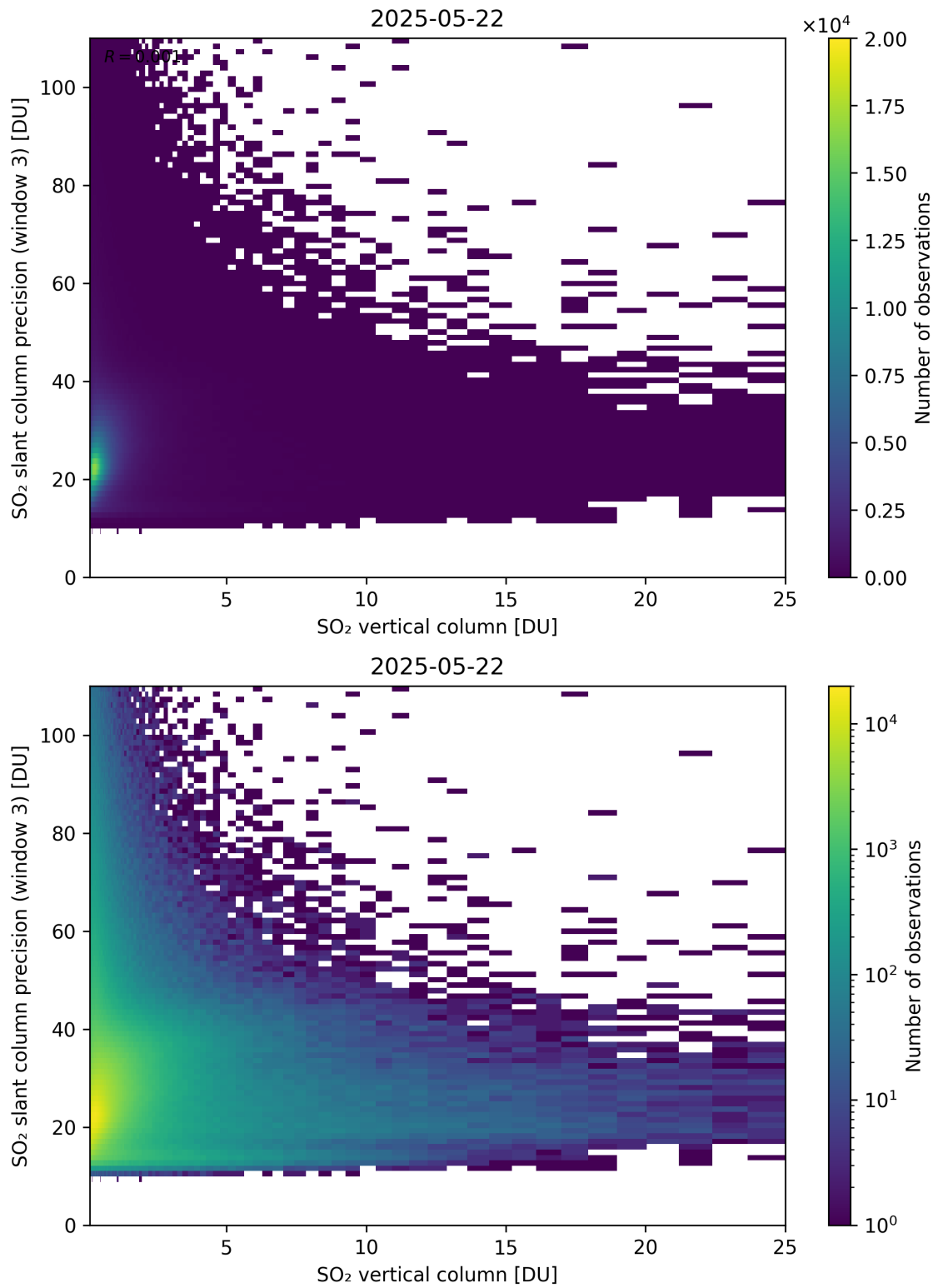
Figure 358: Scatter density plot of “SO 2 vertical column” against “SO 2 slant column precision (window 3)” for 2025-05-21 to 2025-05-23.
