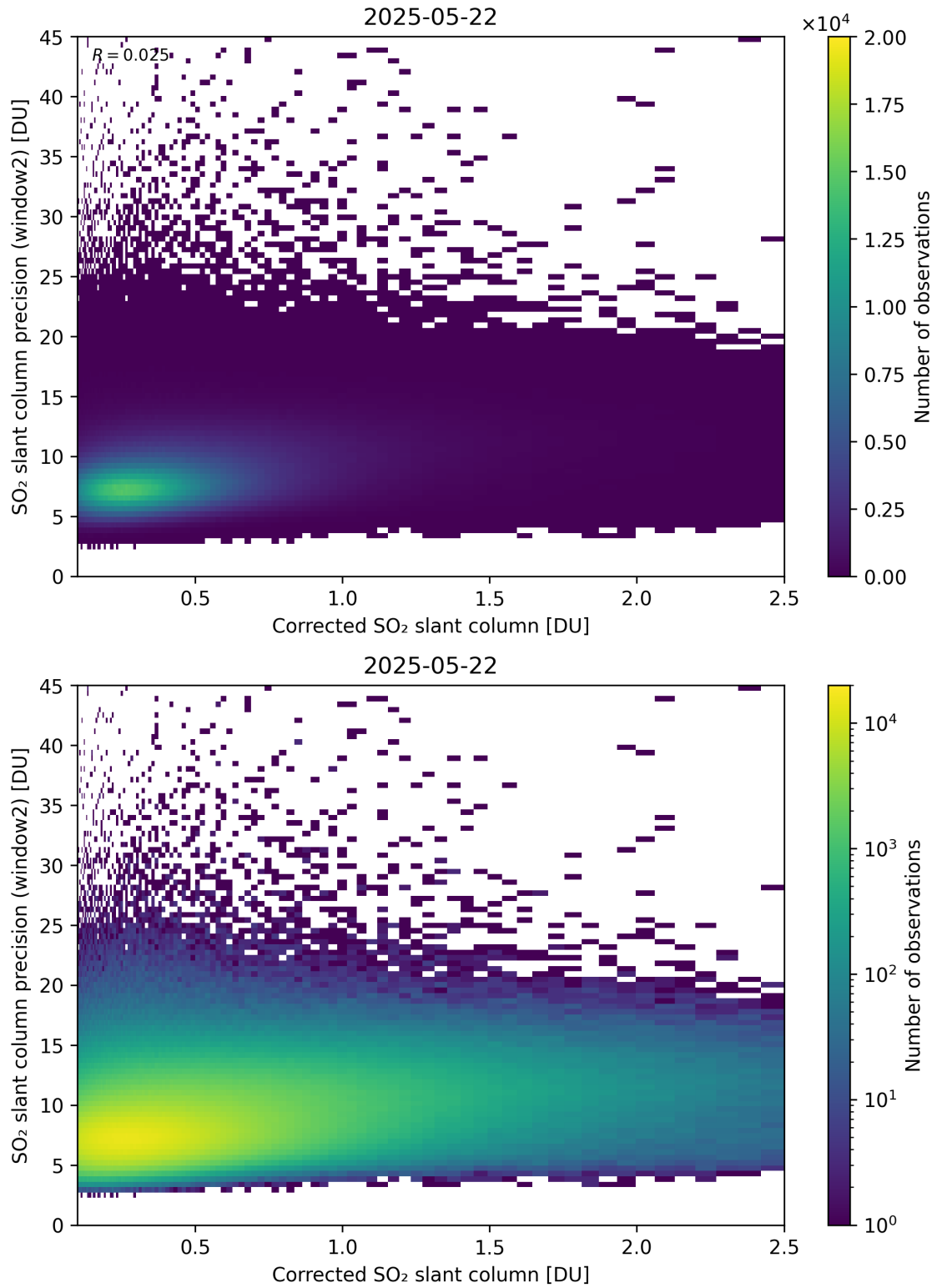
Figure 239: Scatter density plot of “Corrected SO 2 slant column” against “SO 2 slant column precision (window2)” for 2025-05-21 to 2025-05-23.
