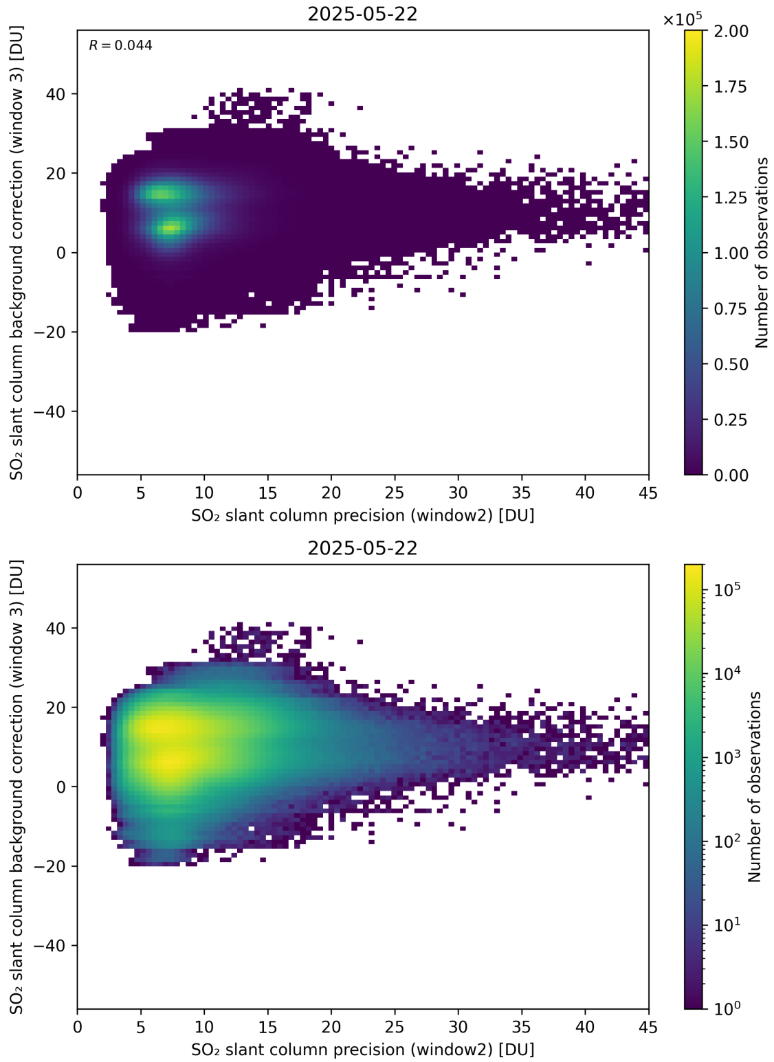
Figure 292: Scatter density plot of “SO 2 slant column precision (window2)” against “SO 2 slant column background correction (window 3)” for 2025-05-21 to 2025-05-23.
