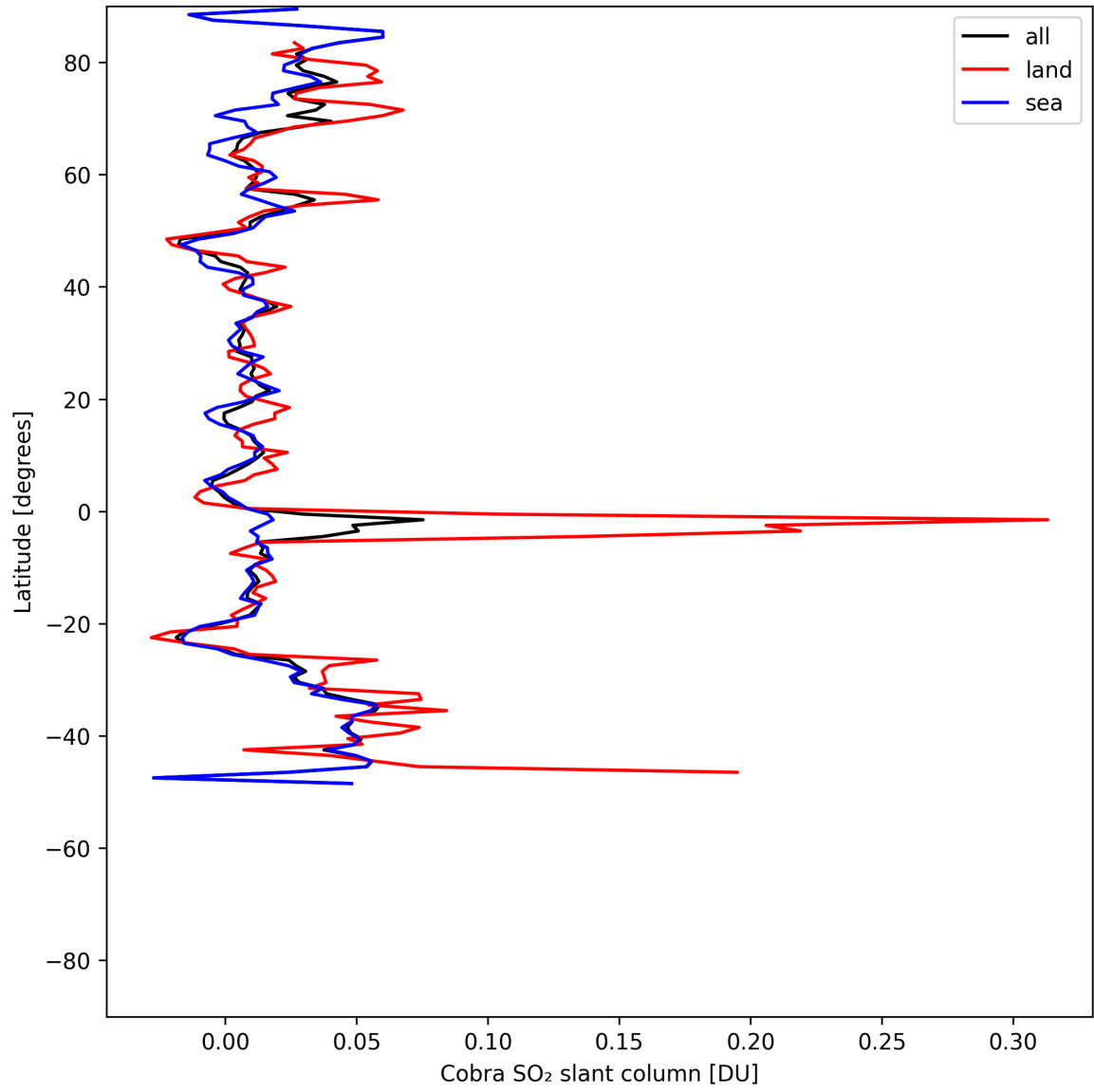
Figure 35: Zonal average of “Cobra SO 2 slant column” for 2025-05-21 to 2025-05-23.
