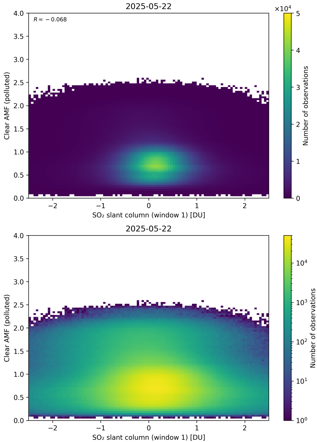
Figure 282: Scatter density plot of “SO 2 slant column (window 1)” against “Clear AMF (polluted)” for 2025-05-21 to 2025-05-23.
