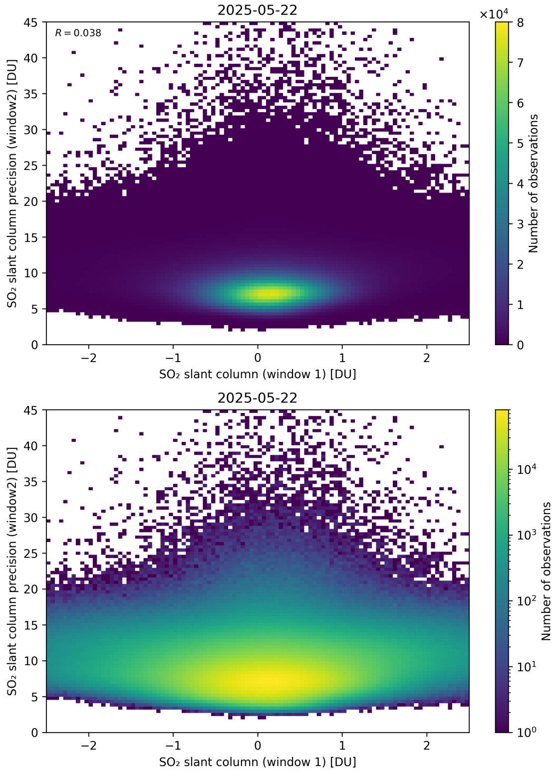
Figure 286: Scatter density plot of “SO 2 slant column (window 1)” against “SO 2 slant column precision (window2)” for 2025-05-21 to 2025-05-23.
