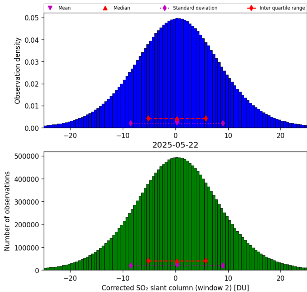
Figure 69: Histogram of “Corrected SO 2 slant column (window 2)” for 2025-05-21 to 2025-05-23
