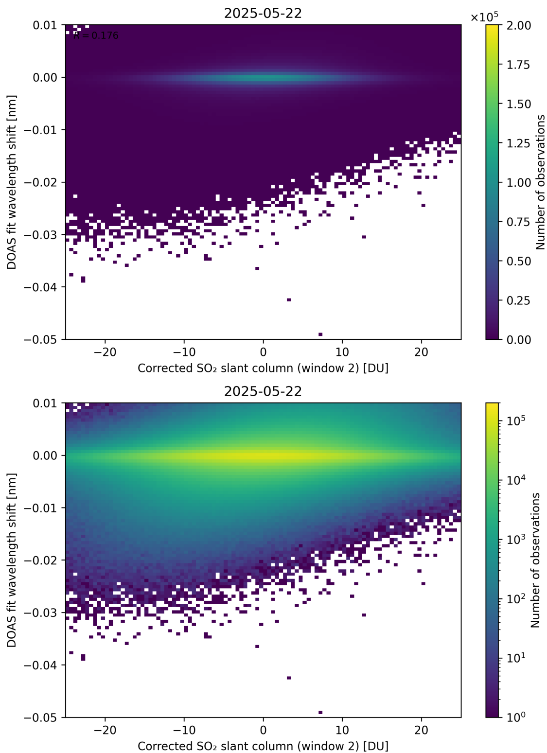
Figure 246: Scatter density plot of “Corrected SO 2 slant column (window 2)” against “DOAS fit wavelength shift” for 2025-05-21 to 2025-05-23.
