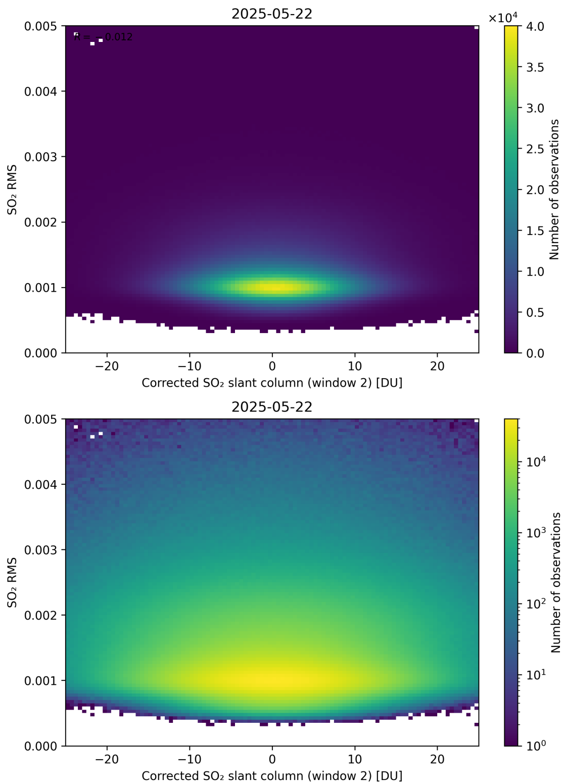
Figure 248: Scatter density plot of “Corrected SO 2 slant column (window 2)” against “SO 2 RMS” for 2025-05-21 to 2025-05-23.
