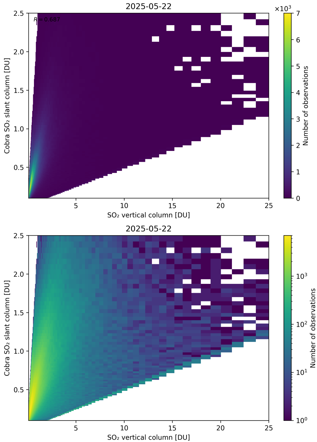
Figure 349: Scatter density plot of “SO 2 vertical column” against “Cobra SO 2 slant column” for 2025-05-21 to 2025-05-23.
