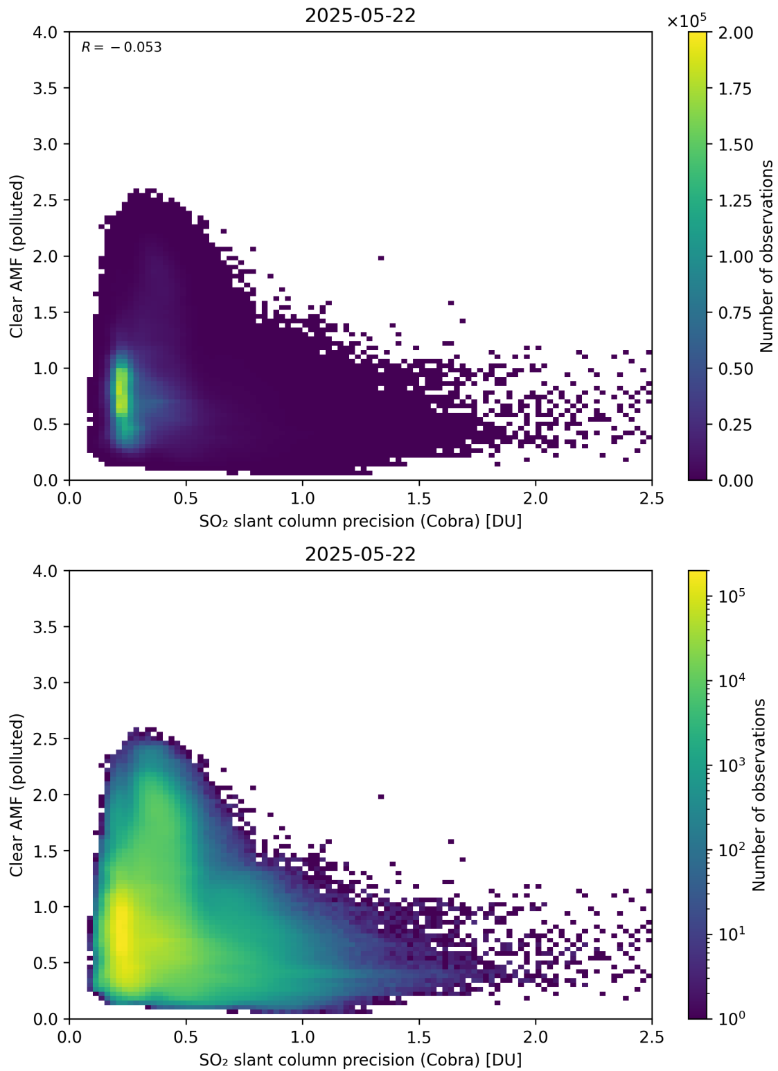
Figure 205: Scatter density plot of “SO 2 slant column precision (Cobra)” against “Clear AMF (polluted)” for 2025-05-21 to 2025-05-23.
