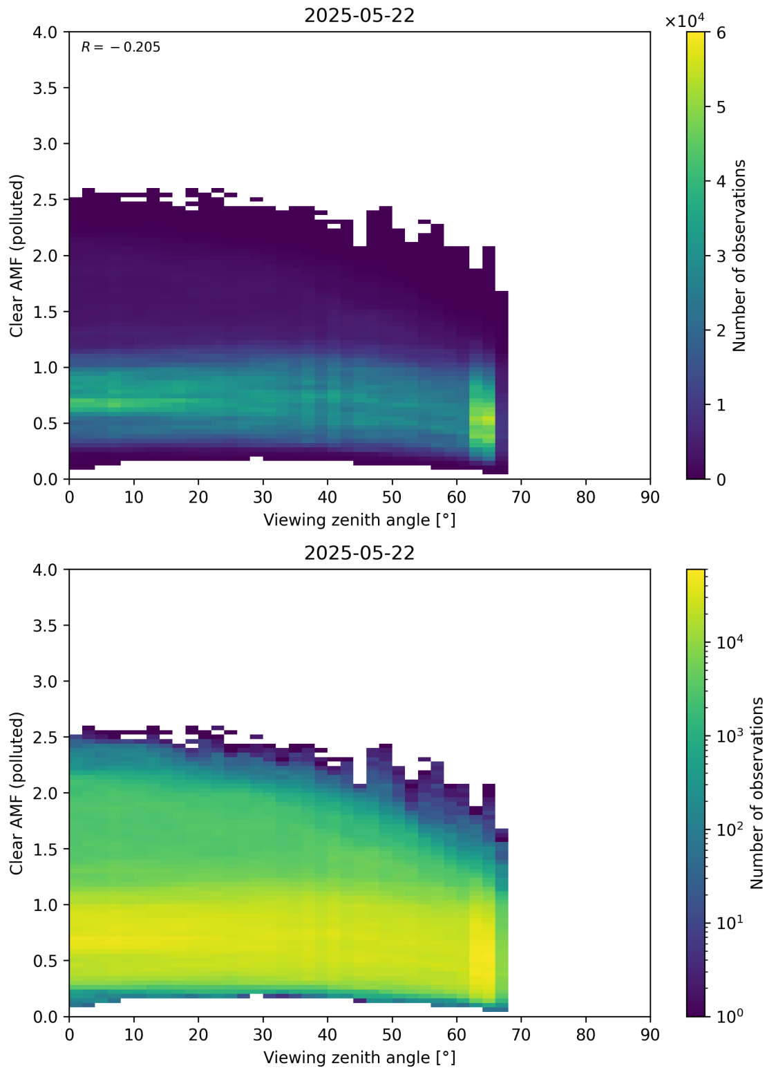
Figure 370: Scatter density plot of “Viewing zenith angle” against “Clear AMF (polluted)” for 2025-05-21 to 2025-05-23.
