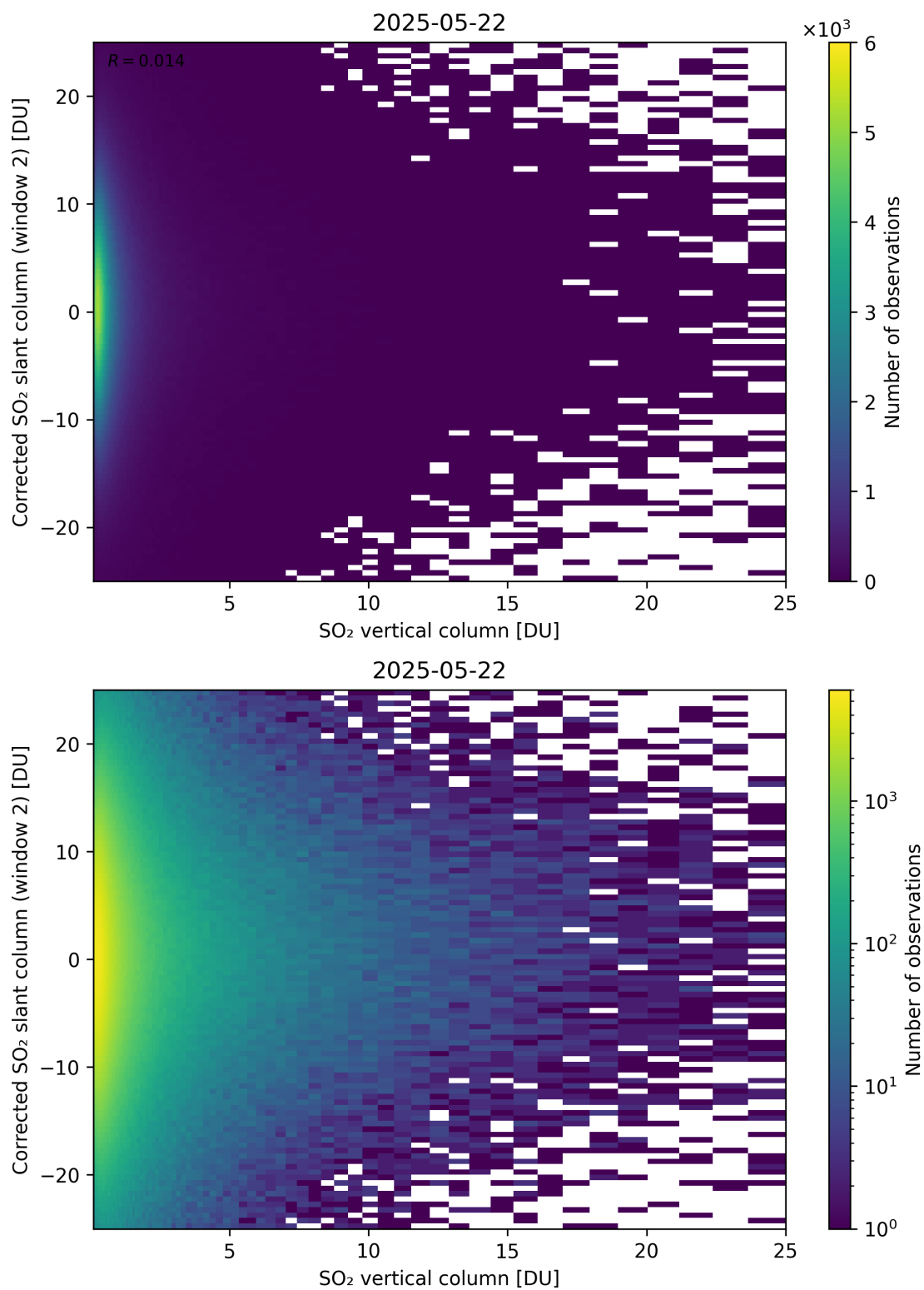
Figure 352: Scatter density plot of “SO 2 vertical column” against “Corrected SO 2 slant column (window 2)” for 2025-05-21 to 2025-05-23.
