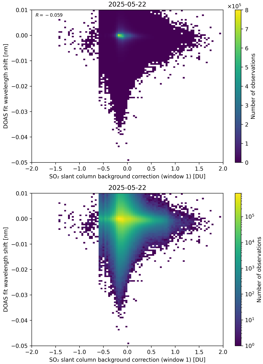
Figure 111: Scatter density plot of “SO 2 slant column background correction (window 1)” against “DOAS fit wavelength shift” for 2025-05-21 to 2025-05-23.
