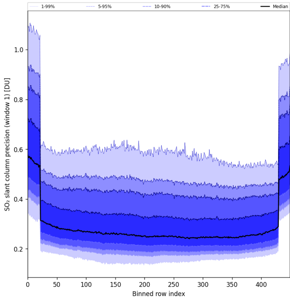
Figure 90: Along track statistics of “SO 2 slant column precision (window 1)” for 2025-05-21 to 2025-05-23
