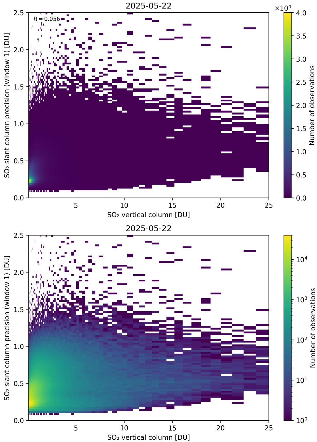
Figure 355: Scatter density plot of “SO 2 vertical column” against “SO 2 slant column precision (window 1)” for 2025-05-21 to 2025-05-23.
