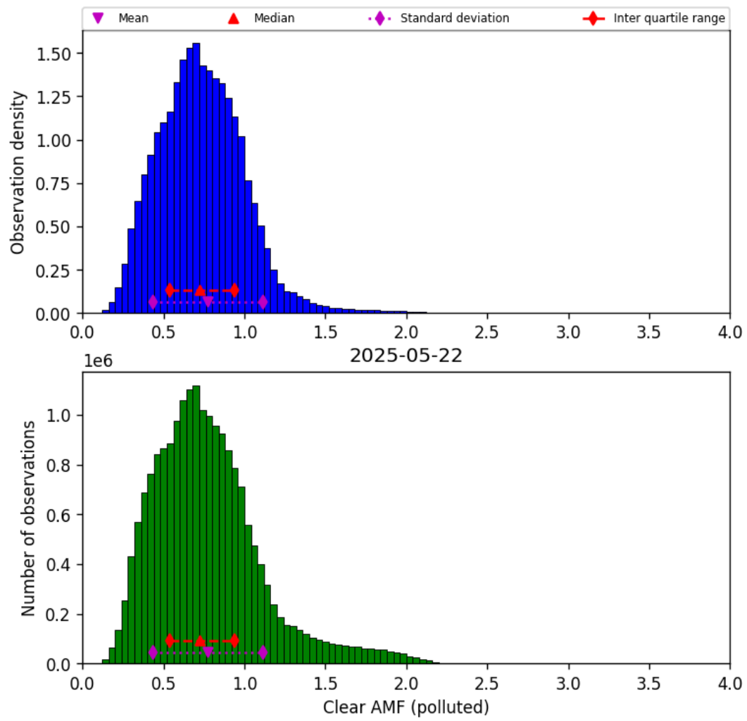
Figure 81: Histogram of “Clear AMF (polluted)” for 2025-05-21 to 2025-05-23
