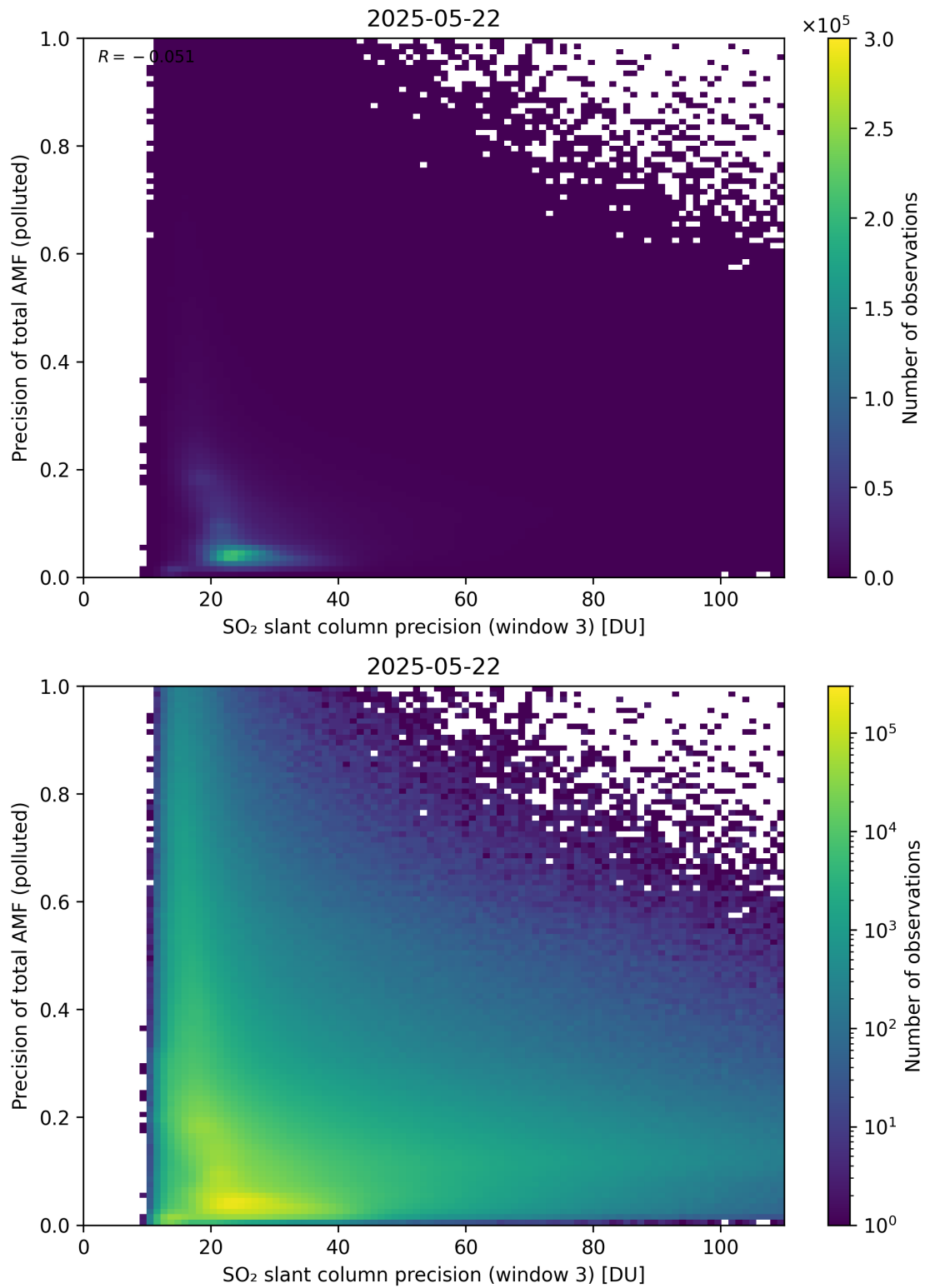
Figure 314: Scatter density plot of “SO 2 slant column precision (window 3)” against “Precision of total AMF (polluted)” for 2025-05-21 to 2025-05-23.
