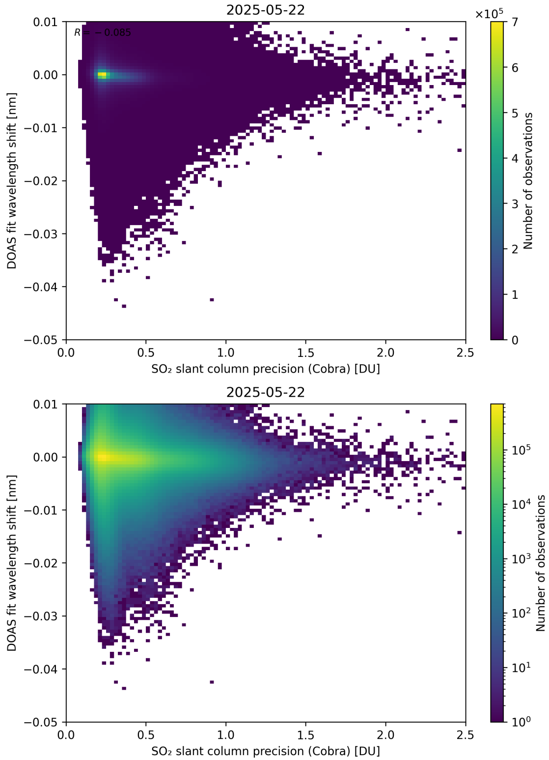
Figure 202: Scatter density plot of “SO 2 slant column precision (Cobra)” against “DOAS fit wavelength shift” for 2025-05-21 to 2025-05-23.
