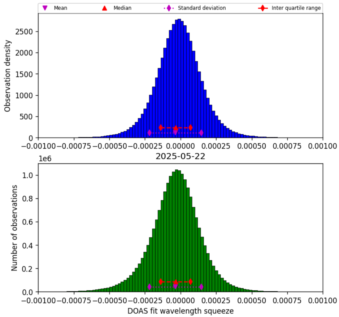
Figure 77: Histogram of “DOAS fit wavelength squeeze” for 2025-05-21 to 2025-05-23
