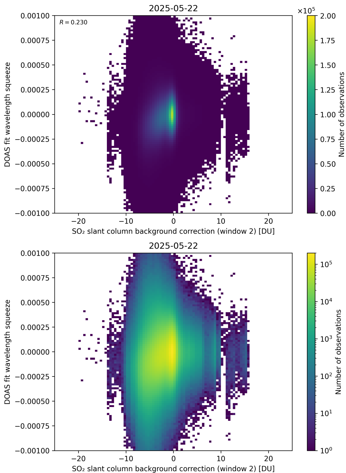
Figure 124: Scatter density plot of “SO 2 slant column background correction (window 2)” against “DOAS fit wavelength squeeze” for 2025-05-21 to 2025-05-23.
