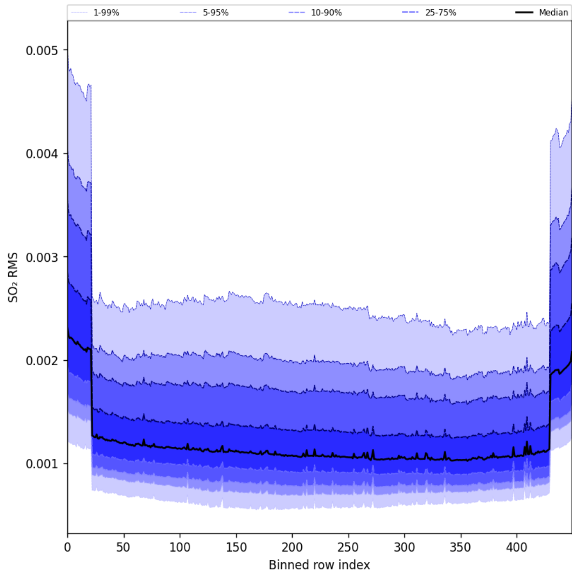
Figure 104: Along track statistics of “SO 2 RMS” for 2025-05-21 to 2025-05-23
