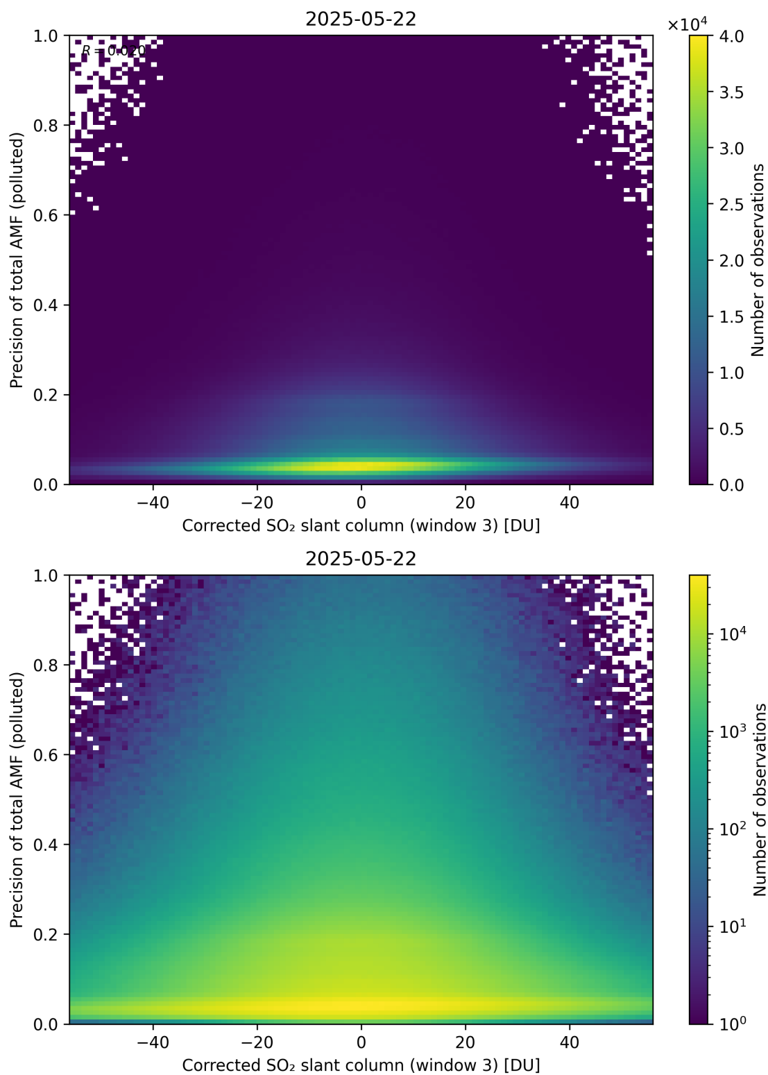
Figure 261: Scatter density plot of “Corrected SO 2 slant column (window 3)” against “Precision of total AMF (polluted)” for 2025-05-21 to 2025-05-23.
