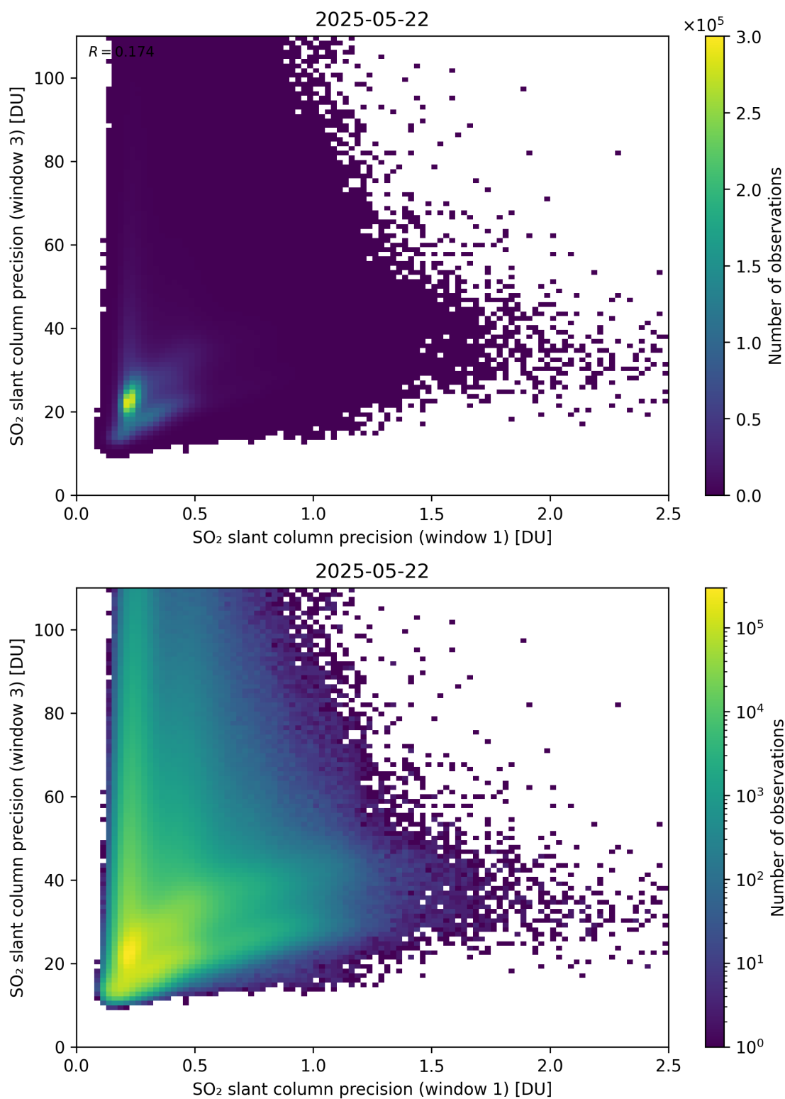
Figure 279: Scatter density plot of “SO 2 slant column precision (window 1)” against “SO 2 slant column precision (window 3)” for 2025-05-21 to 2025-05-23.
