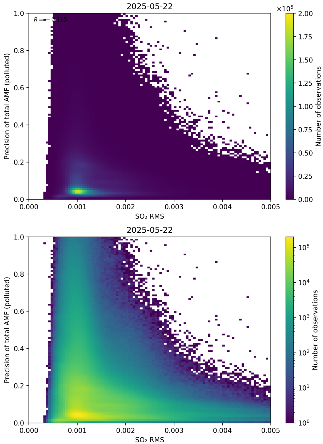
Figure 149: Scatter density plot of “SO 2 RMS” against “Precision of total AMF (polluted)” for 2025-05-21 to 2025-05-23.
