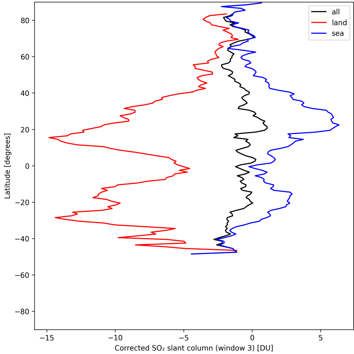
Figure 47: Zonal average of “Corrected SO 2 slant column (window 3)” for 2025-05-21 to 2025-05-23.
