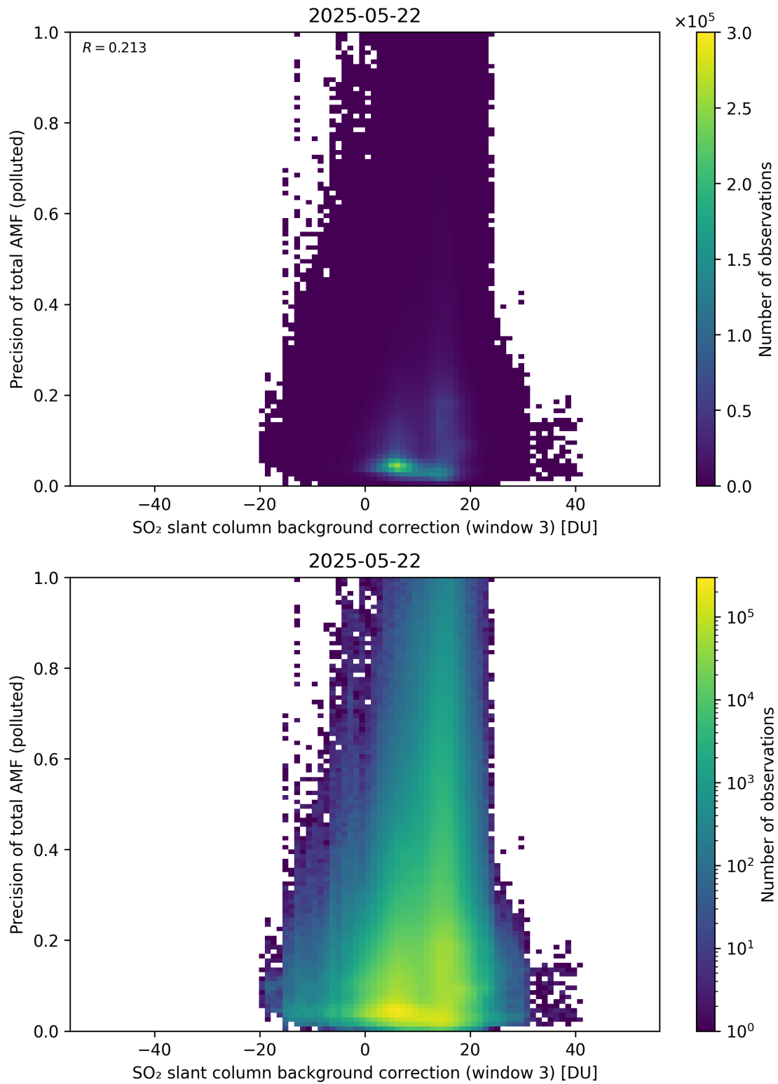
Figure 137: Scatter density plot of “SO 2 slant column background correction (window 3)” against “Precision of total AMF (polluted)” for 2025-05-21 to 2025-05-23.
