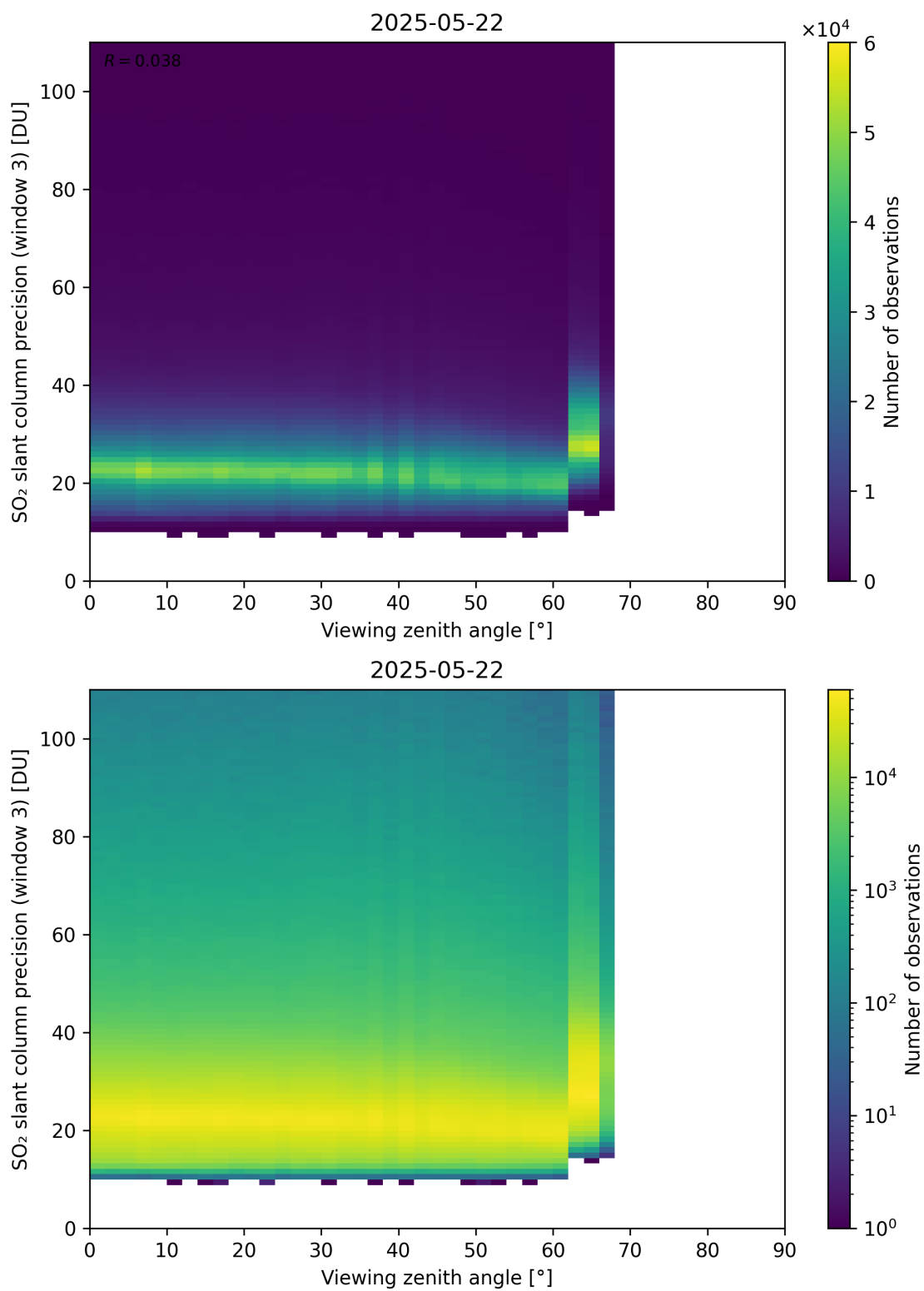
Figure 380: Scatter density plot of “Viewing zenith angle” against “SO 2 slant column precision (window 3)” for 2025-05-21 to 2025-05-23.
