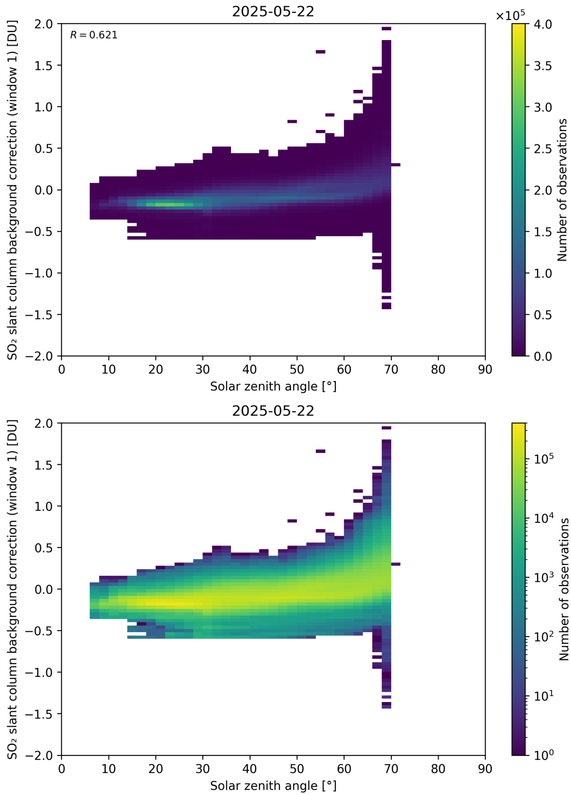
Figure 171: Scatter density plot of “Solar zenith angle” against “SO 2 slant column background correction (window 1)” for 2025-05-21 to 2025-05-23.
