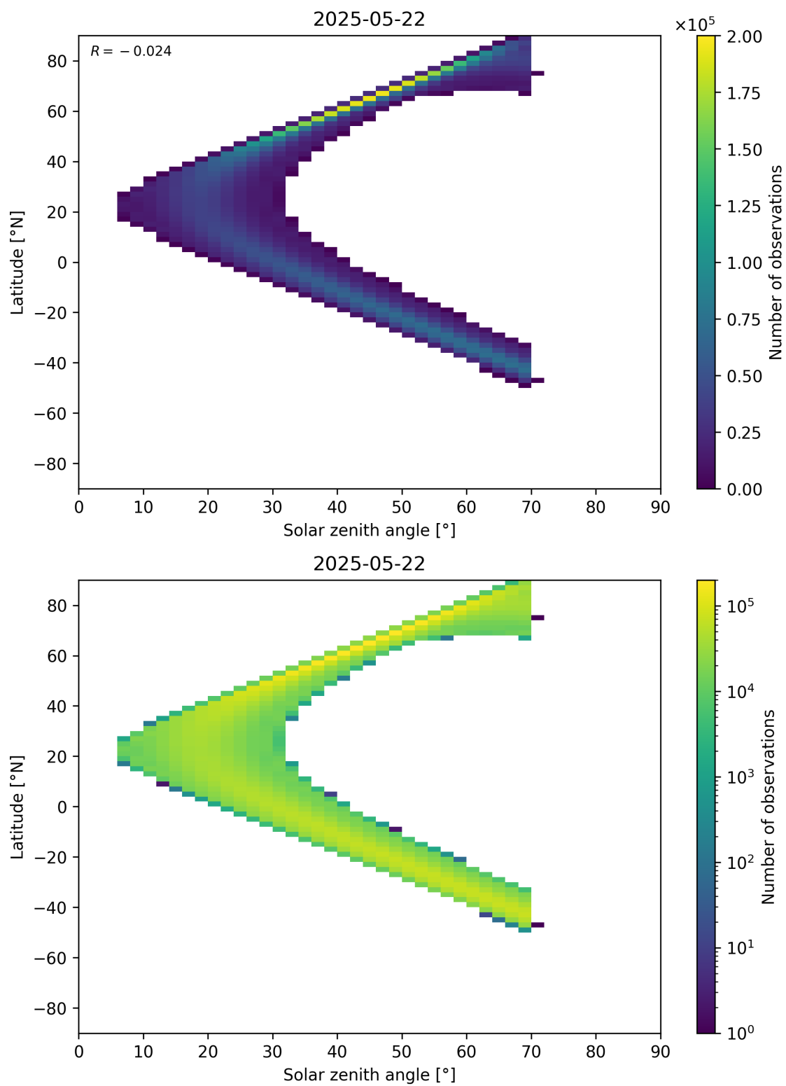
Figure 177: Scatter density plot of “Solar zenith angle” against “Latitude” for 2025-05-21 to 2025-05-23.
