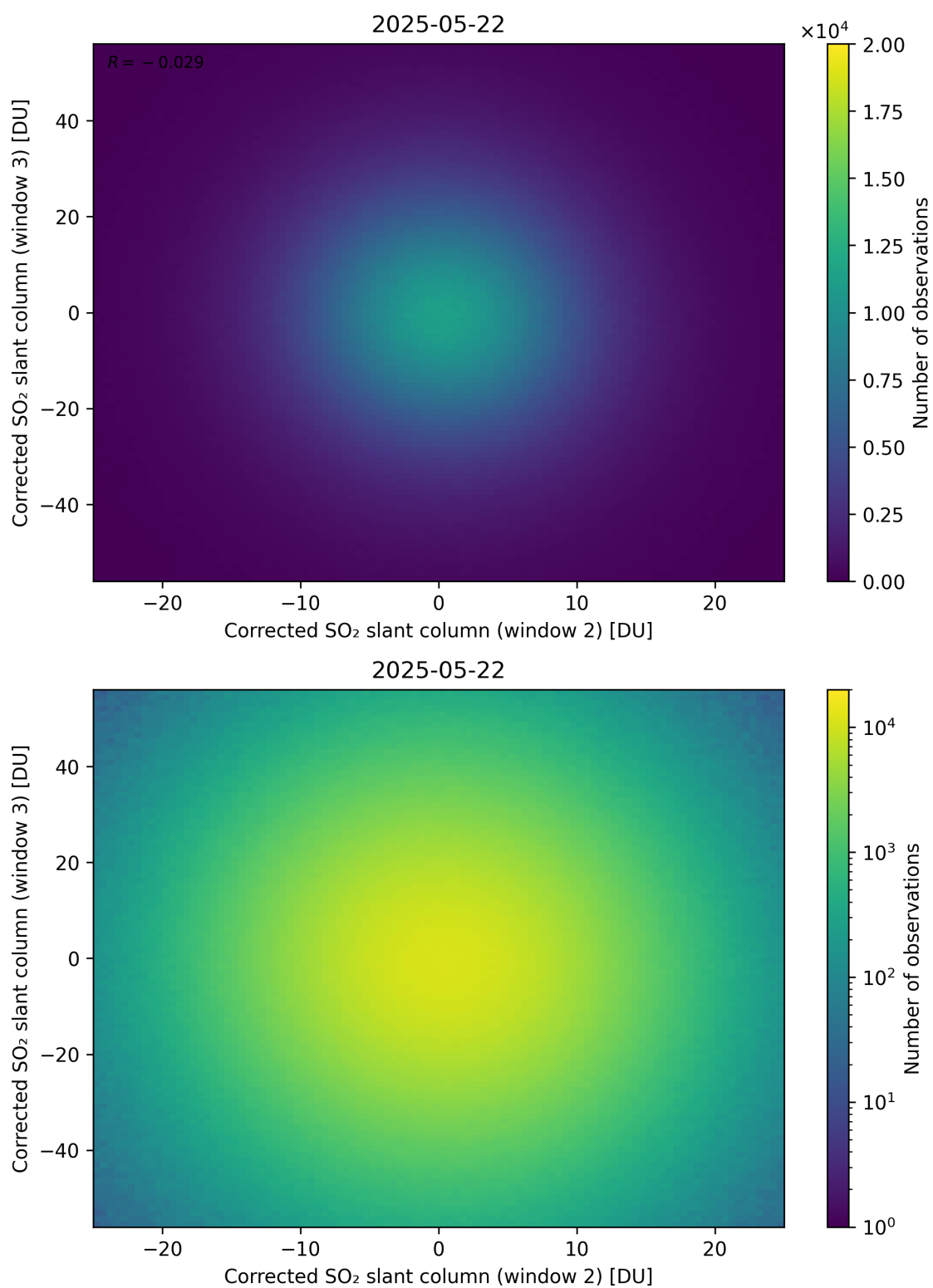
Figure 250: Scatter density plot of “Corrected SO 2 slant column (window 2)” against “Corrected SO 2 slant column (window 3)” for 2025-05-21 to 2025-05-23.
