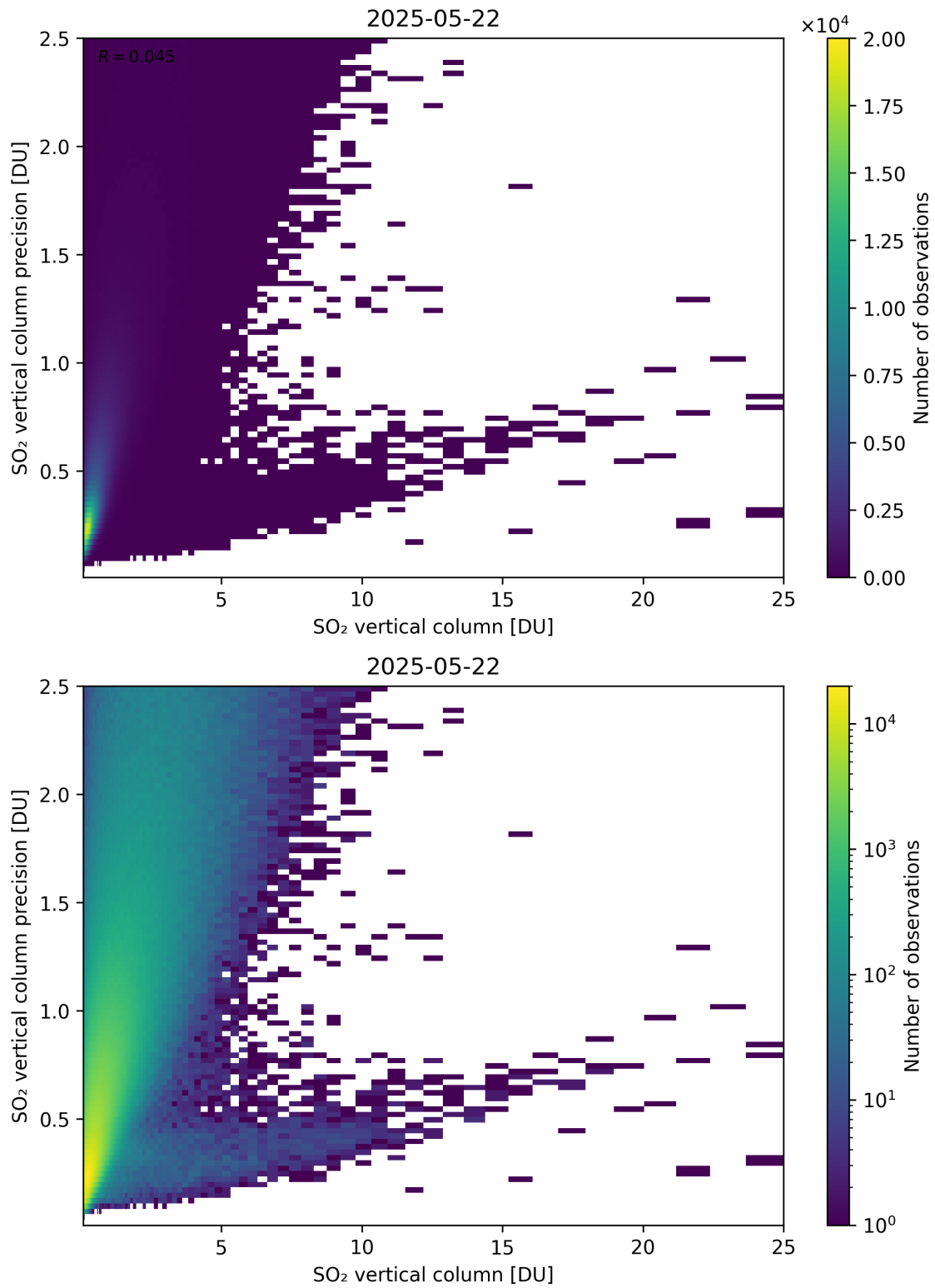
Figure 361: Scatter density plot of “SO 2 vertical column” against “SO 2 vertical column precision” for 2025-05-21 to 2025-05-23.
