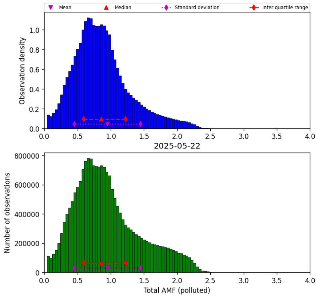
Figure 79: Histogram of “Total AMF (polluted)” for 2025-05-21 to 2025-05-23
