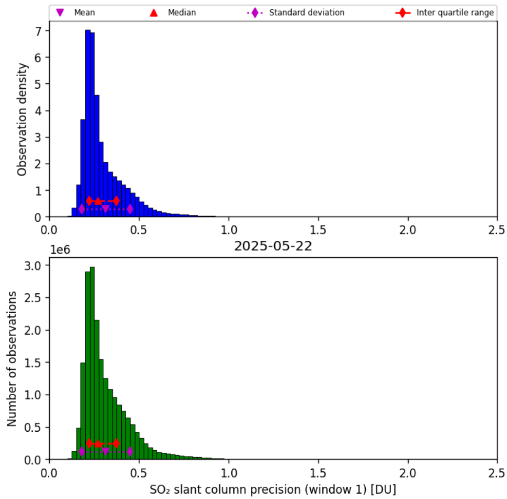
Figure 64: Histogram of “SO 2 slant column precision (window 1)” for 2025-05-21 to 2025-05-23
