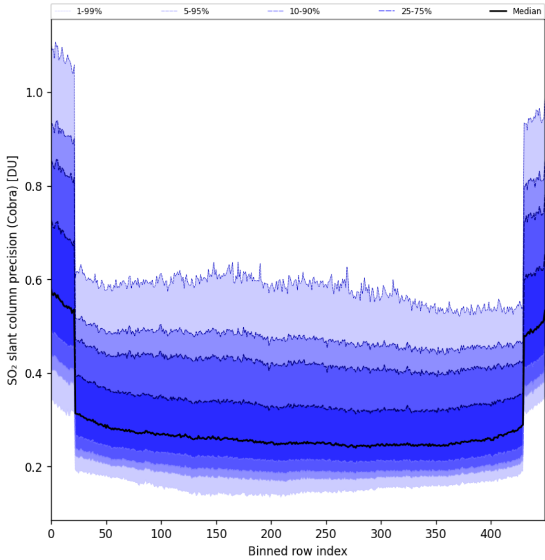
Figure 88: Along track statistics of “SO 2 slant column precision (Cobra)” for 2025-05-21 to 2025-05-23
