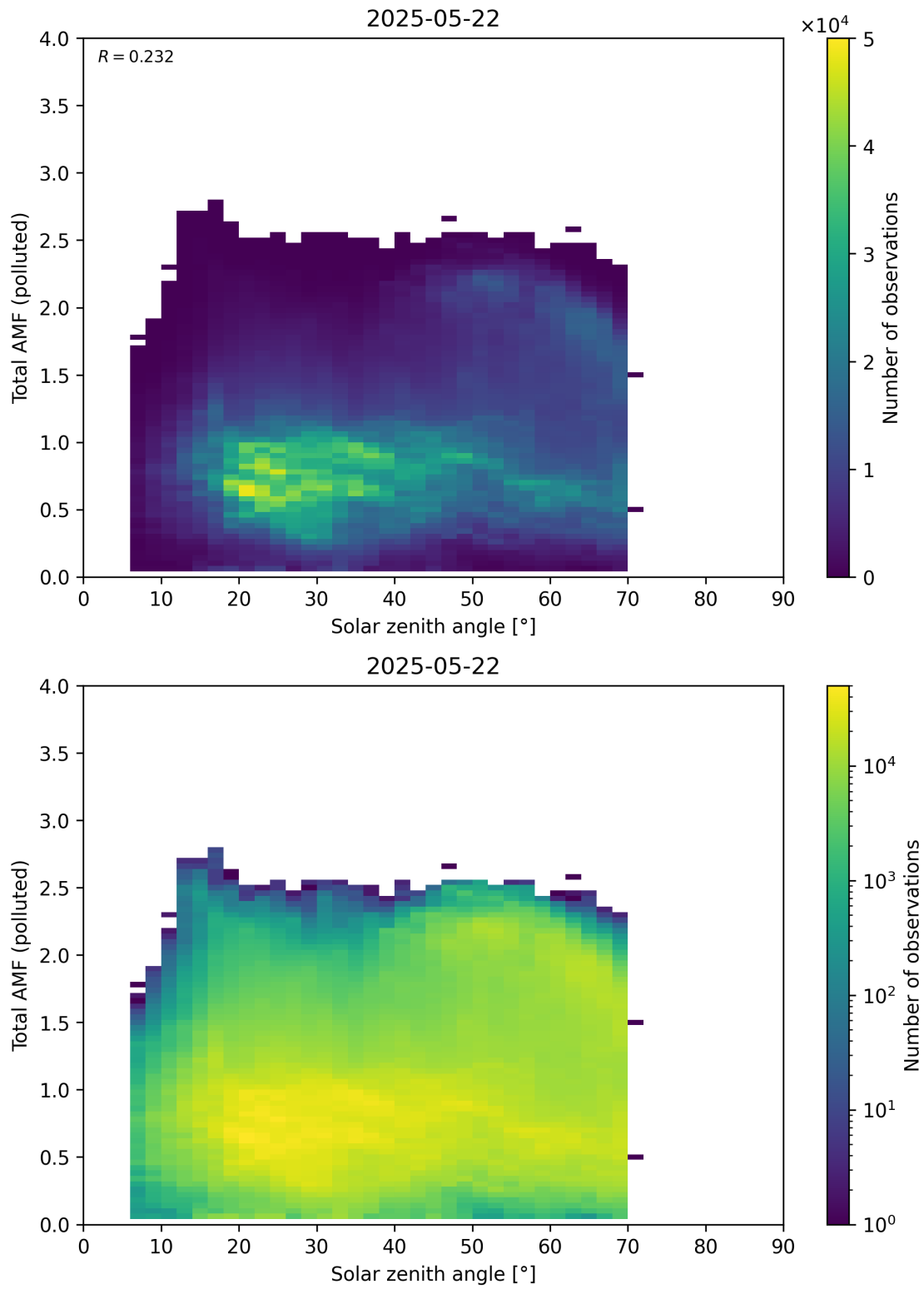
Figure 189: Scatter density plot of “Solar zenith angle” against “Total AMF (polluted)” for 2025-05-21 to 2025-05-23.
