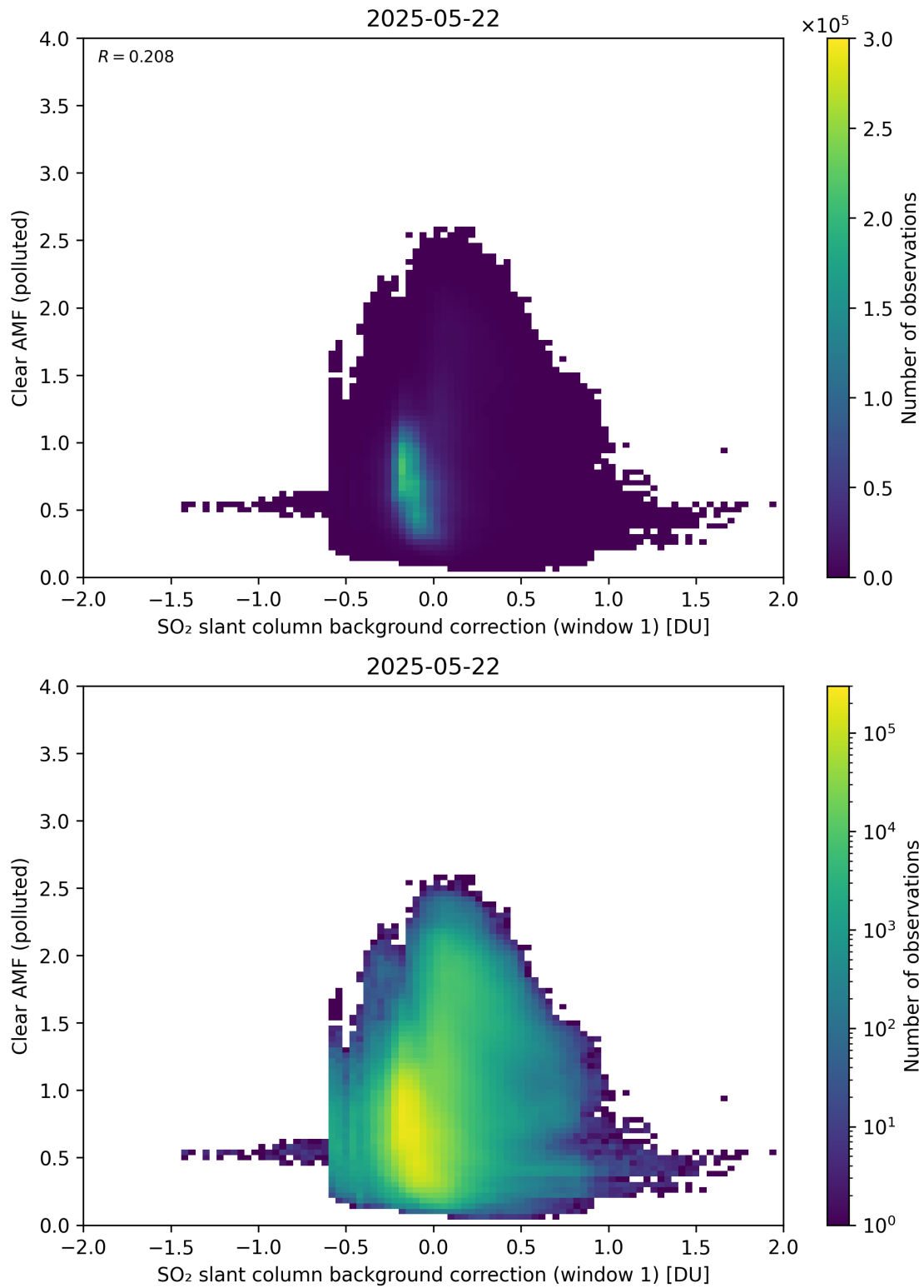
Figure 114: Scatter density plot of “SO 2 slant column background correction (window 1)” against “Clear AMF (polluted)” for 2025-05-21 to 2025-05-23.
