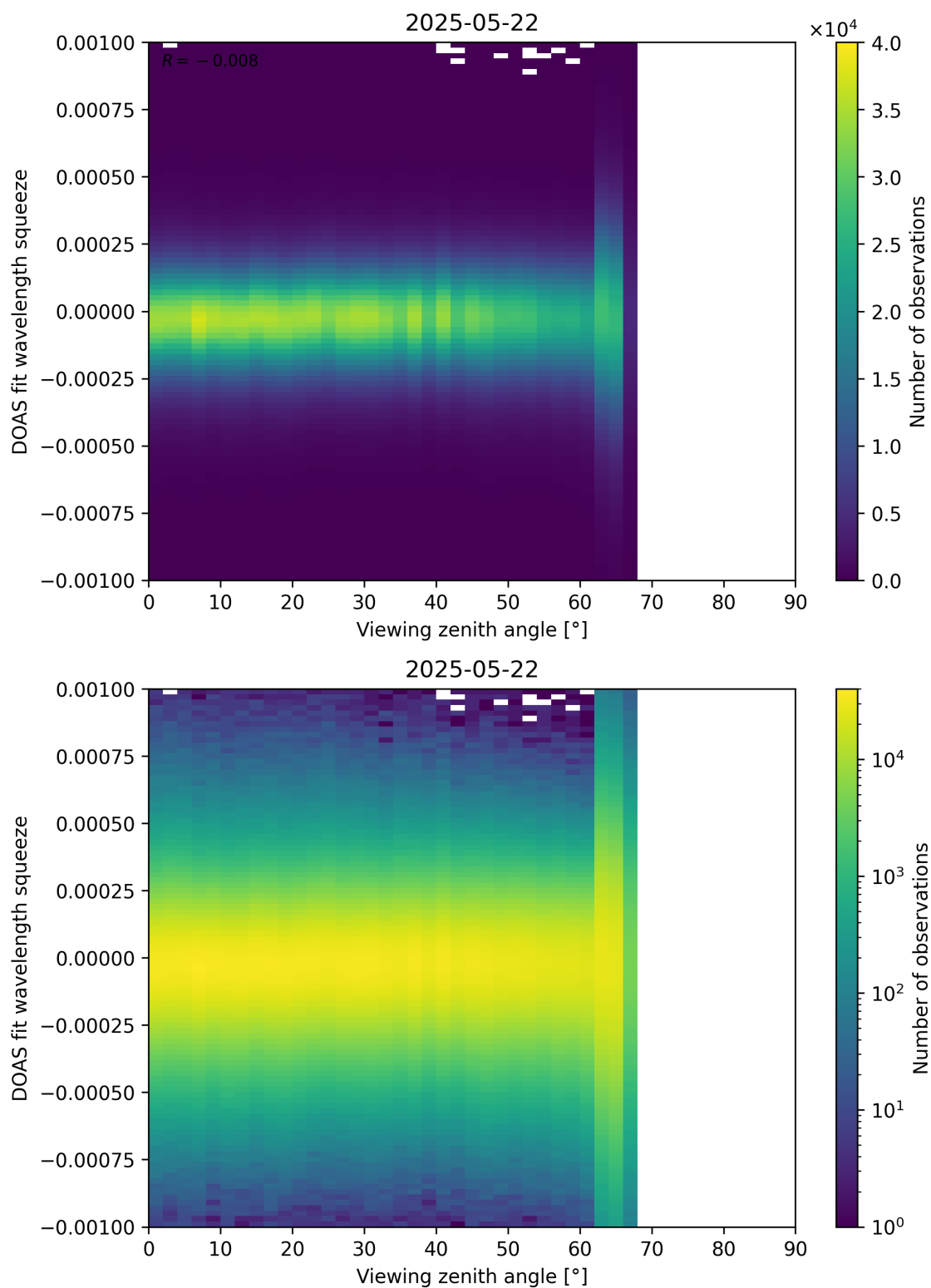
Figure 366: Scatter density plot of “Viewing zenith angle” against “DOAS fit wavelength squeeze” for 2025-05-21 to 2025-05-23.
