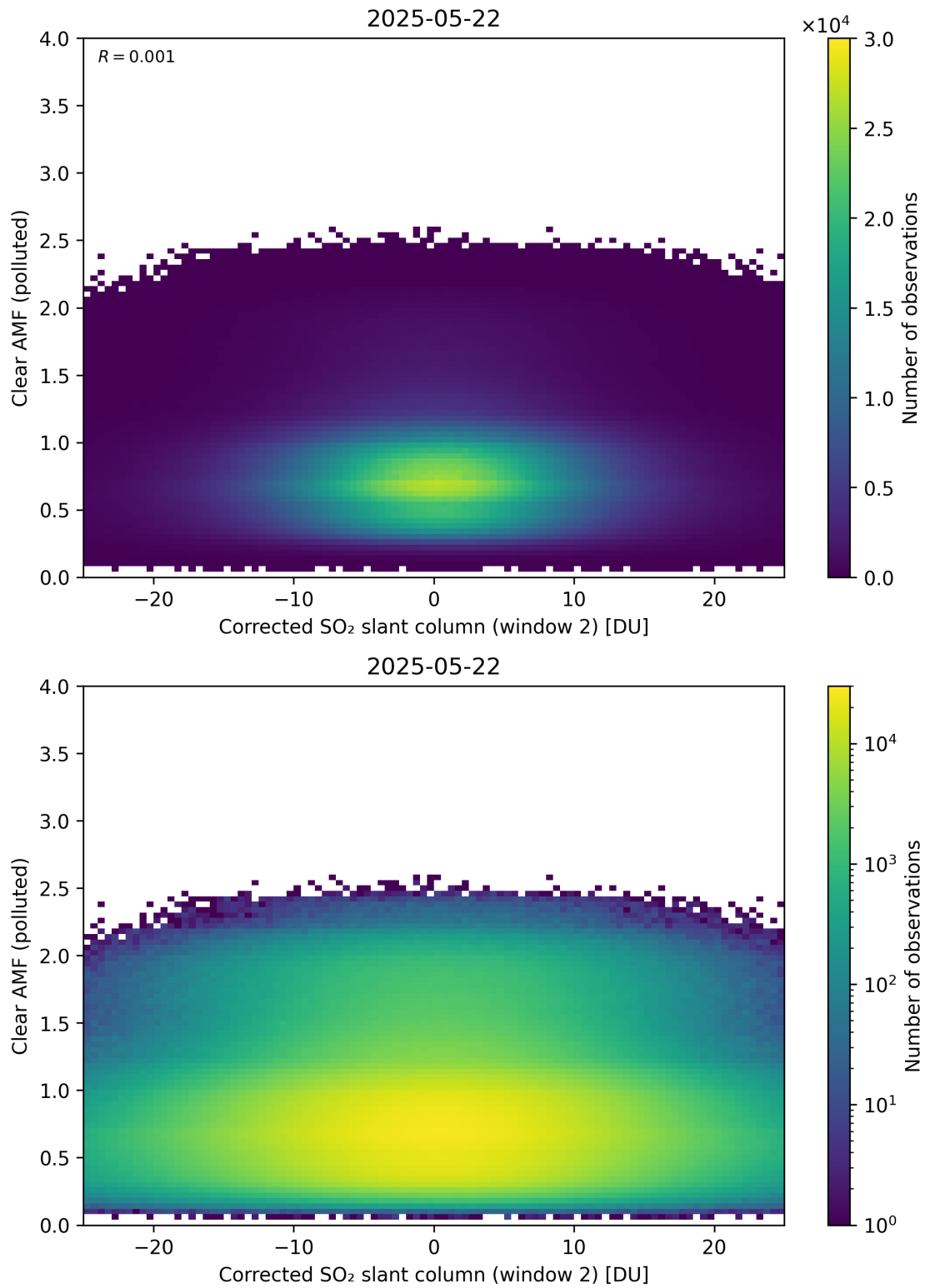
Figure 249: Scatter density plot of “Corrected SO 2 slant column (window 2)” against “Clear AMF (polluted)” for 2025-05-21 to 2025-05-23.
