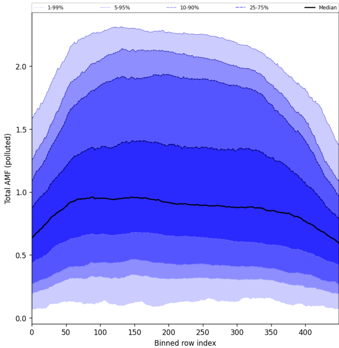
Figure 105: Along track statistics of “Total AMF (polluted)” for 2025-05-21 to 2025-05-23
