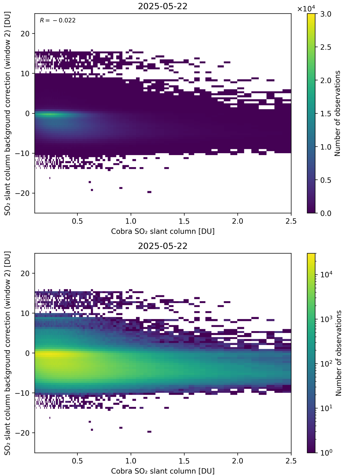
Figure 194: Scatter density plot of “Cobra SO 2 slant column” against “SO 2 slant column background correction (window 2)” for 2025-05-21 to 2025-05-23.
