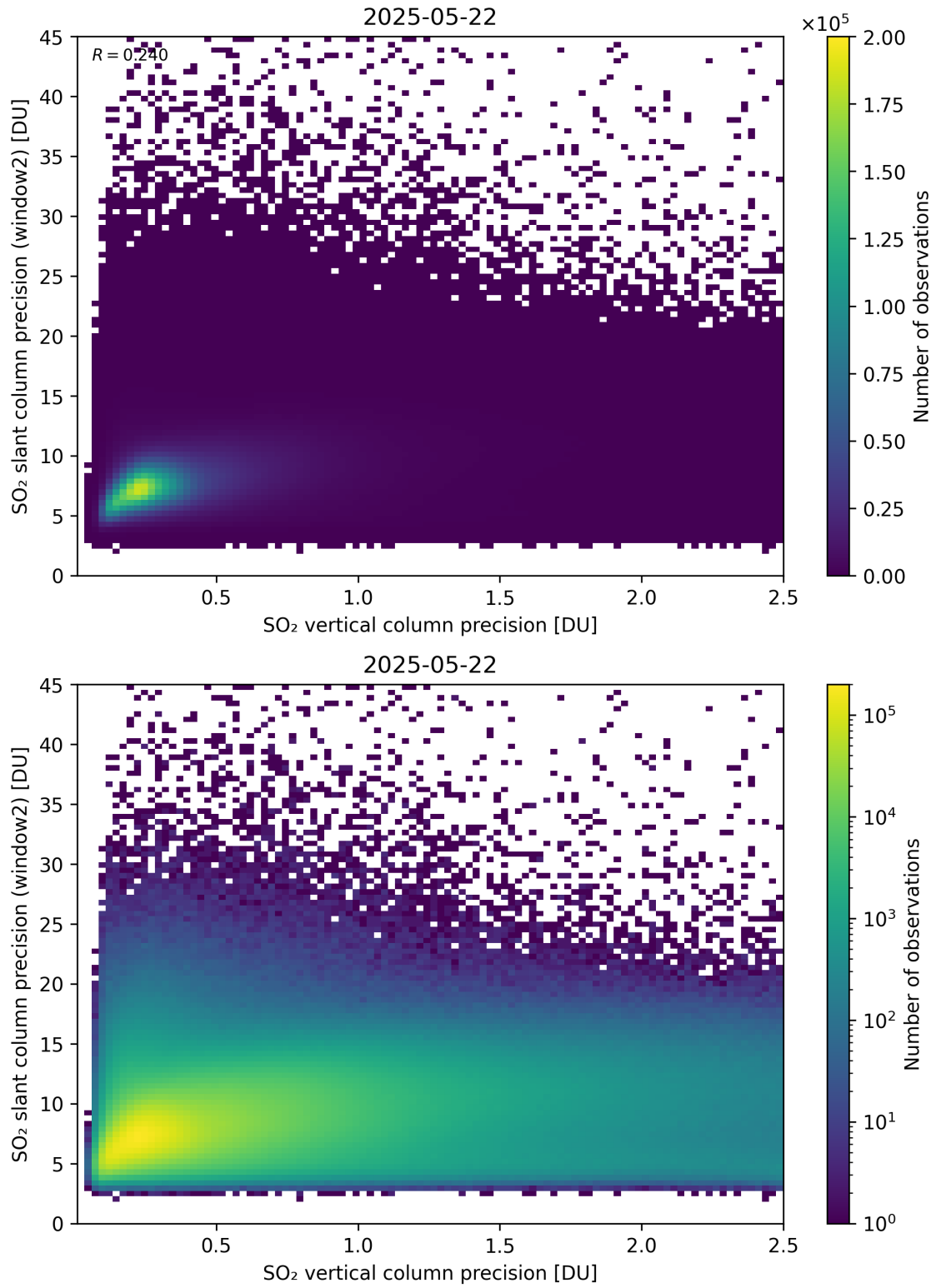
Figure 343: Scatter density plot of “SO 2 vertical column precision” against “SO 2 slant column precision (window2)” for 2025-05-21 to 2025-05-23.
