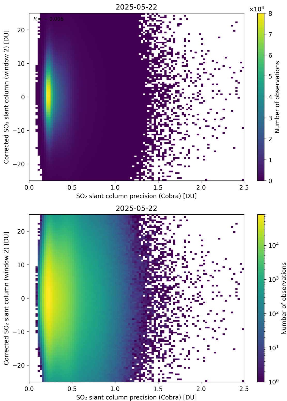
Figure 206: Scatter density plot of “SO 2 slant column precision (Cobra)” against “Corrected SO 2 slant column (window 2)” for 2025-05-21 to 2025-05-23.
