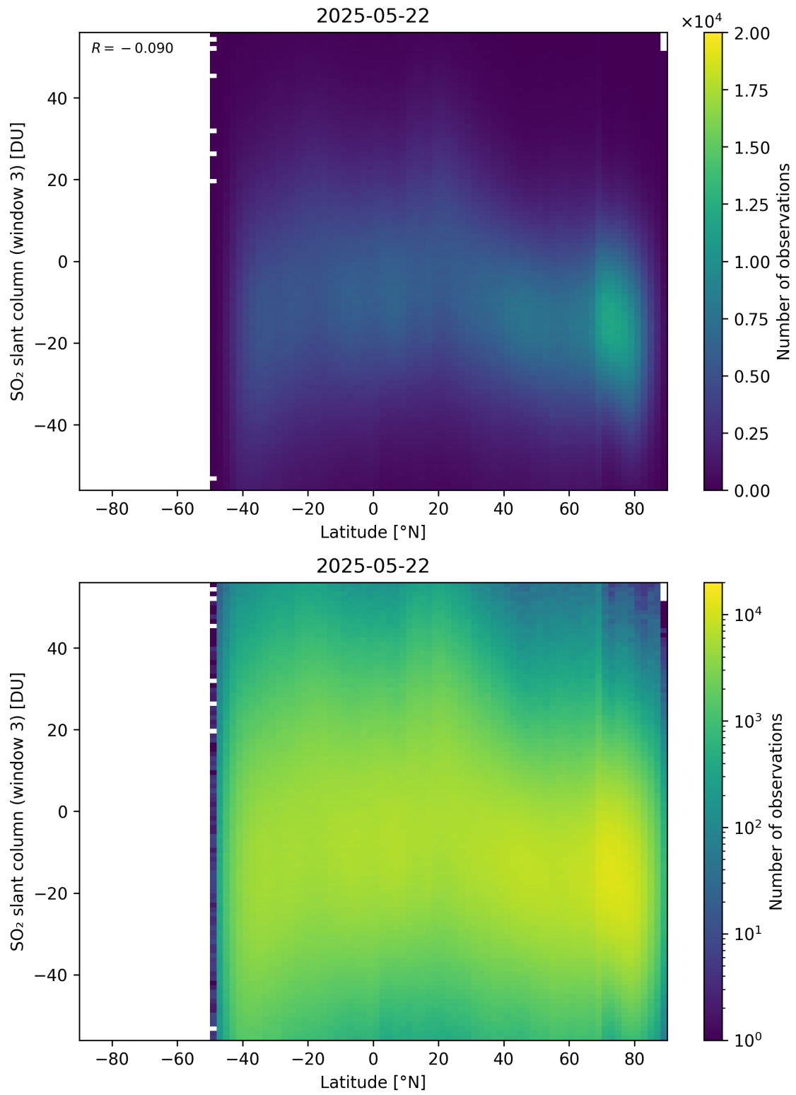
Figure 165: Scatter density plot of “Latitude” against “SO 2 slant column (window 3)” for 2025-05-21 to 2025-05-23.
