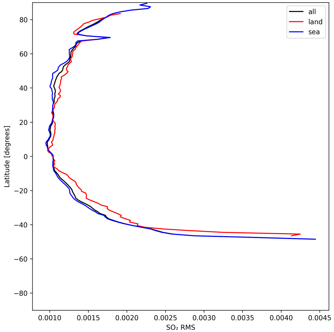
Figure 52: Zonal average of “SO 2 RMS” for 2025-05-21 to 2025-05-23.
