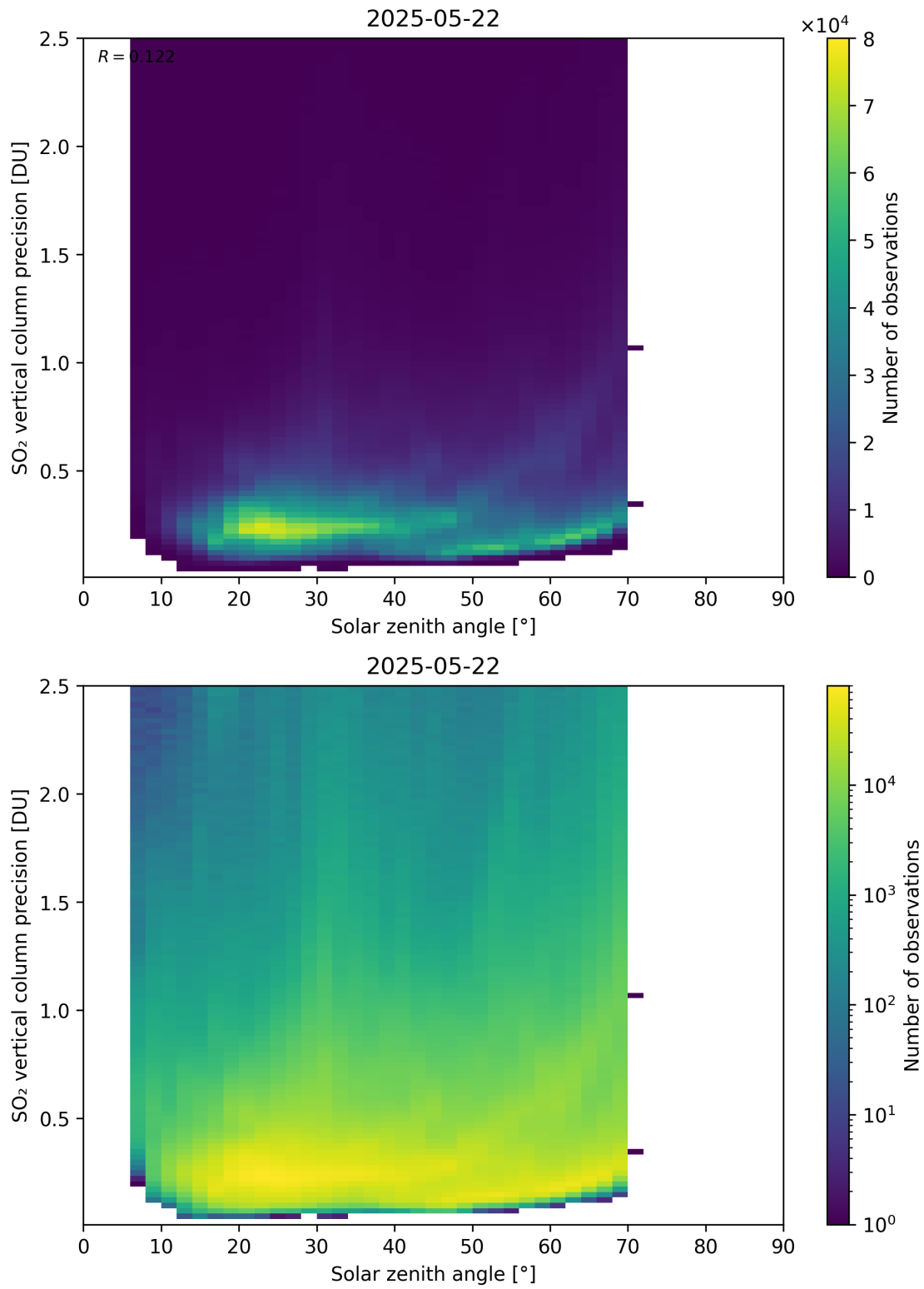
Figure 192: Scatter density plot of “Solar zenith angle” against “SO 2 vertical column precision” for 2025-05-21 to 2025-05-23.
