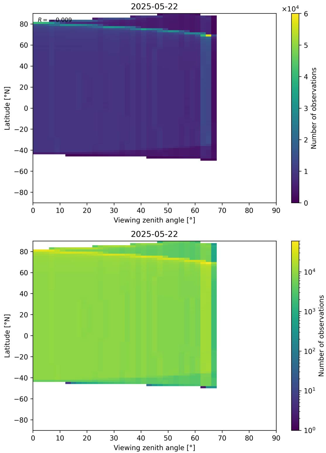
Figure 368: Scatter density plot of “Viewing zenith angle” against “Latitude” for 2025-05-21 to 2025-05-23.
