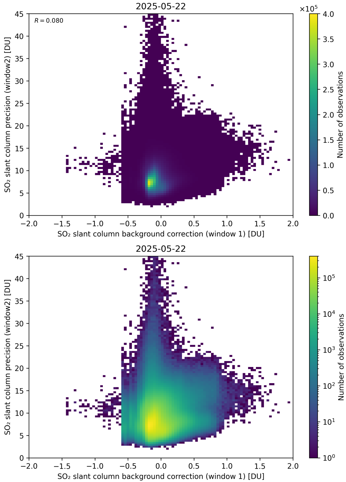
Figure 117: Scatter density plot of “SO 2 slant column background correction (window 1)” against “SO 2 slant column precision (window2)” for 2025-05-21 to 2025-05-23.
