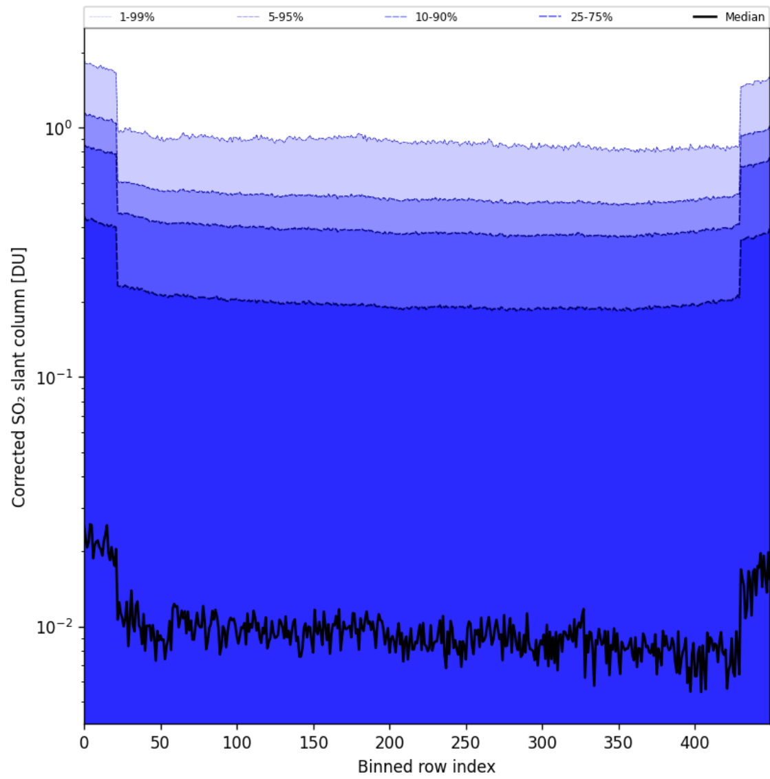
Figure 86: Along track statistics of “Corrected SO 2 slant column” for 2025-05-21 to 2025-05-23
