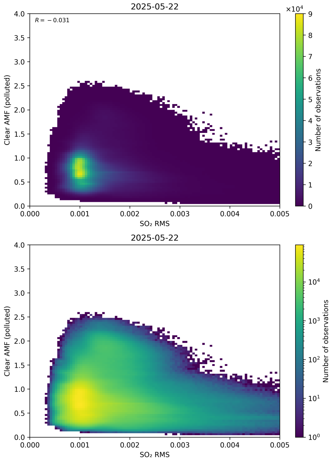
Figure 147: Scatter density plot of “SO 2 RMS” against “Clear AMF (polluted)” for 2025-05-21 to 2025-05-23.
