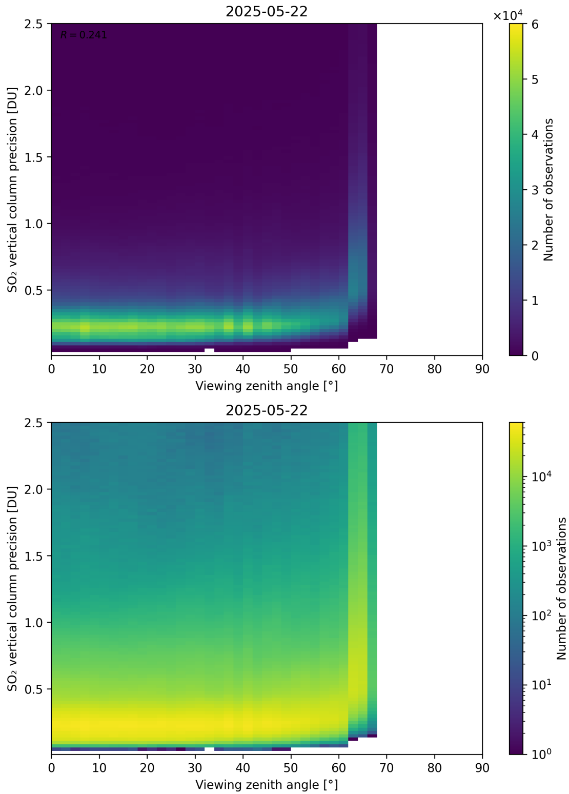
Figure 384: Scatter density plot of “Viewing zenith angle” against “SO 2 vertical column precision” for 2025-05-21 to 2025-05-23.
