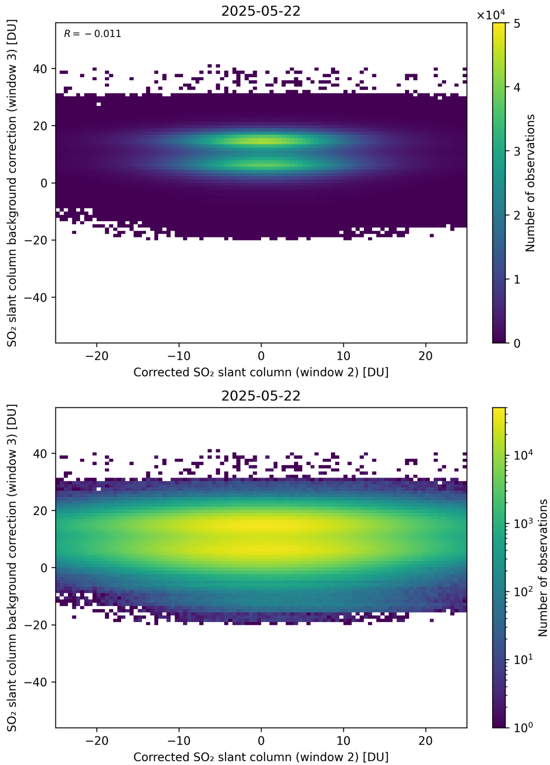
Figure 245: Scatter density plot of “Corrected SO 2 slant column (window 2)” against “SO 2 slant column background correction (window 3)” for 2025-05-21 to 2025-05-23.
