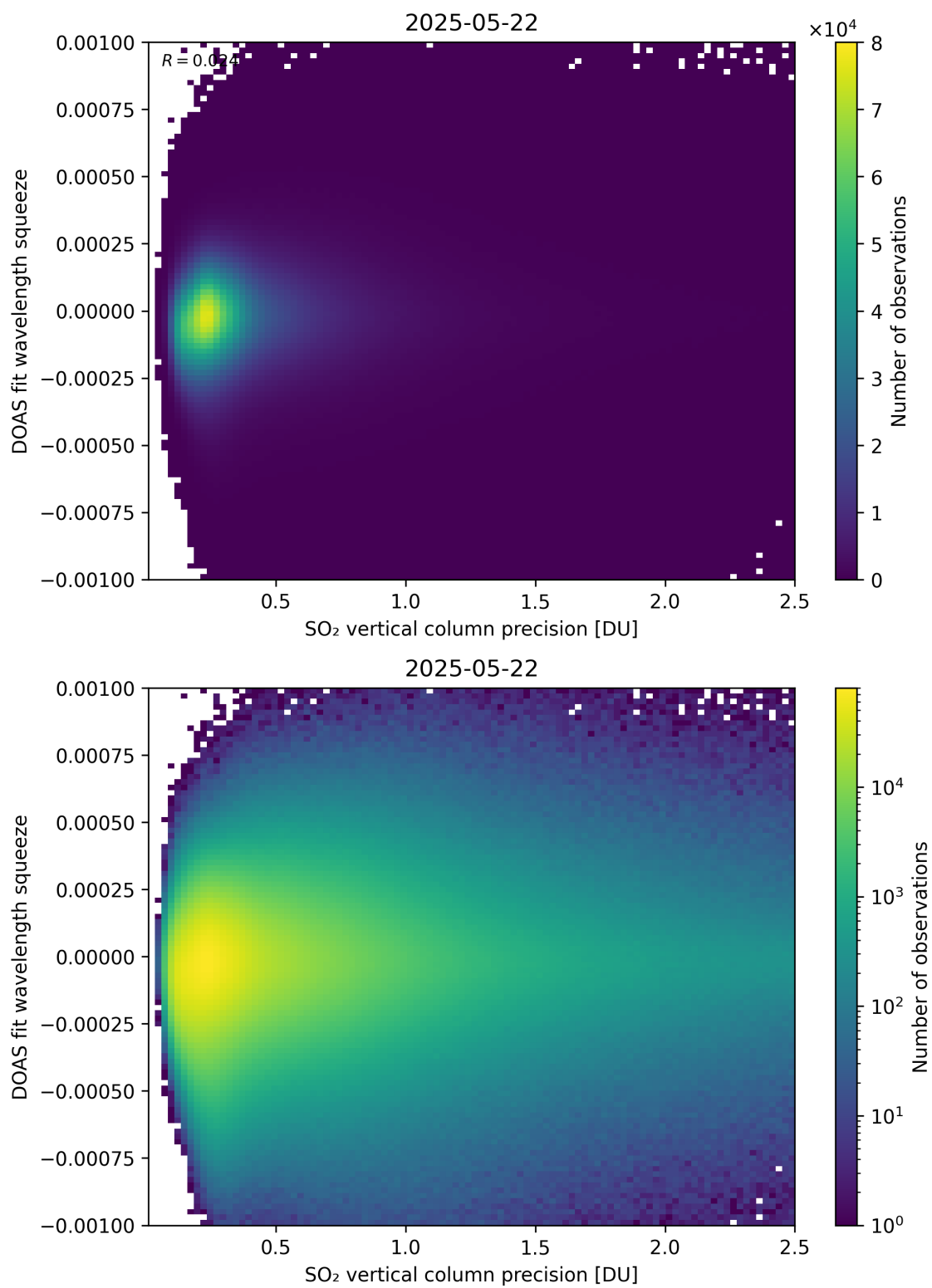
Figure 333: Scatter density plot of “SO 2 vertical column precision” against “DOAS fit wavelength squeeze” for 2025-05-21 to 2025-05-23.
