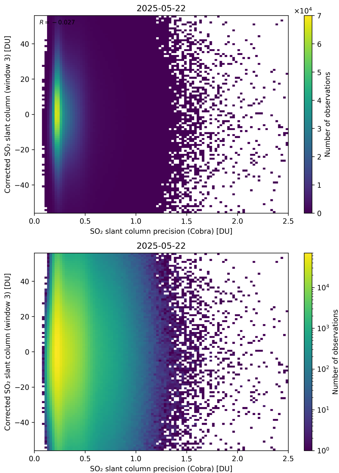
Figure 207: Scatter density plot of “SO 2 slant column precision (Cobra)” against “Corrected SO 2 slant column (window 3)” for 2025-05-21 to 2025-05-23.
