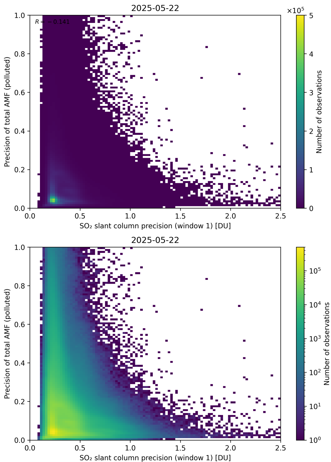
Figure 281: Scatter density plot of “SO 2 slant column precision (window 1)” against “Precision of total AMF (polluted)” for 2025-05-21 to 2025-05-23.
