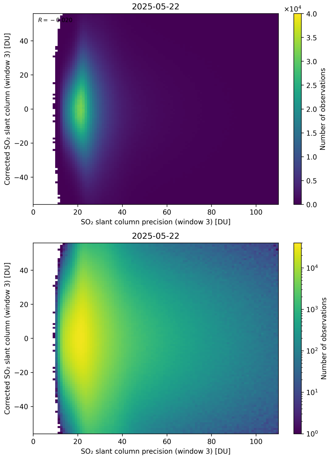
Figure 312: Scatter density plot of “SO 2 slant column precision (window 3)” against “Corrected SO 2 slant column (window 3)” for 2025-05-21 to 2025-05-23.
