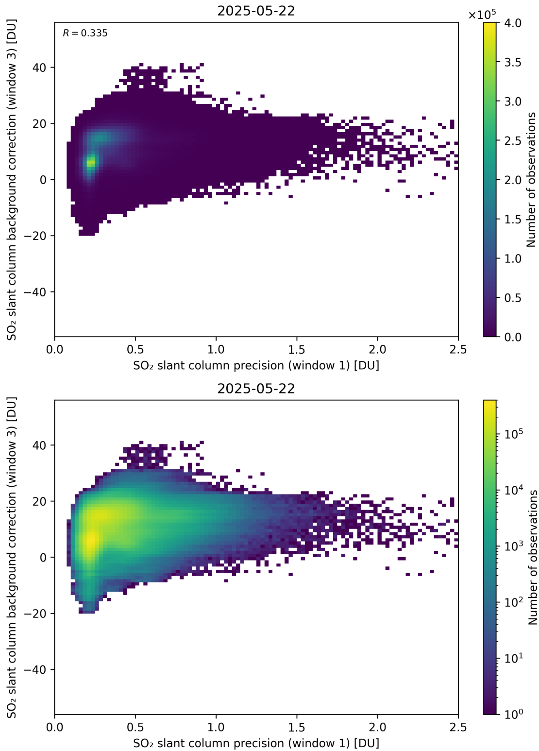
Figure 270: Scatter density plot of “SO 2 slant column precision (window 1)” against “SO 2 slant column background correction (window 3)” for 2025-05-21 to 2025-05-23.
