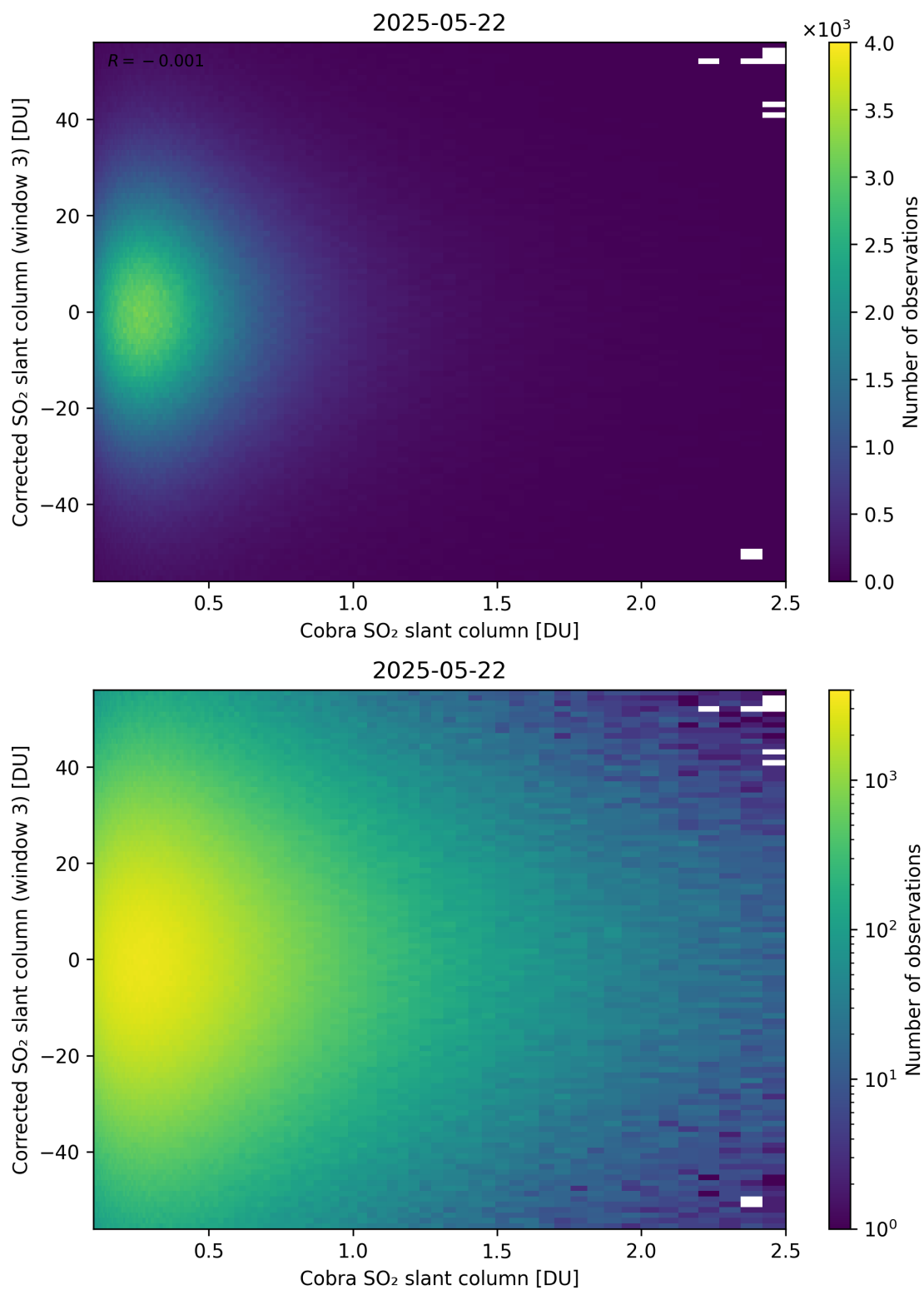
Figure 218: Scatter density plot of “Cobra SO 2 slant column” against “Corrected SO 2 slant column (window 3)” for 2025-05-21 to 2025-05-23.
