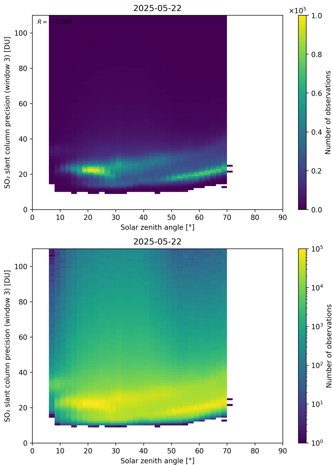
Figure 188: Scatter density plot of “Solar zenith angle” against “SO 2 slant column precision (window 3)” for 2025-05-21 to 2025-05-23.
