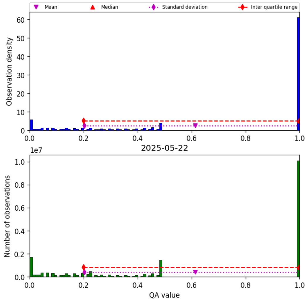
Figure 57: Histogram of “QA value” for 2025-05-21 to 2025-05-23
