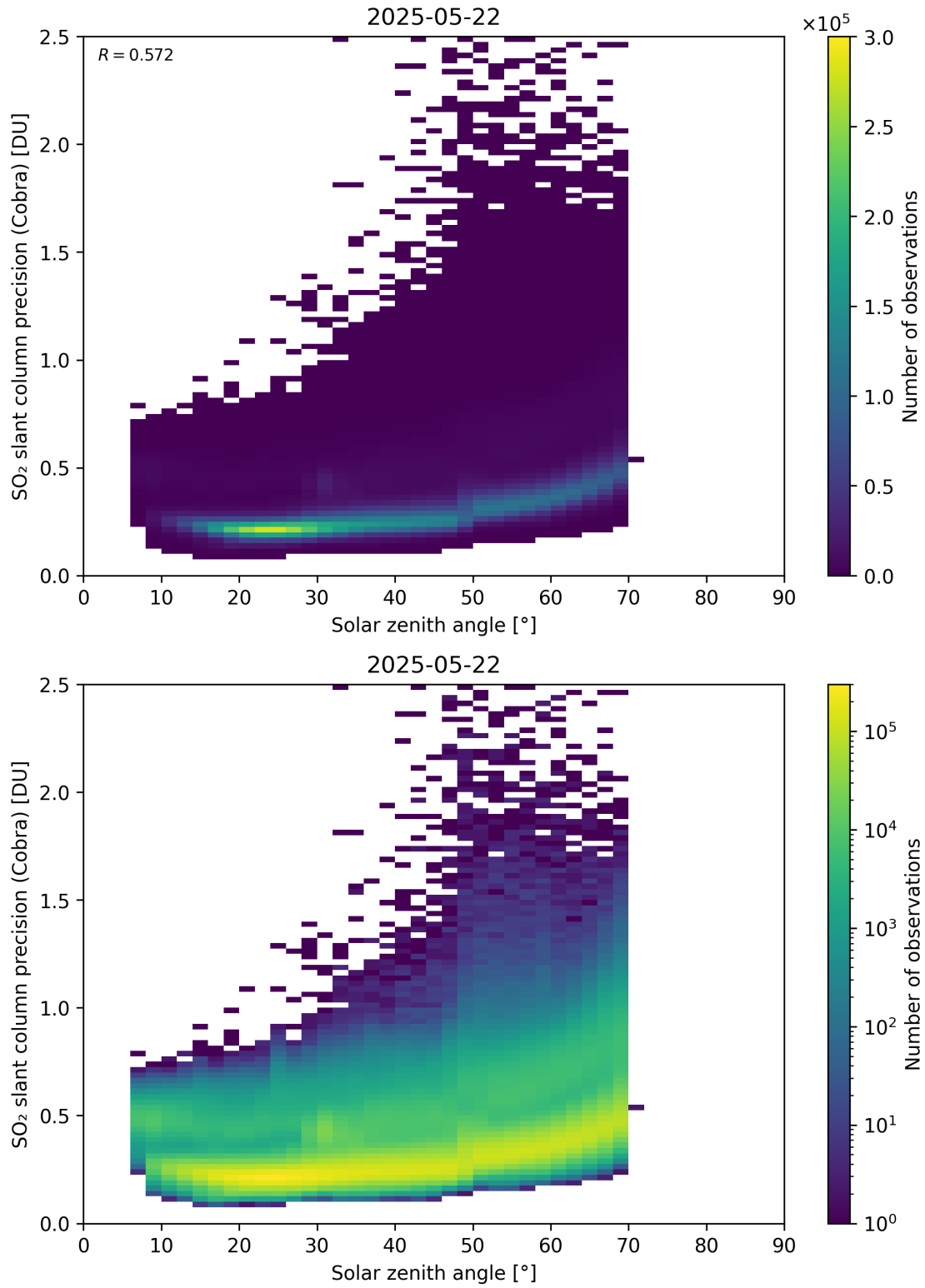
Figure 180: Scatter density plot of “Solar zenith angle” against “SO 2 slant column precision (Cobra)” for 2025-05-21 to 2025-05-23.
