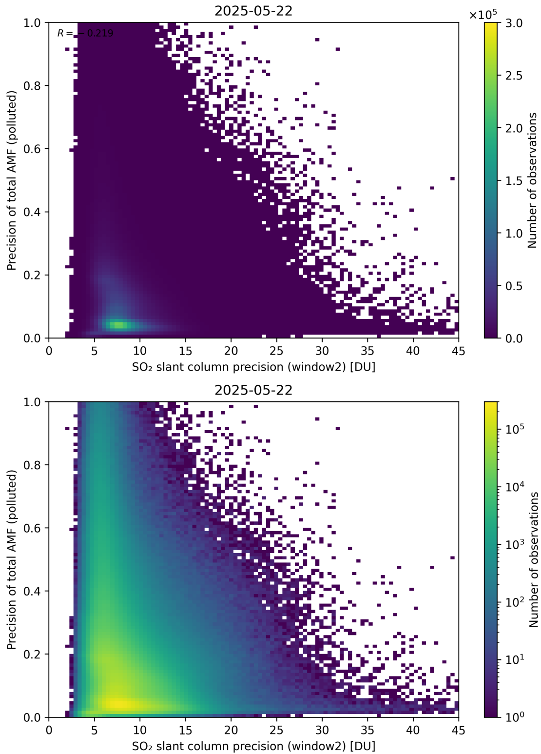
Figure 302: Scatter density plot of “SO 2 slant column precision (window2)” against “Precision of total AMF (polluted)” for 2025-05-21 to 2025-05-23.
