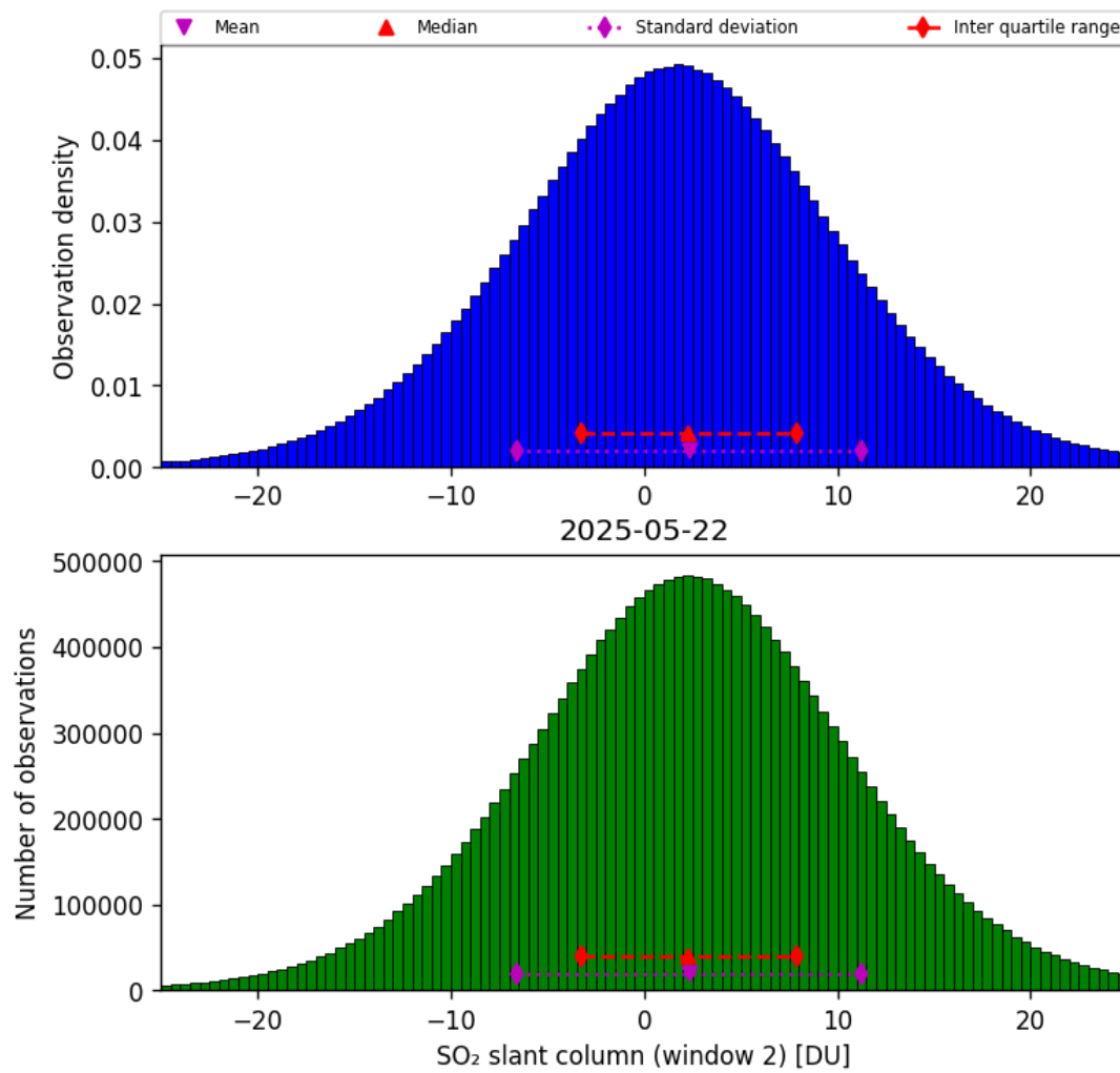
Figure 67: Histogram of “SO 2 slant column (window 2)” for 2025-05-21 to 2025-05-23
