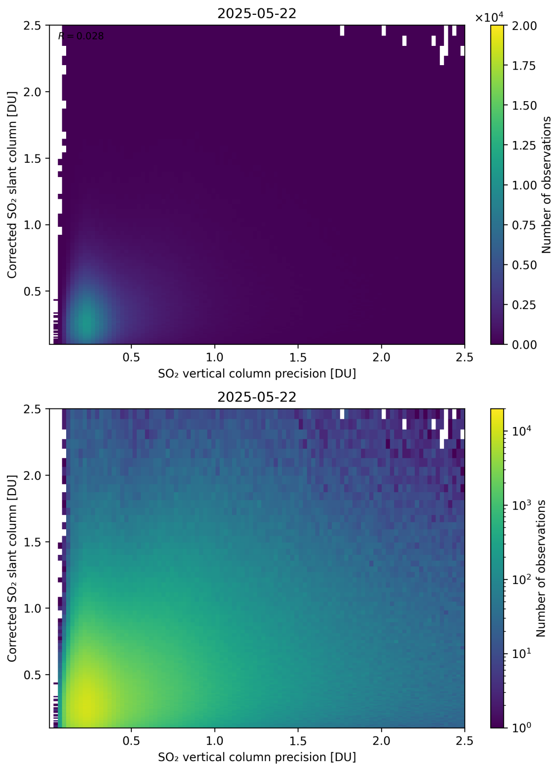
Figure 338: Scatter density plot of “SO 2 vertical column precision” against “Corrected SO 2 slant column” for 2025-05-21 to 2025-05-23.
