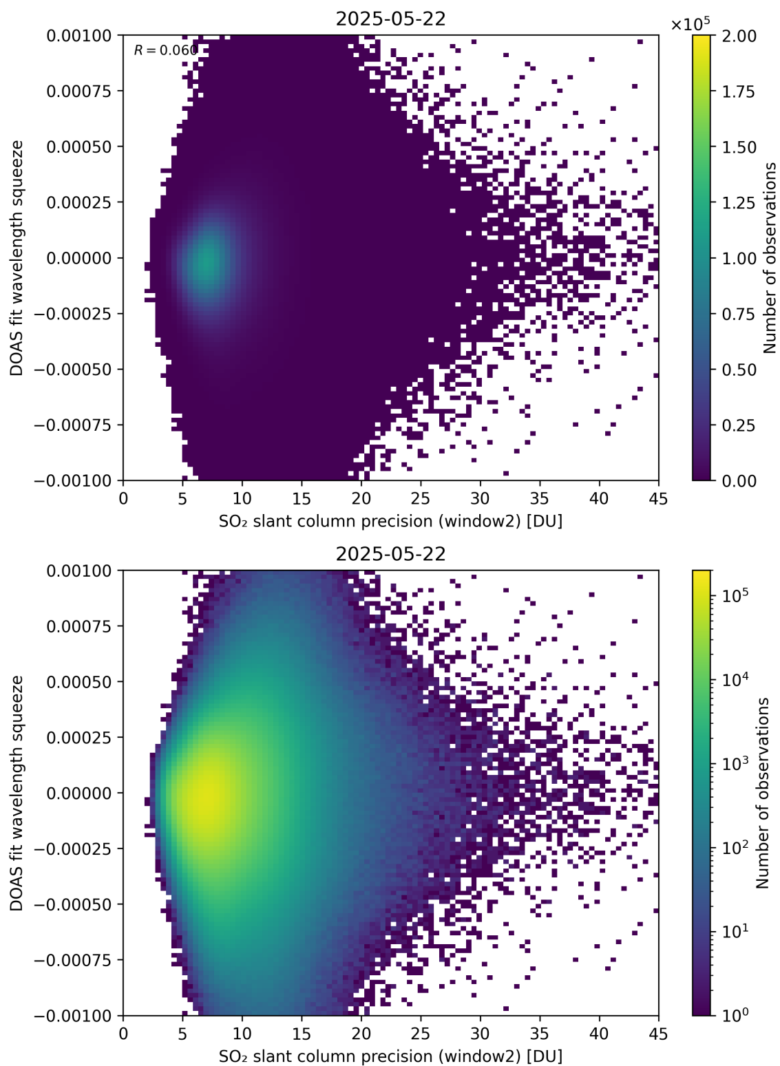
Figure 294: Scatter density plot of “SO 2 slant column precision (window2)” against “DOAS fit wavelength squeeze” for 2025-05-21 to 2025-05-23.
