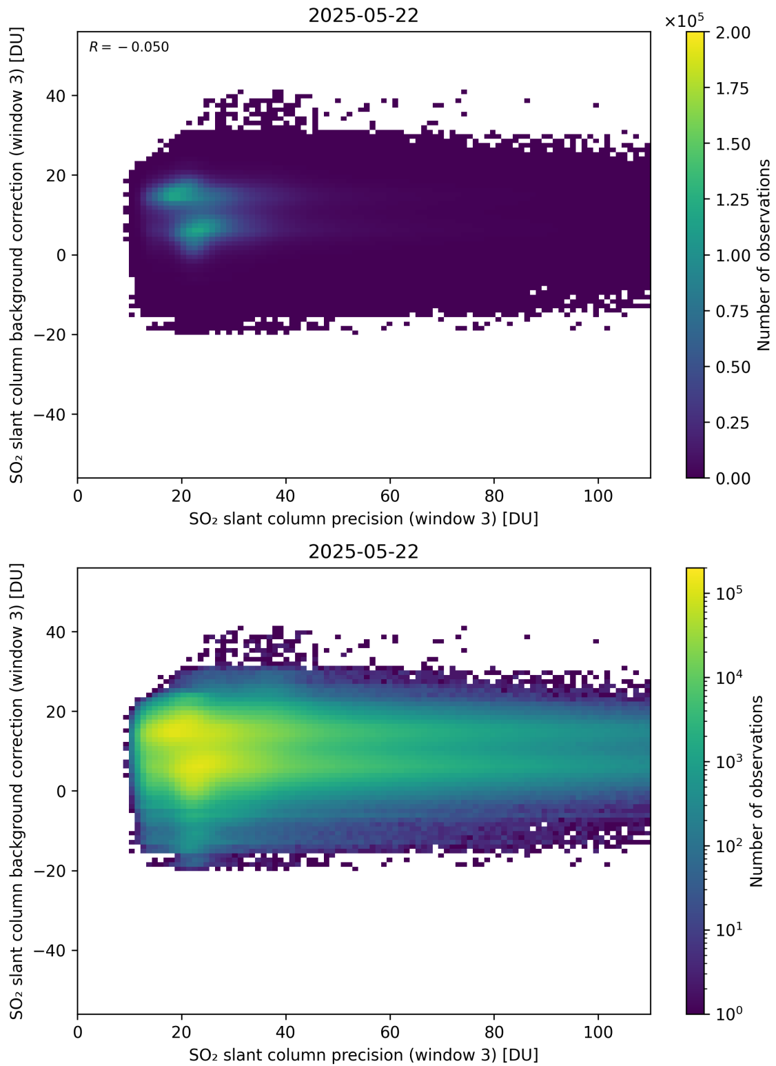
Figure 307: Scatter density plot of “SO 2 slant column precision (window 3)” against “SO 2 slant column background correction (window 3)” for 2025-05-21 to 2025-05-23.
