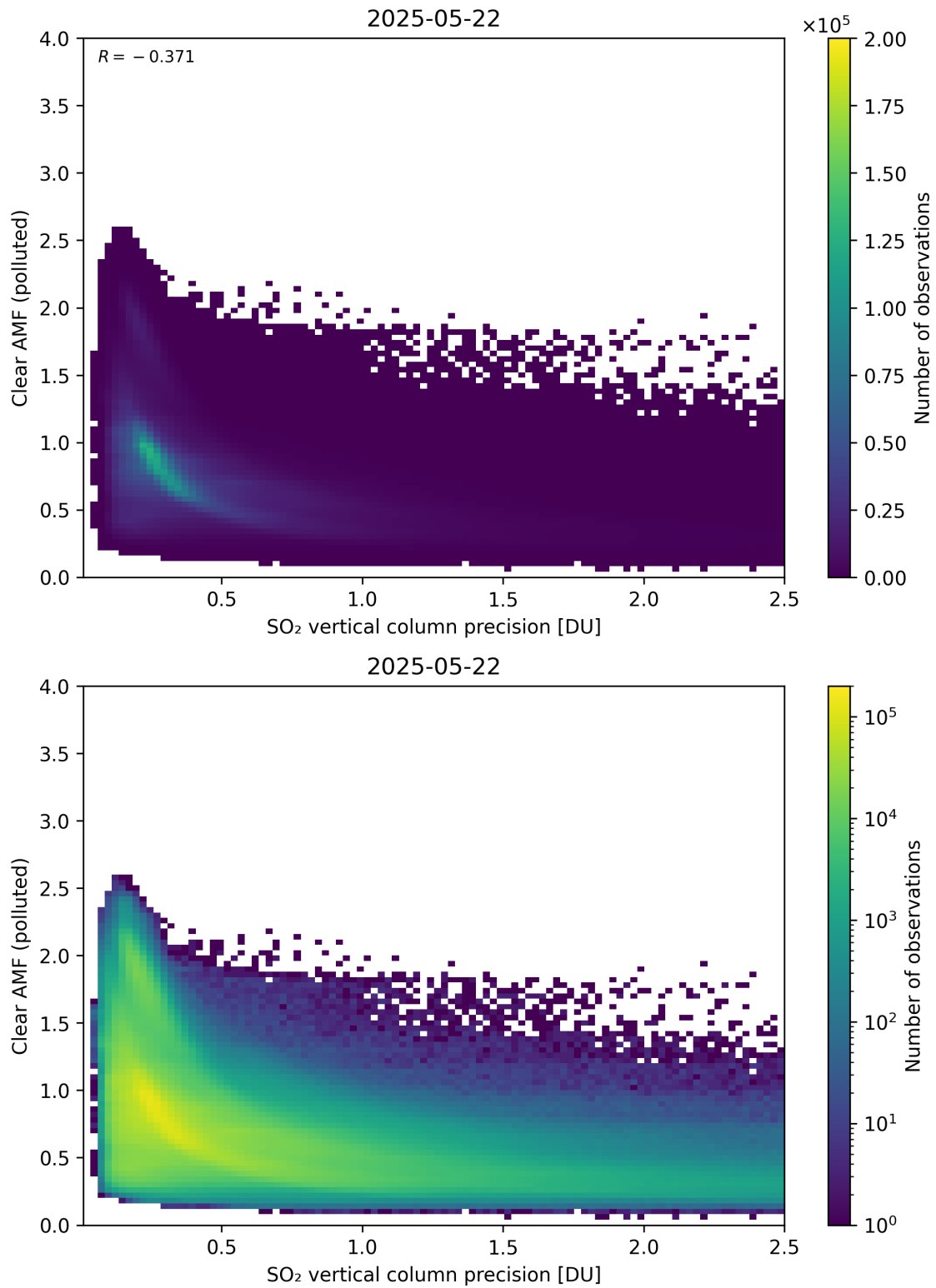
Figure 335: Scatter density plot of “SO 2 vertical column precision” against “Clear AMF (polluted)” for 2025-05-21 to 2025-05-23.
