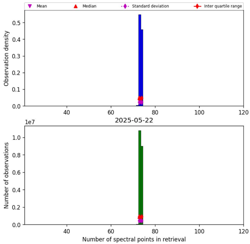
Figure 82: Histogram of “Number of spectral points in retrieval” for 2025-05-21 to 2025-05-23
