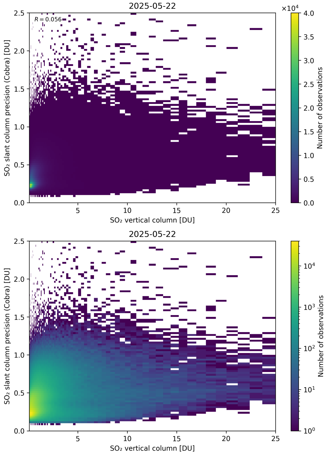
Figure 350: Scatter density plot of “SO 2 vertical column” against “SO 2 slant column precision (Cobra)” for 2025-05-21 to 2025-05-23.
