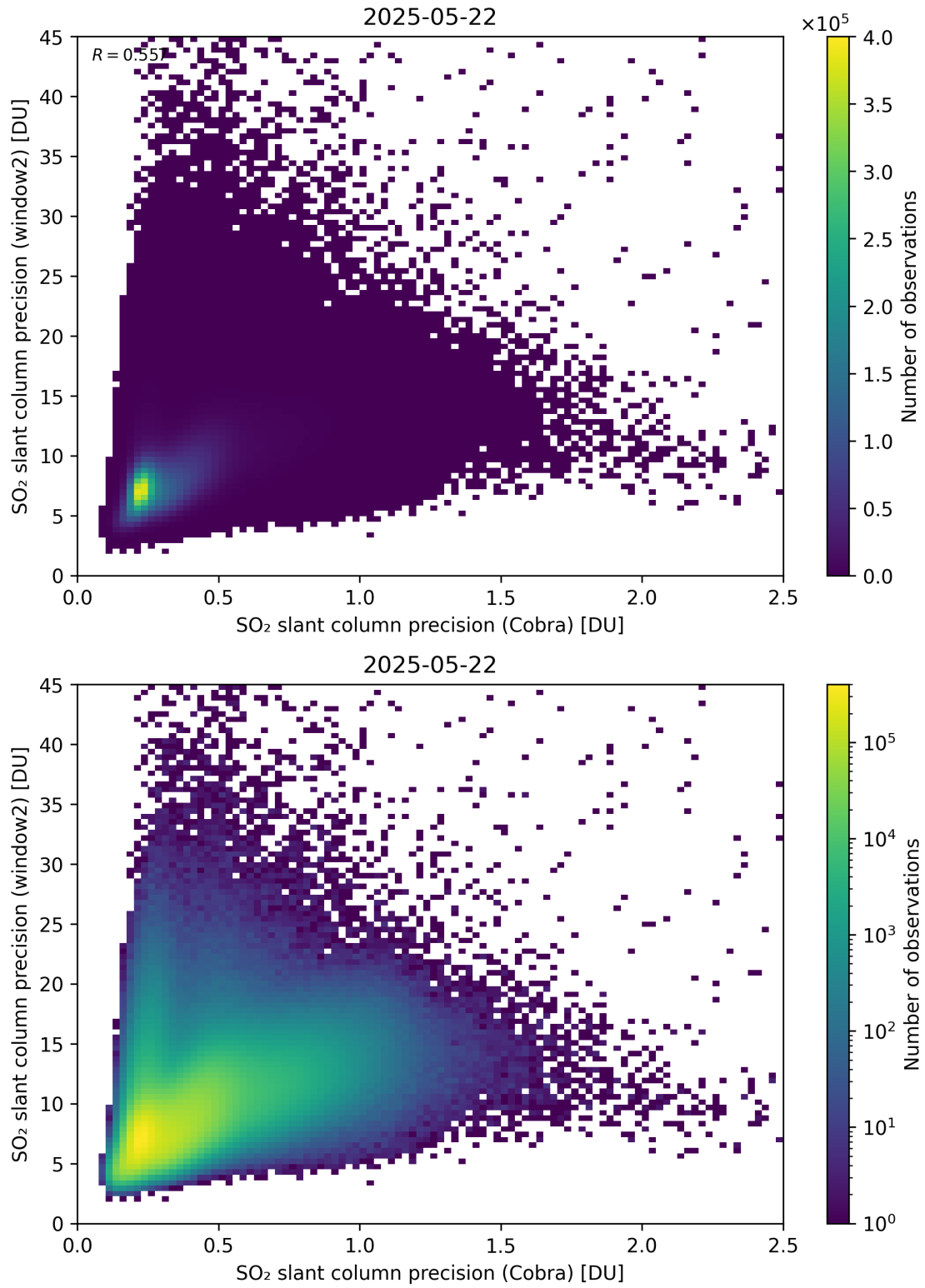
Figure 210: Scatter density plot of “SO 2 slant column precision (Cobra)” against “SO 2 slant column precision (window2)” for 2025-05-21 to 2025-05-23.
