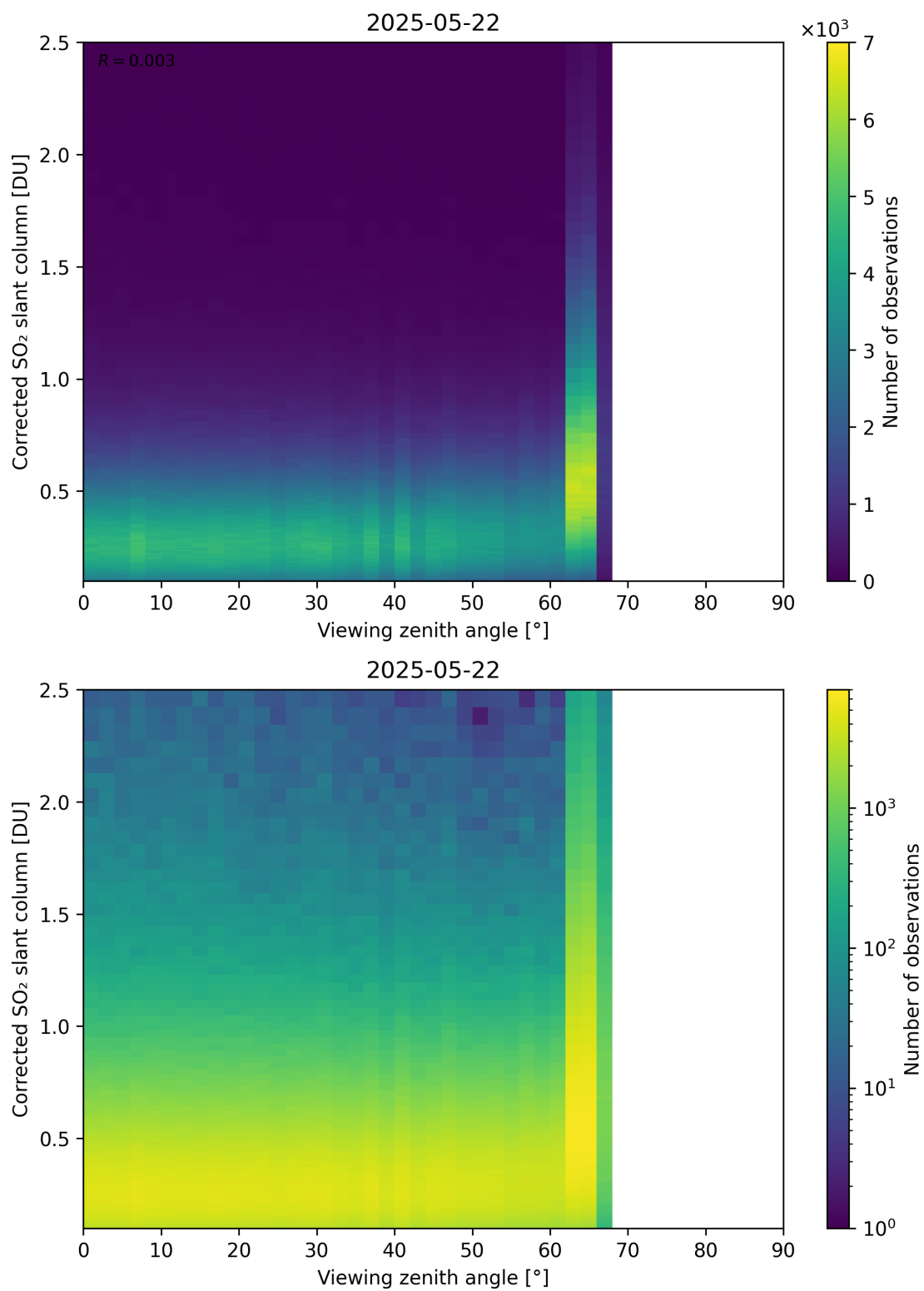
Figure 373: Scatter density plot of “Viewing zenith angle” against “Corrected SO 2 slant column” for 2025-05-21 to 2025-05-23.
