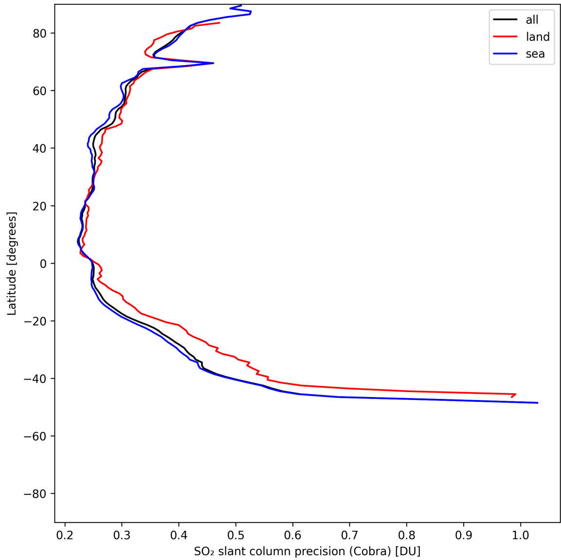
Figure 36: Zonal average of “SO 2 slant column precision (Cobra)” for 2025-05-21 to 2025-05-23.
