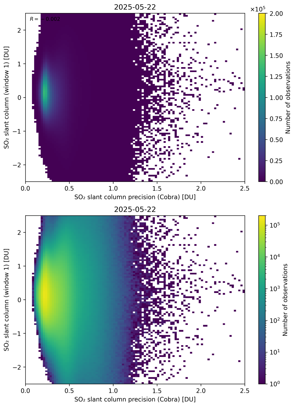
Figure 208: Scatter density plot of “SO 2 slant column precision (Cobra)” against “SO 2 slant column (window 1)” for 2025-05-21 to 2025-05-23.
