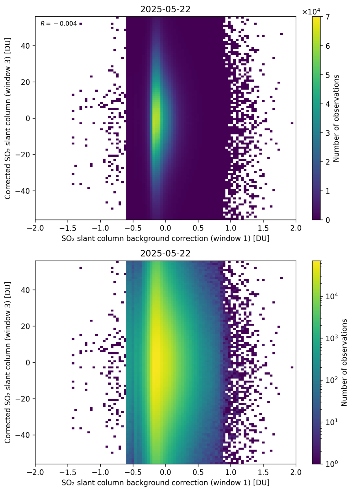
Figure 116: Scatter density plot of “SO 2 slant column background correction (window 1)” against “Corrected SO 2 slant column (window 3)” for 2025-05-21 to 2025-05-23.
