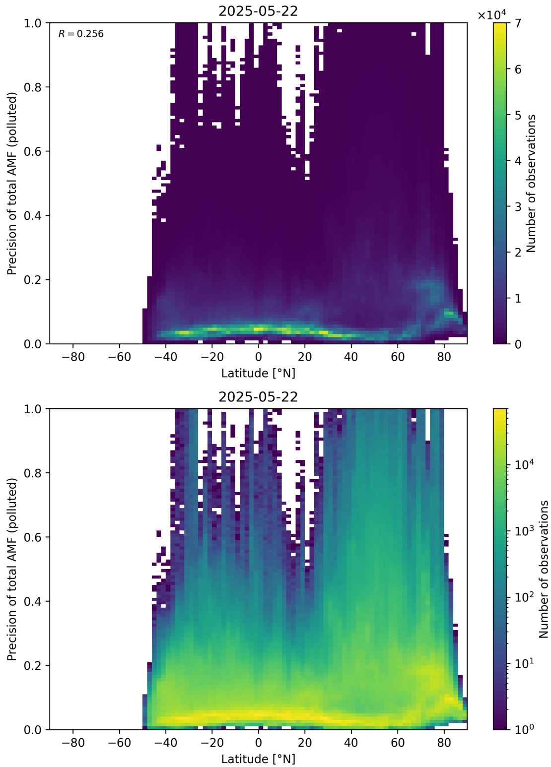
Figure 168: Scatter density plot of “Latitude” against “Precision of total AMF (polluted)” for 2025-05-21 to 2025-05-23.
