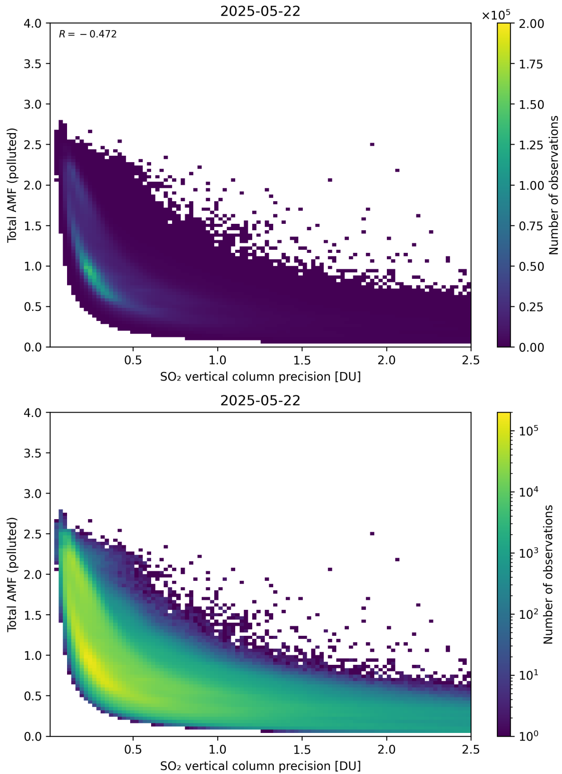
Figure 346: Scatter density plot of “SO 2 vertical column precision” against “Total AMF (polluted)” for 2025-05-21 to 2025-05-23.
