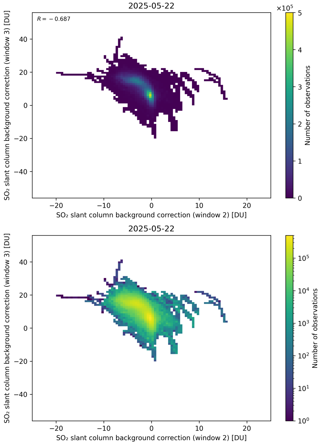
Figure 122: Scatter density plot of “SO 2 slant column background correction (window 2)” against “SO 2 slant column background correction (window 3)” for 2025-05-21 to 2025-05-23.
