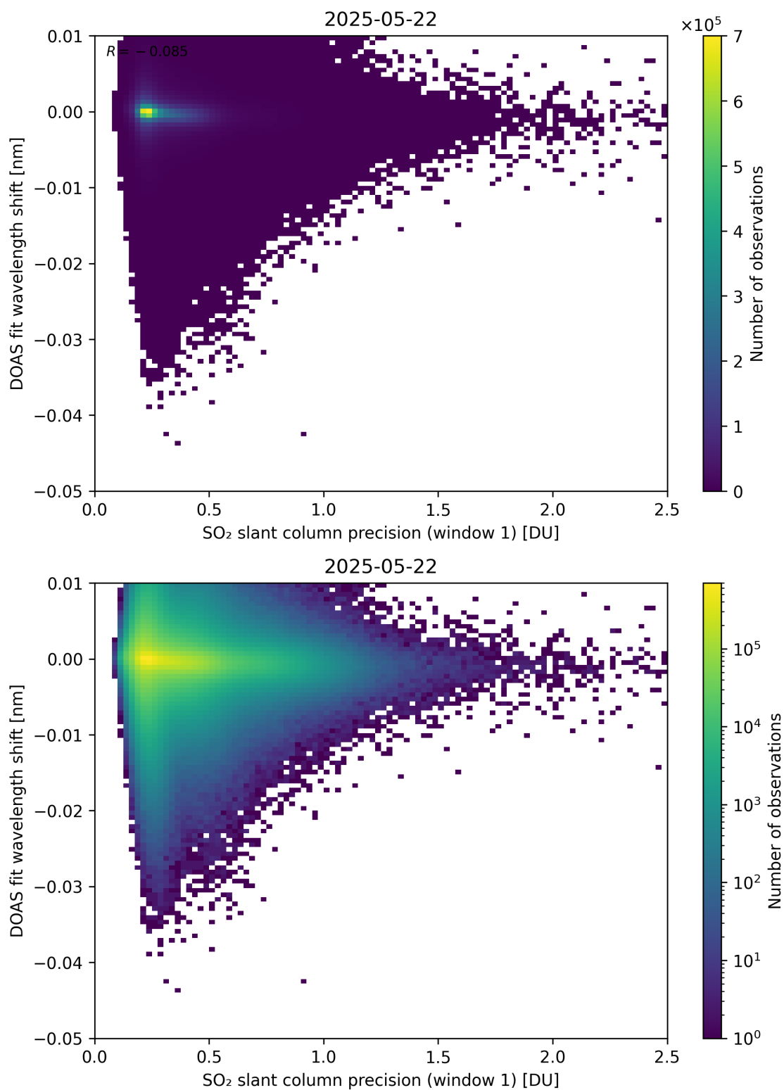
Figure 271: Scatter density plot of “SO 2 slant column precision (window 1)” against “DOAS fit wavelength shift” for 2025-05-21 to 2025-05-23.
