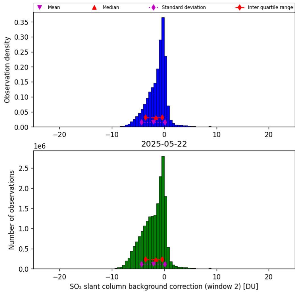
Figure 70: Histogram of “SO 2 slant column background correction (window 2)” for 2025-05-21 to 2025-05-23
