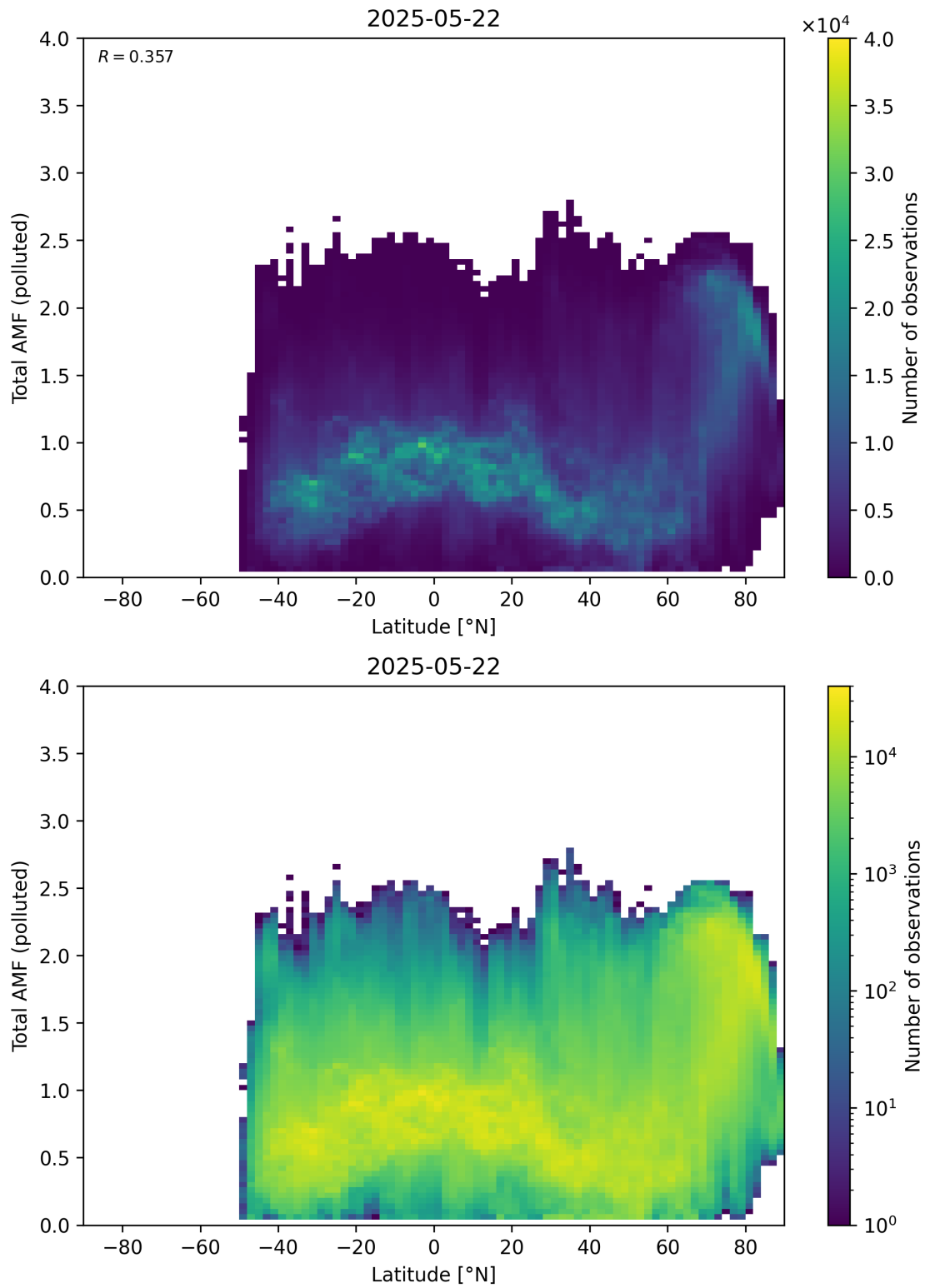
Figure 167: Scatter density plot of “Latitude” against “Total AMF (polluted)” for 2025-05-21 to 2025-05-23.
