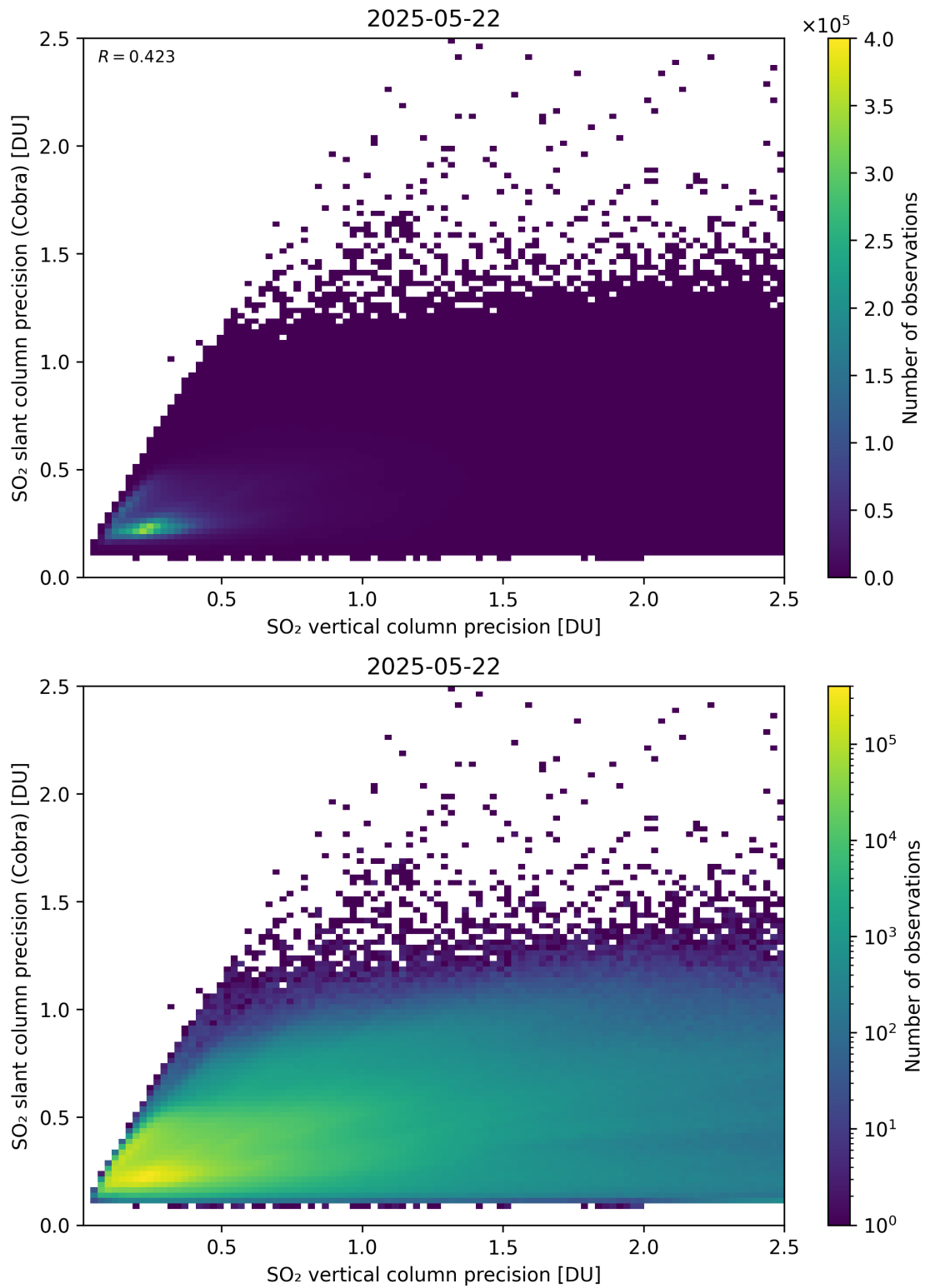
Figure 337: Scatter density plot of “SO 2 vertical column precision” against “SO 2 slant column precision (Cobra)” for 2025-05-21 to 2025-05-23.
