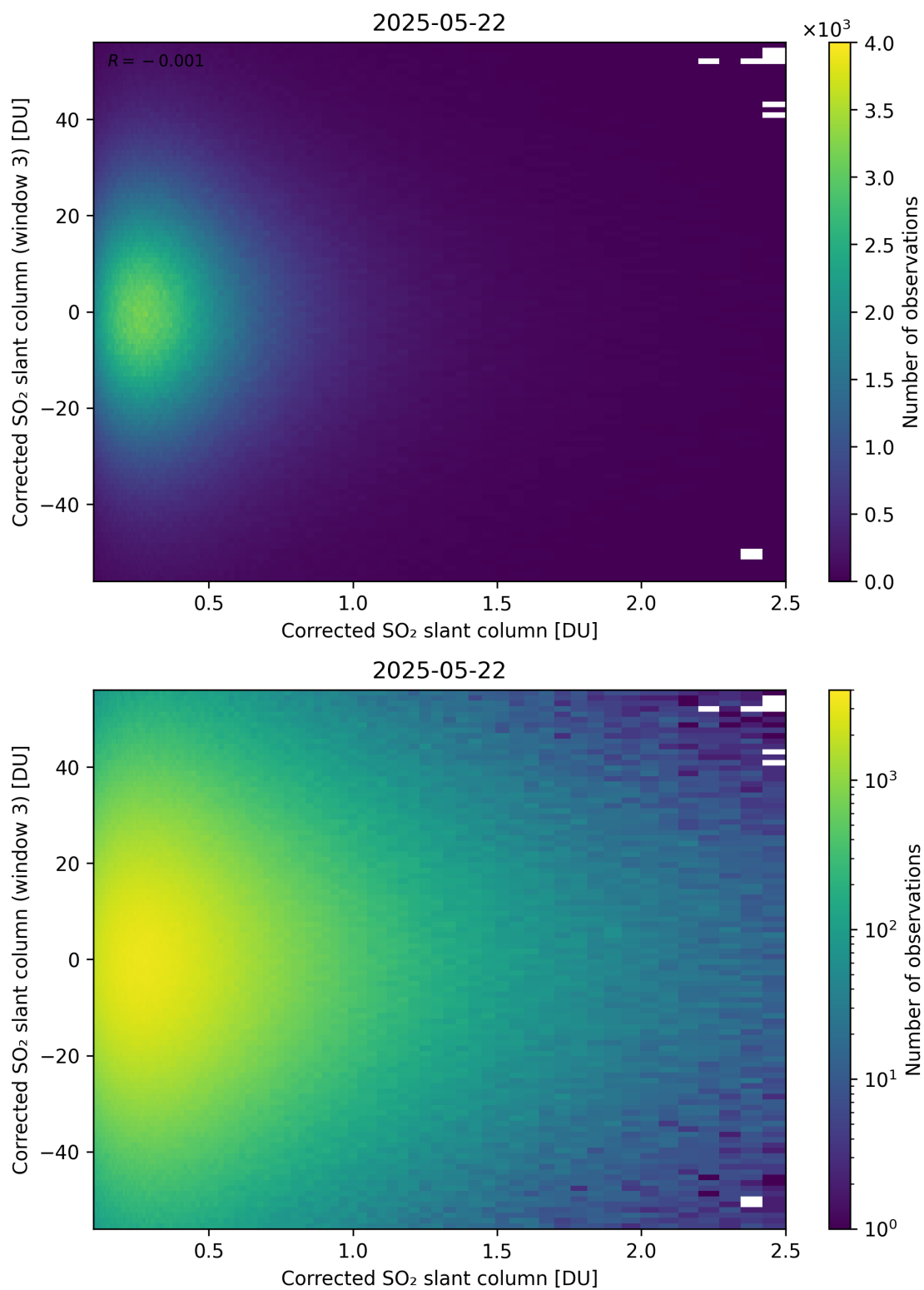
Figure 236: Scatter density plot of “Corrected SO 2 slant column” against “Corrected SO 2 slant column (window 3)” for 2025-05-21 to 2025-05-23.
