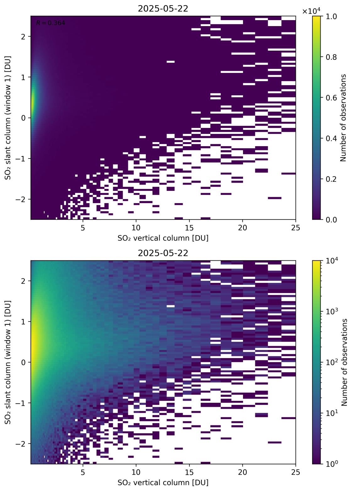
Figure 354: Scatter density plot of “SO 2 vertical column” against “SO 2 slant column (window 1)” for 2025-05-21 to 2025-05-23.
