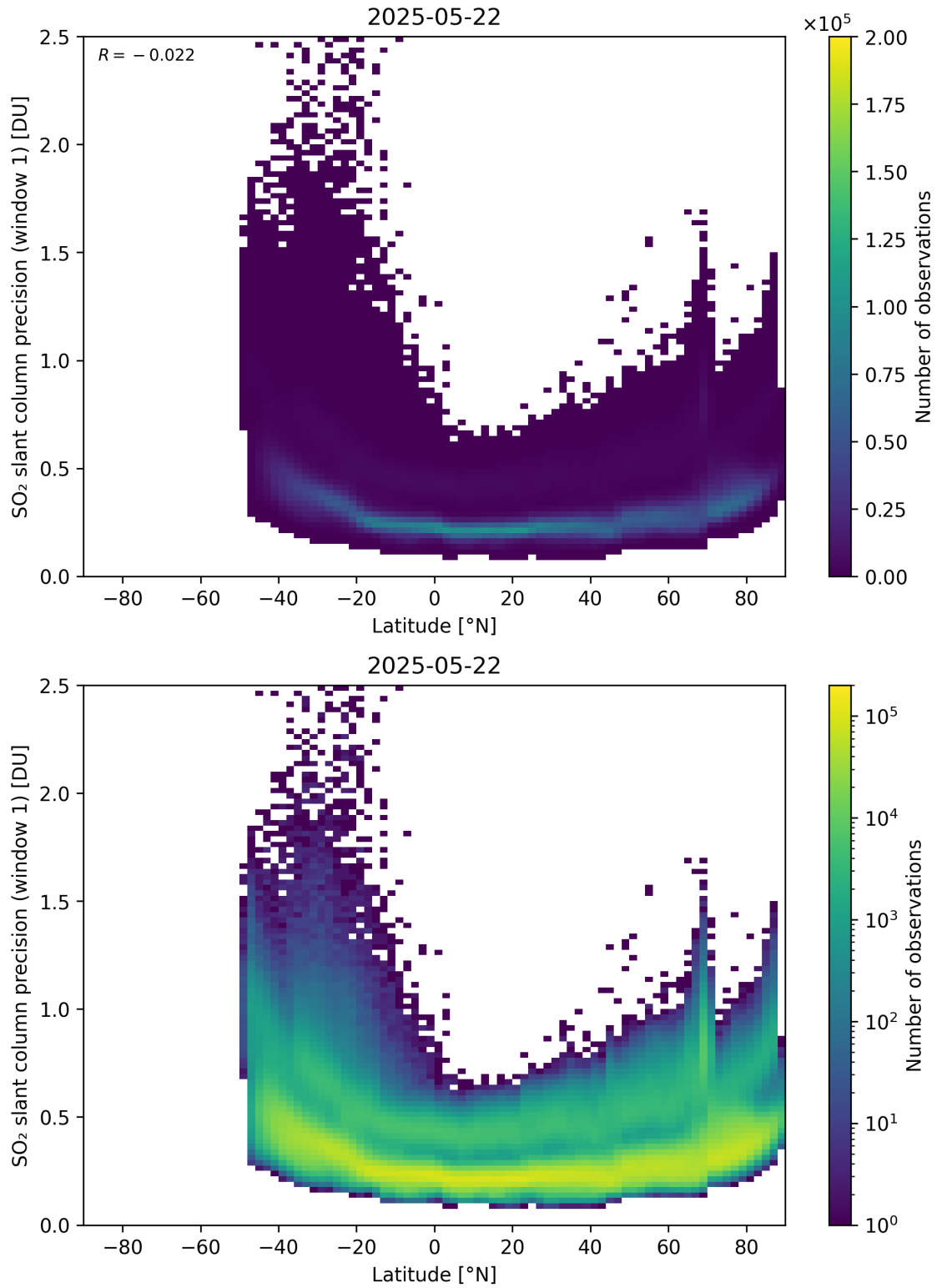
Figure 163: Scatter density plot of “Latitude” against “SO 2 slant column precision (window 1)” for 2025-05-21 to 2025-05-23.
