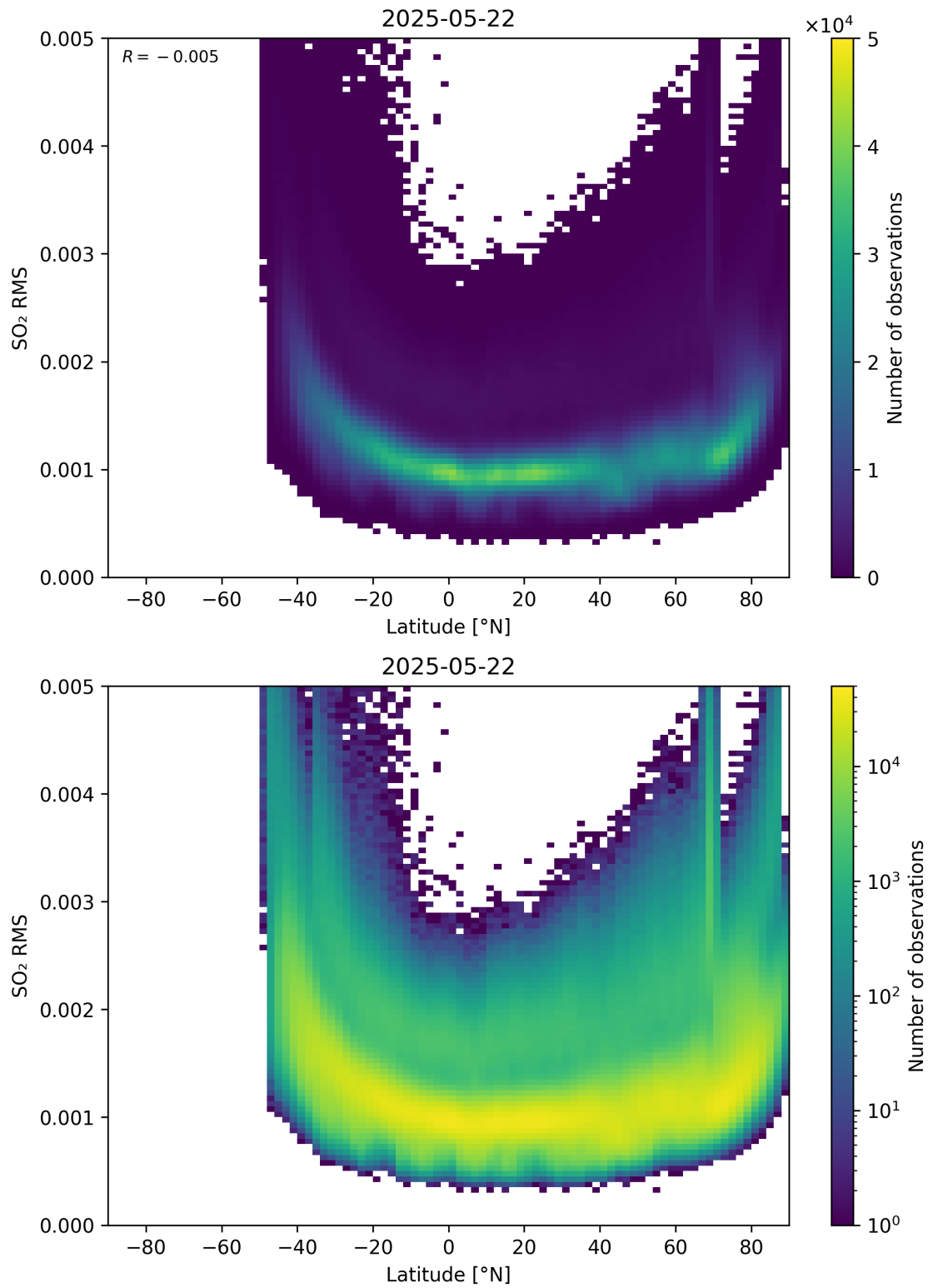
Figure 155: Scatter density plot of “Latitude” against “SO 2 RMS” for 2025-05-21 to 2025-05-23.
