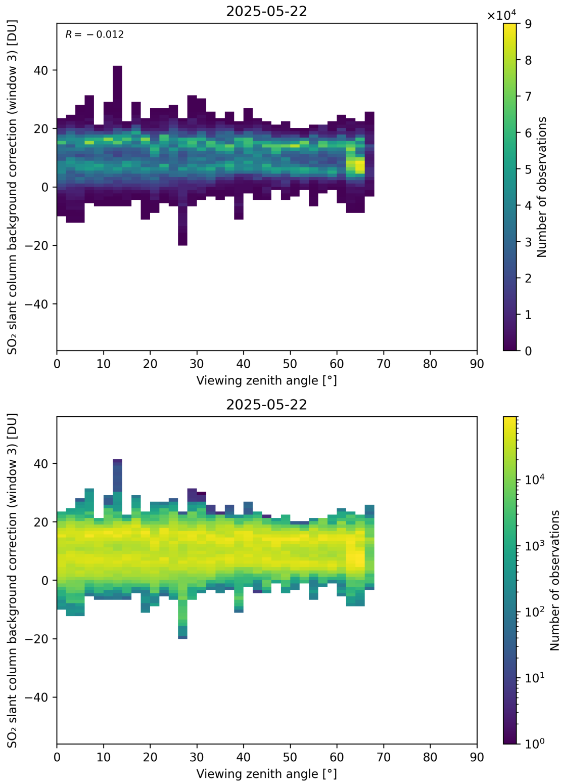
Figure 364: Scatter density plot of “Viewing zenith angle” against “SO 2 slant column background correction (window 3)” for 2025-05-21 to 2025-05-23.
