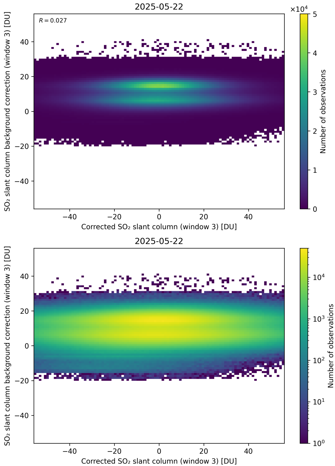
Figure 255: Scatter density plot of “Corrected SO 2 slant column (window 3)” against “SO 2 slant column background correction (window 3)” for 2025-05-21 to 2025-05-23.
