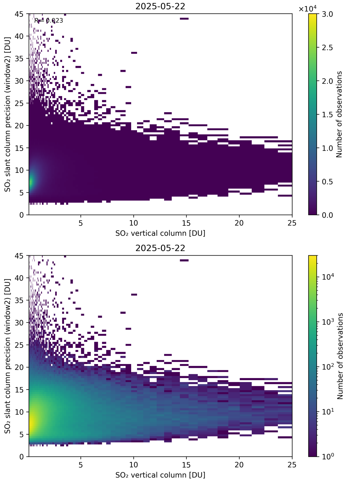
Figure 356: Scatter density plot of “SO 2 vertical column” against “SO 2 slant column precision (window2)” for 2025-05-21 to 2025-05-23.
