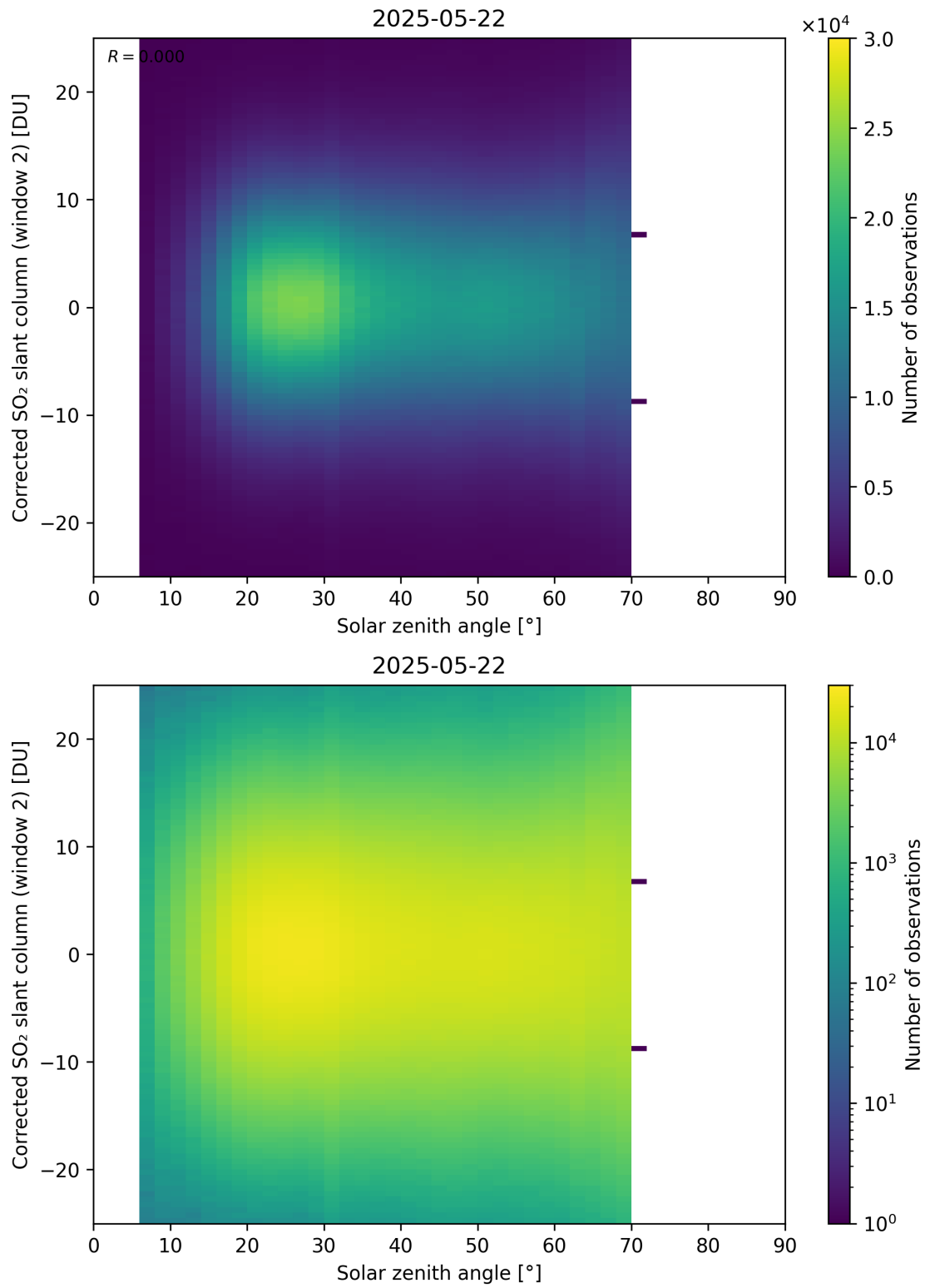
Figure 182: Scatter density plot of “Solar zenith angle” against “Corrected SO 2 slant column (window 2)” for 2025-05-21 to 2025-05-23.
