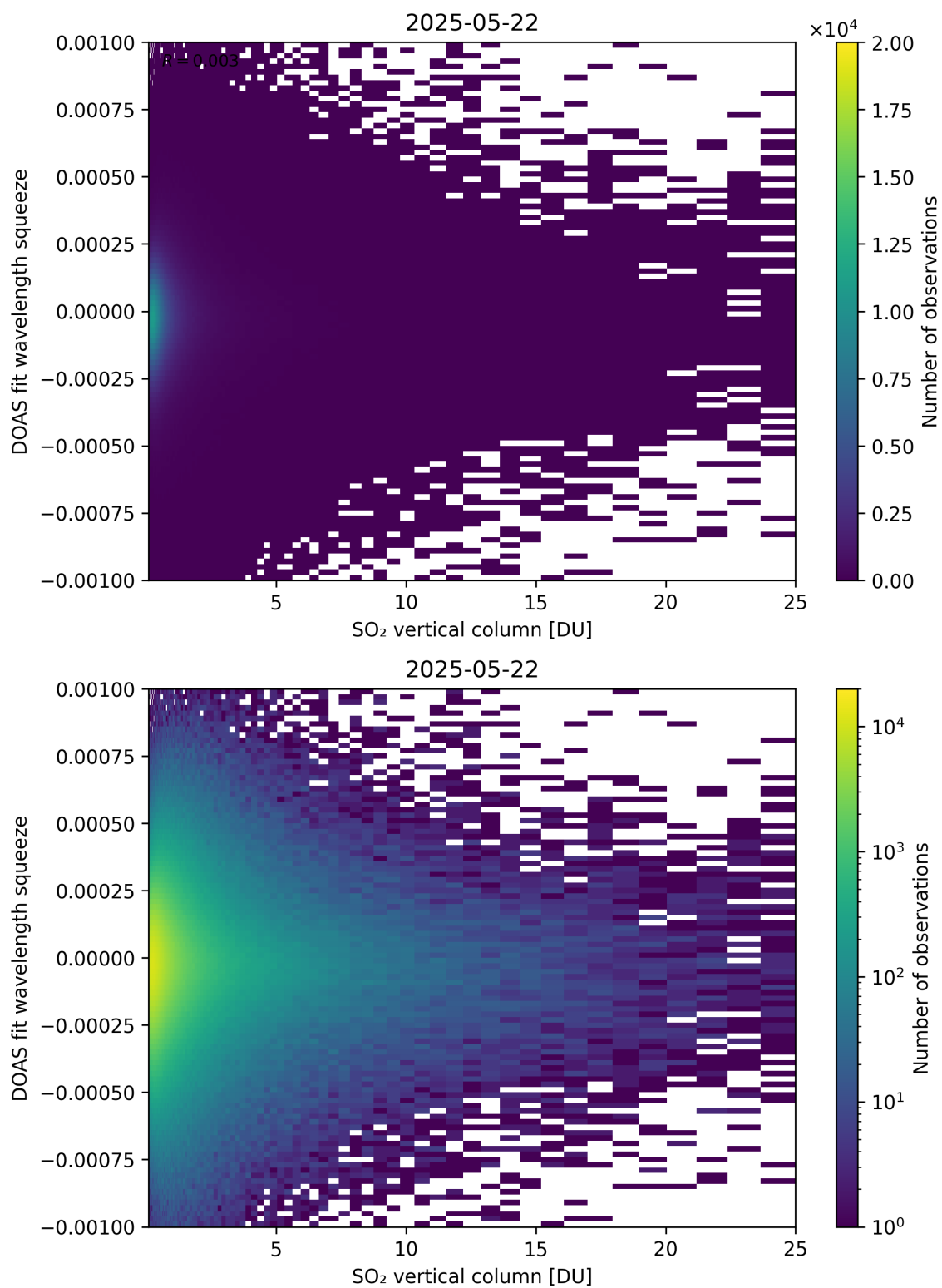
Figure 327: Scatter density plot of “SO 2 vertical column” against “DOAS fit wavelength squeeze” for 2025-05-21 to 2025-05-23.
