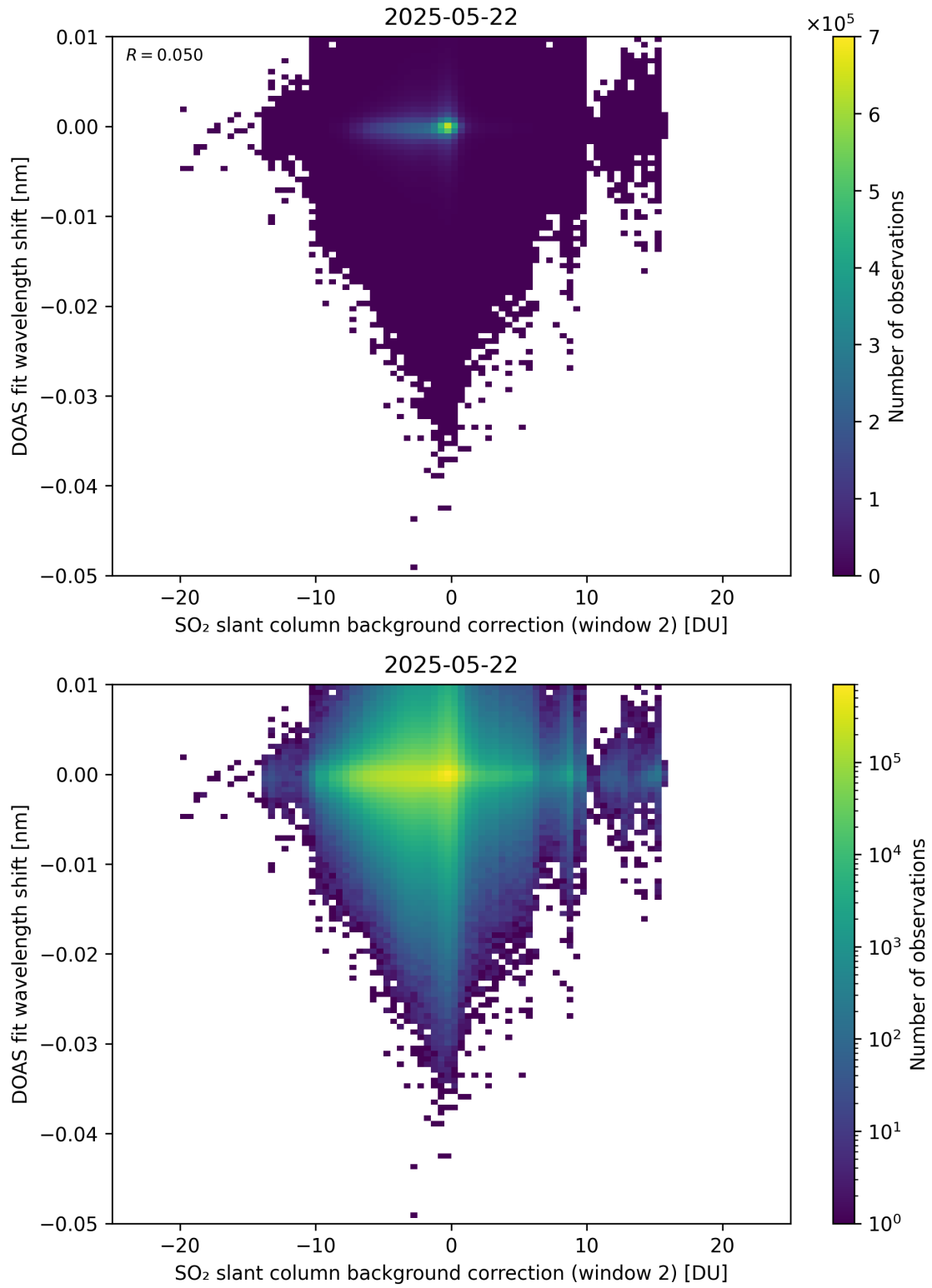
Figure 123: Scatter density plot of “SO 2 slant column background correction (window 2)” against “DOAS fit wavelength shift” for 2025-05-21 to 2025-05-23.
