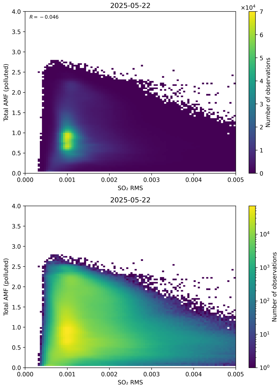
Figure 148: Scatter density plot of “SO 2 RMS” against “Total AMF (polluted)” for 2025-05-21 to 2025-05-23.
