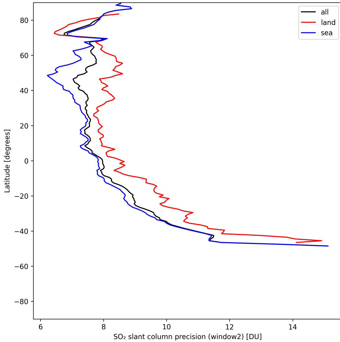
Figure 42: Zonal average of “SO 2 slant column precision (window2)” for 2025-05-21 to 2025-05-23.
