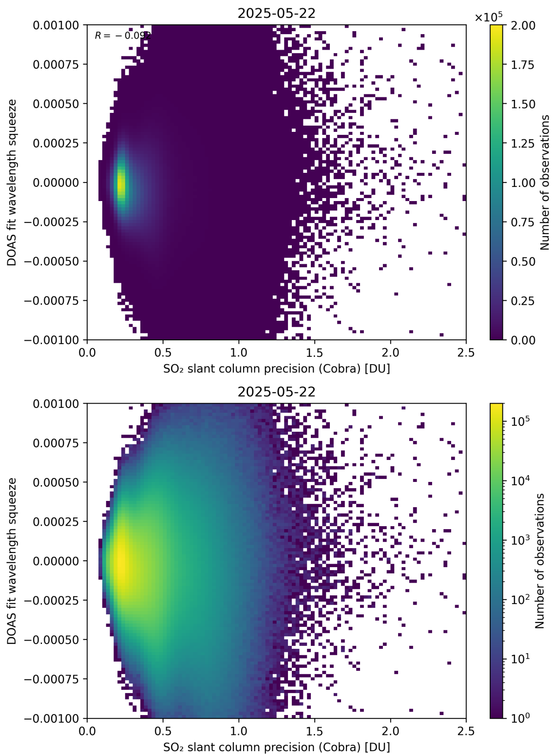
Figure 203: Scatter density plot of “SO 2 slant column precision (Cobra)” against “DOAS fit wavelength squeeze” for 2025-05-21 to 2025-05-23.
