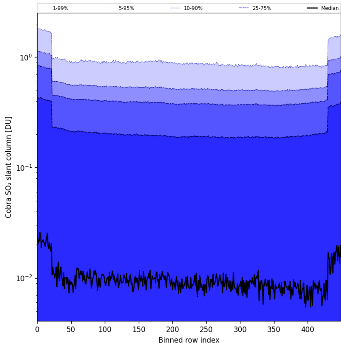
Figure 87: Along track statistics of “Cobra SO 2 slant column” for 2025-05-21 to 2025-05-23
