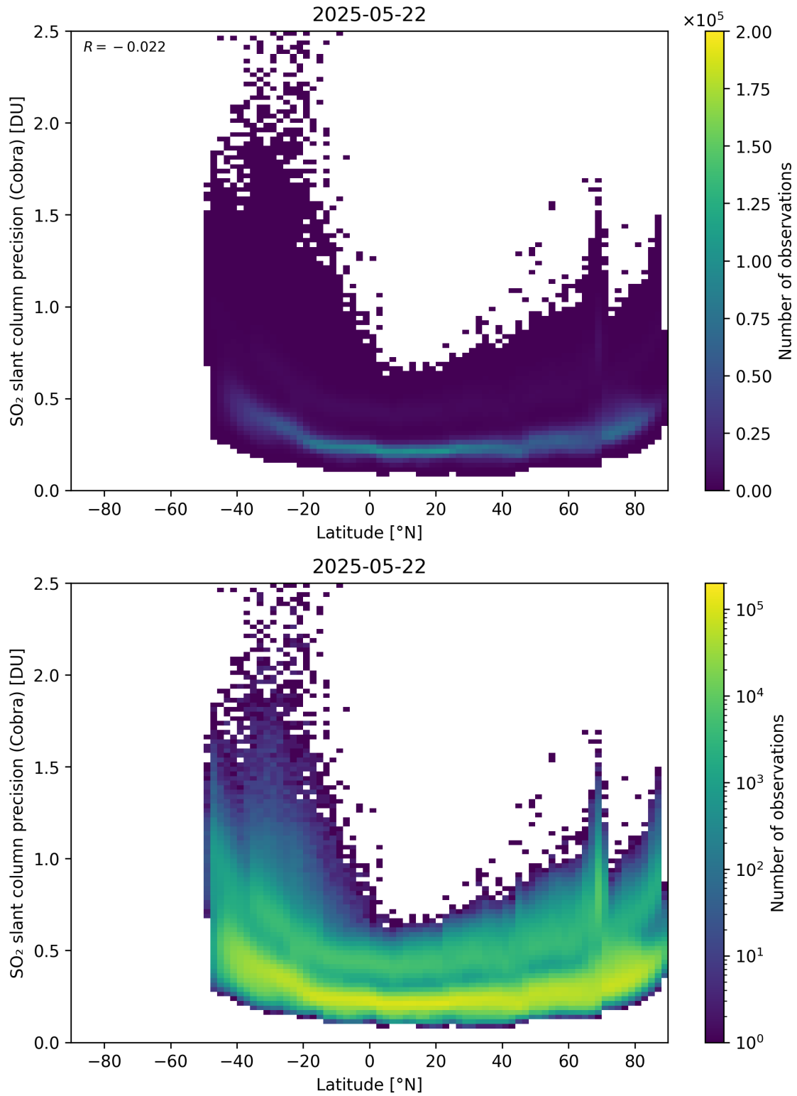
Figure 158: Scatter density plot of “Latitude” against “SO 2 slant column precision (Cobra)” for 2025-05-21 to 2025-05-23.
