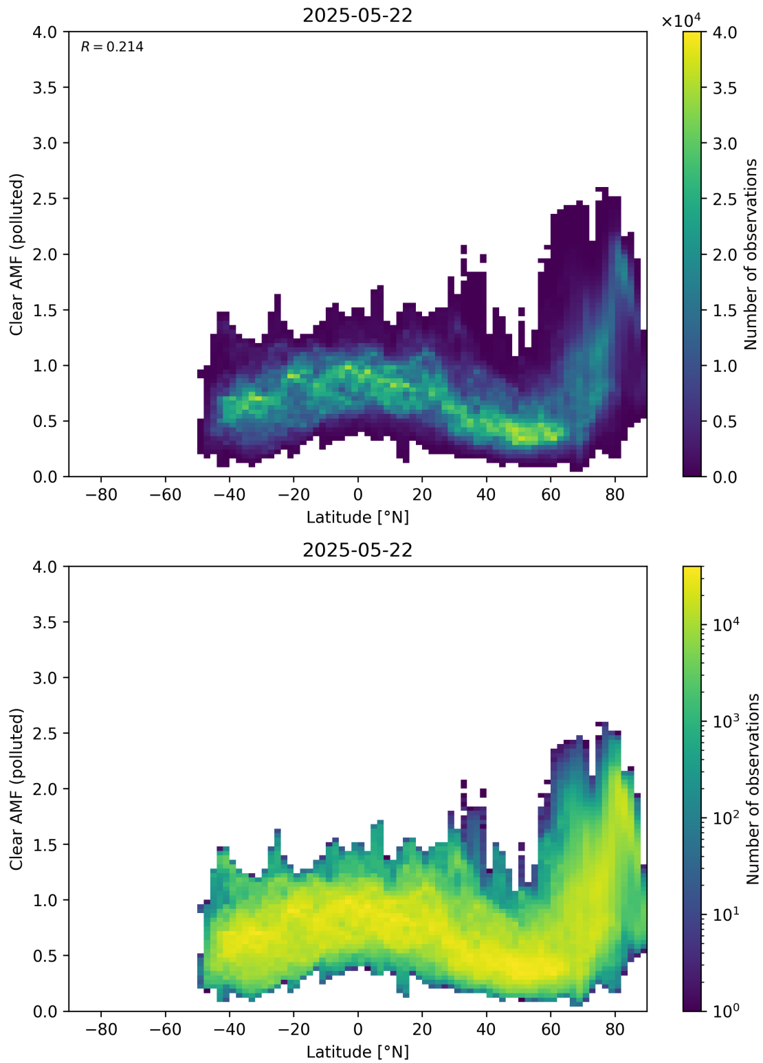
Figure 156: Scatter density plot of “Latitude” against “Clear AMF (polluted)” for 2025-05-21 to 2025-05-23.
