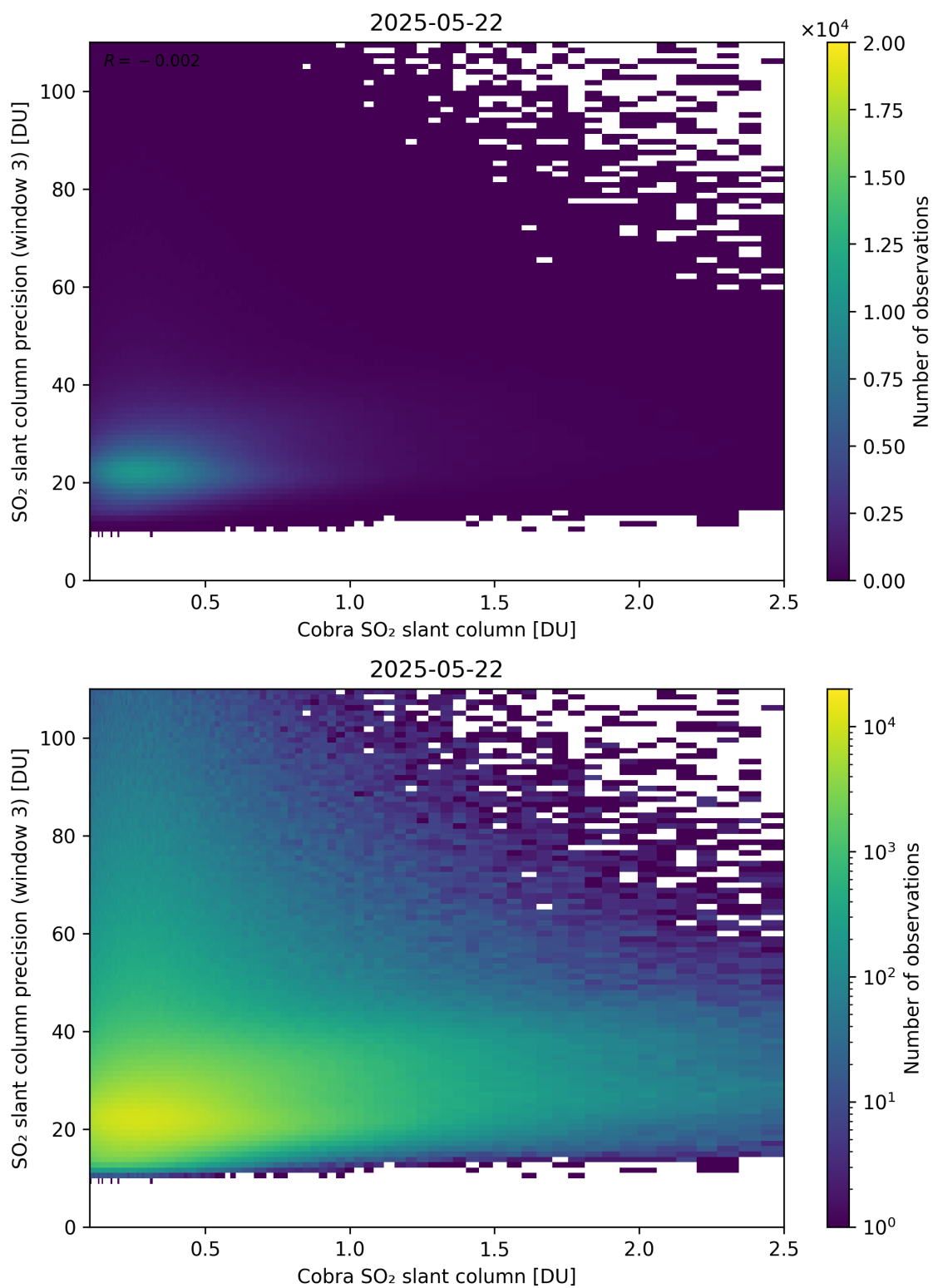
Figure 223: Scatter density plot of “Cobra SO 2 slant column” against “SO 2 slant column precision (window 3)” for 2025-05-21 to 2025-05-23.
