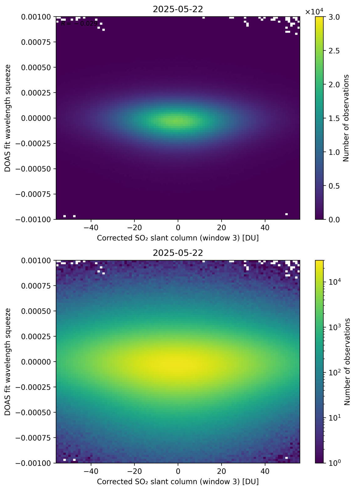
Figure 257: Scatter density plot of “Corrected SO 2 slant column (window 3)” against “DOAS fit wavelength squeeze” for 2025-05-21 to 2025-05-23.
