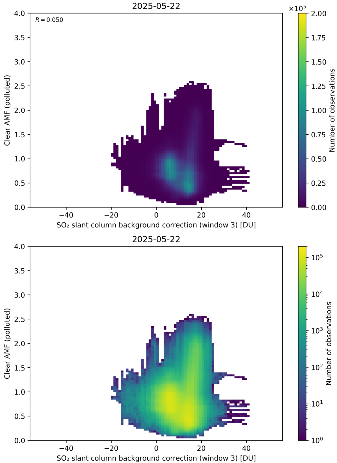
Figure 135: Scatter density plot of “SO 2 slant column background correction (window 3)” against “Clear AMF (polluted)” for 2025-05-21 to 2025-05-23.
