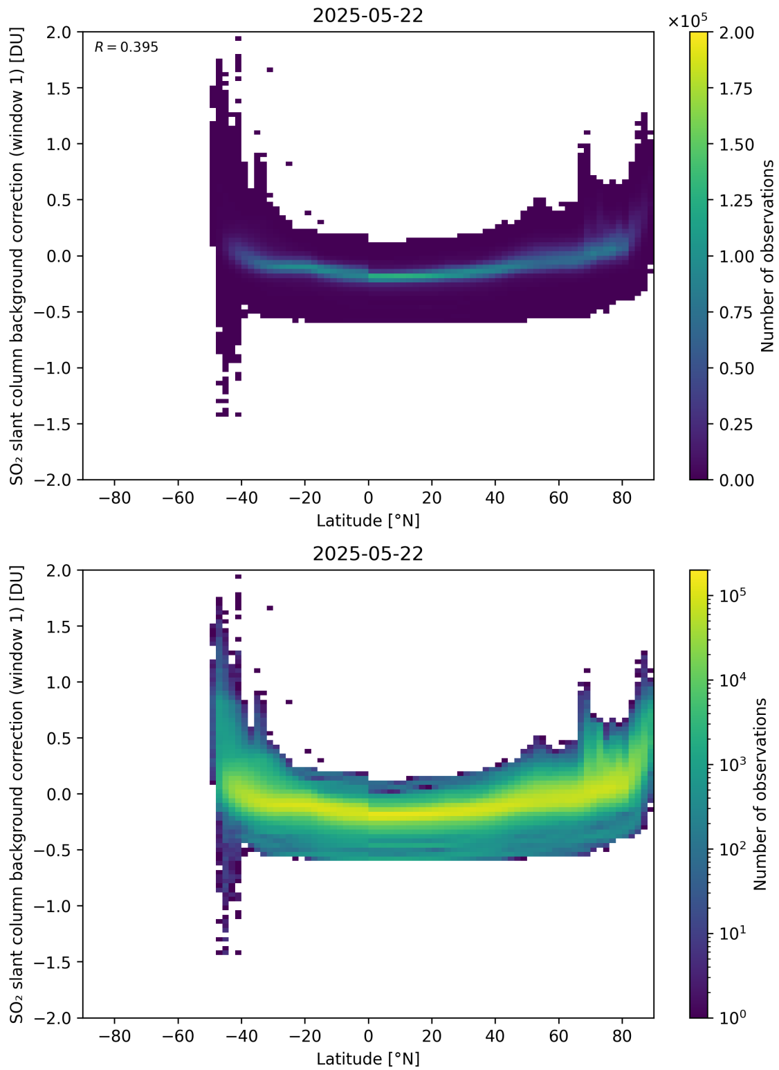
Figure 150: Scatter density plot of “Latitude” against “SO 2 slant column background correction (window 1)” for 2025-05-21 to 2025-05-23.
