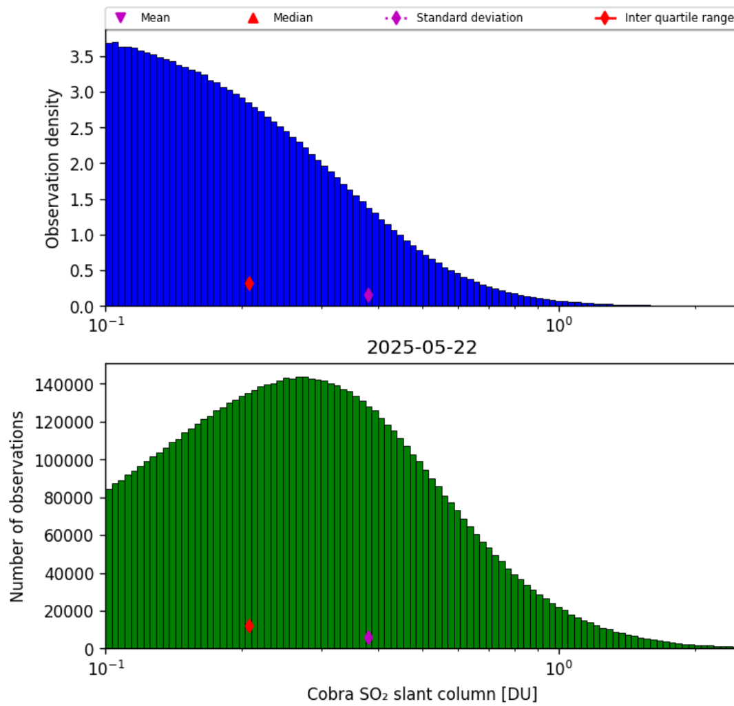
Figure 61: Histogram of “Cobra SO 2 slant column” for 2025-05-21 to 2025-05-23
