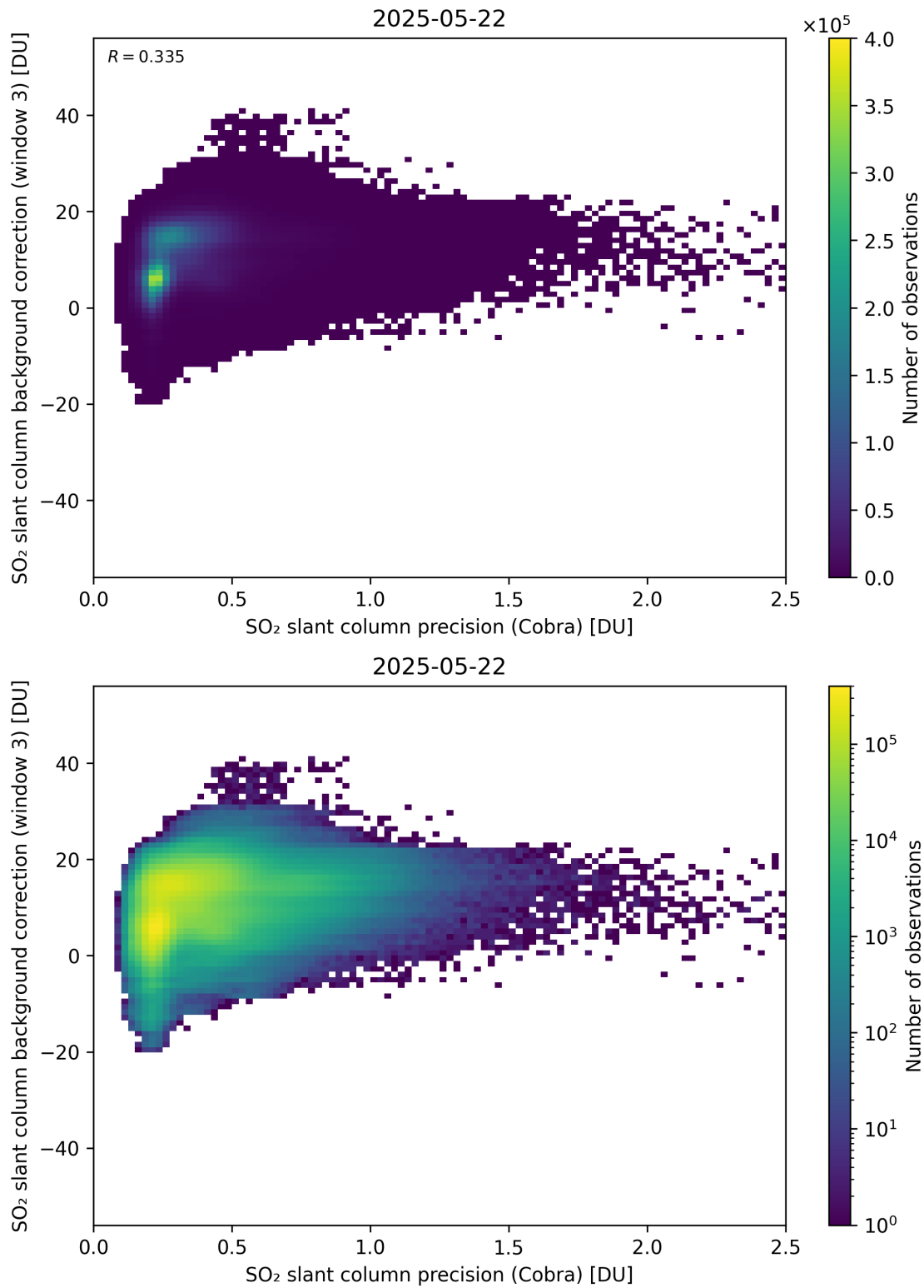
Figure 201: Scatter density plot of “SO 2 slant column precision (Cobra)” against “SO 2 slant column background correction (window 3)” for 2025-05-21 to 2025-05-23.
