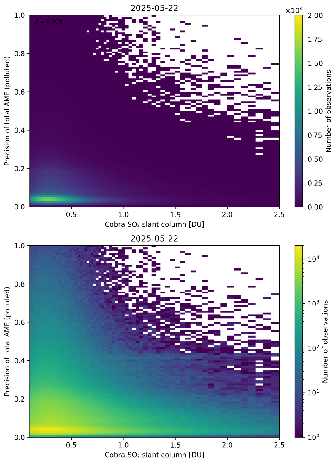
Figure 225: Scatter density plot of “Cobra SO 2 slant column” against “Precision of total AMF (polluted)” for 2025-05-21 to 2025-05-23.
