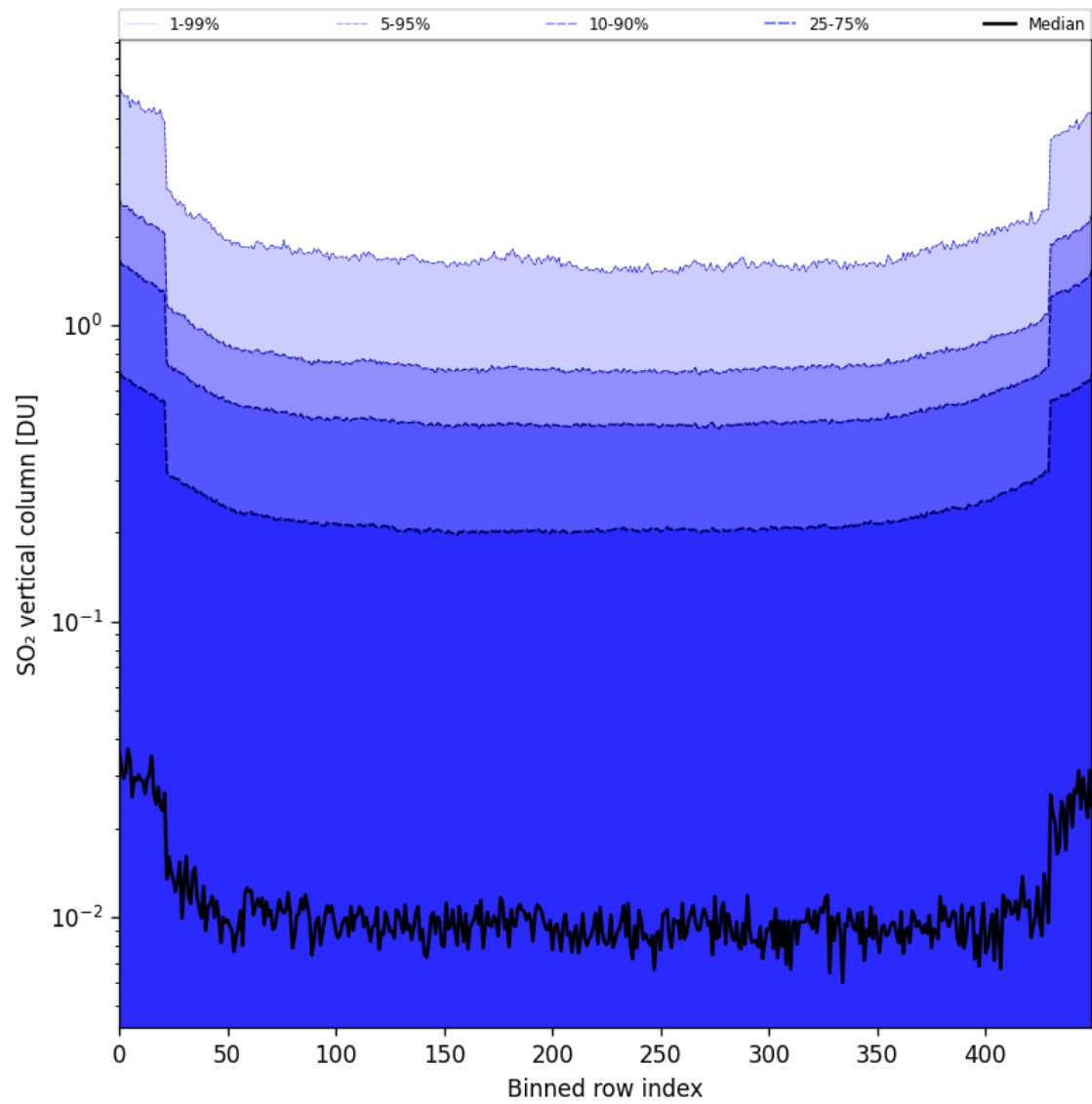
Figure 84: Along track statistics of “SO 2 vertical column” for 2025-05-21 to 2025-05-23
