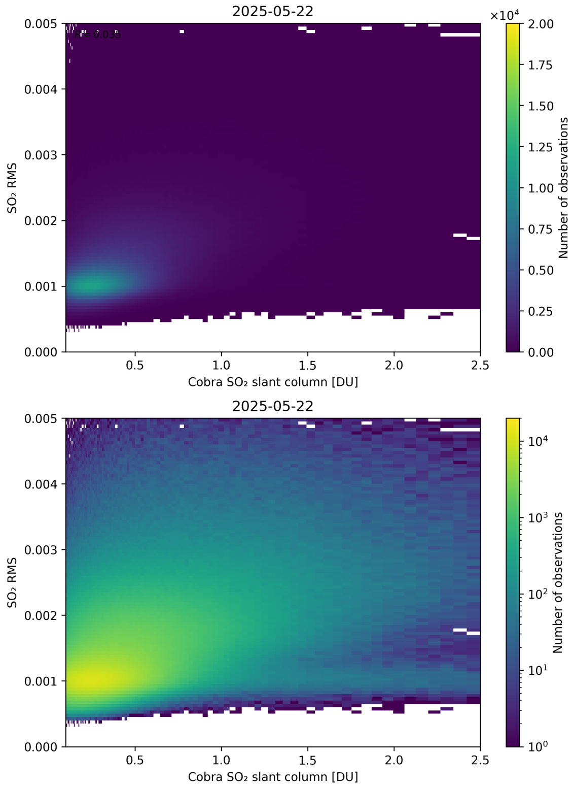
Figure 198: Scatter density plot of “Cobra SO 2 slant column” against “SO 2 RMS” for 2025-05-21 to 2025-05-23.
