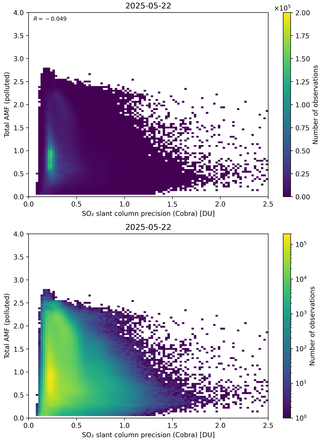
Figure 213: Scatter density plot of “SO 2 slant column precision (Cobra)” against “Total AMF (polluted)” for 2025-05-21 to 2025-05-23.
