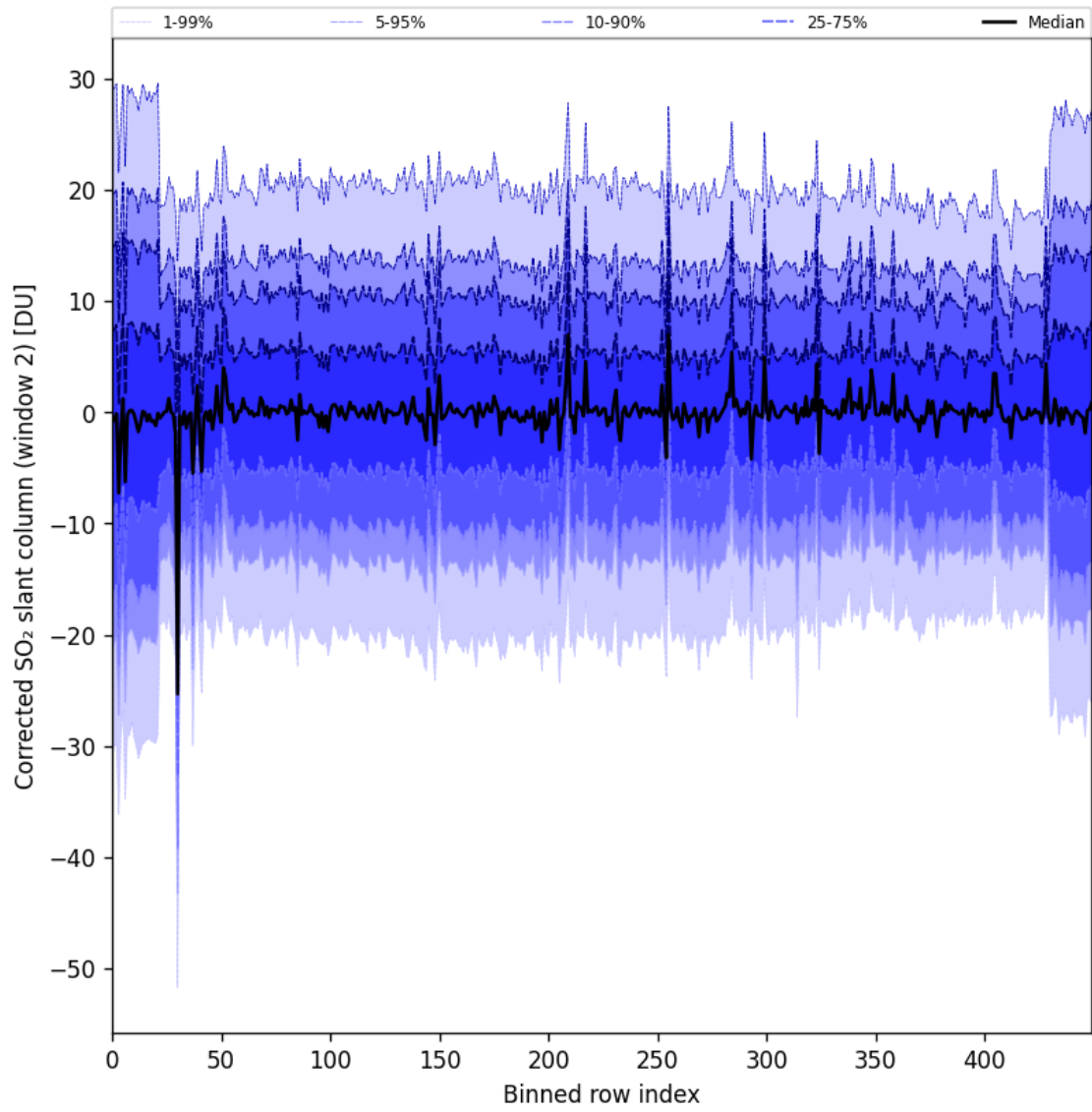
Figure 95: Along track statistics of “Corrected SO 2 slant column (window 2)” for 2025-05-22 to 2025-05-24
