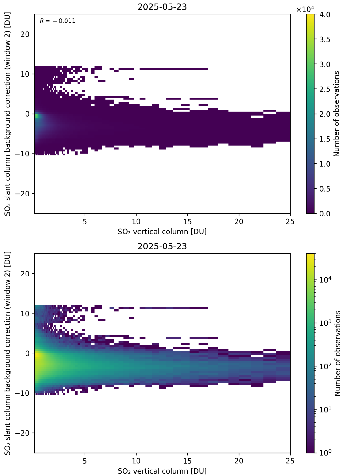
Figure 324: Scatter density plot of “SO 2 vertical column” against “SO 2 slant column background correction (window 2)” for 2025-05-22 to 2025-05-24.
