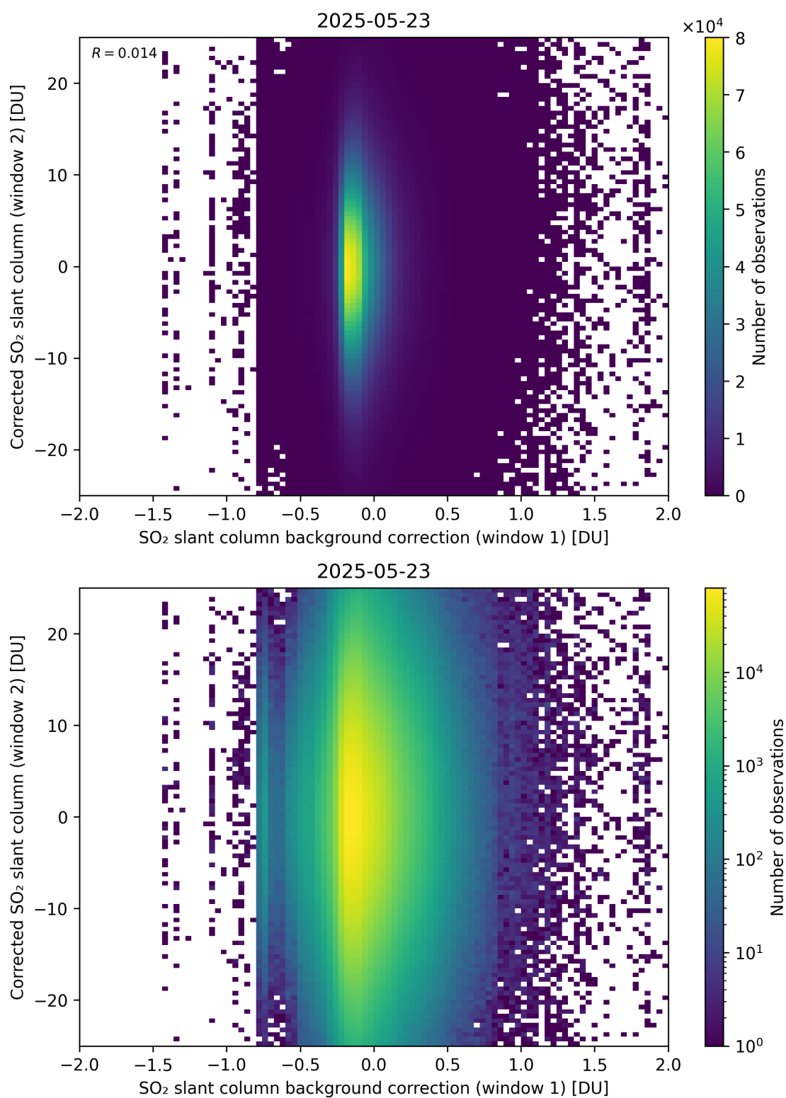
Figure 115: Scatter density plot of “SO 2 slant column background correction (window 1)” against “Corrected SO 2 slant column (window 2)” for 2025-05-22 to 2025-05-24.
