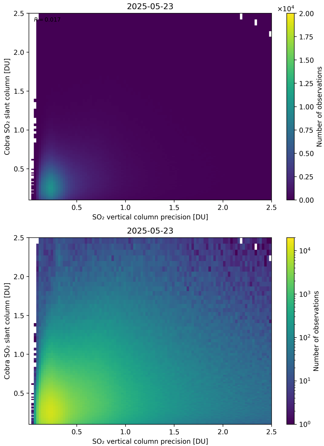
Figure 336: Scatter density plot of “SO 2 vertical column precision” against “Cobra SO 2 slant column” for 2025-05-22 to 2025-05-24.
