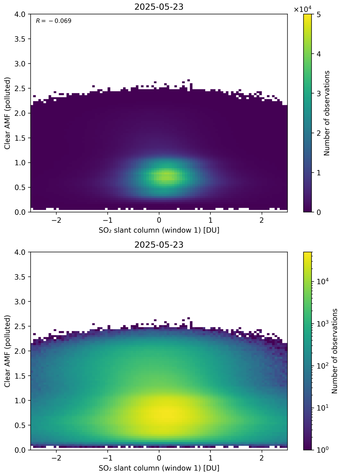
Figure 282: Scatter density plot of “SO 2 slant column (window 1)” against “Clear AMF (polluted)” for 2025-05-22 to 2025-05-24.
