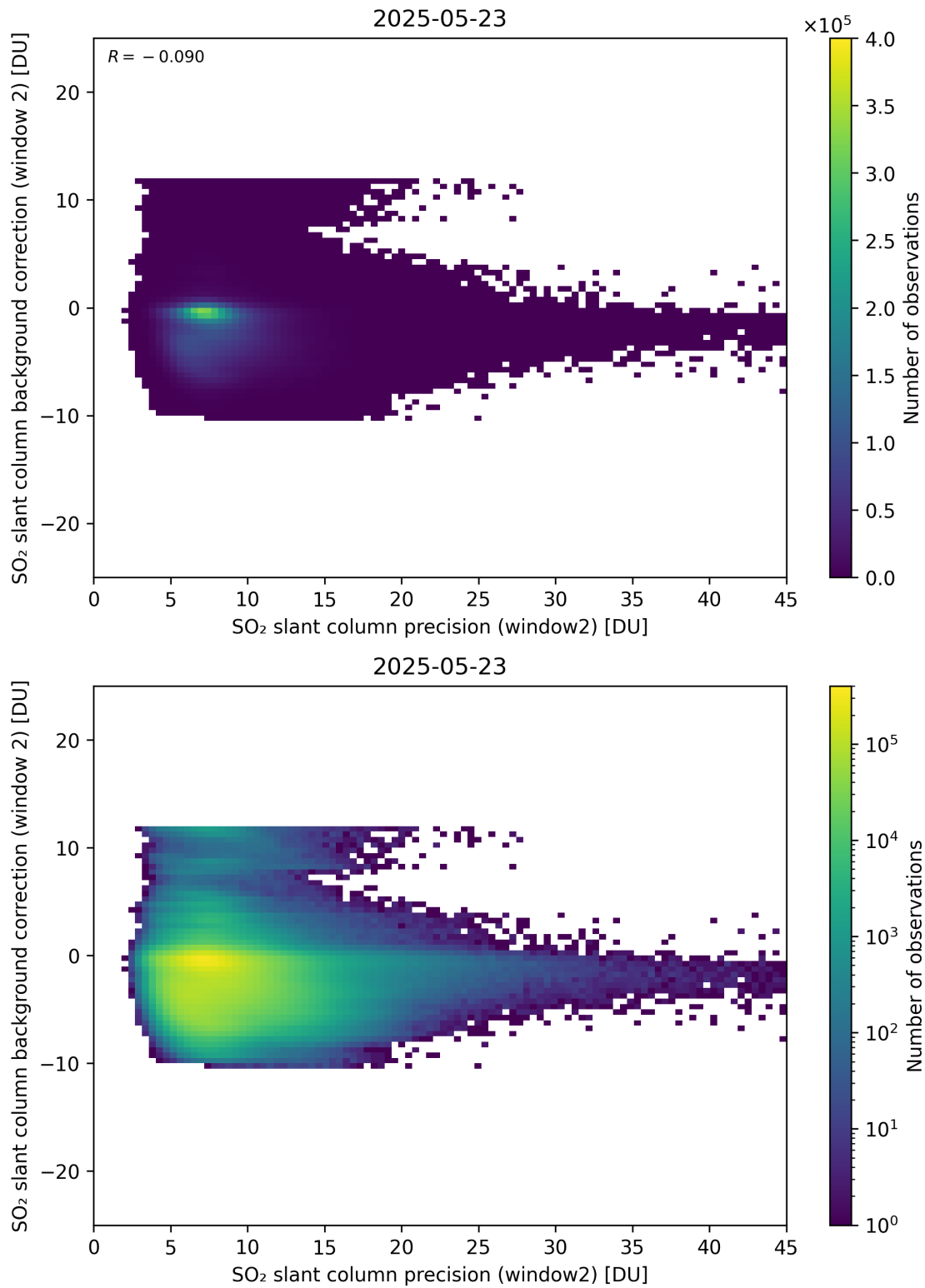
Figure 291: Scatter density plot of “SO 2 slant column precision (window2)” against “SO 2 slant column background correction (window 2)” for 2025-05-22 to 2025-05-24.
