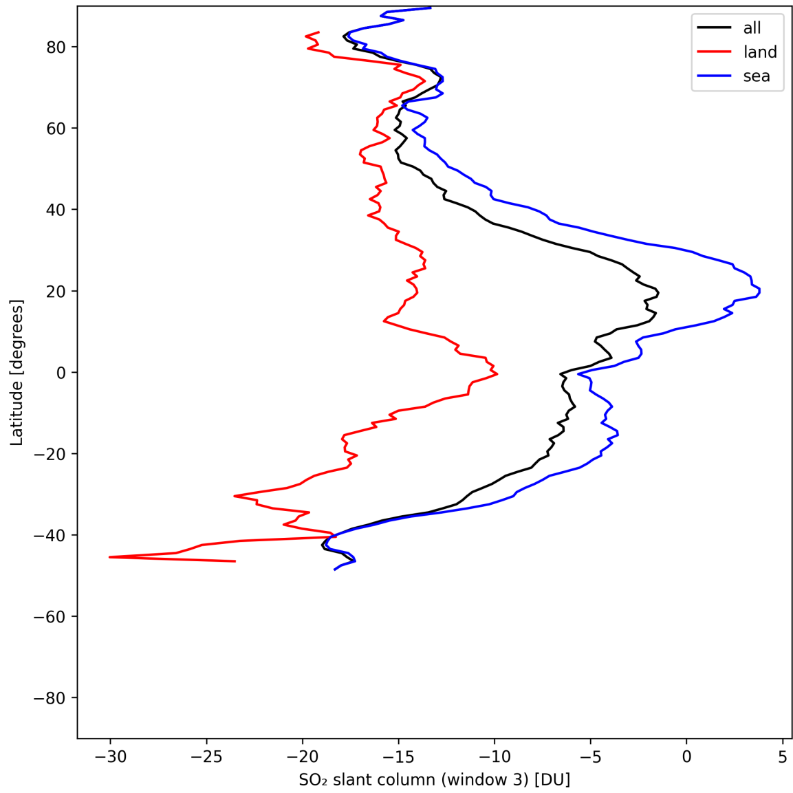
Figure 45: Zonal average of “SO 2 slant column (window 3)” for 2025-05-22 to 2025-05-24.
