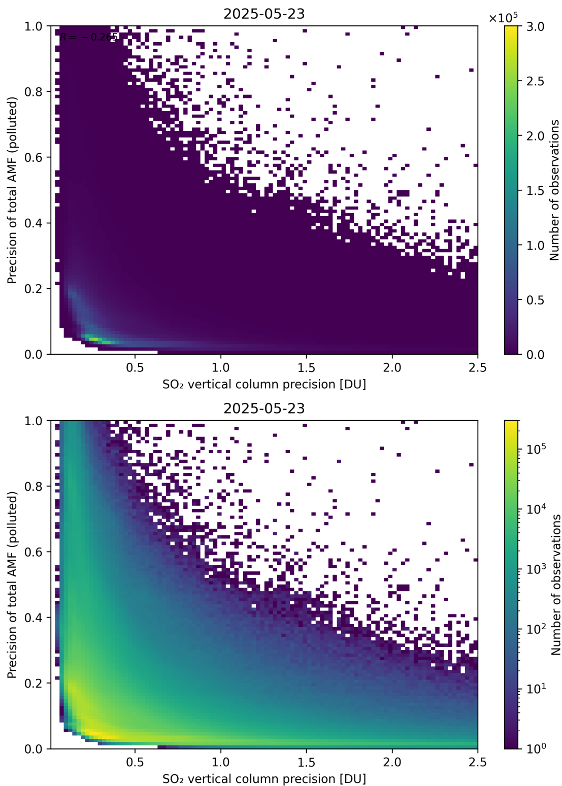
Figure 347: Scatter density plot of “SO 2 vertical column precision” against “Precision of total AMF (polluted)” for 2025-05-22 to 2025-05-24.
