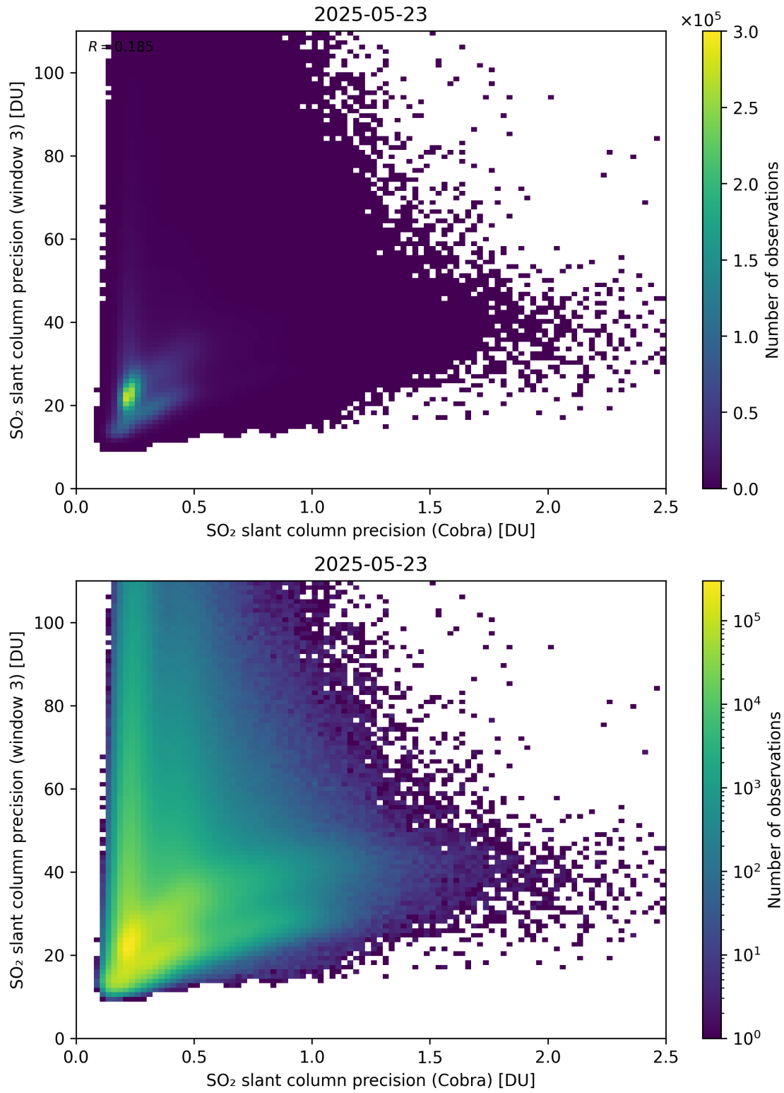
Figure 212: Scatter density plot of “SO 2 slant column precision (Cobra)” against “SO 2 slant column precision (window 3)” for 2025-05-22 to 2025-05-24.
