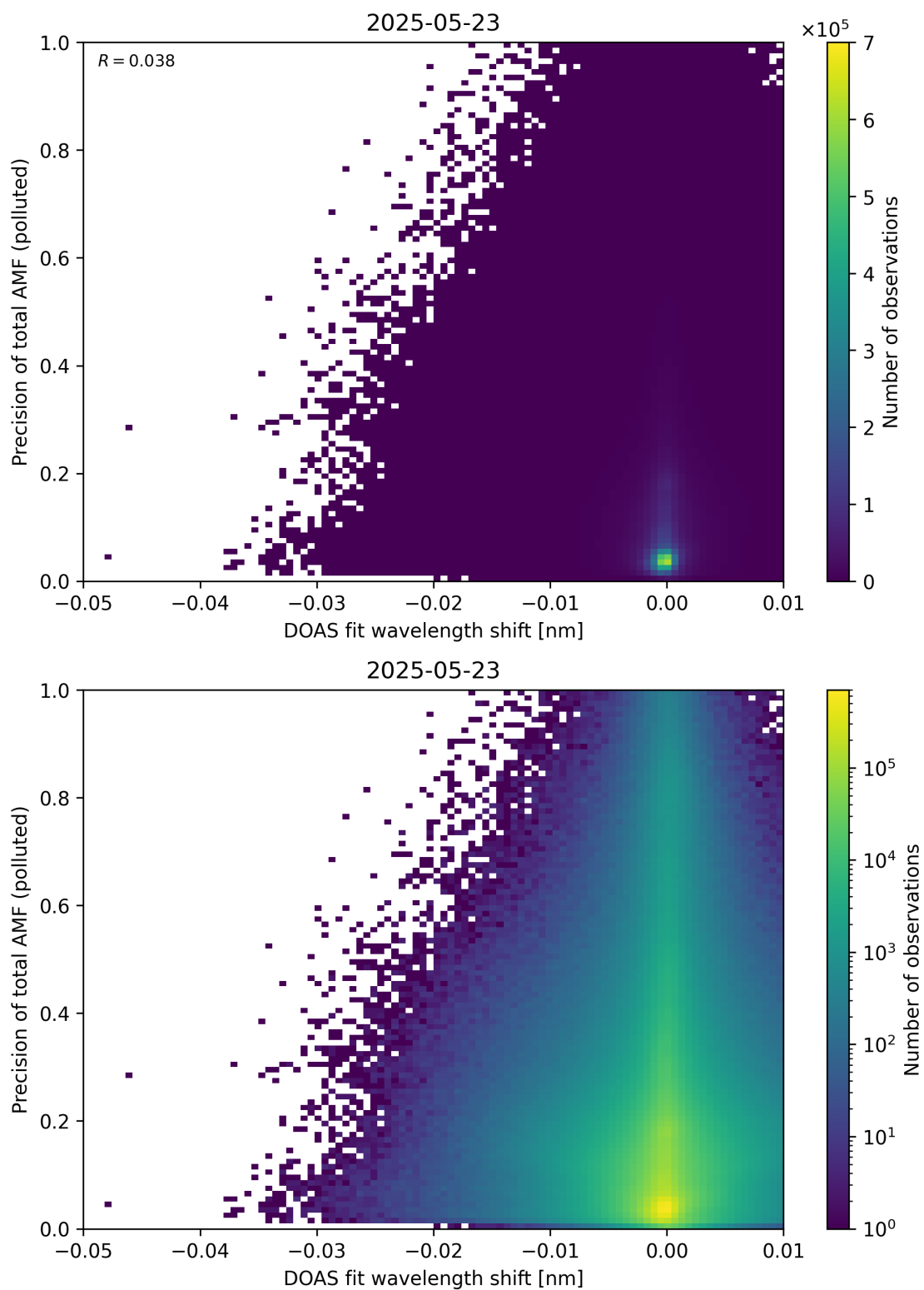
Figure 142: Scatter density plot of “DOAS fit wavelength shift” against “Precision of total AMF (polluted)” for 2025-05-22 to 2025-05-24.
