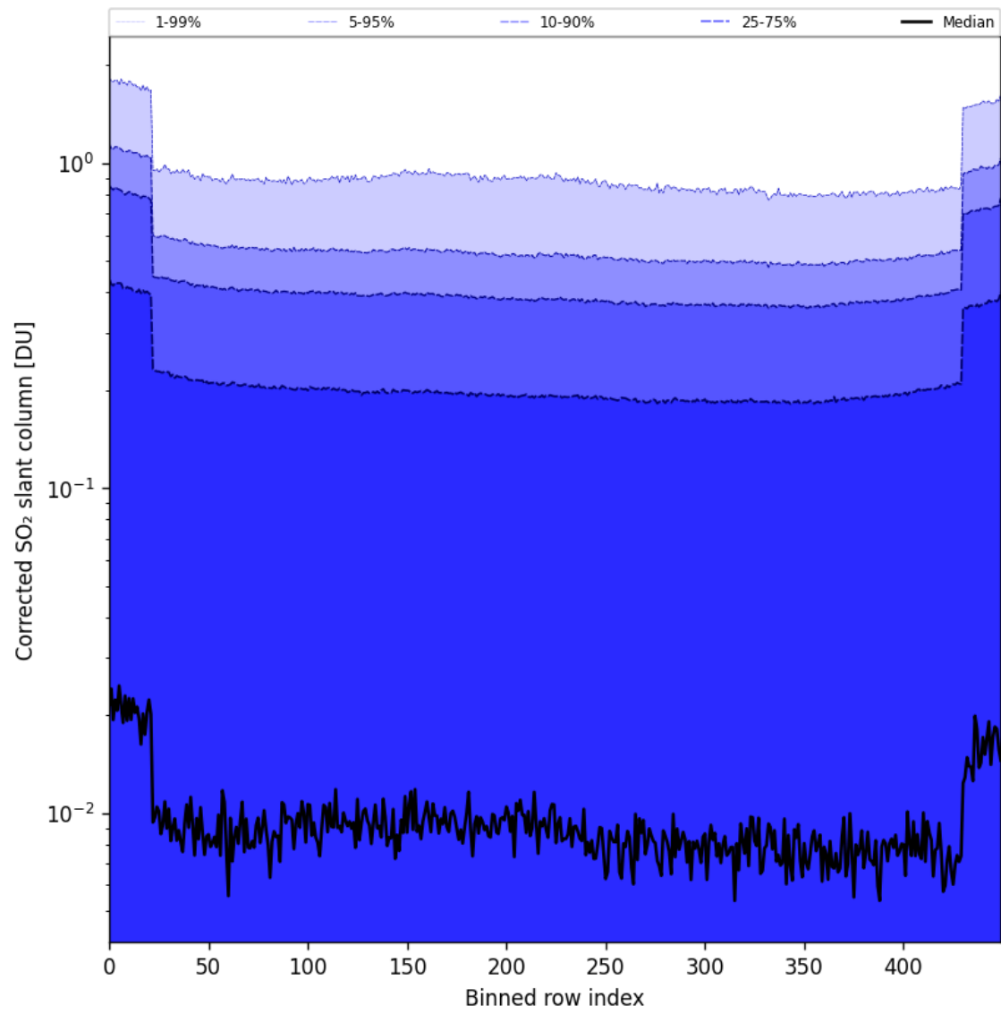
Figure 86: Along track statistics of “Corrected SO 2 slant column” for 2025-05-22 to 2025-05-24
