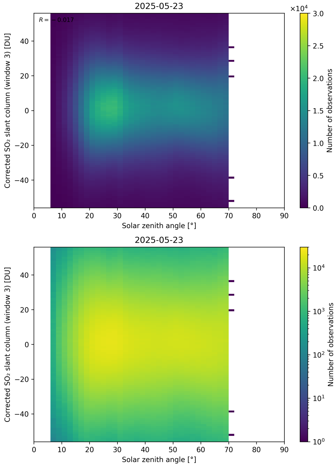
Figure 183: Scatter density plot of “Solar zenith angle” against “Corrected SO 2 slant column (window 3)” for 2025-05-22 to 2025-05-24.
