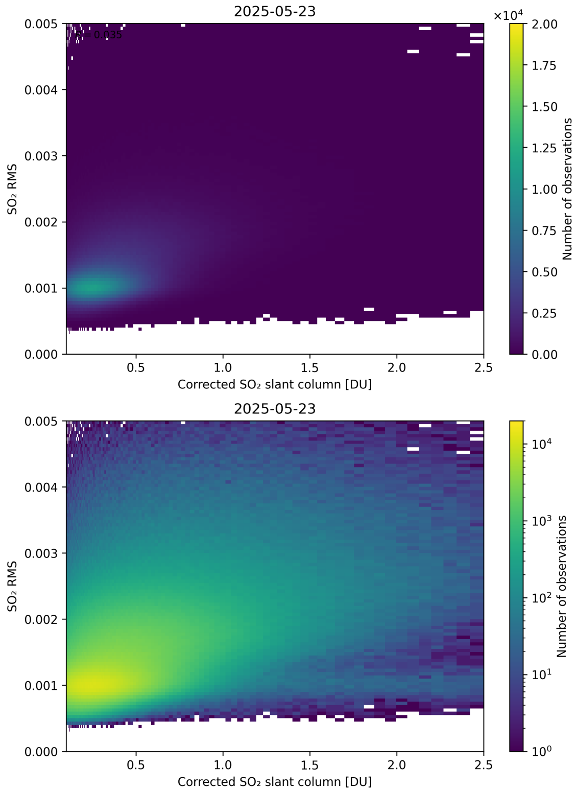
Figure 231: Scatter density plot of “Corrected SO 2 slant column” against “SO 2 RMS” for 2025-05-22 to 2025-05-24.
