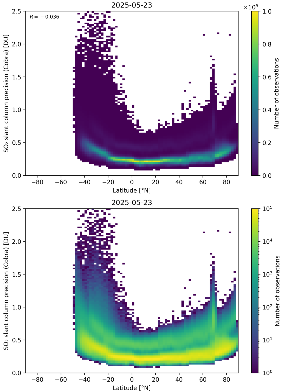
Figure 158: Scatter density plot of “Latitude” against “SO 2 slant column precision (Cobra)” for 2025-05-22 to 2025-05-24.
