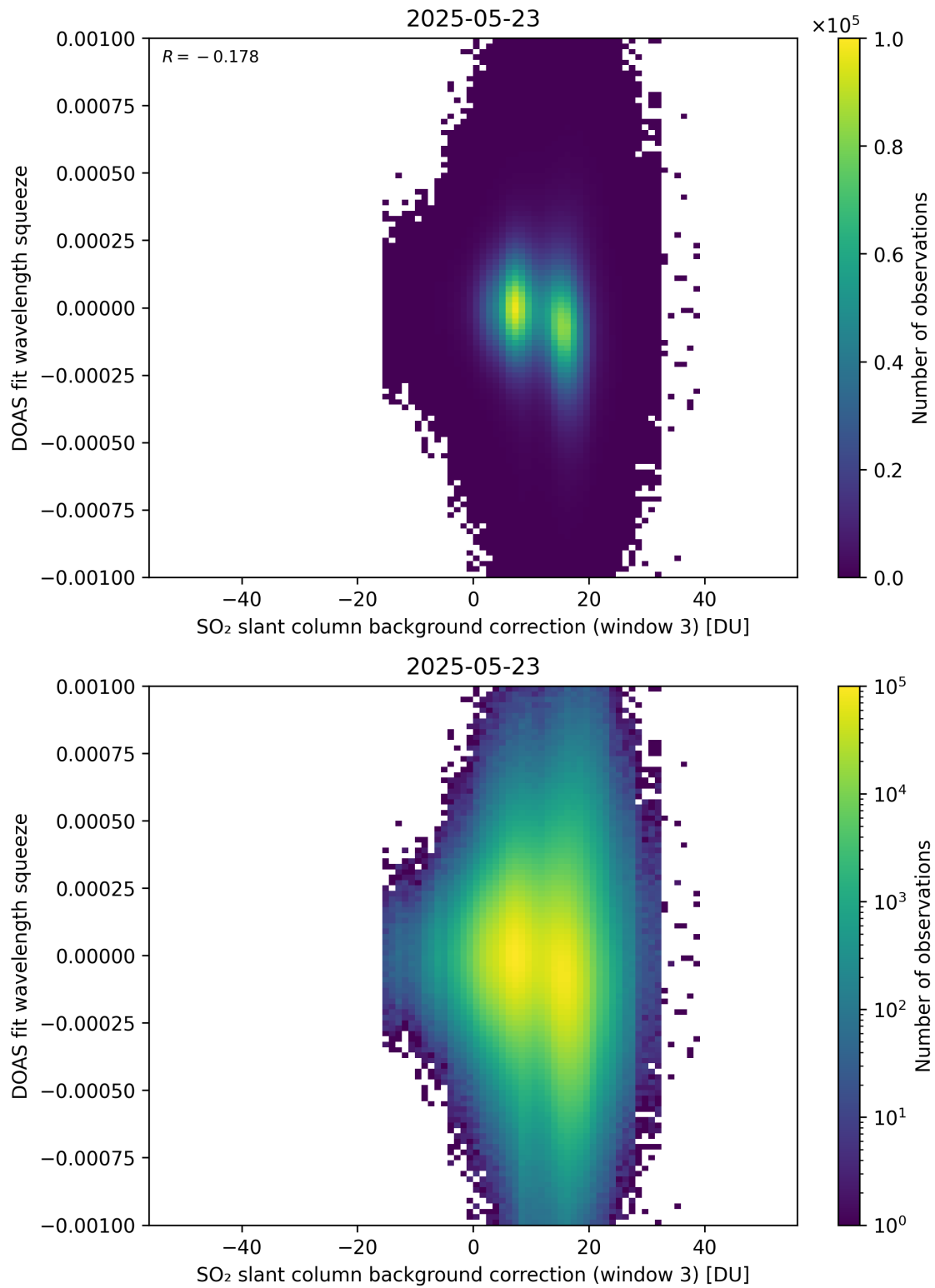
Figure 133: Scatter density plot of “SO 2 slant column background correction (window 3)” against “DOAS fit wavelength squeeze” for 2025-05-22 to 2025-05-24.
