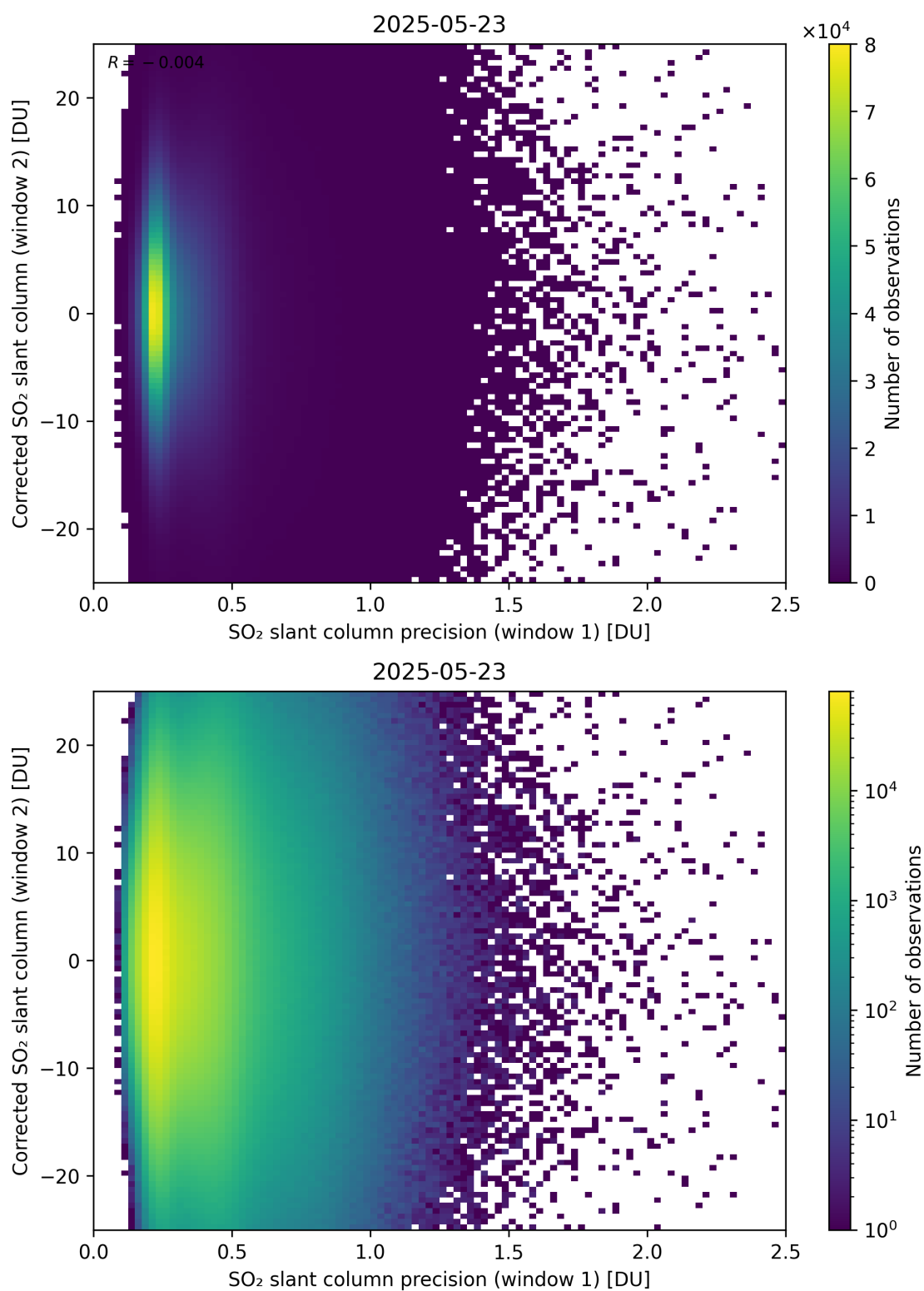
Figure 275: Scatter density plot of “SO 2 slant column precision (window 1)” against “Corrected SO 2 slant column (window 2)” for 2025-05-22 to 2025-05-24.
