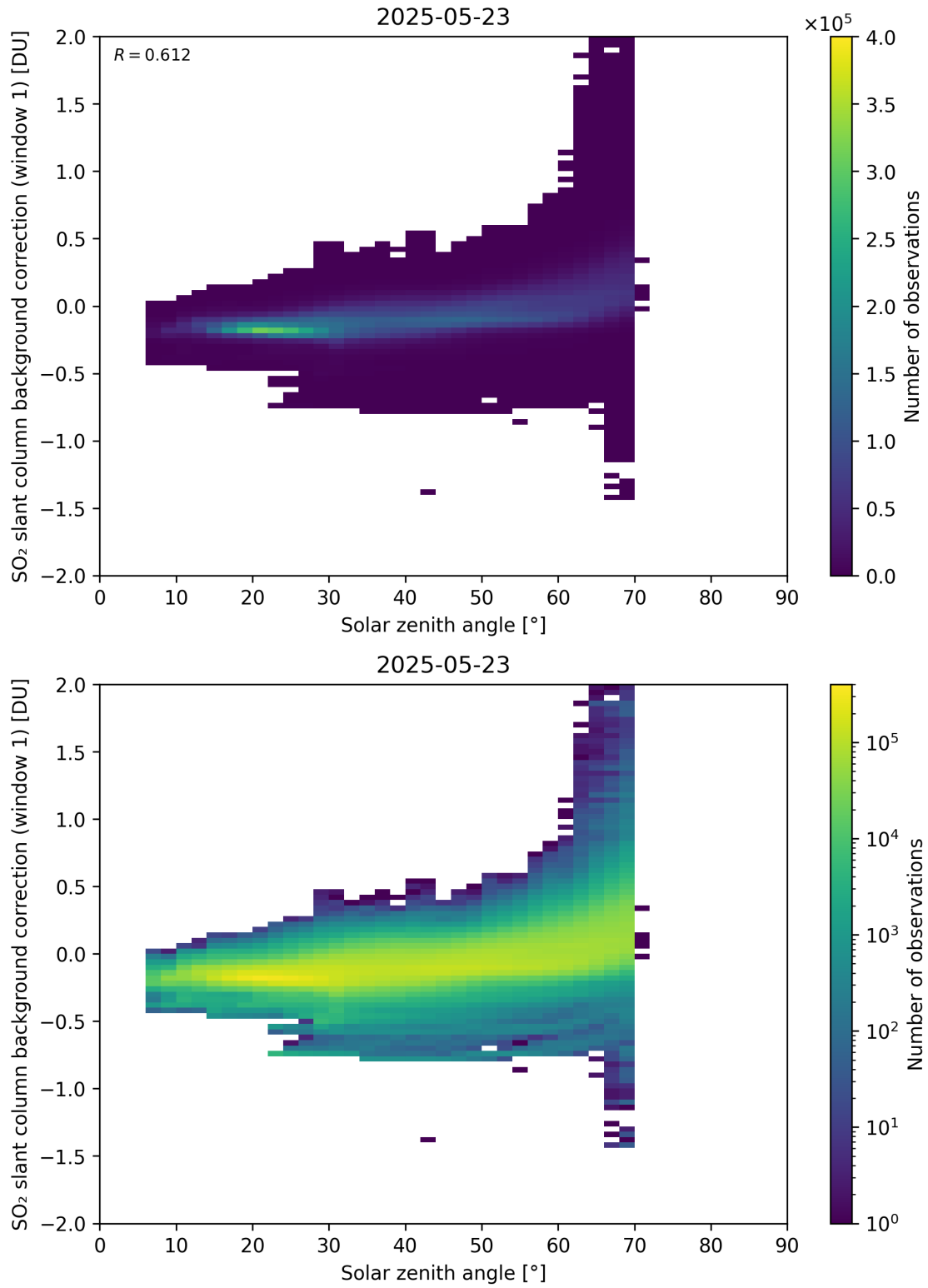
Figure 171: Scatter density plot of “Solar zenith angle” against “SO 2 slant column background correction (window 1)” for 2025-05-22 to 2025-05-24.
