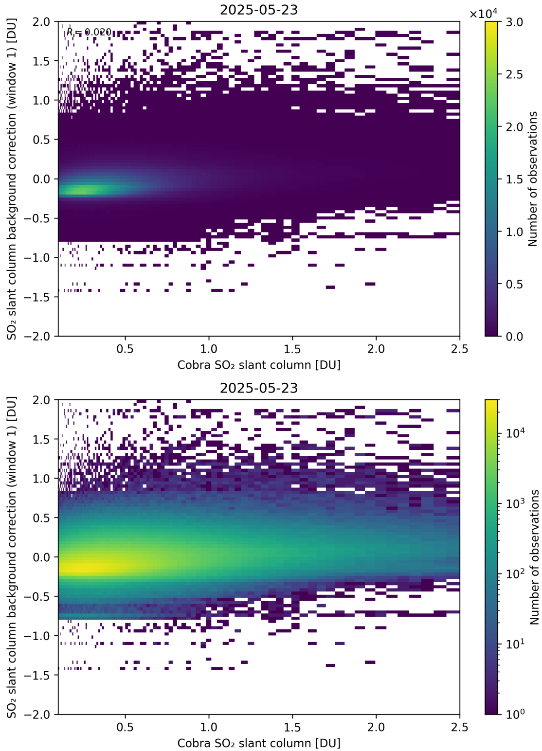
Figure 193: Scatter density plot of “Cobra SO 2 slant column” against “SO 2 slant column background correction (window 1)” for 2025-05-22 to 2025-05-24.
