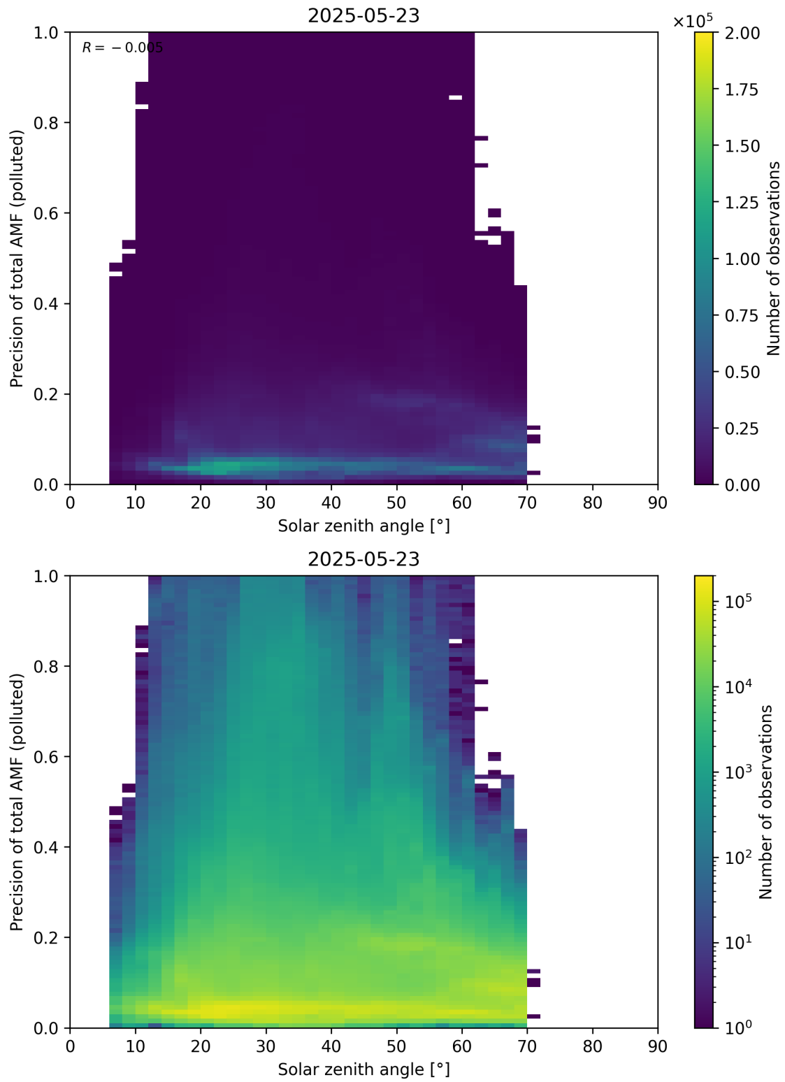
Figure 190: Scatter density plot of “Solar zenith angle” against “Precision of total AMF (polluted)” for 2025-05-22 to 2025-05-24.
