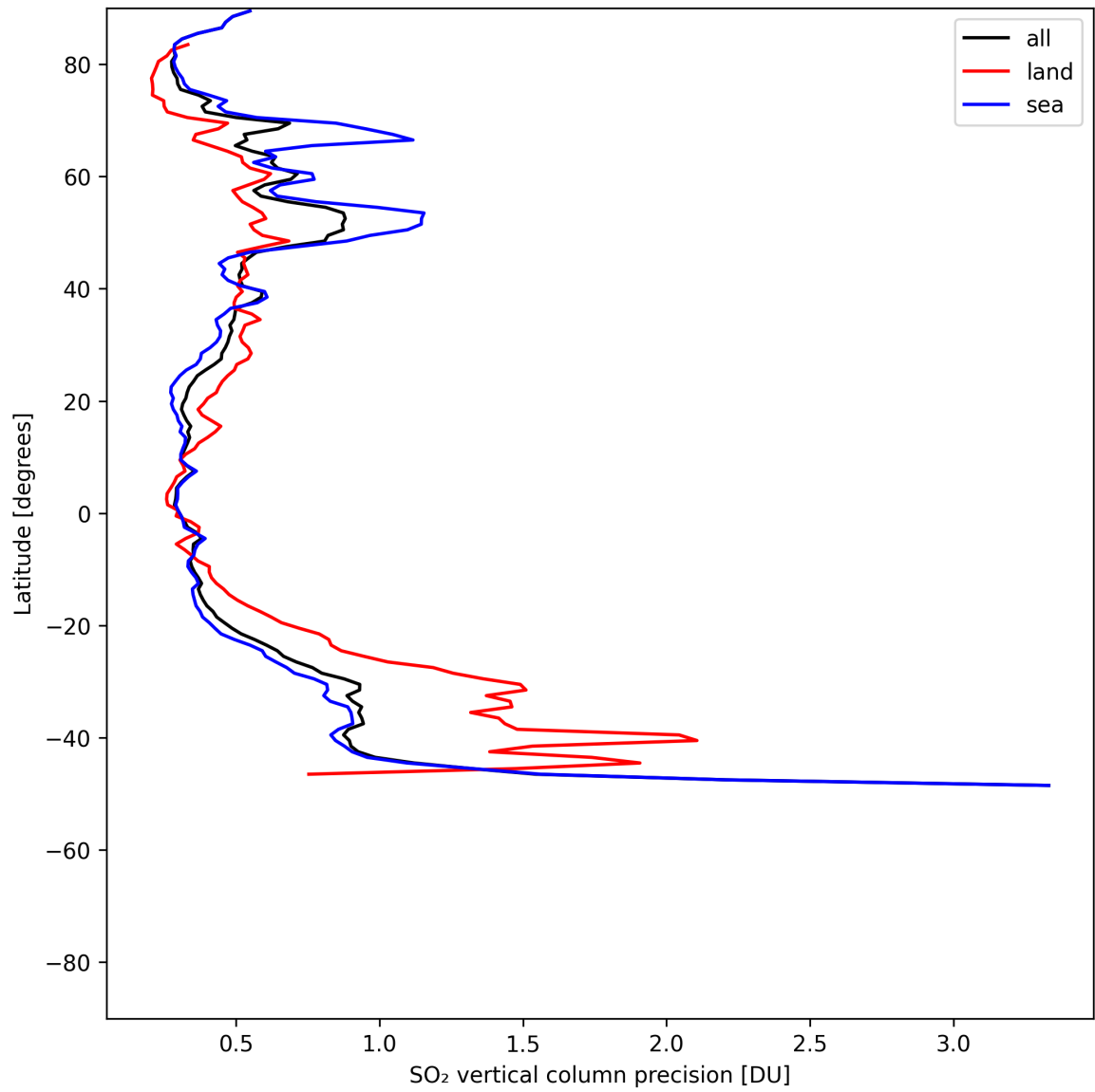
Figure 33: Zonal average of “SO 2 vertical column precision” for 2025-05-22 to 2025-05-24.
