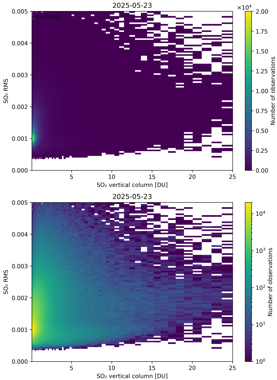
Figure 328: Scatter density plot of “SO 2 vertical column” against “SO 2 RMS” for 2025-05-22 to 2025-05-24.
