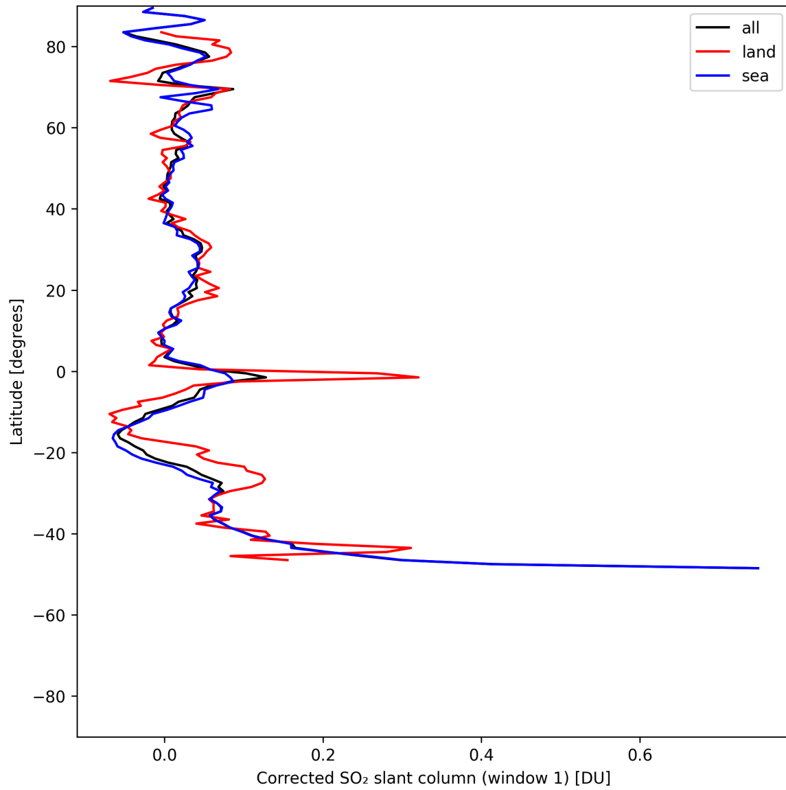
Figure 39: Zonal average of “Corrected SO 2 slant column (window 1)” for 2025-05-22 to 2025-05-24.
