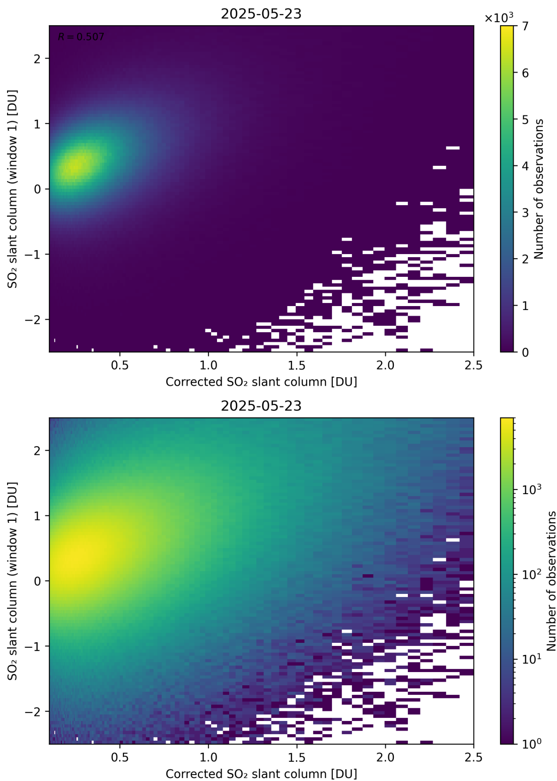
Figure 237: Scatter density plot of “Corrected SO 2 slant column” against “SO 2 slant column (window 1)” for 2025-05-22 to 2025-05-24.
