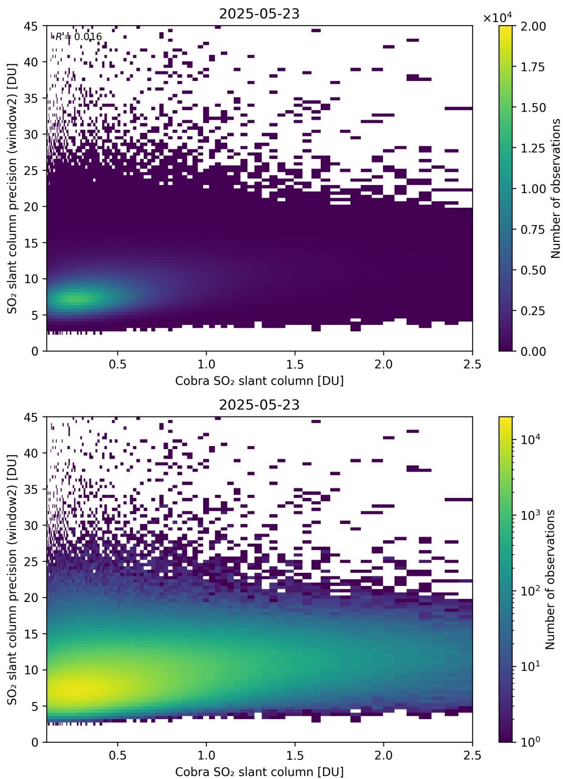
Figure 221: Scatter density plot of “Cobra SO 2 slant column” against “SO 2 slant column precision (window2)” for 2025-05-22 to 2025-05-24.
