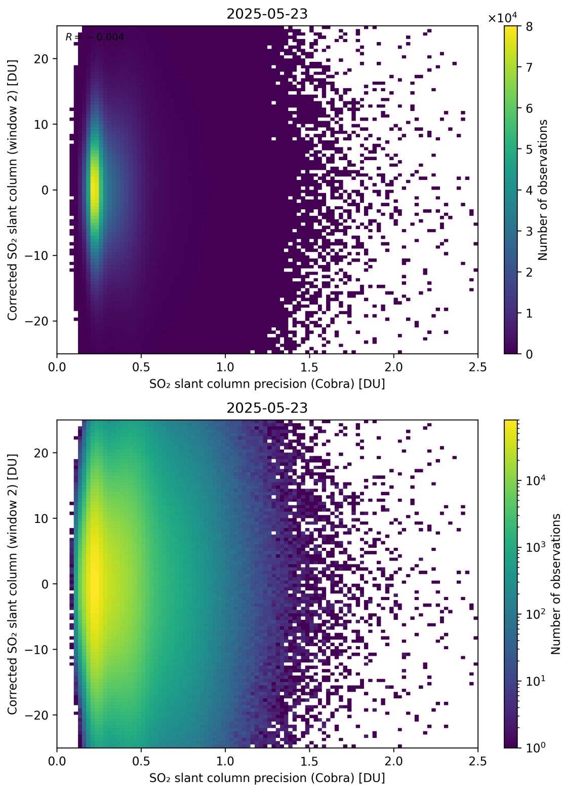
Figure 206: Scatter density plot of “SO 2 slant column precision (Cobra)” against “Corrected SO 2 slant column (window 2)” for 2025-05-22 to 2025-05-24.
