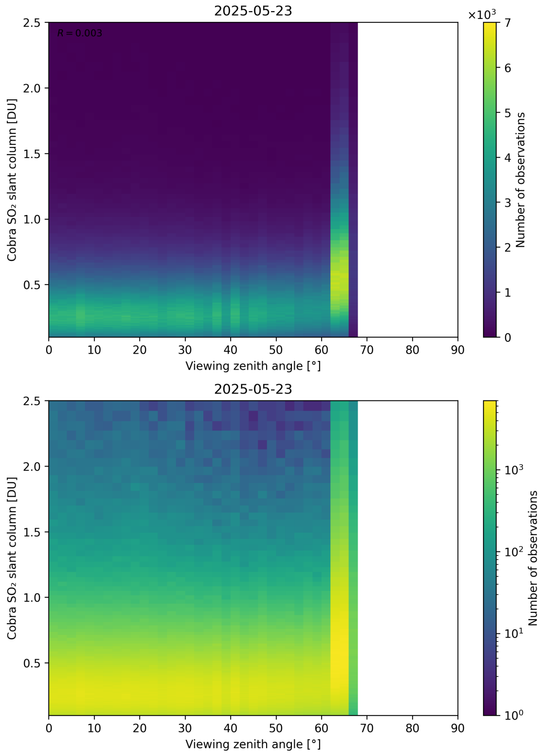
Figure 371: Scatter density plot of “Viewing zenith angle” against “Cobra SO 2 slant column” for 2025-05-22 to 2025-05-24.
