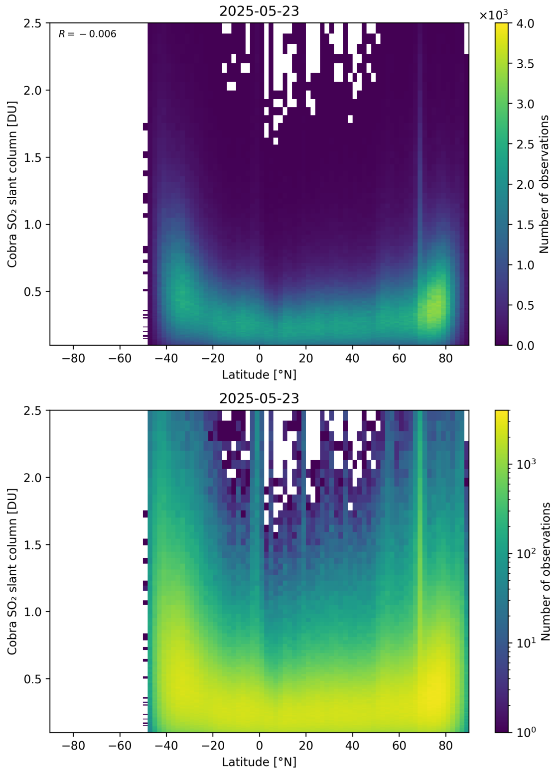
Figure 157: Scatter density plot of “Latitude” against “Cobra SO 2 slant column” for 2025-05-22 to 2025-05-24.
