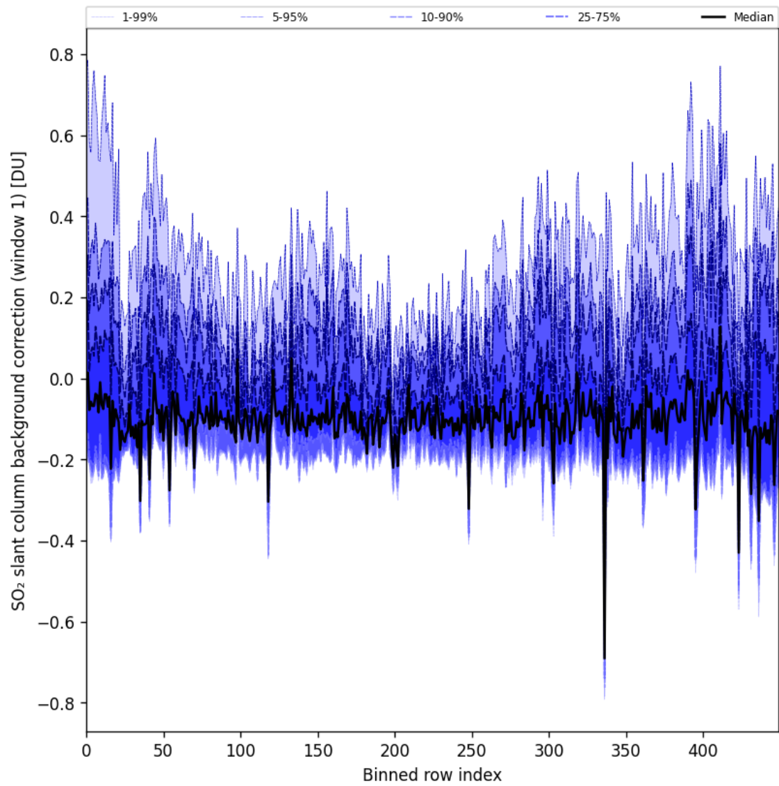
Figure 92: Along track statistics of “SO 2 slant column background correction (window 1)” for 2025-05-22 to 2025-05-24
