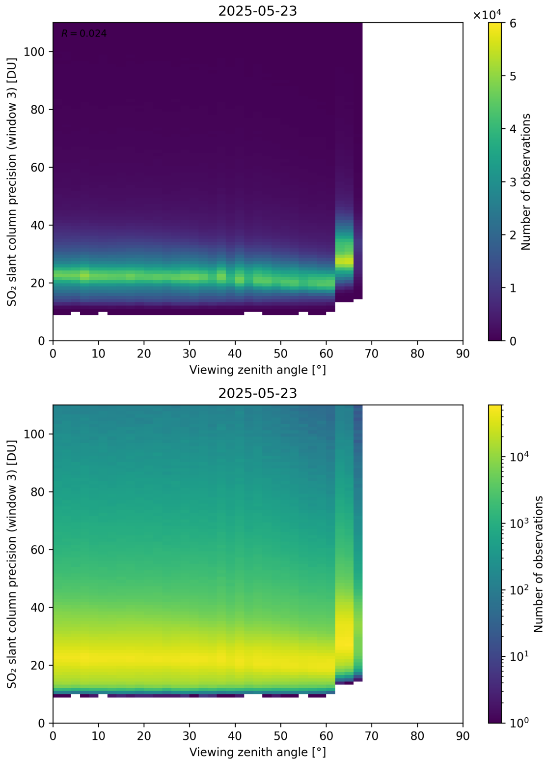
Figure 380: Scatter density plot of “Viewing zenith angle” against “SO 2 slant column precision (window 3)” for 2025-05-22 to 2025-05-24.
