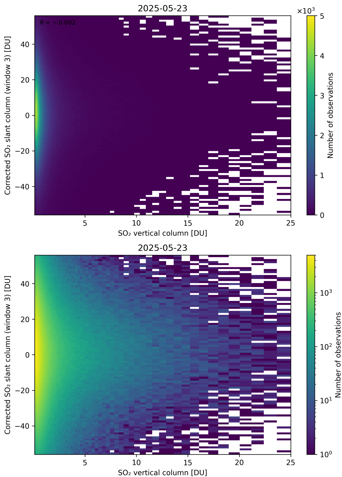
Figure 353: Scatter density plot of “SO 2 vertical column” against “Corrected SO 2 slant column (window 3)” for 2025-05-22 to 2025-05-24.
