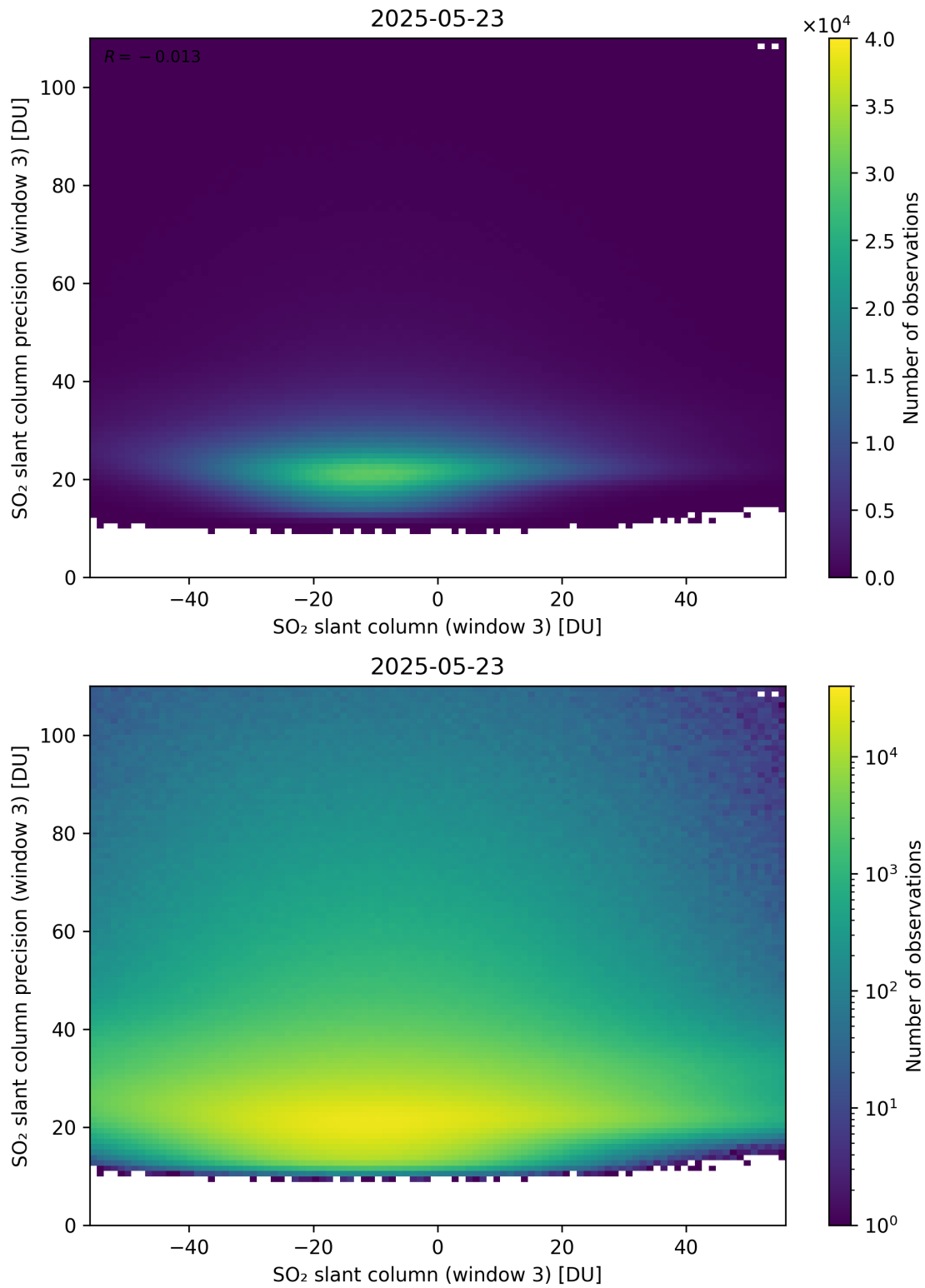
Figure 317: Scatter density plot of “SO 2 slant column (window 3)” against “SO 2 slant column precision (window 3)” for 2025-05-22 to 2025-05-24.
