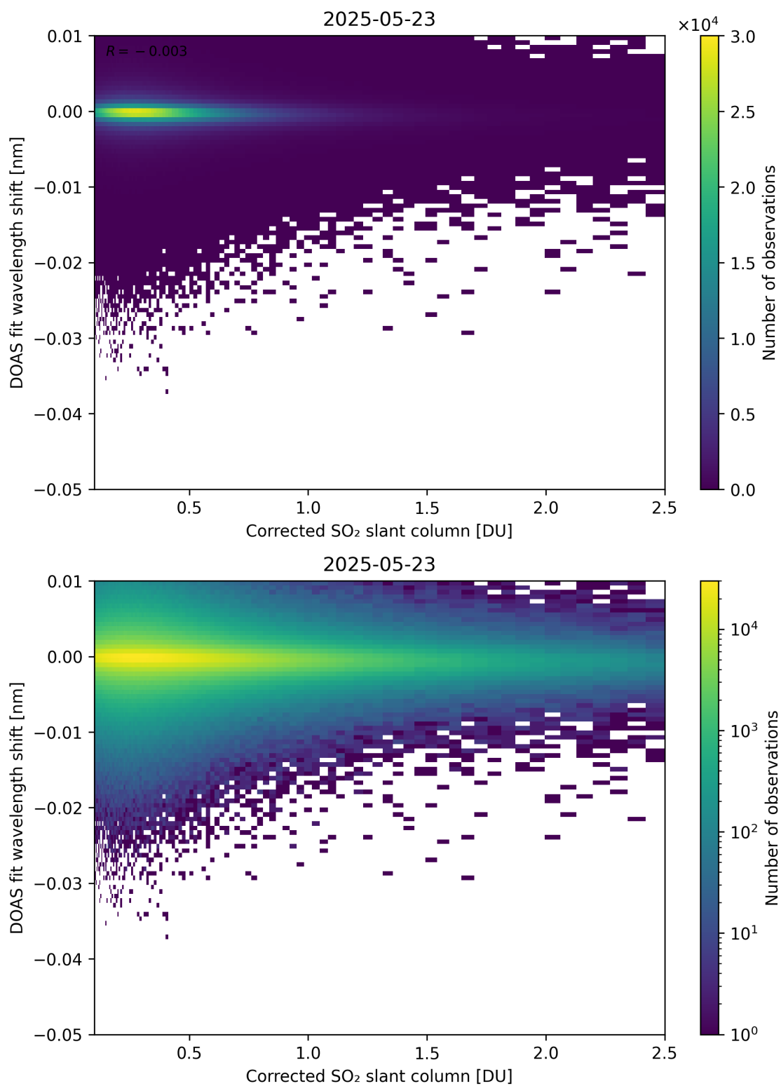
Figure 229: Scatter density plot of “Corrected SO 2 slant column” against “DOAS fit wavelength shift” for 2025-05-22 to 2025-05-24.
