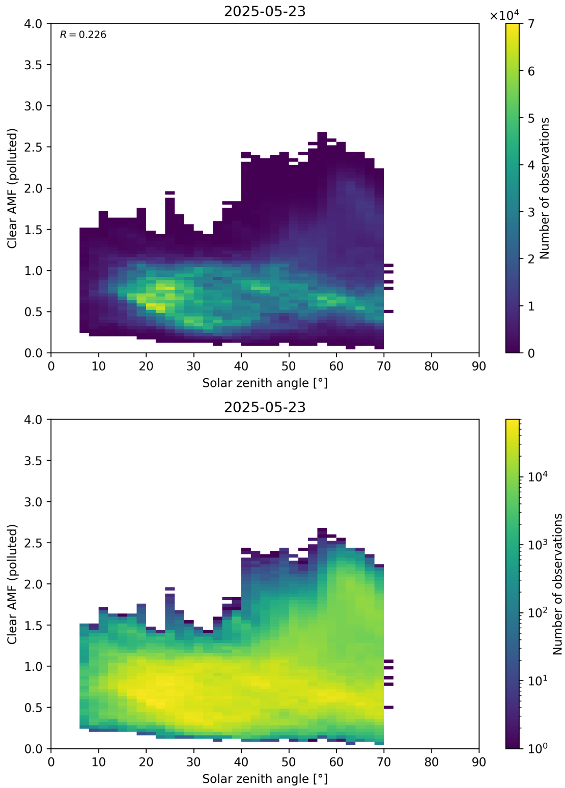
Figure 178: Scatter density plot of “Solar zenith angle” against “Clear AMF (polluted)” for 2025-05-22 to 2025-05-24.
