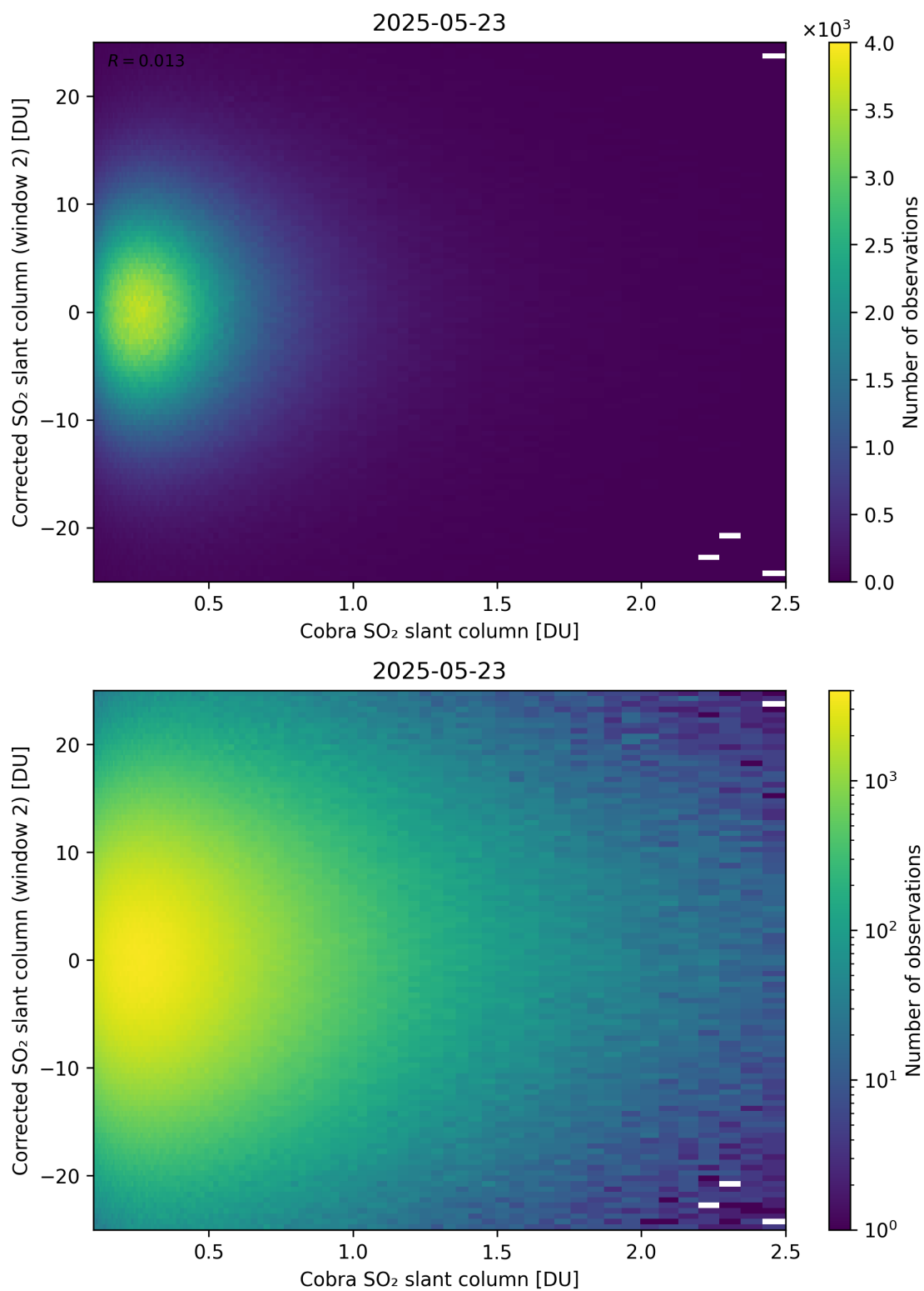
Figure 217: Scatter density plot of “Cobra SO 2 slant column” against “Corrected SO 2 slant column (window 2)” for 2025-05-22 to 2025-05-24.
