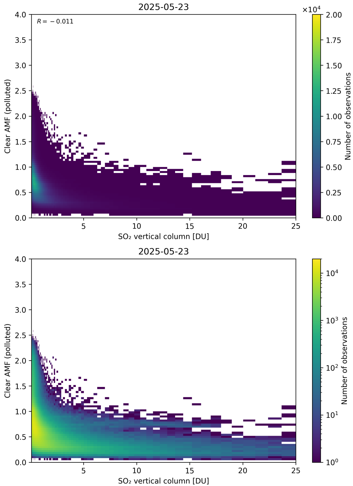
Figure 348: Scatter density plot of “SO 2 vertical column” against “Clear AMF (polluted)” for 2025-05-22 to 2025-05-24.
