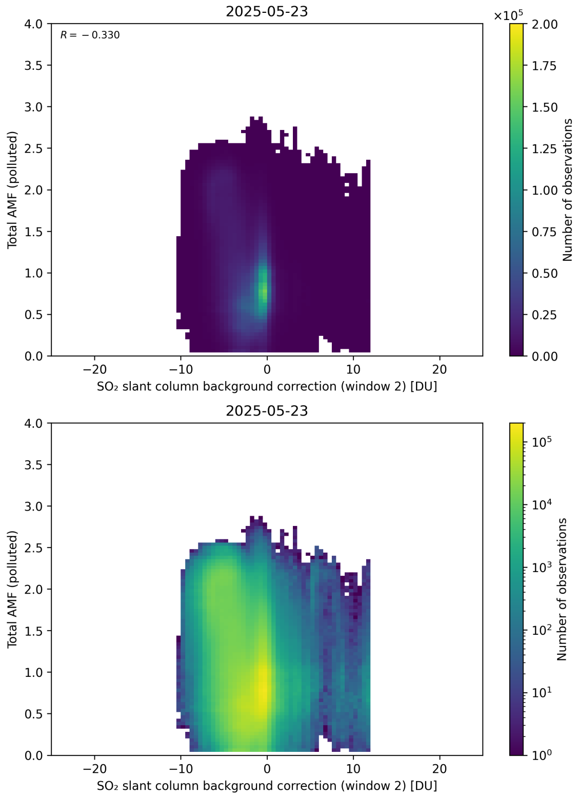
Figure 130: Scatter density plot of “SO 2 slant column background correction (window 2)” against “Total AMF (polluted)” for 2025-05-22 to 2025-05-24.
