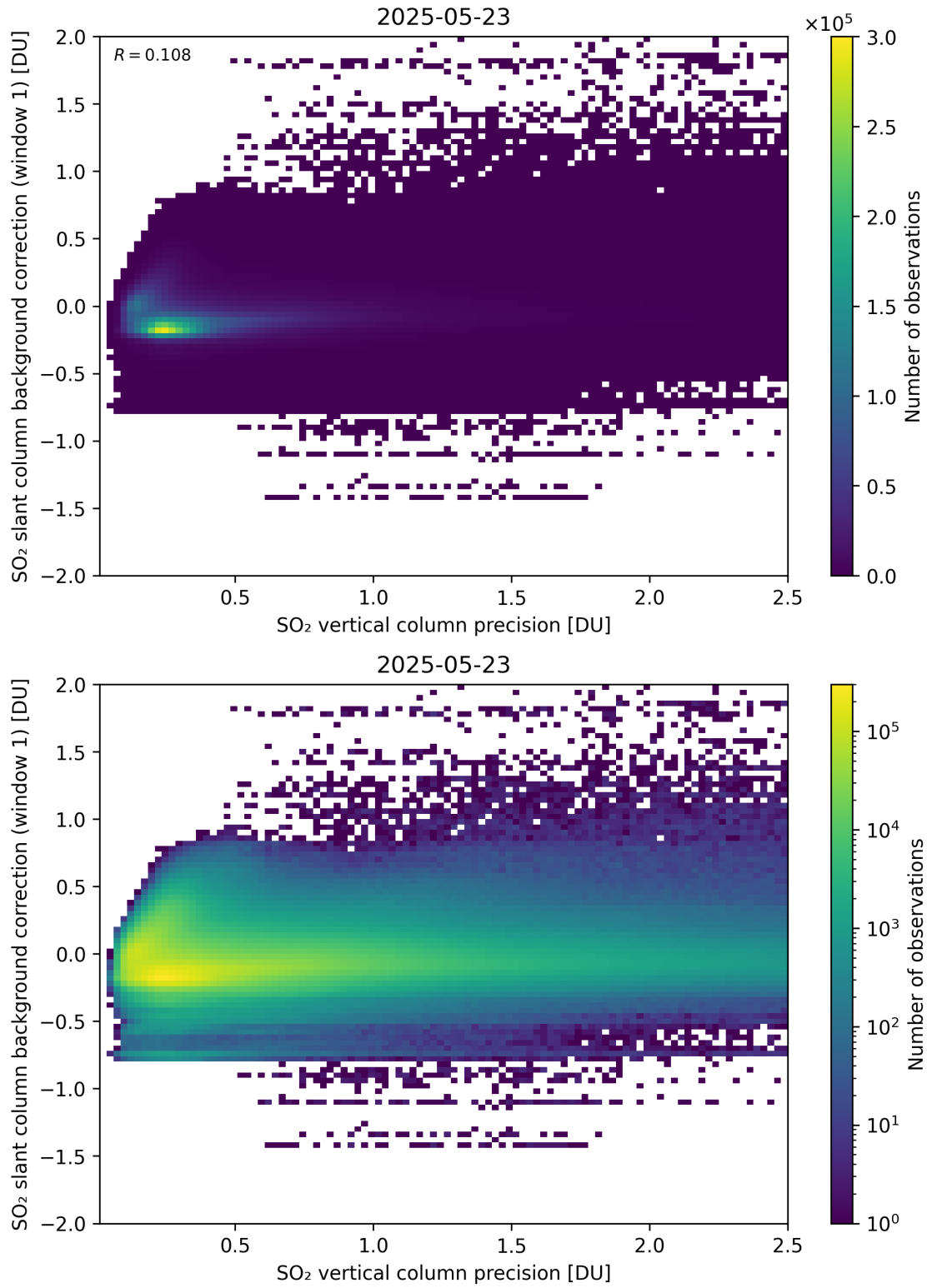
Figure 329: Scatter density plot of “SO 2 vertical column precision” against “SO 2 slant column background correction (window 1)” for 2025-05-22 to 2025-05-24.
