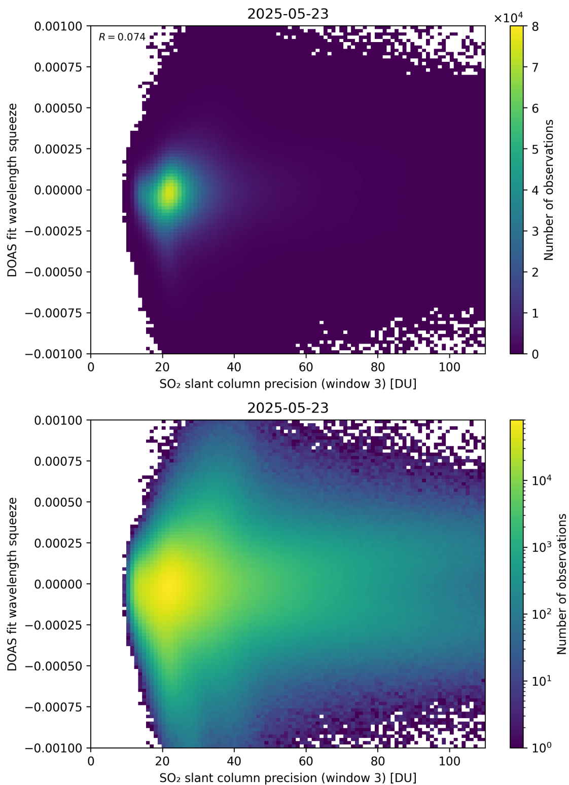
Figure 309: Scatter density plot of “SO 2 slant column precision (window 3)” against “DOAS fit wavelength squeeze” for 2025-05-22 to 2025-05-24.
