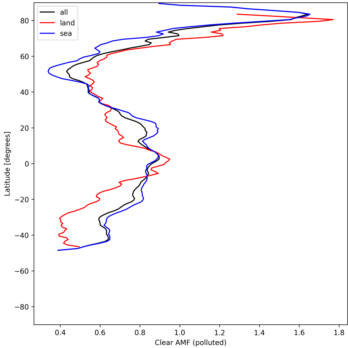
Figure 55: Zonal average of “Clear AMF (polluted)” for 2025-05-22 to 2025-05-24.
