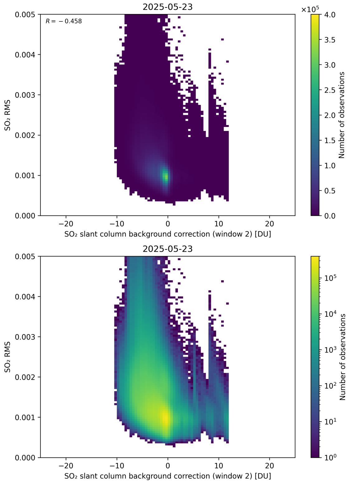
Figure 125: Scatter density plot of “SO 2 slant column background correction (window 2)” against “SO 2 RMS” for 2025-05-22 to 2025-05-24.
