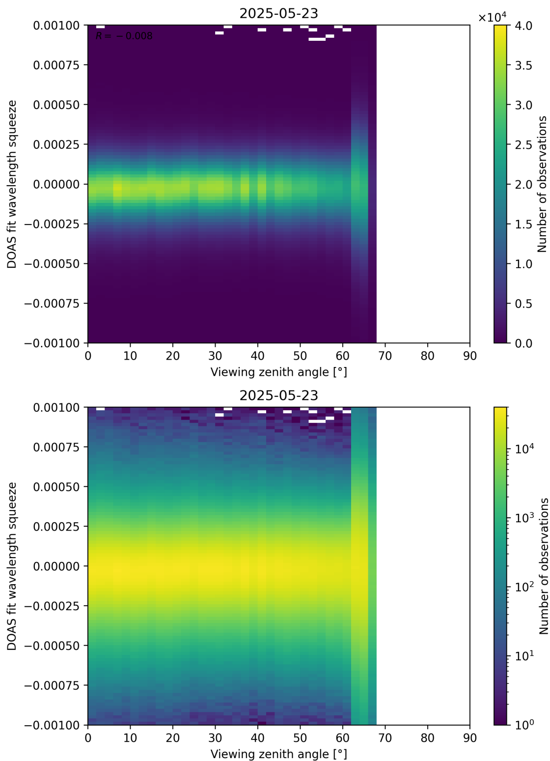
Figure 366: Scatter density plot of “Viewing zenith angle” against “DOAS fit wavelength squeeze” for 2025-05-22 to 2025-05-24.
