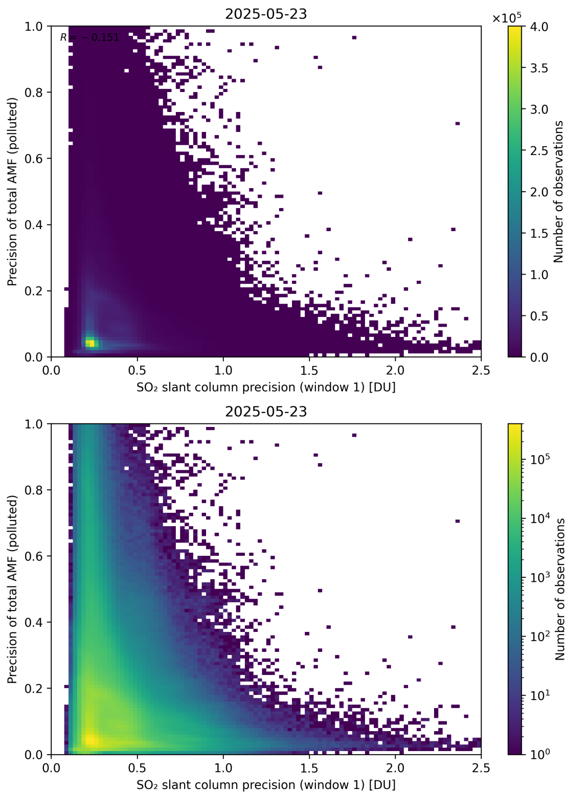
Figure 281: Scatter density plot of “SO 2 slant column precision (window 1)” against “Precision of total AMF (polluted)” for 2025-05-22 to 2025-05-24.
