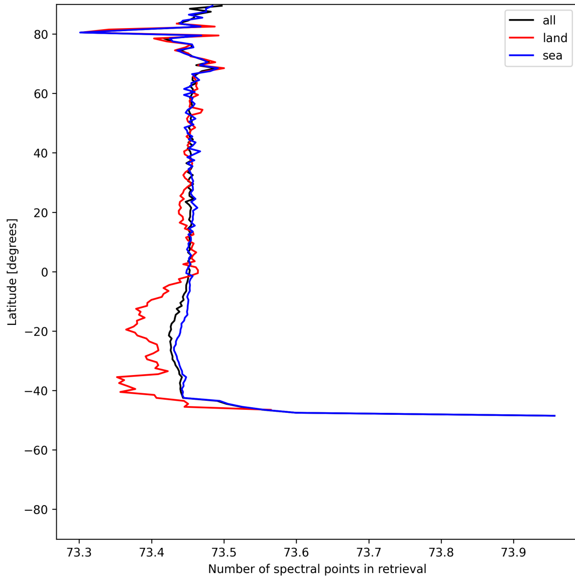
Figure 56: Zonal average of “Number of spectral points in retrieval” for 2025-05-22 to 2025-05-24.
