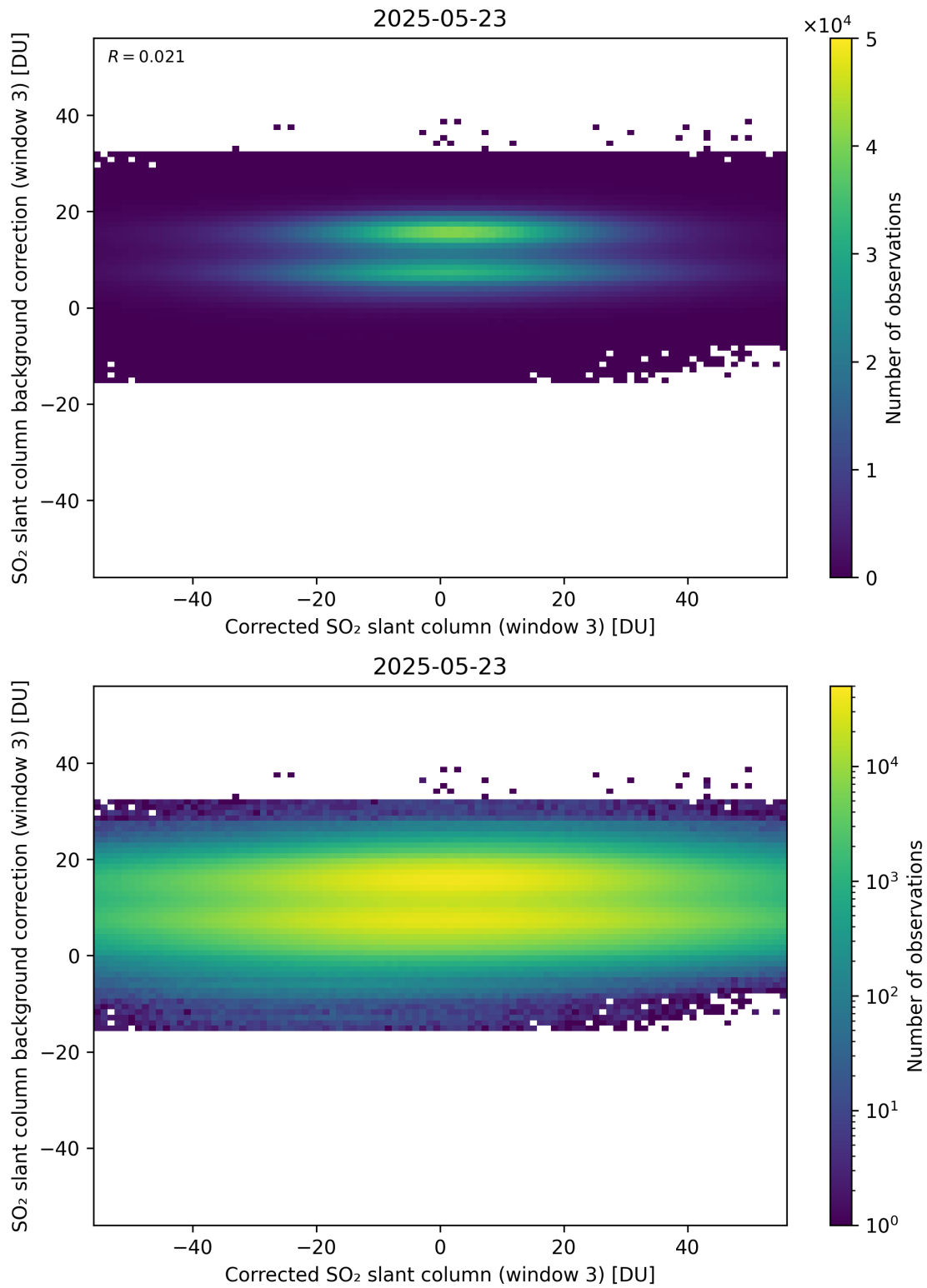
Figure 255: Scatter density plot of “Corrected SO 2 slant column (window 3)” against “SO 2 slant column background correction (window 3)” for 2025-05-22 to 2025-05-24.
