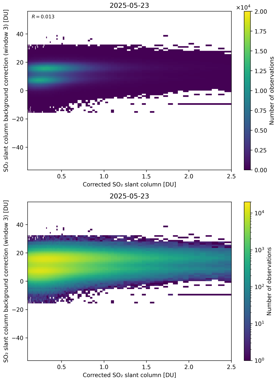
Figure 228: Scatter density plot of “Corrected SO 2 slant column” against “SO 2 slant column background correction (window 3)” for 2025-05-22 to 2025-05-24.
