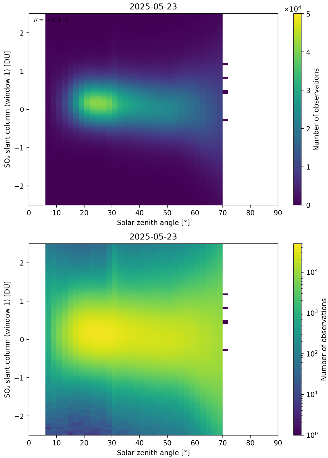
Figure 184: Scatter density plot of “Solar zenith angle” against “SO 2 slant column (window 1)” for 2025-05-22 to 2025-05-24.
