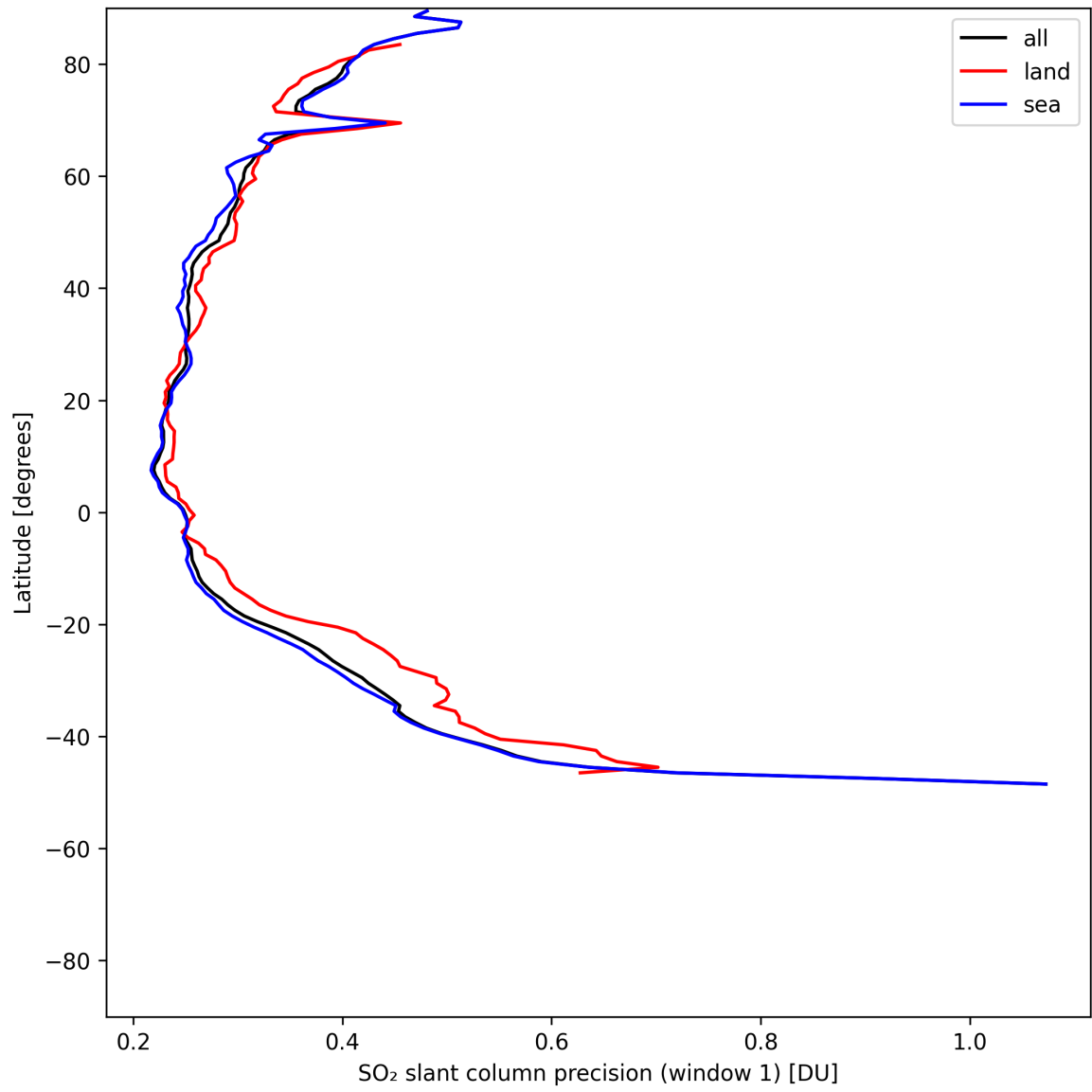
Figure 38: Zonal average of “SO 2 slant column precision (window 1)” for 2025-05-22 to 2025-05-24.
