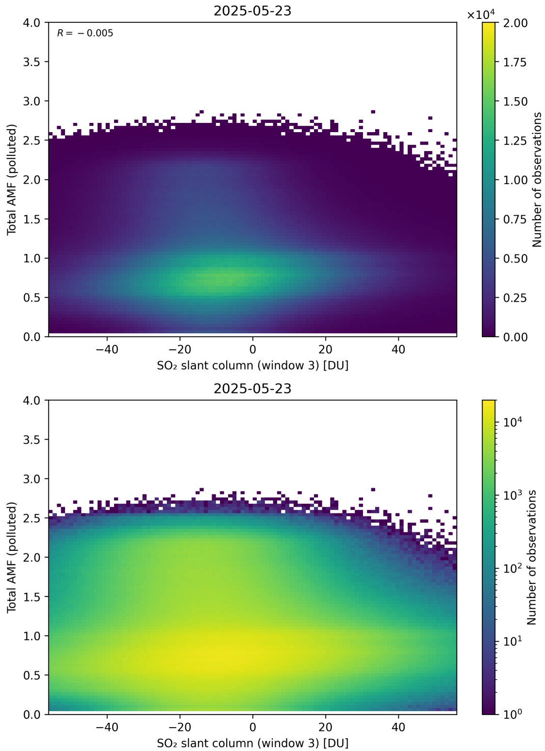
Figure 318: Scatter density plot of “SO 2 slant column (window 3)” against “Total AMF (polluted)” for 2025-05-22 to 2025-05-24.
