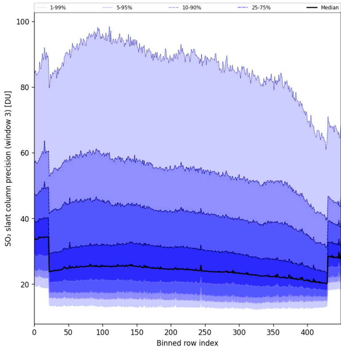
Figure 98: Along track statistics of “SO 2 slant column precision (window 3)” for 2025-05-22 to 2025-05-24
