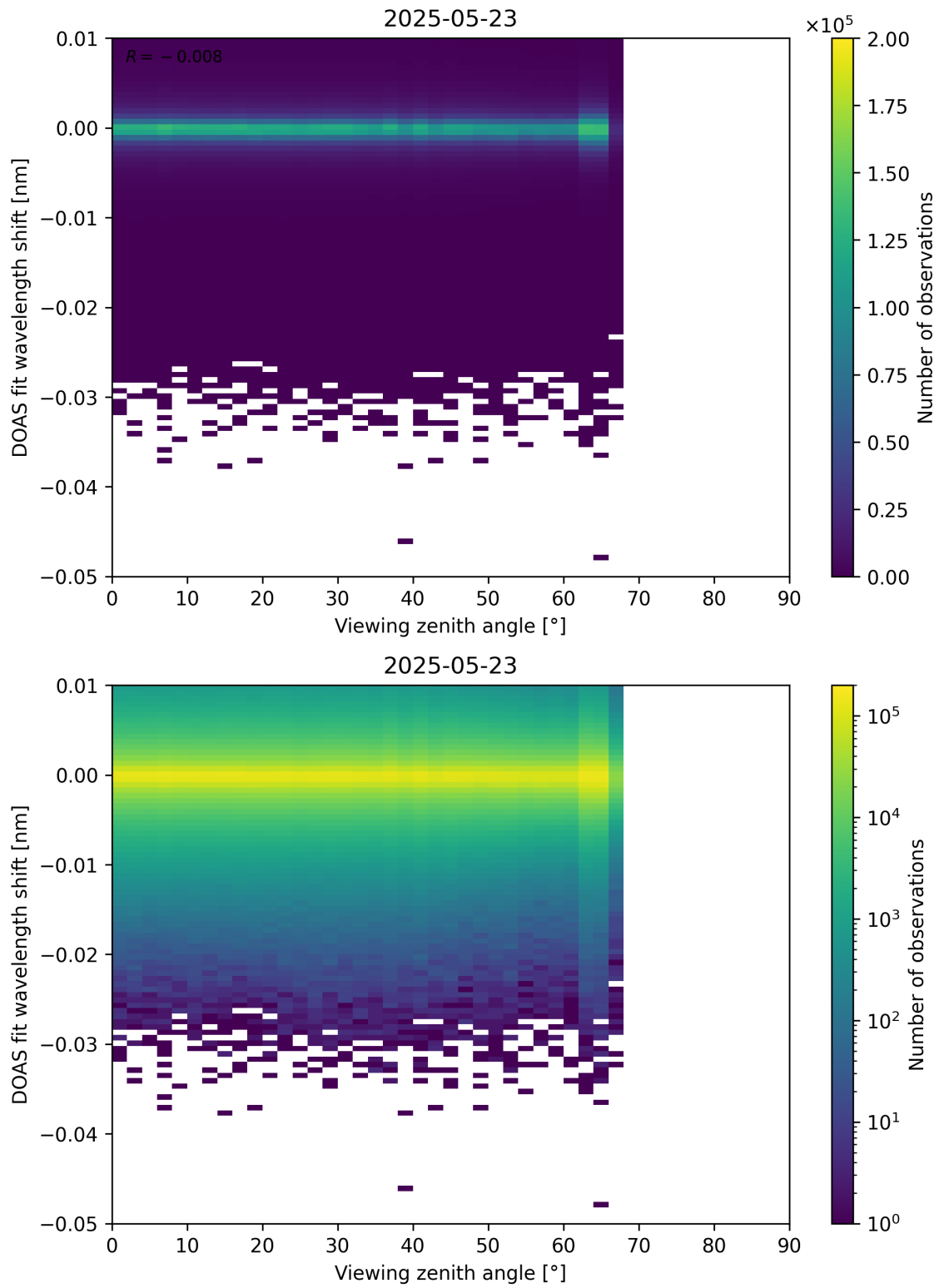
Figure 365: Scatter density plot of “Viewing zenith angle” against “DOAS fit wavelength shift” for 2025-05-22 to 2025-05-24.
