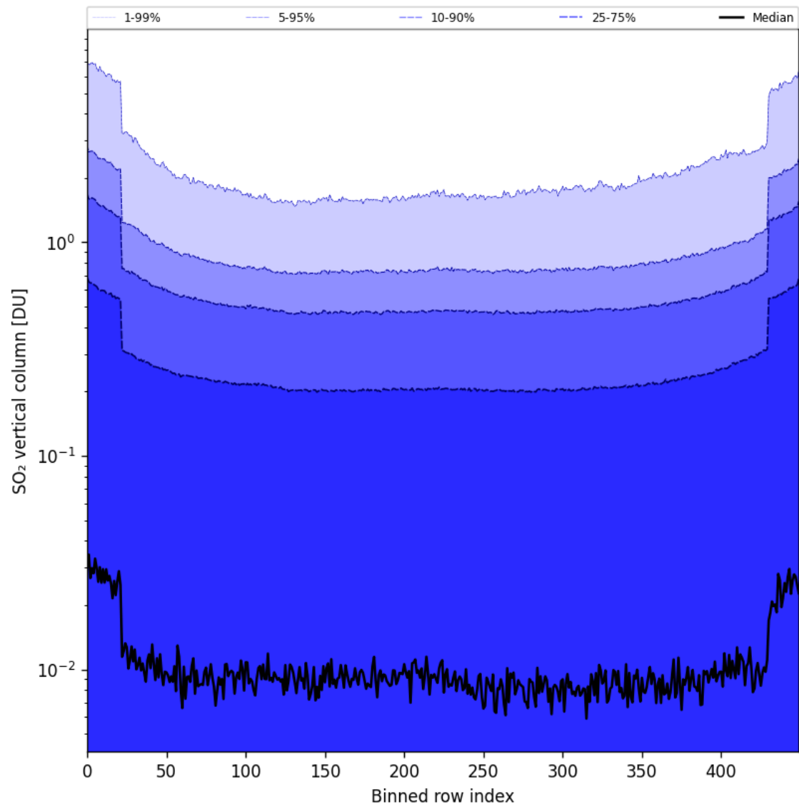
Figure 84: Along track statistics of “SO 2 vertical column” for 2025-05-22 to 2025-05-24
