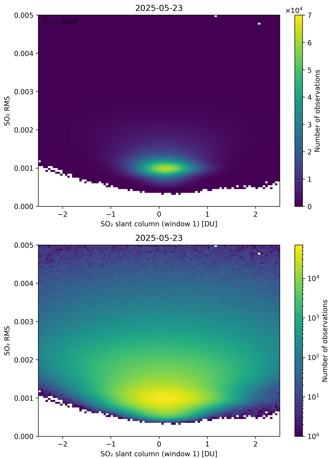
Figure 267: Scatter density plot of “SO 2 slant column (window 1)” against “SO 2 RMS” for 2025-05-22 to 2025-05-24.
