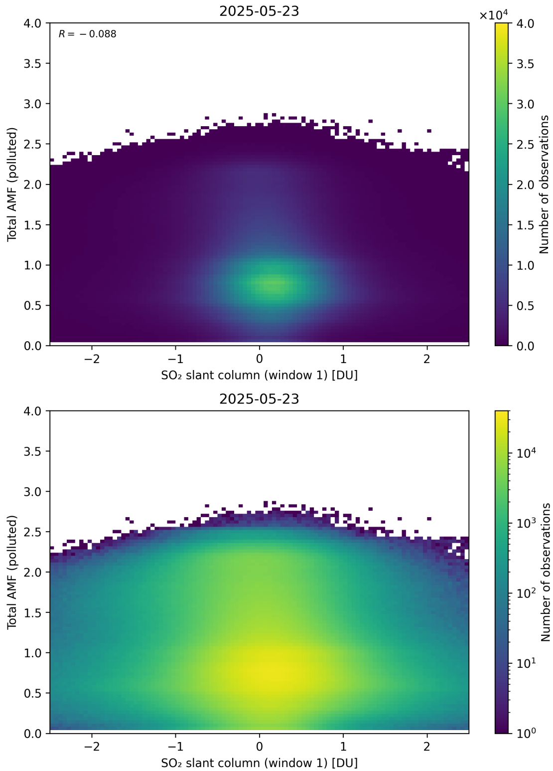
Figure 289: Scatter density plot of “SO 2 slant column (window 1)” against “Total AMF (polluted)” for 2025-05-22 to 2025-05-24.
