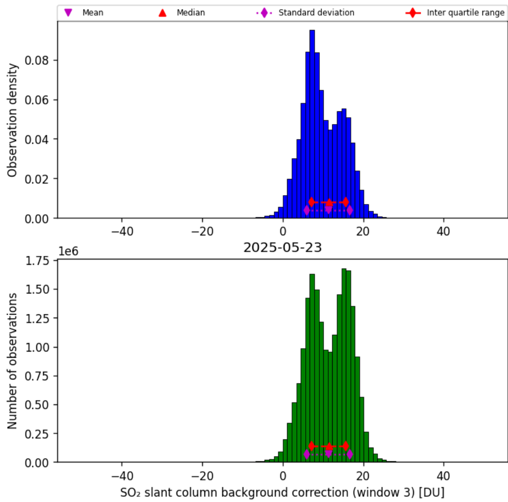
Figure 74: Histogram of “SO 2 slant column background correction (window 3)” for 2025-05-22 to 2025-05-24
