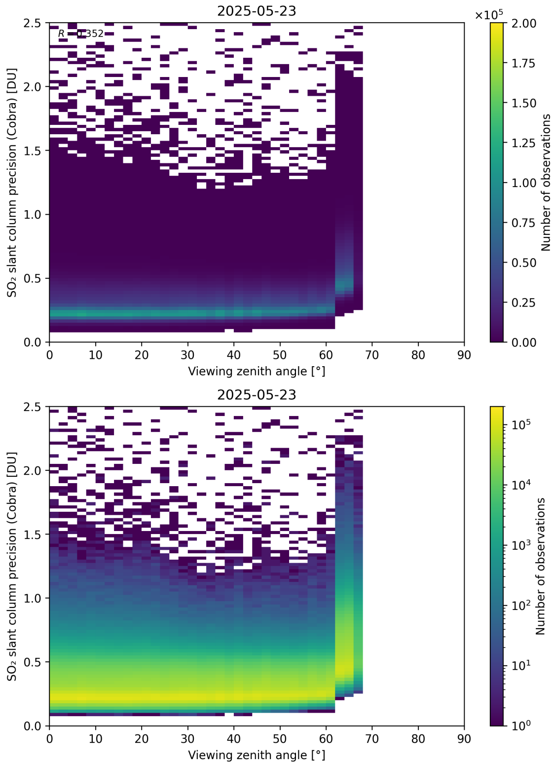
Figure 372: Scatter density plot of “Viewing zenith angle” against “SO 2 slant column precision (Cobra)” for 2025-05-22 to 2025-05-24.
