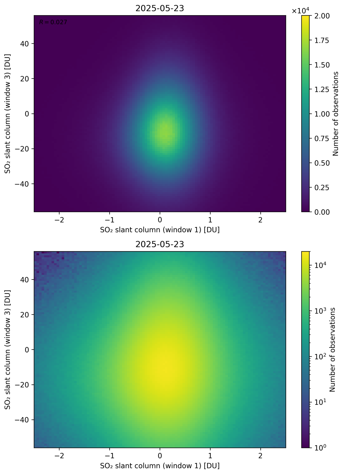
Figure 287: Scatter density plot of “SO 2 slant column (window 1)” against “SO 2 slant column (window 3)” for 2025-05-22 to 2025-05-24.
