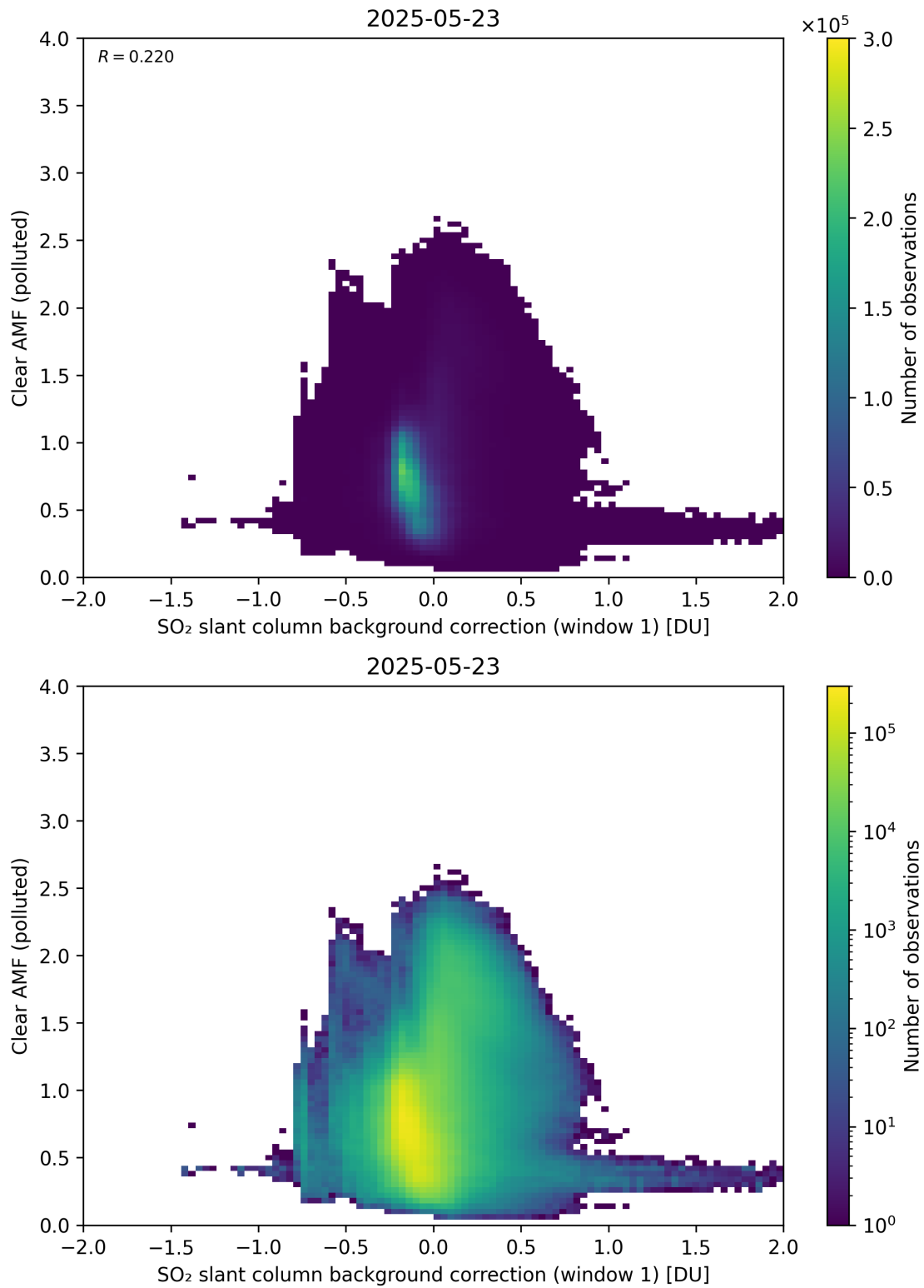
Figure 114: Scatter density plot of “SO 2 slant column background correction (window 1)” against “Clear AMF (polluted)” for 2025-05-22 to 2025-05-24.
