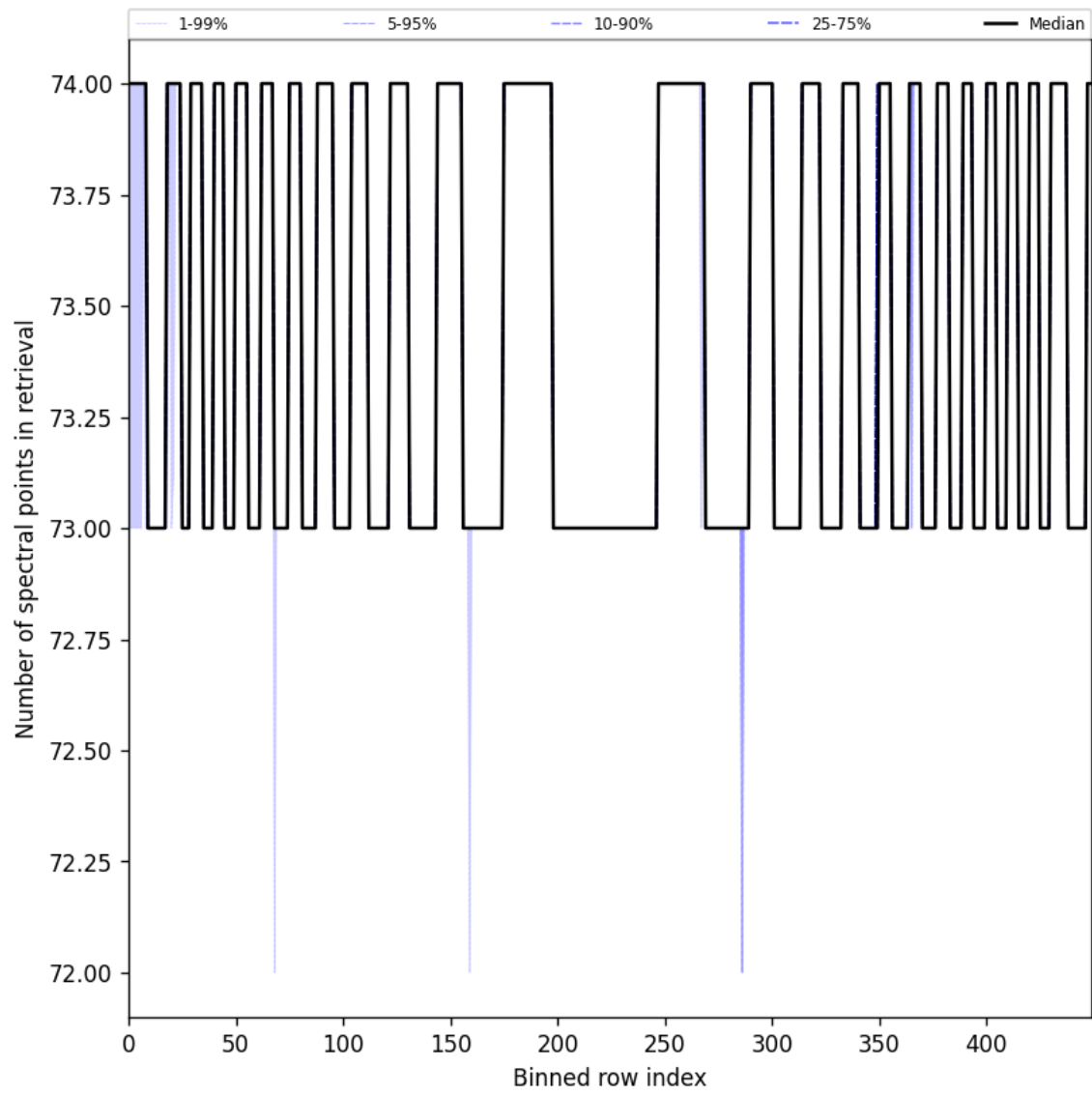
Figure 108: Along track statistics of “Number of spectral points in retrieval” for 2025-05-22 to 2025-05-24
