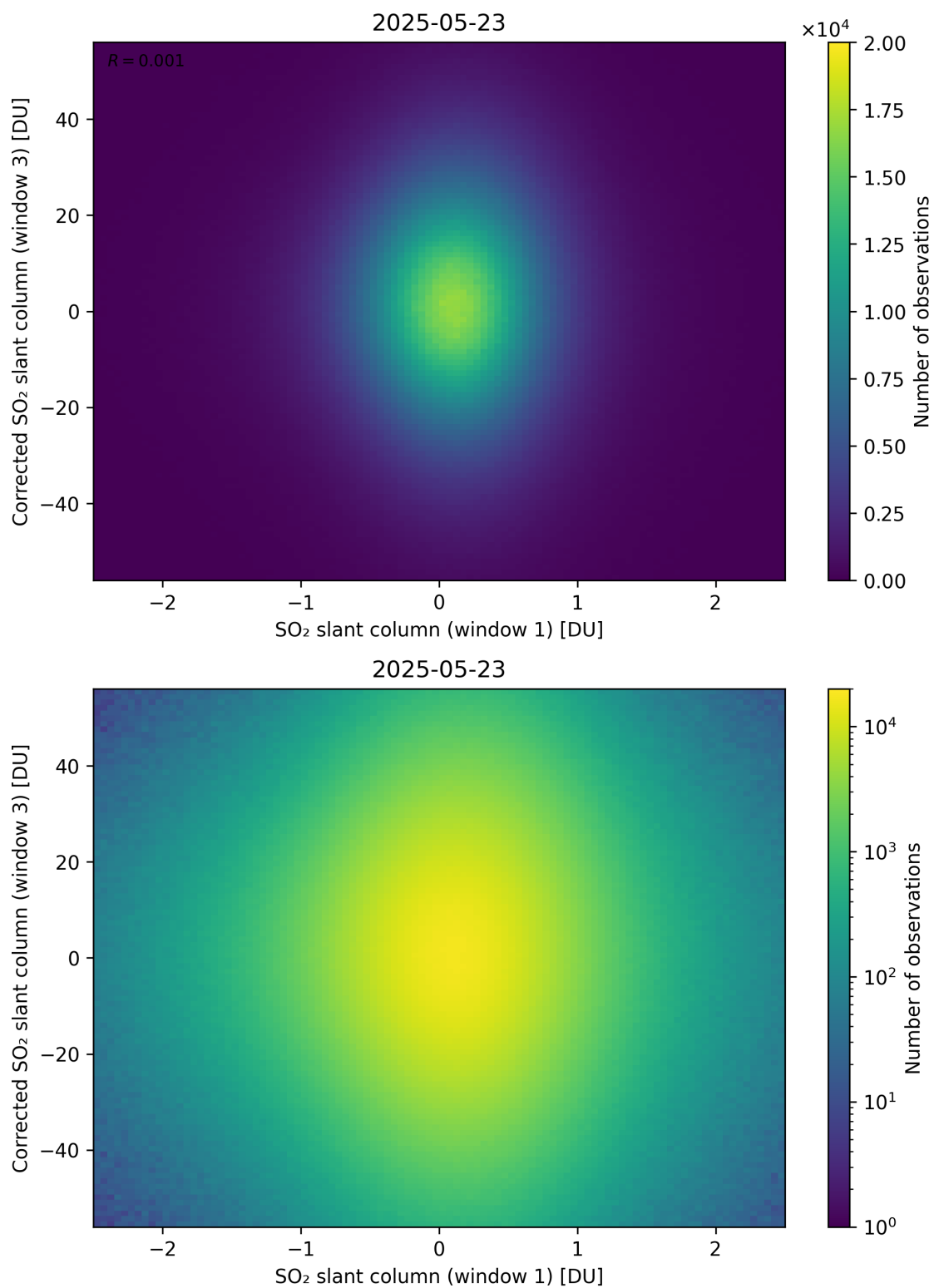
Figure 284: Scatter density plot of “SO 2 slant column (window 1)” against “Corrected SO 2 slant column (window 3)” for 2025-05-22 to 2025-05-24.
