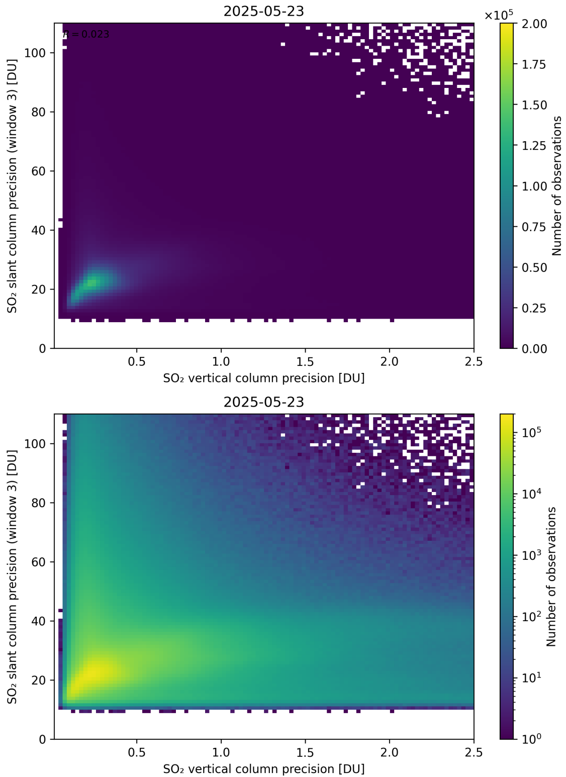
Figure 345: Scatter density plot of “SO 2 vertical column precision” against “SO 2 slant column precision (window 3)” for 2025-05-22 to 2025-05-24.
