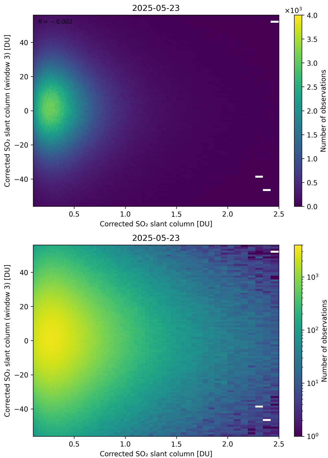
Figure 236: Scatter density plot of “Corrected SO 2 slant column” against “Corrected SO 2 slant column (window 3)” for 2025-05-22 to 2025-05-24.
