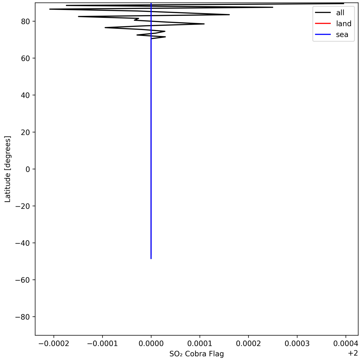
Figure 49: Zonal average of "SO 2 Cobra Flag" for 2025-05-22 to 2025-05-24.
