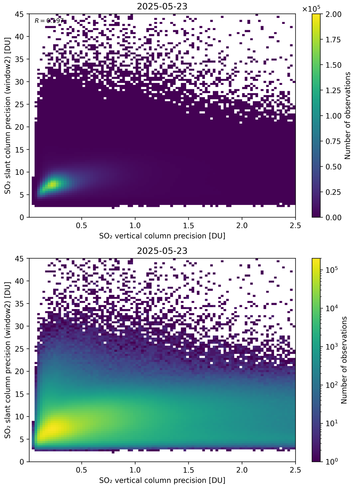
Figure 343: Scatter density plot of “SO 2 vertical column precision” against “SO 2 slant column precision (window2)” for 2025-05-22 to 2025-05-24.
