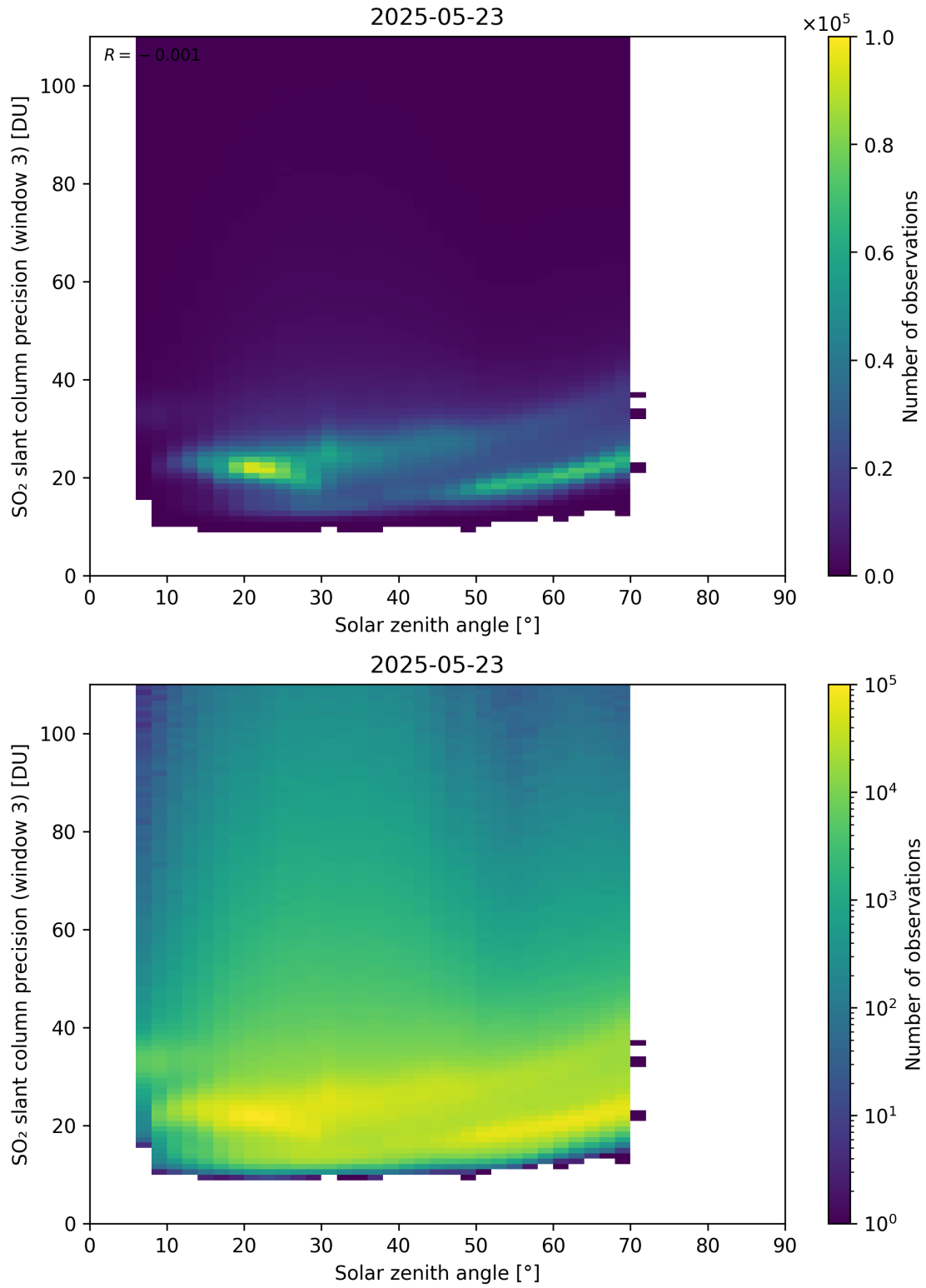
Figure 188: Scatter density plot of “Solar zenith angle” against “SO 2 slant column precision (window 3)” for 2025-05-22 to 2025-05-24.
