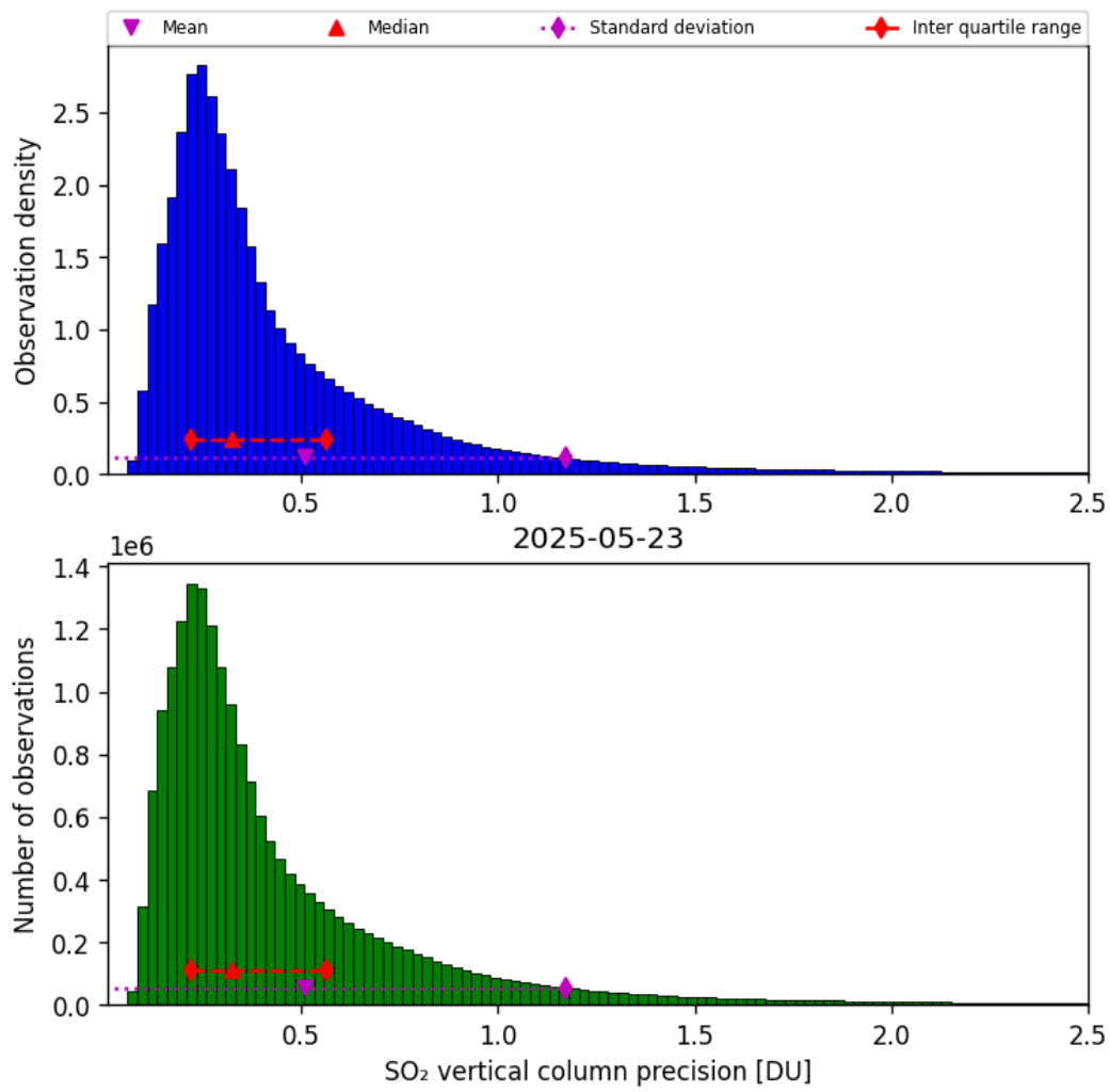
Figure 59: Histogram of “SO 2 vertical column precision” for 2025-05-22 to 2025-05-24
