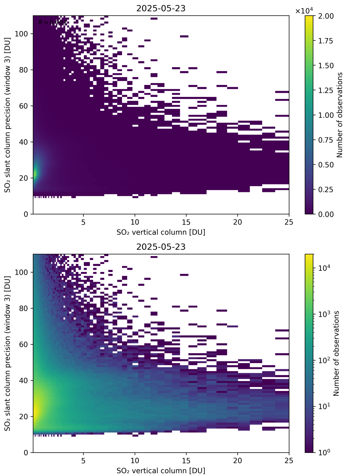
Figure 358: Scatter density plot of “SO 2 vertical column” against “SO 2 slant column precision (window 3)” for 2025-05-22 to 2025-05-24.
