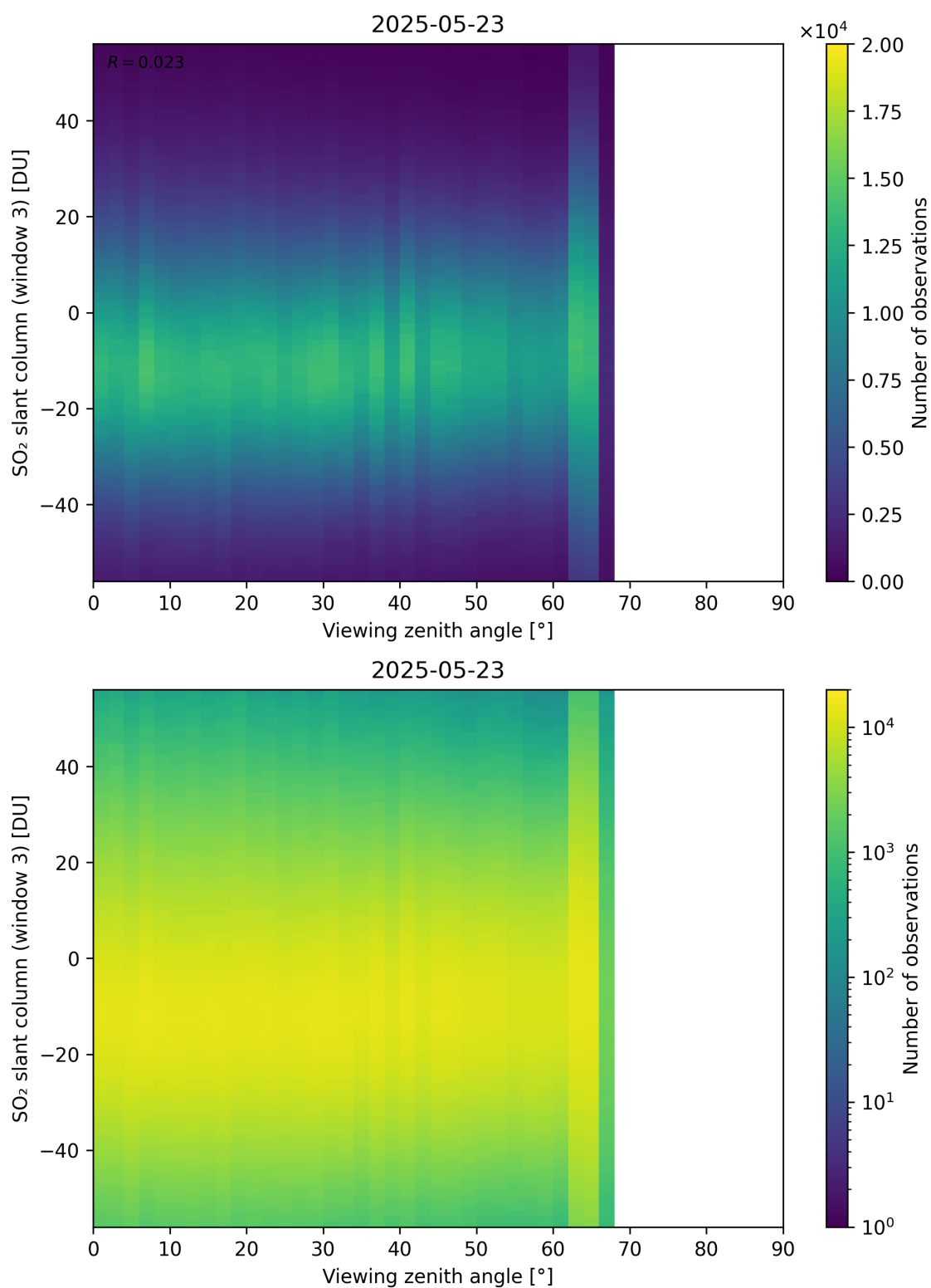
Figure 379: Scatter density plot of “Viewing zenith angle” against “SO 2 slant column (window 3)” for 2025-05-22 to 2025-05-24.
