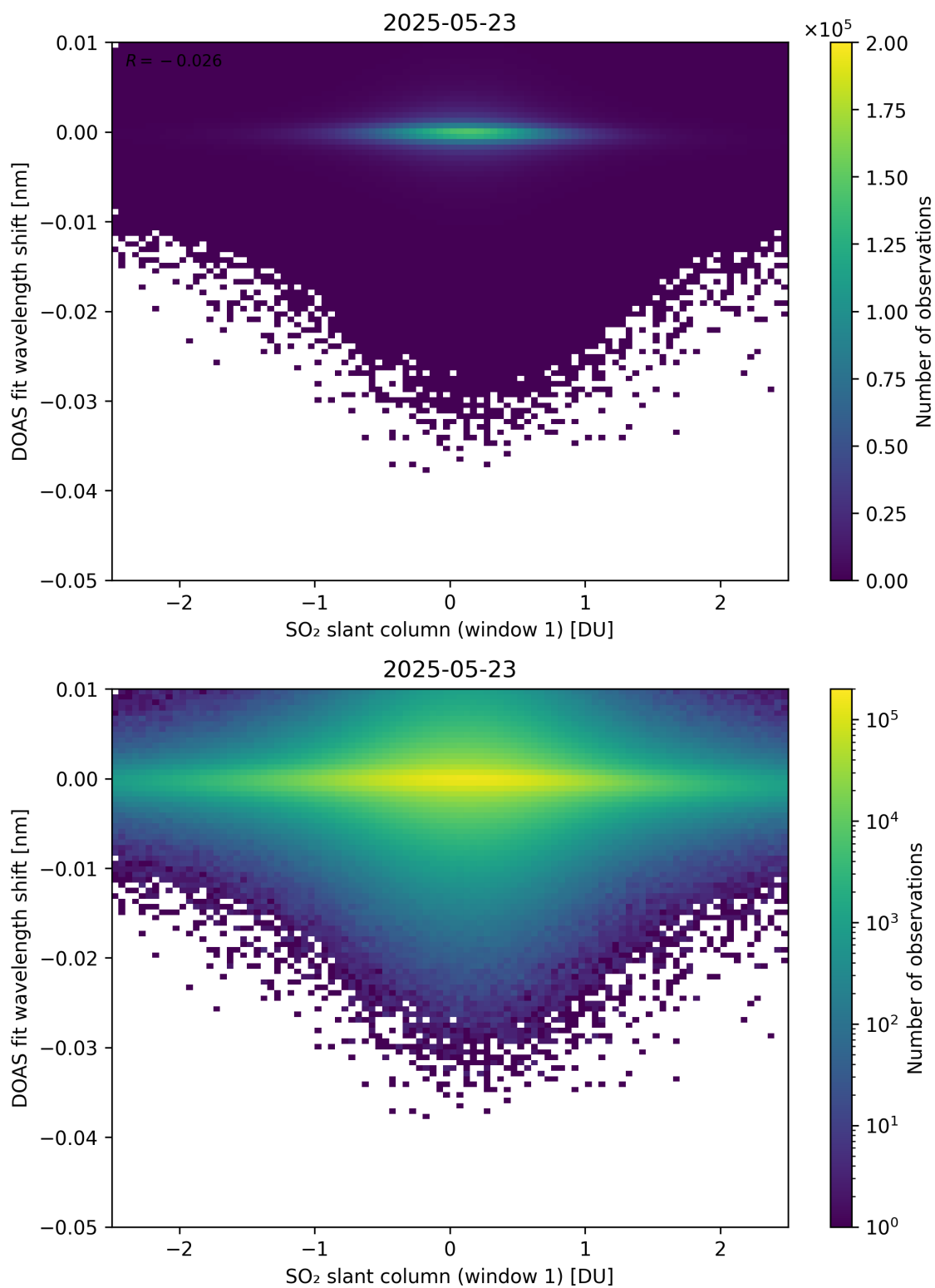
Figure 265: Scatter density plot of “SO 2 slant column (window 1)” against “DOAS fit wavelength shift” for 2025-05-22 to 2025-05-24.
