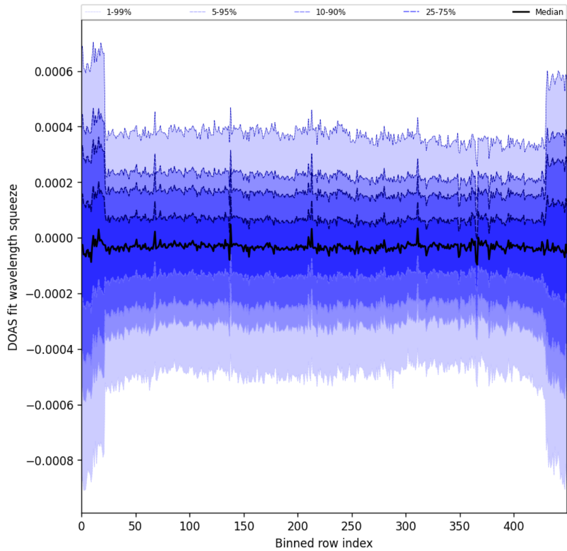
Figure 103: Along track statistics of “DOAS fit wavelength squeeze” for 2025-05-22 to 2025-05-24
