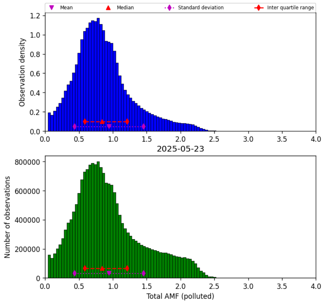
Figure 79: Histogram of “Total AMF (polluted)” for 2025-05-22 to 2025-05-24
