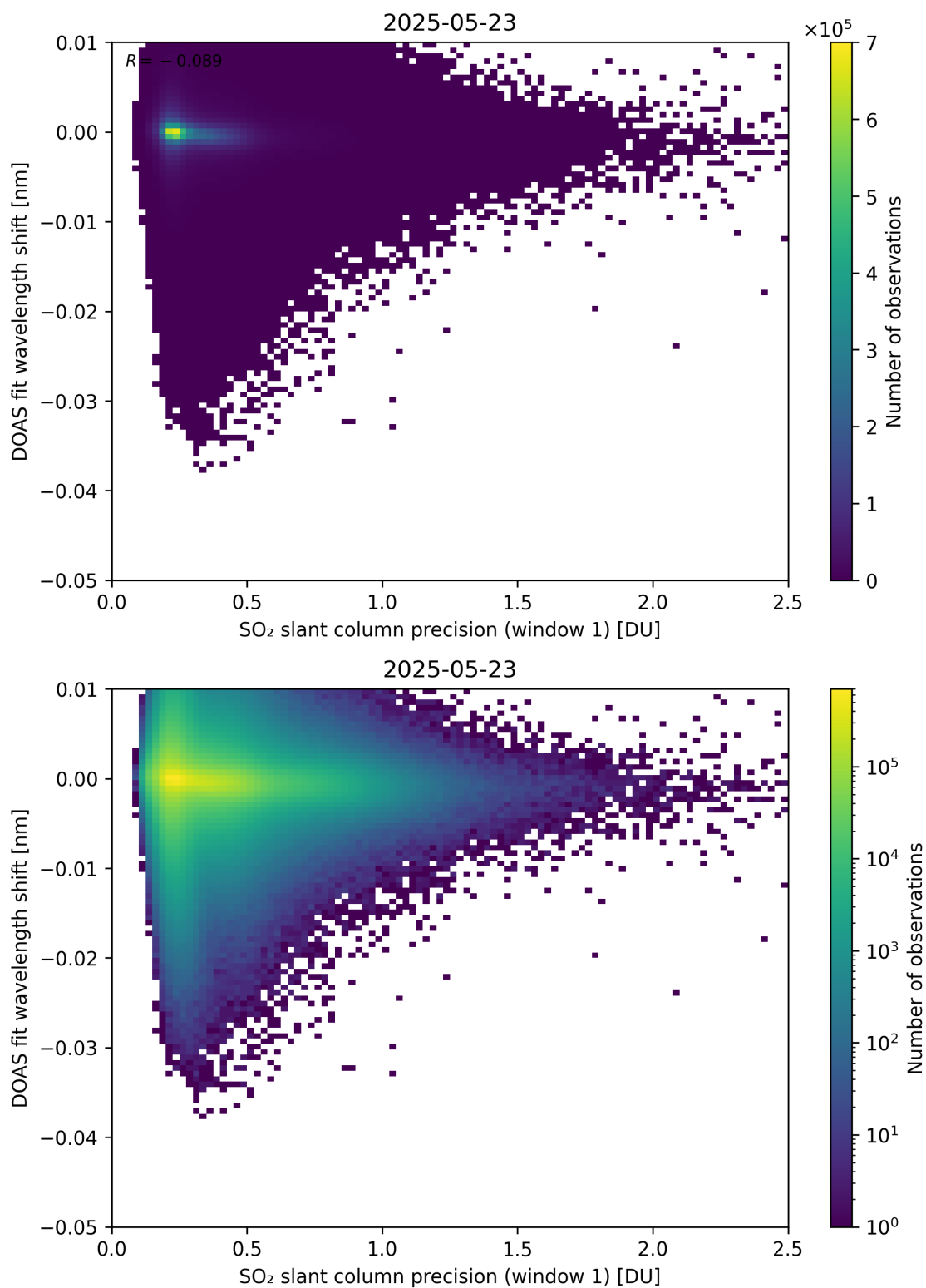
Figure 271: Scatter density plot of “SO 2 slant column precision (window 1)” against “DOAS fit wavelength shift” for 2025-05-22 to 2025-05-24.
