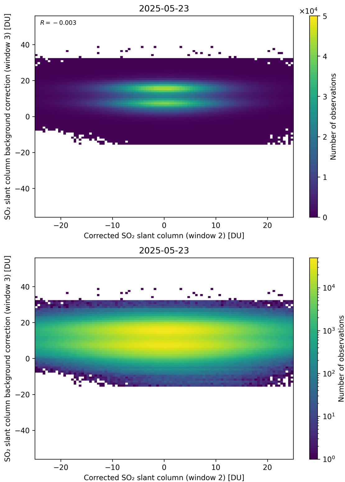
Figure 245: Scatter density plot of “Corrected SO 2 slant column (window 2)” against “SO 2 slant column background correction (window 3)” for 2025-05-22 to 2025-05-24.
