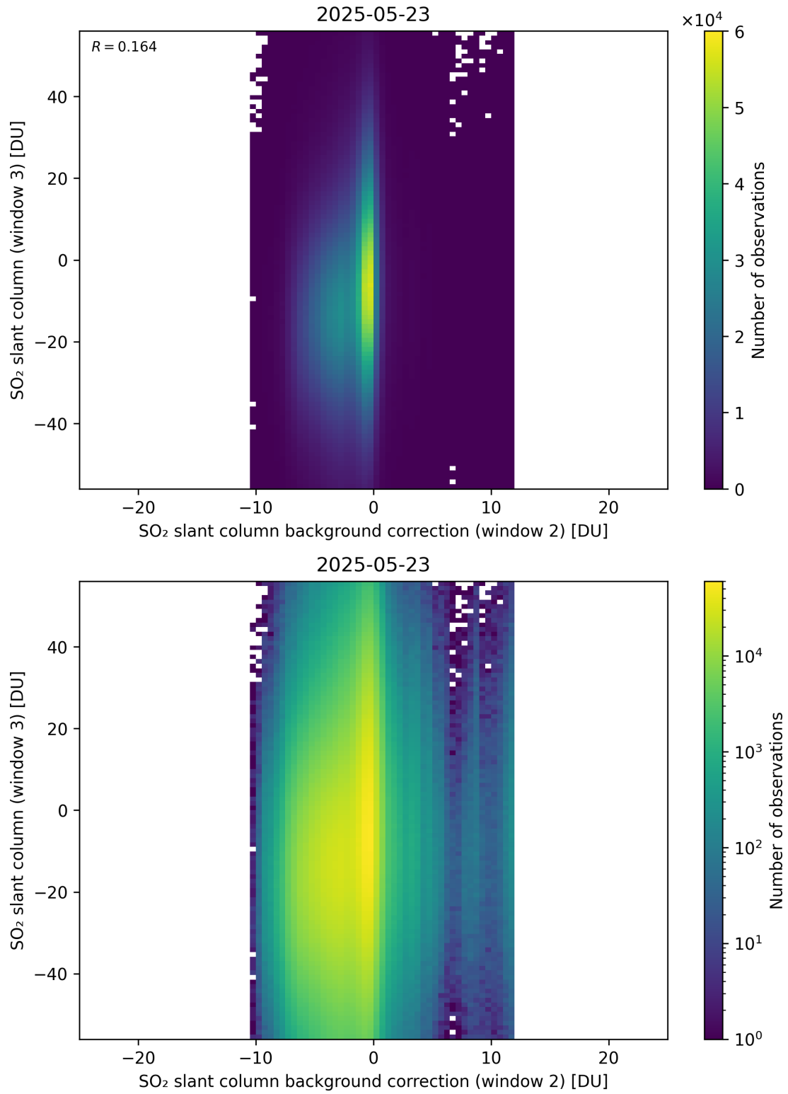
Figure 128: Scatter density plot of “SO 2 slant column background correction (window 2)” against “SO 2 slant column (window 3)” for 2025-05-22 to 2025-05-24.
