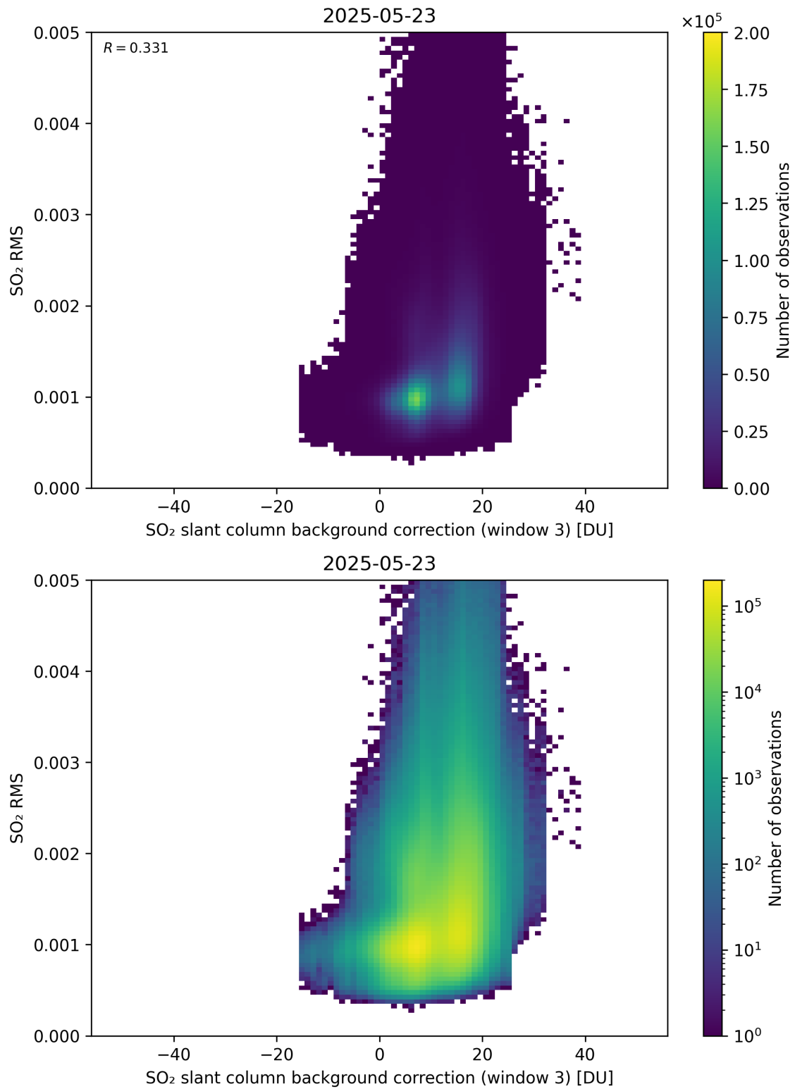
Figure 134: Scatter density plot of “SO 2 slant column background correction (window 3)” against “SO 2 RMS” for 2025-05-22 to 2025-05-24.
