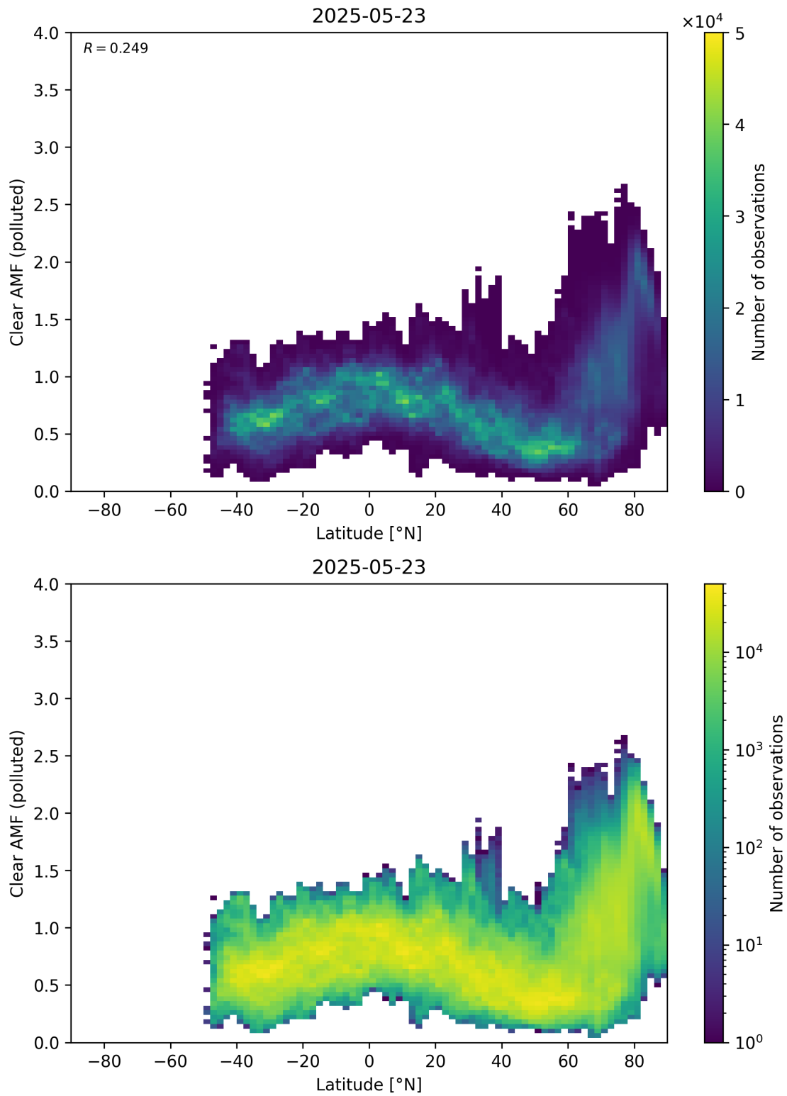
Figure 156: Scatter density plot of “Latitude” against “Clear AMF (polluted)” for 2025-05-22 to 2025-05-24.
