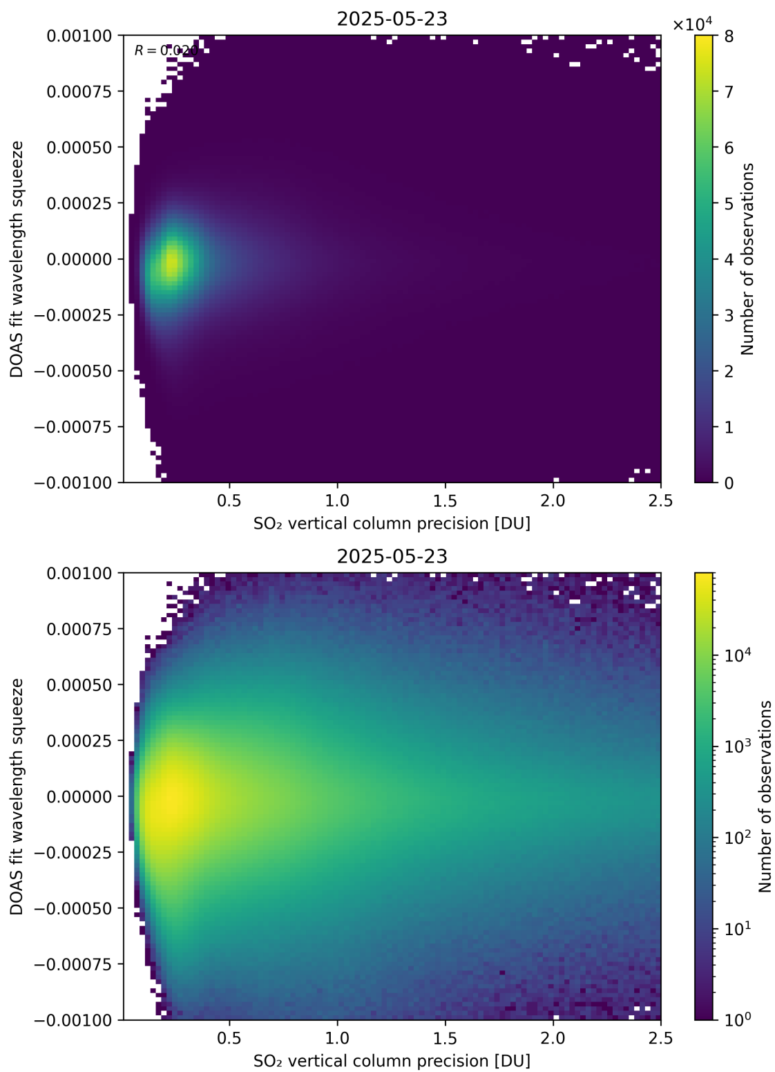
Figure 333: Scatter density plot of “SO 2 vertical column precision” against “DOAS fit wavelength squeeze” for 2025-05-22 to 2025-05-24.
