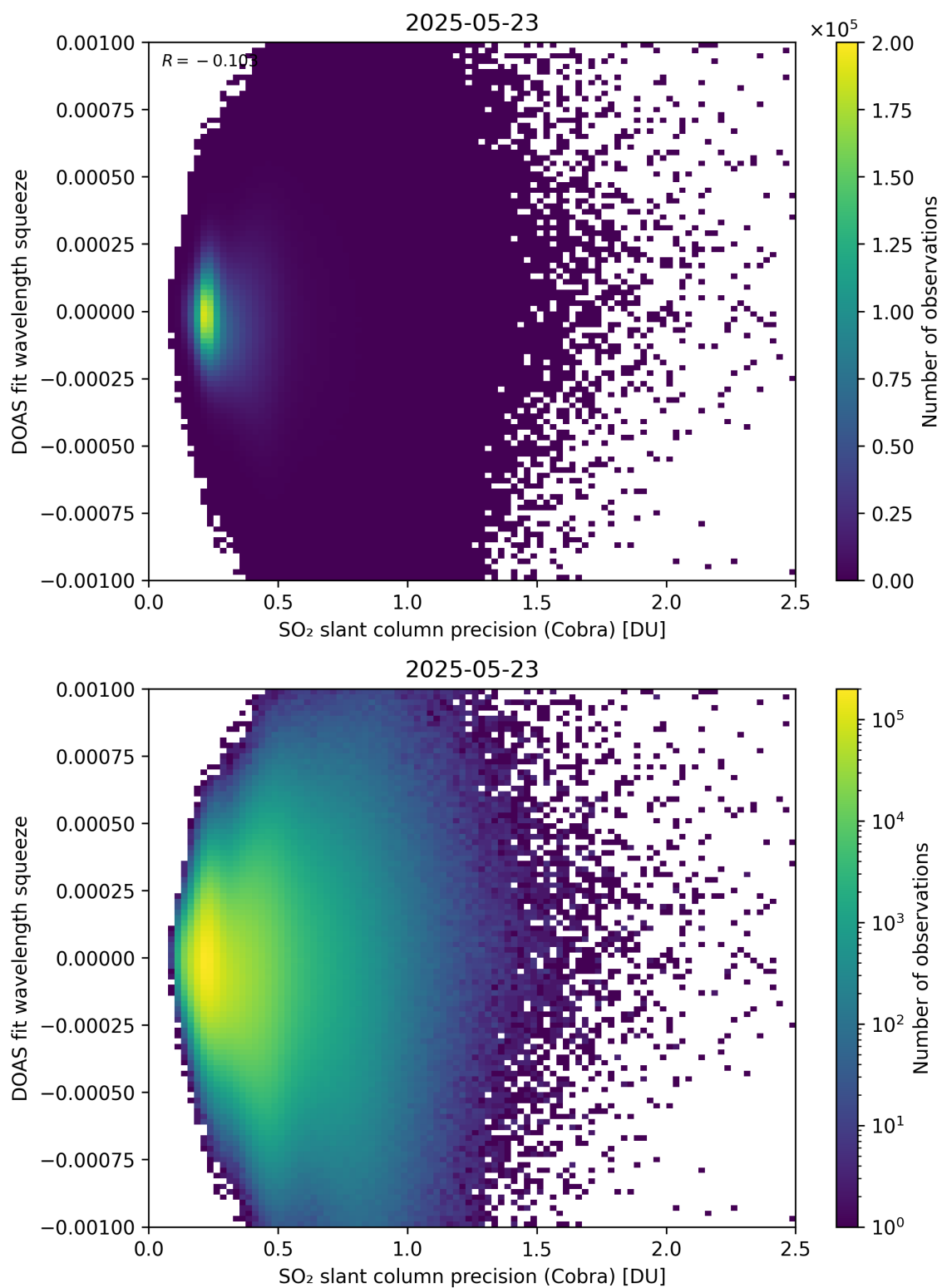
Figure 203: Scatter density plot of “SO 2 slant column precision (Cobra)” against “DOAS fit wavelength squeeze” for 2025-05-22 to 2025-05-24.
