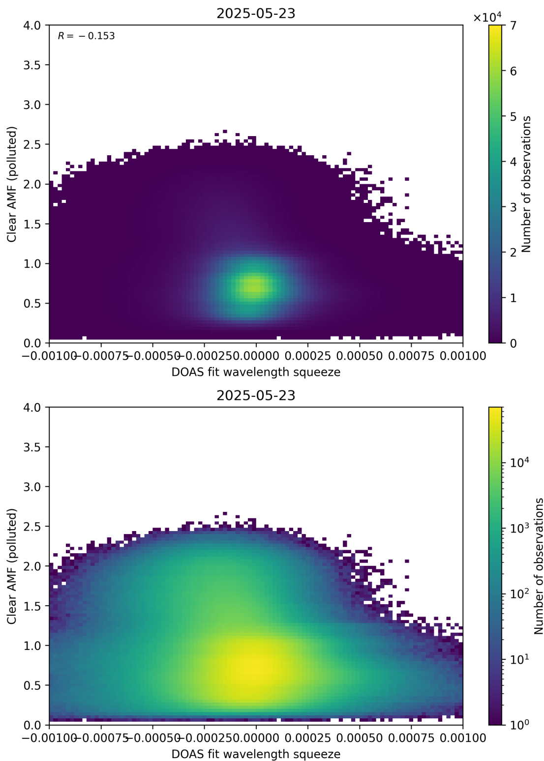
Figure 144: Scatter density plot of “DOAS fit wavelength squeeze” against “Clear AMF (polluted)” for 2025-05-22 to 2025-05-24.
