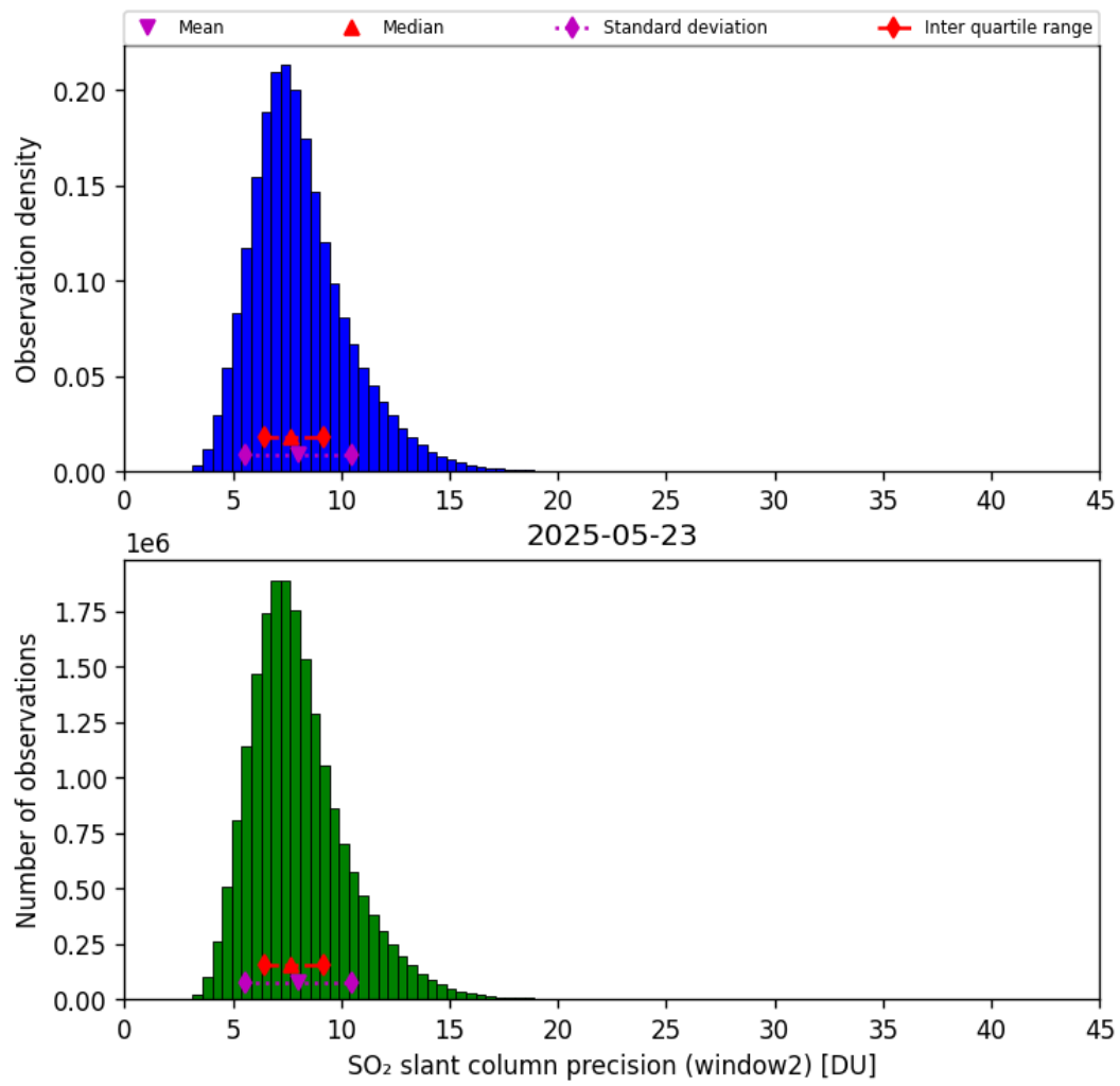
Figure 68: Histogram of “SO 2 slant column precision (window2)” for 2025-05-22 to 2025-05-24
