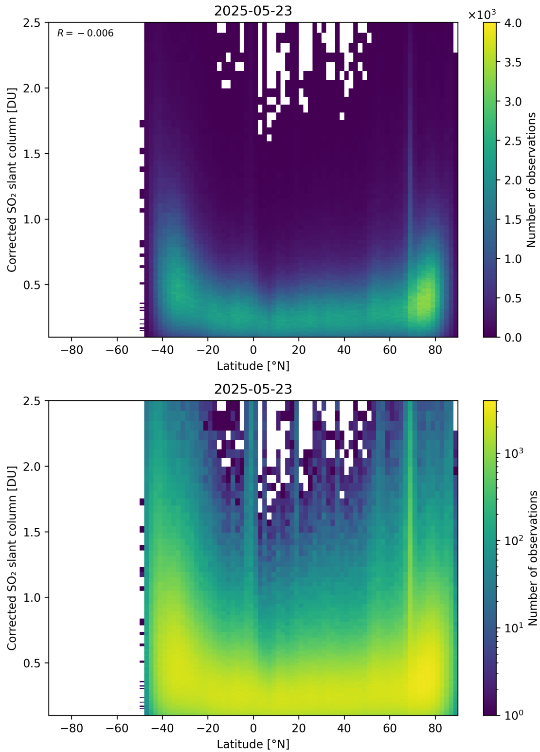
Figure 159: Scatter density plot of “Latitude” against “Corrected SO 2 slant column” for 2025-05-22 to 2025-05-24.
