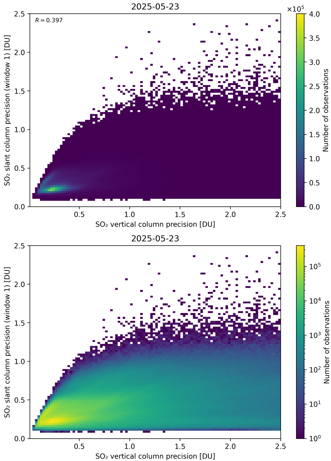
Figure 342: Scatter density plot of “SO 2 vertical column precision” against “SO 2 slant column precision (window 1)” for 2025-05-22 to 2025-05-24.
