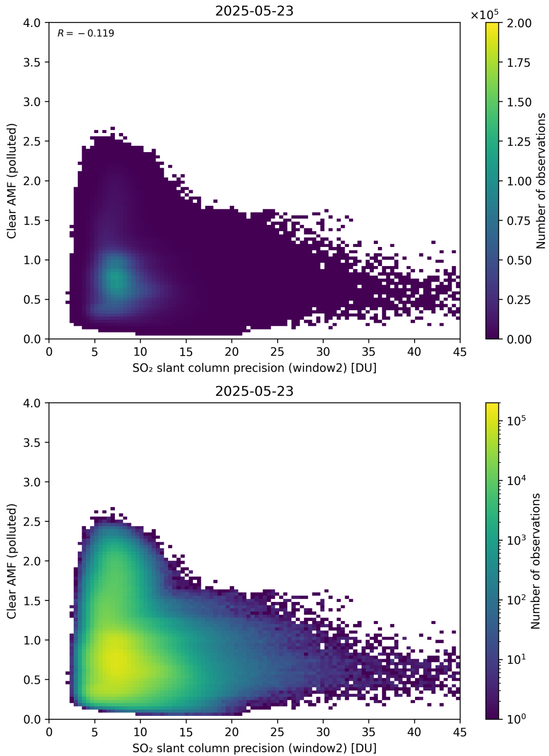
Figure 296: Scatter density plot of “SO 2 slant column precision (window2)” against “Clear AMF (polluted)” for 2025-05-22 to 2025-05-24.
