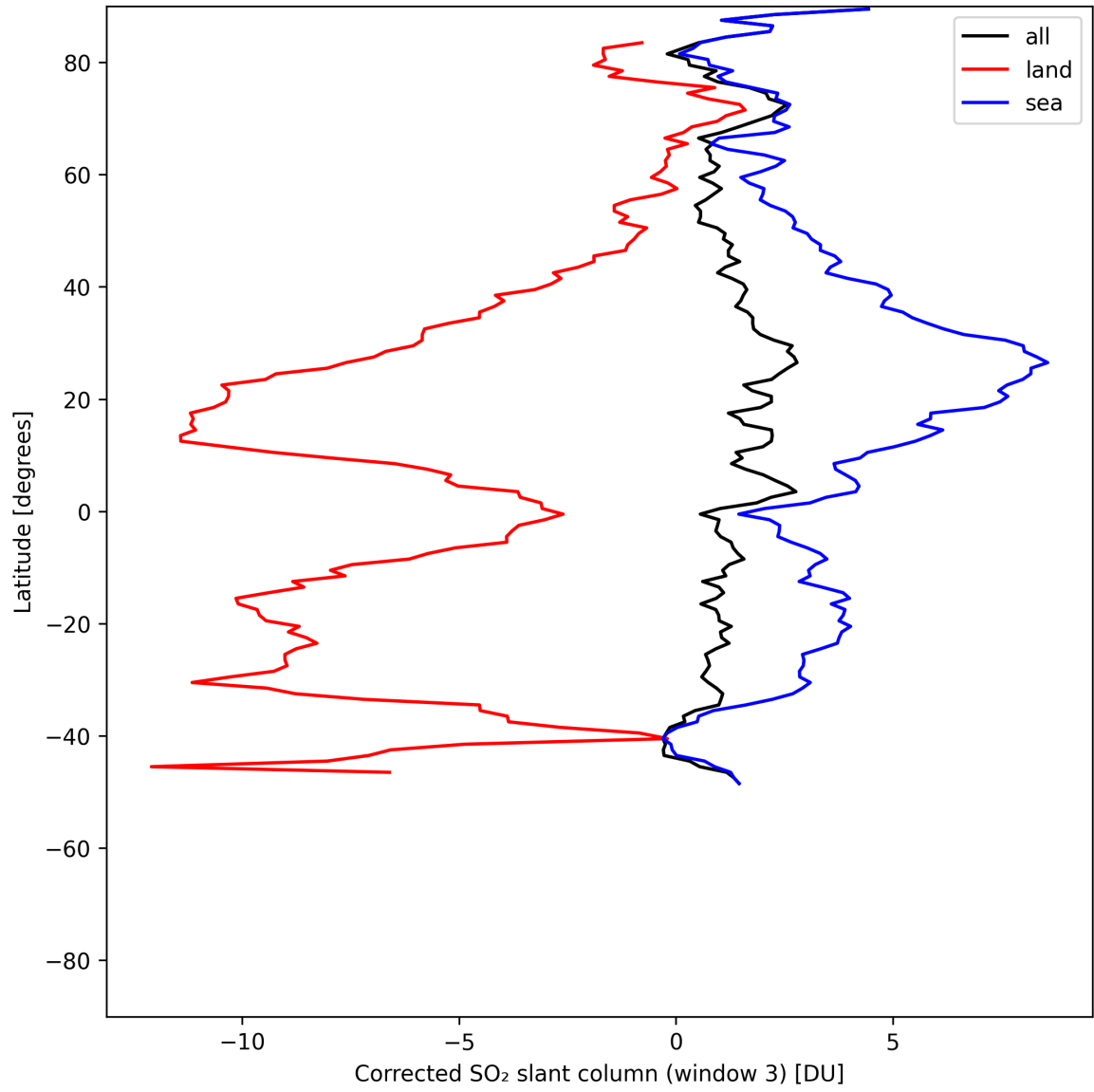
Figure 47: Zonal average of “Corrected SO 2 slant column (window 3)” for 2025-05-22 to 2025-05-24.
