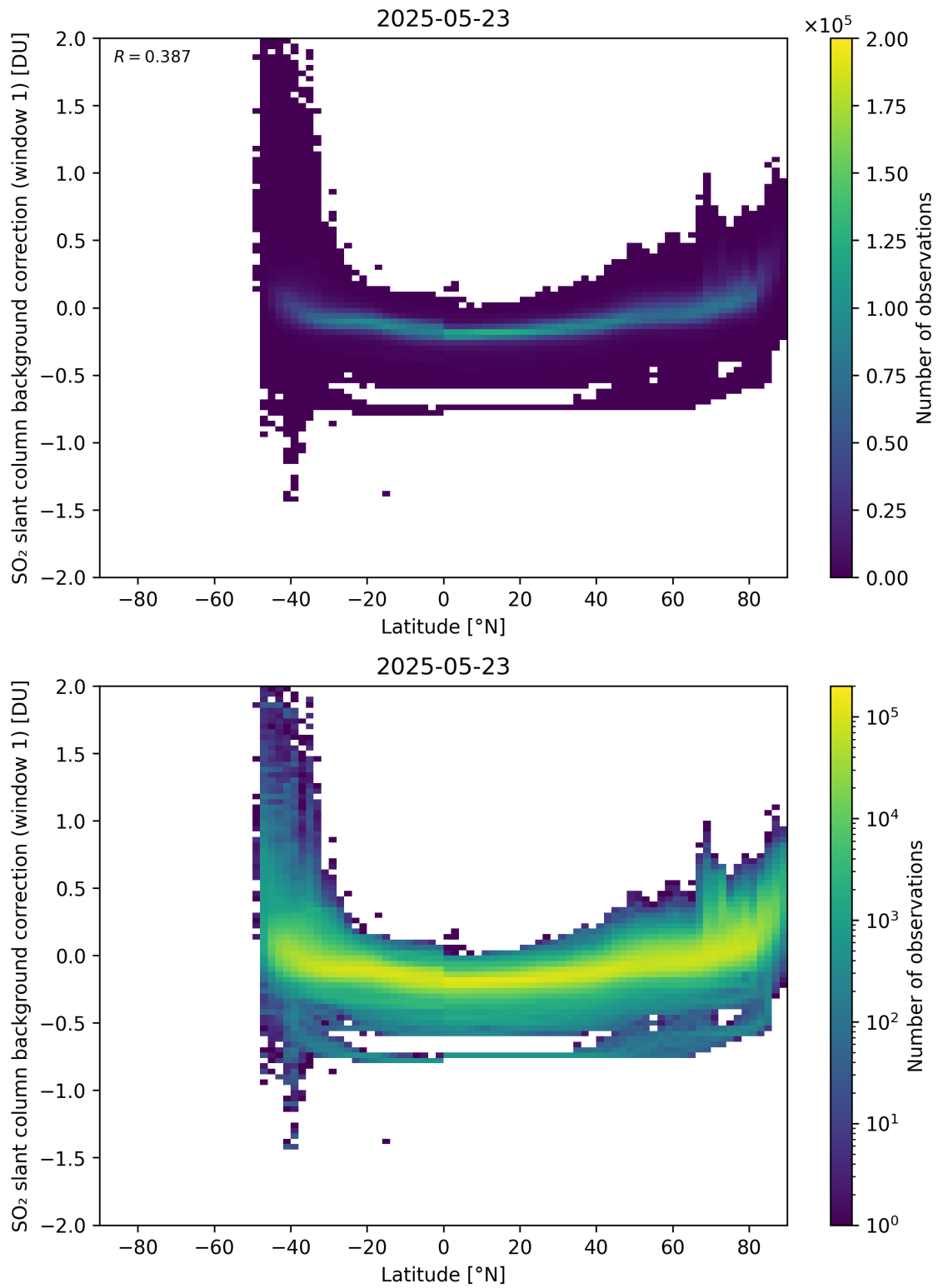
Figure 150: Scatter density plot of “Latitude” against “SO 2 slant column background correction (window 1)” for 2025-05-22 to 2025-05-24.
