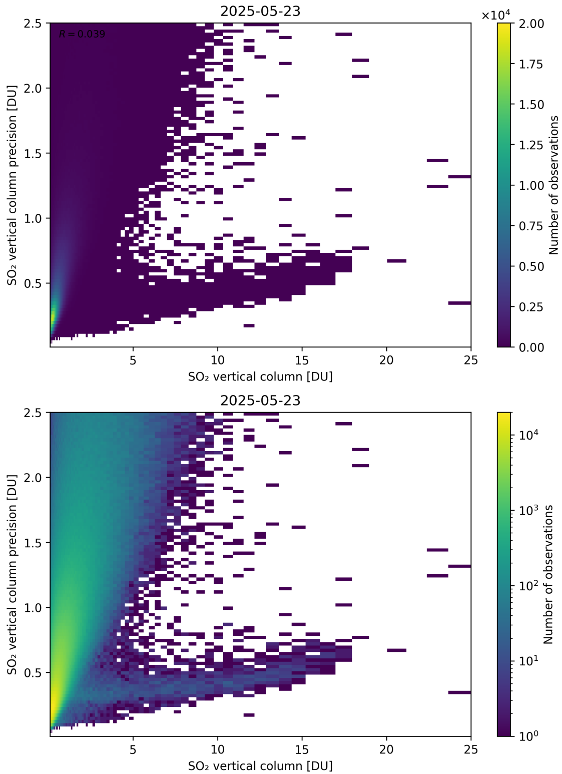
Figure 361: Scatter density plot of “SO 2 vertical column” against “SO 2 vertical column precision” for 2025-05-22 to 2025-05-24.
