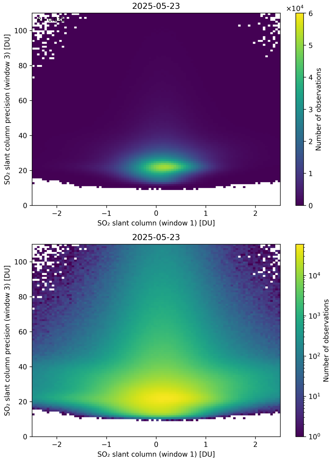
Figure 288: Scatter density plot of “SO 2 slant column (window 1)” against “SO 2 slant column precision (window 3)” for 2025-05-22 to 2025-05-24.
