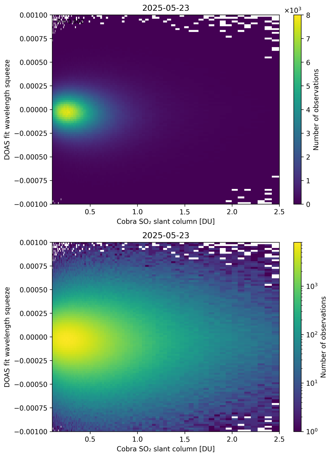
Figure 197: Scatter density plot of “Cobra SO 2 slant column” against “DOAS fit wavelength squeeze” for 2025-05-22 to 2025-05-24.
