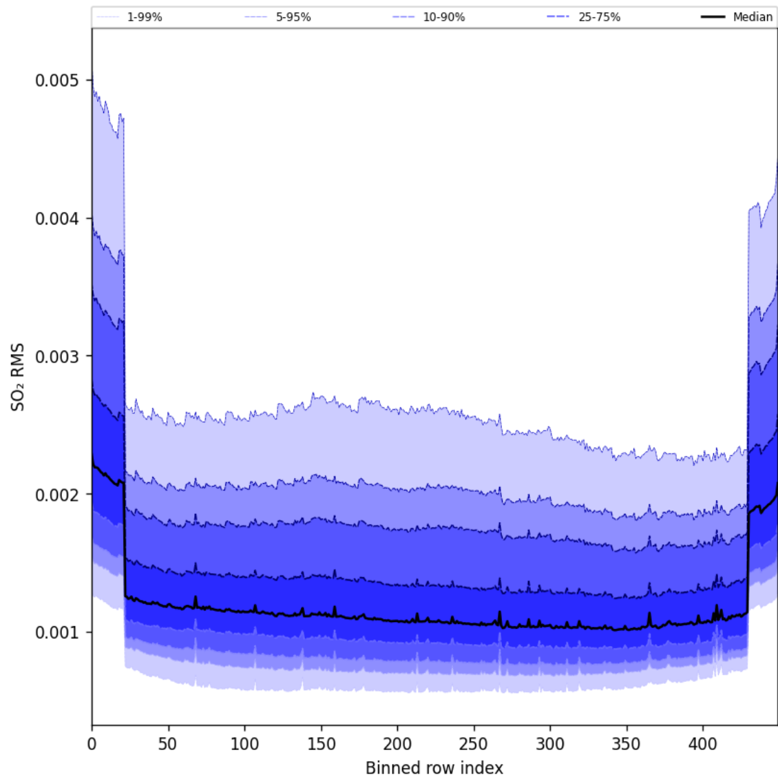
Figure 104: Along track statistics of “SO 2 RMS” for 2025-05-22 to 2025-05-24
