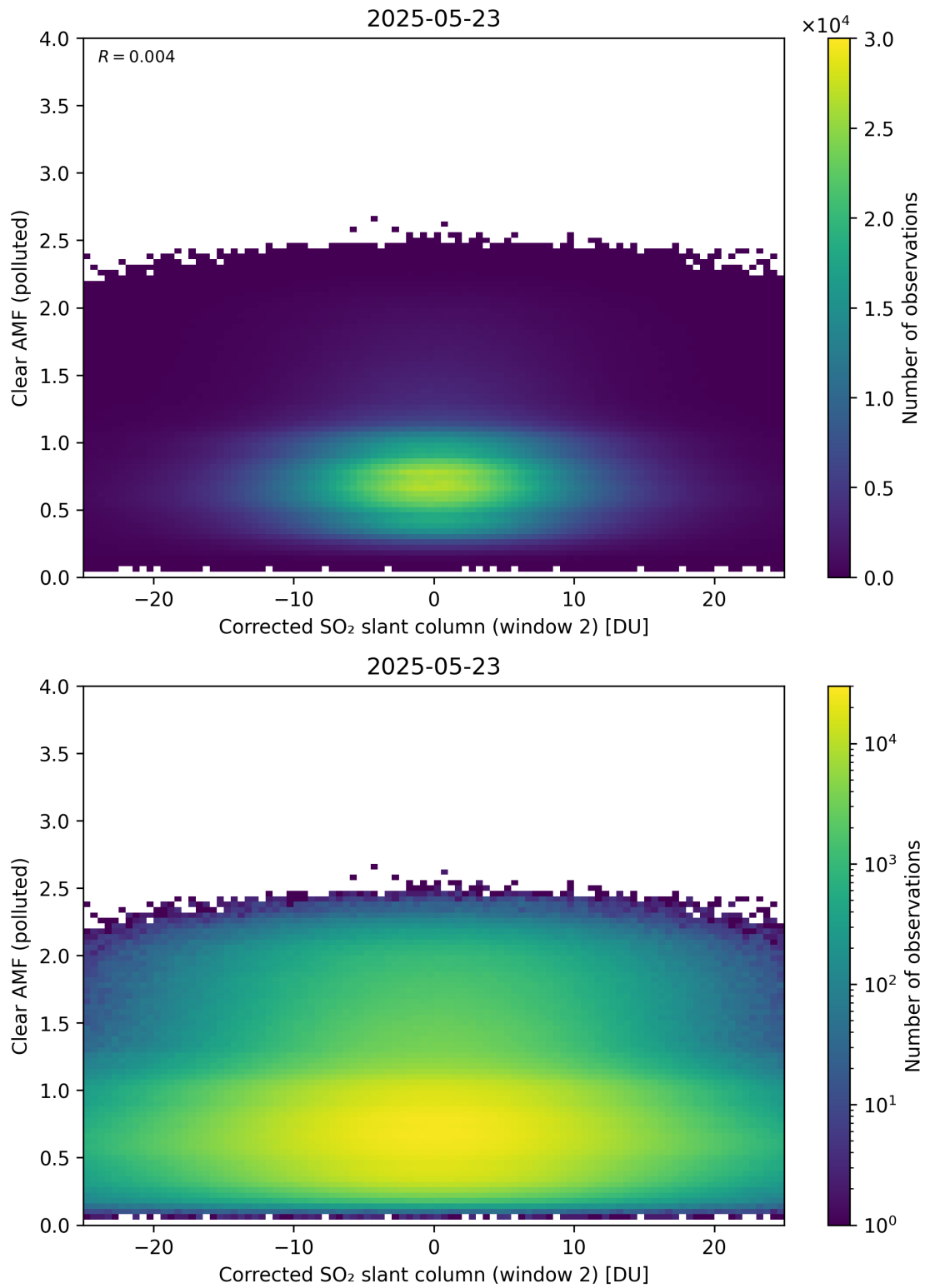
Figure 249: Scatter density plot of “Corrected SO 2 slant column (window 2)” against “Clear AMF (polluted)” for 2025-05-22 to 2025-05-24.
