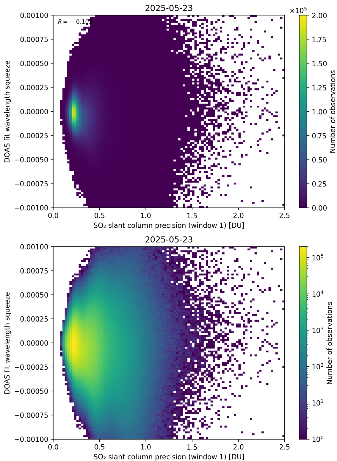
Figure 272: Scatter density plot of “SO 2 slant column precision (window 1)” against “DOAS fit wavelength squeeze” for 2025-05-22 to 2025-05-24.
