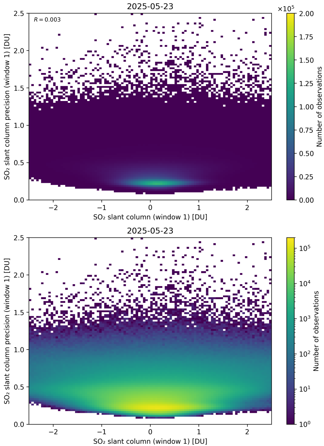
Figure 285: Scatter density plot of “SO 2 slant column (window 1)” against “SO 2 slant column precision (window 1)” for 2025-05-22 to 2025-05-24.
