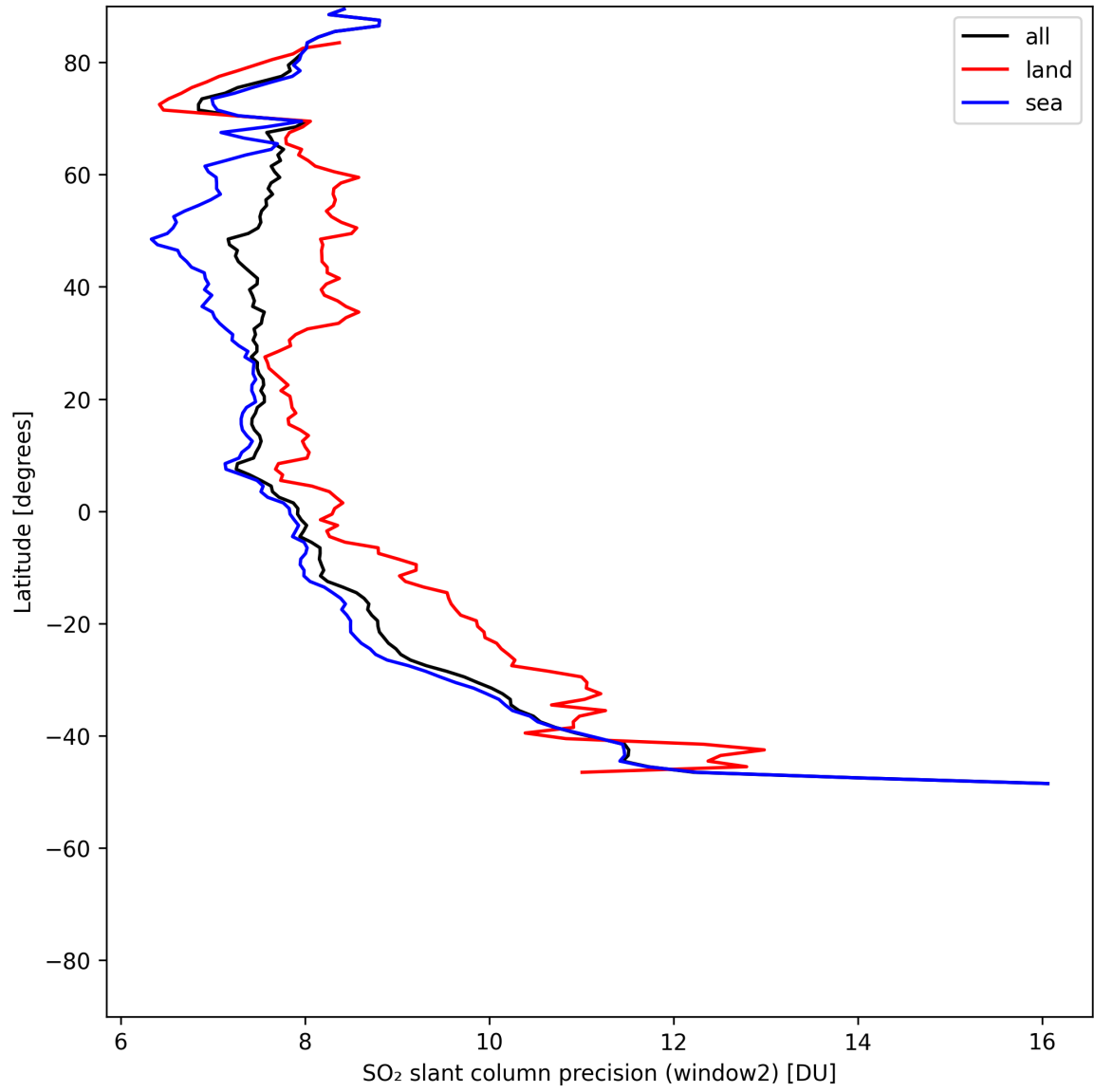
Figure 42: Zonal average of “SO 2 slant column precision (window2)” for 2025-05-22 to 2025-05-24.
