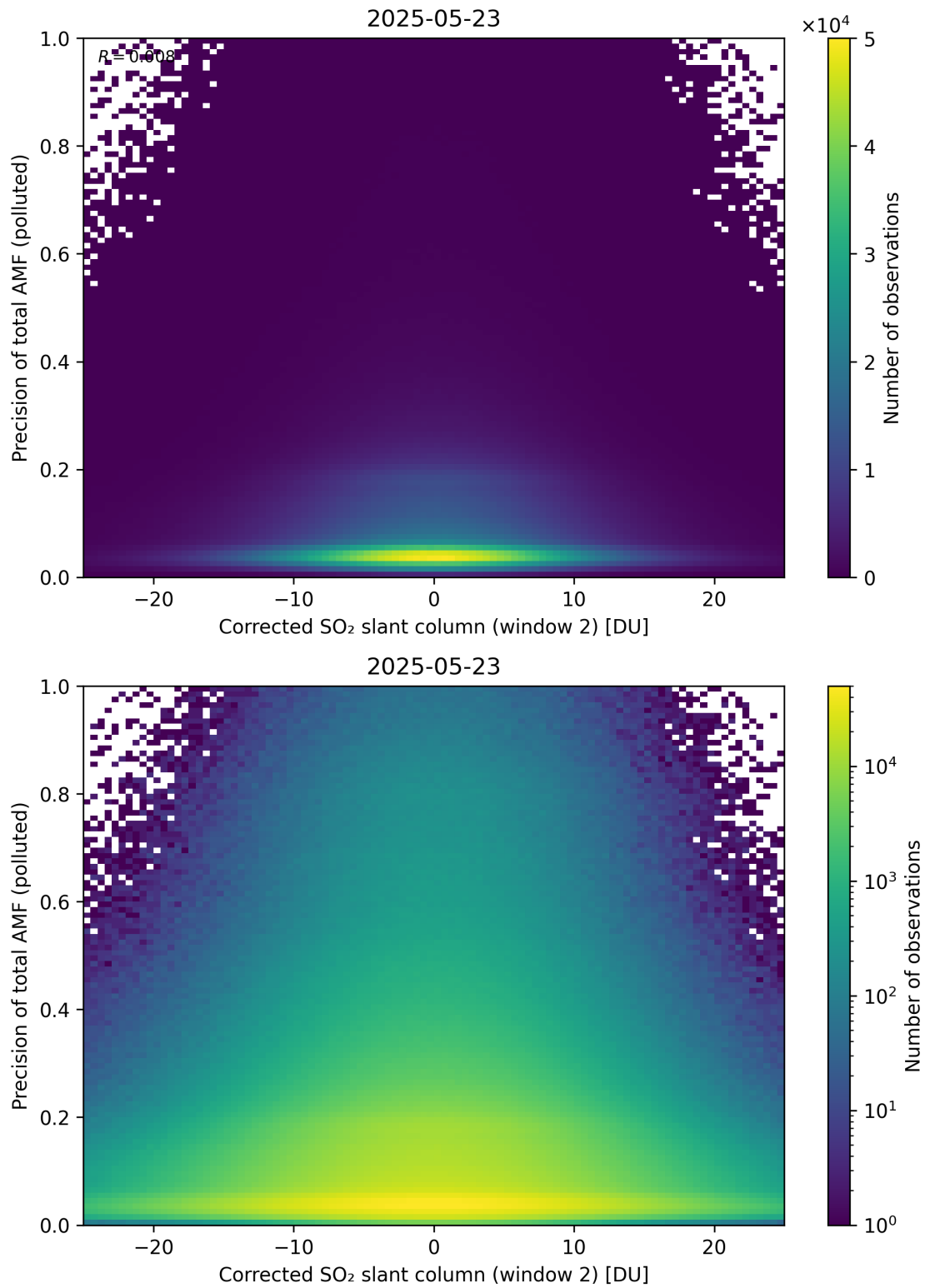
Figure 254: Scatter density plot of “Corrected SO 2 slant column (window 2)” against “Precision of total AMF (polluted)” for 2025-05-22 to 2025-05-24.
