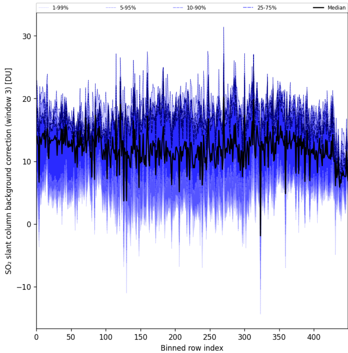
Figure 100: Along track statistics of “SO 2 slant column background correction (window 3)” for 2025-05-22 to 2025-05-24
