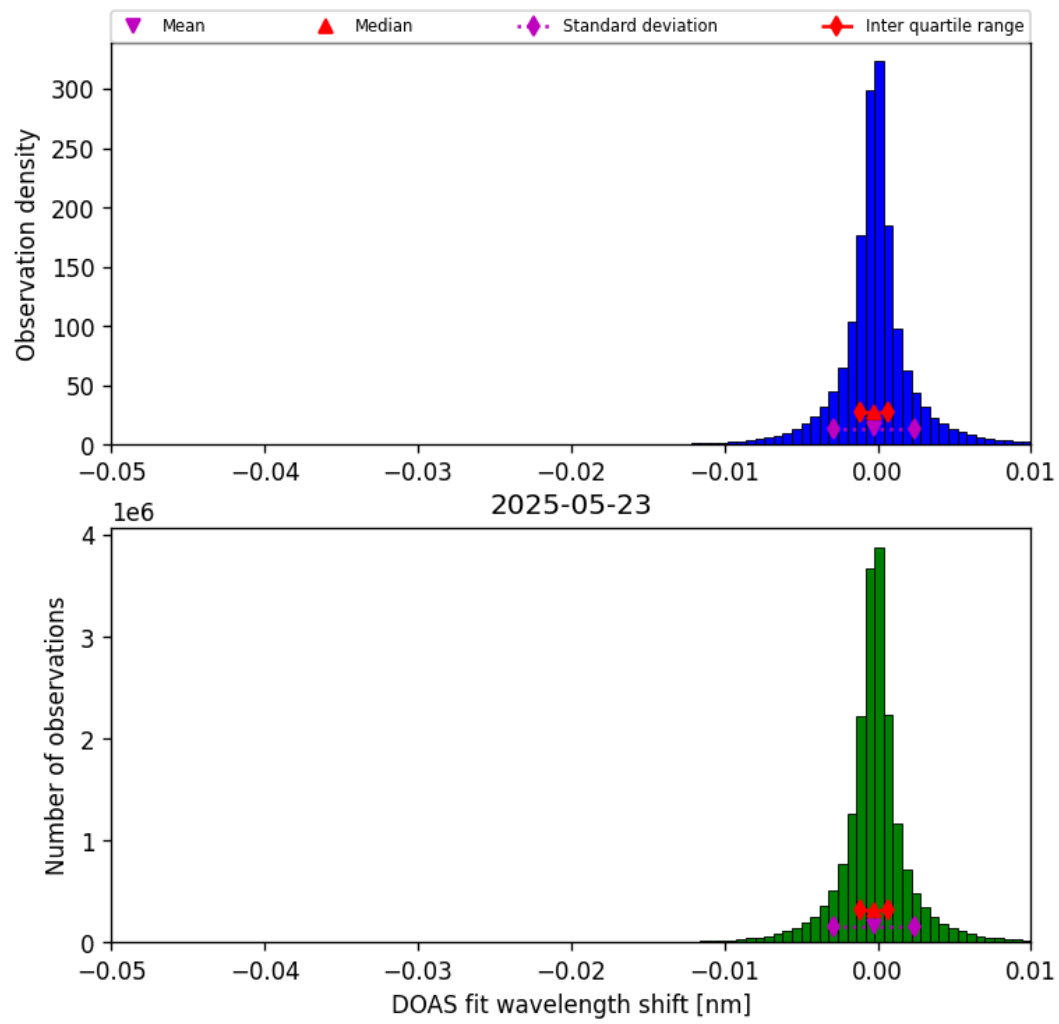
Figure 76: Histogram of “DOAS fit wavelength shift” for 2025-05-22 to 2025-05-24
