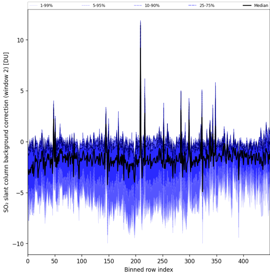
Figure 96: Along track statistics of “SO 2 slant column background correction (window 2)” for 2025-05-22 to 2025-05-24
