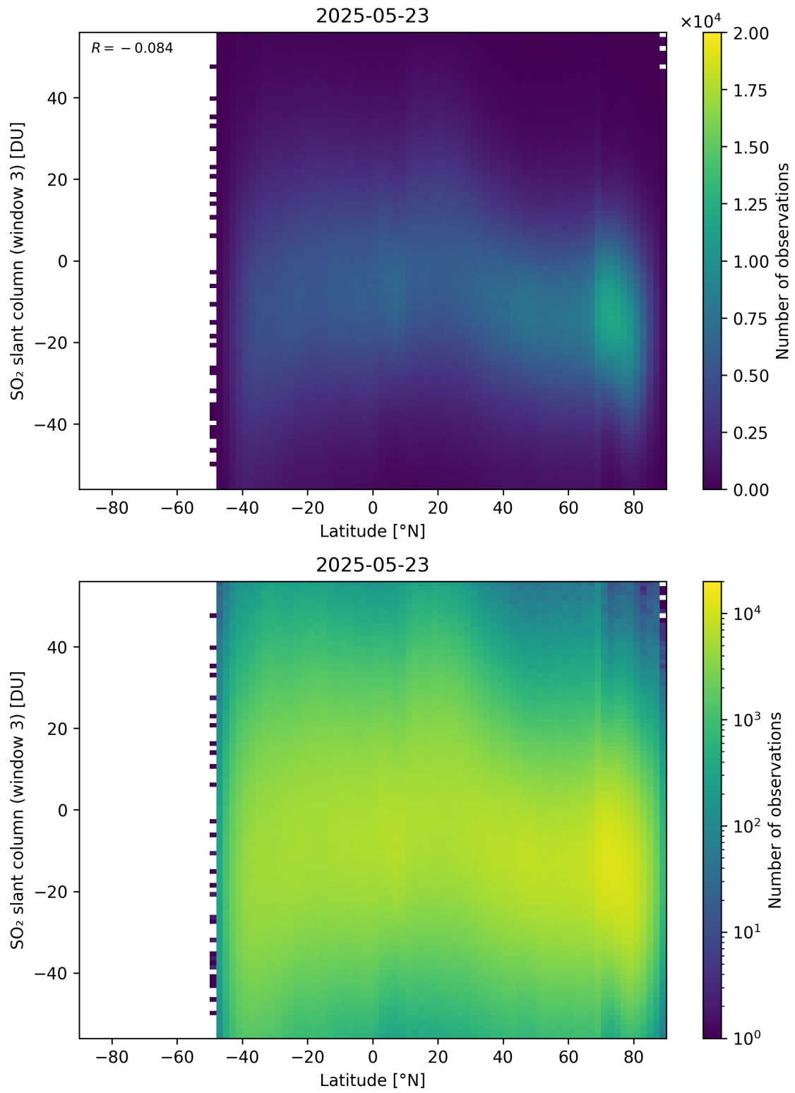
Figure 165: Scatter density plot of “Latitude” against “SO 2 slant column (window 3)” for 2025-05-22 to 2025-05-24.
