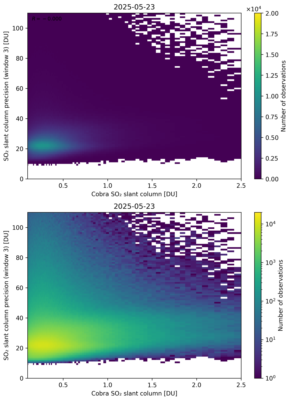
Figure 223: Scatter density plot of “Cobra SO 2 slant column” against “SO 2 slant column precision (window 3)” for 2025-05-22 to 2025-05-24.
