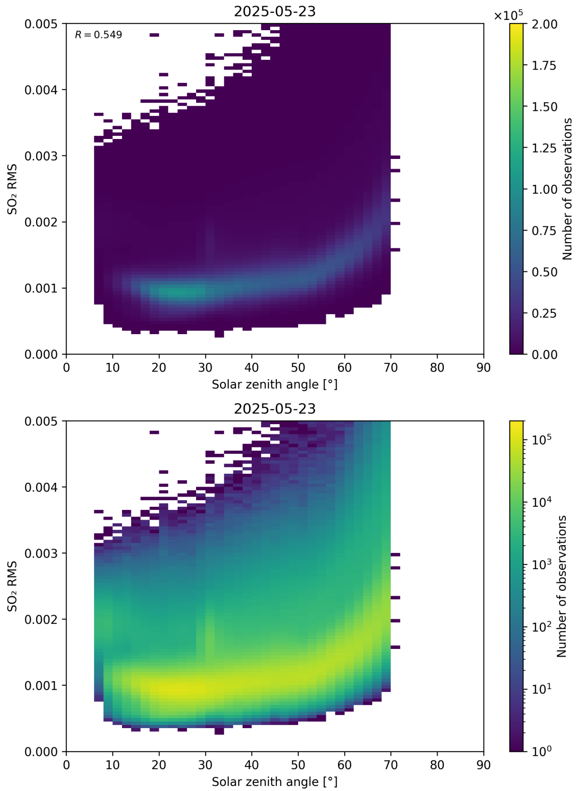
Figure 176: Scatter density plot of “Solar zenith angle” against “SO 2 RMS” for 2025-05-22 to 2025-05-24.
