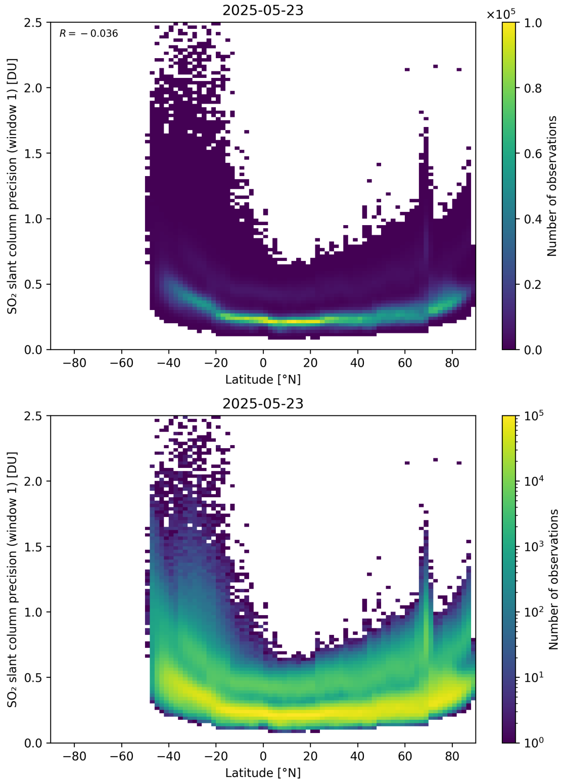
Figure 163: Scatter density plot of “Latitude” against “SO 2 slant column precision (window 1)” for 2025-05-22 to 2025-05-24.
