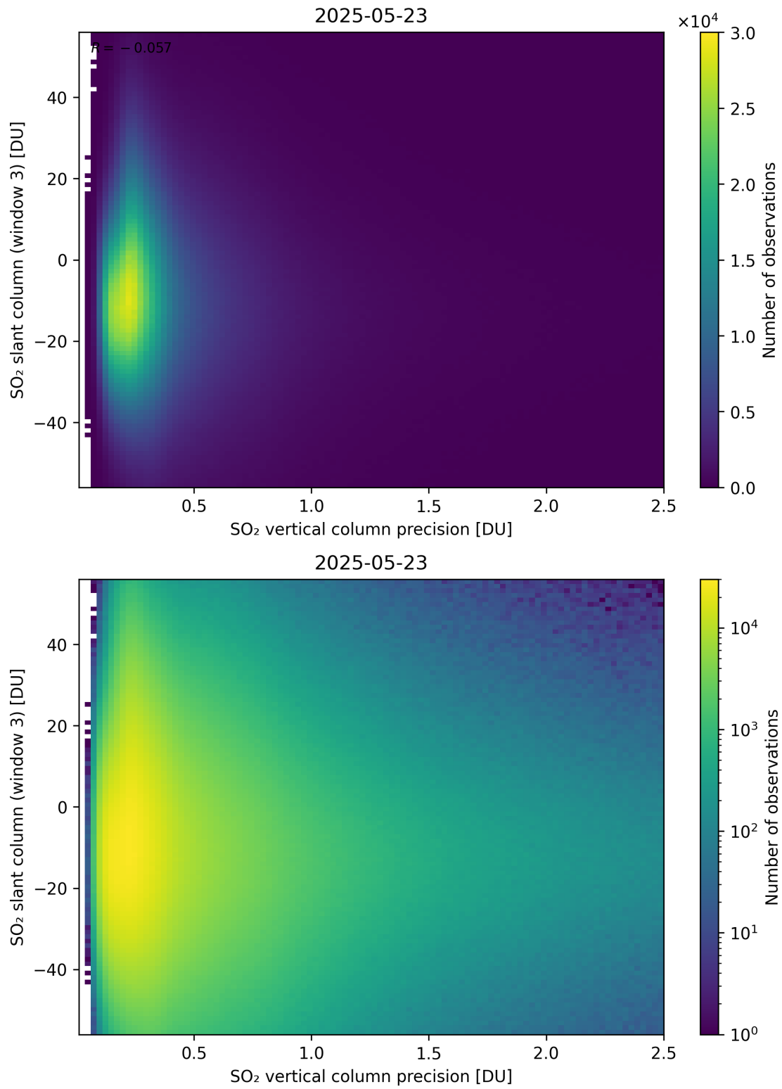
Figure 344: Scatter density plot of “SO 2 vertical column precision” against “SO 2 slant column (window 3)” for 2025-05-22 to 2025-05-24.
