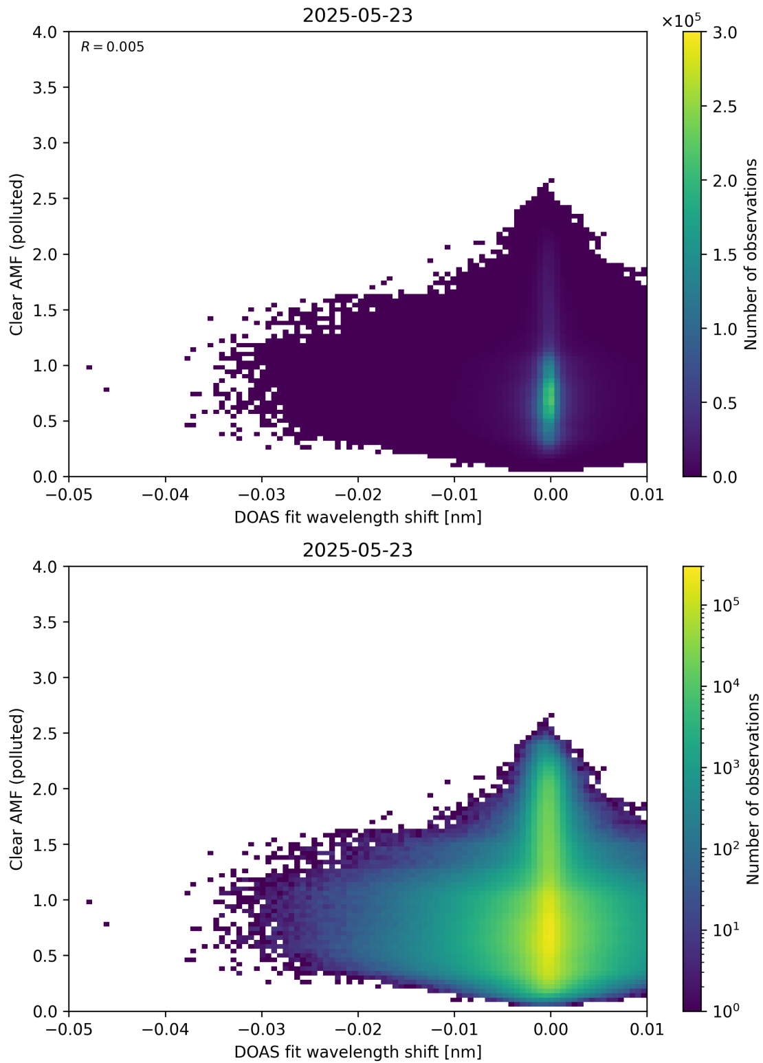
Figure 140: Scatter density plot of “DOAS fit wavelength shift” against “Clear AMF (polluted)” for 2025-05-22 to 2025-05-24.
