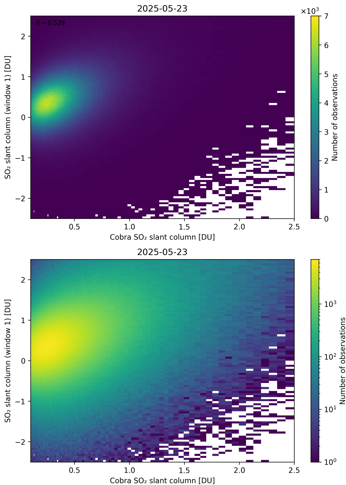
Figure 219: Scatter density plot of “Cobra SO 2 slant column” against “SO 2 slant column (window 1)” for 2025-05-22 to 2025-05-24.
