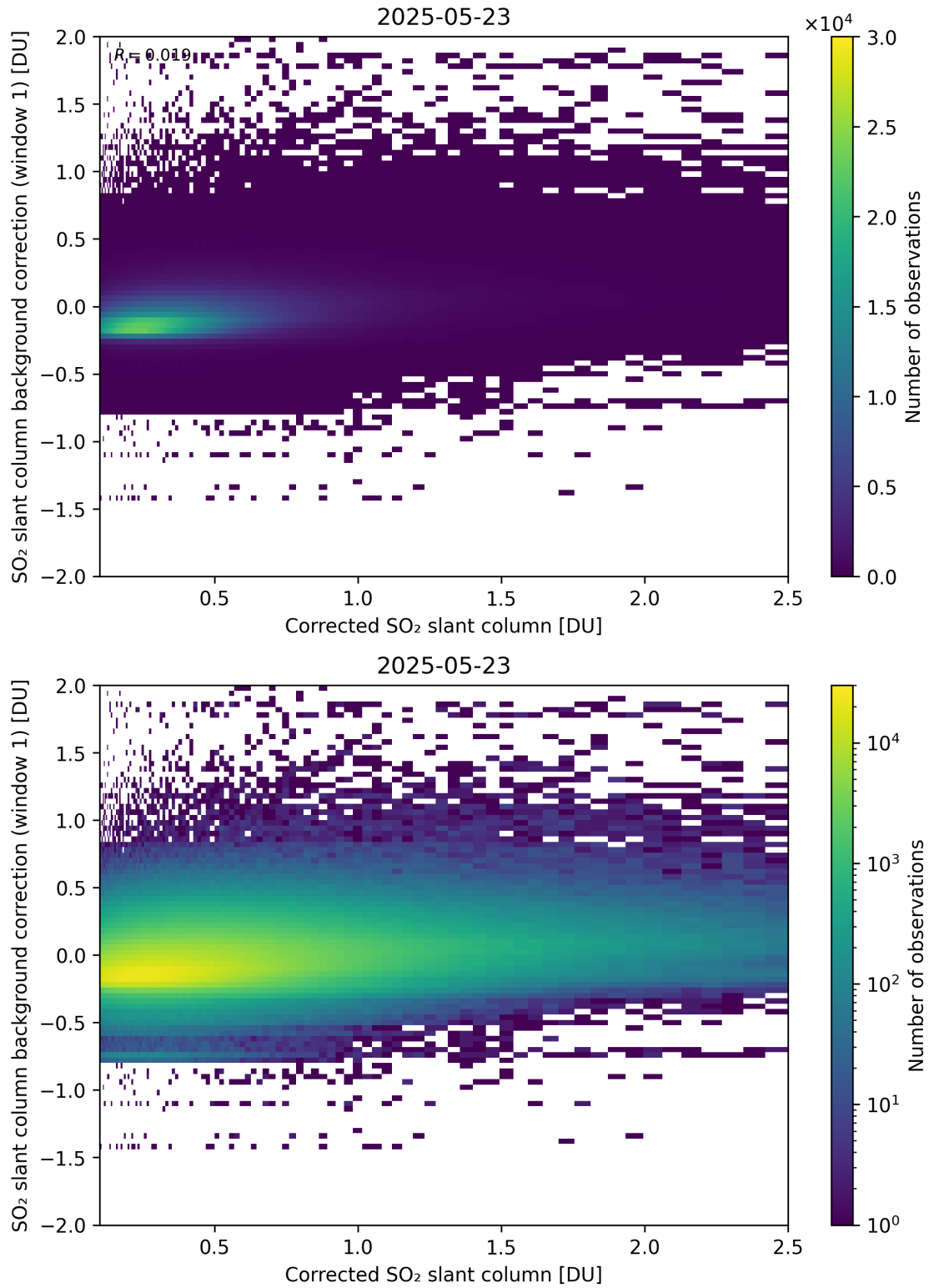
Figure 226: Scatter density plot of “Corrected SO 2 slant column” against “SO 2 slant column background correction (window 1)” for 2025-05-22 to 2025-05-24.
