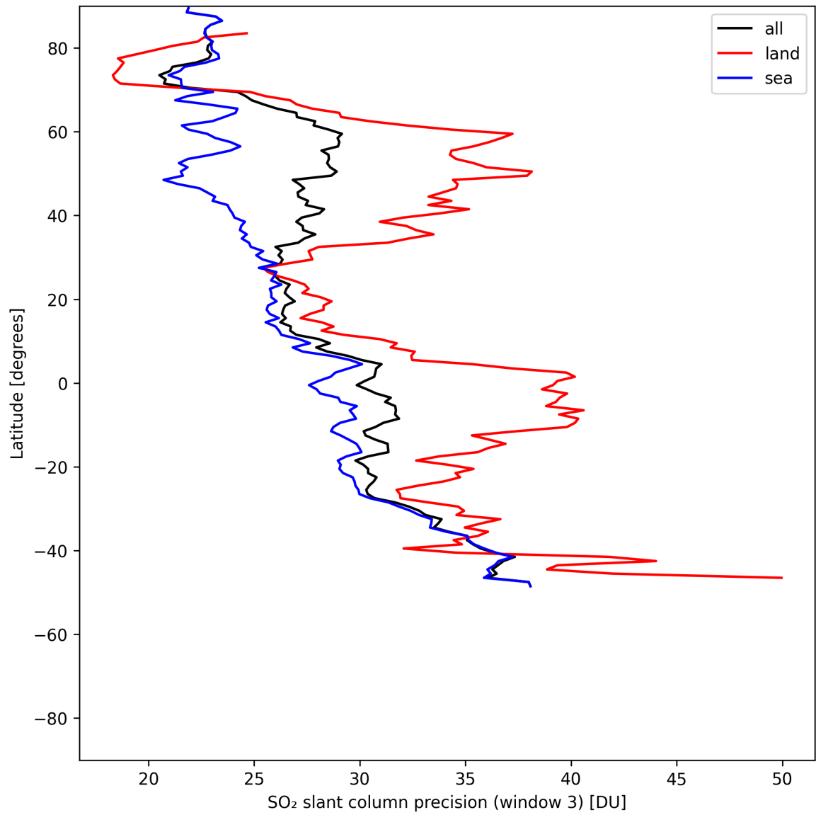
Figure 46: Zonal average of “SO 2 slant column precision (window 3)” for 2025-05-22 to 2025-05-24.
