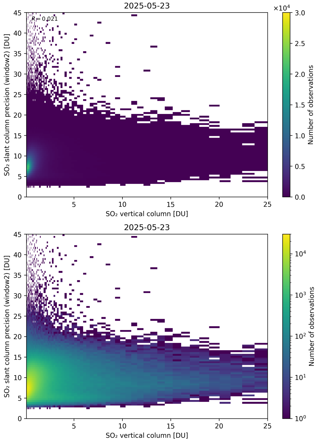
Figure 356: Scatter density plot of “SO 2 vertical column” against “SO 2 slant column precision (window2)” for 2025-05-22 to 2025-05-24.
