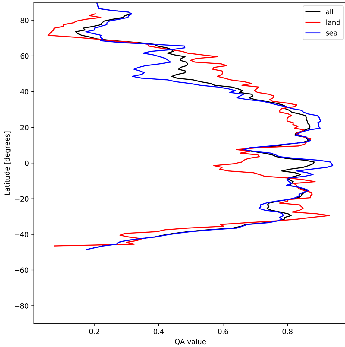
Figure 31: Zonal average of “QA value” for 2025-05-22 to 2025-05-24.
