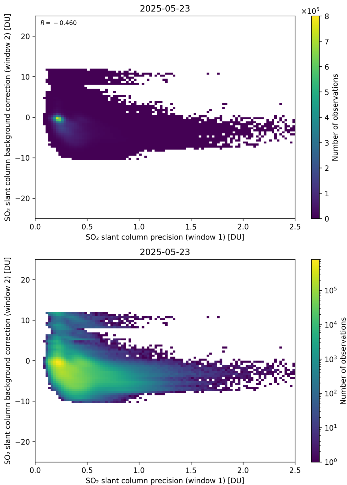
Figure 269: Scatter density plot of “SO 2 slant column precision (window 1)” against “SO 2 slant column background correction (window 2)” for 2025-05-22 to 2025-05-24.
