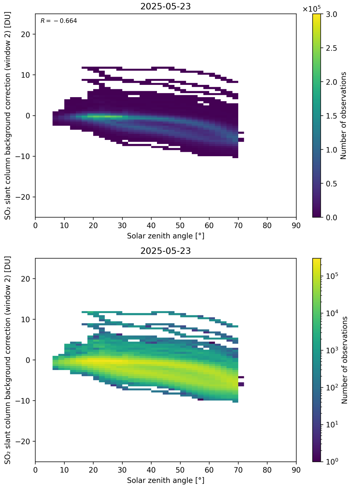
Figure 172: Scatter density plot of “Solar zenith angle” against “SO 2 slant column background correction (window 2)” for 2025-05-22 to 2025-05-24.
