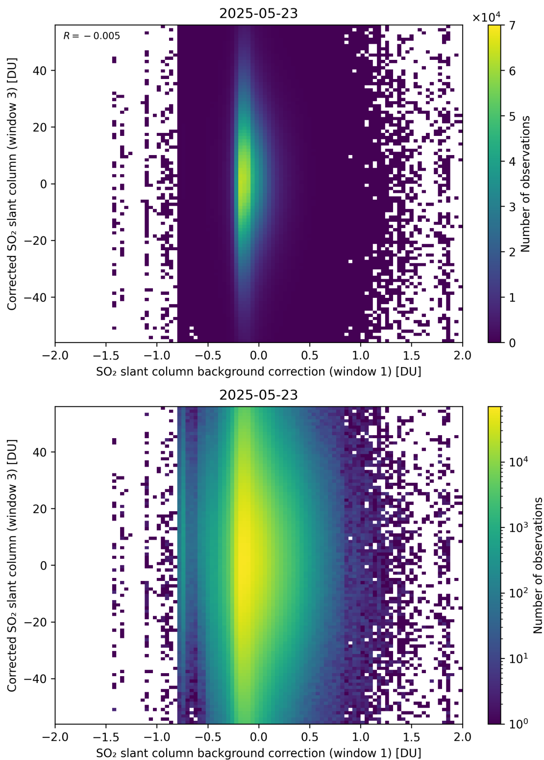
Figure 116: Scatter density plot of “SO 2 slant column background correction (window 1)” against “Corrected SO 2 slant column (window 3)” for 2025-05-22 to 2025-05-24.
