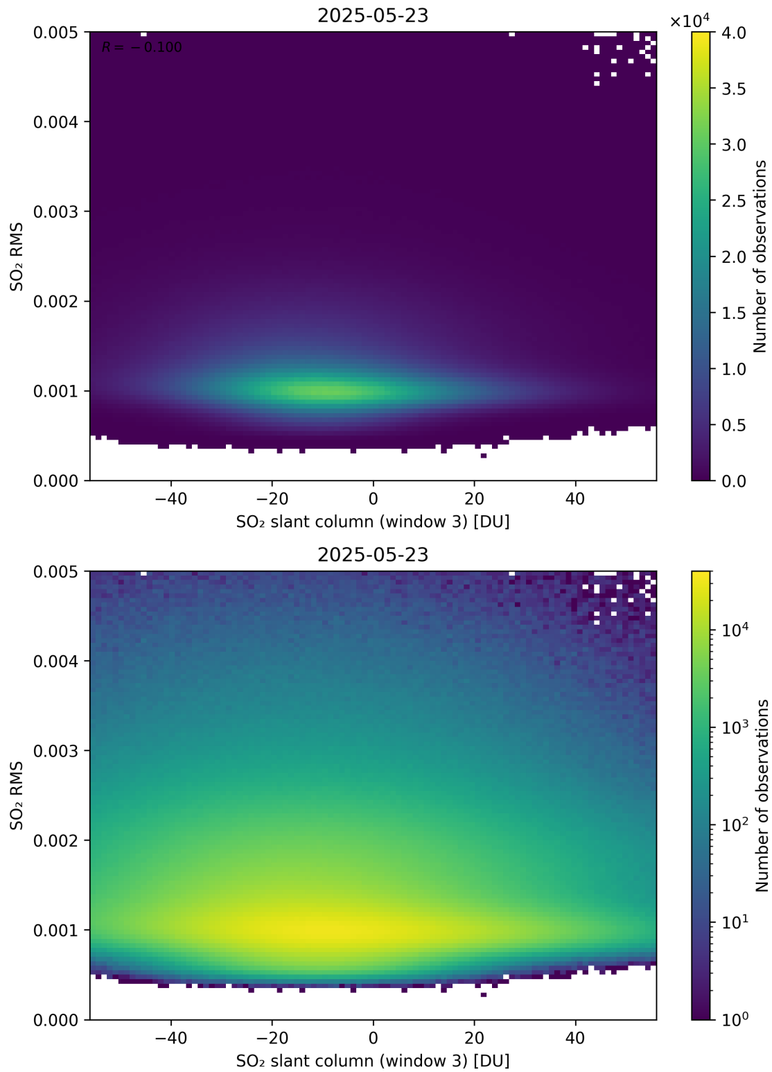
Figure 306: Scatter density plot of “SO 2 slant column (window 3)” against “SO 2 RMS” for 2025-05-22 to 2025-05-24.
