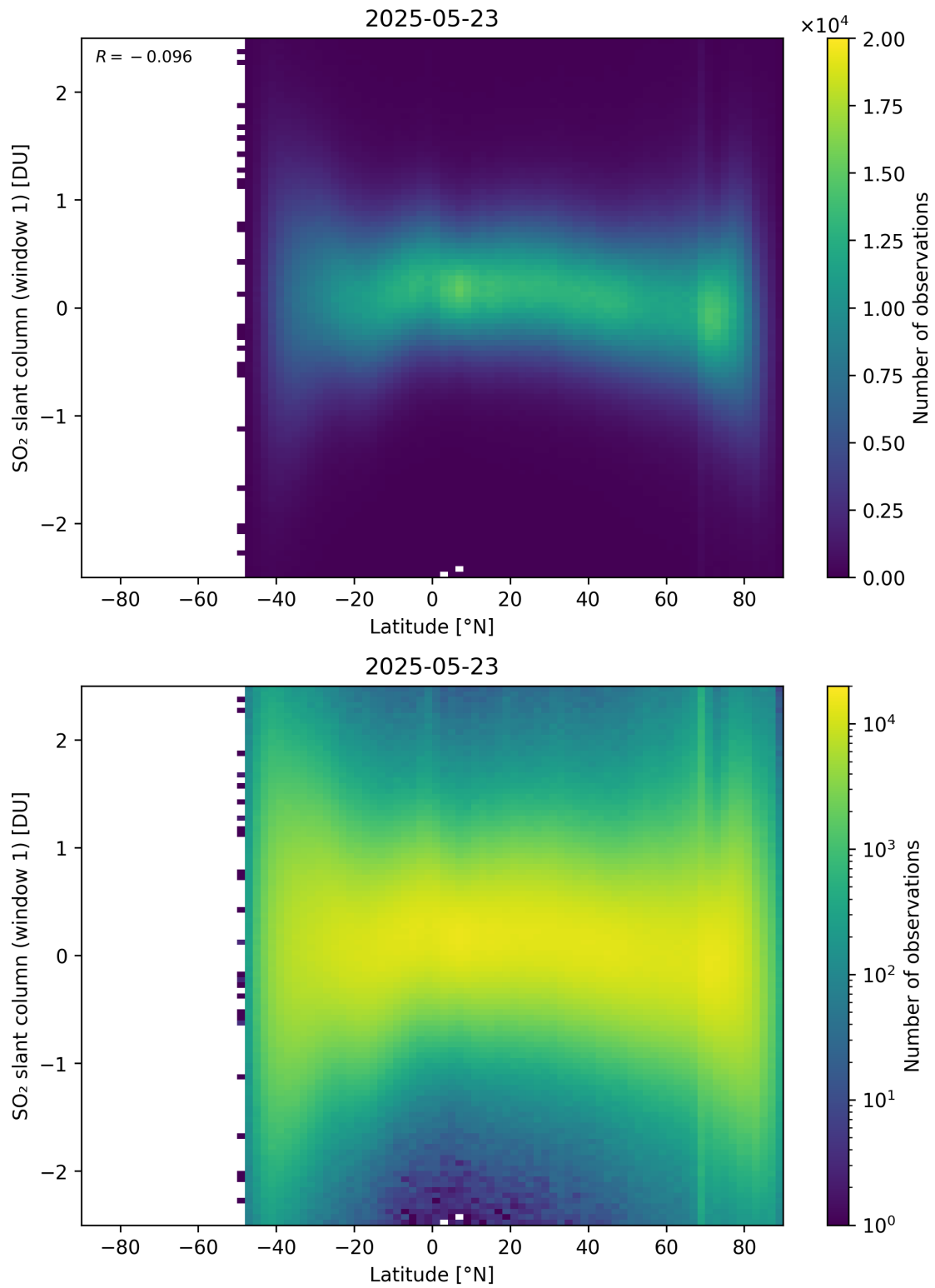
Figure 162: Scatter density plot of “Latitude” against “SO 2 slant column (window 1)” for 2025-05-22 to 2025-05-24.
