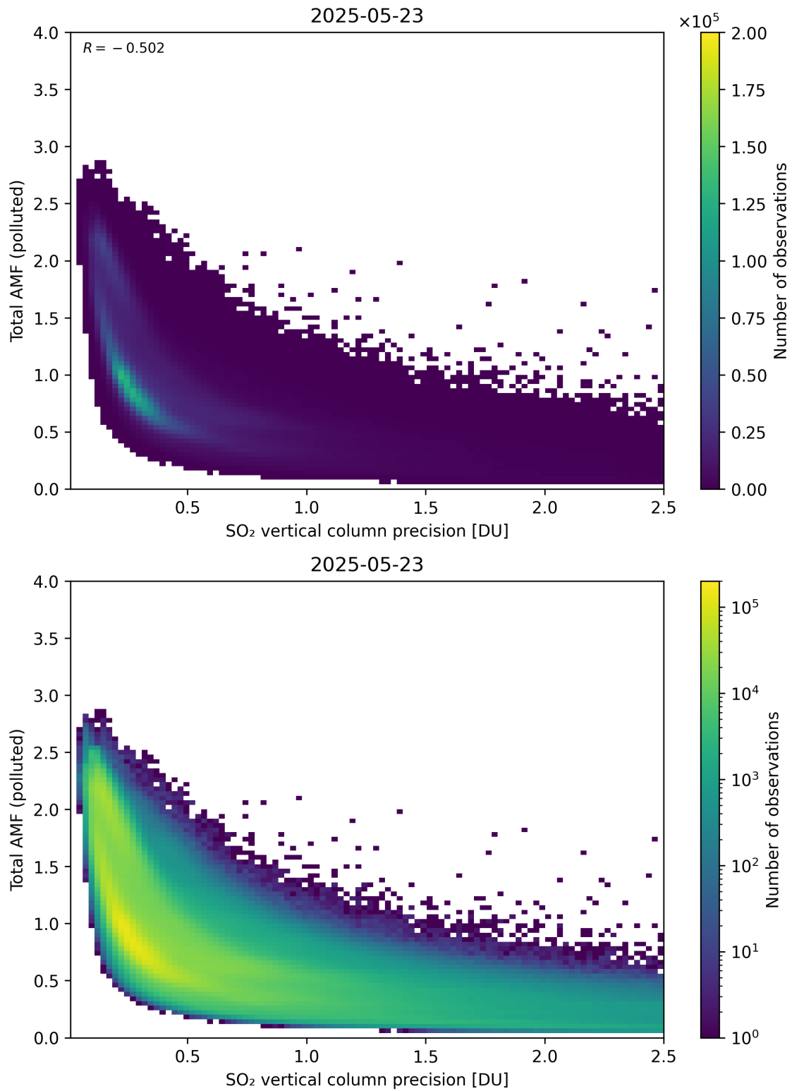
Figure 346: Scatter density plot of “SO 2 vertical column precision” against “Total AMF (polluted)” for 2025-05-22 to 2025-05-24.
