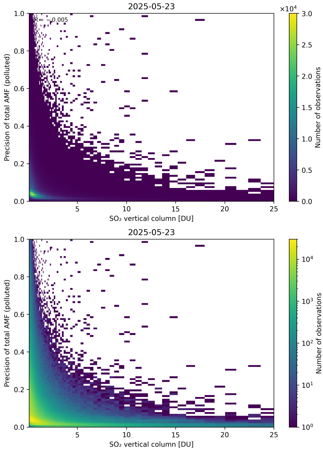
Figure 360: Scatter density plot of “SO 2 vertical column” against “Precision of total AMF (polluted)” for 2025-05-22 to 2025-05-24.
