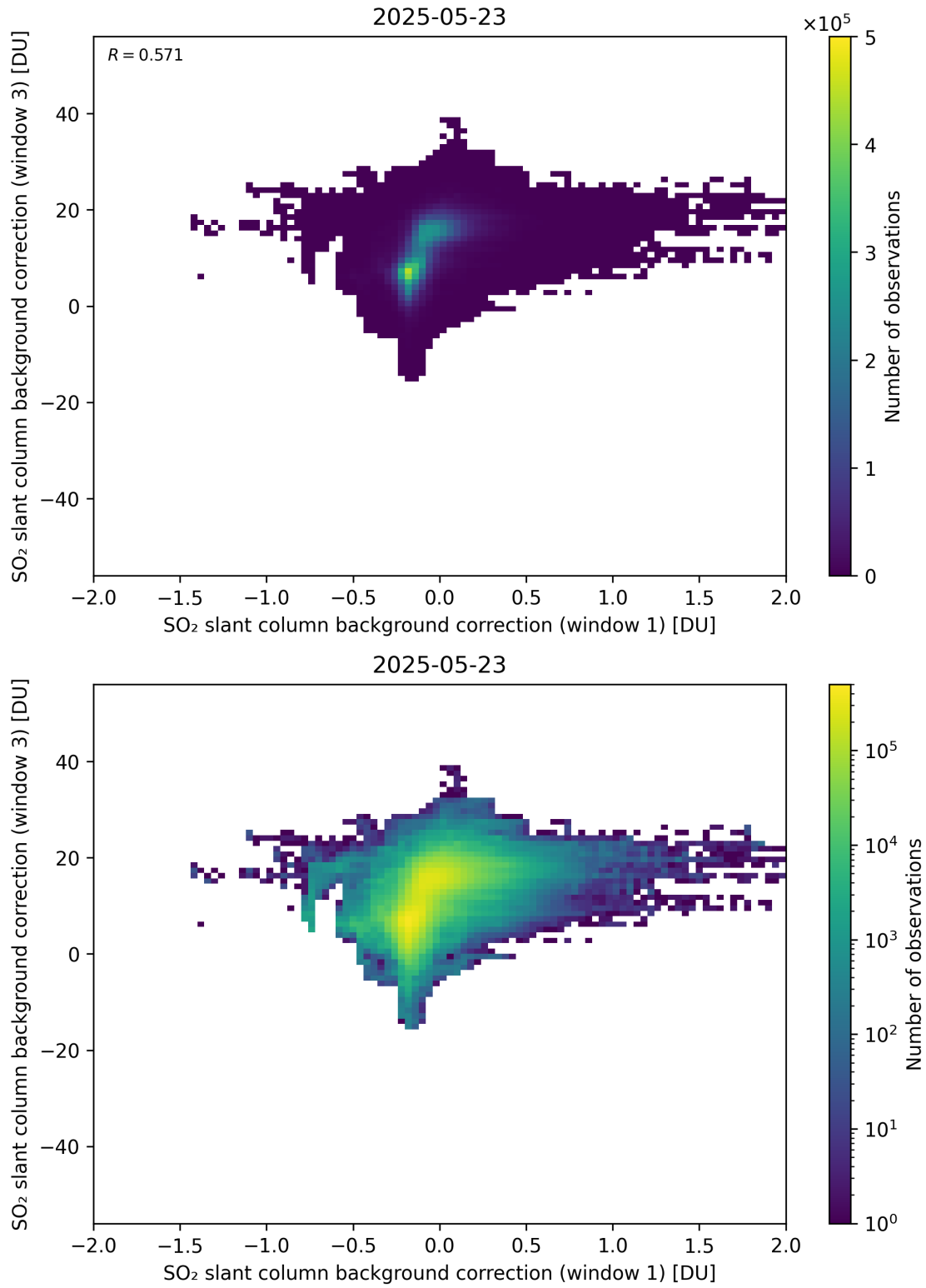
Figure 110: Scatter density plot of “SO 2 slant column background correction (window 1)” against “SO 2 slant column background correction (window 3)” for 2025-05-22 to 2025-05-24.
