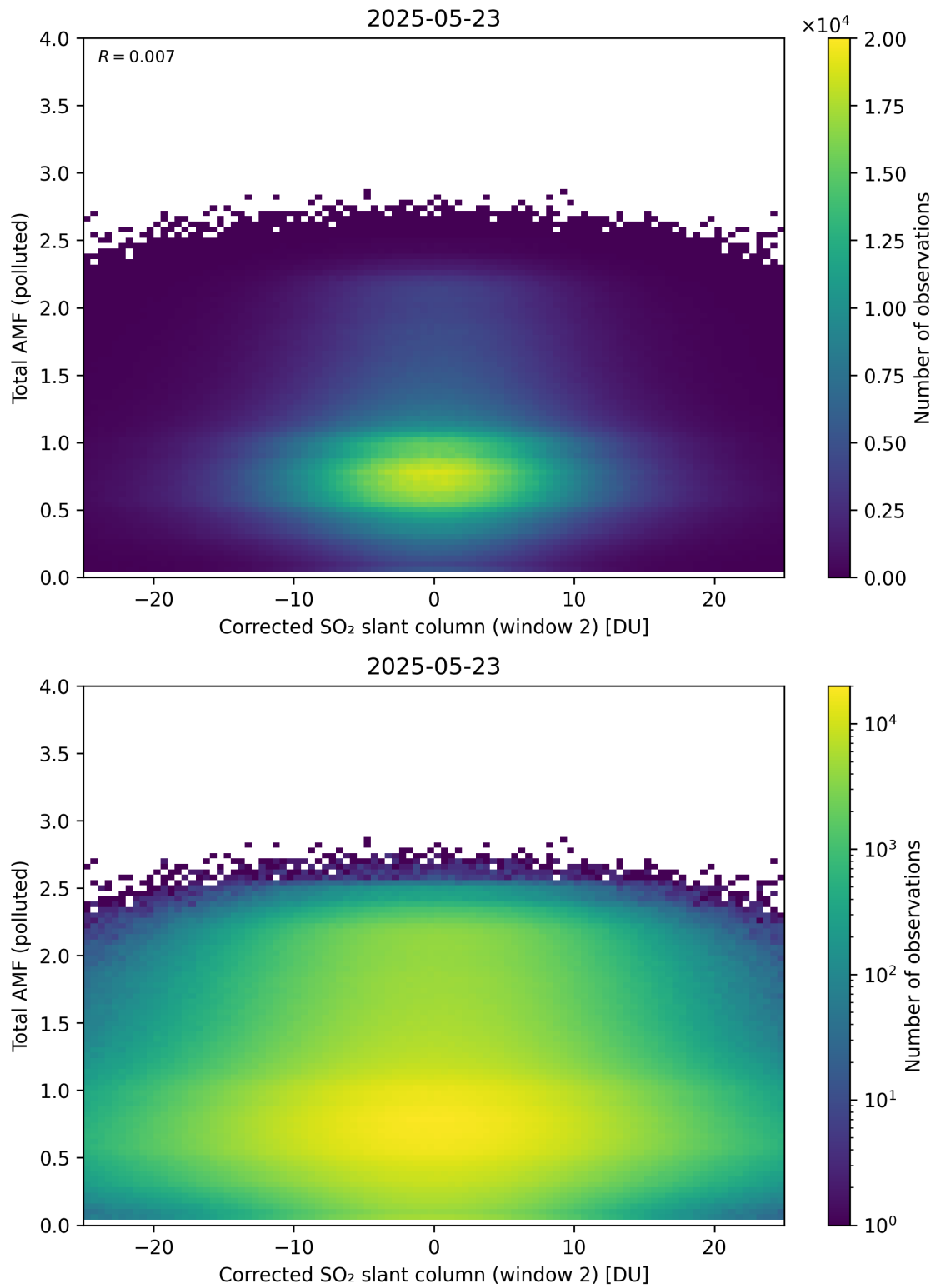
Figure 253: Scatter density plot of “Corrected SO 2 slant column (window 2)” against “Total AMF (polluted)” for 2025-05-22 to 2025-05-24.
