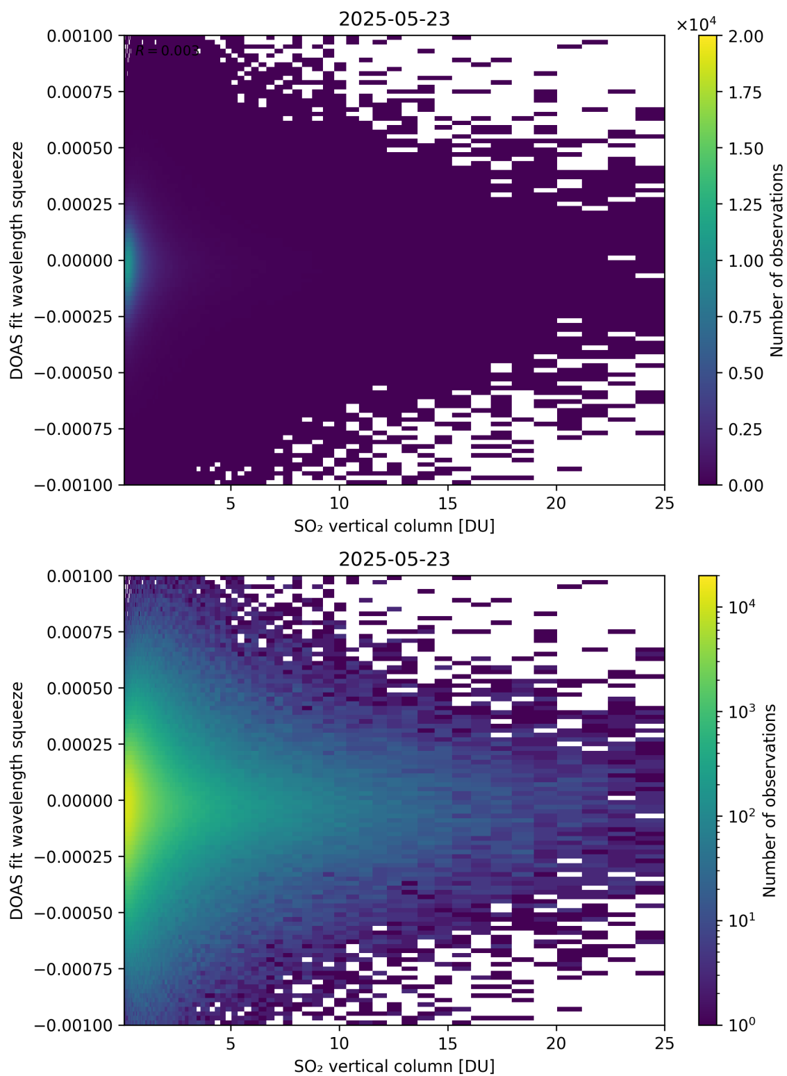
Figure 327: Scatter density plot of “SO 2 vertical column” against “DOAS fit wavelength squeeze” for 2025-05-22 to 2025-05-24.
