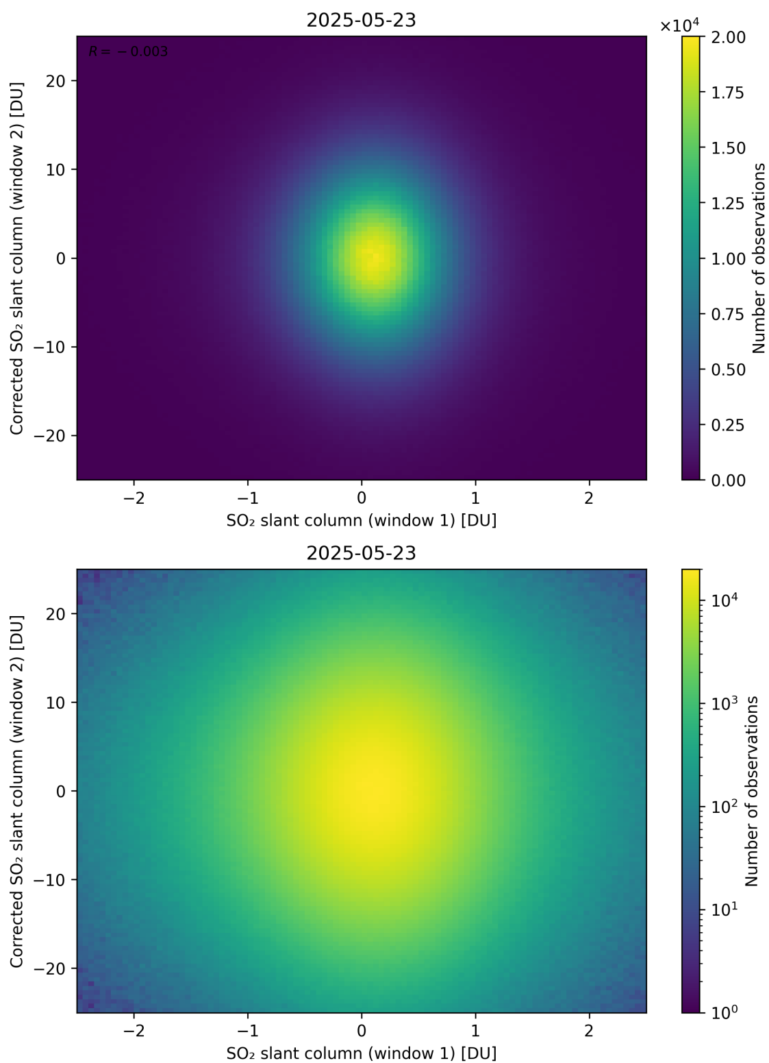
Figure 283: Scatter density plot of “SO 2 slant column (window 1)” against “Corrected SO 2 slant column (window 2)” for 2025-05-22 to 2025-05-24.
