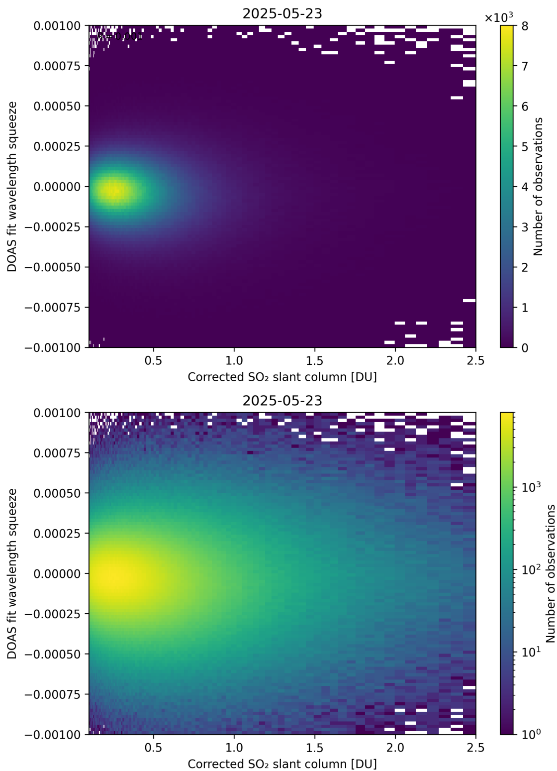
Figure 230: Scatter density plot of “Corrected SO 2 slant column” against “DOAS fit wavelength squeeze” for 2025-05-22 to 2025-05-24.
