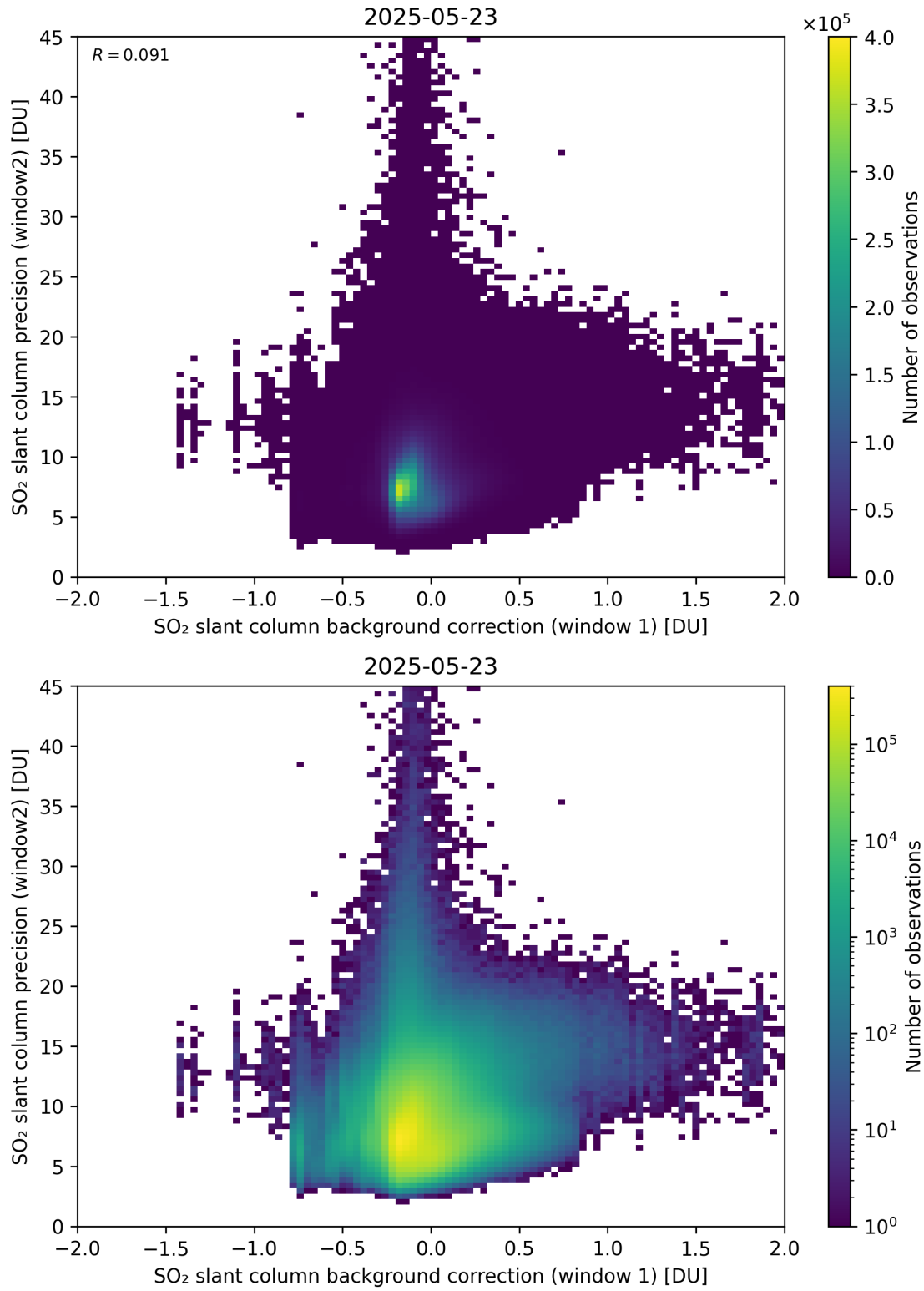
Figure 117: Scatter density plot of “SO 2 slant column background correction (window 1)” against “SO 2 slant column precision (window2)” for 2025-05-22 to 2025-05-24.
