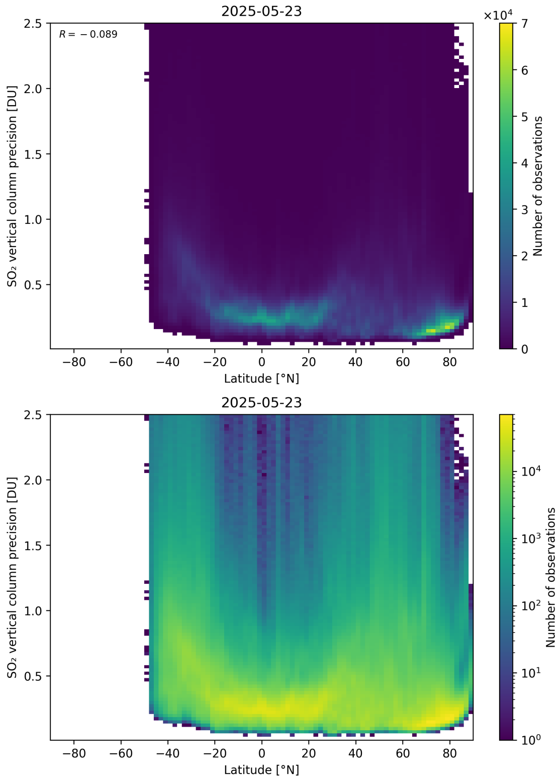
Figure 170: Scatter density plot of “Latitude” against “SO 2 vertical column precision” for 2025-05-22 to 2025-05-24.
