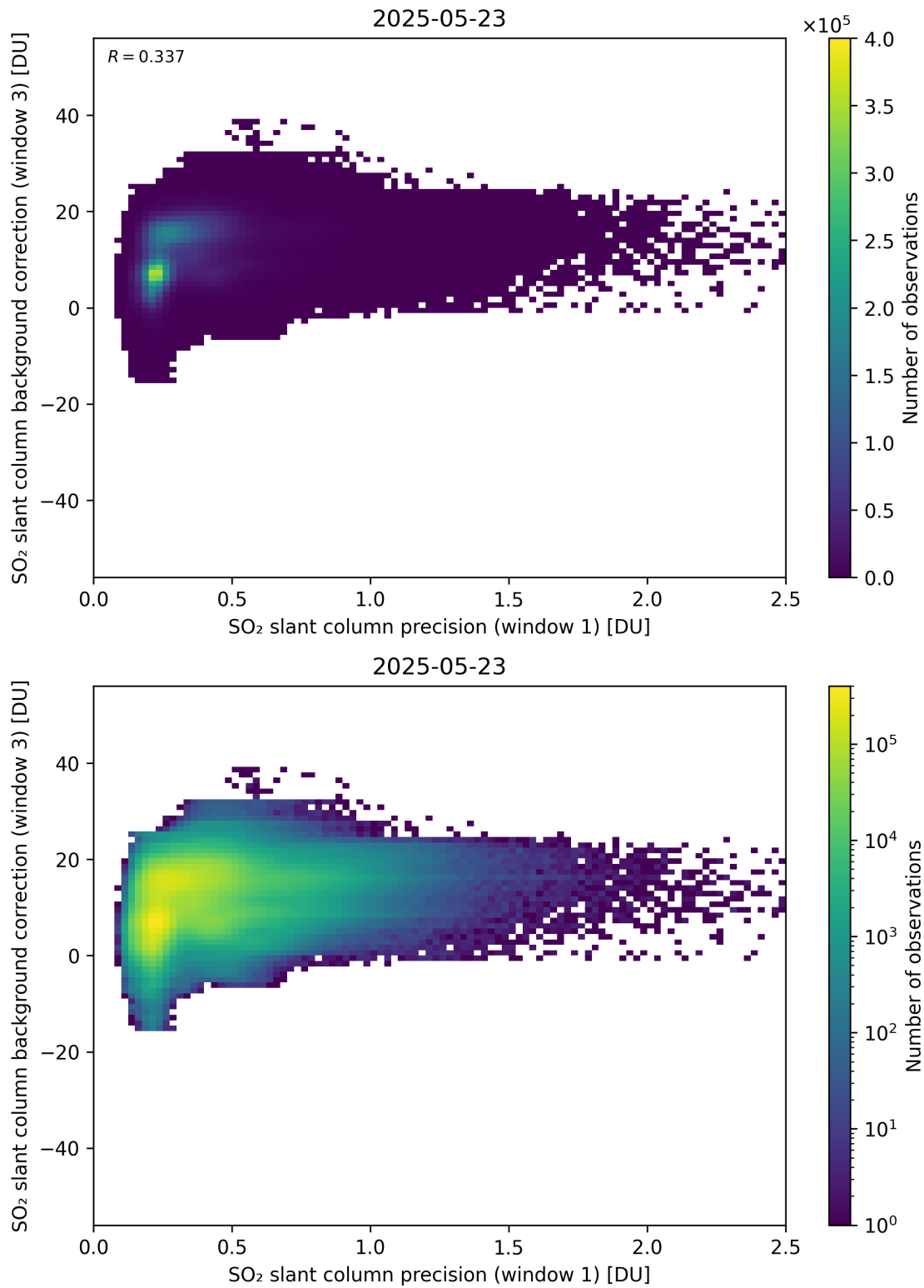
Figure 270: Scatter density plot of “SO 2 slant column precision (window 1)” against “SO 2 slant column background correction (window 3)” for 2025-05-22 to 2025-05-24.
