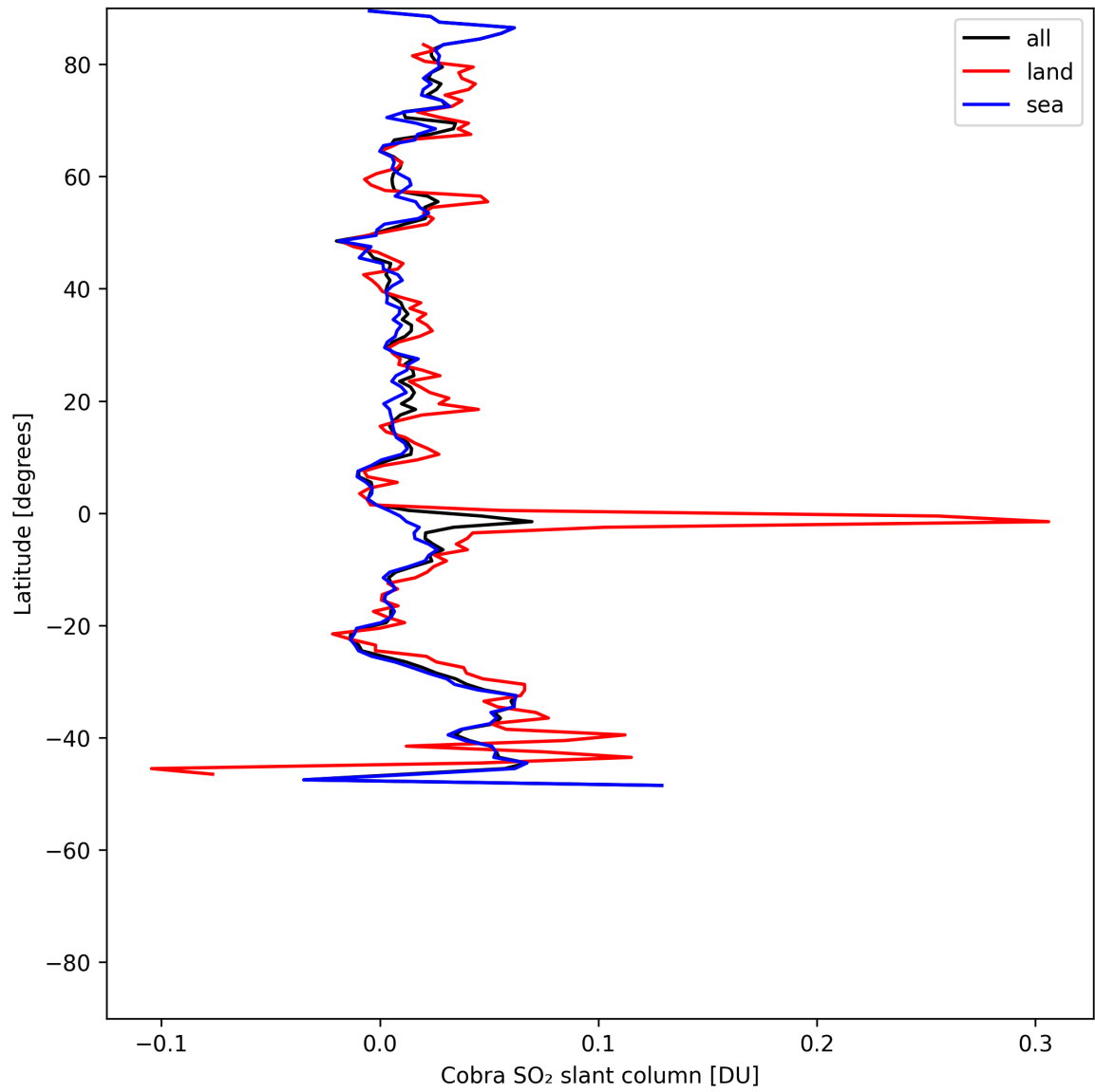
Figure 35: Zonal average of “Cobra SO 2 slant column” for 2025-05-22 to 2025-05-24.
