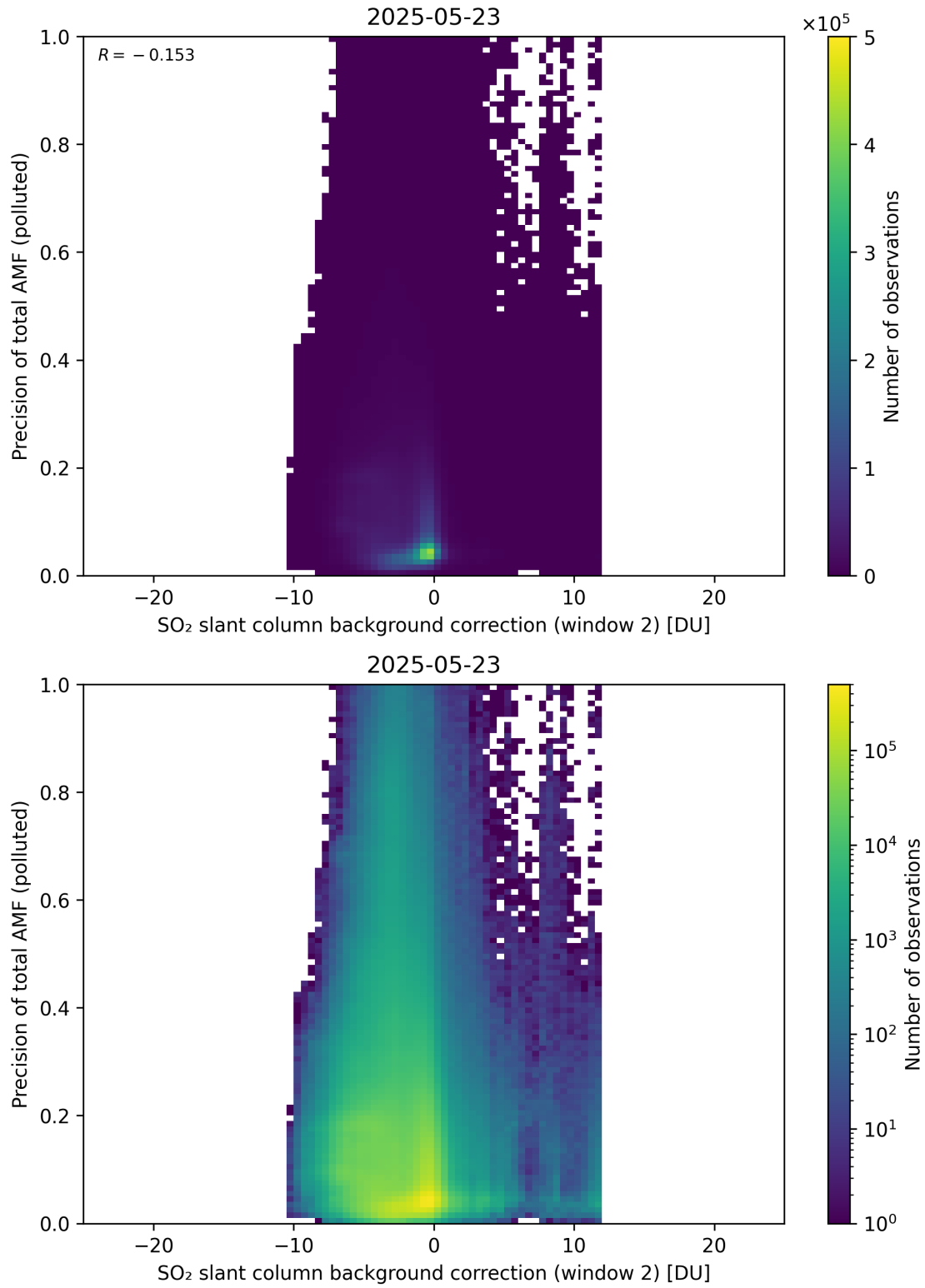
Figure 131: Scatter density plot of “SO 2 slant column background correction (window 2)” against “Precision of total AMF (polluted)” for 2025-05-22 to 2025-05-24.
