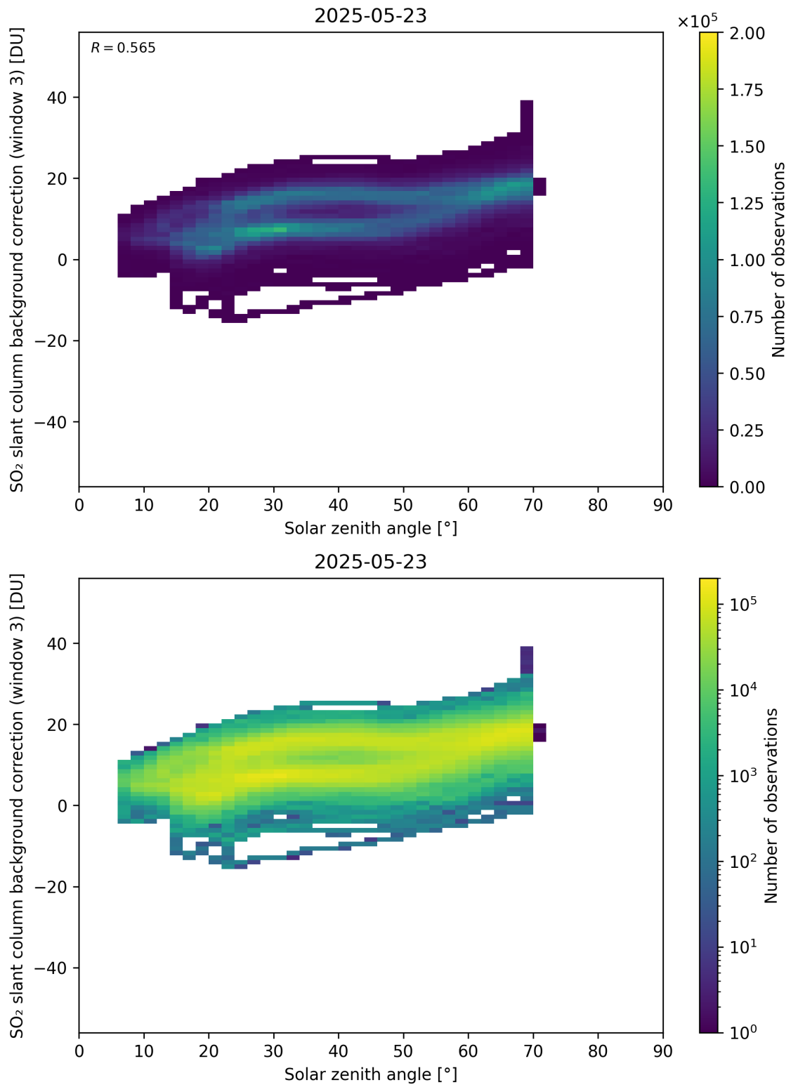
Figure 173: Scatter density plot of “Solar zenith angle” against “SO 2 slant column background correction (window 3)” for 2025-05-22 to 2025-05-24.
