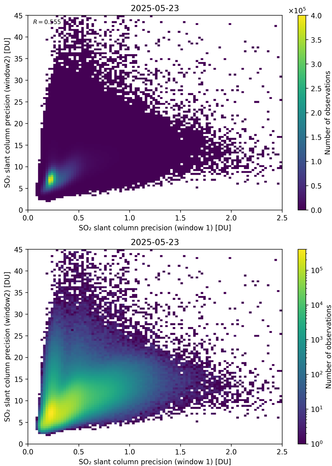
Figure 277: Scatter density plot of “SO 2 slant column precision (window 1)” against “SO 2 slant column precision (window2)” for 2025-05-22 to 2025-05-24.
