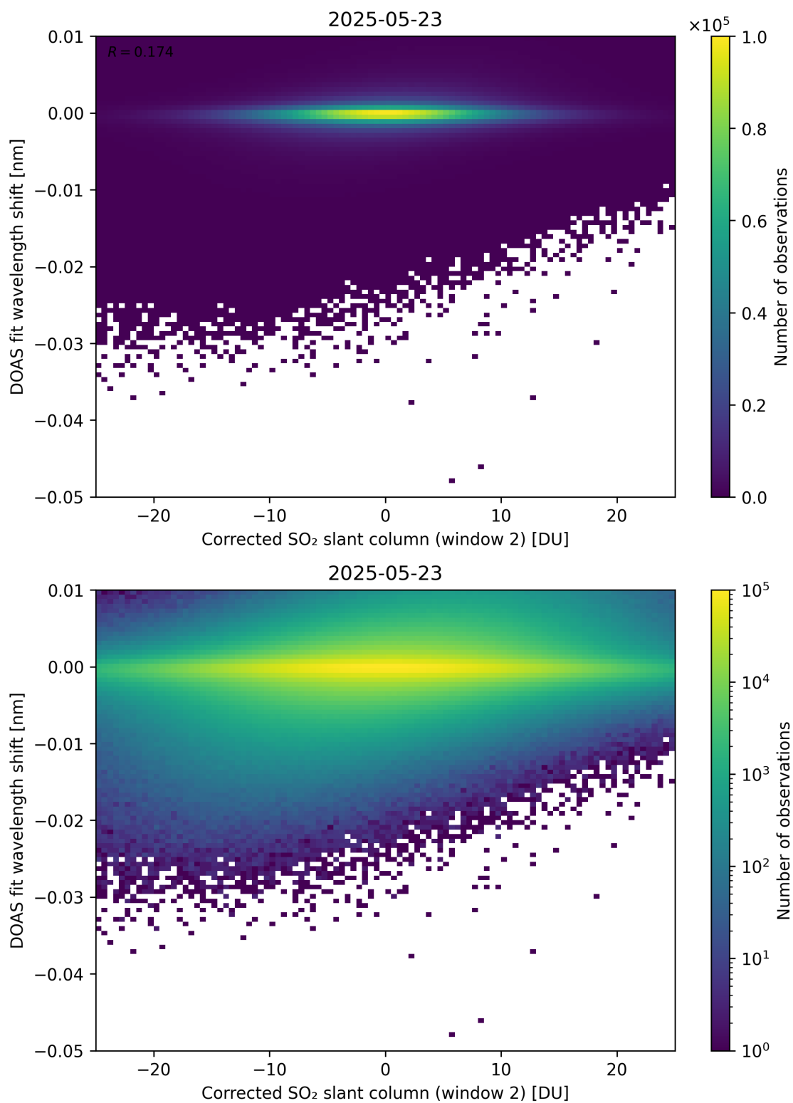
Figure 246: Scatter density plot of “Corrected SO 2 slant column (window 2)” against “DOAS fit wavelength shift” for 2025-05-22 to 2025-05-24.
