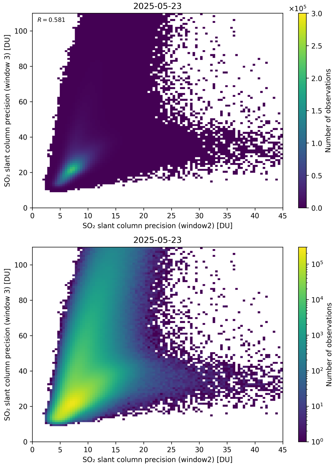
Figure 300: Scatter density plot of “SO 2 slant column precision (window2)” against “SO 2 slant column precision (window 3)” for 2025-05-22 to 2025-05-24.
