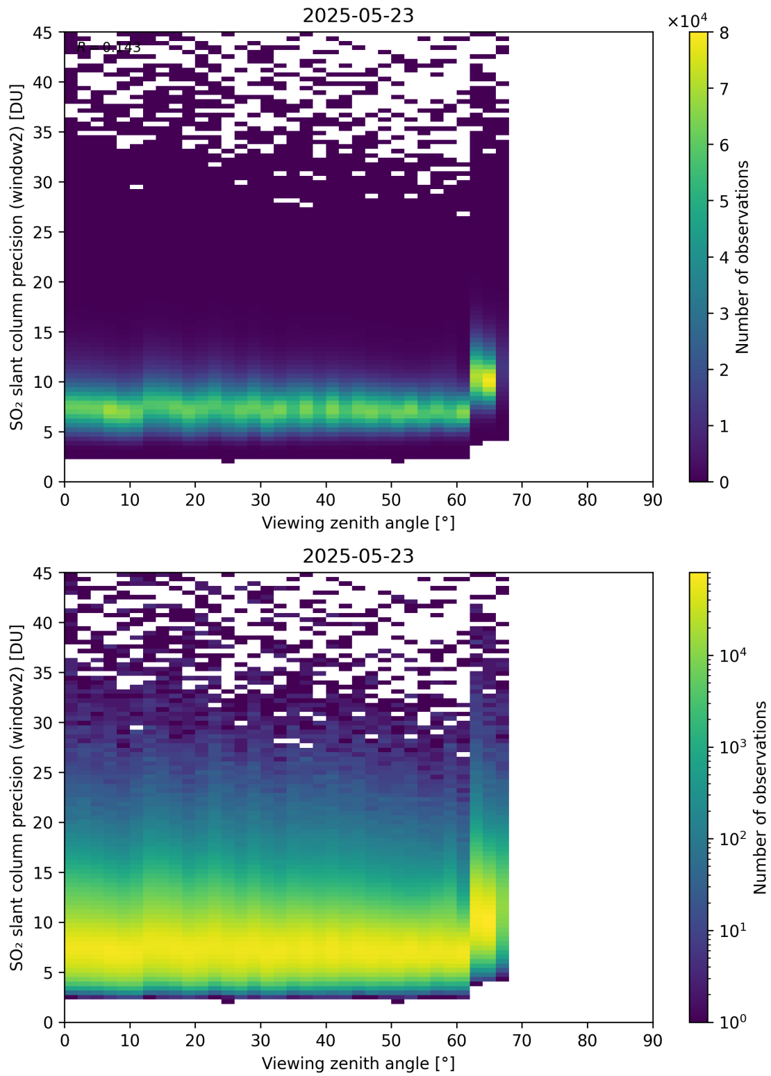
Figure 378: Scatter density plot of “Viewing zenith angle” against “SO 2 slant column precision (window2)” for 2025-05-22 to 2025-05-24.
