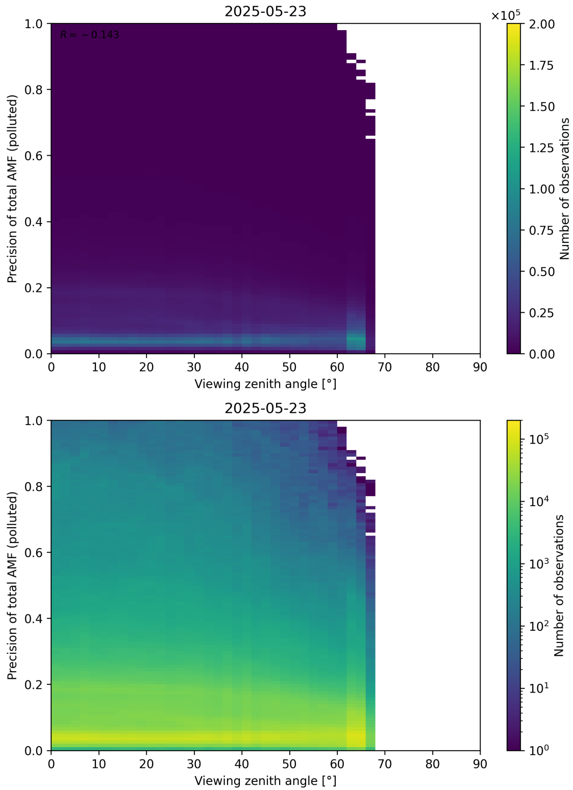
Figure 382: Scatter density plot of “Viewing zenith angle” against “Precision of total AMF (polluted)” for 2025-05-22 to 2025-05-24.
