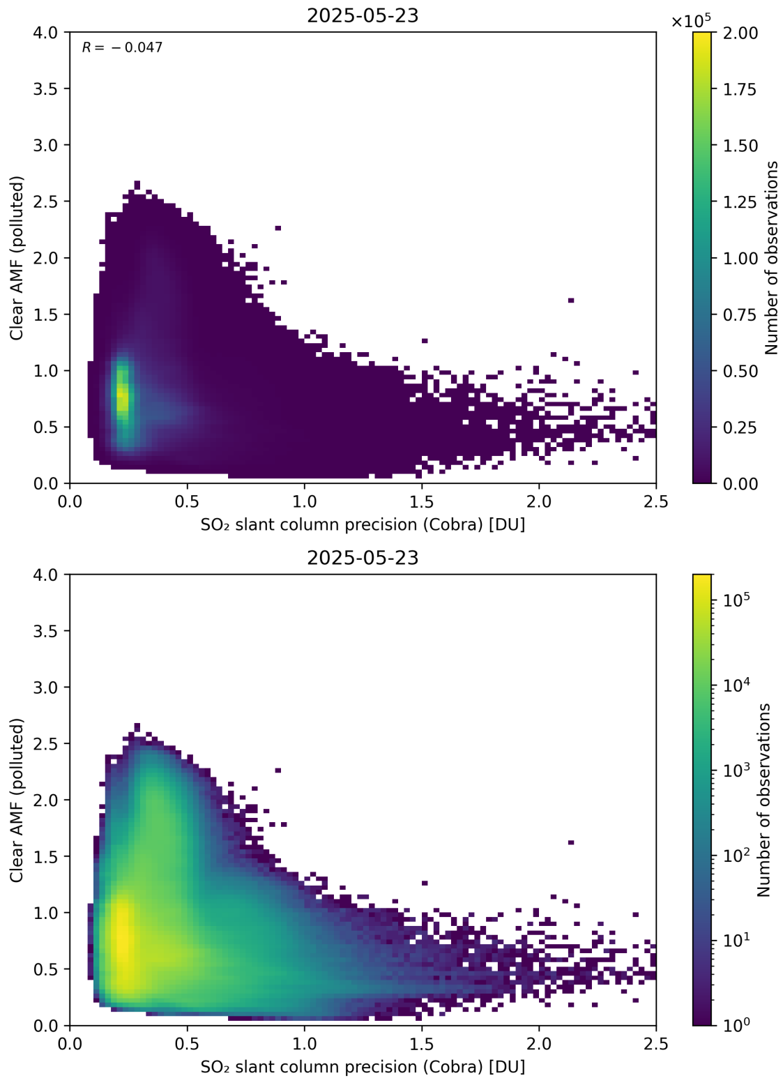
Figure 205: Scatter density plot of “SO 2 slant column precision (Cobra)” against “Clear AMF (polluted)” for 2025-05-22 to 2025-05-24.
