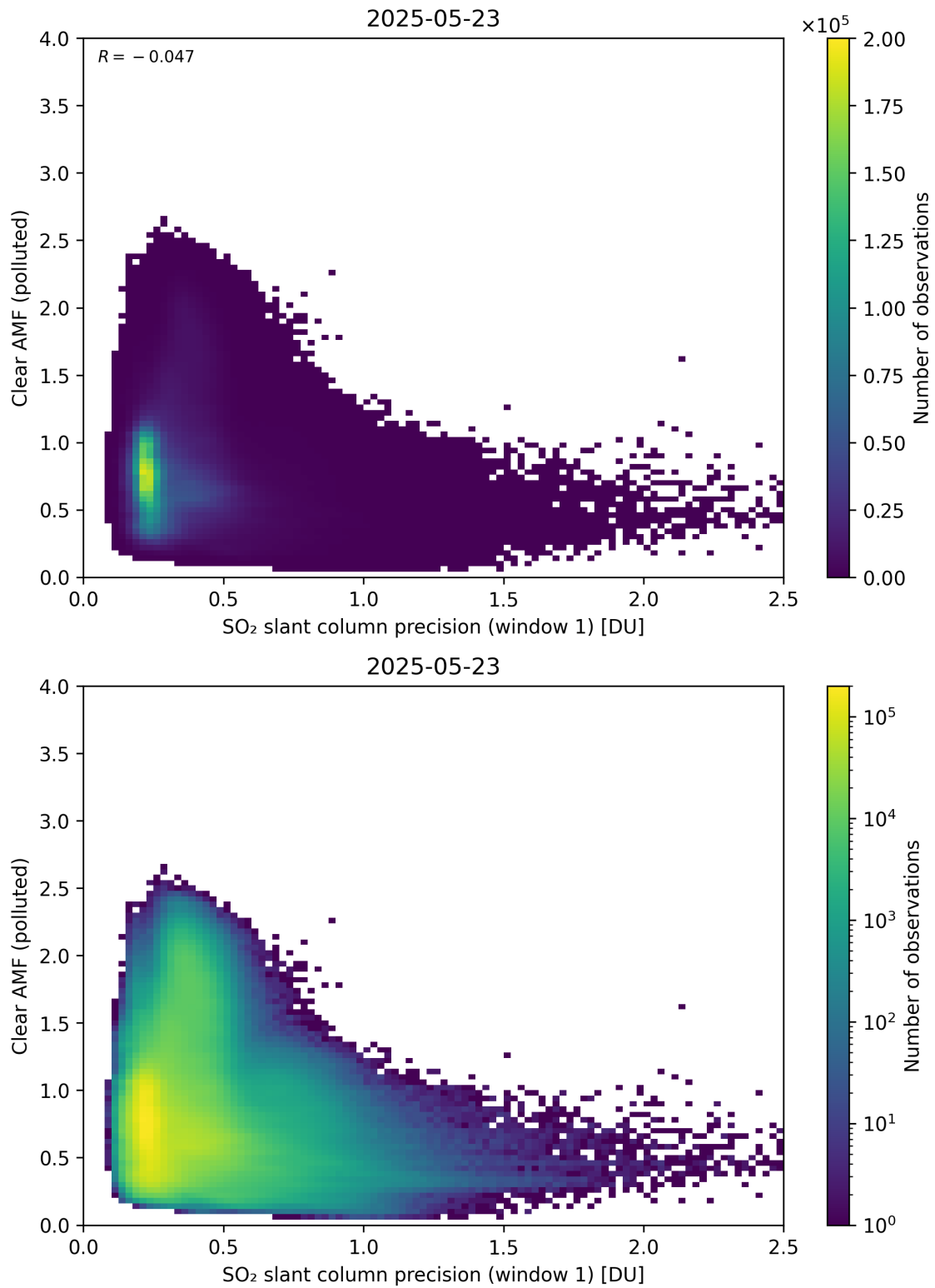
Figure 274: Scatter density plot of “SO 2 slant column precision (window 1)” against “Clear AMF (polluted)” for 2025-05-22 to 2025-05-24.
