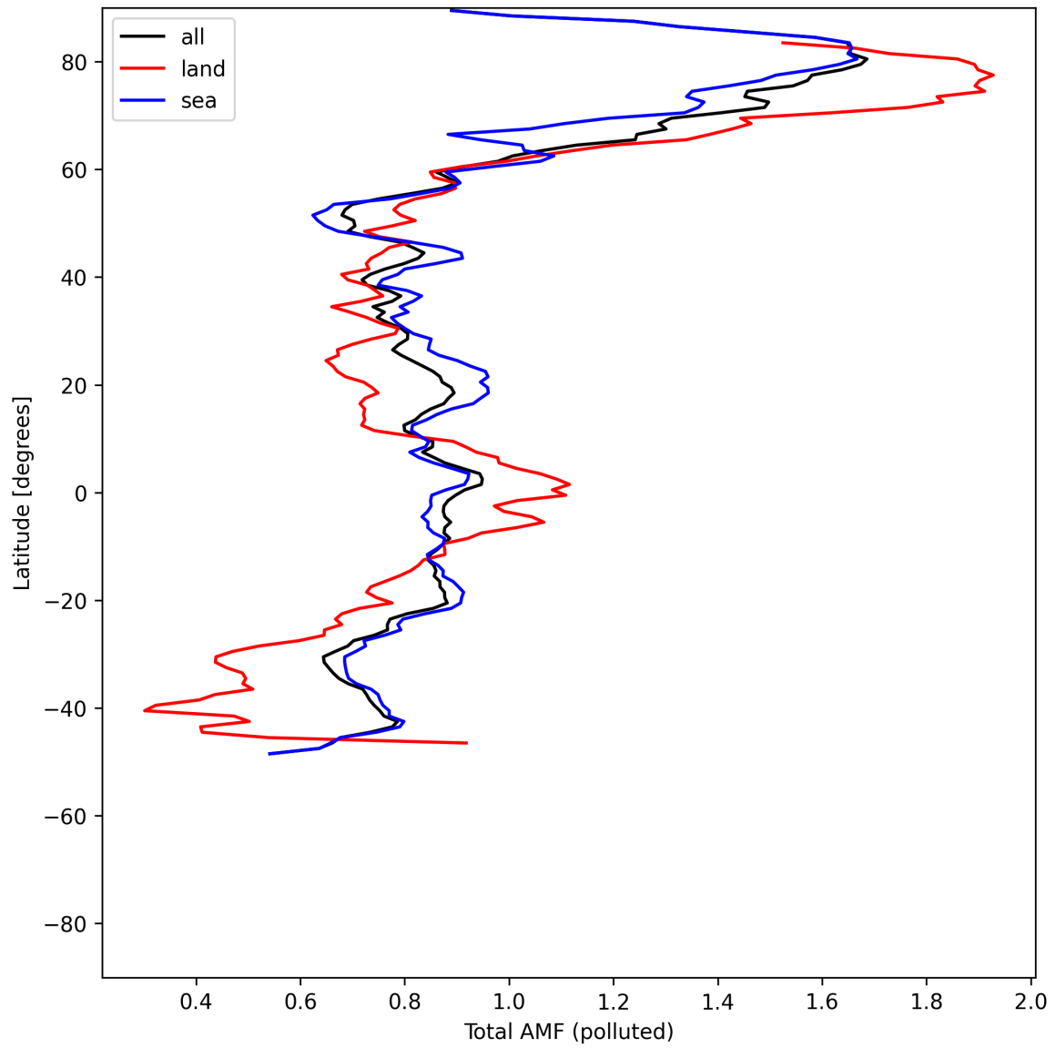
Figure 53: Zonal average of “Total AMF (polluted)” for 2025-05-22 to 2025-05-24.
