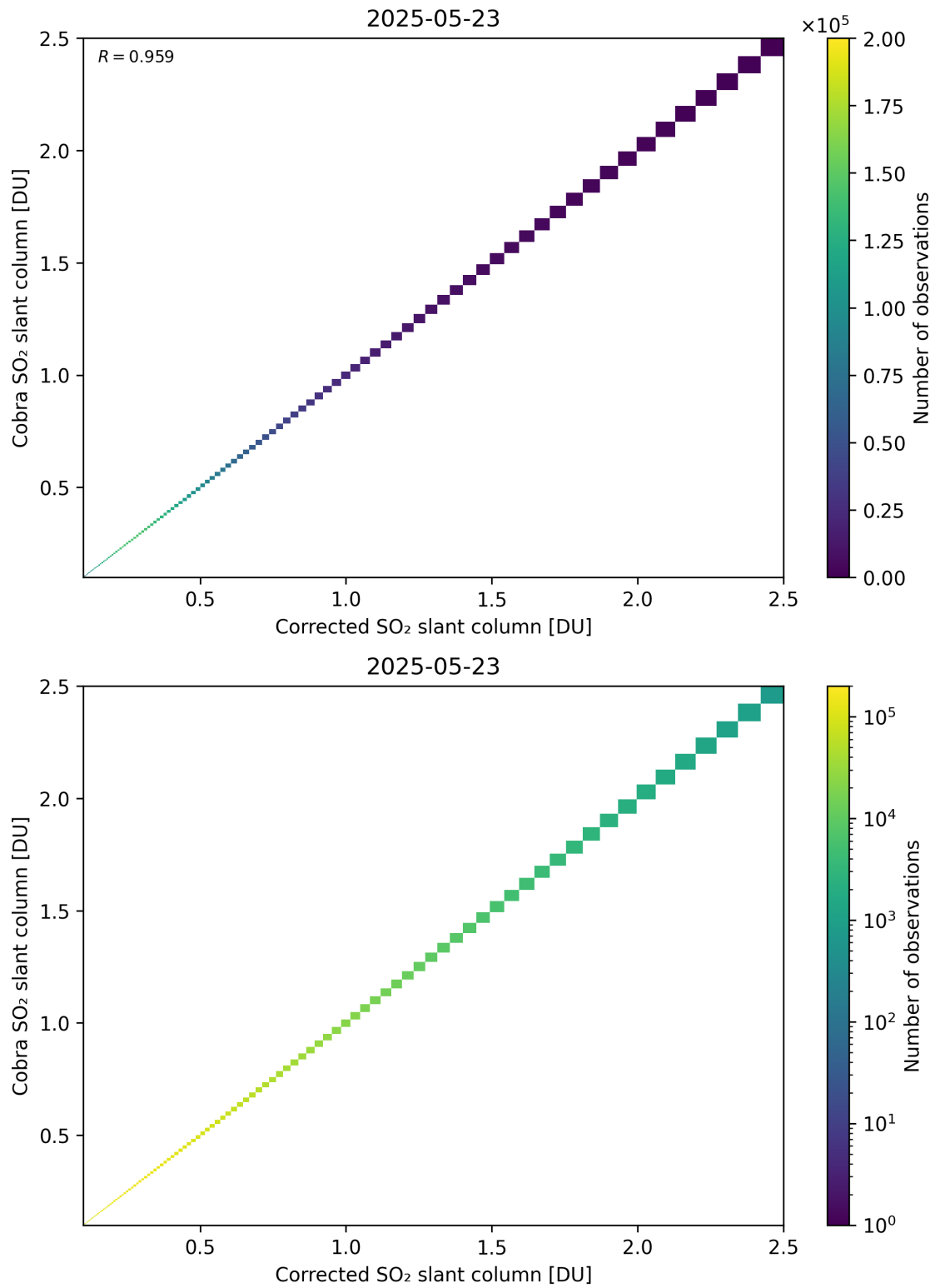
Figure 233: Scatter density plot of “Corrected SO 2 slant column” against “Cobra SO 2 slant column” for 2025-05-22 to 2025-05-24.
