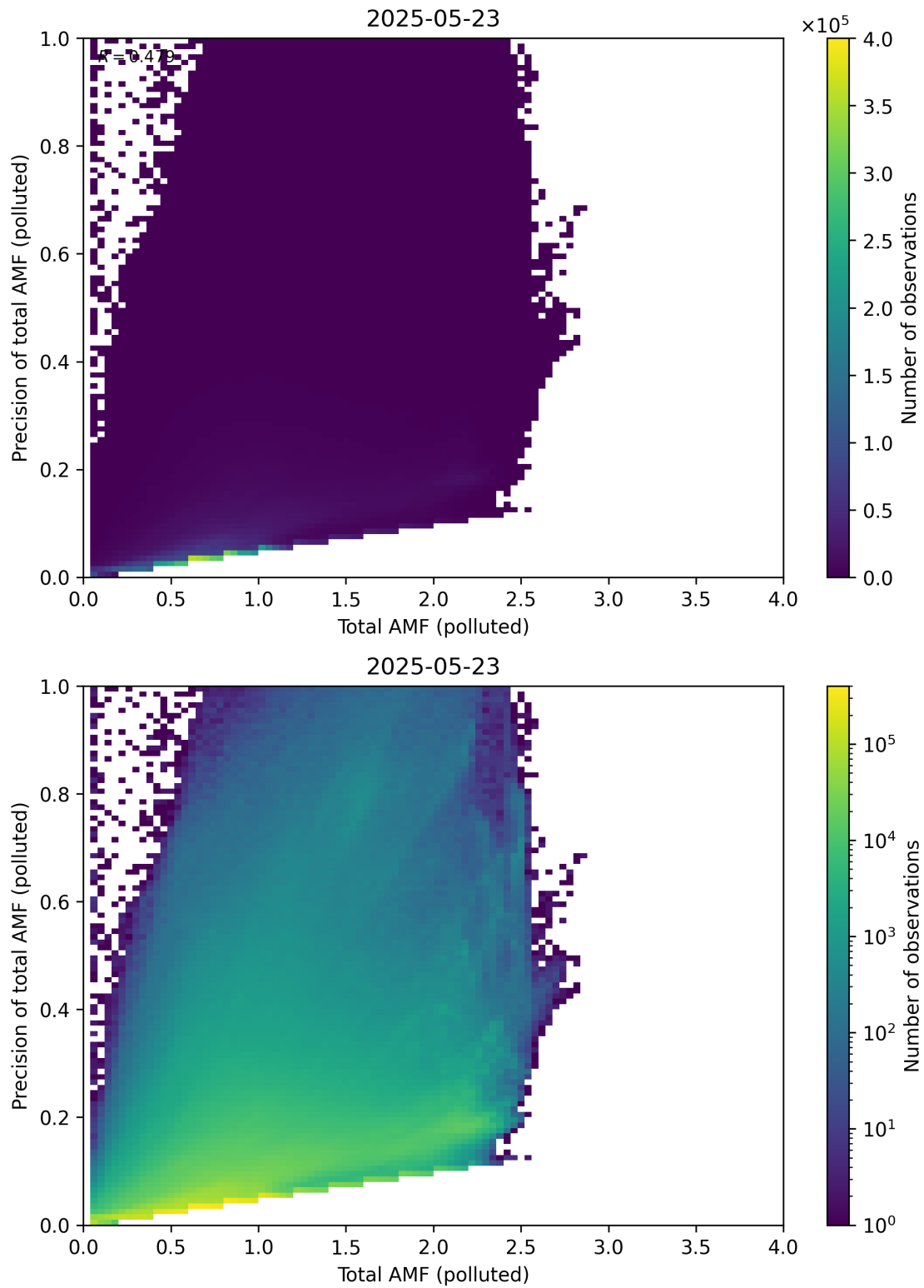
Figure 322: Scatter density plot of “Total AMF (polluted)” against “Precision of total AMF (polluted)” for 2025-05-22 to 2025-05-24.
