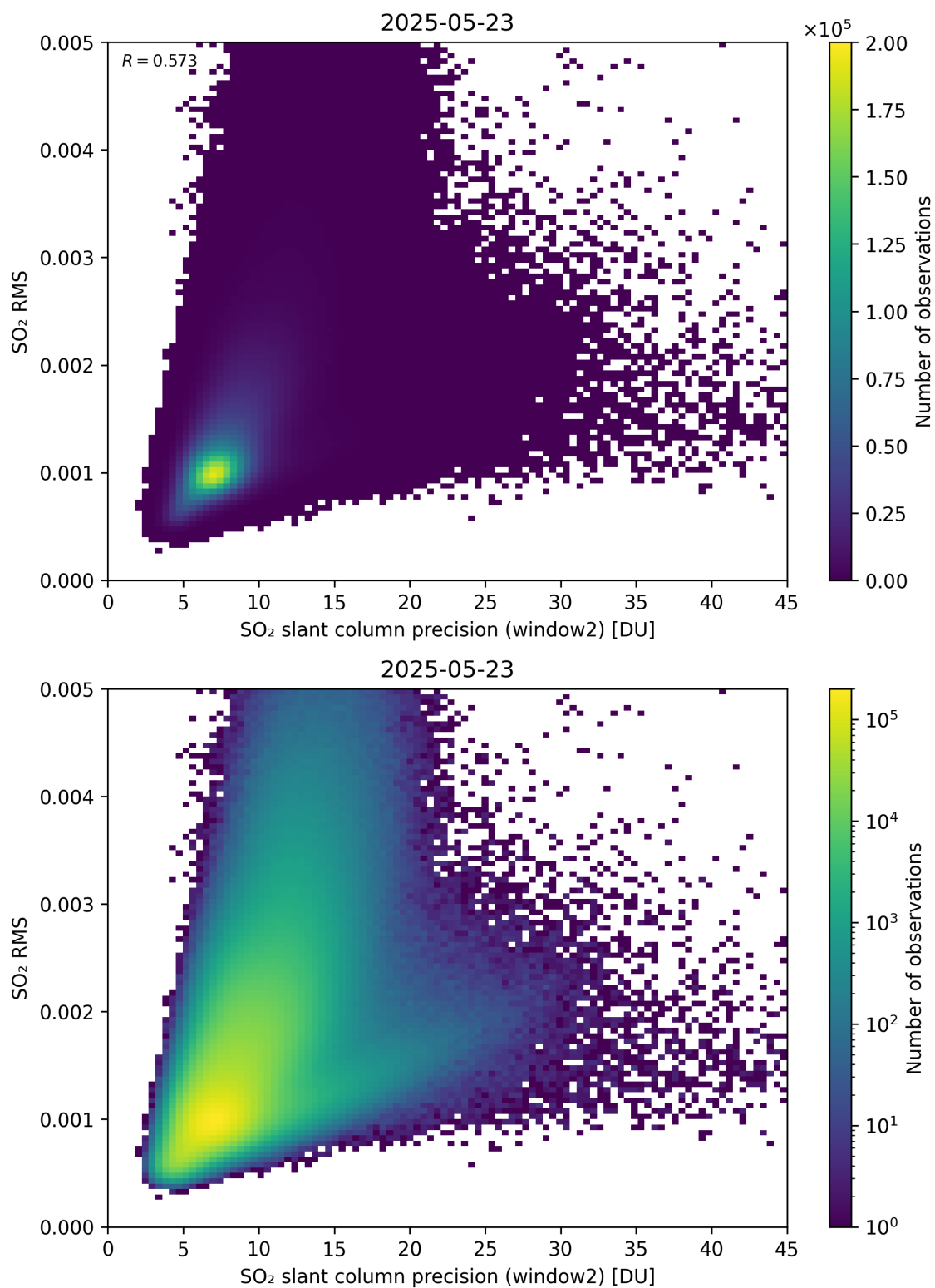
Figure 295: Scatter density plot of “SO 2 slant column precision (window2)” against “SO 2 RMS” for 2025-05-22 to 2025-05-24.
