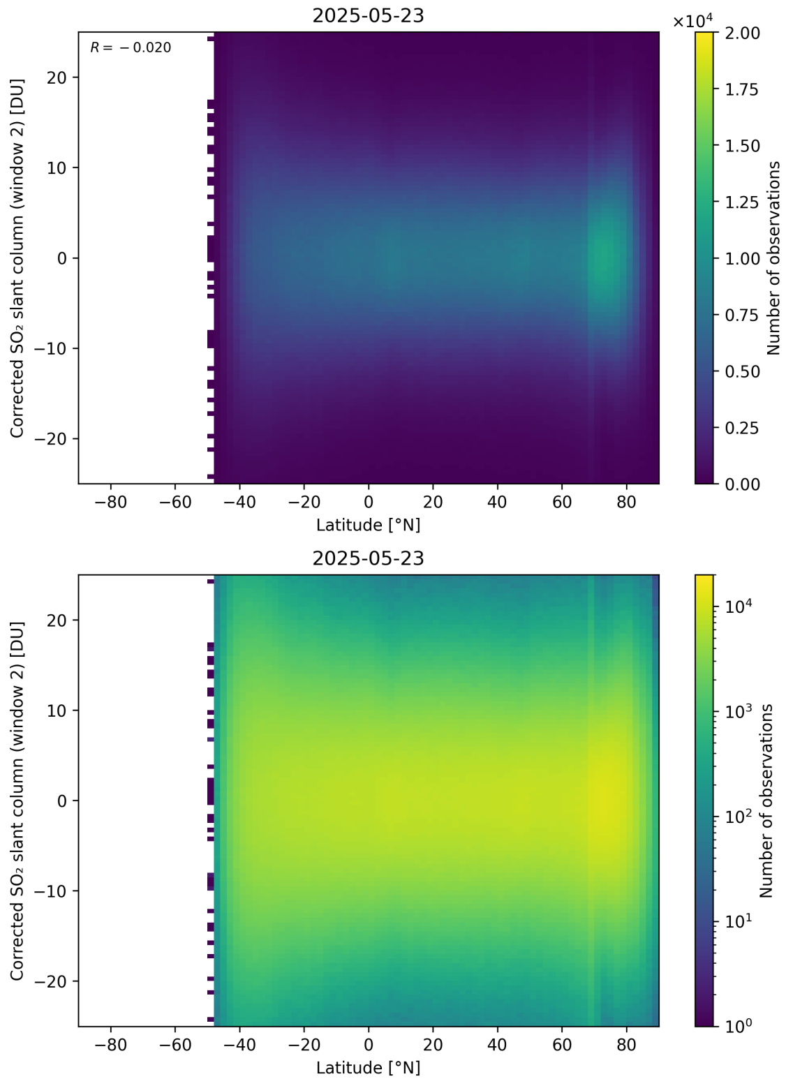
Figure 160: Scatter density plot of “Latitude” against “Corrected SO 2 slant column (window 2)” for 2025-05-22 to 2025-05-24.
