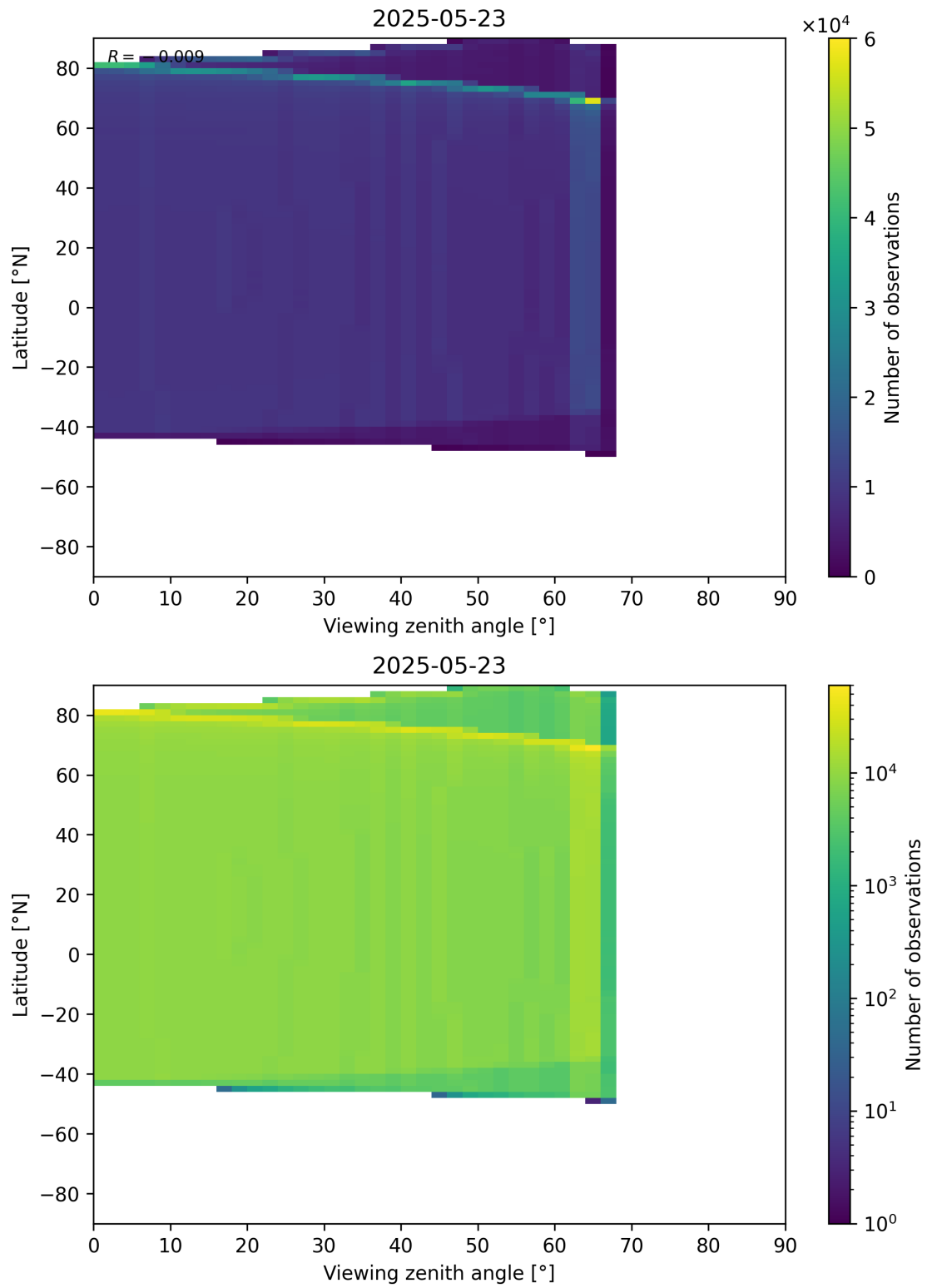
Figure 368: Scatter density plot of “Viewing zenith angle” against “Latitude” for 2025-05-22 to 2025-05-24.
