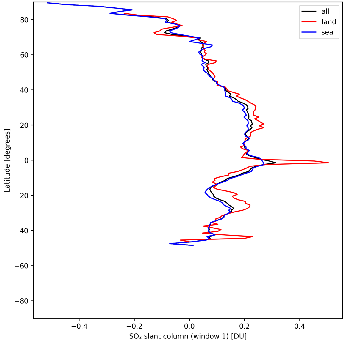
Figure 37: Zonal average of “SO 2 slant column (window 1)” for 2025-05-22 to 2025-05-24.
