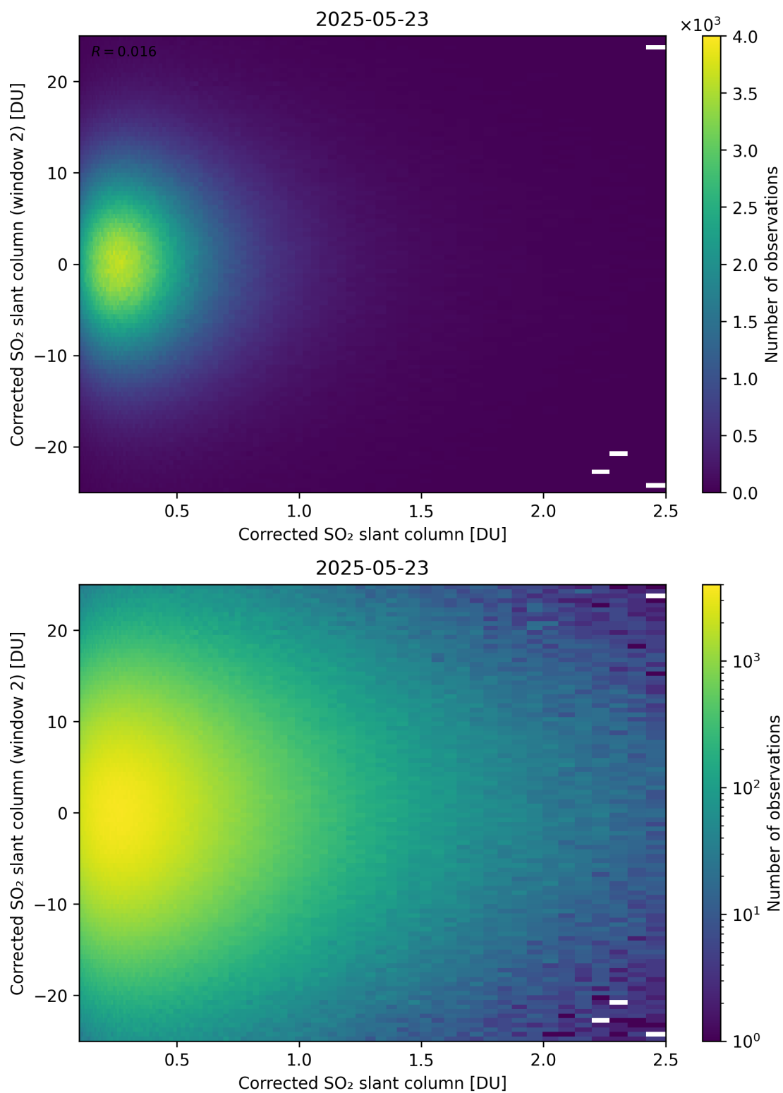
Figure 235: Scatter density plot of “Corrected SO 2 slant column” against “Corrected SO 2 slant column (window 2)” for 2025-05-22 to 2025-05-24.
