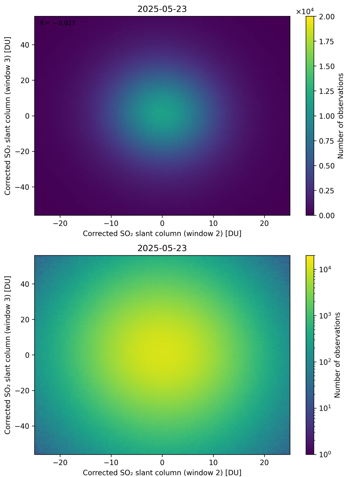
Figure 250: Scatter density plot of “Corrected SO 2 slant column (window 2)” against “Corrected SO 2 slant column (window 3)” for 2025-05-22 to 2025-05-24.
