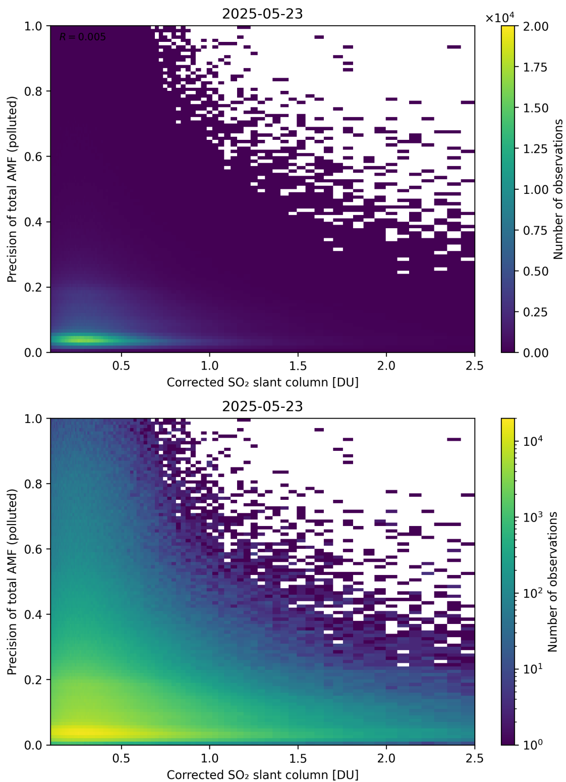
Figure 243: Scatter density plot of “Corrected SO 2 slant column” against “Precision of total AMF (polluted)” for 2025-05-22 to 2025-05-24.
