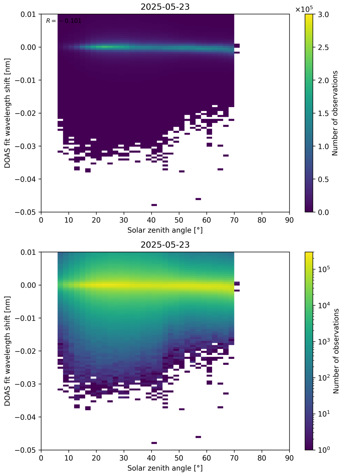
Figure 174: Scatter density plot of “Solar zenith angle” against “DOAS fit wavelength shift” for 2025-05-22 to 2025-05-24.
