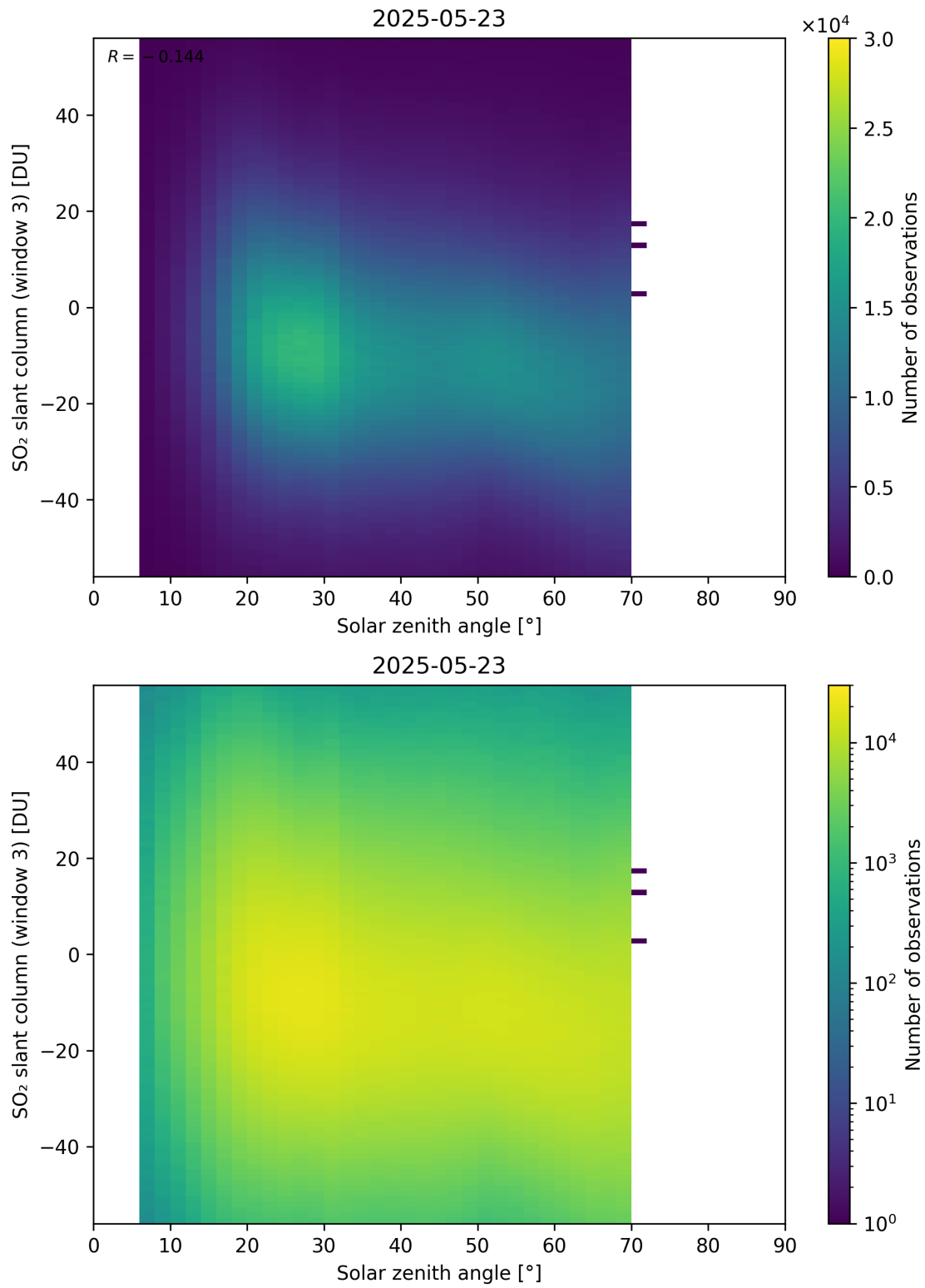
Figure 187: Scatter density plot of “Solar zenith angle” against “SO 2 slant column (window 3)” for 2025-05-22 to 2025-05-24.
