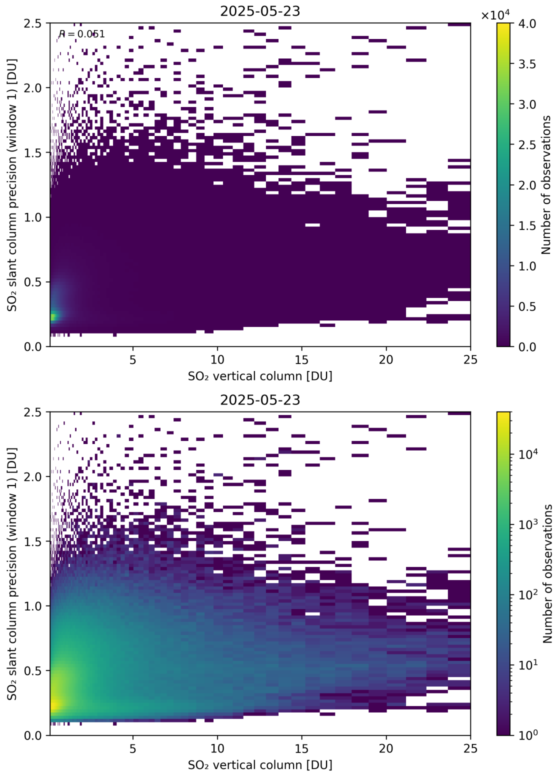
Figure 355: Scatter density plot of “SO 2 vertical column” against “SO 2 slant column precision (window 1)” for 2025-05-22 to 2025-05-24.
