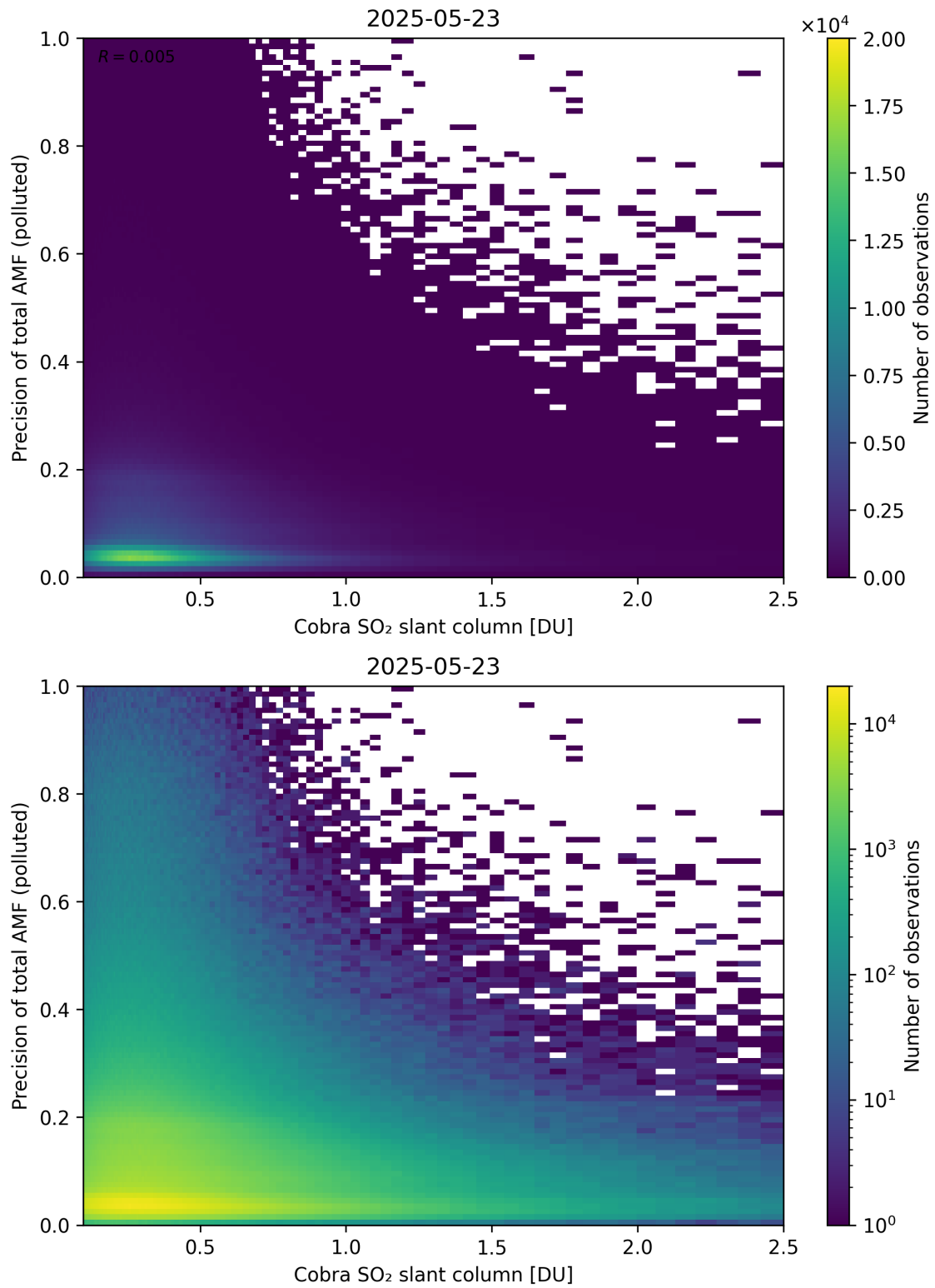
Figure 225: Scatter density plot of “Cobra SO 2 slant column” against “Precision of total AMF (polluted)” for 2025-05-22 to 2025-05-24.
