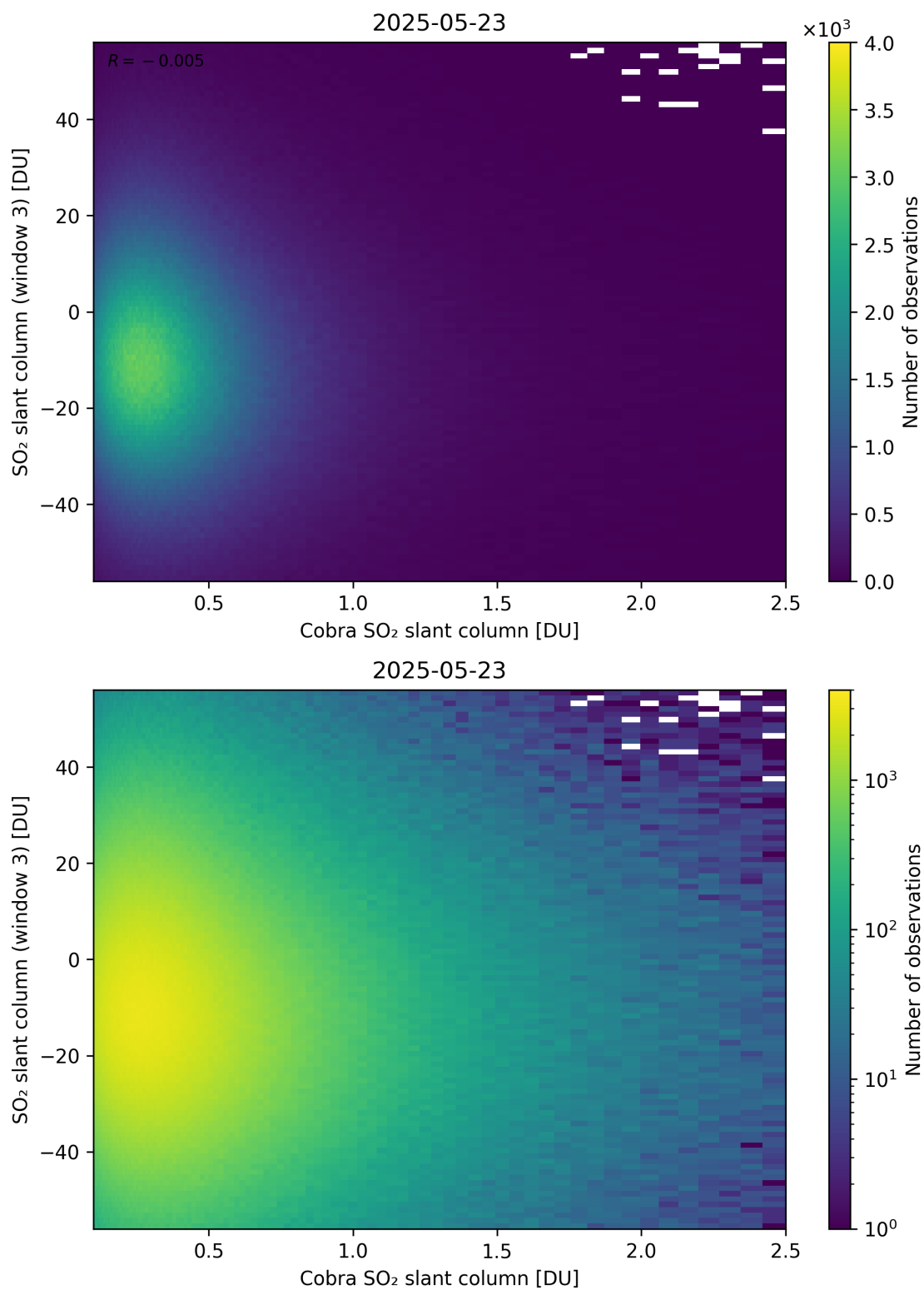
Figure 222: Scatter density plot of “Cobra SO 2 slant column” against “SO 2 slant column (window 3)” for 2025-05-22 to 2025-05-24.
