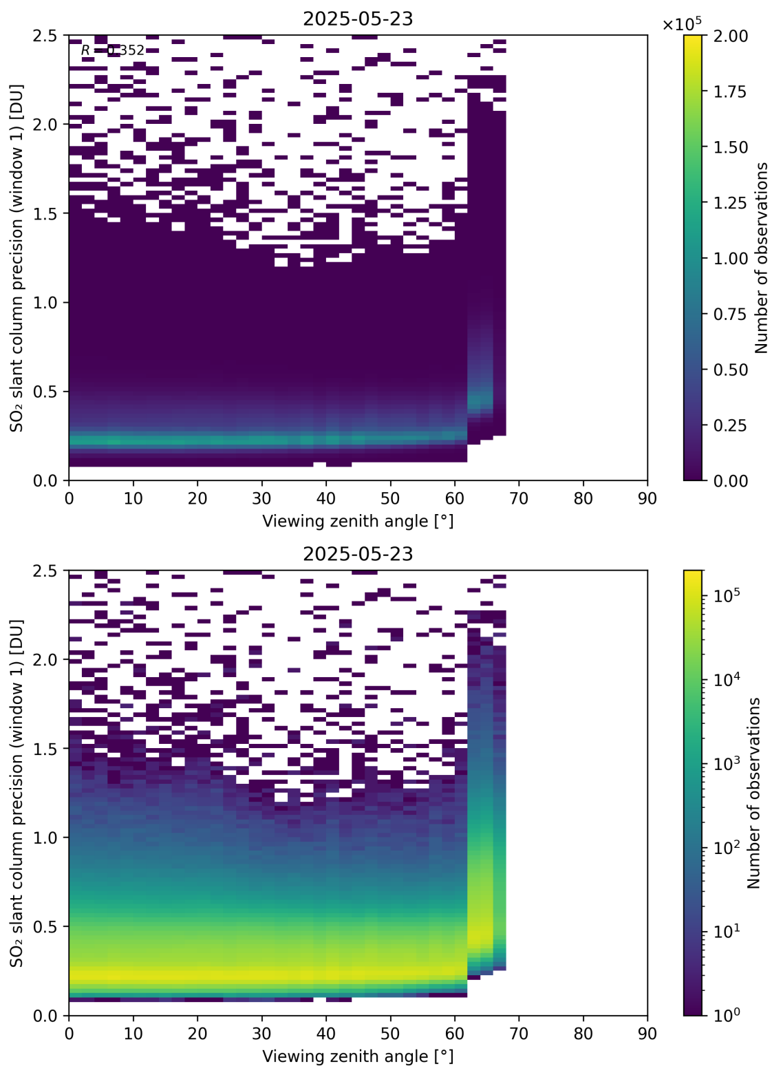
Figure 377: Scatter density plot of “Viewing zenith angle” against “SO 2 slant column precision (window 1)” for 2025-05-22 to 2025-05-24.
