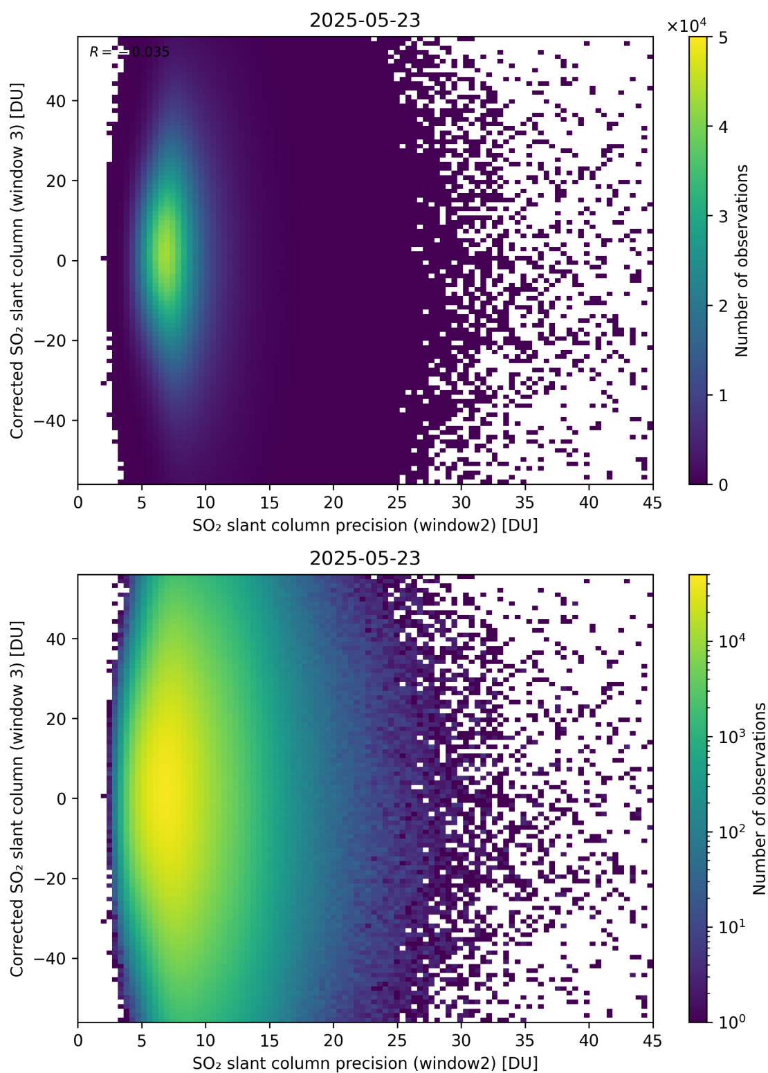
Figure 298: Scatter density plot of “SO 2 slant column precision (window2)” against “Corrected SO 2 slant column (window 3)” for 2025-05-22 to 2025-05-24.
