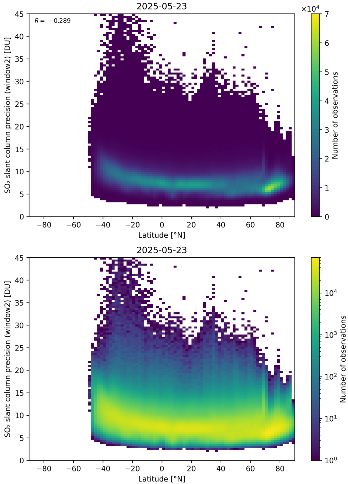
Figure 164: Scatter density plot of “Latitude” against “SO 2 slant column precision (window2)” for 2025-05-22 to 2025-05-24.
