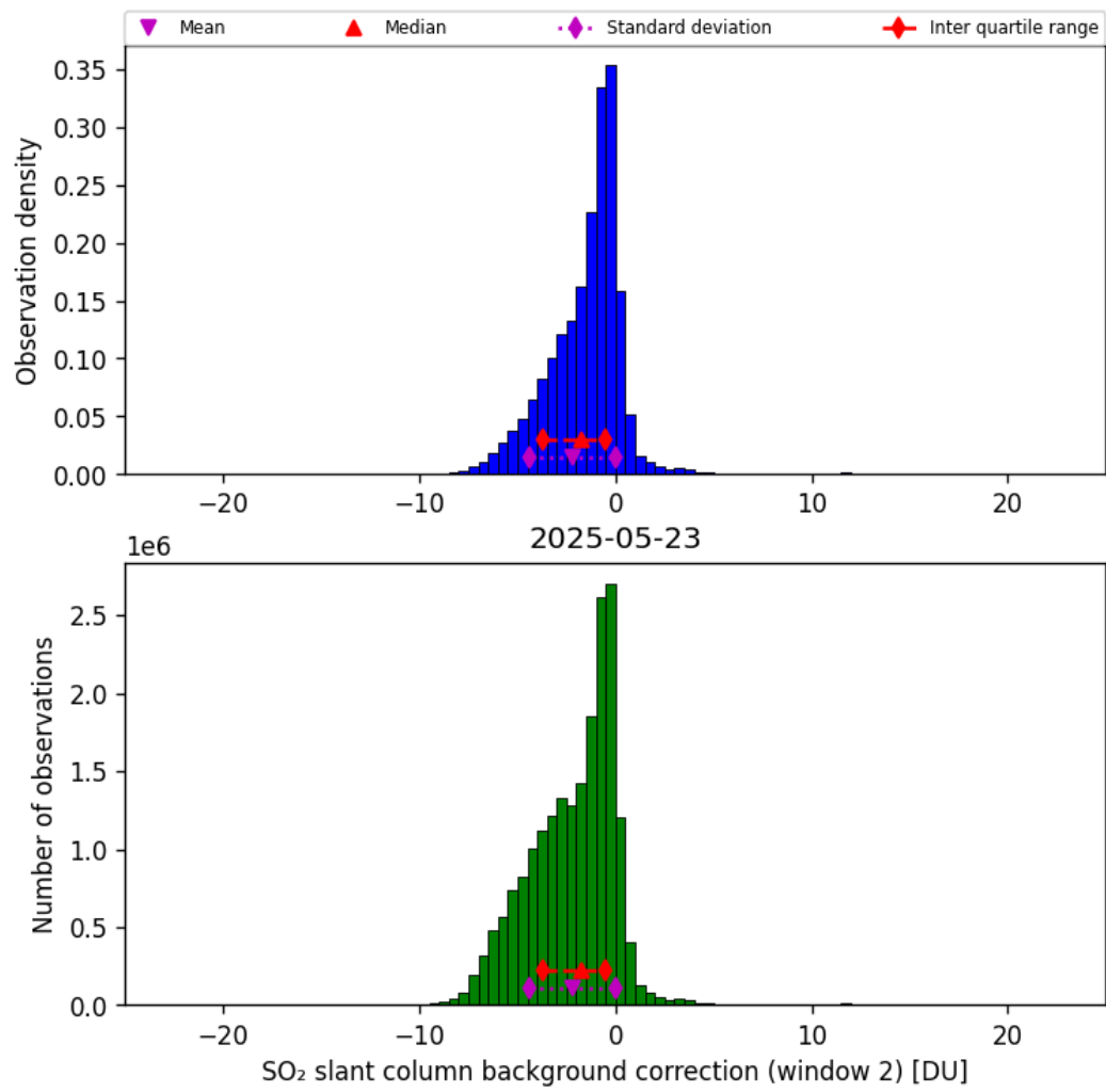
Figure 70: Histogram of “SO 2 slant column background correction (window 2)” for 2025-05-22 to 2025-05-24
