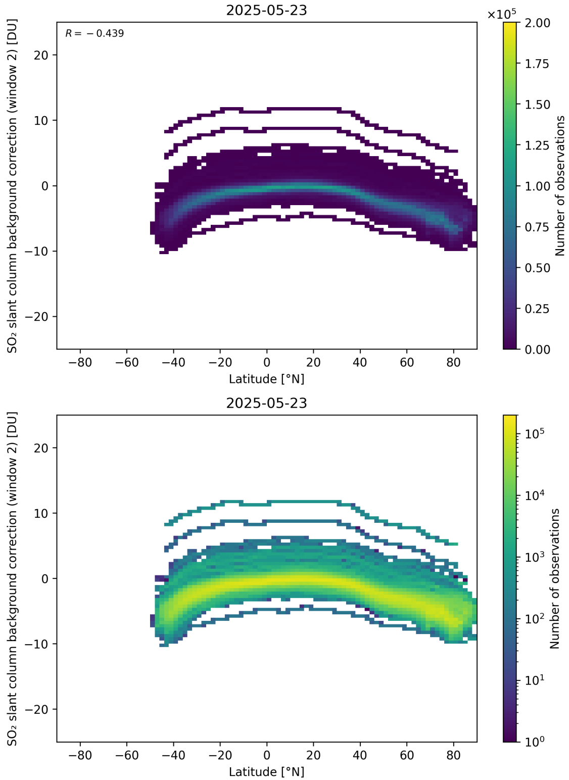
Figure 151: Scatter density plot of “Latitude” against “SO 2 slant column background correction (window 2)” for 2025-05-22 to 2025-05-24.
