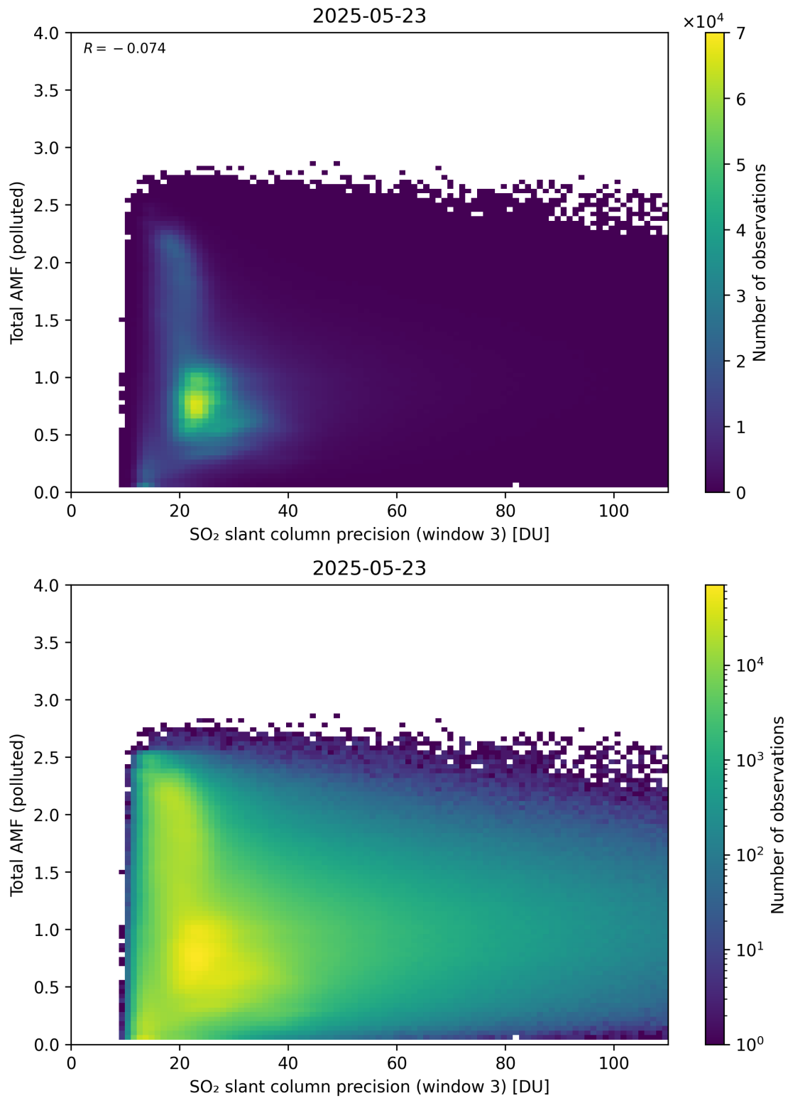
Figure 313: Scatter density plot of “SO 2 slant column precision (window 3)” against “Total AMF (polluted)” for 2025-05-22 to 2025-05-24.
