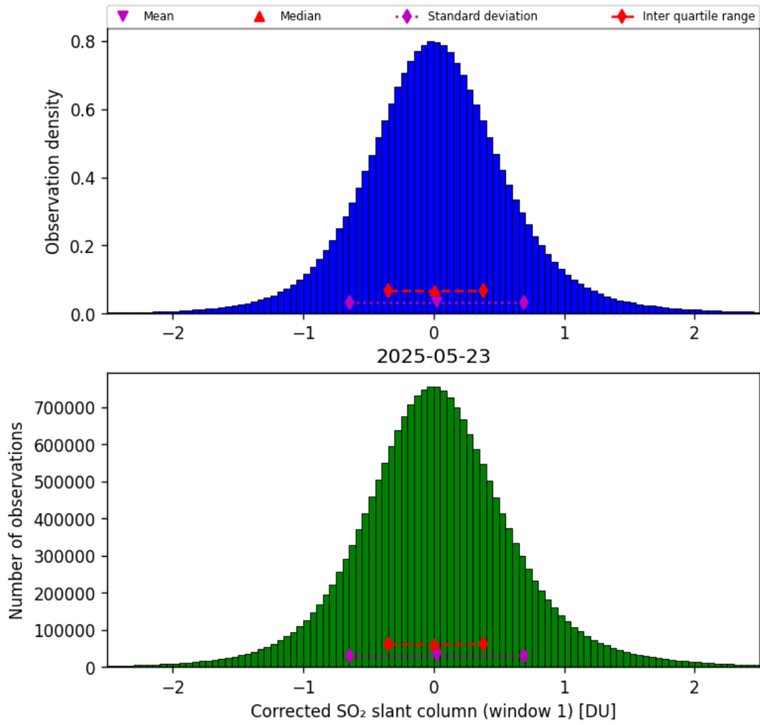
Figure 65: Histogram of “Corrected SO 2 slant column (window 1)” for 2025-05-22 to 2025-05-24
