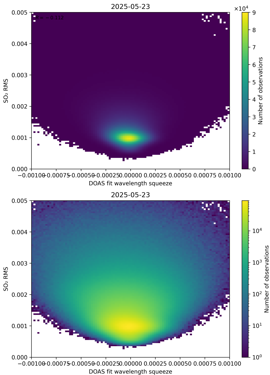
Figure 143: Scatter density plot of “DOAS fit wavelength squeeze” against “SO 2 RMS” for 2025-05-22 to 2025-05-24.
