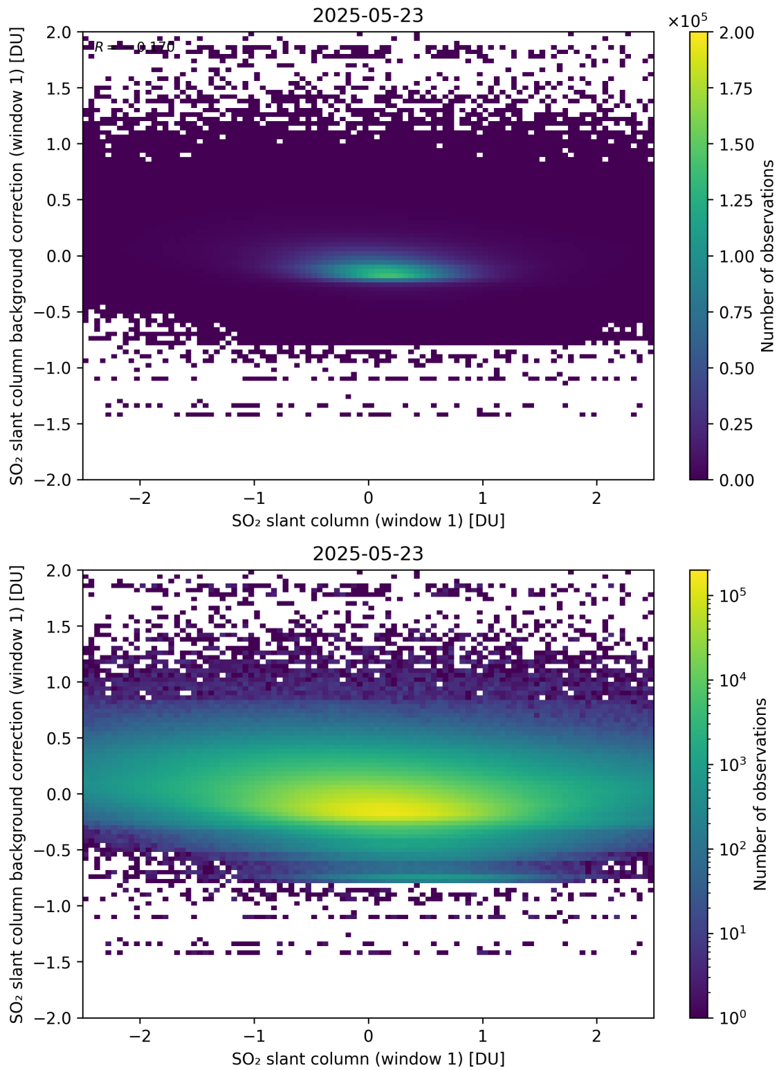
Figure 262: Scatter density plot of “SO 2 slant column (window 1)” against “SO 2 slant column background correction (window 1)” for 2025-05-22 to 2025-05-24.
