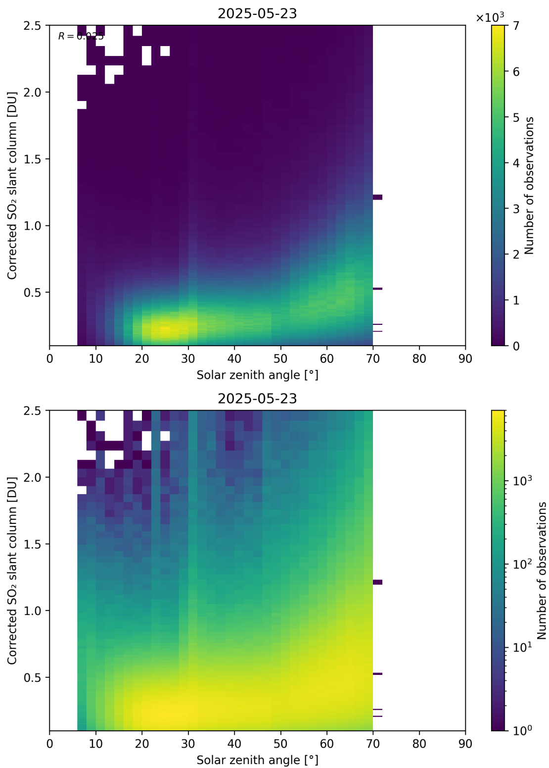
Figure 181: Scatter density plot of “Solar zenith angle” against “Corrected SO 2 slant column” for 2025-05-22 to 2025-05-24.
