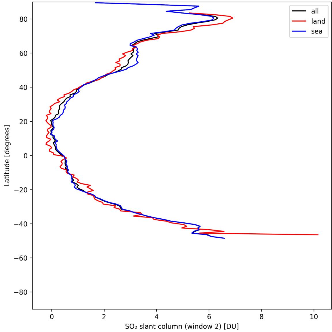
Figure 41: Zonal average of “SO 2 slant column (window 2)” for 2025-05-22 to 2025-05-24.
