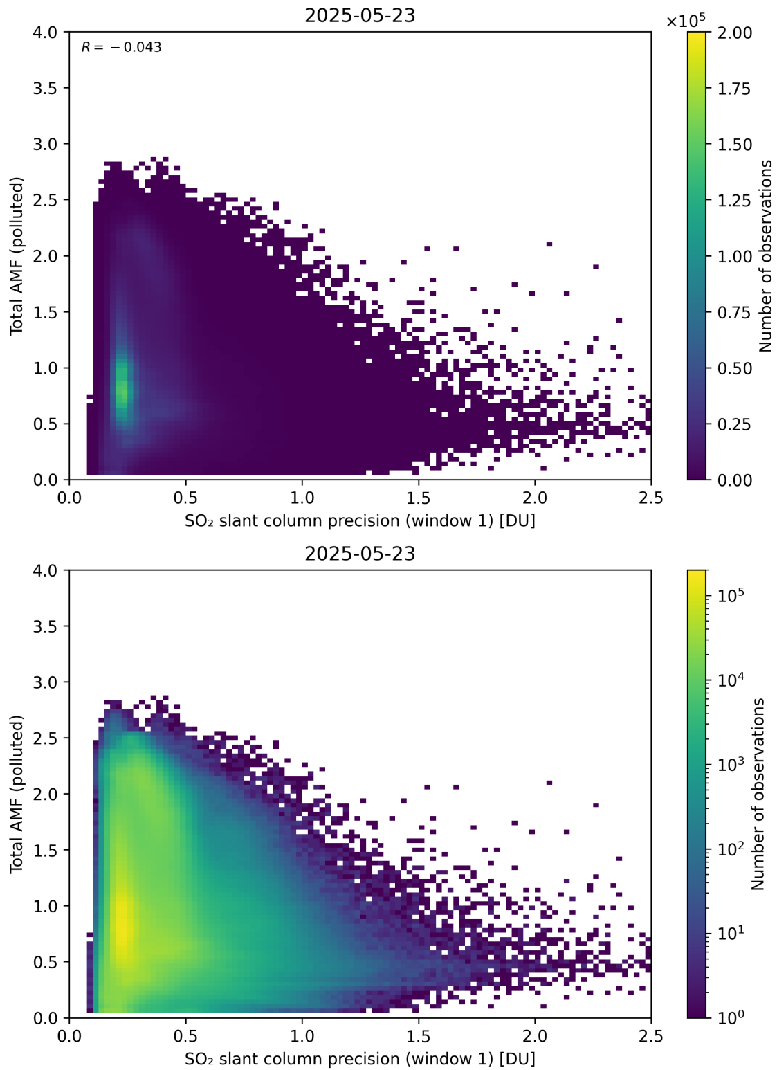
Figure 280: Scatter density plot of “SO 2 slant column precision (window 1)” against “Total AMF (polluted)” for 2025-05-22 to 2025-05-24.
