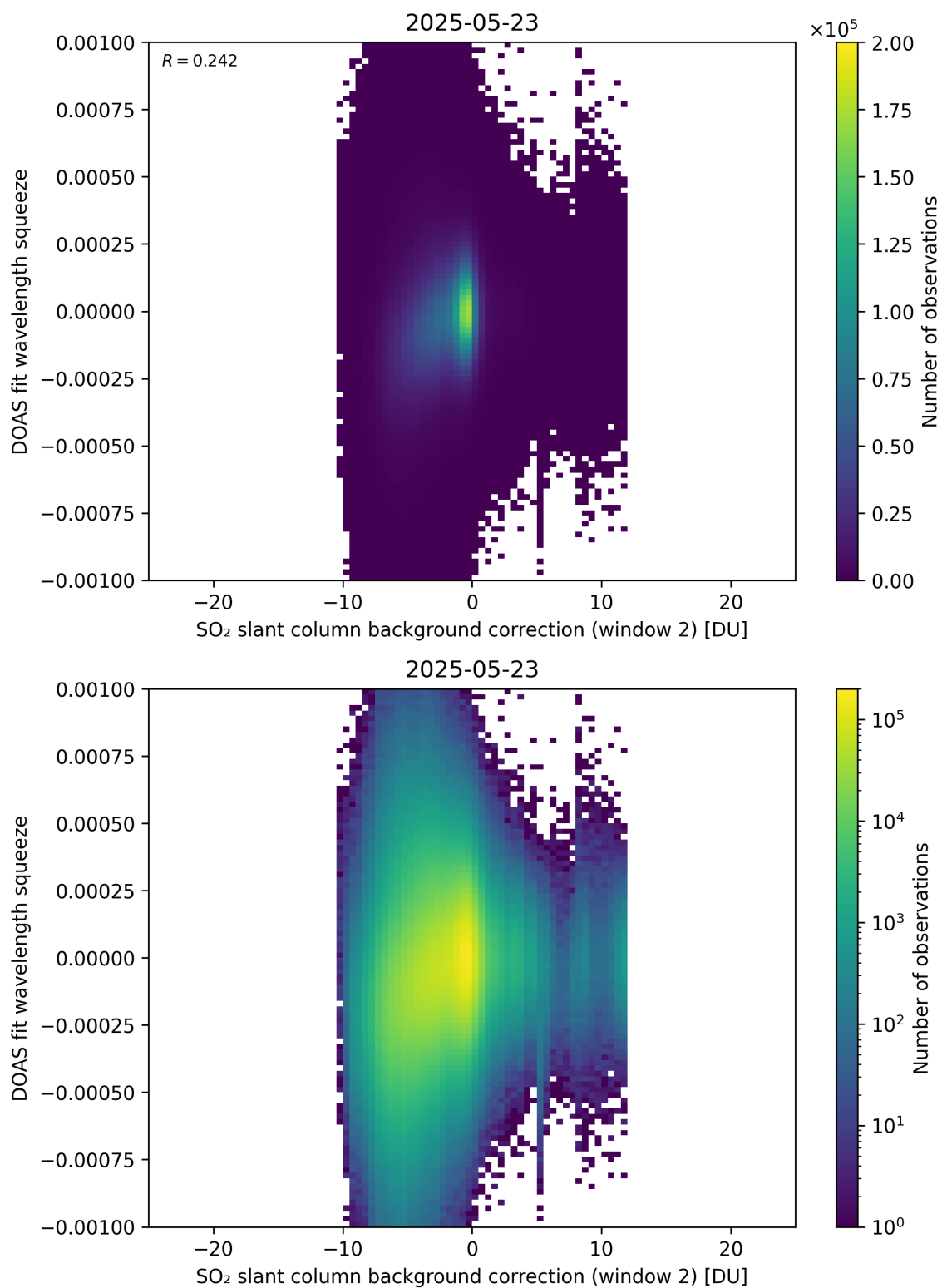
Figure 124: Scatter density plot of “SO 2 slant column background correction (window 2)” against “DOAS fit wavelength squeeze” for 2025-05-22 to 2025-05-24.
