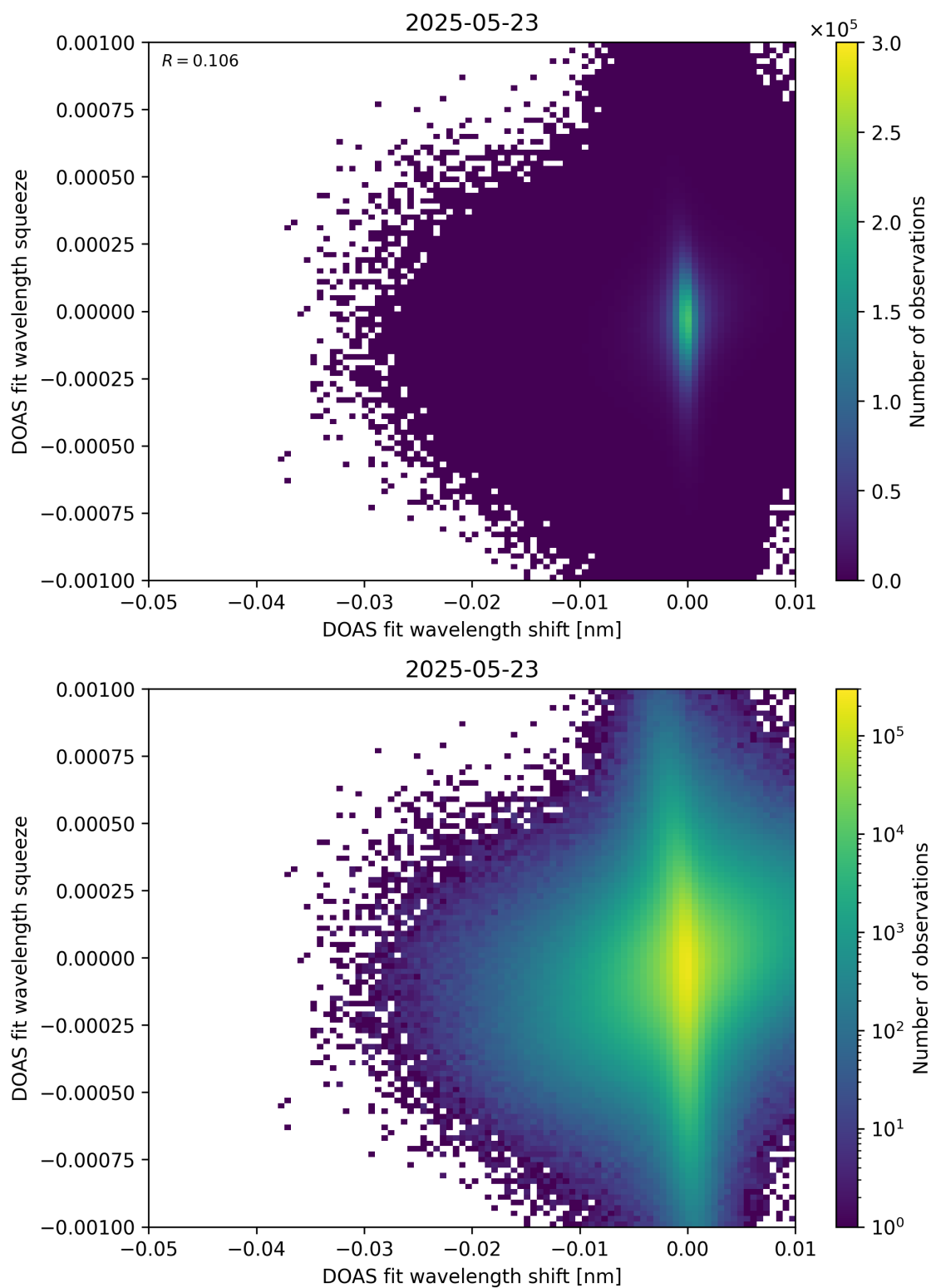
Figure 138: Scatter density plot of “DOAS fit wavelength shift” against “DOAS fit wavelength squeeze” for 2025-05-22 to 2025-05-24.
