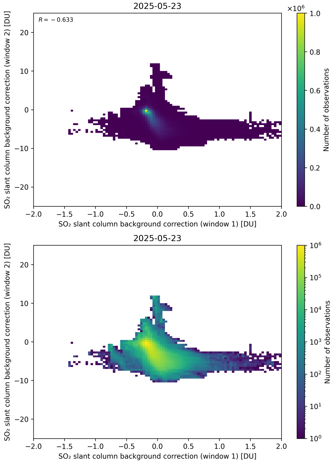
Figure 109: Scatter density plot of “SO 2 slant column background correction (window 1)” against “SO 2 slant column background correction (window 2)” for 2025-05-22 to 2025-05-24.
