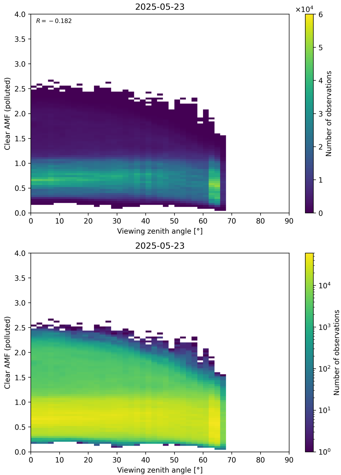
Figure 370: Scatter density plot of “Viewing zenith angle” against “Clear AMF (polluted)” for 2025-05-22 to 2025-05-24.
