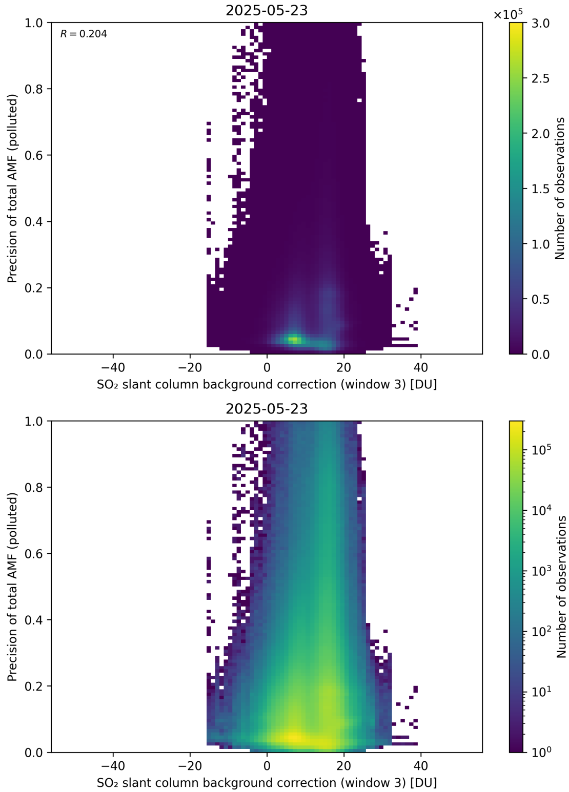
Figure 137: Scatter density plot of “SO 2 slant column background correction (window 3)” against “Precision of total AMF (polluted)” for 2025-05-22 to 2025-05-24.
