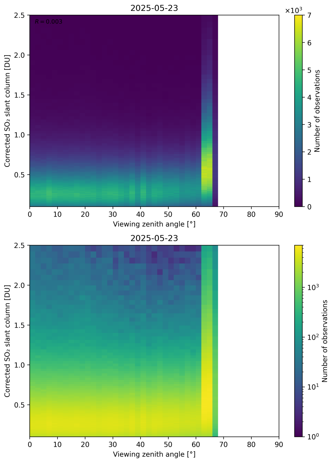
Figure 373: Scatter density plot of “Viewing zenith angle” against “Corrected SO 2 slant column” for 2025-05-22 to 2025-05-24.
