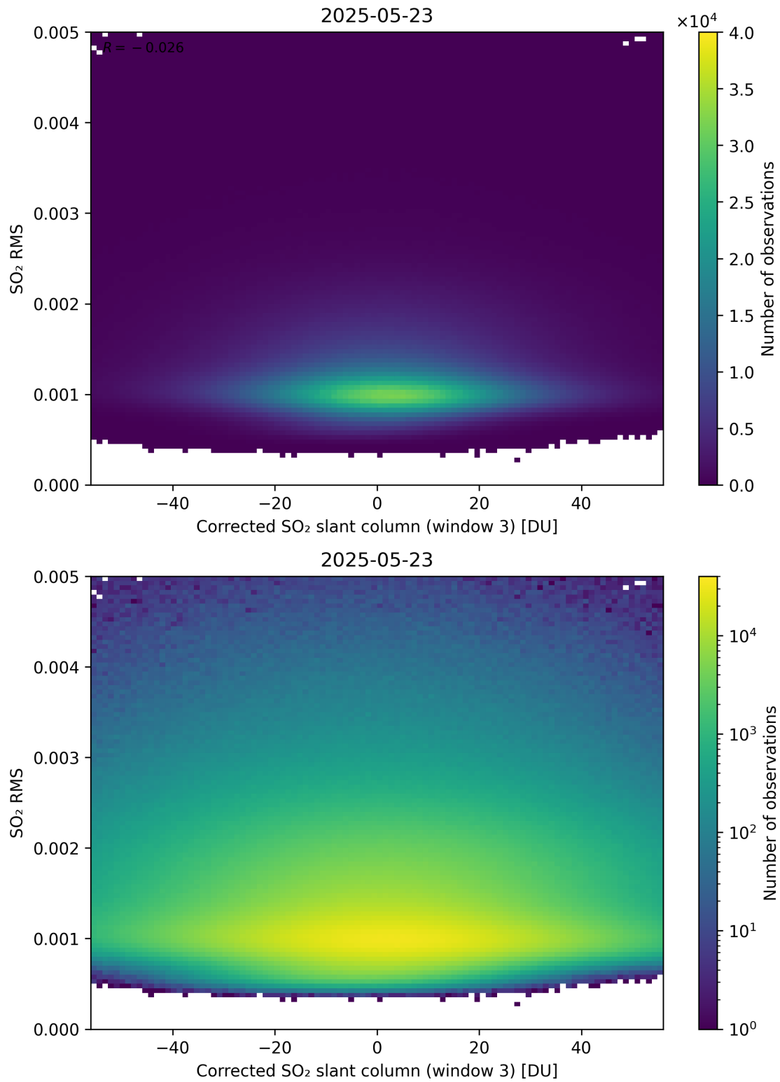
Figure 258: Scatter density plot of “Corrected SO 2 slant column (window 3)” against “SO 2 RMS” for 2025-05-22 to 2025-05-24.
