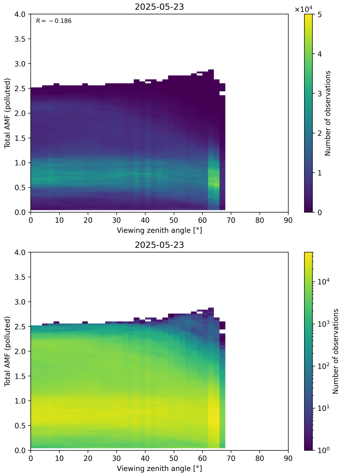
Figure 381: Scatter density plot of “Viewing zenith angle” against “Total AMF (polluted)” for 2025-05-22 to 2025-05-24.
