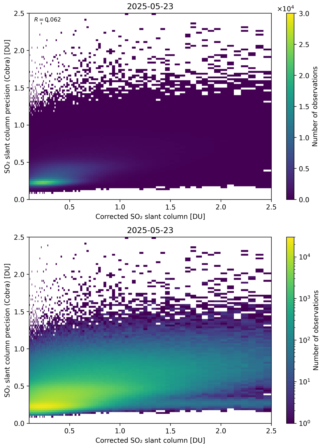
Figure 234: Scatter density plot of “Corrected SO 2 slant column” against “SO 2 slant column precision (Cobra)” for 2025-05-22 to 2025-05-24.
