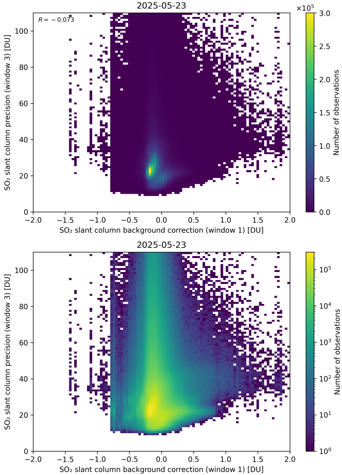
Figure 119: Scatter density plot of “SO 2 slant column background correction (window 1)” against “SO 2 slant column precision (window 3)” for 2025-05-22 to 2025-05-24.
