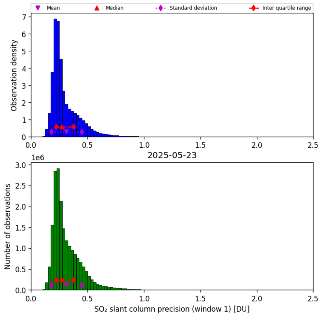
Figure 64: Histogram of “SO 2 slant column precision (window 1)” for 2025-05-22 to 2025-05-24
