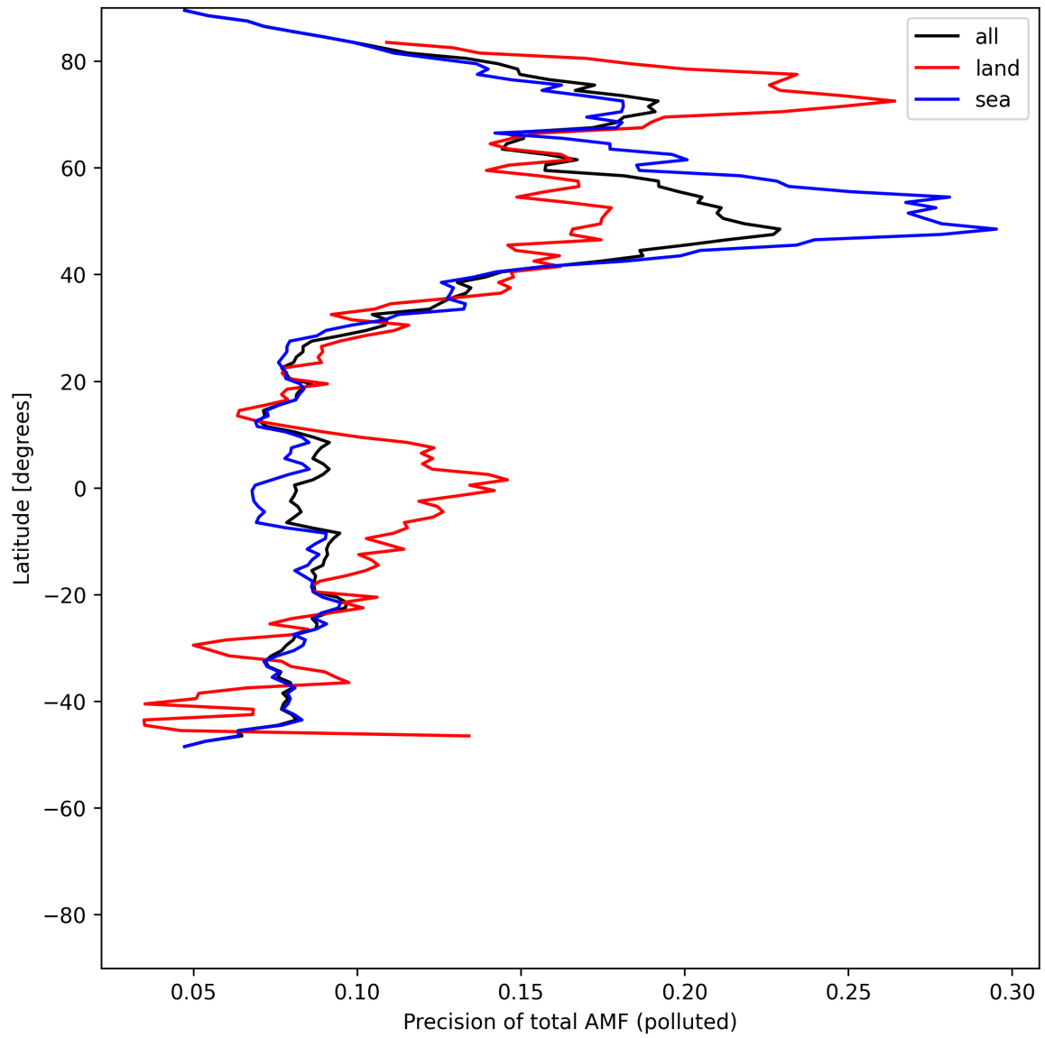
Figure 54: Zonal average of “Precision of total AMF (polluted)” for 2025-05-22 to 2025-05-24.
