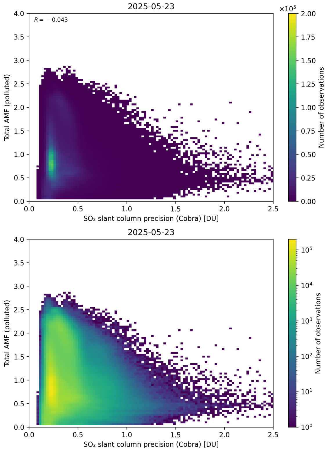
Figure 213: Scatter density plot of “SO 2 slant column precision (Cobra)” against “Total AMF (polluted)” for 2025-05-22 to 2025-05-24.
