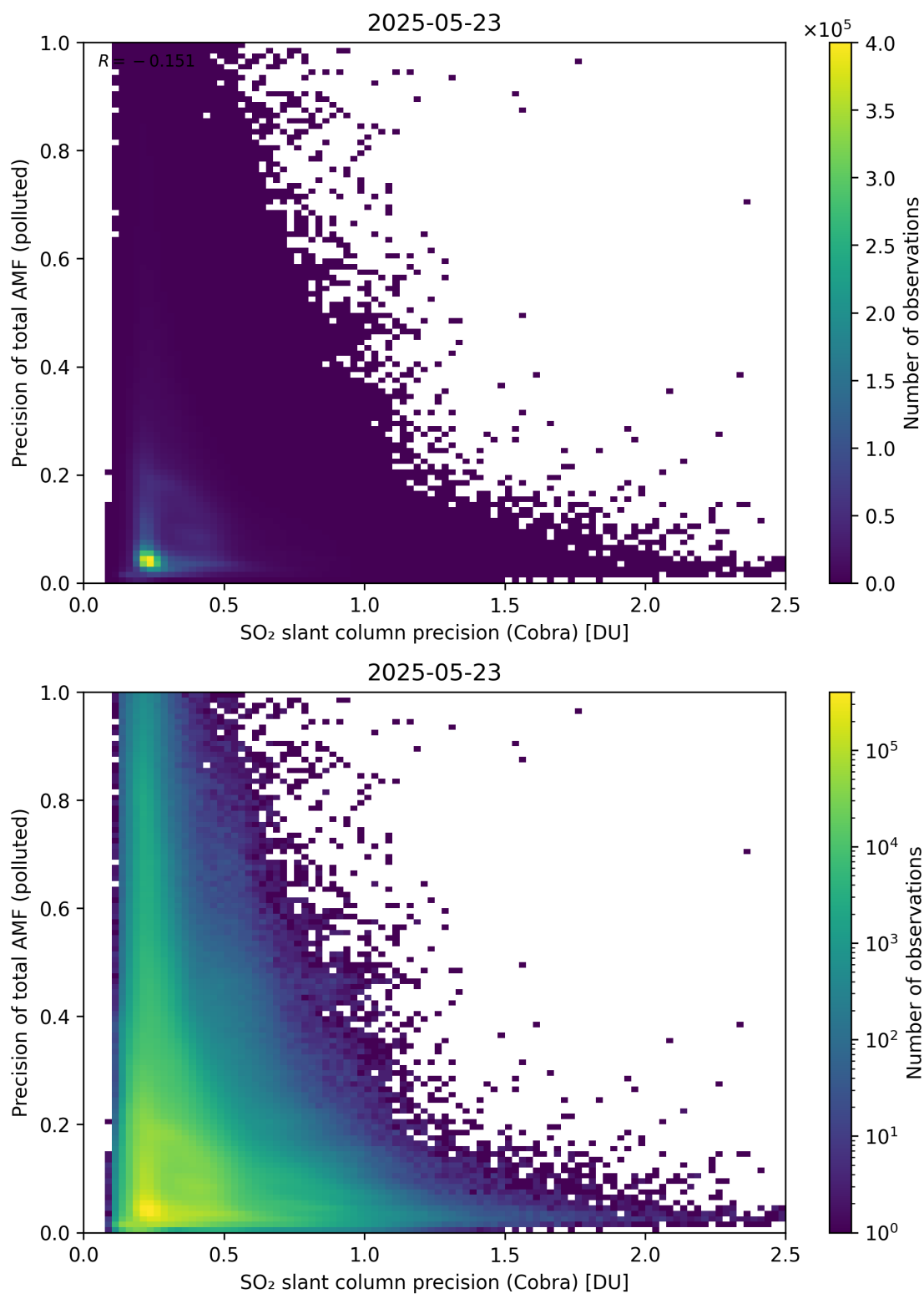
Figure 214: Scatter density plot of “SO 2 slant column precision (Cobra)” against “Precision of total AMF (polluted)” for 2025-05-22 to 2025-05-24.
