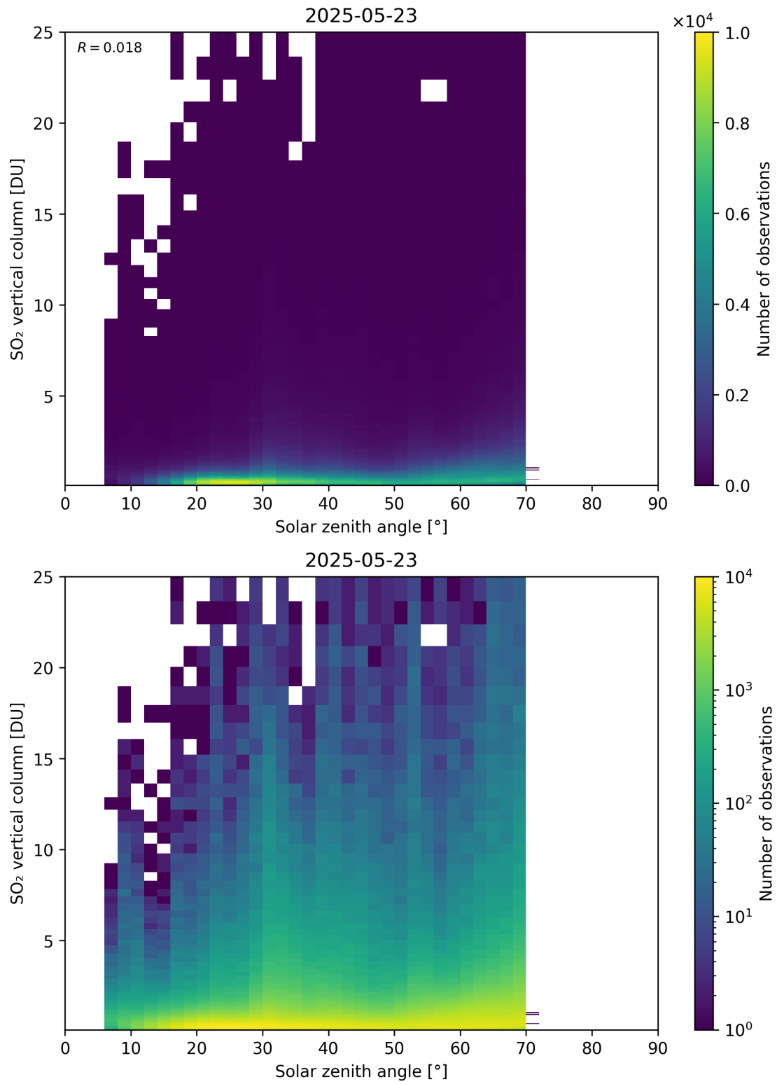
Figure 191: Scatter density plot of “Solar zenith angle” against “SO 2 vertical column” for 2025-05-22 to 2025-05-24.
