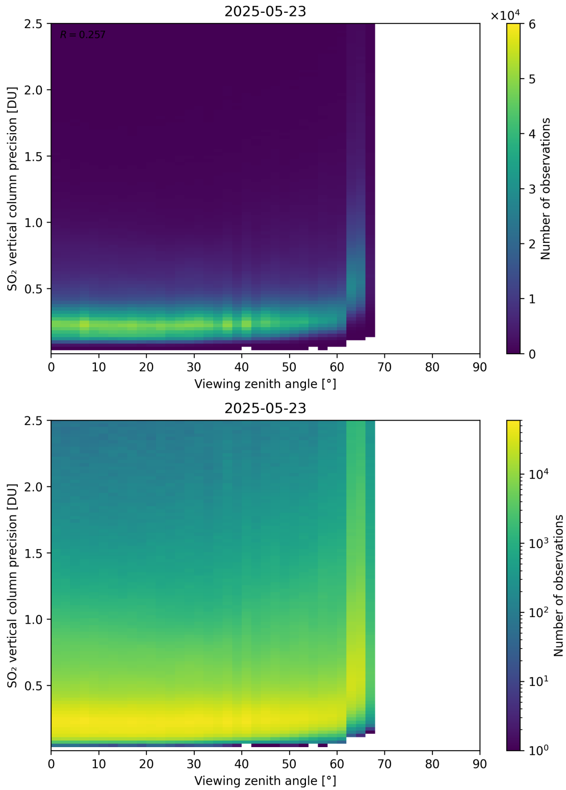
Figure 384: Scatter density plot of “Viewing zenith angle” against “SO 2 vertical column precision” for 2025-05-22 to 2025-05-24.
