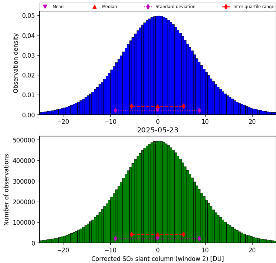
Figure 69: Histogram of “Corrected SO 2 slant column (window 2)” for 2025-05-22 to 2025-05-24
