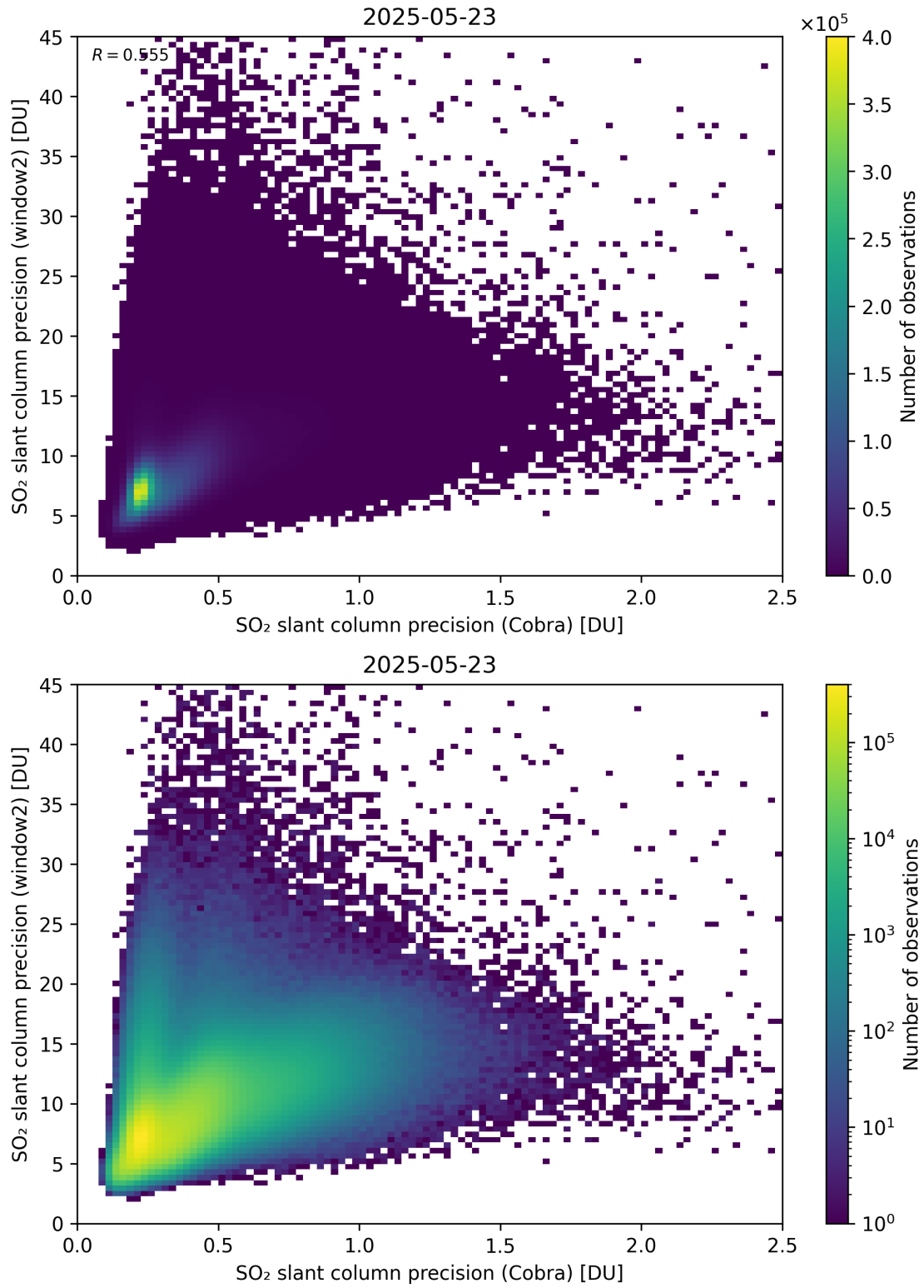
Figure 210: Scatter density plot of “SO 2 slant column precision (Cobra)” against “SO 2 slant column precision (window2)” for 2025-05-22 to 2025-05-24.
