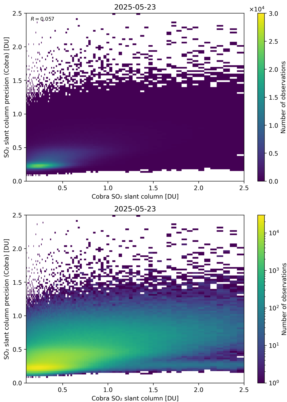
Figure 216: Scatter density plot of “Cobra SO 2 slant column” against “SO 2 slant column precision (Cobra)” for 2025-05-22 to 2025-05-24.
