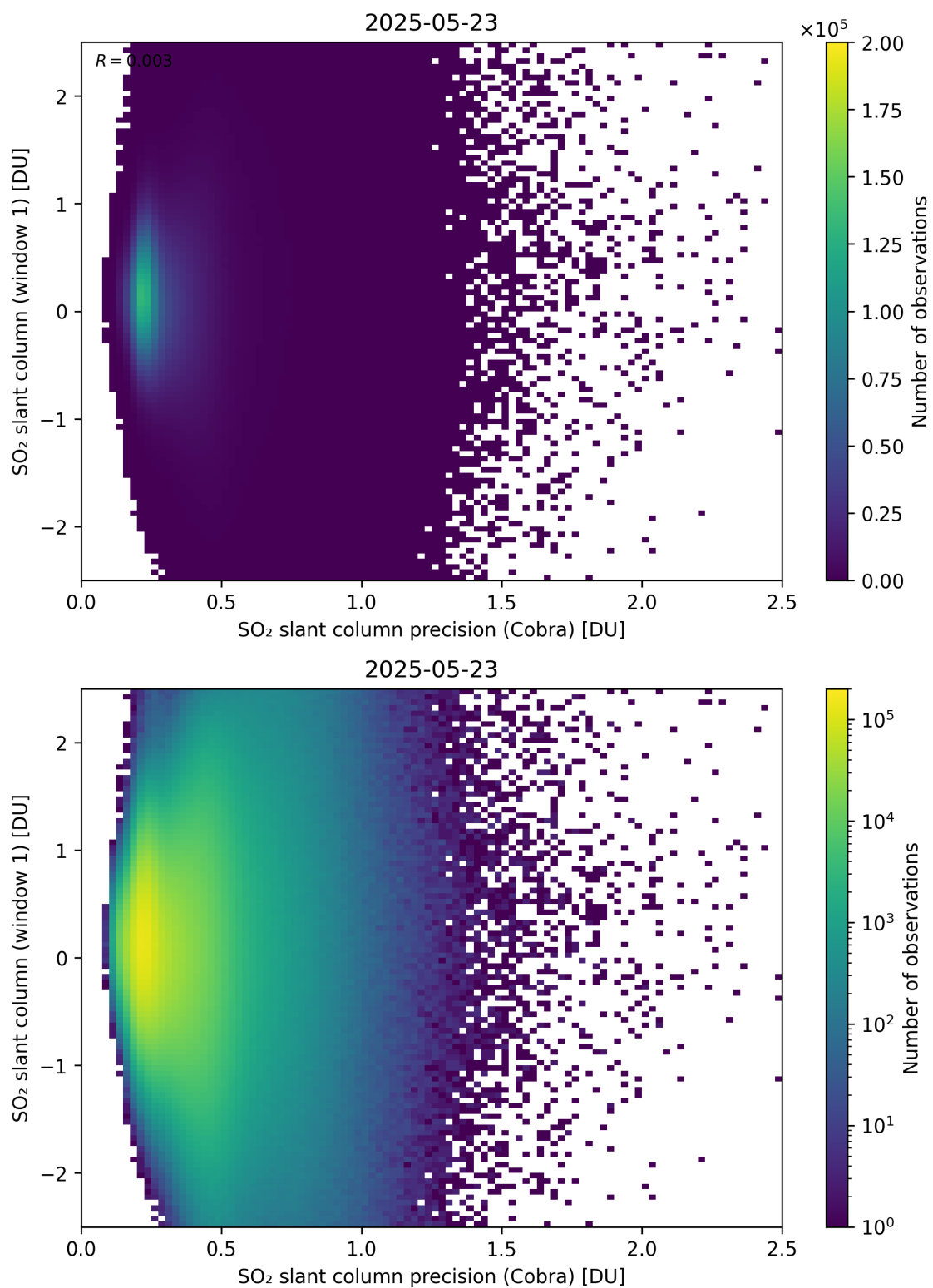
Figure 208: Scatter density plot of “SO 2 slant column precision (Cobra)” against “SO 2 slant column (window 1)” for 2025-05-22 to 2025-05-24.
