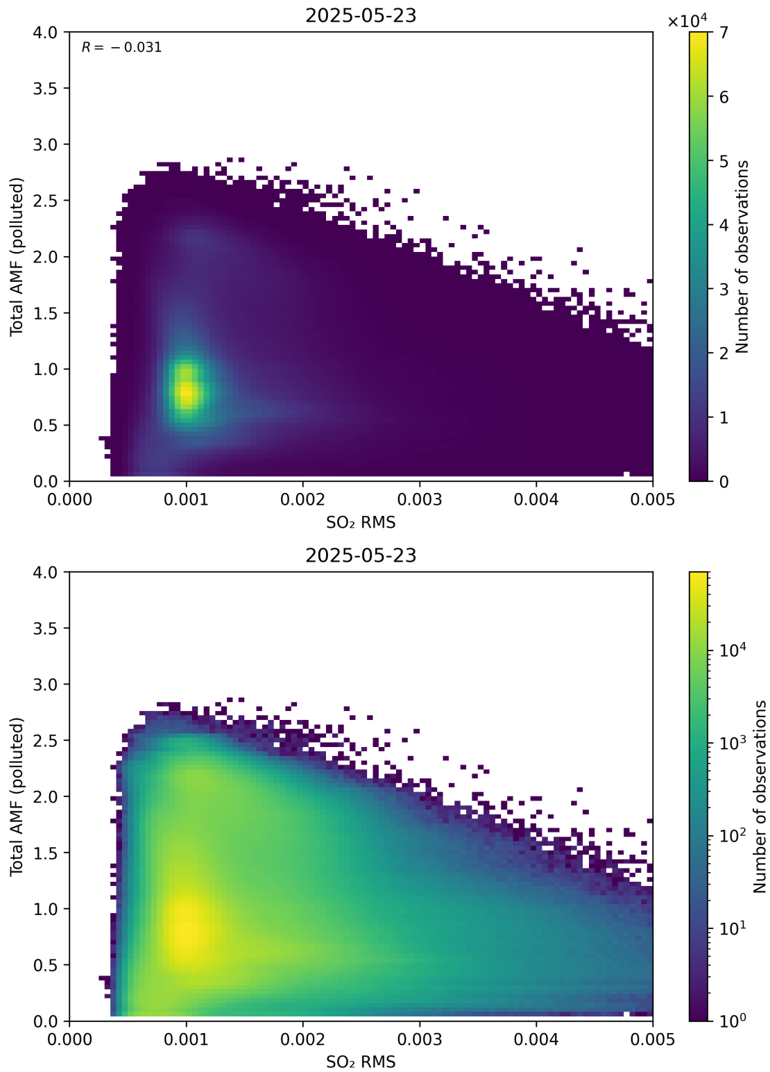
Figure 148: Scatter density plot of “SO 2 RMS” against “Total AMF (polluted)” for 2025-05-22 to 2025-05-24.
