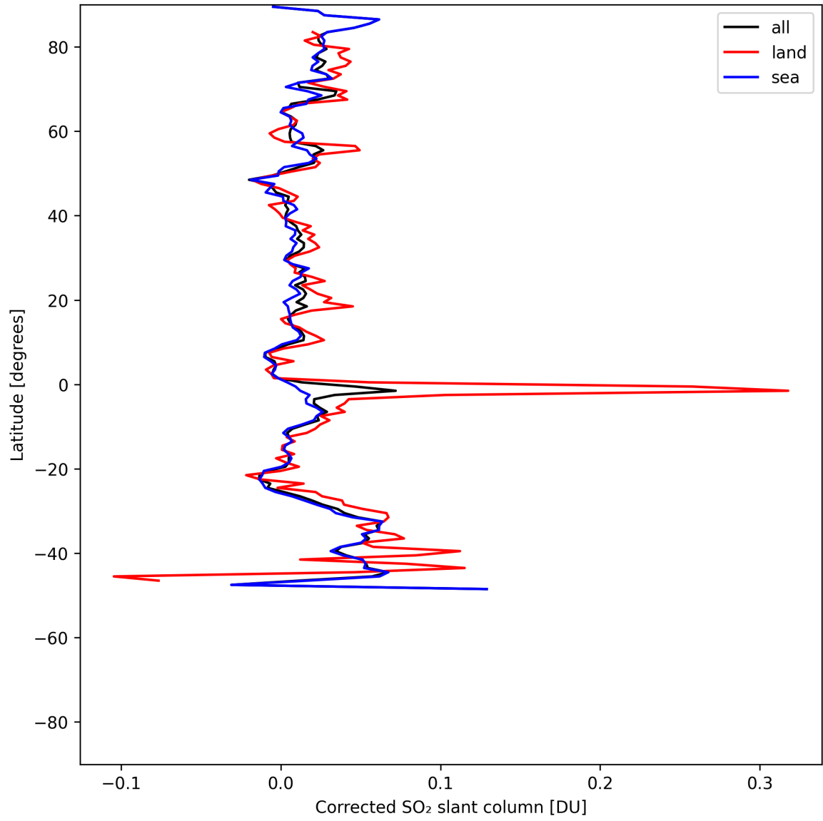
Figure 34: Zonal average of “Corrected SO 2 slant column” for 2025-05-22 to 2025-05-24.
