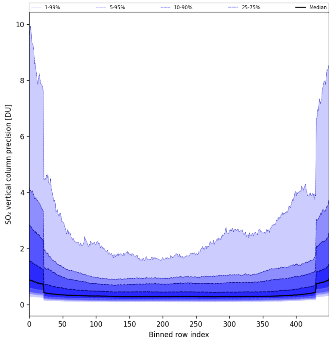
Figure 85: Along track statistics of “SO 2 vertical column precision” for 2025-05-22 to 2025-05-24
