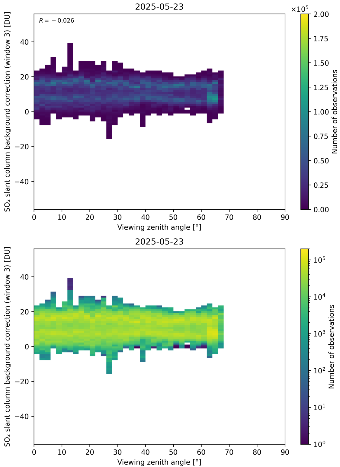
Figure 364: Scatter density plot of “Viewing zenith angle” against “SO 2 slant column background correction (window 3)” for 2025-05-22 to 2025-05-24.
