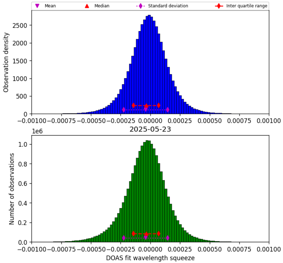
Figure 77: Histogram of “DOAS fit wavelength squeeze” for 2025-05-22 to 2025-05-24
