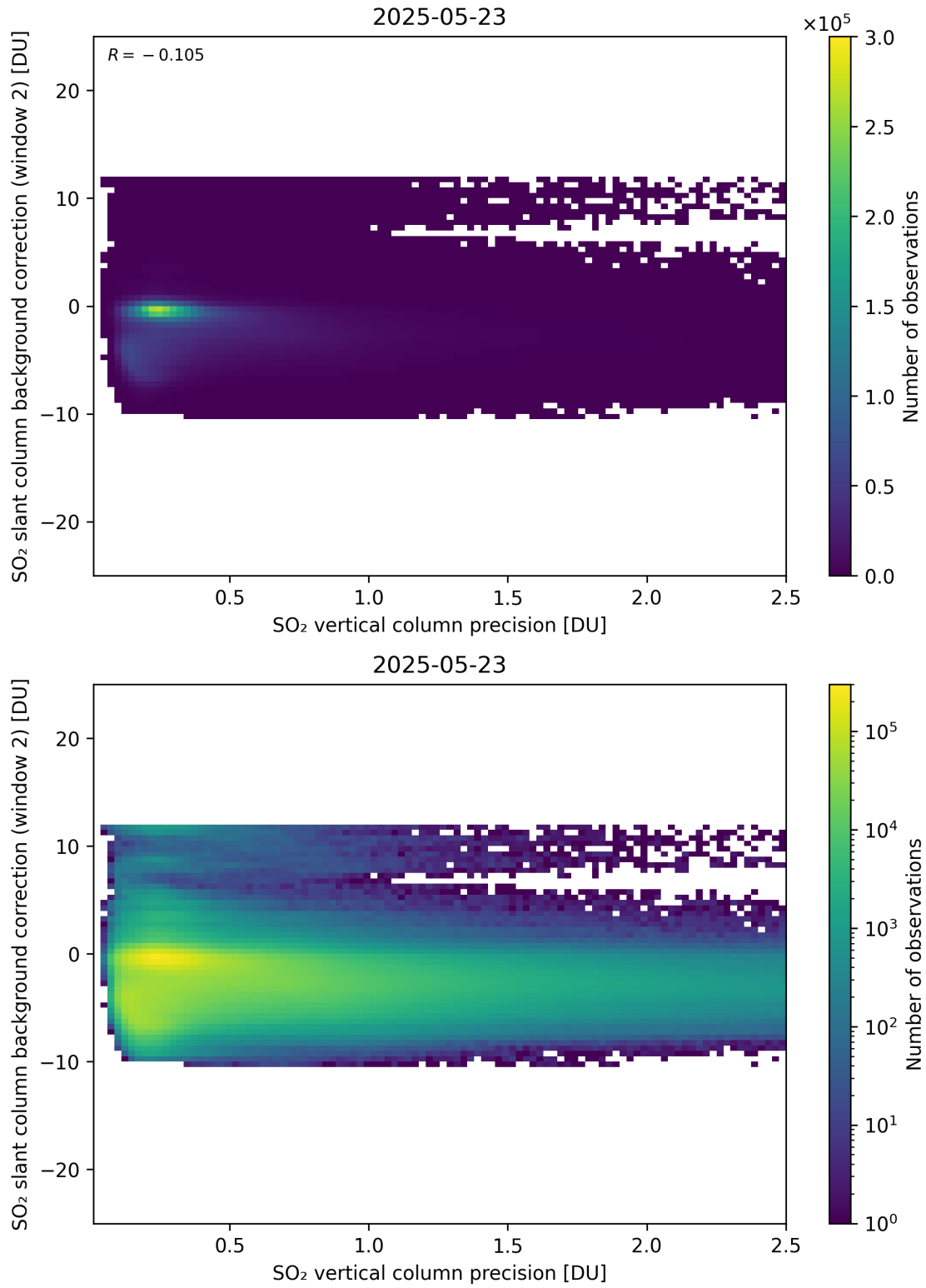
Figure 330: Scatter density plot of “SO 2 vertical column precision” against “SO 2 slant column background correction (window 2)” for 2025-05-22 to 2025-05-24.
