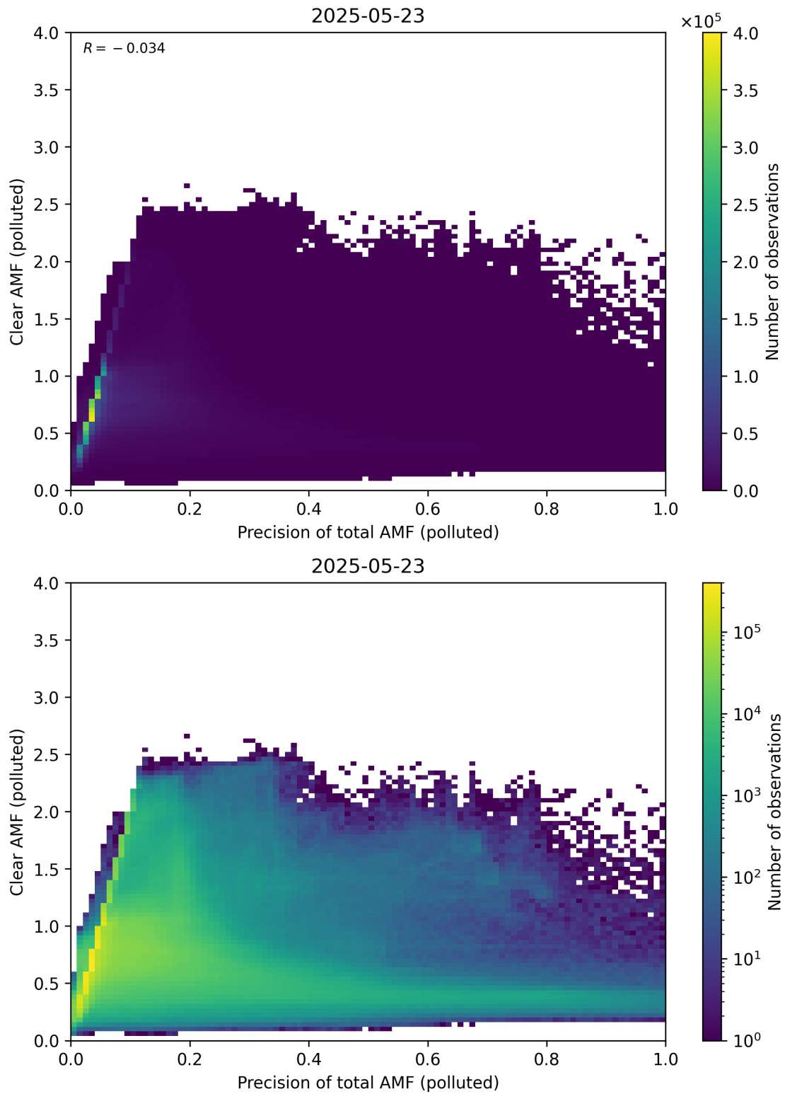
Figure 320: Scatter density plot of “Precision of total AMF (polluted)” against “Clear AMF (polluted)” for 2025-05-22 to 2025-05-24.
