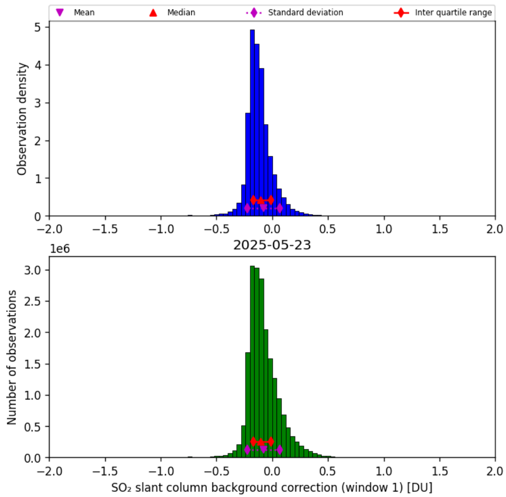
Figure 66: Histogram of “SO 2 slant column background correction (window 1)” for 2025-05-22 to 2025-05-24
