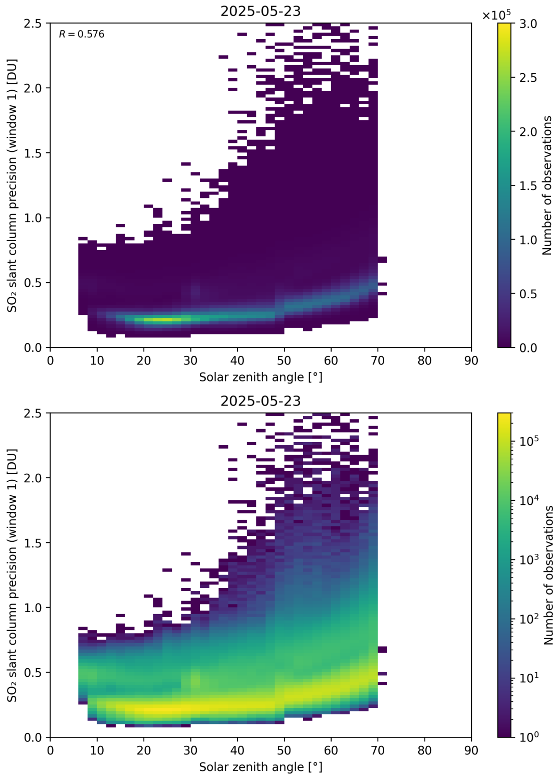
Figure 185: Scatter density plot of “Solar zenith angle” against “SO 2 slant column precision (window 1)” for 2025-05-22 to 2025-05-24.
