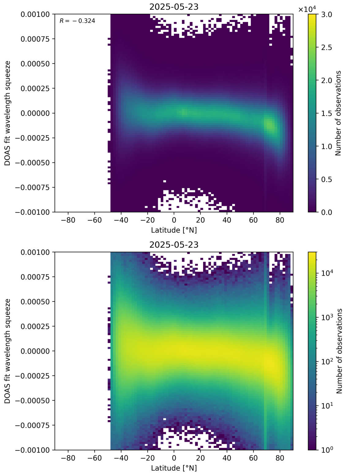
Figure 154: Scatter density plot of “Latitude” against “DOAS fit wavelength squeeze” for 2025-05-22 to 2025-05-24.
