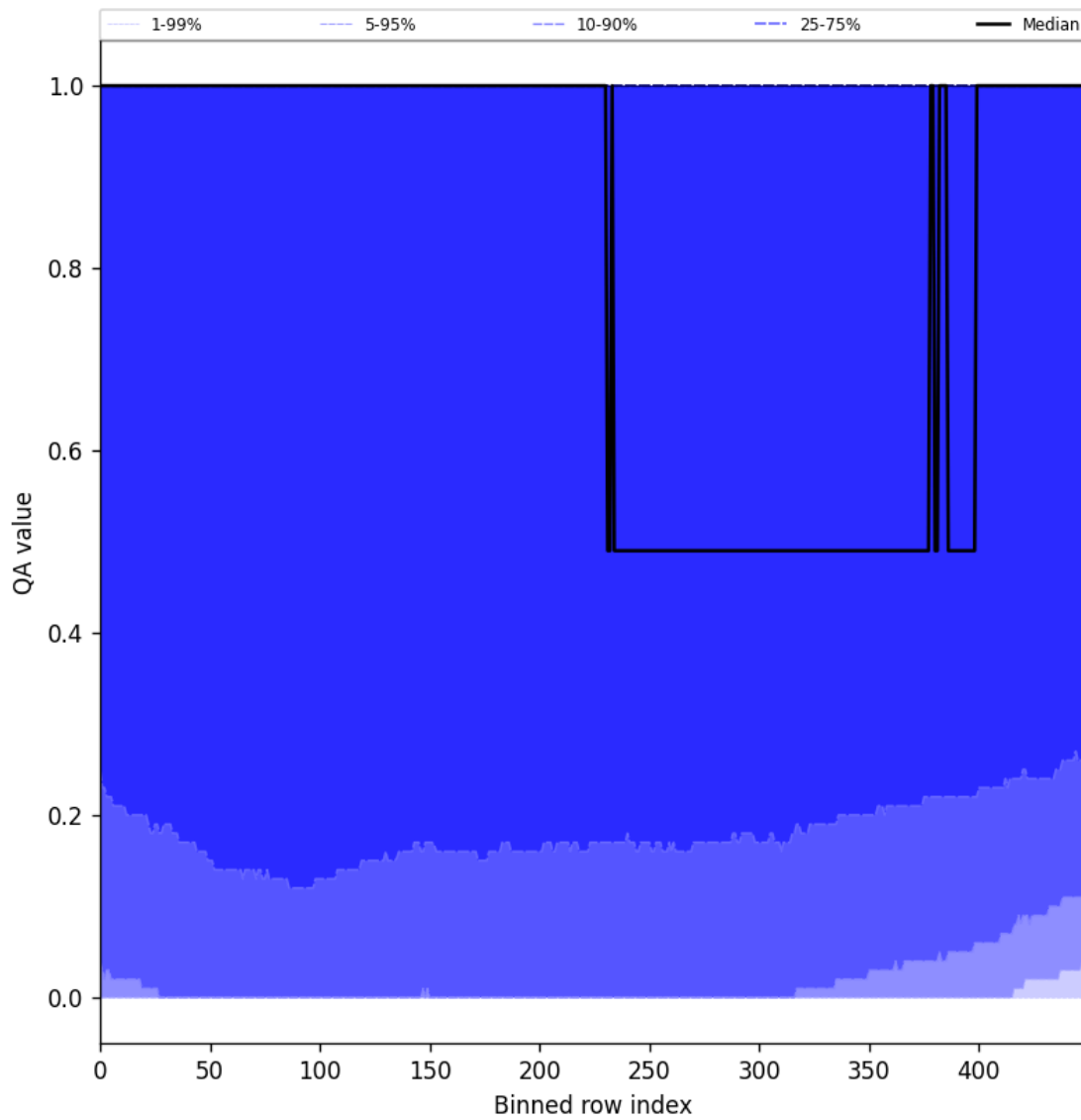
Figure 83: Along track statistics of “QA value” for 2025-05-22 to 2025-05-24
