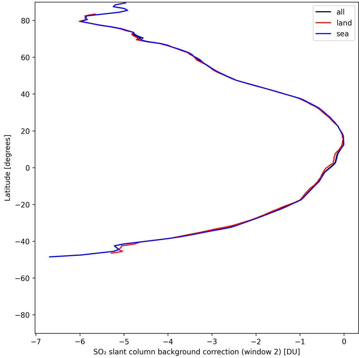
Figure 44: Zonal average of “SO 2 slant column background correction (window 2)” for 2025-05-22 to 2025-05-24.
