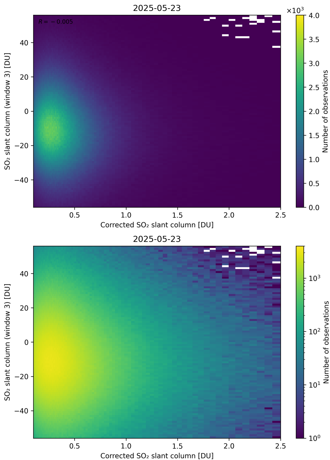
Figure 240: Scatter density plot of “Corrected SO 2 slant column” against “SO 2 slant column (window 3)” for 2025-05-22 to 2025-05-24.
