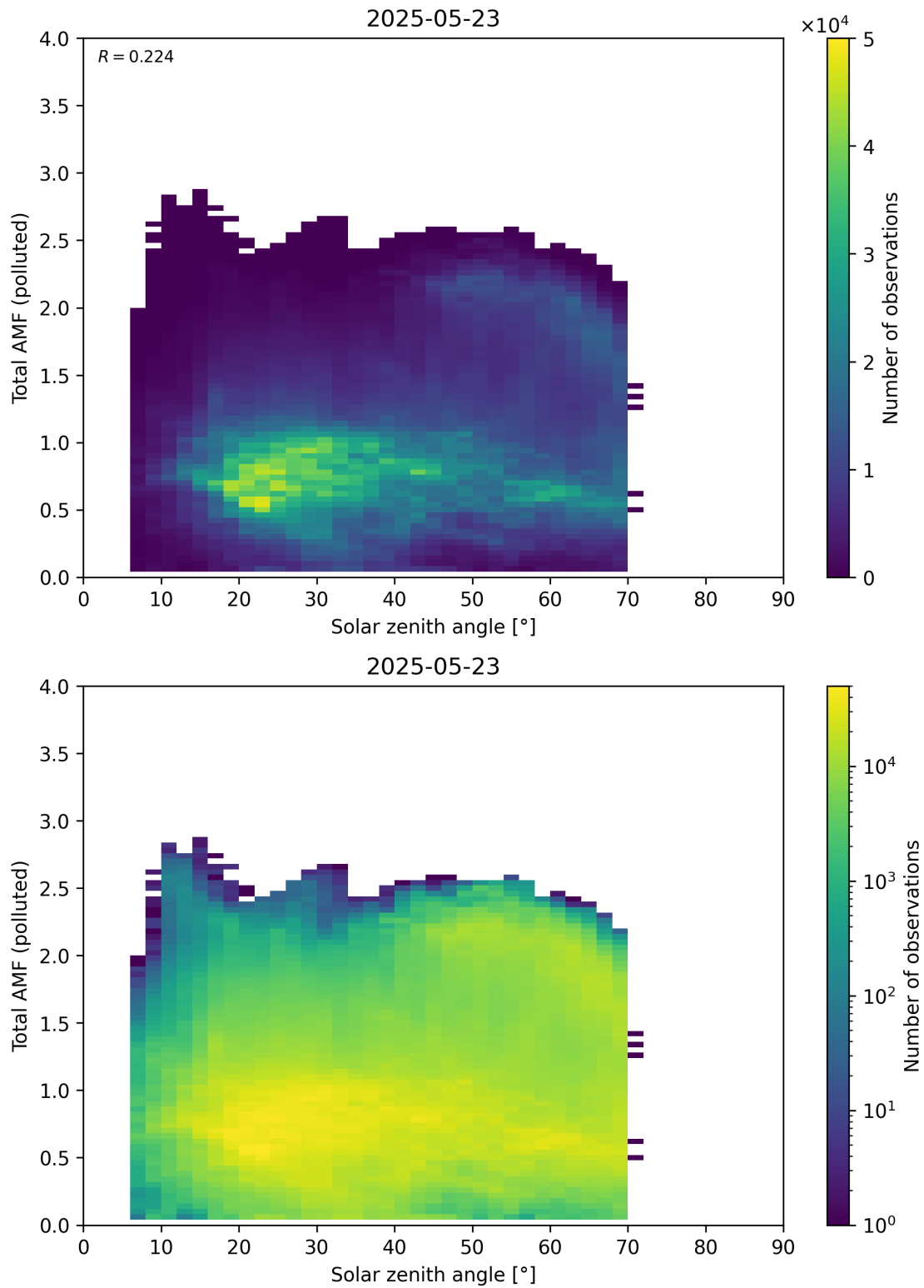
Figure 189: Scatter density plot of “Solar zenith angle” against “Total AMF (polluted)” for 2025-05-22 to 2025-05-24.
