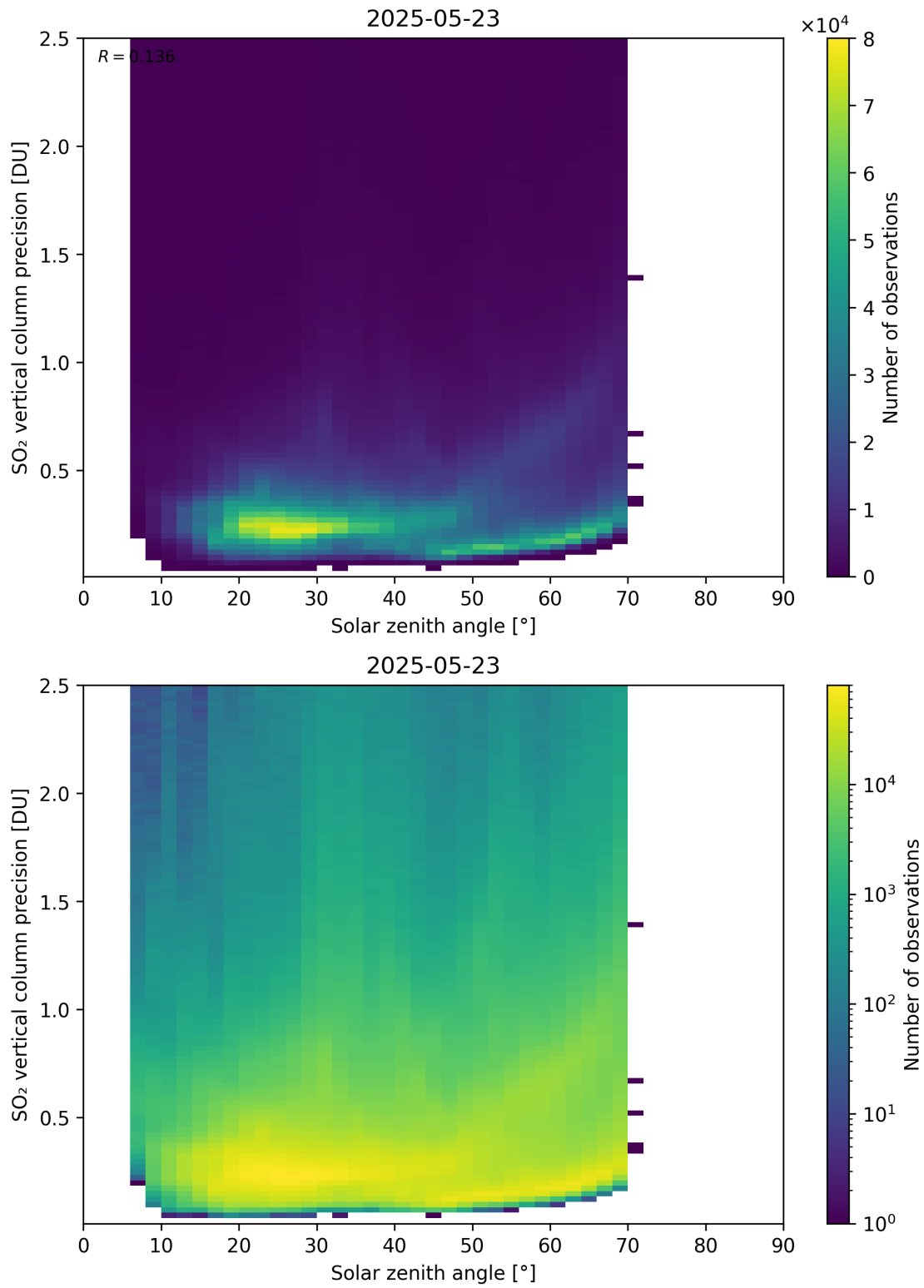
Figure 192: Scatter density plot of “Solar zenith angle” against “SO 2 vertical column precision” for 2025-05-22 to 2025-05-24.
