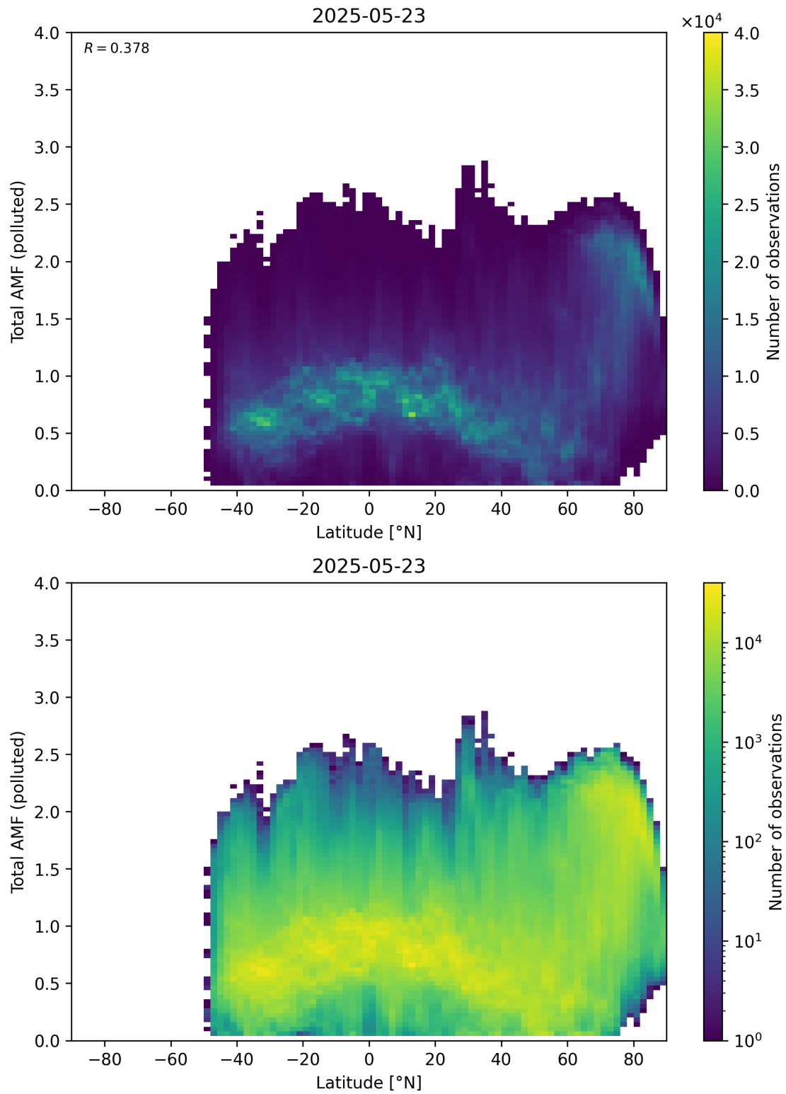
Figure 167: Scatter density plot of “Latitude” against “Total AMF (polluted)” for 2025-05-22 to 2025-05-24.
