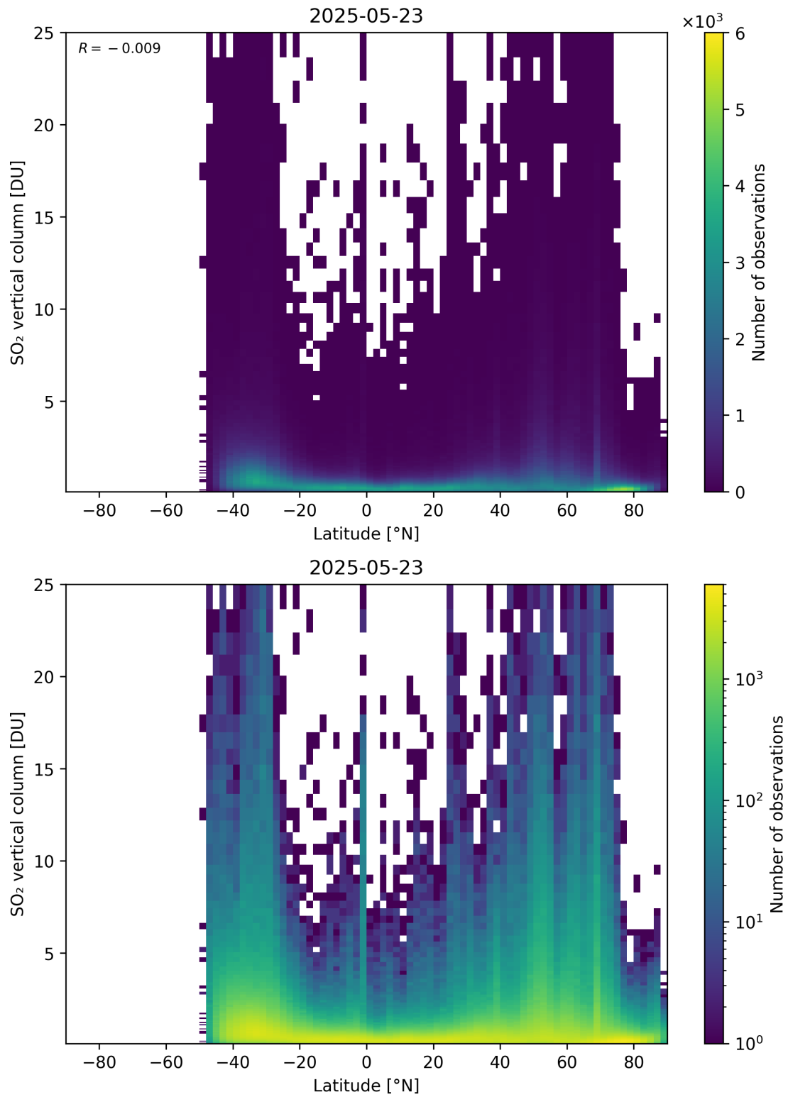
Figure 169: Scatter density plot of “Latitude” against “SO 2 vertical column” for 2025-05-22 to 2025-05-24.
