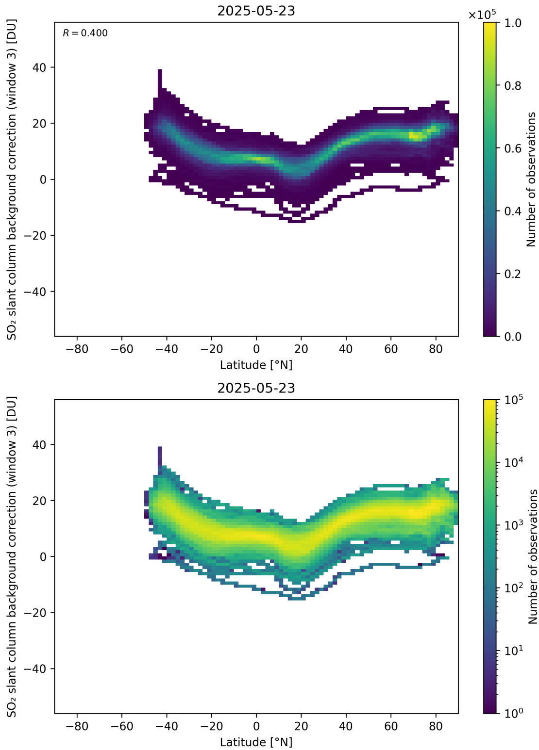
Figure 152: Scatter density plot of “Latitude” against “SO 2 slant column background correction (window 3)” for 2025-05-22 to 2025-05-24.
