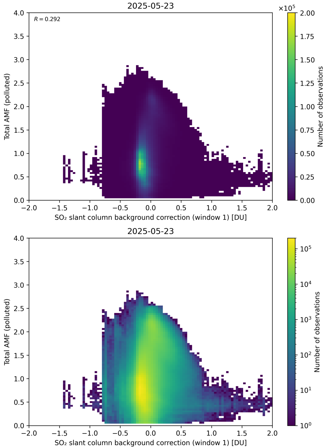
Figure 120: Scatter density plot of “SO 2 slant column background correction (window 1)” against “Total AMF (polluted)” for 2025-05-22 to 2025-05-24.
