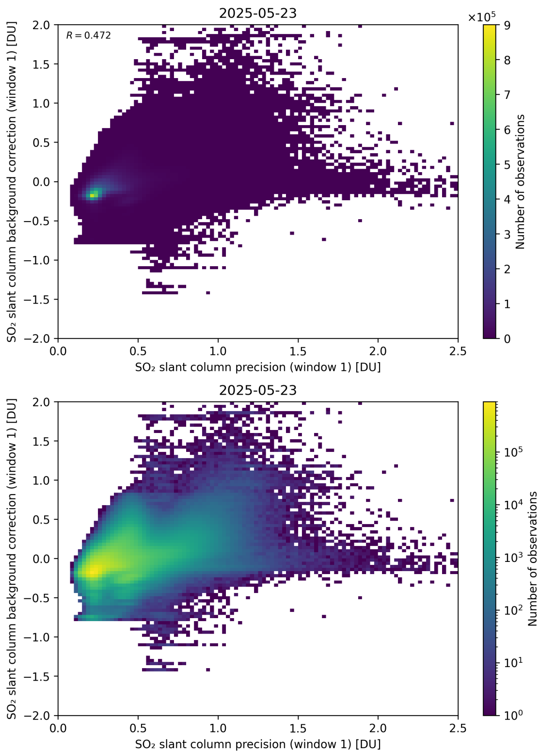
Figure 268: Scatter density plot of “SO 2 slant column precision (window 1)” against “SO 2 slant column background correction (window 1)” for 2025-05-22 to 2025-05-24.
