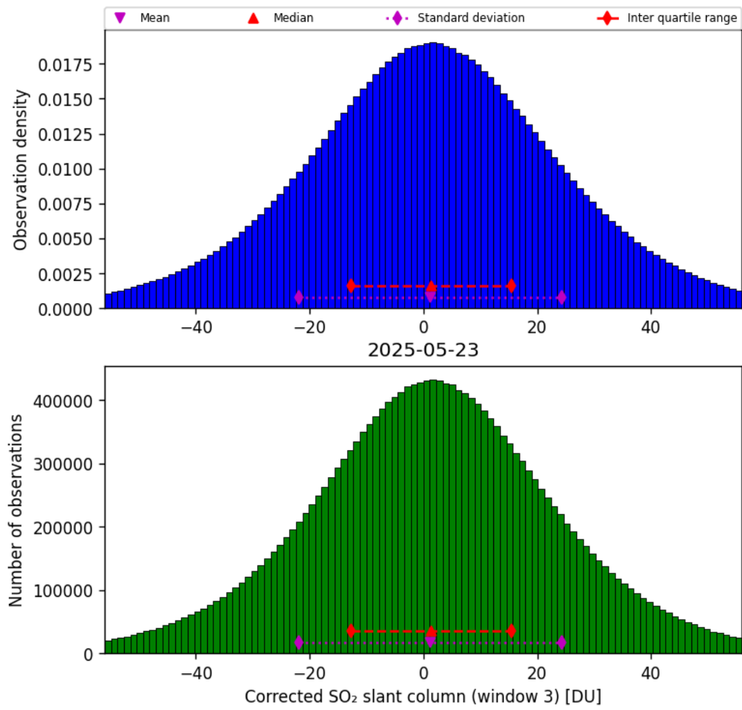
Figure 73: Histogram of “Corrected SO 2 slant column (window 3)” for 2025-05-22 to 2025-05-24
