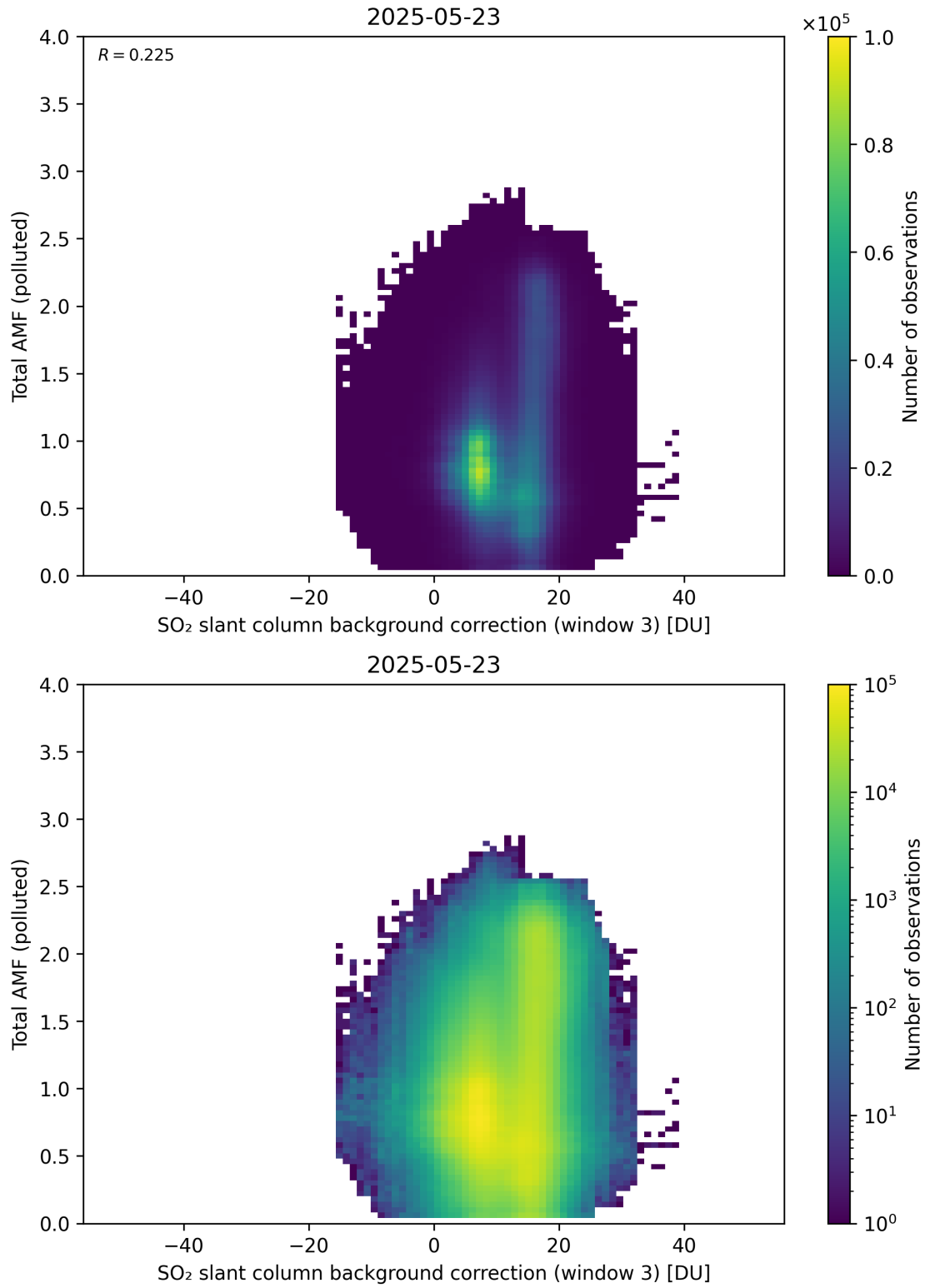
Figure 136: Scatter density plot of “SO 2 slant column background correction (window 3)” against “Total AMF (polluted)” for 2025-05-22 to 2025-05-24.
