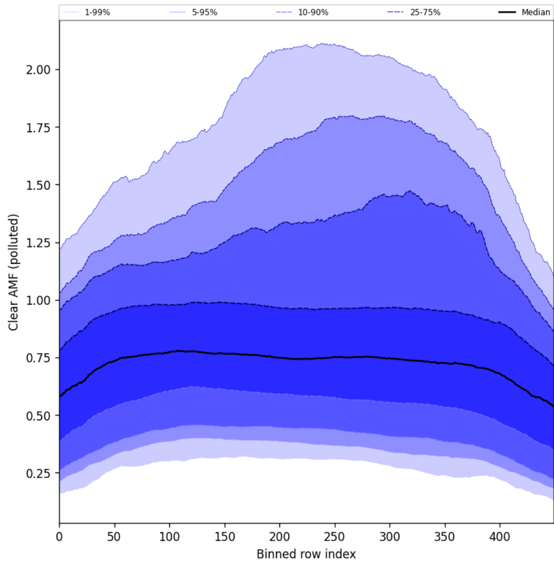
Figure 107: Along track statistics of “Clear AMF (polluted)” for 2025-05-22 to 2025-05-24
