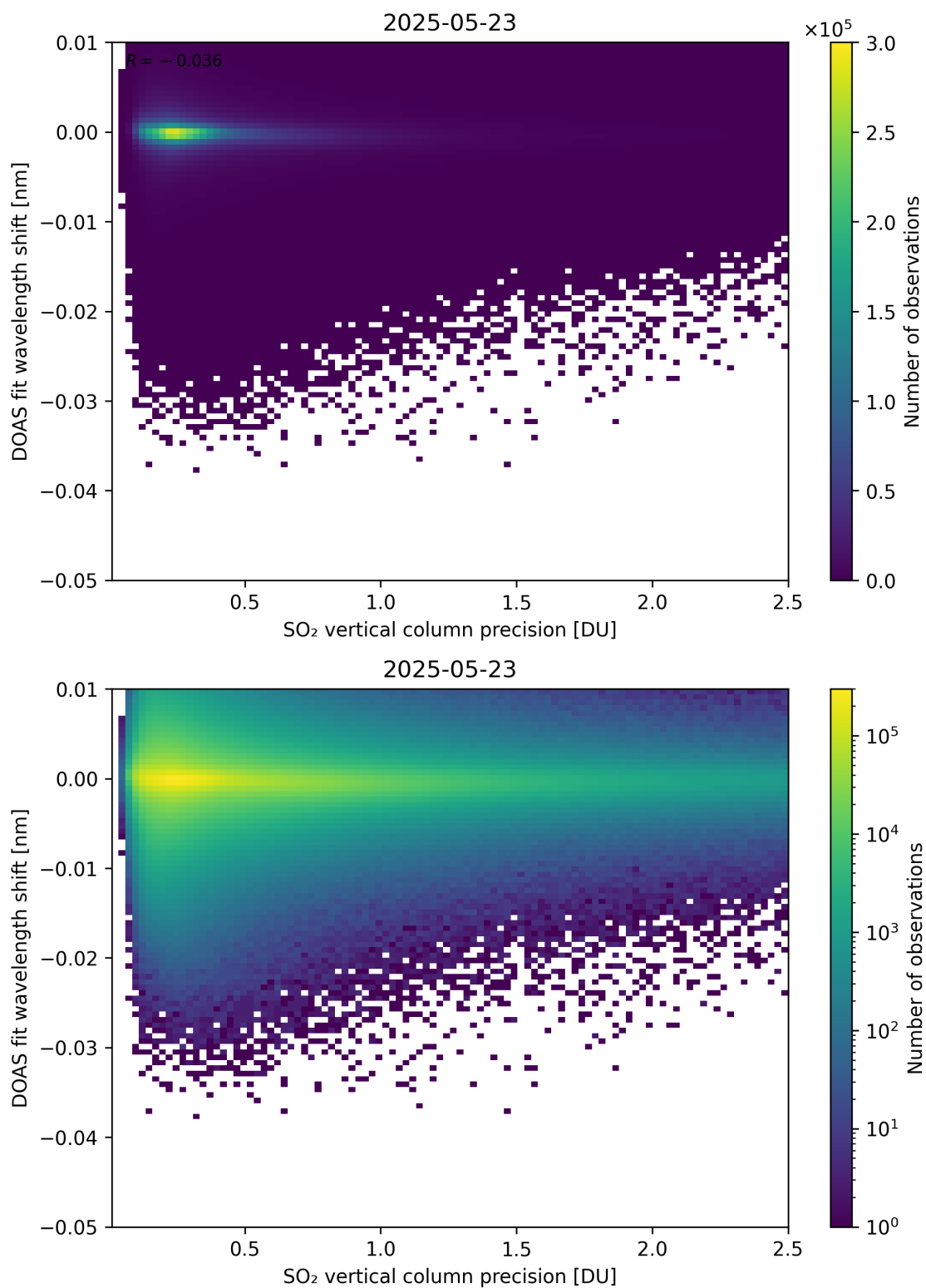
Figure 332: Scatter density plot of “SO 2 vertical column precision” against “DOAS fit wavelength shift” for 2025-05-22 to 2025-05-24.
