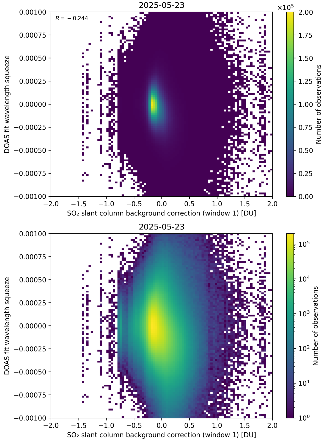
Figure 112: Scatter density plot of “SO 2 slant column background correction (window 1)” against “DOAS fit wavelength squeeze” for 2025-05-22 to 2025-05-24.
