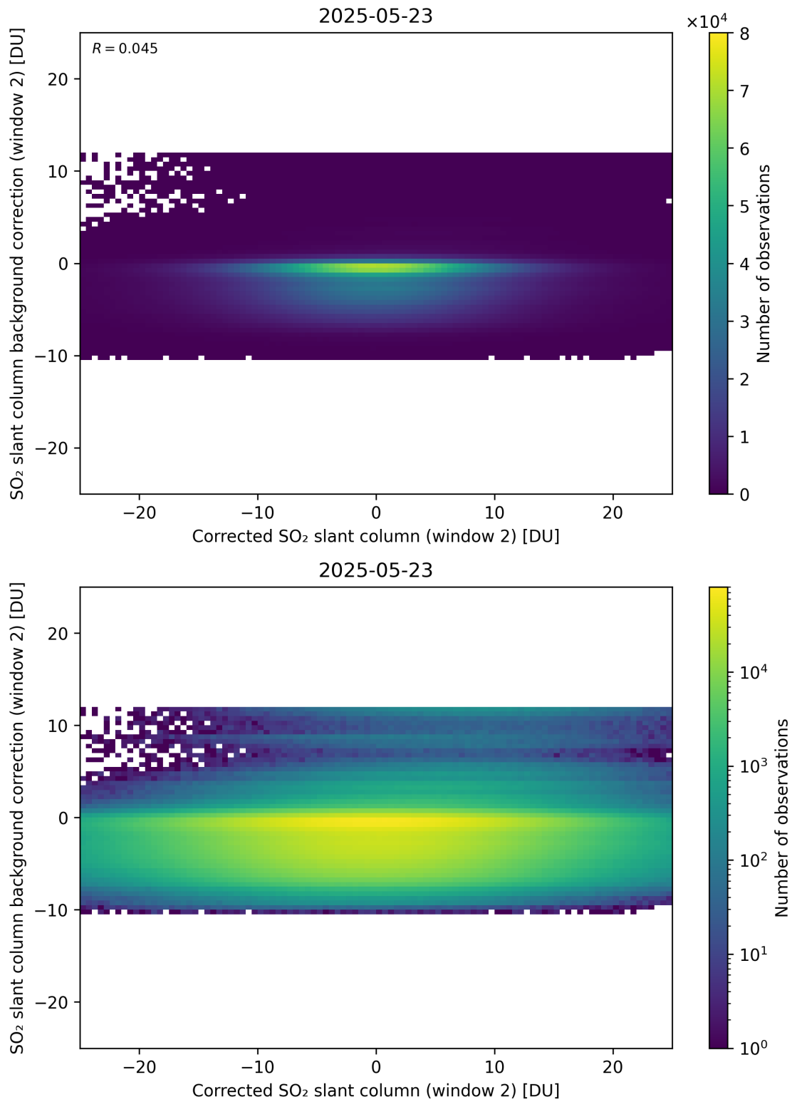
Figure 244: Scatter density plot of “Corrected SO 2 slant column (window 2)” against “SO 2 slant column background correction (window 2)” for 2025-05-22 to 2025-05-24.
