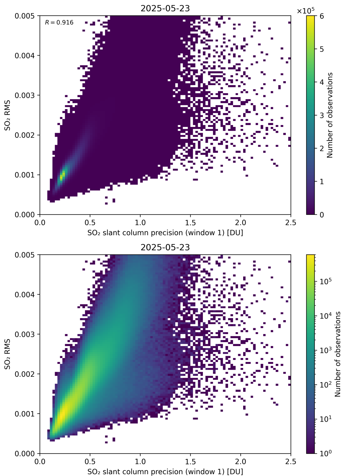
Figure 273: Scatter density plot of “SO 2 slant column precision (window 1)” against “SO 2 RMS” for 2025-05-22 to 2025-05-24.
