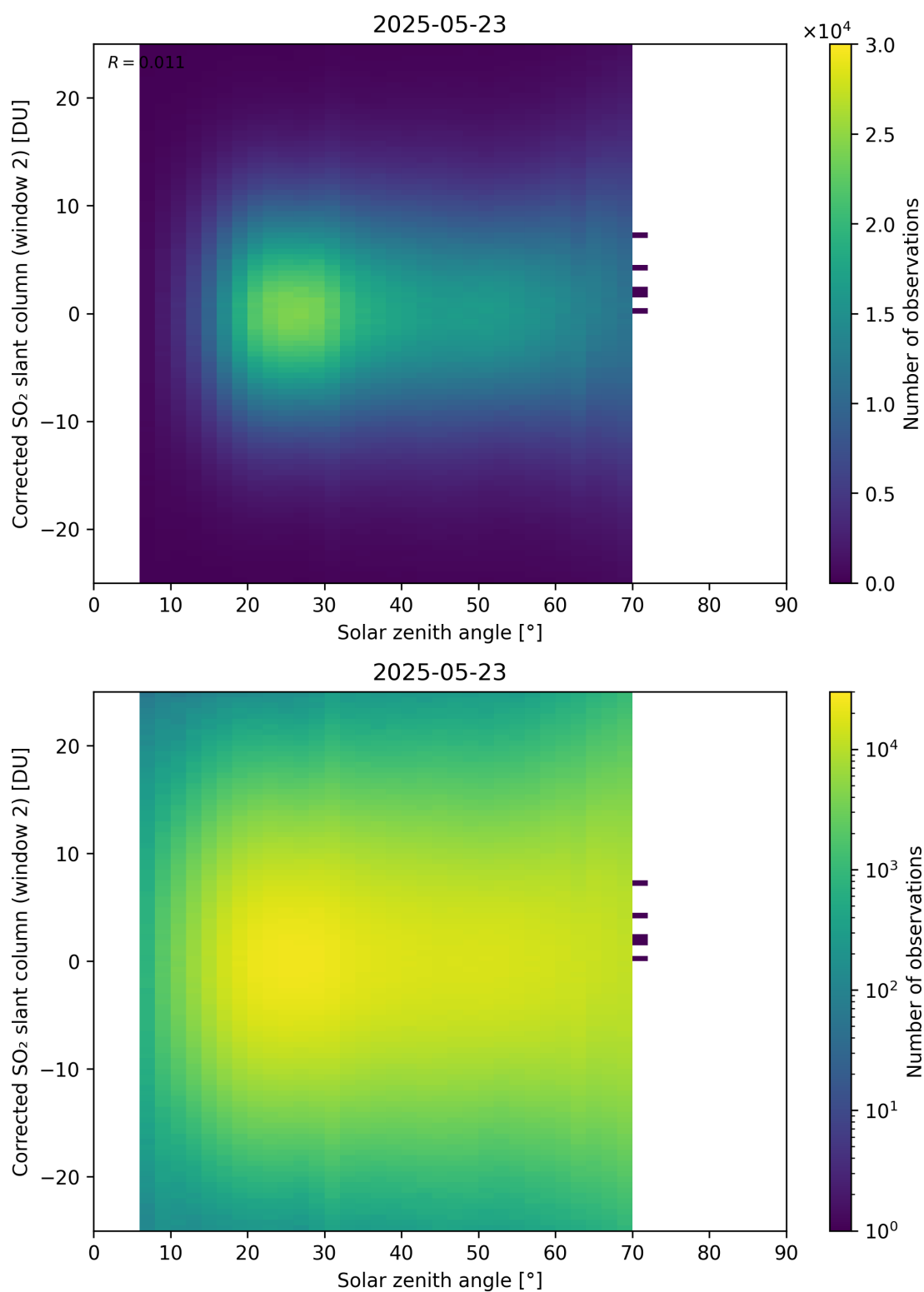
Figure 182: Scatter density plot of “Solar zenith angle” against “Corrected SO 2 slant column (window 2)” for 2025-05-22 to 2025-05-24.
