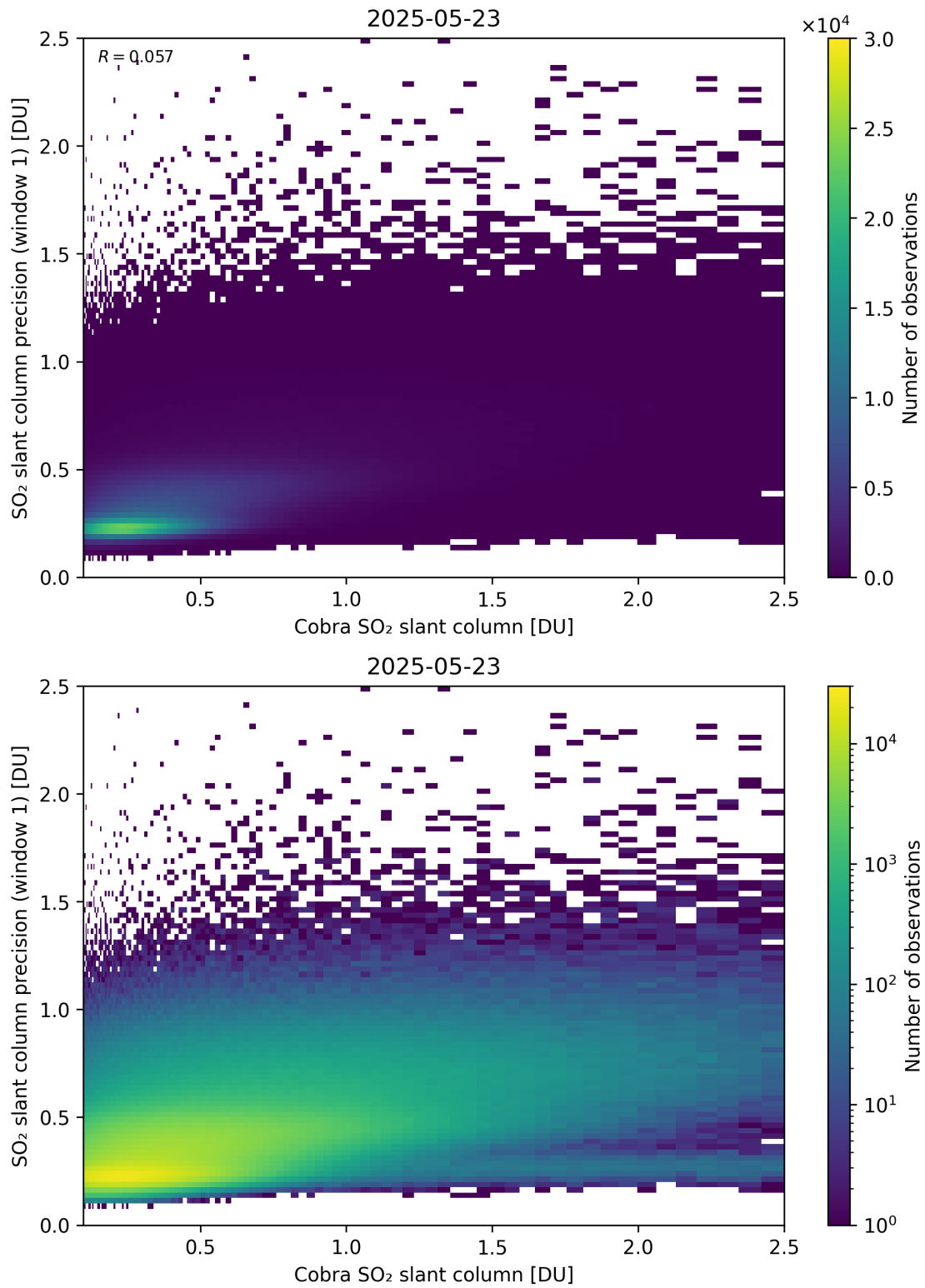
Figure 220: Scatter density plot of “Cobra SO 2 slant column” against “SO 2 slant column precision (window 1)” for 2025-05-22 to 2025-05-24.
