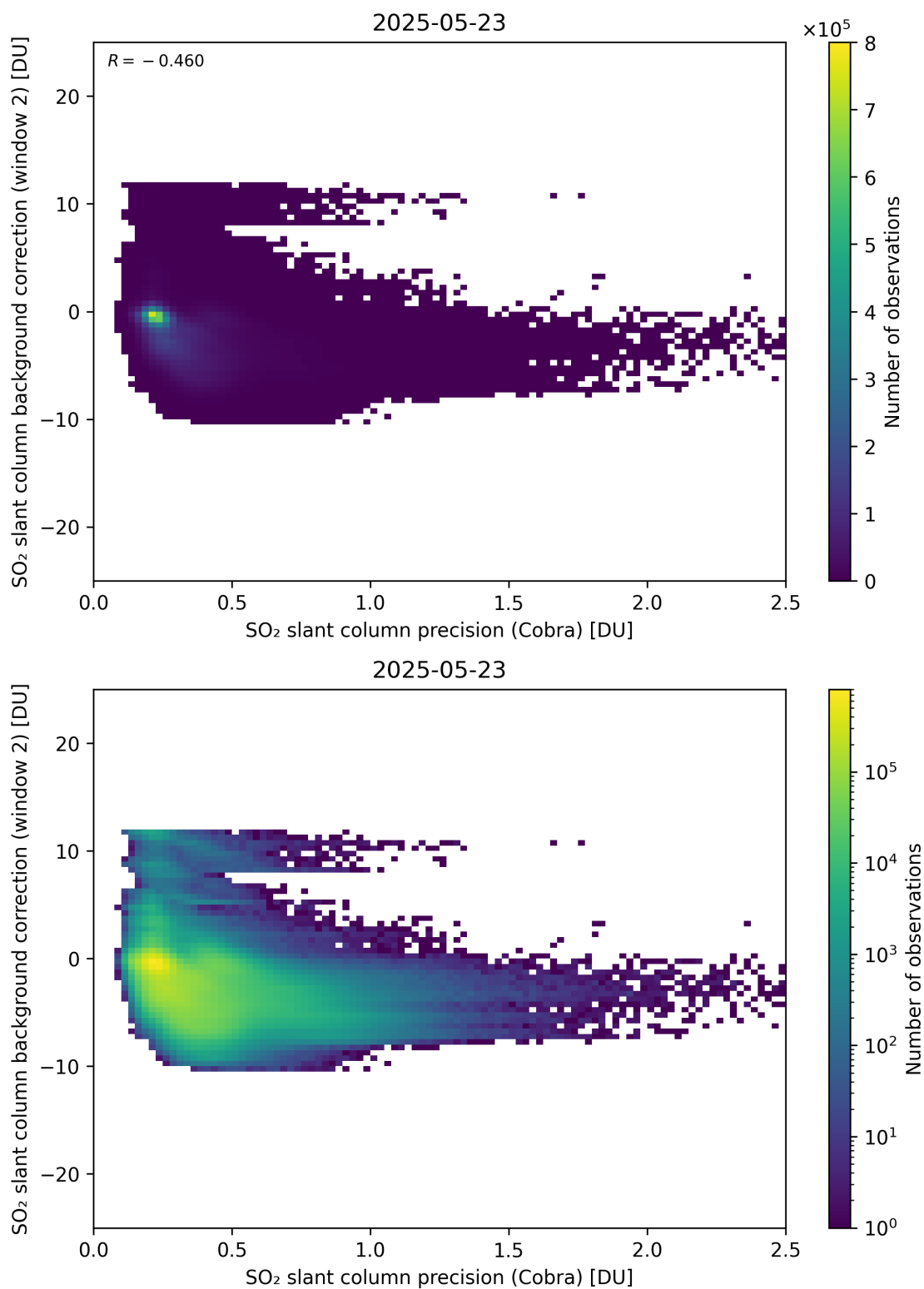
Figure 200: Scatter density plot of “SO 2 slant column precision (Cobra)” against “SO 2 slant column background correction (window 2)” for 2025-05-22 to 2025-05-24.
