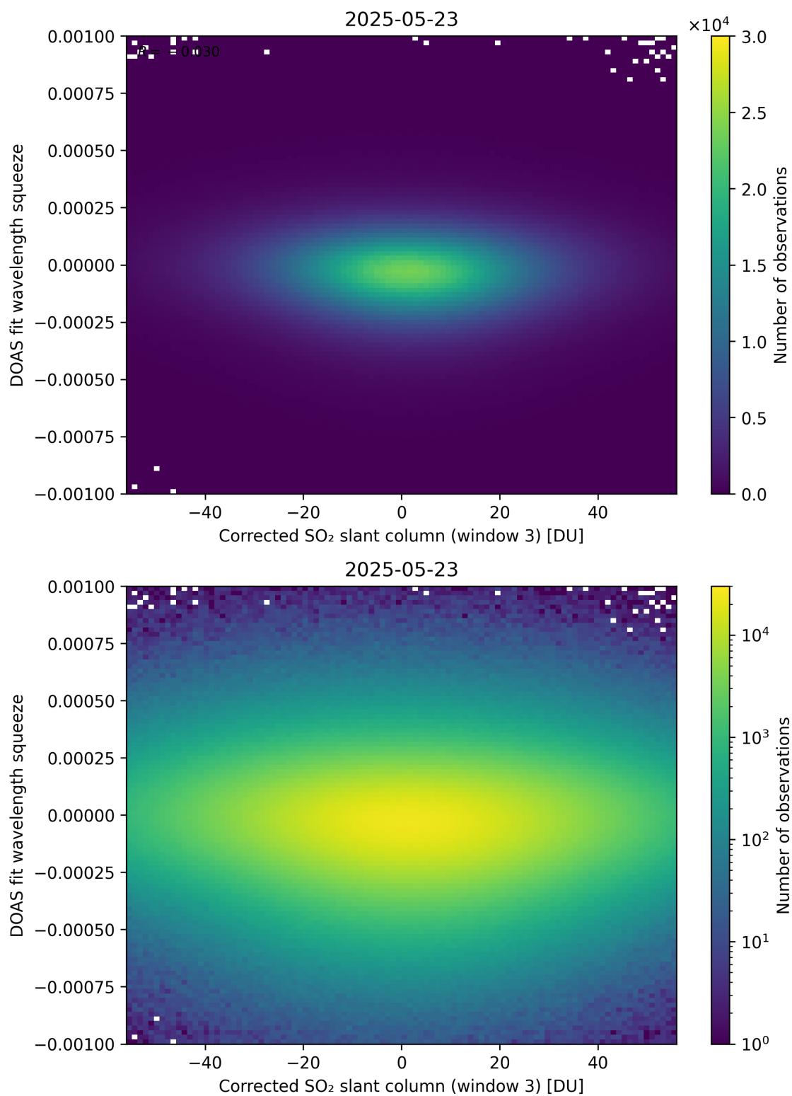
Figure 257: Scatter density plot of “Corrected SO 2 slant column (window 3)” against “DOAS fit wavelength squeeze” for 2025-05-22 to 2025-05-24.
