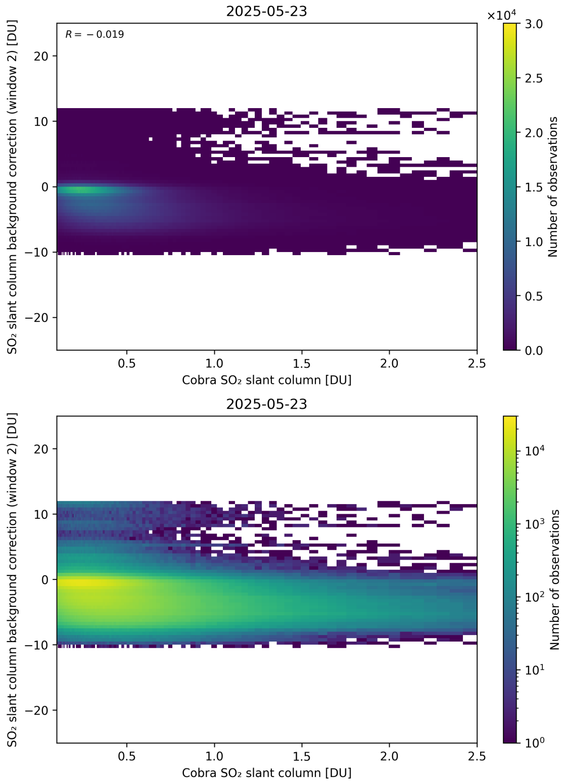
Figure 194: Scatter density plot of “Cobra SO 2 slant column” against “SO 2 slant column background correction (window 2)” for 2025-05-22 to 2025-05-24.
