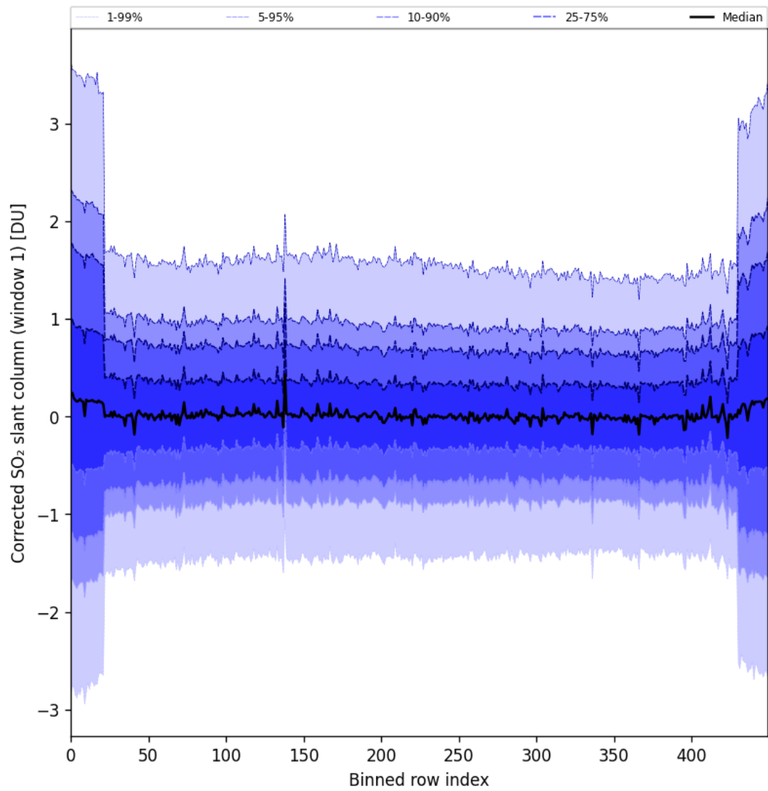
Figure 91: Along track statistics of “Corrected SO 2 slant column (window 1)” for 2025-05-22 to 2025-05-24
