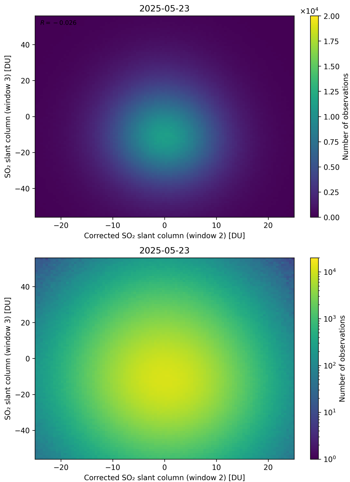
Figure 251: Scatter density plot of “Corrected SO 2 slant column (window 2)” against “SO 2 slant column (window 3)” for 2025-05-22 to 2025-05-24.
