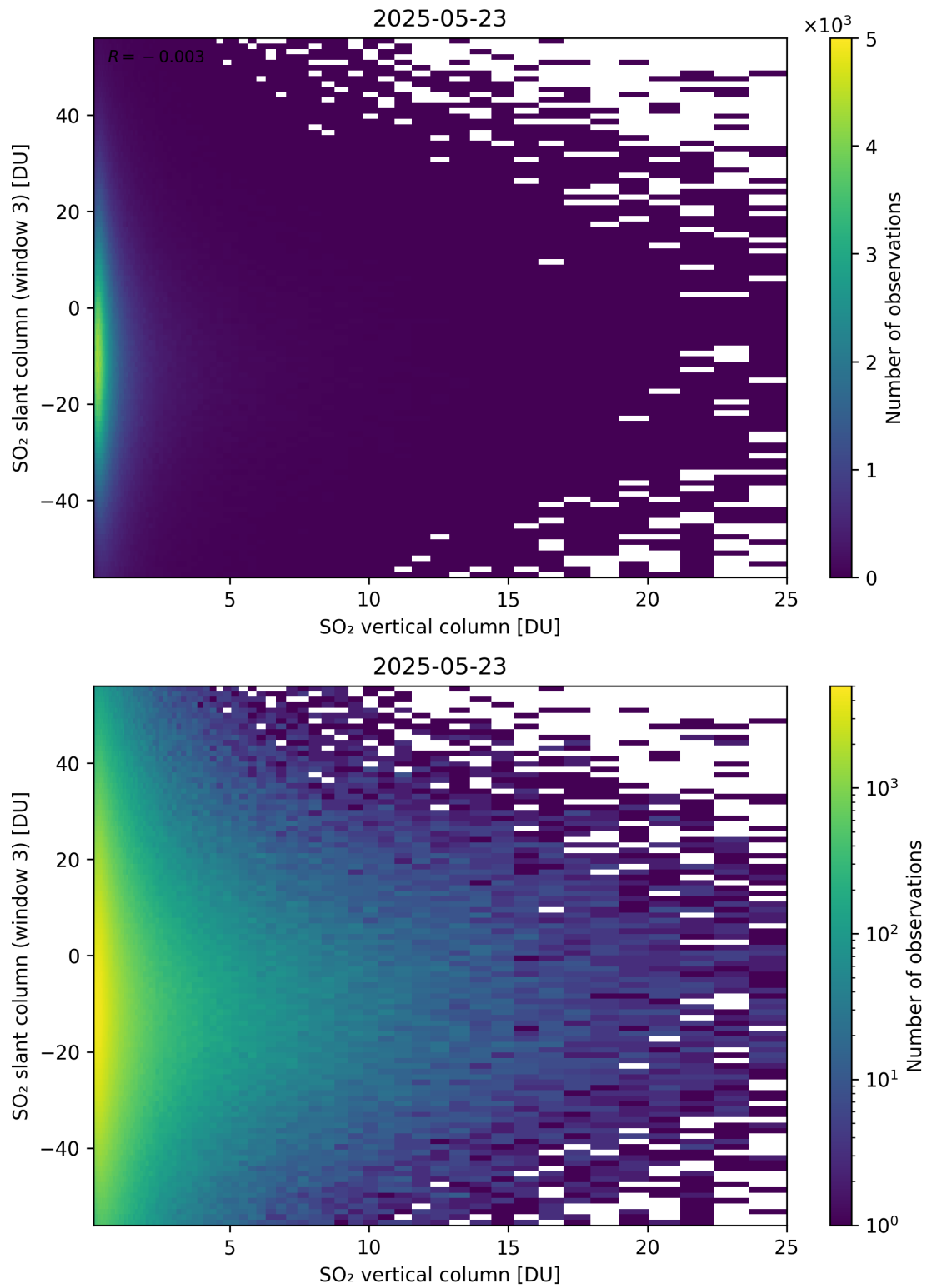
Figure 357: Scatter density plot of “SO 2 vertical column” against “SO 2 slant column (window 3)” for 2025-05-22 to 2025-05-24.
