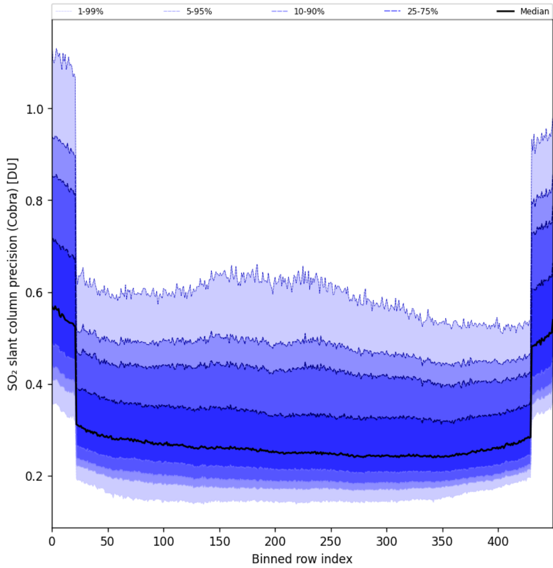
Figure 88: Along track statistics of “SO 2 slant column precision (Cobra)” for 2025-05-22 to 2025-05-24
