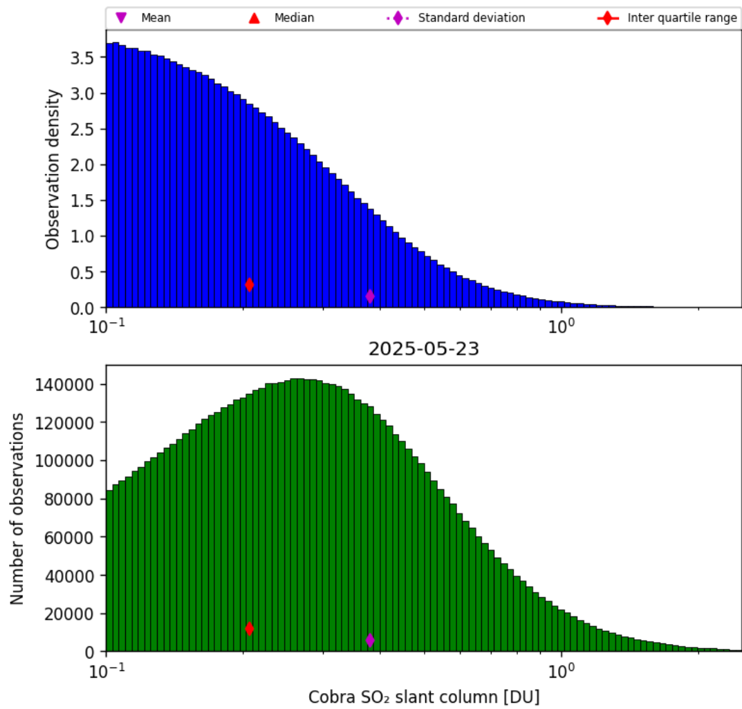
Figure 61: Histogram of “Cobra SO 2 slant column” for 2025-05-22 to 2025-05-24
