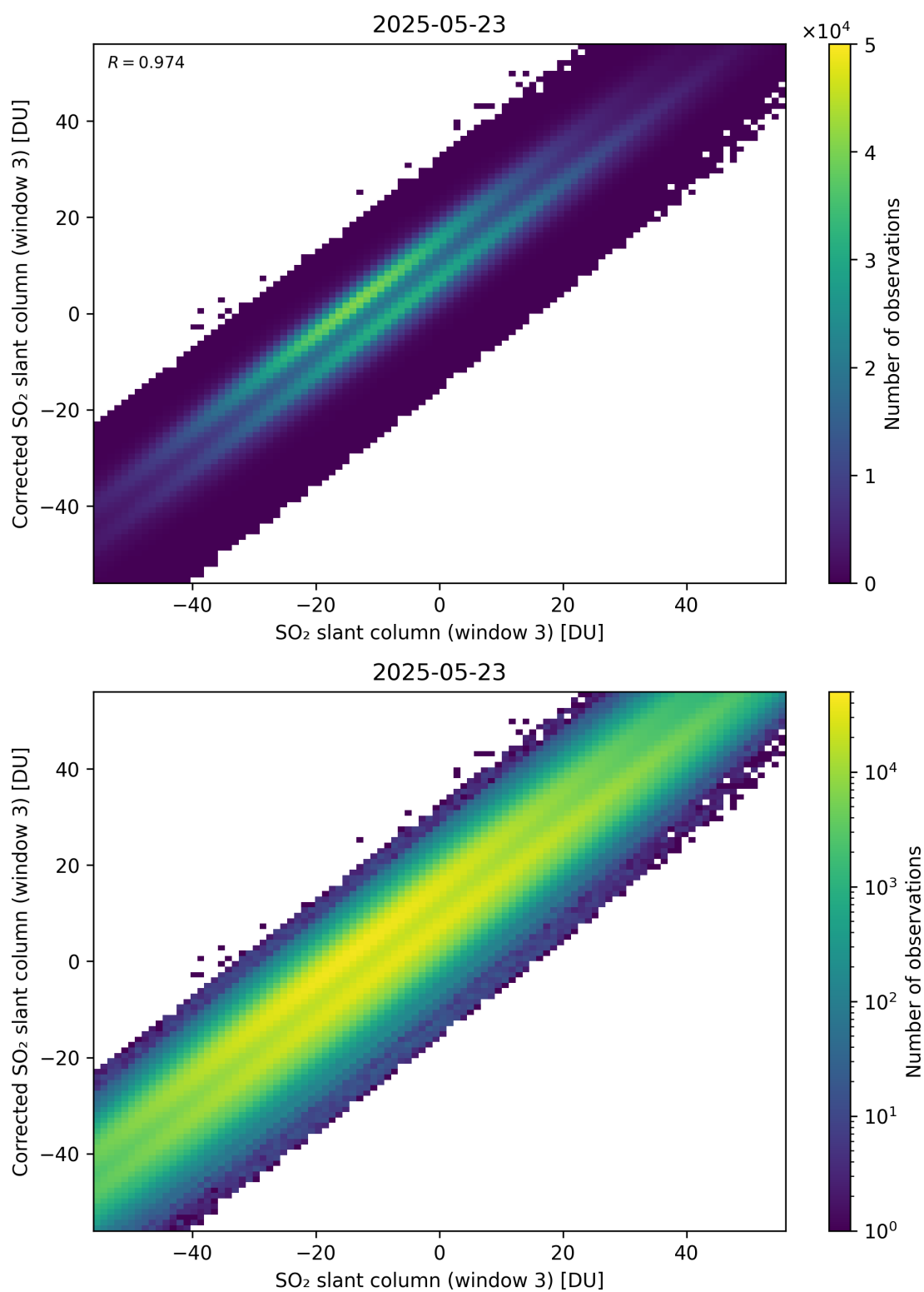
Figure 316: Scatter density plot of “SO 2 slant column (window 3)” against “Corrected SO 2 slant column (window 3)” for 2025-05-22 to 2025-05-24.
