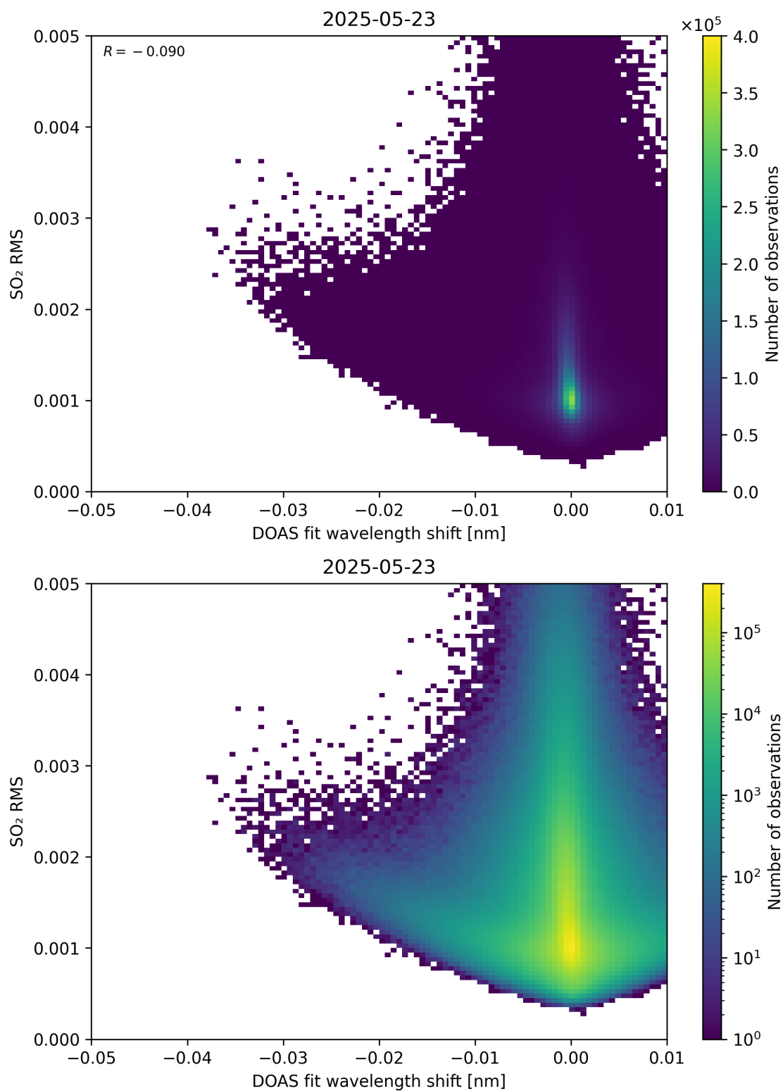
Figure 139: Scatter density plot of “DOAS fit wavelength shift” against “SO 2 RMS” for 2025-05-22 to 2025-05-24.
