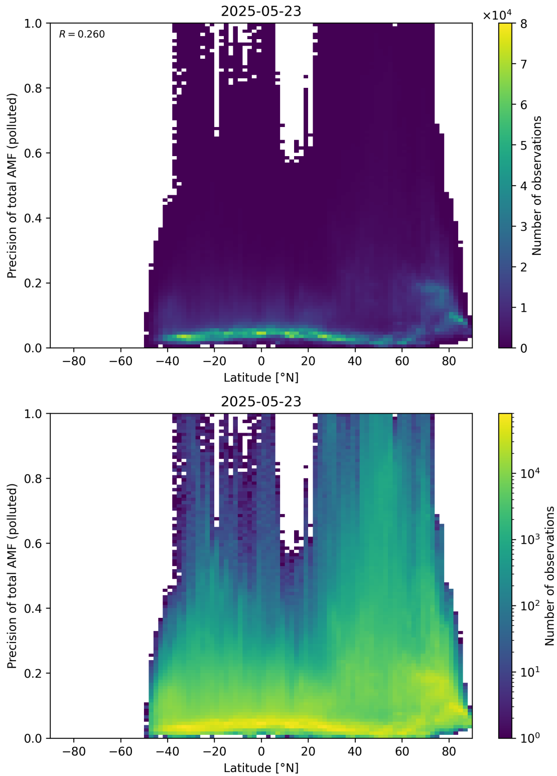
Figure 168: Scatter density plot of “Latitude” against “Precision of total AMF (polluted)” for 2025-05-22 to 2025-05-24.
