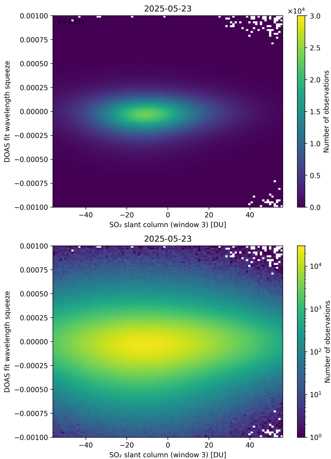
Figure 305: Scatter density plot of “SO 2 slant column (window 3)” against “DOAS fit wavelength squeeze” for 2025-05-22 to 2025-05-24.
