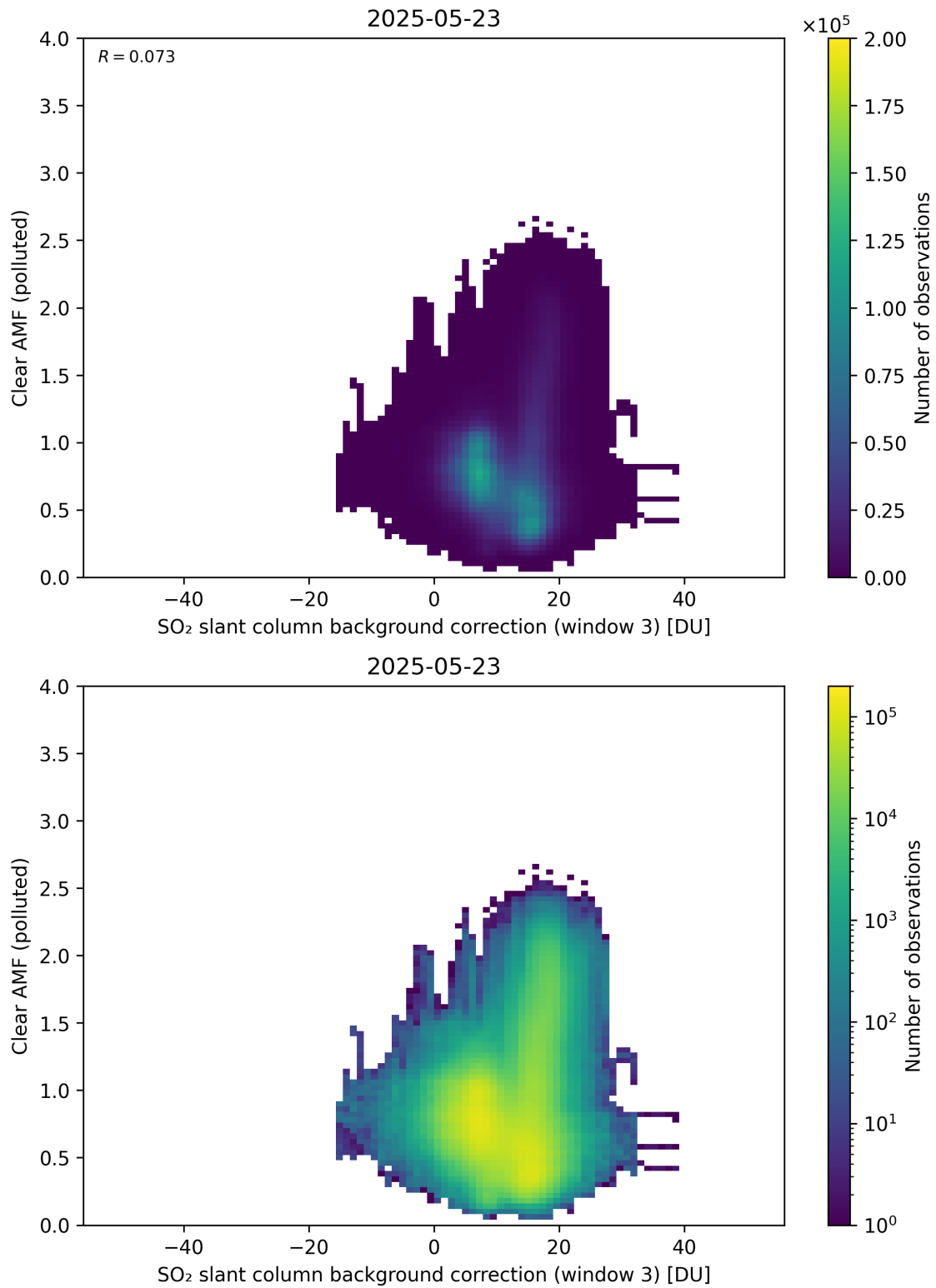
Figure 135: Scatter density plot of “SO 2 slant column background correction (window 3)” against “Clear AMF (polluted)” for 2025-05-22 to 2025-05-24.
