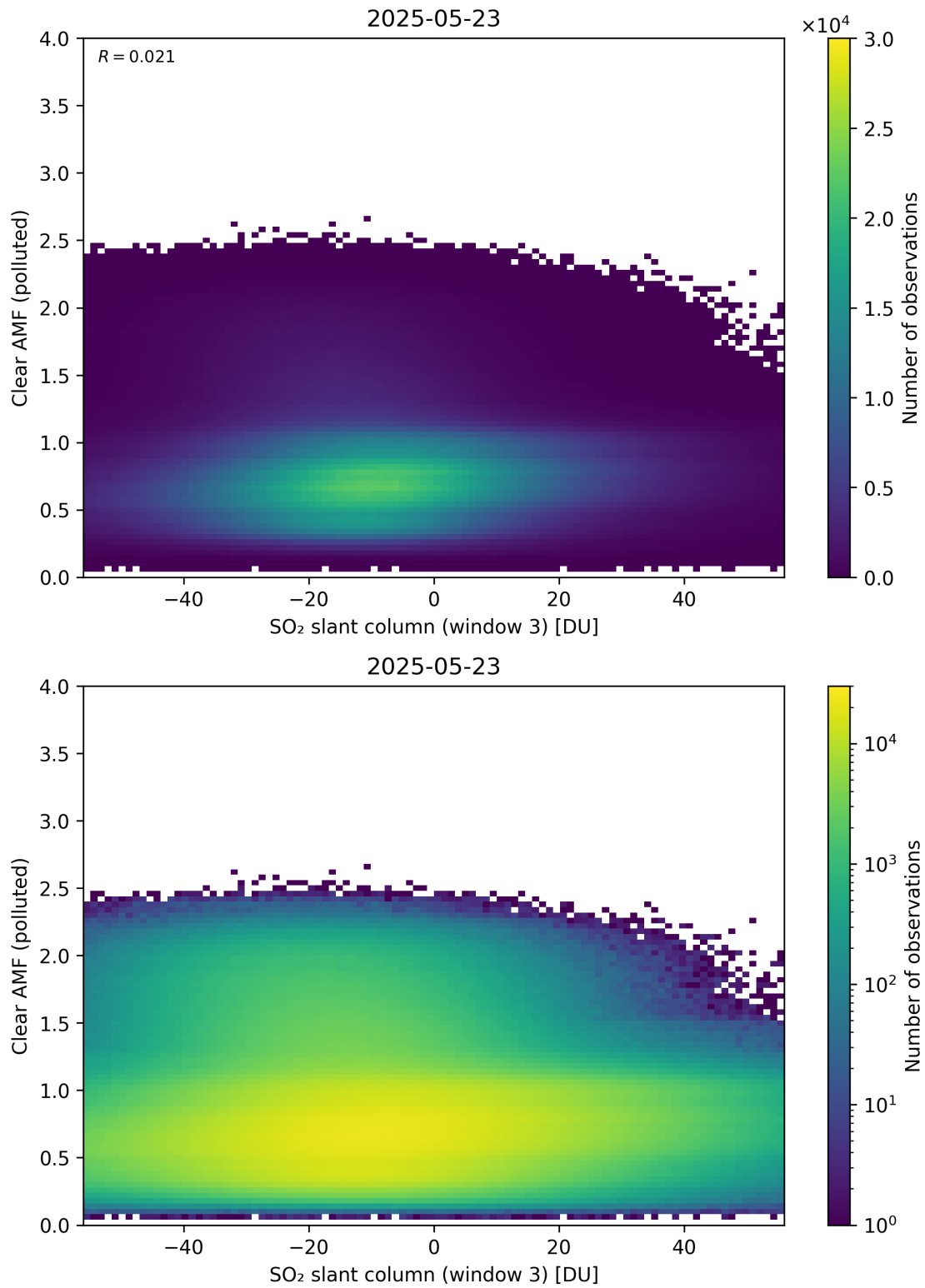
Figure 315: Scatter density plot of “SO 2 slant column (window 3)” against “Clear AMF (polluted)” for 2025-05-22 to 2025-05-24.
