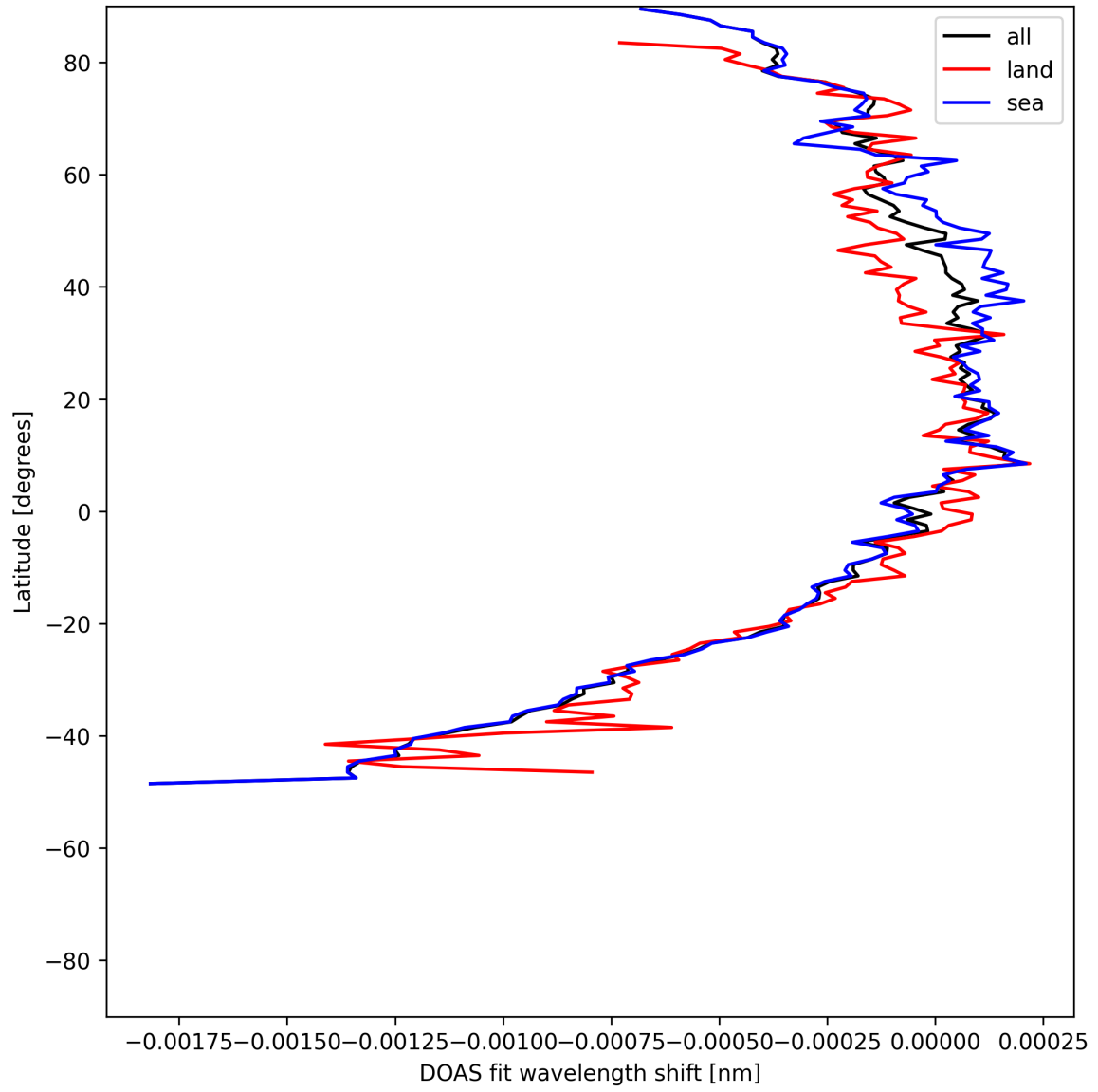
Figure 50: Zonal average of “DOAS fit wavelength shift” for 2025-05-22 to 2025-05-24.
