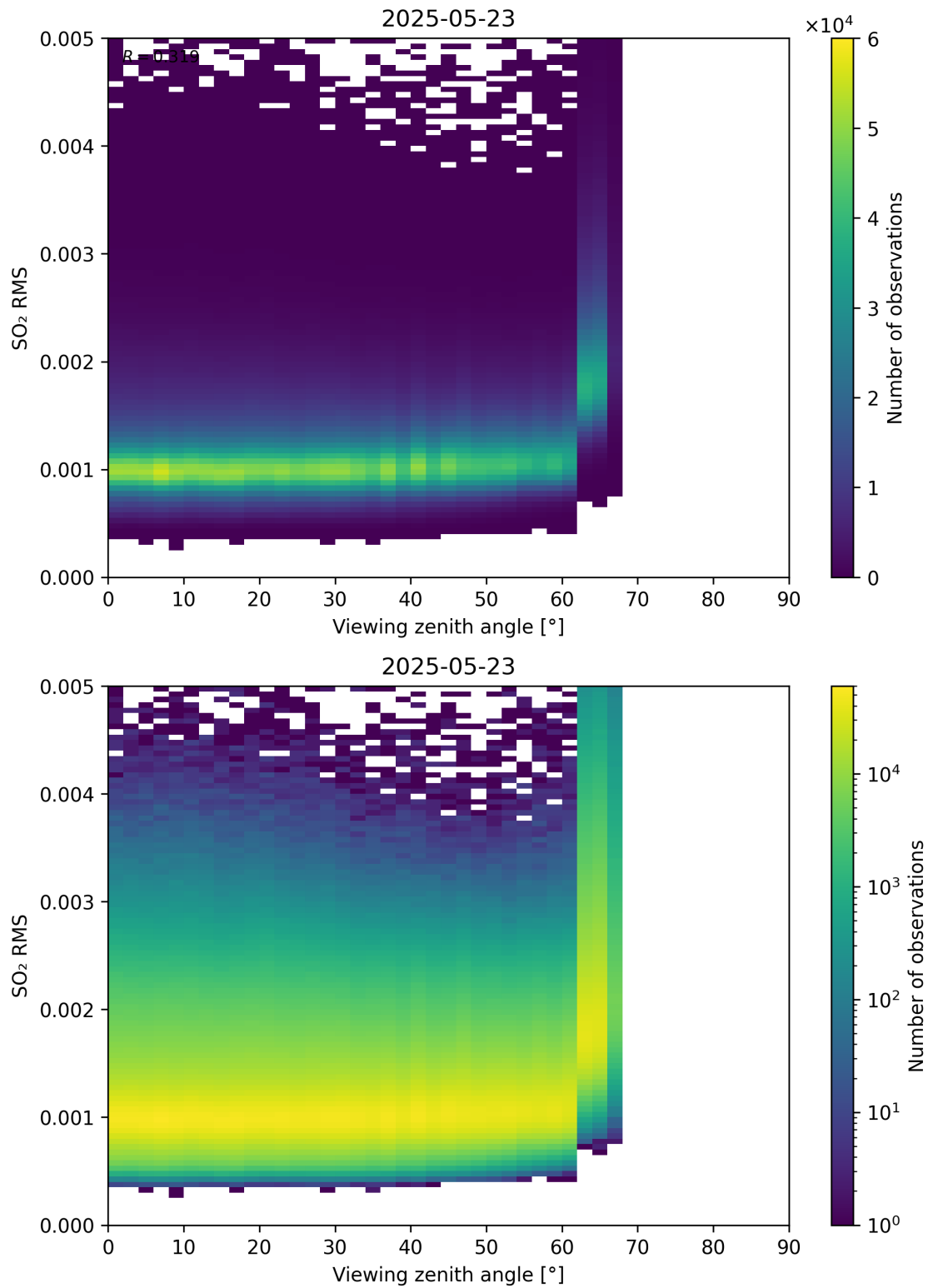
Figure 367: Scatter density plot of “Viewing zenith angle” against “SO 2 RMS” for 2025-05-22 to 2025-05-24.
