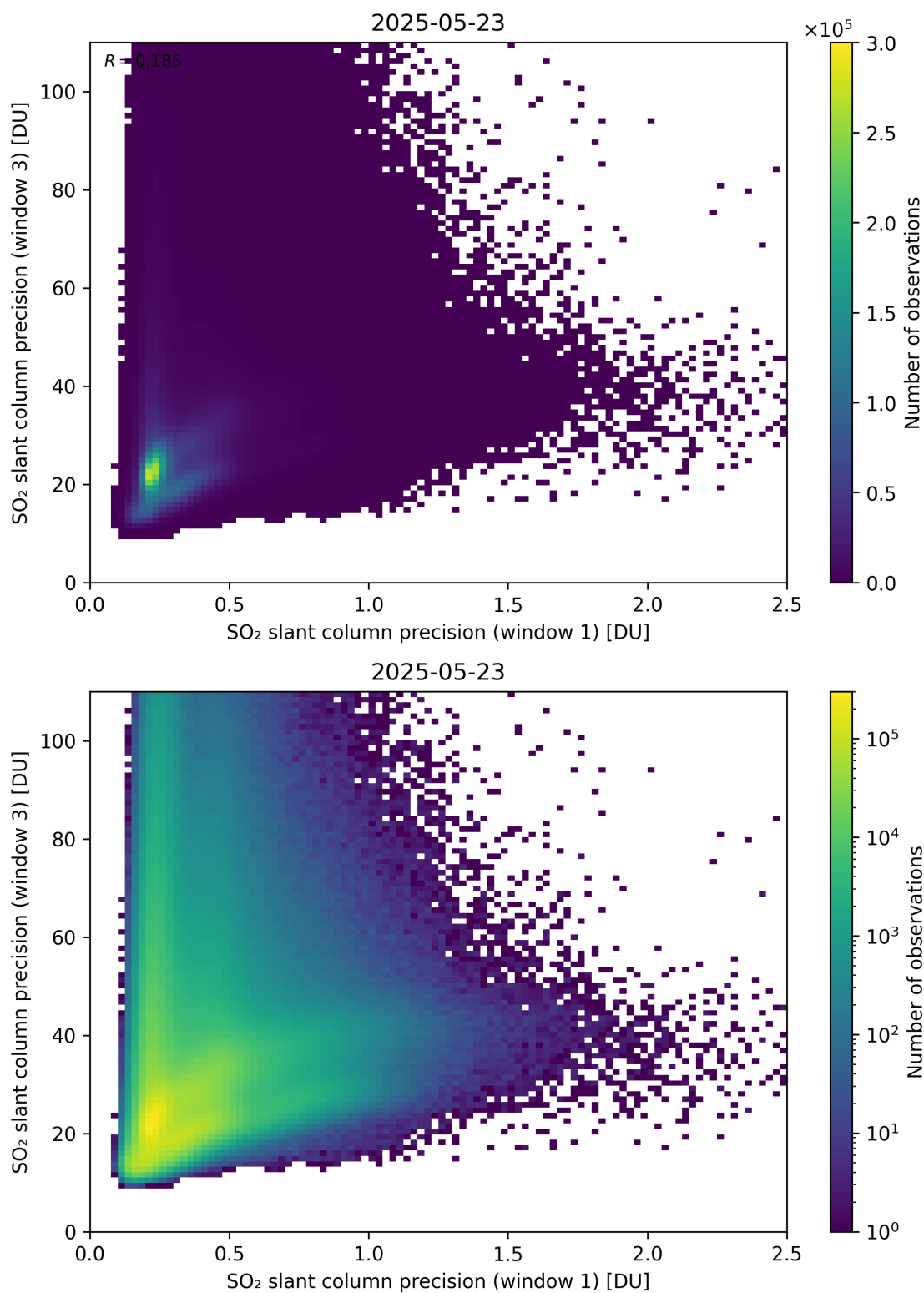
Figure 279: Scatter density plot of “SO 2 slant column precision (window 1)” against “SO 2 slant column precision (window 3)” for 2025-05-22 to 2025-05-24.
