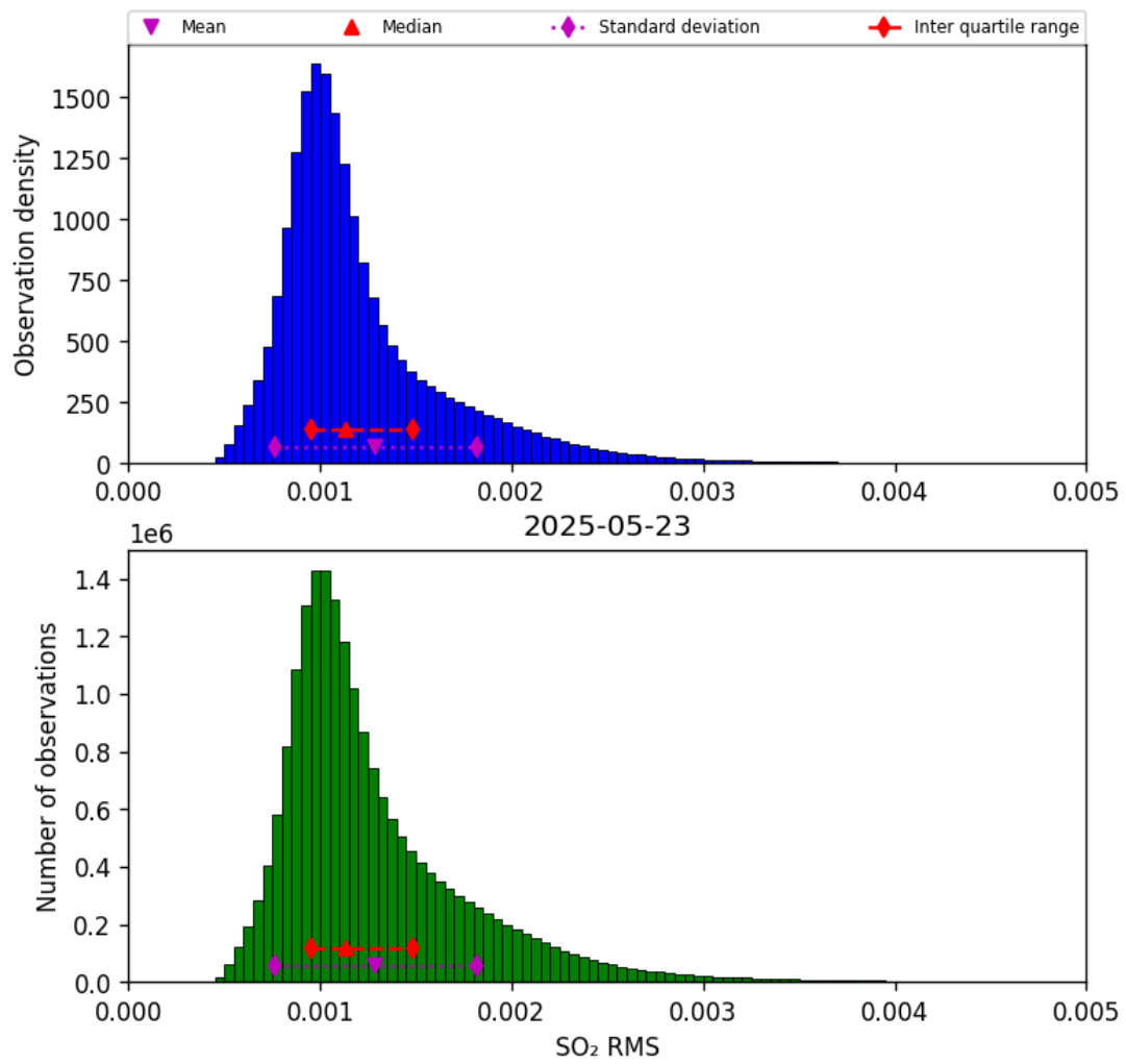
Figure 78: Histogram of “SO 2 RMS” for 2025-05-22 to 2025-05-24
