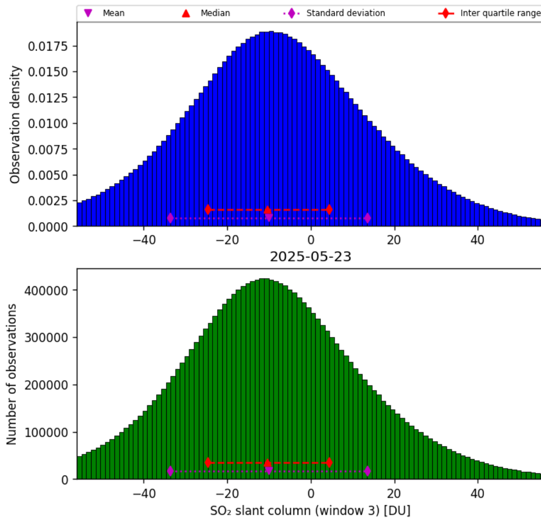
Figure 71: Histogram of “SO 2 slant column (window 3)” for 2025-05-22 to 2025-05-24
