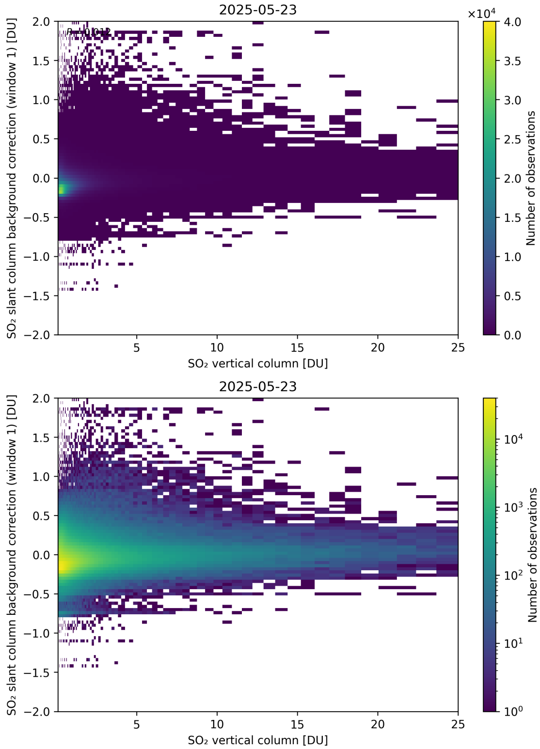
Figure 323: Scatter density plot of “SO 2 vertical column” against “SO 2 slant column background correction (window 1)” for 2025-05-22 to 2025-05-24.
