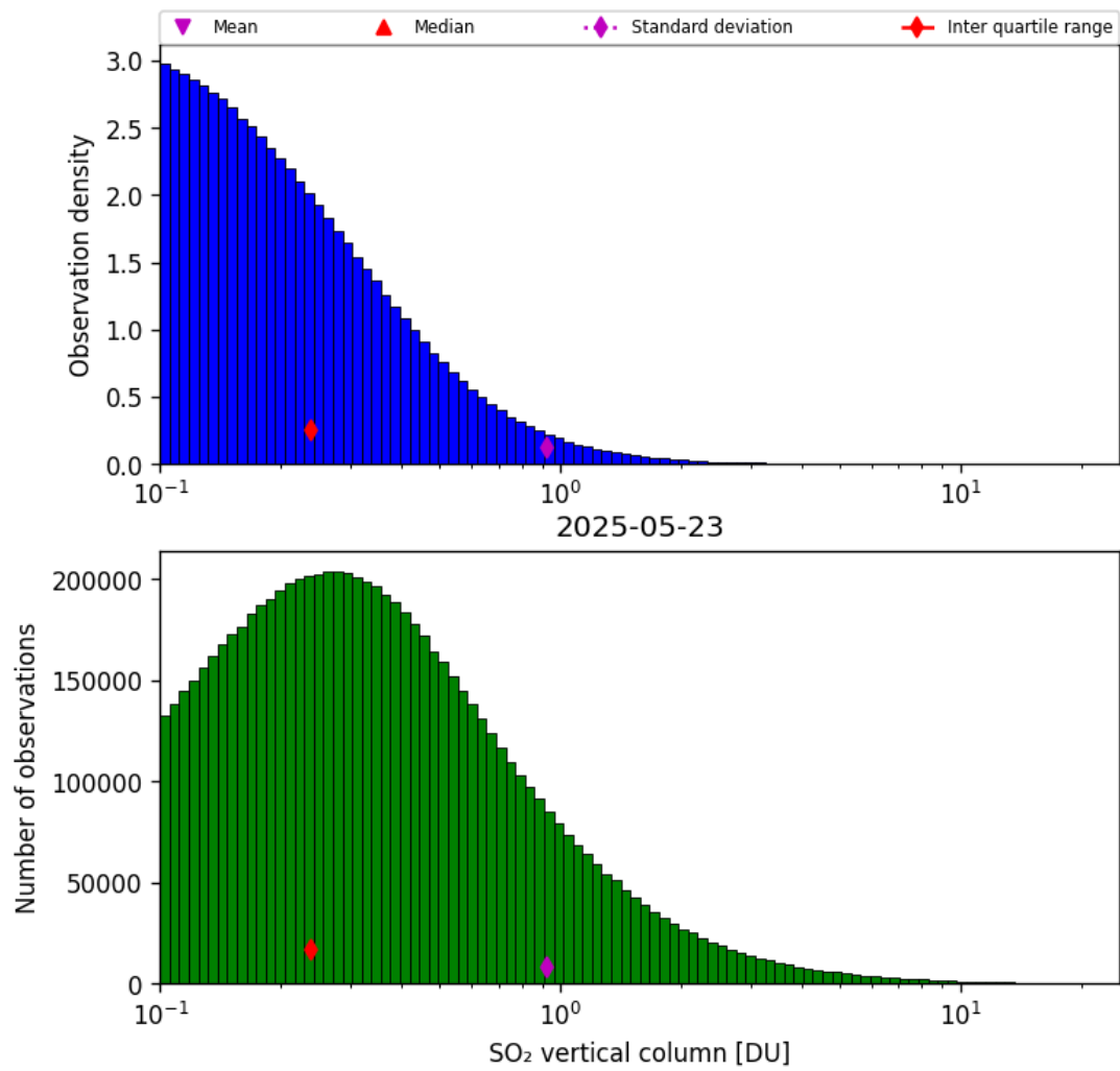
Figure 58: Histogram of “SO 2 vertical column” for 2025-05-22 to 2025-05-24
