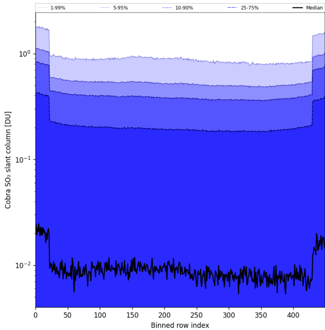
Figure 87: Along track statistics of “Cobra SO 2 slant column” for 2025-05-22 to 2025-05-24
