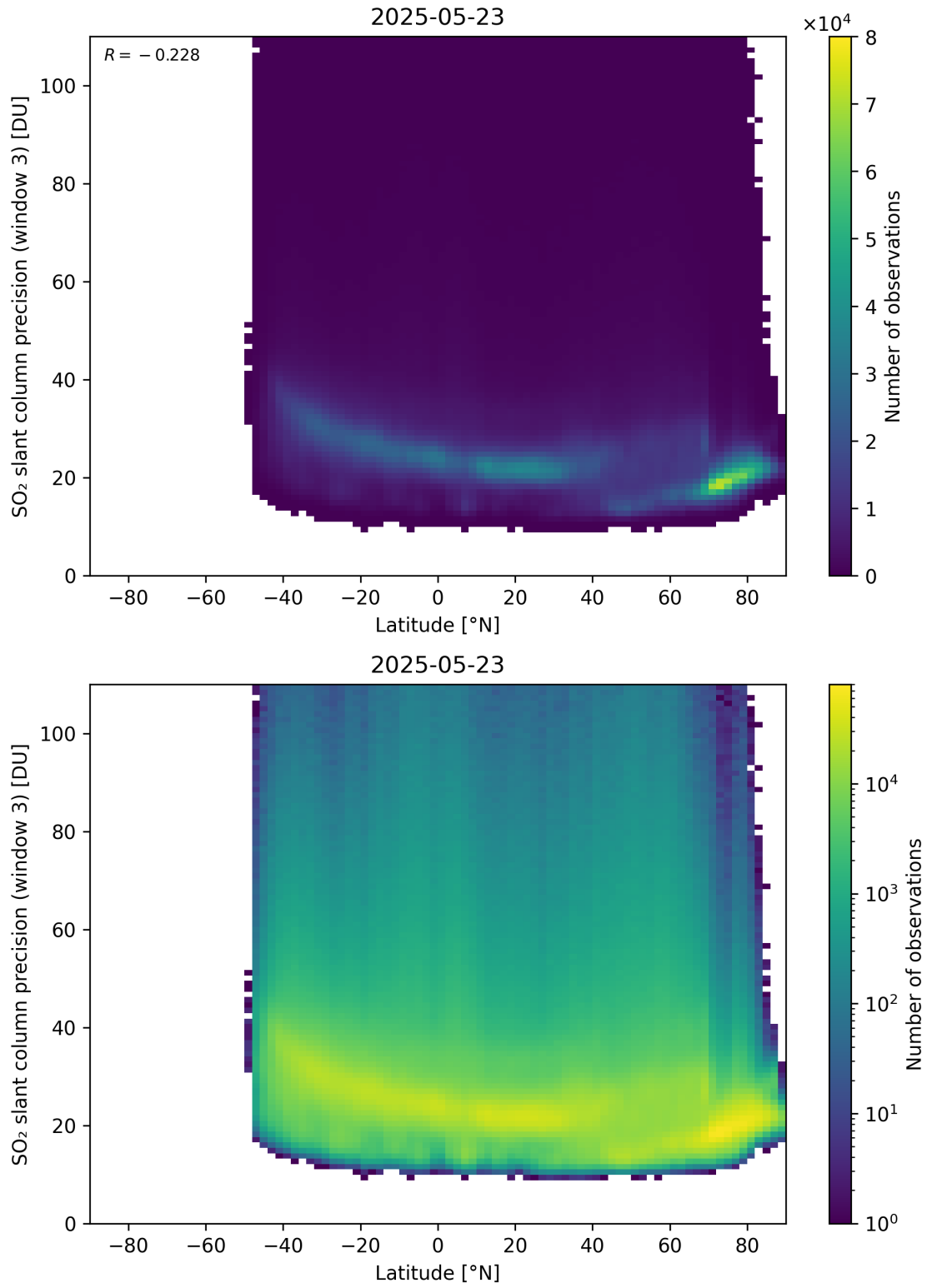
Figure 166: Scatter density plot of “Latitude” against “SO 2 slant column precision (window 3)” for 2025-05-22 to 2025-05-24.
