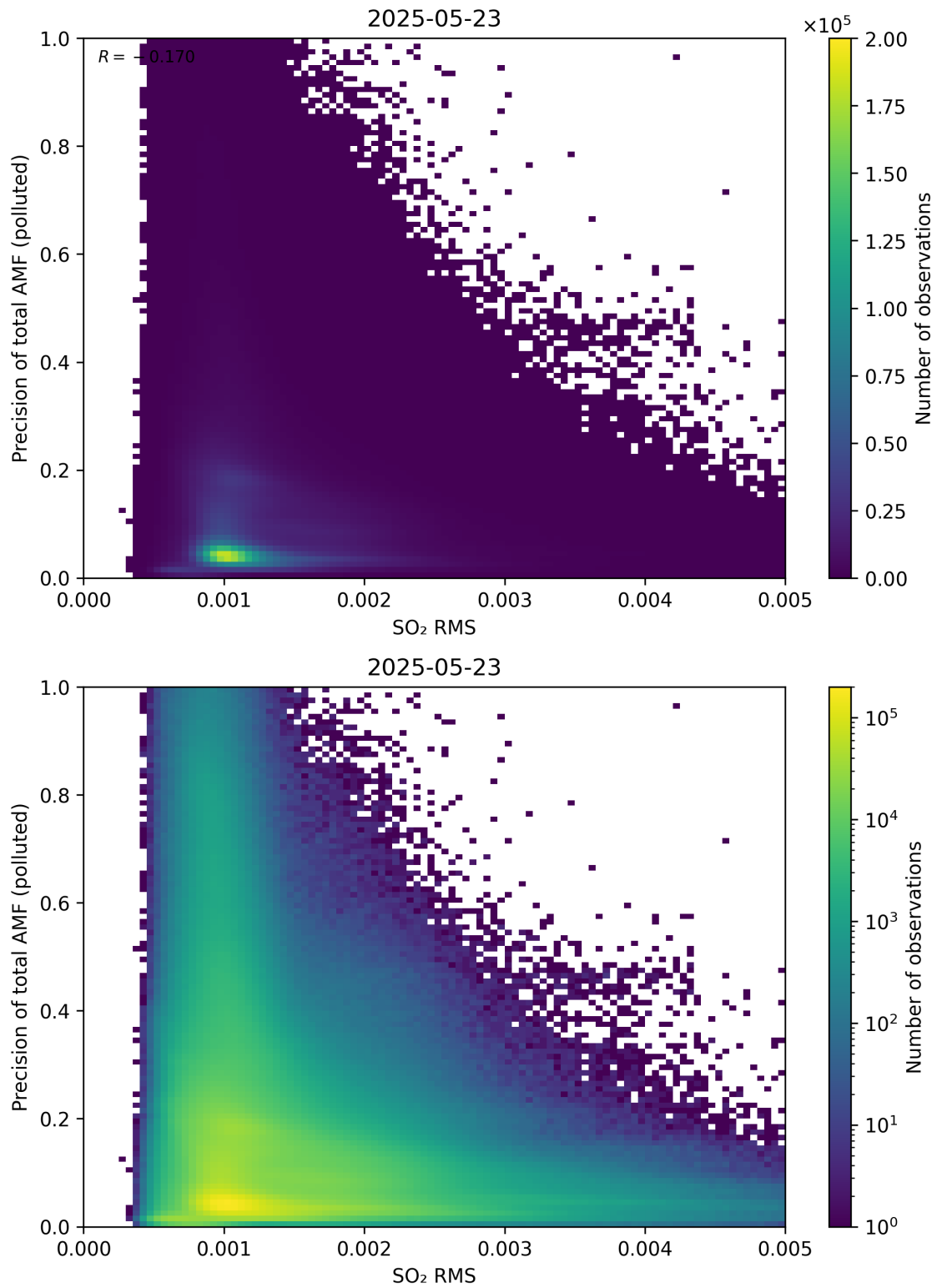
Figure 149: Scatter density plot of “SO 2 RMS” against “Precision of total AMF (polluted)” for 2025-05-22 to 2025-05-24.
