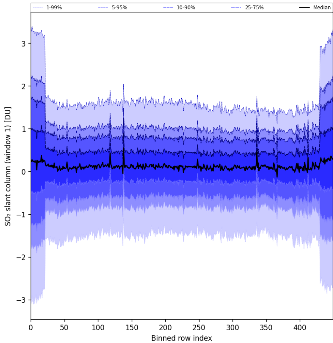
Figure 89: Along track statistics of “SO 2 slant column (window 1)” for 2025-05-22 to 2025-05-24
