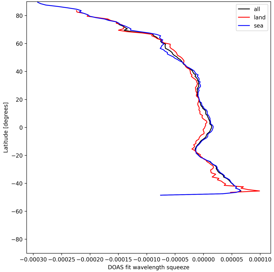
Figure 51: Zonal average of “DOAS fit wavelength squeeze” for 2025-05-22 to 2025-05-24.
