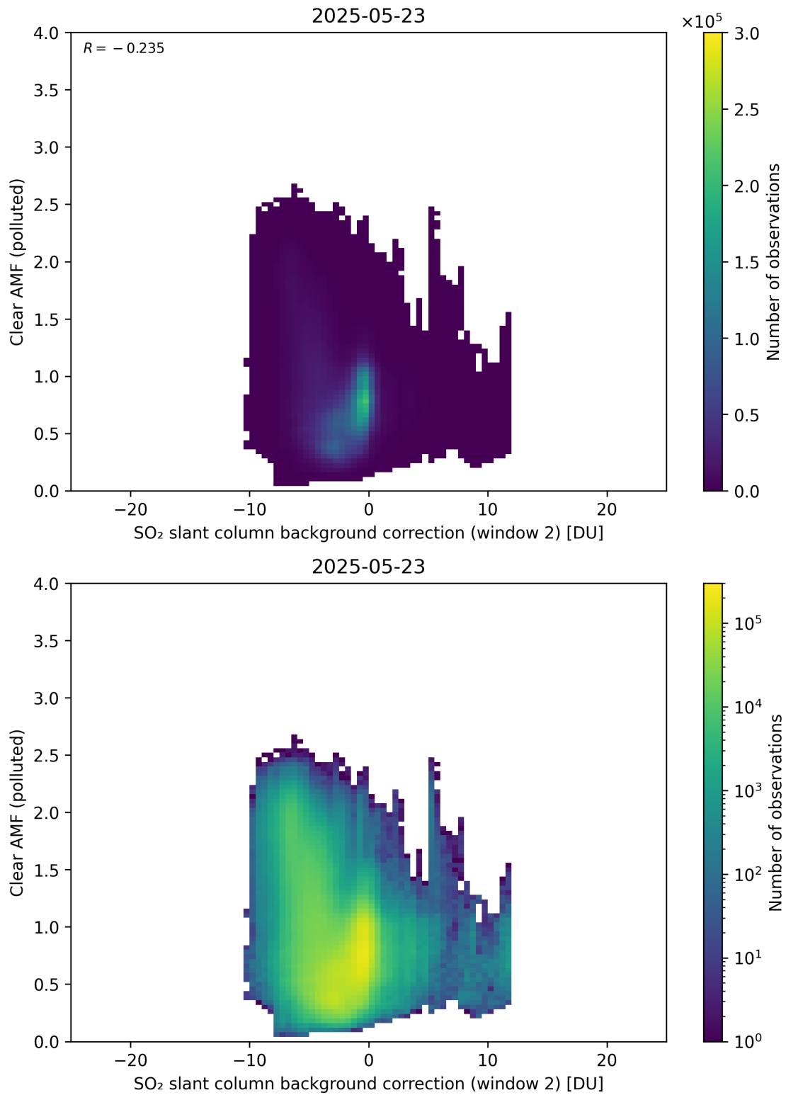
Figure 126: Scatter density plot of “SO 2 slant column background correction (window 2)” against “Clear AMF (polluted)” for 2025-05-22 to 2025-05-24.
