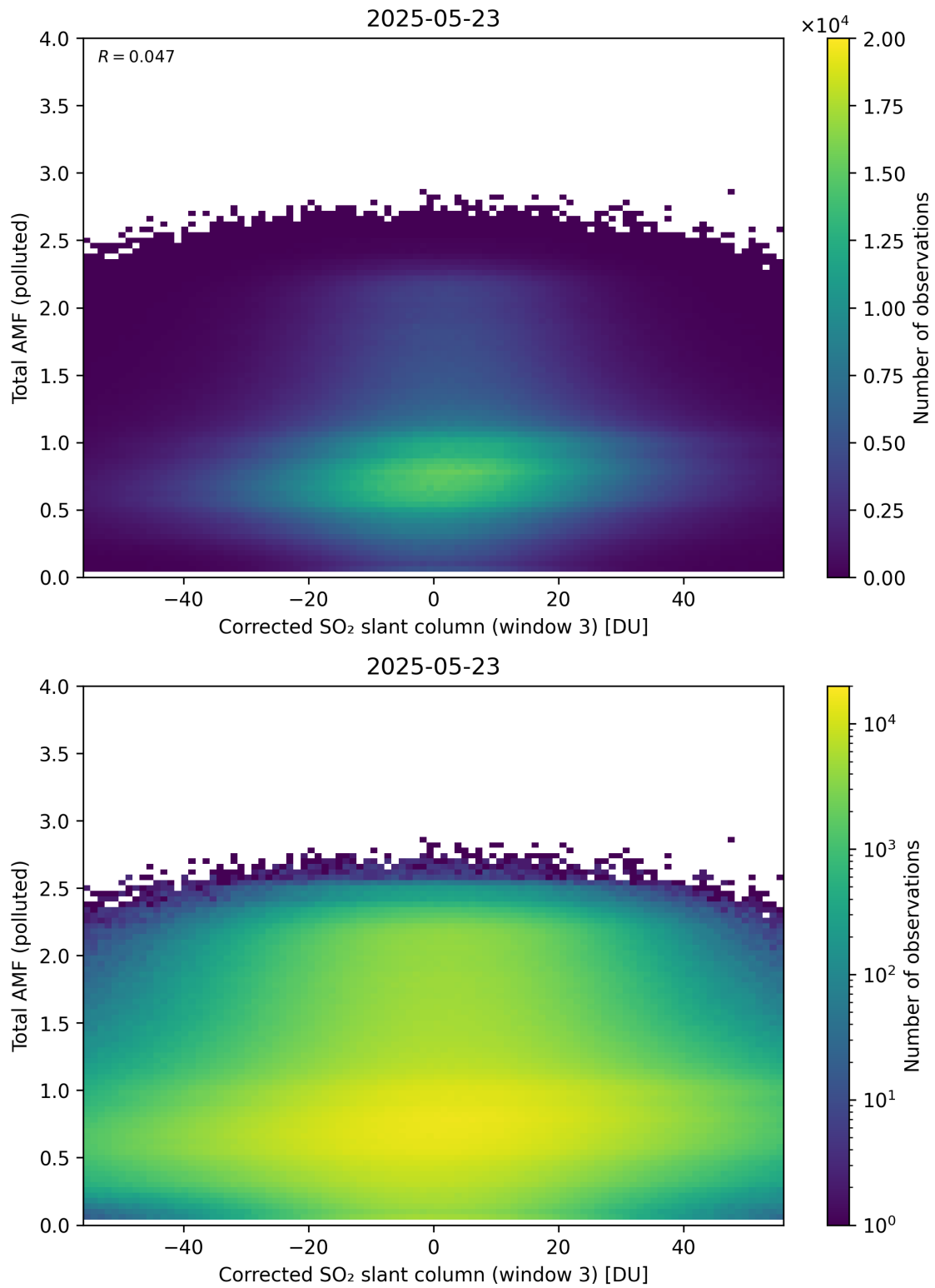
Figure 260: Scatter density plot of “Corrected SO 2 slant column (window 3)” against “Total AMF (polluted)” for 2025-05-22 to 2025-05-24.
