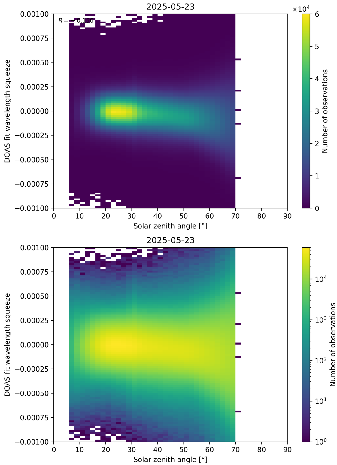
Figure 175: Scatter density plot of “Solar zenith angle” against “DOAS fit wavelength squeeze” for 2025-05-22 to 2025-05-24.
