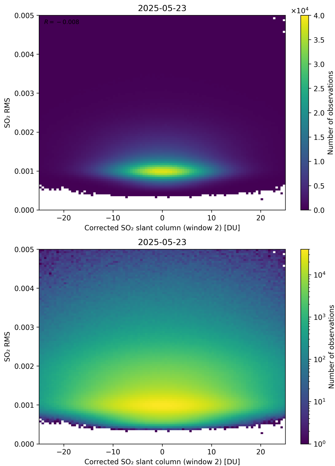
Figure 248: Scatter density plot of “Corrected SO 2 slant column (window 2)” against “SO 2 RMS” for 2025-05-22 to 2025-05-24.
