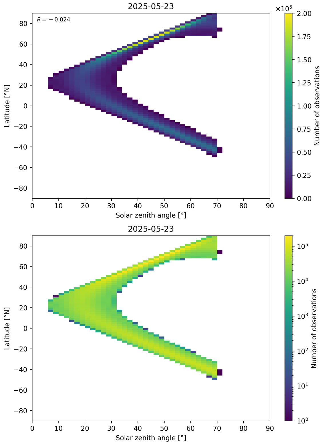
Figure 177: Scatter density plot of “Solar zenith angle” against “Latitude” for 2025-05-22 to 2025-05-24.
