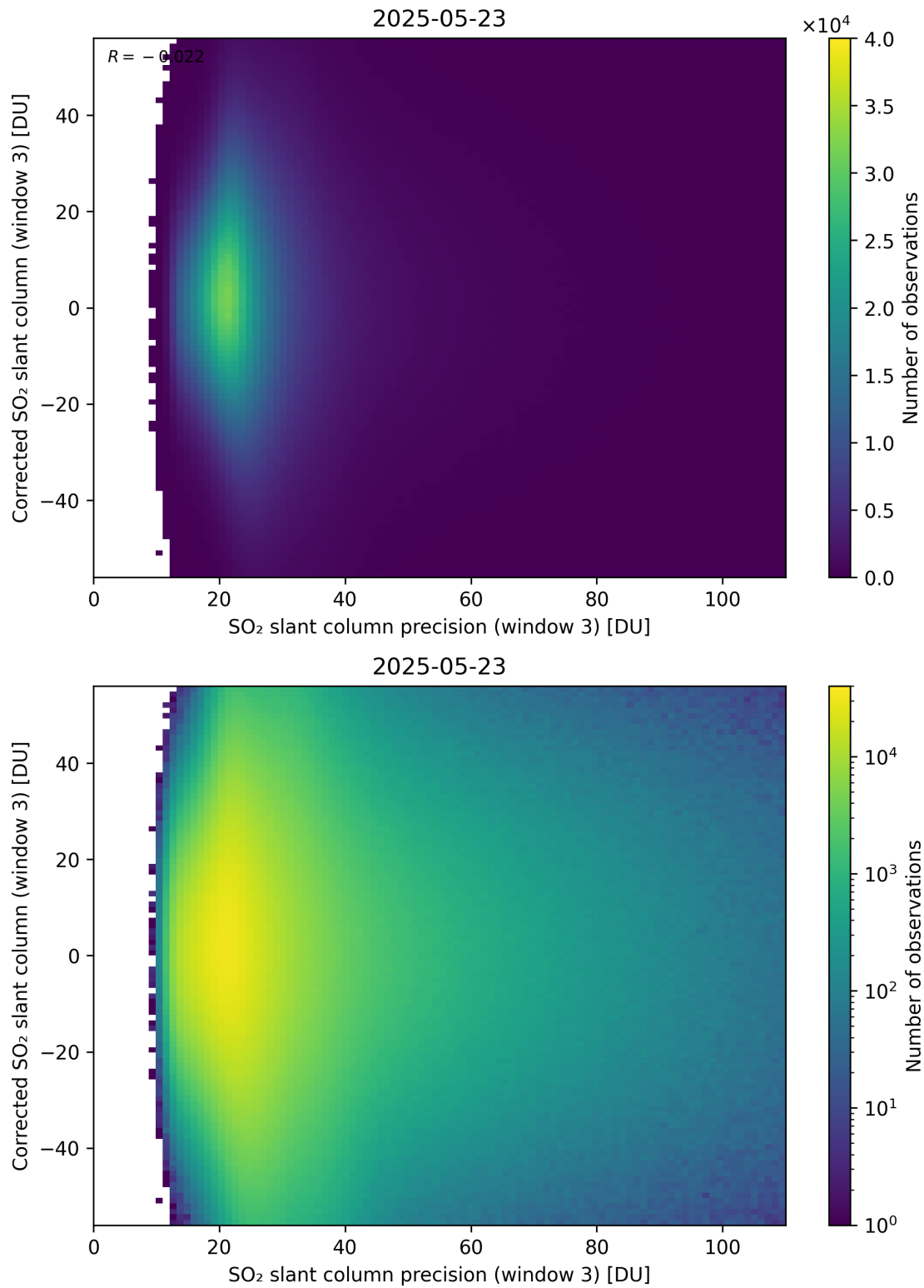
Figure 312: Scatter density plot of “SO 2 slant column precision (window 3)” against “Corrected SO 2 slant column (window 3)” for 2025-05-22 to 2025-05-24.
