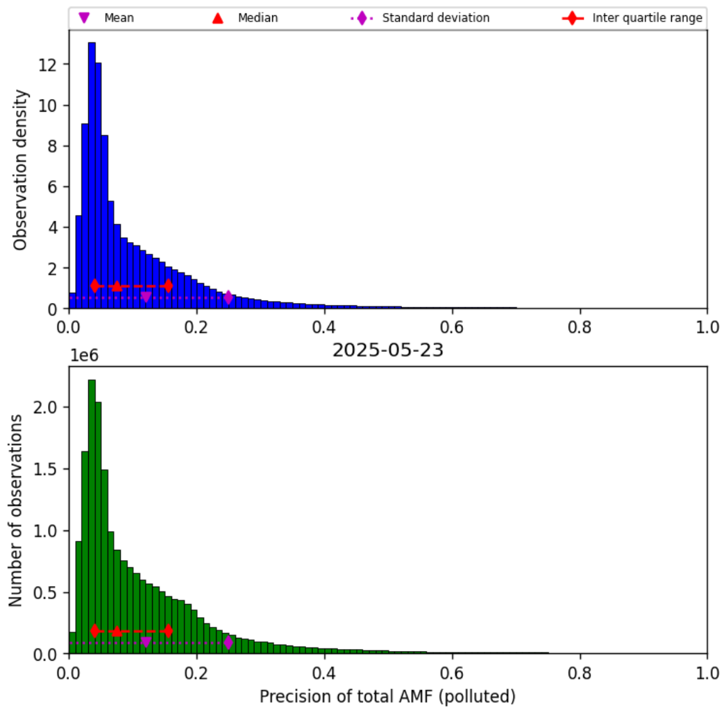
Figure 80: Histogram of “Precision of total AMF (polluted)” for 2025-05-22 to 2025-05-24
