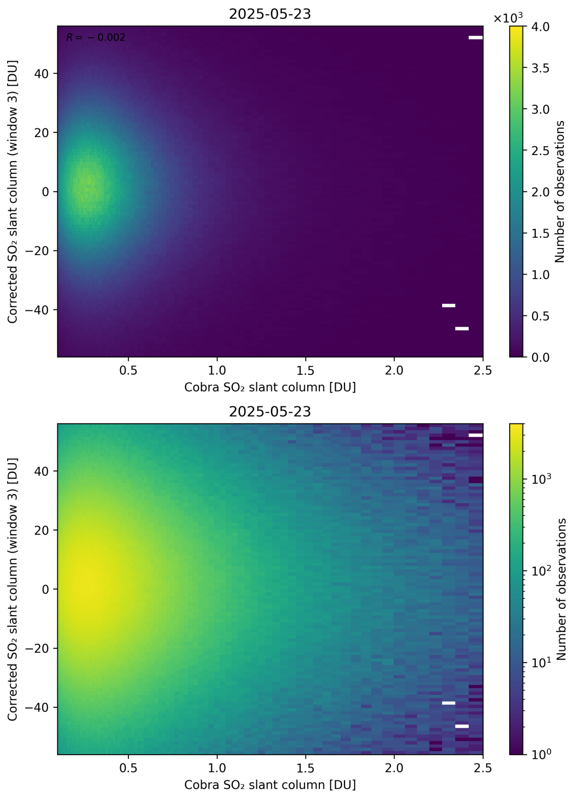
Figure 218: Scatter density plot of “Cobra SO 2 slant column” against “Corrected SO 2 slant column (window 3)” for 2025-05-22 to 2025-05-24.
