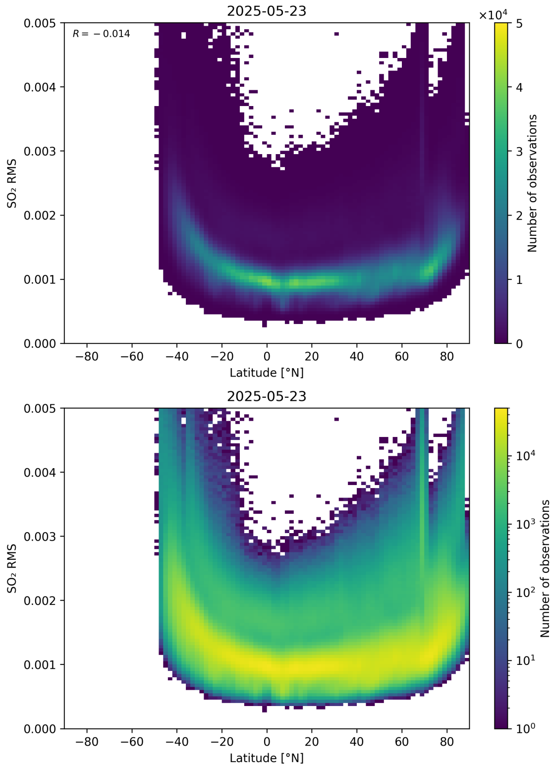
Figure 155: Scatter density plot of “Latitude” against “SO 2 RMS” for 2025-05-22 to 2025-05-24.
