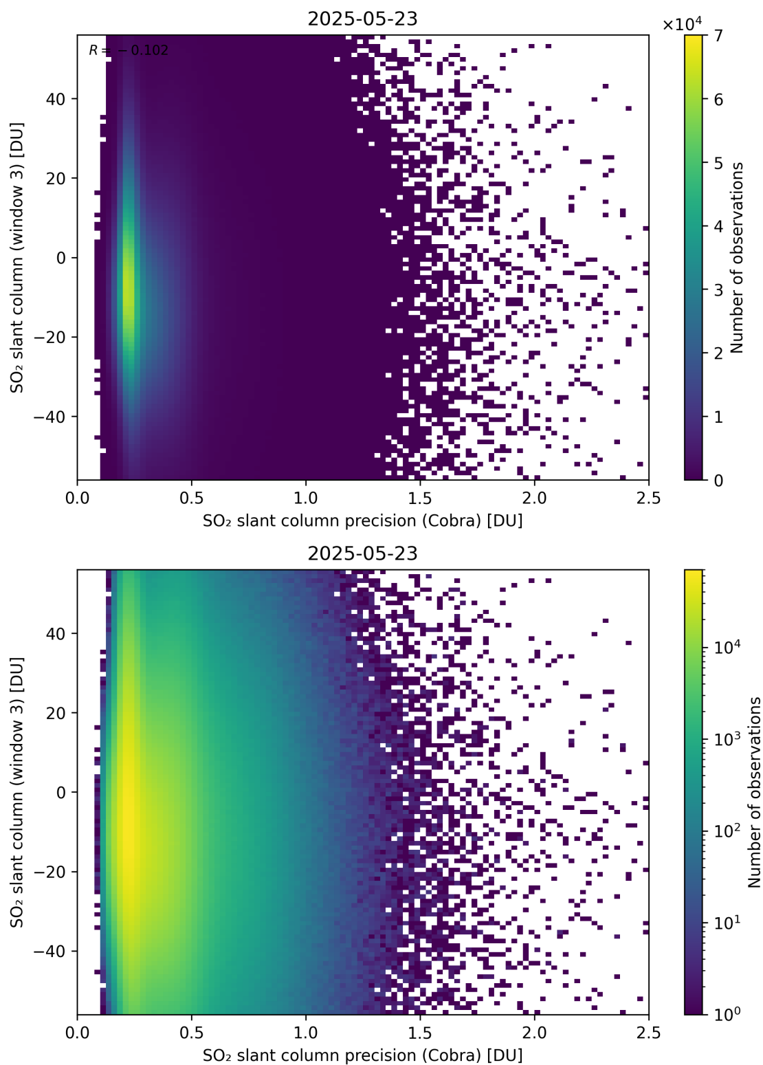
Figure 211: Scatter density plot of “SO 2 slant column precision (Cobra)” against “SO 2 slant column (window 3)” for 2025-05-22 to 2025-05-24.
