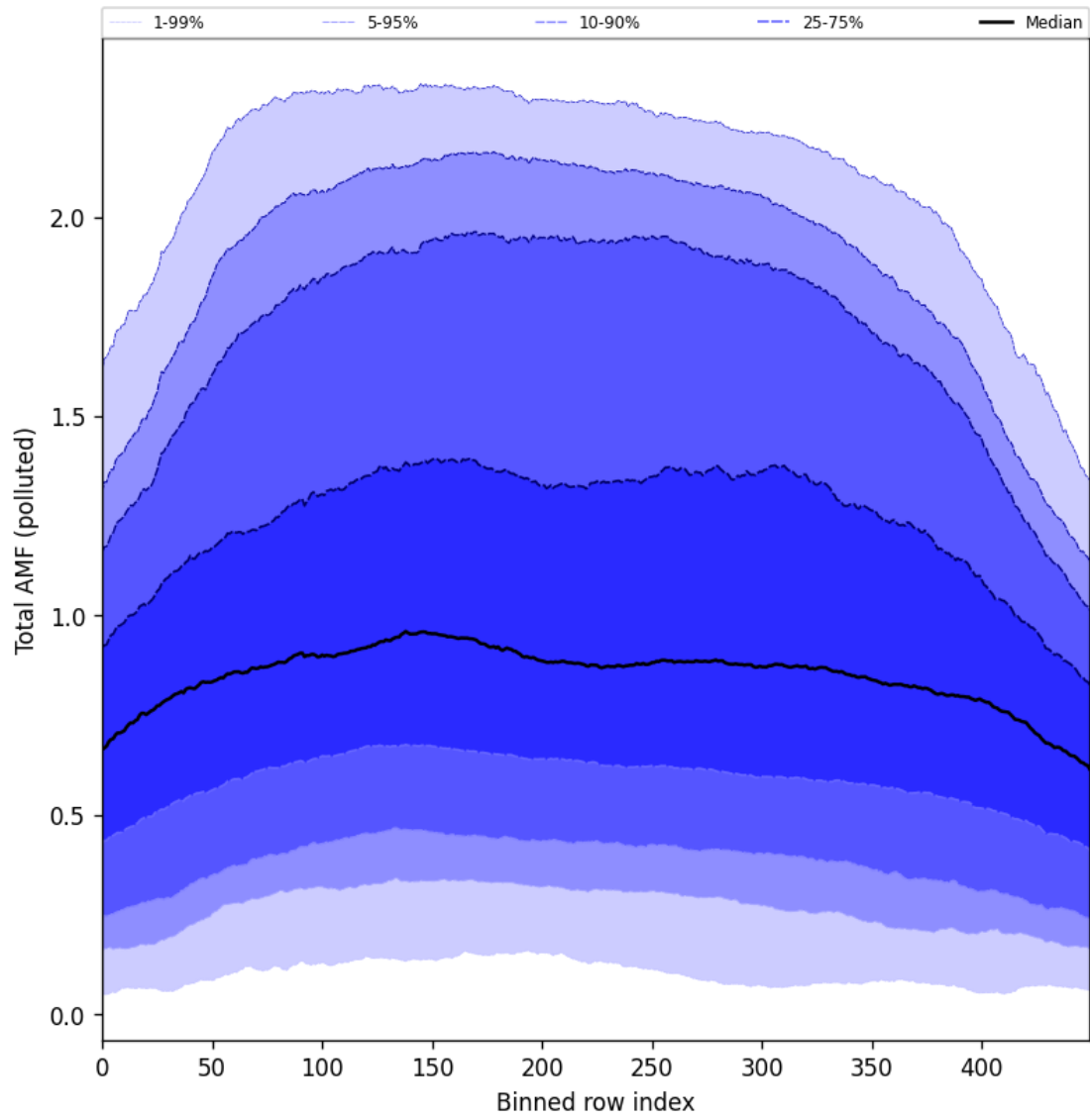
Figure 105: Along track statistics of “Total AMF (polluted)” for 2025-05-22 to 2025-05-24
