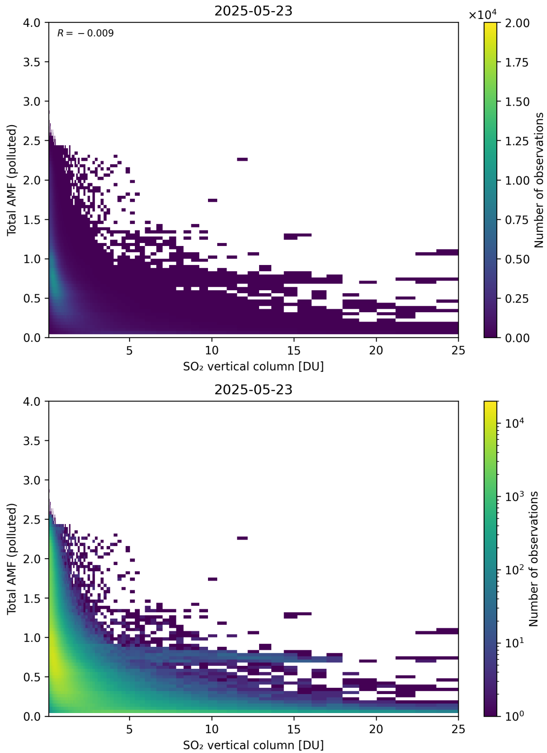
Figure 359: Scatter density plot of “SO 2 vertical column” against “Total AMF (polluted)” for 2025-05-22 to 2025-05-24.
