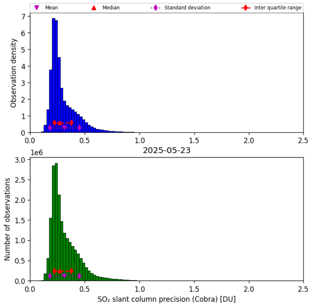
Figure 62: Histogram of “SO 2 slant column precision (Cobra)” for 2025-05-22 to 2025-05-24
