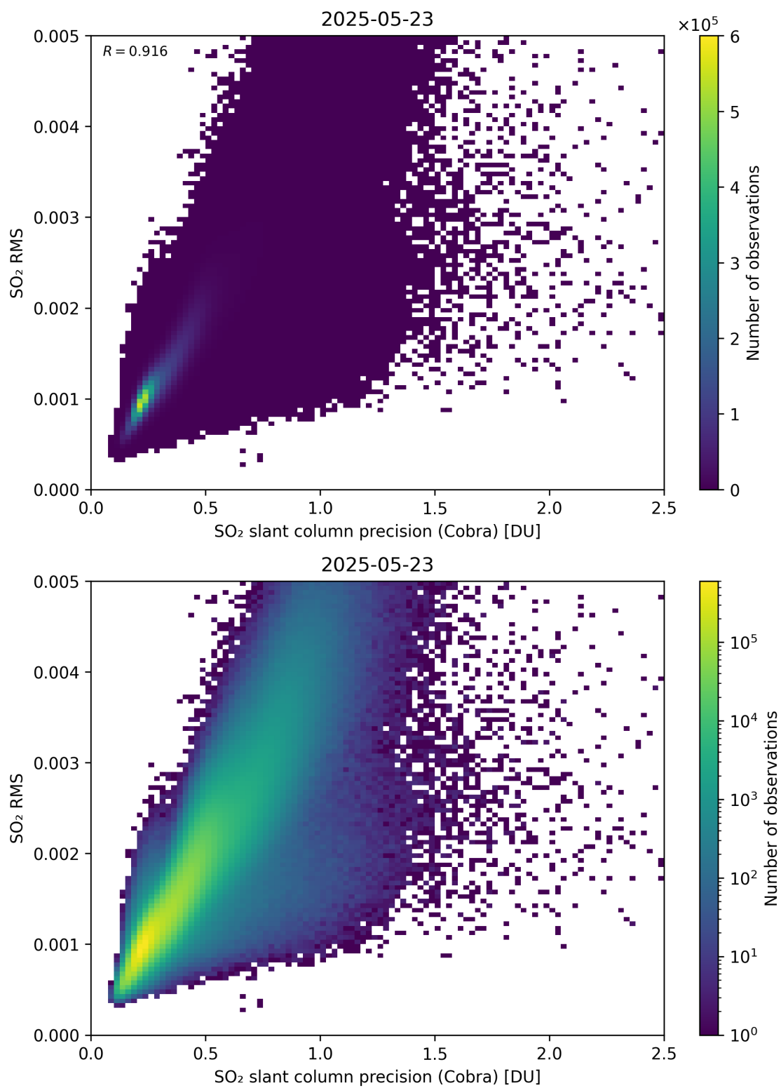
Figure 204: Scatter density plot of “SO 2 slant column precision (Cobra)” against “SO 2 RMS” for 2025-05-22 to 2025-05-24.
