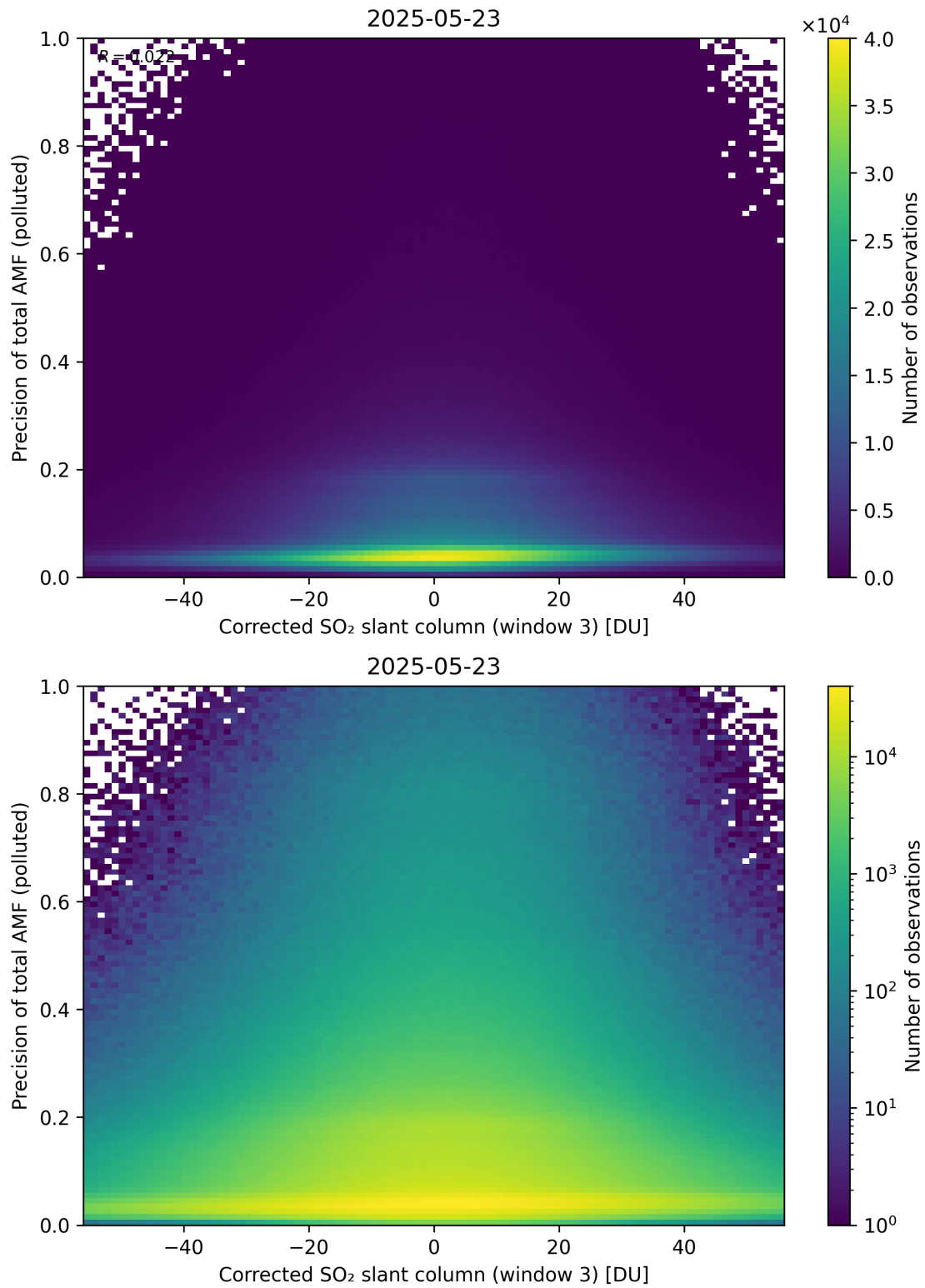
Figure 261: Scatter density plot of “Corrected SO 2 slant column (window 3)” against “Precision of total AMF (polluted)” for 2025-05-22 to 2025-05-24.
