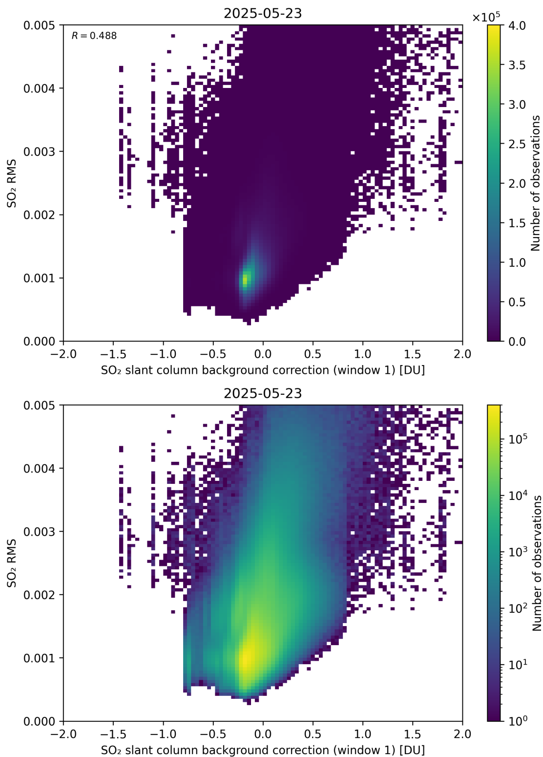
Figure 113: Scatter density plot of “SO 2 slant column background correction (window 1)” against “SO 2 RMS” for 2025-05-22 to 2025-05-24.
