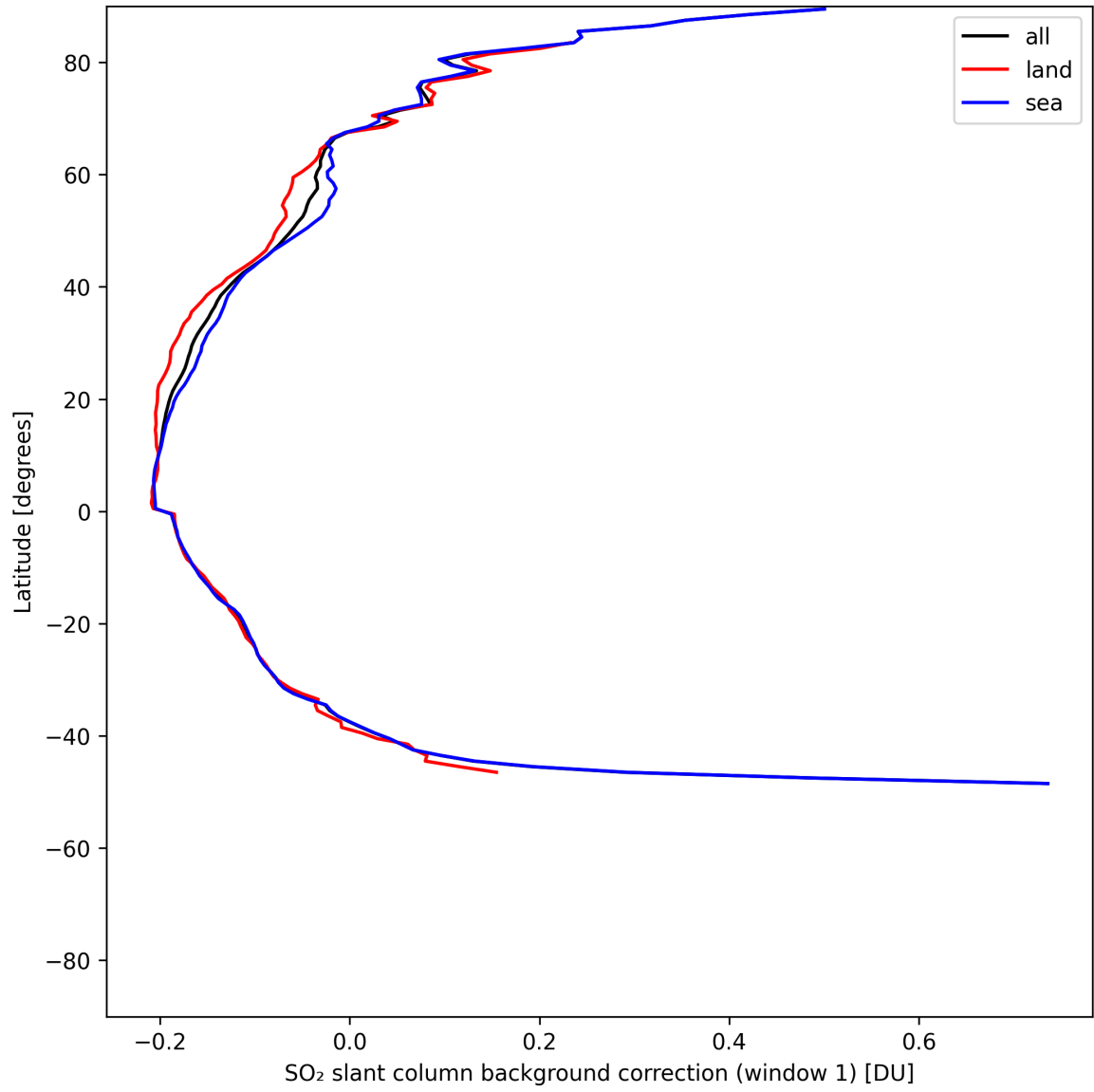
Figure 40: Zonal average of “SO 2 slant column background correction (window 1)” for 2025-05-22 to 2025-05-24.
