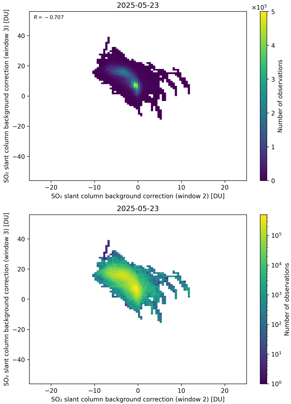
Figure 122: Scatter density plot of “SO 2 slant column background correction (window 2)” against “SO 2 slant column background correction (window 3)” for 2025-05-22 to 2025-05-24.
