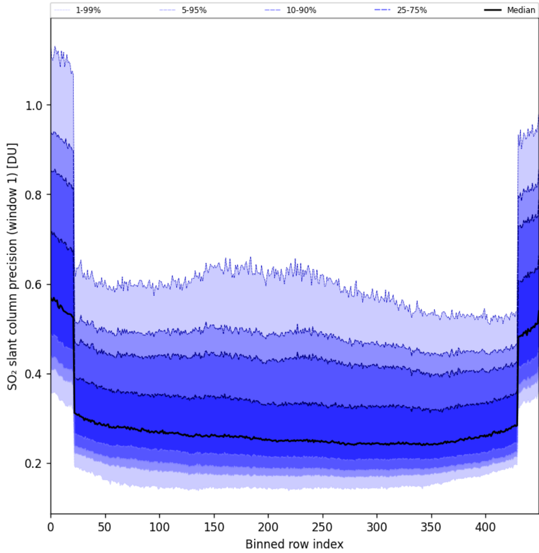
Figure 90: Along track statistics of “SO 2 slant column precision (window 1)” for 2025-05-22 to 2025-05-24
