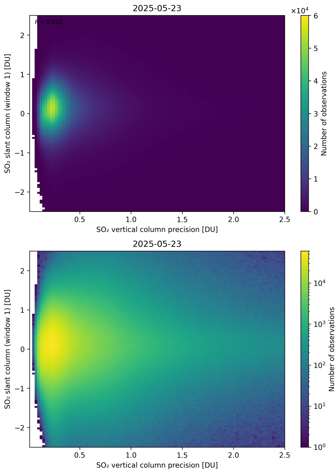
Figure 341: Scatter density plot of “SO 2 vertical column precision” against “SO 2 slant column (window 1)” for 2025-05-22 to 2025-05-24.
