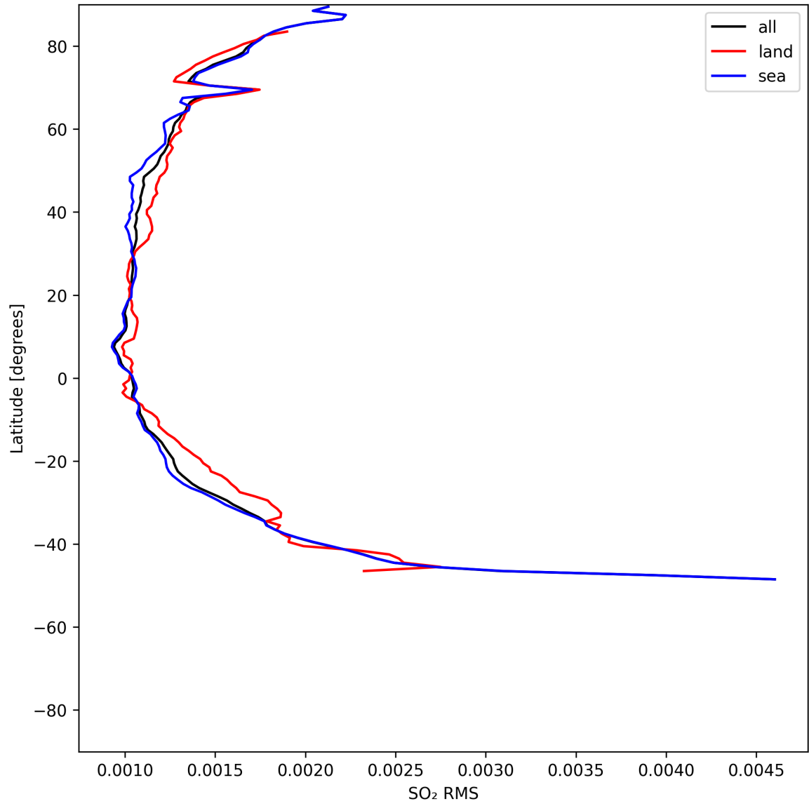
Figure 52: Zonal average of “SO 2 RMS” for 2025-05-22 to 2025-05-24.
