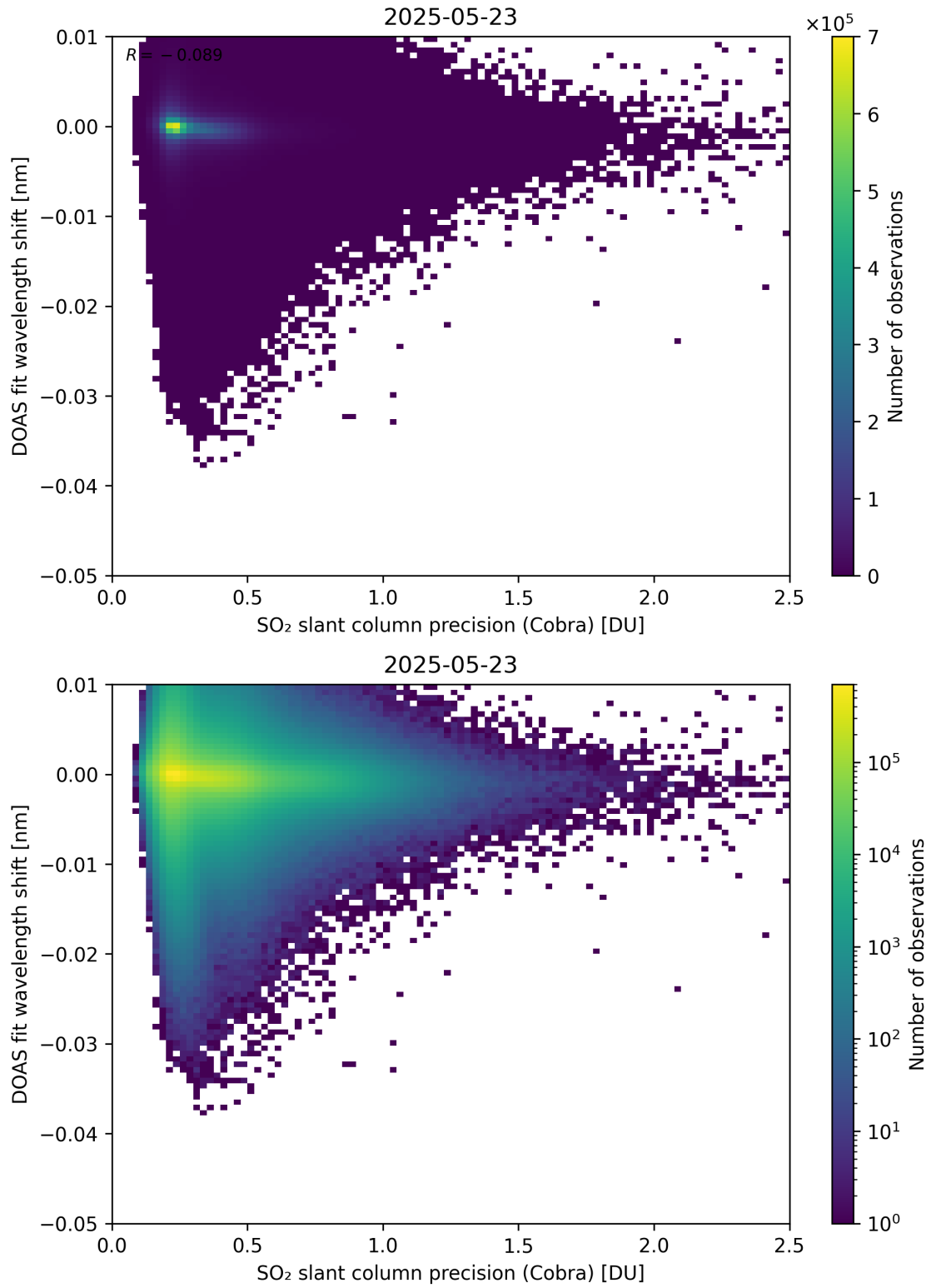
Figure 202: Scatter density plot of “SO 2 slant column precision (Cobra)” against “DOAS fit wavelength shift” for 2025-05-22 to 2025-05-24.
