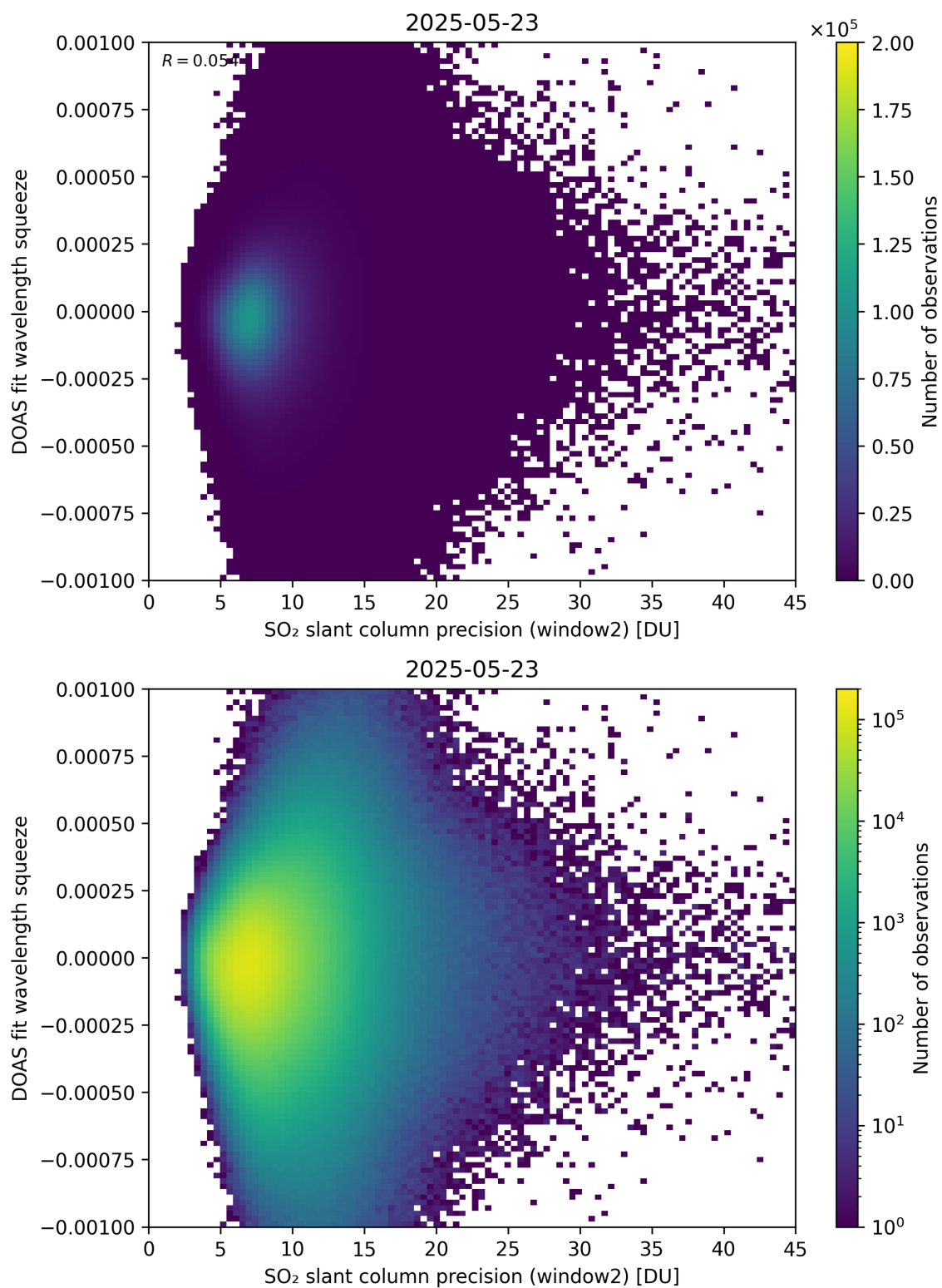
Figure 294: Scatter density plot of “SO 2 slant column precision (window2)” against “DOAS fit wavelength squeeze” for 2025-05-22 to 2025-05-24.
