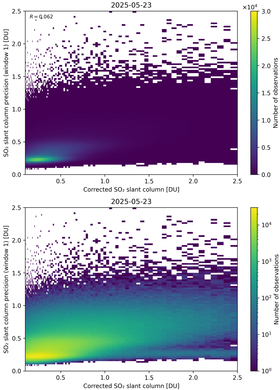
Figure 238: Scatter density plot of “Corrected SO 2 slant column” against “SO 2 slant column precision (window 1)” for 2025-05-22 to 2025-05-24.
