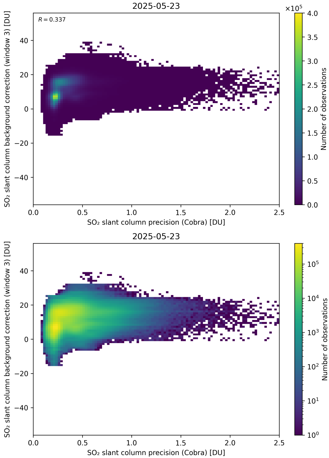
Figure 201: Scatter density plot of “SO 2 slant column precision (Cobra)” against “SO 2 slant column background correction (window 3)” for 2025-05-22 to 2025-05-24.
