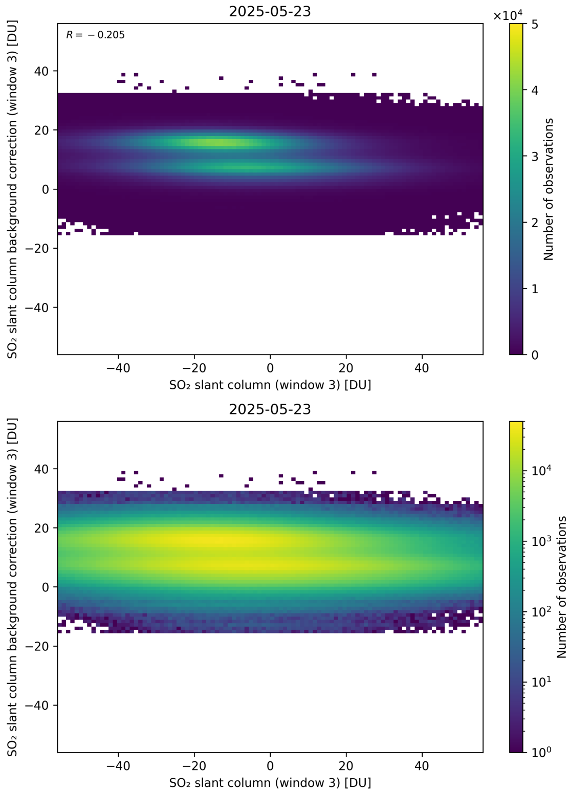
Figure 303: Scatter density plot of “SO 2 slant column (window 3)” against “SO 2 slant column background correction (window 3)” for 2025-05-22 to 2025-05-24.
