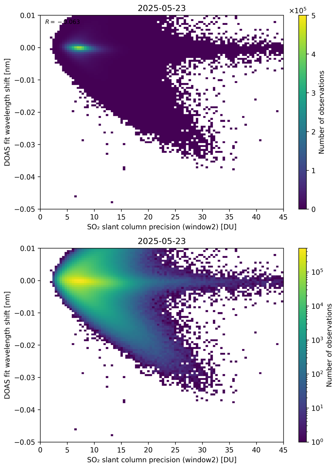
Figure 293: Scatter density plot of “SO 2 slant column precision (window2)” against “DOAS fit wavelength shift” for 2025-05-22 to 2025-05-24.
