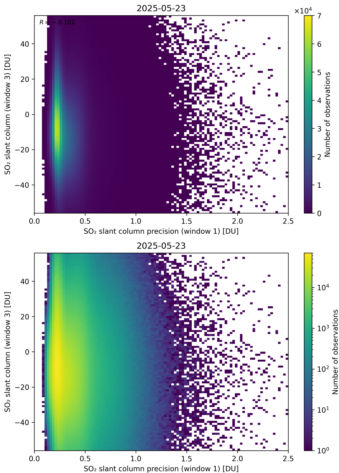
Figure 278: Scatter density plot of “SO 2 slant column precision (window 1)” against “SO 2 slant column (window 3)” for 2025-05-22 to 2025-05-24.
