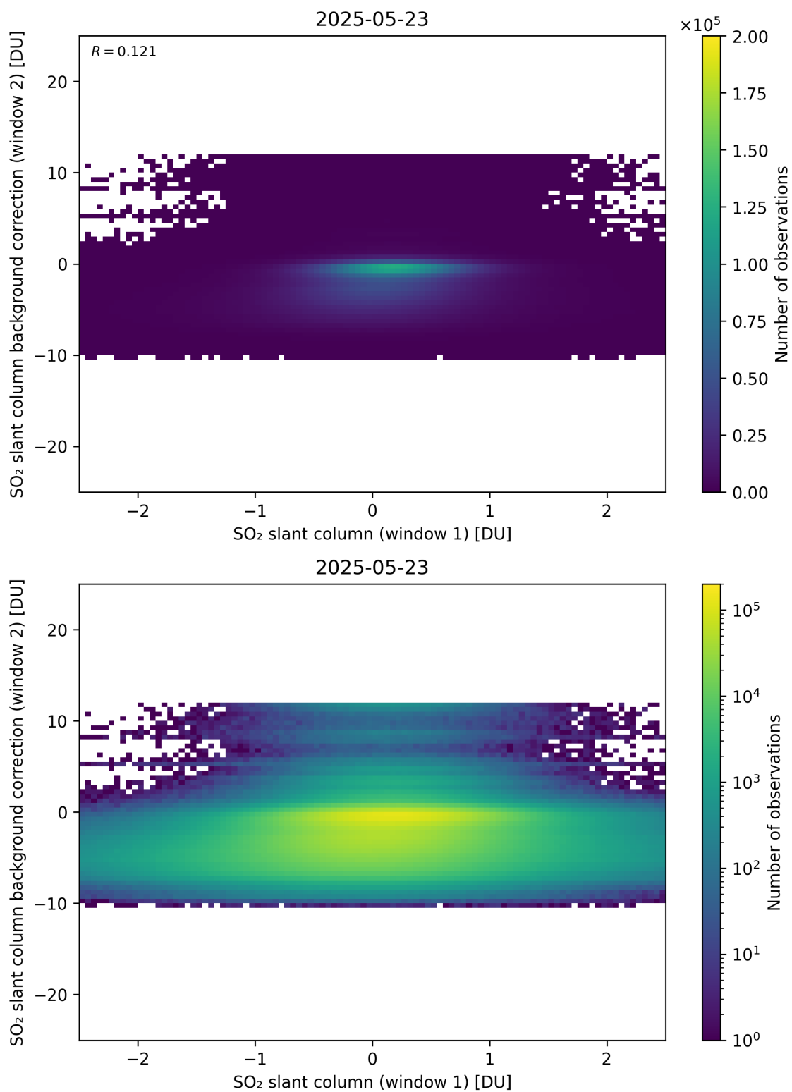
Figure 263: Scatter density plot of “SO 2 slant column (window 1)” against “SO 2 slant column background correction (window 2)” for 2025-05-22 to 2025-05-24.
