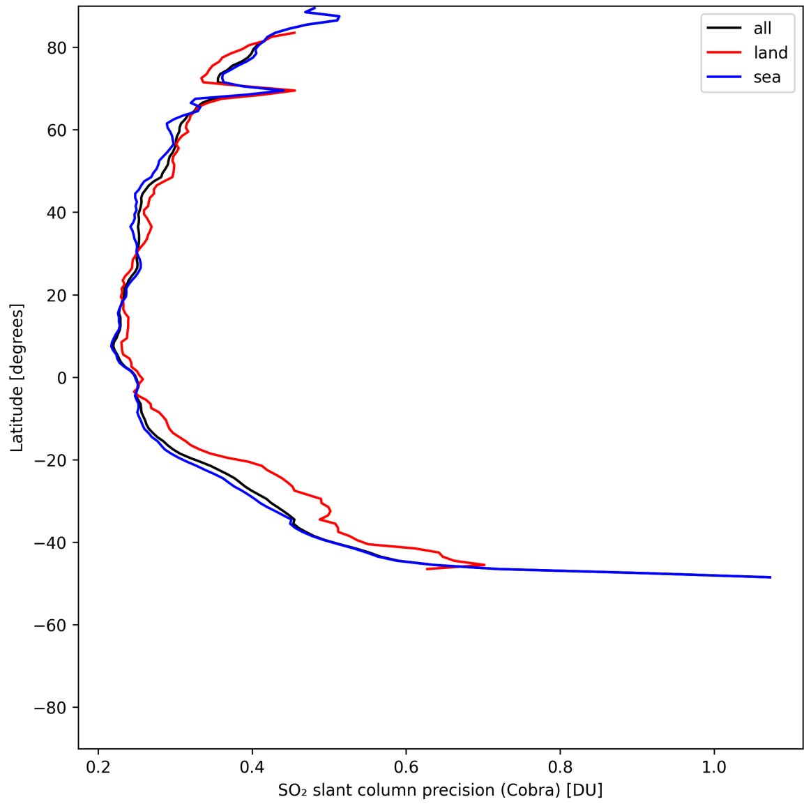
Figure 36: Zonal average of “SO 2 slant column precision (Cobra)” for 2025-05-22 to 2025-05-24.
