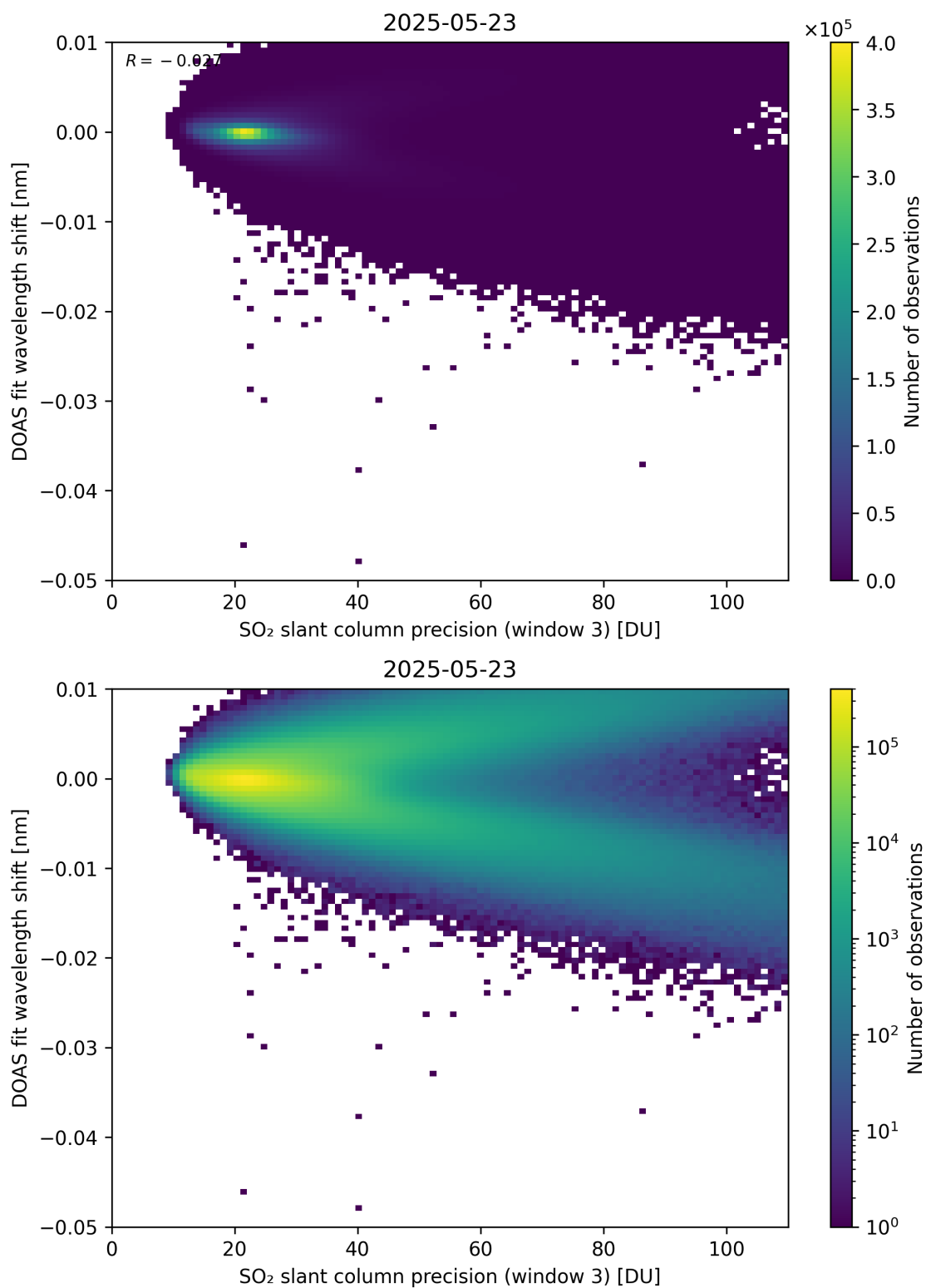
Figure 308: Scatter density plot of “SO 2 slant column precision (window 3)” against “DOAS fit wavelength shift” for 2025-05-22 to 2025-05-24.
