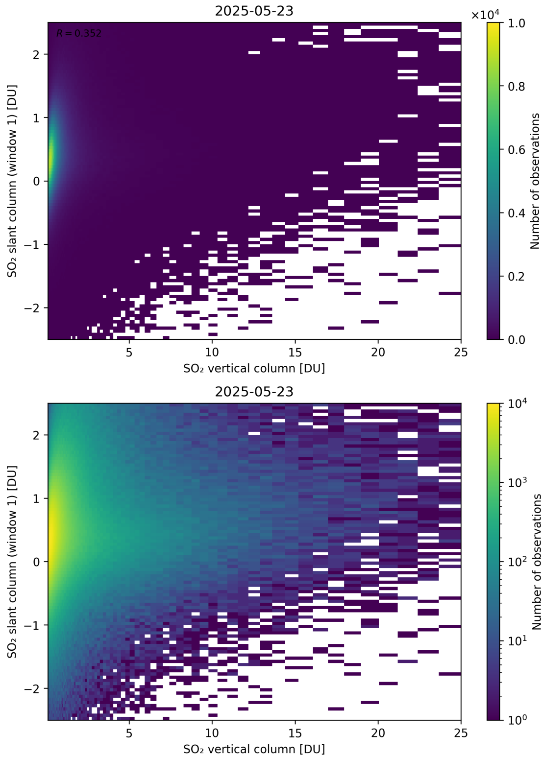
Figure 354: Scatter density plot of “SO 2 vertical column” against “SO 2 slant column (window 1)” for 2025-05-22 to 2025-05-24.
