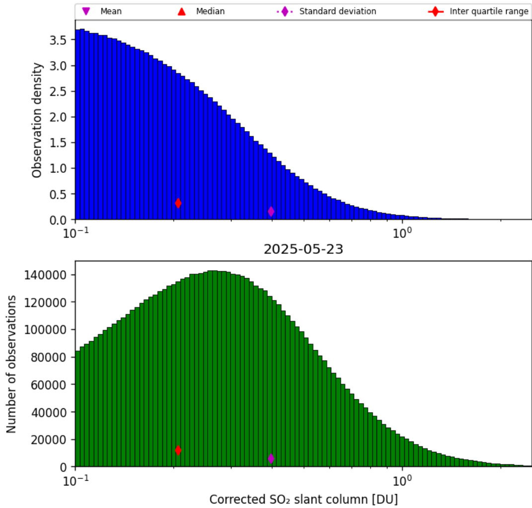
Figure 60: Histogram of “Corrected SO 2 slant column” for 2025-05-22 to 2025-05-24
