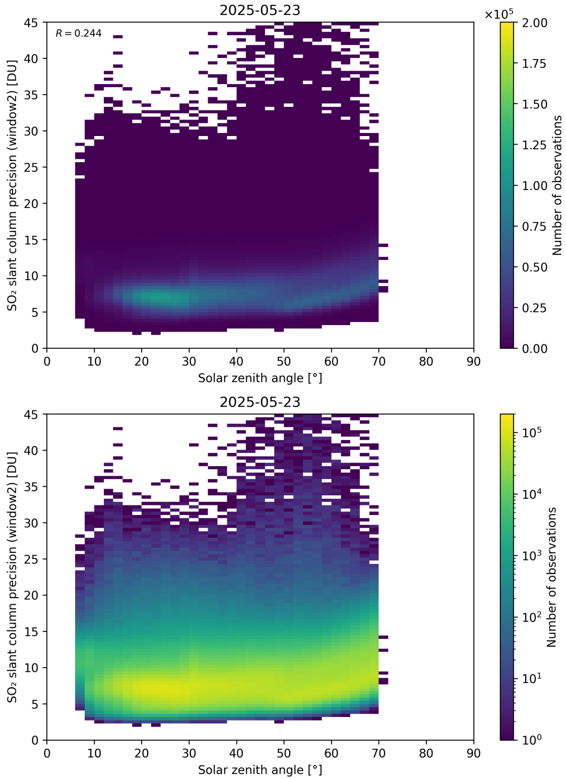
Figure 186: Scatter density plot of “Solar zenith angle” against “SO 2 slant column precision (window2)” for 2025-05-22 to 2025-05-24.
