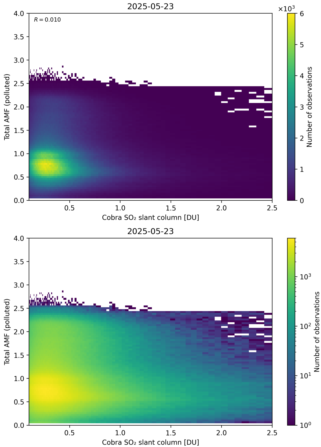
Figure 224: Scatter density plot of “Cobra SO 2 slant column” against “Total AMF (polluted)” for 2025-05-22 to 2025-05-24.
