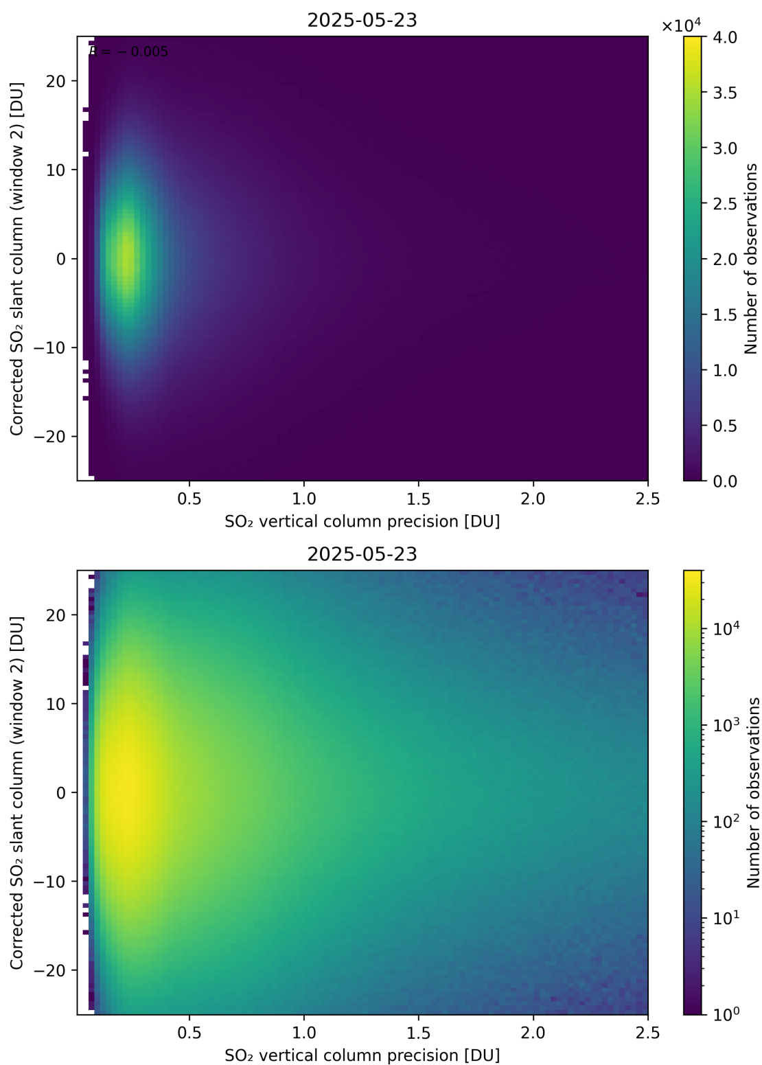
Figure 339: Scatter density plot of “SO 2 vertical column precision” against “Corrected SO 2 slant column (window 2)” for 2025-05-22 to 2025-05-24.
