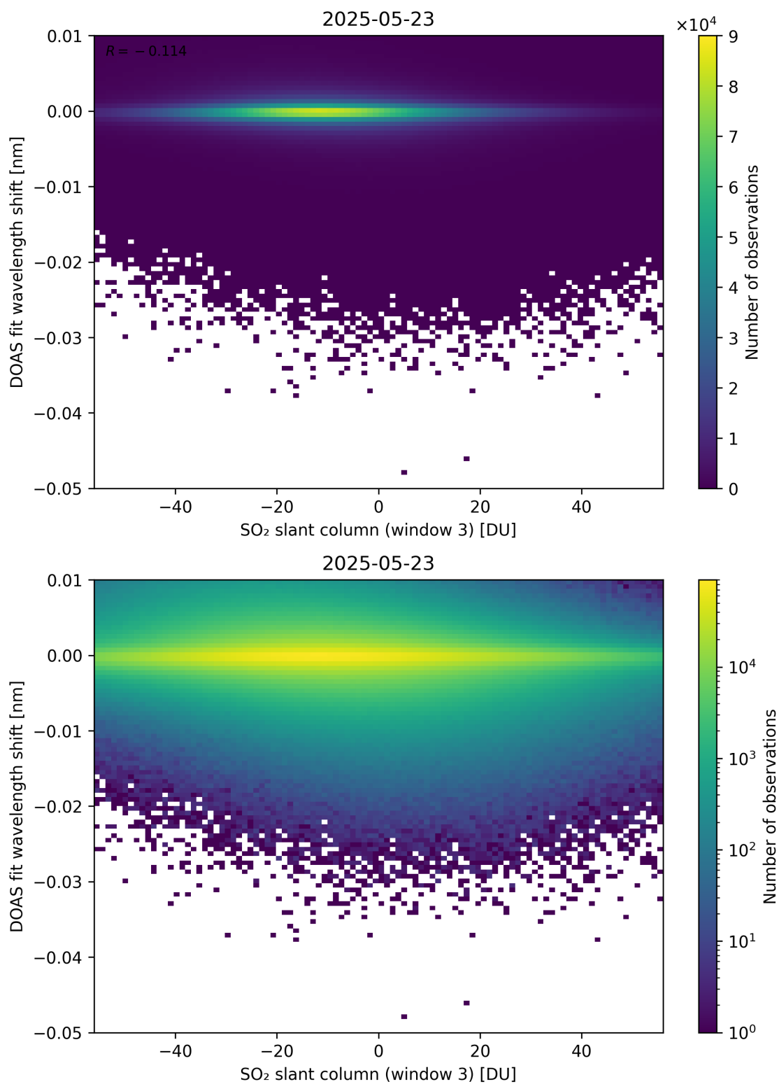
Figure 304: Scatter density plot of “SO 2 slant column (window 3)” against “DOAS fit wavelength shift” for 2025-05-22 to 2025-05-24.
