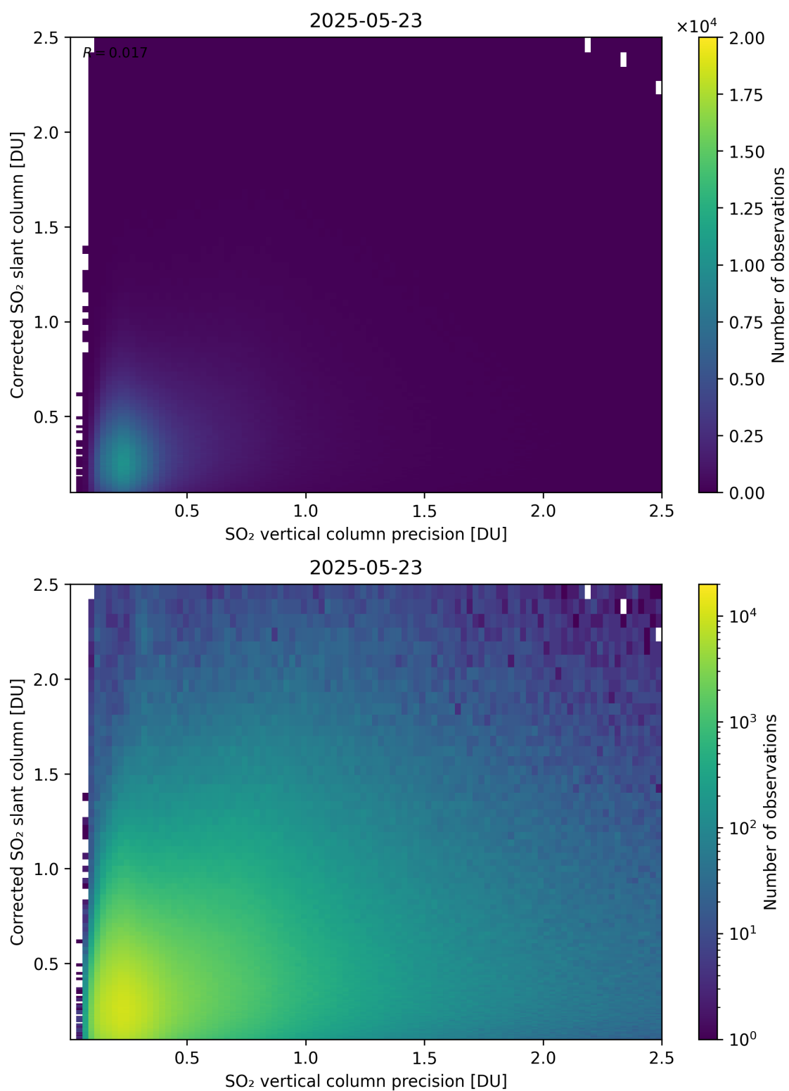
Figure 338: Scatter density plot of “SO 2 vertical column precision” against “Corrected SO 2 slant column” for 2025-05-22 to 2025-05-24.
