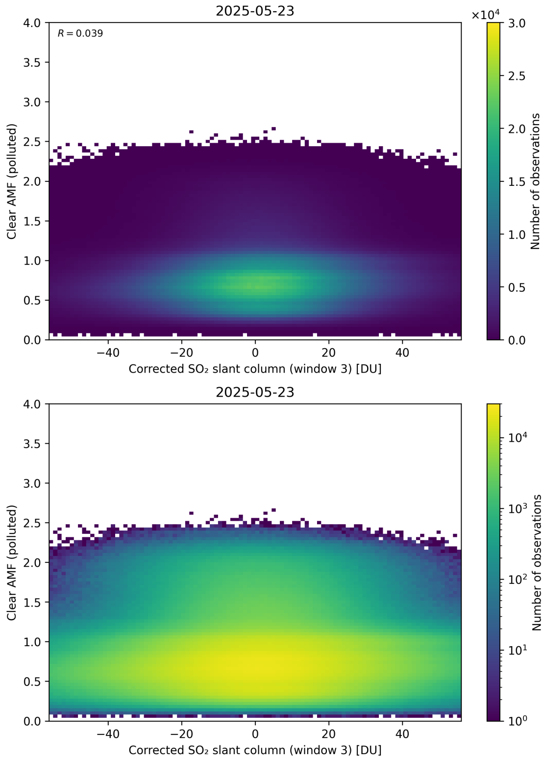
Figure 259: Scatter density plot of “Corrected SO 2 slant column (window 3)” against “Clear AMF (polluted)” for 2025-05-22 to 2025-05-24.
