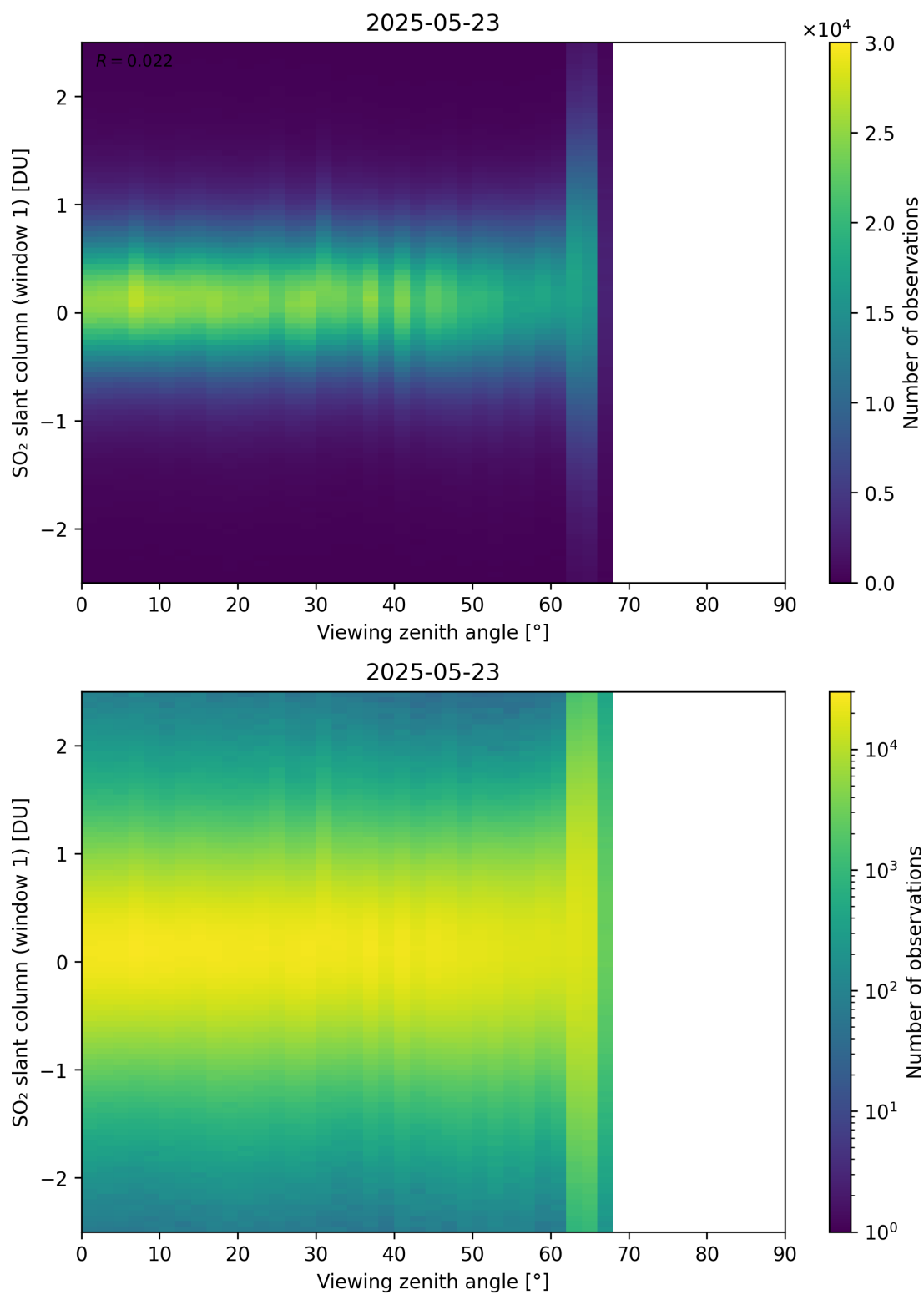
Figure 376: Scatter density plot of “Viewing zenith angle” against “SO 2 slant column (window 1)” for 2025-05-22 to 2025-05-24.
