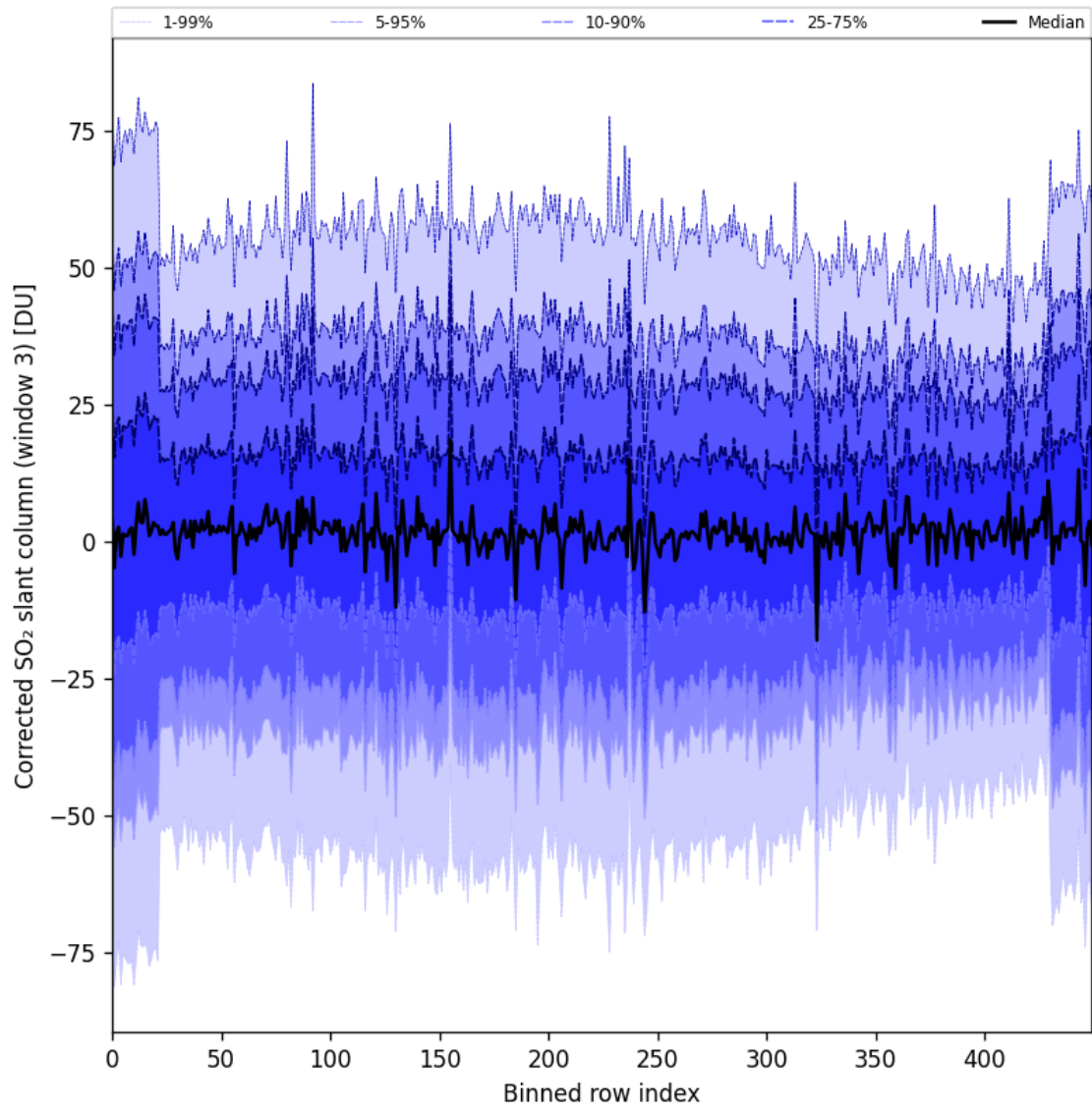
Figure 99: Along track statistics of “Corrected SO 2 slant column (window 3)” for 2025-05-22 to 2025-05-24
