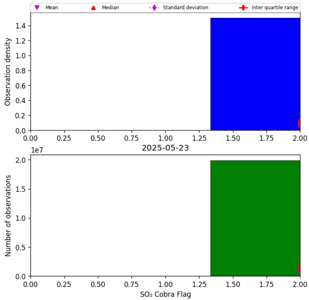
Figure 75: Histogram of “SO 2 Cobra Flag” for 2025-05-22 to 2025-05-24
