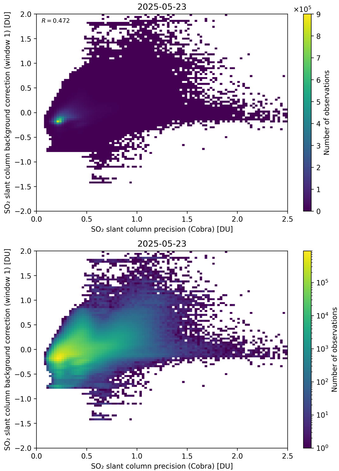
Figure 199: Scatter density plot of “SO 2 slant column precision (Cobra)” against “SO 2 slant column background correction (window 1)” for 2025-05-22 to 2025-05-24.
