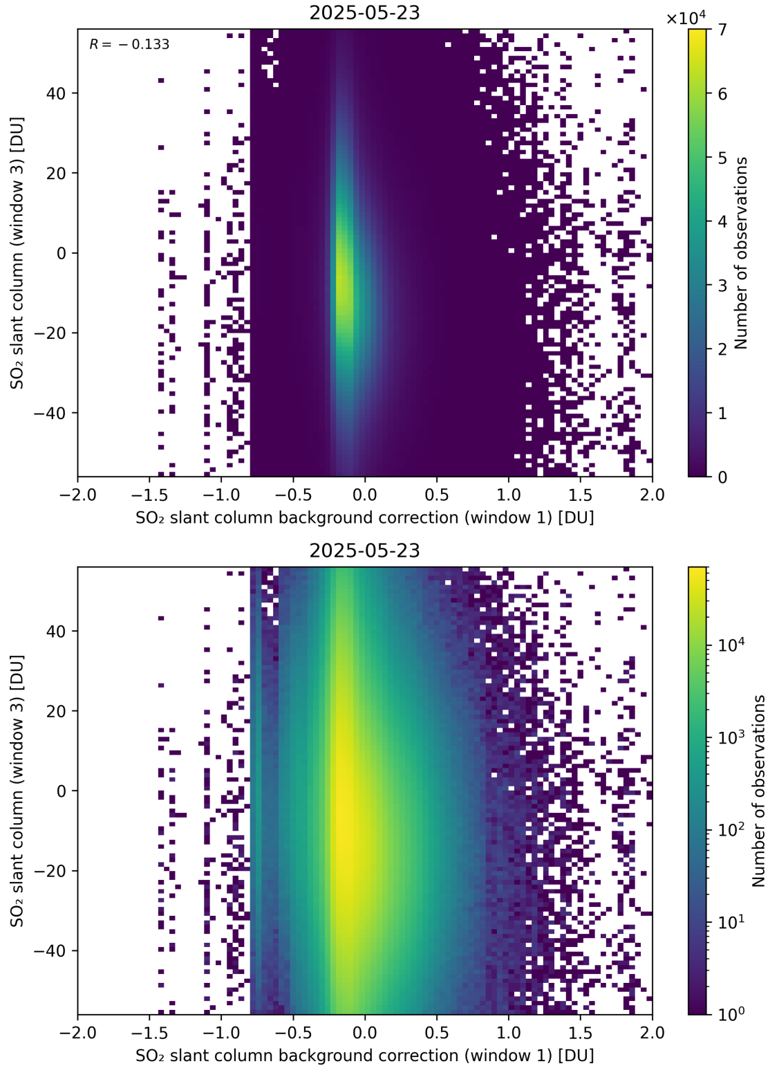
Figure 118: Scatter density plot of “SO 2 slant column background correction (window 1)” against “SO 2 slant column (window 3)” for 2025-05-22 to 2025-05-24.
