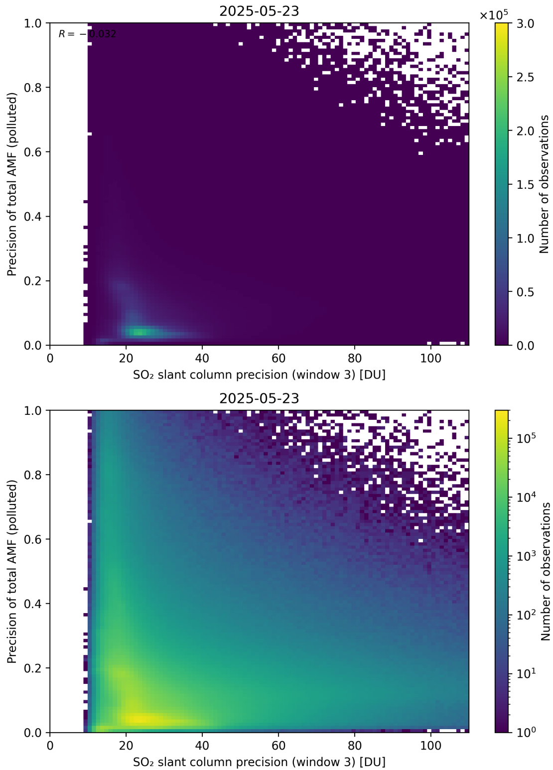
Figure 314: Scatter density plot of “SO 2 slant column precision (window 3)” against “Precision of total AMF (polluted)” for 2025-05-22 to 2025-05-24.
