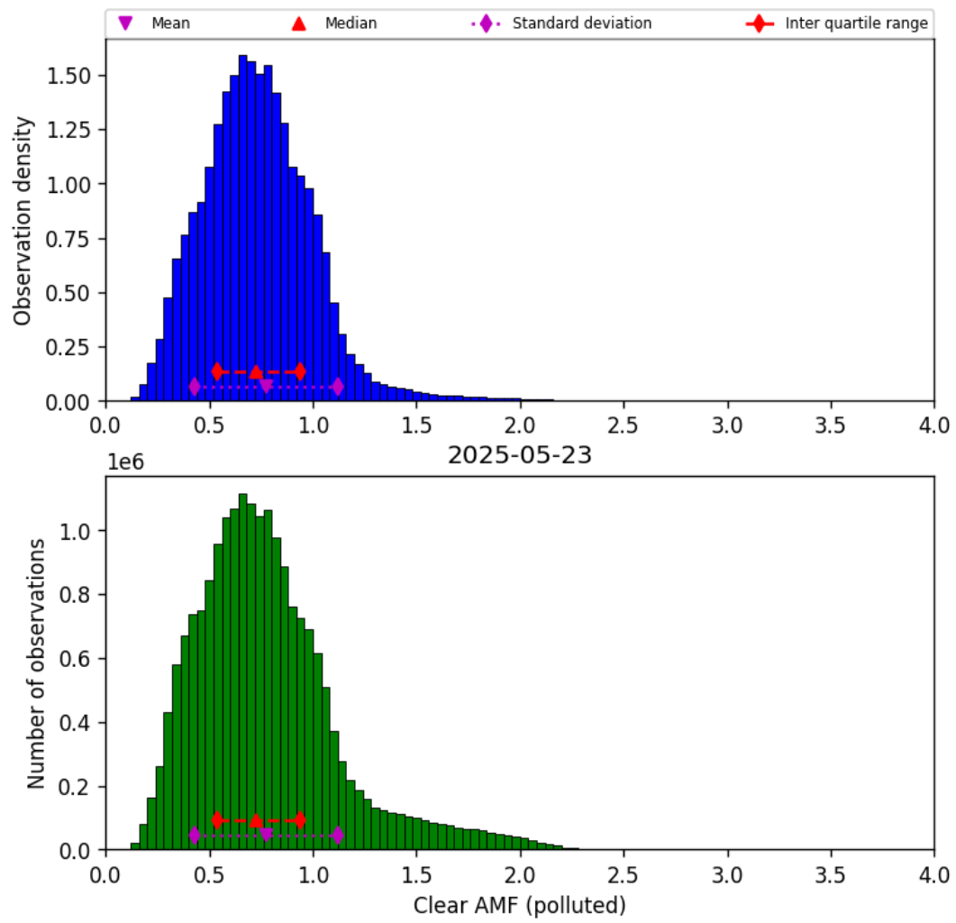
Figure 81: Histogram of “Clear AMF (polluted)” for 2025-05-22 to 2025-05-24
