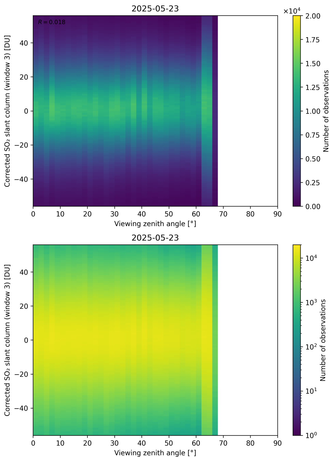
Figure 375: Scatter density plot of “Viewing zenith angle” against “Corrected SO 2 slant column (window 3)” for 2025-05-22 to 2025-05-24.
