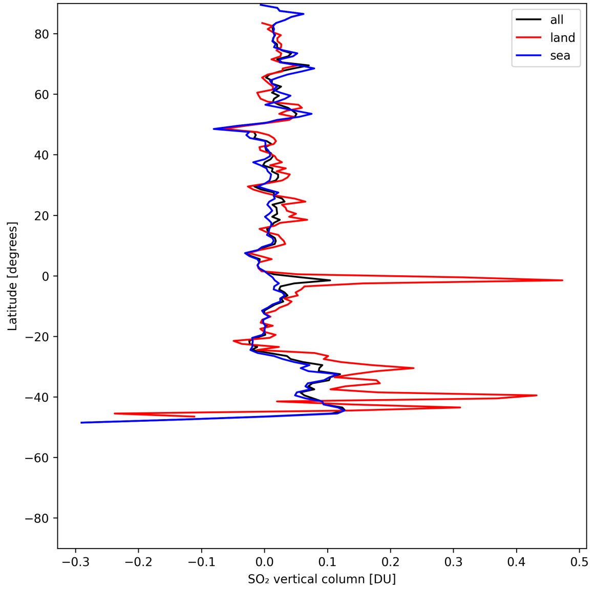
Figure 32: Zonal average of “SO 2 vertical column” for 2025-05-22 to 2025-05-24.
