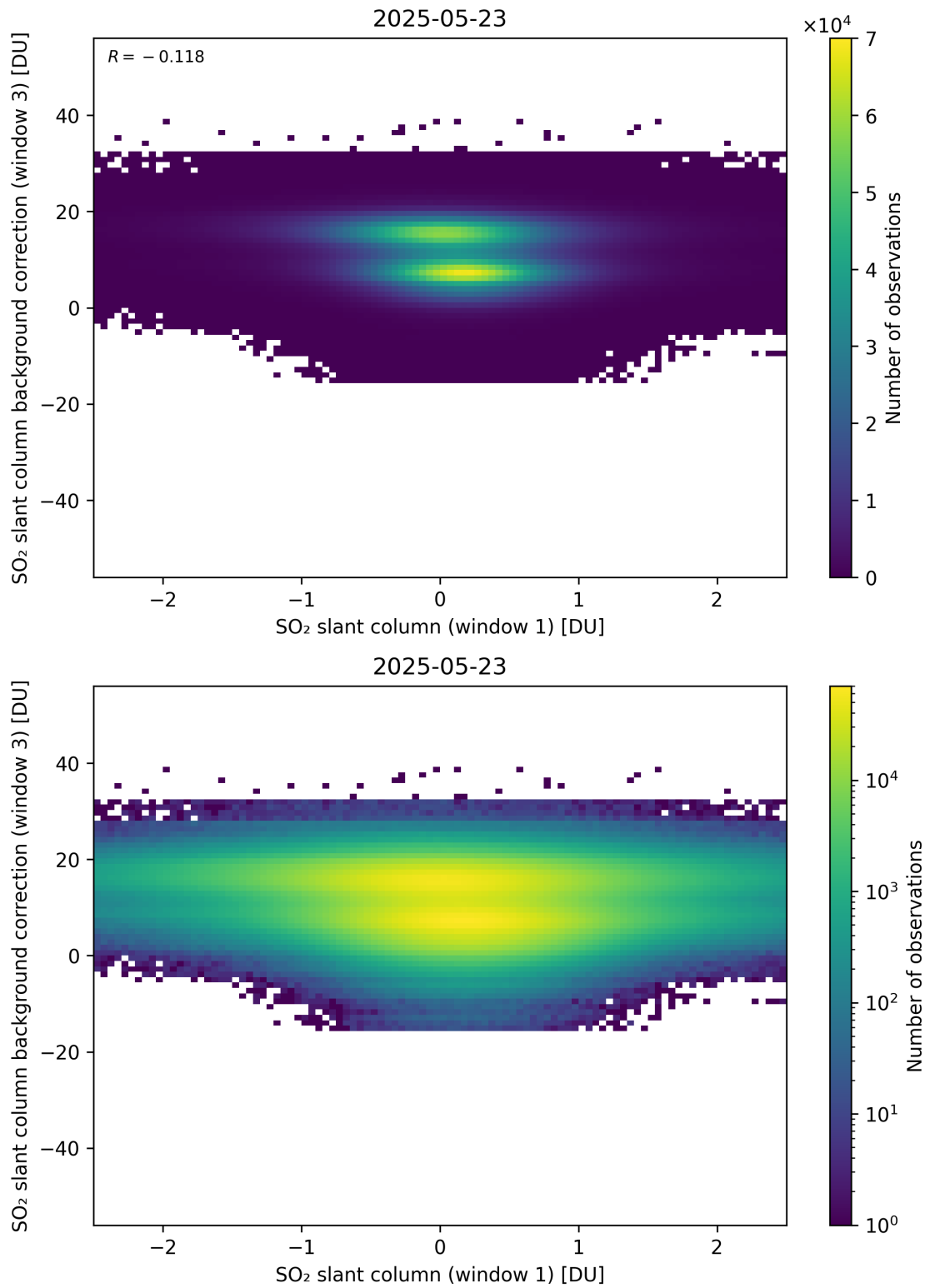
Figure 264: Scatter density plot of “SO 2 slant column (window 1)” against “SO 2 slant column background correction (window 3)” for 2025-05-22 to 2025-05-24.
