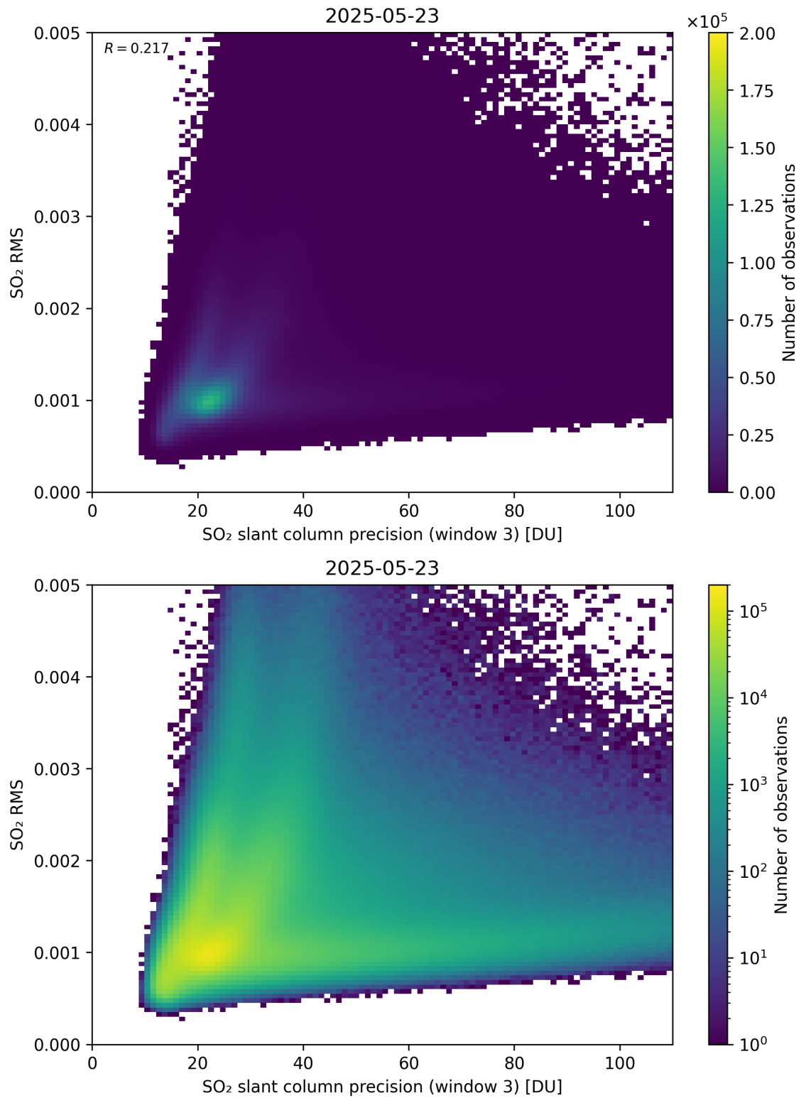
Figure 310: Scatter density plot of “SO 2 slant column precision (window 3)” against “SO 2 RMS” for 2025-05-22 to 2025-05-24.
