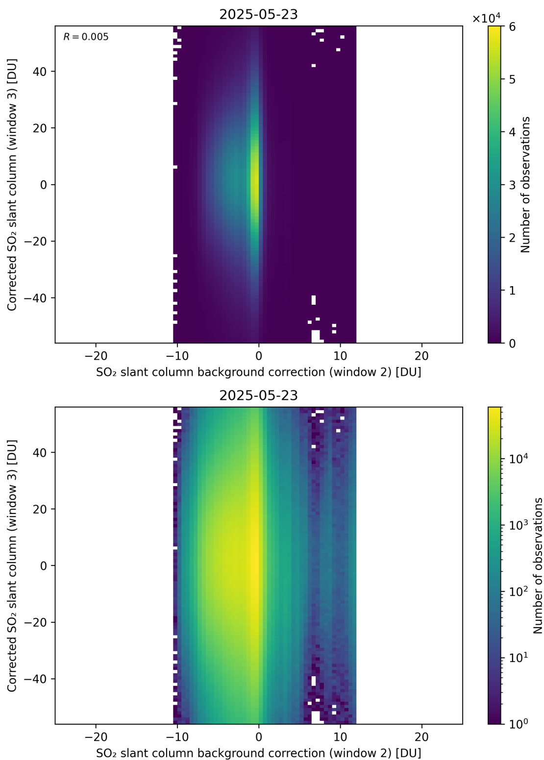
Figure 127: Scatter density plot of “SO 2 slant column background correction (window 2)” against “Corrected SO 2 slant column (window 3)” for 2025-05-22 to 2025-05-24.
