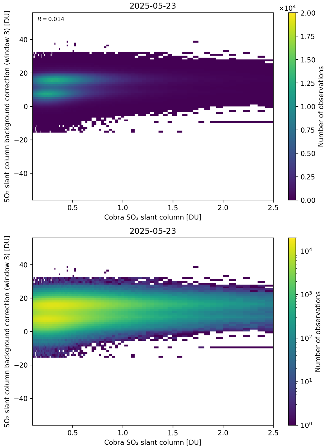
Figure 195: Scatter density plot of “Cobra SO 2 slant column” against “SO 2 slant column background correction (window 3)” for 2025-05-22 to 2025-05-24.
