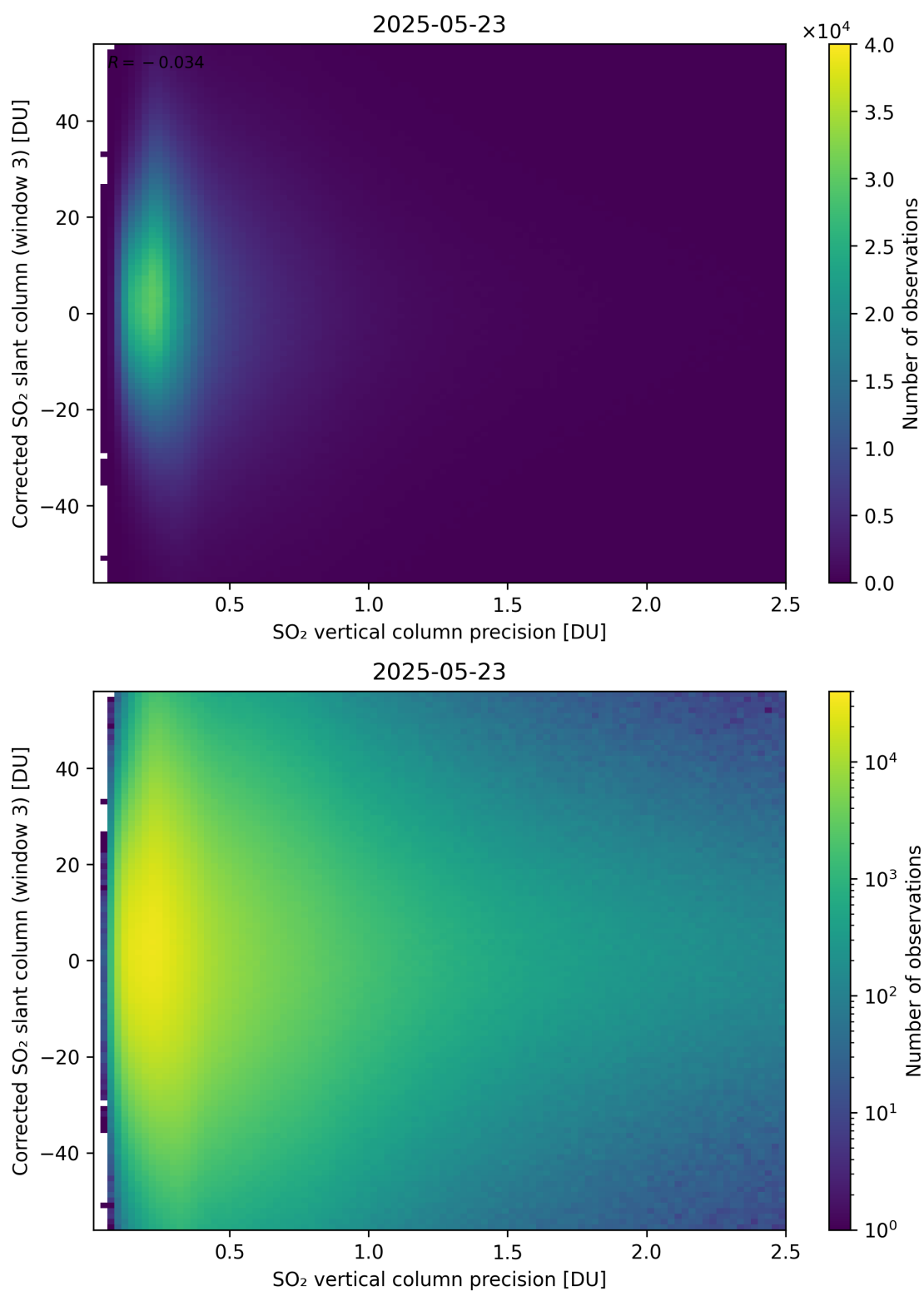
Figure 340: Scatter density plot of “SO 2 vertical column precision” against “Corrected SO 2 slant column (window 3)” for 2025-05-22 to 2025-05-24.
