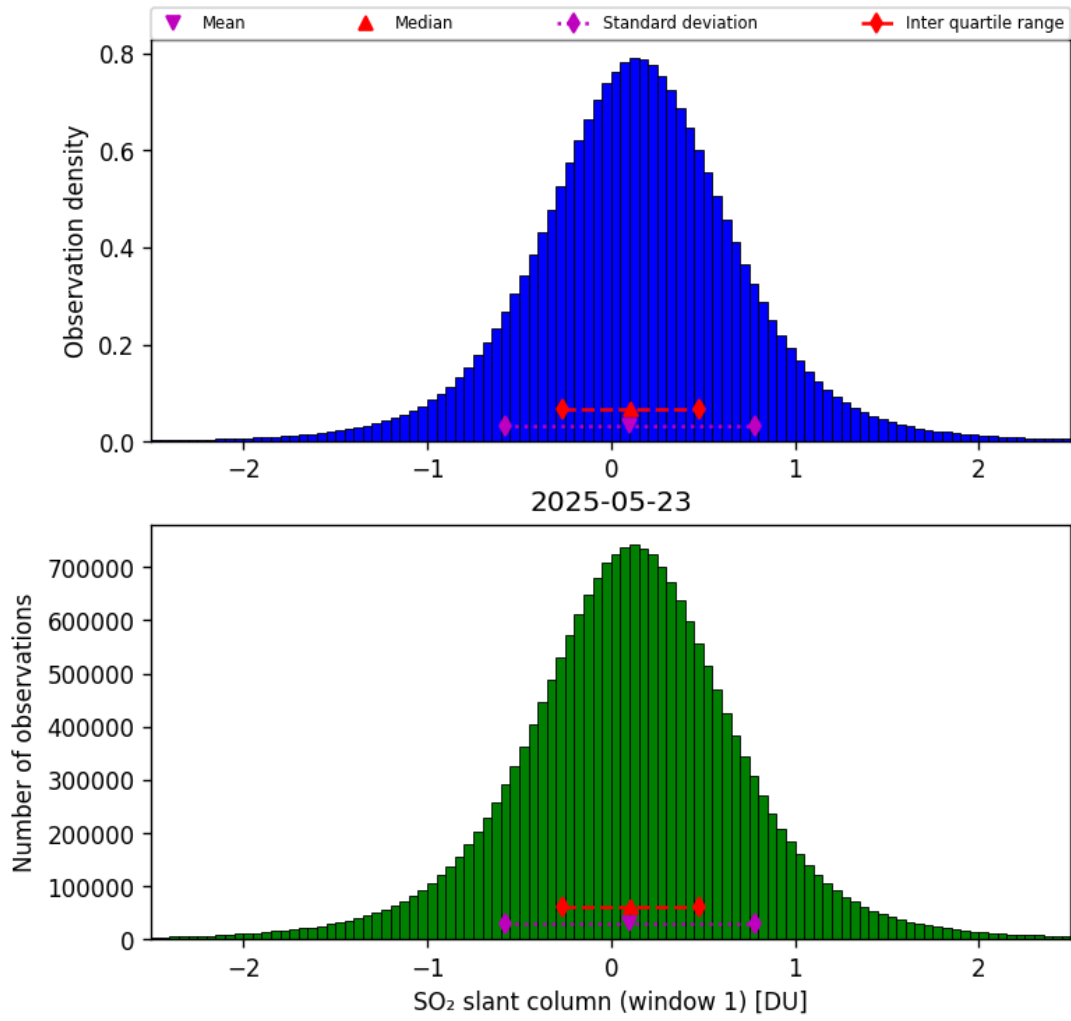
Figure 63: Histogram of “SO 2 slant column (window 1)” for 2025-05-22 to 2025-05-24
