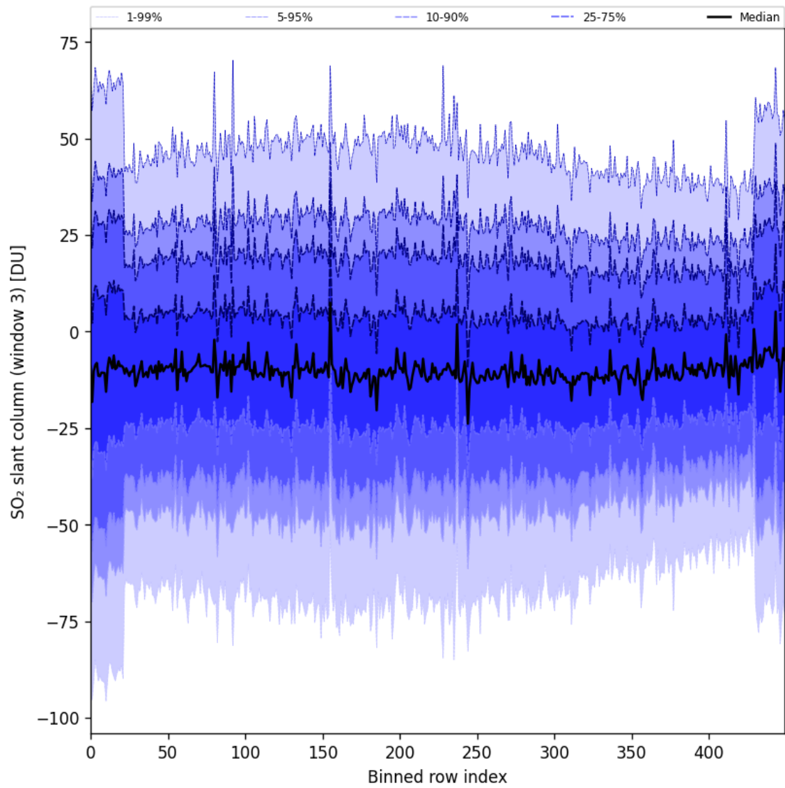
Figure 97: Along track statistics of “SO 2 slant column (window 3)” for 2025-05-22 to 2025-05-24
