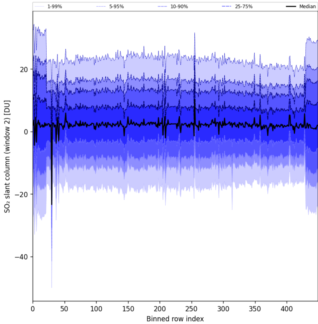
Figure 93: Along track statistics of “SO 2 slant column (window 2)” for 2025-05-22 to 2025-05-24
