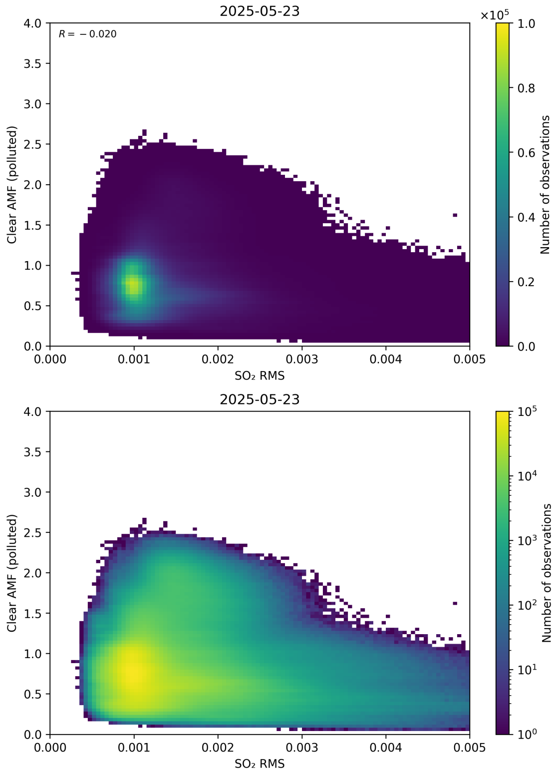
Figure 147: Scatter density plot of “SO 2 RMS” against “Clear AMF (polluted)” for 2025-05-22 to 2025-05-24.
