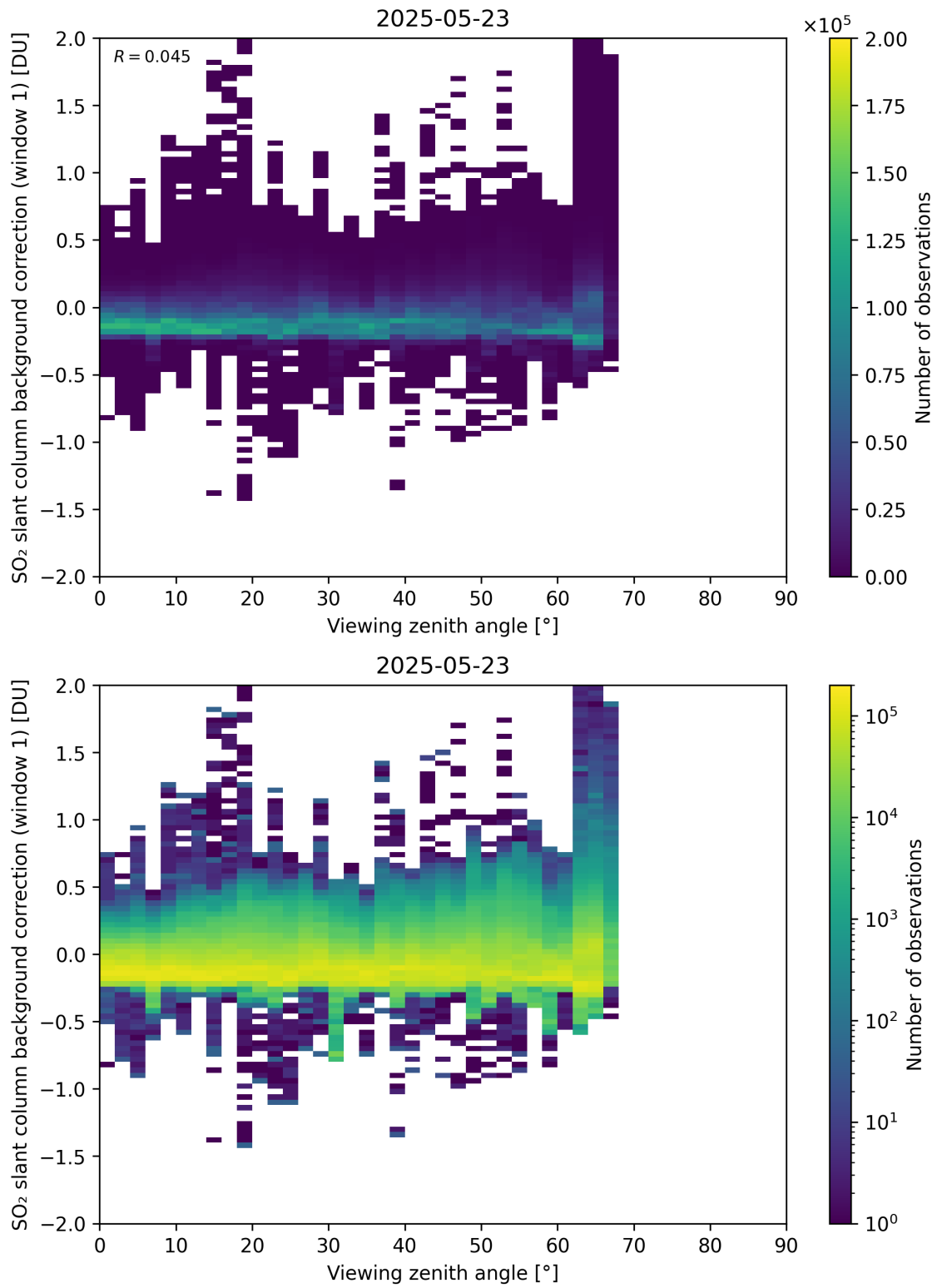
Figure 362: Scatter density plot of “Viewing zenith angle” against “SO 2 slant column background correction (window 1)” for 2025-05-22 to 2025-05-24.
