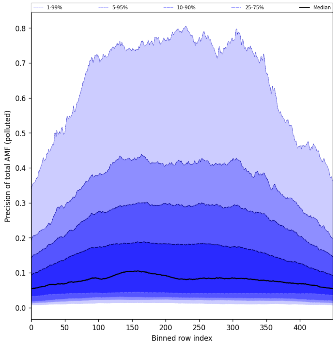
Figure 106: Along track statistics of “Precision of total AMF (polluted)” for 2025-05-22 to 2025-05-24
