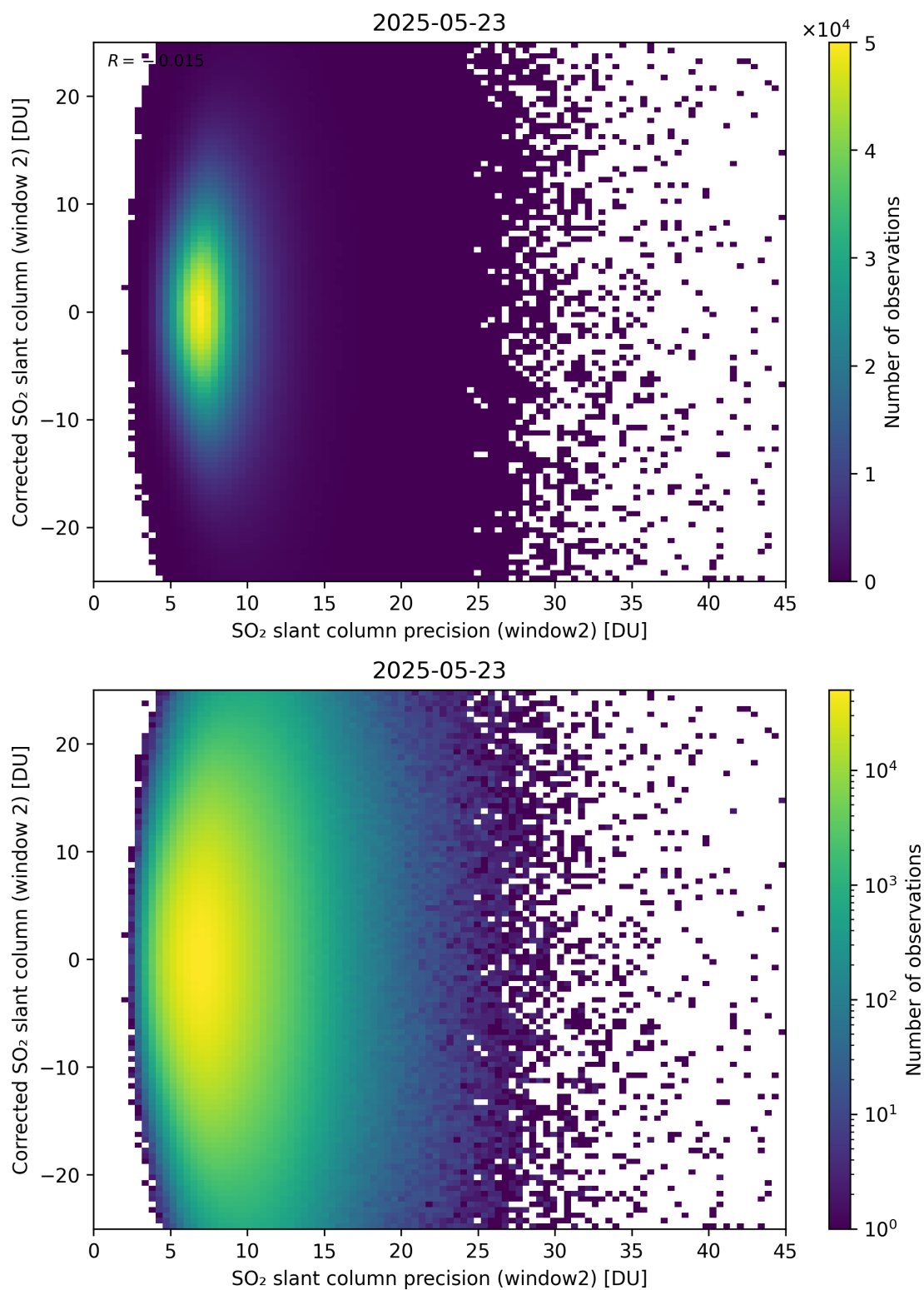
Figure 297: Scatter density plot of “SO 2 slant column precision (window2)” against “Corrected SO 2 slant column (window 2)” for 2025-05-22 to 2025-05-24.
