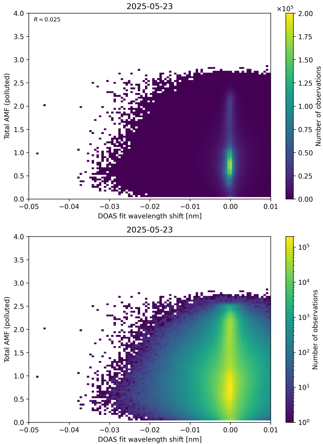
Figure 141: Scatter density plot of “DOAS fit wavelength shift” against “Total AMF (polluted)” for 2025-05-22 to 2025-05-24.
