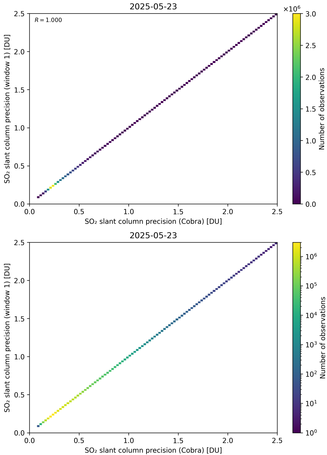
Figure 209: Scatter density plot of “SO 2 slant column precision (Cobra)” against “SO 2 slant column precision (window 1)” for 2025-05-22 to 2025-05-24.
