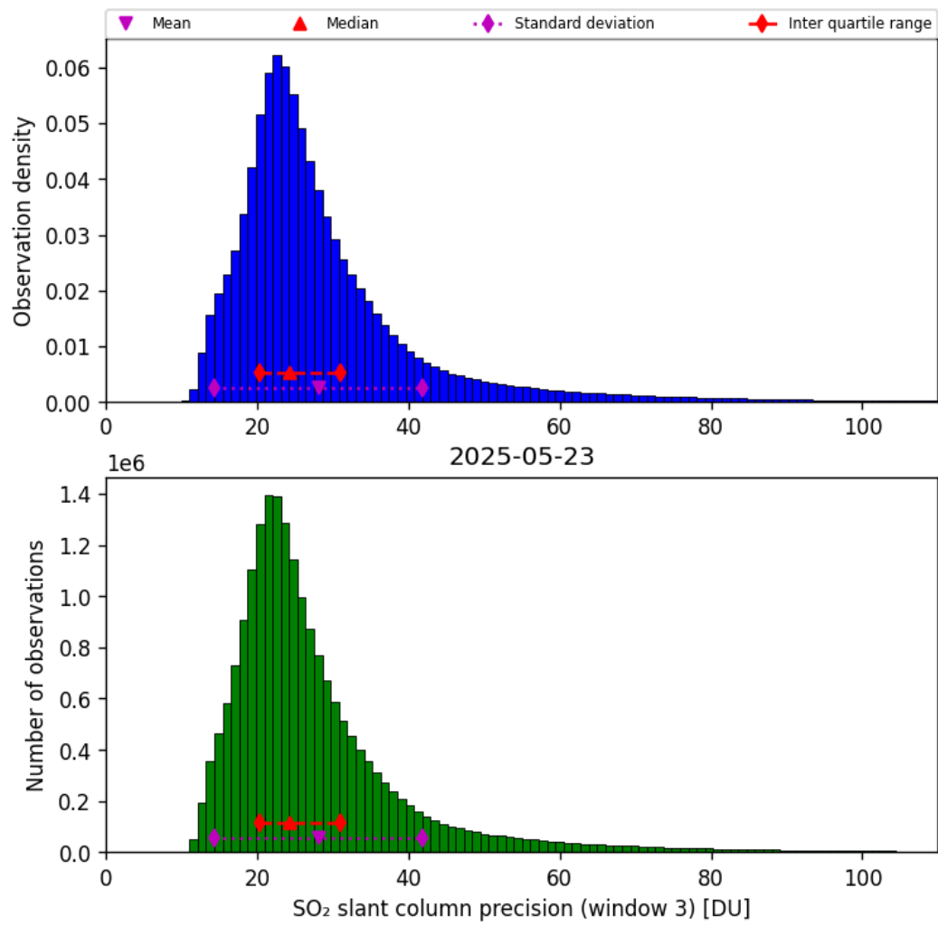
Figure 72: Histogram of “SO 2 slant column precision (window 3)” for 2025-05-22 to 2025-05-24
