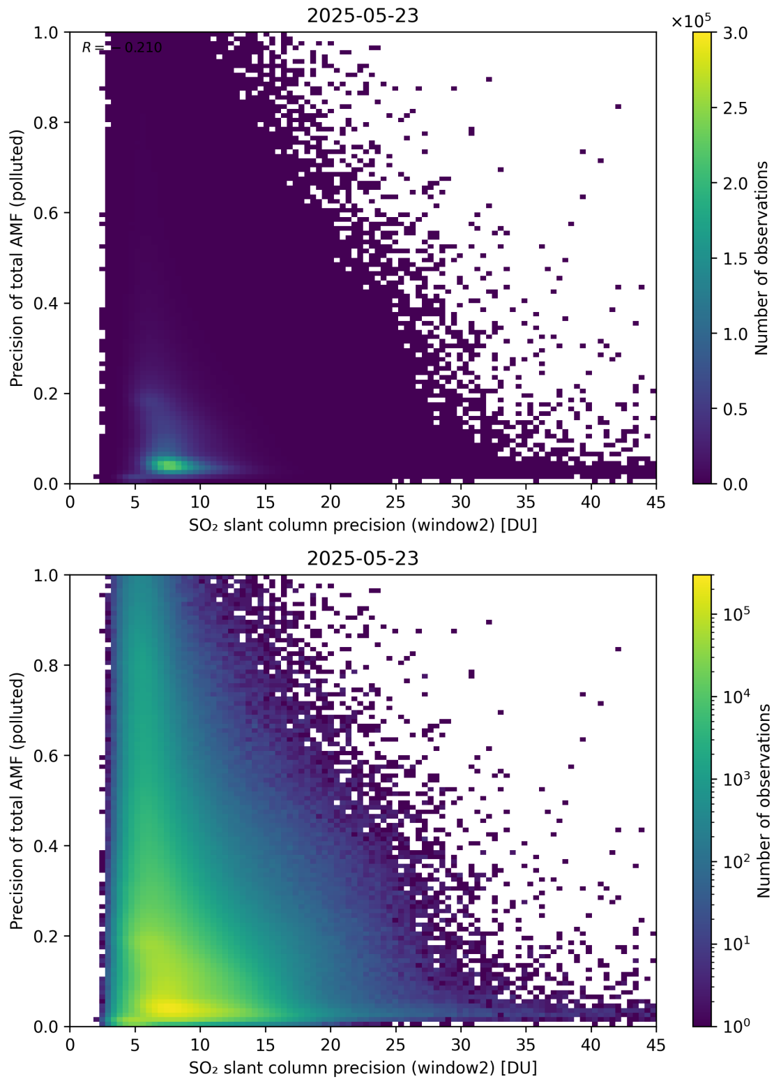
Figure 302: Scatter density plot of “SO 2 slant column precision (window2)” against “Precision of total AMF (polluted)” for 2025-05-22 to 2025-05-24.
