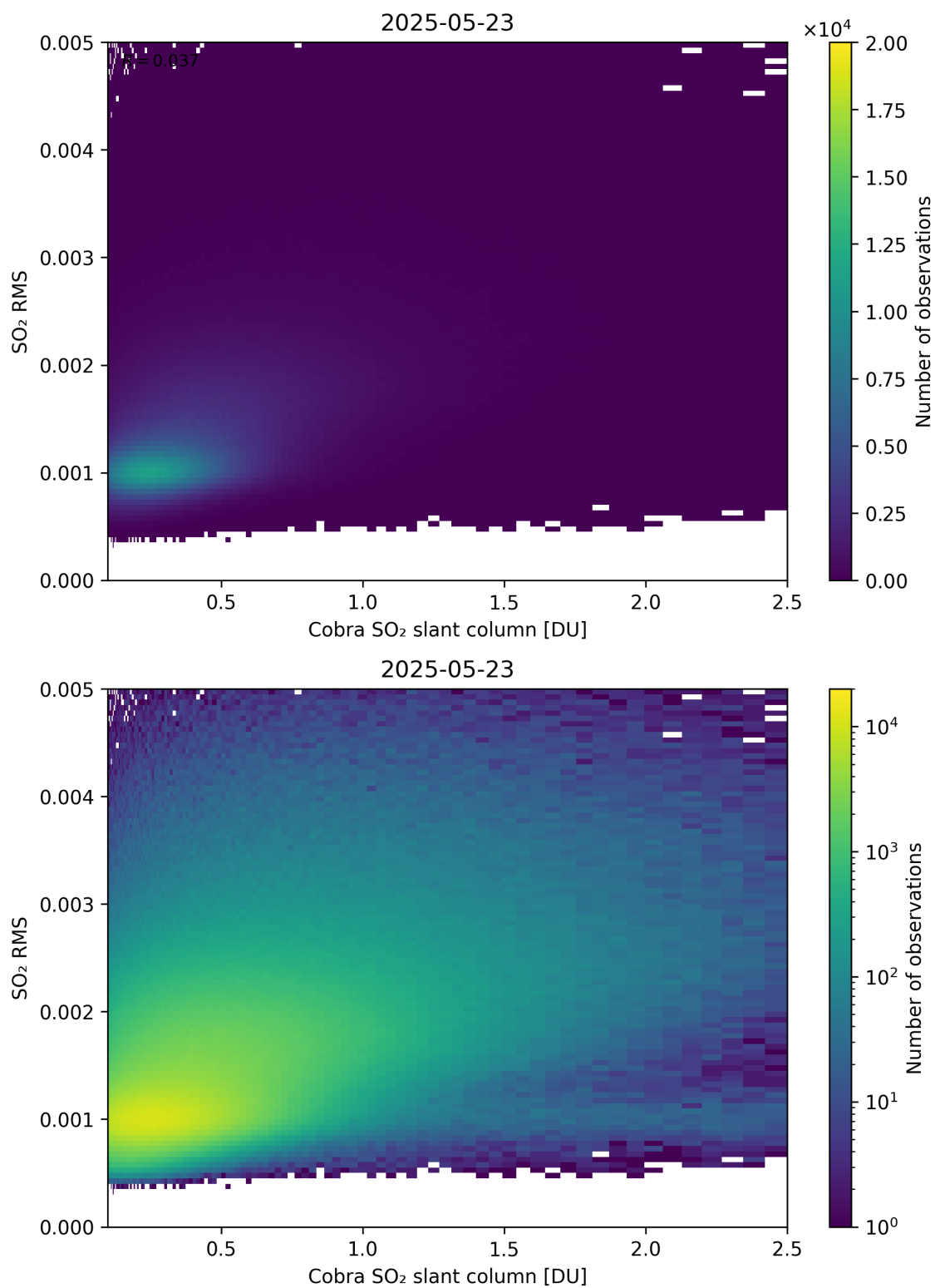
Figure 198: Scatter density plot of “Cobra SO 2 slant column” against “SO 2 RMS” for 2025-05-22 to 2025-05-24.
