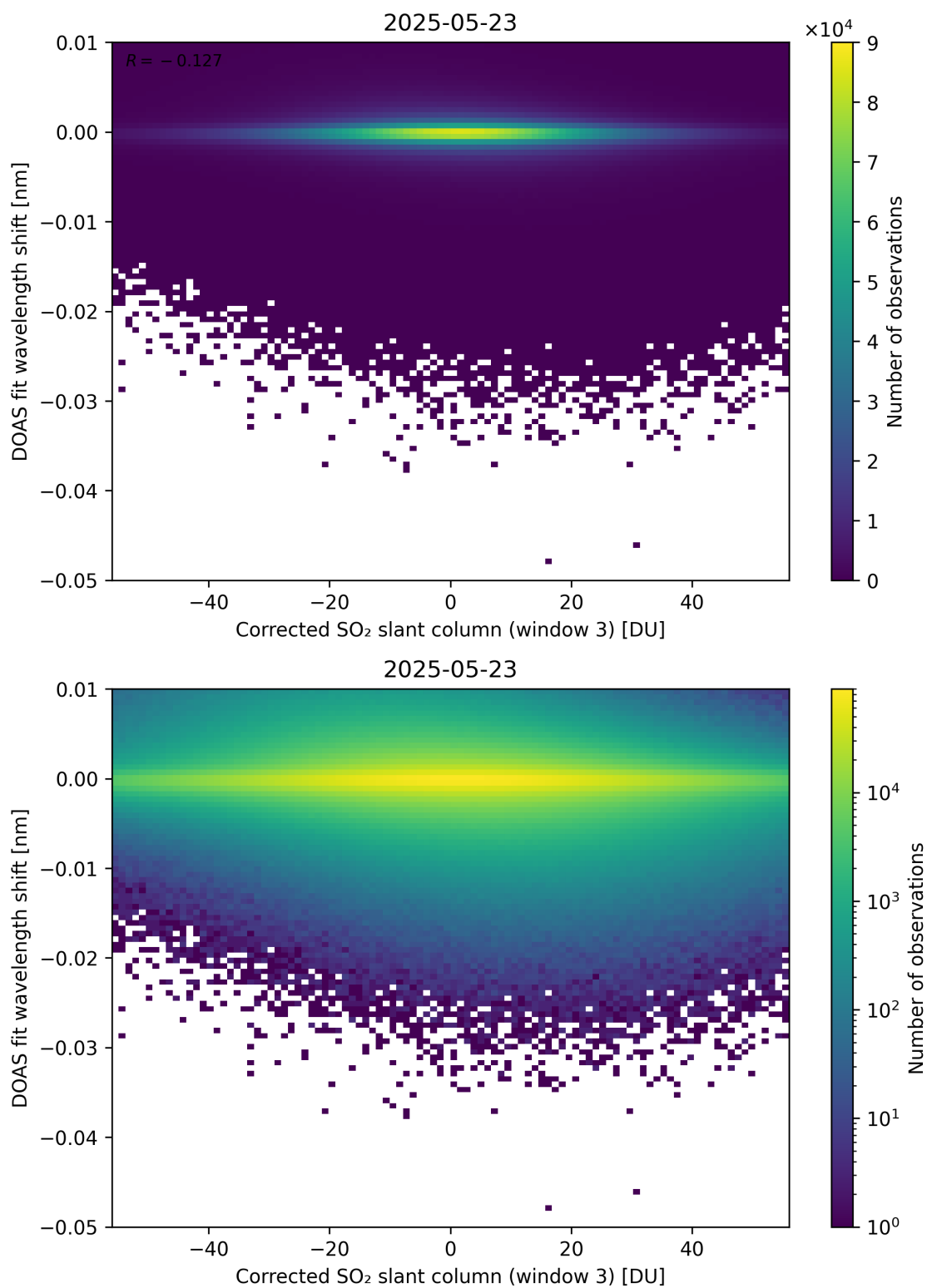
Figure 256: Scatter density plot of “Corrected SO 2 slant column (window 3)” against “DOAS fit wavelength shift” for 2025-05-22 to 2025-05-24.
