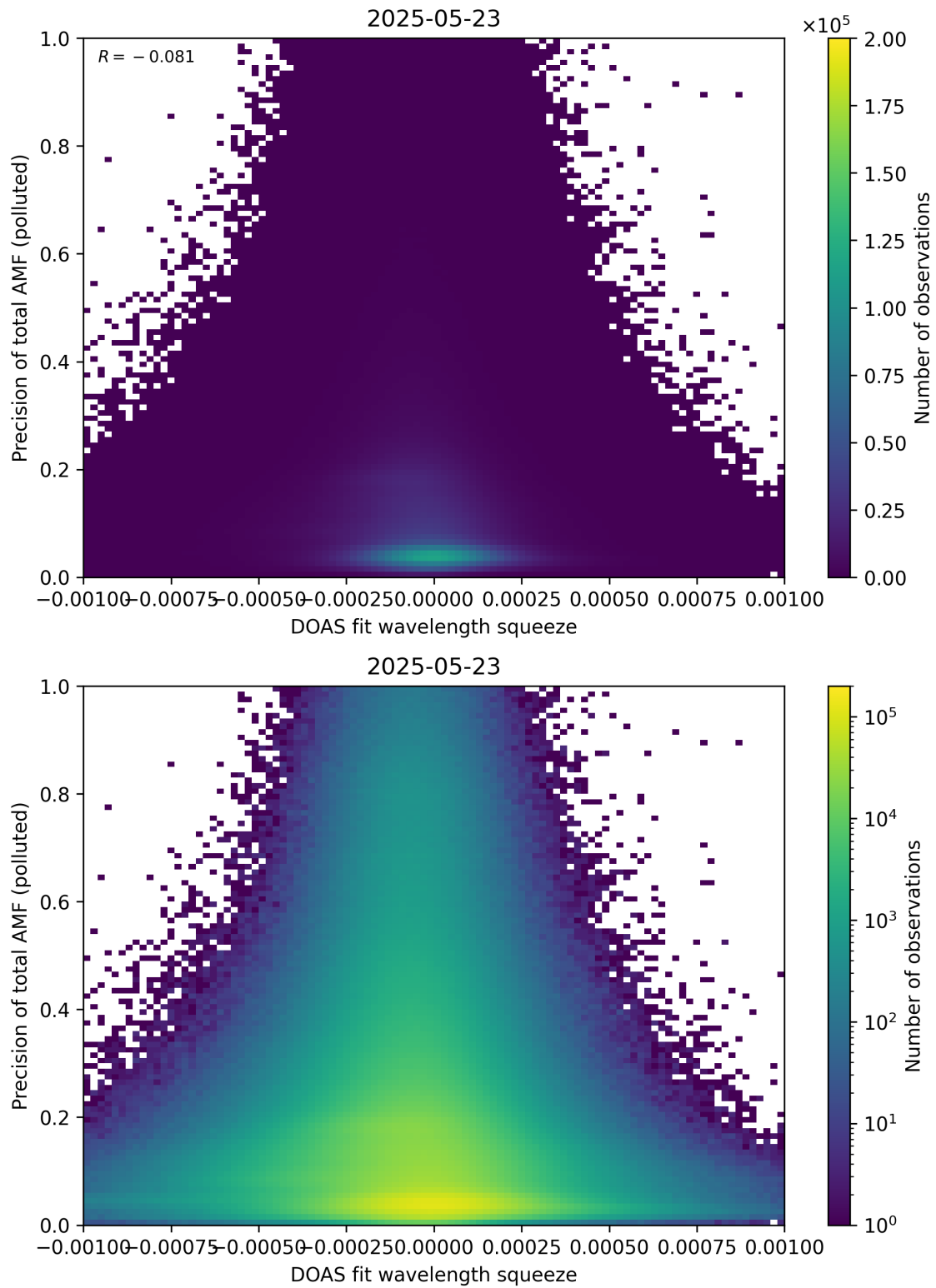
Figure 146: Scatter density plot of “DOAS fit wavelength squeeze” against “Precision of total AMF (polluted)” for 2025-05-22 to 2025-05-24.
