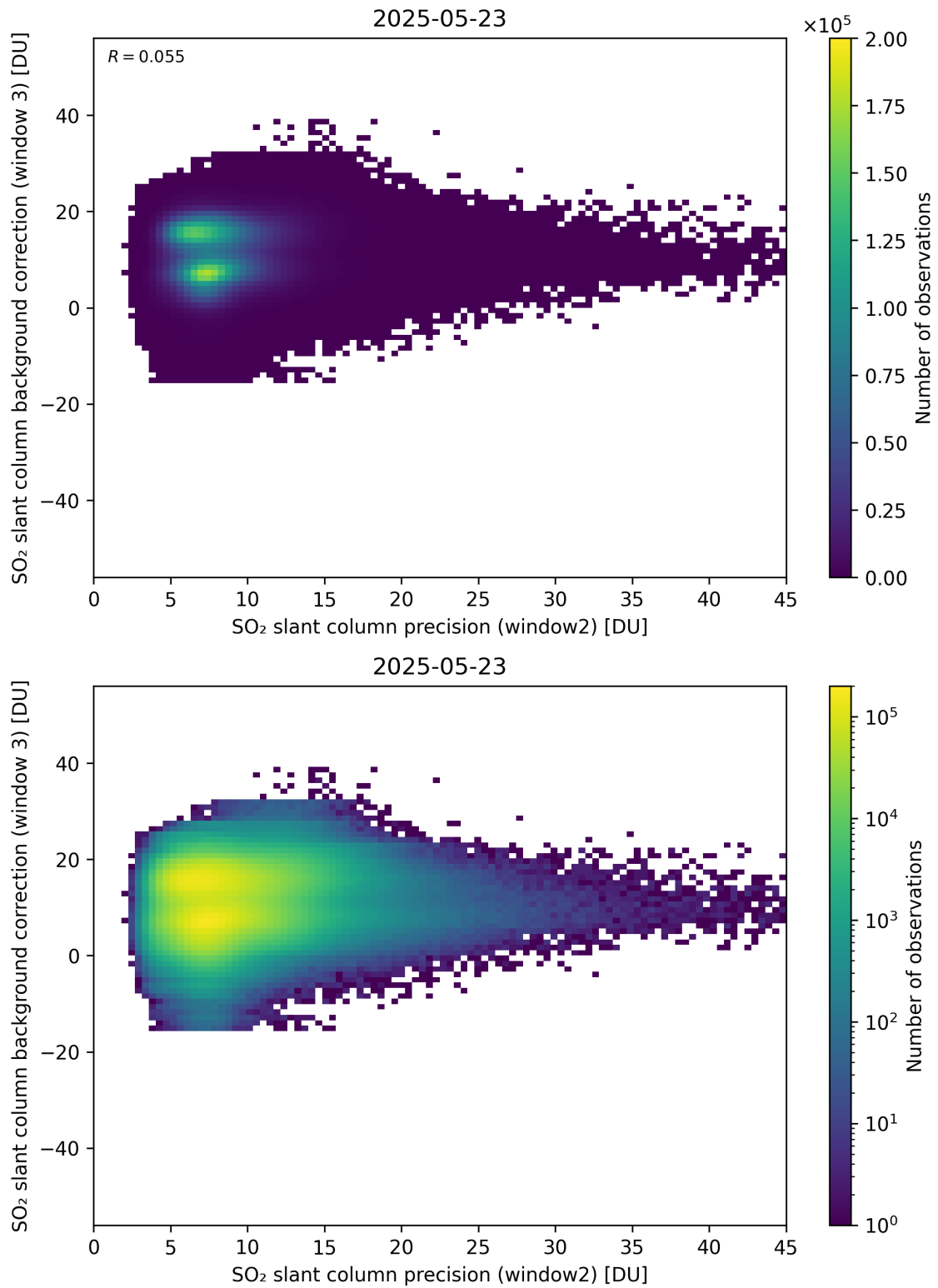
Figure 292: Scatter density plot of “SO 2 slant column precision (window2)” against “SO 2 slant column background correction (window 3)” for 2025-05-22 to 2025-05-24.
