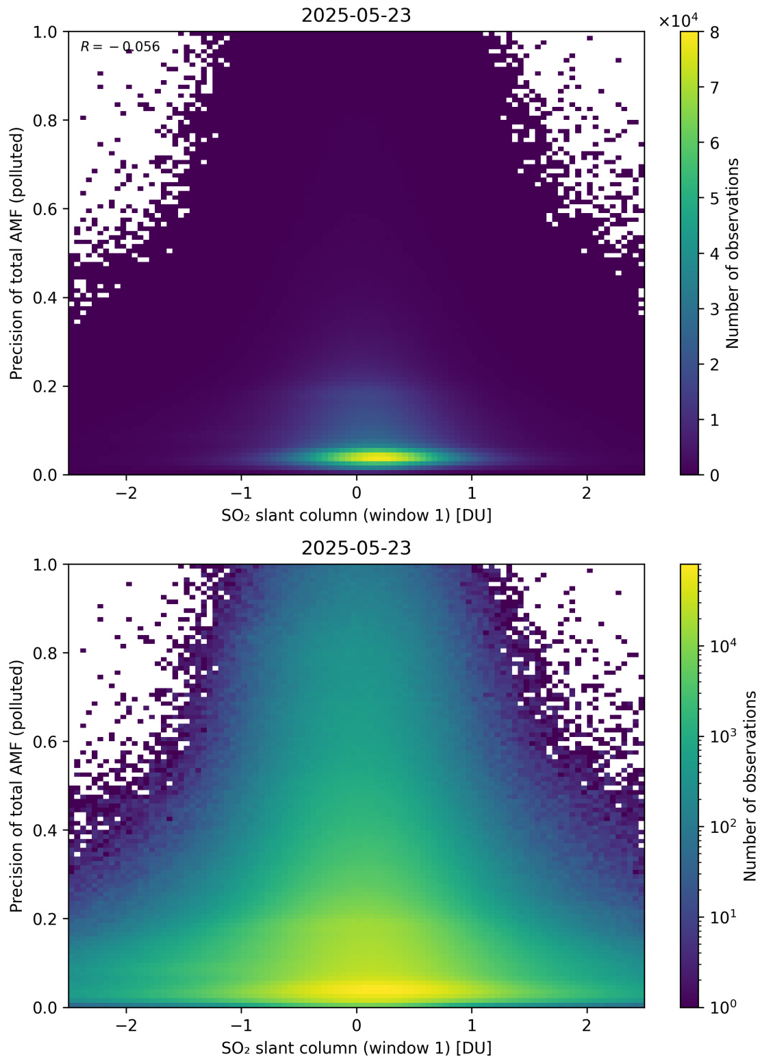
Figure 290: Scatter density plot of “SO 2 slant column (window 1)” against “Precision of total AMF (polluted)” for 2025-05-22 to 2025-05-24.
