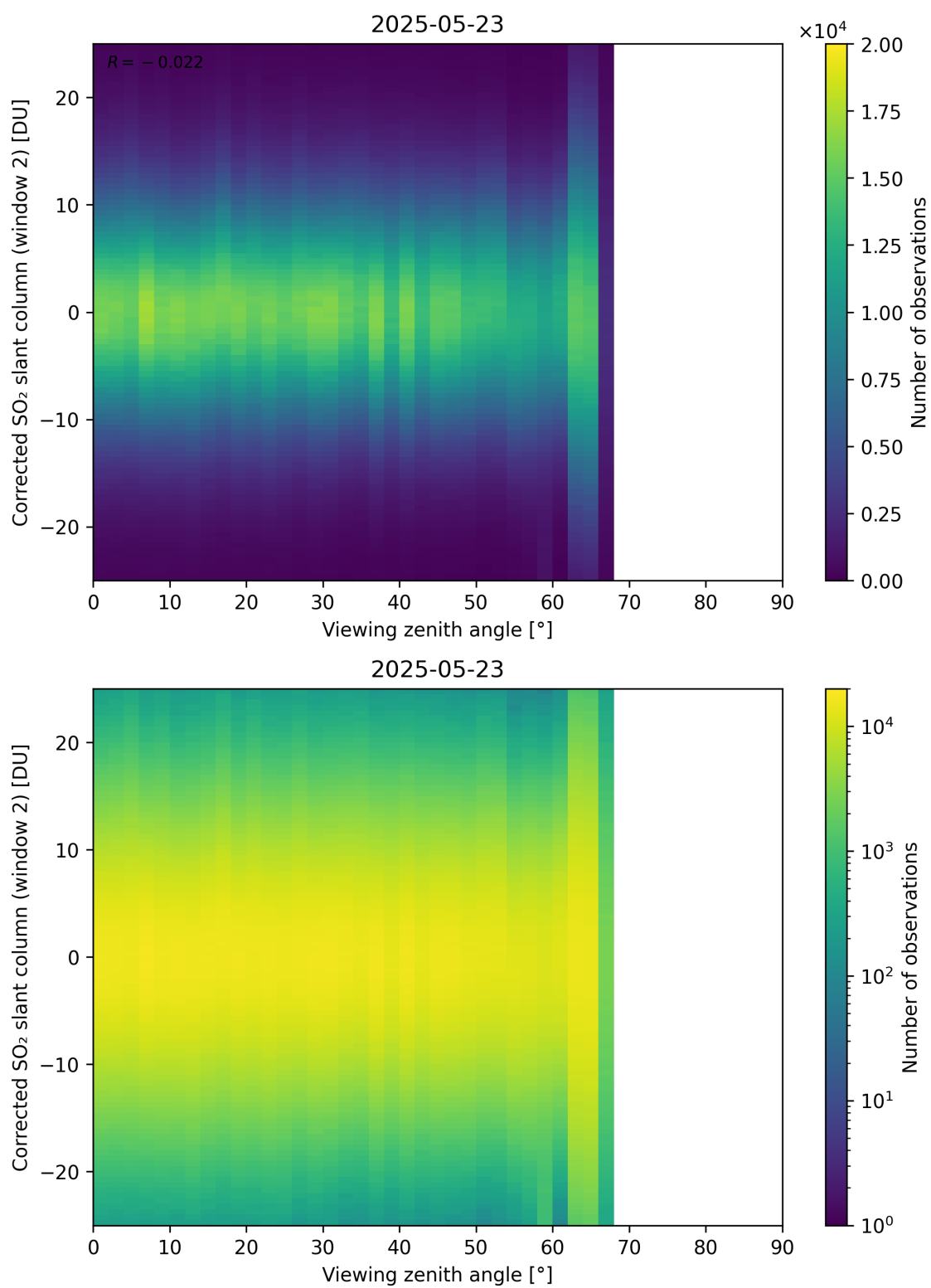
Figure 374: Scatter density plot of “Viewing zenith angle” against “Corrected SO 2 slant column (window 2)” for 2025-05-22 to 2025-05-24.
