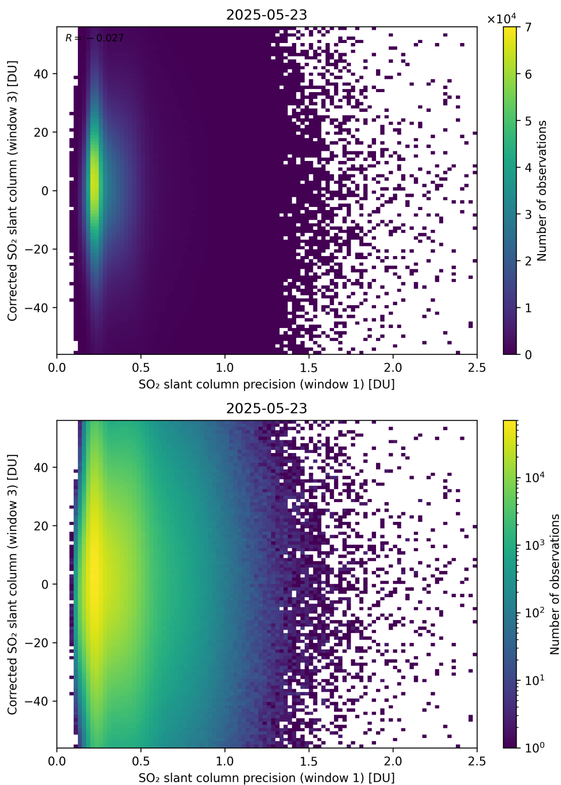
Figure 276: Scatter density plot of “SO 2 slant column precision (window 1)” against “Corrected SO 2 slant column (window 3)” for 2025-05-22 to 2025-05-24.
