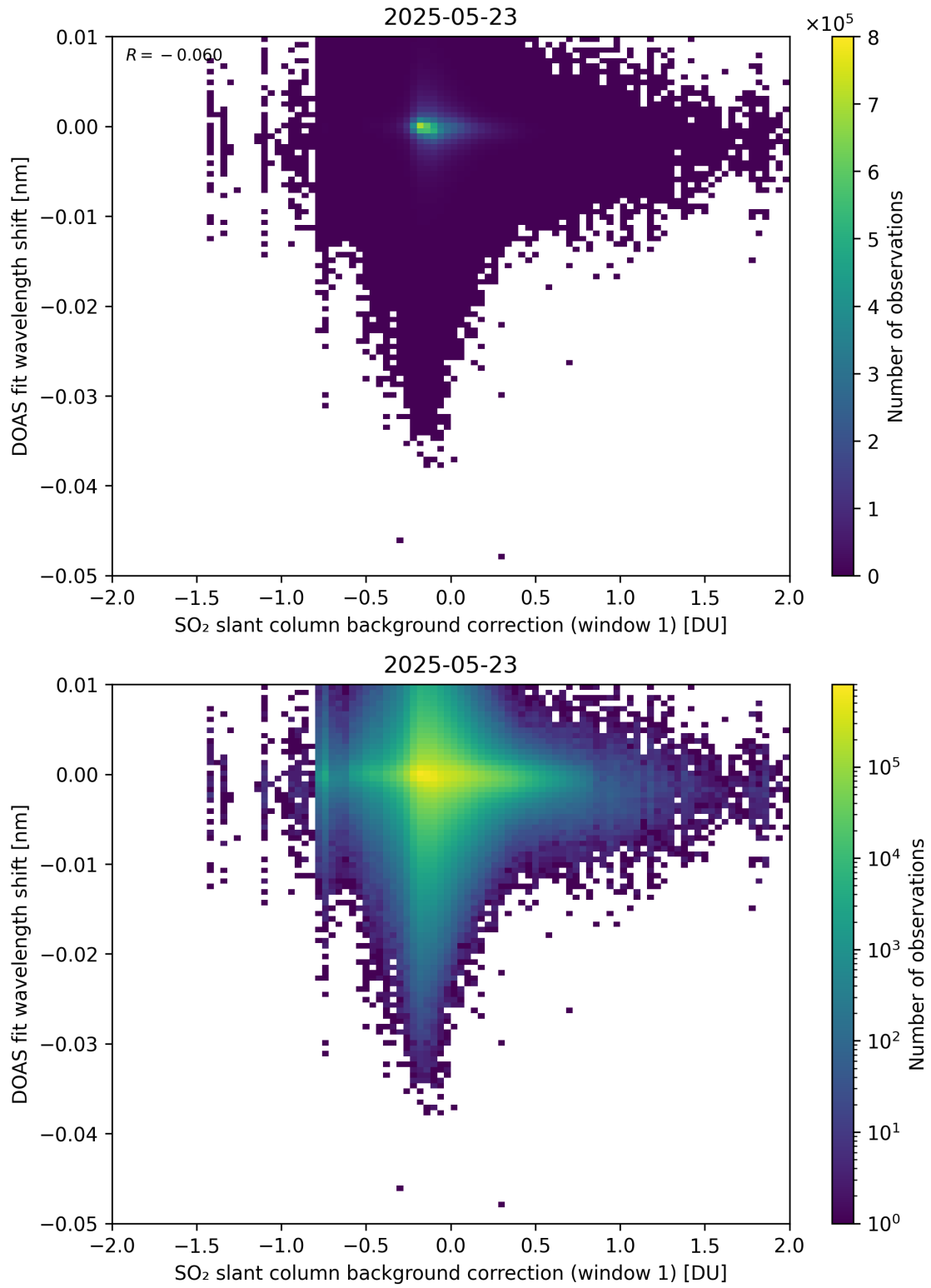
Figure 111: Scatter density plot of “SO 2 slant column background correction (window 1)” against “DOAS fit wavelength shift” for 2025-05-22 to 2025-05-24.
