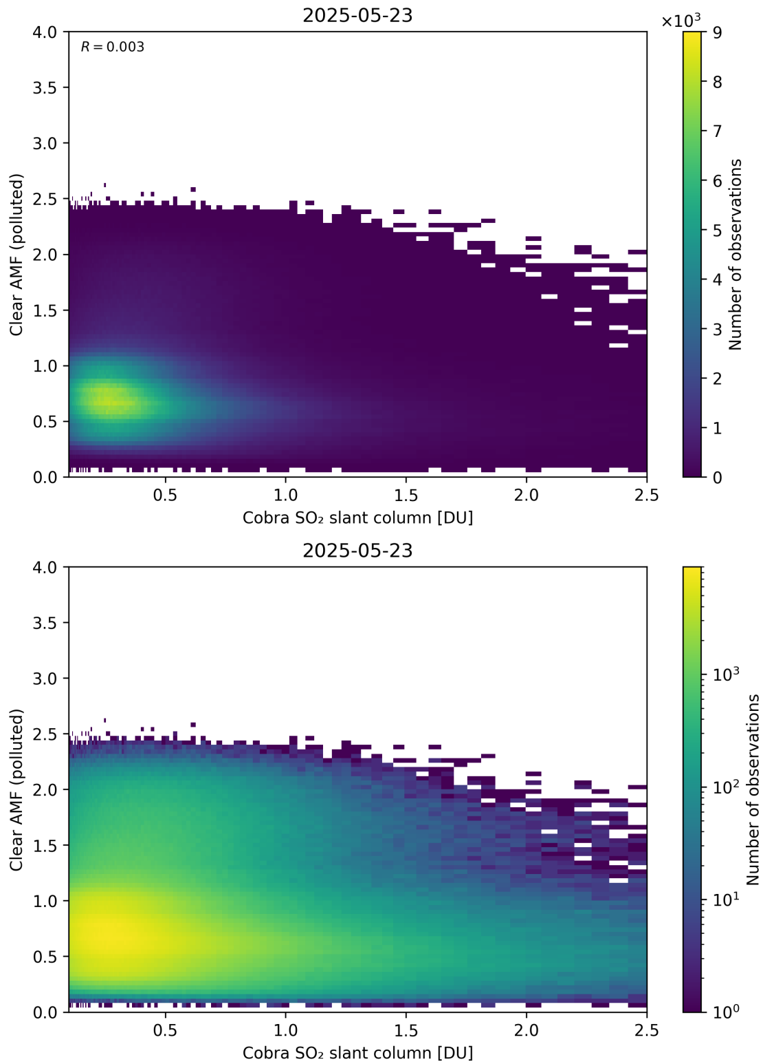
Figure 215: Scatter density plot of “Cobra SO 2 slant column” against “Clear AMF (polluted)” for 2025-05-22 to 2025-05-24.
