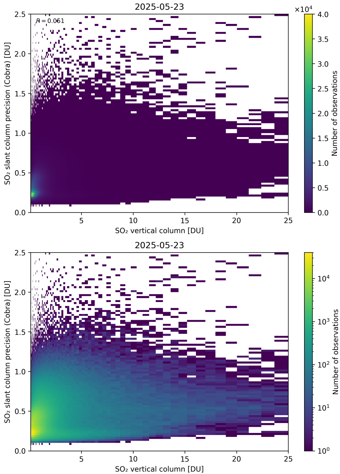
Figure 350: Scatter density plot of “SO 2 vertical column” against “SO 2 slant column precision (Cobra)” for 2025-05-22 to 2025-05-24.
