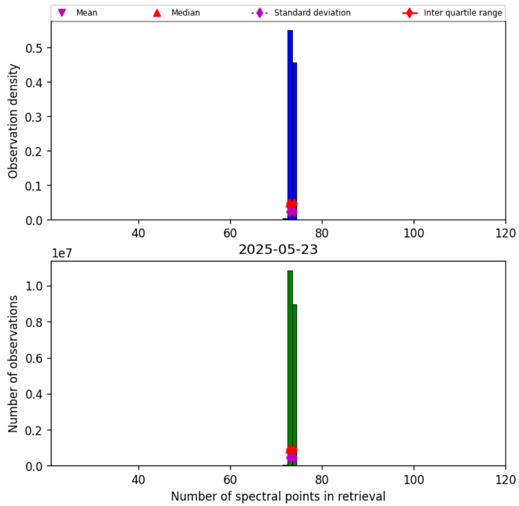
Figure 82: Histogram of “Number of spectral points in retrieval” for 2025-05-22 to 2025-05-24
