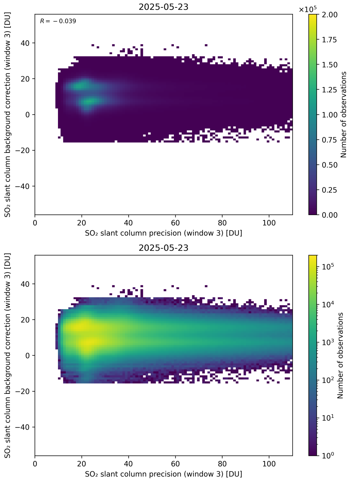
Figure 307: Scatter density plot of “SO 2 slant column precision (window 3)” against “SO 2 slant column background correction (window 3)” for 2025-05-22 to 2025-05-24.
