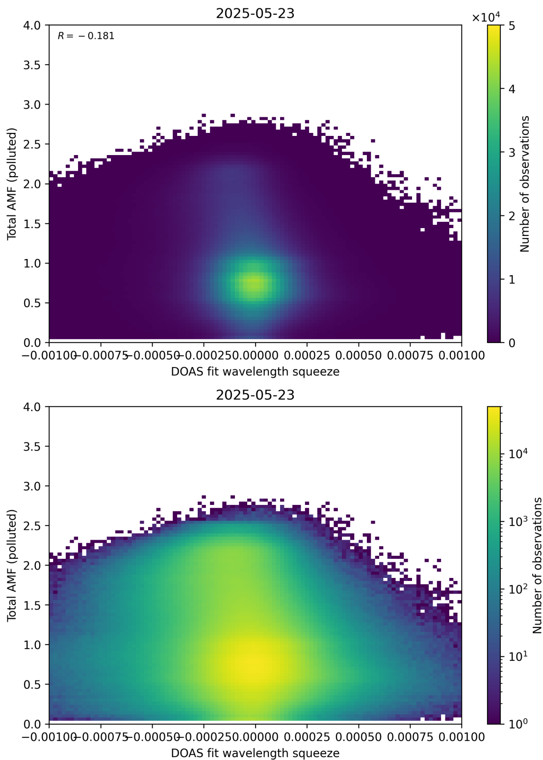
Figure 145: Scatter density plot of “DOAS fit wavelength squeeze” against “Total AMF (polluted)” for 2025-05-22 to 2025-05-24.
