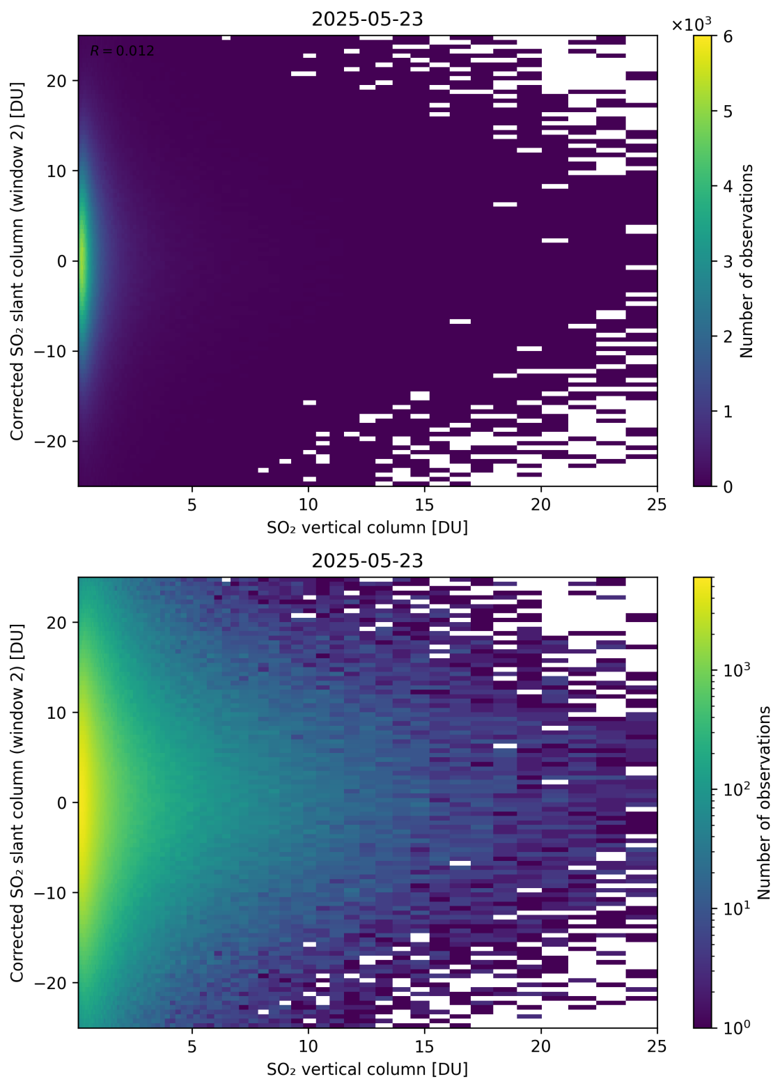
Figure 352: Scatter density plot of “SO 2 vertical column” against “Corrected SO 2 slant column (window 2)” for 2025-05-22 to 2025-05-24.
