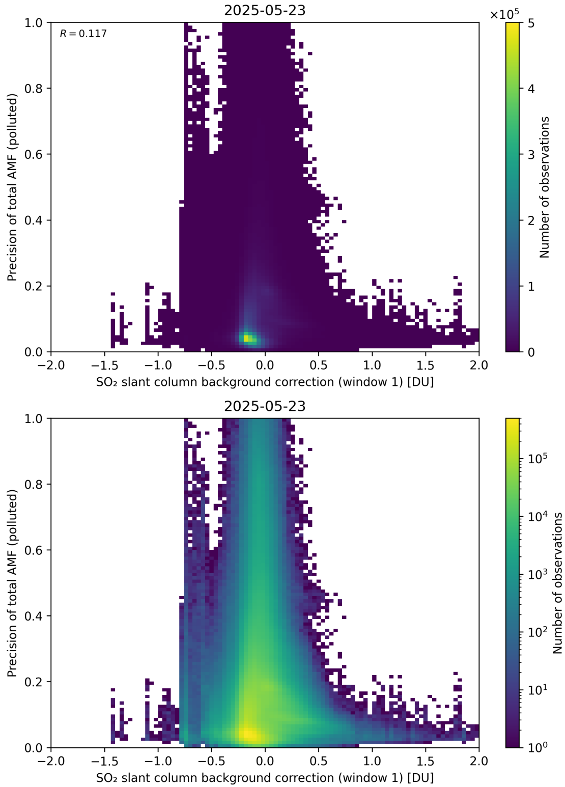
Figure 121: Scatter density plot of “SO 2 slant column background correction (window 1)” against “Precision of total AMF (polluted)” for 2025-05-22 to 2025-05-24.
