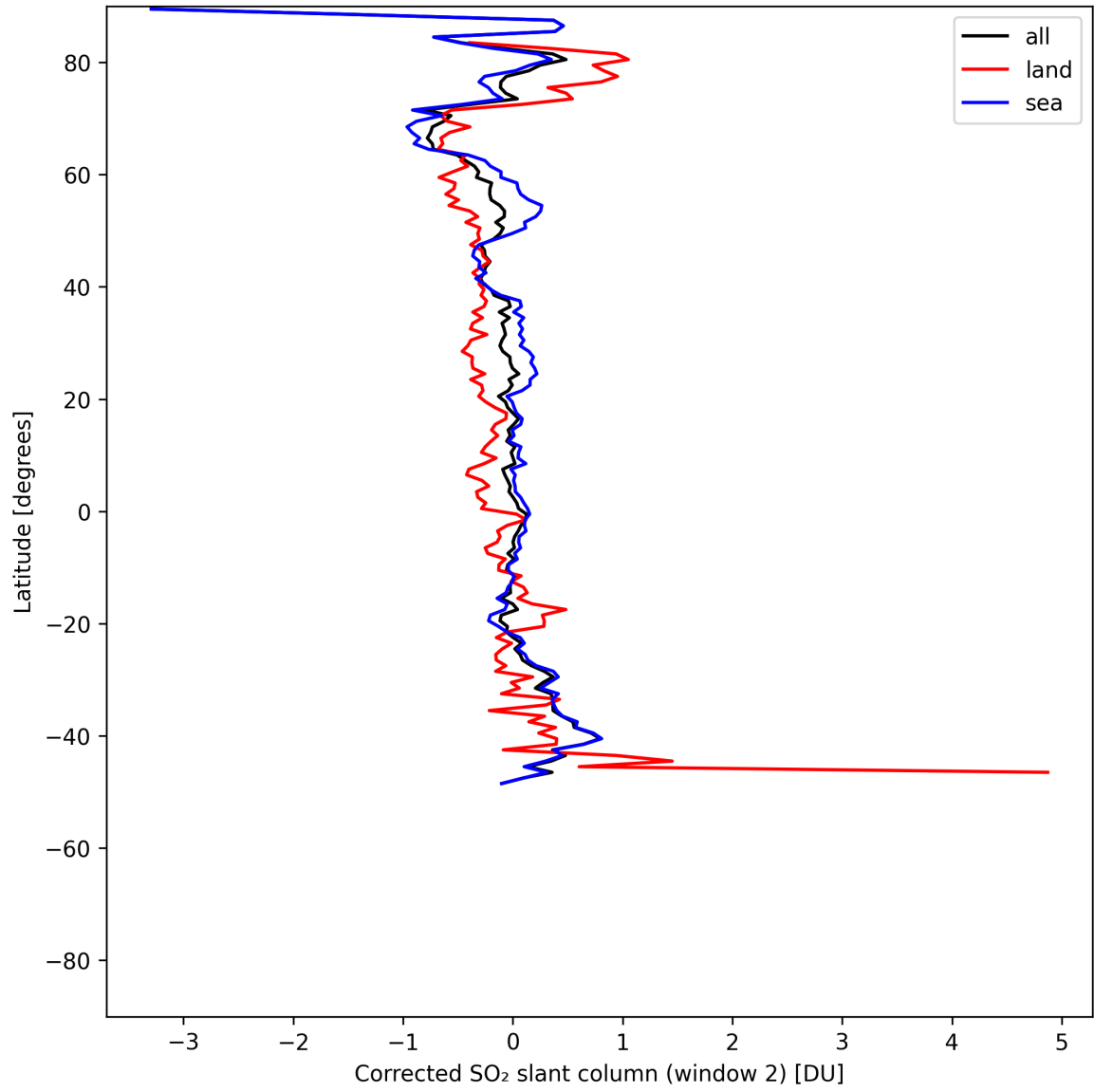
Figure 43: Zonal average of “Corrected SO 2 slant column (window 2)” for 2025-05-22 to 2025-05-24.
