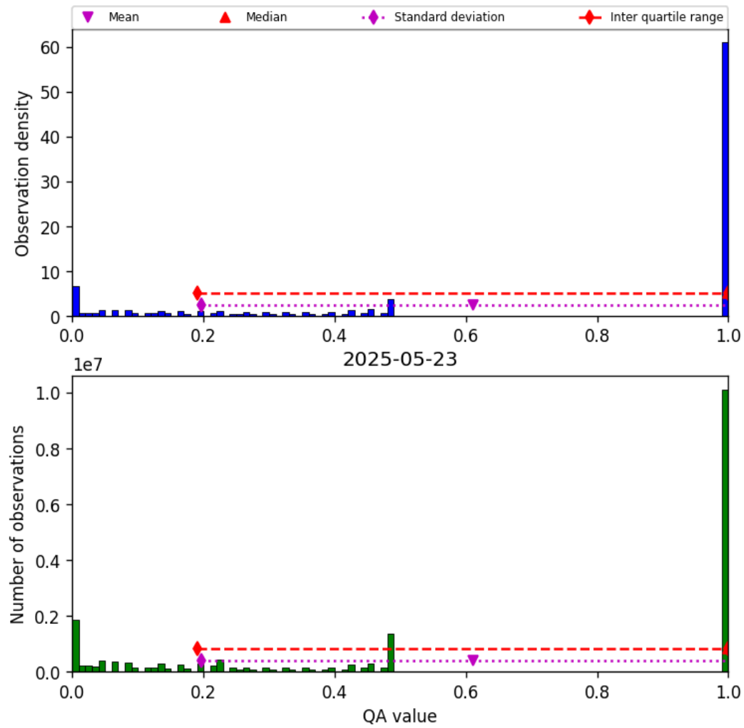
Figure 57: Histogram of “QA value” for 2025-05-22 to 2025-05-24
