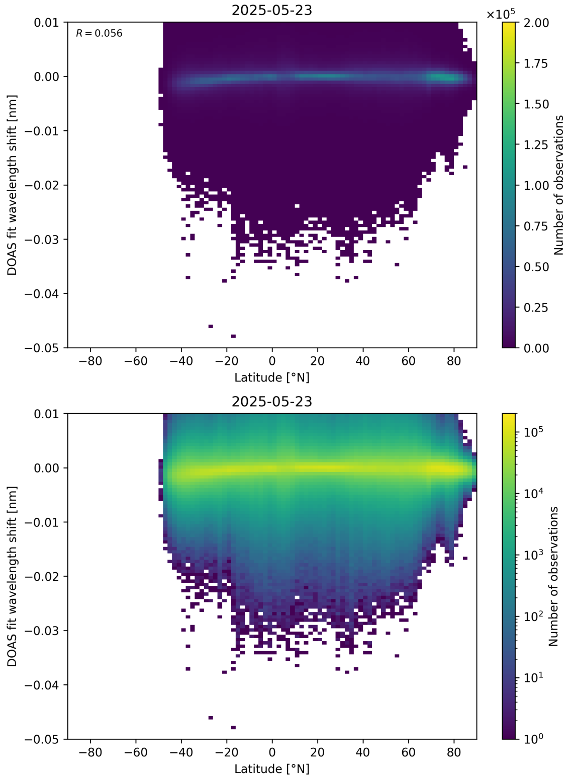
Figure 153: Scatter density plot of “Latitude” against “DOAS fit wavelength shift” for 2025-05-22 to 2025-05-24.
