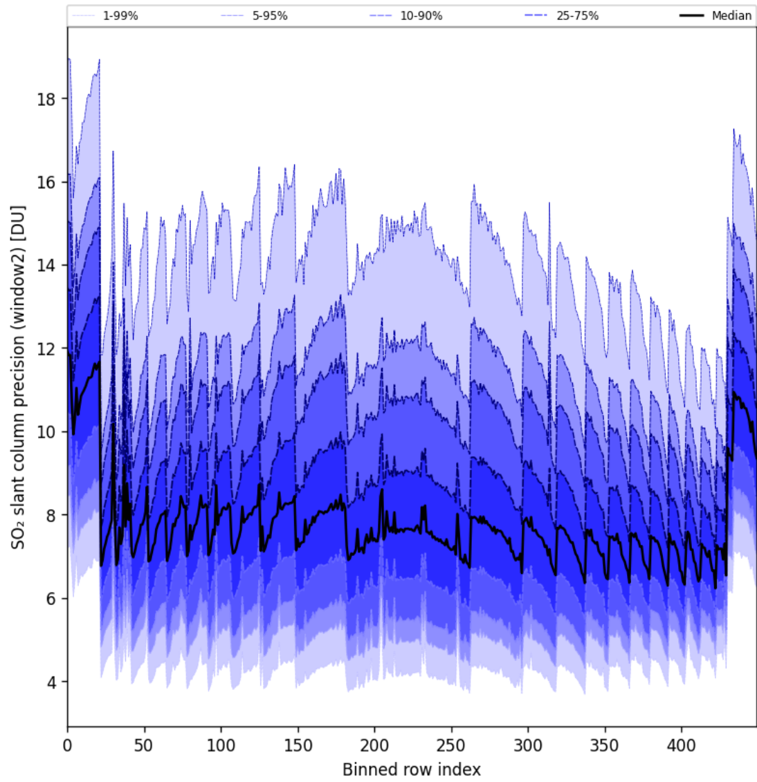
Figure 94: Along track statistics of “SO 2 slant column precision (window2)” for 2025-05-22 to 2025-05-24
