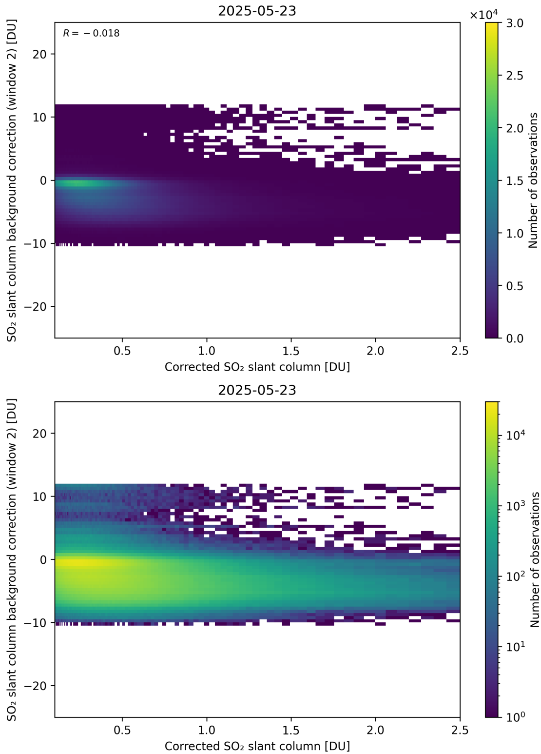
Figure 227: Scatter density plot of “Corrected SO 2 slant column” against “SO 2 slant column background correction (window 2)” for 2025-05-22 to 2025-05-24.
