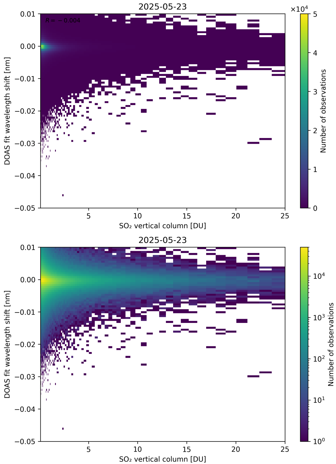
Figure 326: Scatter density plot of “SO 2 vertical column” against “DOAS fit wavelength shift” for 2025-05-22 to 2025-05-24.
