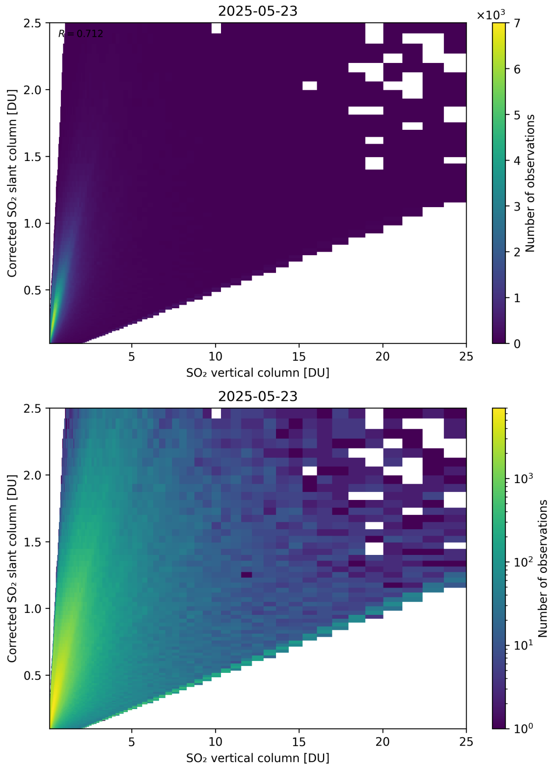
Figure 351: Scatter density plot of “SO 2 vertical column” against “Corrected SO 2 slant column” for 2025-05-22 to 2025-05-24.
