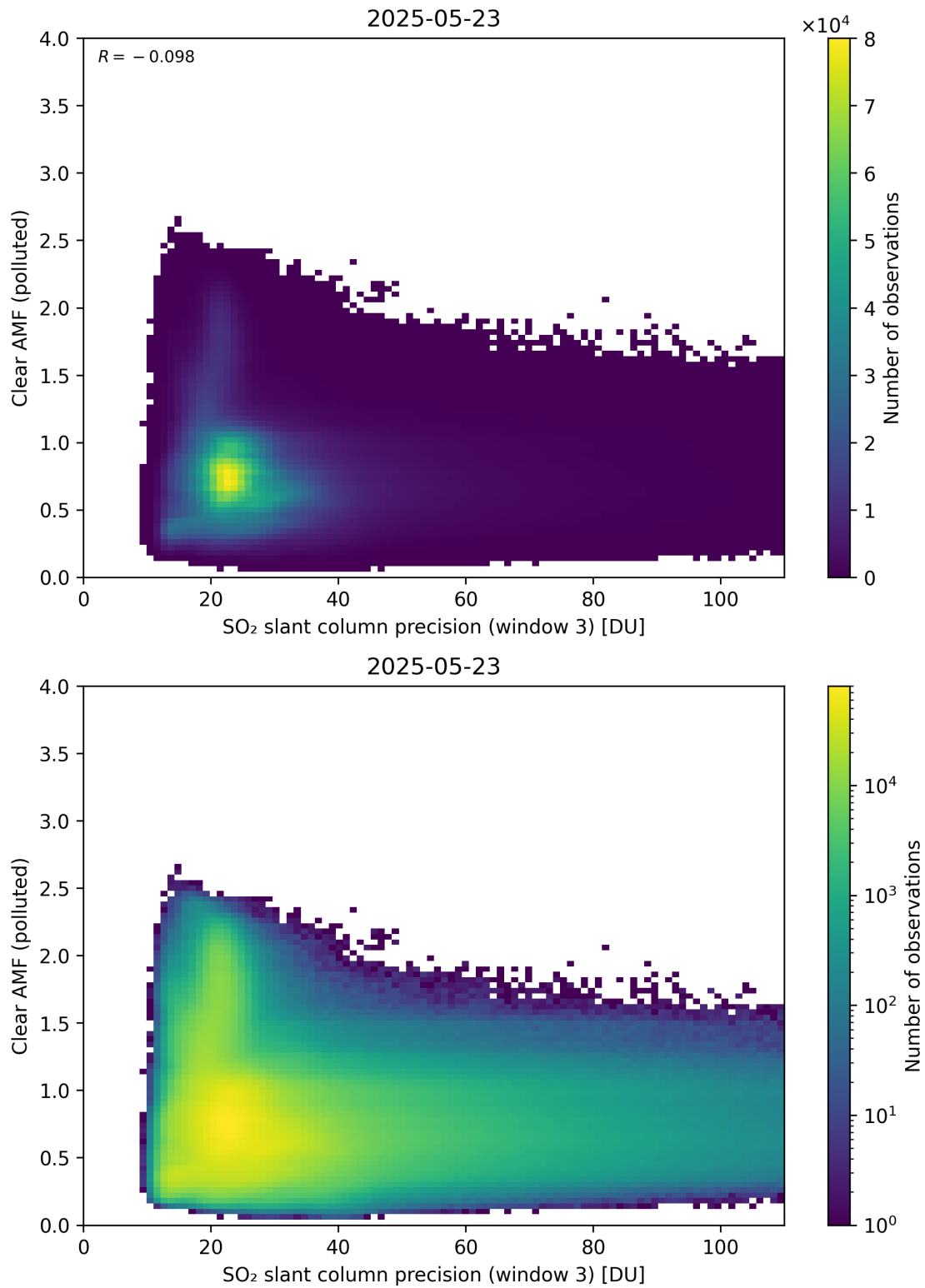
Figure 311: Scatter density plot of “SO 2 slant column precision (window 3)” against “Clear AMF (polluted)” for 2025-05-22 to 2025-05-24.
