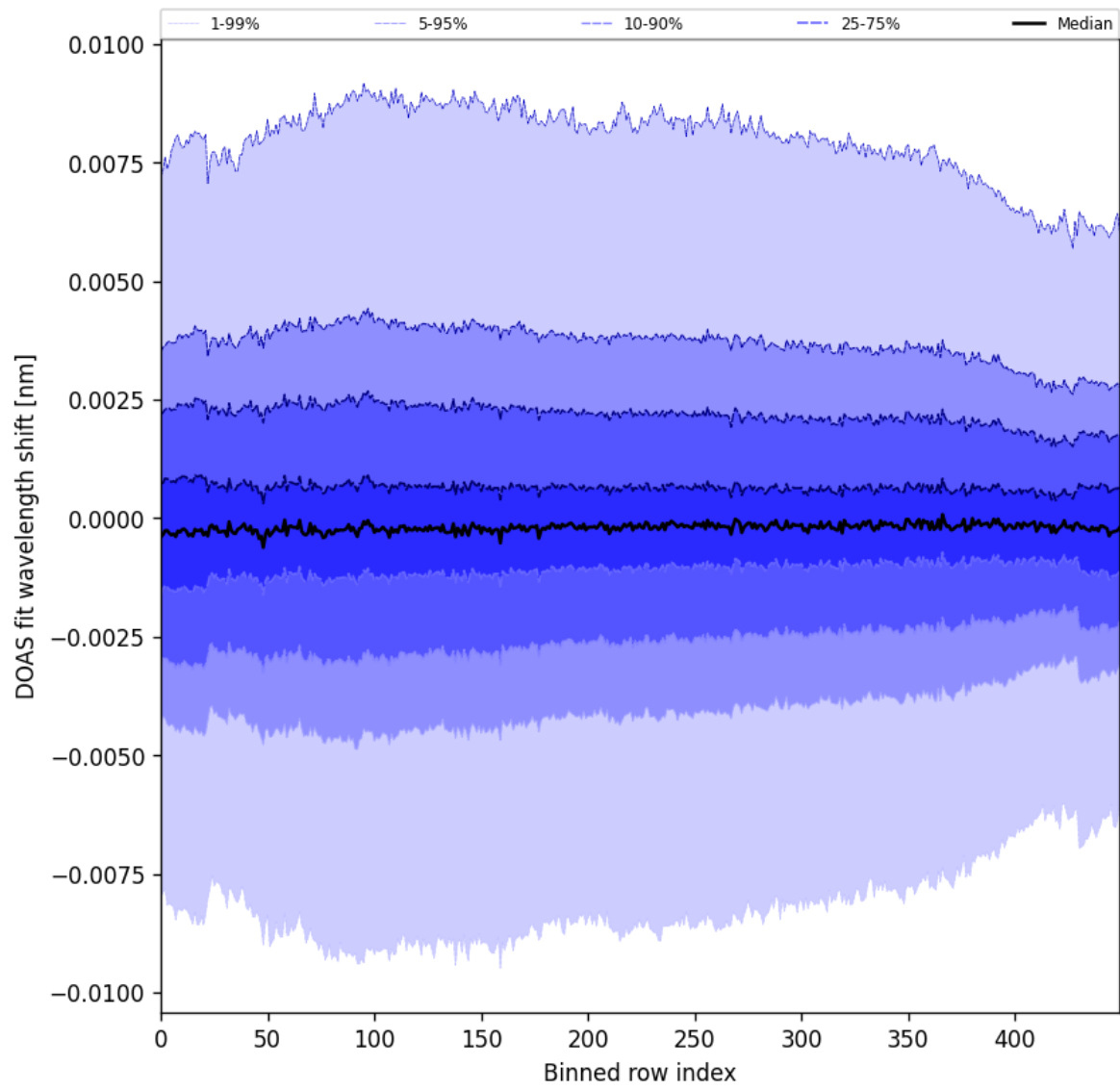
Figure 102: Along track statistics of “DOAS fit wavelength shift” for 2025-05-22 to 2025-05-24
