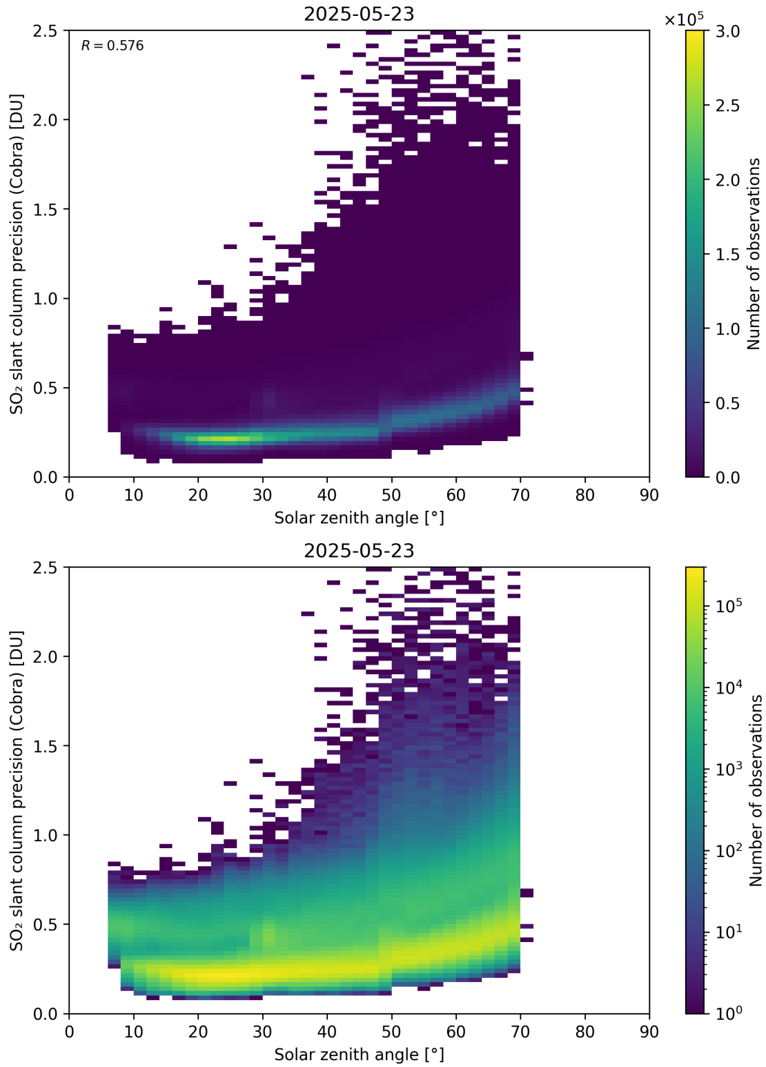
Figure 180: Scatter density plot of “Solar zenith angle” against “SO 2 slant column precision (Cobra)” for 2025-05-22 to 2025-05-24.
