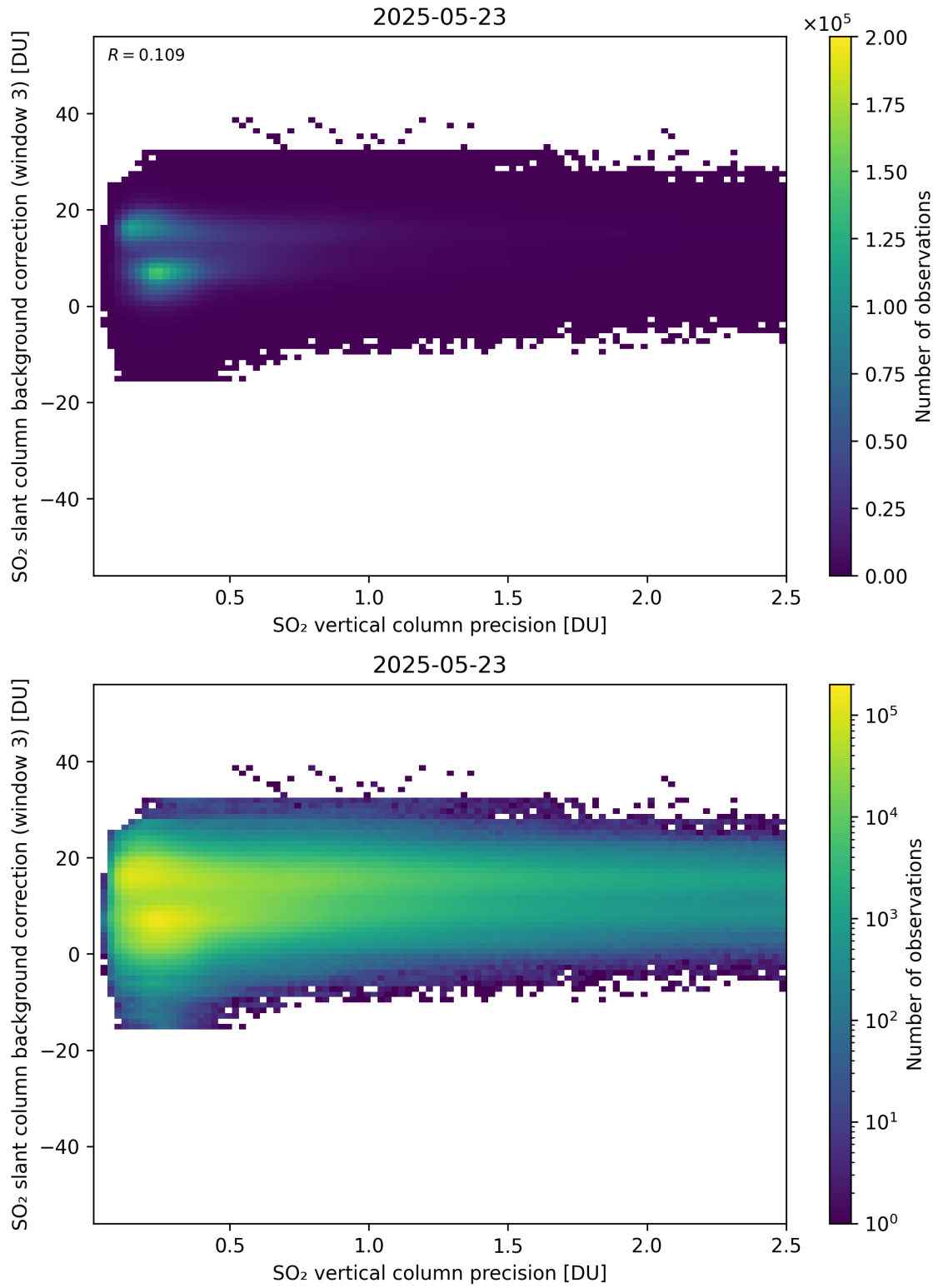
Figure 331: Scatter density plot of “SO 2 vertical column precision” against “SO 2 slant column background correction (window 3)” for 2025-05-22 to 2025-05-24.
