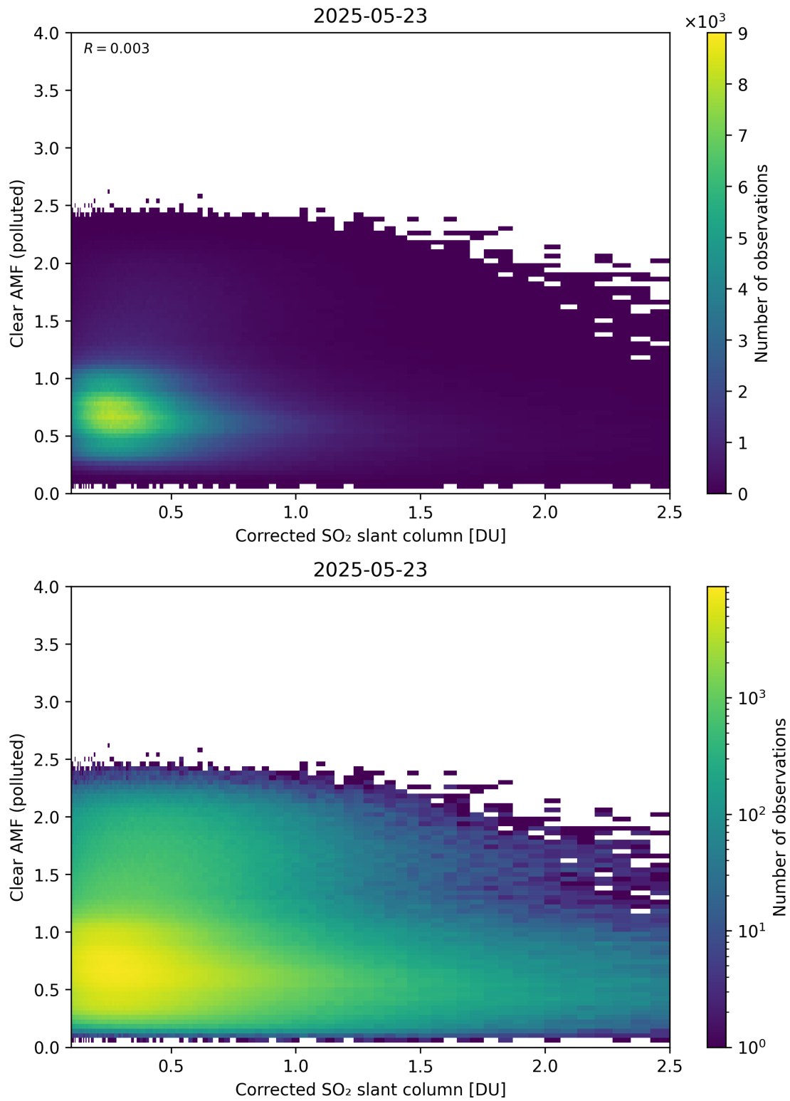
Figure 232: Scatter density plot of “Corrected SO 2 slant column” against “Clear AMF (polluted)” for 2025-05-22 to 2025-05-24.
