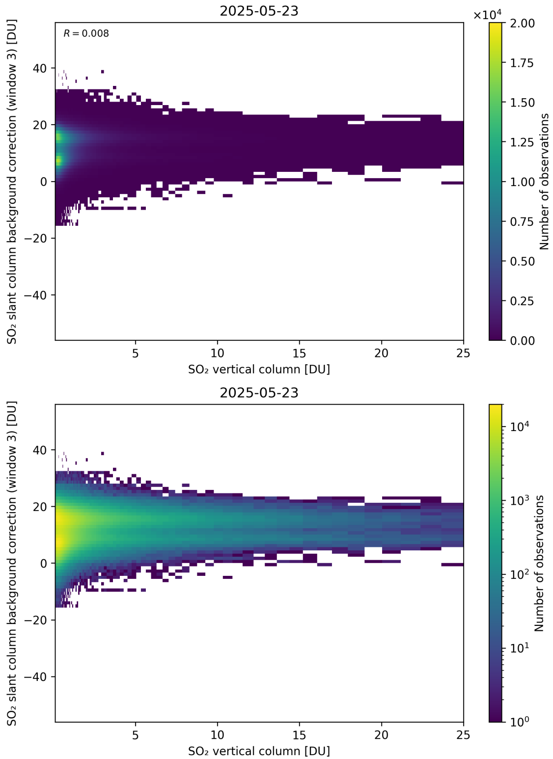
Figure 325: Scatter density plot of “SO 2 vertical column” against “SO 2 slant column background correction (window 3)” for 2025-05-22 to 2025-05-24.
