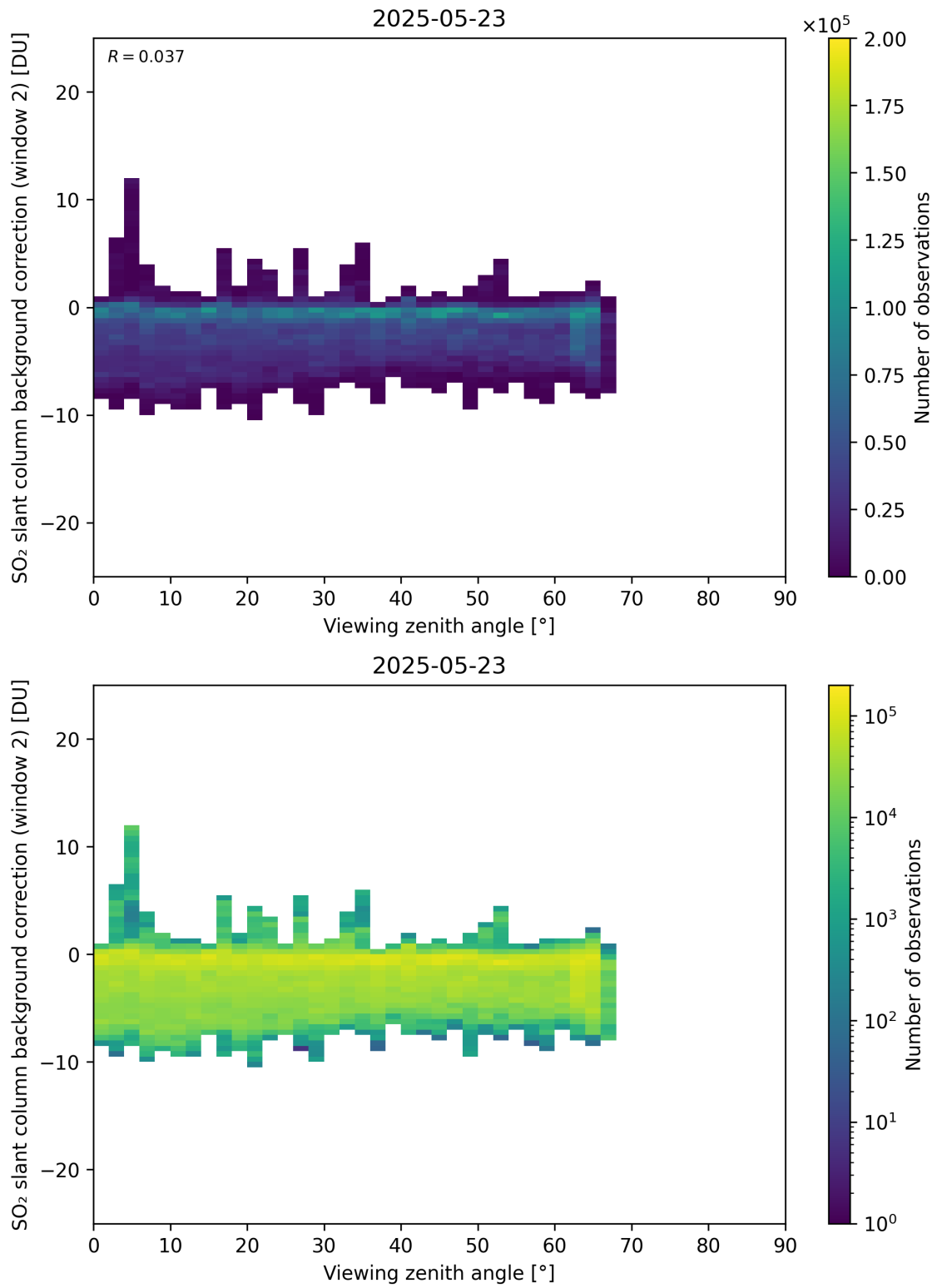
Figure 363: Scatter density plot of “Viewing zenith angle” against “SO 2 slant column background correction (window 2)” for 2025-05-22 to 2025-05-24.
