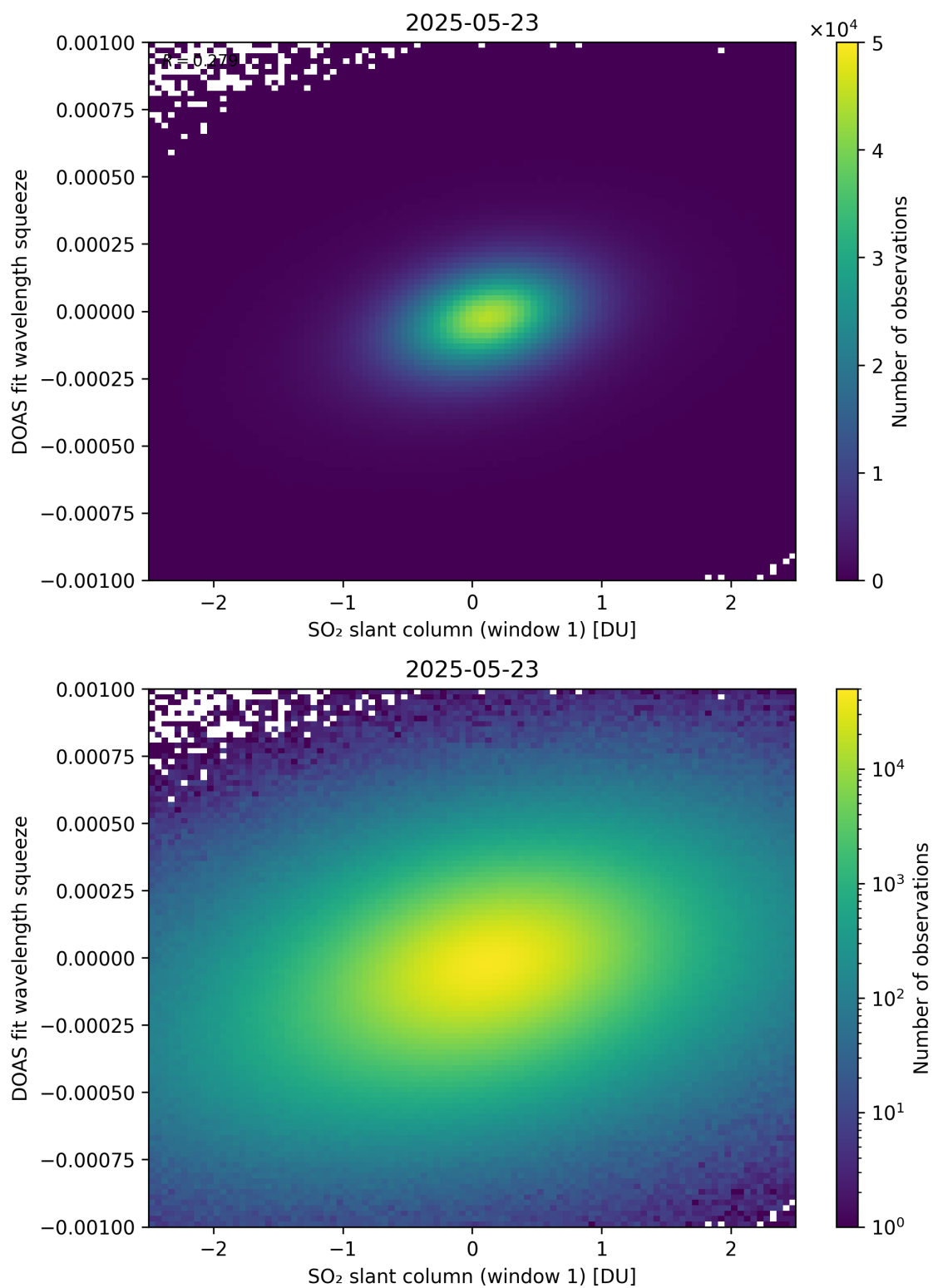
Figure 266: Scatter density plot of “SO 2 slant column (window 1)” against “DOAS fit wavelength squeeze” for 2025-05-22 to 2025-05-24.
