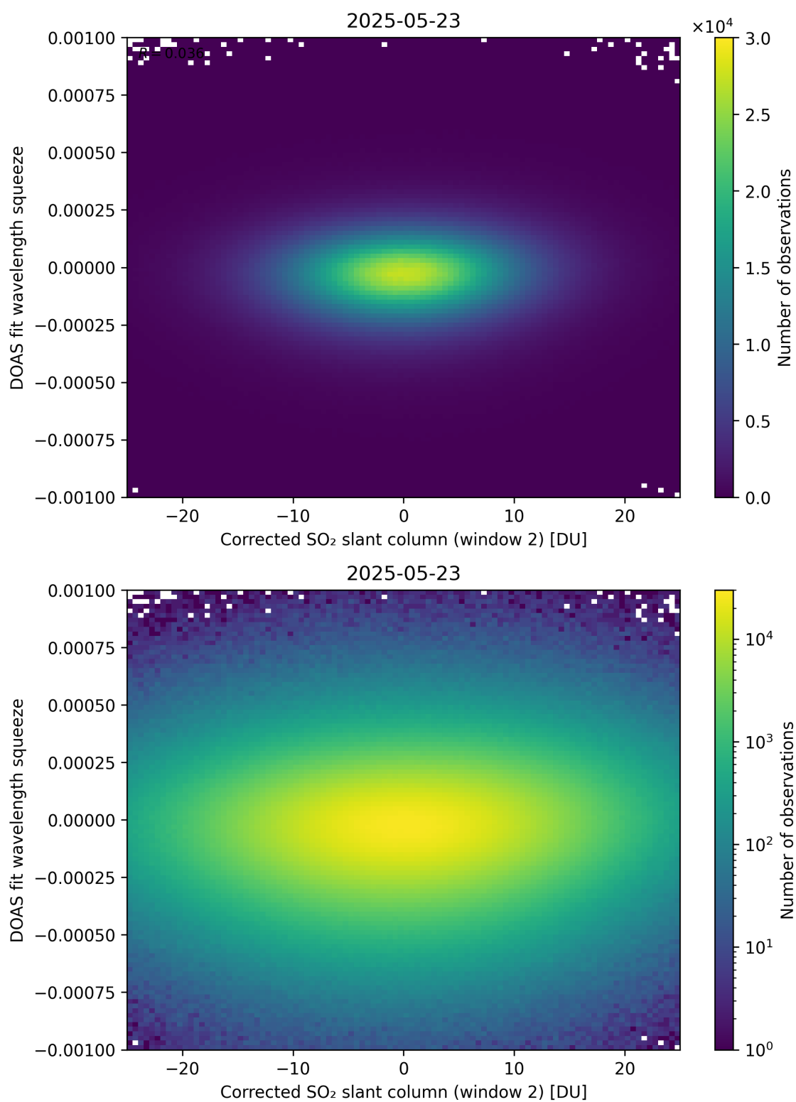
Figure 247: Scatter density plot of “Corrected SO 2 slant column (window 2)” against “DOAS fit wavelength squeeze” for 2025-05-22 to 2025-05-24.
