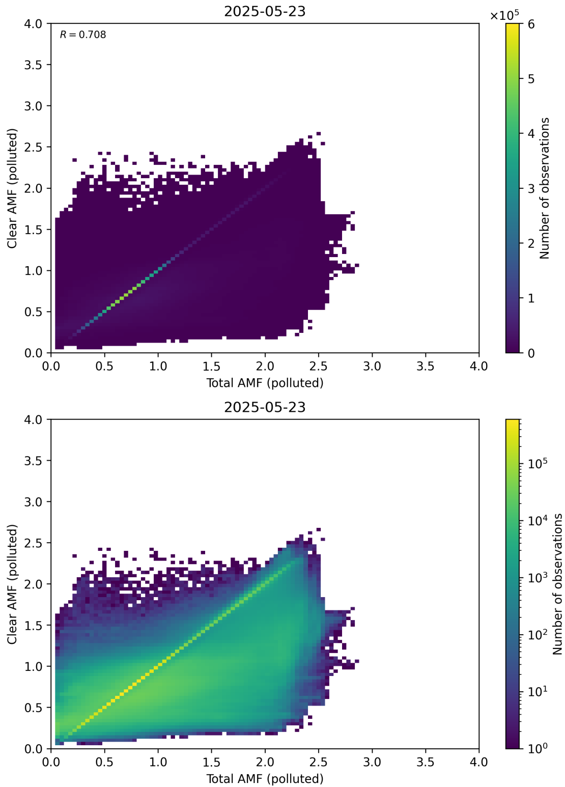
Figure 321: Scatter density plot of “Total AMF (polluted)” against “Clear AMF (polluted)” for 2025-05-22 to 2025-05-24.
