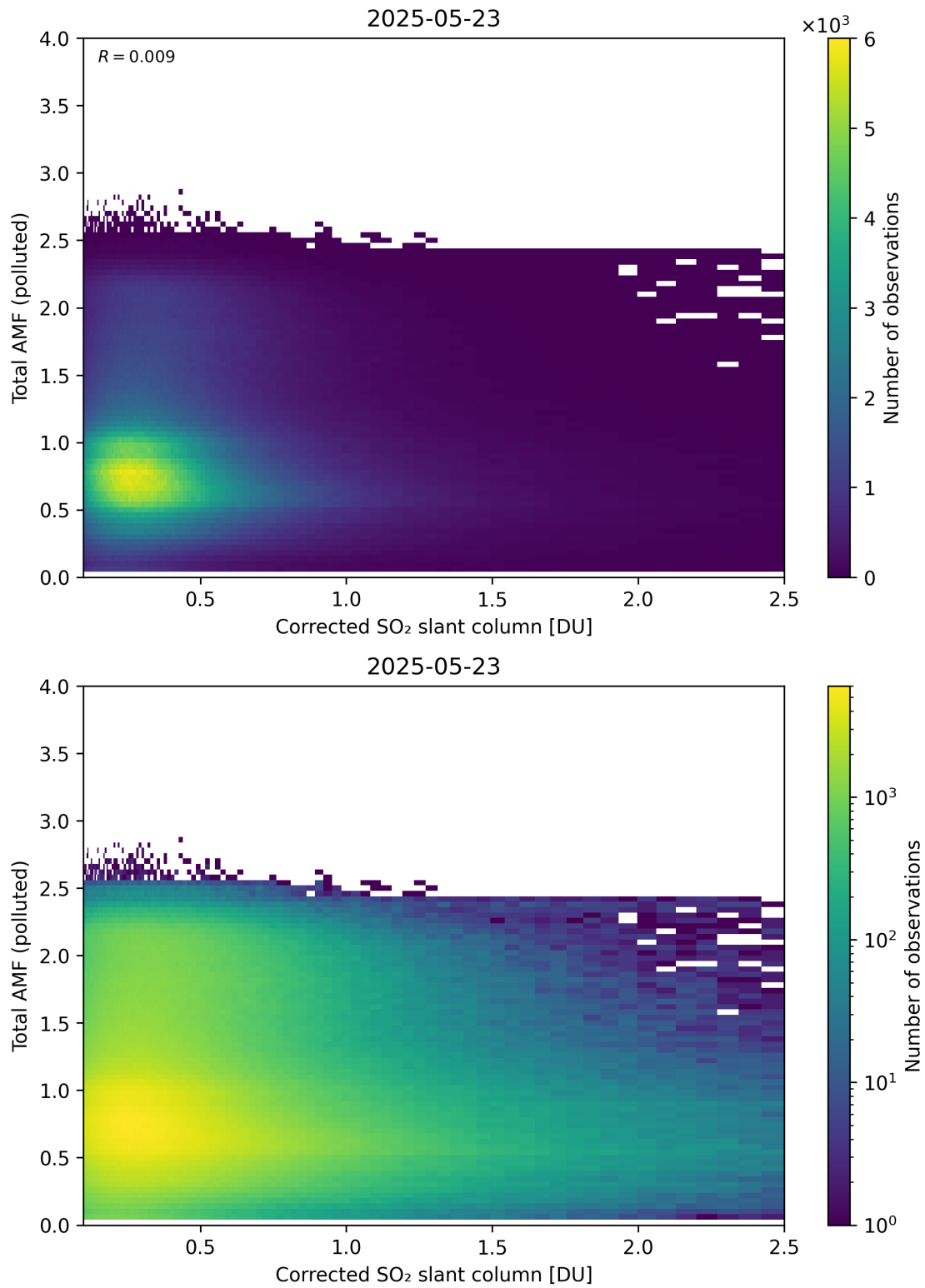
Figure 242: Scatter density plot of “Corrected SO 2 slant column” against “Total AMF (polluted)” for 2025-05-22 to 2025-05-24.
