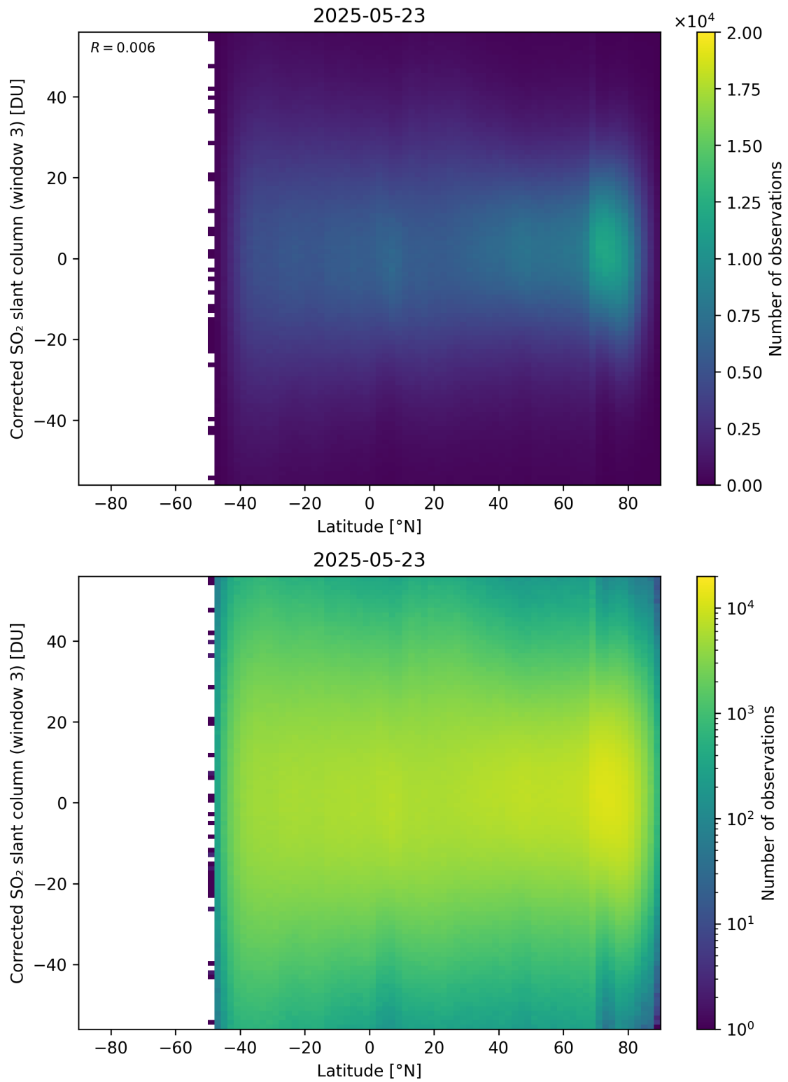
Figure 161: Scatter density plot of “Latitude” against “Corrected SO 2 slant column (window 3)” for 2025-05-22 to 2025-05-24.
