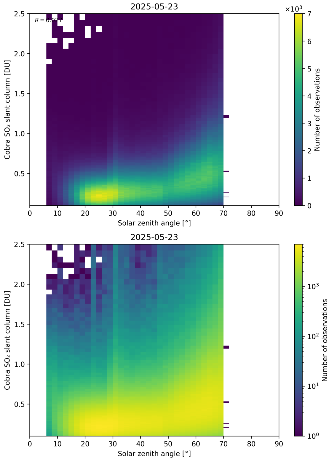
Figure 179: Scatter density plot of “Solar zenith angle” against “Cobra SO 2 slant column” for 2025-05-22 to 2025-05-24.
