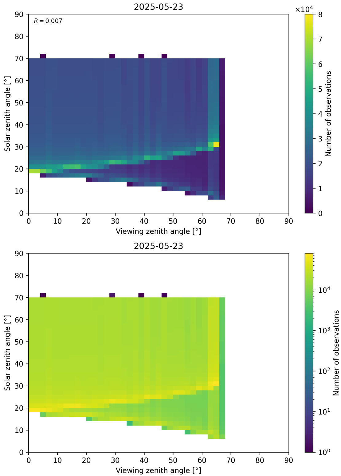
Figure 369: Scatter density plot of “Viewing zenith angle” against “Solar zenith angle” for 2025-05-22 to 2025-05-24.
