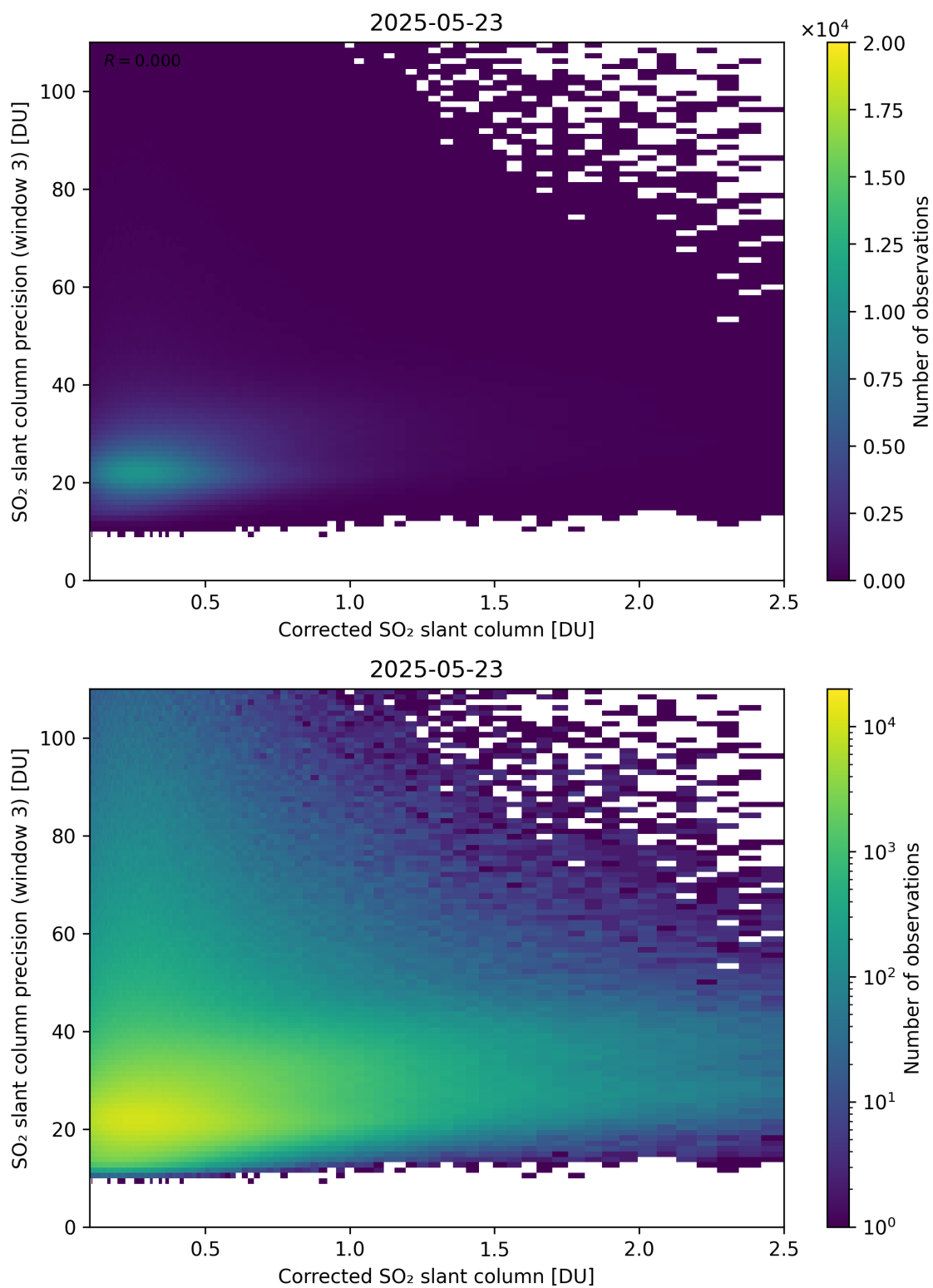
Figure 241: Scatter density plot of “Corrected SO 2 slant column” against “SO 2 slant column precision (window 3)” for 2025-05-22 to 2025-05-24.
