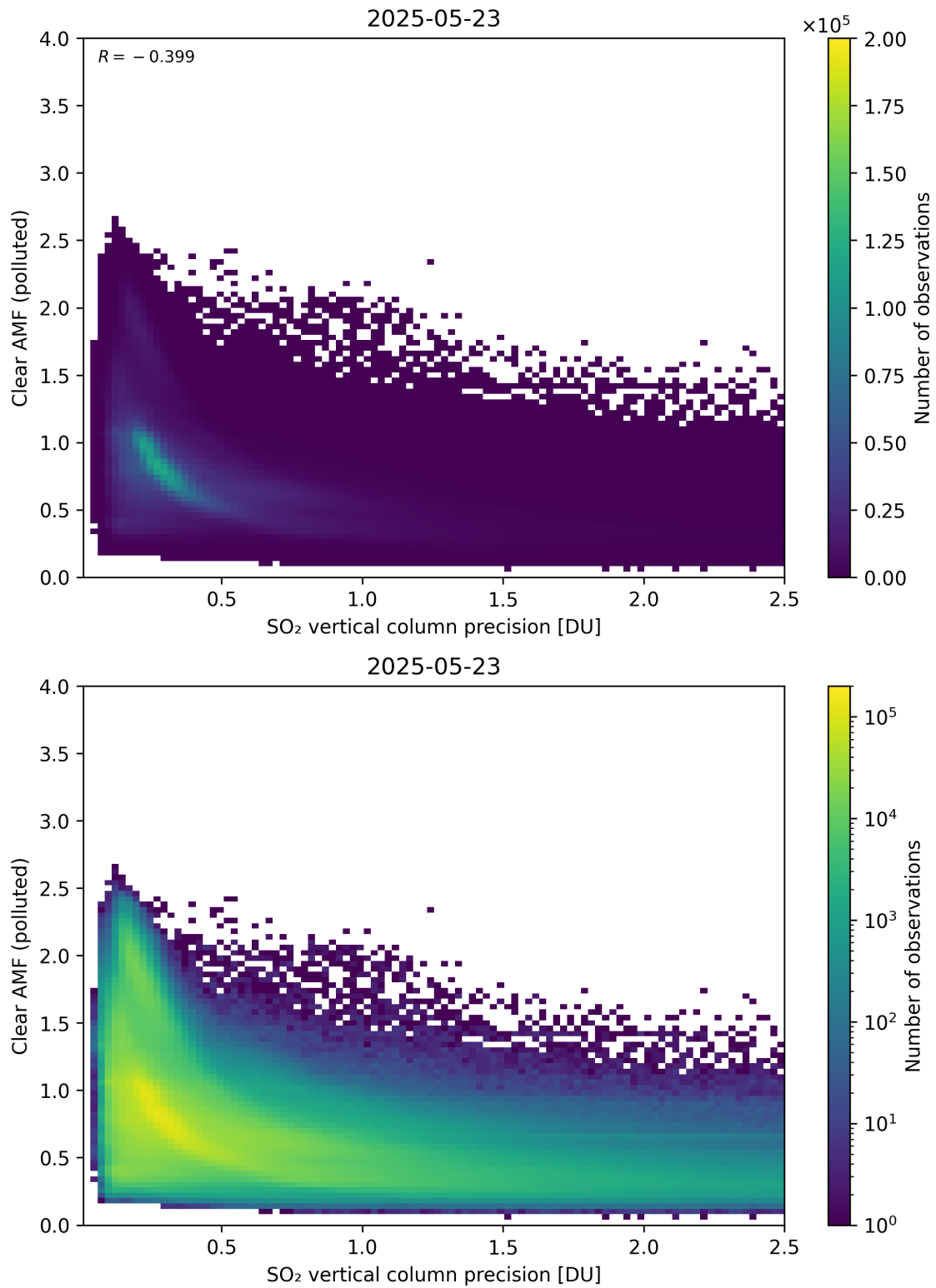
Figure 335: Scatter density plot of “SO 2 vertical column precision” against “Clear AMF (polluted)” for 2025-05-22 to 2025-05-24.
