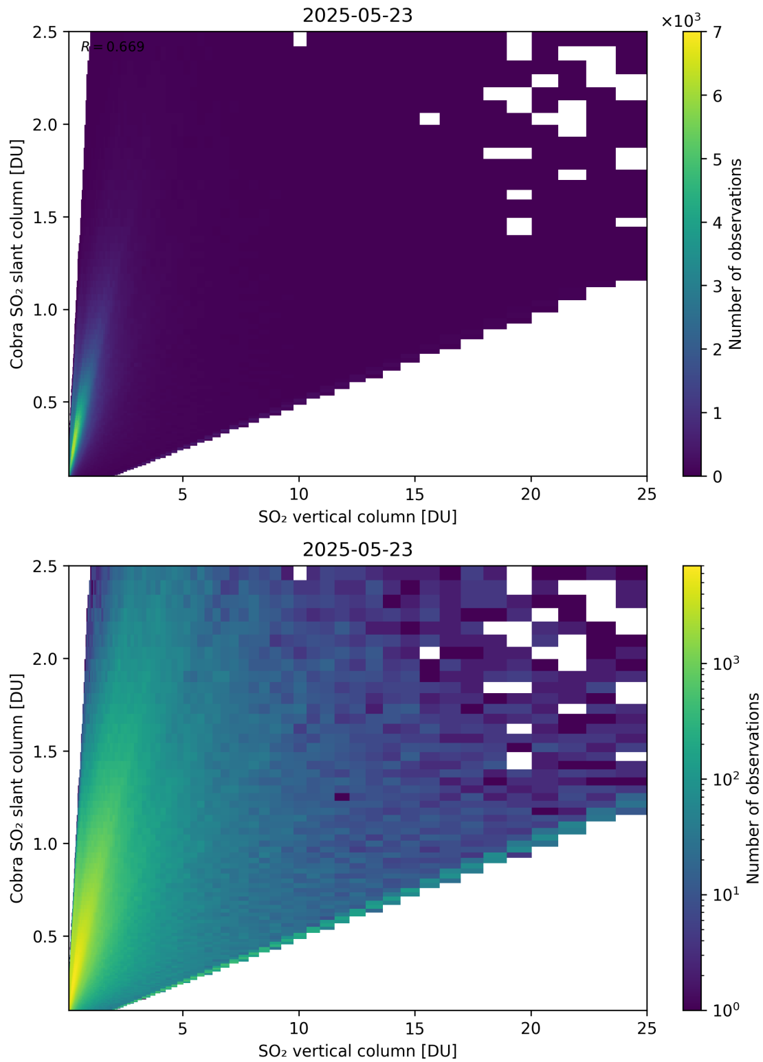
Figure 349: Scatter density plot of “SO 2 vertical column” against “Cobra SO 2 slant column” for 2025-05-22 to 2025-05-24.
