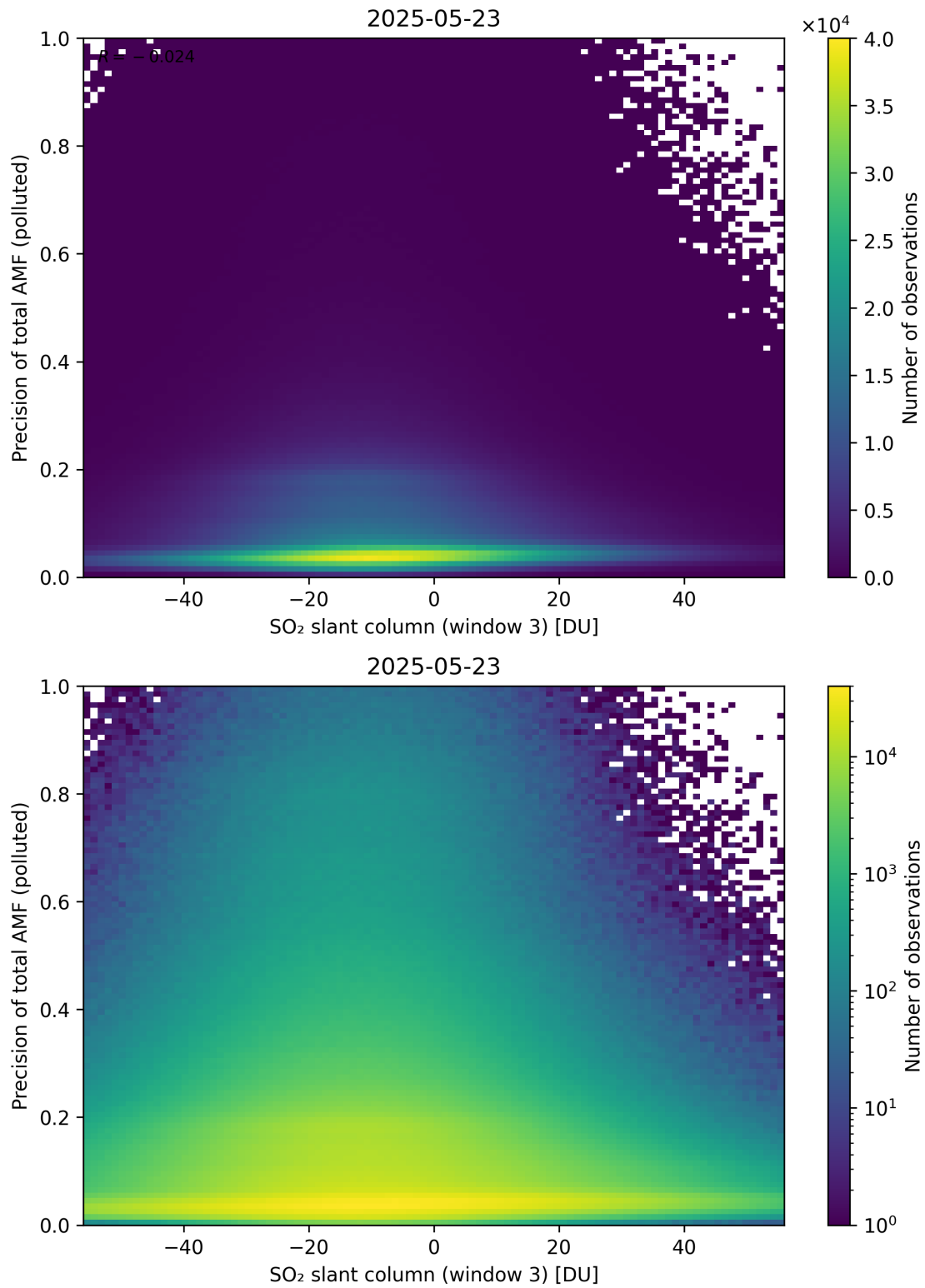
Figure 319: Scatter density plot of “SO 2 slant column (window 3)” against “Precision of total AMF (polluted)” for 2025-05-22 to 2025-05-24.
