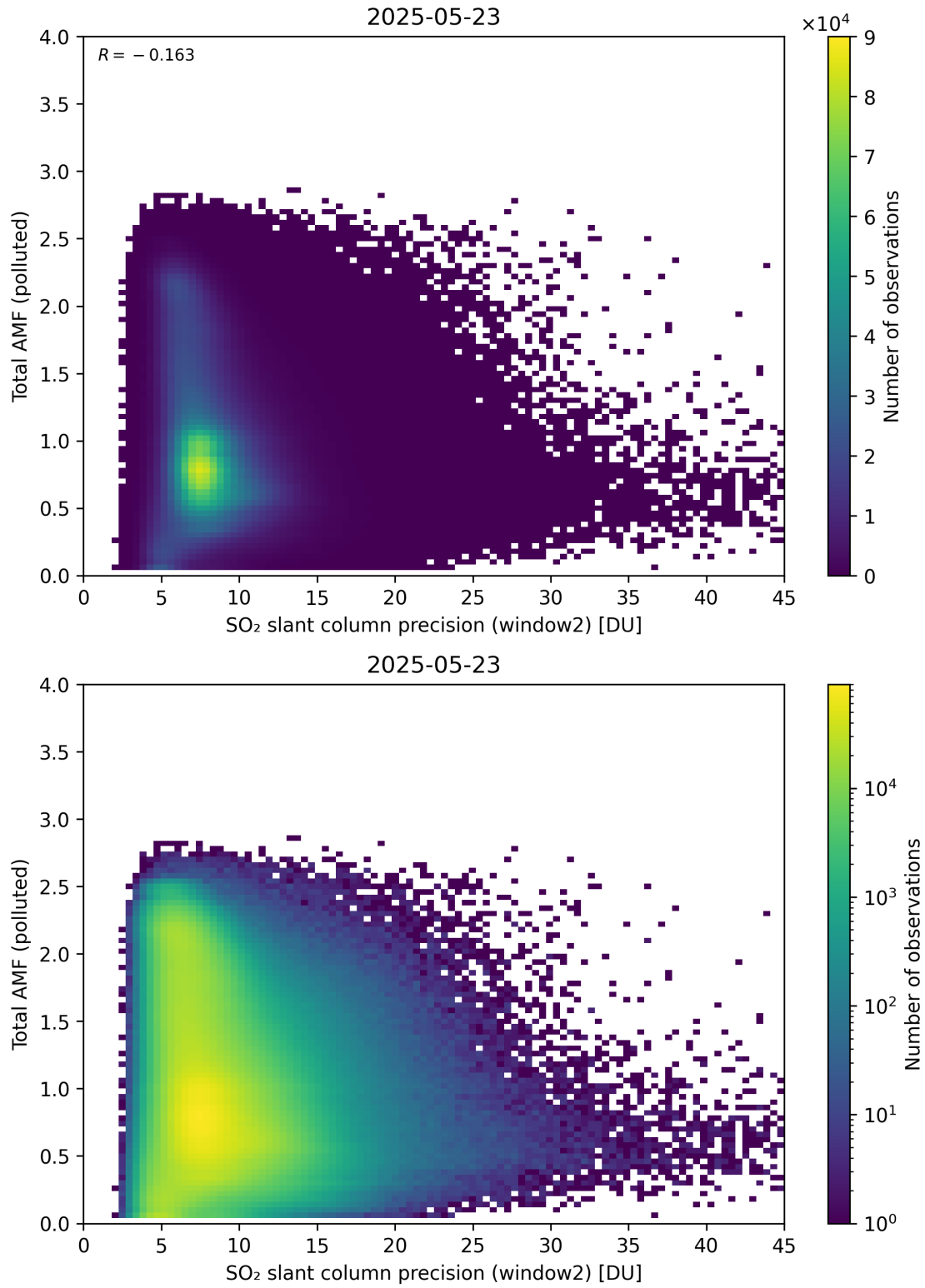
Figure 301: Scatter density plot of “SO 2 slant column precision (window2)” against “Total AMF (polluted)” for 2025-05-22 to 2025-05-24.
