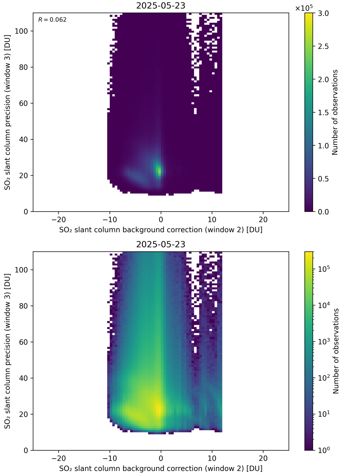
Figure 129: Scatter density plot of “SO 2 slant column background correction (window 2)” against “SO 2 slant column precision (window 3)” for 2025-05-22 to 2025-05-24.
