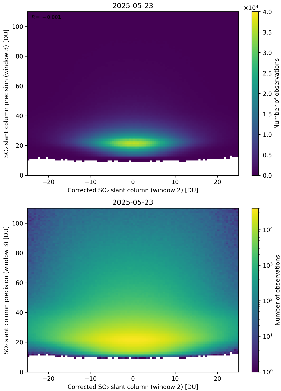
Figure 252: Scatter density plot of “Corrected SO 2 slant column (window 2)” against “SO 2 slant column precision (window 3)” for 2025-05-22 to 2025-05-24.
