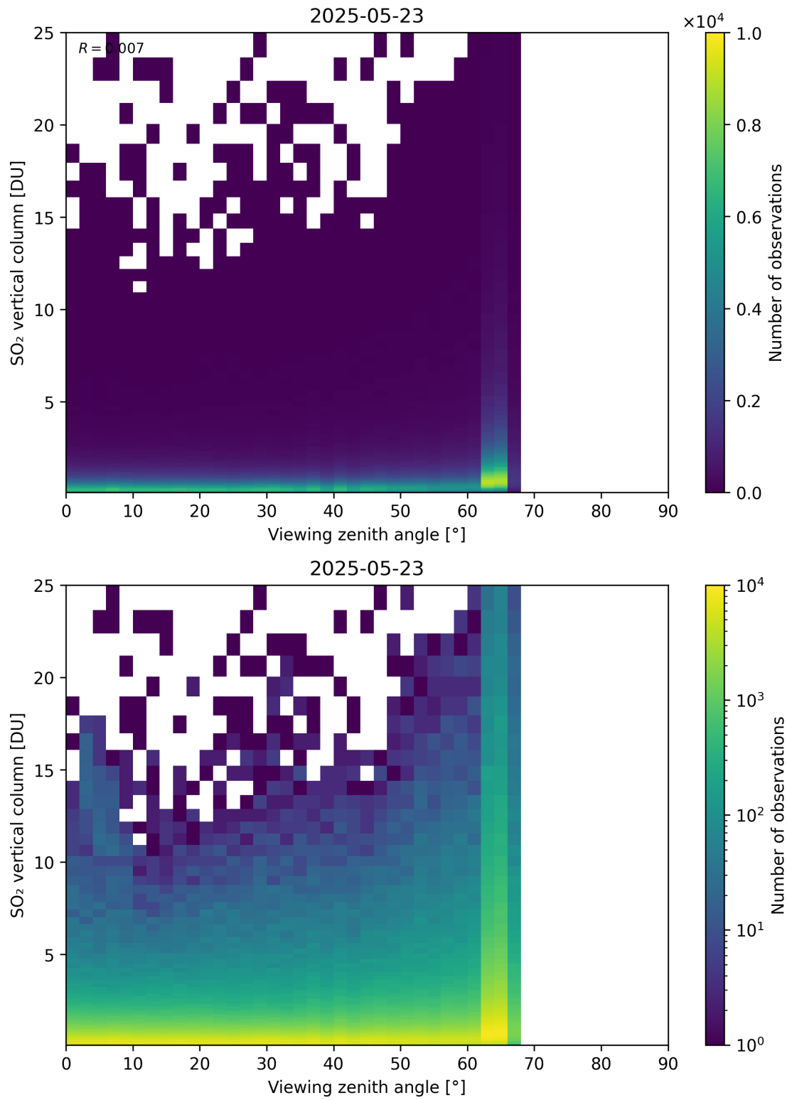
Figure 383: Scatter density plot of “Viewing zenith angle” against “SO 2 vertical column” for 2025-05-22 to 2025-05-24.
