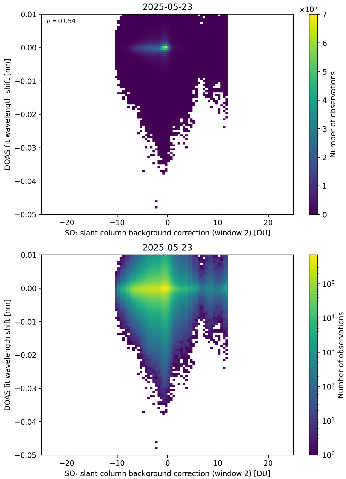
Figure 123: Scatter density plot of “SO 2 slant column background correction (window 2)” against “DOAS fit wavelength shift” for 2025-05-22 to 2025-05-24.
