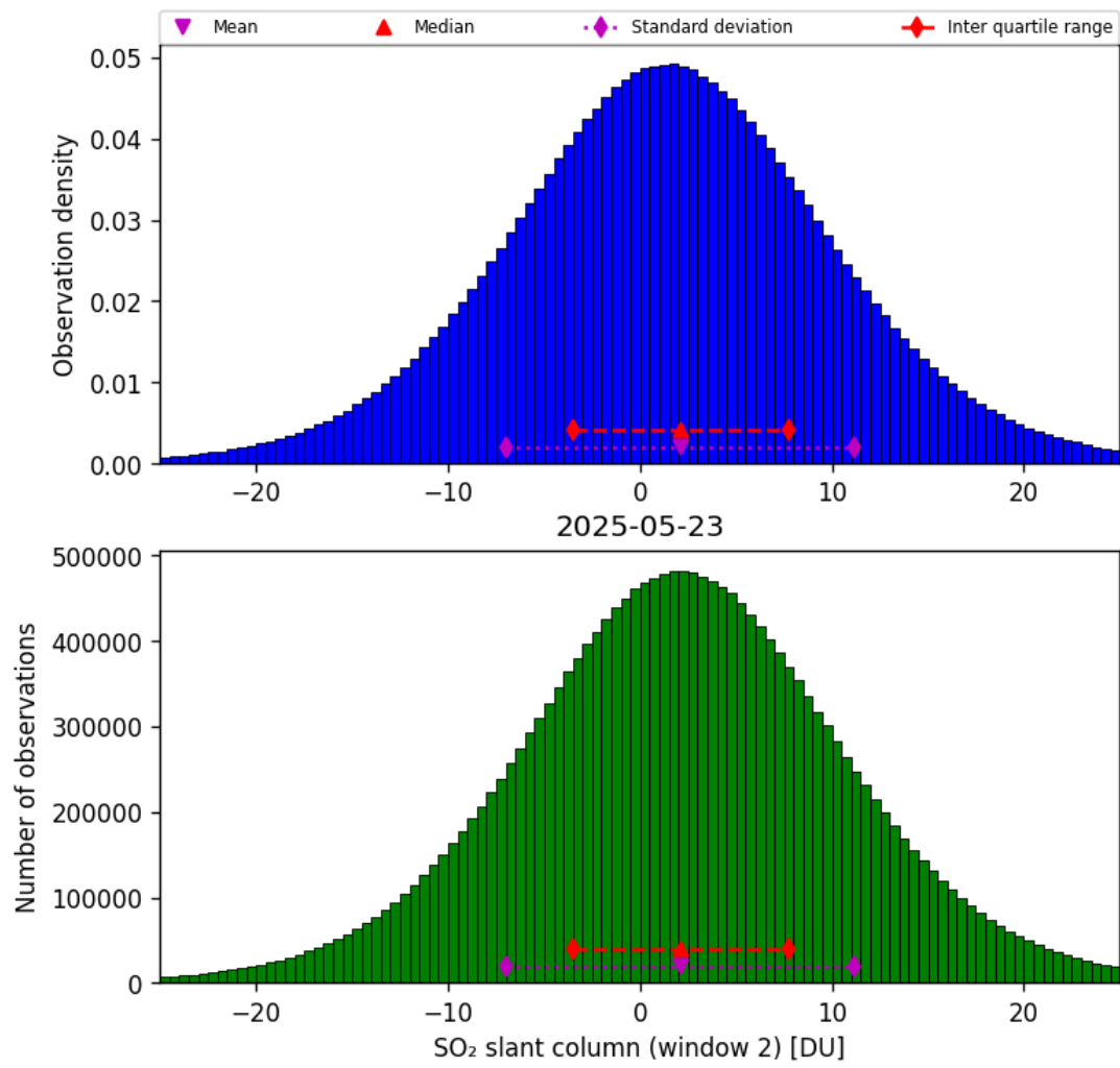
Figure 67: Histogram of “SO 2 slant column (window 2)” for 2025-05-22 to 2025-05-24
