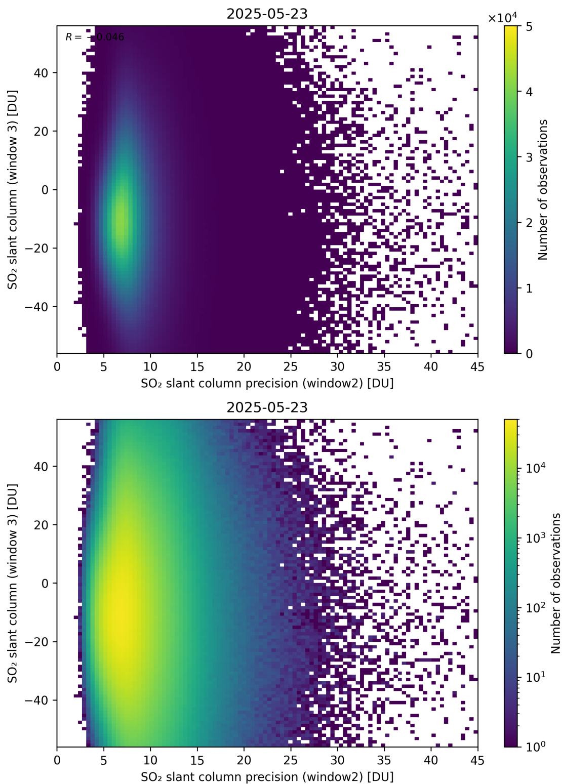
Figure 299: Scatter density plot of “SO 2 slant column precision (window2)” against “SO 2 slant column (window 3)” for 2025-05-22 to 2025-05-24.
