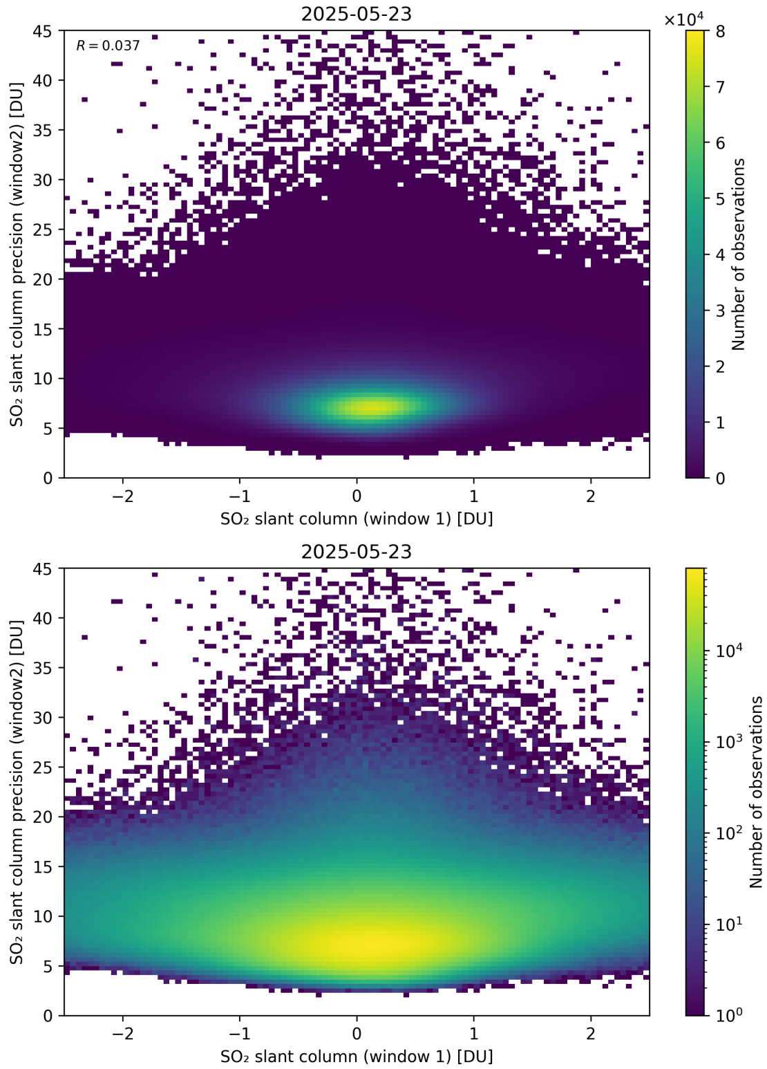
Figure 286: Scatter density plot of “SO 2 slant column (window 1)” against “SO 2 slant column precision (window2)” for 2025-05-22 to 2025-05-24.
