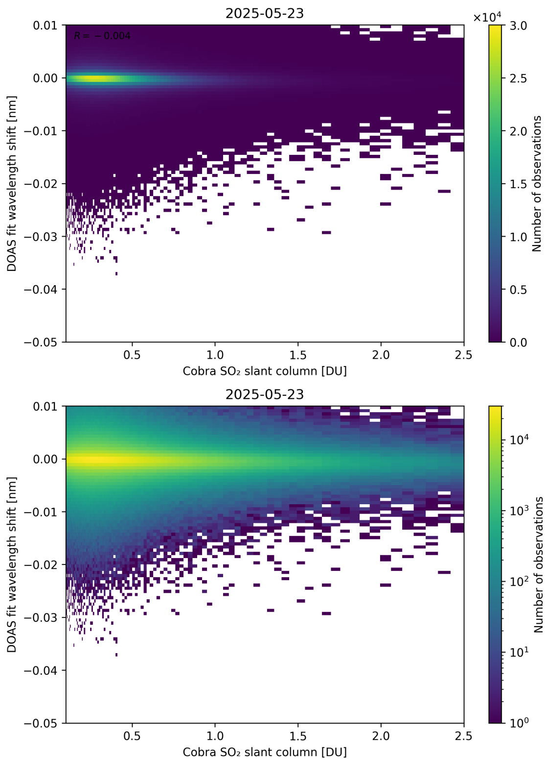
Figure 196: Scatter density plot of “Cobra SO 2 slant column” against “DOAS fit wavelength shift” for 2025-05-22 to 2025-05-24.
