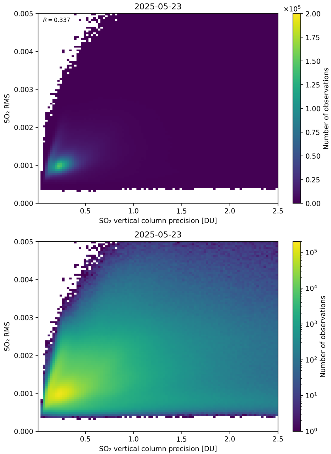
Figure 334: Scatter density plot of “SO 2 vertical column precision” against “SO 2 RMS” for 2025-05-22 to 2025-05-24.
