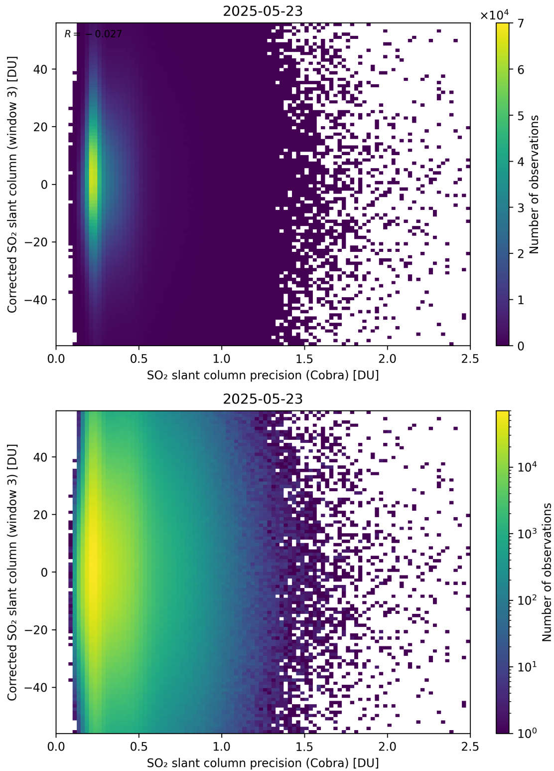
Figure 207: Scatter density plot of “SO 2 slant column precision (Cobra)” against “Corrected SO 2 slant column (window 3)” for 2025-05-22 to 2025-05-24.
