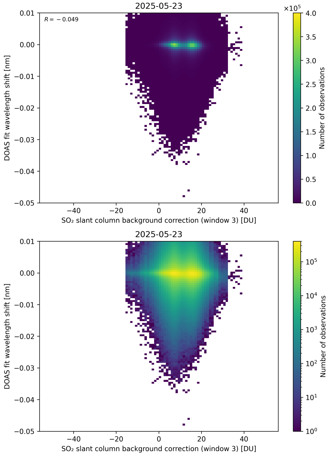
Figure 132: Scatter density plot of “SO 2 slant column background correction (window 3)” against “DOAS fit wavelength shift” for 2025-05-22 to 2025-05-24.
