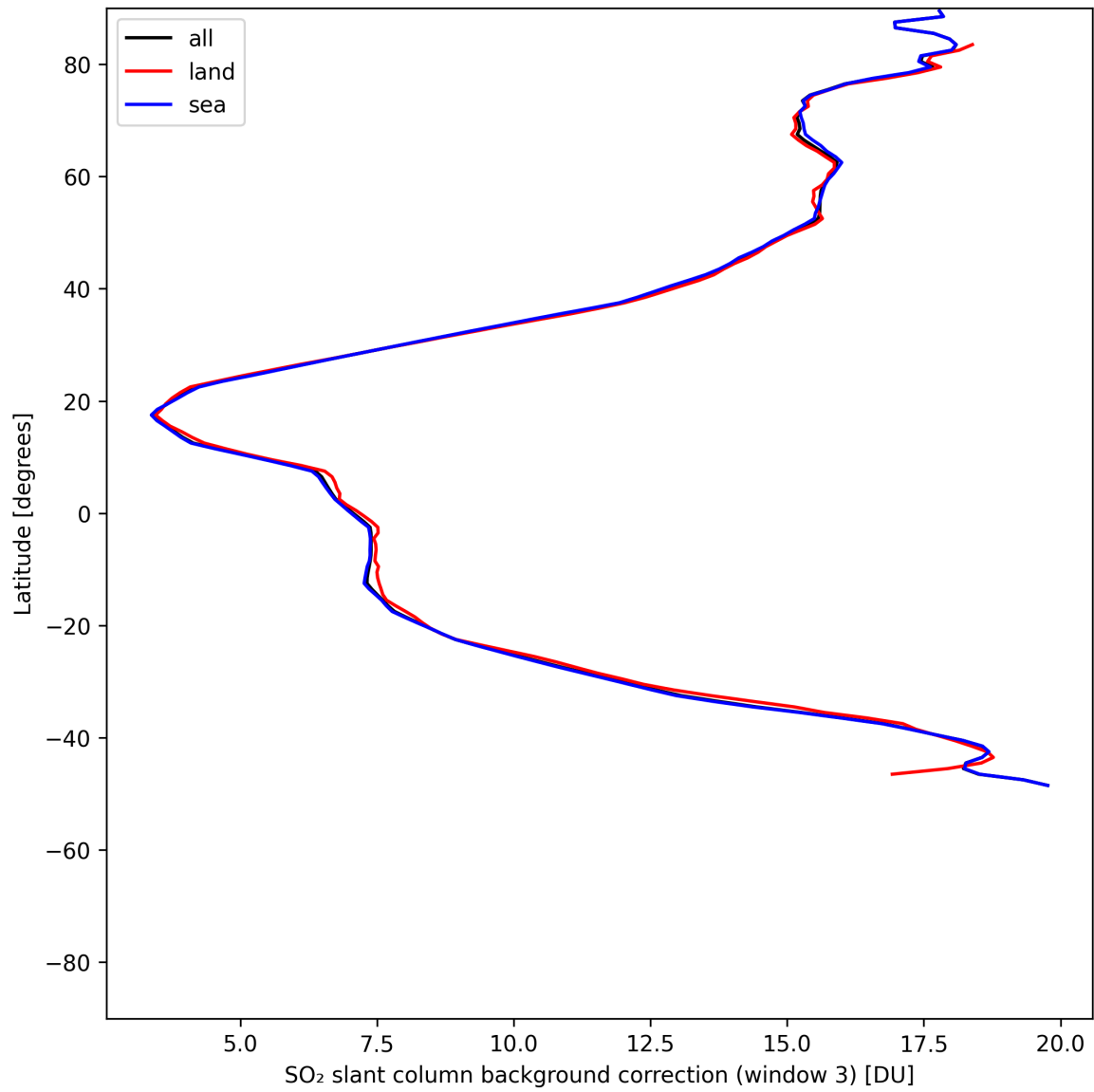
Figure 48: Zonal average of “SO 2 slant column background correction (window 3)” for 2025-05-22 to 2025-05-24.
