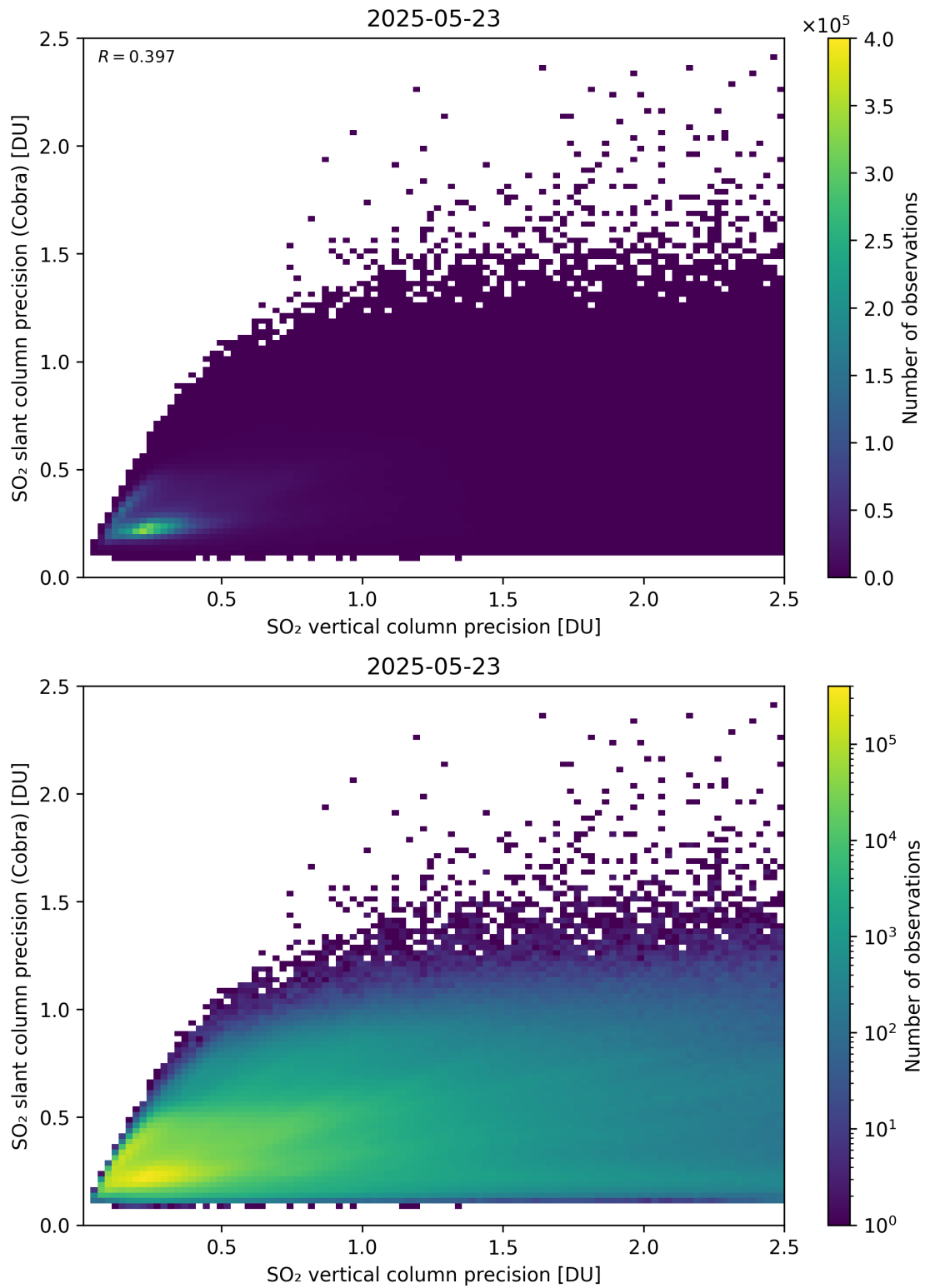
Figure 337: Scatter density plot of “SO 2 vertical column precision” against “SO 2 slant column precision (Cobra)” for 2025-05-22 to 2025-05-24.
