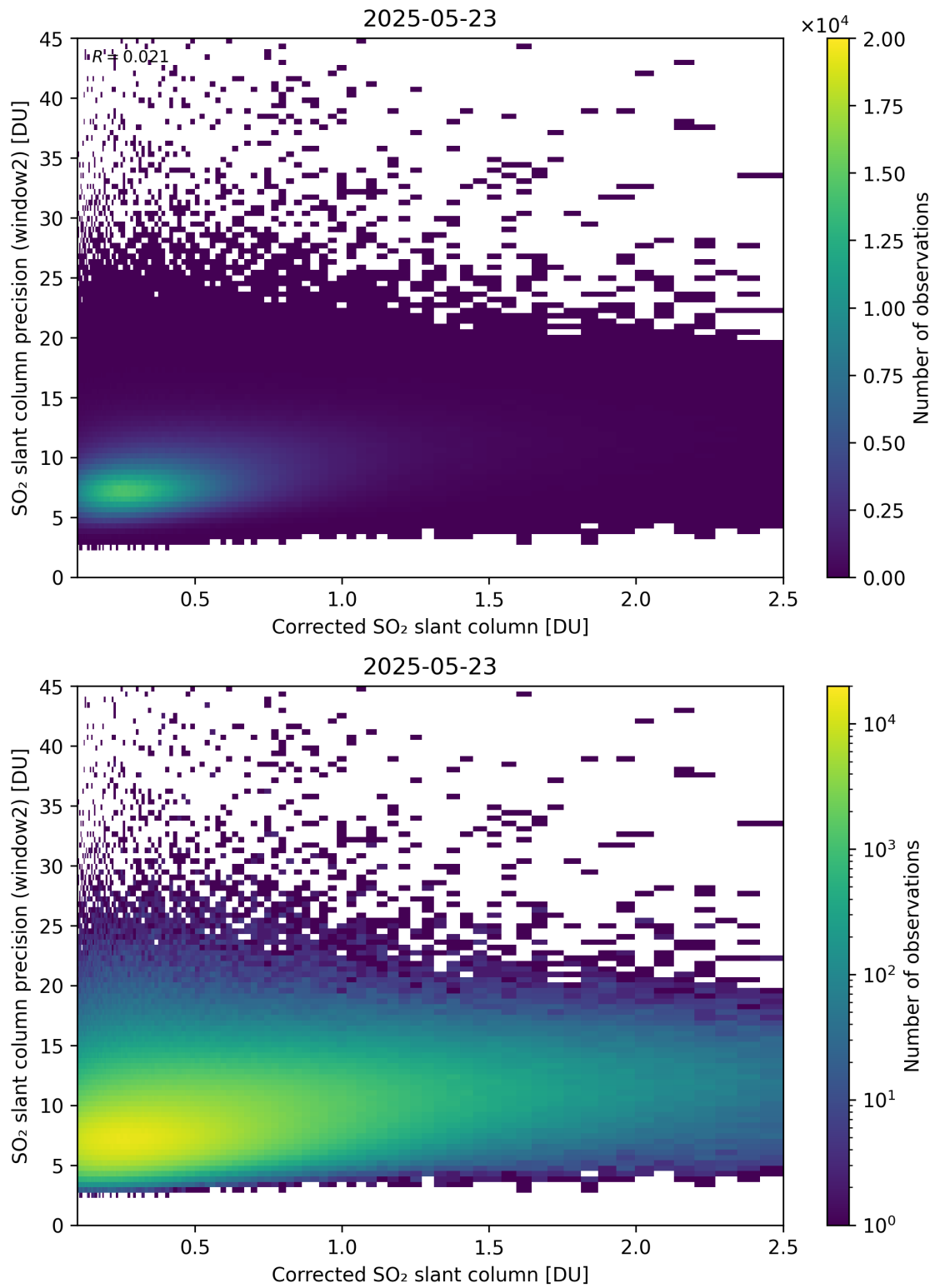
Figure 239: Scatter density plot of “Corrected SO 2 slant column” against “SO 2 slant column precision (window2)” for 2025-05-22 to 2025-05-24.
