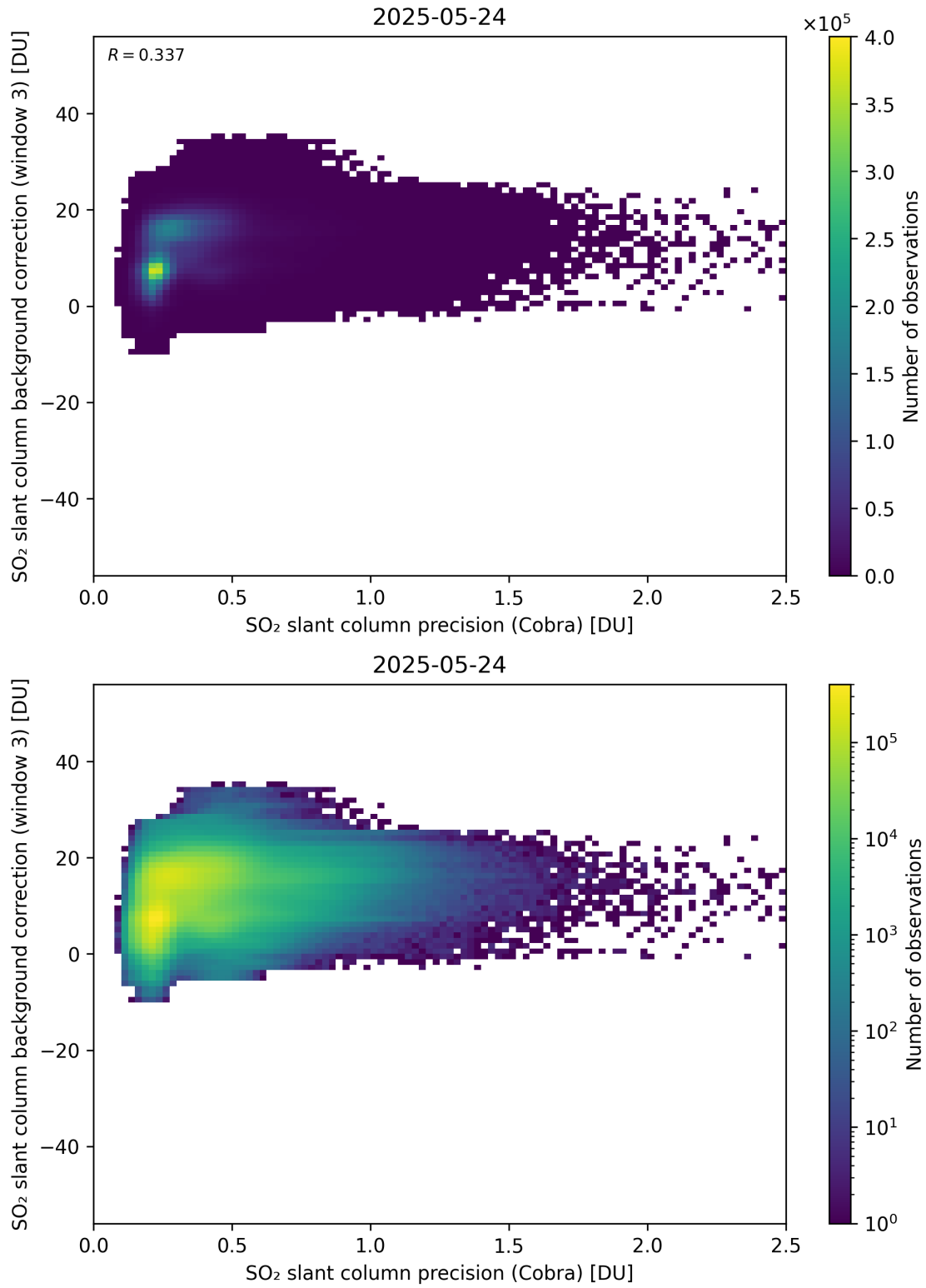
Figure 201: Scatter density plot of “SO 2 slant column precision (Cobra)” against “SO 2 slant column background correction (window 3)” for 2025-05-23 to 2025-05-25.
