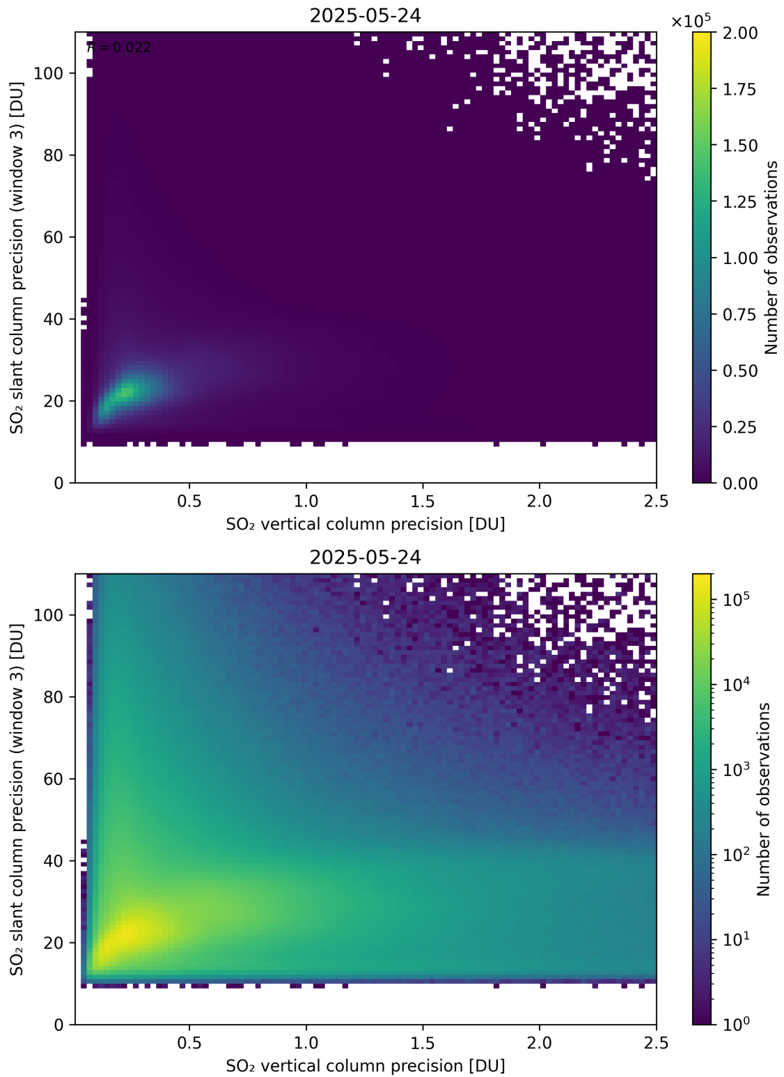
Figure 345: Scatter density plot of “SO 2 vertical column precision” against “SO 2 slant column precision (window 3)” for 2025-05-23 to 2025-05-25.
