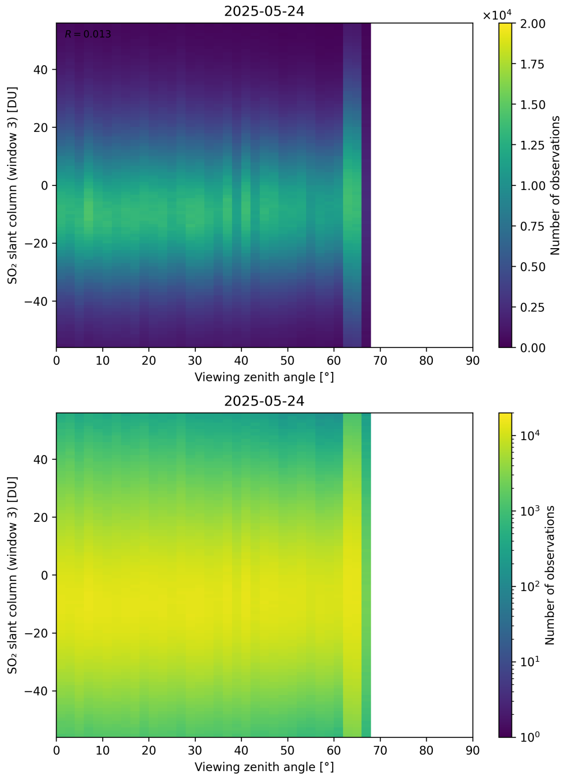
Figure 379: Scatter density plot of “Viewing zenith angle” against “SO 2 slant column (window 3)” for 2025-05-23 to 2025-05-25.
