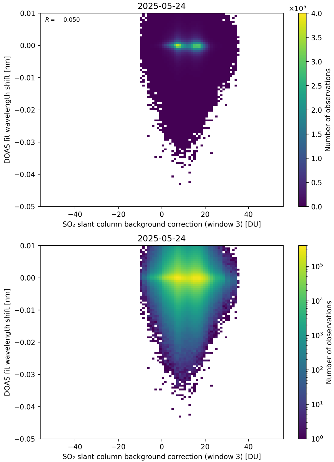
Figure 132: Scatter density plot of “SO 2 slant column background correction (window 3)” against “DOAS fit wavelength shift” for 2025-05-23 to 2025-05-25.
