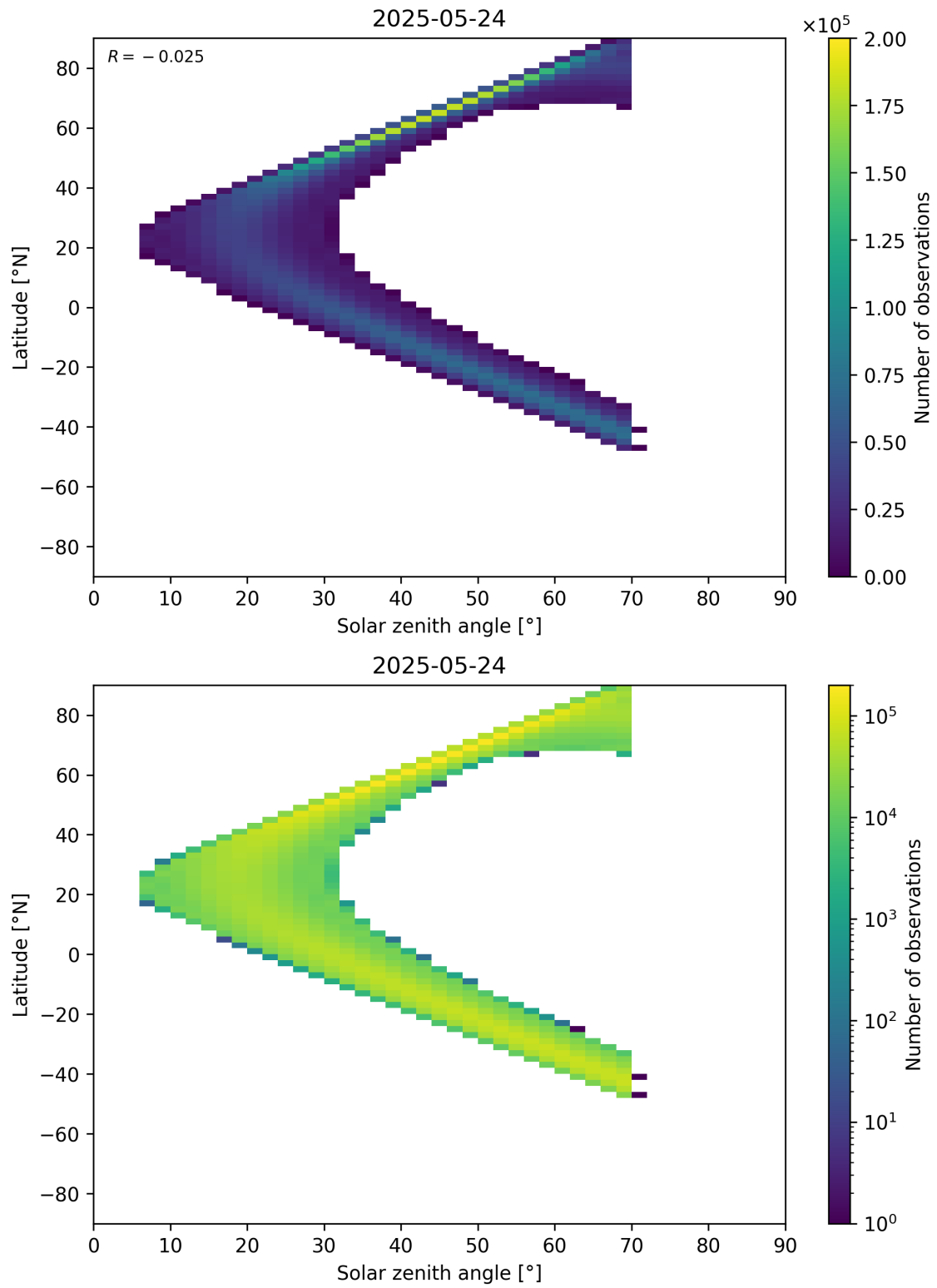
Figure 177: Scatter density plot of “Solar zenith angle” against “Latitude” for 2025-05-23 to 2025-05-25.
