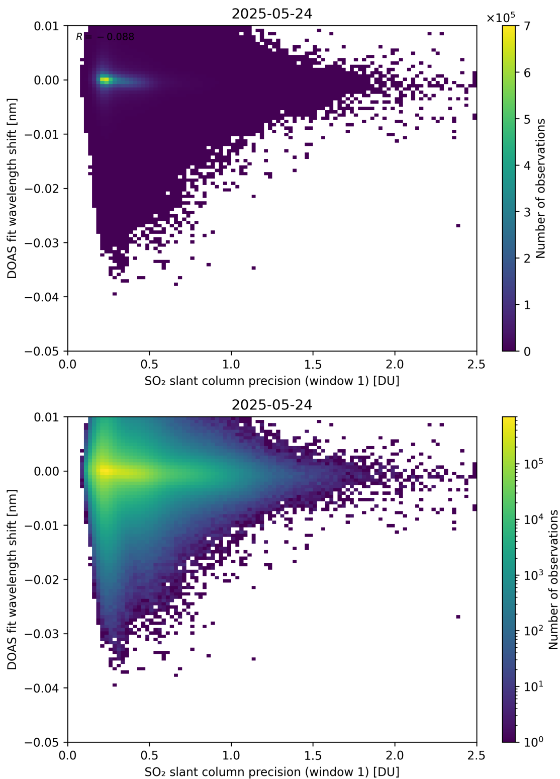
Figure 271: Scatter density plot of “SO 2 slant column precision (window 1)” against “DOAS fit wavelength shift” for 2025-05-23 to 2025-05-25.
