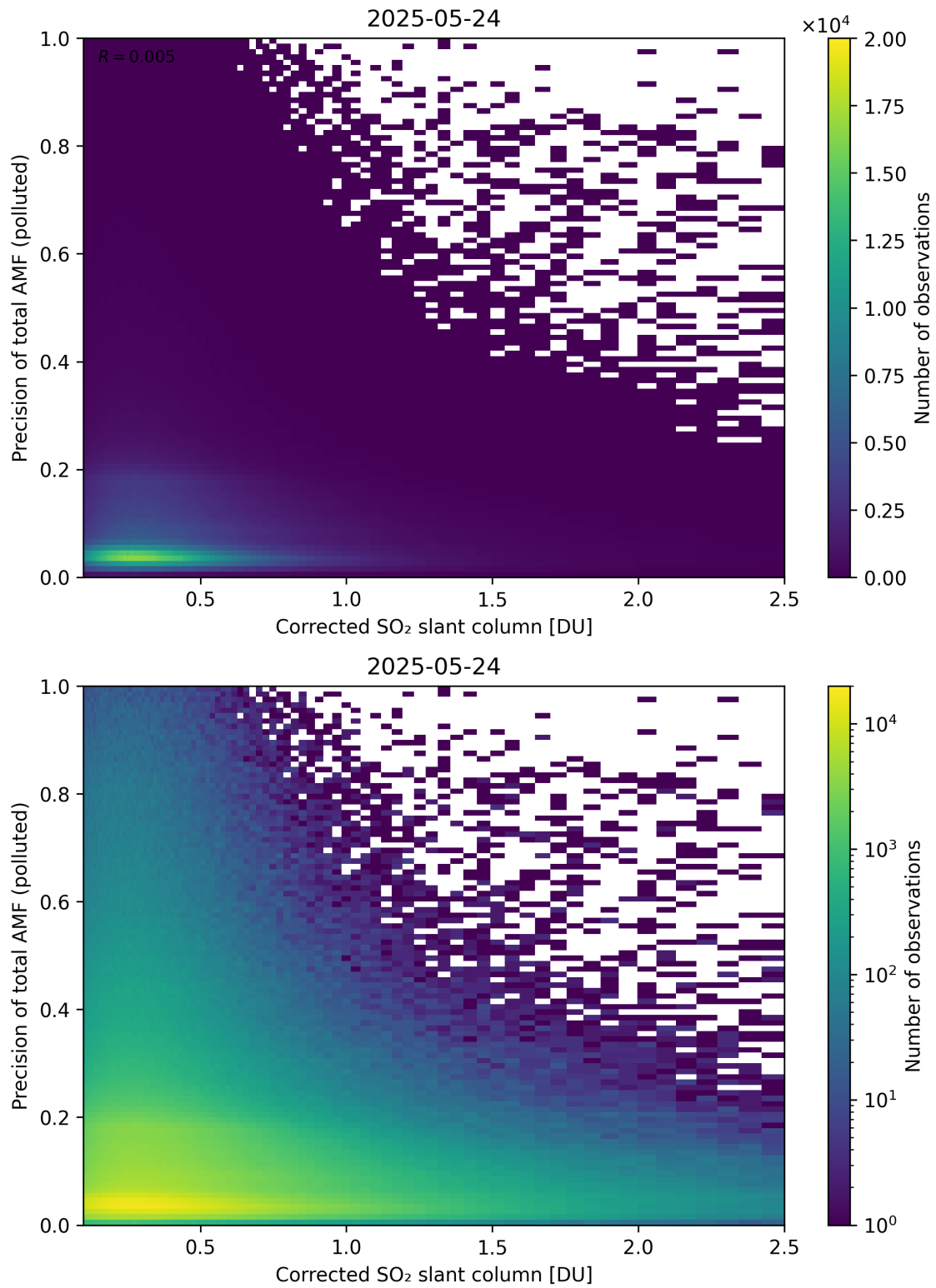
Figure 243: Scatter density plot of “Corrected SO 2 slant column” against “Precision of total AMF (polluted)” for 2025-05-23 to 2025-05-25.
