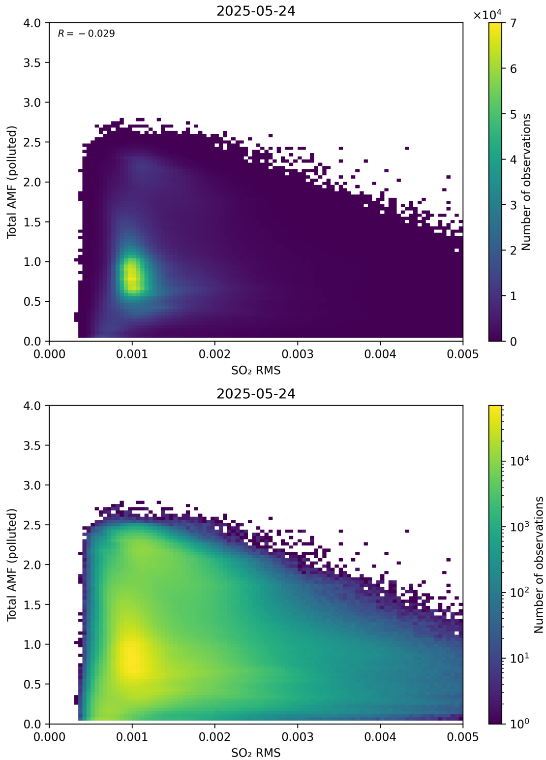
Figure 148: Scatter density plot of “SO 2 RMS” against “Total AMF (polluted)” for 2025-05-23 to 2025-05-25.
