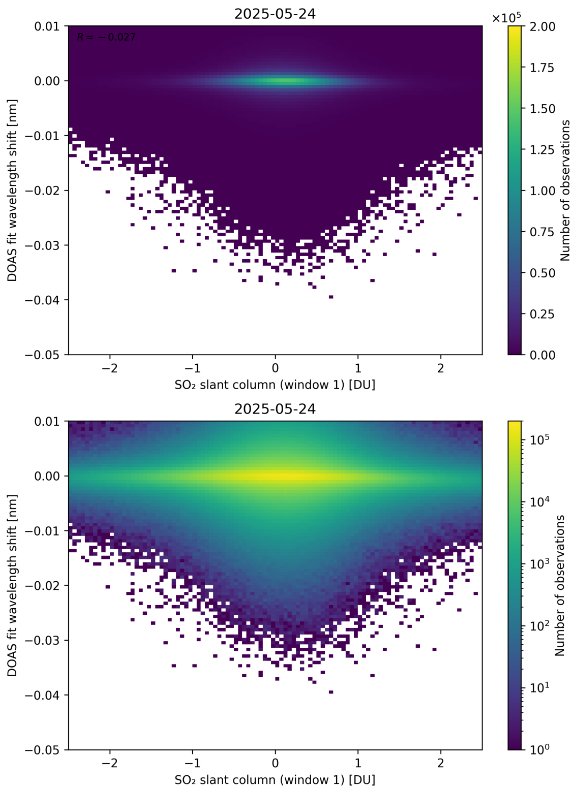
Figure 265: Scatter density plot of “SO 2 slant column (window 1)” against “DOAS fit wavelength shift” for 2025-05-23 to 2025-05-25.
