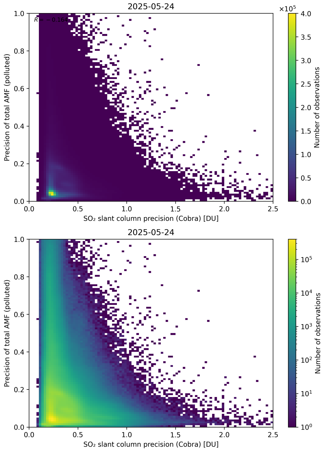
Figure 214: Scatter density plot of “SO 2 slant column precision (Cobra)” against “Precision of total AMF (polluted)” for 2025-05-23 to 2025-05-25.
