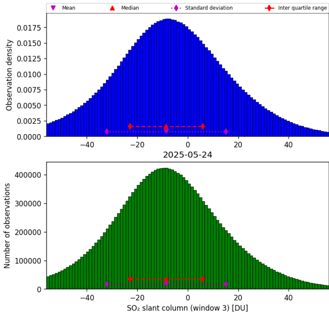
Figure 71: Histogram of “SO 2 slant column (window 3)” for 2025-05-23 to 2025-05-25
