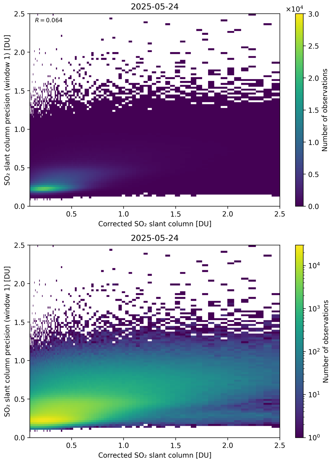
Figure 238: Scatter density plot of “Corrected SO 2 slant column” against “SO 2 slant column precision (window 1)” for 2025-05-23 to 2025-05-25.
