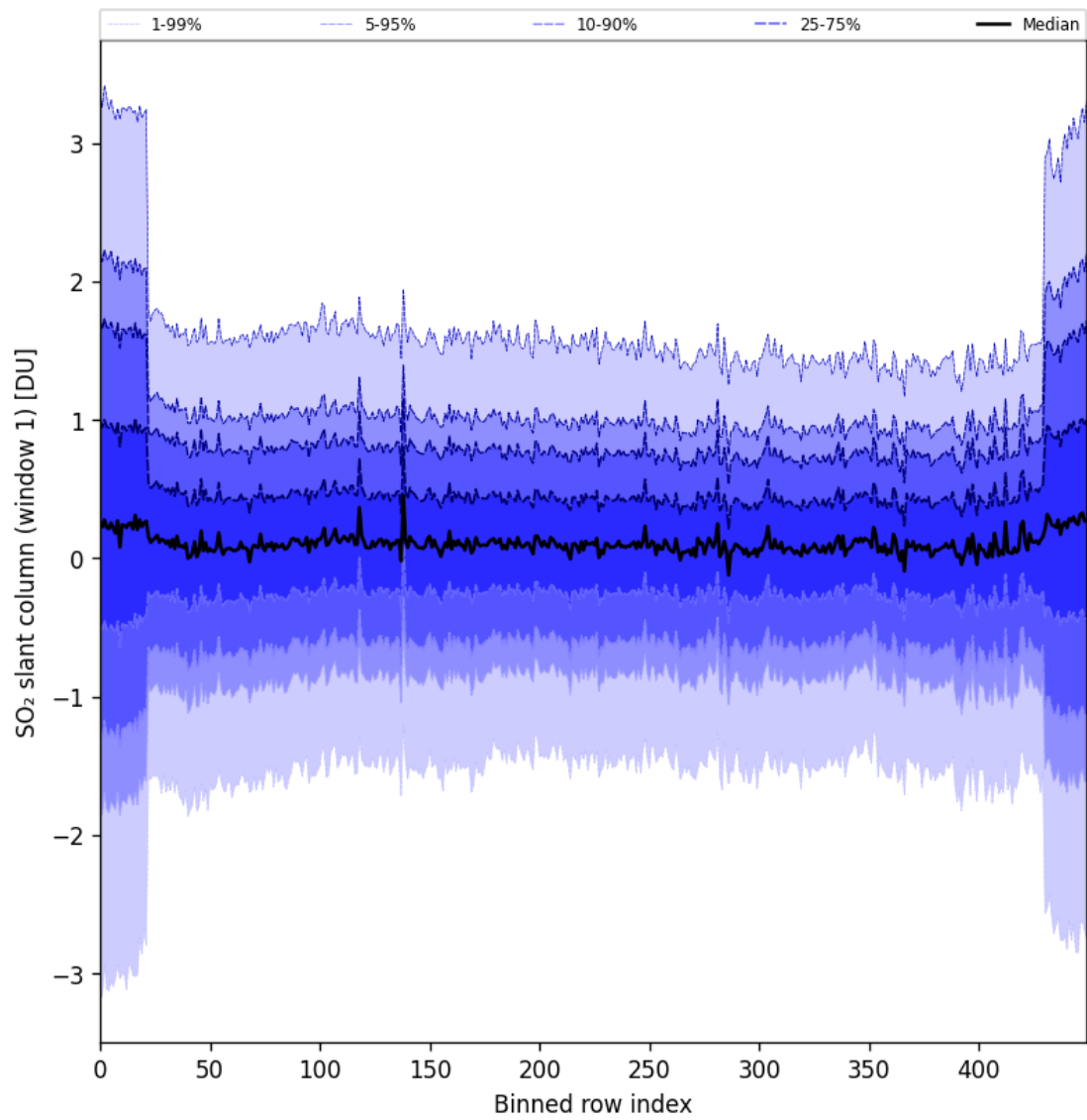
Figure 89: Along track statistics of “SO 2 slant column (window 1)” for 2025-05-23 to 2025-05-25
