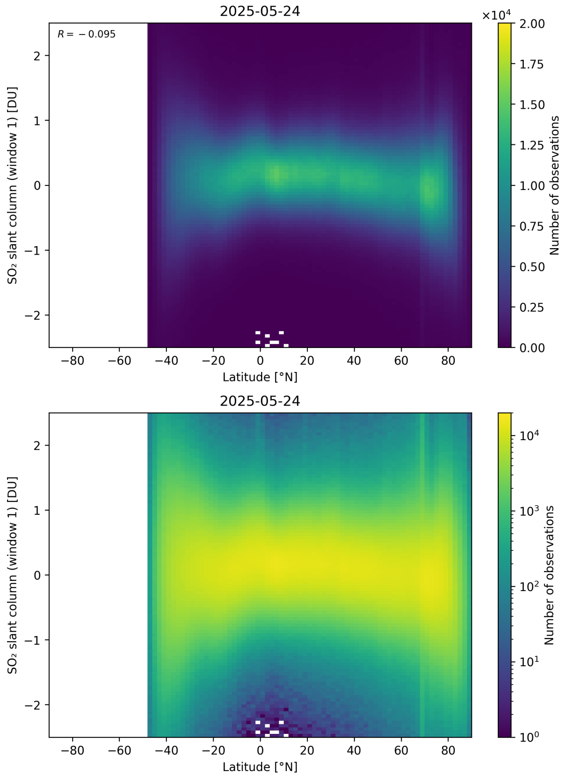
Figure 162: Scatter density plot of “Latitude” against “SO 2 slant column (window 1)” for 2025-05-23 to 2025-05-25.
