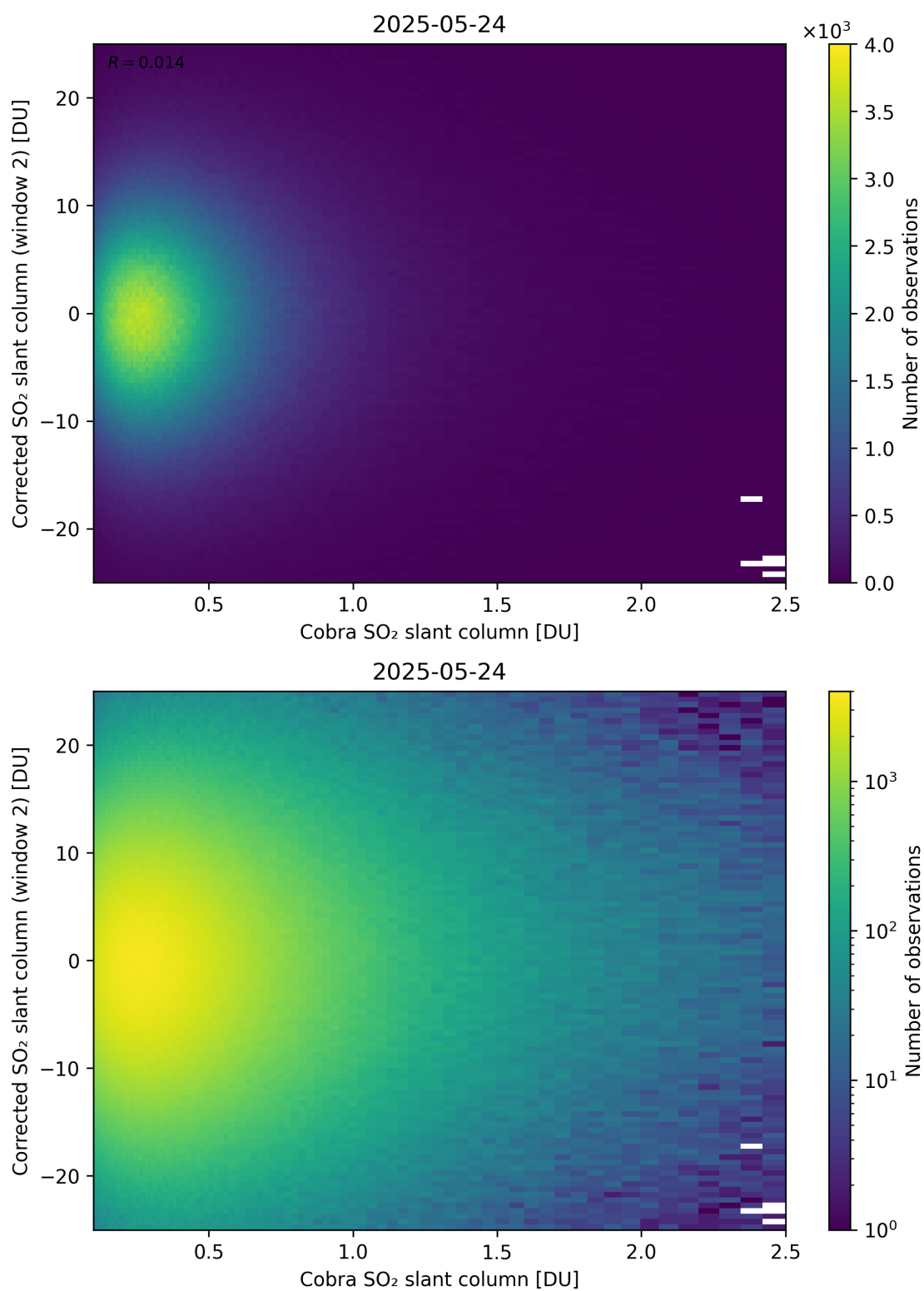
Figure 217: Scatter density plot of “Cobra SO 2 slant column” against “Corrected SO 2 slant column (window 2)” for 2025-05-23 to 2025-05-25.
