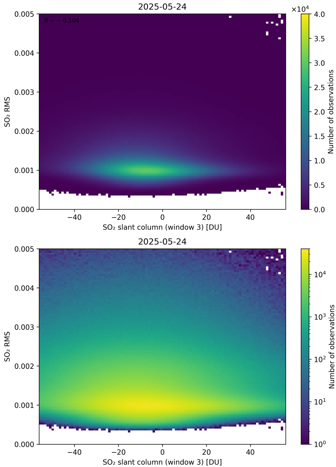
Figure 306: Scatter density plot of “SO 2 slant column (window 3)” against “SO 2 RMS” for 2025-05-23 to 2025-05-25.
