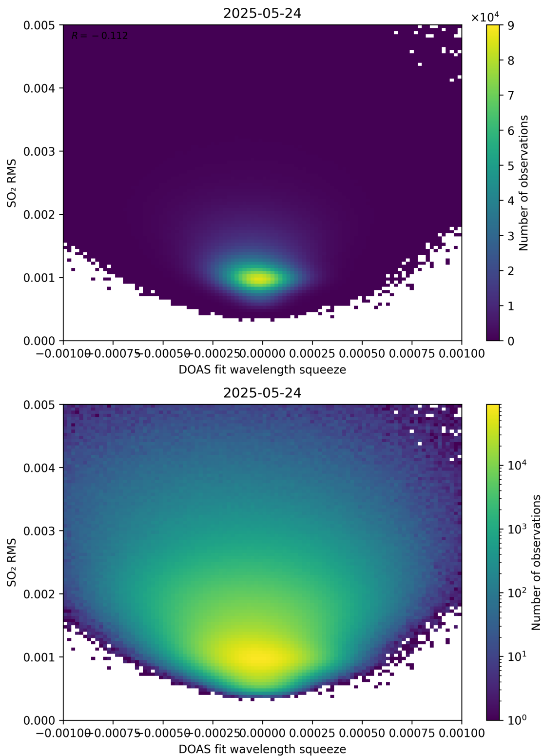
Figure 143: Scatter density plot of “DOAS fit wavelength squeeze” against “SO 2 RMS” for 2025-05-23 to 2025-05-25.
