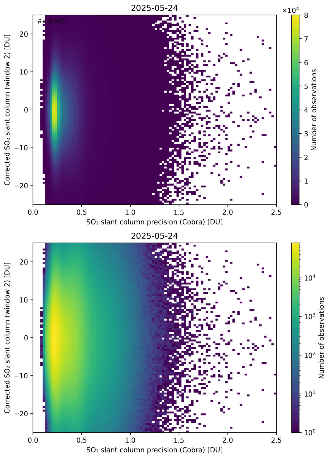
Figure 206: Scatter density plot of “SO 2 slant column precision (Cobra)” against “Corrected SO 2 slant column (window 2)” for 2025-05-23 to 2025-05-25.
