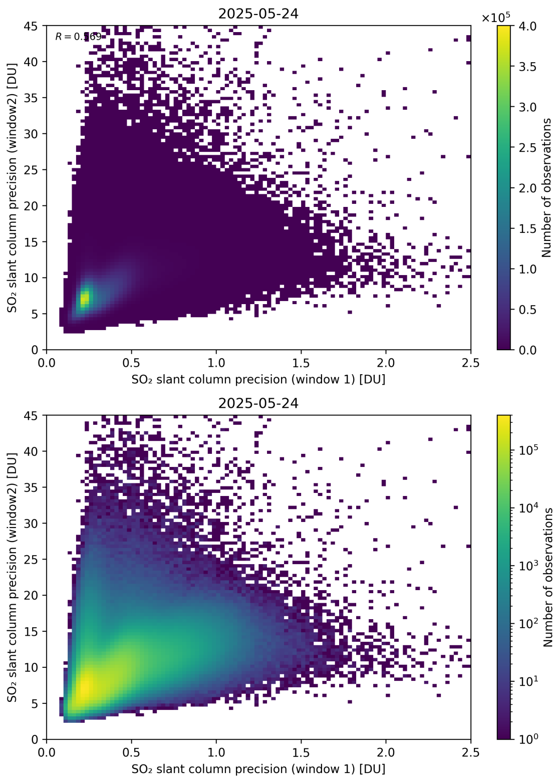
Figure 277: Scatter density plot of “SO 2 slant column precision (window 1)” against “SO 2 slant column precision (window2)” for 2025-05-23 to 2025-05-25.
