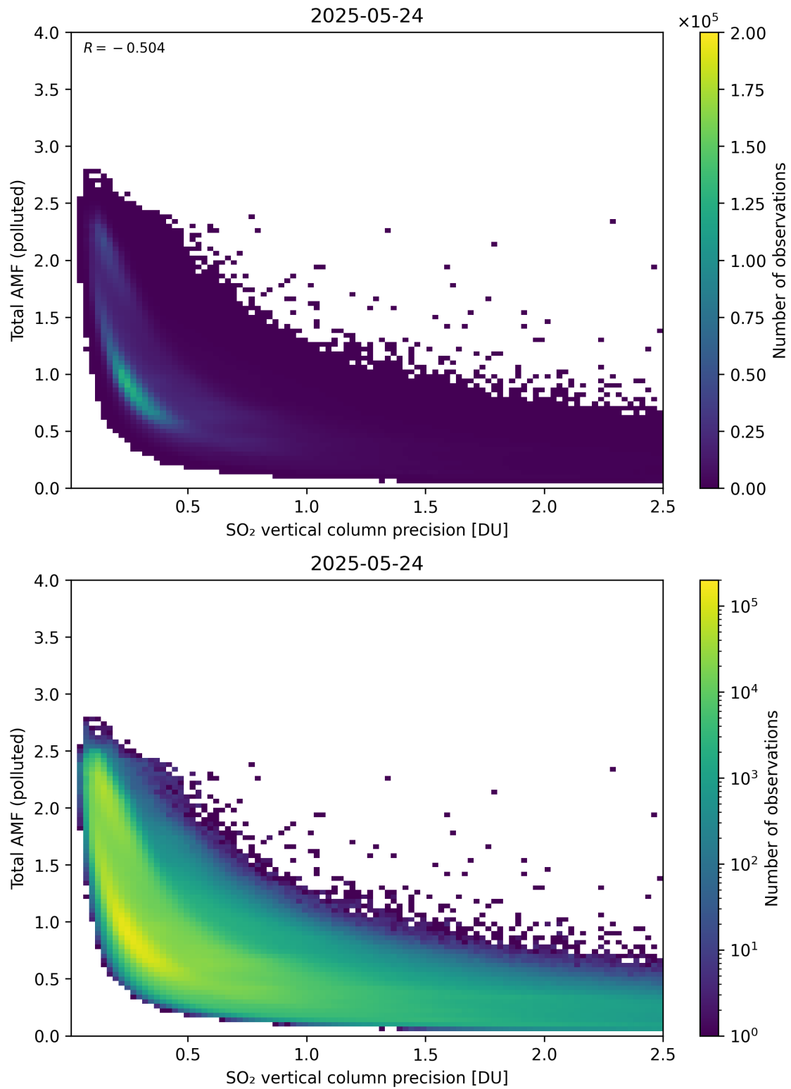
Figure 346: Scatter density plot of “SO 2 vertical column precision” against “Total AMF (polluted)” for 2025-05-23 to 2025-05-25.
