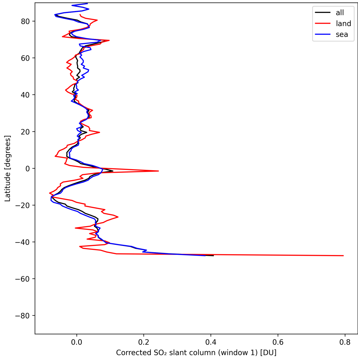
Figure 39: Zonal average of “Corrected SO 2 slant column (window 1)” for 2025-05-23 to 2025-05-25.
