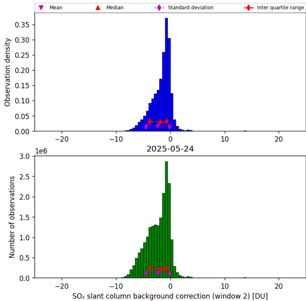
Figure 70: Histogram of “SO 2 slant column background correction (window 2)” for 2025-05-23 to 2025-05-25
