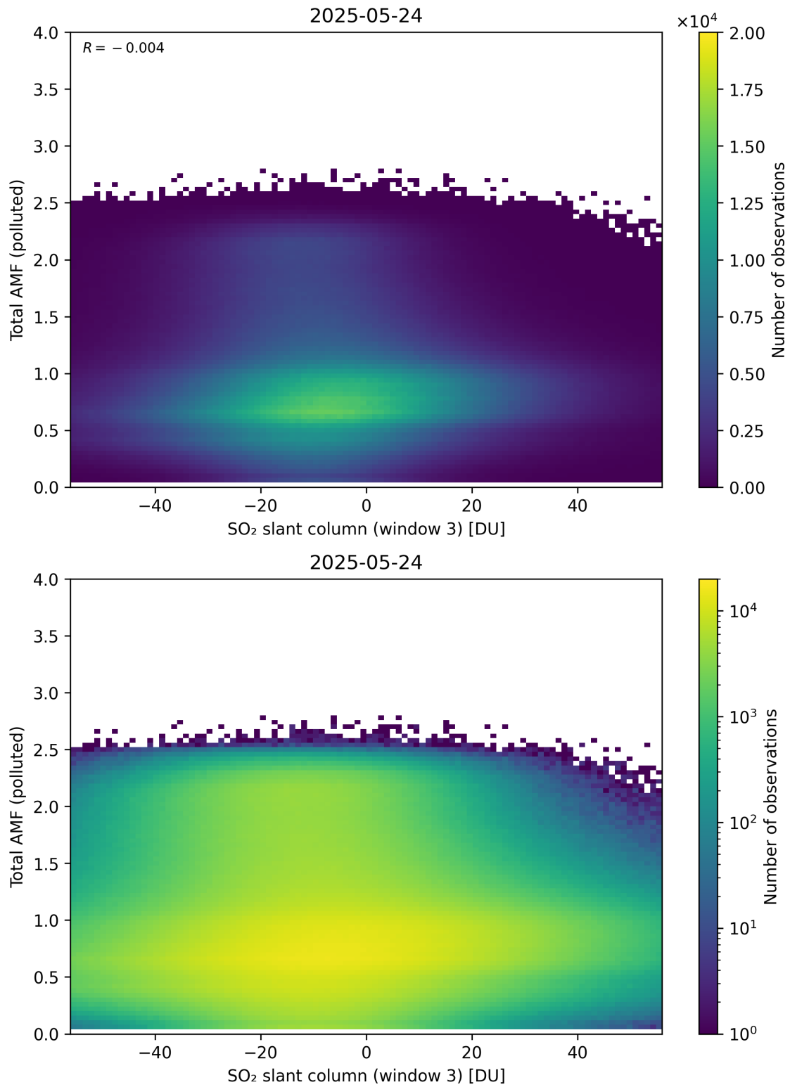
Figure 318: Scatter density plot of “SO 2 slant column (window 3)” against “Total AMF (polluted)” for 2025-05-23 to 2025-05-25.
