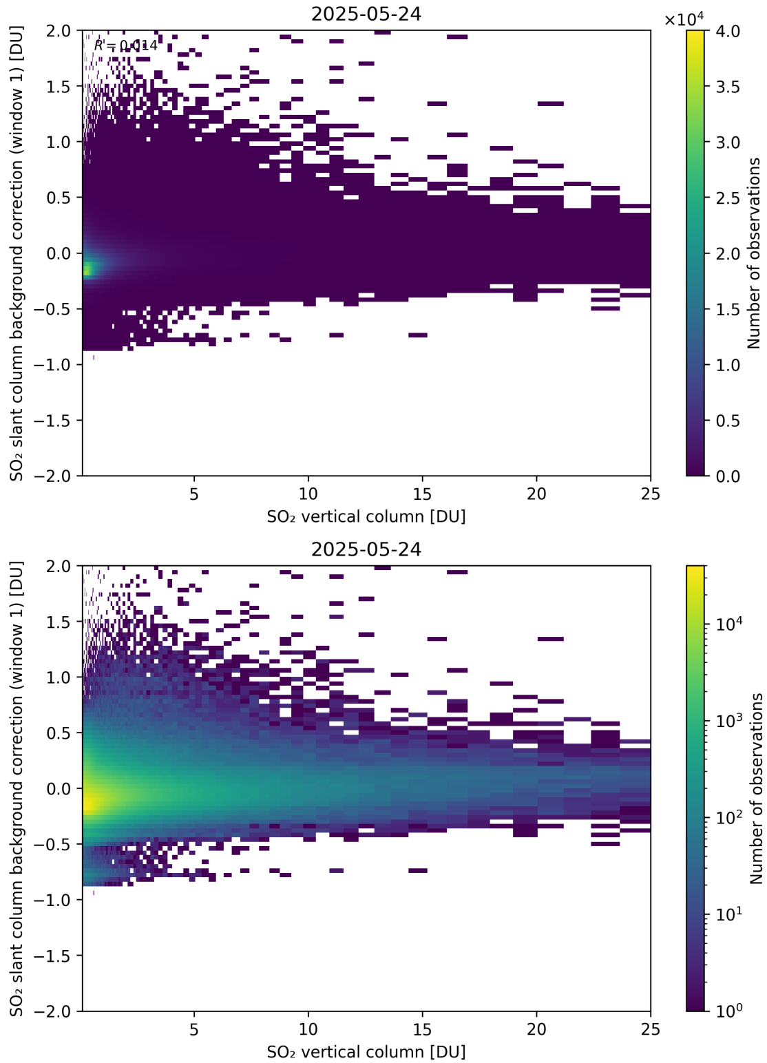
Figure 323: Scatter density plot of “SO 2 vertical column” against “SO 2 slant column background correction (window 1)” for 2025-05-23 to 2025-05-25.
