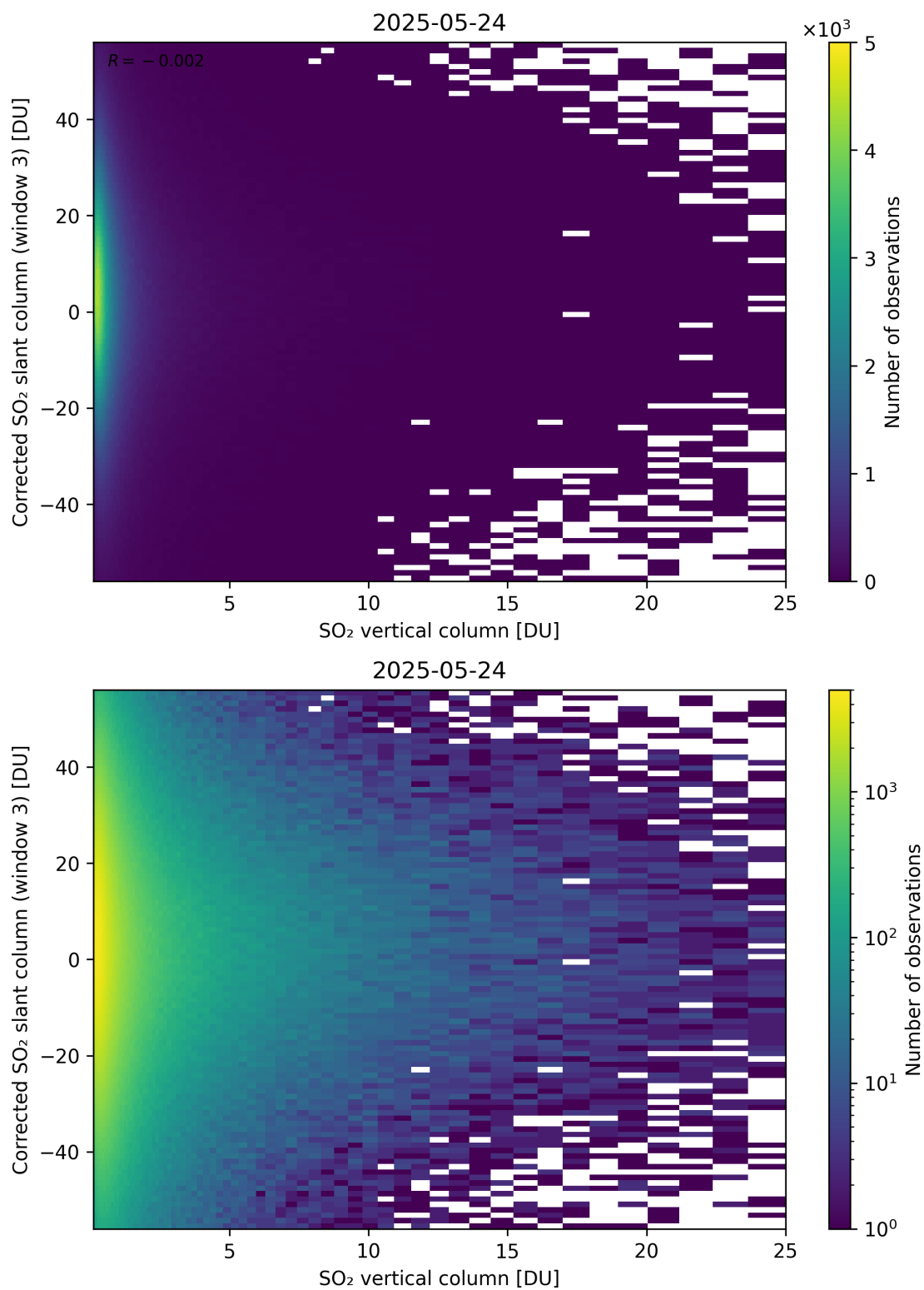
Figure 353: Scatter density plot of “SO 2 vertical column” against “Corrected SO 2 slant column (window 3)” for 2025-05-23 to 2025-05-25.
