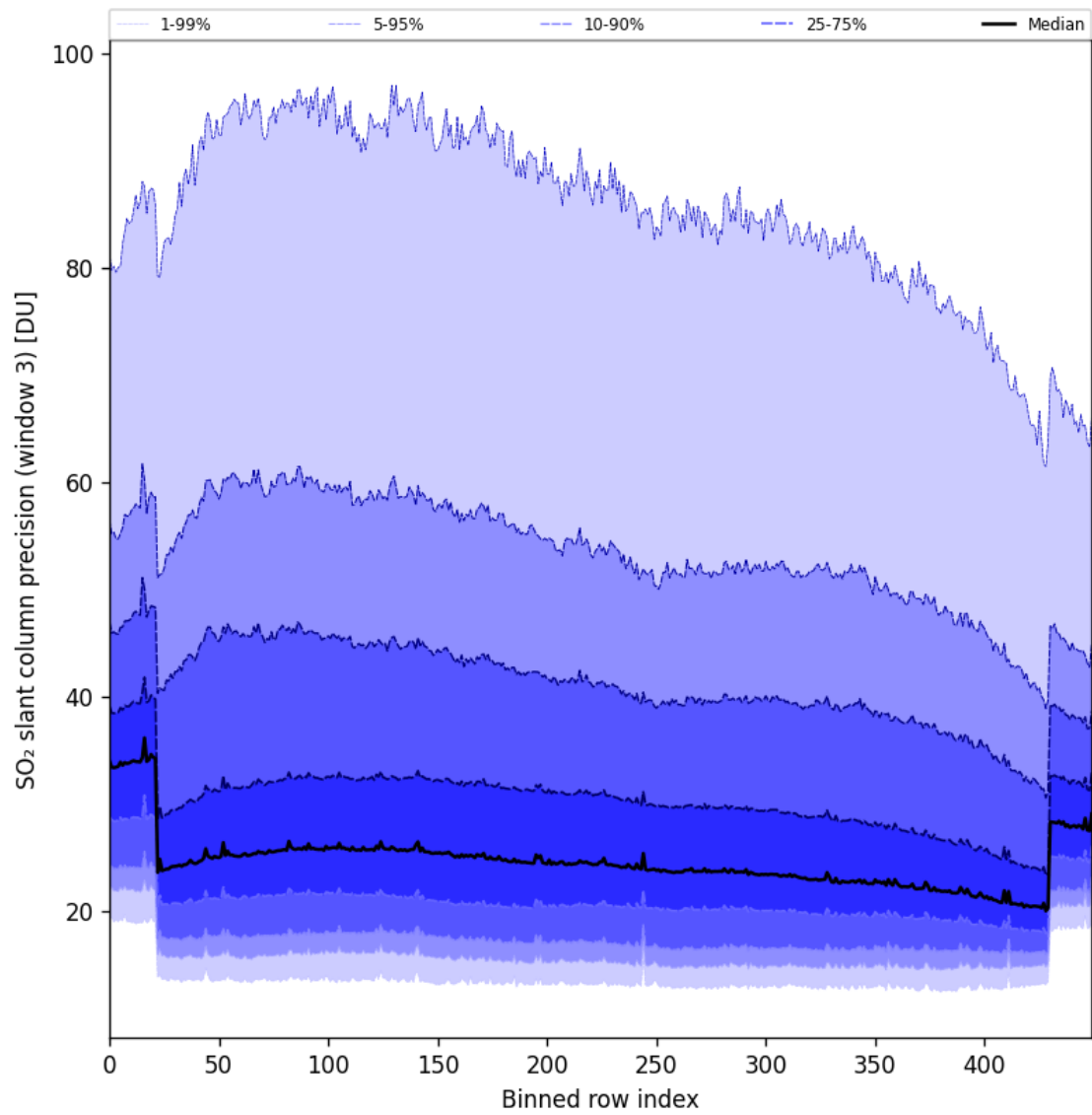
Figure 98: Along track statistics of “SO 2 slant column precision (window 3)” for 2025-05-23 to 2025-05-25
