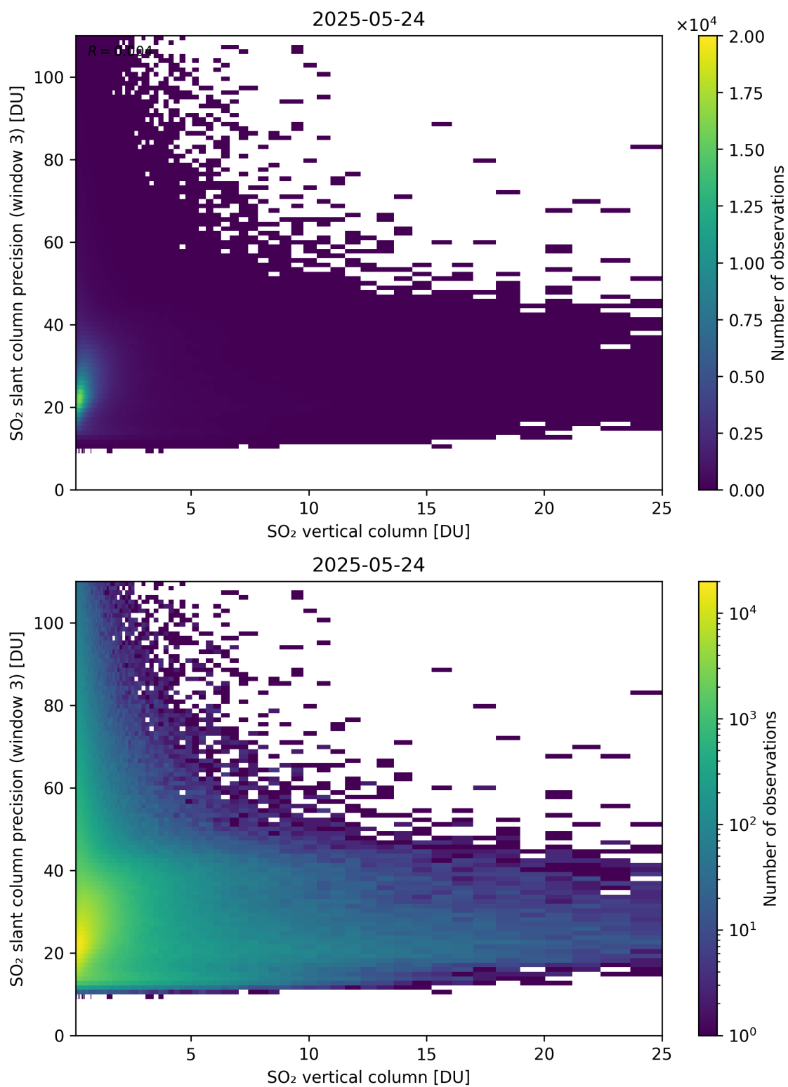
Figure 358: Scatter density plot of “SO 2 vertical column” against “SO 2 slant column precision (window 3)” for 2025-05-23 to 2025-05-25.
