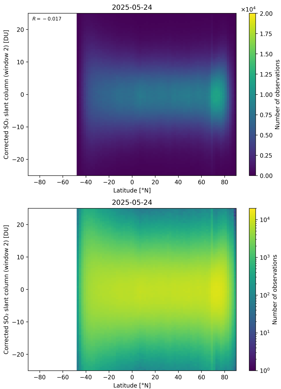
Figure 160: Scatter density plot of “Latitude” against “Corrected SO 2 slant column (window 2)” for 2025-05-23 to 2025-05-25.
