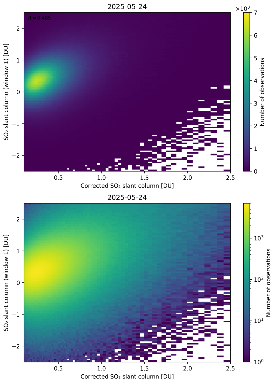
Figure 237: Scatter density plot of “Corrected SO 2 slant column” against “SO 2 slant column (window 1)” for 2025-05-23 to 2025-05-25.
