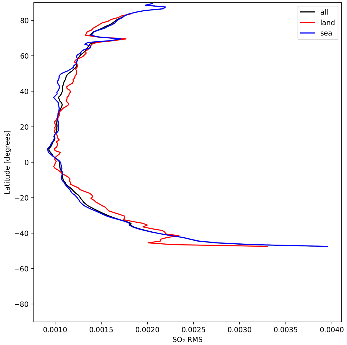
Figure 52: Zonal average of “SO 2 RMS” for 2025-05-23 to 2025-05-25.
