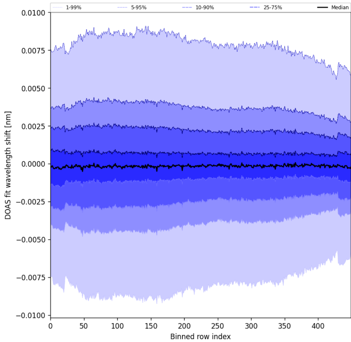
Figure 102: Along track statistics of “DOAS fit wavelength shift” for 2025-05-23 to 2025-05-25
