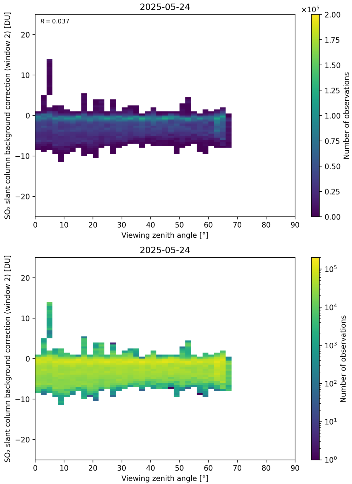
Figure 363: Scatter density plot of “Viewing zenith angle” against “SO 2 slant column background correction (window 2)” for 2025-05-23 to 2025-05-25.
