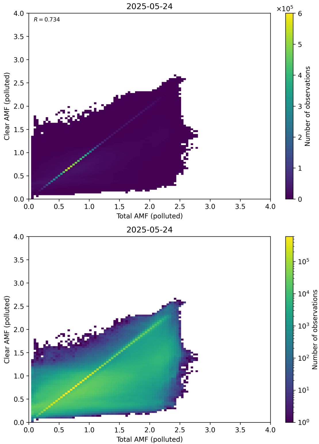
Figure 321: Scatter density plot of “Total AMF (polluted)” against “Clear AMF (polluted)” for 2025-05-23 to 2025-05-25.
