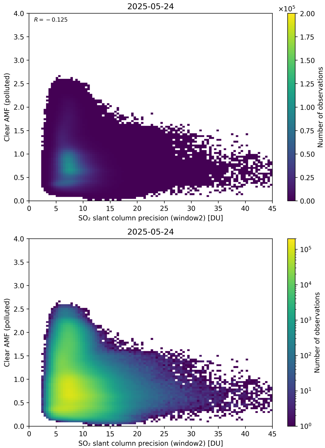
Figure 296: Scatter density plot of “SO 2 slant column precision (window2)” against “Clear AMF (polluted)” for 2025-05-23 to 2025-05-25.
