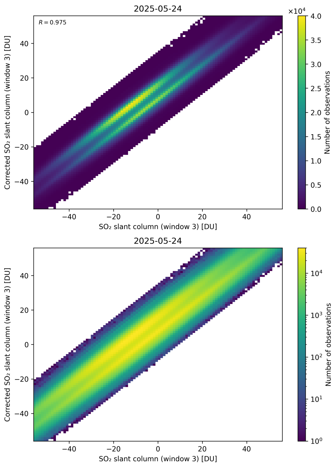
Figure 316: Scatter density plot of “SO 2 slant column (window 3)” against “Corrected SO 2 slant column (window 3)” for 2025-05-23 to 2025-05-25.
