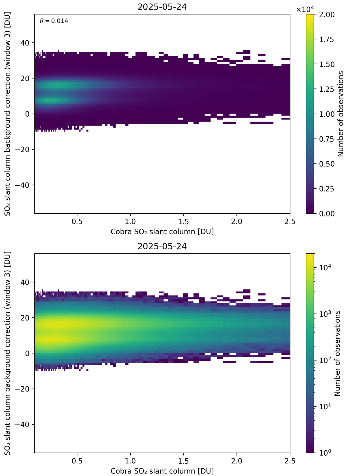
Figure 195: Scatter density plot of “Cobra SO 2 slant column” against “SO 2 slant column background correction (window 3)” for 2025-05-23 to 2025-05-25.
