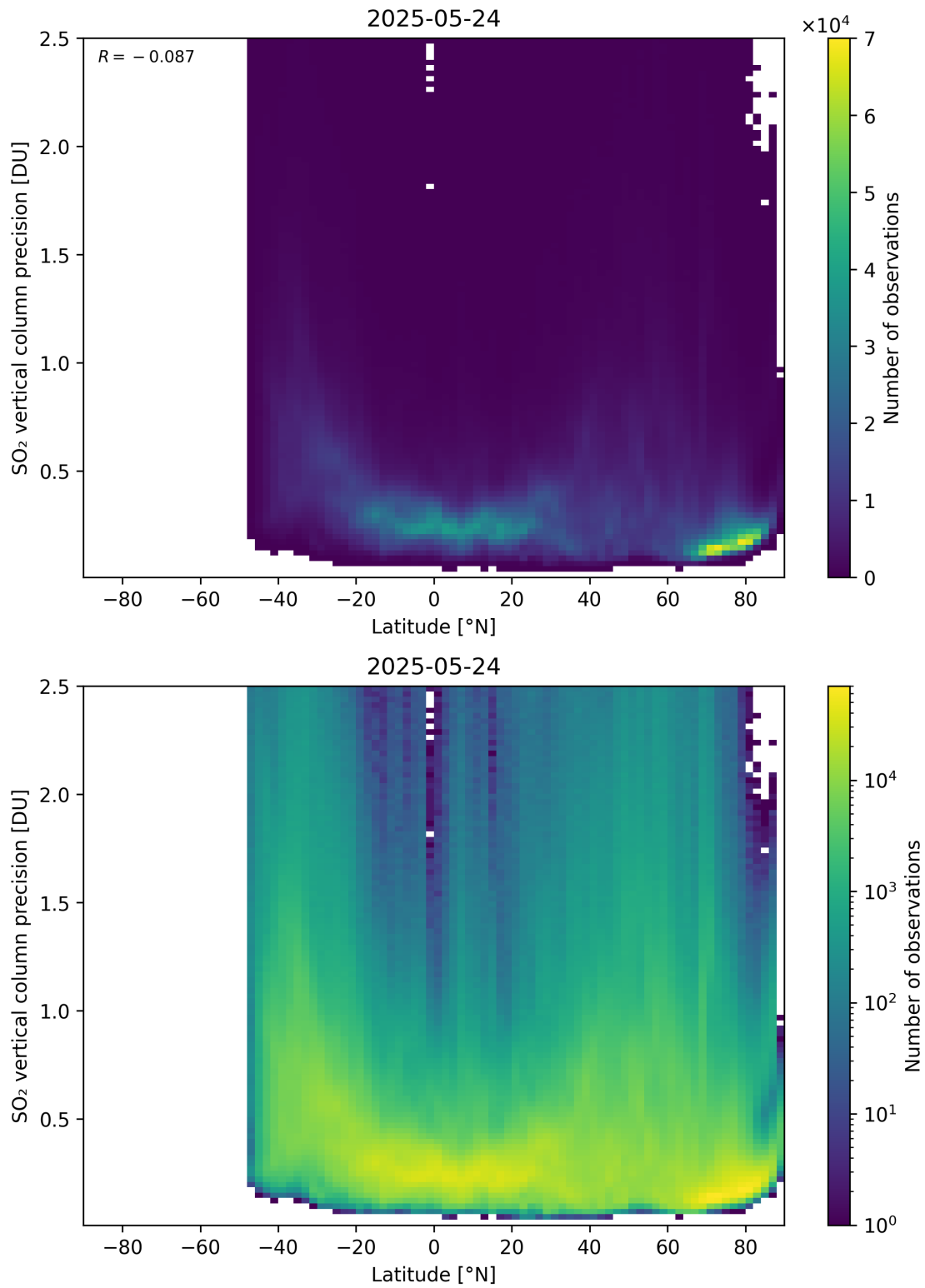
Figure 170: Scatter density plot of “Latitude” against “SO 2 vertical column precision” for 2025-05-23 to 2025-05-25.
