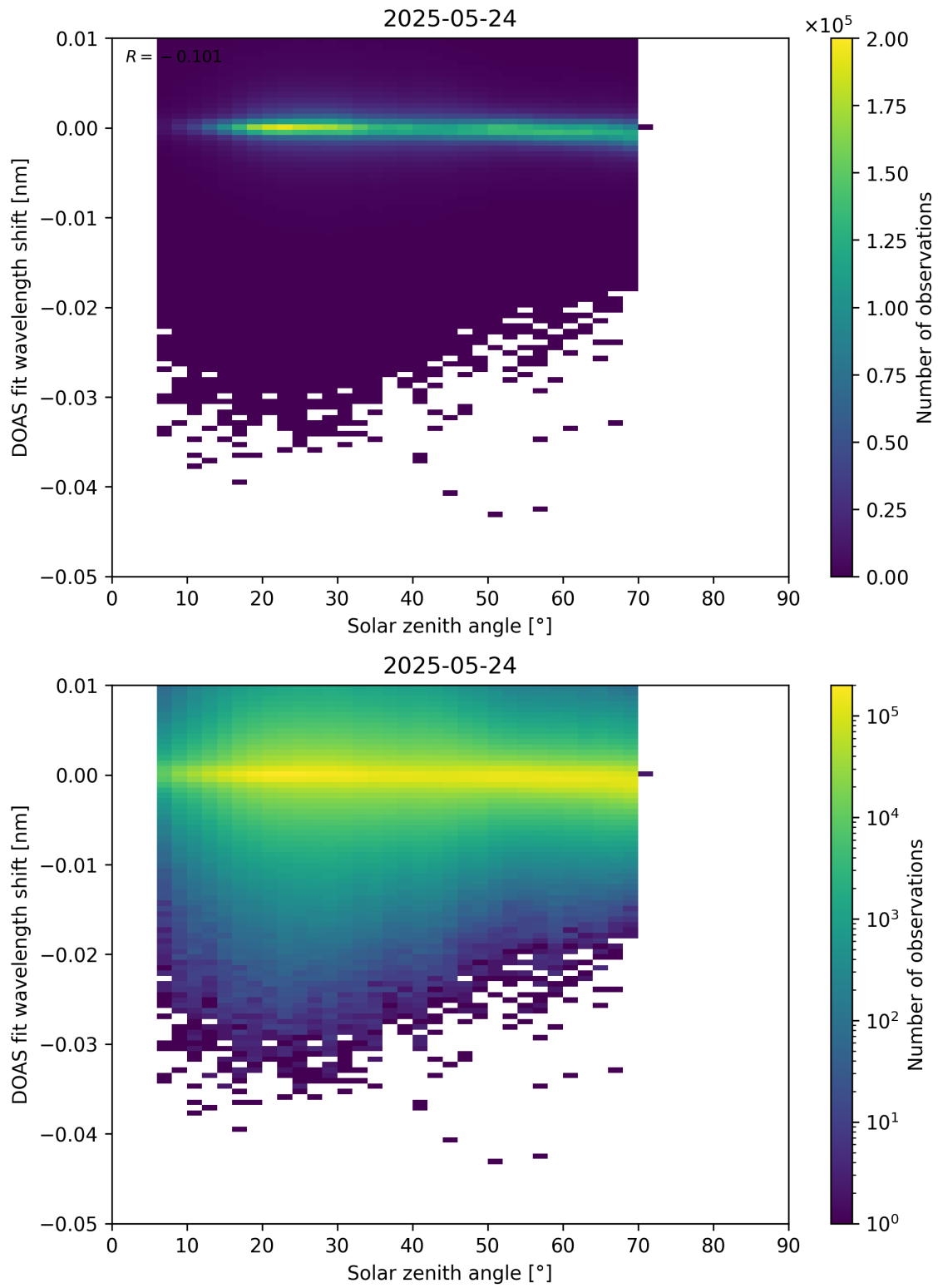
Figure 174: Scatter density plot of “Solar zenith angle” against “DOAS fit wavelength shift” for 2025-05-23 to 2025-05-25.
