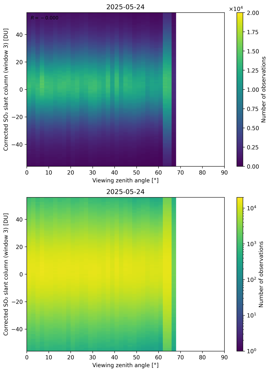
Figure 375: Scatter density plot of “Viewing zenith angle” against “Corrected SO 2 slant column (window 3)” for 2025-05-23 to 2025-05-25.
