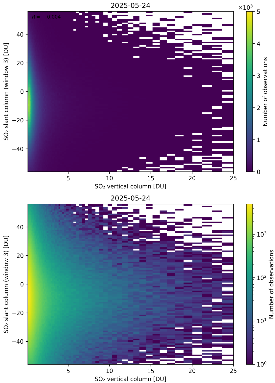
Figure 357: Scatter density plot of “SO 2 vertical column” against “SO 2 slant column (window 3)” for 2025-05-23 to 2025-05-25.
