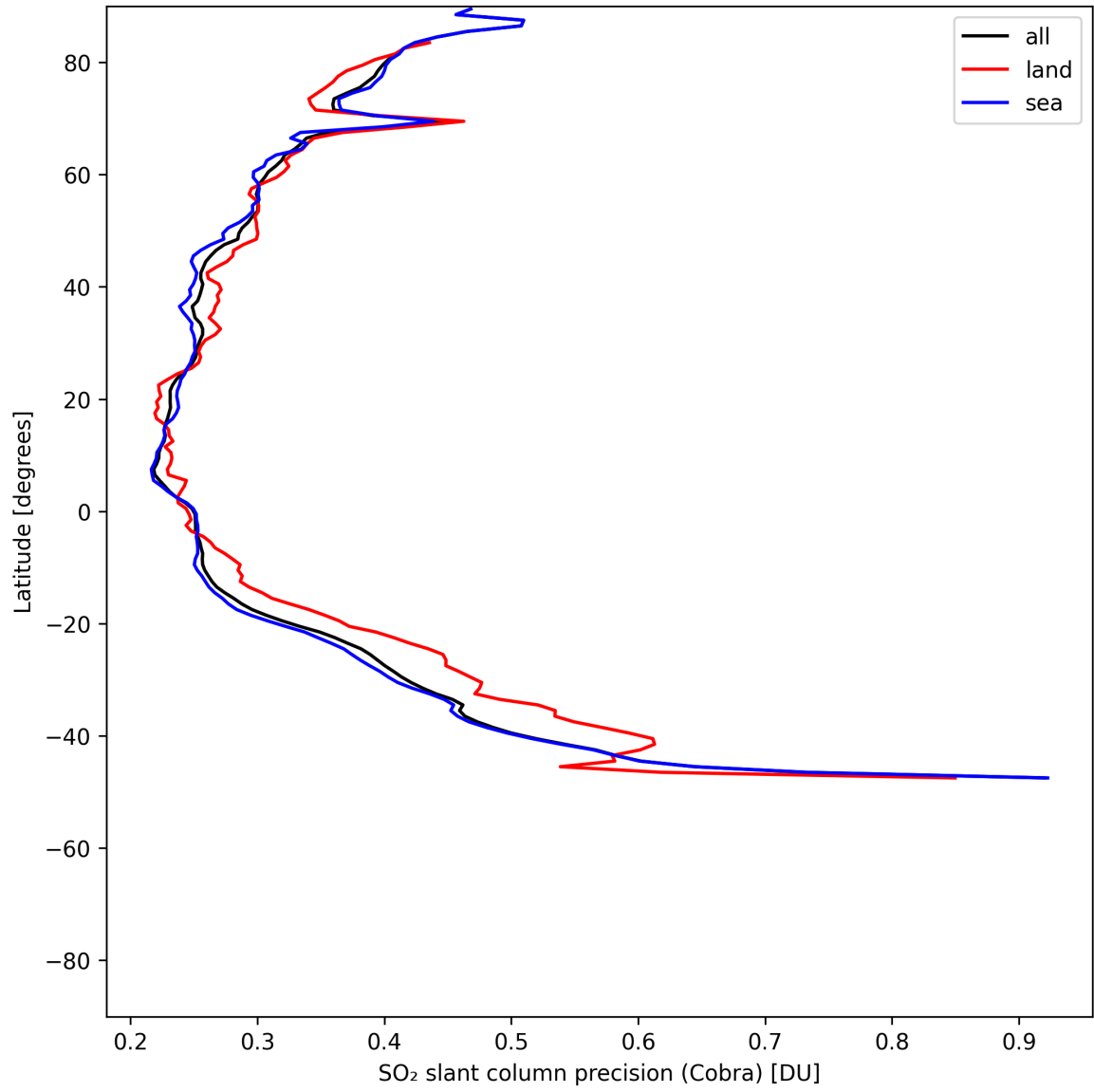
Figure 36: Zonal average of “SO 2 slant column precision (Cobra)” for 2025-05-23 to 2025-05-25.
