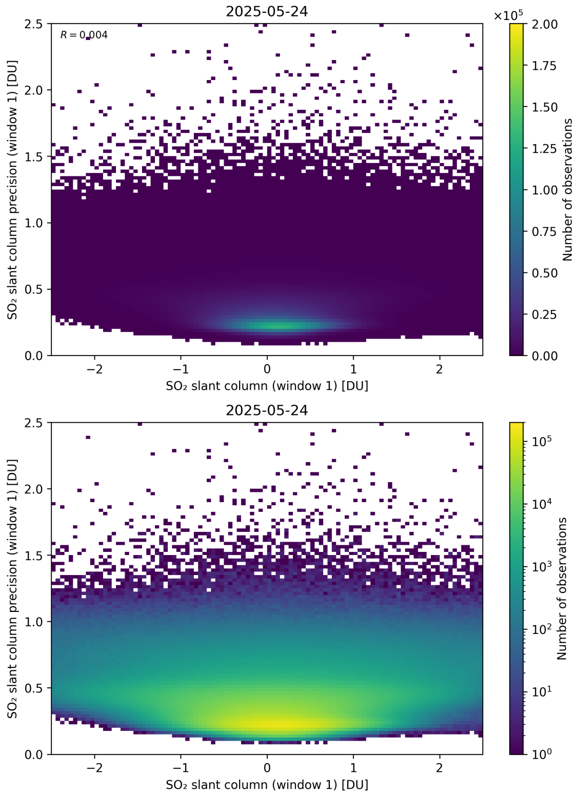
Figure 285: Scatter density plot of “SO 2 slant column (window 1)” against “SO 2 slant column precision (window 1)” for 2025-05-23 to 2025-05-25.
