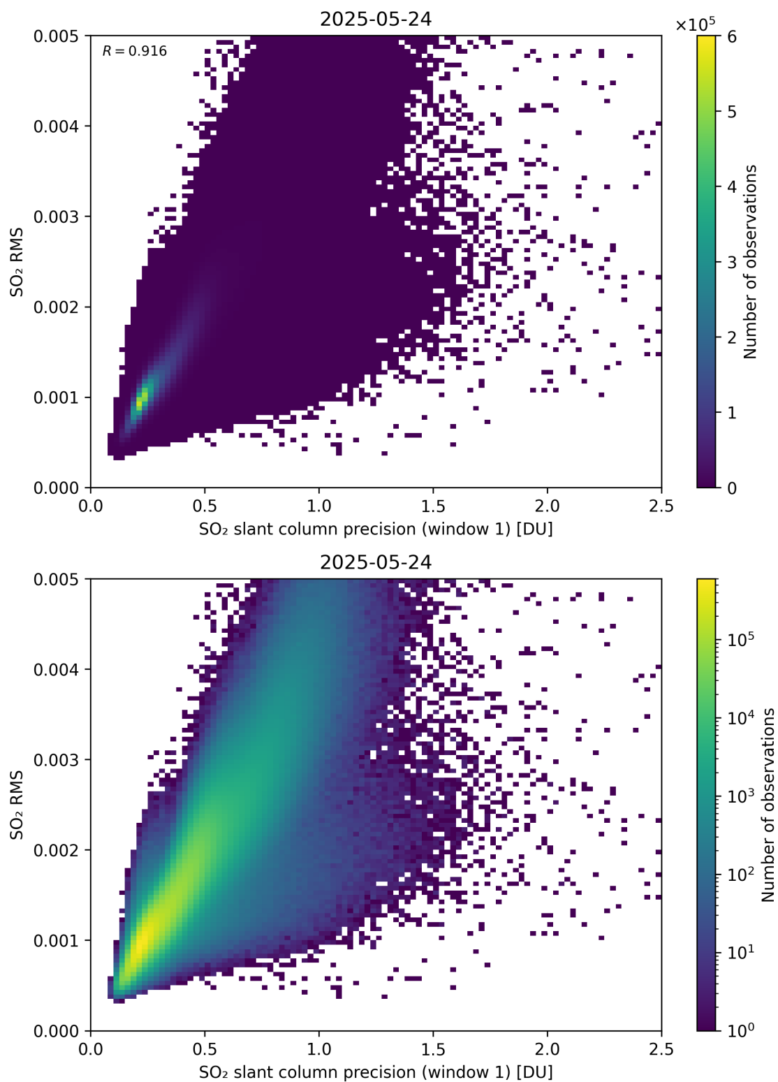
Figure 273: Scatter density plot of “SO 2 slant column precision (window 1)” against “SO 2 RMS” for 2025-05-23 to 2025-05-25.
