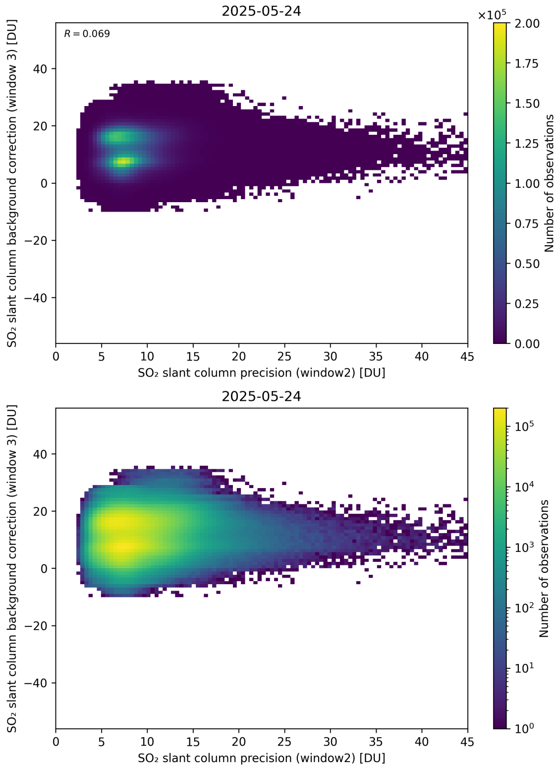
Figure 292: Scatter density plot of “SO 2 slant column precision (window2)” against “SO 2 slant column background correction (window 3)” for 2025-05-23 to 2025-05-25.
