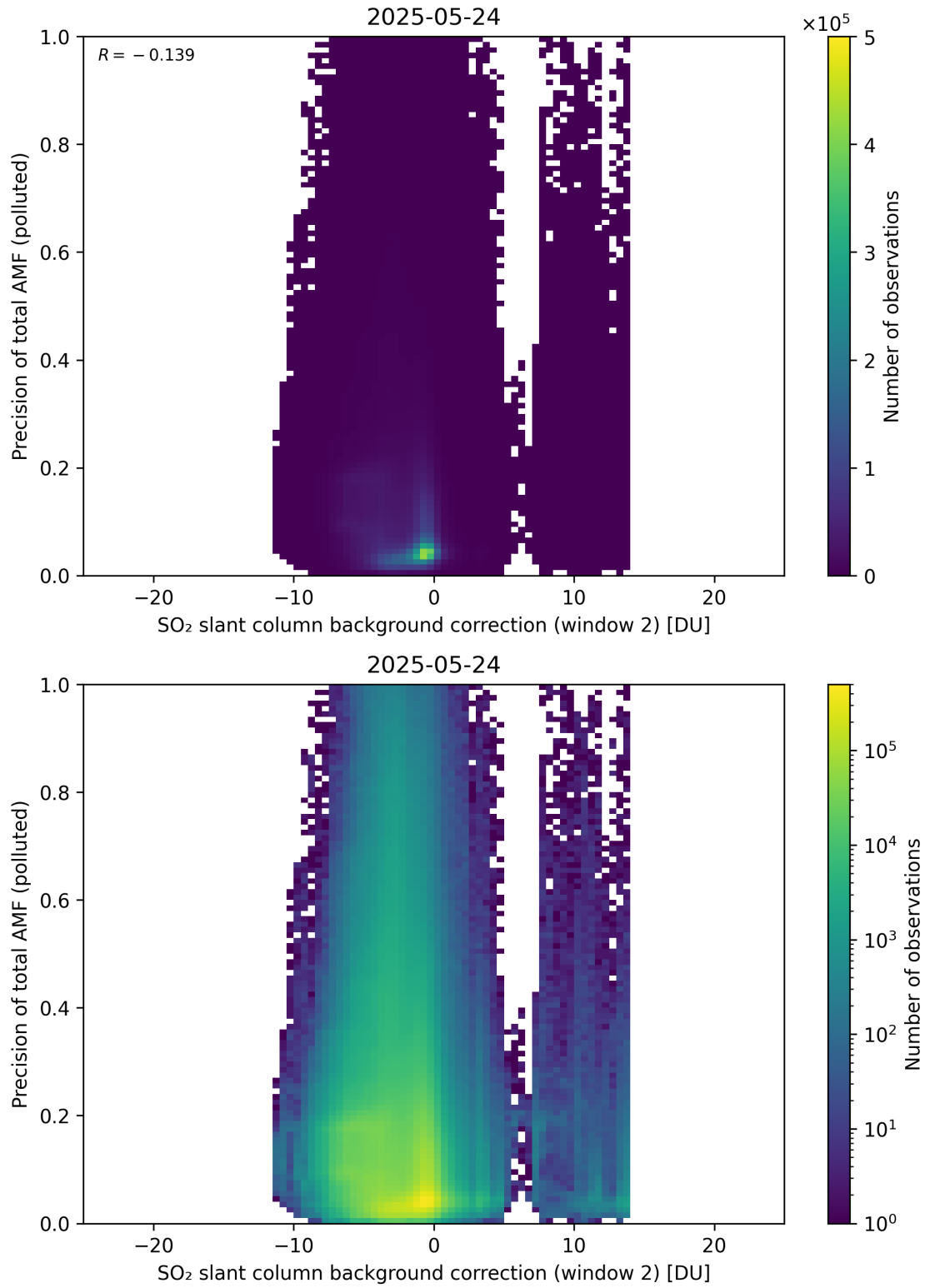
Figure 131: Scatter density plot of “SO 2 slant column background correction (window 2)” against “Precision of total AMF (polluted)” for 2025-05-23 to 2025-05-25.
