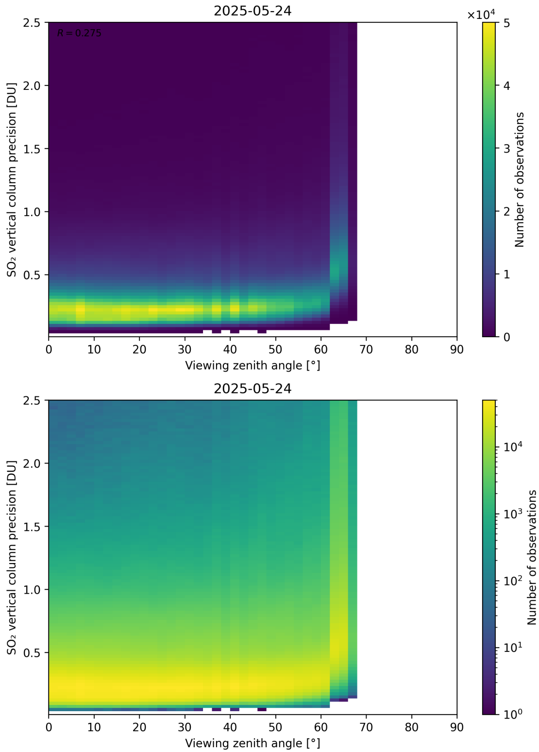
Figure 384: Scatter density plot of “Viewing zenith angle” against “SO 2 vertical column precision” for 2025-05-23 to 2025-05-25.
