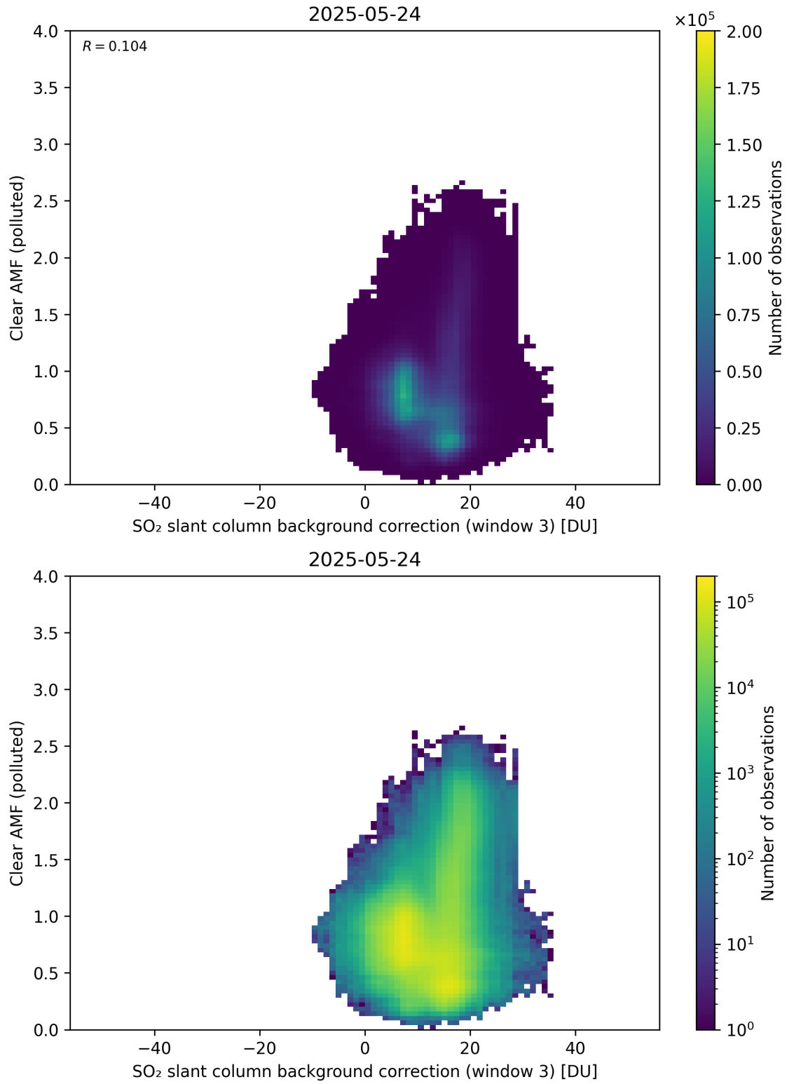
Figure 135: Scatter density plot of “SO 2 slant column background correction (window 3)” against “Clear AMF (polluted)” for 2025-05-23 to 2025-05-25.
