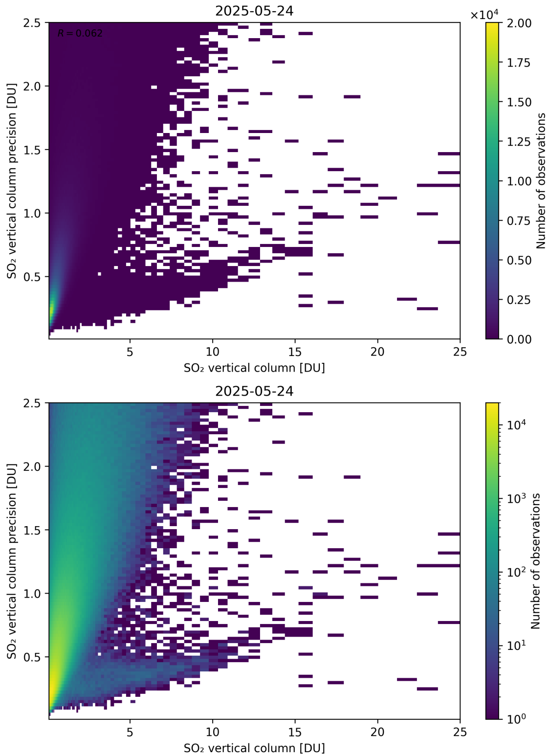
Figure 361: Scatter density plot of “SO 2 vertical column” against “SO 2 vertical column precision” for 2025-05-23 to 2025-05-25.
