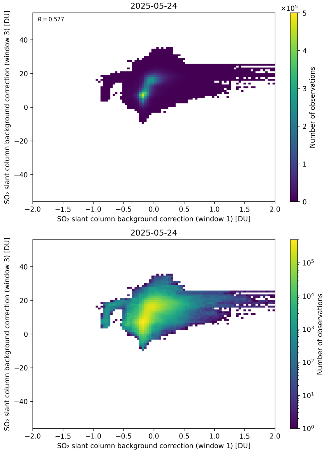
Figure 110: Scatter density plot of “SO 2 slant column background correction (window 1)” against “SO 2 slant column background correction (window 3)” for 2025-05-23 to 2025-05-25.
