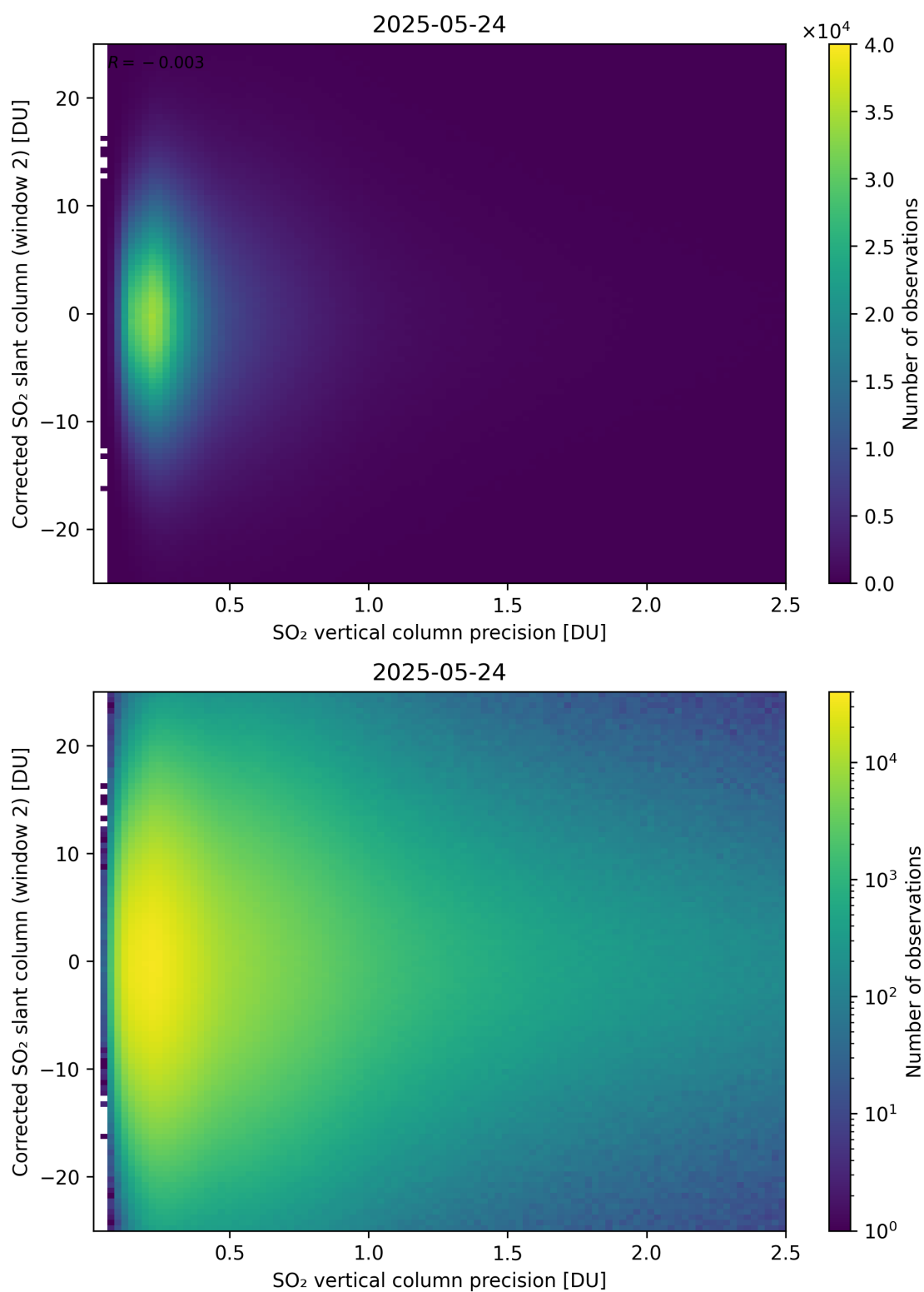
Figure 339: Scatter density plot of “SO 2 vertical column precision” against “Corrected SO 2 slant column (window 2)” for 2025-05-23 to 2025-05-25.
