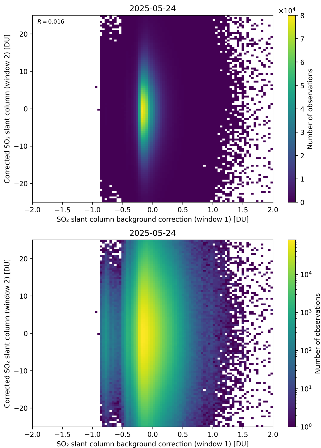
Figure 115: Scatter density plot of “SO 2 slant column background correction (window 1)” against “Corrected SO 2 slant column (window 2)” for 2025-05-23 to 2025-05-25.
