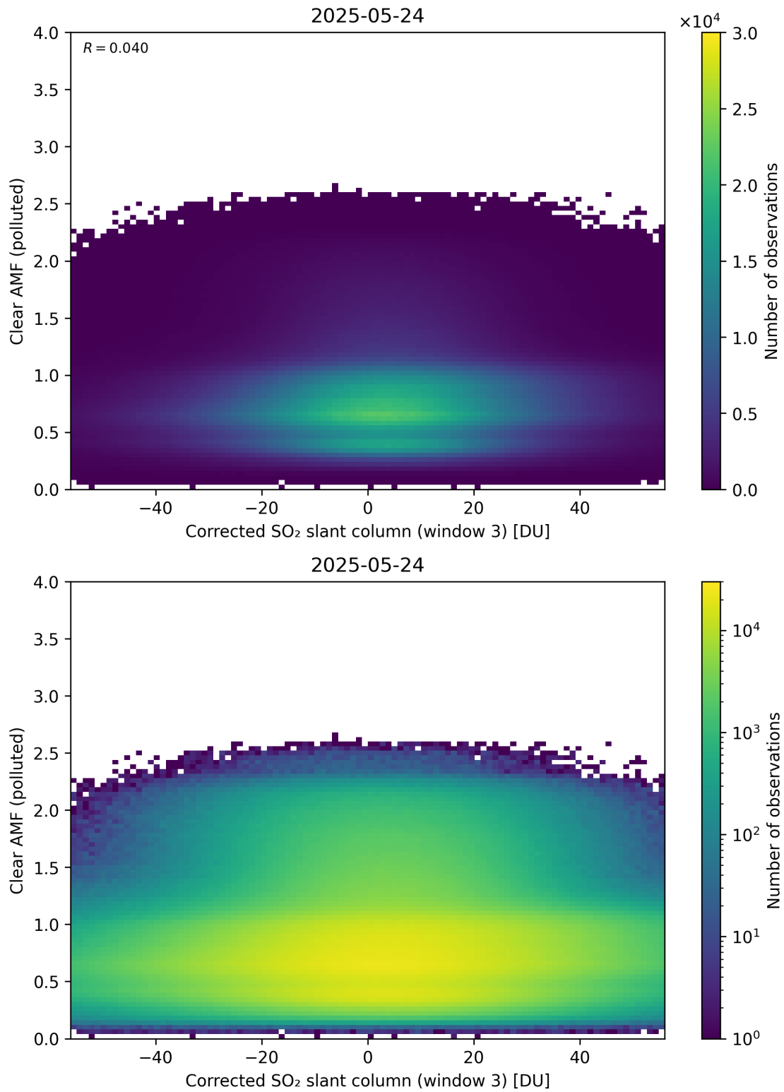
Figure 259: Scatter density plot of “Corrected SO 2 slant column (window 3)” against “Clear AMF (polluted)” for 2025-05-23 to 2025-05-25.
