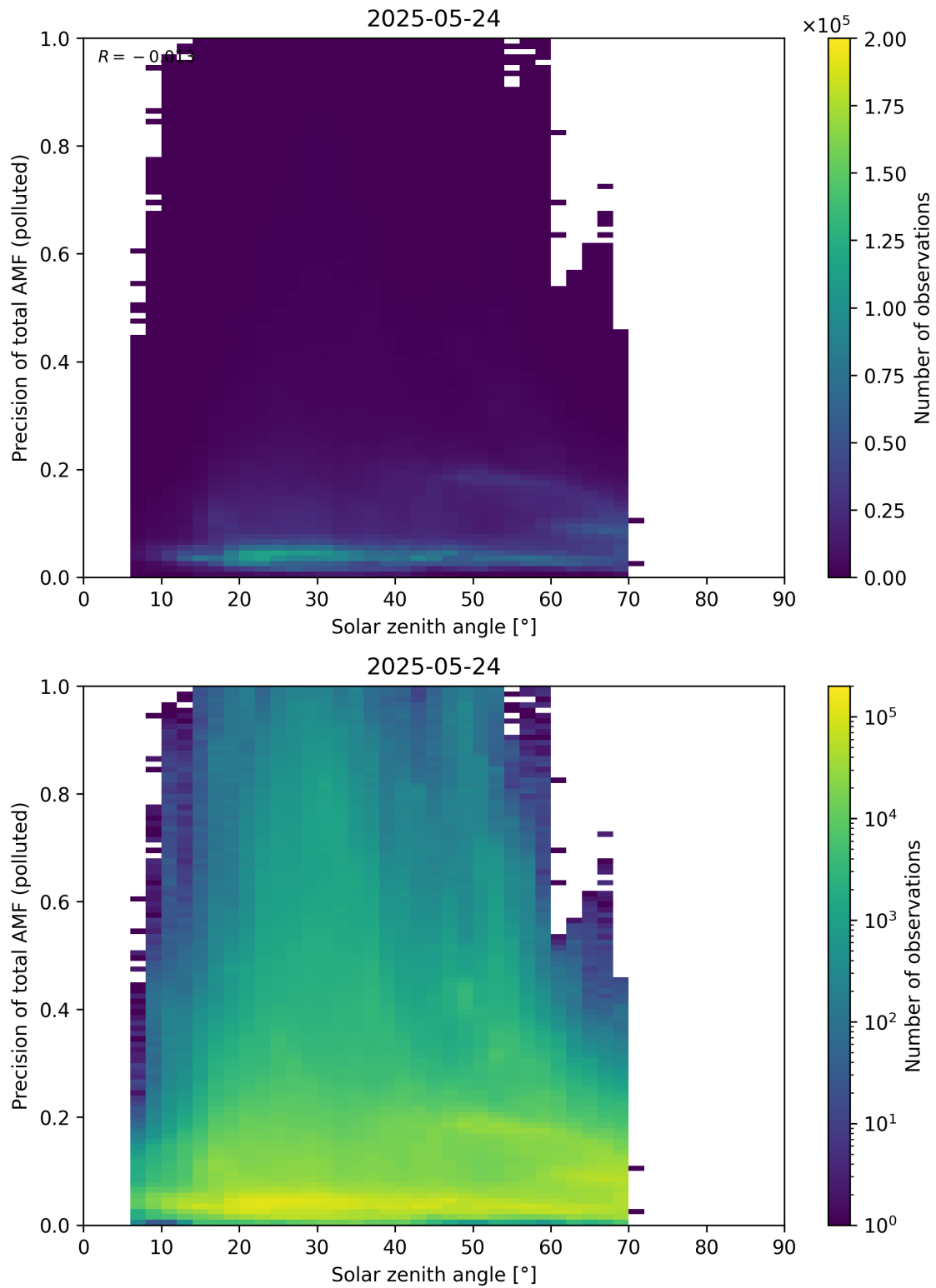
Figure 190: Scatter density plot of “Solar zenith angle” against “Precision of total AMF (polluted)” for 2025-05-23 to 2025-05-25.
