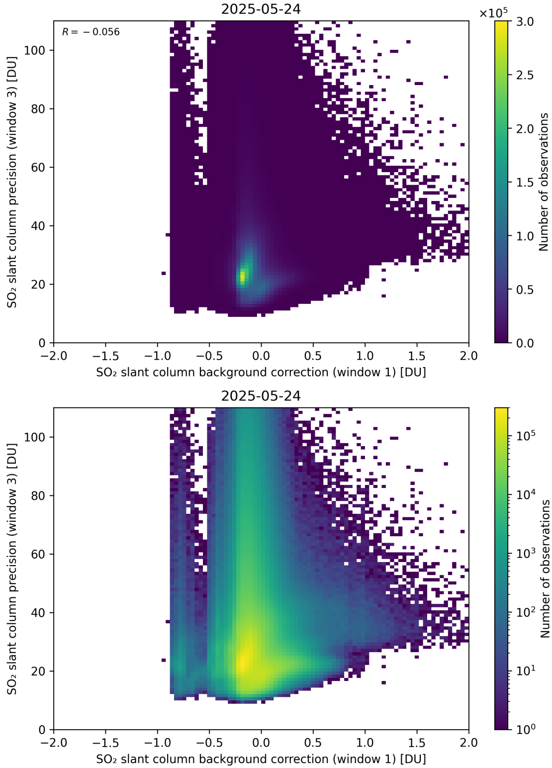
Figure 119: Scatter density plot of “SO 2 slant column background correction (window 1)” against “SO 2 slant column precision (window 3)” for 2025-05-23 to 2025-05-25.
