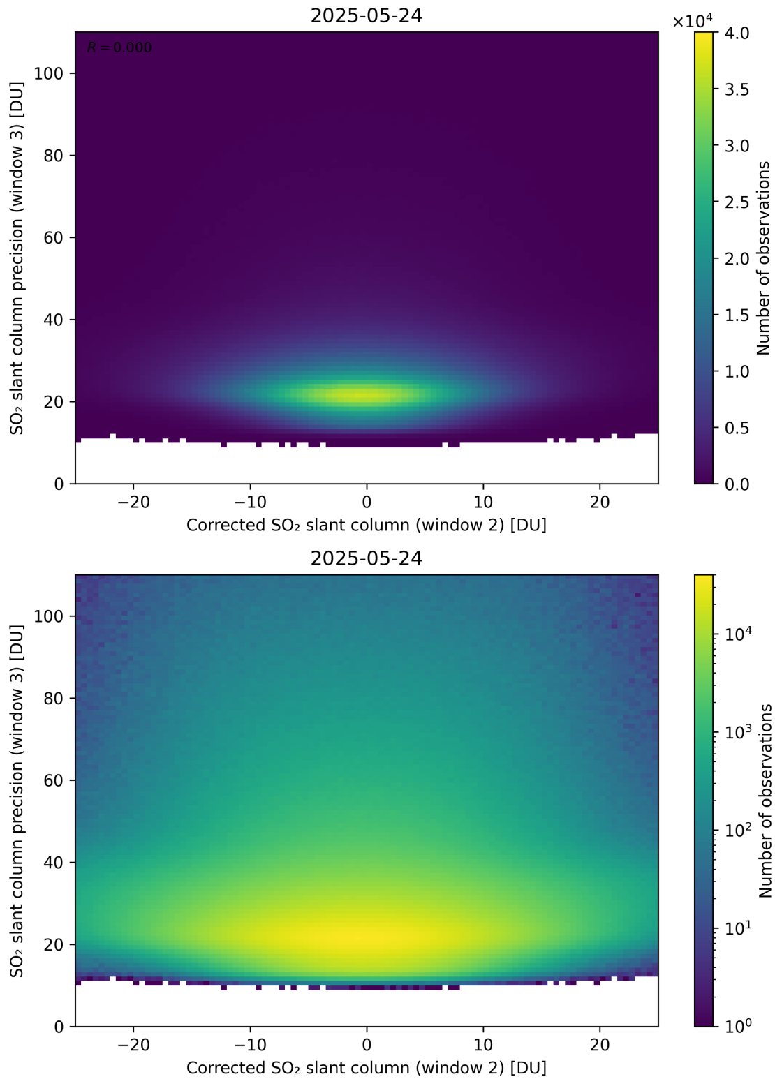
Figure 252: Scatter density plot of “Corrected SO 2 slant column (window 2)” against “SO 2 slant column precision (window 3)” for 2025-05-23 to 2025-05-25.
