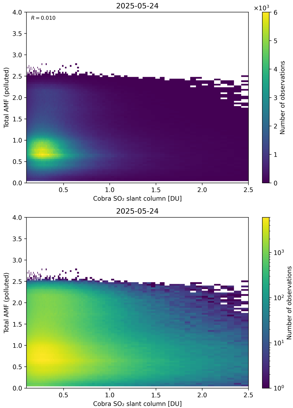
Figure 224: Scatter density plot of “Cobra SO 2 slant column” against “Total AMF (polluted)” for 2025-05-23 to 2025-05-25.
