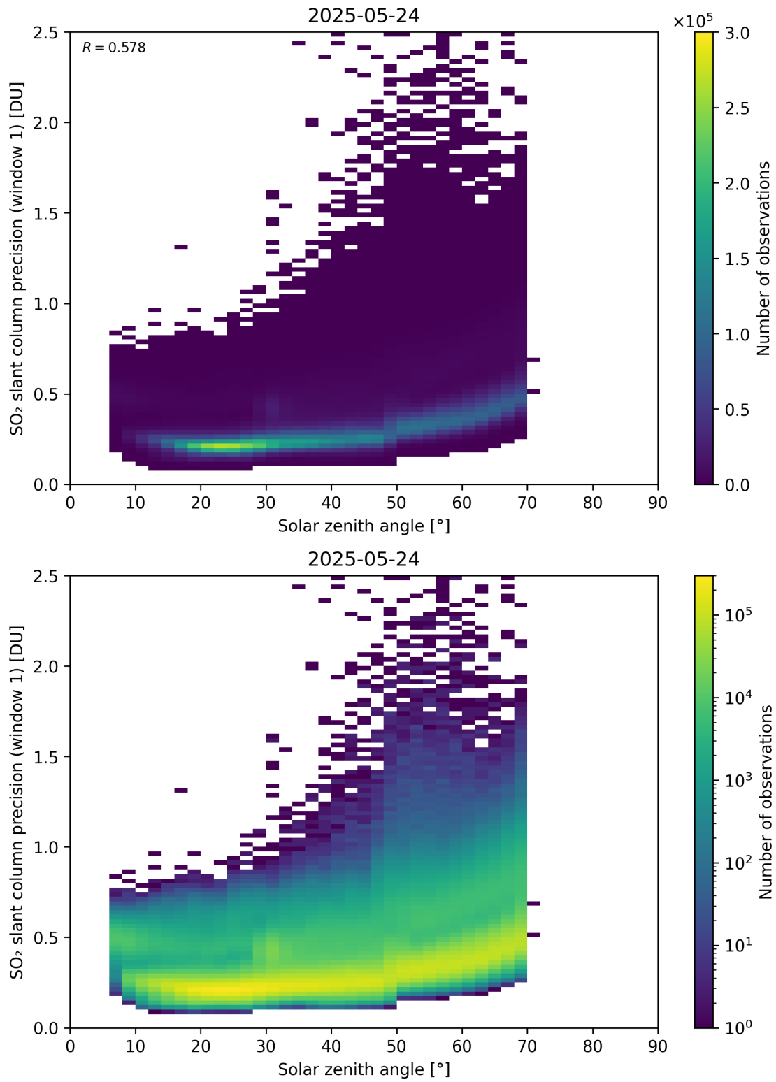
Figure 185: Scatter density plot of “Solar zenith angle” against “SO 2 slant column precision (window 1)” for 2025-05-23 to 2025-05-25.
