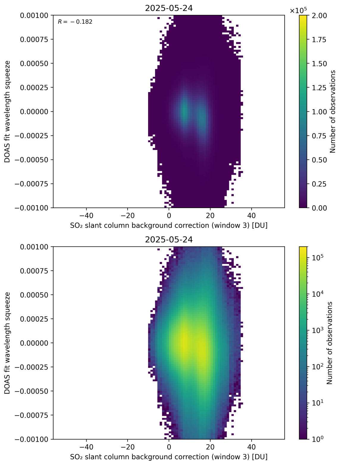
Figure 133: Scatter density plot of “SO 2 slant column background correction (window 3)” against “DOAS fit wavelength squeeze” for 2025-05-23 to 2025-05-25.
