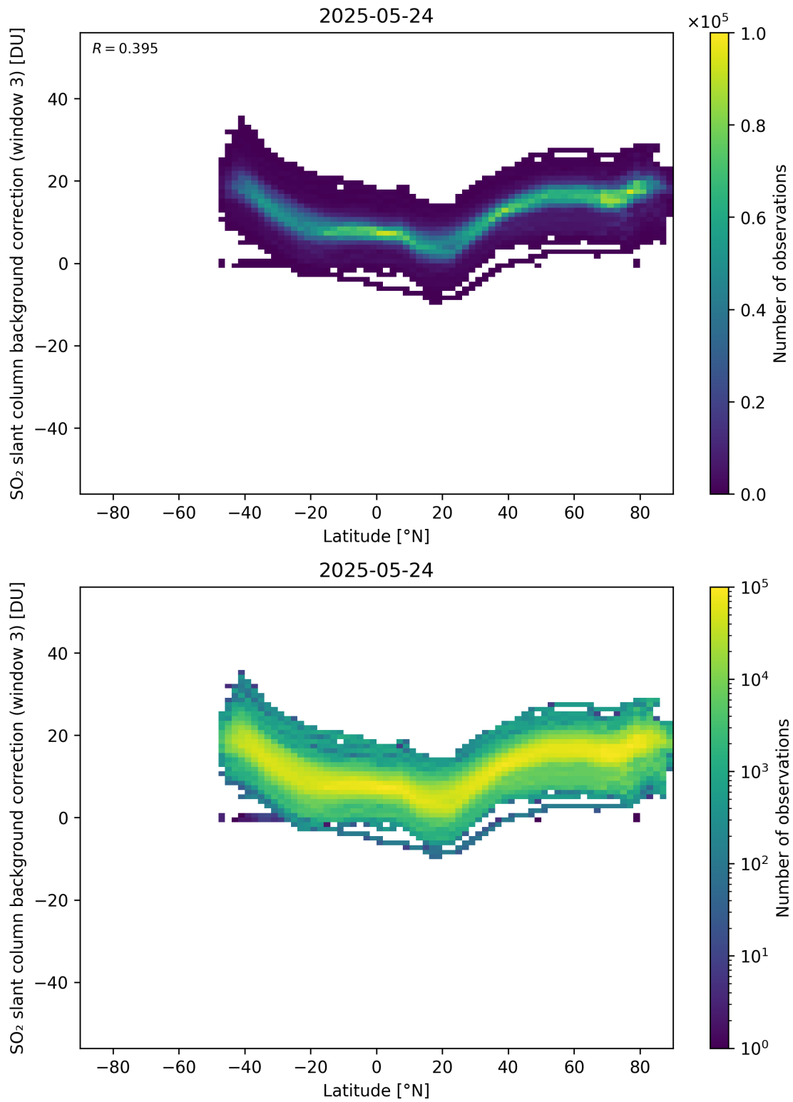
Figure 152: Scatter density plot of “Latitude” against “SO 2 slant column background correction (window 3)” for 2025-05-23 to 2025-05-25.
