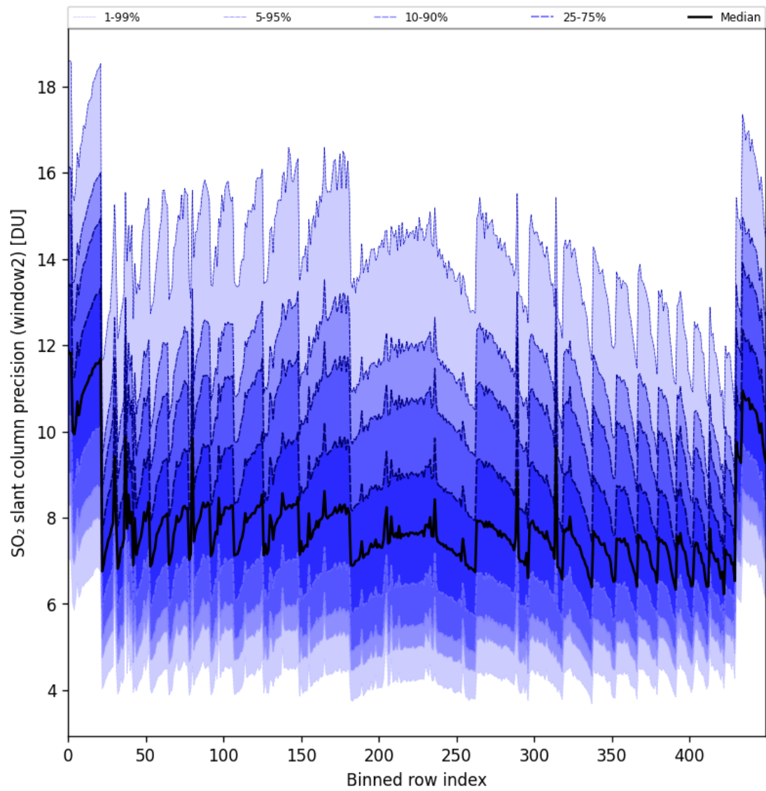
Figure 94: Along track statistics of “SO 2 slant column precision (window2)” for 2025-05-23 to 2025-05-25
