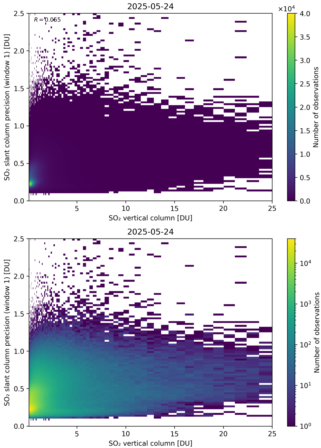
Figure 355: Scatter density plot of “SO 2 vertical column” against “SO 2 slant column precision (window 1)” for 2025-05-23 to 2025-05-25.
