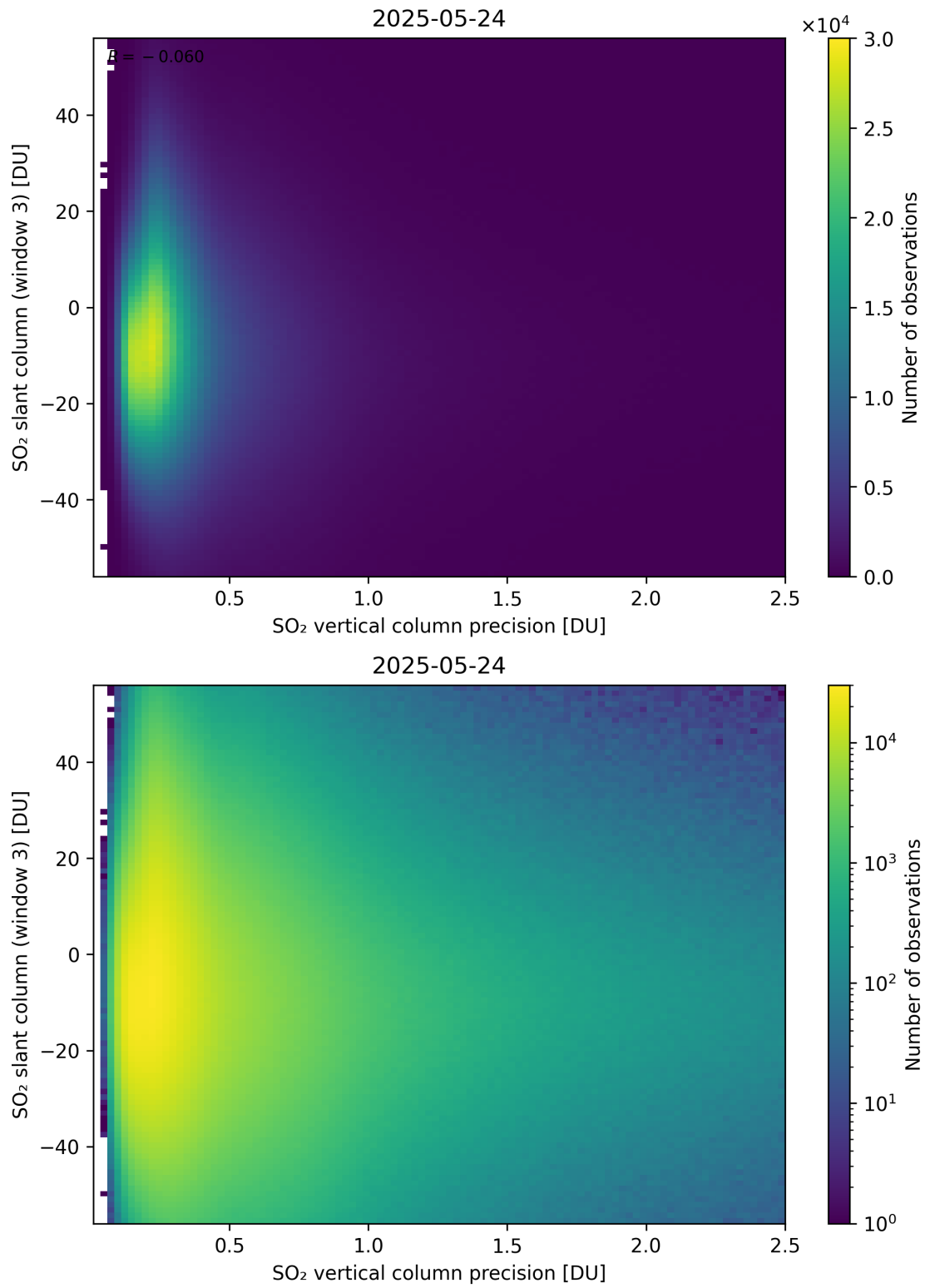
Figure 344: Scatter density plot of “SO 2 vertical column precision” against “SO 2 slant column (window 3)” for 2025-05-23 to 2025-05-25.
