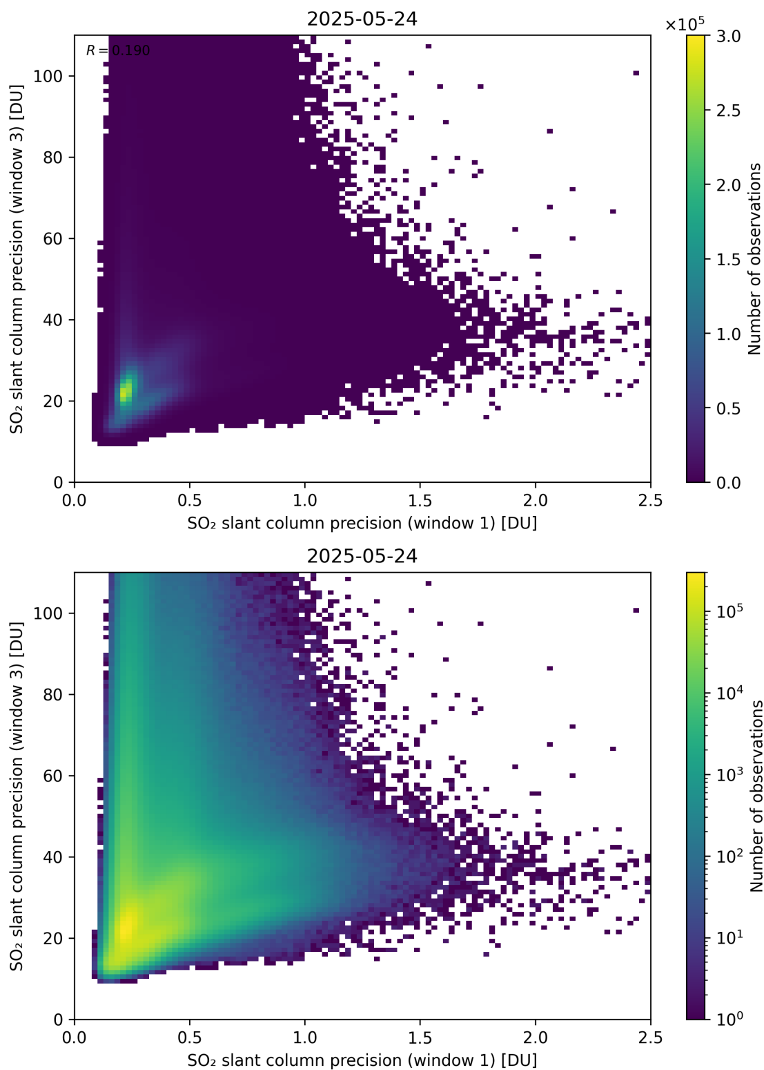
Figure 279: Scatter density plot of “SO 2 slant column precision (window 1)” against “SO 2 slant column precision (window 3)” for 2025-05-23 to 2025-05-25.
