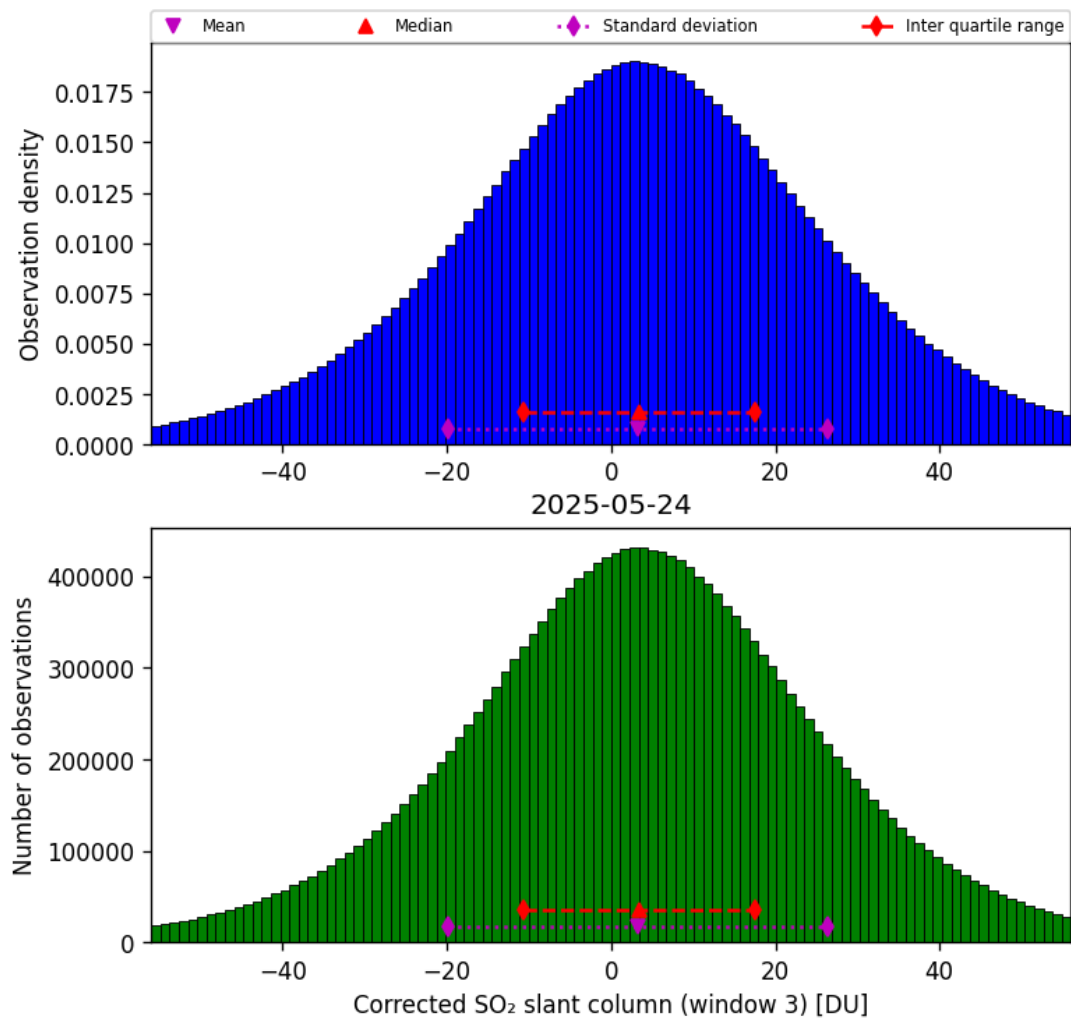
Figure 73: Histogram of "Corrected SO 2 slant column (window 3)" for 2025-05-23 to 2025-05-25
