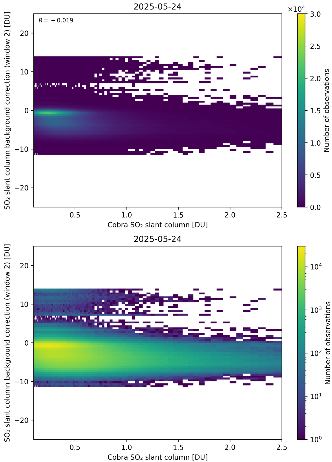
Figure 194: Scatter density plot of “Cobra SO 2 slant column” against “SO 2 slant column background correction (window 2)” for 2025-05-23 to 2025-05-25.
