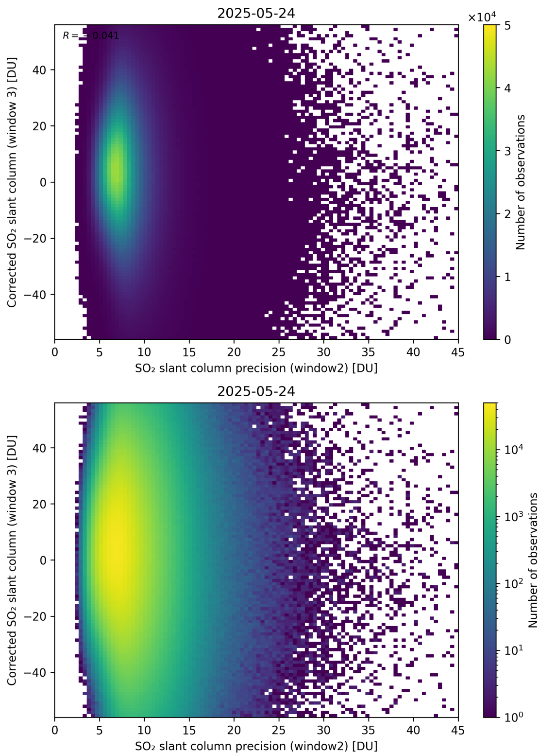
Figure 298: Scatter density plot of “SO 2 slant column precision (window2)” against “Corrected SO 2 slant column (window 3)” for 2025-05-23 to 2025-05-25.
