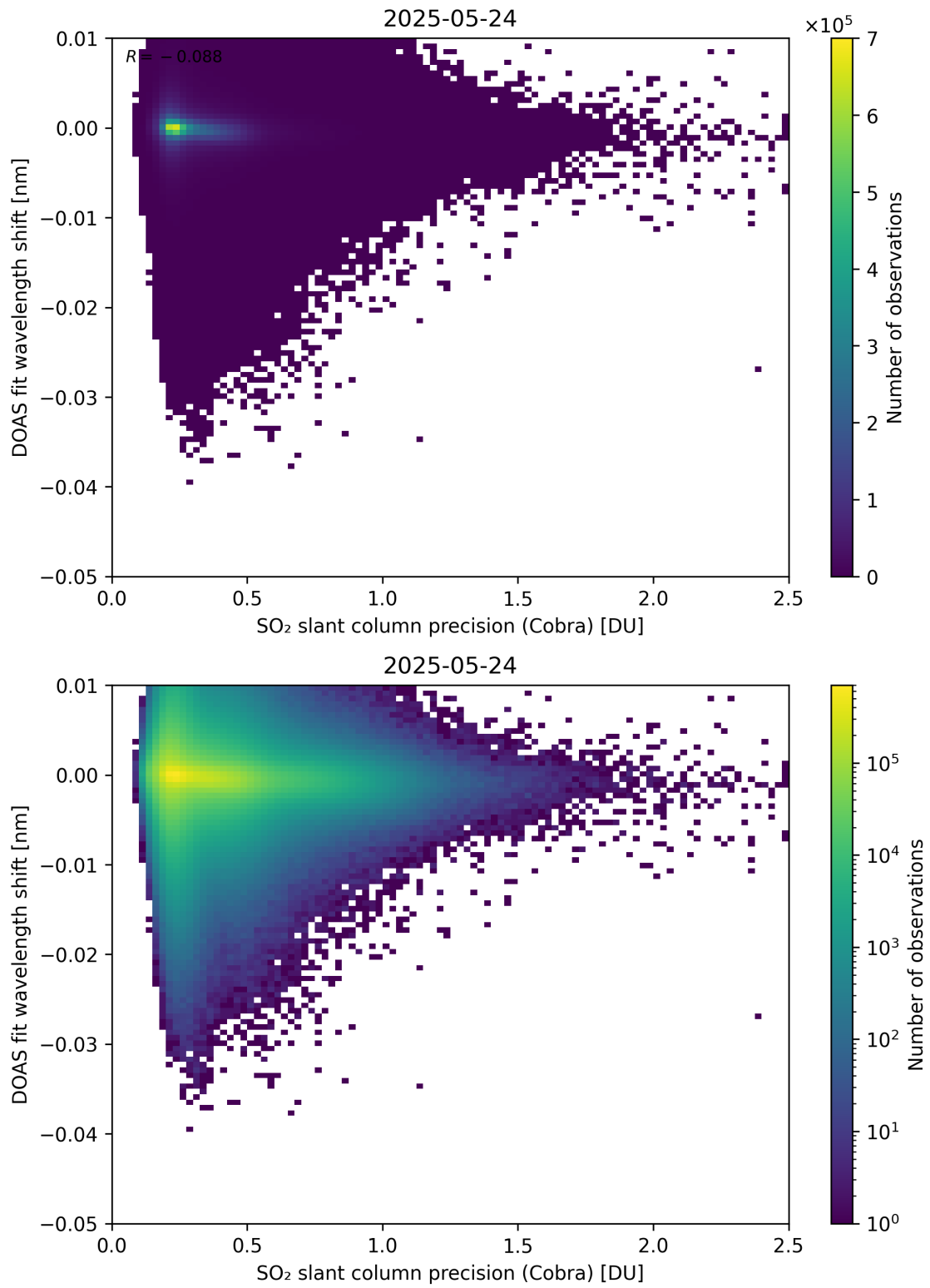
Figure 202: Scatter density plot of “SO 2 slant column precision (Cobra)” against “DOAS fit wavelength shift” for 2025-05-23 to 2025-05-25.
