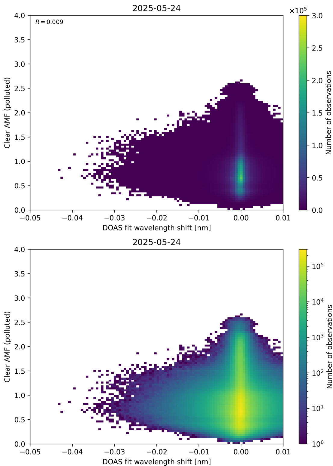
Figure 140: Scatter density plot of “DOAS fit wavelength shift” against “Clear AMF (polluted)” for 2025-05-23 to 2025-05-25.
