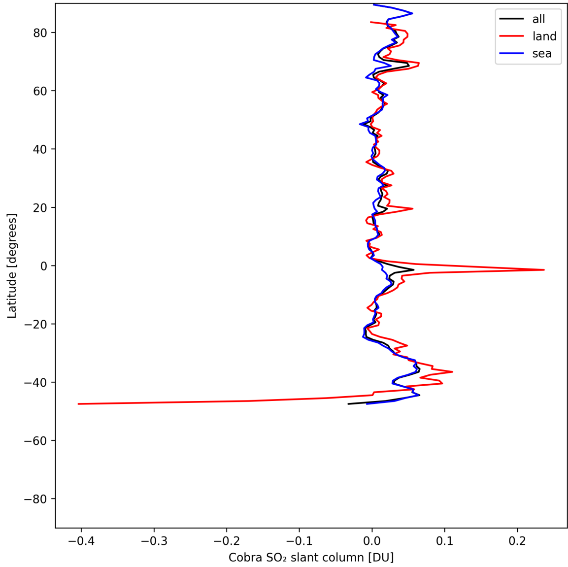
Figure 35: Zonal average of “Cobra SO 2 slant column” for 2025-05-23 to 2025-05-25.
