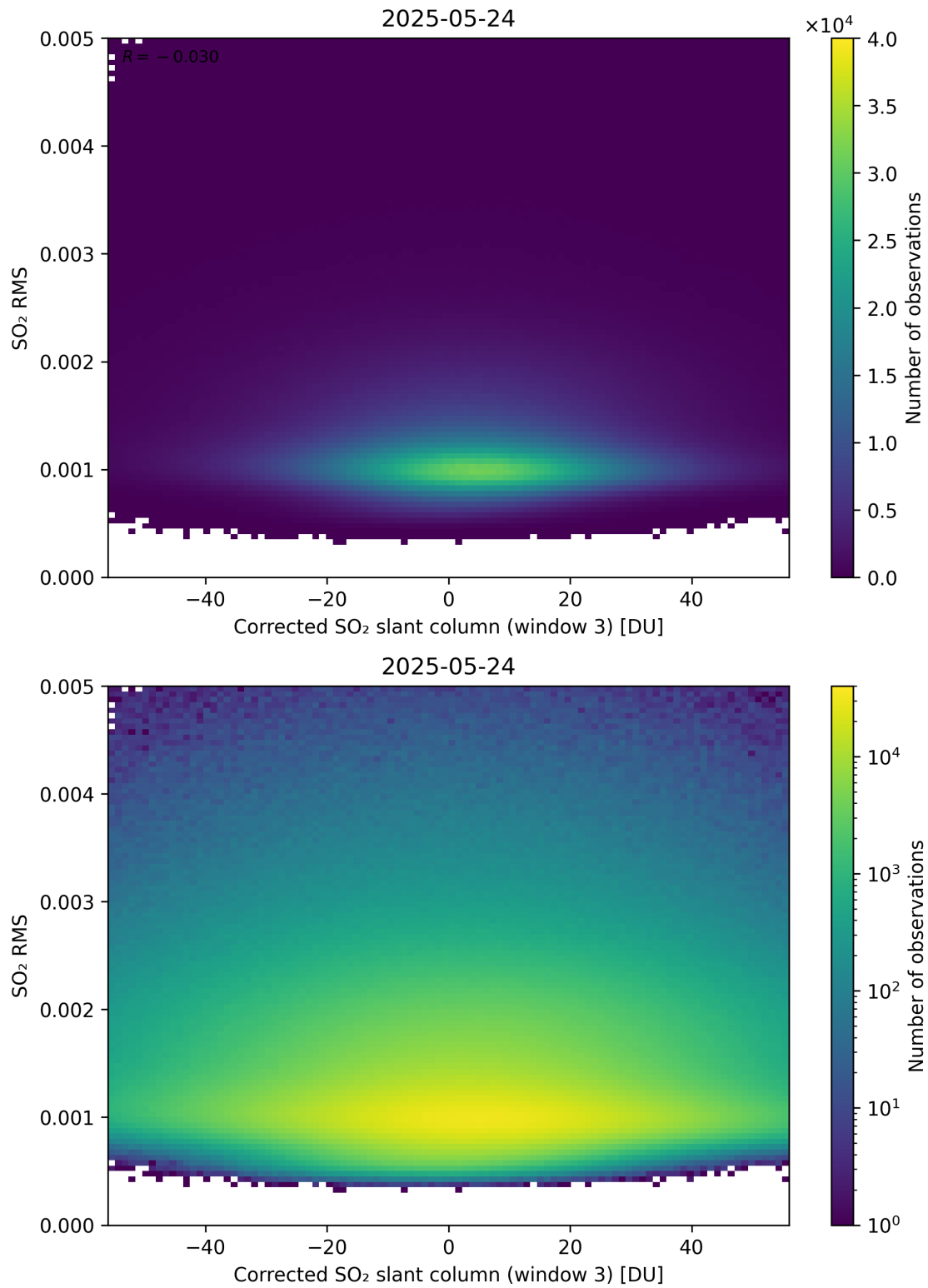
Figure 258: Scatter density plot of “Corrected SO 2 slant column (window 3)” against “SO 2 RMS” for 2025-05-23 to 2025-05-25.
