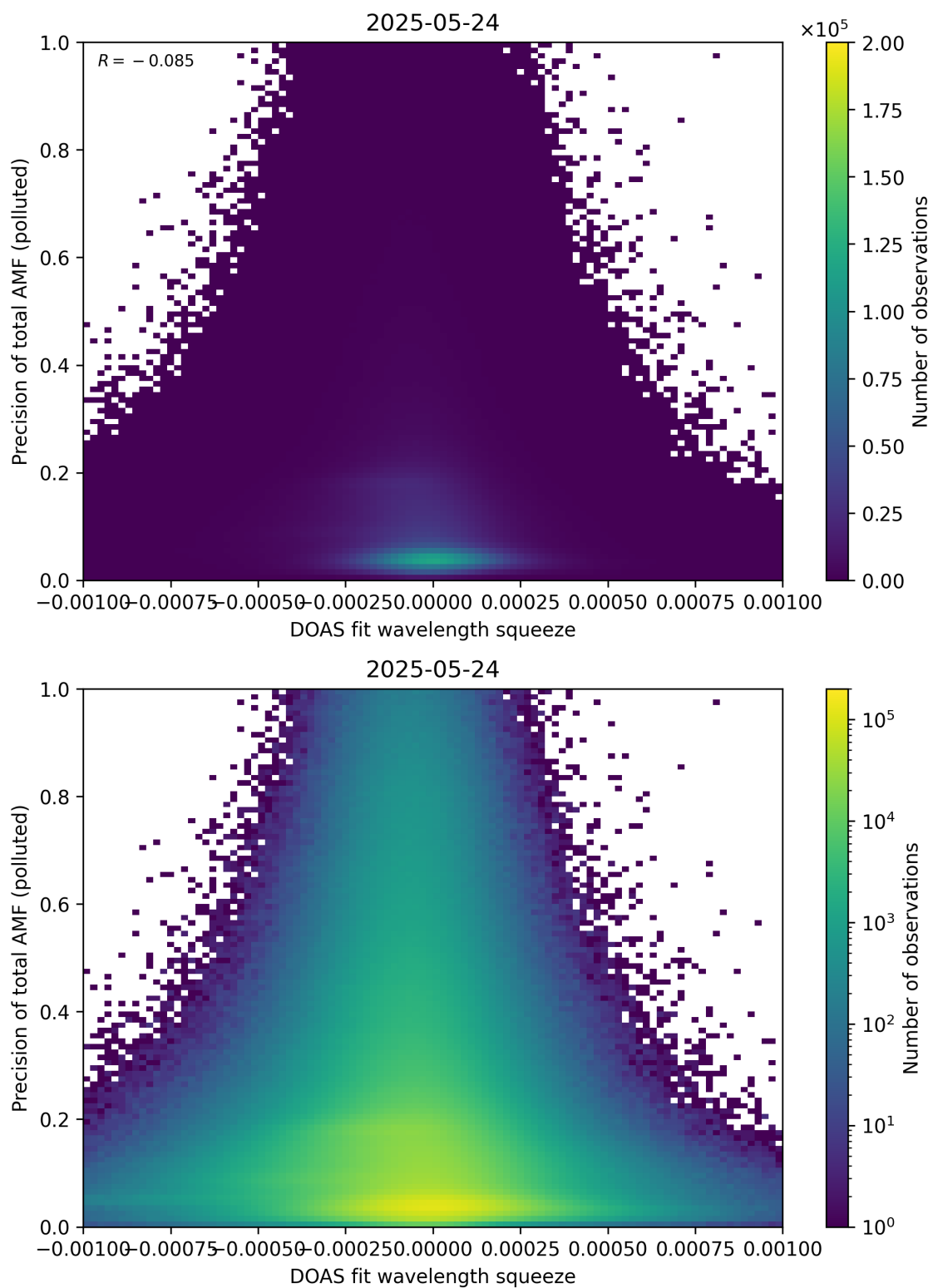
Figure 146: Scatter density plot of “DOAS fit wavelength squeeze” against “Precision of total AMF (polluted)” for 2025-05-23 to 2025-05-25.
