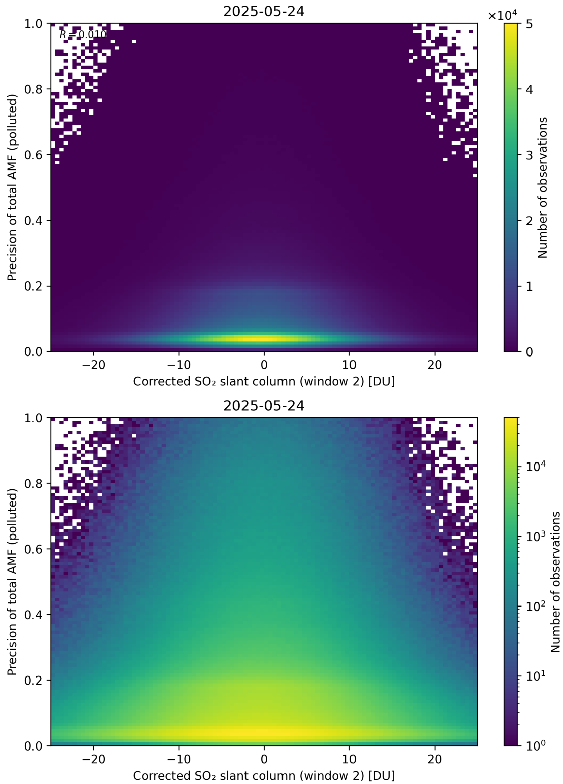
Figure 254: Scatter density plot of “Corrected SO 2 slant column (window 2)” against “Precision of total AMF (polluted)” for 2025-05-23 to 2025-05-25.
