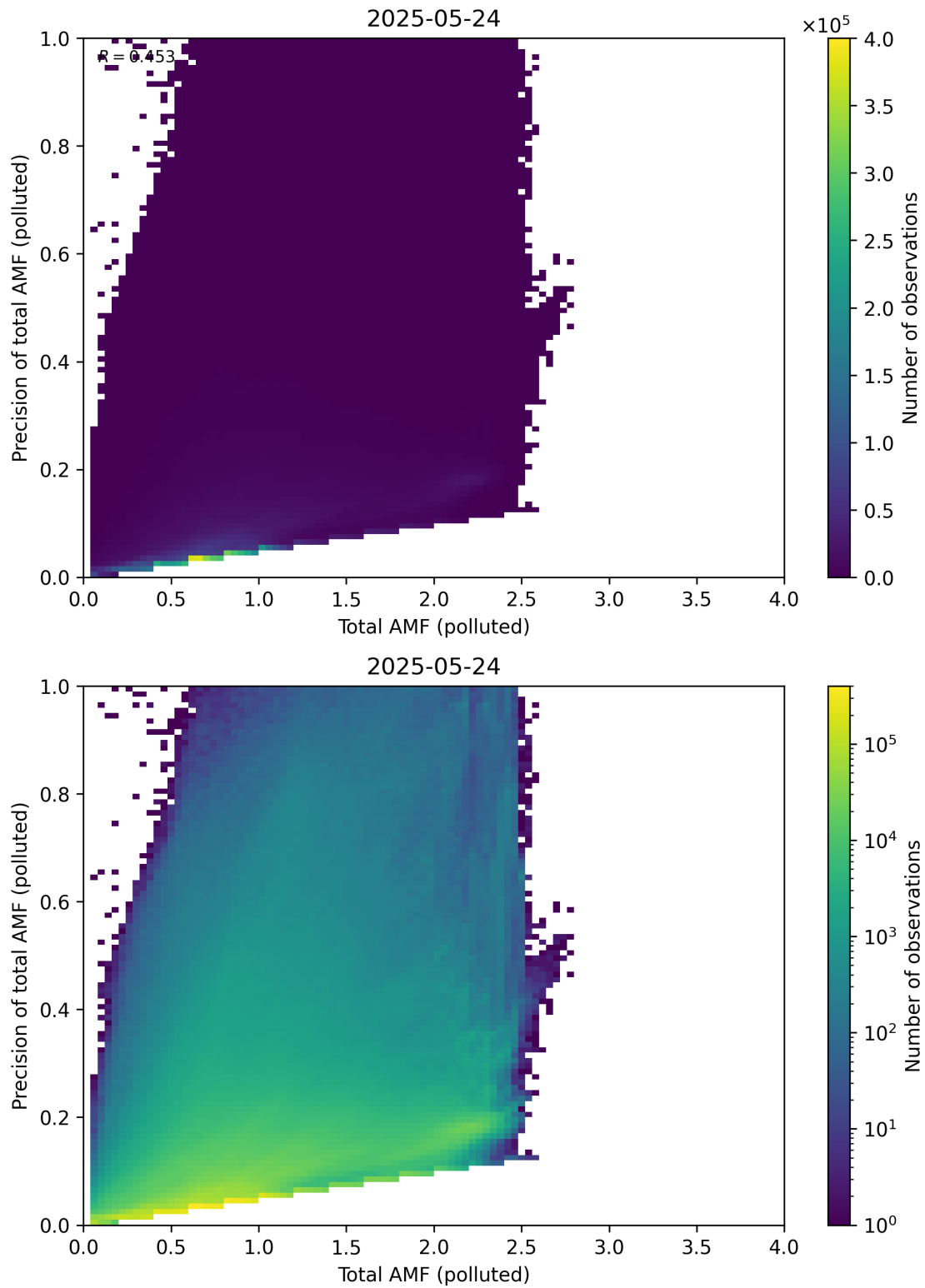
Figure 322: Scatter density plot of “Total AMF (polluted)” against “Precision of total AMF (polluted)” for 2025-05-23 to 2025-05-25.
