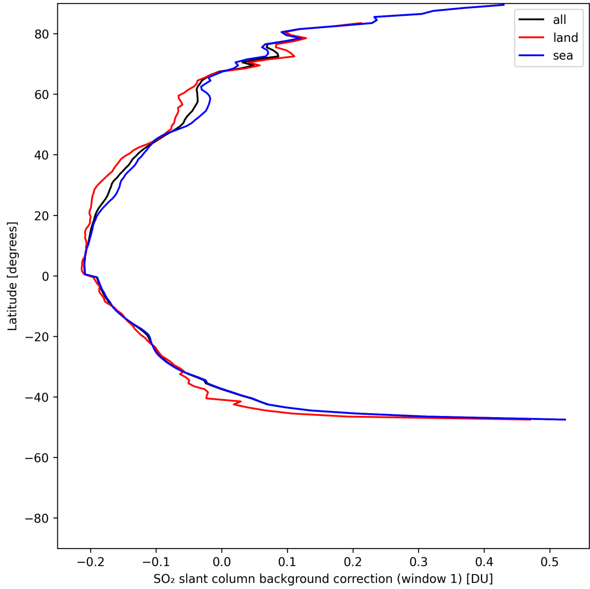
Figure 40: Zonal average of “SO 2 slant column background correction (window 1)” for 2025-05-23 to 2025-05-25.
