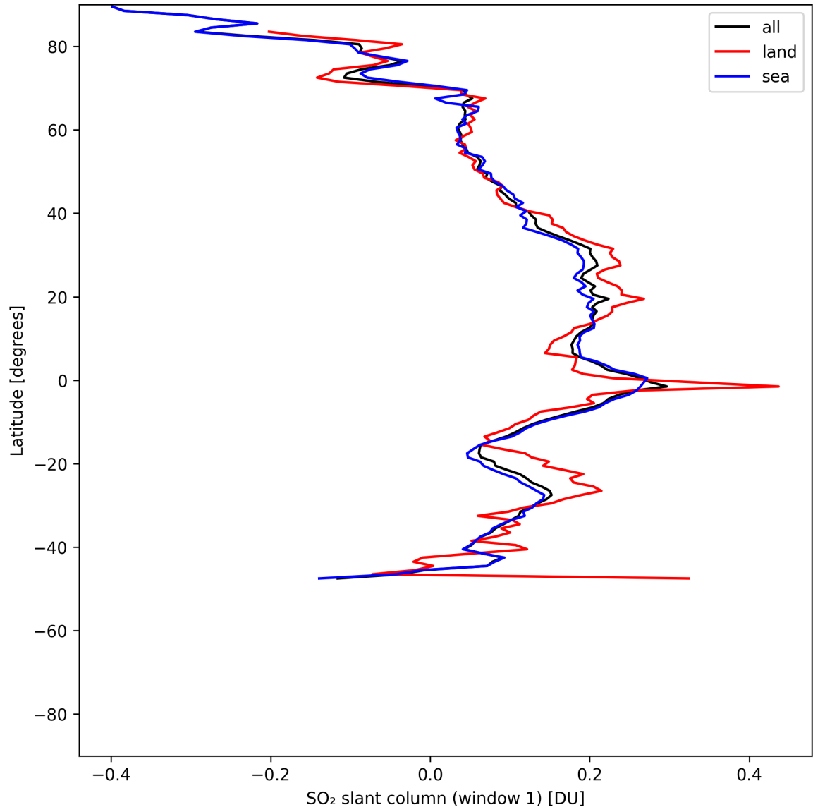
Figure 37: Zonal average of “SO 2 slant column (window 1)” for 2025-05-23 to 2025-05-25.
