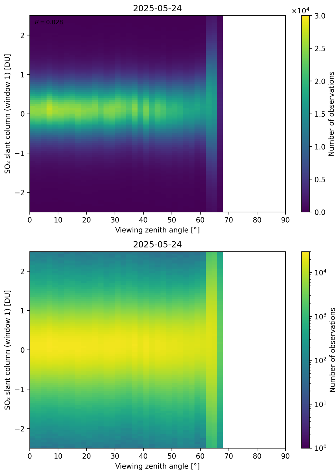
Figure 376: Scatter density plot of “Viewing zenith angle” against “SO 2 slant column (window 1)” for 2025-05-23 to 2025-05-25.
