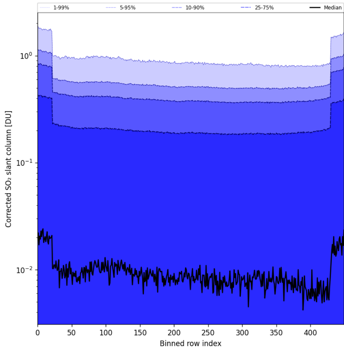
Figure 86: Along track statistics of “Corrected SO 2 slant column” for 2025-05-23 to 2025-05-25
