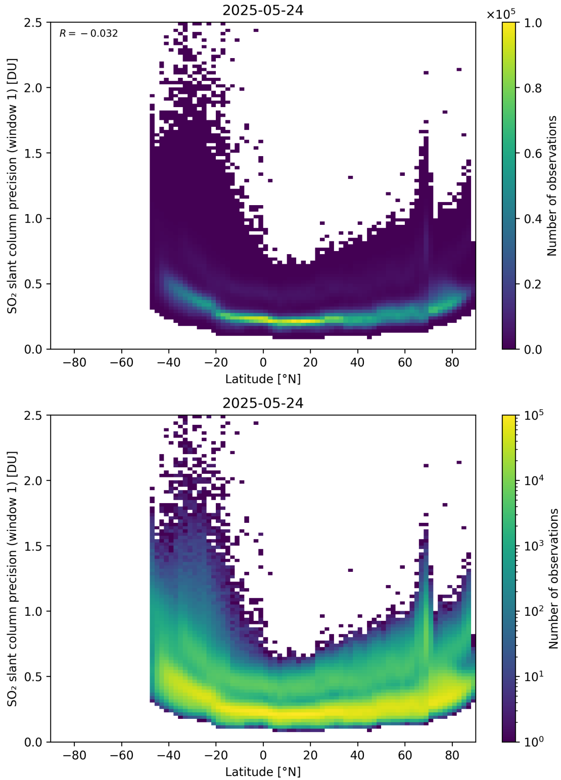
Figure 163: Scatter density plot of “Latitude” against “SO 2 slant column precision (window 1)” for 2025-05-23 to 2025-05-25.
