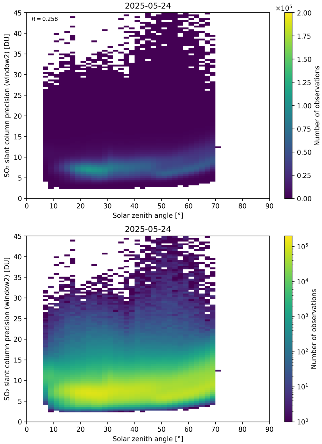
Figure 186: Scatter density plot of “Solar zenith angle” against “SO 2 slant column precision (window2)” for 2025-05-23 to 2025-05-25.
