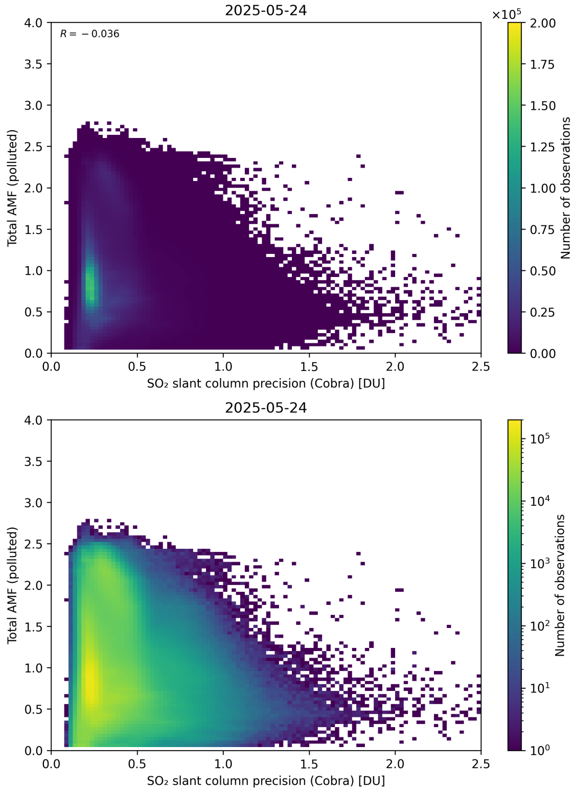
Figure 213: Scatter density plot of “SO 2 slant column precision (Cobra)” against “Total AMF (polluted)” for 2025-05-23 to 2025-05-25.
