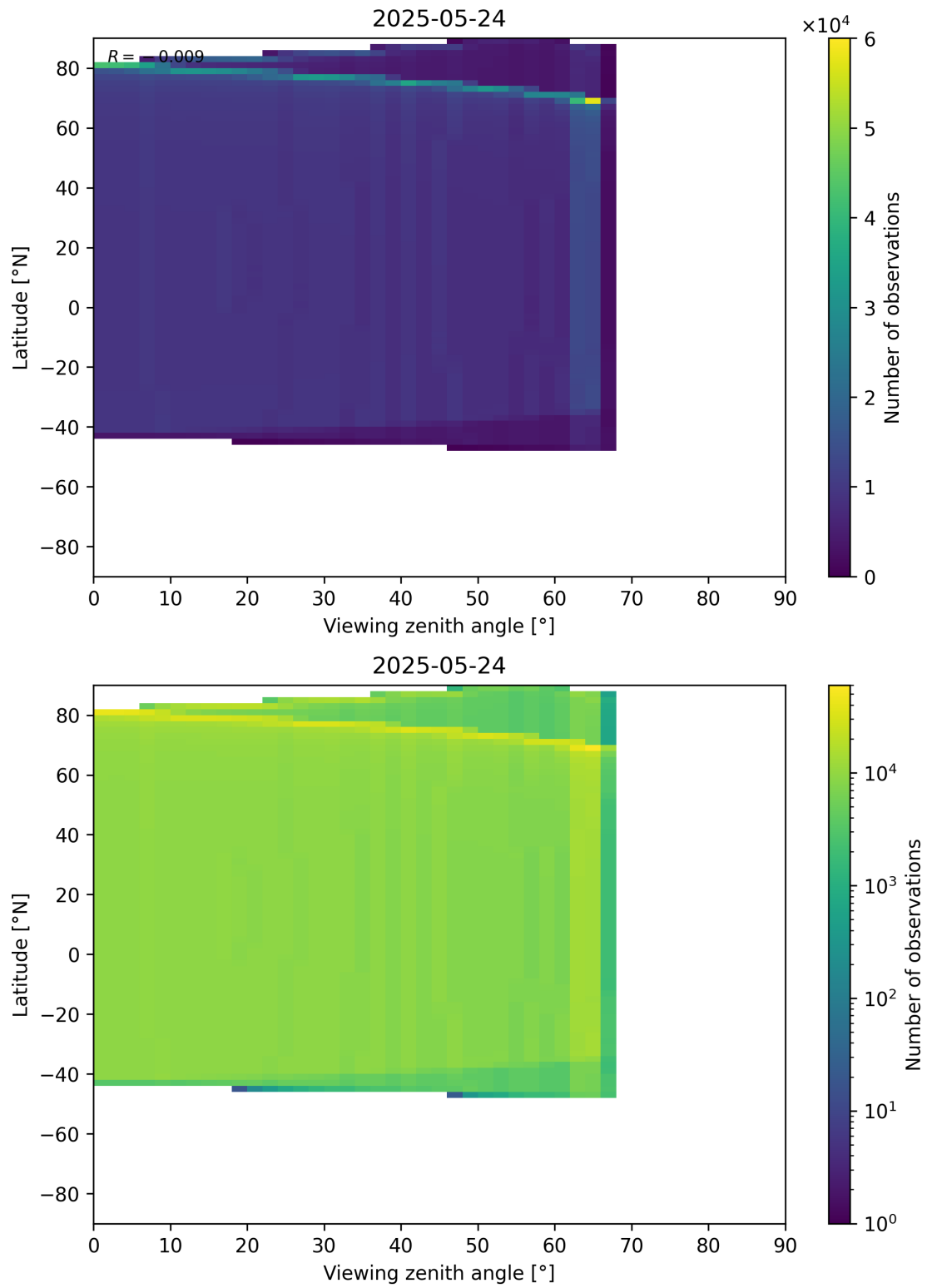
Figure 368: Scatter density plot of “Viewing zenith angle” against “Latitude” for 2025-05-23 to 2025-05-25.
