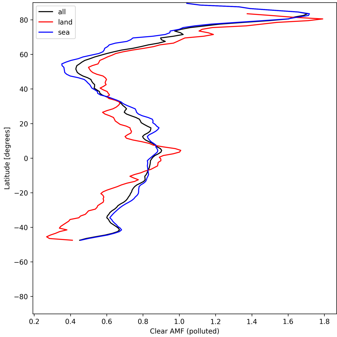
Figure 55: Zonal average of “Clear AMF (polluted)” for 2025-05-23 to 2025-05-25.
