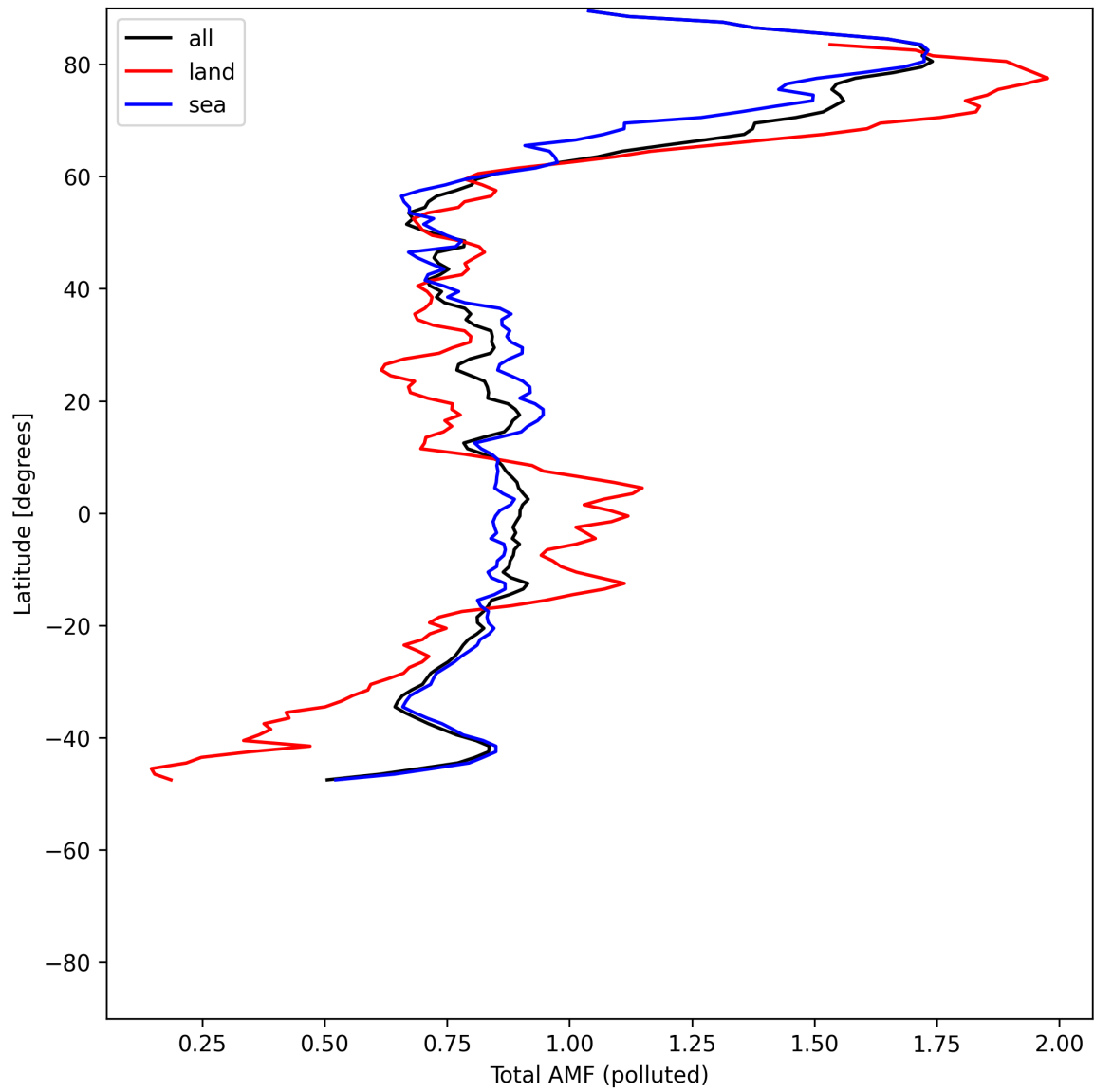
Figure 53: Zonal average of “Total AMF (polluted)” for 2025-05-23 to 2025-05-25.
