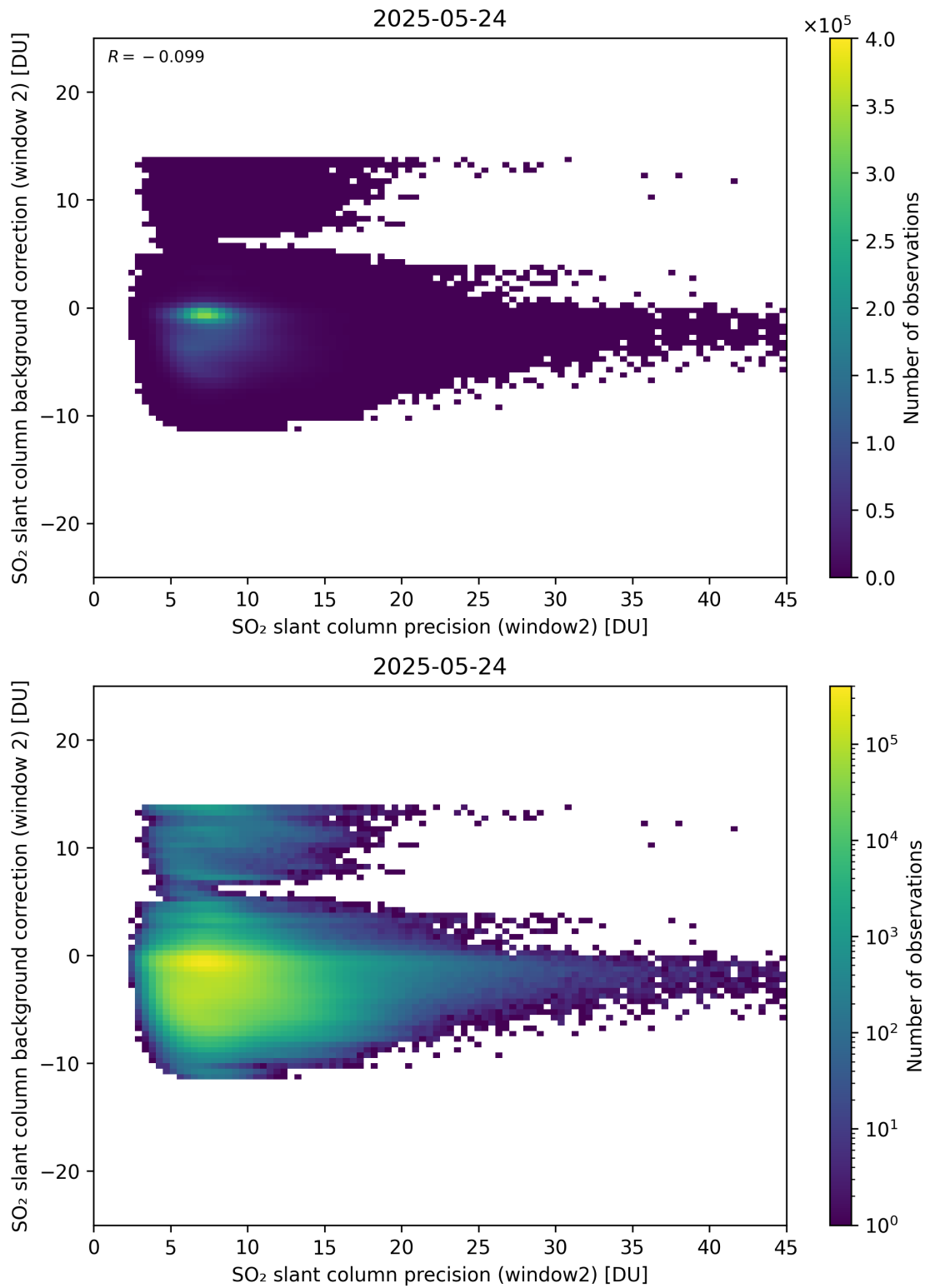
Figure 291: Scatter density plot of “SO 2 slant column precision (window2)” against “SO 2 slant column background correction (window 2)” for 2025-05-23 to 2025-05-25.
