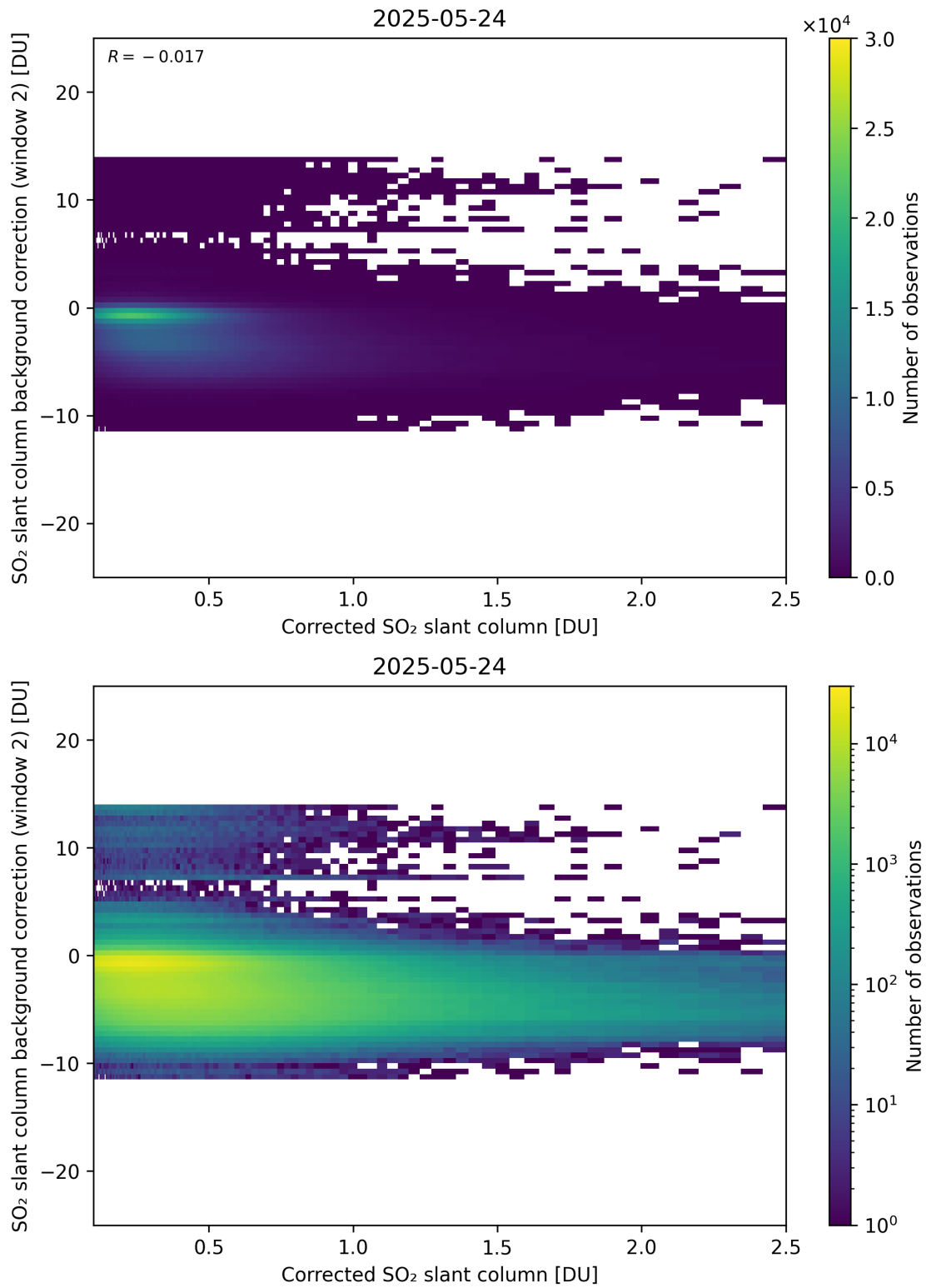
Figure 227: Scatter density plot of “Corrected SO 2 slant column” against “SO 2 slant column background correction (window 2)” for 2025-05-23 to 2025-05-25.
