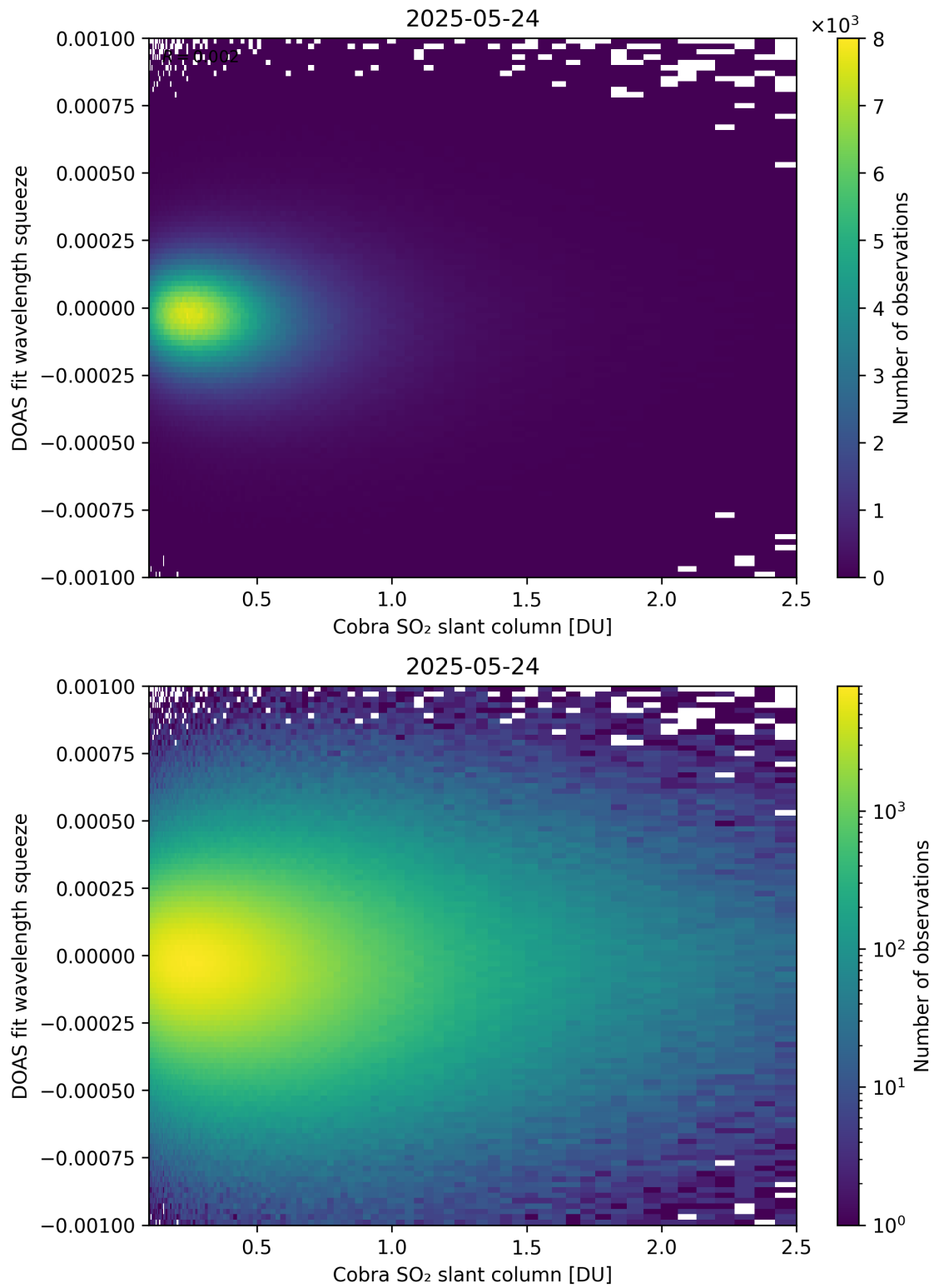
Figure 197: Scatter density plot of “Cobra SO 2 slant column” against “DOAS fit wavelength squeeze” for 2025-05-23 to 2025-05-25.
