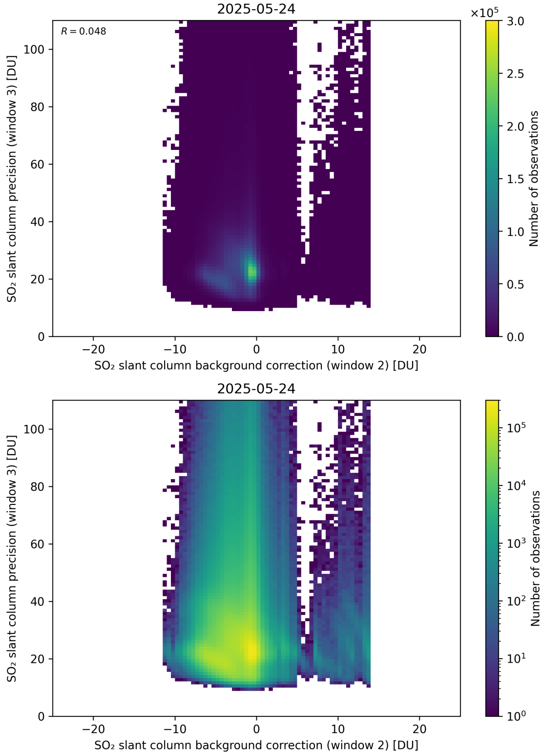
Figure 129: Scatter density plot of “SO 2 slant column background correction (window 2)” against “SO 2 slant column precision (window 3)” for 2025-05-23 to 2025-05-25.
