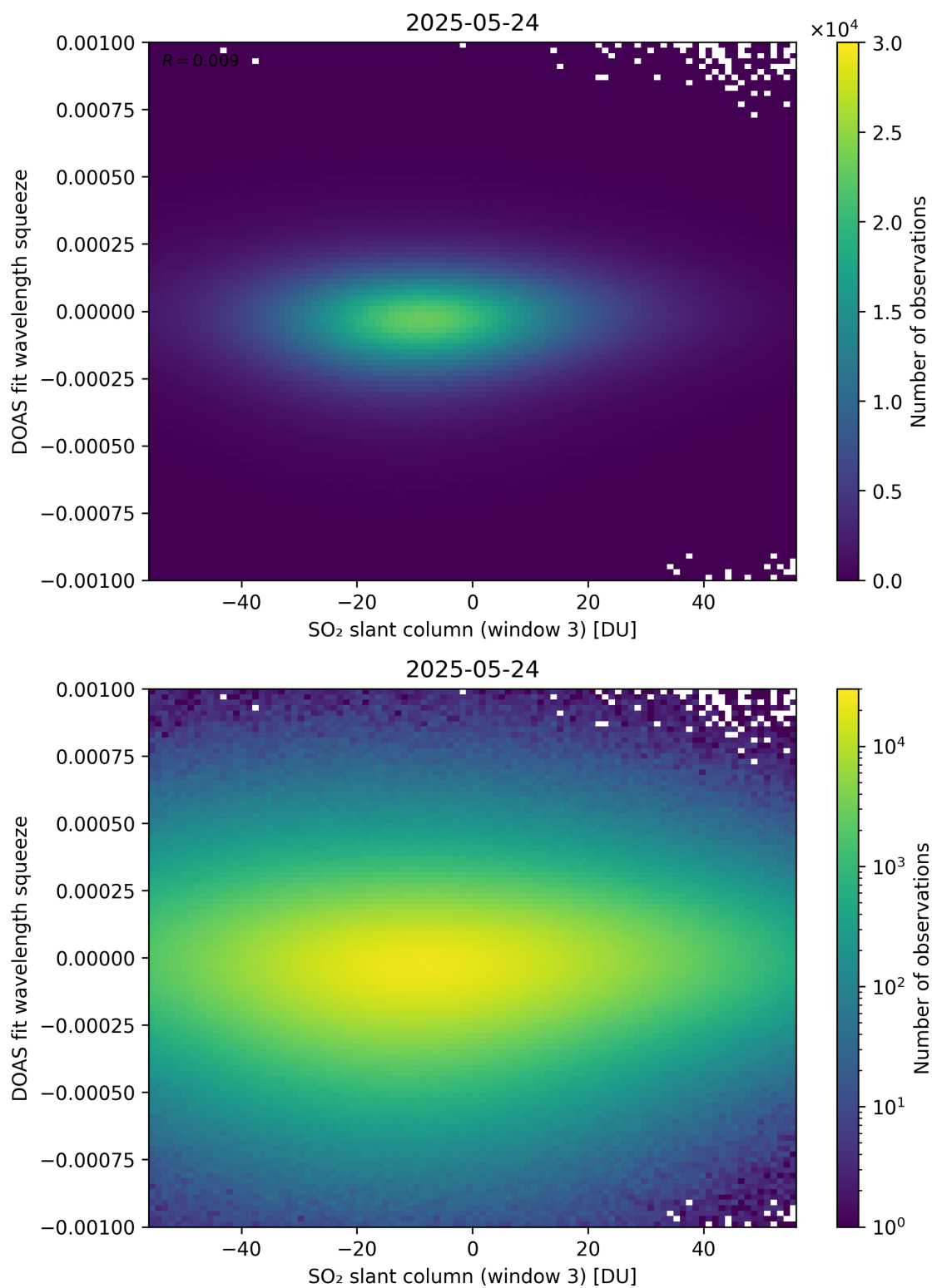
Figure 305: Scatter density plot of “SO 2 slant column (window 3)” against “DOAS fit wavelength squeeze” for 2025-05-23 to 2025-05-25.
