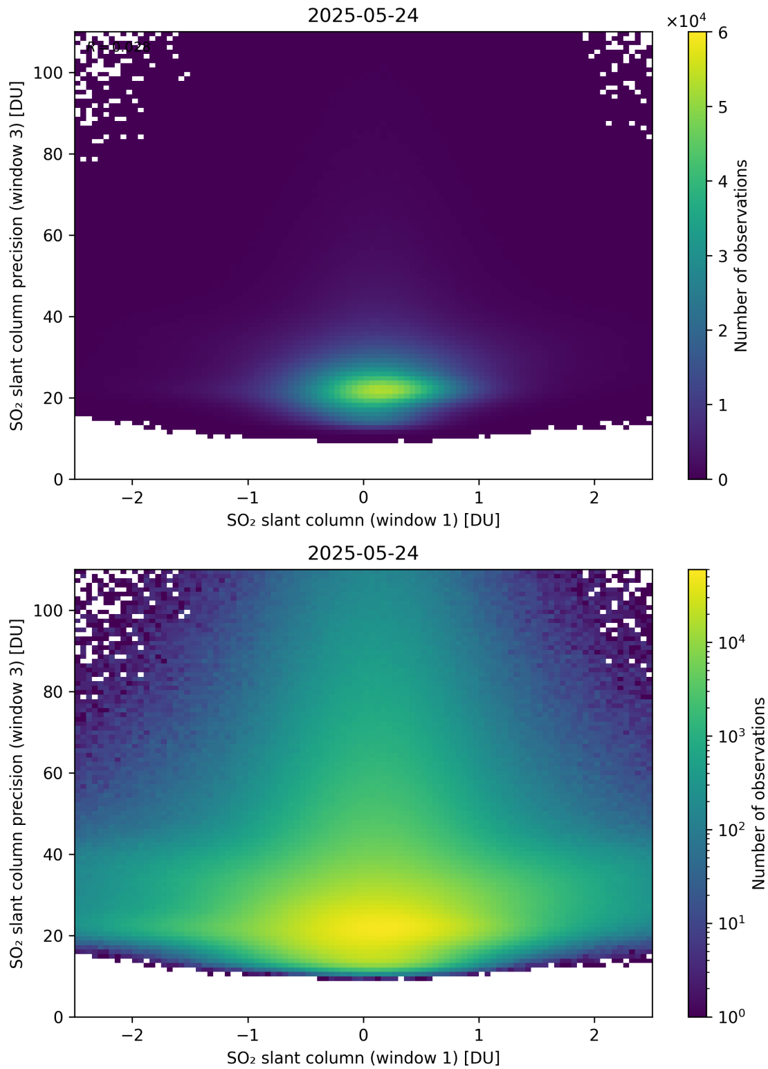
Figure 288: Scatter density plot of “SO 2 slant column (window 1)” against “SO 2 slant column precision (window 3)” for 2025-05-23 to 2025-05-25.
