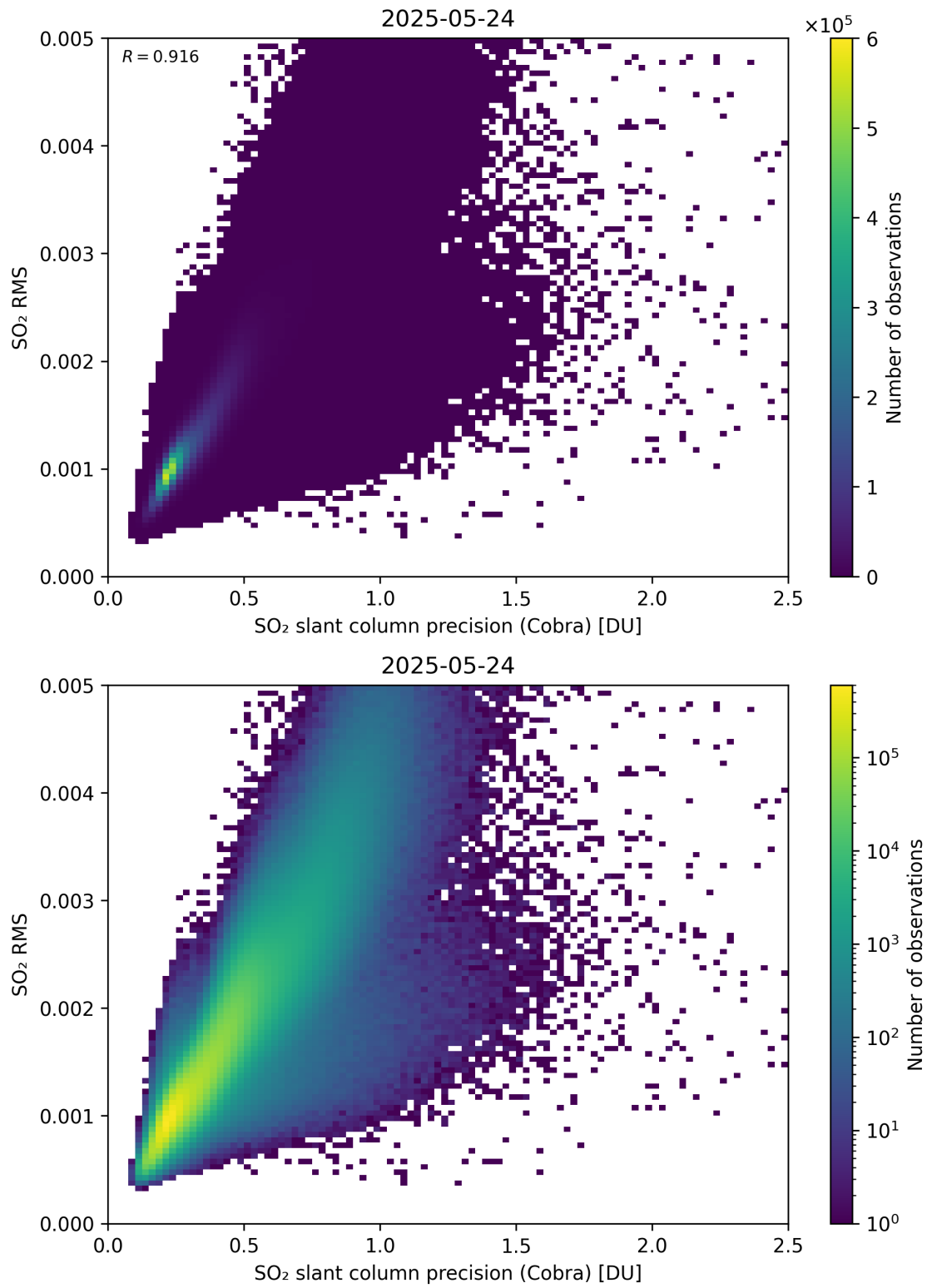
Figure 204: Scatter density plot of “SO 2 slant column precision (Cobra)” against “SO 2 RMS” for 2025-05-23 to 2025-05-25.
