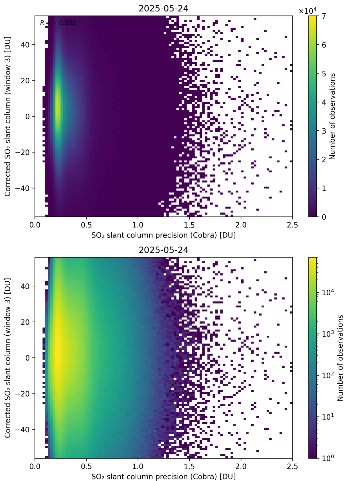
Figure 207: Scatter density plot of “SO 2 slant column precision (Cobra)” against “Corrected SO 2 slant column (window 3)” for 2025-05-23 to 2025-05-25.
