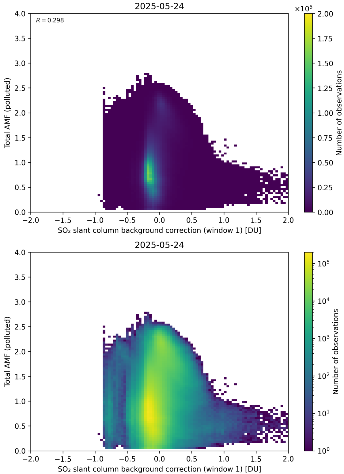
Figure 120: Scatter density plot of “SO 2 slant column background correction (window 1)” against “Total AMF (polluted)” for 2025-05-23 to 2025-05-25.
