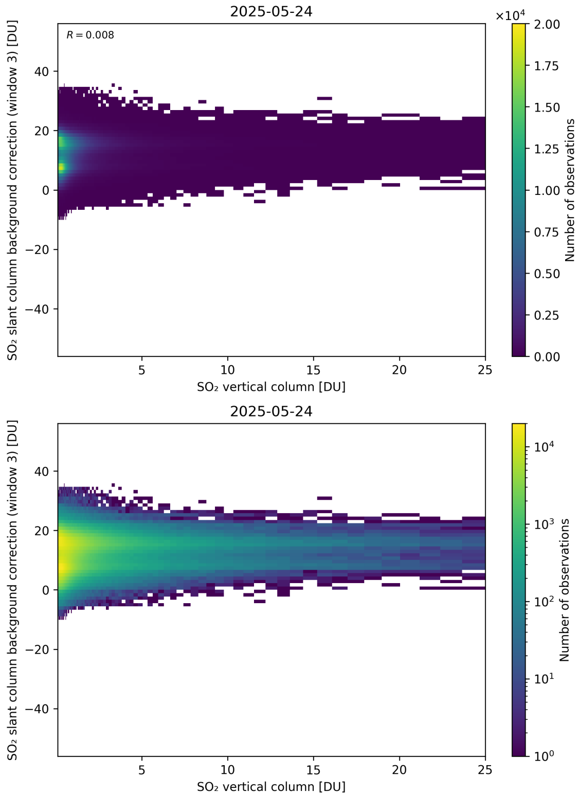
Figure 325: Scatter density plot of “SO 2 vertical column” against “SO 2 slant column background correction (window 3)” for 2025-05-23 to 2025-05-25.
