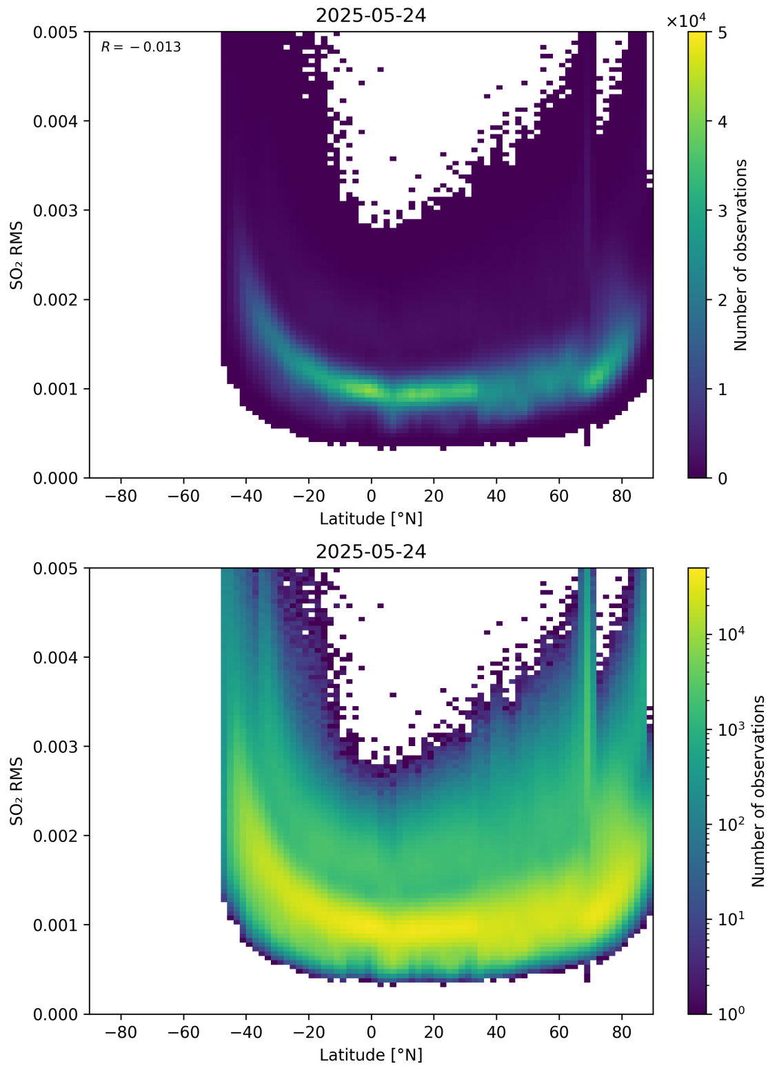
Figure 155: Scatter density plot of “Latitude” against “SO 2 RMS” for 2025-05-23 to 2025-05-25.
