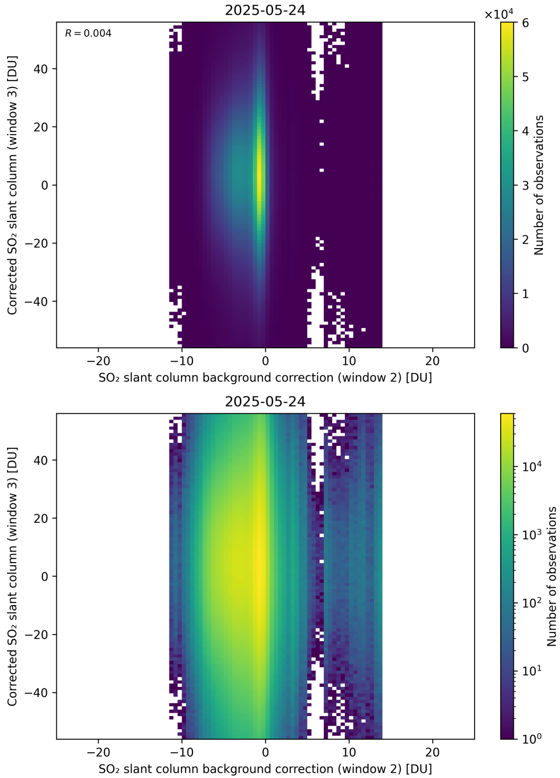
Figure 127: Scatter density plot of “SO 2 slant column background correction (window 2)” against “Corrected SO 2 slant column (window 3)” for 2025-05-23 to 2025-05-25.
