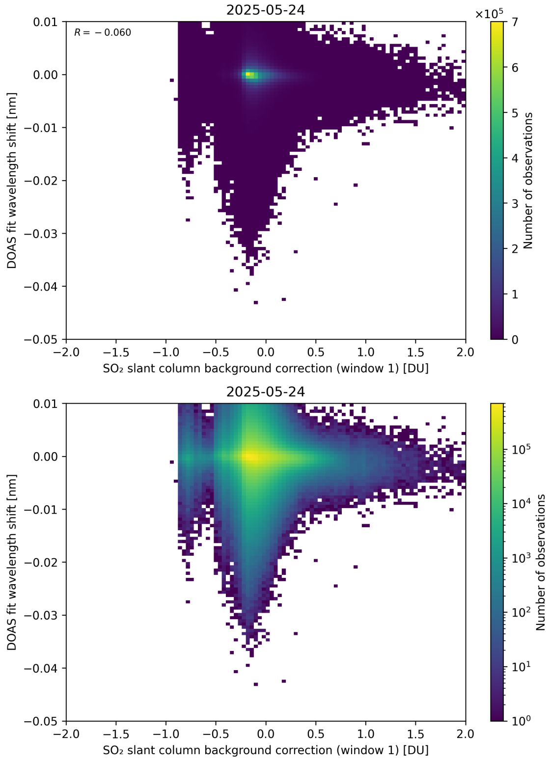
Figure 111: Scatter density plot of “SO 2 slant column background correction (window 1)” against “DOAS fit wavelength shift” for 2025-05-23 to 2025-05-25.
