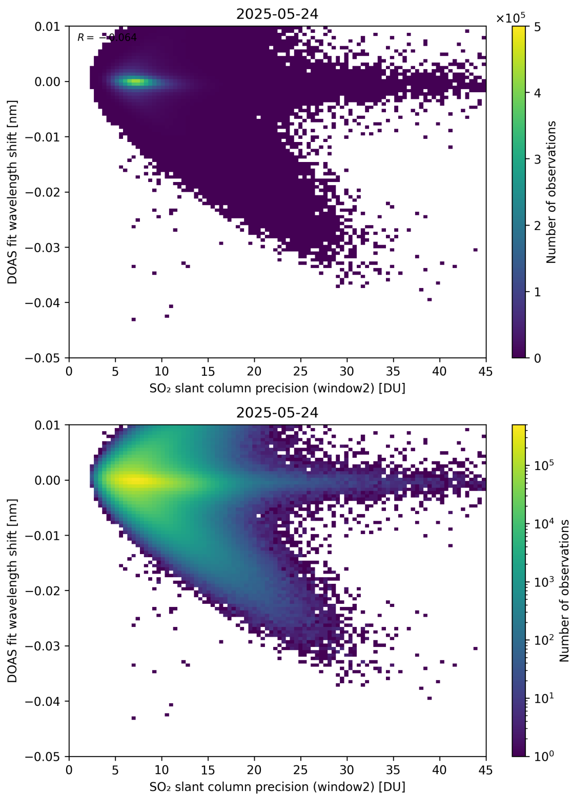
Figure 293: Scatter density plot of “SO 2 slant column precision (window2)” against “DOAS fit wavelength shift” for 2025-05-23 to 2025-05-25.
