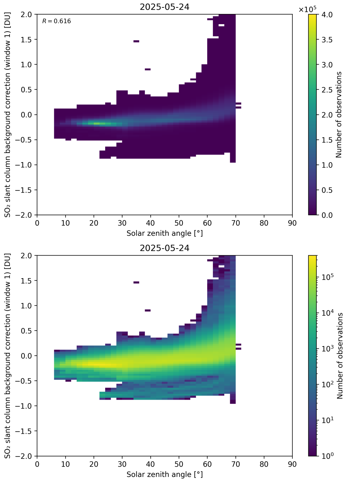
Figure 171: Scatter density plot of “Solar zenith angle” against “SO 2 slant column background correction (window 1)” for 2025-05-23 to 2025-05-25.
