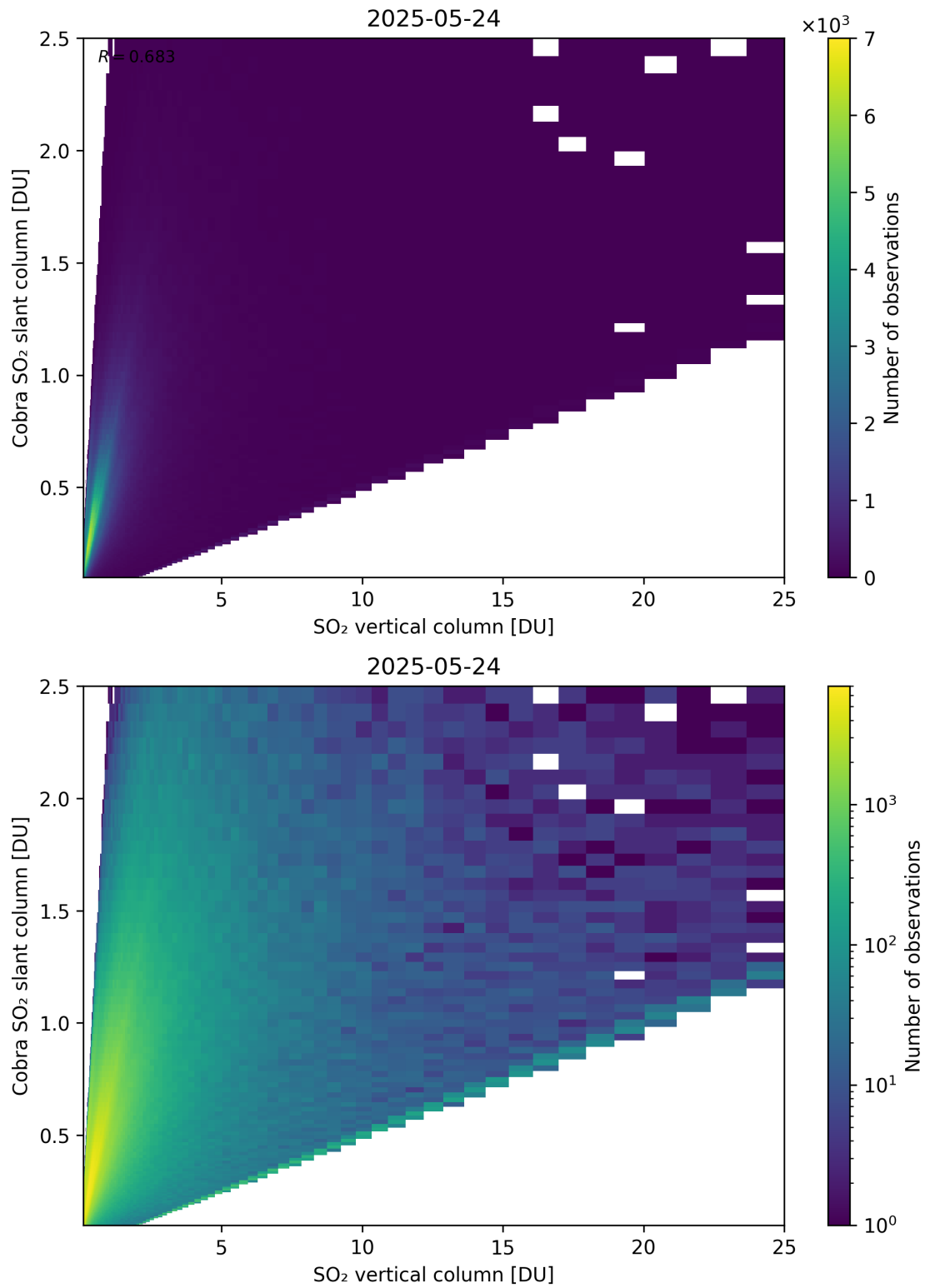
Figure 349: Scatter density plot of “SO 2 vertical column” against “Cobra SO 2 slant column” for 2025-05-23 to 2025-05-25.
