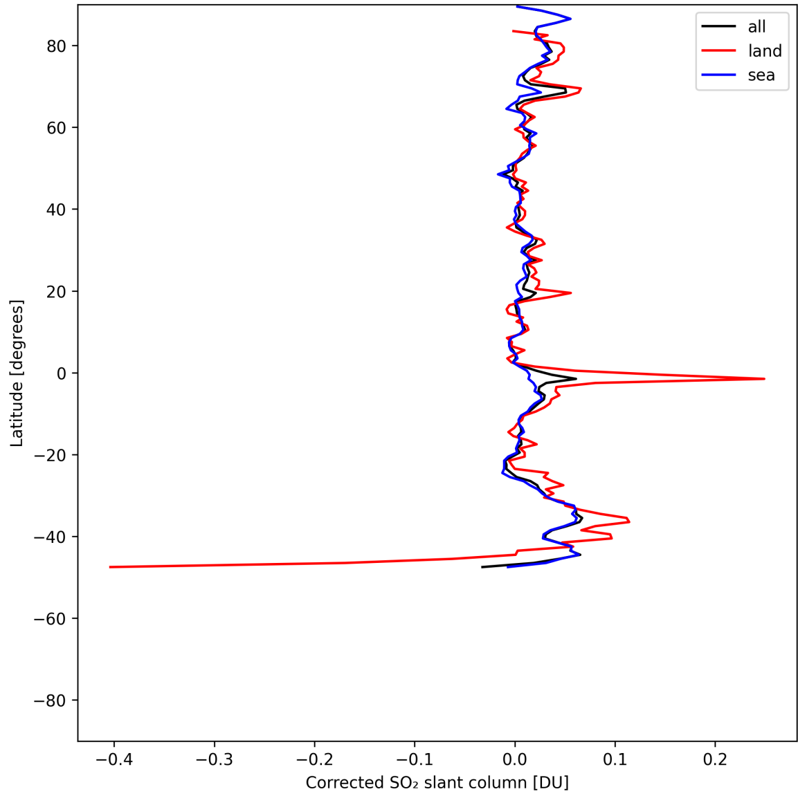
Figure 34: Zonal average of “Corrected SO 2 slant column” for 2025-05-23 to 2025-05-25.
