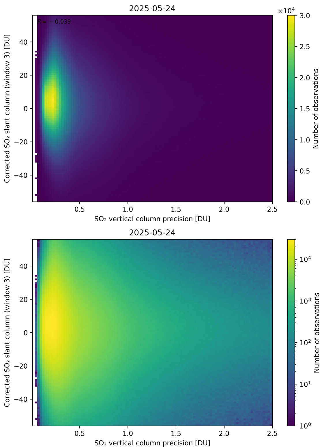
Figure 340: Scatter density plot of “SO 2 vertical column precision” against “Corrected SO 2 slant column (window 3)” for 2025-05-23 to 2025-05-25.
