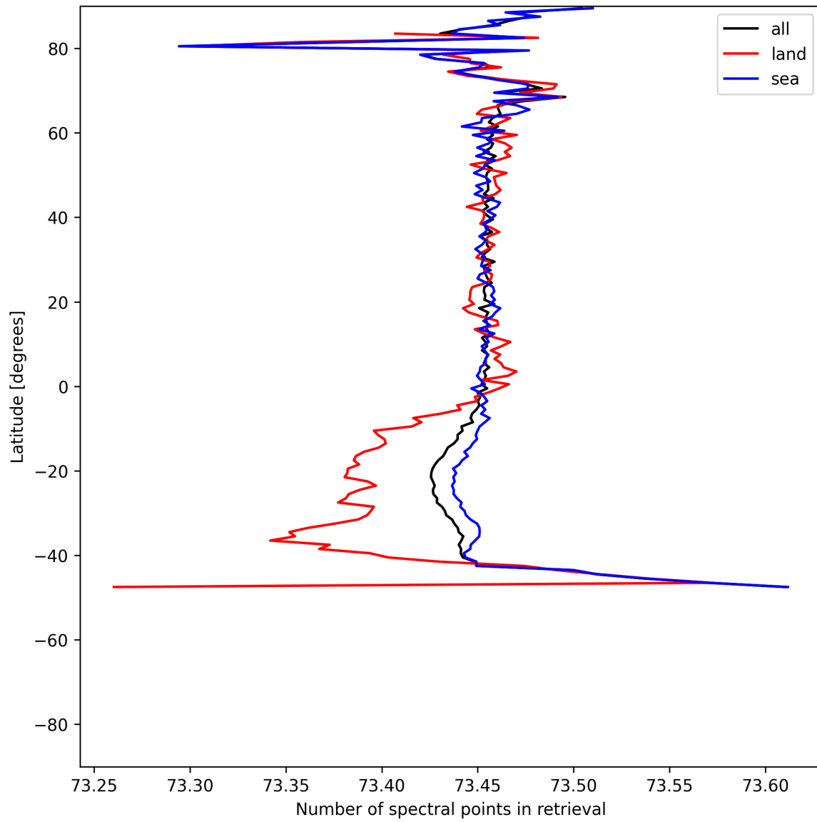
Figure 56: Zonal average of “Number of spectral points in retrieval” for 2025-05-23 to 2025-05-25.
