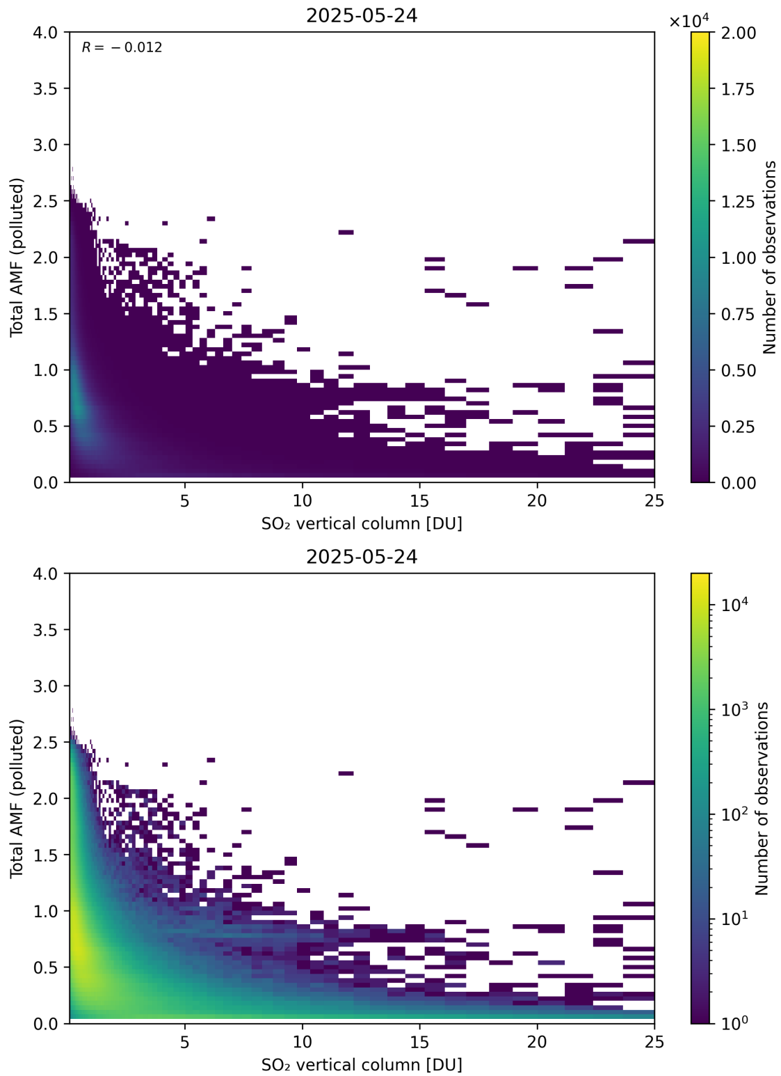
Figure 359: Scatter density plot of “SO 2 vertical column” against “Total AMF (polluted)” for 2025-05-23 to 2025-05-25.
