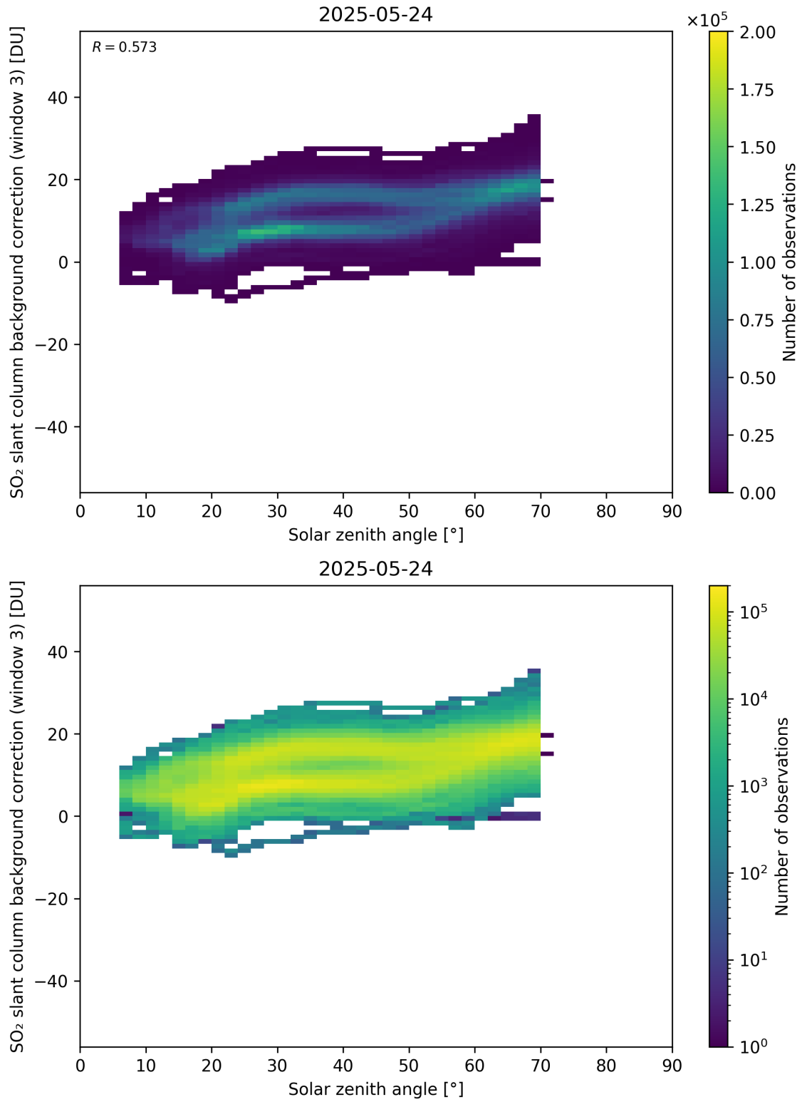
Figure 173: Scatter density plot of “Solar zenith angle” against “SO 2 slant column background correction (window 3)” for 2025-05-23 to 2025-05-25.
