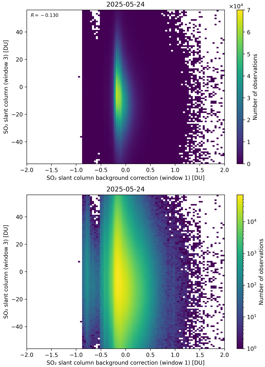
Figure 118: Scatter density plot of “SO 2 slant column background correction (window 1)” against “SO 2 slant column (window 3)” for 2025-05-23 to 2025-05-25.
