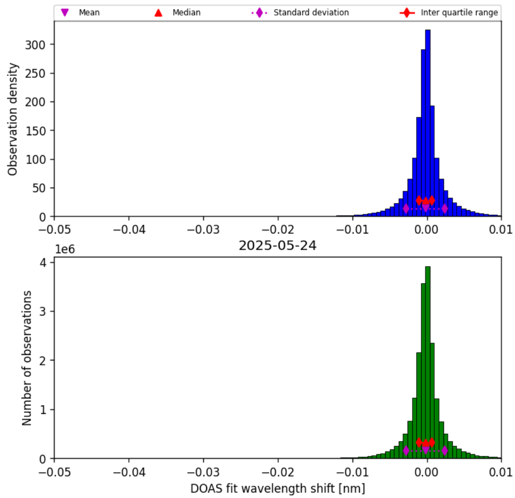
Figure 76: Histogram of “DOAS fit wavelength shift” for 2025-05-23 to 2025-05-25
