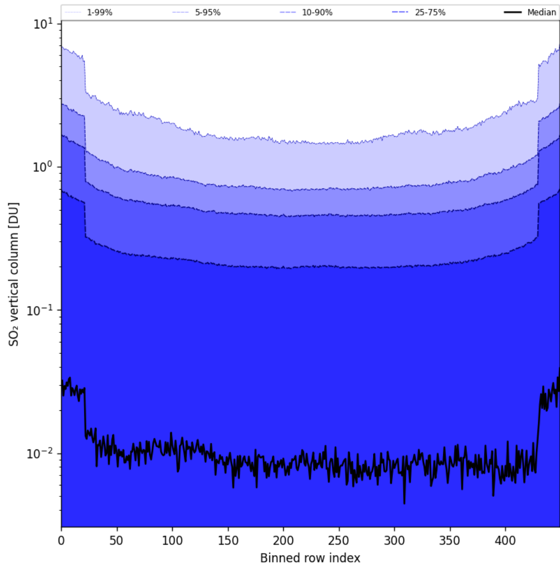
Figure 84: Along track statistics of “SO 2 vertical column” for 2025-05-23 to 2025-05-25
