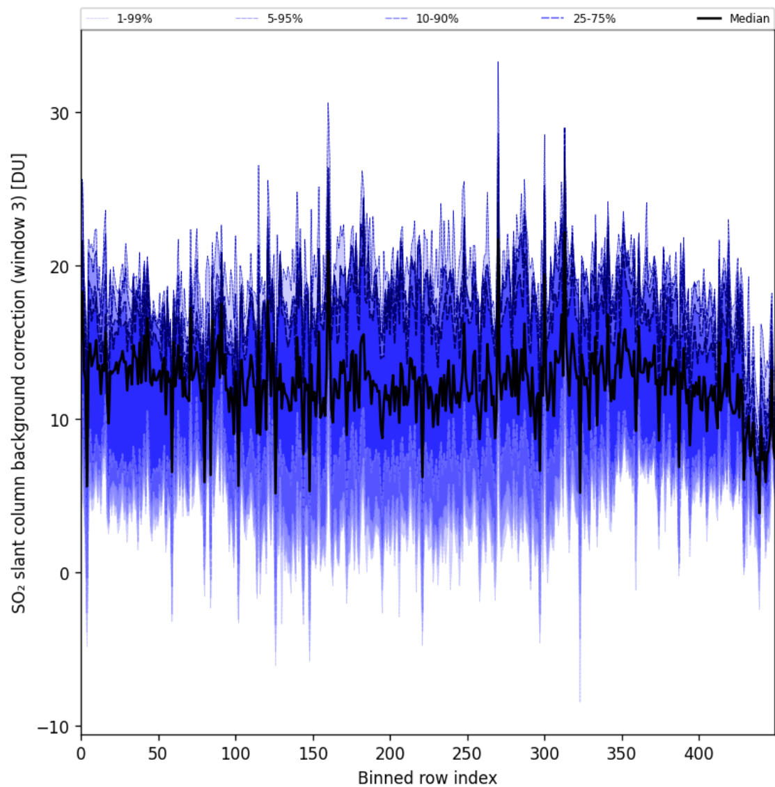
Figure 100: Along track statistics of “SO 2 slant column background correction (window 3)” for 2025-05-23 to 2025-05-25
