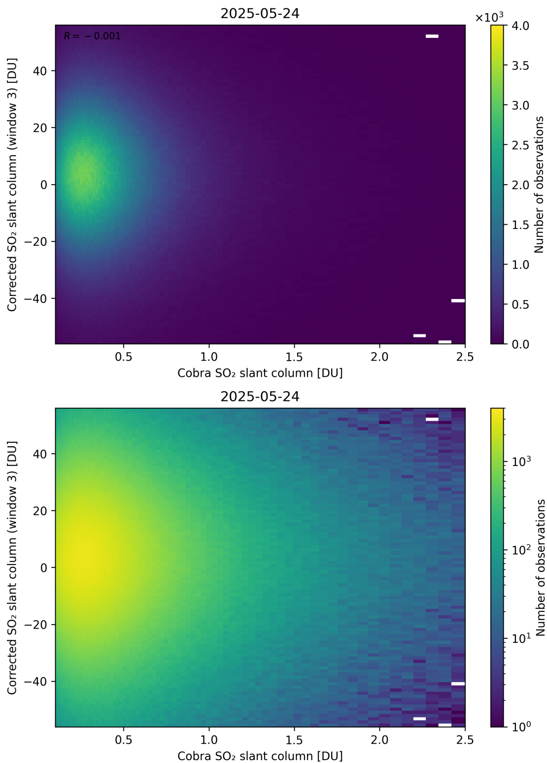
Figure 218: Scatter density plot of “Cobra SO 2 slant column” against “Corrected SO 2 slant column (window 3)” for 2025-05-23 to 2025-05-25.
