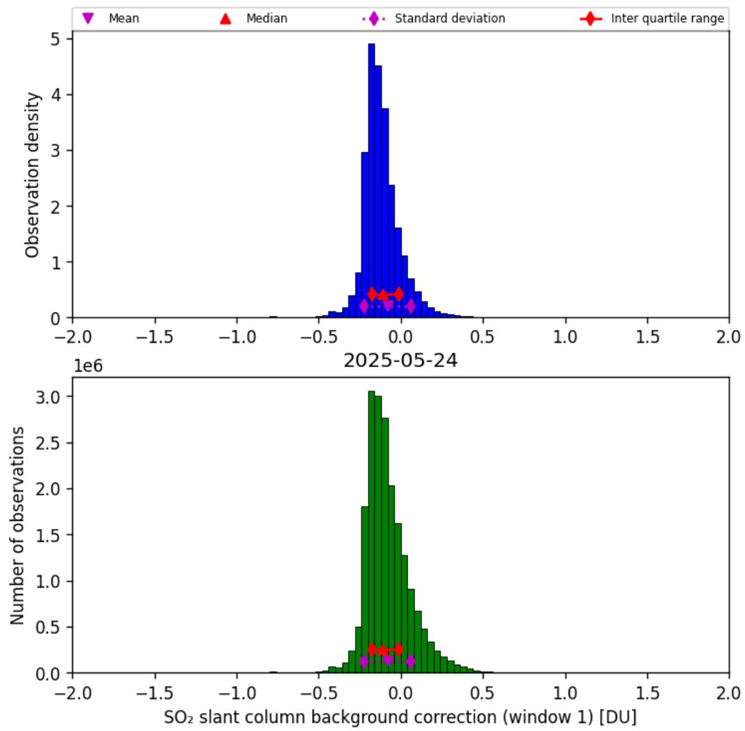
Figure 66: Histogram of “SO 2 slant column background correction (window 1)” for 2025-05-23 to 2025-05-25
