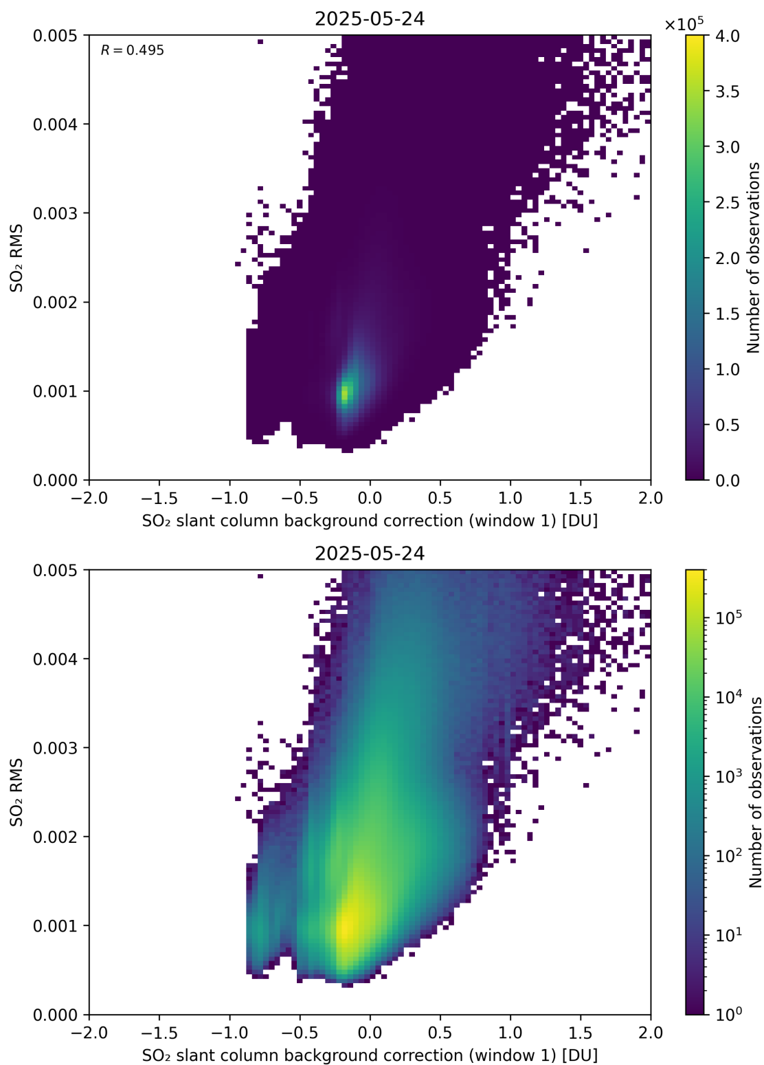
Figure 113: Scatter density plot of “SO 2 slant column background correction (window 1)” against “SO 2 RMS” for 2025-05-23 to 2025-05-25.
