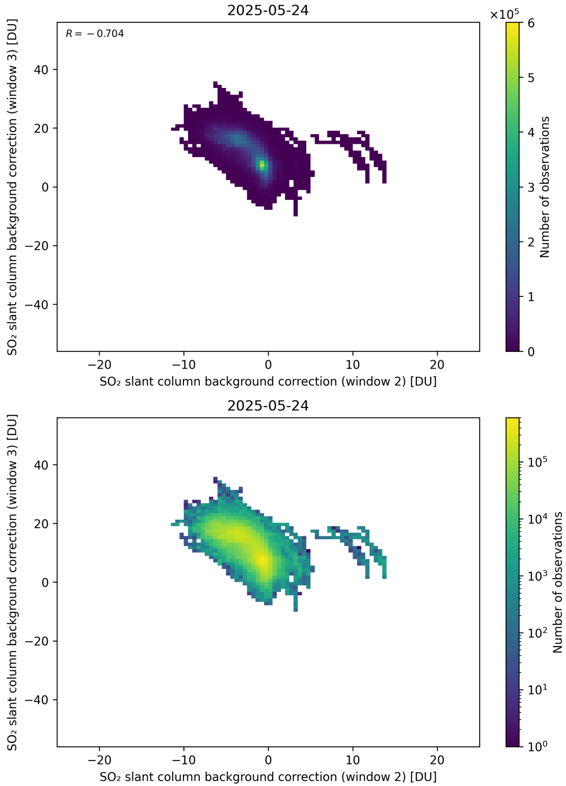
Figure 122: Scatter density plot of “SO 2 slant column background correction (window 2)” against “SO 2 slant column background correction (window 3)” for 2025-05-23 to 2025-05-25.
