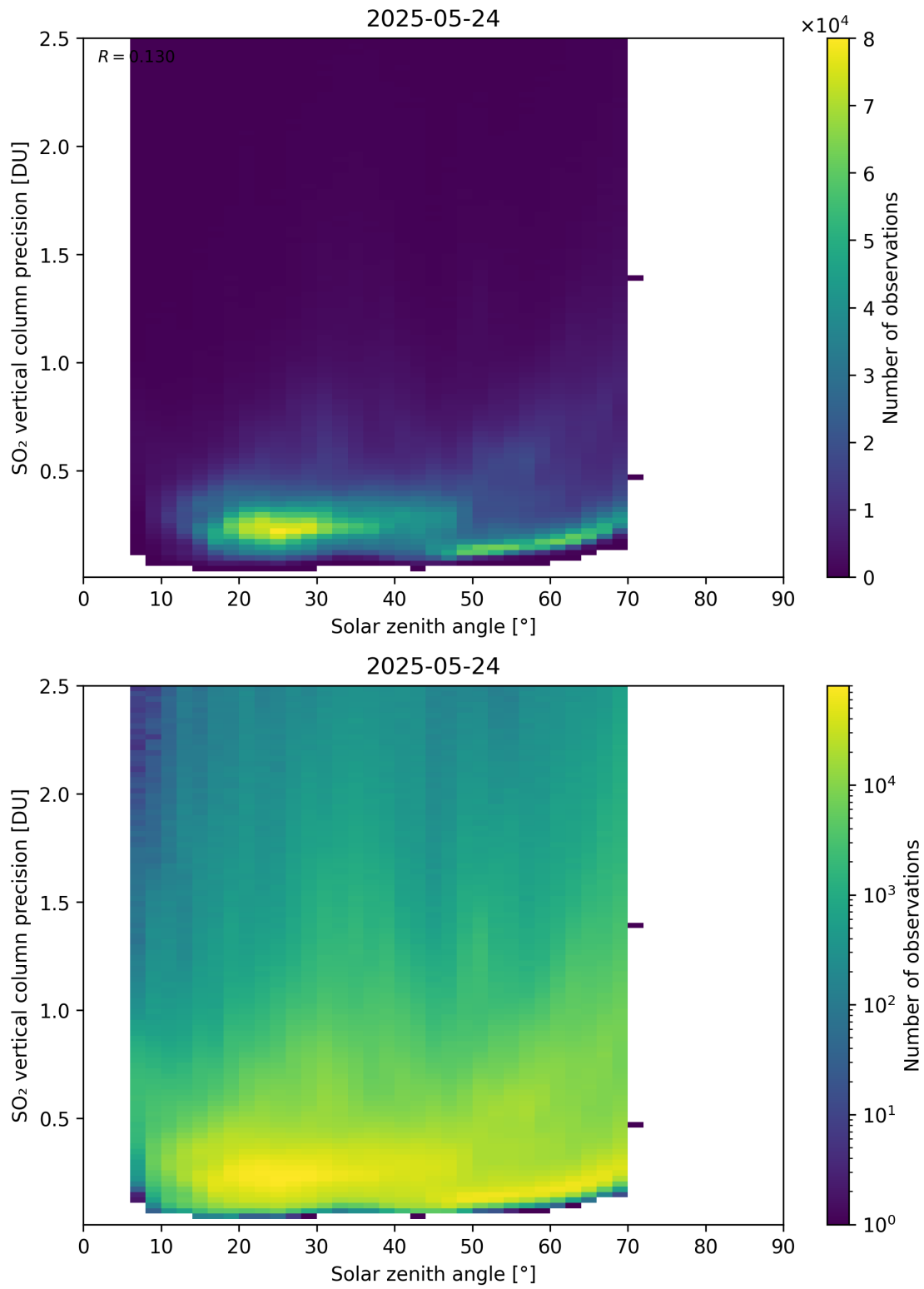
Figure 192: Scatter density plot of “Solar zenith angle” against “SO 2 vertical column precision” for 2025-05-23 to 2025-05-25.
