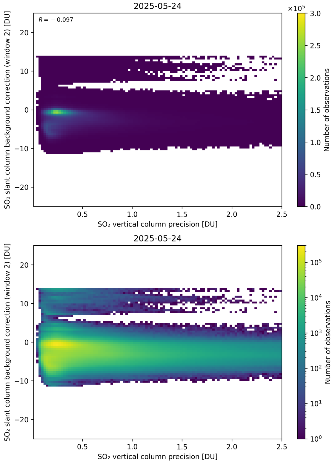
Figure 330: Scatter density plot of “SO 2 vertical column precision” against “SO 2 slant column background correction (window 2)” for 2025-05-23 to 2025-05-25.
