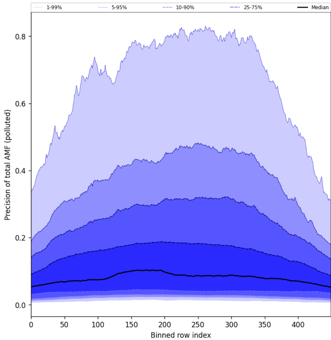
Figure 106: Along track statistics of “Precision of total AMF (polluted)” for 2025-05-23 to 2025-05-25
