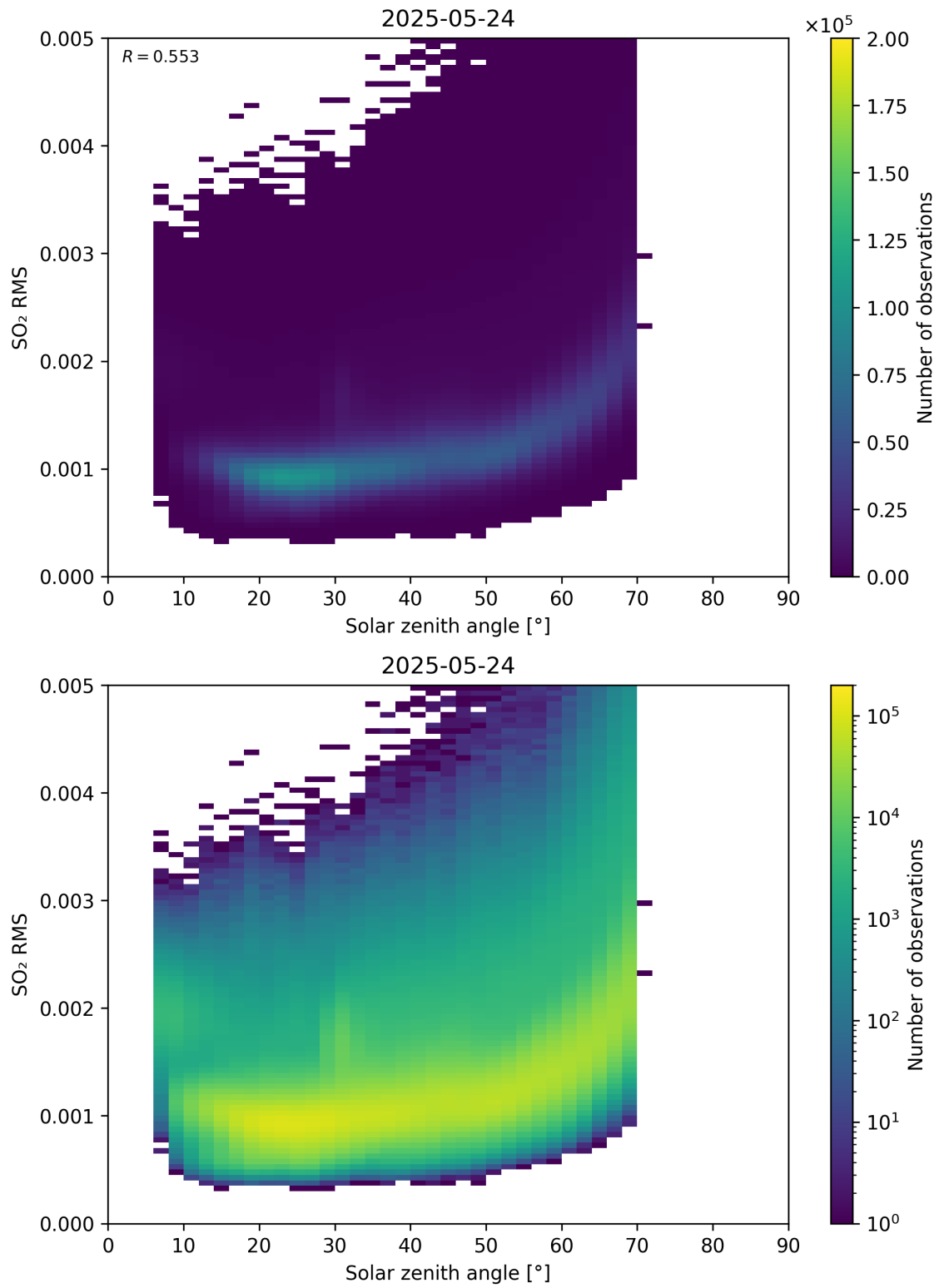
Figure 176: Scatter density plot of “Solar zenith angle” against “SO 2 RMS” for 2025-05-23 to 2025-05-25.
