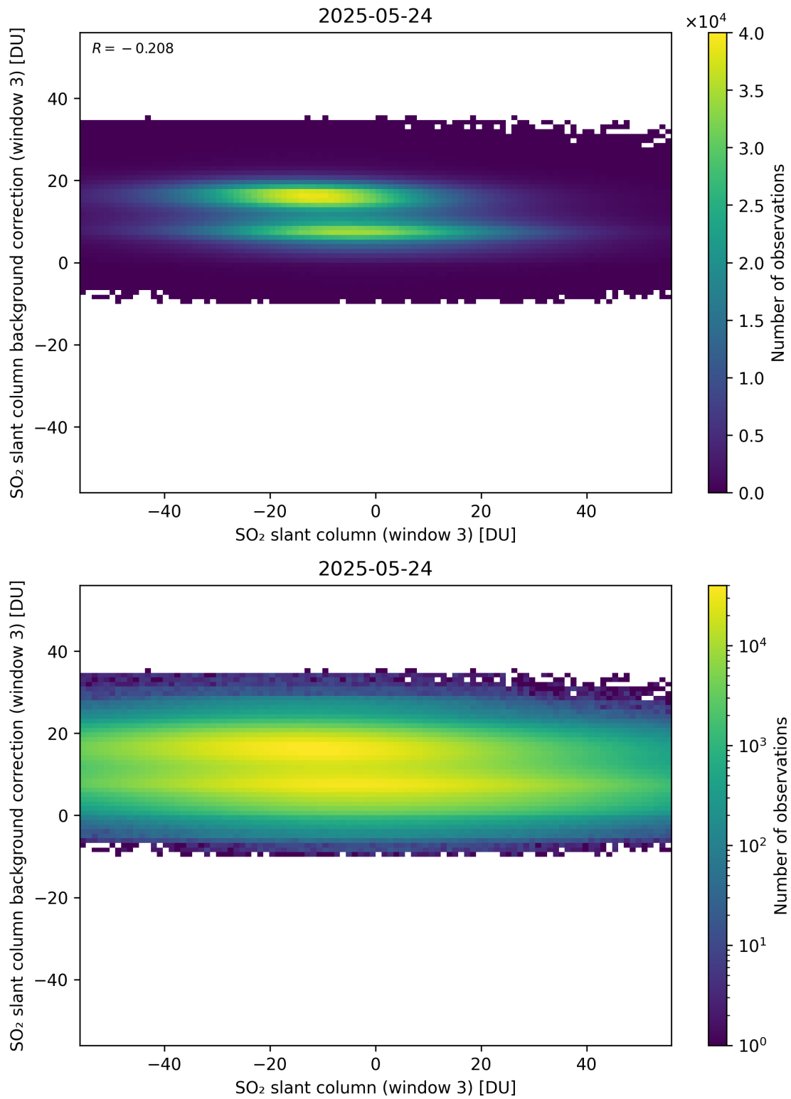
Figure 303: Scatter density plot of “SO 2 slant column (window 3)” against “SO 2 slant column background correction (window 3)” for 2025-05-23 to 2025-05-25.
