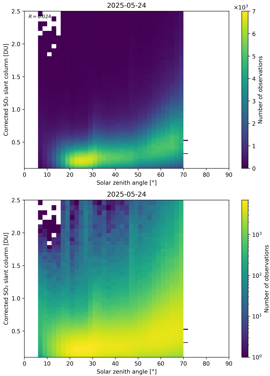
Figure 181: Scatter density plot of “Solar zenith angle” against “Corrected SO 2 slant column” for 2025-05-23 to 2025-05-25.
