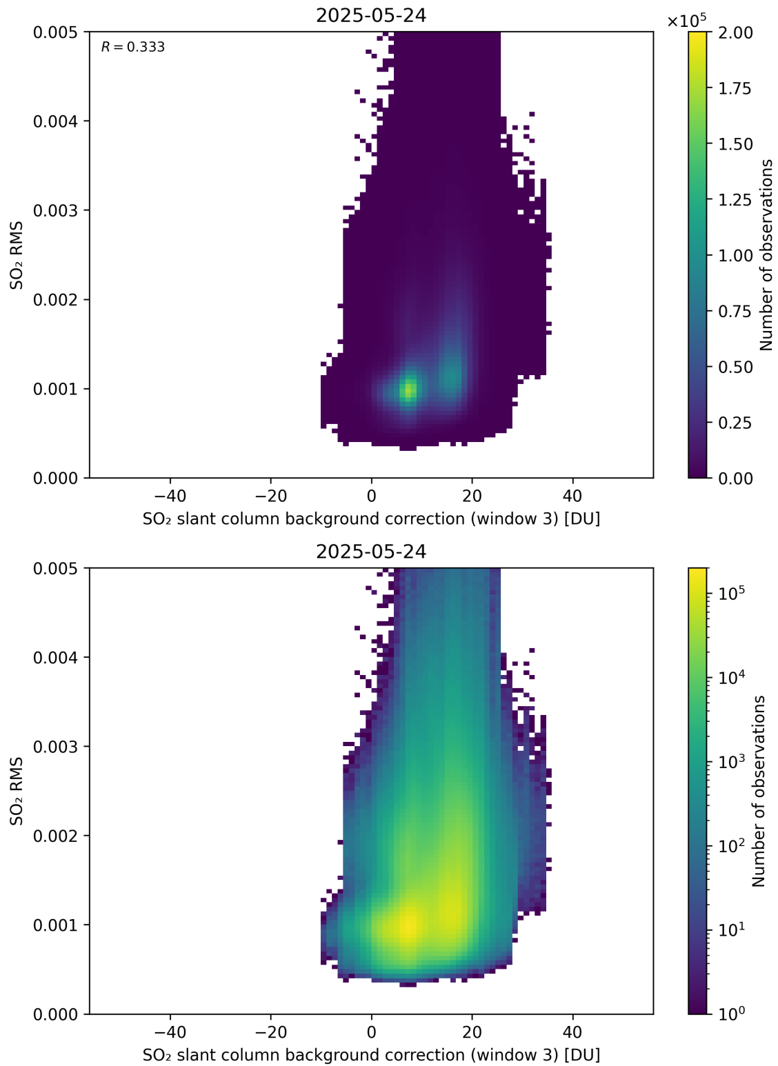
Figure 134: Scatter density plot of “SO 2 slant column background correction (window 3)” against “SO 2 RMS” for 2025-05-23 to 2025-05-25.
