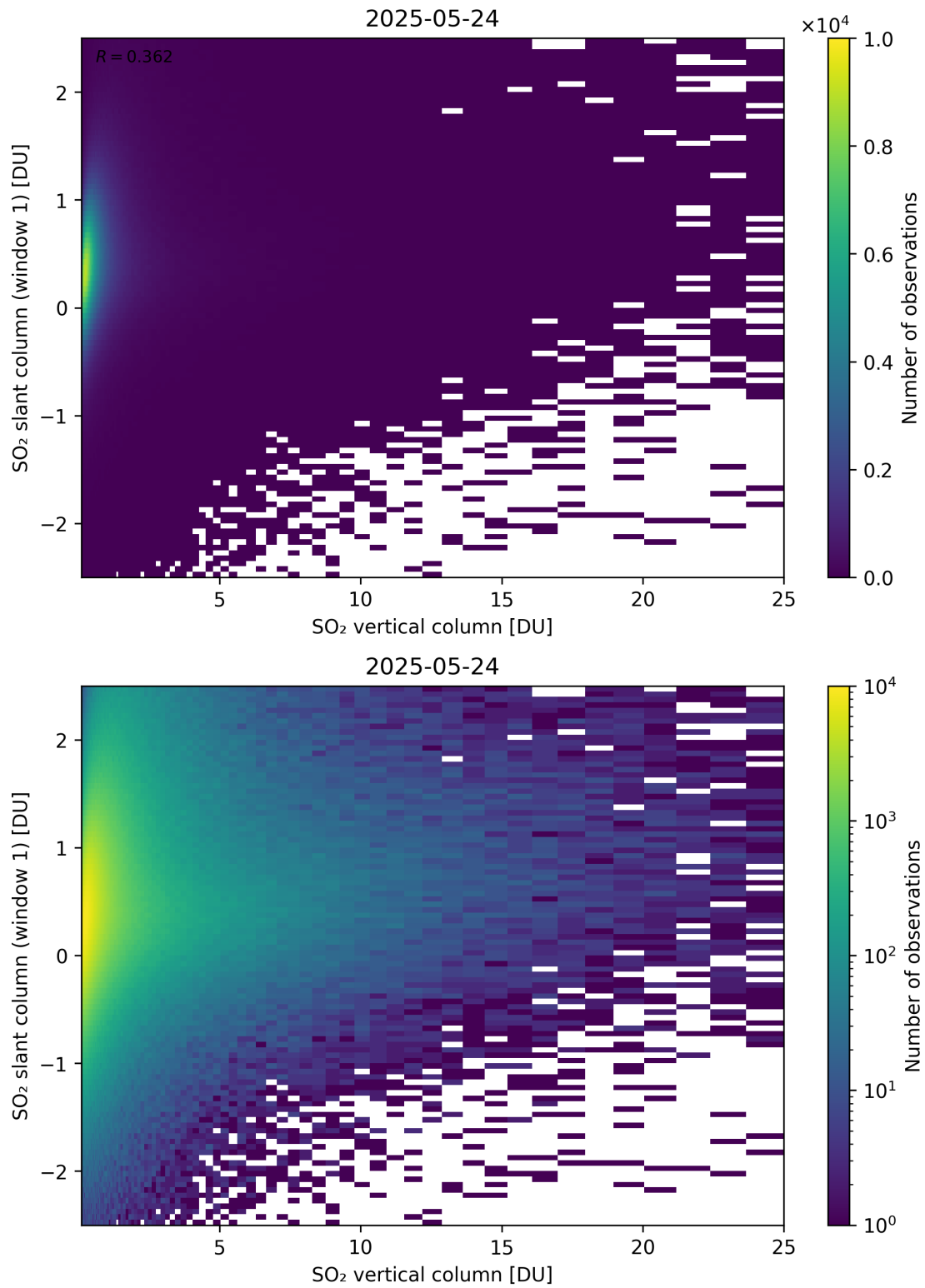
Figure 354: Scatter density plot of “SO 2 vertical column” against “SO 2 slant column (window 1)” for 2025-05-23 to 2025-05-25.
