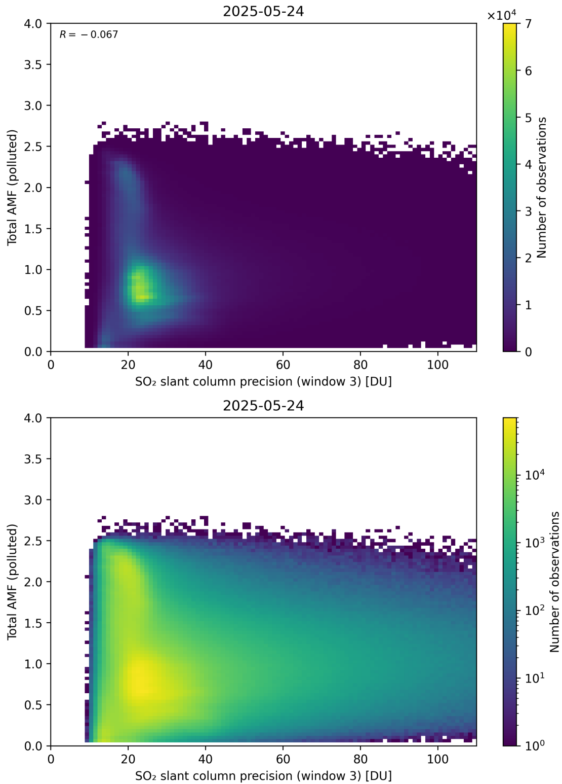
Figure 313: Scatter density plot of “SO 2 slant column precision (window 3)” against “Total AMF (polluted)” for 2025-05-23 to 2025-05-25.
