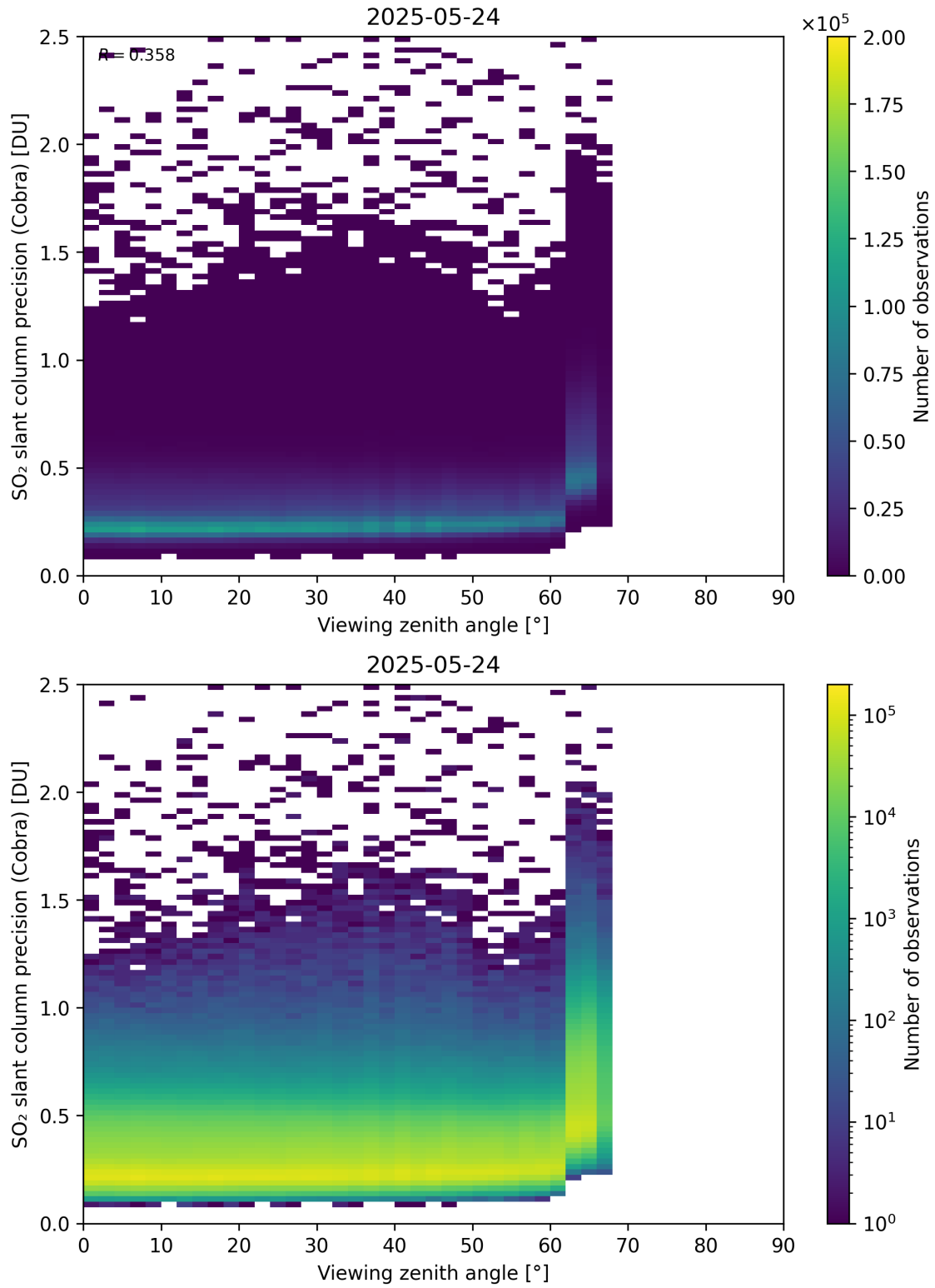
Figure 372: Scatter density plot of “Viewing zenith angle” against “SO 2 slant column precision (Cobra)” for 2025-05-23 to 2025-05-25.
