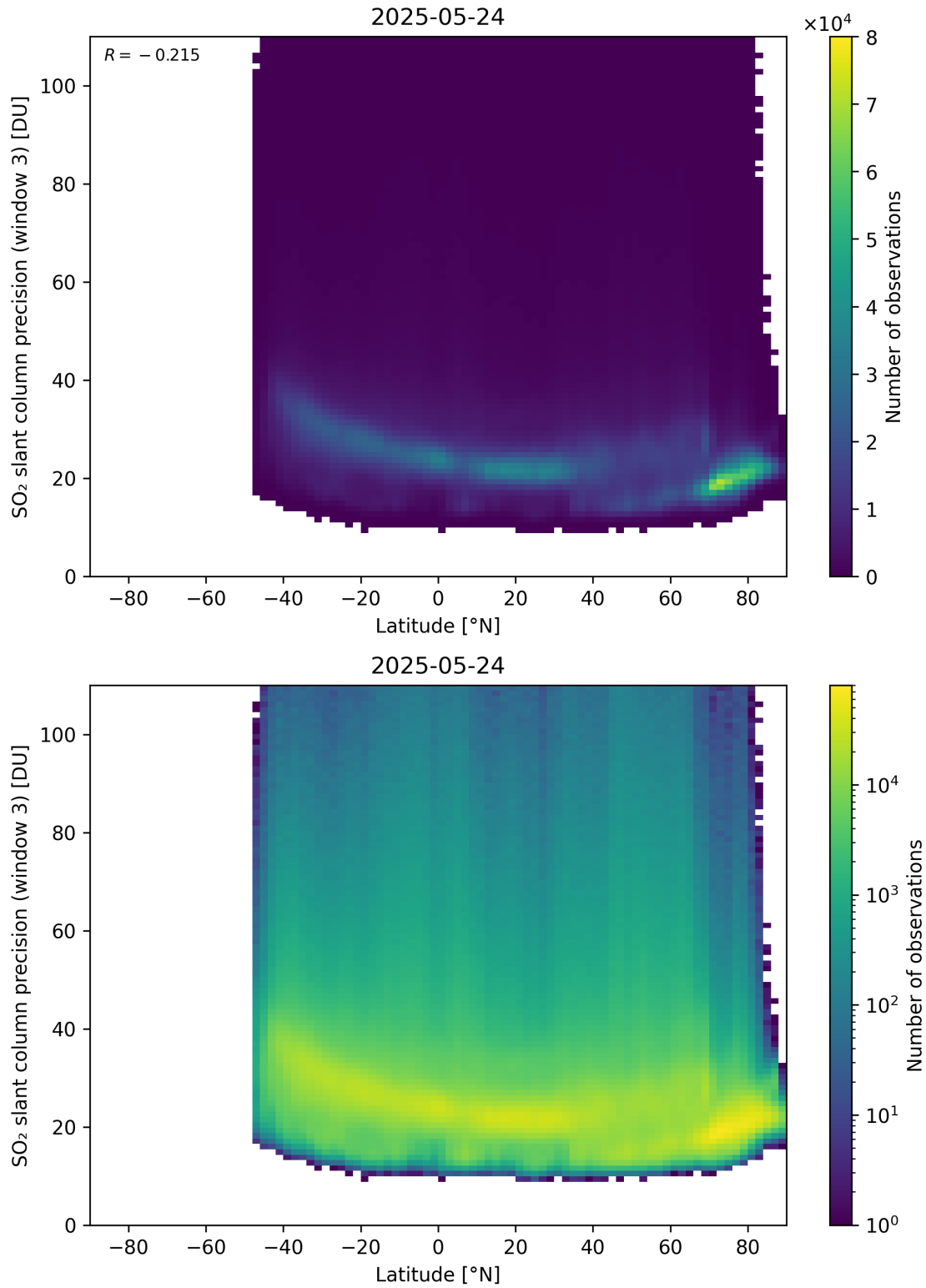
Figure 166: Scatter density plot of “Latitude” against “SO 2 slant column precision (window 3)” for 2025-05-23 to 2025-05-25.
