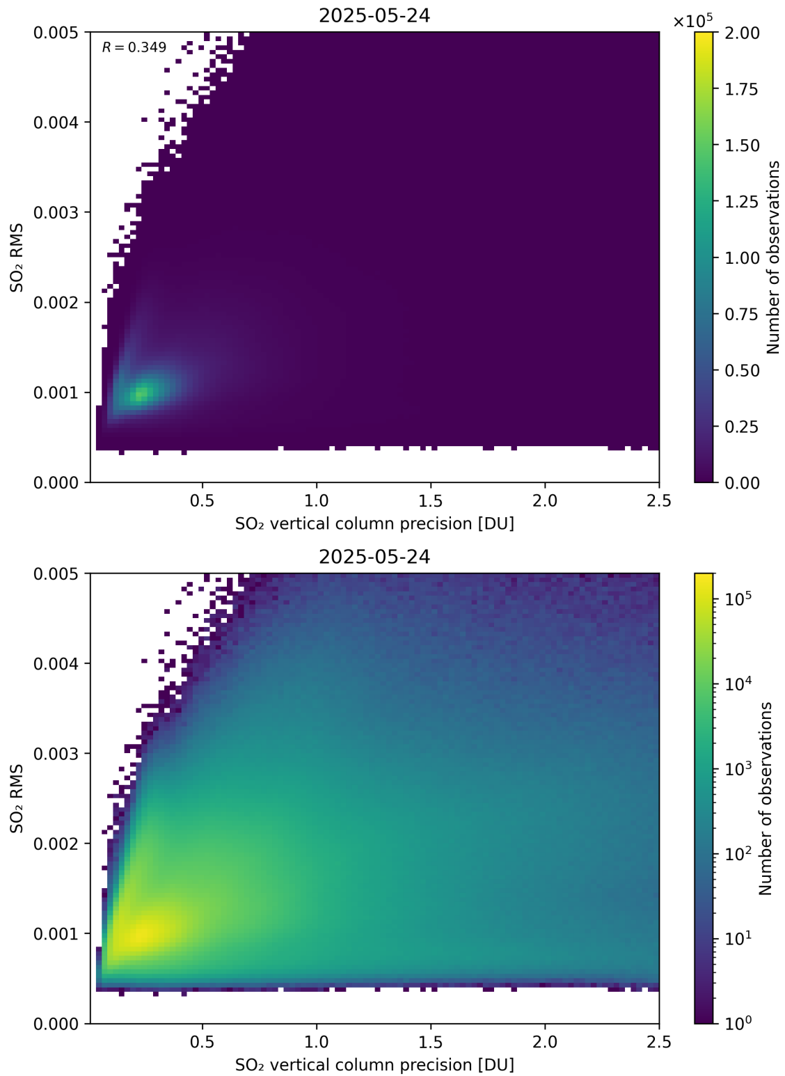
Figure 334: Scatter density plot of “SO 2 vertical column precision” against “SO 2 RMS” for 2025-05-23 to 2025-05-25.
