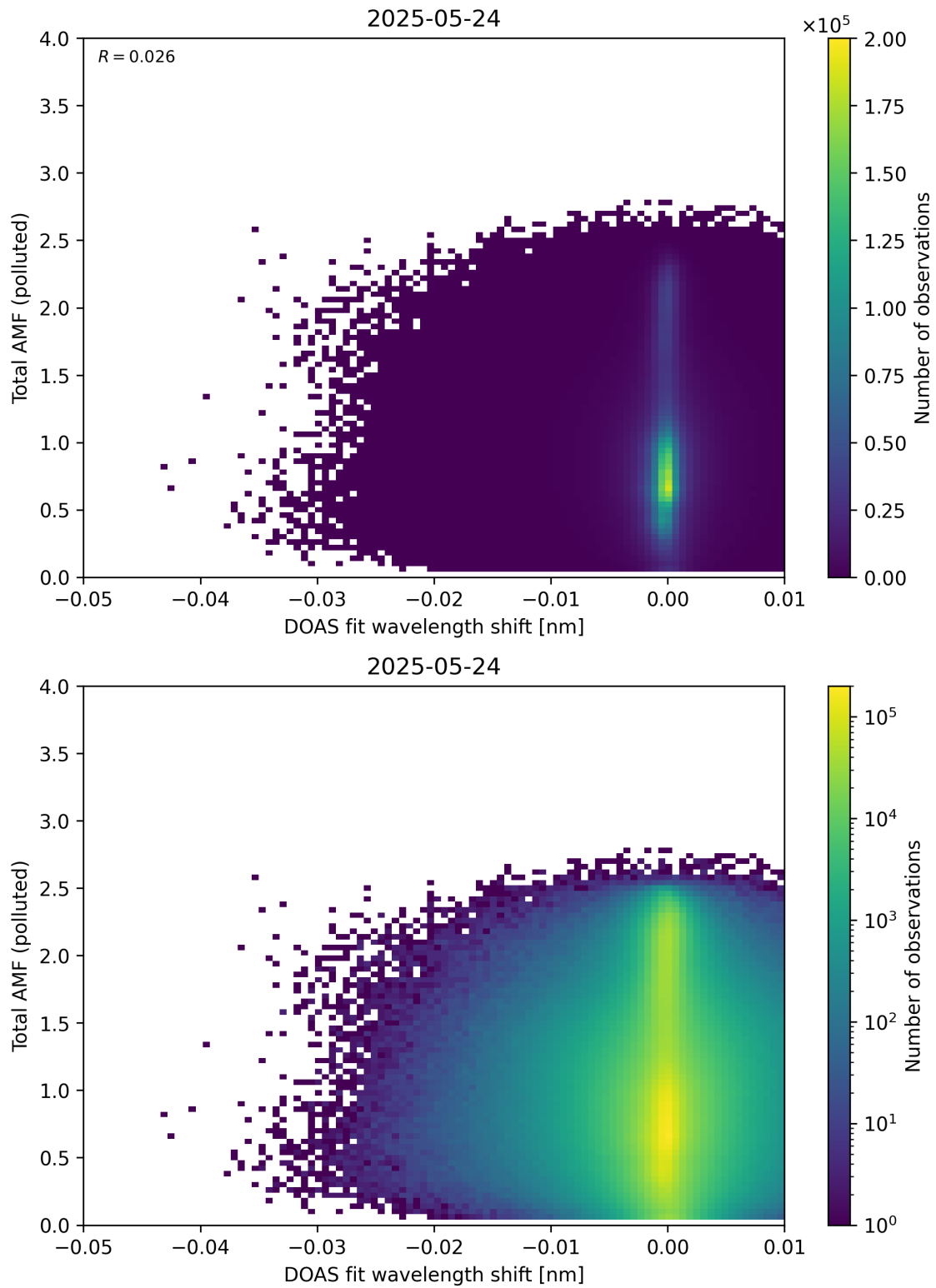
Figure 141: Scatter density plot of “DOAS fit wavelength shift” against “Total AMF (polluted)” for 2025-05-23 to 2025-05-25.
