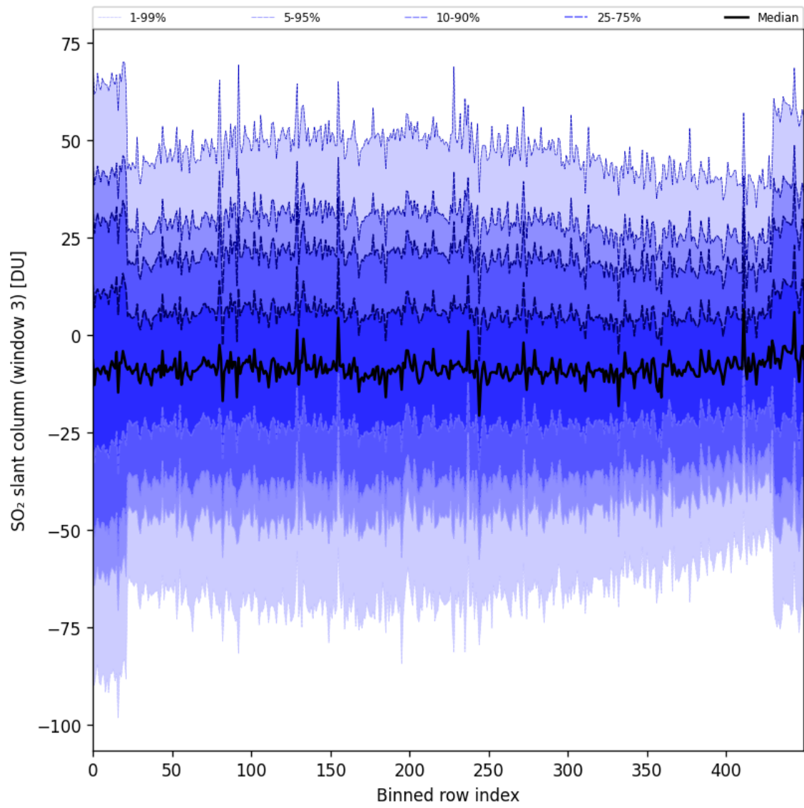
Figure 97: Along track statistics of “SO 2 slant column (window 3)” for 2025-05-23 to 2025-05-25
