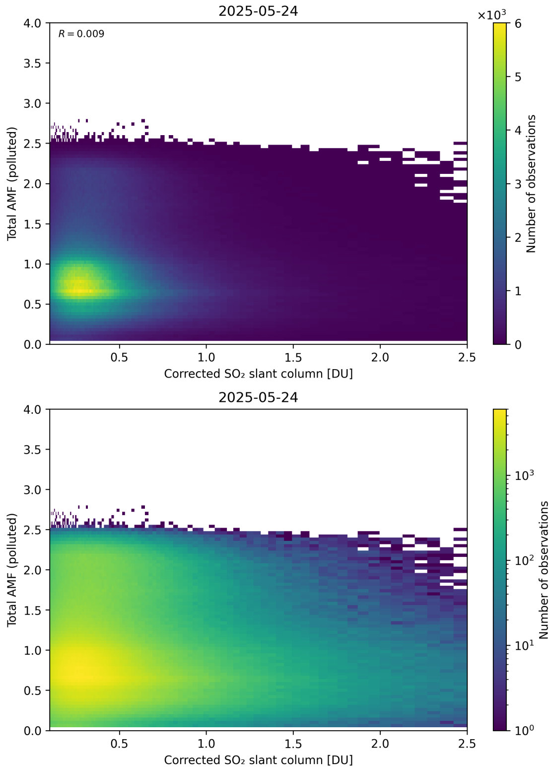
Figure 242: Scatter density plot of “Corrected SO 2 slant column” against “Total AMF (polluted)” for 2025-05-23 to 2025-05-25.
