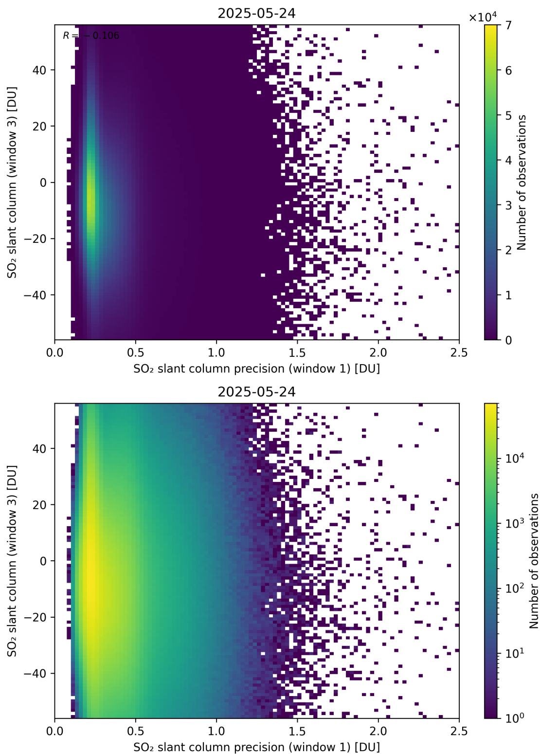
Figure 278: Scatter density plot of “SO 2 slant column precision (window 1)” against “SO 2 slant column (window 3)” for 2025-05-23 to 2025-05-25.
