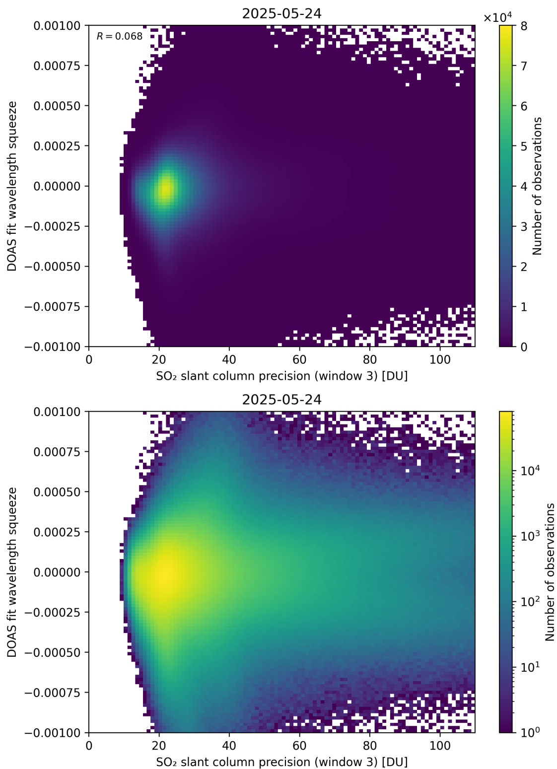
Figure 309: Scatter density plot of “SO 2 slant column precision (window 3)” against “DOAS fit wavelength squeeze” for 2025-05-23 to 2025-05-25.
