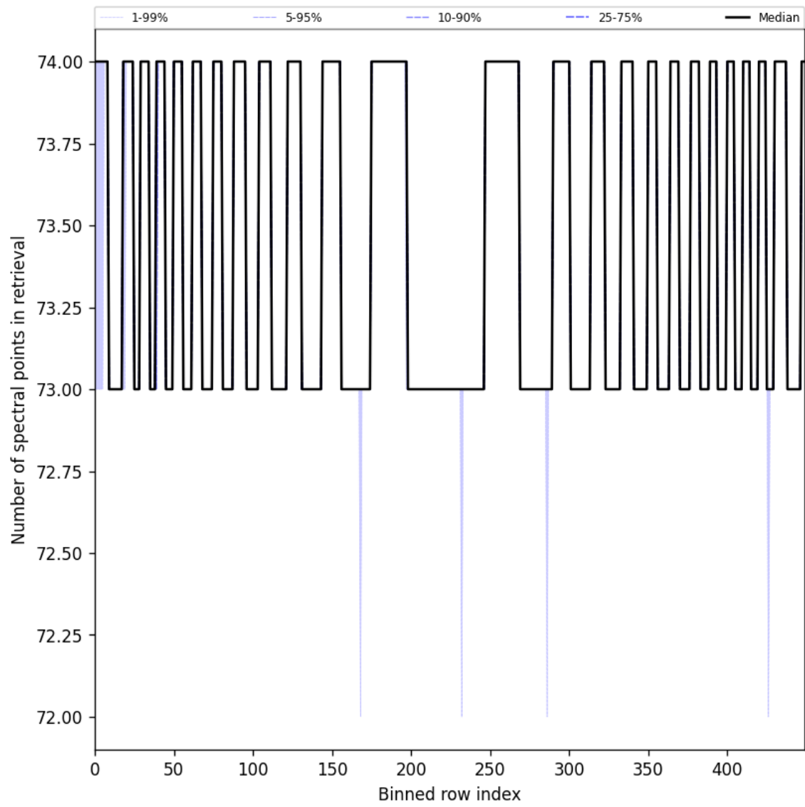
Figure 108: Along track statistics of “Number of spectral points in retrieval” for 2025-05-23 to 2025-05-25
