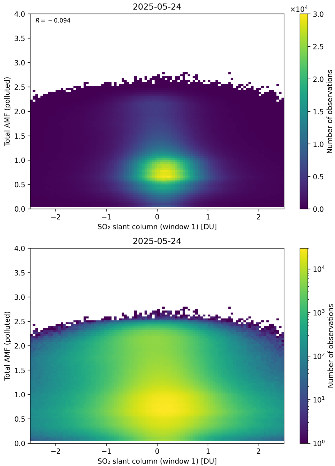
Figure 289: Scatter density plot of “SO 2 slant column (window 1)” against “Total AMF (polluted)” for 2025-05-23 to 2025-05-25.
