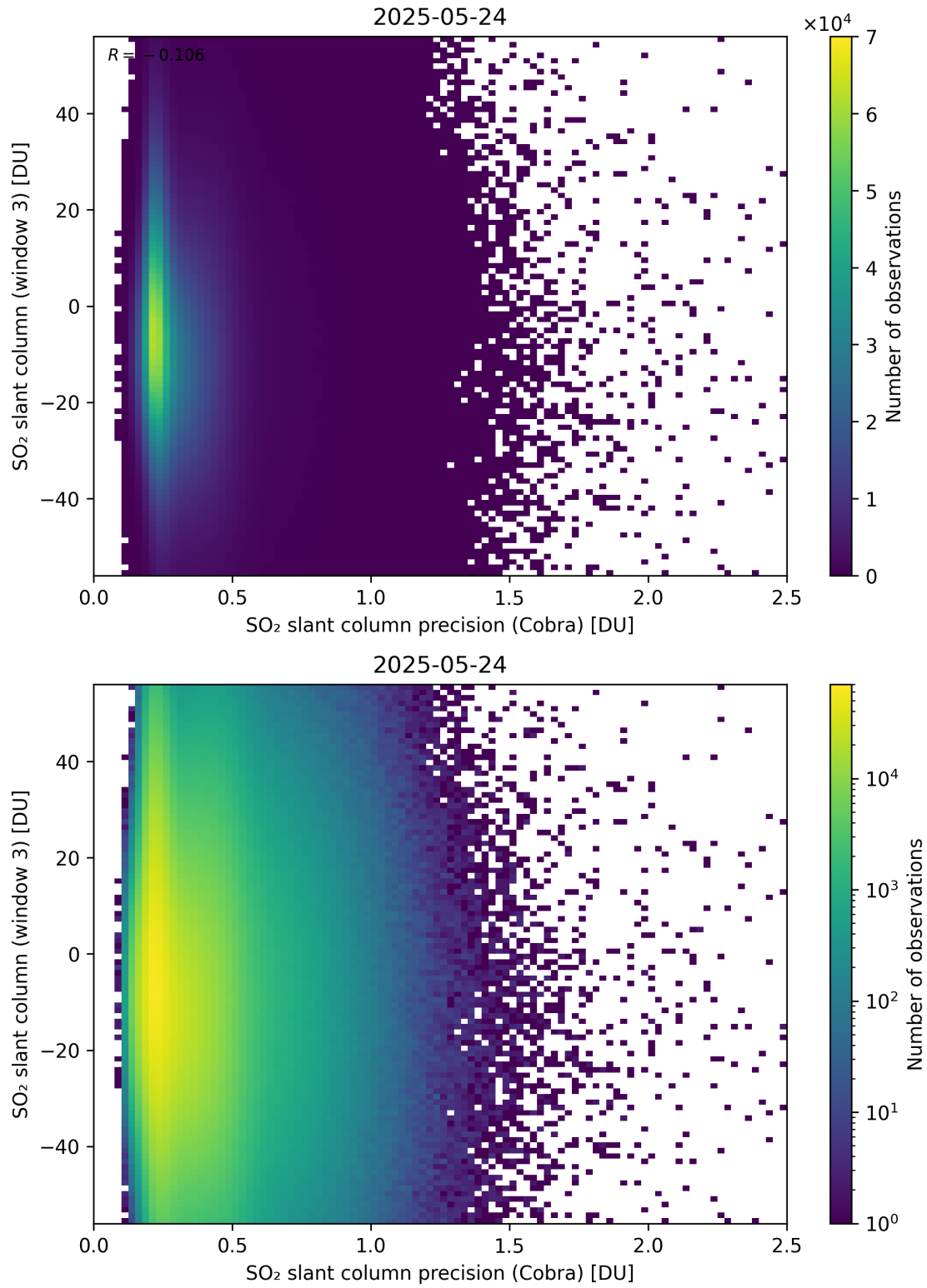
Figure 211: Scatter density plot of “SO 2 slant column precision (Cobra)” against “SO 2 slant column (window 3)” for 2025-05-23 to 2025-05-25.
