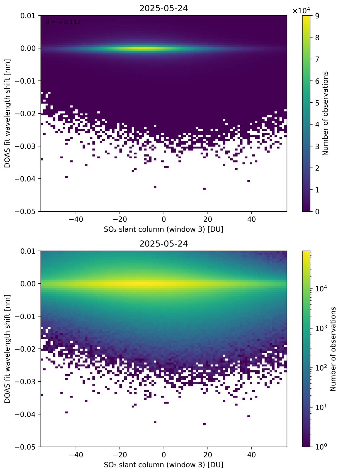
Figure 304: Scatter density plot of “SO 2 slant column (window 3)” against “DOAS fit wavelength shift” for 2025-05-23 to 2025-05-25.
