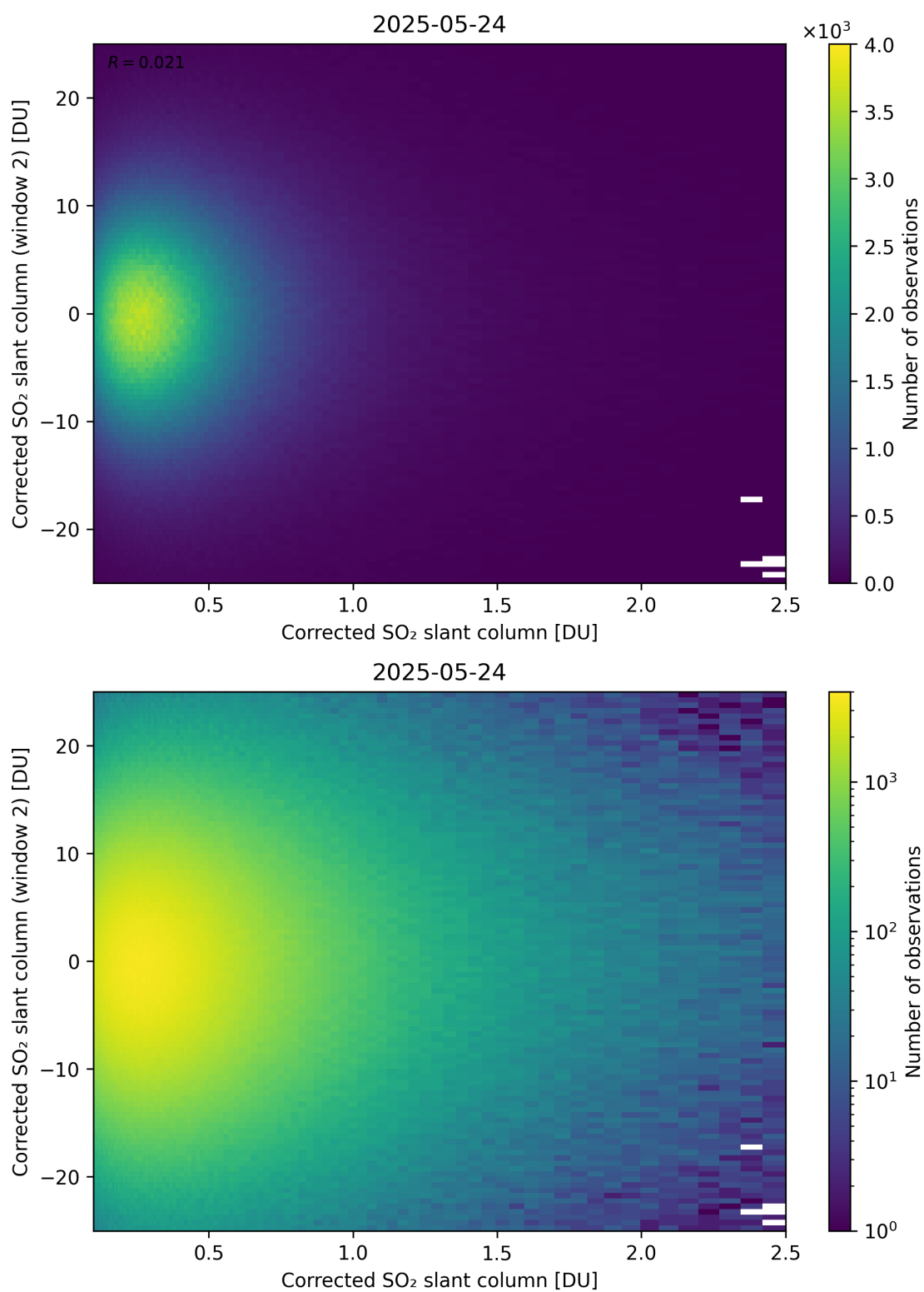
Figure 235: Scatter density plot of “Corrected SO 2 slant column” against “Corrected SO 2 slant column (window 2)” for 2025-05-23 to 2025-05-25.
