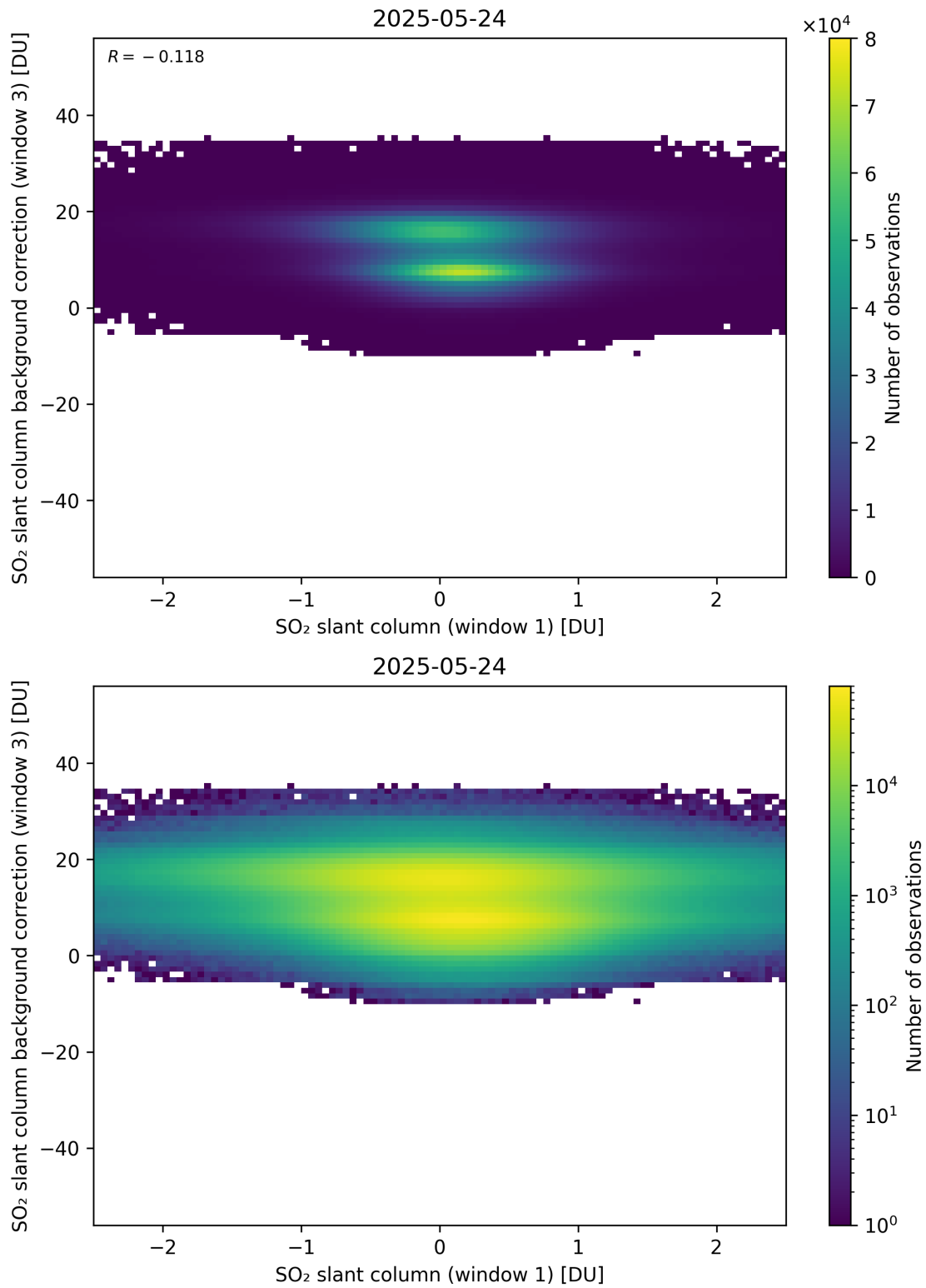
Figure 264: Scatter density plot of “SO 2 slant column (window 1)” against “SO 2 slant column background correction (window 3)” for 2025-05-23 to 2025-05-25.
