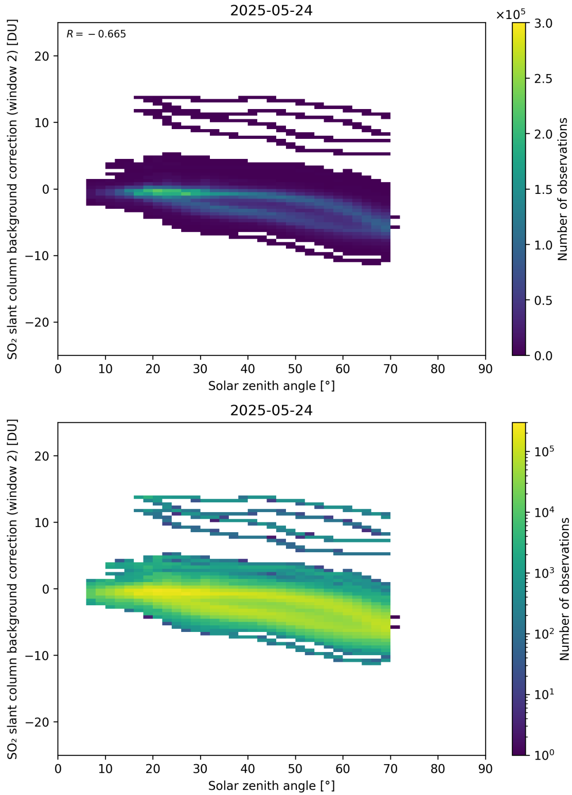
Figure 172: Scatter density plot of “Solar zenith angle” against “SO 2 slant column background correction (window 2)” for 2025-05-23 to 2025-05-25.
