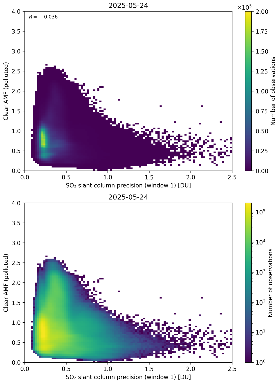
Figure 274: Scatter density plot of “SO 2 slant column precision (window 1)” against “Clear AMF (polluted)” for 2025-05-23 to 2025-05-25.
