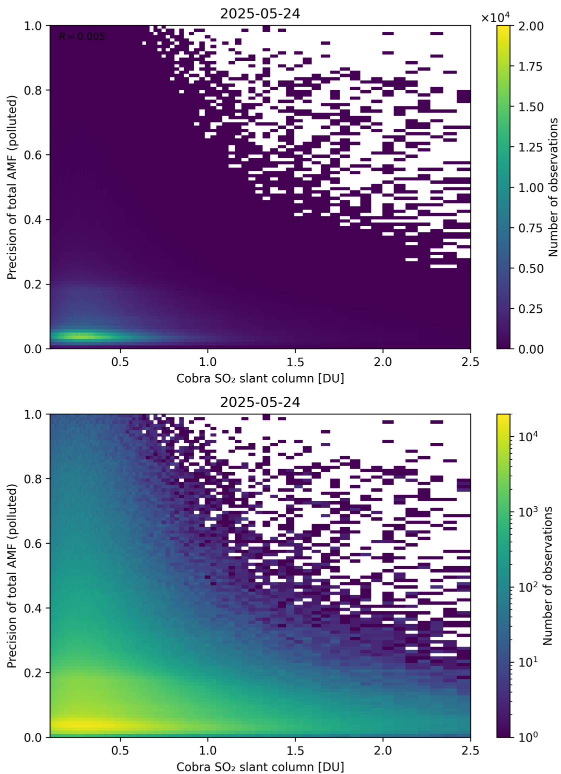
Figure 225: Scatter density plot of “Cobra SO 2 slant column” against “Precision of total AMF (polluted)” for 2025-05-23 to 2025-05-25.
