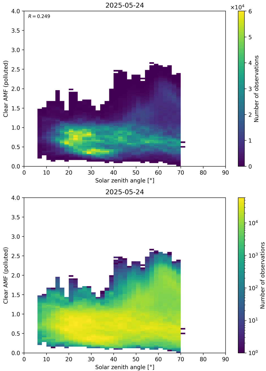
Figure 178: Scatter density plot of “Solar zenith angle” against “Clear AMF (polluted)” for 2025-05-23 to 2025-05-25.
