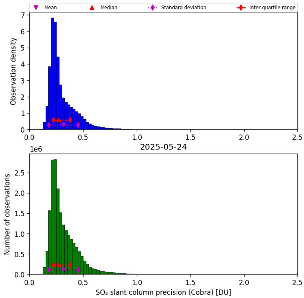
Figure 62: Histogram of “SO 2 slant column precision (Cobra)” for 2025-05-23 to 2025-05-25
