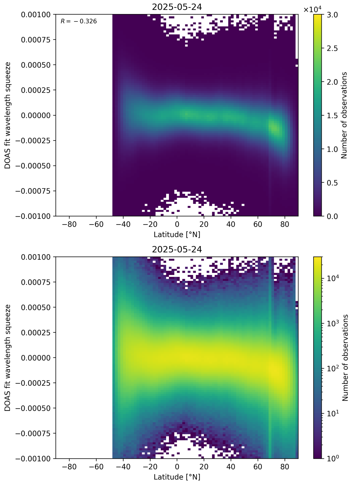
Figure 154: Scatter density plot of “Latitude” against “DOAS fit wavelength squeeze” for 2025-05-23 to 2025-05-25.
