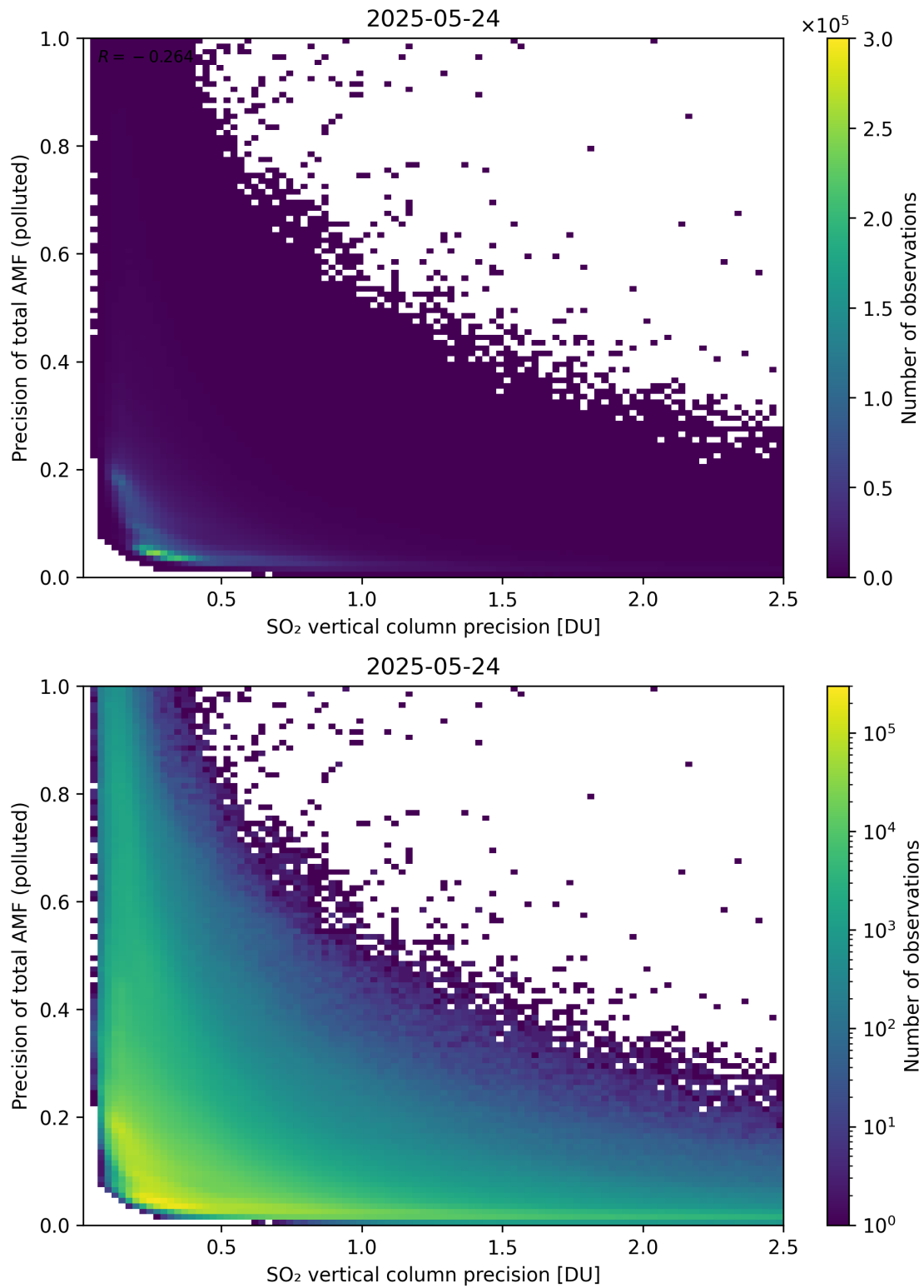
Figure 347: Scatter density plot of “SO 2 vertical column precision” against “Precision of total AMF (polluted)” for 2025-05-23 to 2025-05-25.
