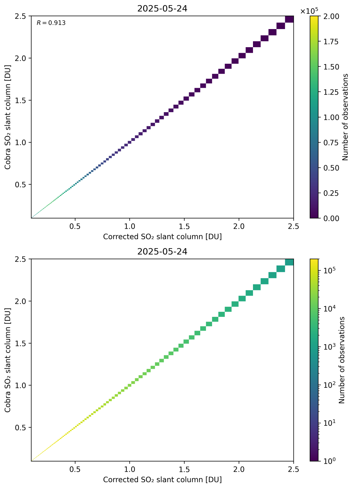
Figure 233: Scatter density plot of “Corrected SO 2 slant column” against “Cobra SO 2 slant column” for 2025-05-23 to 2025-05-25.
