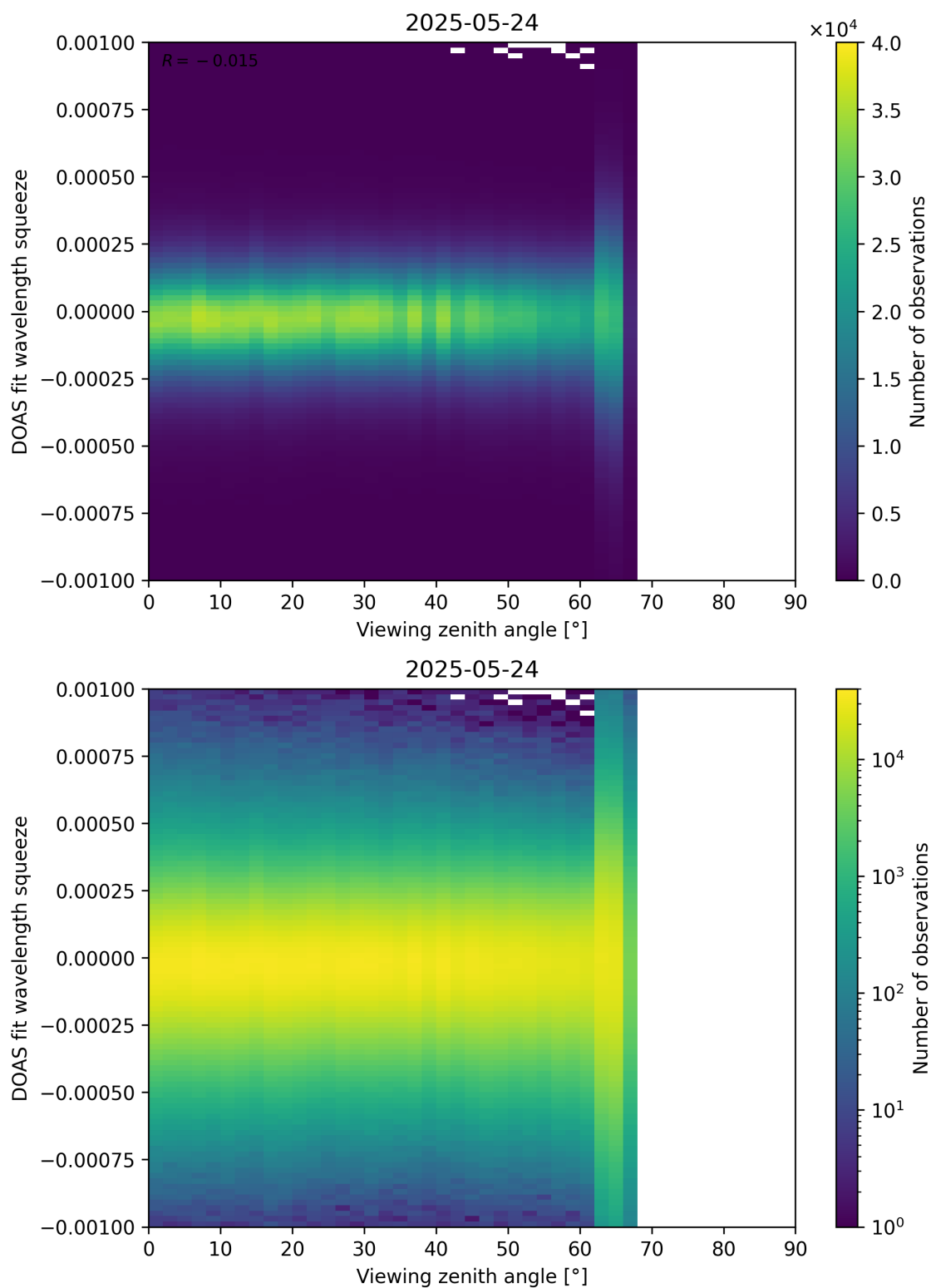
Figure 366: Scatter density plot of “Viewing zenith angle” against “DOAS fit wavelength squeeze” for 2025-05-23 to 2025-05-25.
