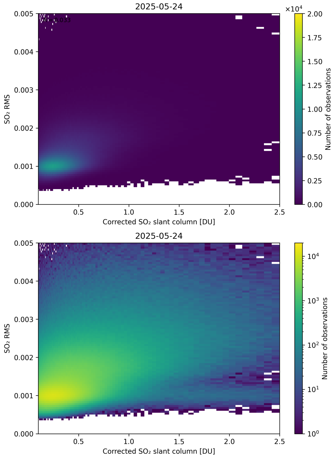
Figure 231: Scatter density plot of “Corrected SO 2 slant column” against “SO 2 RMS” for 2025-05-23 to 2025-05-25.
