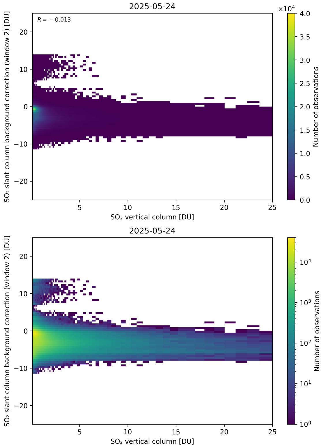
Figure 324: Scatter density plot of “SO 2 vertical column” against “SO 2 slant column background correction (window 2)” for 2025-05-23 to 2025-05-25.
