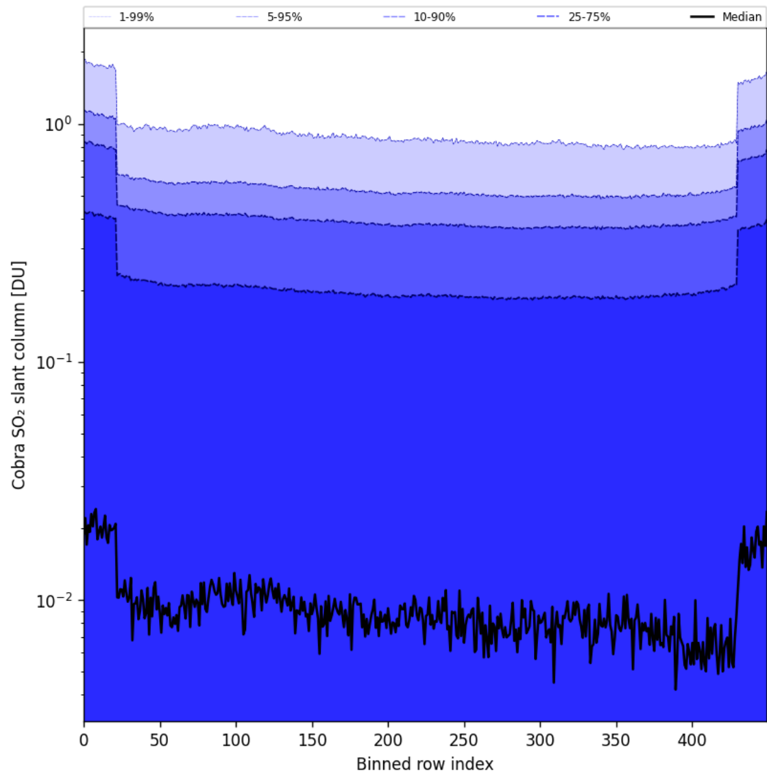
Figure 87: Along track statistics of “Cobra SO 2 slant column” for 2025-05-23 to 2025-05-25
