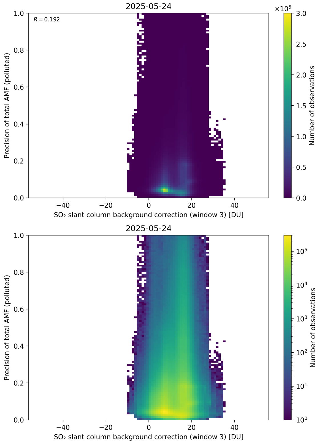
Figure 137: Scatter density plot of “SO 2 slant column background correction (window 3)” against “Precision of total AMF (polluted)” for 2025-05-23 to 2025-05-25.
