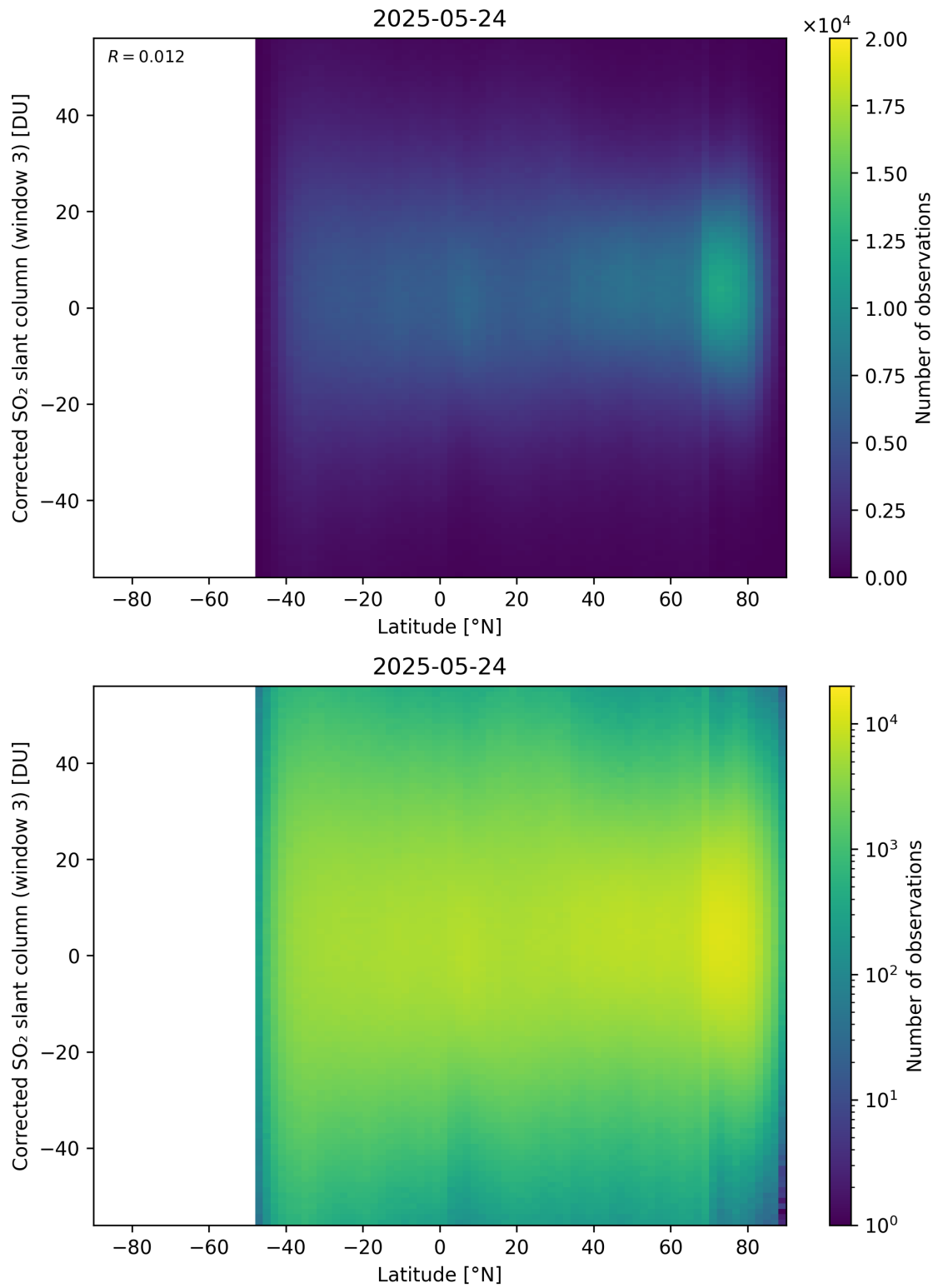
Figure 161: Scatter density plot of “Latitude” against “Corrected SO 2 slant column (window 3)” for 2025-05-23 to 2025-05-25.
