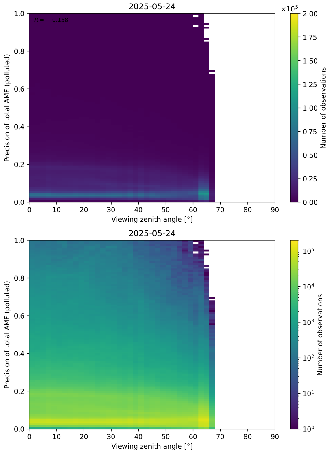
Figure 382: Scatter density plot of “Viewing zenith angle” against “Precision of total AMF (polluted)” for 2025-05-23 to 2025-05-25.
