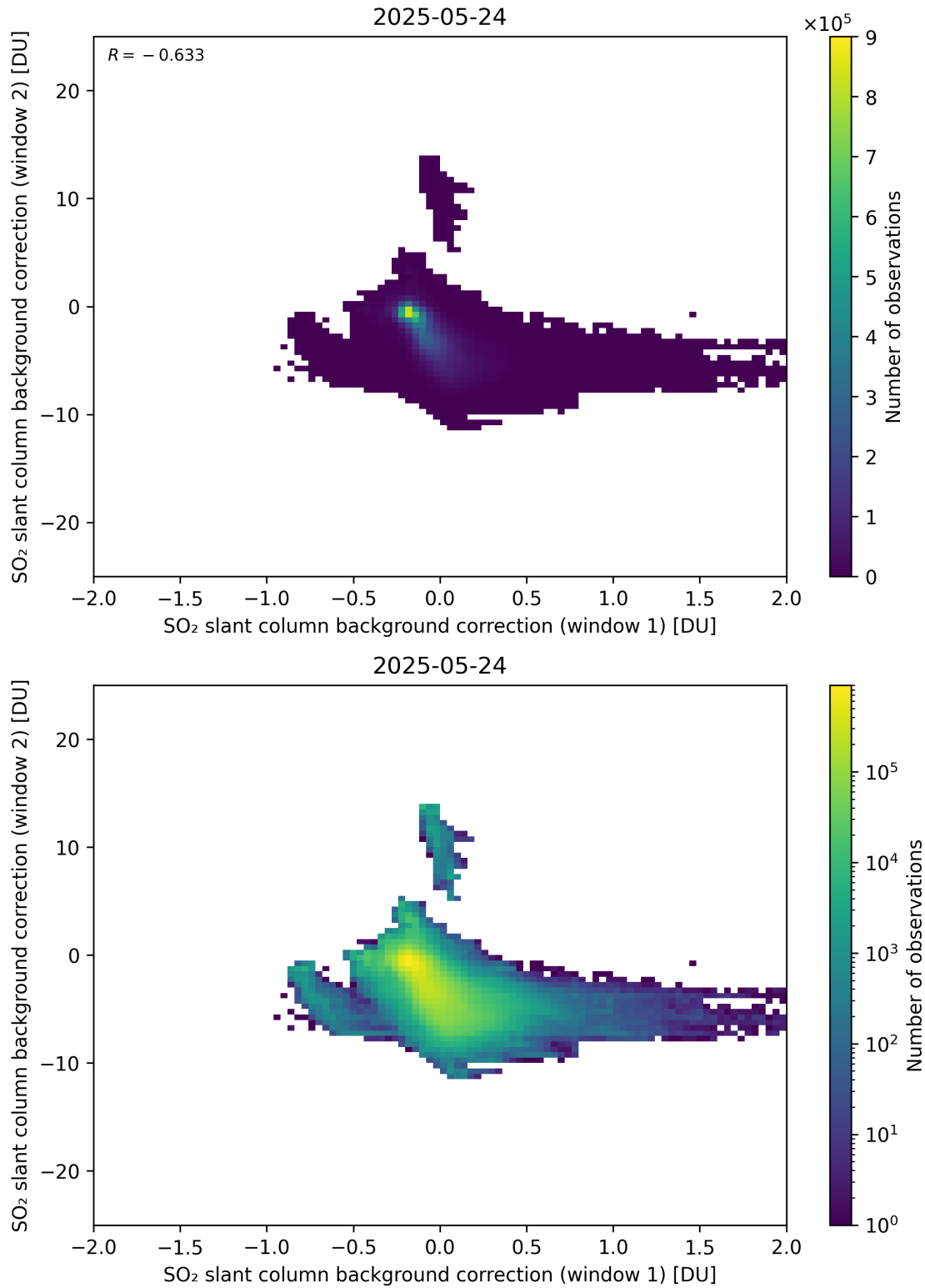
Figure 109: Scatter density plot of “SO 2 slant column background correction (window 1)” against “SO 2 slant column background correction (window 2)” for 2025-05-23 to 2025-05-25.
