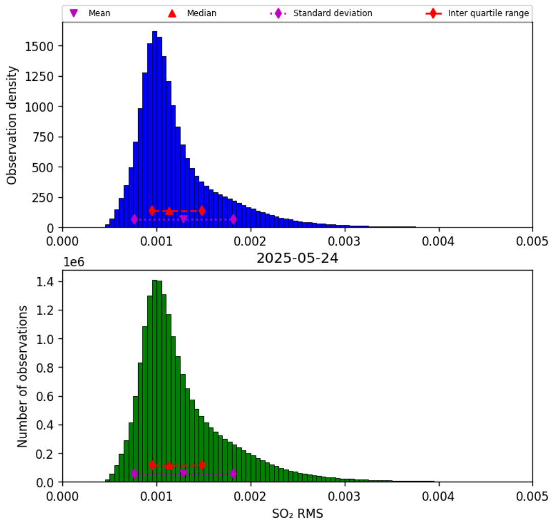
Figure 78: Histogram of “SO 2 RMS” for 2025-05-23 to 2025-05-25
