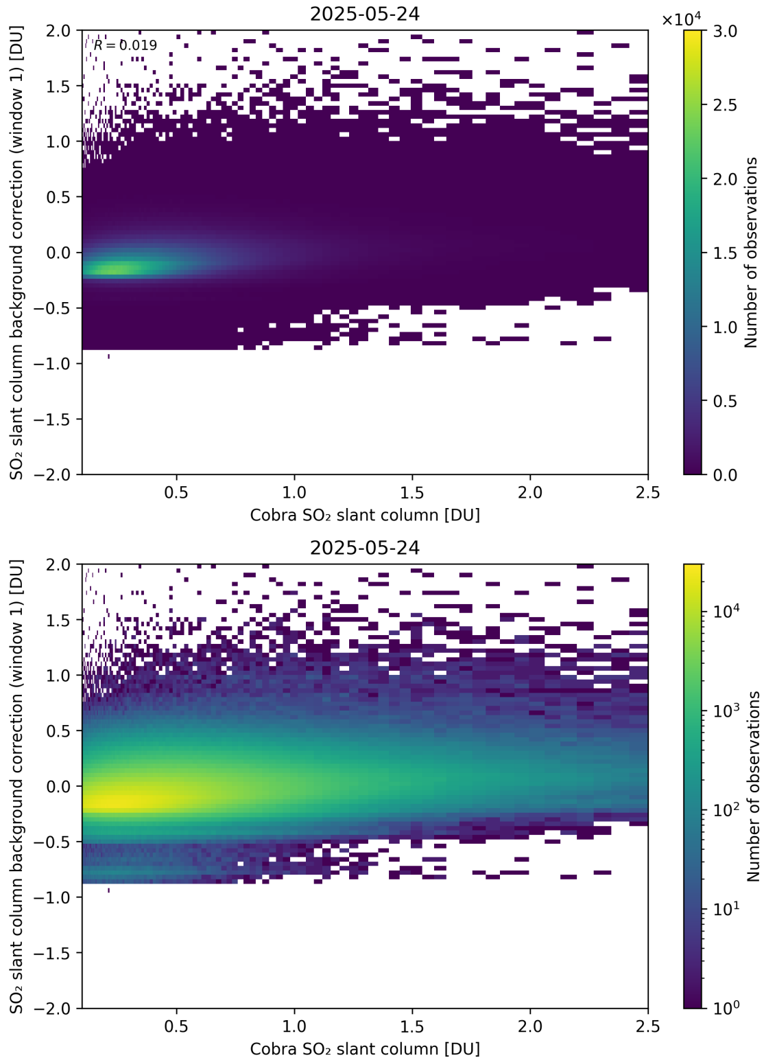
Figure 193: Scatter density plot of “Cobra SO 2 slant column” against “SO 2 slant column background correction (window 1)” for 2025-05-23 to 2025-05-25.
