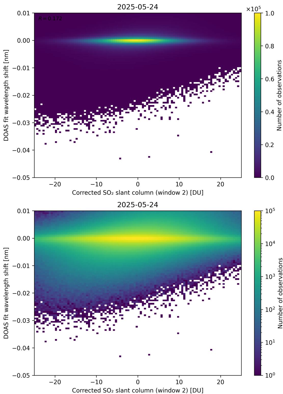
Figure 246: Scatter density plot of “Corrected SO 2 slant column (window 2)” against “DOAS fit wavelength shift” for 2025-05-23 to 2025-05-25.
