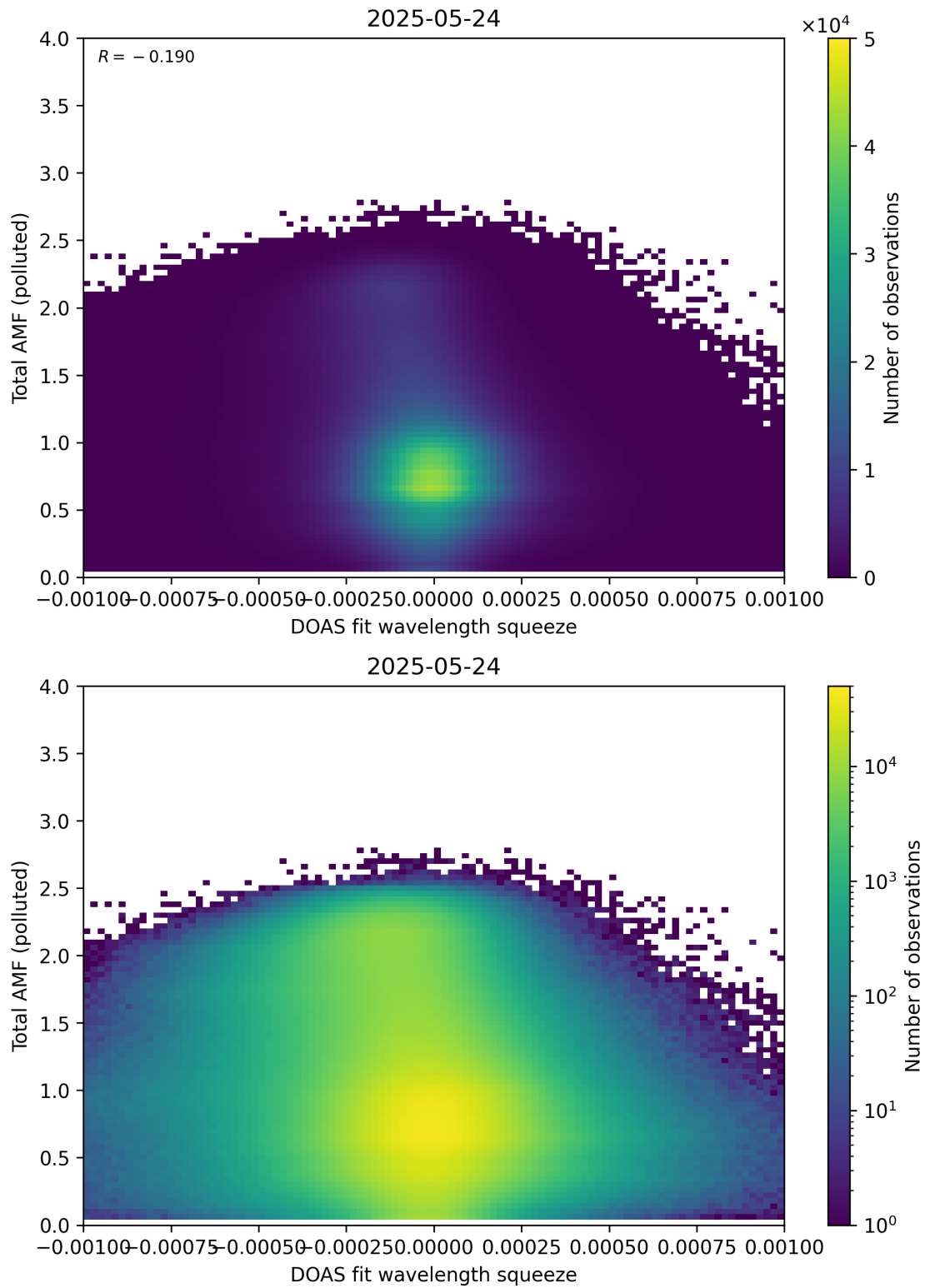
Figure 145: Scatter density plot of “DOAS fit wavelength squeeze” against “Total AMF (polluted)” for 2025-05-23 to 2025-05-25.
