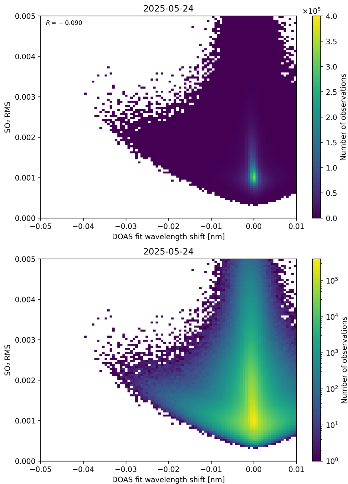
Figure 139: Scatter density plot of “DOAS fit wavelength shift” against “SO 2 RMS” for 2025-05-23 to 2025-05-25.
