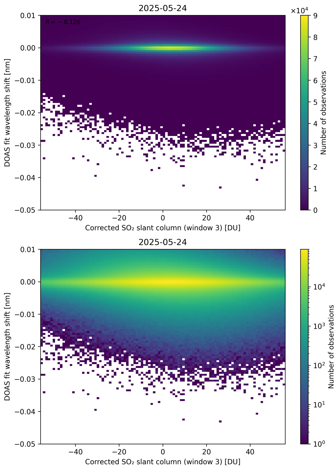
Figure 256: Scatter density plot of “Corrected SO 2 slant column (window 3)” against “DOAS fit wavelength shift” for 2025-05-23 to 2025-05-25.
