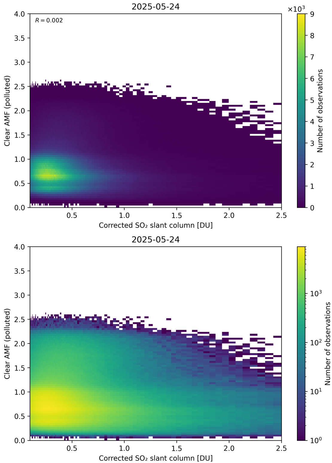
Figure 232: Scatter density plot of “Corrected SO 2 slant column” against “Clear AMF (polluted)” for 2025-05-23 to 2025-05-25.
