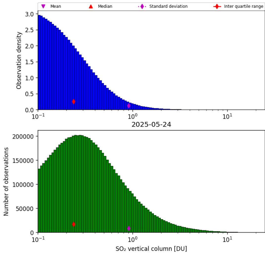
Figure 58: Histogram of “SO 2 vertical column” for 2025-05-23 to 2025-05-25
