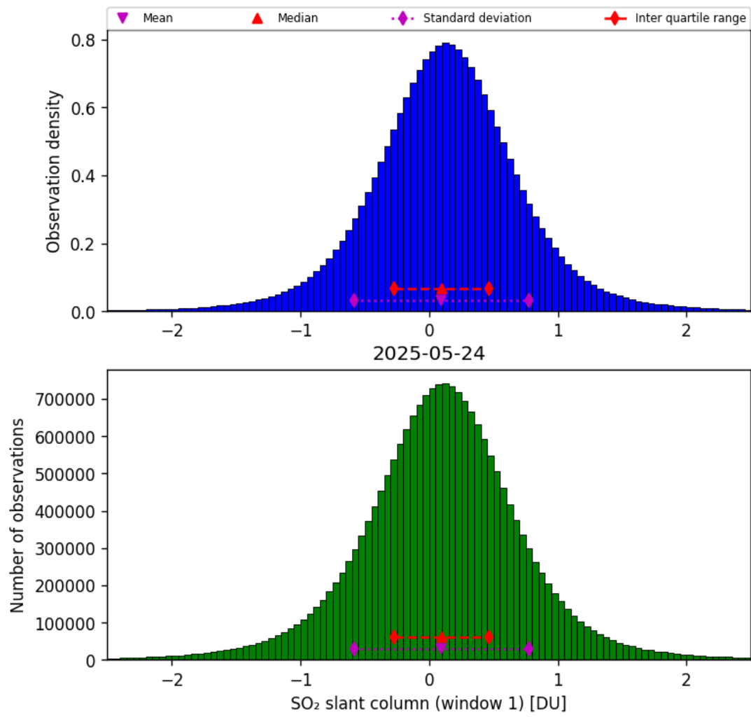
Figure 63: Histogram of “SO 2 slant column (window 1)” for 2025-05-23 to 2025-05-25
