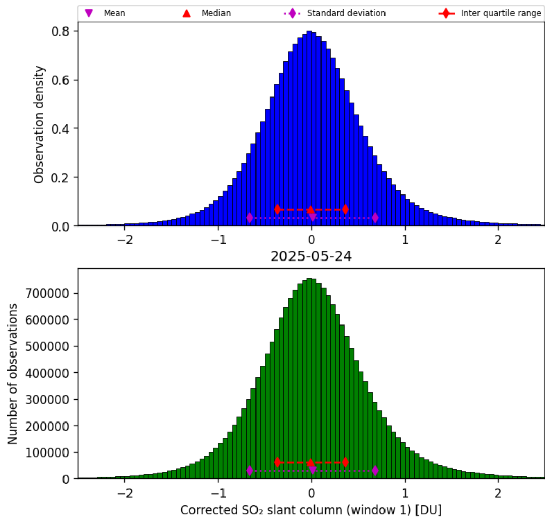
Figure 65: Histogram of “Corrected SO 2 slant column (window 1)” for 2025-05-23 to 2025-05-25
