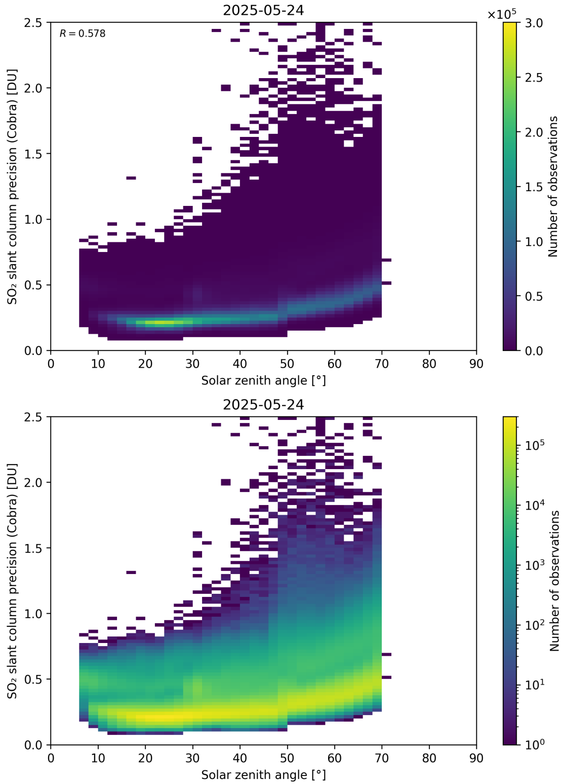
Figure 180: Scatter density plot of “Solar zenith angle” against “SO 2 slant column precision (Cobra)” for 2025-05-23 to 2025-05-25.
