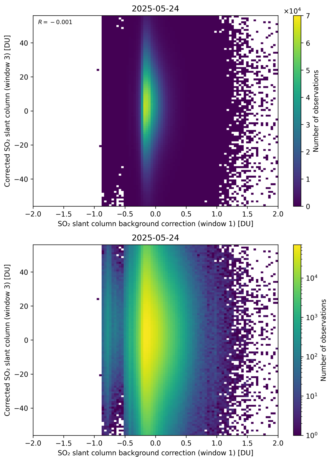
Figure 116: Scatter density plot of “SO 2 slant column background correction (window 1)” against “Corrected SO 2 slant column (window 3)” for 2025-05-23 to 2025-05-25.
