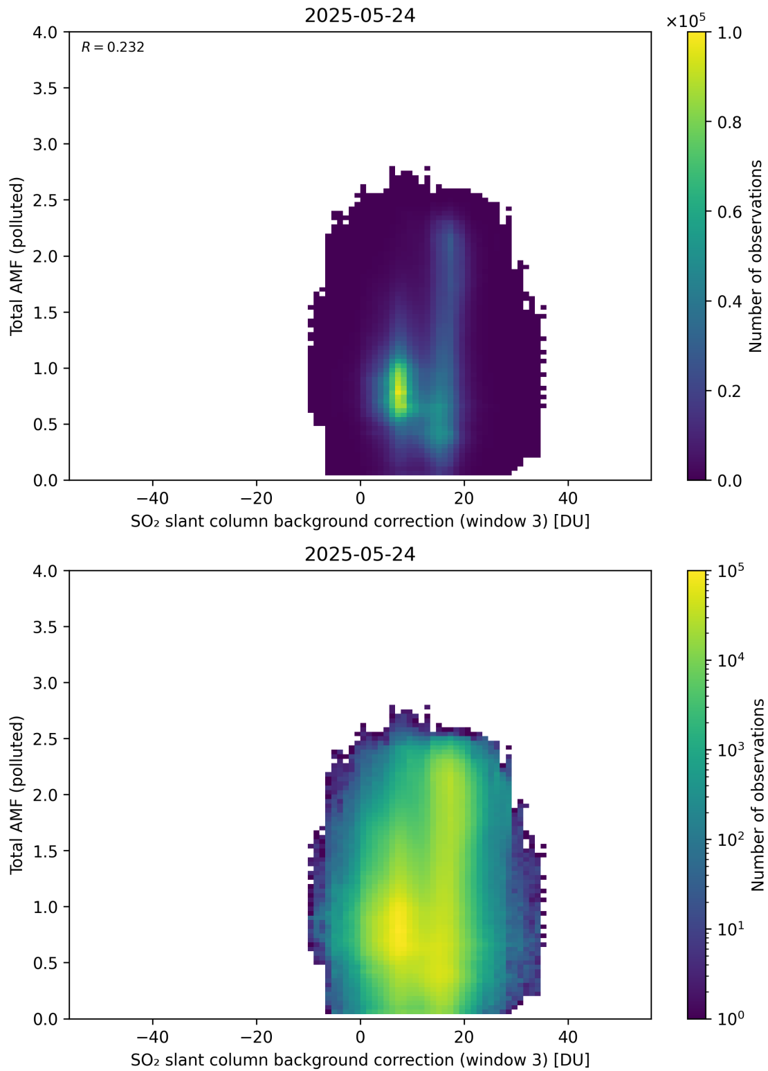
Figure 136: Scatter density plot of “SO 2 slant column background correction (window 3)” against “Total AMF (polluted)” for 2025-05-23 to 2025-05-25.
