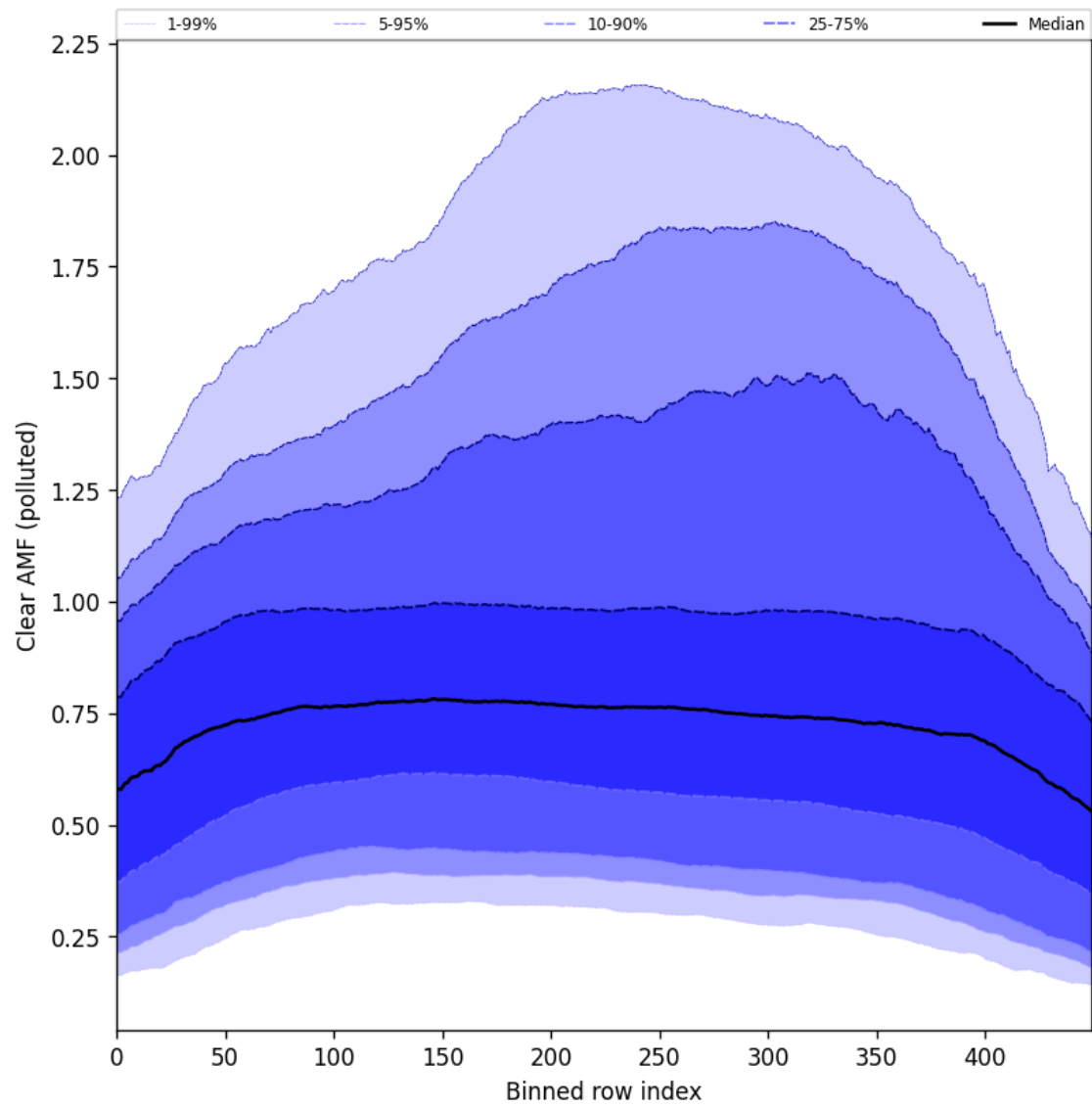
Figure 107: Along track statistics of “Clear AMF (polluted)” for 2025-05-23 to 2025-05-25
