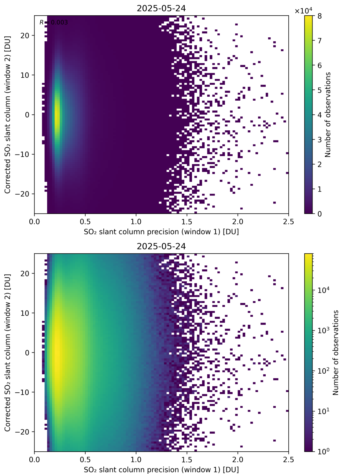
Figure 275: Scatter density plot of “SO 2 slant column precision (window 1)” against “Corrected SO 2 slant column (window 2)” for 2025-05-23 to 2025-05-25.
