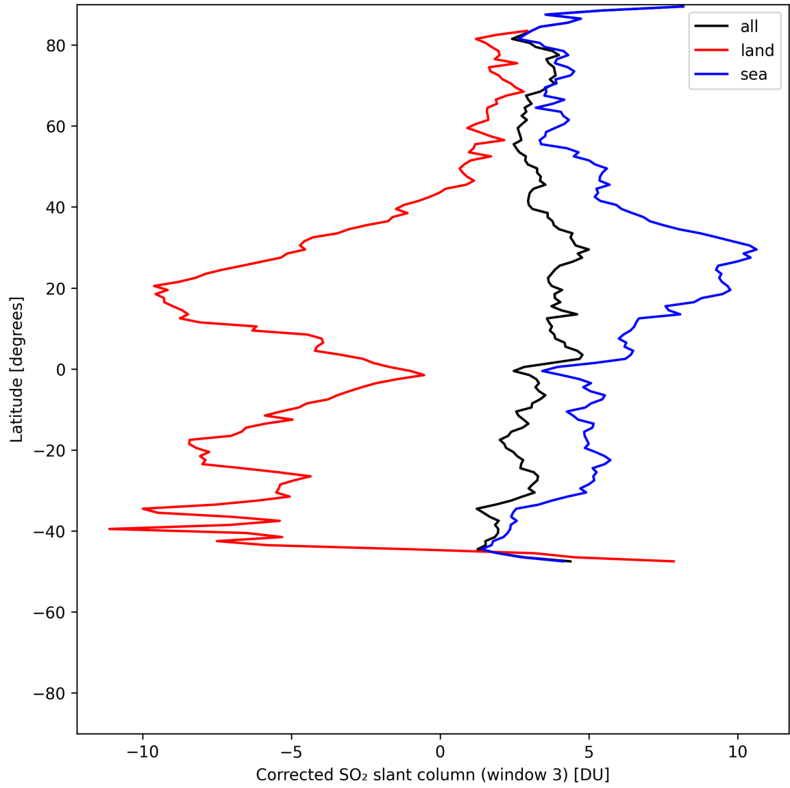
Figure 47: Zonal average of “Corrected SO 2 slant column (window 3)” for 2025-05-23 to 2025-05-25.
