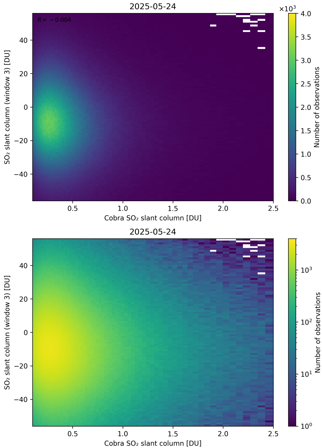
Figure 222: Scatter density plot of “Cobra SO 2 slant column” against “SO 2 slant column (window 3)” for 2025-05-23 to 2025-05-25.
