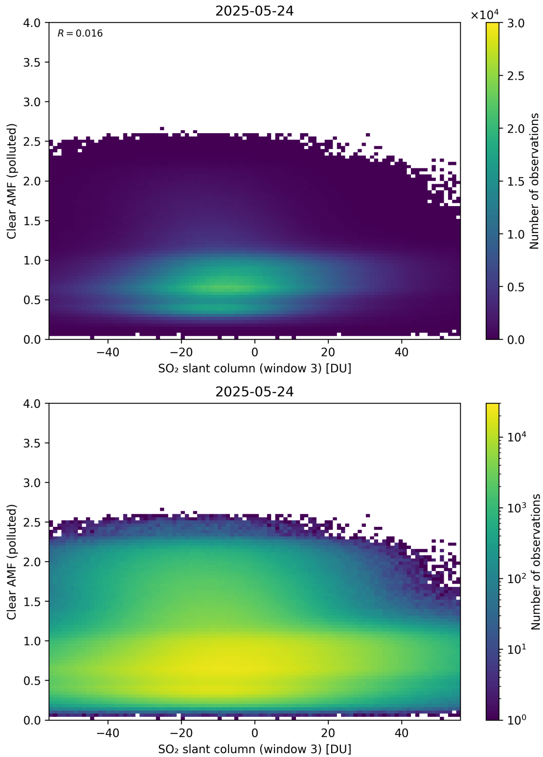
Figure 315: Scatter density plot of “SO 2 slant column (window 3)” against “Clear AMF (polluted)” for 2025-05-23 to 2025-05-25.
