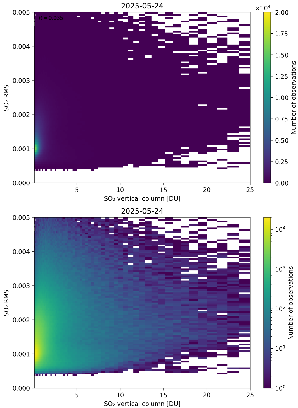
Figure 328: Scatter density plot of “SO 2 vertical column” against “SO 2 RMS” for 2025-05-23 to 2025-05-25.
