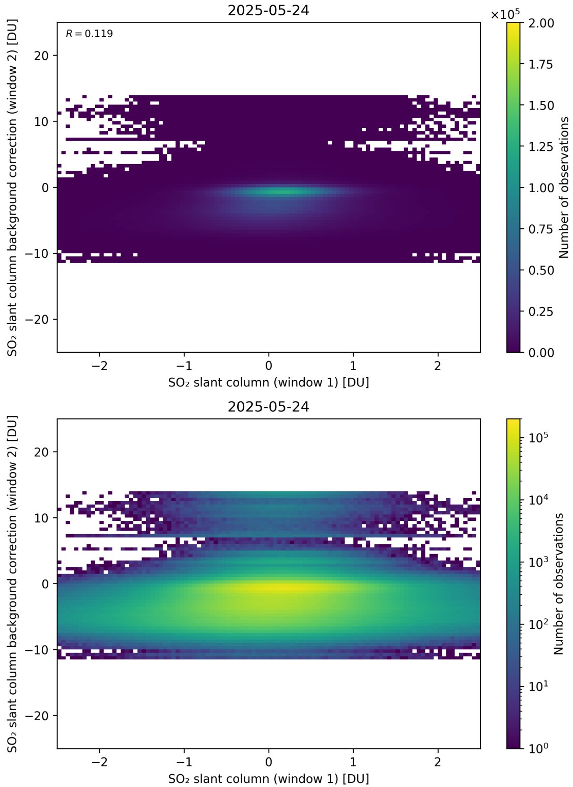
Figure 263: Scatter density plot of “SO 2 slant column (window 1)” against “SO 2 slant column background correction (window 2)” for 2025-05-23 to 2025-05-25.
