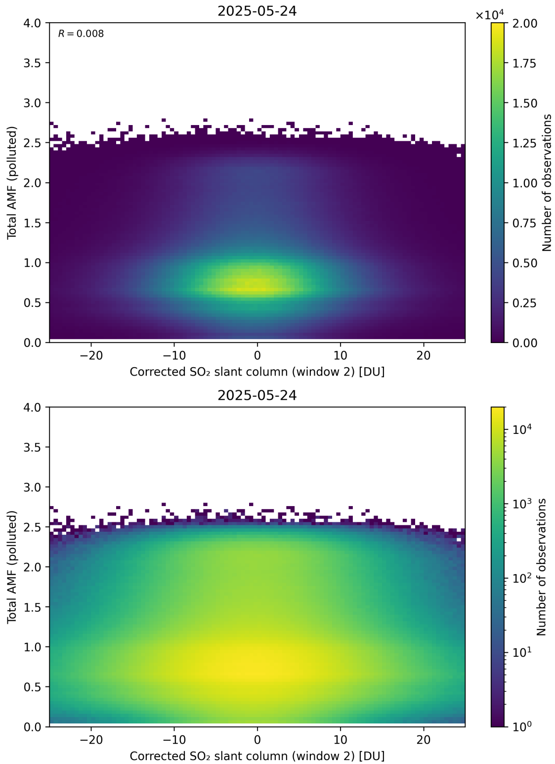
Figure 253: Scatter density plot of “Corrected SO 2 slant column (window 2)” against “Total AMF (polluted)” for 2025-05-23 to 2025-05-25.
