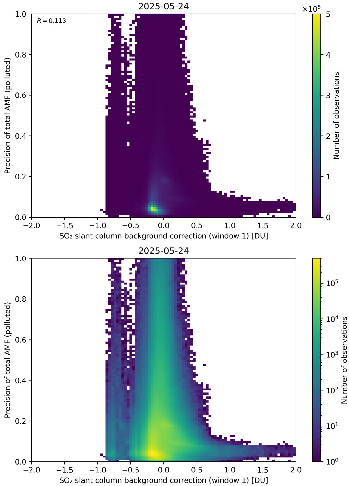
Figure 121: Scatter density plot of “SO 2 slant column background correction (window 1)” against “Precision of total AMF (polluted)” for 2025-05-23 to 2025-05-25.
