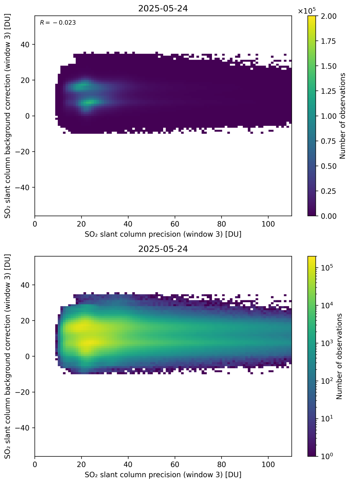
Figure 307: Scatter density plot of “SO 2 slant column precision (window 3)” against “SO 2 slant column background correction (window 3)” for 2025-05-23 to 2025-05-25.
