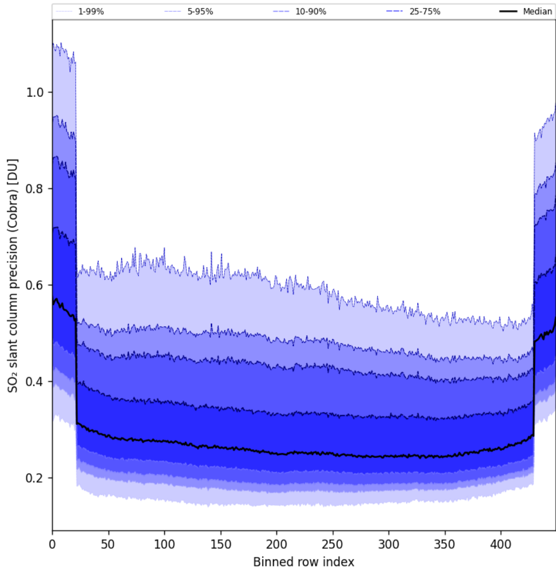
Figure 88: Along track statistics of “SO 2 slant column precision (Cobra)” for 2025-05-23 to 2025-05-25
