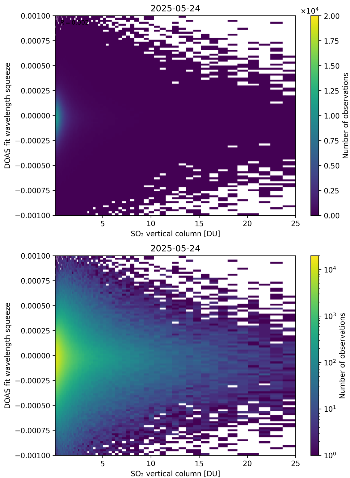
Figure 327: Scatter density plot of “SO 2 vertical column” against “DOAS fit wavelength squeeze” for 2025-05-23 to 2025-05-25.
