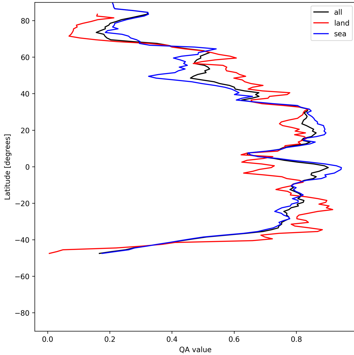
Figure 31: Zonal average of “QA value” for 2025-05-23 to 2025-05-25.
