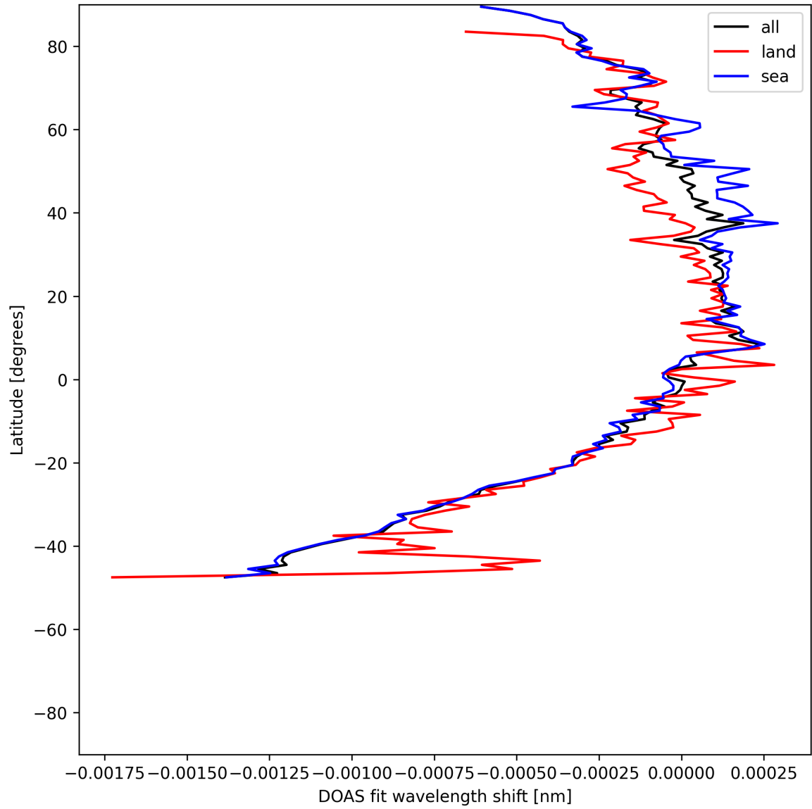
Figure 50: Zonal average of “DOAS fit wavelength shift” for 2025-05-23 to 2025-05-25.
