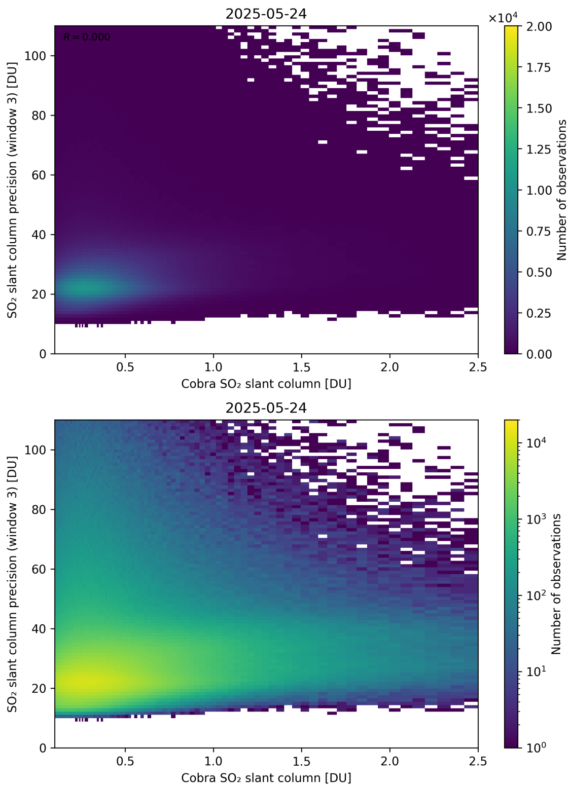
Figure 223: Scatter density plot of “Cobra SO 2 slant column” against “SO 2 slant column precision (window 3)” for 2025-05-23 to 2025-05-25.
