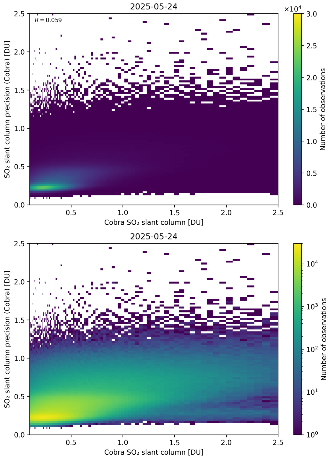
Figure 216: Scatter density plot of “Cobra SO 2 slant column” against “SO 2 slant column precision (Cobra)” for 2025-05-23 to 2025-05-25.
