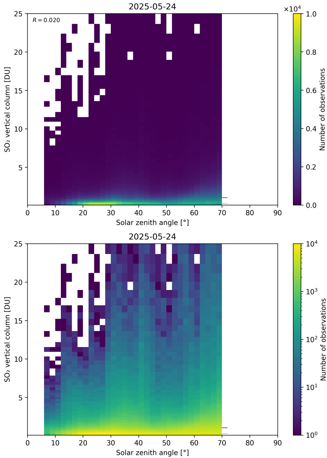
Figure 191: Scatter density plot of “Solar zenith angle” against “SO 2 vertical column” for 2025-05-23 to 2025-05-25.
