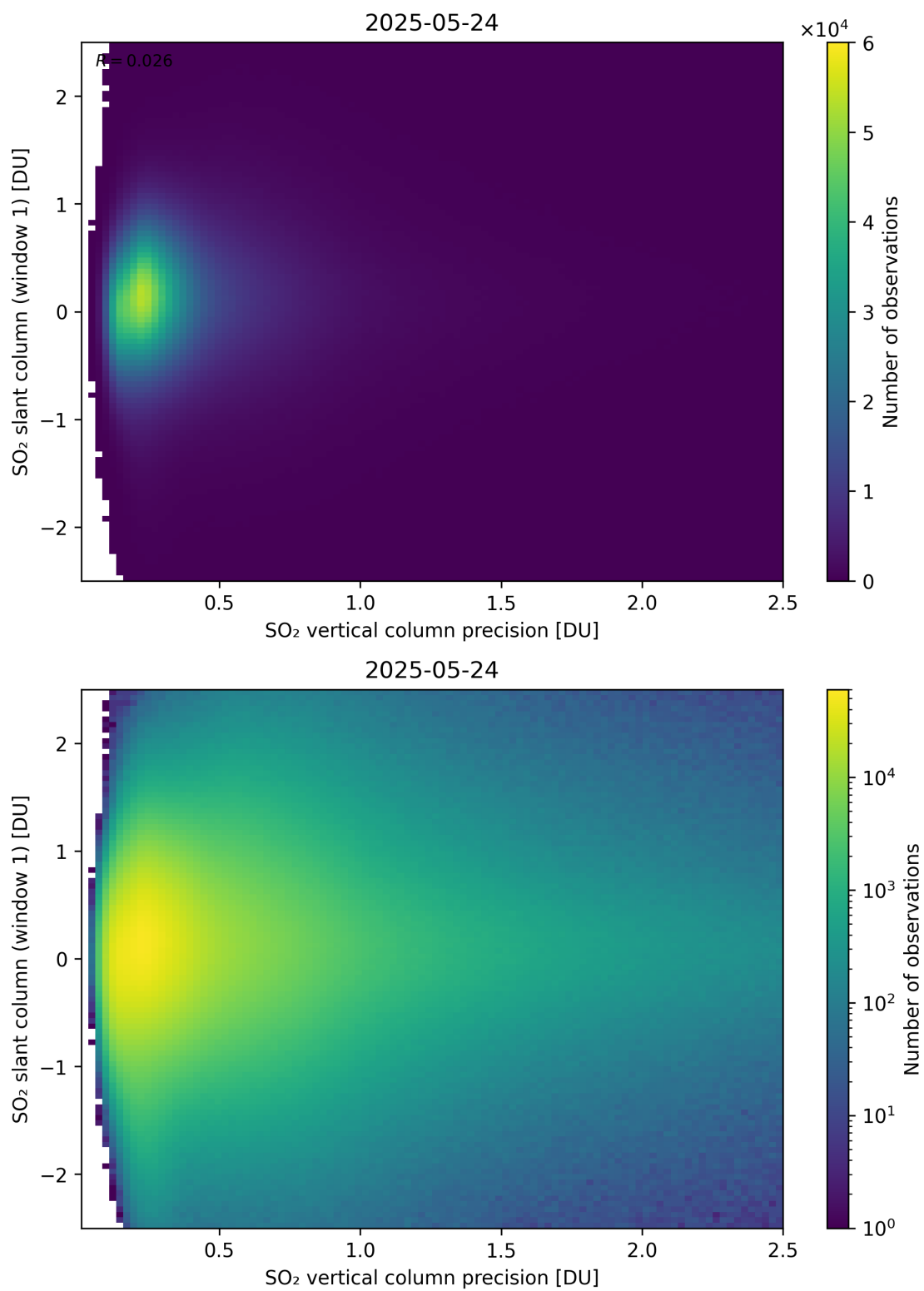
Figure 341: Scatter density plot of “SO 2 vertical column precision” against “SO 2 slant column (window 1)” for 2025-05-23 to 2025-05-25.
