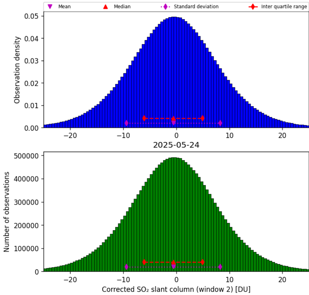
Figure 69: Histogram of “Corrected SO 2 slant column (window 2)” for 2025-05-23 to 2025-05-25
