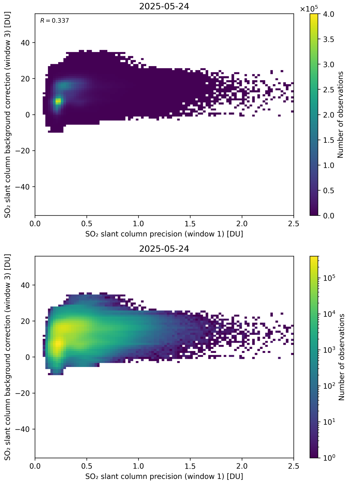
Figure 270: Scatter density plot of “SO 2 slant column precision (window 1)” against “SO 2 slant column background correction (window 3)” for 2025-05-23 to 2025-05-25.
