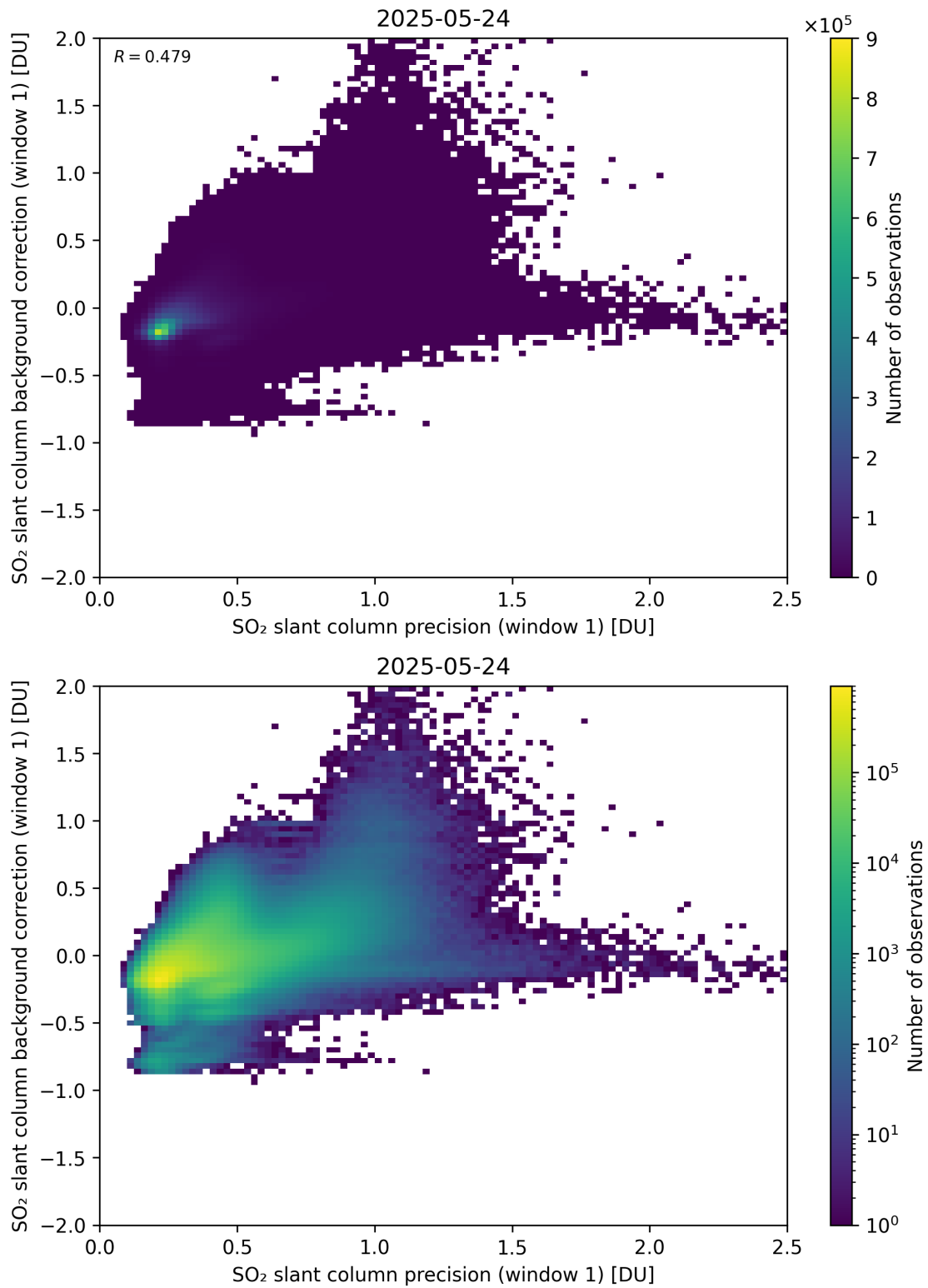
Figure 268: Scatter density plot of “SO 2 slant column precision (window 1)” against “SO 2 slant column background correction (window 1)” for 2025-05-23 to 2025-05-25.
