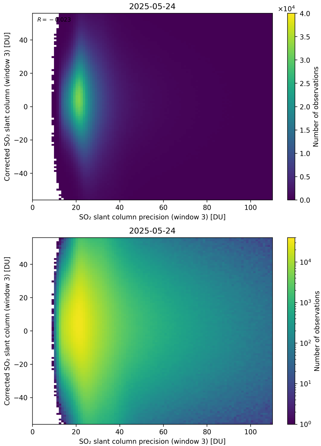
Figure 312: Scatter density plot of “SO 2 slant column precision (window 3)” against “Corrected SO 2 slant column (window 3)” for 2025-05-23 to 2025-05-25.
