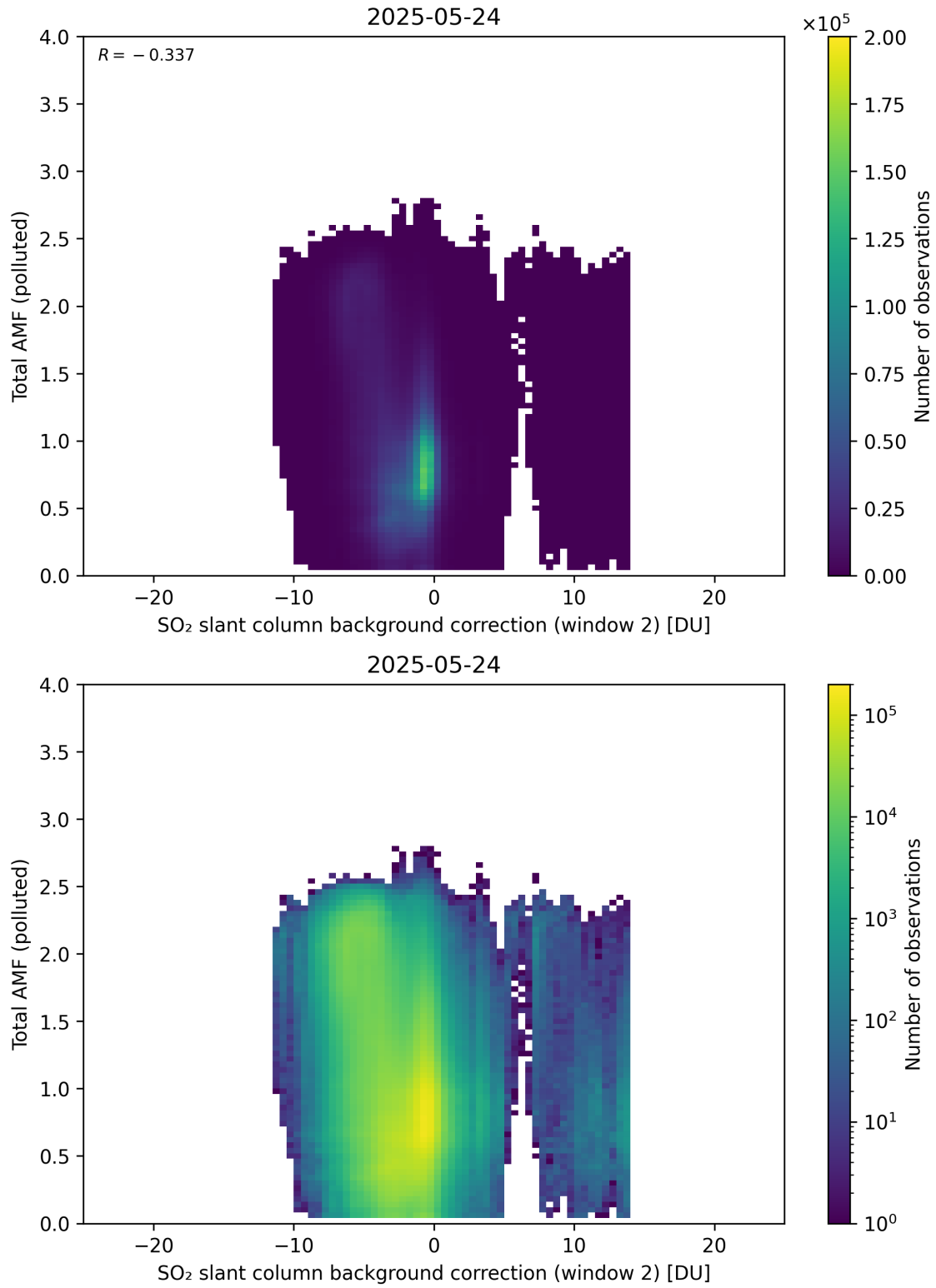
Figure 130: Scatter density plot of “SO 2 slant column background correction (window 2)” against “Total AMF (polluted)” for 2025-05-23 to 2025-05-25.
