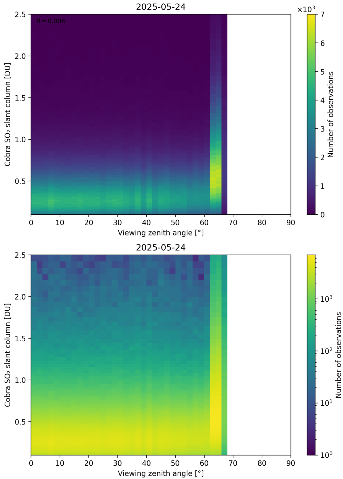
Figure 371: Scatter density plot of “Viewing zenith angle” against “Cobra SO 2 slant column” for 2025-05-23 to 2025-05-25.
