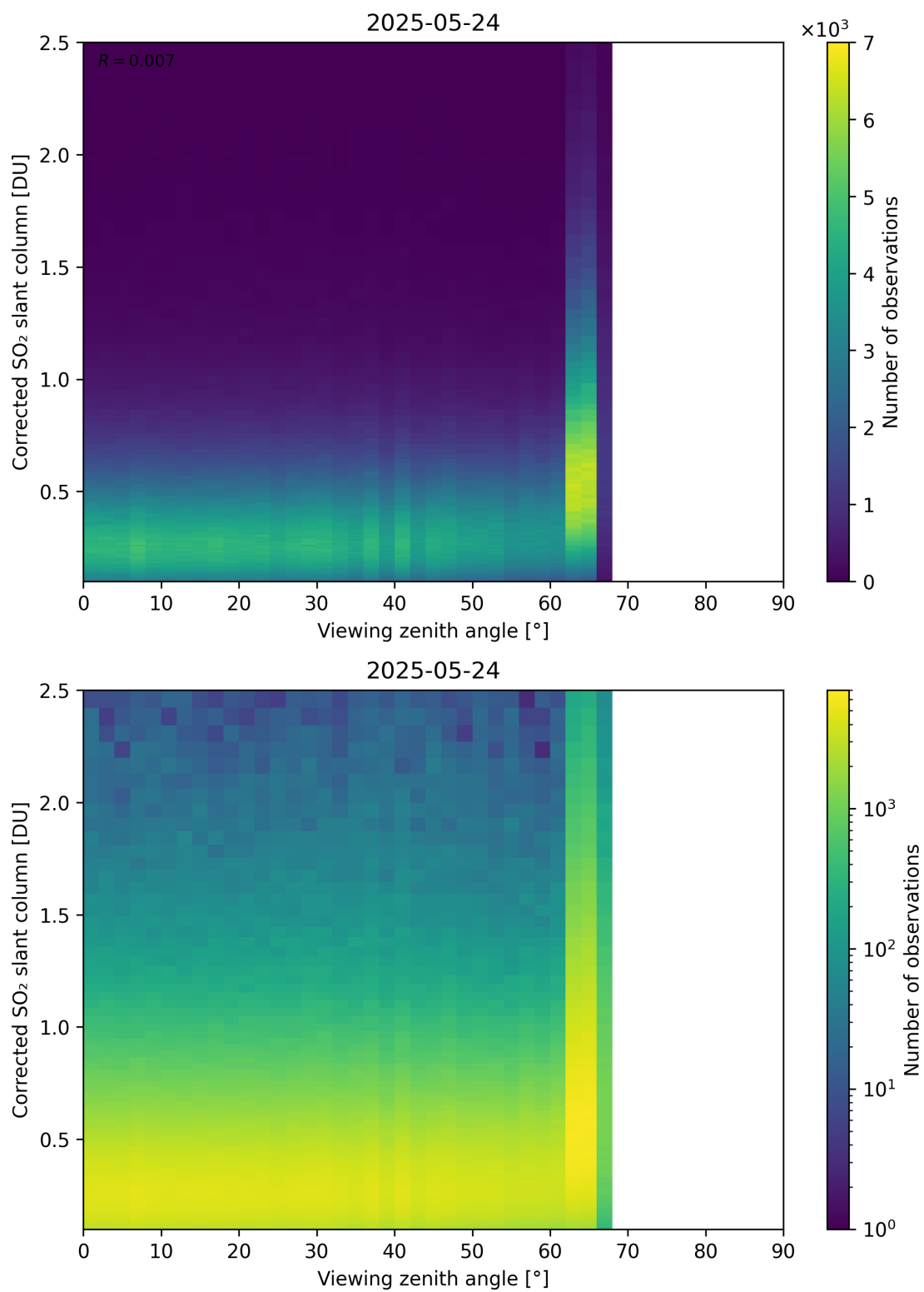
Figure 373: Scatter density plot of “Viewing zenith angle” against “Corrected SO 2 slant column” for 2025-05-23 to 2025-05-25.
