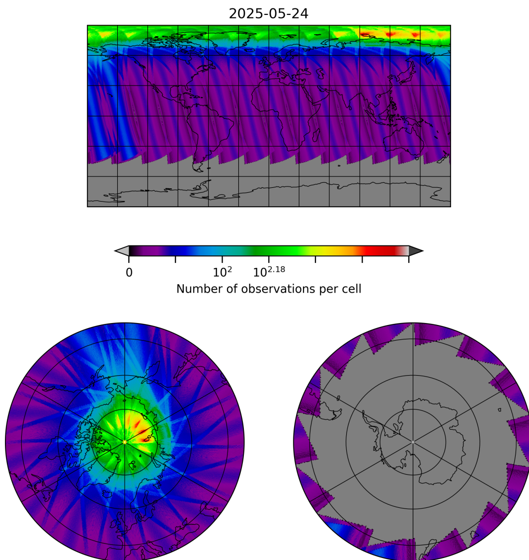
Figure 30: Map of the number of observations for 2025-05-23 to 2025-05-25
