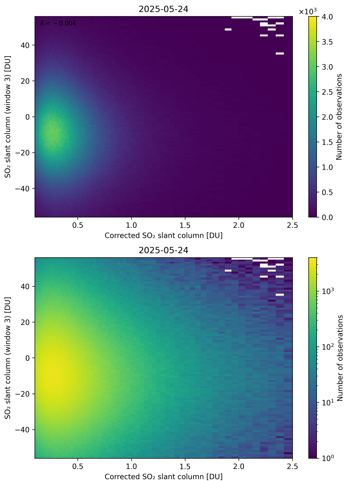
Figure 240: Scatter density plot of “Corrected SO 2 slant column” against “SO 2 slant column (window 3)” for 2025-05-23 to 2025-05-25.
