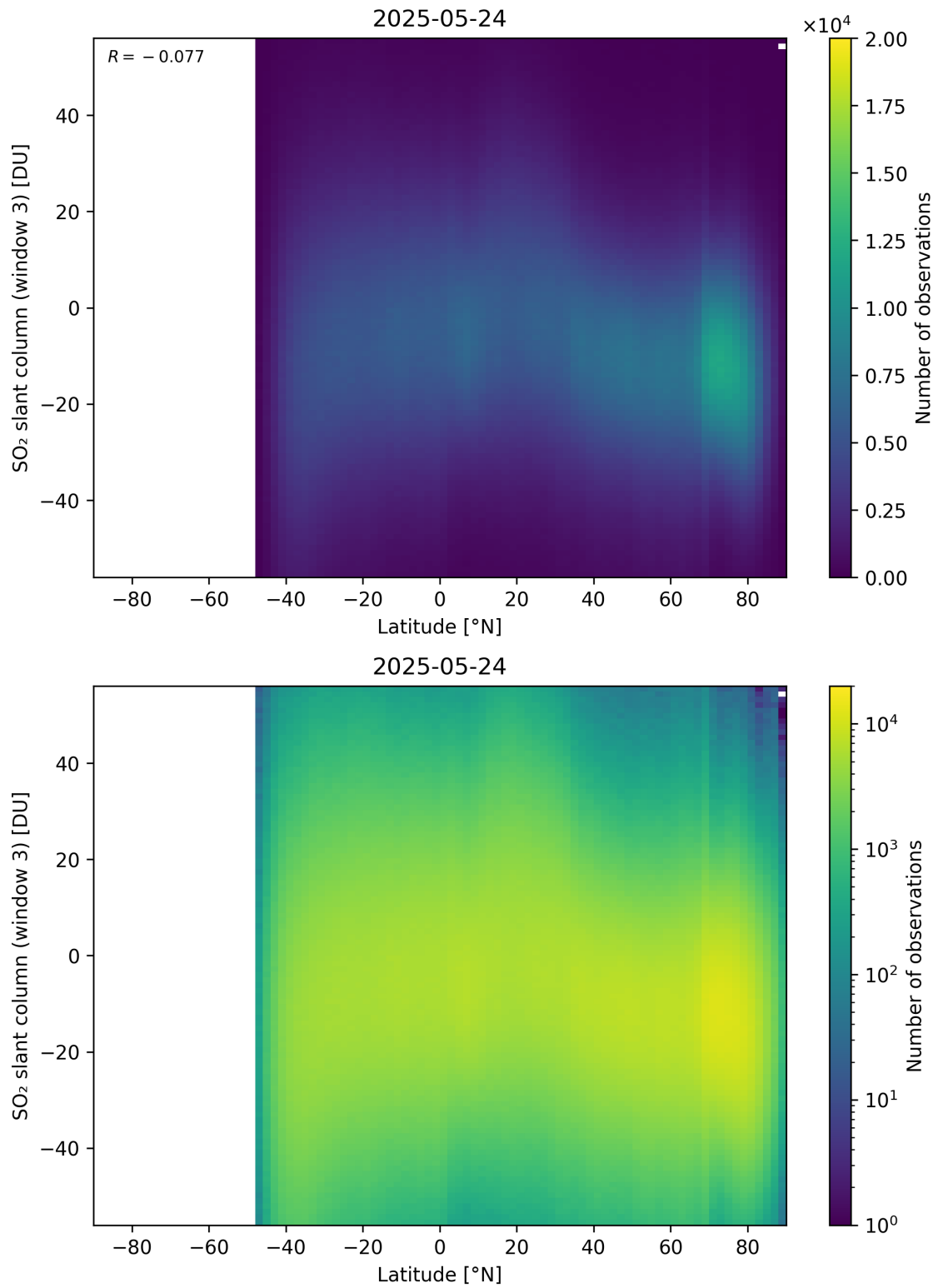
Figure 165: Scatter density plot of “Latitude” against “SO 2 slant column (window 3)” for 2025-05-23 to 2025-05-25.
