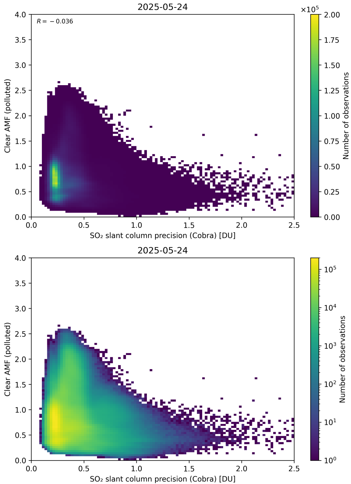
Figure 205: Scatter density plot of “SO 2 slant column precision (Cobra)” against “Clear AMF (polluted)” for 2025-05-23 to 2025-05-25.
