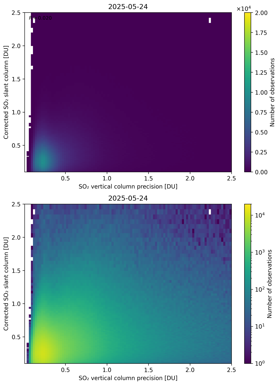
Figure 338: Scatter density plot of “SO 2 vertical column precision” against “Corrected SO 2 slant column” for 2025-05-23 to 2025-05-25.
