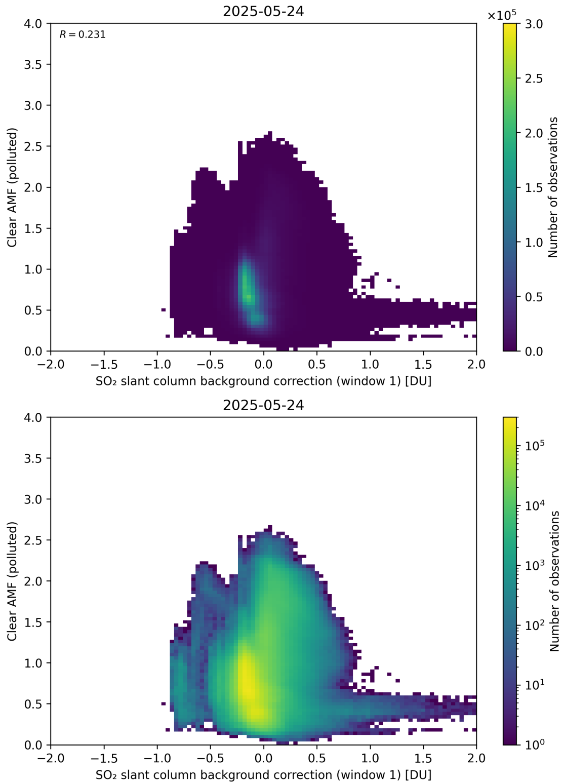
Figure 114: Scatter density plot of “SO 2 slant column background correction (window 1)” against “Clear AMF (polluted)” for 2025-05-23 to 2025-05-25.
