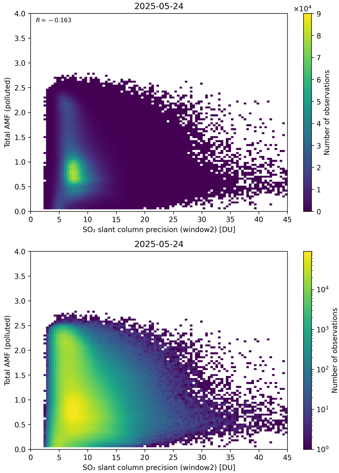
Figure 301: Scatter density plot of “SO 2 slant column precision (window2)” against “Total AMF (polluted)” for 2025-05-23 to 2025-05-25.
