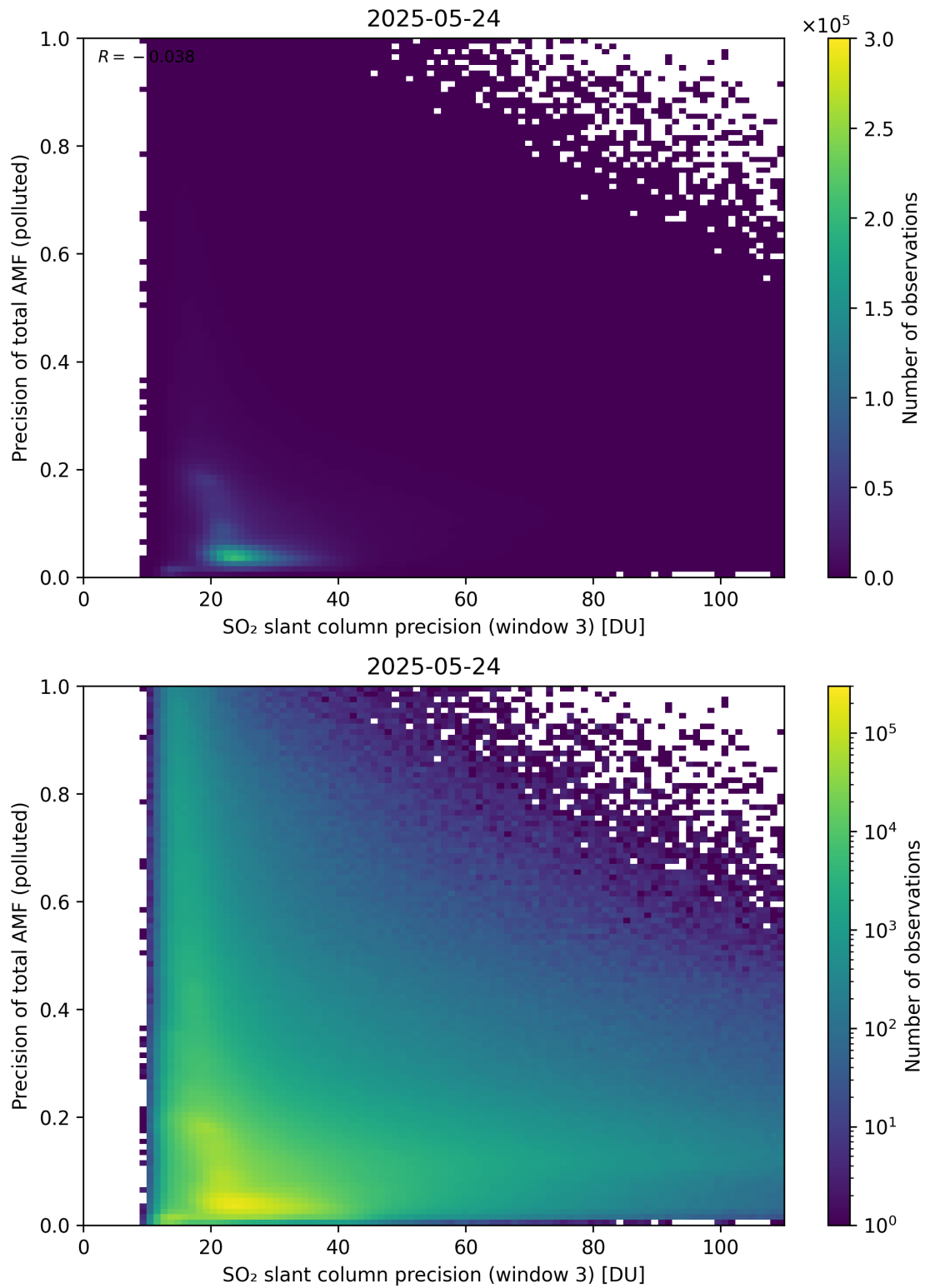
Figure 314: Scatter density plot of “SO 2 slant column precision (window 3)” against “Precision of total AMF (polluted)” for 2025-05-23 to 2025-05-25.
