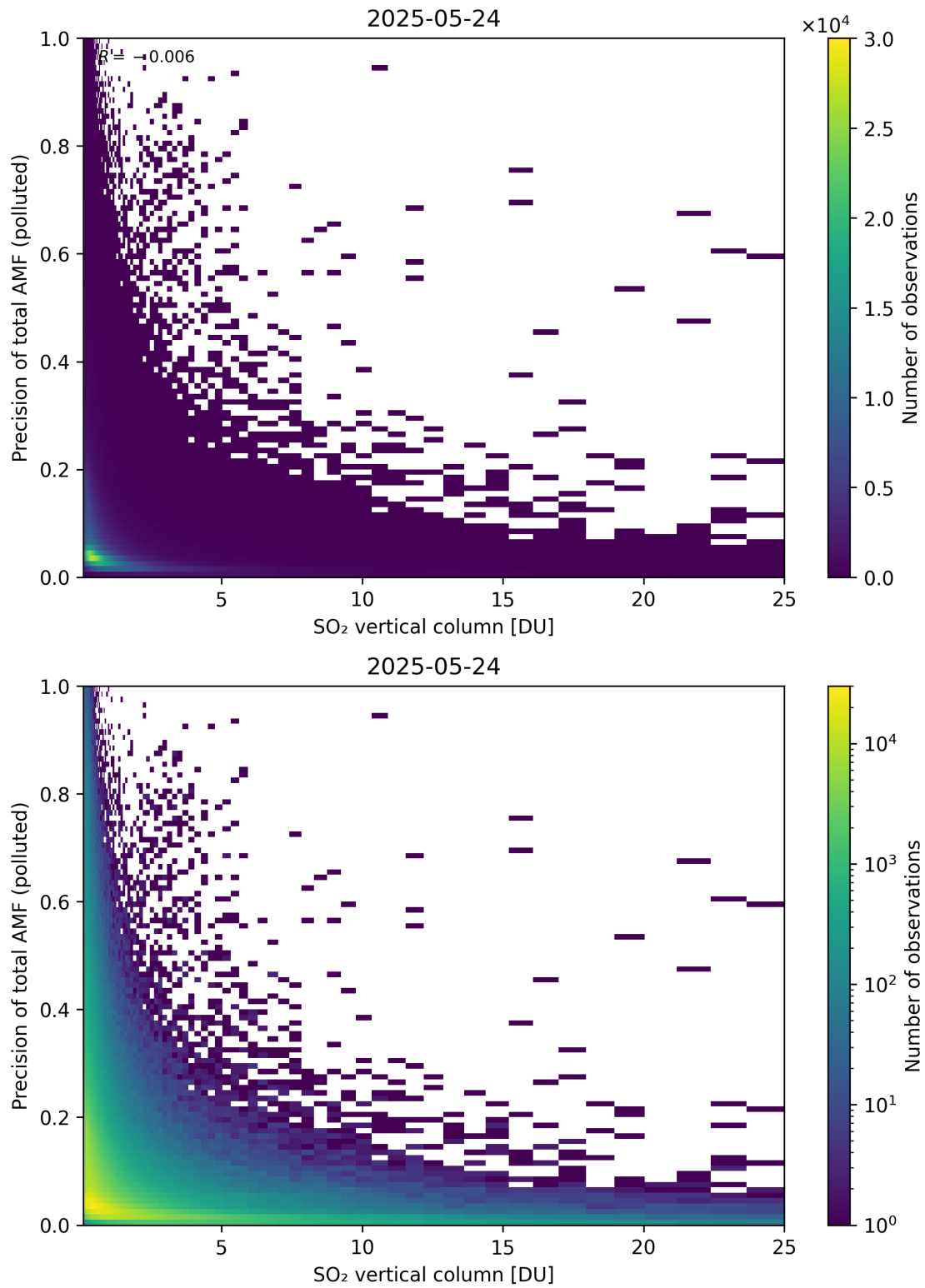
Figure 360: Scatter density plot of “SO 2 vertical column” against “Precision of total AMF (polluted)” for 2025-05-23 to 2025-05-25.
