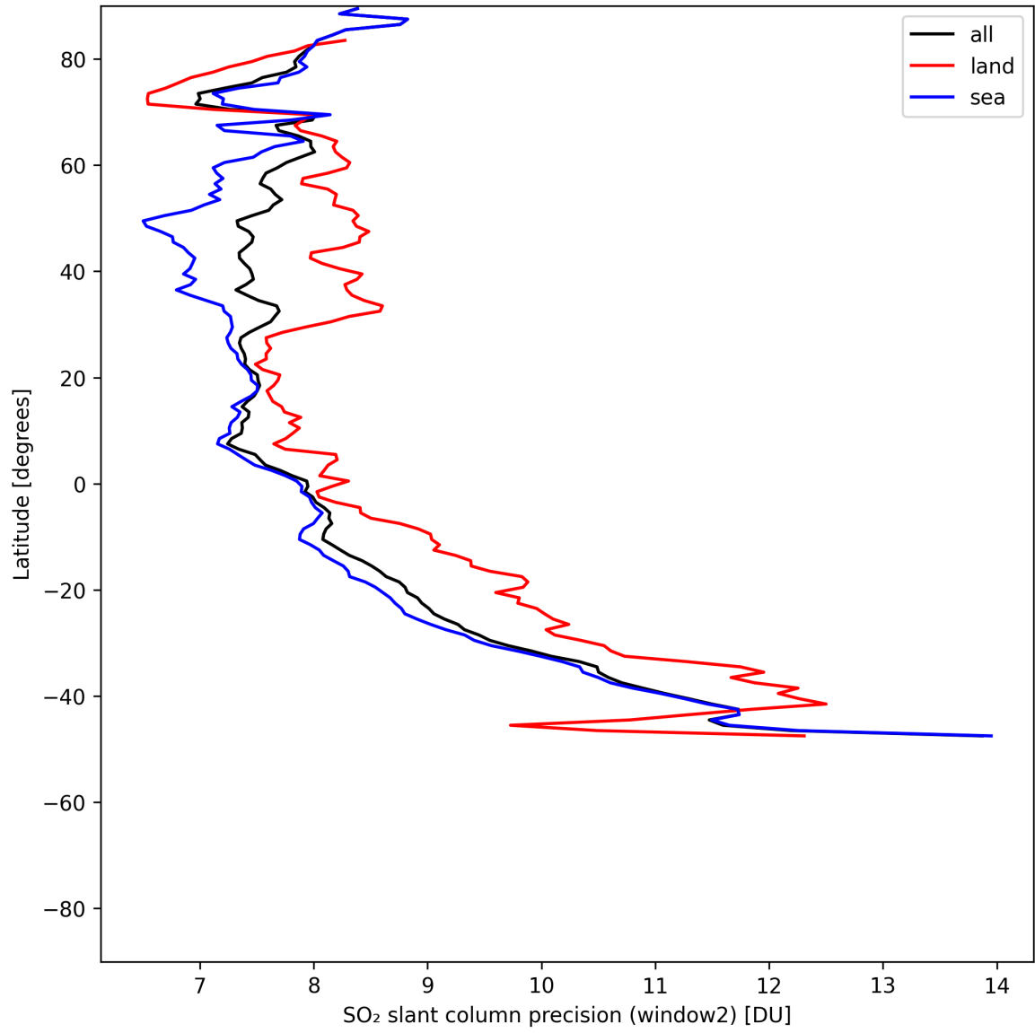
Figure 42: Zonal average of “SO 2 slant column precision (window2)” for 2025-05-23 to 2025-05-25.
