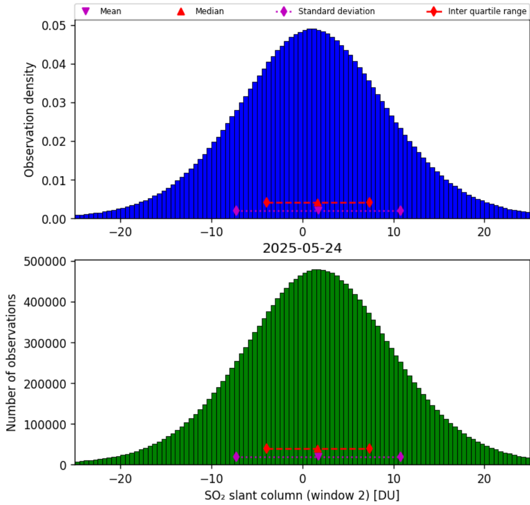
Figure 67: Histogram of “SO 2 slant column (window 2)” for 2025-05-23 to 2025-05-25
