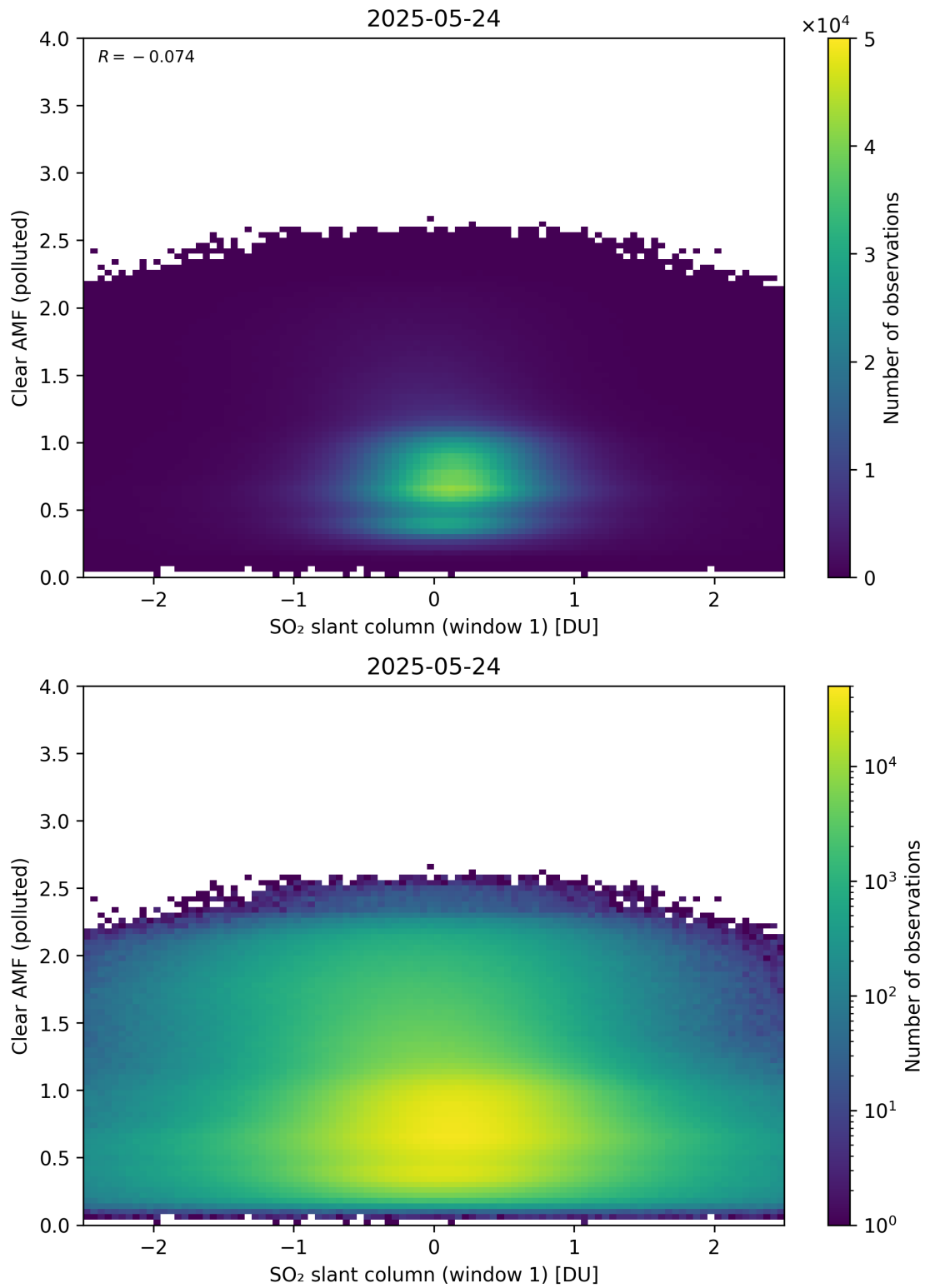
Figure 282: Scatter density plot of “SO 2 slant column (window 1)” against “Clear AMF (polluted)” for 2025-05-23 to 2025-05-25.
