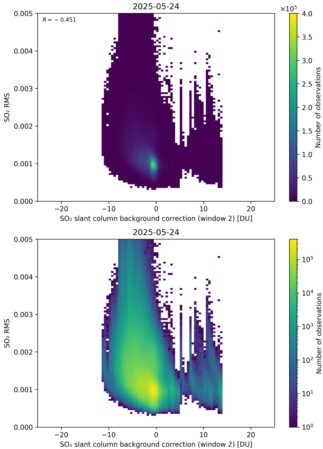
Figure 125: Scatter density plot of “SO 2 slant column background correction (window 2)” against “SO 2 RMS” for 2025-05-23 to 2025-05-25.
