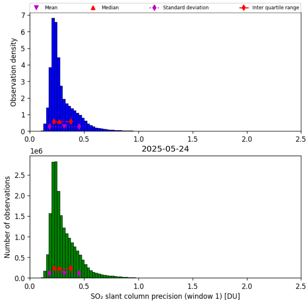
Figure 64: Histogram of “SO 2 slant column precision (window 1)” for 2025-05-23 to 2025-05-25
