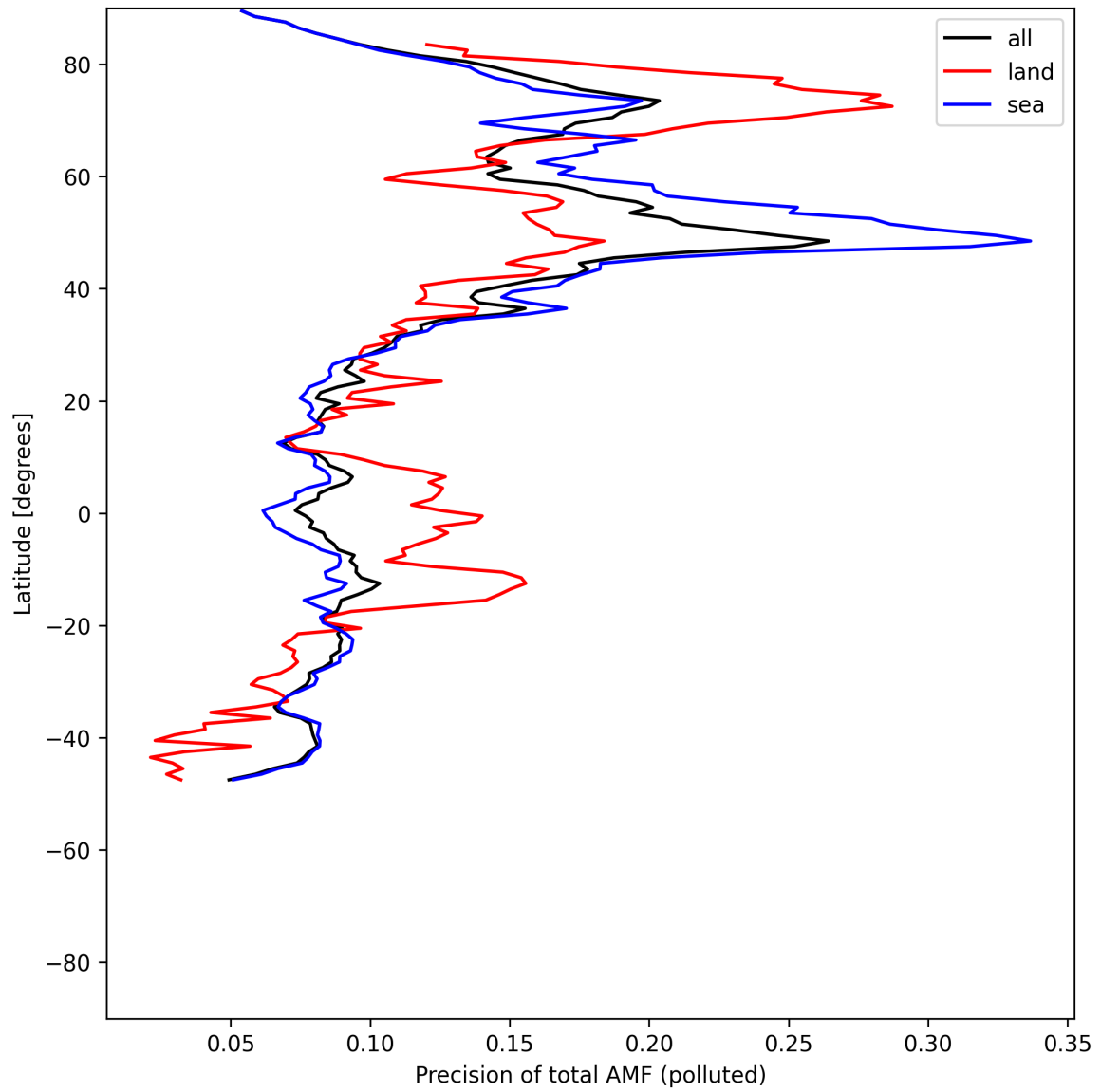
Figure 54: Zonal average of “Precision of total AMF (polluted)” for 2025-05-23 to 2025-05-25.
