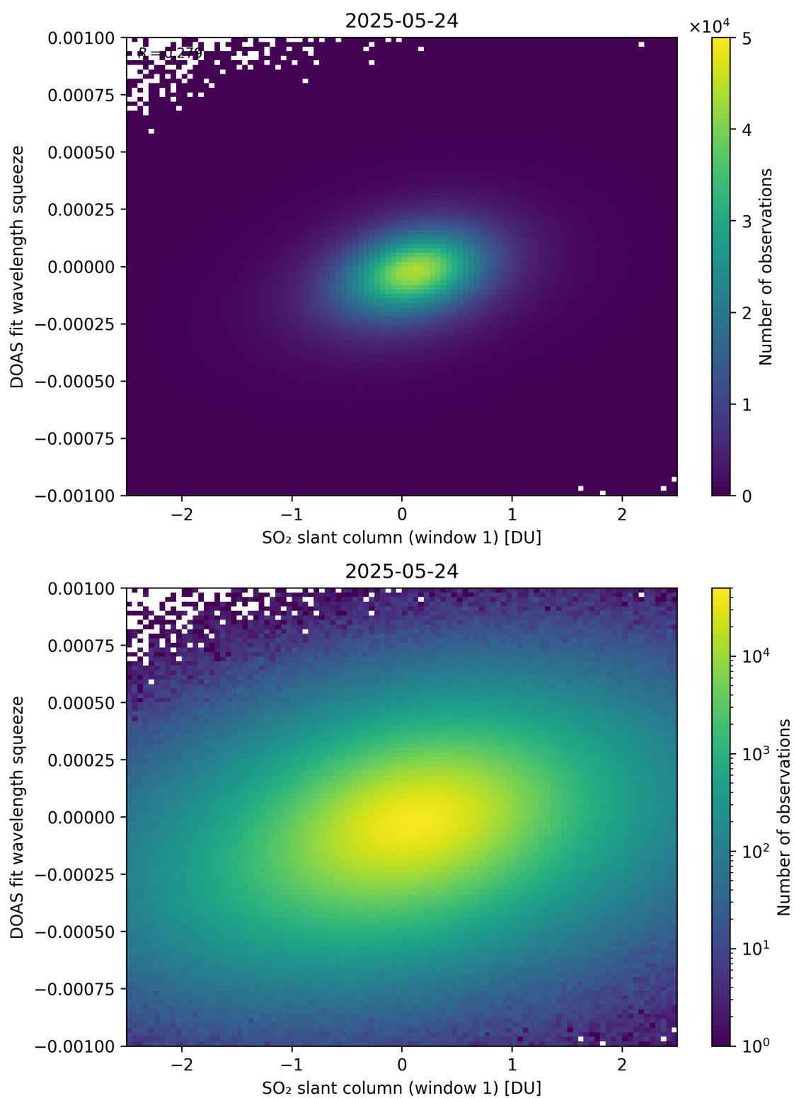
Figure 266: Scatter density plot of “SO 2 slant column (window 1)” against “DOAS fit wavelength squeeze” for 2025-05-23 to 2025-05-25.
