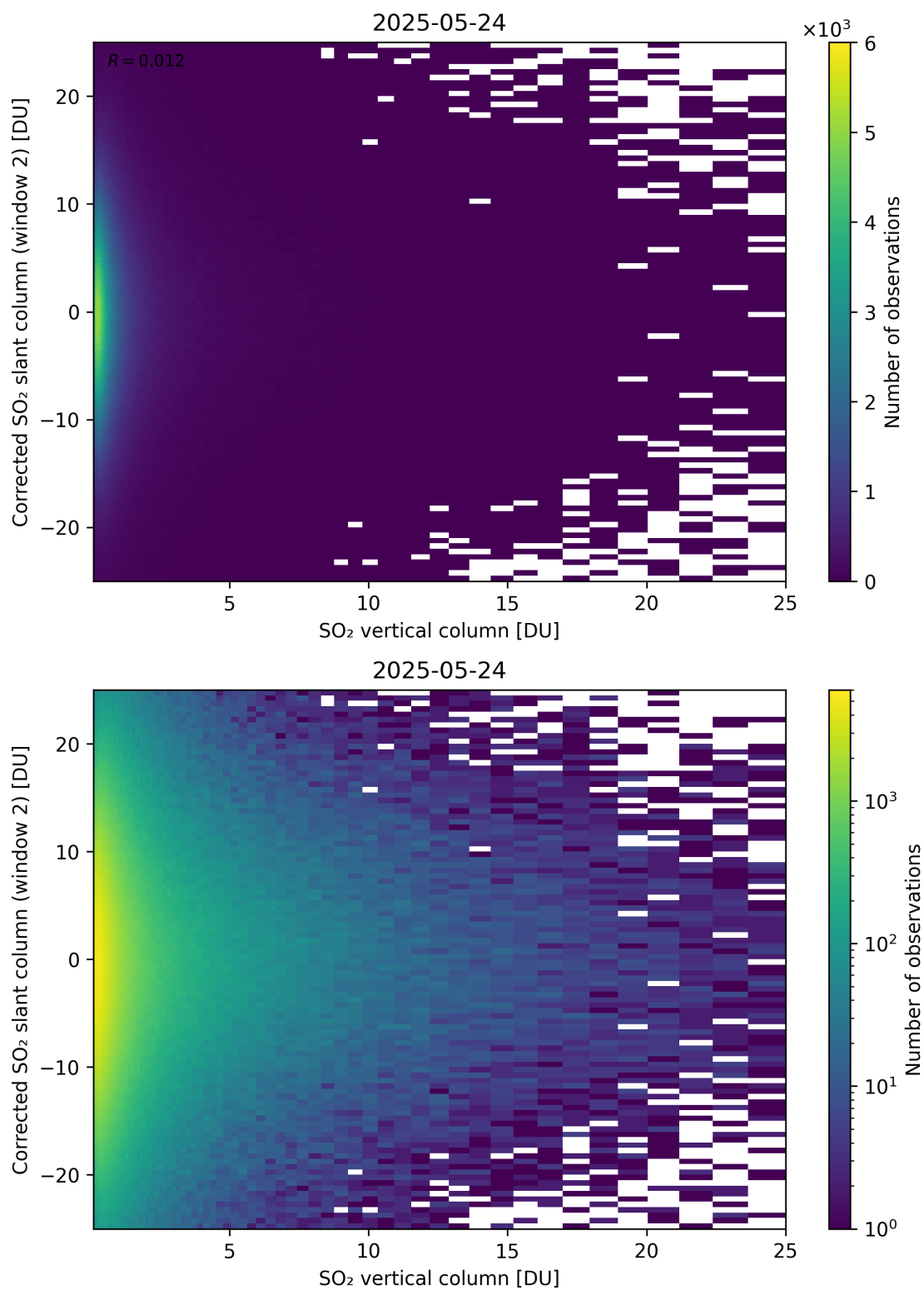
Figure 352: Scatter density plot of “SO 2 vertical column” against “Corrected SO 2 slant column (window 2)” for 2025-05-23 to 2025-05-25.
