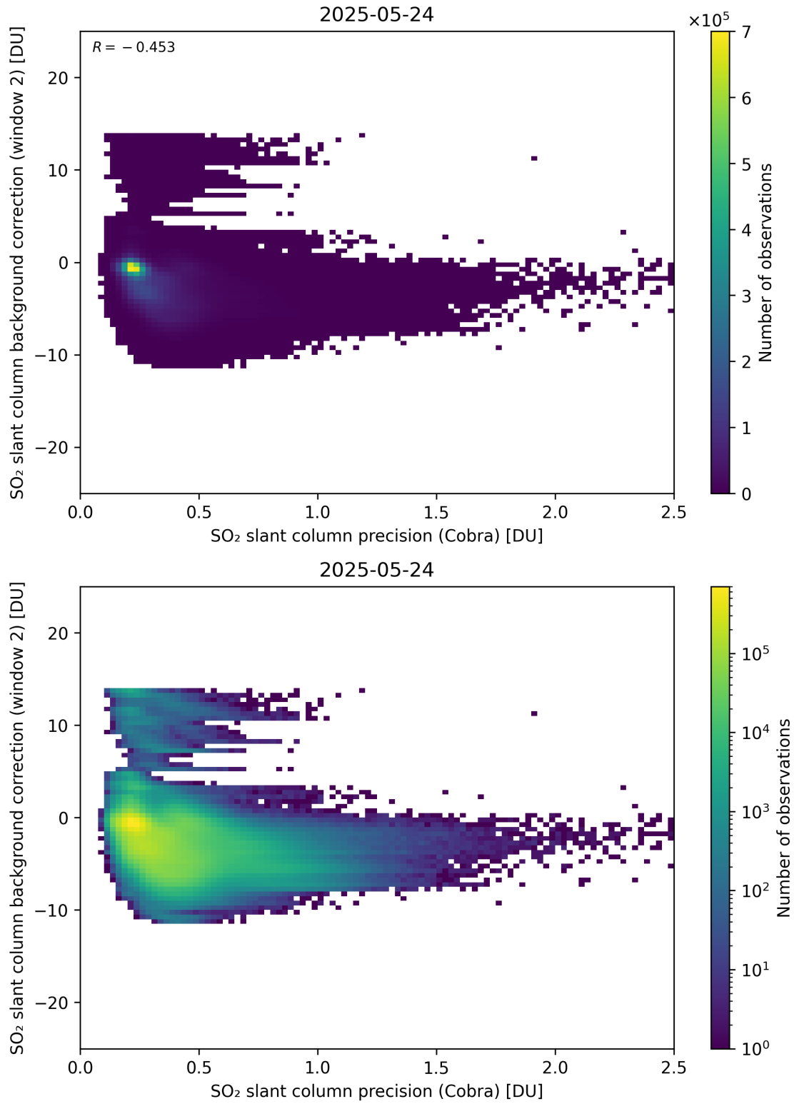
Figure 200: Scatter density plot of “SO 2 slant column precision (Cobra)” against “SO 2 slant column background correction (window 2)” for 2025-05-23 to 2025-05-25.
