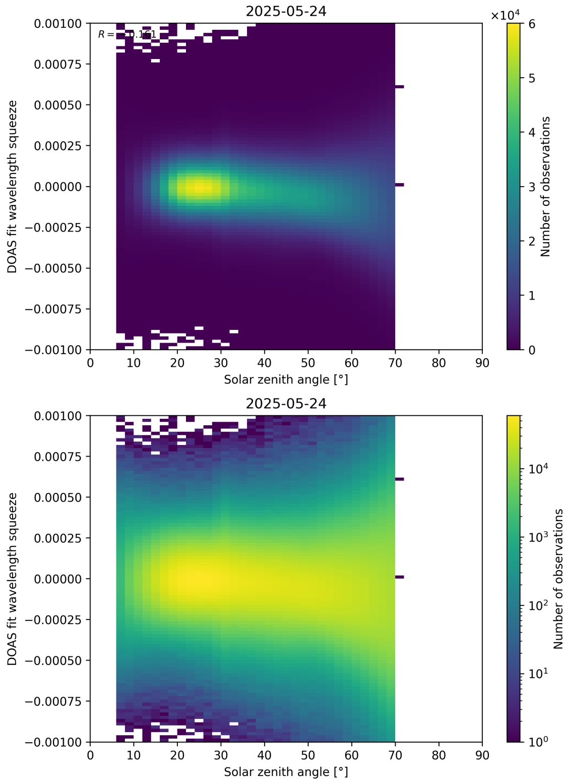
Figure 175: Scatter density plot of “Solar zenith angle” against “DOAS fit wavelength squeeze” for 2025-05-23 to 2025-05-25.
