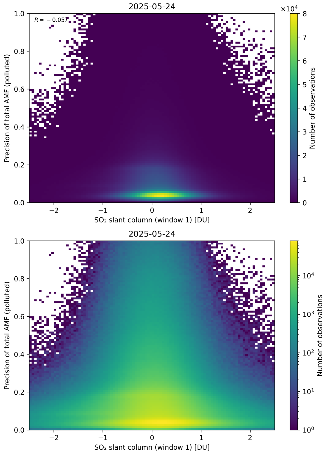
Figure 290: Scatter density plot of “SO 2 slant column (window 1)” against “Precision of total AMF (polluted)” for 2025-05-23 to 2025-05-25.
