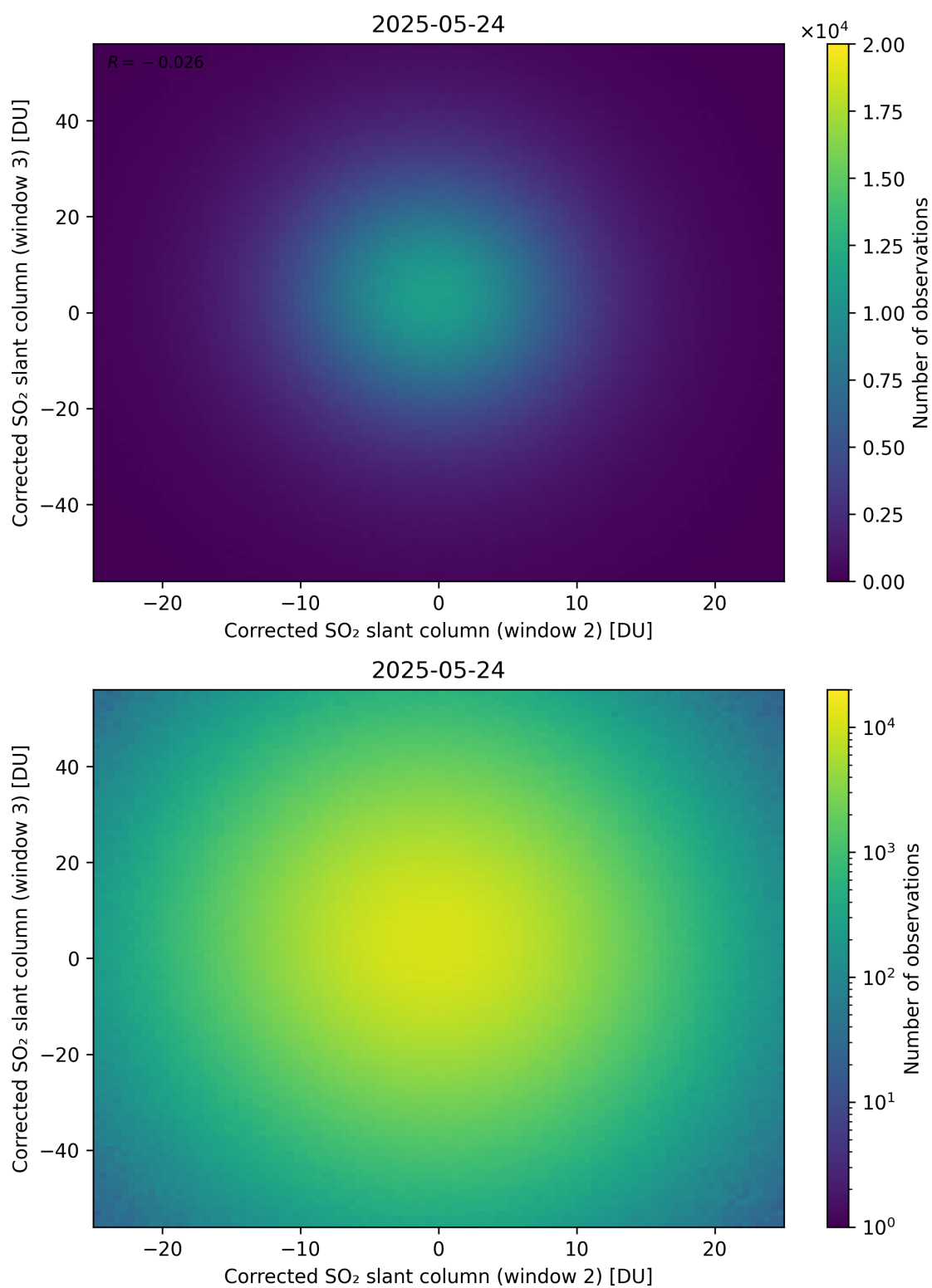
Figure 250: Scatter density plot of “Corrected SO 2 slant column (window 2)” against “Corrected SO 2 slant column (window 3)” for 2025-05-23 to 2025-05-25.
