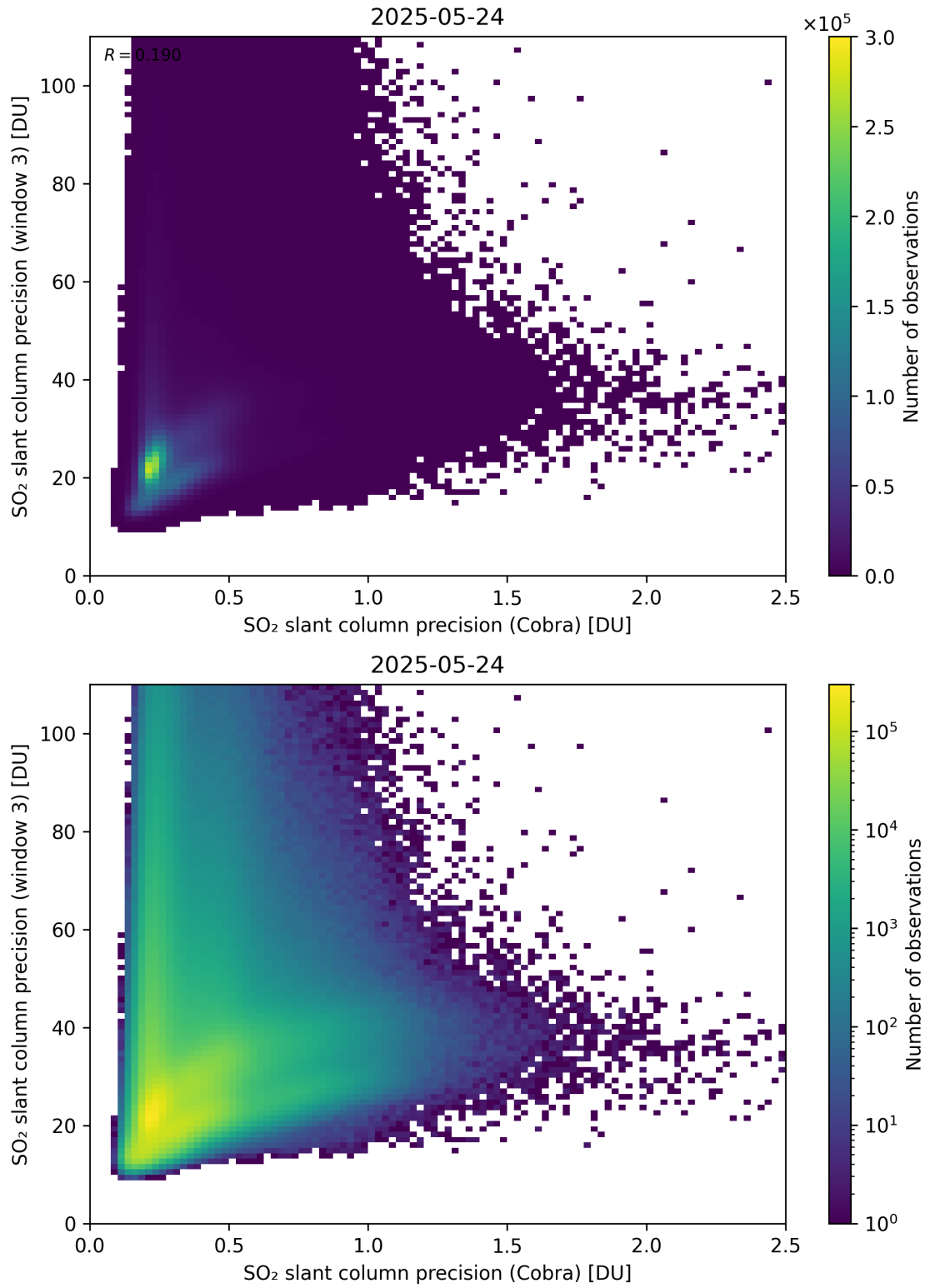
Figure 212: Scatter density plot of “SO 2 slant column precision (Cobra)” against “SO 2 slant column precision (window 3)” for 2025-05-23 to 2025-05-25.
