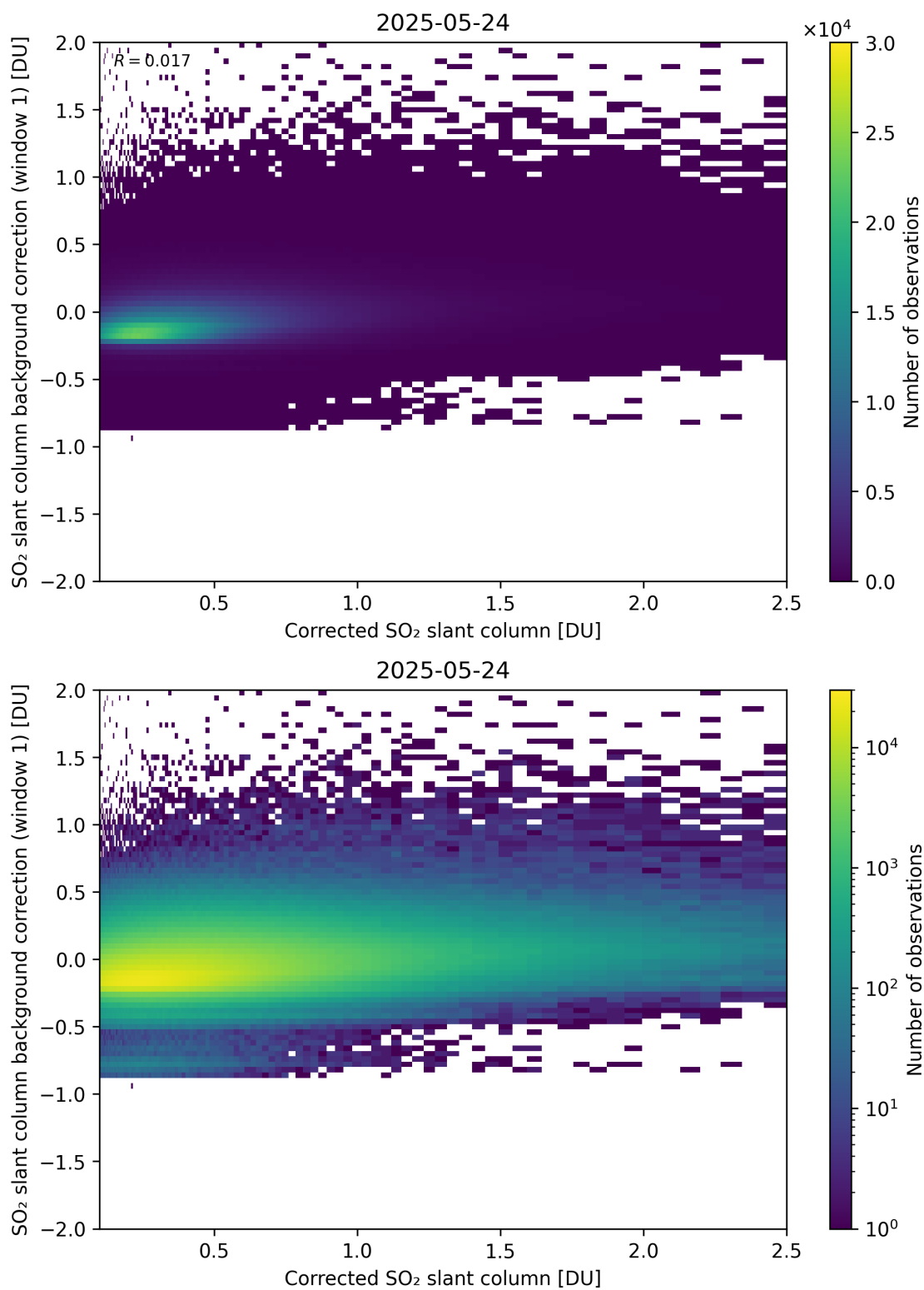
Figure 226: Scatter density plot of “Corrected SO 2 slant column” against “SO 2 slant column background correction (window 1)” for 2025-05-23 to 2025-05-25.
