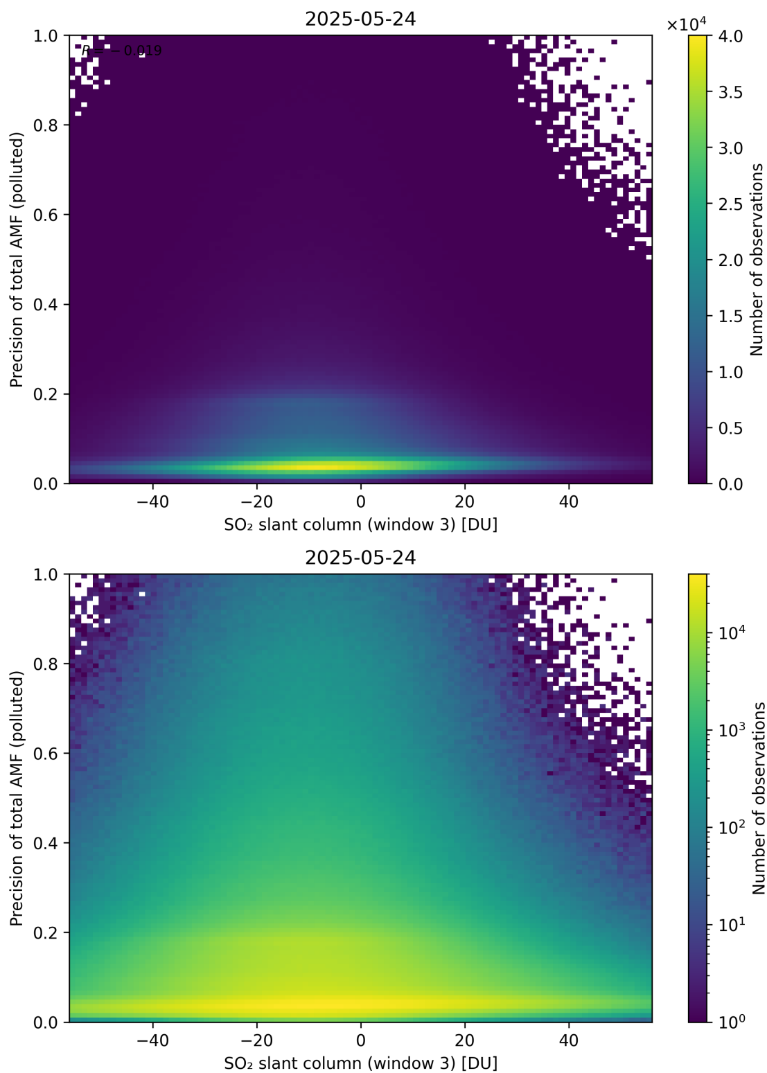
Figure 319: Scatter density plot of “SO 2 slant column (window 3)” against “Precision of total AMF (polluted)” for 2025-05-23 to 2025-05-25.
