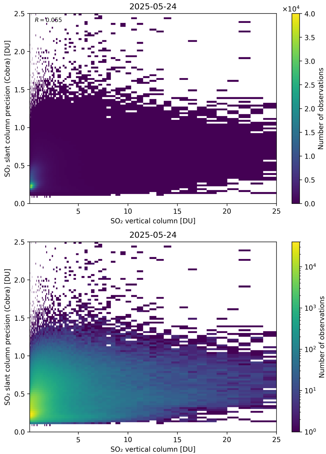
Figure 350: Scatter density plot of “SO 2 vertical column” against “SO 2 slant column precision (Cobra)” for 2025-05-23 to 2025-05-25.
