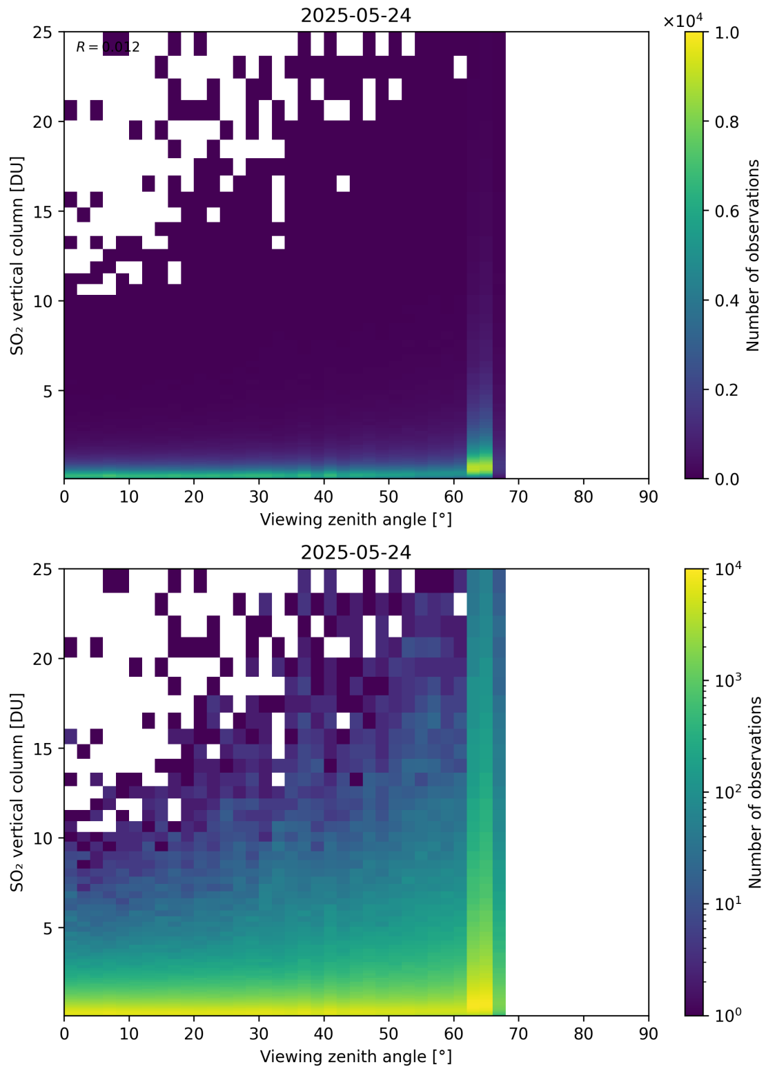
Figure 383: Scatter density plot of “Viewing zenith angle” against “SO 2 vertical column” for 2025-05-23 to 2025-05-25.
