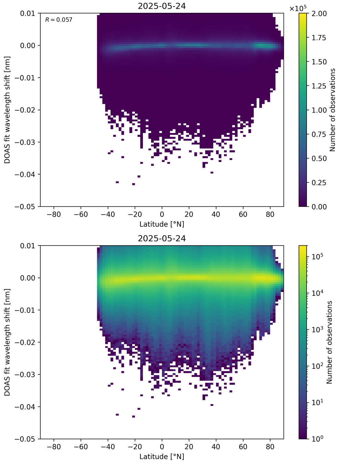
Figure 153: Scatter density plot of “Latitude” against “DOAS fit wavelength shift” for 2025-05-23 to 2025-05-25.
