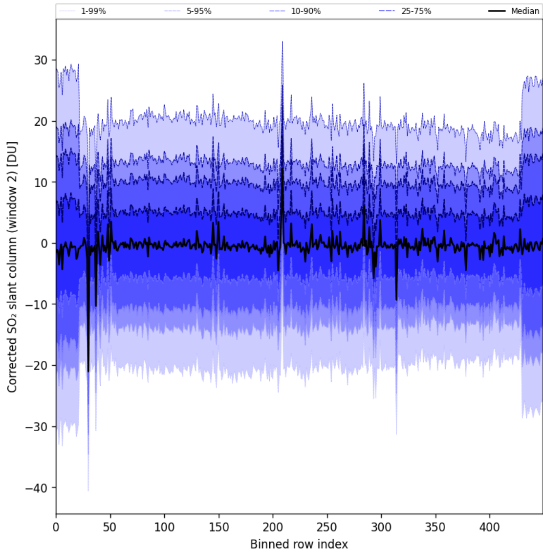
Figure 95: Along track statistics of "Corrected SO 2 slant column (window 2)" for 2025-05-23 to 2025-05-25
