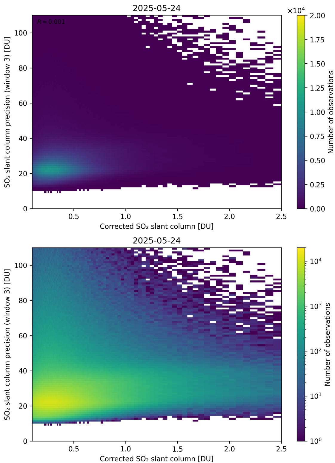
Figure 241: Scatter density plot of “Corrected SO 2 slant column” against “SO 2 slant column precision (window 3)” for 2025-05-23 to 2025-05-25.
