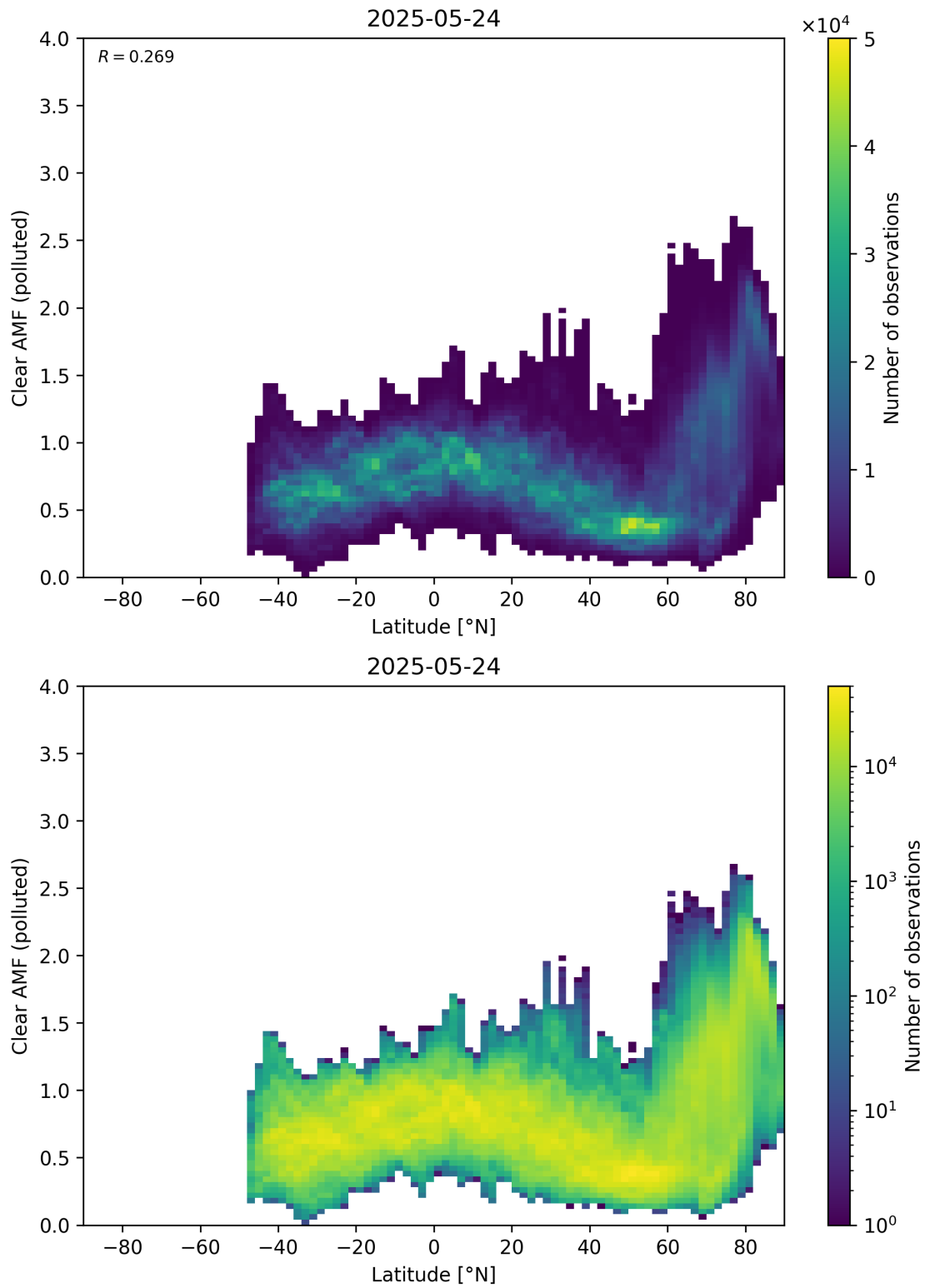
Figure 156: Scatter density plot of “Latitude” against “Clear AMF (polluted)” for 2025-05-23 to 2025-05-25.
