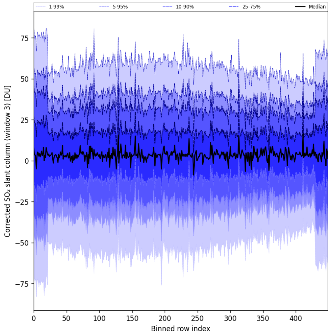
Figure 99: Along track statistics of “Corrected SO 2 slant column (window 3)” for 2025-05-23 to 2025-05-25
