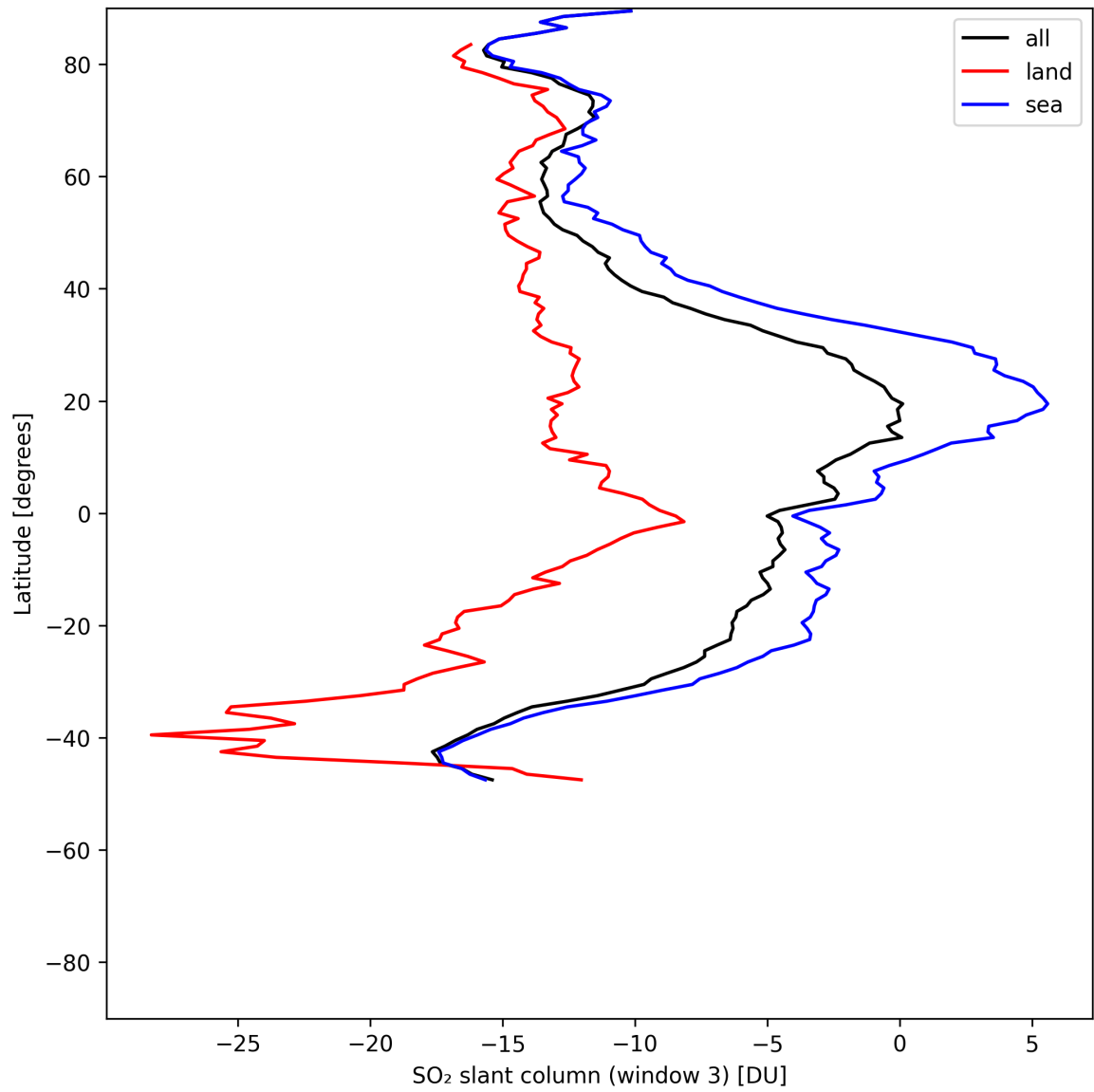
Figure 45: Zonal average of “SO 2 slant column (window 3)” for 2025-05-23 to 2025-05-25.
