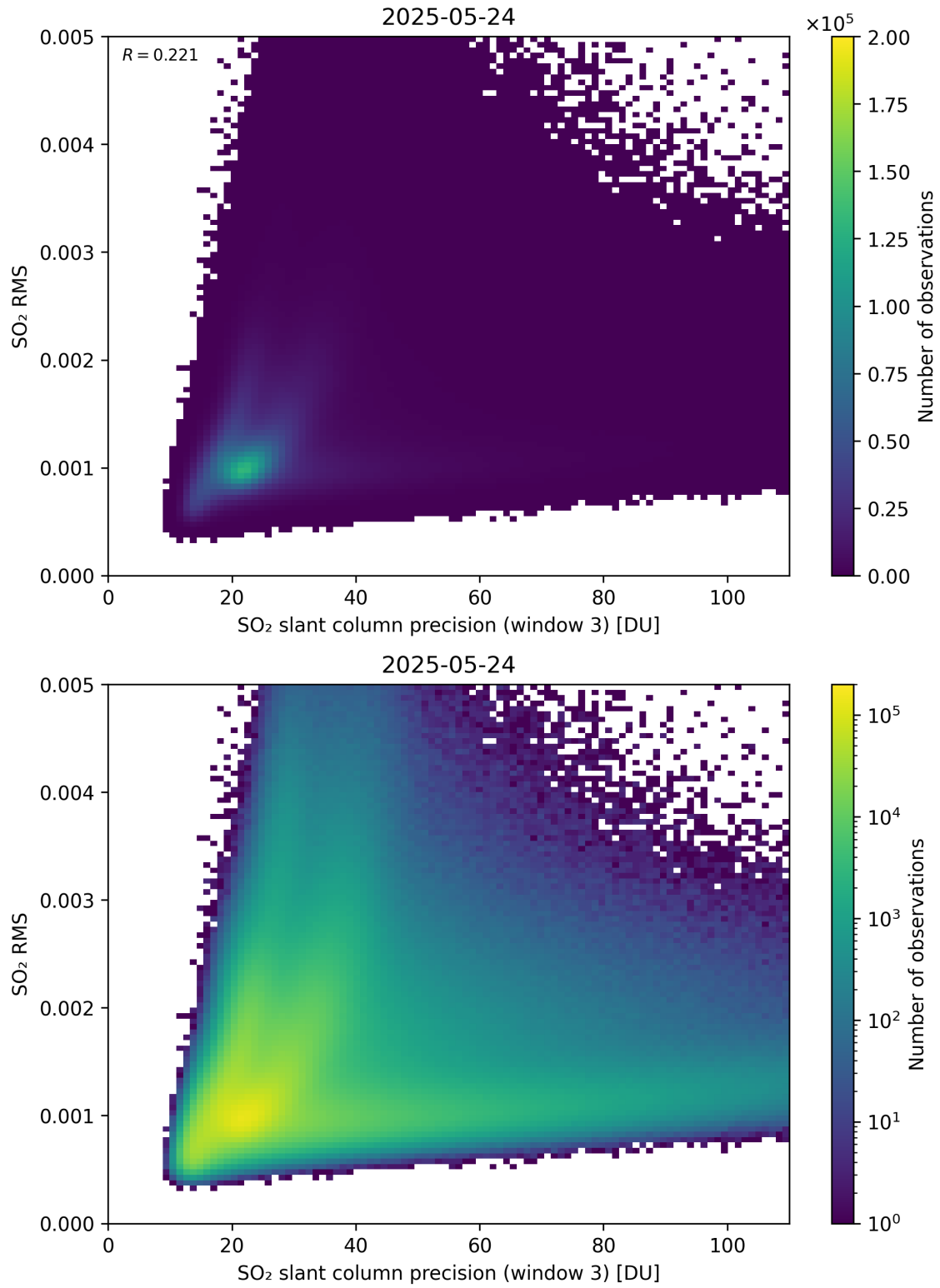
Figure 310: Scatter density plot of “SO 2 slant column precision (window 3)” against “SO 2 RMS” for 2025-05-23 to 2025-05-25.
