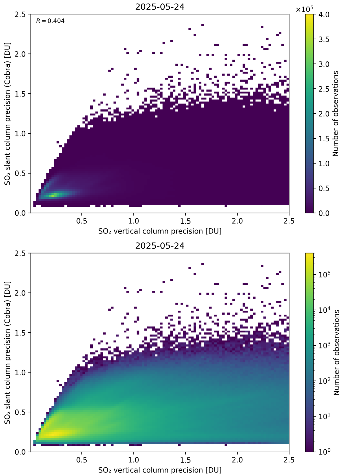
Figure 337: Scatter density plot of “SO 2 vertical column precision” against “SO 2 slant column precision (Cobra)” for 2025-05-23 to 2025-05-25.
