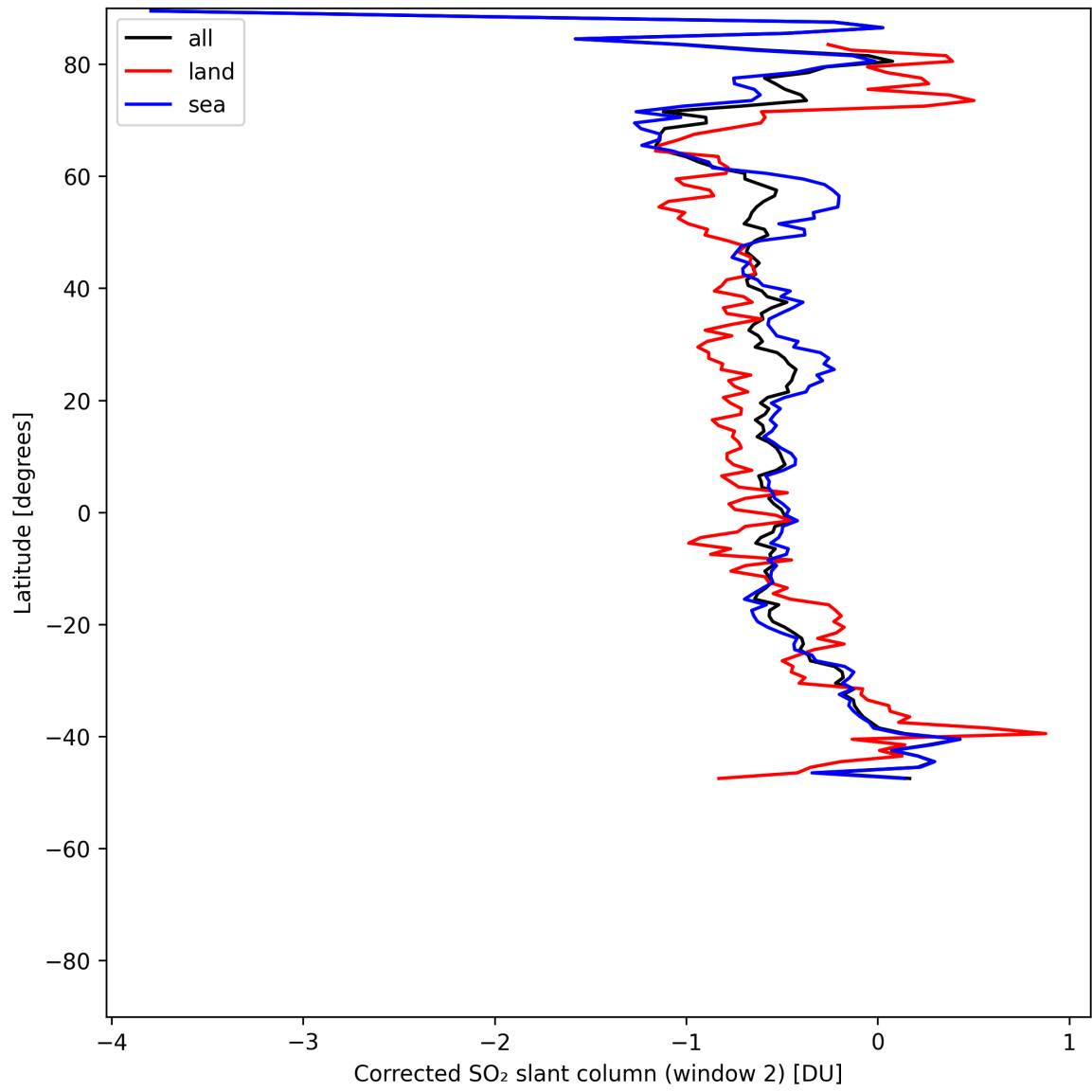
Figure 43: Zonal average of “Corrected SO 2 slant column (window 2)” for 2025-05-23 to 2025-05-25.
