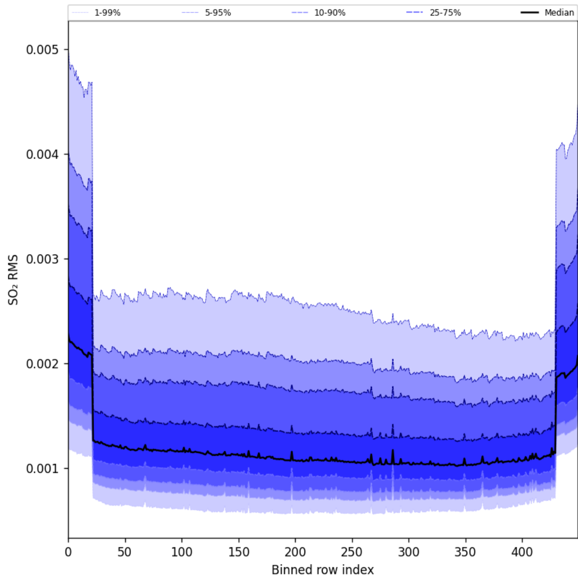
Figure 104: Along track statistics of “SO 2 RMS” for 2025-05-23 to 2025-05-25
