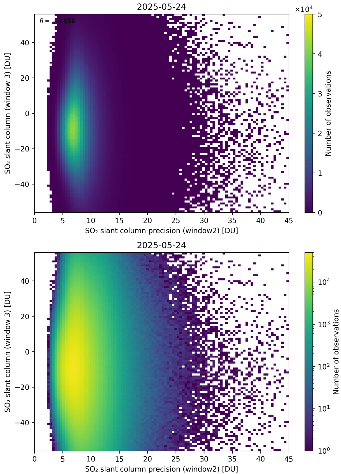
Figure 299: Scatter density plot of “SO 2 slant column precision (window2)” against “SO 2 slant column (window 3)” for 2025-05-23 to 2025-05-25.
