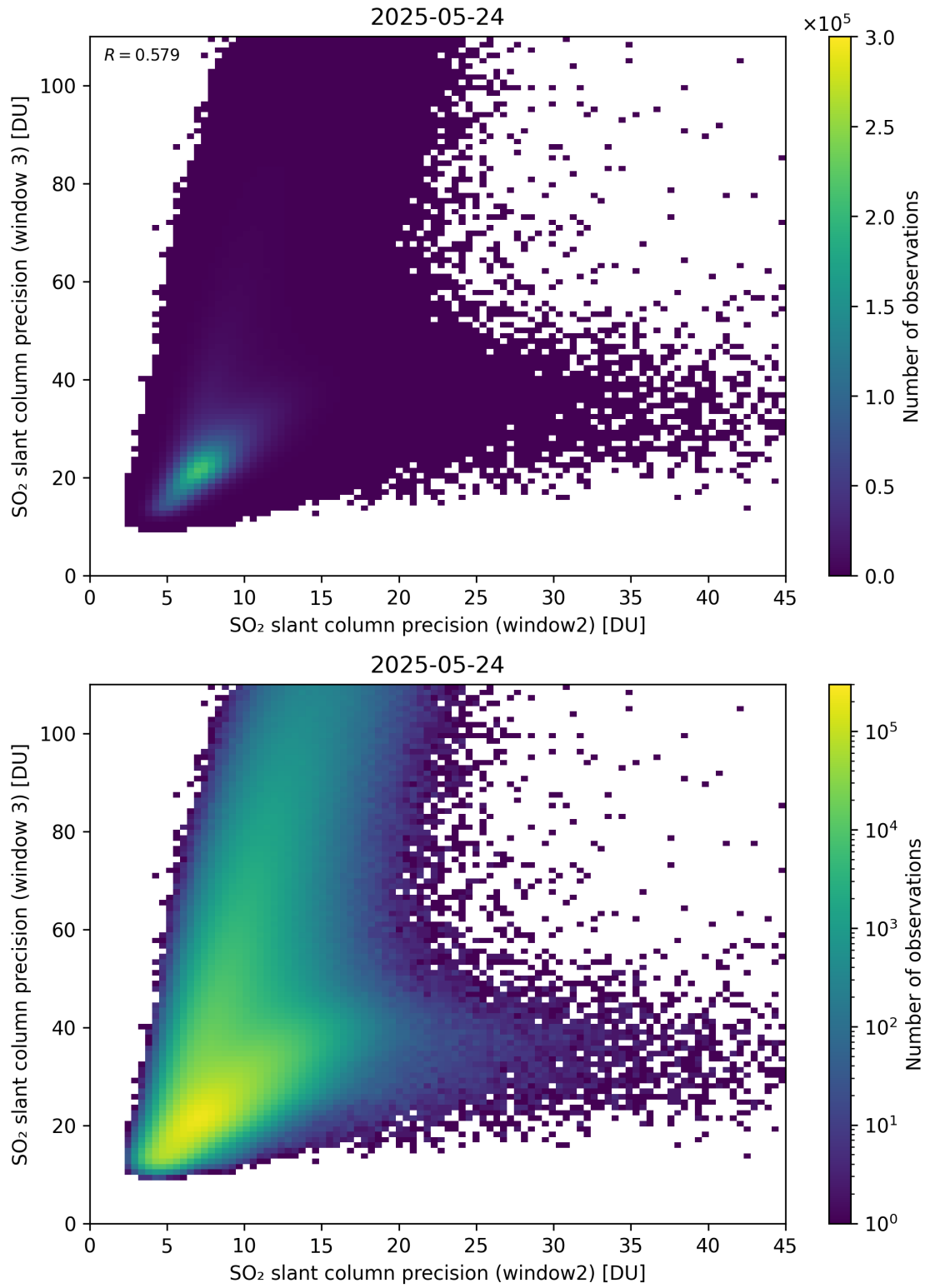
Figure 300: Scatter density plot of “SO 2 slant column precision (window2)” against “SO 2 slant column precision (window 3)” for 2025-05-23 to 2025-05-25.
