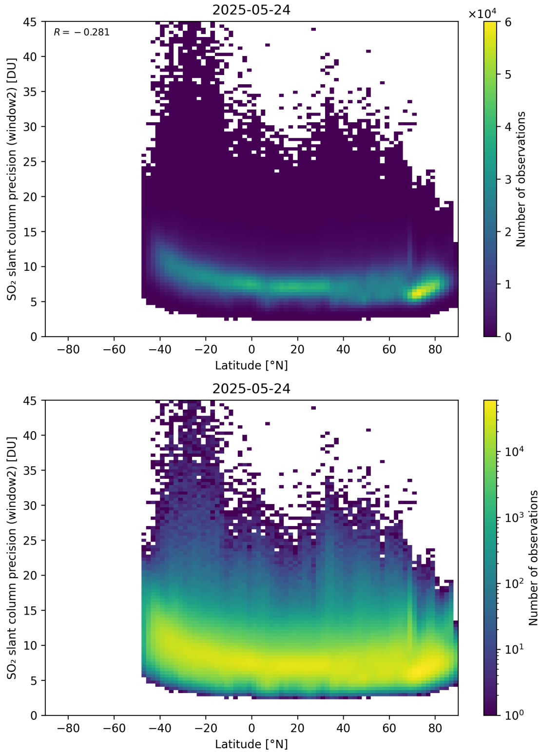
Figure 164: Scatter density plot of “Latitude” against “SO 2 slant column precision (window2)” for 2025-05-23 to 2025-05-25.
