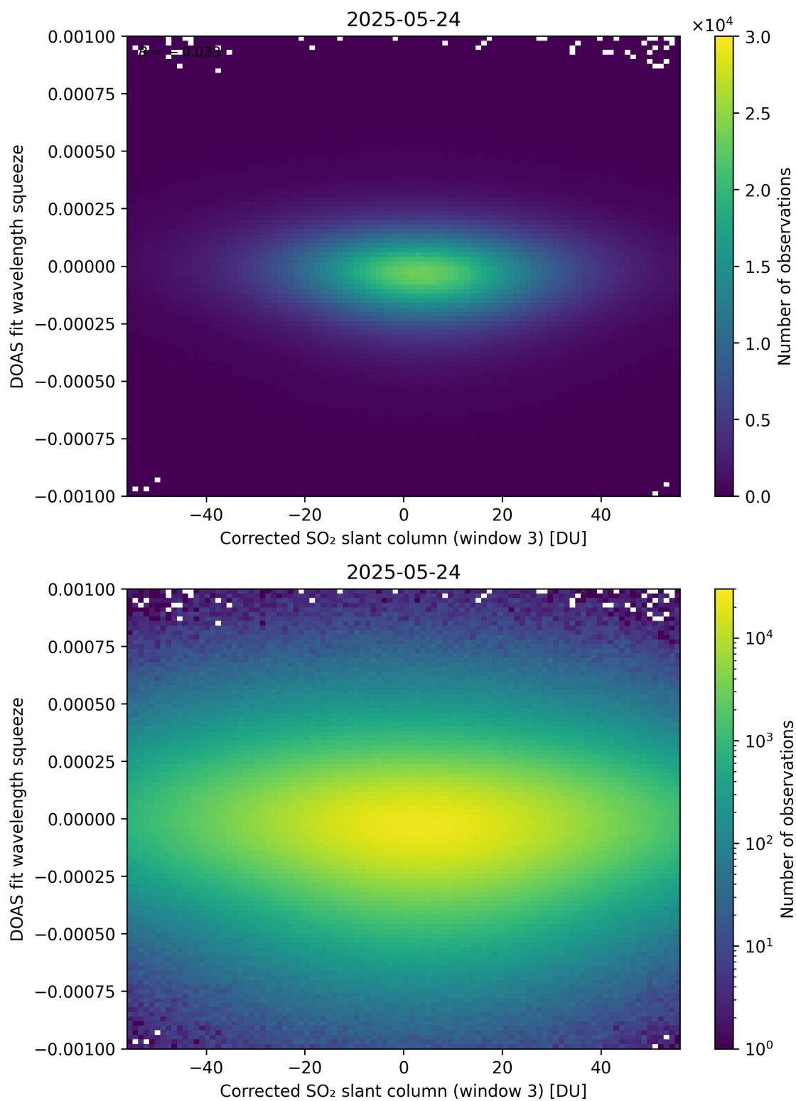
Figure 257: Scatter density plot of “Corrected SO 2 slant column (window 3)” against “DOAS fit wavelength squeeze” for 2025-05-23 to 2025-05-25.
