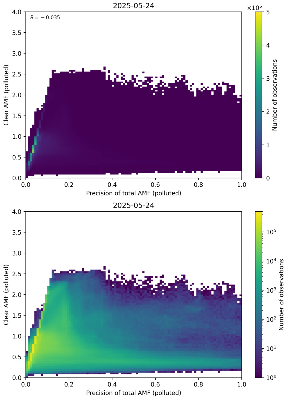
Figure 320: Scatter density plot of “Precision of total AMF (polluted)” against “Clear AMF (polluted)” for 2025-05-23 to 2025-05-25.
