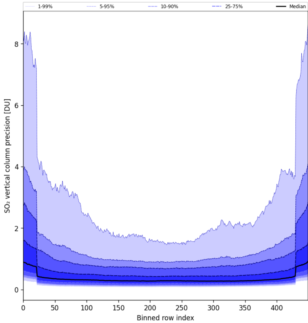
Figure 85: Along track statistics of “SO 2 vertical column precision” for 2025-05-23 to 2025-05-25
