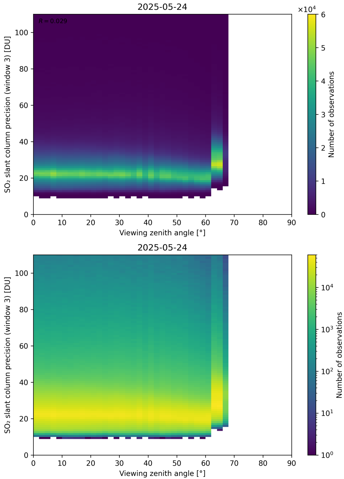
Figure 380: Scatter density plot of “Viewing zenith angle” against “SO 2 slant column precision (window 3)” for 2025-05-23 to 2025-05-25.
