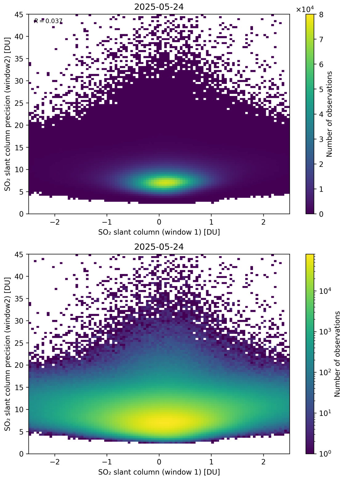
Figure 286: Scatter density plot of “SO 2 slant column (window 1)” against “SO 2 slant column precision (window2)” for 2025-05-23 to 2025-05-25.
