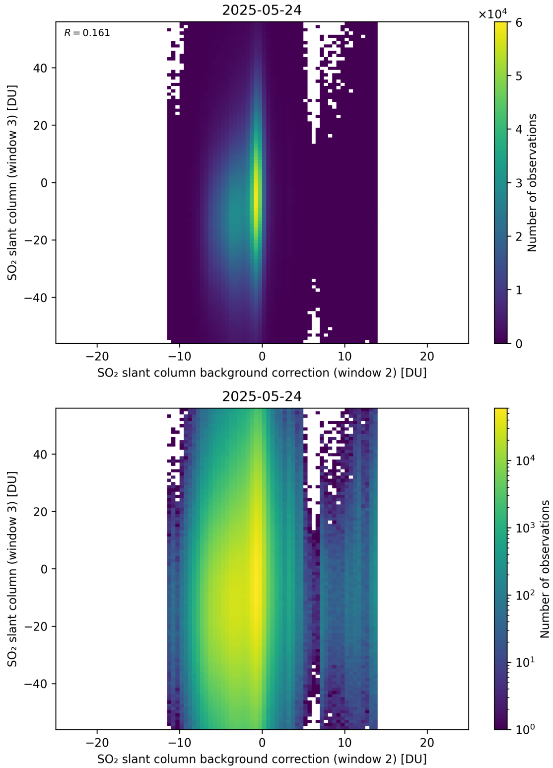
Figure 128: Scatter density plot of “SO 2 slant column background correction (window 2)” against “SO 2 slant column (window 3)” for 2025-05-23 to 2025-05-25.
