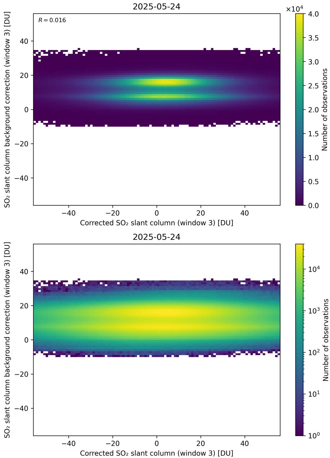
Figure 255: Scatter density plot of “Corrected SO 2 slant column (window 3)” against “SO 2 slant column background correction (window 3)” for 2025-05-23 to 2025-05-25.
