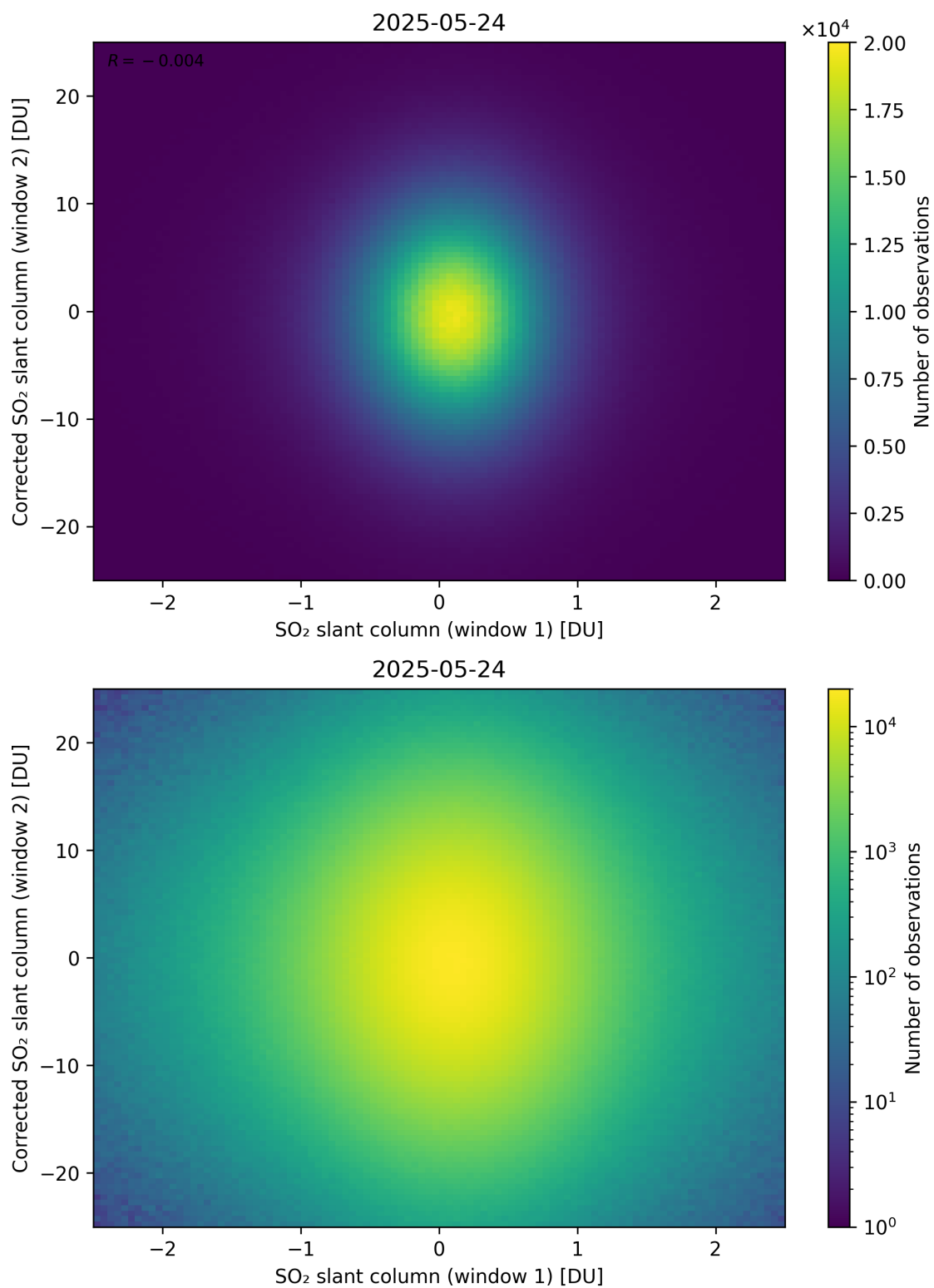
Figure 283: Scatter density plot of “SO 2 slant column (window 1)” against “Corrected SO 2 slant column (window 2)” for 2025-05-23 to 2025-05-25.
