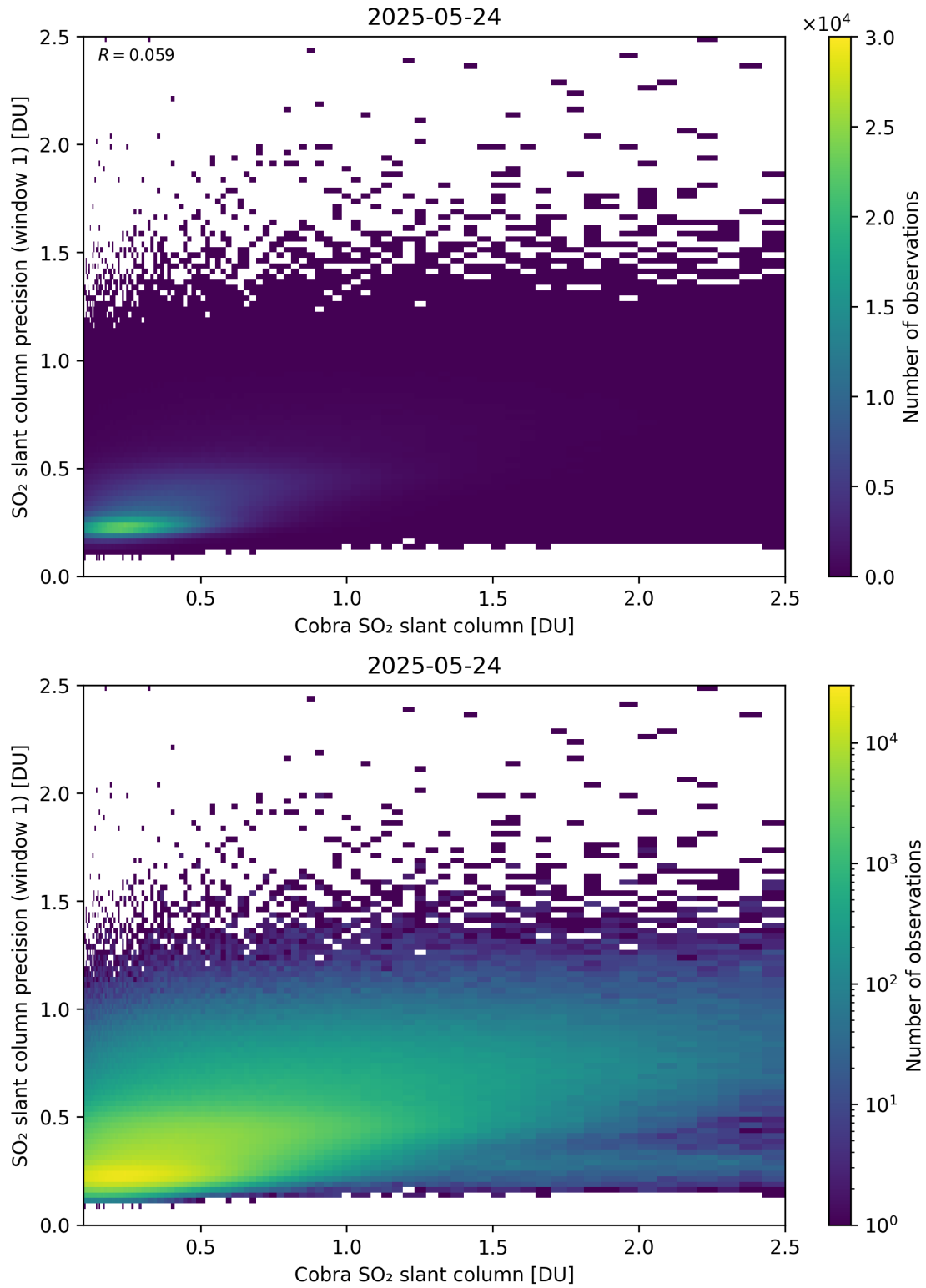
Figure 220: Scatter density plot of “Cobra SO 2 slant column” against “SO 2 slant column precision (window 1)” for 2025-05-23 to 2025-05-25.
