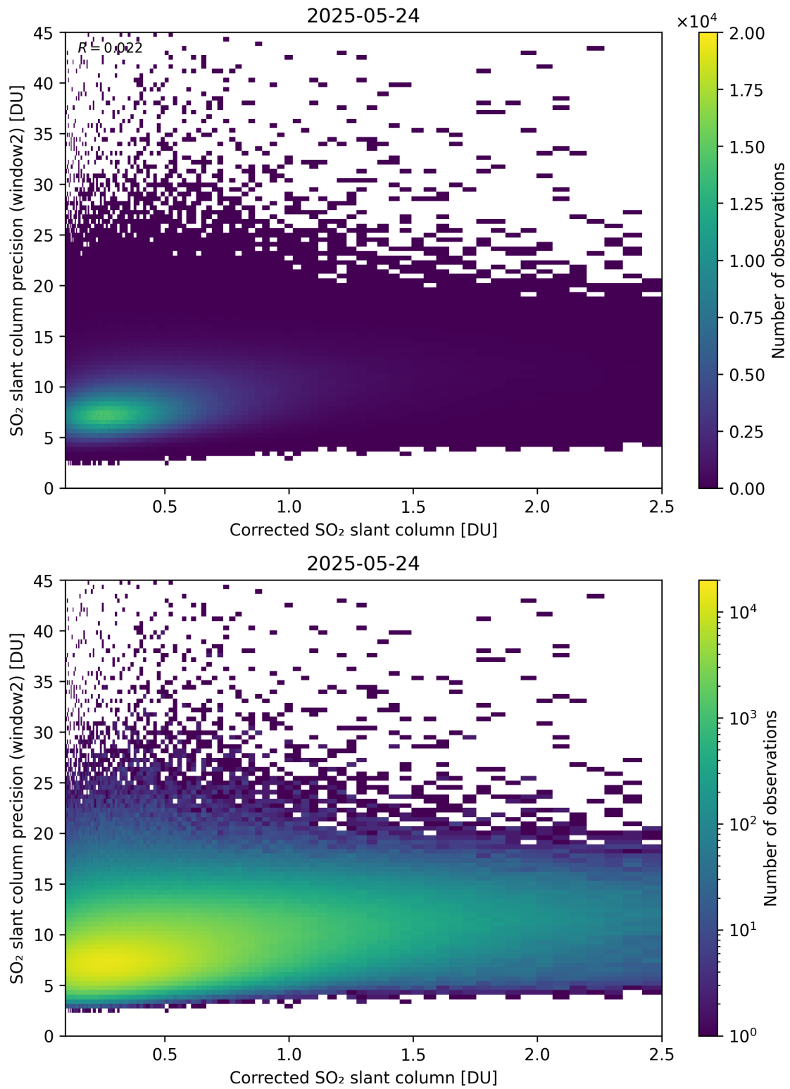
Figure 239: Scatter density plot of “Corrected SO 2 slant column” against “SO 2 slant column precision (window2)” for 2025-05-23 to 2025-05-25.
