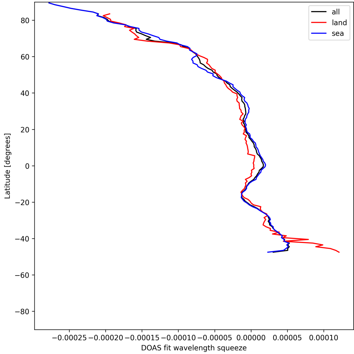
Figure 51: Zonal average of “DOAS fit wavelength squeeze” for 2025-05-23 to 2025-05-25.
