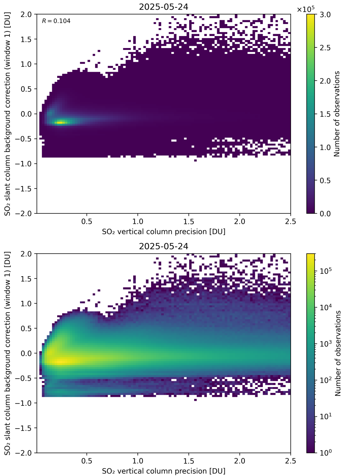
Figure 329: Scatter density plot of “SO 2 vertical column precision” against “SO 2 slant column background correction (window 1)” for 2025-05-23 to 2025-05-25.
