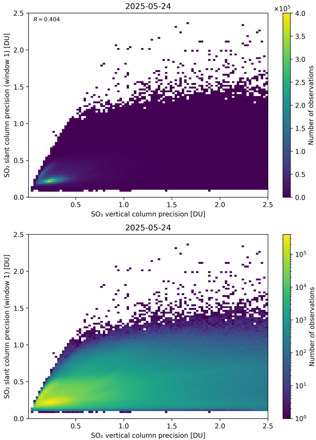
Figure 342: Scatter density plot of “SO 2 vertical column precision” against “SO 2 slant column precision (window 1)” for 2025-05-23 to 2025-05-25.
