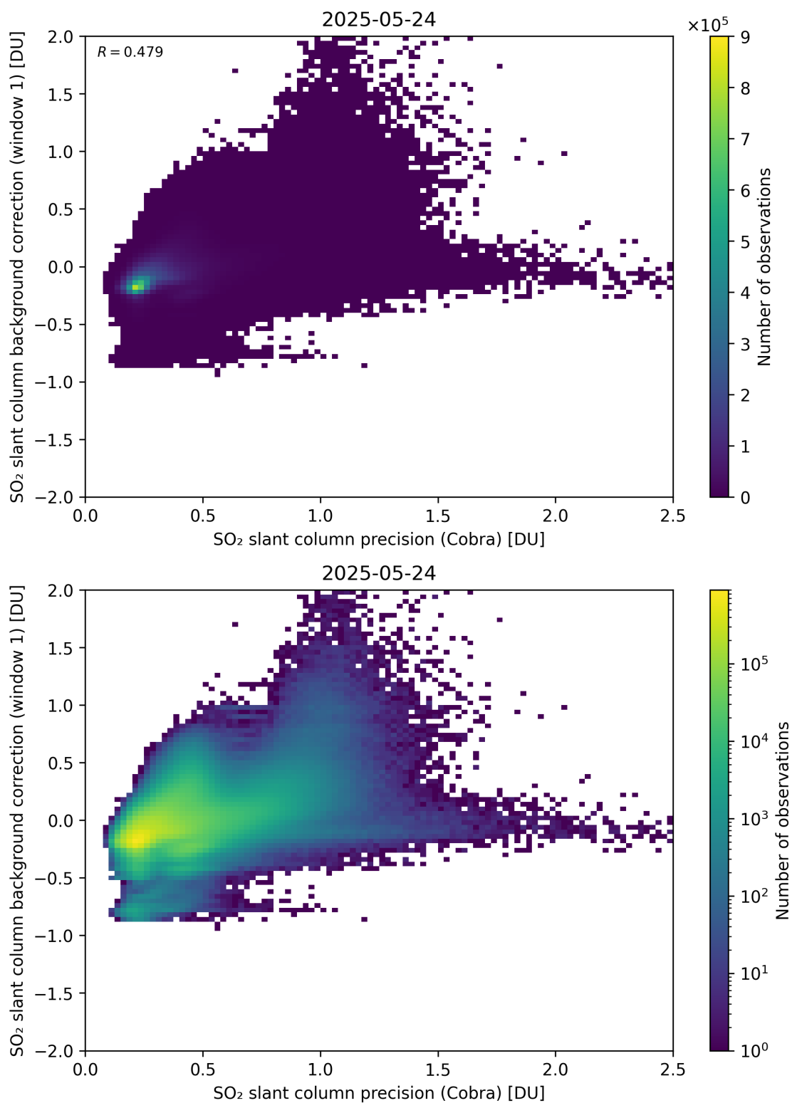
Figure 199: Scatter density plot of “SO 2 slant column precision (Cobra)” against “SO 2 slant column background correction (window 1)” for 2025-05-23 to 2025-05-25.
