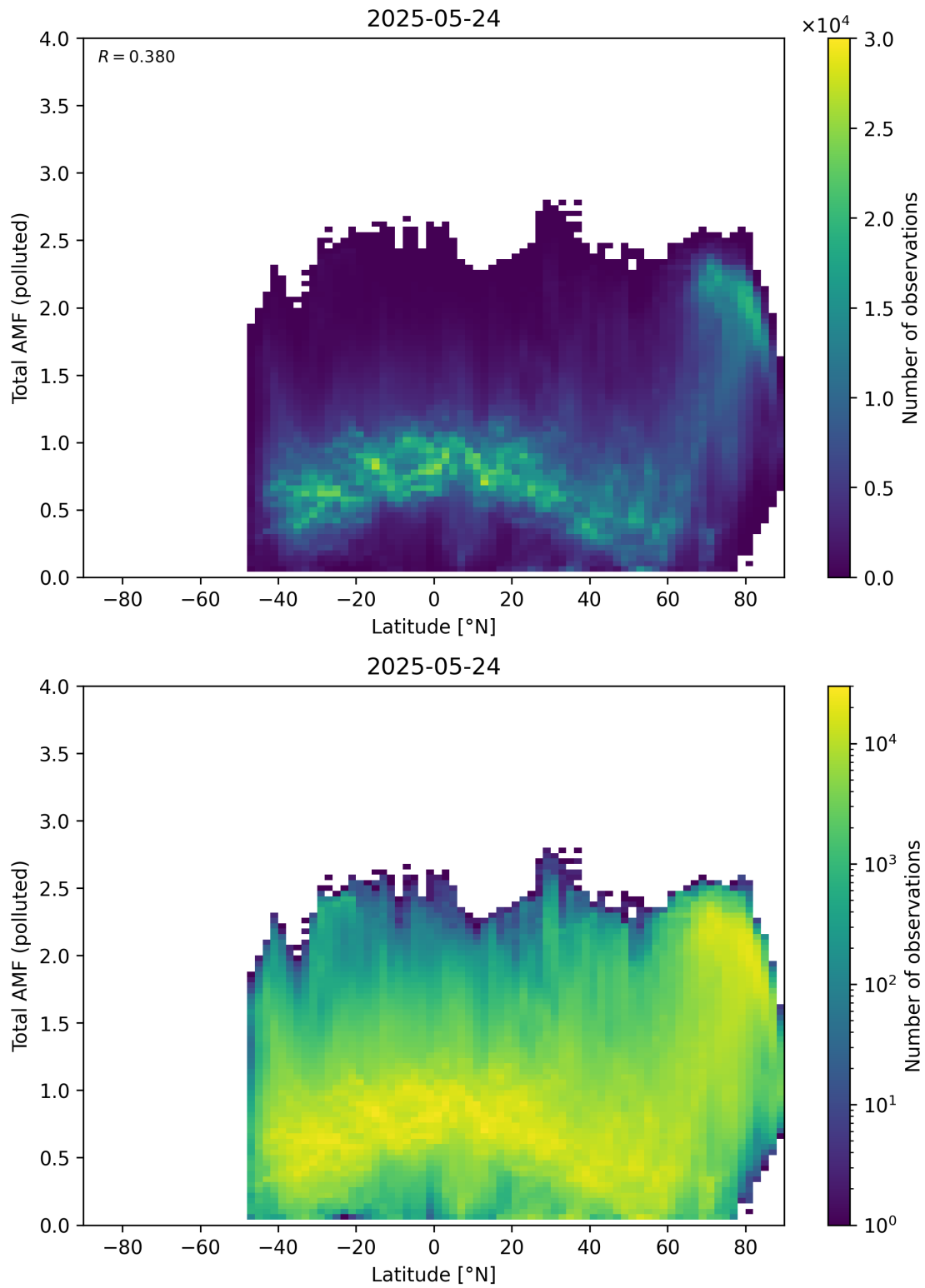
Figure 167: Scatter density plot of “Latitude” against “Total AMF (polluted)” for 2025-05-23 to 2025-05-25.
