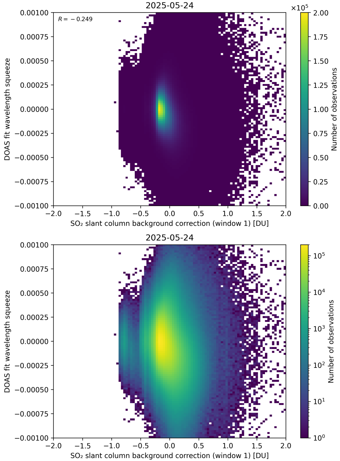
Figure 112: Scatter density plot of “SO 2 slant column background correction (window 1)” against “DOAS fit wavelength squeeze” for 2025-05-23 to 2025-05-25.
