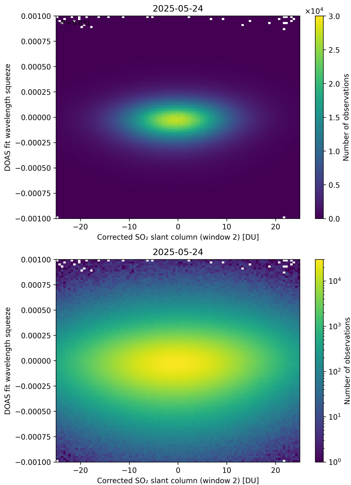
Figure 247: Scatter density plot of “Corrected SO 2 slant column (window 2)” against “DOAS fit wavelength squeeze” for 2025-05-23 to 2025-05-25.
