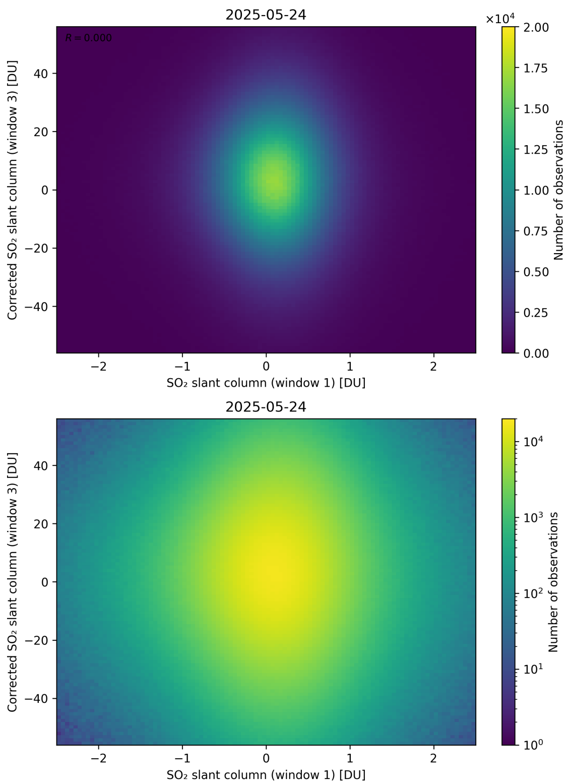
Figure 284: Scatter density plot of “SO 2 slant column (window 1)” against “Corrected SO 2 slant column (window 3)” for 2025-05-23 to 2025-05-25.
