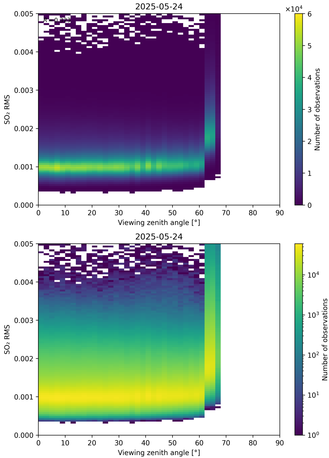
Figure 367: Scatter density plot of “Viewing zenith angle” against “SO 2 RMS” for 2025-05-23 to 2025-05-25.
