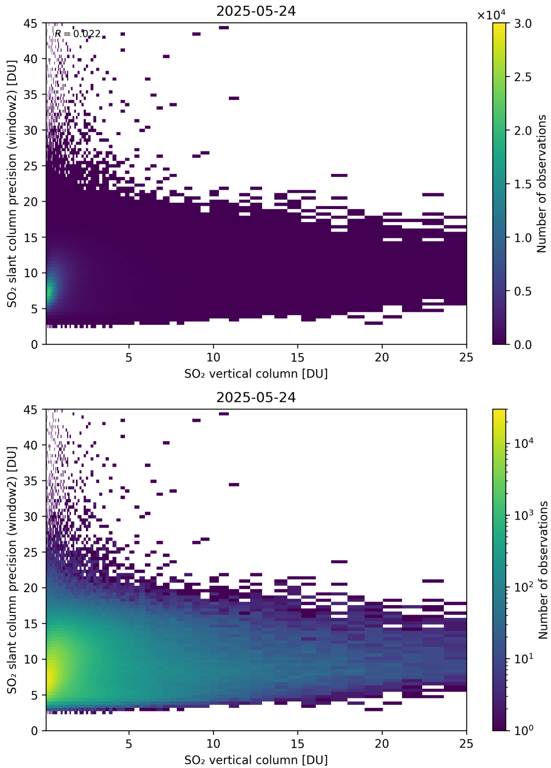
Figure 356: Scatter density plot of “SO 2 vertical column” against “SO 2 slant column precision (window2)” for 2025-05-23 to 2025-05-25.
