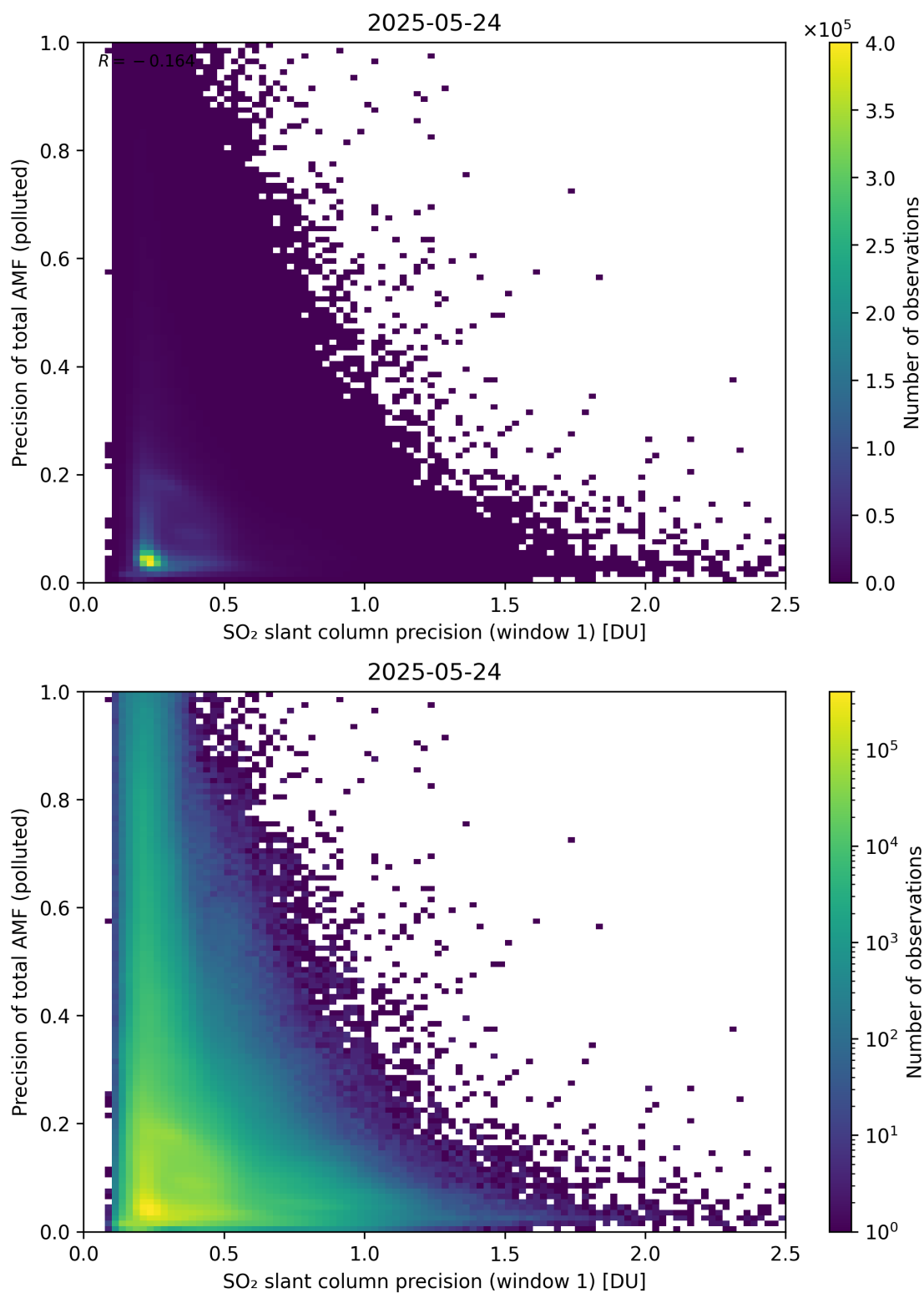
Figure 281: Scatter density plot of “SO 2 slant column precision (window 1)” against “Precision of total AMF (polluted)” for 2025-05-23 to 2025-05-25.
