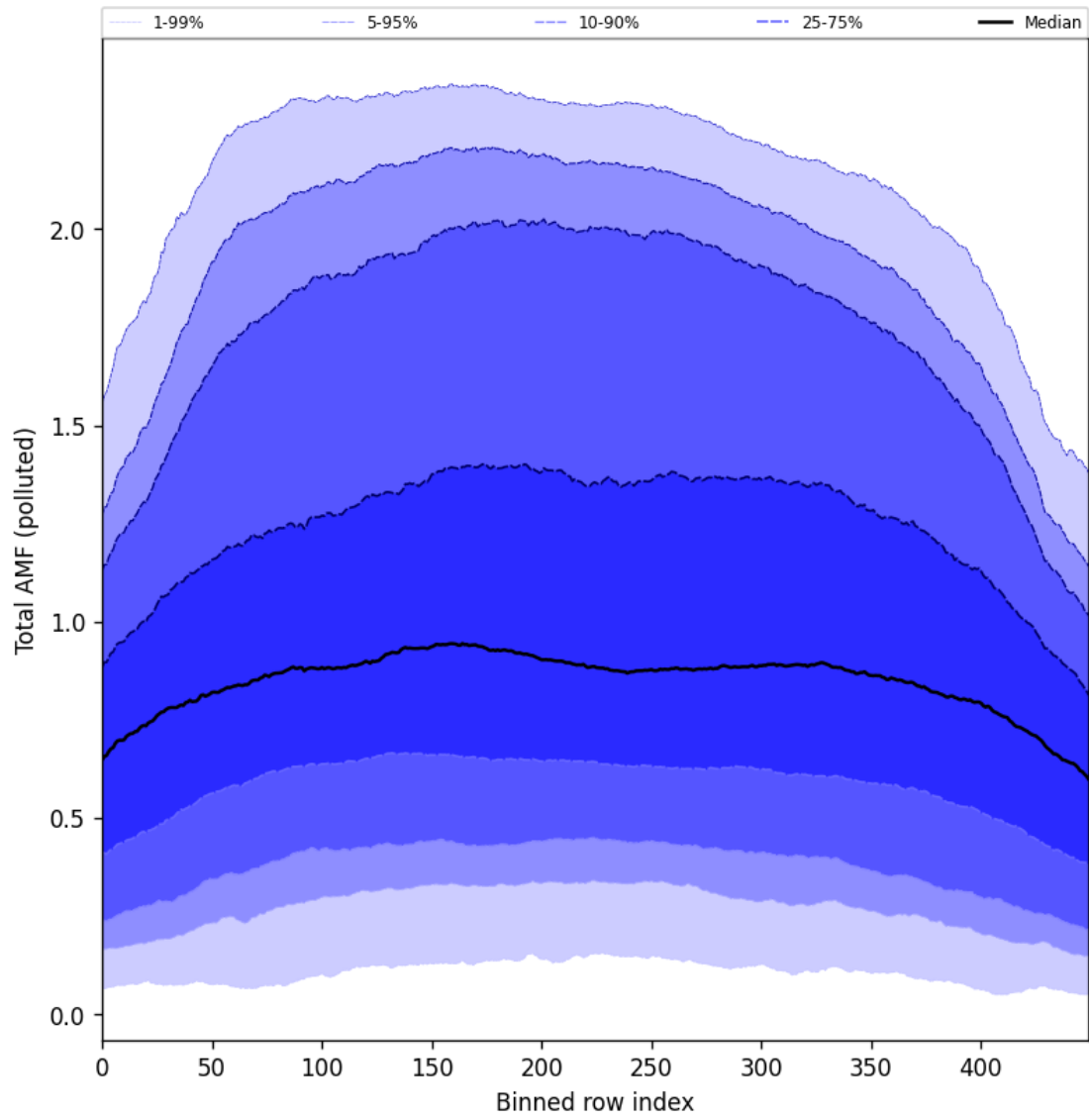
Figure 105: Along track statistics of “Total AMF (polluted)” for 2025-05-23 to 2025-05-25
