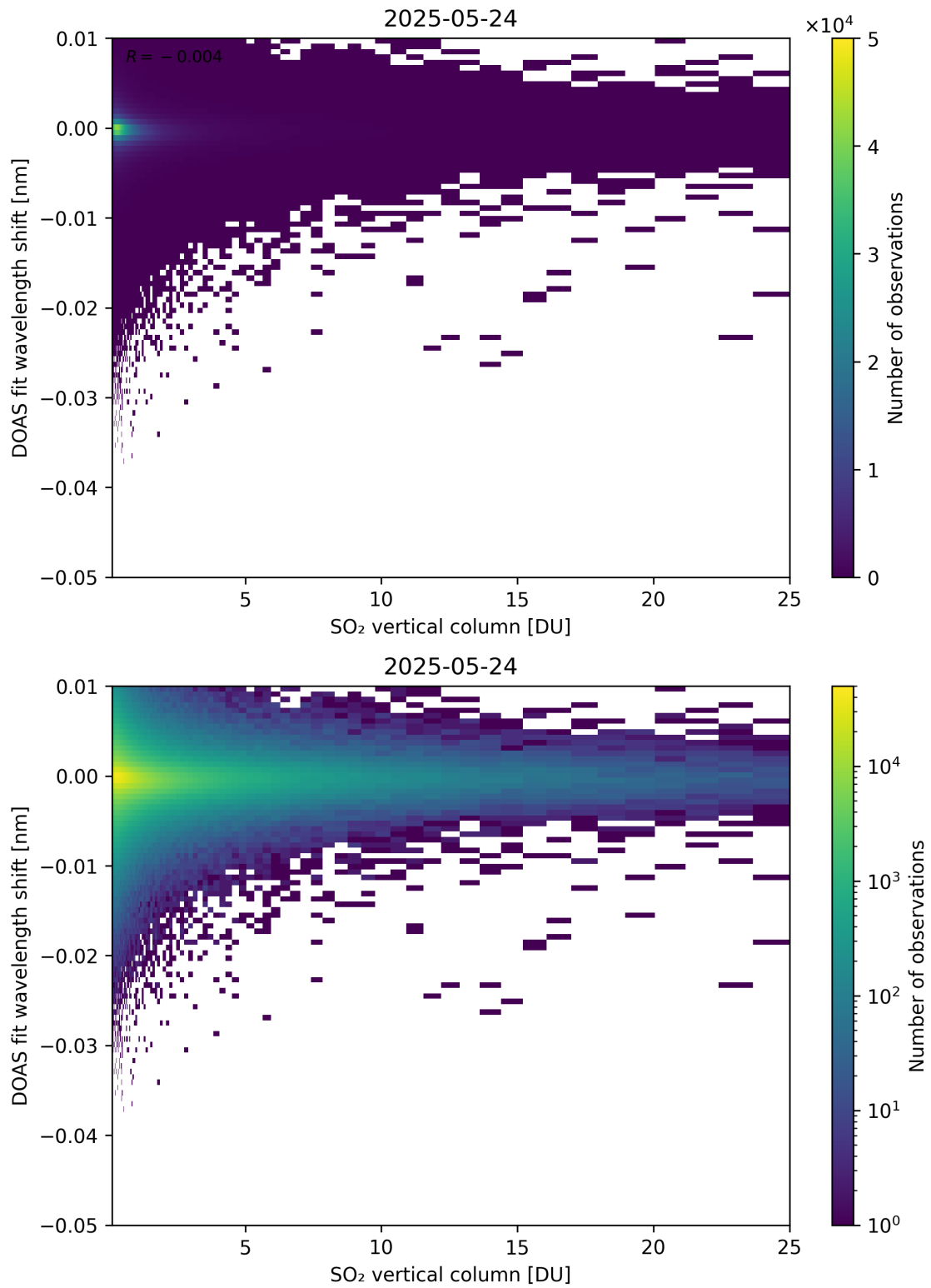
Figure 326: Scatter density plot of “SO 2 vertical column” against “DOAS fit wavelength shift” for 2025-05-23 to 2025-05-25.
