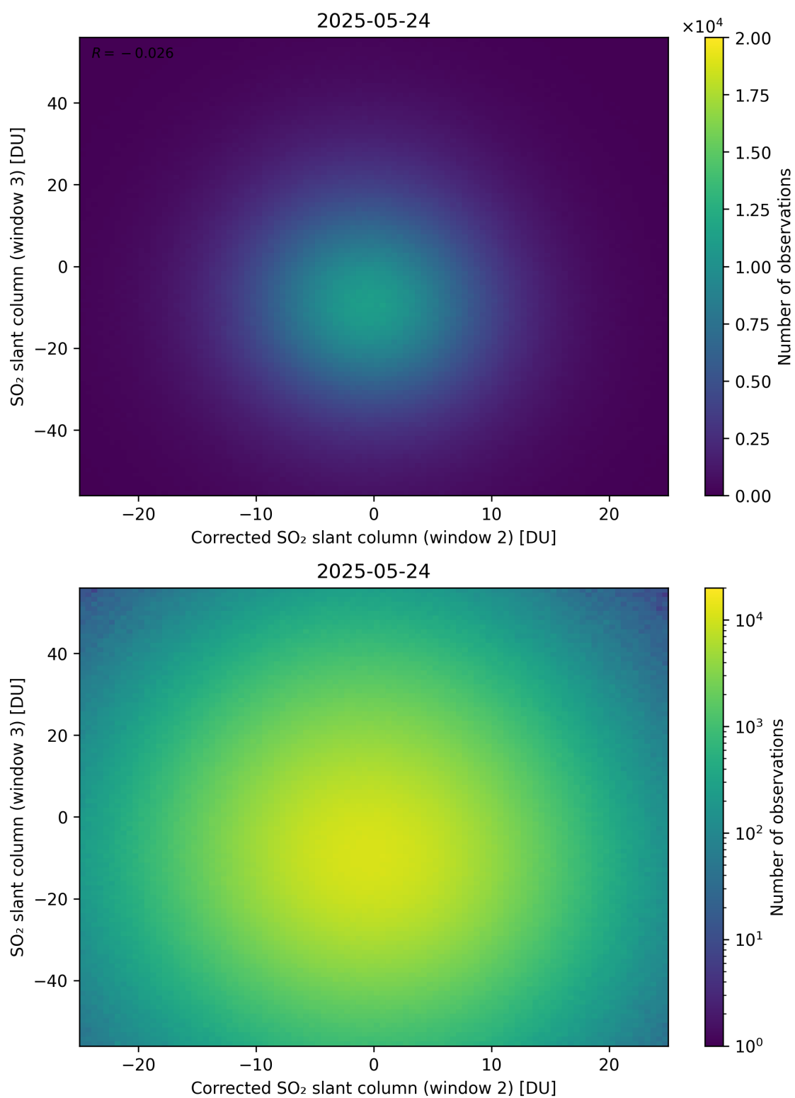
Figure 251: Scatter density plot of “Corrected SO 2 slant column (window 2)” against “SO 2 slant column (window 3)” for 2025-05-23 to 2025-05-25.
