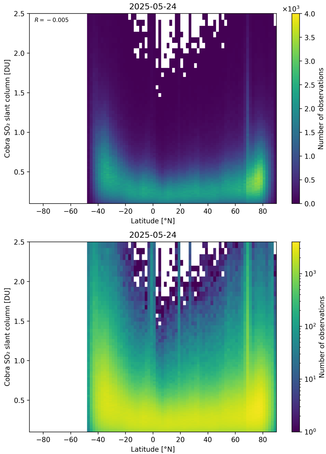
Figure 157: Scatter density plot of “Latitude” against “Cobra SO 2 slant column” for 2025-05-23 to 2025-05-25.
