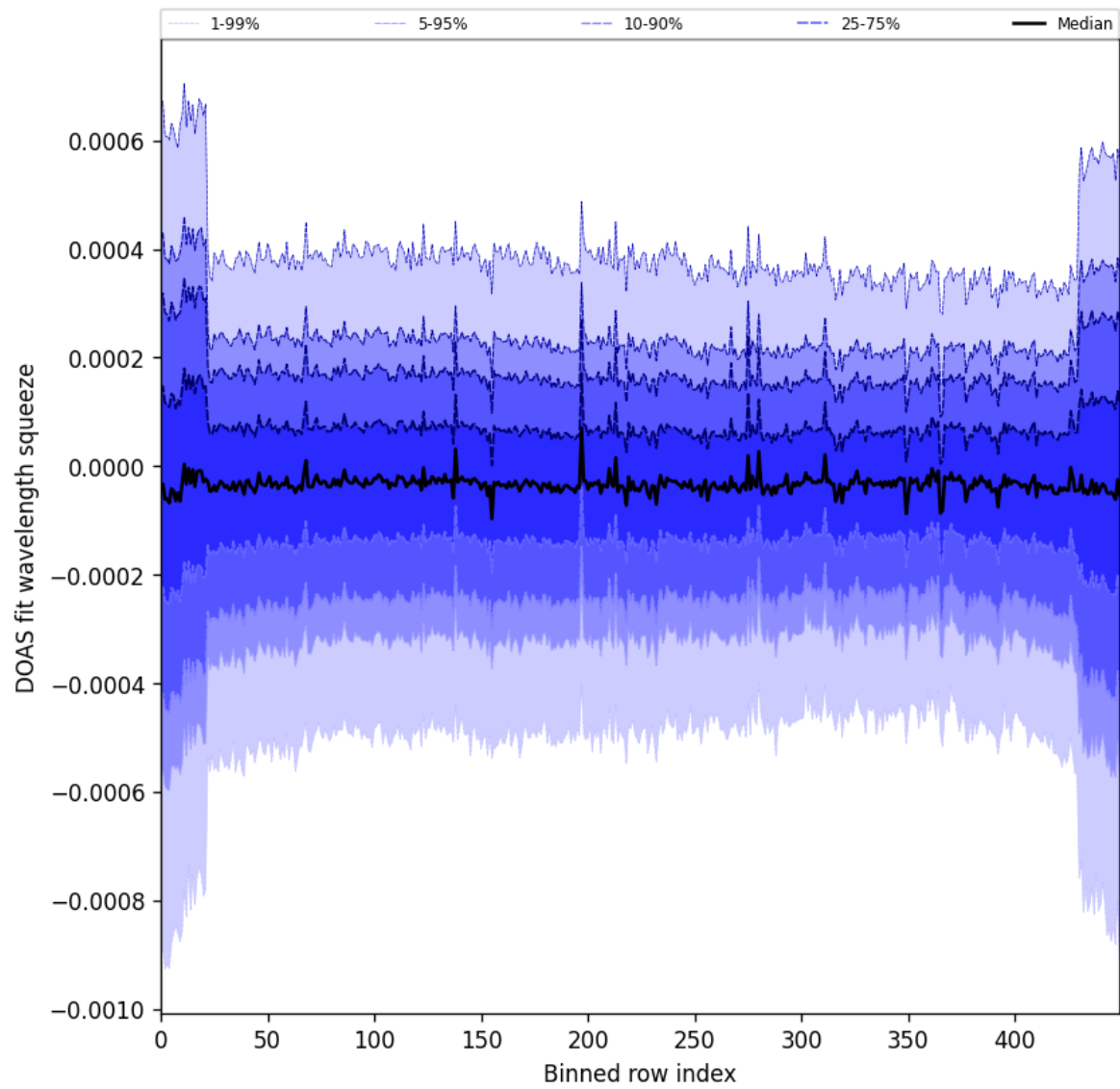
Figure 103: Along track statistics of “DOAS fit wavelength squeeze” for 2025-05-23 to 2025-05-25
