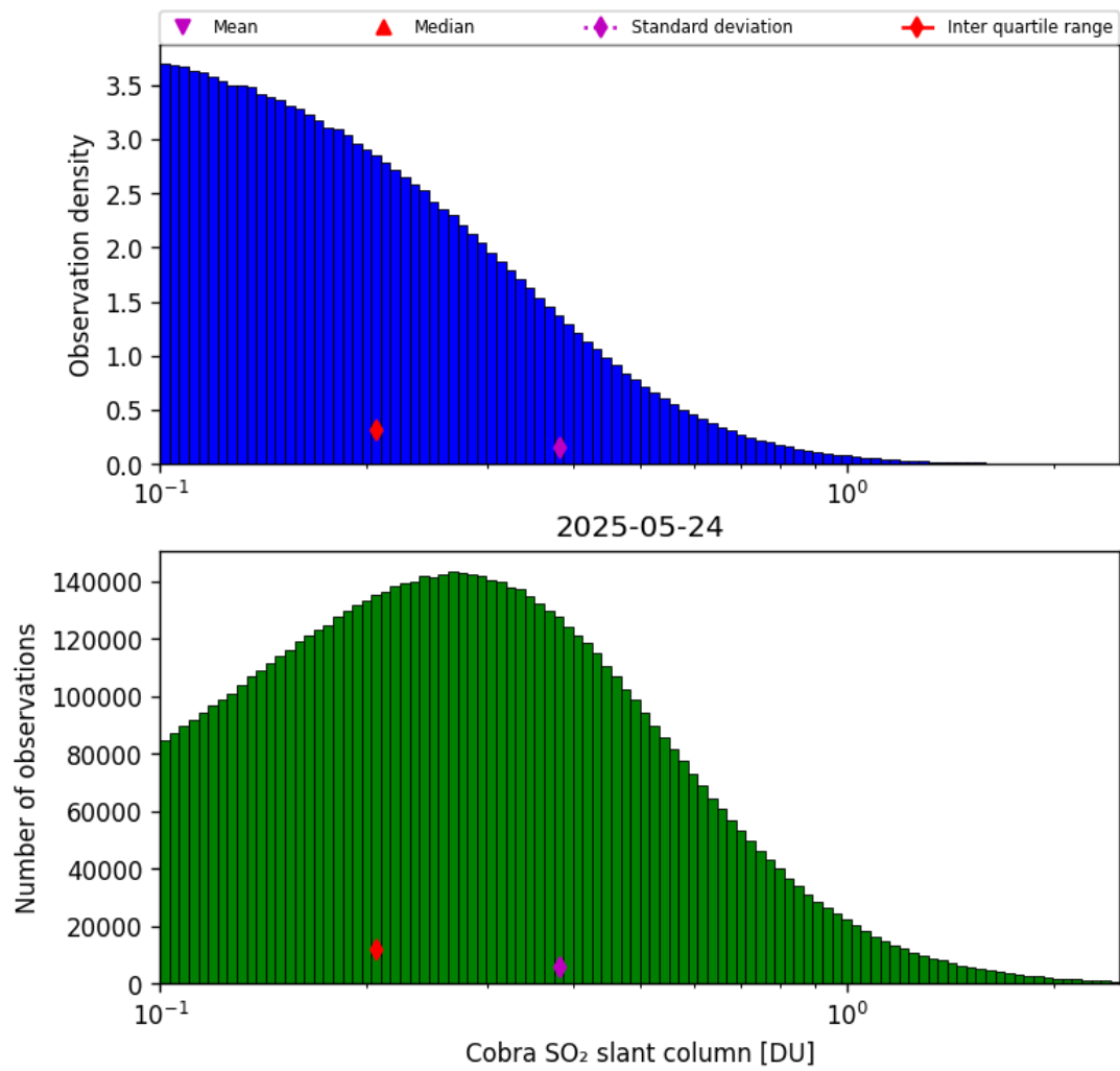
Figure 61: Histogram of “Cobra SO 2 slant column” for 2025-05-23 to 2025-05-25
