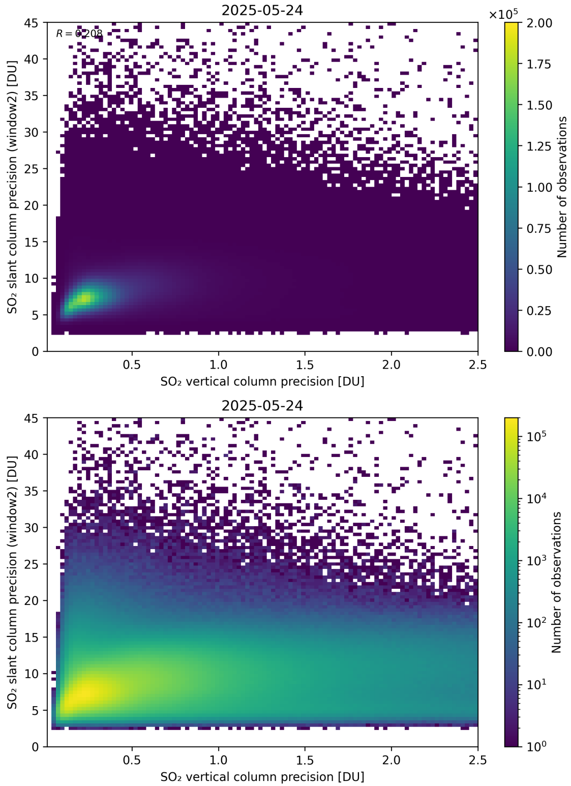
Figure 343: Scatter density plot of “SO 2 vertical column precision” against “SO 2 slant column precision (window2)” for 2025-05-23 to 2025-05-25.
