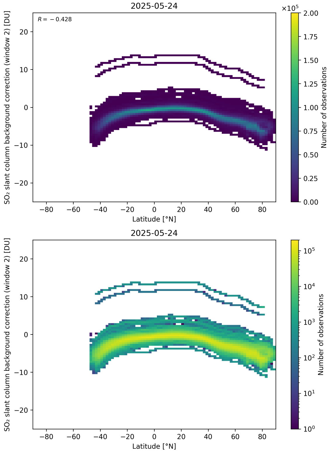
Figure 151: Scatter density plot of “Latitude” against “SO 2 slant column background correction (window 2)” for 2025-05-23 to 2025-05-25.
