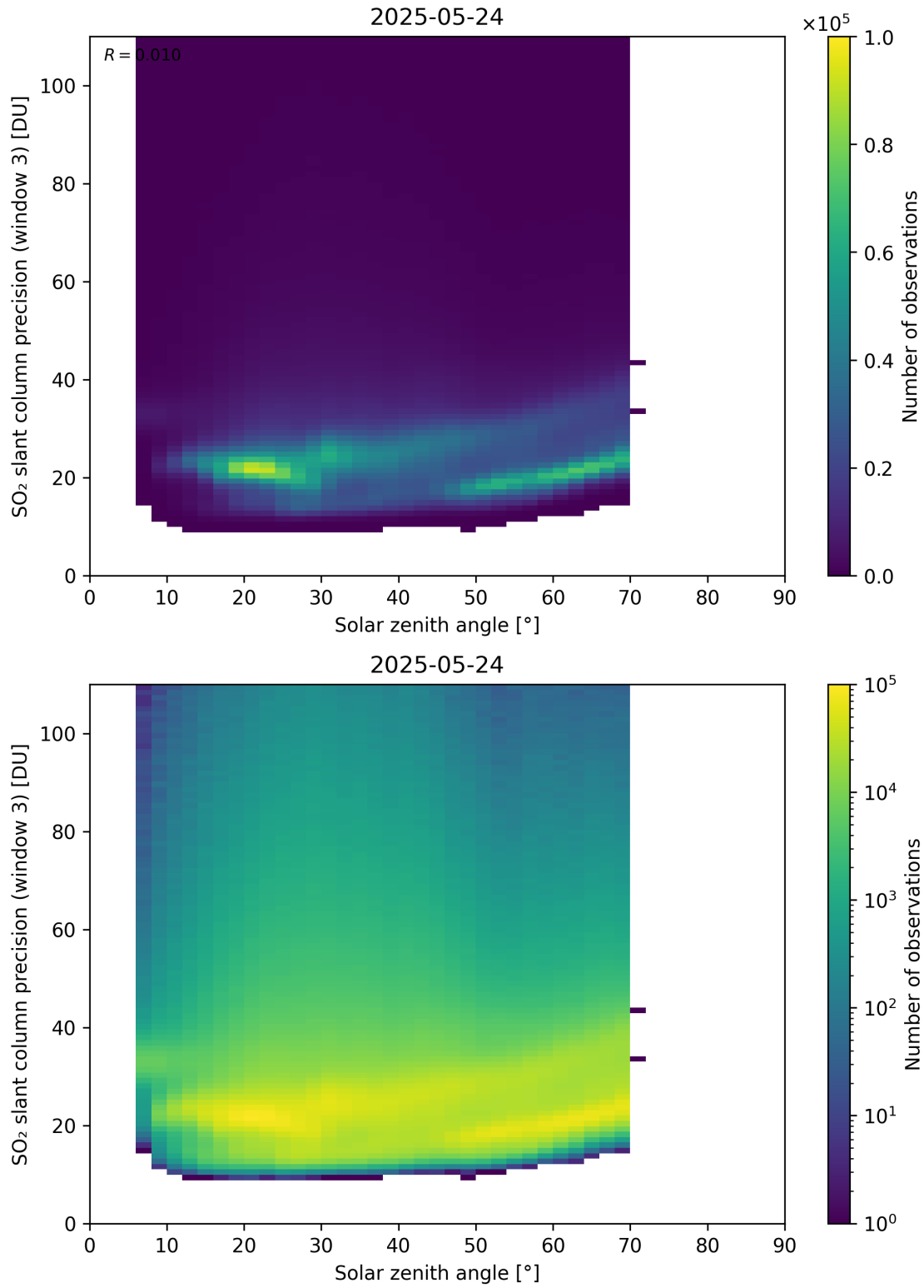
Figure 188: Scatter density plot of “Solar zenith angle” against “SO 2 slant column precision (window 3)” for 2025-05-23 to 2025-05-25.
