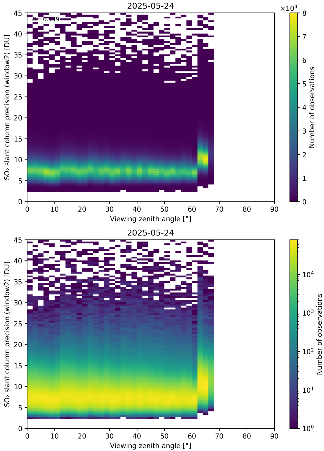
Figure 378: Scatter density plot of “Viewing zenith angle” against “SO 2 slant column precision (window2)” for 2025-05-23 to 2025-05-25.
