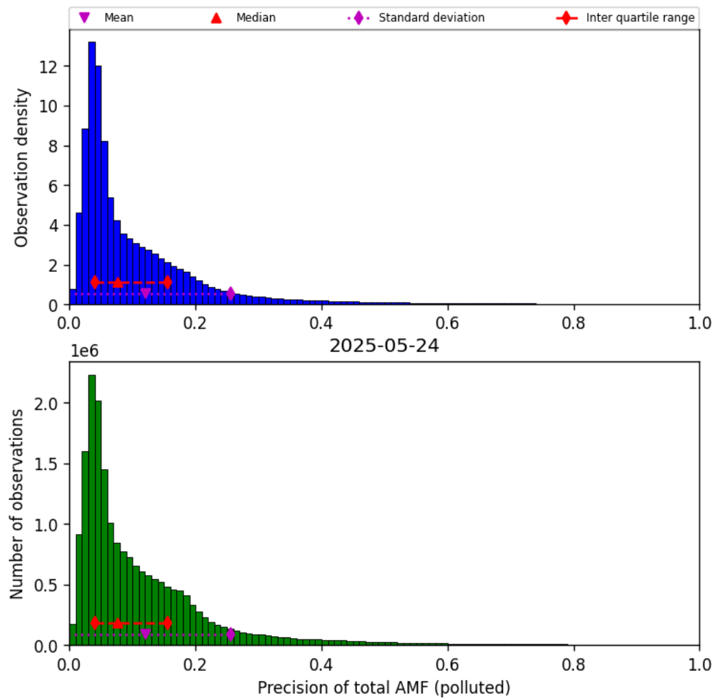
Figure 80: Histogram of “Precision of total AMF (polluted)” for 2025-05-23 to 2025-05-25
