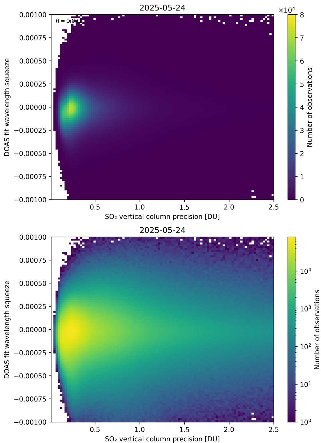
Figure 333: Scatter density plot of “SO 2 vertical column precision” against “DOAS fit wavelength squeeze” for 2025-05-23 to 2025-05-25.
