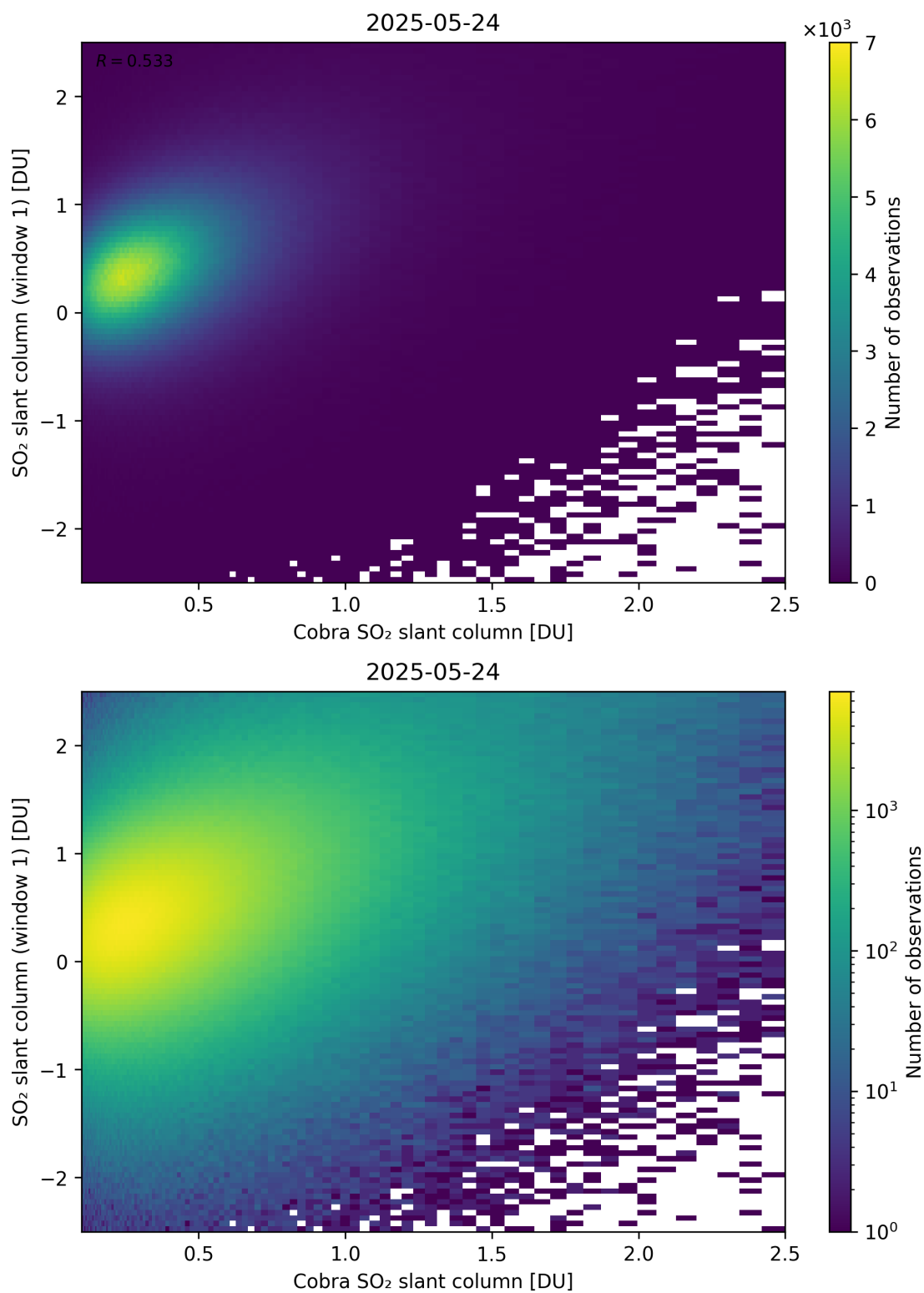
Figure 219: Scatter density plot of “Cobra SO 2 slant column” against “SO 2 slant column (window 1)” for 2025-05-23 to 2025-05-25.
