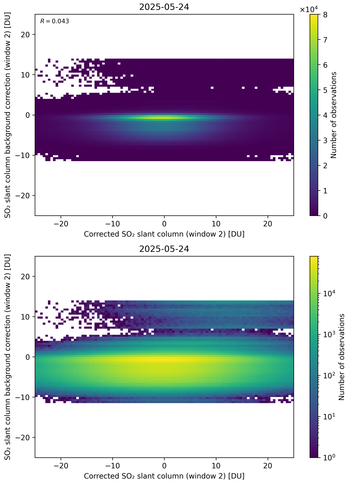
Figure 244: Scatter density plot of “Corrected SO 2 slant column (window 2)” against “SO 2 slant column background correction (window 2)” for 2025-05-23 to 2025-05-25.
