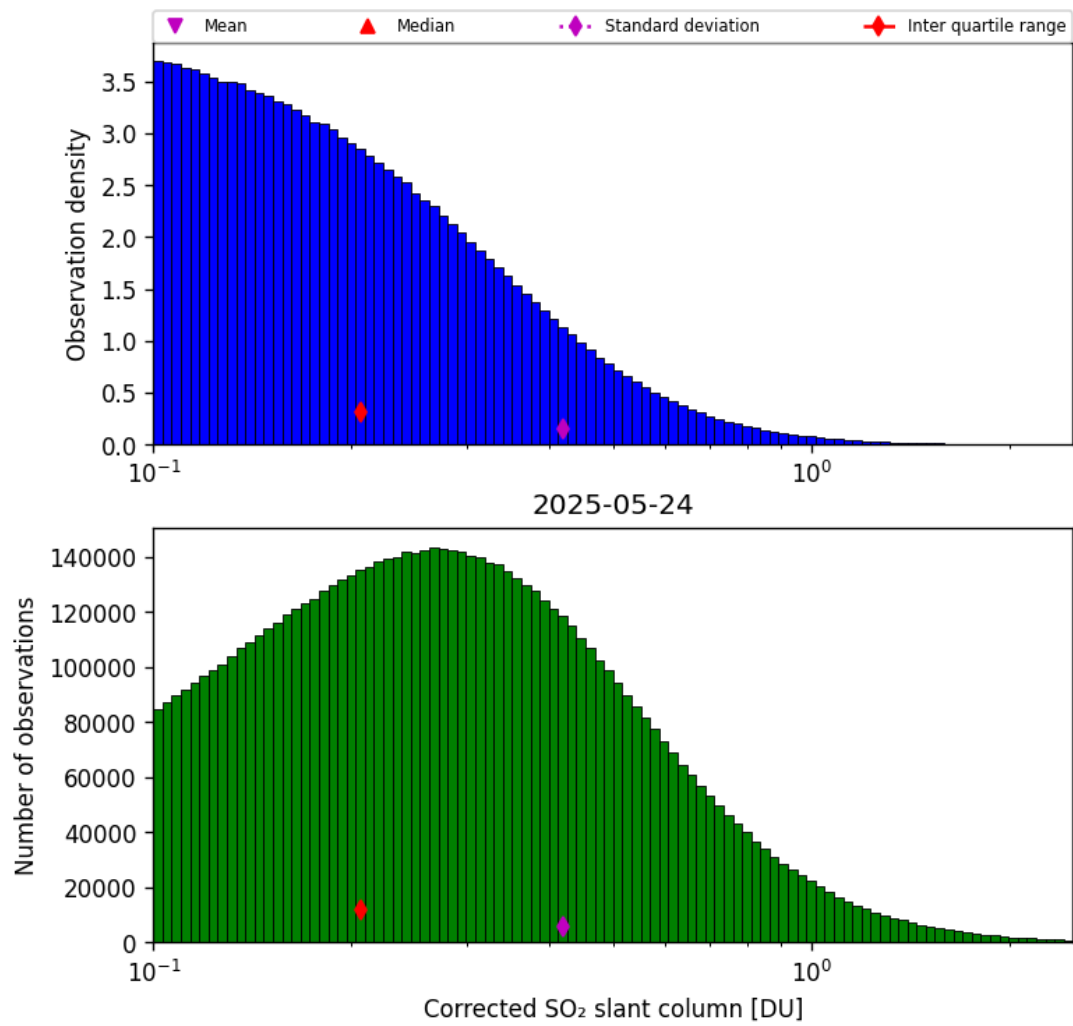
Figure 60: Histogram of “Corrected SO 2 slant column” for 2025-05-23 to 2025-05-25
