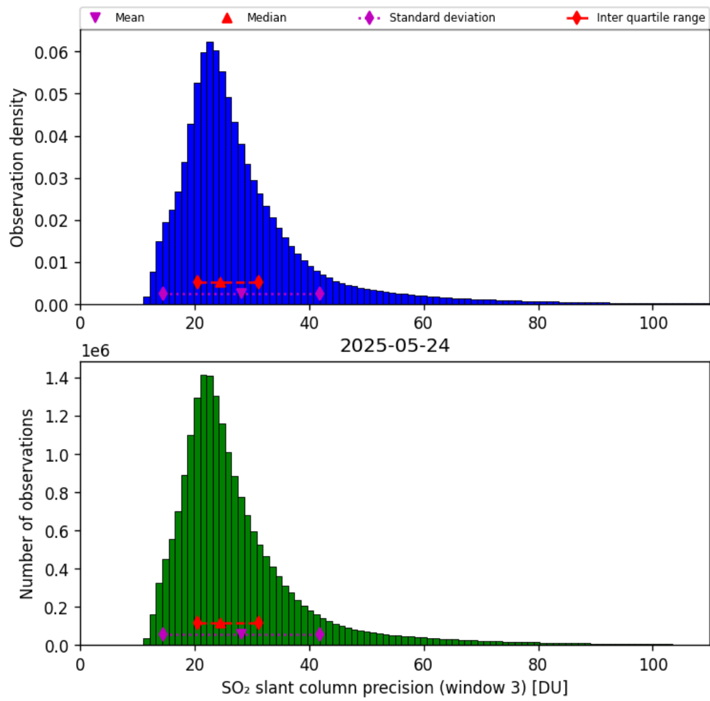
Figure 72: Histogram of “SO 2 slant column precision (window 3)” for 2025-05-23 to 2025-05-25
