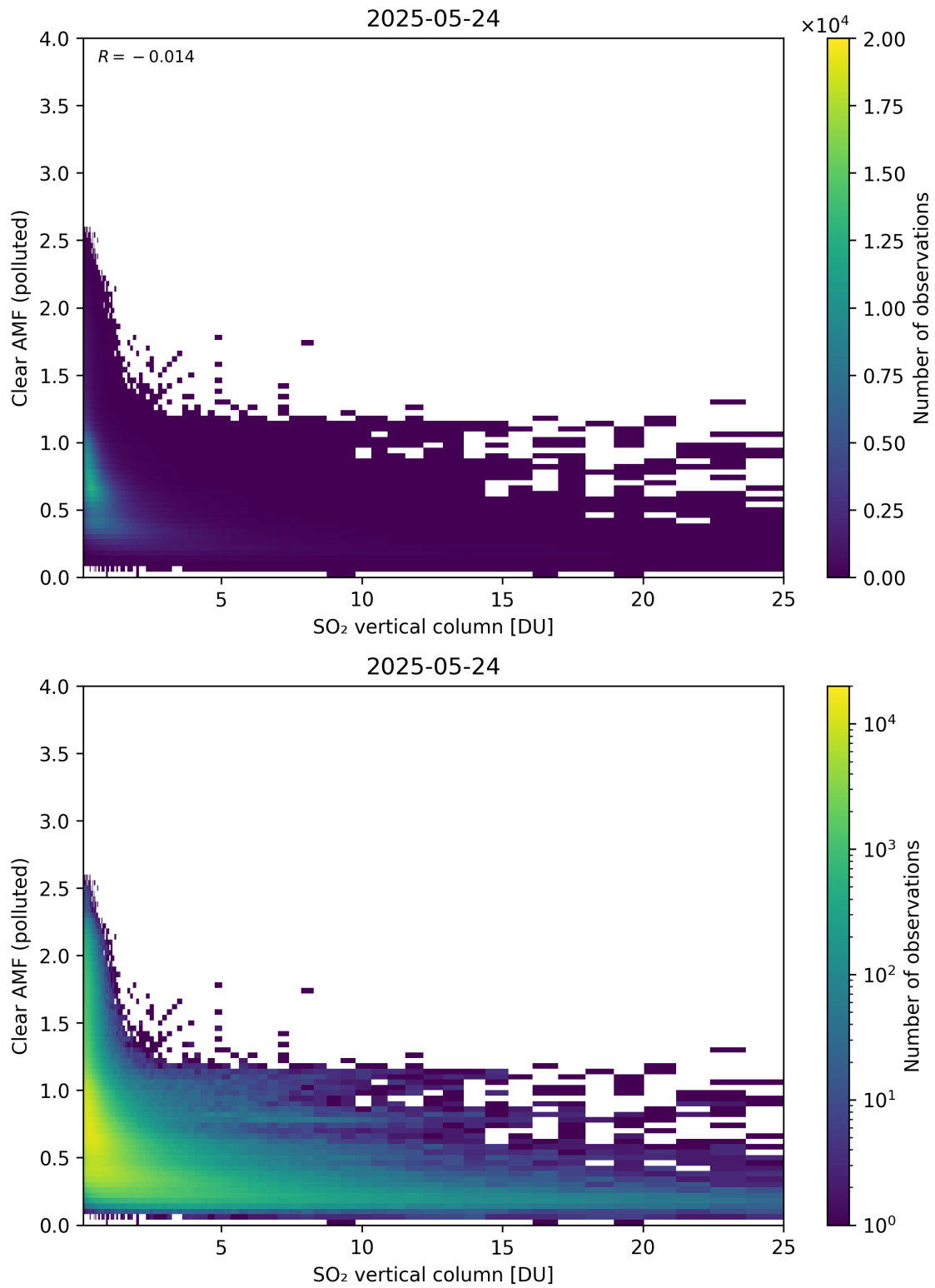
Figure 348: Scatter density plot of “SO 2 vertical column” against “Clear AMF (polluted)” for 2025-05-23 to 2025-05-25.
