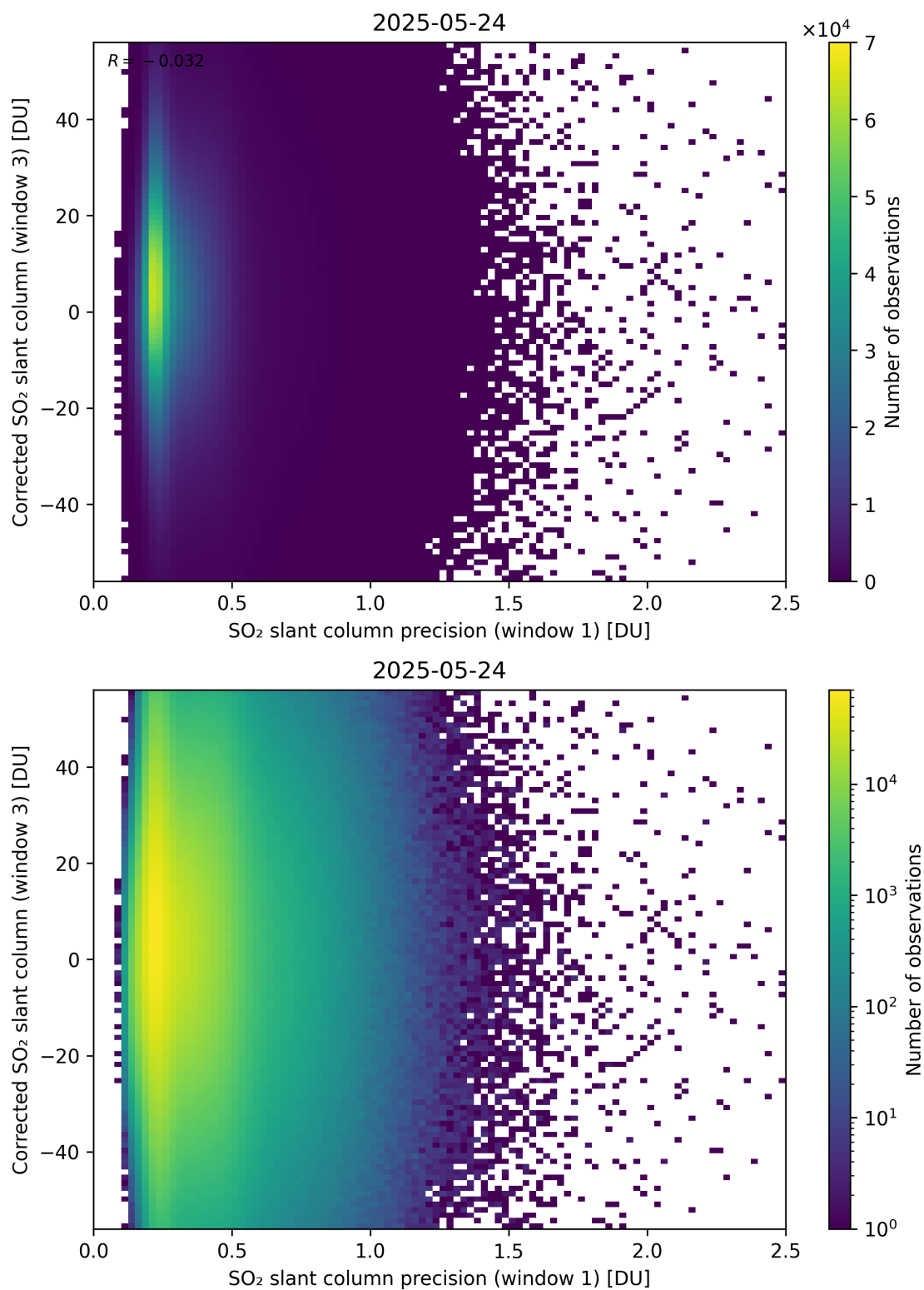
Figure 276: Scatter density plot of “SO 2 slant column precision (window 1)” against “Corrected SO 2 slant column (window 3)” for 2025-05-23 to 2025-05-25.
