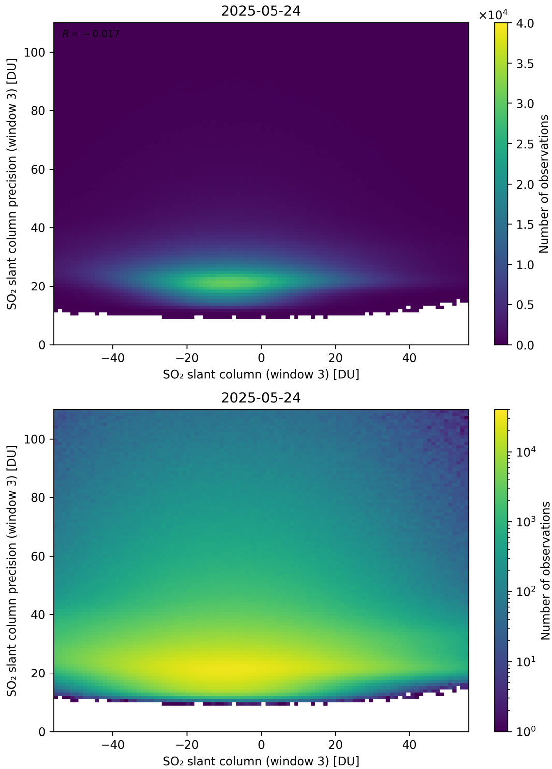
Figure 317: Scatter density plot of “SO 2 slant column (window 3)” against “SO 2 slant column precision (window 3)” for 2025-05-23 to 2025-05-25.
