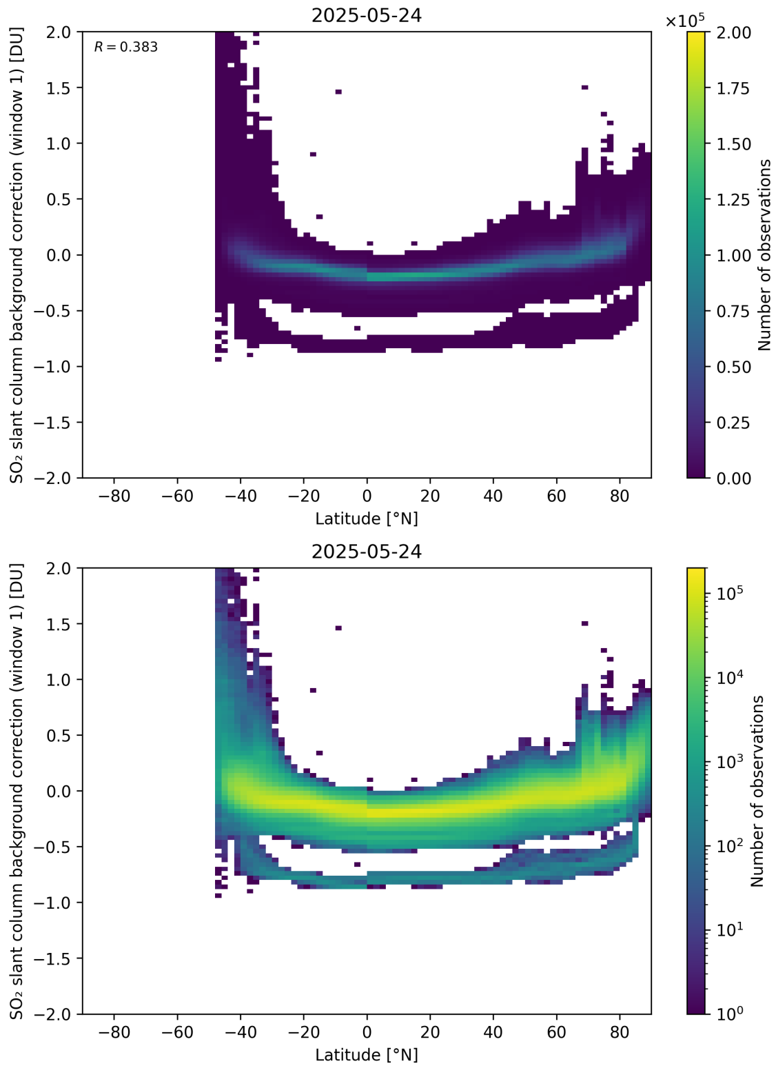
Figure 150: Scatter density plot of “Latitude” against “SO 2 slant column background correction (window 1)” for 2025-05-23 to 2025-05-25.
