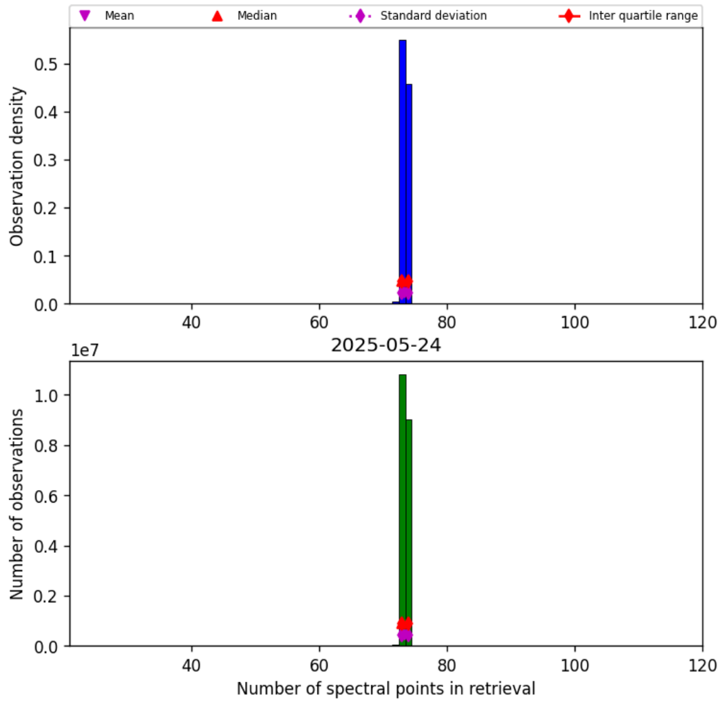
Figure 82: Histogram of “Number of spectral points in retrieval” for 2025-05-23 to 2025-05-25
