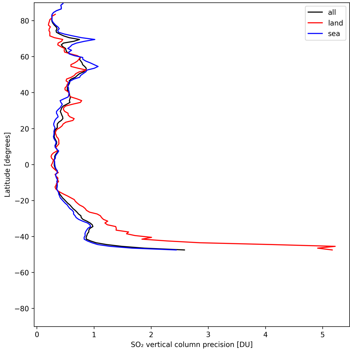
Figure 33: Zonal average of “SO 2 vertical column precision” for 2025-05-23 to 2025-05-25.
