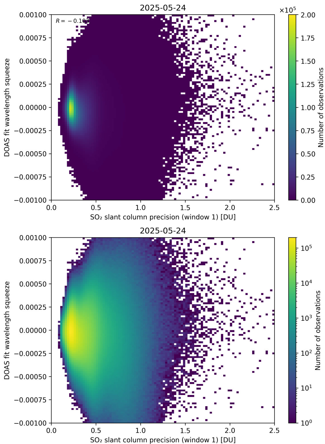
Figure 272: Scatter density plot of “SO 2 slant column precision (window 1)” against “DOAS fit wavelength squeeze” for 2025-05-23 to 2025-05-25.
