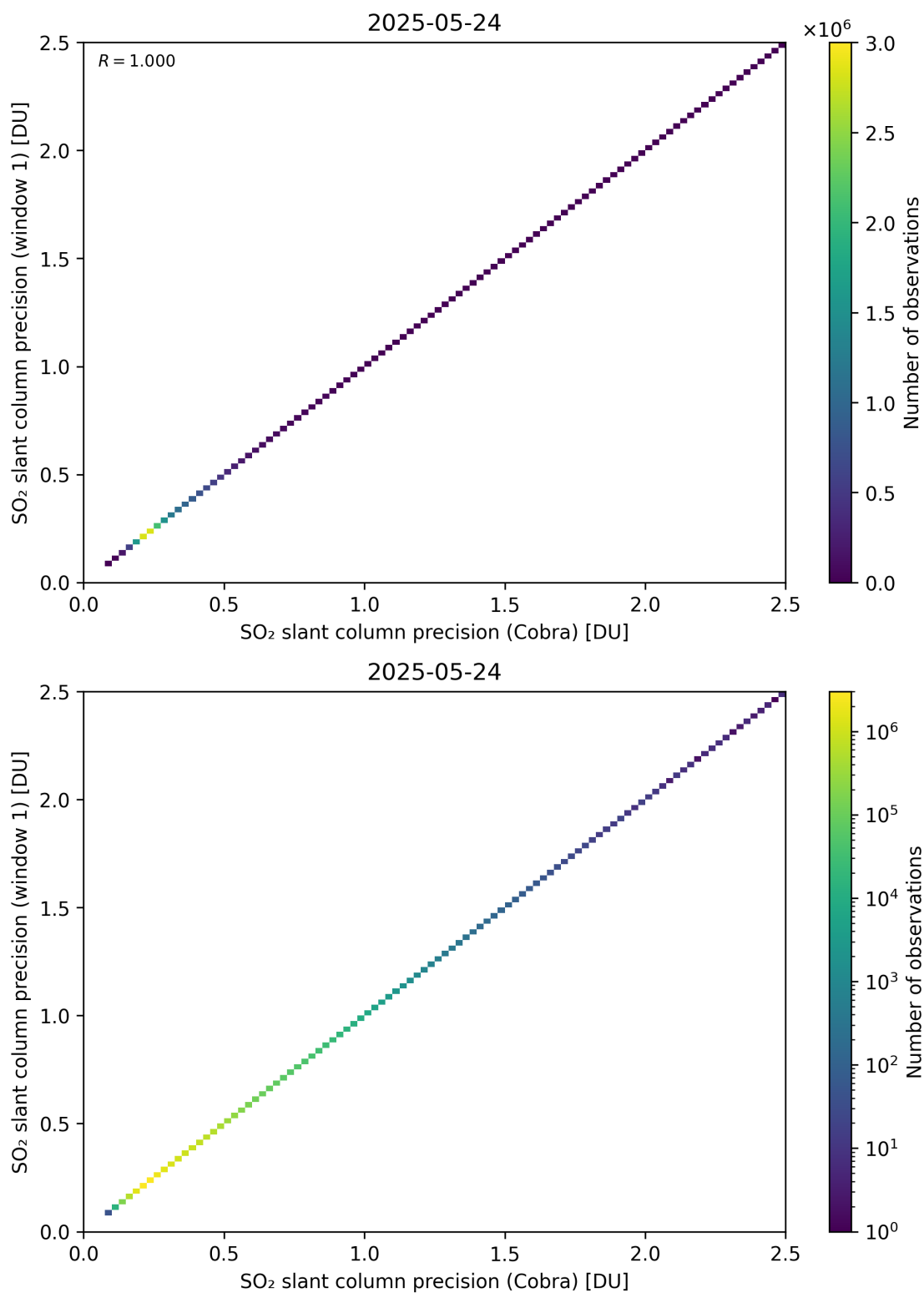
Figure 209: Scatter density plot of “SO 2 slant column precision (Cobra)” against “SO 2 slant column precision (window 1)” for 2025-05-23 to 2025-05-25.
