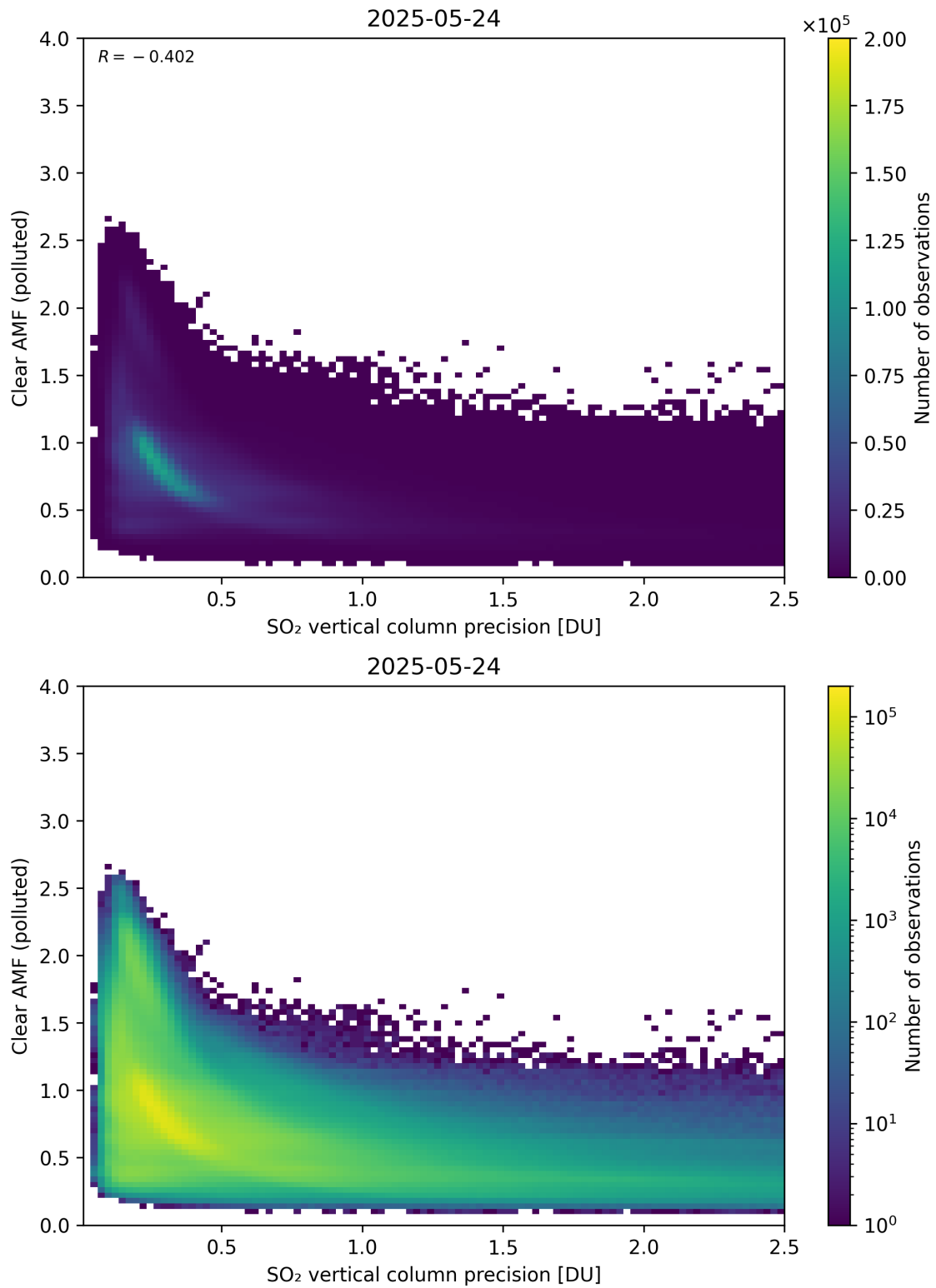
Figure 335: Scatter density plot of “SO 2 vertical column precision” against “Clear AMF (polluted)” for 2025-05-23 to 2025-05-25.
