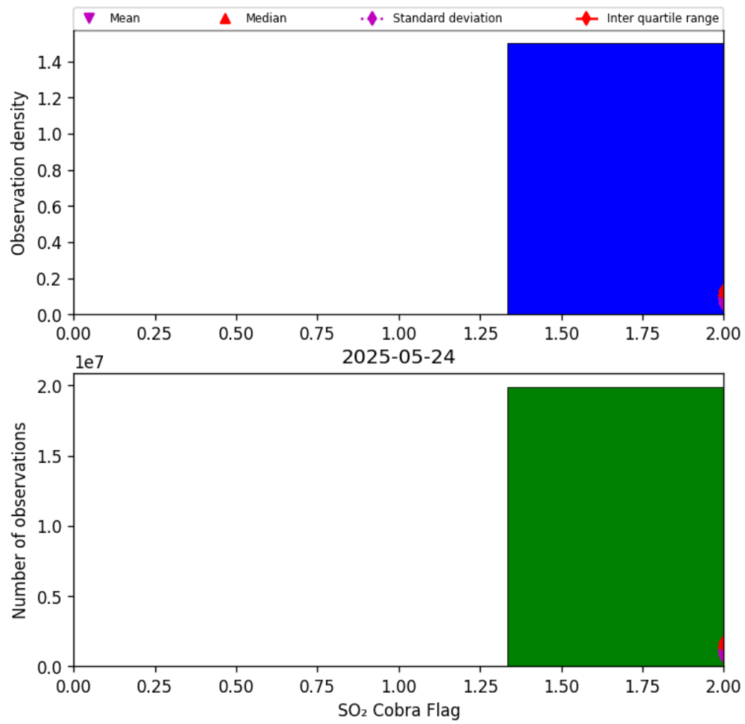
Figure 75: Histogram of “SO 2 Cobra Flag” for 2025-05-23 to 2025-05-25
