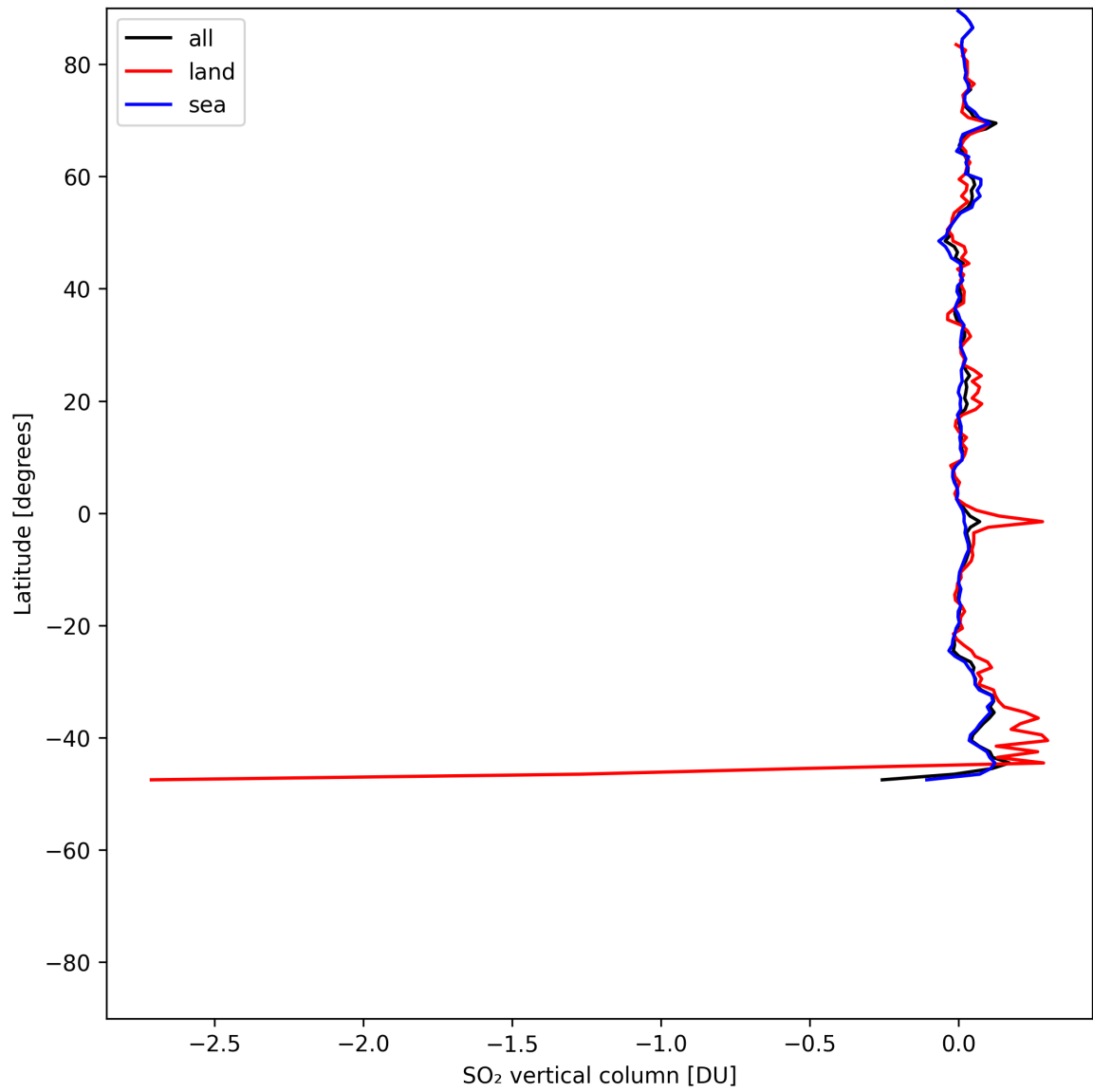
Figure 32: Zonal average of “SO 2 vertical column” for 2025-05-23 to 2025-05-25.
