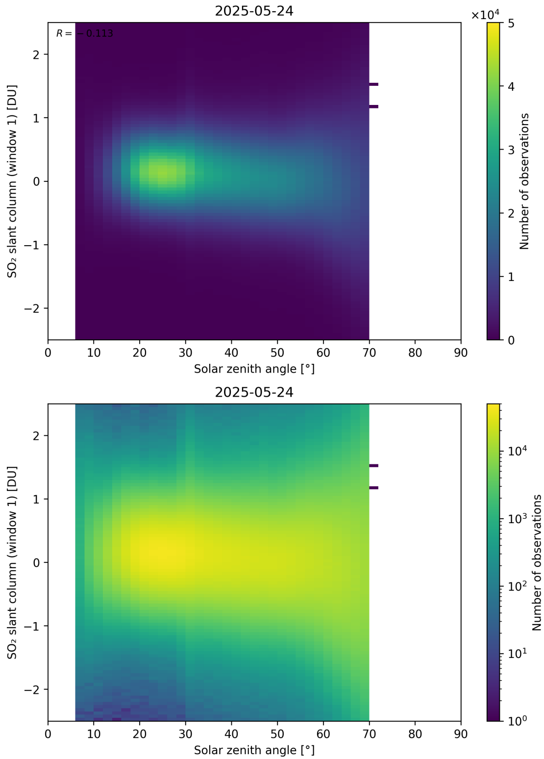
Figure 184: Scatter density plot of “Solar zenith angle” against “SO 2 slant column (window 1)” for 2025-05-23 to 2025-05-25.
