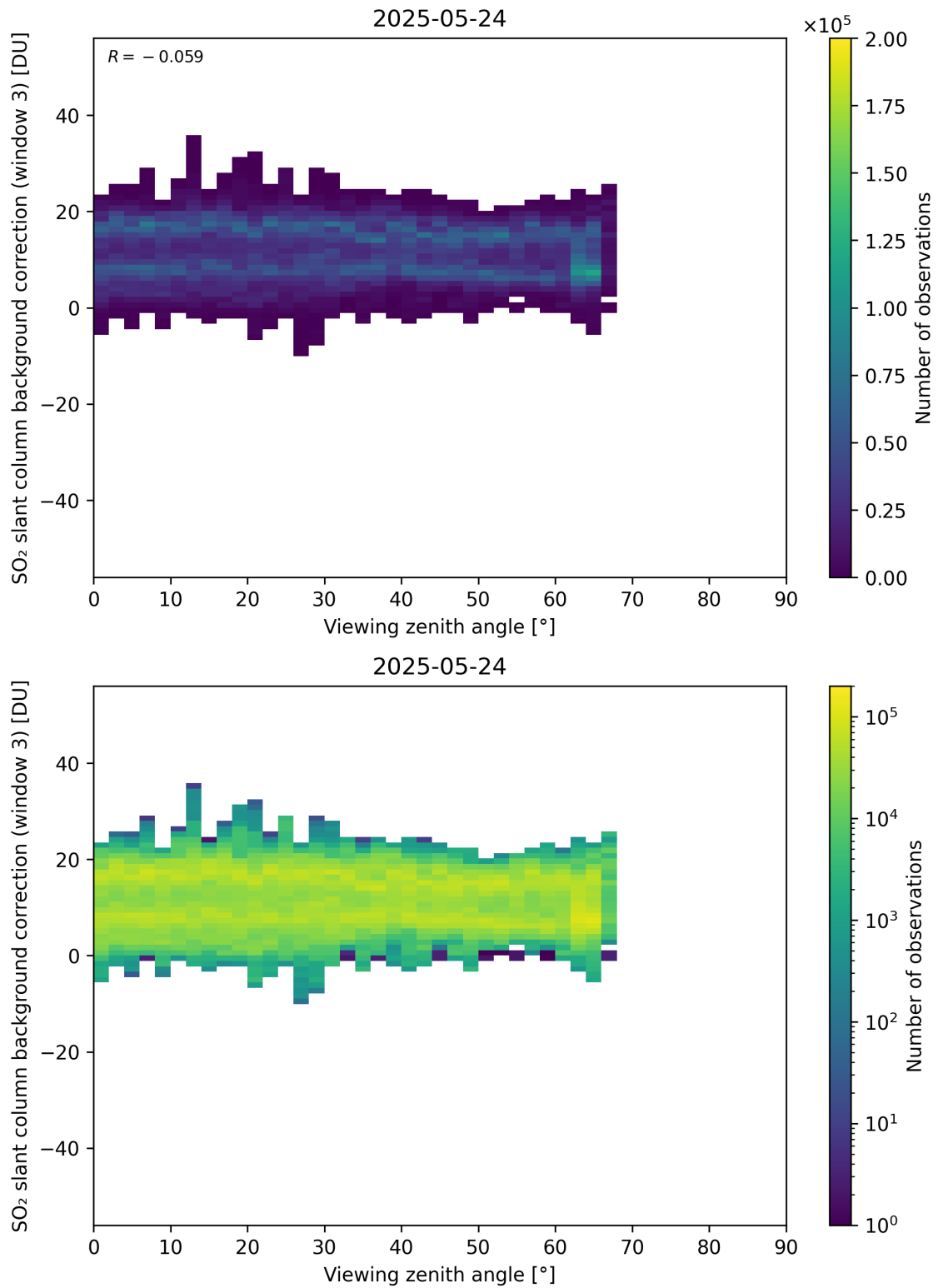
Figure 364: Scatter density plot of “Viewing zenith angle” against “SO 2 slant column background correction (window 3)” for 2025-05-23 to 2025-05-25.
