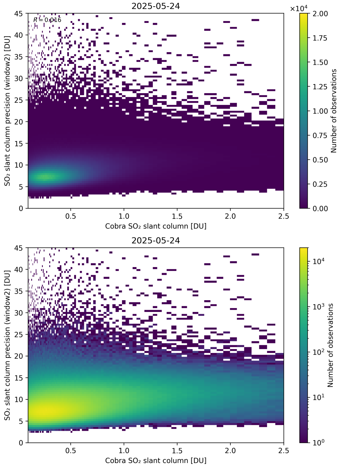
Figure 221: Scatter density plot of “Cobra SO 2 slant column” against “SO 2 slant column precision (window2)” for 2025-05-23 to 2025-05-25.
