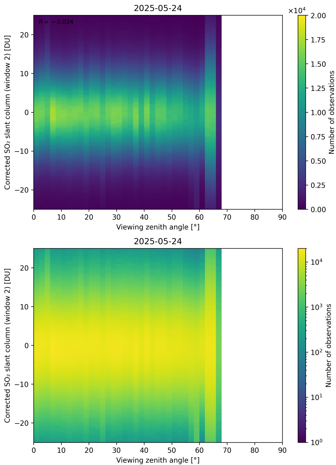
Figure 374: Scatter density plot of “Viewing zenith angle” against “Corrected SO 2 slant column (window 2)” for 2025-05-23 to 2025-05-25.
