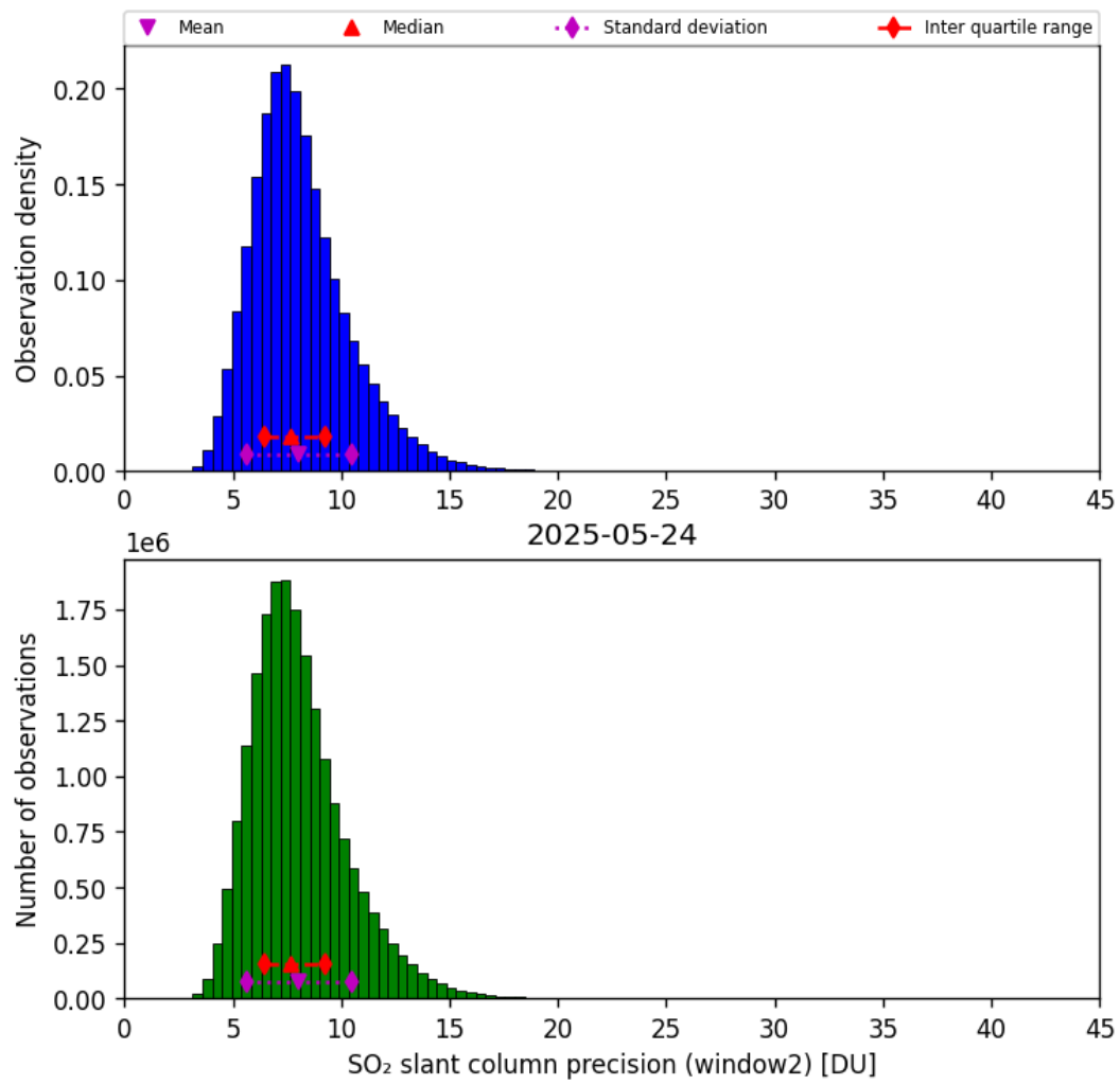
Figure 68: Histogram of “SO 2 slant column precision (window2)” for 2025-05-23 to 2025-05-25
