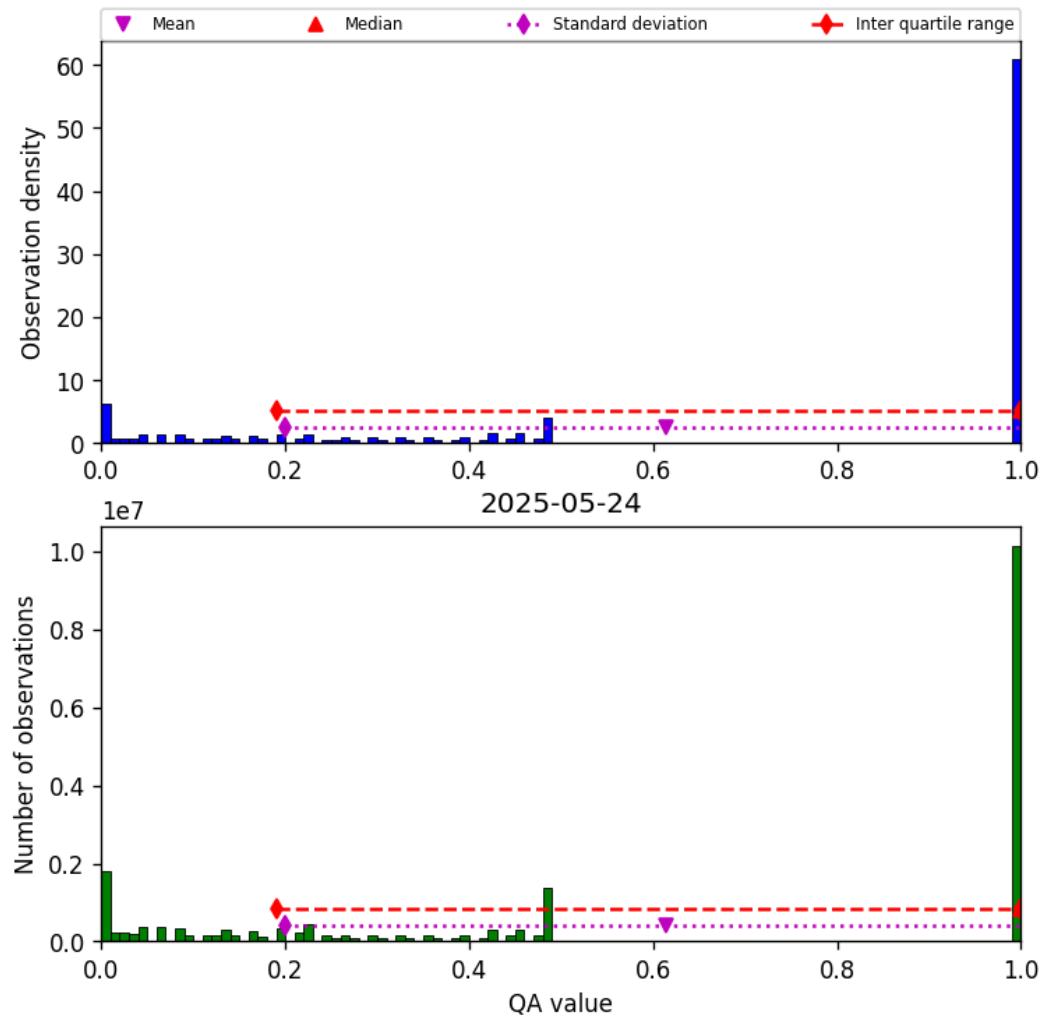
Figure 57: Histogram of “QA value” for 2025-05-23 to 2025-05-25
