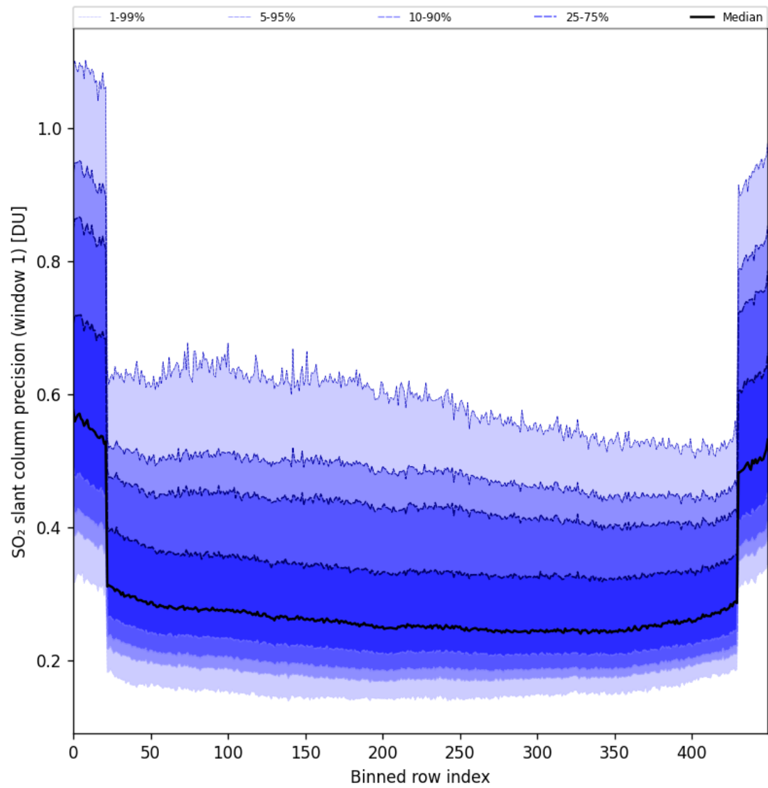
Figure 90: Along track statistics of “SO 2 slant column precision (window 1)” for 2025-05-23 to 2025-05-25
