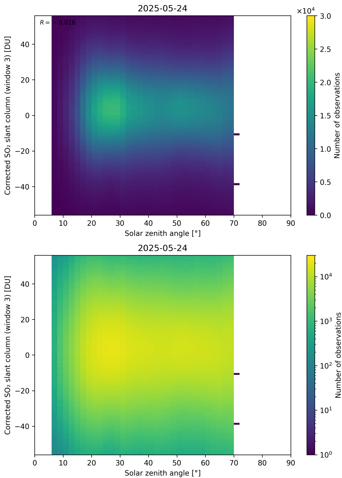
Figure 183: Scatter density plot of “Solar zenith angle” against “Corrected SO 2 slant column (window 3)” for 2025-05-23 to 2025-05-25.
