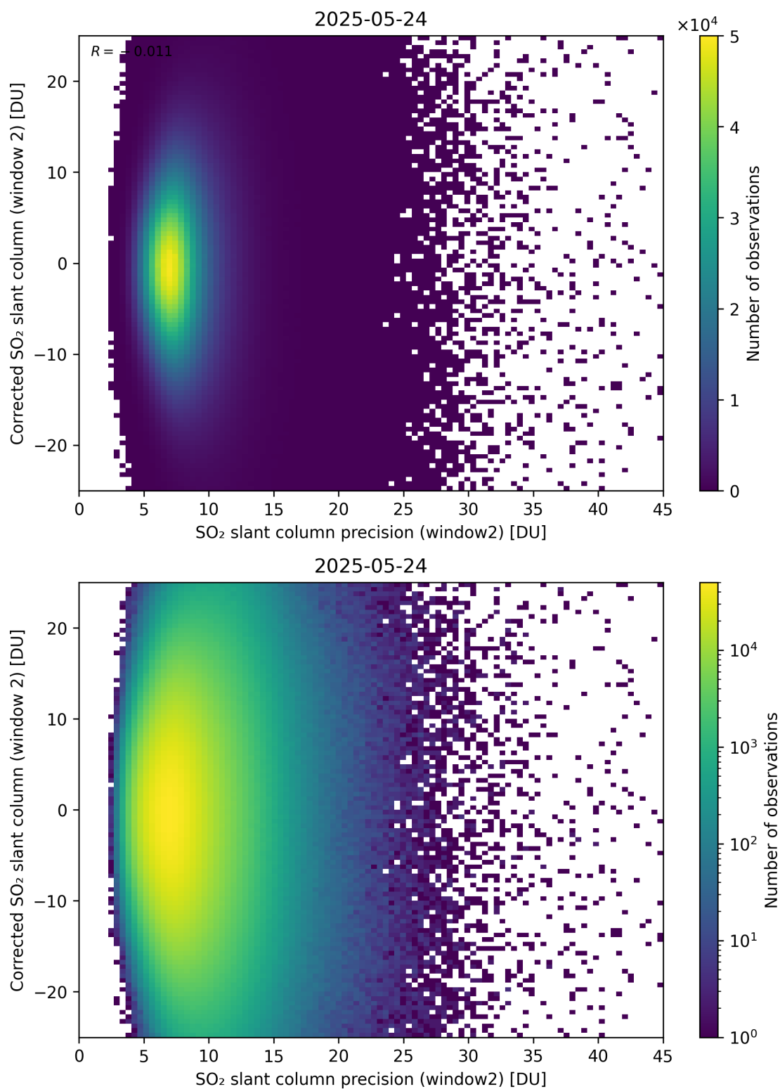
Figure 297: Scatter density plot of “SO 2 slant column precision (window2)” against “Corrected SO 2 slant column (window 2)” for 2025-05-23 to 2025-05-25.
