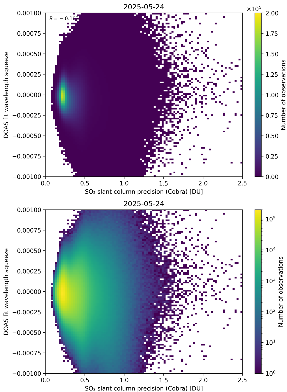
Figure 203: Scatter density plot of “SO 2 slant column precision (Cobra)” against “DOAS fit wavelength squeeze” for 2025-05-23 to 2025-05-25.
