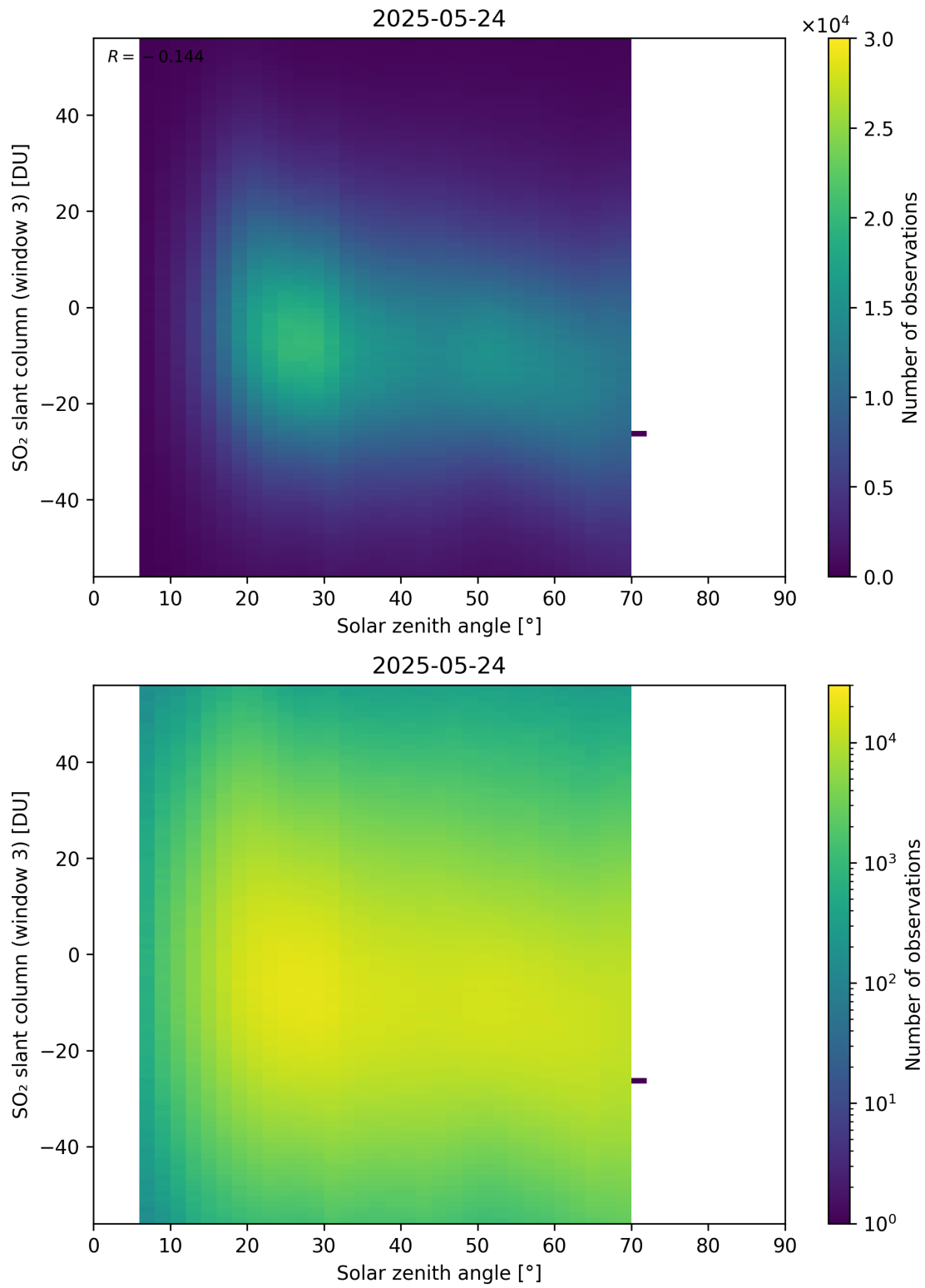
Figure 187: Scatter density plot of “Solar zenith angle” against “SO 2 slant column (window 3)” for 2025-05-23 to 2025-05-25.
