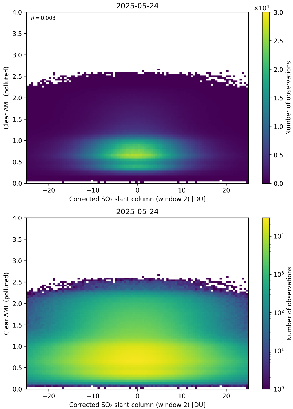
Figure 249: Scatter density plot of “Corrected SO 2 slant column (window 2)” against “Clear AMF (polluted)” for 2025-05-23 to 2025-05-25.
