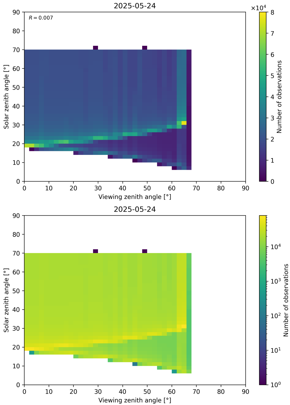
Figure 369: Scatter density plot of “Viewing zenith angle” against “Solar zenith angle” for 2025-05-23 to 2025-05-25.
