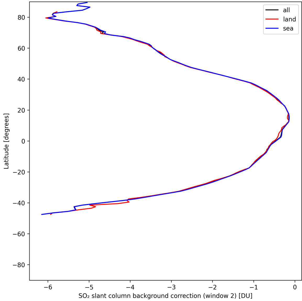
Figure 44: Zonal average of “SO 2 slant column background correction (window 2)” for 2025-05-23 to 2025-05-25.
