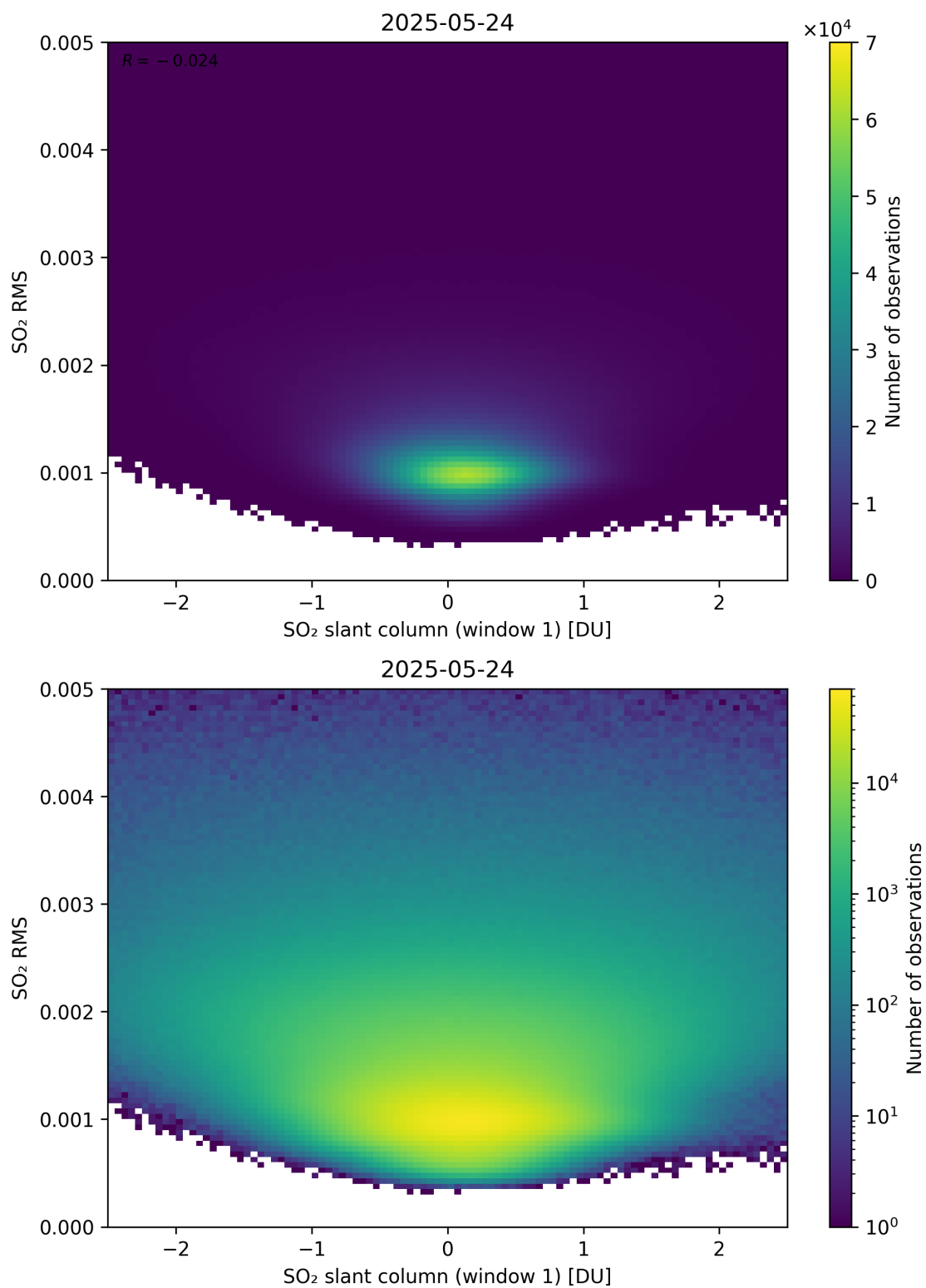
Figure 267: Scatter density plot of “SO 2 slant column (window 1)” against “SO 2 RMS” for 2025-05-23 to 2025-05-25.
