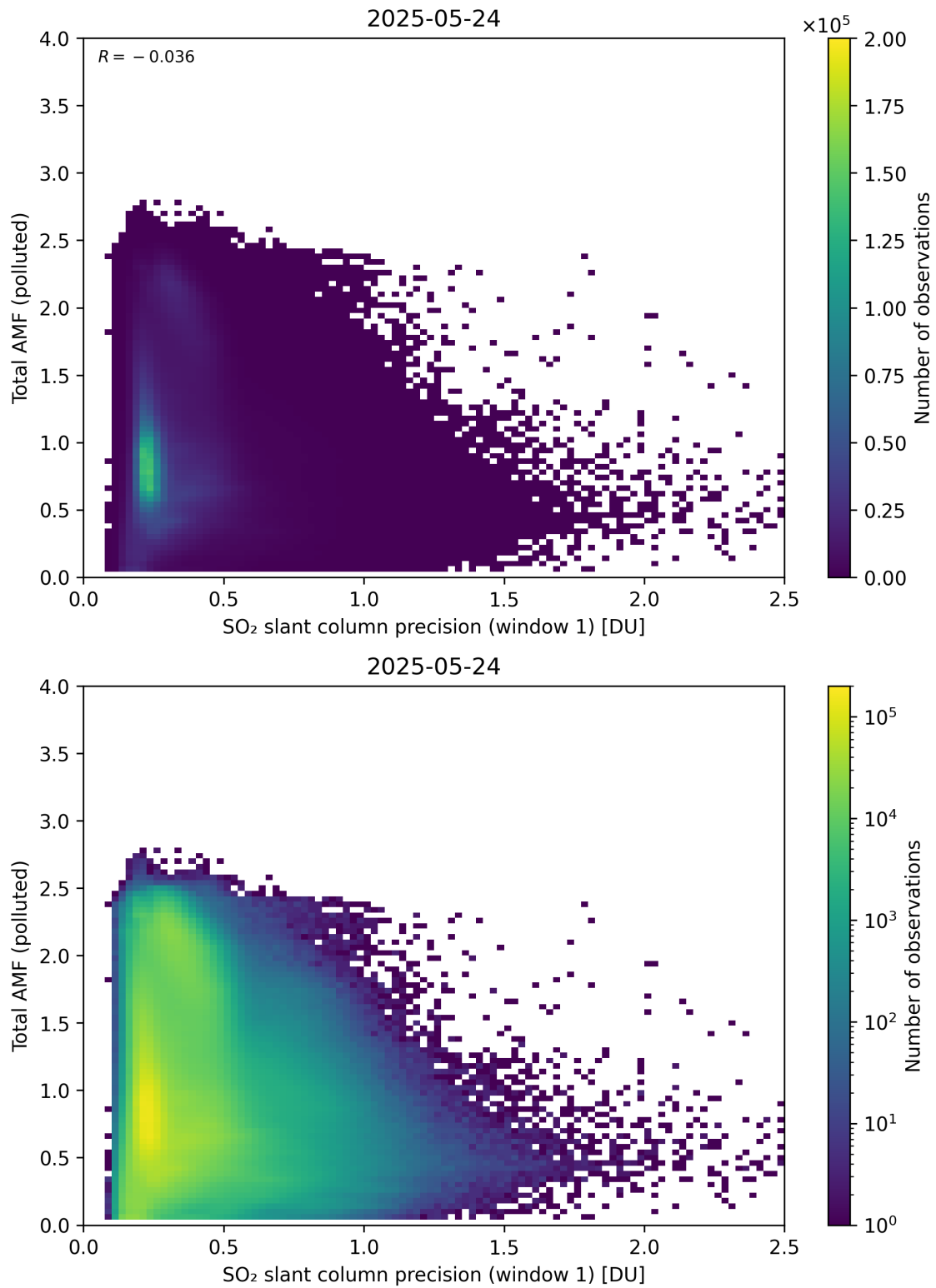
Figure 280: Scatter density plot of “SO 2 slant column precision (window 1)” against “Total AMF (polluted)” for 2025-05-23 to 2025-05-25.
