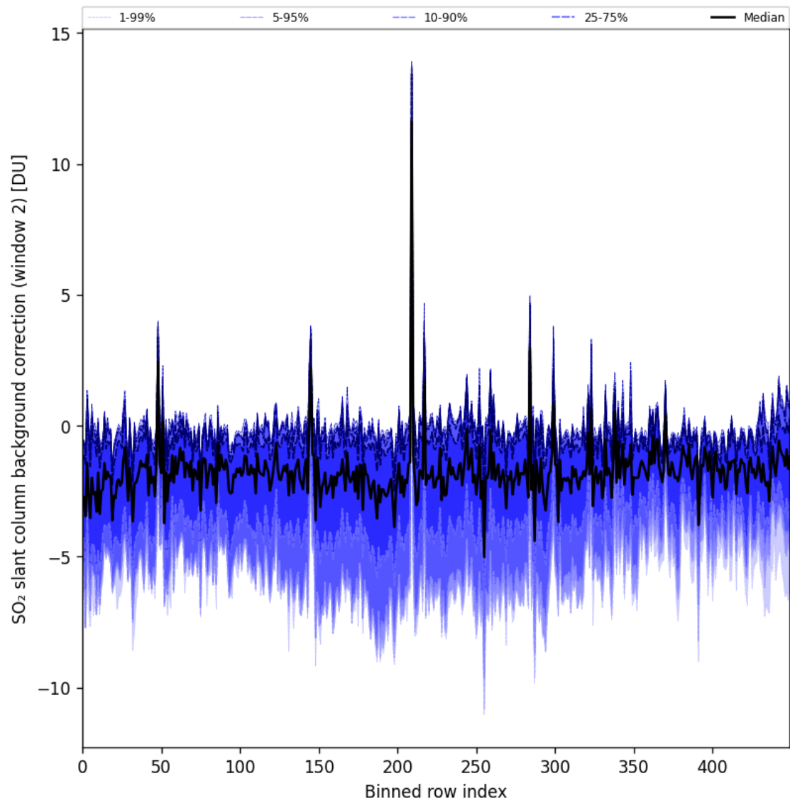
Figure 96: Along track statistics of “SO 2 slant column background correction (window 2)” for 2025-05-23 to 2025-05-25
