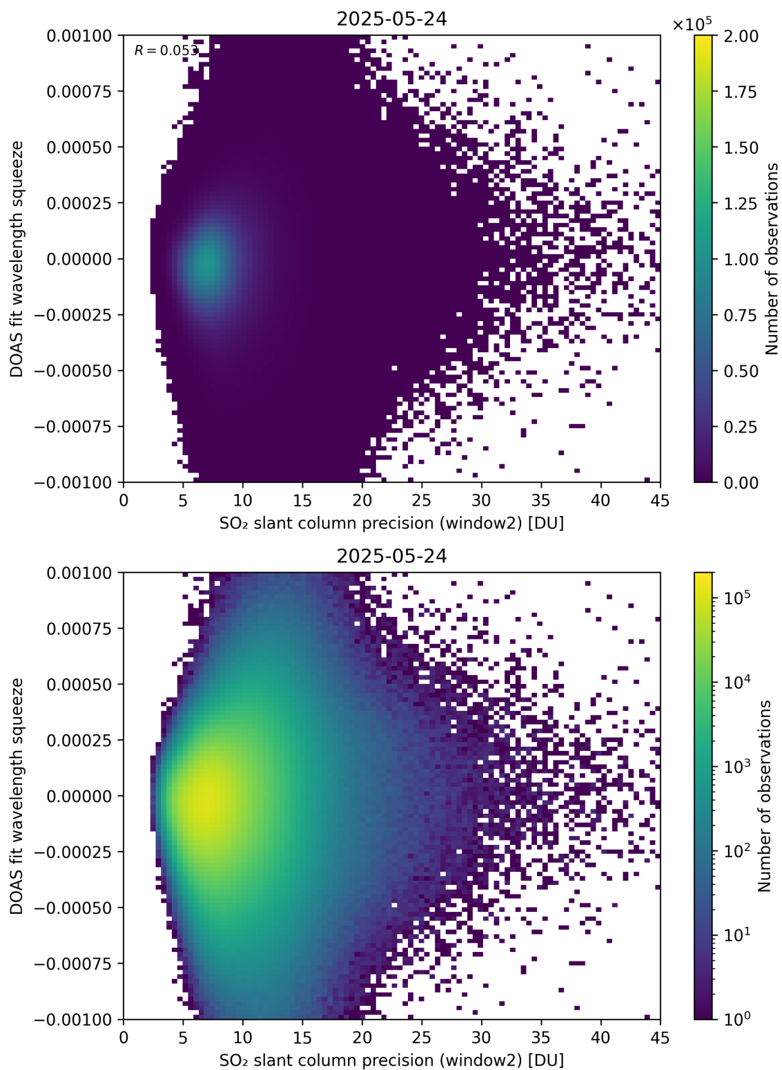
Figure 294: Scatter density plot of “SO 2 slant column precision (window2)” against “DOAS fit wavelength squeeze” for 2025-05-23 to 2025-05-25.
