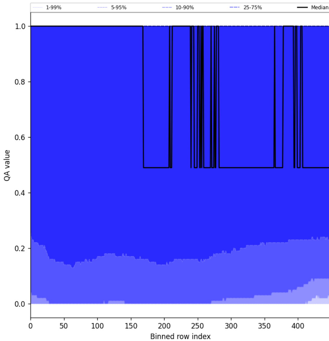
Figure 83: Along track statistics of “QA value” for 2025-05-23 to 2025-05-25
