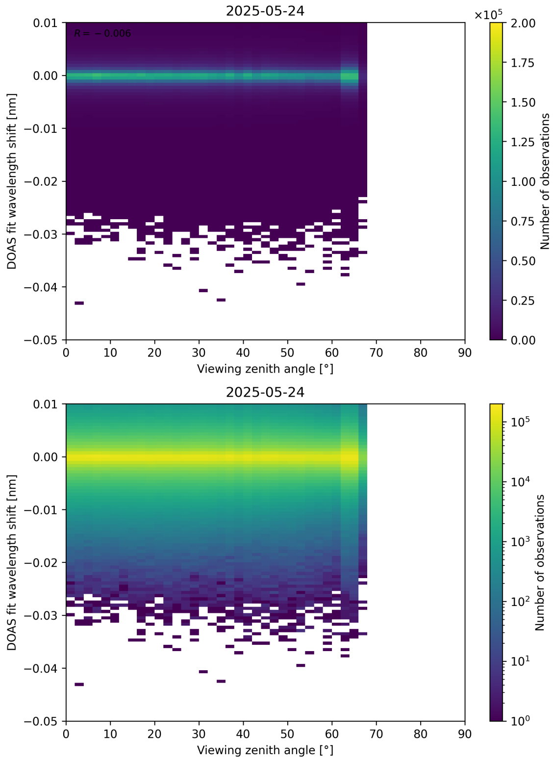
Figure 365: Scatter density plot of “Viewing zenith angle” against “DOAS fit wavelength shift” for 2025-05-23 to 2025-05-25.
