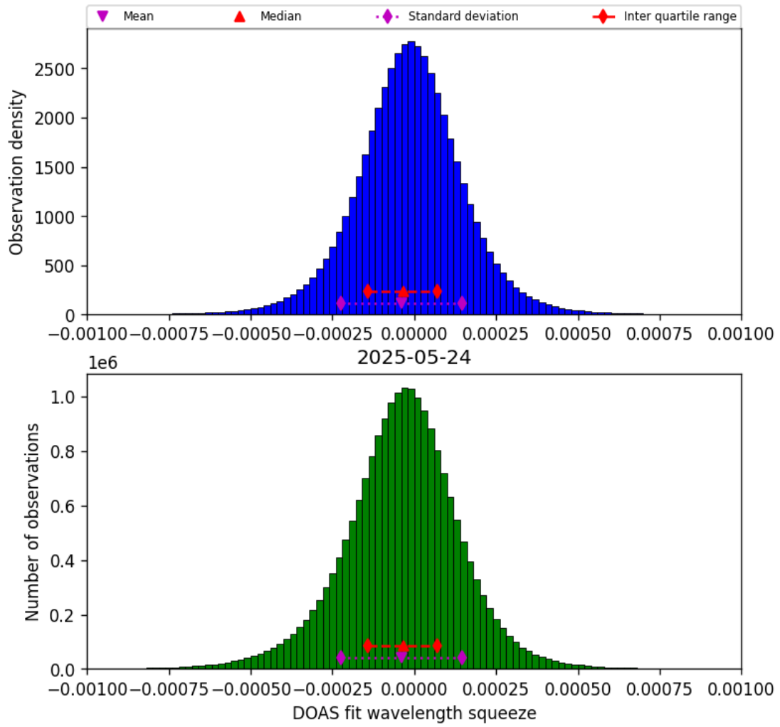
Figure 77: Histogram of “DOAS fit wavelength squeeze” for 2025-05-23 to 2025-05-25
