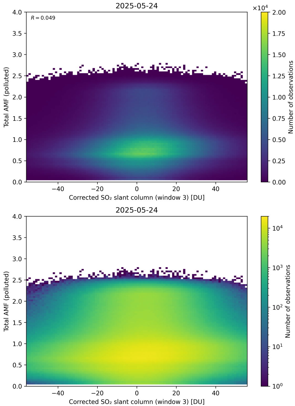
Figure 260: Scatter density plot of “Corrected SO 2 slant column (window 3)” against “Total AMF (polluted)” for 2025-05-23 to 2025-05-25.
