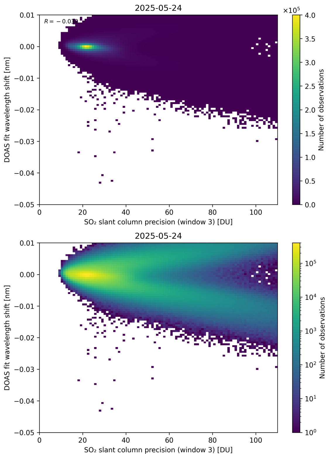
Figure 308: Scatter density plot of “SO 2 slant column precision (window 3)” against “DOAS fit wavelength shift” for 2025-05-23 to 2025-05-25.
