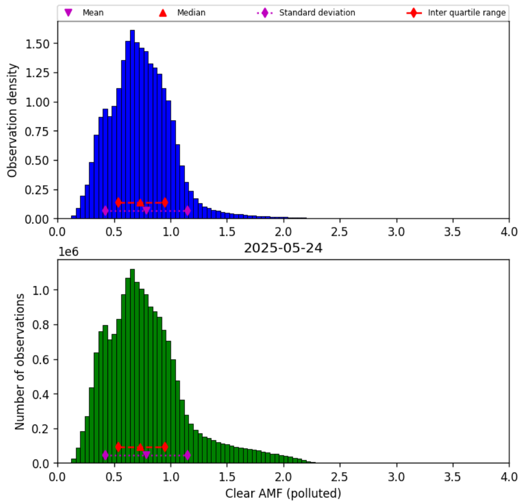
Figure 81: Histogram of “Clear AMF (polluted)” for 2025-05-23 to 2025-05-25
