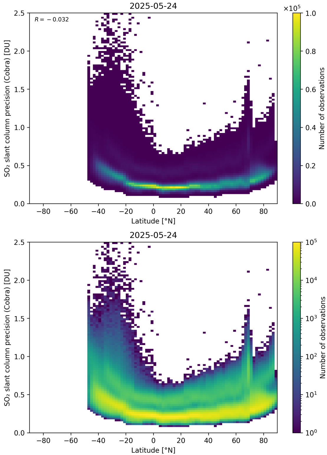
Figure 158: Scatter density plot of “Latitude” against “SO 2 slant column precision (Cobra)” for 2025-05-23 to 2025-05-25.
