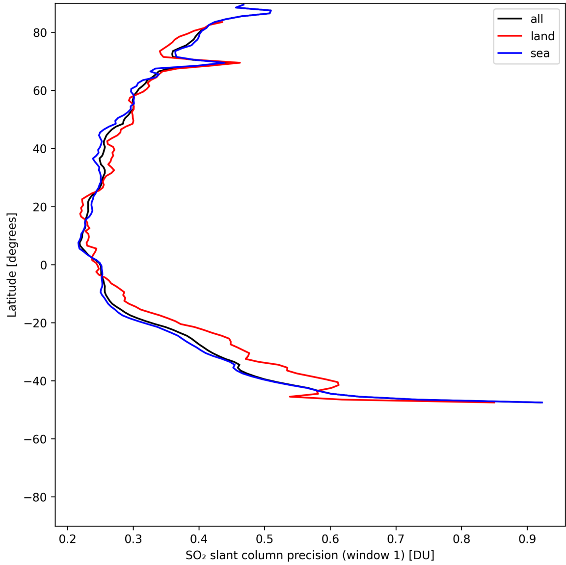
Figure 38: Zonal average of “SO 2 slant column precision (window 1)” for 2025-05-23 to 2025-05-25.
