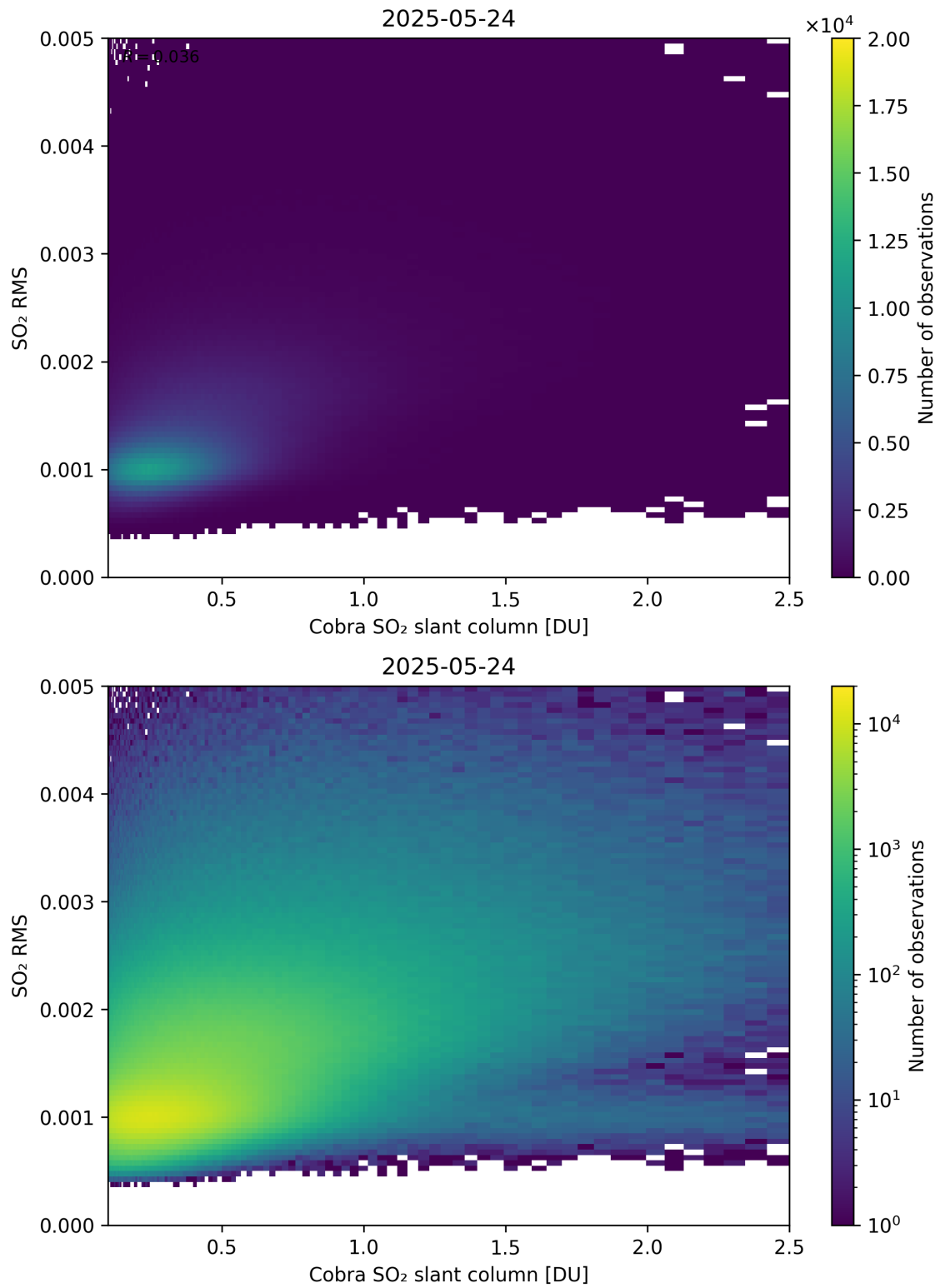
Figure 198: Scatter density plot of “Cobra SO 2 slant column” against “SO 2 RMS” for 2025-05-23 to 2025-05-25.
