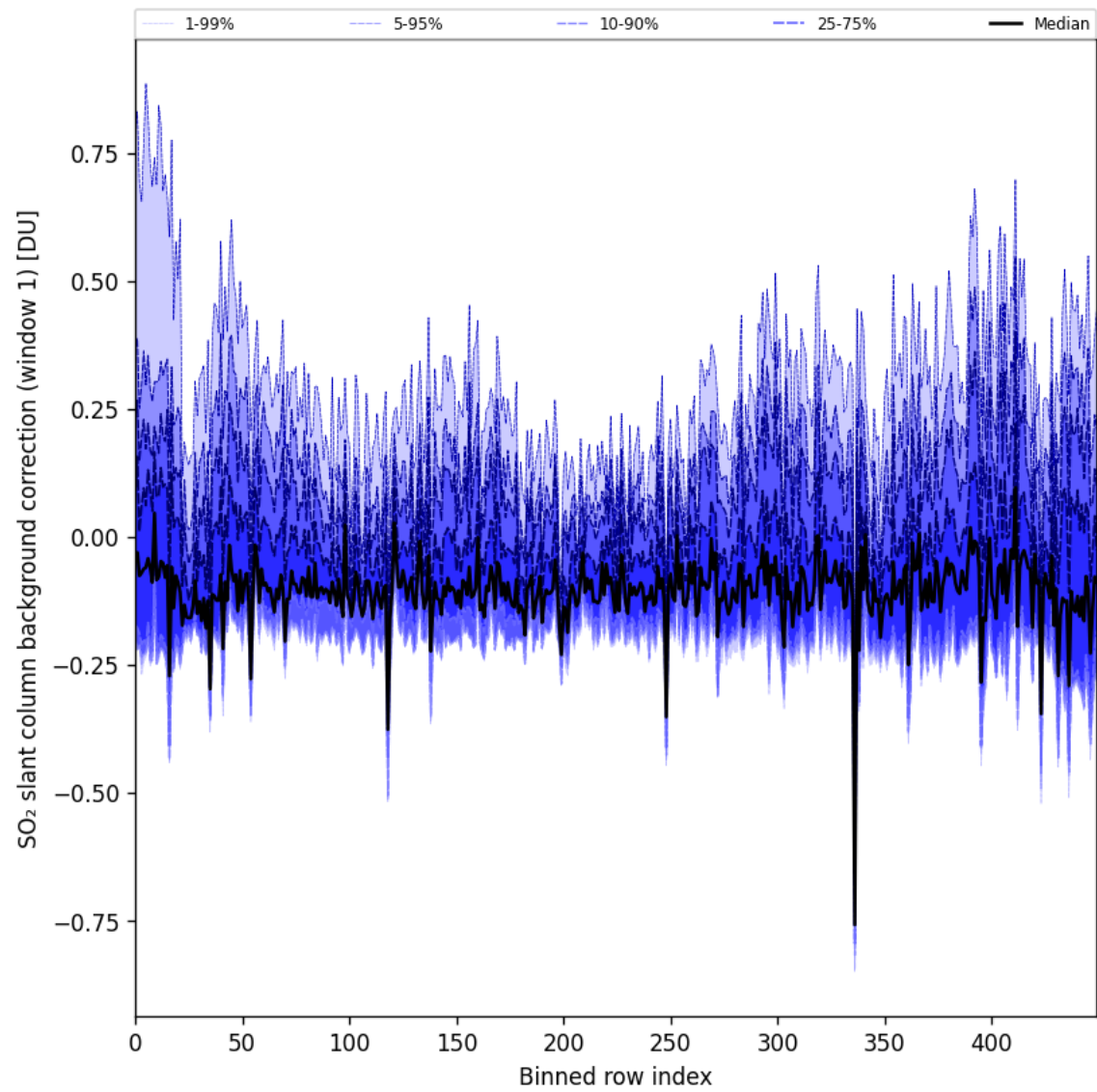
Figure 92: Along track statistics of “SO 2 slant column background correction (window 1)” for 2025-05-23 to 2025-05-25
