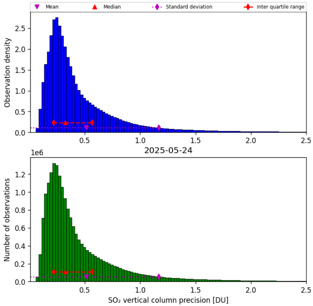
Figure 59: Histogram of “SO 2 vertical column precision” for 2025-05-23 to 2025-05-25
