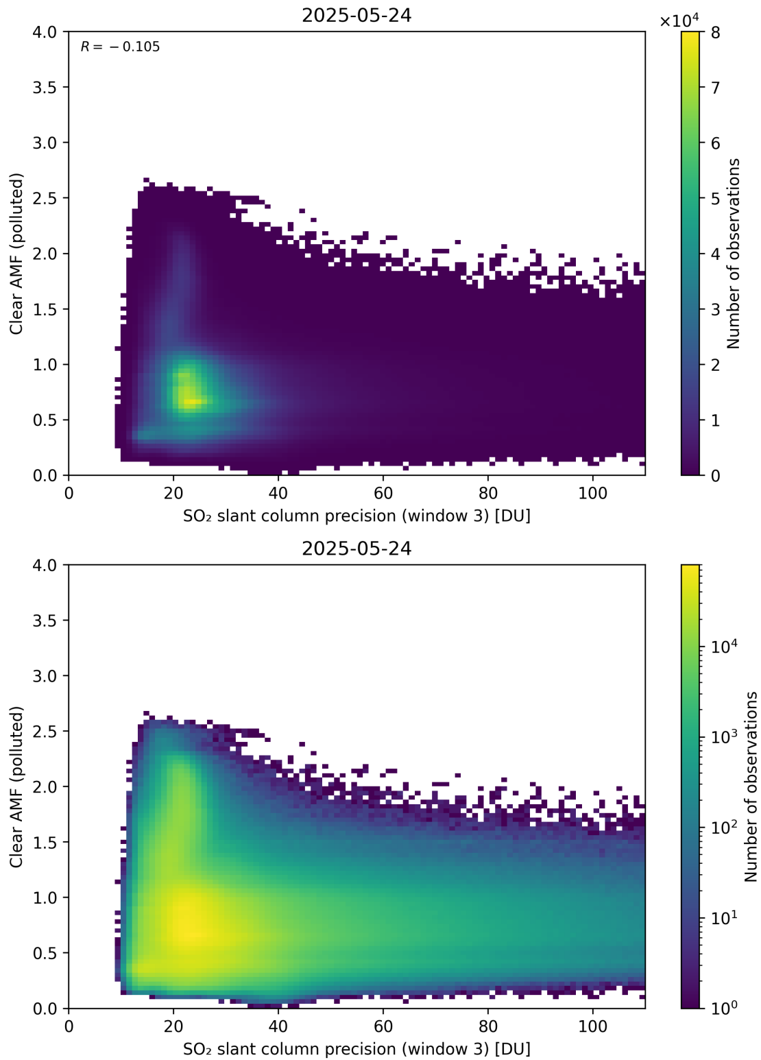
Figure 311: Scatter density plot of “SO 2 slant column precision (window 3)” against “Clear AMF (polluted)” for 2025-05-23 to 2025-05-25.
