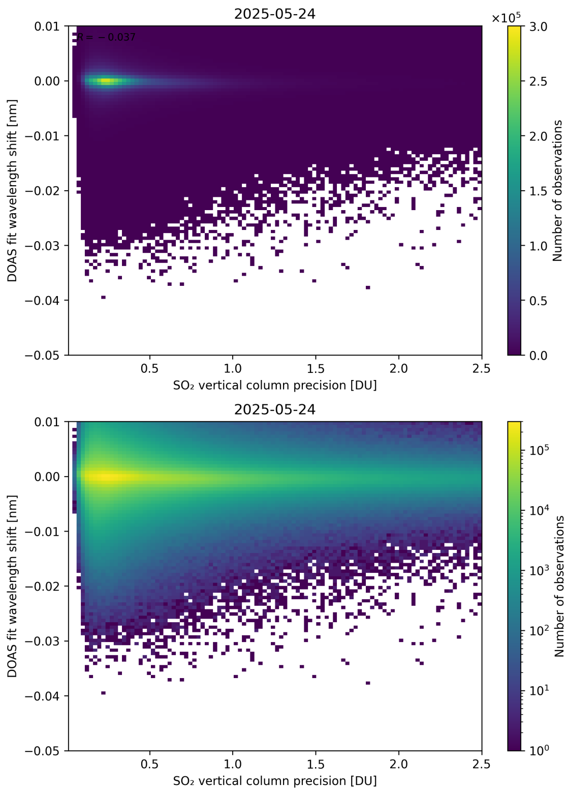
Figure 332: Scatter density plot of “SO 2 vertical column precision” against “DOAS fit wavelength shift” for 2025-05-23 to 2025-05-25.
