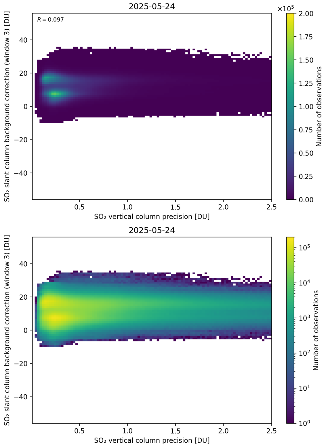
Figure 331: Scatter density plot of “SO 2 vertical column precision” against “SO 2 slant column background correction (window 3)” for 2025-05-23 to 2025-05-25.
