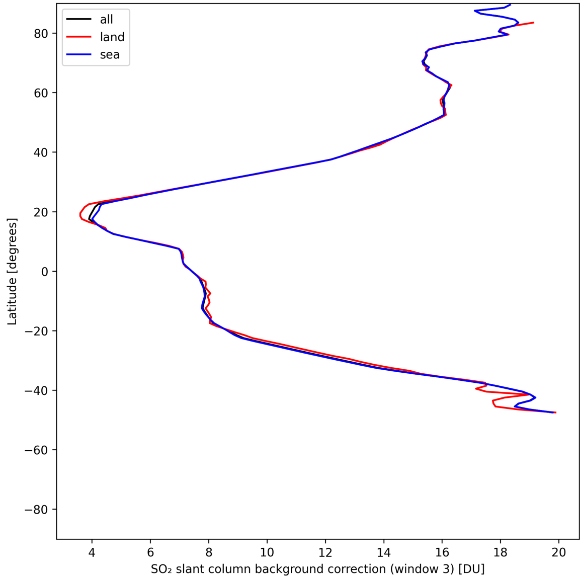
Figure 48: Zonal average of “SO 2 slant column background correction (window 3)” for 2025-05-23 to 2025-05-25.
