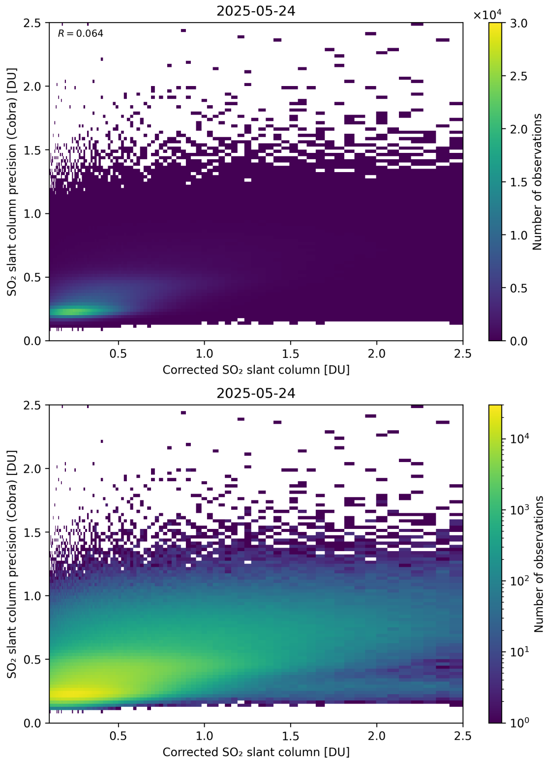
Figure 234: Scatter density plot of “Corrected SO 2 slant column” against “SO 2 slant column precision (Cobra)” for 2025-05-23 to 2025-05-25.
