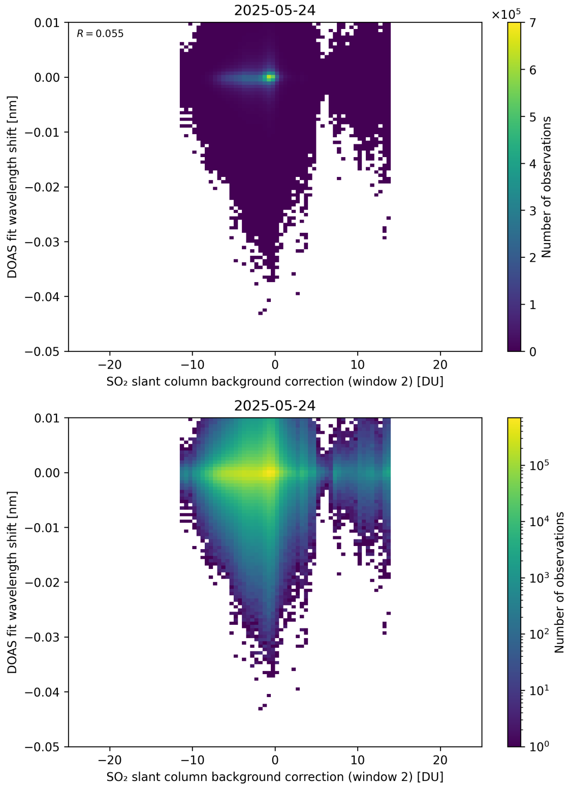
Figure 123: Scatter density plot of “SO 2 slant column background correction (window 2)” against “DOAS fit wavelength shift” for 2025-05-23 to 2025-05-25.
