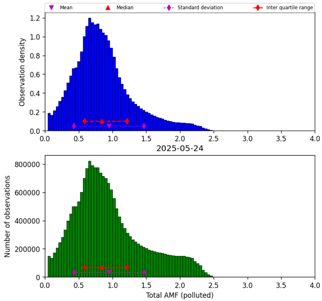
Figure 79: Histogram of “Total AMF (polluted)” for 2025-05-23 to 2025-05-25
