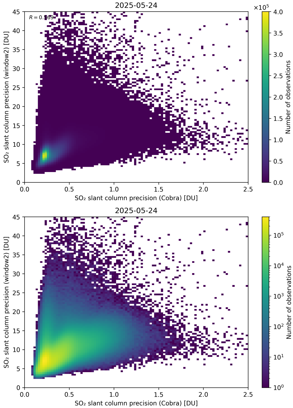
Figure 210: Scatter density plot of “SO 2 slant column precision (Cobra)” against “SO 2 slant column precision (window2)” for 2025-05-23 to 2025-05-25.
