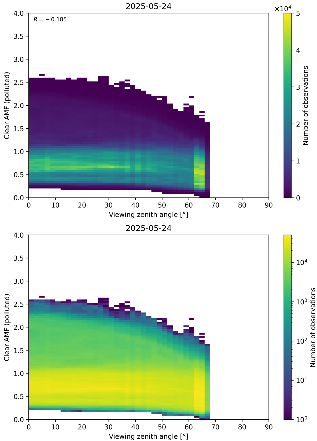
Figure 370: Scatter density plot of “Viewing zenith angle” against “Clear AMF (polluted)” for 2025-05-23 to 2025-05-25.
