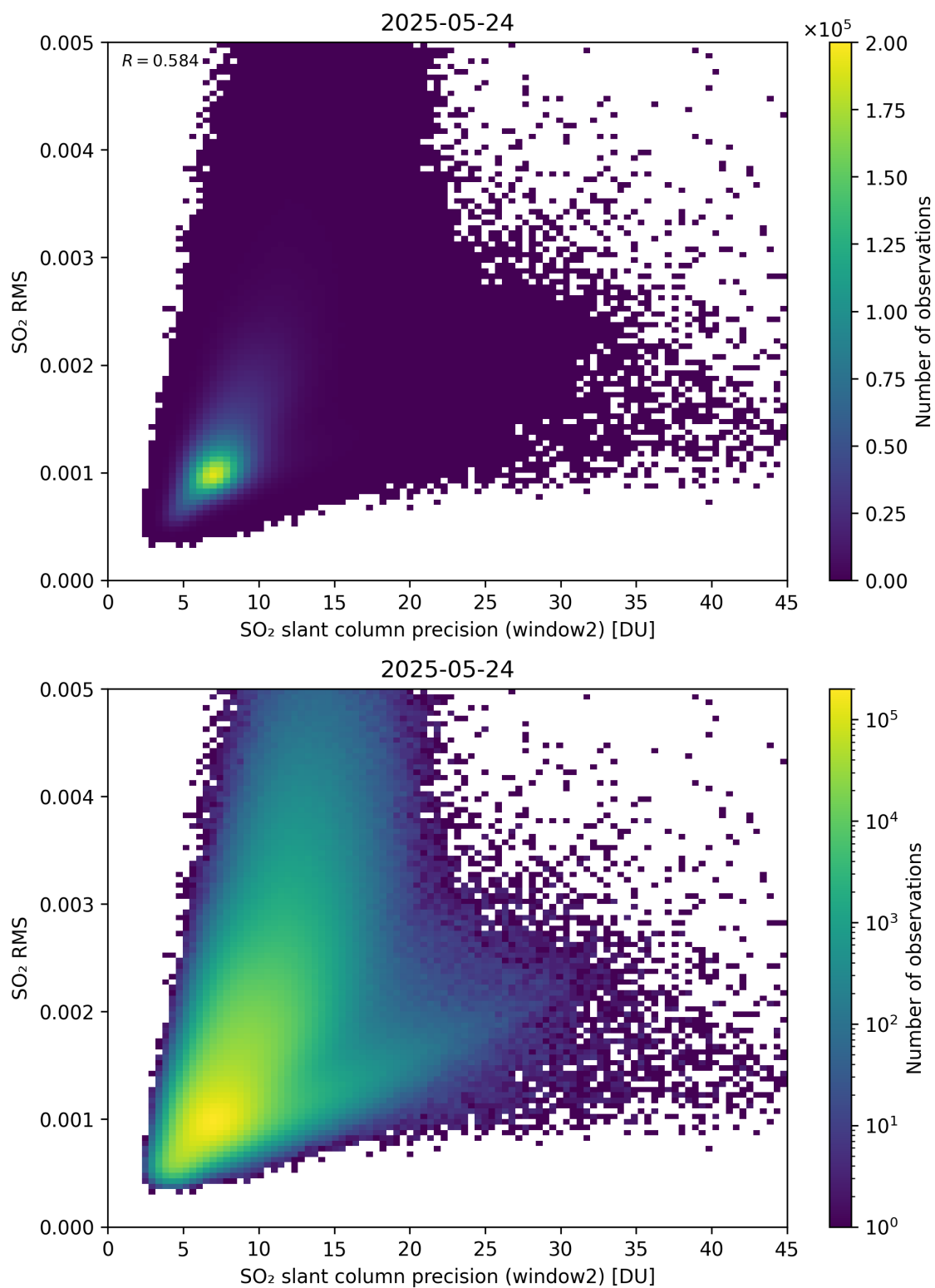
Figure 295: Scatter density plot of “SO 2 slant column precision (window2)” against “SO 2 RMS” for 2025-05-23 to 2025-05-25.
