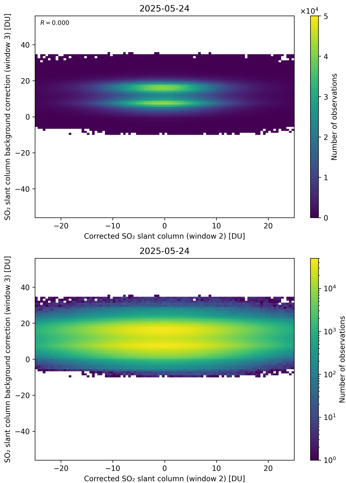
Figure 245: Scatter density plot of “Corrected SO 2 slant column (window 2)” against “SO 2 slant column background correction (window 3)” for 2025-05-23 to 2025-05-25.
