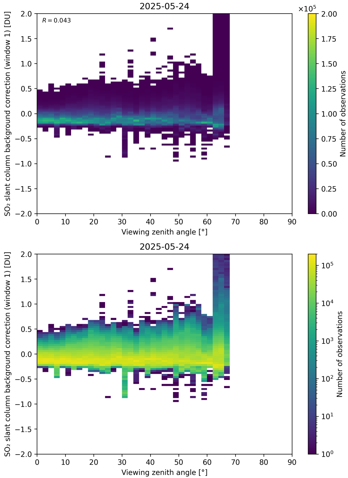
Figure 362: Scatter density plot of “Viewing zenith angle” against “SO 2 slant column background correction (window 1)” for 2025-05-23 to 2025-05-25.
