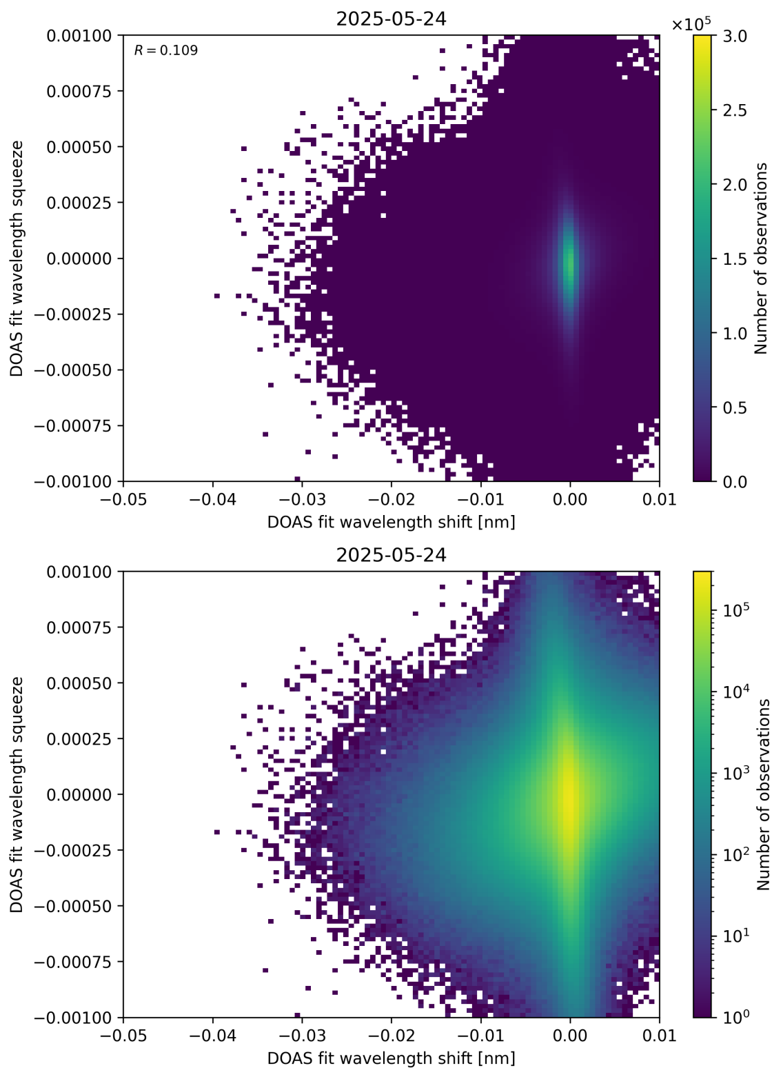
Figure 138: Scatter density plot of “DOAS fit wavelength shift” against “DOAS fit wavelength squeeze” for 2025-05-23 to 2025-05-25.
