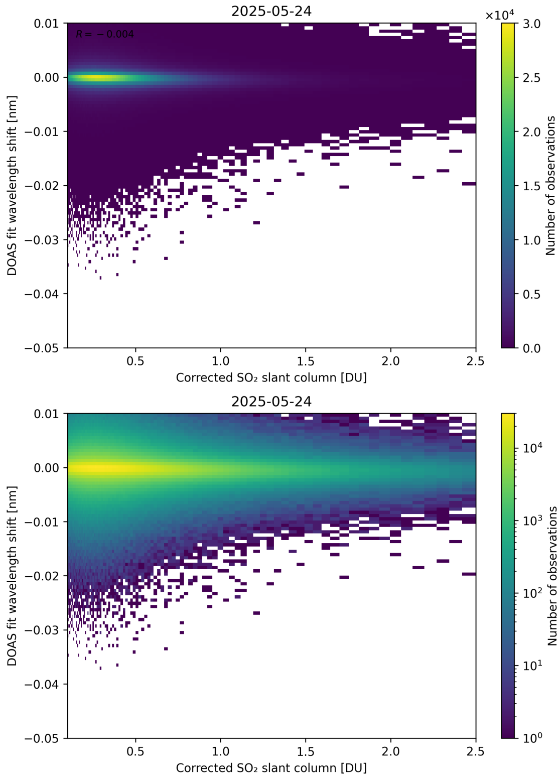
Figure 229: Scatter density plot of “Corrected SO 2 slant column” against “DOAS fit wavelength shift” for 2025-05-23 to 2025-05-25.
