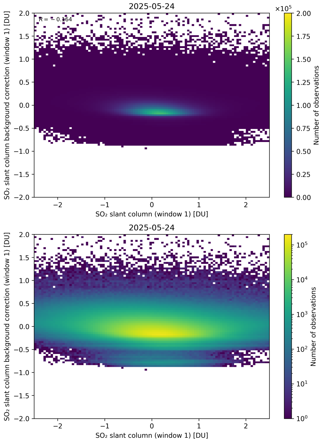
Figure 262: Scatter density plot of “SO 2 slant column (window 1)” against “SO 2 slant column background correction (window 1)” for 2025-05-23 to 2025-05-25.
