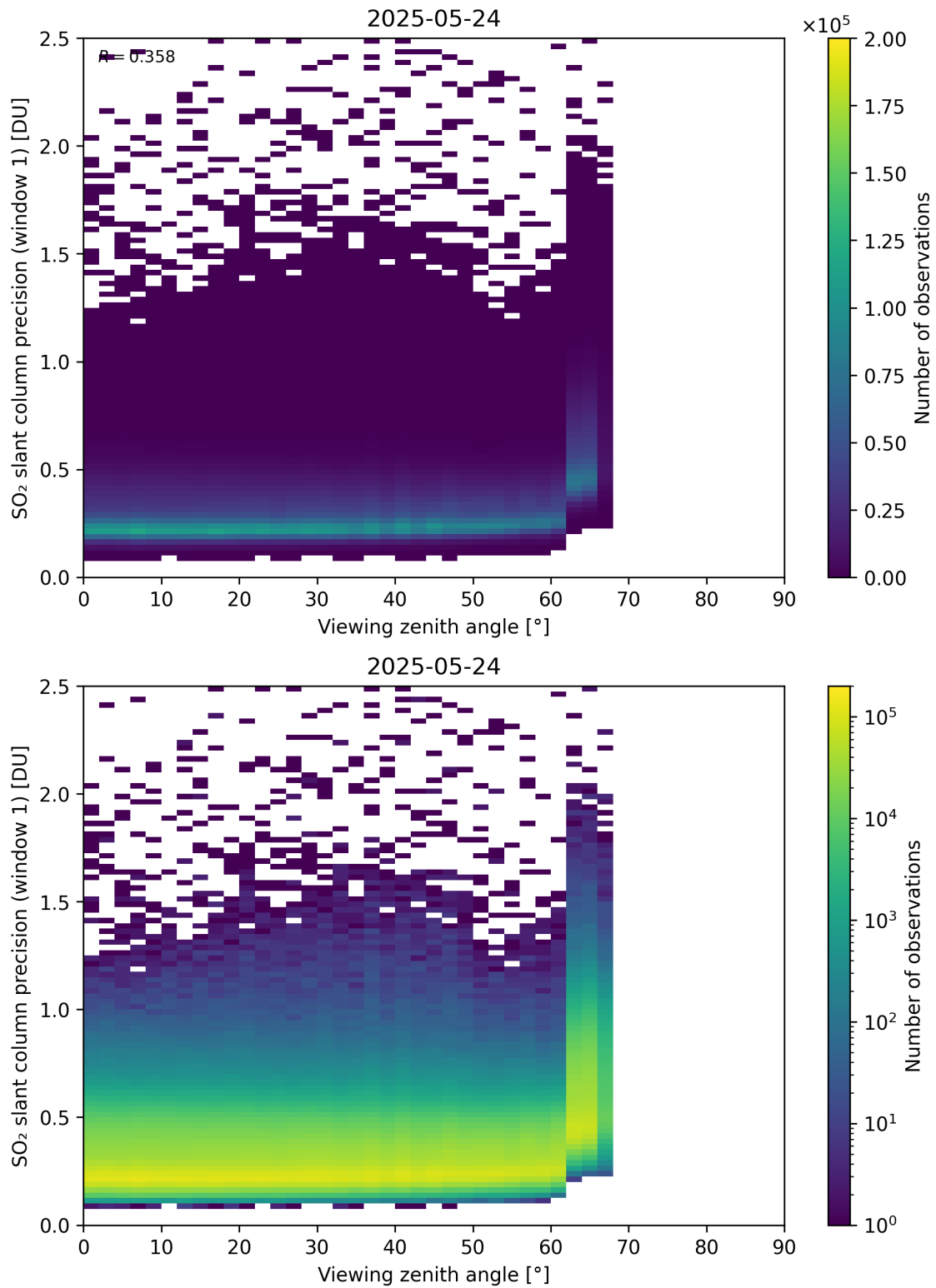
Figure 377: Scatter density plot of “Viewing zenith angle” against “SO 2 slant column precision (window 1)” for 2025-05-23 to 2025-05-25.
