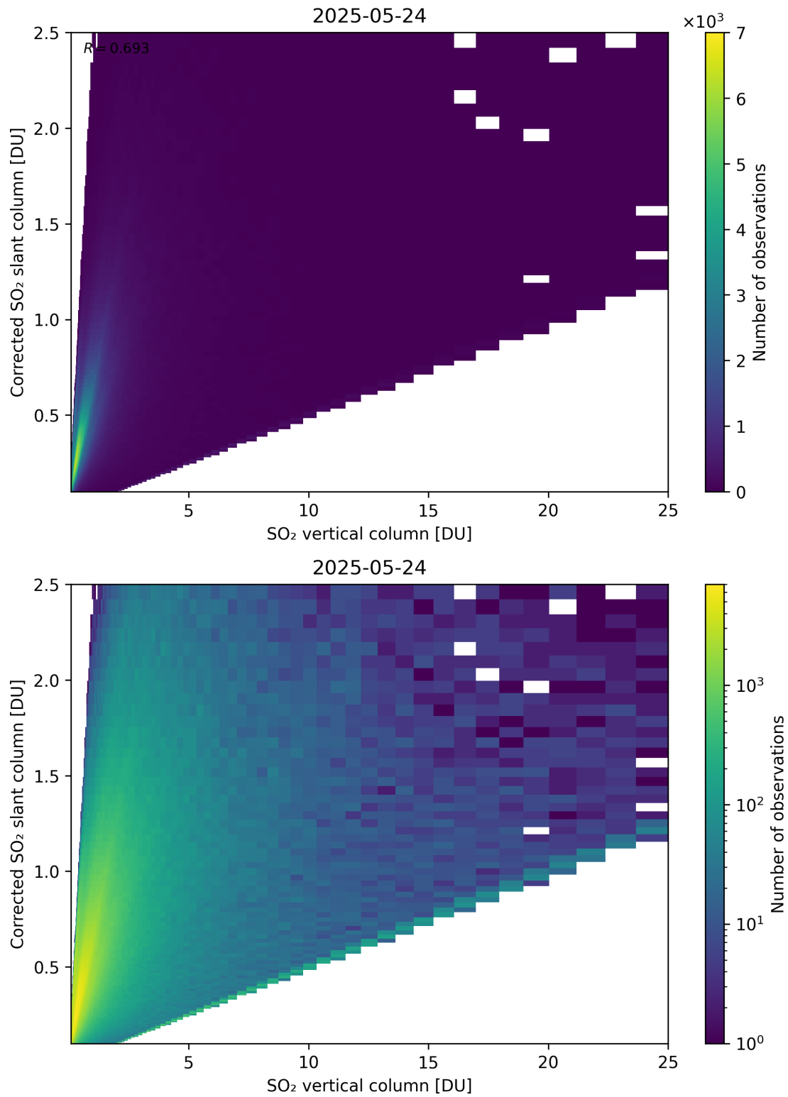
Figure 351: Scatter density plot of “SO 2 vertical column” against “Corrected SO 2 slant column” for 2025-05-23 to 2025-05-25.
