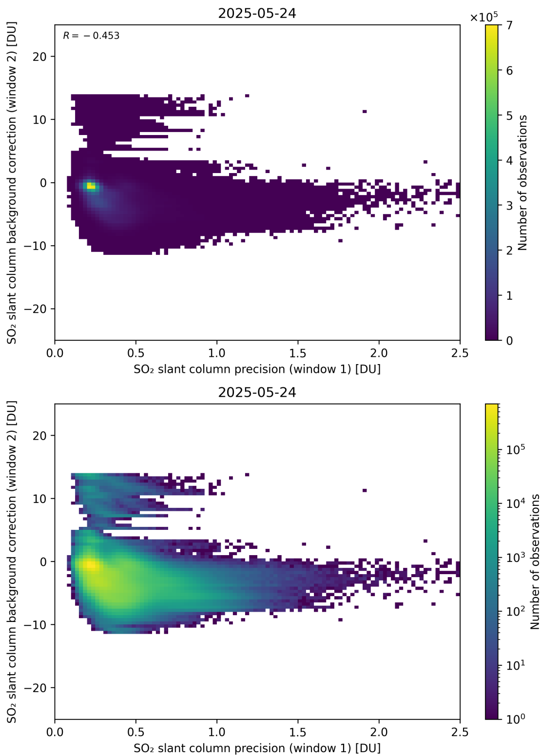
Figure 269: Scatter density plot of “SO 2 slant column precision (window 1)” against “SO 2 slant column background correction (window 2)” for 2025-05-23 to 2025-05-25.
