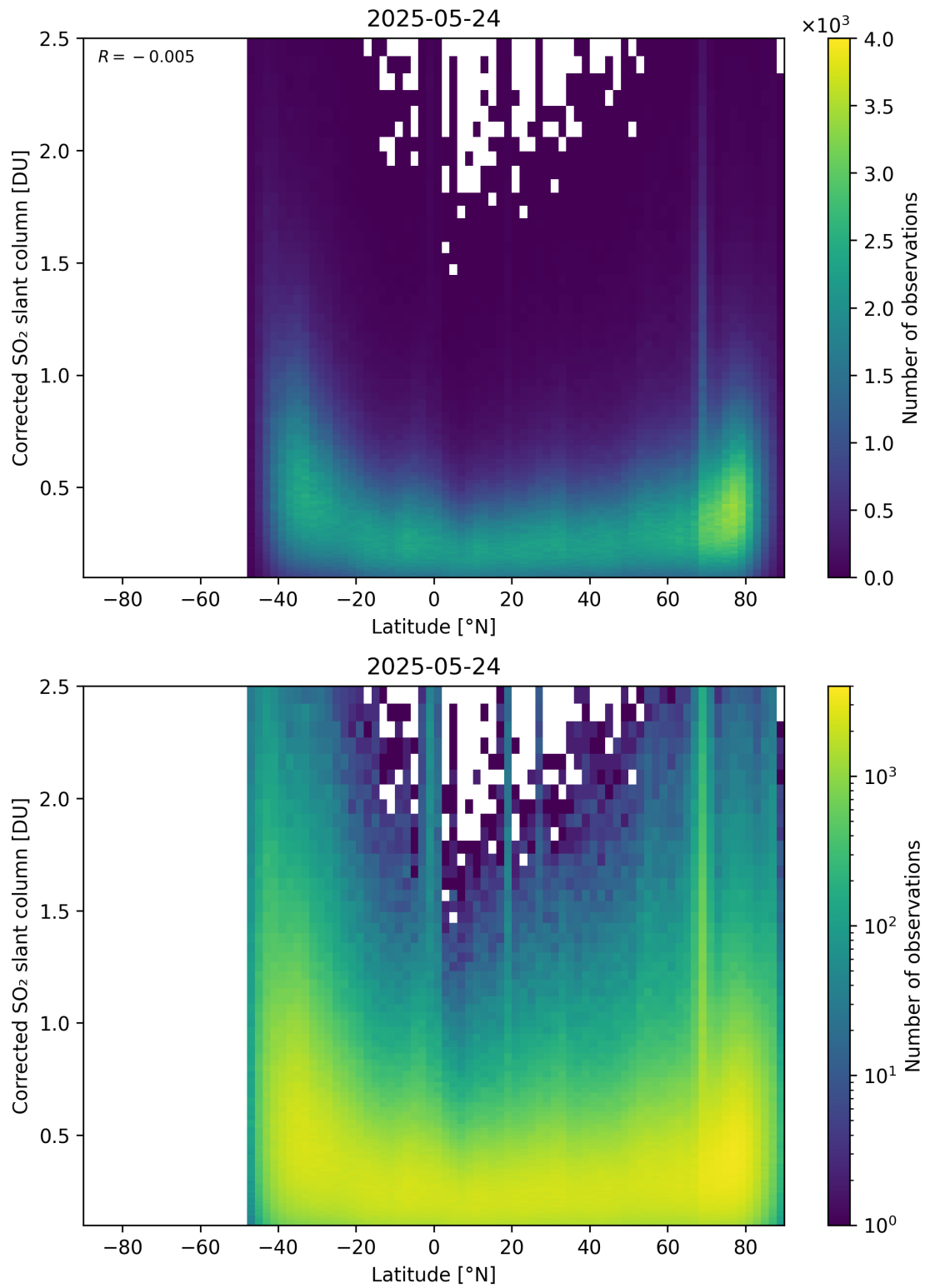
Figure 159: Scatter density plot of “Latitude” against “Corrected SO 2 slant column” for 2025-05-23 to 2025-05-25.
