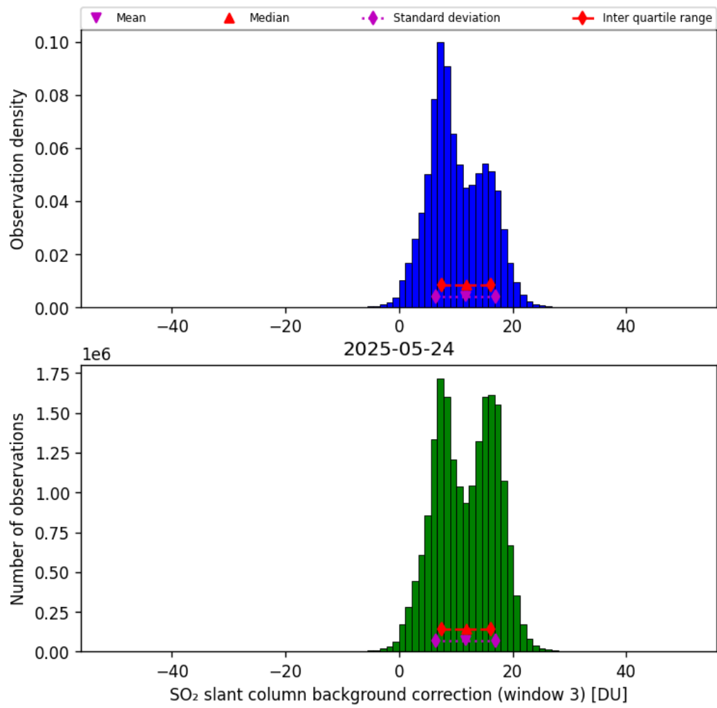
Figure 74: Histogram of “SO 2 slant column background correction (window 3)” for 2025-05-23 to 2025-05-25
