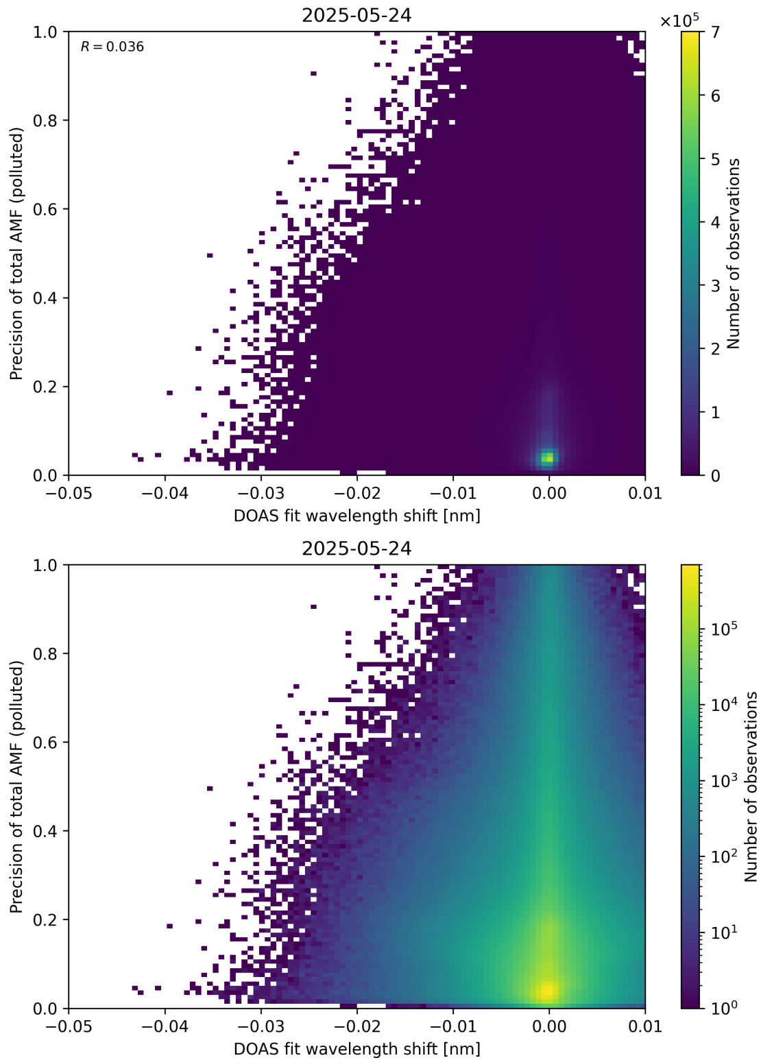
Figure 142: Scatter density plot of “DOAS fit wavelength shift” against “Precision of total AMF (polluted)” for 2025-05-23 to 2025-05-25.
