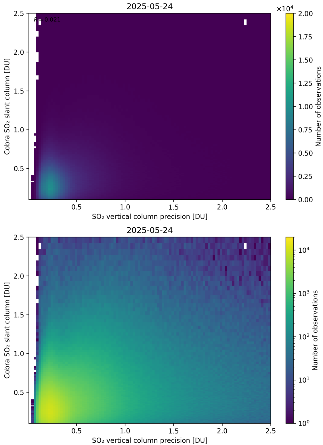
Figure 336: Scatter density plot of “SO 2 vertical column precision” against “Cobra SO 2 slant column” for 2025-05-23 to 2025-05-25.
