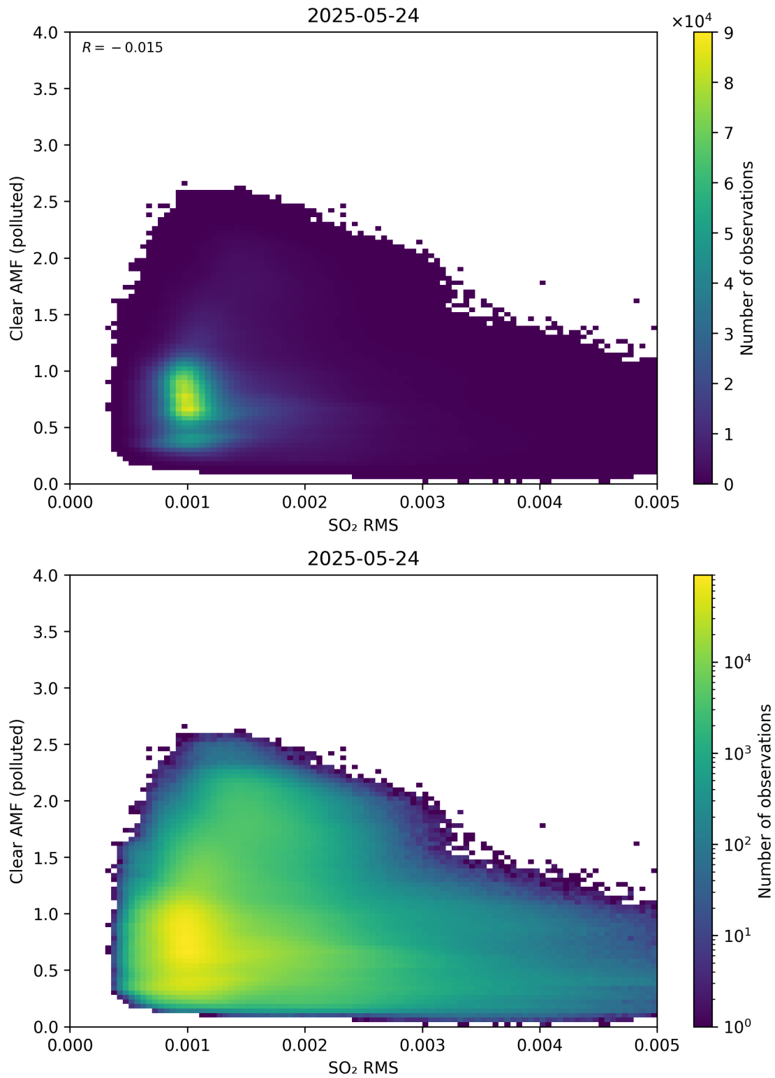
Figure 147: Scatter density plot of “SO 2 RMS” against “Clear AMF (polluted)” for 2025-05-23 to 2025-05-25.
