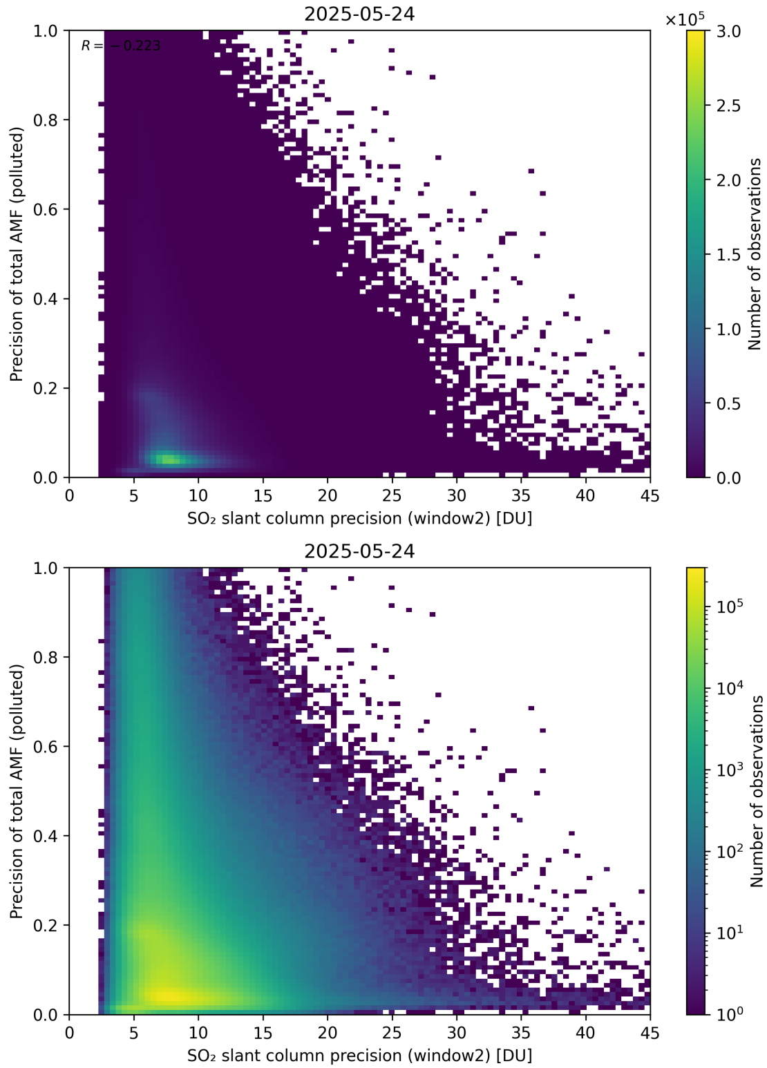
Figure 302: Scatter density plot of “SO 2 slant column precision (window2)” against “Precision of total AMF (polluted)” for 2025-05-23 to 2025-05-25.
