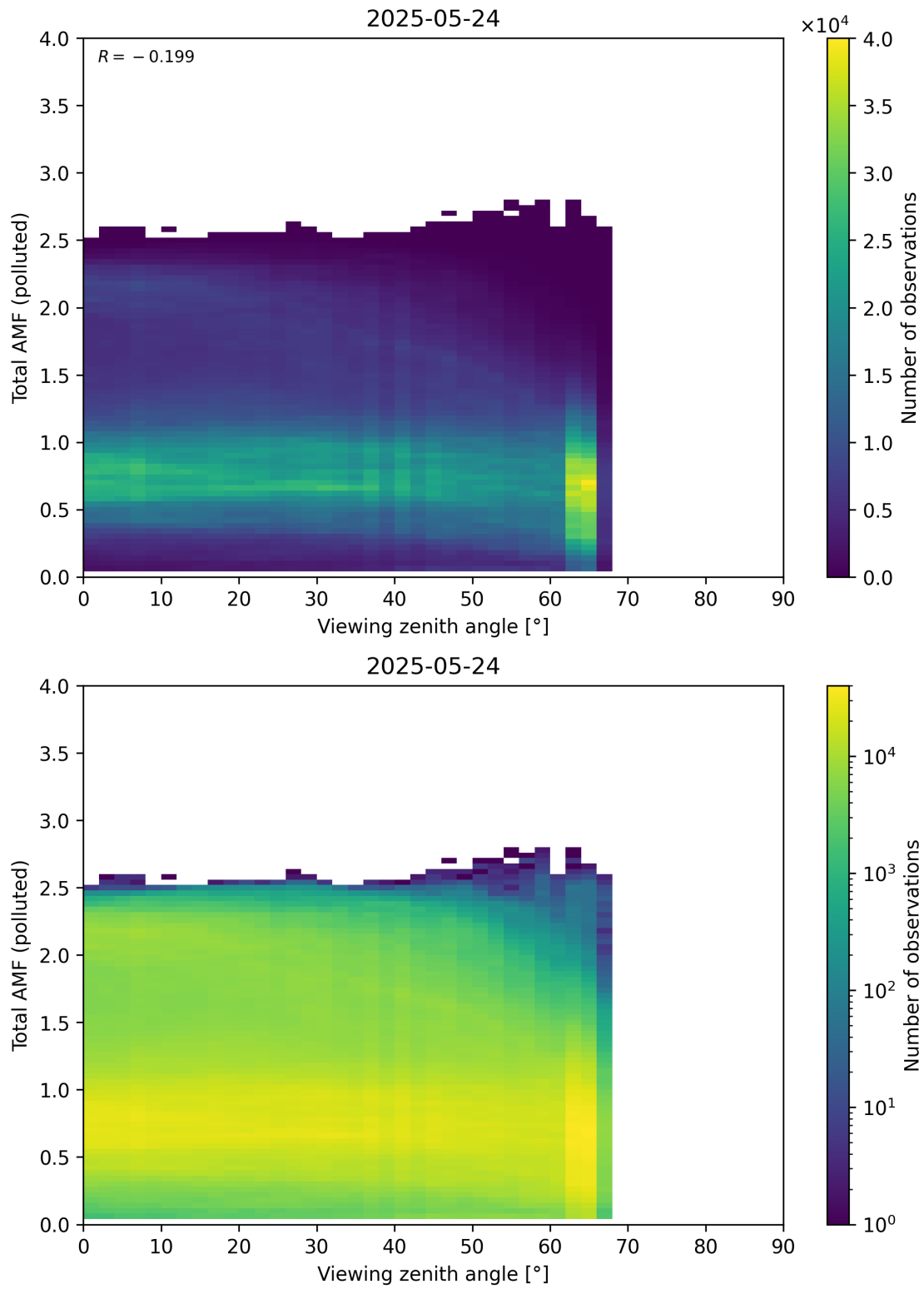
Figure 381: Scatter density plot of “Viewing zenith angle” against “Total AMF (polluted)” for 2025-05-23 to 2025-05-25.
