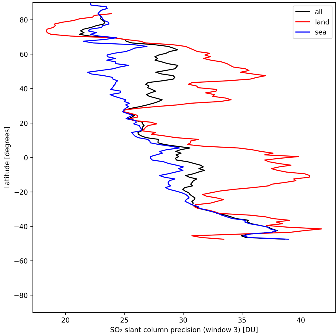
Figure 46: Zonal average of “SO 2 slant column precision (window 3)” for 2025-05-23 to 2025-05-25.
