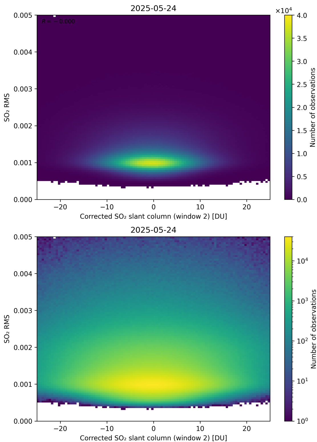
Figure 248: Scatter density plot of “Corrected SO 2 slant column (window 2)” against “SO 2 RMS” for 2025-05-23 to 2025-05-25.
