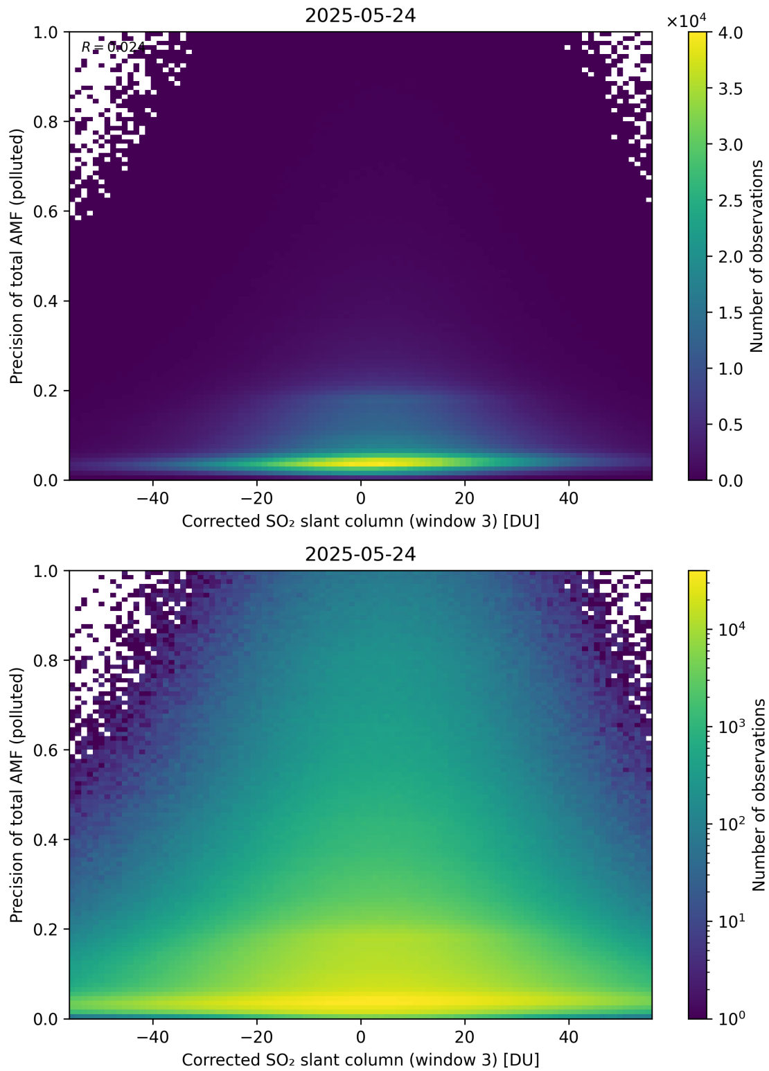
Figure 261: Scatter density plot of “Corrected SO 2 slant column (window 3)” against “Precision of total AMF (polluted)” for 2025-05-23 to 2025-05-25.
