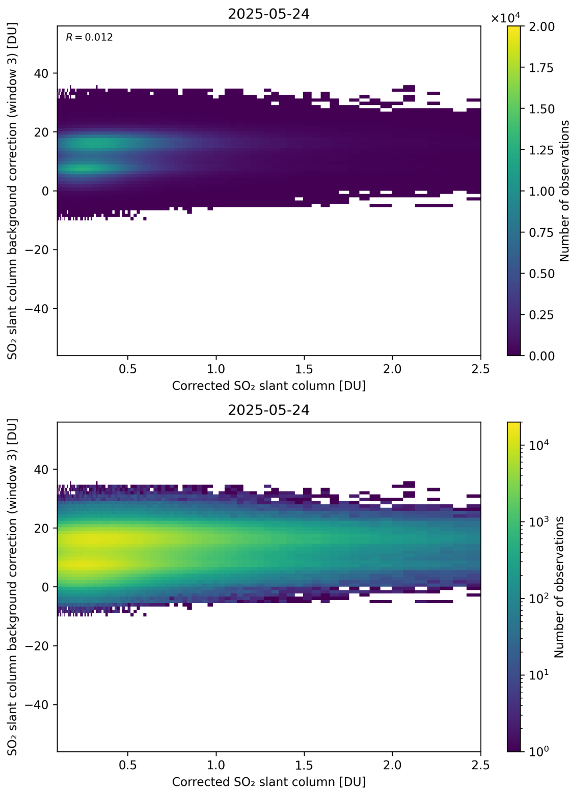
Figure 228: Scatter density plot of “Corrected SO 2 slant column” against “SO 2 slant column background correction (window 3)” for 2025-05-23 to 2025-05-25.
