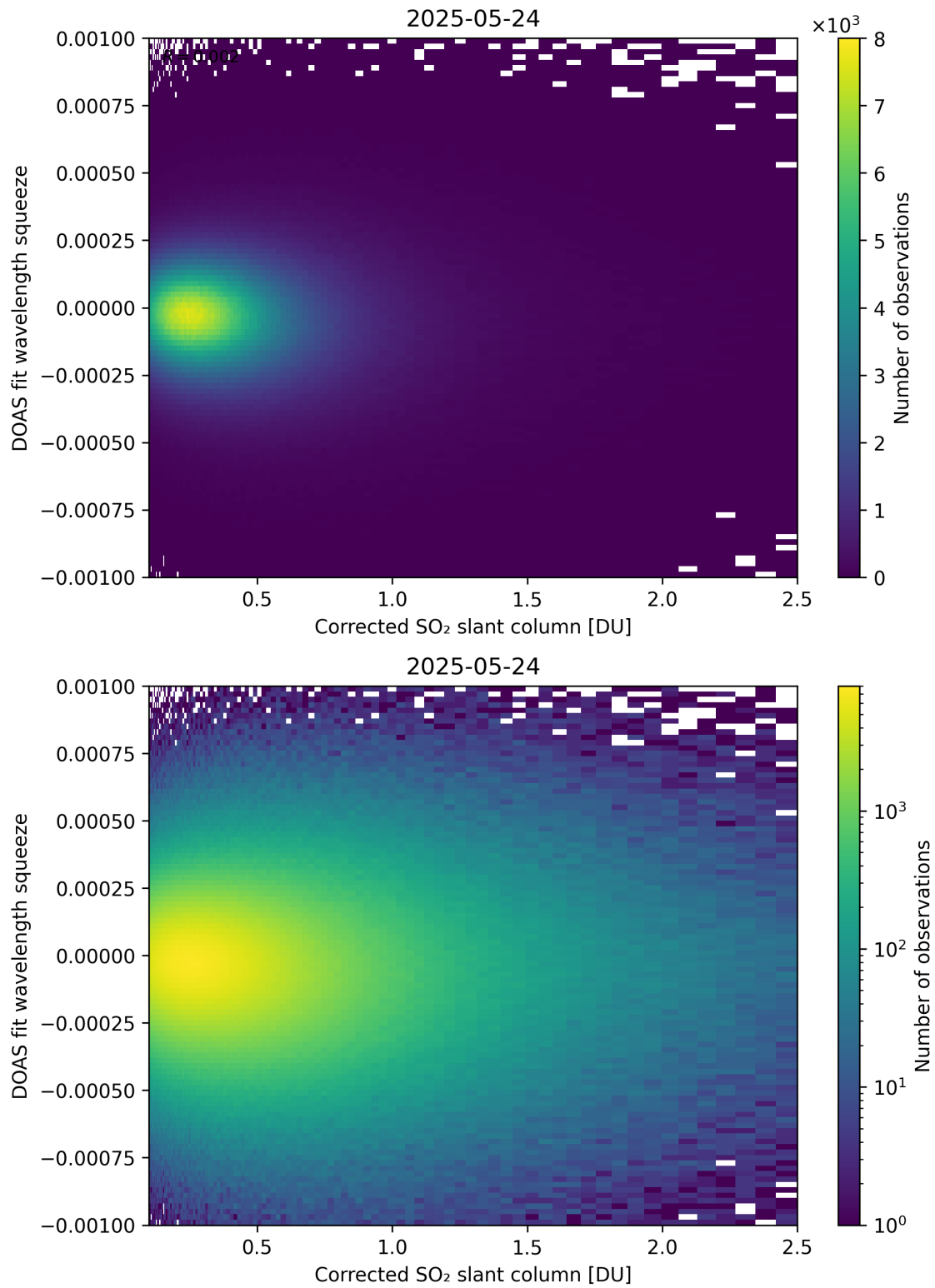
Figure 230: Scatter density plot of “Corrected SO 2 slant column” against “DOAS fit wavelength squeeze” for 2025-05-23 to 2025-05-25.
