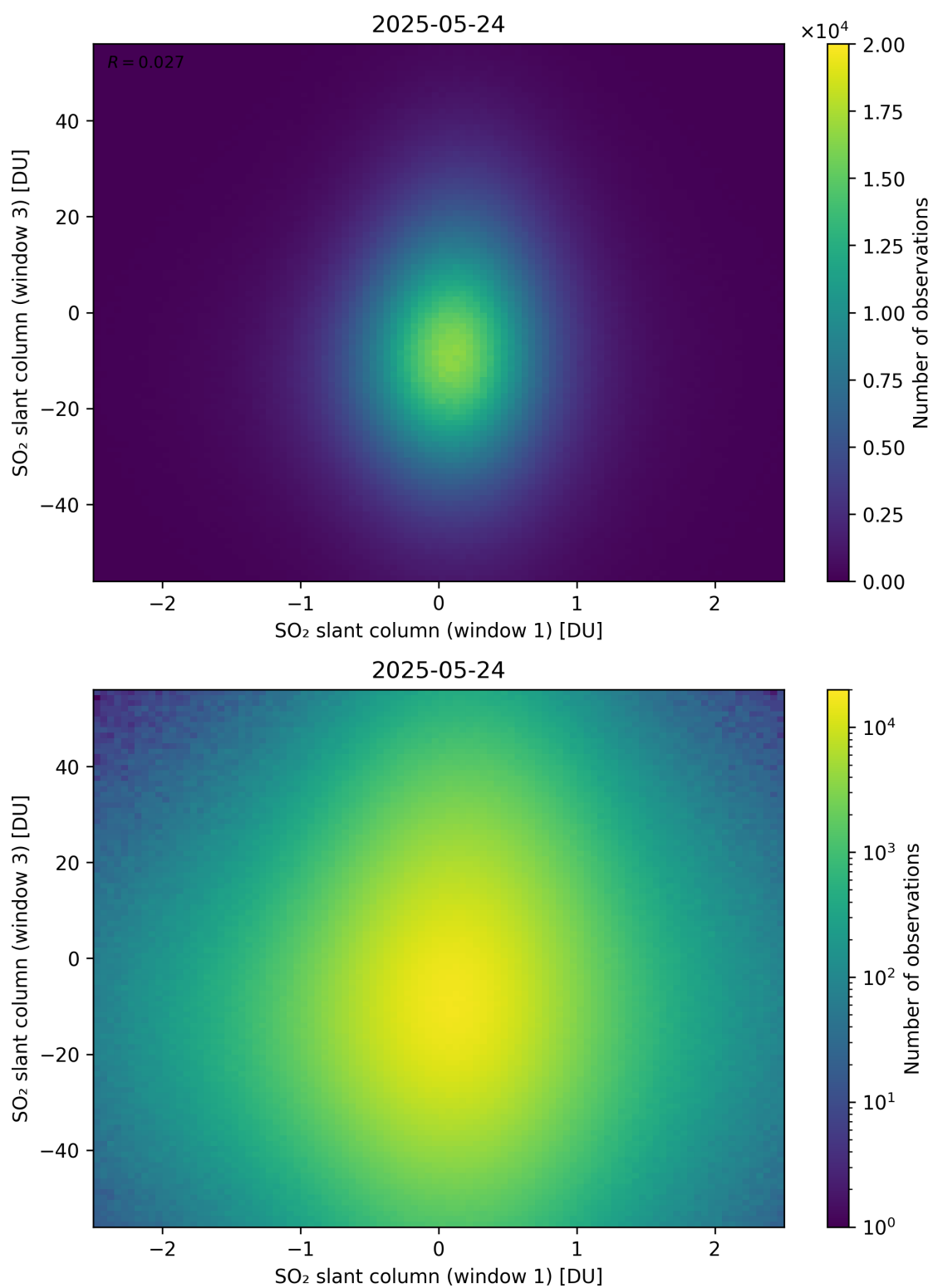
Figure 287: Scatter density plot of “SO 2 slant column (window 1)” against “SO 2 slant column (window 3)” for 2025-05-23 to 2025-05-25.
