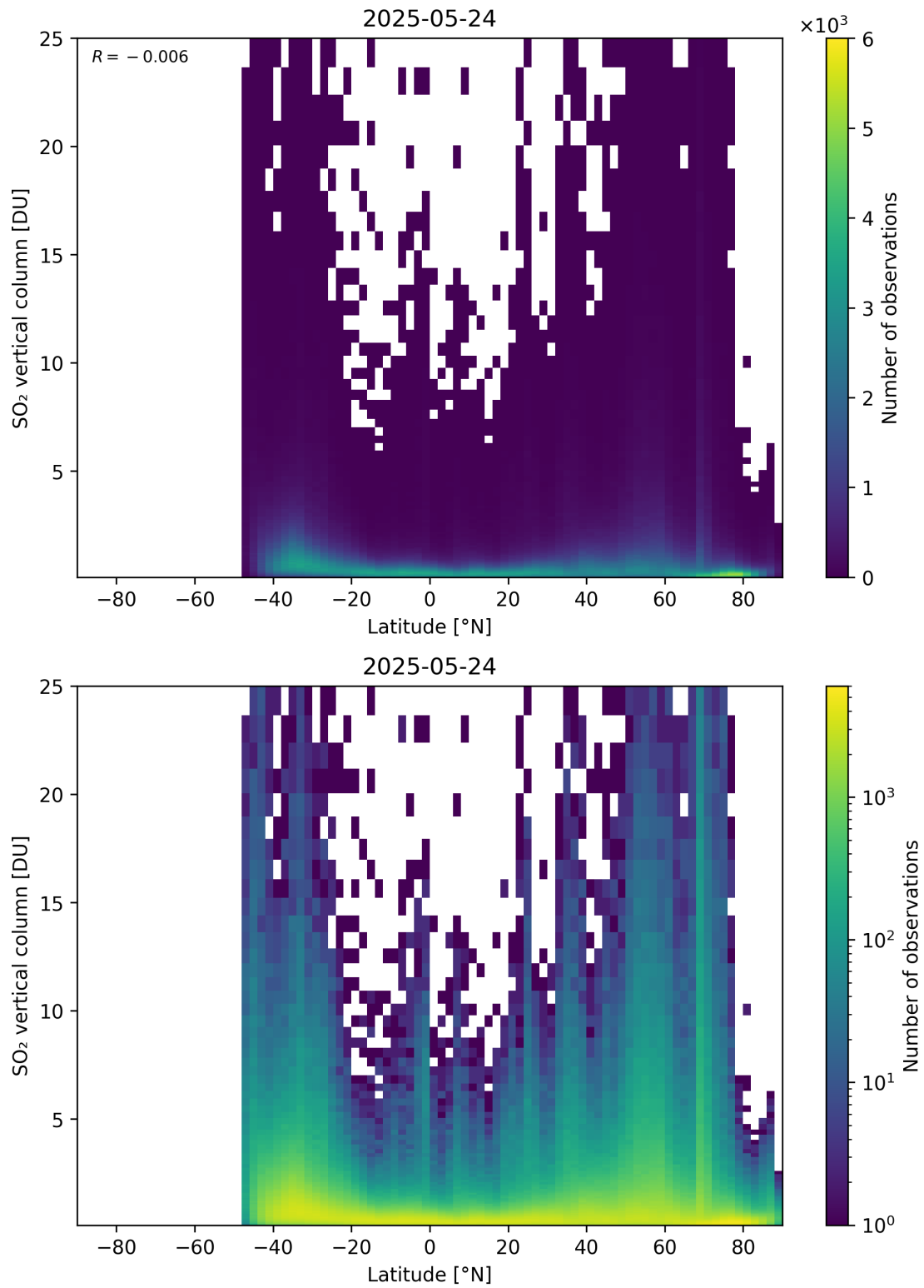
Figure 169: Scatter density plot of “Latitude” against “SO 2 vertical column” for 2025-05-23 to 2025-05-25.
