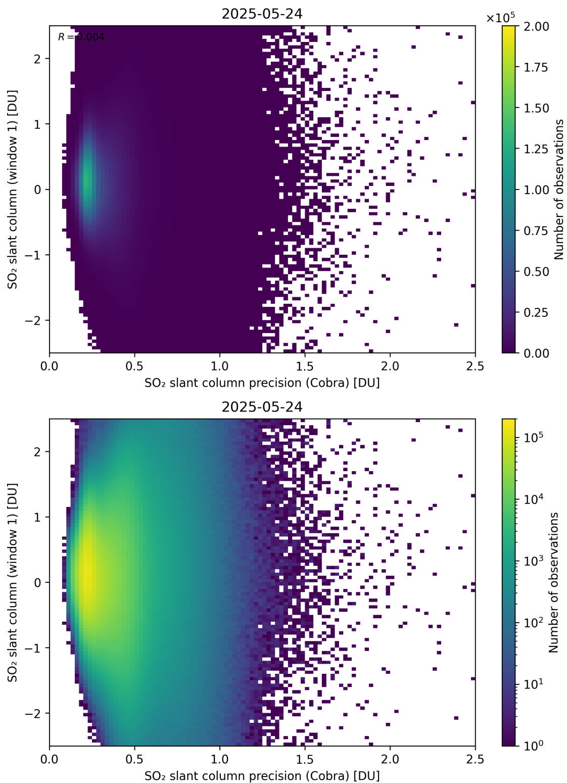
Figure 208: Scatter density plot of “SO 2 slant column precision (Cobra)” against “SO 2 slant column (window 1)” for 2025-05-23 to 2025-05-25.
