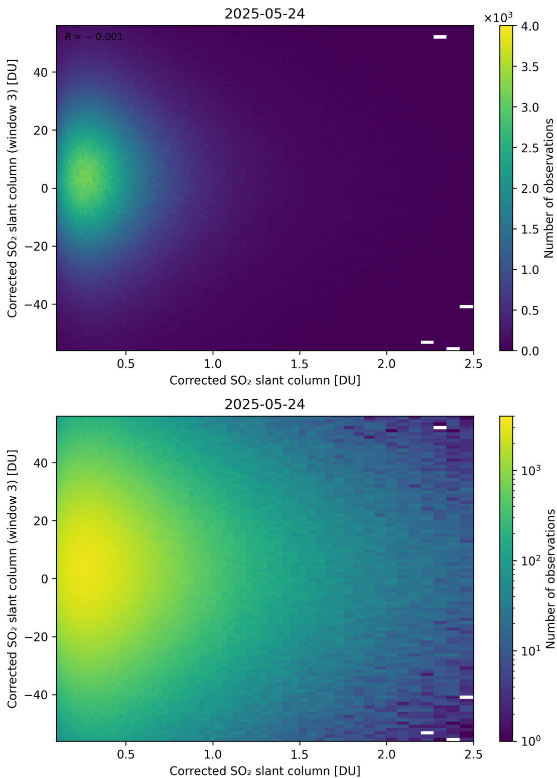
Figure 236: Scatter density plot of “Corrected SO 2 slant column” against “Corrected SO 2 slant column (window 3)” for 2025-05-23 to 2025-05-25.
