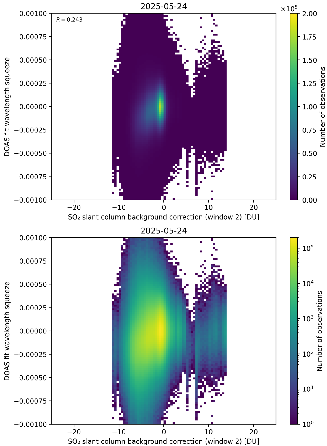
Figure 124: Scatter density plot of “SO 2 slant column background correction (window 2)” against “DOAS fit wavelength squeeze” for 2025-05-23 to 2025-05-25.
