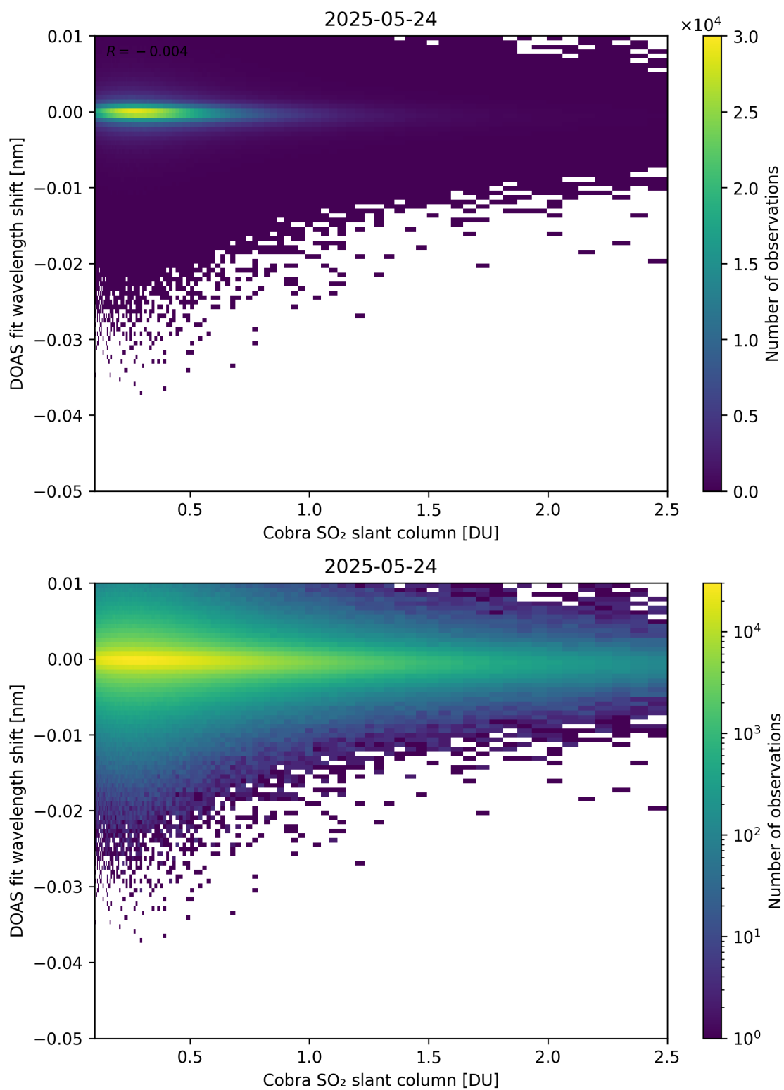
Figure 196: Scatter density plot of “Cobra SO 2 slant column” against “DOAS fit wavelength shift” for 2025-05-23 to 2025-05-25.
