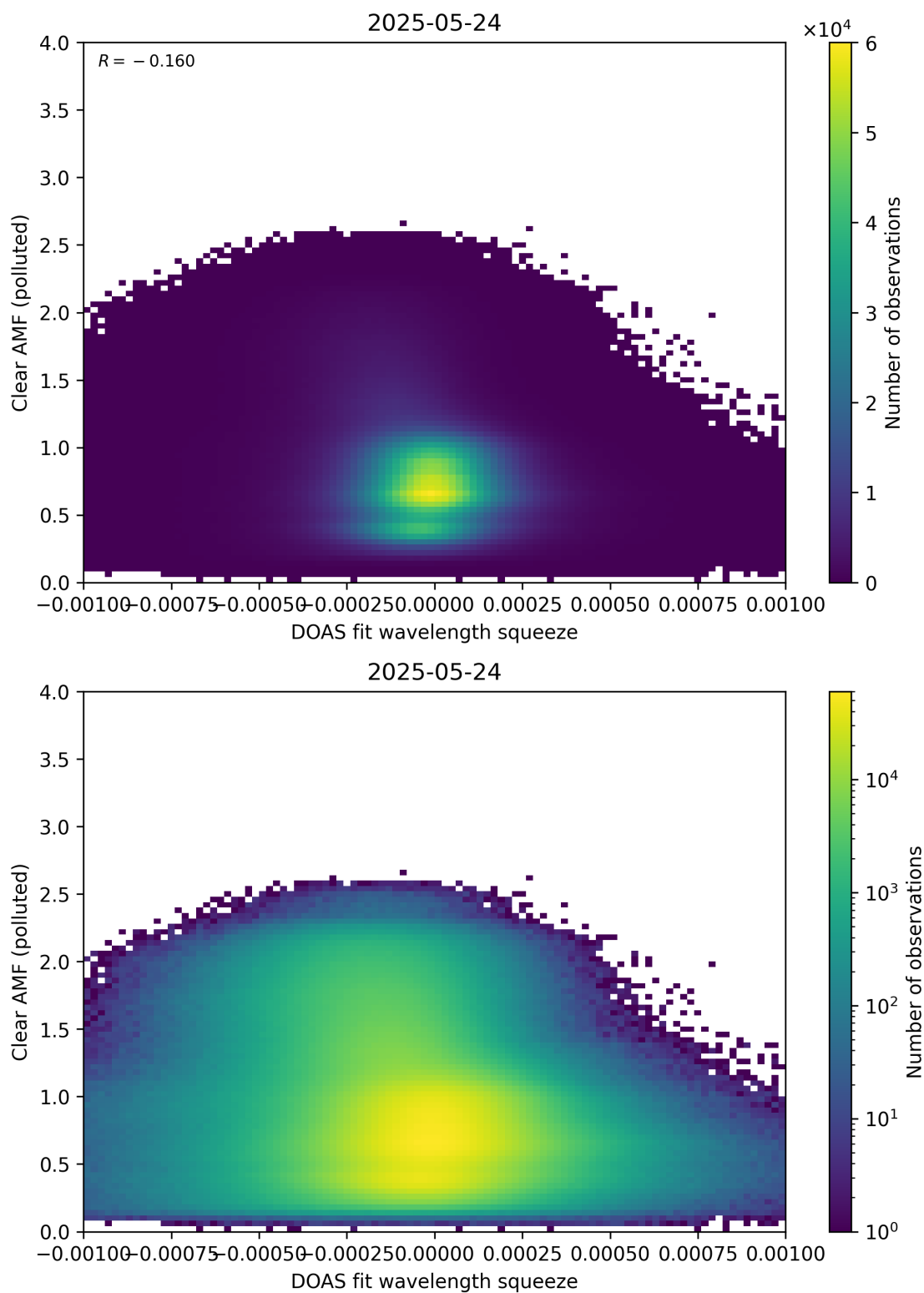
Figure 144: Scatter density plot of “DOAS fit wavelength squeeze” against “Clear AMF (polluted)” for 2025-05-23 to 2025-05-25.
