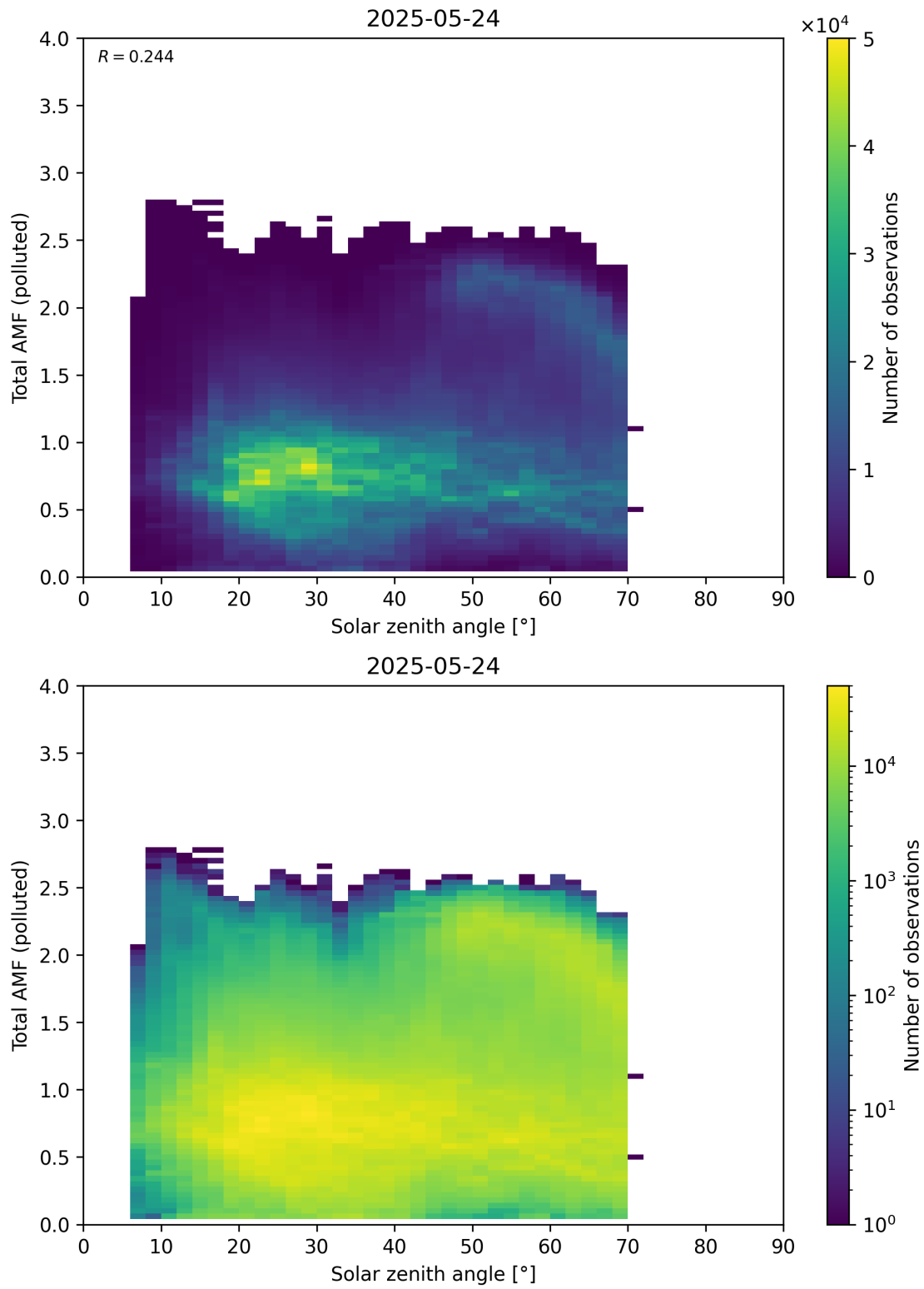
Figure 189: Scatter density plot of “Solar zenith angle” against “Total AMF (polluted)” for 2025-05-23 to 2025-05-25.
