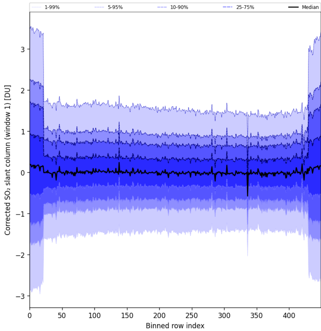
Figure 91: Along track statistics of “Corrected SO 2 slant column (window 1)” for 2025-05-23 to 2025-05-25
