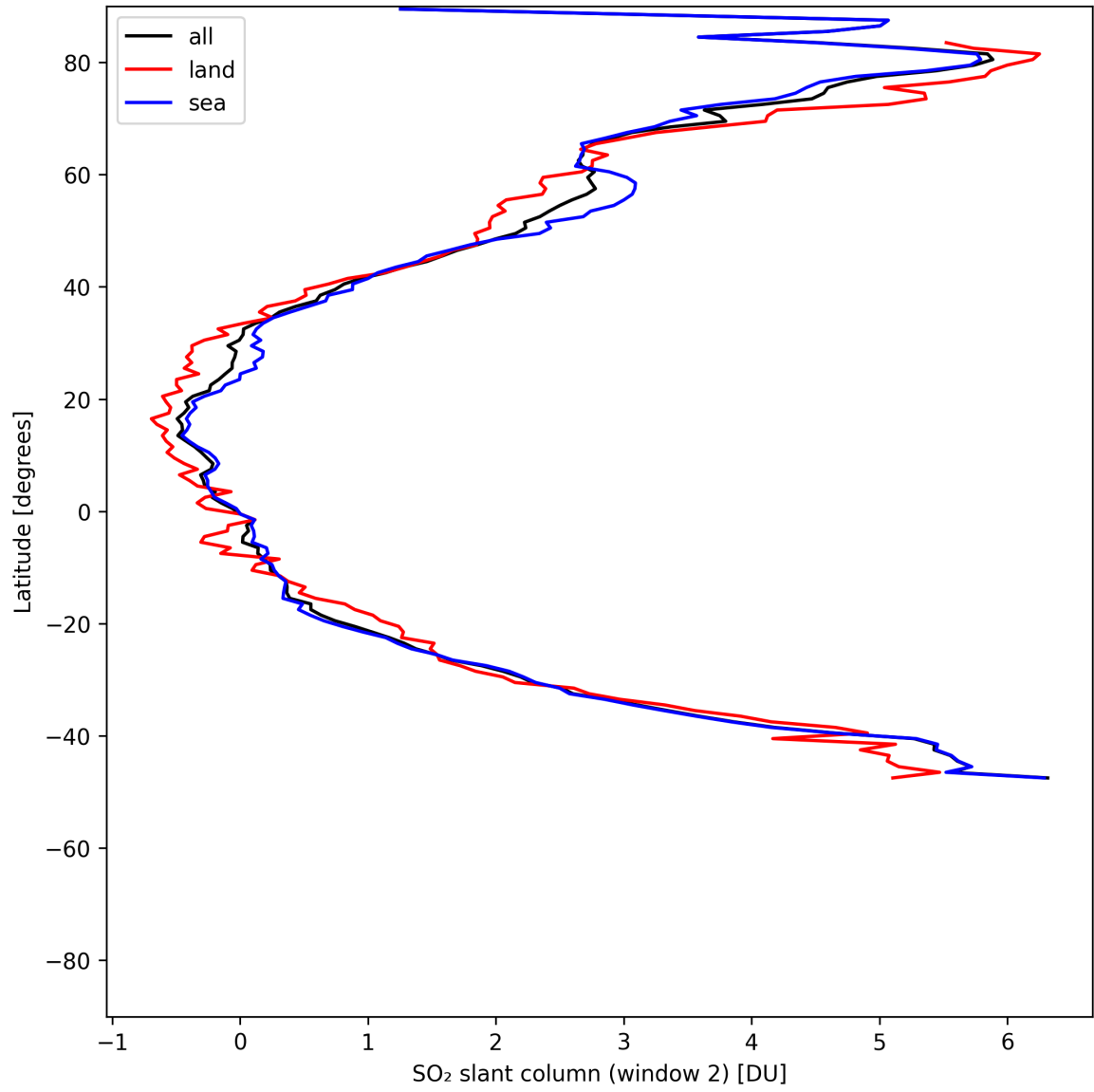
Figure 41: Zonal average of “SO 2 slant column (window 2)” for 2025-05-23 to 2025-05-25.
