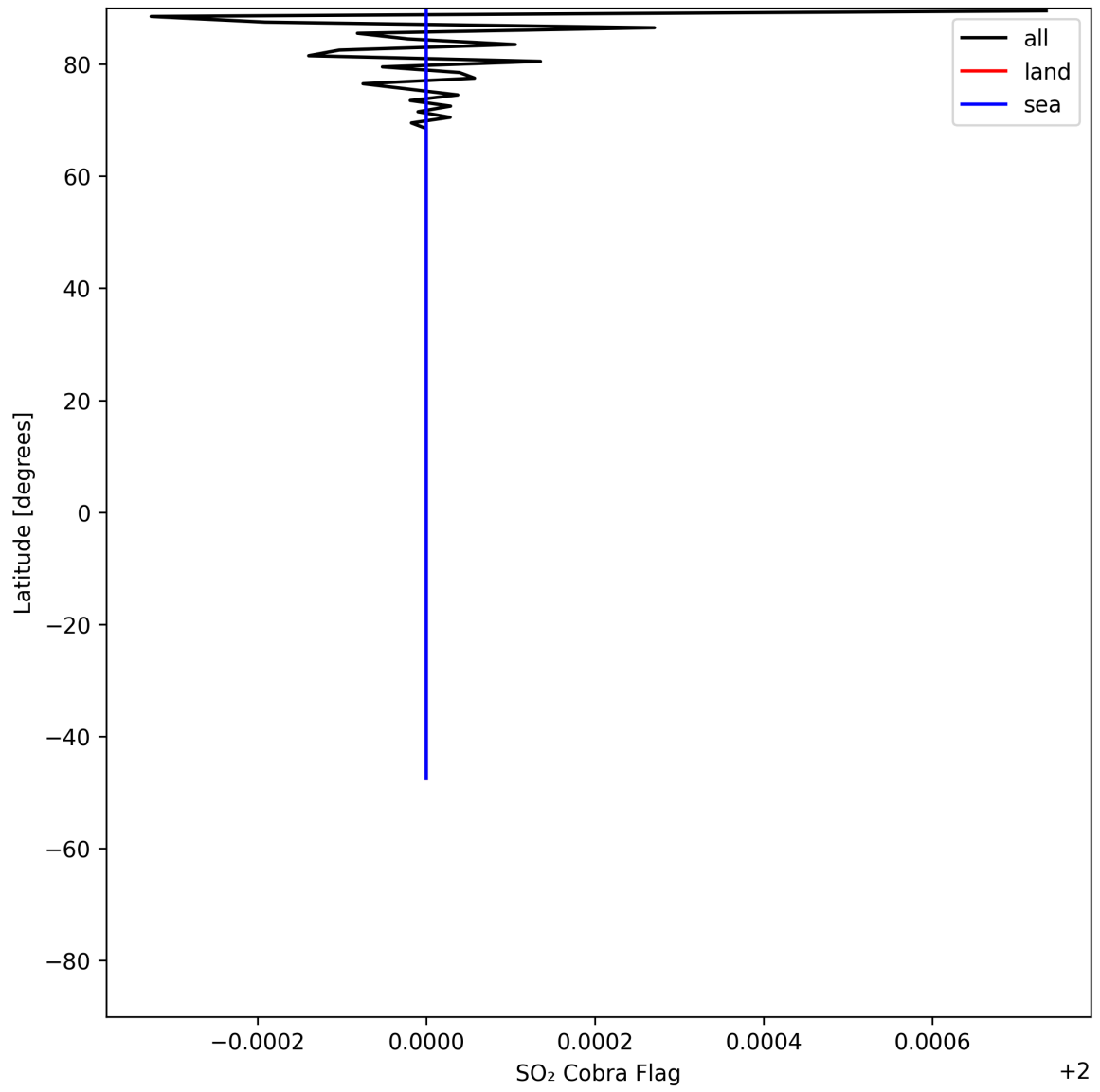
Figure 49: Zonal average of “SO 2 Cobra Flag” for 2025-05-23 to 2025-05-25.
