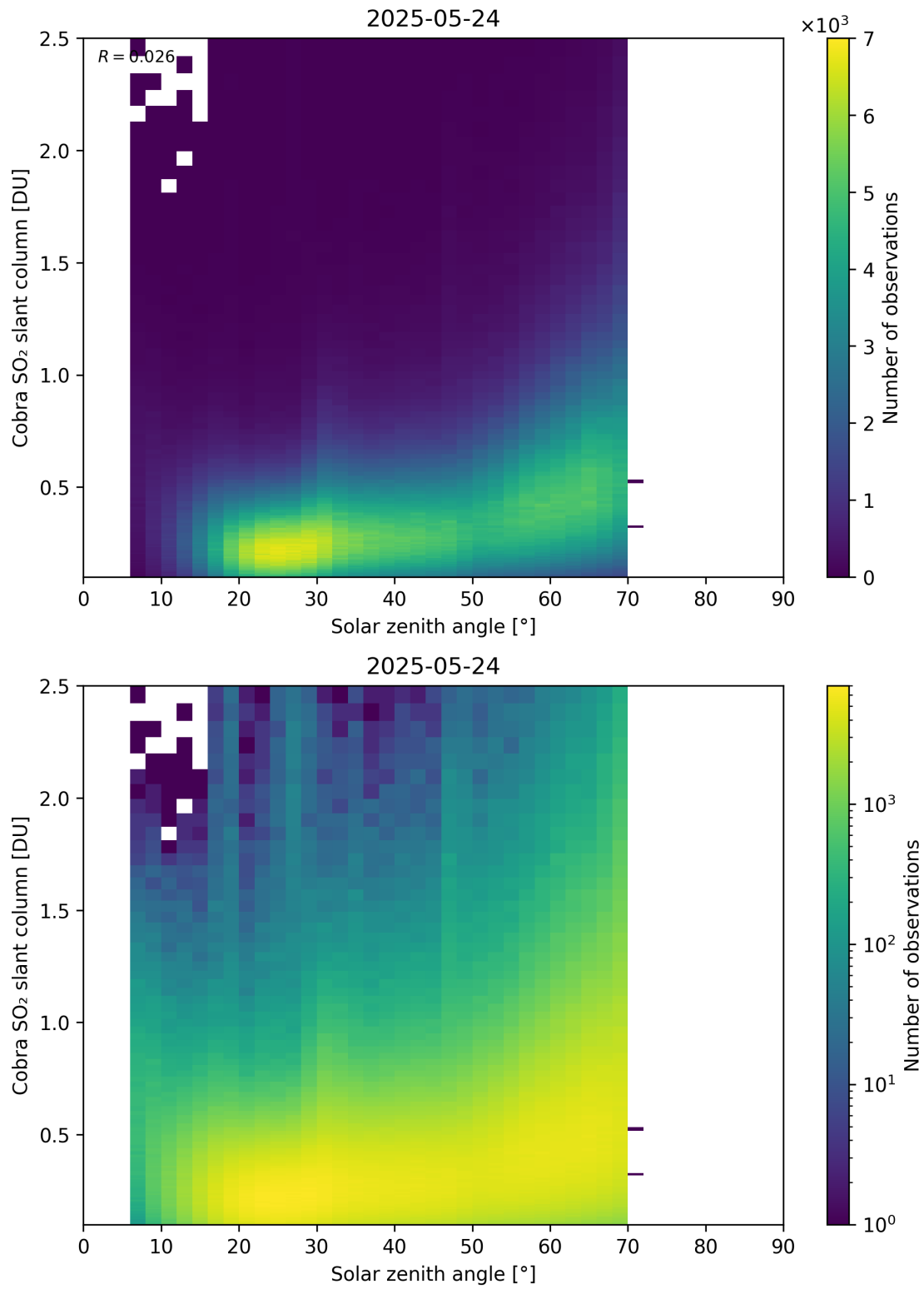
Figure 179: Scatter density plot of “Solar zenith angle” against “Cobra SO 2 slant column” for 2025-05-23 to 2025-05-25.
