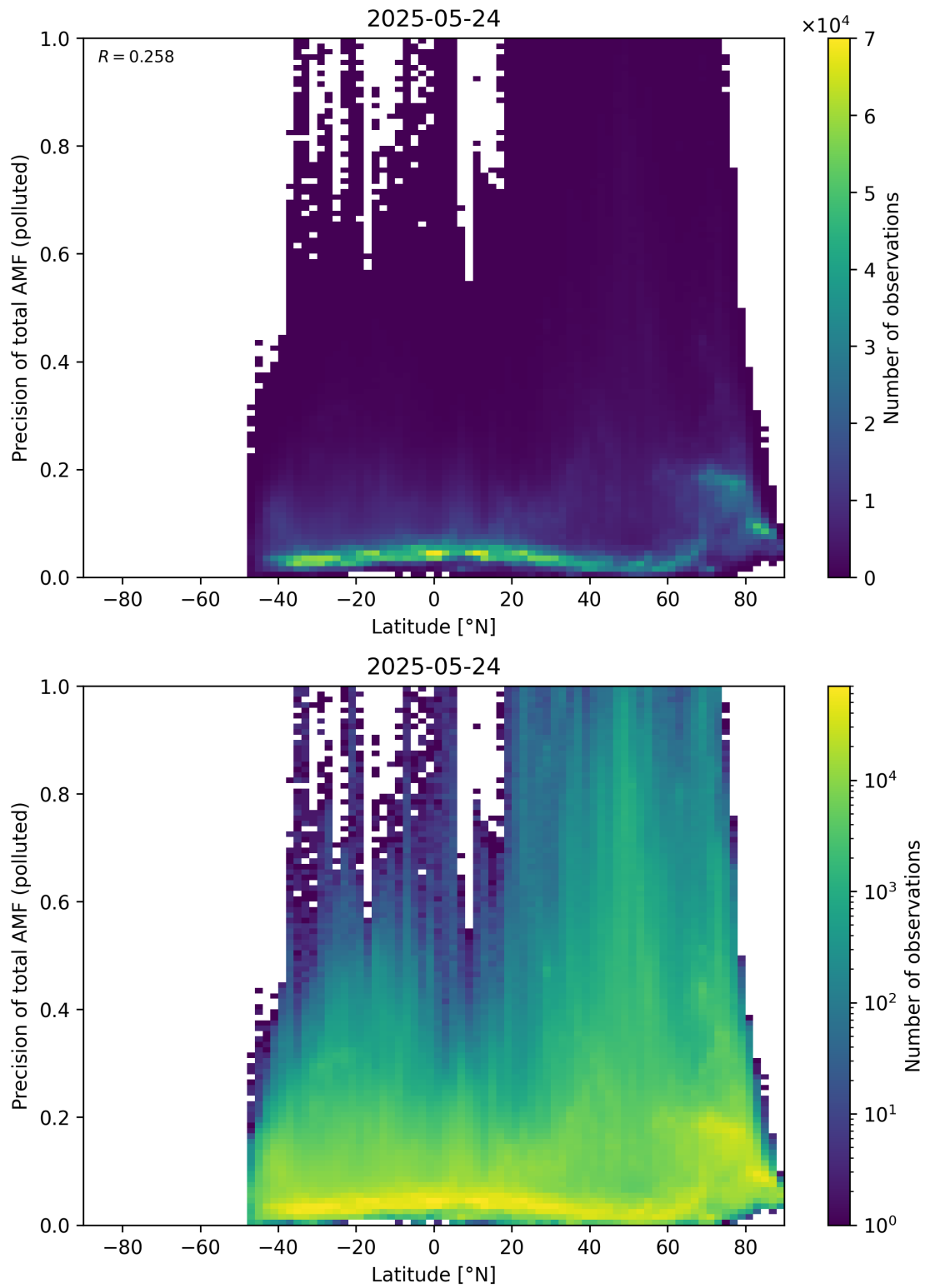
Figure 168: Scatter density plot of “Latitude” against “Precision of total AMF (polluted)” for 2025-05-23 to 2025-05-25.
