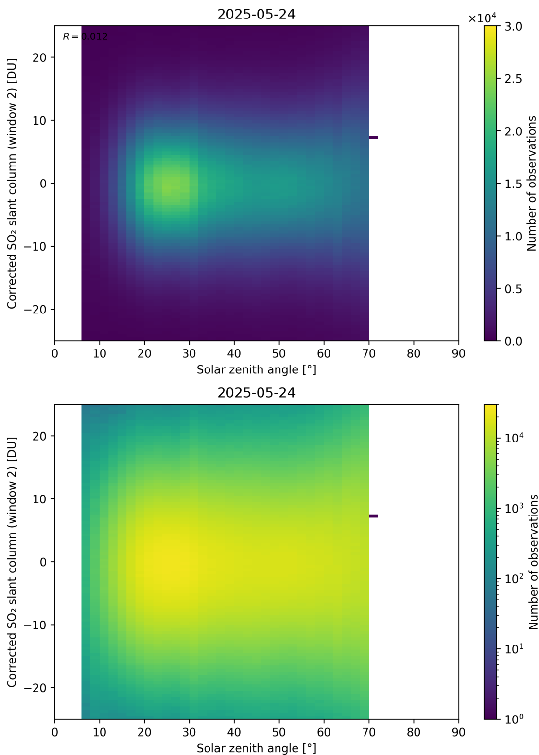
Figure 182: Scatter density plot of “Solar zenith angle” against “Corrected SO 2 slant column (window 2)” for 2025-05-23 to 2025-05-25.
