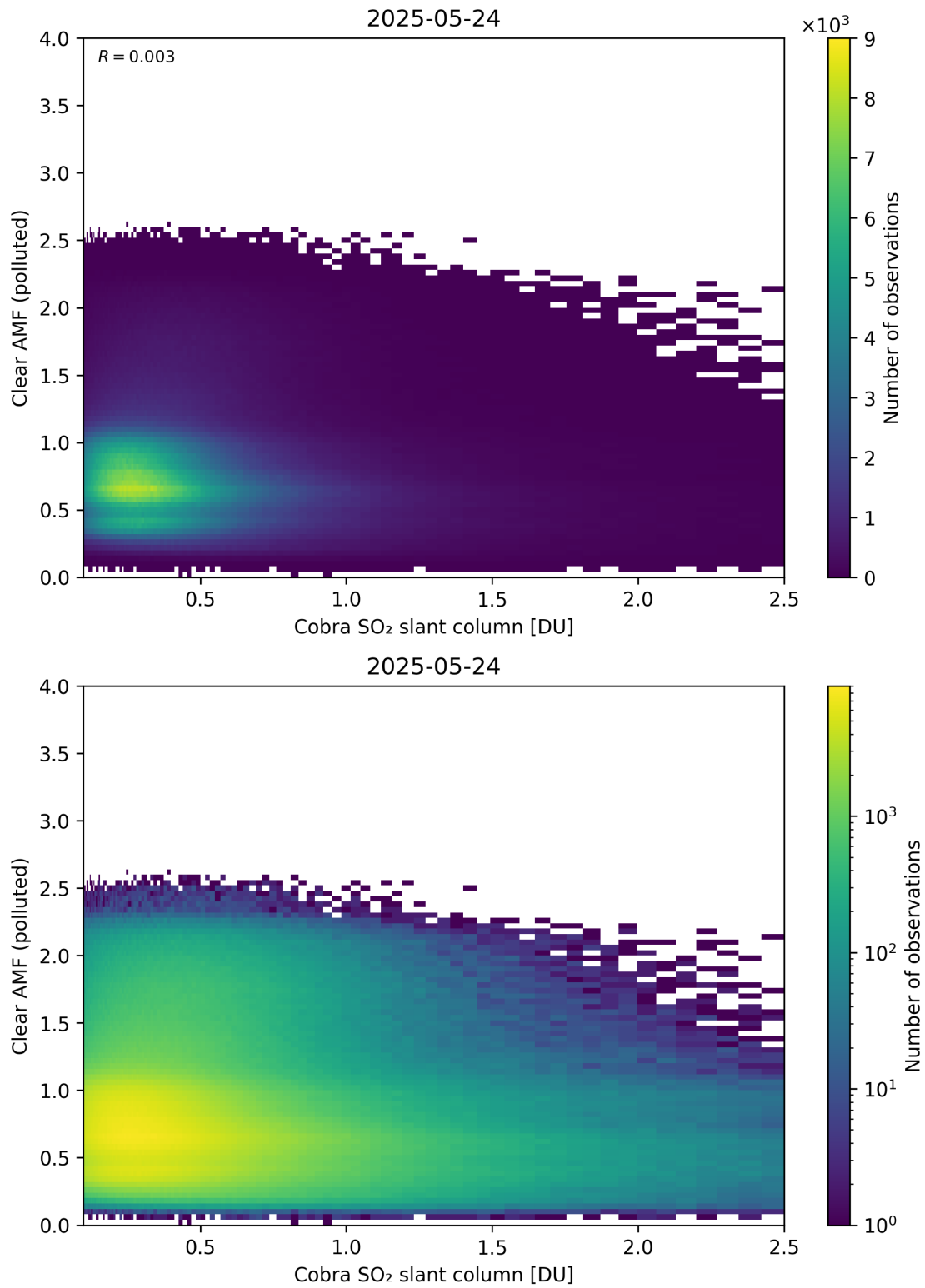
Figure 215: Scatter density plot of “Cobra SO 2 slant column” against “Clear AMF (polluted)” for 2025-05-23 to 2025-05-25.
