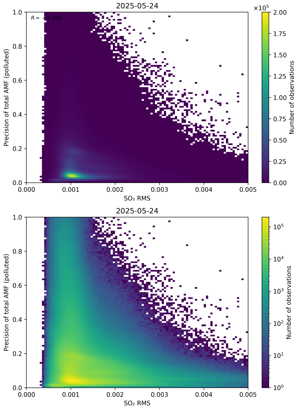
Figure 149: Scatter density plot of “SO 2 RMS” against “Precision of total AMF (polluted)” for 2025-05-23 to 2025-05-25.
