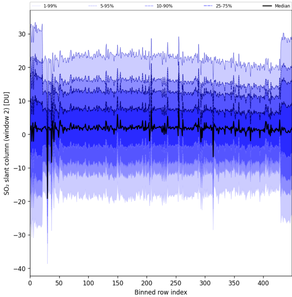
Figure 93: Along track statistics of “SO 2 slant column (window 2)” for 2025-05-23 to 2025-05-25
