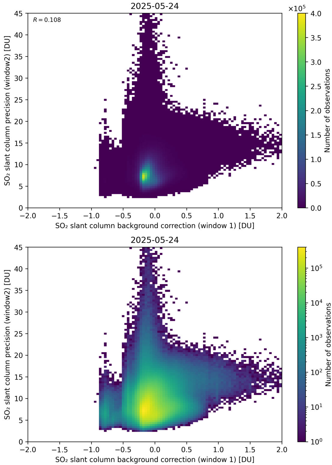
Figure 117: Scatter density plot of “SO 2 slant column background correction (window 1)” against “SO 2 slant column precision (window2)” for 2025-05-23 to 2025-05-25.
