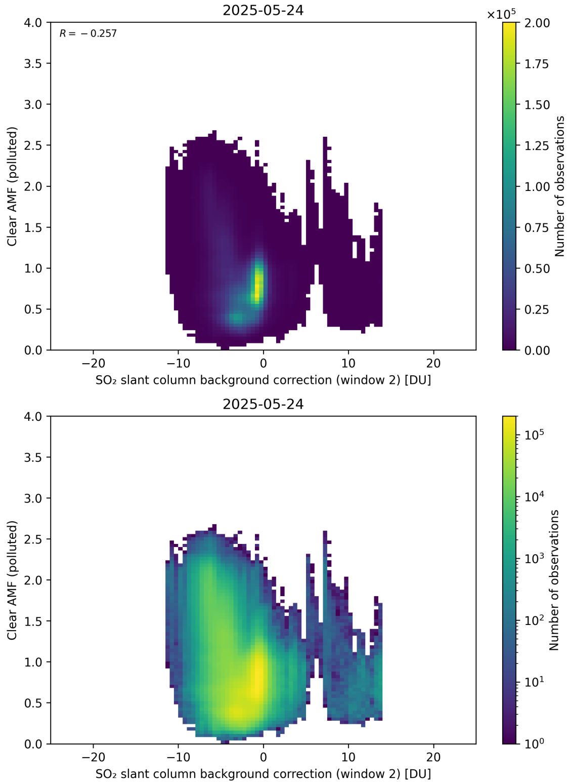
Figure 126: Scatter density plot of “SO 2 slant column background correction (window 2)” against “Clear AMF (polluted)” for 2025-05-23 to 2025-05-25.
